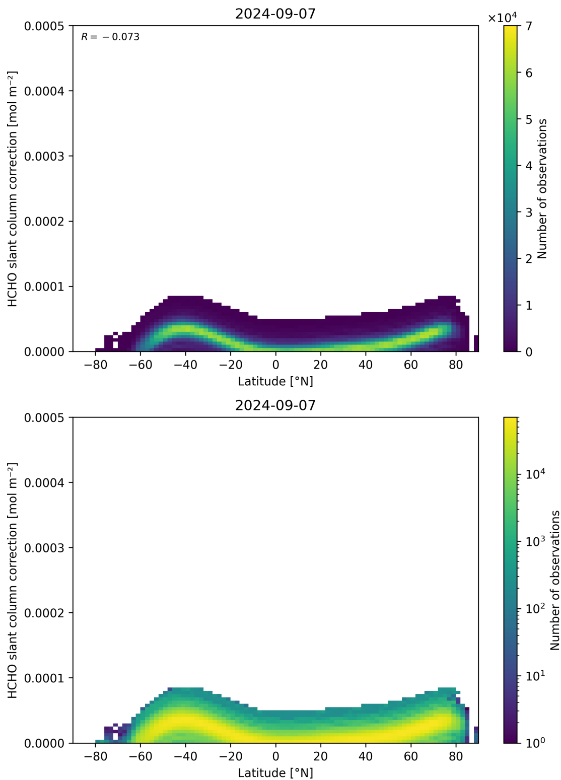
Figure 158: Scatter density plot of “Latitude” against “HCHO slant column correction” for 2024-09-06 to 2024-09-08.
