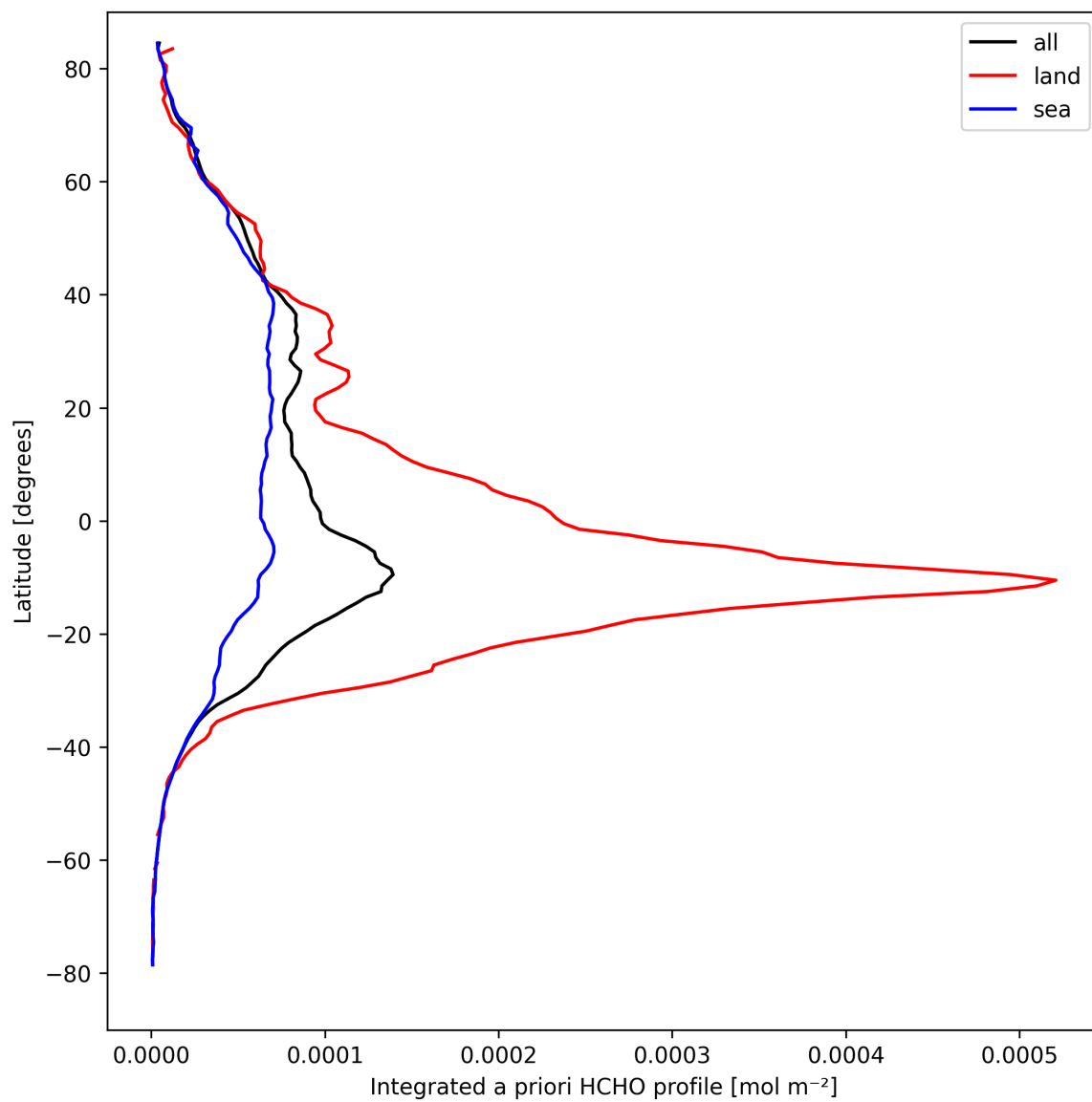
Figure 29: Zonal average of “Integrated a priori HCHO profile” for 2024-09-06 to 2024-09-08.
