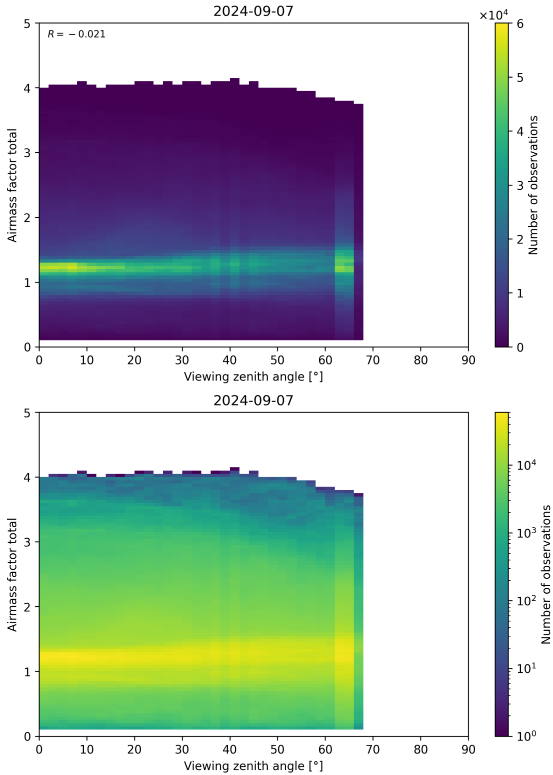
Figure 190: Scatter density plot of “Viewing zenith angle” against “Airmass factor total” for 2024-09-06 to 2024-09-08.
