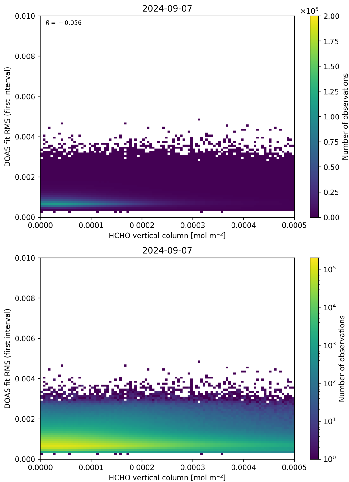
Figure 123: Scatter density plot of “HCHO vertical column” against “DOAS fit RMS (first interval)” for 2024-09-06 to 2024-09-08.
