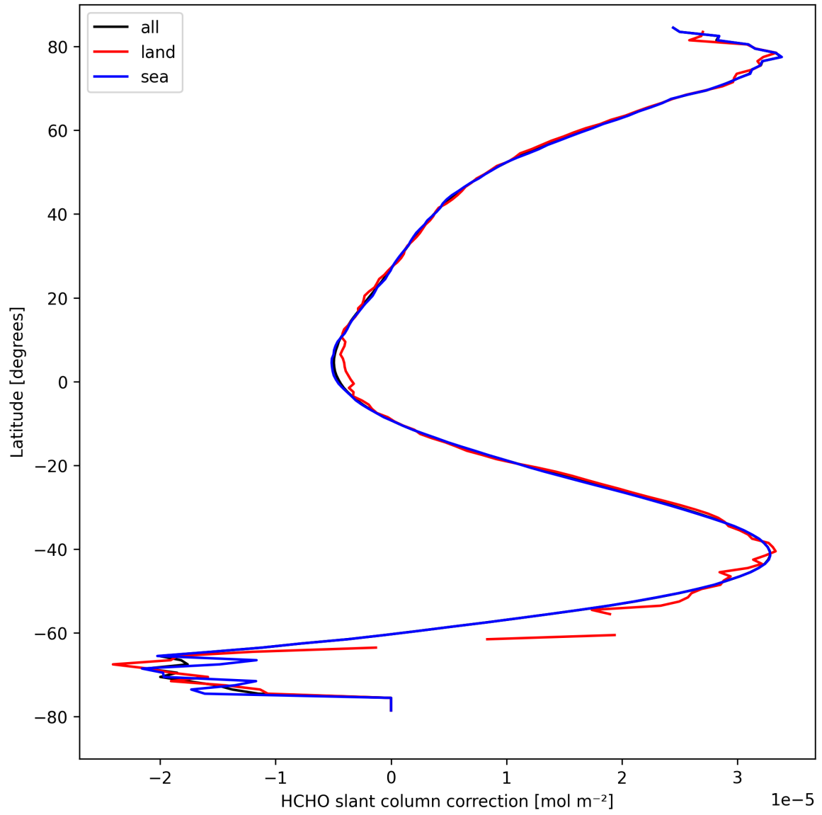
Figure 33: Zonal average of “HCHO slant column correction” for 2024-09-06 to 2024-09-08.
