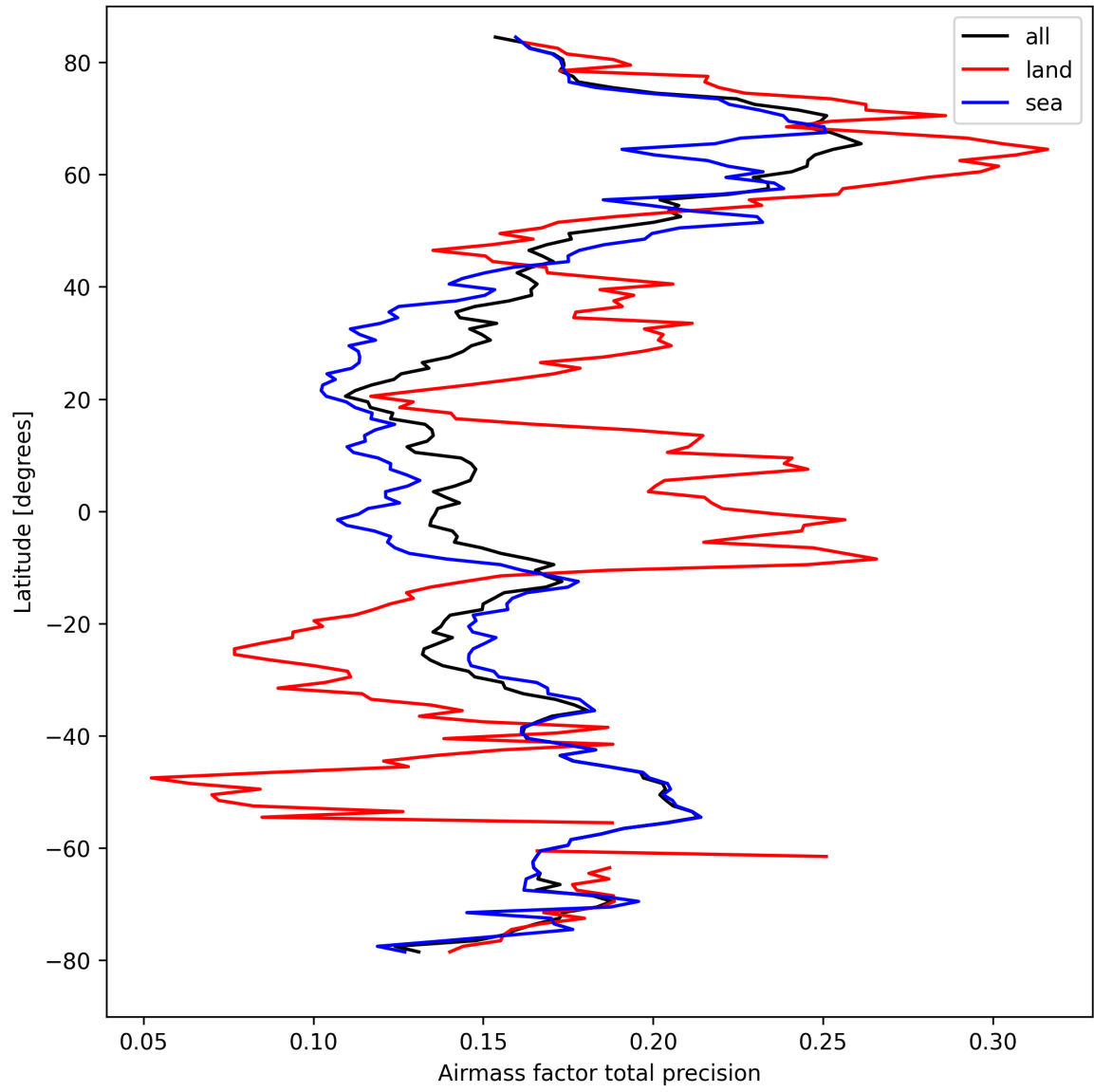
Figure 27: Zonal average of “Airmass factor total precision” for 2024-09-06 to 2024-09-08.
