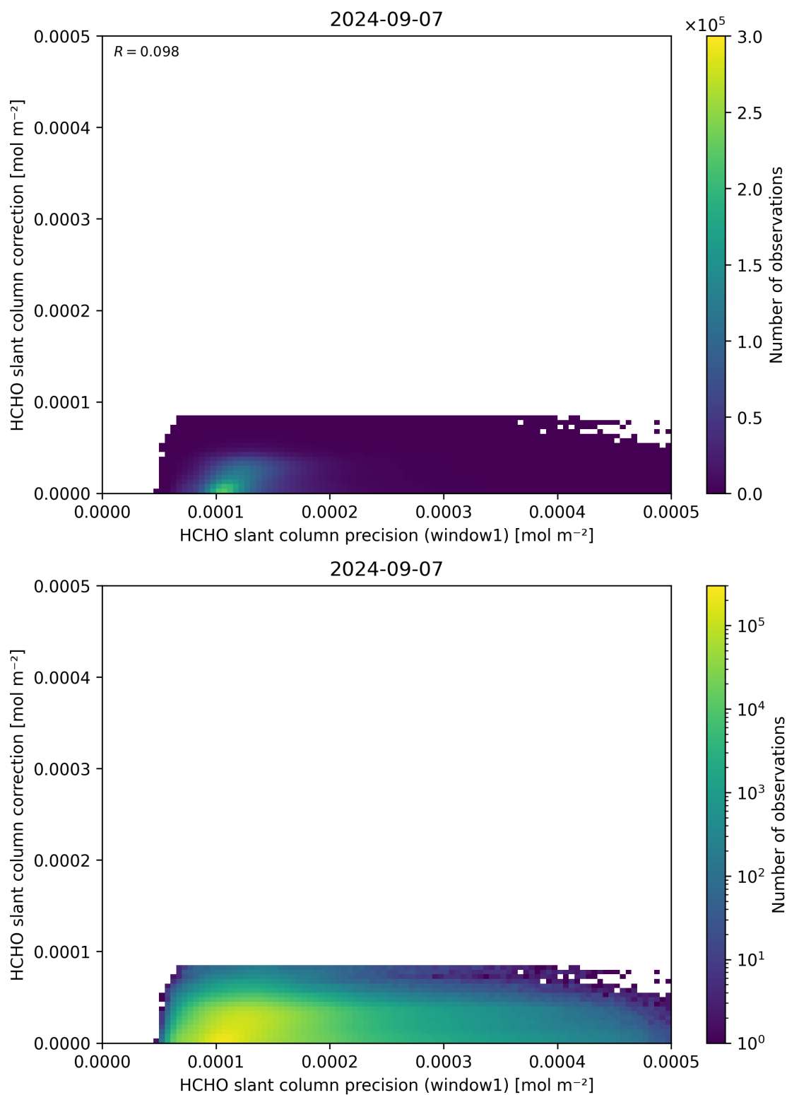
Figure 93: Scatter density plot of “HCHO slant column precision (window1)” against “HCHO slant column correction” for 2024-09-06 to 2024-09-08.
