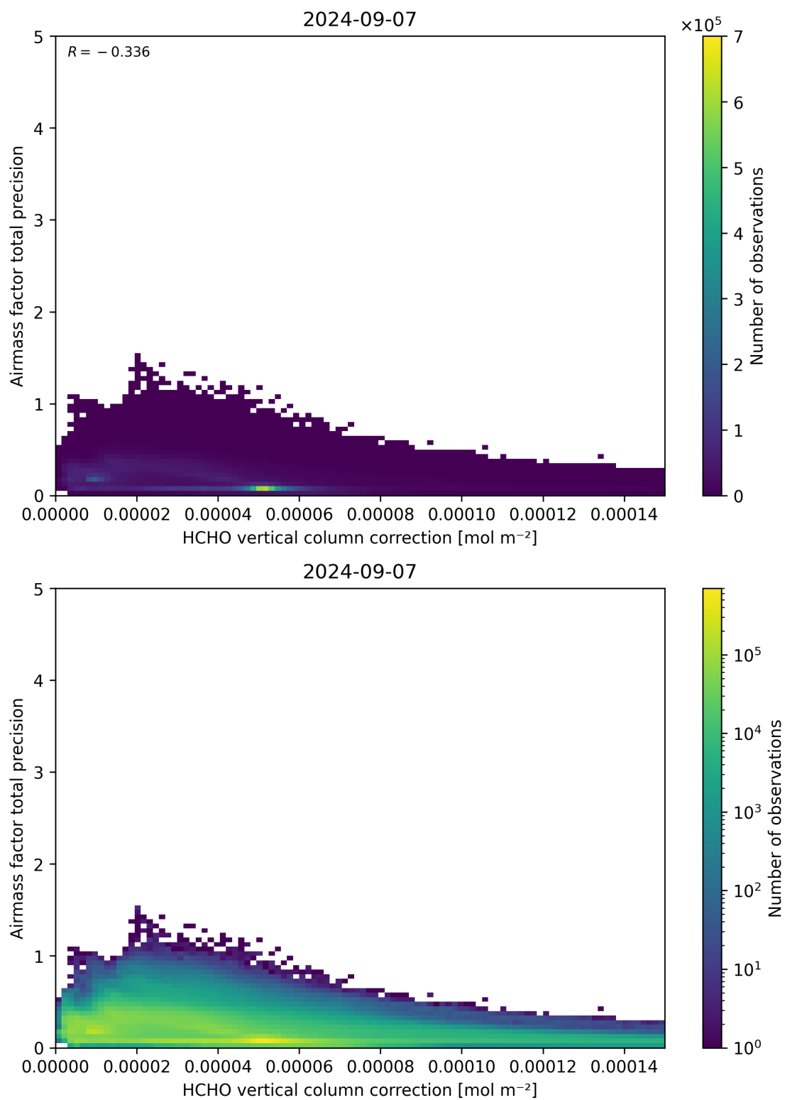
Figure 121: Scatter density plot of “HCHO vertical column correction” against “Airmass factor total precision” for 2024-09-06 to 2024-09-08.
