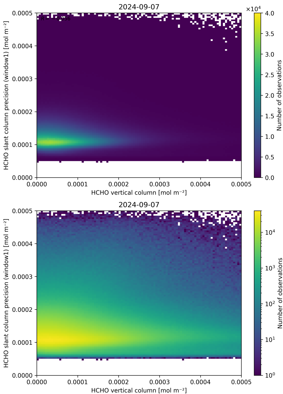
Figure 130: Scatter density plot of “HCHO vertical column” against “HCHO slant column precision (window1)” for 2024-09-06 to 2024-09-08.
