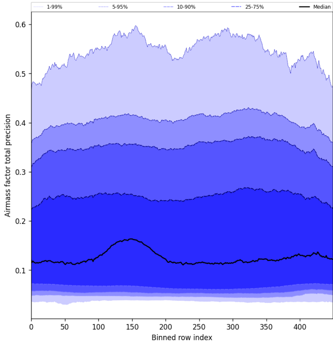
Figure 55: Along track statistics of “Airmass factor total precision” for 2024-09-06 to 2024-09-08
