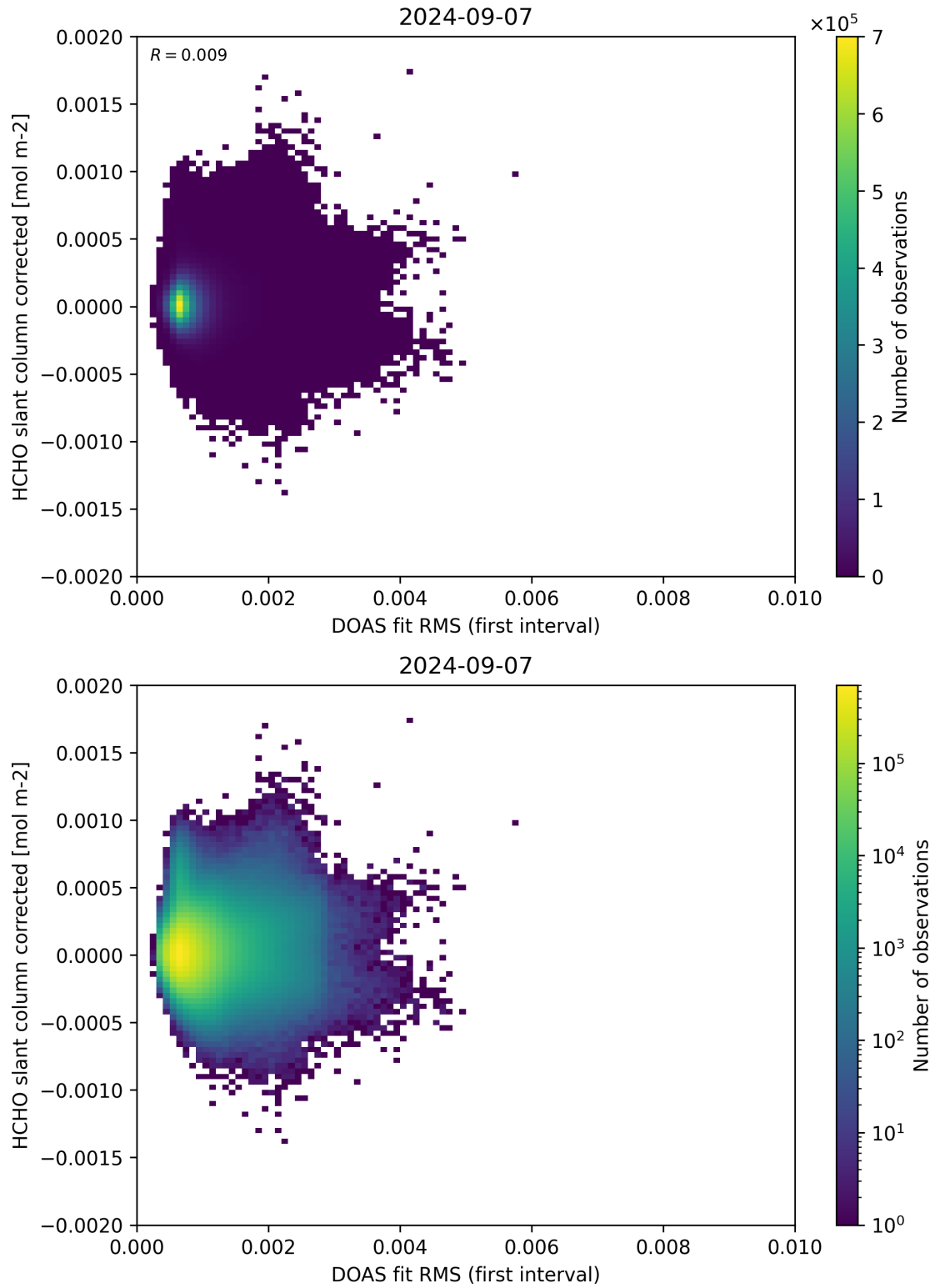
Figure 62: Scatter density plot of “DOAS fit RMS (first interval)” against “HCHO slant column corrected” for 2024-09-06 to 2024-09-08.
