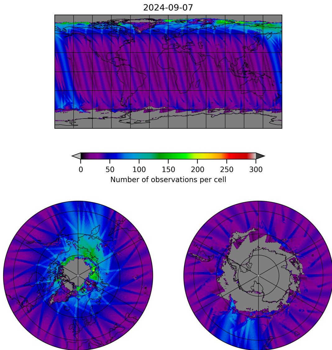
Figure 19: Map of the number of observations for 2024-09-06 to 2024-09-08
