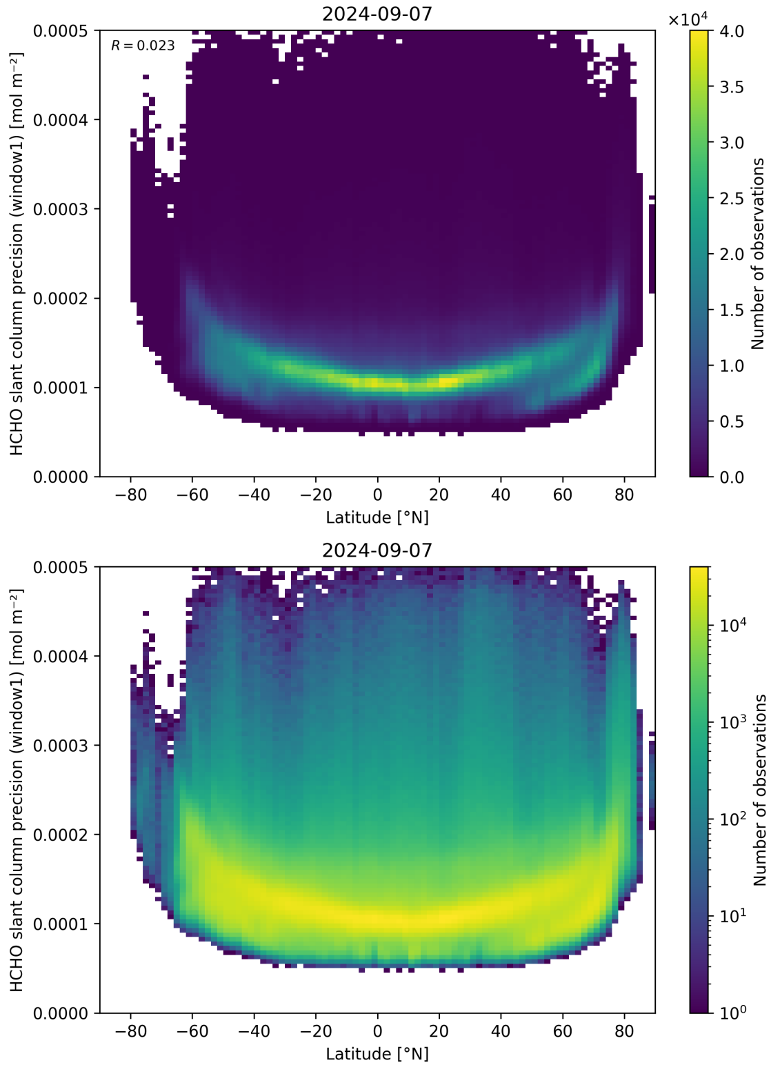
Figure 160: Scatter density plot of “Latitude” against “HCHO slant column precision (window1)” for 2024-09-06 to 2024-09-08.
