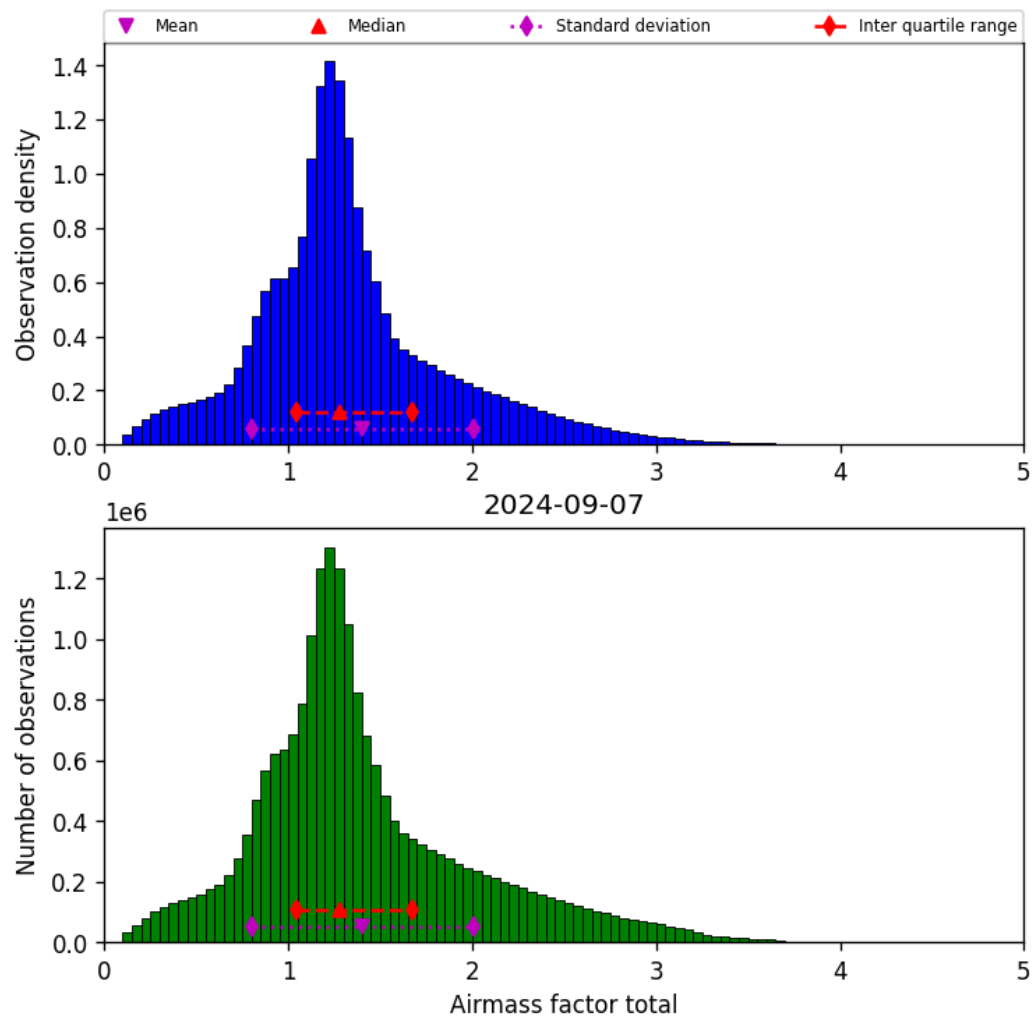
Figure 40: Histogram of “Airmass factor total” for 2024-09-06 to 2024-09-08
