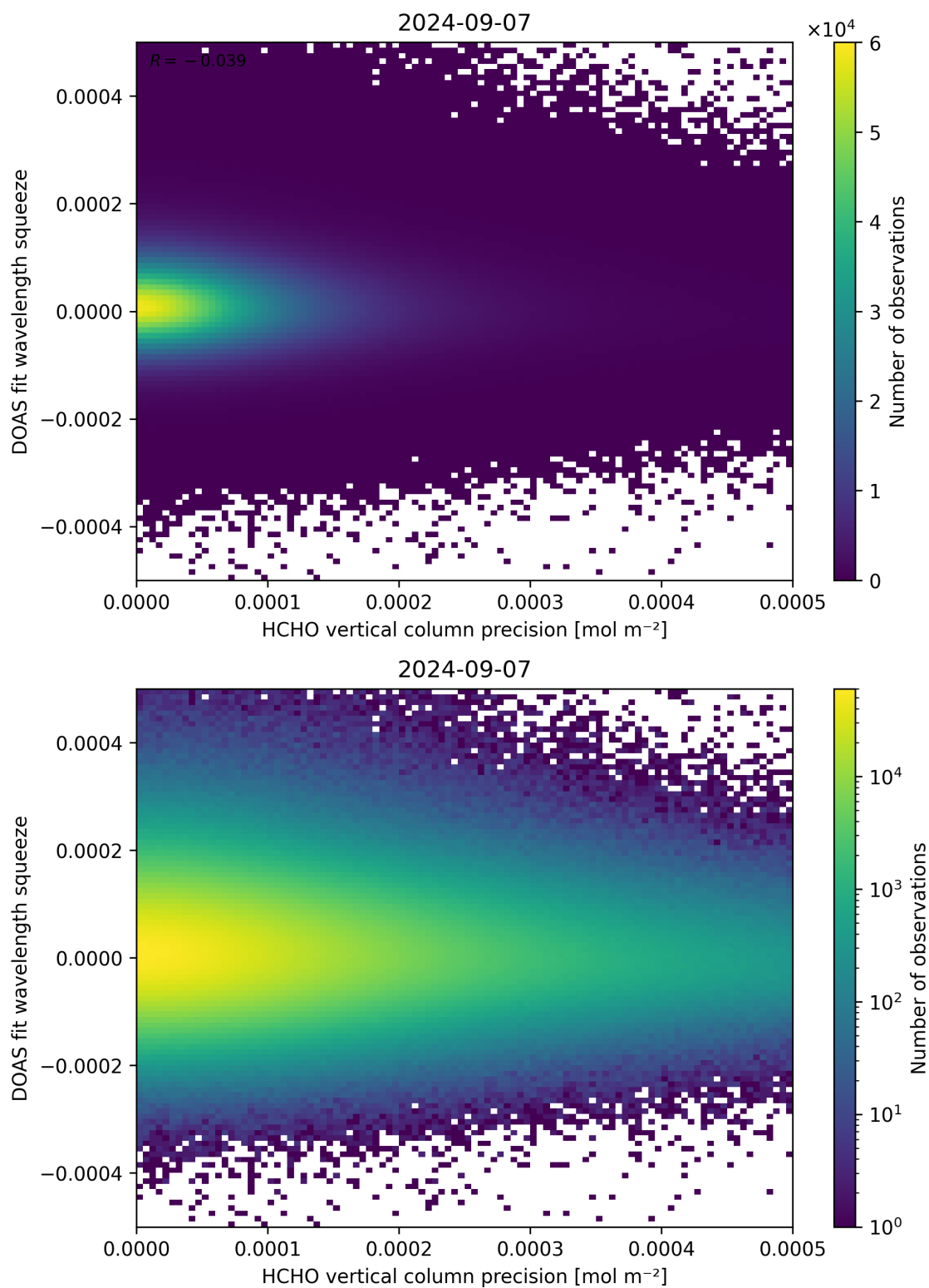
Figure 138: Scatter density plot of “HCHO vertical column precision” against “DOAS fit wavelength squeeze” for 2024-09-06 to 2024-09-08.
