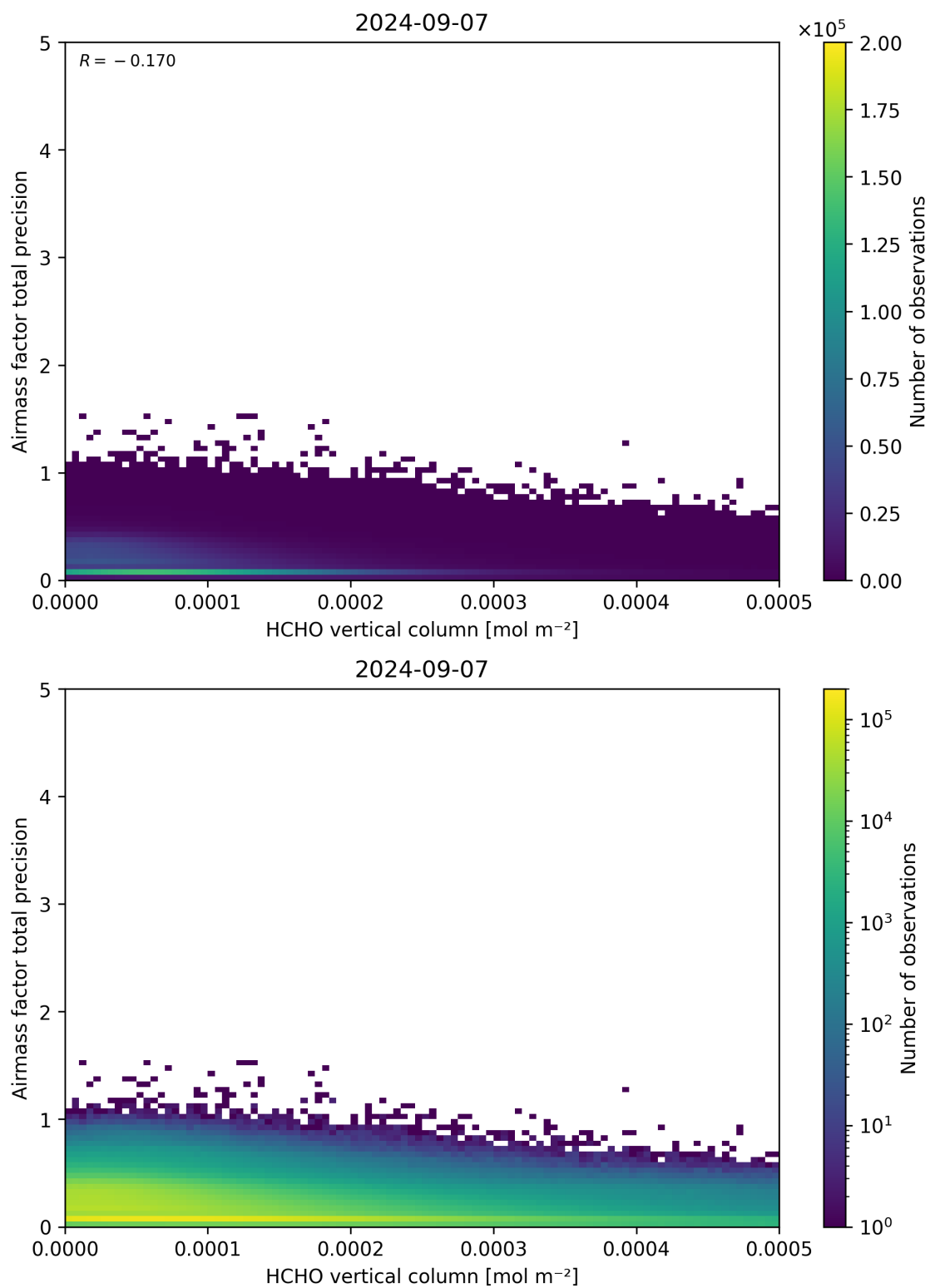
Figure 132: Scatter density plot of “HCHO vertical column” against “Airmass factor total precision” for 2024-09-06 to 2024-09-08.
