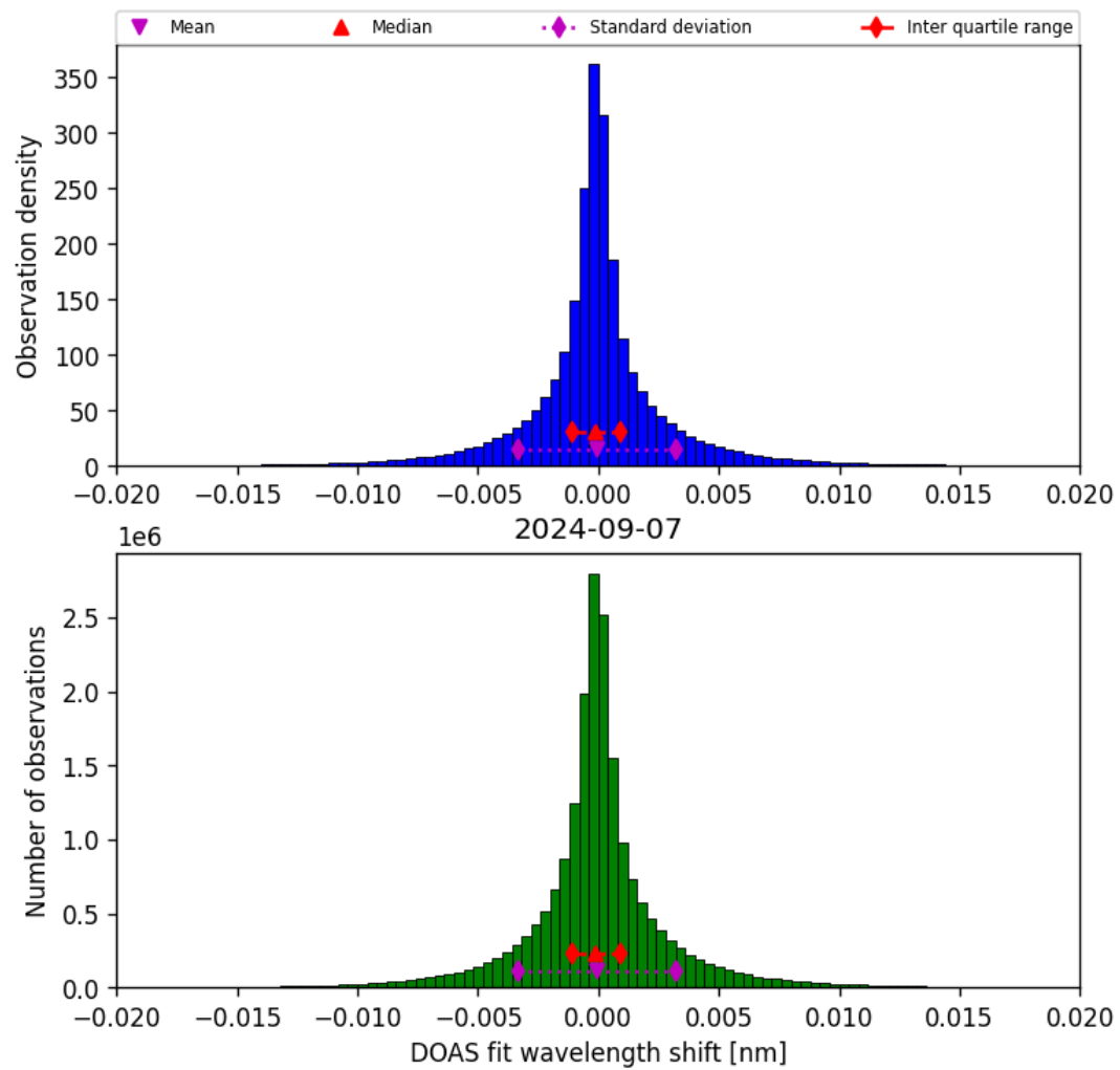
Figure 44: Histogram of “DOAS fit wavelength shift” for 2024-09-06 to 2024-09-08
