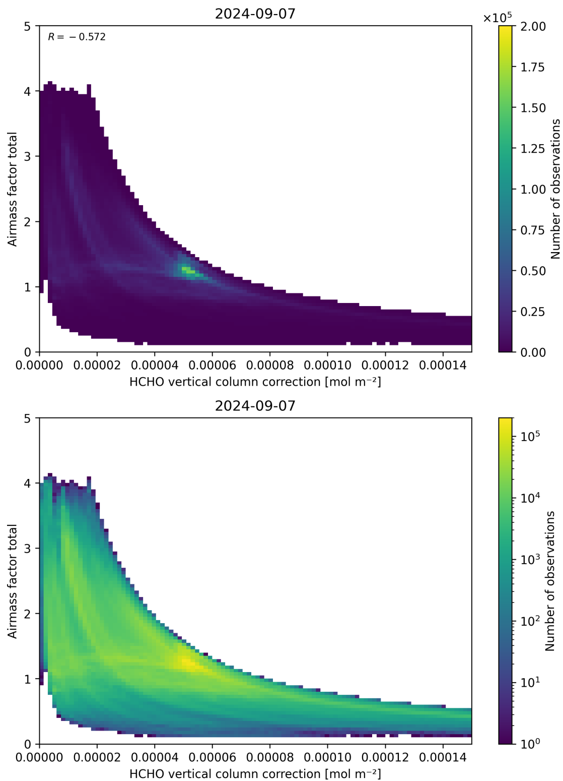
Figure 120: Scatter density plot of “HCHO vertical column correction” against “Airmass factor total” for 2024-09-06 to 2024-09-08.
