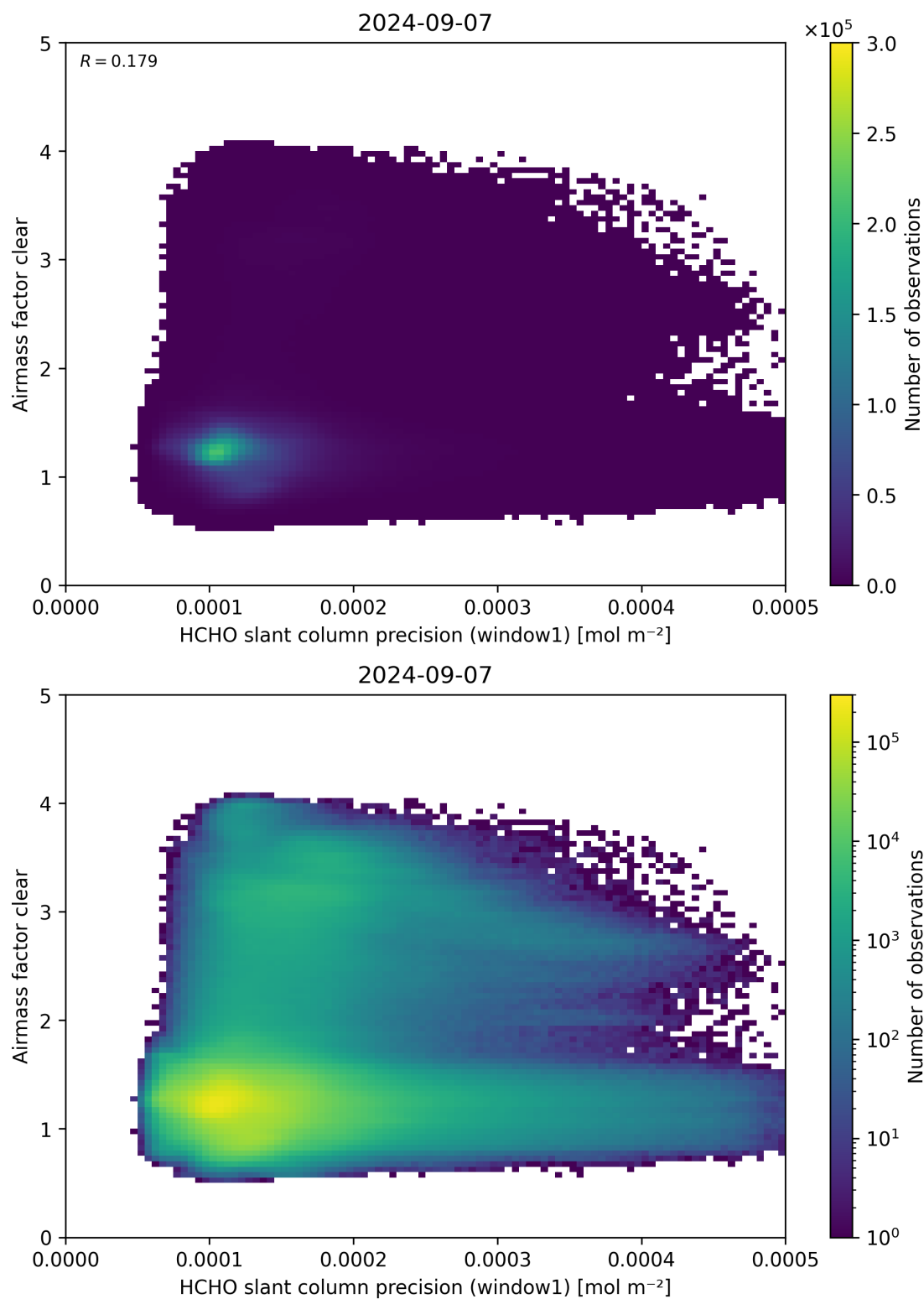
Figure 91: Scatter density plot of “HCHO slant column precision (window1)” against “Airmass factor clear” for 2024-09-06 to 2024-09-08.
