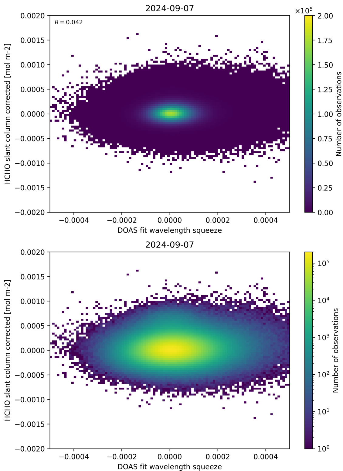
Figure 69: Scatter density plot of “DOAS fit wavelength squeeze” against “HCHO slant column corrected” for 2024-09-06 to 2024-09-08.
