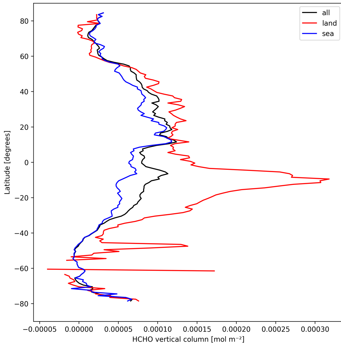
Figure 21: Zonal average of “HCHO vertical column” for 2024-09-06 to 2024-09-08.
