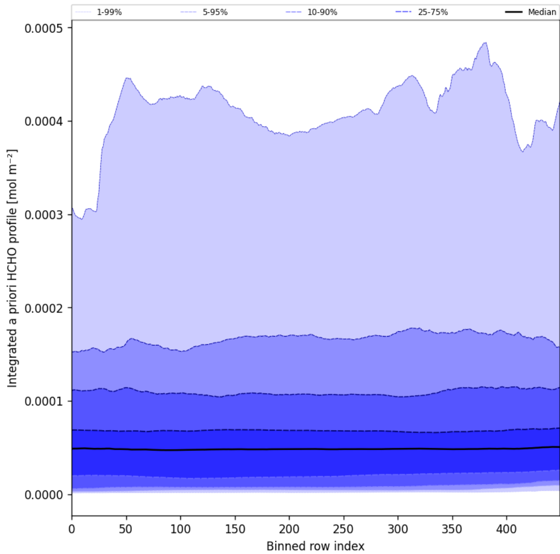
Figure 57: Along track statistics of “Integrated a priori HCHO profile” for 2024-09-06 to 2024-09-08
