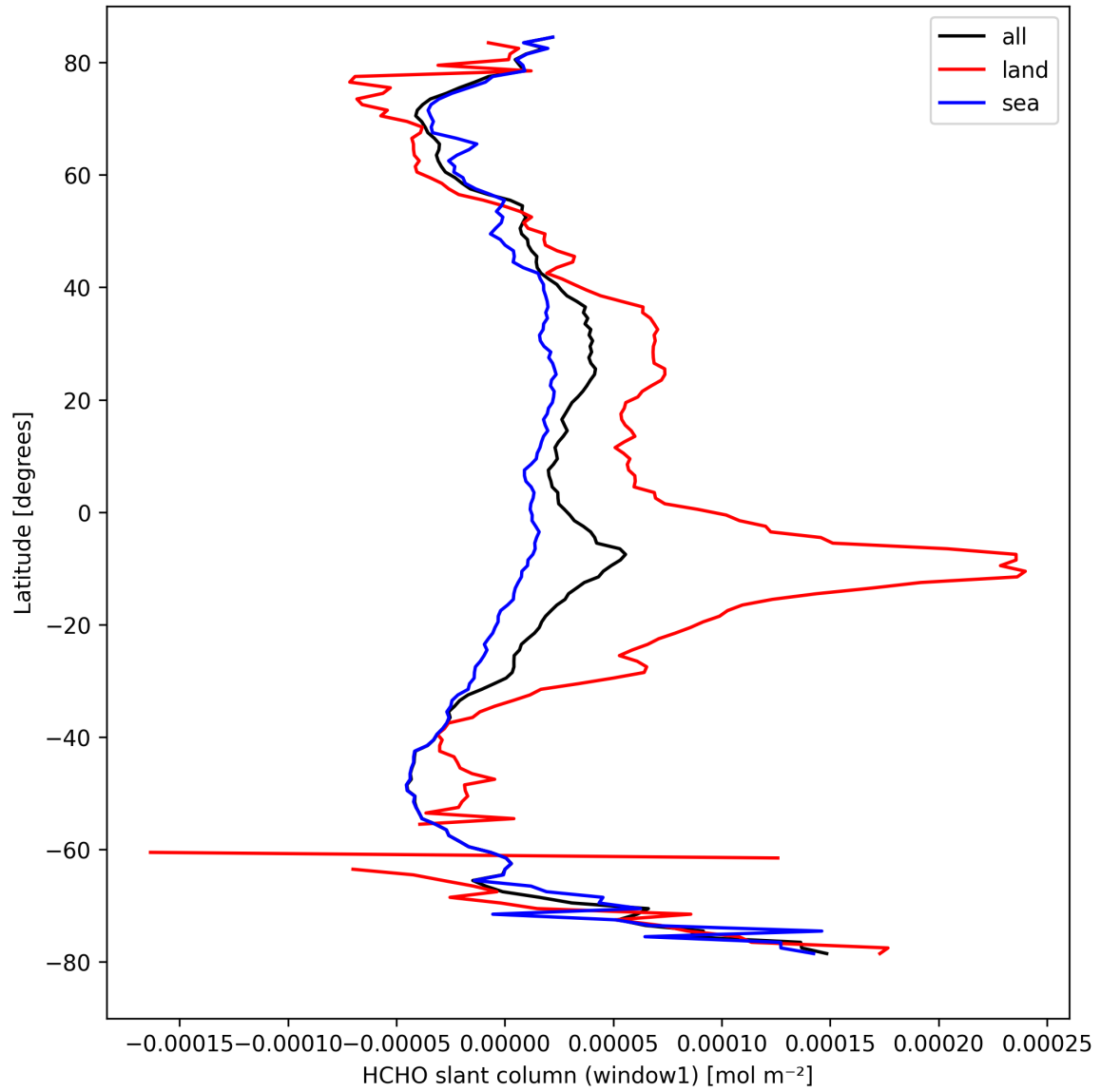
Figure 24: Zonal average of “HCHO slant column (window1)” for 2024-09-06 to 2024-09-08.
