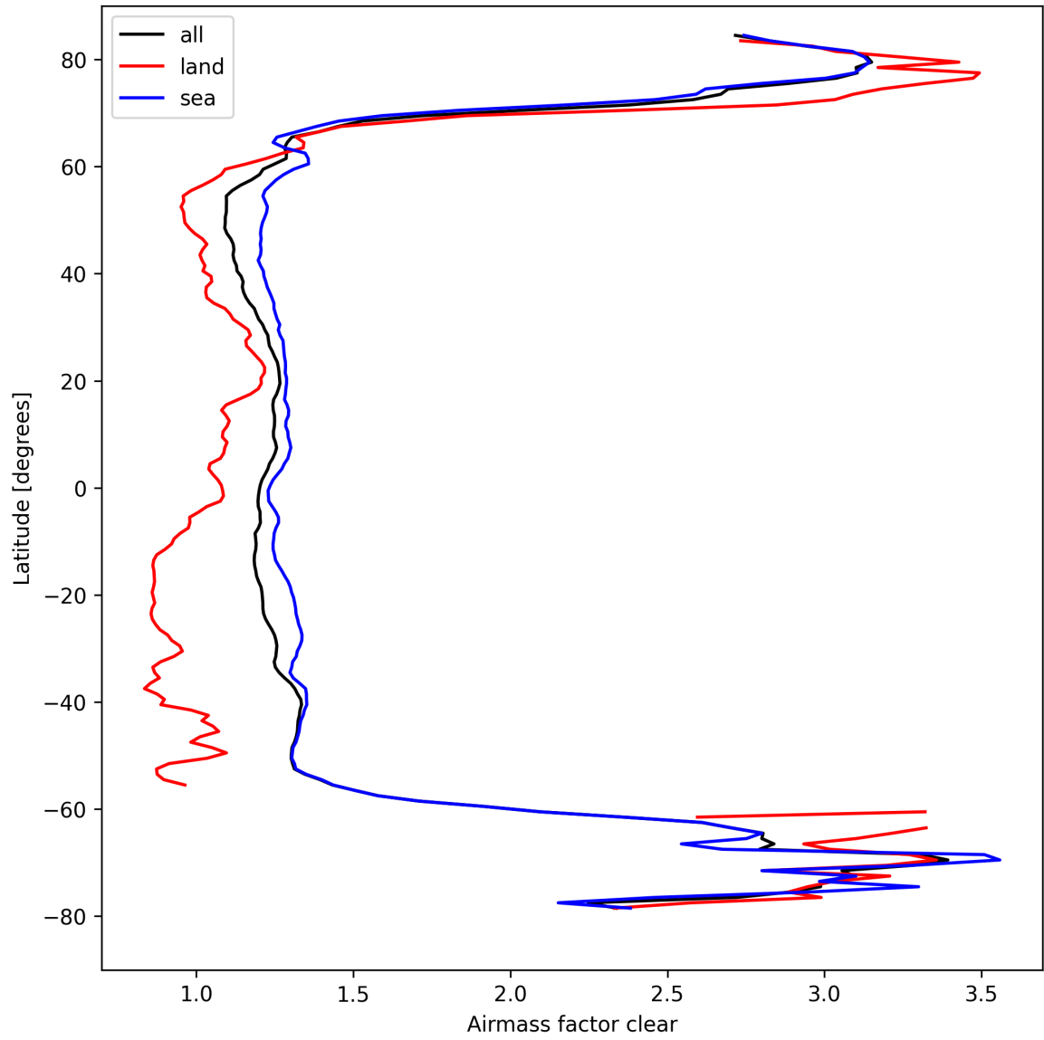
Figure 28: Zonal average of “Airmass factor clear” for 2024-09-06 to 2024-09-08.
