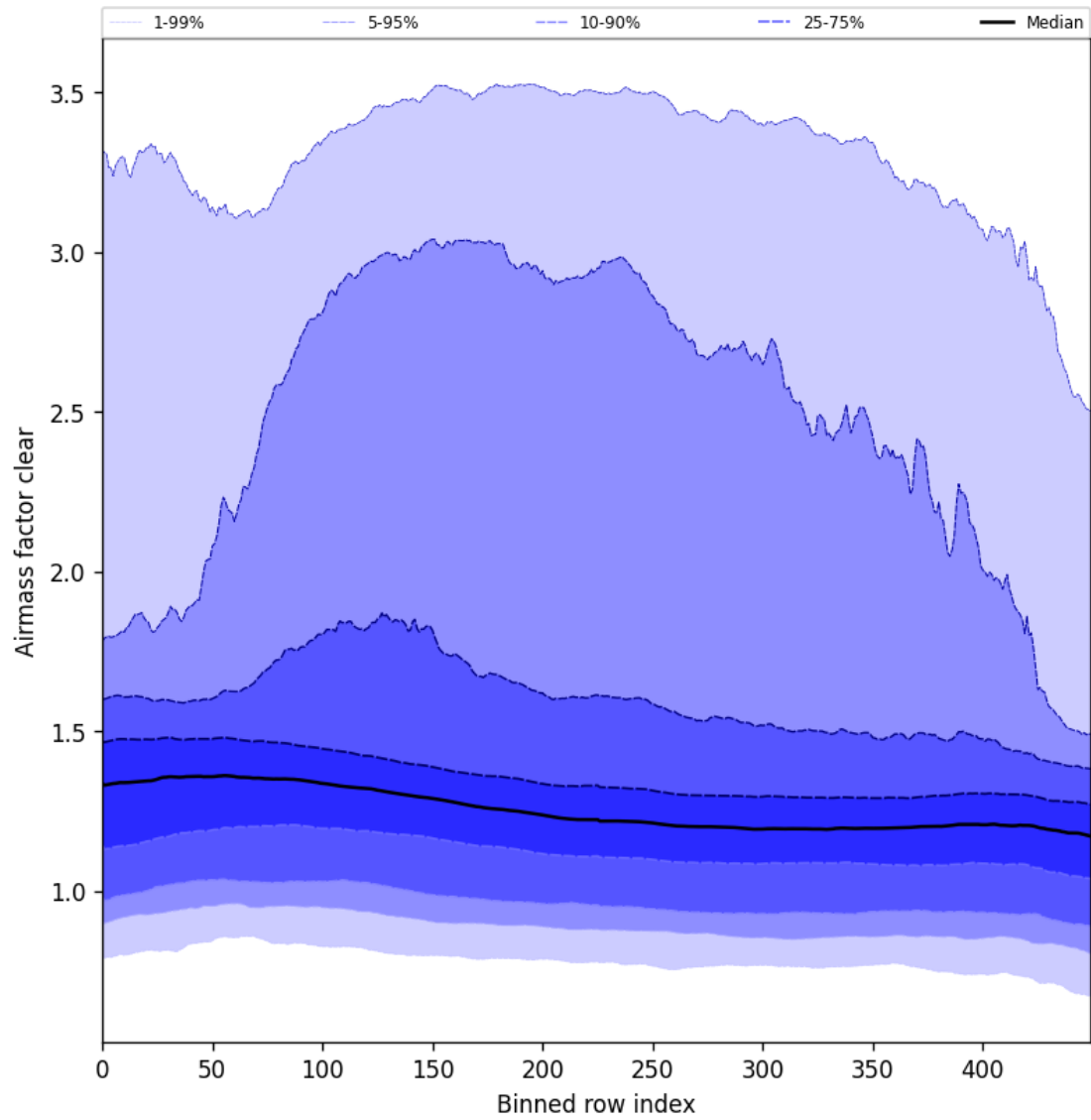
Figure 56: Along track statistics of “Airmass factor clear” for 2024-09-06 to 2024-09-08
