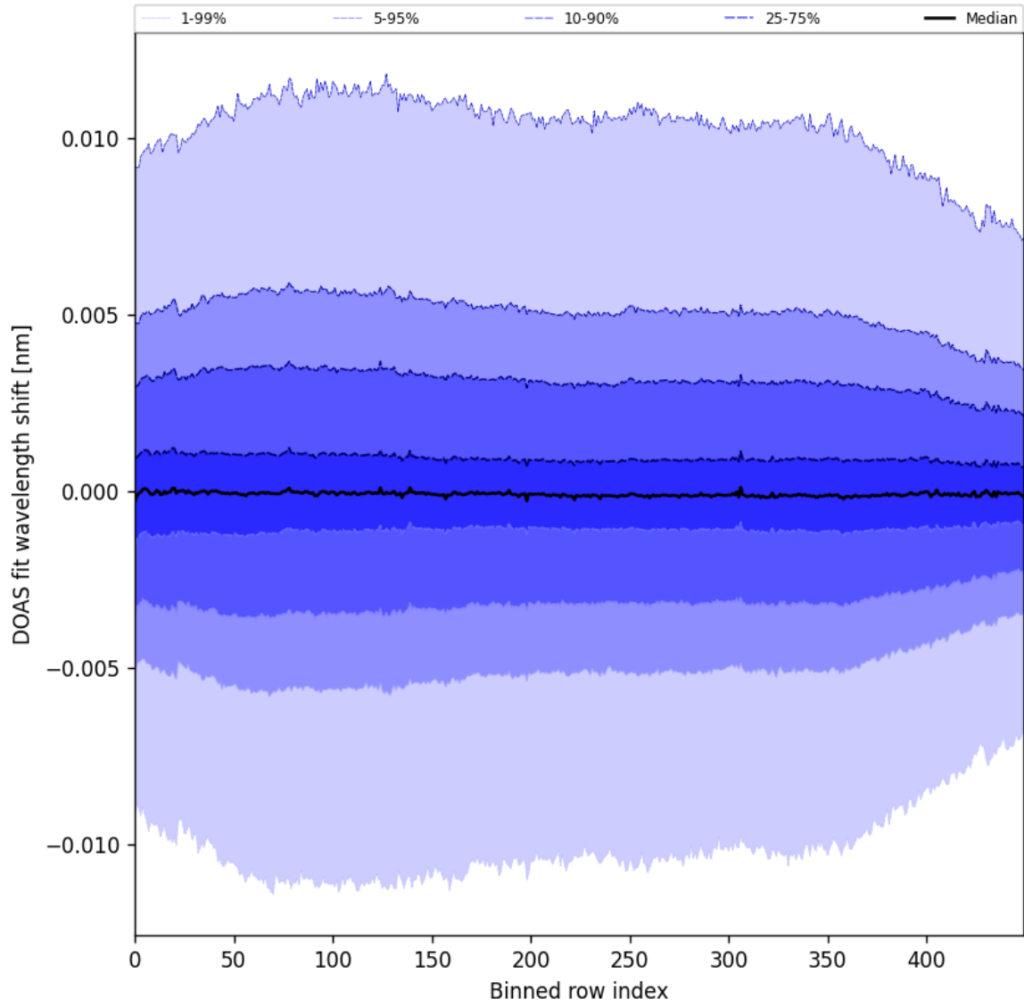
Figure 58: Along track statistics of “DOAS fit wavelength shift” for 2024-09-06 to 2024-09-08
