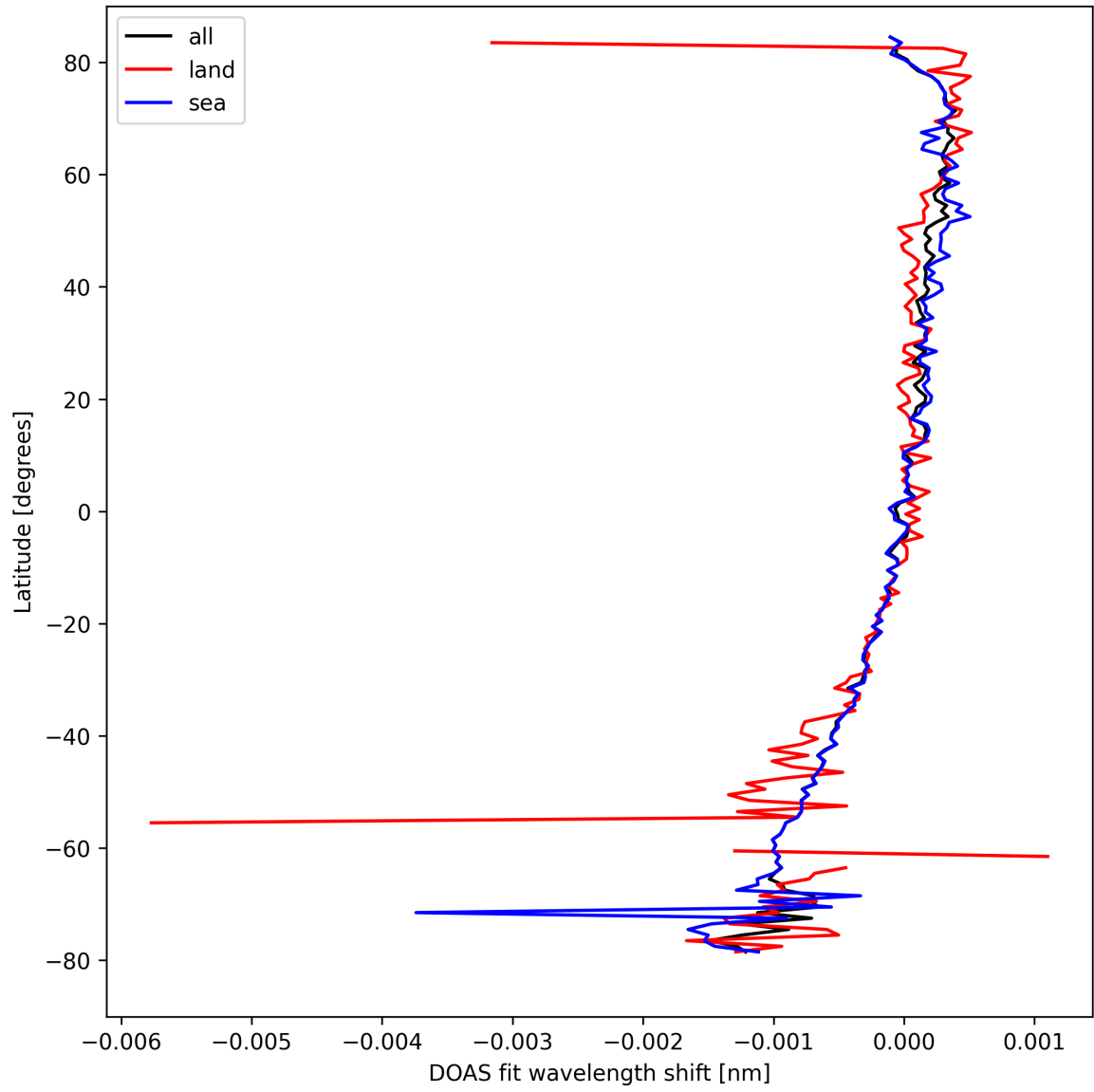
Figure 30: Zonal average of “DOAS fit wavelength shift” for 2024-09-06 to 2024-09-08.
