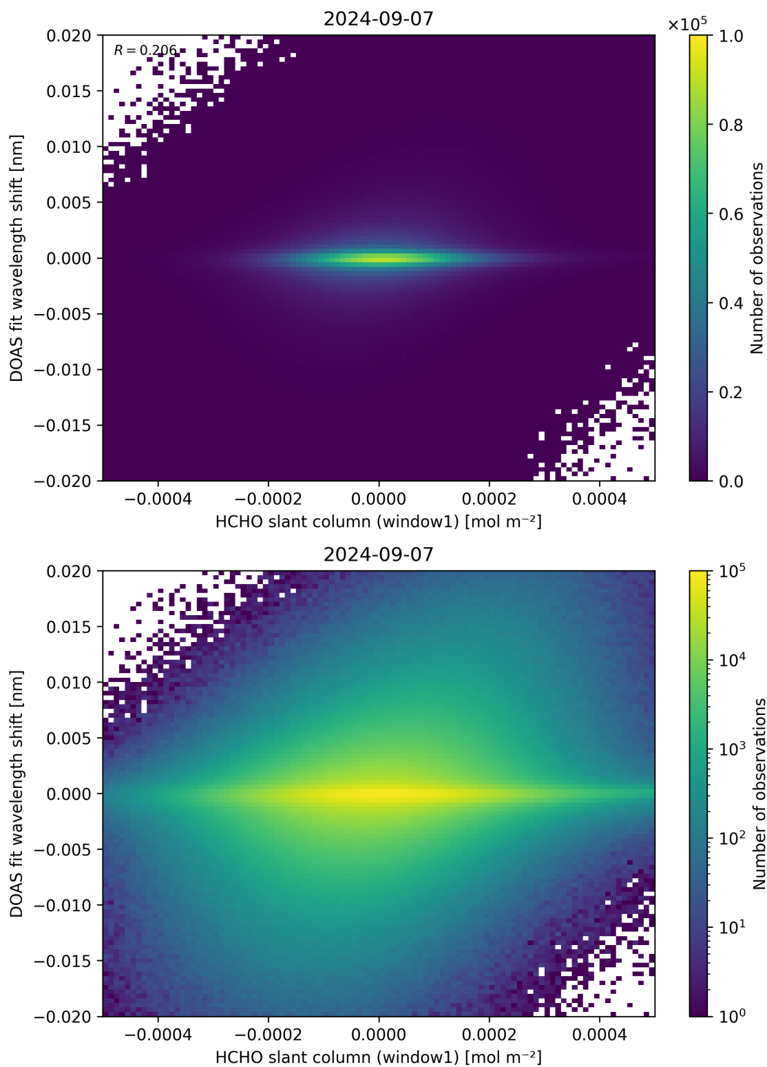
Figure 79: Scatter density plot of “HCHO slant column (window1)” against “DOAS fit wavelength shift” for 2024-09-06 to 2024-09-08.
