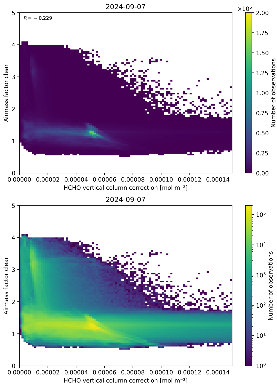
Figure 115: Scatter density plot of “HCHO vertical column correction” against “Airmass factor clear” for 2024-09-06 to 2024-09-08.
