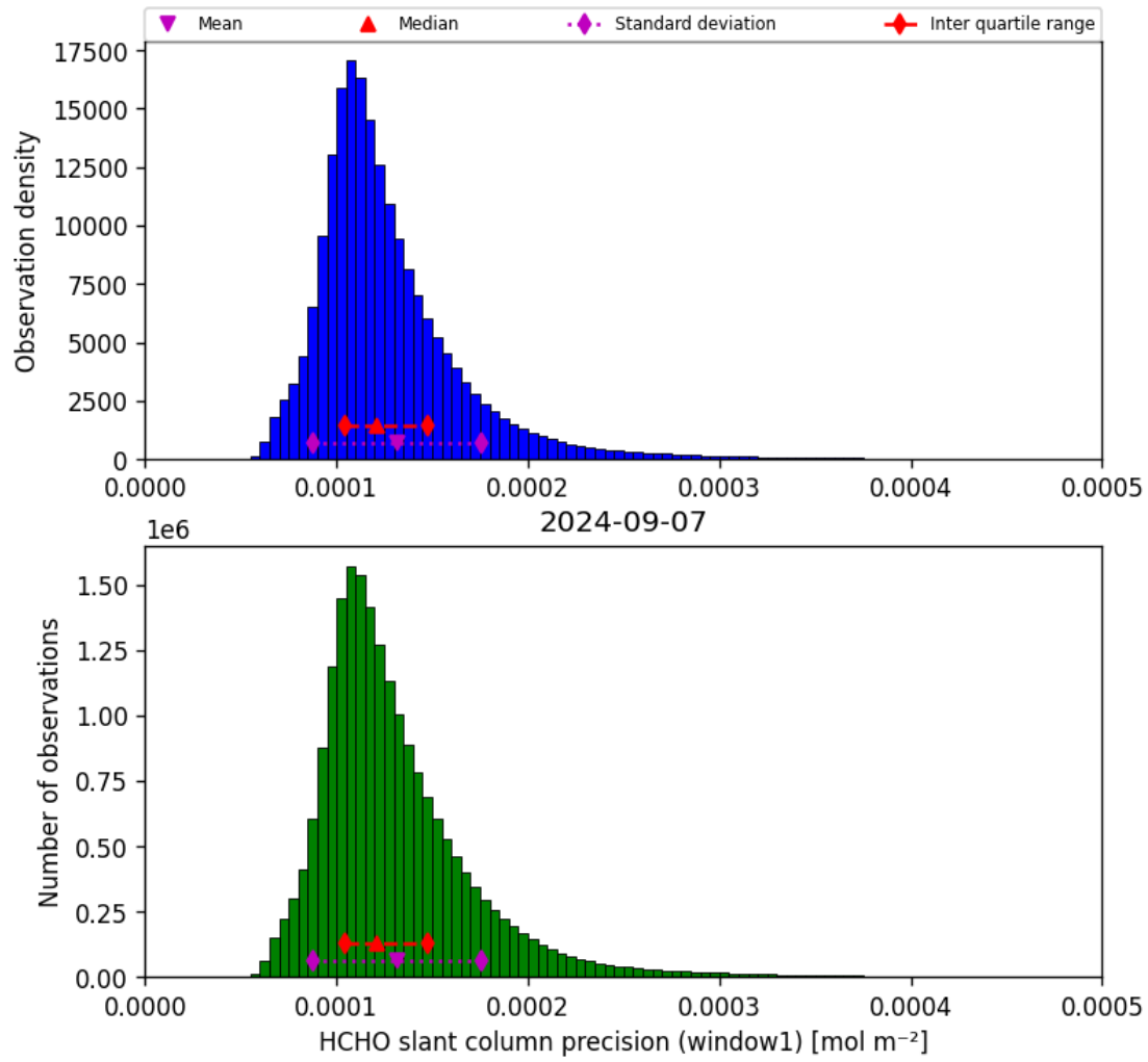
Figure 39: Histogram of “HCHO slant column precision (window1)” for 2024-09-06 to 2024-09-08
