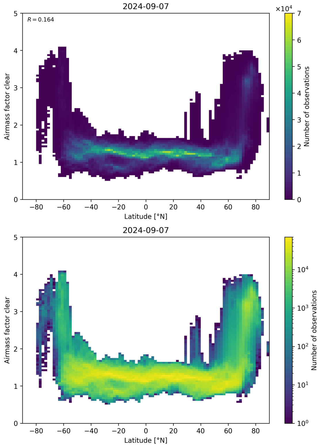
Figure 156: Scatter density plot of “Latitude” against “Airmass factor clear” for 2024-09-06 to 2024-09-08.
