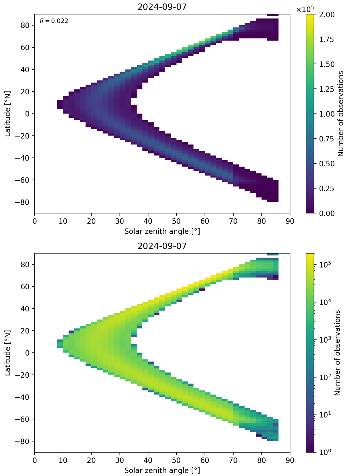
Figure 181: Scatter density plot of “Solar zenith angle” against “Latitude” for 2024-09-06 to 2024-09-08.
