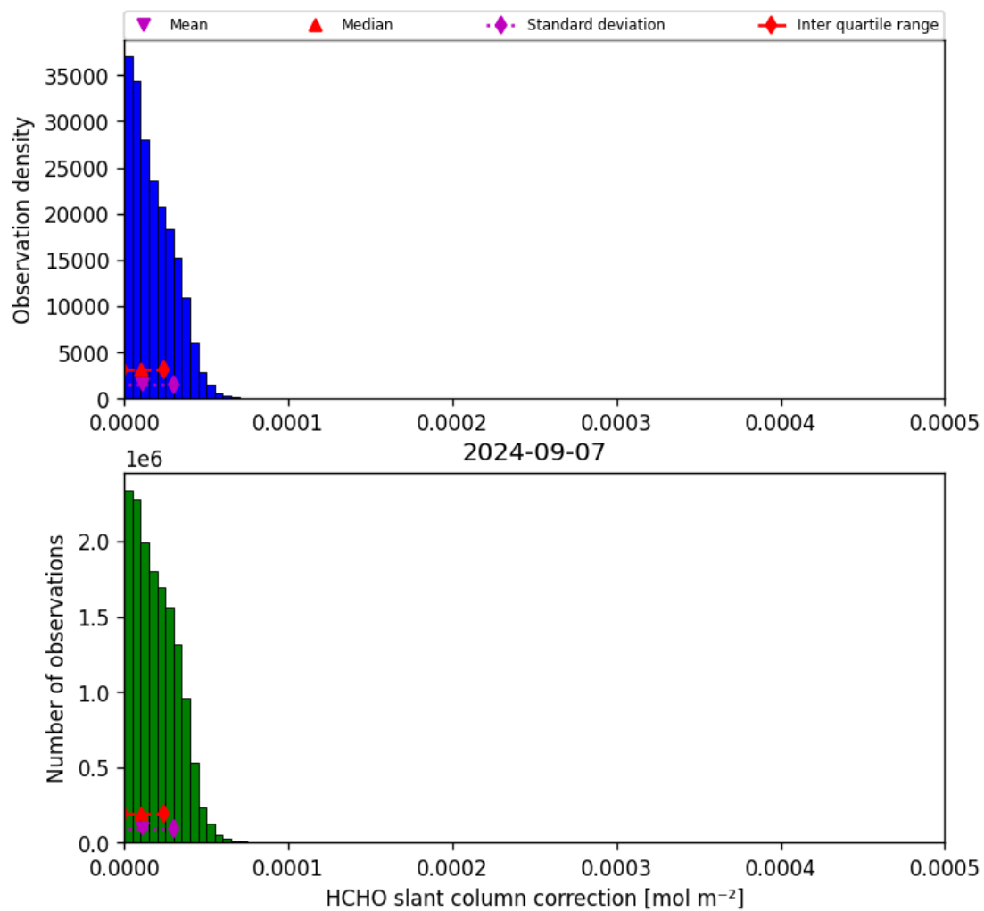
Figure 47: Histogram of “HCHO slant column correction” for 2024-09-06 to 2024-09-08
