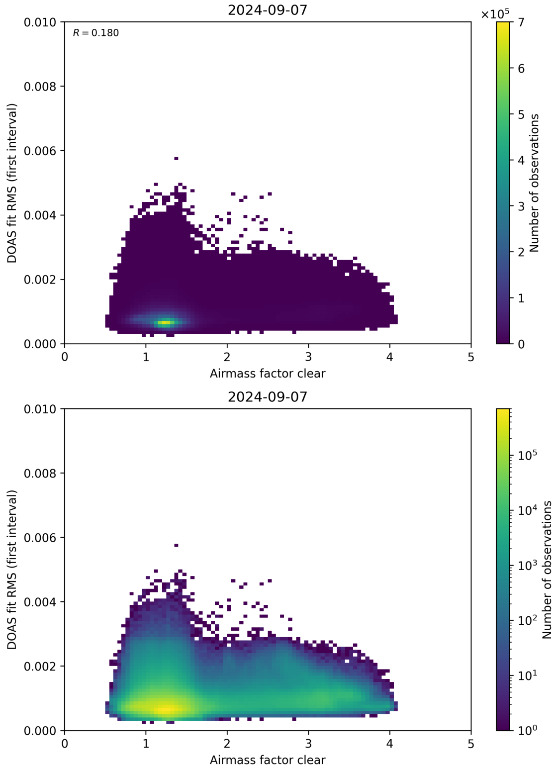
Figure 71: Scatter density plot of “Airmass factor clear” against “DOAS fit RMS (first interval)” for 2024-09-06 to 2024-09-08.
