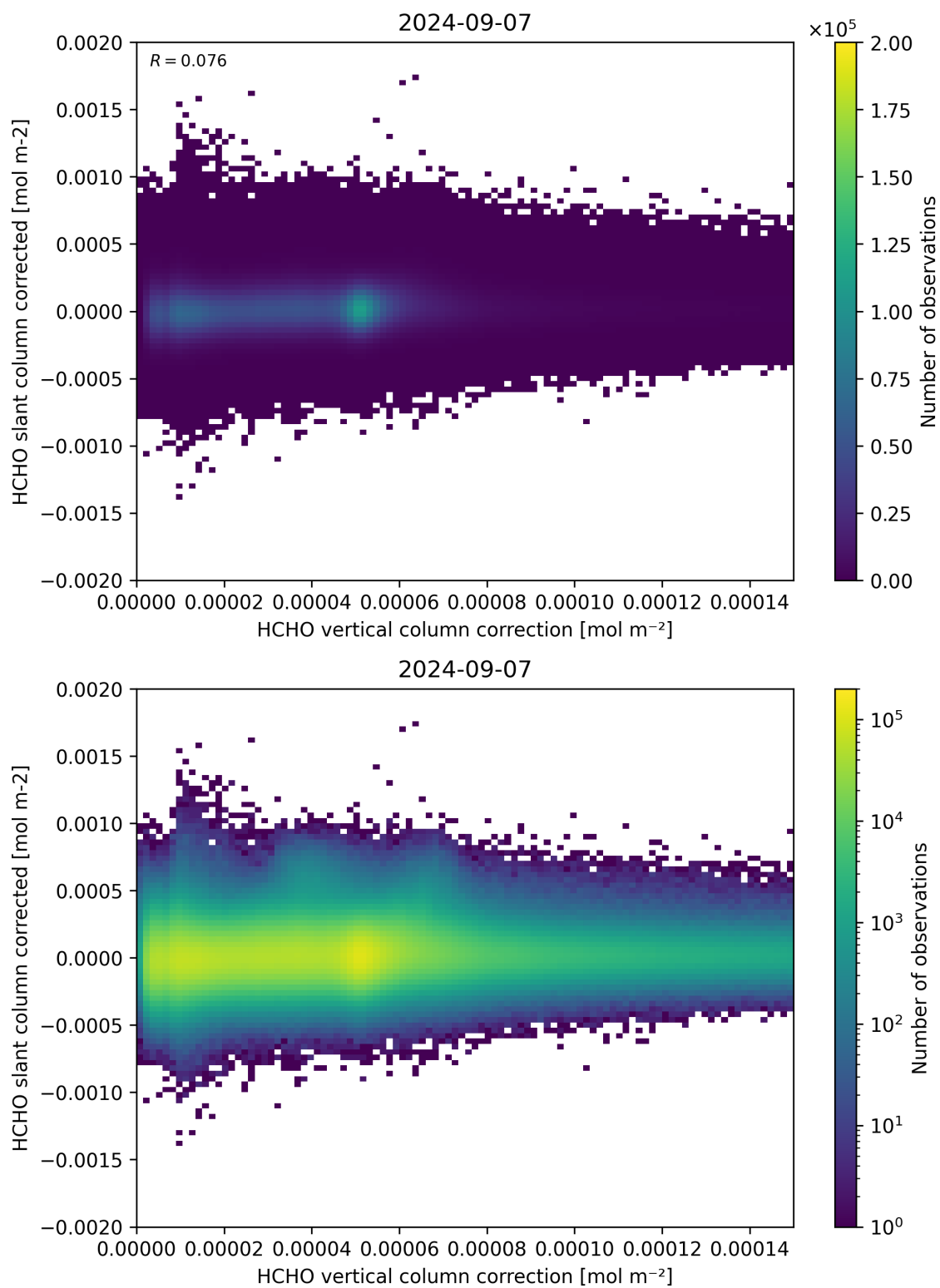
Figure 116: Scatter density plot of “HCHO vertical column correction” against “HCHO slant column corrected” for 2024-09-06 to 2024-09-08.
