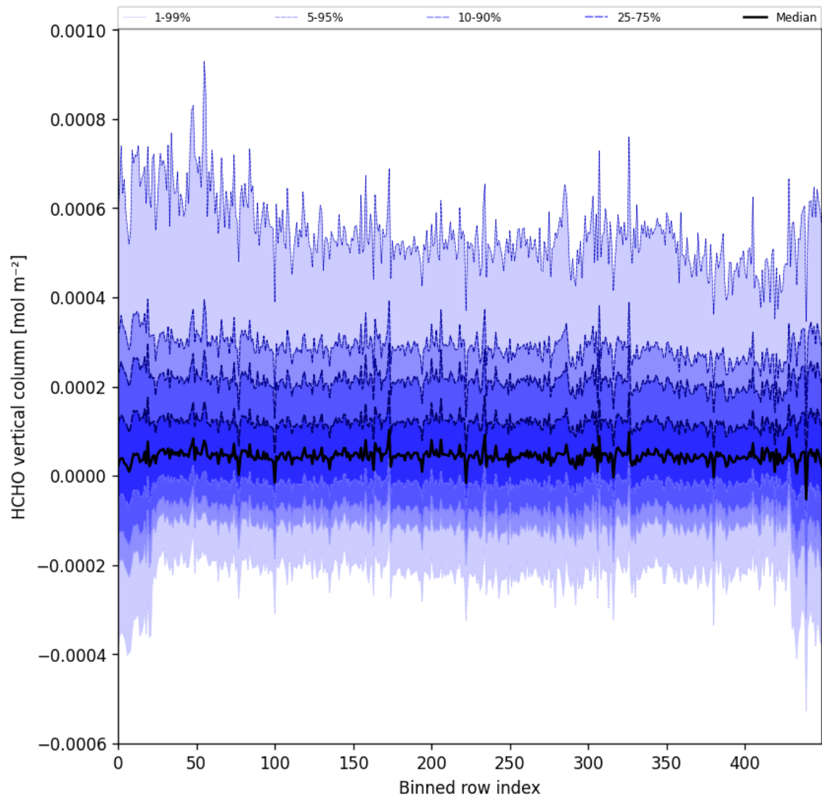
Figure 49: Along track statistics of “HCHO vertical column” for 2024-09-06 to 2024-09-08
