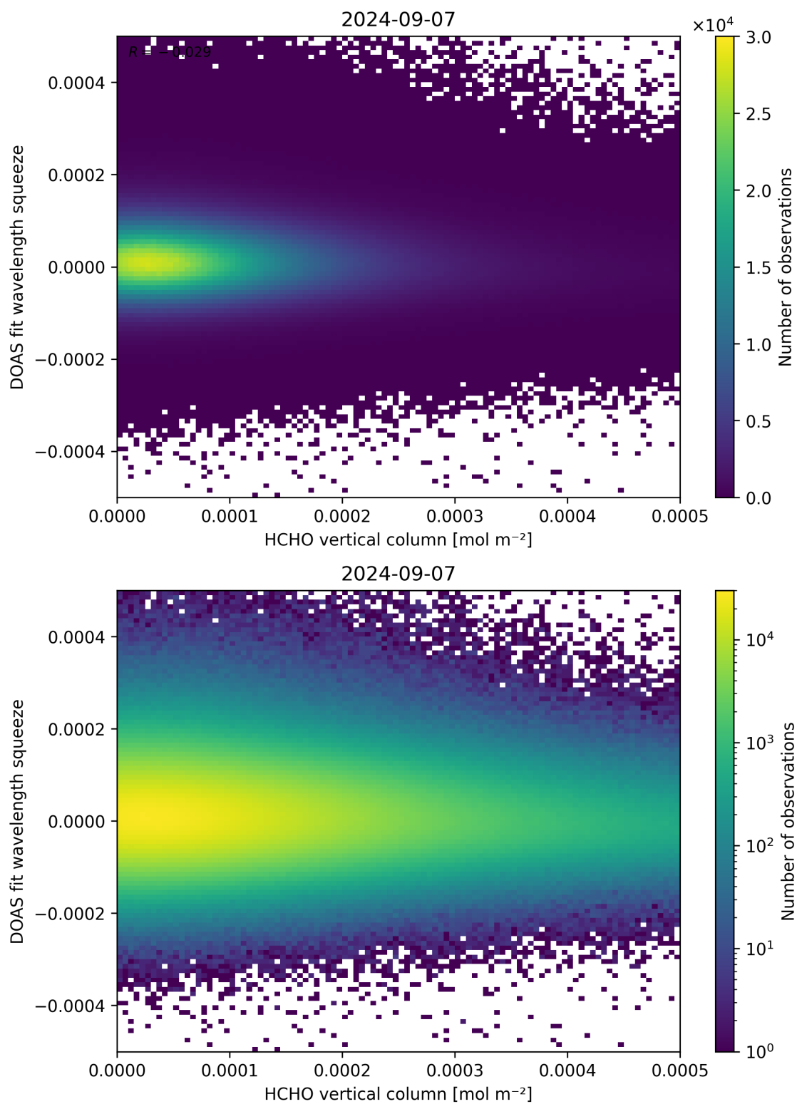
Figure 125: Scatter density plot of “HCHO vertical column” against “DOAS fit wavelength squeeze” for 2024-09-06 to 2024-09-08.
