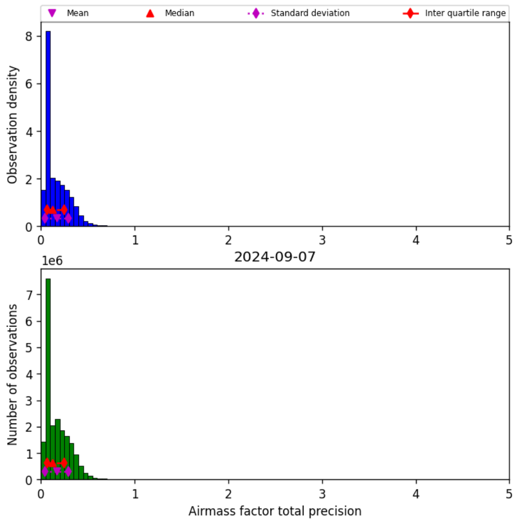
Figure 41: Histogram of “Airmass factor total precision” for 2024-09-06 to 2024-09-08
