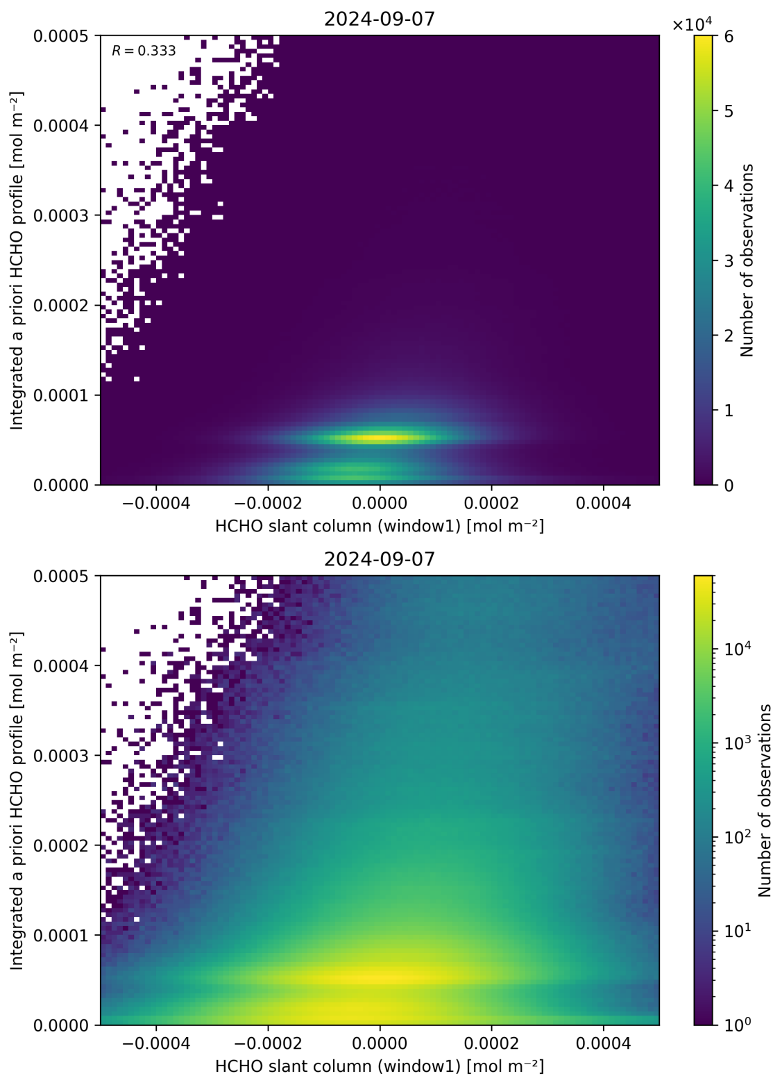
Figure 87: Scatter density plot of “HCHO slant column (window1)” against “Integrated a priori HCHO profile” for 2024-09-06 to 2024-09-08.
