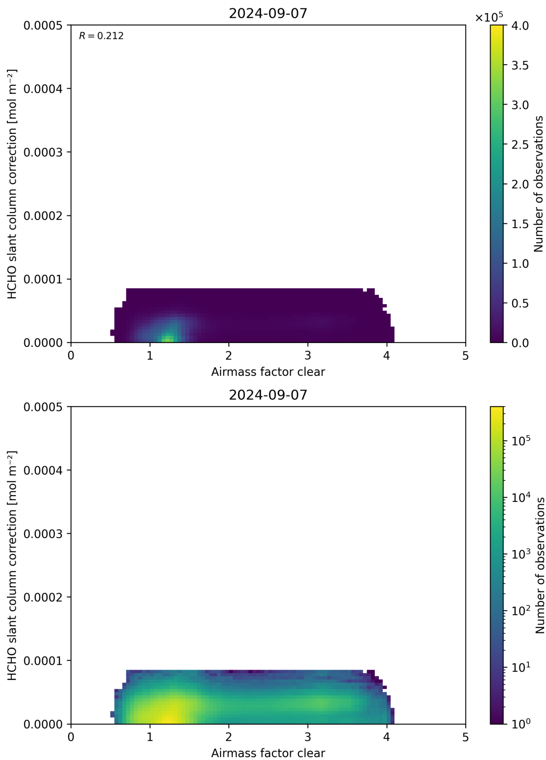
Figure 75: Scatter density plot of “Airmass factor clear” against “HCHO slant column correction” for 2024-09-06 to 2024-09-08.
