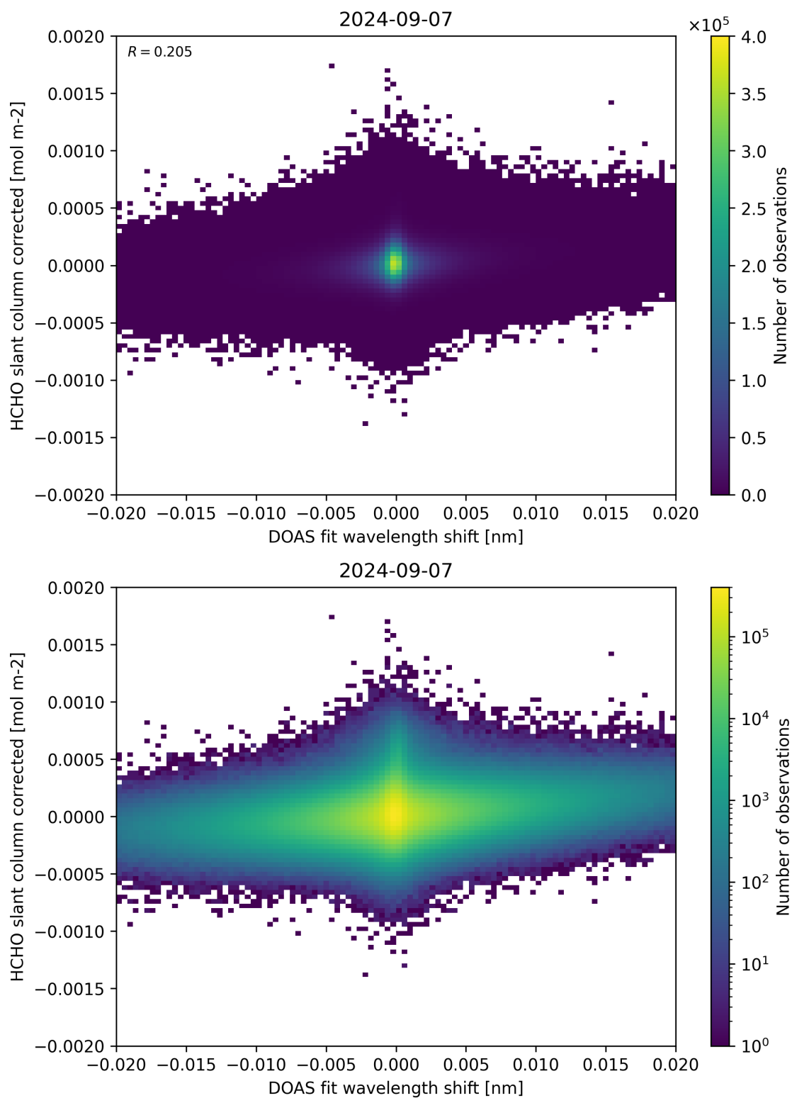
Figure 66: Scatter density plot of “DOAS fit wavelength shift” against “HCHO slant column corrected” for 2024-09-06 to 2024-09-08.
