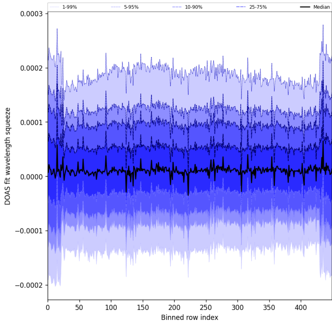
Figure 59: Along track statistics of “DOAS fit wavelength squeeze” for 2024-09-06 to 2024-09-08
