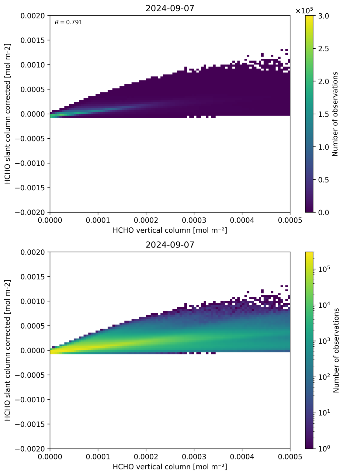
Figure 127: Scatter density plot of “HCHO vertical column” against “HCHO slant column corrected” for 2024-09-06 to 2024-09-08.
