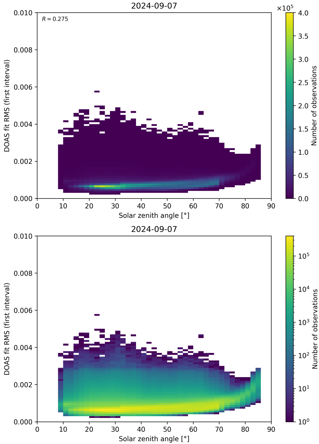
Figure 167: Scatter density plot of “Solar zenith angle” against “DOAS fit RMS (first interval)” for 2024-09-06 to 2024-09-08.
