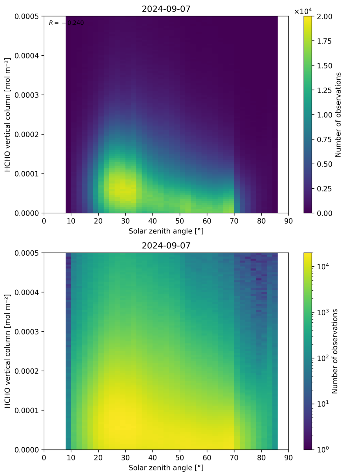
Figure 177: Scatter density plot of “Solar zenith angle” against “HCHO vertical column” for 2024-09-06 to 2024-09-08.
