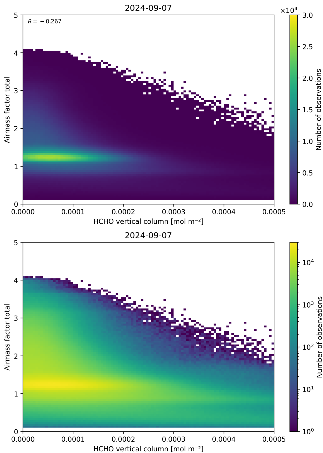
Figure 131: Scatter density plot of “HCHO vertical column” against “Airmass factor total” for 2024-09-06 to 2024-09-08.
