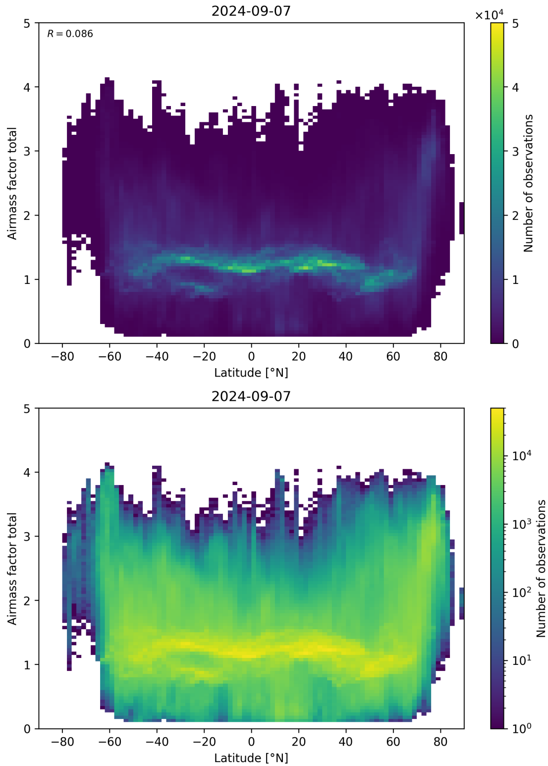
Figure 161: Scatter density plot of “Latitude” against “Airmass factor total” for 2024-09-06 to 2024-09-08.
