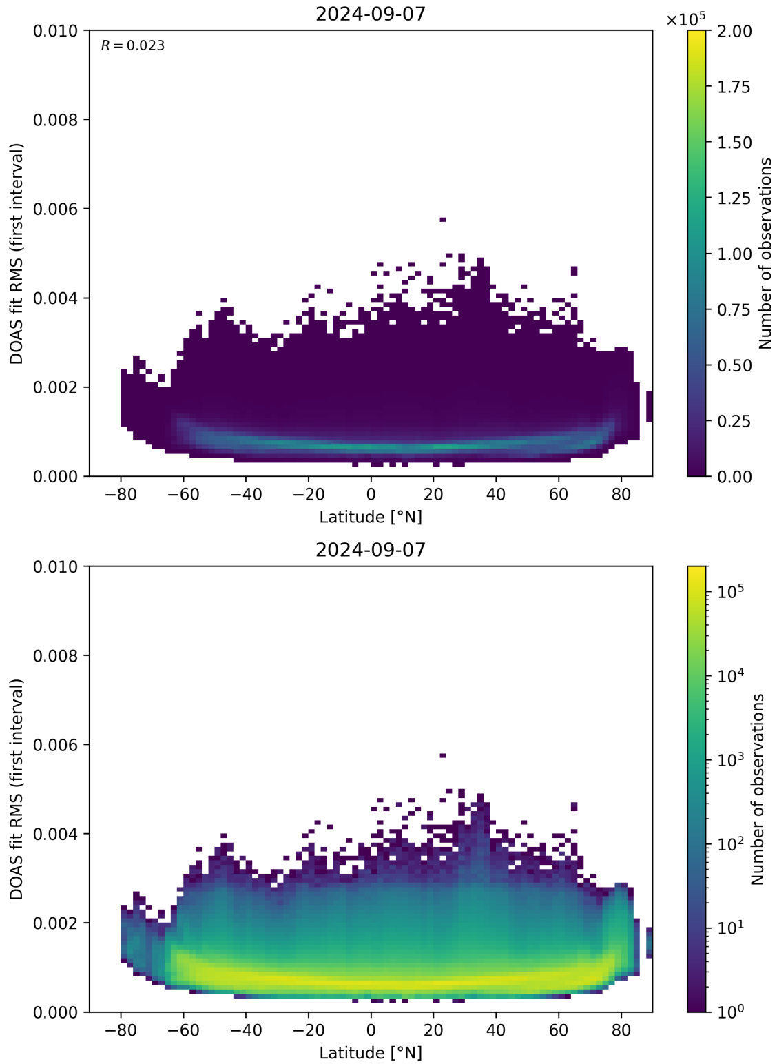
Figure 153: Scatter density plot of “Latitude” against “DOAS fit RMS (first interval)” for 2024-09-06 to 2024-09-08.
