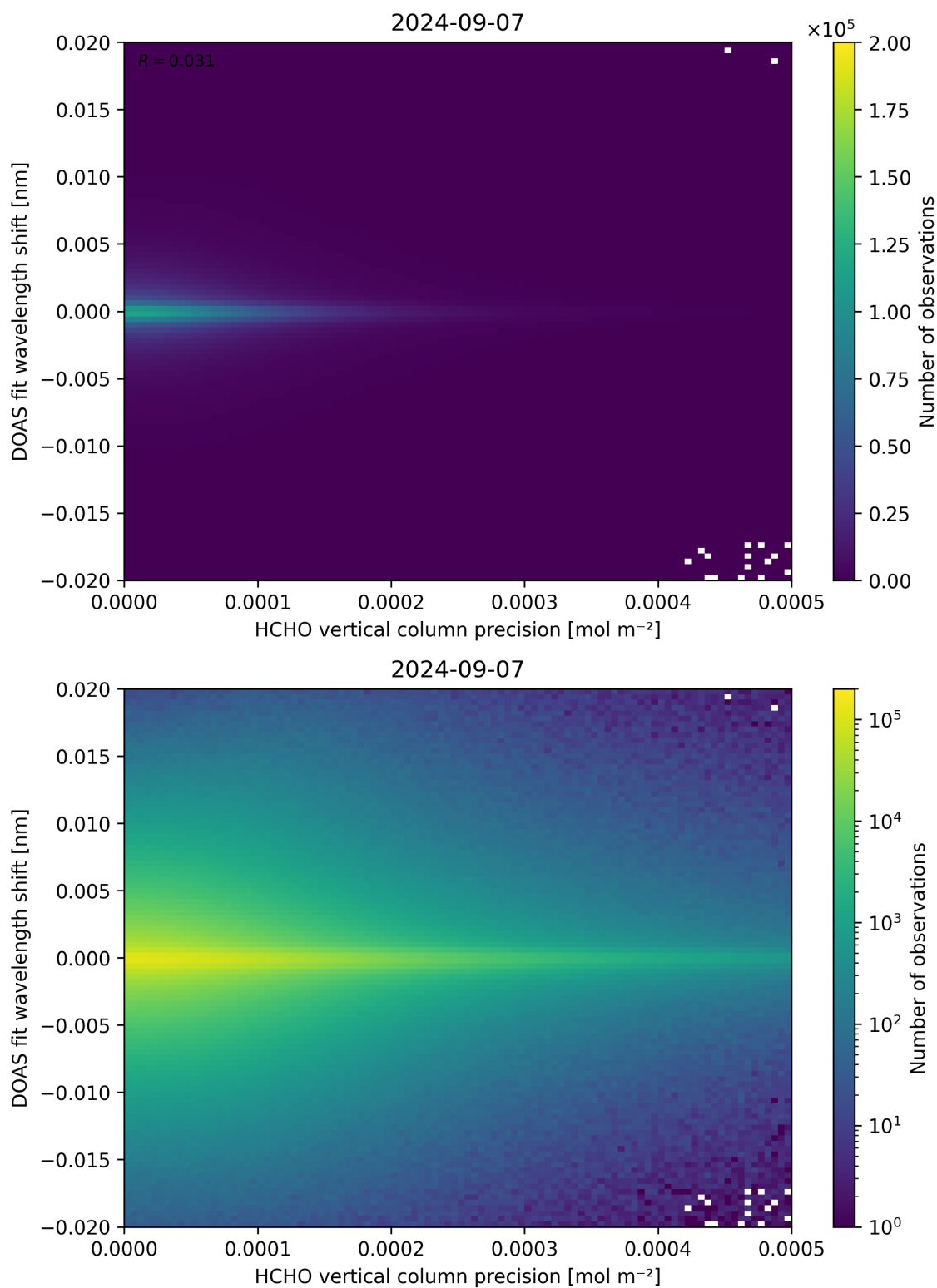
Figure 137: Scatter density plot of “HCHO vertical column precision” against “DOAS fit wavelength shift” for 2024-09-06 to 2024-09-08.
