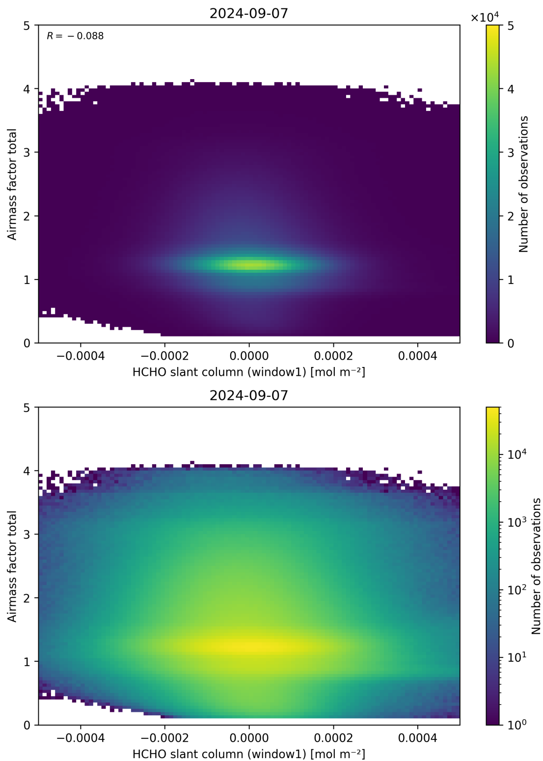
Figure 85: Scatter density plot of “HCHO slant column (window1)” against “Airmass factor total” for 2024-09-06 to 2024-09-08.
