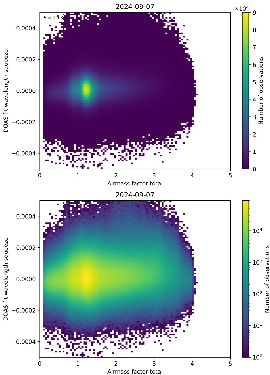
Figure 99: Scatter density plot of “Airmass factor total” against “DOAS fit wavelength squeeze” for 2024-09-06 to 2024-09-08.
