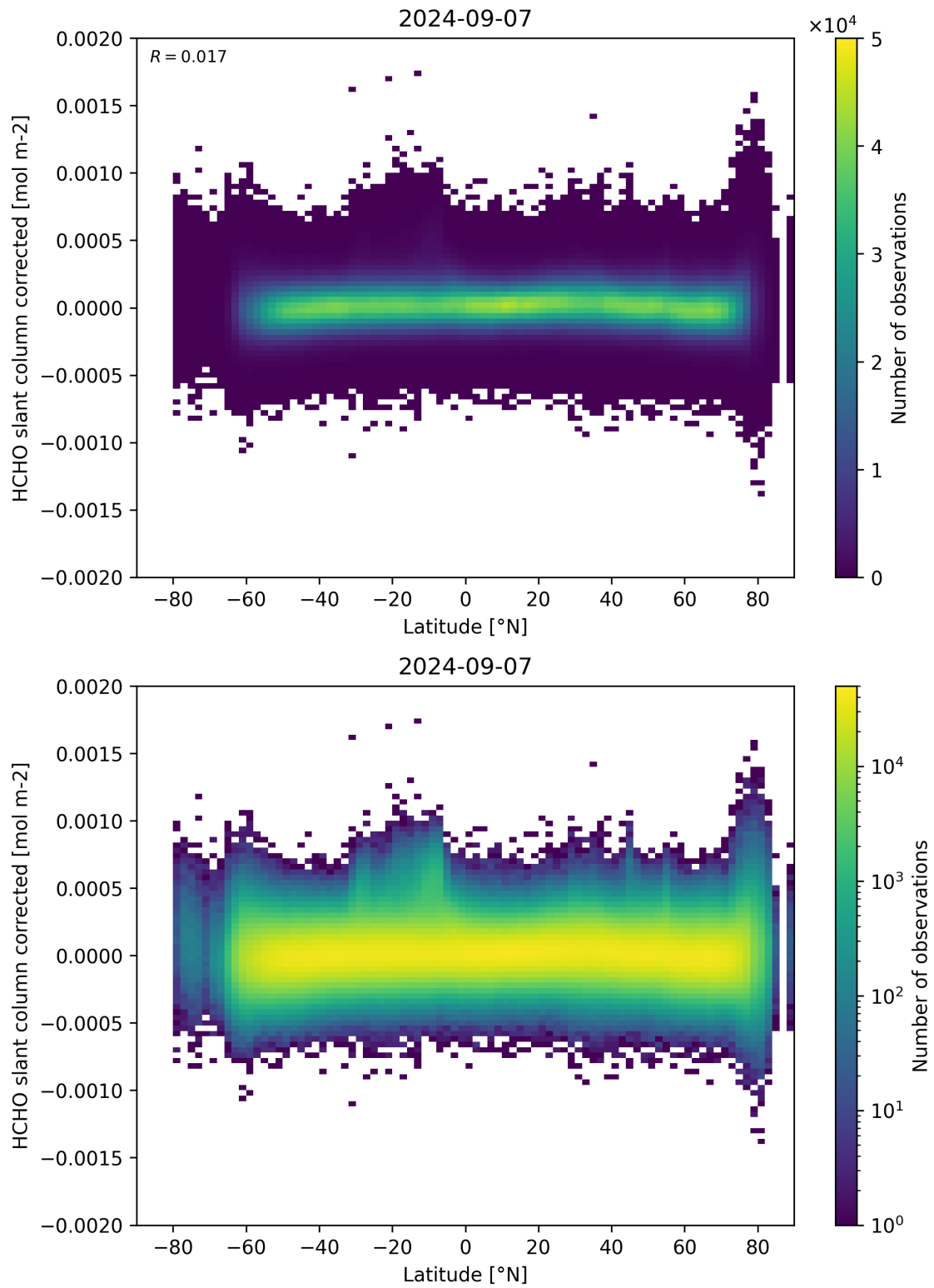
Figure 157: Scatter density plot of “Latitude” against “HCHO slant column corrected” for 2024-09-06 to 2024-09-08.
