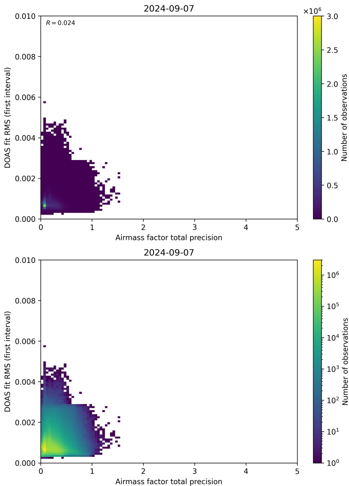
Figure 105: Scatter density plot of “Airmass factor total precision” against “DOAS fit RMS (first interval)” for 2024-09-06 to 2024-09-08.
