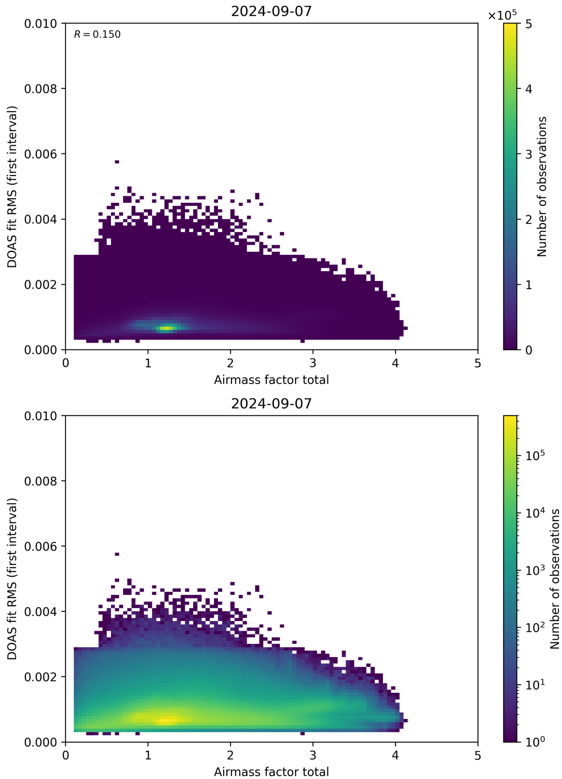
Figure 97: Scatter density plot of “Airmass factor total” against “DOAS fit RMS (first interval)” for 2024-09-06 to 2024-09-08.
