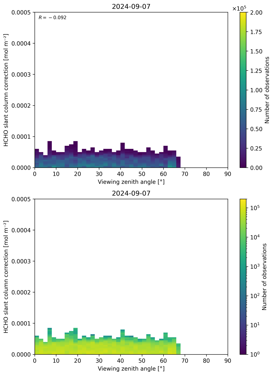
Figure 187: Scatter density plot of “Viewing zenith angle” against “HCHO slant column correction” for 2024-09-06 to 2024-09-08.
