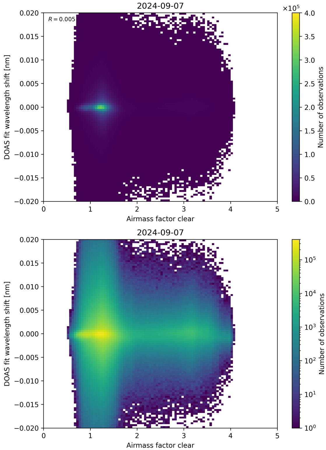
Figure 72: Scatter density plot of “Airmass factor clear” against “DOAS fit wavelength shift” for 2024-09-06 to 2024-09-08.
