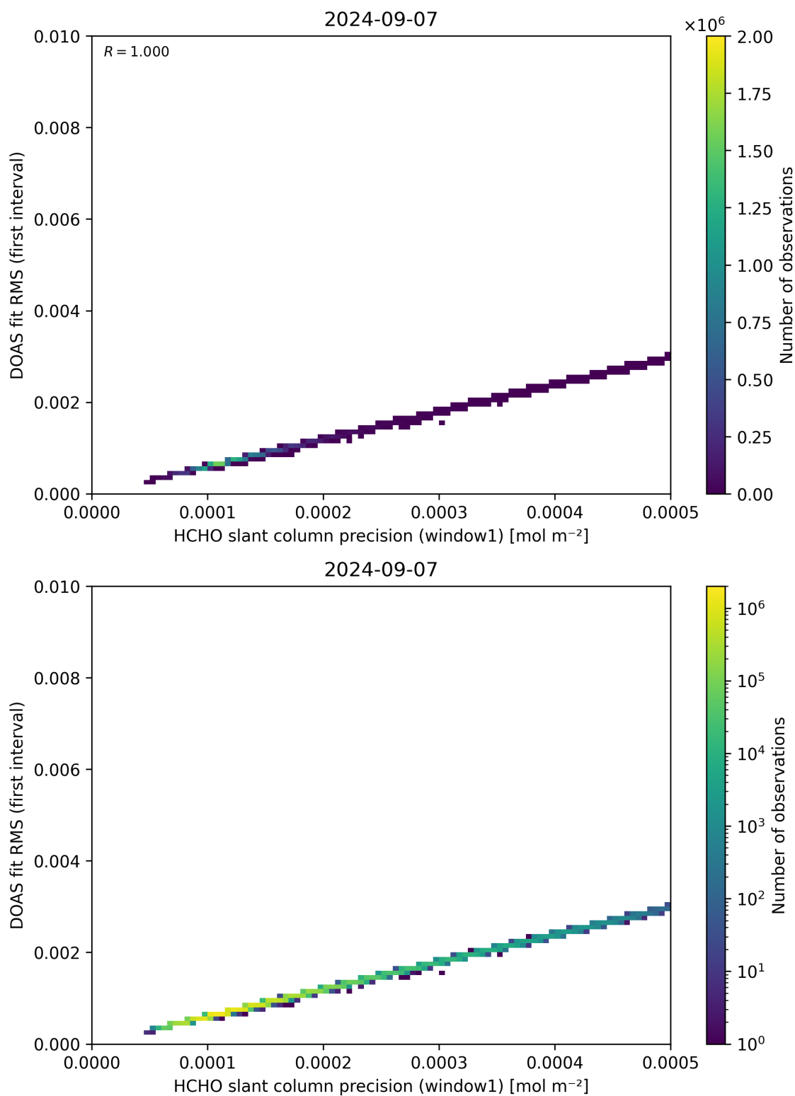
Figure 88: Scatter density plot of “HCHO slant column precision (window1)” against “DOAS fit RMS (first interval)” for 2024-09-06 to 2024-09-08.
