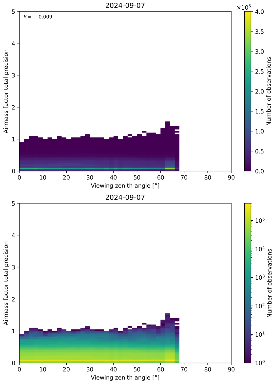
Figure 191: Scatter density plot of “Viewing zenith angle” against “Airmass factor total precision” for 2024-09-06 to 2024-09-08.
