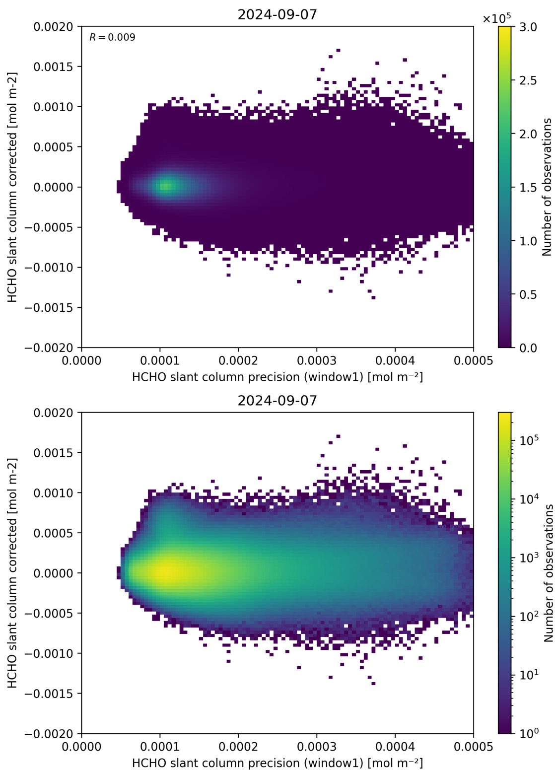
Figure 92: Scatter density plot of “HCHO slant column precision (window1)” against “HCHO slant column corrected” for 2024-09-06 to 2024-09-08.
