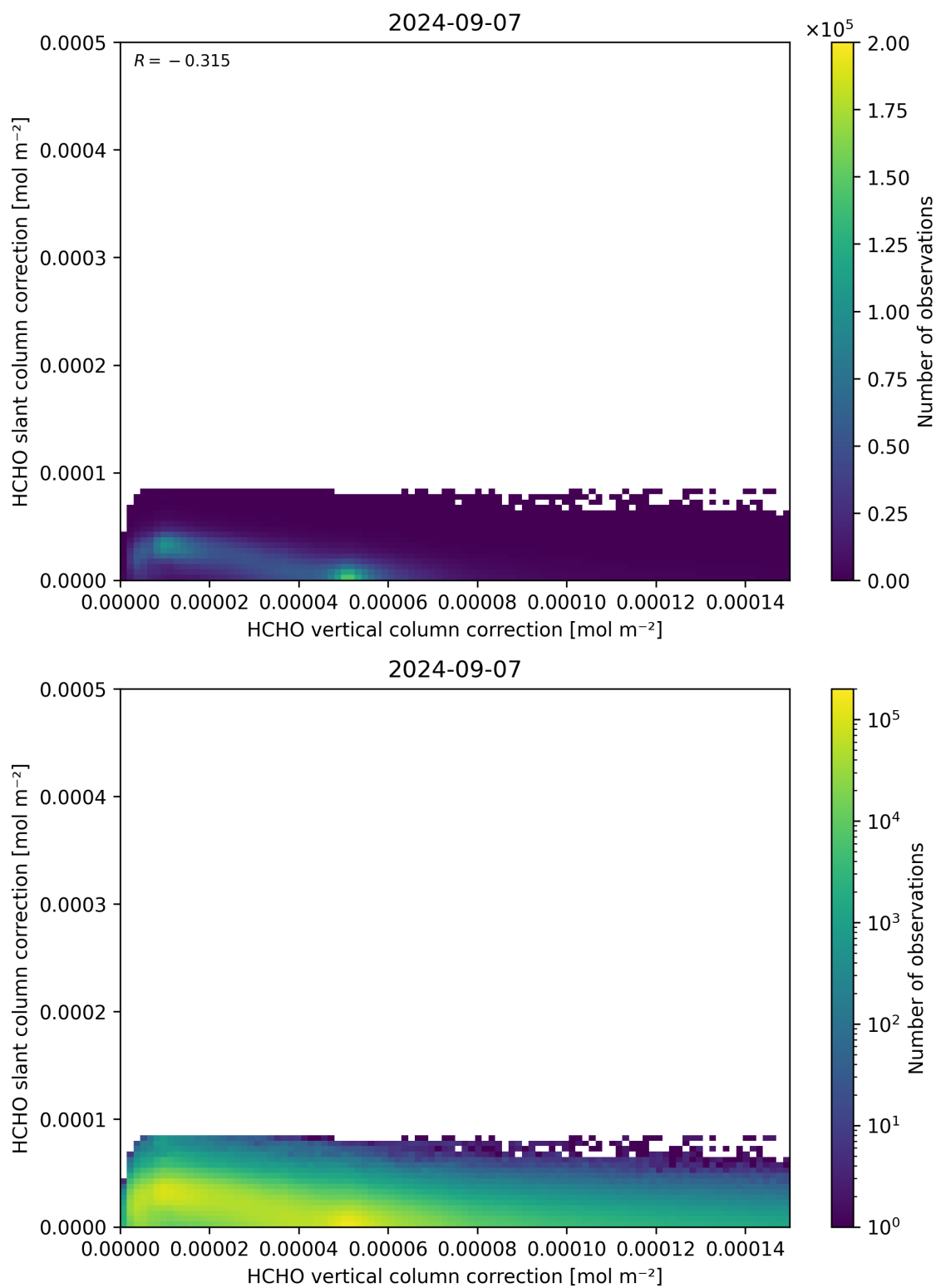
Figure 117: Scatter density plot of “HCHO vertical column correction” against “HCHO slant column correction” for 2024-09-06 to 2024-09-08.
