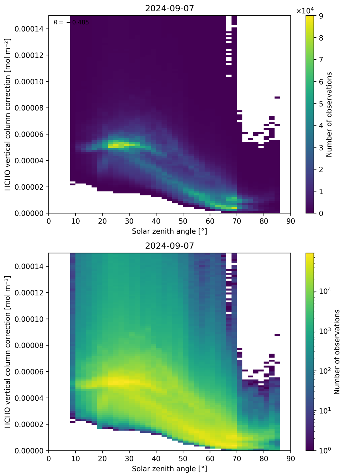
Figure 178: Scatter density plot of “Solar zenith angle” against “HCHO vertical column correction” for 2024-09-06 to 2024-09-08.
