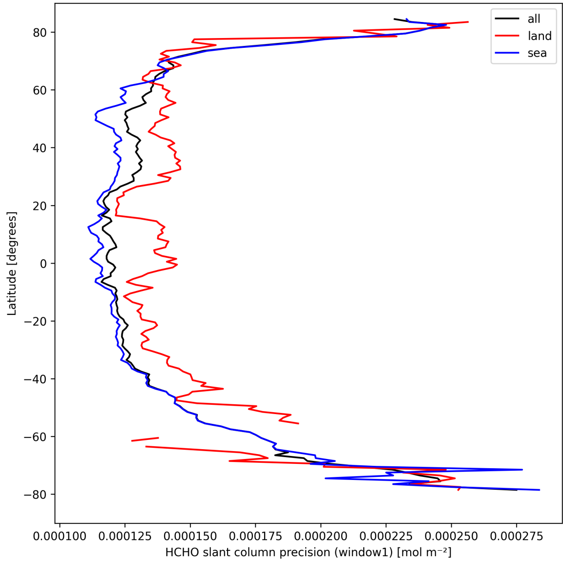
Figure 25: Zonal average of “HCHO slant column precision (window1)” for 2024-09-06 to 2024-09-08.
