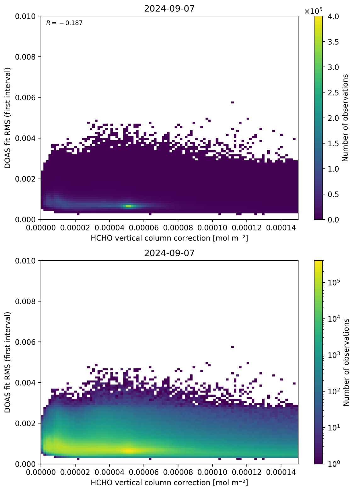
Figure 112: Scatter density plot of “HCHO vertical column correction” against “DOAS fit RMS (first interval)” for 2024-09-06 to 2024-09-08.
