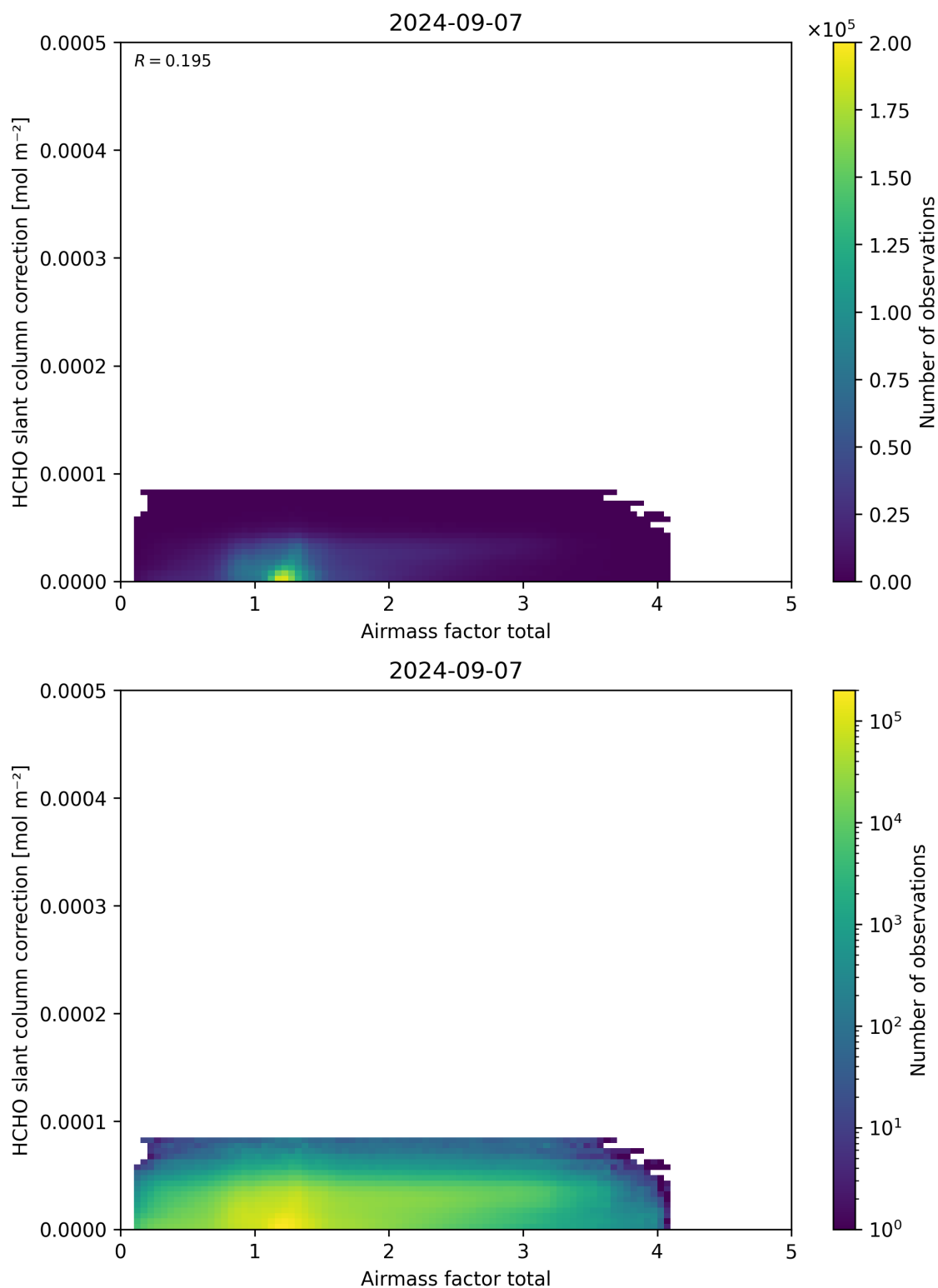
Figure 102: Scatter density plot of “Airmass factor total” against “HCHO slant column correction” for 2024-09-06 to 2024-09-08.
