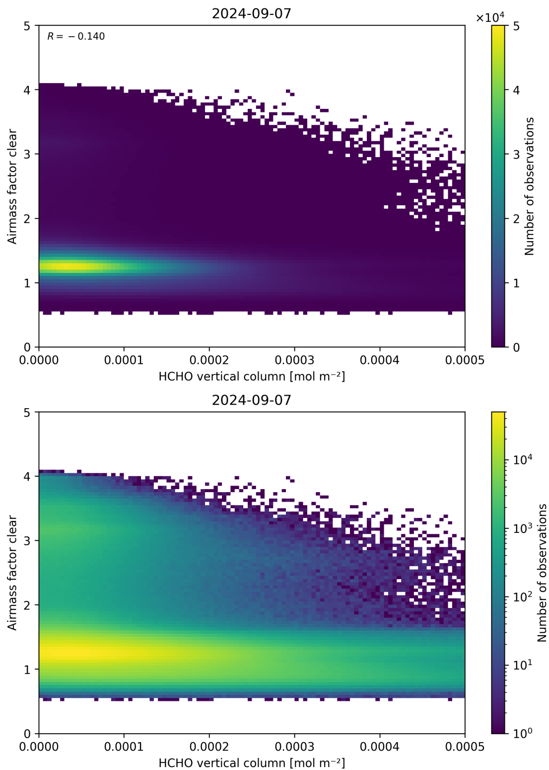
Figure 126: Scatter density plot of “HCHO vertical column” against “Airmass factor clear” for 2024-09-06 to 2024-09-08.
