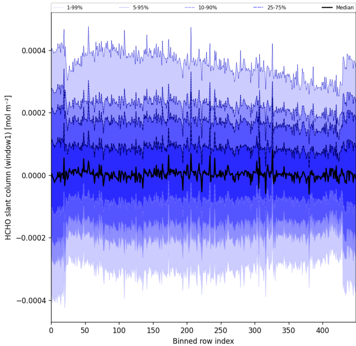
Figure 52: Along track statistics of “HCHO slant column (window1)” for 2024-09-06 to 2024-09-08
