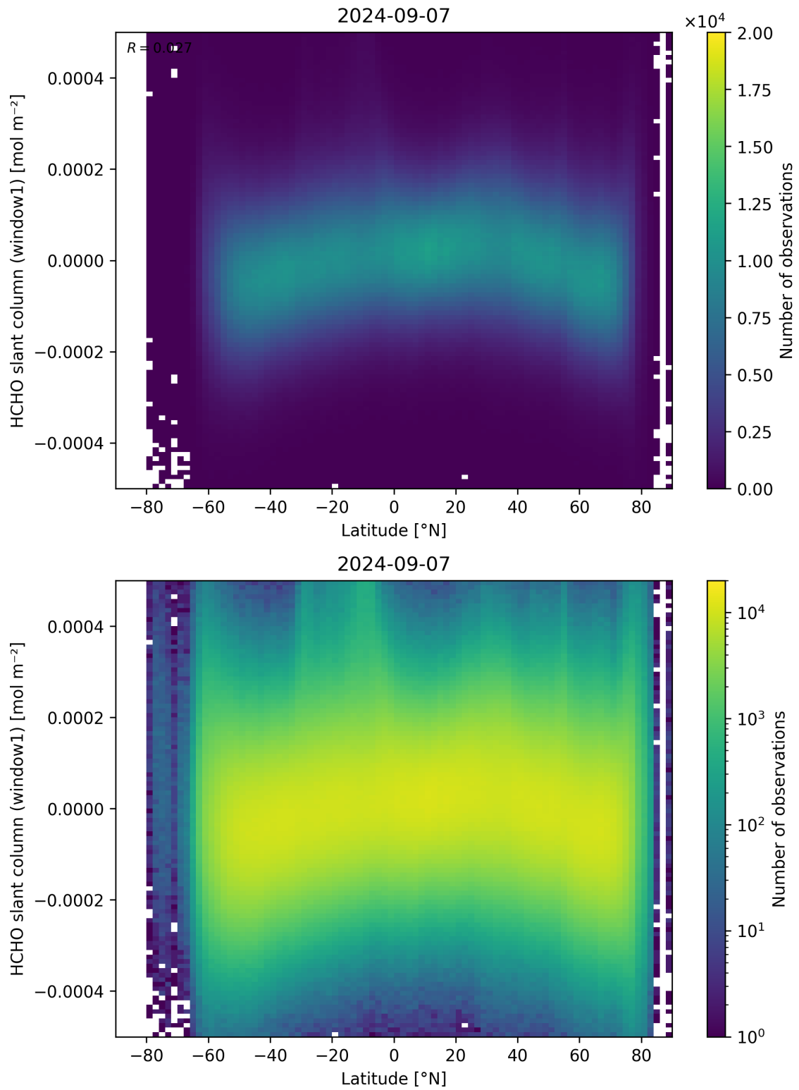
Figure 159: Scatter density plot of “Latitude” against “HCHO slant column (window1)” for 2024-09-06 to 2024-09-08.
