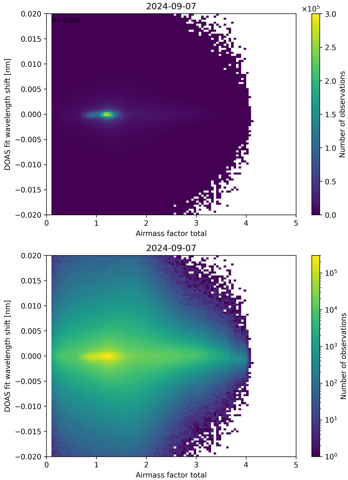
Figure 98: Scatter density plot of “Airmass factor total” against “DOAS fit wavelength shift” for 2024-09-06 to 2024-09-08.
