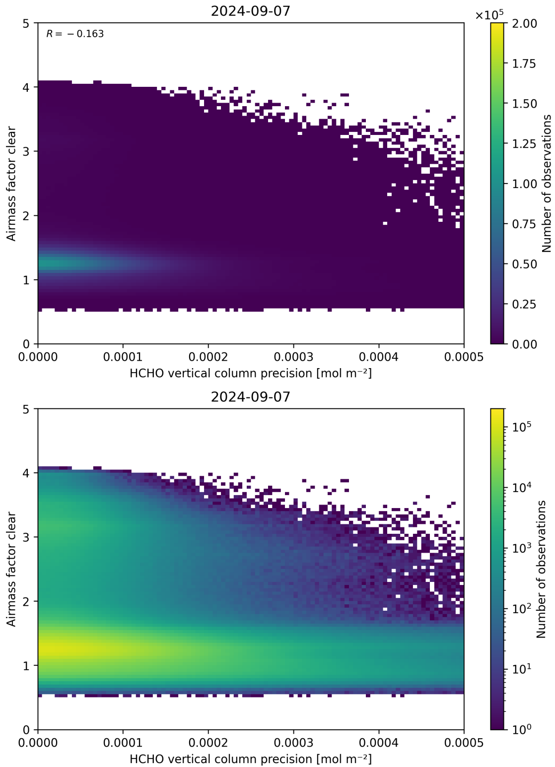
Figure 139: Scatter density plot of “HCHO vertical column precision” against “Airmass factor clear” for 2024-09-06 to 2024-09-08.
