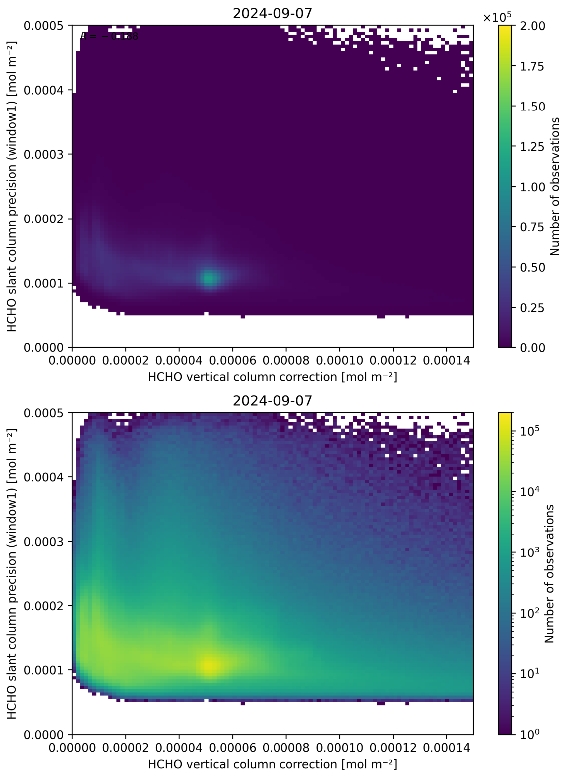
Figure 119: Scatter density plot of “HCHO vertical column correction” against “HCHO slant column precision (window1)” for 2024-09-06 to 2024-09-08.
