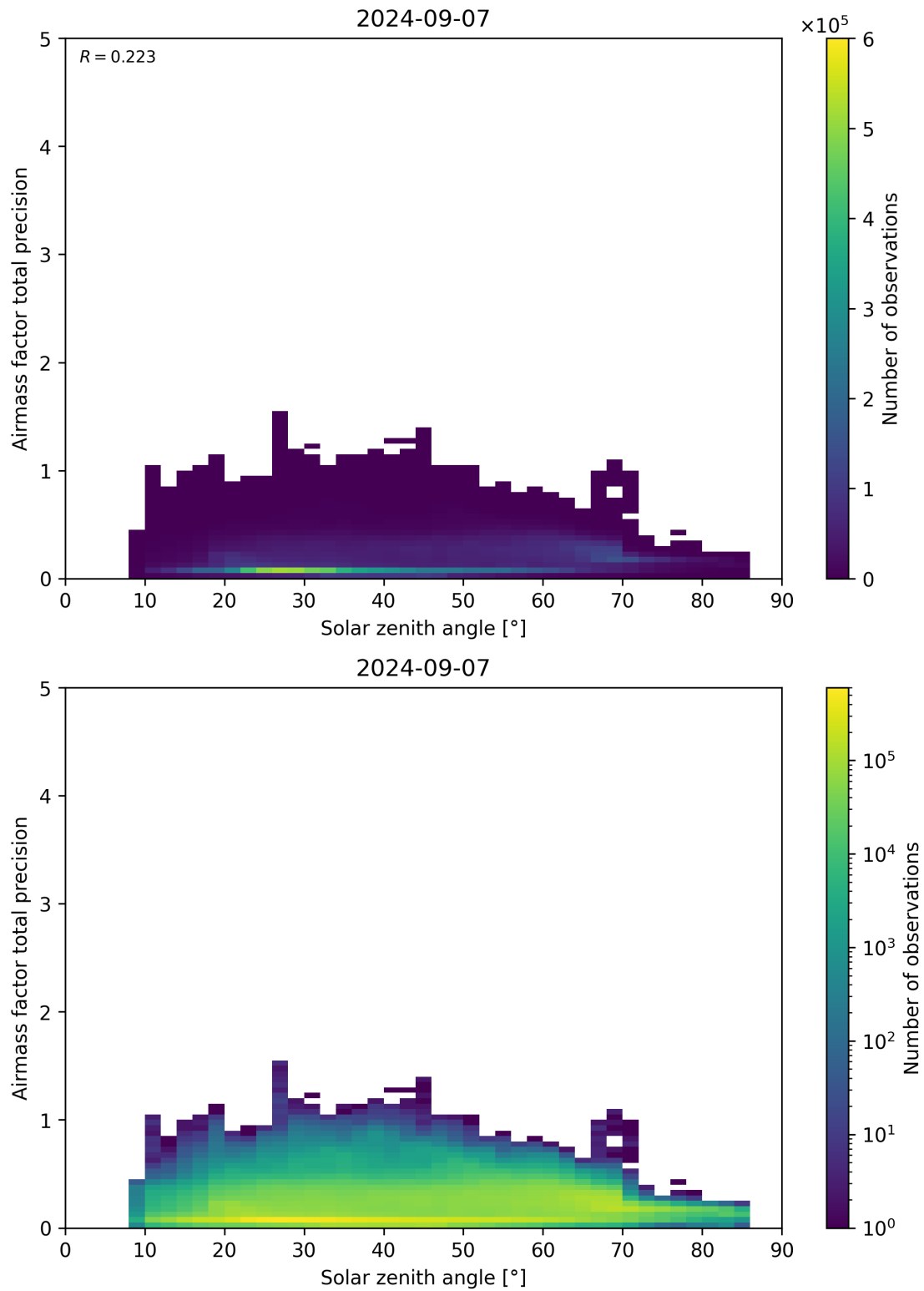
Figure 176: Scatter density plot of “Solar zenith angle” against “Airmass factor total precision” for 2024-09-06 to 2024-09-08.
