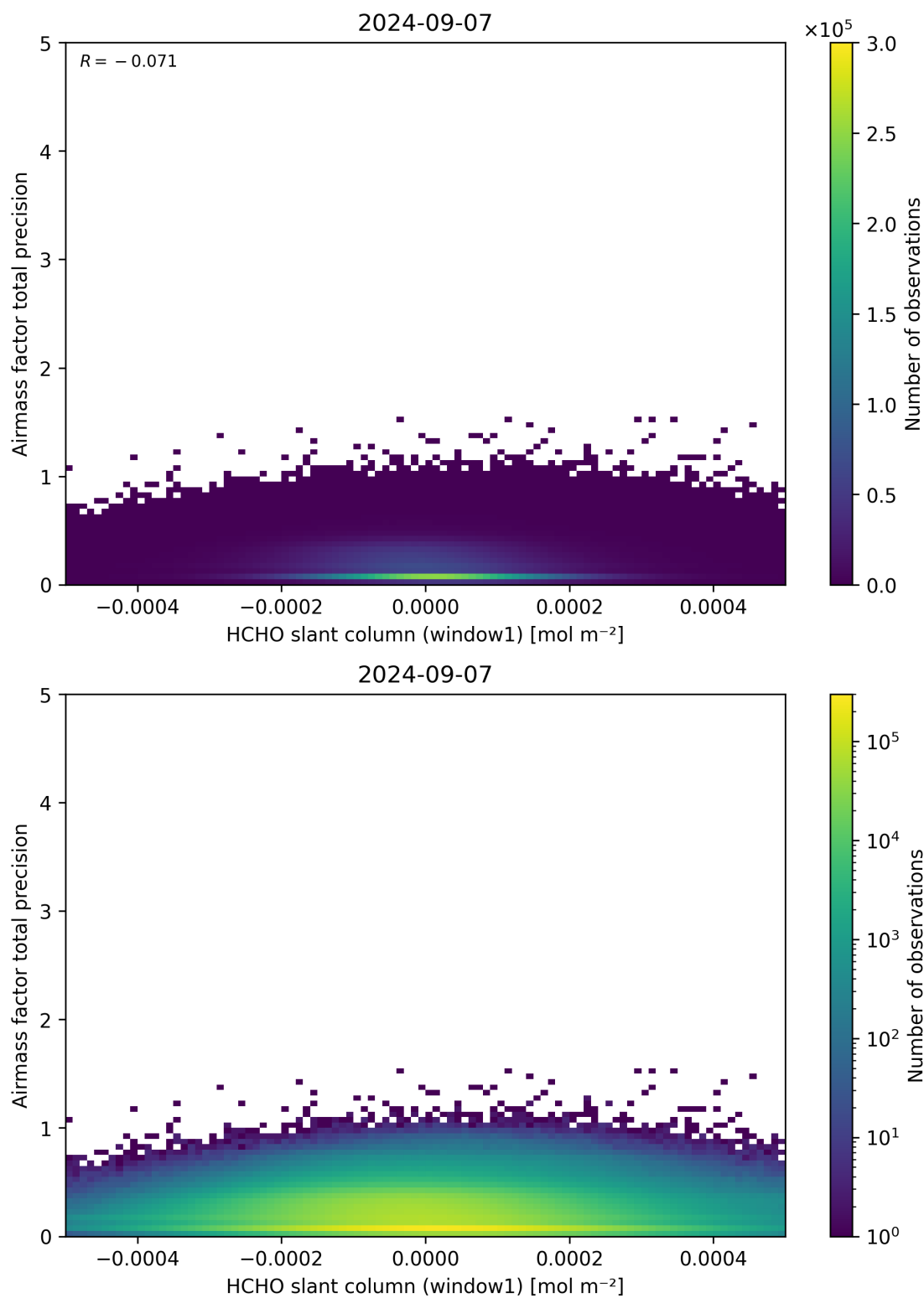
Figure 86: Scatter density plot of “HCHO slant column (window1)” against “Airmass factor total precision” for 2024-09-06 to 2024-09-08.
