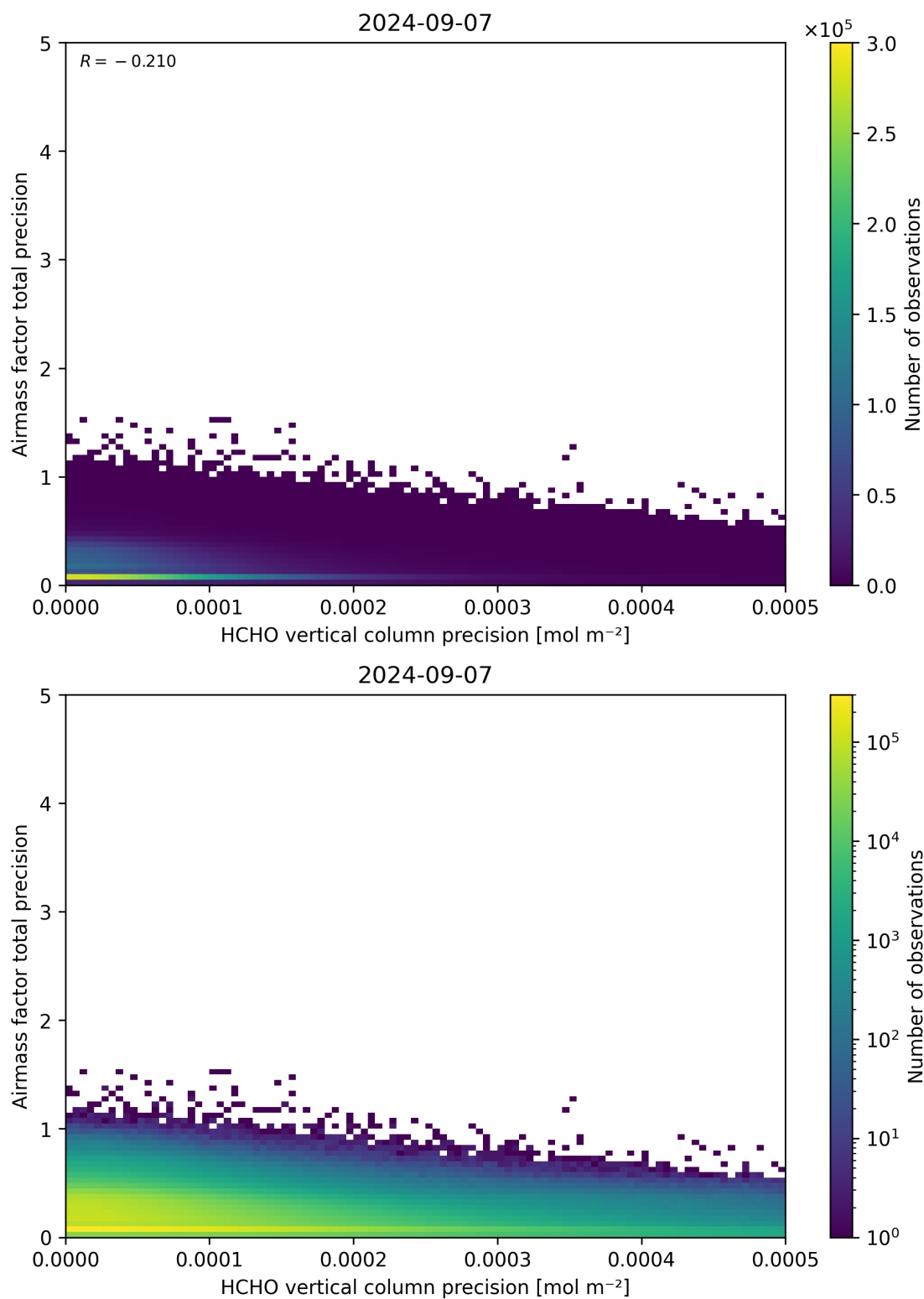
Figure 145: Scatter density plot of “HCHO vertical column precision” against “Airmass factor total precision” for 2024-09-06 to 2024-09-08.
