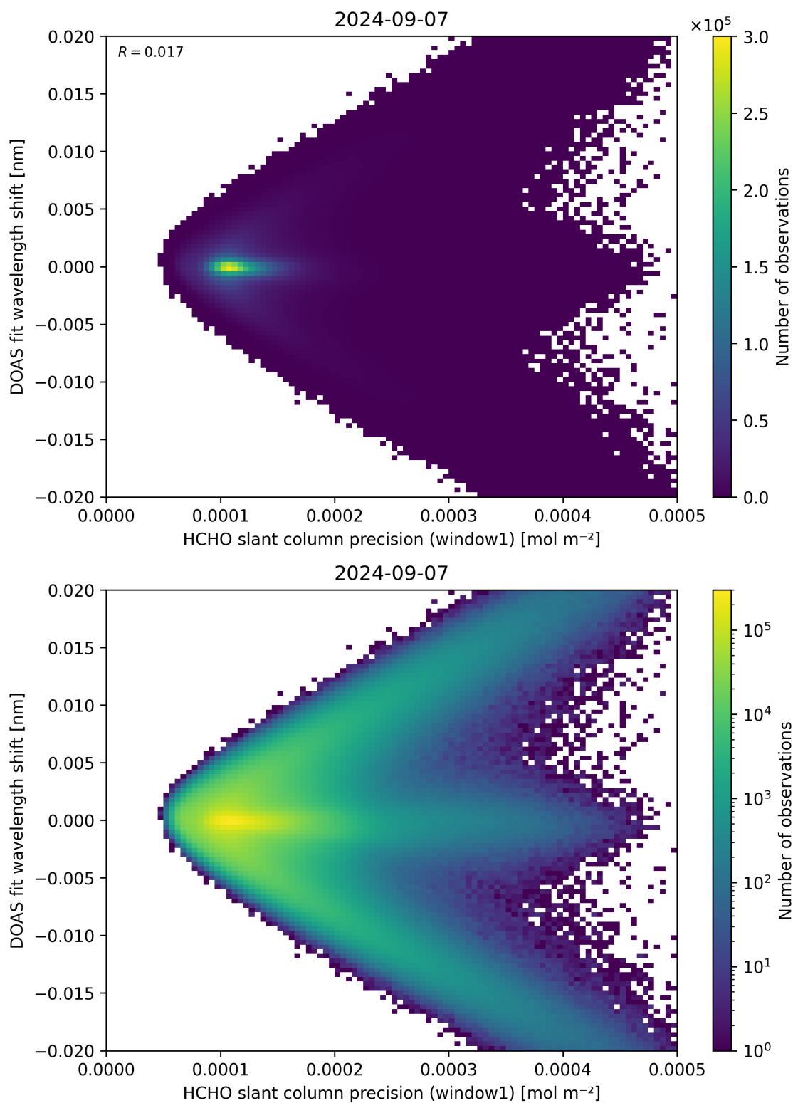
Figure 89: Scatter density plot of “HCHO slant column precision (window1)” against “DOAS fit wavelength shift” for 2024-09-06 to 2024-09-08.
