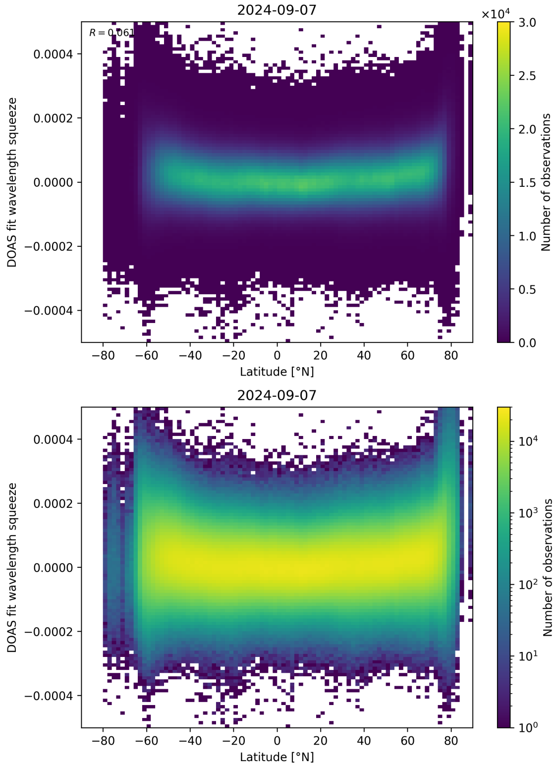
Figure 155: Scatter density plot of “Latitude” against “DOAS fit wavelength squeeze” for 2024-09-06 to 2024-09-08.
