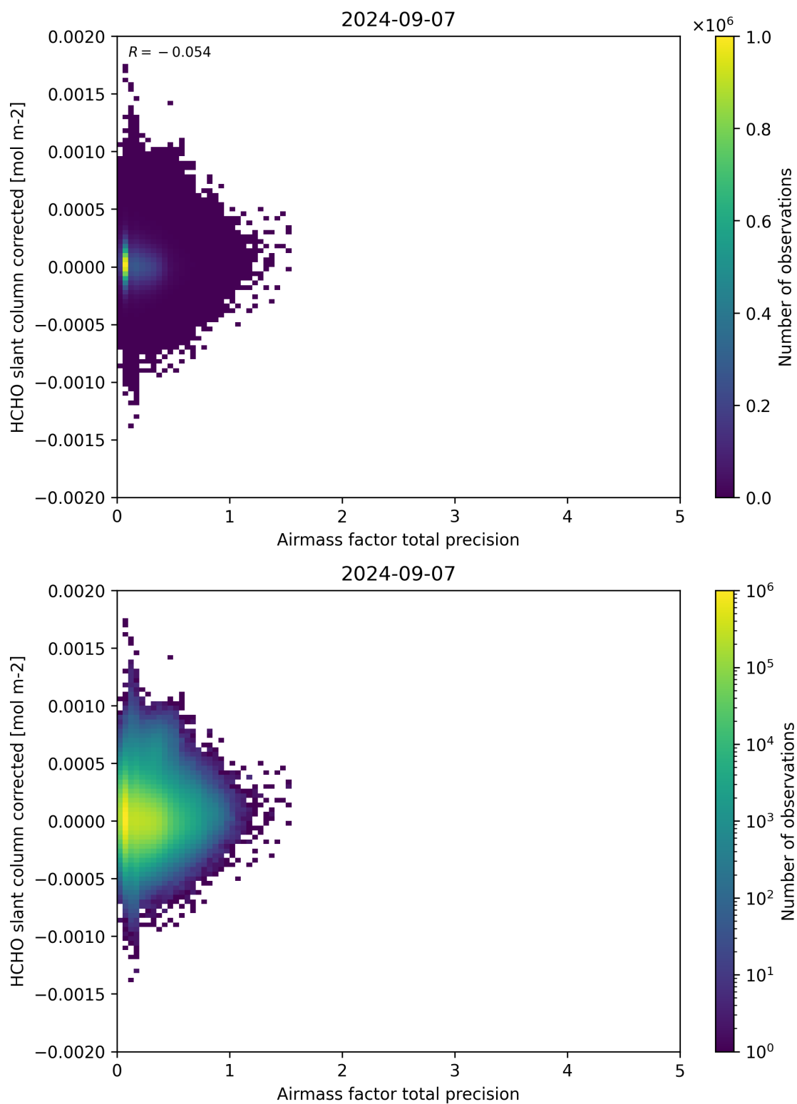
Figure 109: Scatter density plot of “Airmass factor total precision” against “HCHO slant column corrected” for 2024-09-06 to 2024-09-08.
