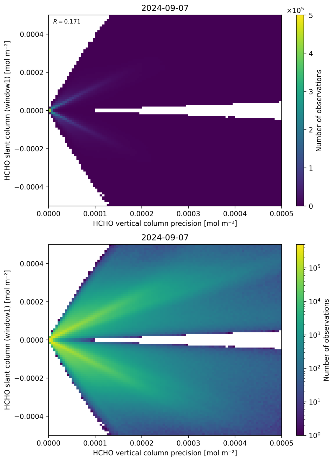
Figure 142: Scatter density plot of “HCHO vertical column precision” against “HCHO slant column (window1)” for 2024-09-06 to 2024-09-08.
