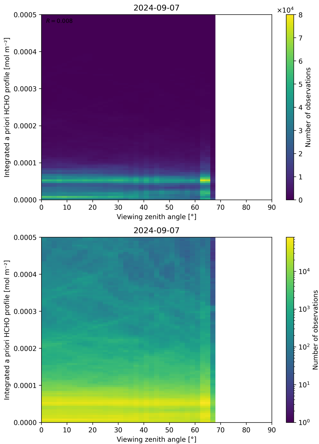
Figure 195: Scatter density plot of “Viewing zenith angle” against “Integrated a priori HCHO profile” for 2024-09-06 to 2024-09-08.
