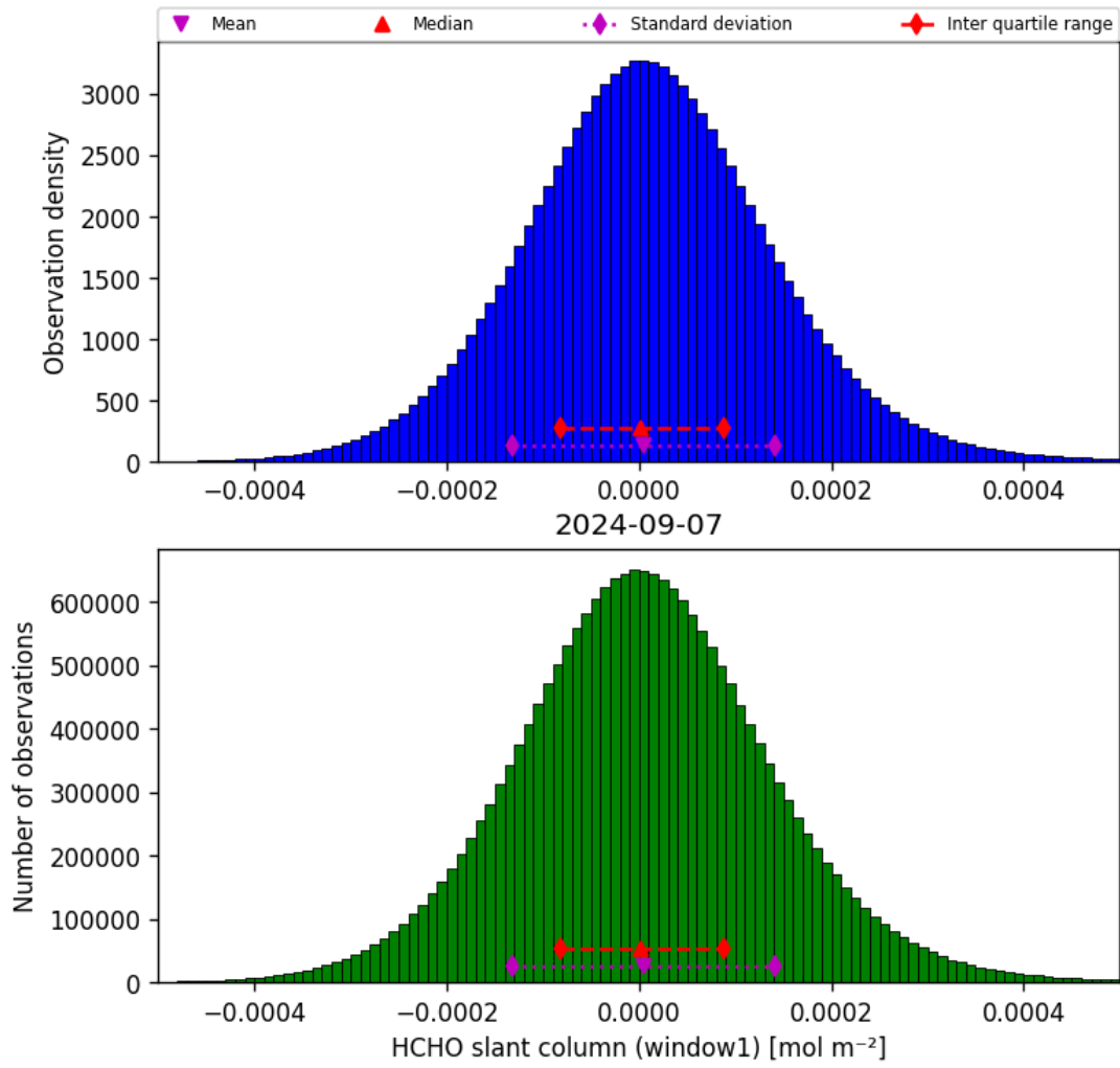
Figure 38: Histogram of “HCHO slant column (window1)” for 2024-09-06 to 2024-09-08
