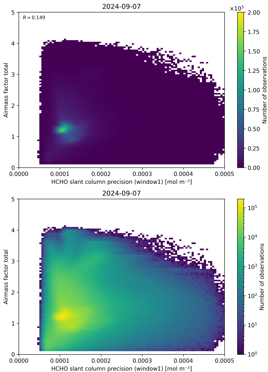
Figure 94: Scatter density plot of “HCHO slant column precision (window1)” against “Airmass factor total” for 2024-09-06 to 2024-09-08.
