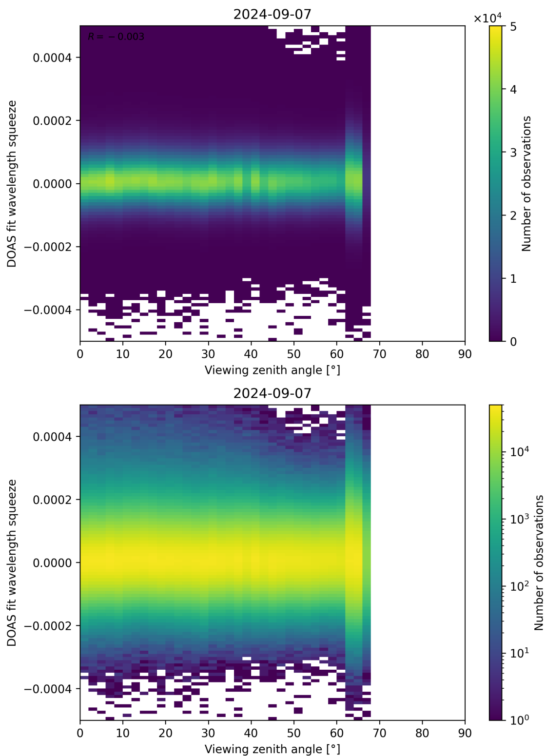
Figure 184: Scatter density plot of “Viewing zenith angle” against “DOAS fit wavelength squeeze” for 2024-09-06 to 2024-09-08.
