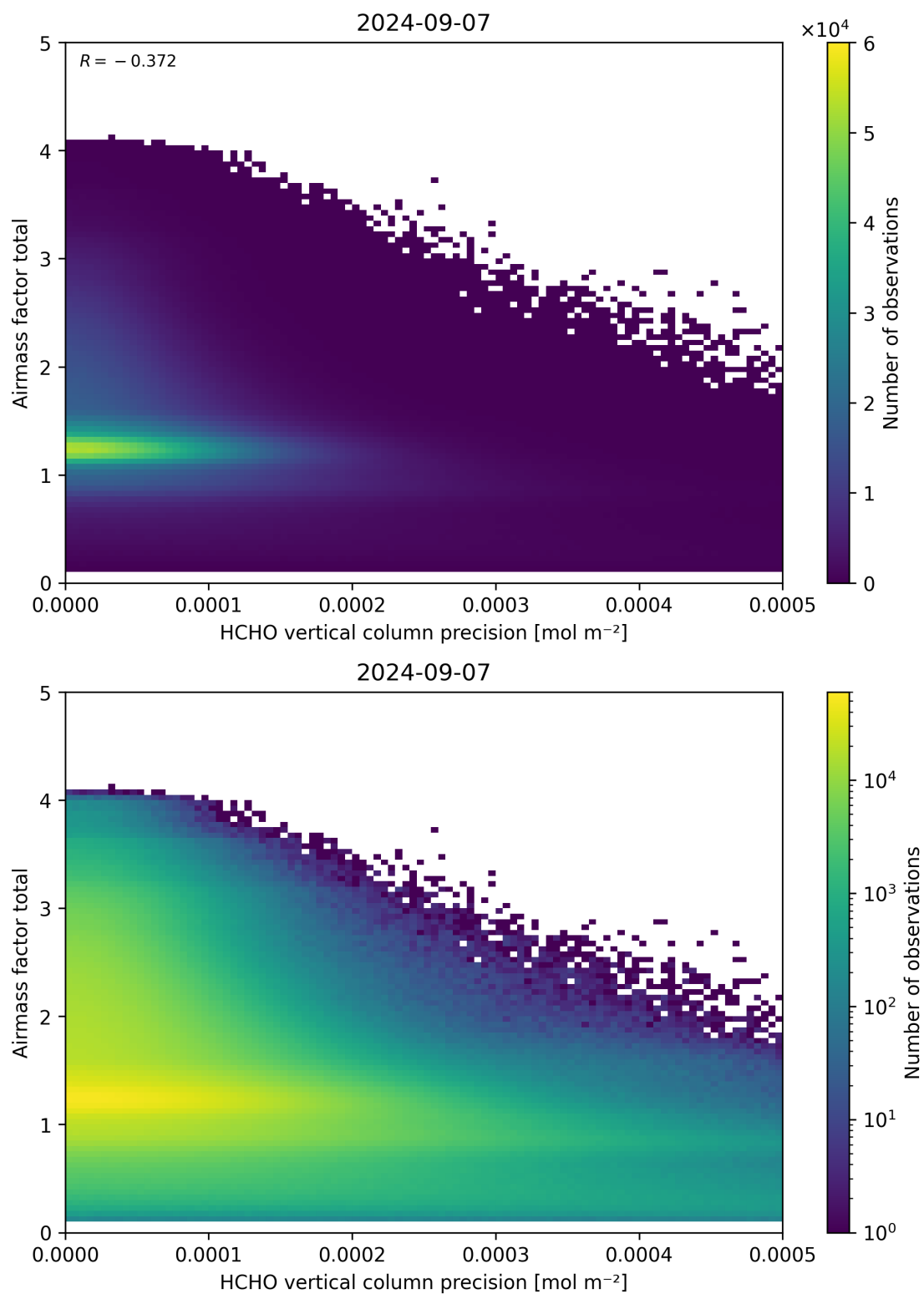
Figure 144: Scatter density plot of “HCHO vertical column precision” against “Airmass factor total” for 2024-09-06 to 2024-09-08.
