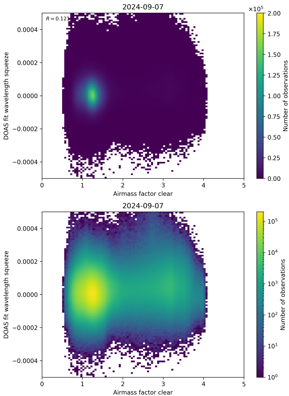
Figure 73: Scatter density plot of “Airmass factor clear” against “DOAS fit wavelength squeeze” for 2024-09-06 to 2024-09-08.
