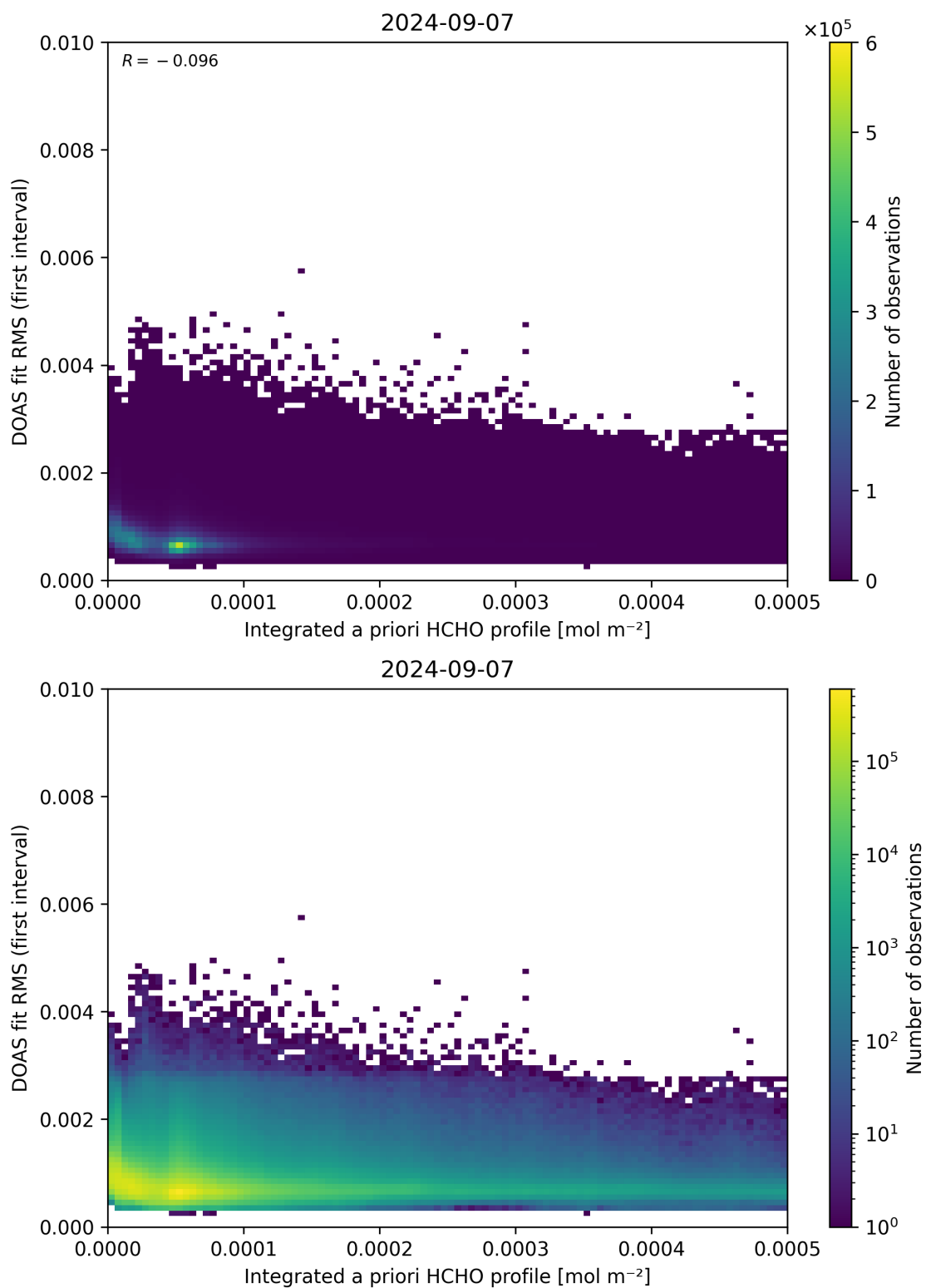
Figure 148: Scatter density plot of “Integrated a priori HCHO profile” against “DOAS fit RMS (first interval)” for 2024-09-06 to 2024-09-08.
