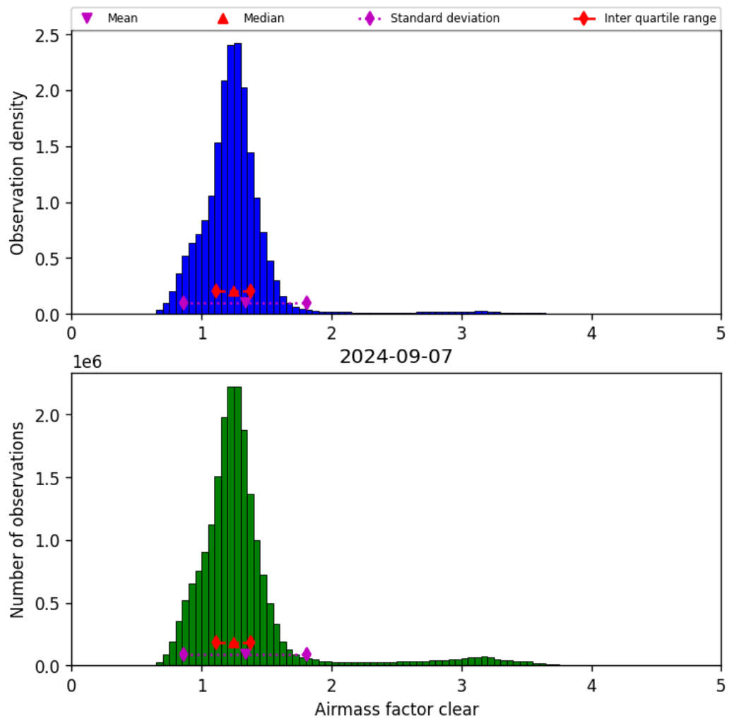
Figure 42: Histogram of “Airmass factor clear” for 2024-09-06 to 2024-09-08
