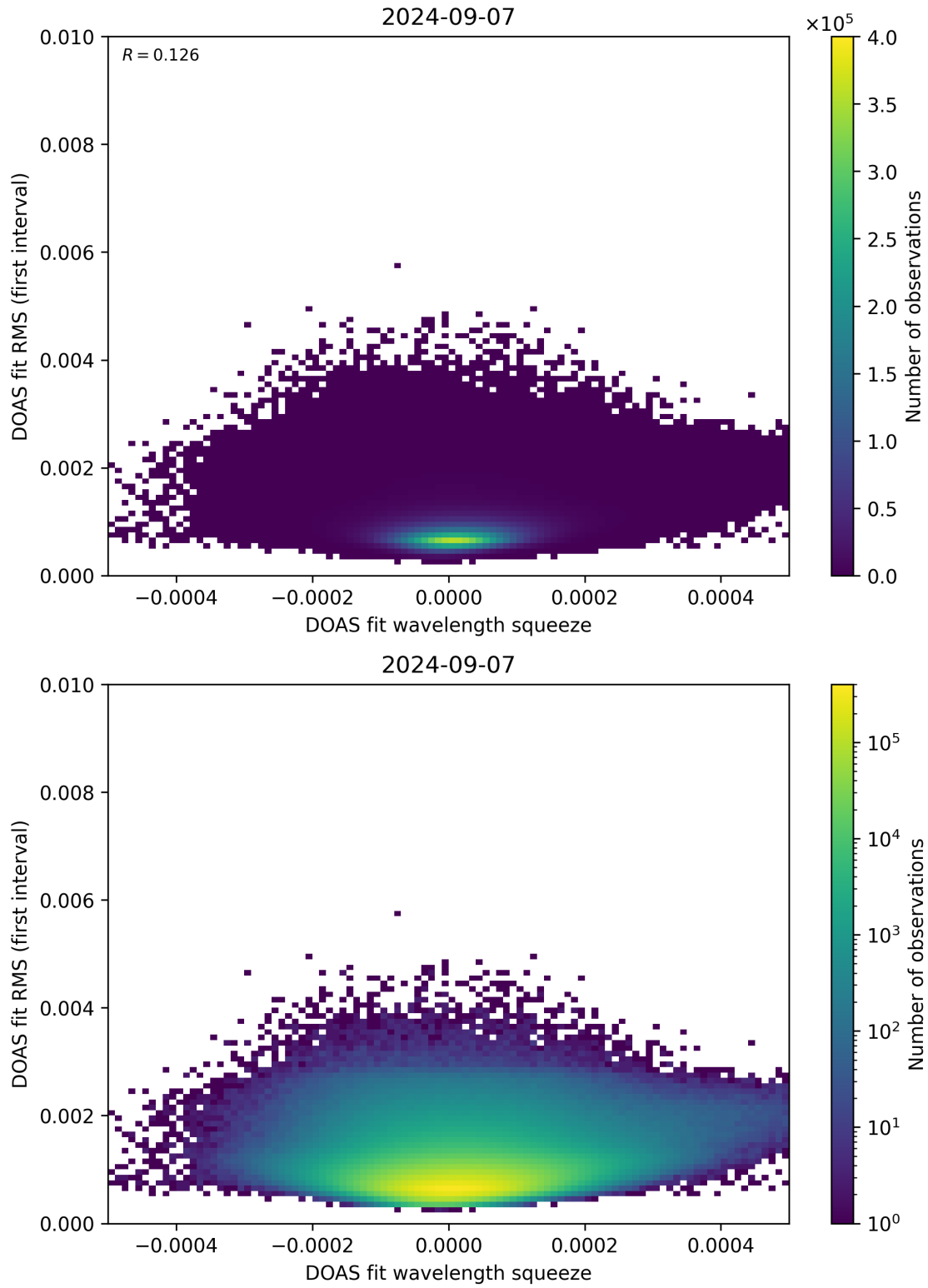
Figure 68: Scatter density plot of “DOAS fit wavelength squeeze” against “DOAS fit RMS (first interval)” for 2024-09-06 to 2024-09-08.
