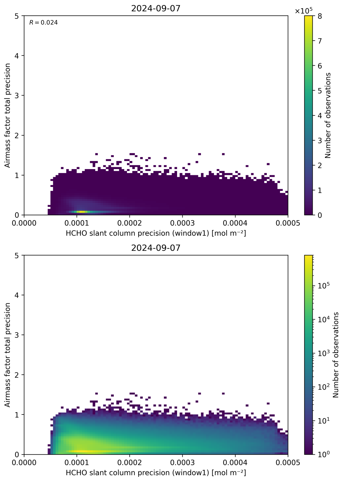
Figure 95: Scatter density plot of “HCHO slant column precision (window1)” against “Airmass factor total precision” for 2024-09-06 to 2024-09-08.
