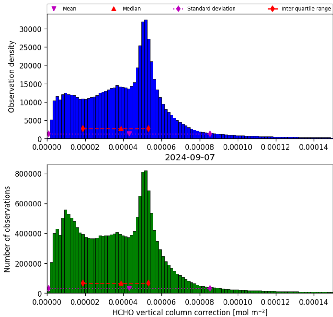
Figure 37: Histogram of “HCHO vertical column correction” for 2024-09-06 to 2024-09-08
