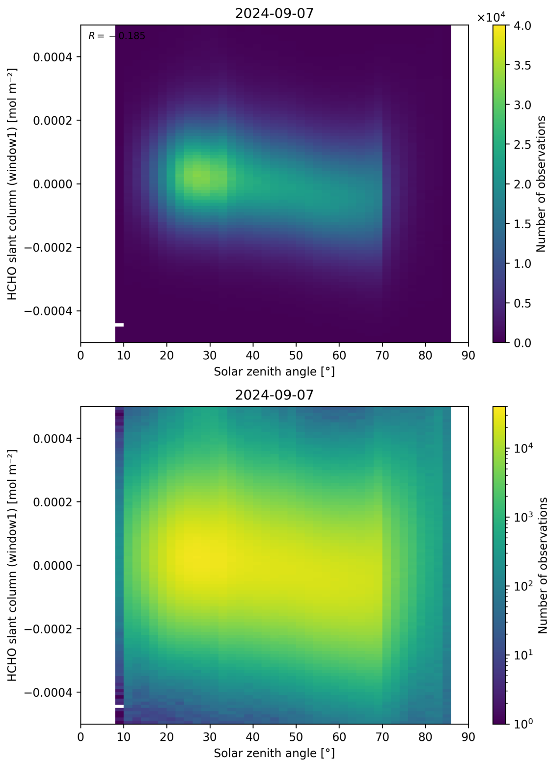
Figure 173: Scatter density plot of “Solar zenith angle” against “HCHO slant column (window1)” for 2024-09-06 to 2024-09-08.
