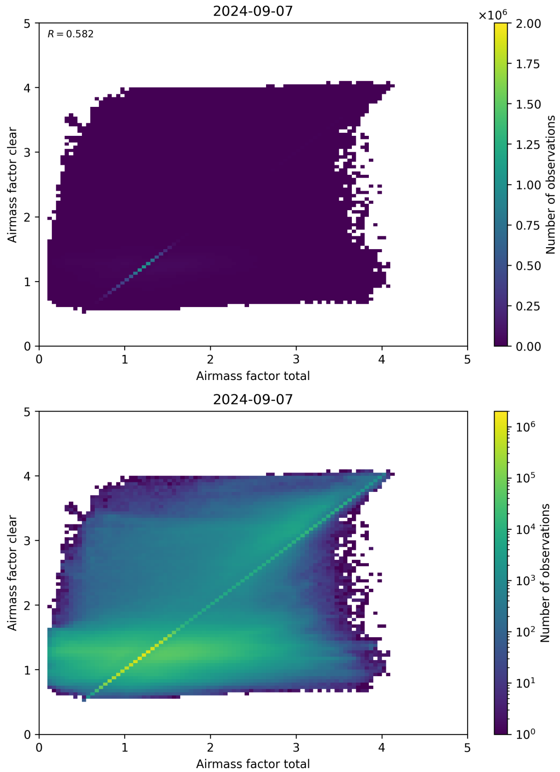
Figure 100: Scatter density plot of “Airmass factor total” against “Airmass factor clear” for 2024-09-06 to 2024-09-08.
