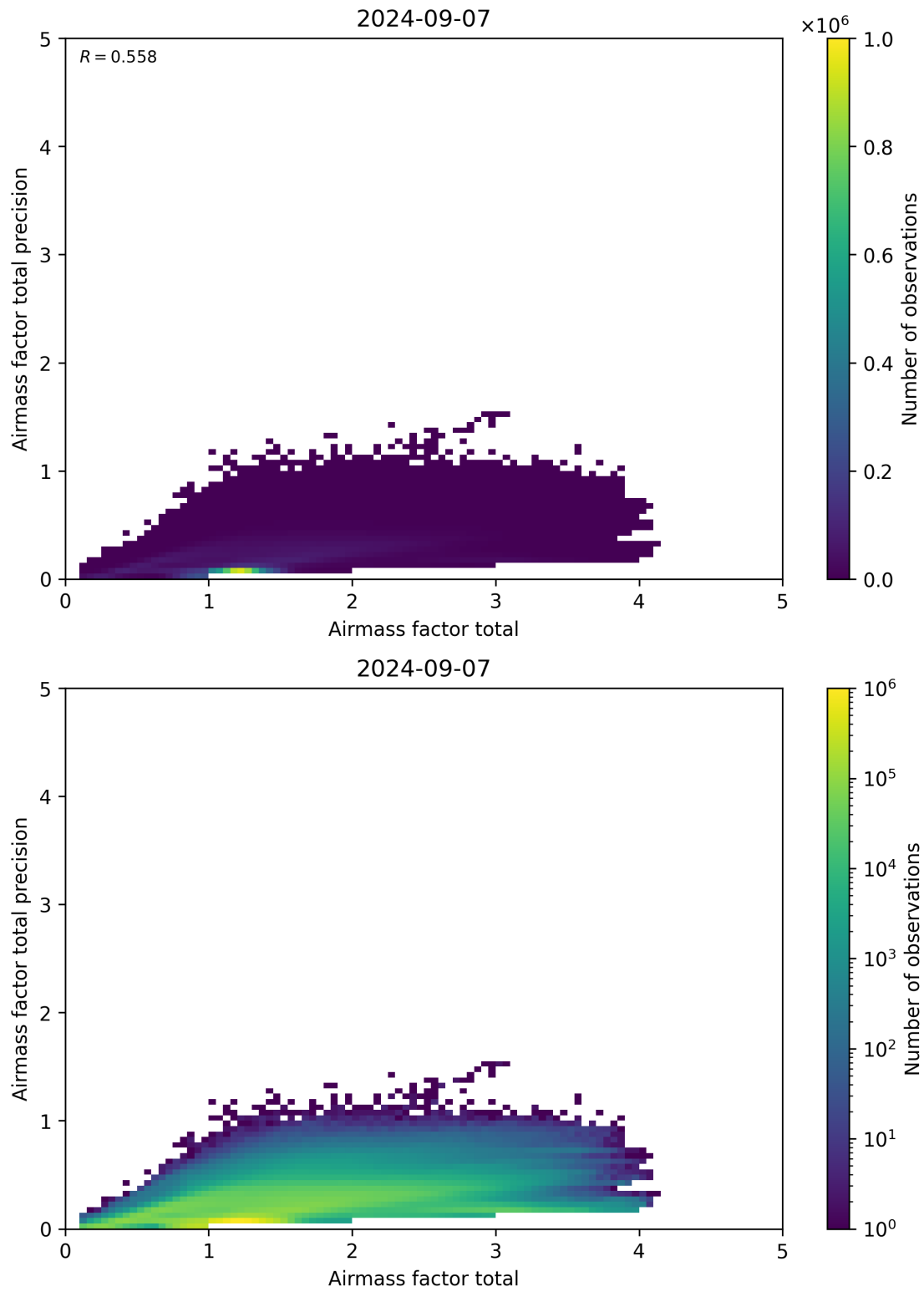
Figure 103: Scatter density plot of “Airmass factor total” against “Airmass factor total precision” for 2024-09-06 to 2024-09-08.
