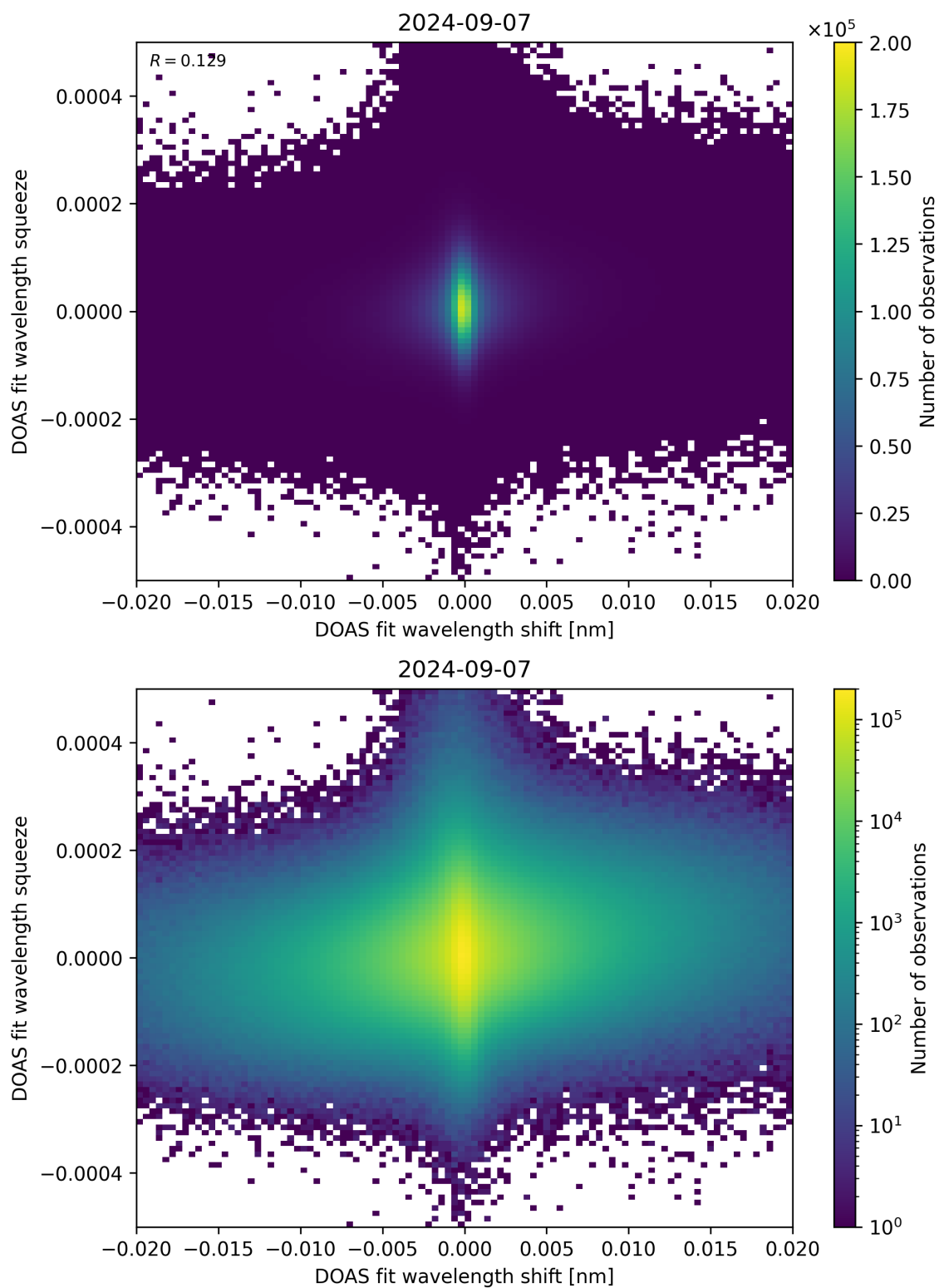
Figure 65: Scatter density plot of “DOAS fit wavelength shift” against “DOAS fit wavelength squeeze” for 2024-09-06 to 2024-09-08.
