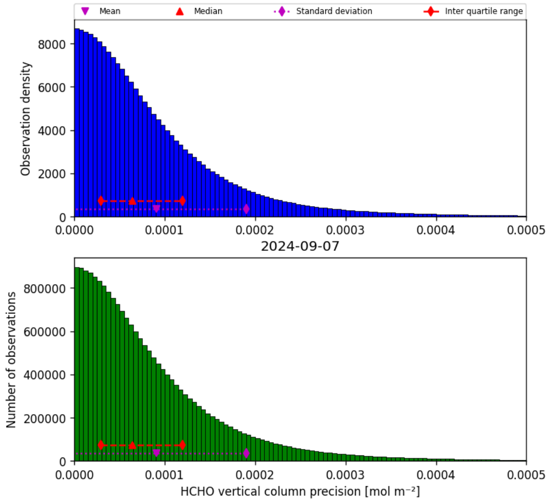
Figure 36: Histogram of “HCHO vertical column precision” for 2024-09-06 to 2024-09-08
