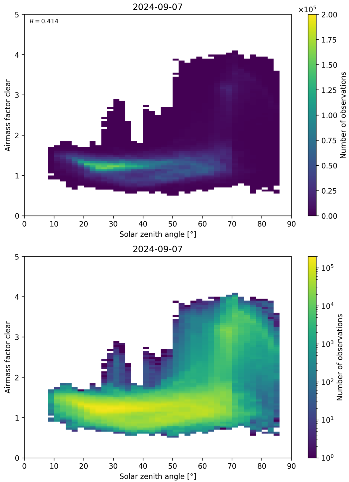
Figure 170: Scatter density plot of “Solar zenith angle” against “Airmass factor clear” for 2024-09-06 to 2024-09-08.
