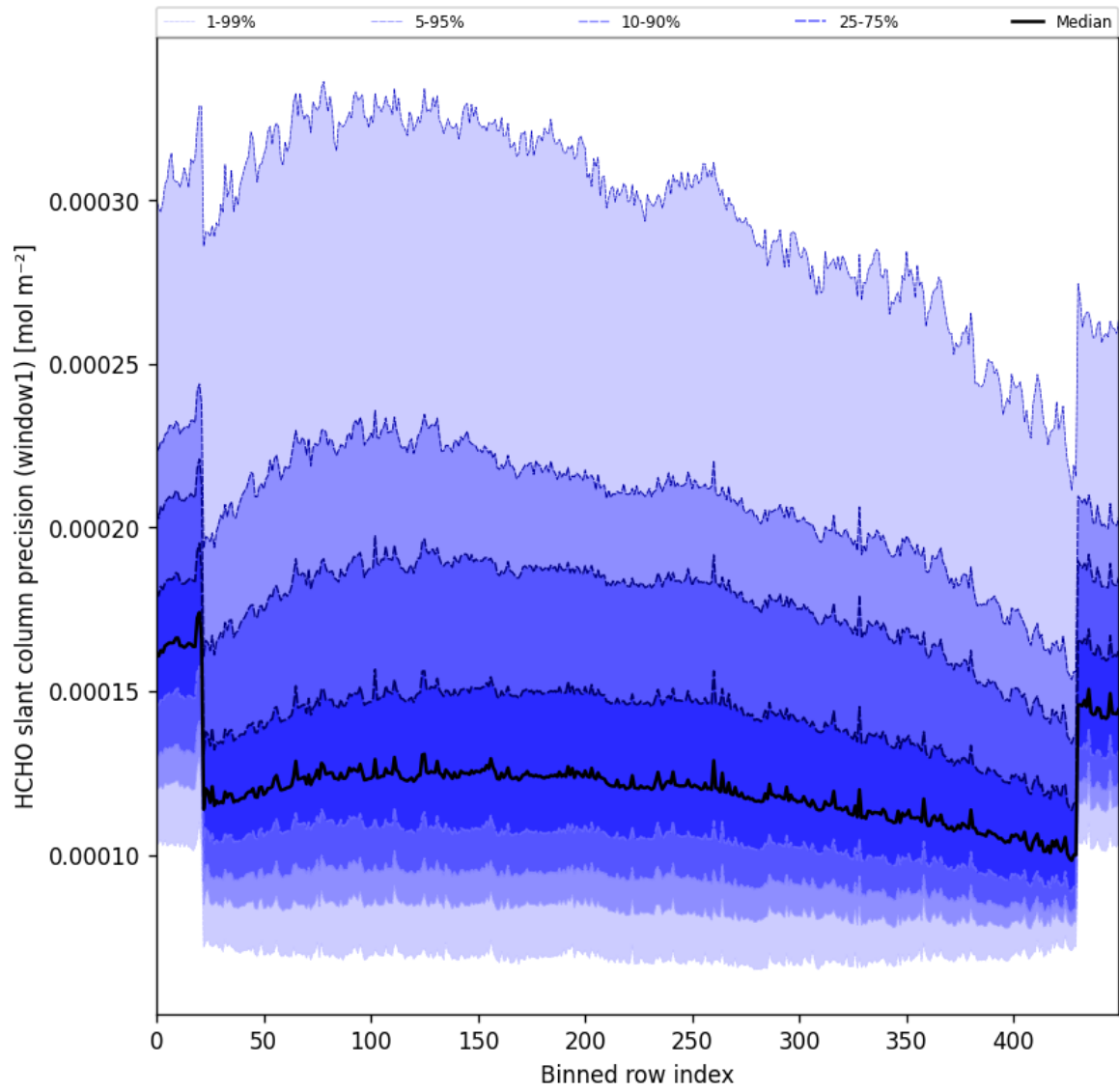
Figure 53: Along track statistics of “HCHO slant column precision (window1)” for 2024-09-06 to 2024-09-08
