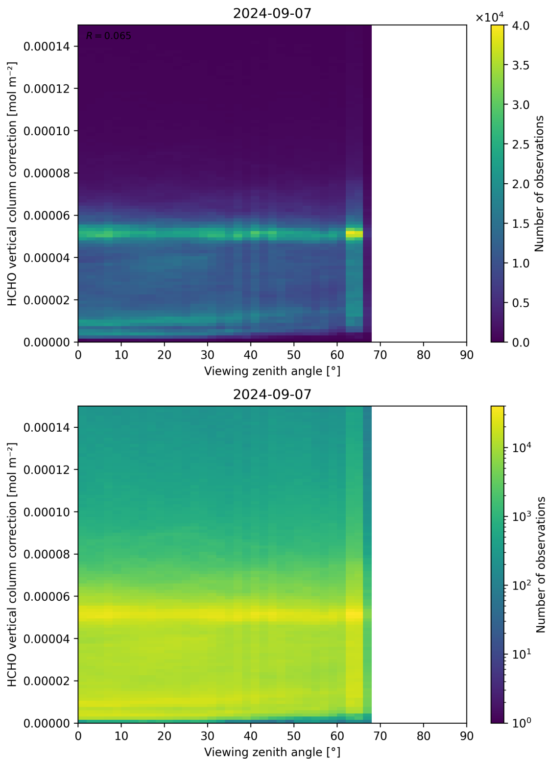
Figure 193: Scatter density plot of “Viewing zenith angle” against “HCHO vertical column correction” for 2024-09-06 to 2024-09-08.
