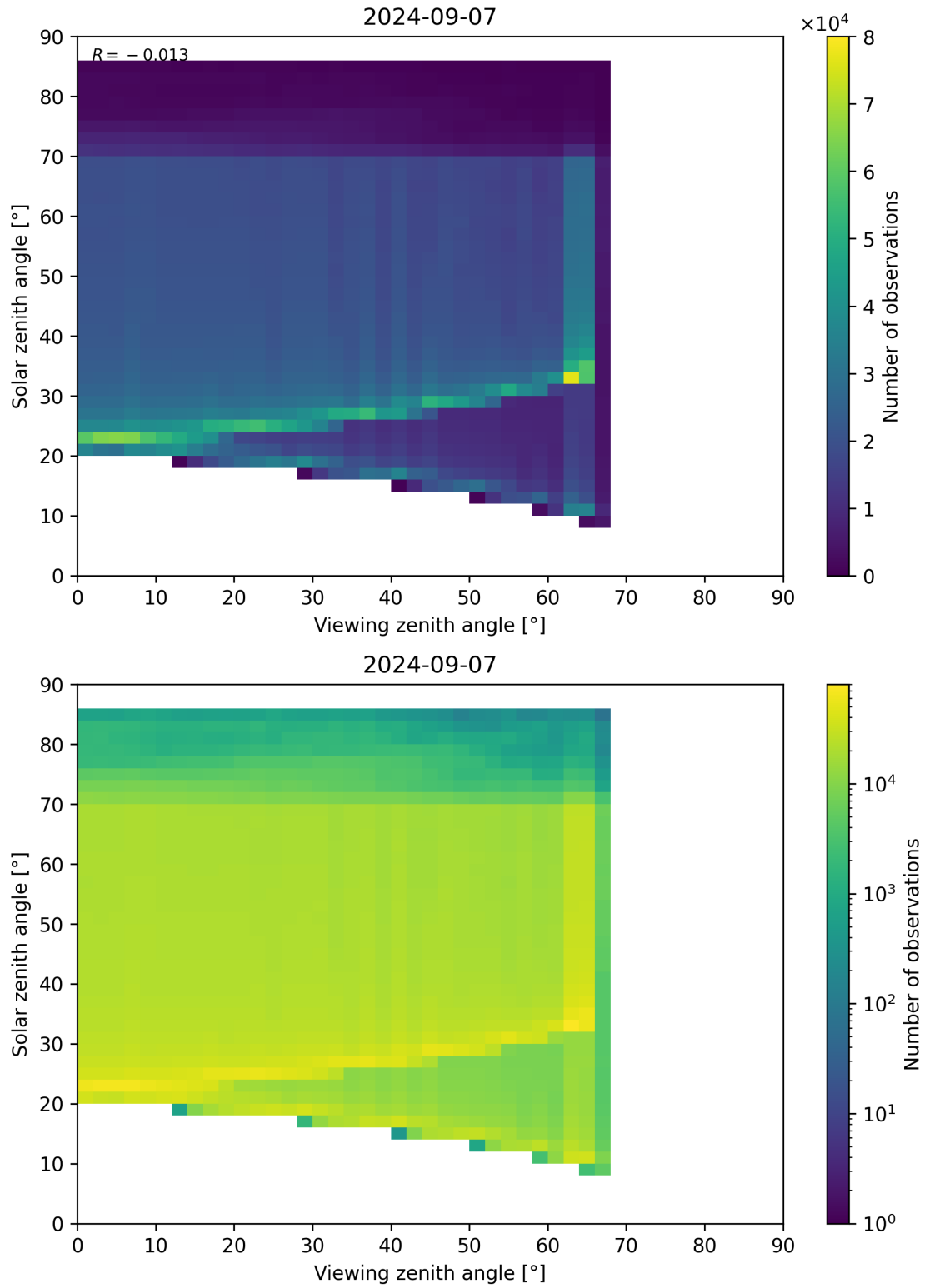
Figure 197: Scatter density plot of “Viewing zenith angle” against “Solar zenith angle” for 2024-09-06 to 2024-09-08.
