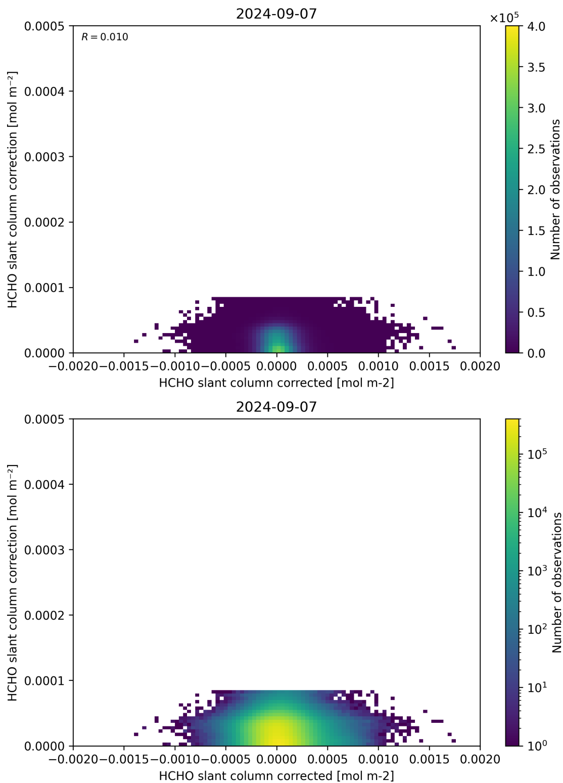
Figure 77: Scatter density plot of “HCHO slant column corrected” against “HCHO slant column correction” for 2024-09-06 to 2024-09-08.
