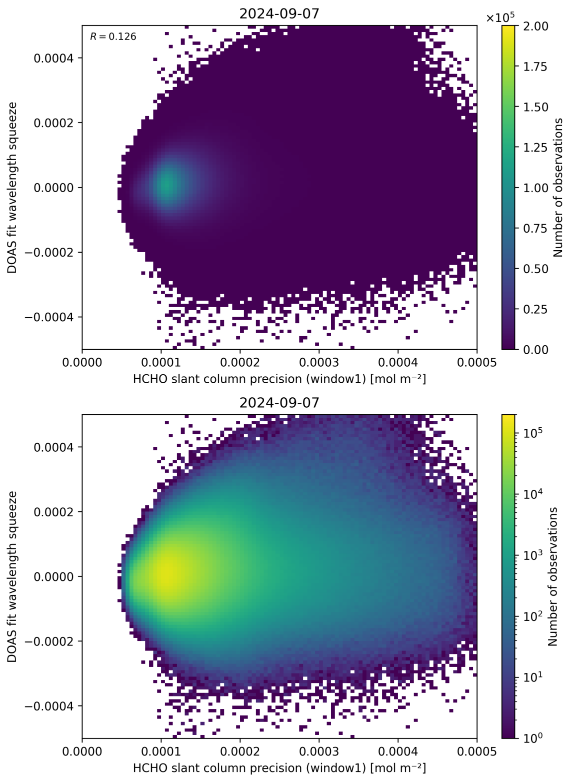
Figure 90: Scatter density plot of “HCHO slant column precision (window1)” against “DOAS fit wavelength squeeze” for 2024-09-06 to 2024-09-08.
