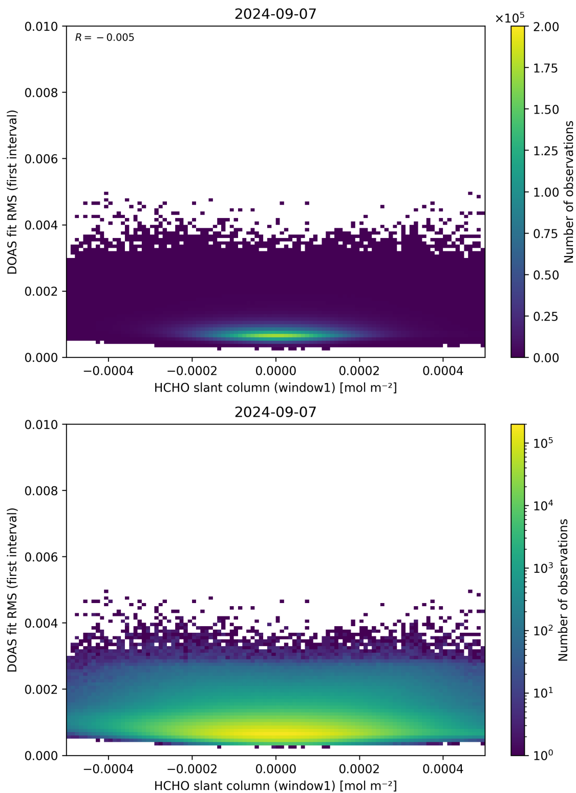
Figure 78: Scatter density plot of “HCHO slant column (window1)” against “DOAS fit RMS (first interval)” for 2024-09-06 to 2024-09-08.
