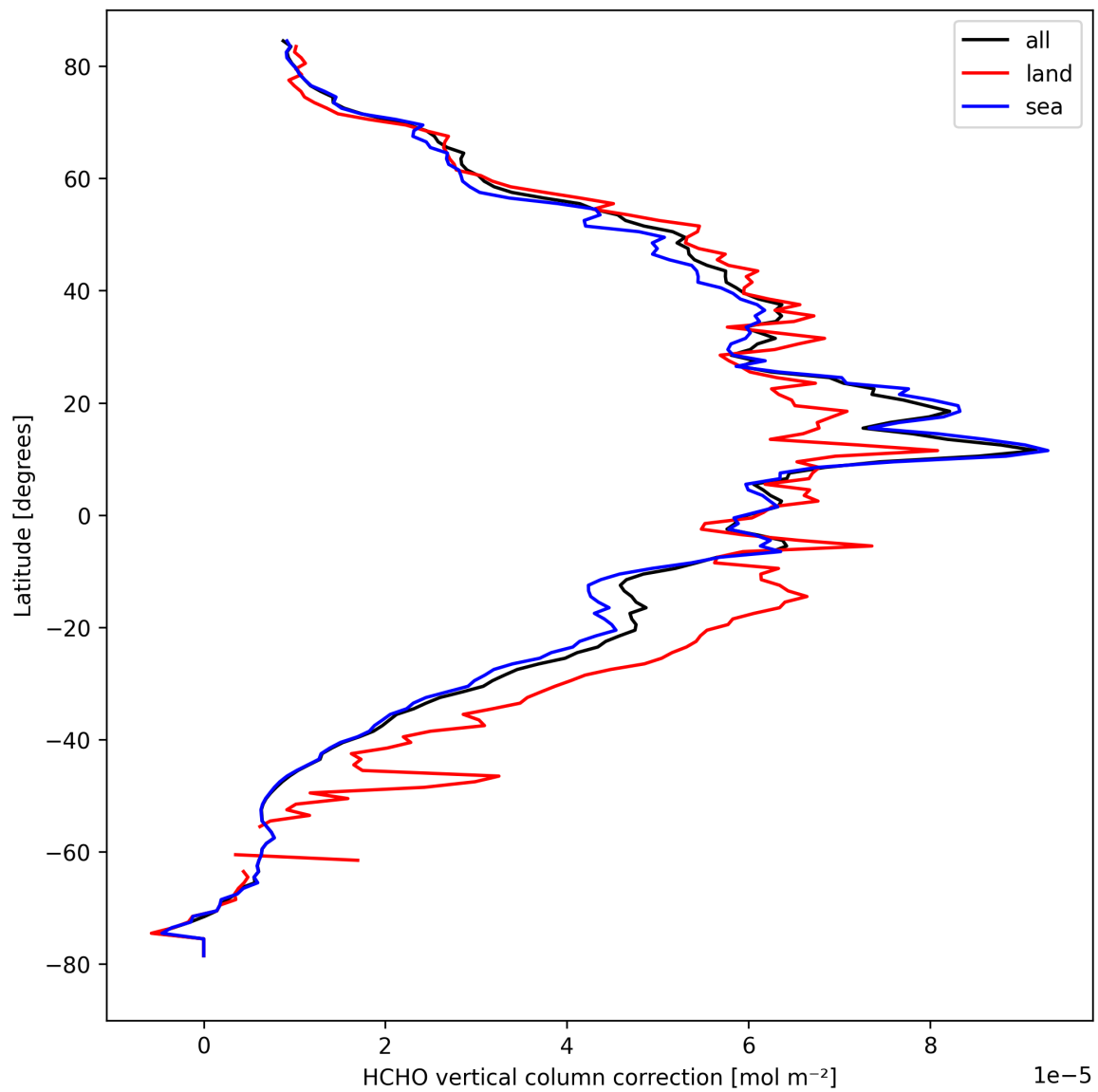
Figure 23: Zonal average of “HCHO vertical column correction” for 2024-09-06 to 2024-09-08.
