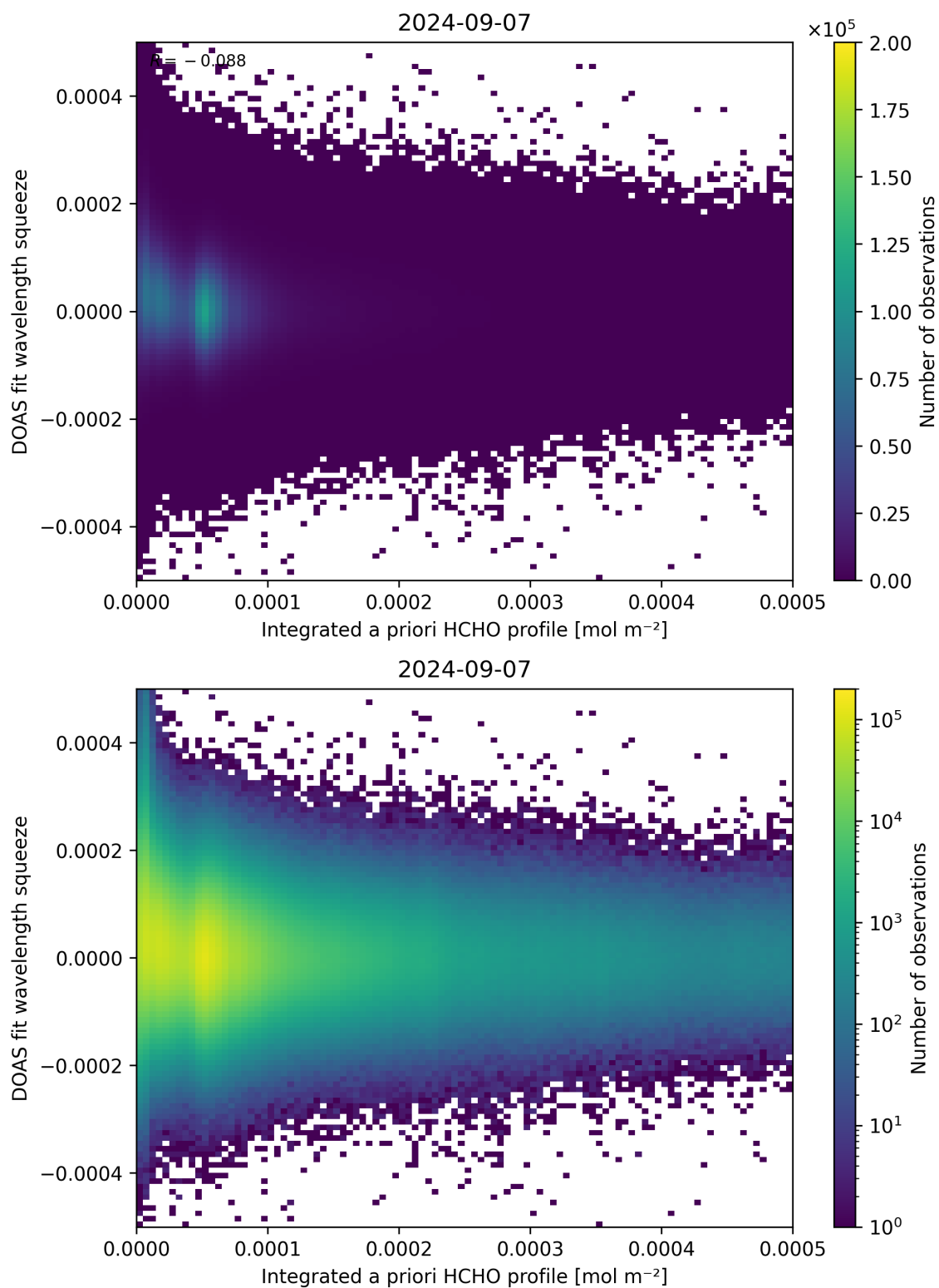
Figure 150: Scatter density plot of “Integrated a priori HCHO profile” against “DOAS fit wavelength squeeze” for 2024-09-06 to 2024-09-08.
