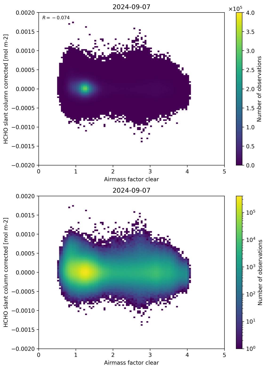
Figure 74: Scatter density plot of “Airmass factor clear” against “HCHO slant column corrected” for 2024-09-06 to 2024-09-08.
