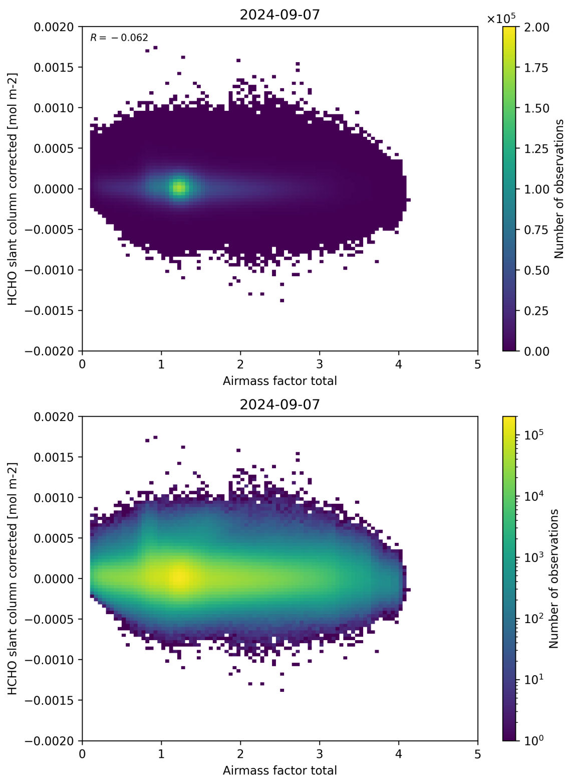
Figure 101: Scatter density plot of “Airmass factor total” against “HCHO slant column corrected” for 2024-09-06 to 2024-09-08.
