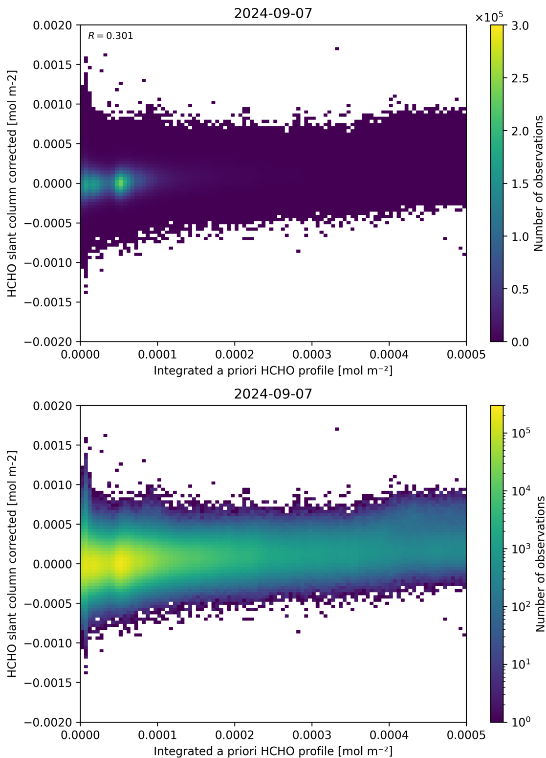
Figure 151: Scatter density plot of “Integrated a priori HCHO profile” against “HCHO slant column corrected” for 2024-09-06 to 2024-09-08.
