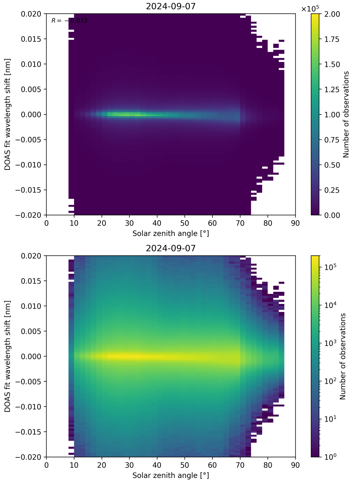
Figure 168: Scatter density plot of “Solar zenith angle” against “DOAS fit wavelength shift” for 2024-09-06 to 2024-09-08.
