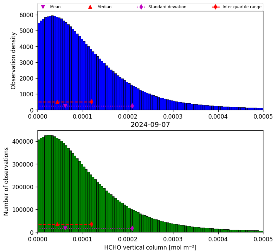
Figure 35: Histogram of “HCHO vertical column” for 2024-09-06 to 2024-09-08
