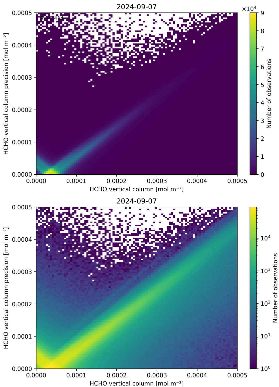
Figure 134: Scatter density plot of “HCHO vertical column” against “HCHO vertical column precision” for 2024-09-06 to 2024-09-08.
