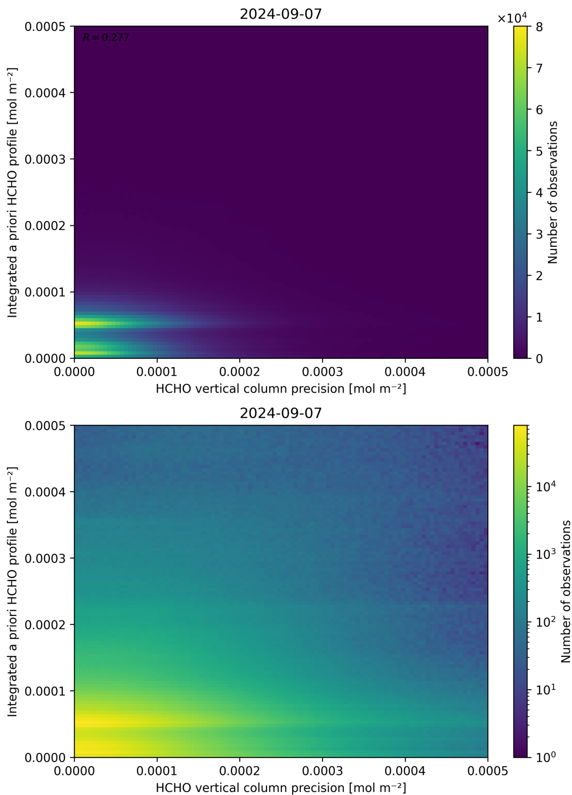
Figure 147: Scatter density plot of “HCHO vertical column precision” against “Integrated a priori HCHO profile” for 2024-09-06 to 2024-09-08.
