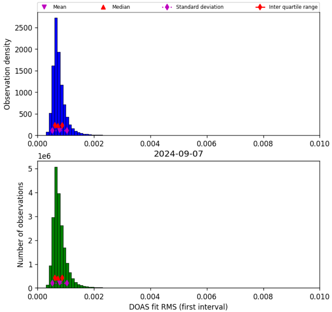
Figure 46: Histogram of “DOAS fit RMS (first interval)” for 2024-09-06 to 2024-09-08
