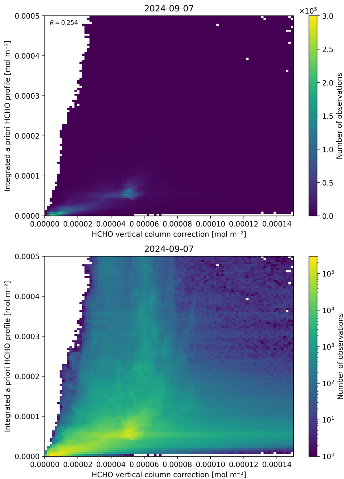
Figure 122: Scatter density plot of “HCHO vertical column correction” against “Integrated a priori HCHO profile” for 2024-09-06 to 2024-09-08.
