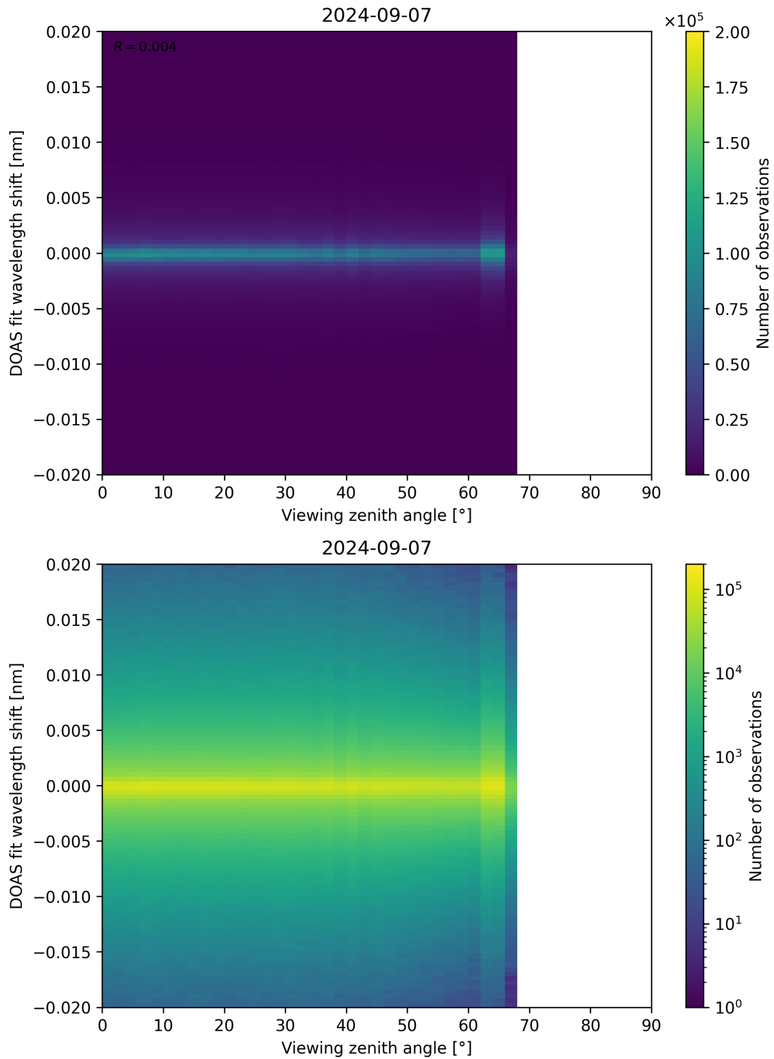
Figure 183: Scatter density plot of “Viewing zenith angle” against “DOAS fit wavelength shift” for 2024-09-06 to 2024-09-08.
