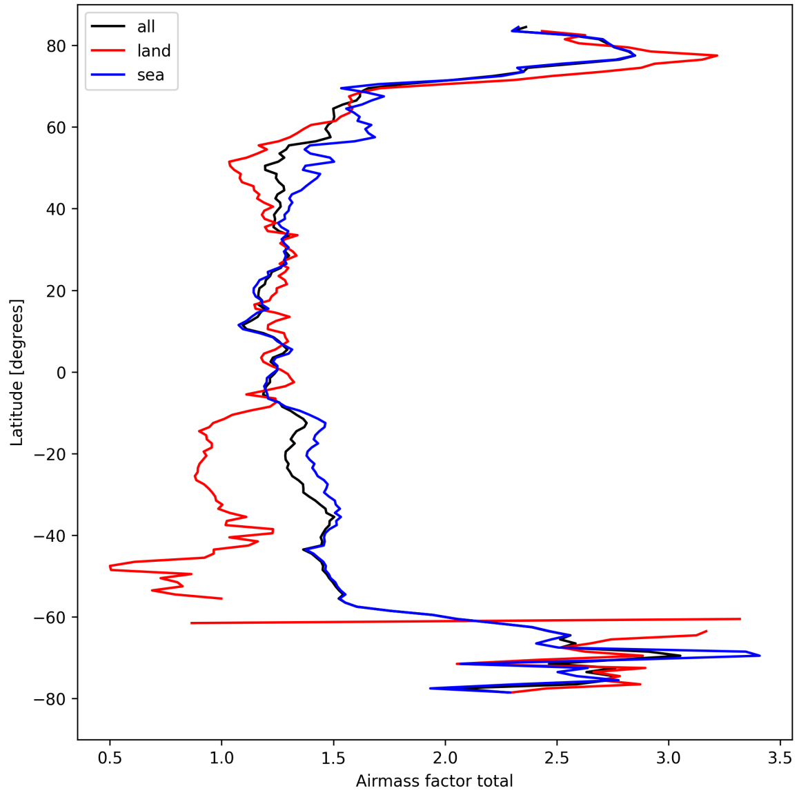
Figure 26: Zonal average of “Airmass factor total” for 2024-09-06 to 2024-09-08.
