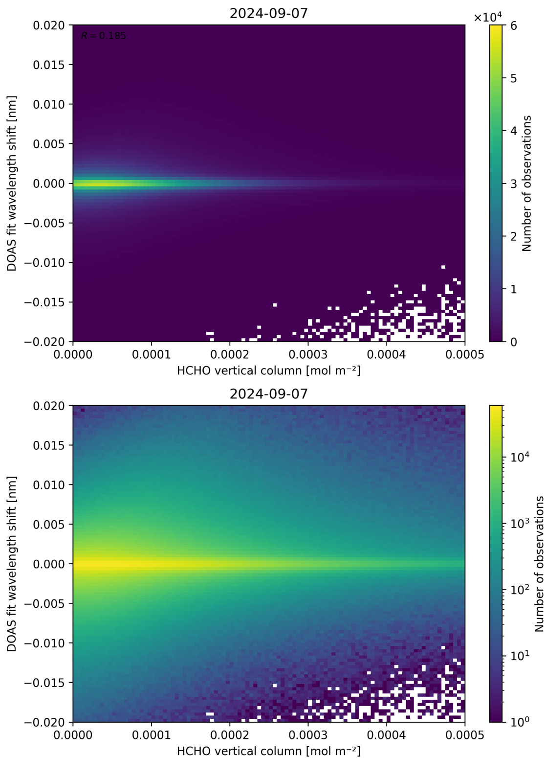
Figure 124: Scatter density plot of “HCHO vertical column” against “DOAS fit wavelength shift” for 2024-09-06 to 2024-09-08.
