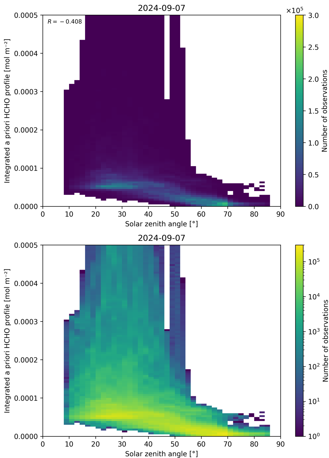
Figure 180: Scatter density plot of “Solar zenith angle” against “Integrated a priori HCHO profile” for 2024-09-06 to 2024-09-08.
