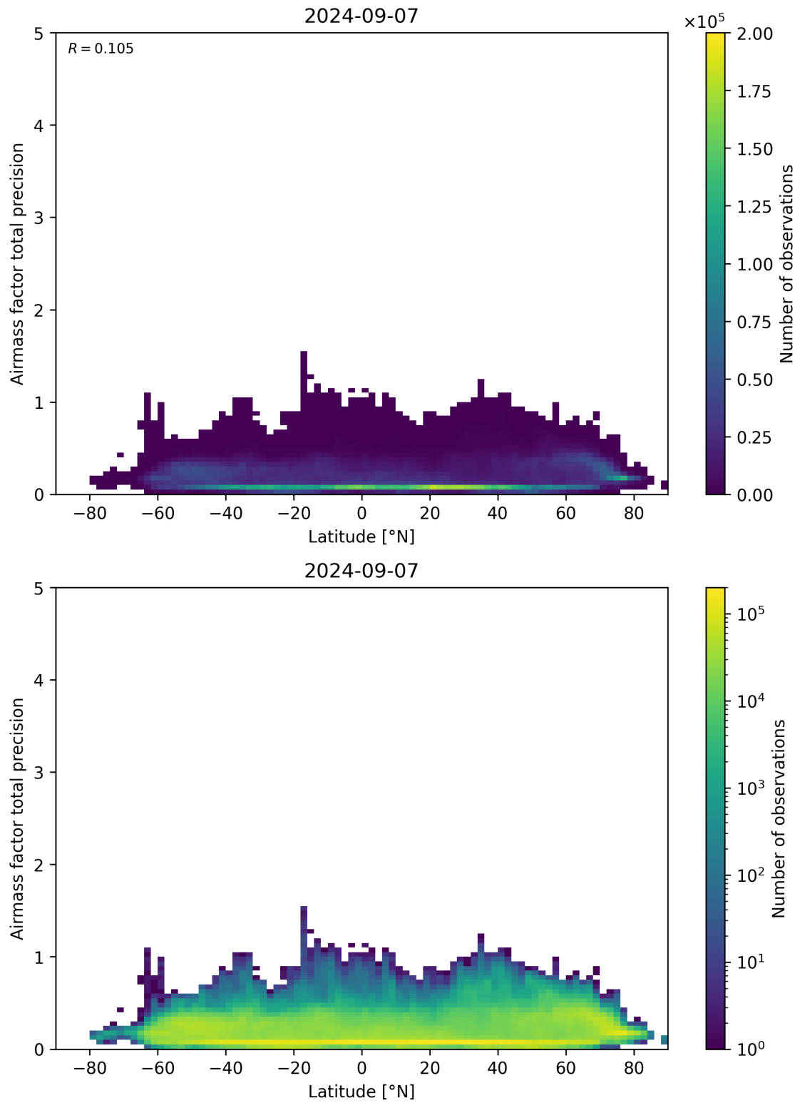
Figure 162: Scatter density plot of “Latitude” against “Airmass factor total precision” for 2024-09-06 to 2024-09-08.
