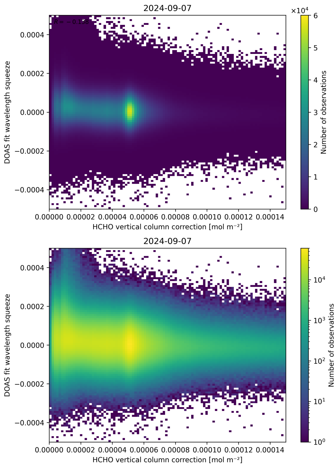
Figure 114: Scatter density plot of “HCHO vertical column correction” against “DOAS fit wavelength squeeze” for 2024-09-06 to 2024-09-08.
