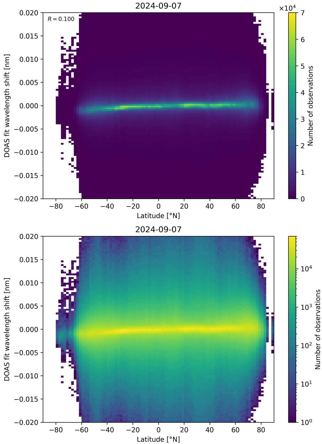
Figure 154: Scatter density plot of “Latitude” against “DOAS fit wavelength shift” for 2024-09-06 to 2024-09-08.
