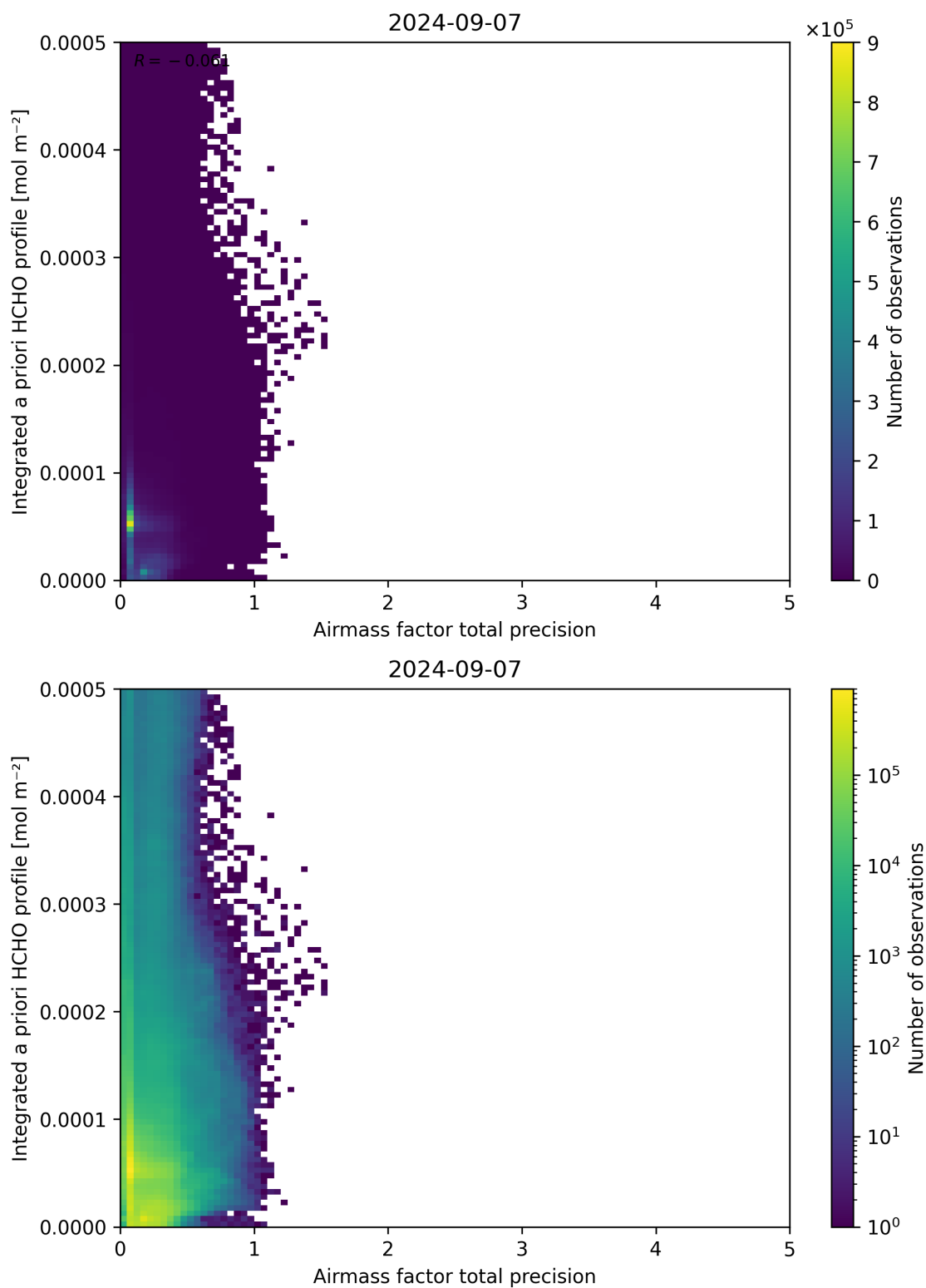
Figure 111: Scatter density plot of “Airmass factor total precision” against “Integrated a priori HCHO profile” for 2024-09-06 to 2024-09-08.
