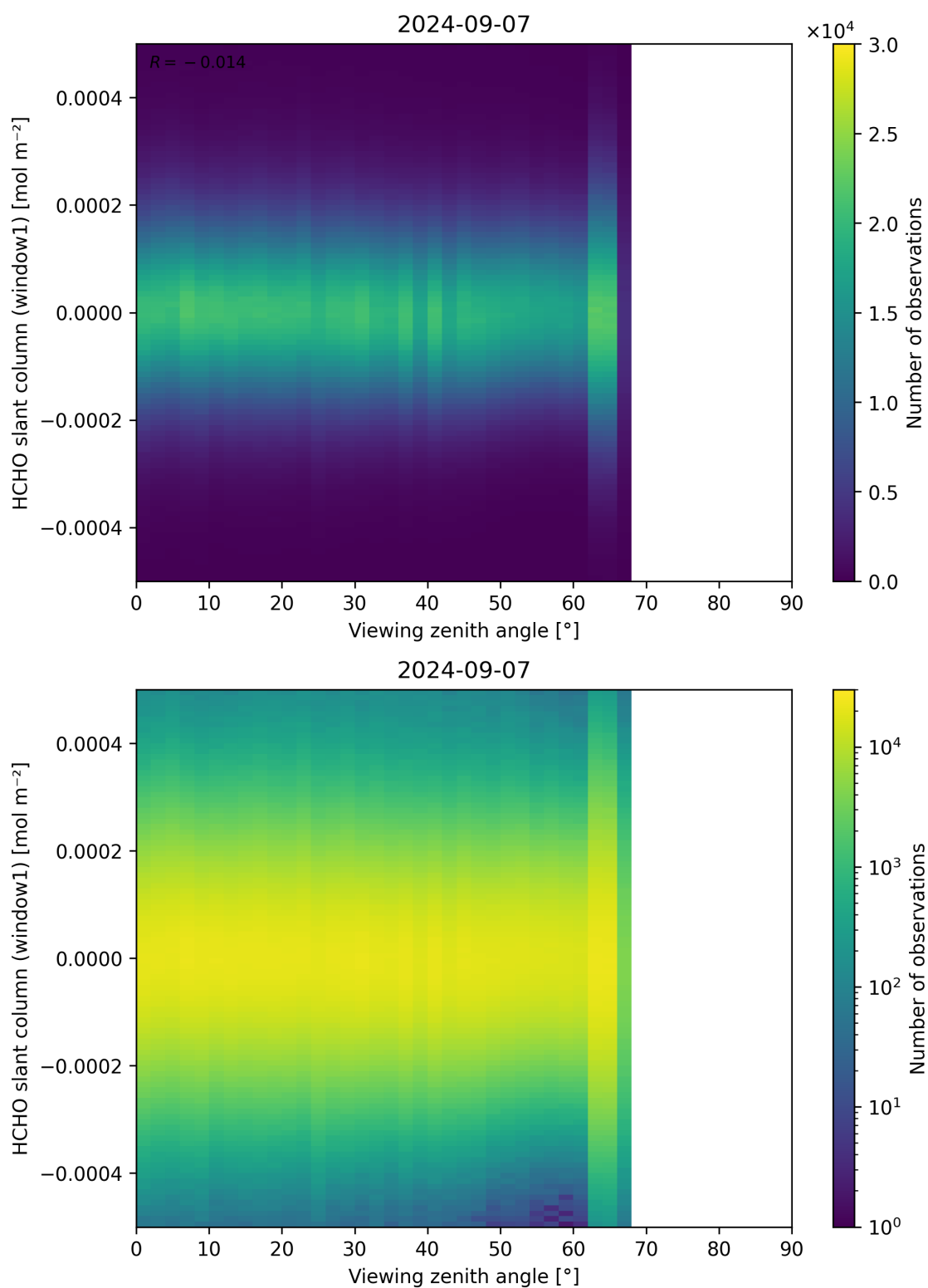
Figure 188: Scatter density plot of “Viewing zenith angle” against “HCHO slant column (window1)” for 2024-09-06 to 2024-09-08.
