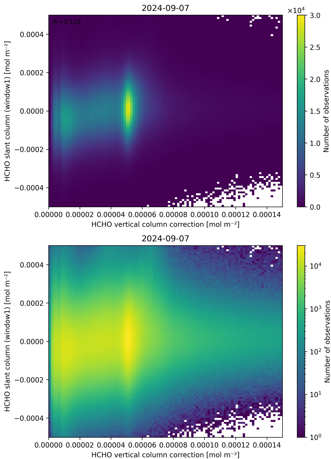
Figure 118: Scatter density plot of “HCHO vertical column correction” against “HCHO slant column (window1)” for 2024-09-06 to 2024-09-08.
