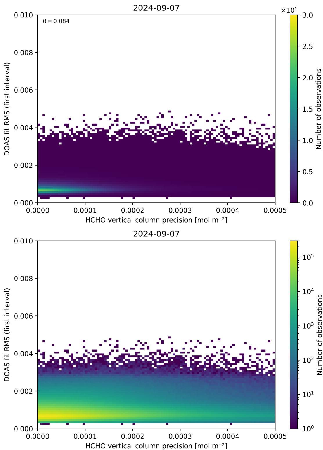
Figure 136: Scatter density plot of “HCHO vertical column precision” against “DOAS fit RMS (first interval)” for 2024-09-06 to 2024-09-08.
