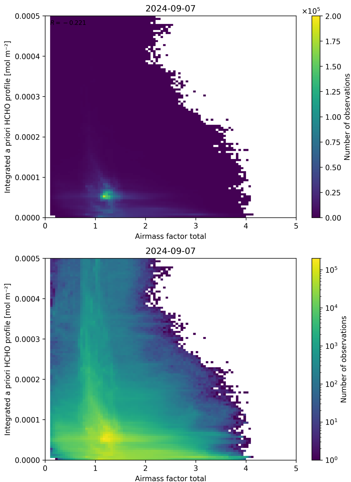
Figure 104: Scatter density plot of “Airmass factor total” against “Integrated a priori HCHO profile” for 2024-09-06 to 2024-09-08.
