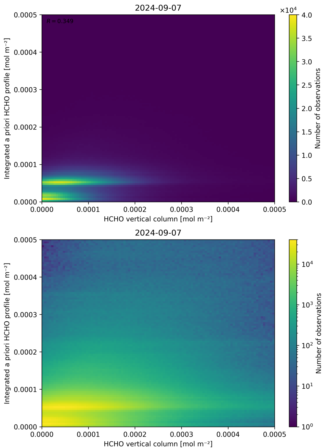
Figure 135: Scatter density plot of “HCHO vertical column” against “Integrated a priori HCHO profile” for 2024-09-06 to 2024-09-08.
