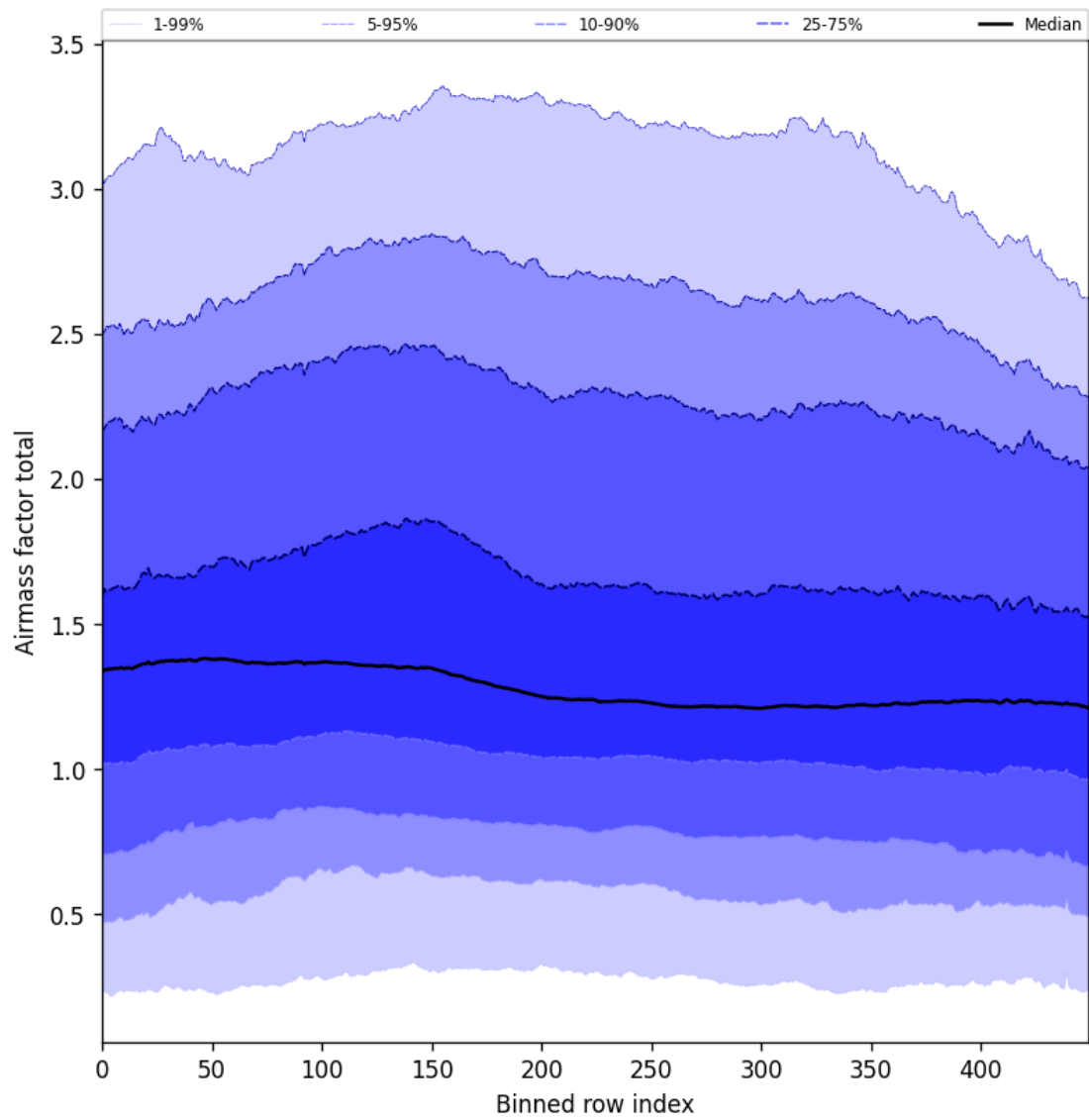
Figure 54: Along track statistics of “Airmass factor total” for 2024-09-06 to 2024-09-08
