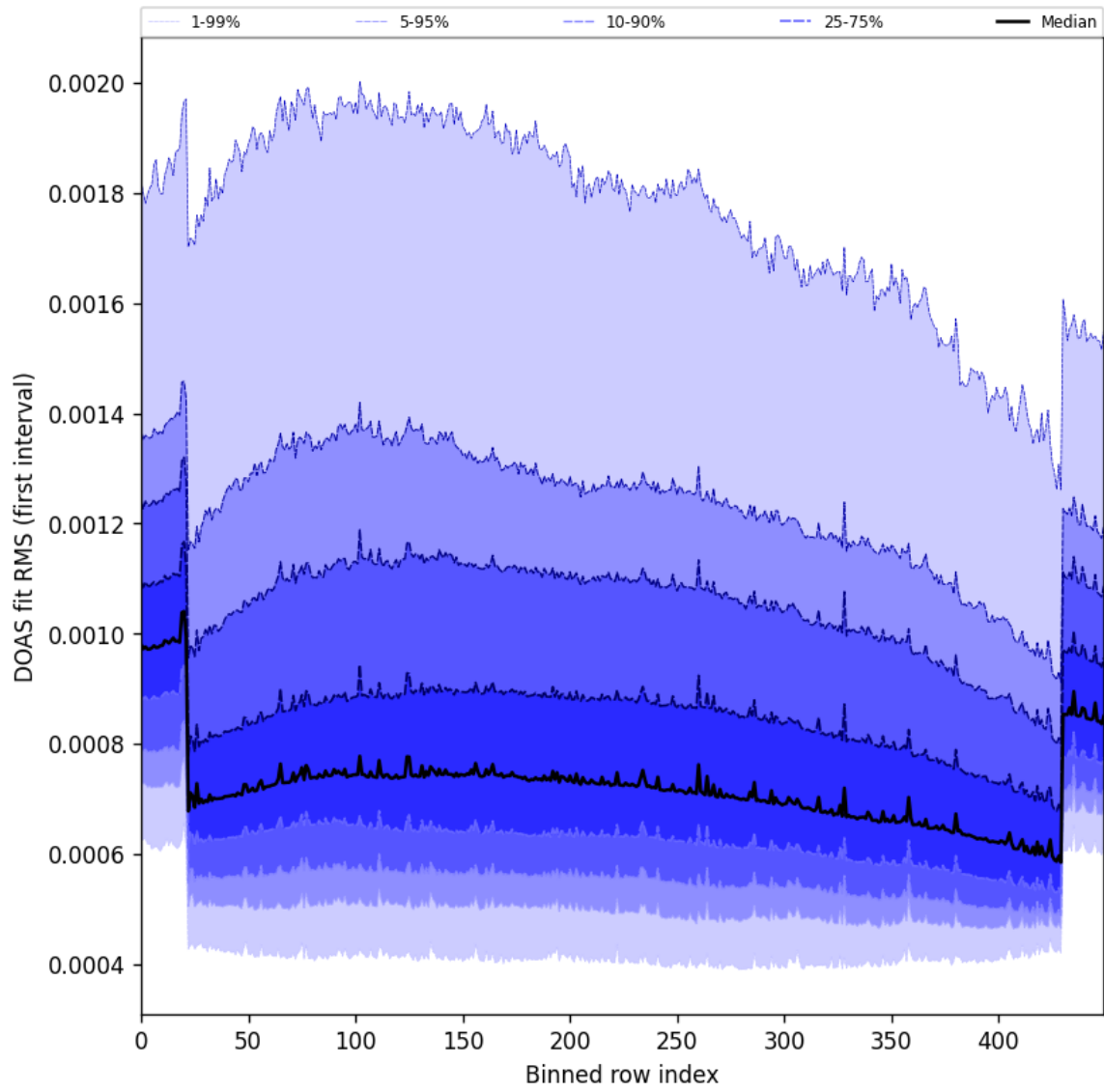
Figure 60: Along track statistics of “DOAS fit RMS (first interval)” for 2024-09-06 to 2024-09-08
