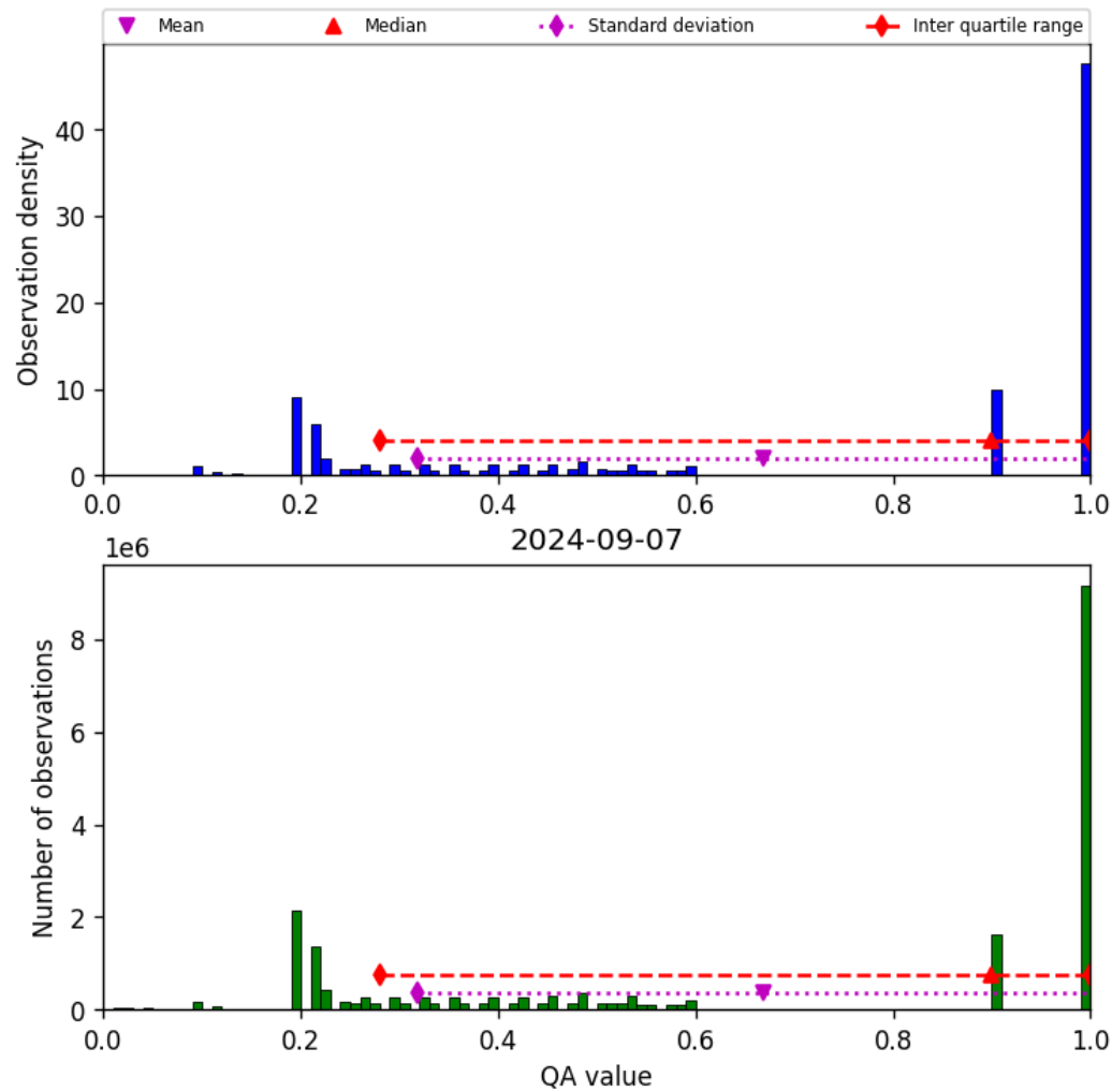
Figure 34: Histogram of “QA value” for 2024-09-06 to 2024-09-08
