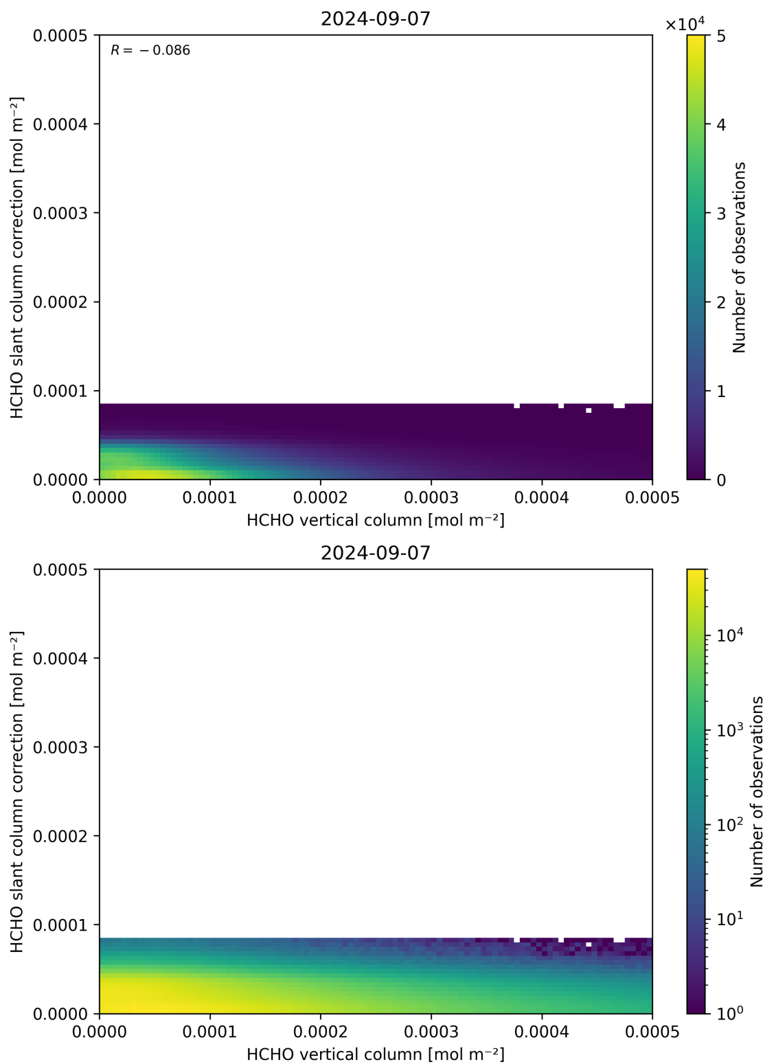
Figure 128: Scatter density plot of “HCHO vertical column” against “HCHO slant column correction” for 2024-09-06 to 2024-09-08.
