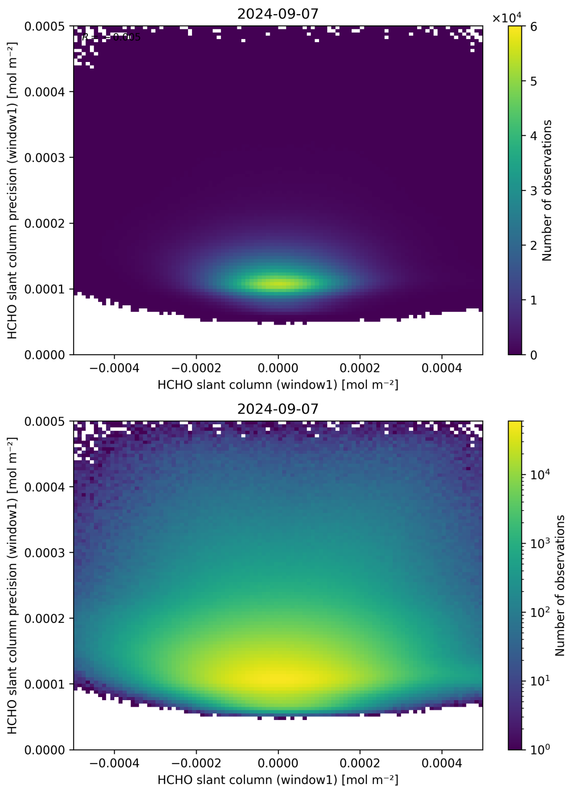
Figure 84: Scatter density plot of “HCHO slant column (window1)” against “HCHO slant column precision (window1)” for 2024-09-06 to 2024-09-08.
