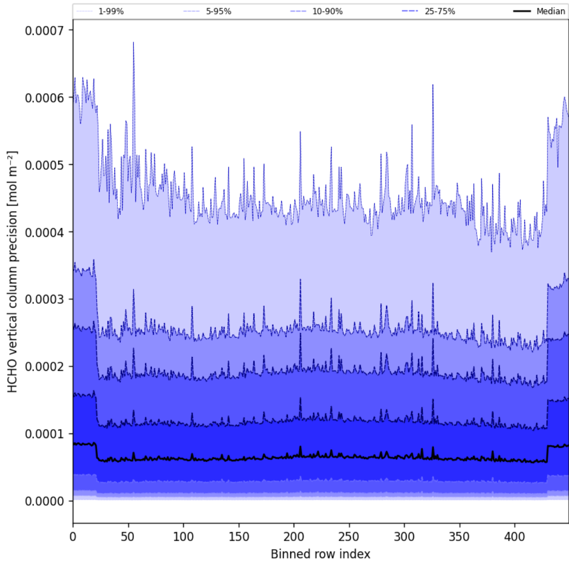
Figure 50: Along track statistics of “HCHO vertical column precision” for 2024-09-06 to 2024-09-08
