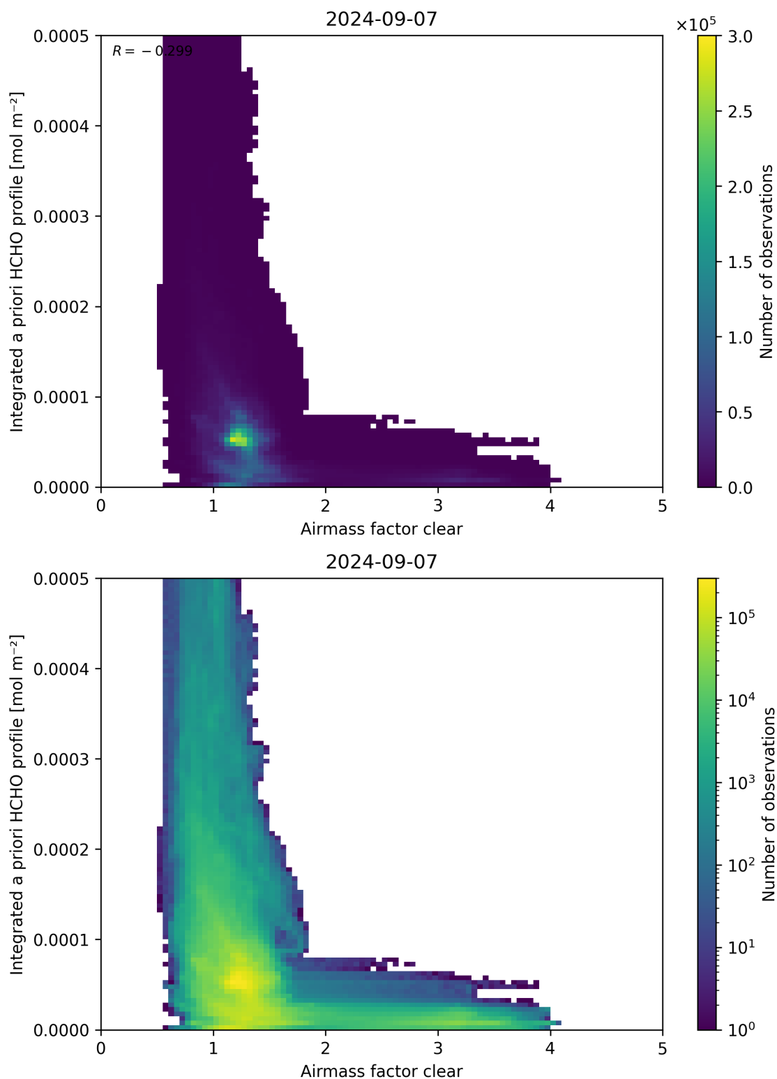
Figure 76: Scatter density plot of “Airmass factor clear” against “Integrated a priori HCHO profile” for 2024-09-06 to 2024-09-08.
