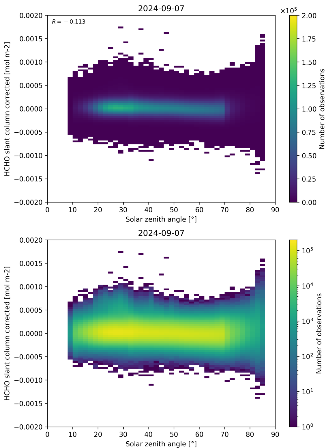
Figure 171: Scatter density plot of “Solar zenith angle” against “HCHO slant column corrected” for 2024-09-06 to 2024-09-08.
