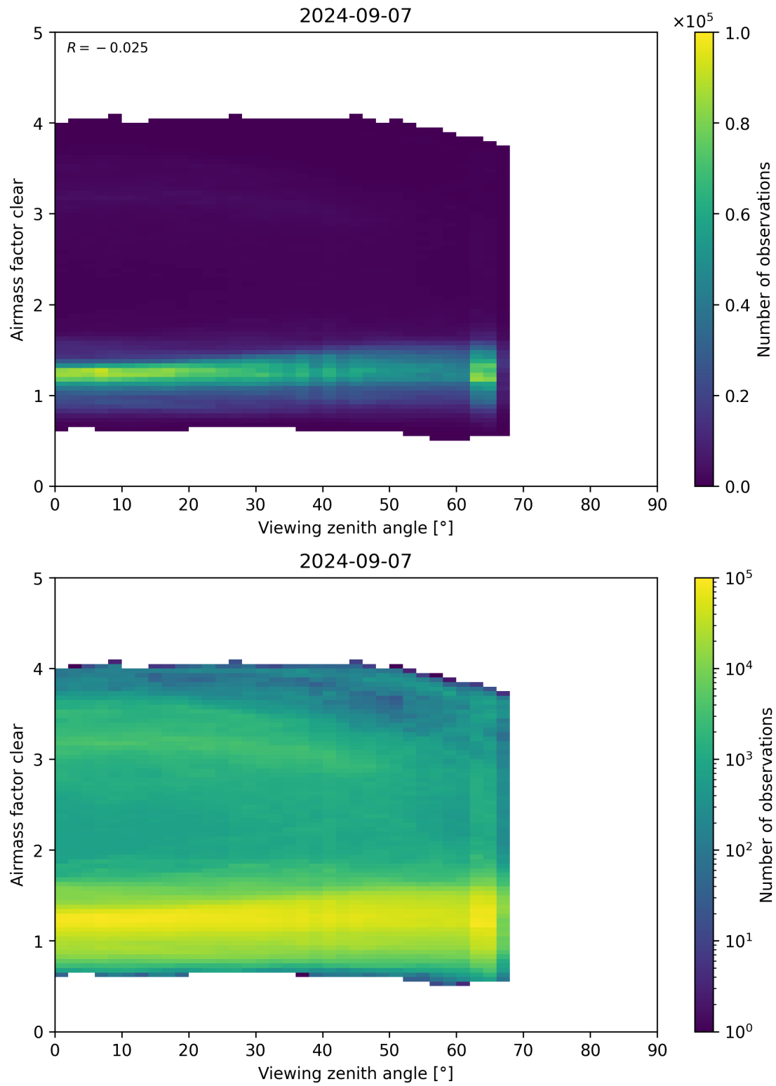
Figure 185: Scatter density plot of “Viewing zenith angle” against “Airmass factor clear” for 2024-09-06 to 2024-09-08.
