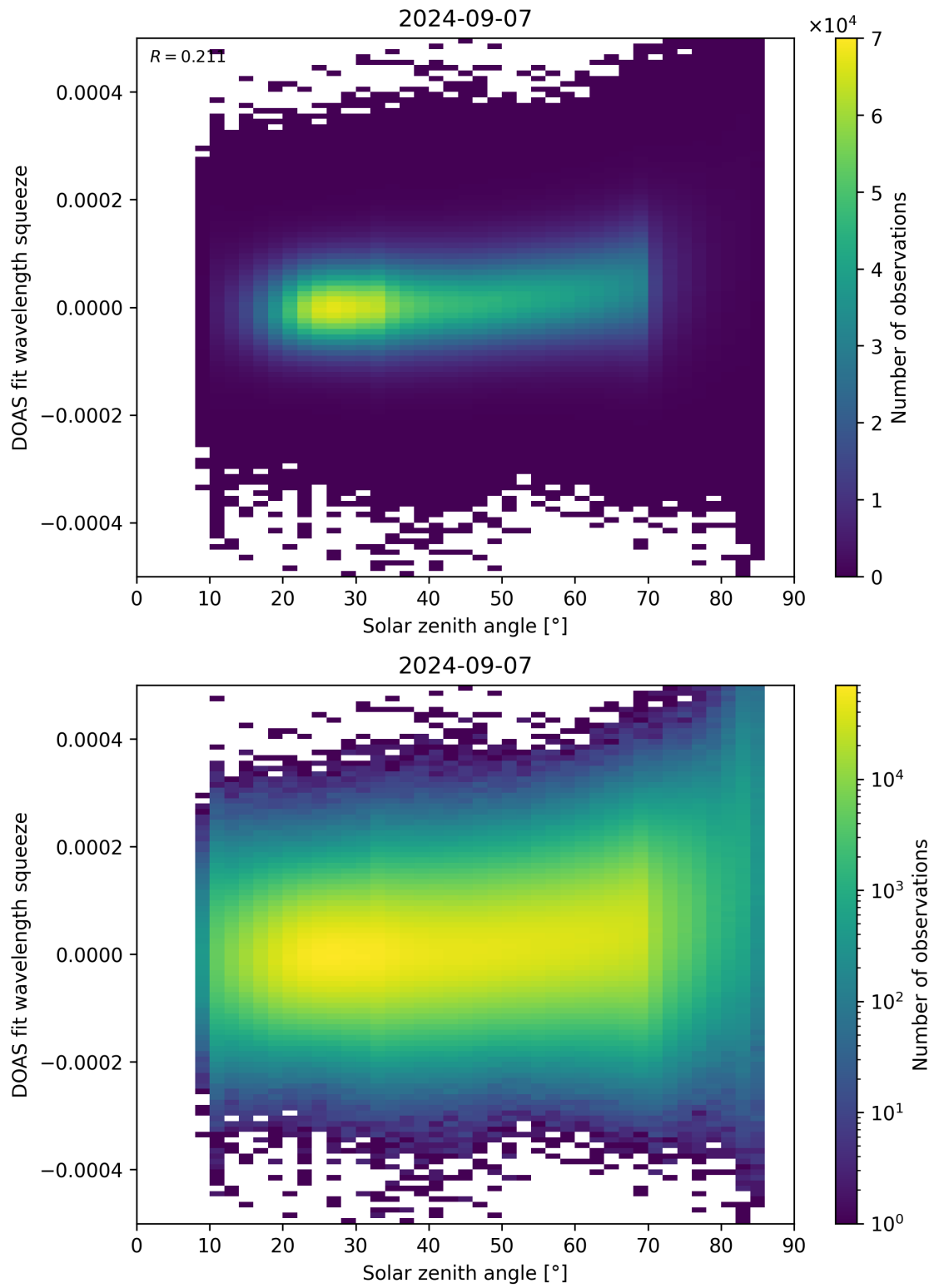
Figure 169: Scatter density plot of “Solar zenith angle” against “DOAS fit wavelength squeeze” for 2024-09-06 to 2024-09-08.
