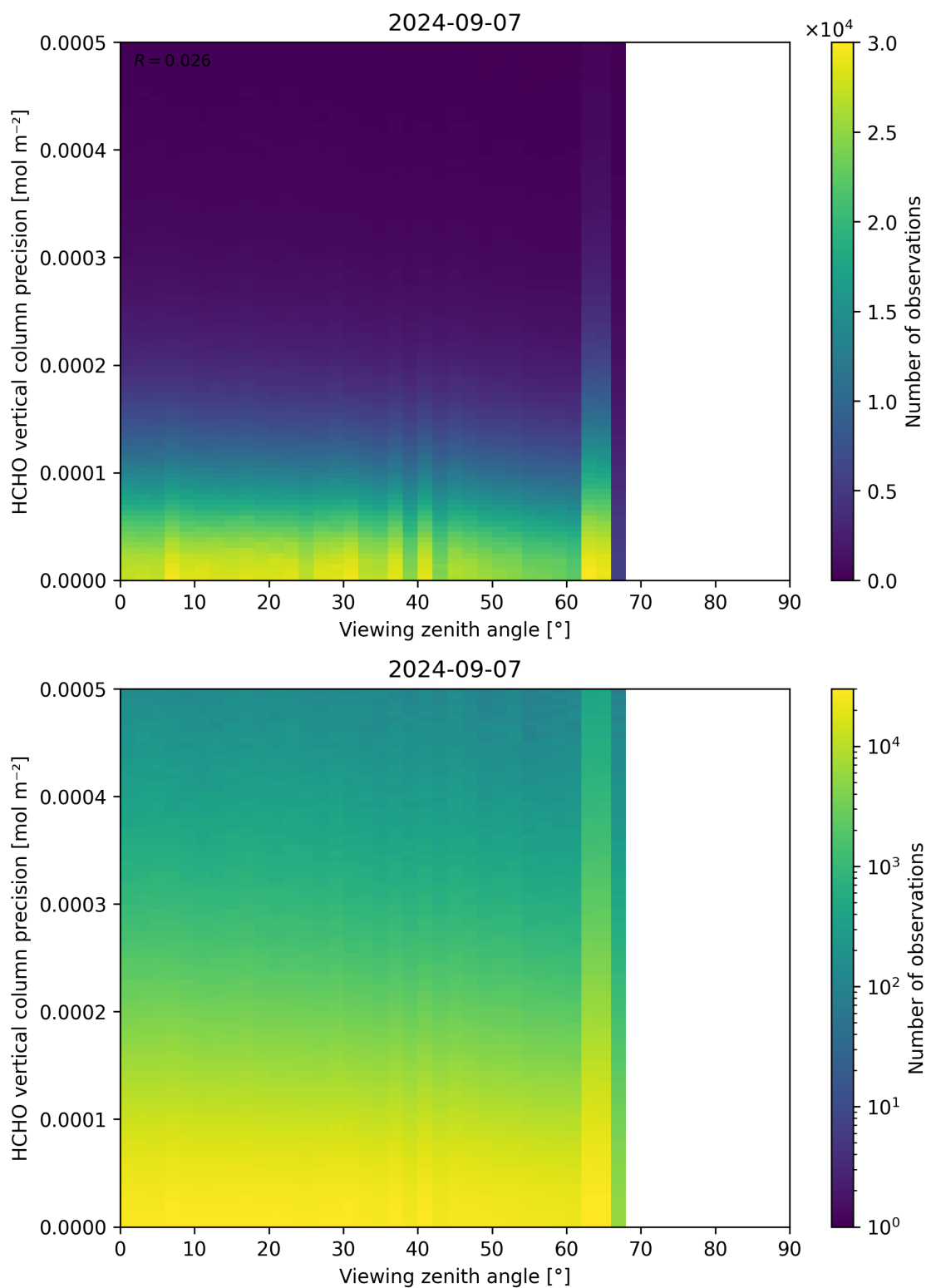
Figure 194: Scatter density plot of “Viewing zenith angle” against “HCHO vertical column precision” for 2024-09-06 to 2024-09-08.
