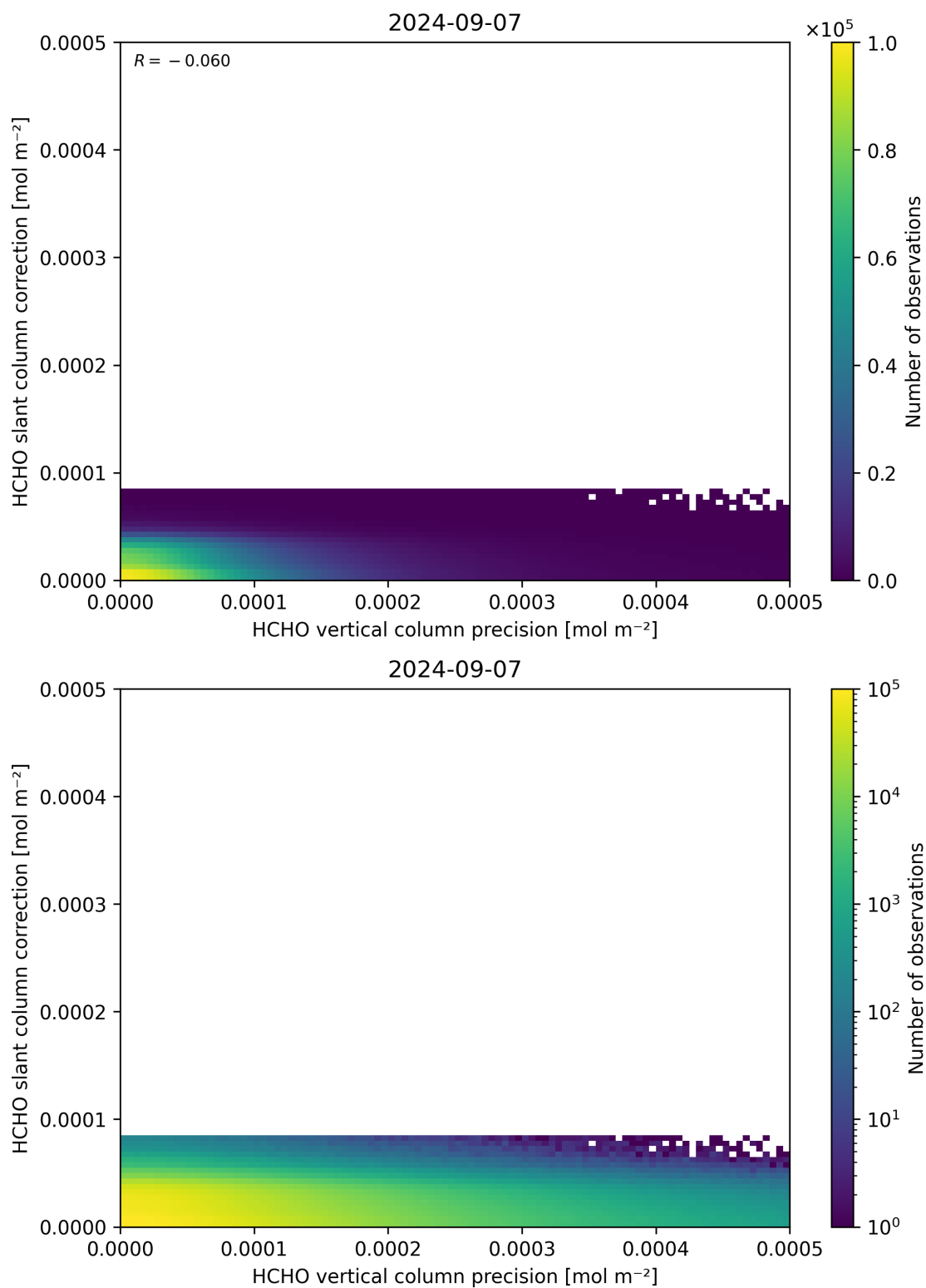
Figure 141: Scatter density plot of “HCHO vertical column precision” against “HCHO slant column correction” for 2024-09-06 to 2024-09-08.
