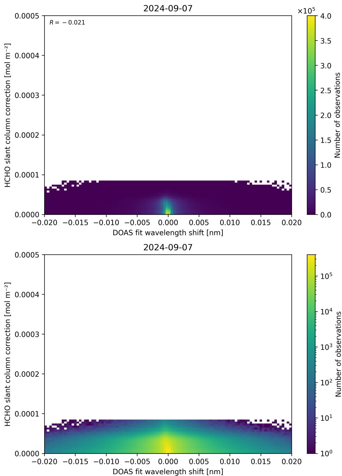
Figure 67: Scatter density plot of “DOAS fit wavelength shift” against “HCHO slant column correction” for 2024-09-06 to 2024-09-08.
