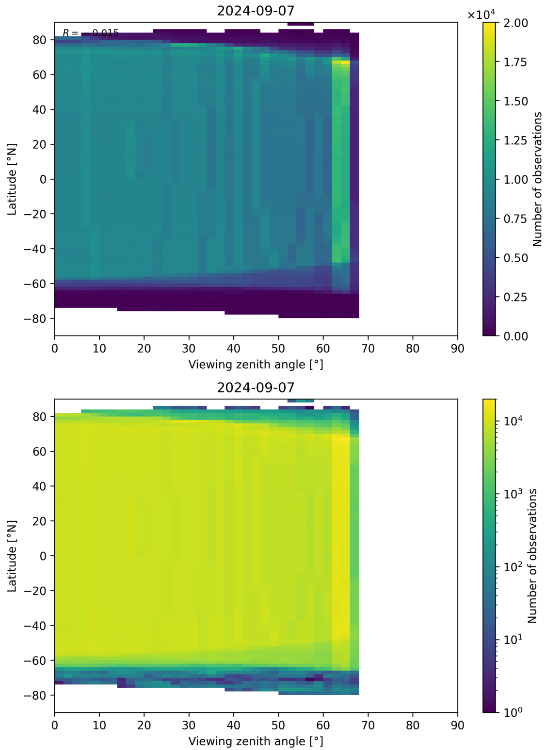
Figure 196: Scatter density plot of “Viewing zenith angle” against “Latitude” for 2024-09-06 to 2024-09-08.
