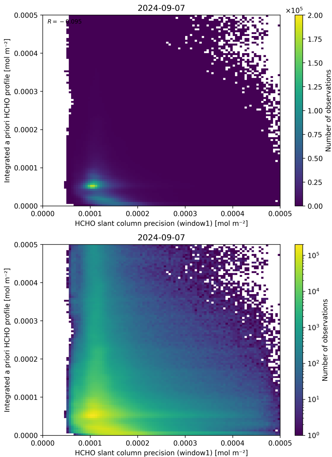
Figure 96: Scatter density plot of “HCHO slant column precision (window1)” against “Integrated a priori HCHO profile” for 2024-09-06 to 2024-09-08.
