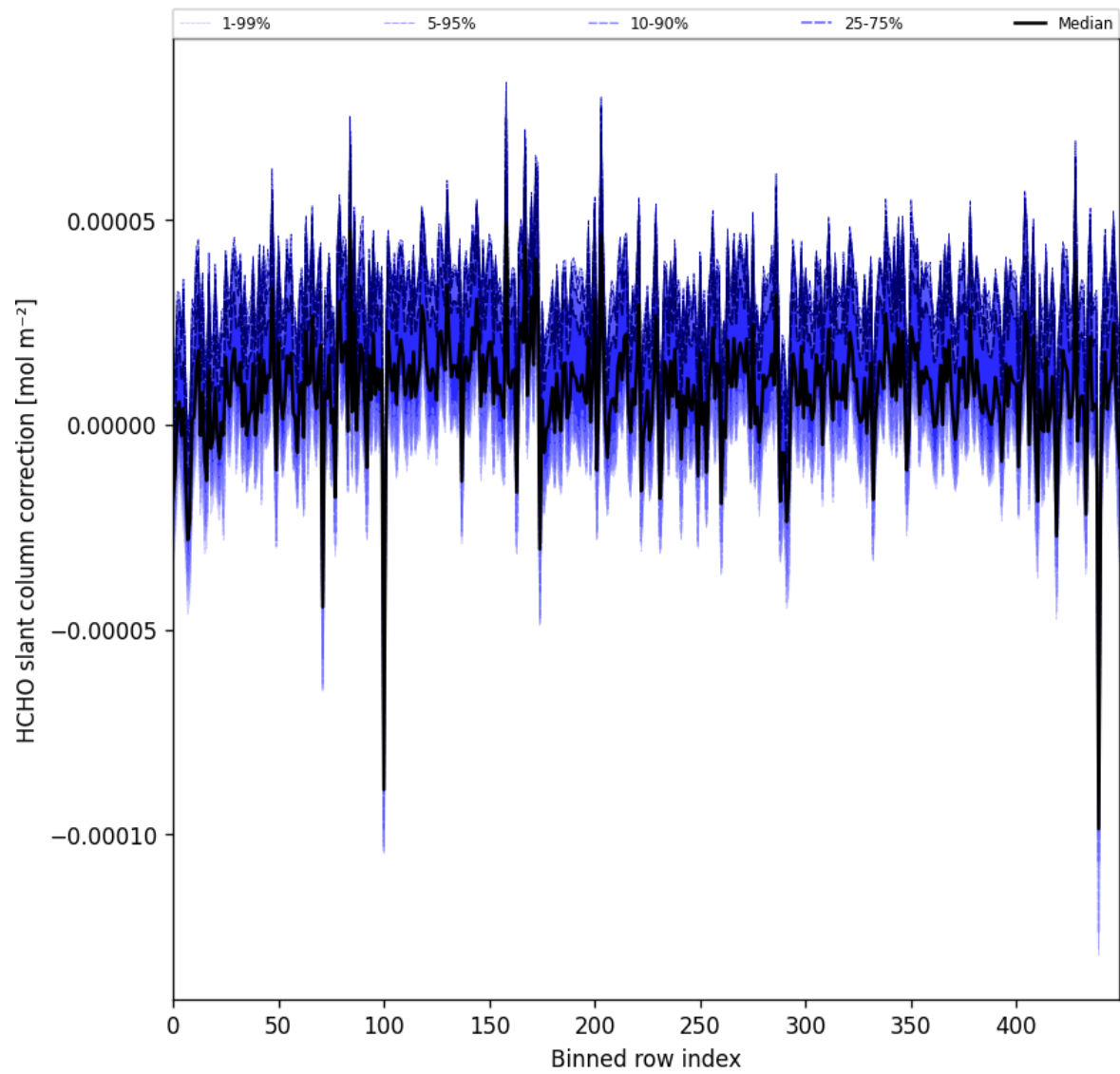
Figure 61: Along track statistics of “HCHO slant column correction” for 2024-09-06 to 2024-09-08
