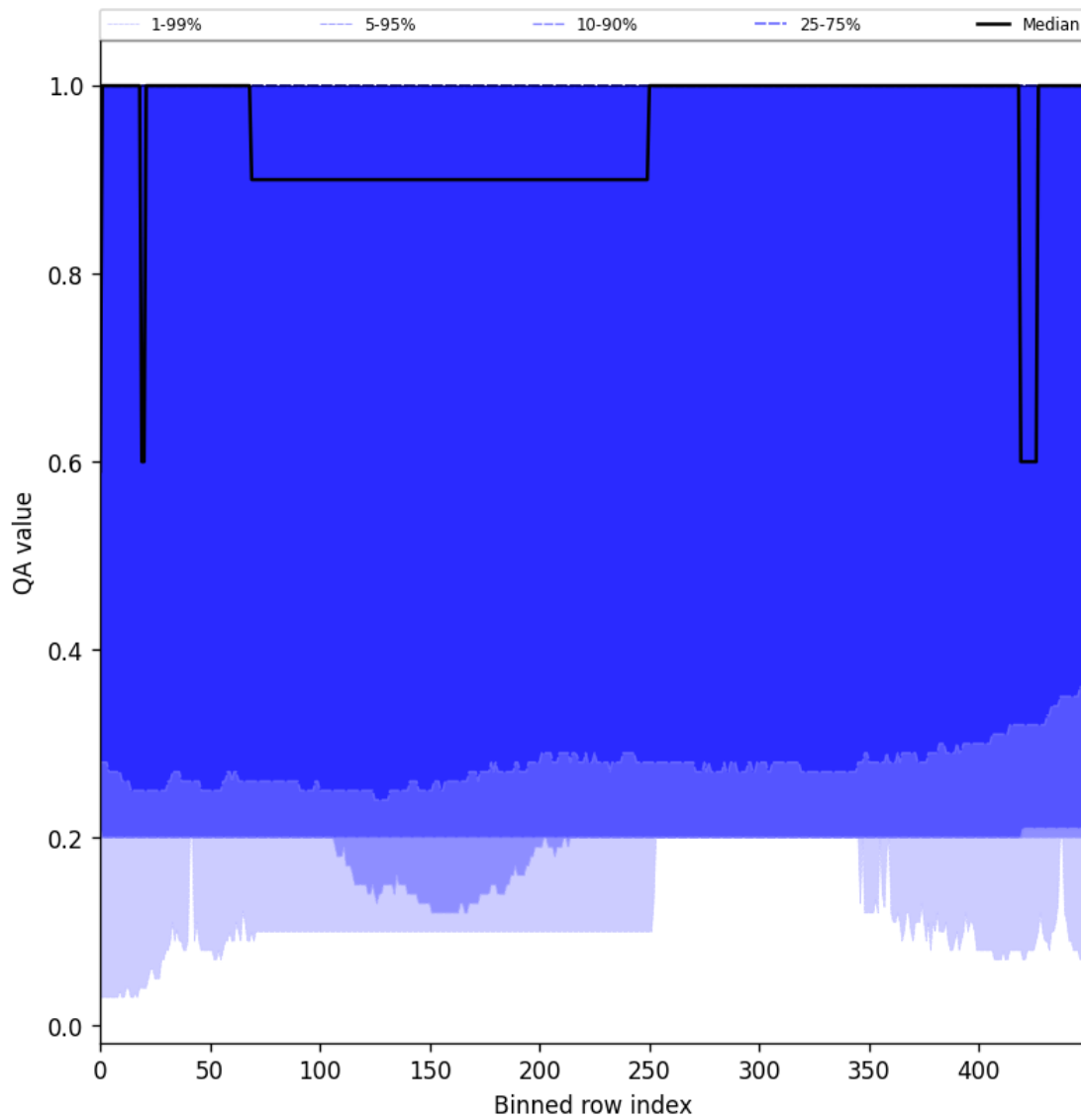
Figure 48: Along track statistics of “QA value” for 2024-09-06 to 2024-09-08
