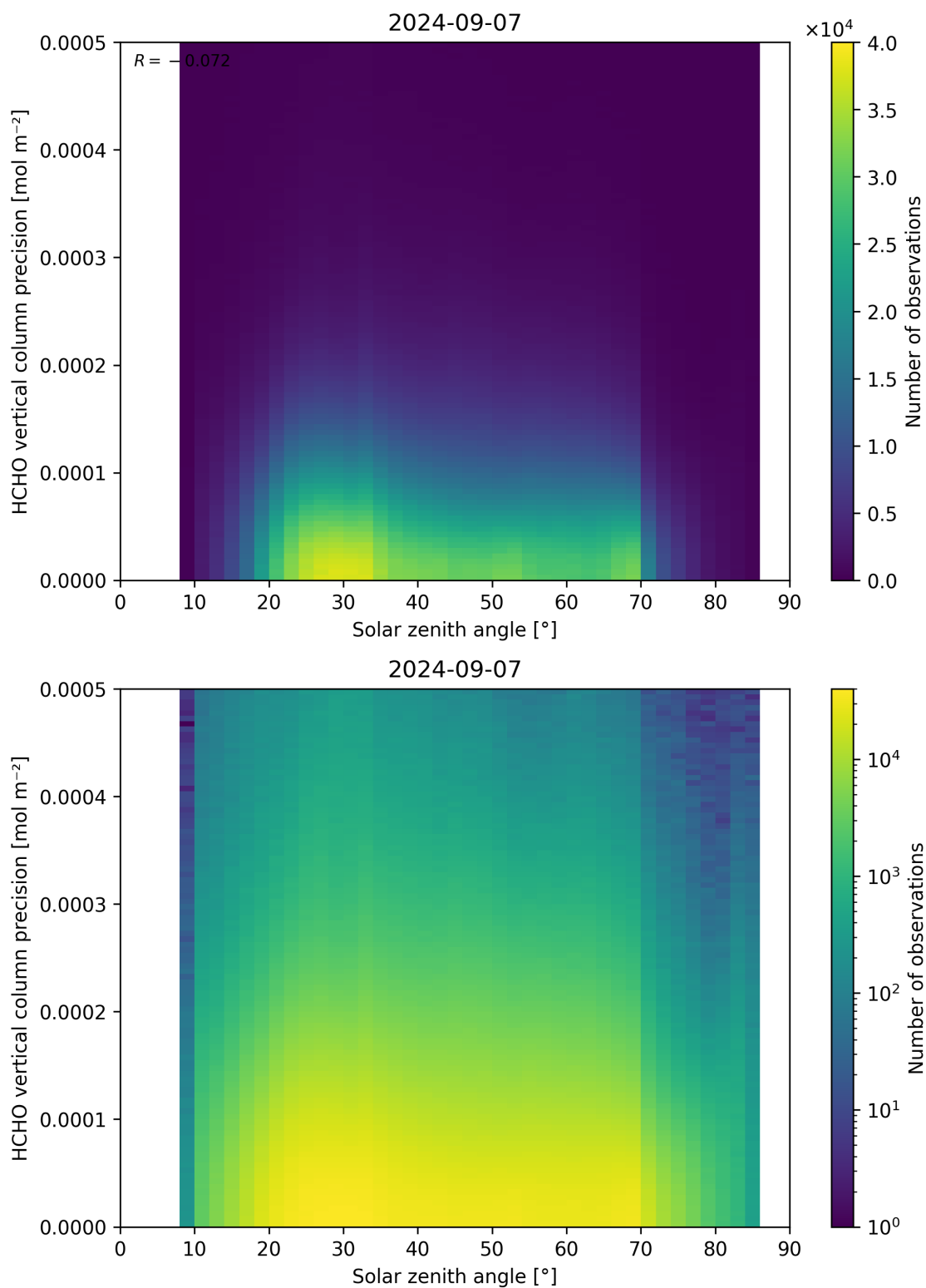
Figure 179: Scatter density plot of “Solar zenith angle” against “HCHO vertical column precision” for 2024-09-06 to 2024-09-08.
