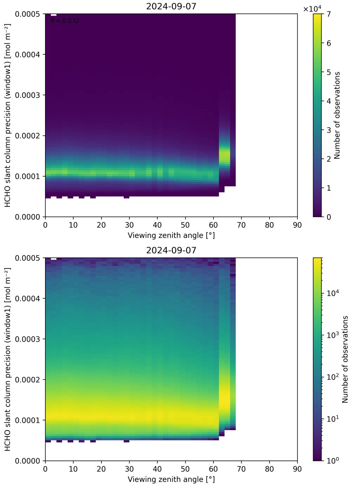
Figure 189: Scatter density plot of “Viewing zenith angle” against “HCHO slant column precision (window1)” for 2024-09-06 to 2024-09-08.
