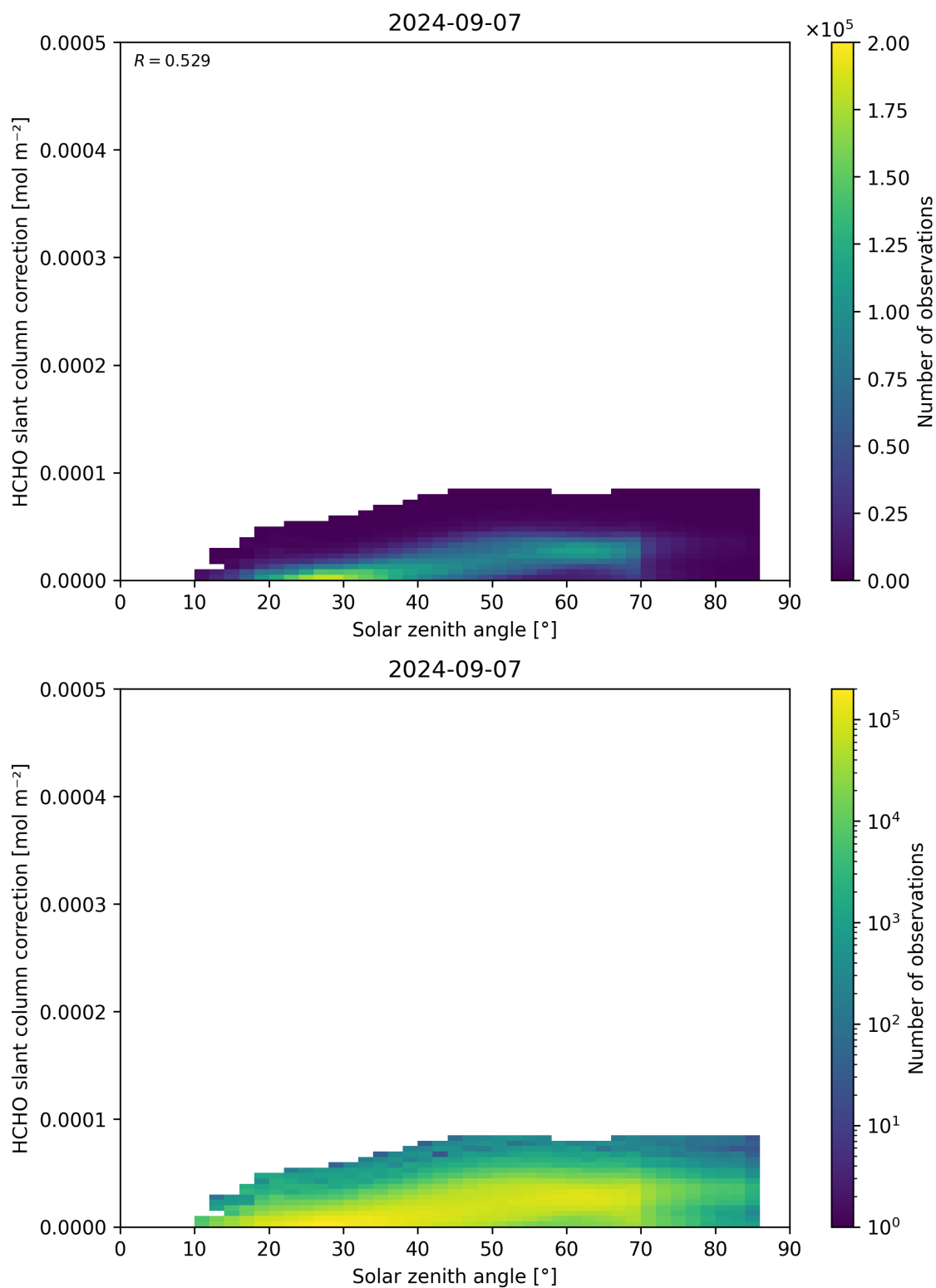
Figure 172: Scatter density plot of “Solar zenith angle” against “HCHO slant column correction” for 2024-09-06 to 2024-09-08.
