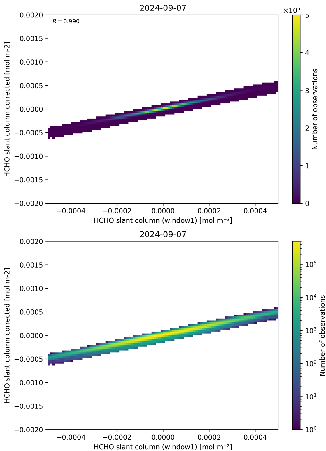
Figure 82: Scatter density plot of “HCHO slant column (window1)” against “HCHO slant column corrected” for 2024-09-06 to 2024-09-08.
