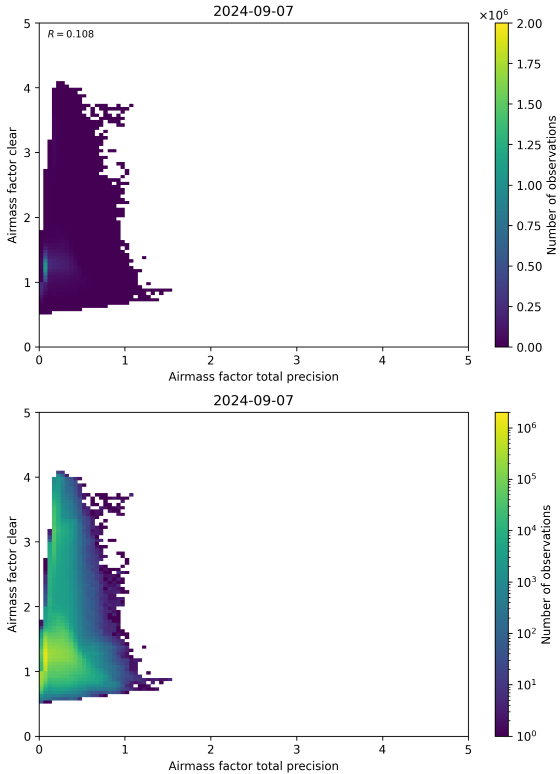
Figure 108: Scatter density plot of “Airmass factor total precision” against “Airmass factor clear” for 2024-09-06 to 2024-09-08.
