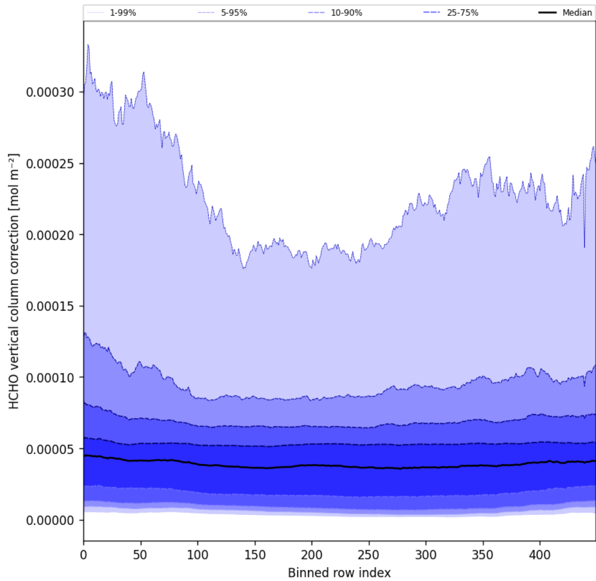
Figure 51: Along track statistics of “HCHO vertical column correction” for 2024-09-06 to 2024-09-08
