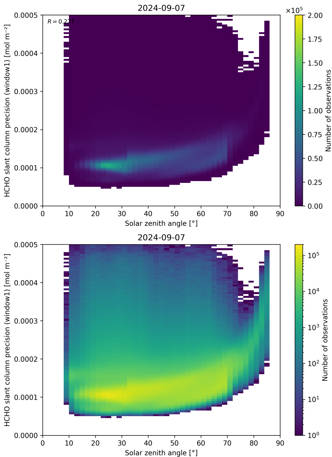
Figure 174: Scatter density plot of “Solar zenith angle” against “HCHO slant column precision (window1)” for 2024-09-06 to 2024-09-08.
