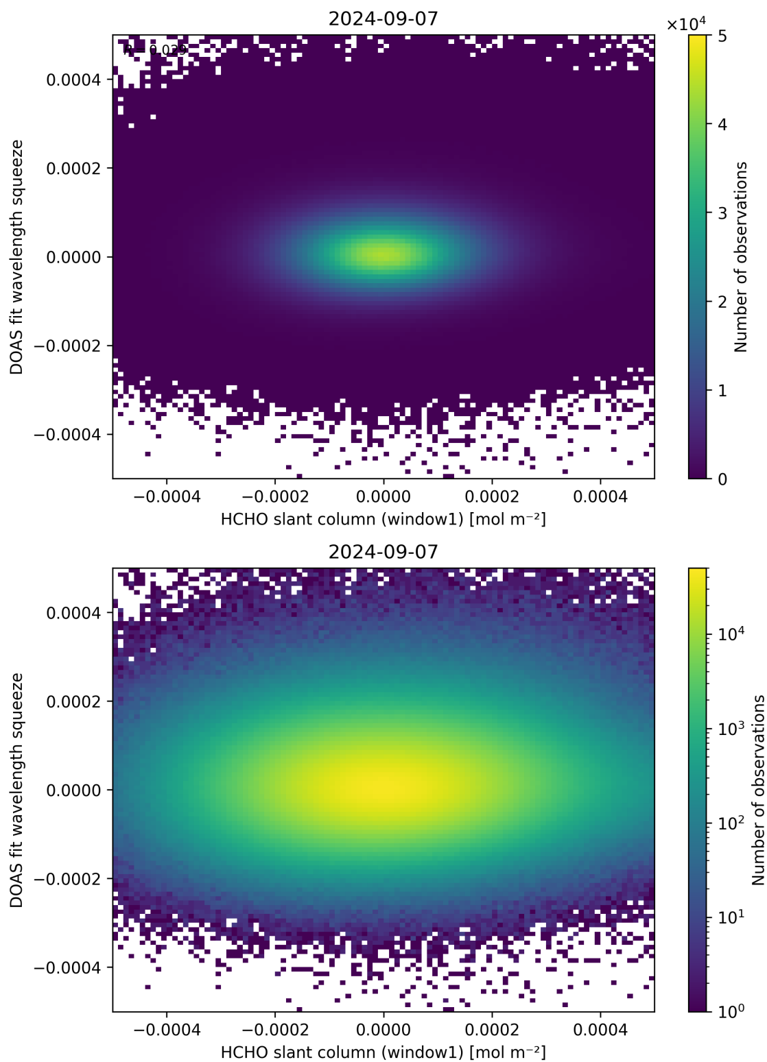
Figure 80: Scatter density plot of “HCHO slant column (window1)” against “DOAS fit wavelength squeeze” for 2024-09-06 to 2024-09-08.
