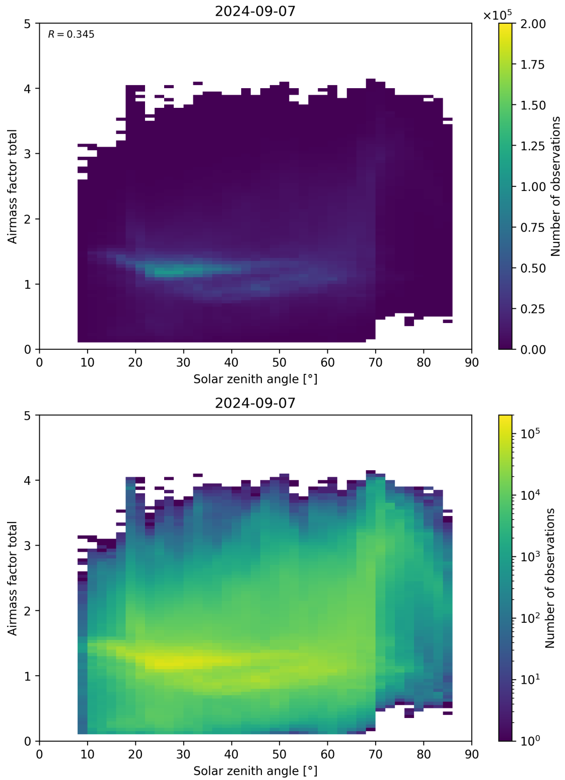
Figure 175: Scatter density plot of “Solar zenith angle” against “Airmass factor total” for 2024-09-06 to 2024-09-08.
