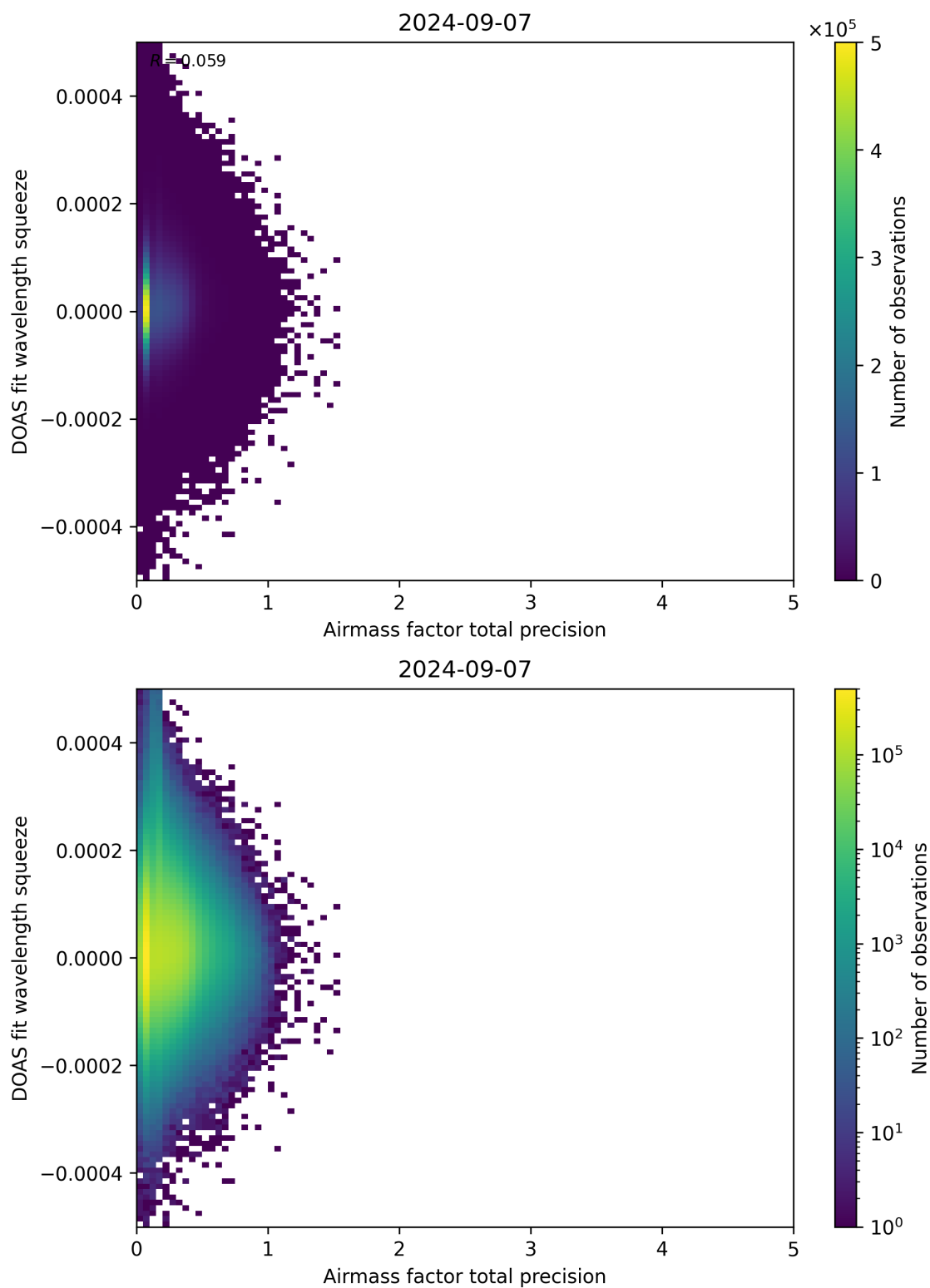
Figure 107: Scatter density plot of “Airmass factor total precision” against “DOAS fit wavelength squeeze” for 2024-09-06 to 2024-09-08.
