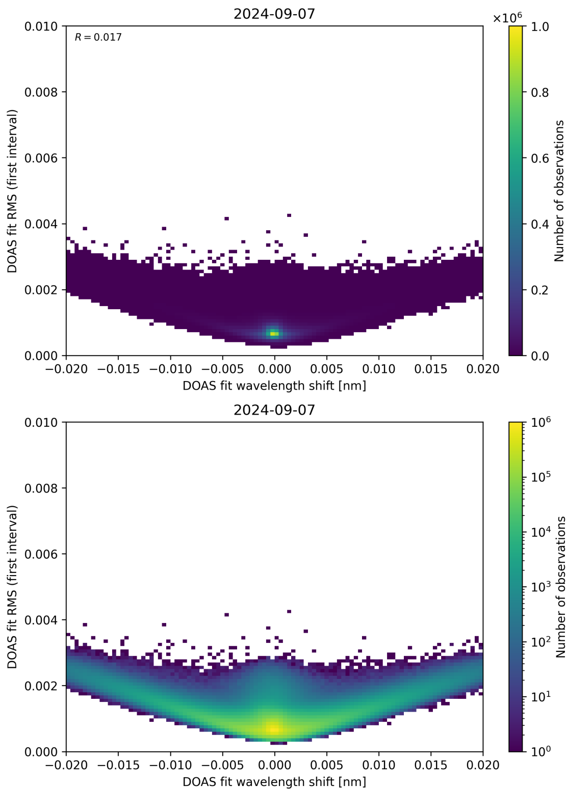
Figure 64: Scatter density plot of “DOAS fit wavelength shift” against “DOAS fit RMS (first interval)” for 2024-09-06 to 2024-09-08.
