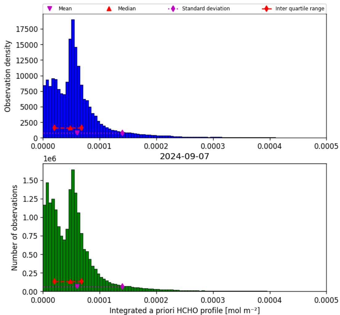
Figure 43: Histogram of “Integrated a priori HCHO profile” for 2024-09-06 to 2024-09-08
