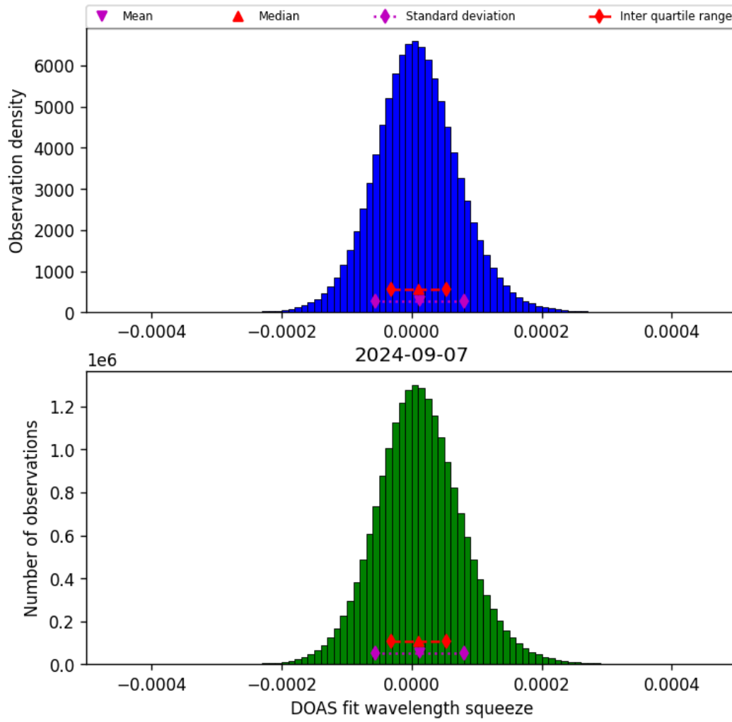
Figure 45: Histogram of “DOAS fit wavelength squeeze” for 2024-09-06 to 2024-09-08
