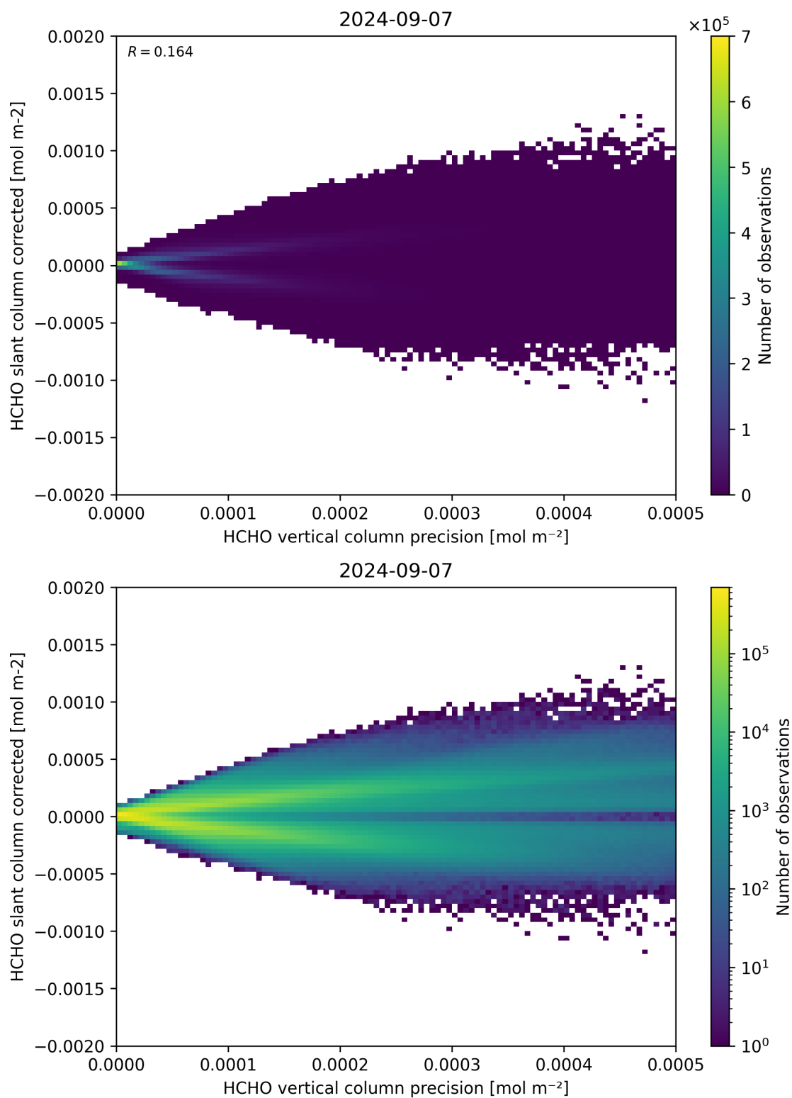
Figure 140: Scatter density plot of “HCHO vertical column precision” against “HCHO slant column corrected” for 2024-09-06 to 2024-09-08.
