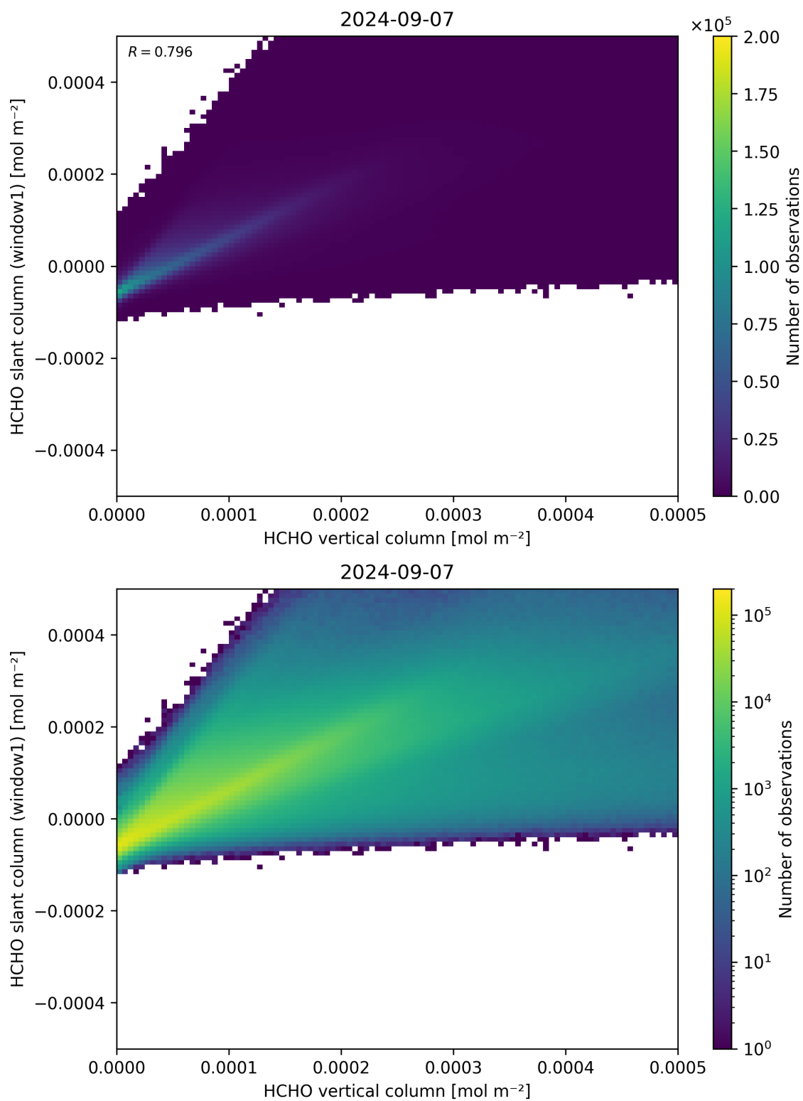
Figure 129: Scatter density plot of “HCHO vertical column” against “HCHO slant column (window1)” for 2024-09-06 to 2024-09-08.
