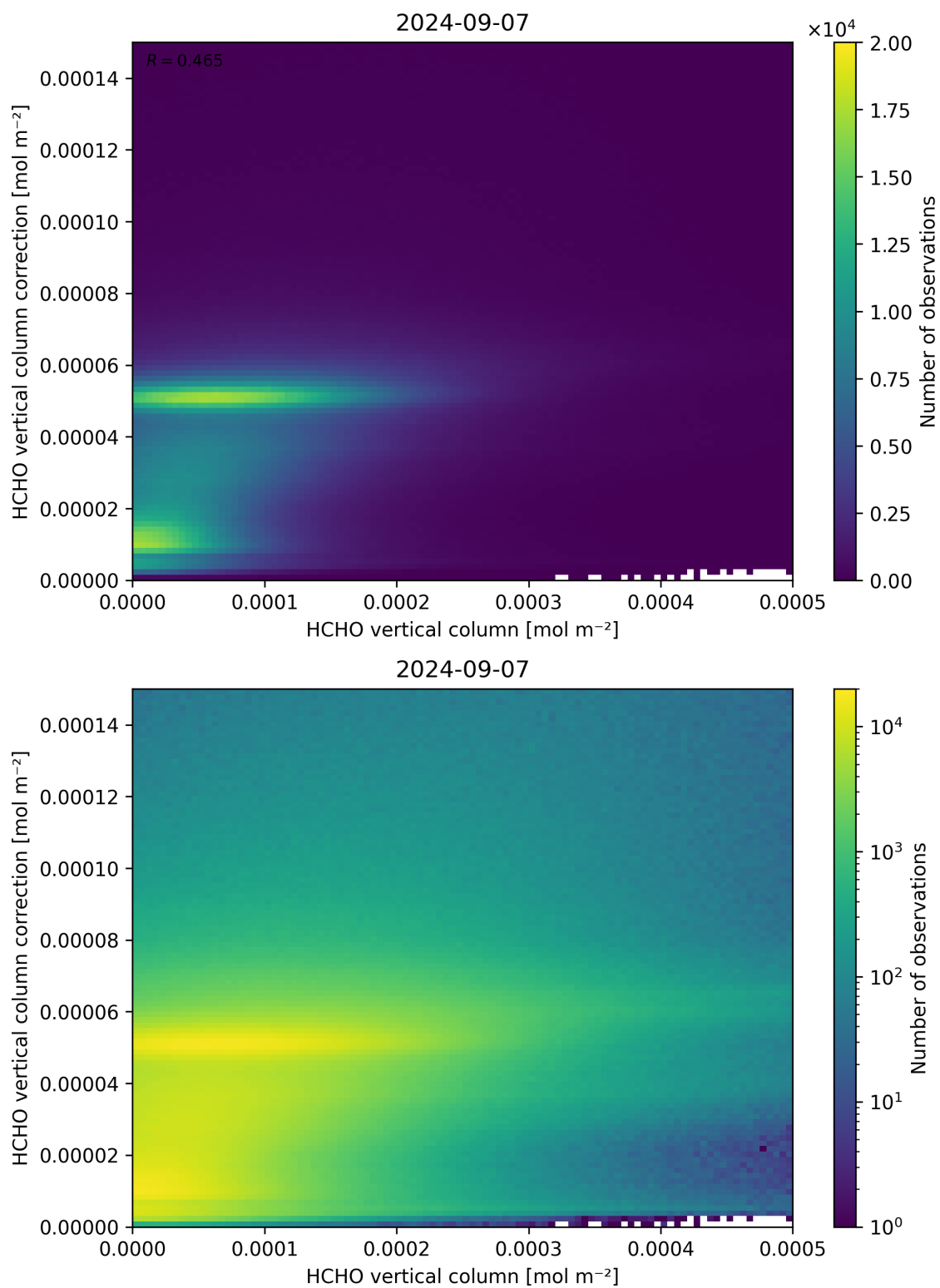
Figure 133: Scatter density plot of “HCHO vertical column” against “HCHO vertical column correction” for 2024-09-06 to 2024-09-08.
