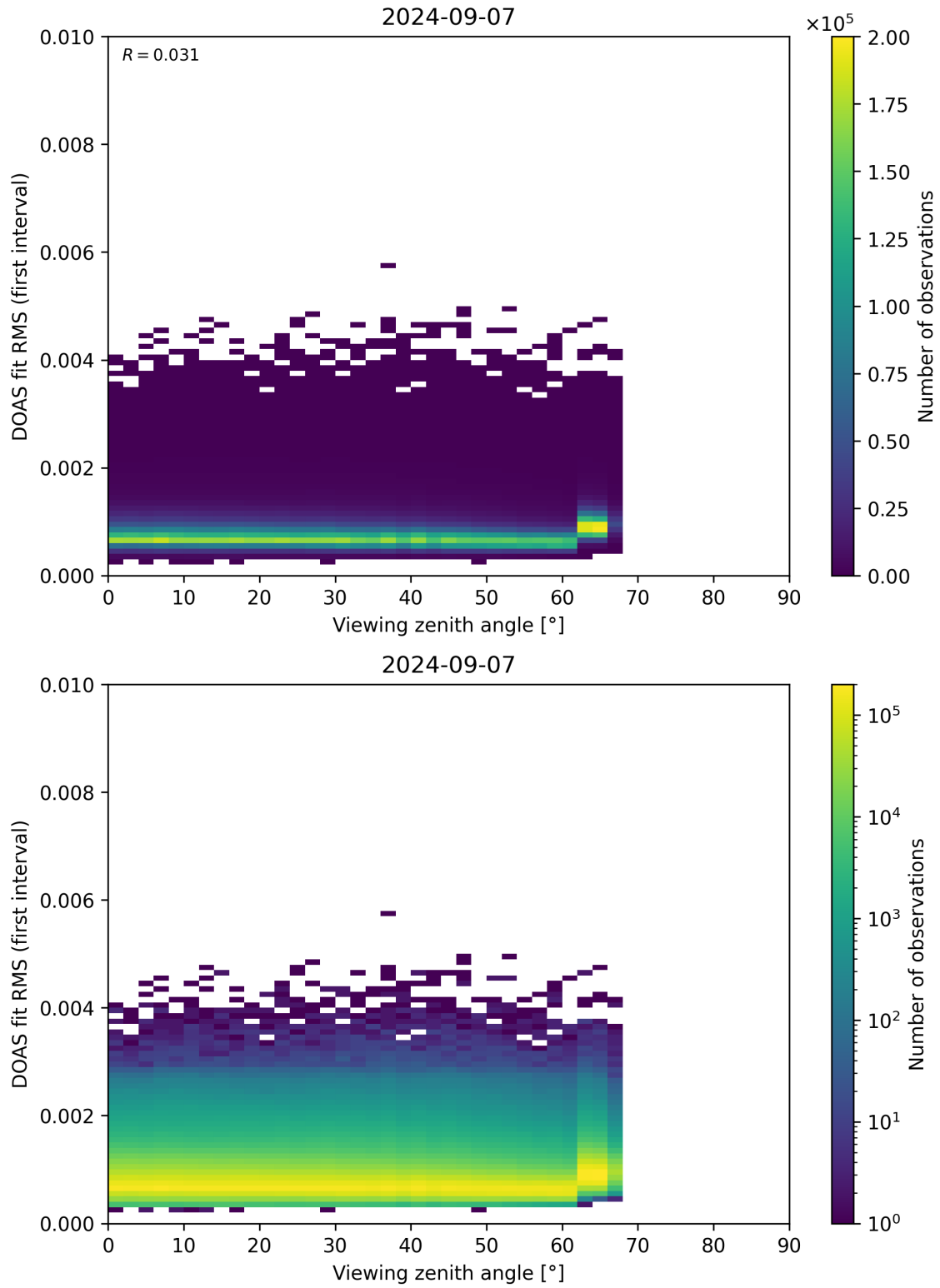
Figure 182: Scatter density plot of “Viewing zenith angle” against “DOAS fit RMS (first interval)” for 2024-09-06 to 2024-09-08.
