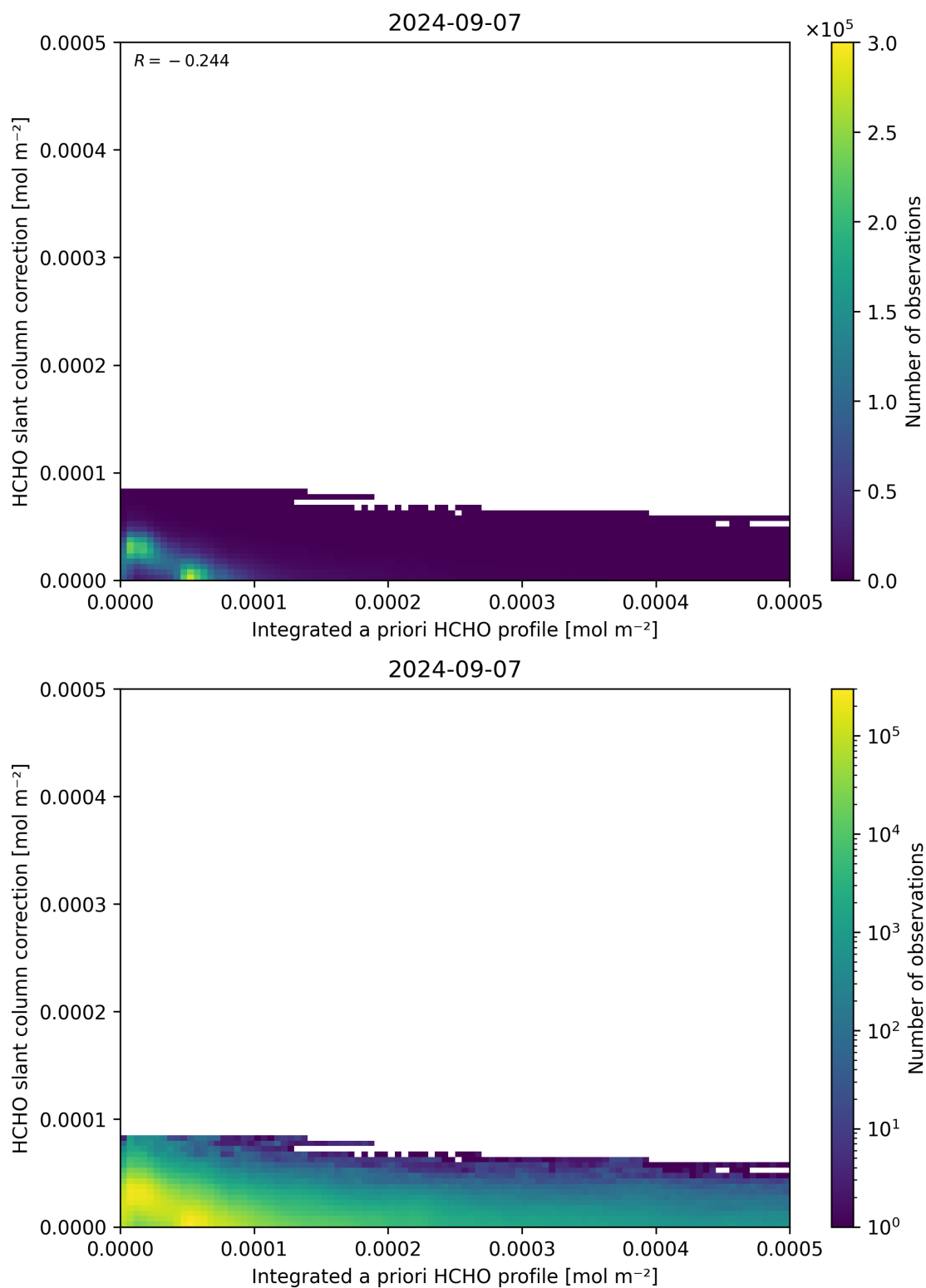
Figure 152: Scatter density plot of “Integrated a priori HCHO profile” against “HCHO slant column correction” for 2024-09-06 to 2024-09-08.
