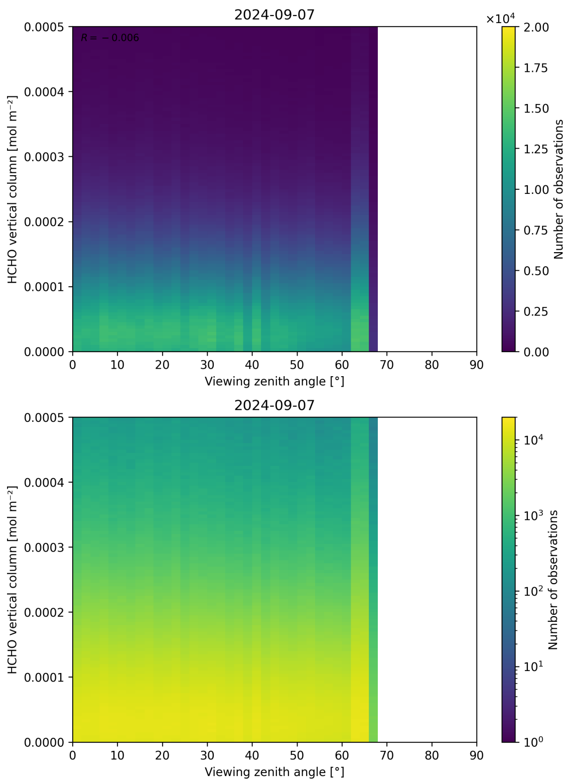
Figure 192: Scatter density plot of “Viewing zenith angle” against “HCHO vertical column” for 2024-09-06 to 2024-09-08.
