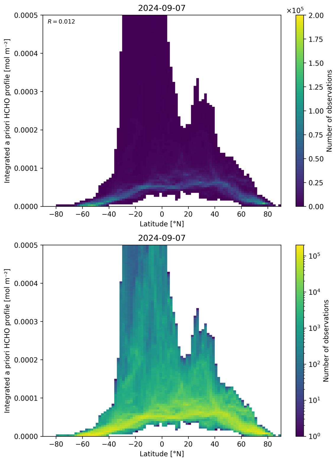
Figure 166: Scatter density plot of “Latitude” against “Integrated a priori HCHO profile” for 2024-09-06 to 2024-09-08.
