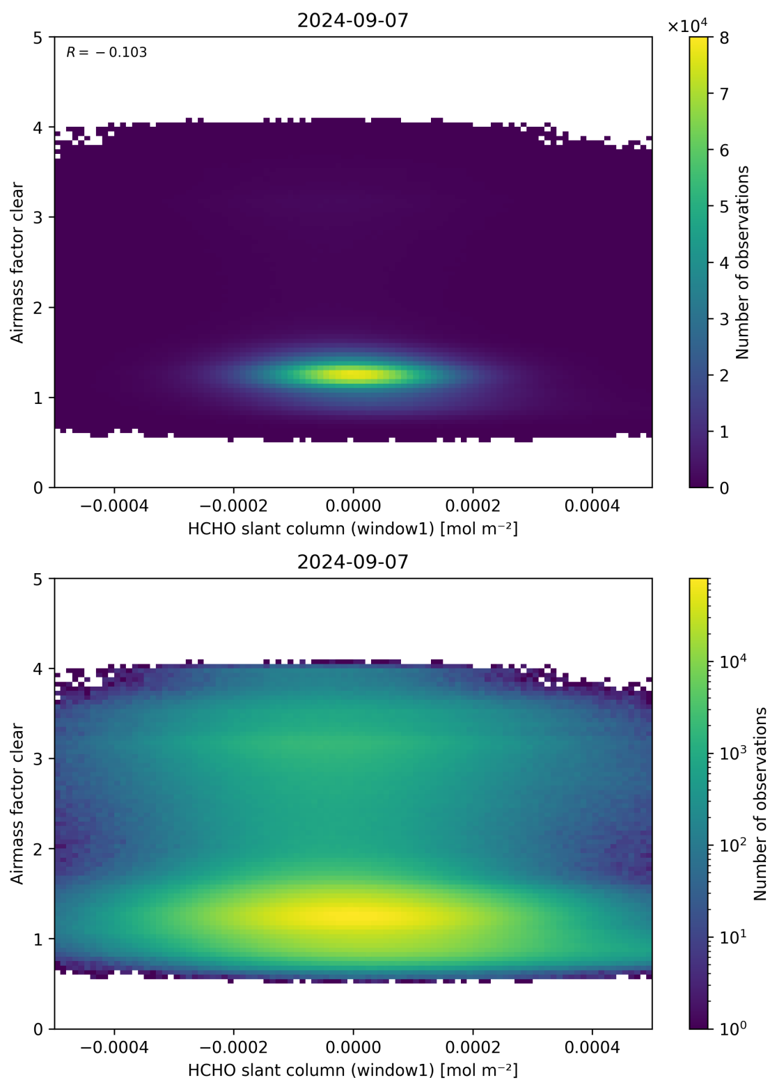
Figure 81: Scatter density plot of “HCHO slant column (window1)” against “Airmass factor clear” for 2024-09-06 to 2024-09-08.
