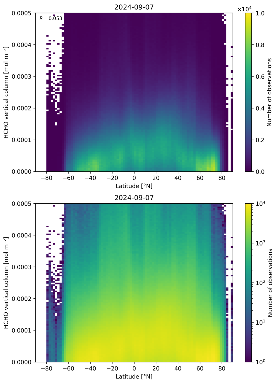
Figure 163: Scatter density plot of “Latitude” against “HCHO vertical column” for 2024-09-06 to 2024-09-08.
