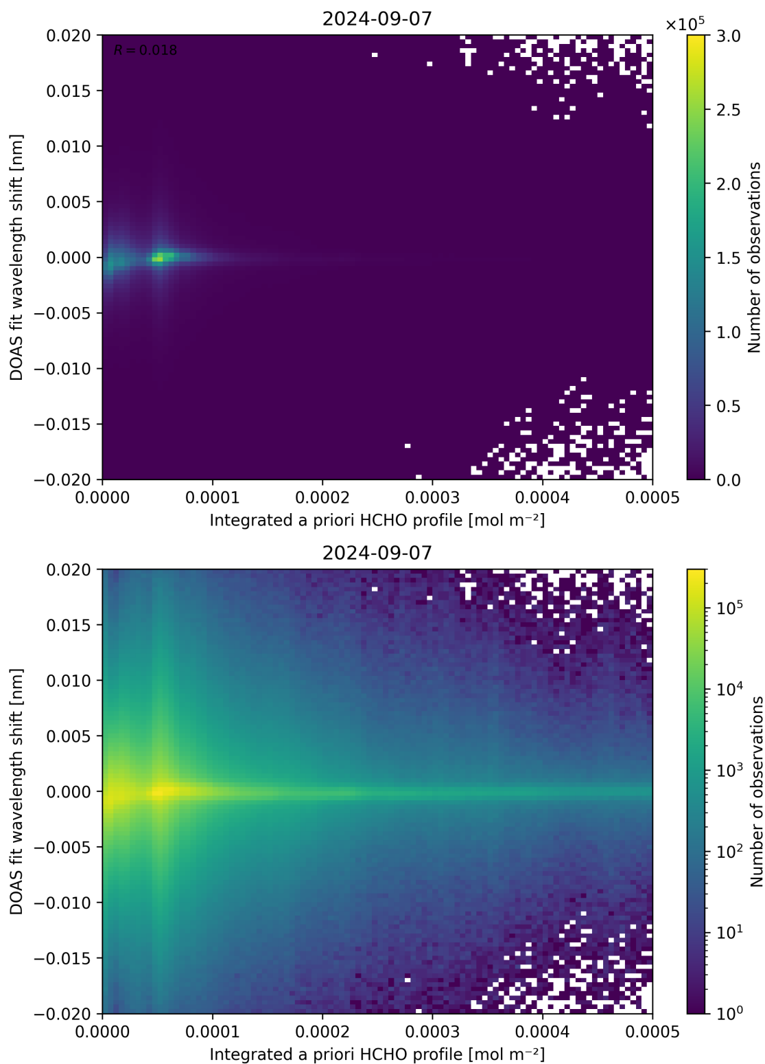
Figure 149: Scatter density plot of “Integrated a priori HCHO profile” against “DOAS fit wavelength shift” for 2024-09-06 to 2024-09-08.
