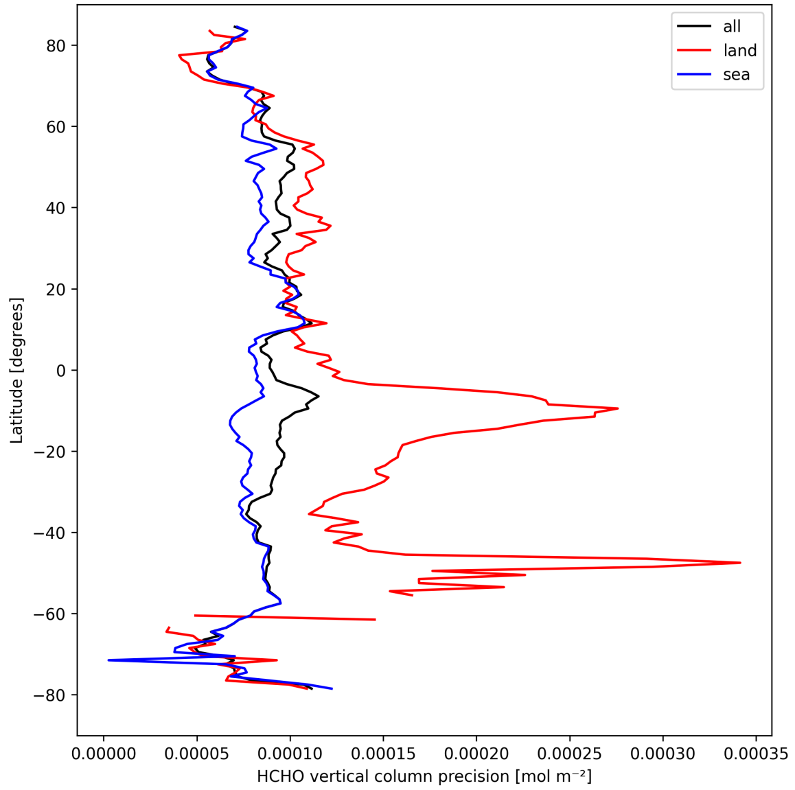
Figure 22: Zonal average of “HCHO vertical column precision” for 2024-09-06 to 2024-09-08.
