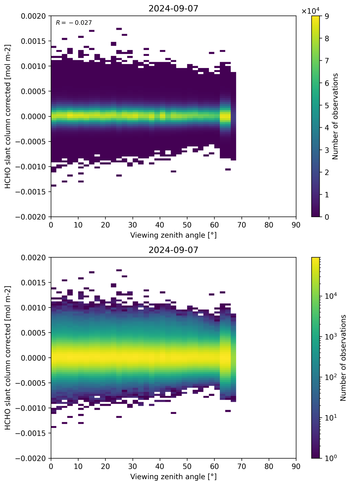
Figure 186: Scatter density plot of “Viewing zenith angle” against “HCHO slant column corrected” for 2024-09-06 to 2024-09-08.
