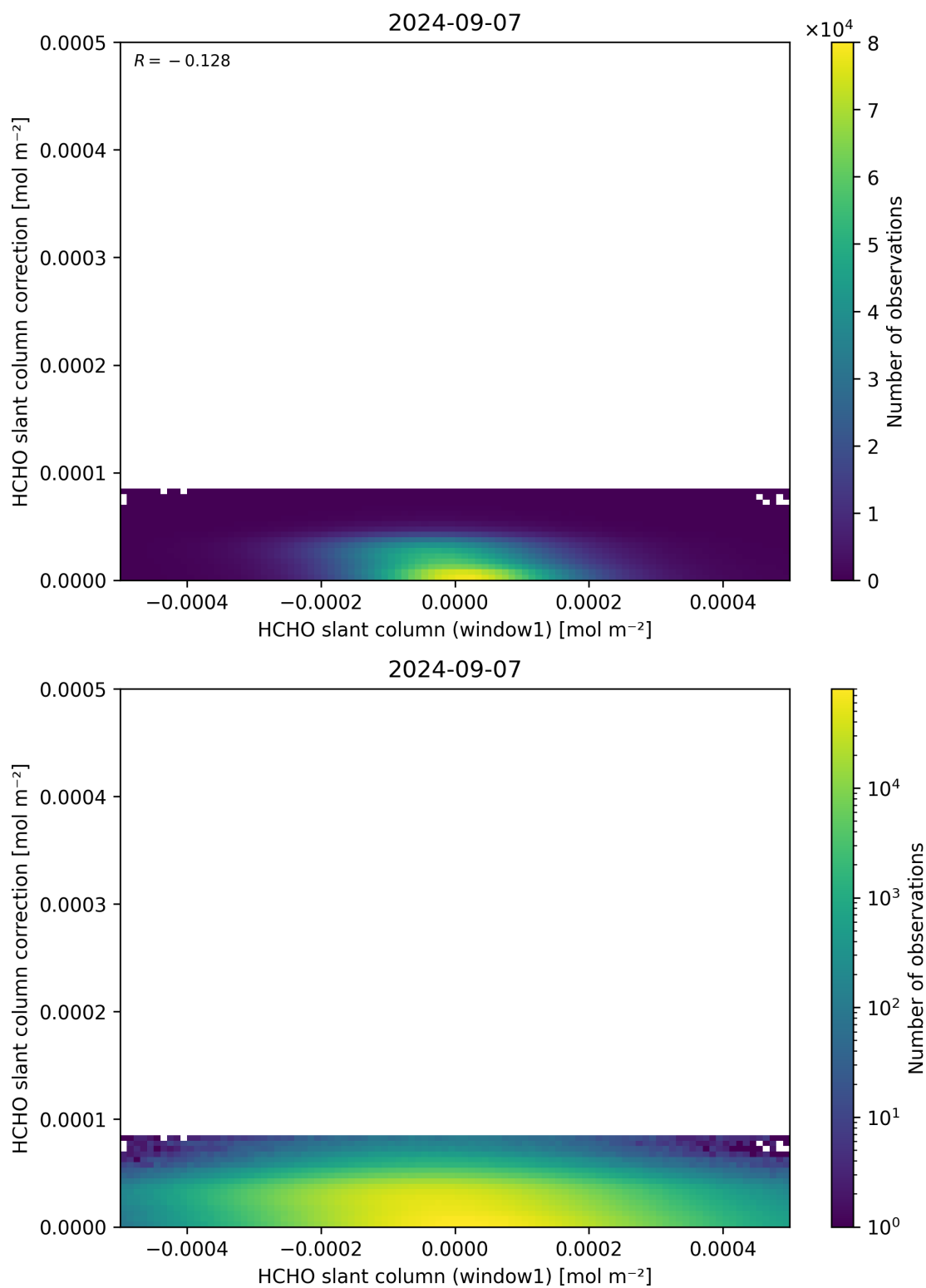
Figure 83: Scatter density plot of “HCHO slant column (window1)” against “HCHO slant column correction” for 2024-09-06 to 2024-09-08.
