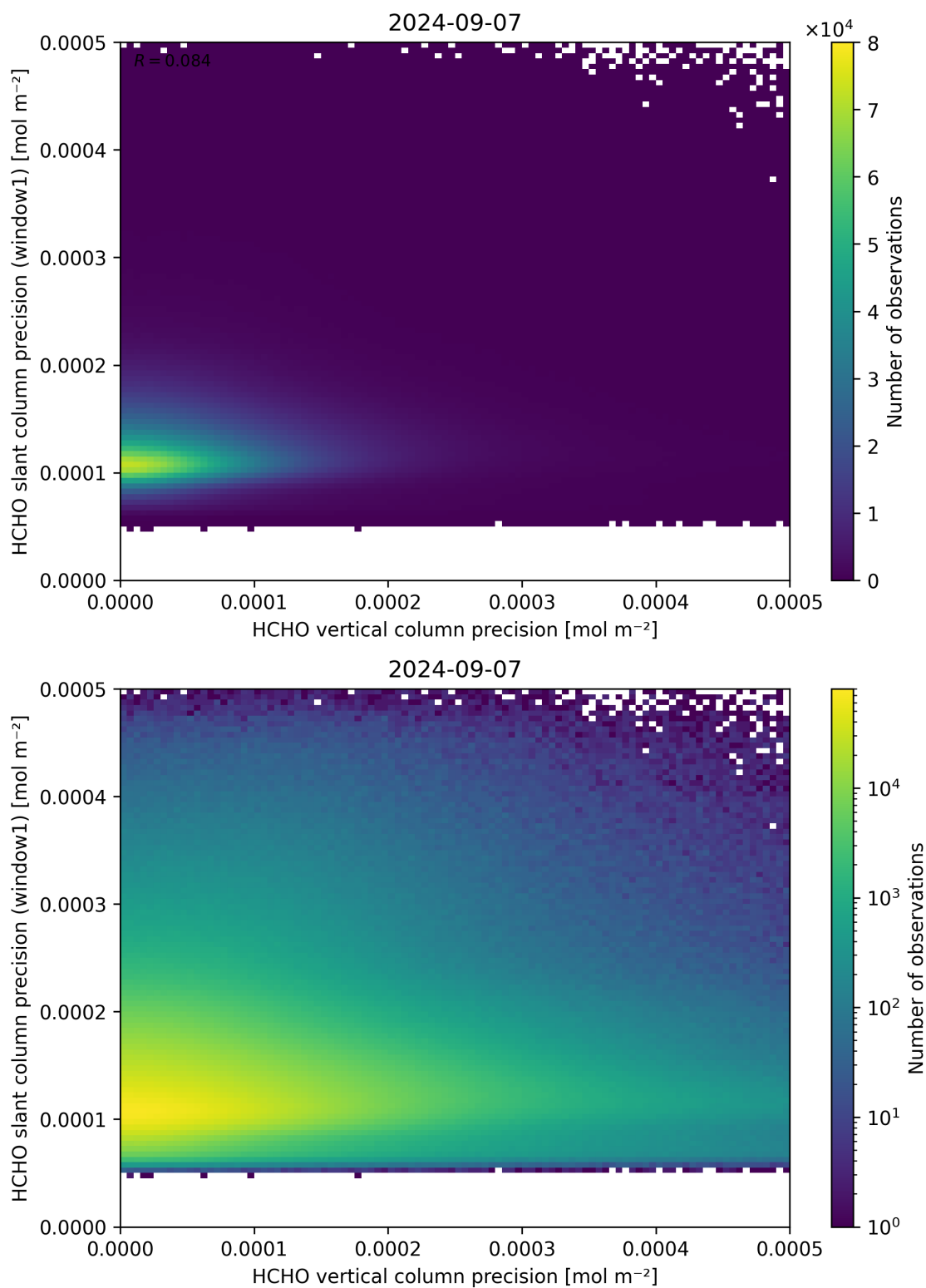
Figure 143: Scatter density plot of “HCHO vertical column precision” against “HCHO slant column precision (window1)” for 2024-09-06 to 2024-09-08.
