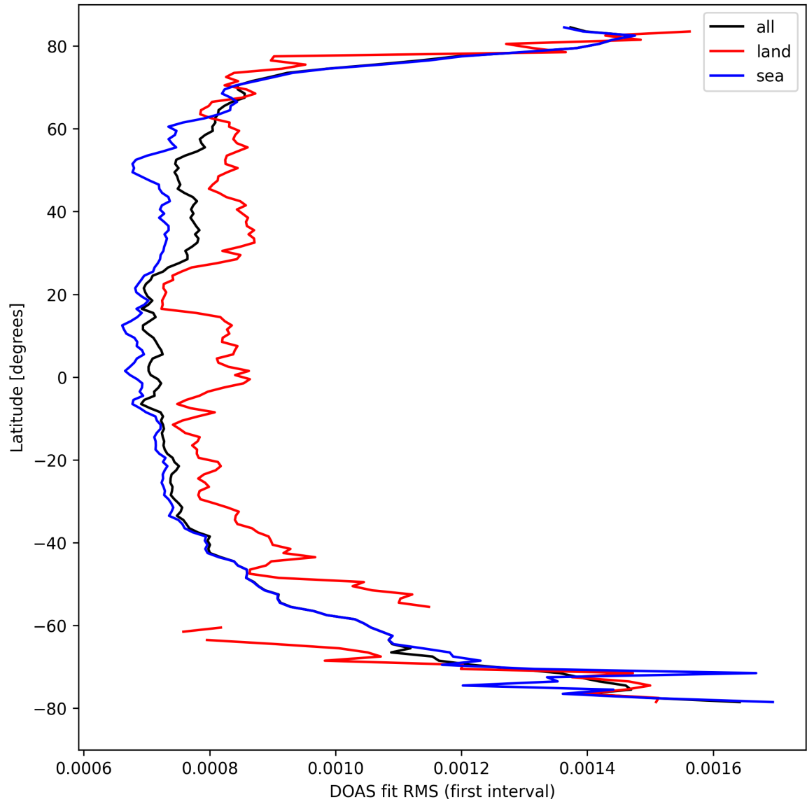
Figure 32: Zonal average of “DOAS fit RMS (first interval)” for 2024-09-06 to 2024-09-08.
