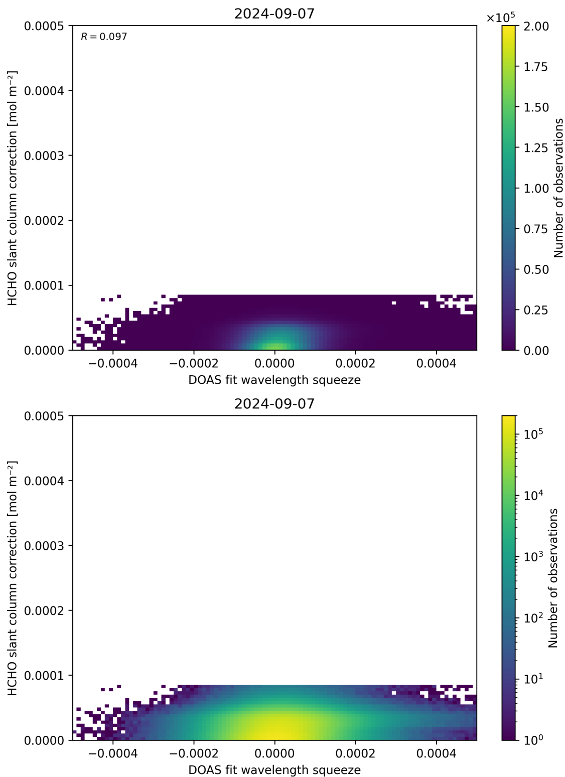
Figure 70: Scatter density plot of “DOAS fit wavelength squeeze” against “HCHO slant column correction” for 2024-09-06 to 2024-09-08.
