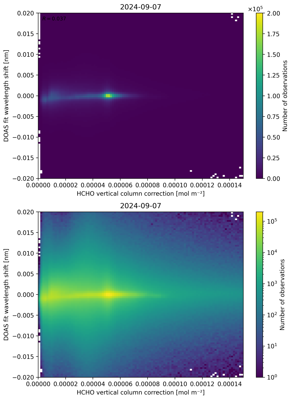
Figure 113: Scatter density plot of “HCHO vertical column correction” against “DOAS fit wavelength shift” for 2024-09-06 to 2024-09-08.
