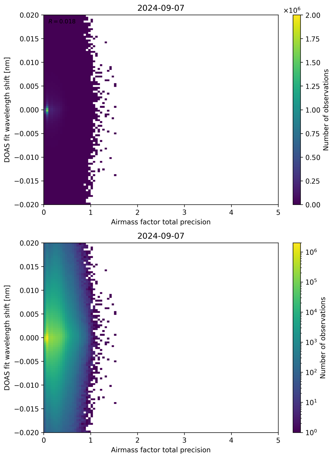
Figure 106: Scatter density plot of “Airmass factor total precision” against “DOAS fit wavelength shift” for 2024-09-06 to 2024-09-08.
