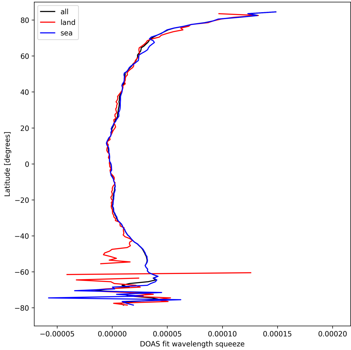
Figure 31: Zonal average of “DOAS fit wavelength squeeze” for 2024-09-06 to 2024-09-08.
