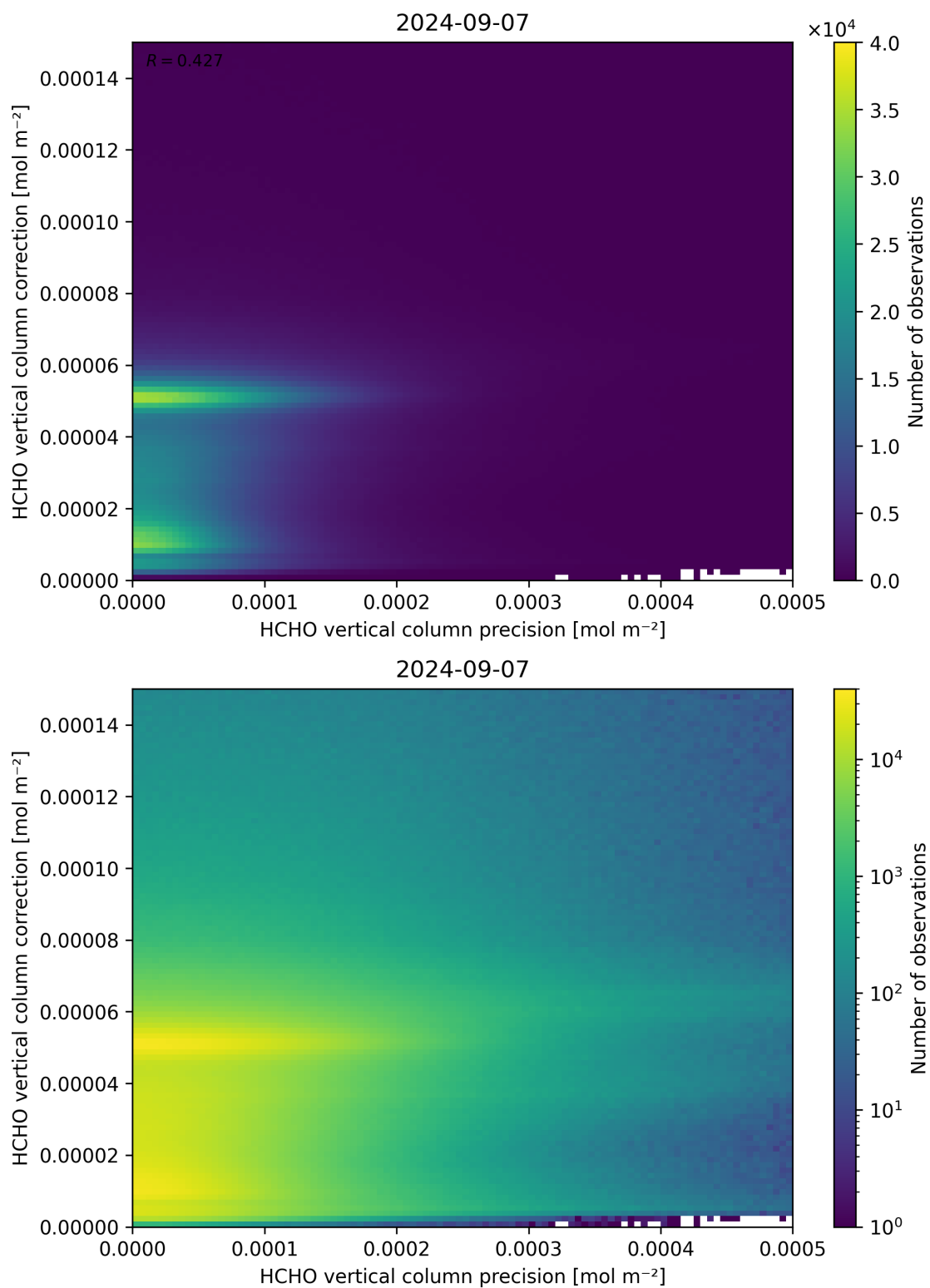
Figure 146: Scatter density plot of “HCHO vertical column precision” against “HCHO vertical column correction” for 2024-09-06 to 2024-09-08.
