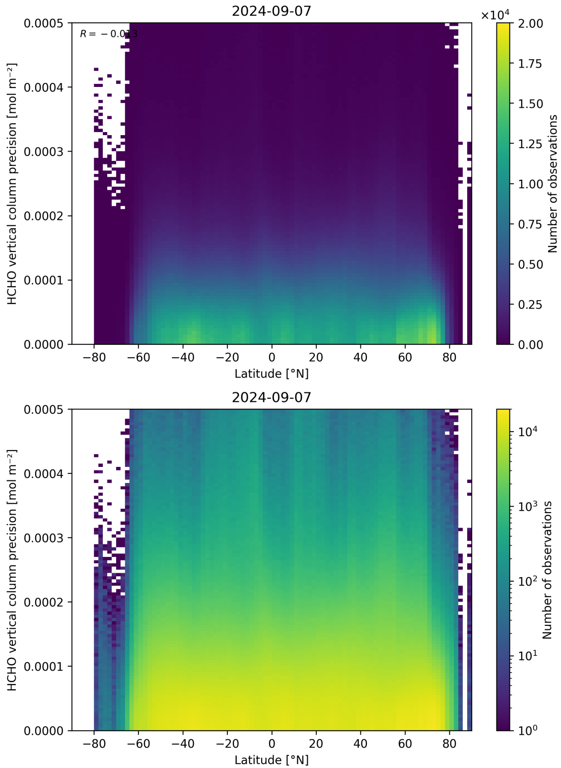
Figure 165: Scatter density plot of “Latitude” against “HCHO vertical column precision” for 2024-09-06 to 2024-09-08.
