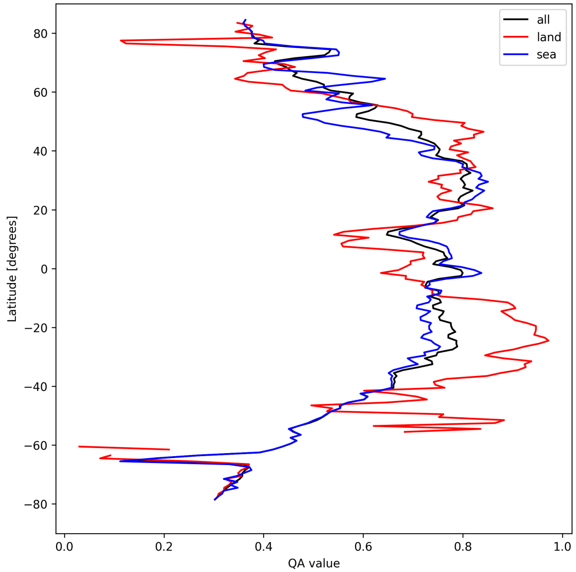
Figure 20: Zonal average of “QA value” for 2024-09-06 to 2024-09-08.
