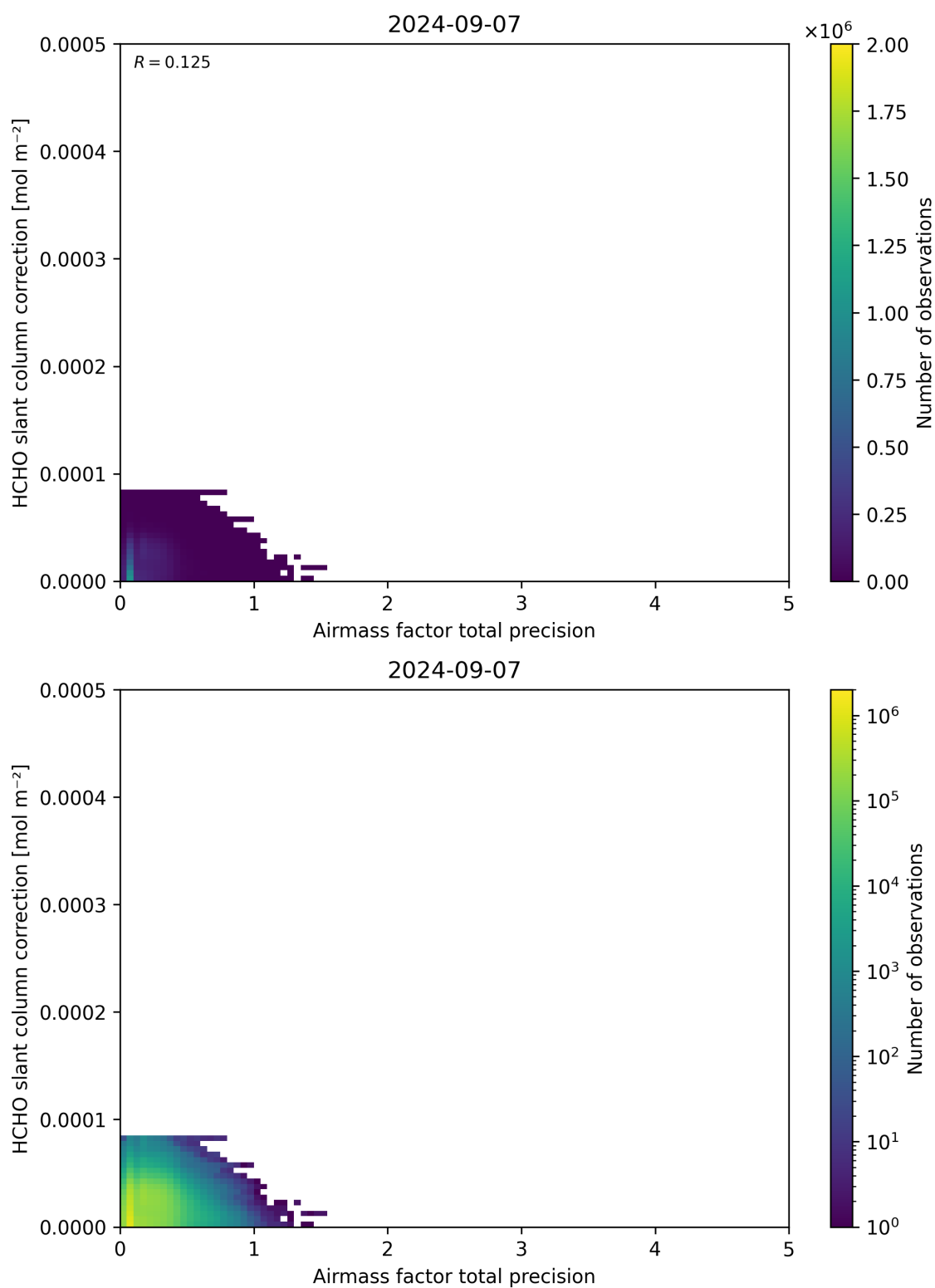
Figure 110: Scatter density plot of “Airmass factor total precision” against “HCHO slant column correction” for 2024-09-06 to 2024-09-08.
