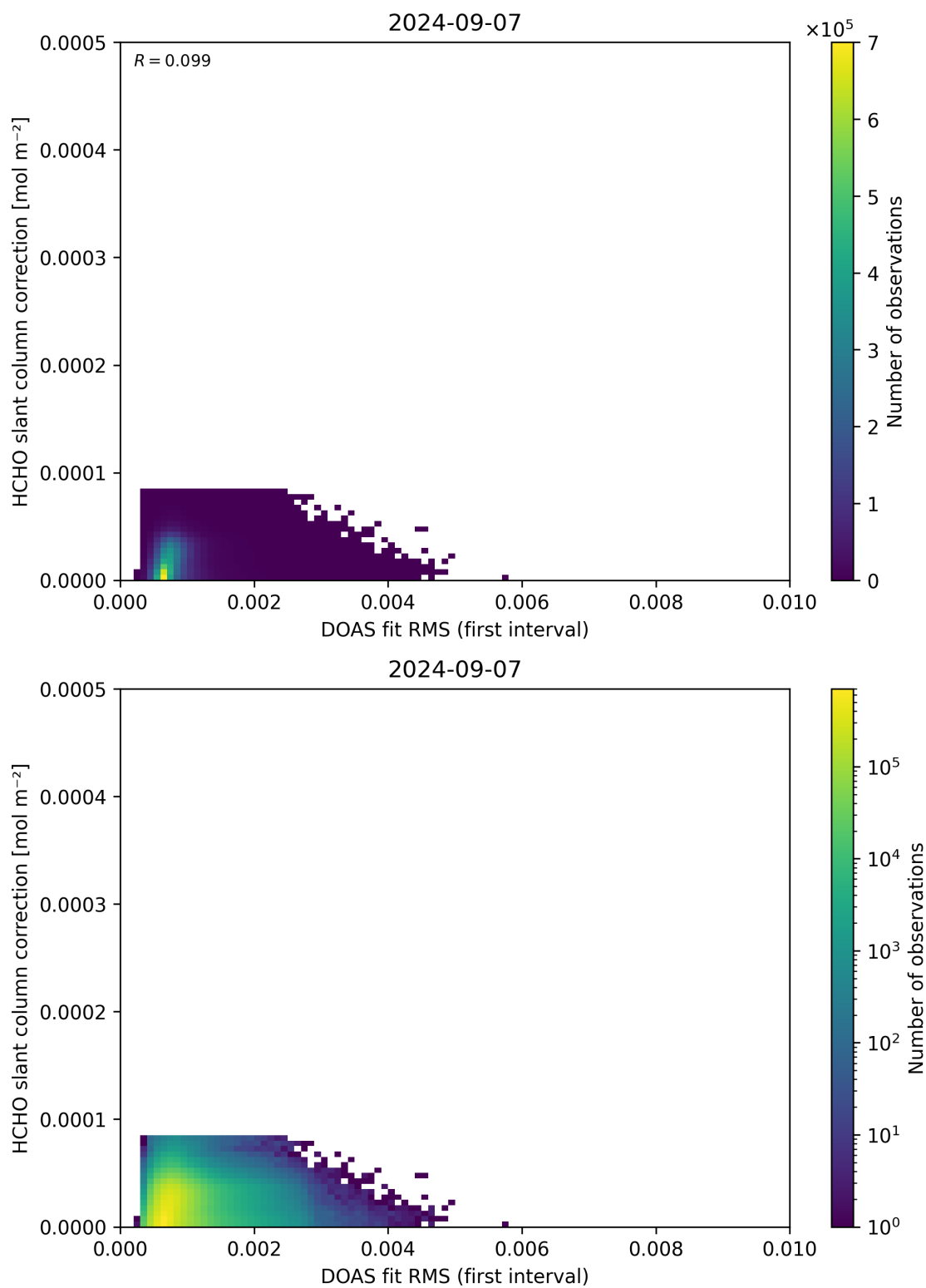
Figure 63: Scatter density plot of “DOAS fit RMS (first interval)” against “HCHO slant column correction” for 2024-09-06 to 2024-09-08.
