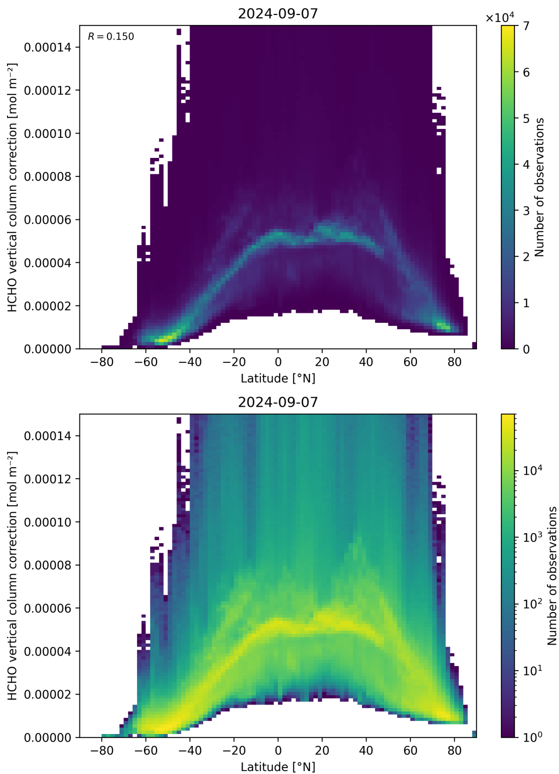
Figure 164: Scatter density plot of “Latitude” against “HCHO vertical column correction” for 2024-09-06 to 2024-09-08.
