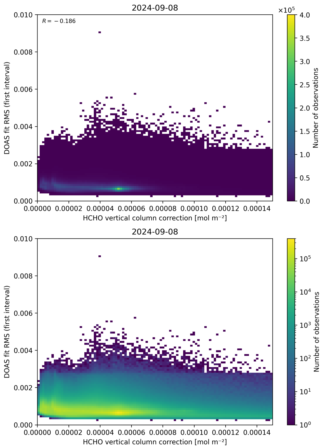
Figure 112: Scatter density plot of “HCHO vertical column correction” against “DOAS fit RMS (first interval)” for 2024-09-07 to 2024-09-09.
