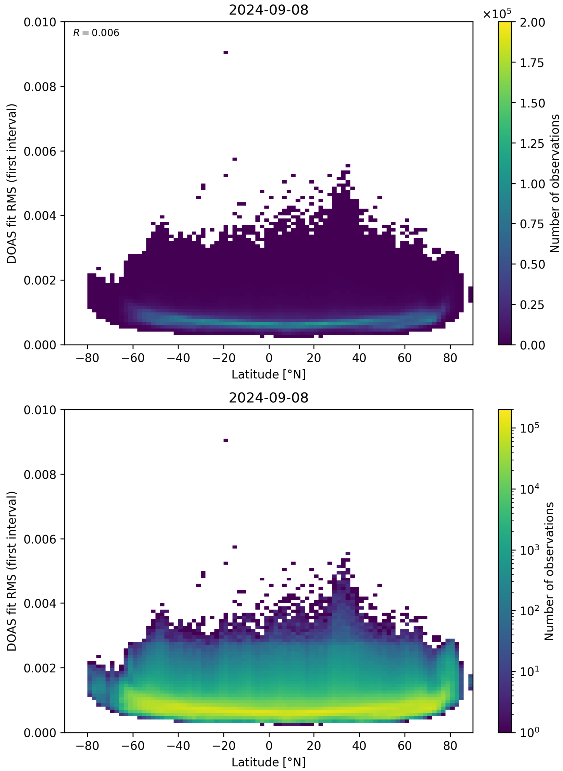
Figure 153: Scatter density plot of “Latitude” against “DOAS fit RMS (first interval)” for 2024-09-07 to 2024-09-09.
