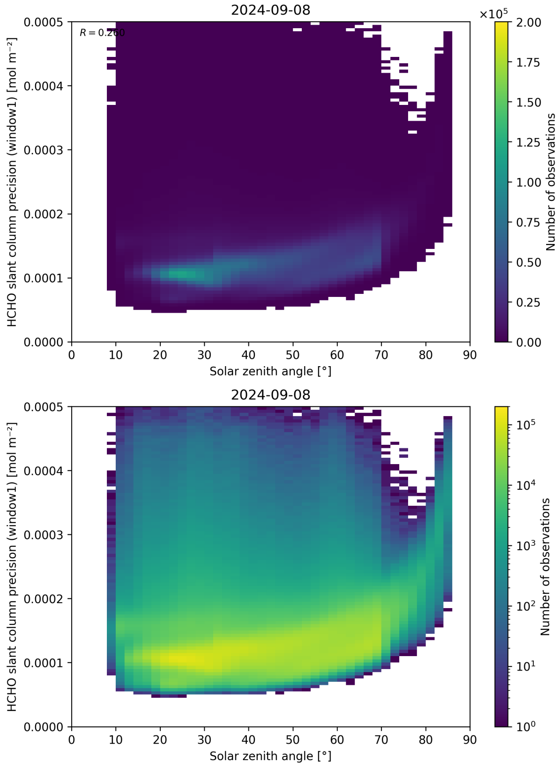
Figure 174: Scatter density plot of “Solar zenith angle” against “HCHO slant column precision (window1)” for 2024-09-07 to 2024-09-09.
