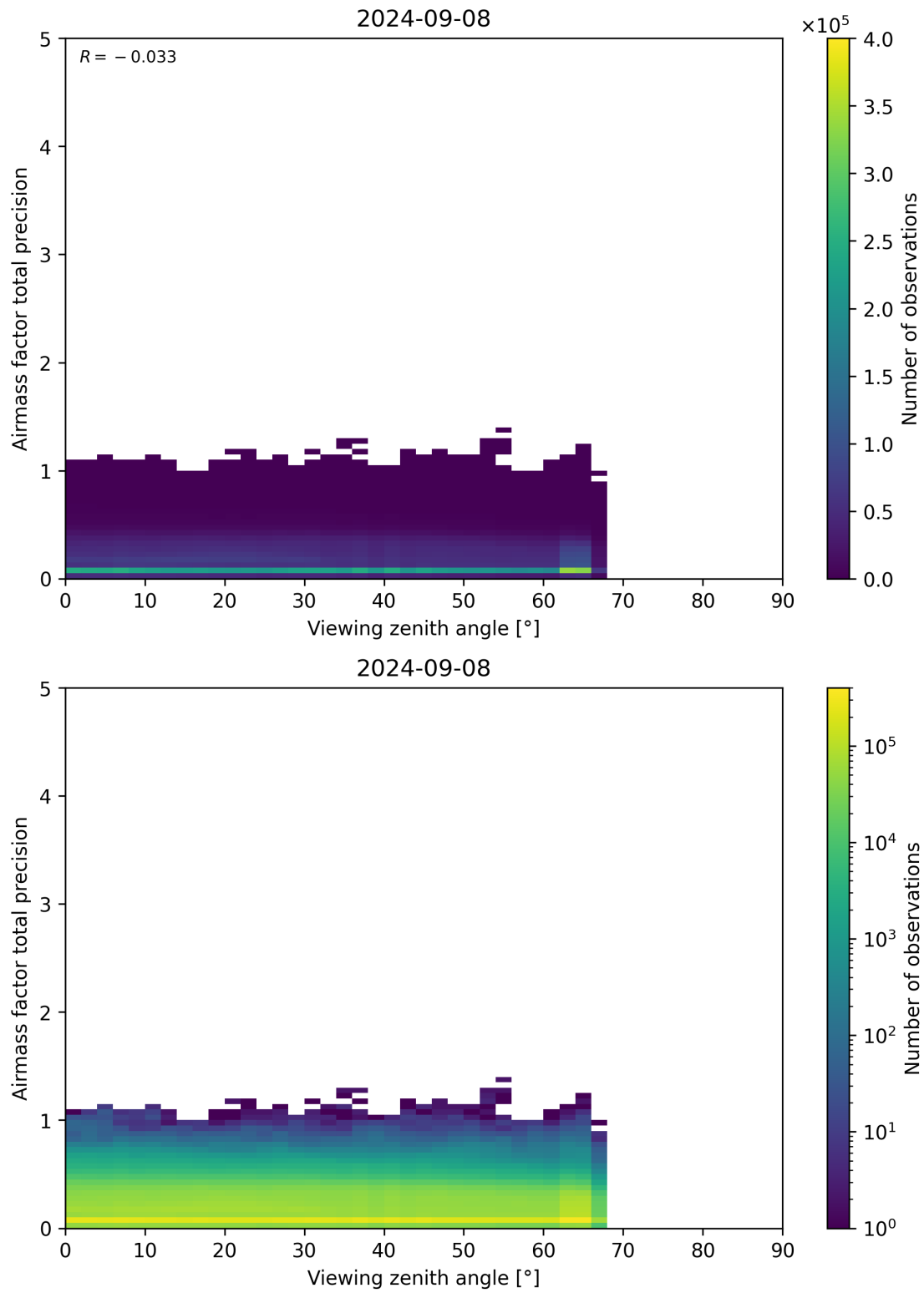
Figure 191: Scatter density plot of “Viewing zenith angle” against “Airmass factor total precision” for 2024-09-07 to 2024-09-09.
