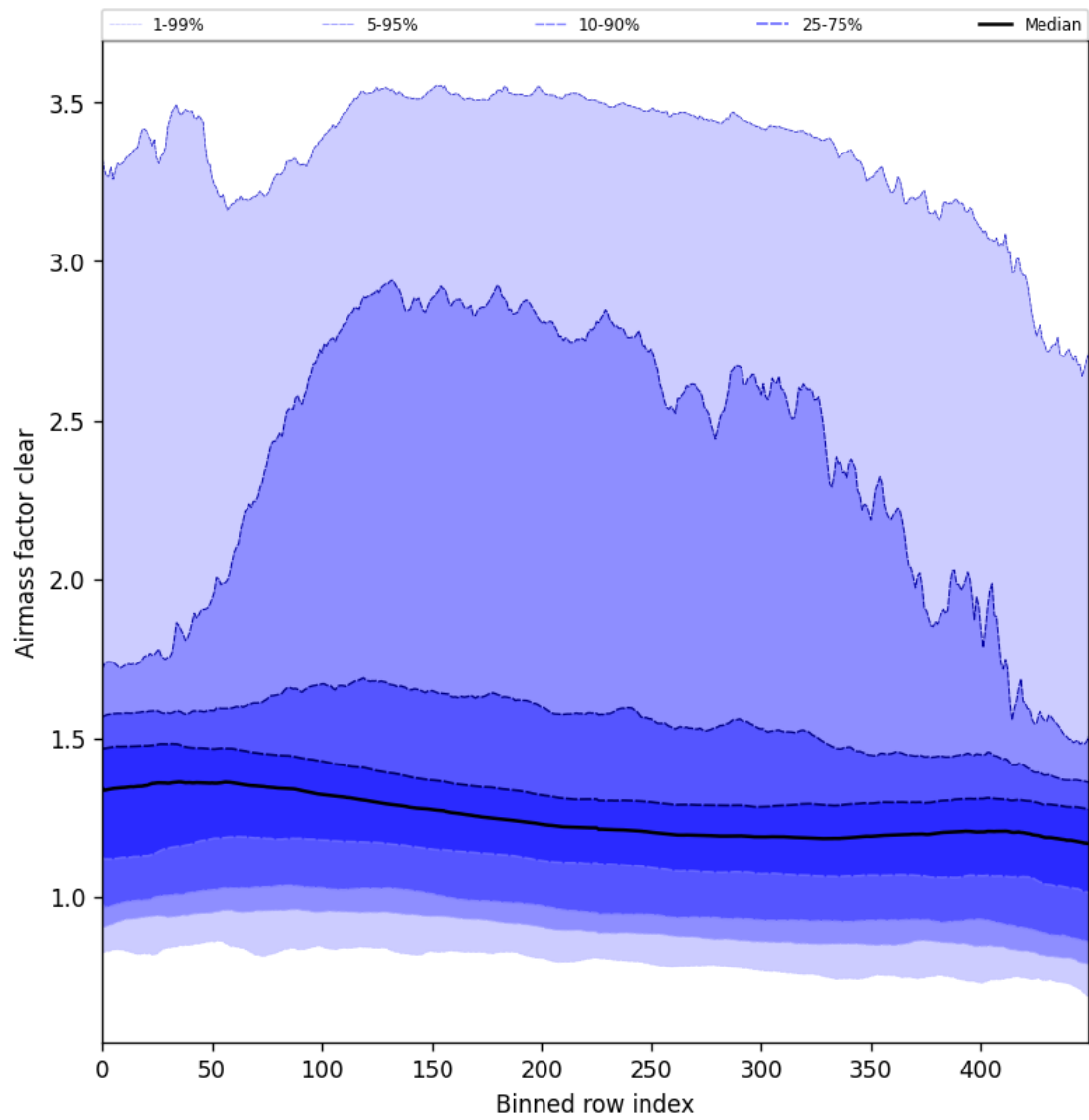
Figure 56: Along track statistics of “Airmass factor clear” for 2024-09-07 to 2024-09-09
