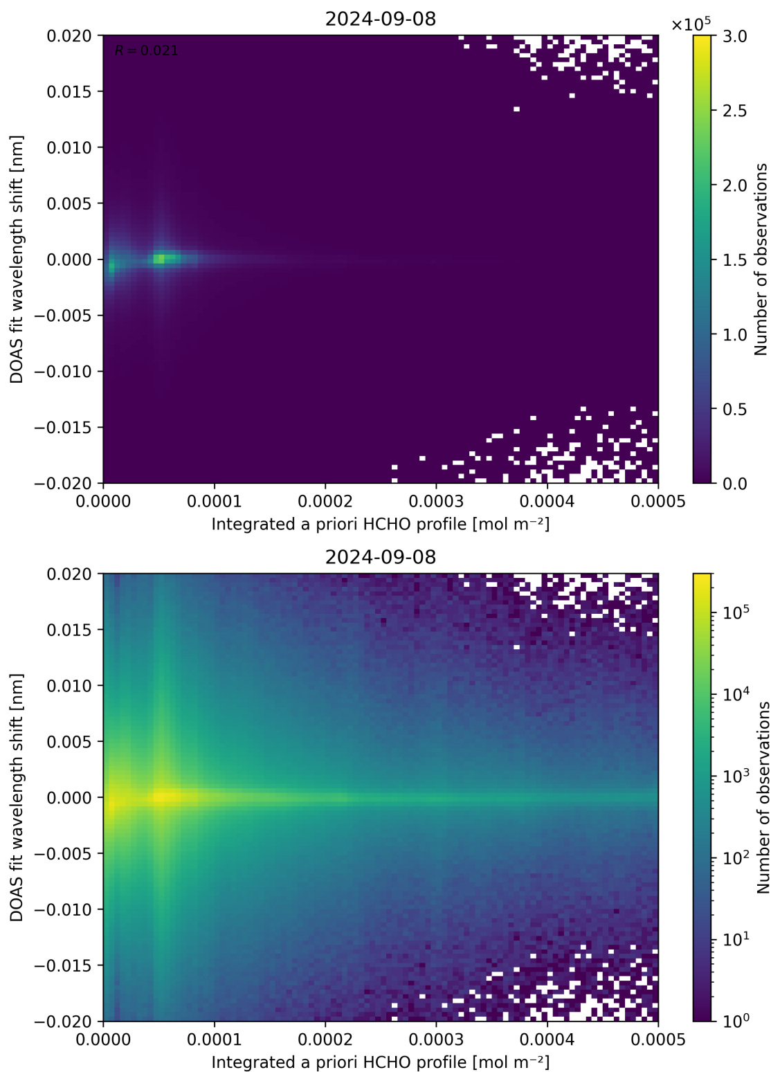
Figure 149: Scatter density plot of “Integrated a priori HCHO profile” against “DOAS fit wavelength shift” for 2024-09-07 to 2024-09-09.
