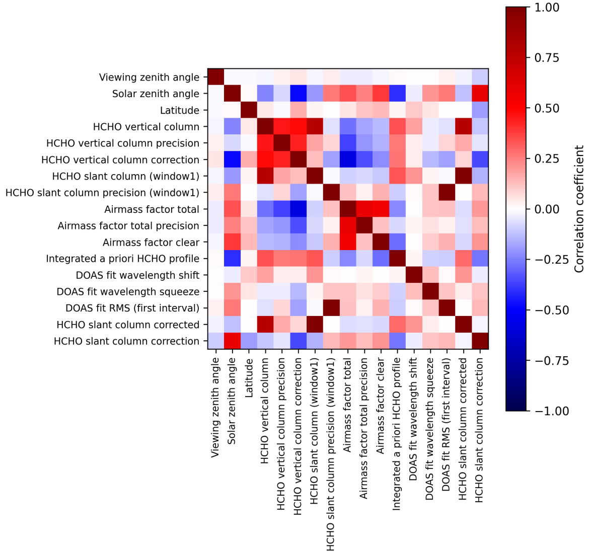
Figure 2: Map of correlation matrix for 2024-09-07 to 2024-09-09.
