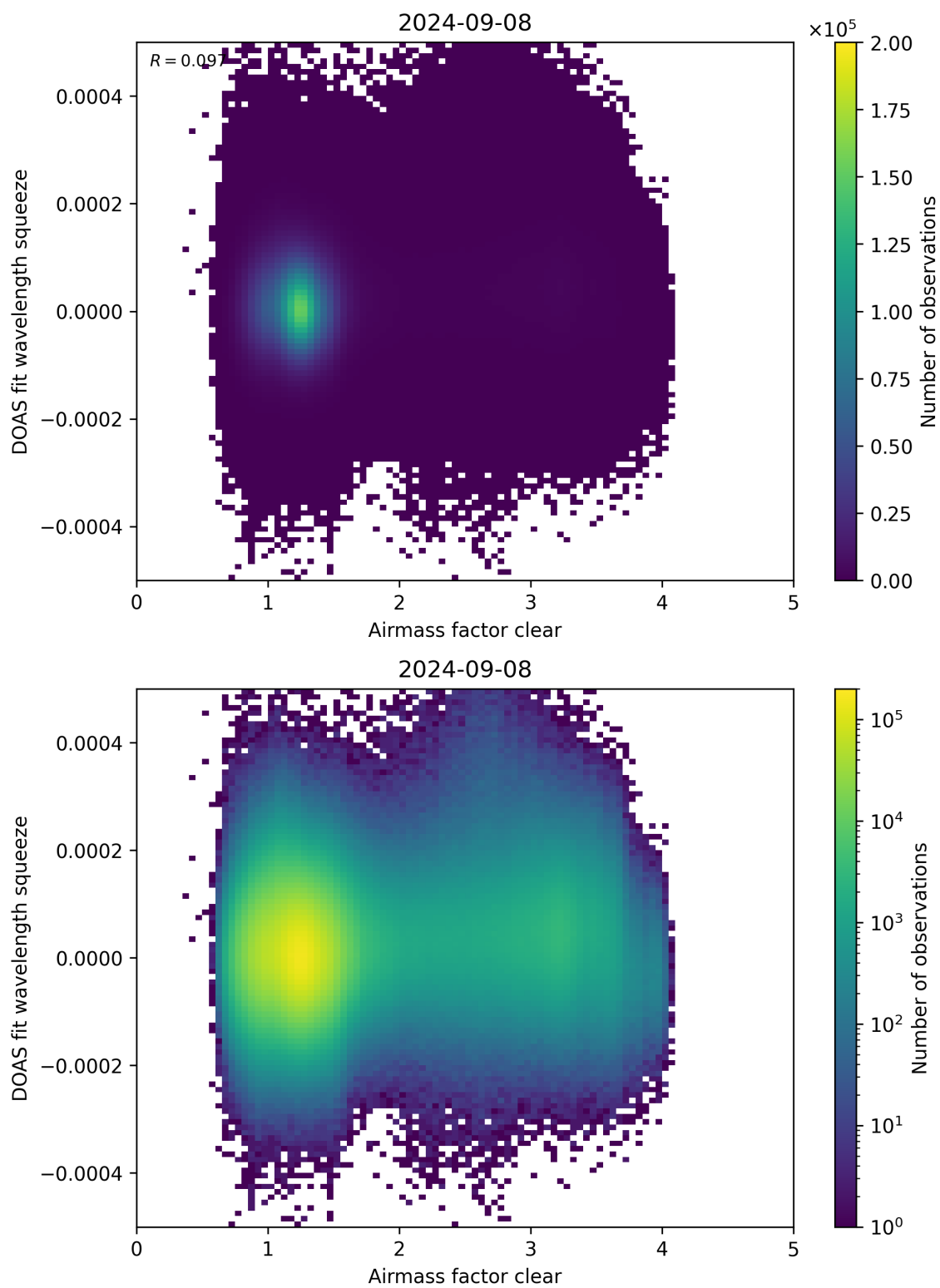
Figure 73: Scatter density plot of “Airmass factor clear” against “DOAS fit wavelength squeeze” for 2024-09-07 to 2024-09-09.
