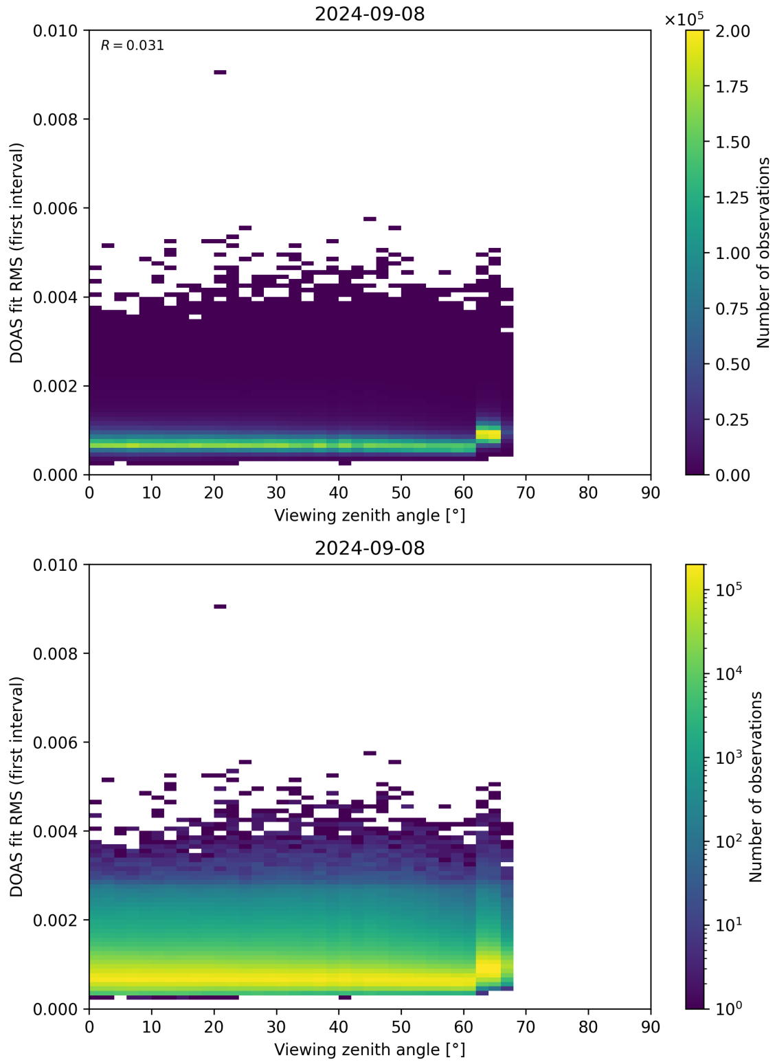
Figure 182: Scatter density plot of “Viewing zenith angle” against “DOAS fit RMS (first interval)” for 2024-09-07 to 2024-09-09.
