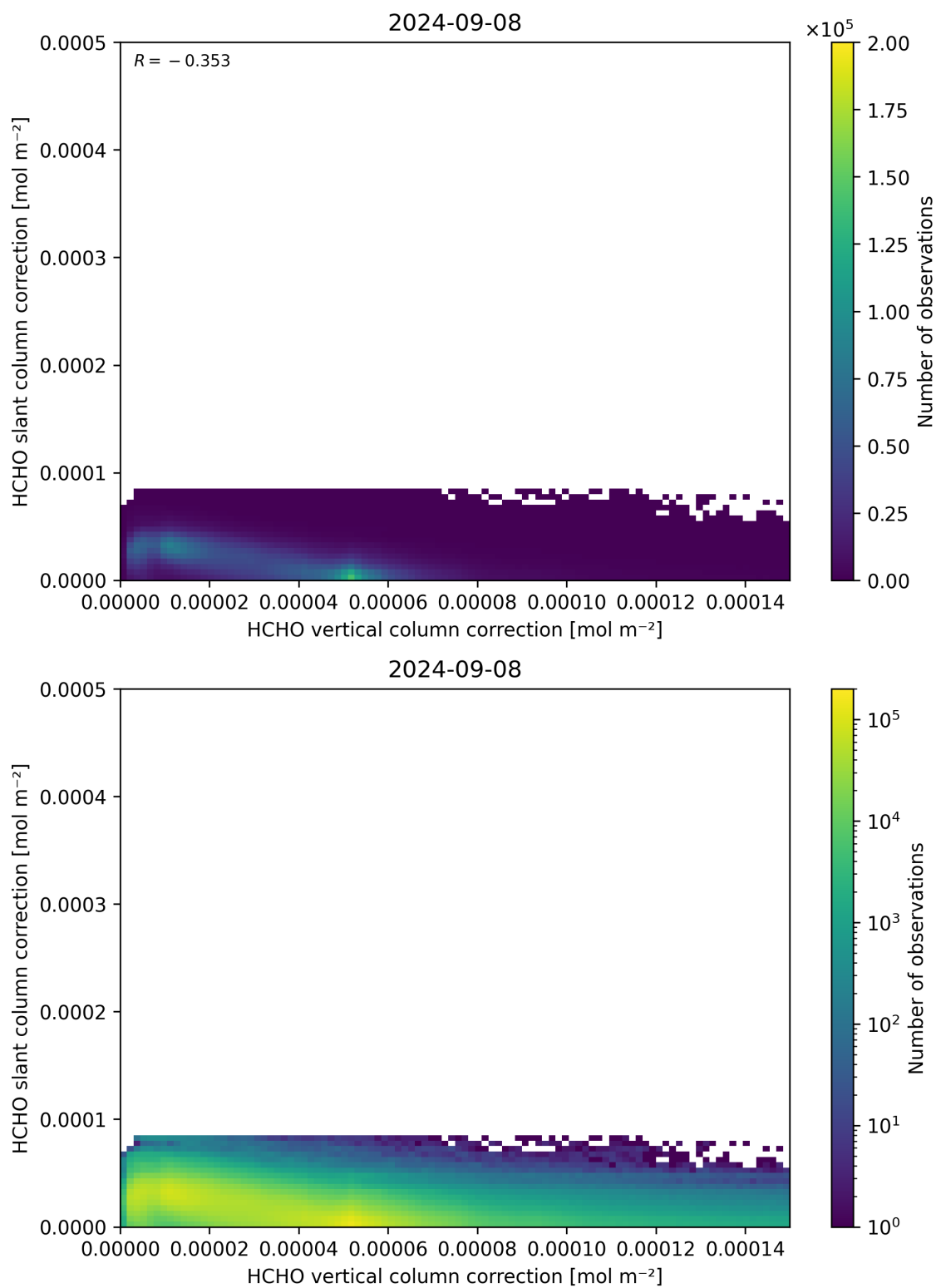
Figure 117: Scatter density plot of “HCHO vertical column correction” against “HCHO slant column correction” for 2024-09-07 to 2024-09-09.
