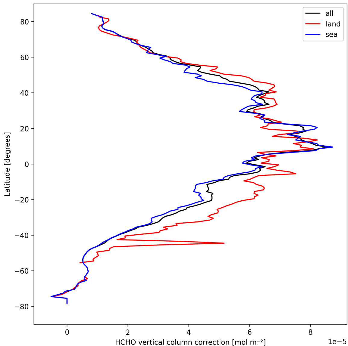
Figure 23: Zonal average of “HCHO vertical column correction” for 2024-09-07 to 2024-09-09.
