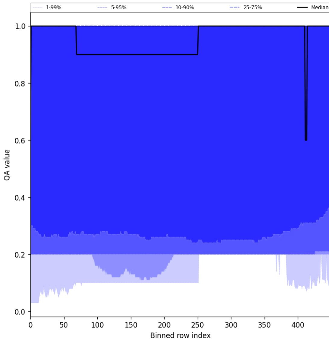
Figure 48: Along track statistics of “QA value” for 2024-09-07 to 2024-09-09
