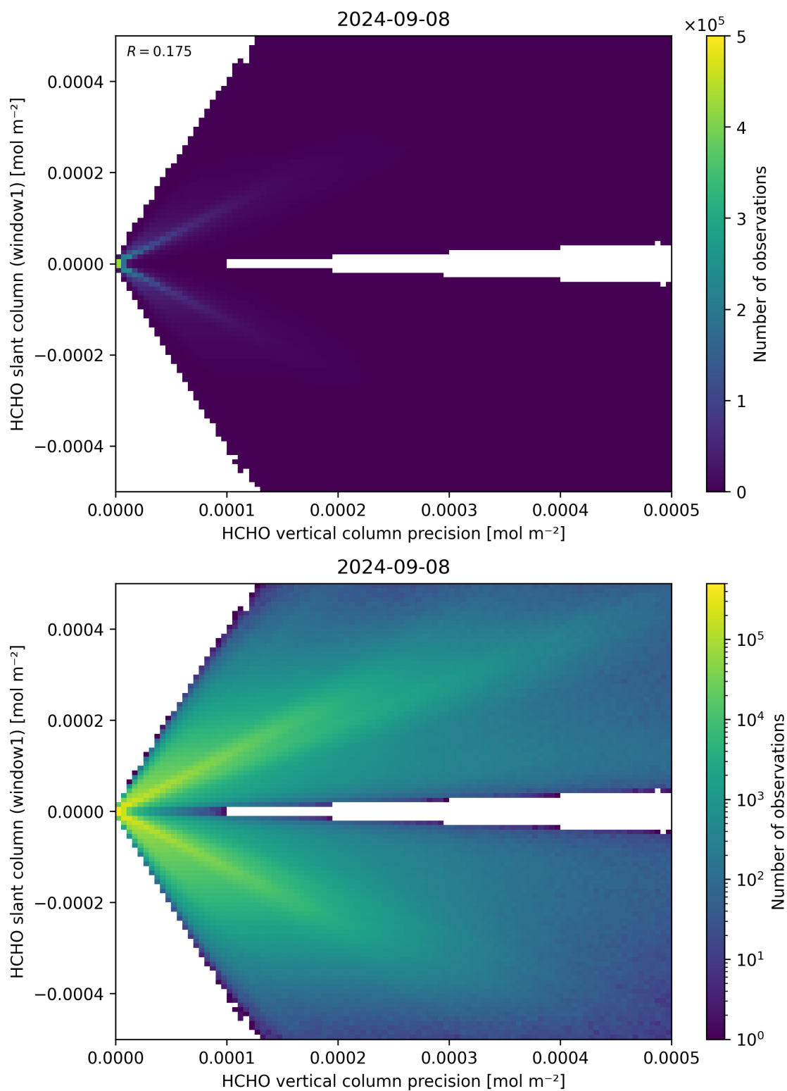
Figure 142: Scatter density plot of “HCHO vertical column precision” against “HCHO slant column (window1)” for 2024-09-07 to 2024-09-09.
