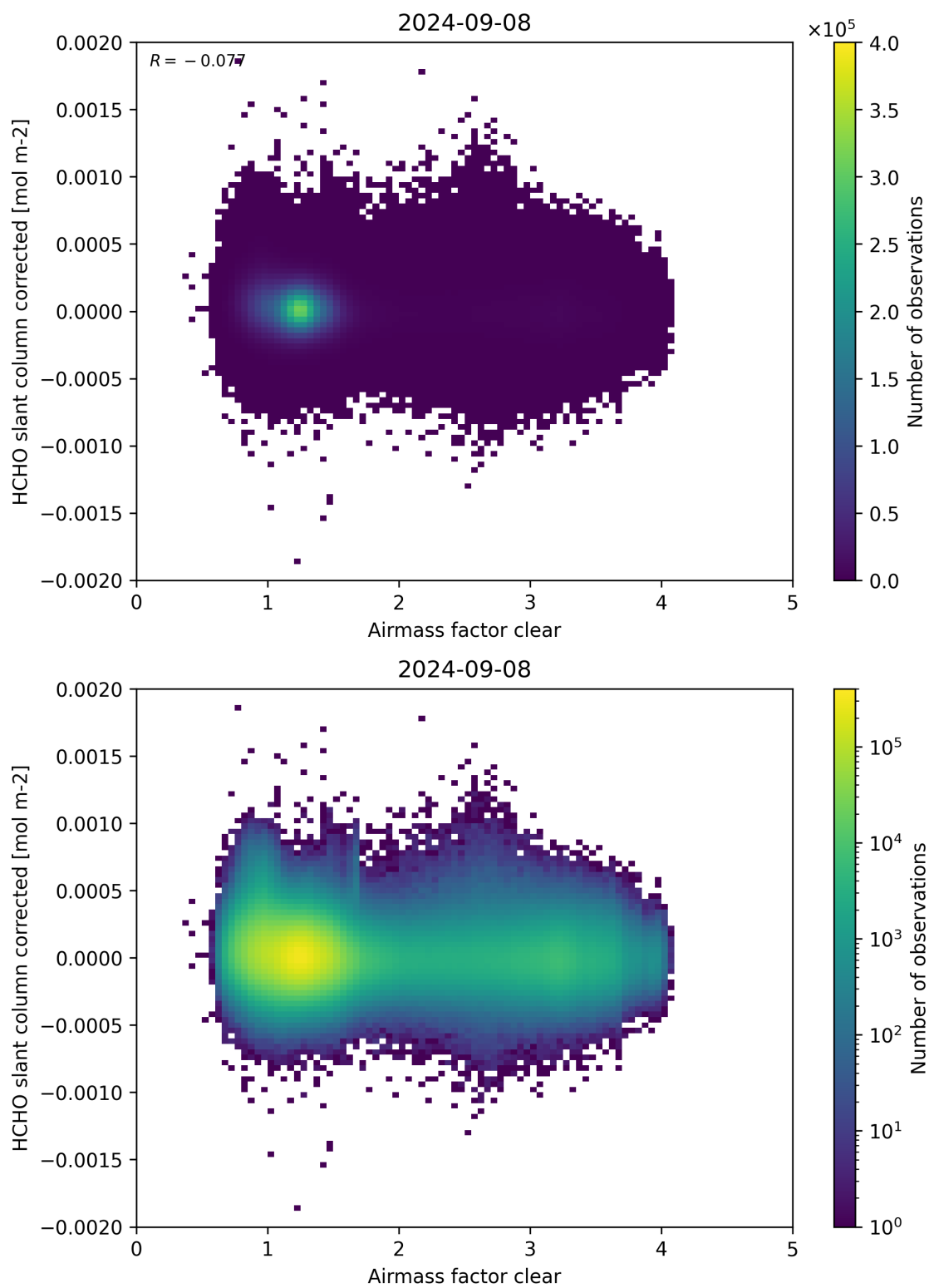
Figure 74: Scatter density plot of “Airmass factor clear” against “HCHO slant column corrected” for 2024-09-07 to 2024-09-09.
