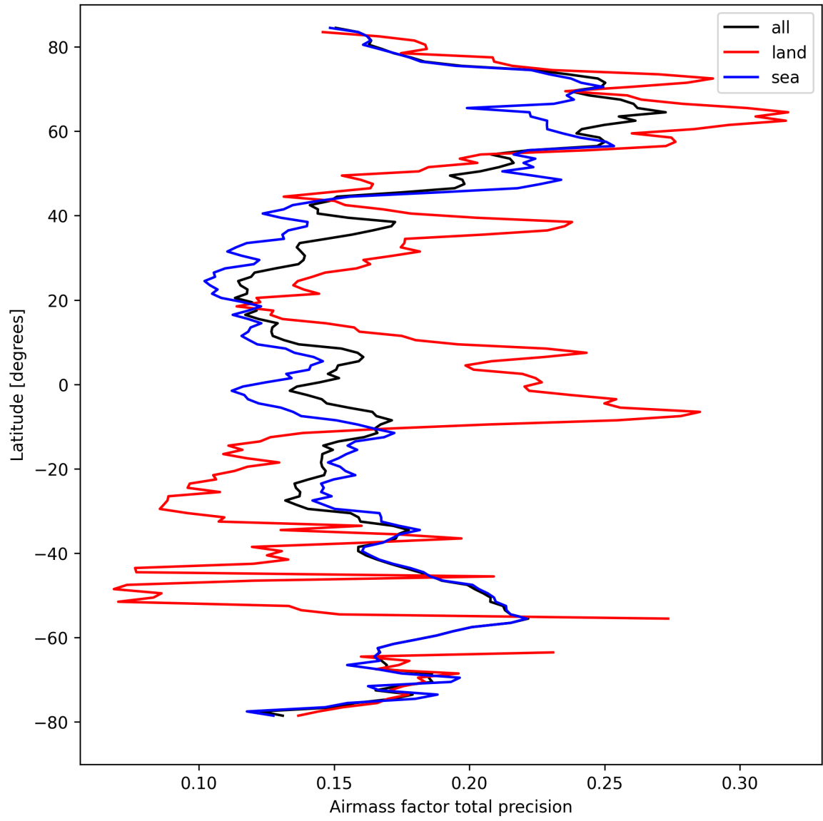
Figure 27: Zonal average of “Airmass factor total precision” for 2024-09-07 to 2024-09-09.
