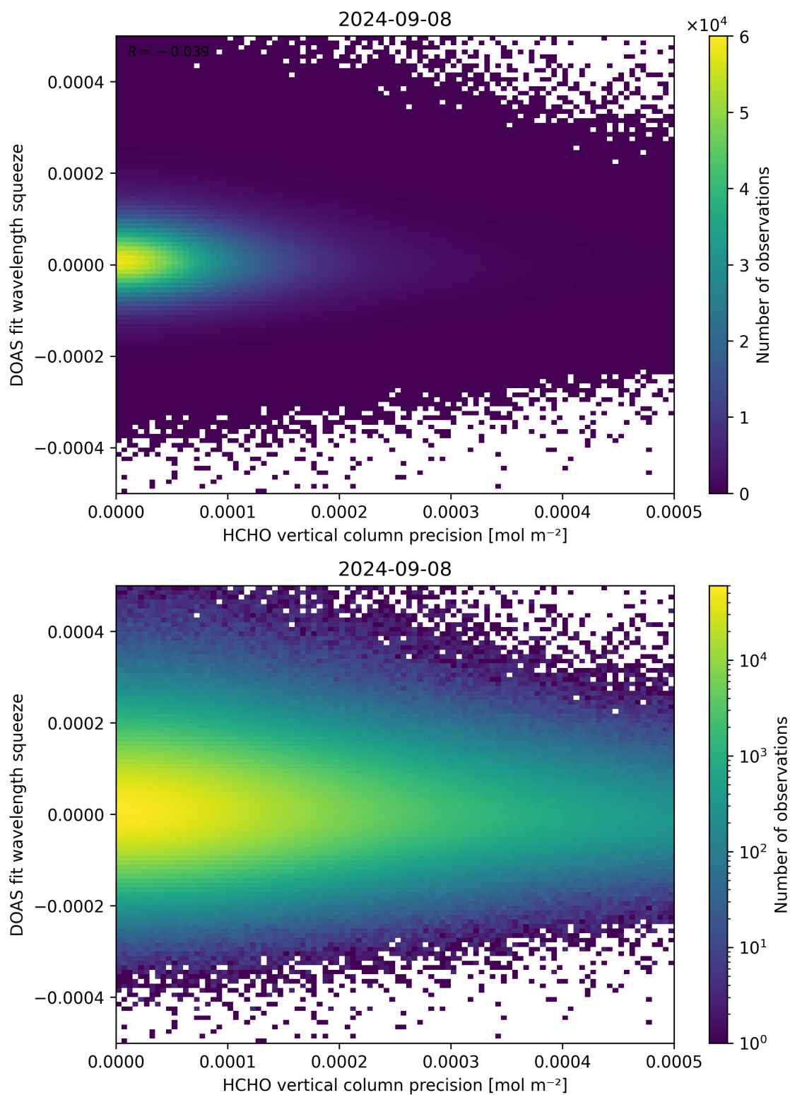
Figure 138: Scatter density plot of “HCHO vertical column precision” against “DOAS fit wavelength squeeze” for 2024-09-07 to 2024-09-09.
