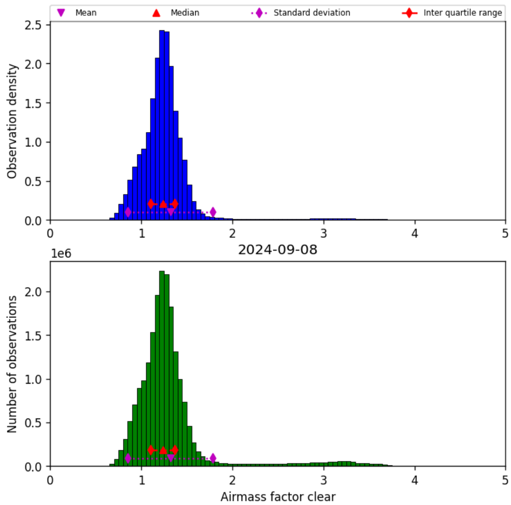
Figure 42: Histogram of “Airmass factor clear” for 2024-09-07 to 2024-09-09
