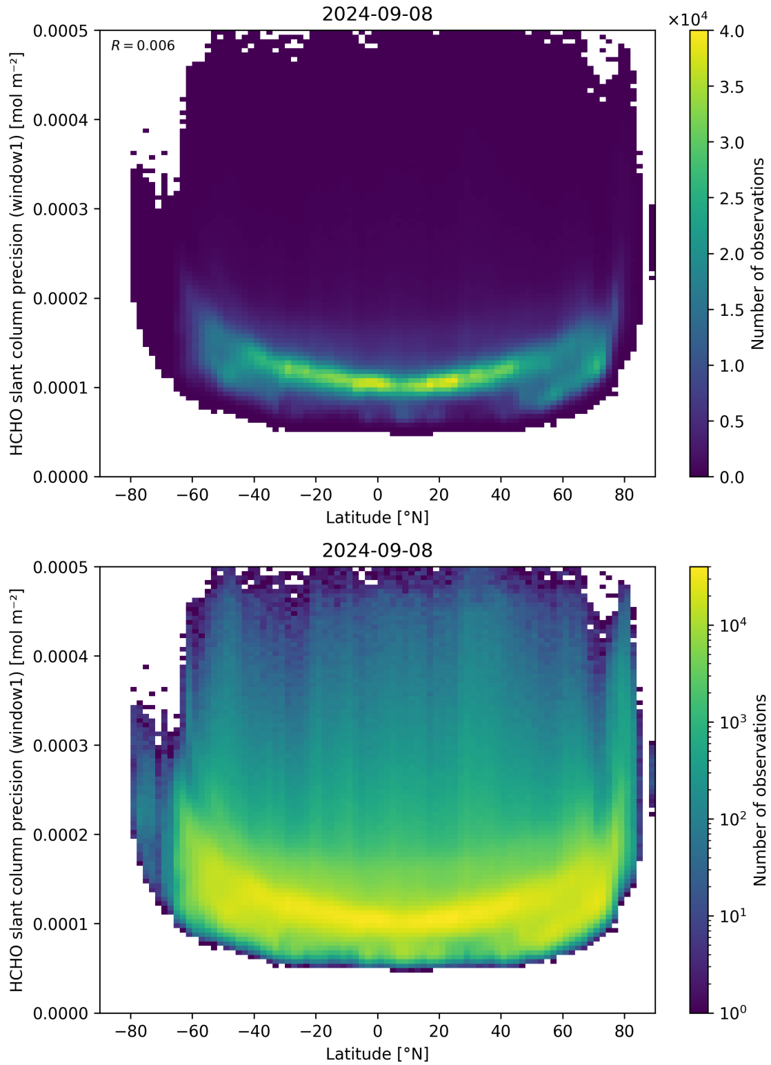
Figure 160: Scatter density plot of “Latitude” against “HCHO slant column precision (window1)” for 2024-09-07 to 2024-09-09.
