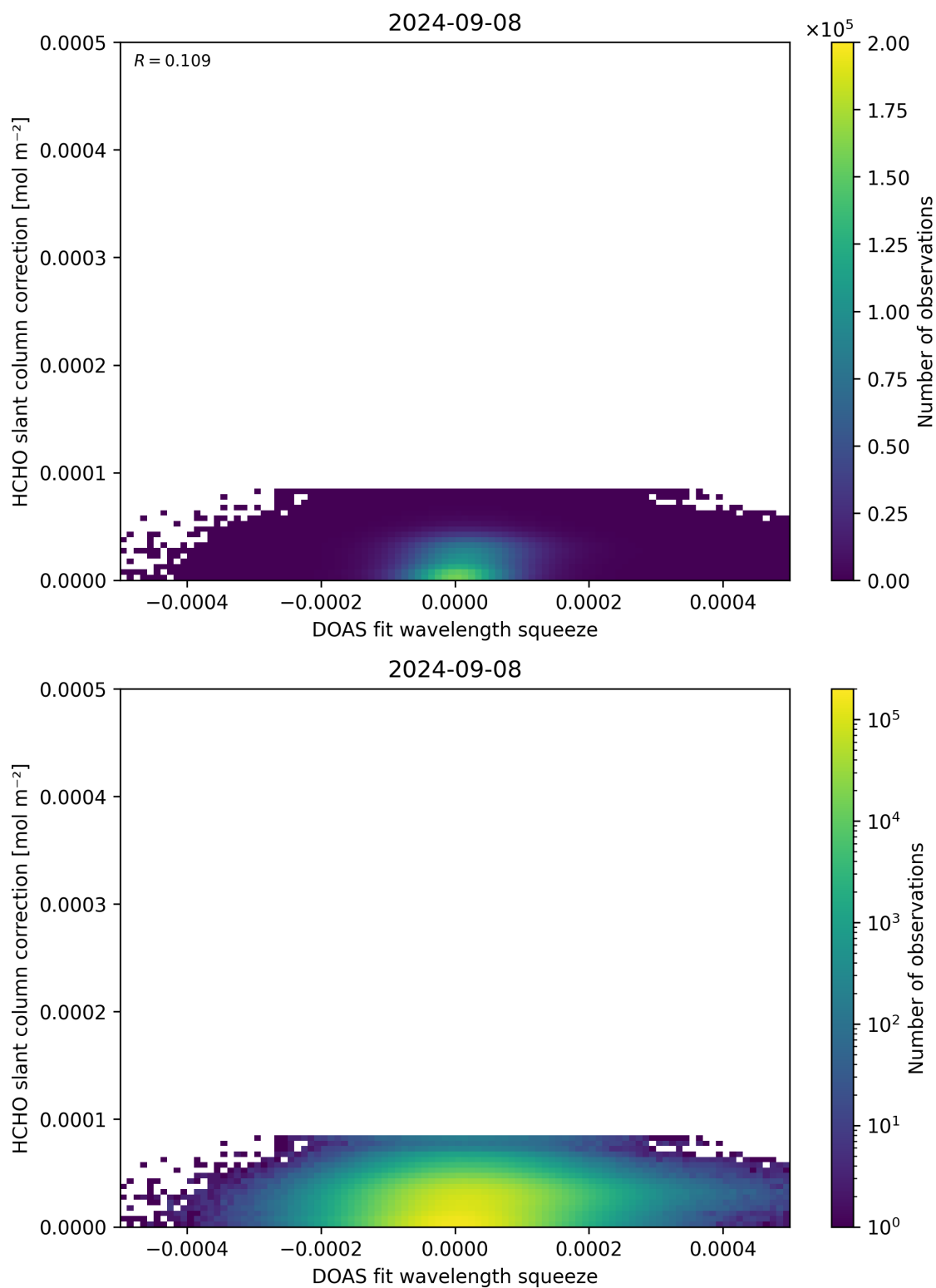
Figure 70: Scatter density plot of “DOAS fit wavelength squeeze” against “HCHO slant column correction” for 2024-09-07 to 2024-09-09.
