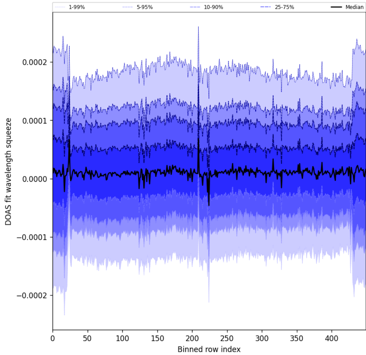
Figure 59: Along track statistics of “DOAS fit wavelength squeeze” for 2024-09-07 to 2024-09-09
