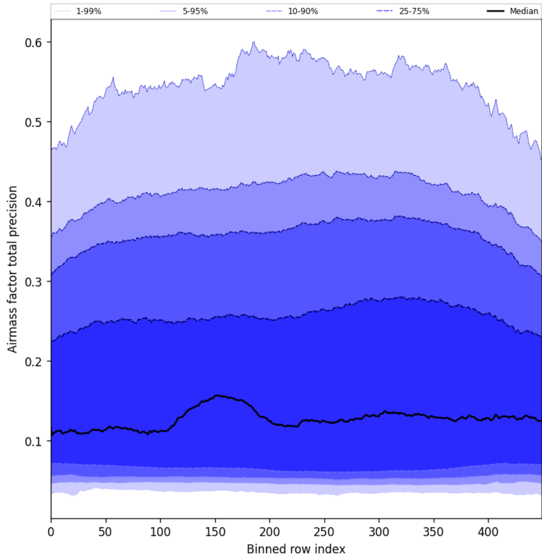
Figure 55: Along track statistics of “Airmass factor total precision” for 2024-09-07 to 2024-09-09
