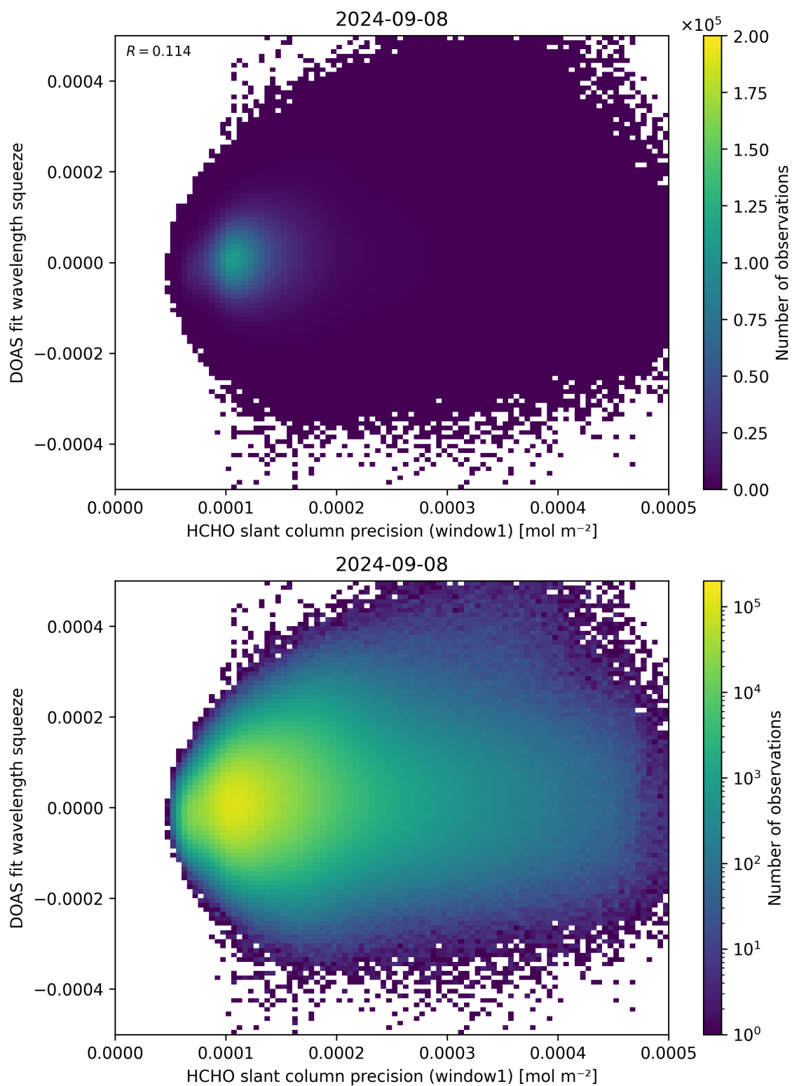
Figure 90: Scatter density plot of “HCHO slant column precision (window1)” against “DOAS fit wavelength squeeze” for 2024-09-07 to 2024-09-09.
