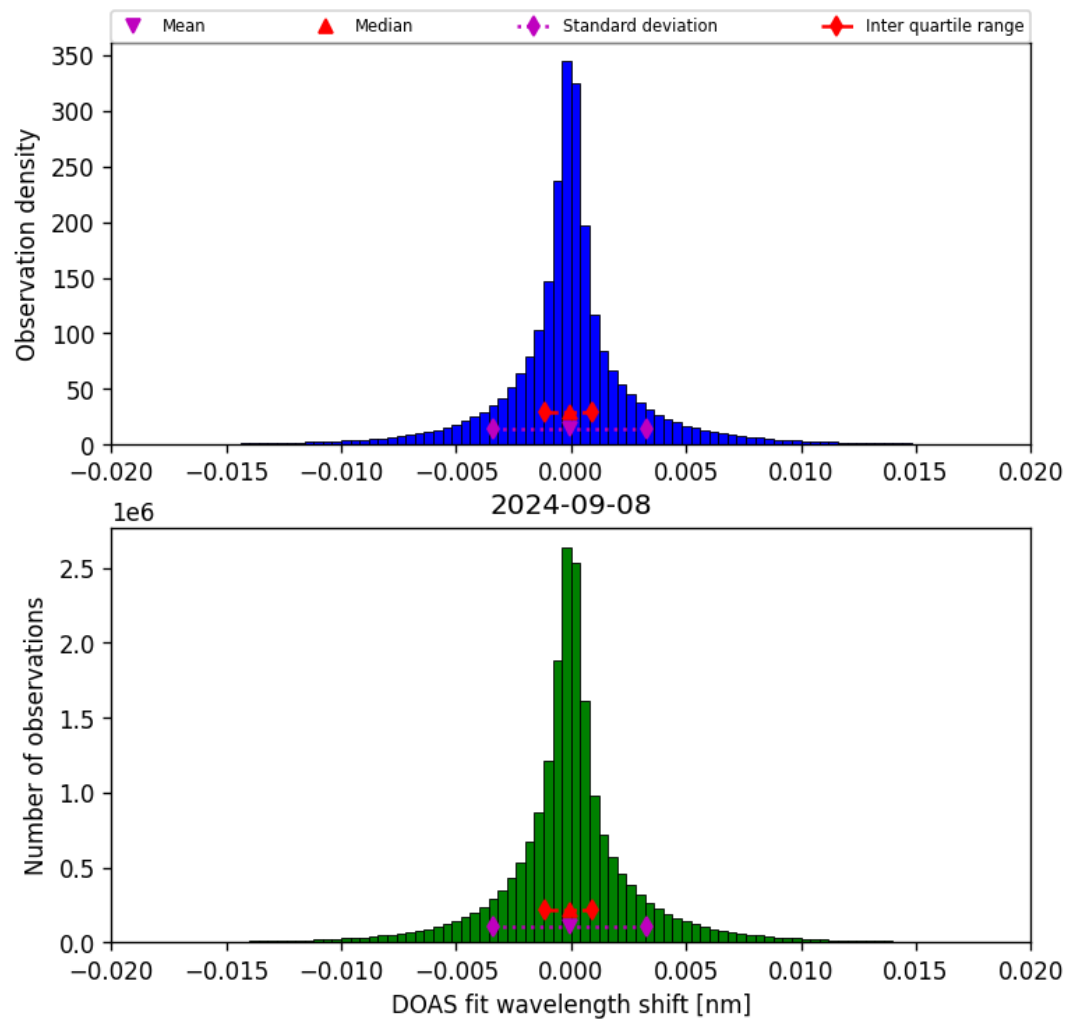
Figure 44: Histogram of “DOAS fit wavelength shift” for 2024-09-07 to 2024-09-09
