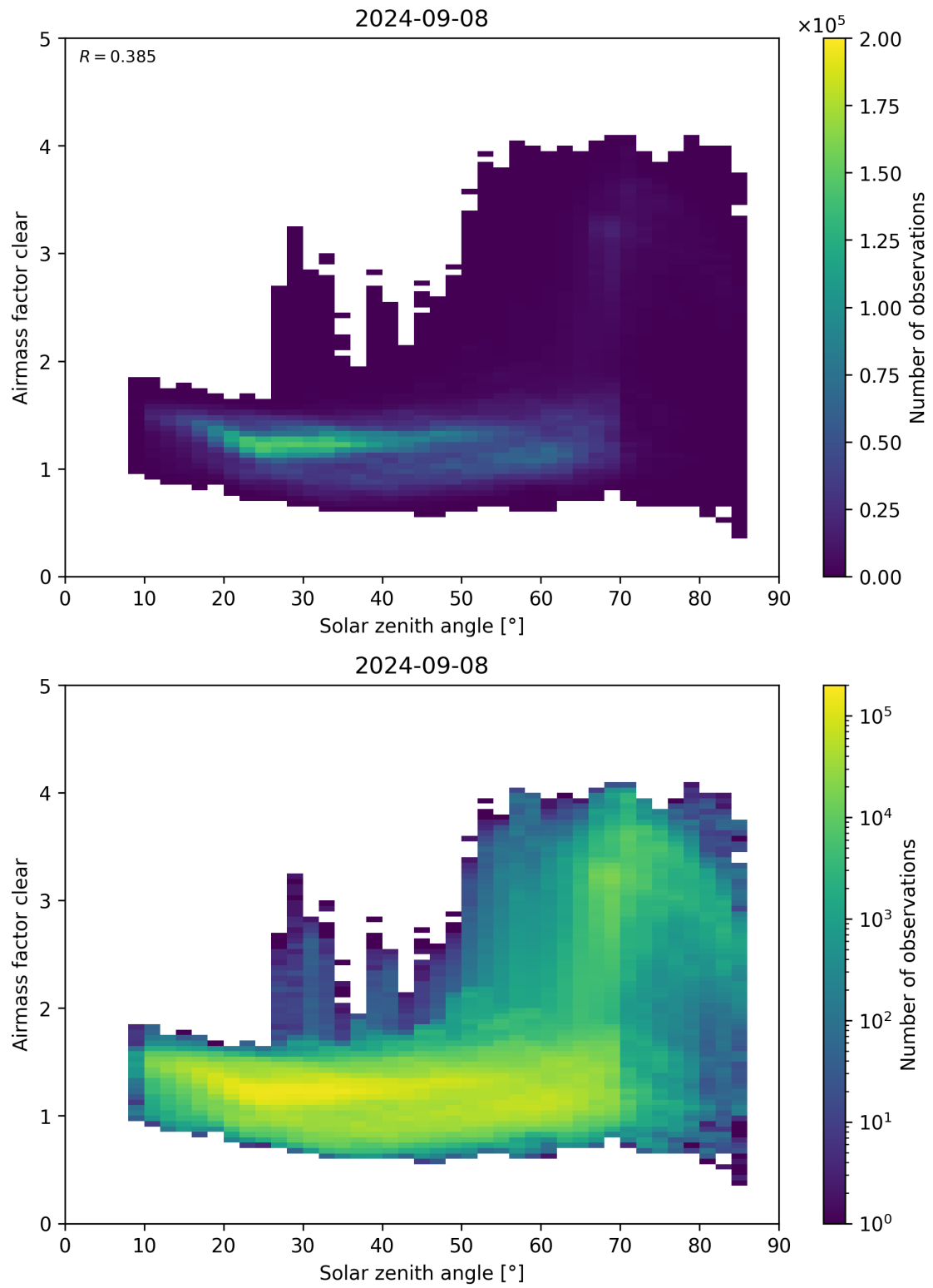
Figure 170: Scatter density plot of “Solar zenith angle” against “Airmass factor clear” for 2024-09-07 to 2024-09-09.
