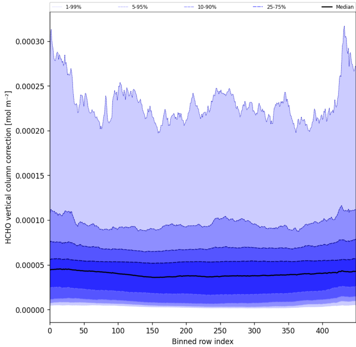
Figure 51: Along track statistics of “HCHO vertical column correction” for 2024-09-07 to 2024-09-09
