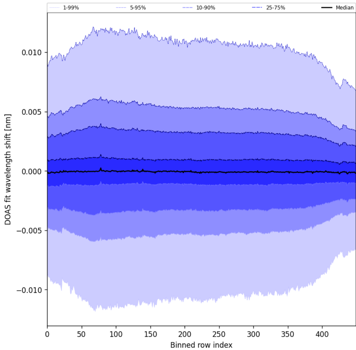
Figure 58: Along track statistics of “DOAS fit wavelength shift” for 2024-09-07 to 2024-09-09
