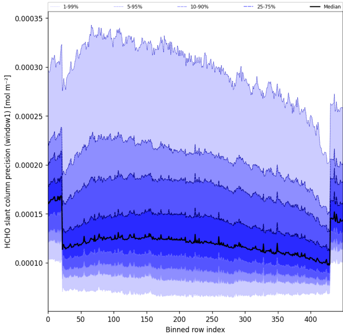
Figure 53: Along track statistics of “HCHO slant column precision (window1)” for 2024-09-07 to 2024-09-09
