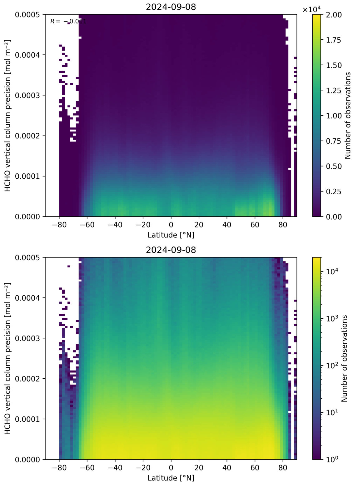
Figure 165: Scatter density plot of “Latitude” against “HCHO vertical column precision” for 2024-09-07 to 2024-09-09.
