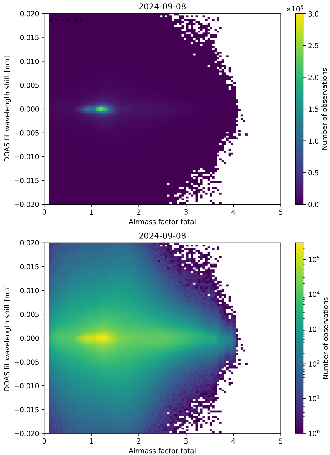
Figure 98: Scatter density plot of “Airmass factor total” against “DOAS fit wavelength shift” for 2024-09-07 to 2024-09-09.
