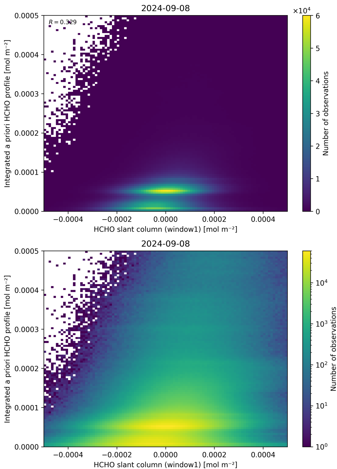
Figure 87: Scatter density plot of “HCHO slant column (window1)” against “Integrated a priori HCHO profile” for 2024-09-07 to 2024-09-09.
