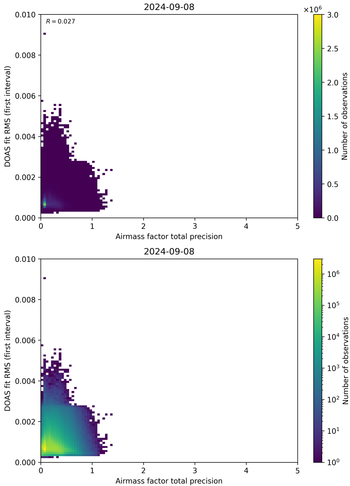
Figure 105: Scatter density plot of “Airmass factor total precision” against “DOAS fit RMS (first interval)” for 2024-09-07 to 2024-09-09.
