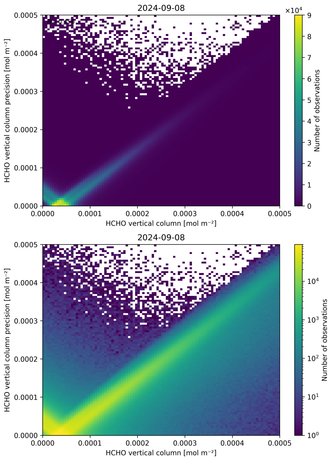
Figure 134: Scatter density plot of “HCHO vertical column” against “HCHO vertical column precision” for 2024-09-07 to 2024-09-09.
