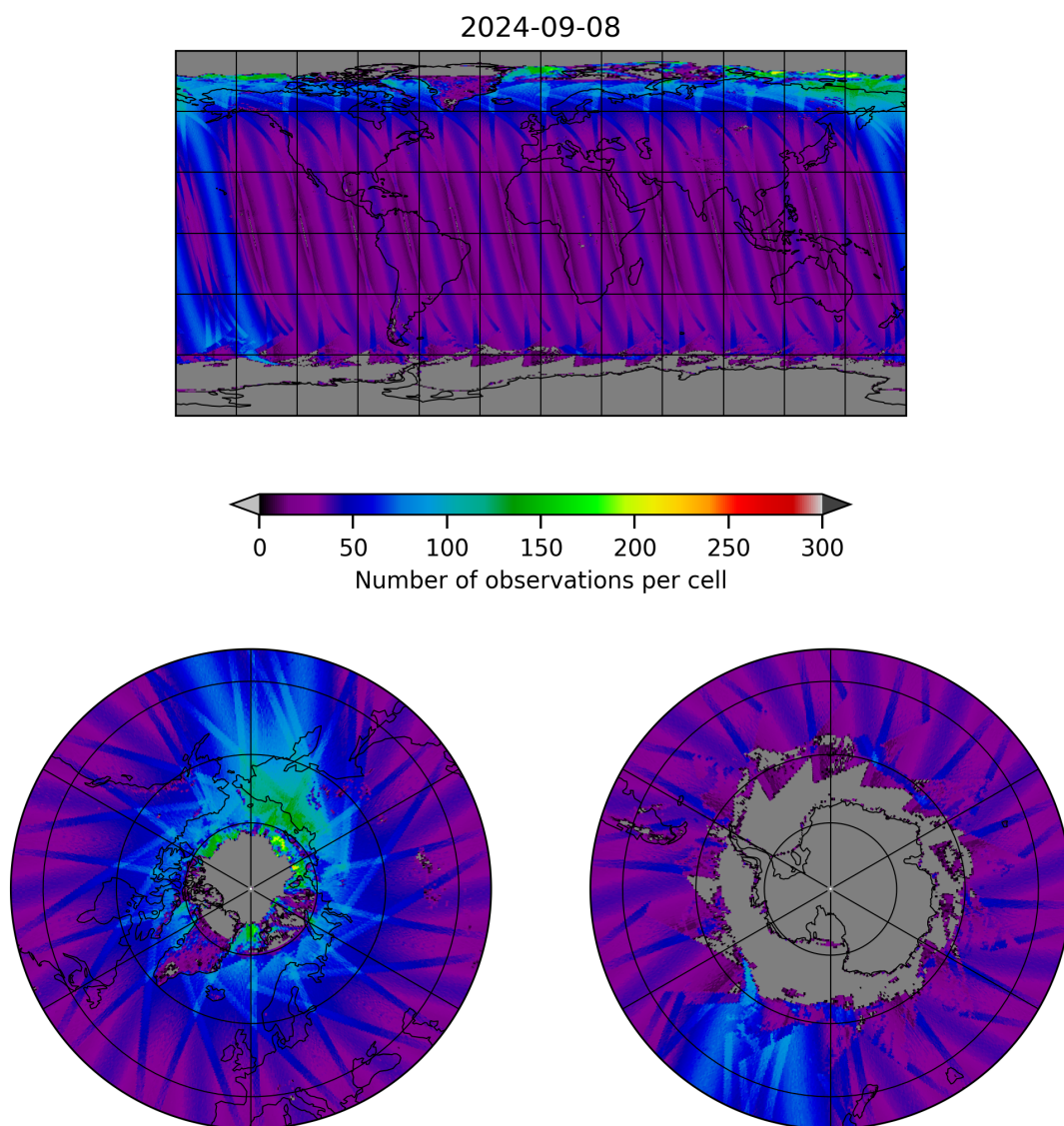
Figure 19: Map of the number of observations for 2024-09-07 to 2024-09-09
