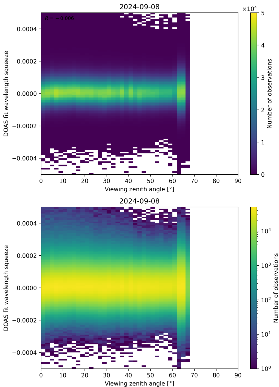
Figure 184: Scatter density plot of “Viewing zenith angle” against “DOAS fit wavelength squeeze” for 2024-09-07 to 2024-09-09.
