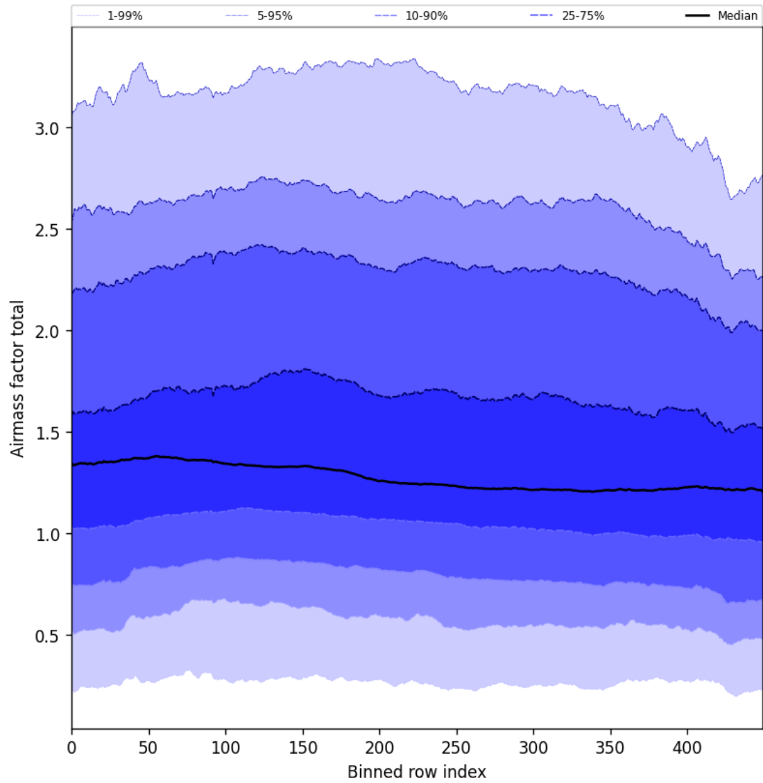
Figure 54: Along track statistics of “Airmass factor total” for 2024-09-07 to 2024-09-09
