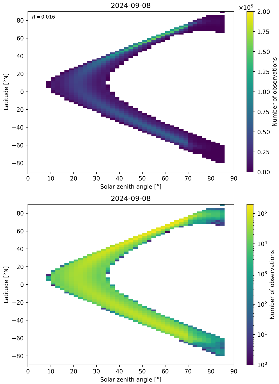
Figure 181: Scatter density plot of “Solar zenith angle” against “Latitude” for 2024-09-07 to 2024-09-09.
