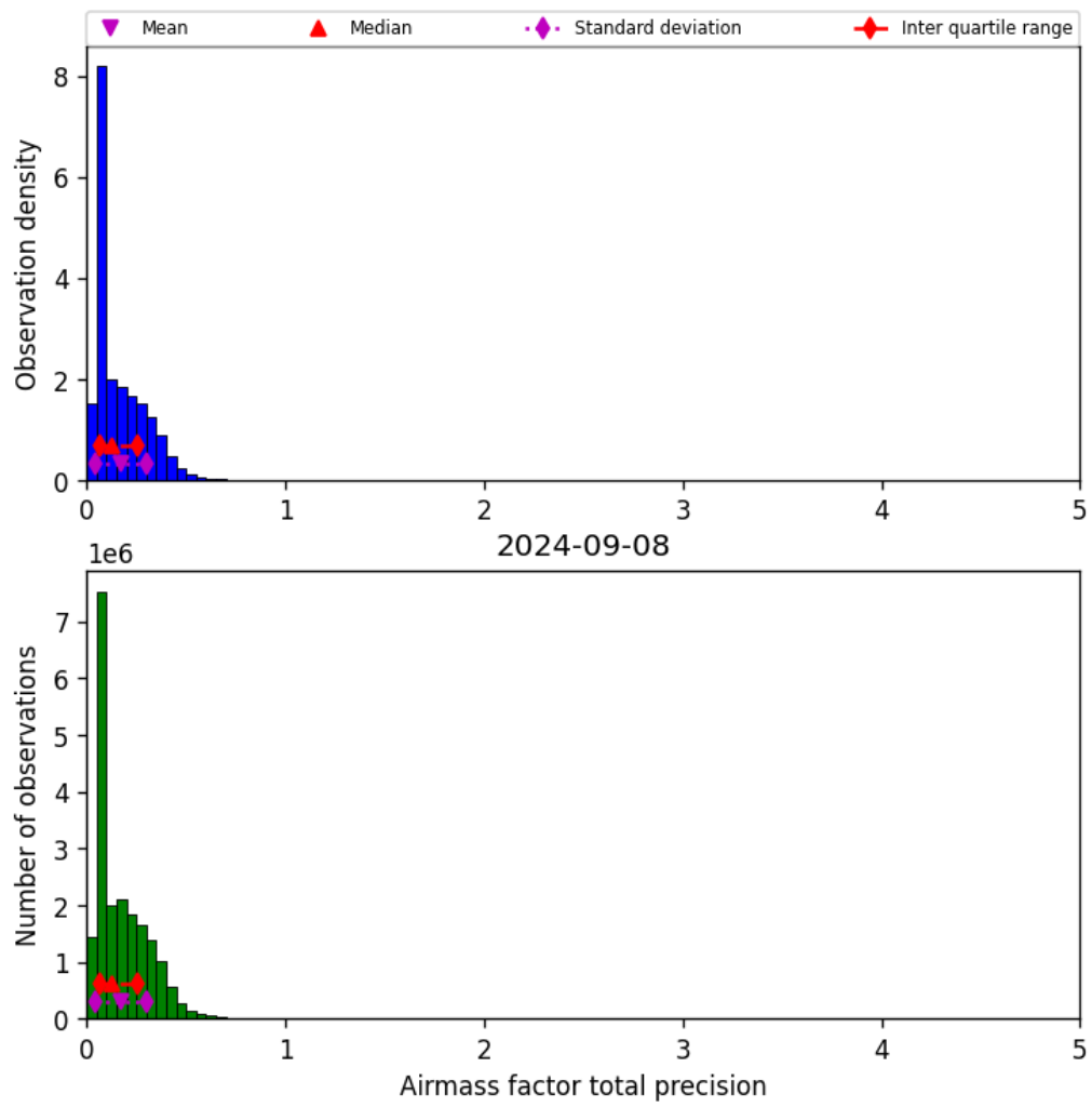
Figure 41: Histogram of “Airmass factor total precision” for 2024-09-07 to 2024-09-09
