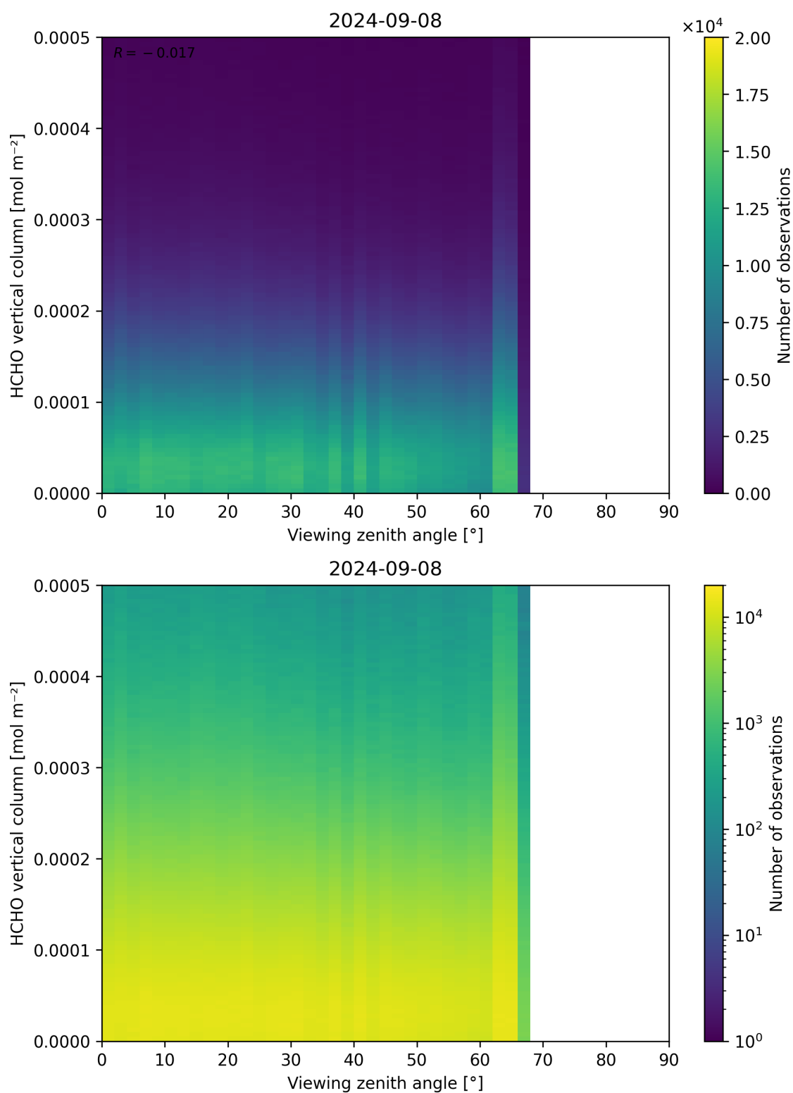
Figure 192: Scatter density plot of “Viewing zenith angle” against “HCHO vertical column” for 2024-09-07 to 2024-09-09.
