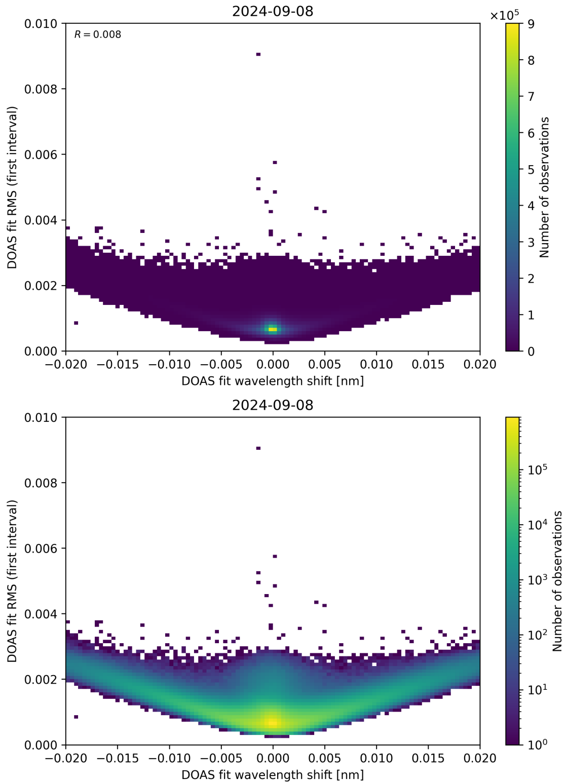
Figure 64: Scatter density plot of “DOAS fit wavelength shift” against “DOAS fit RMS (first interval)” for 2024-09-07 to 2024-09-09.
