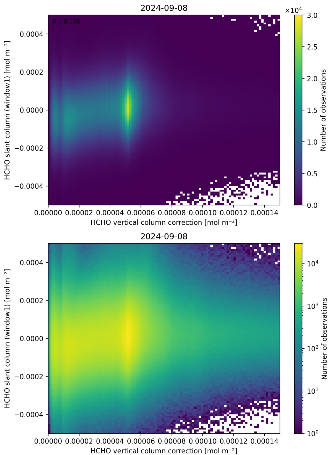
Figure 118: Scatter density plot of “HCHO vertical column correction” against “HCHO slant column (window1)” for 2024-09-07 to 2024-09-09.
