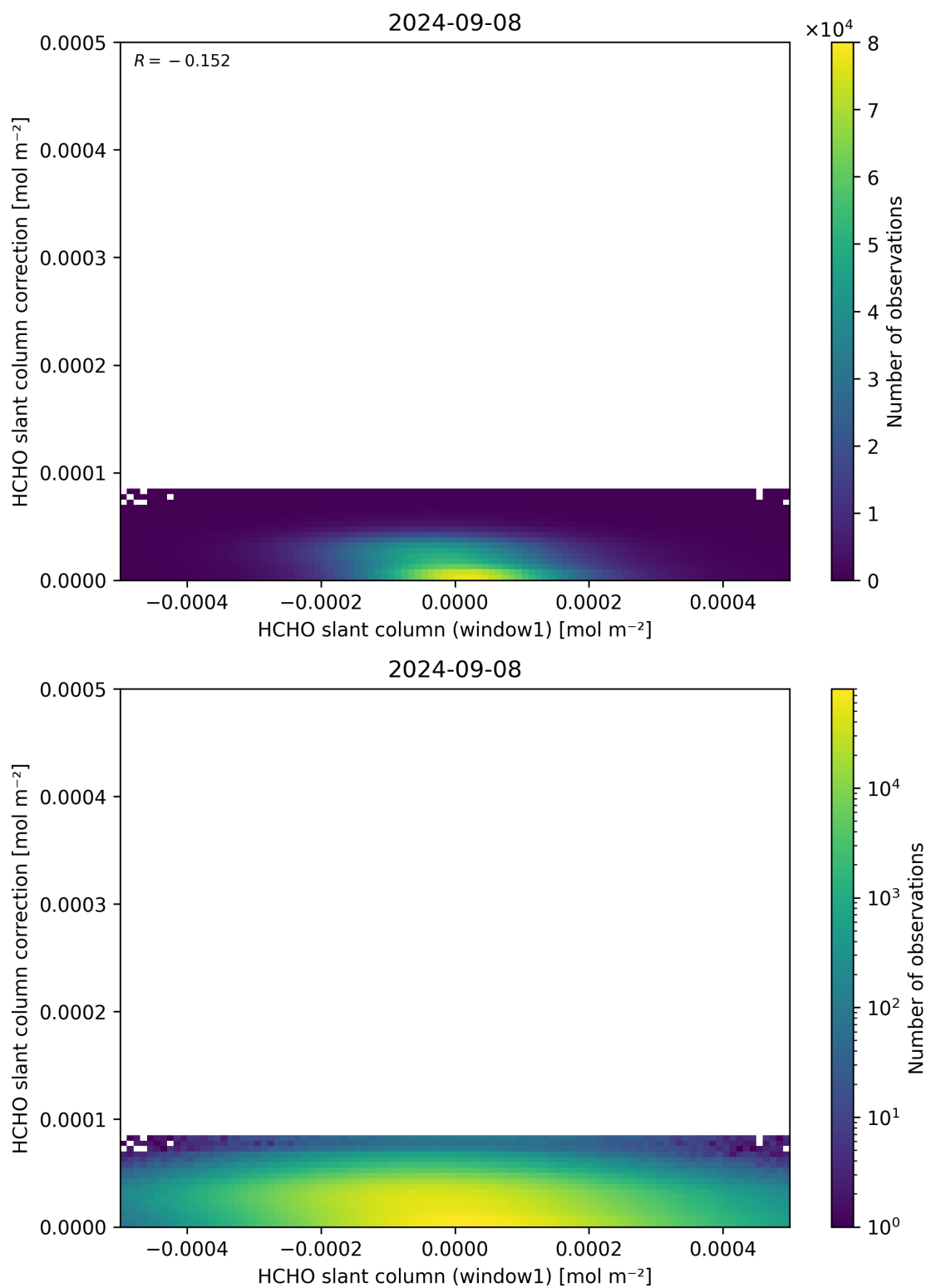
Figure 83: Scatter density plot of “HCHO slant column (window1)” against “HCHO slant column correction” for 2024-09-07 to 2024-09-09.
