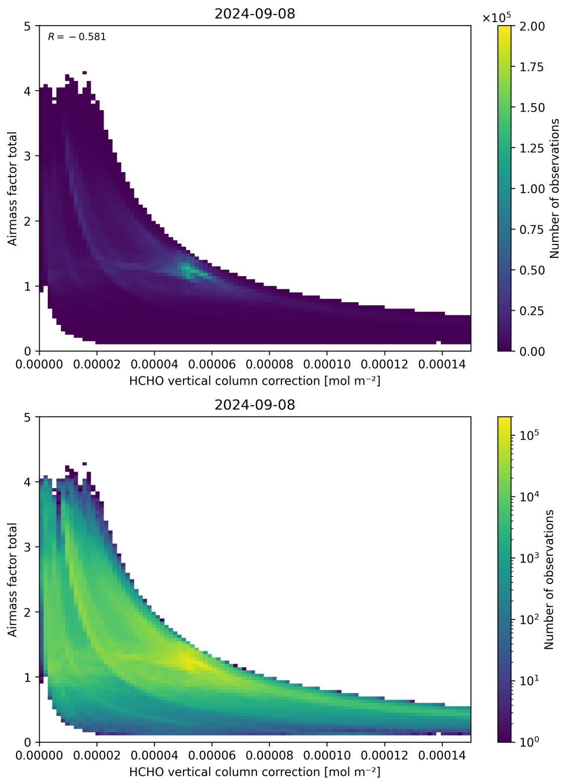
Figure 120: Scatter density plot of “HCHO vertical column correction” against “Airmass factor total” for 2024-09-07 to 2024-09-09.
