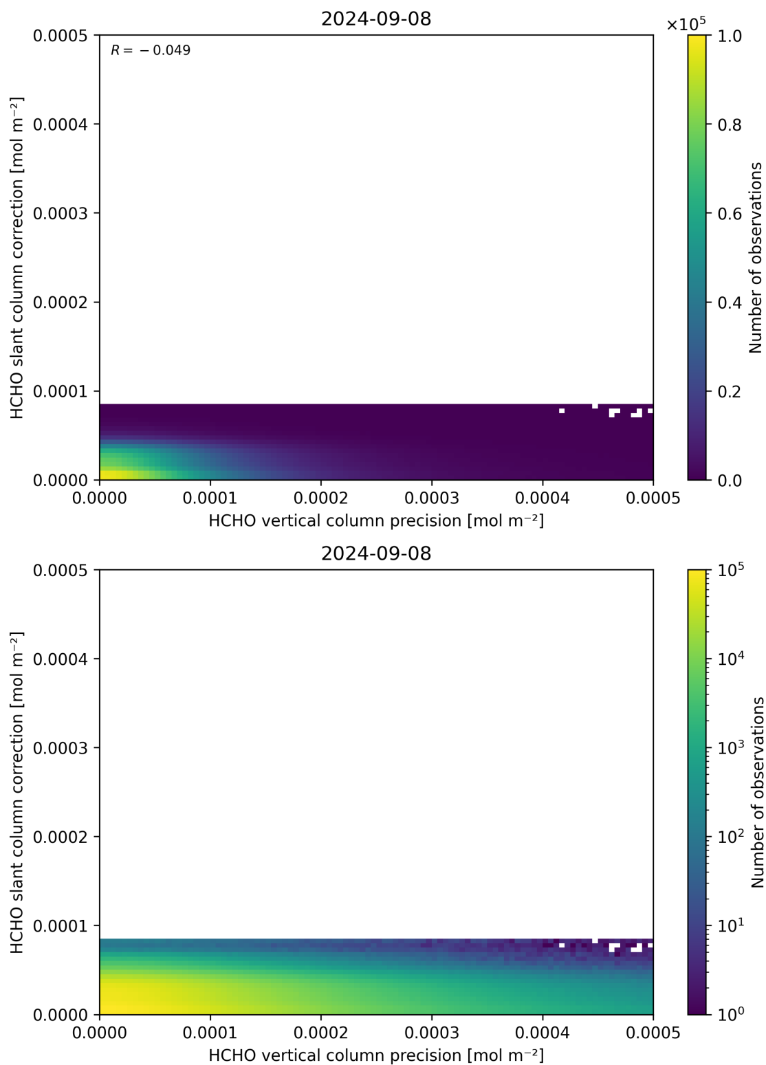
Figure 141: Scatter density plot of “HCHO vertical column precision” against “HCHO slant column correction” for 2024-09-07 to 2024-09-09.
