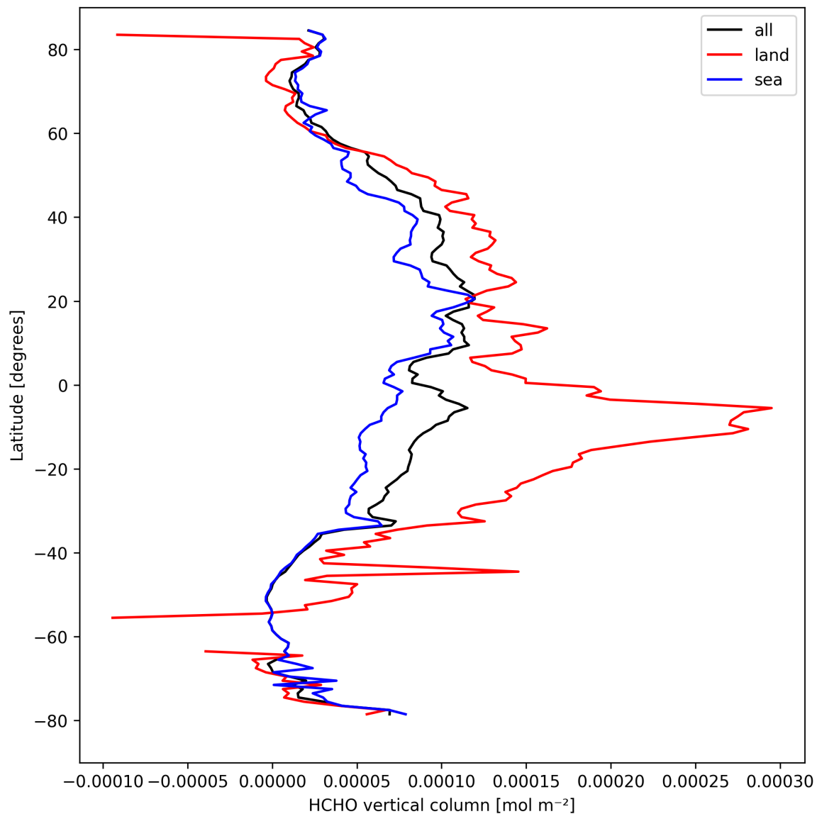
Figure 21: Zonal average of “HCHO vertical column” for 2024-09-07 to 2024-09-09.
