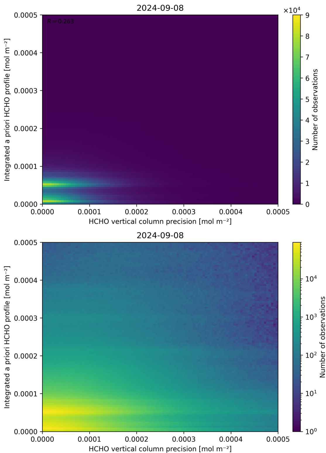
Figure 147: Scatter density plot of “HCHO vertical column precision” against “Integrated a priori HCHO profile” for 2024-09-07 to 2024-09-09.
