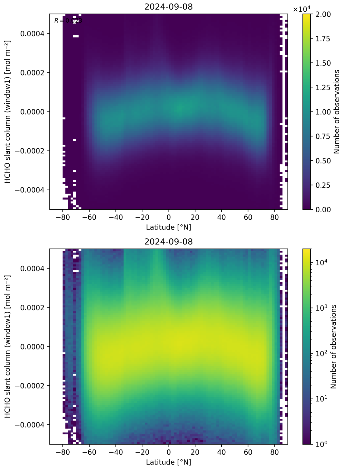
Figure 159: Scatter density plot of “Latitude” against “HCHO slant column (window1)” for 2024-09-07 to 2024-09-09.
