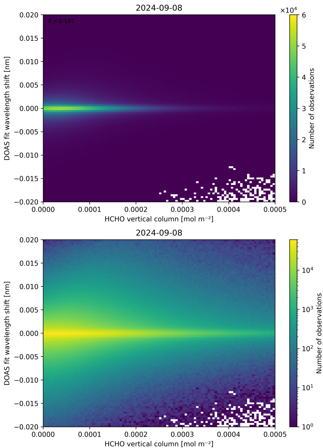
Figure 124: Scatter density plot of “HCHO vertical column” against “DOAS fit wavelength shift” for 2024-09-07 to 2024-09-09.
