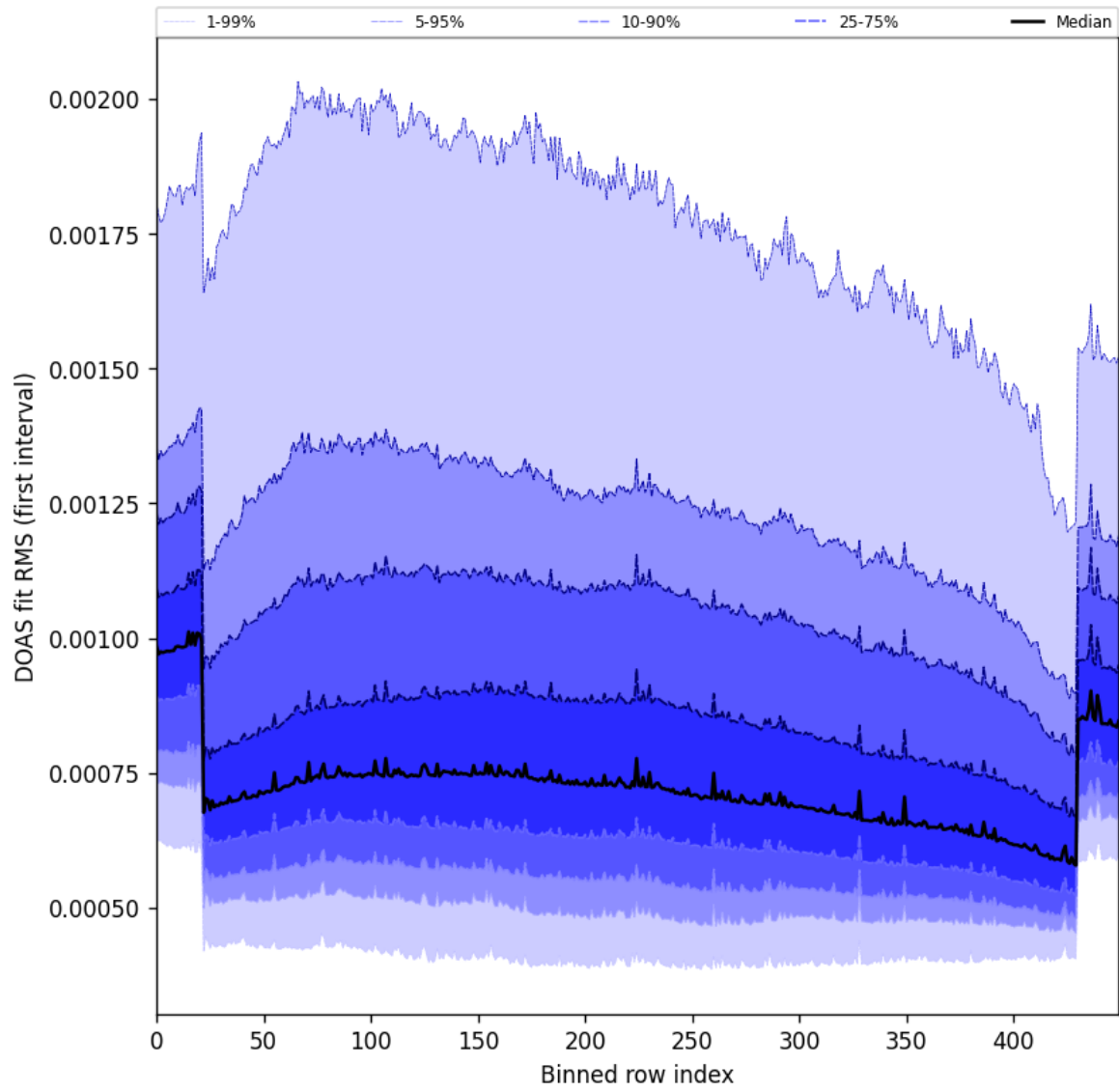
Figure 60: Along track statistics of “DOAS fit RMS (first interval)” for 2024-09-07 to 2024-09-09
