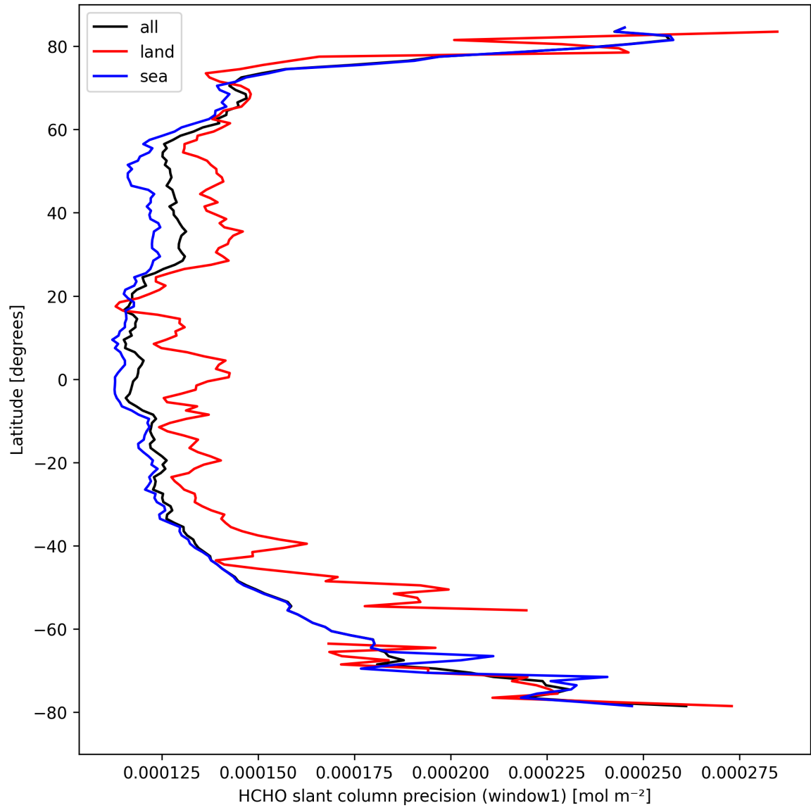
Figure 25: Zonal average of “HCHO slant column precision (window1)” for 2024-09-07 to 2024-09-09.
