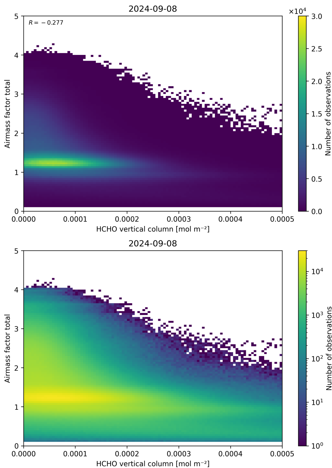
Figure 131: Scatter density plot of “HCHO vertical column” against “Airmass factor total” for 2024-09-07 to 2024-09-09.
