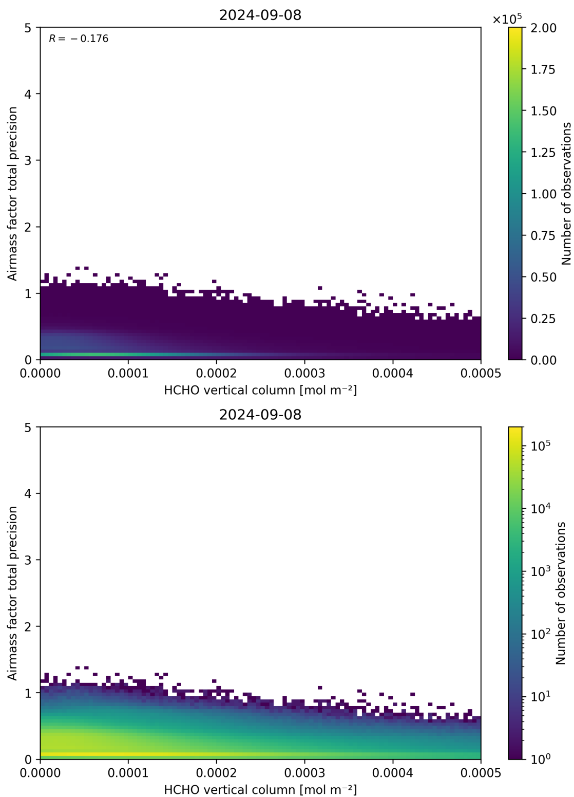
Figure 132: Scatter density plot of “HCHO vertical column” against “Airmass factor total precision” for 2024-09-07 to 2024-09-09.
