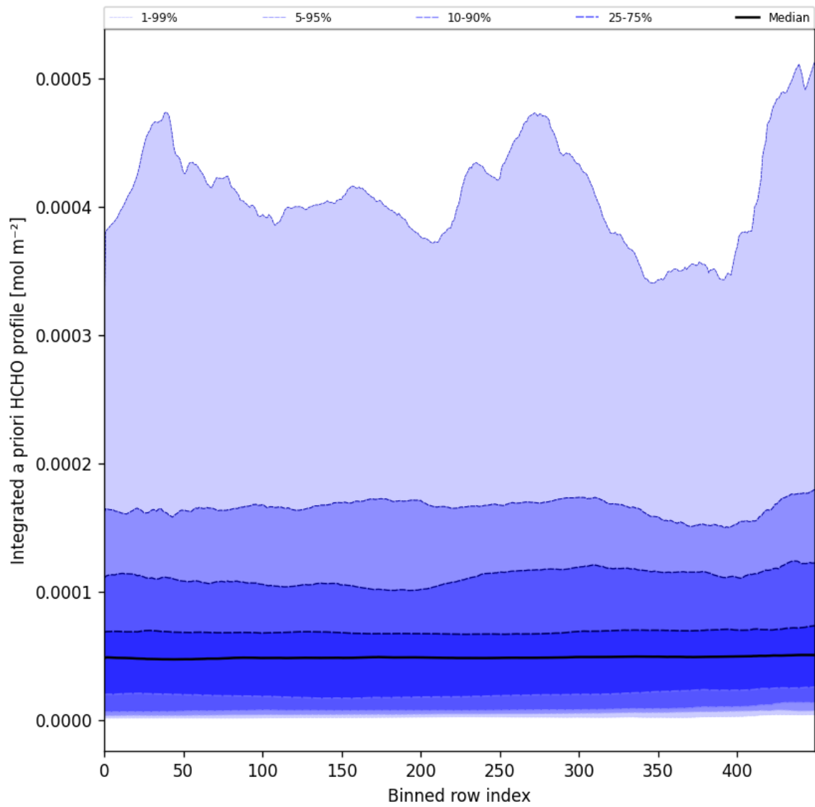
Figure 57: Along track statistics of “Integrated a priori HCHO profile” for 2024-09-07 to 2024-09-09
