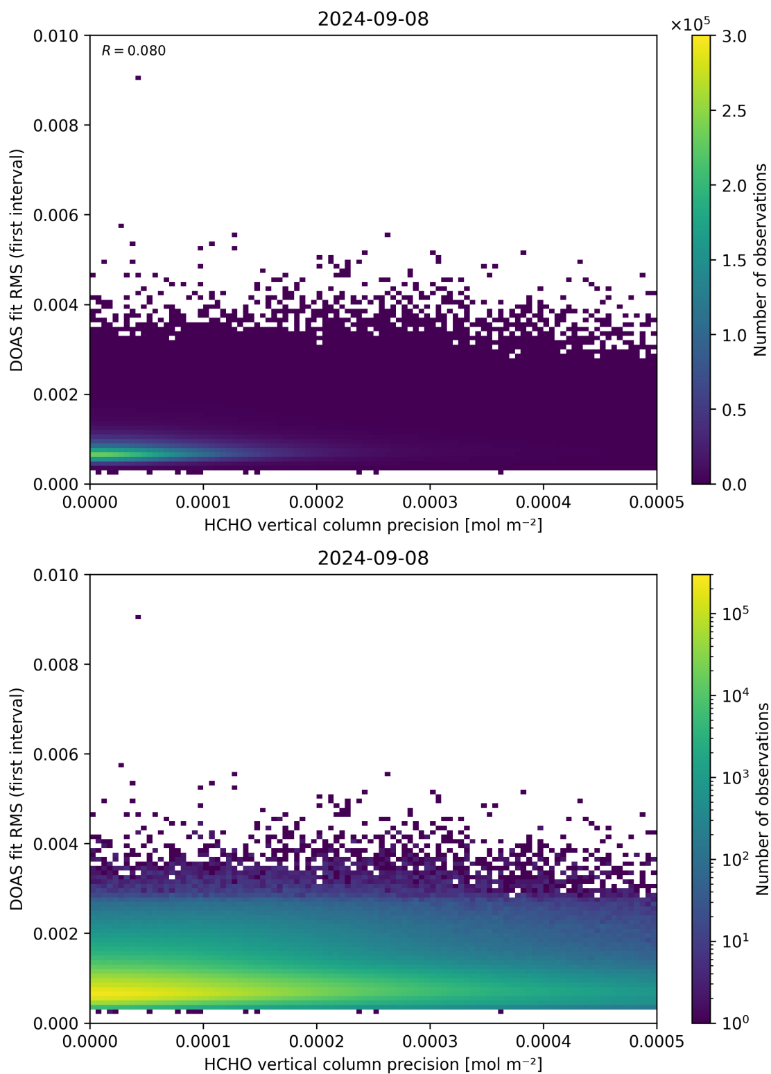
Figure 136: Scatter density plot of “HCHO vertical column precision” against “DOAS fit RMS (first interval)” for 2024-09-07 to 2024-09-09.
