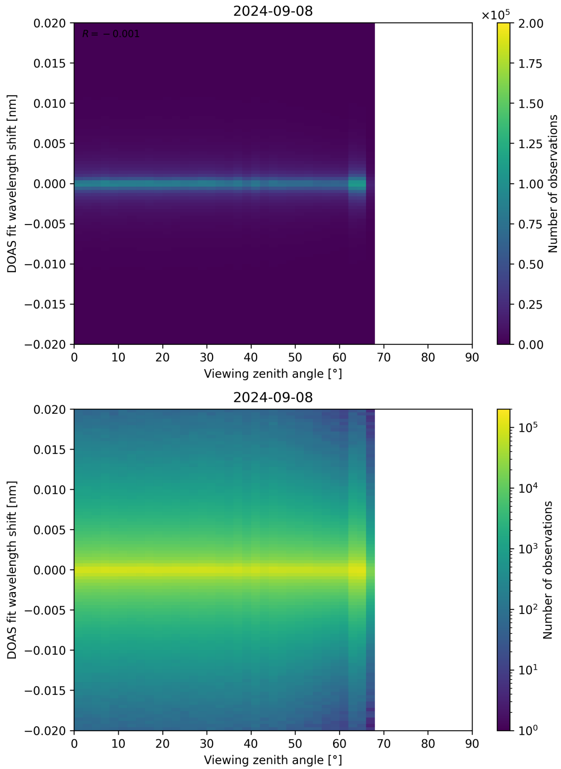
Figure 183: Scatter density plot of “Viewing zenith angle” against “DOAS fit wavelength shift” for 2024-09-07 to 2024-09-09.
