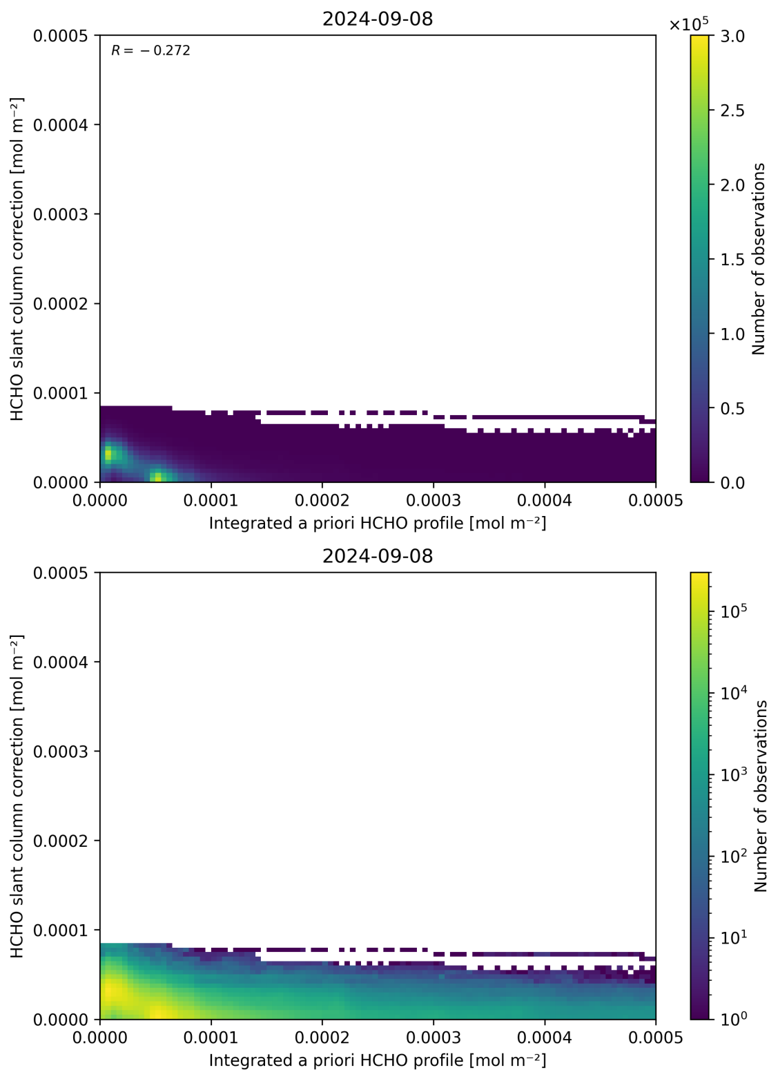
Figure 152: Scatter density plot of “Integrated a priori HCHO profile” against “HCHO slant column correction” for 2024-09-07 to 2024-09-09.
