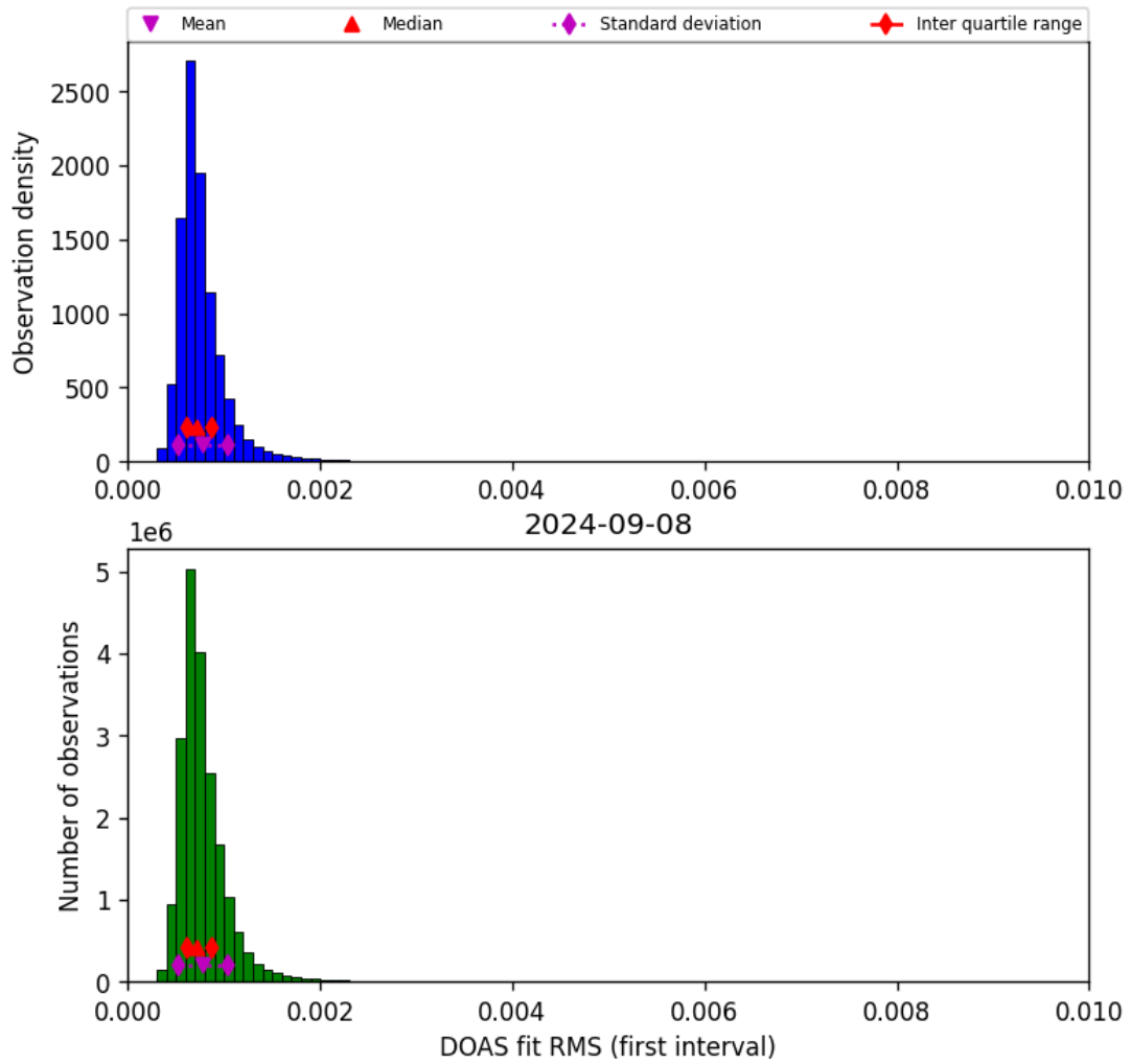
Figure 46: Histogram of “DOAS fit RMS (first interval)” for 2024-09-07 to 2024-09-09
