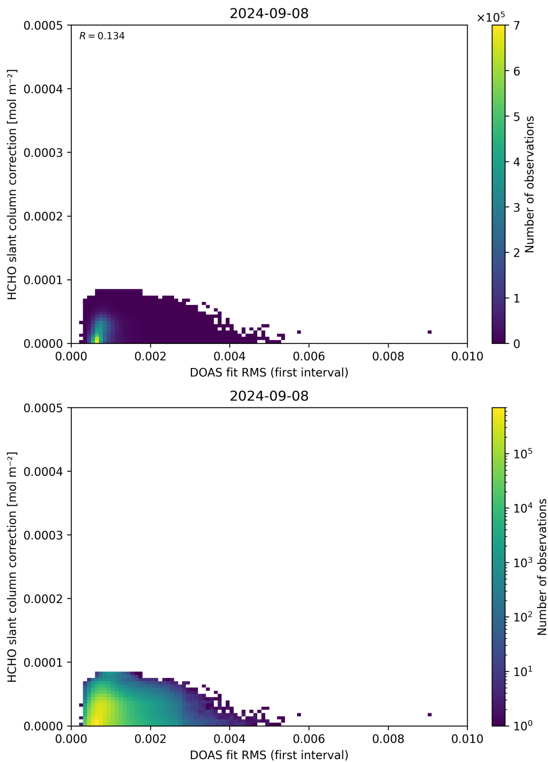
Figure 63: Scatter density plot of “DOAS fit RMS (first interval)” against “HCHO slant column correction” for 2024-09-07 to 2024-09-09.
