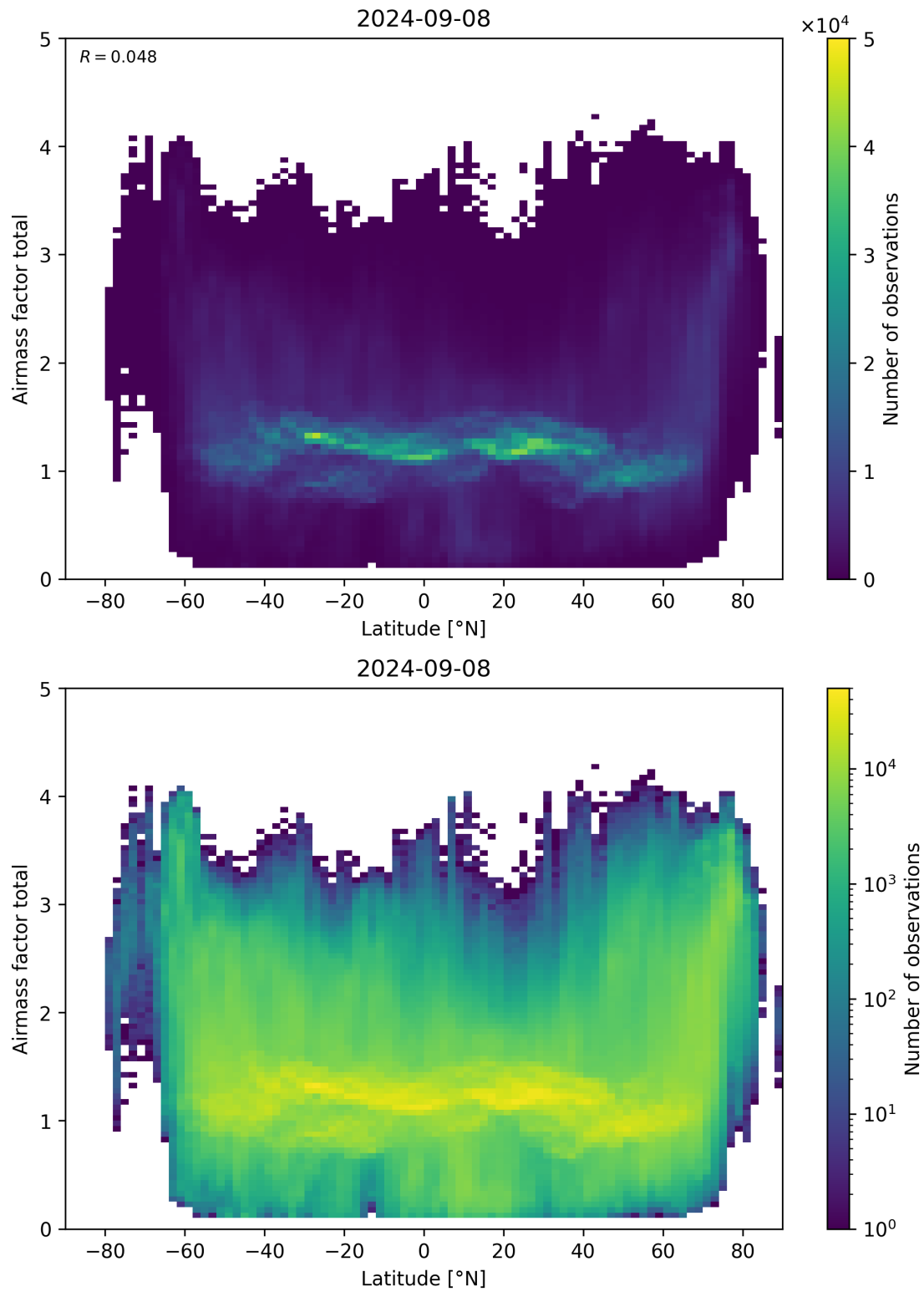
Figure 161: Scatter density plot of “Latitude” against “Airmass factor total” for 2024-09-07 to 2024-09-09.
