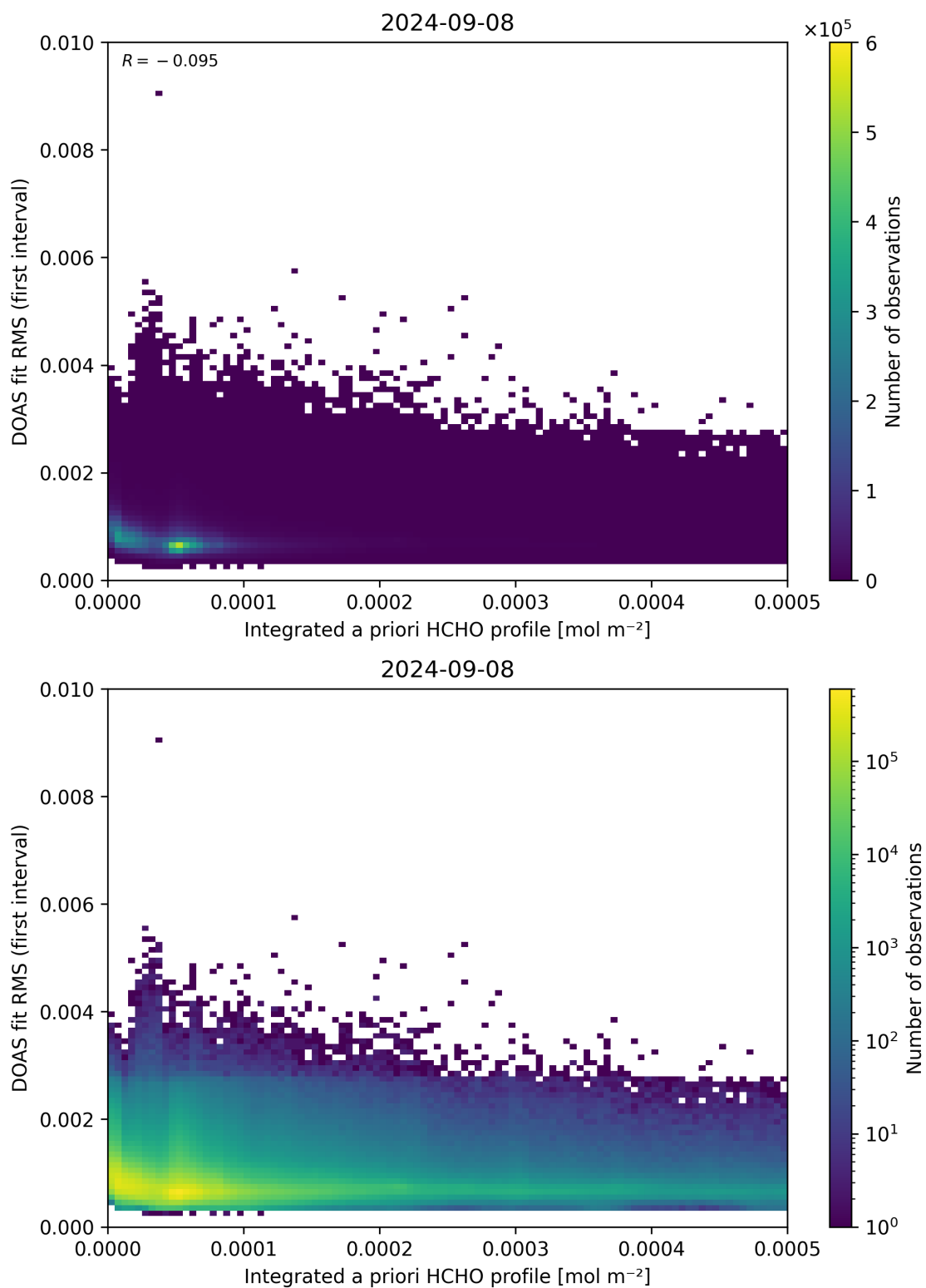
Figure 148: Scatter density plot of “Integrated a priori HCHO profile” against “DOAS fit RMS (first interval)” for 2024-09-07 to 2024-09-09.
