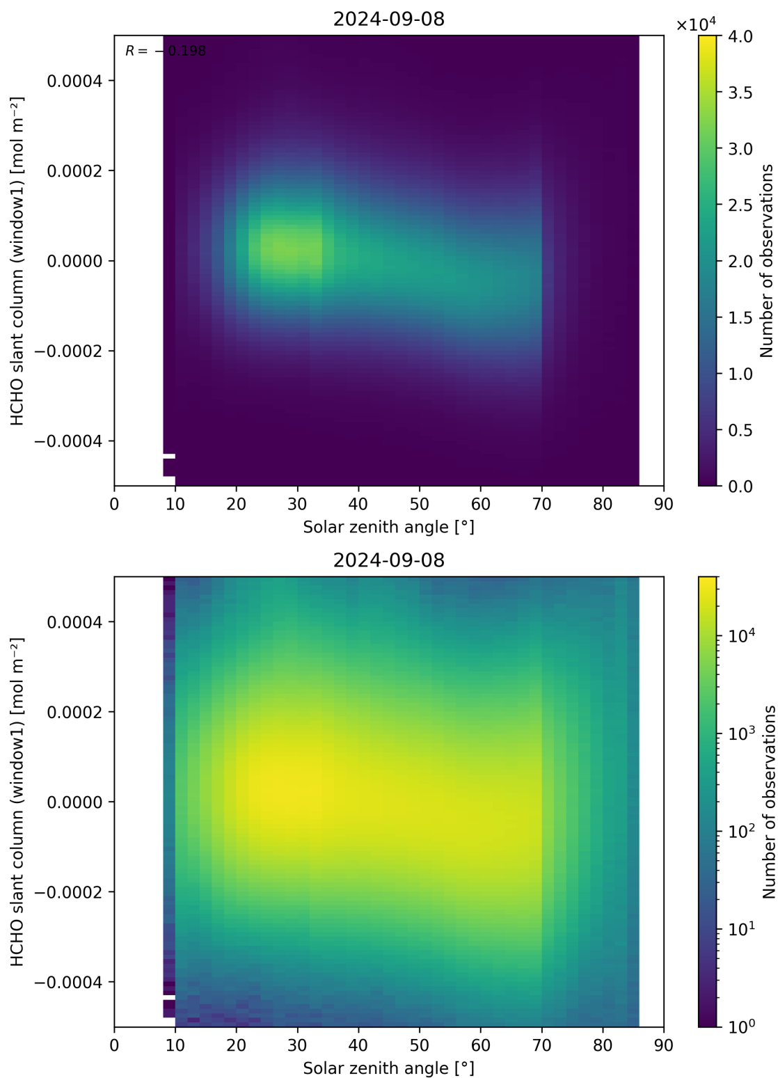
Figure 173: Scatter density plot of “Solar zenith angle” against “HCHO slant column (window1)” for 2024-09-07 to 2024-09-09.
