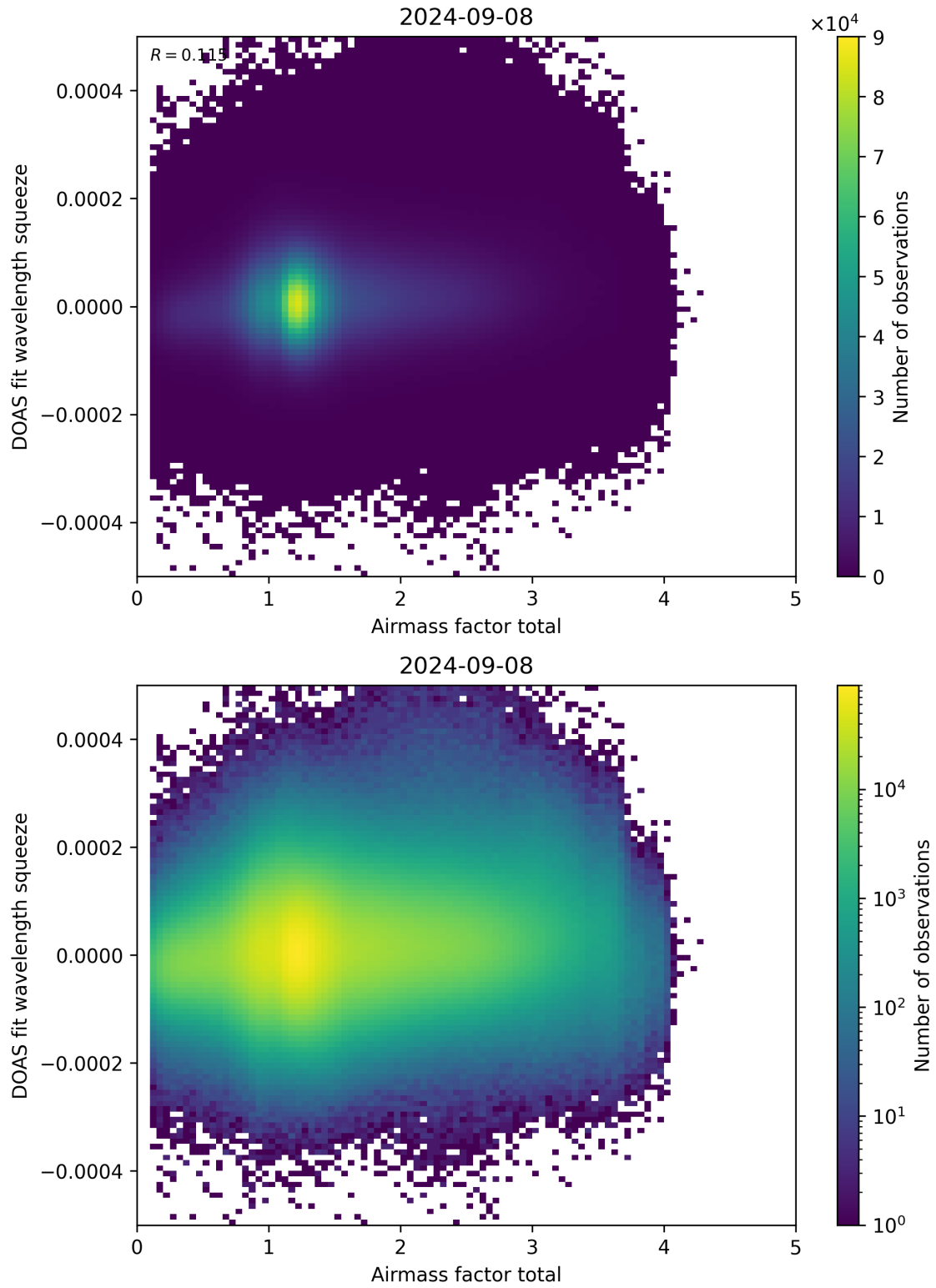
Figure 99: Scatter density plot of “Airmass factor total” against “DOAS fit wavelength squeeze” for 2024-09-07 to 2024-09-09.
