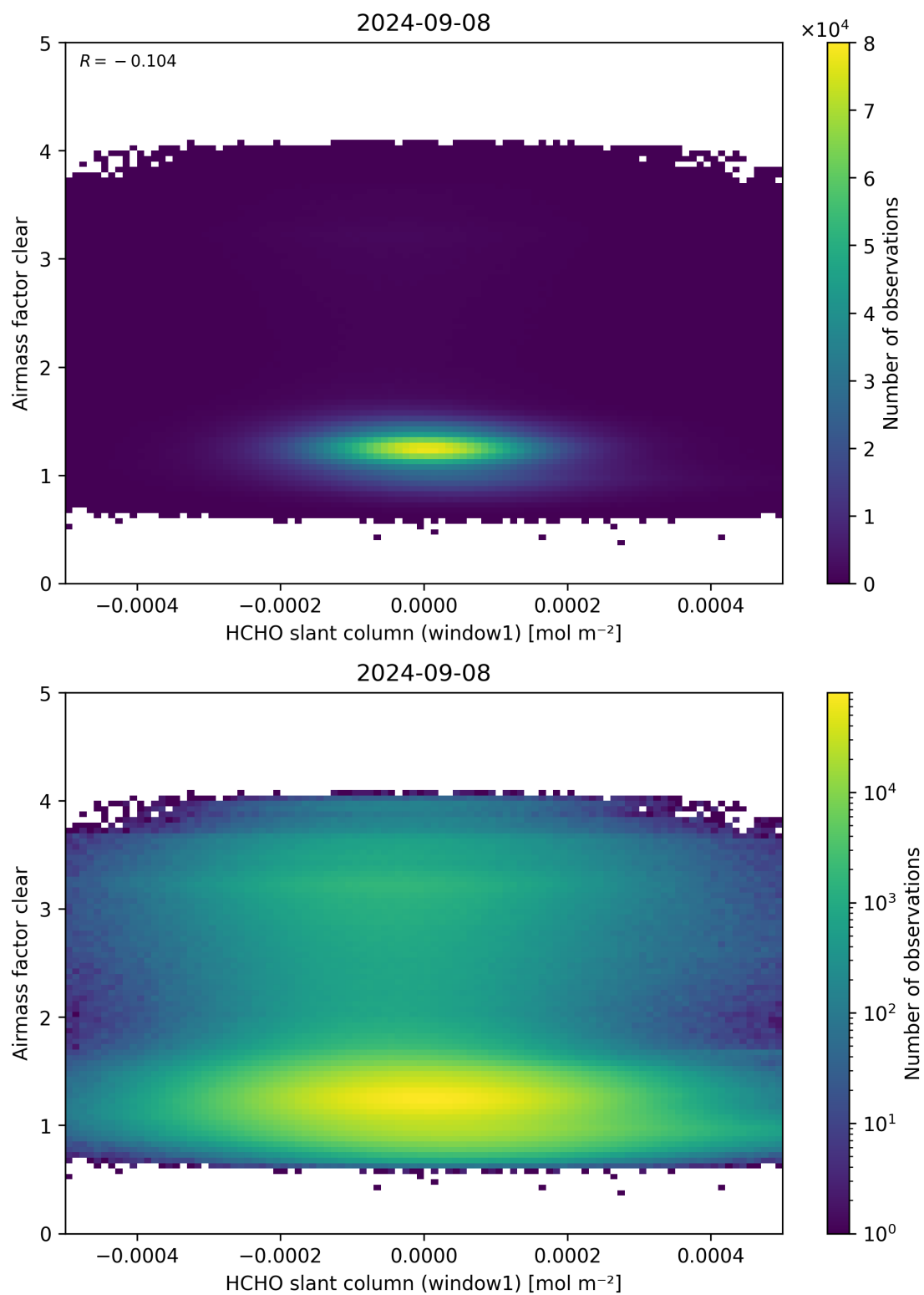
Figure 81: Scatter density plot of “HCHO slant column (window1)” against “Airmass factor clear” for 2024-09-07 to 2024-09-09.
