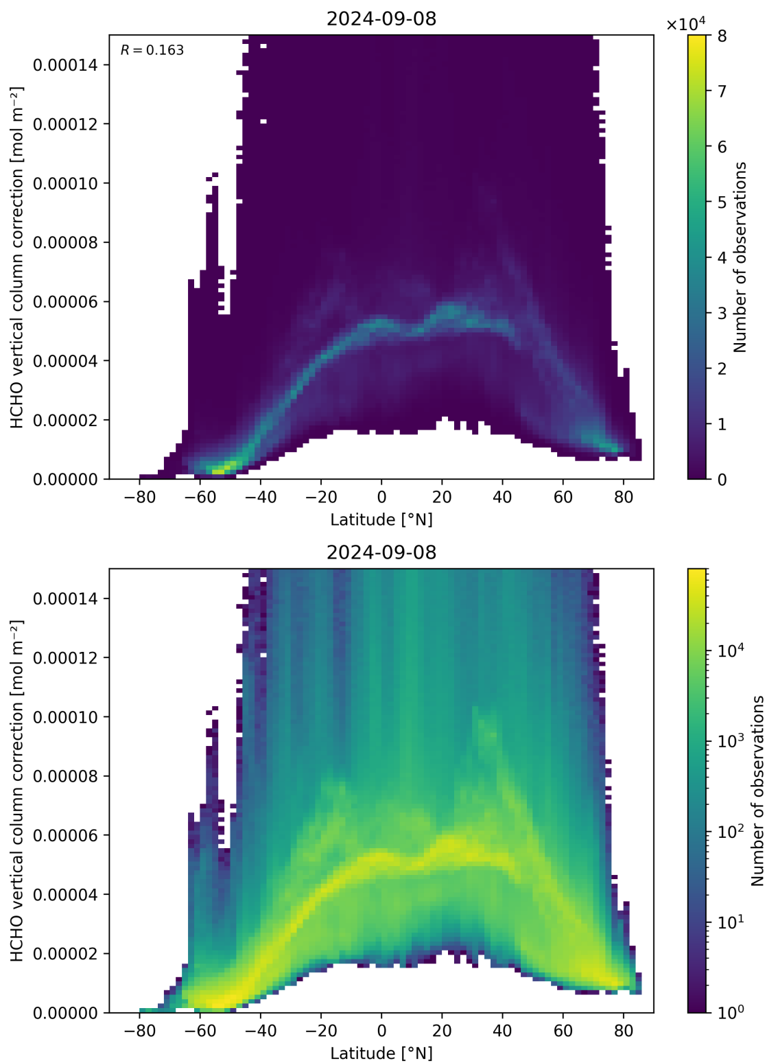
Figure 164: Scatter density plot of “Latitude” against “HCHO vertical column correction” for 2024-09-07 to 2024-09-09.
