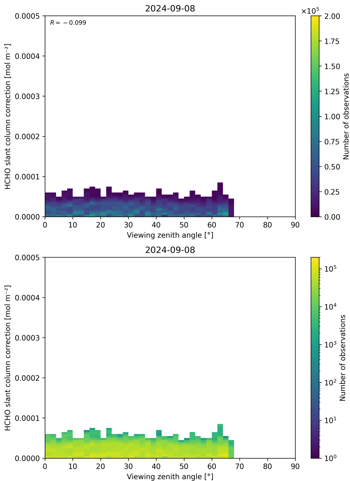
Figure 187: Scatter density plot of “Viewing zenith angle” against “HCHO slant column correction” for 2024-09-07 to 2024-09-09.
