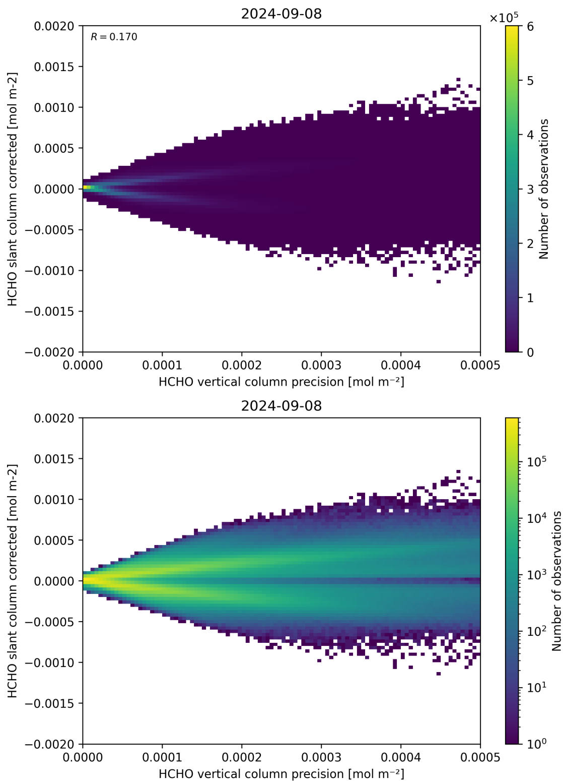
Figure 140: Scatter density plot of “HCHO vertical column precision” against “HCHO slant column corrected” for 2024-09-07 to 2024-09-09.
