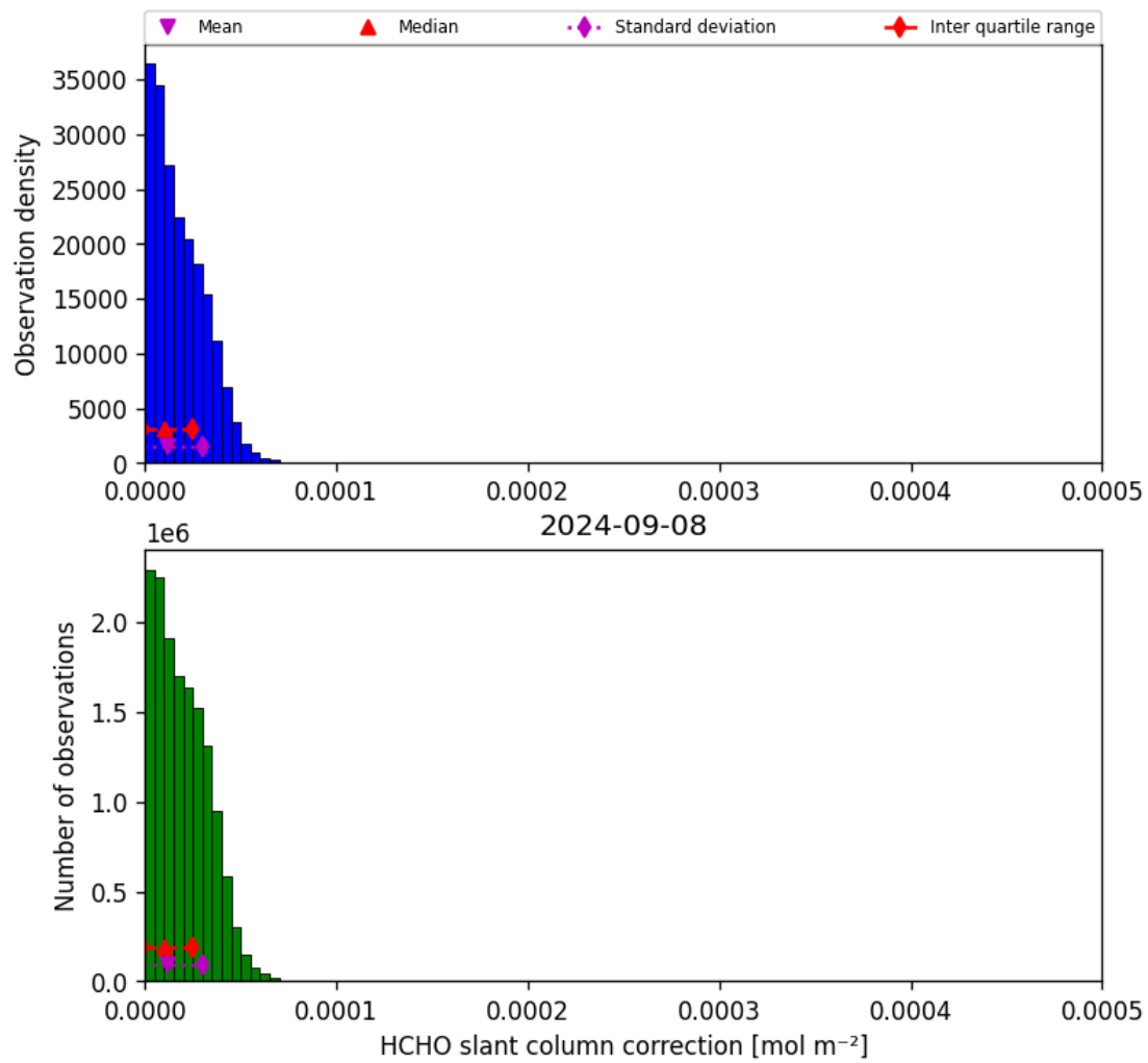
Figure 47: Histogram of “HCHO slant column correction” for 2024-09-07 to 2024-09-09
