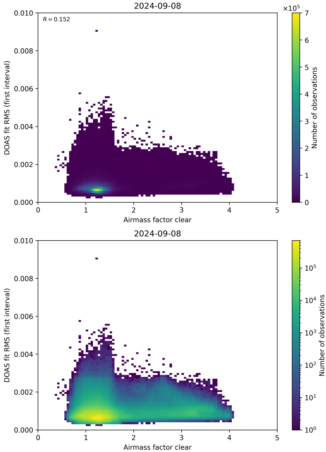
Figure 71: Scatter density plot of “Airmass factor clear” against “DOAS fit RMS (first interval)” for 2024-09-07 to 2024-09-09.
