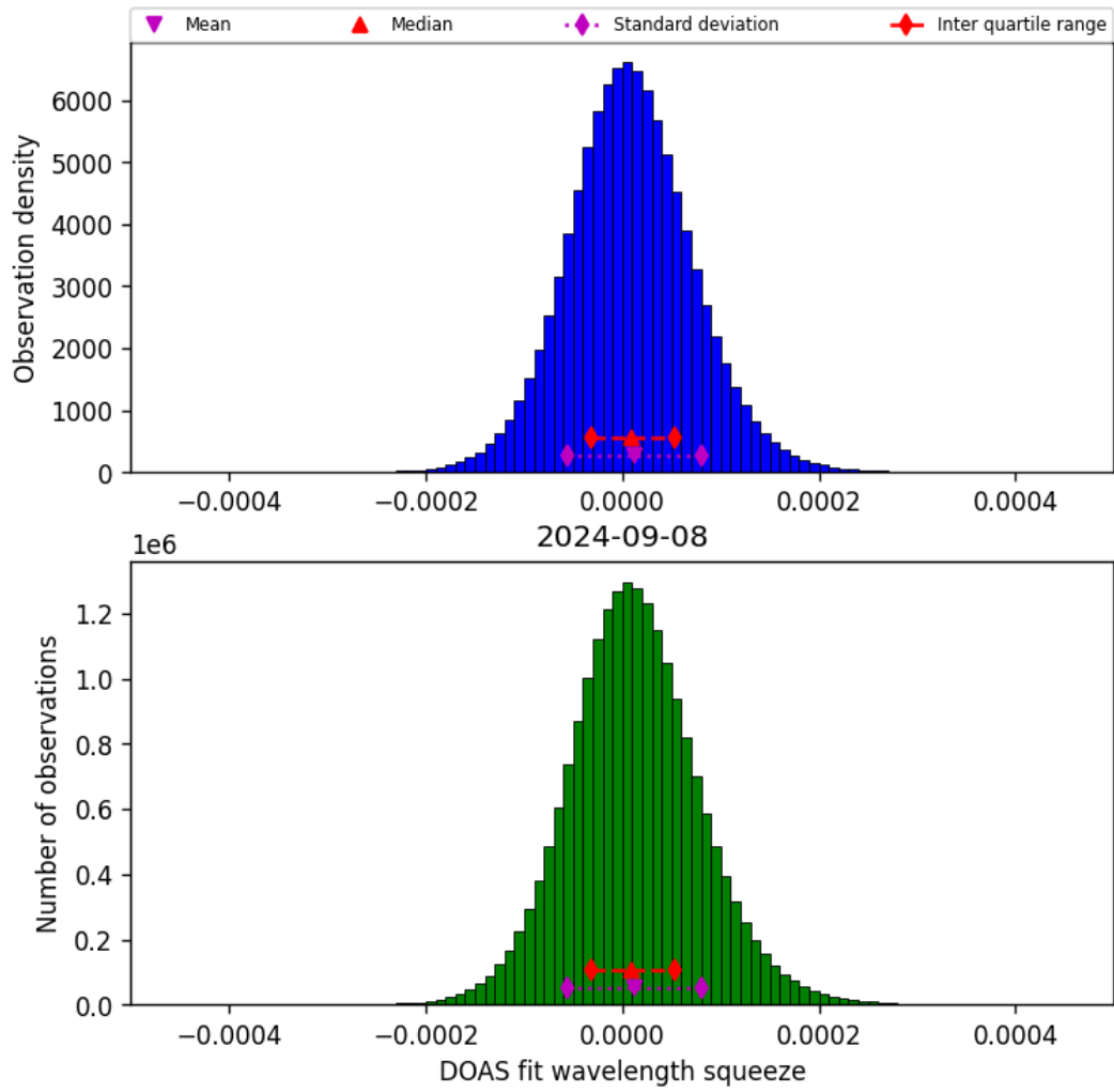
Figure 45: Histogram of “DOAS fit wavelength squeeze” for 2024-09-07 to 2024-09-09
