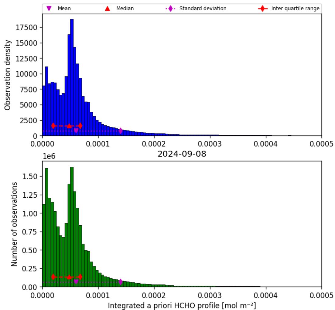
Figure 43: Histogram of “Integrated a priori HCHO profile” for 2024-09-07 to 2024-09-09
