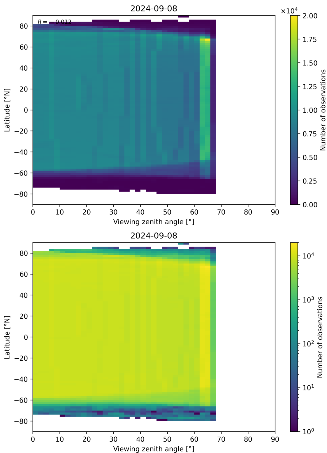
Figure 196: Scatter density plot of “Viewing zenith angle” against “Latitude” for 2024-09-07 to 2024-09-09.
