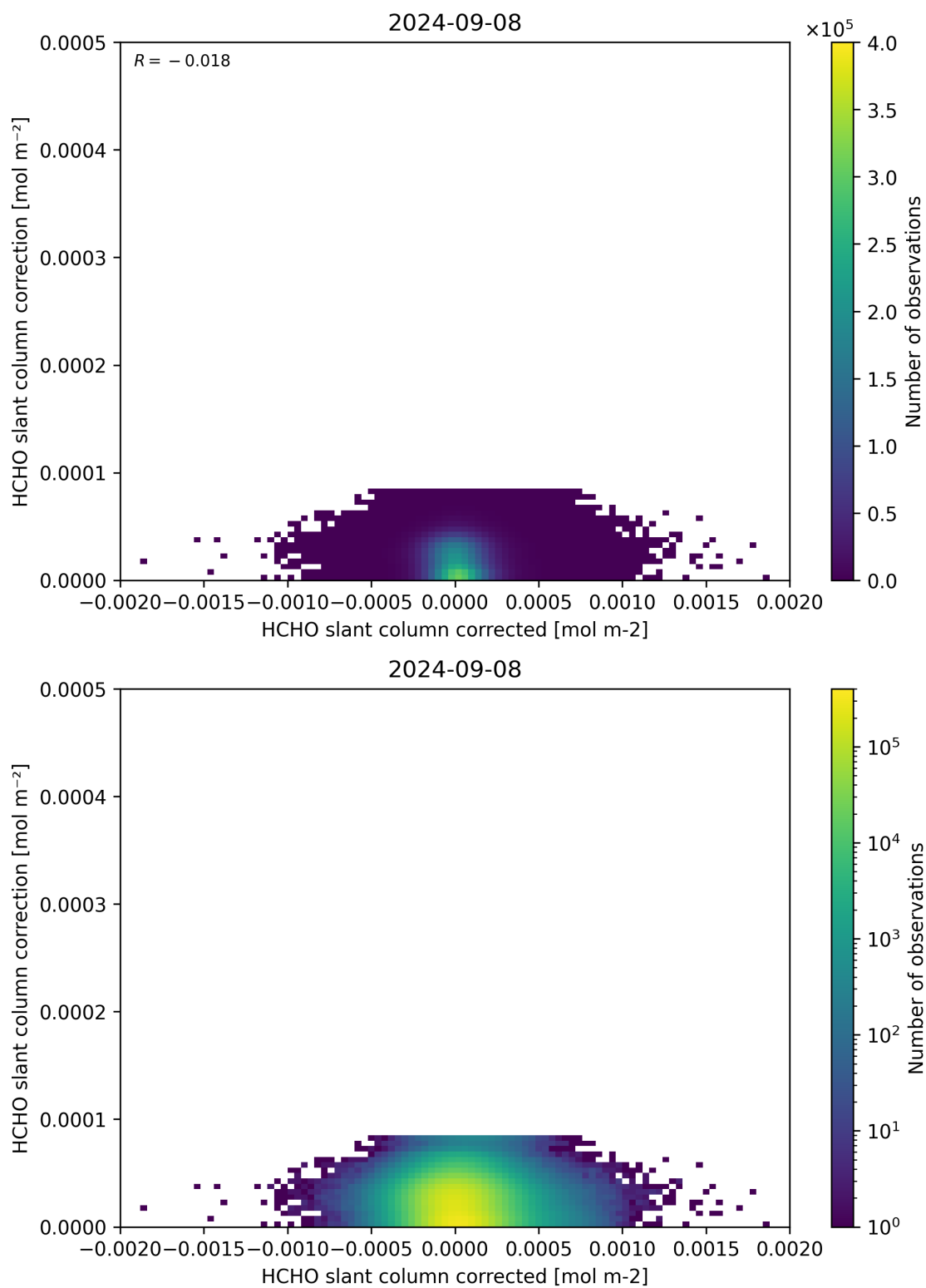
Figure 77: Scatter density plot of “HCHO slant column corrected” against “HCHO slant column correction” for 2024-09-07 to 2024-09-09.
