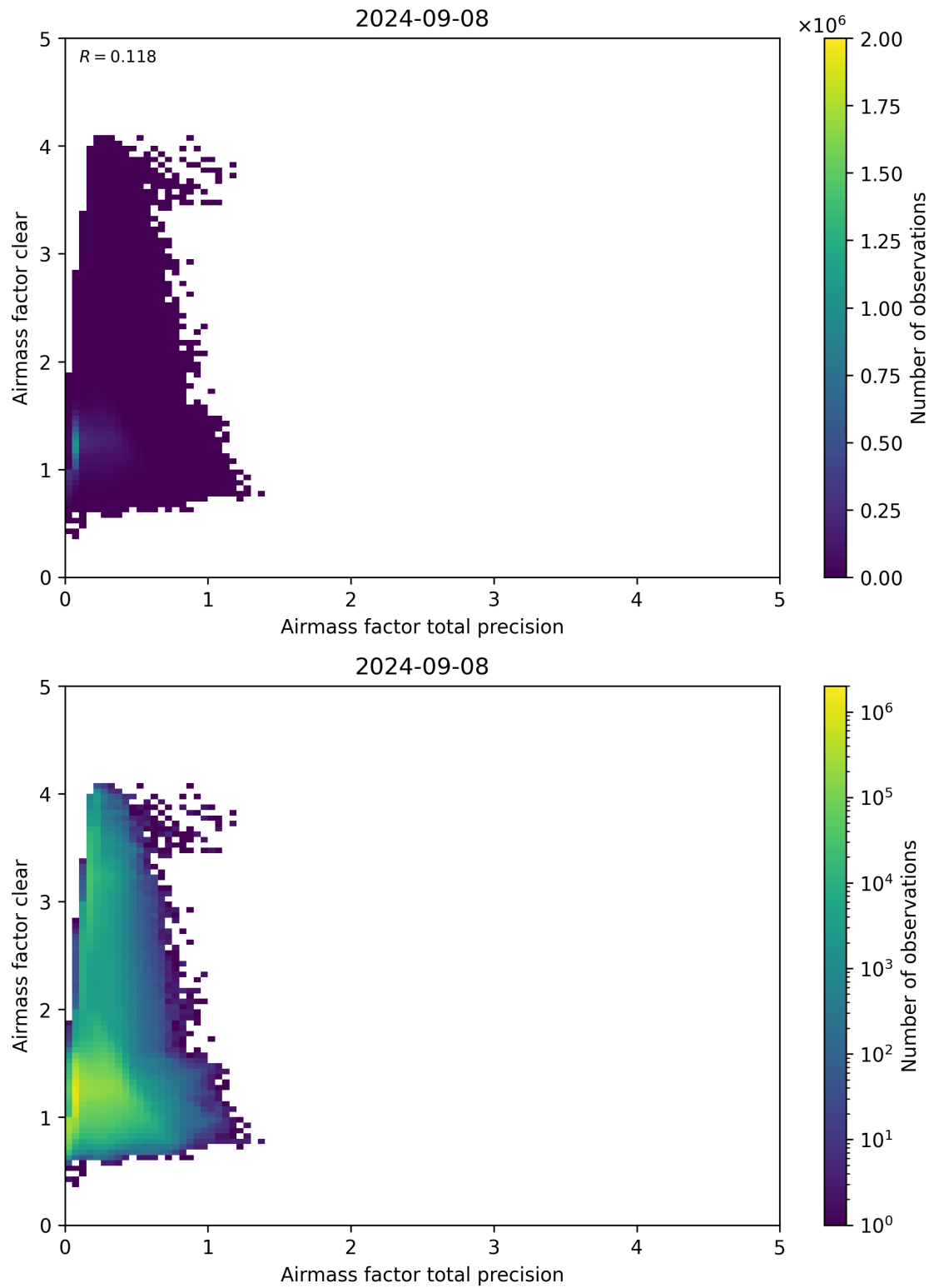
Figure 108: Scatter density plot of “Airmass factor total precision” against “Airmass factor clear” for 2024-09-07 to 2024-09-09.
