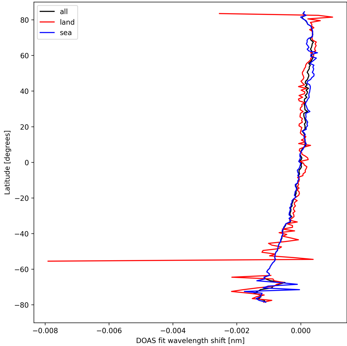
Figure 30: Zonal average of "DOAS fit wavelength shift" for 2024-09-07 to 2024-09-09.
