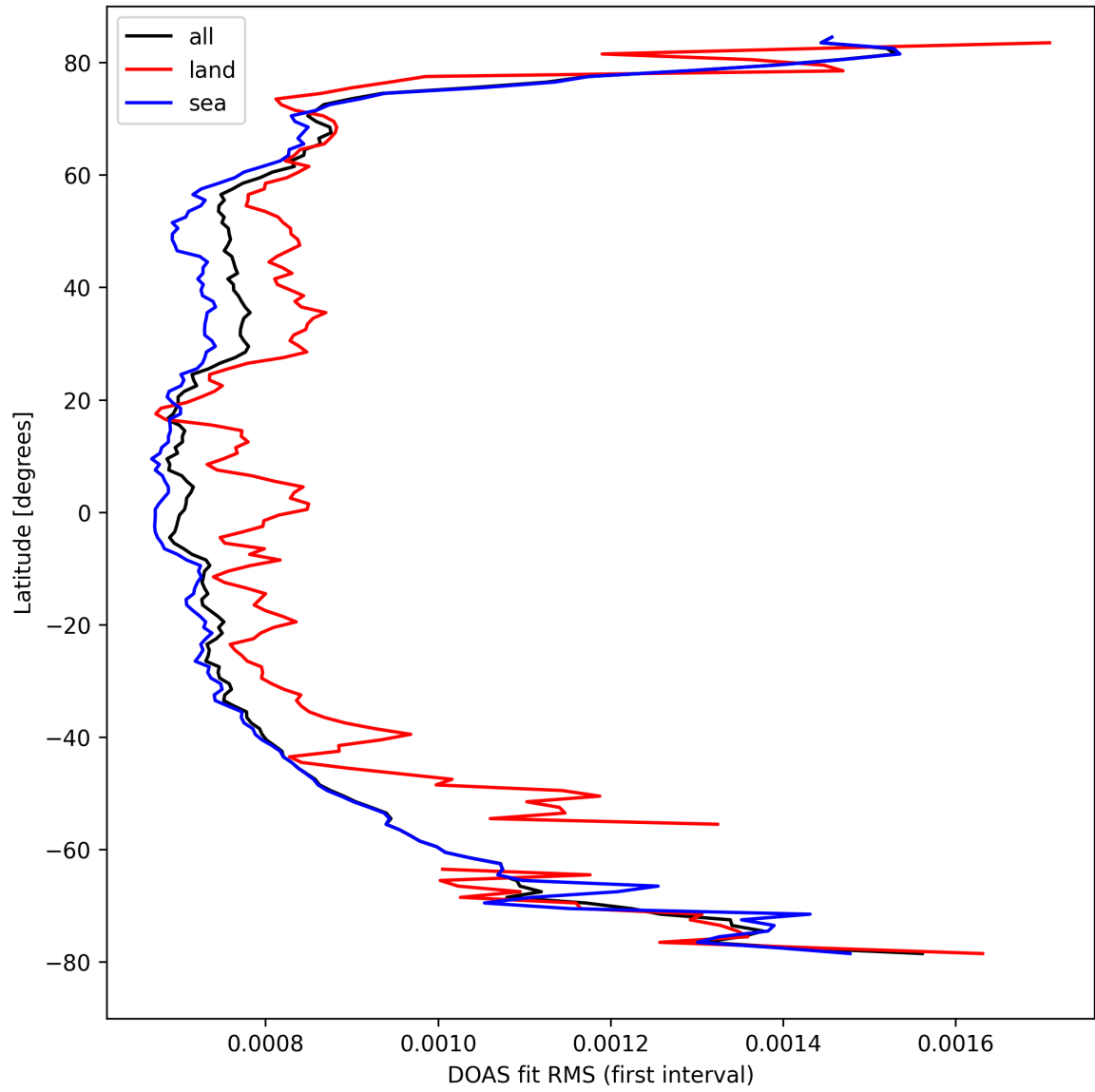
Figure 32: Zonal average of "DOAS fit RMS (first interval)" for 2024-09-07 to 2024-09-09.
