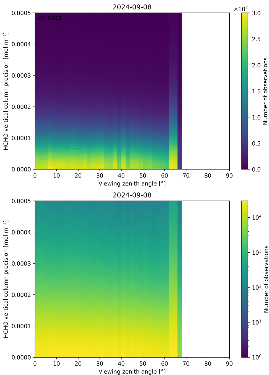
Figure 194: Scatter density plot of “Viewing zenith angle” against “HCHO vertical column precision” for 2024-09-07 to 2024-09-09.
