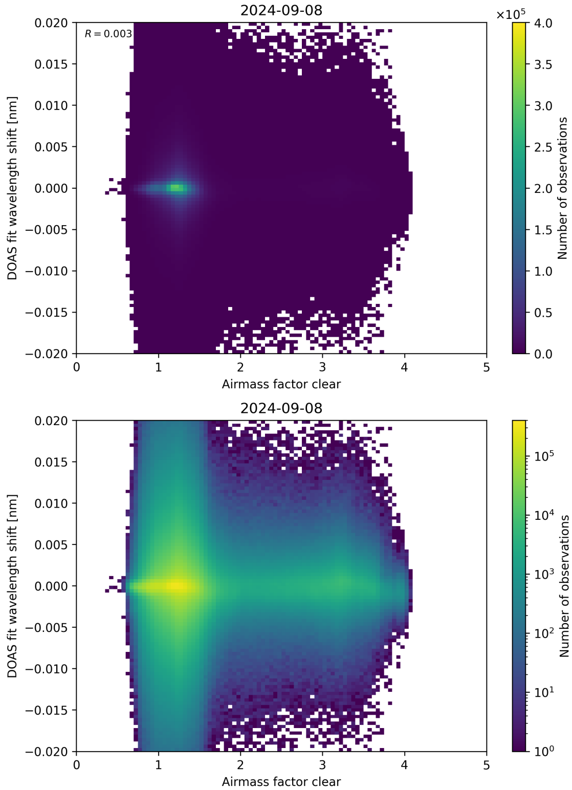
Figure 72: Scatter density plot of “Airmass factor clear” against “DOAS fit wavelength shift” for 2024-09-07 to 2024-09-09.
