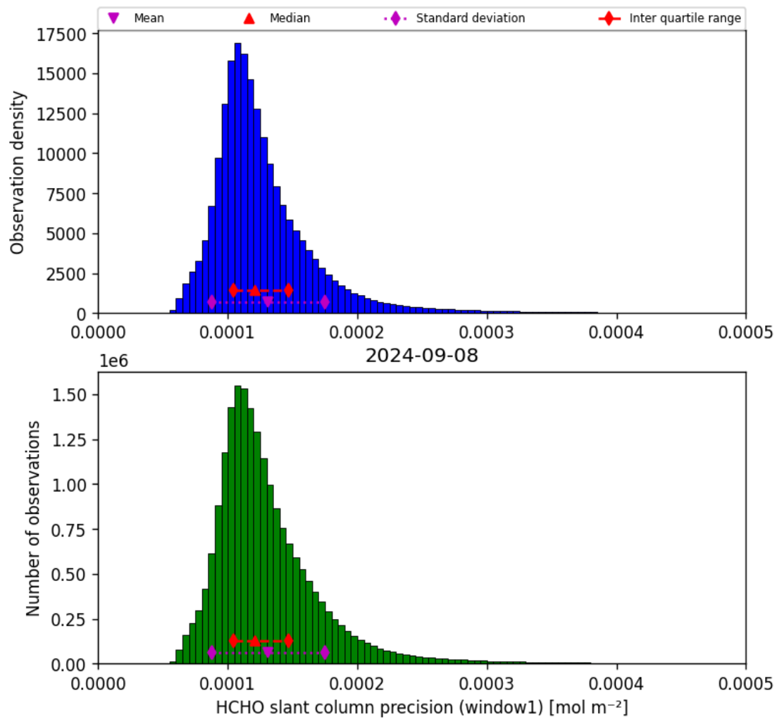
Figure 39: Histogram of “HCHO slant column precision (window1)” for 2024-09-07 to 2024-09-09
