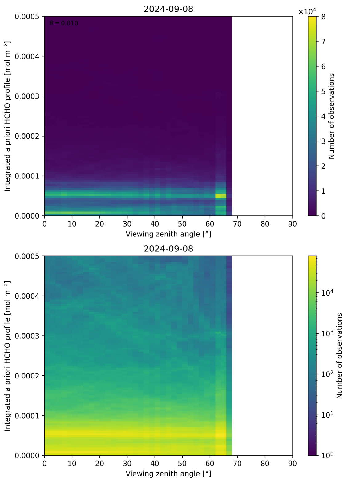
Figure 195: Scatter density plot of “Viewing zenith angle” against “Integrated a priori HCHO profile” for 2024-09-07 to 2024-09-09.
