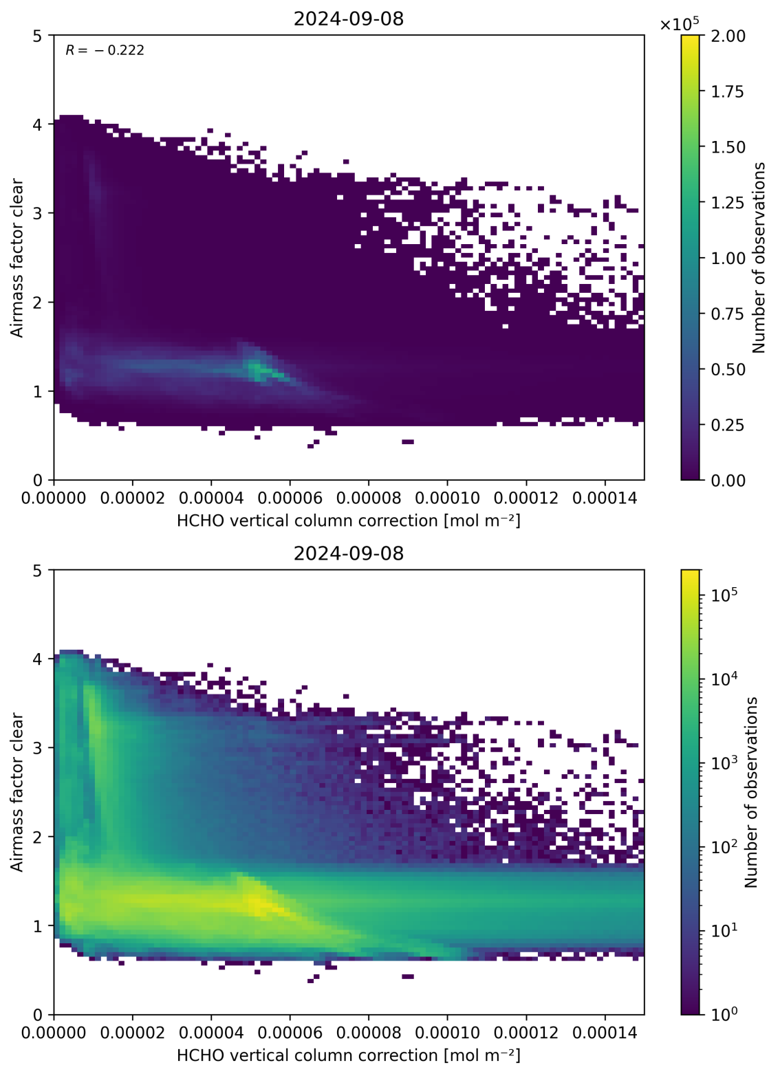
Figure 115: Scatter density plot of “HCHO vertical column correction” against “Airmass factor clear” for 2024-09-07 to 2024-09-09.
