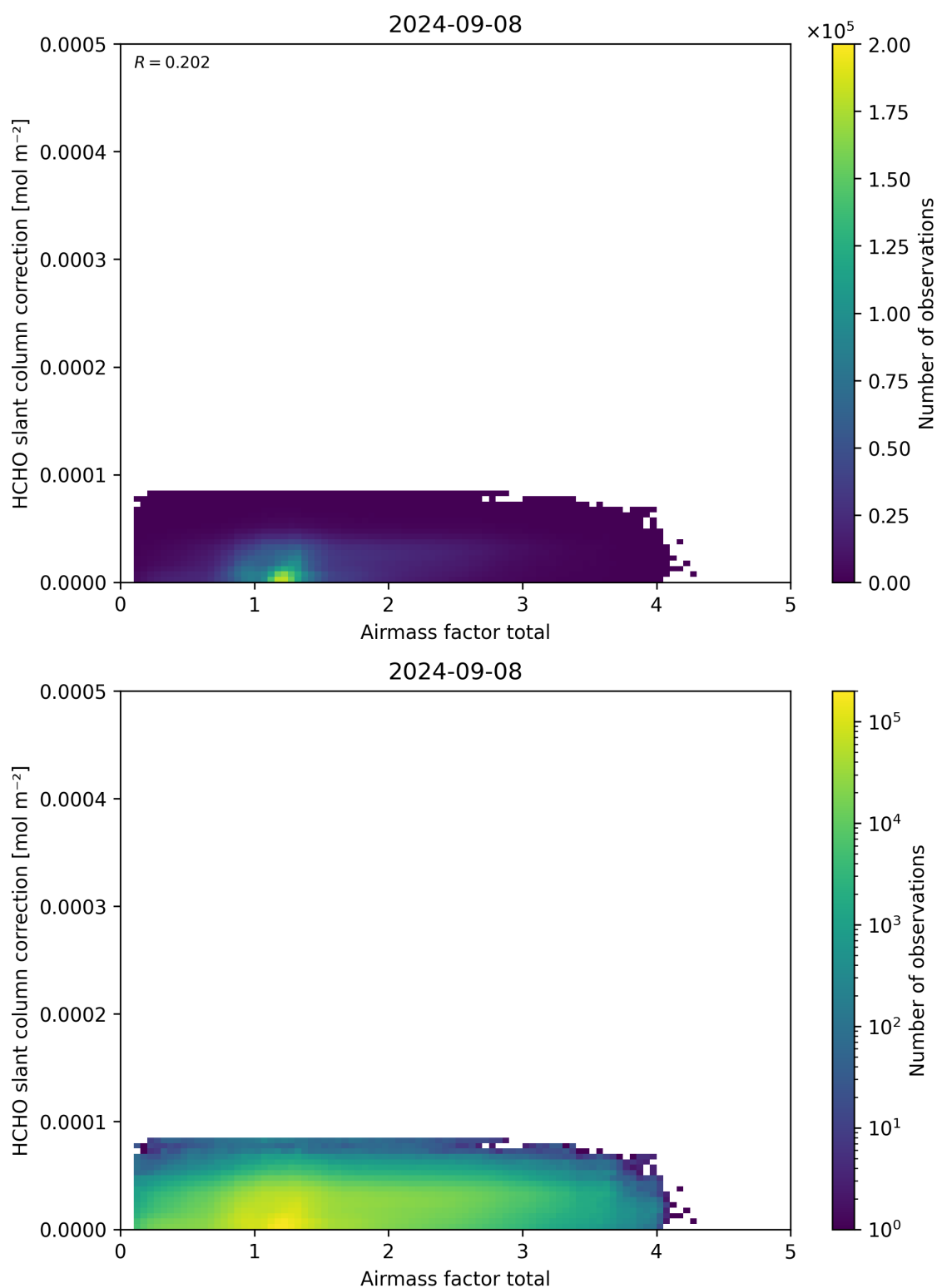
Figure 102: Scatter density plot of “Airmass factor total” against “HCHO slant column correction” for 2024-09-07 to 2024-09-09.
