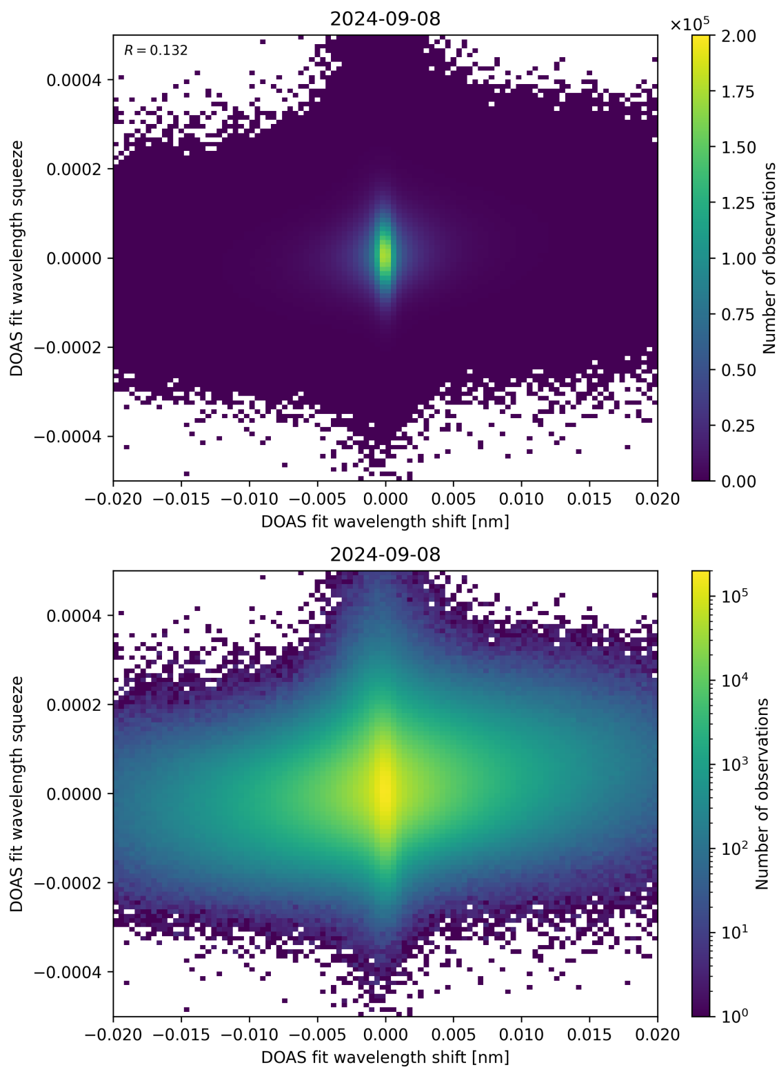
Figure 65: Scatter density plot of “DOAS fit wavelength shift” against “DOAS fit wavelength squeeze” for 2024-09-07 to 2024-09-09.
