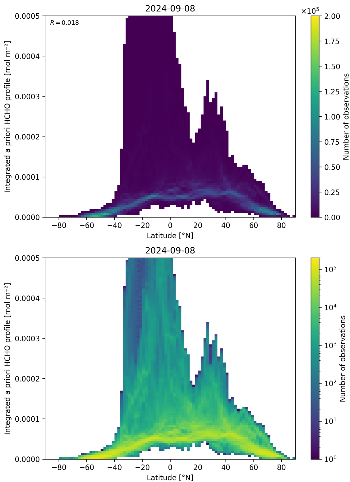
Figure 166: Scatter density plot of “Latitude” against “Integrated a priori HCHO profile” for 2024-09-07 to 2024-09-09.
