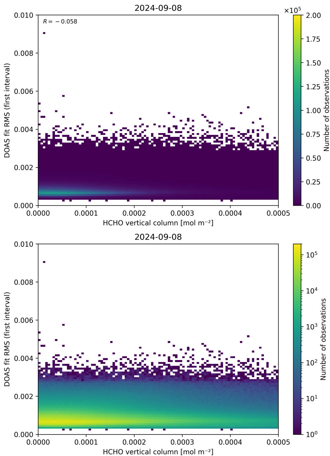
Figure 123: Scatter density plot of “HCHO vertical column” against “DOAS fit RMS (first interval)” for 2024-09-07 to 2024-09-09.
