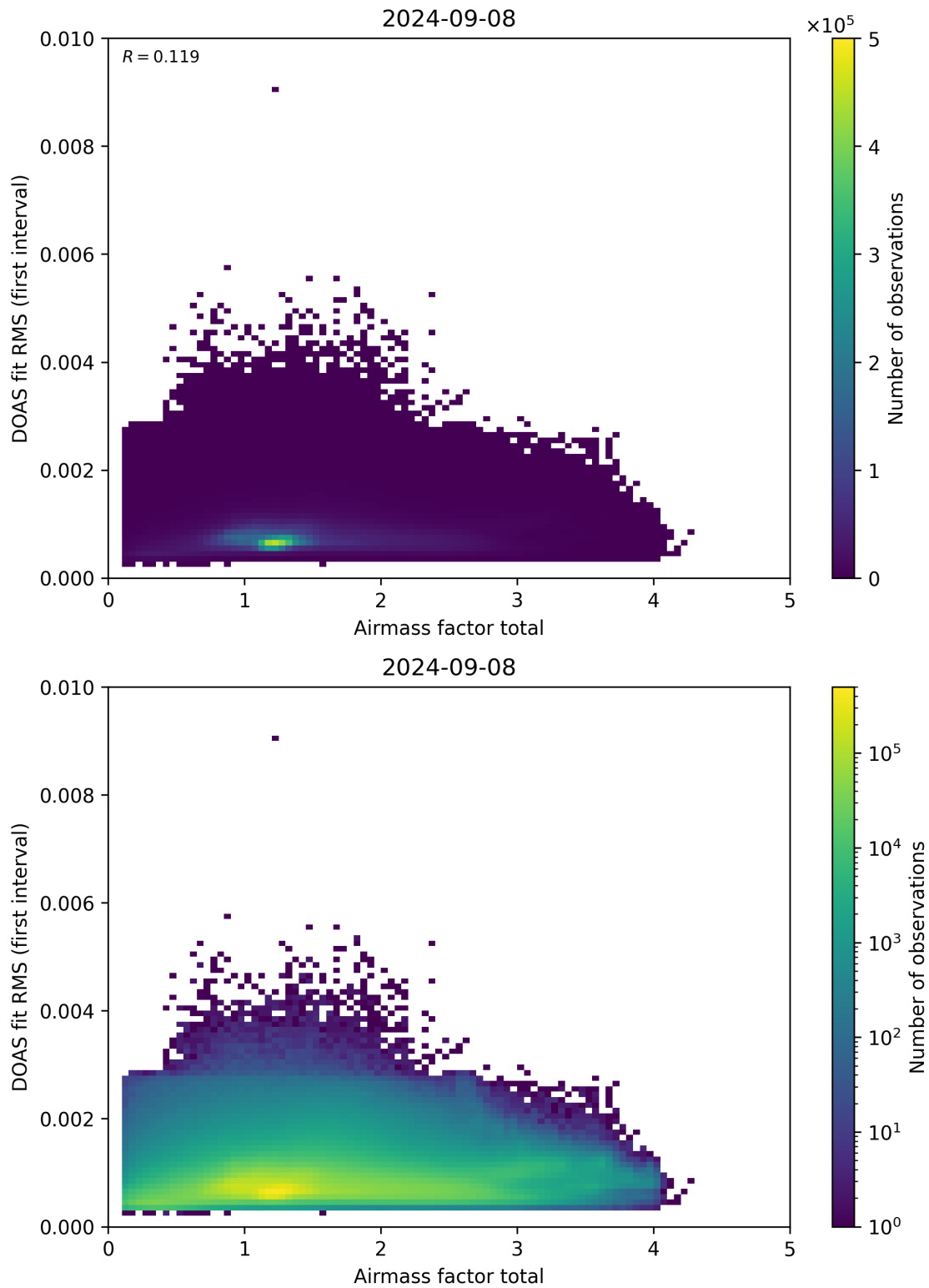
Figure 97: Scatter density plot of “Airmass factor total” against “DOAS fit RMS (first interval)” for 2024-09-07 to 2024-09-09.
