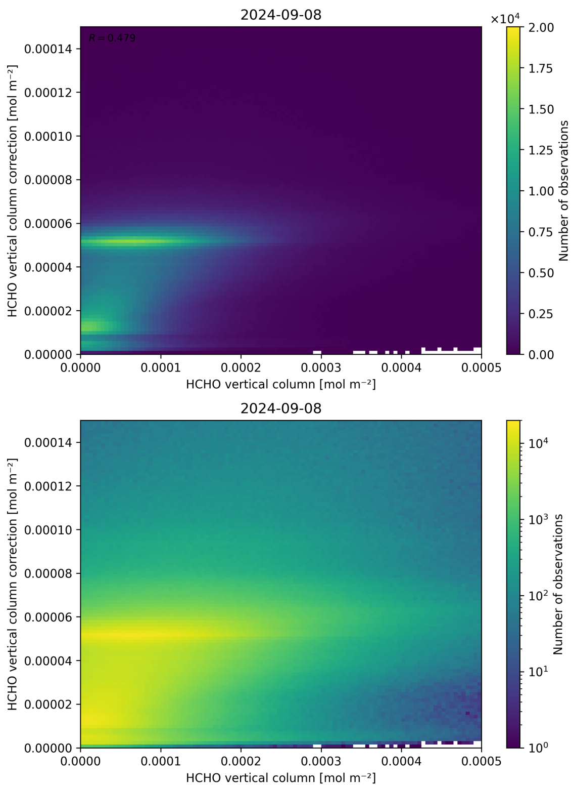
Figure 133: Scatter density plot of “HCHO vertical column” against “HCHO vertical column correction” for 2024-09-07 to 2024-09-09.
