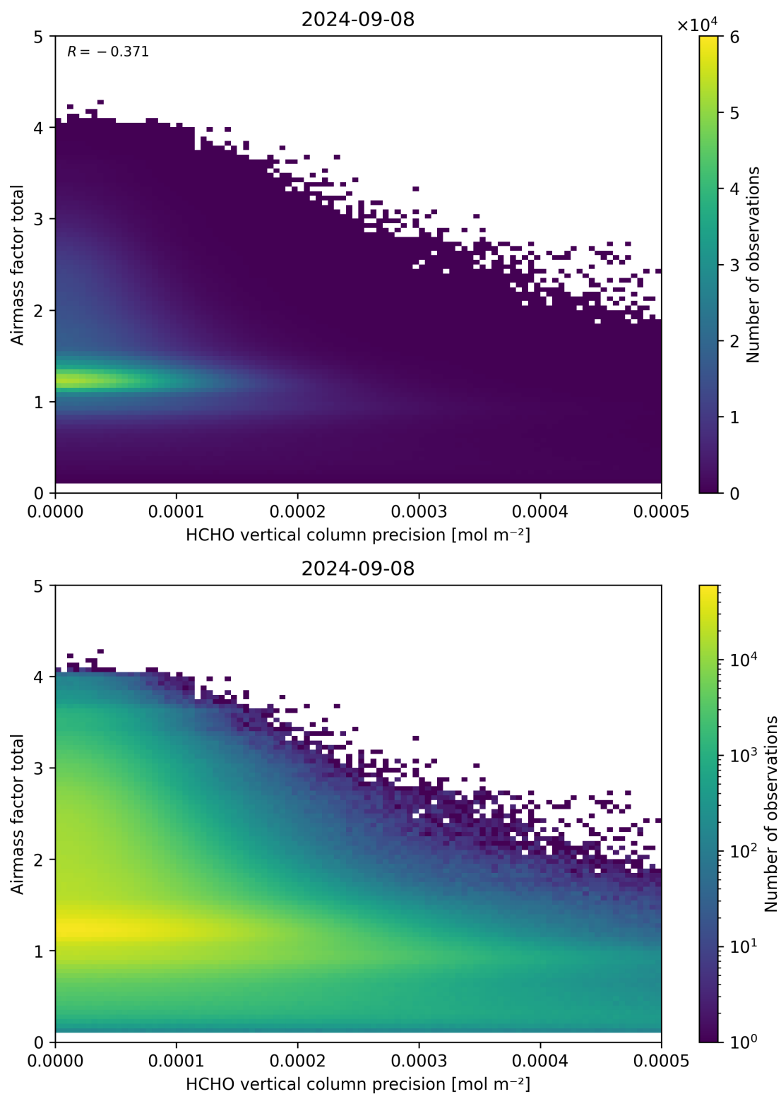
Figure 144: Scatter density plot of “HCHO vertical column precision” against “Airmass factor total” for 2024-09-07 to 2024-09-09.
