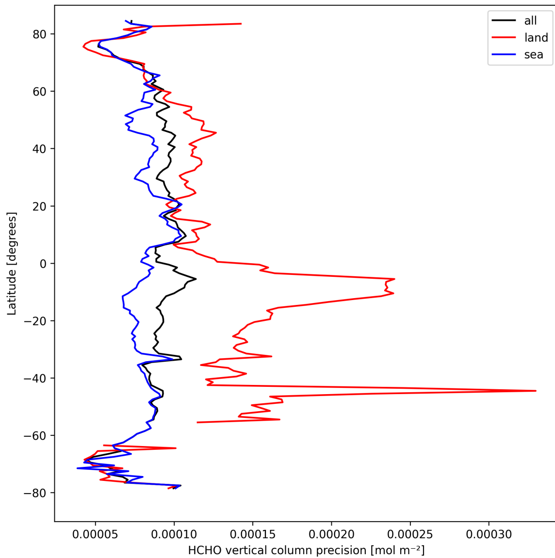
Figure 22: Zonal average of “HCHO vertical column precision” for 2024-09-07 to 2024-09-09.
