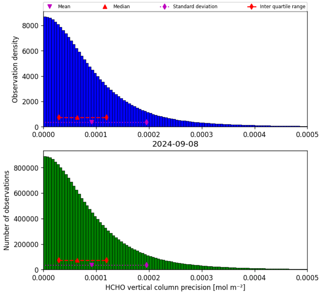
Figure 36: Histogram of “HCHO vertical column precision” for 2024-09-07 to 2024-09-09
