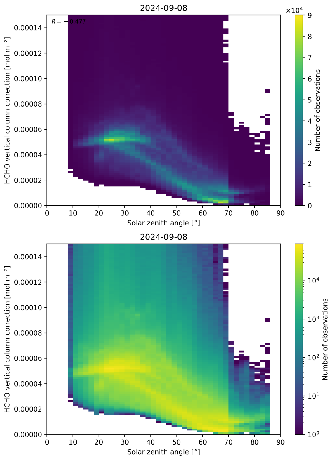
Figure 178: Scatter density plot of “Solar zenith angle” against “HCHO vertical column correction” for 2024-09-07 to 2024-09-09.
