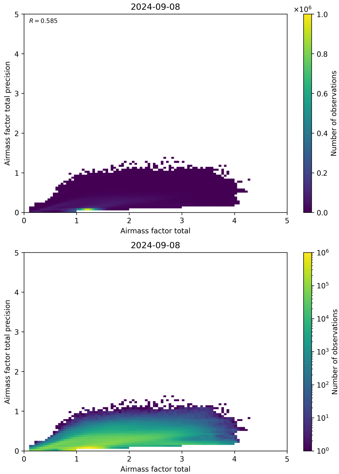
Figure 103: Scatter density plot of “Airmass factor total” against “Airmass factor total precision” for 2024-09-07 to 2024-09-09.
