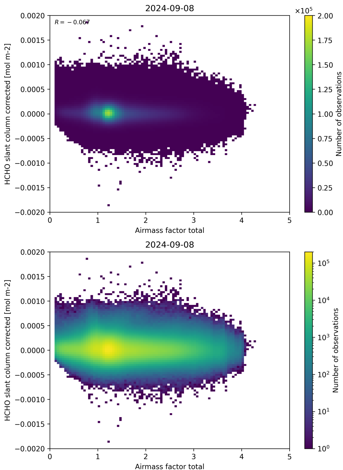
Figure 101: Scatter density plot of “Airmass factor total” against “HCHO slant column corrected” for 2024-09-07 to 2024-09-09.
