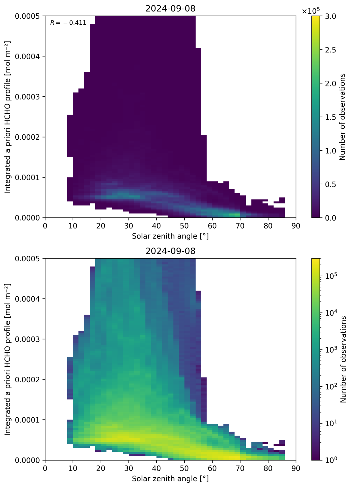
Figure 180: Scatter density plot of “Solar zenith angle” against “Integrated a priori HCHO profile” for 2024-09-07 to 2024-09-09.
