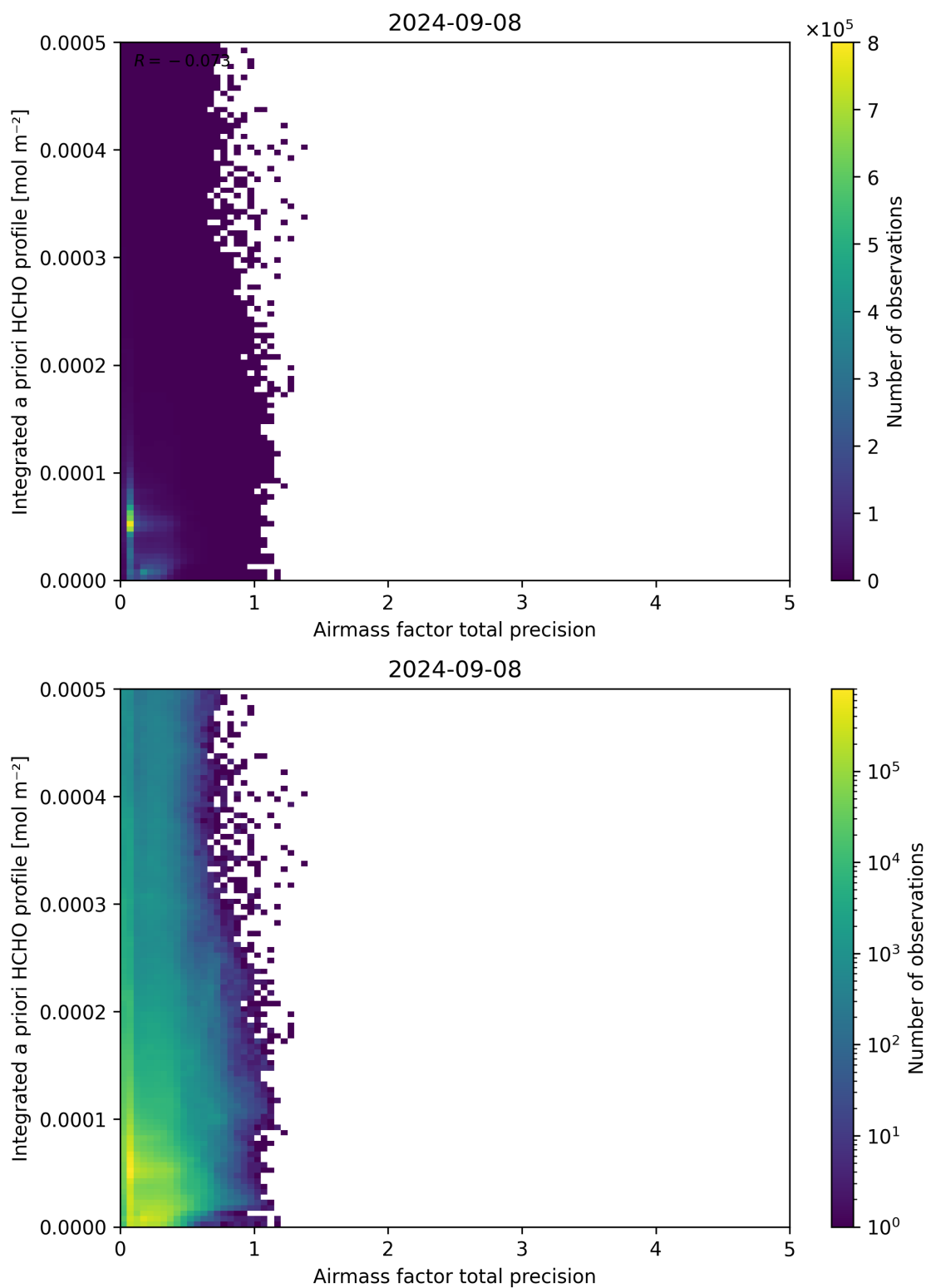
Figure 111: Scatter density plot of “Airmass factor total precision” against “Integrated a priori HCHO profile” for 2024-09-07 to 2024-09-09.
