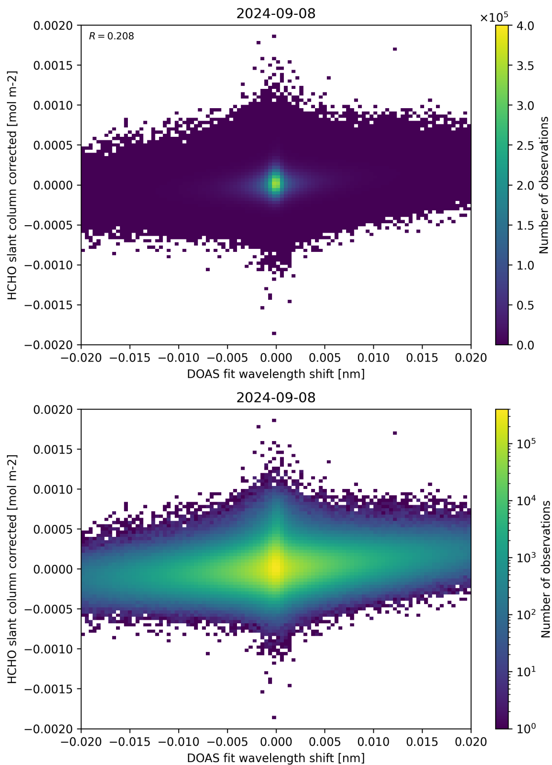
Figure 66: Scatter density plot of “DOAS fit wavelength shift” against “HCHO slant column corrected” for 2024-09-07 to 2024-09-09.
