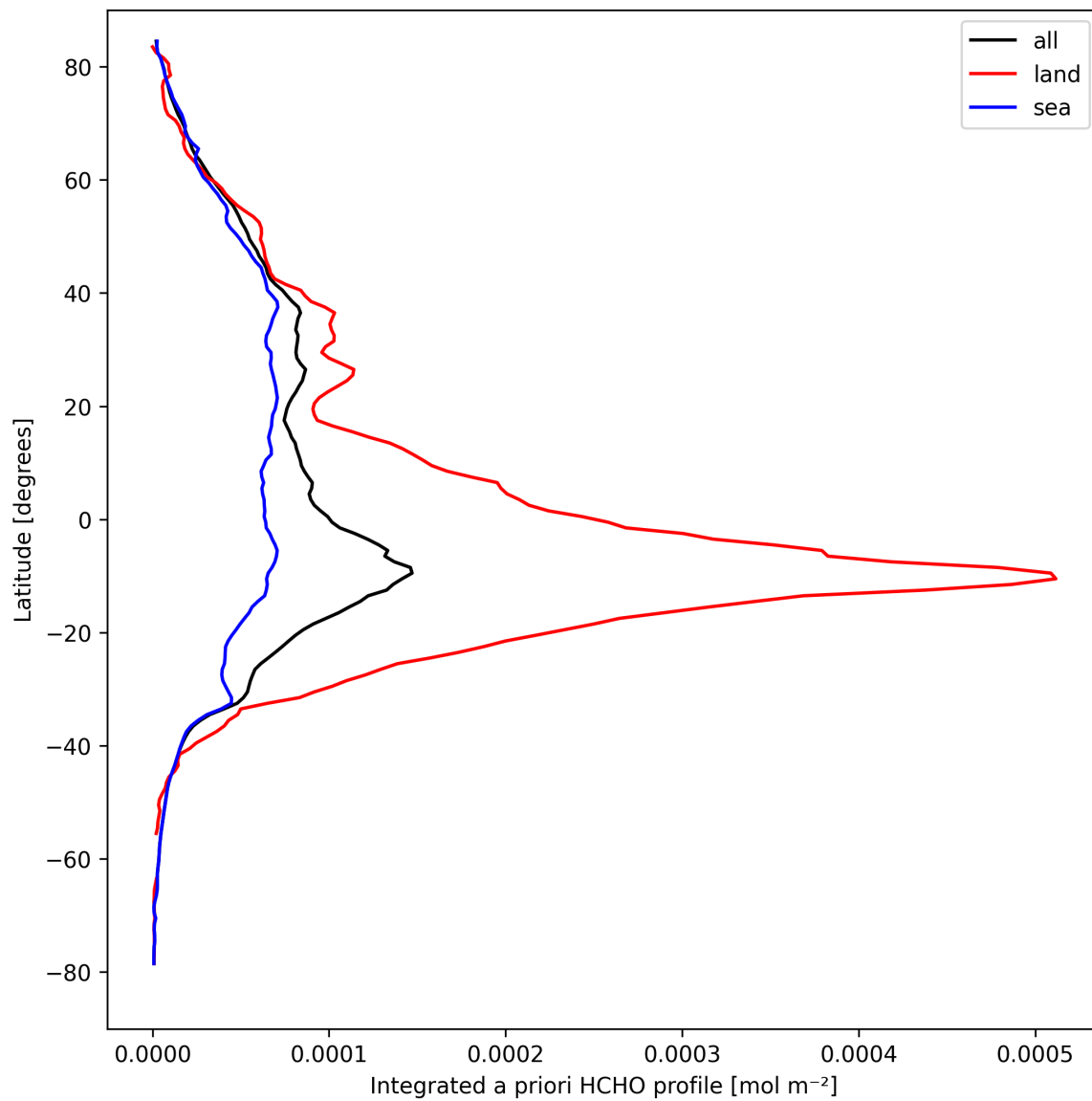
Figure 29: Zonal average of “Integrated a priori HCHO profile” for 2024-09-07 to 2024-09-09.
