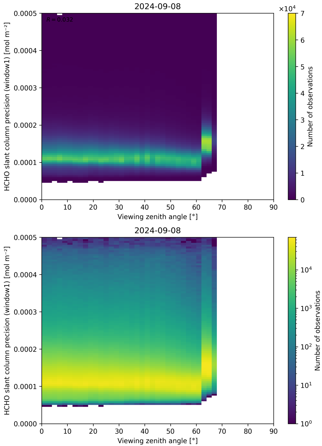
Figure 189: Scatter density plot of “Viewing zenith angle” against “HCHO slant column precision (window1)” for 2024-09-07 to 2024-09-09.
