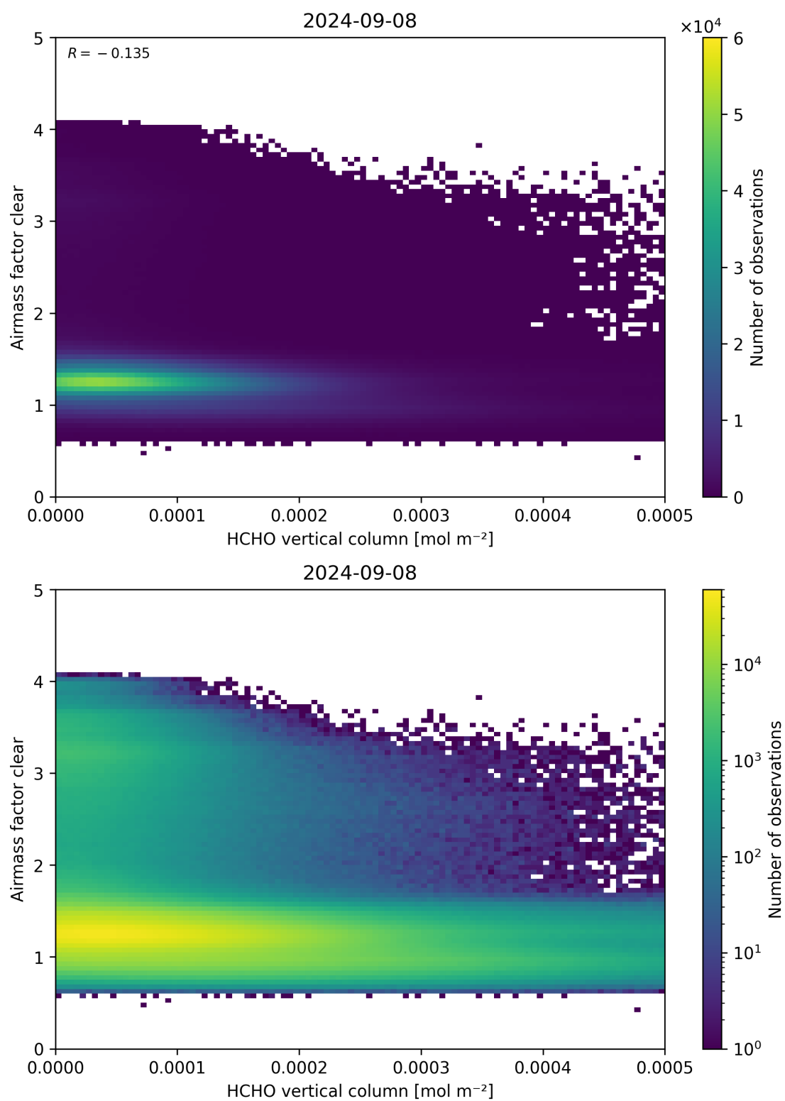
Figure 126: Scatter density plot of “HCHO vertical column” against “Airmass factor clear” for 2024-09-07 to 2024-09-09.
