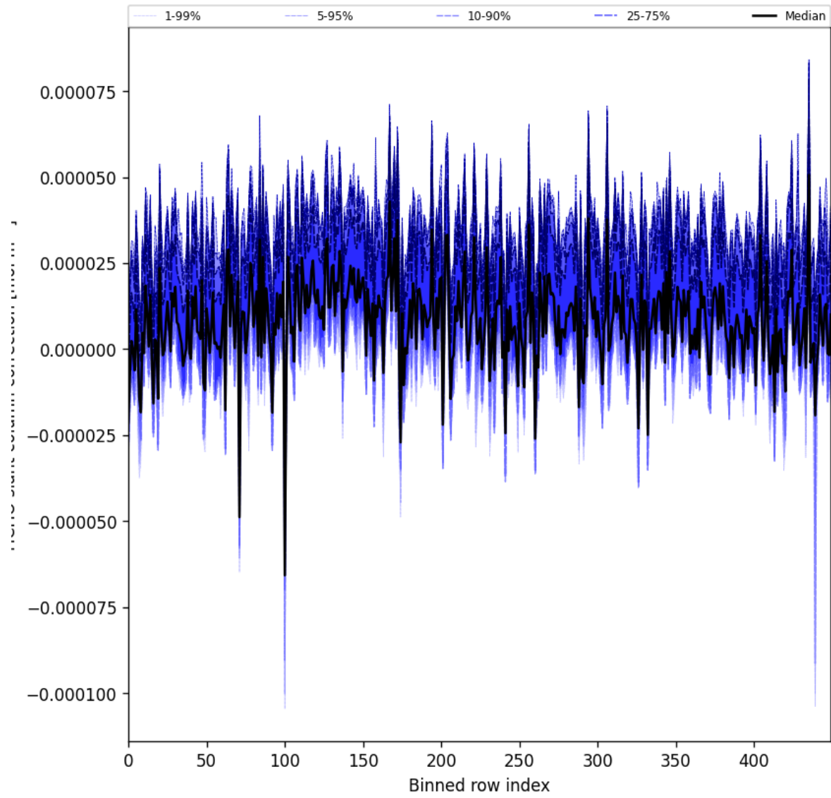
Figure 61: Along track statistics of “HCHO slant column correction” for 2024-09-07 to 2024-09-09
