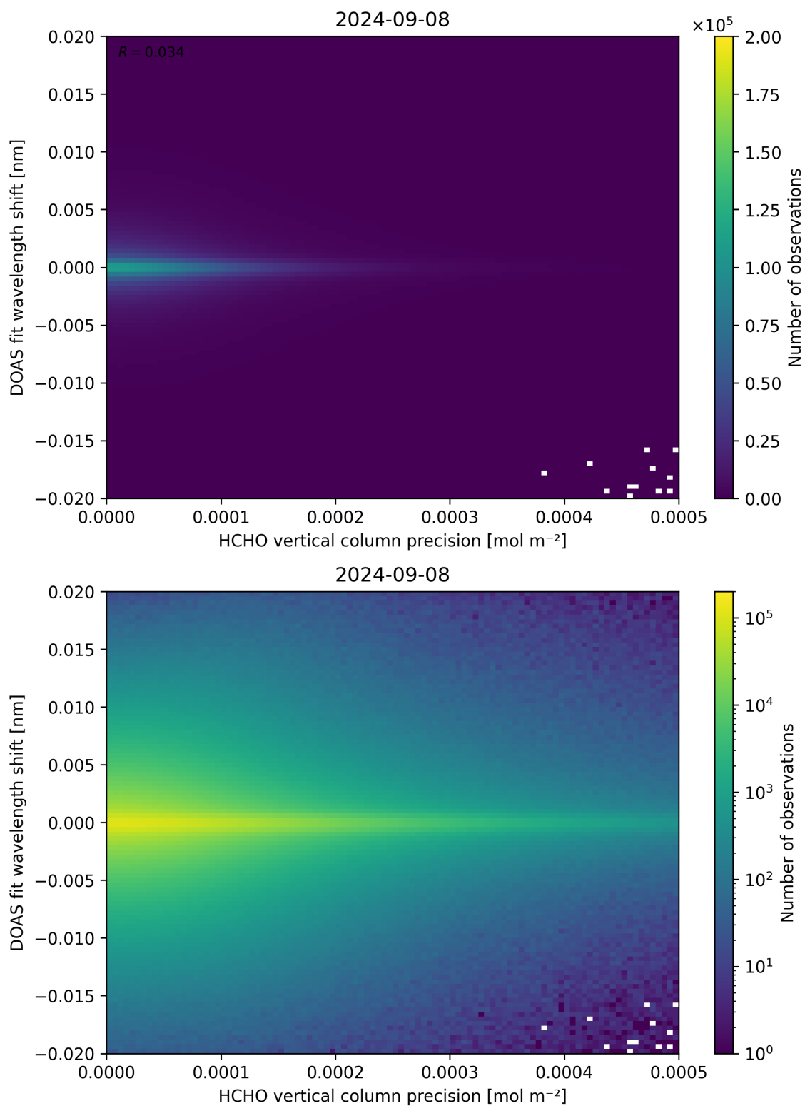
Figure 137: Scatter density plot of “HCHO vertical column precision” against “DOAS fit wavelength shift” for 2024-09-07 to 2024-09-09.
