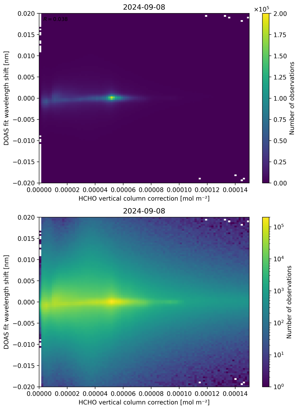
Figure 113: Scatter density plot of “HCHO vertical column correction” against “DOAS fit wavelength shift” for 2024-09-07 to 2024-09-09.
