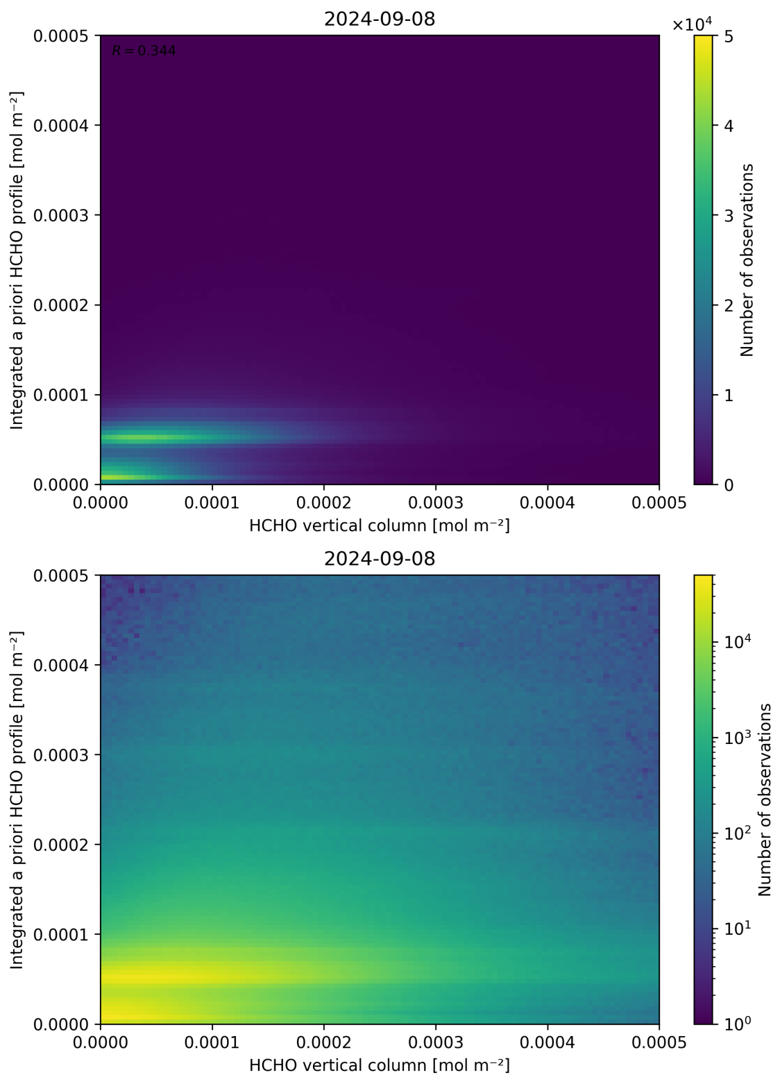
Figure 135: Scatter density plot of “HCHO vertical column” against “Integrated a priori HCHO profile” for 2024-09-07 to 2024-09-09.
