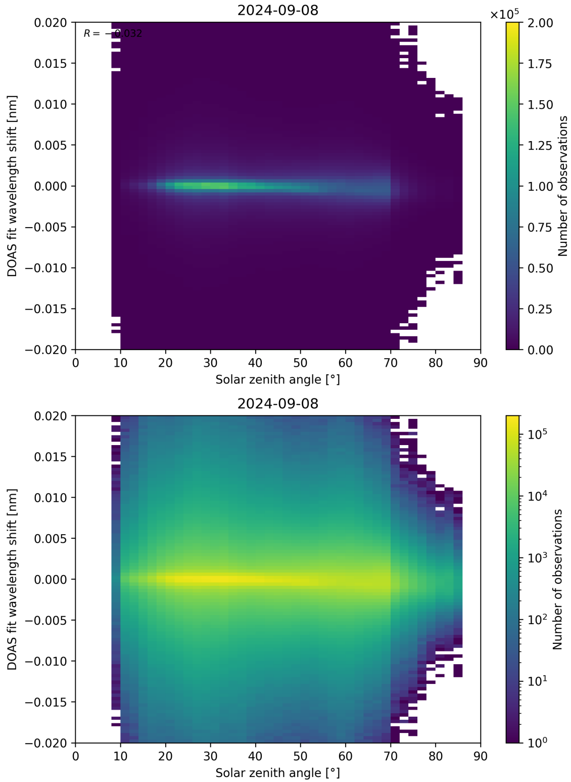
Figure 168: Scatter density plot of “Solar zenith angle” against “DOAS fit wavelength shift” for 2024-09-07 to 2024-09-09.
