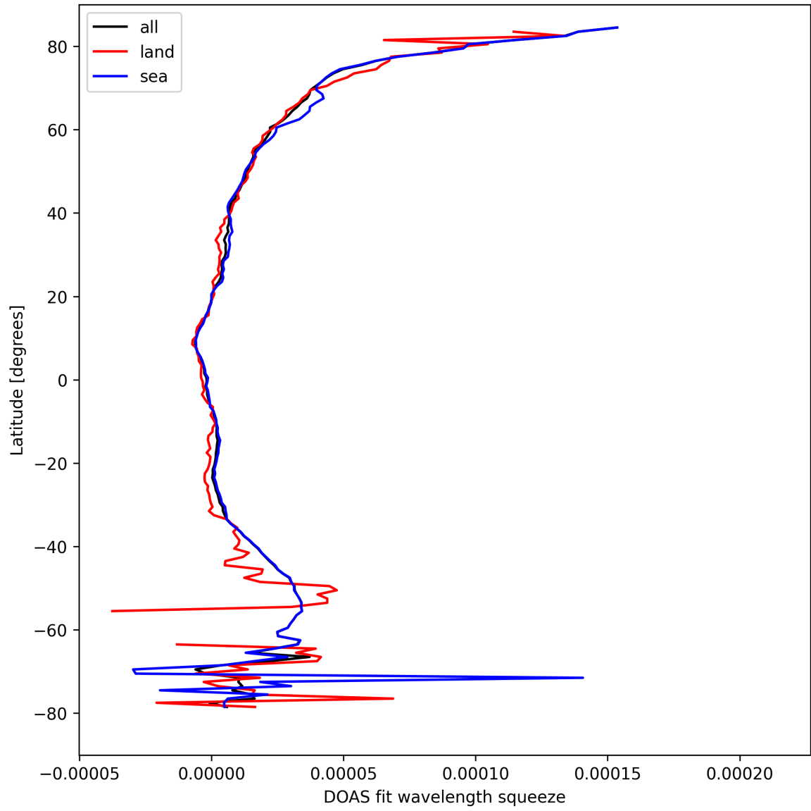
Figure 31: Zonal average of “DOAS fit wavelength squeeze” for 2024-09-07 to 2024-09-09.
