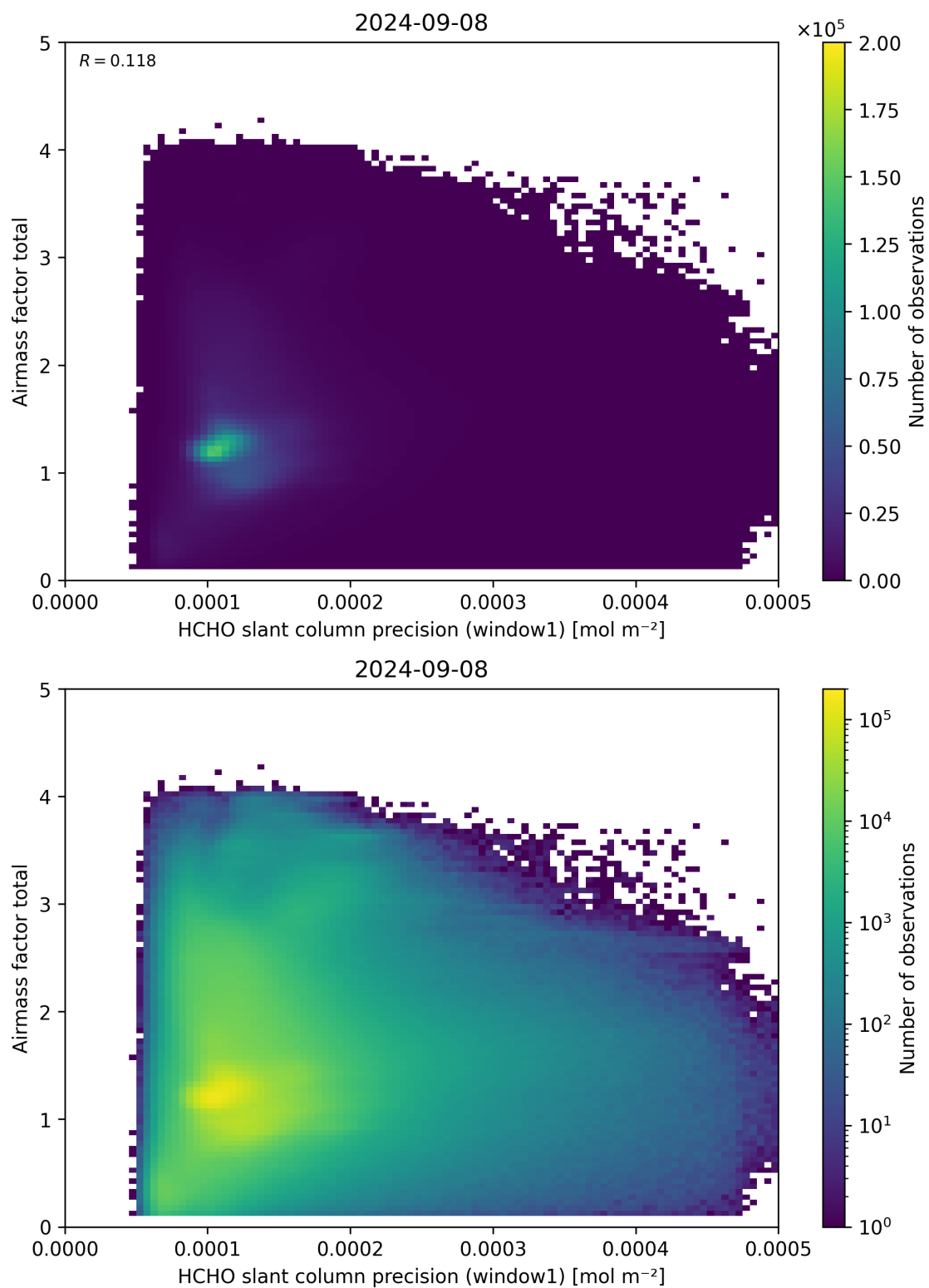
Figure 94: Scatter density plot of “HCHO slant column precision (window1)” against “Airmass factor total” for 2024-09-07 to 2024-09-09.
