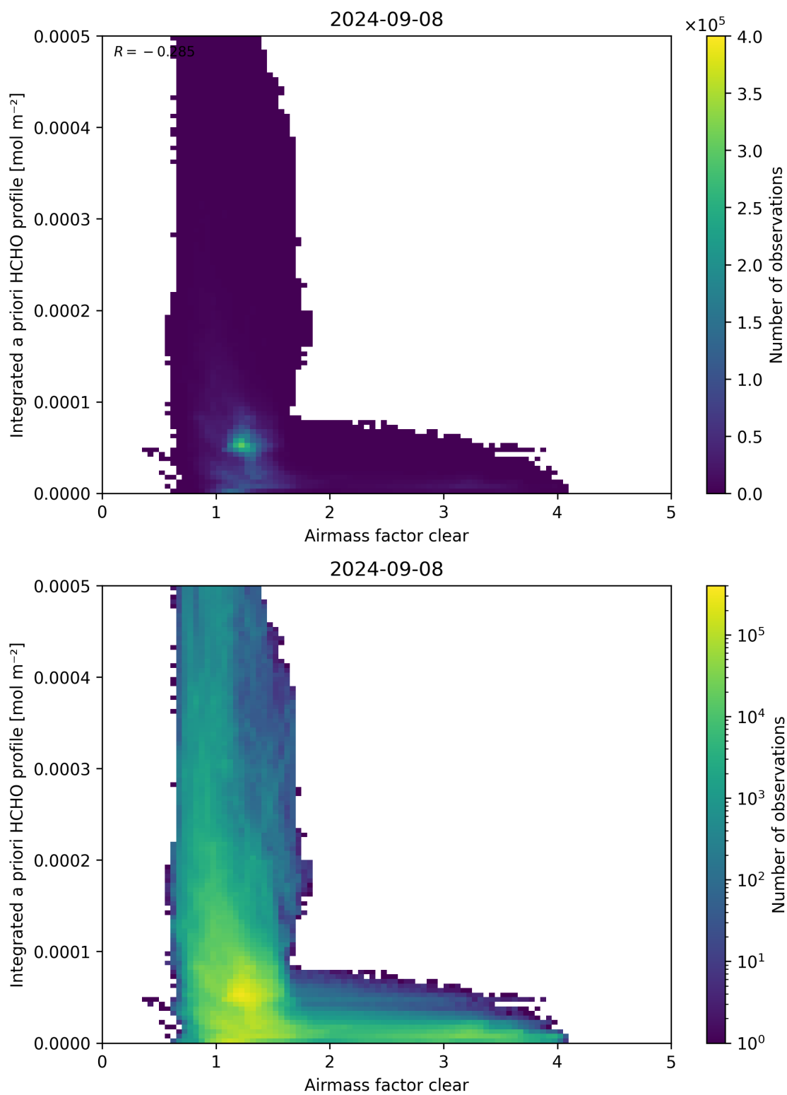
Figure 76: Scatter density plot of “Airmass factor clear” against “Integrated a priori HCHO profile” for 2024-09-07 to 2024-09-09.
