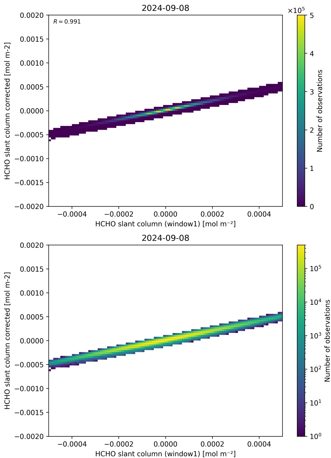
Figure 82: Scatter density plot of “HCHO slant column (window1)” against “HCHO slant column corrected” for 2024-09-07 to 2024-09-09.
