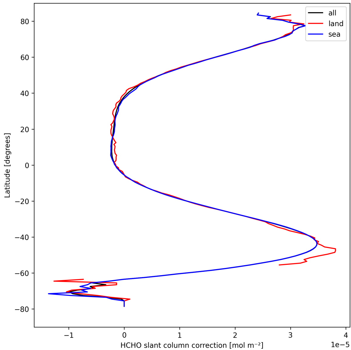
Figure 33: Zonal average of “HCHO slant column correction” for 2024-09-07 to 2024-09-09.
