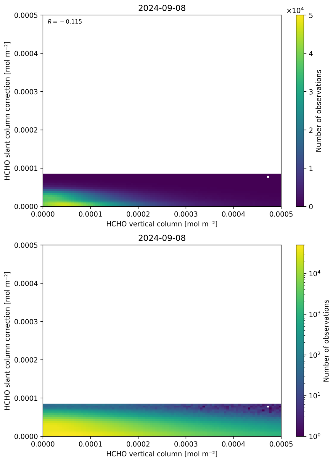
Figure 128: Scatter density plot of “HCHO vertical column” against “HCHO slant column correction” for 2024-09-07 to 2024-09-09.
