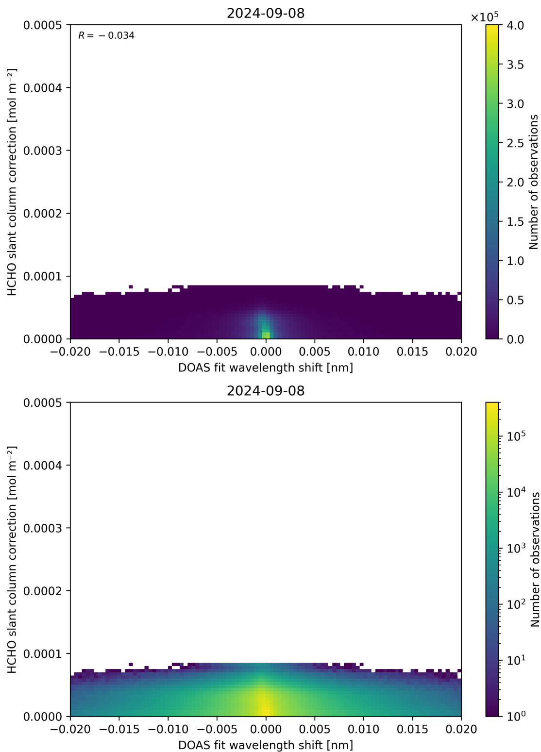
Figure 67: Scatter density plot of “DOAS fit wavelength shift” against “HCHO slant column correction” for 2024-09-07 to 2024-09-09.
