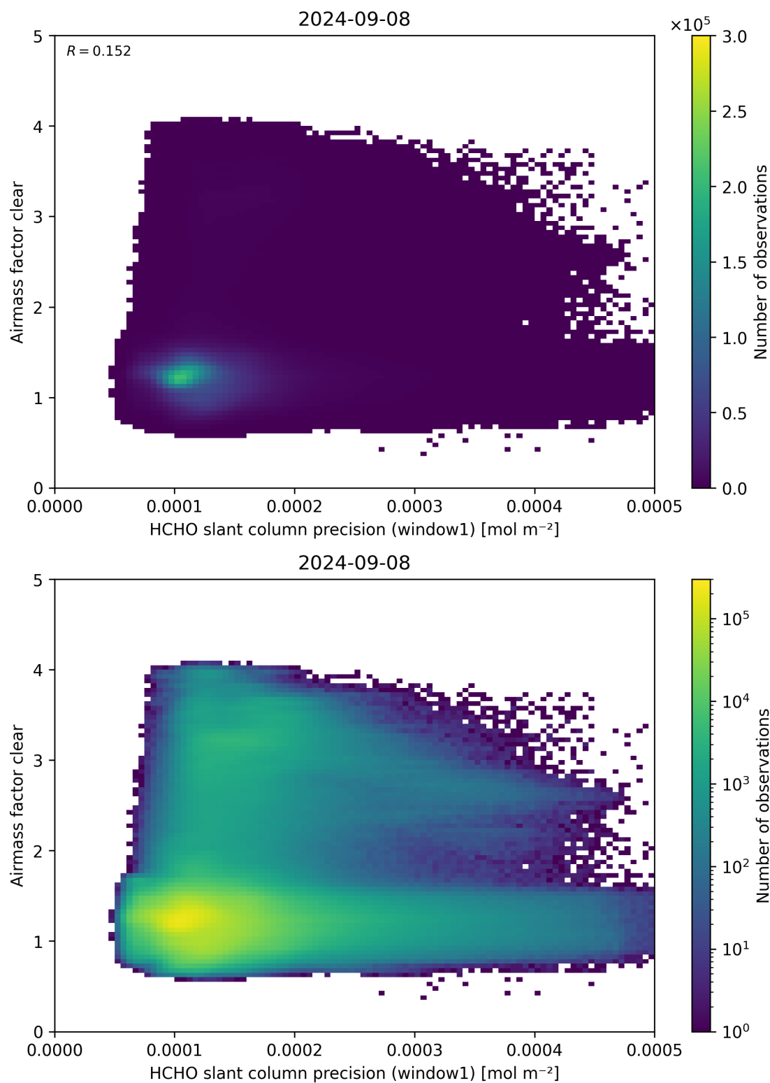
Figure 91: Scatter density plot of “HCHO slant column precision (window1)” against “Airmass factor clear” for 2024-09-07 to 2024-09-09.
