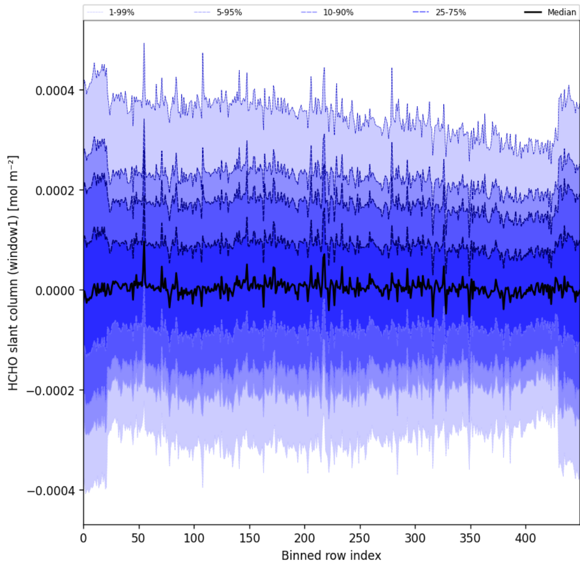
Figure 52: Along track statistics of “HCHO slant column (window1)” for 2024-09-07 to 2024-09-09
