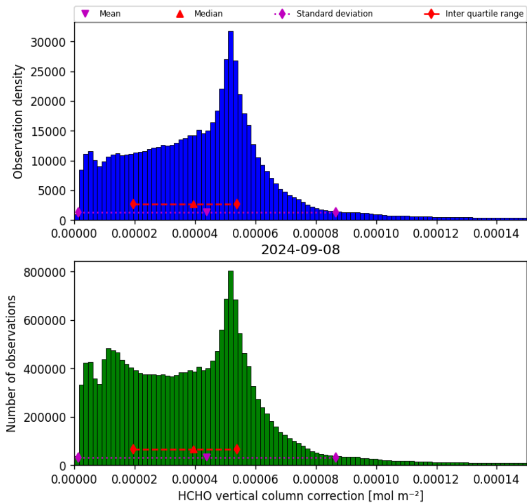
Figure 37: Histogram of “HCHO vertical column correction” for 2024-09-07 to 2024-09-09
