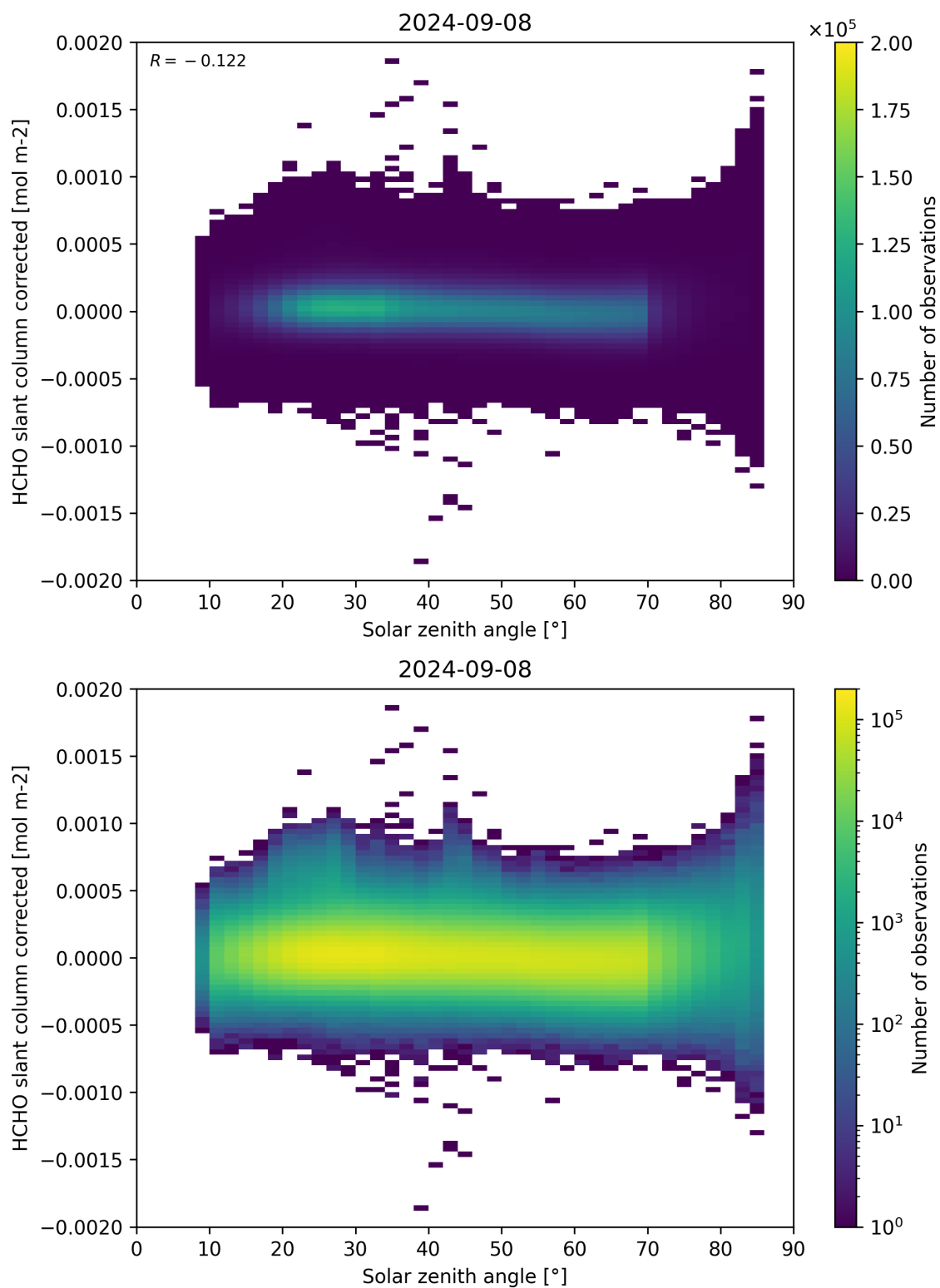
Figure 171: Scatter density plot of “Solar zenith angle” against “HCHO slant column corrected” for 2024-09-07 to 2024-09-09.
