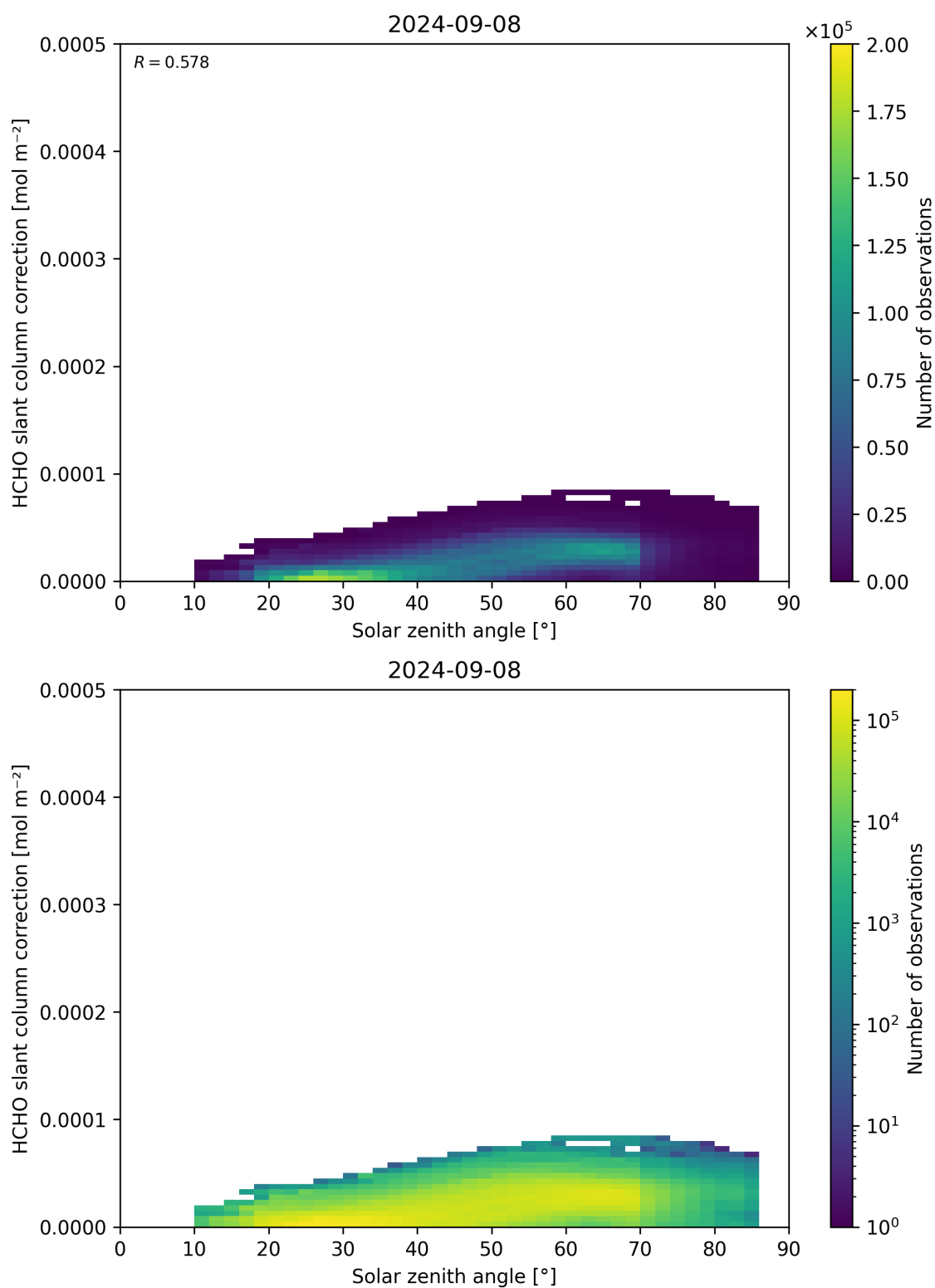
Figure 172: Scatter density plot of “Solar zenith angle” against “HCHO slant column correction” for 2024-09-07 to 2024-09-09.
