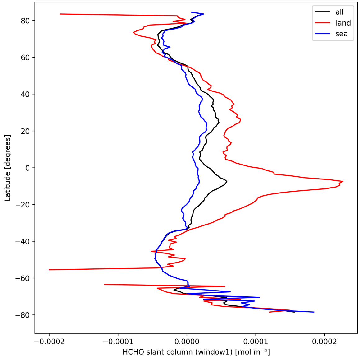
Figure 24: Zonal average of “HCHO slant column (window1)” for 2024-09-07 to 2024-09-09.
