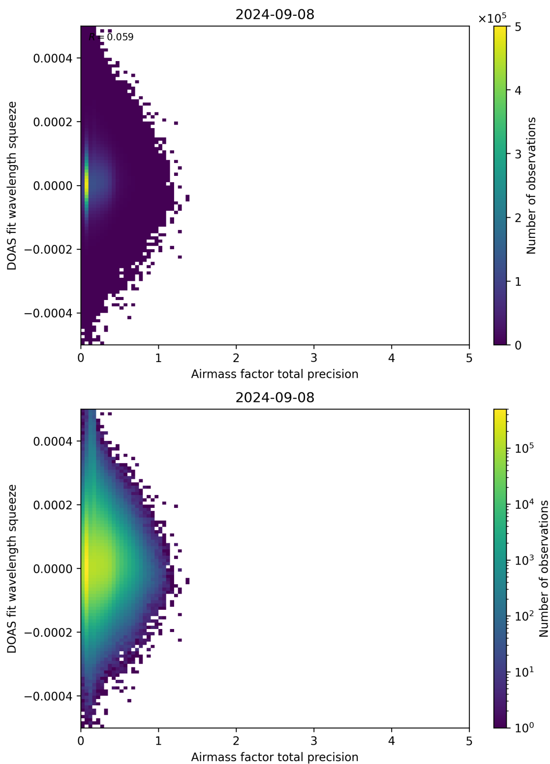
Figure 107: Scatter density plot of “Airmass factor total precision” against “DOAS fit wavelength squeeze” for 2024-09-07 to 2024-09-09.
