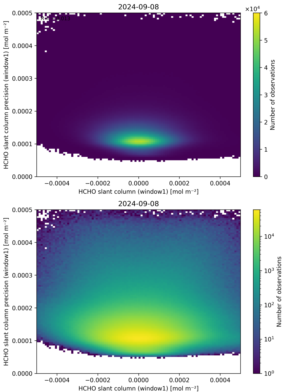
Figure 84: Scatter density plot of “HCHO slant column (window1)” against “HCHO slant column precision (window1)” for 2024-09-07 to 2024-09-09.
