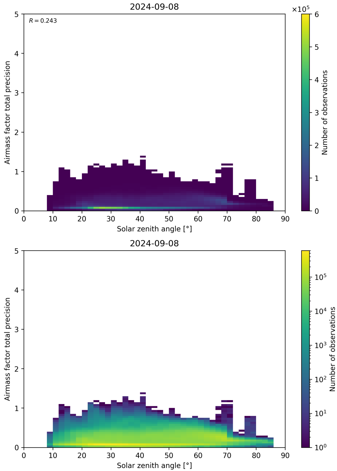
Figure 176: Scatter density plot of “Solar zenith angle” against “Airmass factor total precision” for 2024-09-07 to 2024-09-09.
