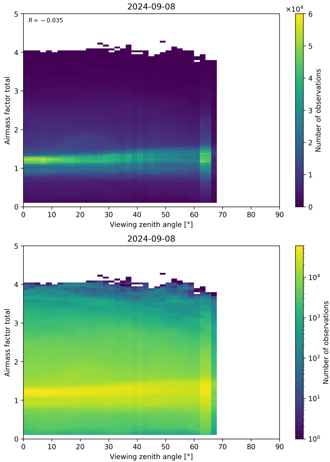
Figure 190: Scatter density plot of “Viewing zenith angle” against “Airmass factor total” for 2024-09-07 to 2024-09-09.
