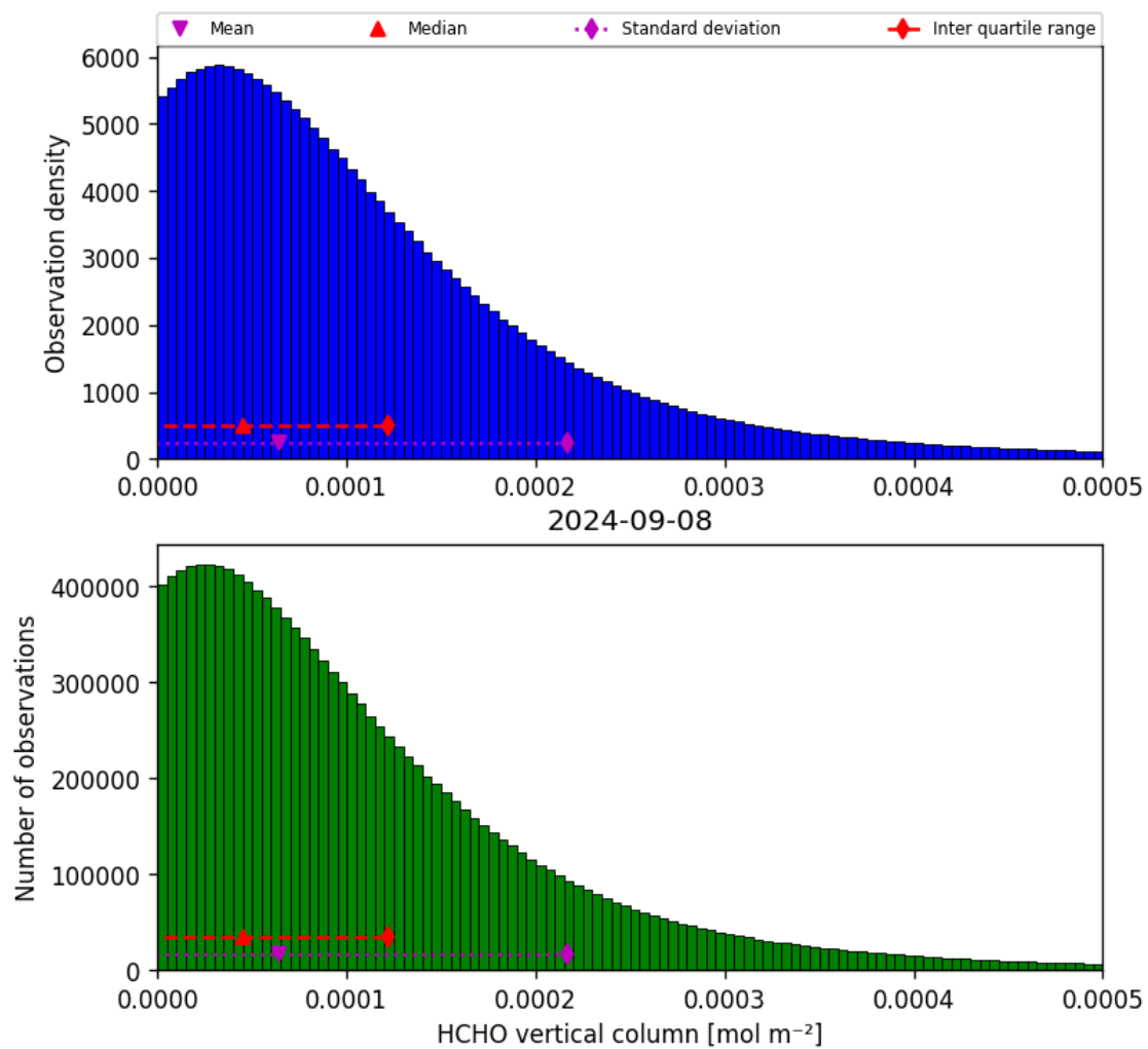
Figure 35: Histogram of “HCHO vertical column” for 2024-09-07 to 2024-09-09
