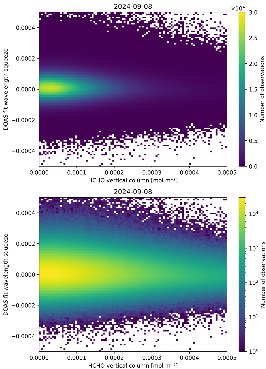
Figure 125: Scatter density plot of “HCHO vertical column” against “DOAS fit wavelength squeeze” for 2024-09-07 to 2024-09-09.
