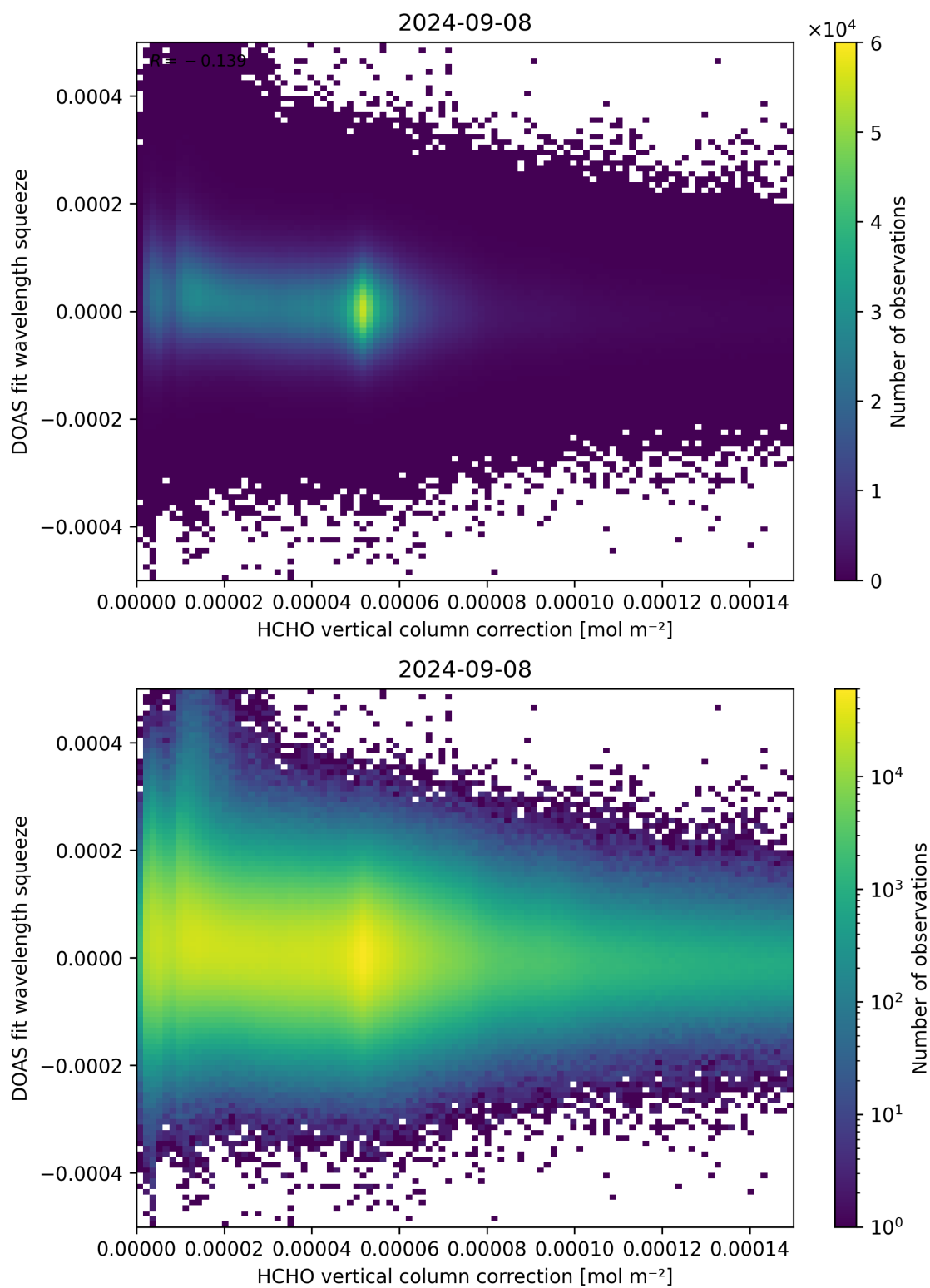
Figure 114: Scatter density plot of “HCHO vertical column correction” against “DOAS fit wavelength squeeze” for 2024-09-07 to 2024-09-09.
