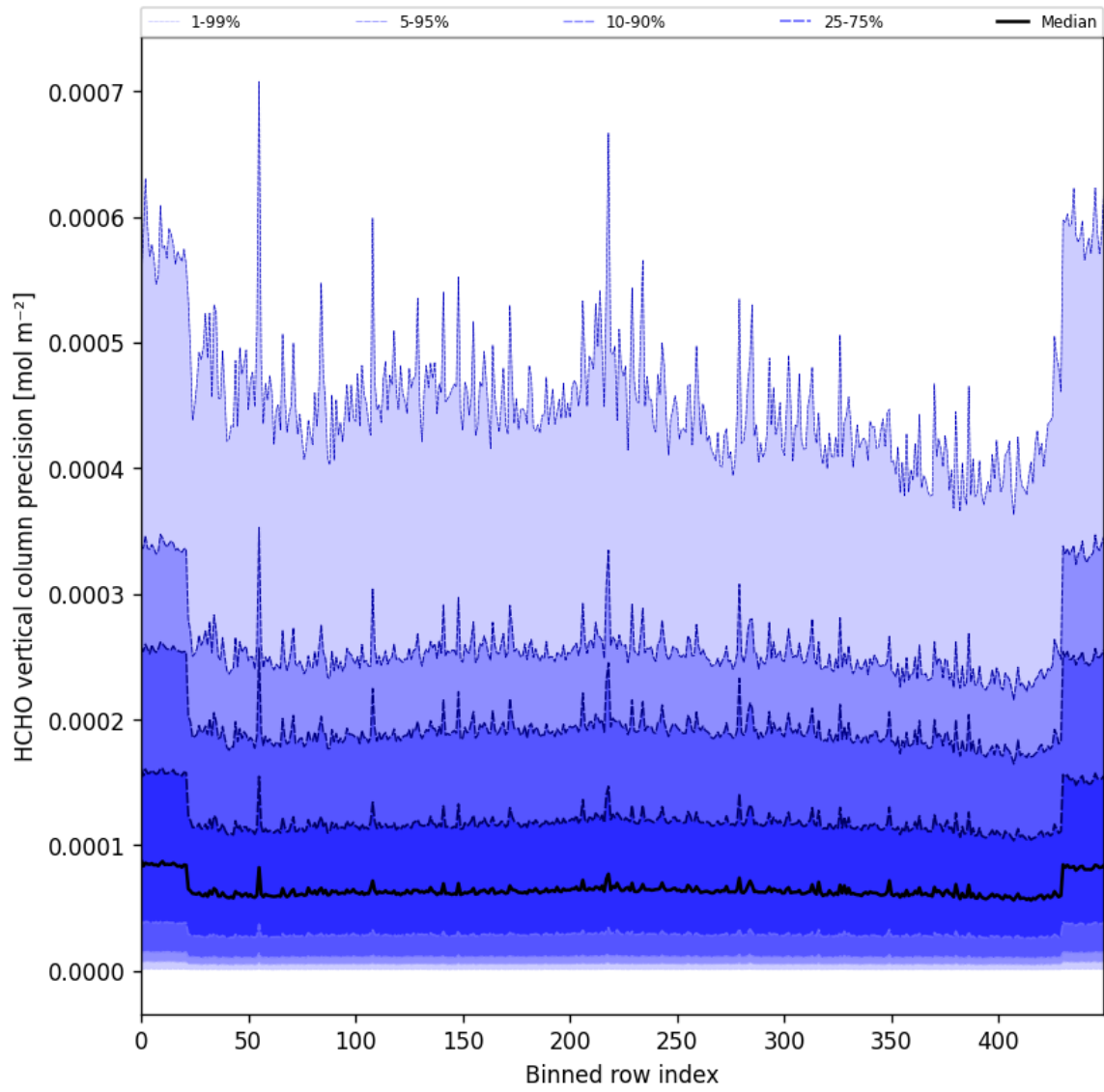
Figure 50: Along track statistics of “HCHO vertical column precision” for 2024-09-07 to 2024-09-09
