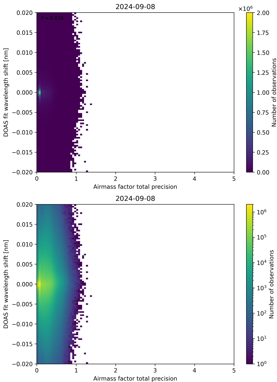
Figure 106: Scatter density plot of “Airmass factor total precision” against “DOAS fit wavelength shift” for 2024-09-07 to 2024-09-09.
