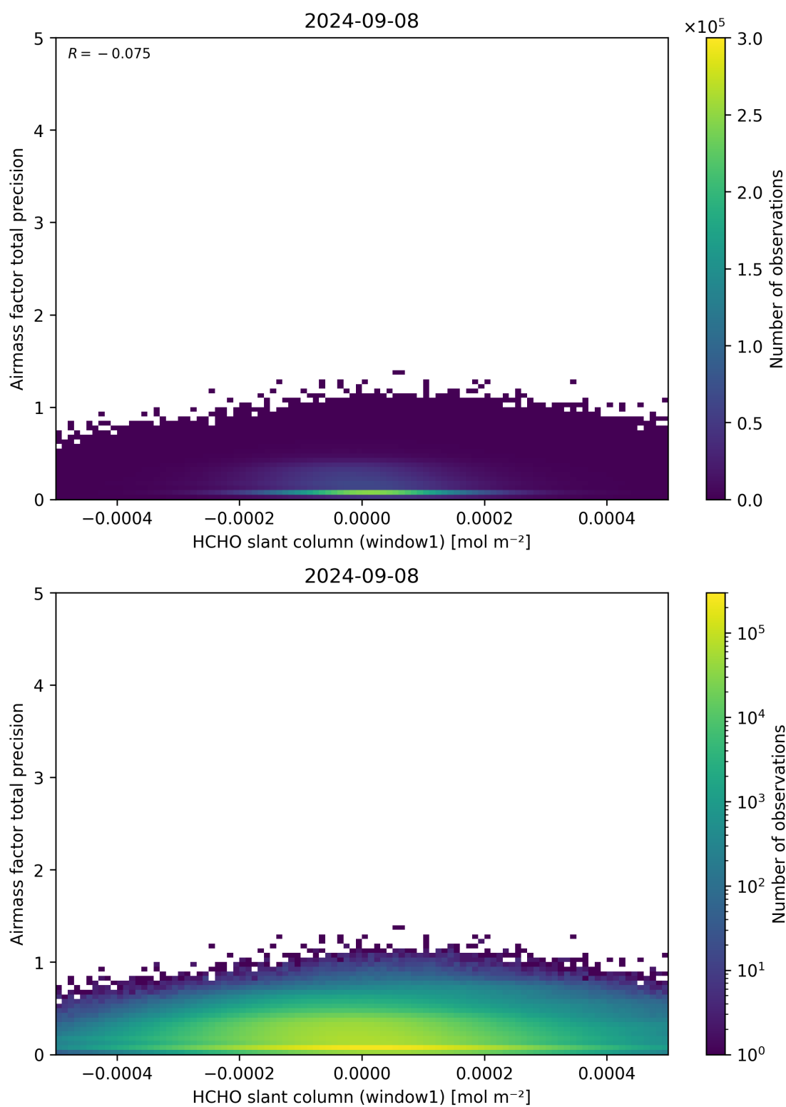
Figure 86: Scatter density plot of “HCHO slant column (window1)” against “Airmass factor total precision” for 2024-09-07 to 2024-09-09.
