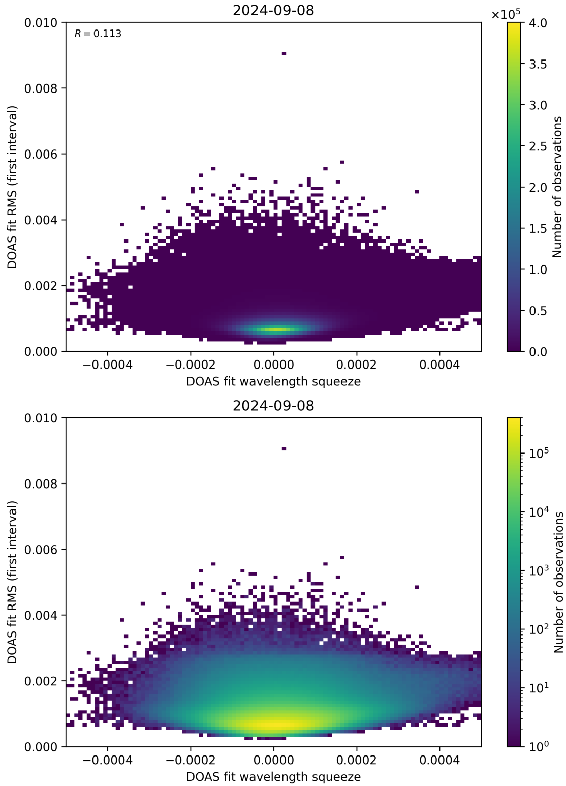
Figure 68: Scatter density plot of “DOAS fit wavelength squeeze” against “DOAS fit RMS (first interval)” for 2024-09-07 to 2024-09-09.
