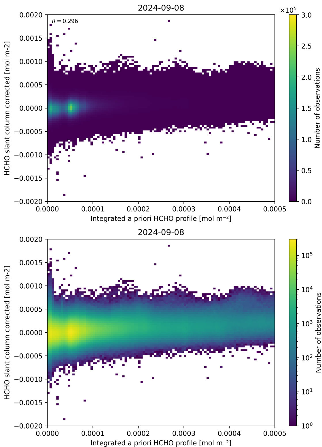
Figure 151: Scatter density plot of “Integrated a priori HCHO profile” against “HCHO slant column corrected” for 2024-09-07 to 2024-09-09.
