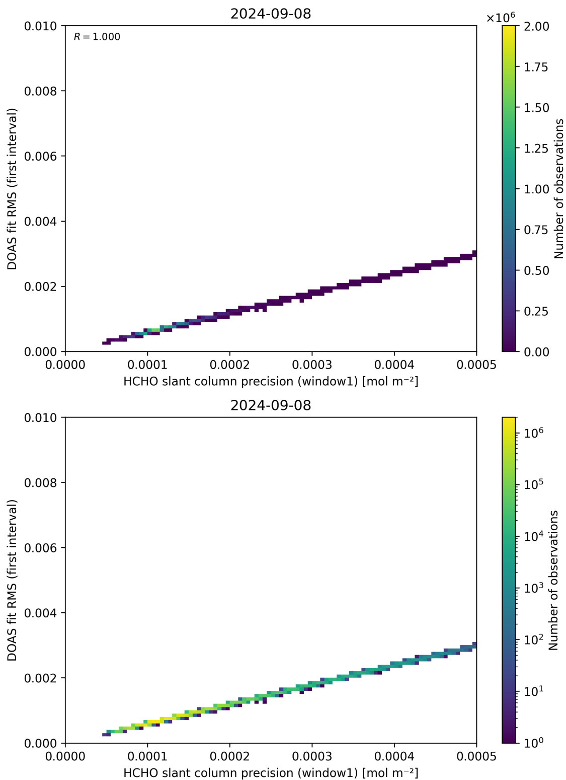
Figure 88: Scatter density plot of “HCHO slant column precision (window1)” against “DOAS fit RMS (first interval)” for 2024-09-07 to 2024-09-09.
