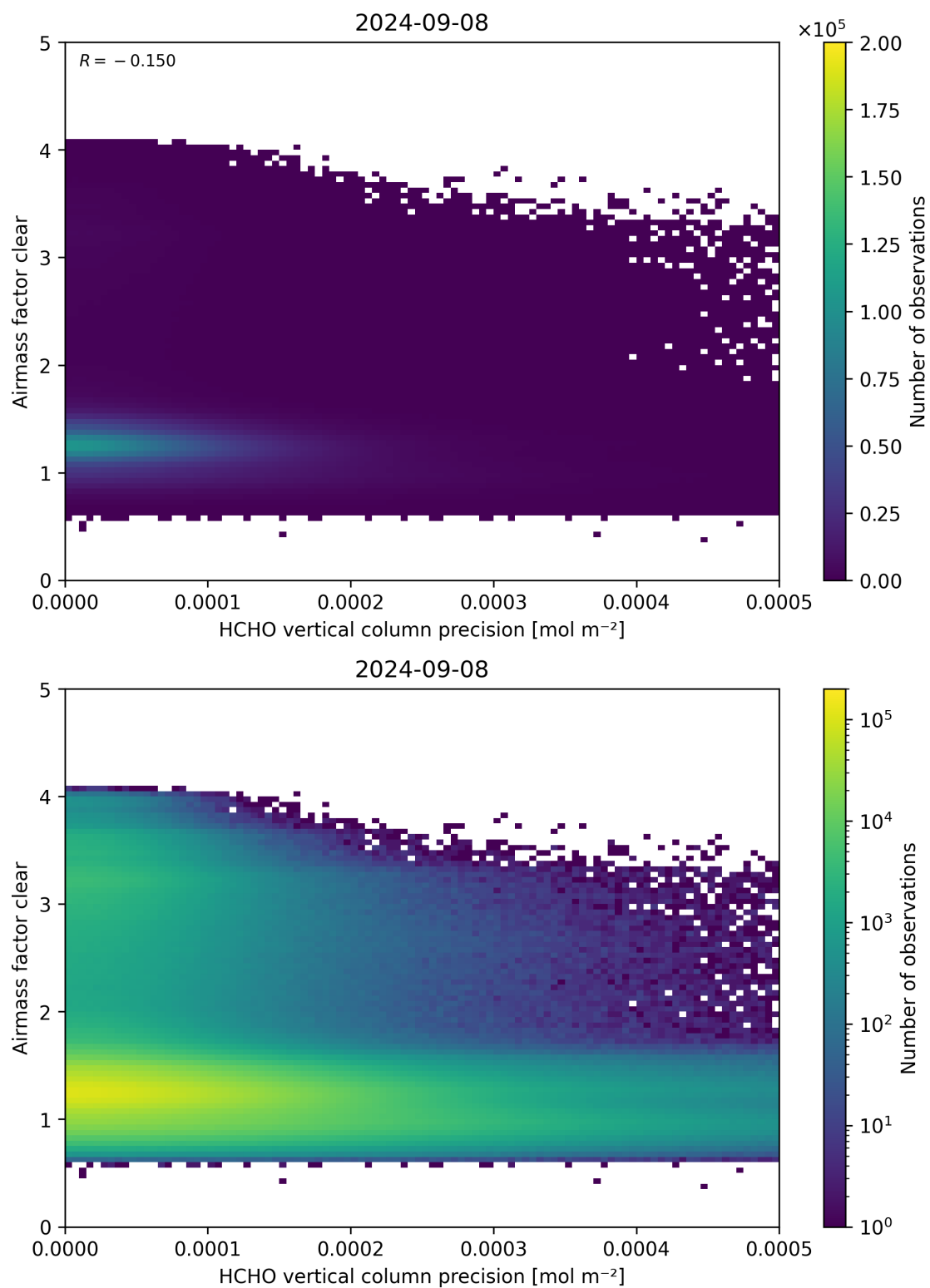
Figure 139: Scatter density plot of “HCHO vertical column precision” against “Airmass factor clear” for 2024-09-07 to 2024-09-09.
