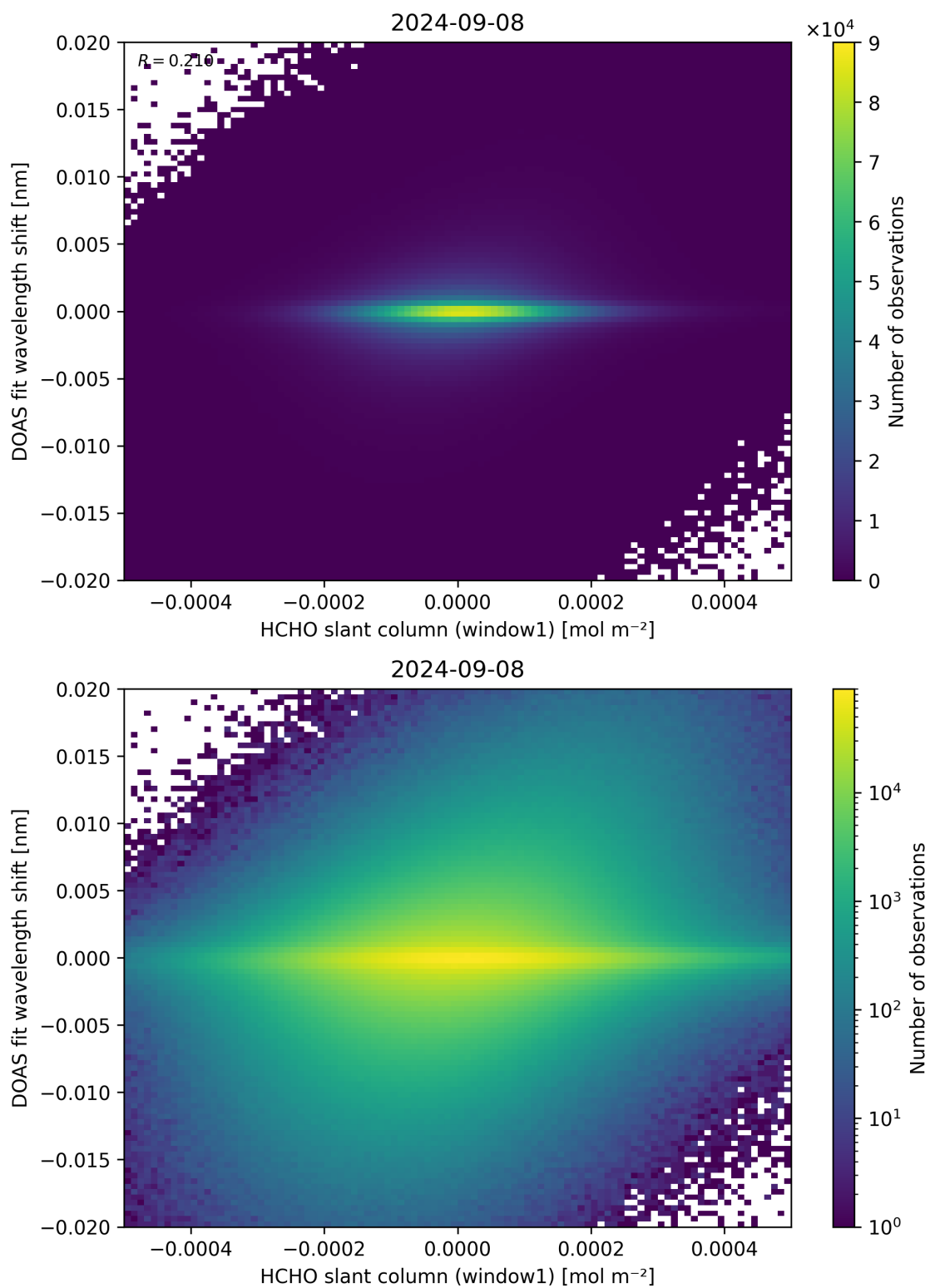
Figure 79: Scatter density plot of “HCHO slant column (window1)” against “DOAS fit wavelength shift” for 2024-09-07 to 2024-09-09.
