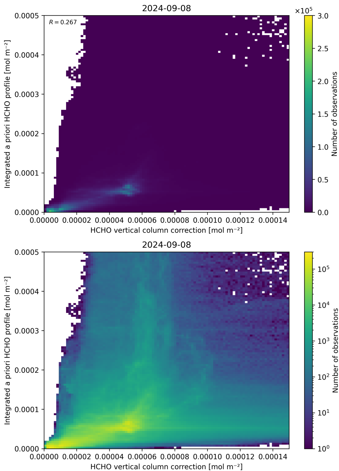
Figure 122: Scatter density plot of “HCHO vertical column correction” against “Integrated a priori HCHO profile” for 2024-09-07 to 2024-09-09.
