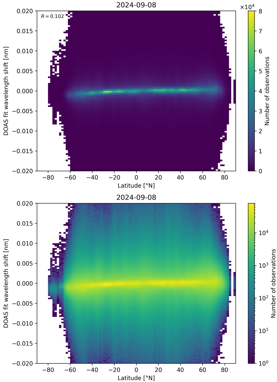
Figure 154: Scatter density plot of “Latitude” against “DOAS fit wavelength shift” for 2024-09-07 to 2024-09-09.
