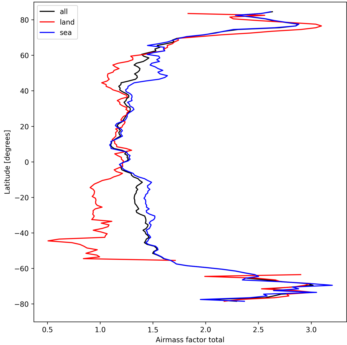
Figure 26: Zonal average of “Airmass factor total” for 2024-09-07 to 2024-09-09.
