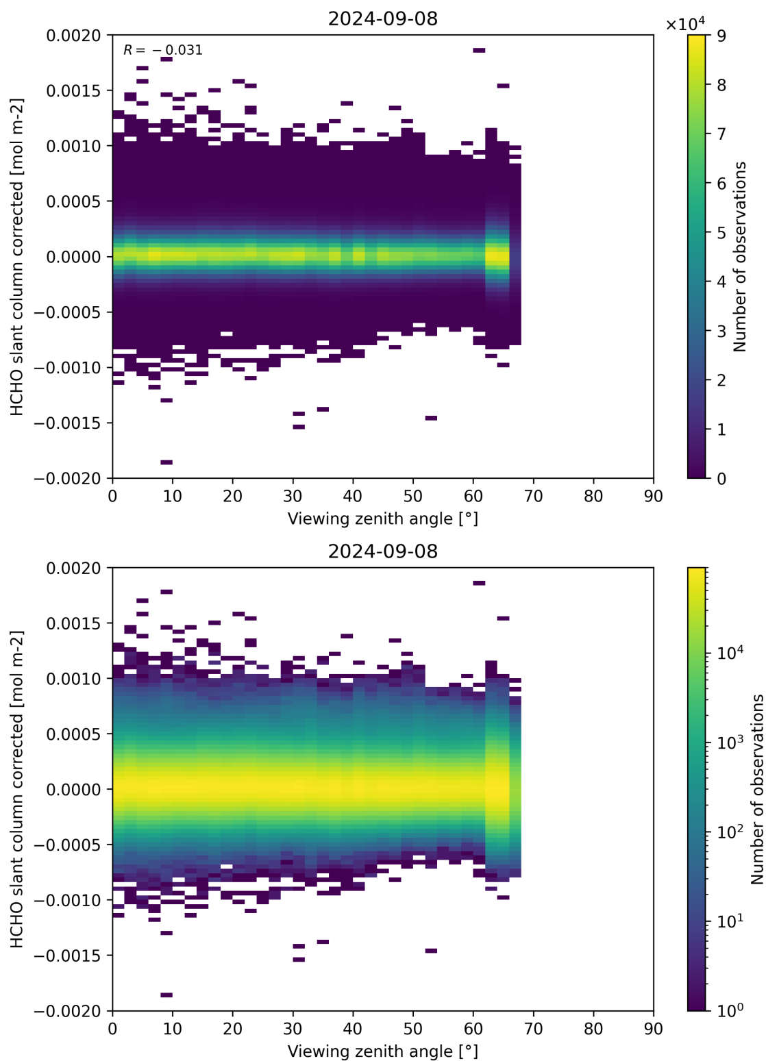
Figure 186: Scatter density plot of “Viewing zenith angle” against “HCHO slant column corrected” for 2024-09-07 to 2024-09-09.
