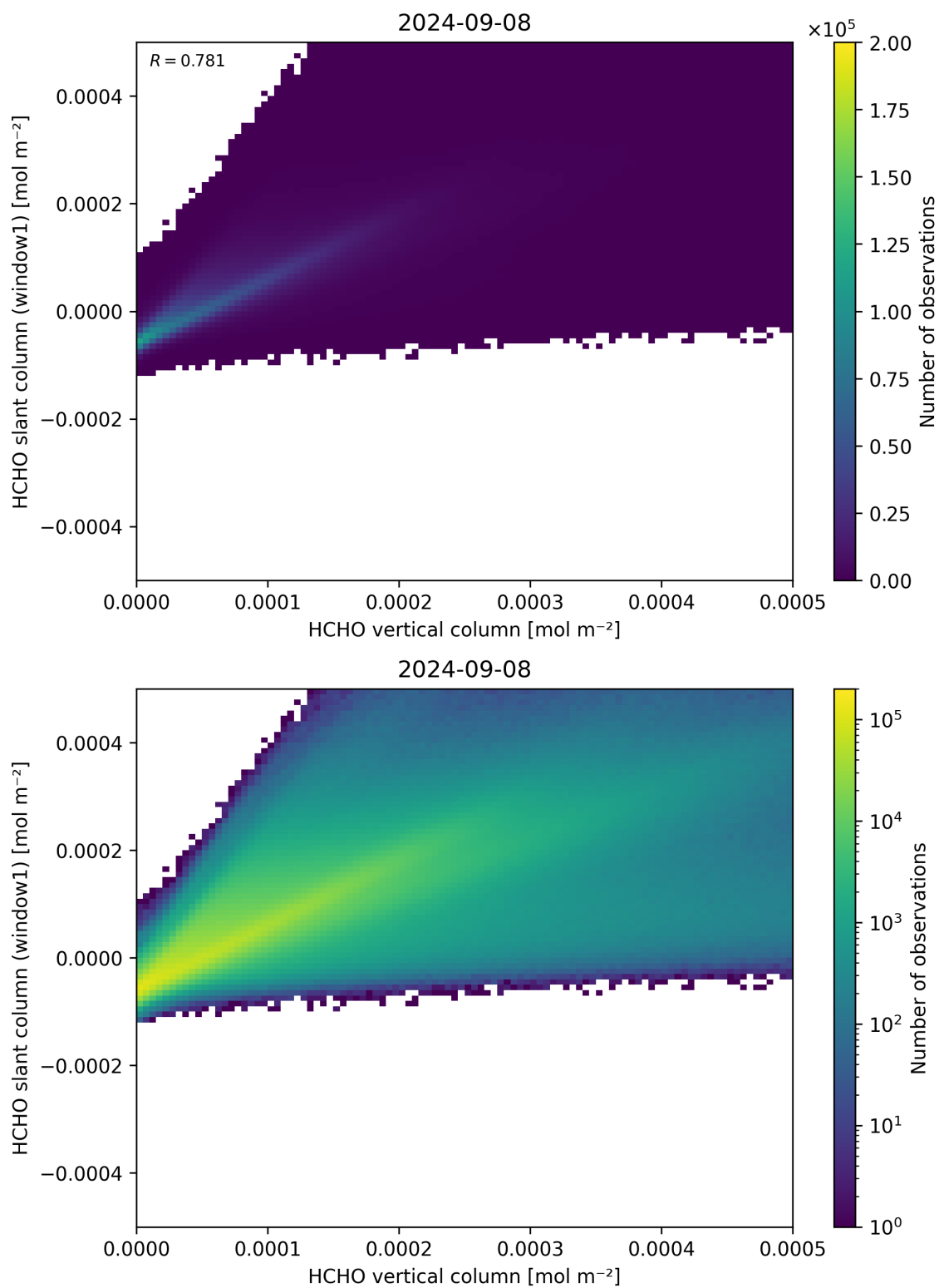
Figure 129: Scatter density plot of “HCHO vertical column” against “HCHO slant column (window1)” for 2024-09-07 to 2024-09-09.
