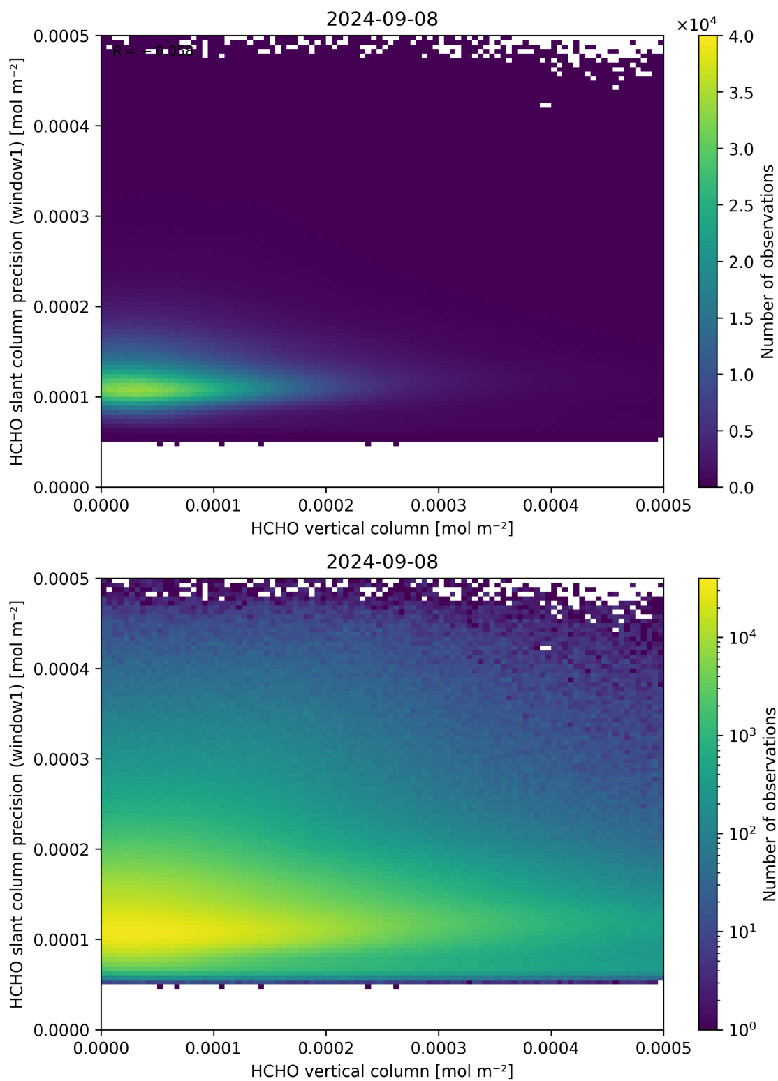
Figure 130: Scatter density plot of “HCHO vertical column” against “HCHO slant column precision (window1)” for 2024-09-07 to 2024-09-09.
