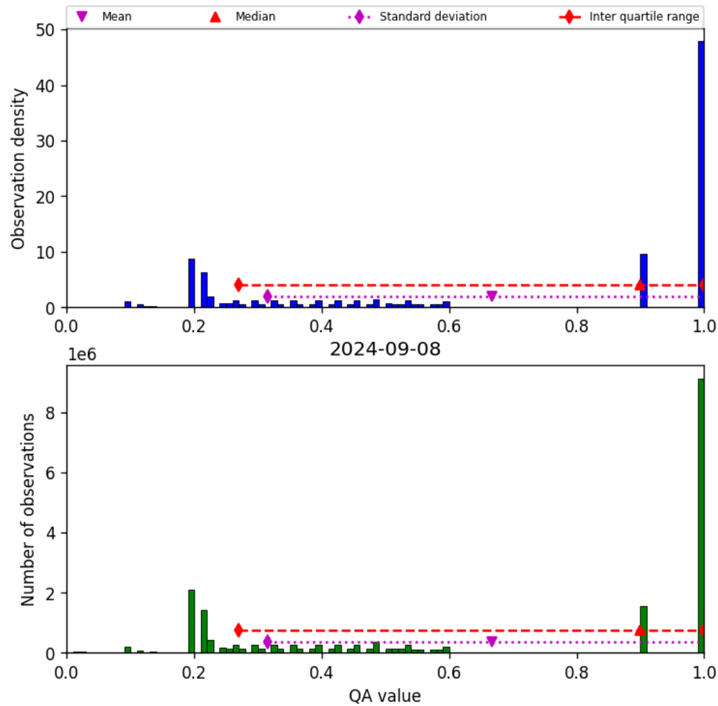
Figure 34: Histogram of “QA value” for 2024-09-07 to 2024-09-09
