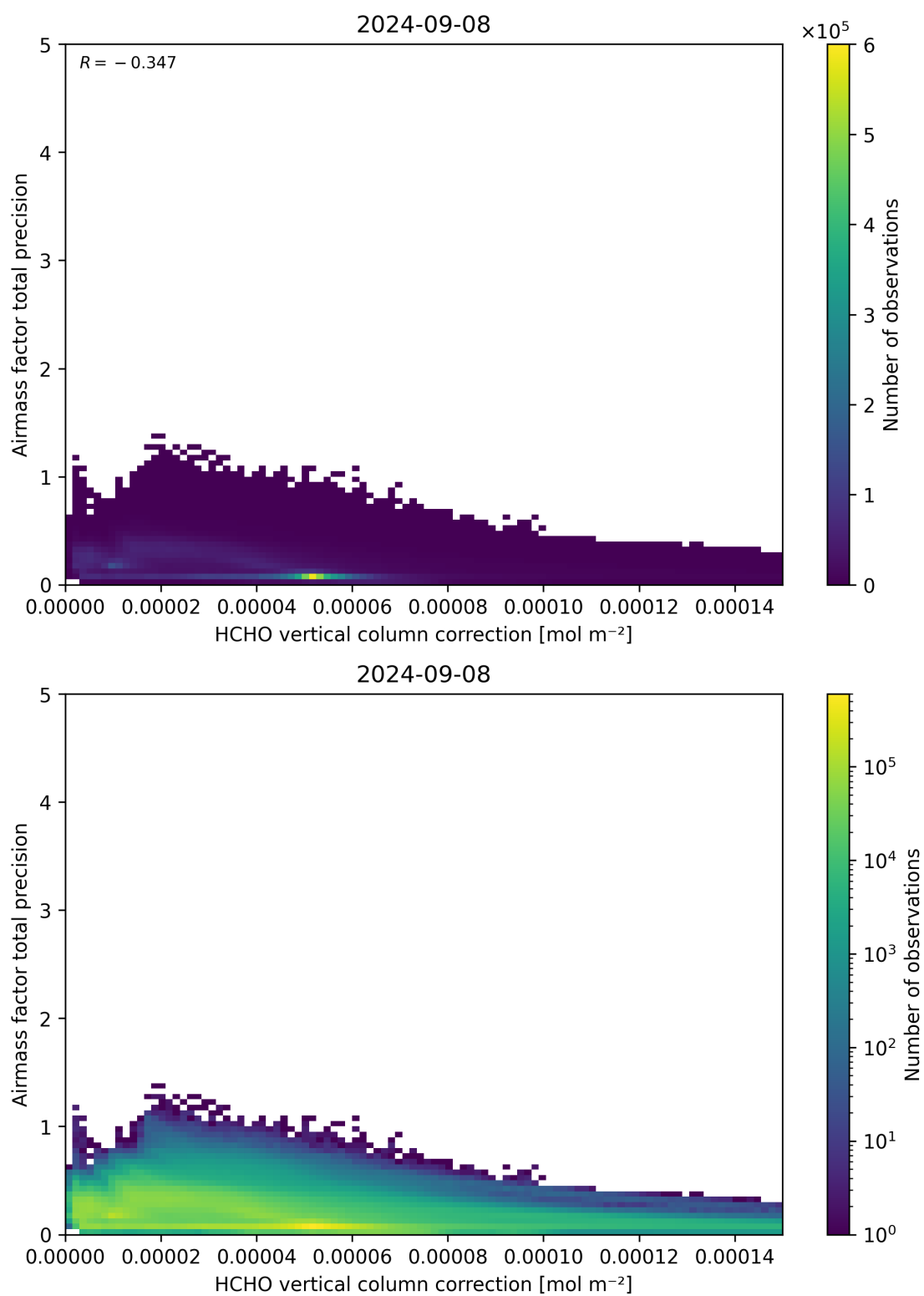
Figure 121: Scatter density plot of “HCHO vertical column correction” against “Airmass factor total precision” for 2024-09-07 to 2024-09-09.
