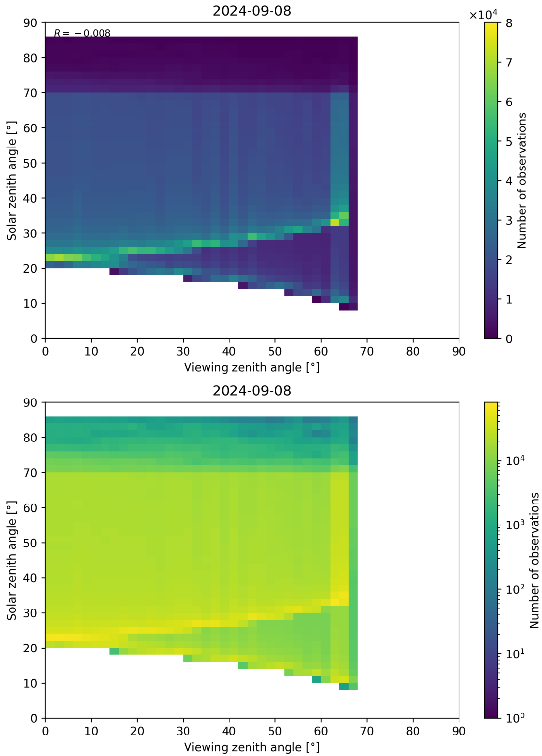
Figure 197: Scatter density plot of “Viewing zenith angle” against “Solar zenith angle” for 2024-09-07 to 2024-09-09.
