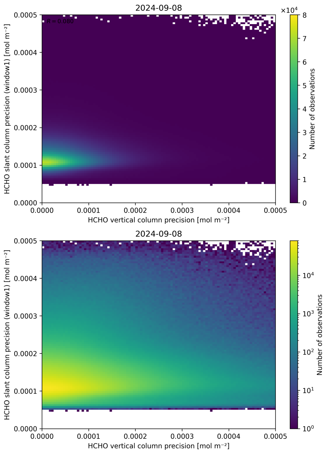
Figure 143: Scatter density plot of “HCHO vertical column precision” against “HCHO slant column precision (window1)” for 2024-09-07 to 2024-09-09.
