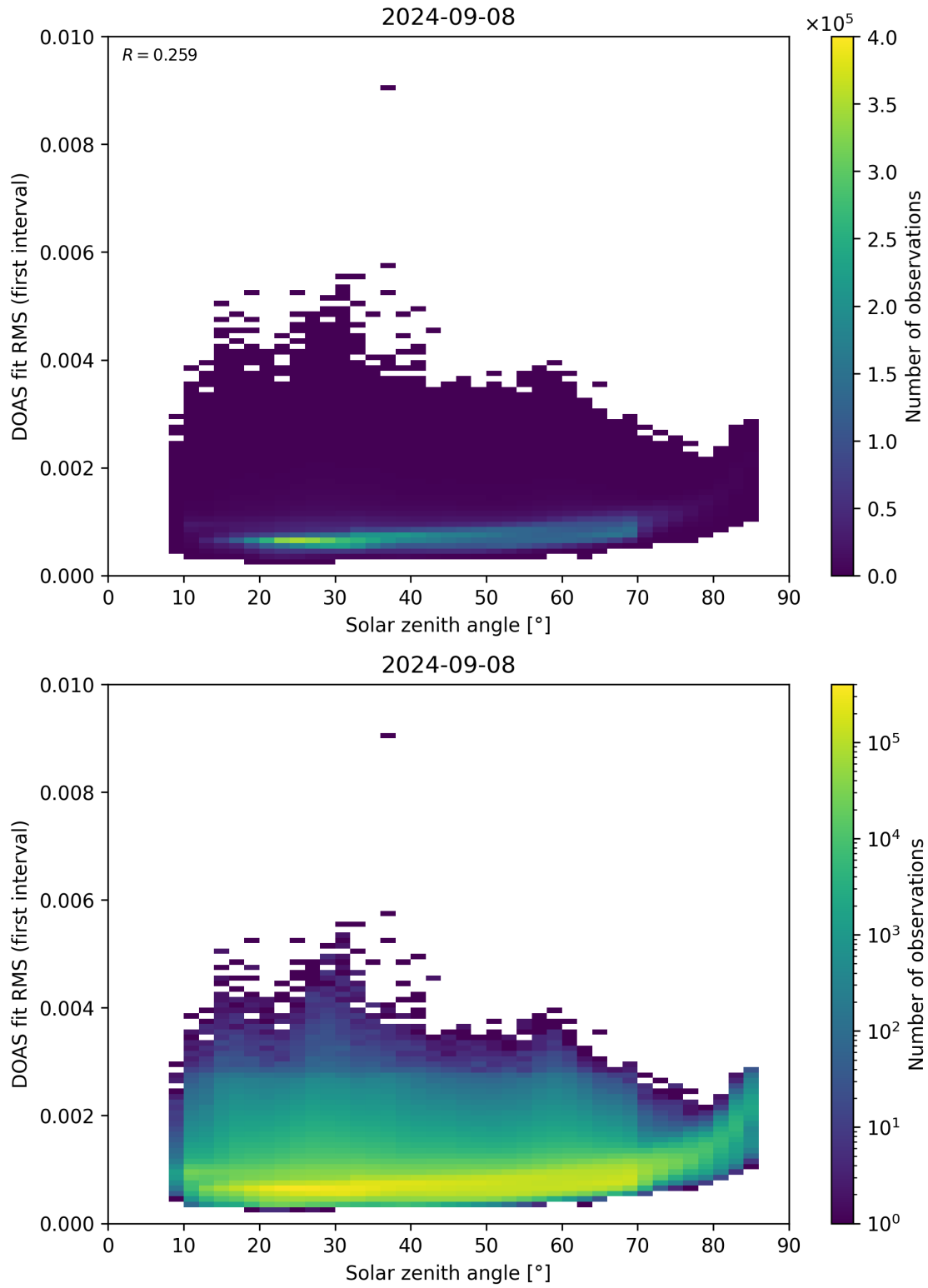
Figure 167: Scatter density plot of “Solar zenith angle” against “DOAS fit RMS (first interval)” for 2024-09-07 to 2024-09-09.
