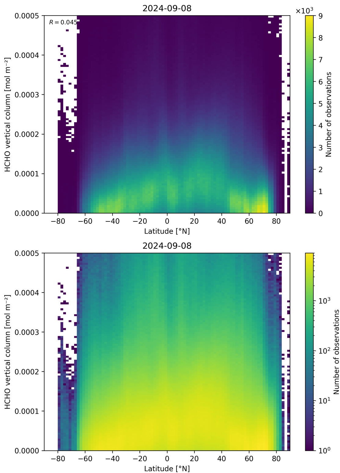
Figure 163: Scatter density plot of “Latitude” against “HCHO vertical column” for 2024-09-07 to 2024-09-09.
