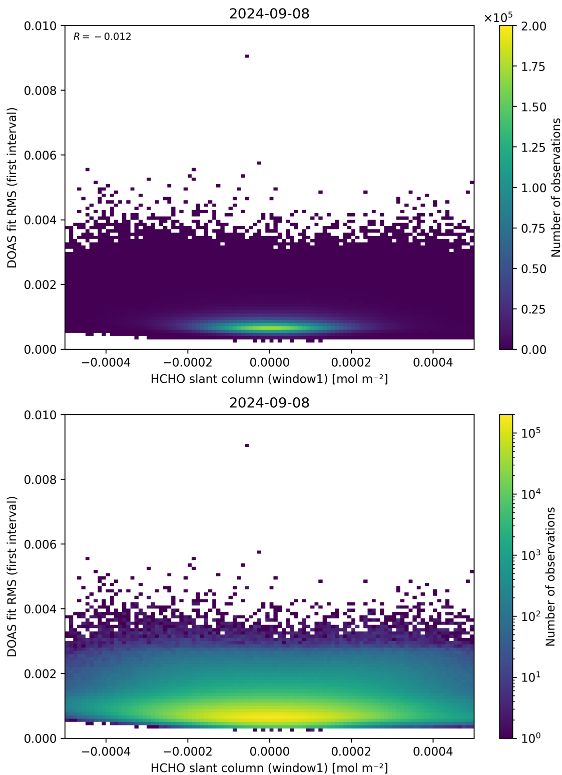
Figure 78: Scatter density plot of “HCHO slant column (window1)” against “DOAS fit RMS (first interval)” for 2024-09-07 to 2024-09-09.
