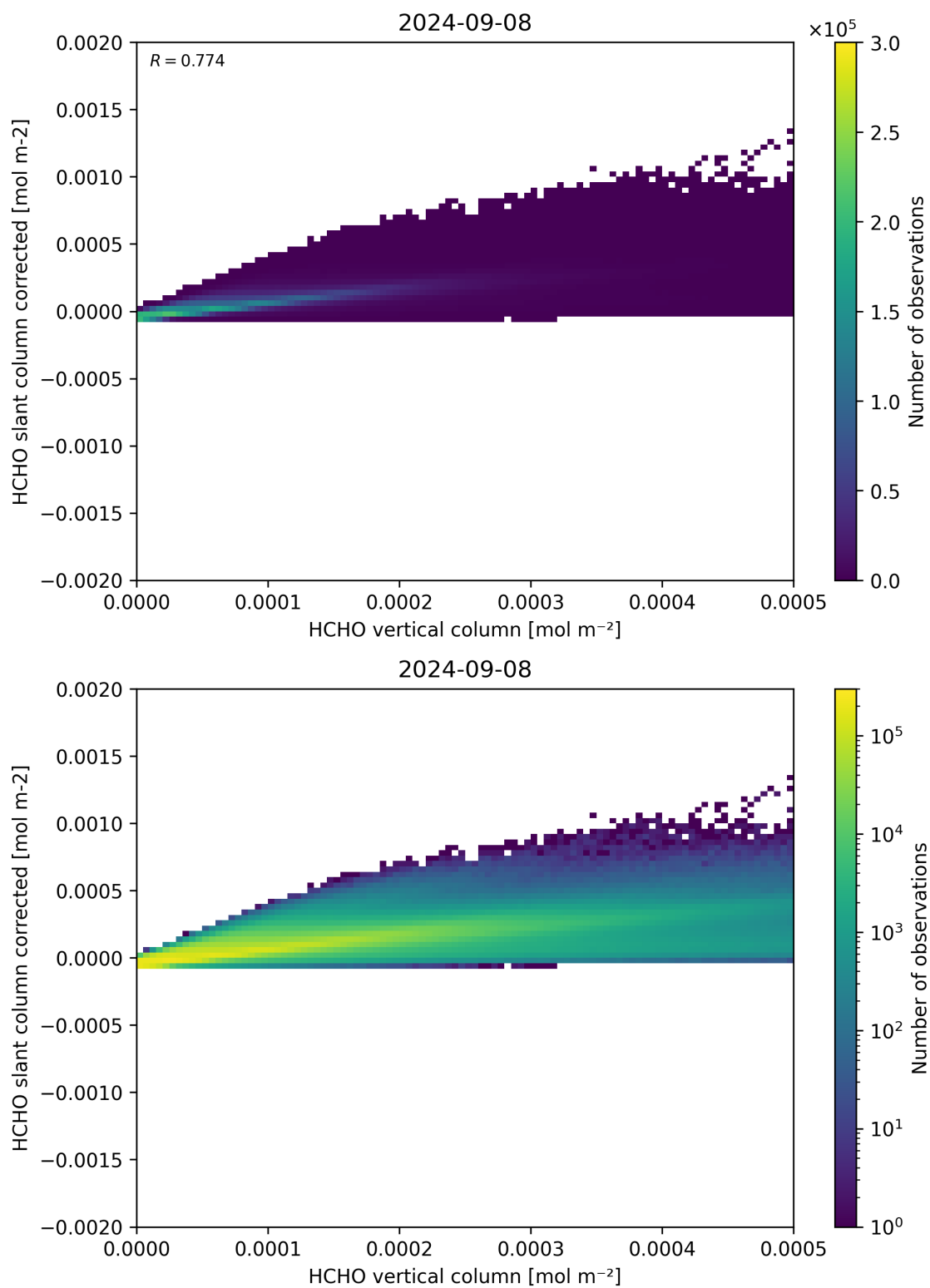
Figure 127: Scatter density plot of “HCHO vertical column” against “HCHO slant column corrected” for 2024-09-07 to 2024-09-09.
