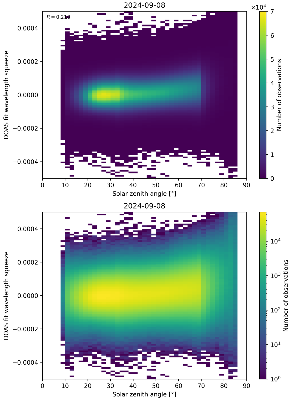
Figure 169: Scatter density plot of “Solar zenith angle” against “DOAS fit wavelength squeeze” for 2024-09-07 to 2024-09-09.
