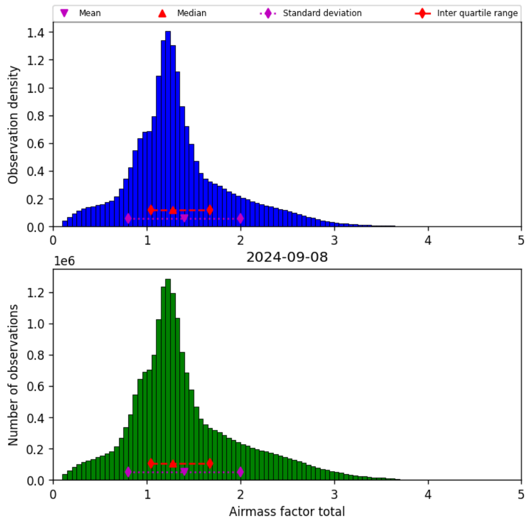
Figure 40: Histogram of “Airmass factor total” for 2024-09-07 to 2024-09-09
