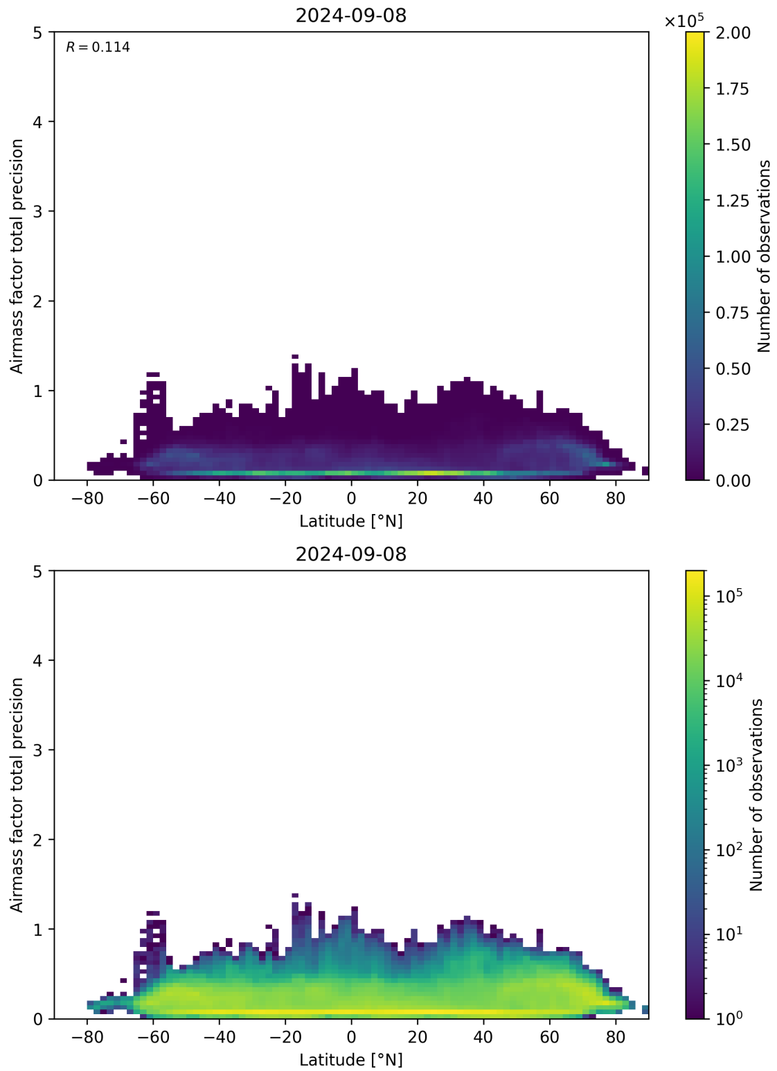
Figure 162: Scatter density plot of “Latitude” against “Airmass factor total precision” for 2024-09-07 to 2024-09-09.
