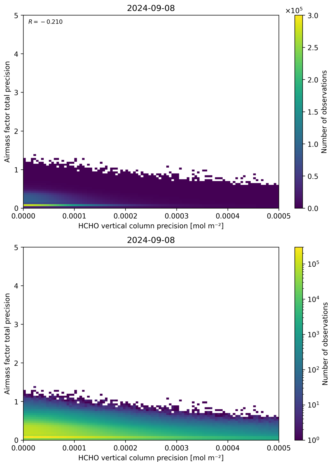
Figure 145: Scatter density plot of “HCHO vertical column precision” against “Airmass factor total precision” for 2024-09-07 to 2024-09-09.
