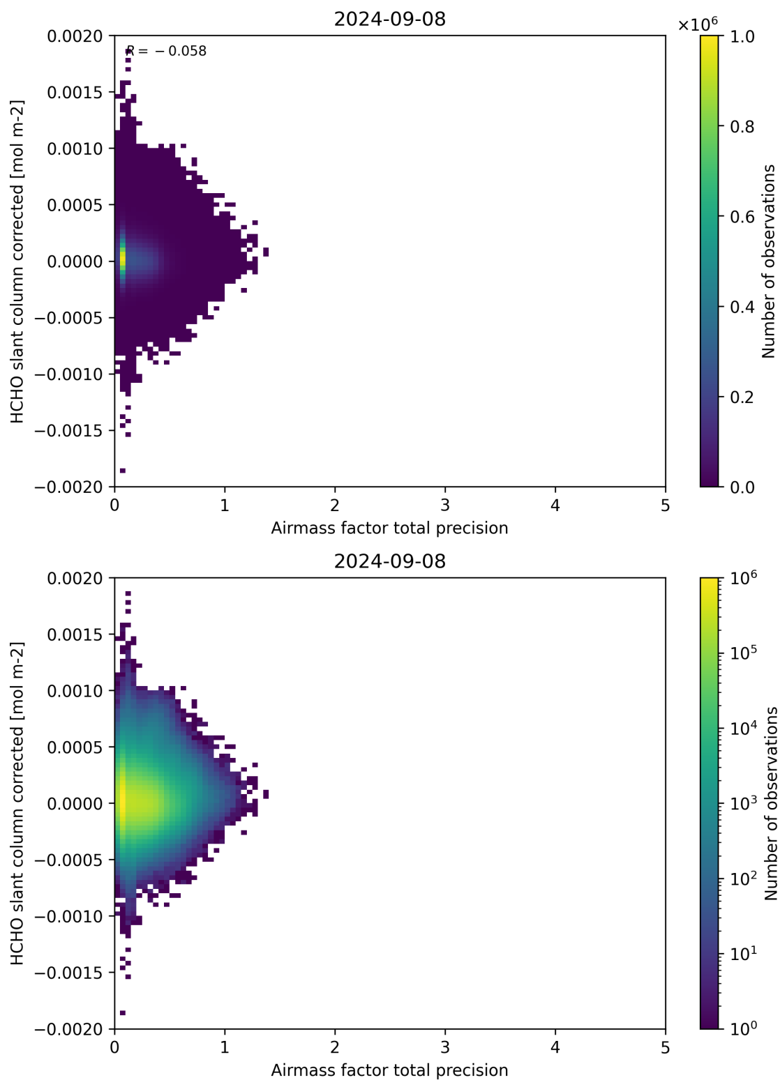
Figure 109: Scatter density plot of “Airmass factor total precision” against “HCHO slant column corrected” for 2024-09-07 to 2024-09-09.
