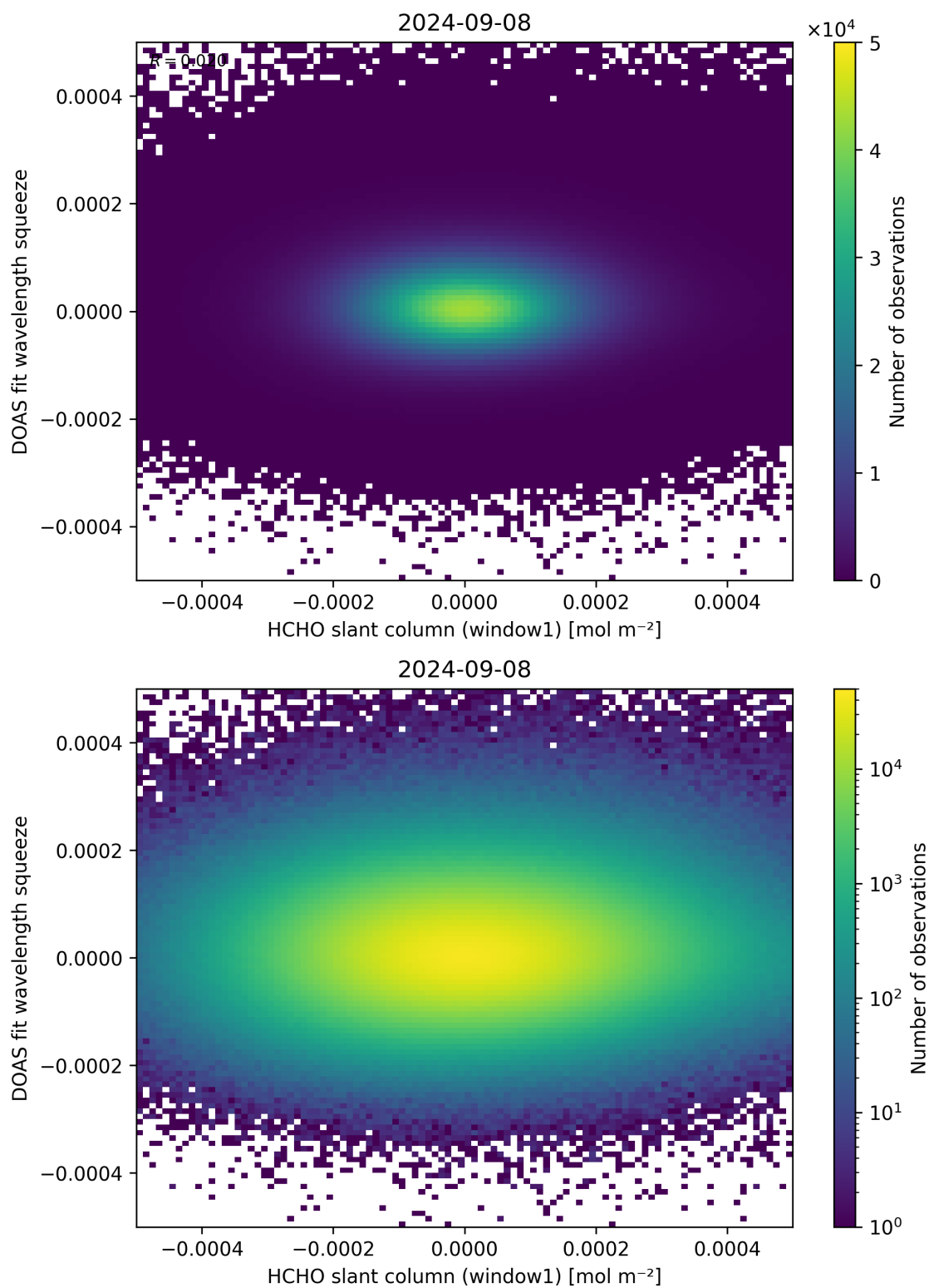
Figure 80: Scatter density plot of “HCHO slant column (window1)” against “DOAS fit wavelength squeeze” for 2024-09-07 to 2024-09-09.
