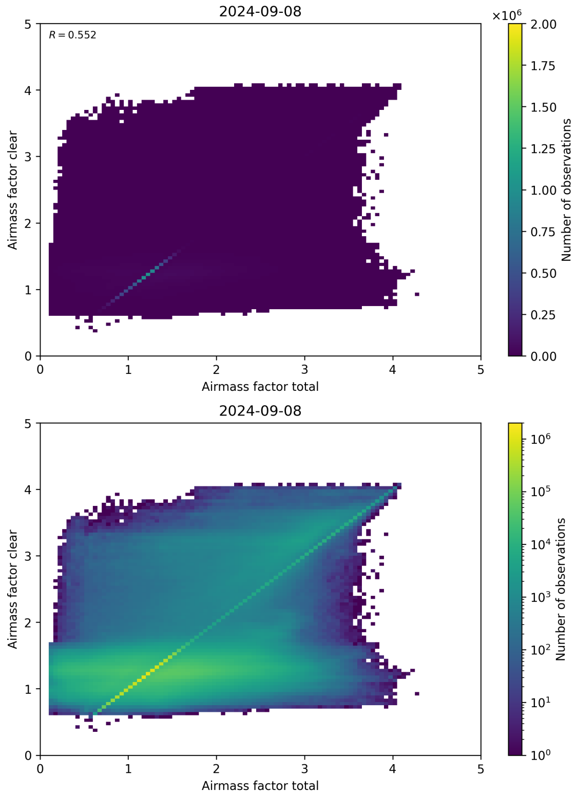
Figure 100: Scatter density plot of “Airmass factor total” against “Airmass factor clear” for 2024-09-07 to 2024-09-09.
