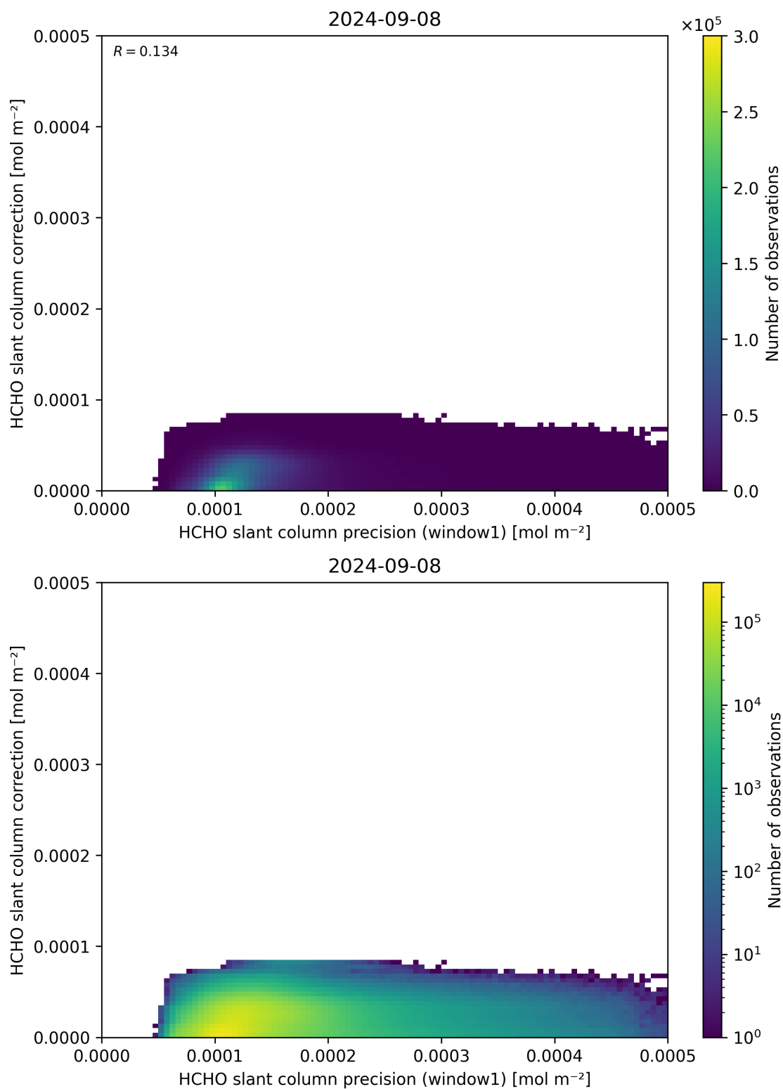
Figure 93: Scatter density plot of “HCHO slant column precision (window1)” against “HCHO slant column correction” for 2024-09-07 to 2024-09-09.
