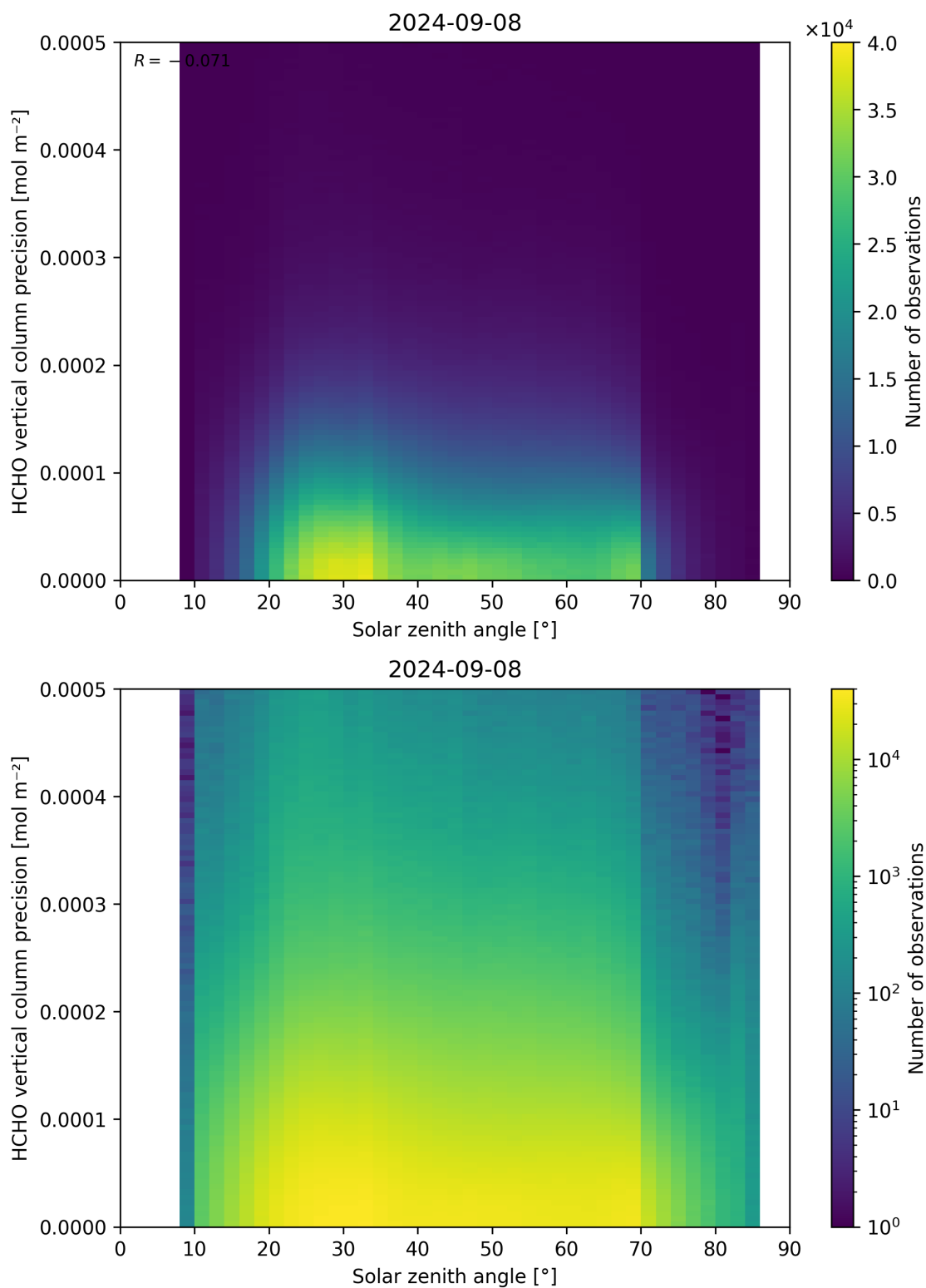
Figure 179: Scatter density plot of “Solar zenith angle” against “HCHO vertical column precision” for 2024-09-07 to 2024-09-09.
