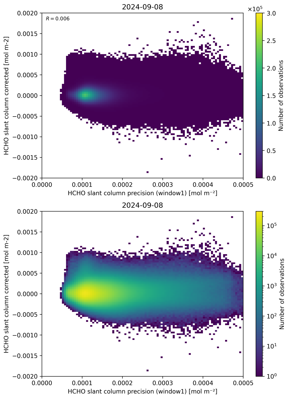
Figure 92: Scatter density plot of “HCHO slant column precision (window1)” against “HCHO slant column corrected” for 2024-09-07 to 2024-09-09.
