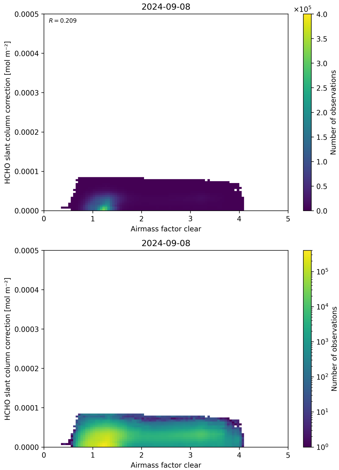
Figure 75: Scatter density plot of “Air mass factor clear” against “HCHO slant column correction” for 2024-09-07 to 2024-09-09.
