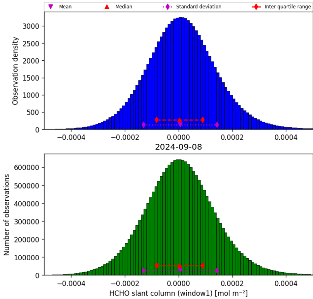
Figure 38: Histogram of “HCHO slant column (window1)” for 2024-09-07 to 2024-09-09
