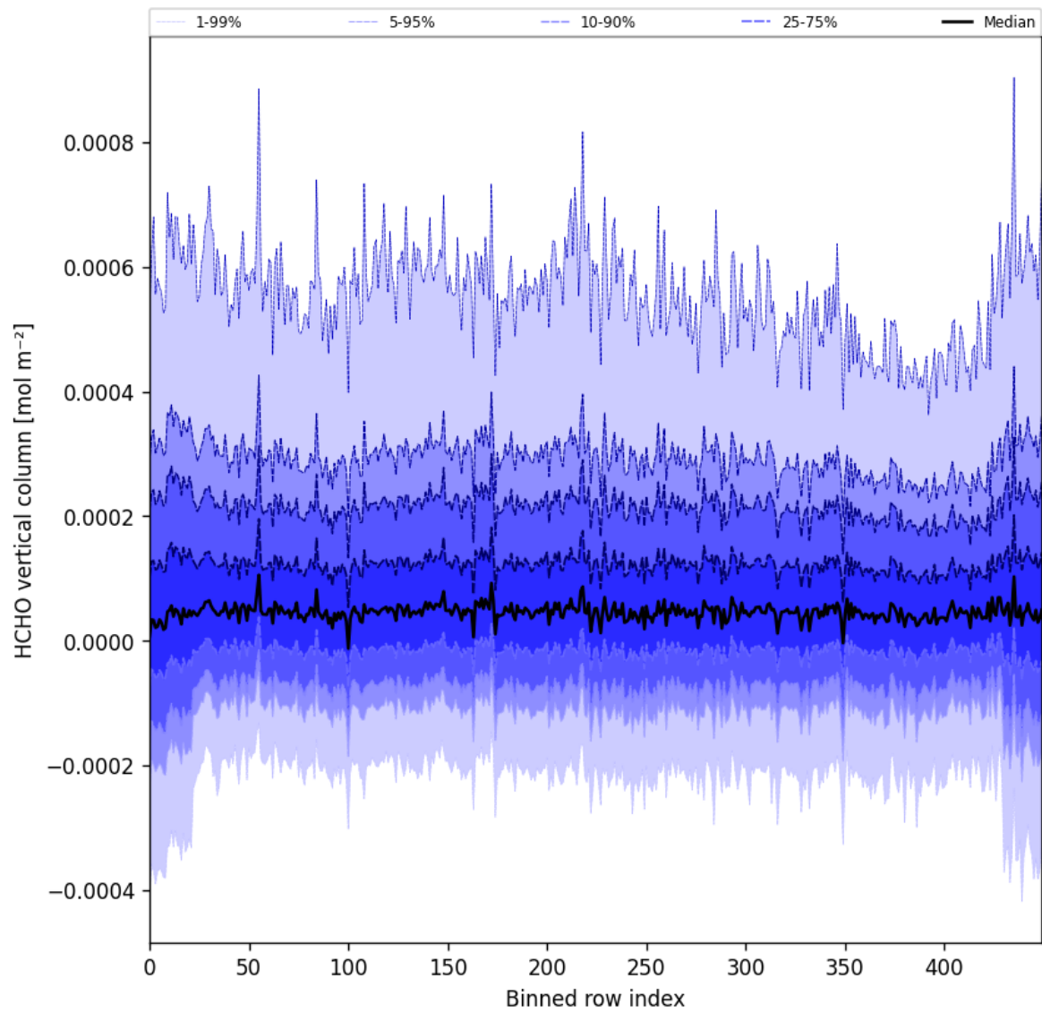
Figure 49: Along track statistics of “HCHO vertical column” for 2024-09-07 to 2024-09-09
