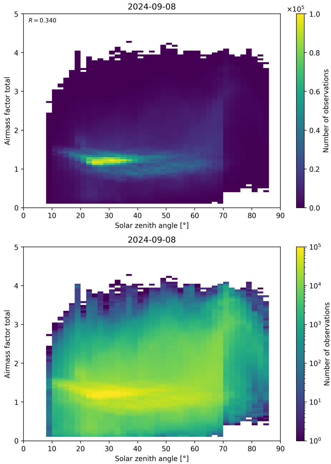
Figure 175: Scatter density plot of “Solar zenith angle” against “Airmass factor total” for 2024-09-07 to 2024-09-09.
