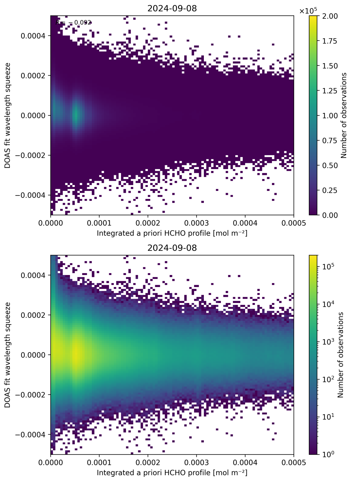
Figure 150: Scatter density plot of “Integrated a priori HCHO profile” against “DOAS fit wavelength squeeze” for 2024-09-07 to 2024-09-09.
