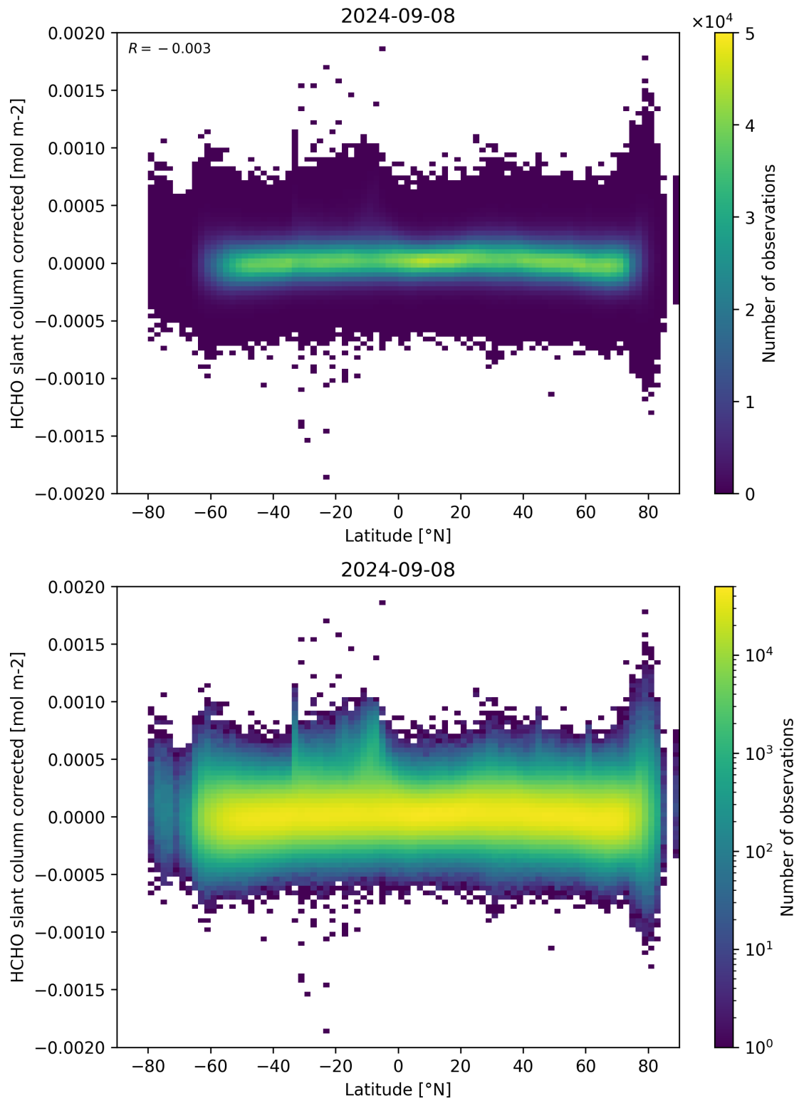
Figure 157: Scatter density plot of “Latitude” against “HCHO slant column corrected” for 2024-09-07 to 2024-09-09.
