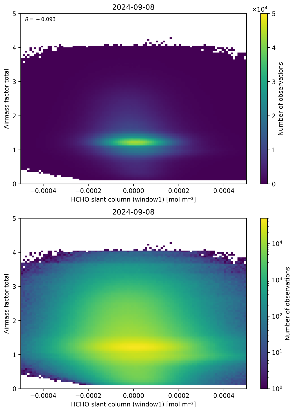
Figure 85: Scatter density plot of “HCHO slant column (window1)” against “Airmass factor total” for 2024-09-07 to 2024-09-09.
