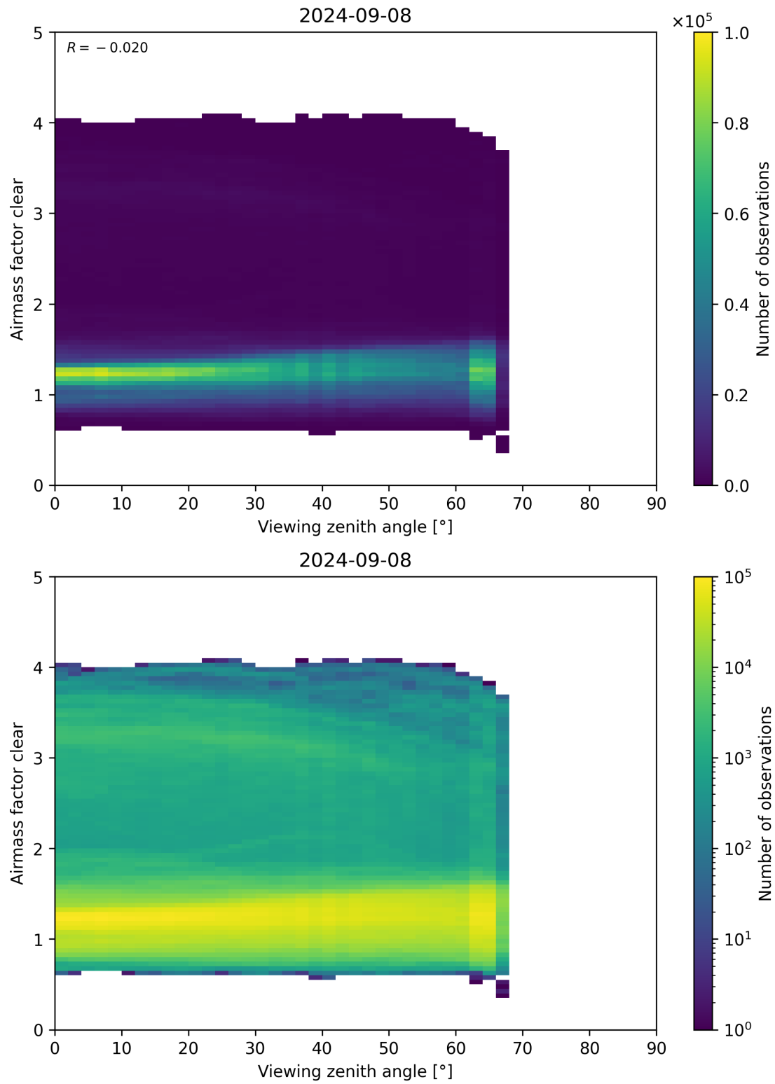
Figure 185: Scatter density plot of “Viewing zenith angle” against “Airmass factor clear” for 2024-09-07 to 2024-09-09.
