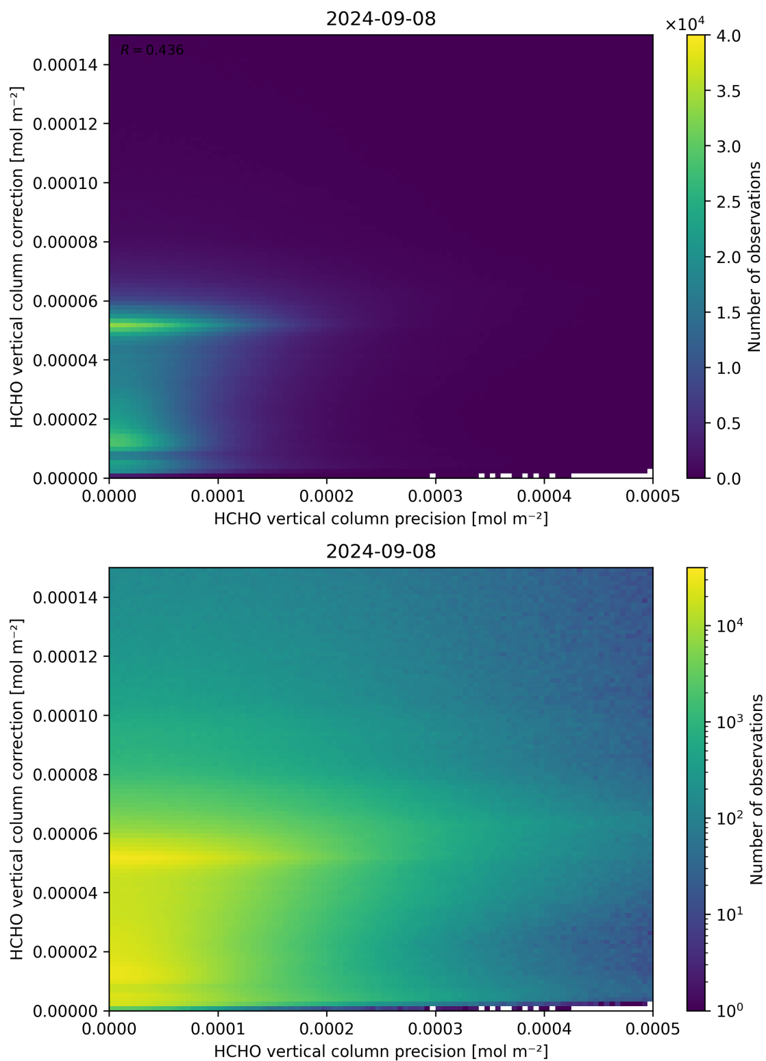
Figure 146: Scatter density plot of “HCHO vertical column precision” against “HCHO vertical column correction” for 2024-09-07 to 2024-09-09.
