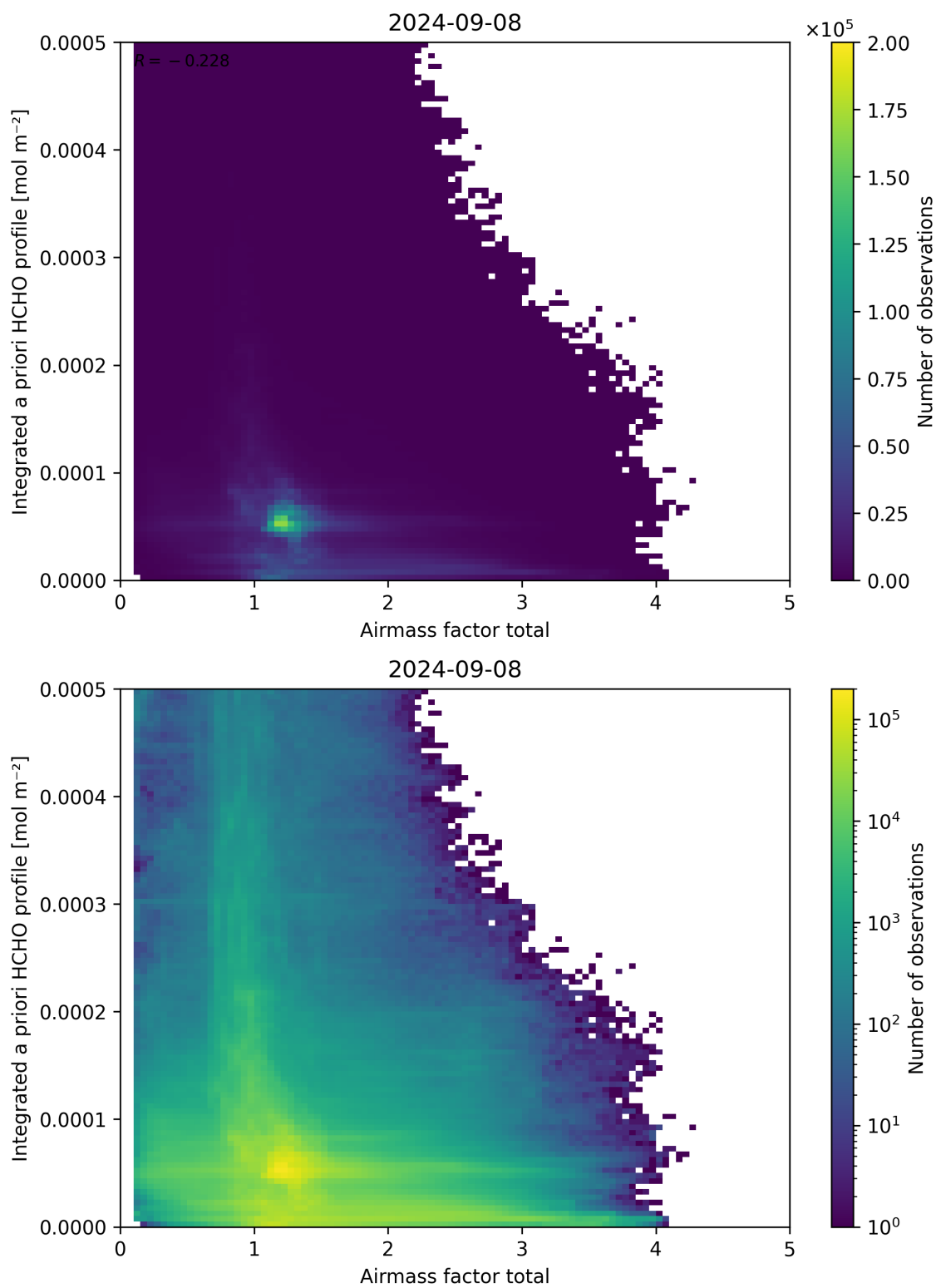
Figure 104: Scatter density plot of “Airmass factor total” against “Integrated a priori HCHO profile” for 2024-09-07 to 2024-09-09.
