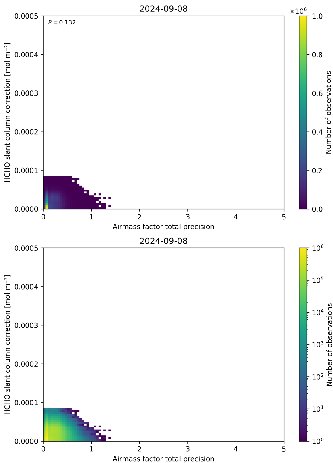
Figure 110: Scatter density plot of “Airmass factor total precision” against “HCHO slant column correction” for 2024-09-07 to 2024-09-09.
