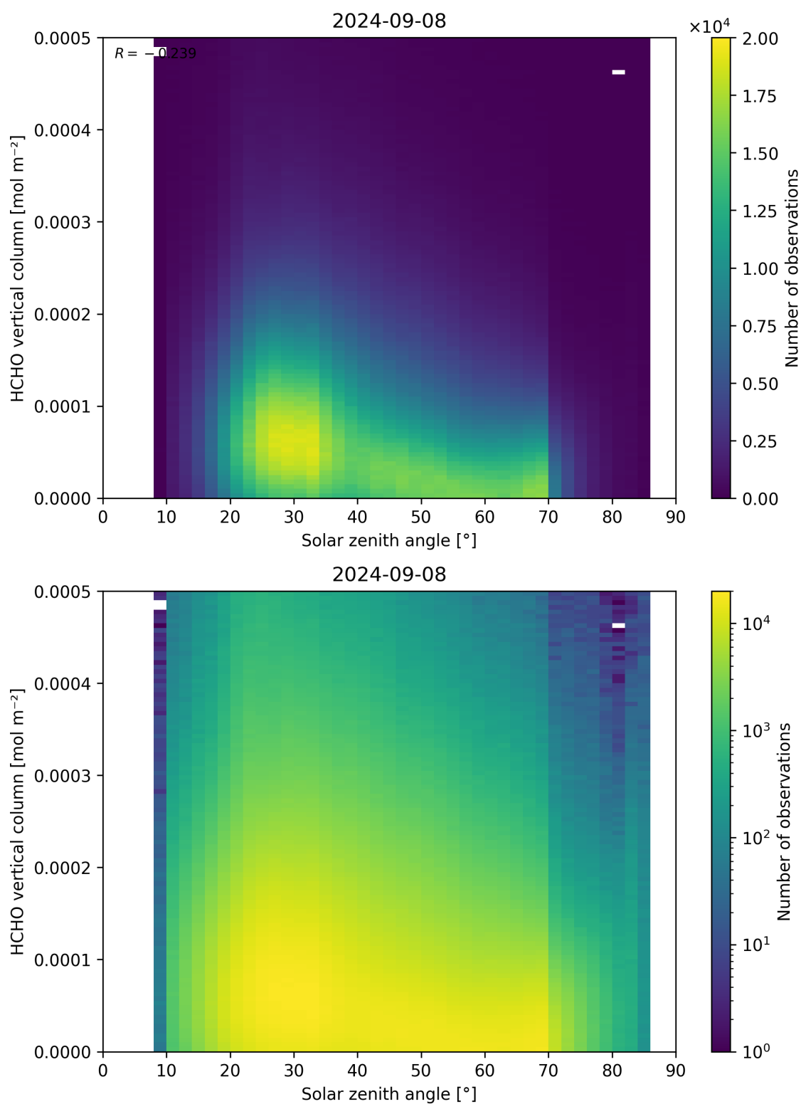
Figure 177: Scatter density plot of “Solar zenith angle” against “HCHO vertical column” for 2024-09-07 to 2024-09-09.
