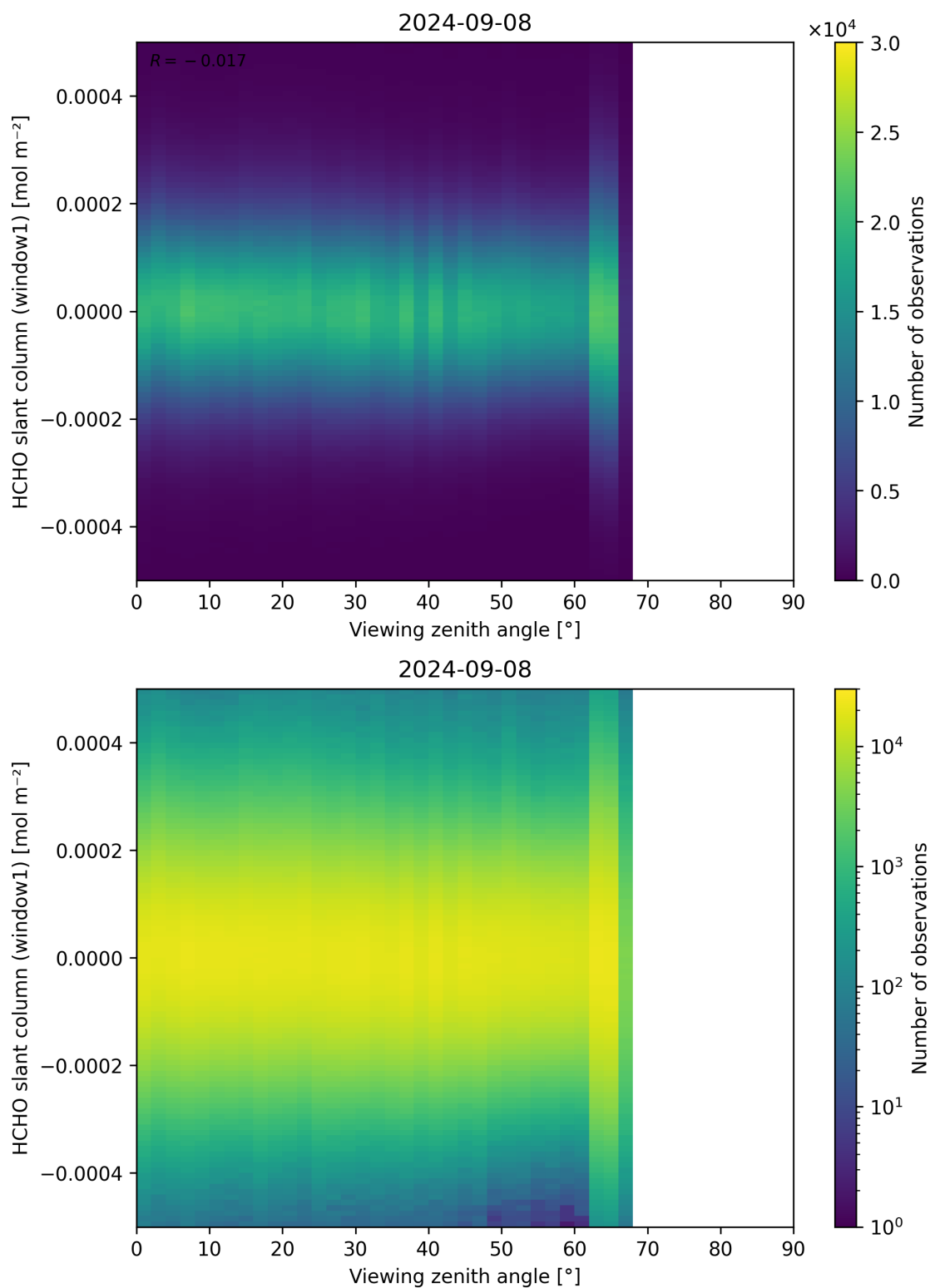
Figure 188: Scatter density plot of “Viewing zenith angle” against “HCHO slant column (window1)” for 2024-09-07 to 2024-09-09.
