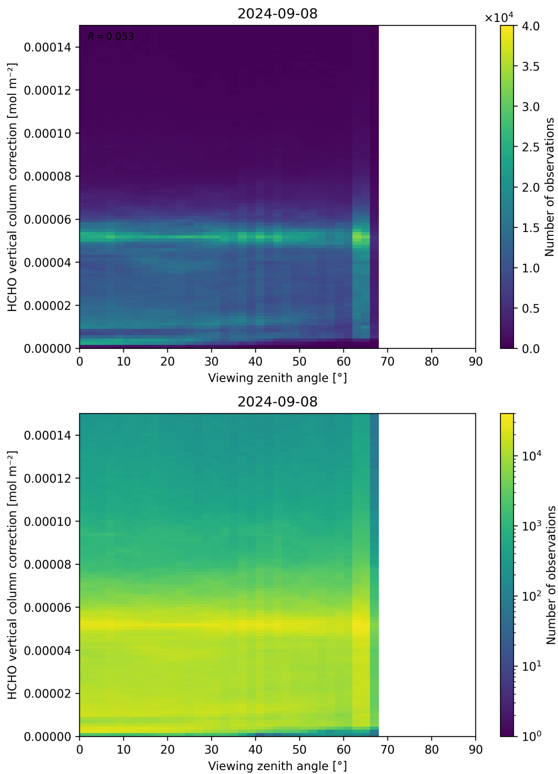
Figure 193: Scatter density plot of “Viewing zenith angle” against “HCHO vertical column correction” for 2024-09-07 to 2024-09-09.
