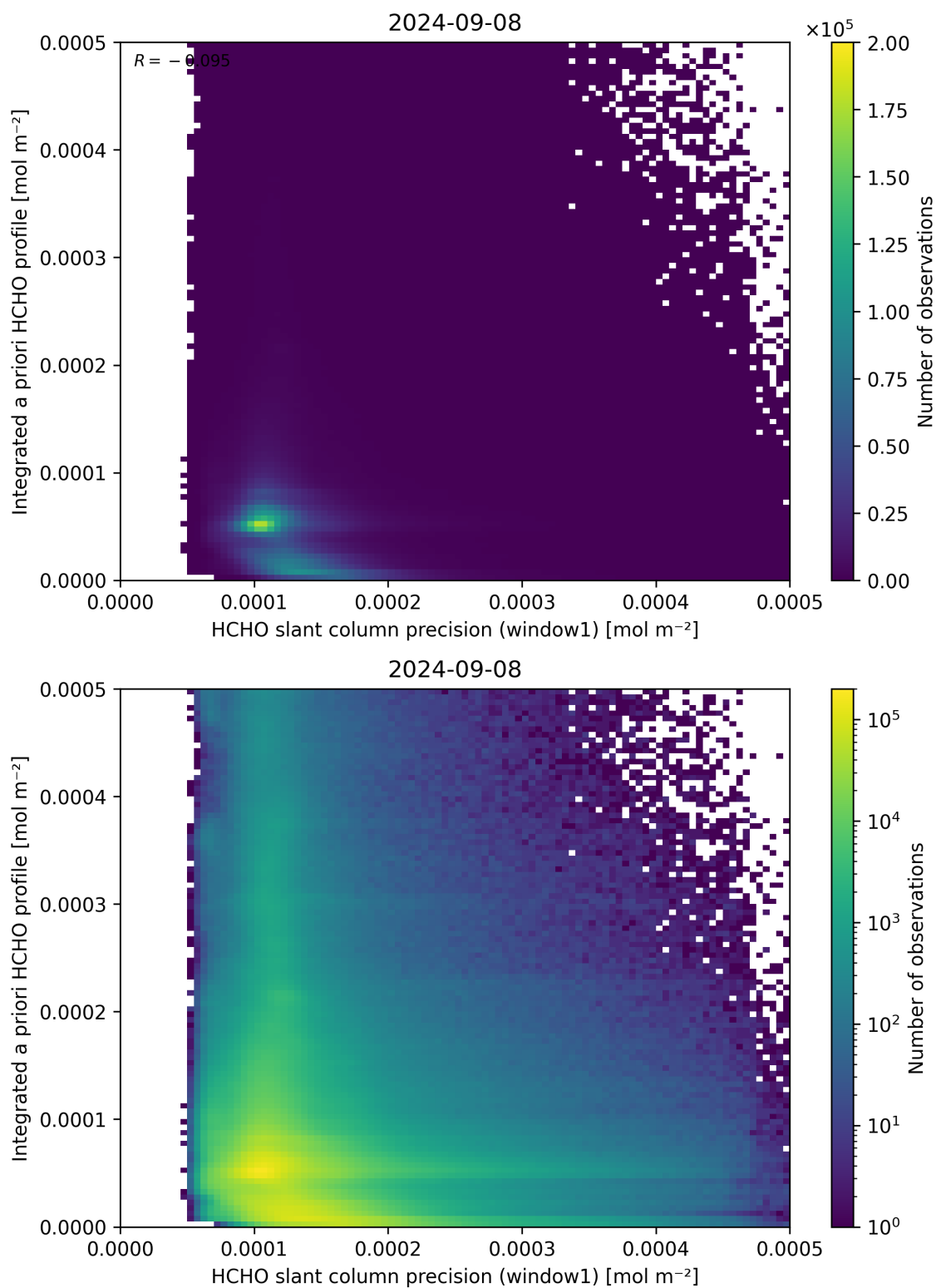
Figure 96: Scatter density plot of “HCHO slant column precision (window1)” against “Integrated a priori HCHO profile” for 2024-09-07 to 2024-09-09.
