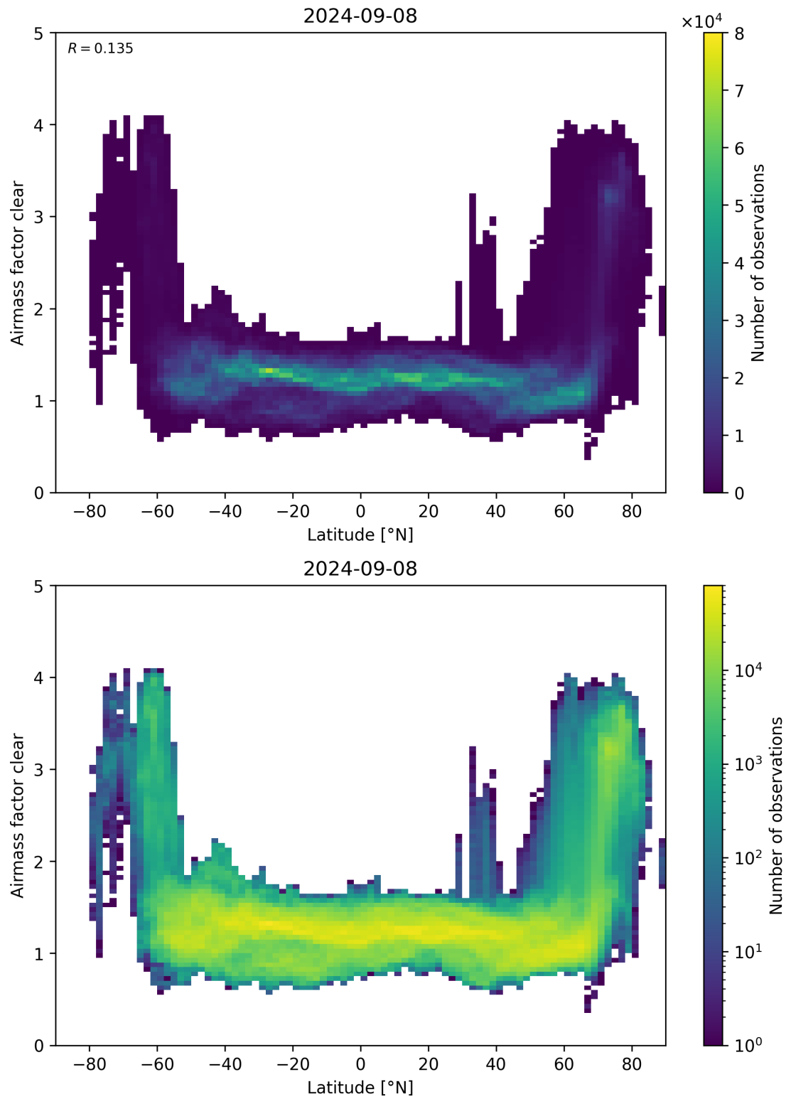
Figure 156: Scatter density plot of “Latitude” against “Airmass factor clear” for 2024-09-07 to 2024-09-09.
