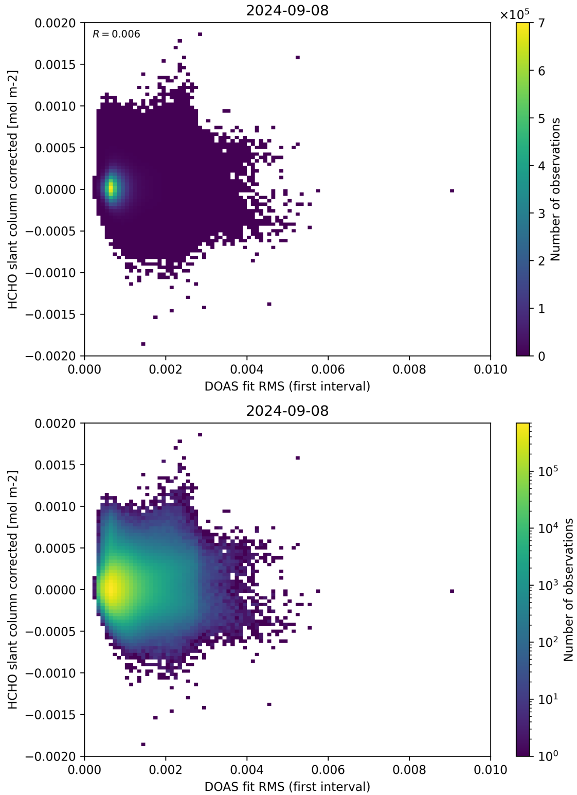
Figure 62: Scatter density plot of “DOAS fit RMS (first interval)” against “HCHO slant column corrected” for 2024-09-07 to 2024-09-09.
