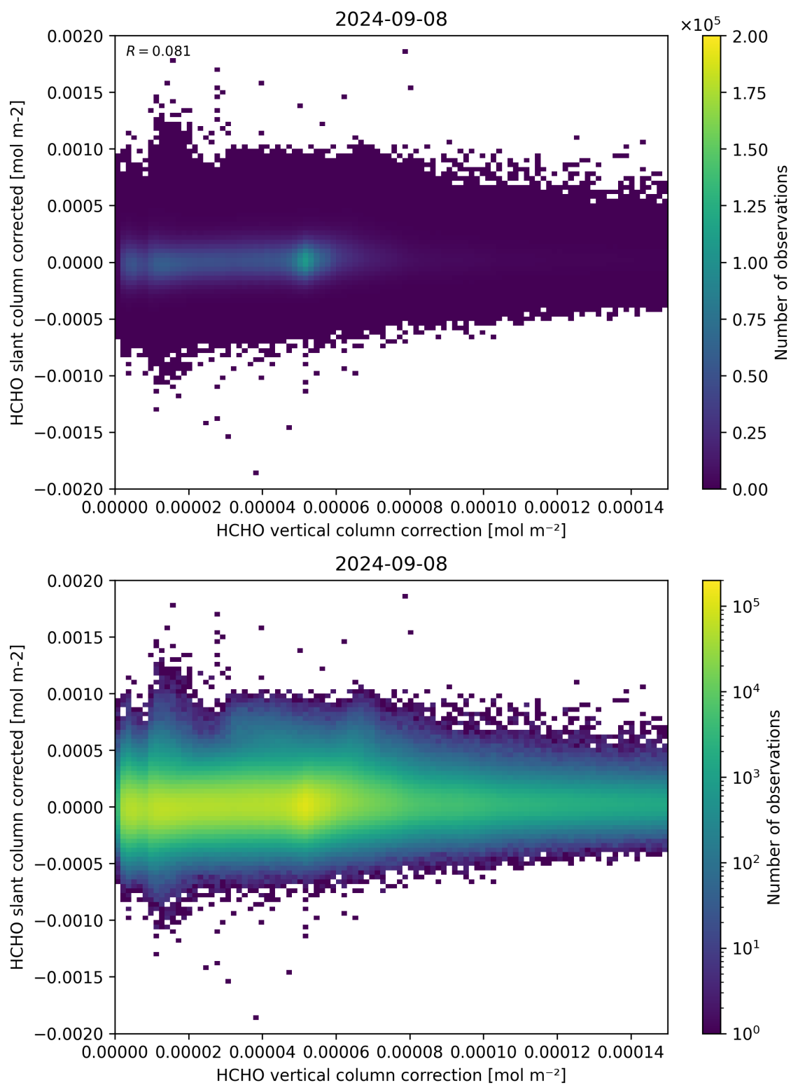
Figure 116: Scatter density plot of “HCHO vertical column correction” against “HCHO slant column corrected” for 2024-09-07 to 2024-09-09.
