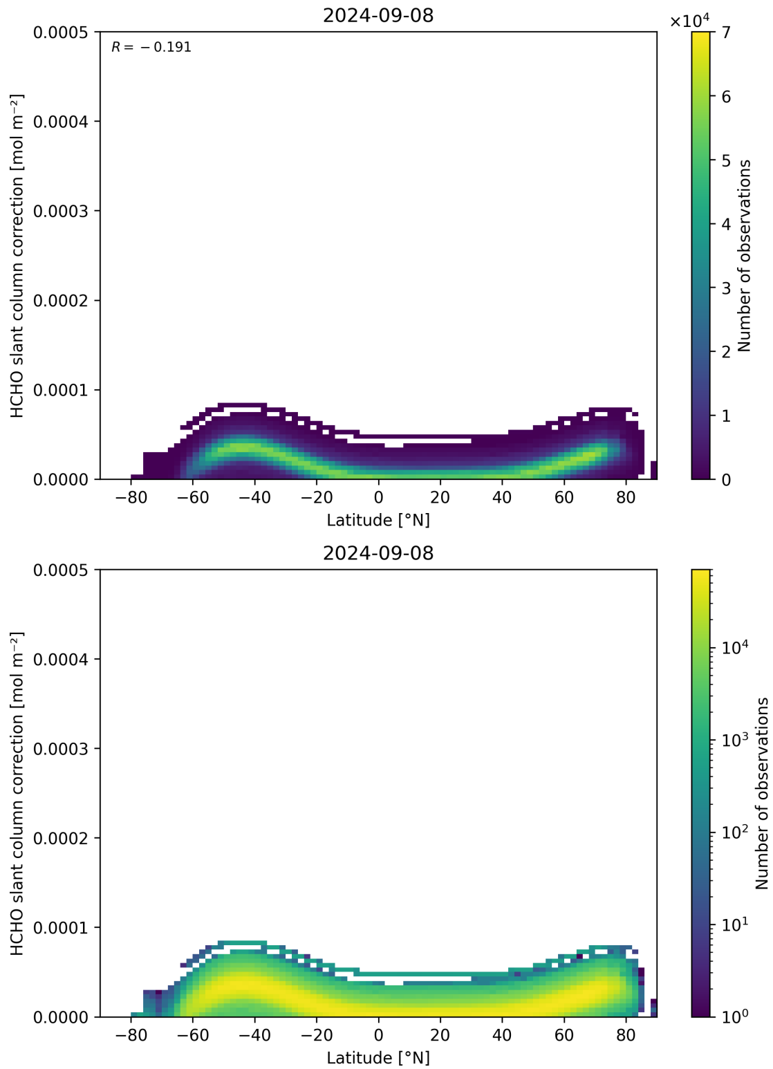
Figure 158: Scatter density plot of “Latitude” against “HCHO slant column correction” for 2024-09-07 to 2024-09-09.
