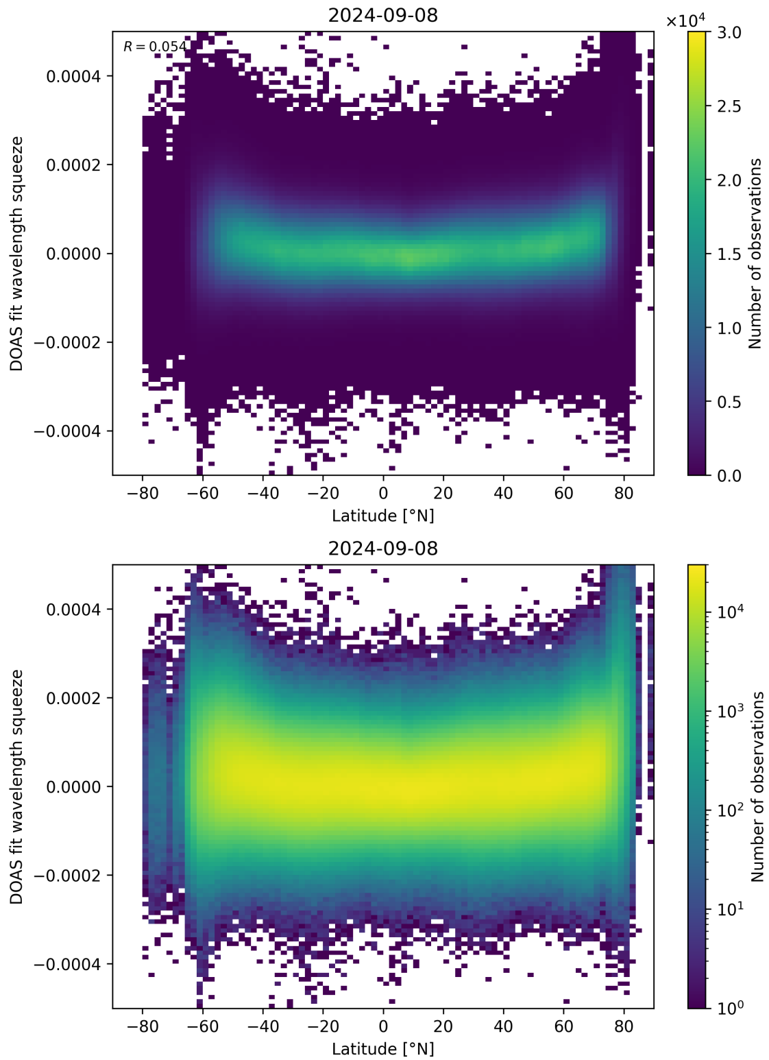
Figure 155: Scatter density plot of “Latitude” against “DOAS fit wavelength squeeze” for 2024-09-07 to 2024-09-09.
