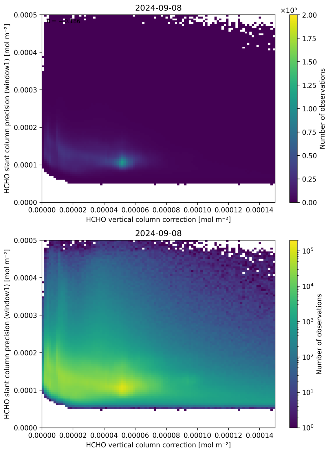
Figure 119: Scatter density plot of “HCHO vertical column correction” against “HCHO slant column precision (window1)” for 2024-09-07 to 2024-09-09.
