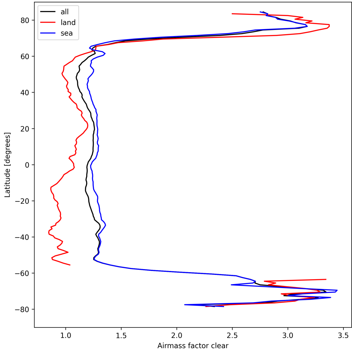
Figure 28: Zonal average of “Airmass factor clear” for 2024-09-07 to 2024-09-09.
