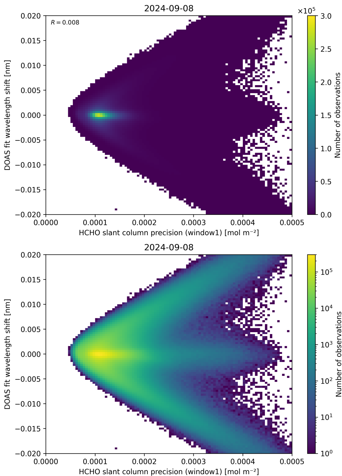
Figure 89: Scatter density plot of “HCHO slant column precision (window1)” against “DOAS fit wavelength shift” for 2024-09-07 to 2024-09-09.
