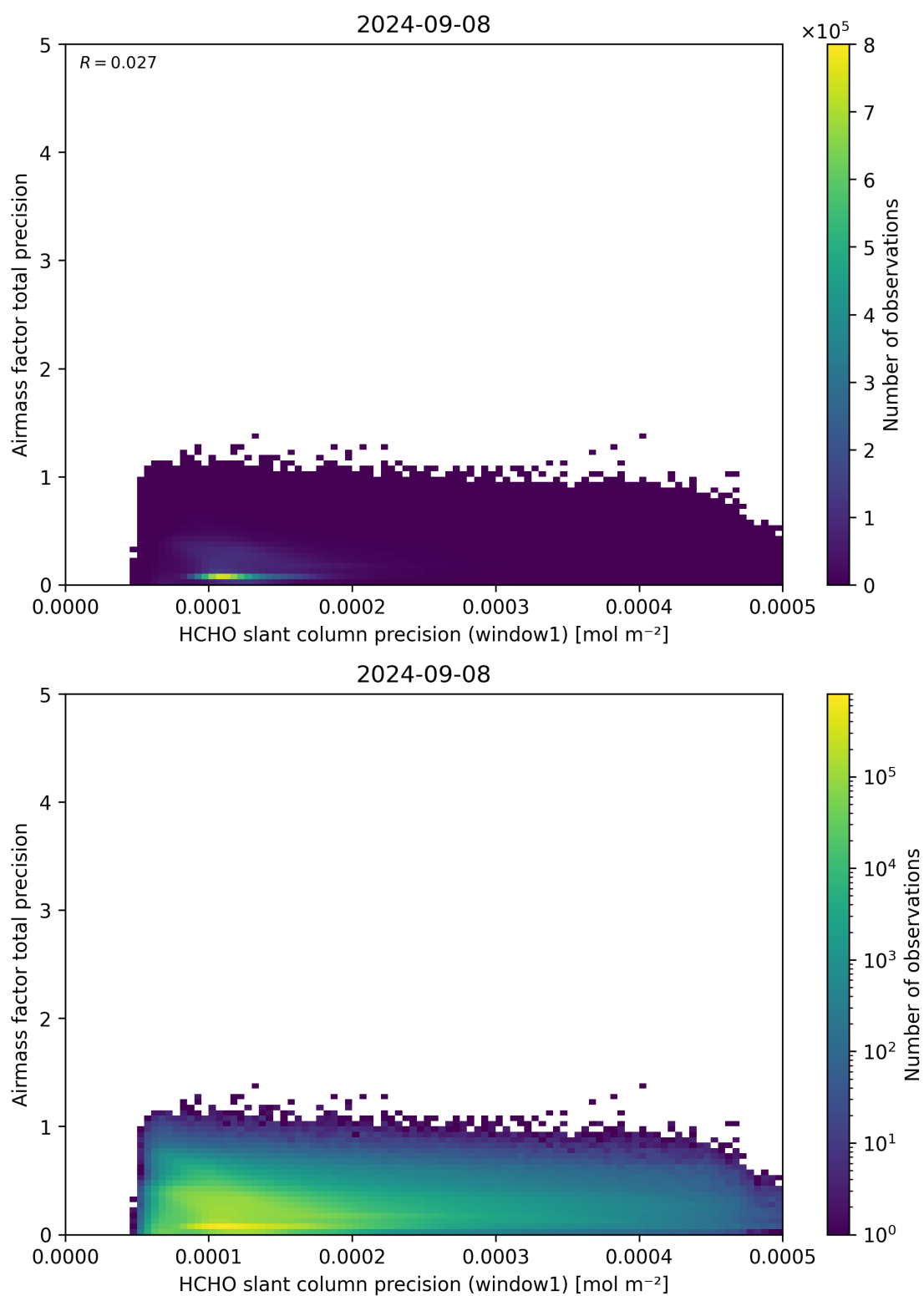
Figure 95: Scatter density plot of “HCHO slant column precision (window1)” against “Airmass factor total precision” for 2024-09-07 to 2024-09-09.
