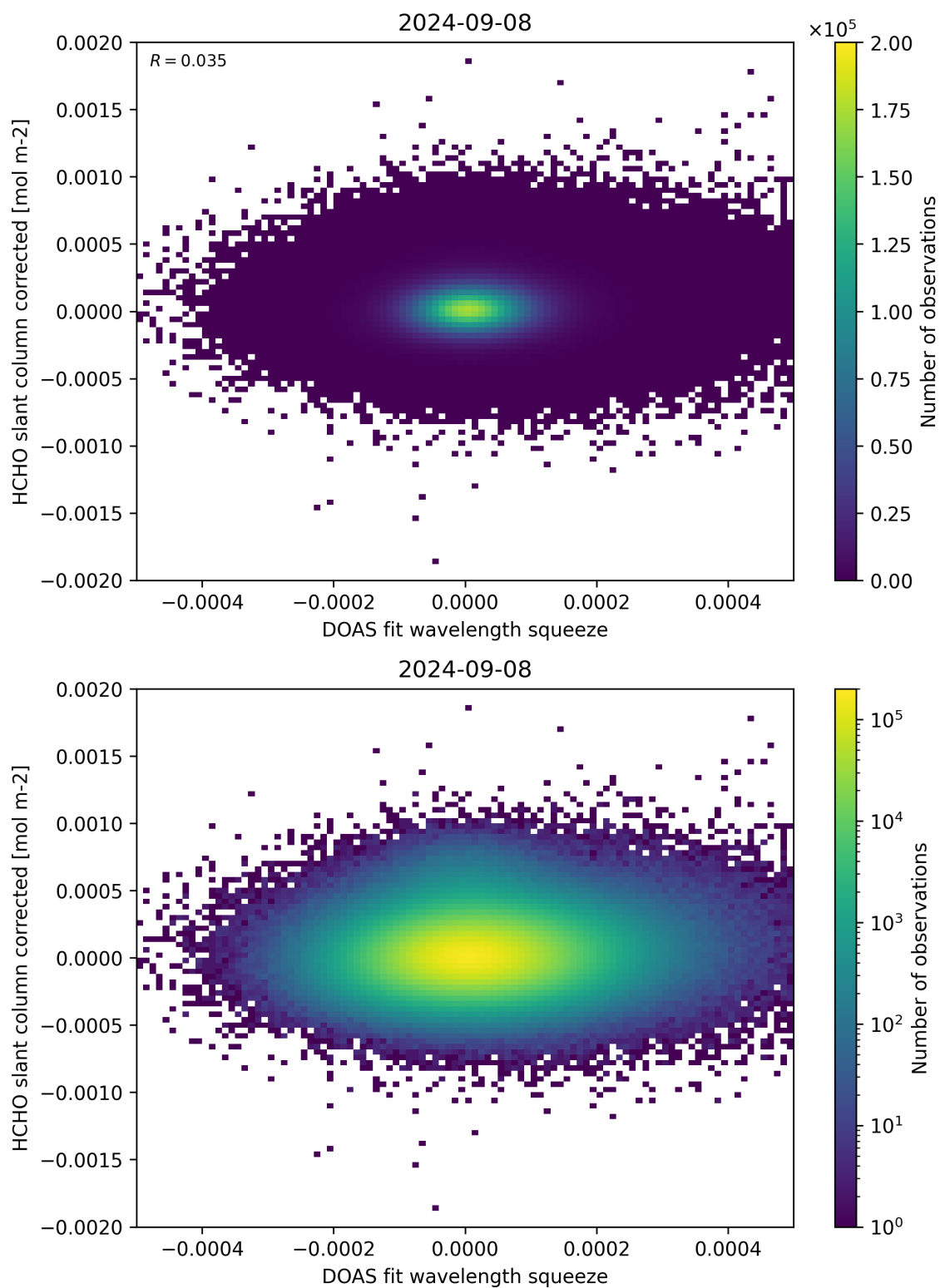
Figure 69: Scatter density plot of “DOAS fit wavelength squeeze” against “HCHO slant column corrected” for 2024-09-07 to 2024-09-09.
