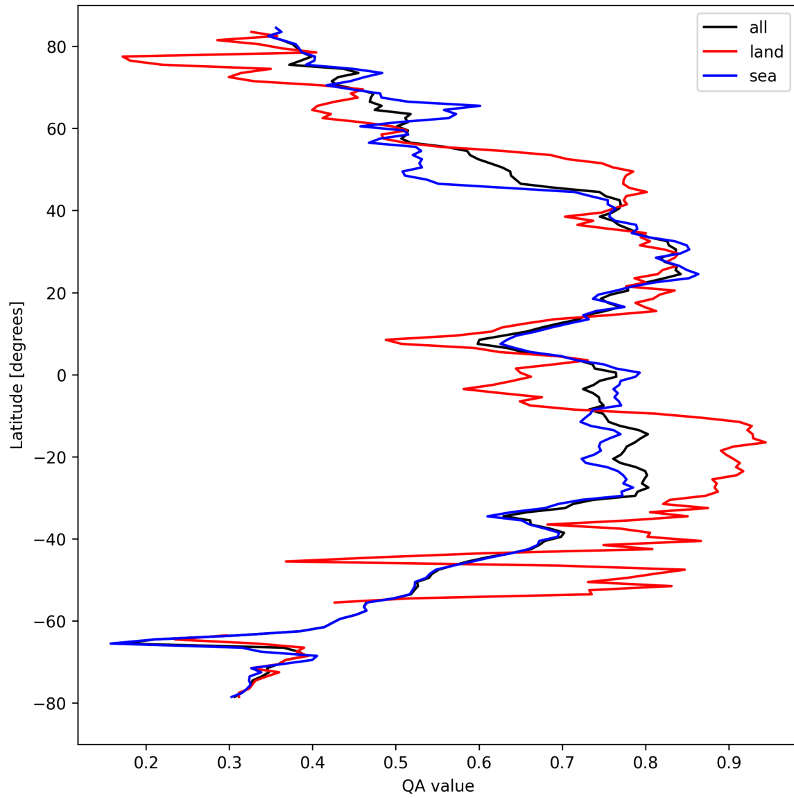
Figure 20: Zonal average of “QA value” for 2024-09-07 to 2024-09-09.
