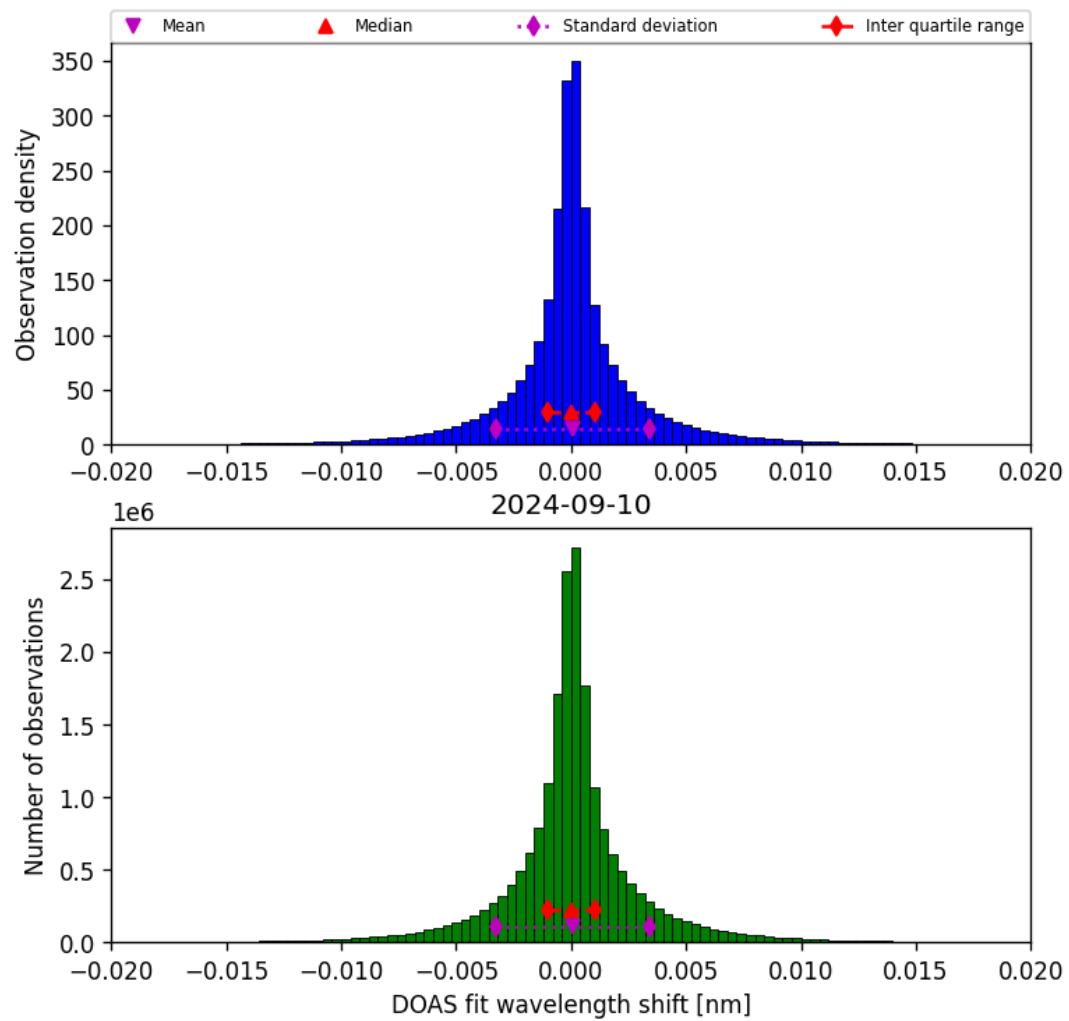
Figure 44: Histogram of “DOAS fit wavelength shift” for 2024-09-09 to 2024-09-11
