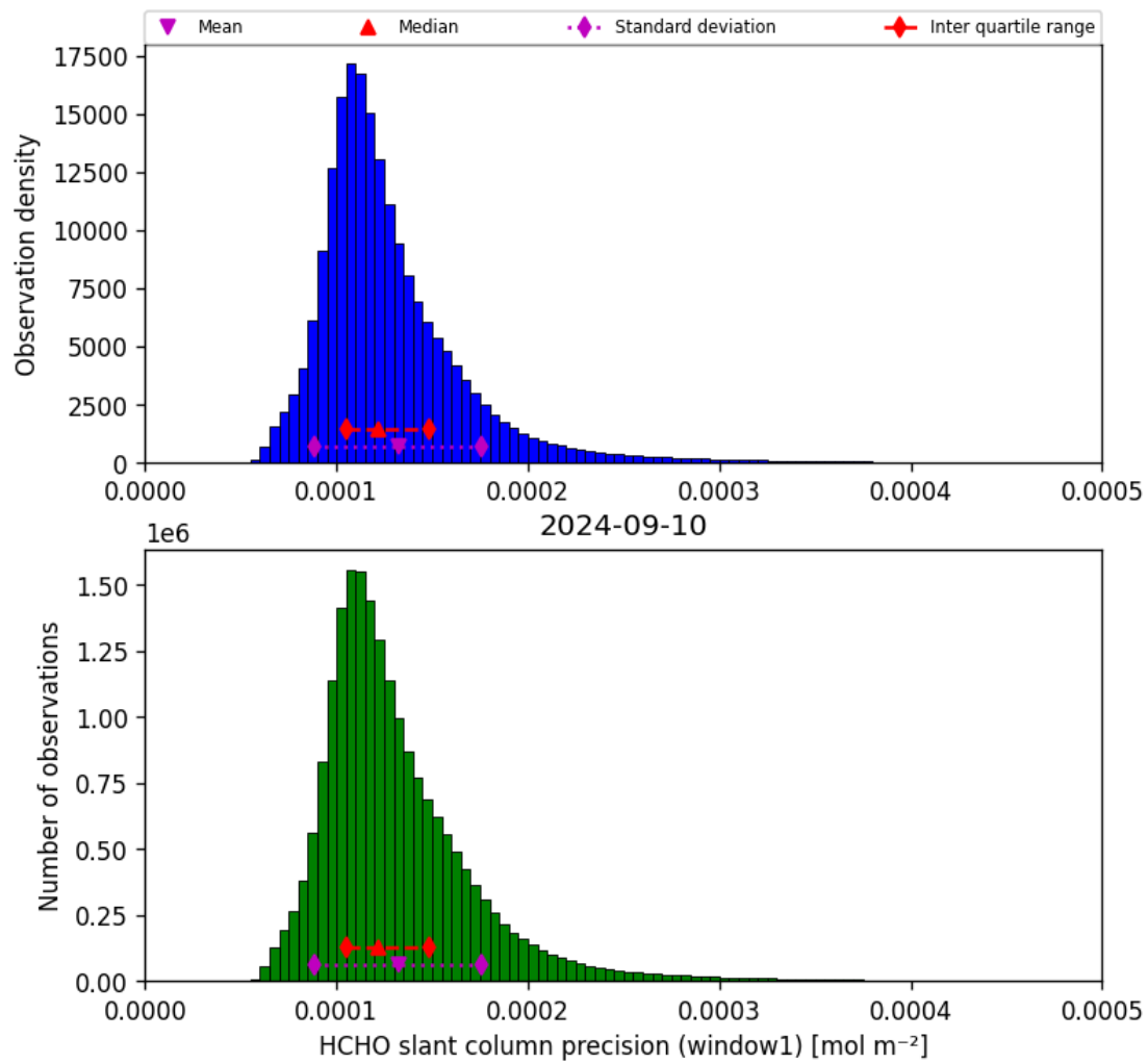
Figure 39: Histogram of “HCHO slant column precision (window1)” for 2024-09-09 to 2024-09-11
