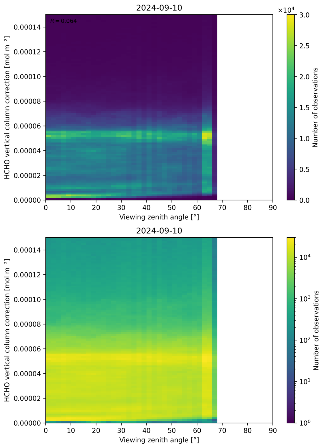
Figure 193: Scatter density plot of “Viewing zenith angle” against “HCHO vertical column correction” for 2024-09-09 to 2024-09-11.
