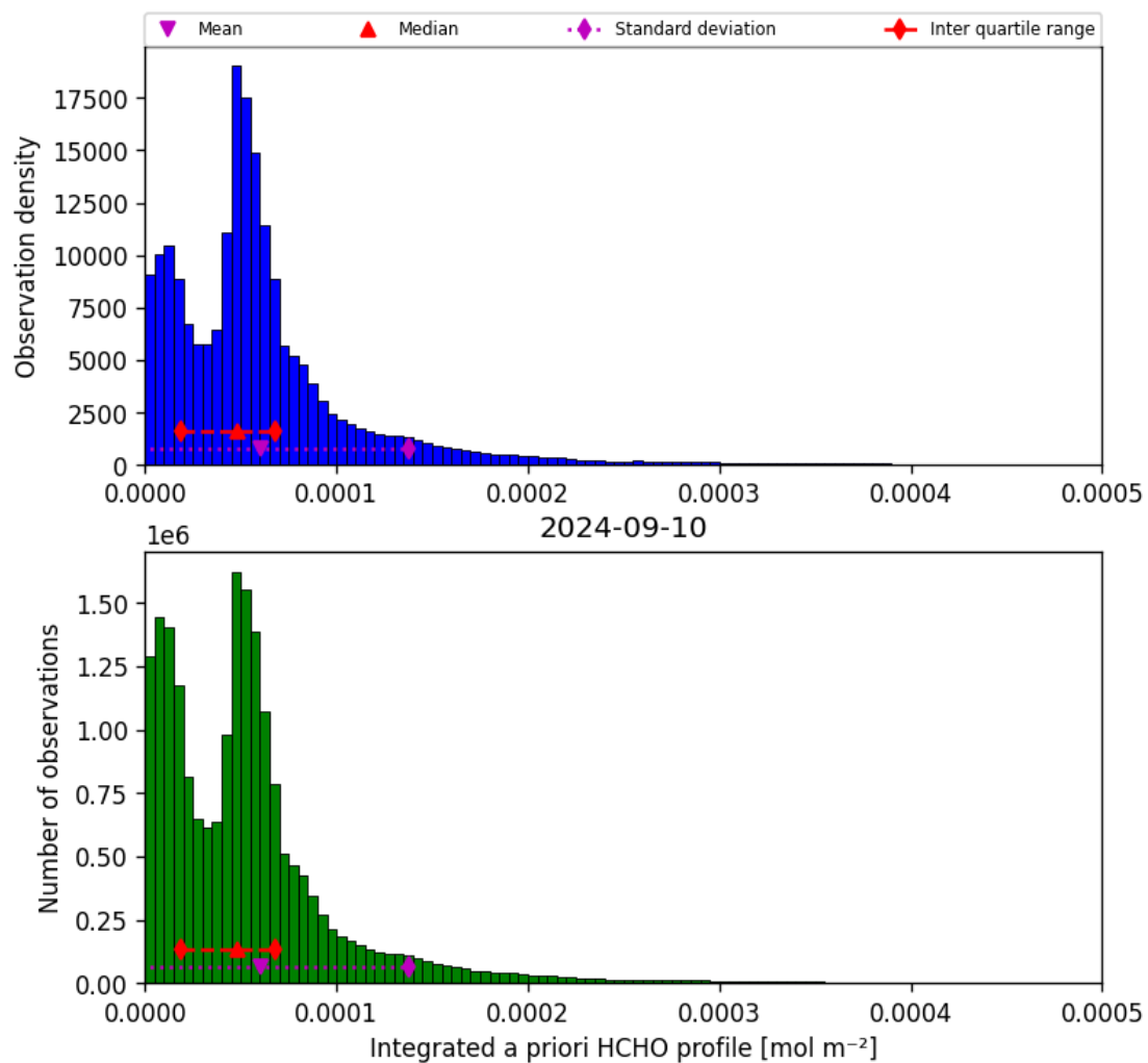
Figure 43: Histogram of “Integrated a priori HCHO profile” for 2024-09-09 to 2024-09-11
