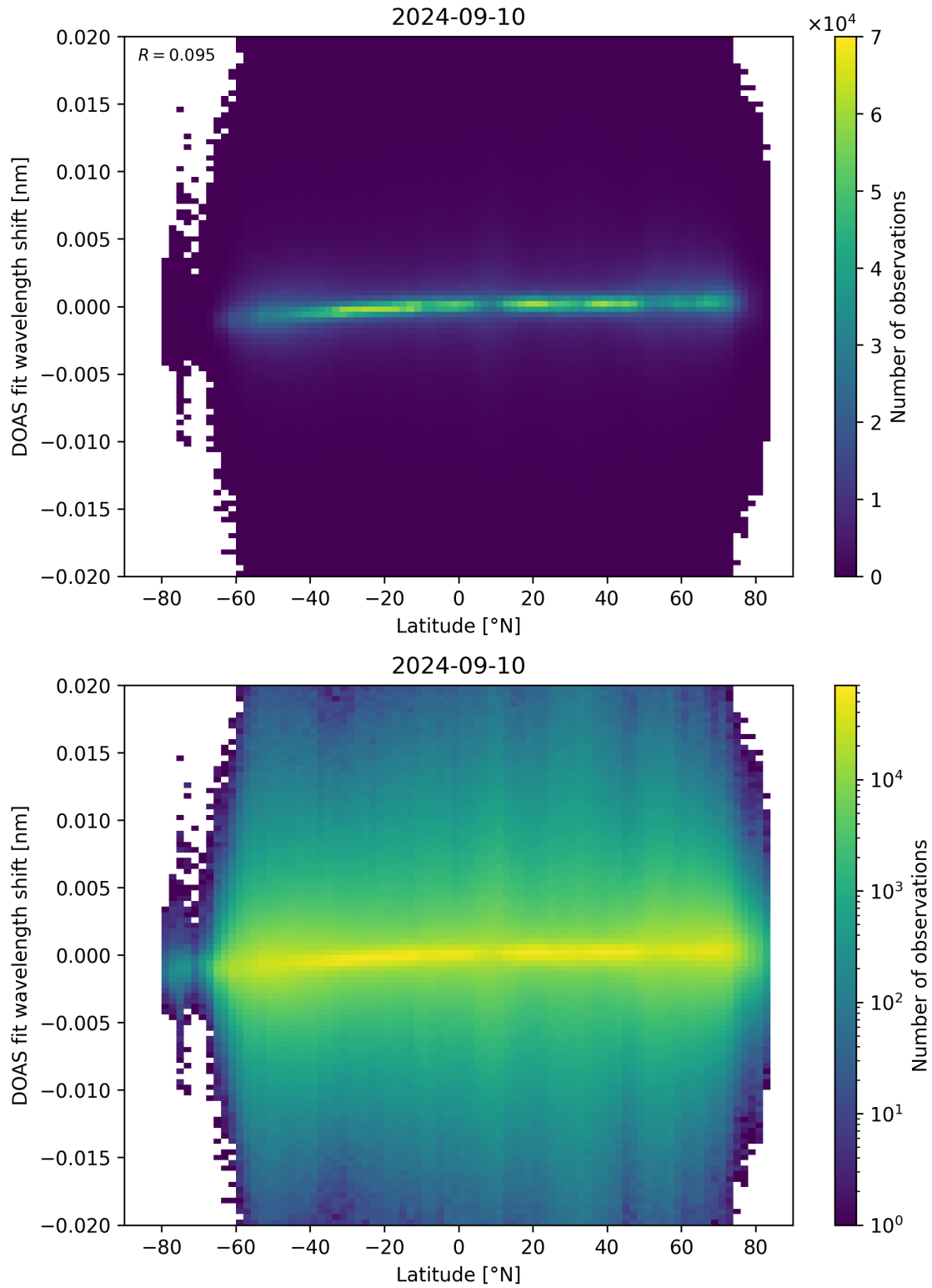
Figure 154: Scatter density plot of “Latitude” against “DOAS fit wavelength shift” for 2024-09-09 to 2024-09-11.
