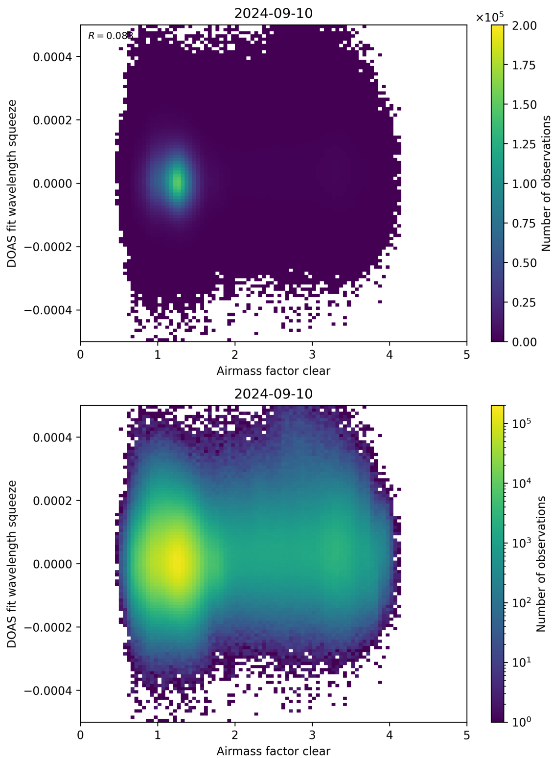
Figure 73: Scatter density plot of “Airmass factor clear” against “DOAS fit wavelength squeeze” for 2024-09-09 to 2024-09-11.
