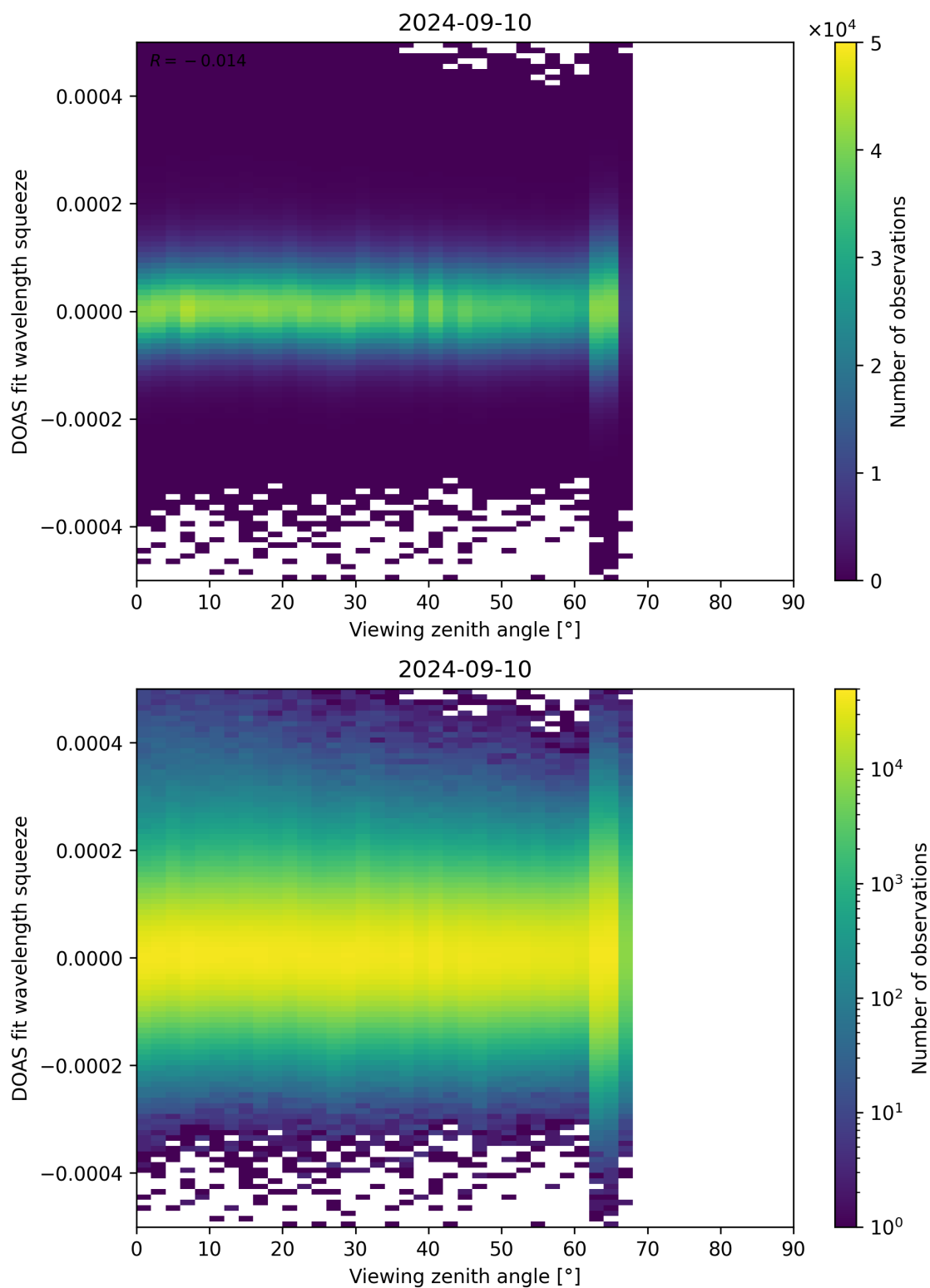
Figure 184: Scatter density plot of “Viewing zenith angle” against “DOAS fit wavelength squeeze” for 2024-09-09 to 2024-09-11.
