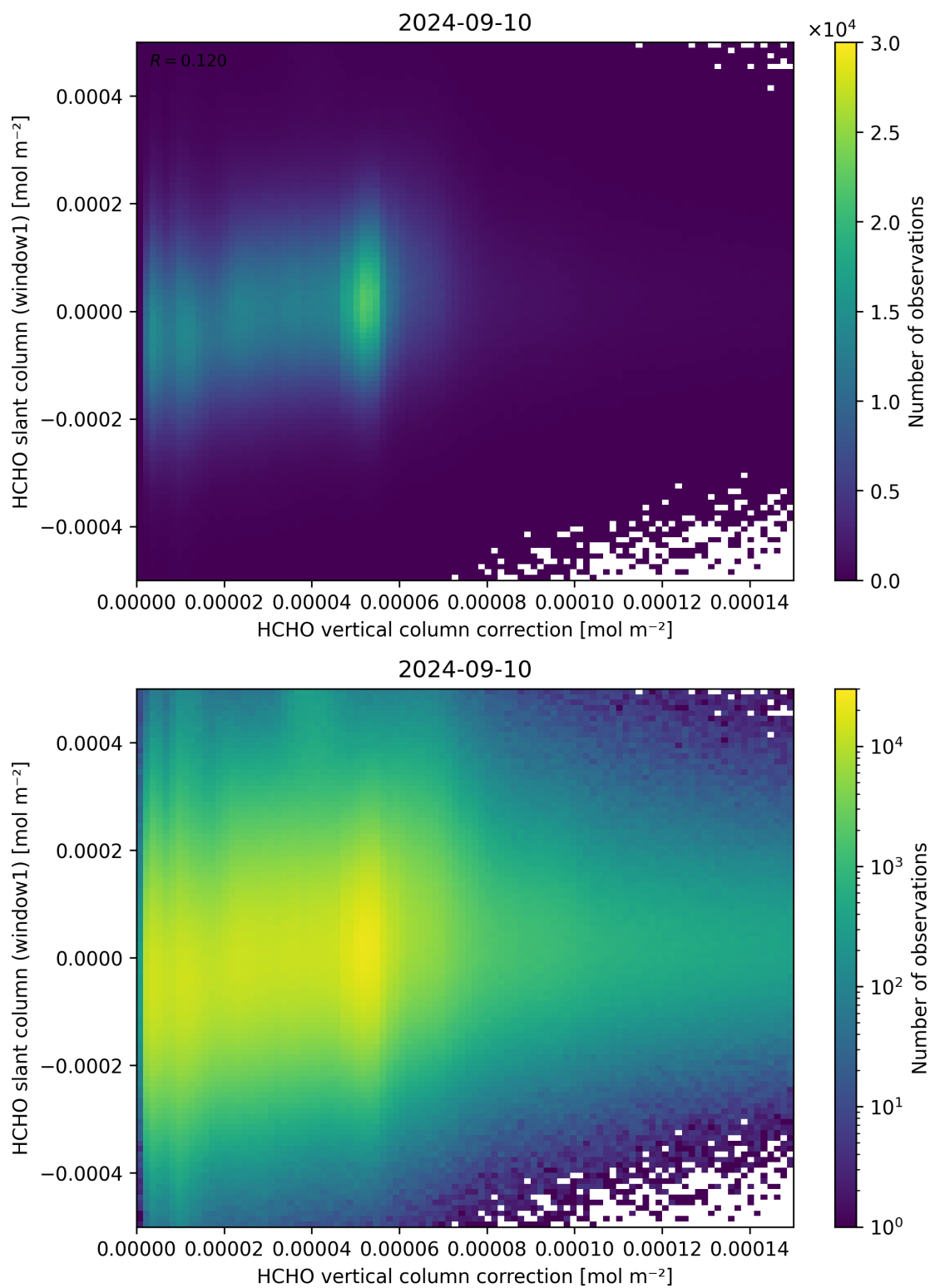
Figure 118: Scatter density plot of “HCHO vertical column correction” against “HCHO slant column (window1)” for 2024-09-09 to 2024-09-11.
