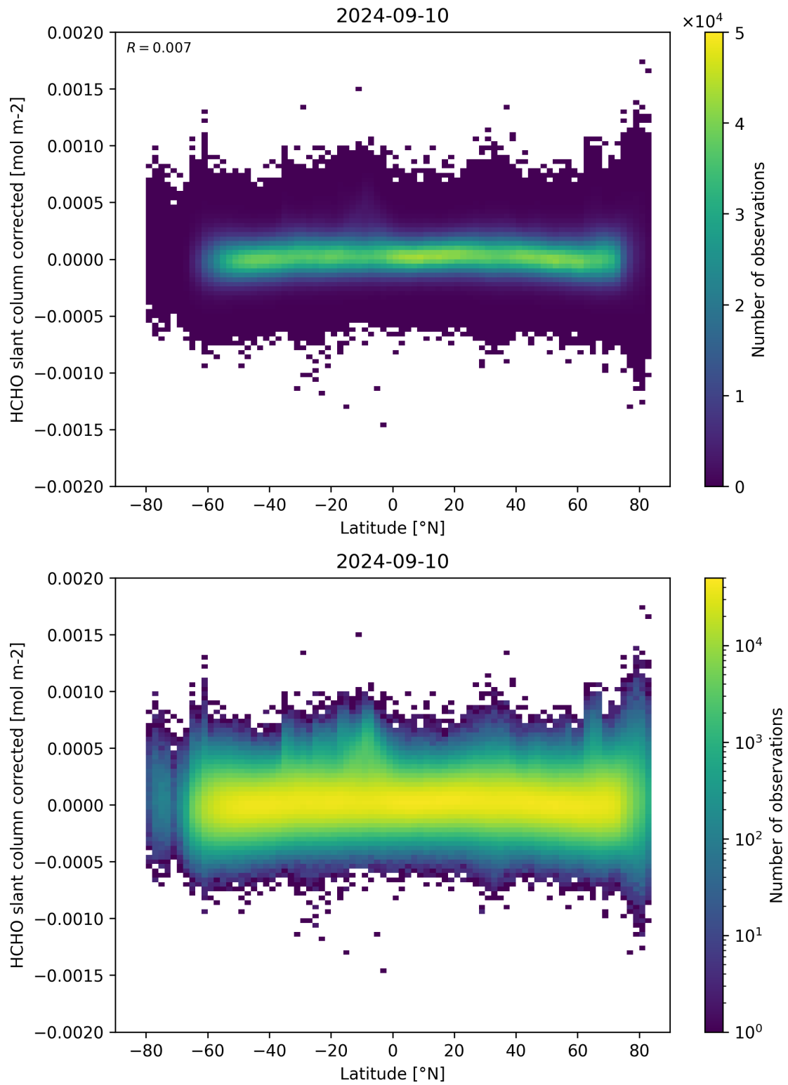
Figure 157: Scatter density plot of “Latitude” against “HCHO slant column corrected” for 2024-09-09 to 2024-09-11.
