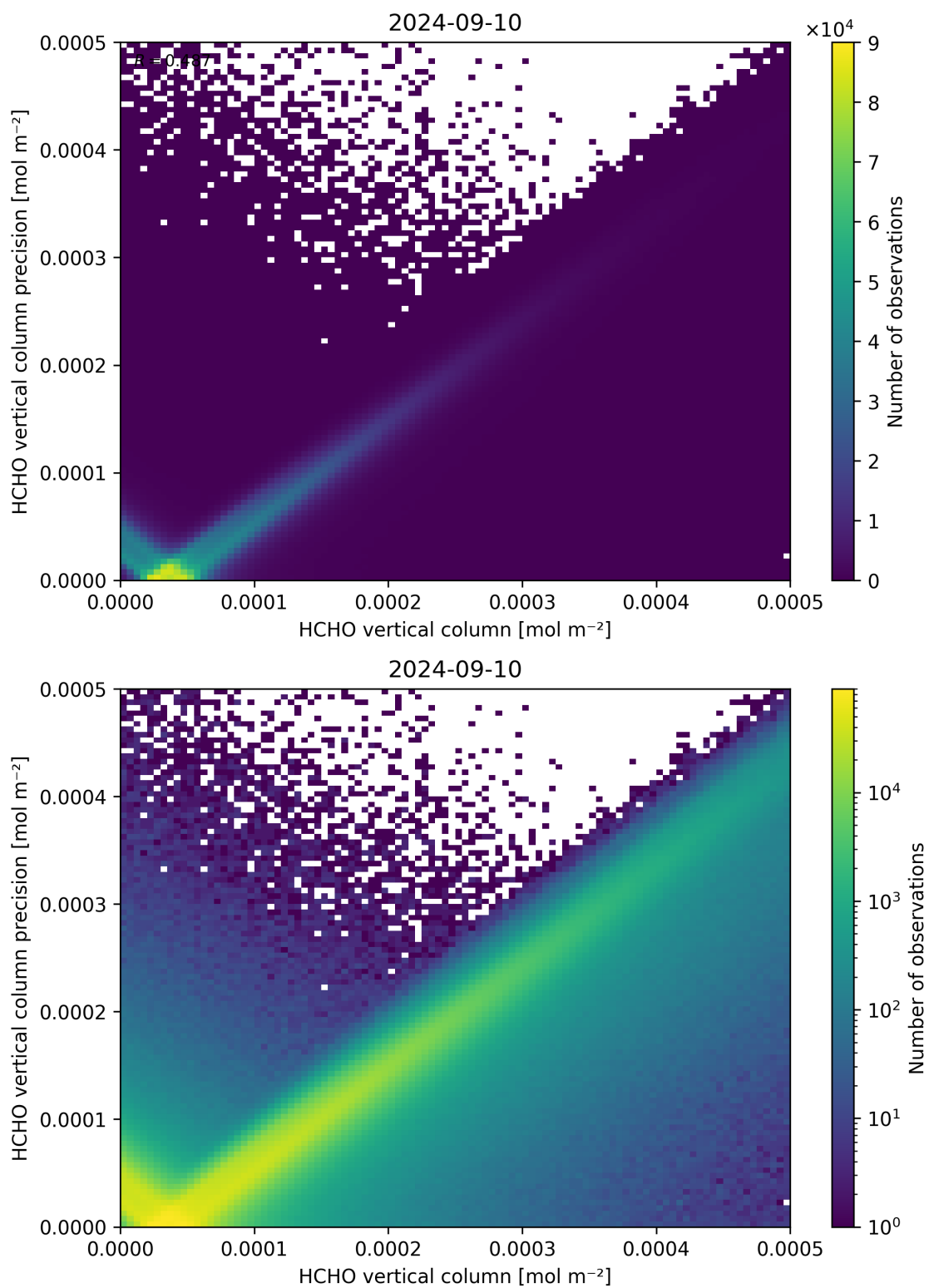
Figure 134: Scatter density plot of “HCHO vertical column” against “HCHO vertical column precision” for 2024-09-09 to 2024-09-11.
