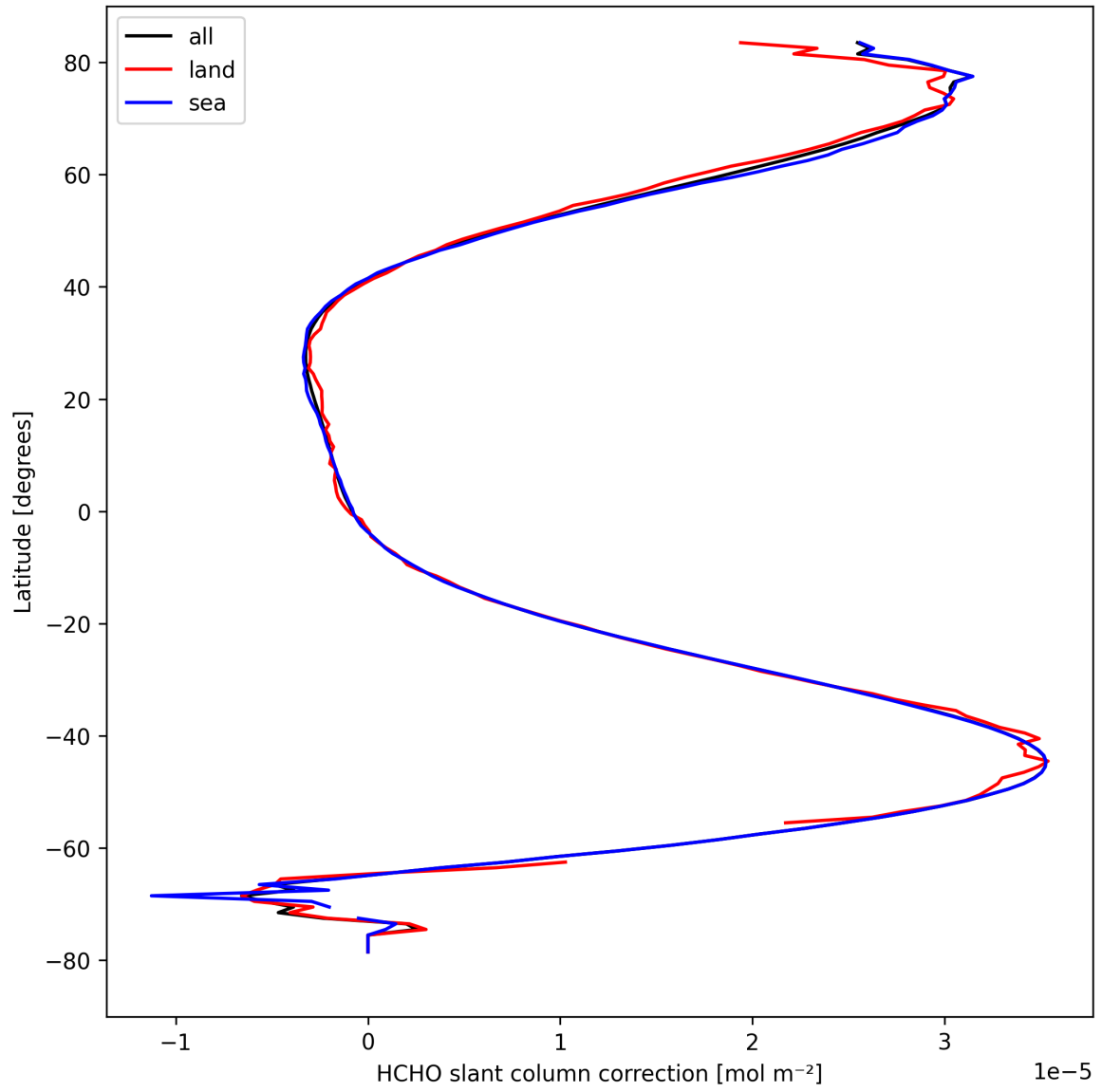
Figure 33: Zonal average of "HCHO slant column correction" for 2024-09-09 to 2024-09-11.
