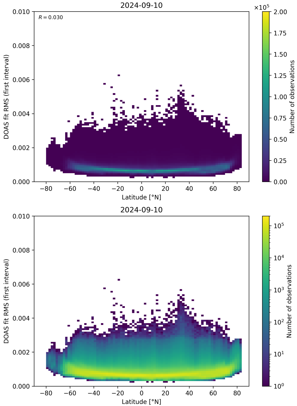
Figure 153: Scatter density plot of “Latitude” against “DOAS fit RMS (first interval)” for 2024-09-09 to 2024-09-11.
