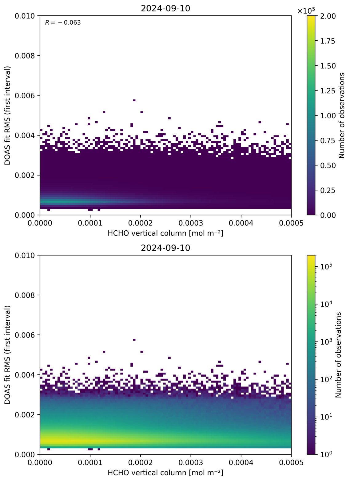
Figure 123: Scatter density plot of “HCHO vertical column” against “DOAS fit RMS (first interval)” for 2024-09-09 to 2024-09-11.
