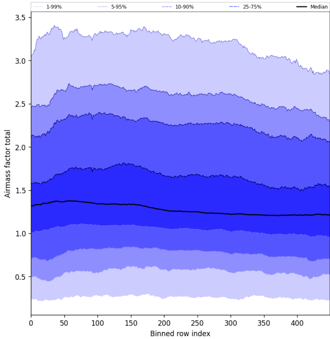
Figure 54: Along track statistics of “Airmass factor total” for 2024-09-09 to 2024-09-11
