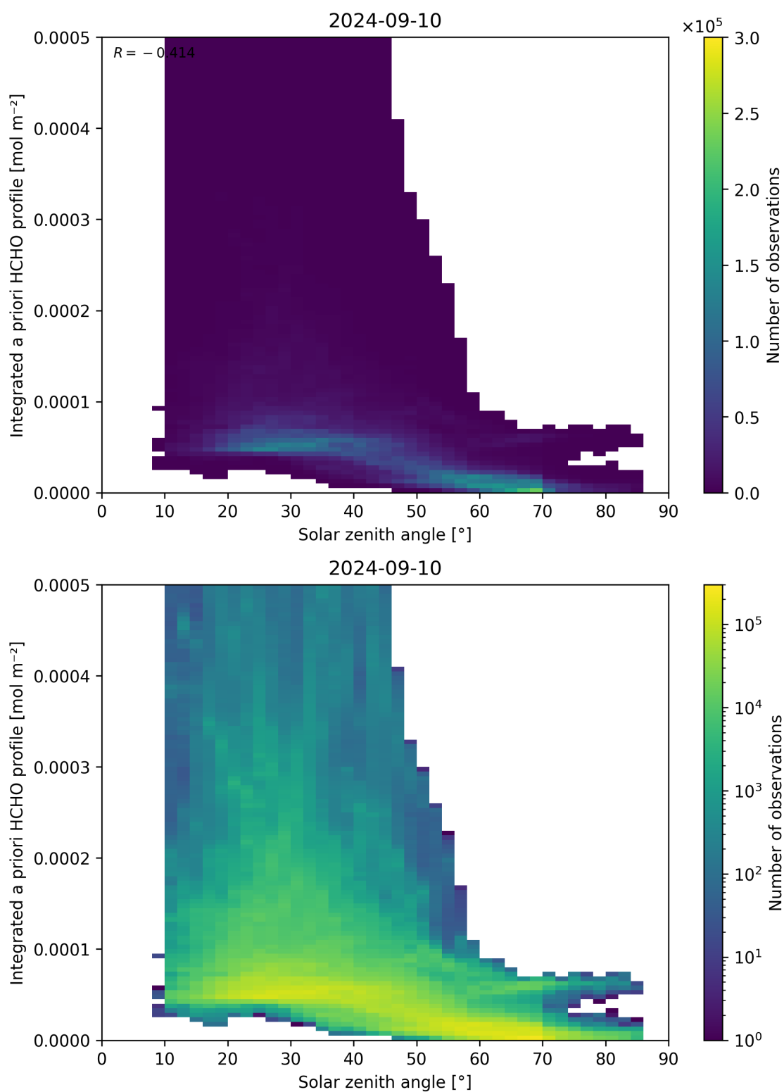
Figure 180: Scatter density plot of “Solar zenith angle” against “Integrated a priori HCHO profile” for 2024-09-09 to 2024-09-11.
