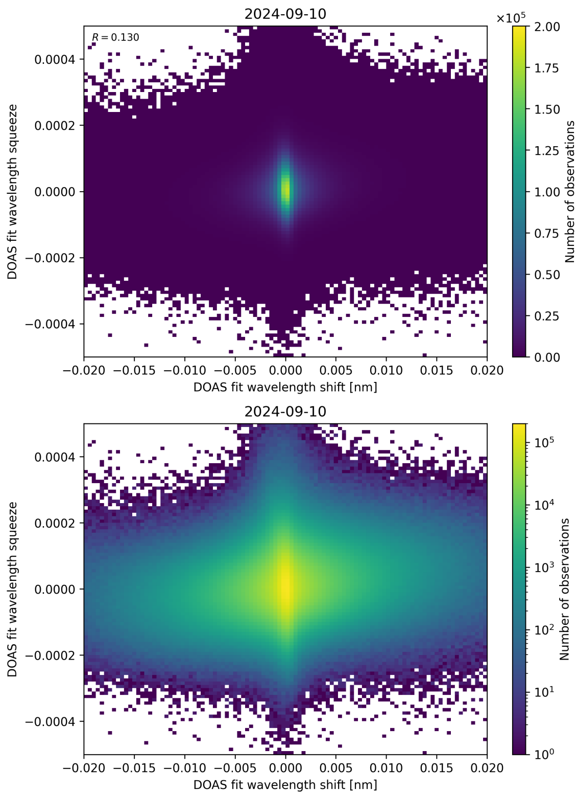
Figure 65: Scatter density plot of “DOAS fit wavelength shift” against “DOAS fit wavelength squeeze” for 2024-09-09 to 2024-09-11.
