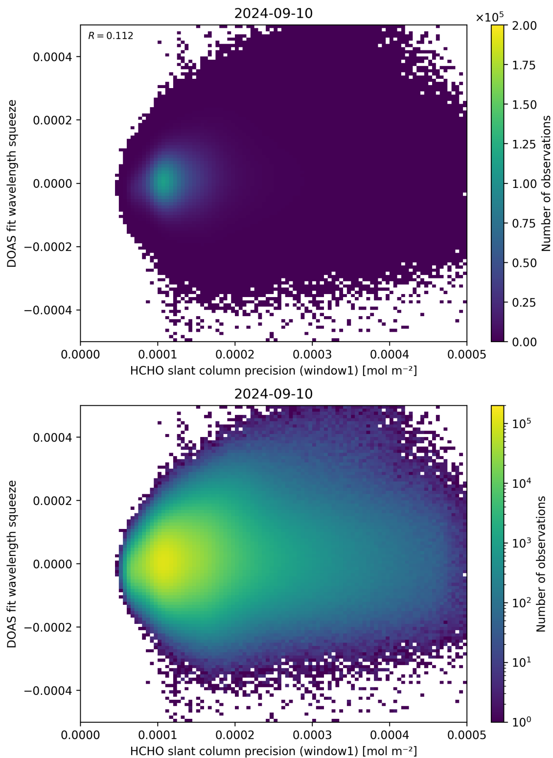
Figure 90: Scatter density plot of “HCHO slant column precision (window1)” against “DOAS fit wavelength squeeze” for 2024-09-09 to 2024-09-11.
