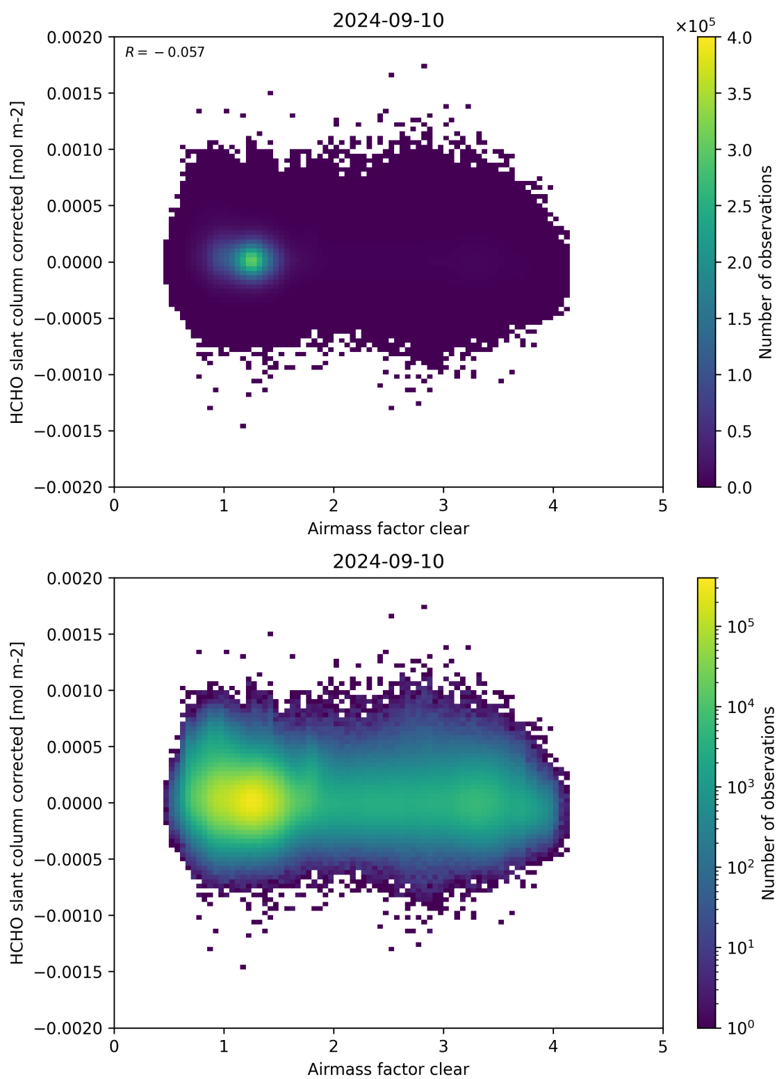
Figure 74: Scatter density plot of “Airmass factor clear” against “HCHO slant column corrected” for 2024-09-09 to 2024-09-11.
