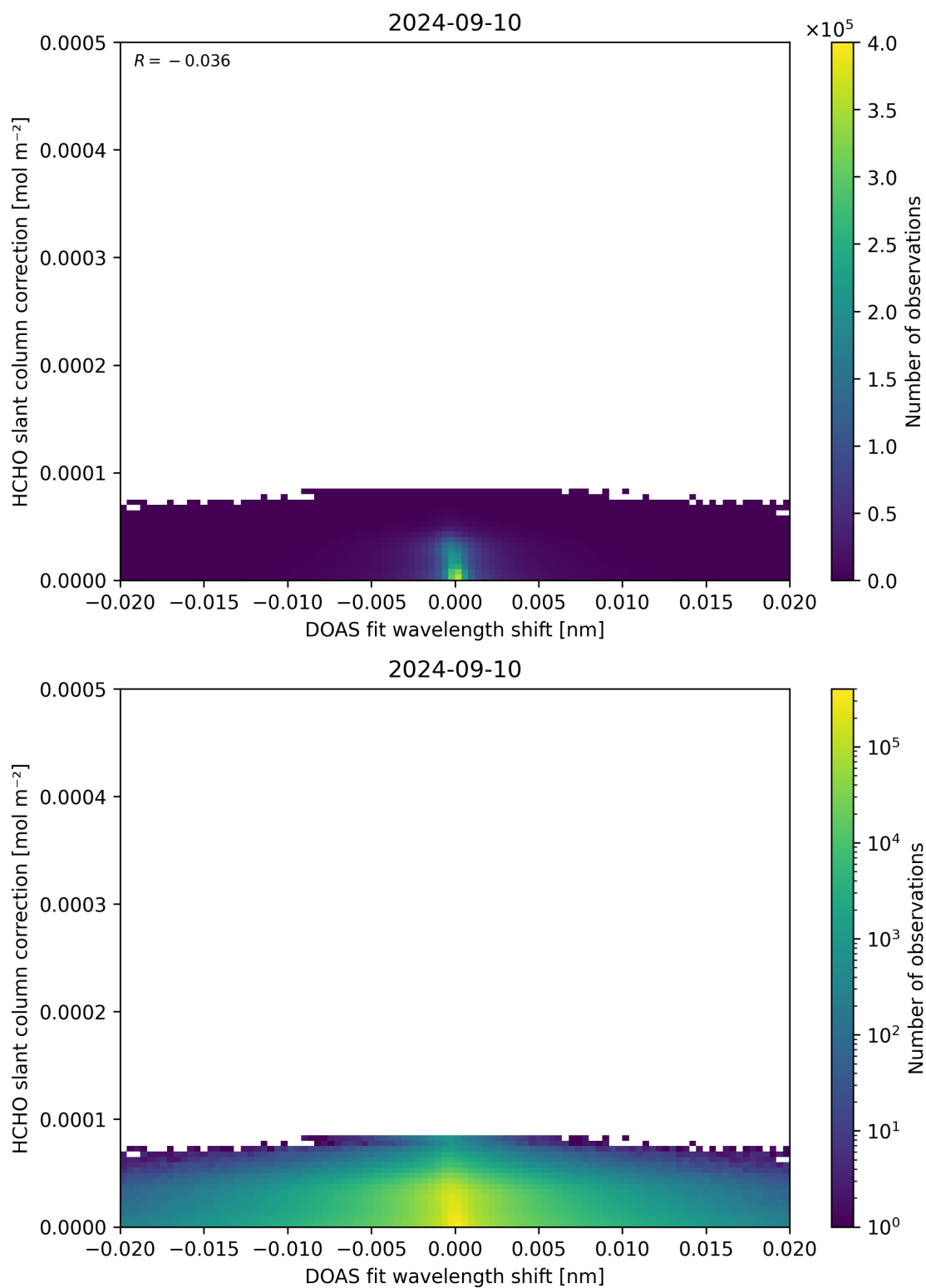
Figure 67: Scatter density plot of “DOAS fit wavelength shift” against “HCHO slant column correction” for 2024-09-09 to 2024-09-11.
