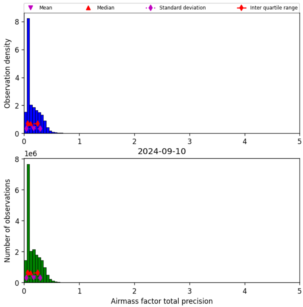
Figure 41: Histogram of “Airmass factor total precision” for 2024-09-09 to 2024-09-11
