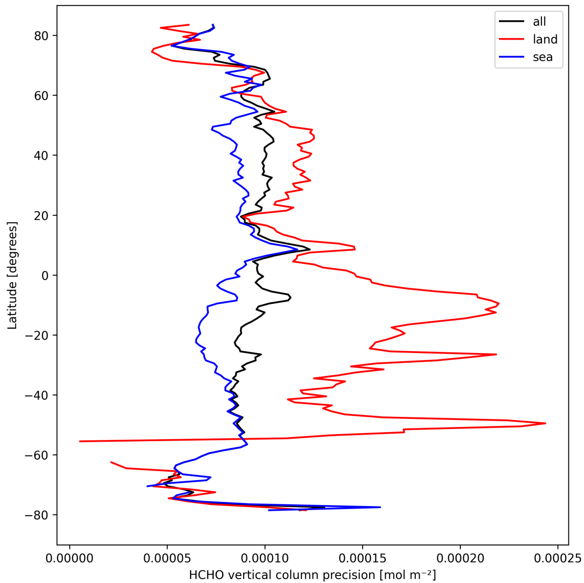
Figure 22: Zonal average of “HCHO vertical column precision” for 2024-09-09 to 2024-09-11.
