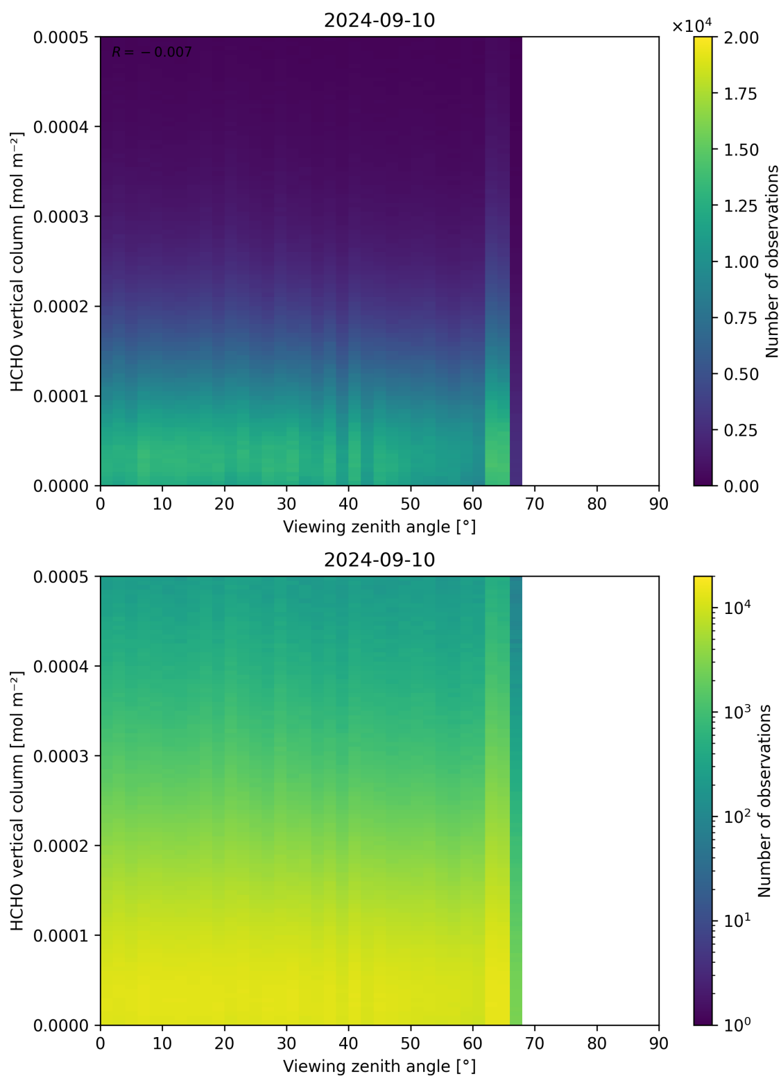
Figure 192: Scatter density plot of “Viewing zenith angle” against “HCHO vertical column” for 2024-09-09 to 2024-09-11.
