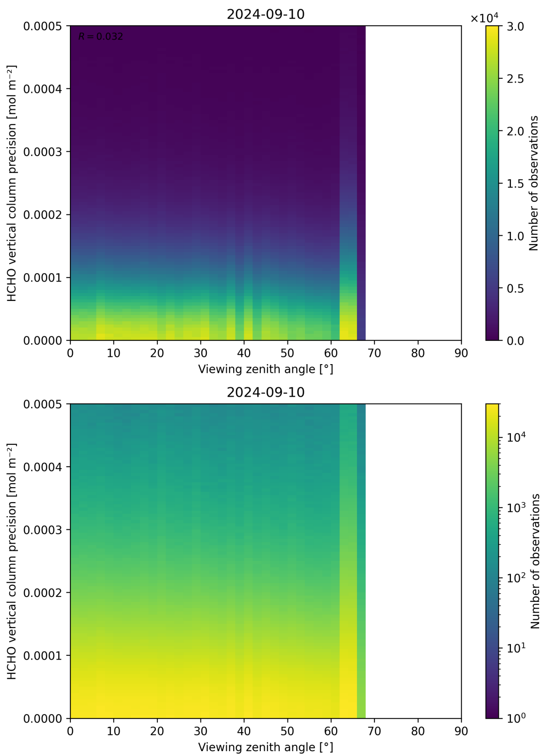
Figure 194: Scatter density plot of “Viewing zenith angle” against “HCHO vertical column precision” for 2024-09-09 to 2024-09-11.
