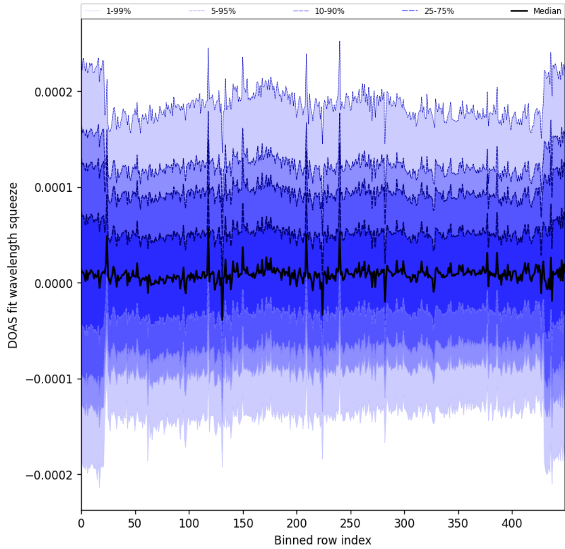
Figure 59: Along track statistics of “DOAS fit wavelength squeeze” for 2024-09-09 to 2024-09-11
