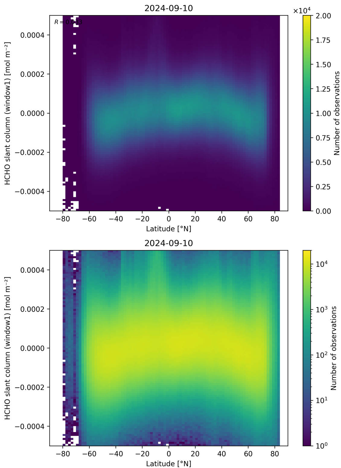
Figure 159: Scatter density plot of “Latitude” against “HCHO slant column (window1)” for 2024-09-09 to 2024-09-11.
