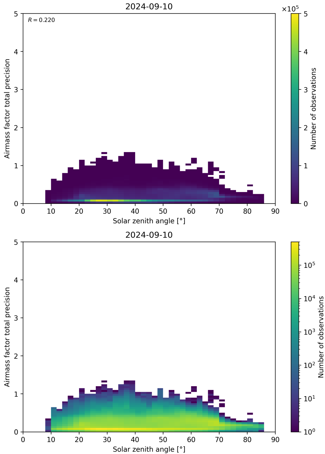
Figure 176: Scatter density plot of “Solar zenith angle” against “Airmass factor total precision” for 2024-09-09 to 2024-09-11.
