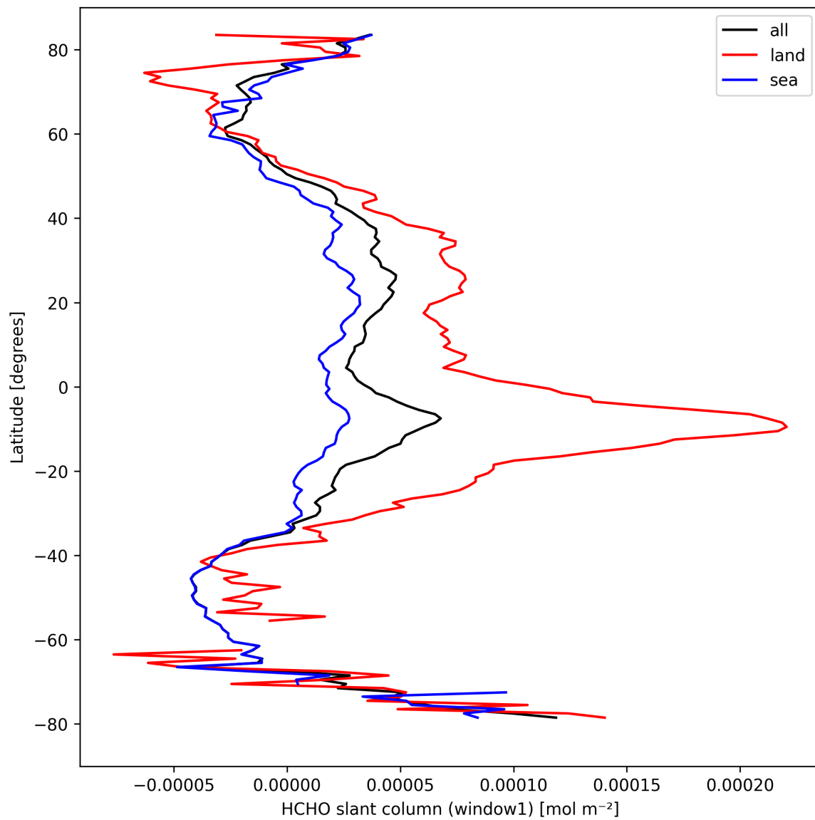
Figure 24: Zonal average of “HCHO slant column (window1)” for 2024-09-09 to 2024-09-11.
