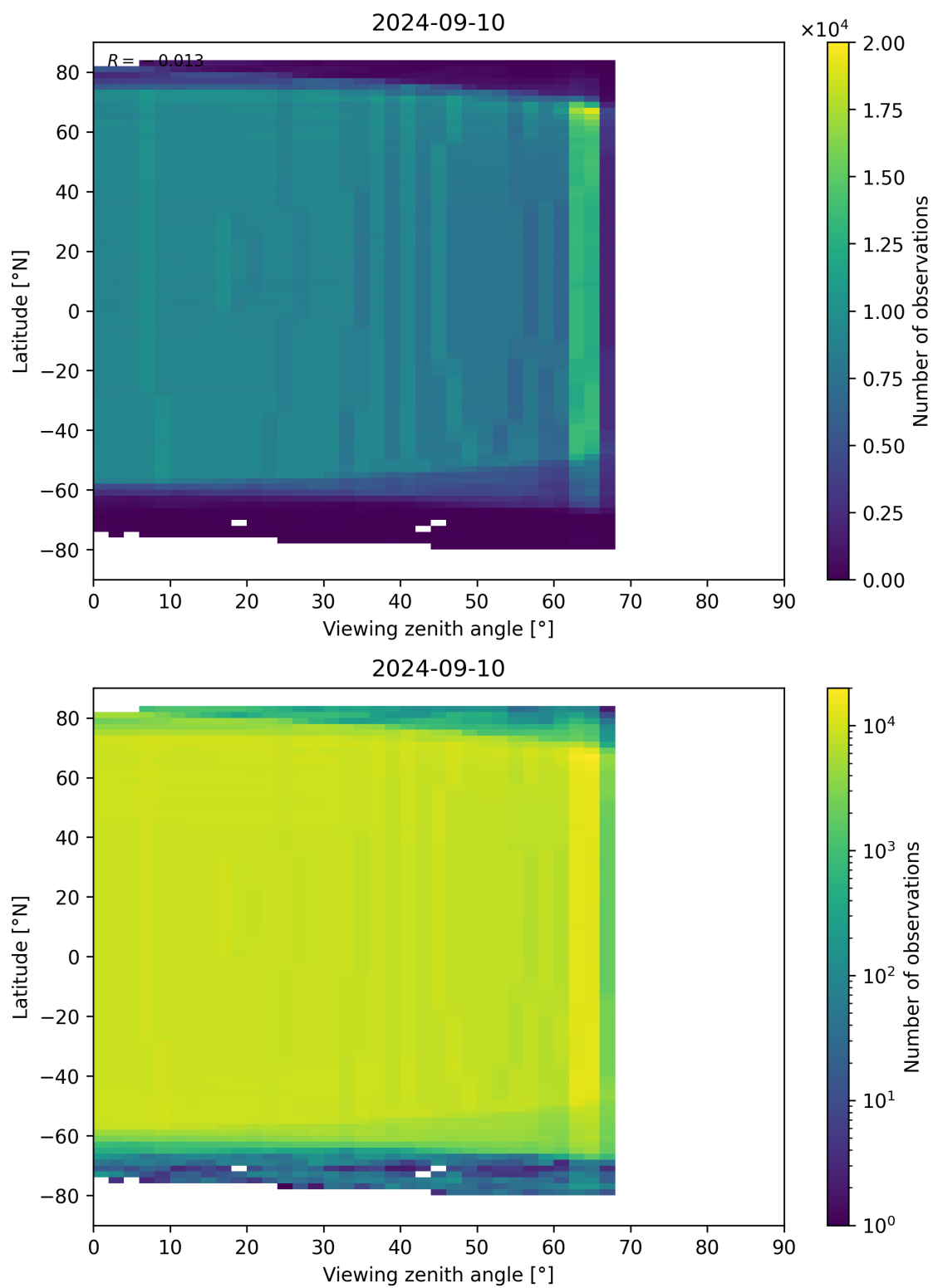
Figure 196: Scatter density plot of “Viewing zenith angle” against “Latitude” for 2024-09-09 to 2024-09-11.
