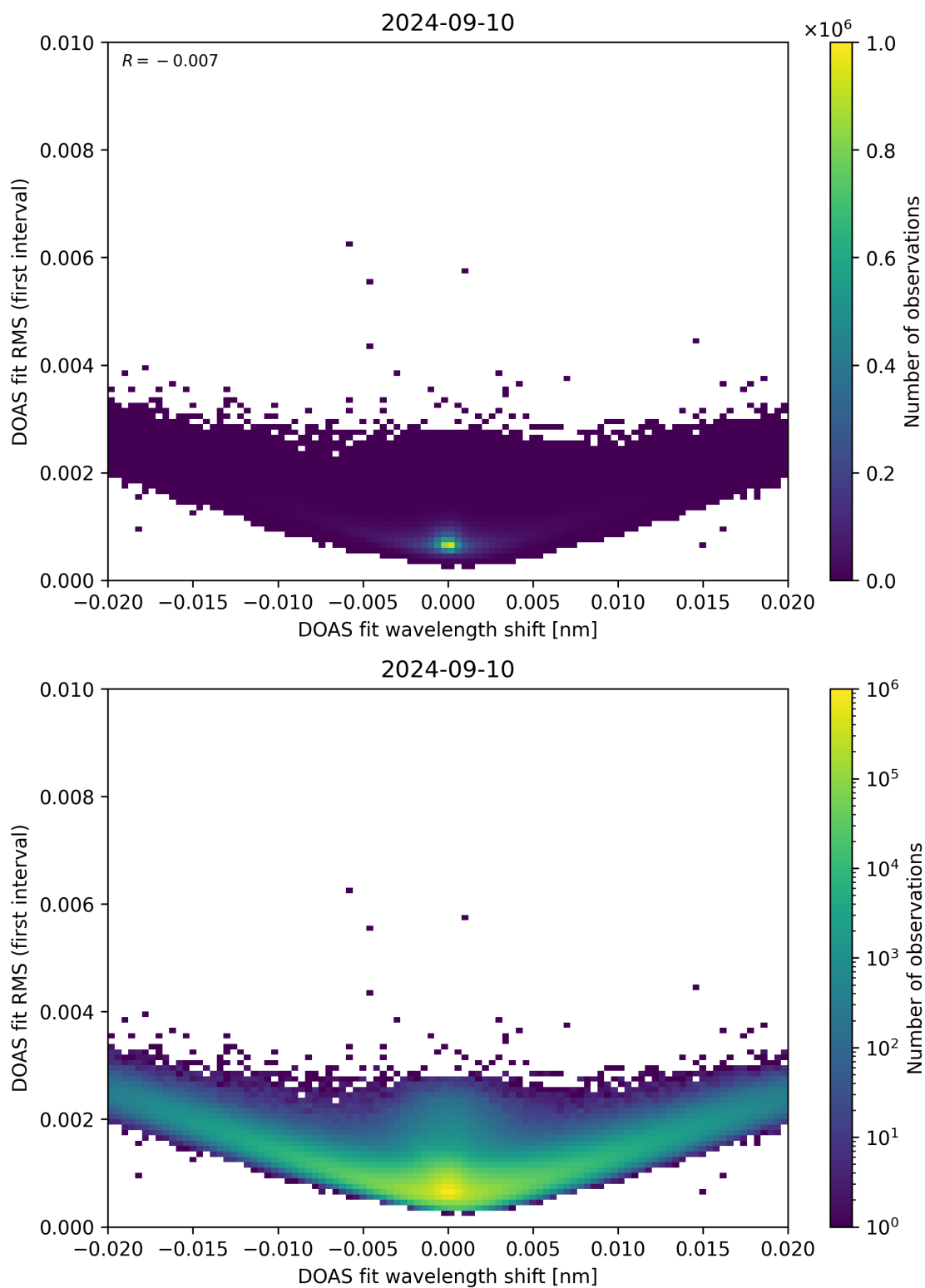
Figure 64: Scatter density plot of “DOAS fit wavelength shift” against “DOAS fit RMS (first interval)” for 2024-09-09 to 2024-09-11.
