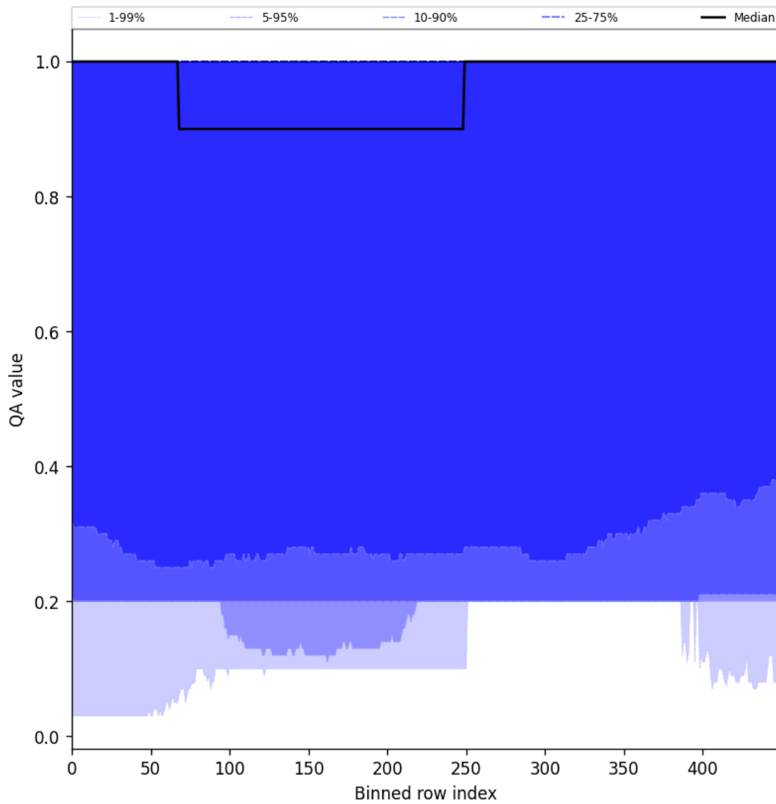
Figure 48: Along track statistics of “QA value” for 2024-09-09 to 2024-09-11
