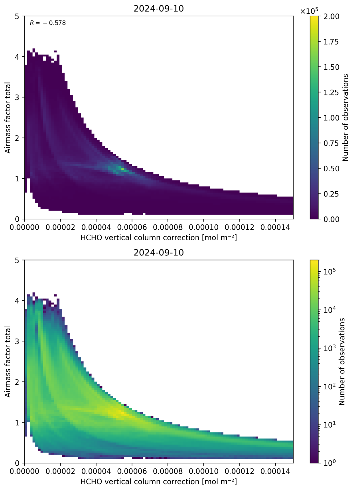
Figure 120: Scatter density plot of “HCHO vertical column correction” against “Airmass factor total” for 2024-09-09 to 2024-09-11.
