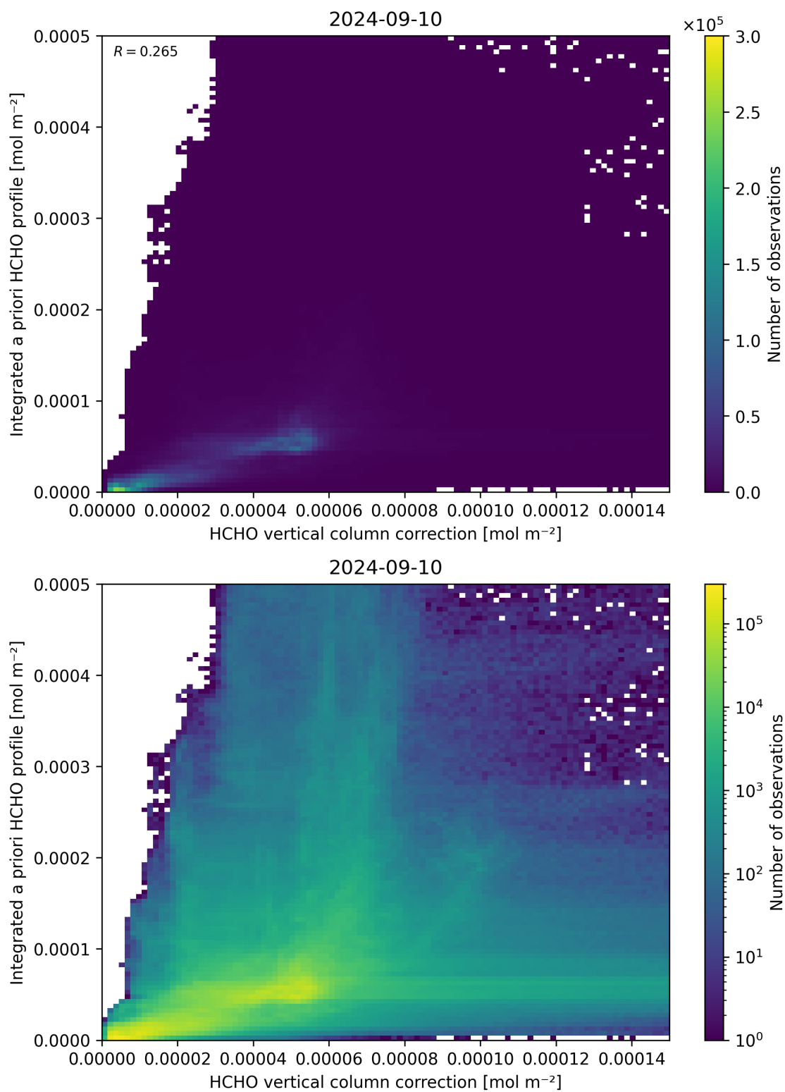
Figure 122: Scatter density plot of “HCHO vertical column correction” against “Integrated a priori HCHO profile” for 2024-09-09 to 2024-09-11.
