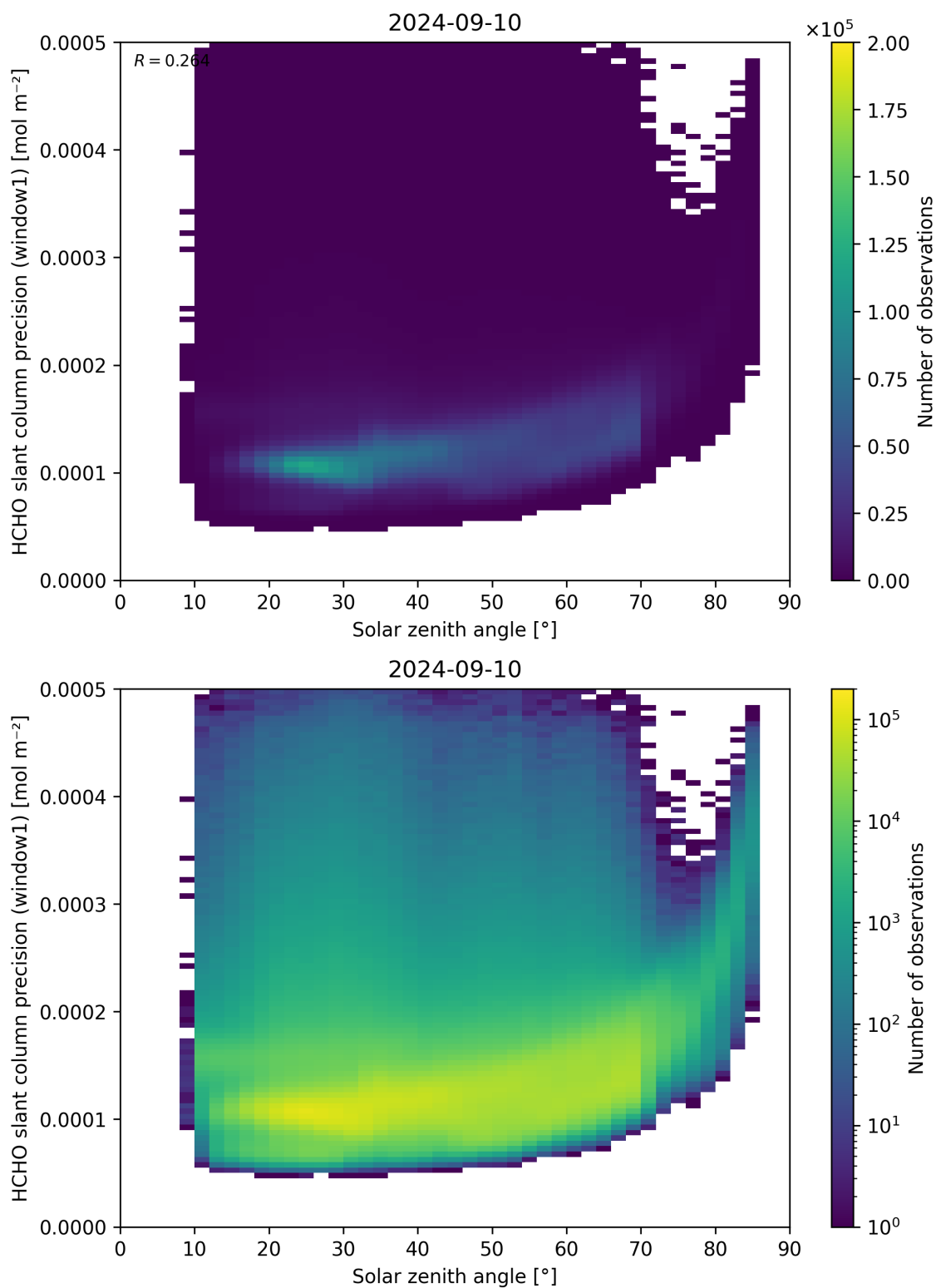
Figure 174: Scatter density plot of “Solar zenith angle” against “HCHO slant column precision (window1)” for 2024-09-09 to 2024-09-11.
