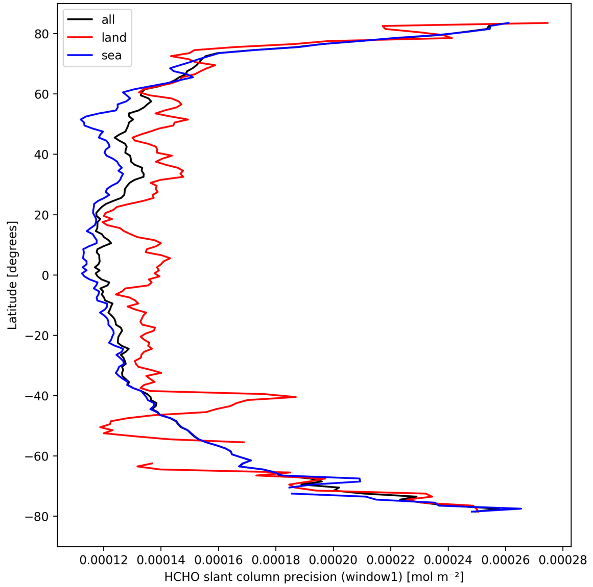
Figure 25: Zonal average of “HCHO slant column precision (window1)” for 2024-09-09 to 2024-09-11.
