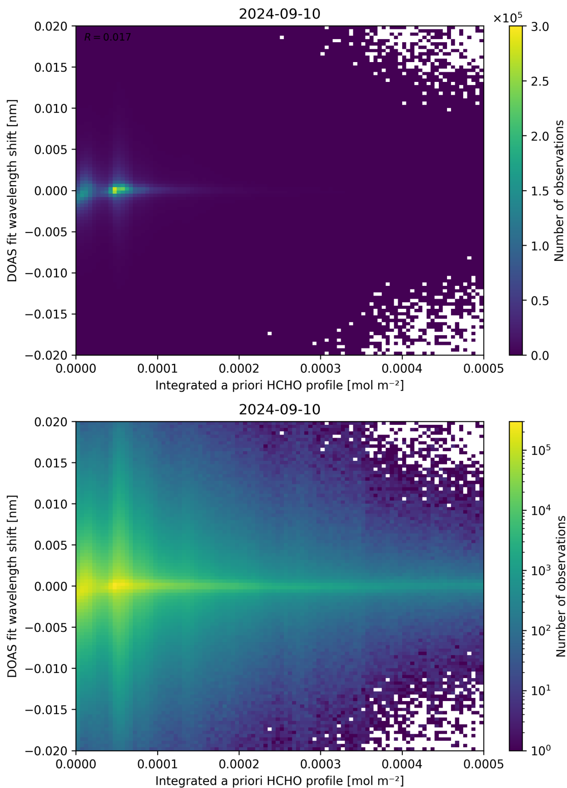
Figure 149: Scatter density plot of “Integrated a priori HCHO profile” against “DOAS fit wavelength shift” for 2024-09-09 to 2024-09-11.
