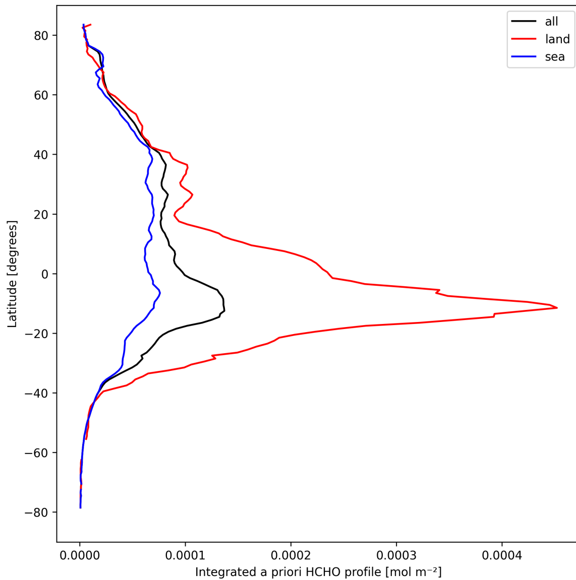
Figure 29: Zonal average of “Integrated a priori HCHO profile” for 2024-09-09 to 2024-09-11.
