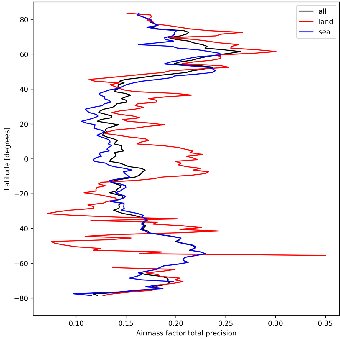
Figure 27: Zonal average of “Airmass factor total precision” for 2024-09-09 to 2024-09-11.
