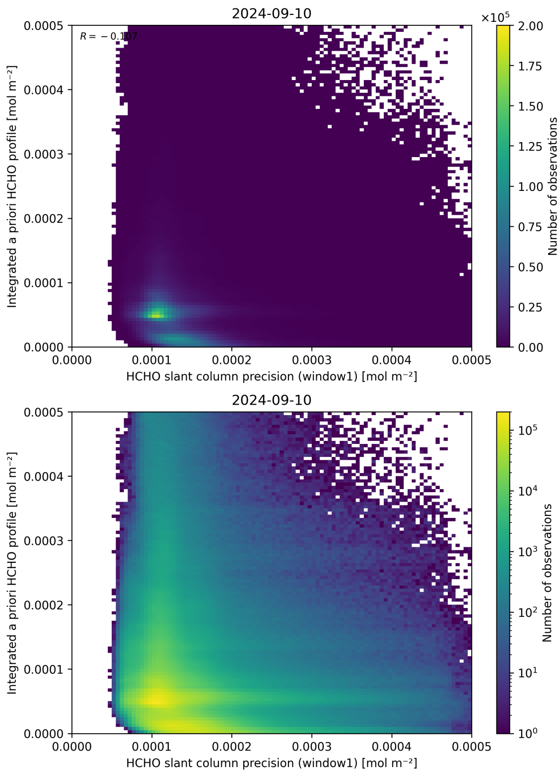
Figure 96: Scatter density plot of “HCHO slant column precision (window1)” against “Integrated a priori HCHO profile” for 2024-09-09 to 2024-09-11.
