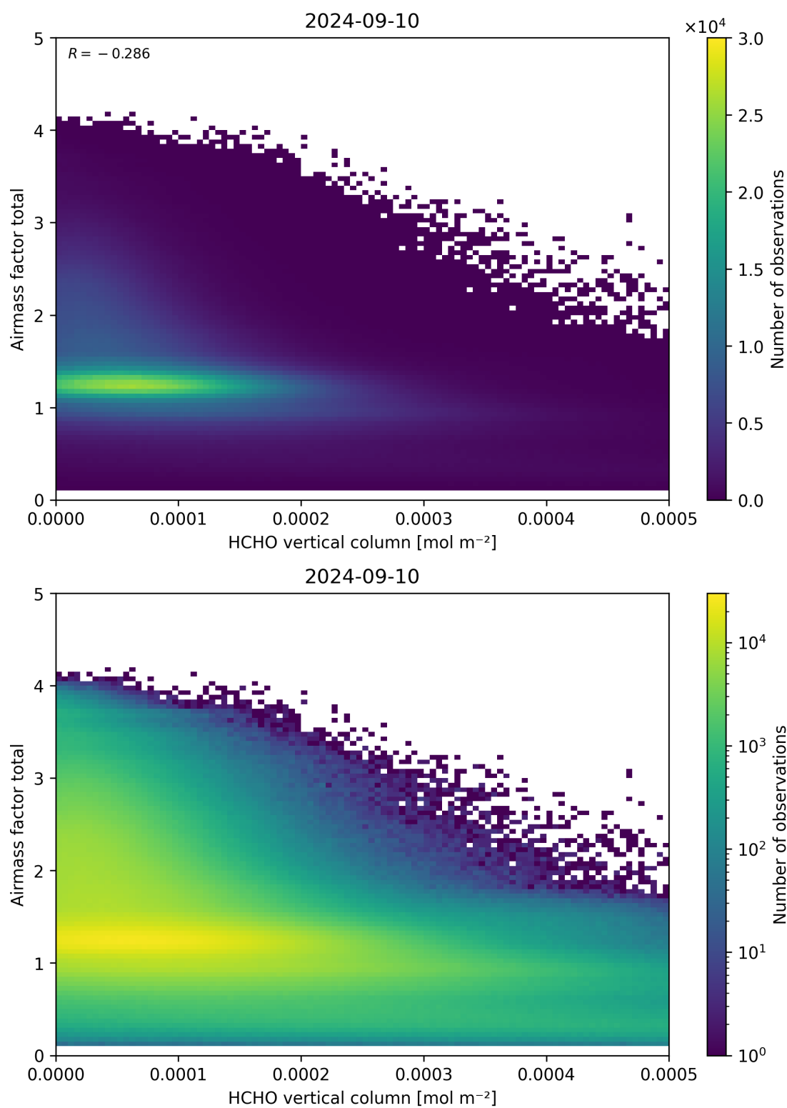
Figure 131: Scatter density plot of “HCHO vertical column” against “Airmass factor total” for 2024-09-09 to 2024-09-11.
