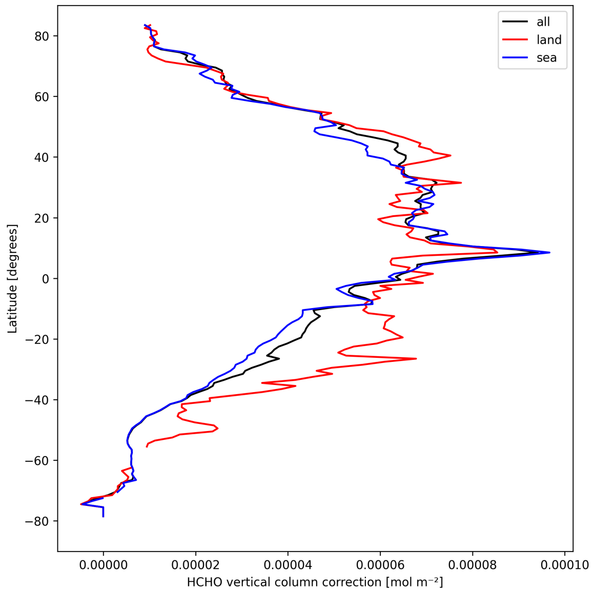
Figure 23: Zonal average of “HCHO vertical column correction” for 2024-09-09 to 2024-09-11.
