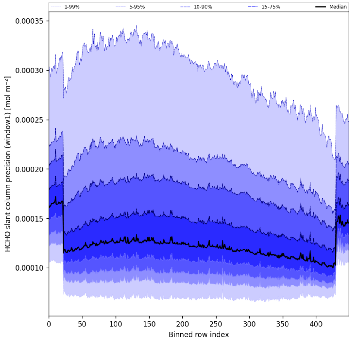
Figure 53: Along track statistics of “HCHO slant column precision (window1)” for 2024-09-09 to 2024-09-11
