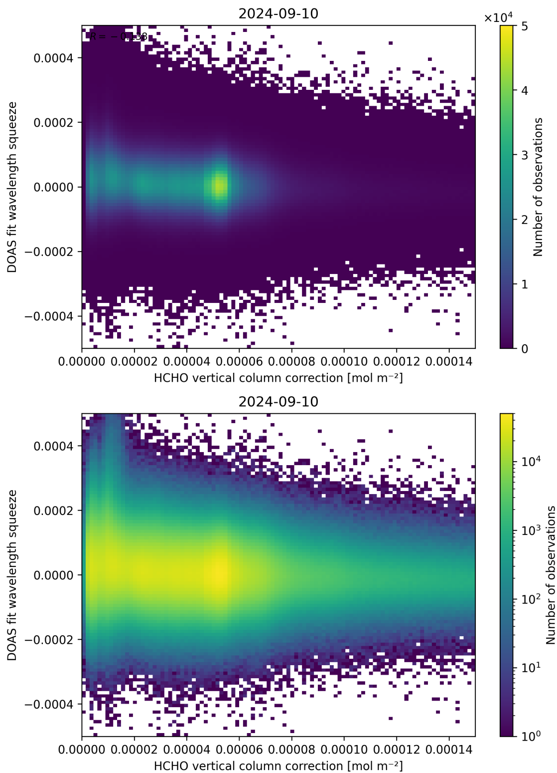
Figure 114: Scatter density plot of “HCHO vertical column correction” against “DOAS fit wavelength squeeze” for 2024-09-09 to 2024-09-11.
