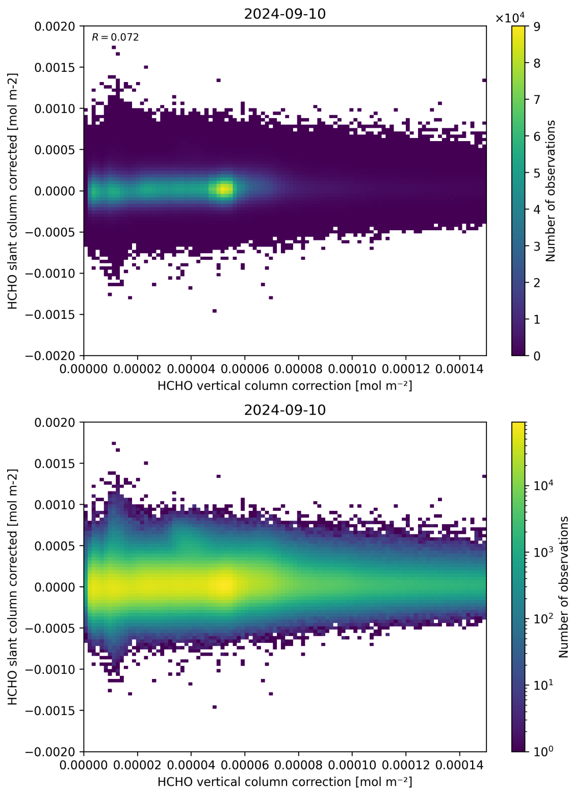
Figure 116: Scatter density plot of “HCHO vertical column correction” against “HCHO slant column corrected” for 2024-09-09 to 2024-09-11.
