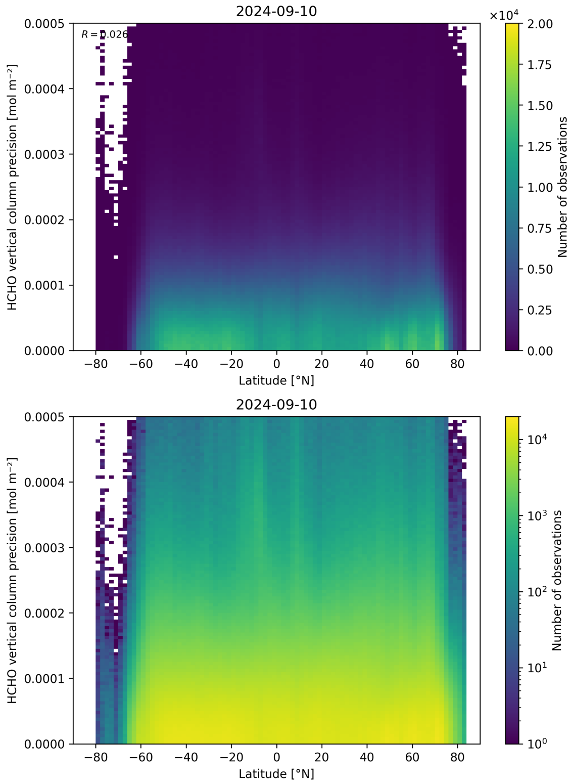
Figure 165: Scatter density plot of “Latitude” against “HCHO vertical column precision” for 2024-09-09 to 2024-09-11.
