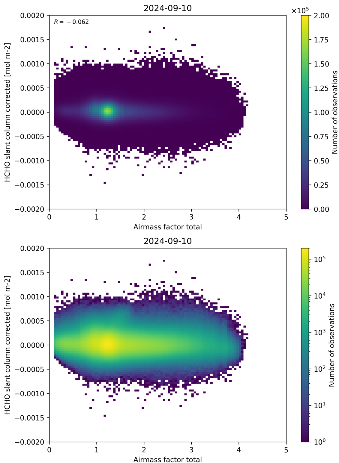
Figure 101: Scatter density plot of “Airmass factor total” against “HCHO slant column corrected” for 2024-09-09 to 2024-09-11.
