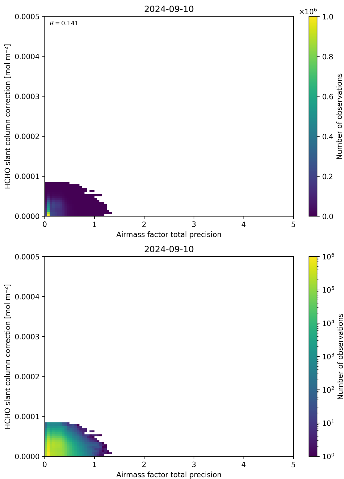
Figure 110: Scatter density plot of “Airmass factor total precision” against “HCHO slant column correction” for 2024-09-09 to 2024-09-11.
