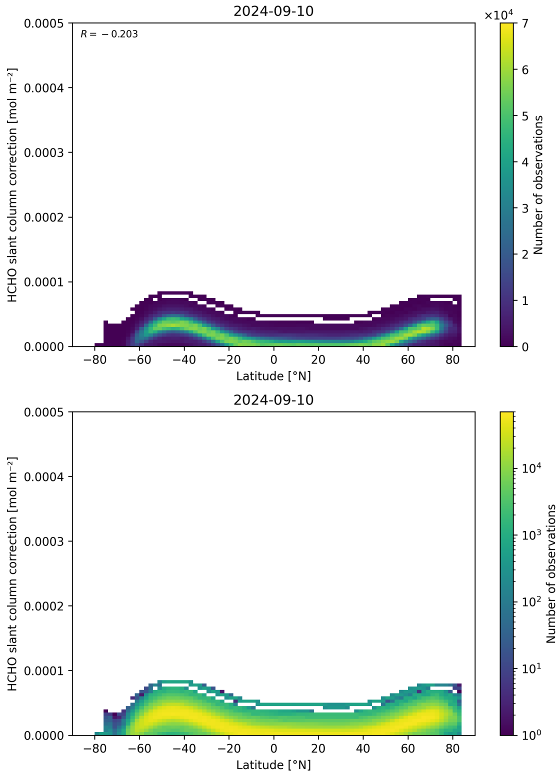
Figure 158: Scatter density plot of “Latitude” against “HCHO slant column correction” for 2024-09-09 to 2024-09-11.
