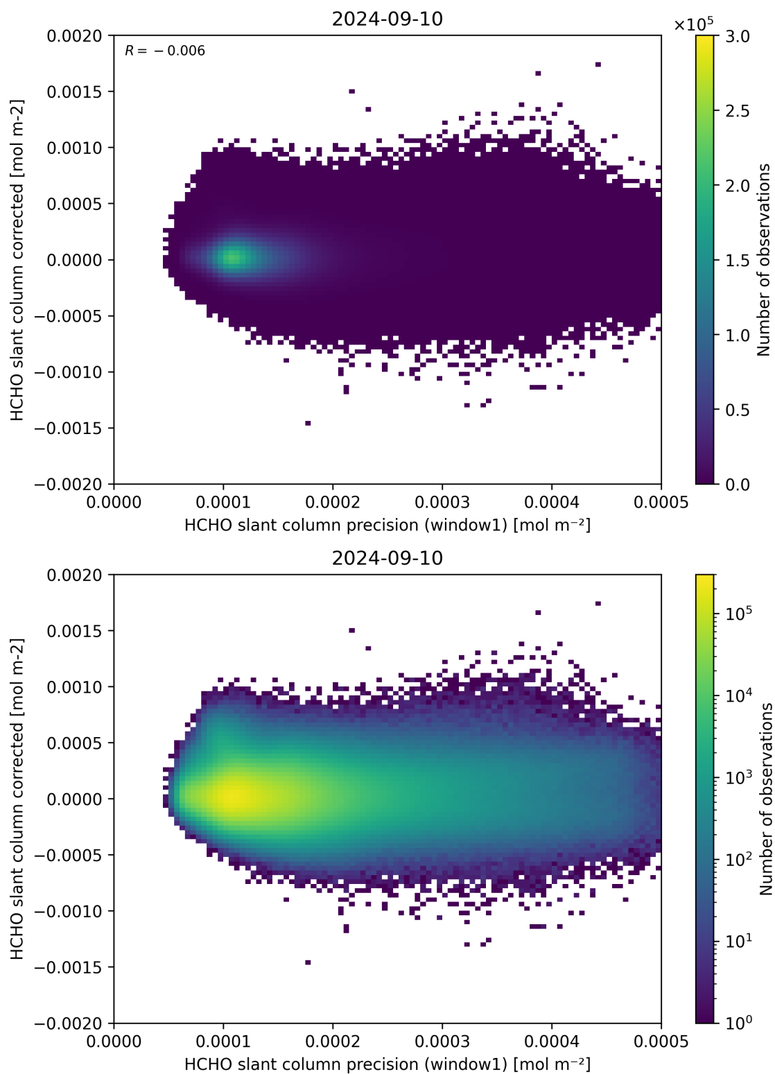
Figure 92: Scatter density plot of “HCHO slant column precision (window1)” against “HCHO slant column corrected” for 2024-09-09 to 2024-09-11.
