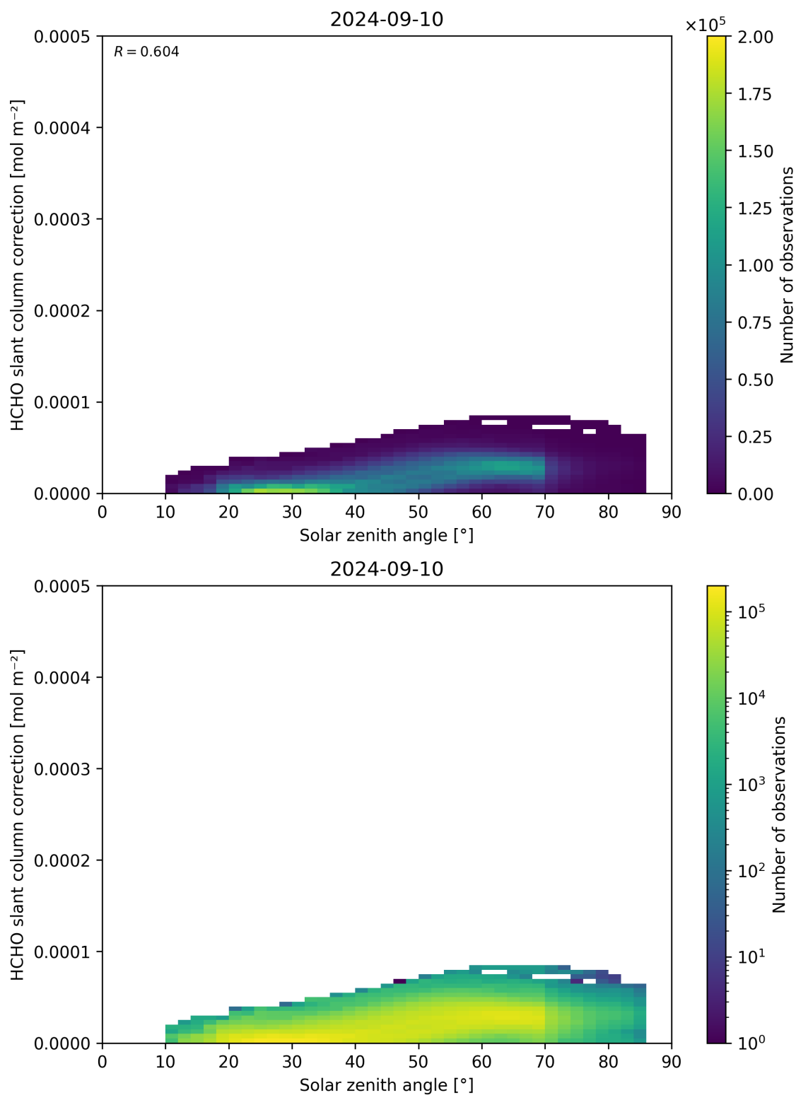
Figure 172: Scatter density plot of “Solar zenith angle” against “HCHO slant column correction” for 2024-09-09 to 2024-09-11.
