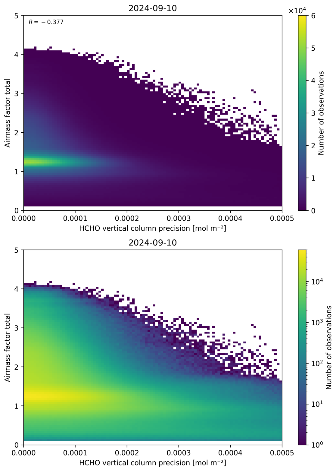
Figure 144: Scatter density plot of “HCHO vertical column precision” against “Airmass factor total” for 2024-09-09 to 2024-09-11.
