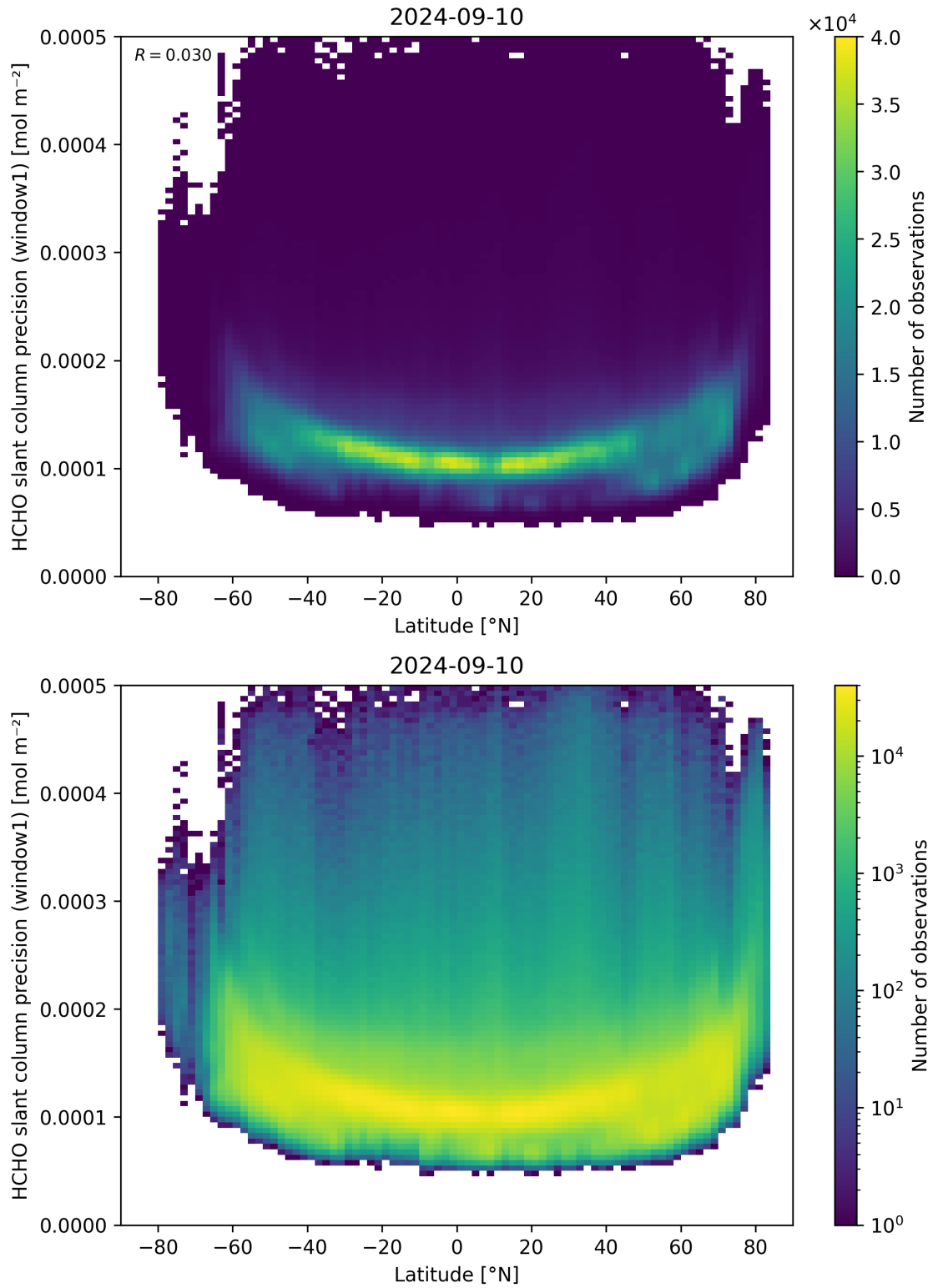
Figure 160: Scatter density plot of “Latitude” against “HCHO slant column precision (window1)” for 2024-09-09 to 2024-09-11.
