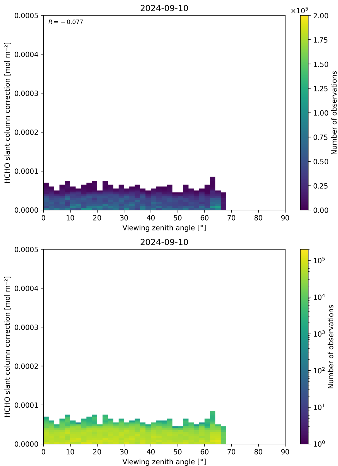
Figure 187: Scatter density plot of “Viewing zenith angle” against “HCHO slant column correction” for 2024-09-09 to 2024-09-11.
