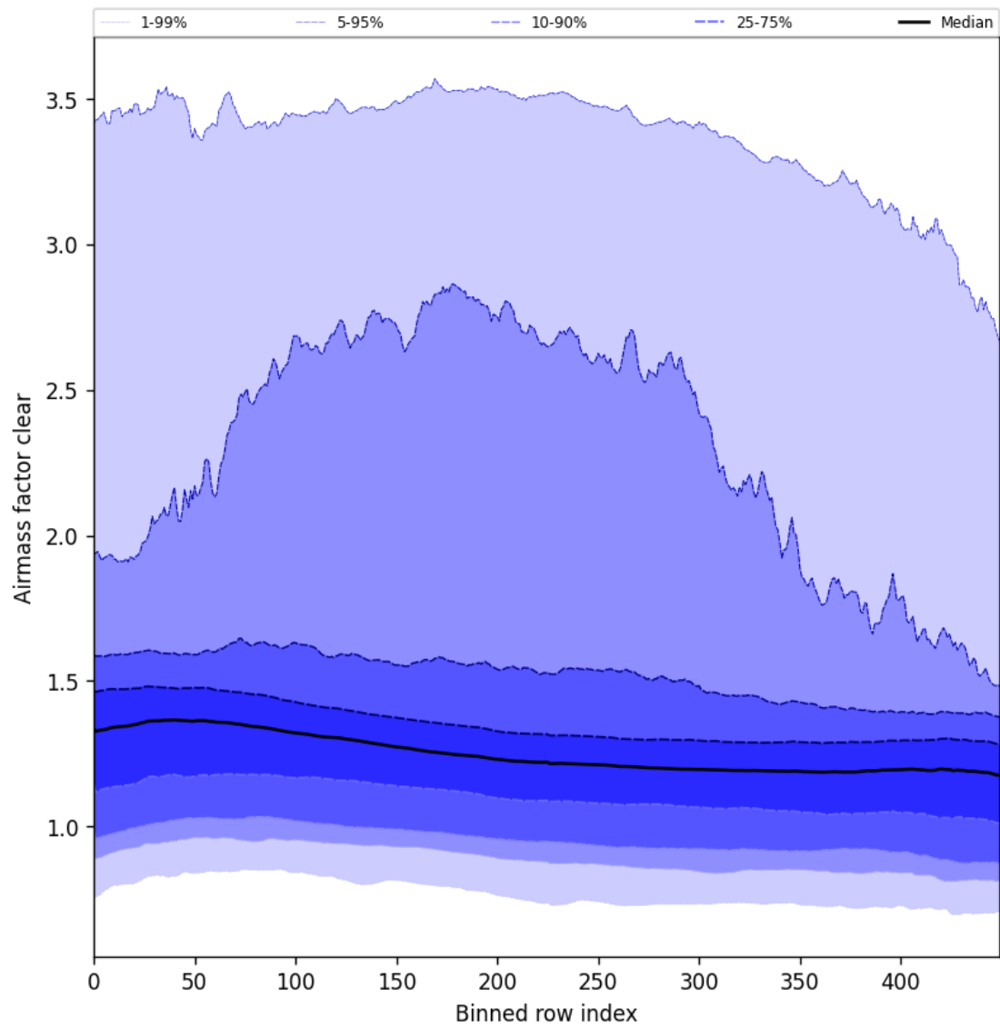
Figure 56: Along track statistics of “Airmass factor clear” for 2024-09-09 to 2024-09-11
