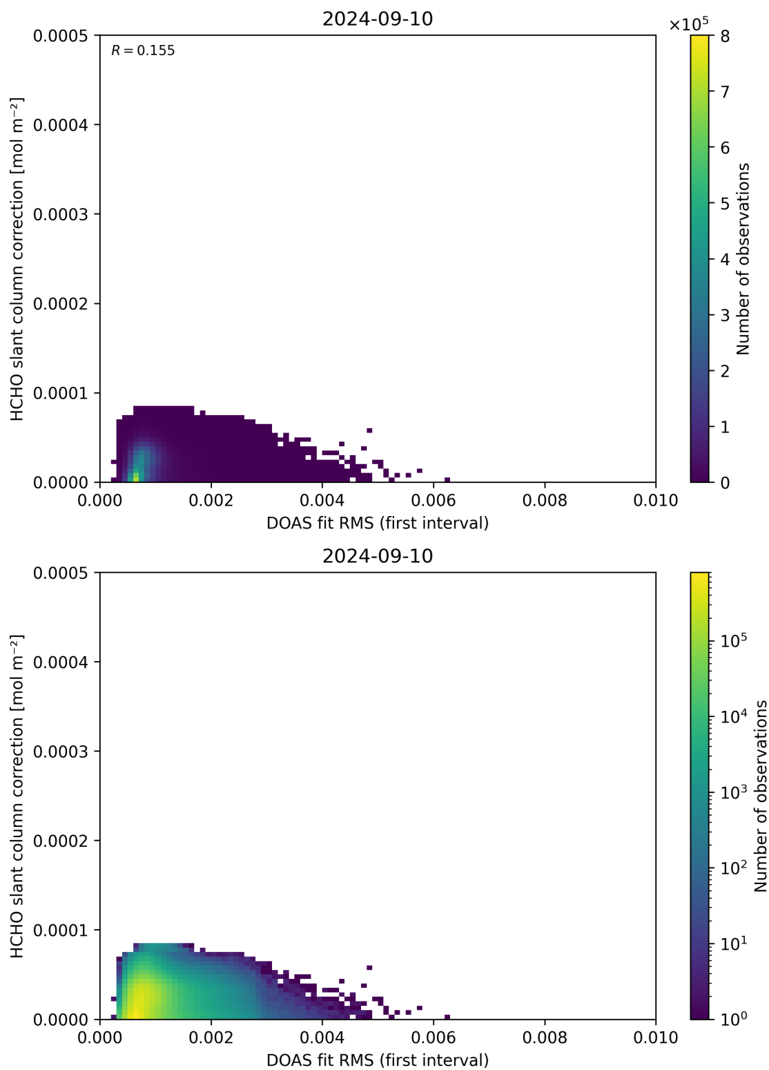
Figure 63: Scatter density plot of “DOAS fit RMS (first interval)” against “HCHO slant column correction” for 2024-09-09 to 2024-09-11.
