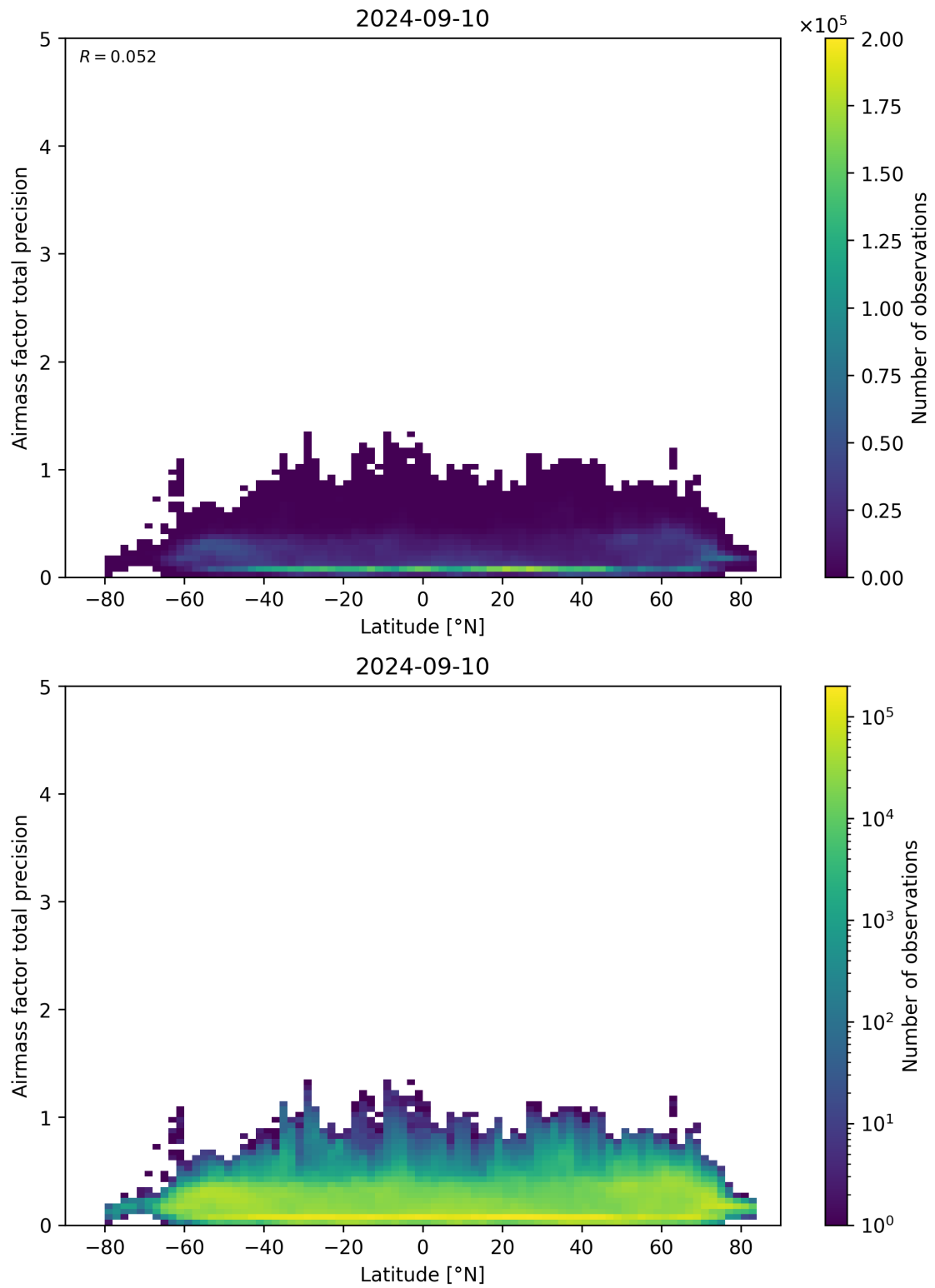
Figure 162: Scatter density plot of “Latitude” against “Airmass factor total precision” for 2024-09-09 to 2024-09-11.
