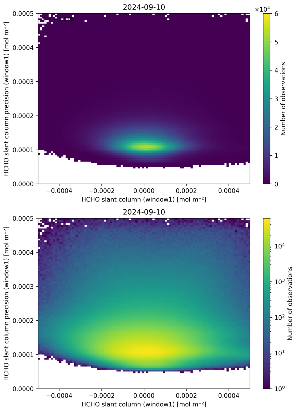
Figure 84: Scatter density plot of “HCHO slant column (window1)” against “HCHO slant column precision (window1)” for 2024-09-09 to 2024-09-11.
