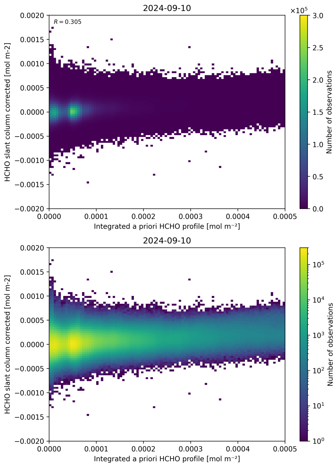
Figure 151: Scatter density plot of “Integrated a priori HCHO profile” against “HCHO slant column corrected” for 2024-09-09 to 2024-09-11.
