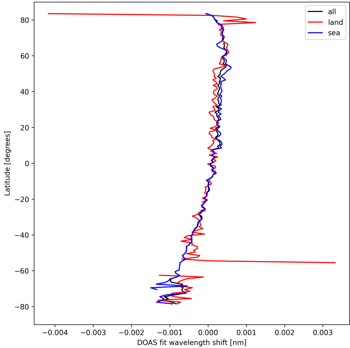
Figure 30: Zonal average of "DOAS fit wavelength shift" for 2024-09-09 to 2024-09-11.
