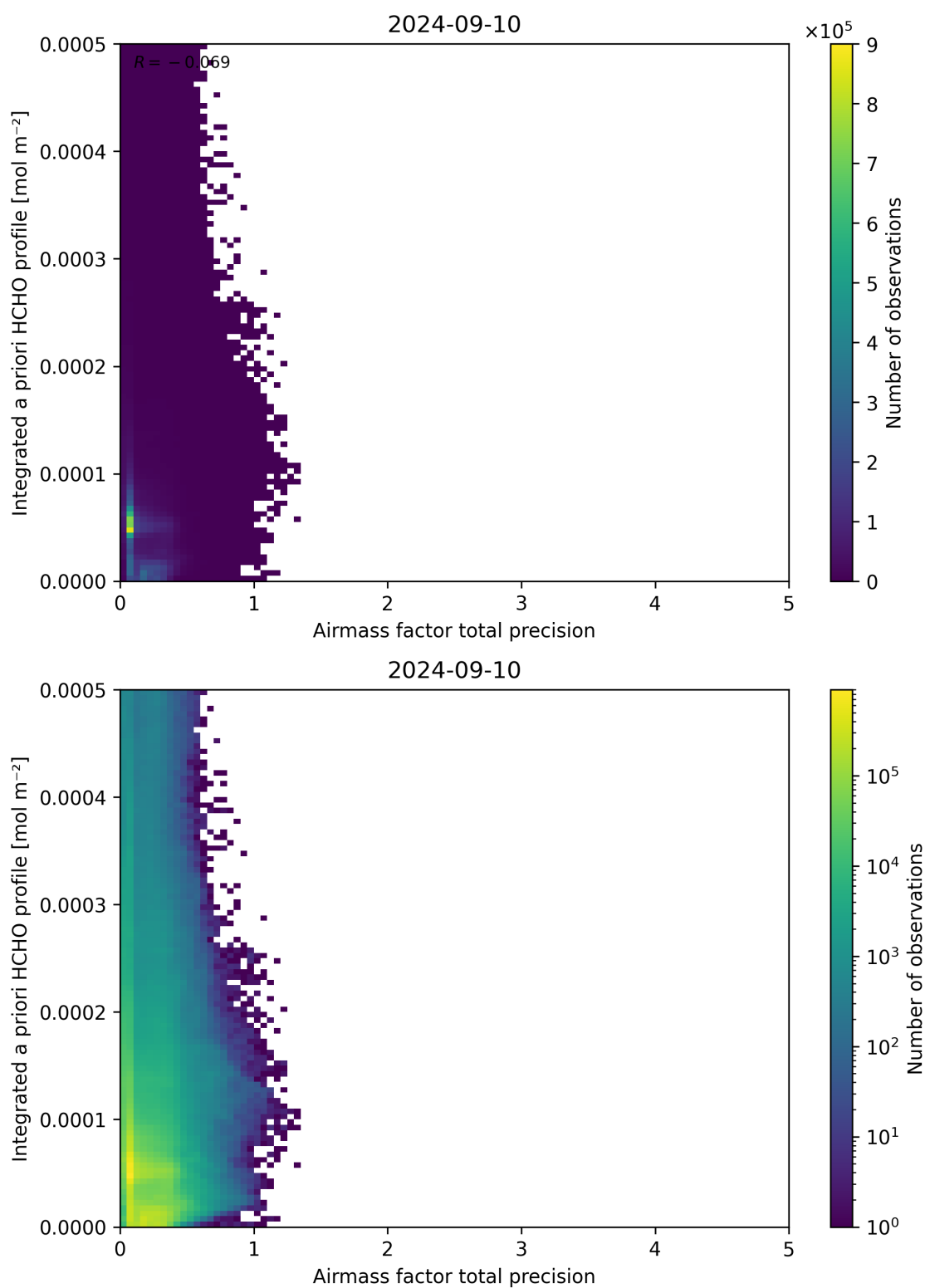
Figure 111: Scatter density plot of “Airmass factor total precision” against “Integrated a priori HCHO profile” for 2024-09-09 to 2024-09-11.
