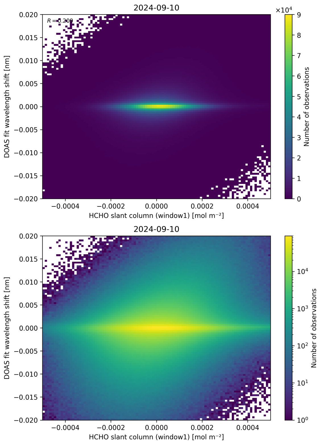
Figure 79: Scatter density plot of “HCHO slant column (window1)” against “DOAS fit wavelength shift” for 2024-09-09 to 2024-09-11.
