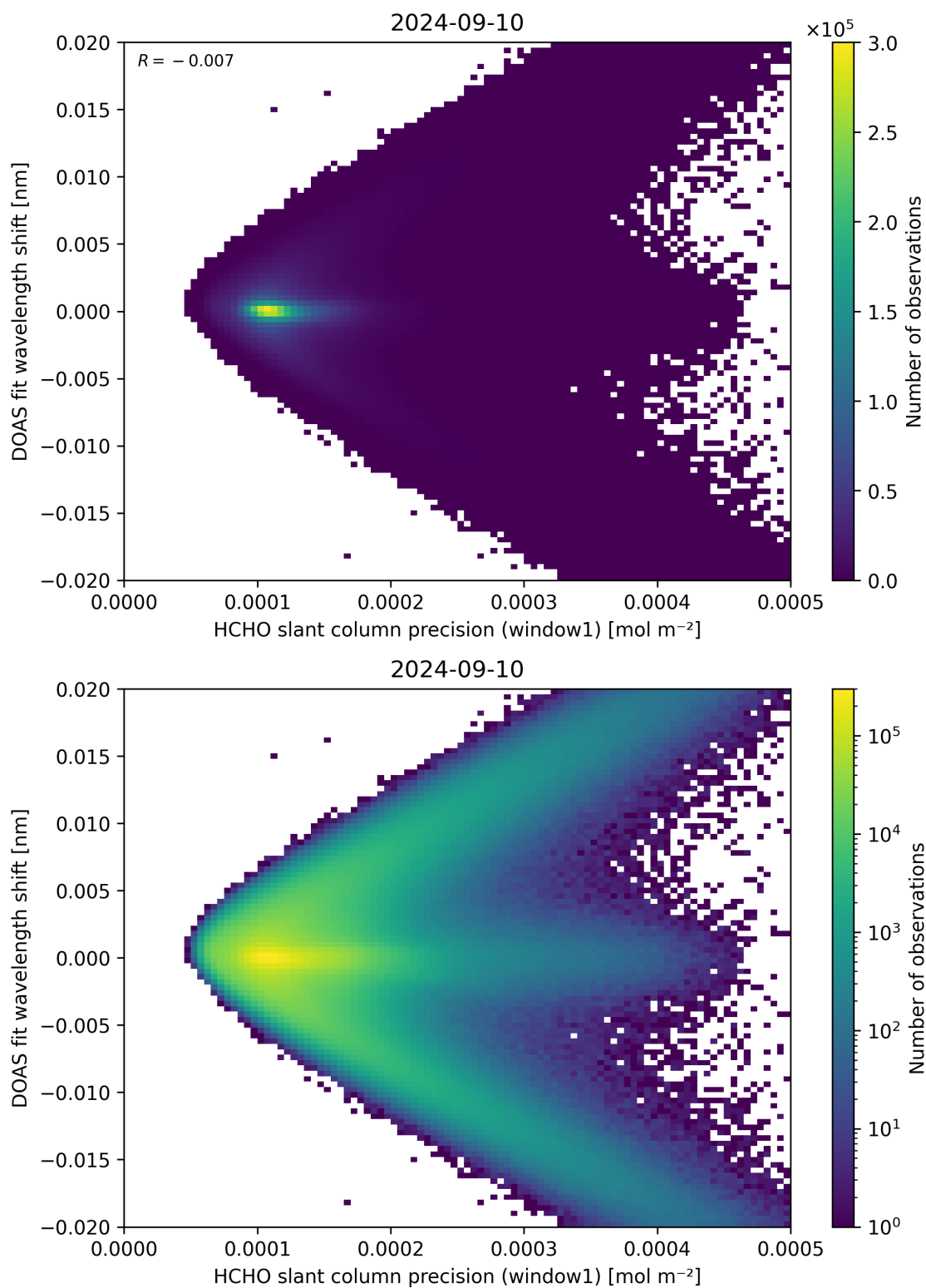
Figure 89: Scatter density plot of “HCHO slant column precision (window1)” against “DOAS fit wavelength shift” for 2024-09-09 to 2024-09-11.
