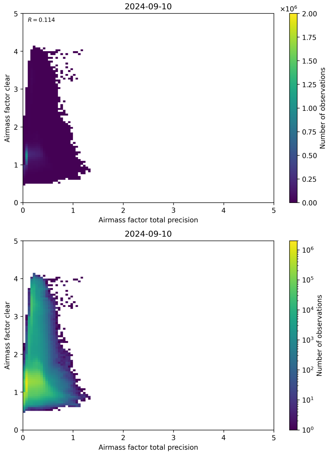
Figure 108: Scatter density plot of “Airmass factor total precision” against “Airmass factor clear” for 2024-09-09 to 2024-09-11.
