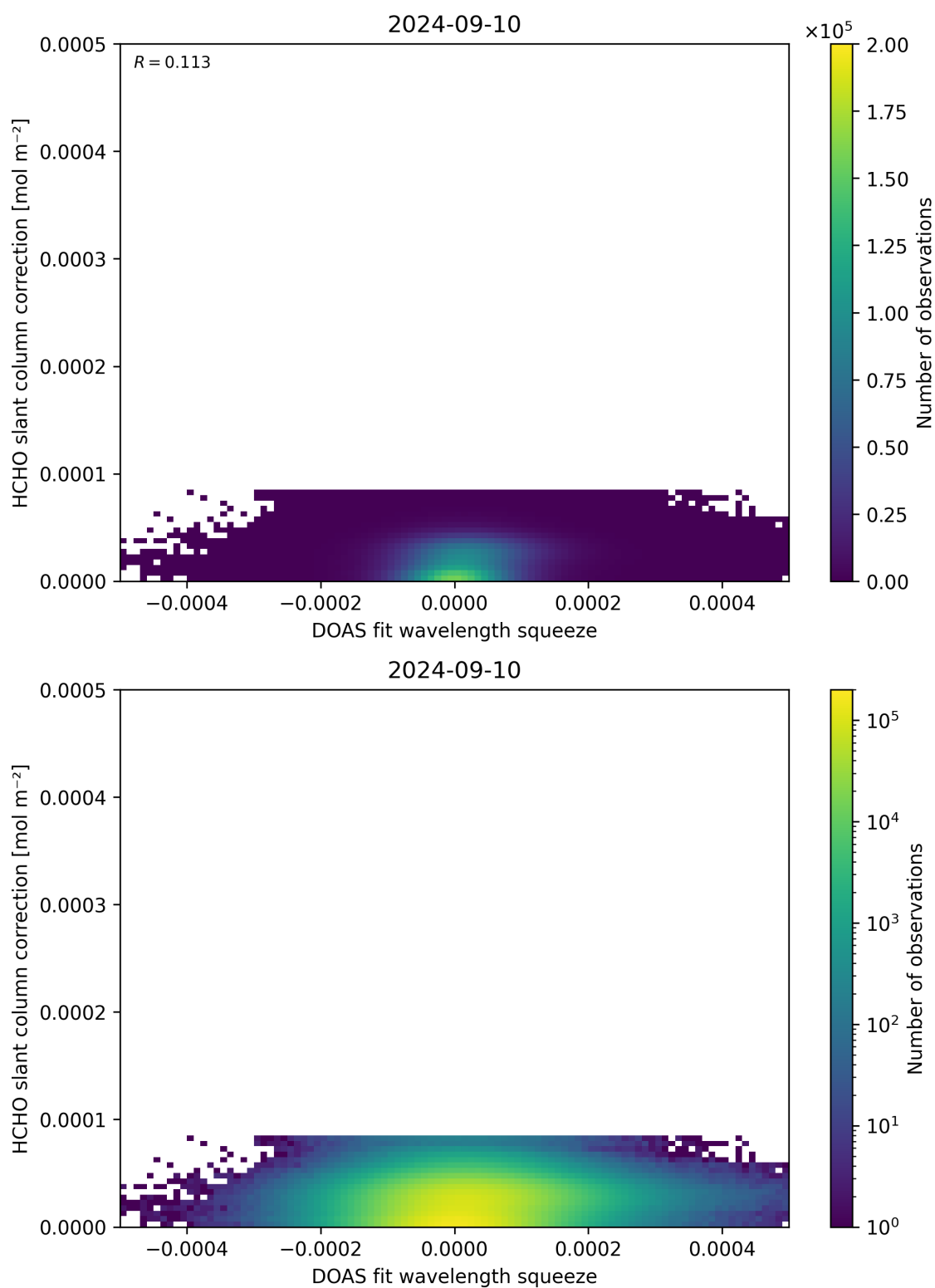
Figure 70: Scatter density plot of “DOAS fit wavelength squeeze” against “HCHO slant column correction” for 2024-09-09 to 2024-09-11.
