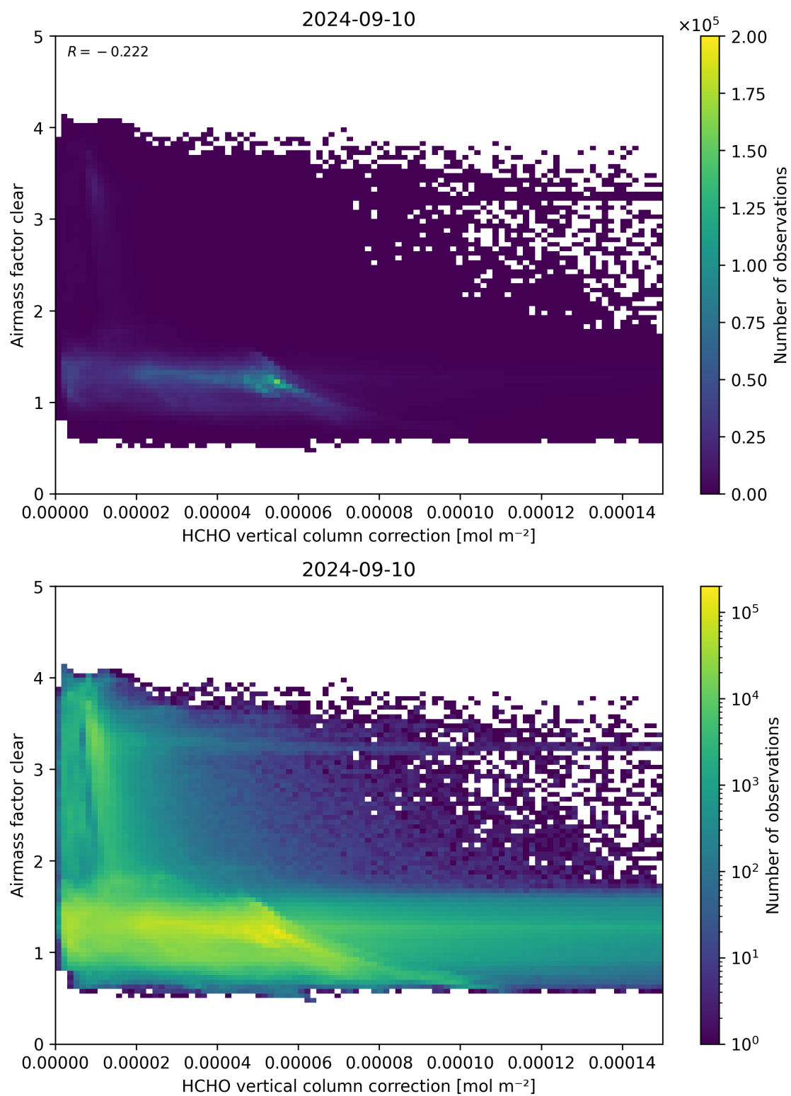
Figure 115: Scatter density plot of “HCHO vertical column correction” against “Airmass factor clear” for 2024-09-09 to 2024-09-11.
