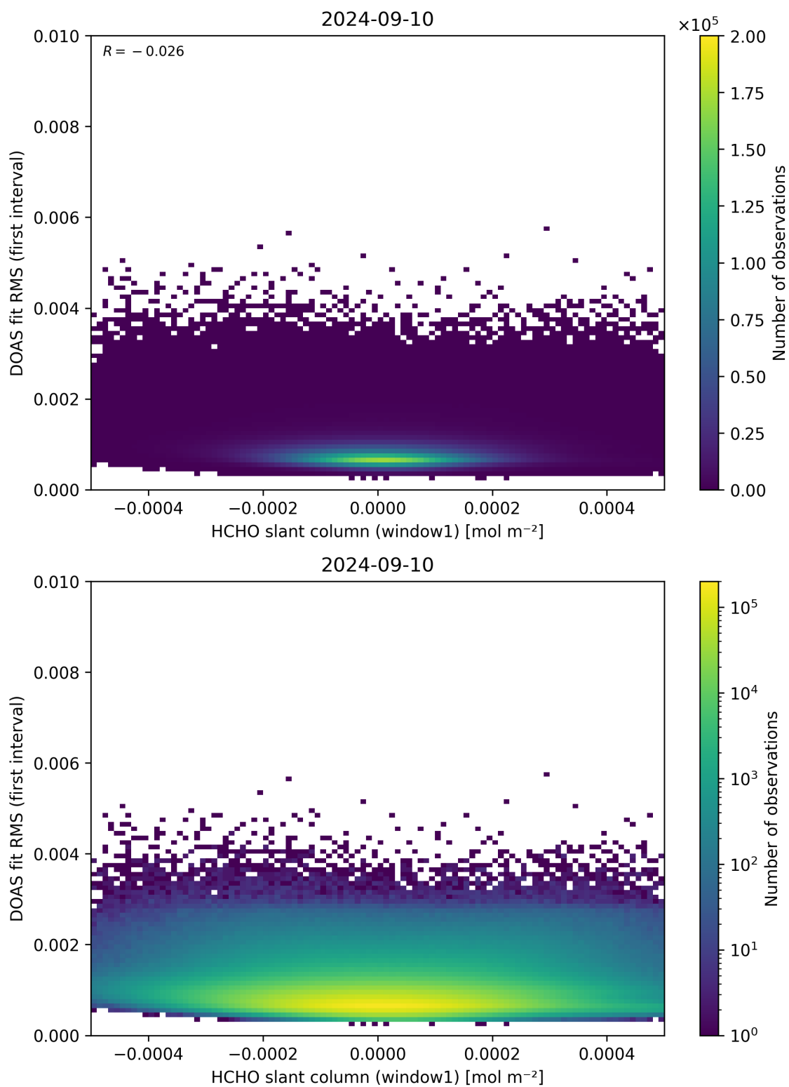
Figure 78: Scatter density plot of “HCHO slant column (window1)” against “DOAS fit RMS (first interval)” for 2024-09-09 to 2024-09-11.
