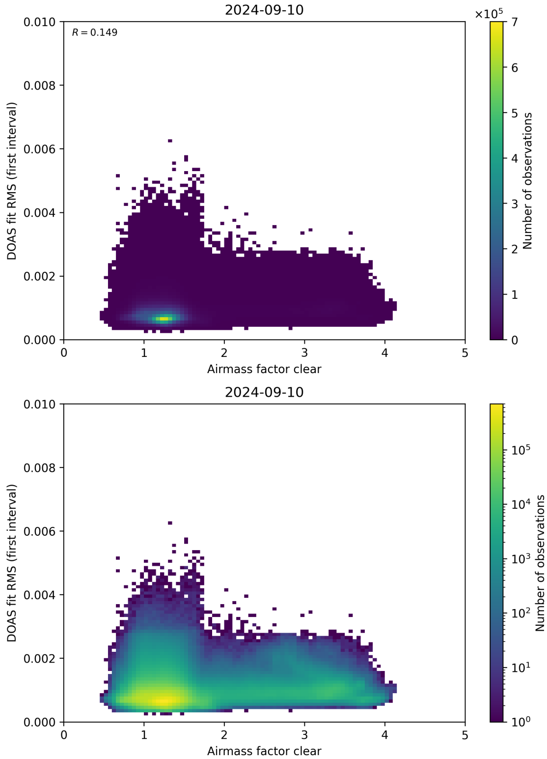
Figure 71: Scatter density plot of “Airmass factor clear” against “DOAS fit RMS (first interval)” for 2024-09-09 to 2024-09-11.
