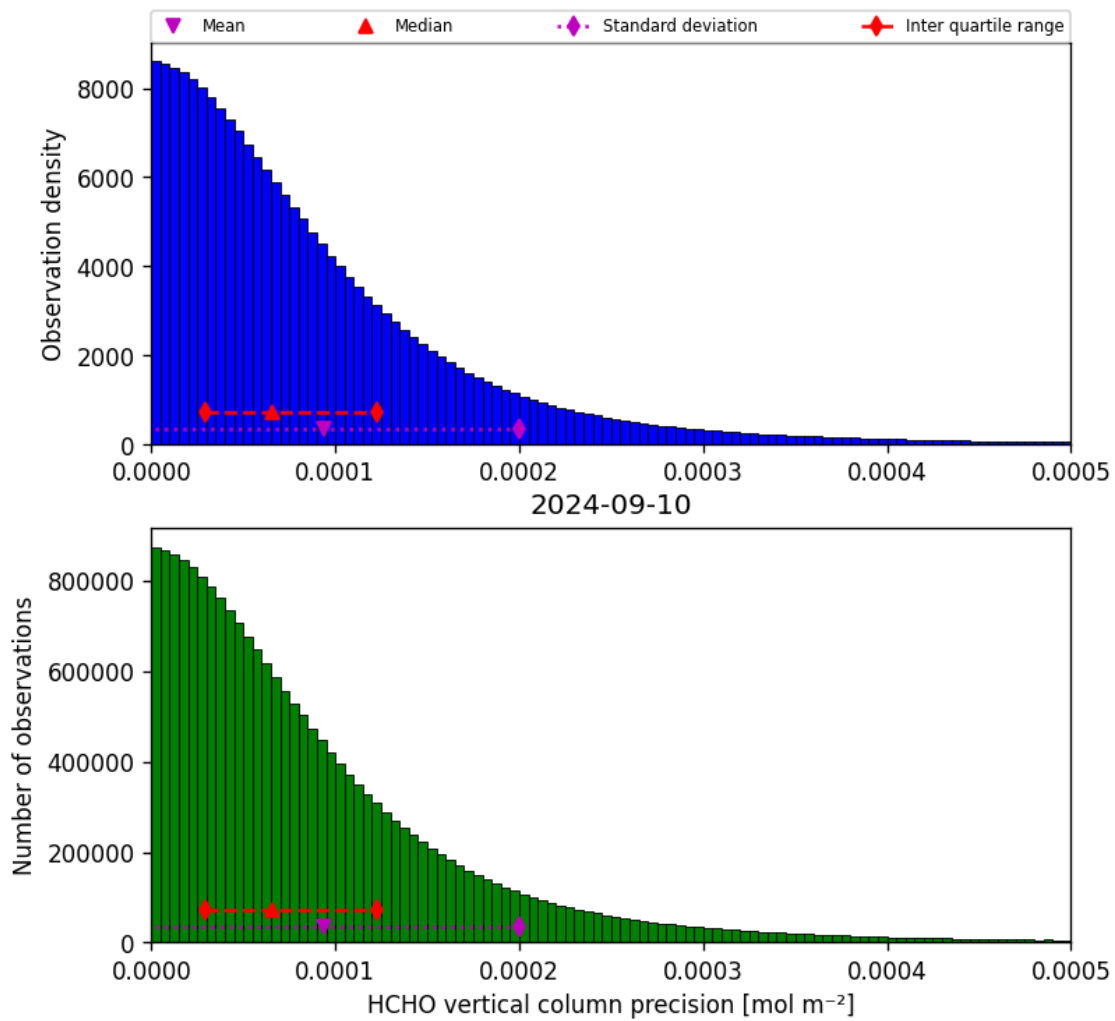
Figure 36: Histogram of “HCHO vertical column precision” for 2024-09-09 to 2024-09-11
