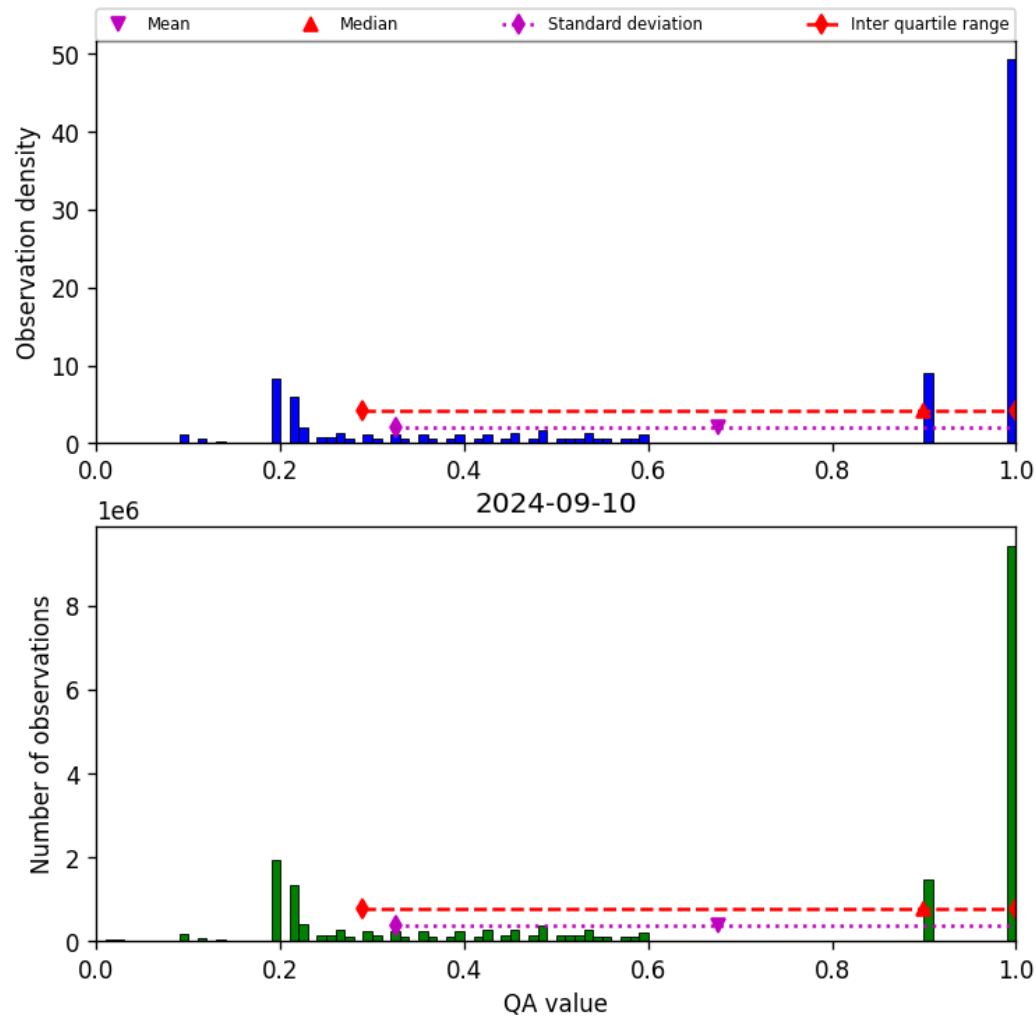
Figure 34: Histogram of “QA value” for 2024-09-09 to 2024-09-11
