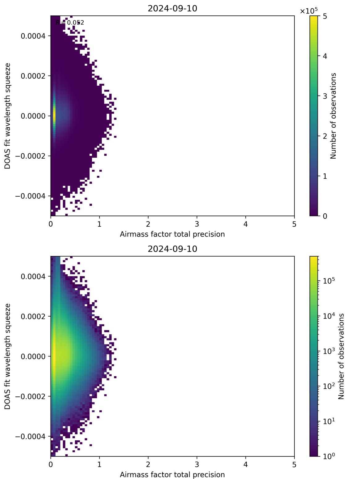
Figure 107: Scatter density plot of “Airmass factor total precision” against “DOAS fit wavelength squeeze” for 2024-09-09 to 2024-09-11.
