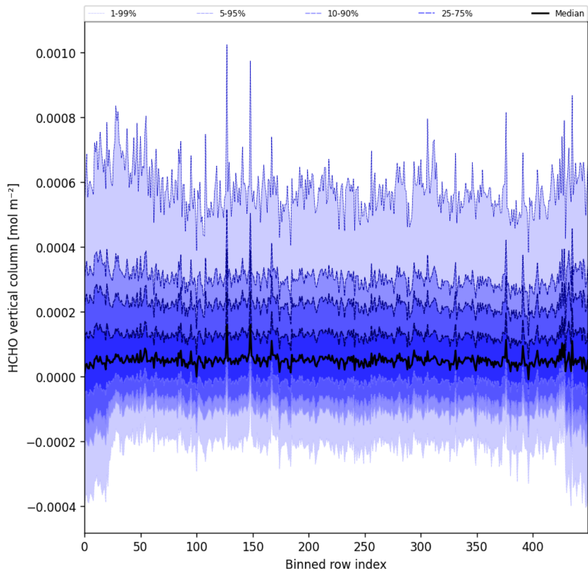
Figure 49: Along track statistics of “HCHO vertical column” for 2024-09-09 to 2024-09-11
