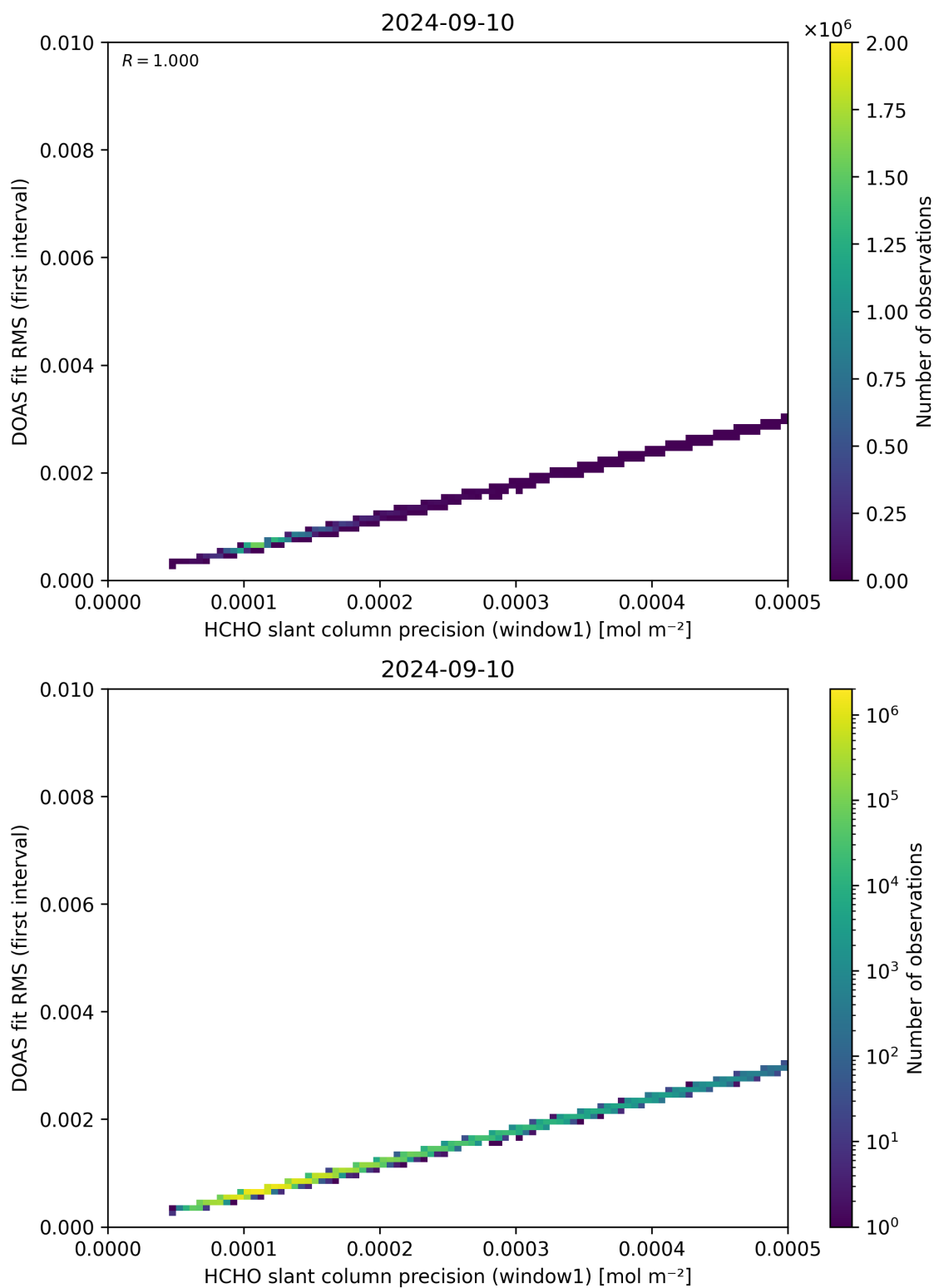
Figure 88: Scatter density plot of “HCHO slant column precision (window1)” against “DOAS fit RMS (first interval)” for 2024-09-09 to 2024-09-11.
