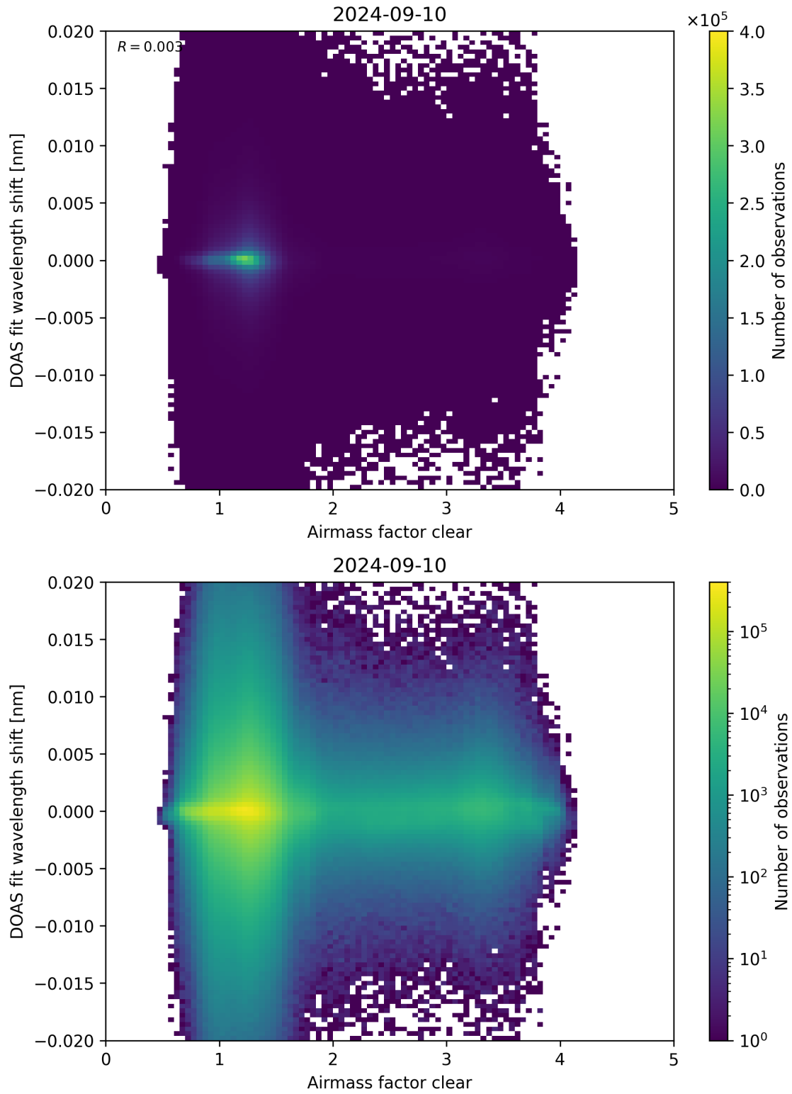
Figure 72: Scatter density plot of “Airmass factor clear” against “DOAS fit wavelength shift” for 2024-09-09 to 2024-09-11.
