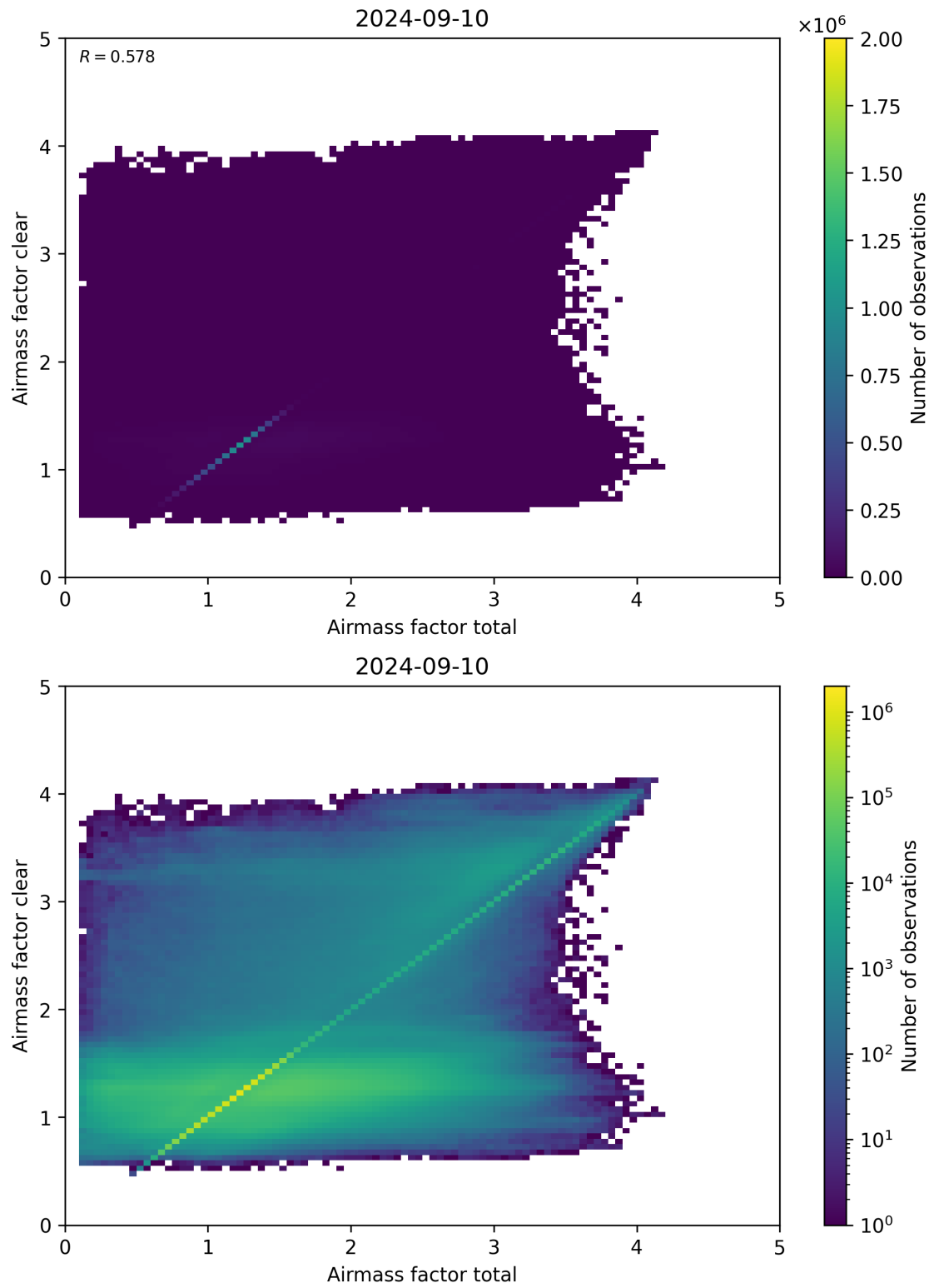
Figure 100: Scatter density plot of “Airmass factor total” against “Airmass factor clear” for 2024-09-09 to 2024-09-11.
