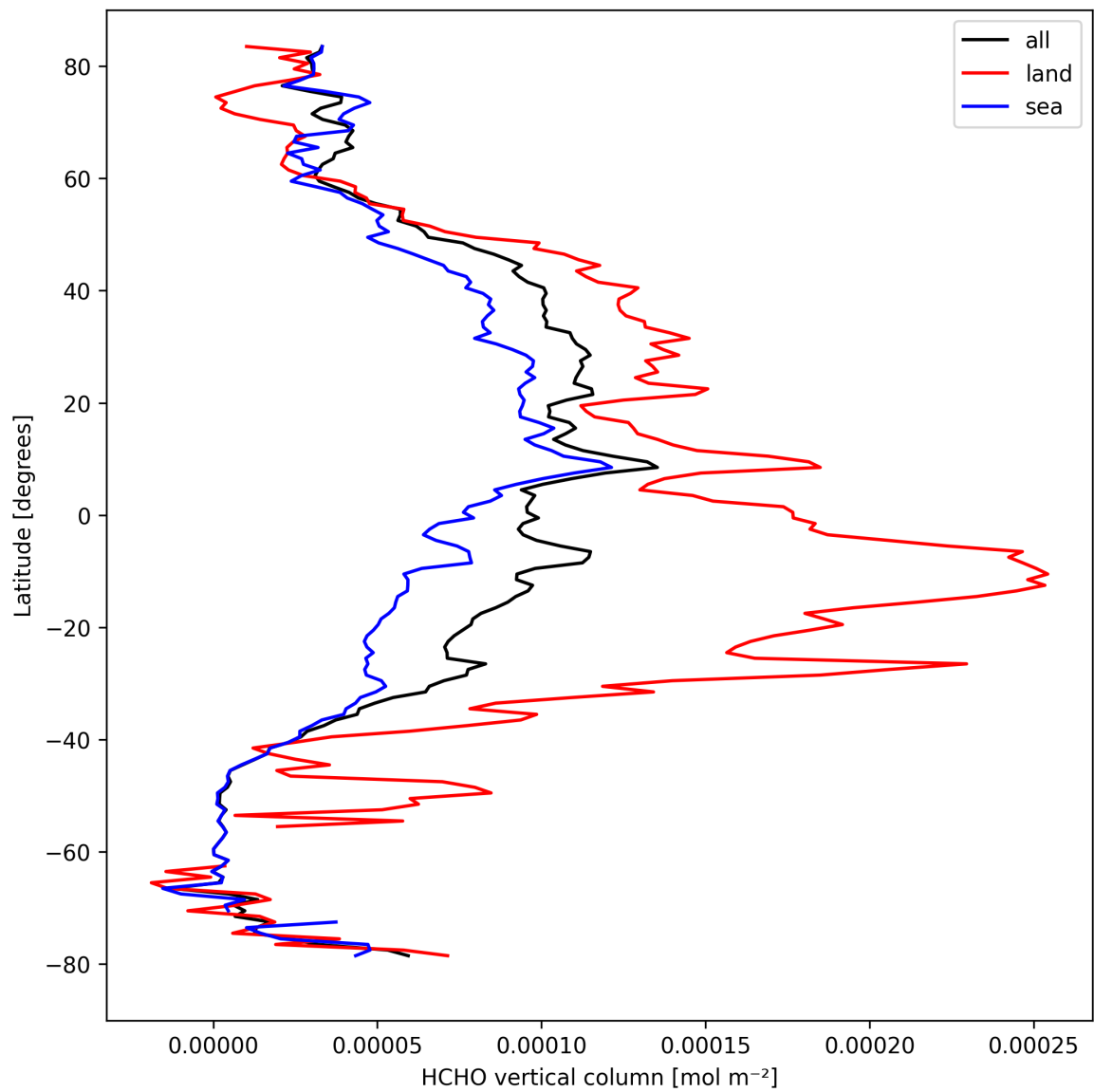
Figure 21: Zonal average of “HCHO vertical column” for 2024-09-09 to 2024-09-11.
