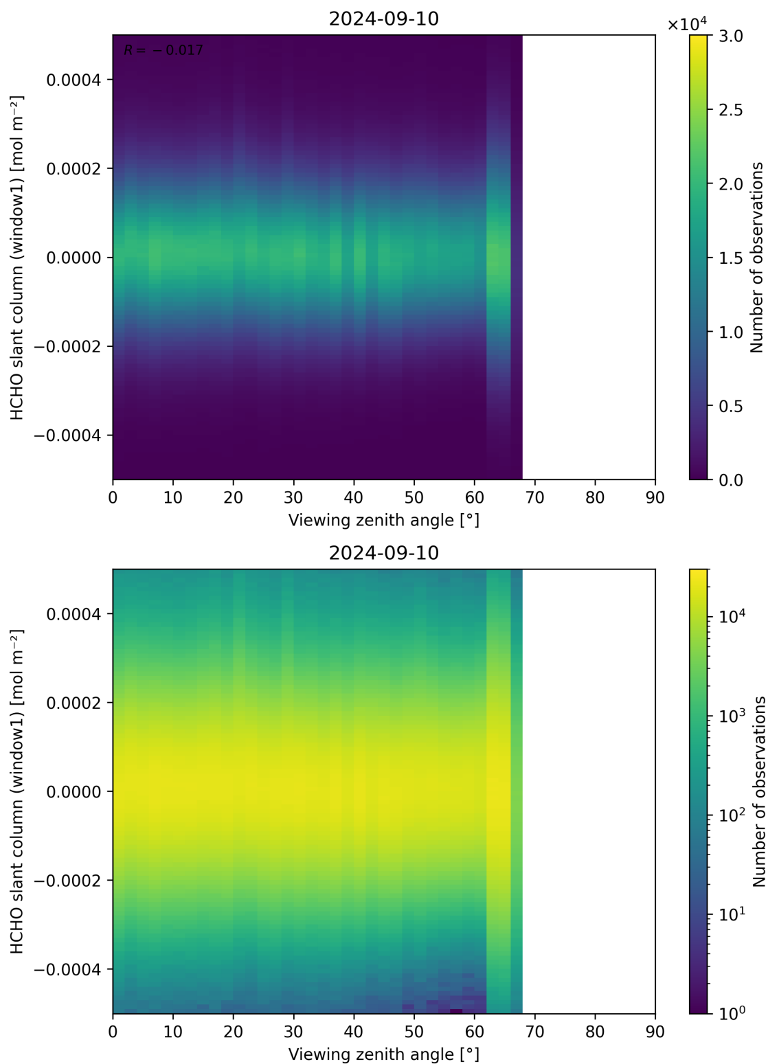
Figure 188: Scatter density plot of “Viewing zenith angle” against “HCHO slant column (window1)” for 2024-09-09 to 2024-09-11.
