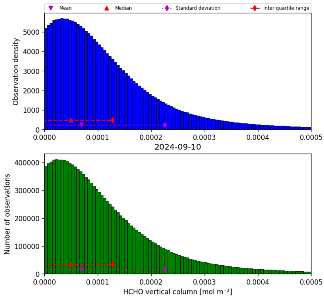
Figure 35: Histogram of “HCHO vertical column” for 2024-09-09 to 2024-09-11
