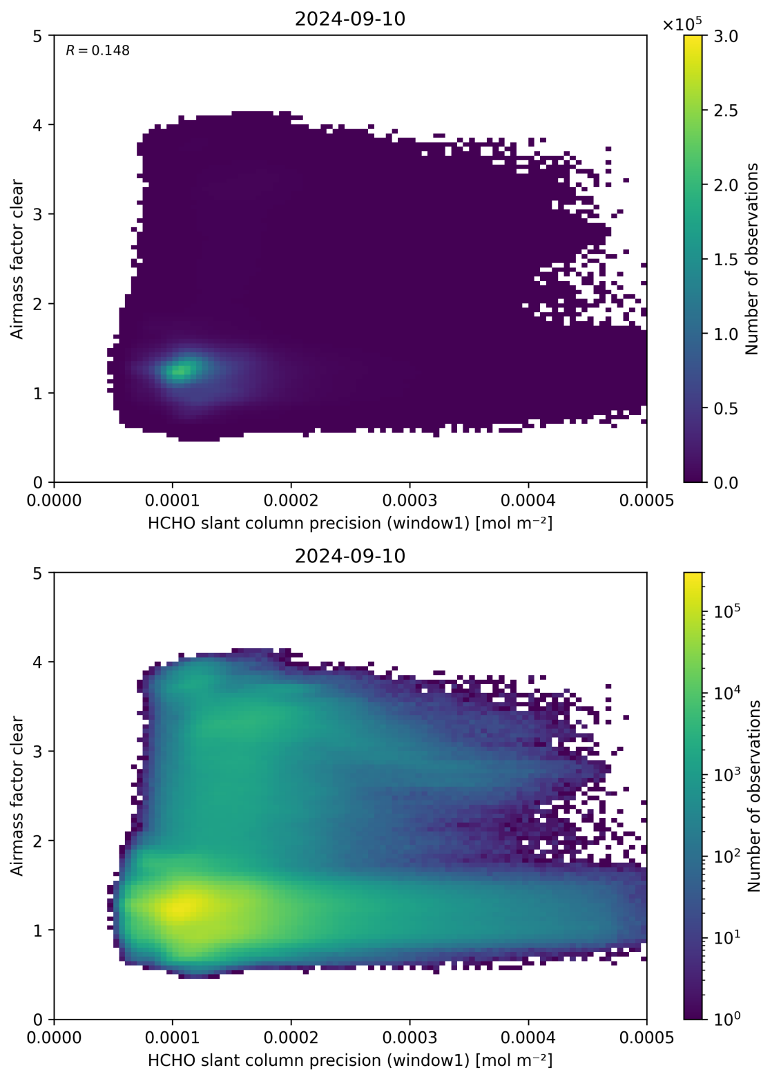
Figure 91: Scatter density plot of “HCHO slant column precision (window1)” against “Airmass factor clear” for 2024-09-09 to 2024-09-11.
