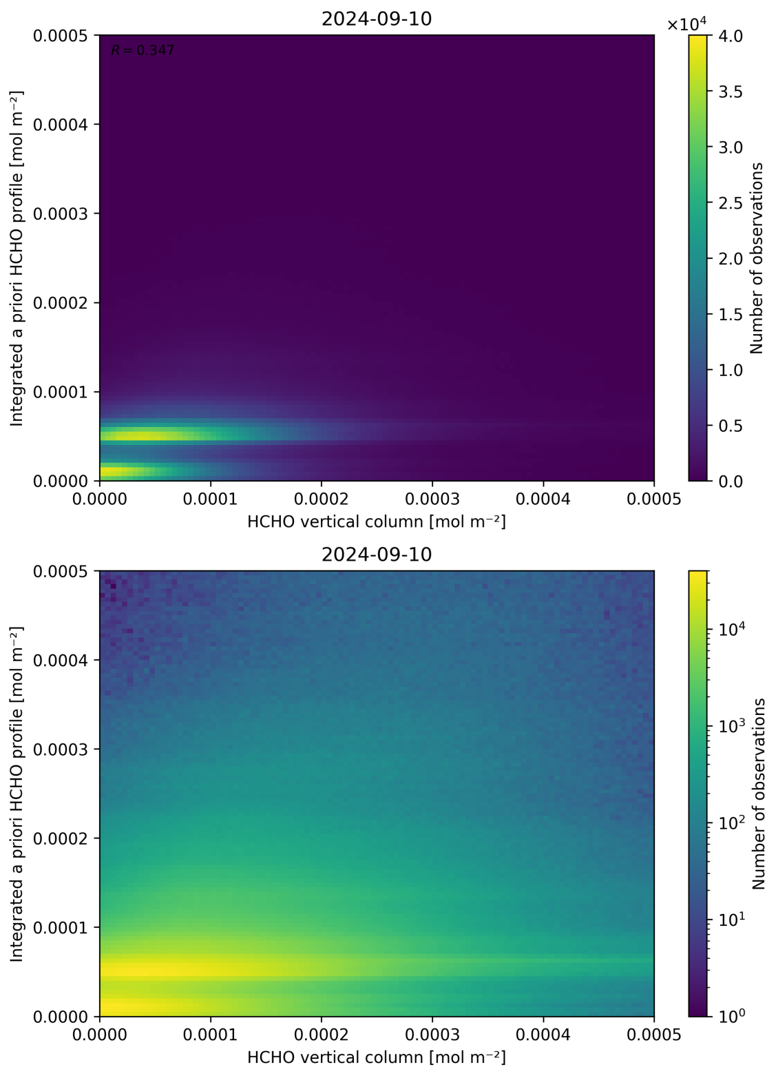
Figure 135: Scatter density plot of “HCHO vertical column” against “Integrated a priori HCHO profile” for 2024-09-09 to 2024-09-11.
