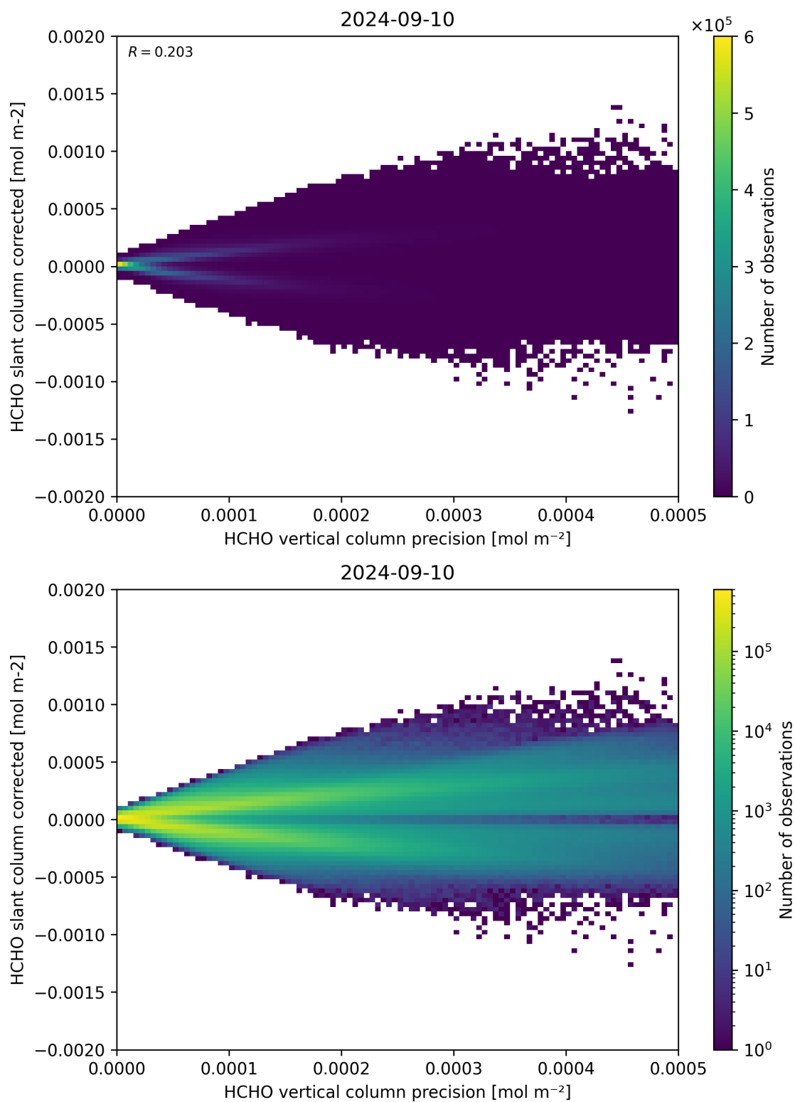
Figure 140: Scatter density plot of “HCHO vertical column precision” against “HCHO slant column corrected” for 2024-09-09 to 2024-09-11.
