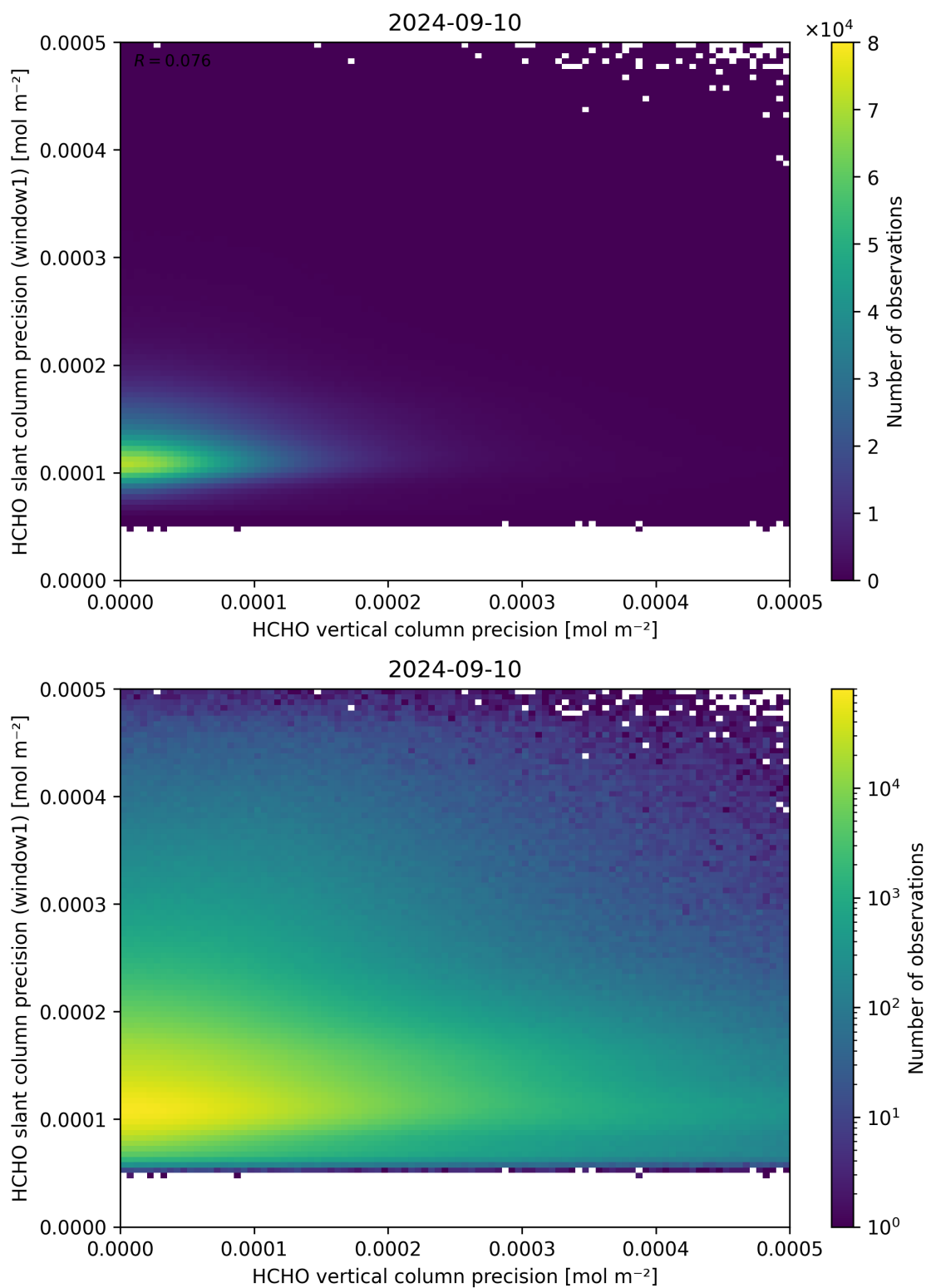
Figure 143: Scatter density plot of “HCHO vertical column precision” against “HCHO slant column precision (window1)” for 2024-09-09 to 2024-09-11.
