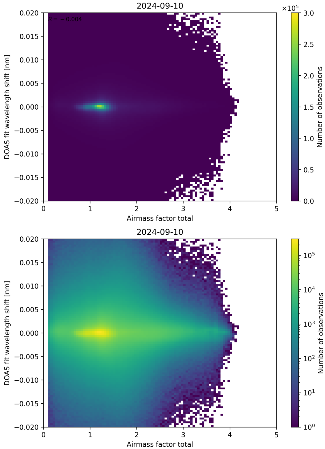
Figure 98: Scatter density plot of “Airmass factor total” against “DOAS fit wavelength shift” for 2024-09-09 to 2024-09-11.
