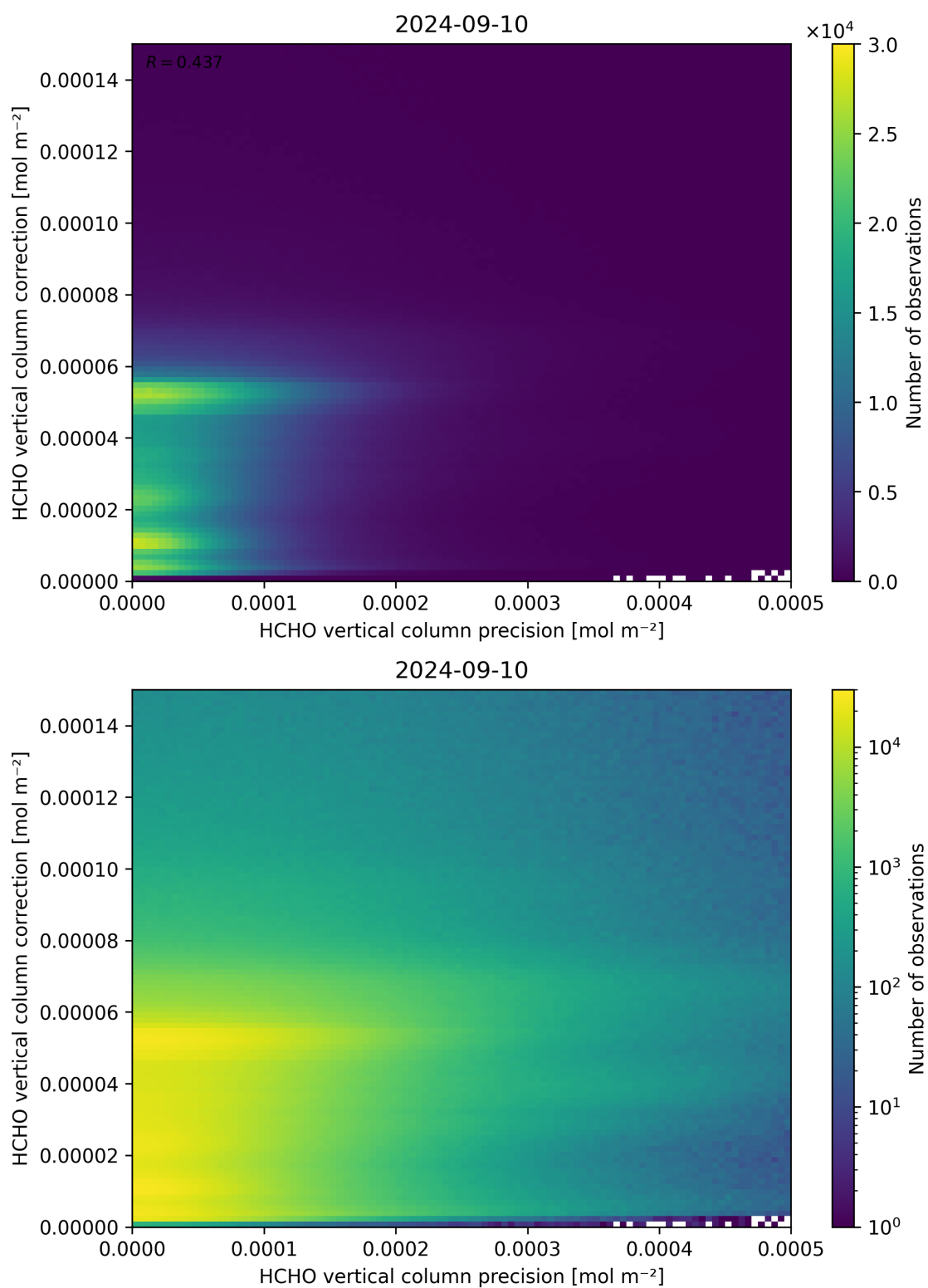
Figure 146: Scatter density plot of “HCHO vertical column precision” against “HCHO vertical column correction” for 2024-09-09 to 2024-09-11.
