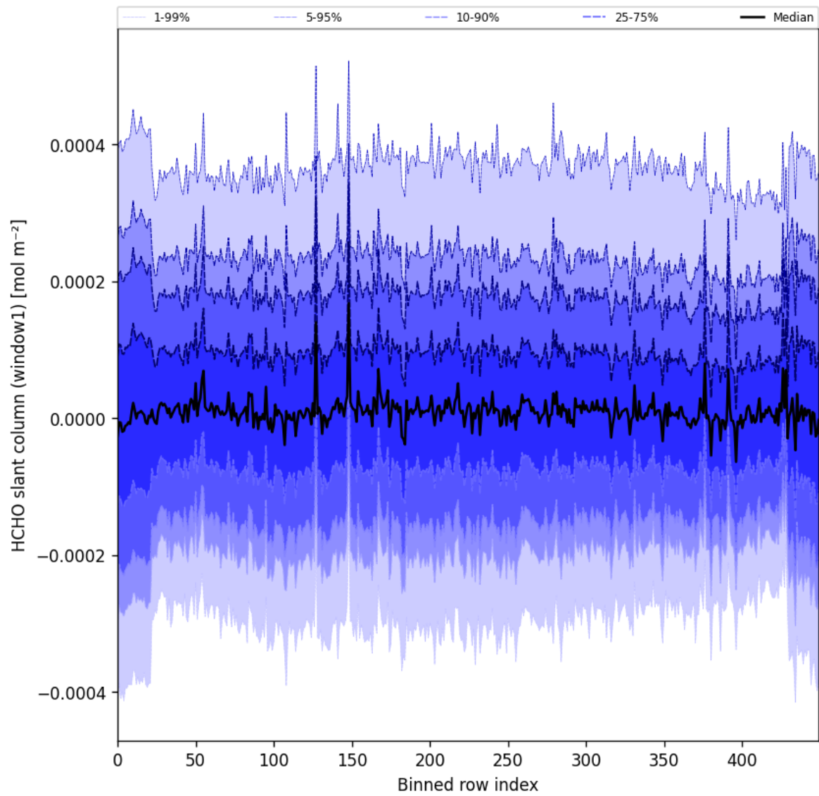
Figure 52: Along track statistics of “HCHO slant column (window1)” for 2024-09-09 to 2024-09-11
