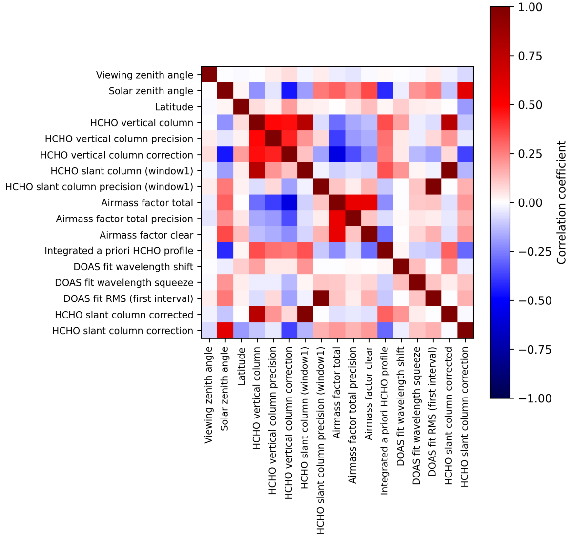
Figure 2: Map of correlation matrix for 2024-09-09 to 2024-09-11.
