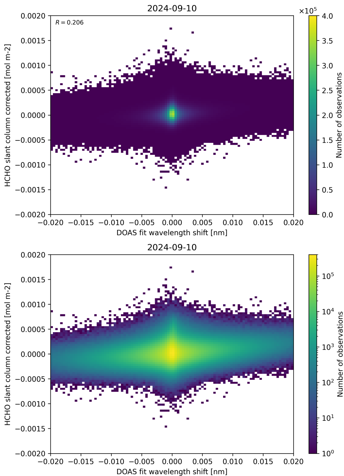
Figure 66: Scatter density plot of “DOAS fit wavelength shift” against “HCHO slant column corrected” for 2024-09-09 to 2024-09-11.
