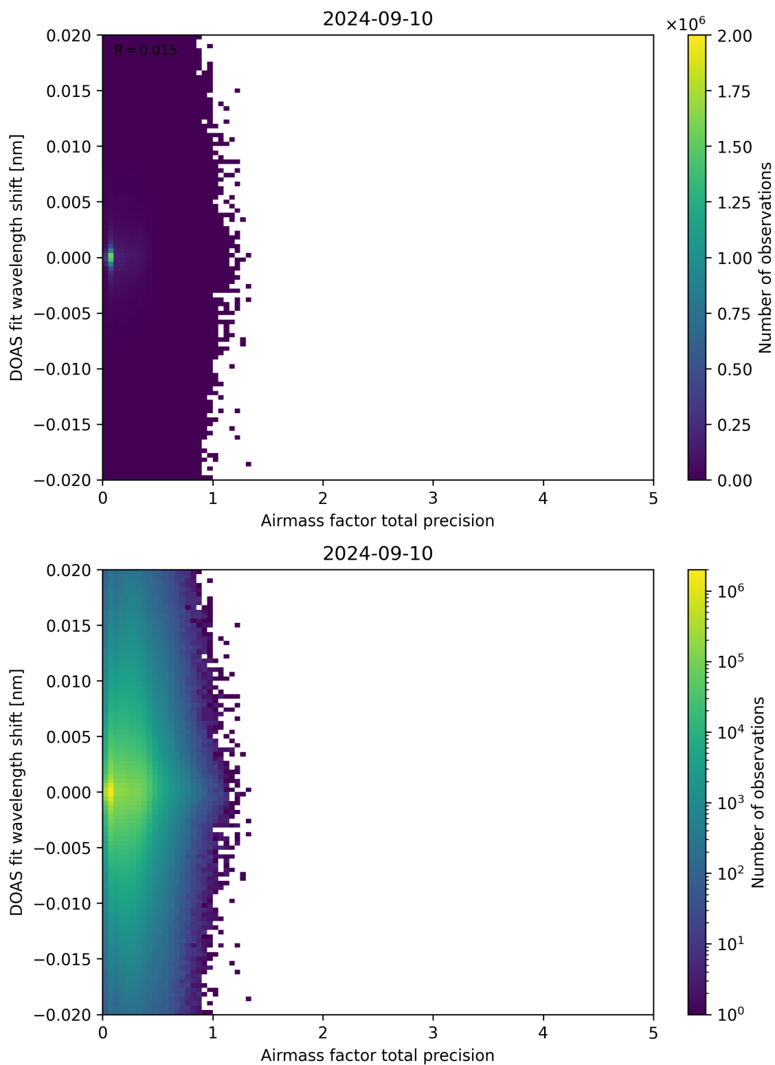
Figure 106: Scatter density plot of “Airmass factor total precision” against “DOAS fit wavelength shift” for 2024-09-09 to 2024-09-11.
