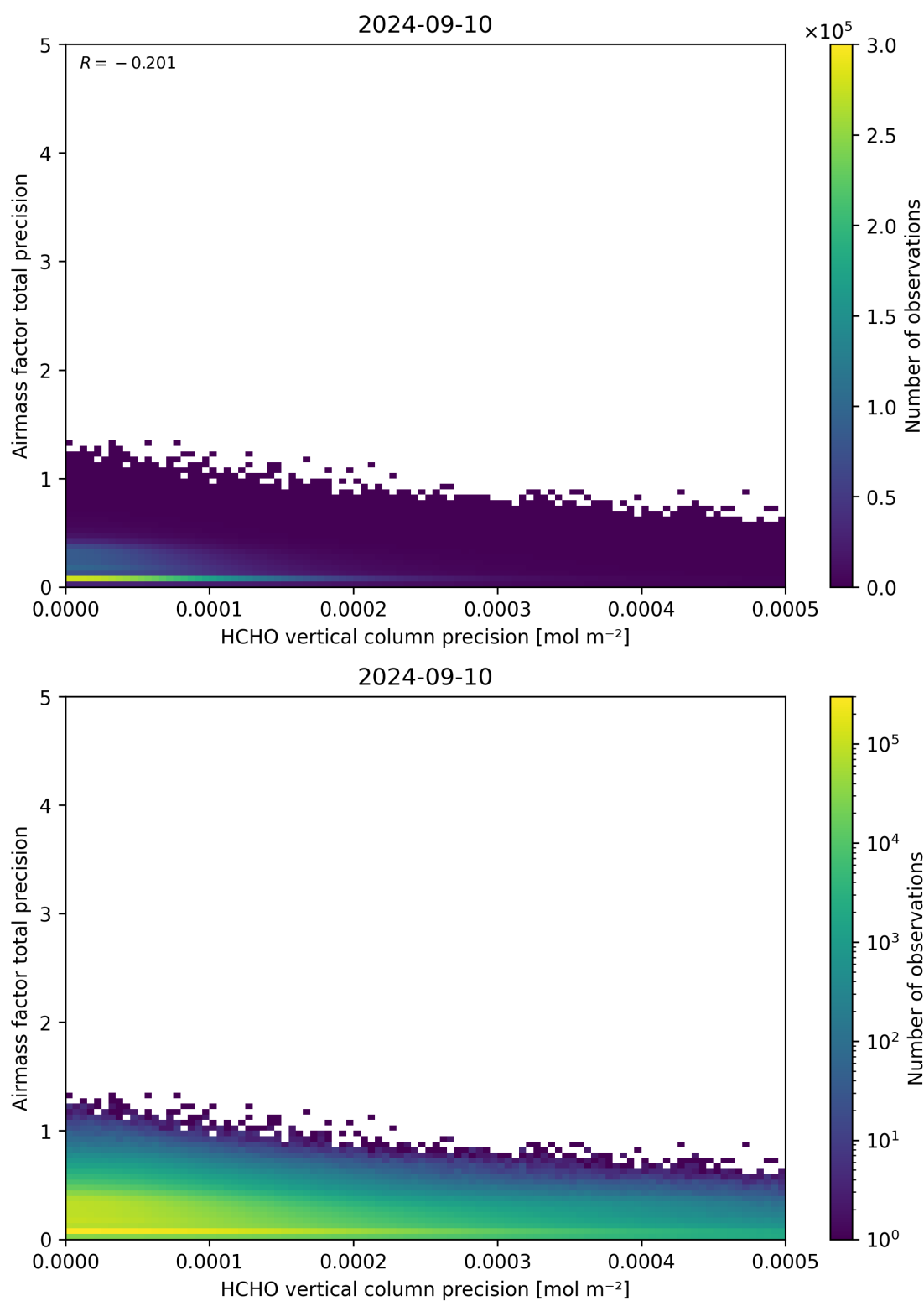
Figure 145: Scatter density plot of “HCHO vertical column precision” against “Airmass factor total precision” for 2024-09-09 to 2024-09-11.
