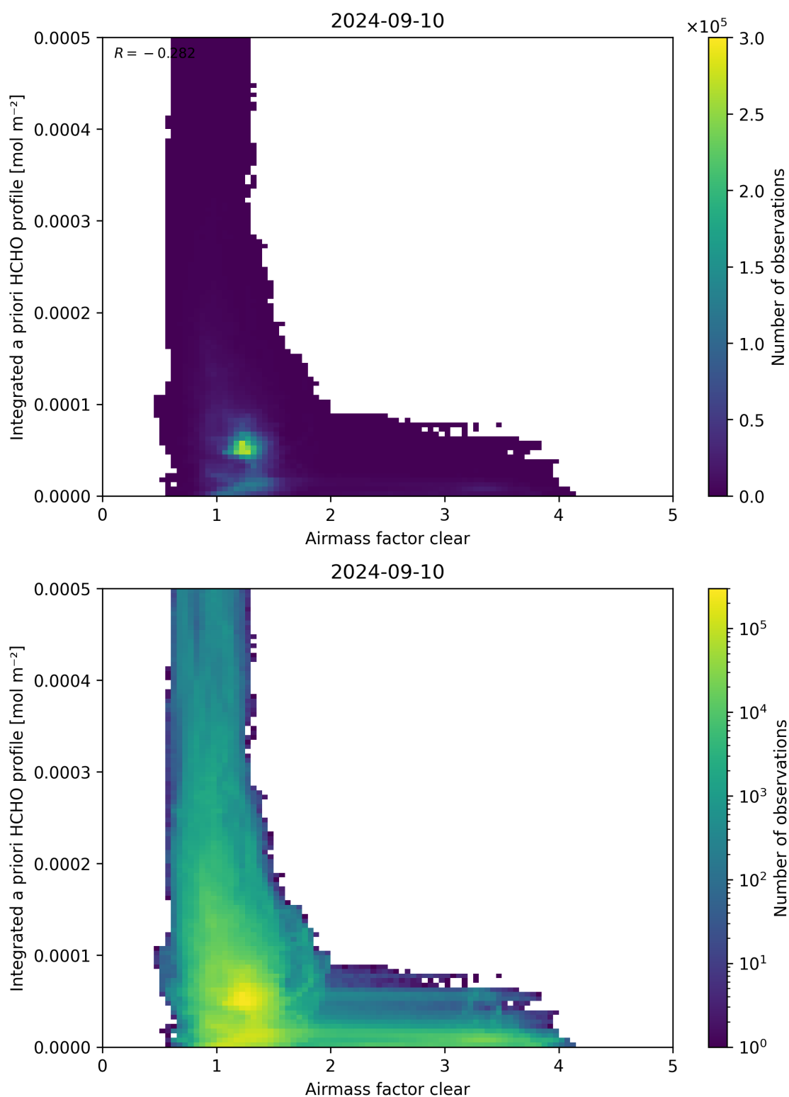
Figure 76: Scatter density plot of “Airmass factor clear” against “Integrated a priori HCHO profile” for 2024-09-09 to 2024-09-11.
