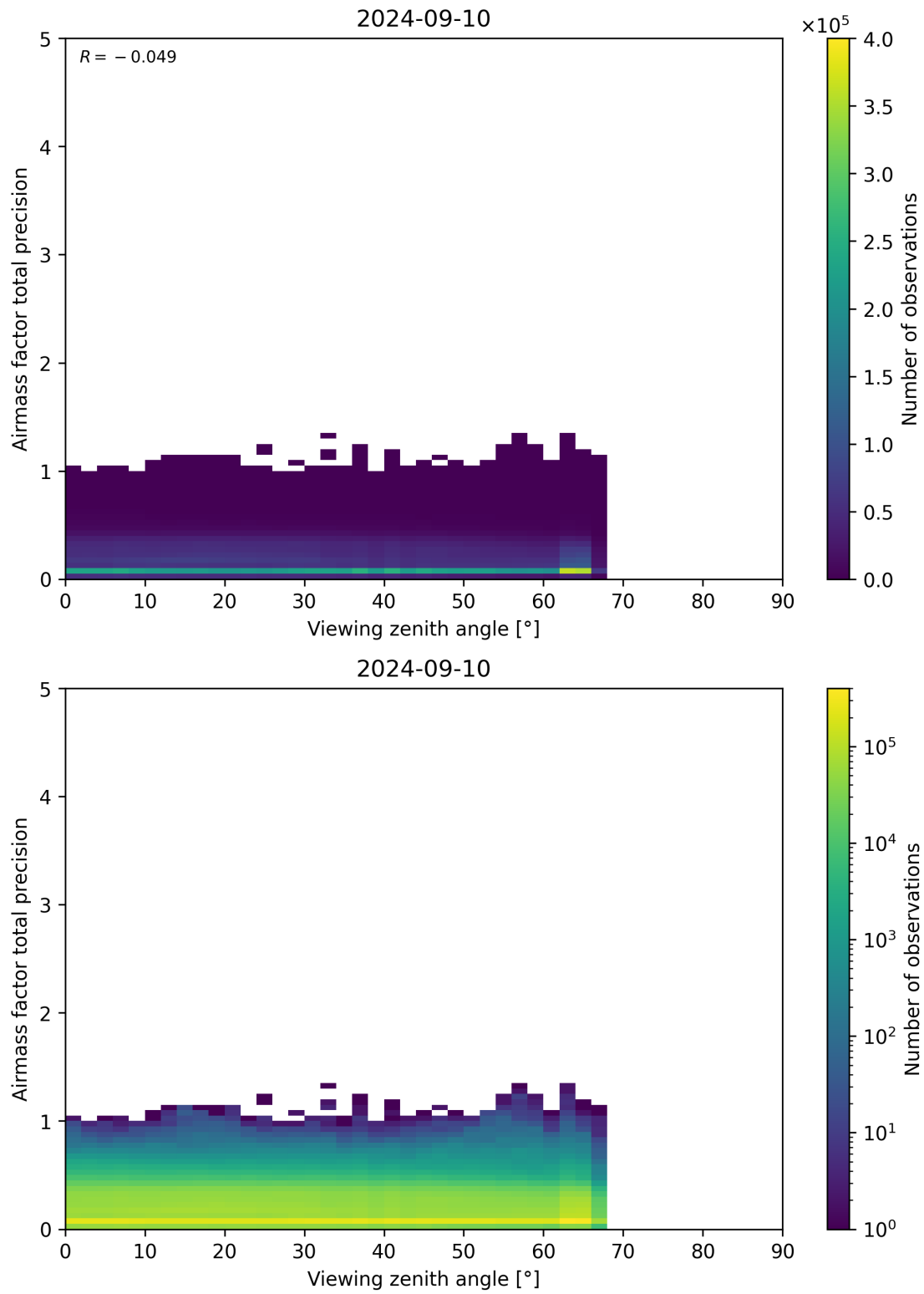
Figure 191: Scatter density plot of “Viewing zenith angle” against “Airmass factor total precision” for 2024-09-09 to 2024-09-11.
