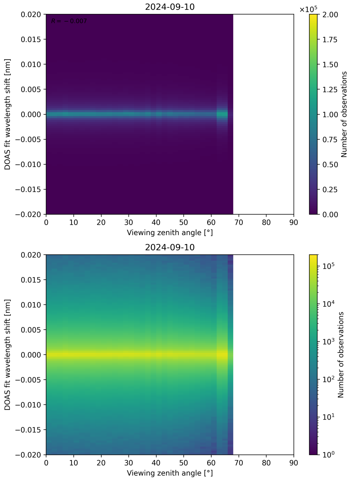
Figure 183: Scatter density plot of “Viewing zenith angle” against “DOAS fit wavelength shift” for 2024-09-09 to 2024-09-11.
