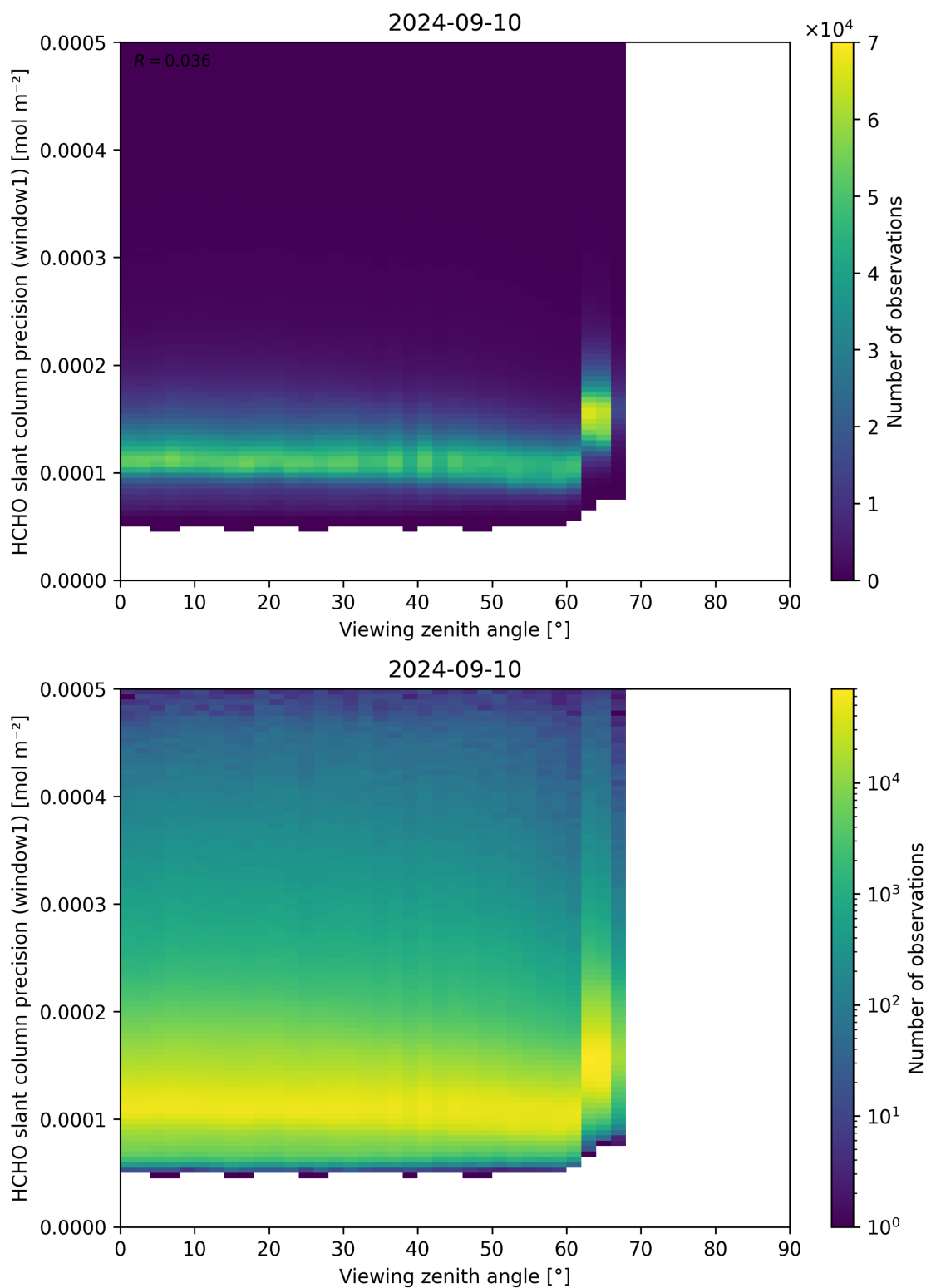
Figure 189: Scatter density plot of “Viewing zenith angle” against “HCHO slant column precision (window1)” for 2024-09-09 to 2024-09-11.
