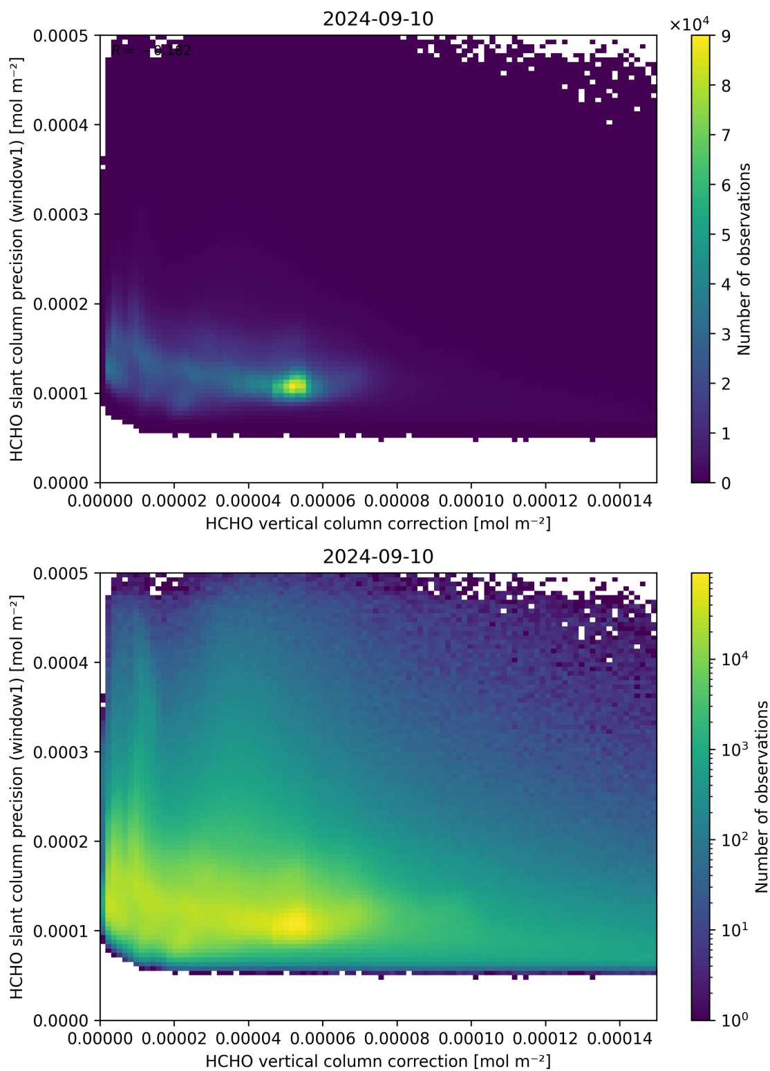
Figure 119: Scatter density plot of “HCHO vertical column correction” against “HCHO slant column precision (window1)” for 2024-09-09 to 2024-09-11.
