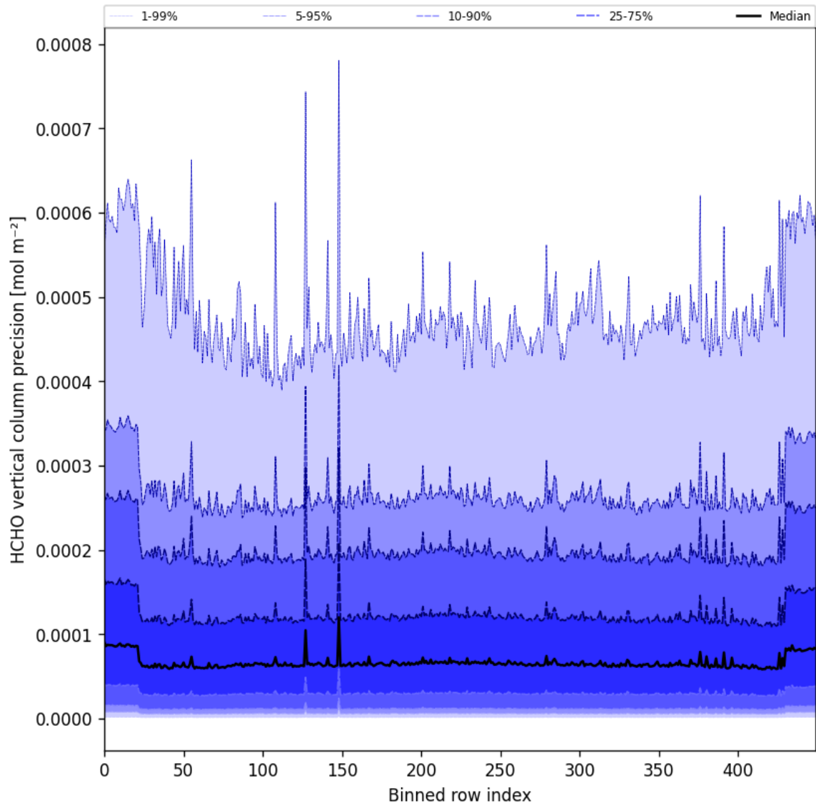
Figure 50: Along track statistics of “HCHO vertical column precision” for 2024-09-09 to 2024-09-11
