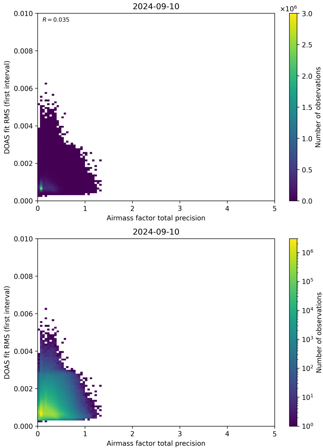
Figure 105: Scatter density plot of “Airmass factor total precision” against “DOAS fit RMS (first interval)” for 2024-09-09 to 2024-09-11.
