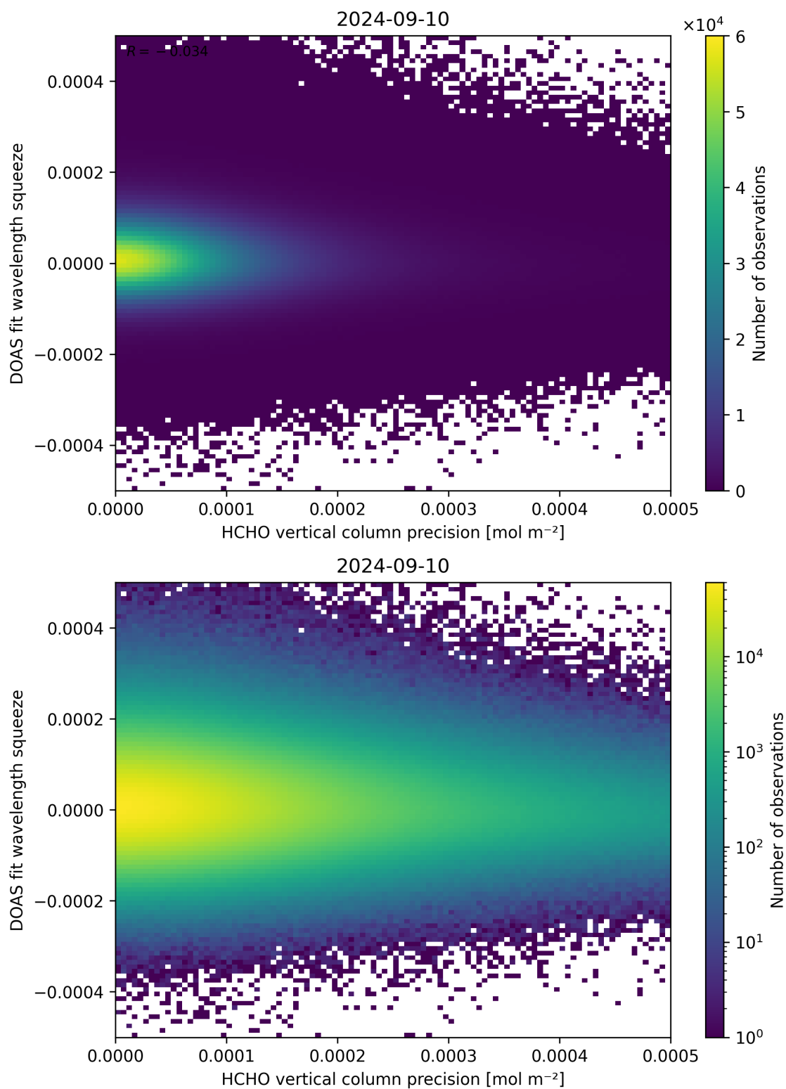
Figure 138: Scatter density plot of “HCHO vertical column precision” against “DOAS fit wavelength squeeze” for 2024-09-09 to 2024-09-11.
