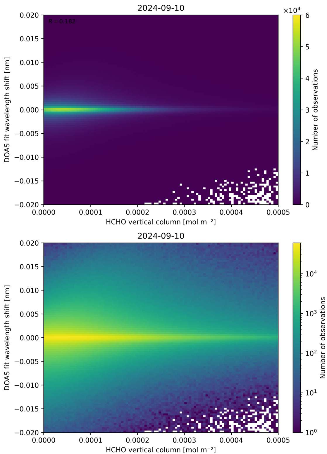
Figure 124: Scatter density plot of “HCHO vertical column” against “DOAS fit wavelength shift” for 2024-09-09 to 2024-09-11.
