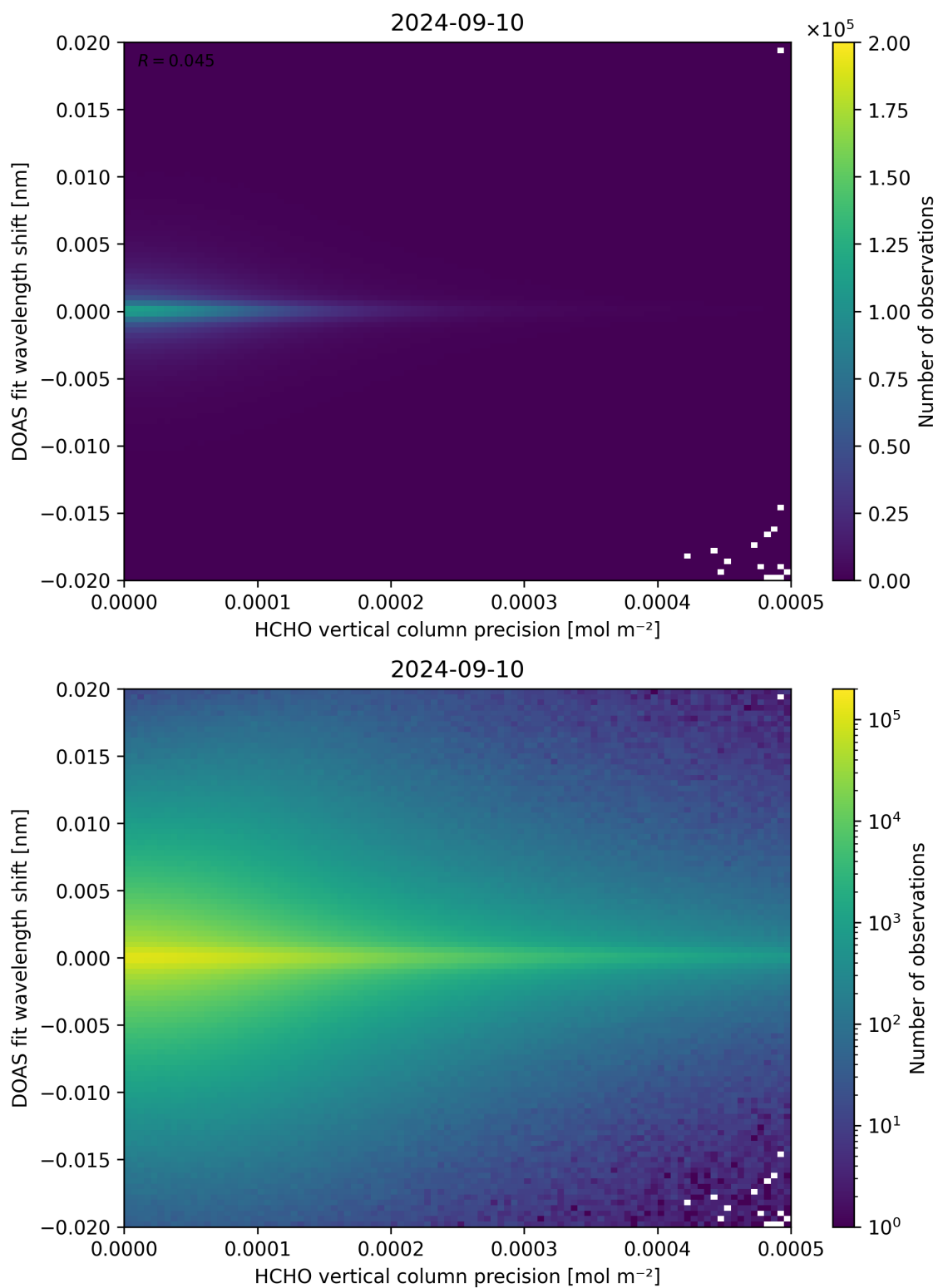
Figure 137: Scatter density plot of “HCHO vertical column precision” against “DOAS fit wavelength shift” for 2024-09-09 to 2024-09-11.
