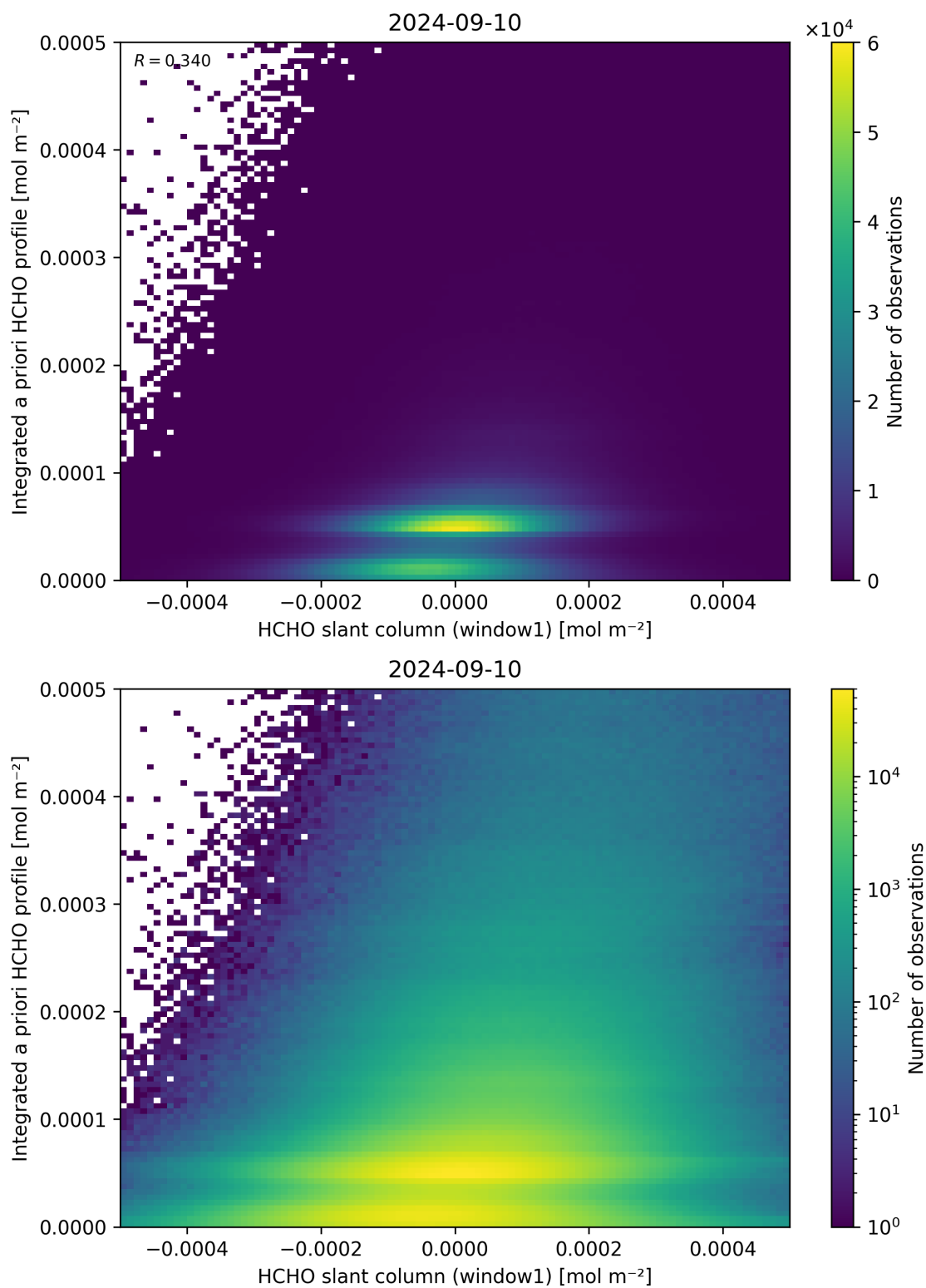
Figure 87: Scatter density plot of “HCHO slant column (window1)” against “Integrated a priori HCHO profile” for 2024-09-09 to 2024-09-11.
