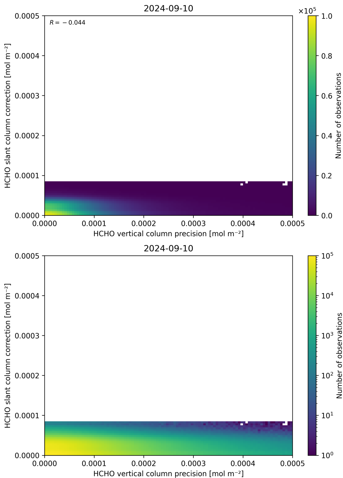
Figure 141: Scatter density plot of “HCHO vertical column precision” against “HCHO slant column correction” for 2024-09-09 to 2024-09-11.
