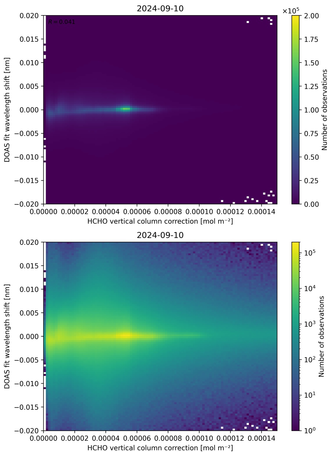
Figure 113: Scatter density plot of “HCHO vertical column correction” against “DOAS fit wavelength shift” for 2024-09-09 to 2024-09-11.
