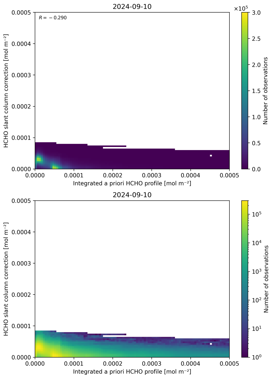
Figure 152: Scatter density plot of “Integrated a priori HCHO profile” against “HCHO slant column correction” for 2024-09-09 to 2024-09-11.
