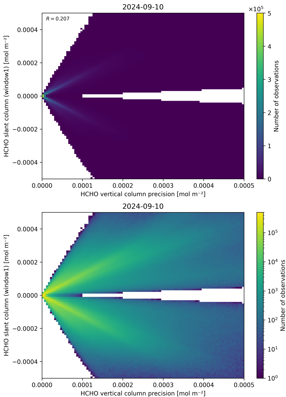
Figure 142: Scatter density plot of “HCHO vertical column precision” against “HCHO slant column (window1)” for 2024-09-09 to 2024-09-11.
