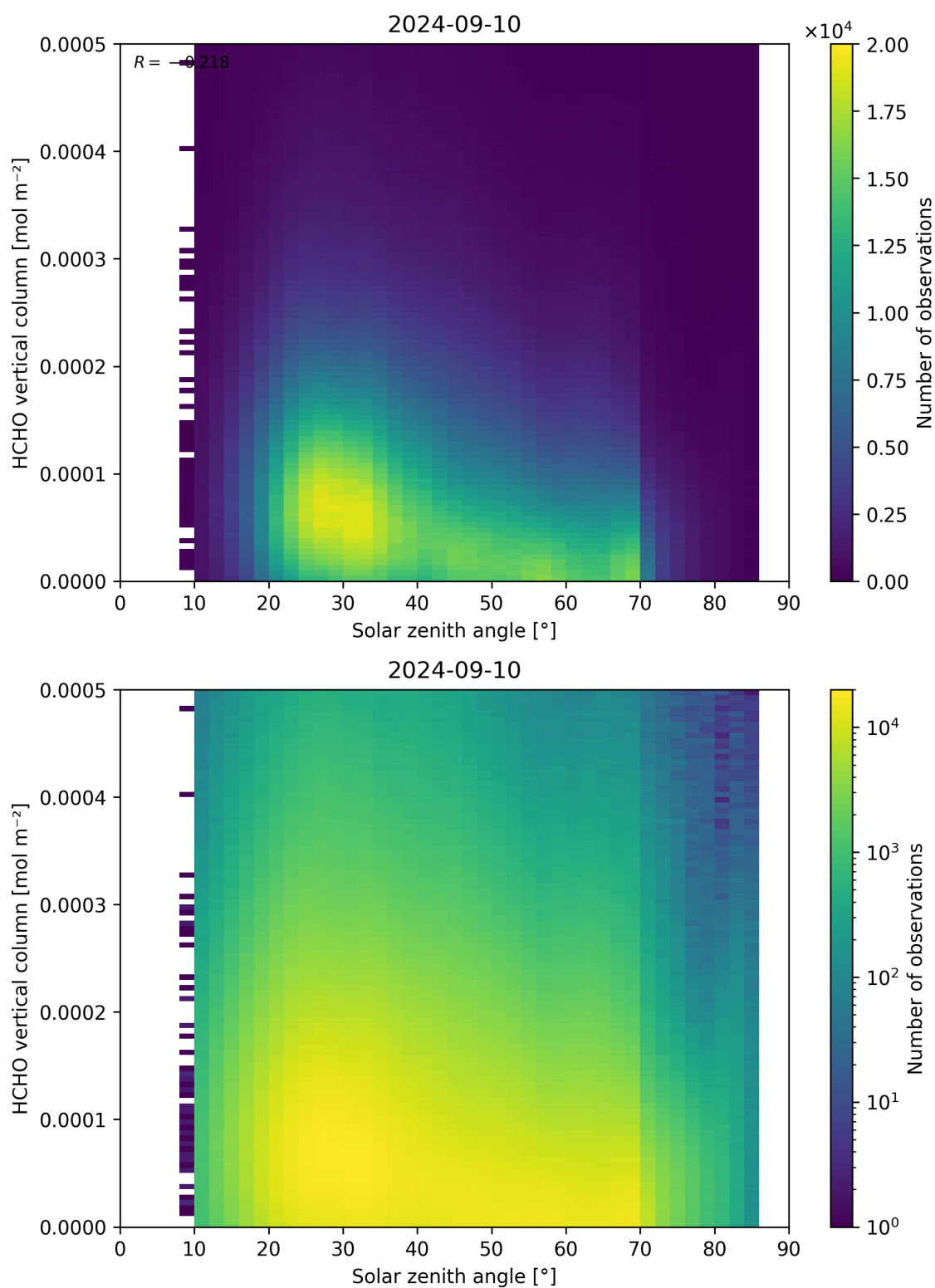
Figure 177: Scatter density plot of “Solar zenith angle” against “HCHO vertical column” for 2024-09-09 to 2024-09-11.
