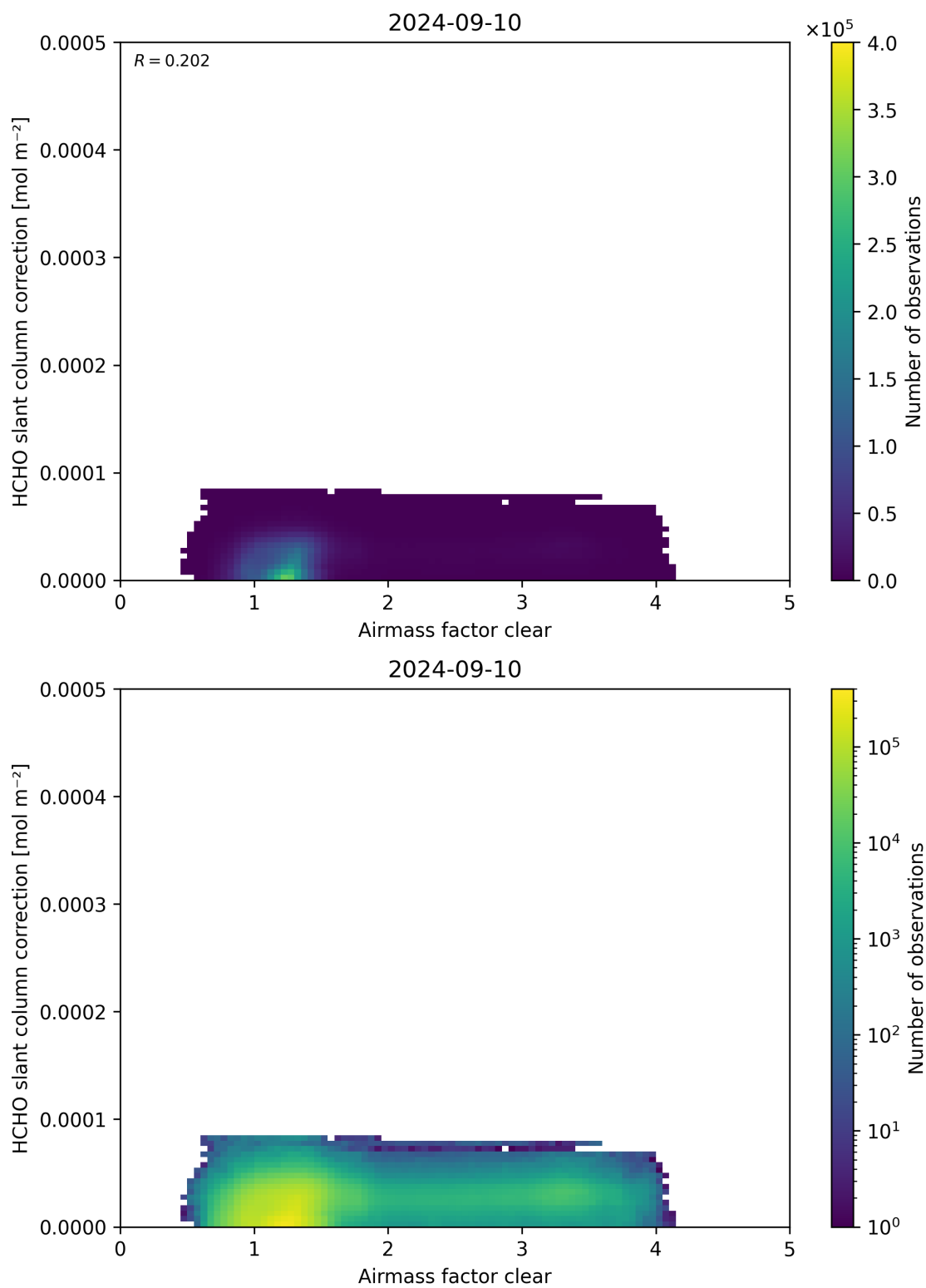
Figure 75: Scatter density plot of “Airmass factor clear” against “HCHO slant column correction” for 2024-09-09 to 2024-09-11.
