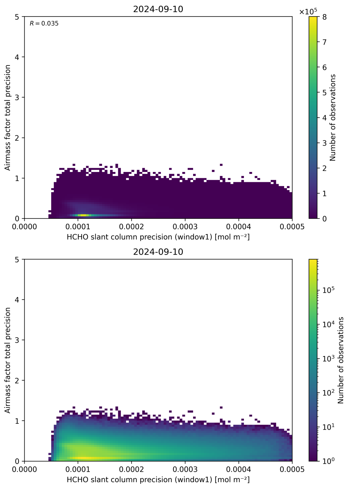
Figure 95: Scatter density plot of “HCHO slant column precision (window1)” against “Airmass factor total precision” for 2024-09-09 to 2024-09-11.
