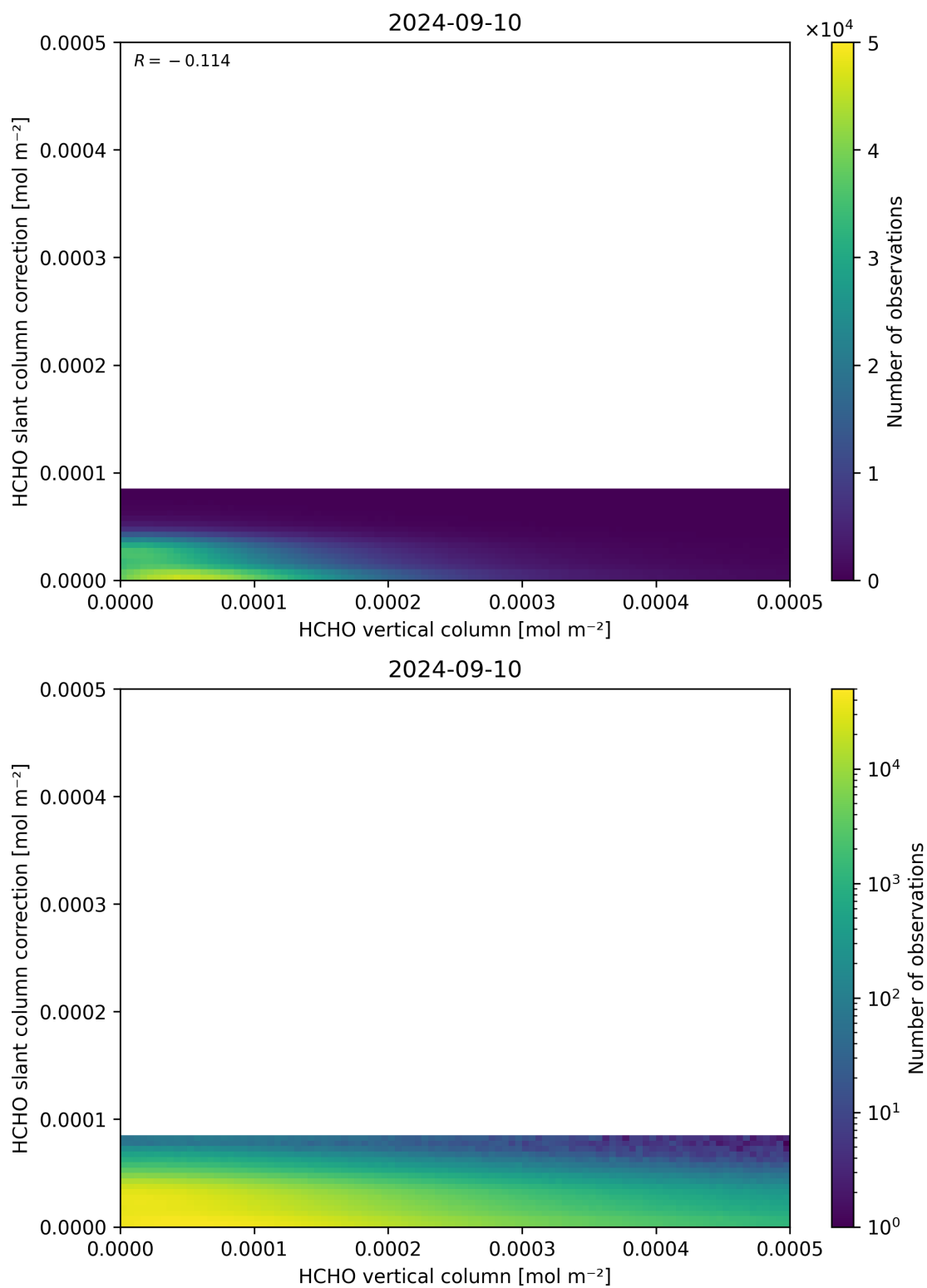
Figure 128: Scatter density plot of “HCHO vertical column” against “HCHO slant column correction” for 2024-09-09 to 2024-09-11.
