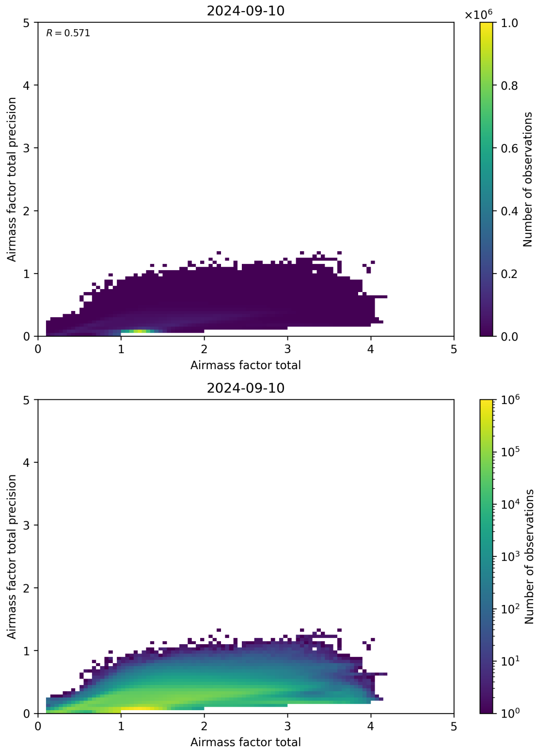
Figure 103: Scatter density plot of “Airmass factor total” against “Airmass factor total precision” for 2024-09-09 to 2024-09-11.
