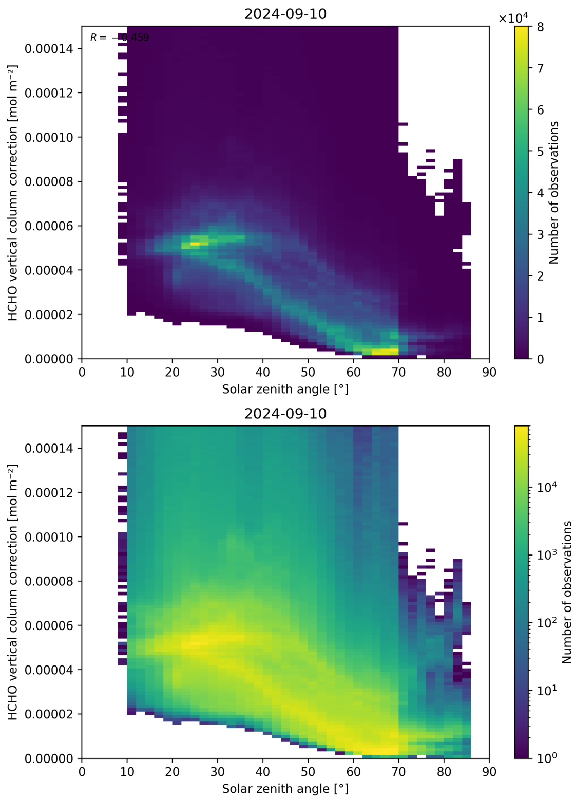
Figure 178: Scatter density plot of “Solar zenith angle” against “HCHO vertical column correction” for 2024-09-09 to 2024-09-11.
