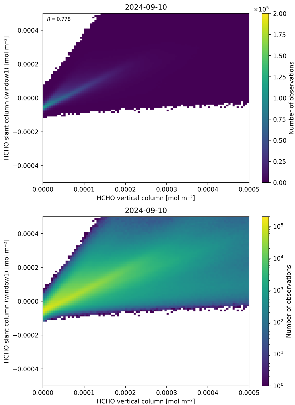
Figure 129: Scatter density plot of “HCHO vertical column” against “HCHO slant column (window1)” for 2024-09-09 to 2024-09-11.
