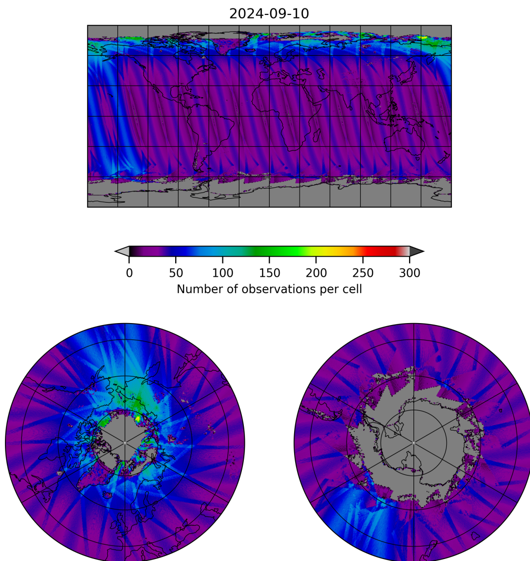
Figure 19: Map of the number of observations for 2024-09-09 to 2024-09-11
