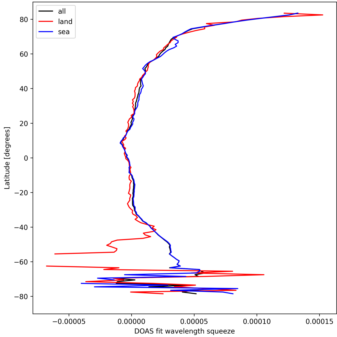
Figure 31: Zonal average of “DOAS fit wavelength squeeze” for 2024-09-09 to 2024-09-11.
