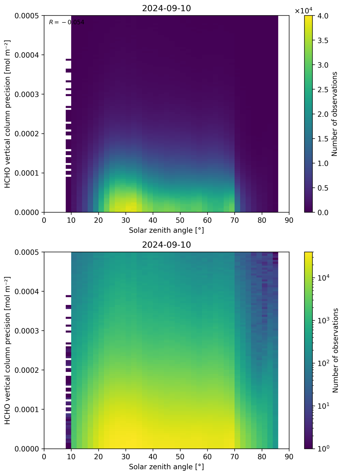
Figure 179: Scatter density plot of “Solar zenith angle” against “HCHO vertical column precision” for 2024-09-09 to 2024-09-11.
