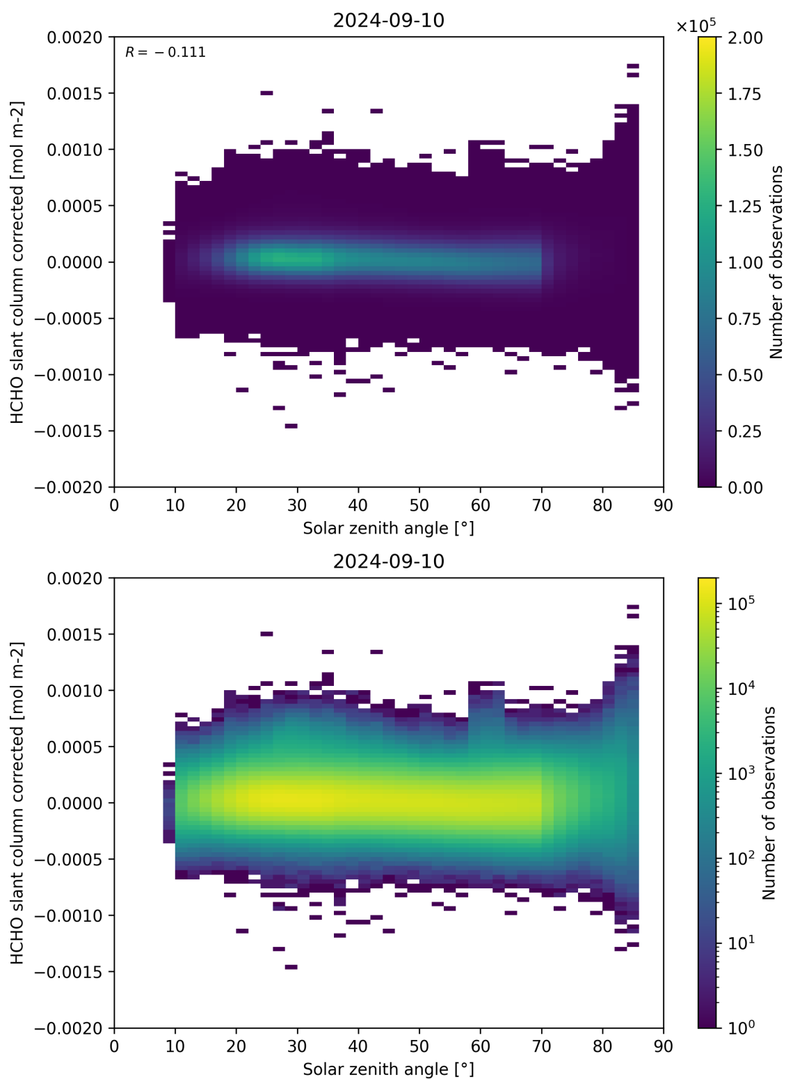
Figure 171: Scatter density plot of “Solar zenith angle” against “HCHO slant column corrected” for 2024-09-09 to 2024-09-11.
