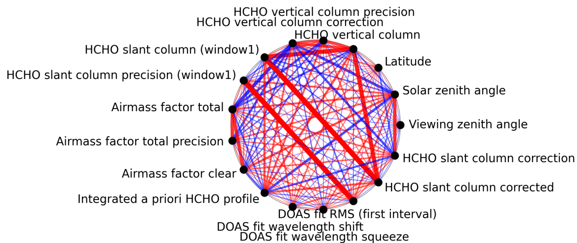
Figure 1: Map of correlation graph for 2024-09-09 to 2024-09-11.
