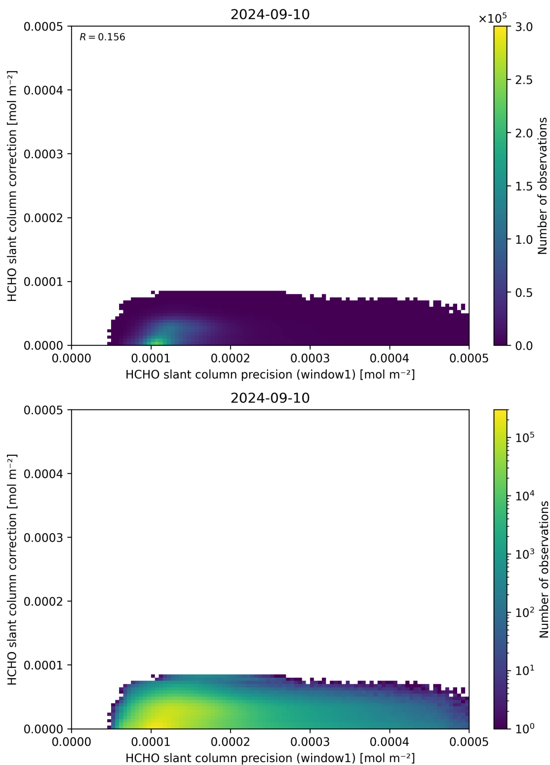
Figure 93: Scatter density plot of “HCHO slant column precision (window1)” against “HCHO slant column correction” for 2024-09-09 to 2024-09-11.
