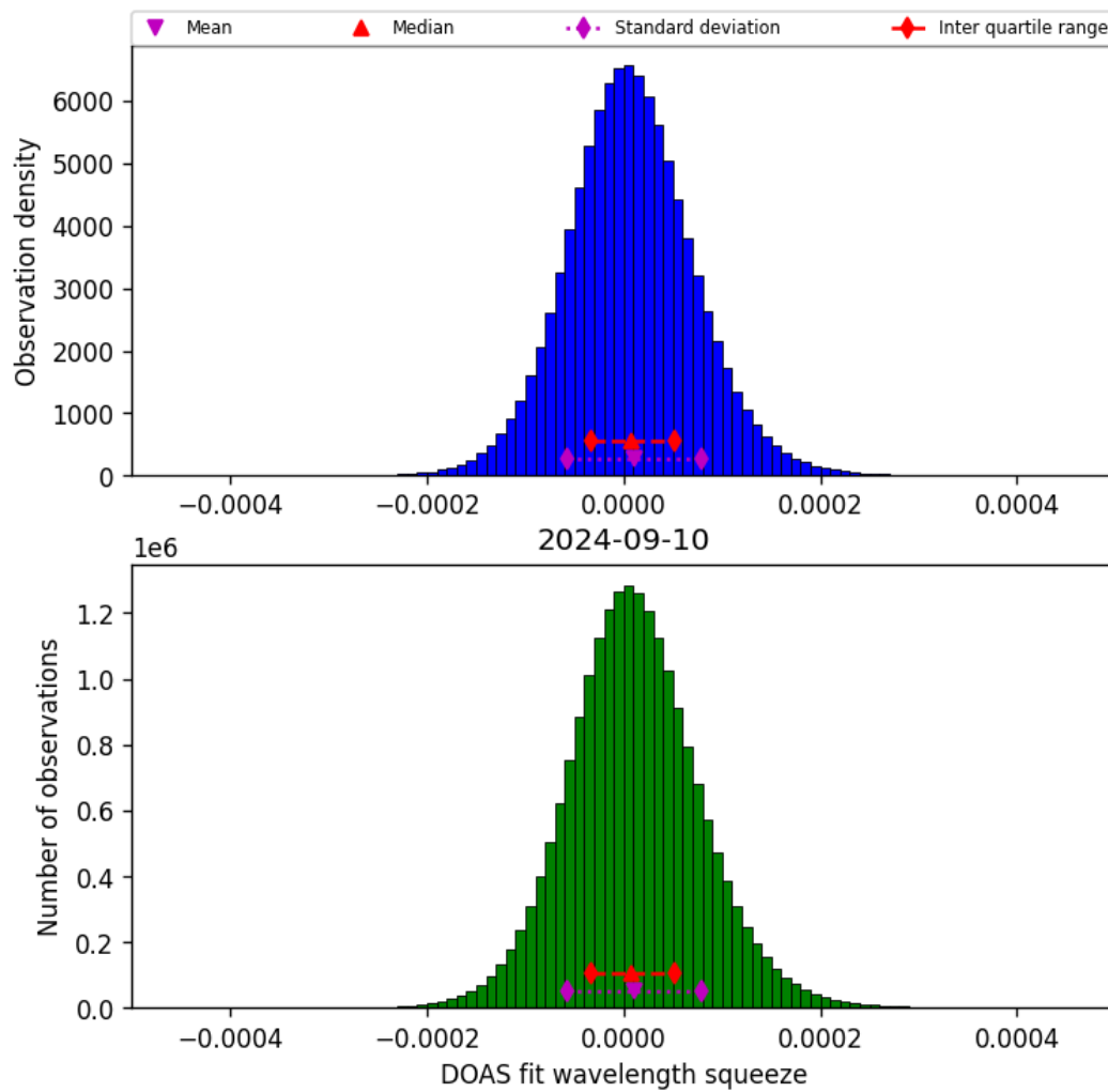
Figure 45: Histogram of “DOAS fit wavelength squeeze” for 2024-09-09 to 2024-09-11
