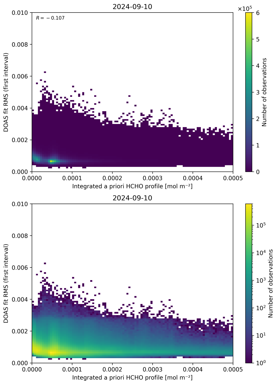
Figure 148: Scatter density plot of “Integrated a priori HCHO profile” against “DOAS fit RMS (first interval)” for 2024-09-09 to 2024-09-11.
