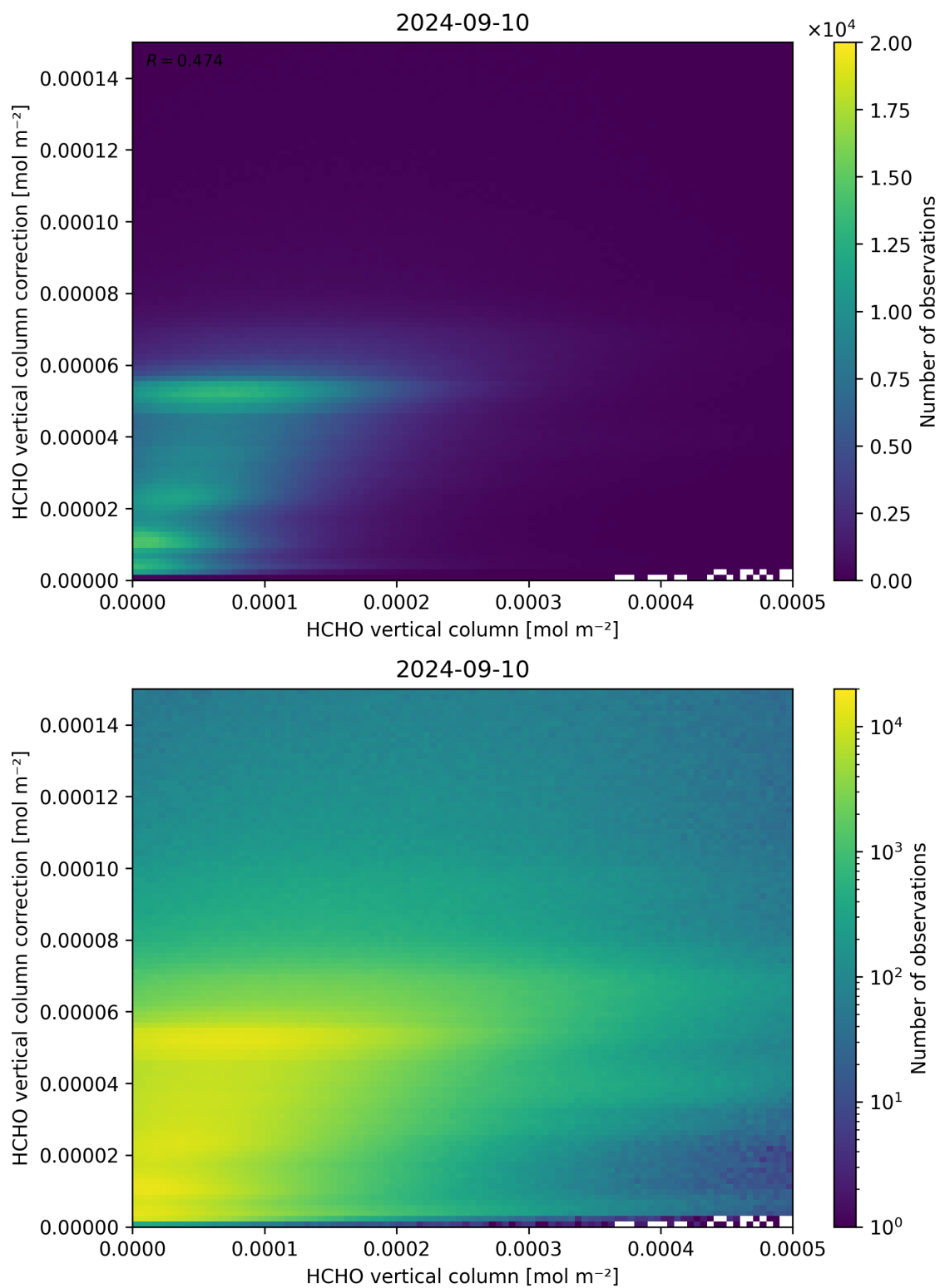
Figure 133: Scatter density plot of “HCHO vertical column” against “HCHO vertical column correction” for 2024-09-09 to 2024-09-11.
