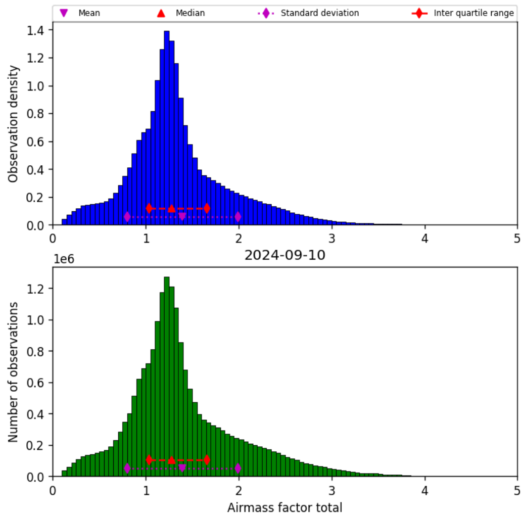
Figure 40: Histogram of “Airmass factor total” for 2024-09-09 to 2024-09-11
