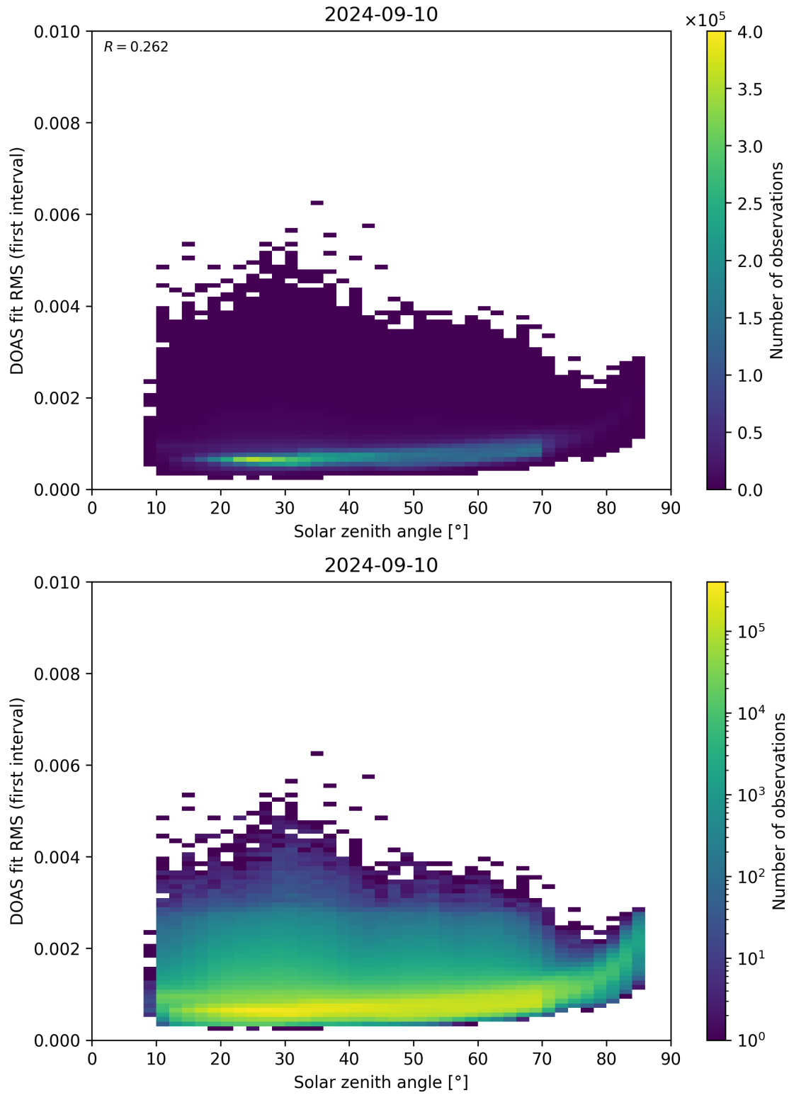
Figure 167: Scatter density plot of “Solar zenith angle” against “DOAS fit RMS (first interval)” for 2024-09-09 to 2024-09-11.
