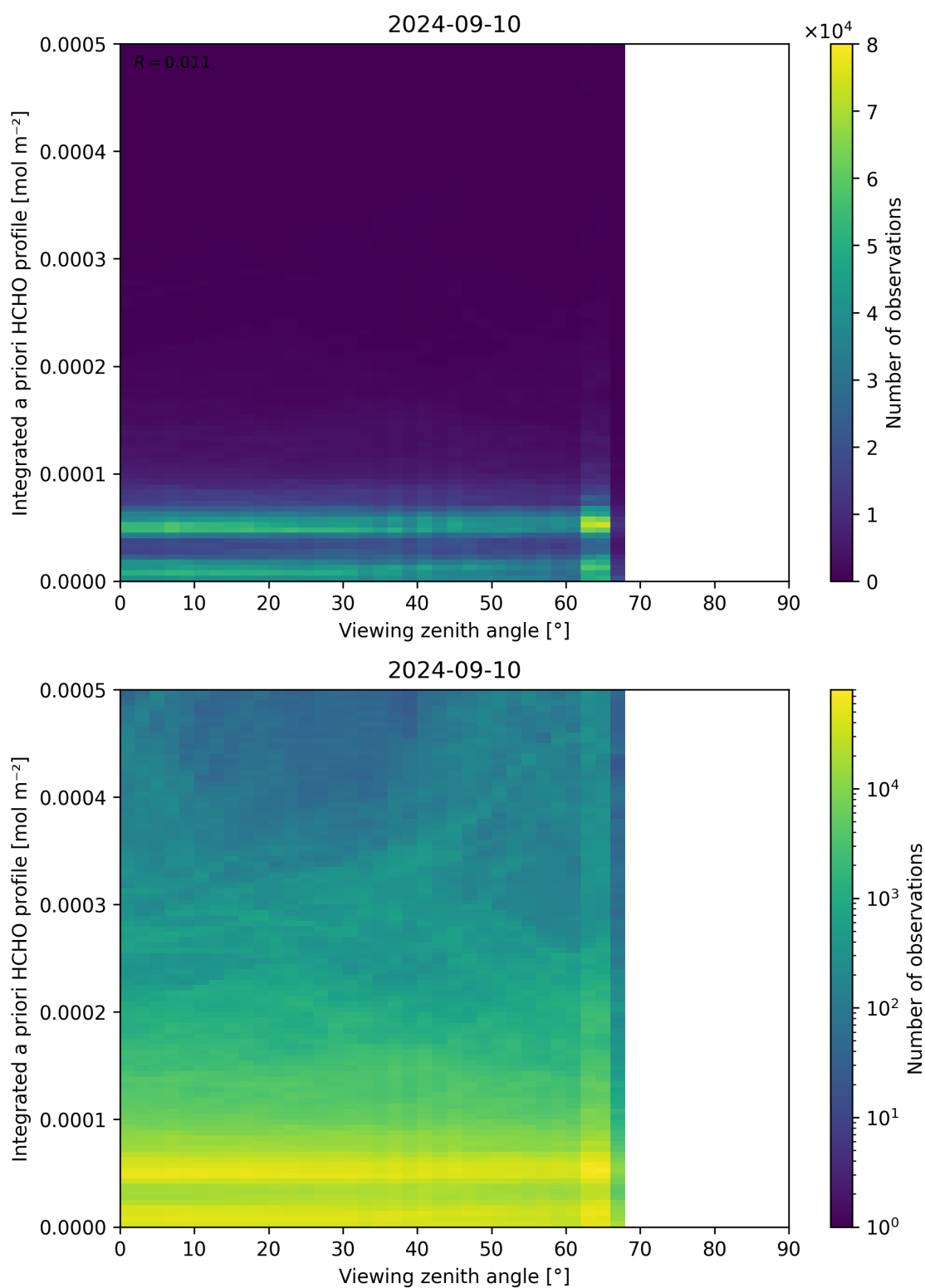
Figure 195: Scatter density plot of “Viewing zenith angle” against “Integrated a priori HCHO profile” for 2024-09-09 to 2024-09-11.
