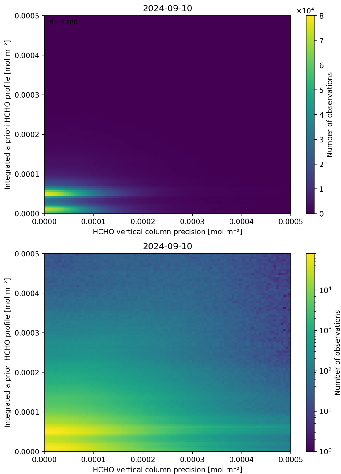
Figure 147: Scatter density plot of “HCHO vertical column precision” against “Integrated a priori HCHO profile” for 2024-09-09 to 2024-09-11.
