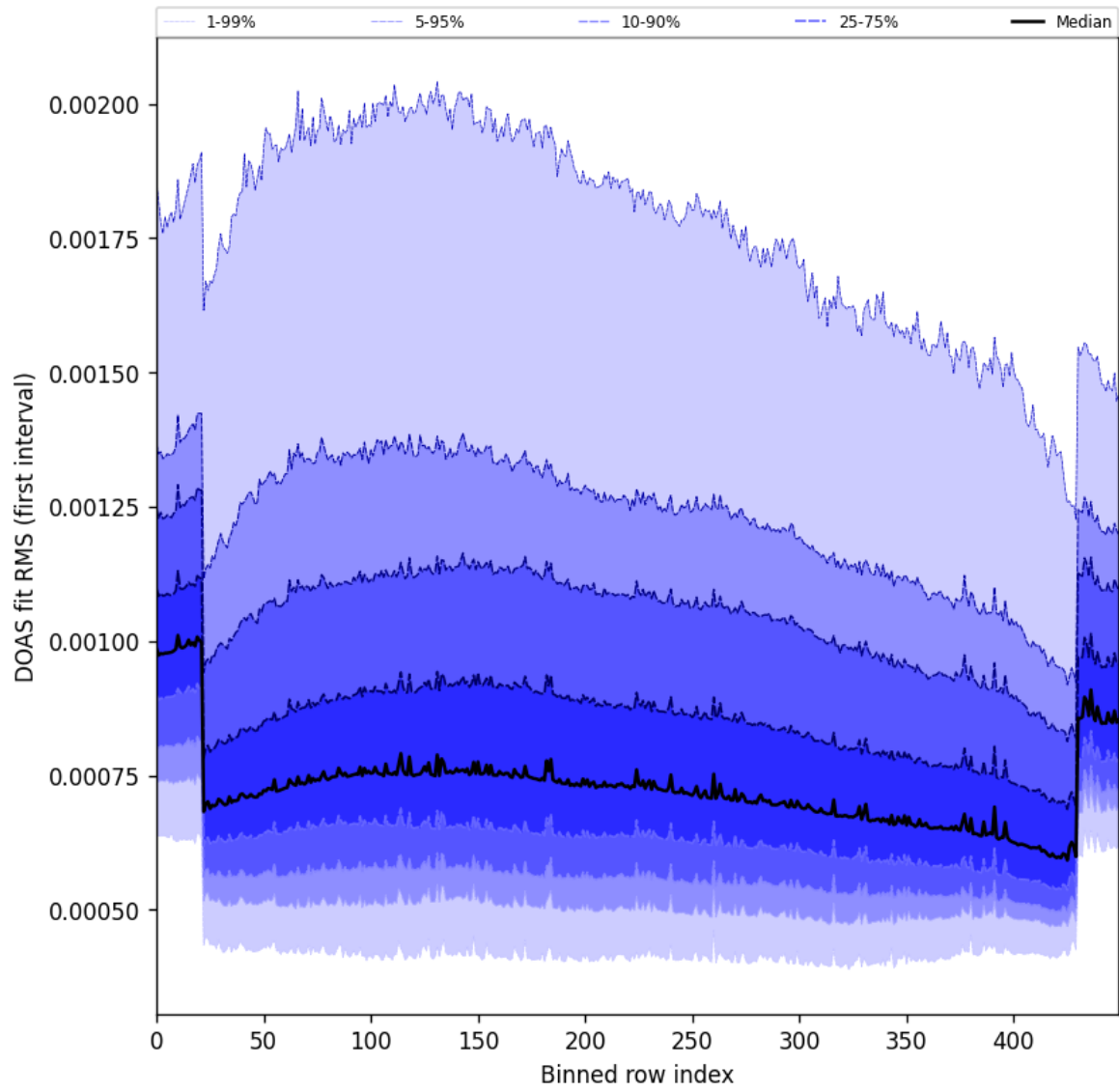
Figure 60: Along track statistics of “DOAS fit RMS (first interval)” for 2024-09-09 to 2024-09-11
