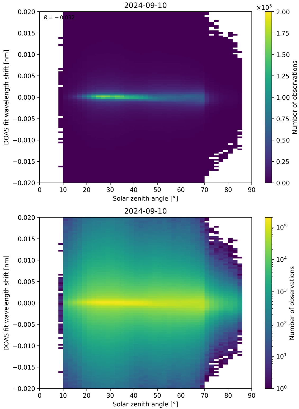
Figure 168: Scatter density plot of “Solar zenith angle” against “DOAS fit wavelength shift” for 2024-09-09 to 2024-09-11.
