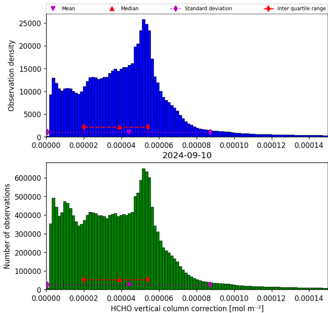
Figure 37: Histogram of “HCHO vertical column correction” for 2024-09-09 to 2024-09-11
