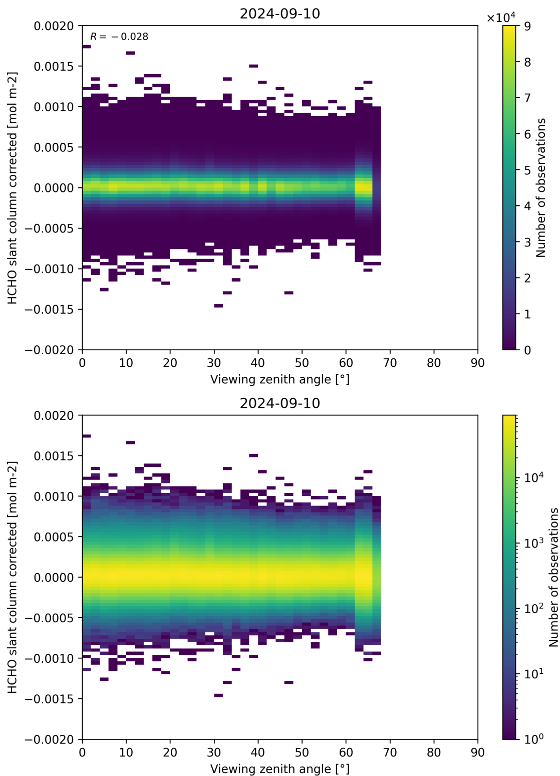
Figure 186: Scatter density plot of “Viewing zenith angle” against “HCHO slant column corrected” for 2024-09-09 to 2024-09-11.
