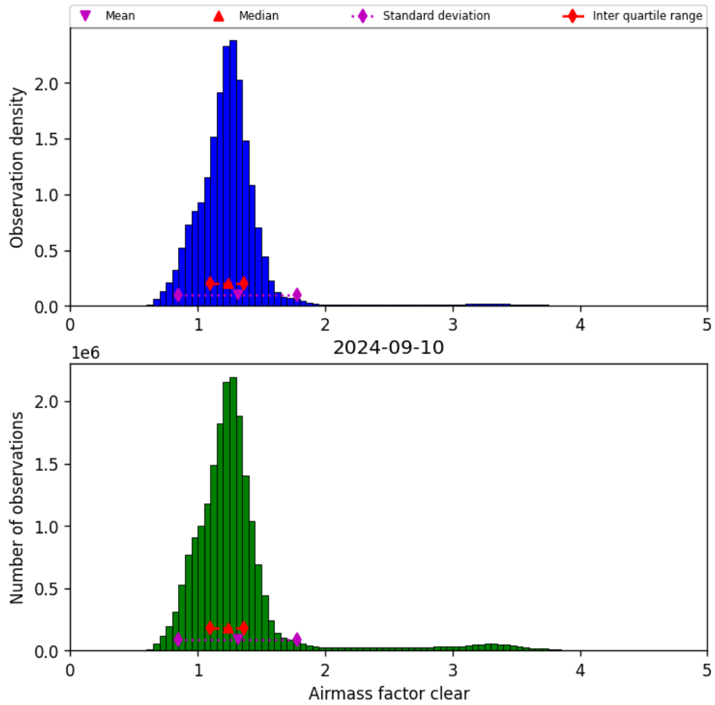
Figure 42: Histogram of “Airmass factor clear” for 2024-09-09 to 2024-09-11
