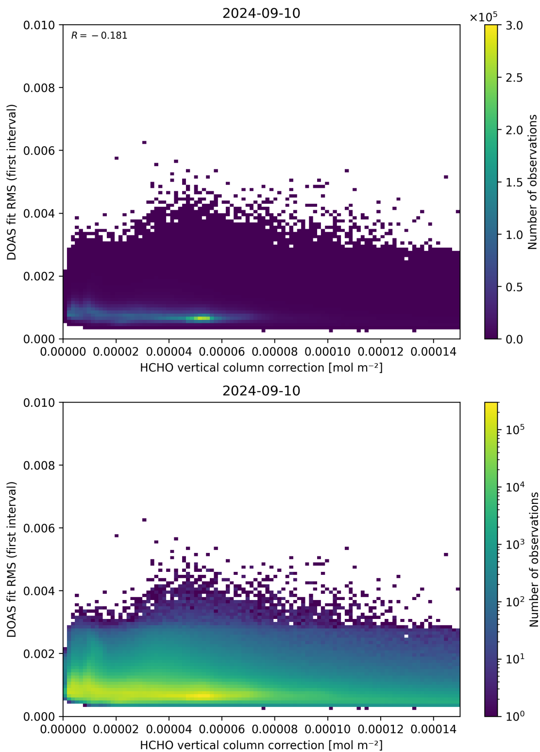
Figure 112: Scatter density plot of “HCHO vertical column correction” against “DOAS fit RMS (first interval)” for 2024-09-09 to 2024-09-11.
