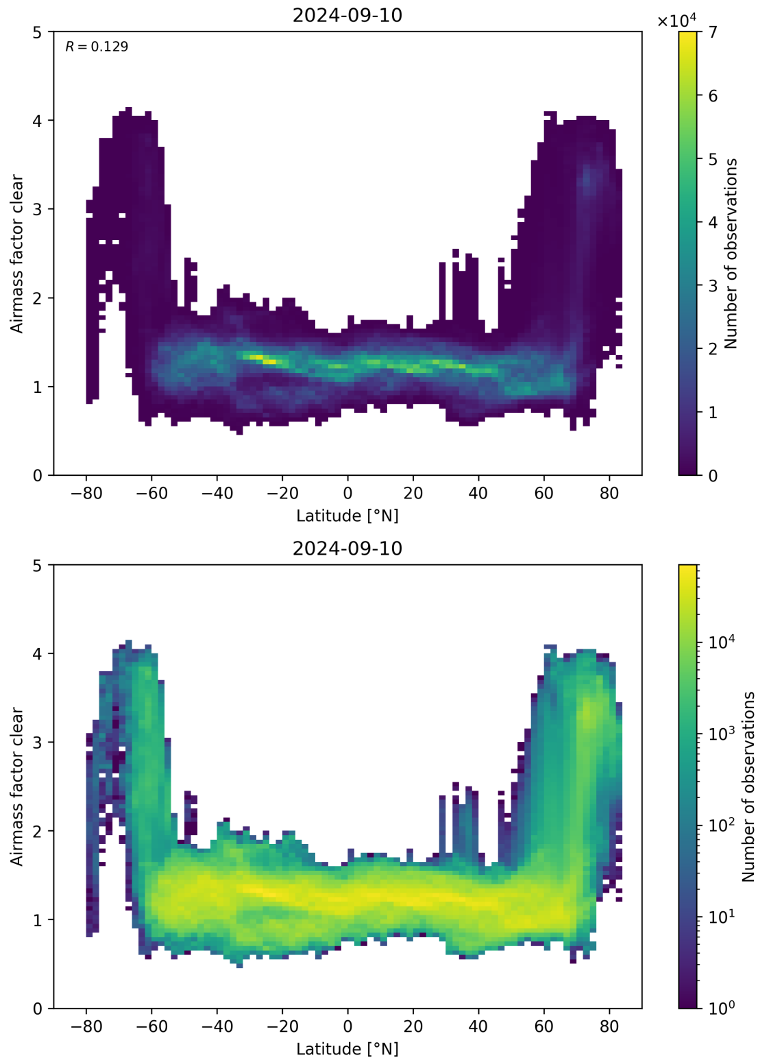
Figure 156: Scatter density plot of “Latitude” against “Airmass factor clear” for 2024-09-09 to 2024-09-11.
