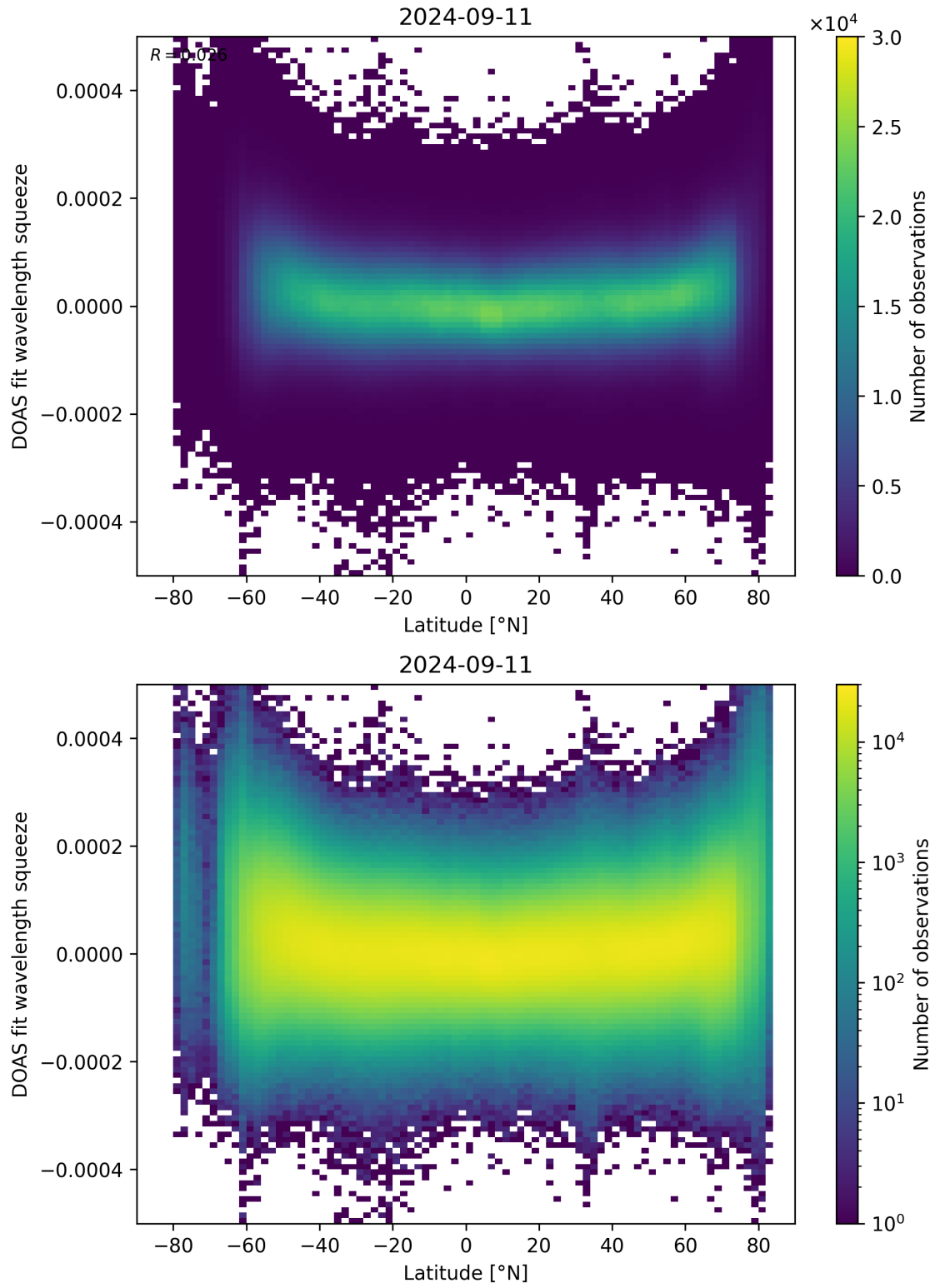
Figure 155: Scatter density plot of “Latitude” against “DOAS fit wavelength squeeze” for 2024-09-10 to 2024-09-12.
