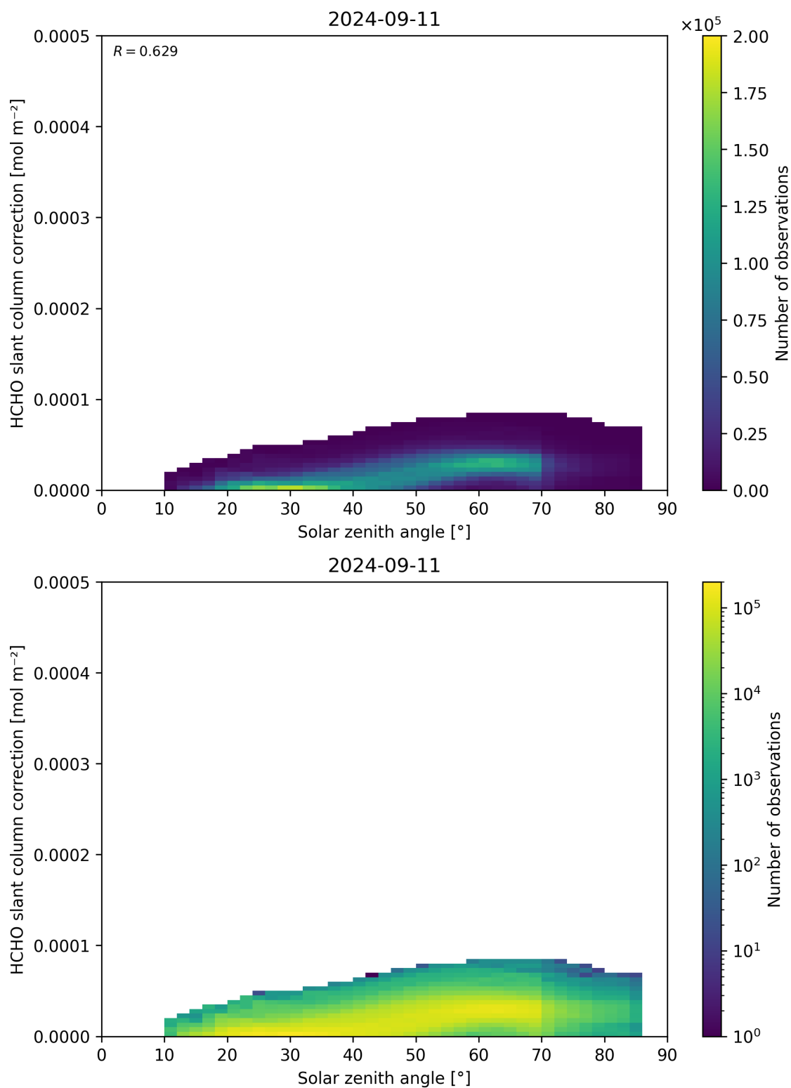
Figure 172: Scatter density plot of “Solar zenith angle” against “HCHO slant column correction” for 2024-09-10 to 2024-09-12.
