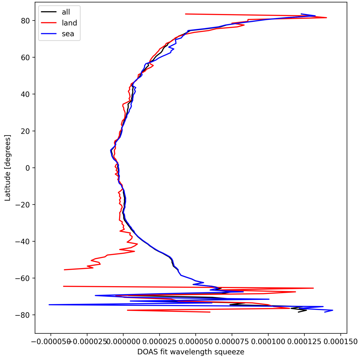
Figure 31: Zonal average of "DOAS fit wavelength squeeze" for 2024-09-10 to 2024-09-12.
