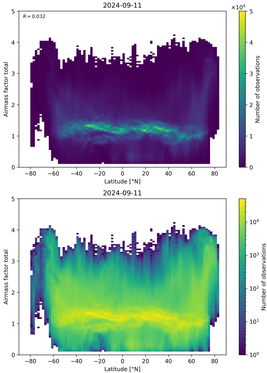
Figure 161: Scatter density plot of “Latitude” against “Airmass factor total” for 2024-09-10 to 2024-09-12.
