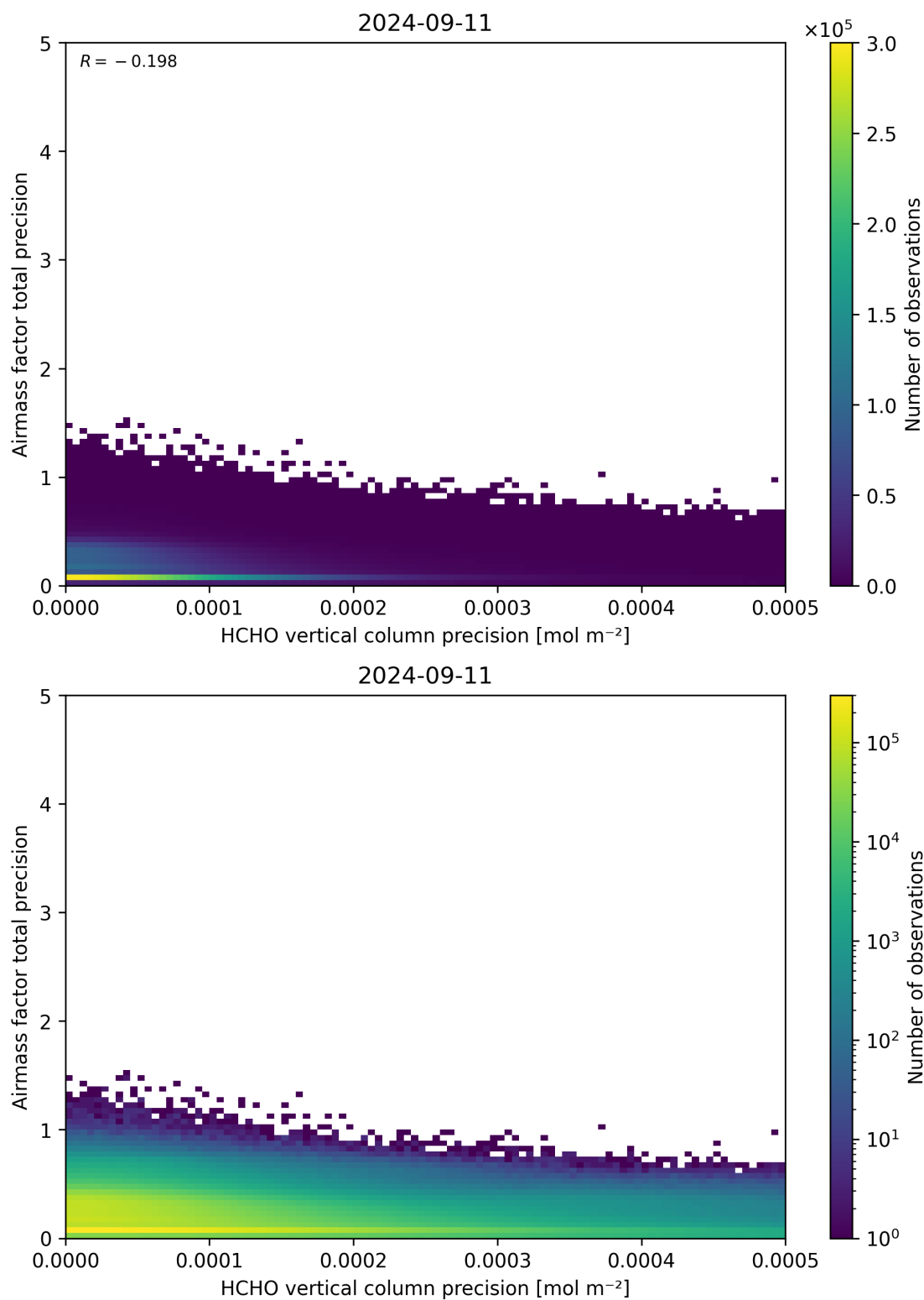
Figure 145: Scatter density plot of “HCHO vertical column precision” against “Airmass factor total precision” for 2024-09-10 to 2024-09-12.
