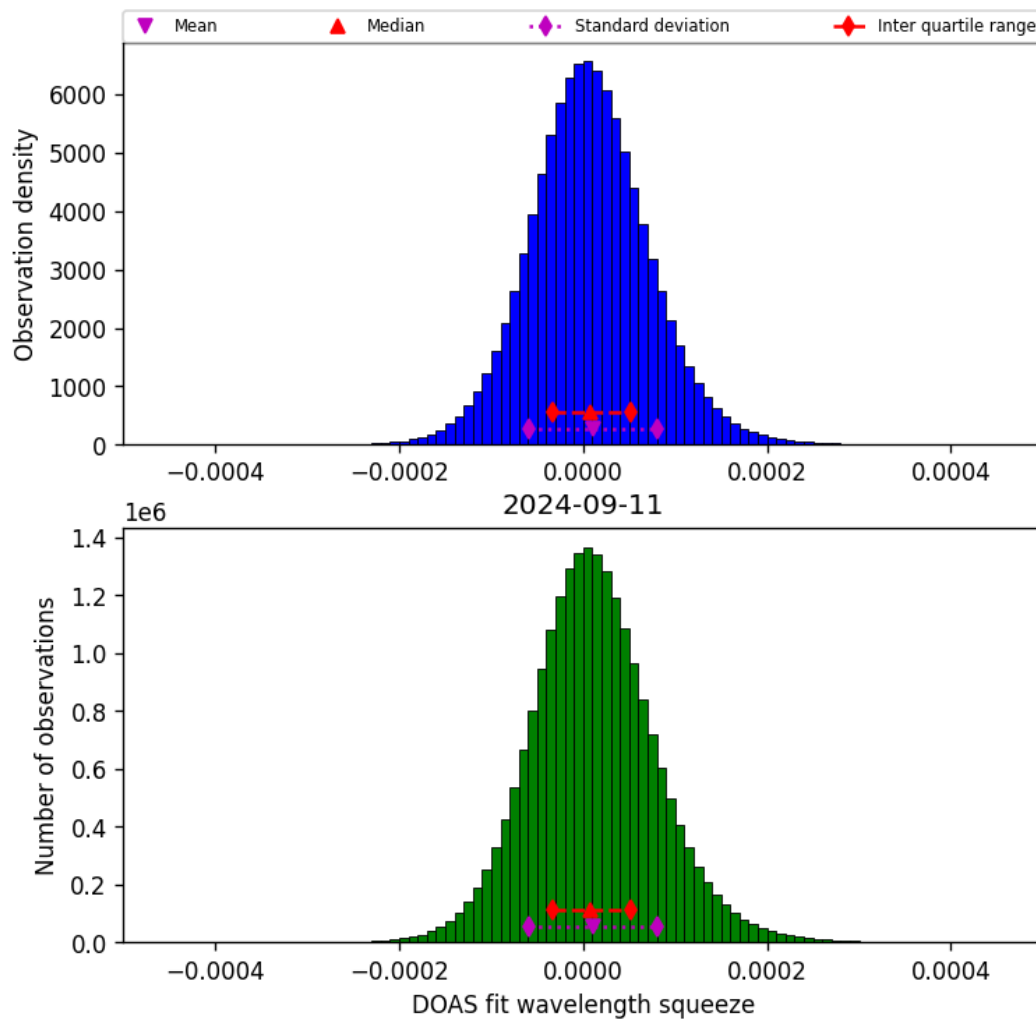
Figure 45: Histogram of “DOAS fit wavelength squeeze” for 2024-09-10 to 2024-09-12
