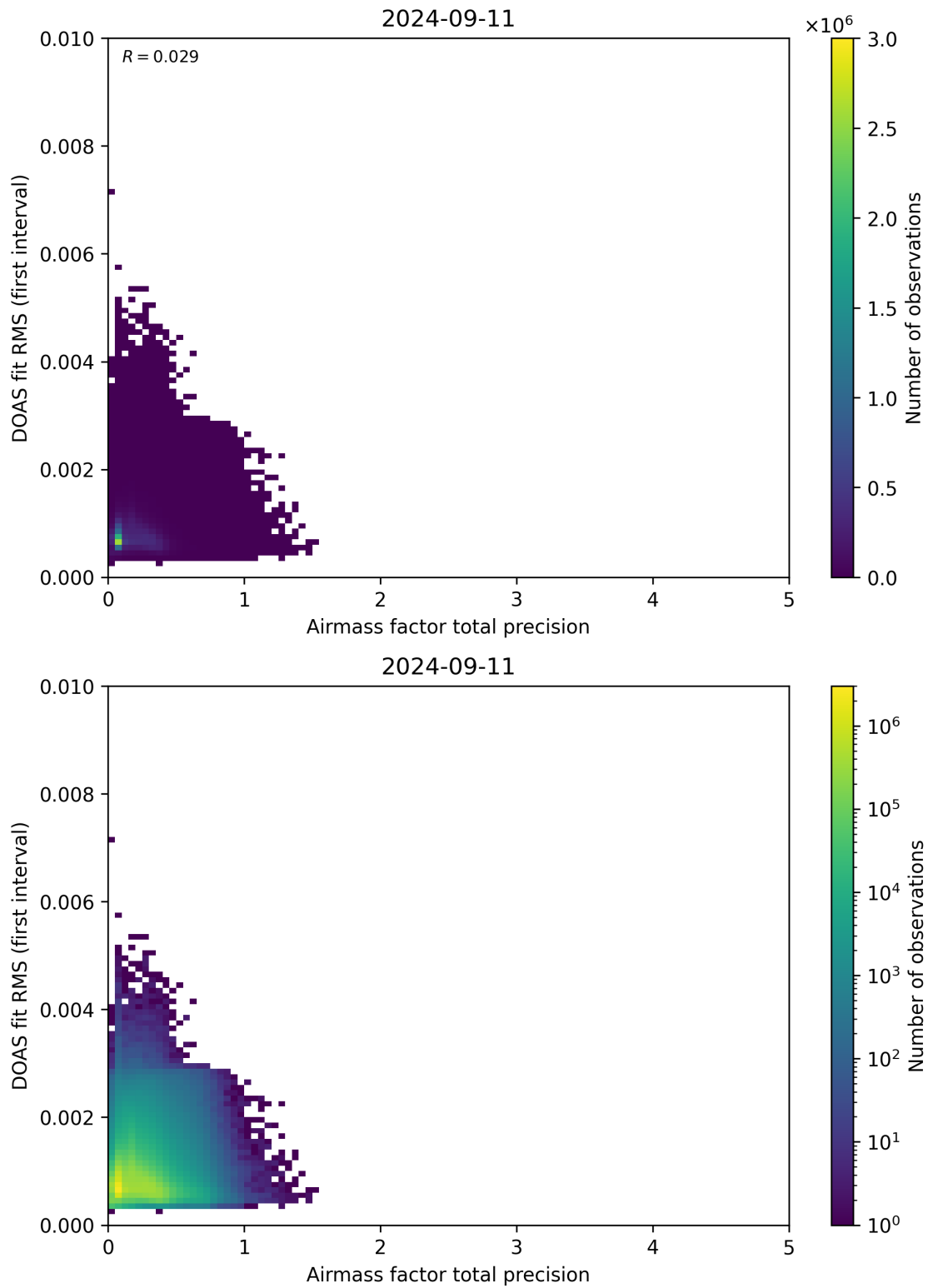
Figure 105: Scatter density plot of “Airmass factor total precision” against “DOAS fit RMS (first interval)” for 2024-09-10 to 2024-09-12.
