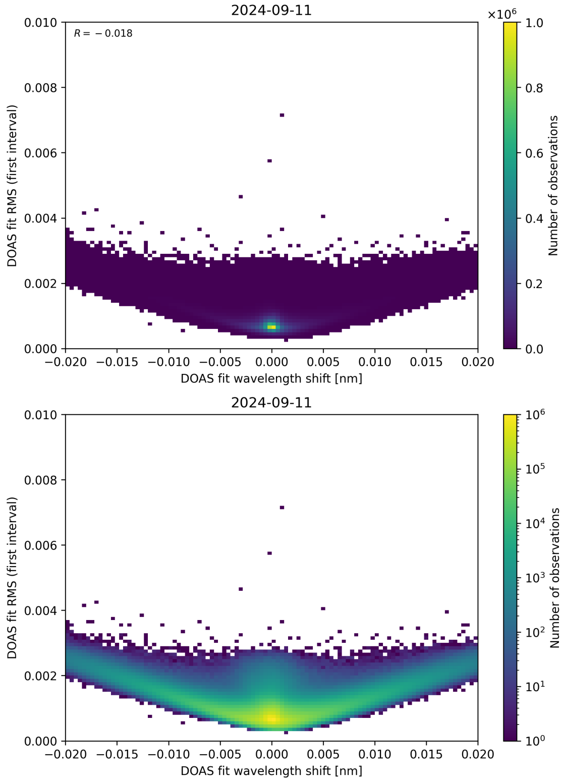
Figure 64: Scatter density plot of “DOAS fit wavelength shift” against “DOAS fit RMS (first interval)” for 2024-09-10 to 2024-09-12.
