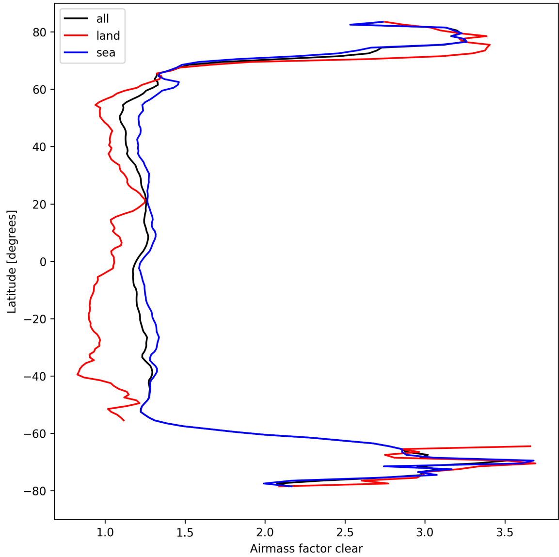
Figure 28: Zonal average of “Airmass factor clear” for 2024-09-10 to 2024-09-12.
