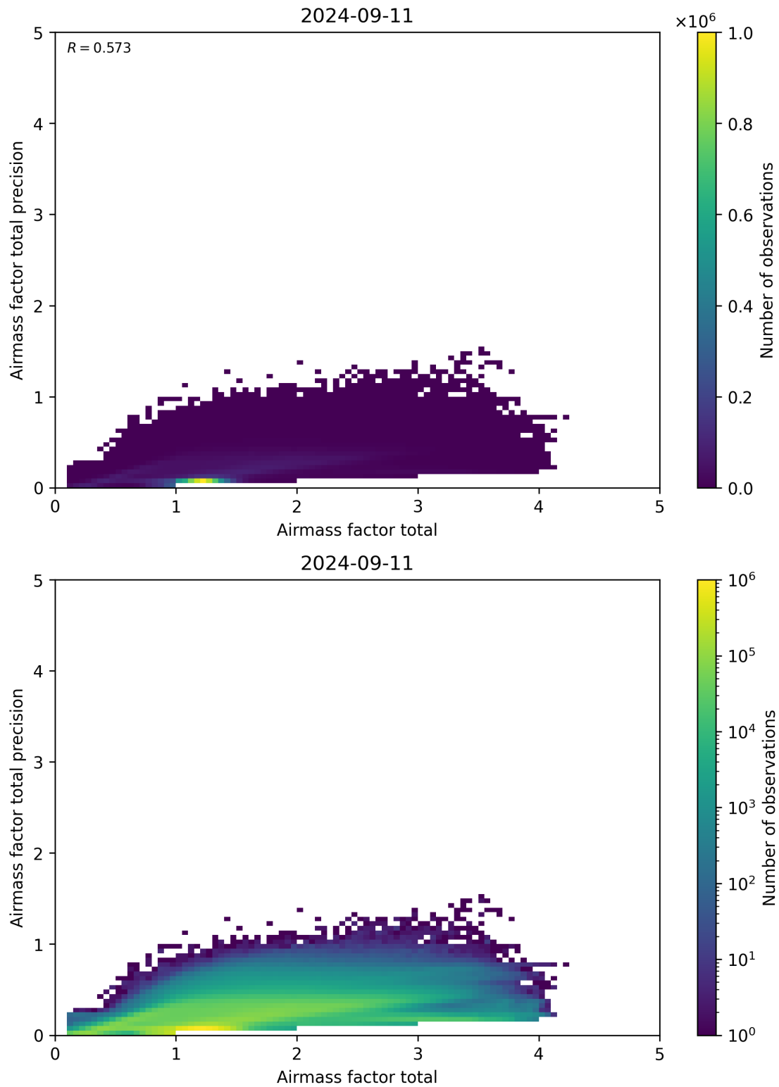
Figure 103: Scatter density plot of “Airmass factor total” against “Airmass factor total precision” for 2024-09-10 to 2024-09-12.
