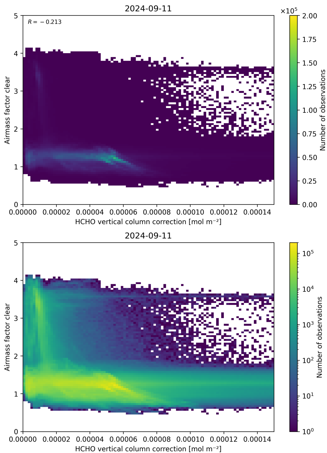
Figure 115: Scatter density plot of “HCHO vertical column correction” against “Airmass factor clear” for 2024-09-10 to 2024-09-12.
