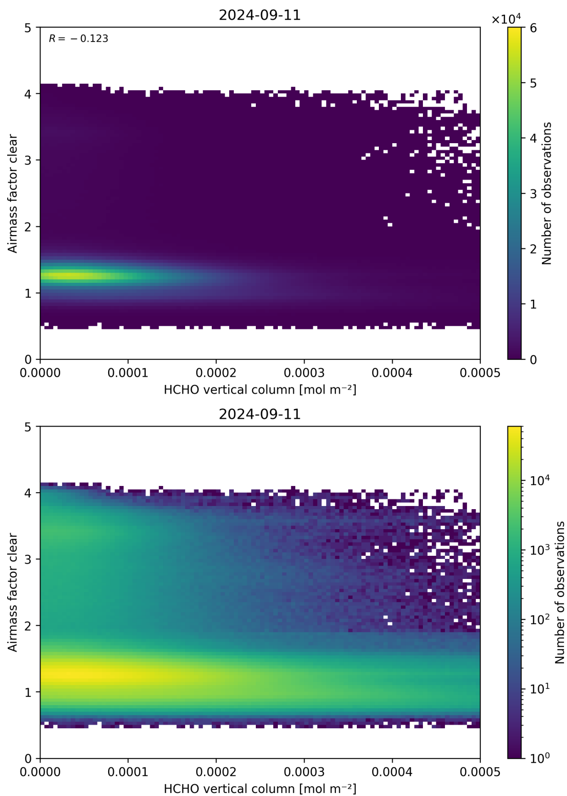
Figure 126: Scatter density plot of “HCHO vertical column” against “Airmass factor clear” for 2024-09-10 to 2024-09-12.
