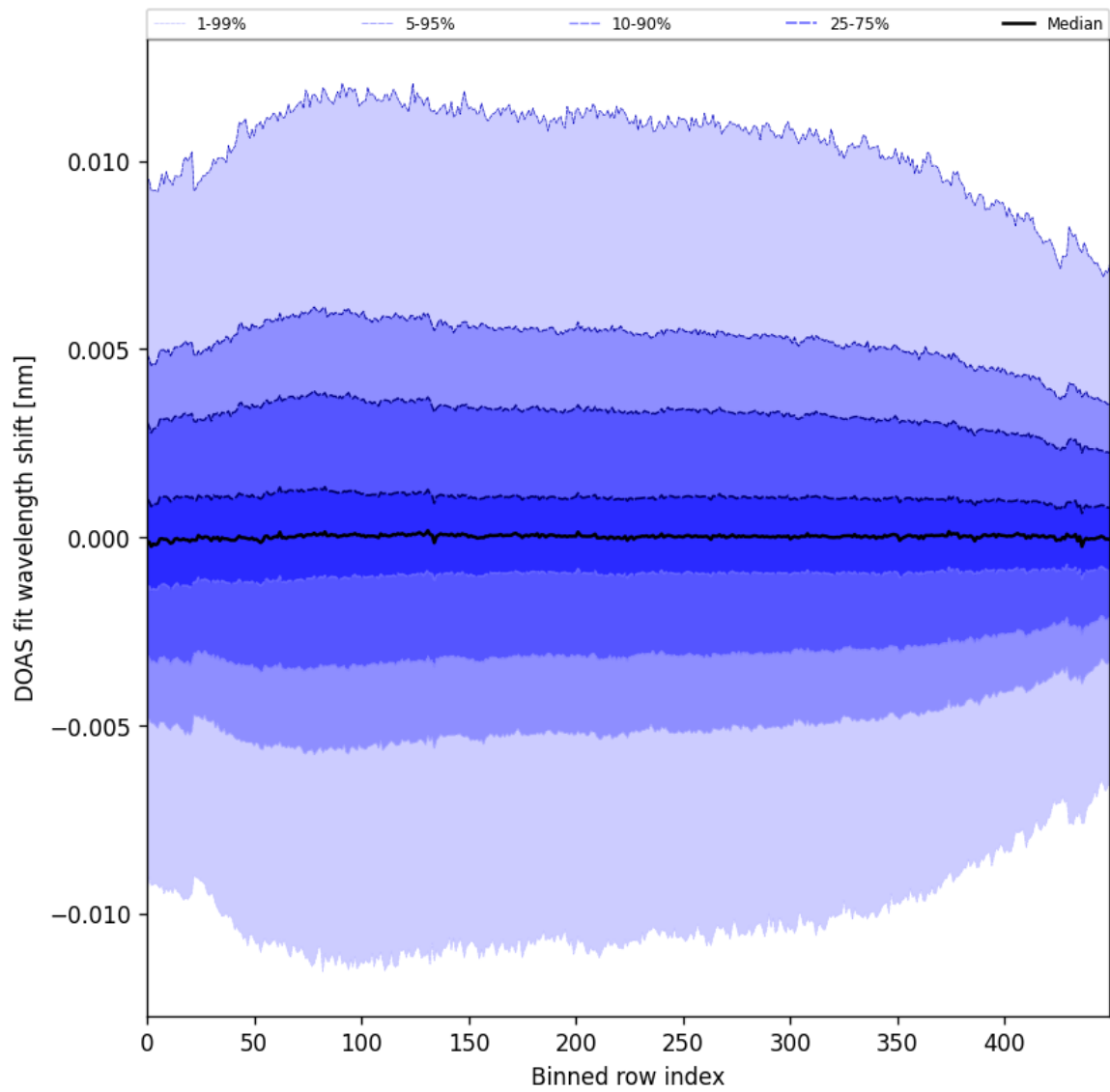
Figure 58: Along track statistics of “DOAS fit wavelength shift” for 2024-09-10 to 2024-09-12
