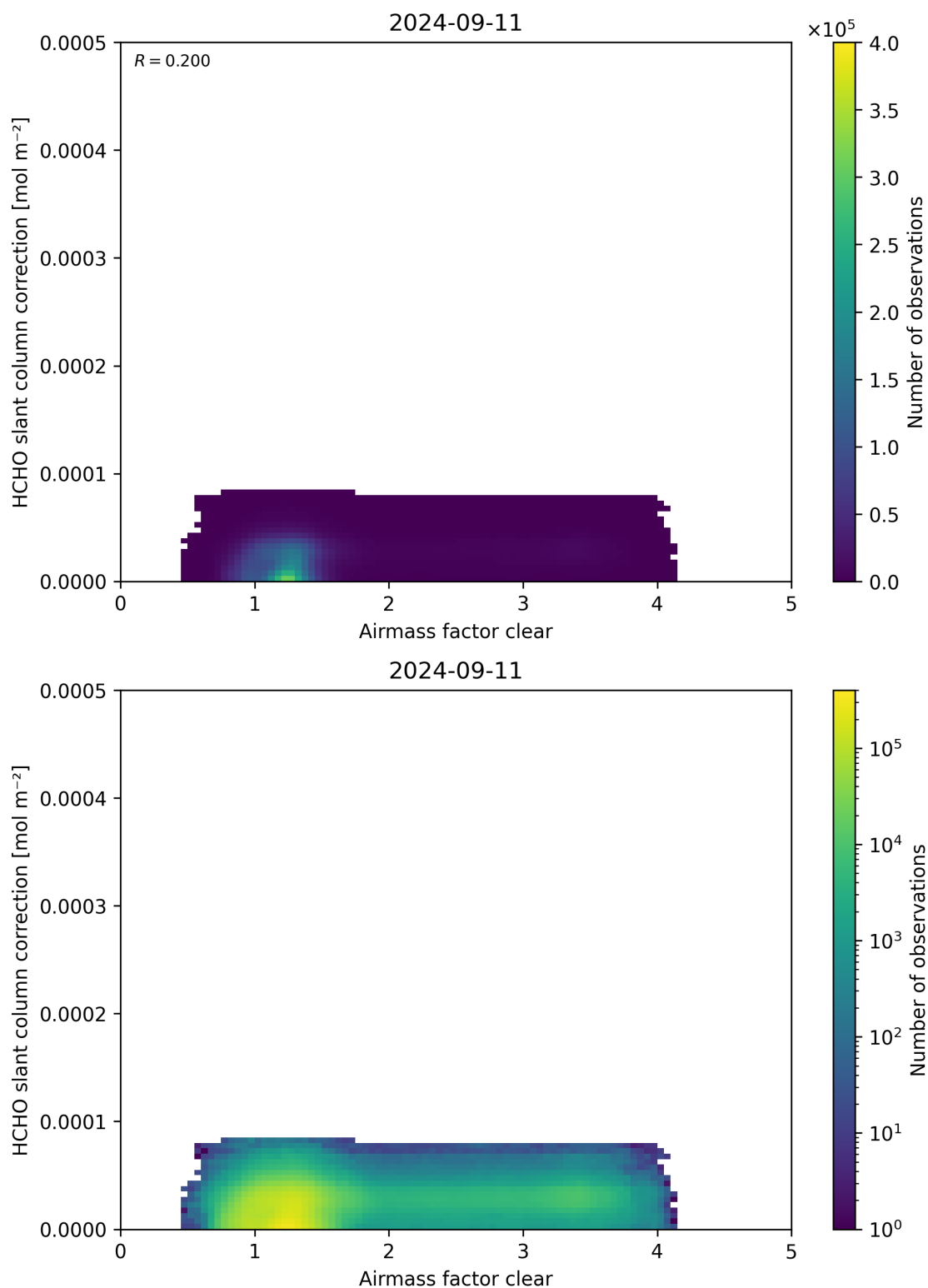
Figure 75: Scatter density plot of “Airmass factor clear” against “HCHO slant column correction” for 2024-09-10 to 2024-09-12.
