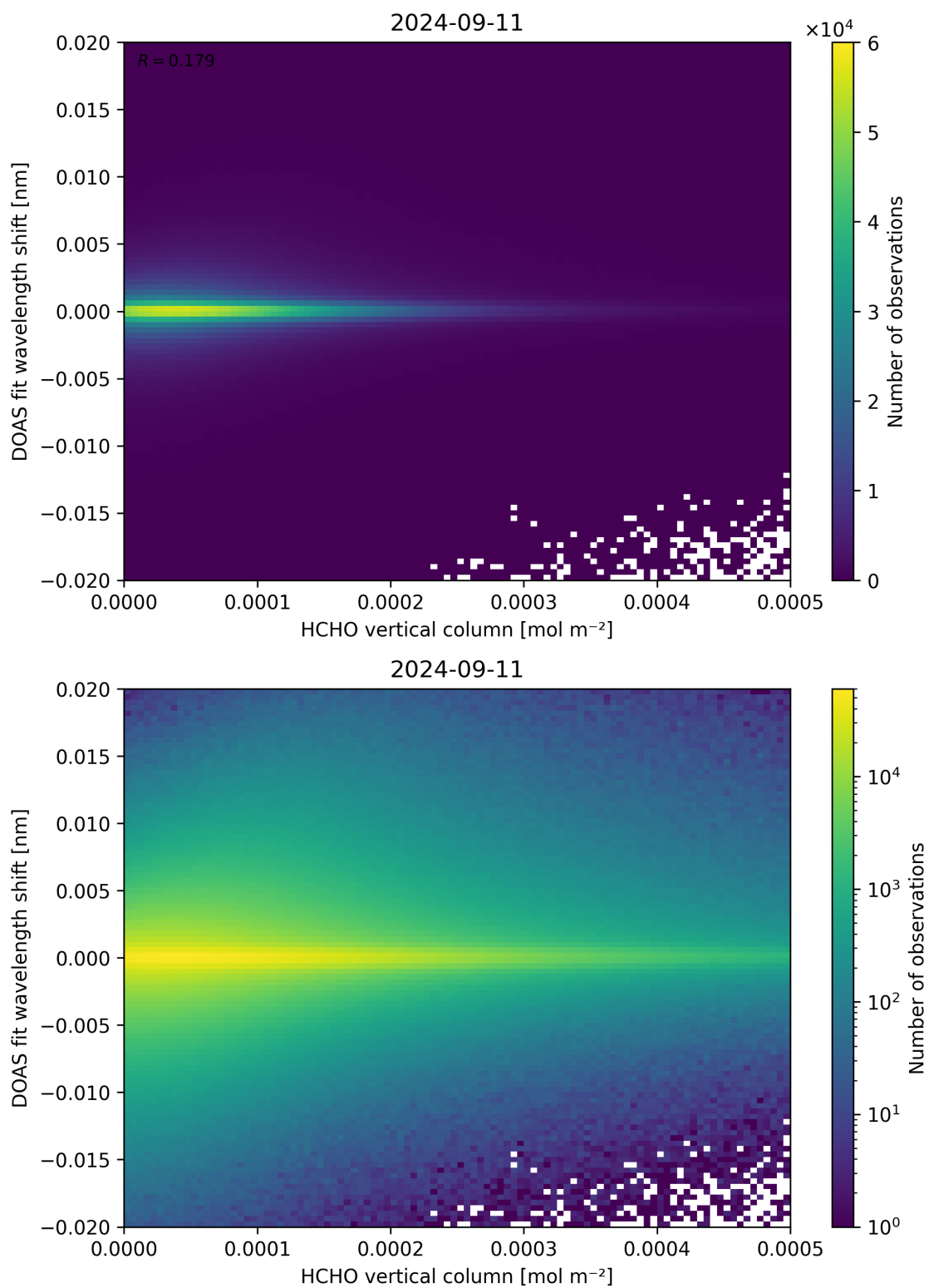
Figure 124: Scatter density plot of “HCHO vertical column” against “DOAS fit wavelength shift” for 2024-09-10 to 2024-09-12.
