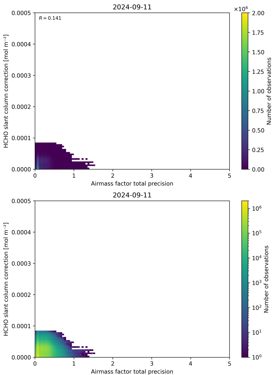
Figure 110: Scatter density plot of “Airmass factor total precision” against “HCHO slant column correction” for 2024-09-10 to 2024-09-12.
