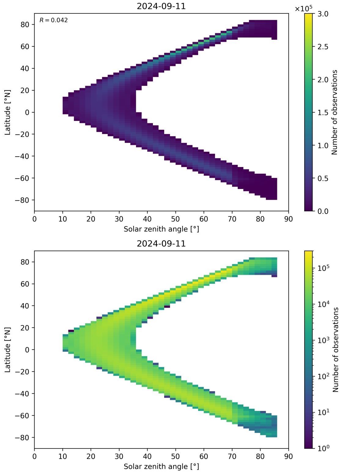
Figure 181: Scatter density plot of “Solar zenith angle” against “Latitude” for 2024-09-10 to 2024-09-12.
