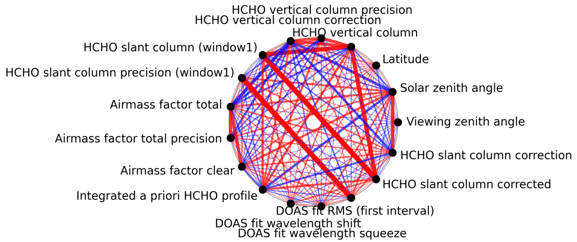
Figure 1: Map of correlation graph for 2024-09-10 to 2024-09-12.
