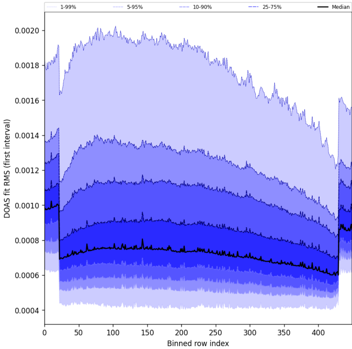
Figure 60: Along track statistics of “DOAS fit RMS (first interval)” for 2024-09-10 to 2024-09-12
