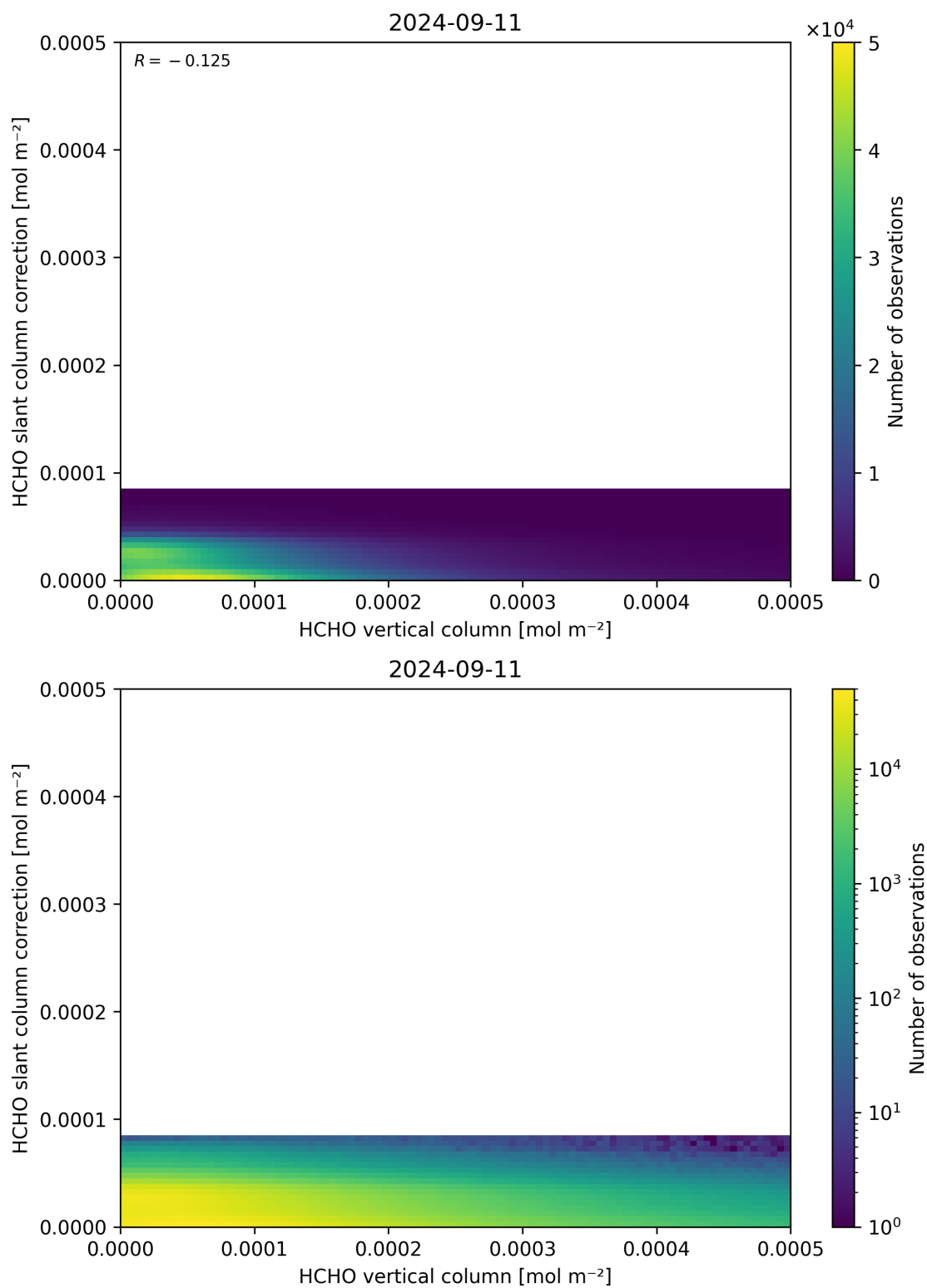
Figure 128: Scatter density plot of “HCHO vertical column” against “HCHO slant column correction” for 2024-09-10 to 2024-09-12.
