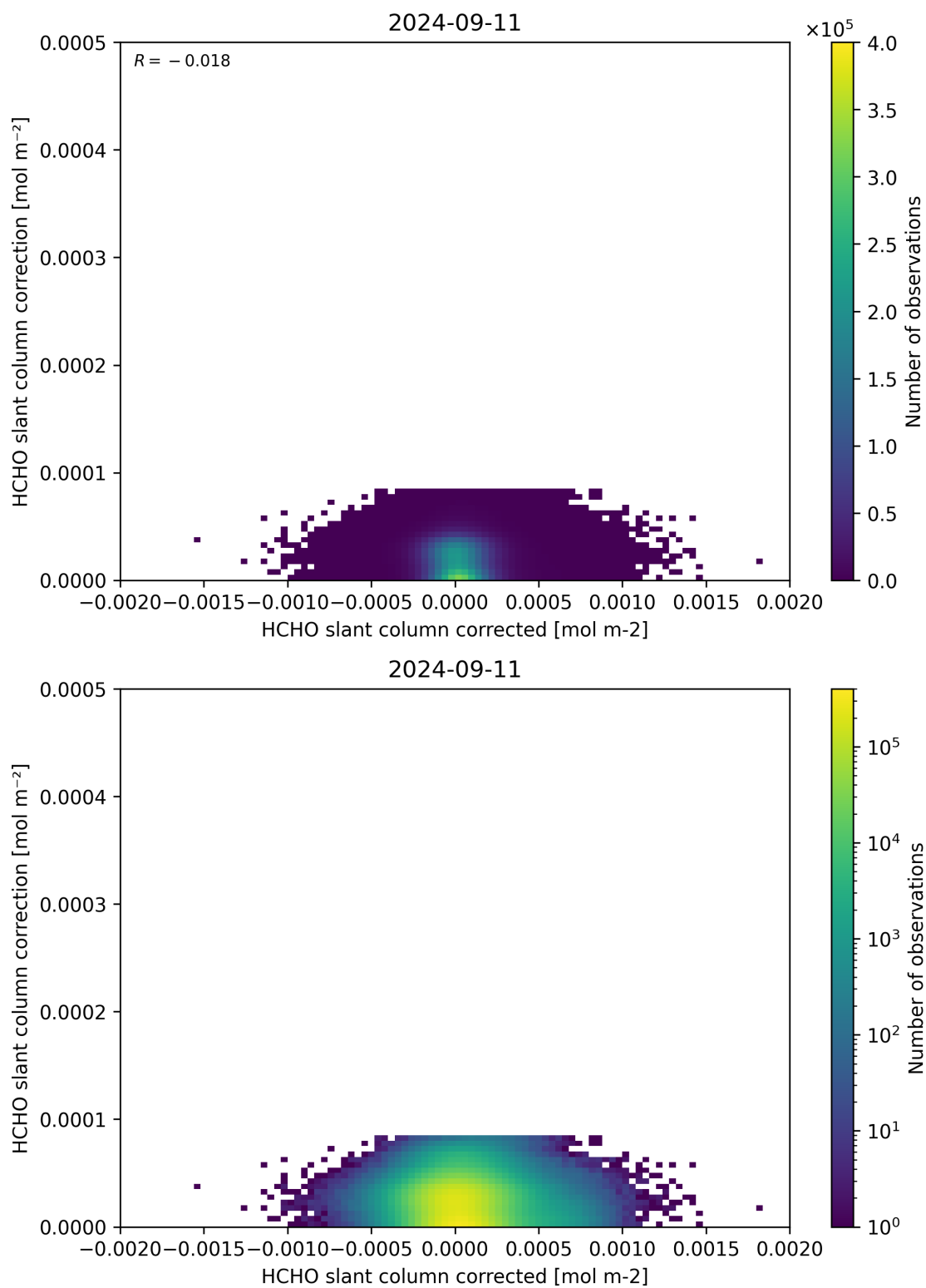
Figure 77: Scatter density plot of “HCHO slant column corrected” against “HCHO slant column correction” for 2024-09-10 to 2024-09-12.
