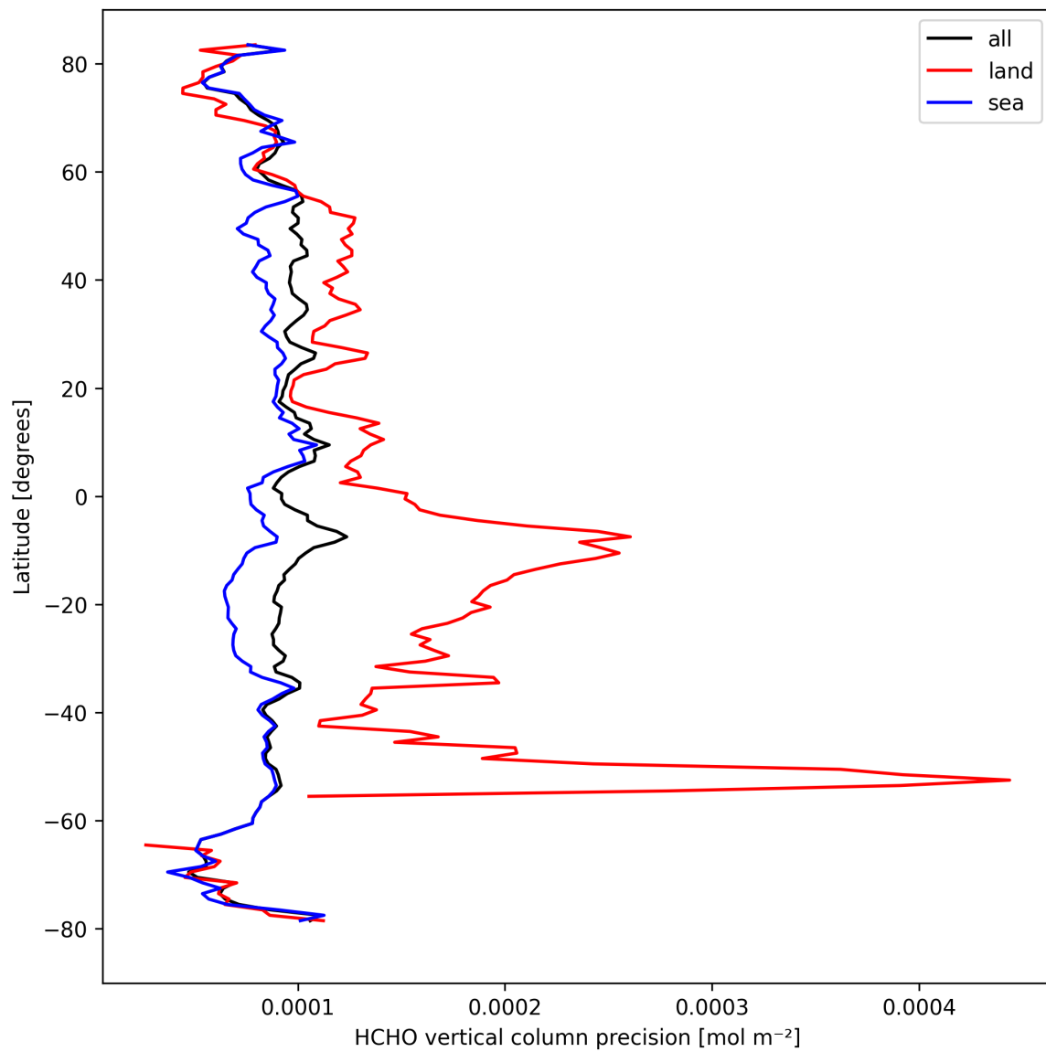
Figure 22: Zonal average of “HCHO vertical column precision” for 2024-09-10 to 2024-09-12.
