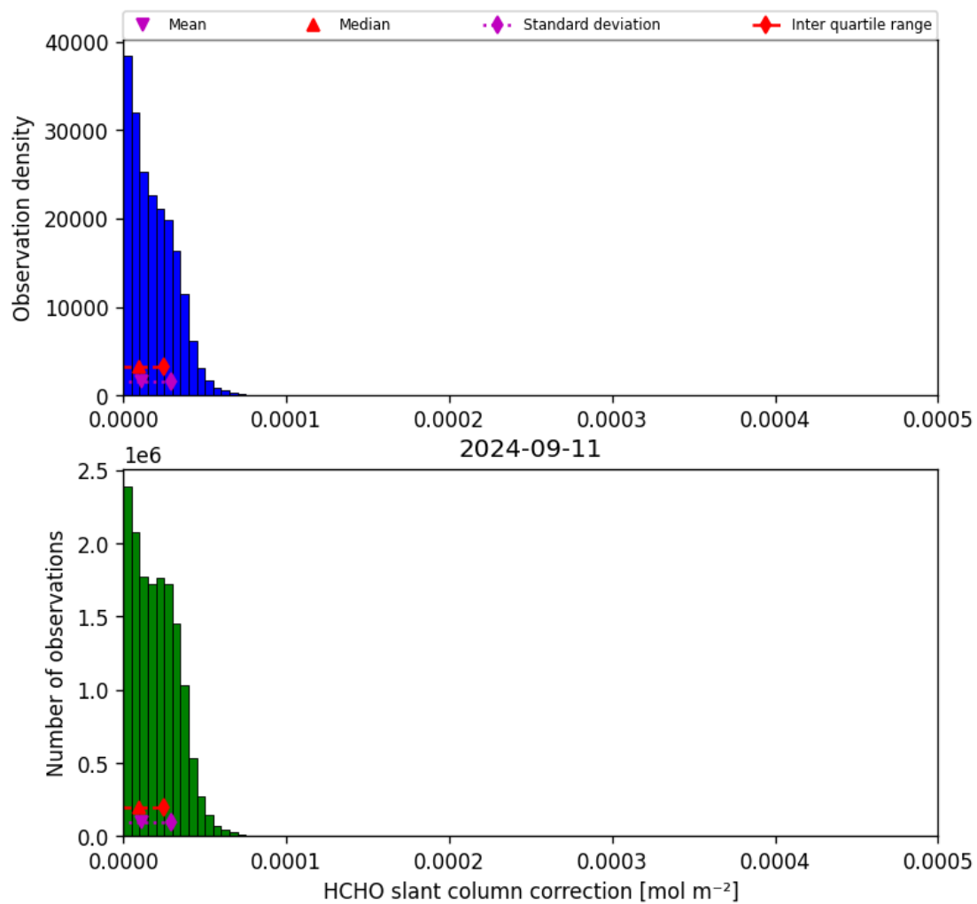
Figure 47: Histogram of “HCHO slant column correction” for 2024-09-10 to 2024-09-12
