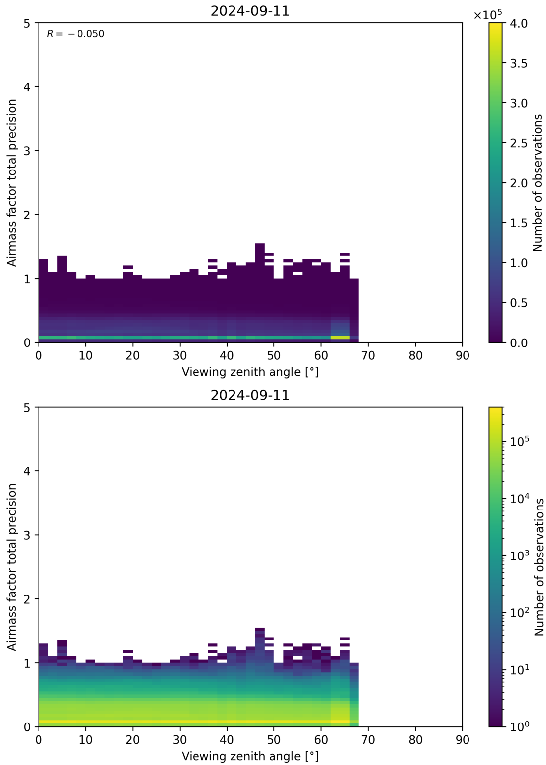
Figure 191: Scatter density plot of “Viewing zenith angle” against “Airmass factor total precision” for 2024-09-10 to 2024-09-12.
