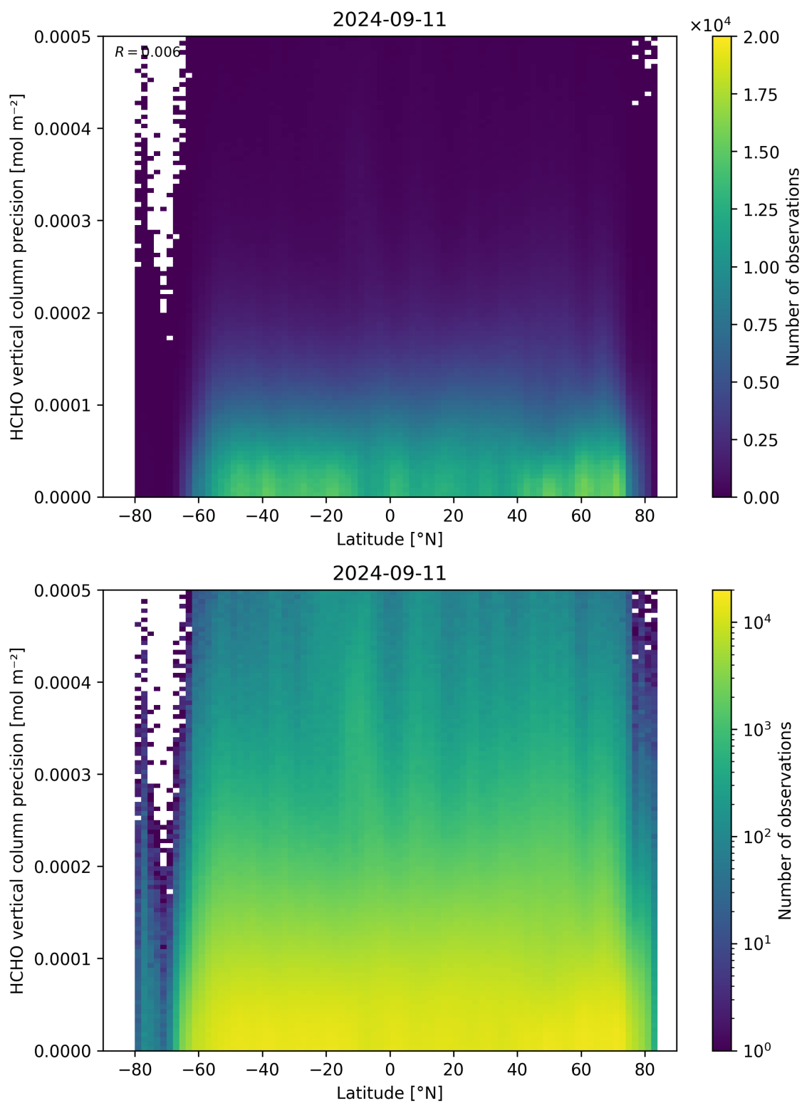
Figure 165: Scatter density plot of “Latitude” against “HCHO vertical column precision” for 2024-09-10 to 2024-09-12.
