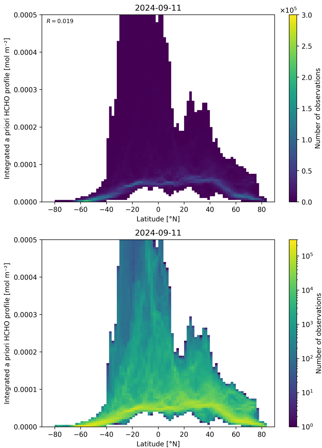
Figure 166: Scatter density plot of “Latitude” against “Integrated a priori HCHO profile” for 2024-09-10 to 2024-09-12.
