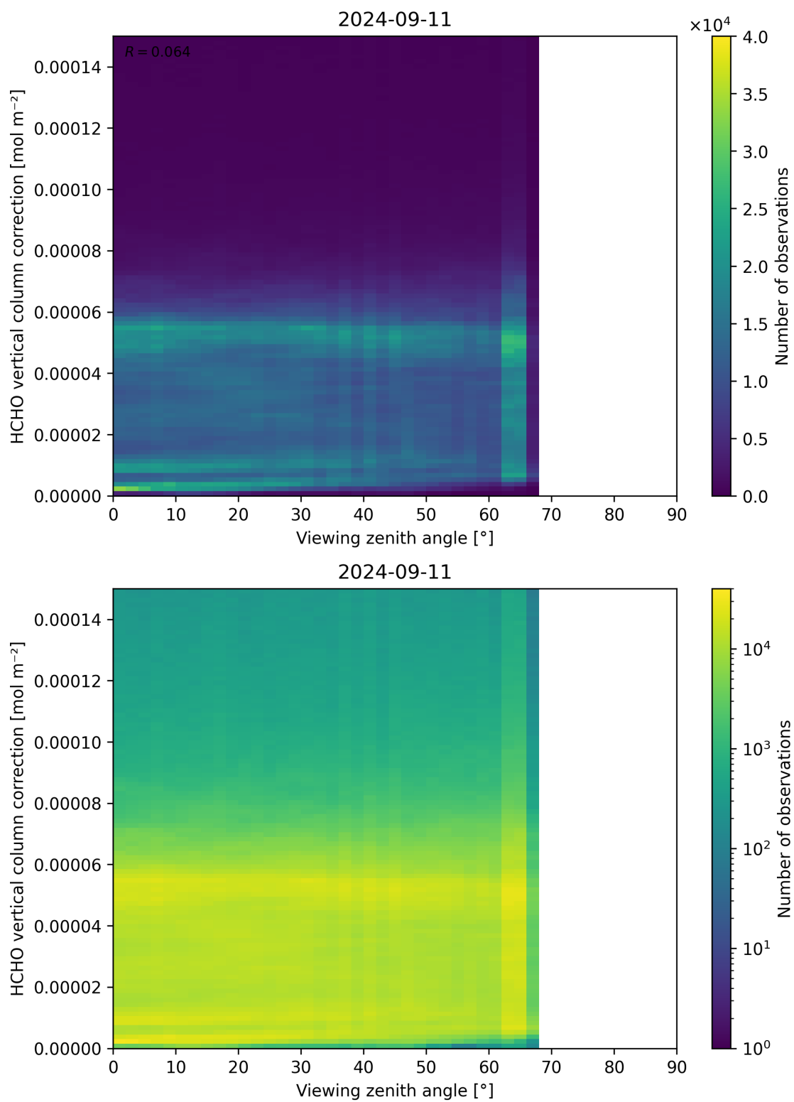
Figure 193: Scatter density plot of “Viewing zenith angle” against “HCHO vertical column correction” for 2024-09-10 to 2024-09-12.
