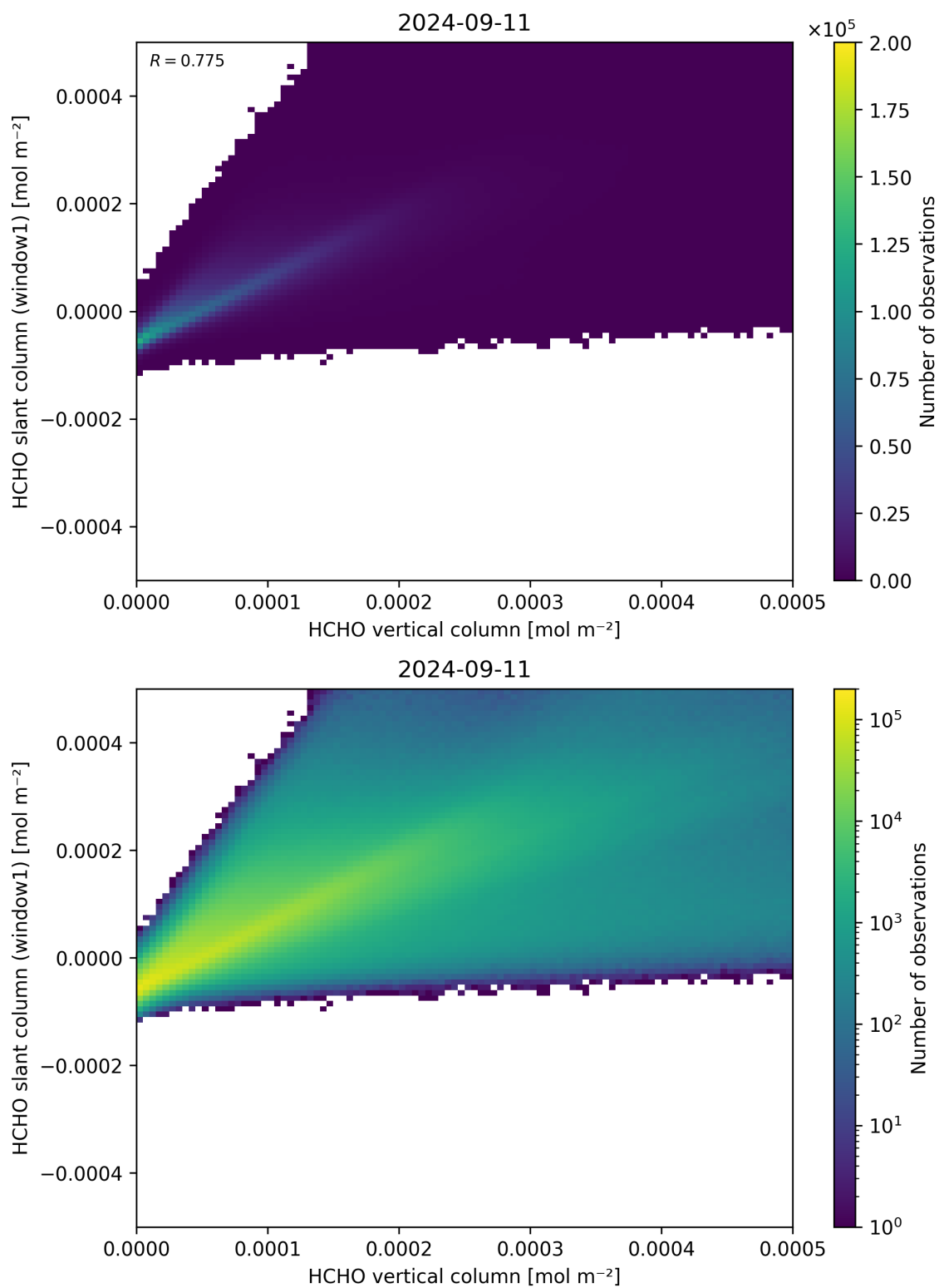
Figure 129: Scatter density plot of “HCHO vertical column” against “HCHO slant column (window1)” for 2024-09-10 to 2024-09-12.
