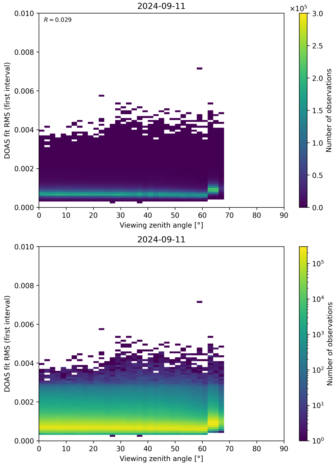
Figure 182: Scatter density plot of “Viewing zenith angle” against “DOAS fit RMS (first interval)” for 2024-09-10 to 2024-09-12.
