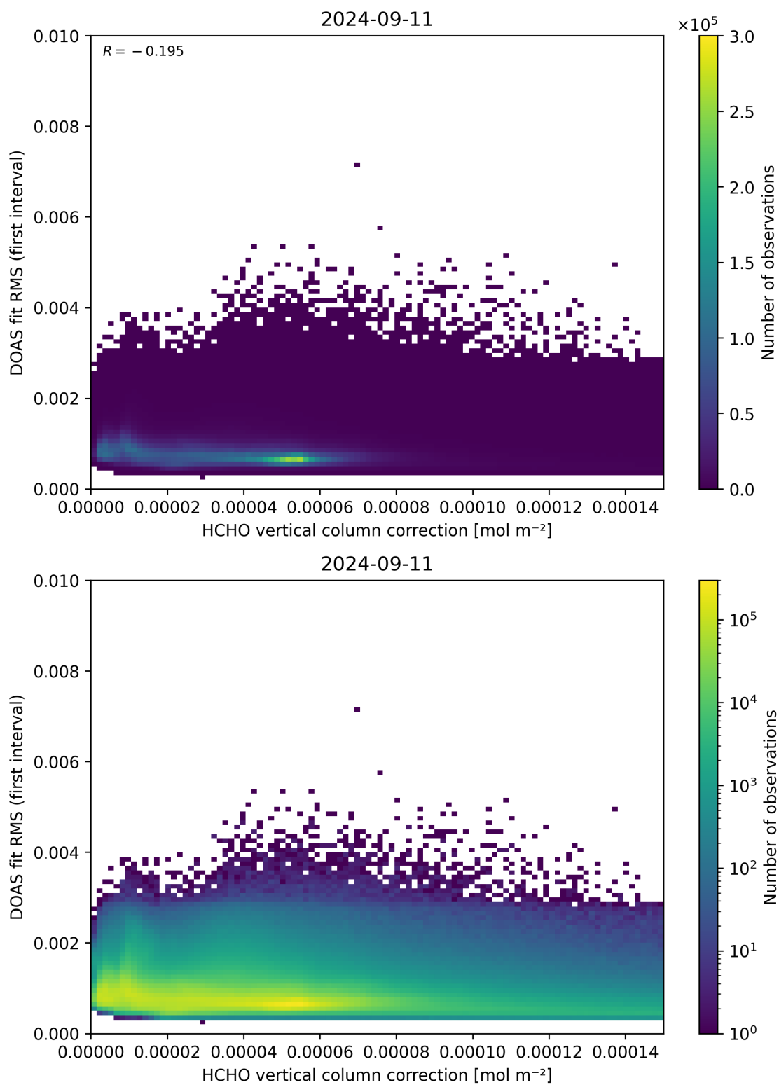
Figure 112: Scatter density plot of “HCHO vertical column correction” against “DOAS fit RMS (first interval)” for 2024-09-10 to 2024-09-12.
