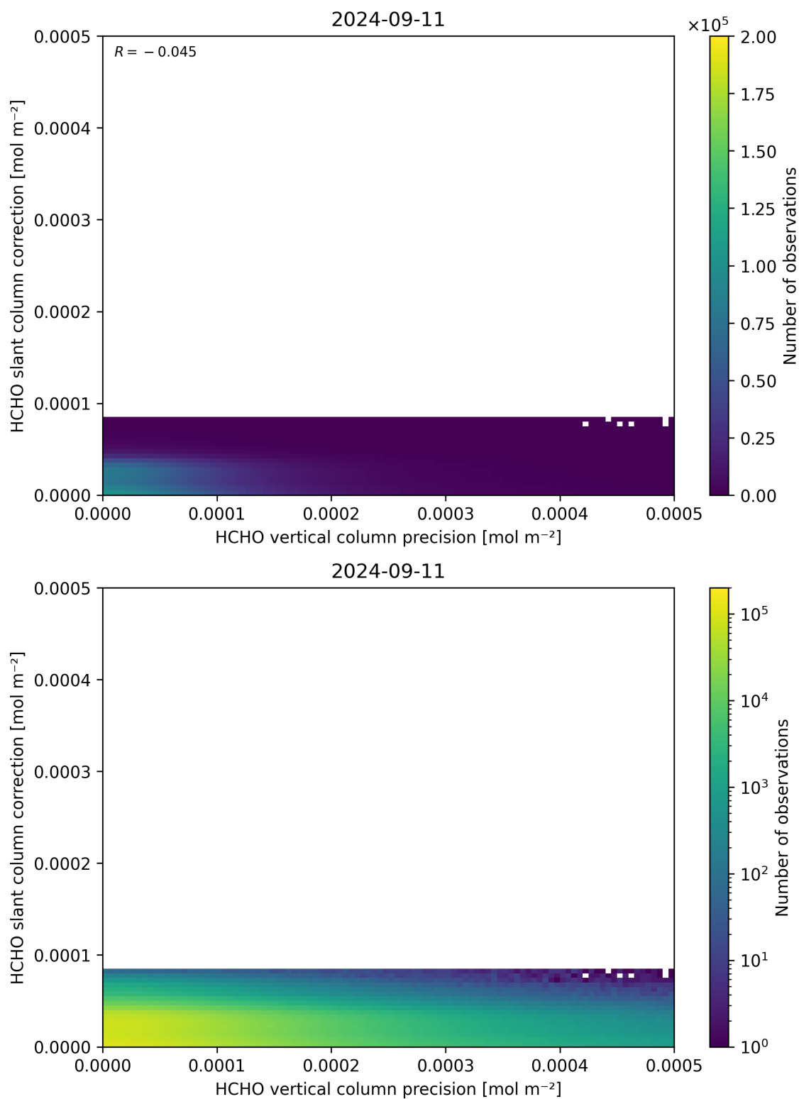
Figure 141: Scatter density plot of “HCHO vertical column precision” against “HCHO slant column correction” for 2024-09-10 to 2024-09-12.
