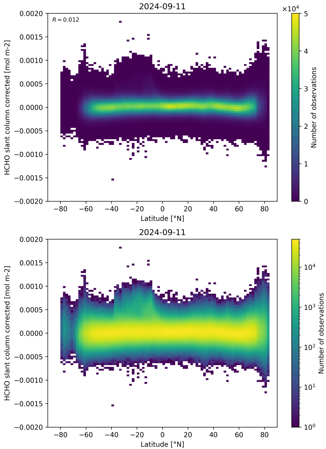
Figure 157: Scatter density plot of “Latitude” against “HCHO slant column corrected” for 2024-09-10 to 2024-09-12.
