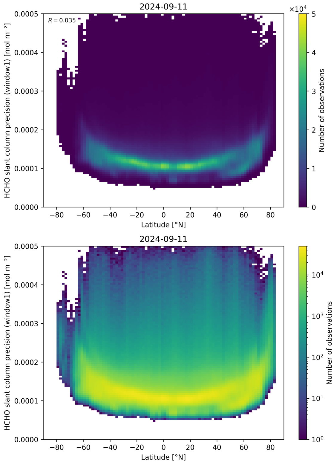
Figure 160: Scatter density plot of “Latitude” against “HCHO slant column precision (window1)” for 2024-09-10 to 2024-09-12.
