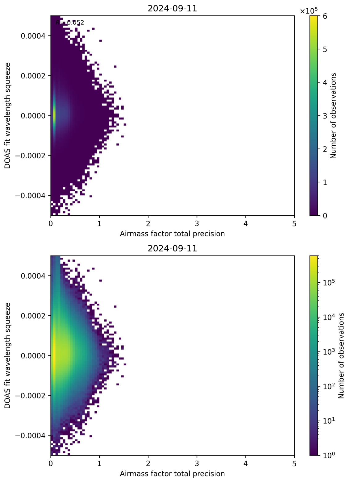
Figure 107: Scatter density plot of “Airmass factor total precision” against “DOAS fit wavelength squeeze” for 2024-09-10 to 2024-09-12.
