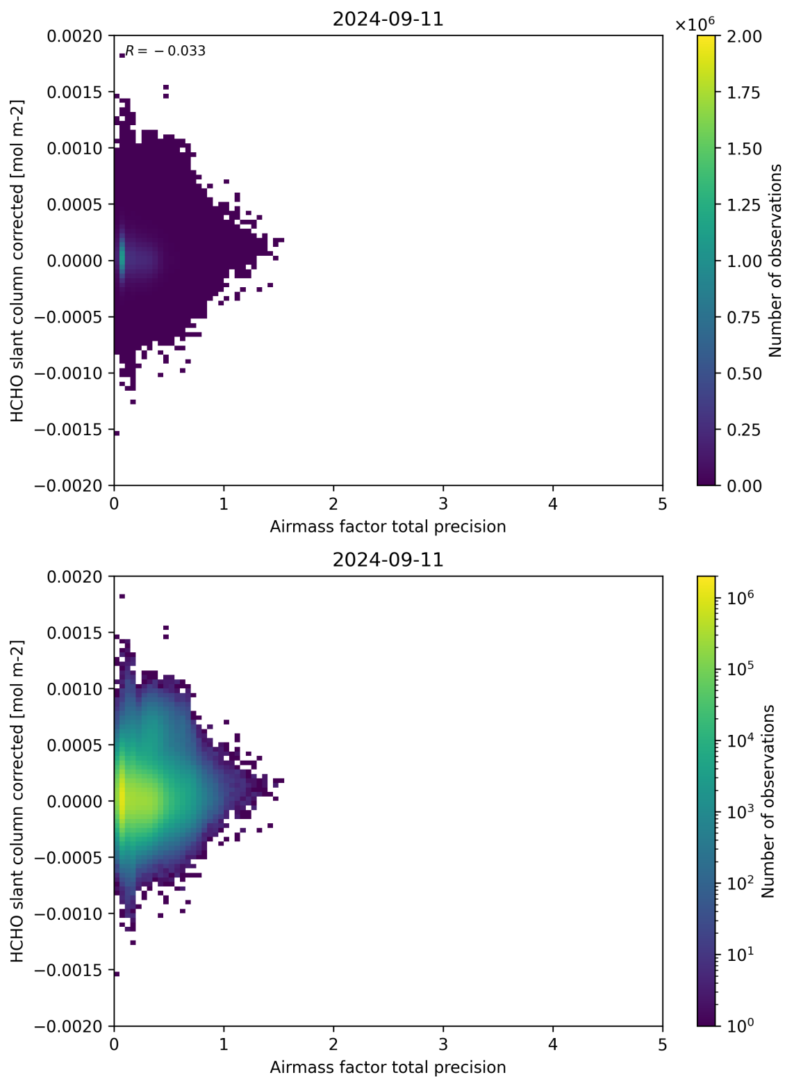
Figure 109: Scatter density plot of “Airmass factor total precision” against “HCHO slant column corrected” for 2024-09-10 to 2024-09-12.
