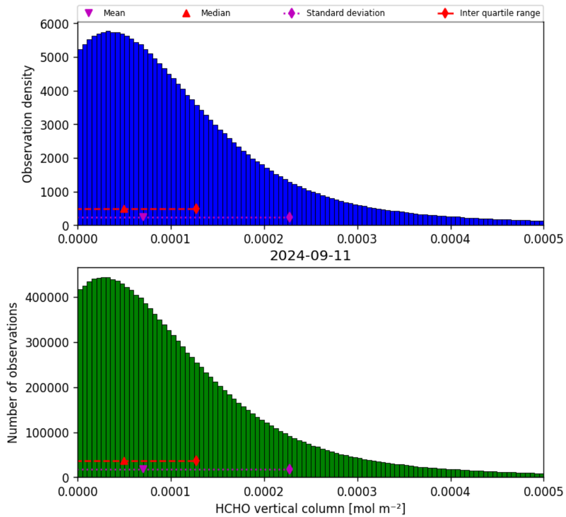
Figure 35: Histogram of “HCHO vertical column” for 2024-09-10 to 2024-09-12
