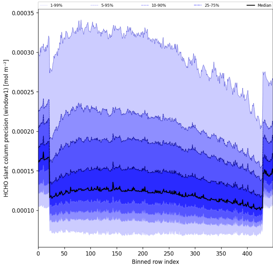
Figure 53: Along track statistics of “HCHO slant column precision (window1)” for 2024-09-10 to 2024-09-12
