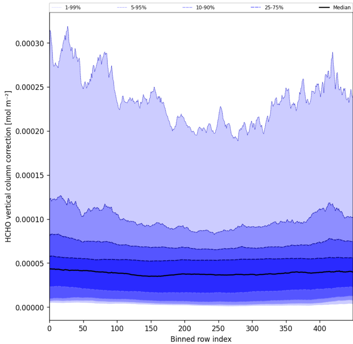
Figure 51: Along track statistics of “HCHO vertical column correction” for 2024-09-10 to 2024-09-12
