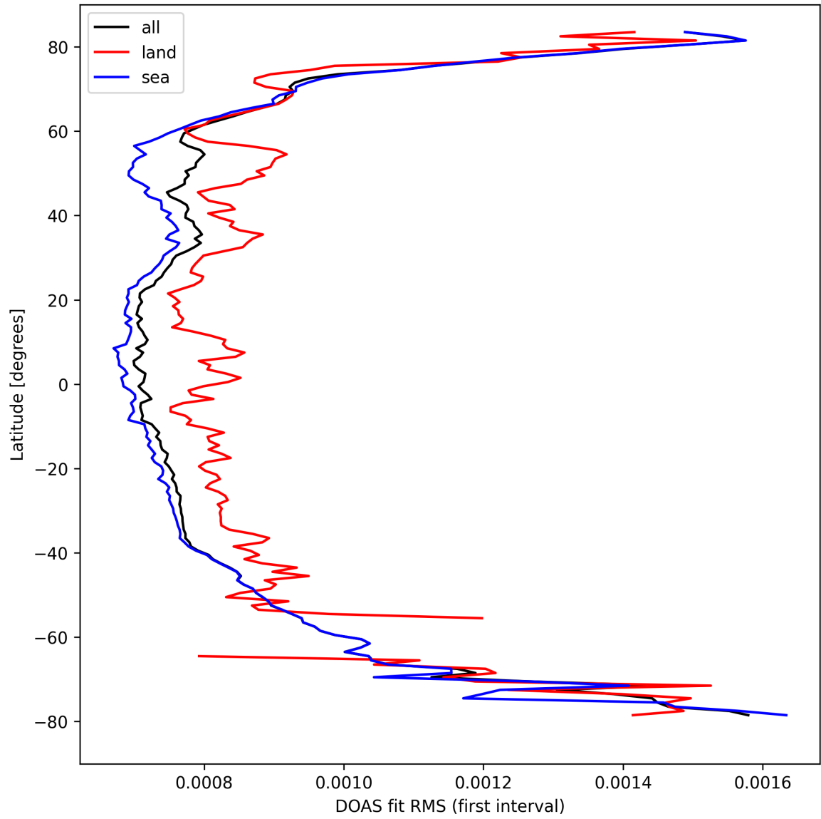
Figure 32: Zonal average of “DOAS fit RMS (first interval)” for 2024-09-10 to 2024-09-12.
