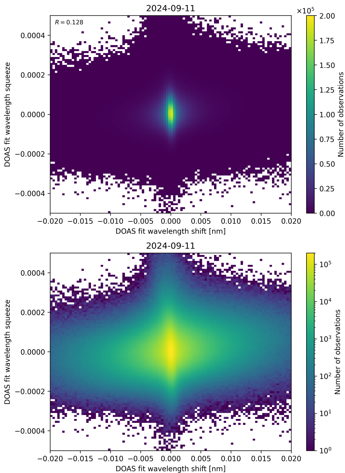
Figure 65: Scatter density plot of “DOAS fit wavelength shift” against “DOAS fit wavelength squeeze” for 2024-09-10 to 2024-09-12.
