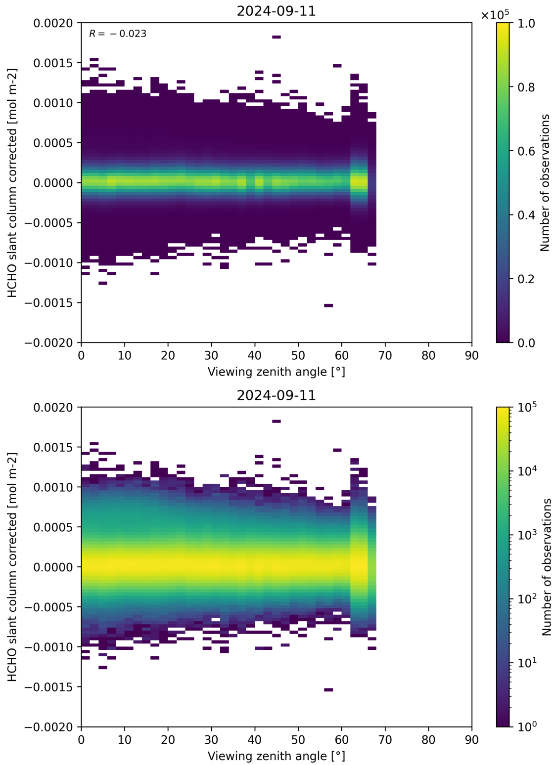
Figure 186: Scatter density plot of “Viewing zenith angle” against “HCHO slant column corrected” for 2024-09-10 to 2024-09-12.
