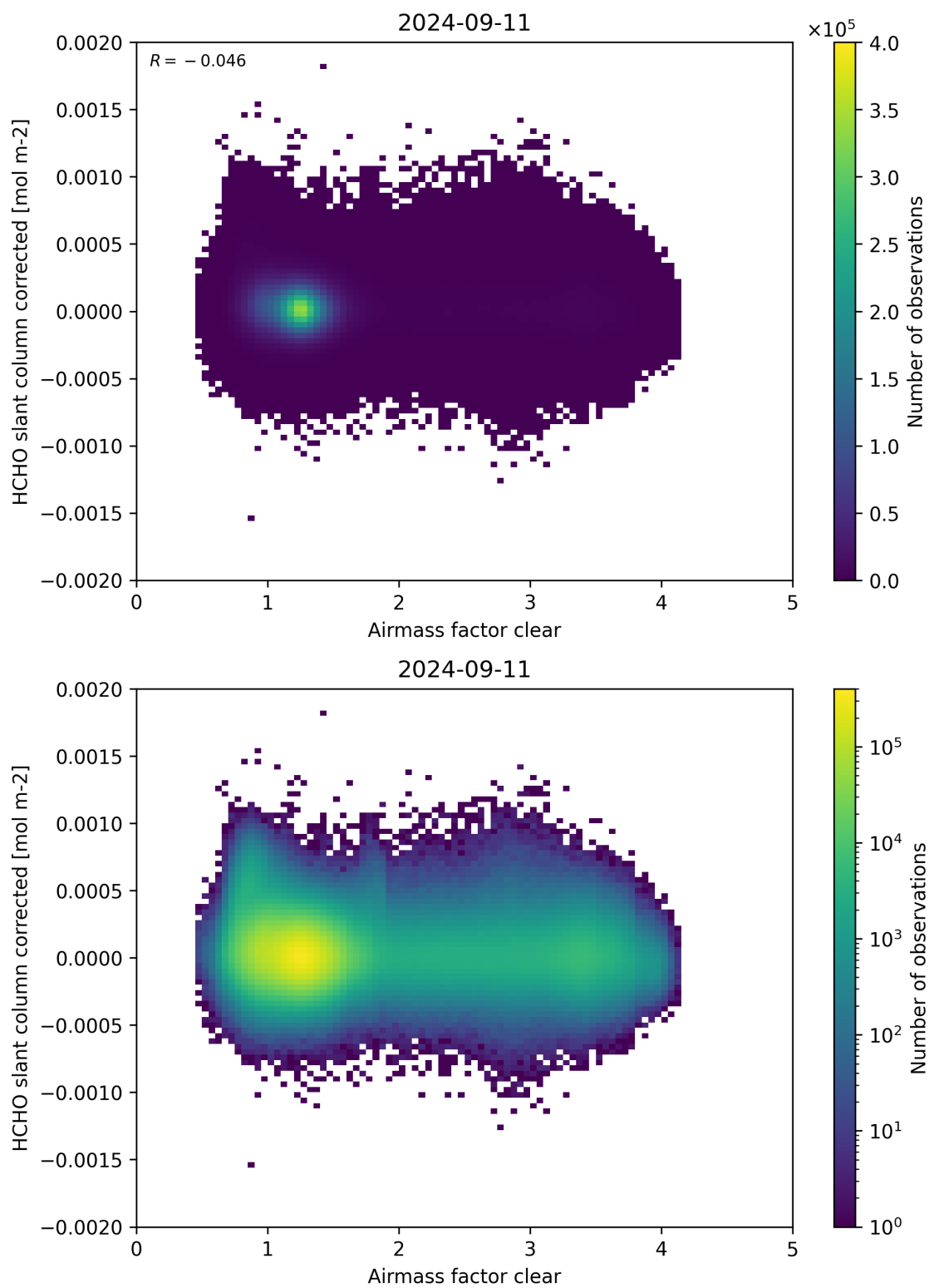
Figure 74: Scatter density plot of “Airmass factor clear” against “HCHO slant column corrected” for 2024-09-10 to 2024-09-12.
