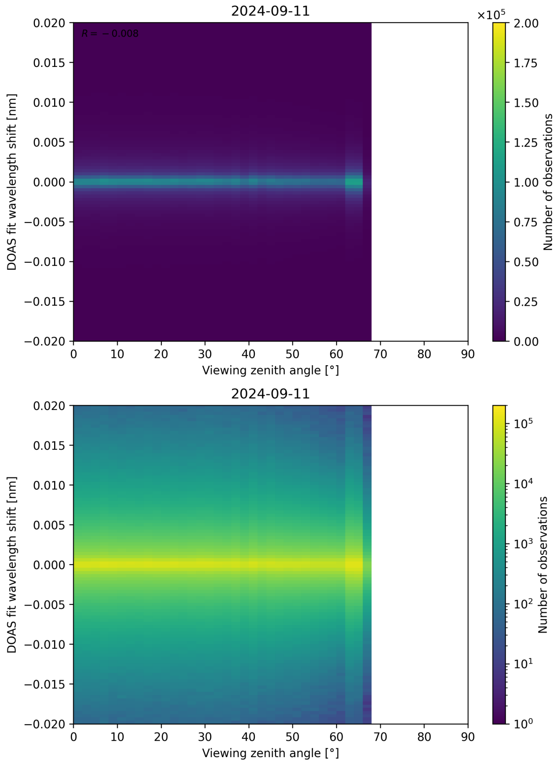
Figure 183: Scatter density plot of “Viewing zenith angle” against “DOAS fit wavelength shift” for 2024-09-10 to 2024-09-12.
