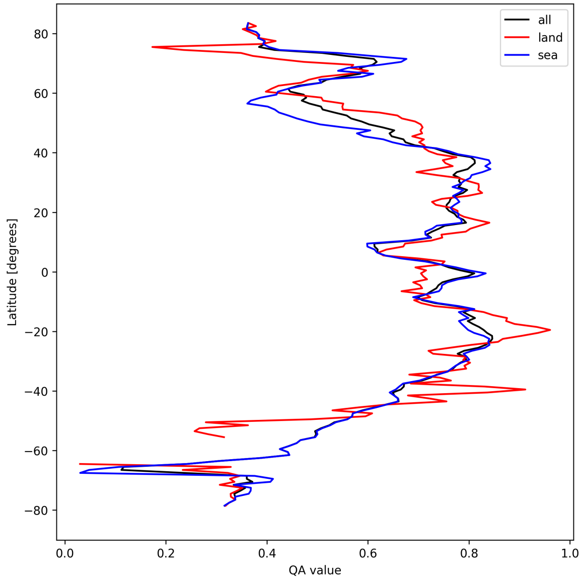
Figure 20: Zonal average of “QA value” for 2024-09-10 to 2024-09-12.
