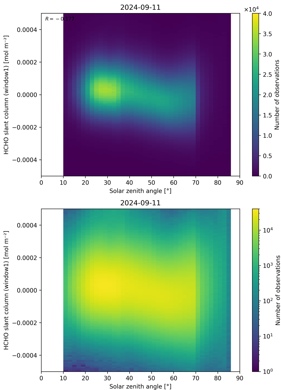
Figure 173: Scatter density plot of “Solar zenith angle” against “HCHO slant column (window1)” for 2024-09-10 to 2024-09-12.
