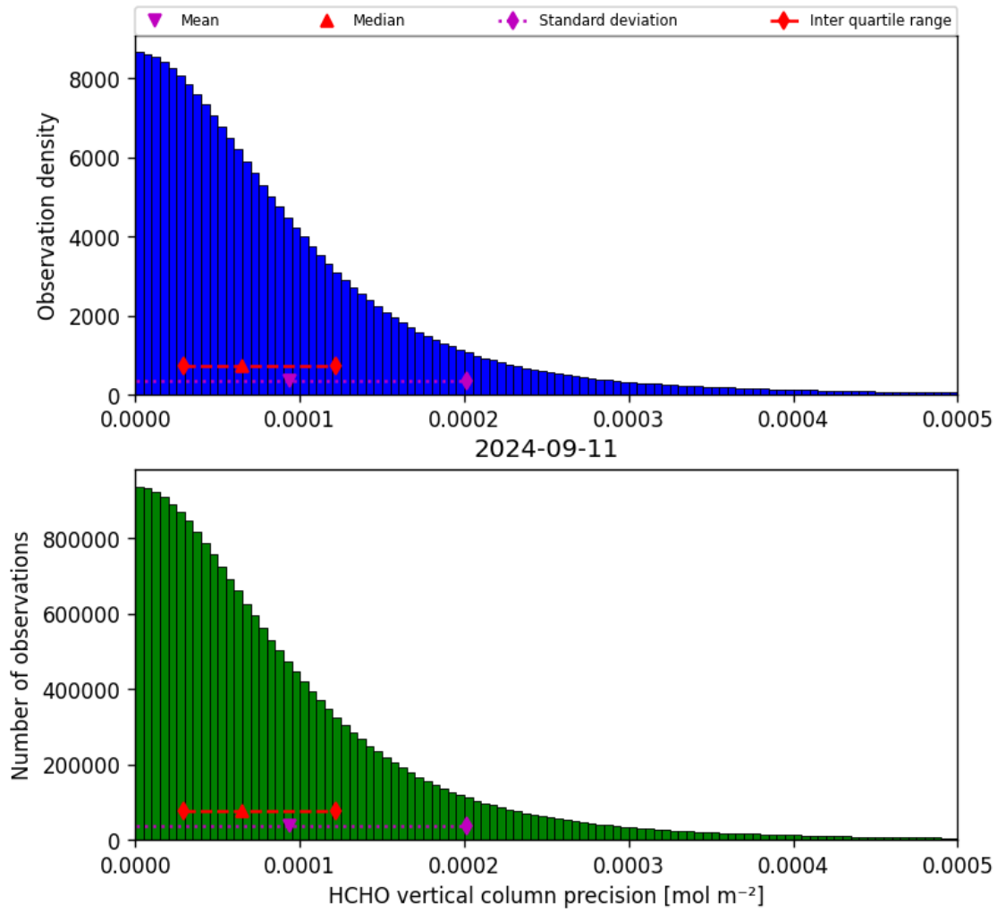
Figure 36: Histogram of “HCHO vertical column precision” for 2024-09-10 to 2024-09-12
