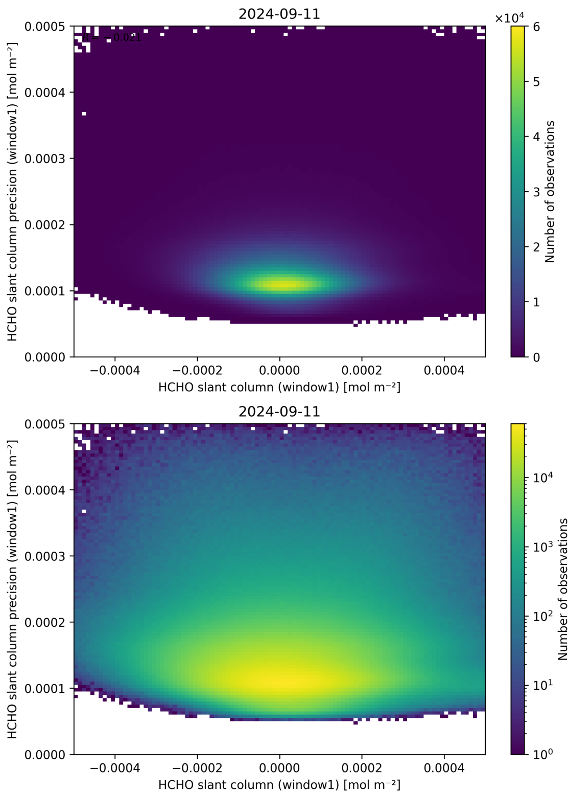
Figure 84: Scatter density plot of “HCHO slant column (window1)” against “HCHO slant column precision (window1)” for 2024-09-10 to 2024-09-12.
