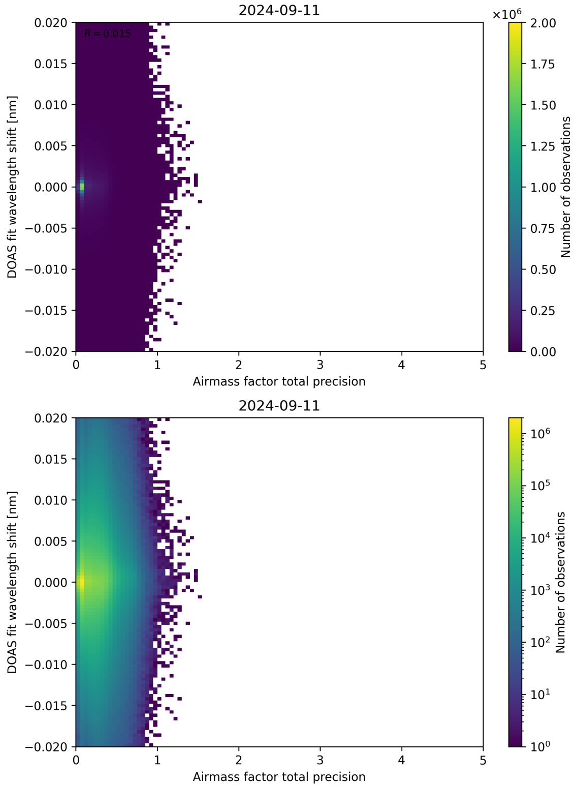
Figure 106: Scatter density plot of “Airmass factor total precision” against “DOAS fit wavelength shift” for 2024-09-10 to 2024-09-12.
