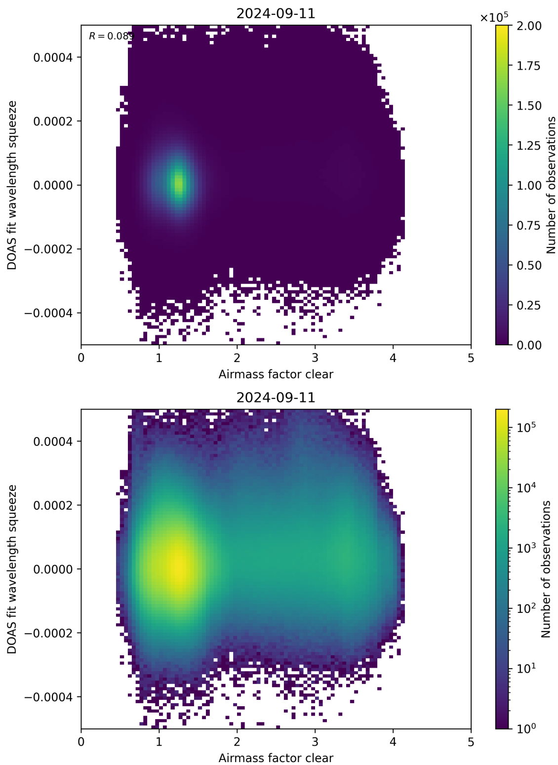
Figure 73: Scatter density plot of “Airmass factor clear” against “DOAS fit wavelength squeeze” for 2024-09-10 to 2024-09-12.
