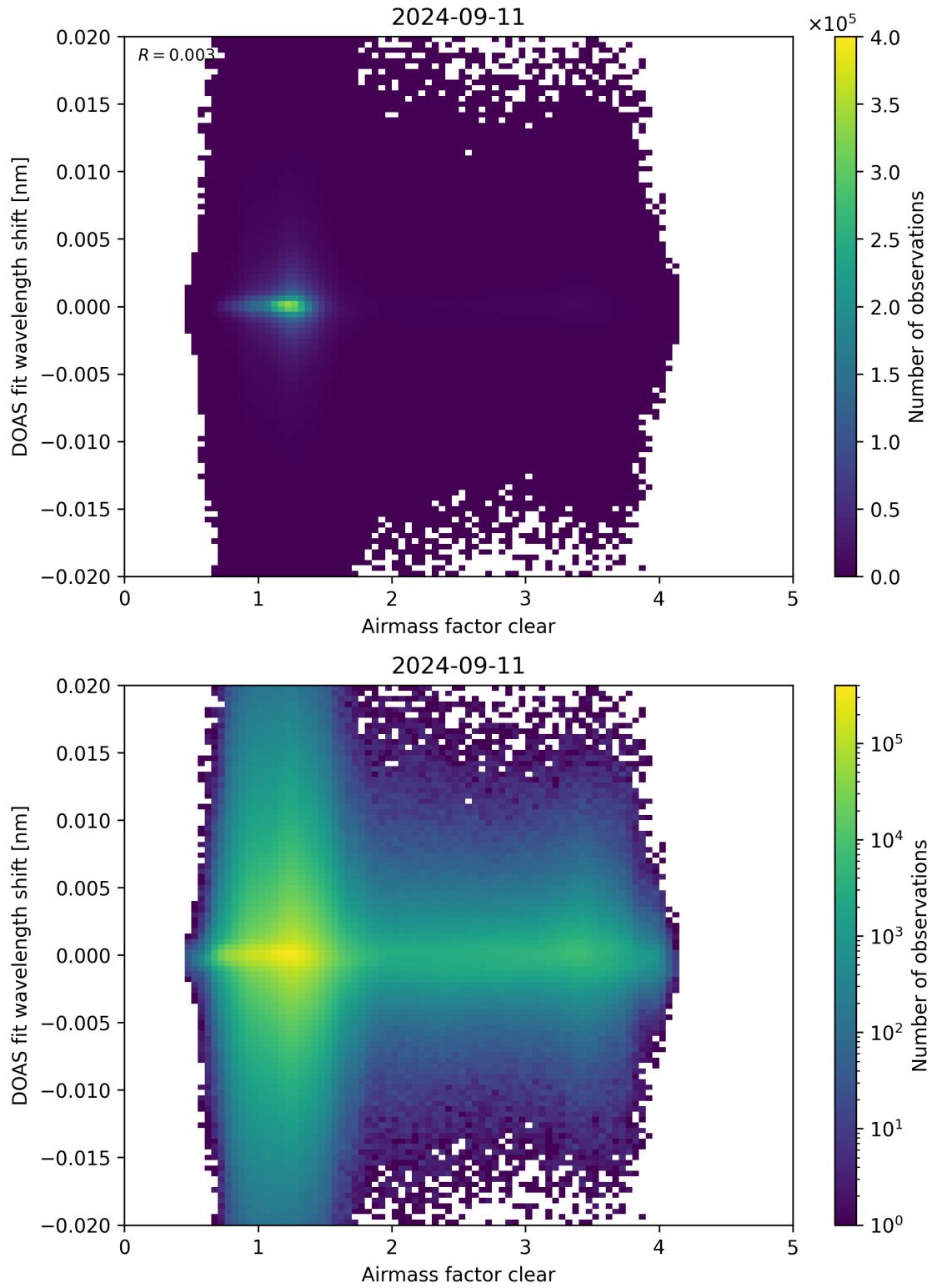
Figure 72: Scatter density plot of “Airmass factor clear” against “DOAS fit wavelength shift” for 2024-09-10 to 2024-09-12.
