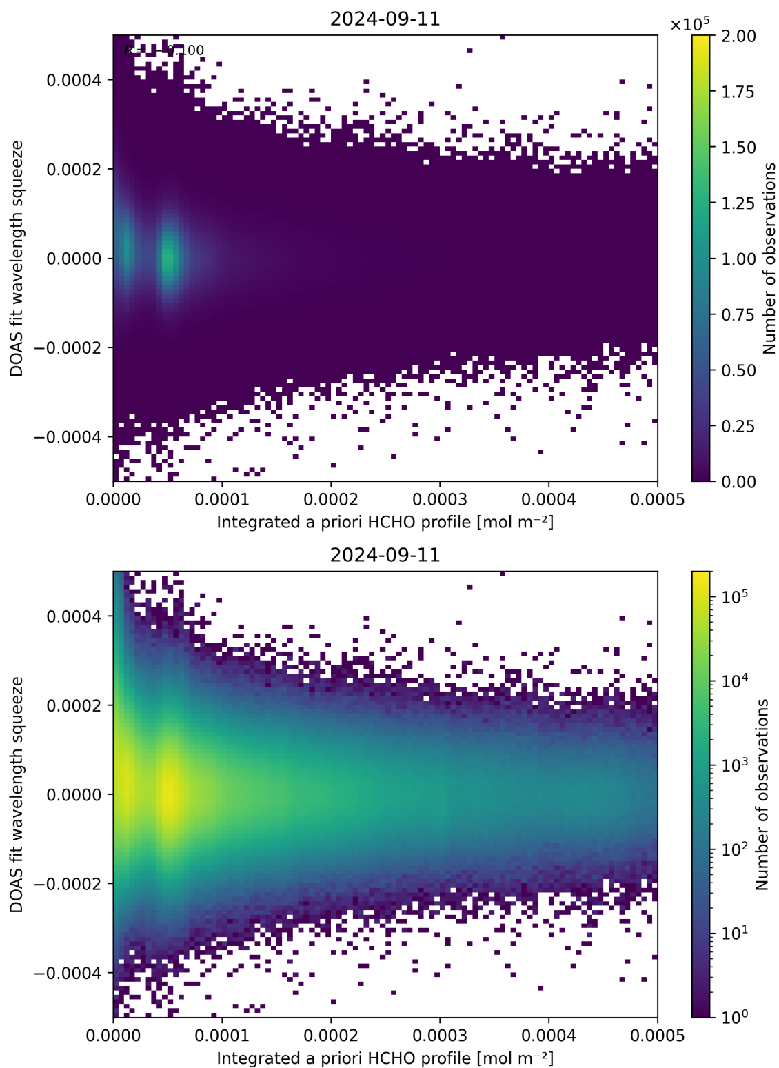
Figure 150: Scatter density plot of “Integrated a priori HCHO profile” against “DOAS fit wavelength squeeze” for 2024-09-10 to 2024-09-12.
