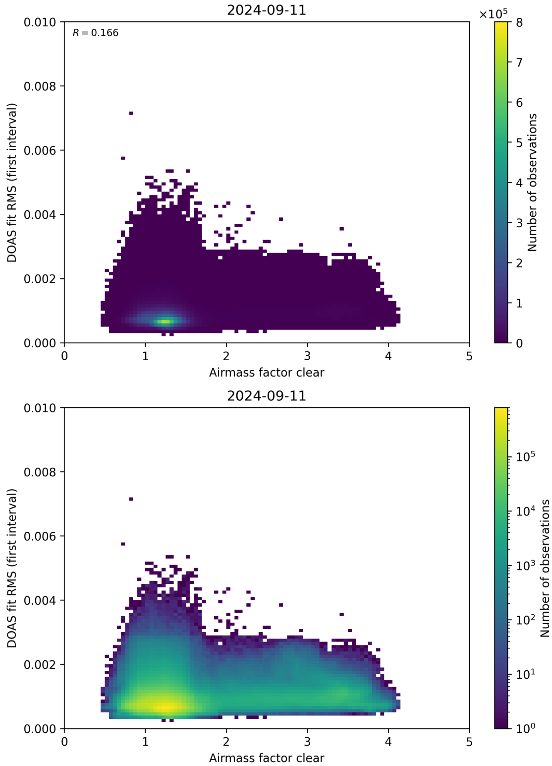
Figure 71: Scatter density plot of “Airmass factor clear” against “DOAS fit RMS (first interval)” for 2024-09-10 to 2024-09-12.
