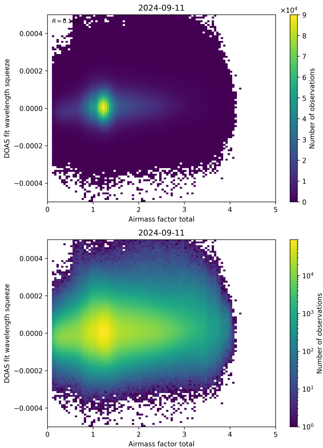
Figure 99: Scatter density plot of “Airmass factor total” against “DOAS fit wavelength squeeze” for 2024-09-10 to 2024-09-12.
