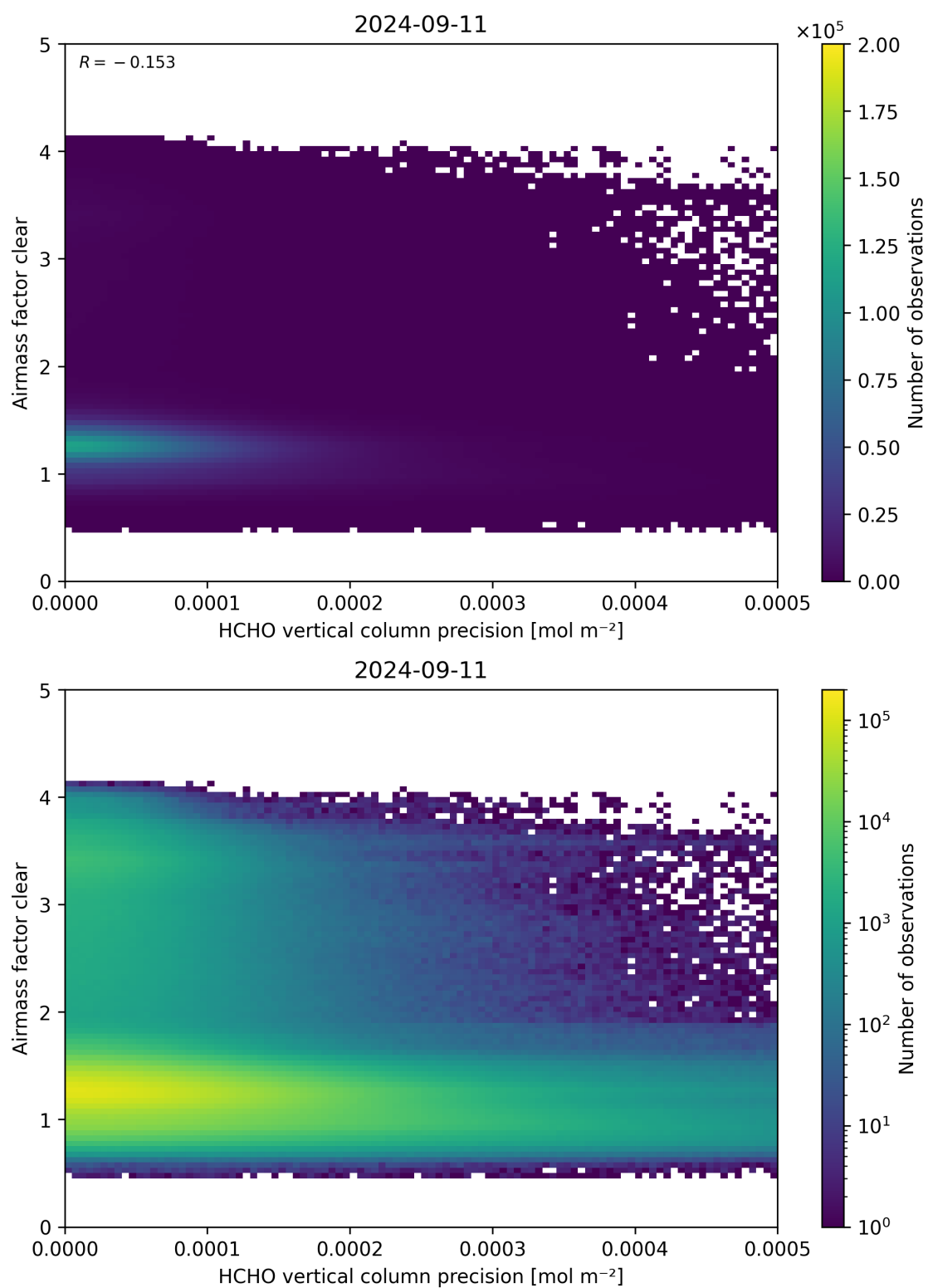
Figure 139: Scatter density plot of “HCHO vertical column precision” against “Airmass factor clear” for 2024-09-10 to 2024-09-12.
