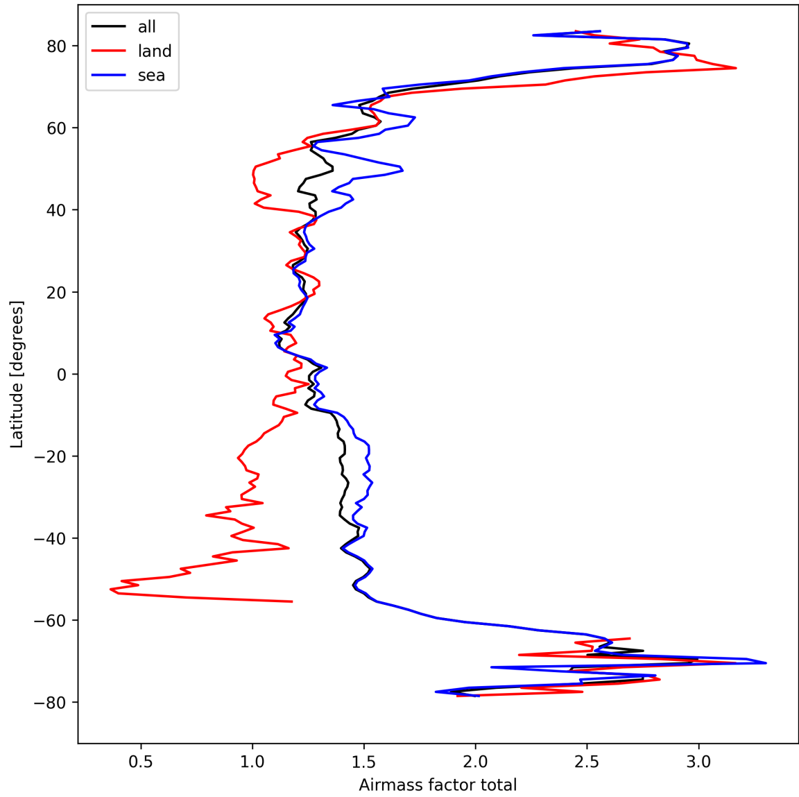
Figure 26: Zonal average of “Airmass factor total” for 2024-09-10 to 2024-09-12.
