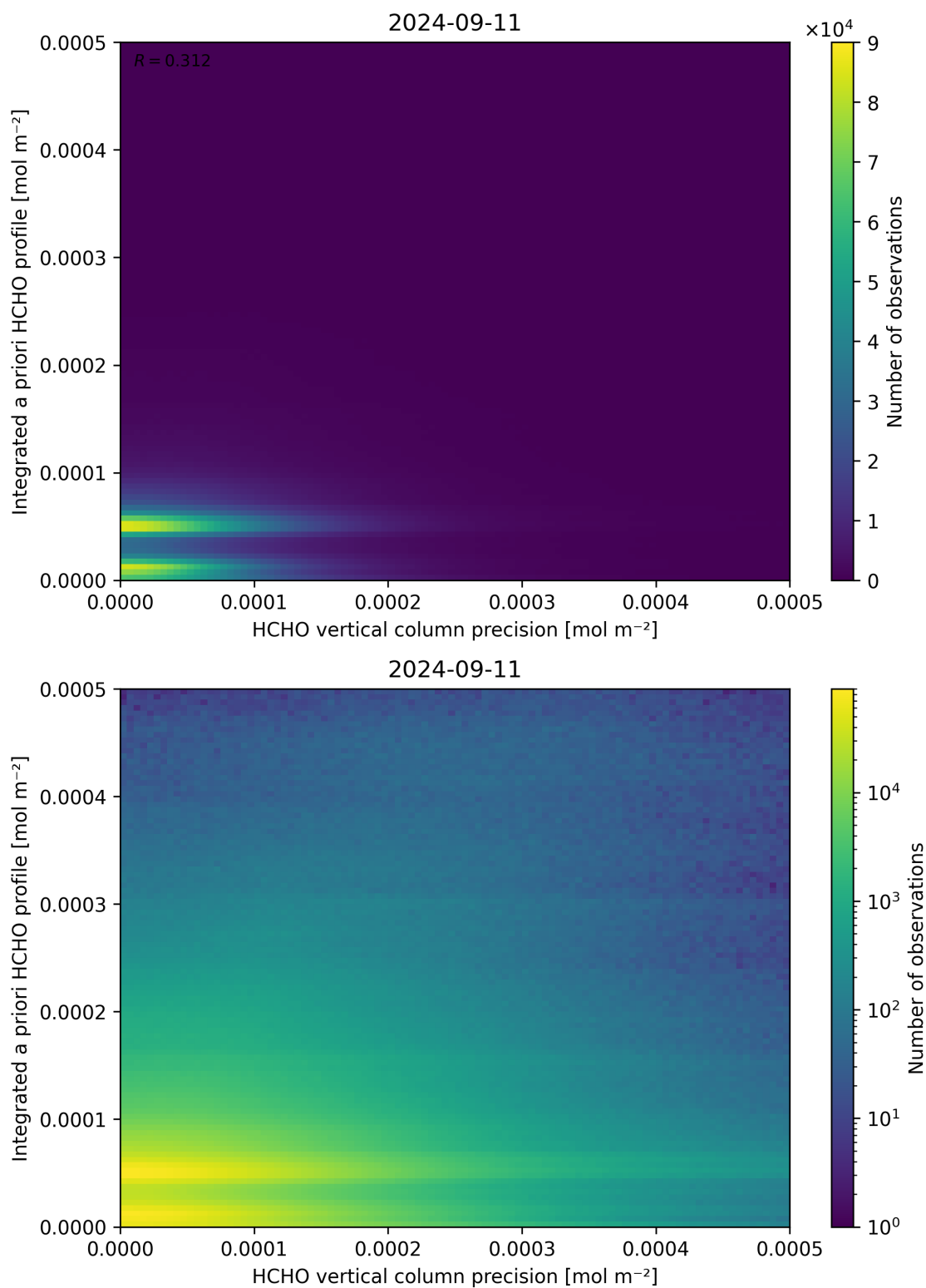
Figure 147: Scatter density plot of “HCHO vertical column precision” against “Integrated a priori HCHO profile” for 2024-09-10 to 2024-09-12.
