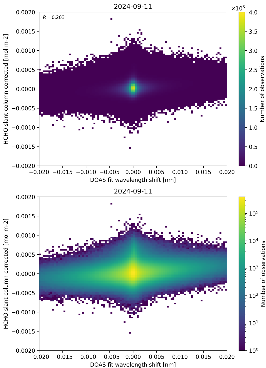
Figure 66: Scatter density plot of “DOAS fit wavelength shift” against “HCHO slant column corrected” for 2024-09-10 to 2024-09-12.
