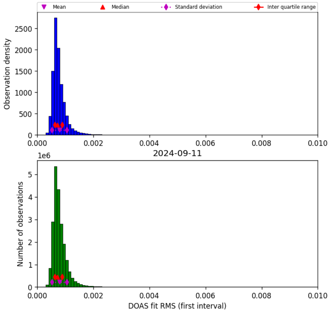
Figure 46: Histogram of “DOAS fit RMS (first interval)” for 2024-09-10 to 2024-09-12
