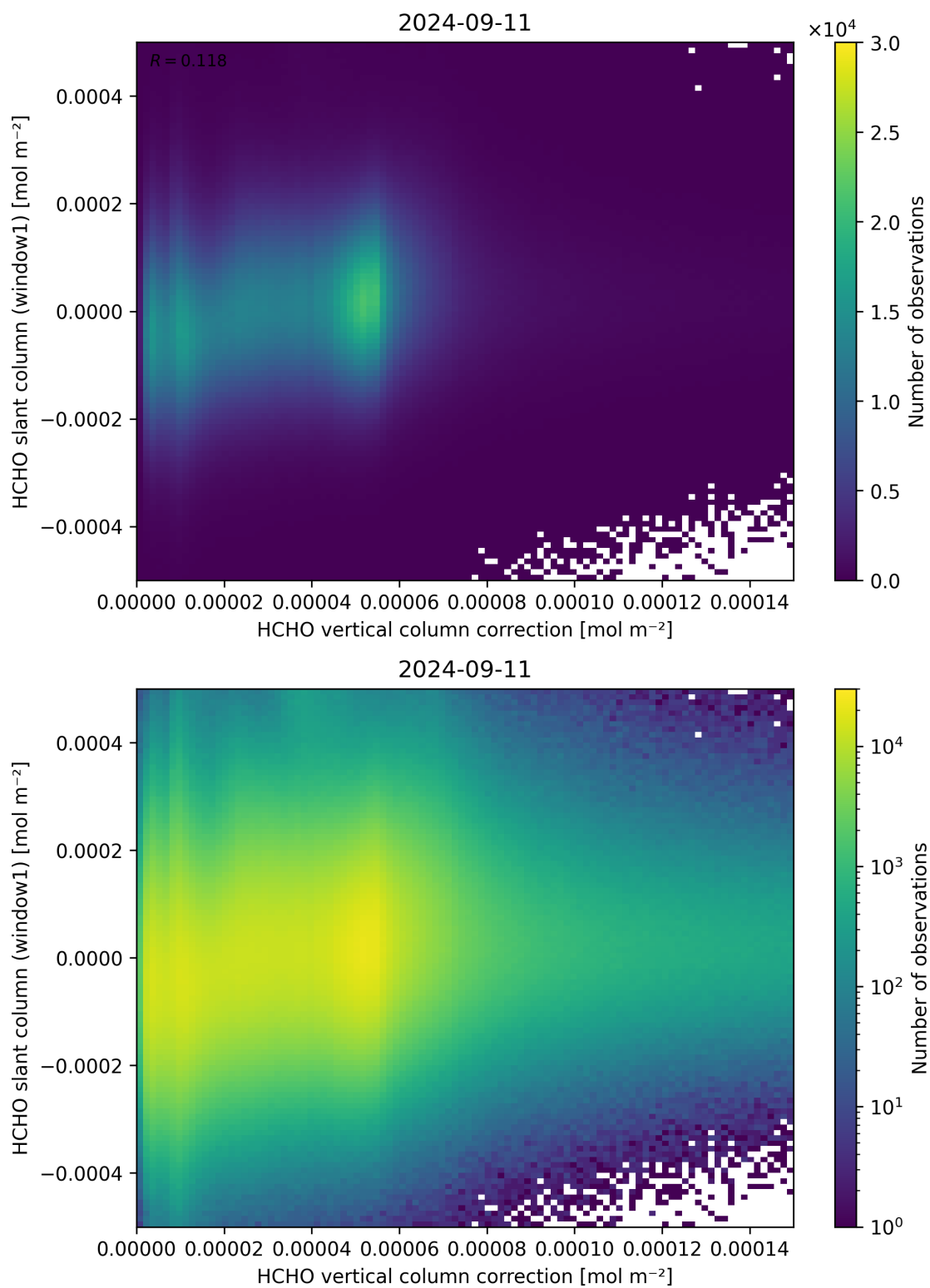
Figure 118: Scatter density plot of “HCHO vertical column correction” against “HCHO slant column (window1)” for 2024-09-10 to 2024-09-12.
