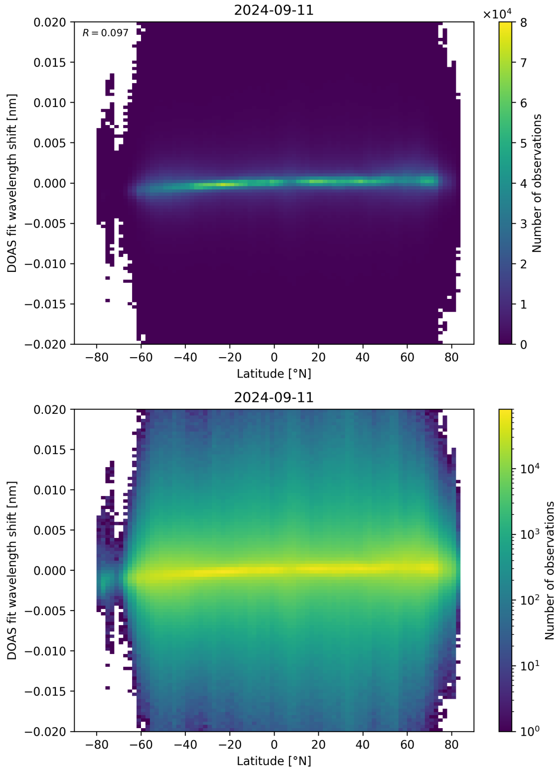
Figure 154: Scatter density plot of “Latitude” against “DOAS fit wavelength shift” for 2024-09-10 to 2024-09-12.
