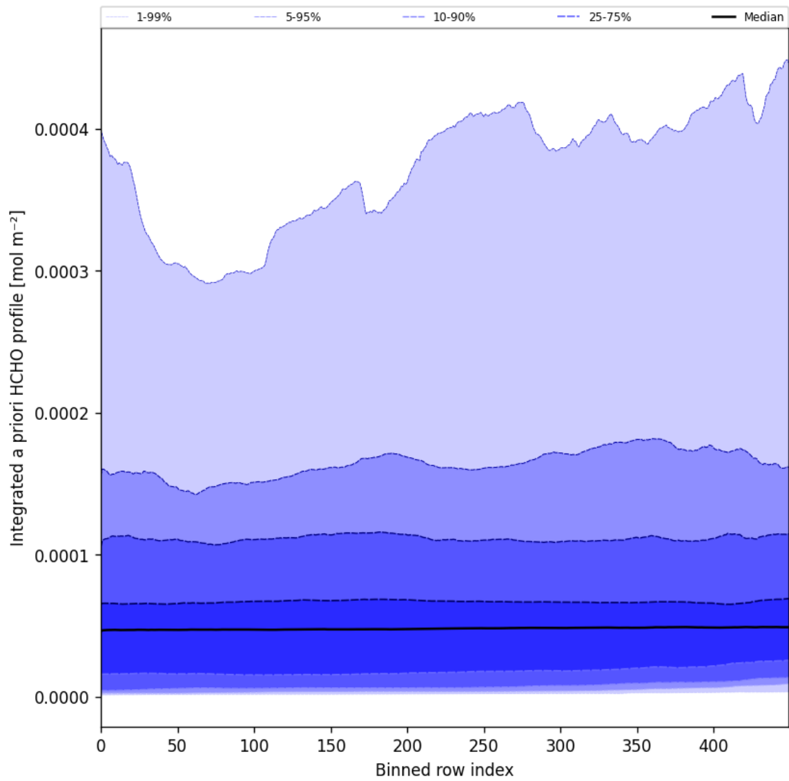
Figure 57: Along track statistics of “Integrated a priori HCHO profile” for 2024-09-10 to 2024-09-12
