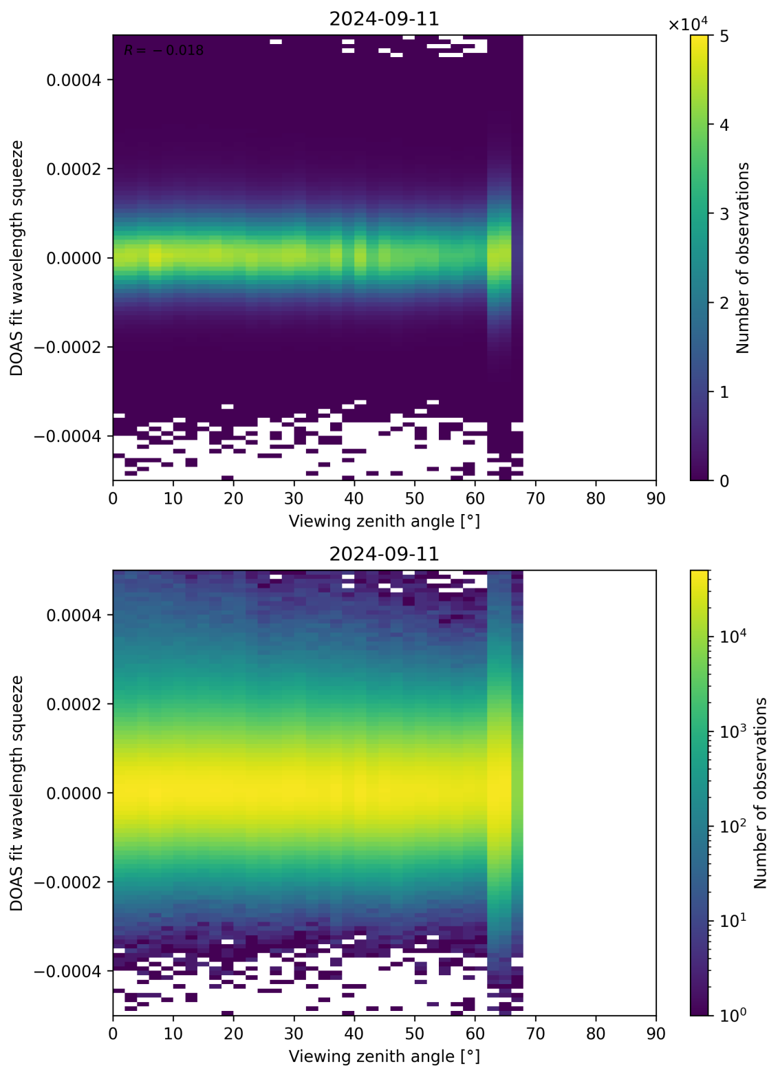
Figure 184: Scatter density plot of “Viewing zenith angle” against “DOAS fit wavelength squeeze” for 2024-09-10 to 2024-09-12.
