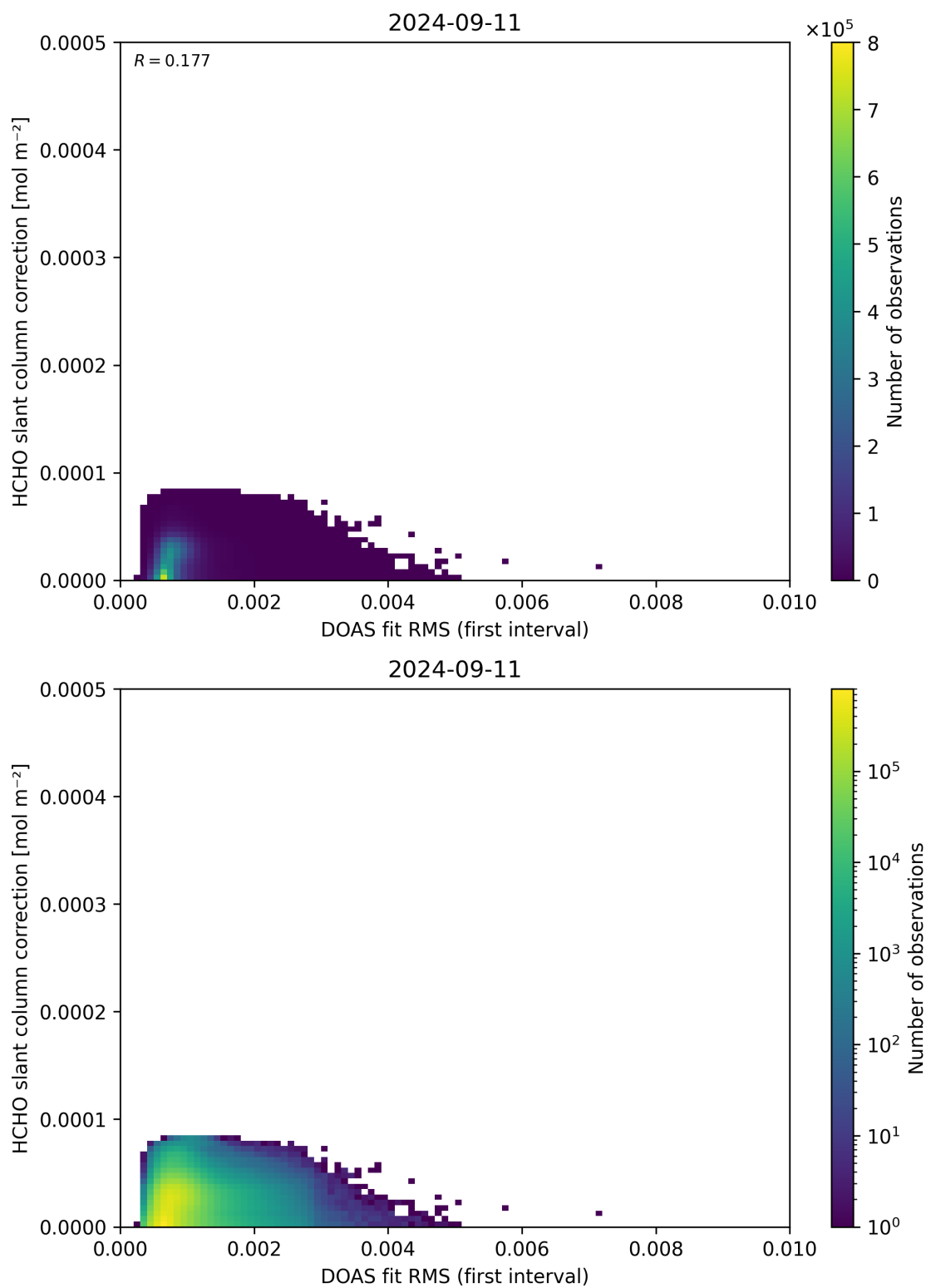
Figure 63: Scatter density plot of “DOAS fit RMS (first interval)” against “HCHO slant column correction” for 2024-09-10 to 2024-09-12.
