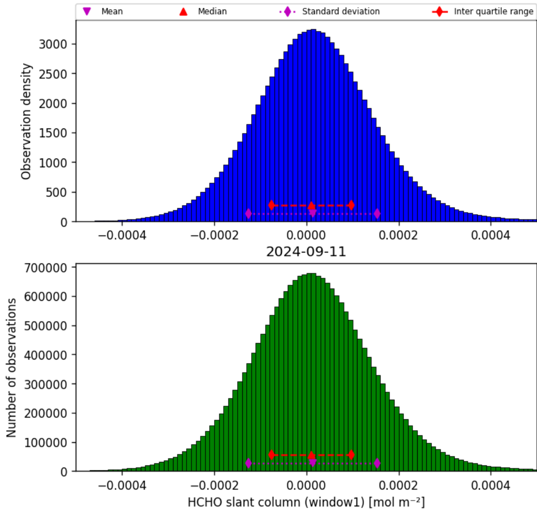
Figure 38: Histogram of “HCHO slant column (window1)” for 2024-09-10 to 2024-09-12
