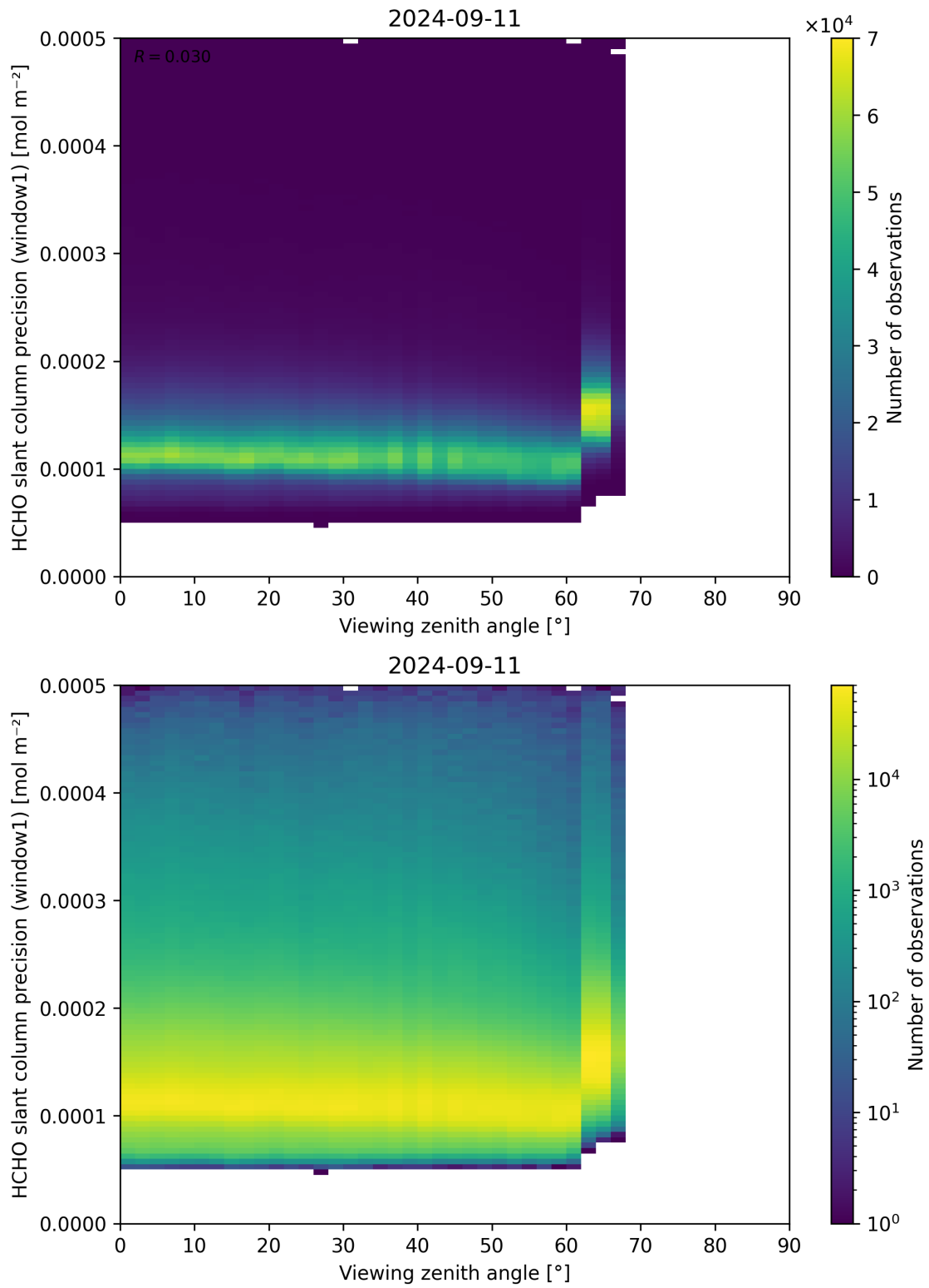
Figure 189: Scatter density plot of “Viewing zenith angle” against “HCHO slant column precision (window1)” for 2024-09-10 to 2024-09-12.
