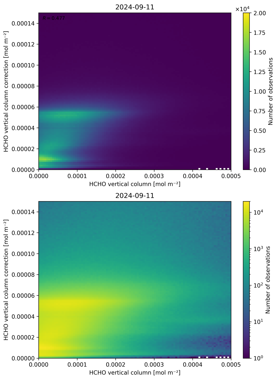
Figure 133: Scatter density plot of “HCHO vertical column” against “HCHO vertical column correction” for 2024-09-10 to 2024-09-12.
