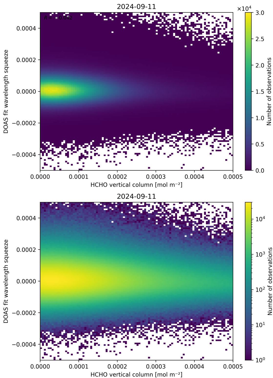
Figure 125: Scatter density plot of “HCHO vertical column” against “DOAS fit wavelength squeeze” for 2024-09-10 to 2024-09-12.
