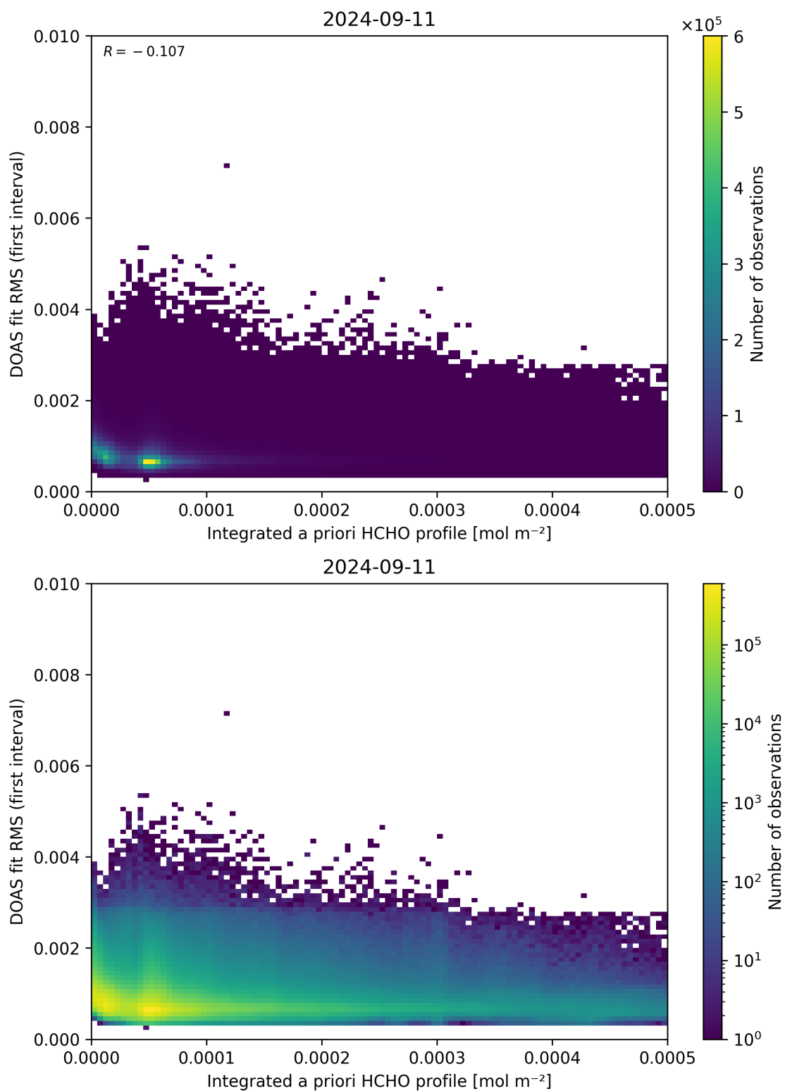
Figure 148: Scatter density plot of “Integrated a priori HCHO profile” against “DOAS fit RMS (first interval)” for 2024-09-10 to 2024-09-12.
