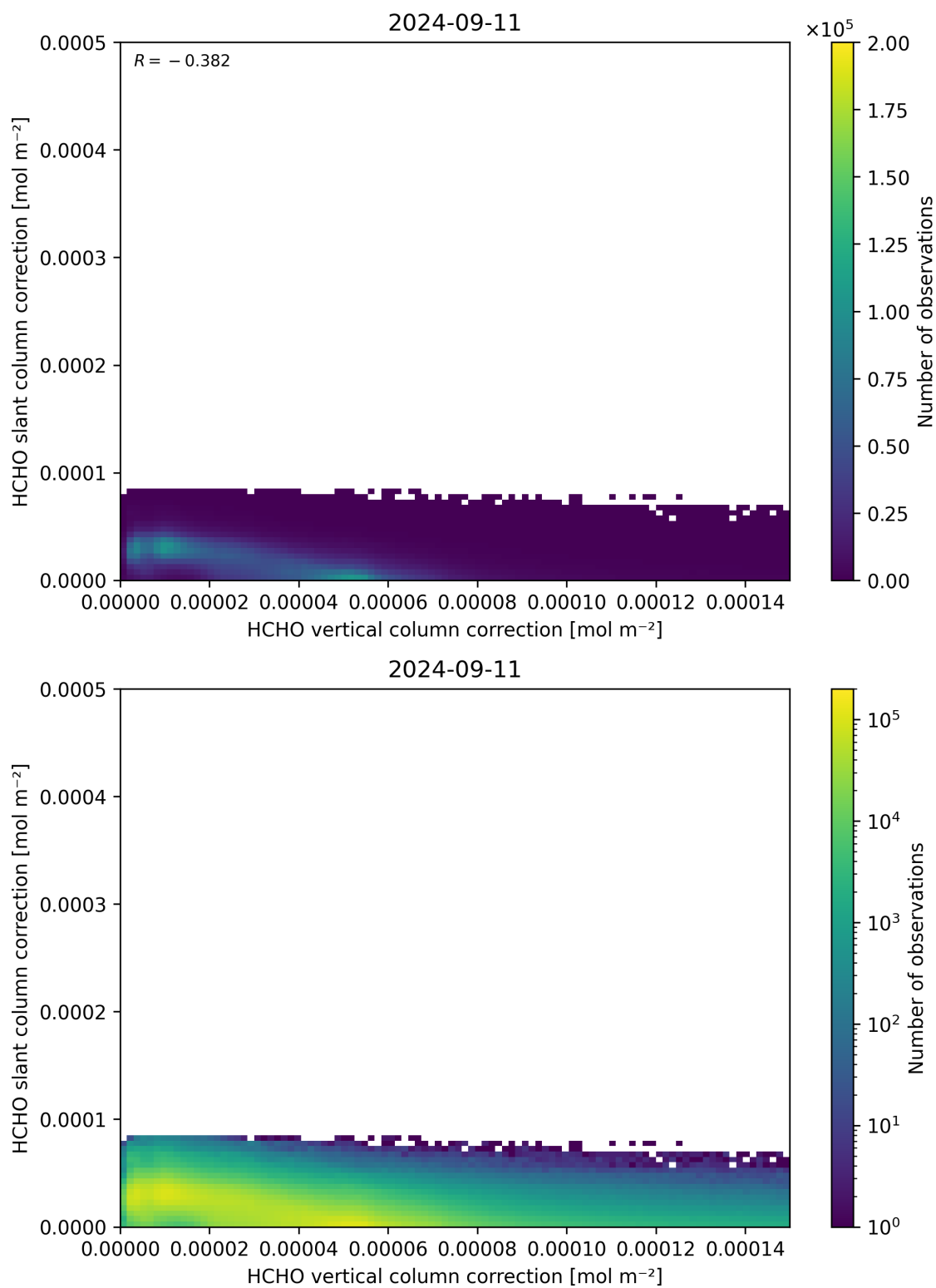
Figure 117: Scatter density plot of “HCHO vertical column correction” against “HCHO slant column correction” for 2024-09-10 to 2024-09-12.
