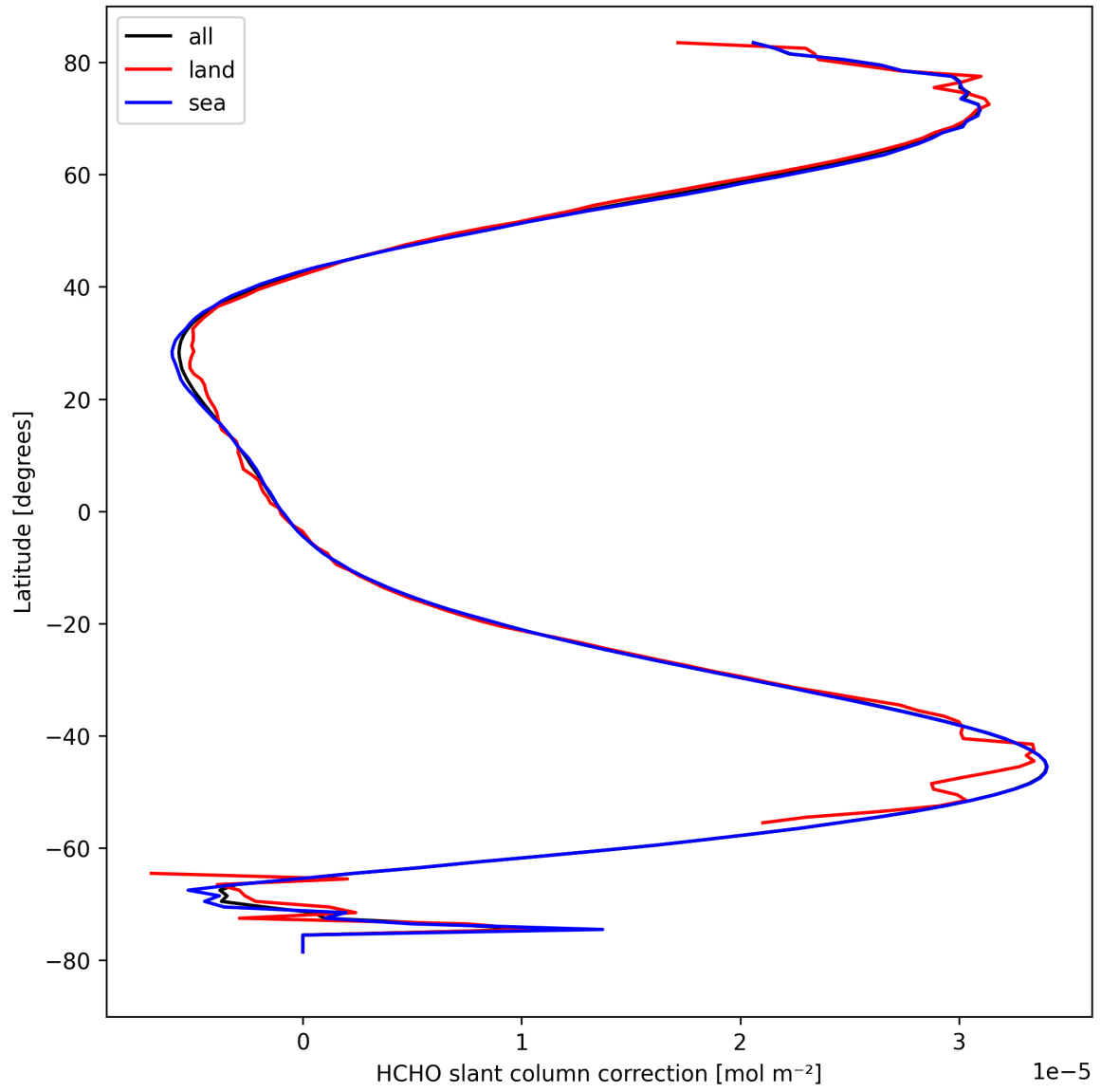
Figure 33: Zonal average of “HCHO slant column correction” for 2024-09-10 to 2024-09-12.
