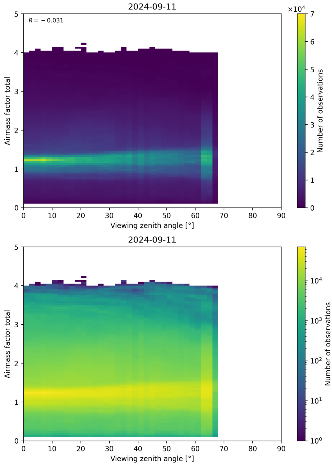
Figure 190: Scatter density plot of “Viewing zenith angle” against “Airmass factor total” for 2024-09-10 to 2024-09-12.
