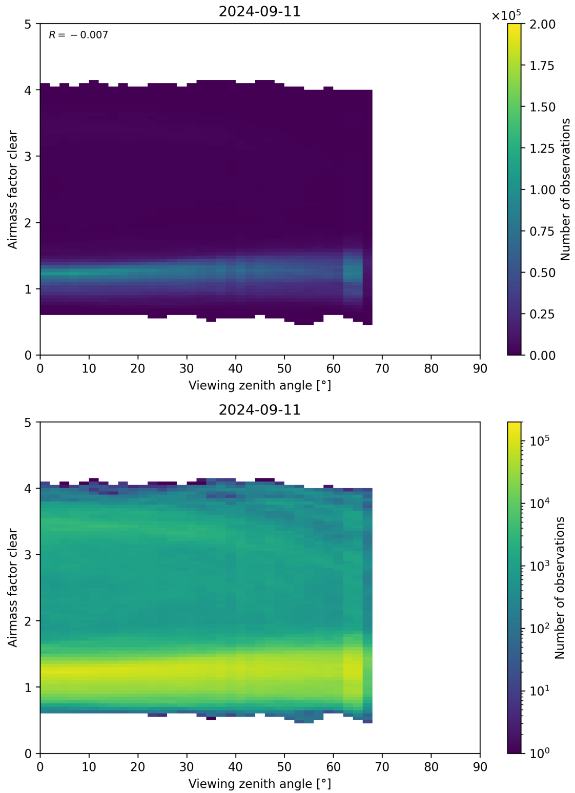
Figure 185: Scatter density plot of “Viewing zenith angle” against “Airmass factor clear” for 2024-09-10 to 2024-09-12.
