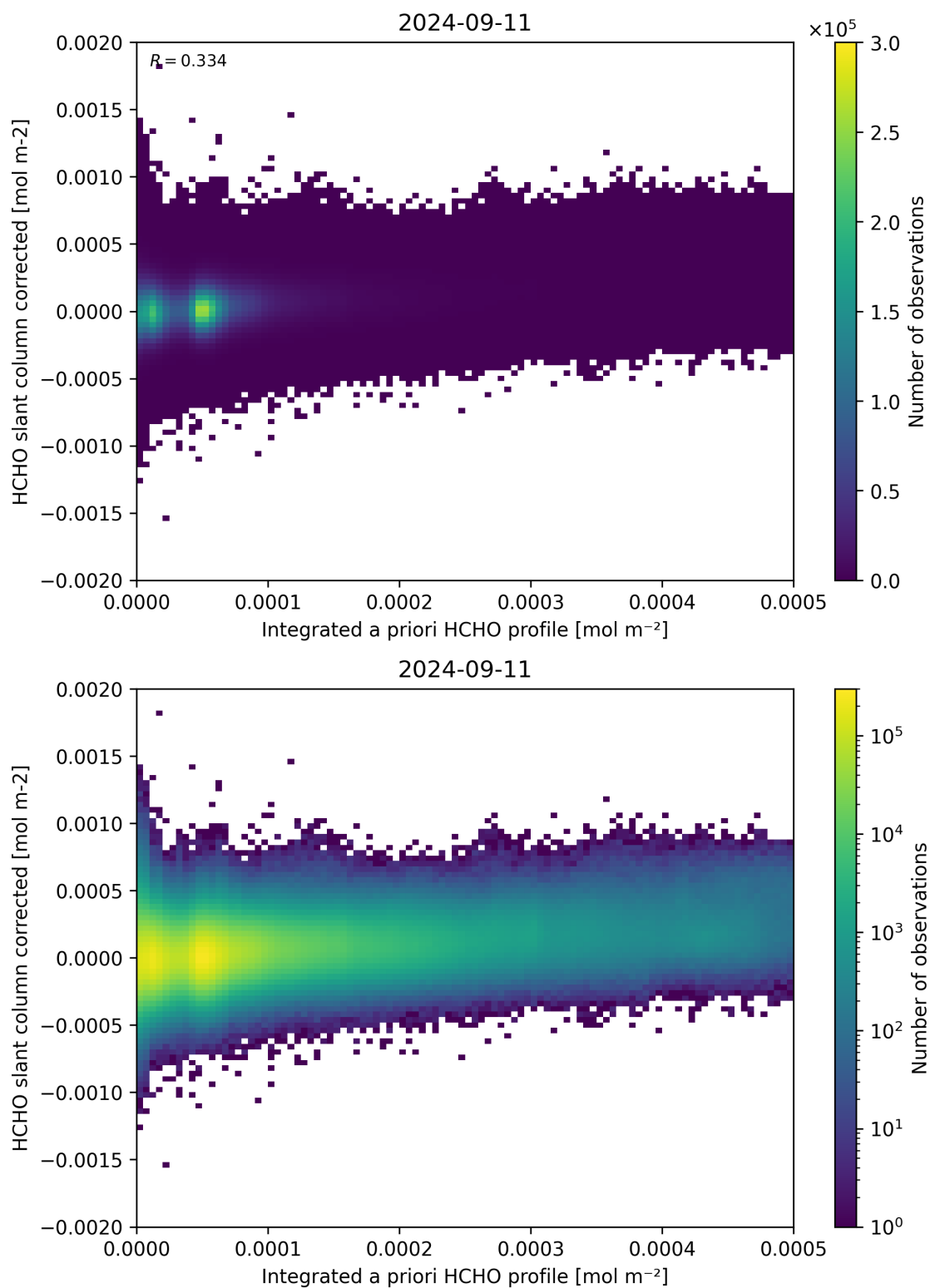
Figure 151: Scatter density plot of “Integrated a priori HCHO profile” against “HCHO slant column corrected” for 2024-09-10 to 2024-09-12.
