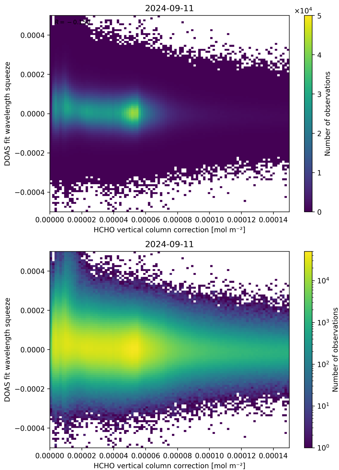
Figure 114: Scatter density plot of “HCHO vertical column correction” against “DOAS fit wavelength squeeze” for 2024-09-10 to 2024-09-12.
