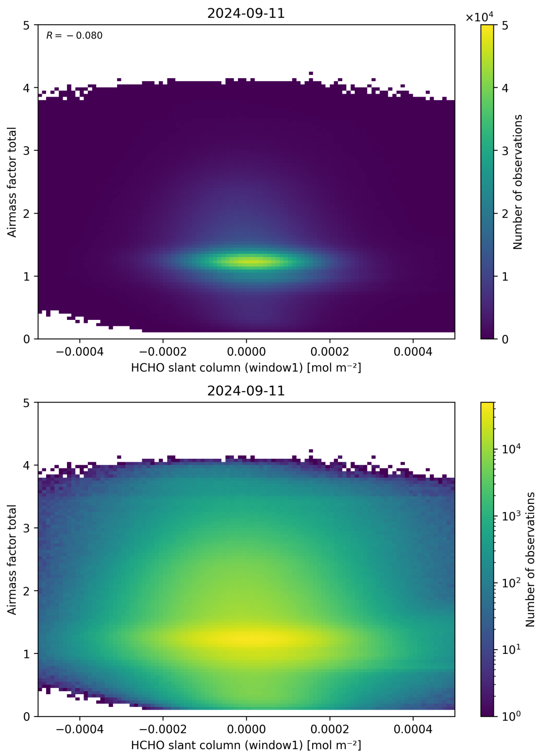
Figure 85: Scatter density plot of “HCHO slant column (window1)” against “Airmass factor total” for 2024-09-10 to 2024-09-12.
