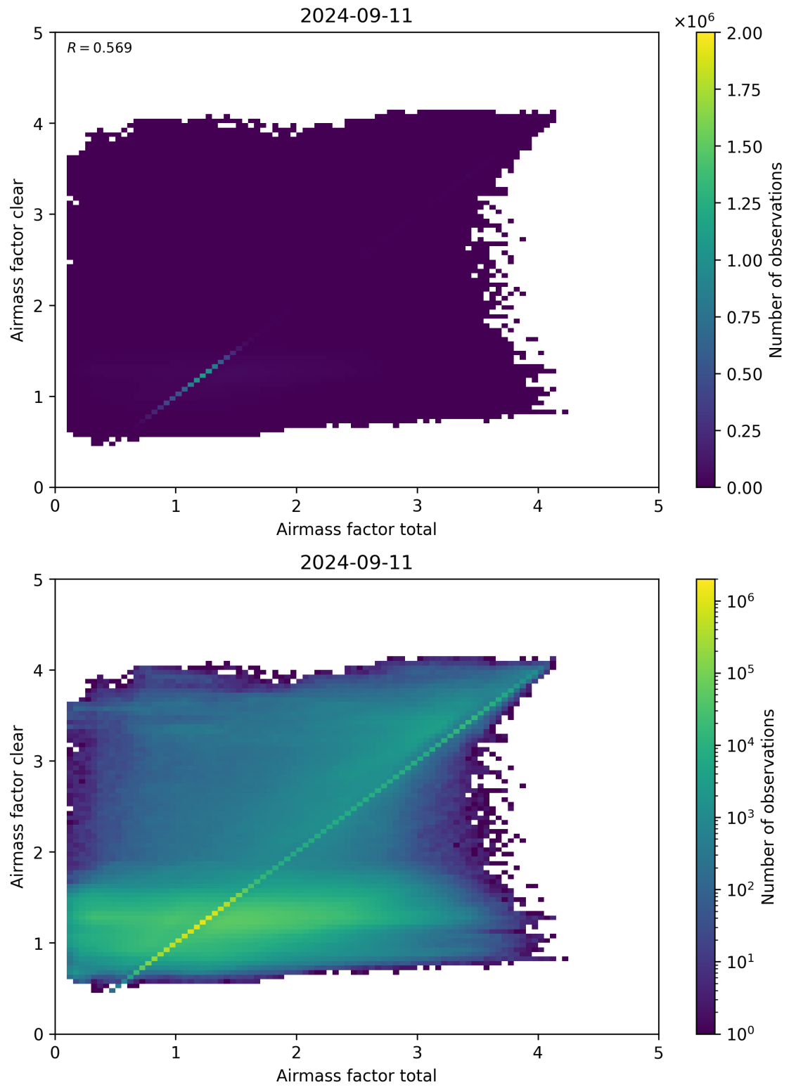
Figure 100: Scatter density plot of “Airmass factor total” against “Airmass factor clear” for 2024-09-10 to 2024-09-12.
