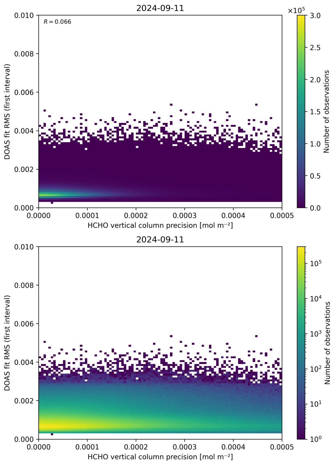
Figure 136: Scatter density plot of “HCHO vertical column precision” against “DOAS fit RMS (first interval)” for 2024-09-10 to 2024-09-12.
