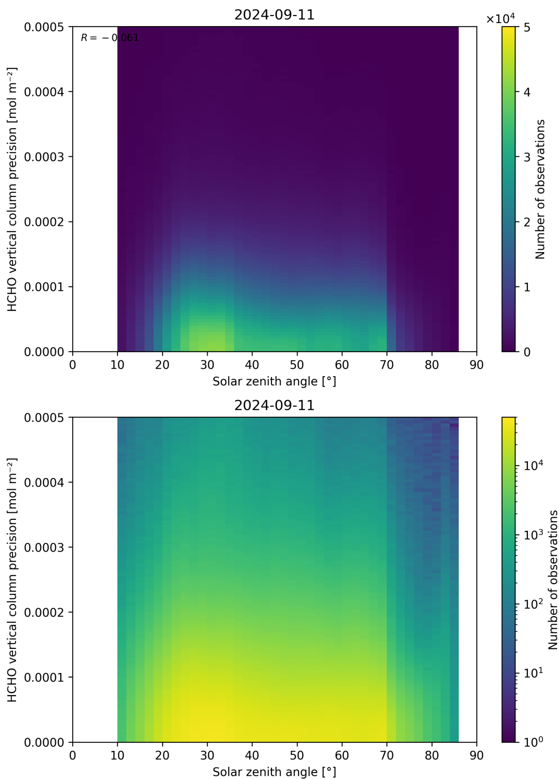
Figure 179: Scatter density plot of “Solar zenith angle” against “HCHO vertical column precision” for 2024-09-10 to 2024-09-12.
