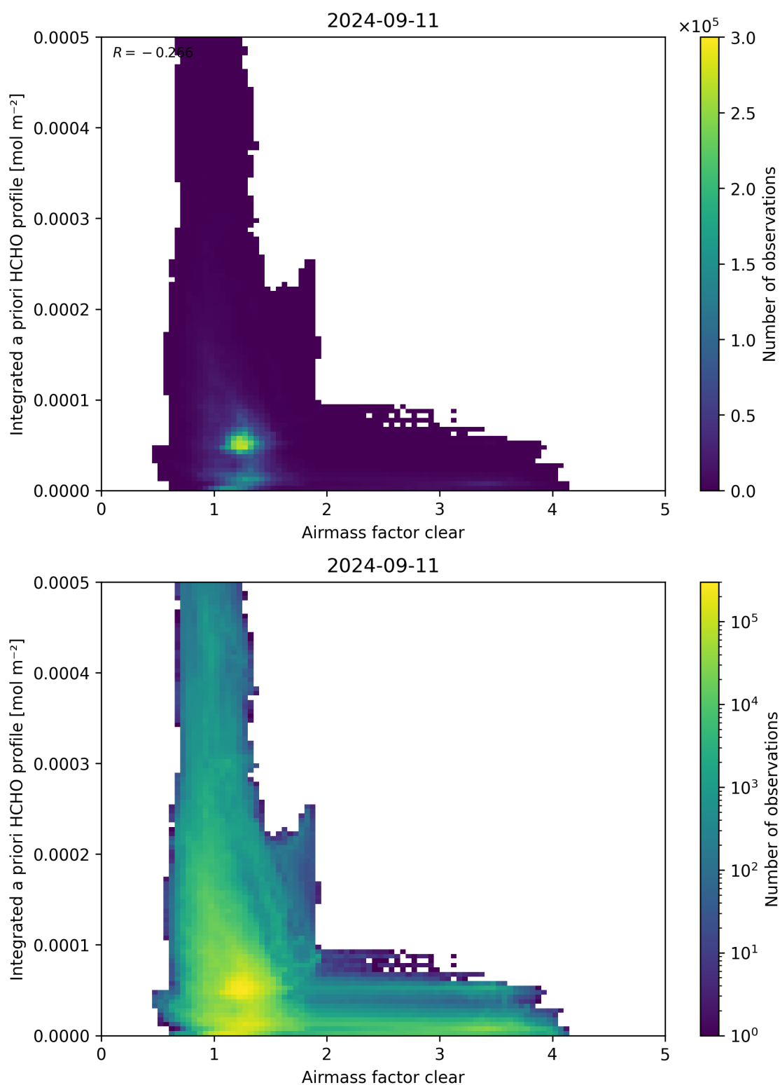
Figure 76: Scatter density plot of “Airmass factor clear” against “Integrated a priori HCHO profile” for 2024-09-10 to 2024-09-12.
