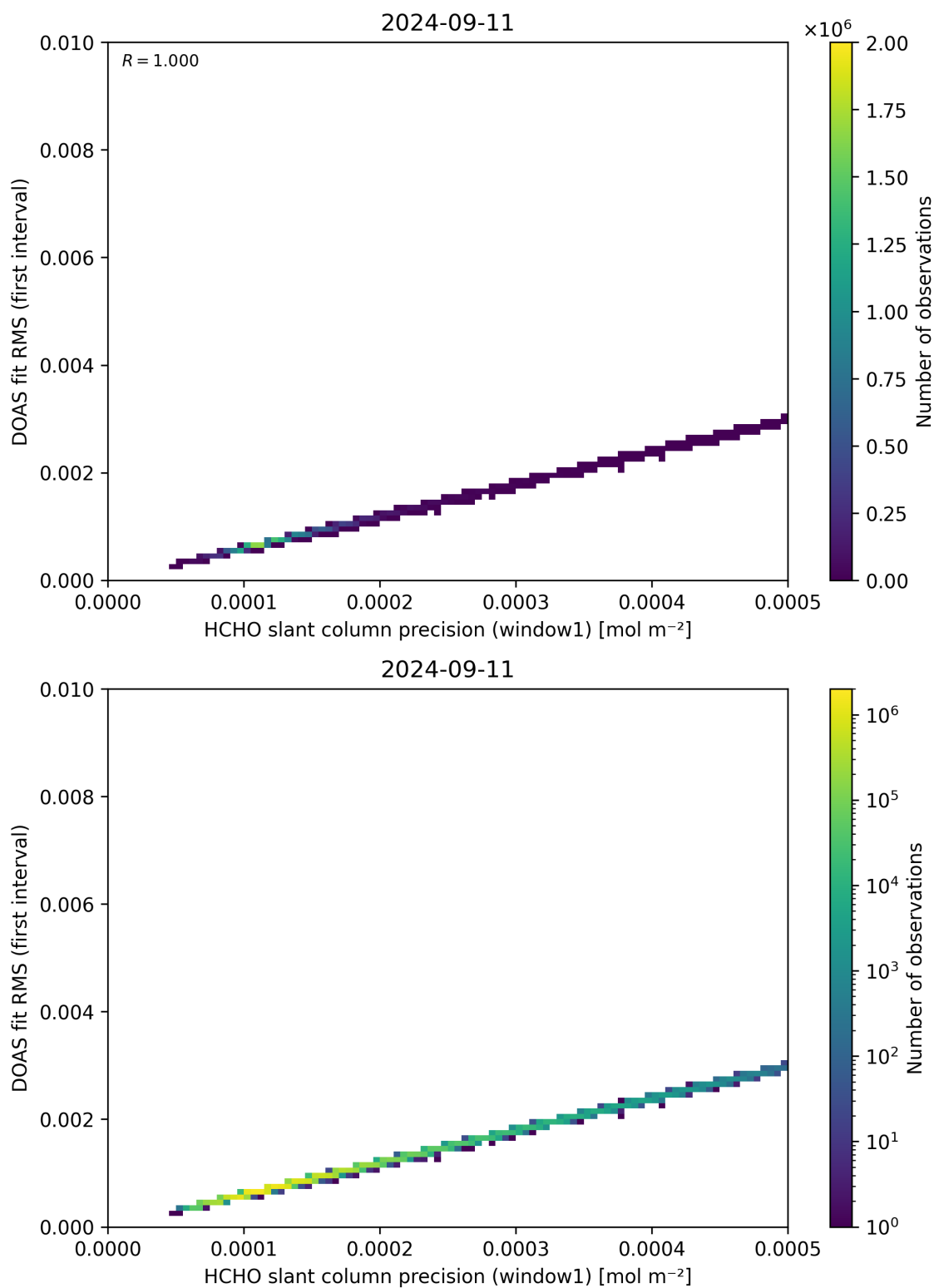
Figure 88: Scatter density plot of “HCHO slant column precision (window1)” against “DOAS fit RMS (first interval)” for 2024-09-10 to 2024-09-12.
