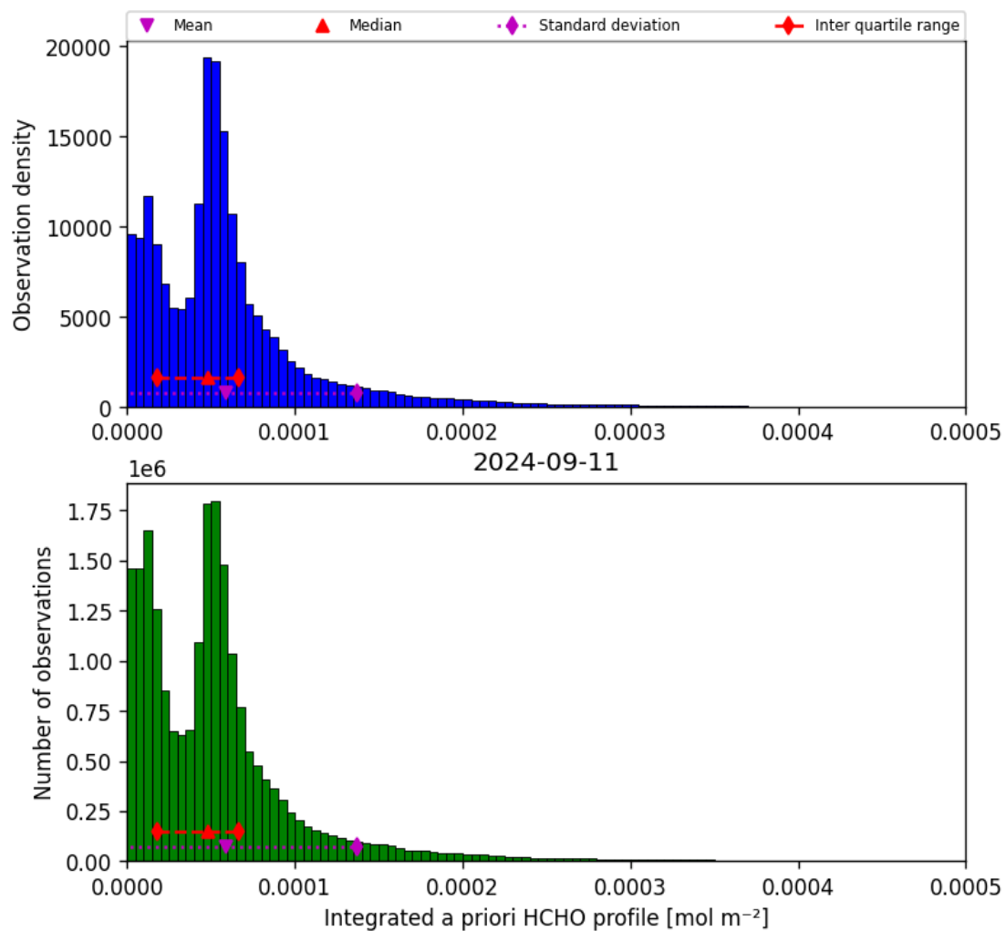
Figure 43: Histogram of “Integrated a priori HCHO profile” for 2024-09-10 to 2024-09-12
