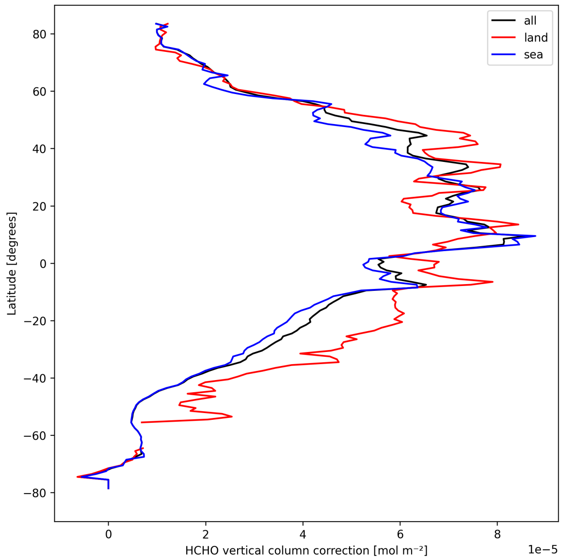
Figure 23: Zonal average of “HCHO vertical column correction” for 2024-09-10 to 2024-09-12.
