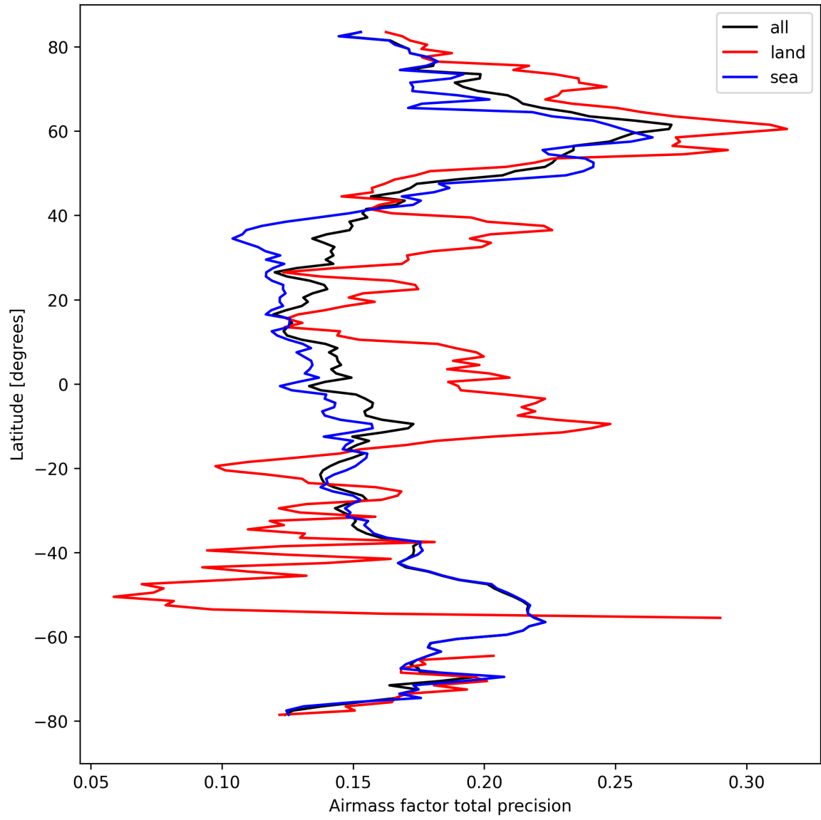
Figure 27: Zonal average of “Airmass factor total precision” for 2024-09-10 to 2024-09-12.
