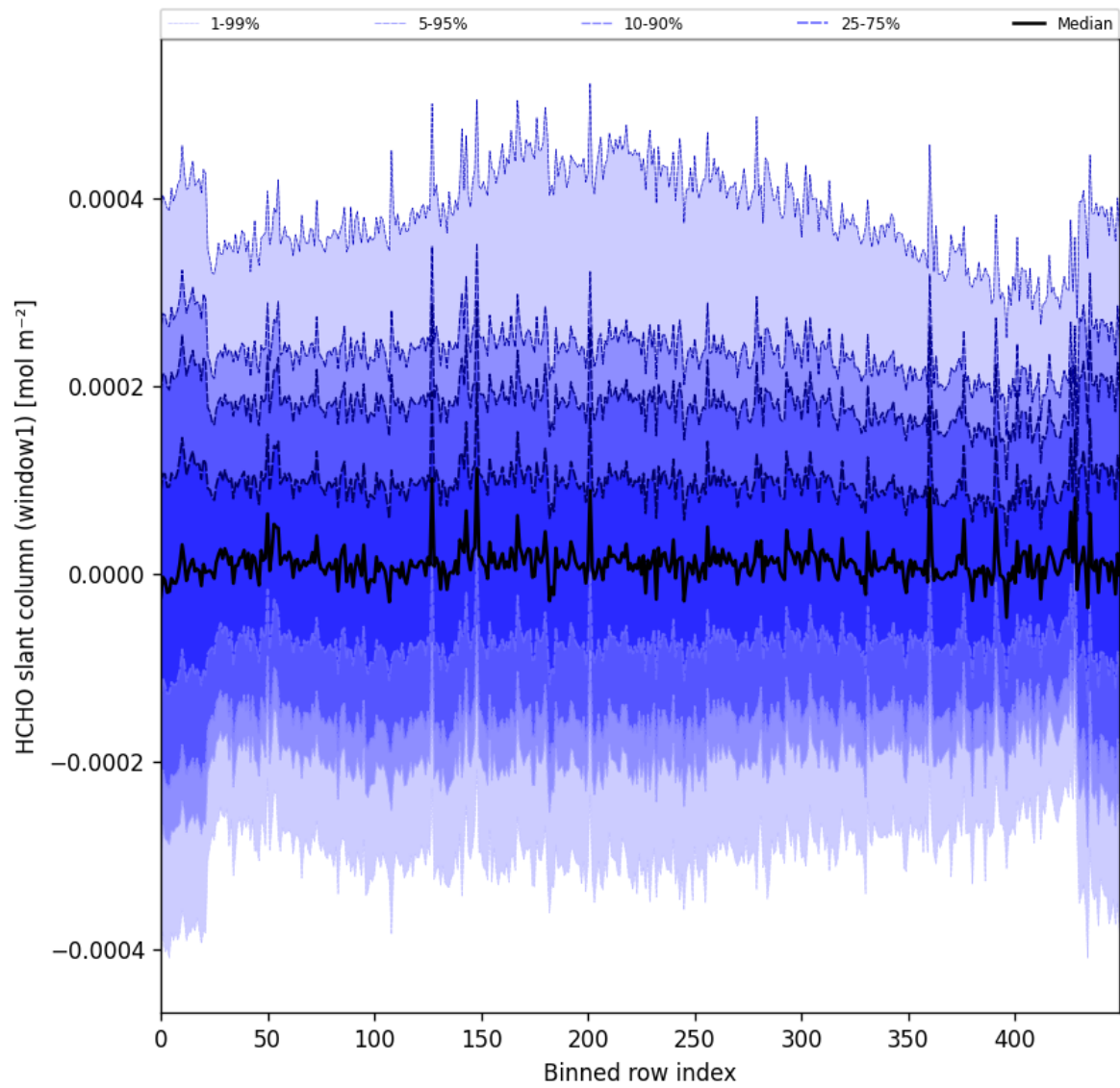
Figure 52: Along track statistics of “HCHO slant column (window1)” for 2024-09-10 to 2024-09-12
