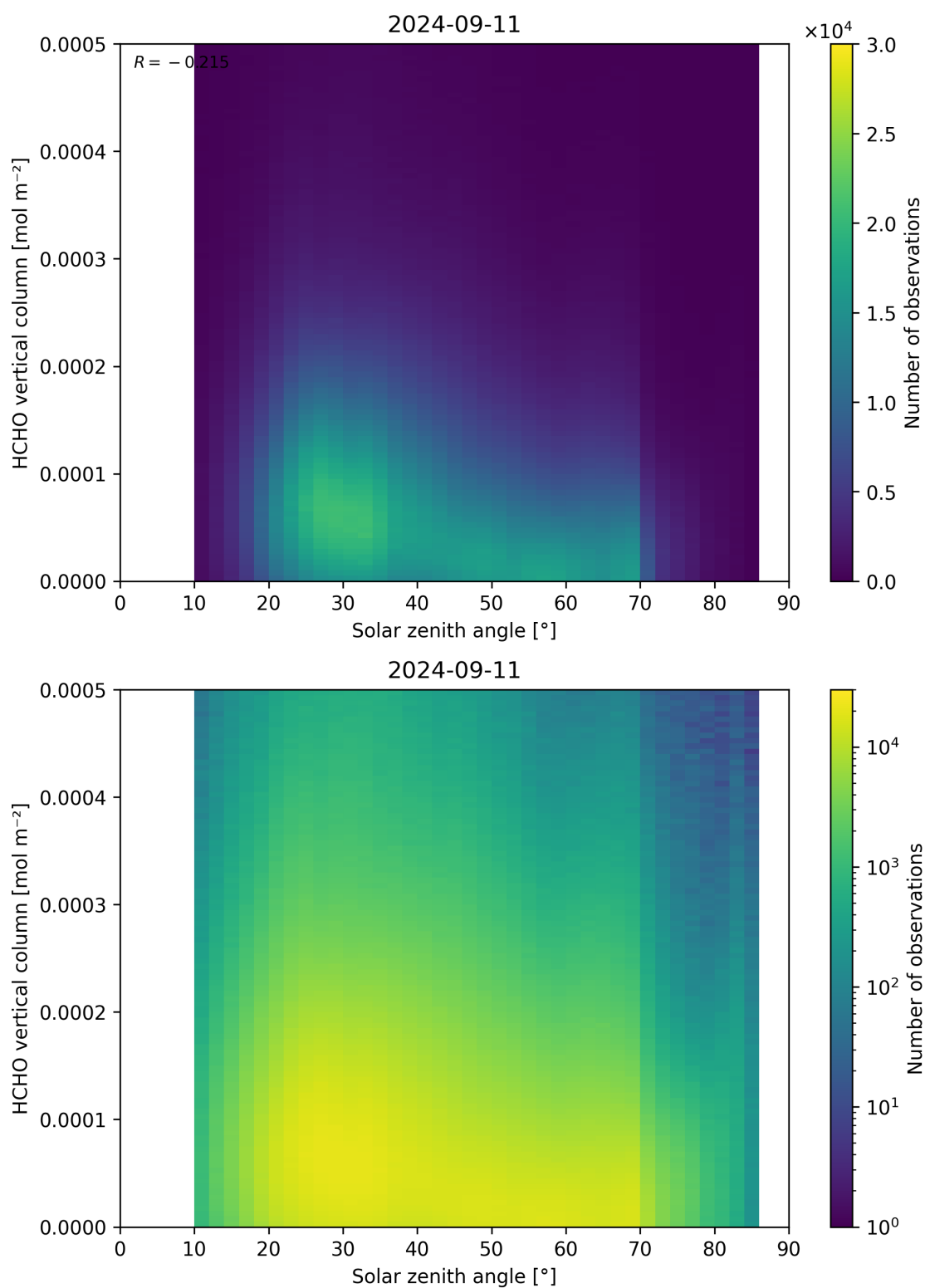
Figure 177: Scatter density plot of “Solar zenith angle” against “HCHO vertical column” for 2024-09-10 to 2024-09-12.
