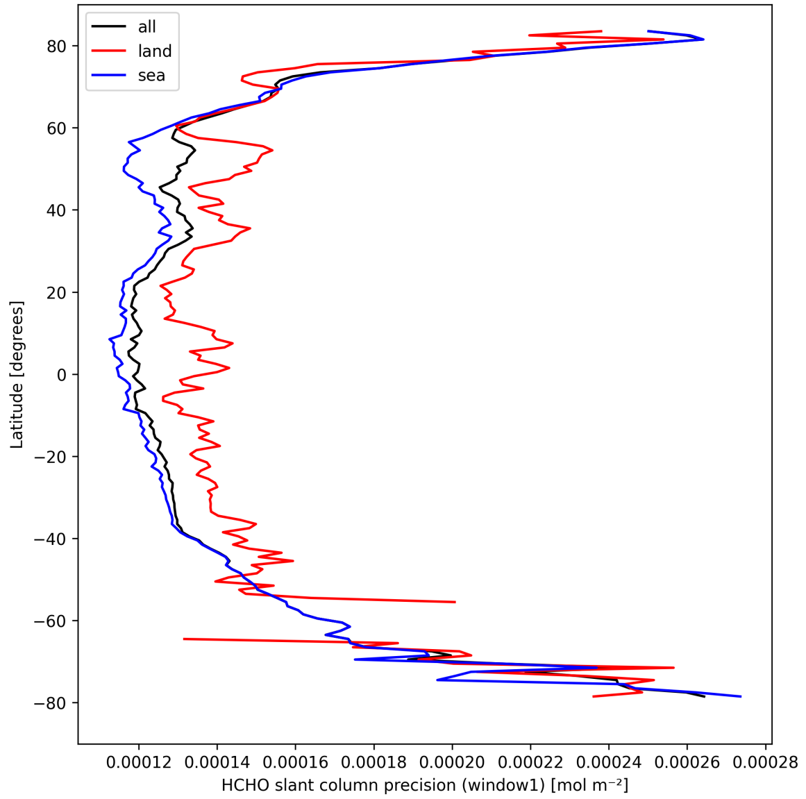
Figure 25: Zonal average of “HCHO slant column precision (window1)” for 2024-09-10 to 2024-09-12.
