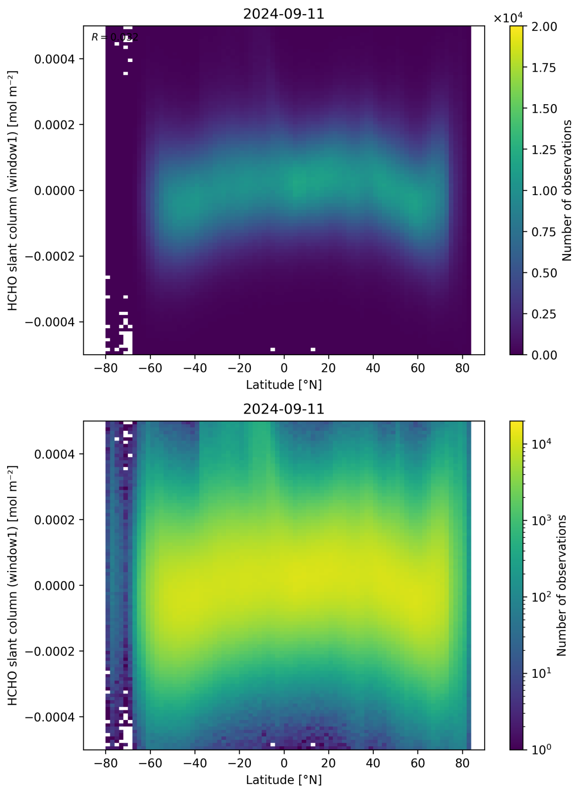
Figure 159: Scatter density plot of “Latitude” against “HCHO slant column (window1)” for 2024-09-10 to 2024-09-12.
