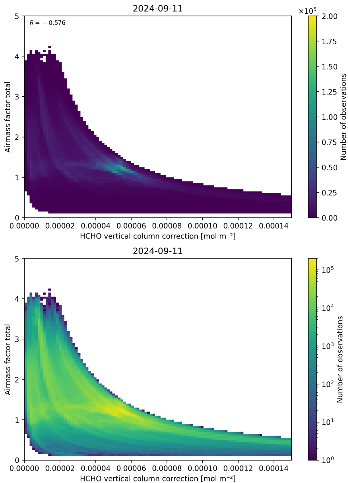
Figure 120: Scatter density plot of “HCHO vertical column correction” against “Airmass factor total” for 2024-09-10 to 2024-09-12.
