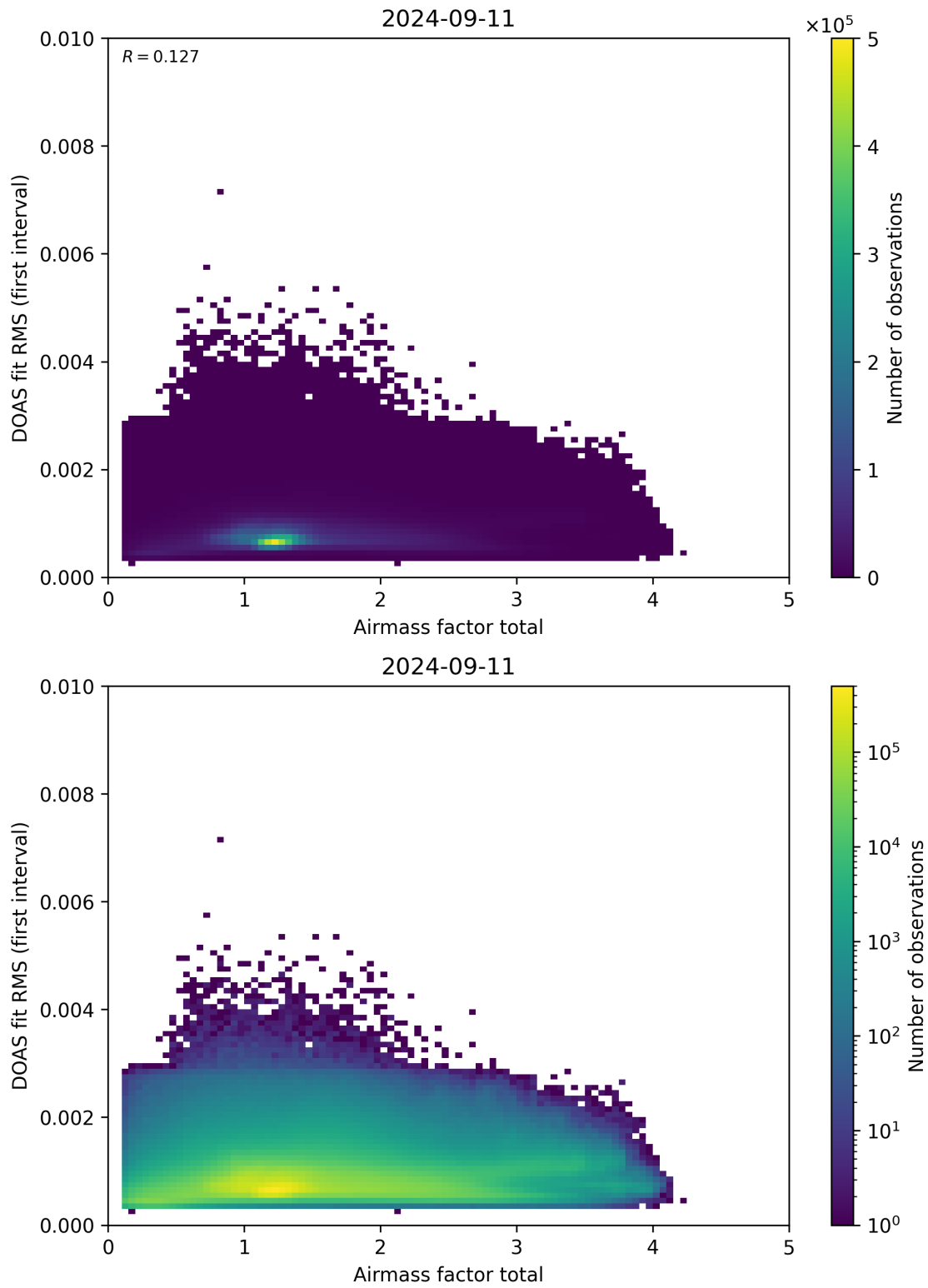
Figure 97: Scatter density plot of “Airmass factor total” against “DOAS fit RMS (first interval)” for 2024-09-10 to 2024-09-12.
