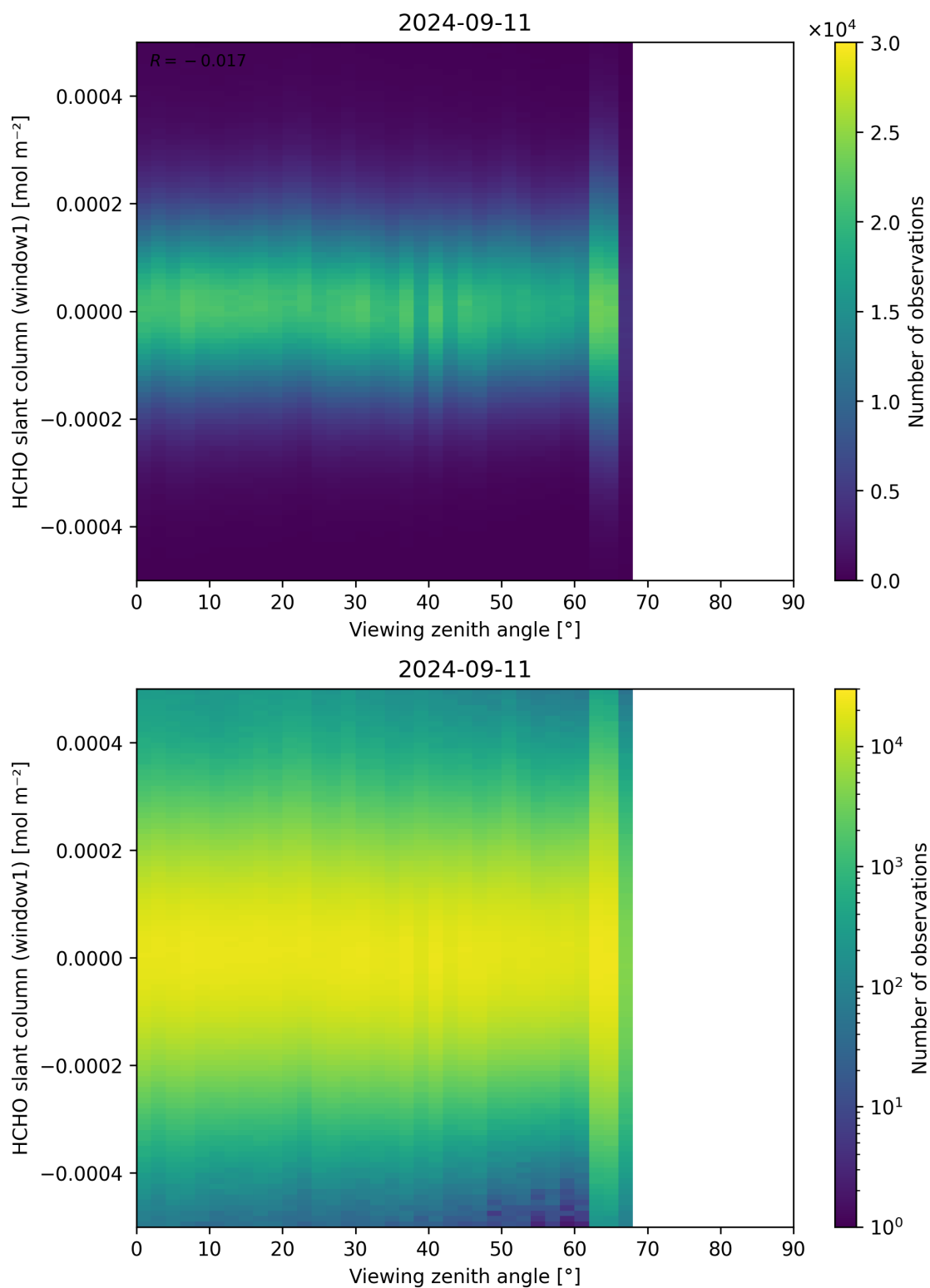
Figure 188: Scatter density plot of “Viewing zenith angle” against “HCHO slant column (window1)” for 2024-09-10 to 2024-09-12.
