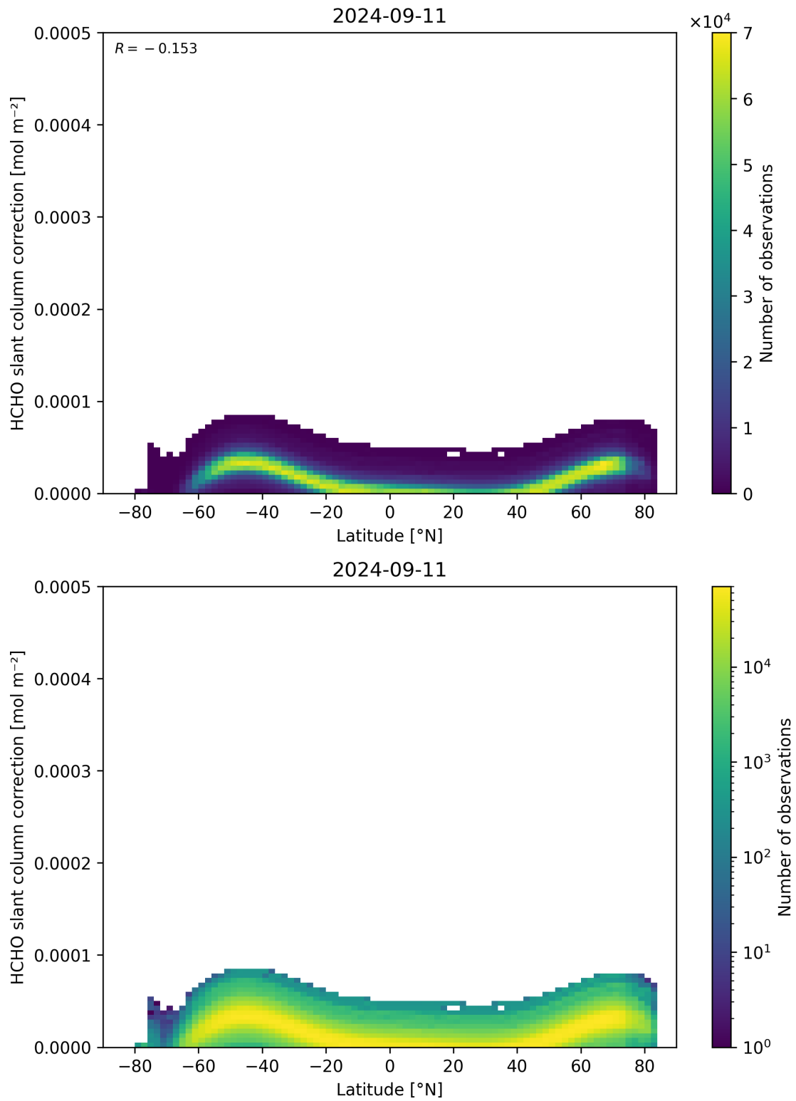
Figure 158: Scatter density plot of “Latitude” against “HCHO slant column correction” for 2024-09-10 to 2024-09-12.
