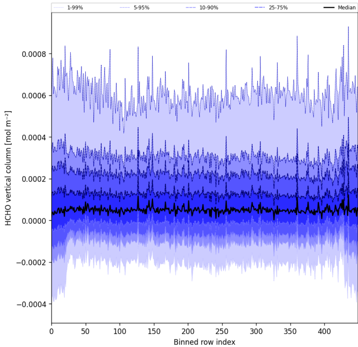
Figure 49: Along track statistics of “HCHO vertical column” for 2024-09-10 to 2024-09-12
