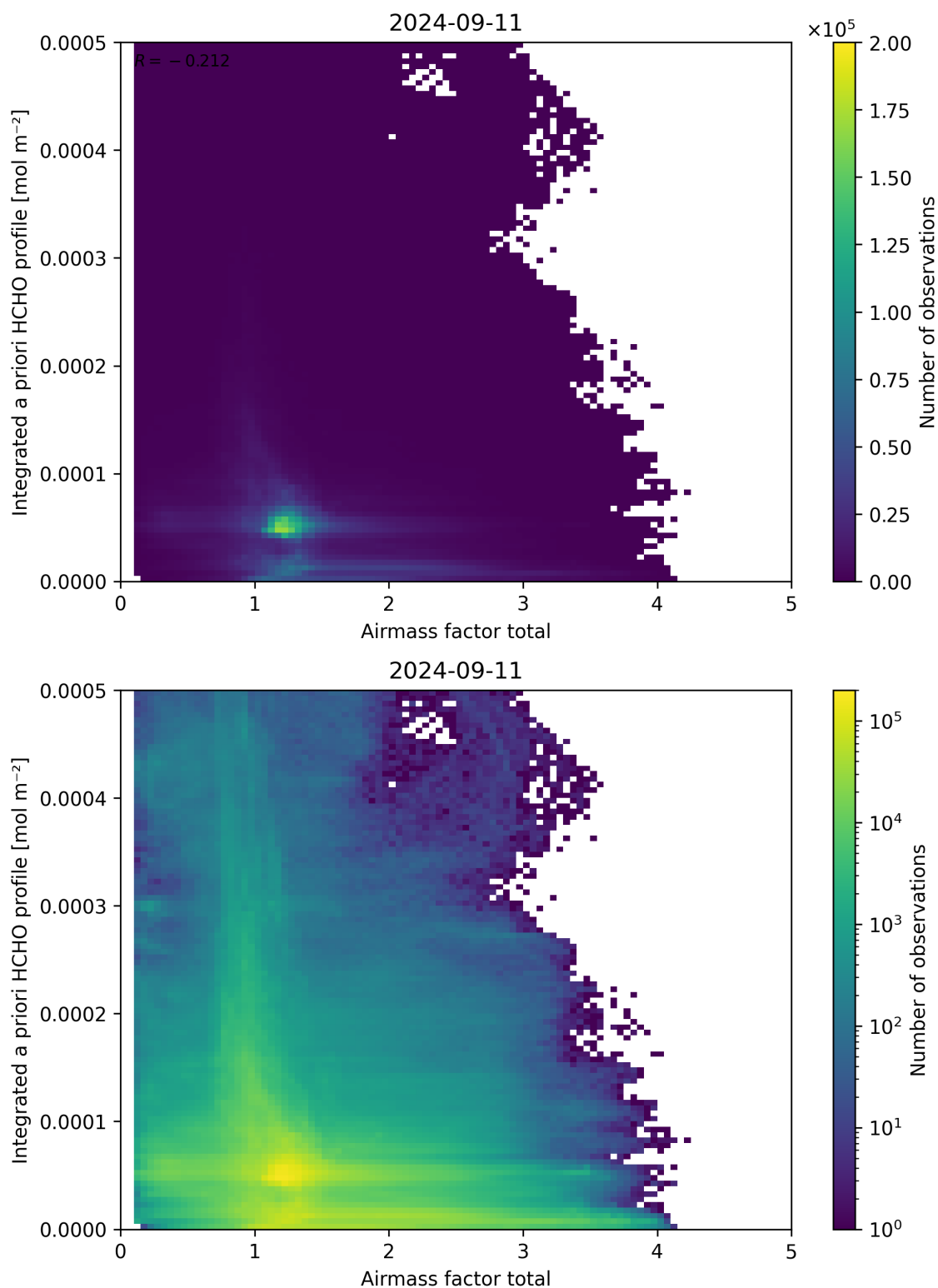
Figure 104: Scatter density plot of “Airmass factor total” against “Integrated a priori HCHO profile” for 2024-09-10 to 2024-09-12.
