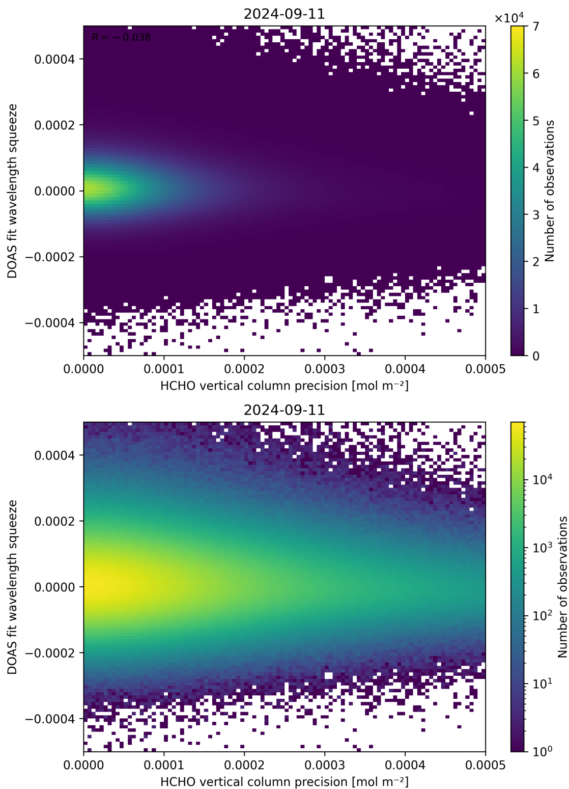
Figure 138: Scatter density plot of “HCHO vertical column precision” against “DOAS fit wavelength squeeze” for 2024-09-10 to 2024-09-12.
