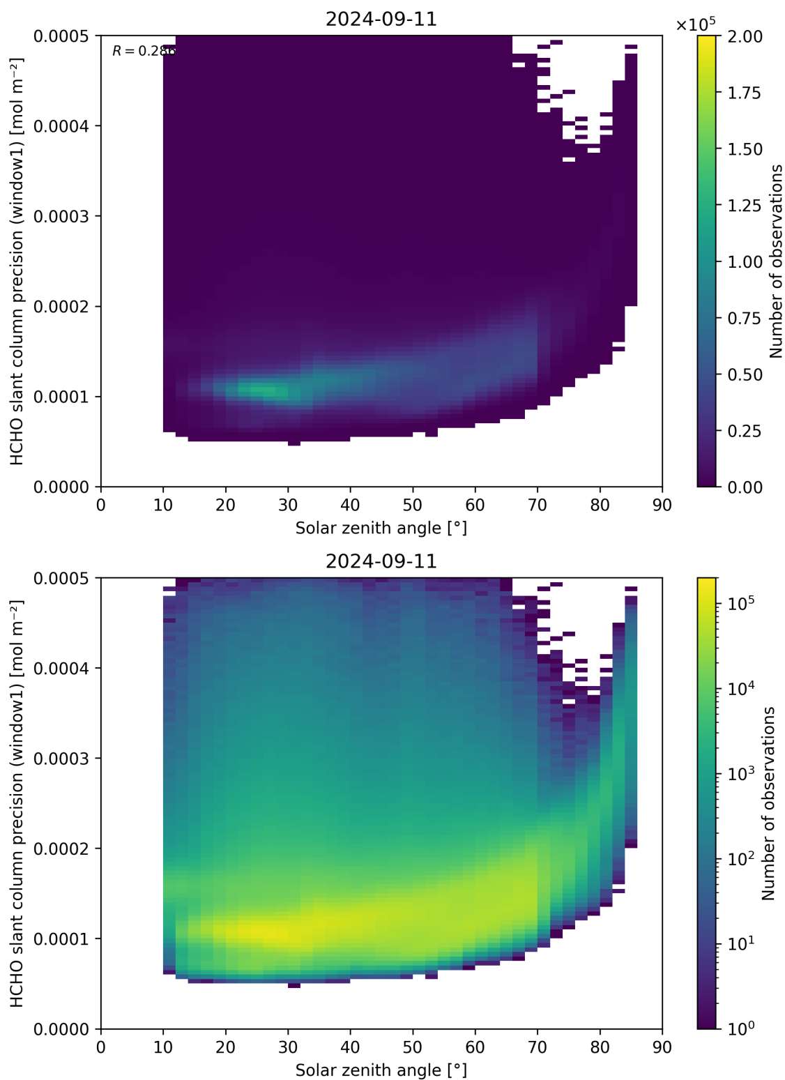
Figure 174: Scatter density plot of “Solar zenith angle” against “HCHO slant column precision (window1)” for 2024-09-10 to 2024-09-12.
