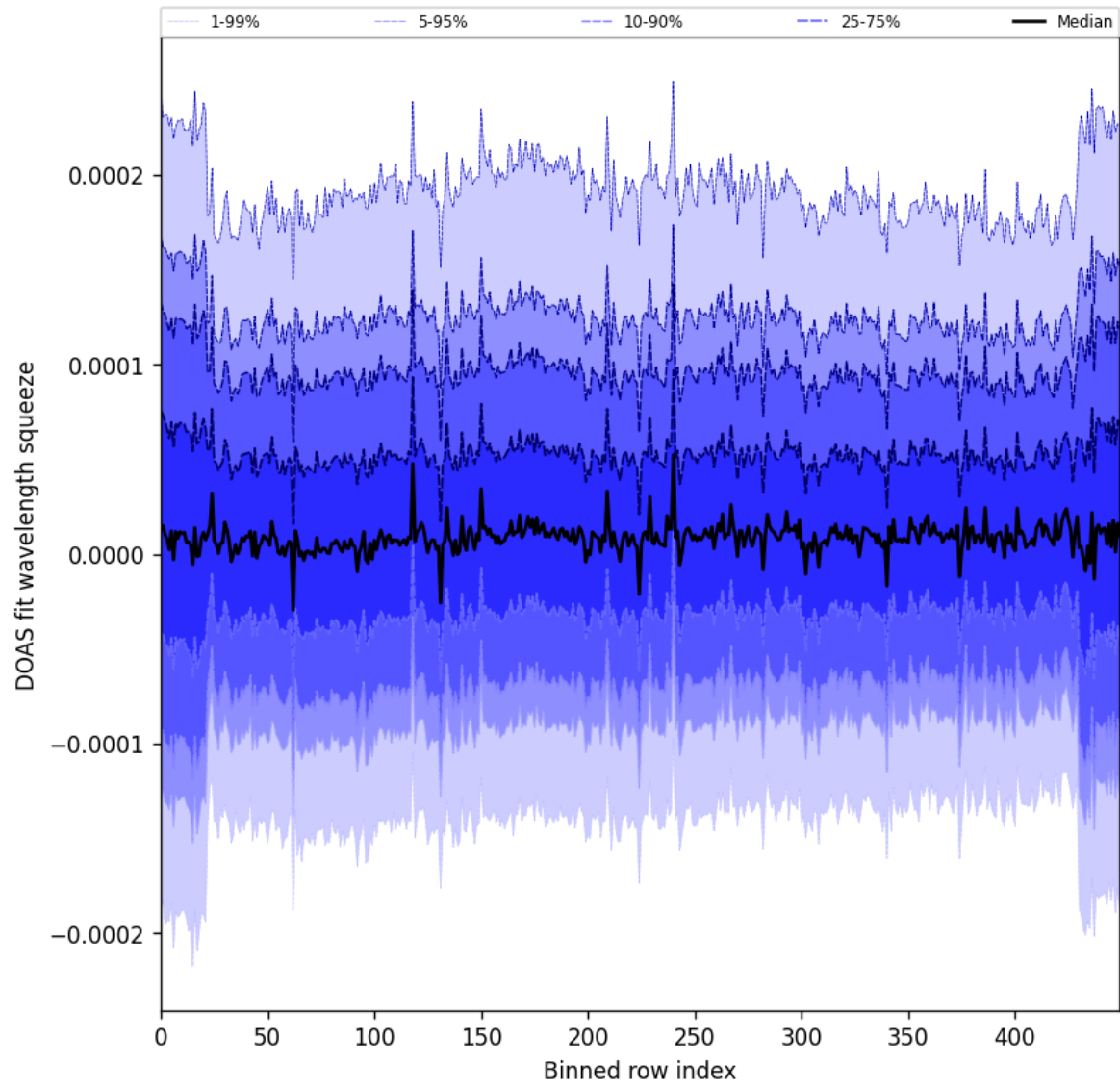
Figure 59: Along track statistics of “DOAS fit wavelength squeeze” for 2024-09-10 to 2024-09-12
