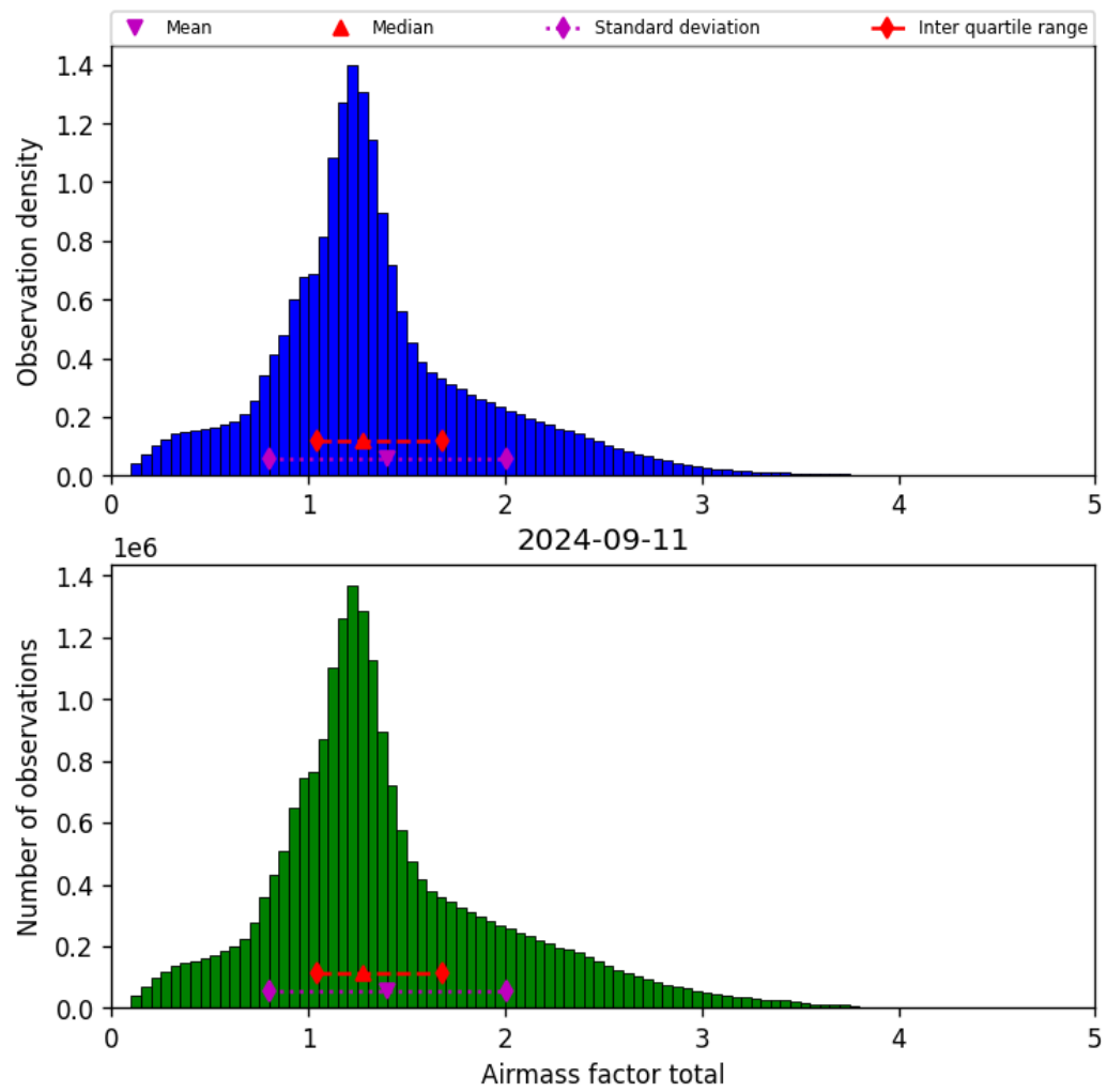
Figure 40: Histogram of “Airmass factor total” for 2024-09-10 to 2024-09-12
