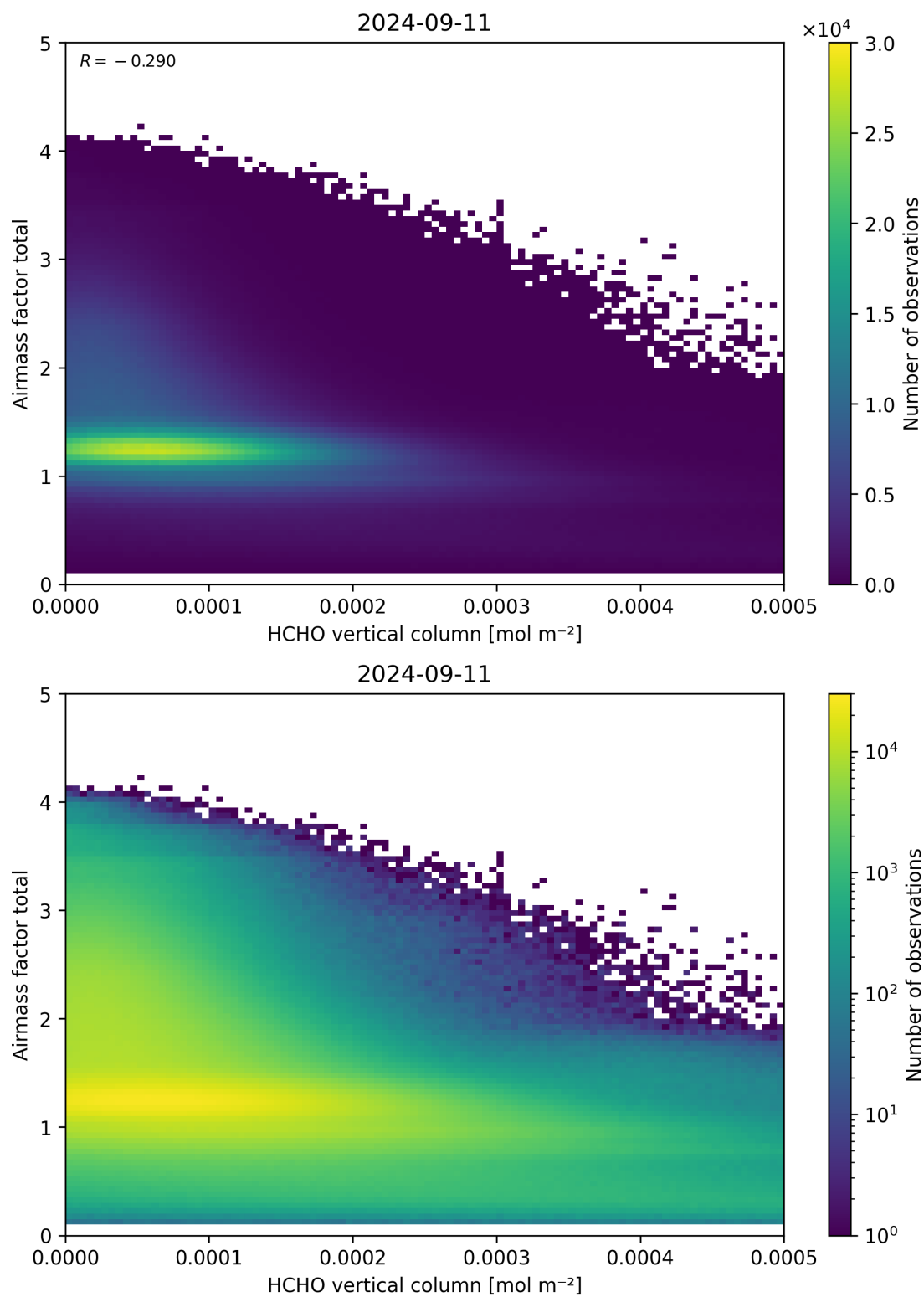
Figure 131: Scatter density plot of “HCHO vertical column” against “Airmass factor total” for 2024-09-10 to 2024-09-12.
