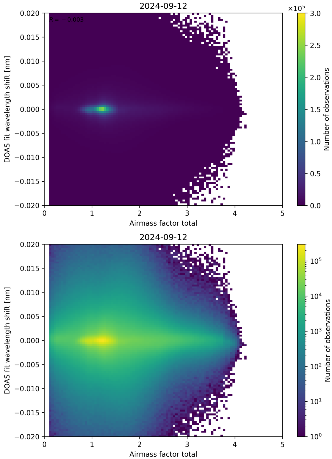
Figure 98: Scatter density plot of “Airmass factor total” against “DOAS fit wavelength shift” for 2024-09-12 to 2024-09-13.
