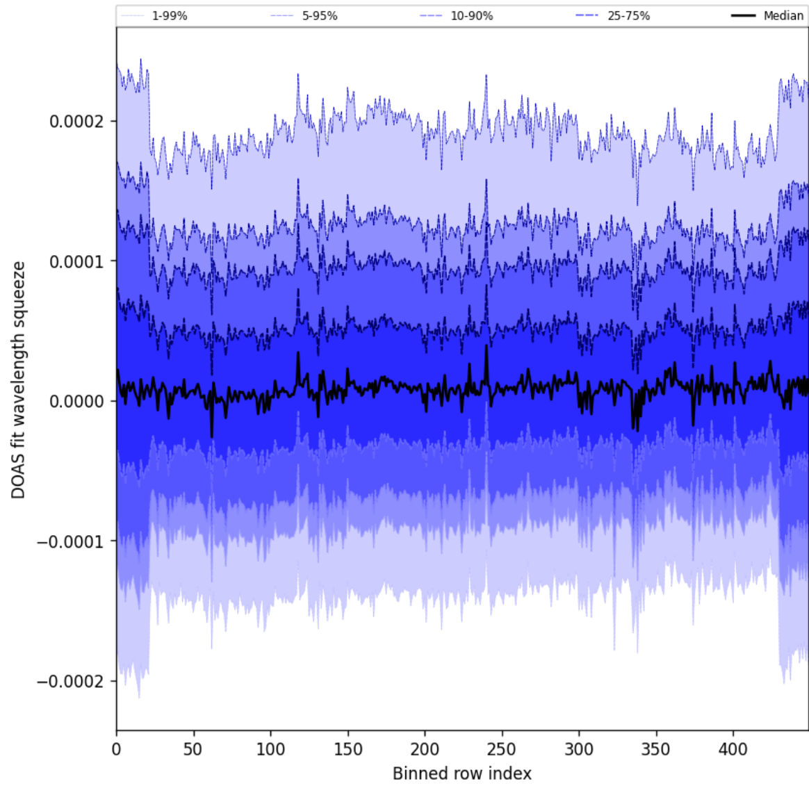
Figure 59: Along track statistics of “DOAS fit wavelength squeeze” for 2024-09-12 to 2024-09-13
