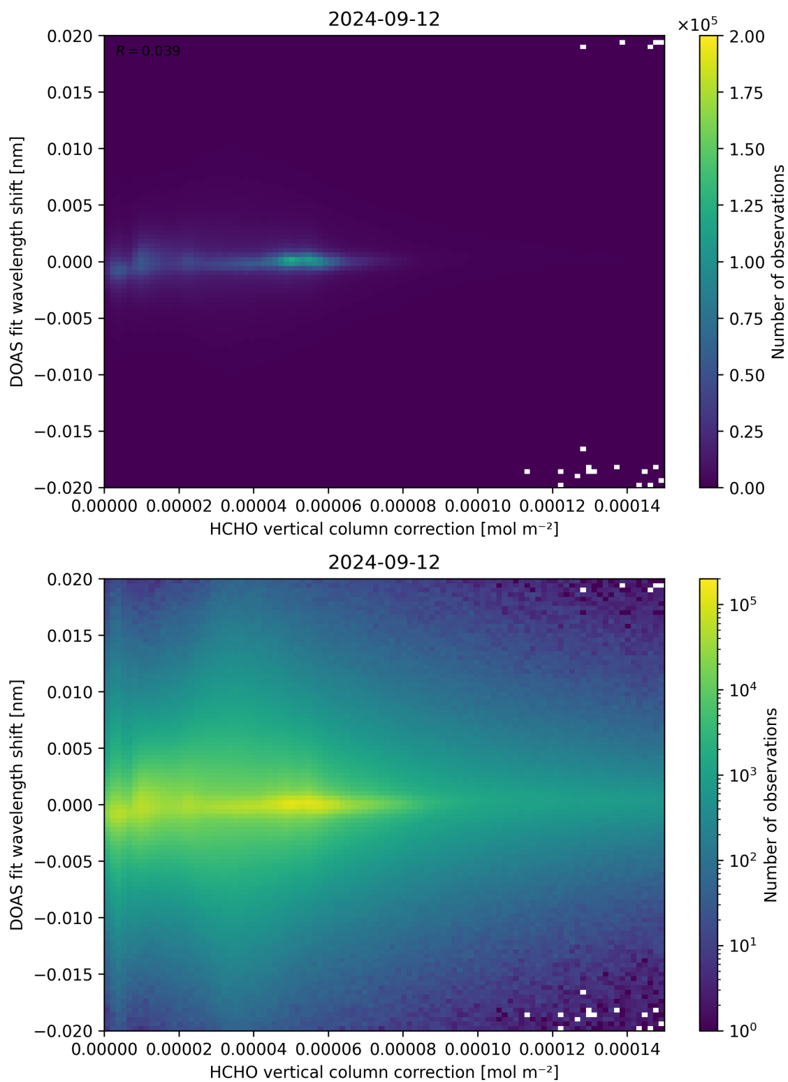
Figure 113: Scatter density plot of “HCHO vertical column correction” against “DOAS fit wavelength shift” for 2024-09-12 to 2024-09-13.
