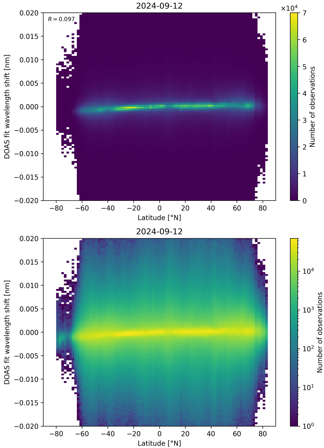
Figure 154: Scatter density plot of “Latitude” against “DOAS fit wavelength shift” for 2024-09-12 to 2024-09-13.
