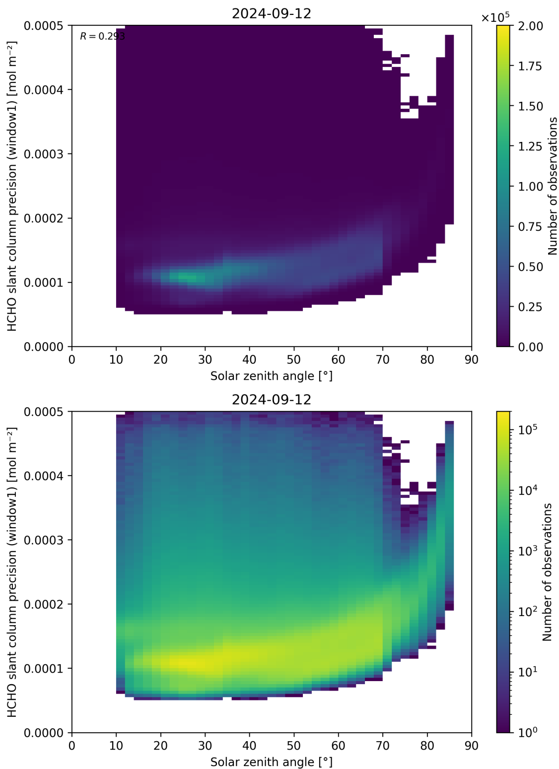
Figure 174: Scatter density plot of “Solar zenith angle” against “HCHO slant column precision (window1)” for 2024-09-12 to 2024-09-13.
