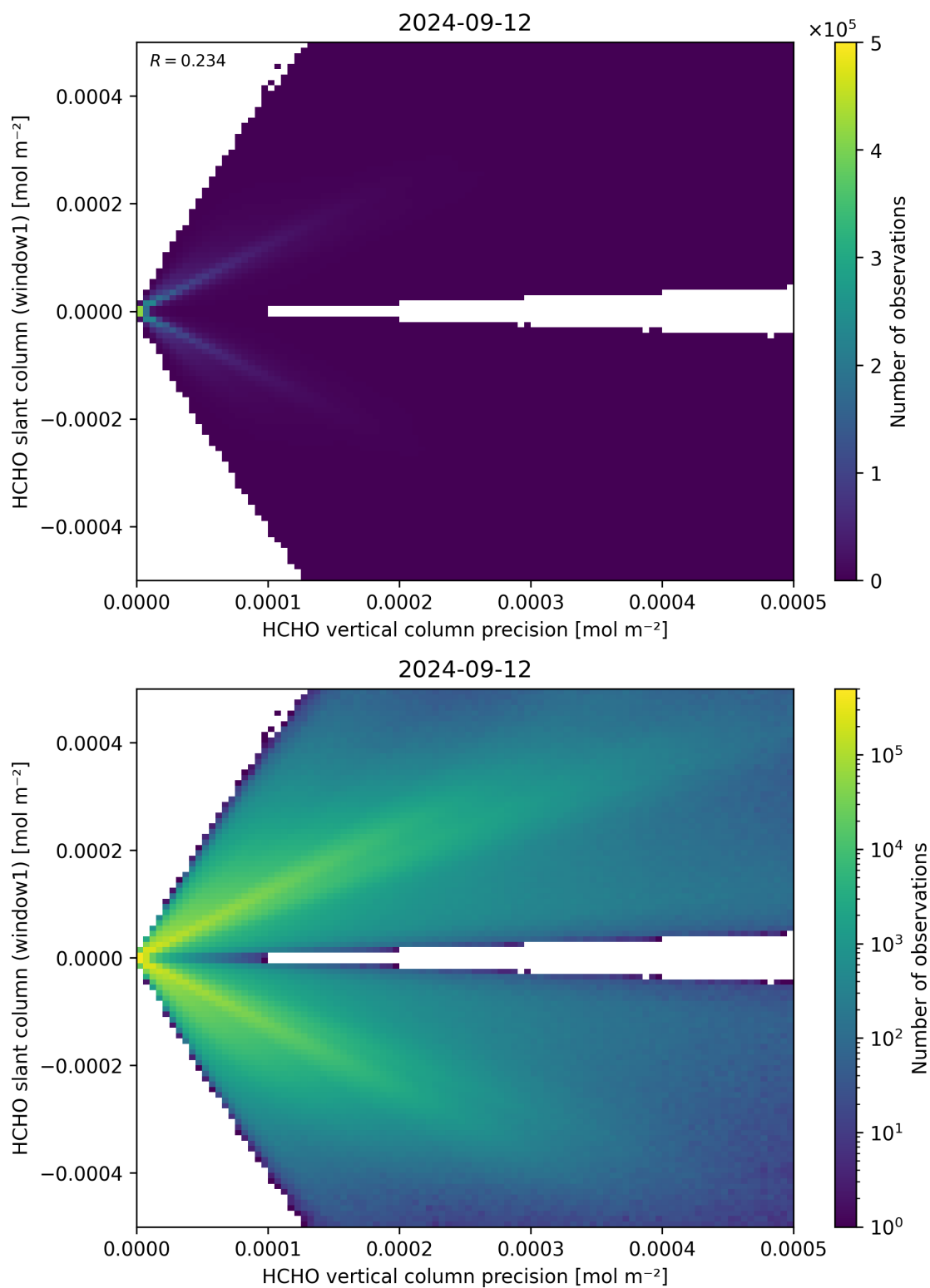
Figure 142: Scatter density plot of “HCHO vertical column precision” against “HCHO slant column (window1)” for 2024-09-12 to 2024-09-13.
