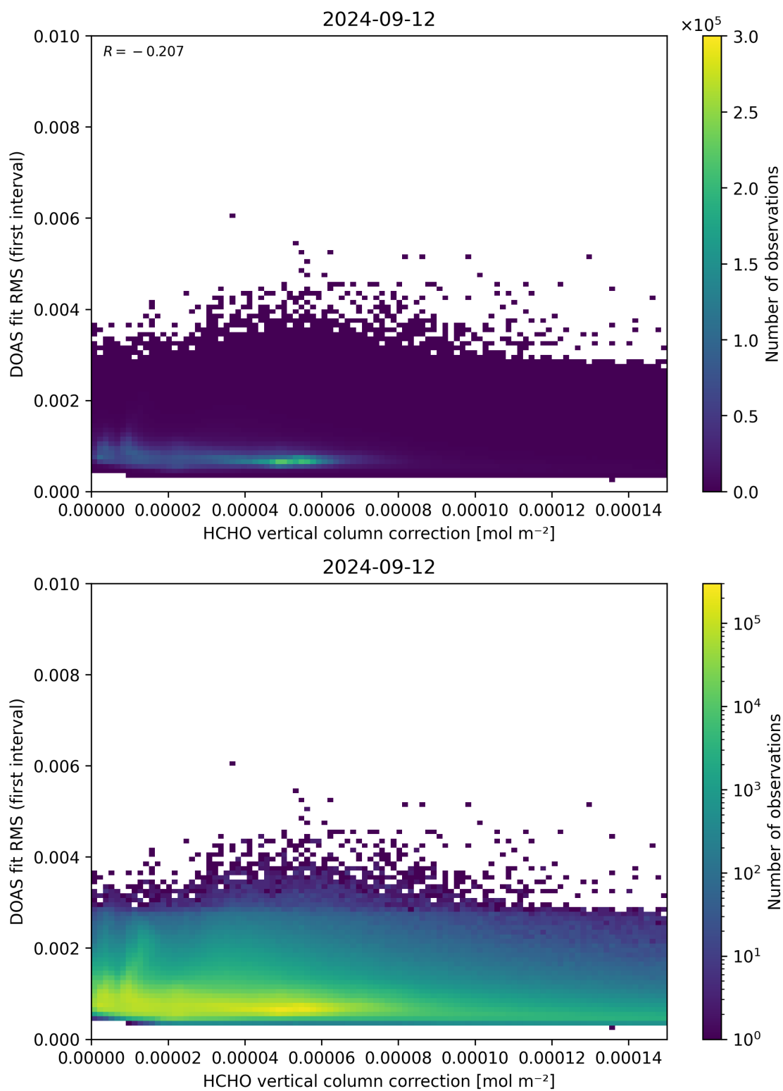
Figure 112: Scatter density plot of “HCHO vertical column correction” against “DOAS fit RMS (first interval)” for 2024-09-12 to 2024-09-13.
