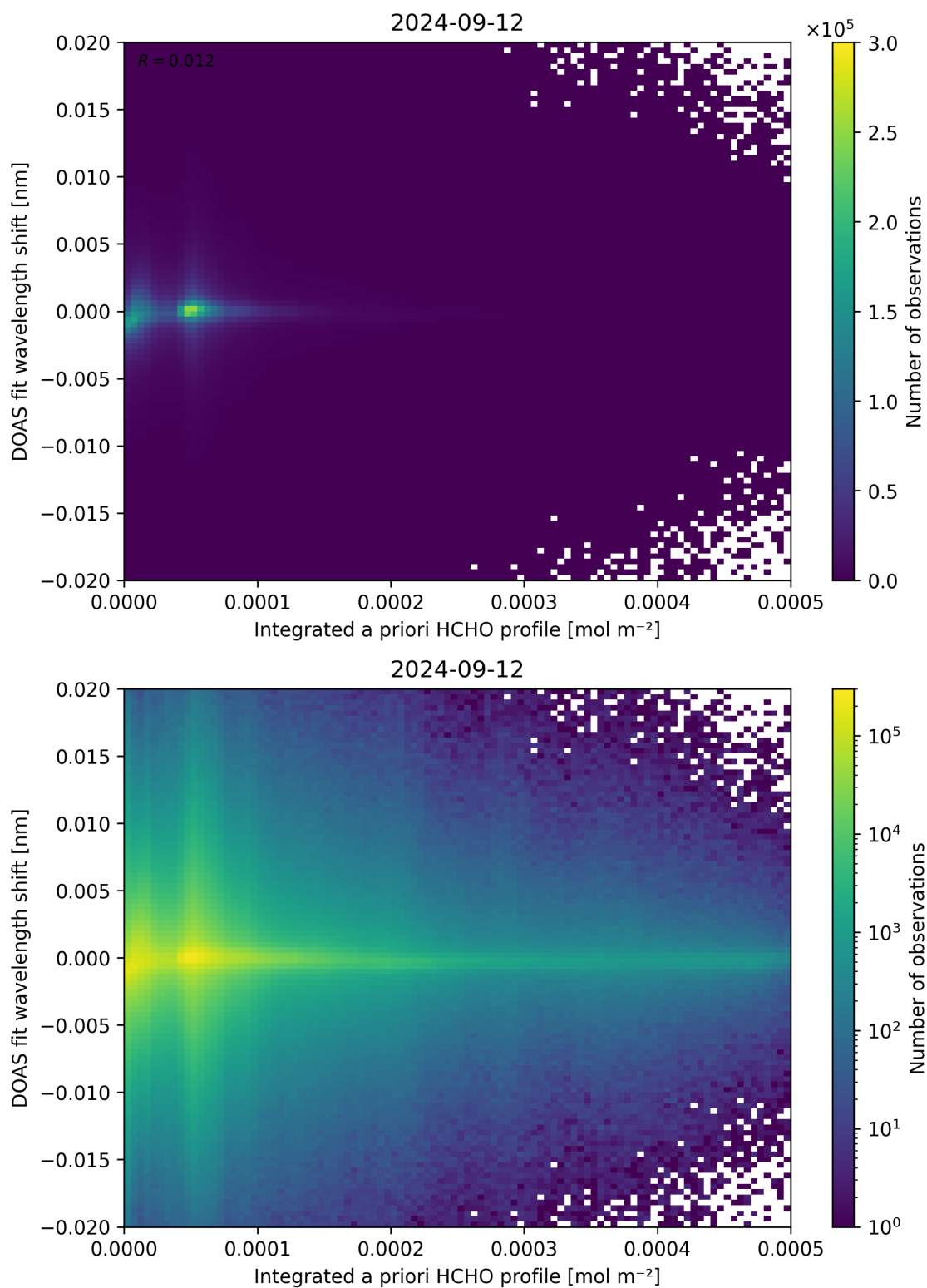
Figure 149: Scatter density plot of “Integrated a priori HCHO profile” against “DOAS fit wavelength shift” for 2024-09-12 to 2024-09-13.
