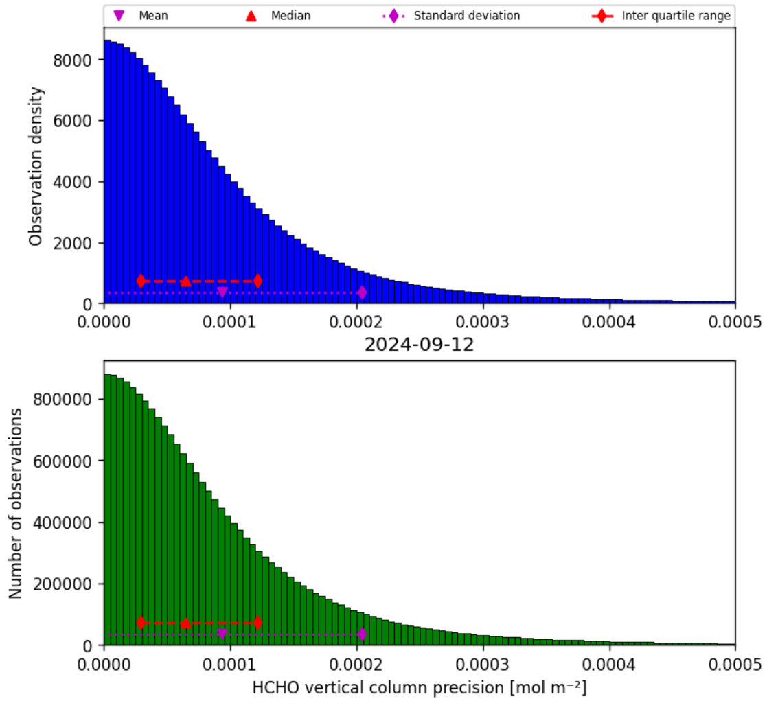
Figure 36: Histogram of “HCHO vertical column precision” for 2024-09-12 to 2024-09-13
