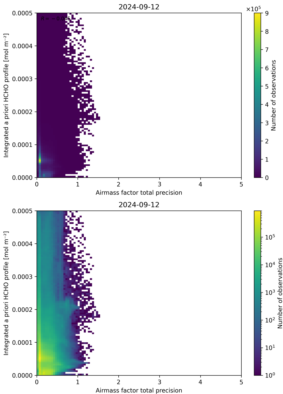
Figure 111: Scatter density plot of “Airmass factor total precision” against “Integrated a priori HCHO profile” for 2024-09-12 to 2024-09-13.
