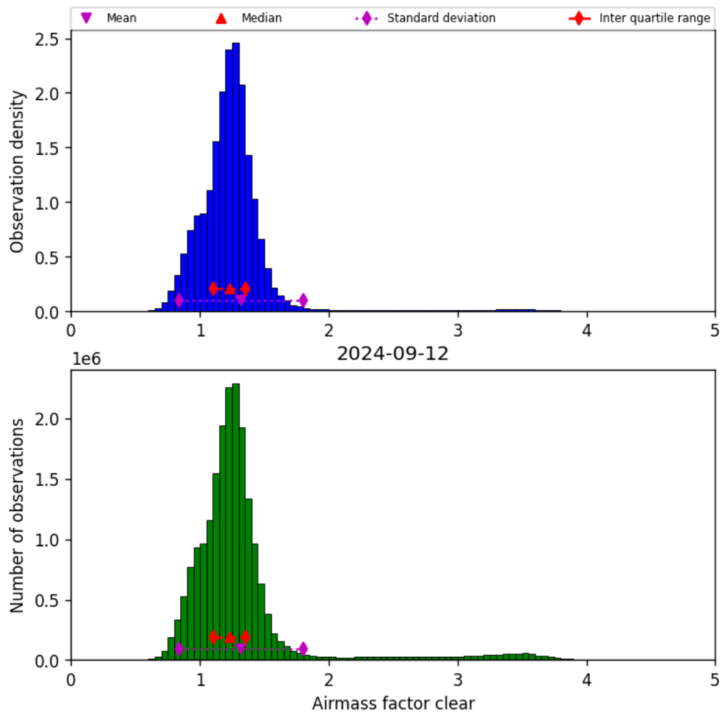
Figure 42: Histogram of “Airmass factor clear” for 2024-09-12 to 2024-09-13
