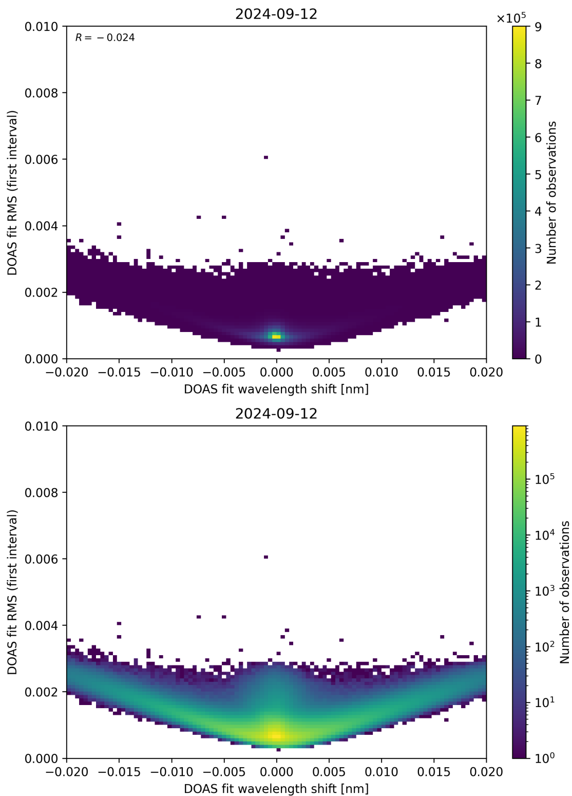
Figure 64: Scatter density plot of “DOAS fit wavelength shift” against “DOAS fit RMS (first interval)” for 2024-09-12 to 2024-09-13.
