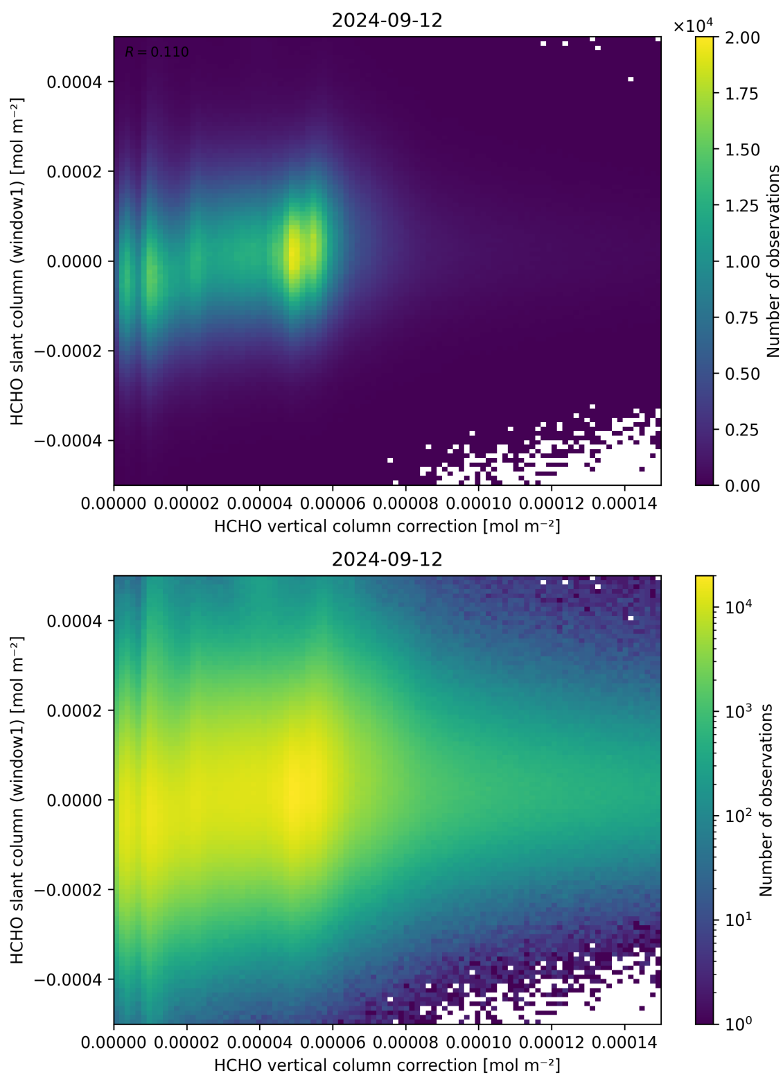
Figure 118: Scatter density plot of “HCHO vertical column correction” against “HCHO slant column (window1)” for 2024-09-12 to 2024-09-13.
