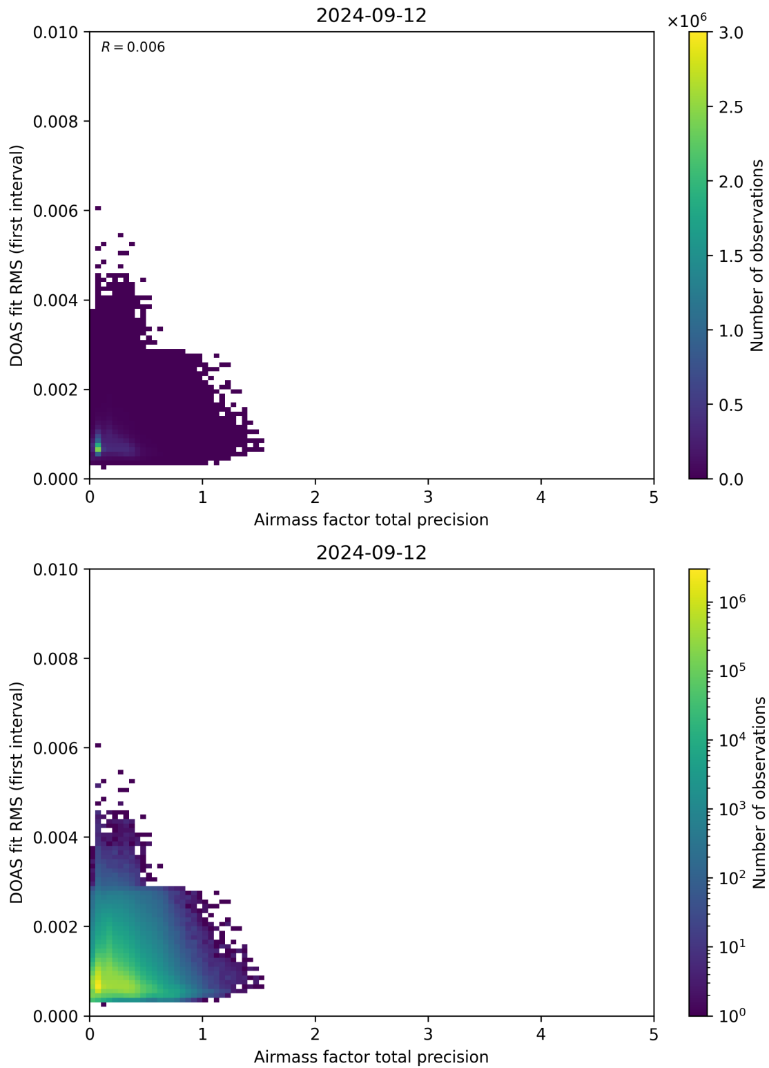
Figure 105: Scatter density plot of “Airmass factor total precision” against “DOAS fit RMS (first interval)” for 2024-09-12 to 2024-09-13.
