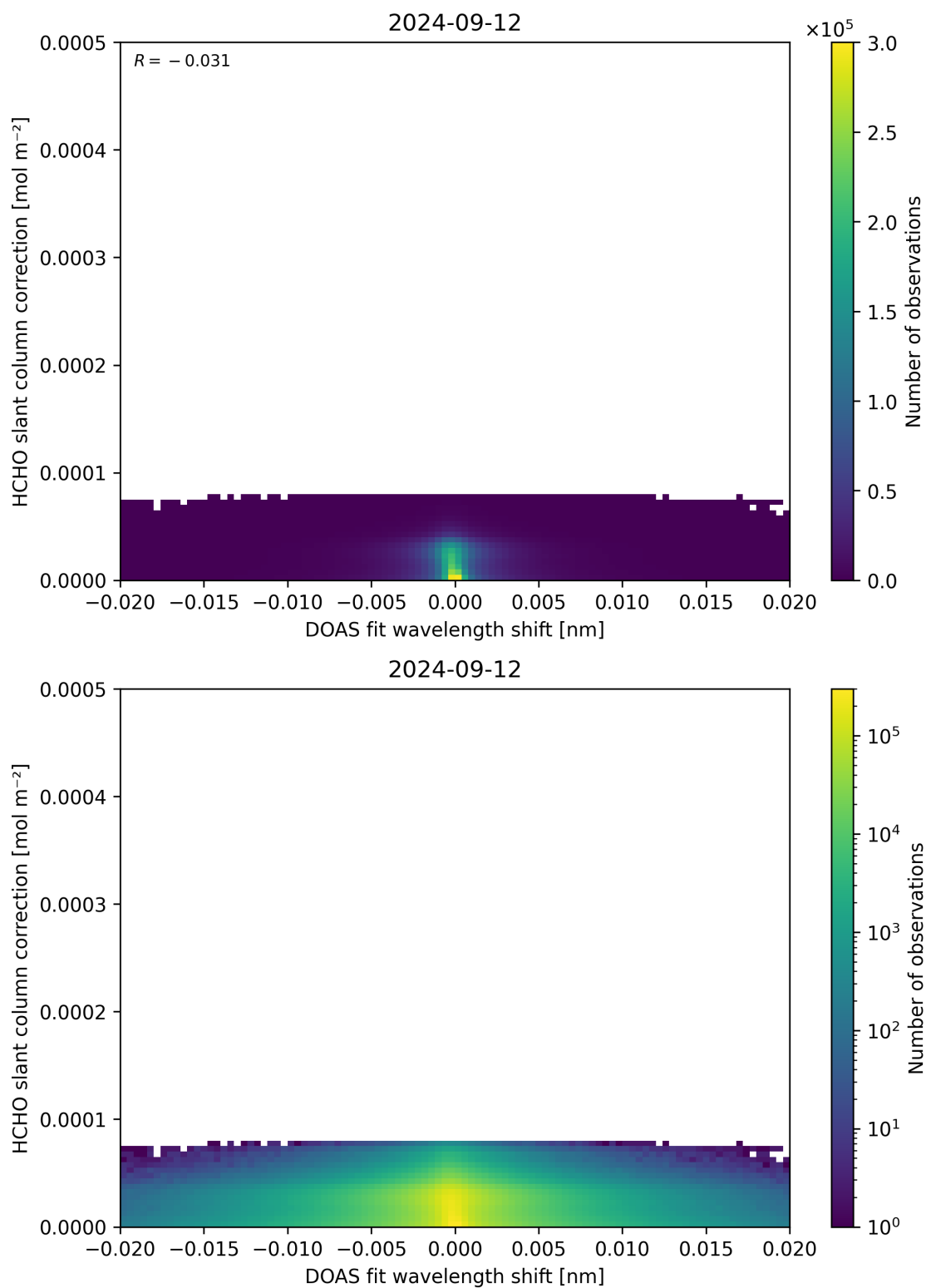
Figure 67: Scatter density plot of “DOAS fit wavelength shift” against “HCHO slant column correction” for 2024-09-12 to 2024-09-13.
