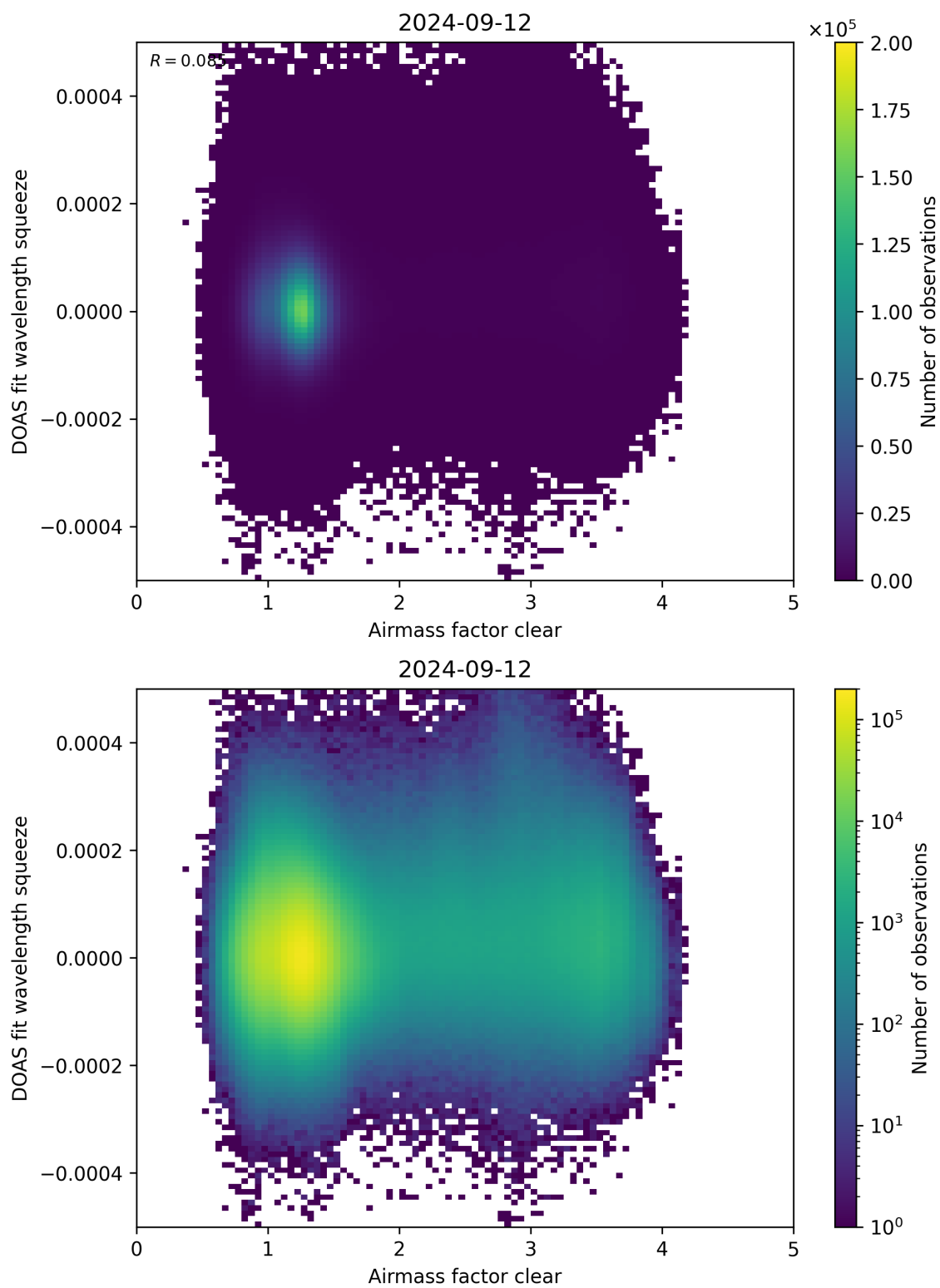
Figure 73: Scatter density plot of “Airmass factor clear” against “DOAS fit wavelength squeeze” for 2024-09-12 to 2024-09-13.
