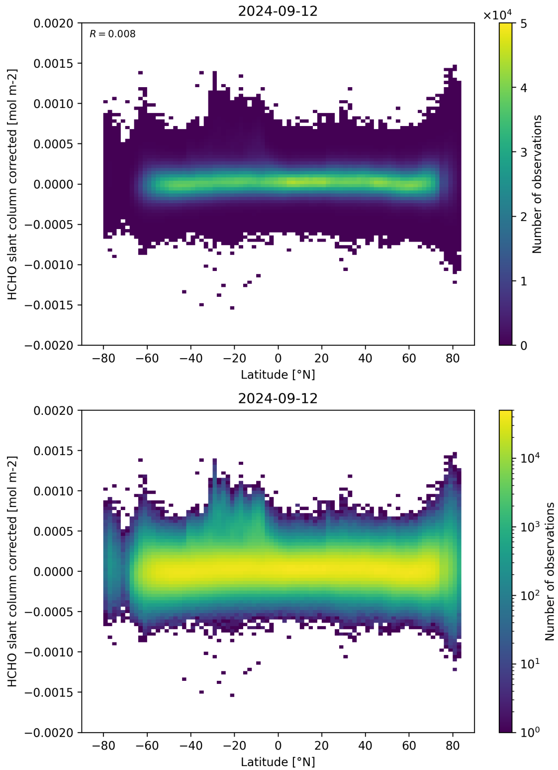
Figure 157: Scatter density plot of “Latitude” against “HCHO slant column corrected” for 2024-09-12 to 2024-09-13.
