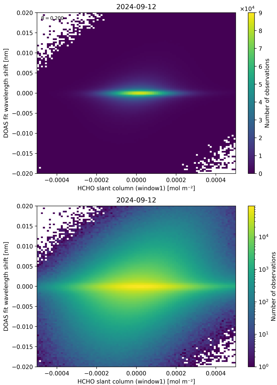
Figure 79: Scatter density plot of “HCHO slant column (window1)” against “DOAS fit wavelength shift” for 2024-09-12 to 2024-09-13.
