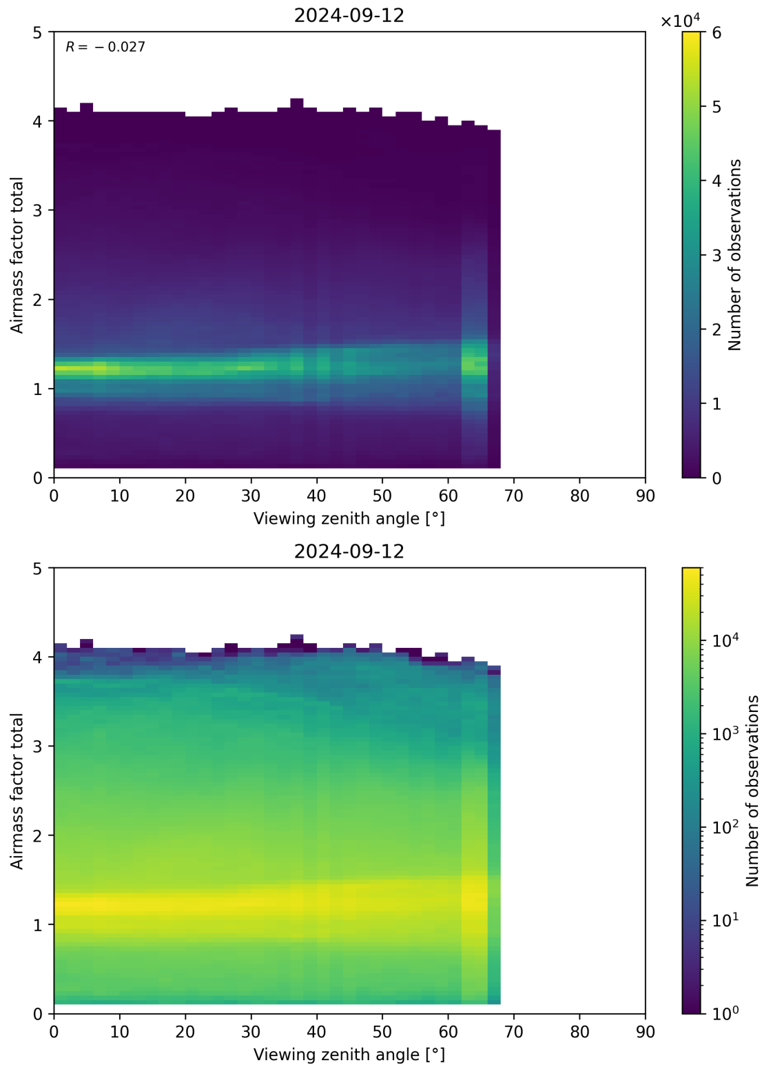
Figure 190: Scatter density plot of “Viewing zenith angle” against “Airmass factor total” for 2024-09-12 to 2024-09-13.
