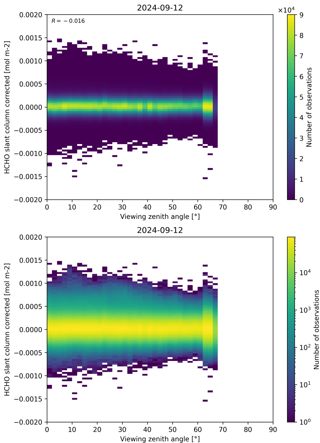
Figure 186: Scatter density plot of “Viewing zenith angle” against “HCHO slant column corrected” for 2024-09-12 to 2024-09-13.
