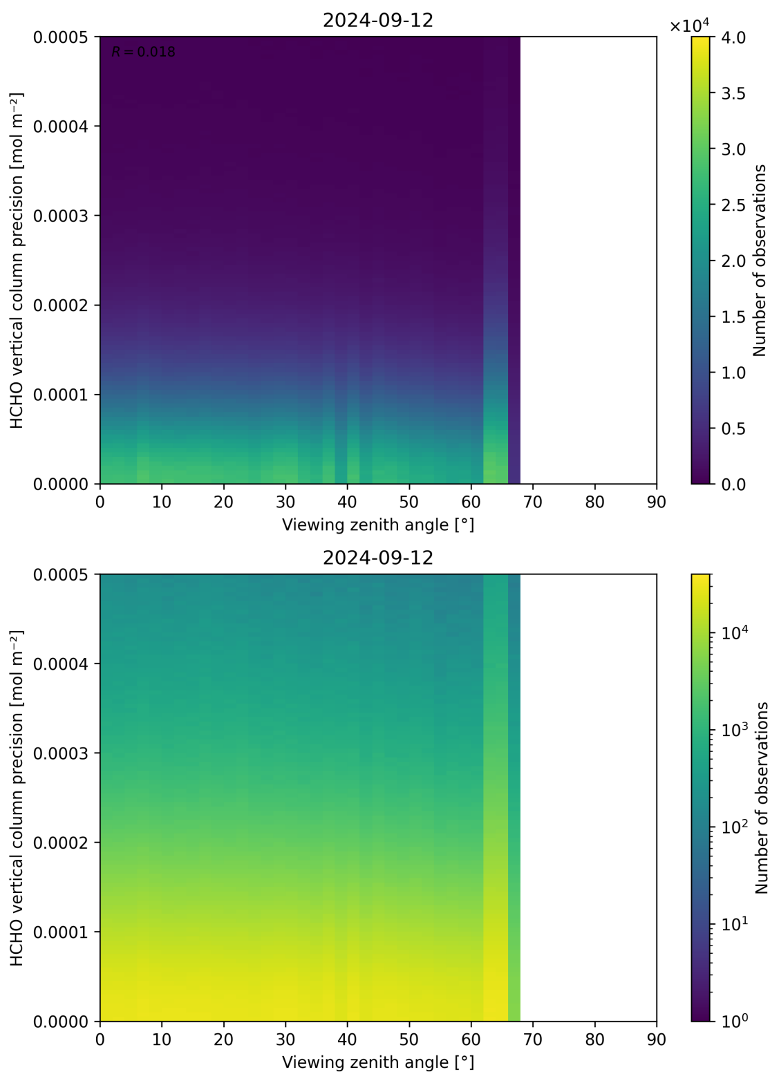
Figure 194: Scatter density plot of “Viewing zenith angle” against “HCHO vertical column precision” for 2024-09-12 to 2024-09-13.
