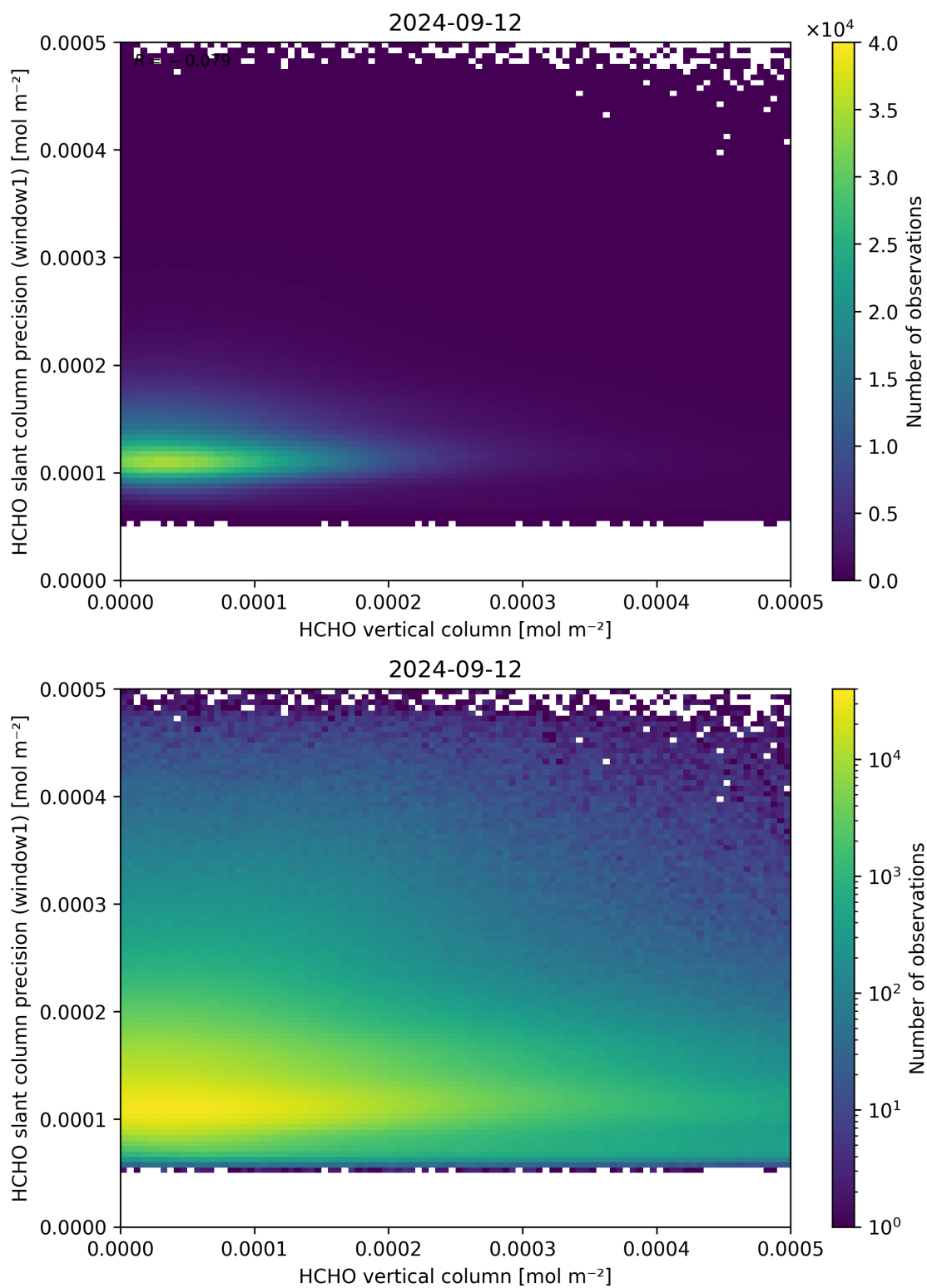
Figure 130: Scatter density plot of “HCHO vertical column” against “HCHO slant column precision (window1)” for 2024-09-12 to 2024-09-13.
