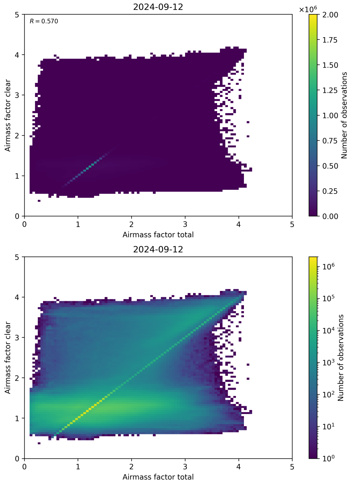
Figure 100: Scatter density plot of “Airmass factor total” against “Airmass factor clear” for 2024-09-12 to 2024-09-13.
