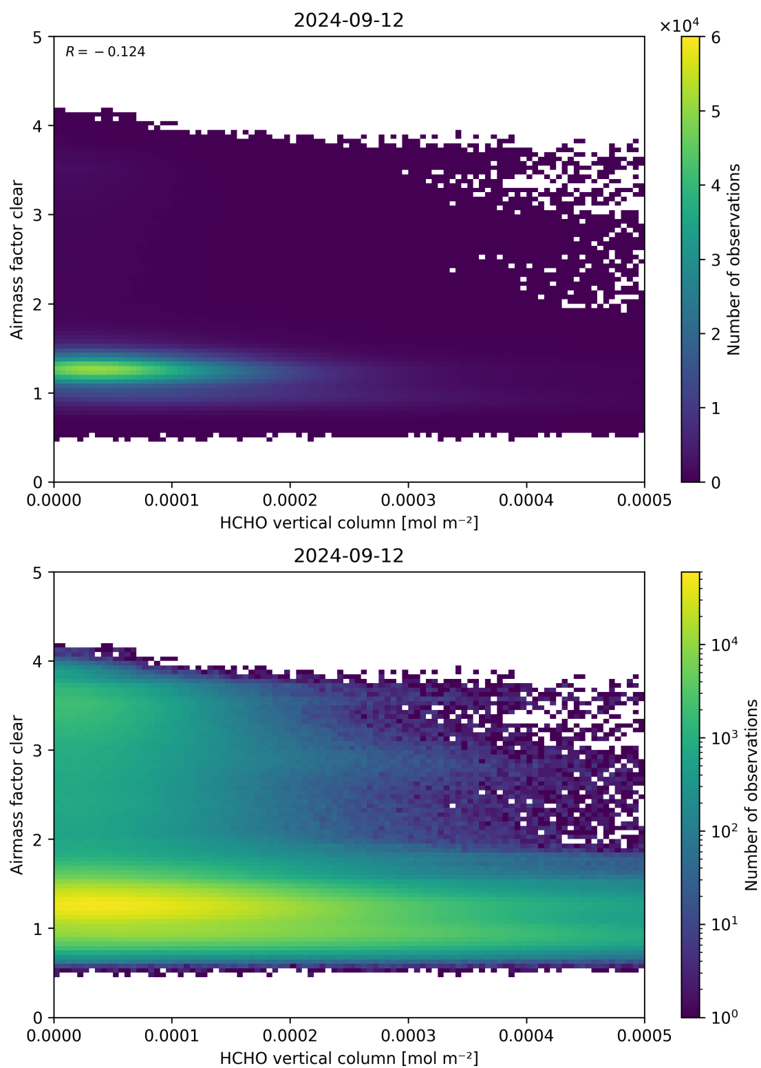
Figure 126: Scatter density plot of “HCHO vertical column” against “Airmass factor clear” for 2024-09-12 to 2024-09-13.
