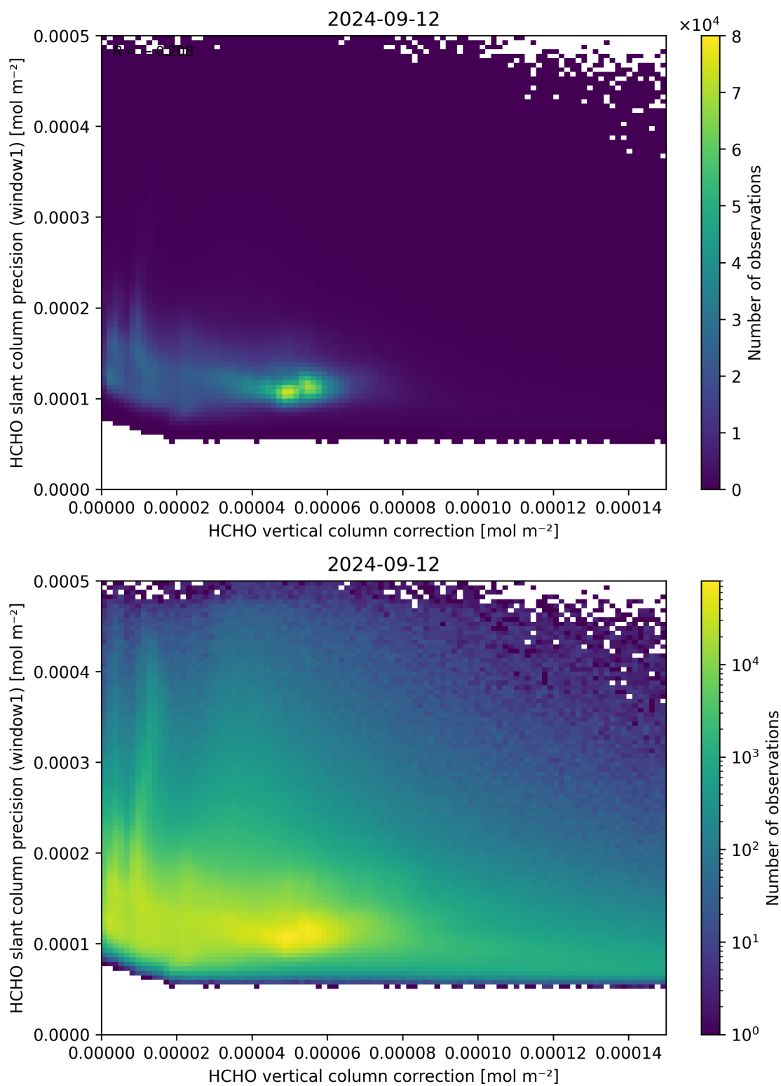
Figure 119: Scatter density plot of “HCHO vertical column correction” against “HCHO slant column precision (window1)” for 2024-09-12 to 2024-09-13.
