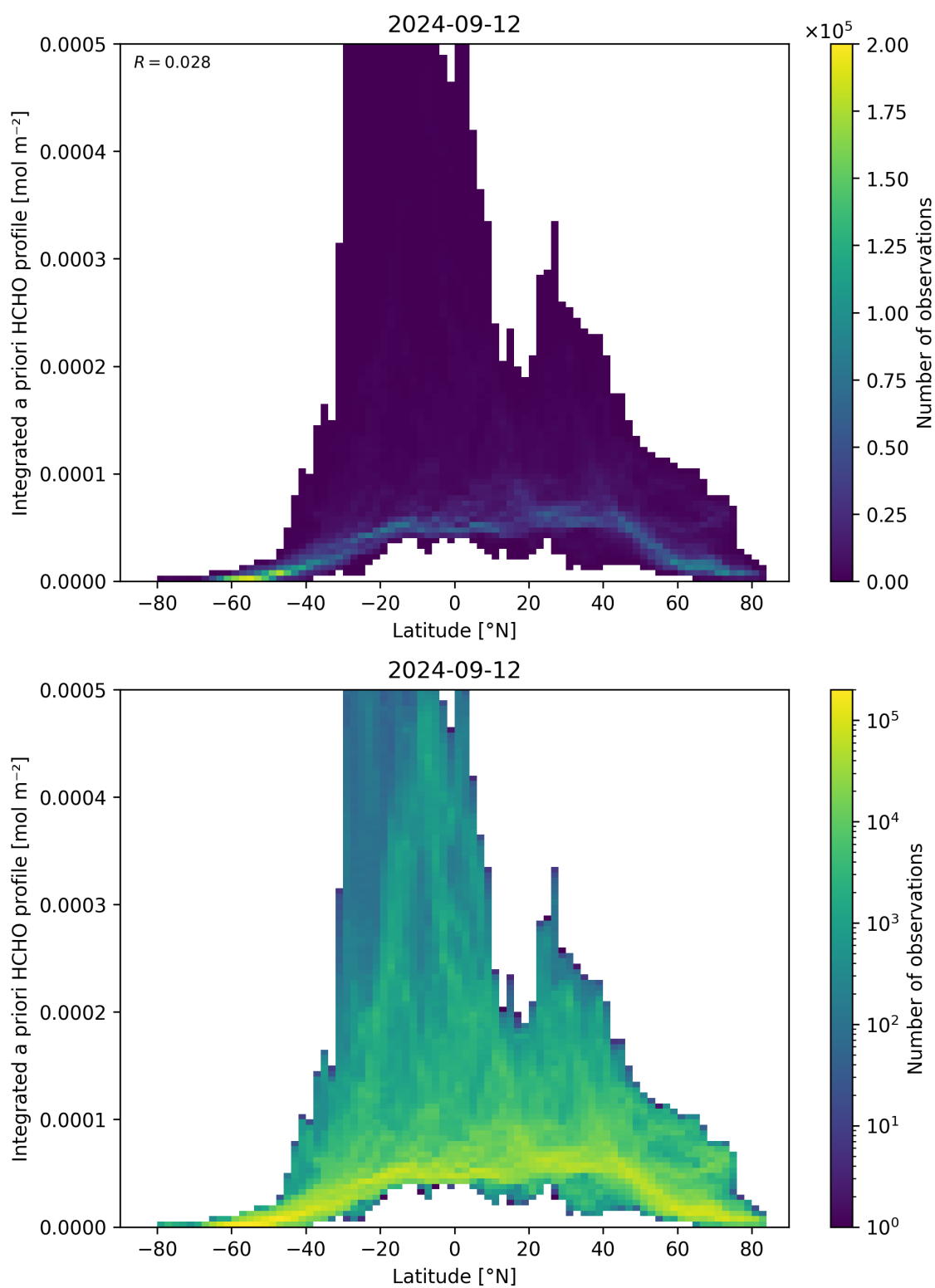
Figure 166: Scatter density plot of “Latitude” against “Integrated a priori HCHO profile” for 2024-09-12 to 2024-09-13.
