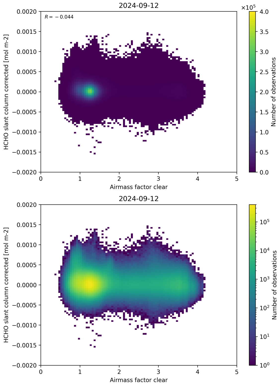
Figure 74: Scatter density plot of “Airmass factor clear” against “HCHO slant column corrected” for 2024-09-12 to 2024-09-13.
