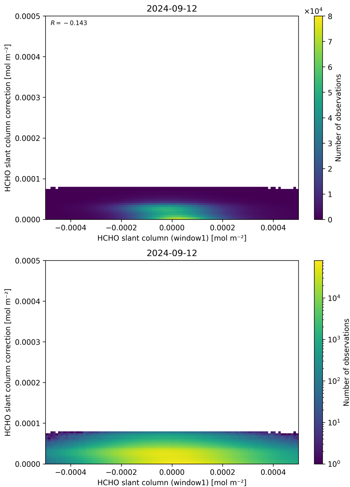
Figure 83: Scatter density plot of “HCHO slant column (window1)” against “HCHO slant column correction” for 2024-09-12 to 2024-09-13.
