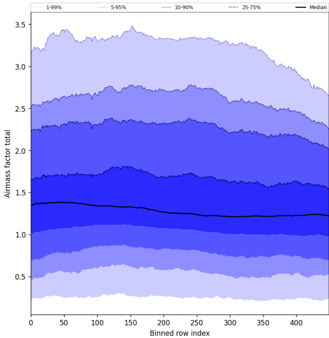
Figure 54: Along track statistics of “Airmass factor total” for 2024-09-12 to 2024-09-13
