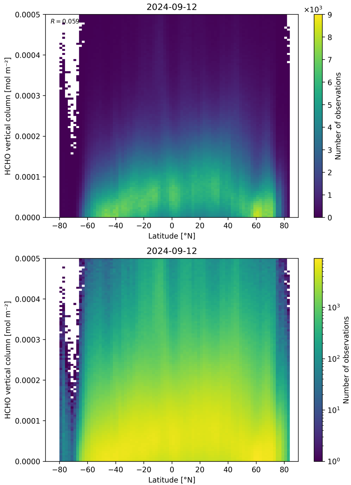
Figure 163: Scatter density plot of “Latitude” against “HCHO vertical column” for 2024-09-12 to 2024-09-13.
