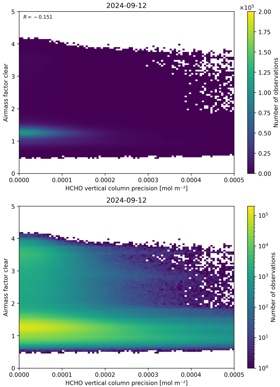
Figure 139: Scatter density plot of “HCHO vertical column precision” against “Airmass factor clear” for 2024-09-12 to 2024-09-13.
