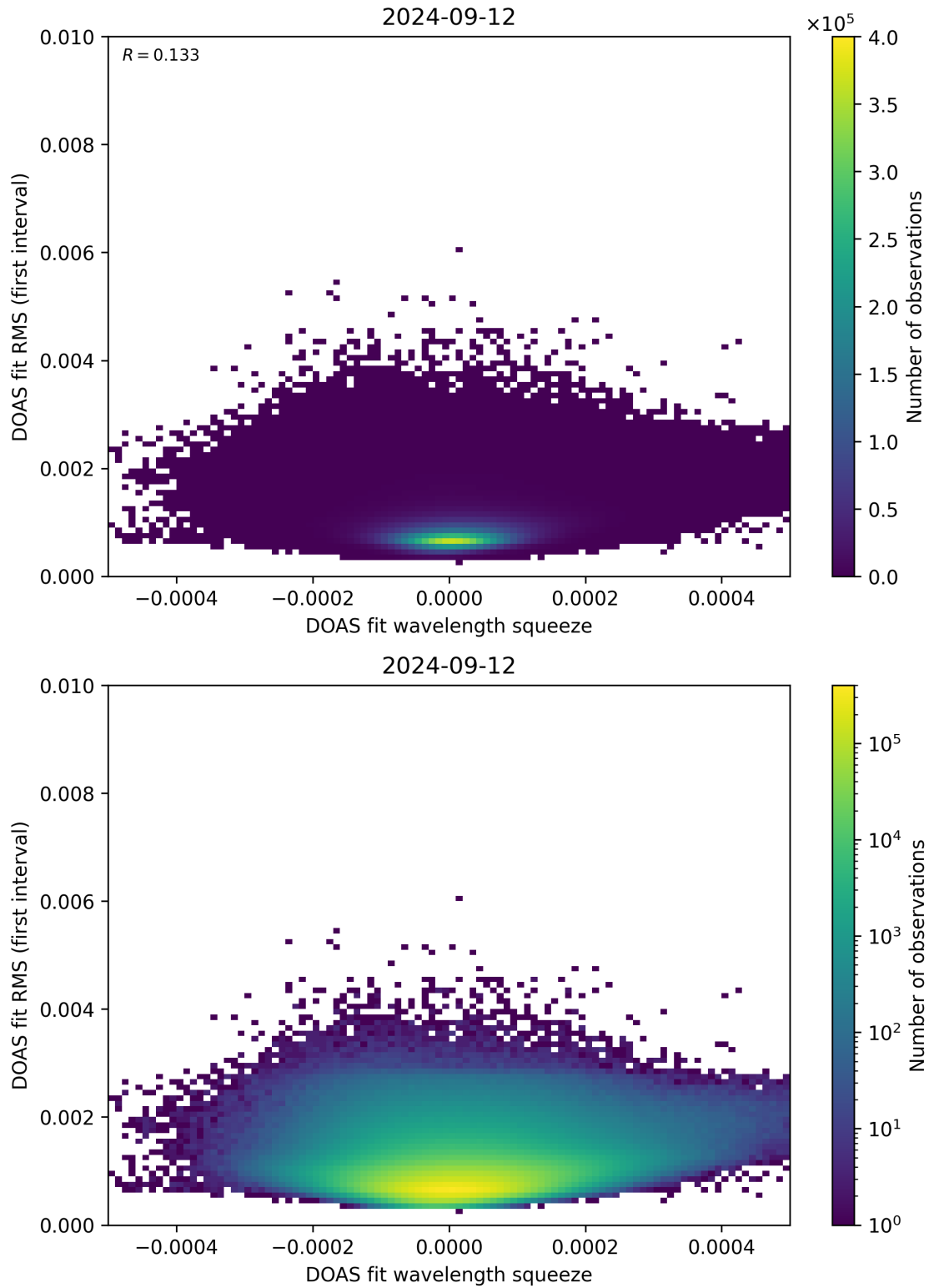
Figure 68: Scatter density plot of “DOAS fit wavelength squeeze” against “DOAS fit RMS (first interval)” for 2024-09-12 to 2024-09-13.
