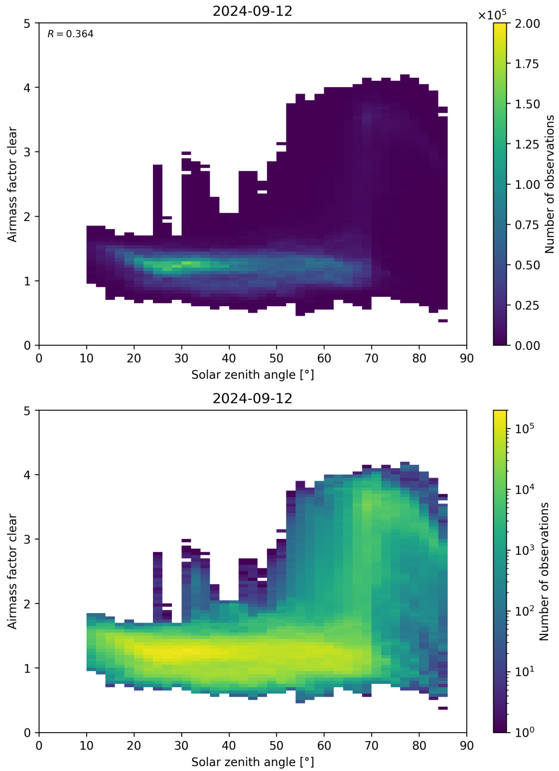
Figure 170: Scatter density plot of “Solar zenith angle” against “Airmass factor clear” for 2024-09-12 to 2024-09-13.
