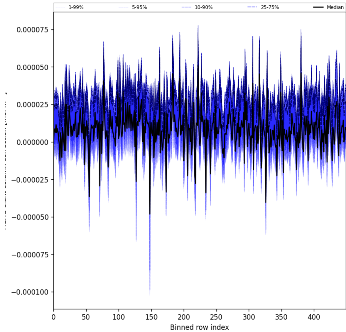
Figure 61: Along track statistics of “HCHO slant column correction” for 2024-09-12 to 2024-09-13
