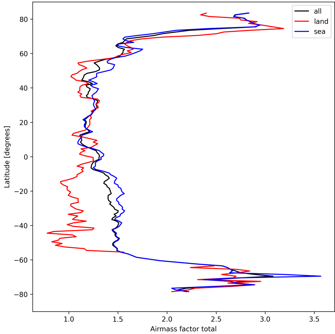
Figure 26: Zonal average of “Airmass factor total” for 2024-09-12 to 2024-09-13.
