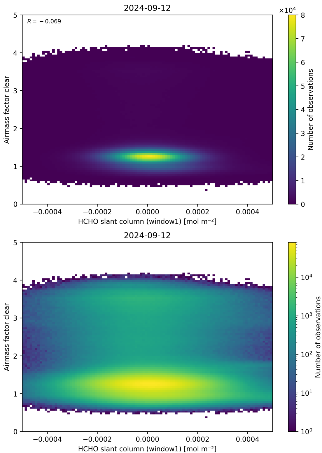
Figure 81: Scatter density plot of “HCHO slant column (window1)” against “Airmass factor clear” for 2024-09-12 to 2024-09-13.
