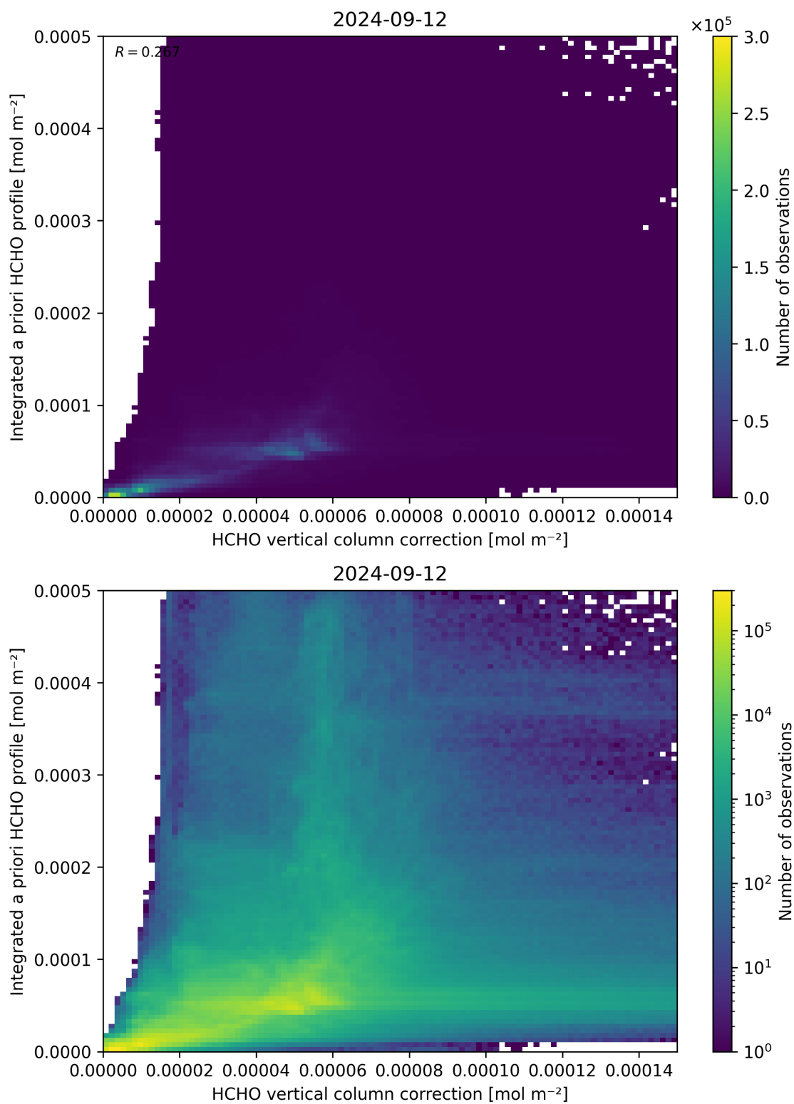
Figure 122: Scatter density plot of “HCHO vertical column correction” against “Integrated a priori HCHO profile” for 2024-09-12 to 2024-09-13.
