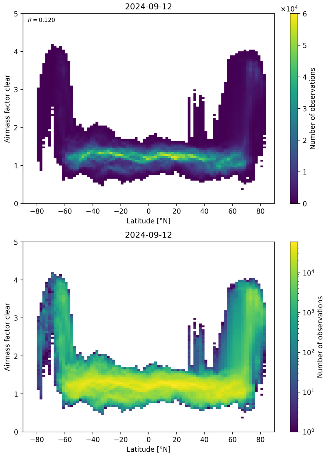
Figure 156: Scatter density plot of “Latitude” against “Airmass factor clear” for 2024-09-12 to 2024-09-13.
