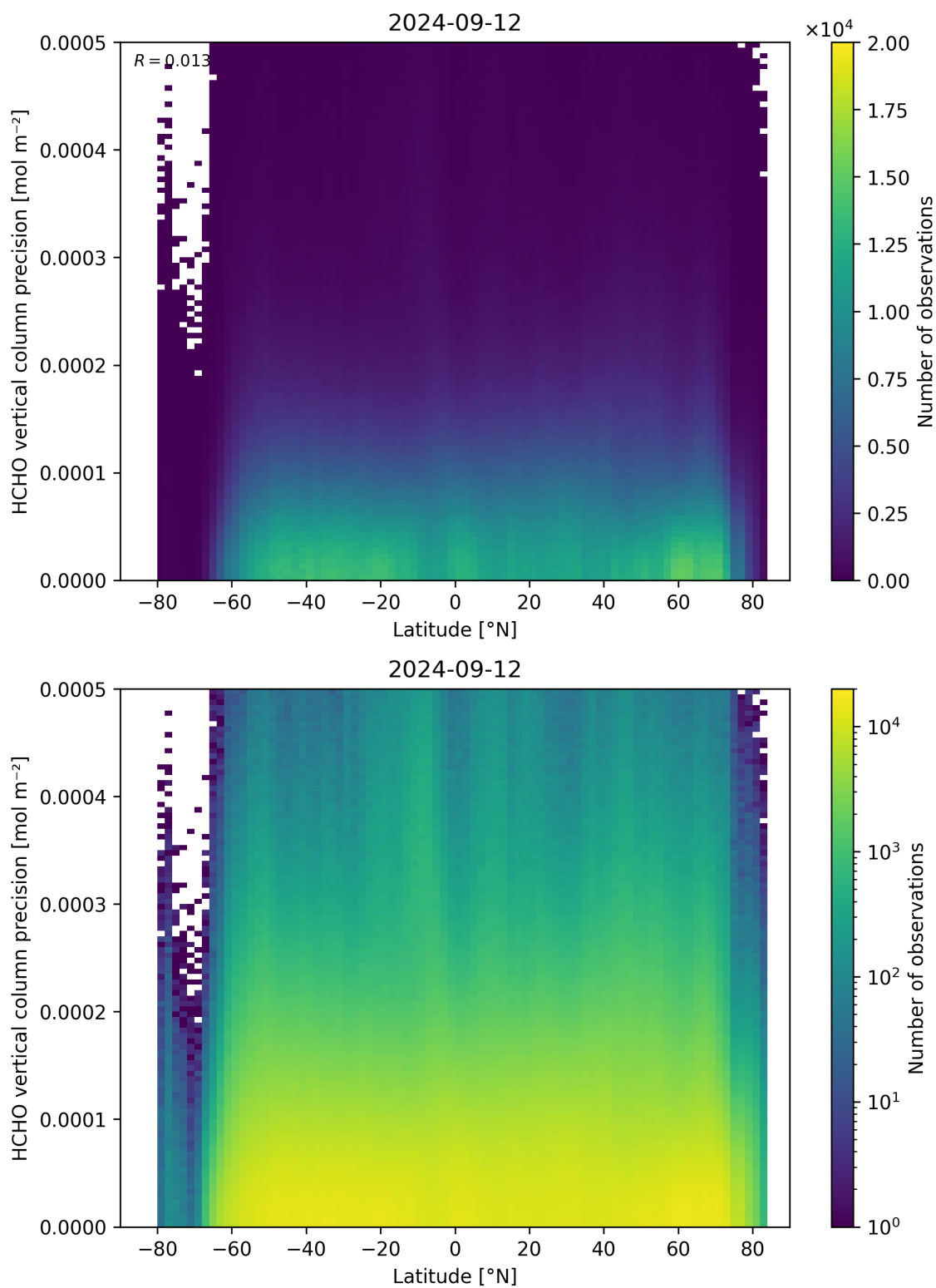
Figure 165: Scatter density plot of “Latitude” against “HCHO vertical column precision” for 2024-09-12 to 2024-09-13.
