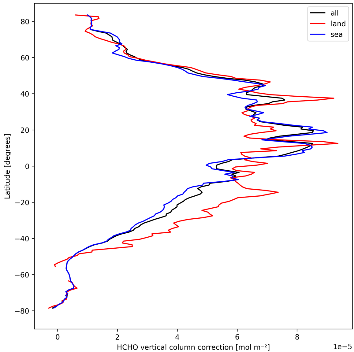
Figure 23: Zonal average of “HCHO vertical column correction” for 2024-09-12 to 2024-09-13.
