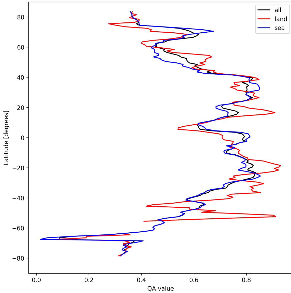
Figure 20: Zonal average of “QA value” for 2024-09-12 to 2024-09-13.
