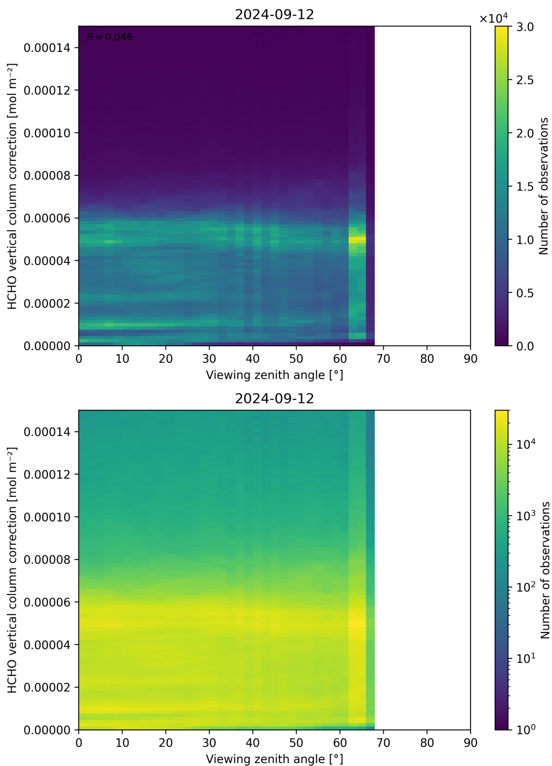
Figure 193: Scatter density plot of “Viewing zenith angle” against “HCHO vertical column correction” for 2024-09-12 to 2024-09-13.
