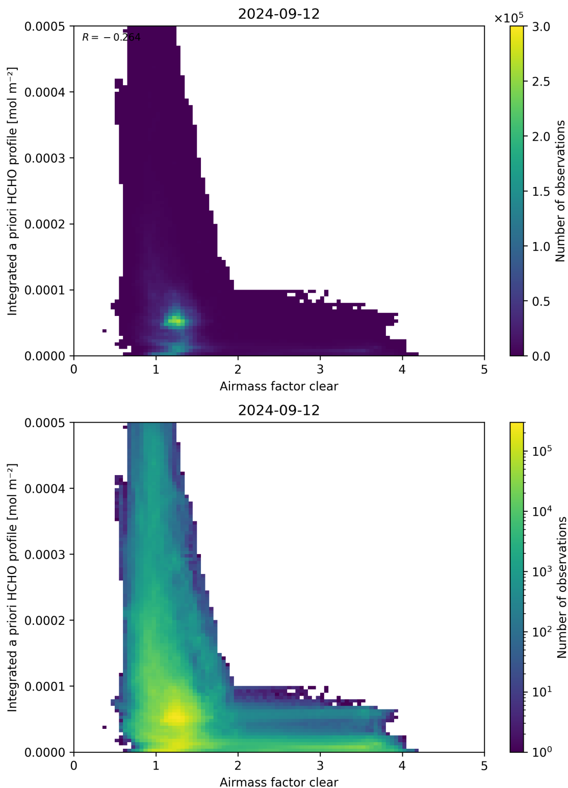
Figure 76: Scatter density plot of “Airmass factor clear” against “Integrated a priori HCHO profile” for 2024-09-12 to 2024-09-13.
