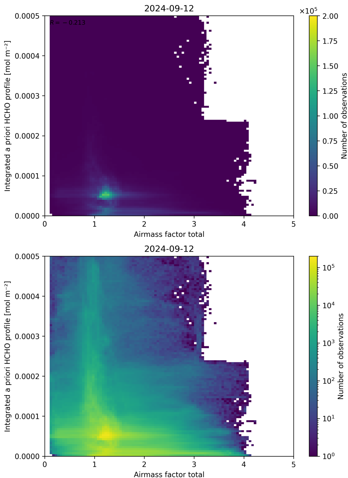
Figure 104: Scatter density plot of “Airmass factor total” against “Integrated a priori HCHO profile” for 2024-09-12 to 2024-09-13.
