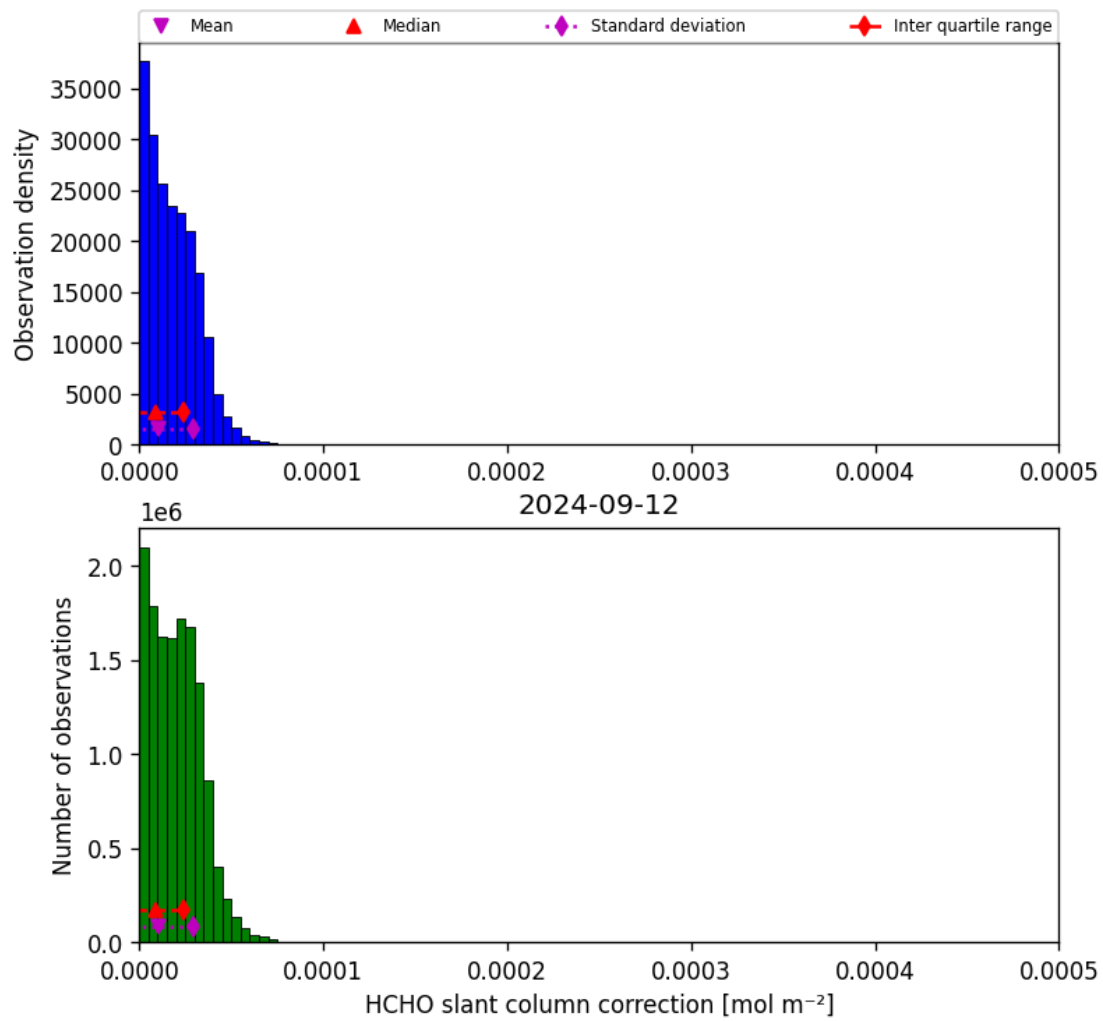
Figure 47: Histogram of “HCHO slant column correction” for 2024-09-12 to 2024-09-13
