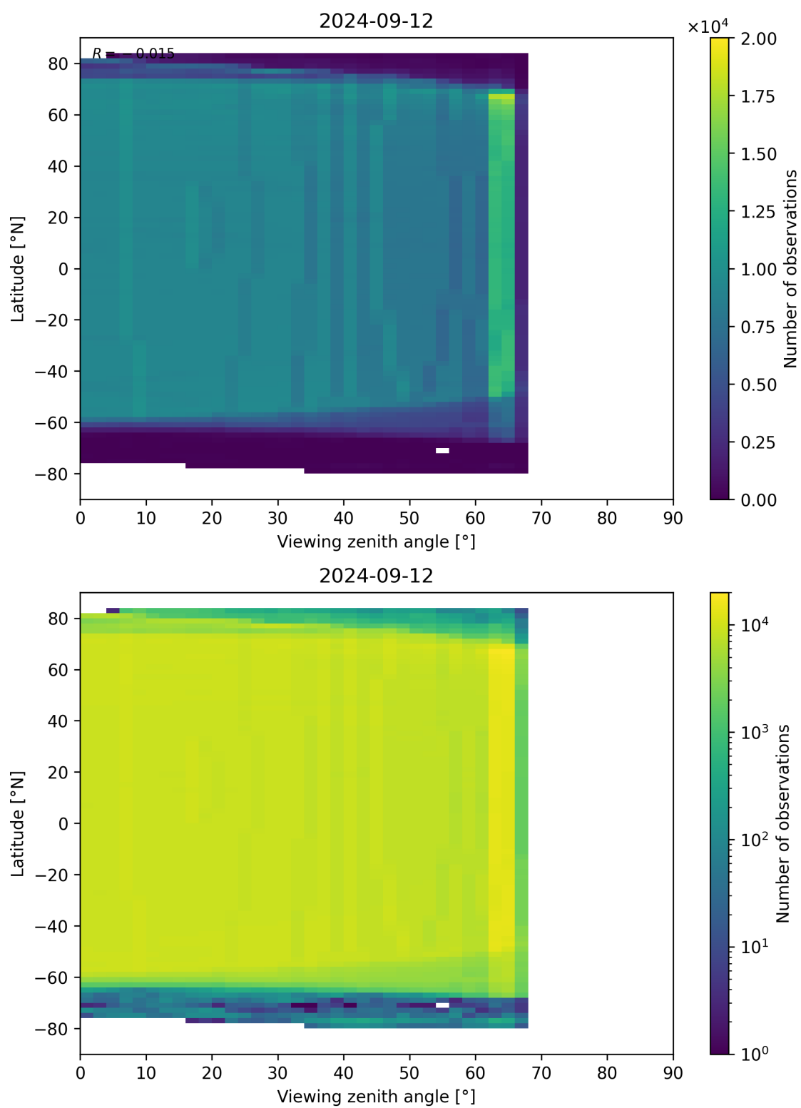
Figure 196: Scatter density plot of “Viewing zenith angle” against “Latitude” for 2024-09-12 to 2024-09-13.
