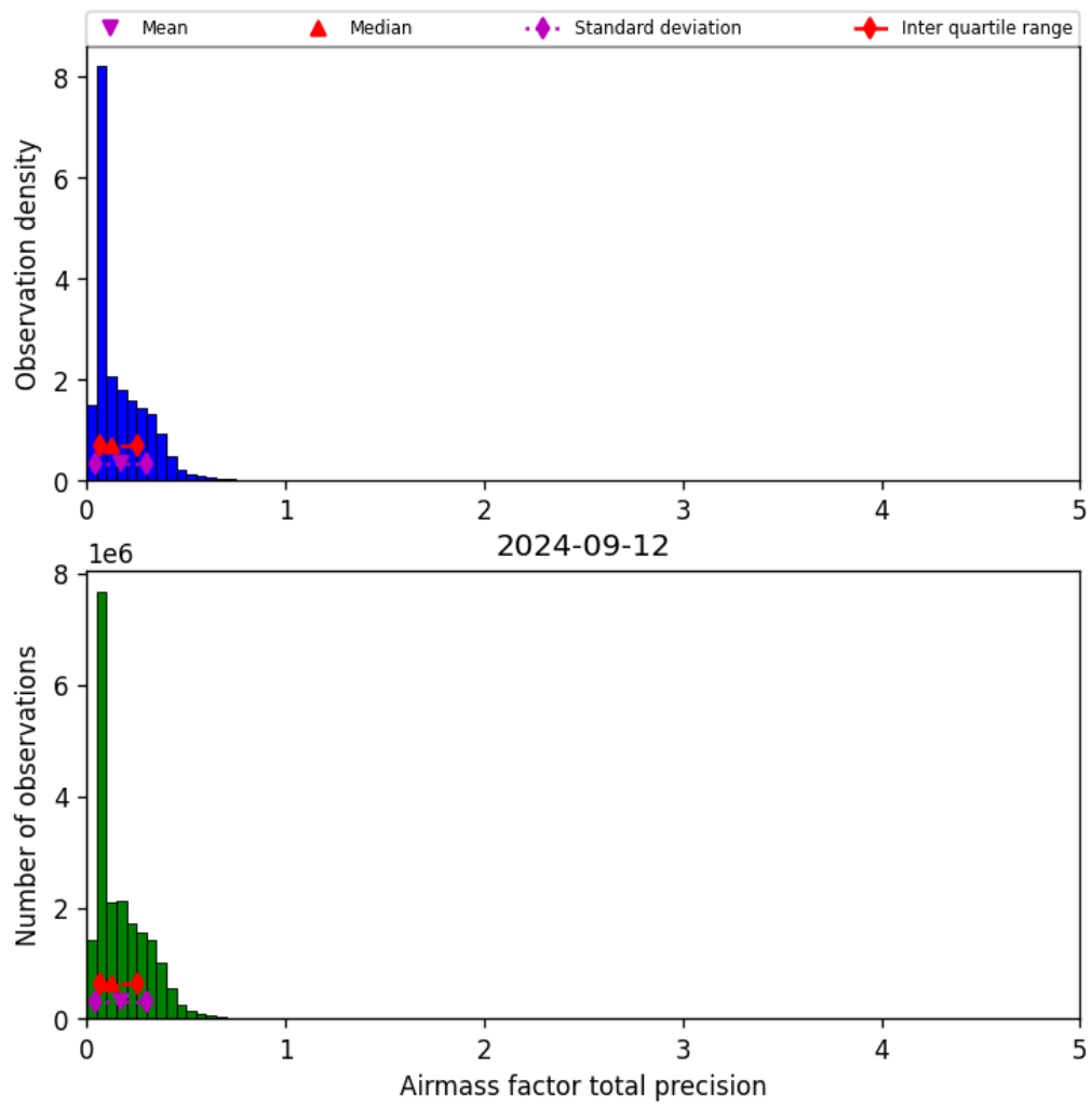
Figure 41: Histogram of “Airmass factor total precision” for 2024-09-12 to 2024-09-13
