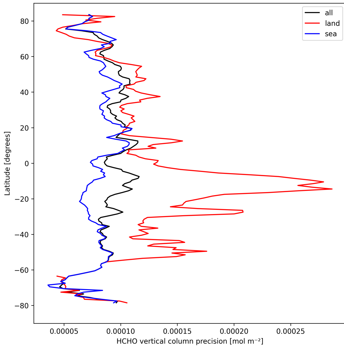
Figure 22: Zonal average of “HCHO vertical column precision” for 2024-09-12 to 2024-09-13.
