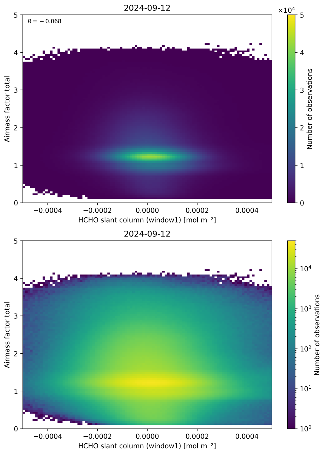
Figure 85: Scatter density plot of “HCHO slant column (window1)” against “Airmass factor total” for 2024-09-12 to 2024-09-13.
