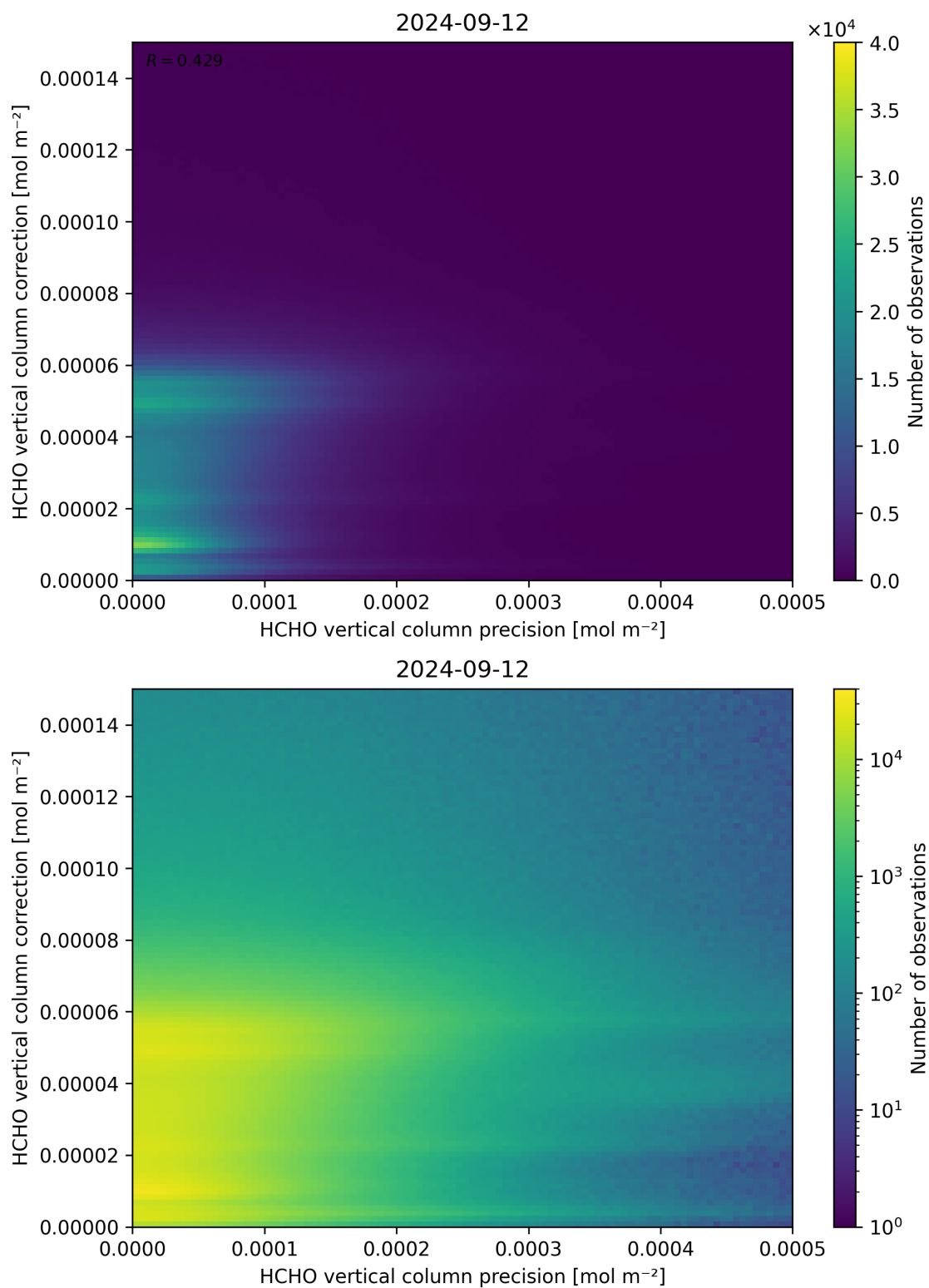
Figure 146: Scatter density plot of “HCHO vertical column precision” against “HCHO vertical column correction” for 2024-09-12 to 2024-09-13.
