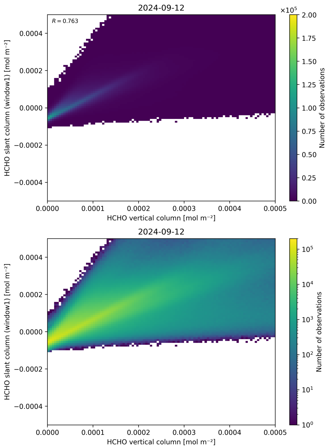
Figure 129: Scatter density plot of “HCHO vertical column” against “HCHO slant column (window1)” for 2024-09-12 to 2024-09-13.
