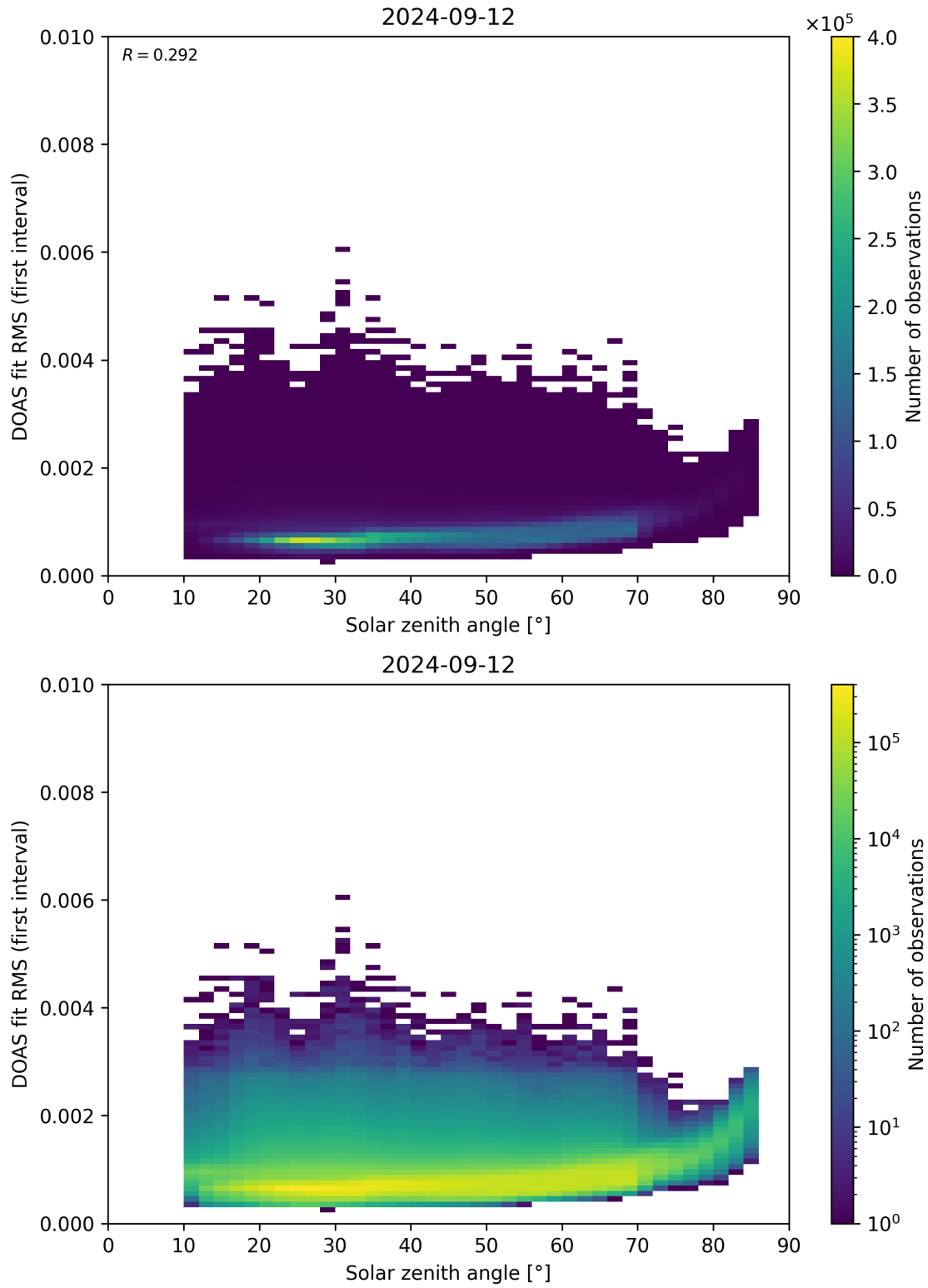
Figure 167: Scatter density plot of “Solar zenith angle” against “DOAS fit RMS (first interval)” for 2024-09-12 to 2024-09-13.
