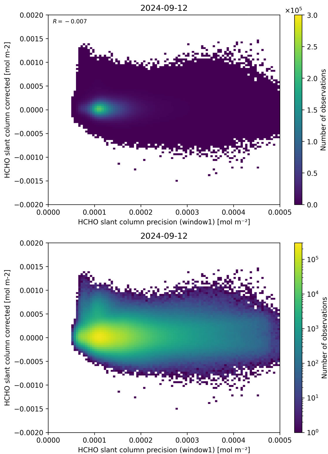
Figure 92: Scatter density plot of “HCHO slant column precision (window1)” against “HCHO slant column corrected” for 2024-09-12 to 2024-09-13.
