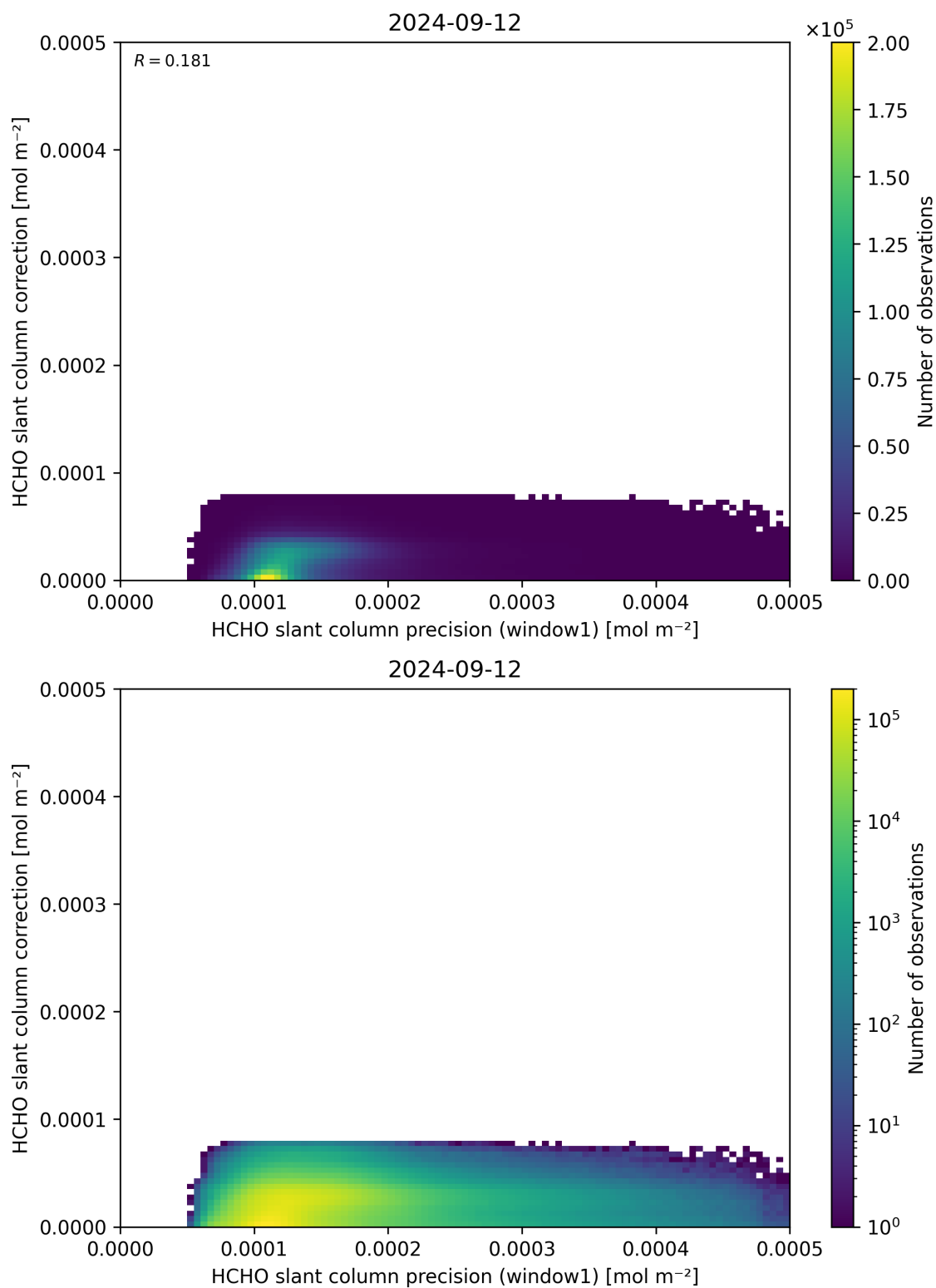
Figure 93: Scatter density plot of “HCHO slant column precision (window1)” against “HCHO slant column correction” for 2024-09-12 to 2024-09-13.
