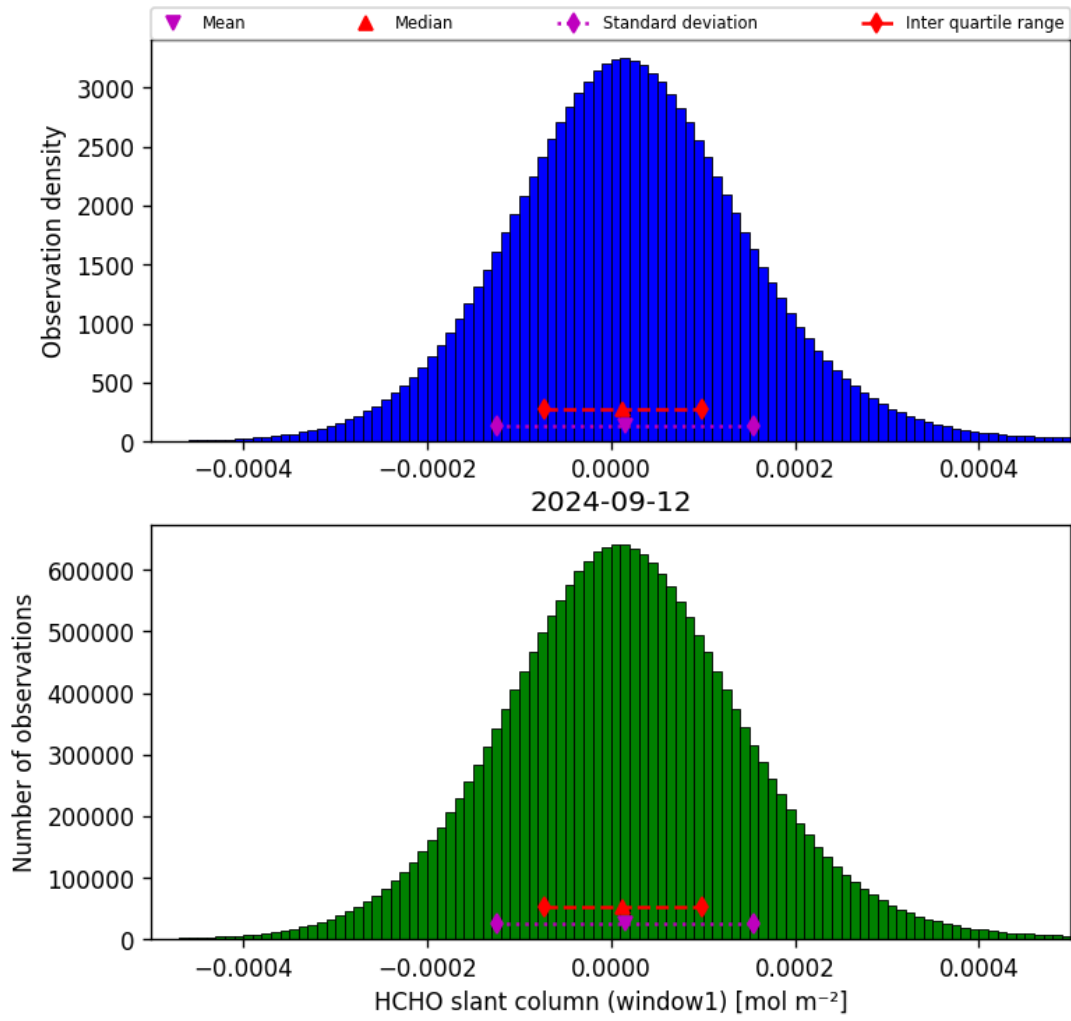
Figure 38: Histogram of “HCHO slant column (window1)” for 2024-09-12 to 2024-09-13
