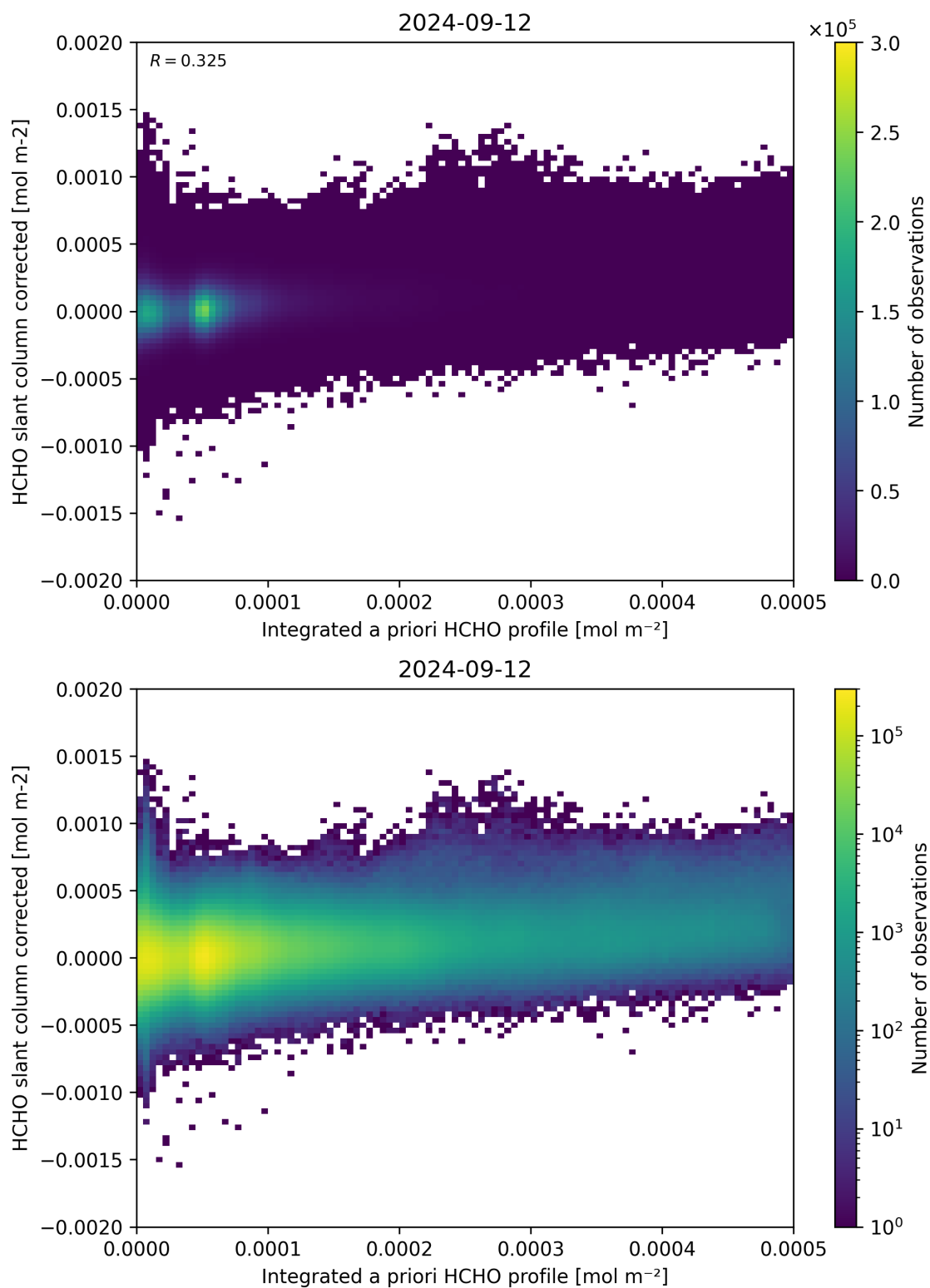
Figure 151: Scatter density plot of “Integrated a priori HCHO profile” against “HCHO slant column corrected” for 2024-09-12 to 2024-09-13.
