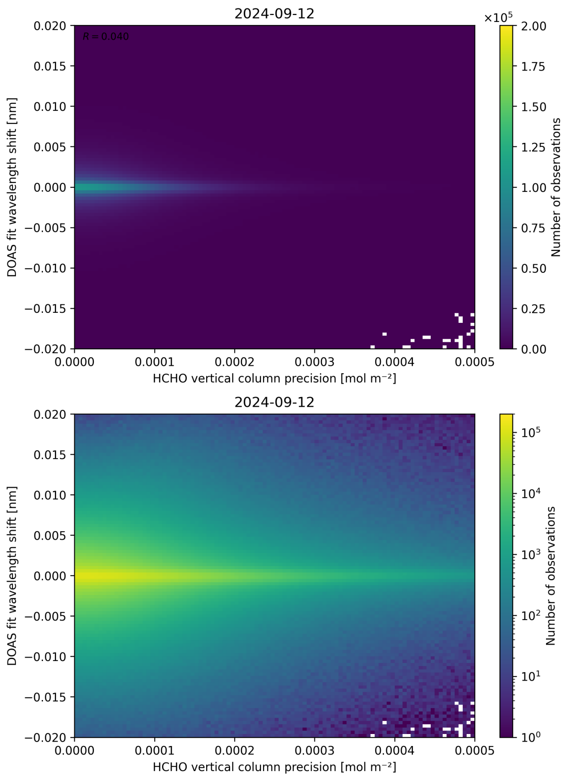
Figure 137: Scatter density plot of “HCHO vertical column precision” against “DOAS fit wavelength shift” for 2024-09-12 to 2024-09-13.
