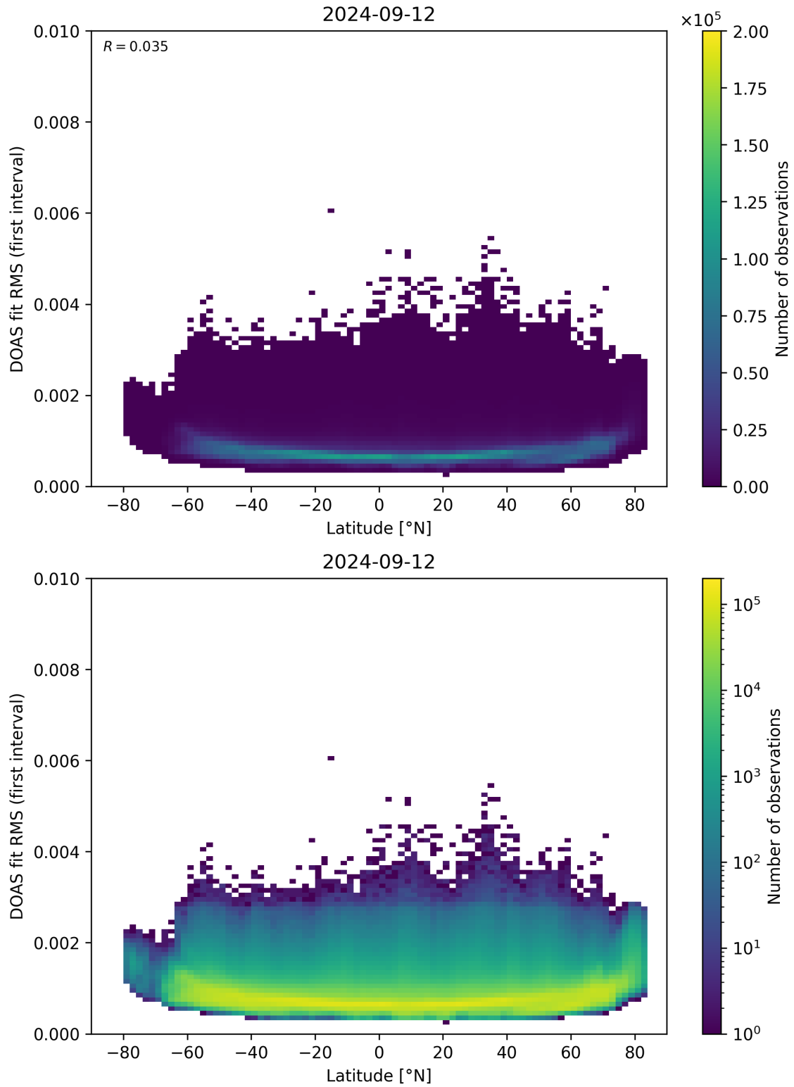
Figure 153: Scatter density plot of “Latitude” against “DOAS fit RMS (first interval)” for 2024-09-12 to 2024-09-13.
