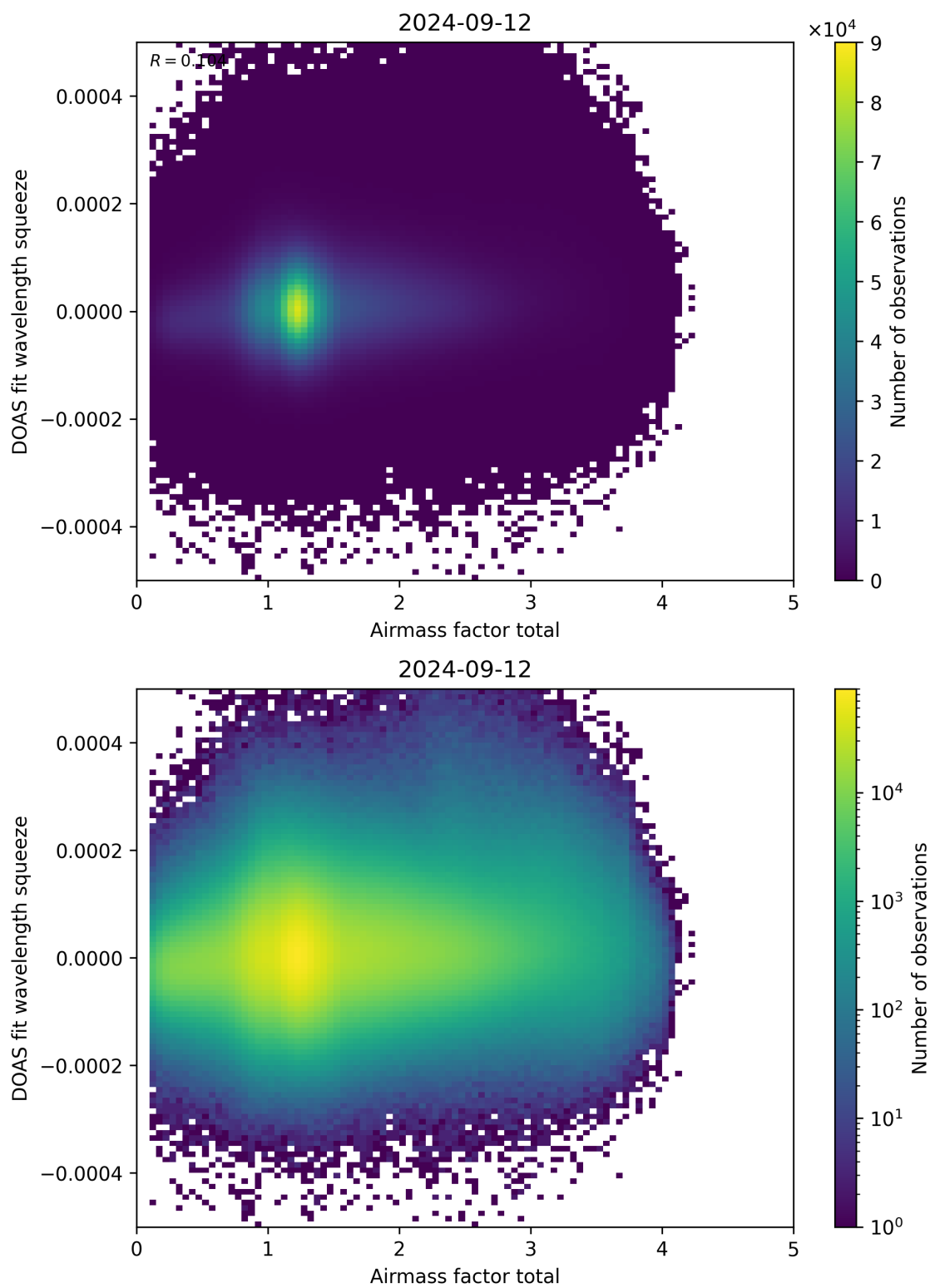
Figure 99: Scatter density plot of “Airmass factor total” against “DOAS fit wavelength squeeze” for 2024-09-12 to 2024-09-13.
