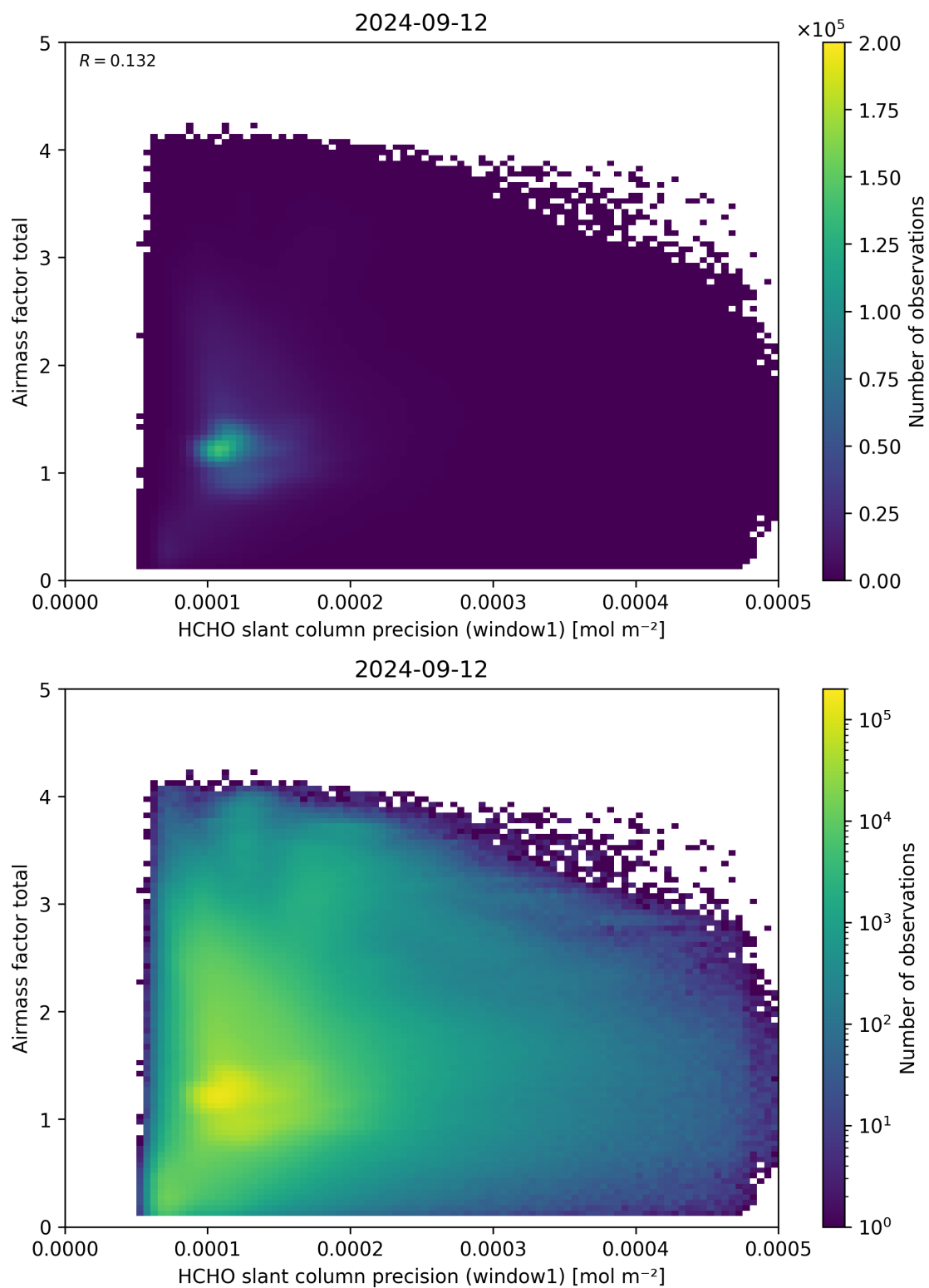
Figure 94: Scatter density plot of “HCHO slant column precision (window1)” against “Airmass factor total” for 2024-09-12 to 2024-09-13.
