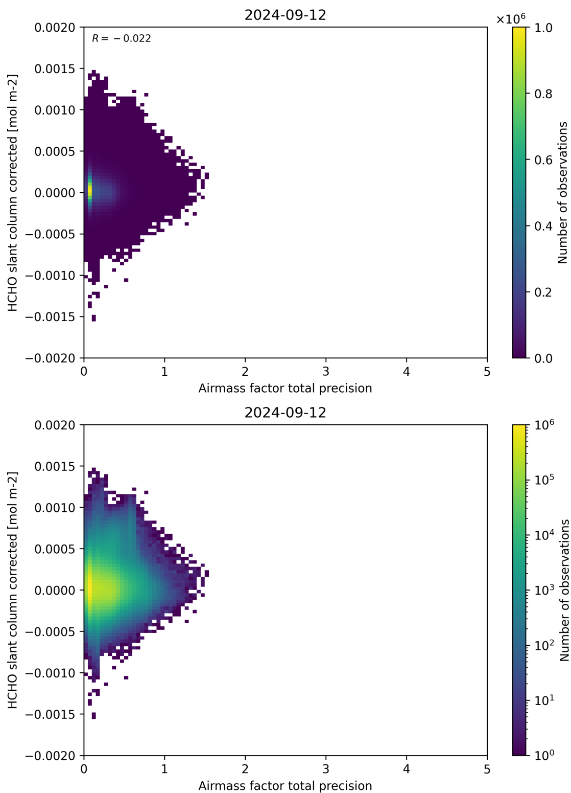
Figure 109: Scatter density plot of “Airmass factor total precision” against “HCHO slant column corrected” for 2024-09-12 to 2024-09-13.
