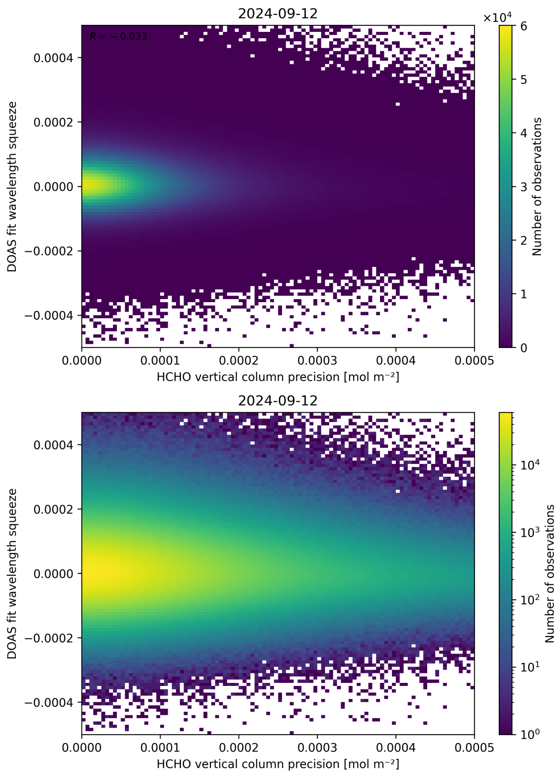
Figure 138: Scatter density plot of “HCHO vertical column precision” against “DOAS fit wavelength squeeze” for 2024-09-12 to 2024-09-13.
