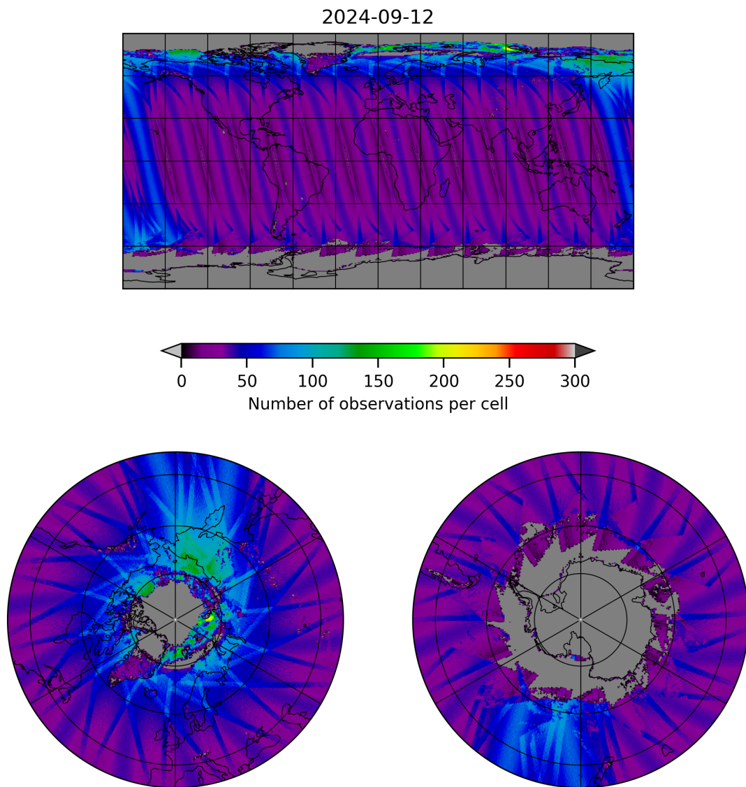
Figure 19: Map of the number of observations for 2024-09-12 to 2024-09-13
