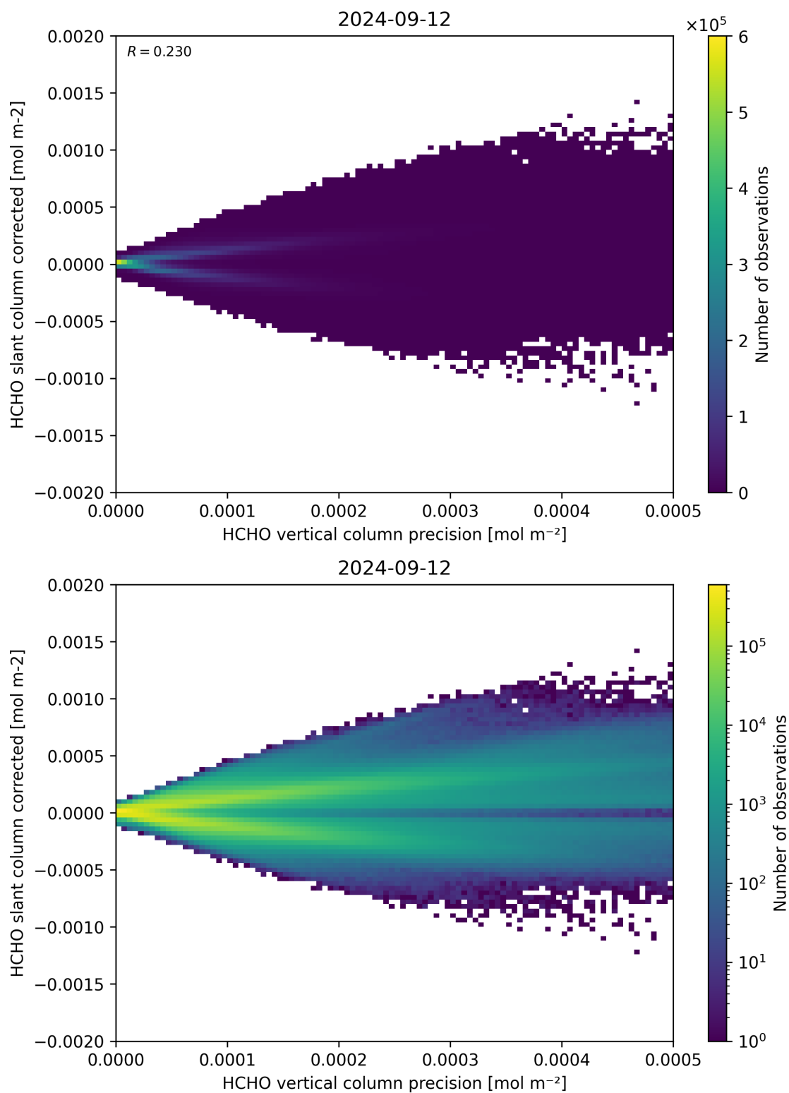
Figure 140: Scatter density plot of “HCHO vertical column precision” against “HCHO slant column corrected” for 2024-09-12 to 2024-09-13.
