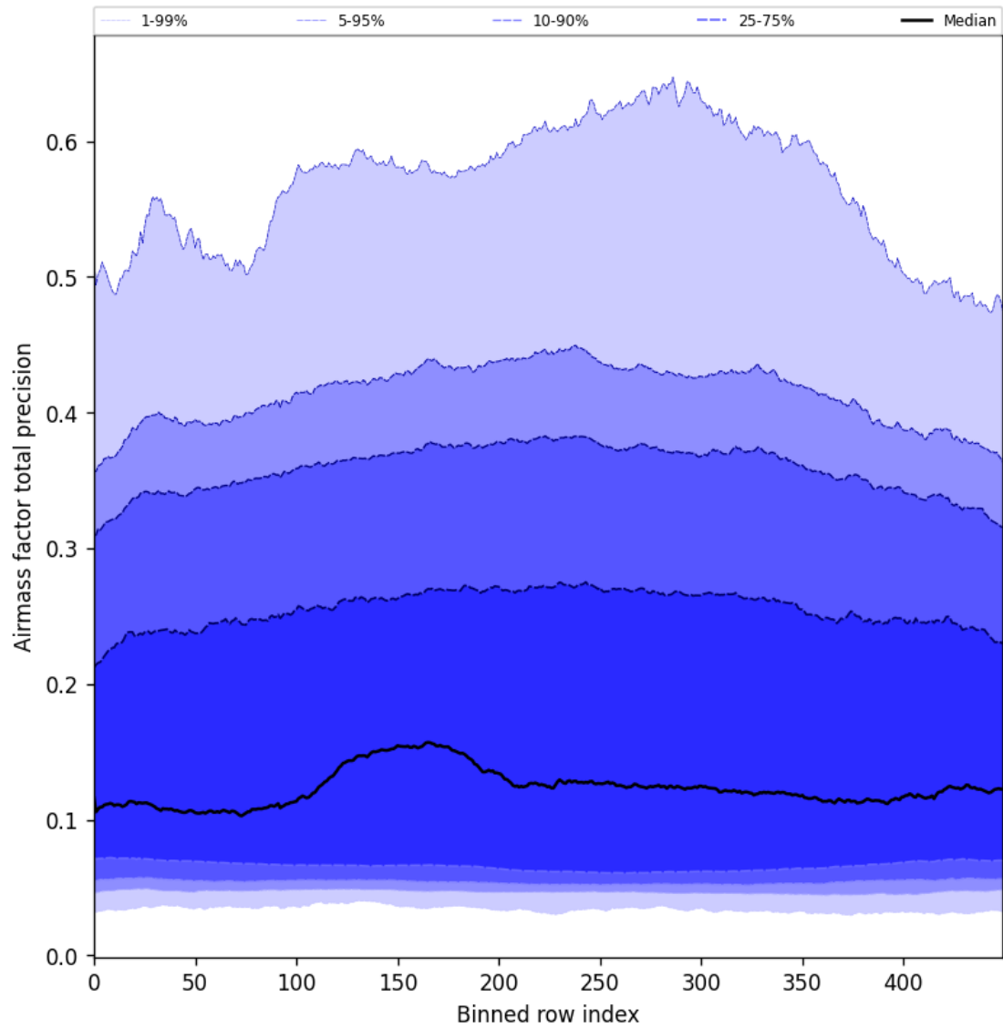
Figure 55: Along track statistics of “Airmass factor total precision” for 2024-09-12 to 2024-09-13
