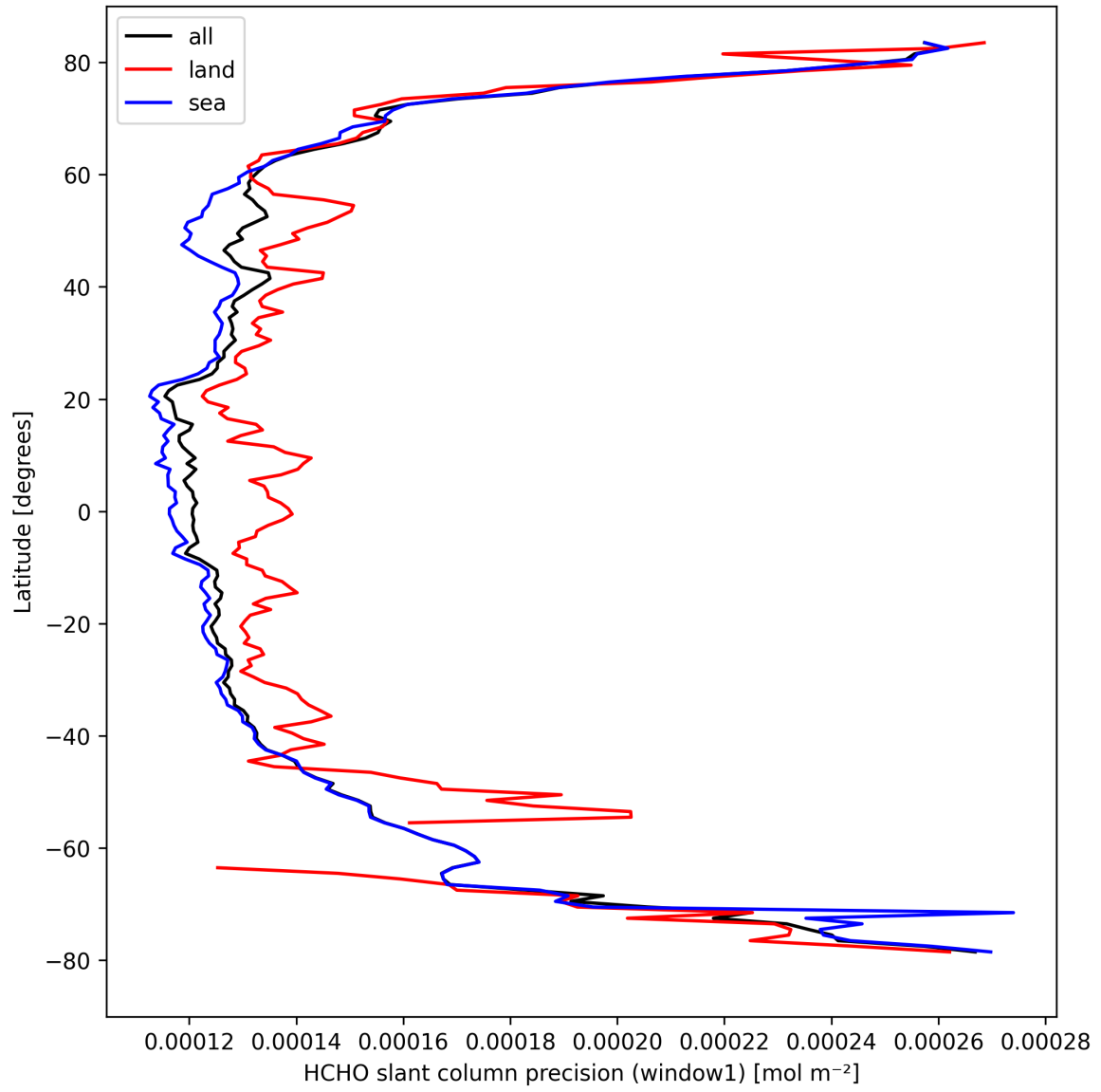
Figure 25: Zonal average of “HCHO slant column precision (window1)” for 2024-09-12 to 2024-09-13.
