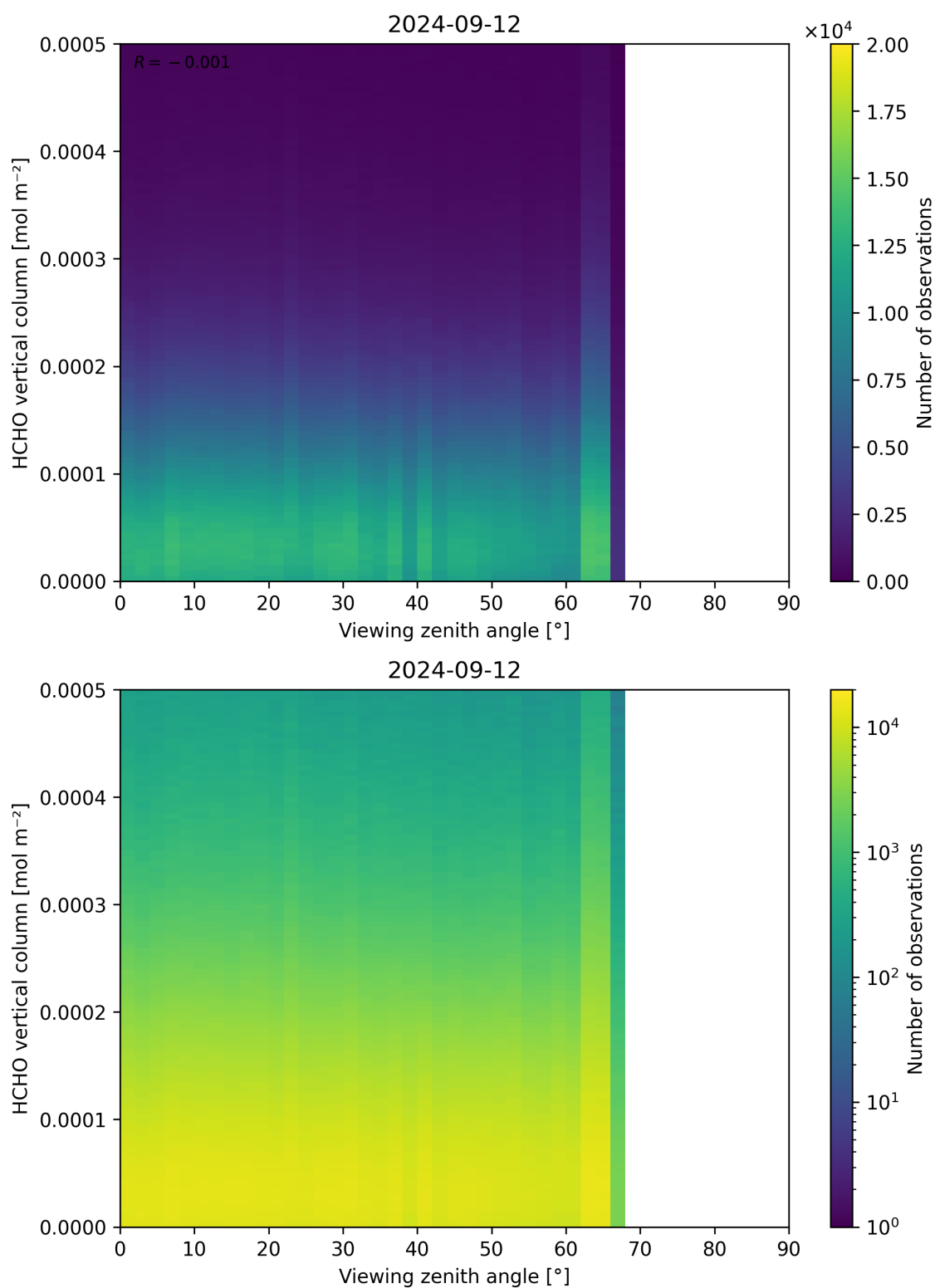
Figure 192: Scatter density plot of “Viewing zenith angle” against “HCHO vertical column” for 2024-09-12 to 2024-09-13.
