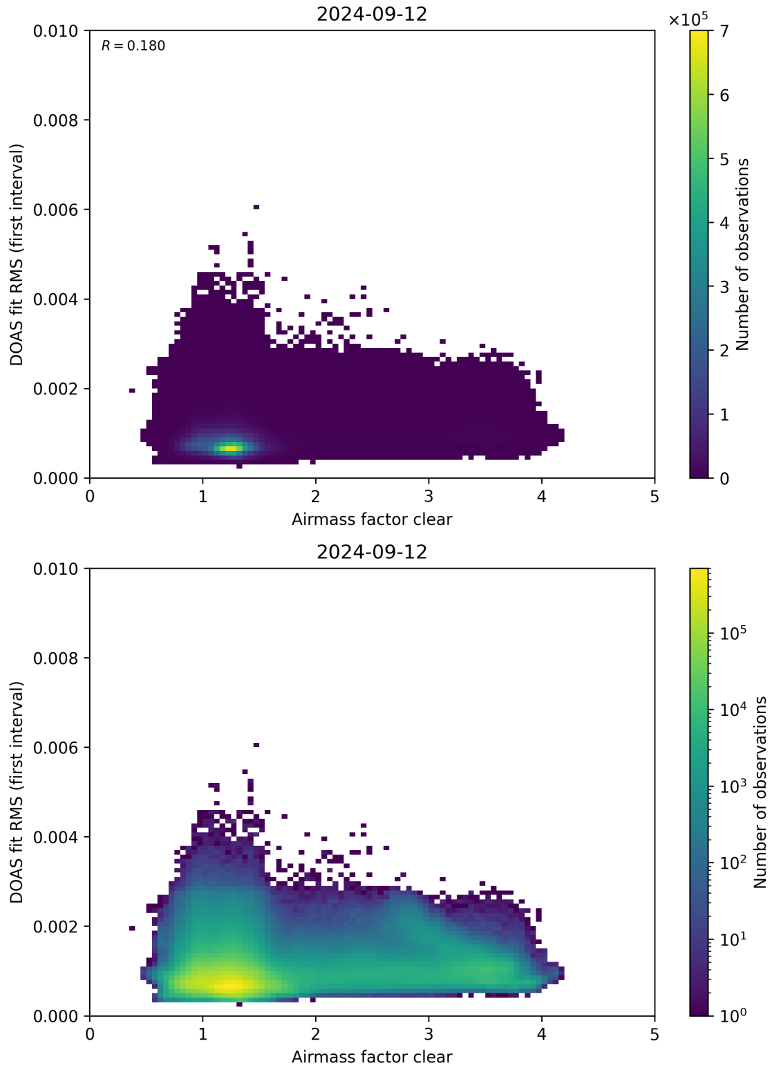
Figure 71: Scatter density plot of “Airmass factor clear” against “DOAS fit RMS (first interval)” for 2024-09-12 to 2024-09-13.
