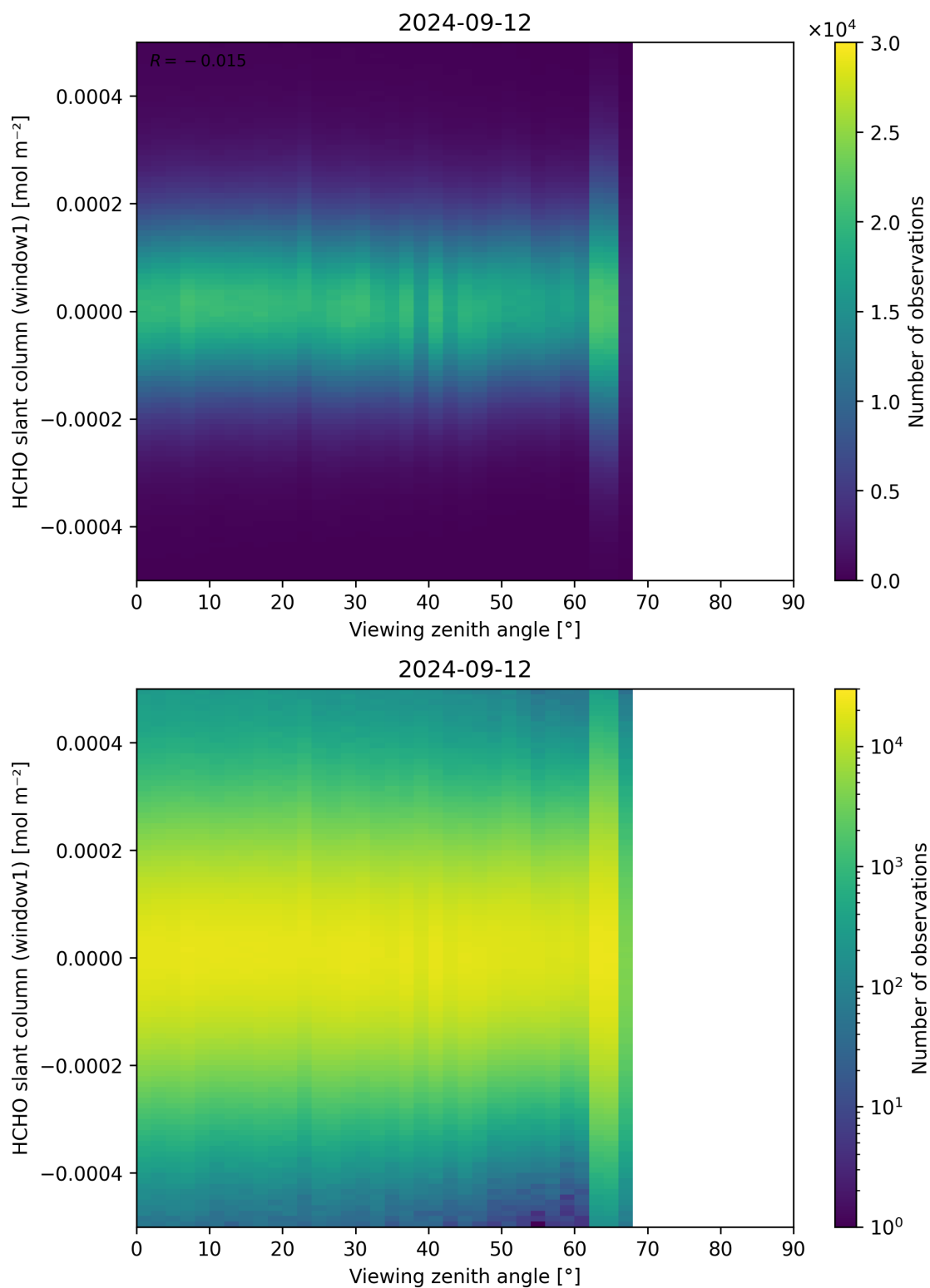
Figure 188: Scatter density plot of “Viewing zenith angle” against “HCHO slant column (window1)” for 2024-09-12 to 2024-09-13.
