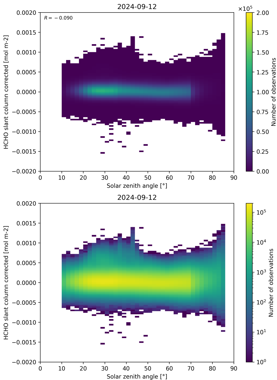
Figure 171: Scatter density plot of “Solar zenith angle” against “HCHO slant column corrected” for 2024-09-12 to 2024-09-13.
