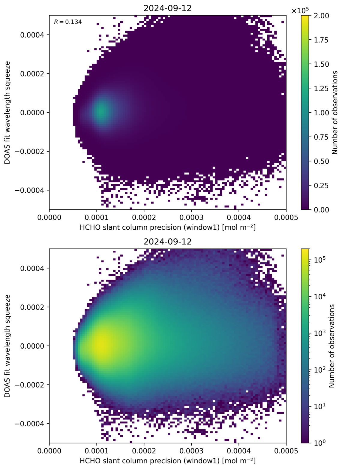
Figure 90: Scatter density plot of “HCHO slant column precision (window1)” against “DOAS fit wavelength squeeze” for 2024-09-12 to 2024-09-13.
