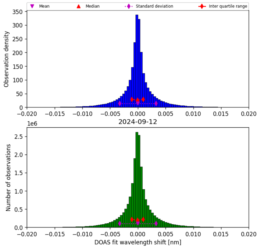
Figure 44: Histogram of “DOAS fit wavelength shift” for 2024-09-12 to 2024-09-13
