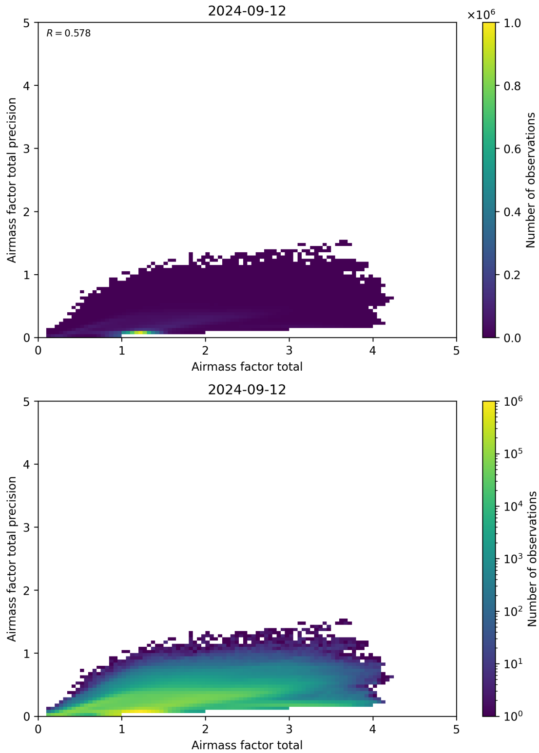
Figure 103: Scatter density plot of “Airmass factor total” against “Airmass factor total precision” for 2024-09-12 to 2024-09-13.
