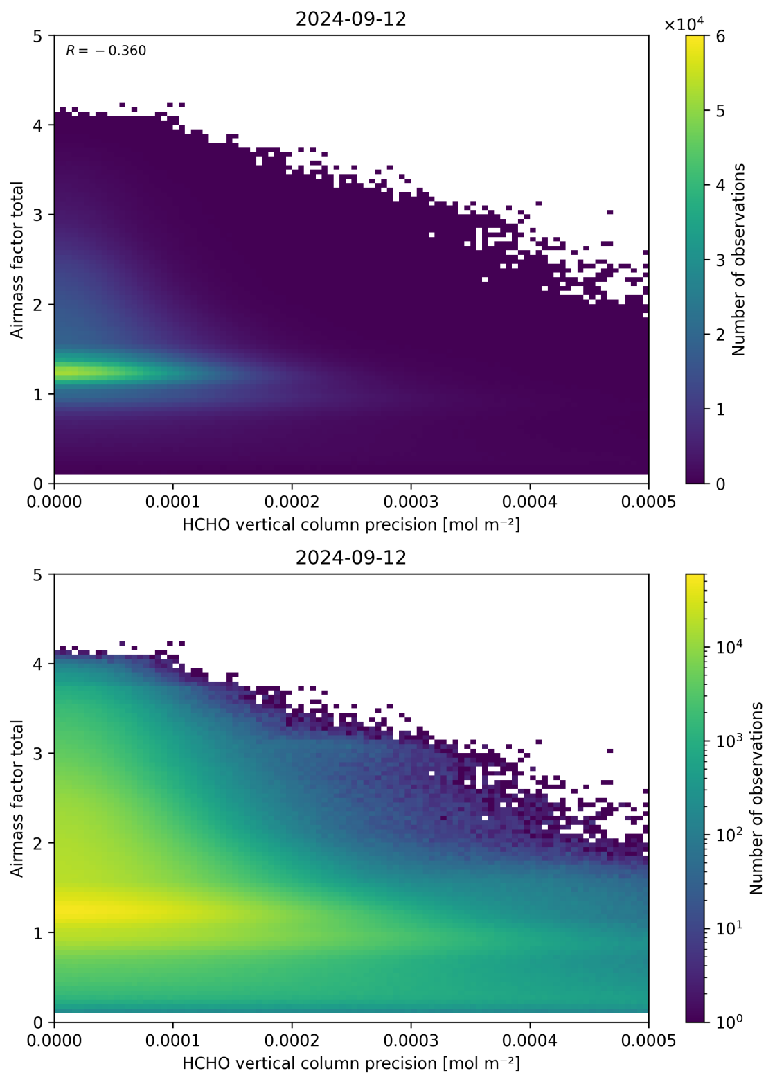
Figure 144: Scatter density plot of “HCHO vertical column precision” against “Airmass factor total” for 2024-09-12 to 2024-09-13.
