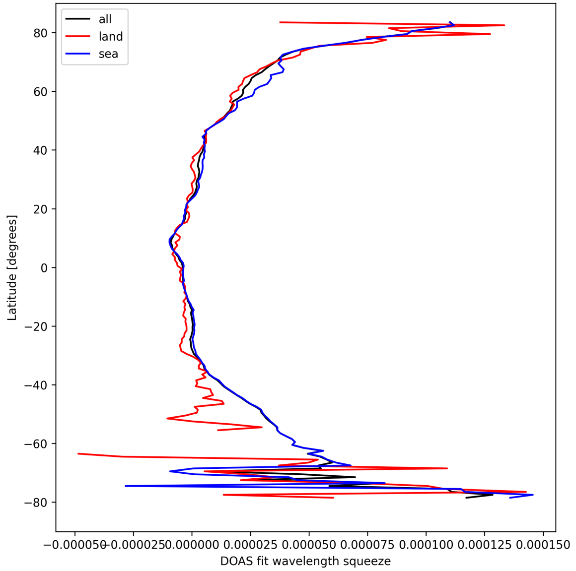
Figure 31: Zonal average of “DOAS fit wavelength squeeze” for 2024-09-12 to 2024-09-13.
