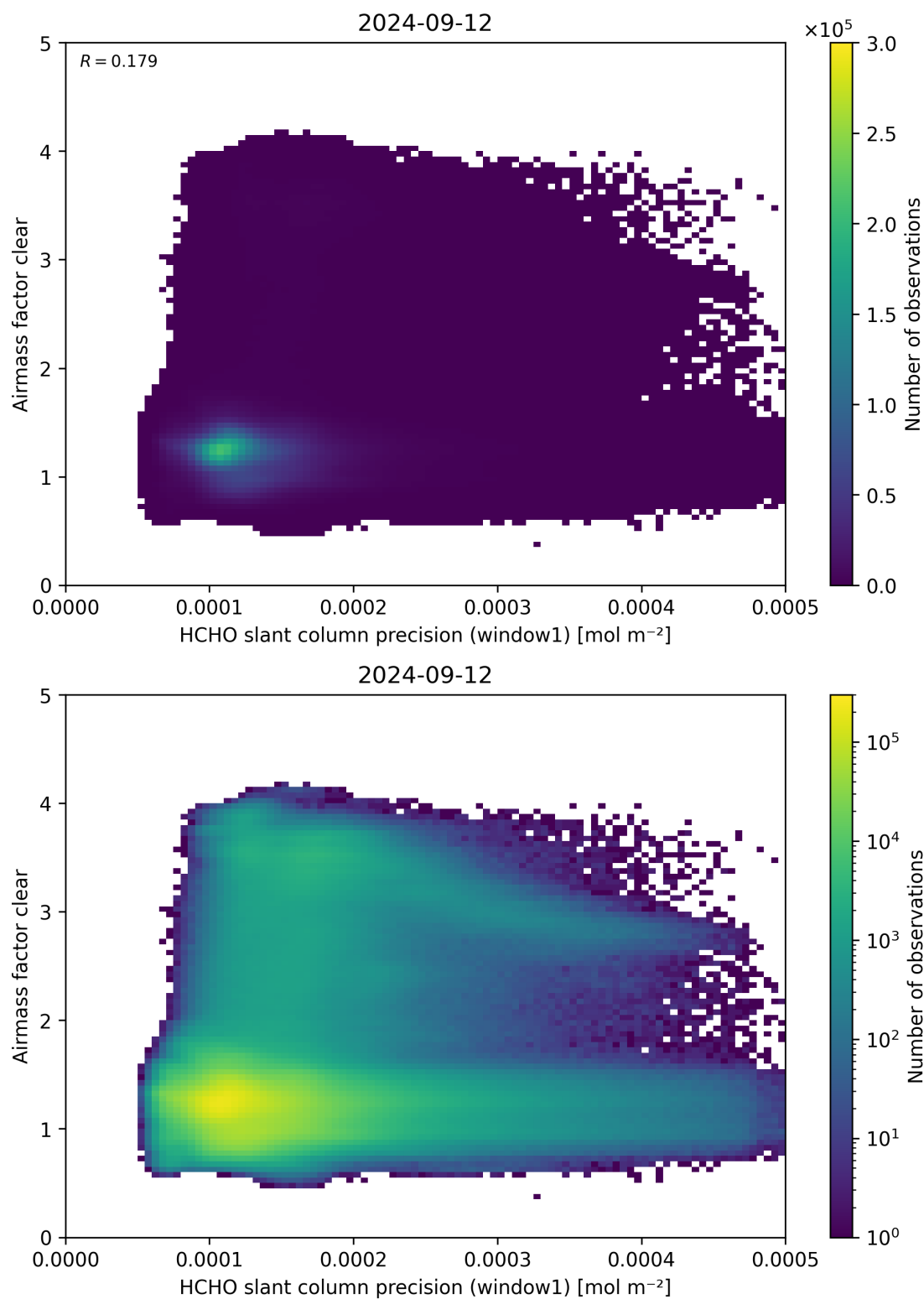
Figure 91: Scatter density plot of “HCHO slant column precision (window1)” against “Airmass factor clear” for 2024-09-12 to 2024-09-13.
