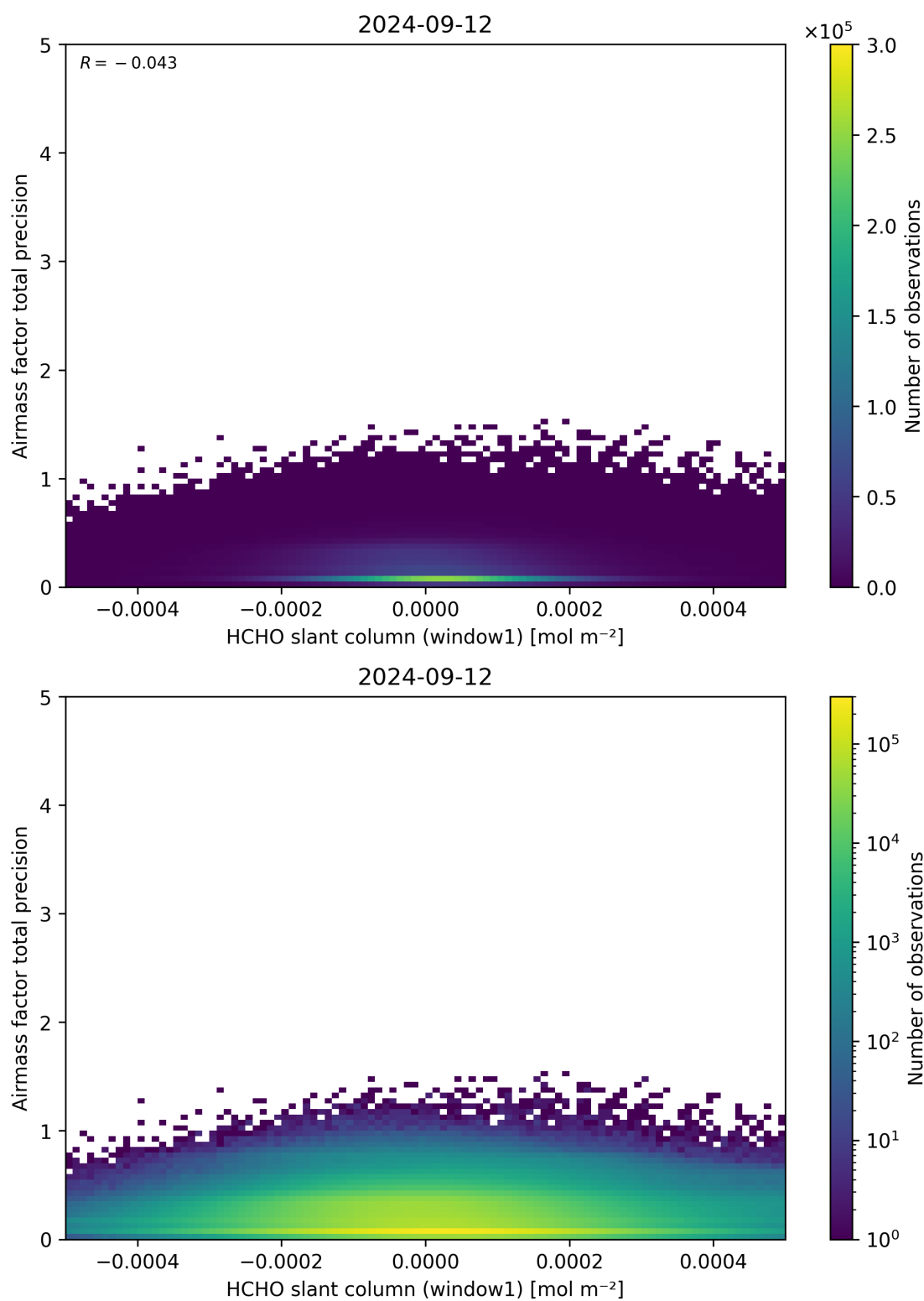
Figure 86: Scatter density plot of “HCHO slant column (window1)” against “Airmass factor total precision” for 2024-09-12 to 2024-09-13.
