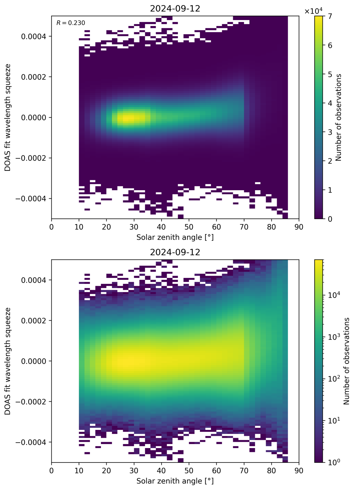
Figure 169: Scatter density plot of “Solar zenith angle” against “DOAS fit wavelength squeeze” for 2024-09-12 to 2024-09-13.
