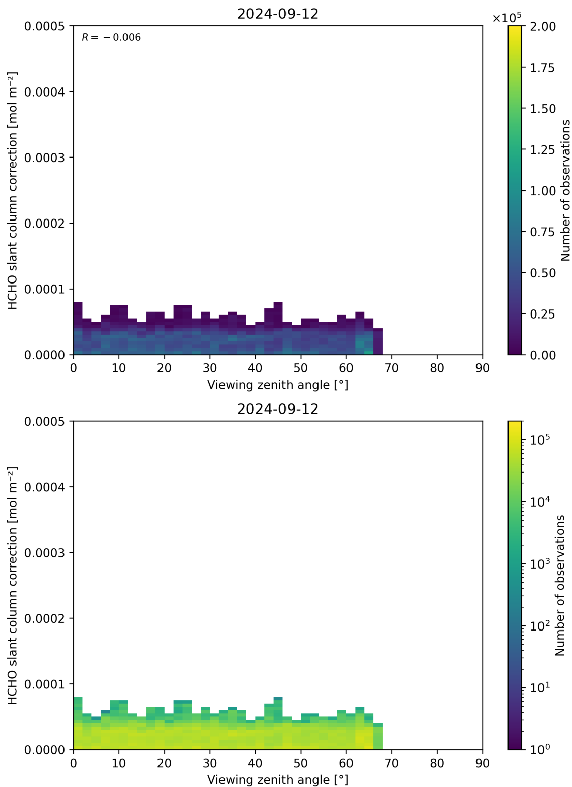
Figure 187: Scatter density plot of “Viewing zenith angle” against “HCHO slant column correction” for 2024-09-12 to 2024-09-13.
