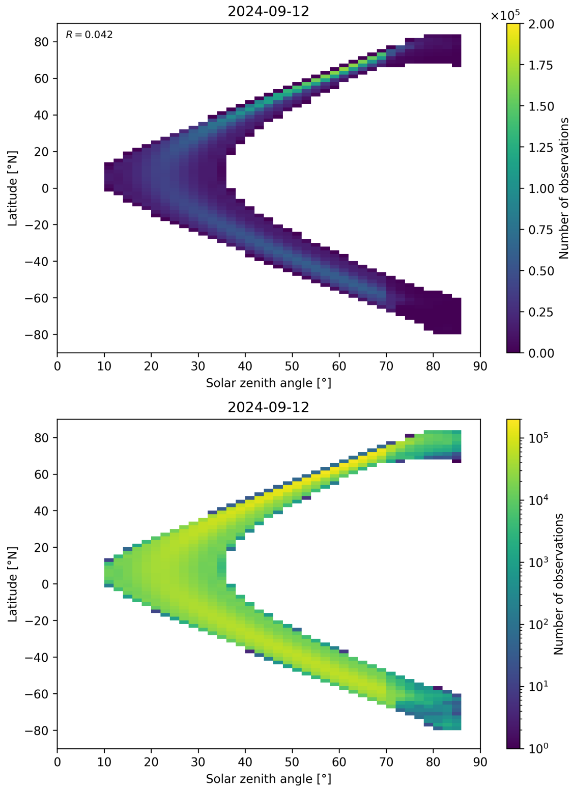
Figure 181: Scatter density plot of “Solar zenith angle” against “Latitude” for 2024-09-12 to 2024-09-13.
