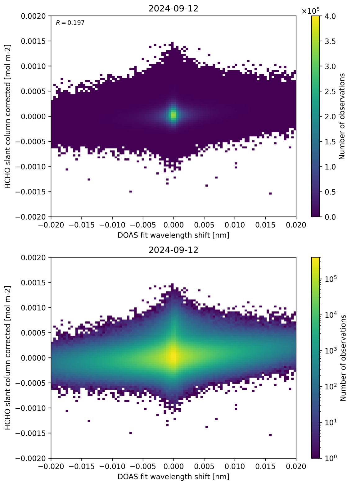
Figure 66: Scatter density plot of “DOAS fit wavelength shift” against “HCHO slant column corrected” for 2024-09-12 to 2024-09-13.
