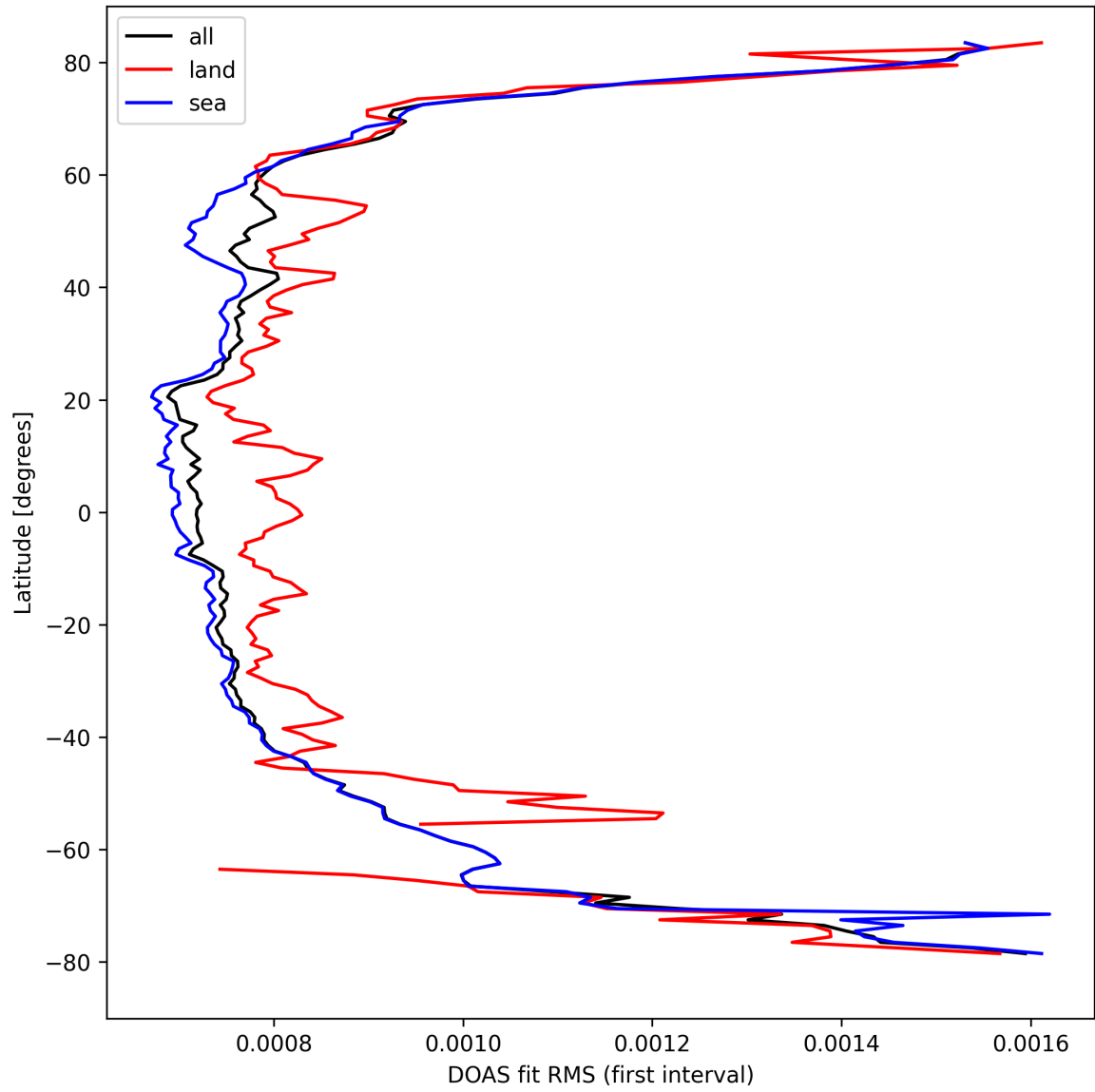
Figure 32: Zonal average of “DOAS fit RMS (first interval)” for 2024-09-12 to 2024-09-13.
