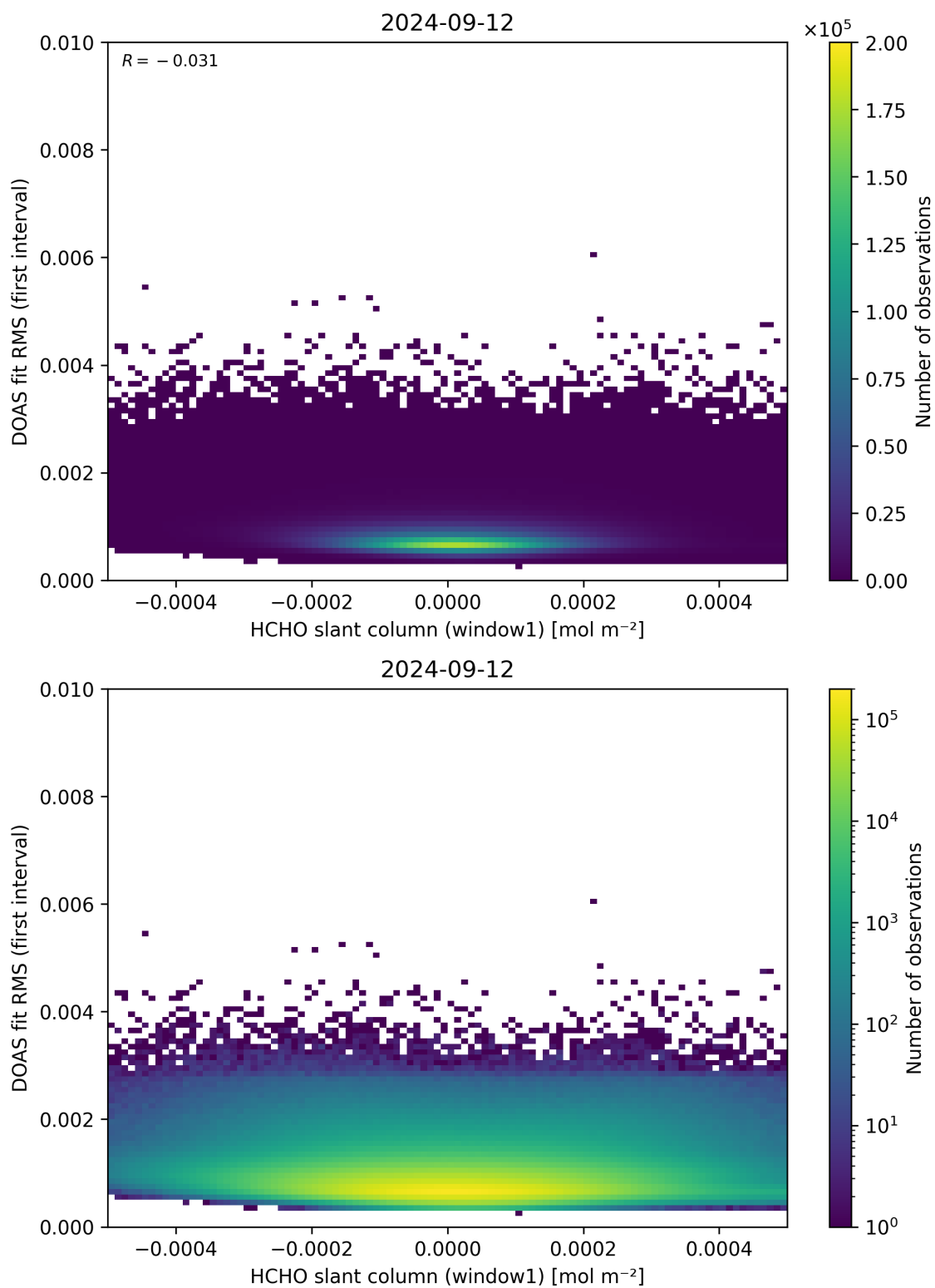
Figure 78: Scatter density plot of “HCHO slant column (window1)” against “DOAS fit RMS (first interval)” for 2024-09-12 to 2024-09-13.
