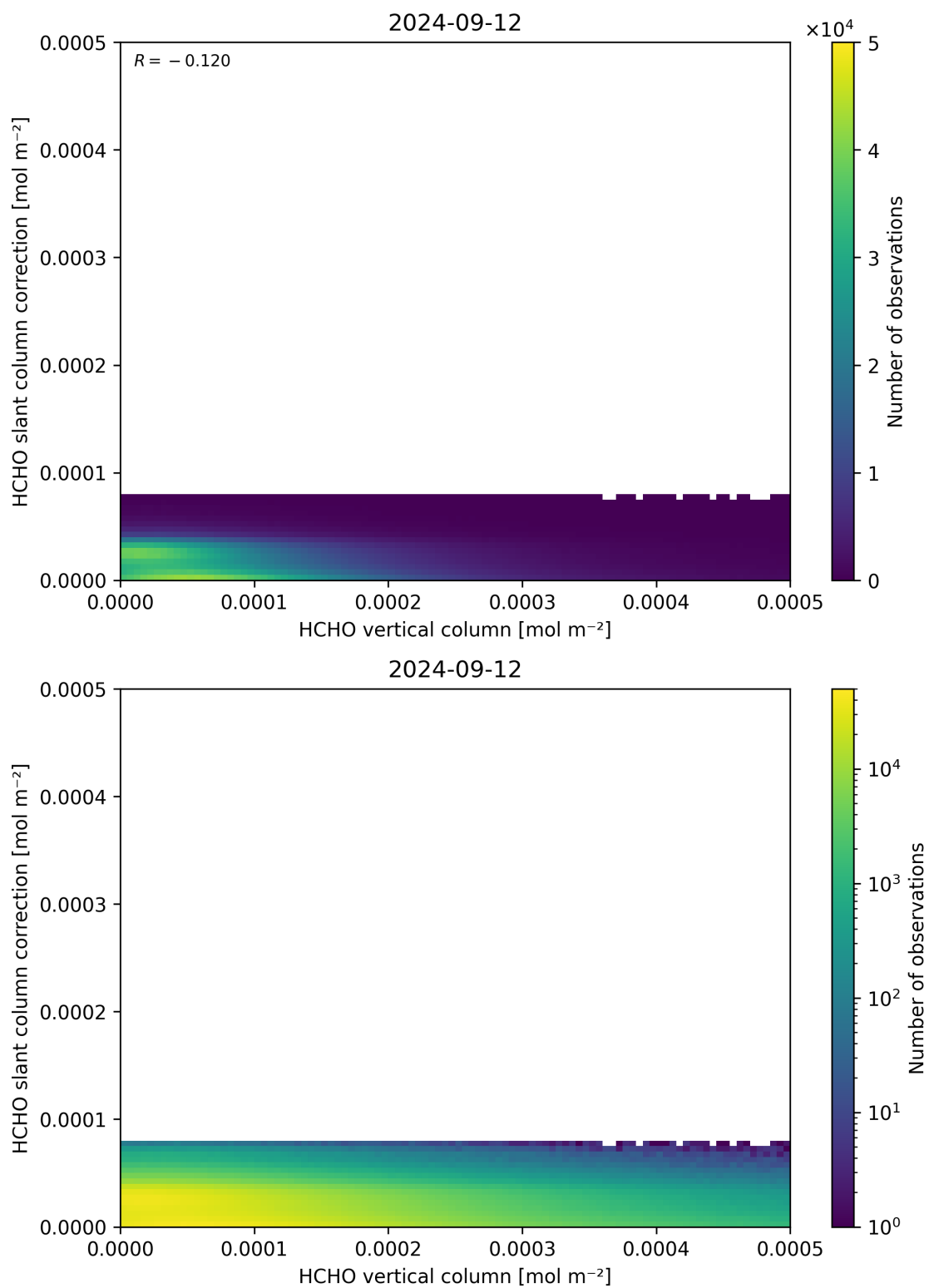
Figure 128: Scatter density plot of “HCHO vertical column” against “HCHO slant column correction” for 2024-09-12 to 2024-09-13.
