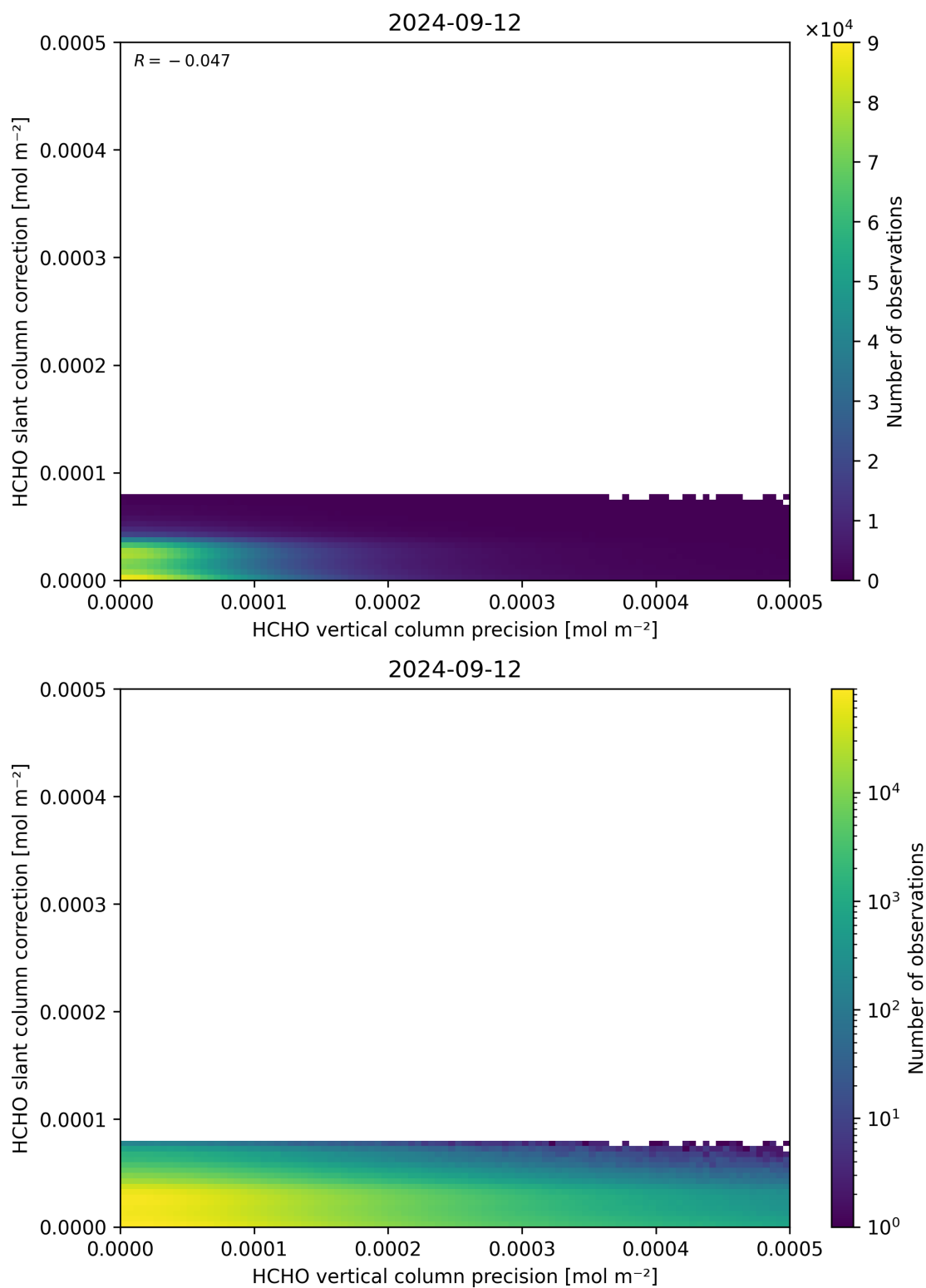
Figure 141: Scatter density plot of “HCHO vertical column precision” against “HCHO slant column correction” for 2024-09-12 to 2024-09-13.
