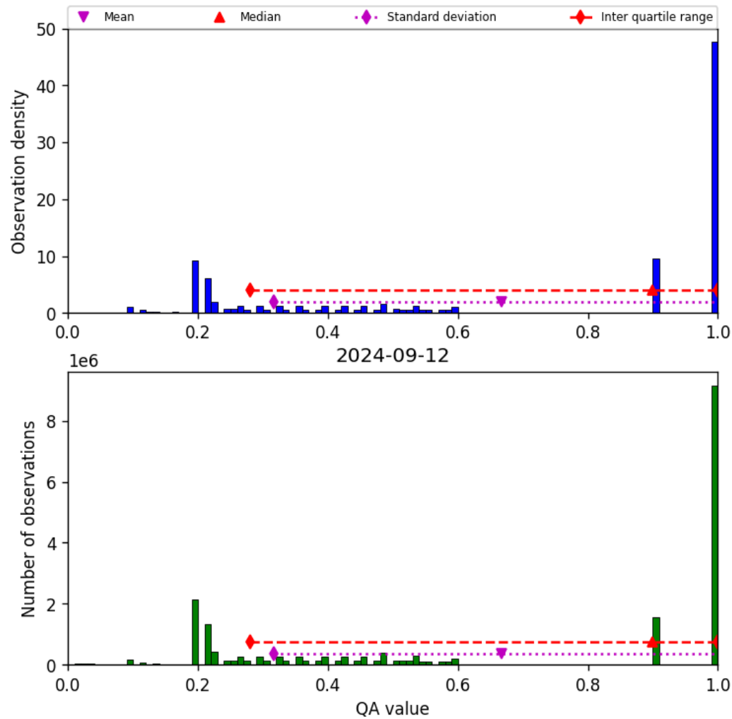
Figure 34: Histogram of “QA value” for 2024-09-12 to 2024-09-13
