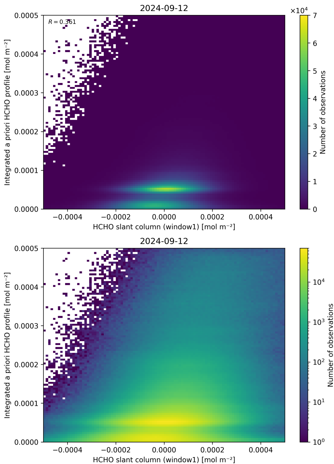
Figure 87: Scatter density plot of “HCHO slant column (window1)” against “Integrated a priori HCHO profile” for 2024-09-12 to 2024-09-13.
