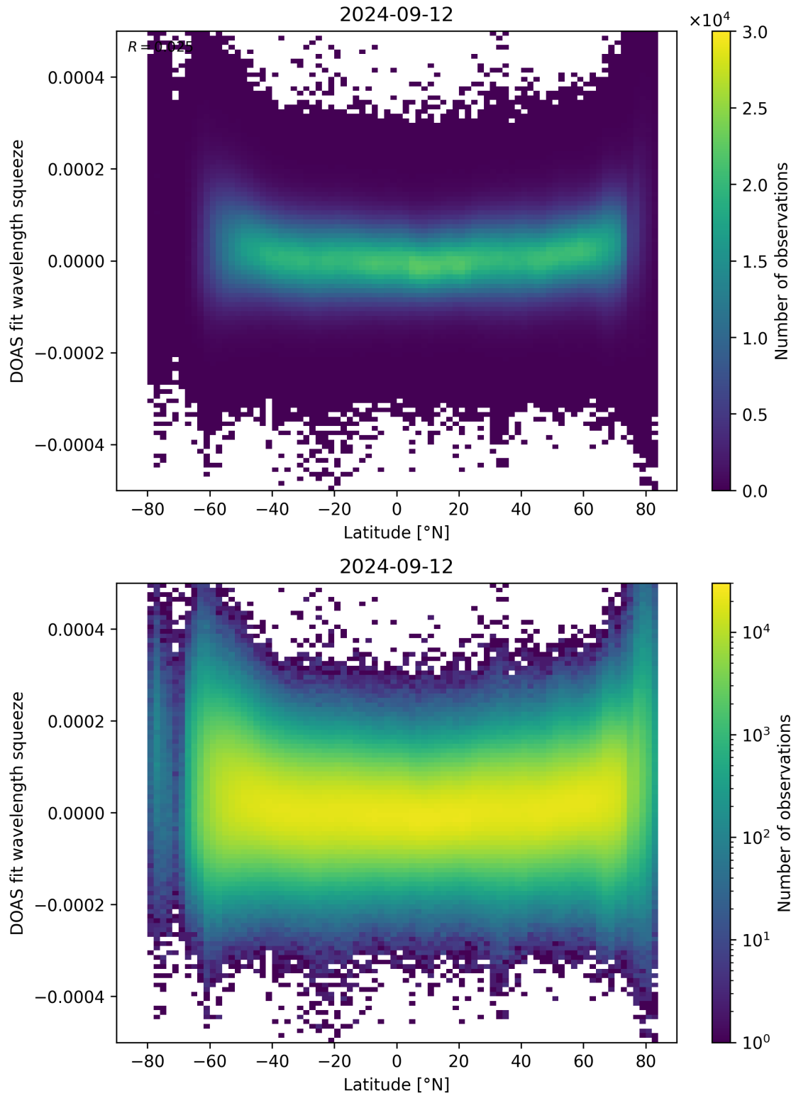
Figure 155: Scatter density plot of “Latitude” against “DOAS fit wavelength squeeze” for 2024-09-12 to 2024-09-13.
