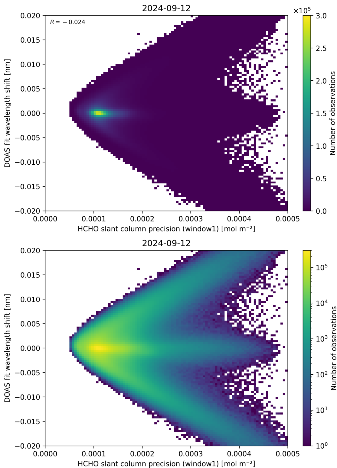
Figure 89: Scatter density plot of “HCHO slant column precision (window1)” against “DOAS fit wavelength shift” for 2024-09-12 to 2024-09-13.
