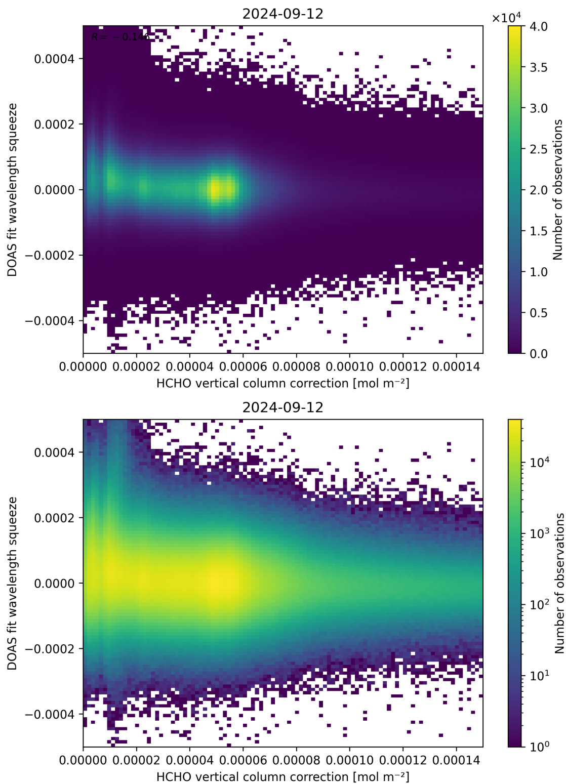
Figure 114: Scatter density plot of “HCHO vertical column correction” against “DOAS fit wavelength squeeze” for 2024-09-12 to 2024-09-13.
