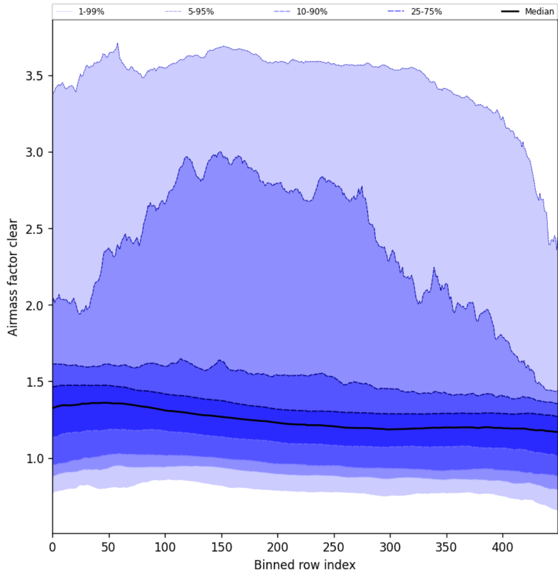
Figure 56: Along track statistics of “Airmass factor clear” for 2024-09-12 to 2024-09-13
