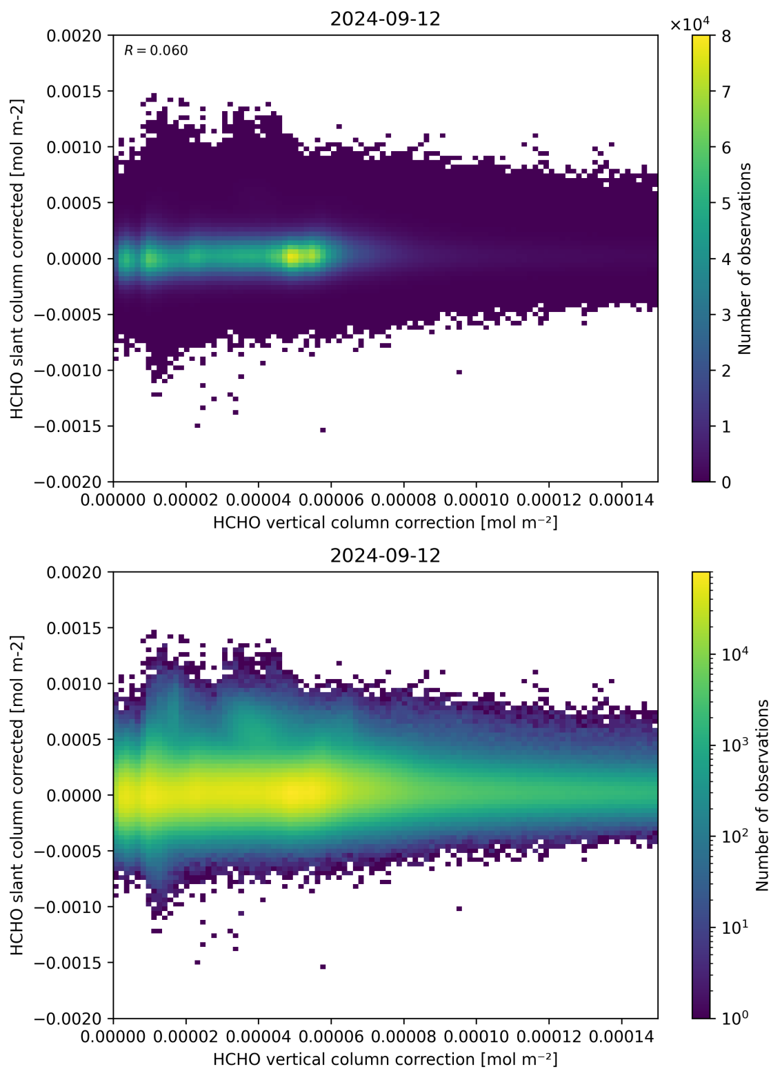
Figure 116: Scatter density plot of “HCHO vertical column correction” against “HCHO slant column corrected” for 2024-09-12 to 2024-09-13.
