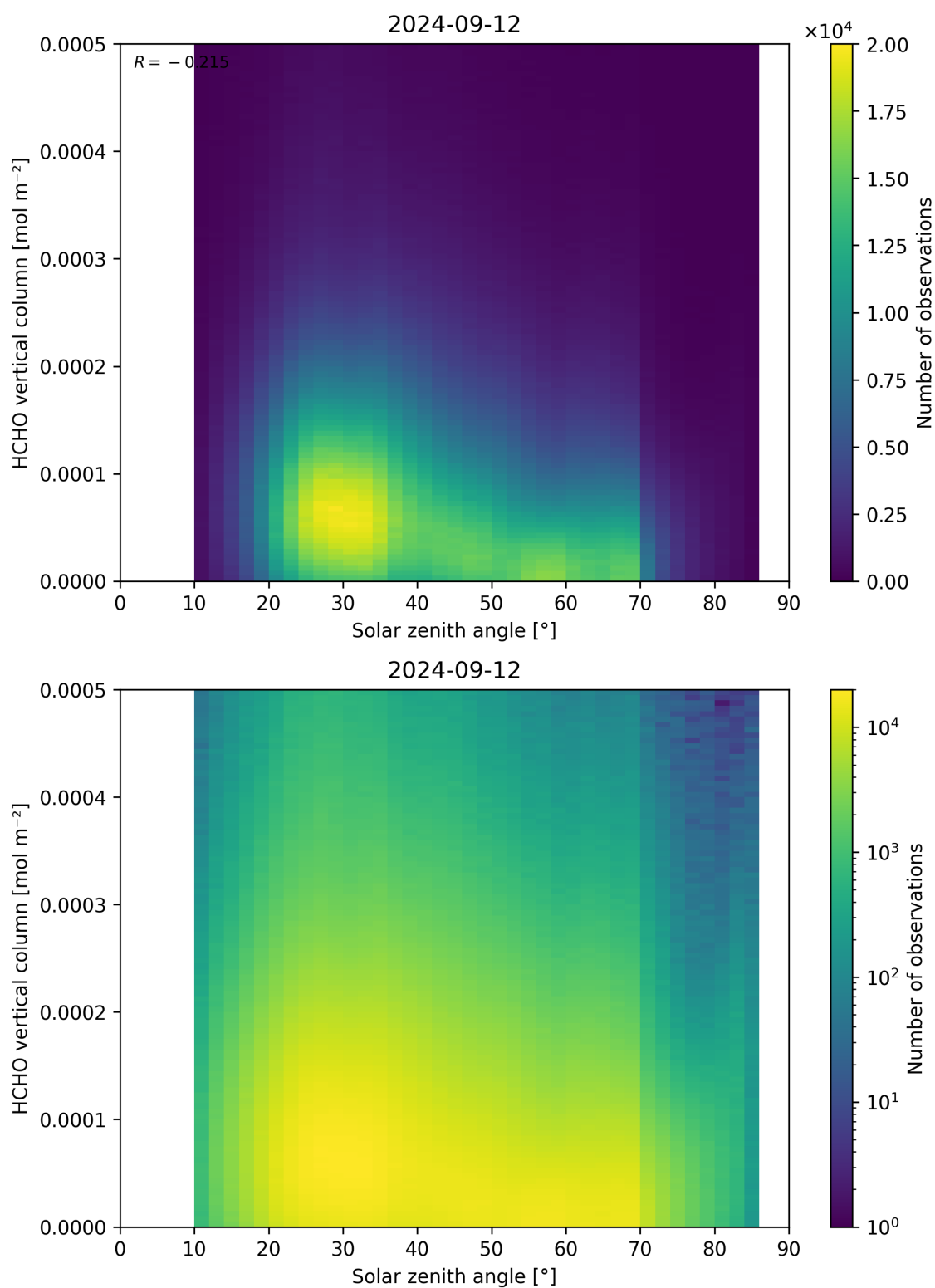
Figure 177: Scatter density plot of “Solar zenith angle” against “HCHO vertical column” for 2024-09-12 to 2024-09-13.
