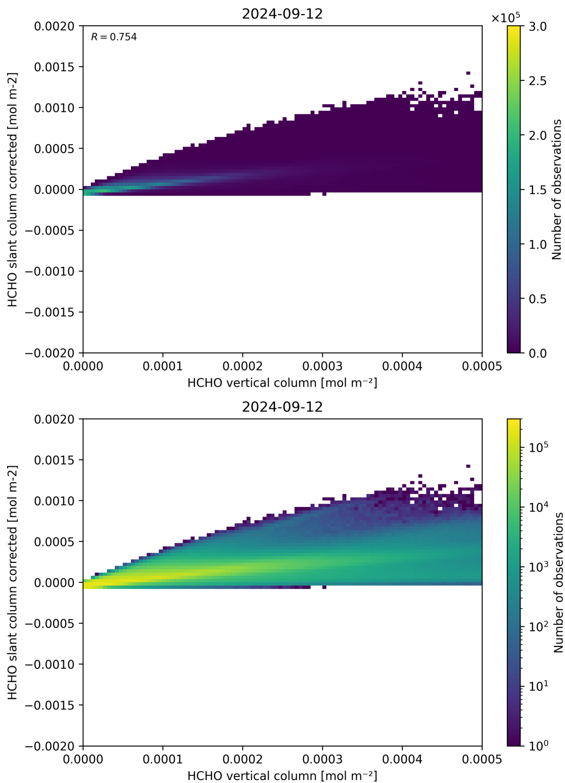
Figure 127: Scatter density plot of “HCHO vertical column” against “HCHO slant column corrected” for 2024-09-12 to 2024-09-13.
