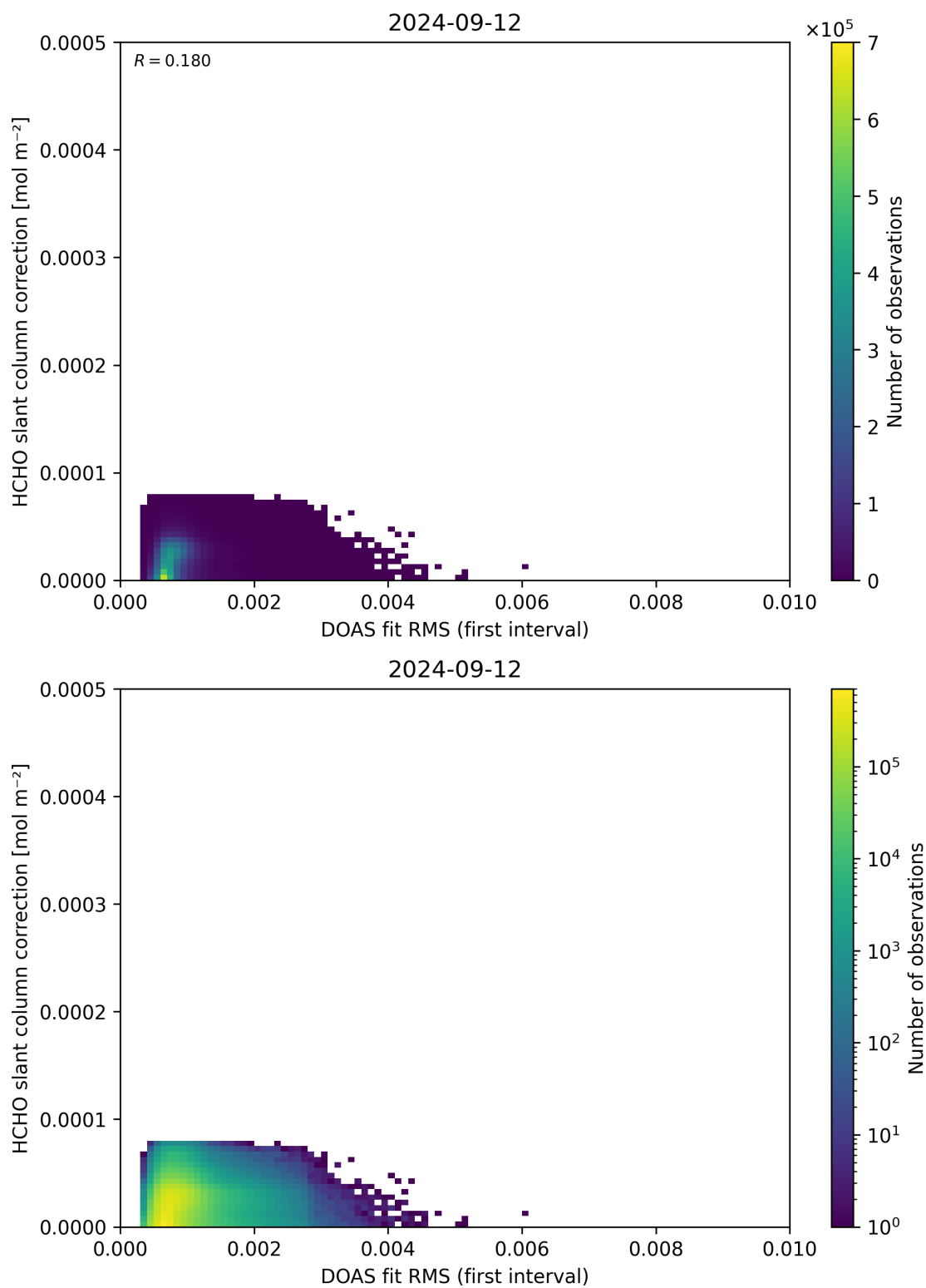
Figure 63: Scatter density plot of “DOAS fit RMS (first interval)” against “HCHO slant column correction” for 2024-09-12 to 2024-09-13.
