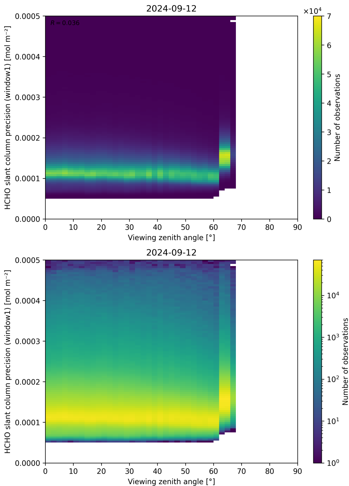
Figure 189: Scatter density plot of “Viewing zenith angle” against “HCHO slant column precision (window1)” for 2024-09-12 to 2024-09-13.
