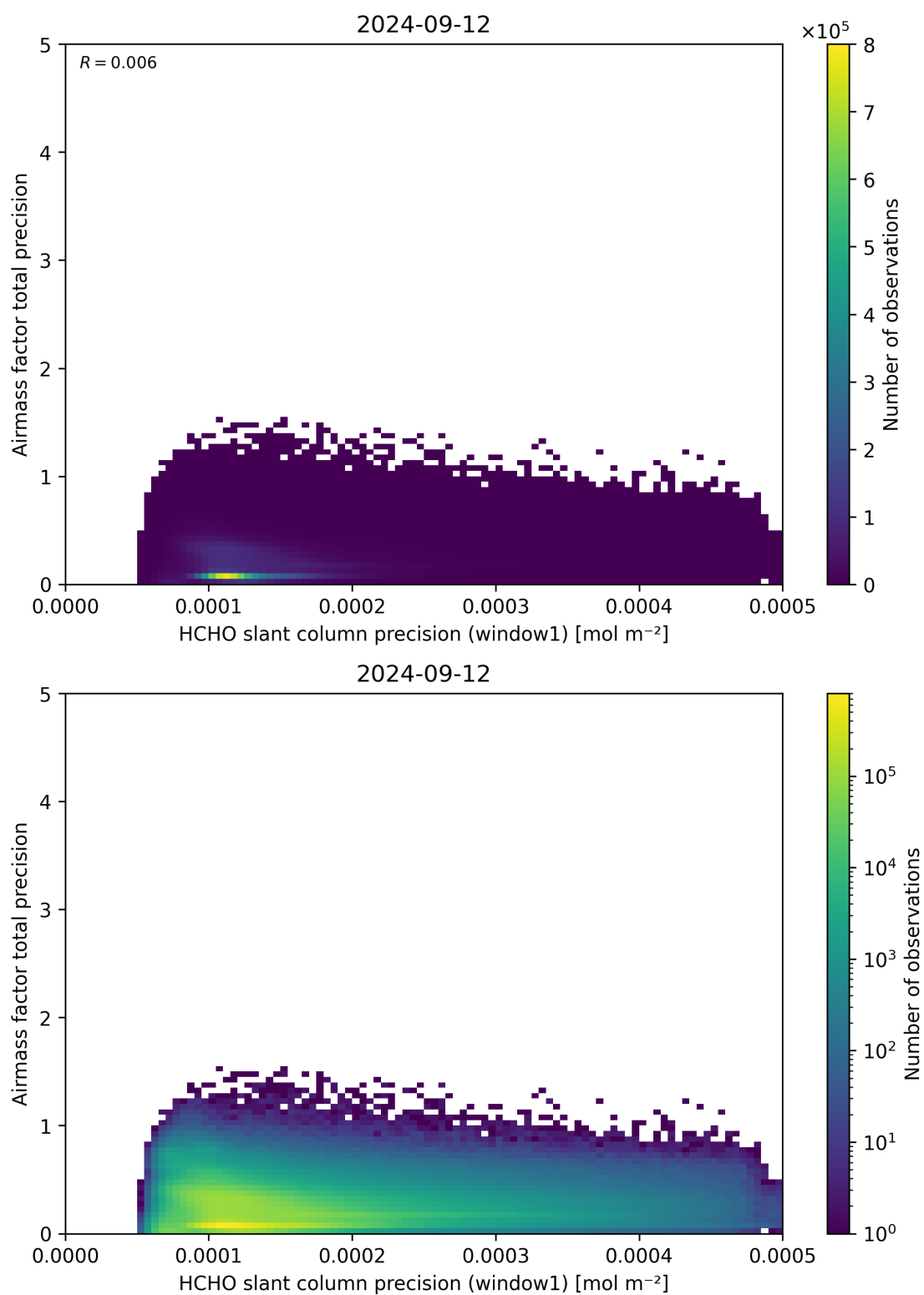
Figure 95: Scatter density plot of “HCHO slant column precision (window1)” against “Airmass factor total precision” for 2024-09-12 to 2024-09-13.
