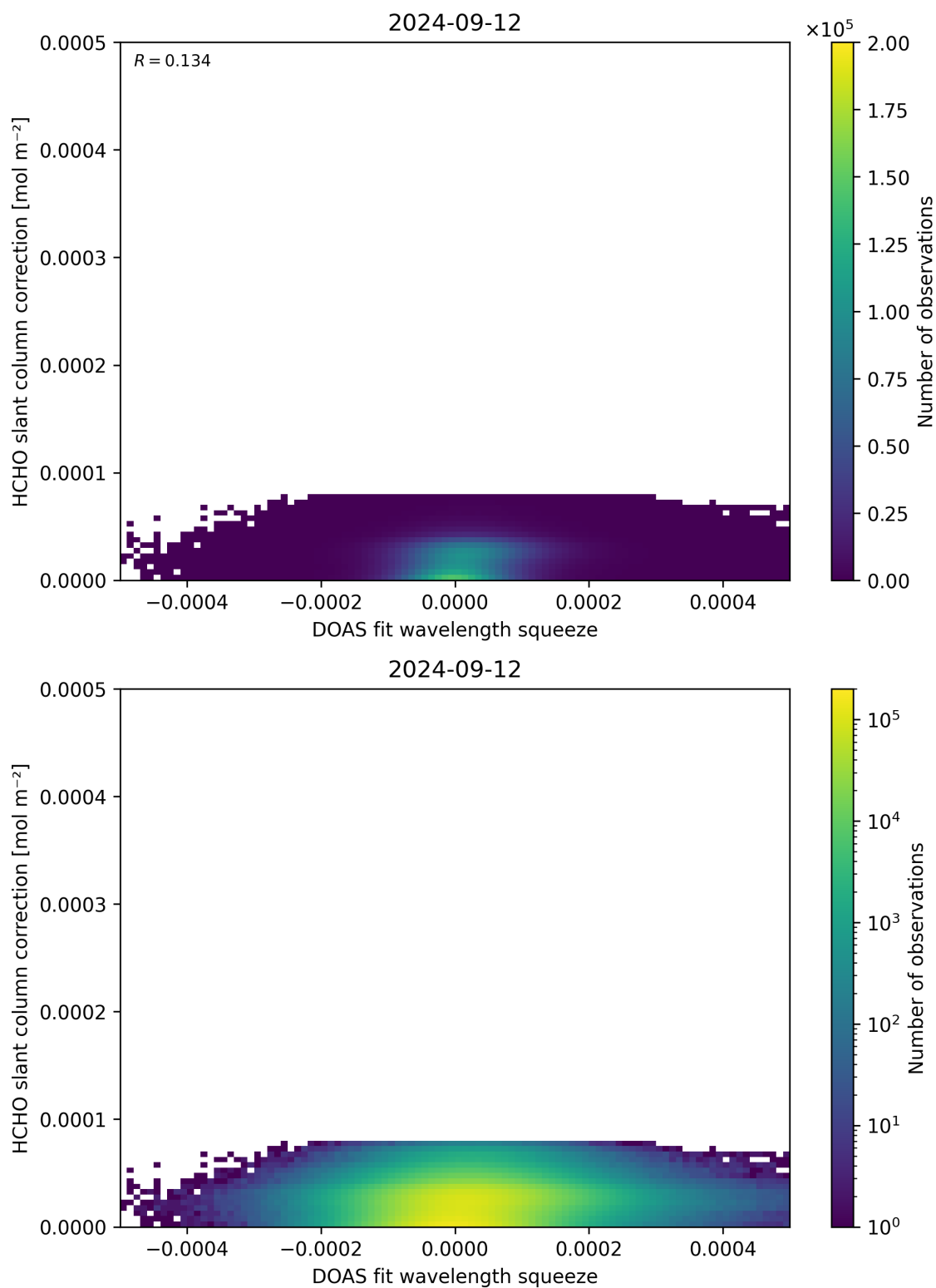
Figure 70: Scatter density plot of “DOAS fit wavelength squeeze” against “HCHO slant column correction” for 2024-09-12 to 2024-09-13.
