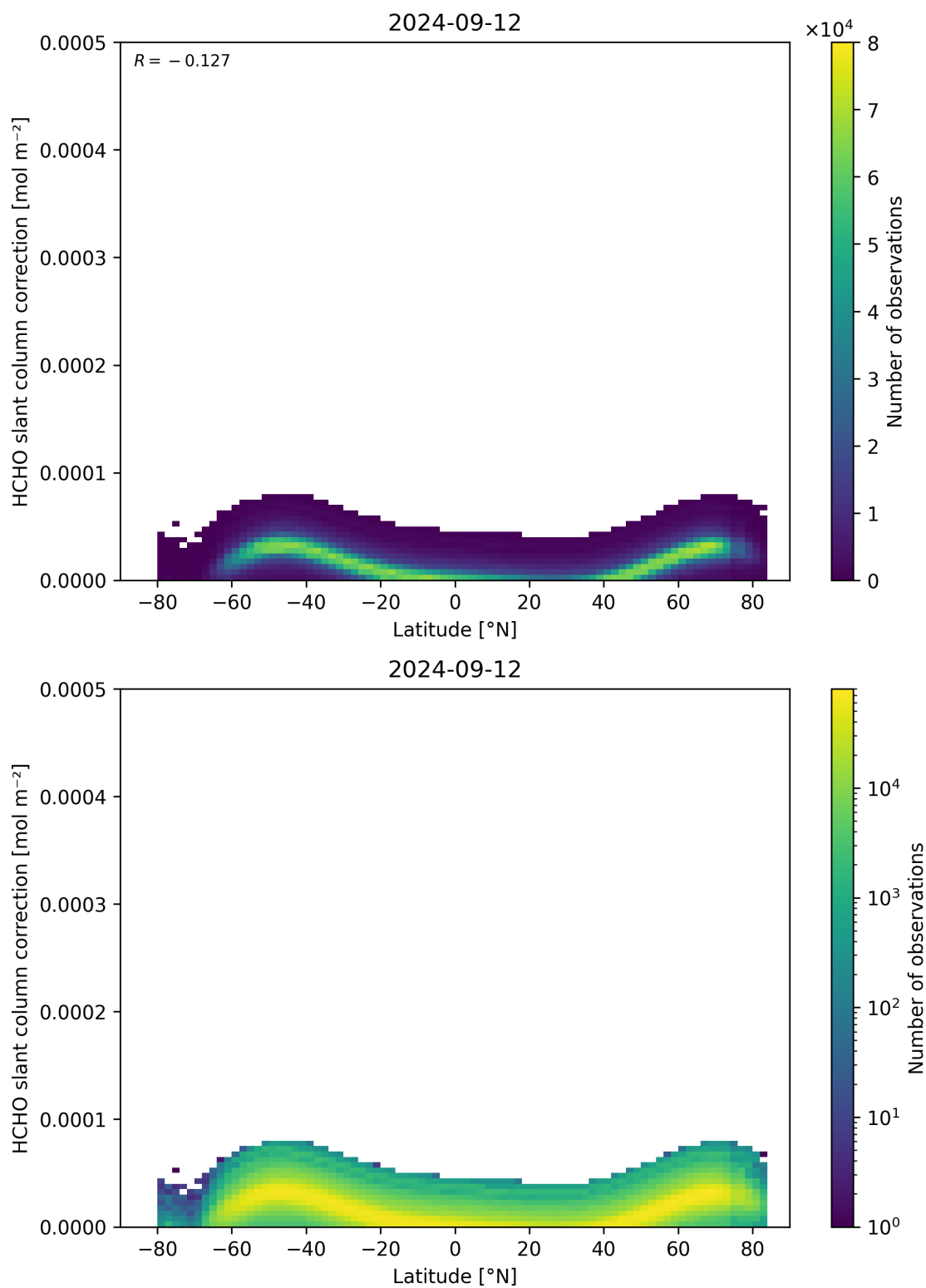
Figure 158: Scatter density plot of “Latitude” against “HCHO slant column correction” for 2024-09-12 to 2024-09-13.
