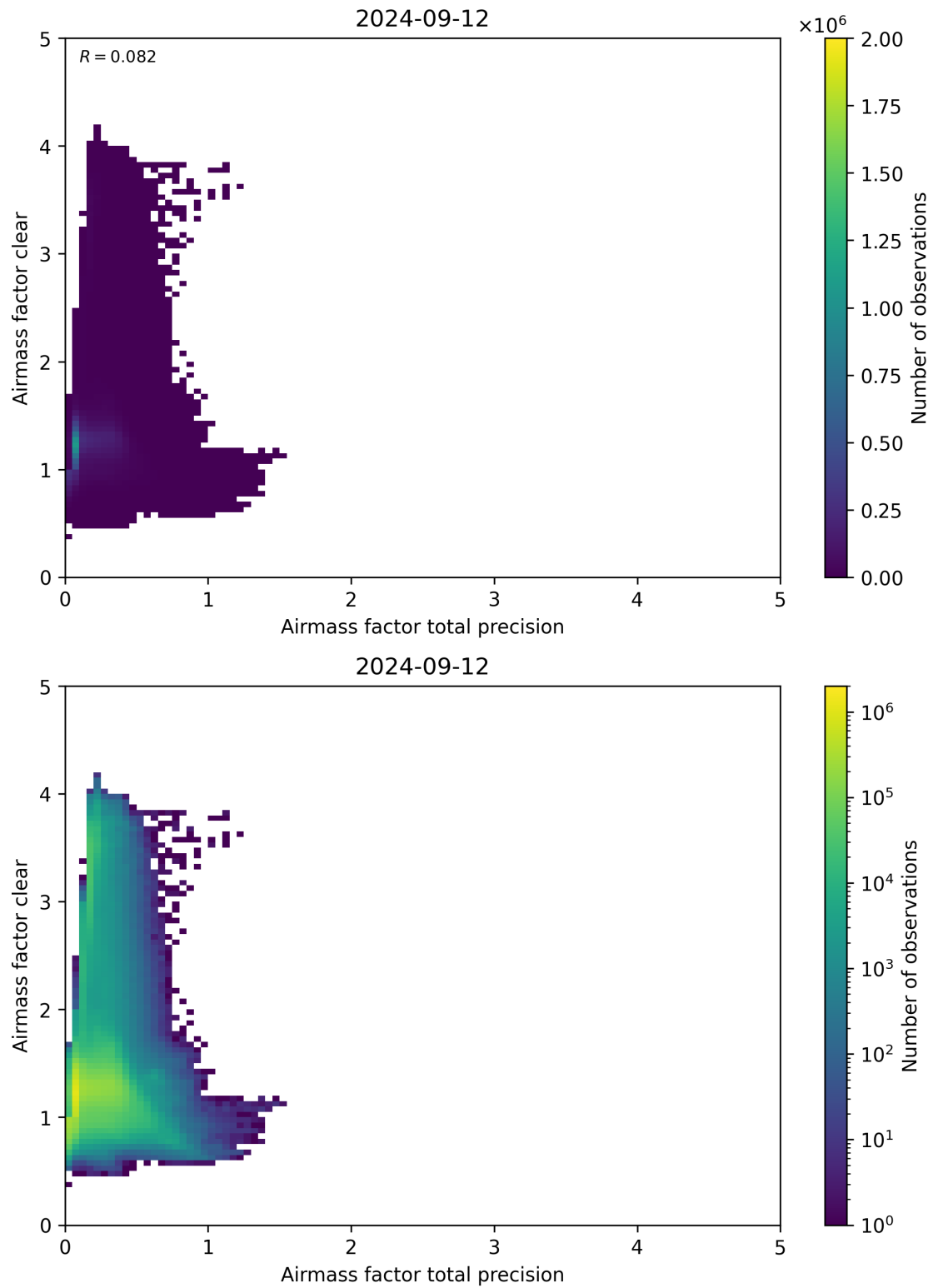
Figure 108: Scatter density plot of “Airmass factor total precision” against “Airmass factor clear” for 2024-09-12 to 2024-09-13.
