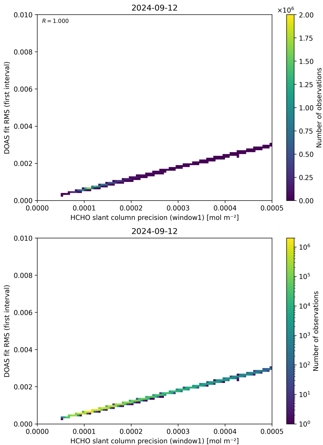
Figure 88: Scatter density plot of “HCHO slant column precision (window1)” against “DOAS fit RMS (first interval)” for 2024-09-12 to 2024-09-13.
