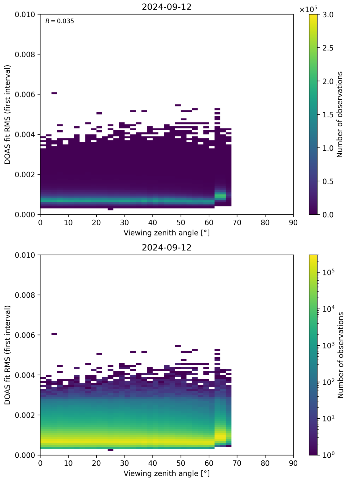
Figure 182: Scatter density plot of “Viewing zenith angle” against “DOAS fit RMS (first interval)” for 2024-09-12 to 2024-09-13.
