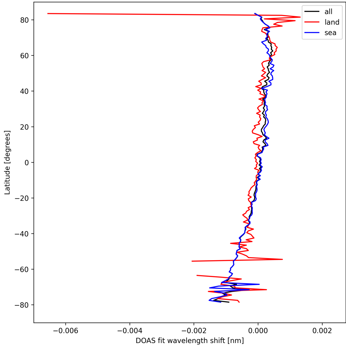
Figure 30: Zonal average of “DOAS fit wavelength shift” for 2024-09-12 to 2024-09-13.
