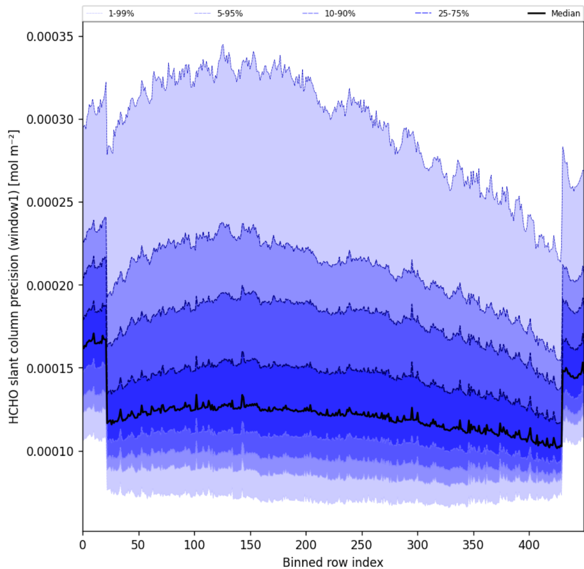
Figure 53: Along track statistics of “HCHO slant column precision (window1)” for 2024-09-12 to 2024-09-13
