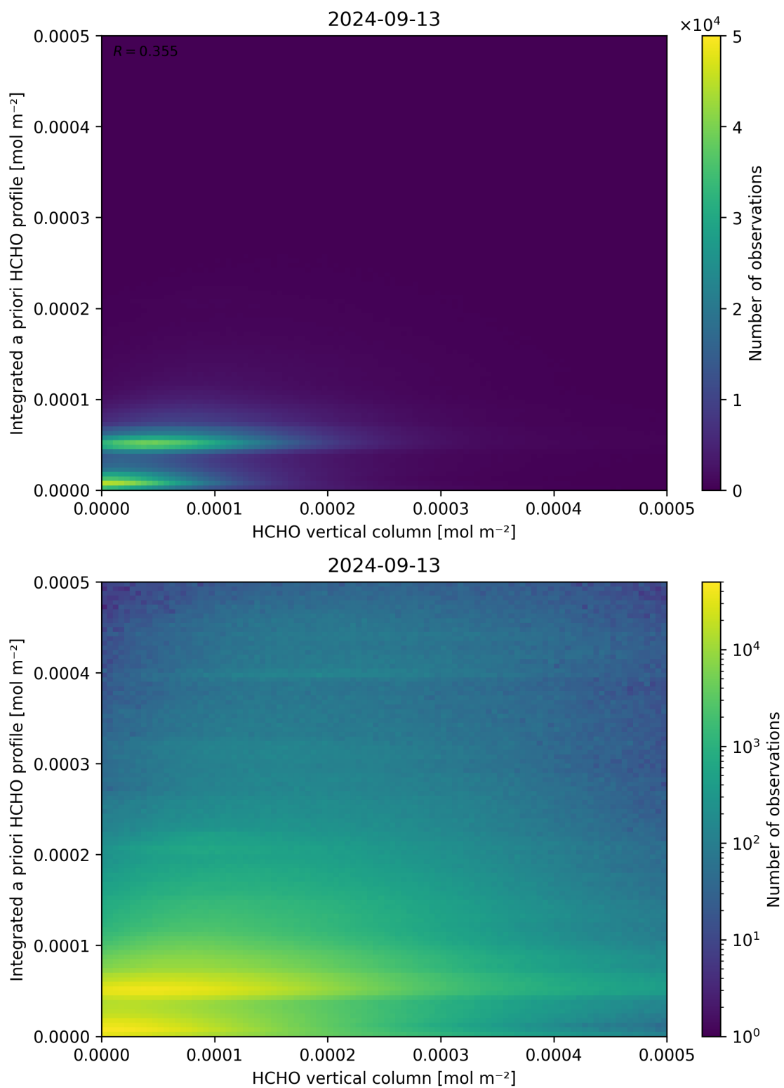
Figure 135: Scatter density plot of “HCHO vertical column” against “Integrated a priori HCHO profile” for 2024-09-12 to 2024-09-14.
