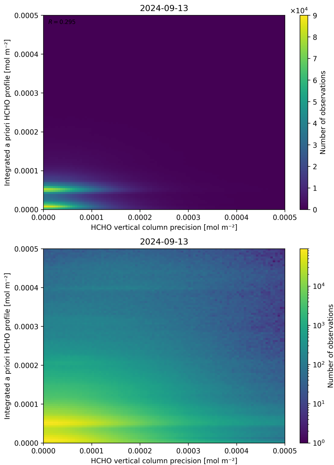
Figure 147: Scatter density plot of “HCHO vertical column precision” against “Integrated a priori HCHO profile” for 2024-09-12 to 2024-09-14.
