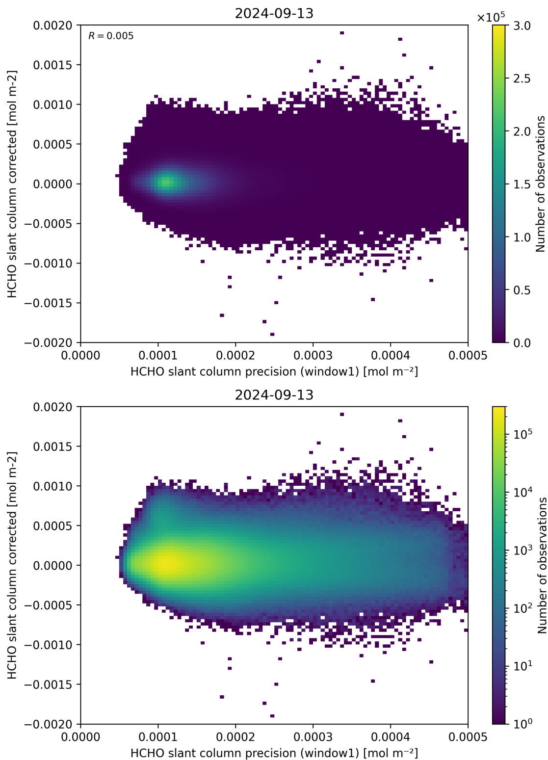
Figure 92: Scatter density plot of “HCHO slant column precision (window1)” against “HCHO slant column corrected” for 2024-09-12 to 2024-09-14.
