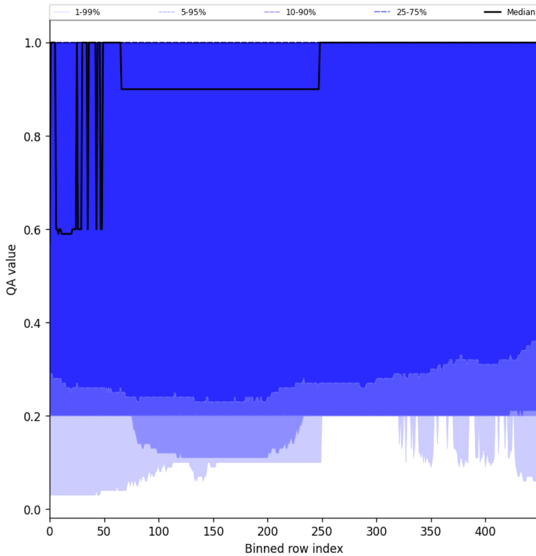
Figure 48: Along track statistics of “QA value” for 2024-09-12 to 2024-09-14
