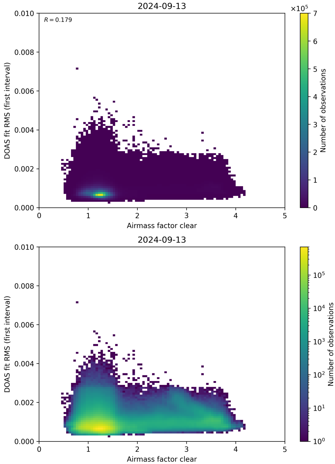
Figure 71: Scatter density plot of “Airmass factor clear” against “DOAS fit RMS (first interval)” for 2024-09-12 to 2024-09-14.
