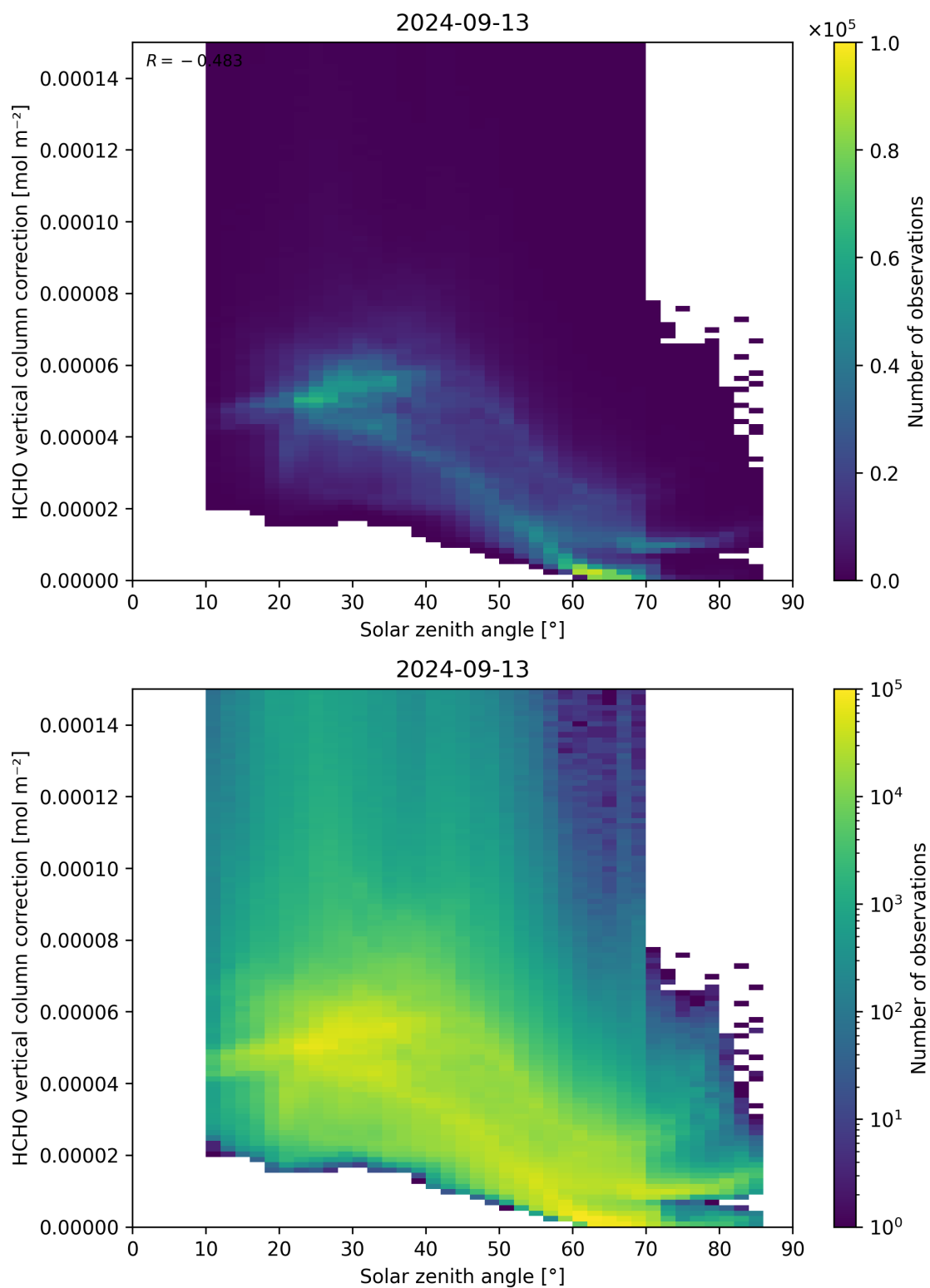
Figure 178: Scatter density plot of “Solar zenith angle” against “HCHO vertical column correction” for 2024-09-12 to 2024-09-14.
