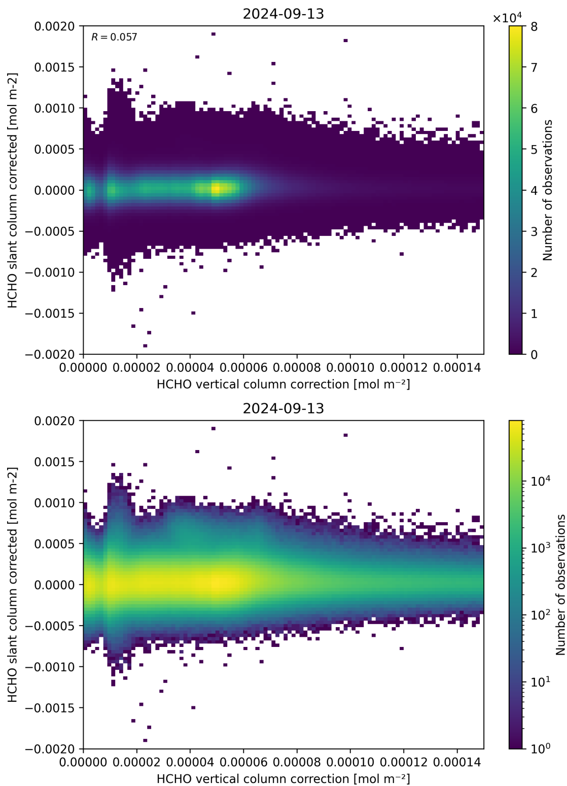
Figure 116: Scatter density plot of “HCHO vertical column correction” against “HCHO slant column corrected” for 2024-09-12 to 2024-09-14.
