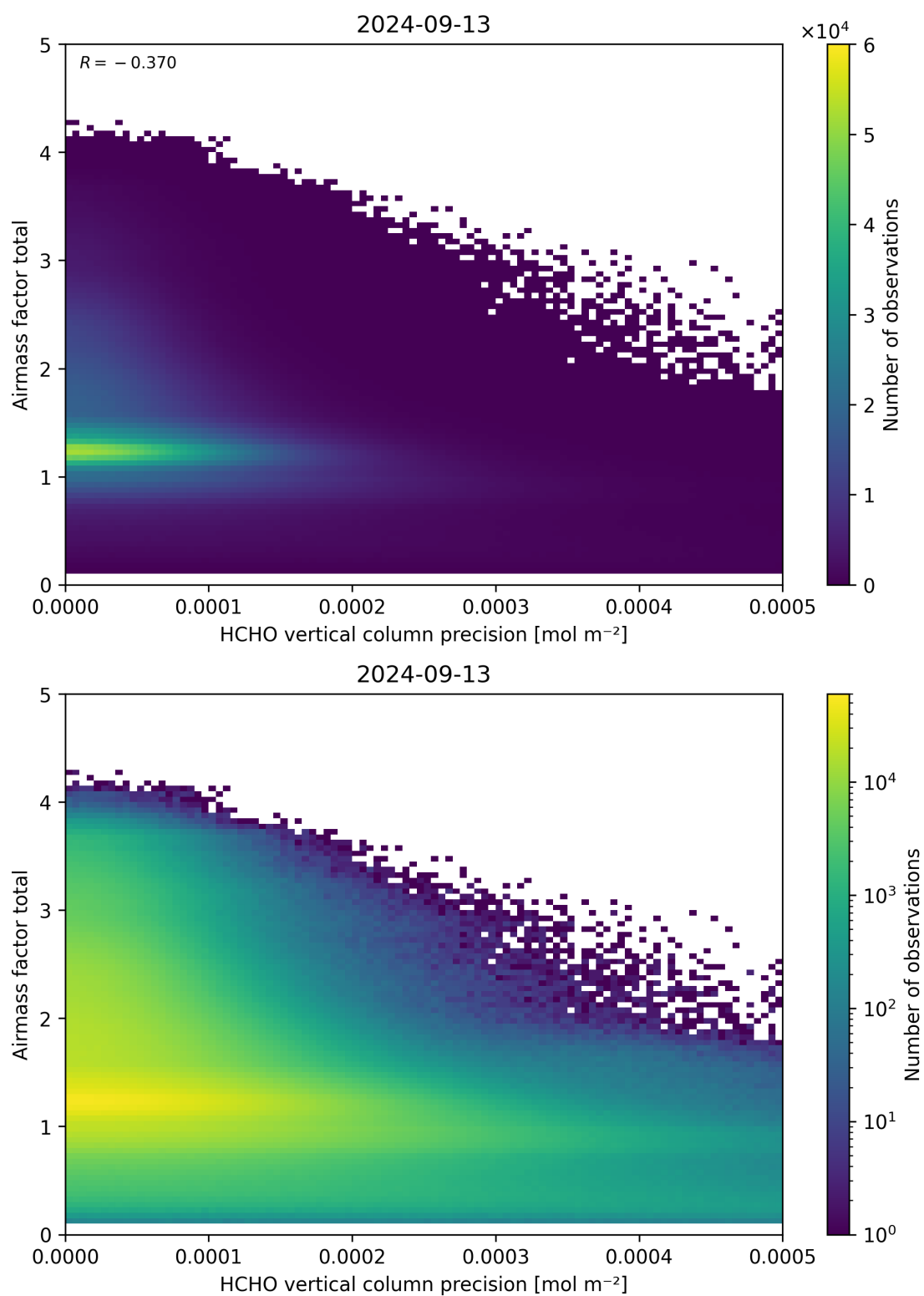
Figure 144: Scatter density plot of “HCHO vertical column precision” against “Airmass factor total” for 2024-09-12 to 2024-09-14.
