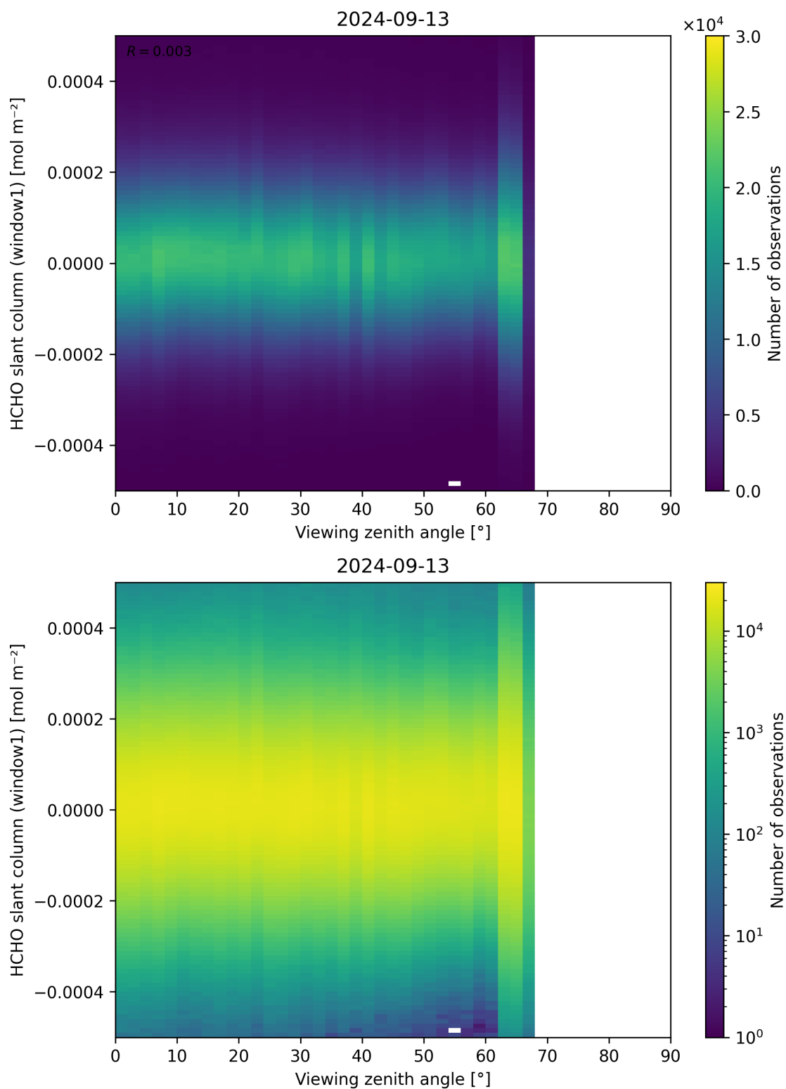
Figure 188: Scatter density plot of “Viewing zenith angle” against “HCHO slant column (window1)” for 2024-09-12 to 2024-09-14.
