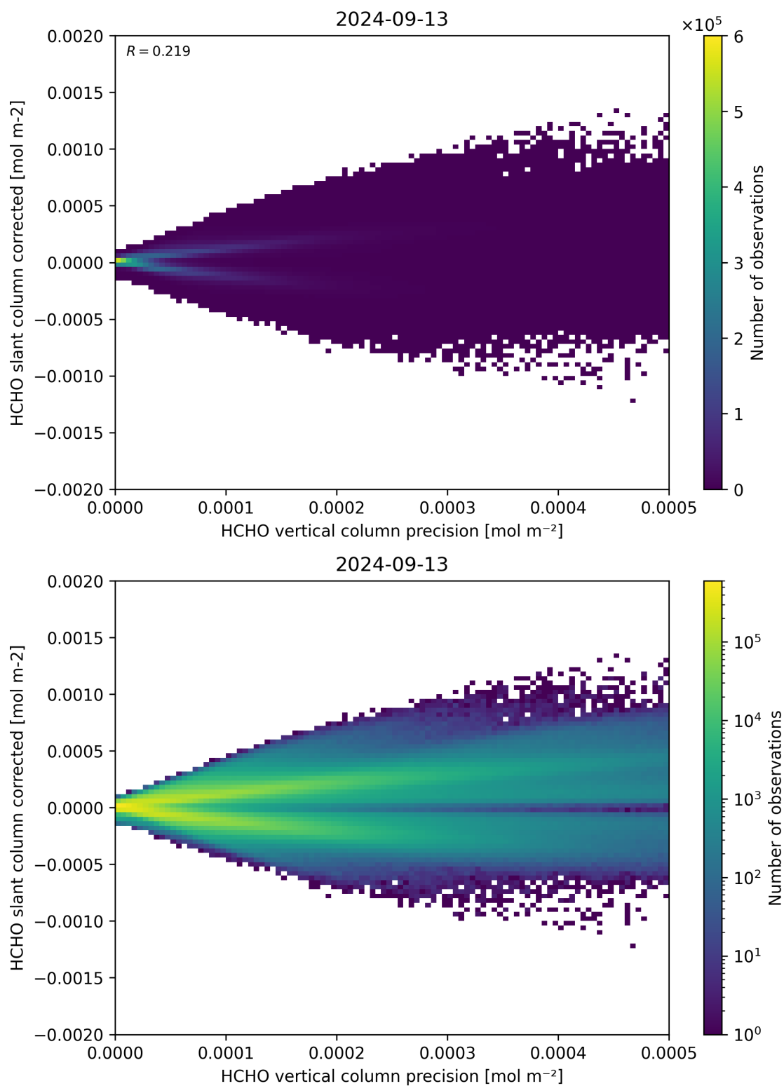
Figure 140: Scatter density plot of “HCHO vertical column precision” against “HCHO slant column corrected” for 2024-09-12 to 2024-09-14.
