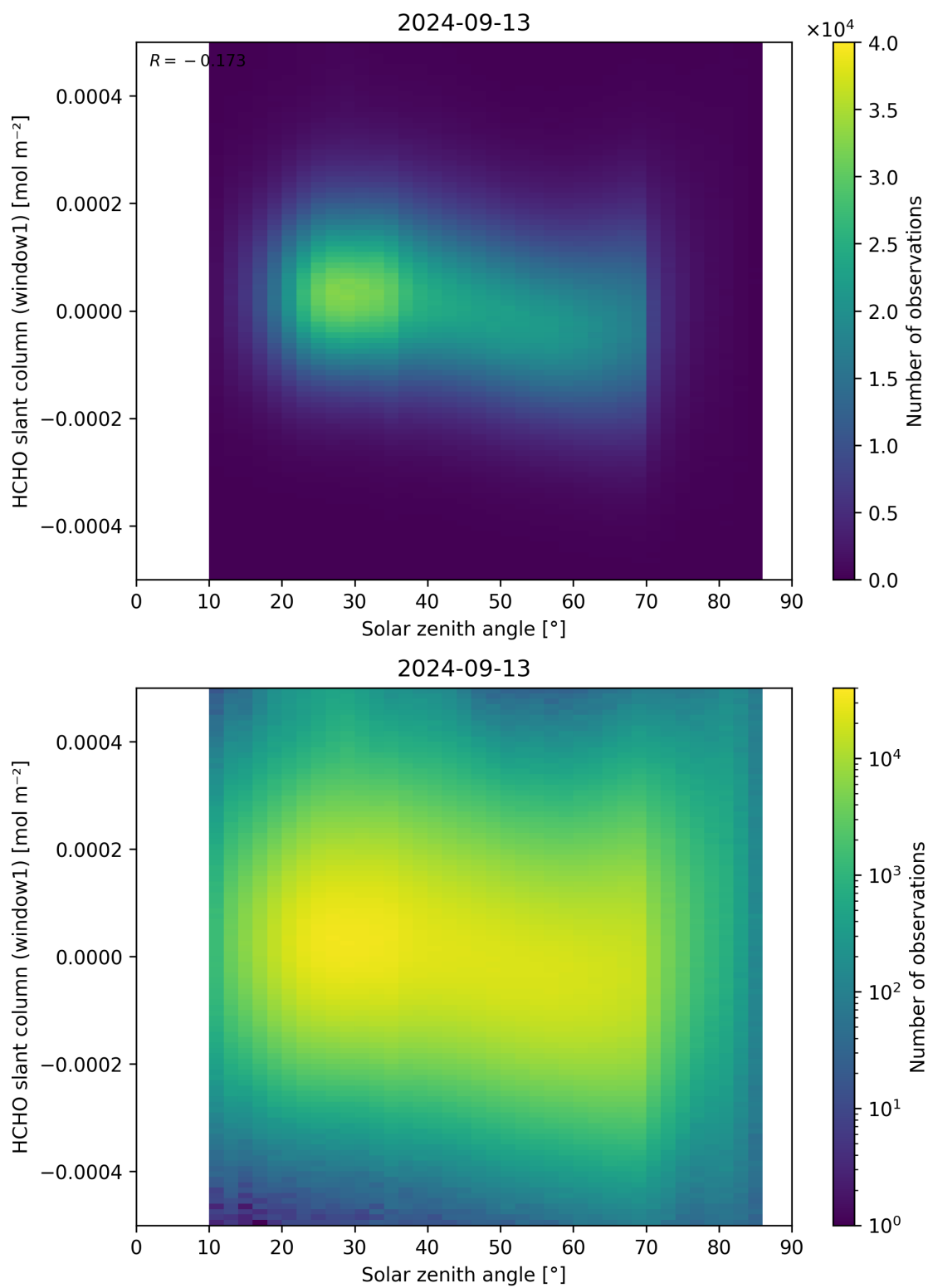
Figure 173: Scatter density plot of “Solar zenith angle” against “HCHO slant column (window1)” for 2024-09-12 to 2024-09-14.
