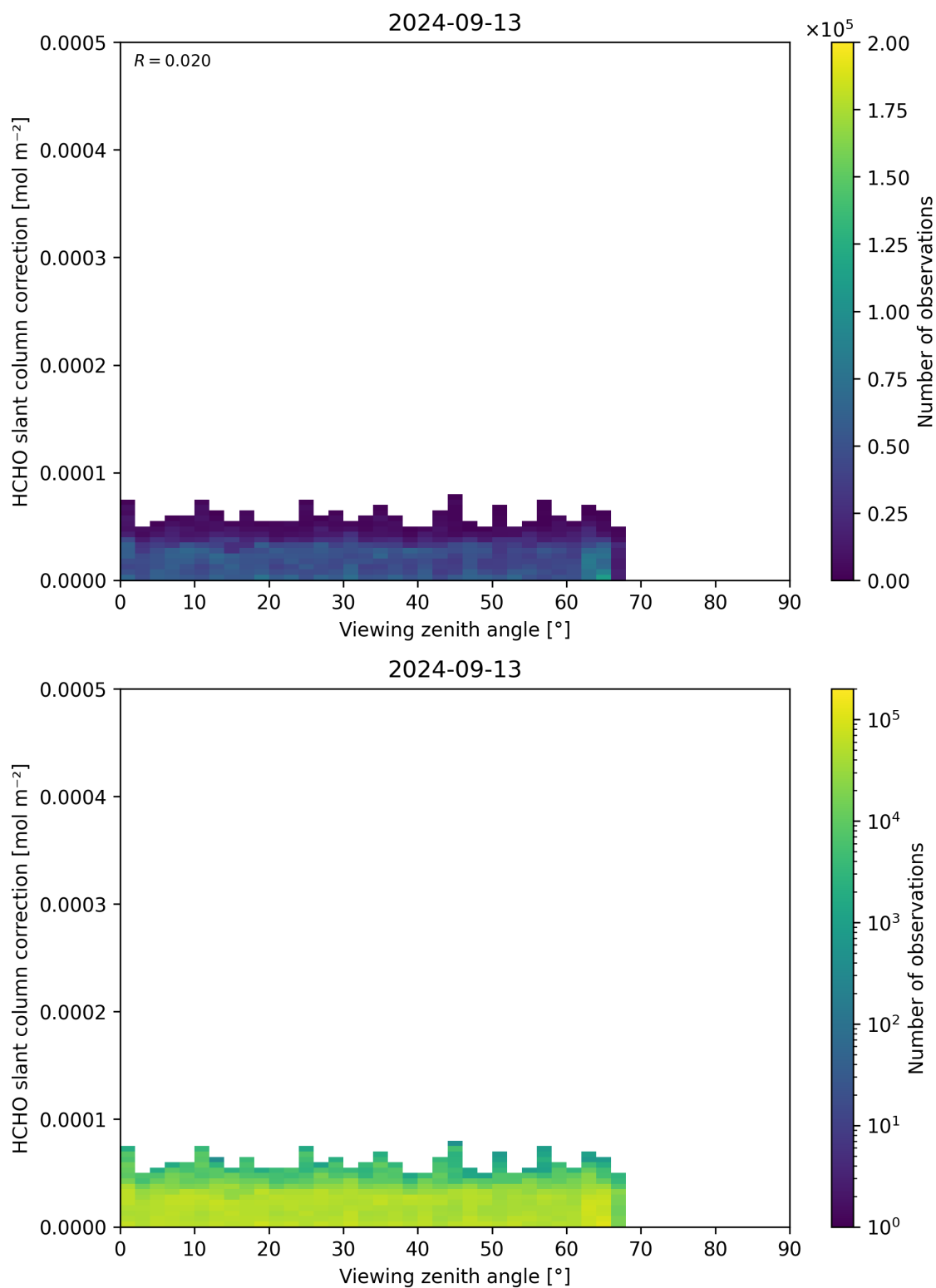
Figure 187: Scatter density plot of “Viewing zenith angle” against “HCHO slant column correction” for 2024-09-12 to 2024-09-14.
