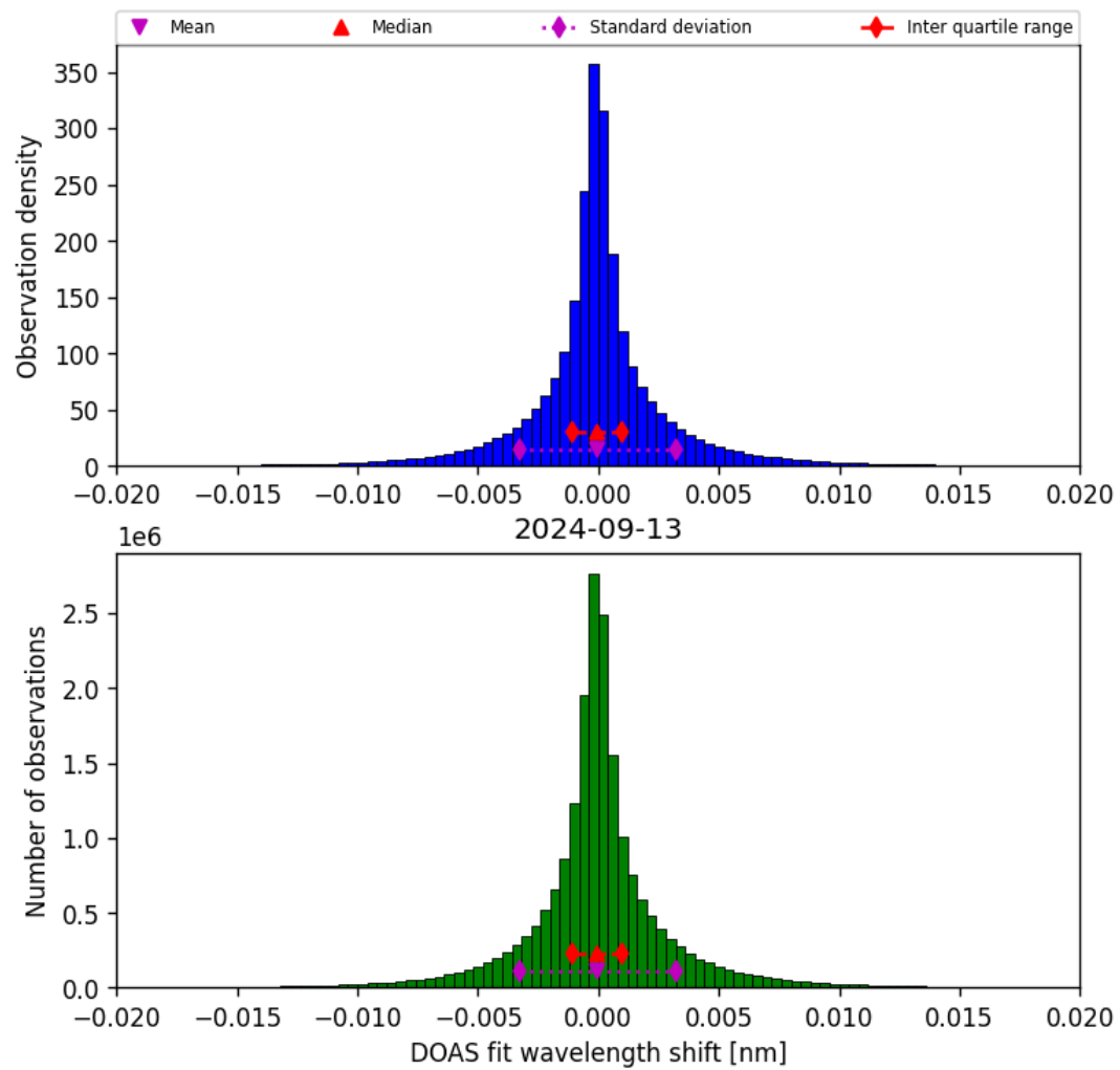
Figure 44: Histogram of “DOAS fit wavelength shift” for 2024-09-12 to 2024-09-14
