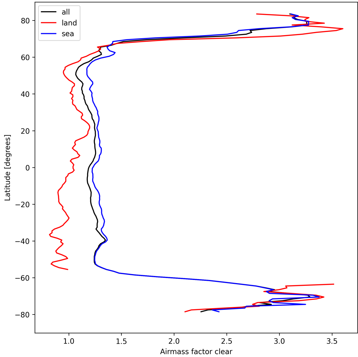
Figure 28: Zonal average of “Airmass factor clear” for 2024-09-12 to 2024-09-14.
