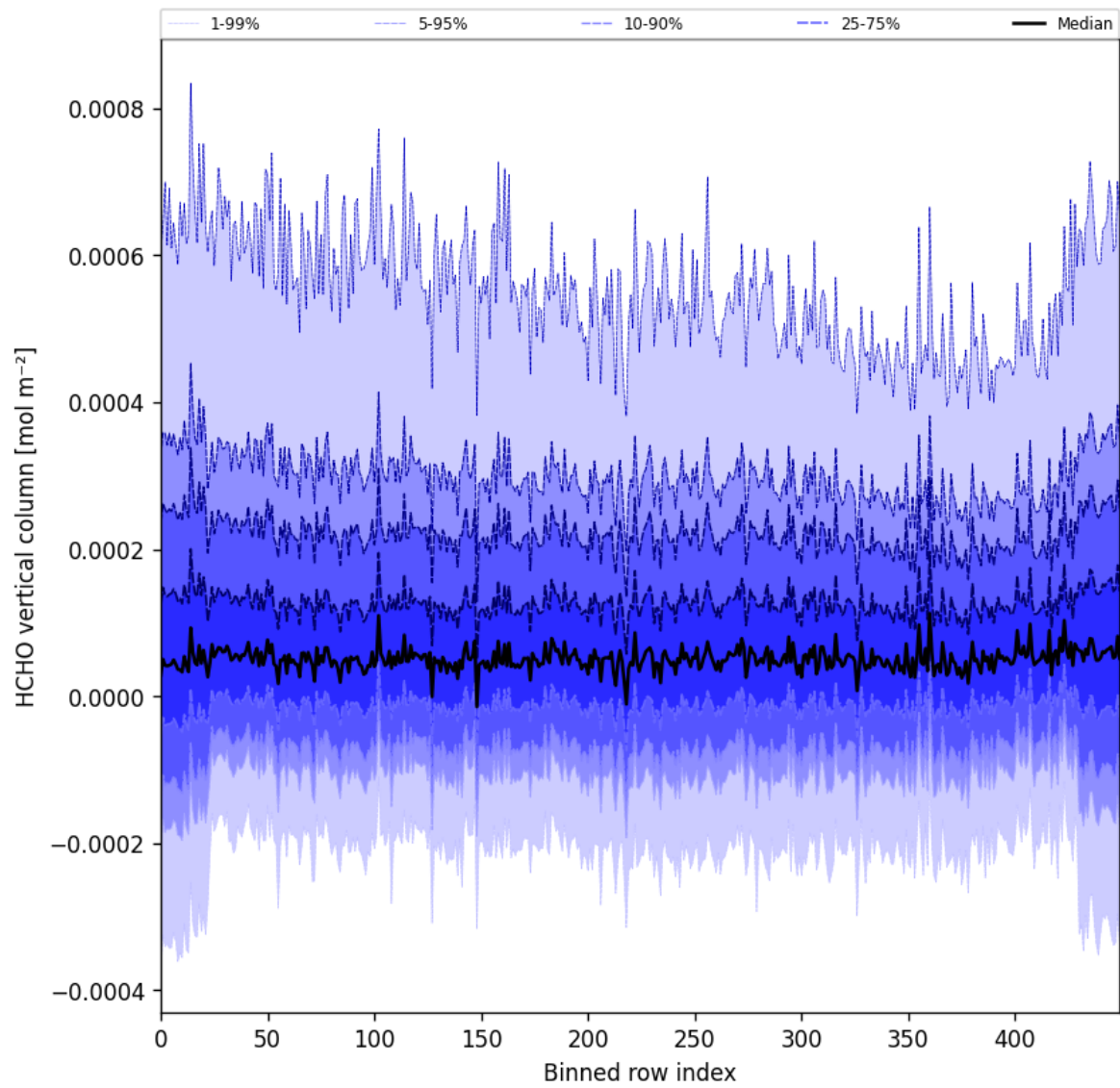
Figure 49: Along track statistics of “HCHO vertical column” for 2024-09-12 to 2024-09-14
