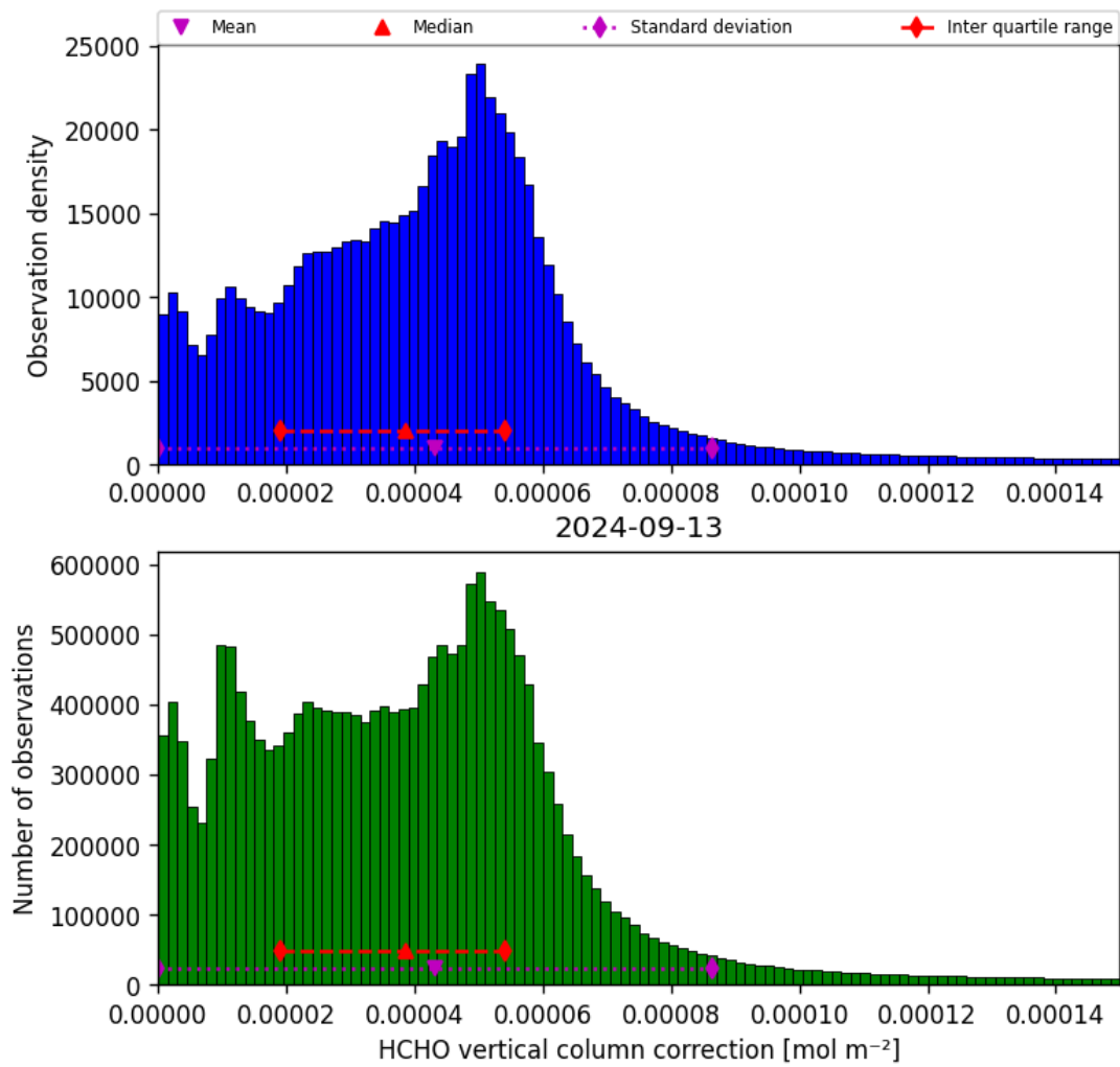
Figure 37: Histogram of “HCHO vertical column correction” for 2024-09-12 to 2024-09-14
