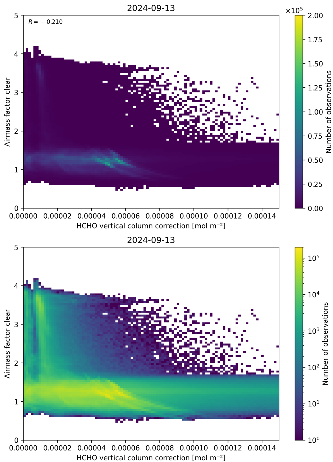
Figure 115: Scatter density plot of “HCHO vertical column correction” against “Airmass factor clear” for 2024-09-12 to 2024-09-14.
