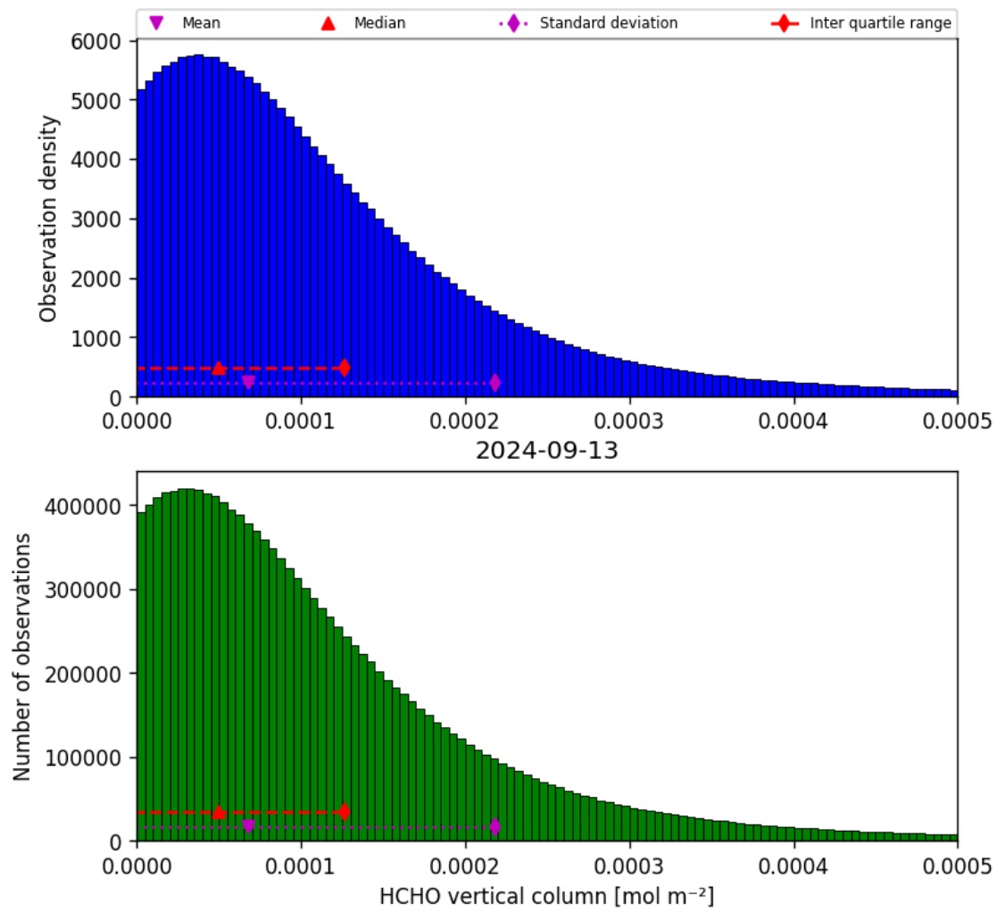
Figure 35: Histogram of “HCHO vertical column” for 2024-09-12 to 2024-09-14
