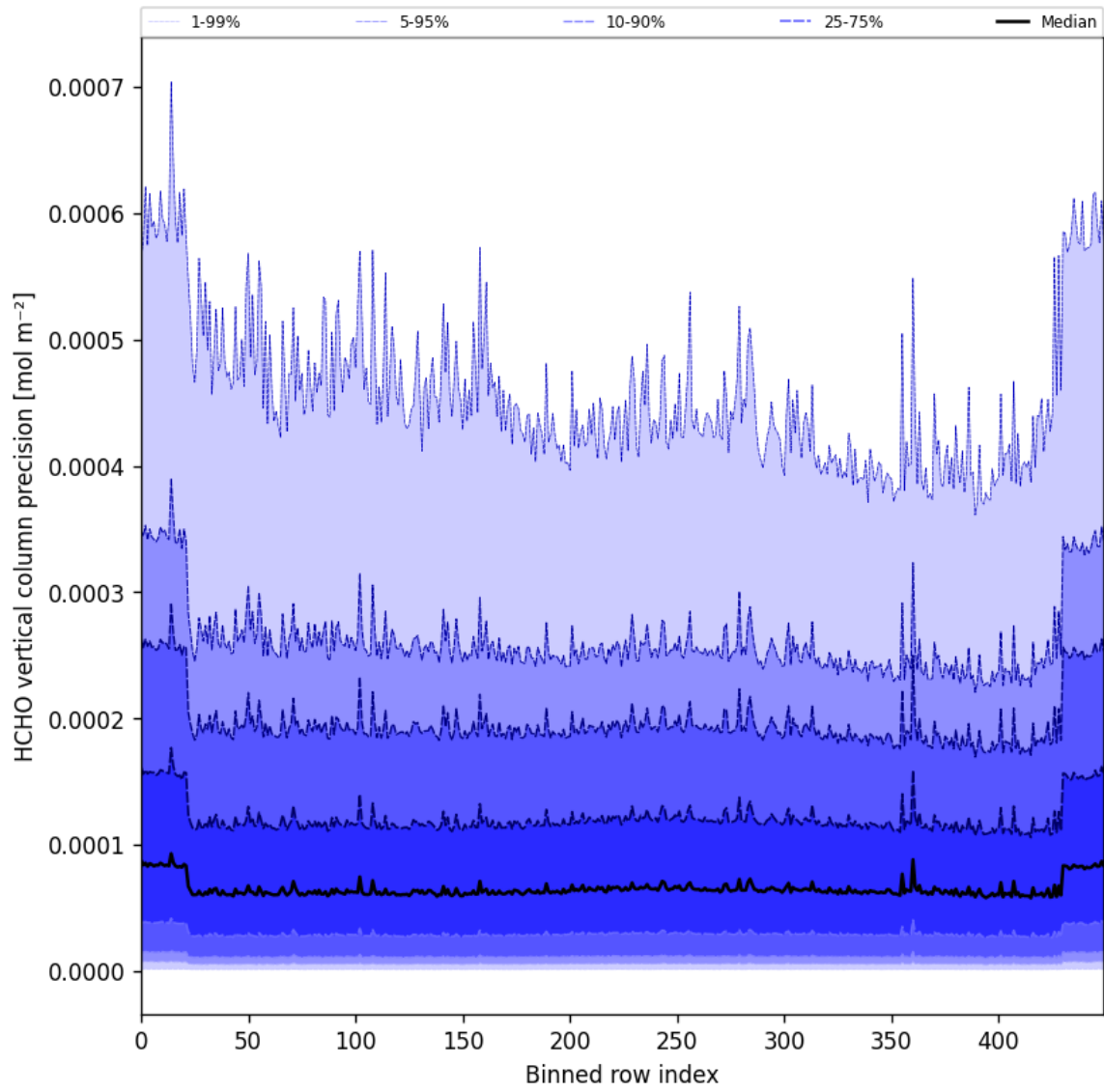
Figure 50: Along track statistics of “HCHO vertical column precision” for 2024-09-12 to 2024-09-14
