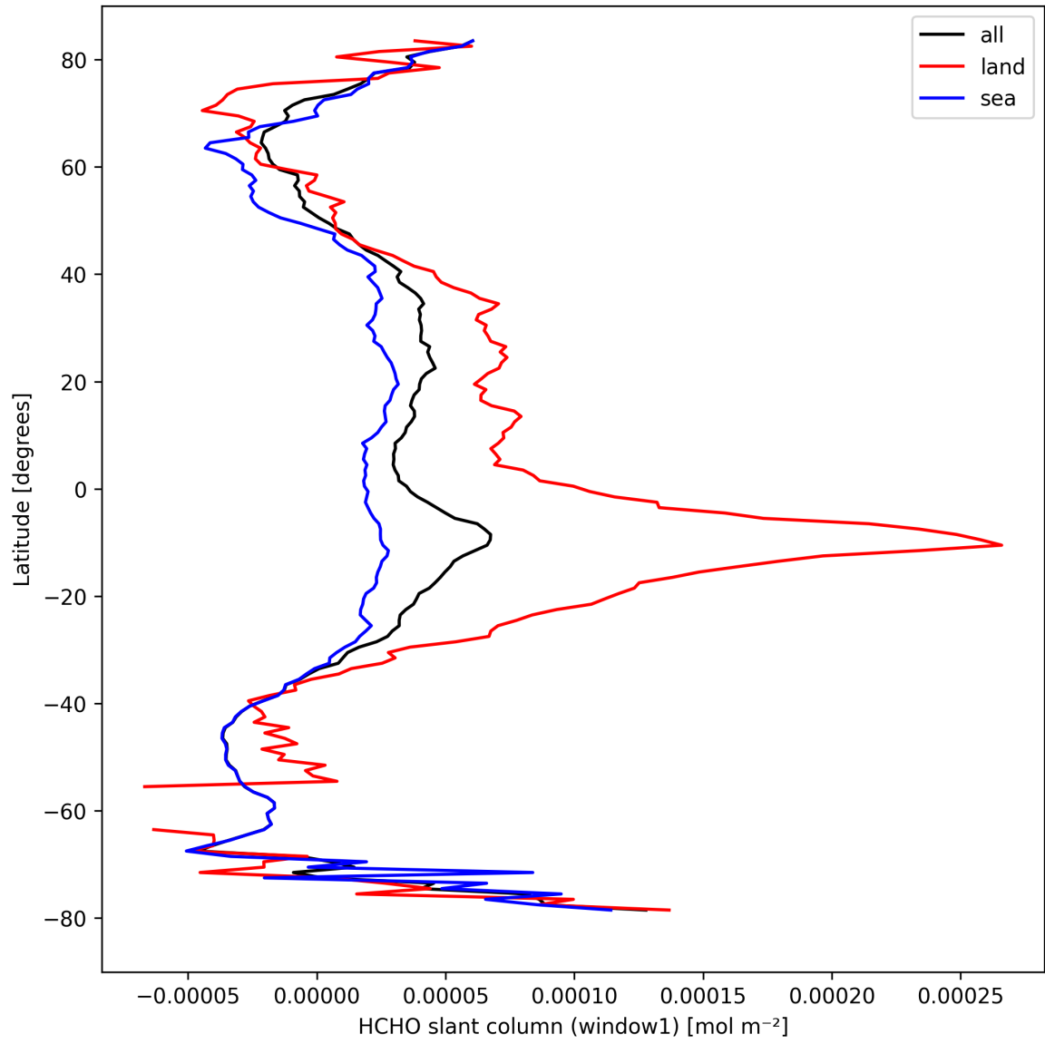
Figure 24: Zonal average of “HCHO slant column (window1)” for 2024-09-12 to 2024-09-14.
