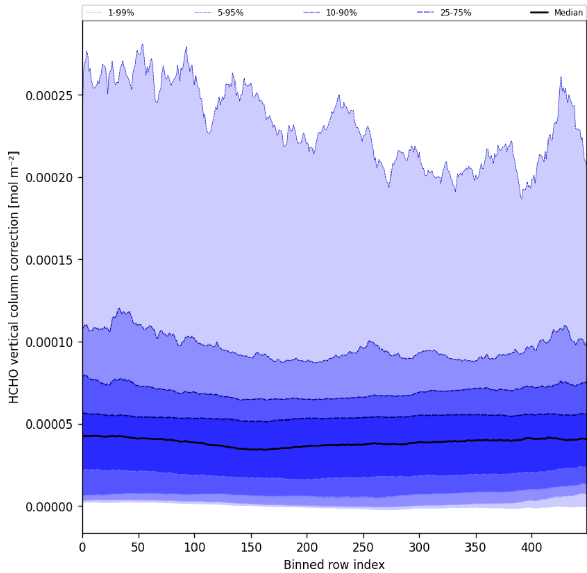
Figure 51: Along track statistics of “HCHO vertical column correction” for 2024-09-12 to 2024-09-14
