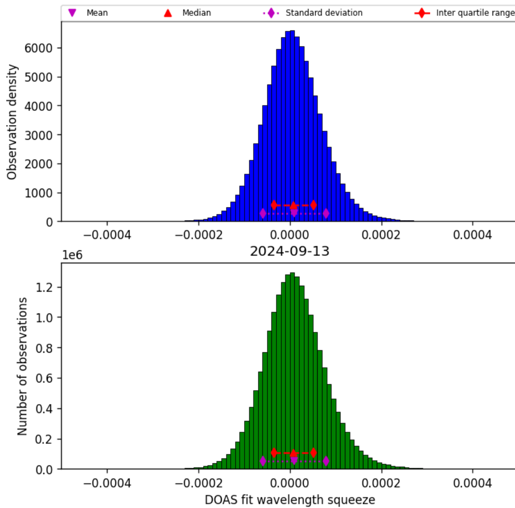
Figure 45: Histogram of “DOAS fit wavelength squeeze” for 2024-09-12 to 2024-09-14
