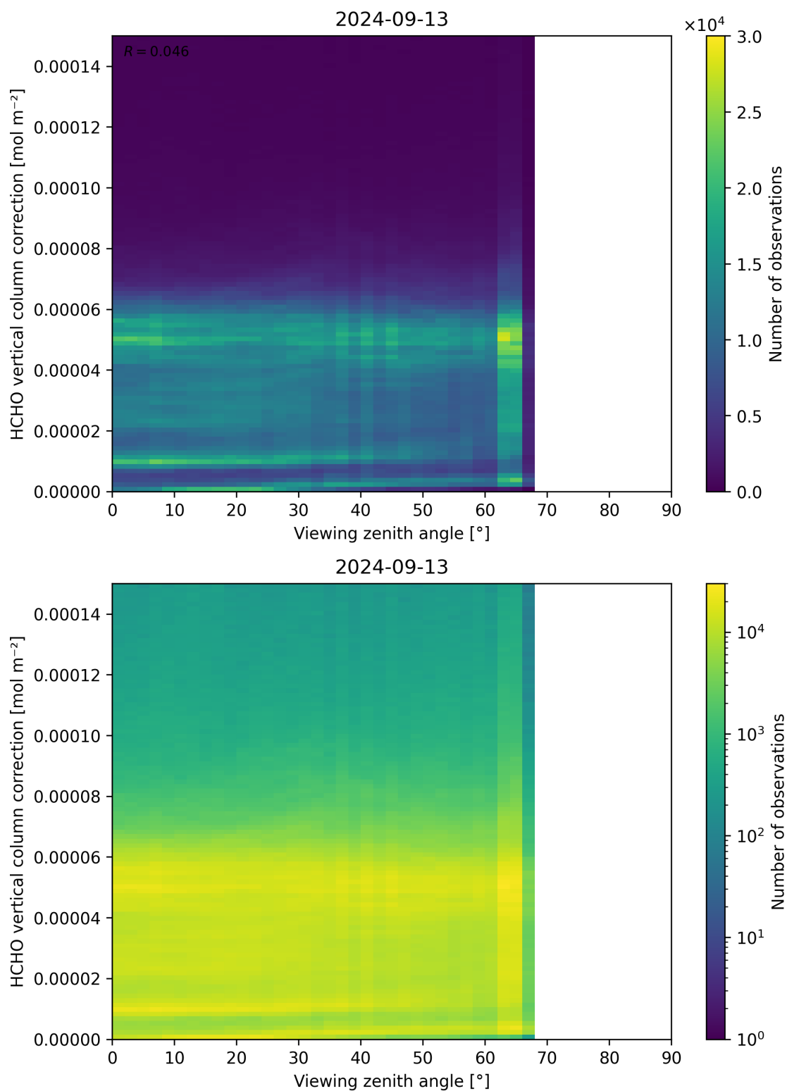
Figure 193: Scatter density plot of “Viewing zenith angle” against “HCHO vertical column correction” for 2024-09-12 to 2024-09-14.
