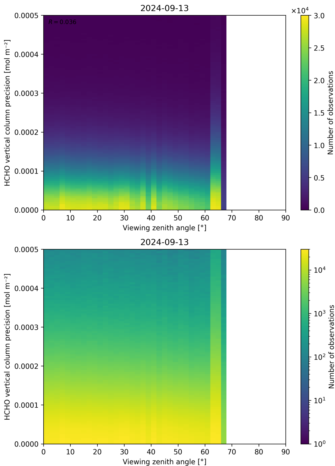
Figure 194: Scatter density plot of “Viewing zenith angle” against “HCHO vertical column precision” for 2024-09-12 to 2024-09-14.
