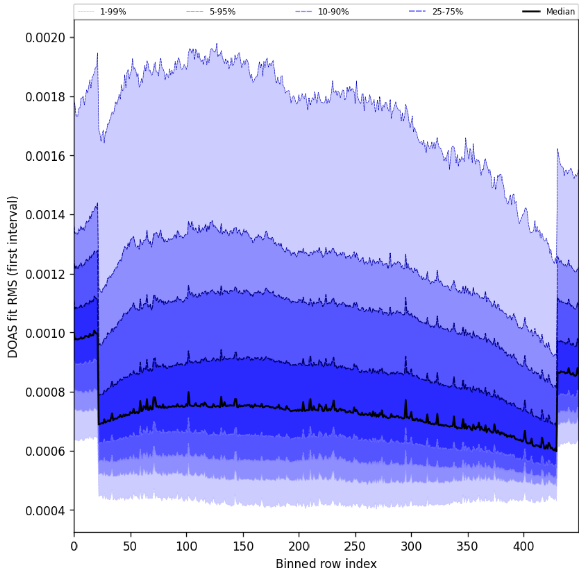
Figure 60: Along track statistics of “DOAS fit RMS (first interval)” for 2024-09-12 to 2024-09-14
