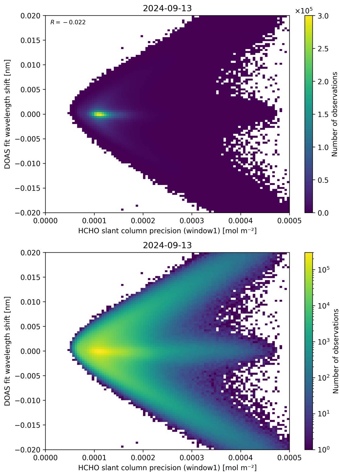
Figure 89: Scatter density plot of “HCHO slant column precision (window1)” against “DOAS fit wavelength shift” for 2024-09-12 to 2024-09-14.
