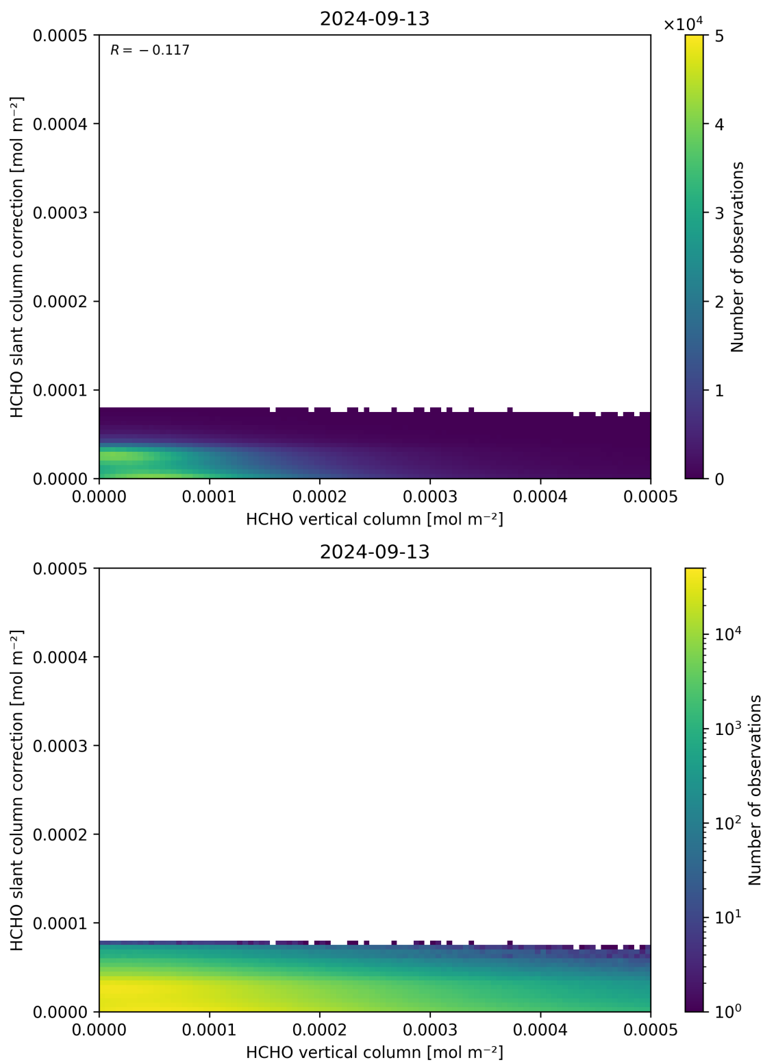
Figure 128: Scatter density plot of “HCHO vertical column” against “HCHO slant column correction” for 2024-09-12 to 2024-09-14.
