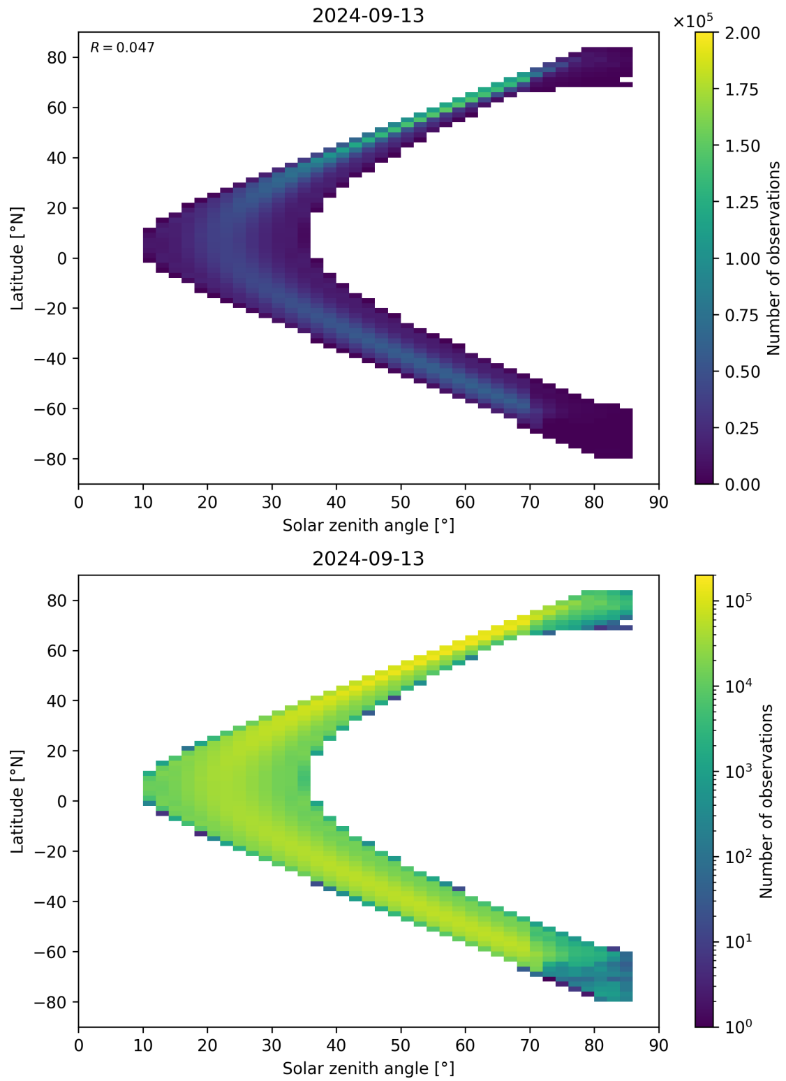
Figure 181: Scatter density plot of “Solar zenith angle” against “Latitude” for 2024-09-12 to 2024-09-14.
