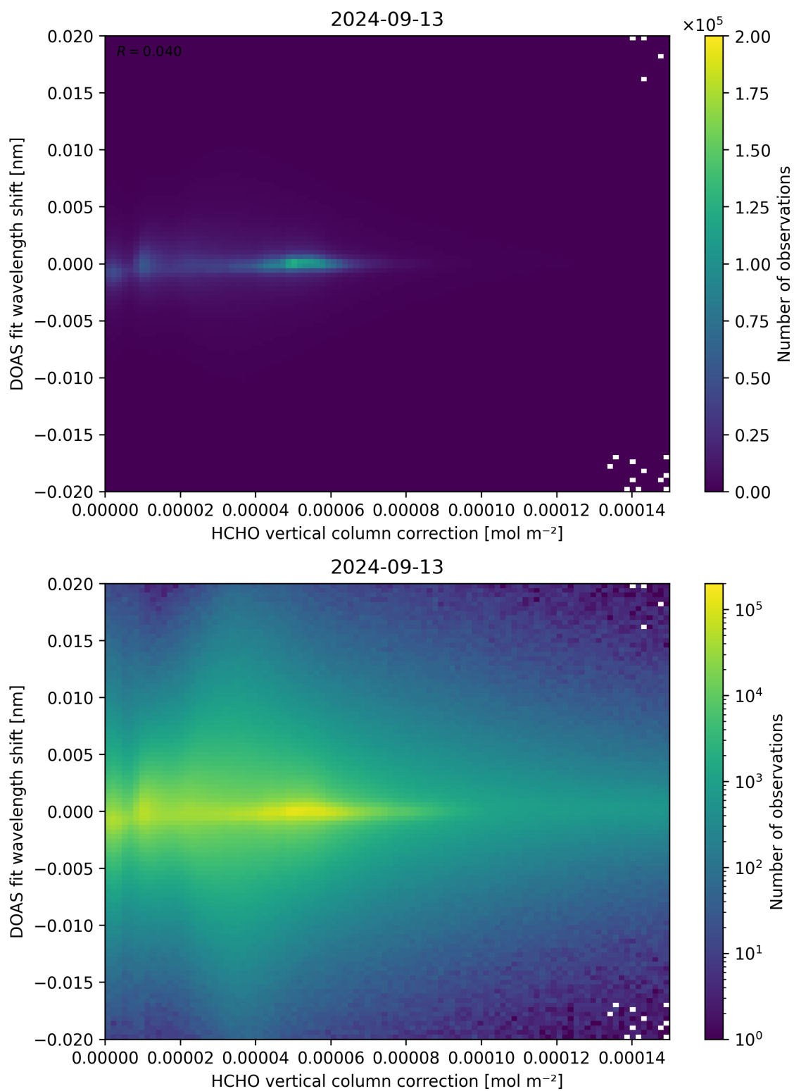
Figure 113: Scatter density plot of “HCHO vertical column correction” against “DOAS fit wavelength shift” for 2024-09-12 to 2024-09-14.
