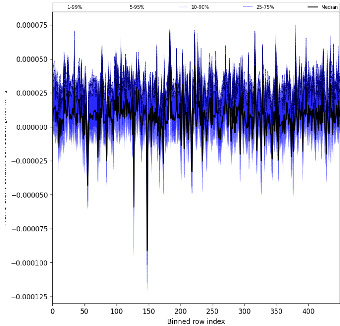
Figure 61: Along track statistics of “HCHO slant column correction” for 2024-09-12 to 2024-09-14
