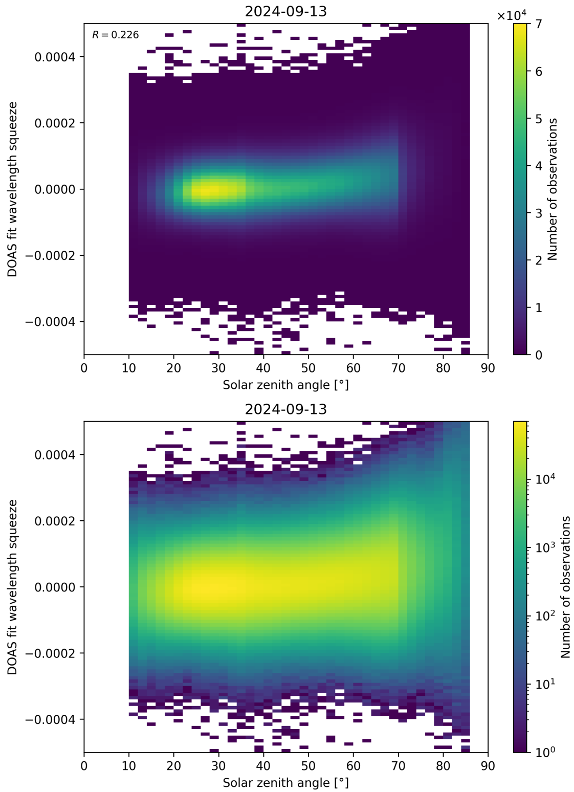
Figure 169: Scatter density plot of “Solar zenith angle” against “DOAS fit wavelength squeeze” for 2024-09-12 to 2024-09-14.
