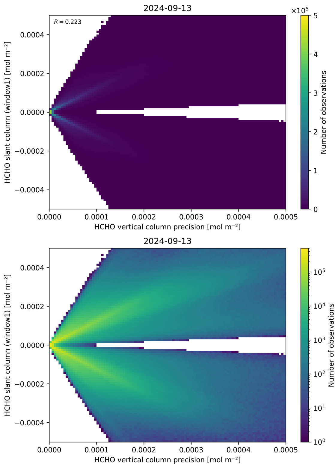
Figure 142: Scatter density plot of “HCHO vertical column precision” against “HCHO slant column (window1)” for 2024-09-12 to 2024-09-14.
