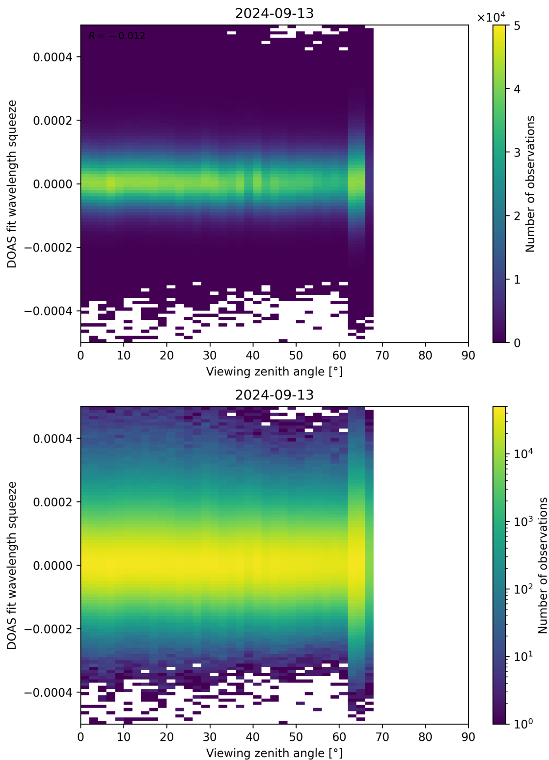
Figure 184: Scatter density plot of “Viewing zenith angle” against “DOAS fit wavelength squeeze” for 2024-09-12 to 2024-09-14.
