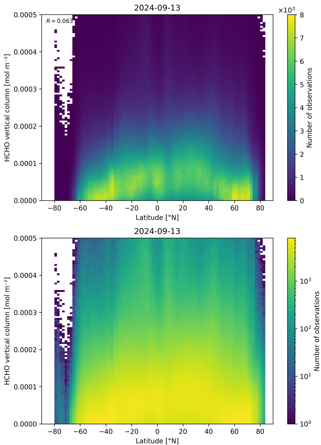
Figure 163: Scatter density plot of “Latitude” against “HCHO vertical column” for 2024-09-12 to 2024-09-14.
