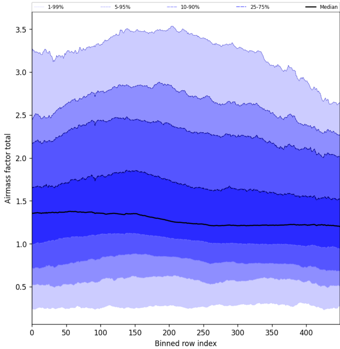
Figure 54: Along track statistics of “Airmass factor total” for 2024-09-12 to 2024-09-14
