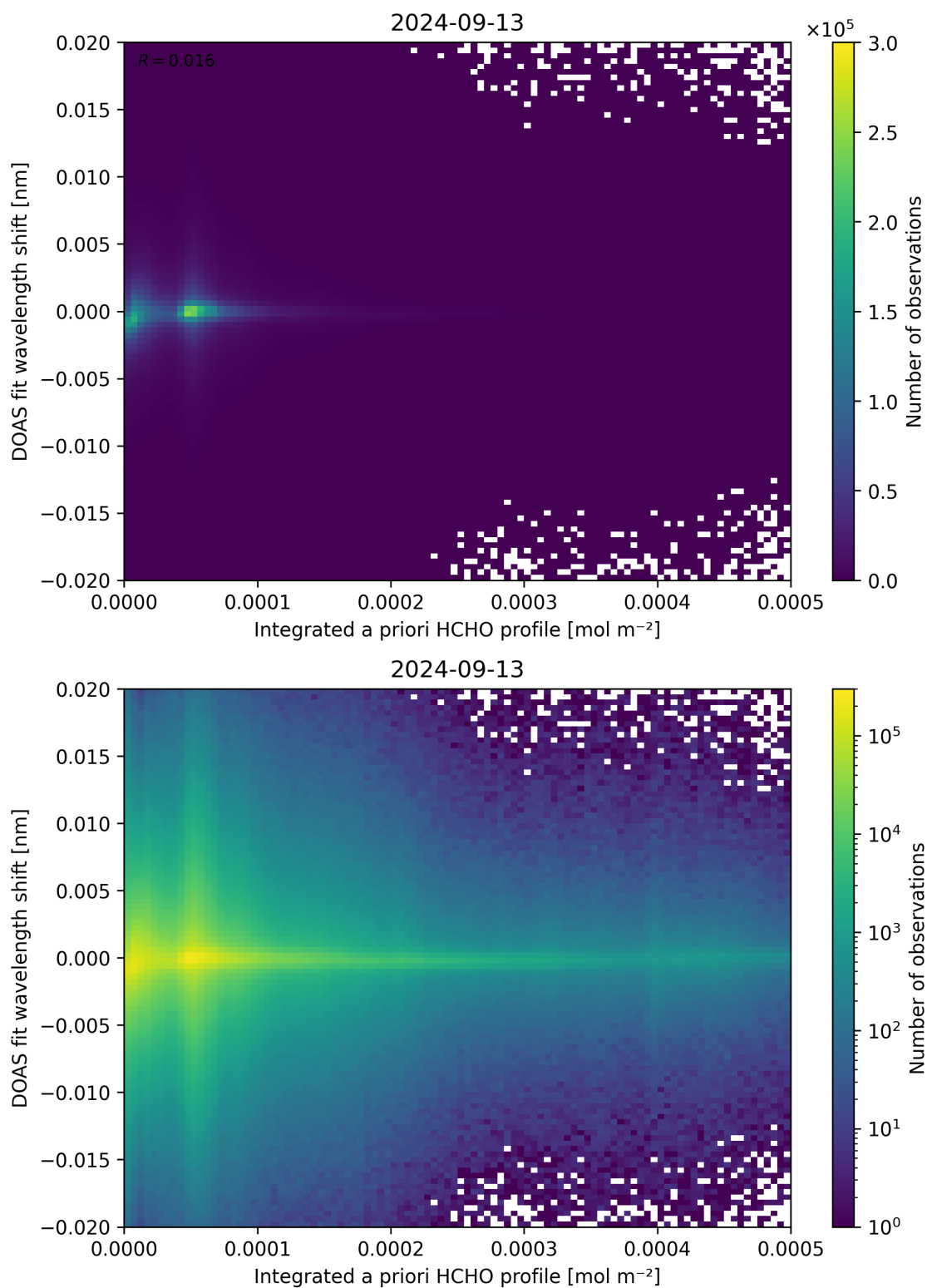
Figure 149: Scatter density plot of “Integrated a priori HCHO profile” against “DOAS fit wavelength shift” for 2024-09-12 to 2024-09-14.
