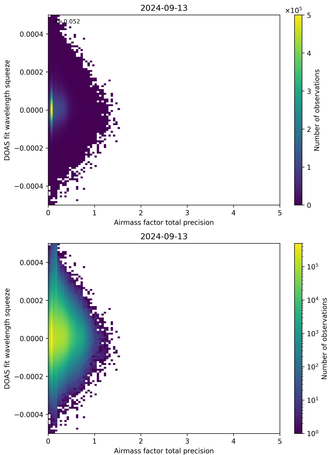
Figure 107: Scatter density plot of “Airmass factor total precision” against “DOAS fit wavelength squeeze” for 2024-09-12 to 2024-09-14.
