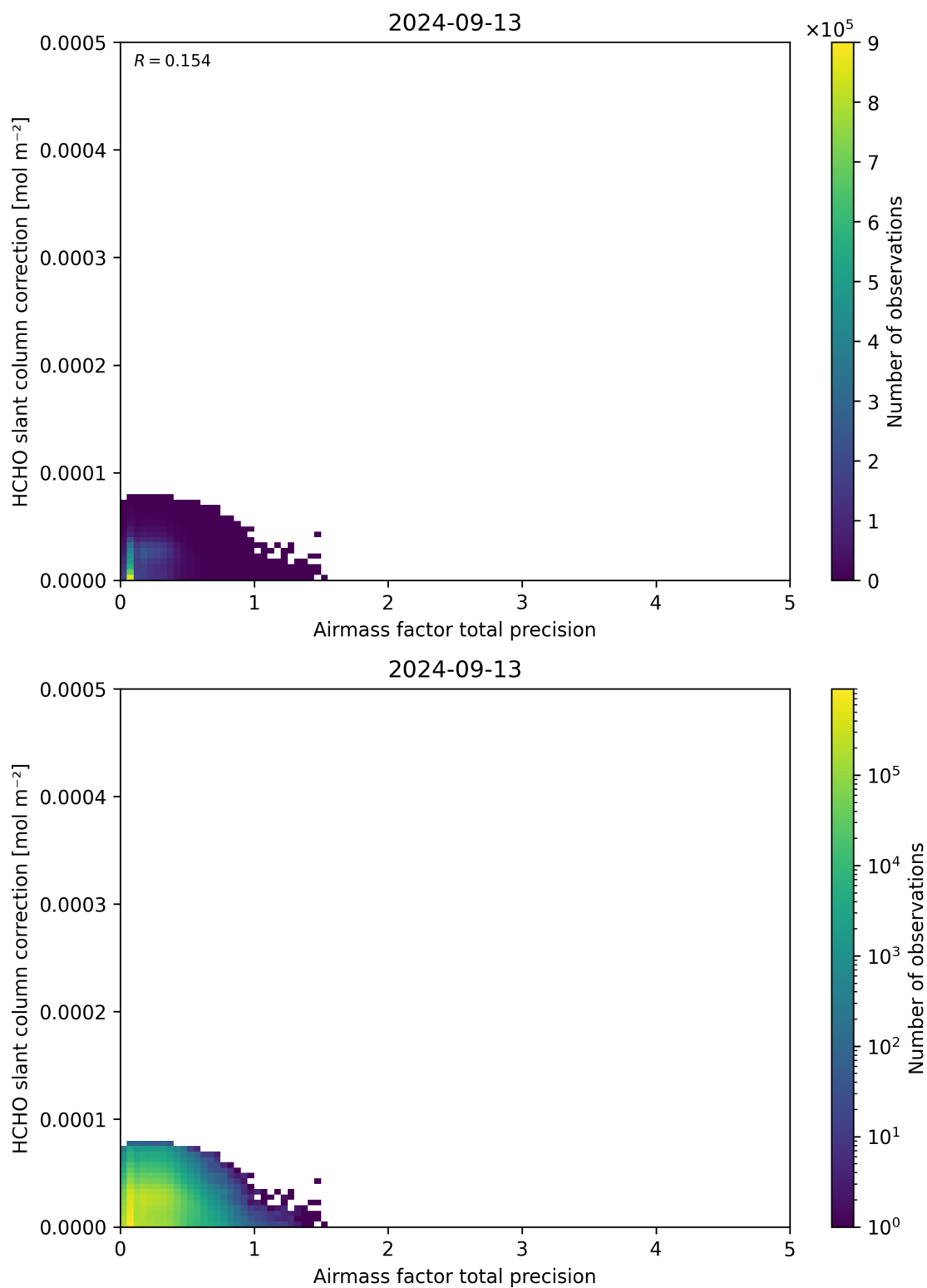
Figure 110: Scatter density plot of “Airmass factor total precision” against “HCHO slant column correction” for 2024-09-12 to 2024-09-14.
