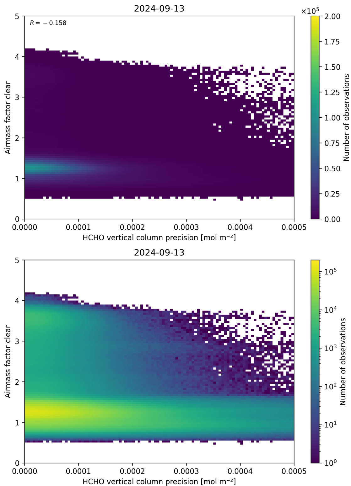
Figure 139: Scatter density plot of “HCHO vertical column precision” against “Airmass factor clear” for 2024-09-12 to 2024-09-14.
