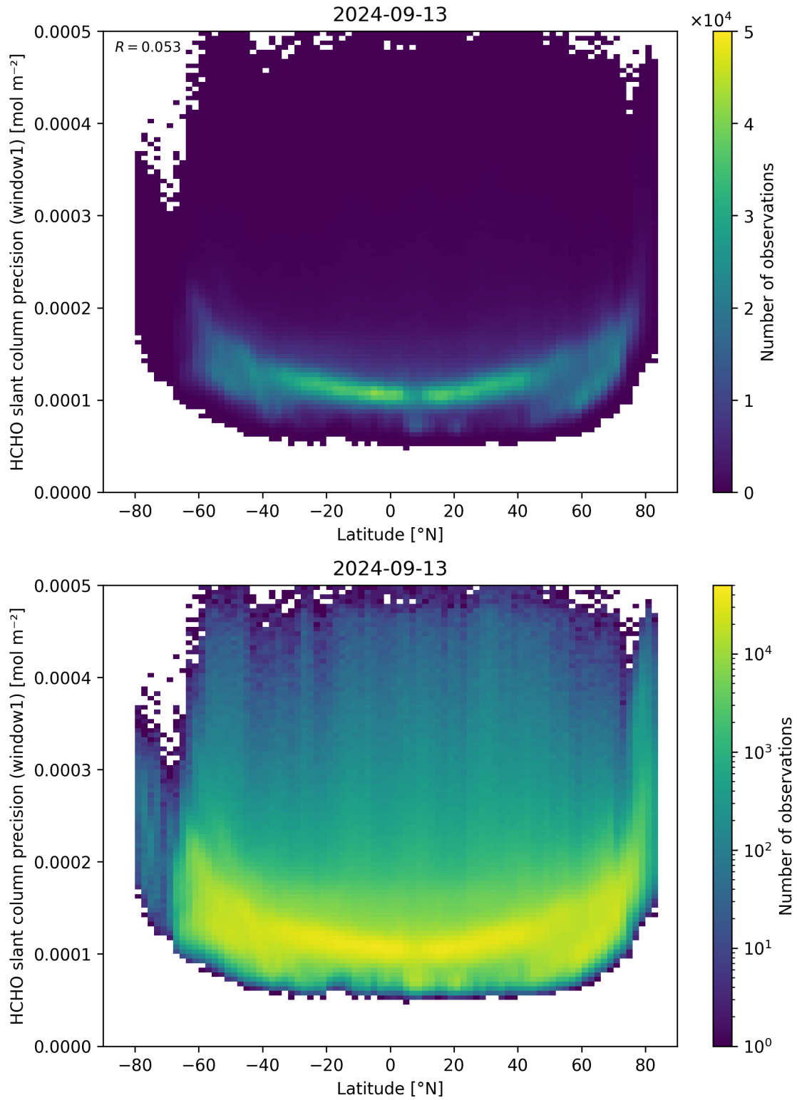
Figure 160: Scatter density plot of “Latitude” against “HCHO slant column precision (window1)” for 2024-09-12 to 2024-09-14.
