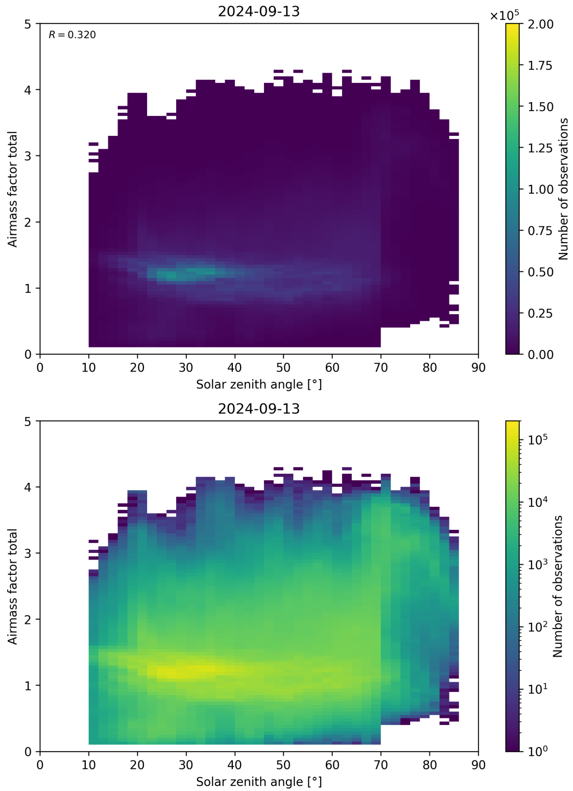
Figure 175: Scatter density plot of “Solar zenith angle” against “Airmass factor total” for 2024-09-12 to 2024-09-14.
