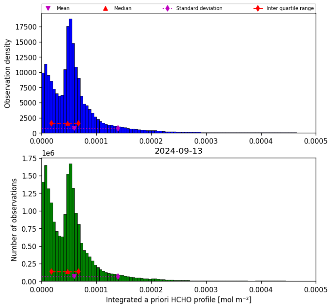
Figure 43: Histogram of “Integrated a priori HCHO profile” for 2024-09-12 to 2024-09-14
