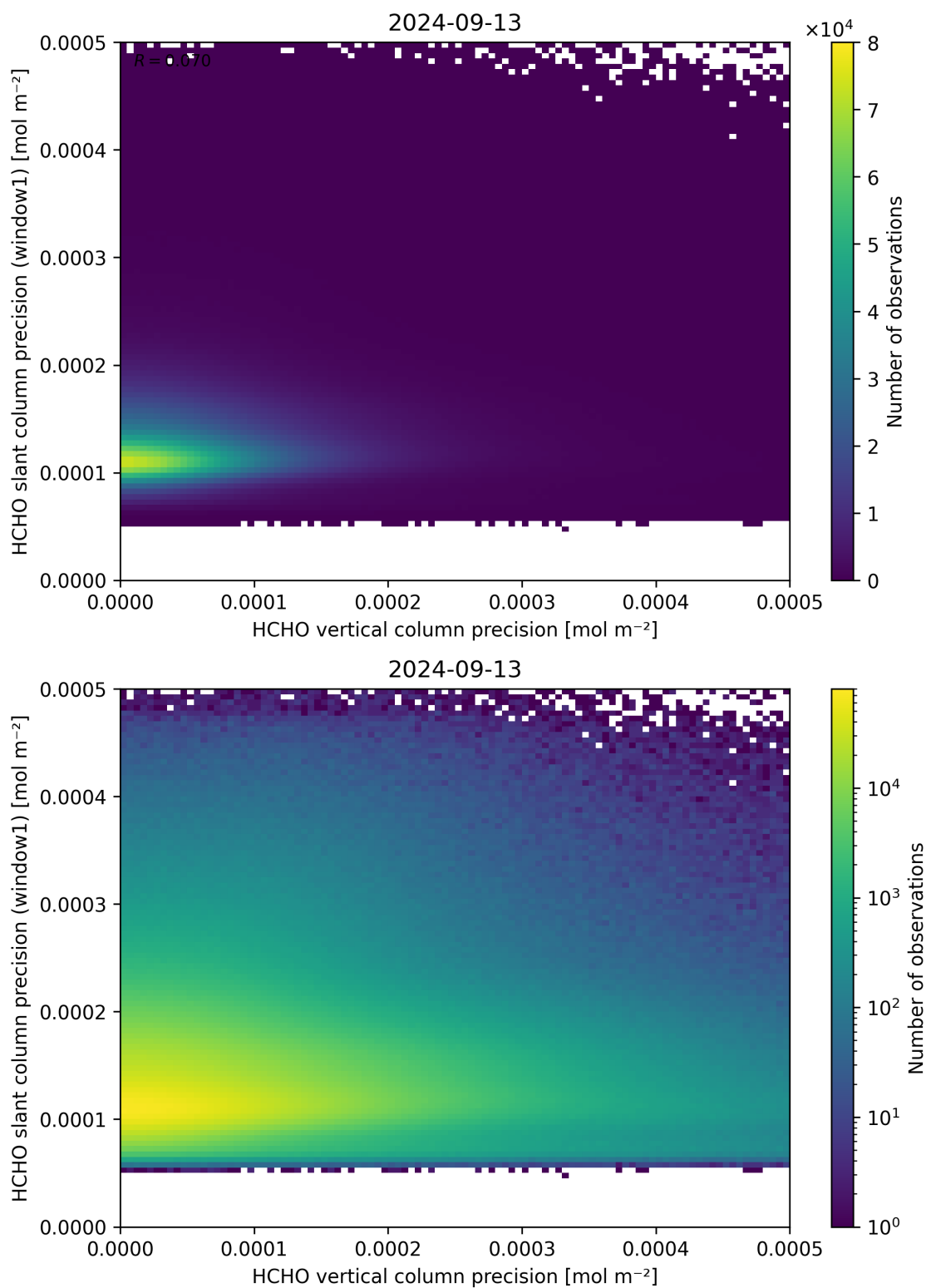
Figure 143: Scatter density plot of “HCHO vertical column precision” against “HCHO slant column precision (window1)” for 2024-09-12 to 2024-09-14.
