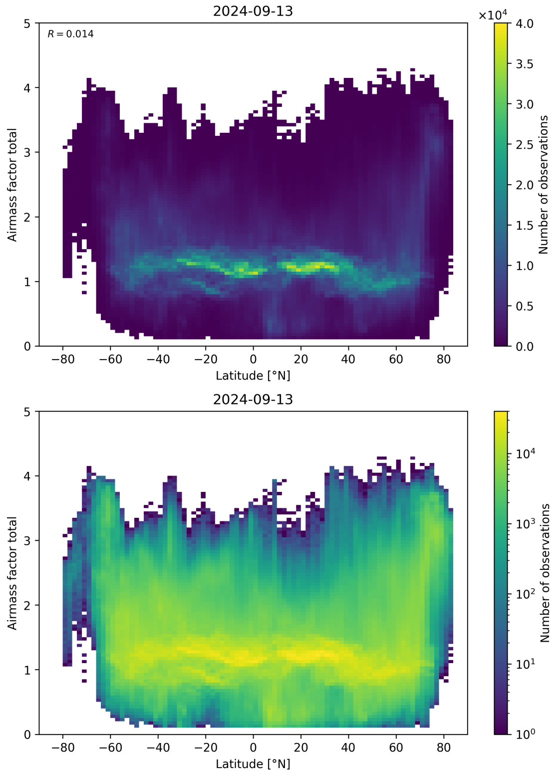
Figure 161: Scatter density plot of “Latitude” against “Airmass factor total” for 2024-09-12 to 2024-09-14.
