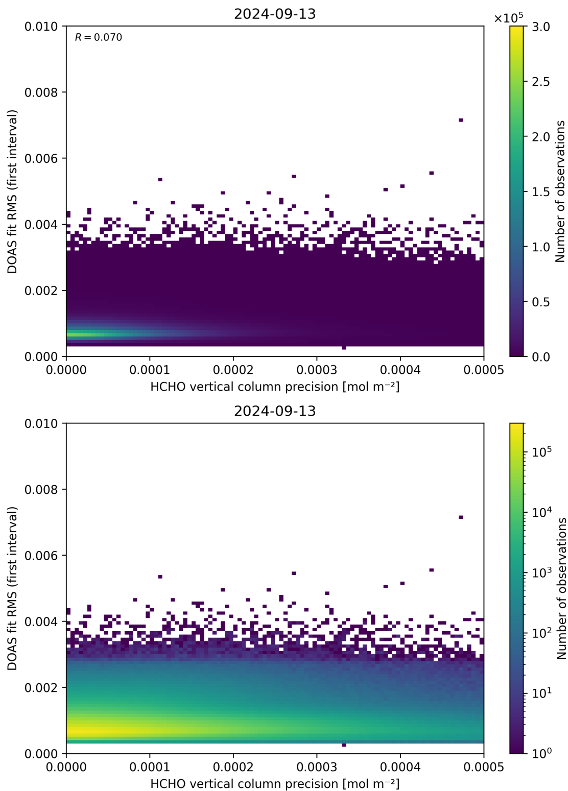
Figure 136: Scatter density plot of “HCHO vertical column precision” against “DOAS fit RMS (first interval)” for 2024-09-12 to 2024-09-14.
