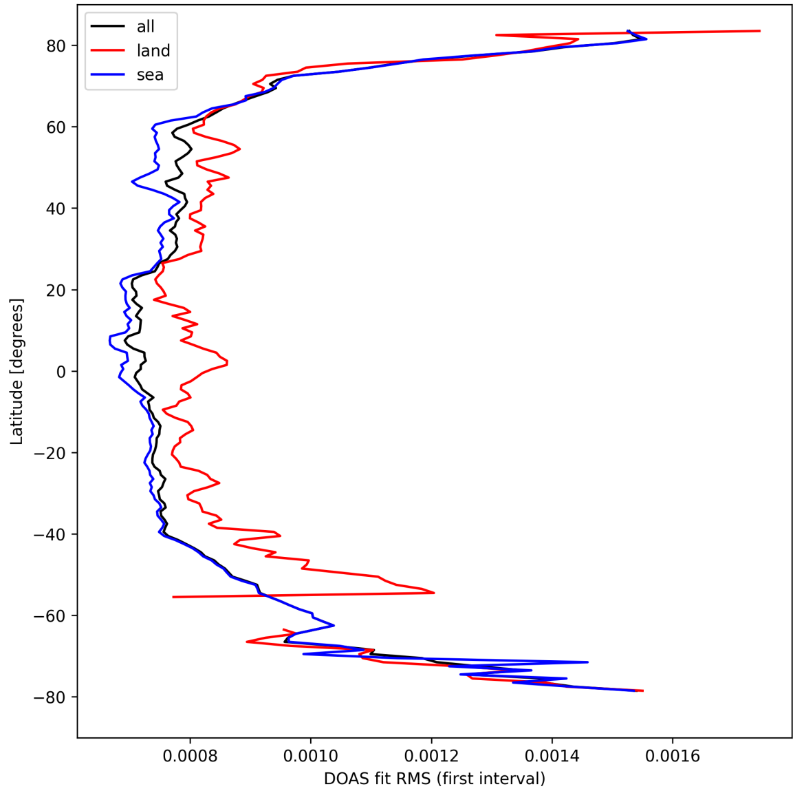
Figure 32: Zonal average of "DOAS fit RMS (first interval)" for 2024-09-12 to 2024-09-14.
