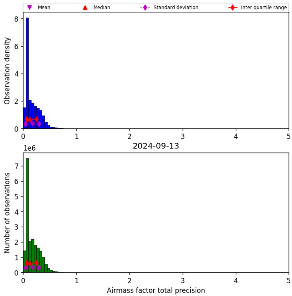
Figure 41: Histogram of “Airmass factor total precision” for 2024-09-12 to 2024-09-14
