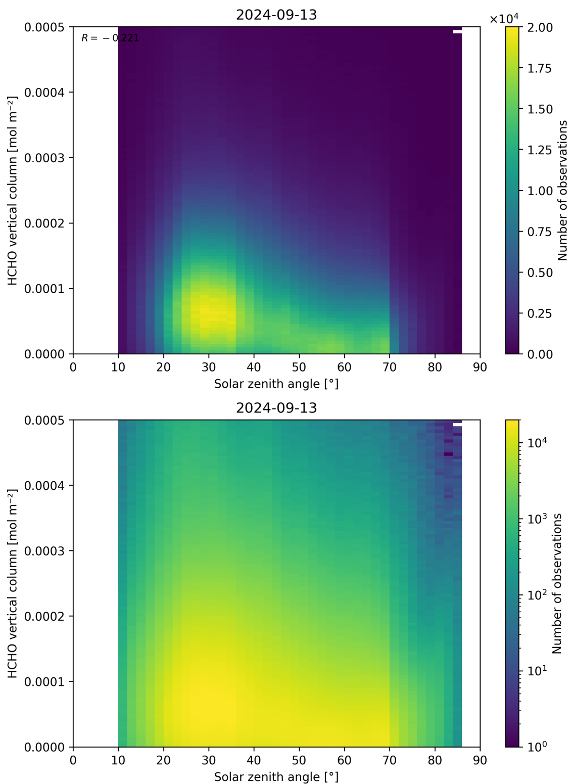
Figure 177: Scatter density plot of “Solar zenith angle” against “HCHO vertical column” for 2024-09-12 to 2024-09-14.
