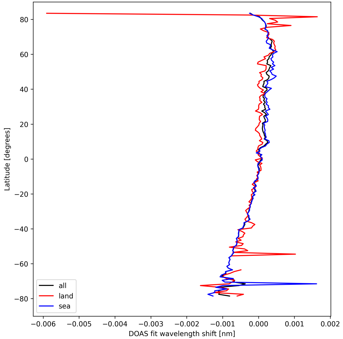
Figure 30: Zonal average of “DOAS fit wavelength shift” for 2024-09-12 to 2024-09-14.
