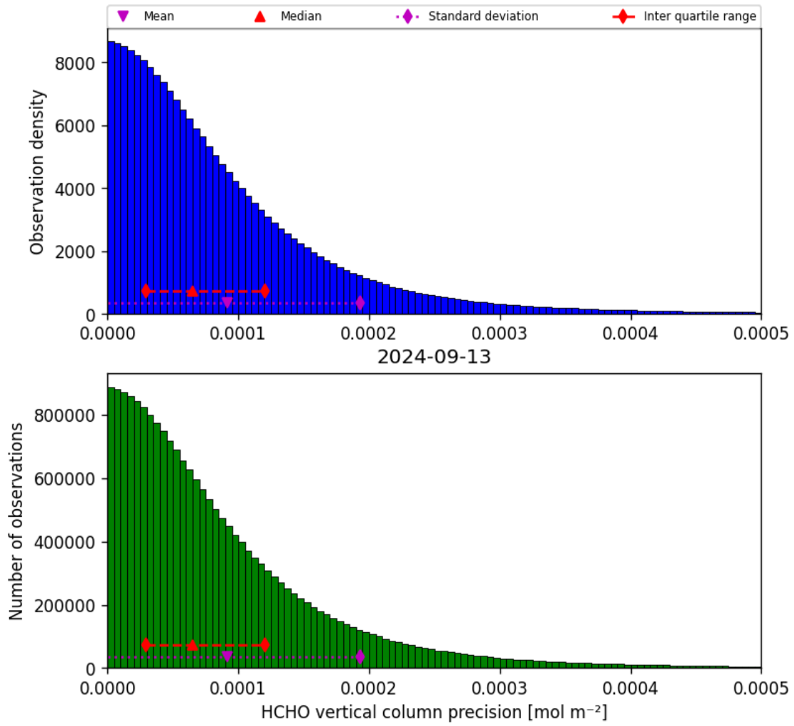
Figure 36: Histogram of “HCHO vertical column precision” for 2024-09-12 to 2024-09-14
