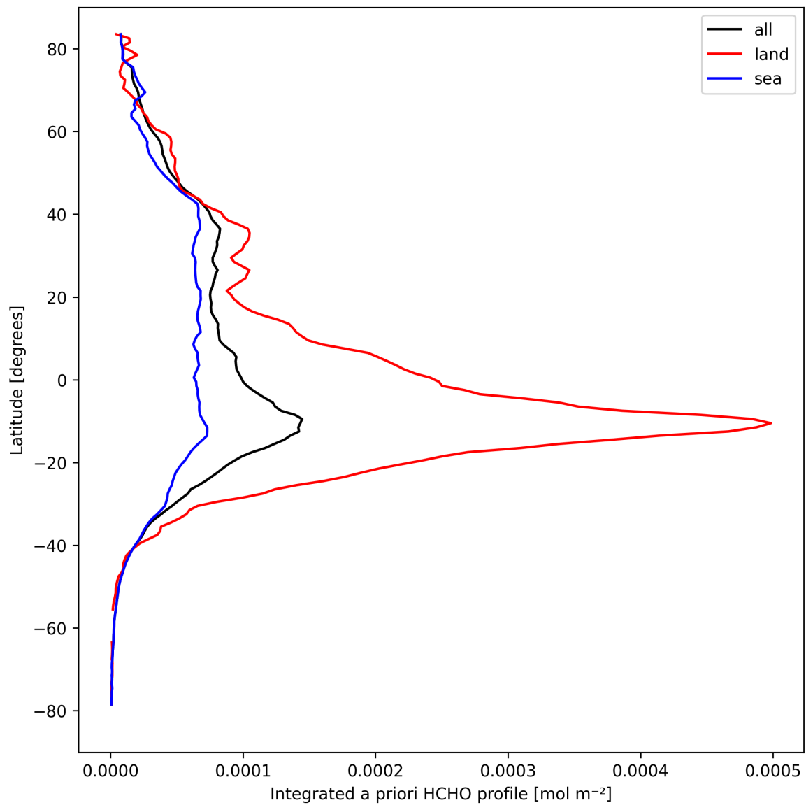
Figure 29: Zonal average of “Integrated a priori HCHO profile” for 2024-09-12 to 2024-09-14.
