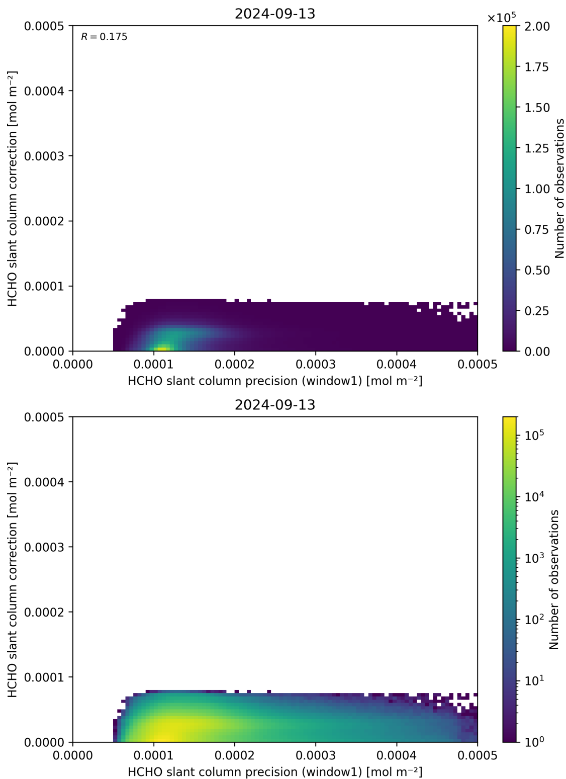
Figure 93: Scatter density plot of “HCHO slant column precision (window1)” against “HCHO slant column correction” for 2024-09-12 to 2024-09-14.
