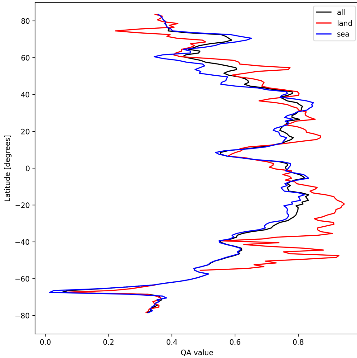
Figure 20: Zonal average of “QA value” for 2024-09-12 to 2024-09-14.
