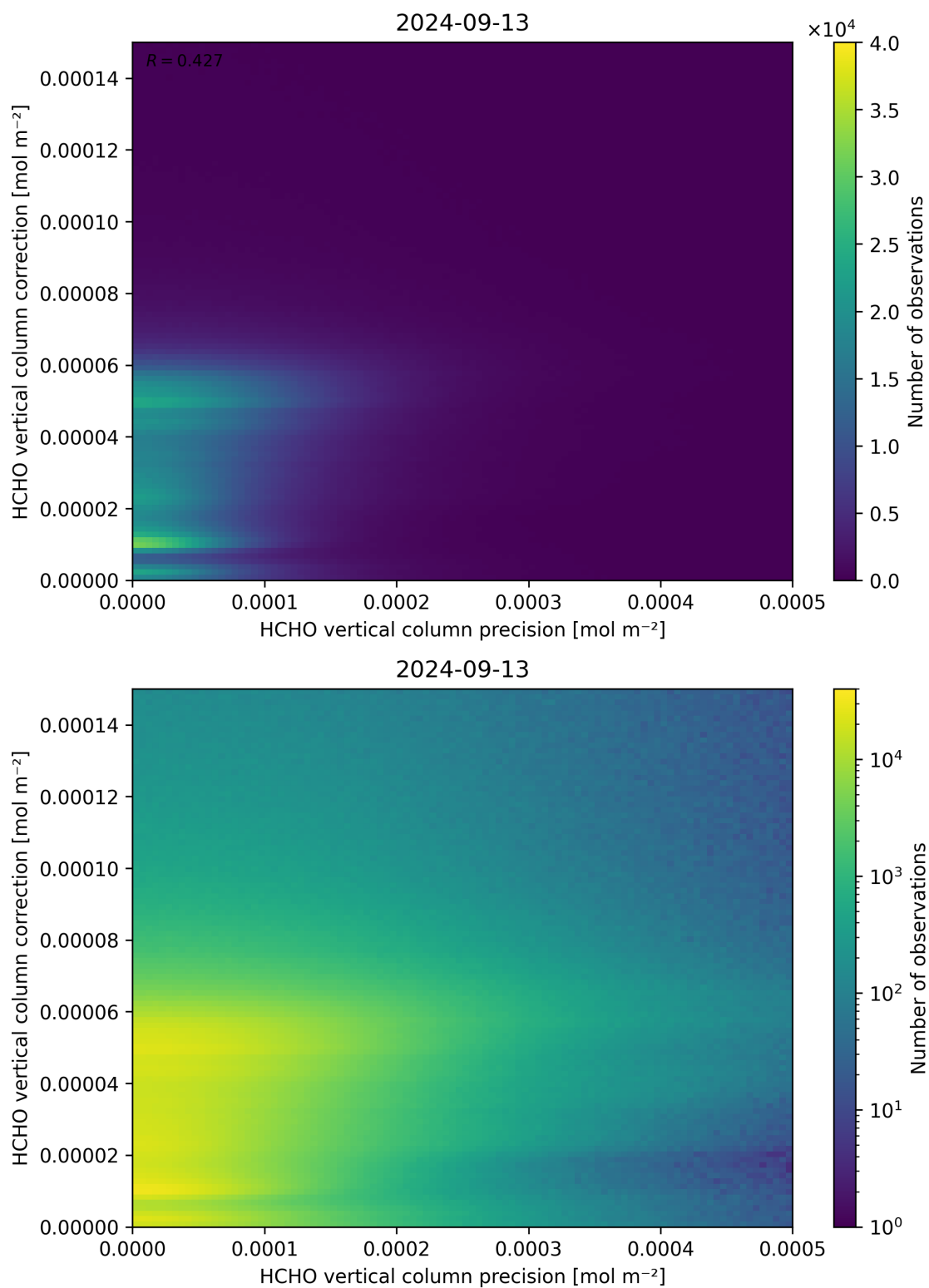
Figure 146: Scatter density plot of “HCHO vertical column precision” against “HCHO vertical column correction” for 2024-09-12 to 2024-09-14.
