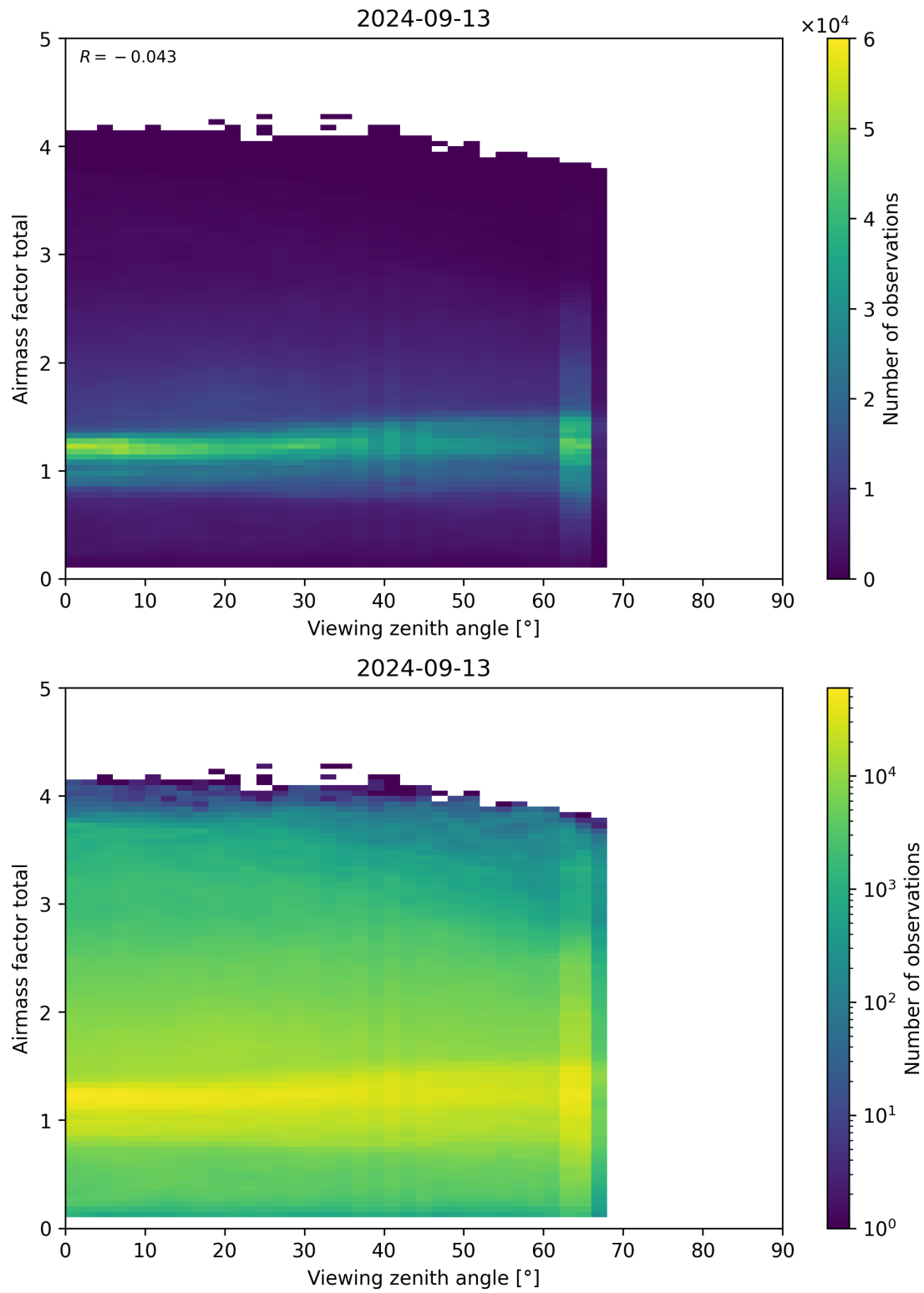
Figure 190: Scatter density plot of “Viewing zenith angle” against “Airmass factor total” for 2024-09-12 to 2024-09-14.
