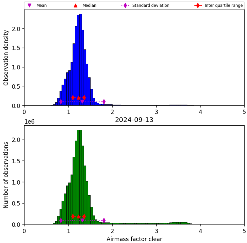
Figure 42: Histogram of “Airmass factor clear” for 2024-09-12 to 2024-09-14
