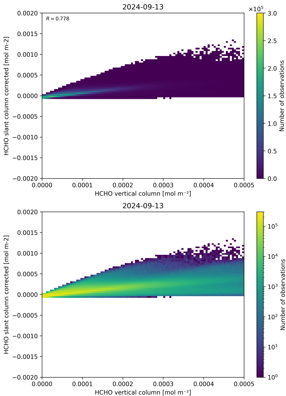
Figure 127: Scatter density plot of “HCHO vertical column” against “HCHO slant column corrected” for 2024-09-12 to 2024-09-14.
