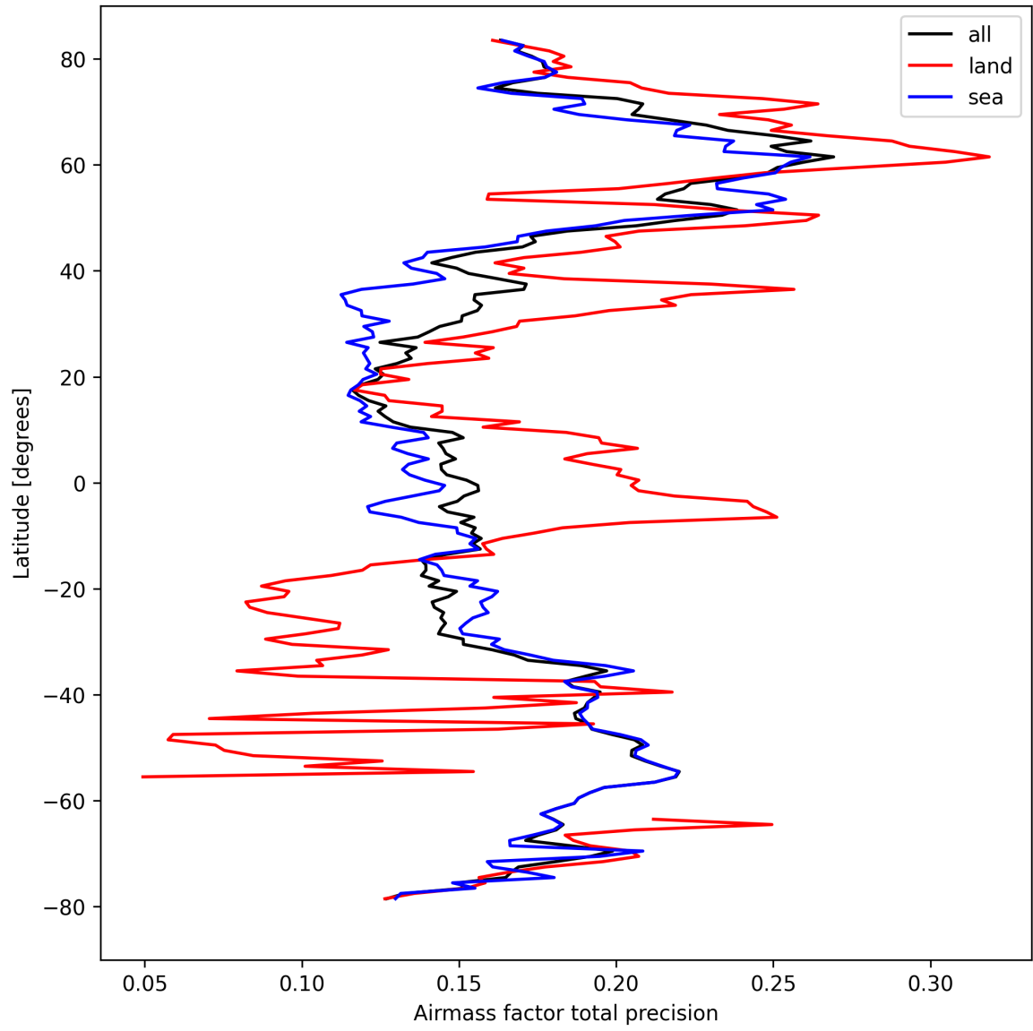
Figure 27: Zonal average of “Airmass factor total precision” for 2024-09-12 to 2024-09-14.
