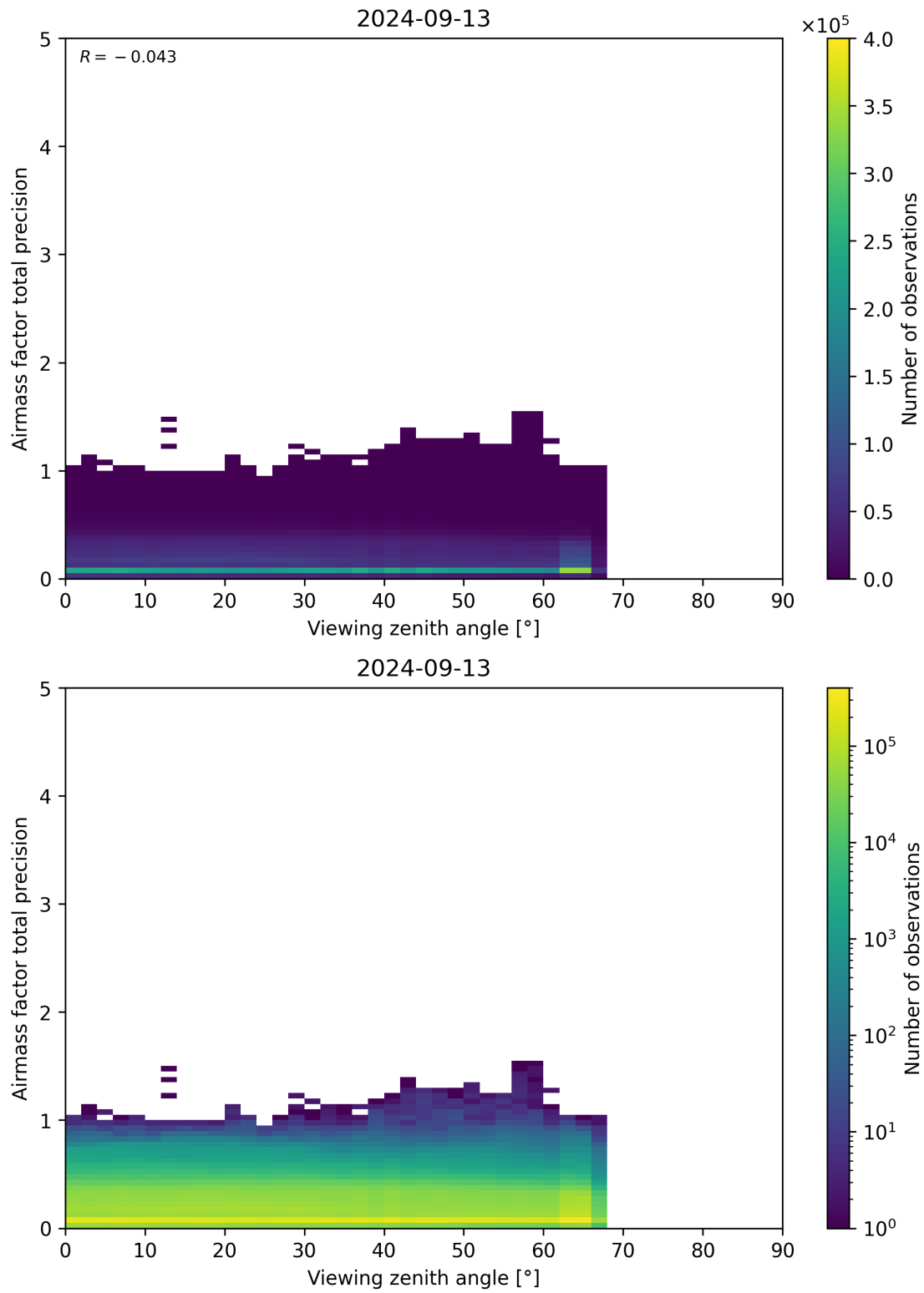
Figure 191: Scatter density plot of “Viewing zenith angle” against “Airmass factor total precision” for 2024-09-12 to 2024-09-14.
