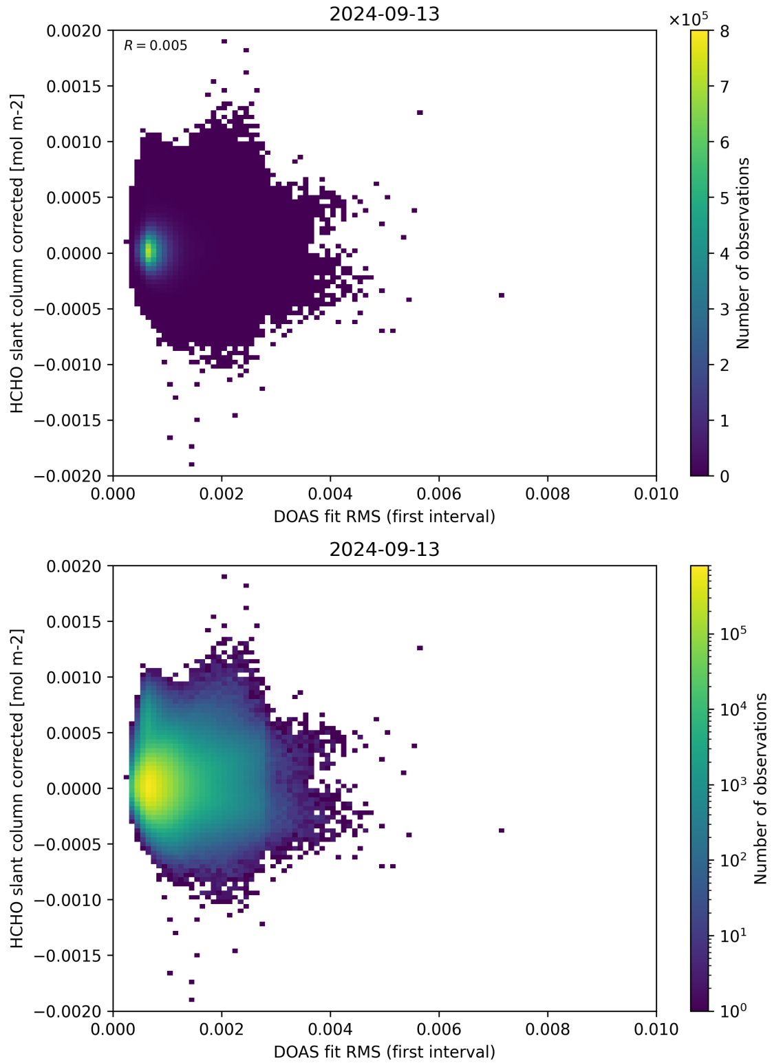
Figure 62: Scatter density plot of “DOAS fit RMS (first interval)” against “HCHO slant column corrected” for 2024-09-12 to 2024-09-14.
