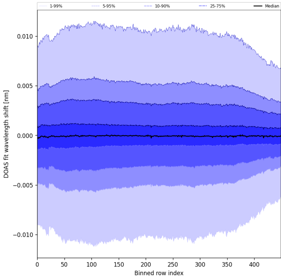
Figure 58: Along track statistics of “DOAS fit wavelength shift” for 2024-09-12 to 2024-09-14
