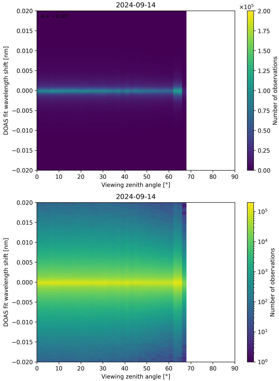
Figure 183: Scatter density plot of “Viewing zenith angle” against “DOAS fit wavelength shift” for 2024-09-13 to 2024-09-15.
