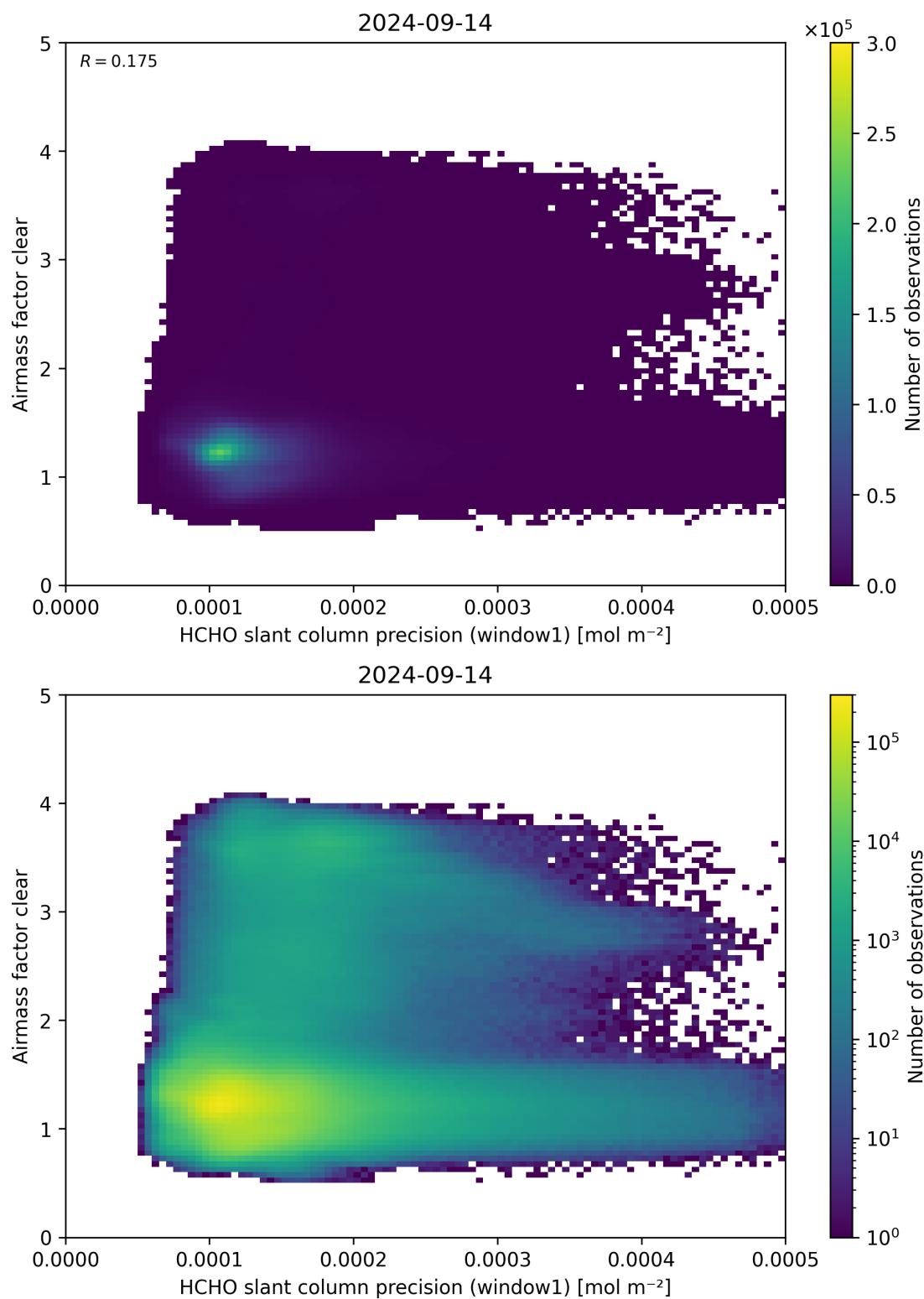
Figure 91: Scatter density plot of “HCHO slant column precision (window1)” against “Airmass factor clear” for 2024-09-13 to 2024-09-15.
