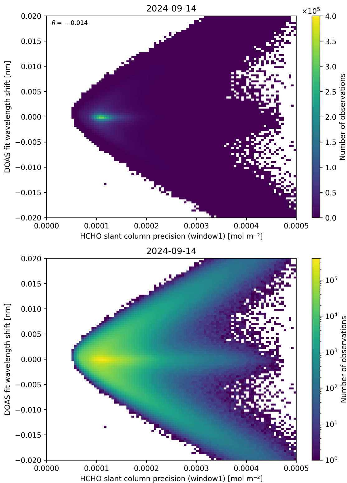
Figure 89: Scatter density plot of “HCHO slant column precision (window1)” against “DOAS fit wavelength shift” for 2024-09-13 to 2024-09-15.
