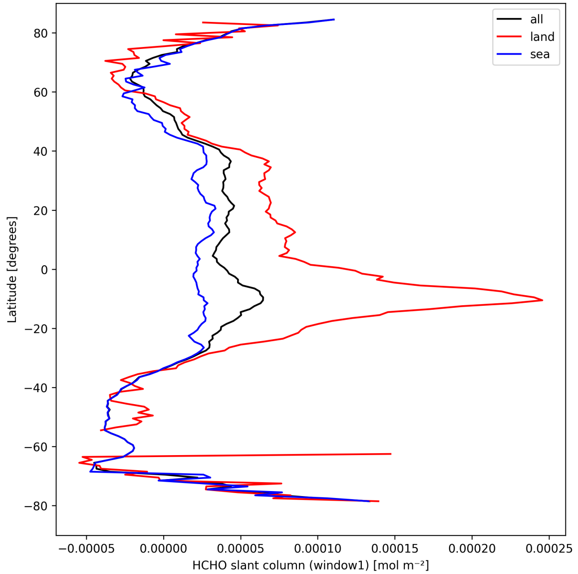
Figure 24: Zonal average of “HCHO slant column (window1)” for 2024-09-13 to 2024-09-15.
