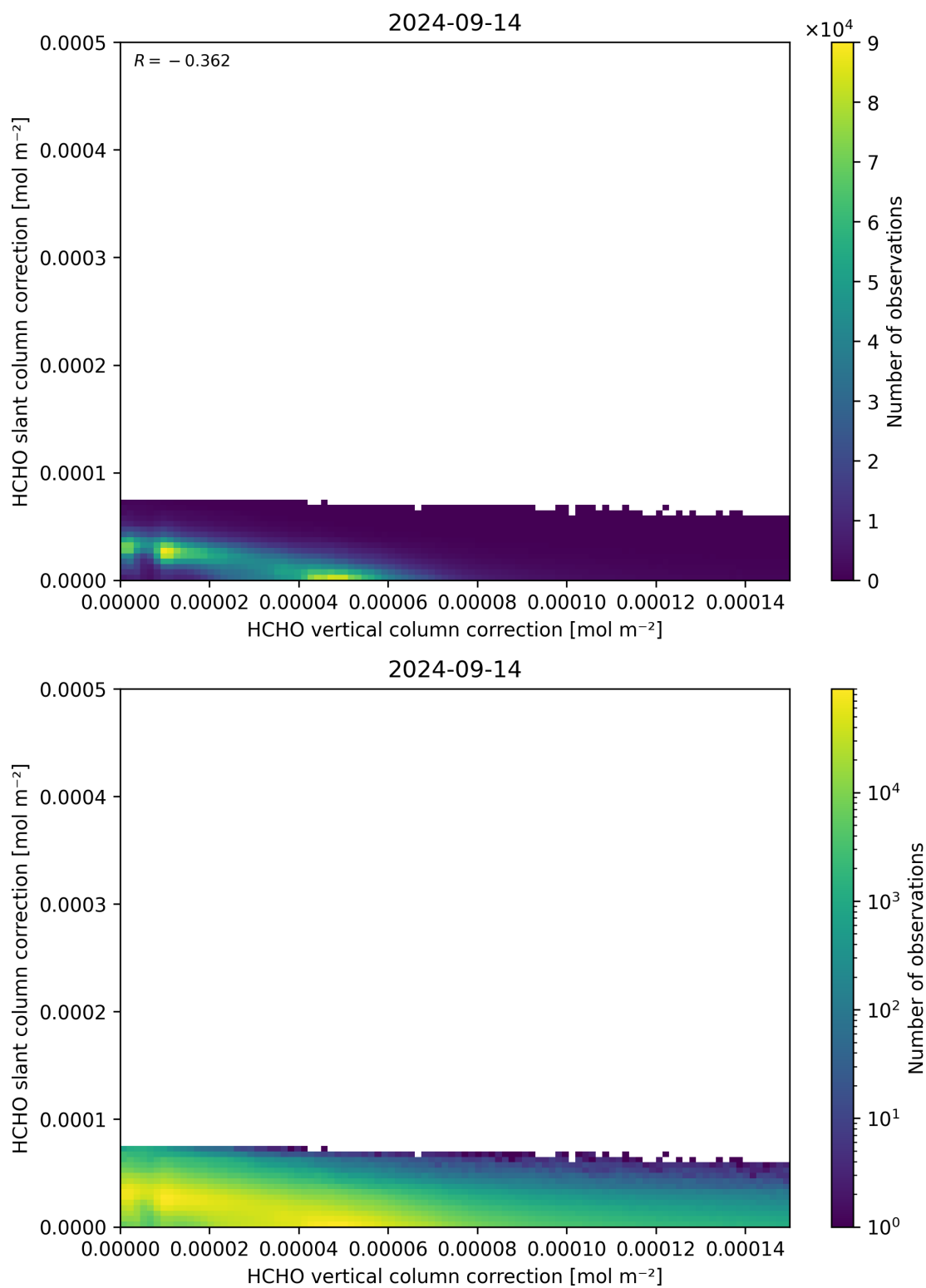
Figure 117: Scatter density plot of “HCHO vertical column correction” against “HCHO slant column correction” for 2024-09-13 to 2024-09-15.
