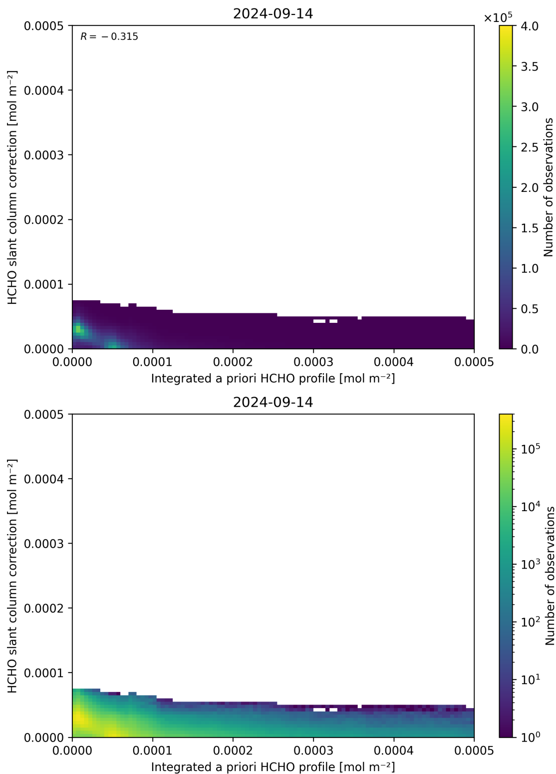
Figure 152: Scatter density plot of “Integrated a priori HCHO profile” against “HCHO slant column correction” for 2024-09-13 to 2024-09-15.
