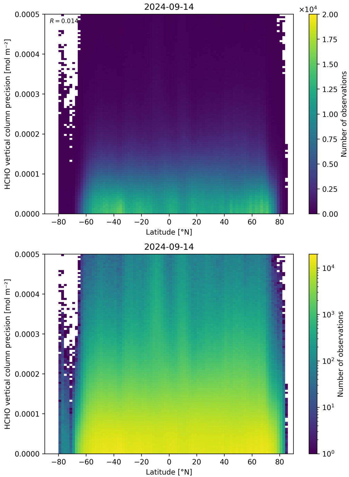
Figure 165: Scatter density plot of “Latitude” against “HCHO vertical column precision” for 2024-09-13 to 2024-09-15.
