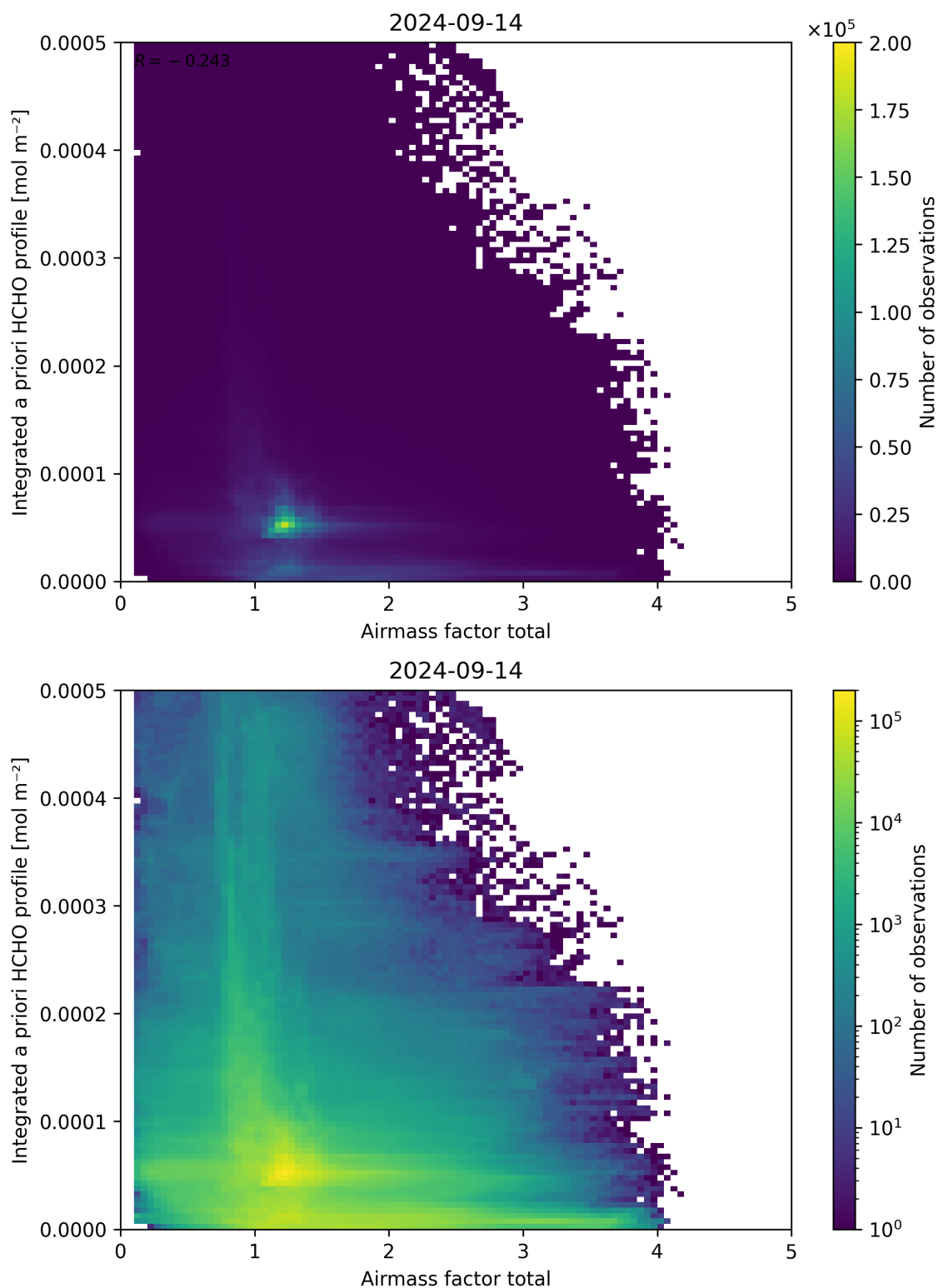
Figure 104: Scatter density plot of “Airmass factor total” against “Integrated a priori HCHO profile” for 2024-09-13 to 2024-09-15.
