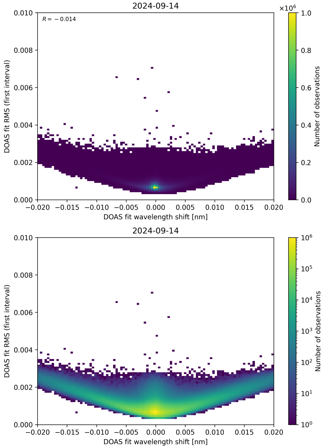
Figure 64: Scatter density plot of “DOAS fit wavelength shift” against “DOAS fit RMS (first interval)” for 2024-09-13 to 2024-09-15.
