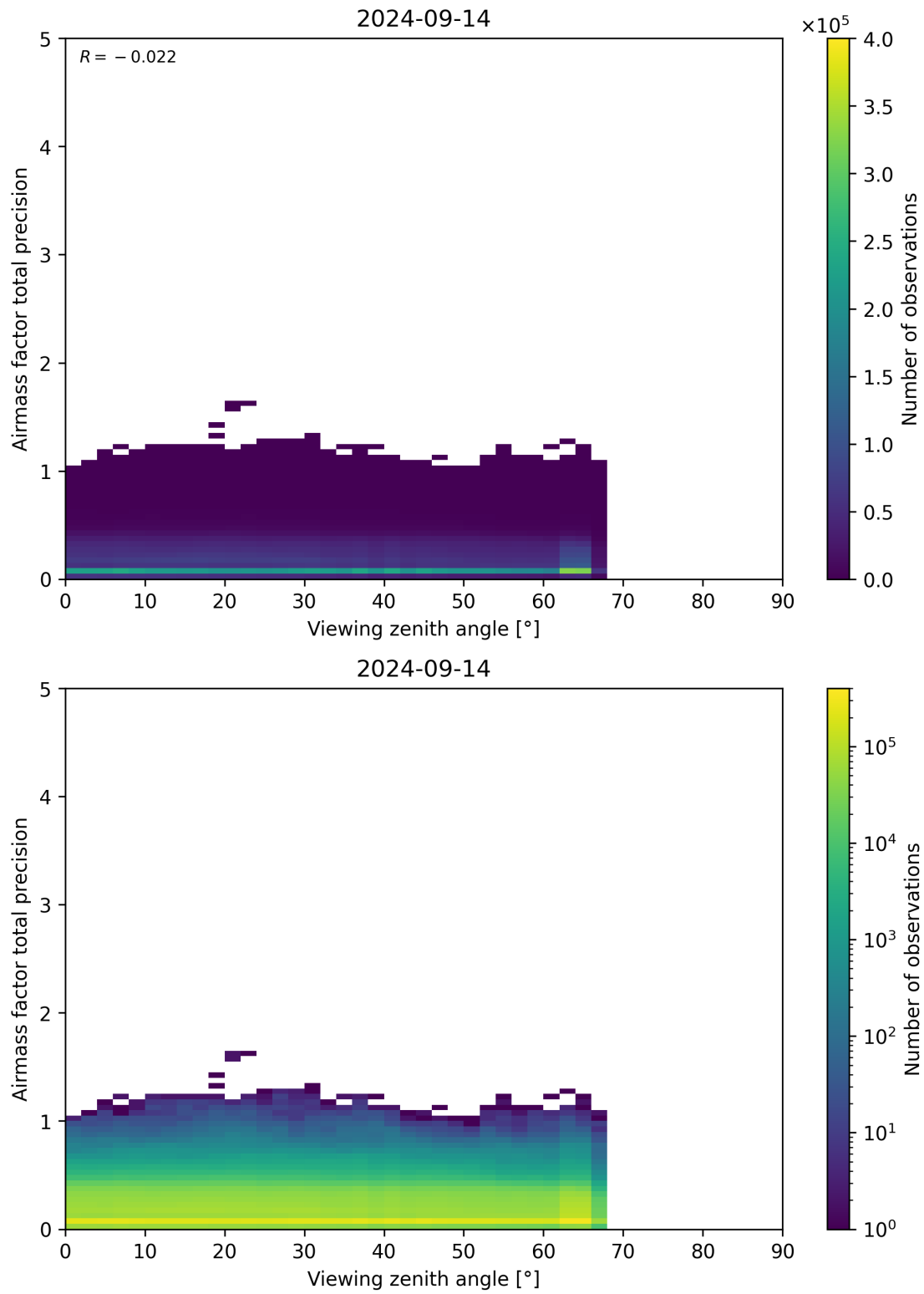
Figure 191: Scatter density plot of “Viewing zenith angle” against “Airmass factor total precision” for 2024-09-13 to 2024-09-15.
