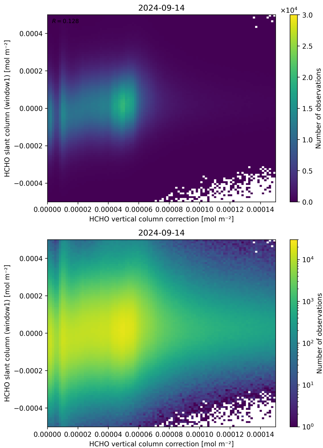
Figure 118: Scatter density plot of “HCHO vertical column correction” against “HCHO slant column (window1)” for 2024-09-13 to 2024-09-15.
