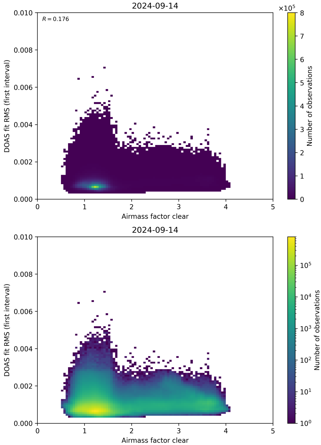
Figure 71: Scatter density plot of “Airmass factor clear” against “DOAS fit RMS (first interval)” for 2024-09-13 to 2024-09-15.
