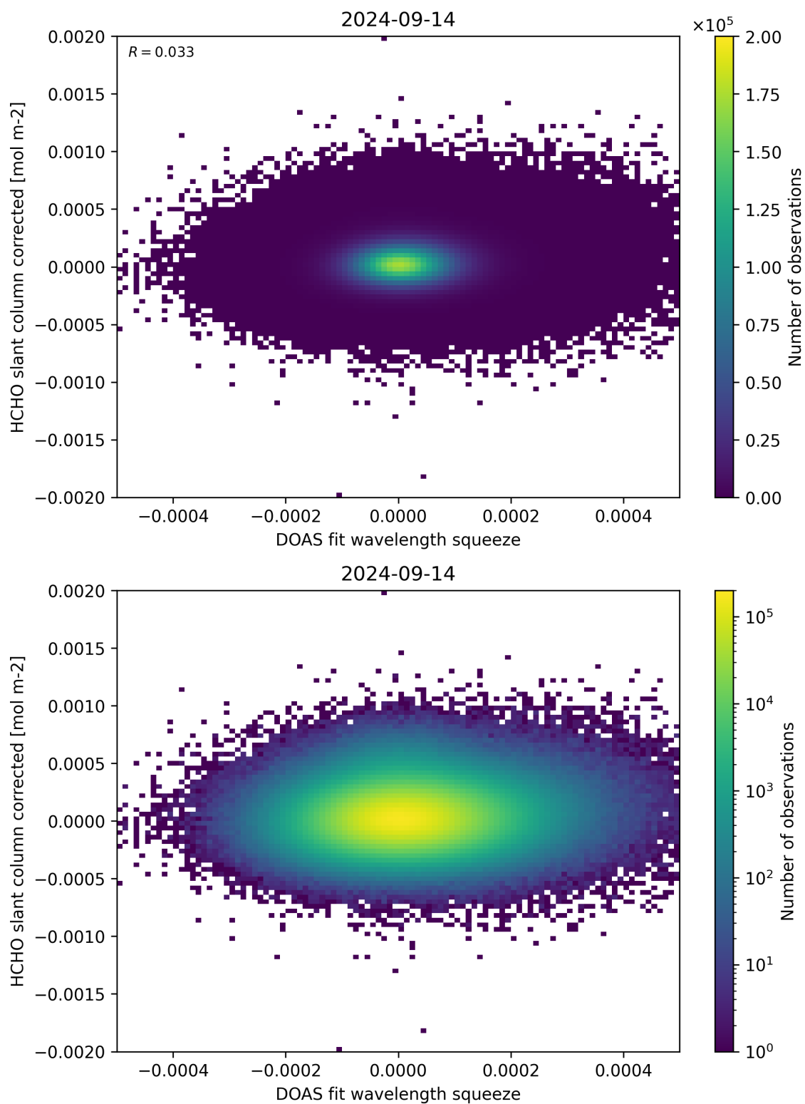
Figure 69: Scatter density plot of “DOAS fit wavelength squeeze” against “HCHO slant column corrected” for 2024-09-13 to 2024-09-15.
