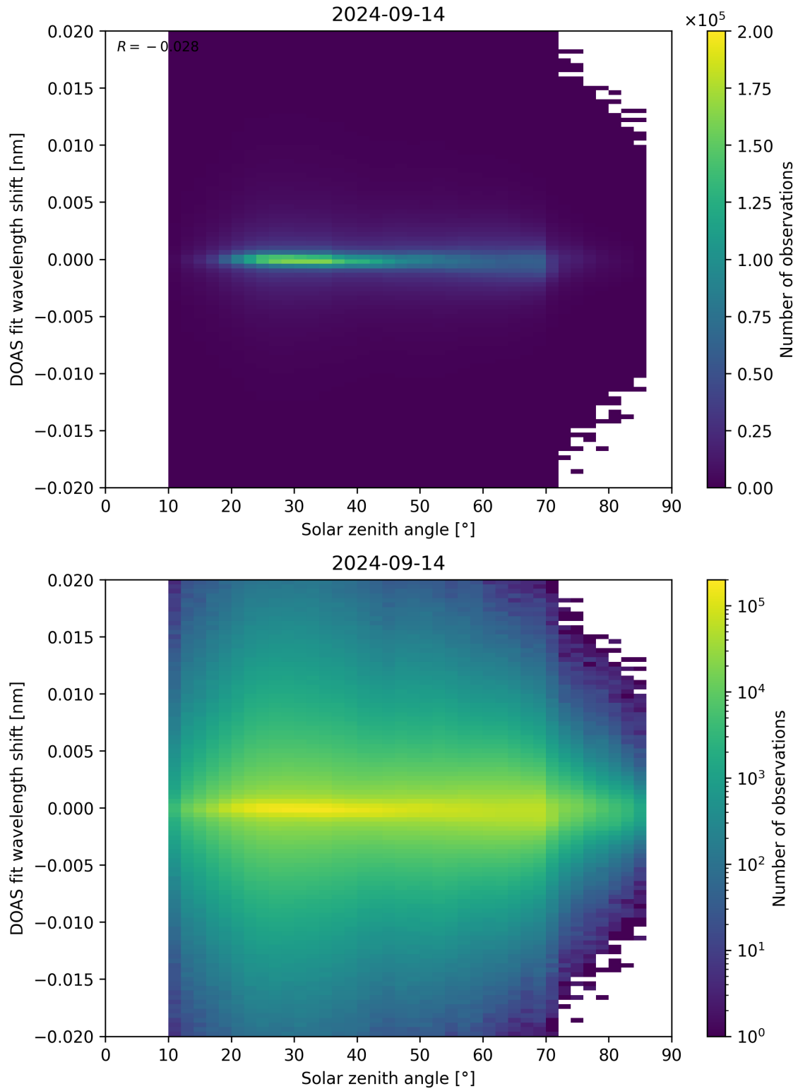
Figure 168: Scatter density plot of “Solar zenith angle” against “DOAS fit wavelength shift” for 2024-09-13 to 2024-09-15.
