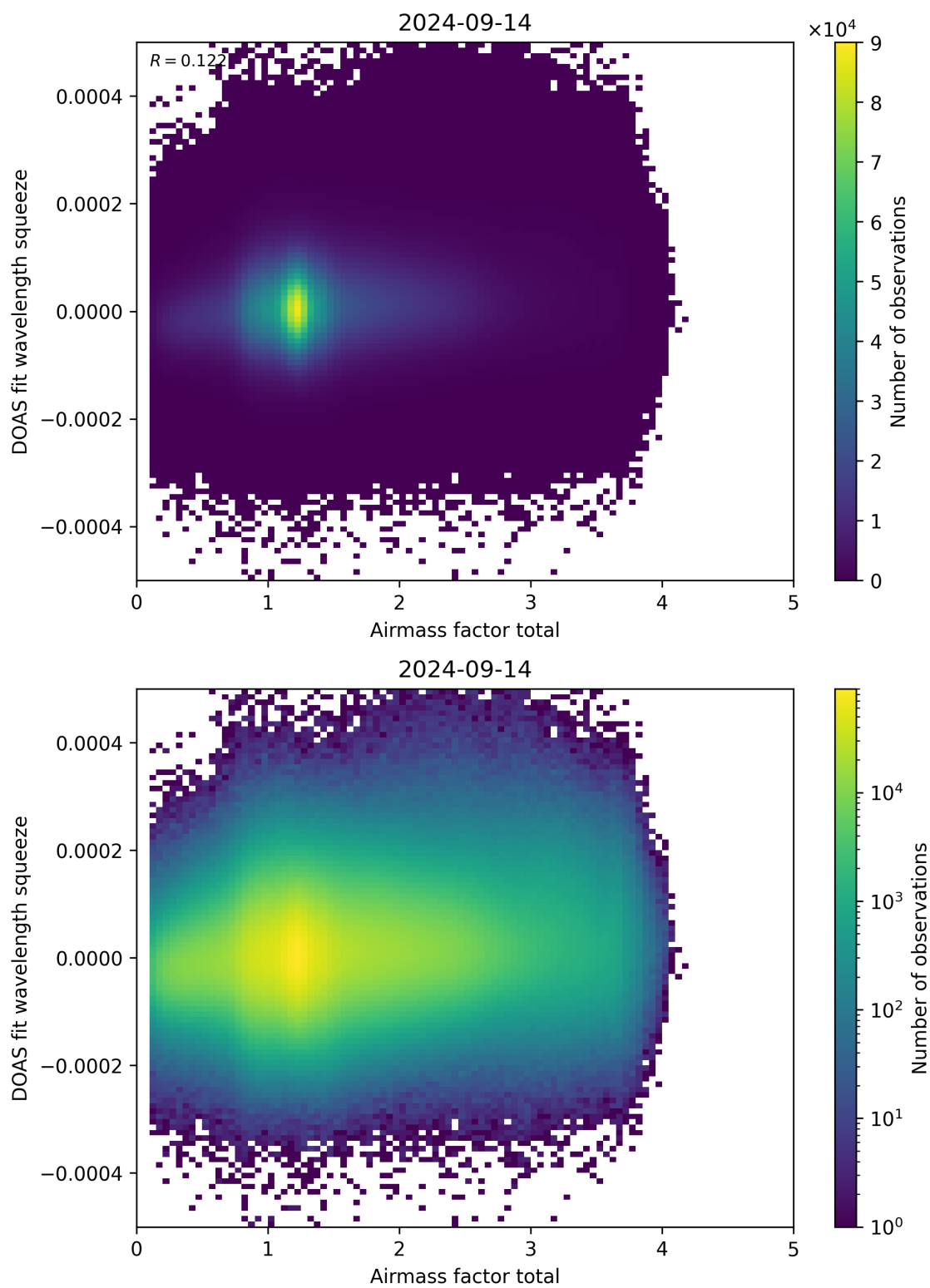
Figure 99: Scatter density plot of “Airmass factor total” against “DOAS fit wavelength squeeze” for 2024-09-13 to 2024-09-15.
