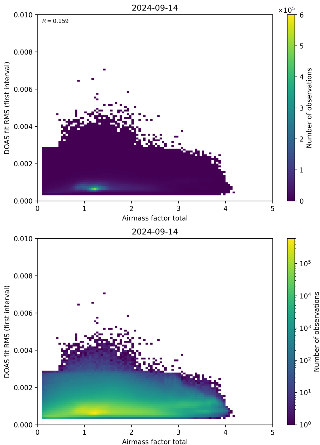
Figure 97: Scatter density plot of “Airmass factor total” against “DOAS fit RMS (first interval)” for 2024-09-13 to 2024-09-15.
