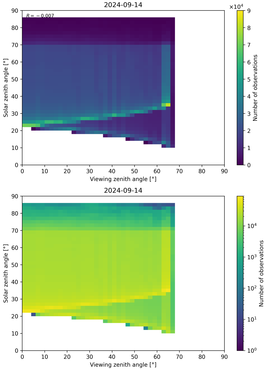
Figure 197: Scatter density plot of “Viewing zenith angle” against “Solar zenith angle” for 2024-09-13 to 2024-09-15.
