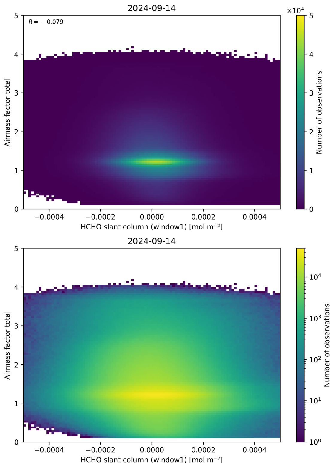
Figure 85: Scatter density plot of “HCHO slant column (window1)” against “Airmass factor total” for 2024-09-13 to 2024-09-15.
