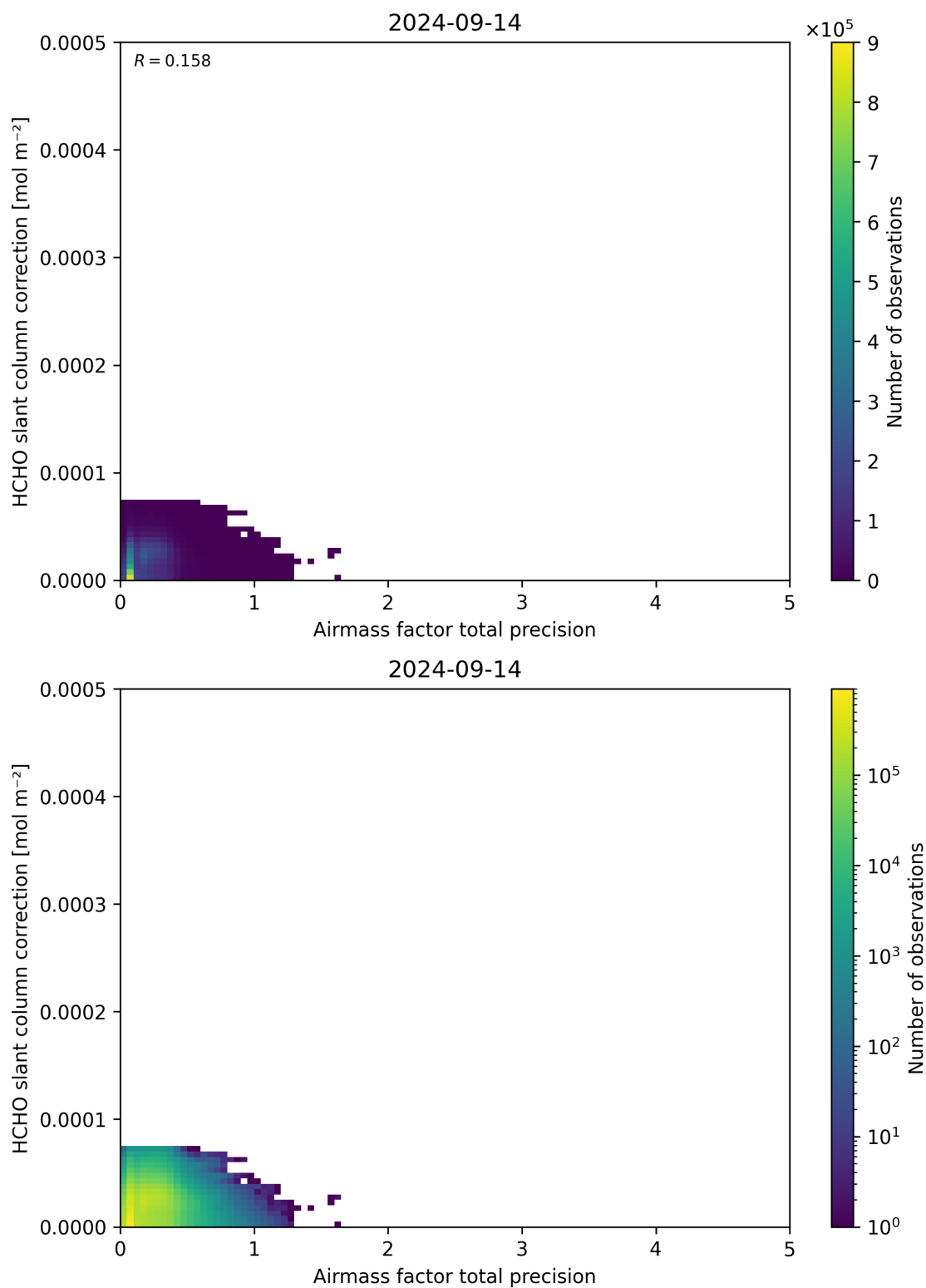
Figure 110: Scatter density plot of “Airmass factor total precision” against “HCHO slant column correction” for 2024-09-13 to 2024-09-15.
