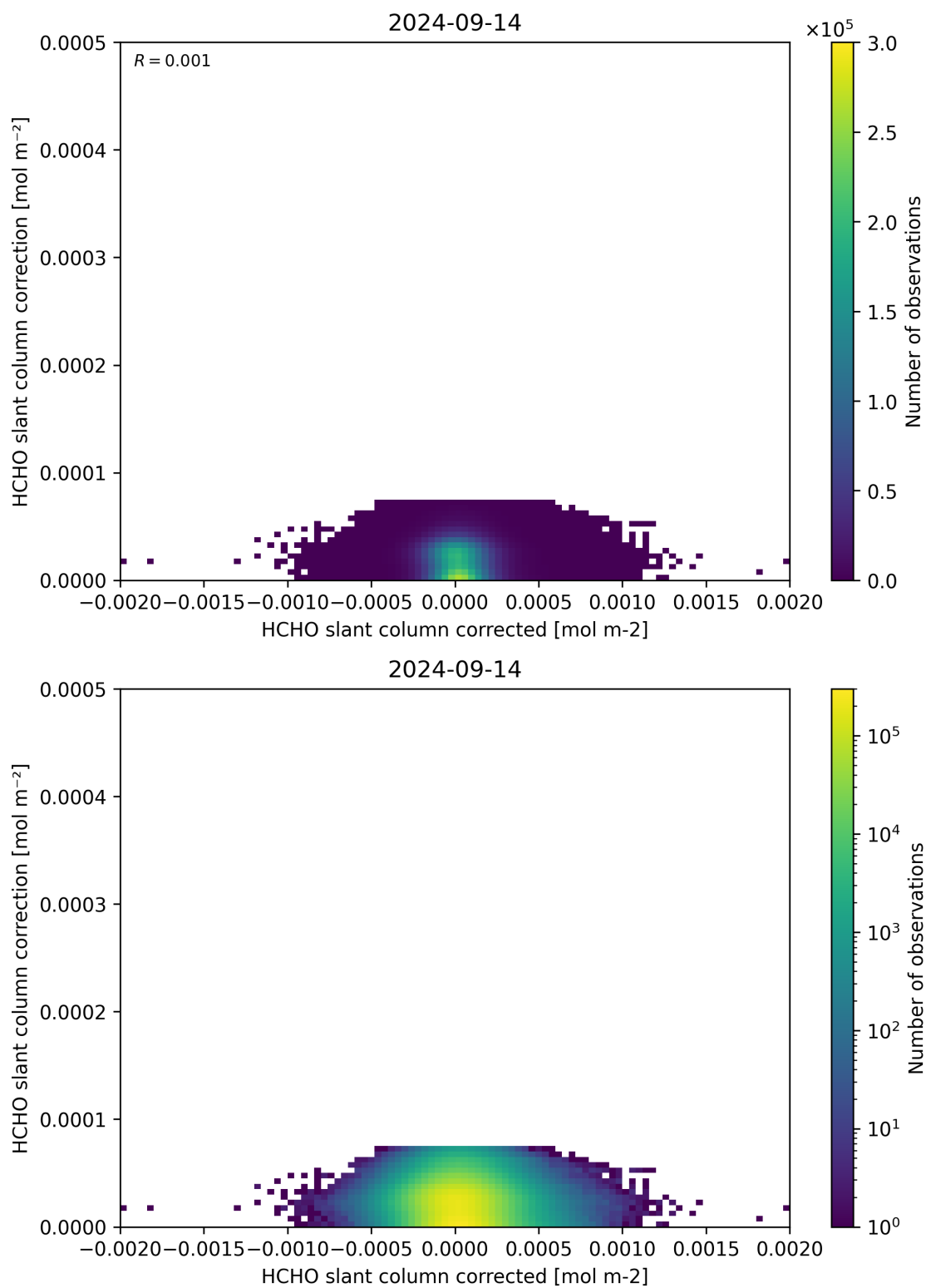
Figure 77: Scatter density plot of “HCHO slant column corrected” against “HCHO slant column correction” for 2024-09-13 to 2024-09-15.
