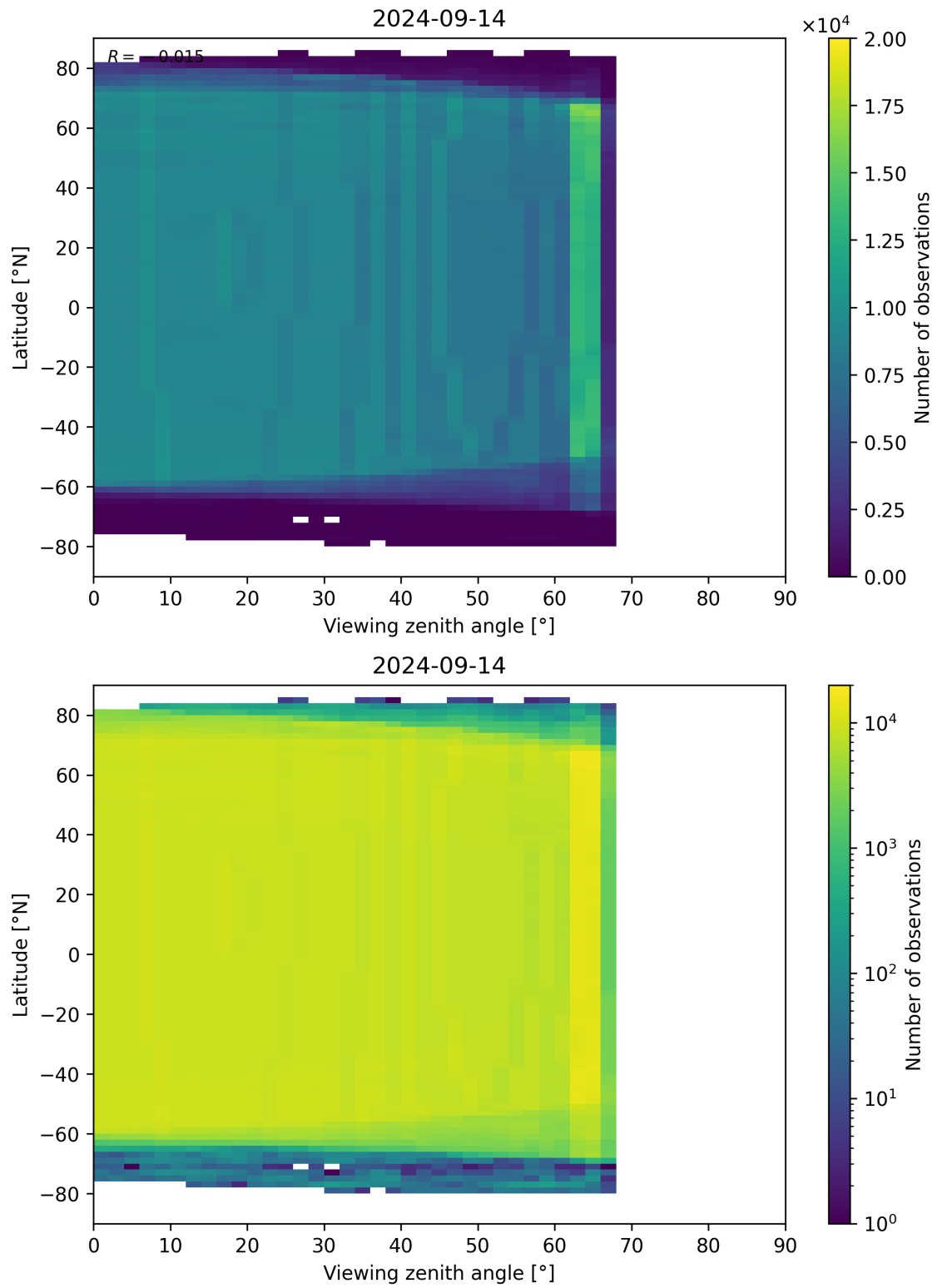
Figure 196: Scatter density plot of “Viewing zenith angle” against “Latitude” for 2024-09-13 to 2024-09-15.
