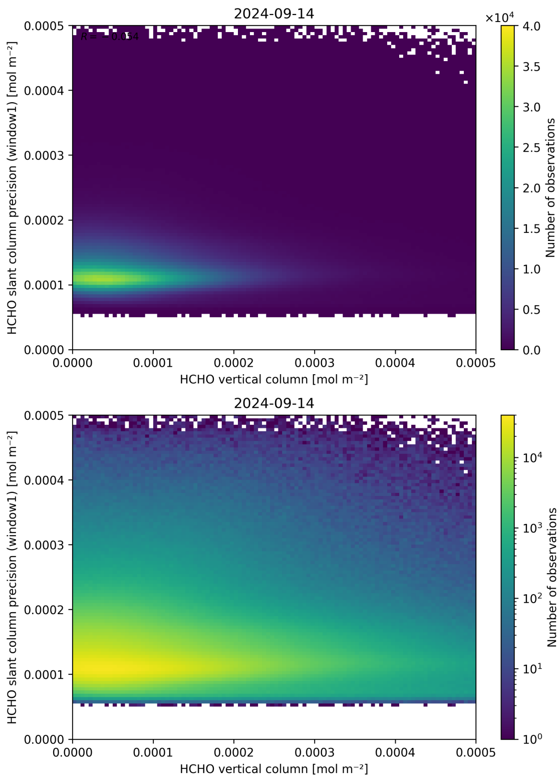
Figure 130: Scatter density plot of “HCHO vertical column” against “HCHO slant column precision (window1)” for 2024-09-13 to 2024-09-15.
