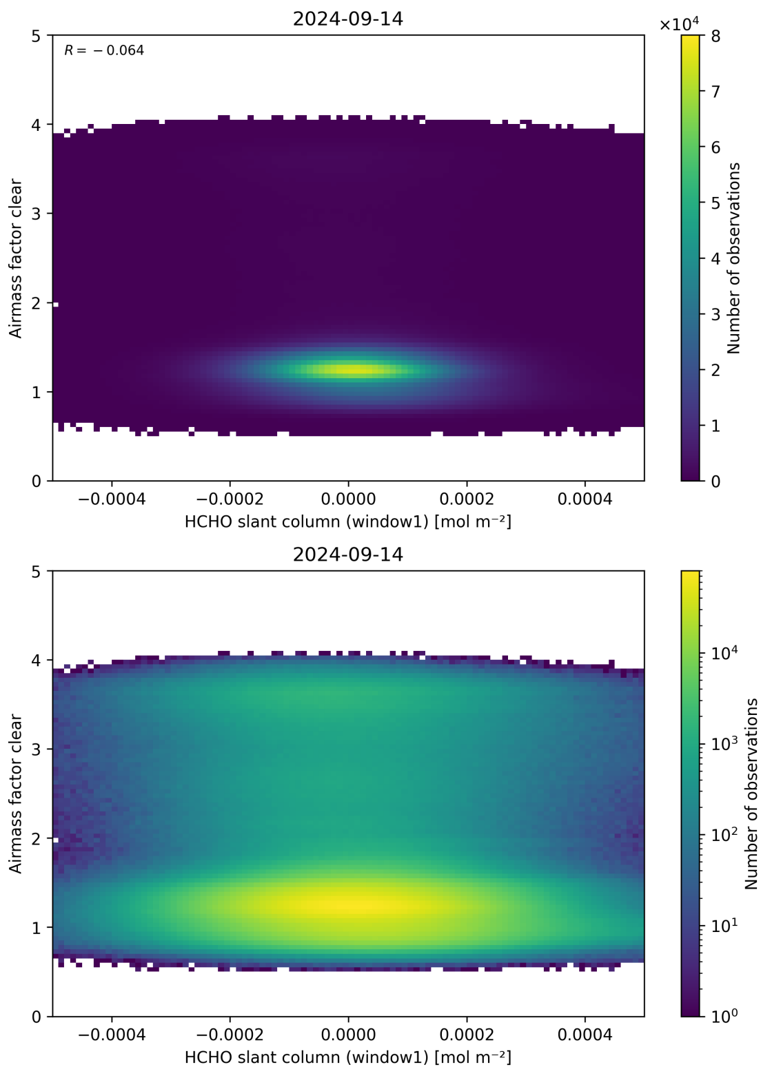
Figure 81: Scatter density plot of “HCHO slant column (window1)” against “Airmass factor clear” for 2024-09-13 to 2024-09-15.
