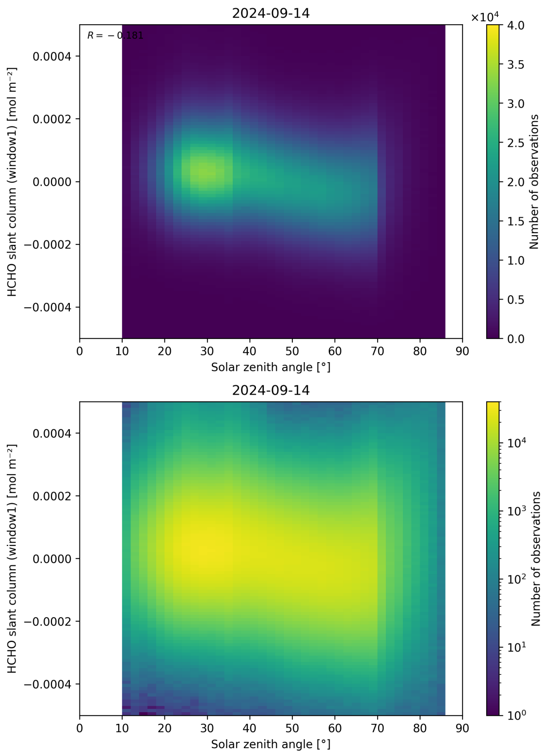
Figure 173: Scatter density plot of “Solar zenith angle” against “HCHO slant column (window1)” for 2024-09-13 to 2024-09-15.
