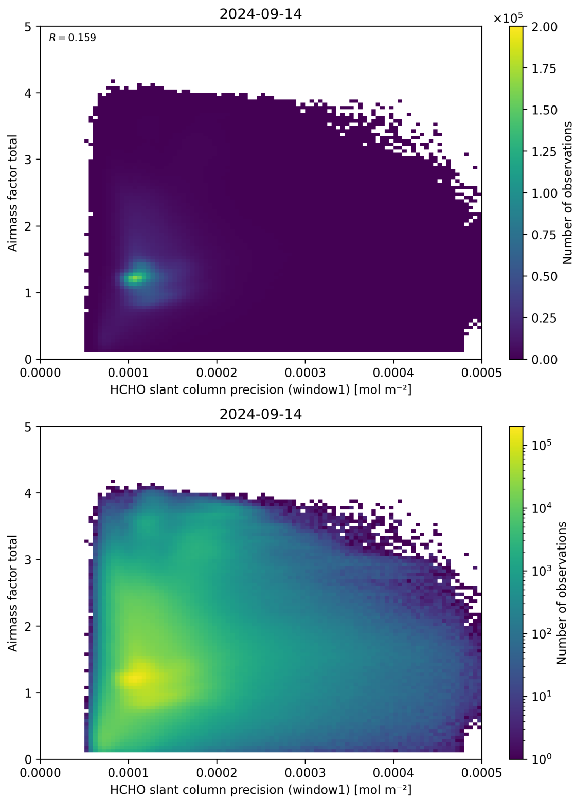
Figure 94: Scatter density plot of “HCHO slant column precision (window1)” against “Airmass factor total” for 2024-09-13 to 2024-09-15.
