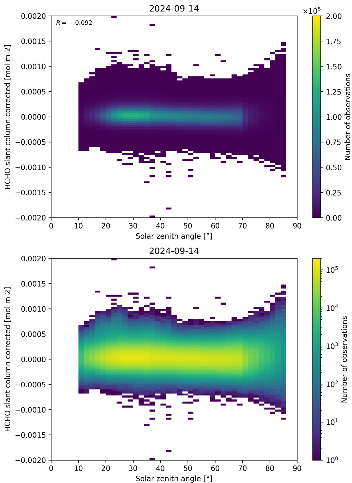
Figure 171: Scatter density plot of “Solar zenith angle” against “HCHO slant column corrected” for 2024-09-13 to 2024-09-15.
