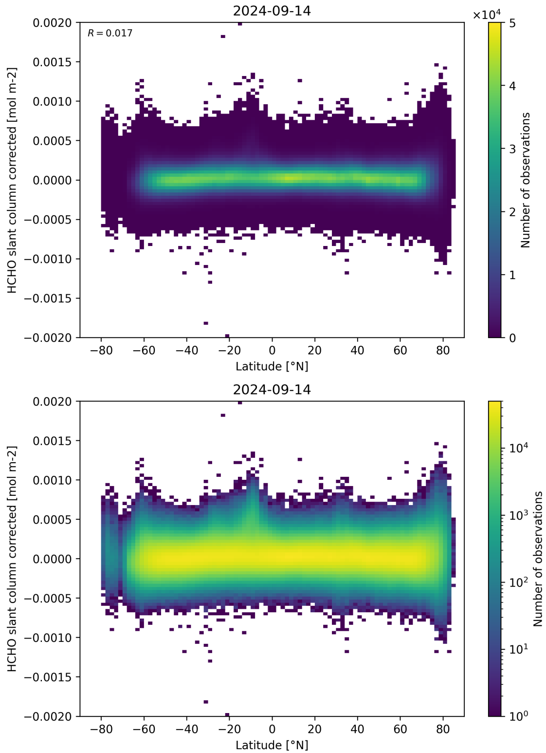
Figure 157: Scatter density plot of “Latitude” against “HCHO slant column corrected” for 2024-09-13 to 2024-09-15.
