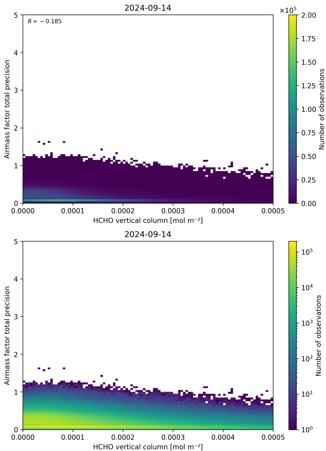
Figure 132: Scatter density plot of “HCHO vertical column” against “Airmass factor total precision” for 2024-09-13 to 2024-09-15.
