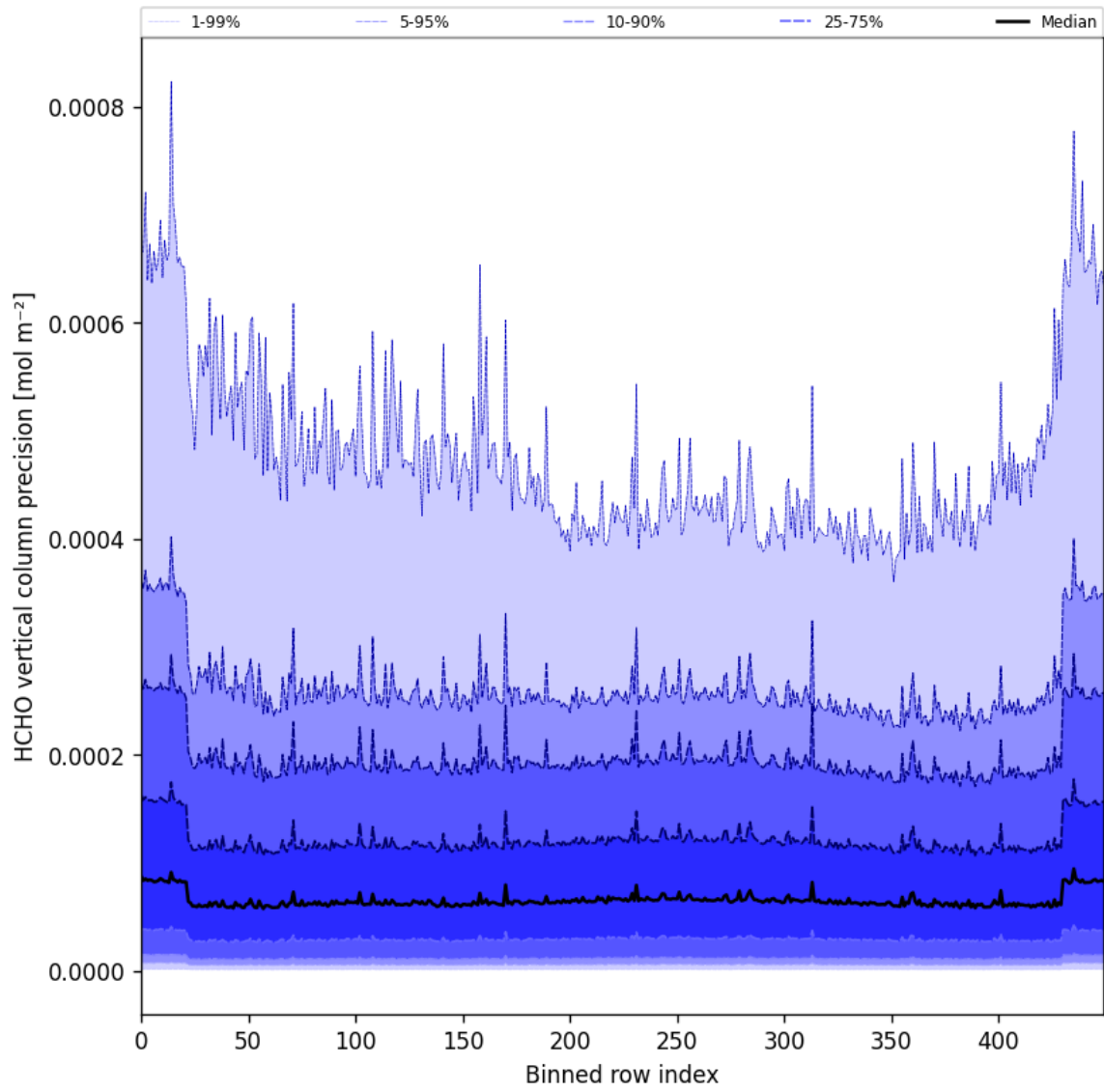
Figure 50: Along track statistics of “HCHO vertical column precision” for 2024-09-13 to 2024-09-15
