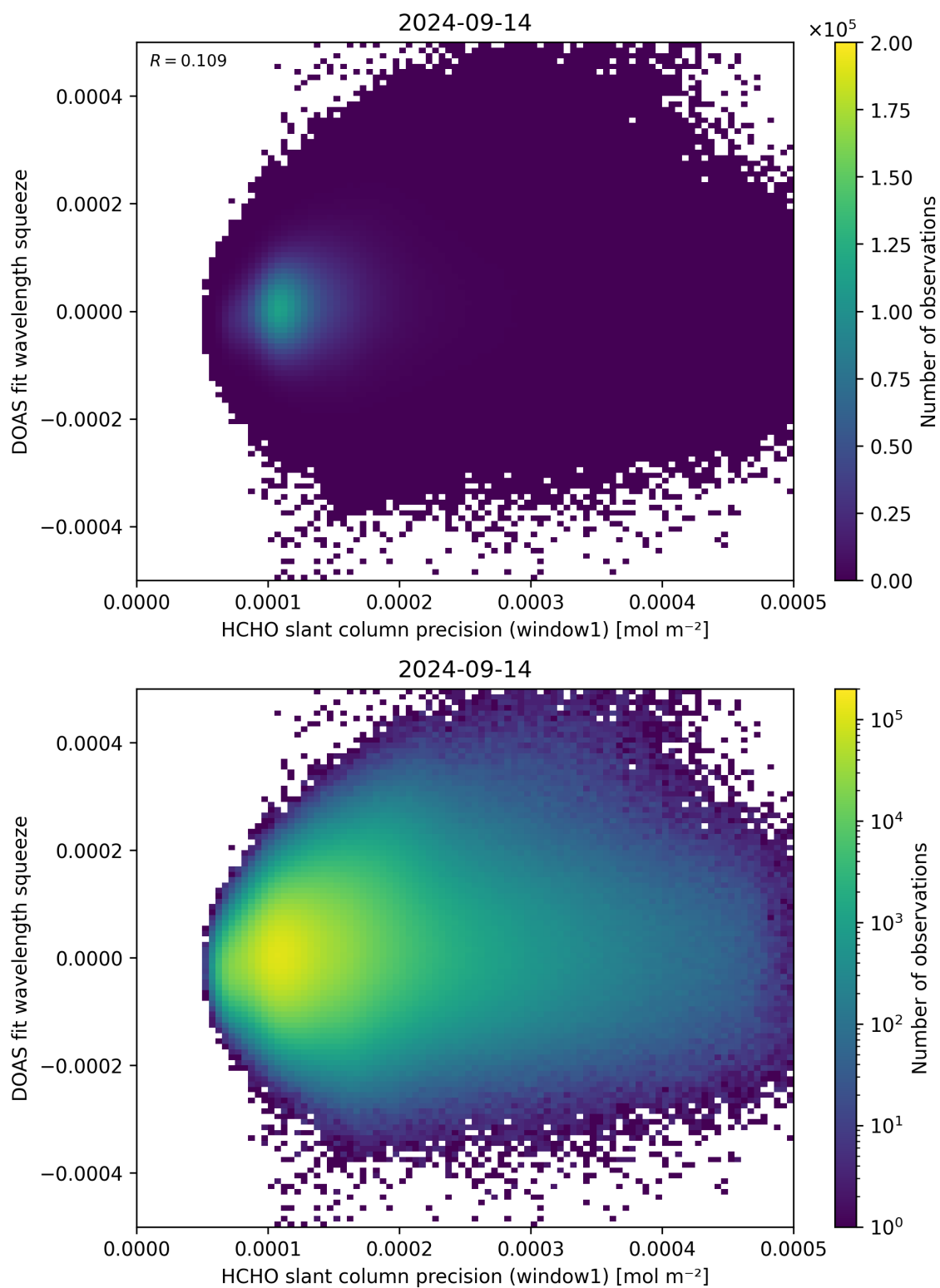
Figure 90: Scatter density plot of “HCHO slant column precision (window1)” against “DOAS fit wavelength squeeze” for 2024-09-13 to 2024-09-15.
