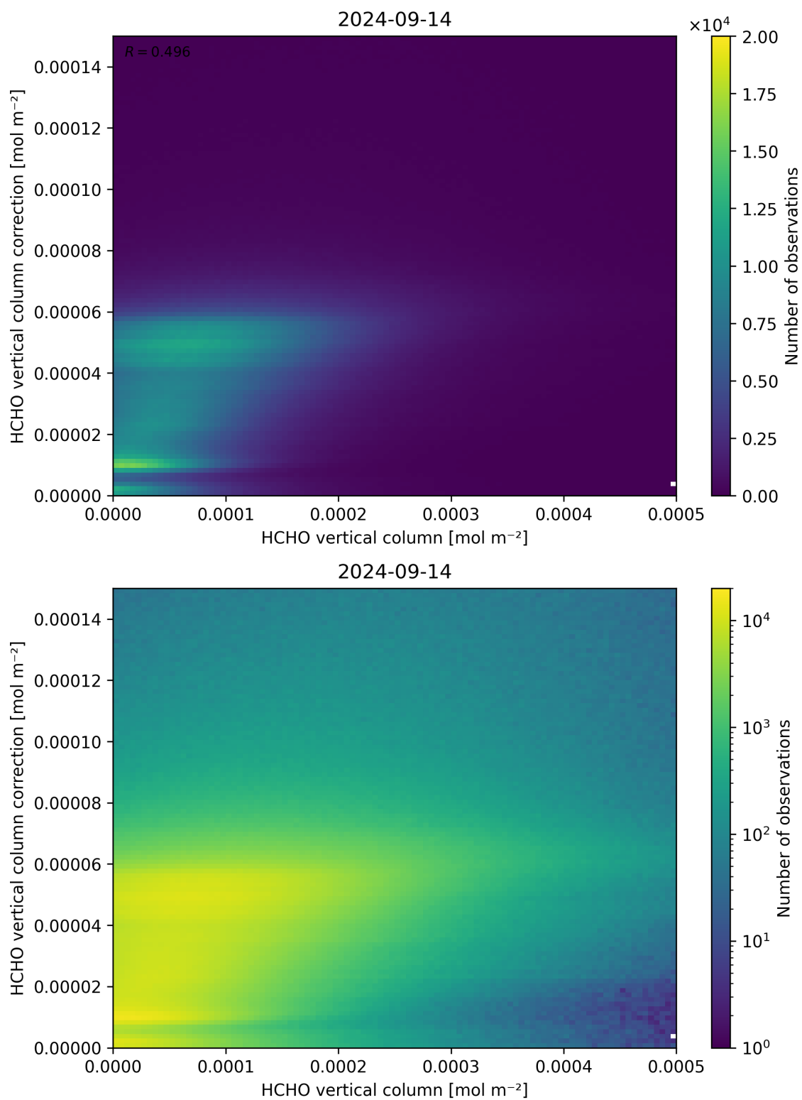
Figure 133: Scatter density plot of “HCHO vertical column” against “HCHO vertical column correction” for 2024-09-13 to 2024-09-15.
