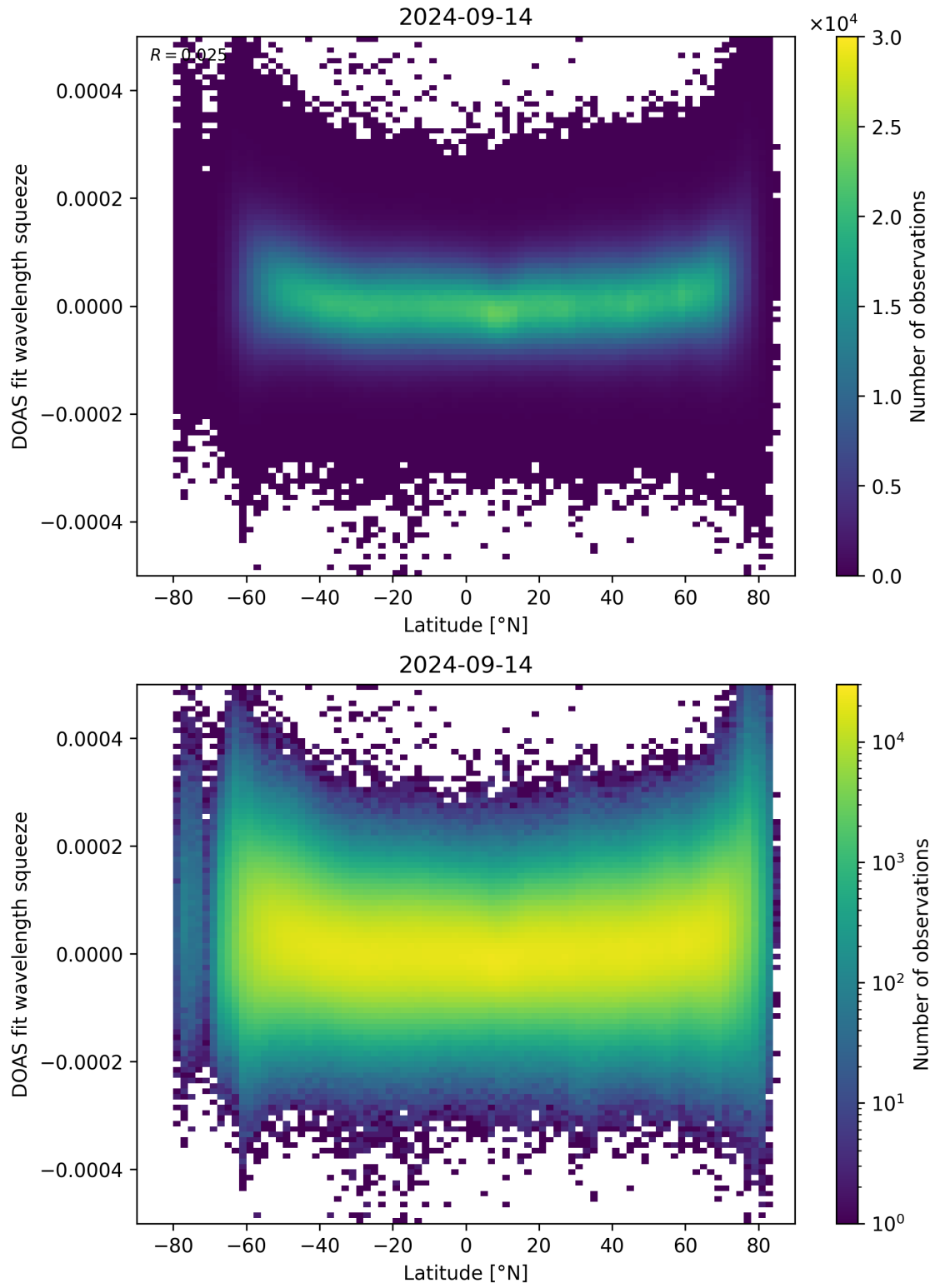
Figure 155: Scatter density plot of “Latitude” against “DOAS fit wavelength squeeze” for 2024-09-13 to 2024-09-15.
