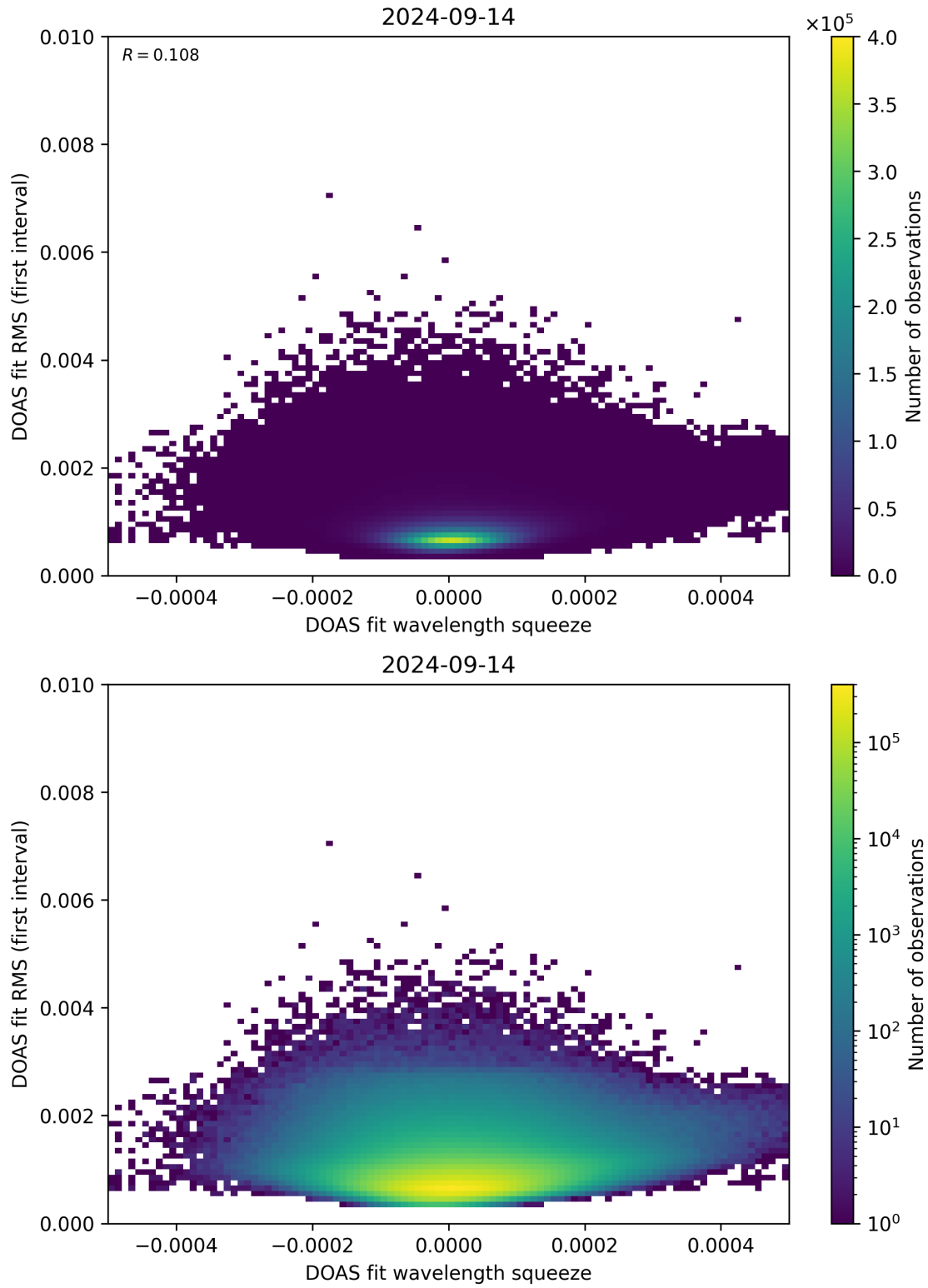
Figure 68: Scatter density plot of “DOAS fit wavelength squeeze” against “DOAS fit RMS (first interval)” for 2024-09-13 to 2024-09-15.
