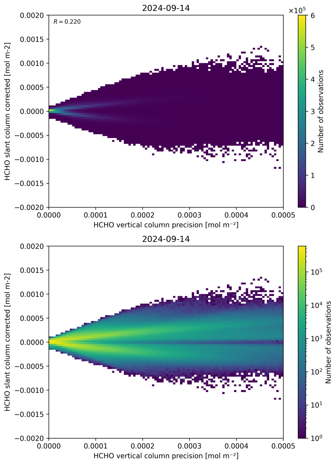
Figure 140: Scatter density plot of “HCHO vertical column precision” against “HCHO slant column corrected” for 2024-09-13 to 2024-09-15.
