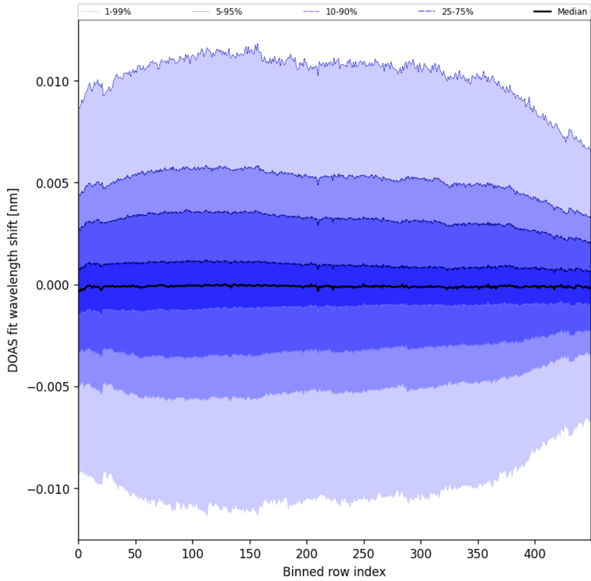
Figure 58: Along track statistics of “DOAS fit wavelength shift” for 2024-09-13 to 2024-09-15
