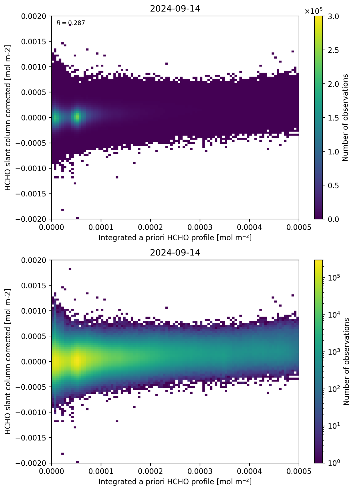
Figure 151: Scatter density plot of “Integrated a priori HCHO profile” against “HCHO slant column corrected” for 2024-09-13 to 2024-09-15.
