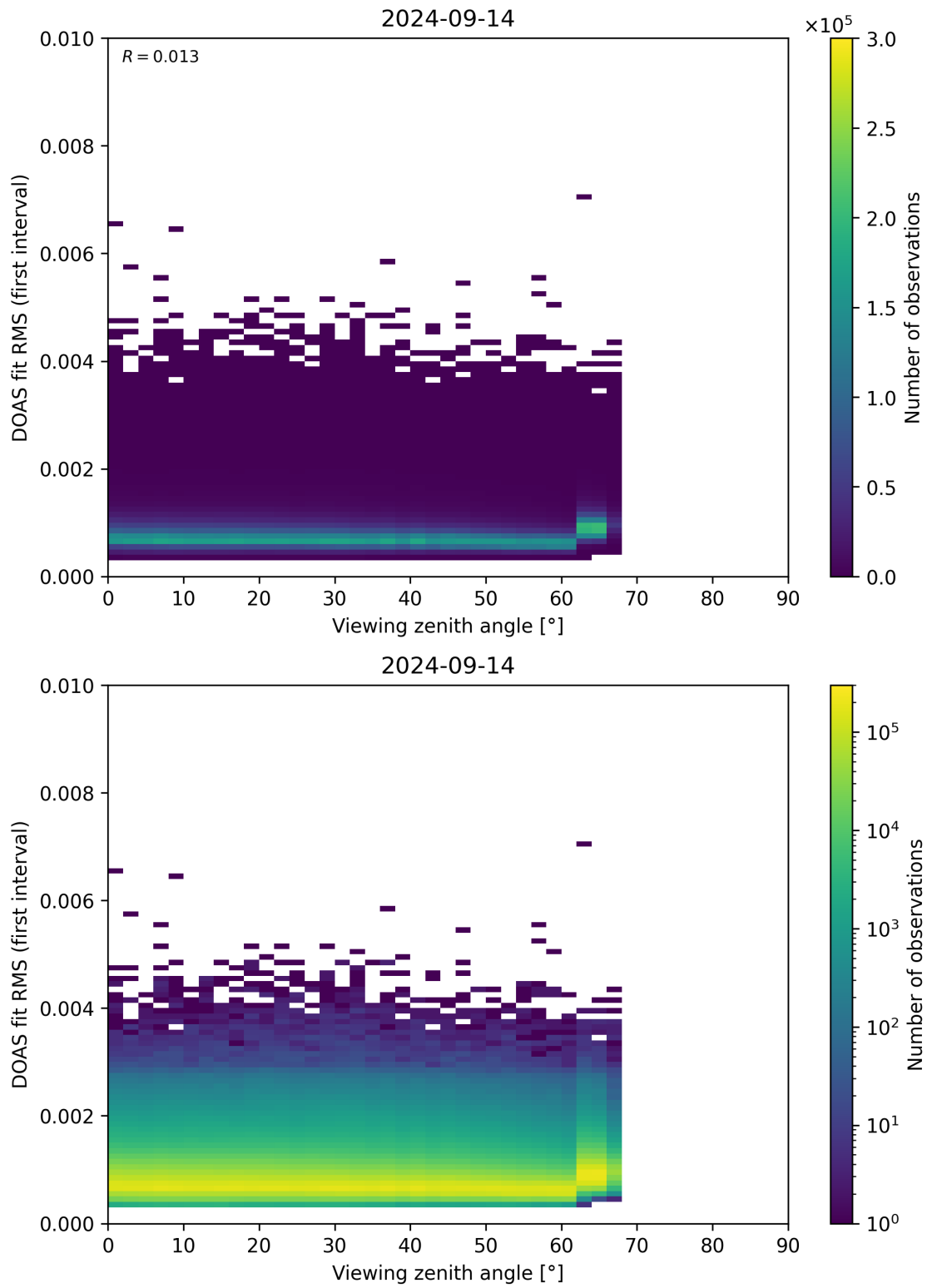
Figure 182: Scatter density plot of “Viewing zenith angle” against “DOAS fit RMS (first interval)” for 2024-09-13 to 2024-09-15.
