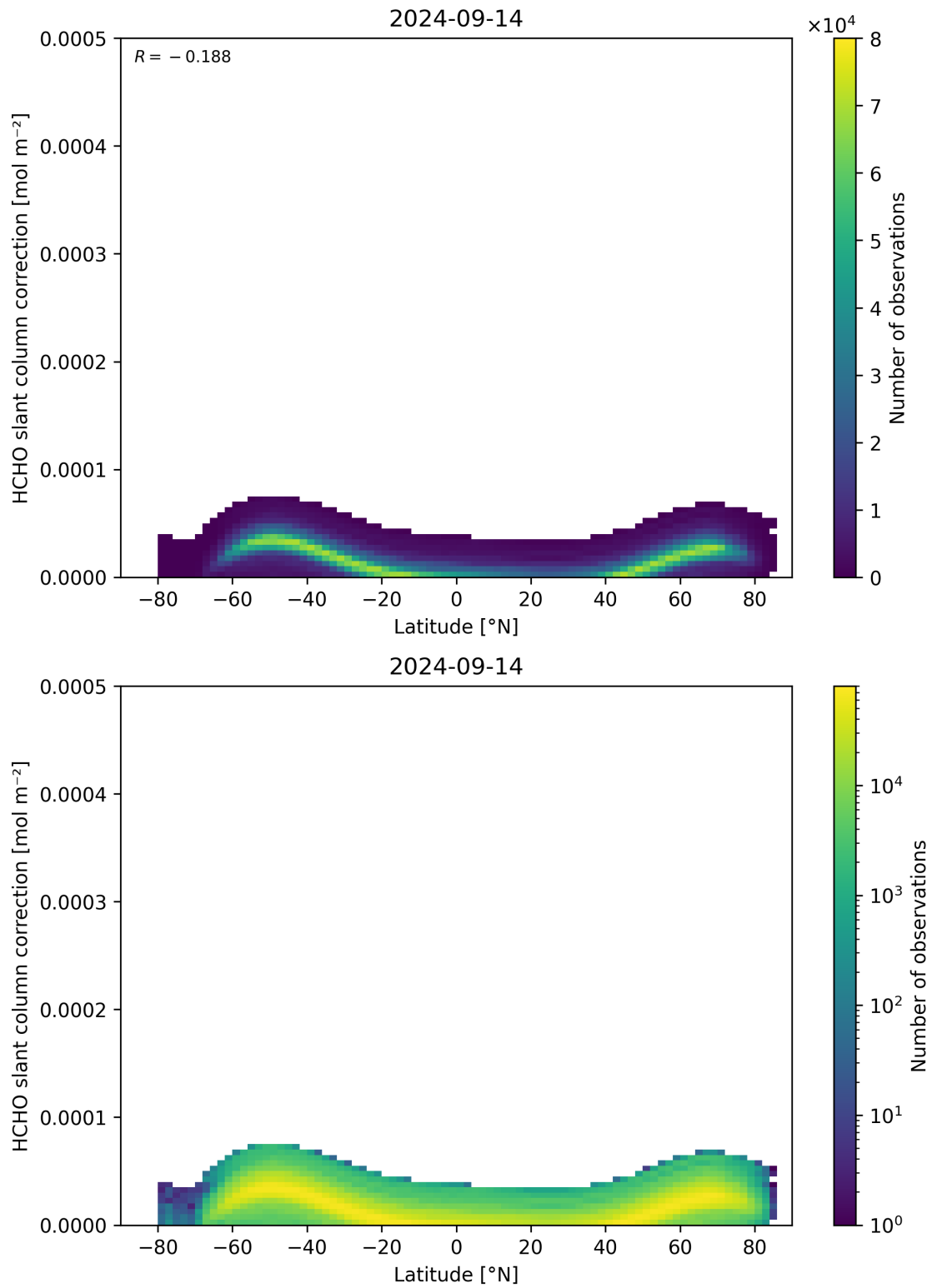
Figure 158: Scatter density plot of “Latitude” against “HCHO slant column correction” for 2024-09-13 to 2024-09-15.
