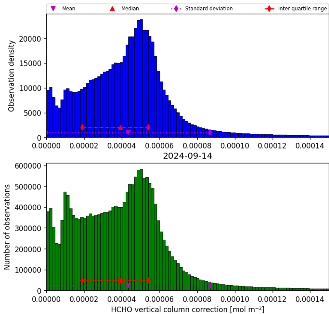
Figure 37: Histogram of “HCHO vertical column correction” for 2024-09-13 to 2024-09-15
