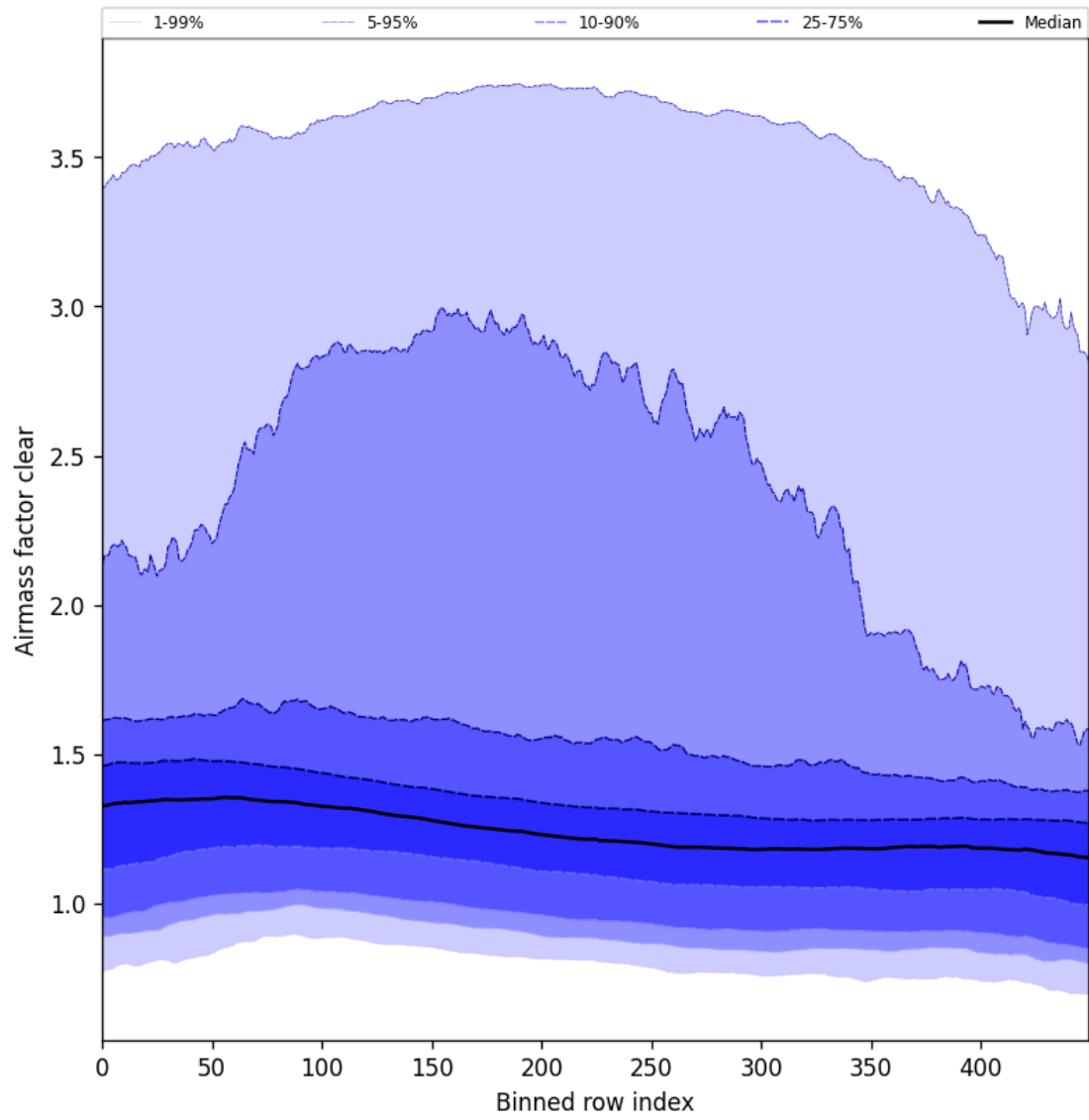
Figure 56: Along track statistics of “Airmass factor clear” for 2024-09-13 to 2024-09-15
