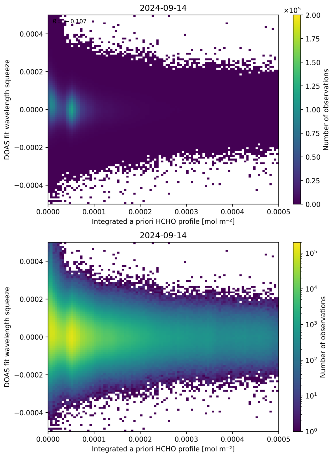
Figure 150: Scatter density plot of “Integrated a priori HCHO profile” against “DOAS fit wavelength squeeze” for 2024-09-13 to 2024-09-15.
