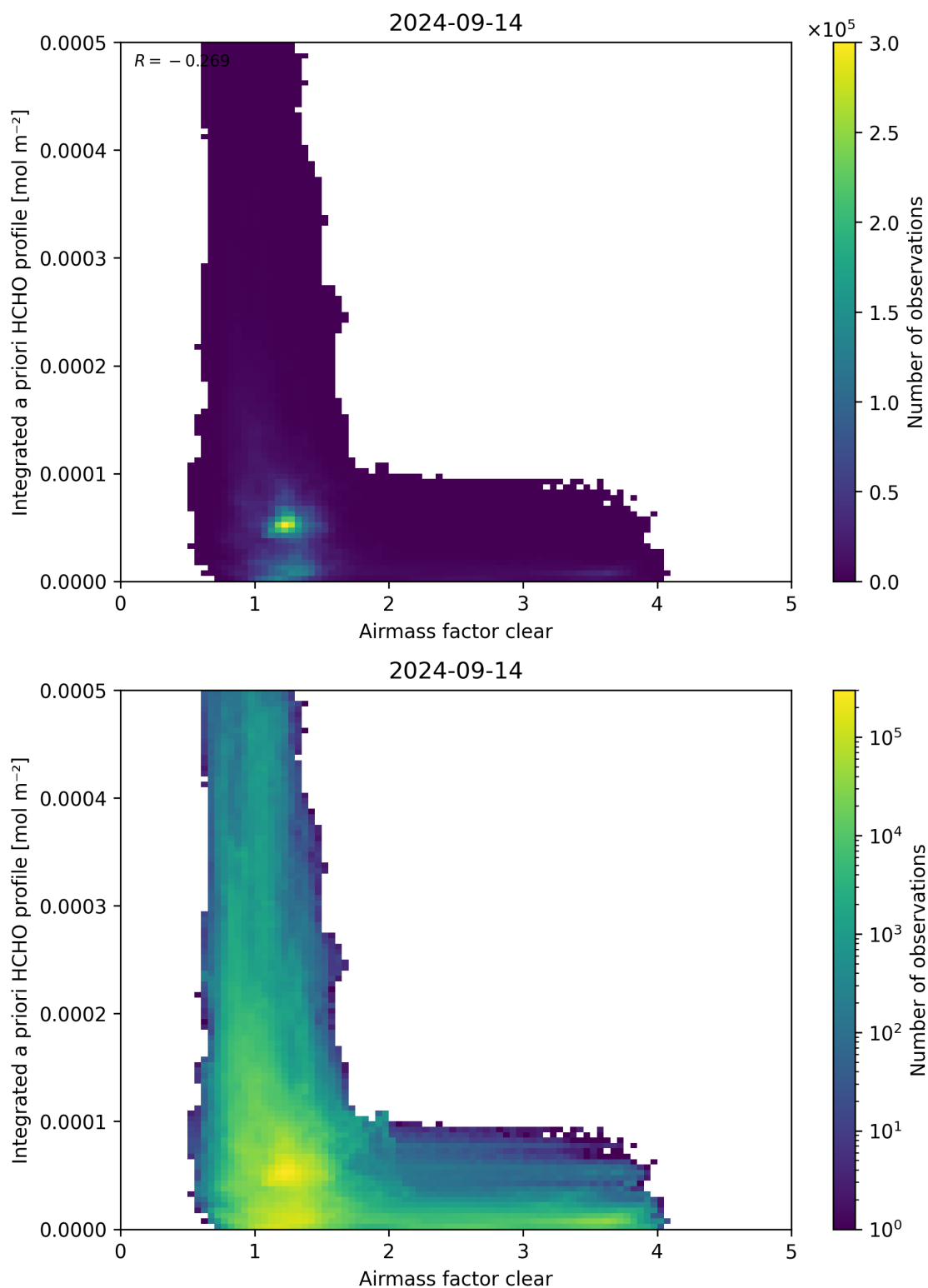
Figure 76: Scatter density plot of “Airmass factor clear” against “Integrated a priori HCHO profile” for 2024-09-13 to 2024-09-15.
