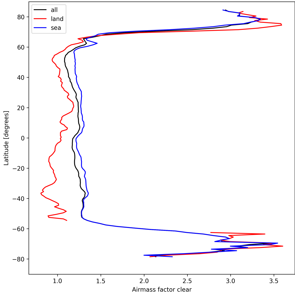
Figure 28: Zonal average of “Airmass factor clear” for 2024-09-13 to 2024-09-15.
