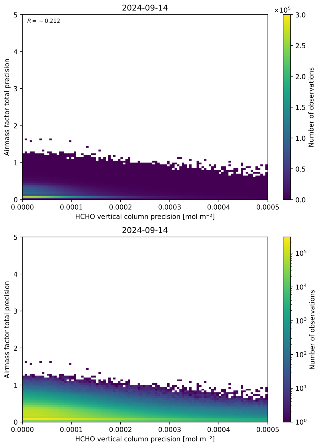
Figure 145: Scatter density plot of “HCHO vertical column precision” against “Airmass factor total precision” for 2024-09-13 to 2024-09-15.
