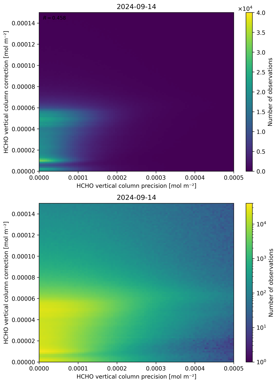
Figure 146: Scatter density plot of “HCHO vertical column precision” against “HCHO vertical column correction” for 2024-09-13 to 2024-09-15.
