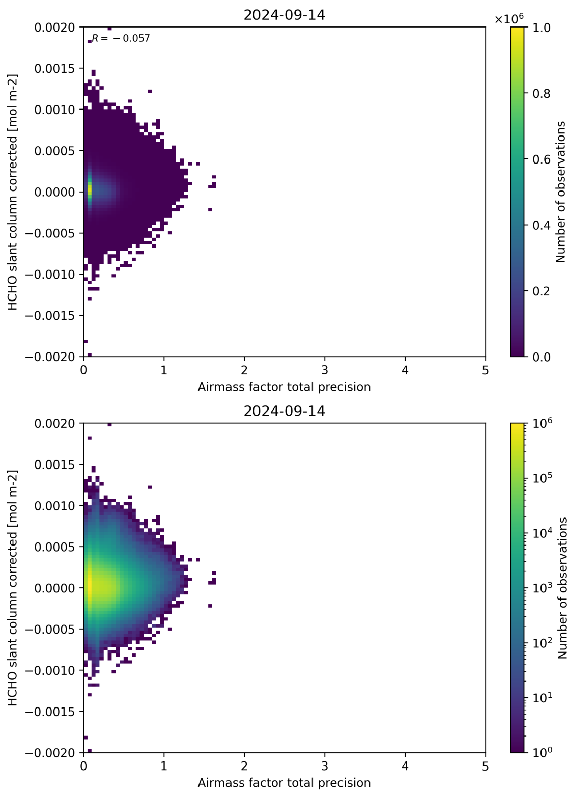
Figure 109: Scatter density plot of “Airmass factor total precision” against “HCHO slant column corrected” for 2024-09-13 to 2024-09-15.
