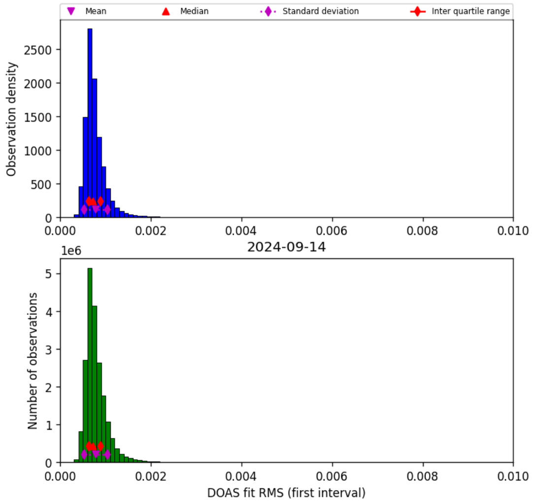
Figure 46: Histogram of “DOAS fit RMS (first interval)” for 2024-09-13 to 2024-09-15
