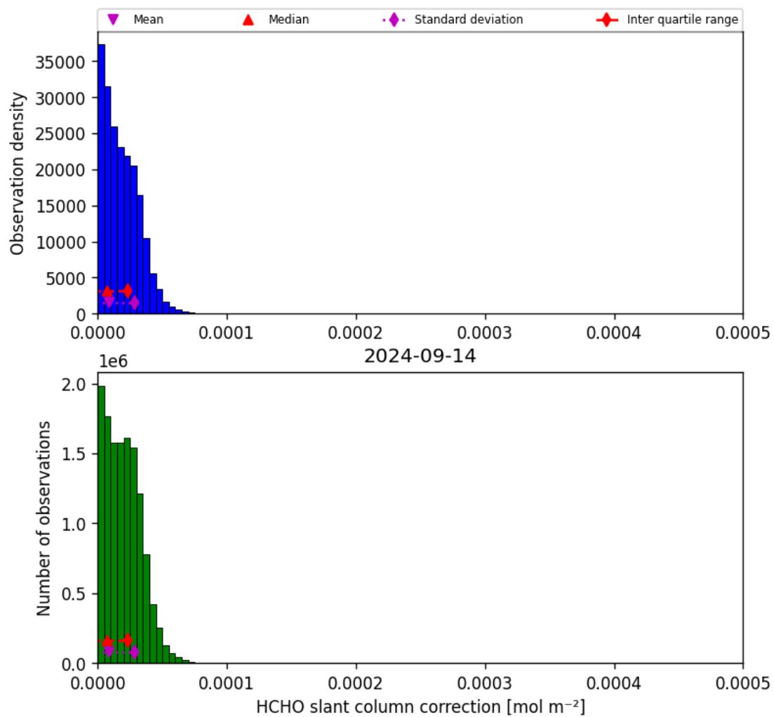
Figure 47: Histogram of “HCHO slant column correction” for 2024-09-13 to 2024-09-15
