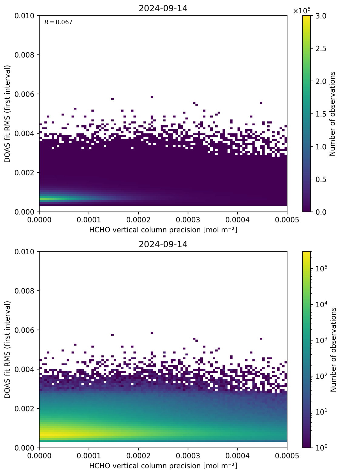
Figure 136: Scatter density plot of “HCHO vertical column precision” against “DOAS fit RMS (first interval)” for 2024-09-13 to 2024-09-15.
