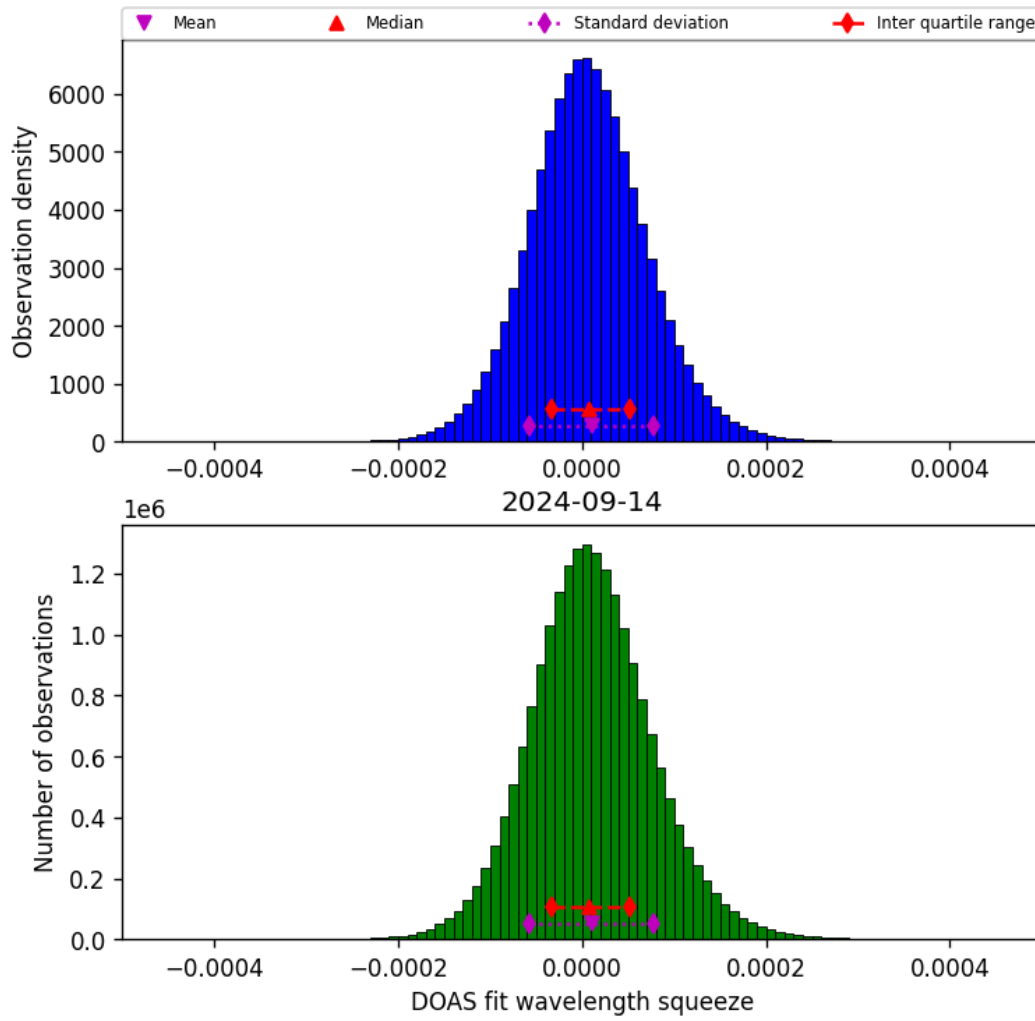
Figure 45: Histogram of “DOAS fit wavelength squeeze” for 2024-09-13 to 2024-09-15
