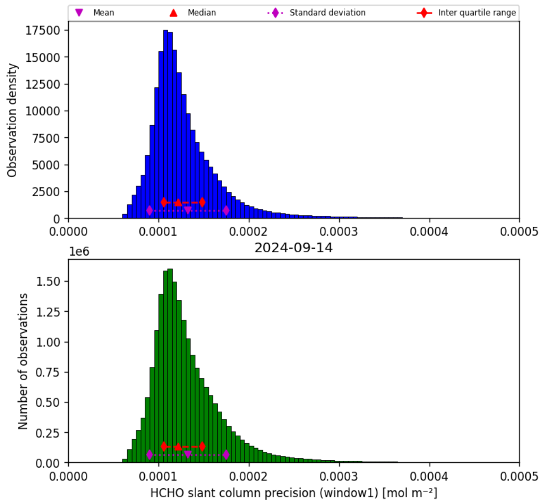
Figure 39: Histogram of “HCHO slant column precision (window1)” for 2024-09-13 to 2024-09-15
