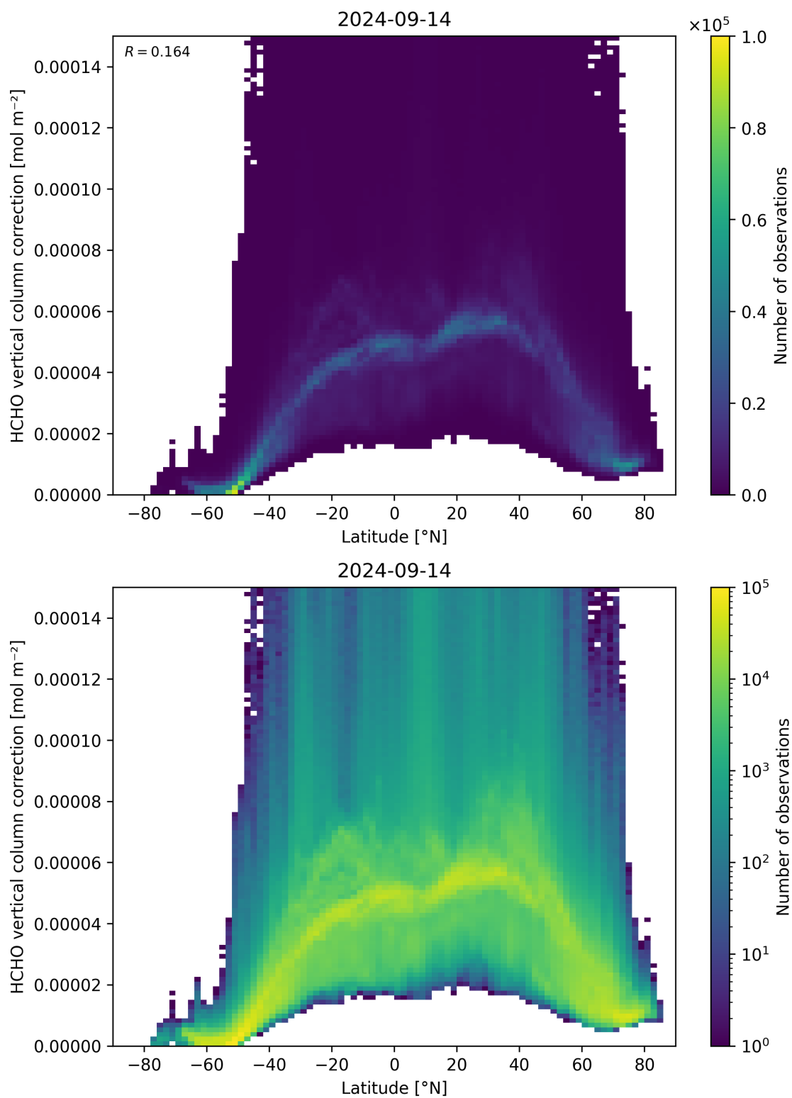
Figure 164: Scatter density plot of “Latitude” against “HCHO vertical column correction” for 2024-09-13 to 2024-09-15.
