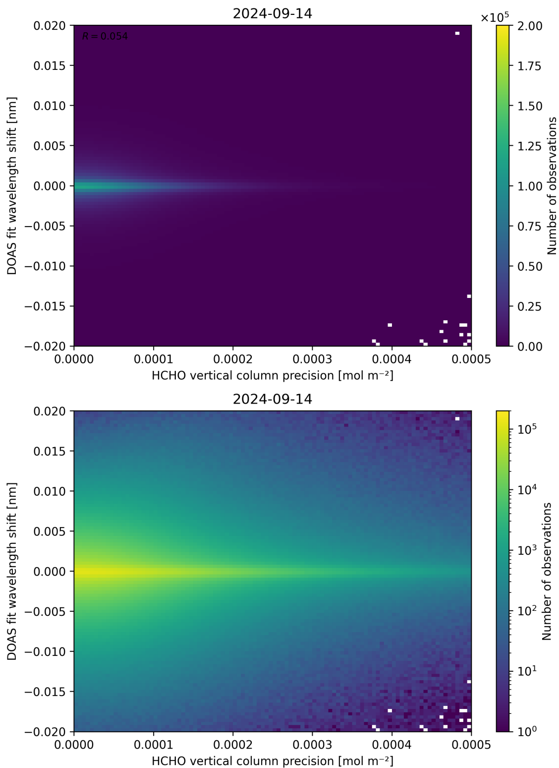
Figure 137: Scatter density plot of “HCHO vertical column precision” against “DOAS fit wavelength shift” for 2024-09-13 to 2024-09-15.
