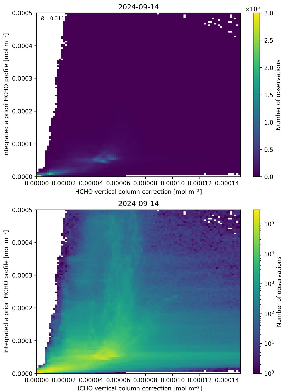
Figure 122: Scatter density plot of “HCHO vertical column correction” against “Integrated a priori HCHO profile” for 2024-09-13 to 2024-09-15.
