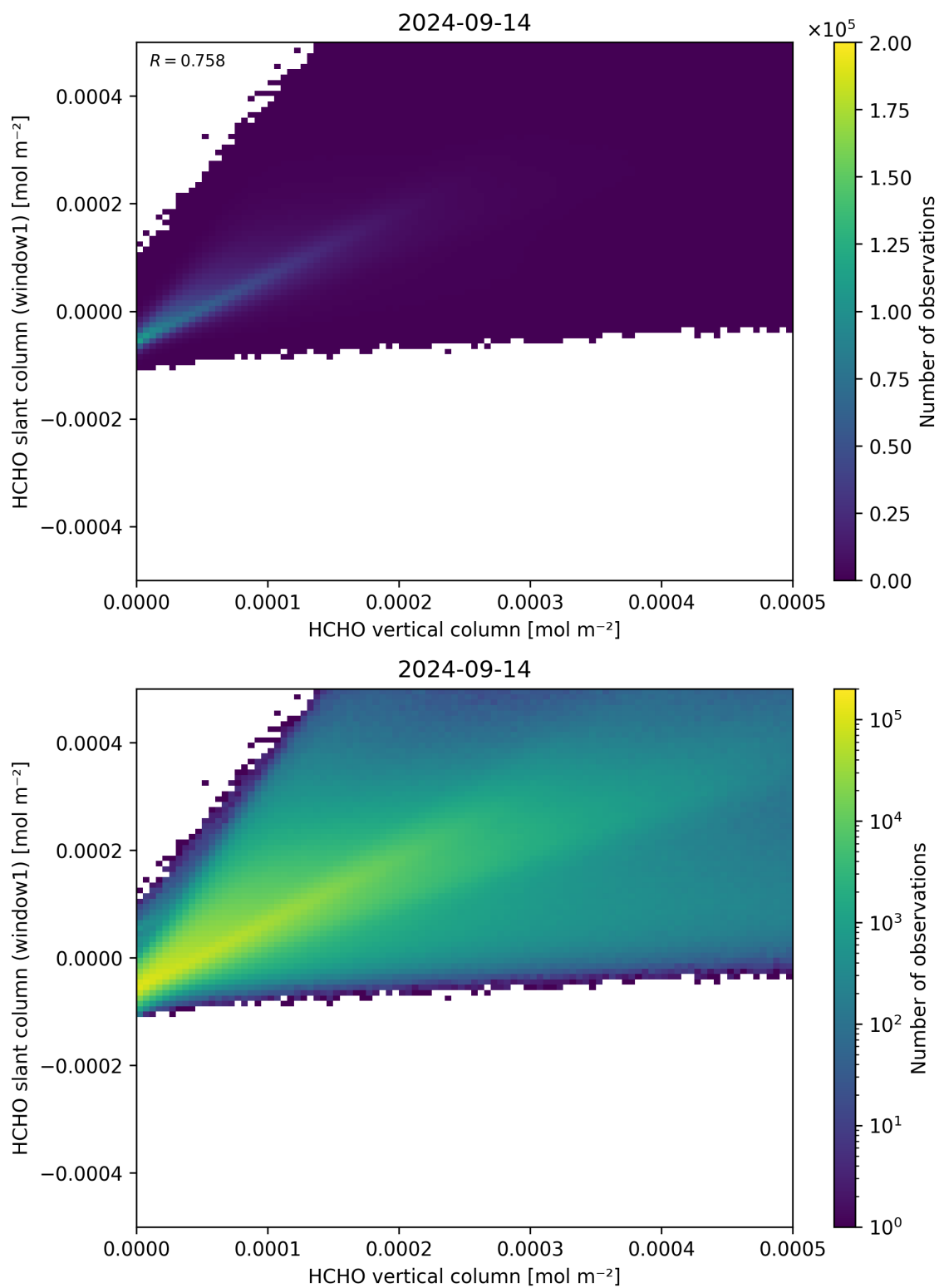
Figure 129: Scatter density plot of “HCHO vertical column” against “HCHO slant column (window1)” for 2024-09-13 to 2024-09-15.
