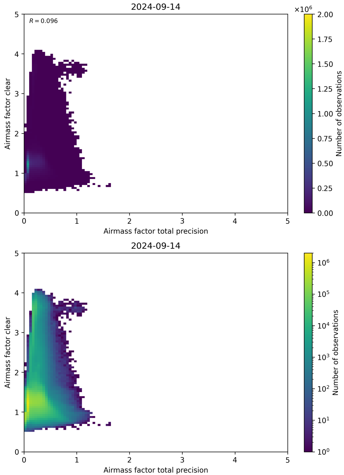
Figure 108: Scatter density plot of “Airmass factor total precision” against “Airmass factor clear” for 2024-09-13 to 2024-09-15.
