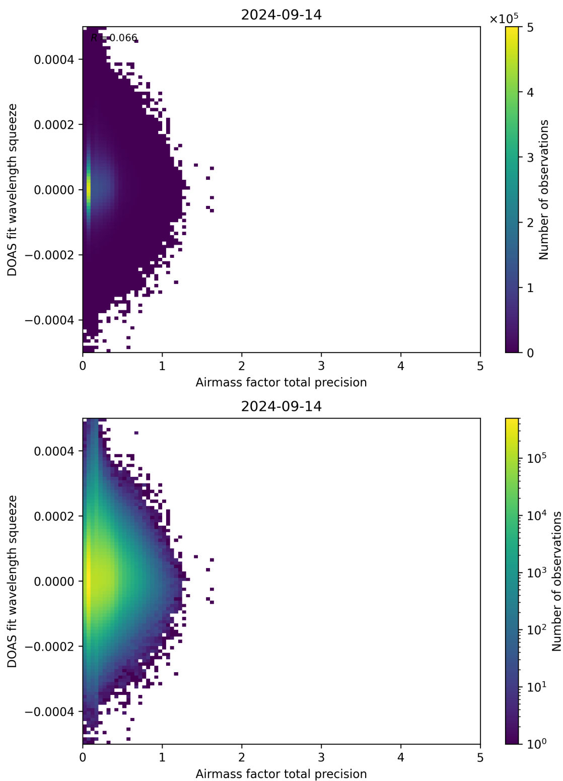
Figure 107: Scatter density plot of “Airmass factor total precision” against “DOAS fit wavelength squeeze” for 2024-09-13 to 2024-09-15.
