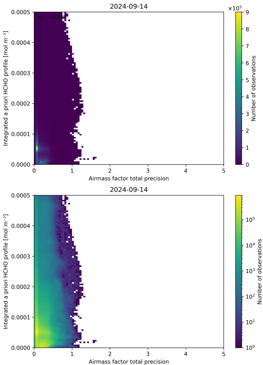
Figure 111: Scatter density plot of “Airmass factor total precision” against “Integrated a priori HCHO profile” for 2024-09-13 to 2024-09-15.
