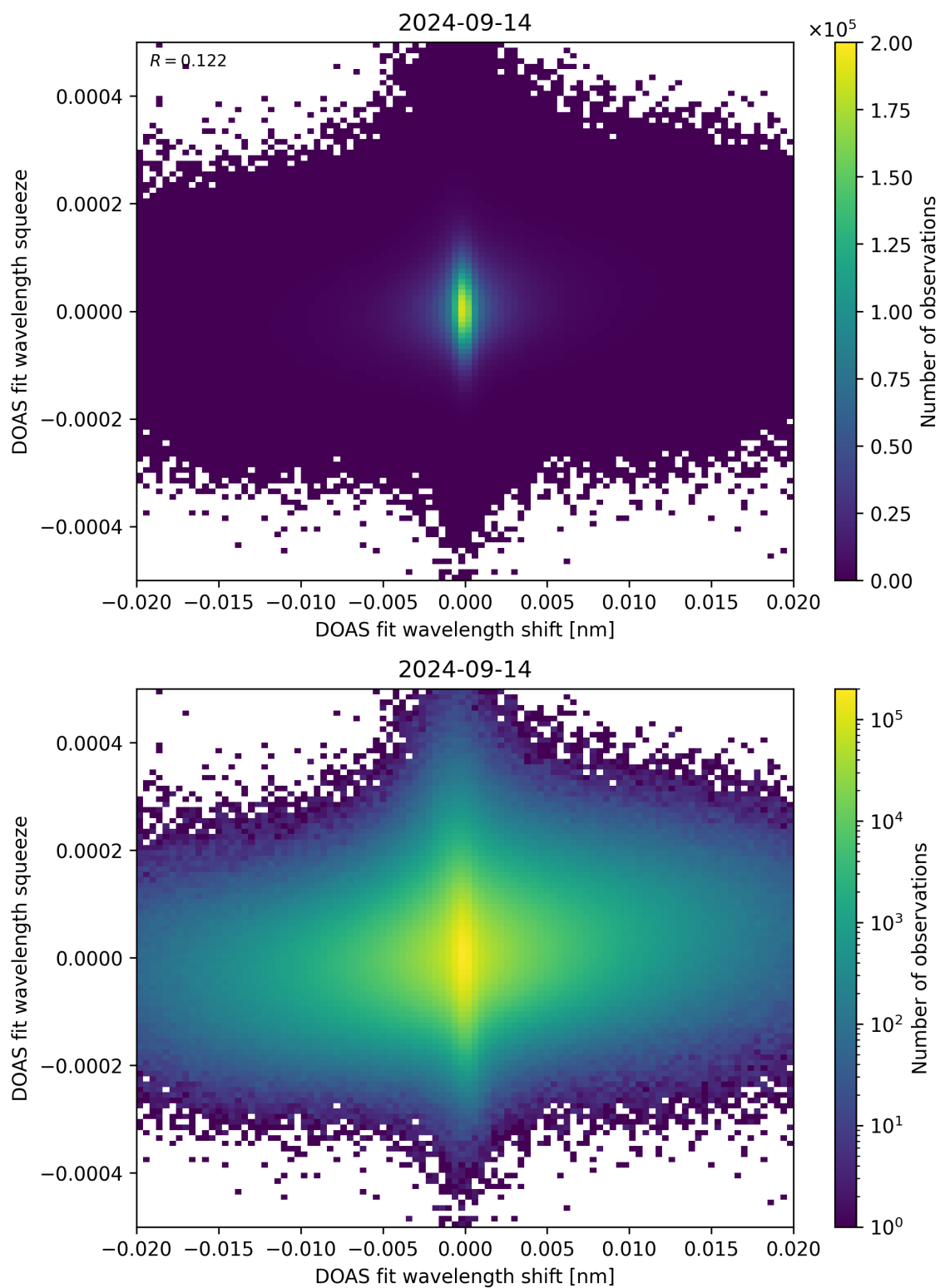
Figure 65: Scatter density plot of “DOAS fit wavelength shift” against “DOAS fit wavelength squeeze” for 2024-09-13 to 2024-09-15.
