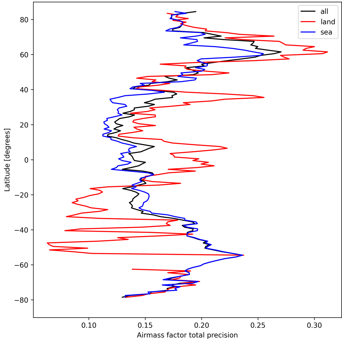
Figure 27: Zonal average of “Airmass factor total precision” for 2024-09-13 to 2024-09-15.
