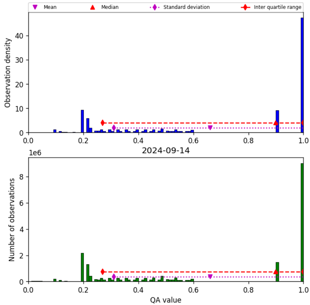
Figure 34: Histogram of “QA value” for 2024-09-13 to 2024-09-15
