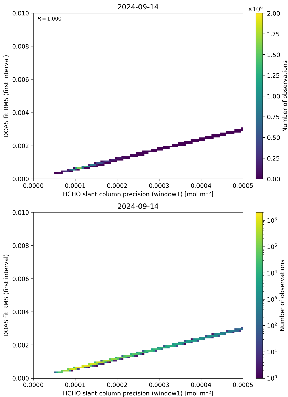
Figure 88: Scatter density plot of “HCHO slant column precision (window1)” against “DOAS fit RMS (first interval)” for 2024-09-13 to 2024-09-15.
