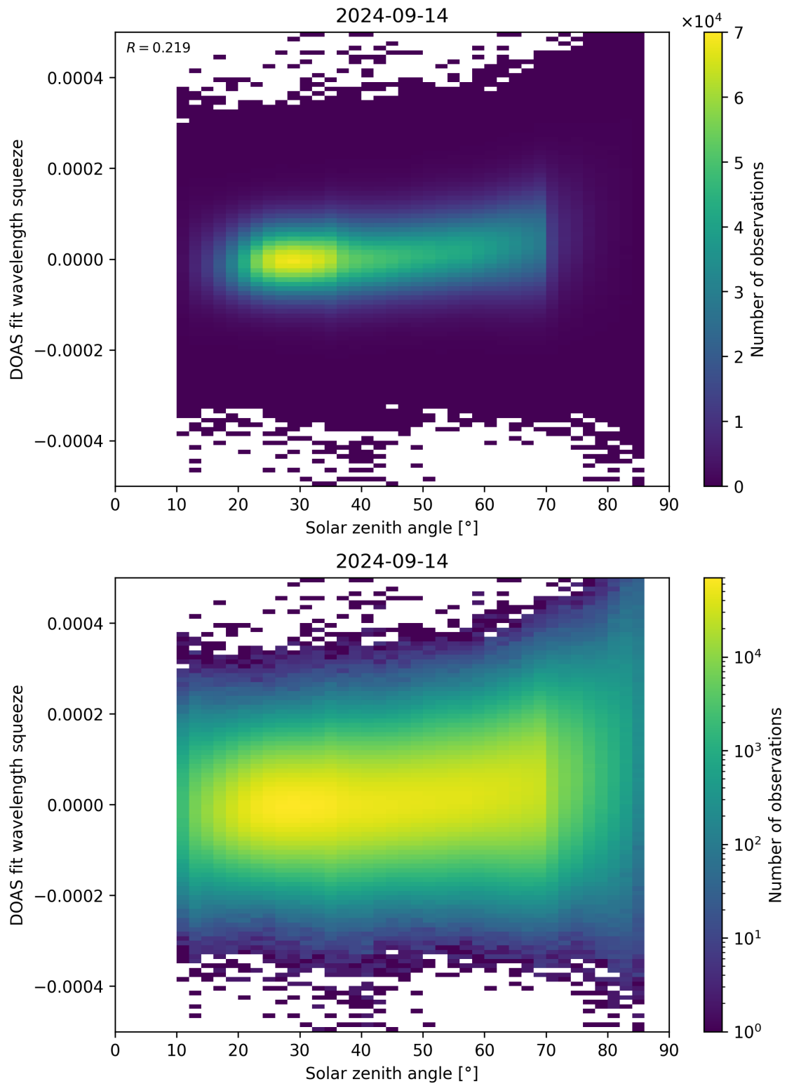
Figure 169: Scatter density plot of “Solar zenith angle” against “DOAS fit wavelength squeeze” for 2024-09-13 to 2024-09-15.
