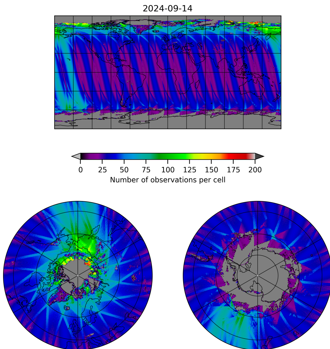
Figure 19: Map of the number of observations for 2024-09-13 to 2024-09-15
