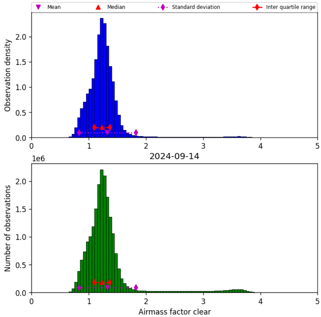
Figure 42: Histogram of “Airmass factor clear” for 2024-09-13 to 2024-09-15
