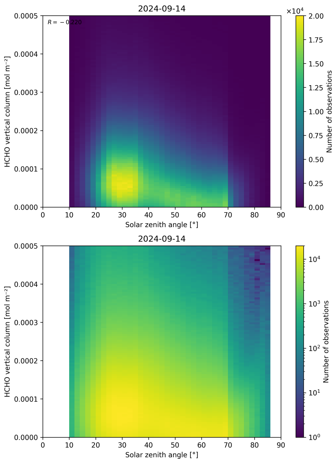
Figure 177: Scatter density plot of “Solar zenith angle” against “HCHO vertical column” for 2024-09-13 to 2024-09-15.
