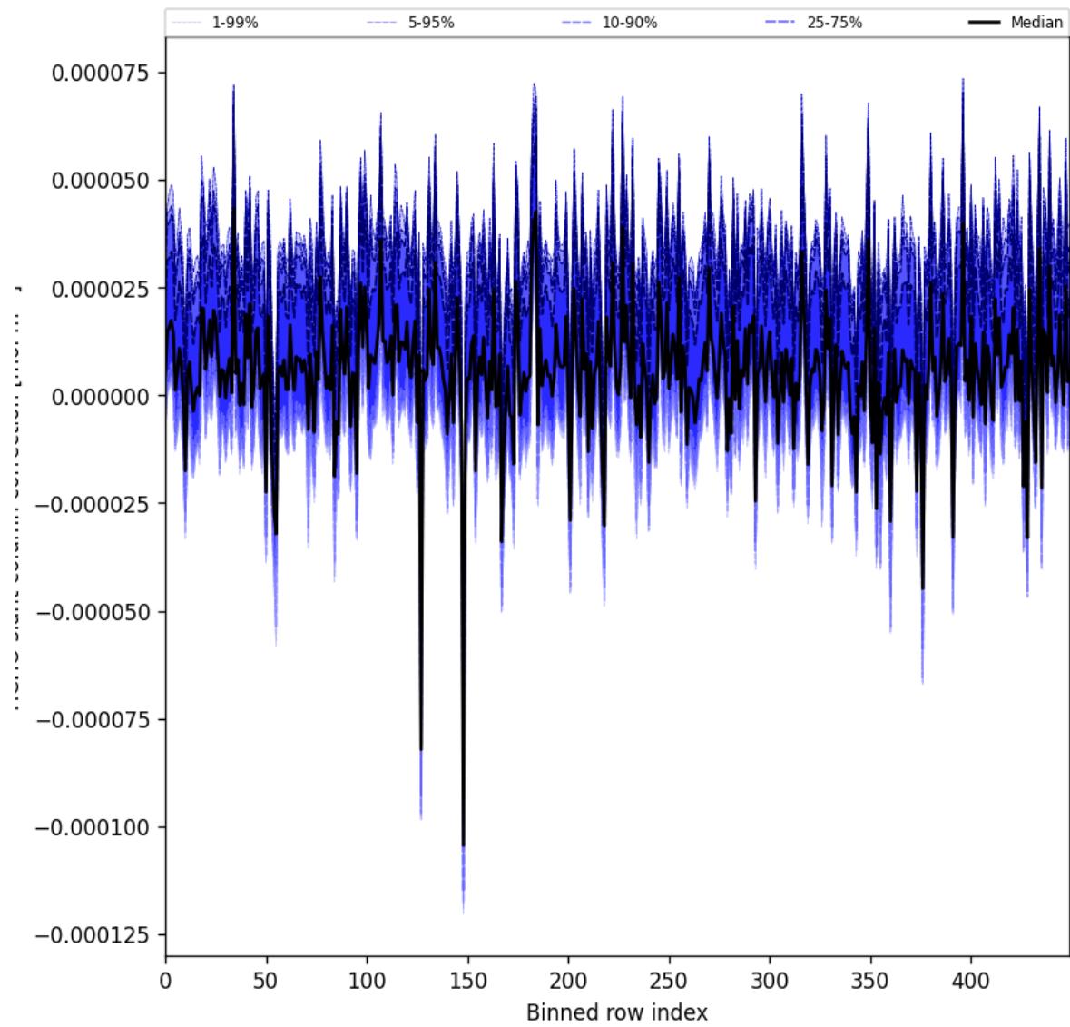
Figure 61: Along track statistics of “HCHO slant column correction” for 2024-09-13 to 2024-09-15
