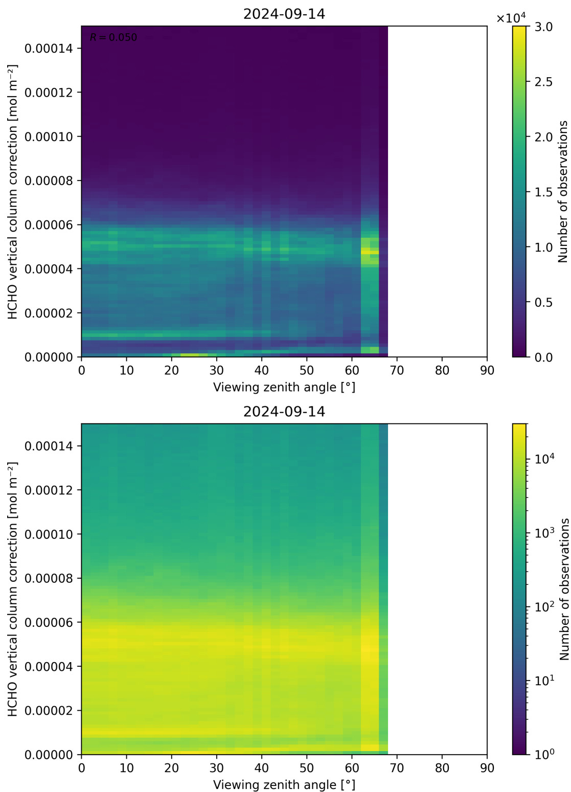
Figure 193: Scatter density plot of “Viewing zenith angle” against “HCHO vertical column correction” for 2024-09-13 to 2024-09-15.
