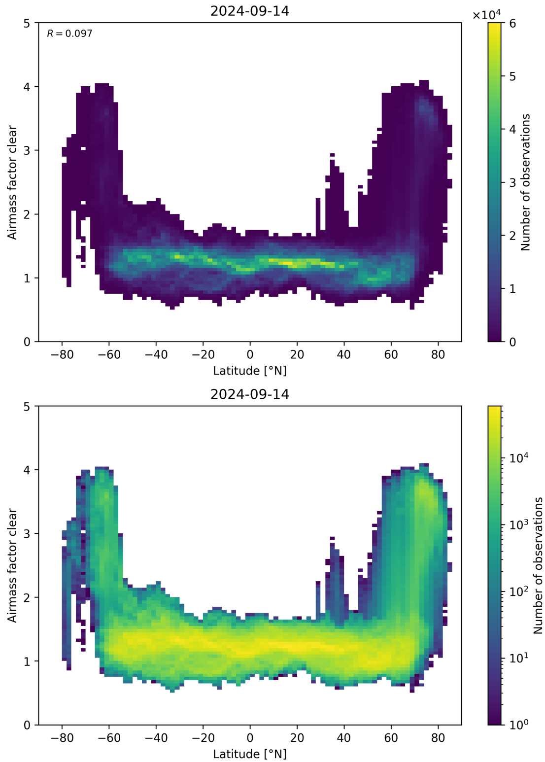
Figure 156: Scatter density plot of “Latitude” against “Airmass factor clear” for 2024-09-13 to 2024-09-15.
