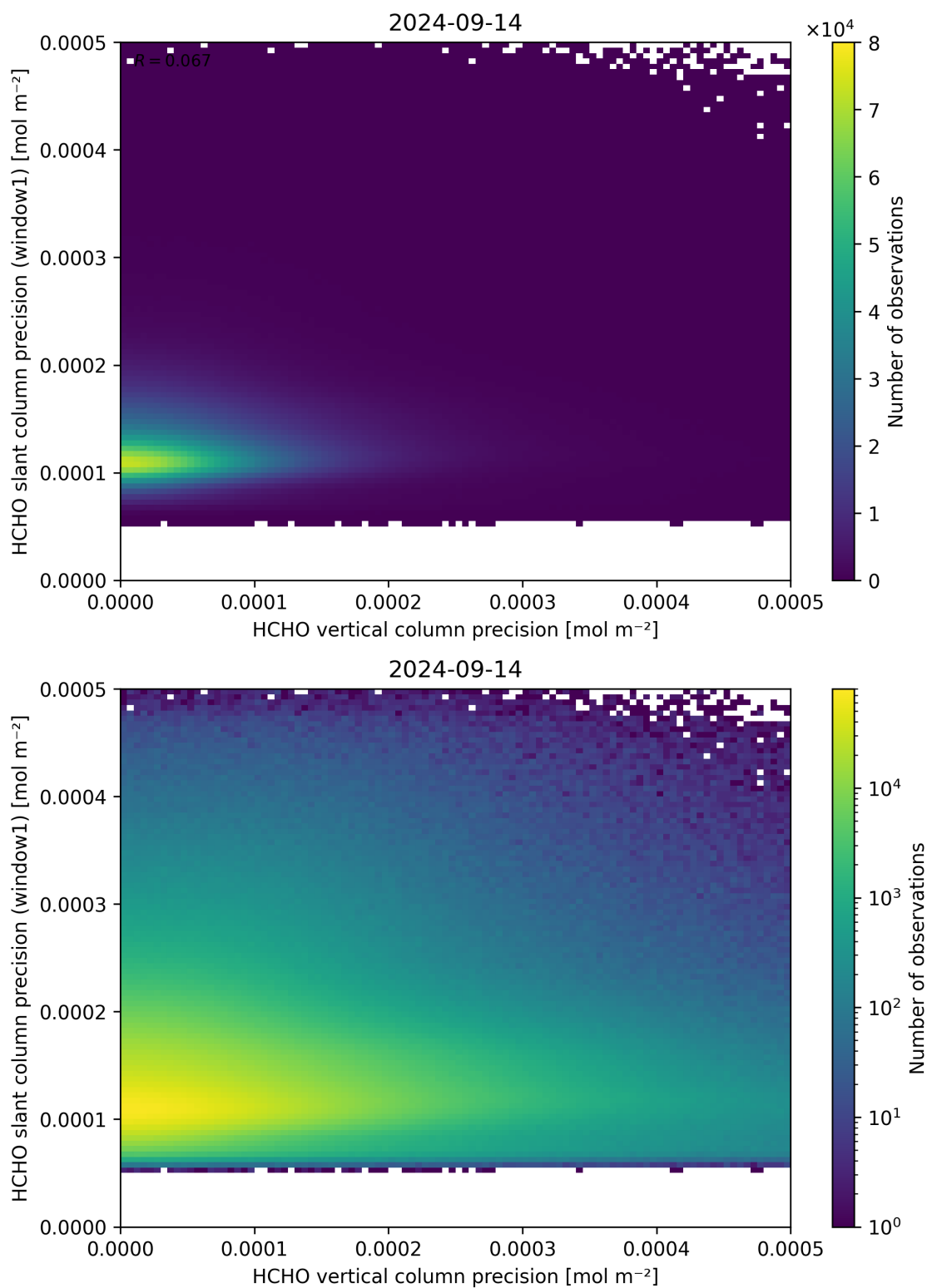
Figure 143: Scatter density plot of “HCHO vertical column precision” against “HCHO slant column precision (window1)” for 2024-09-13 to 2024-09-15.
