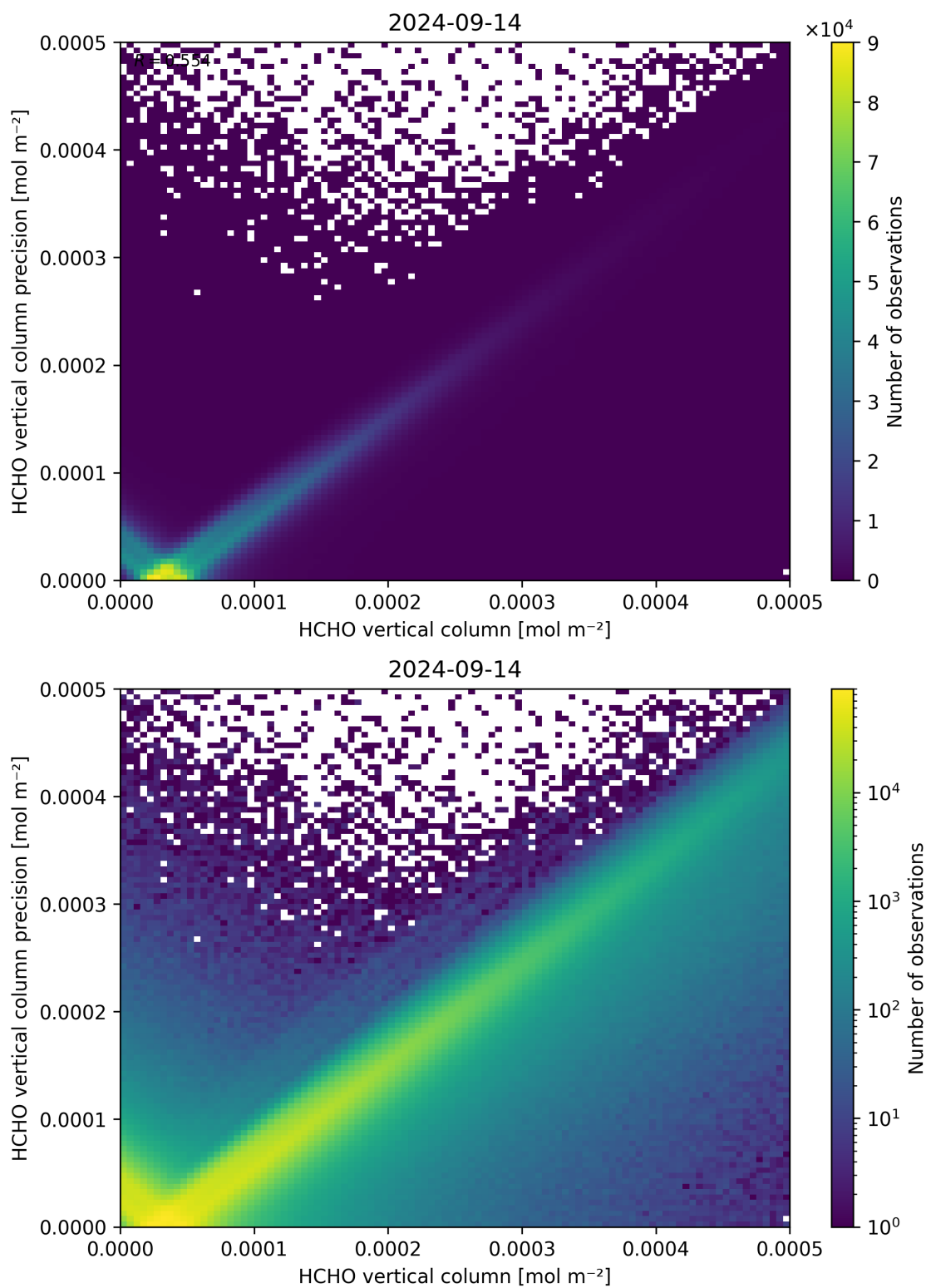
Figure 134: Scatter density plot of “HCHO vertical column” against “HCHO vertical column precision” for 2024-09-13 to 2024-09-15.
