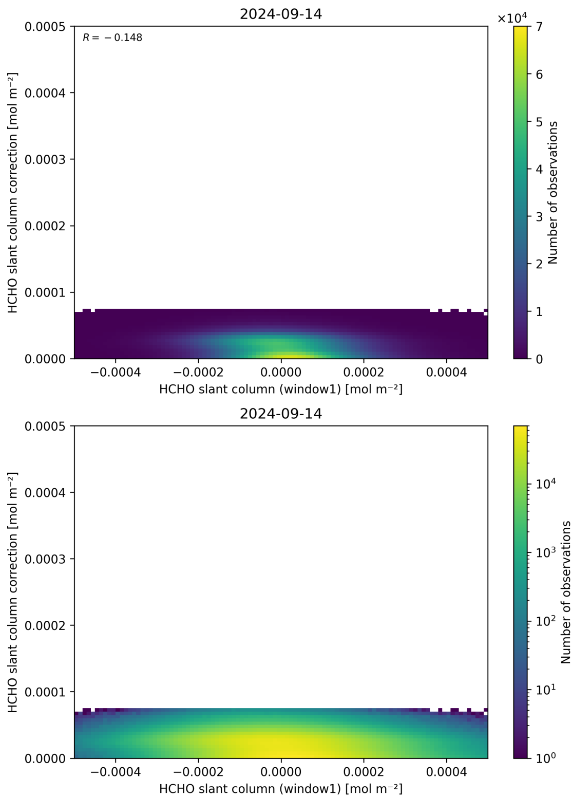
Figure 83: Scatter density plot of “HCHO slant column (window1)” against “HCHO slant column correction” for 2024-09-13 to 2024-09-15.
