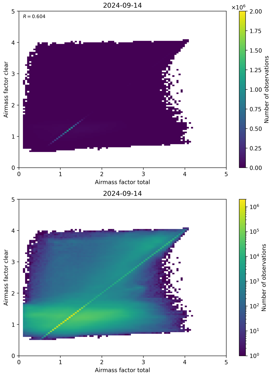
Figure 100: Scatter density plot of “Airmass factor total” against “Airmass factor clear” for 2024-09-13 to 2024-09-15.
