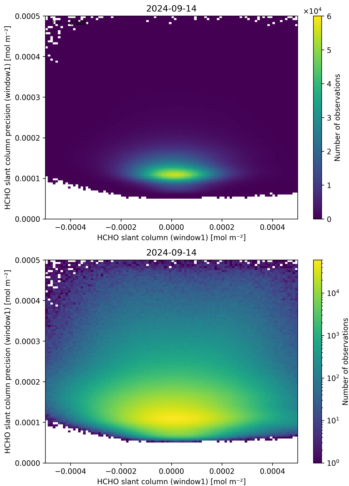
Figure 84: Scatter density plot of “HCHO slant column (window1)” against “HCHO slant column precision (window1)” for 2024-09-13 to 2024-09-15.
