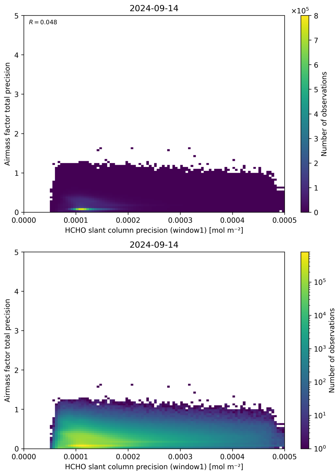
Figure 95: Scatter density plot of “HCHO slant column precision (window1)” against “Airmass factor total precision” for 2024-09-13 to 2024-09-15.
