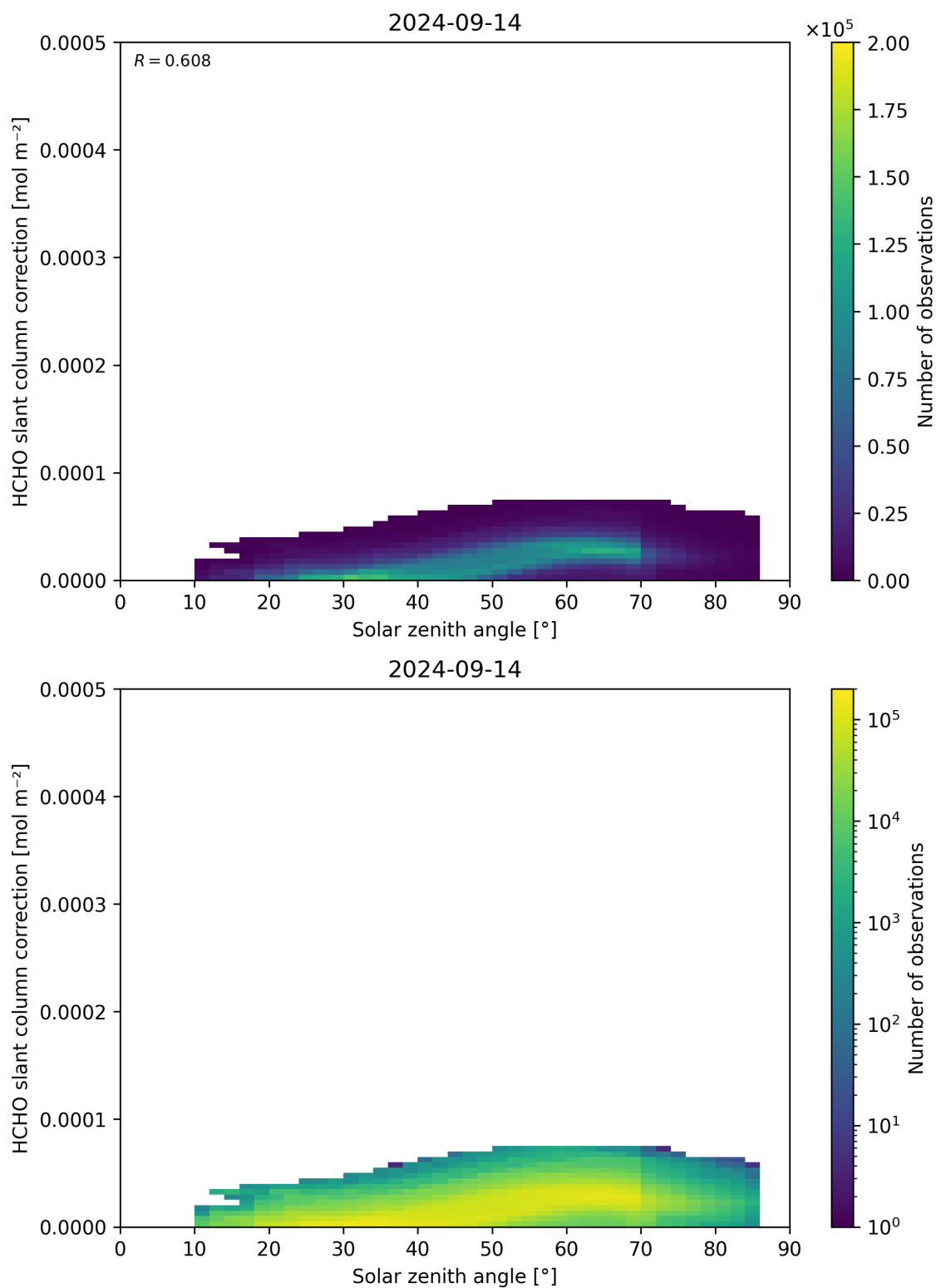
Figure 172: Scatter density plot of “Solar zenith angle” against “HCHO slant column correction” for 2024-09-13 to 2024-09-15.
