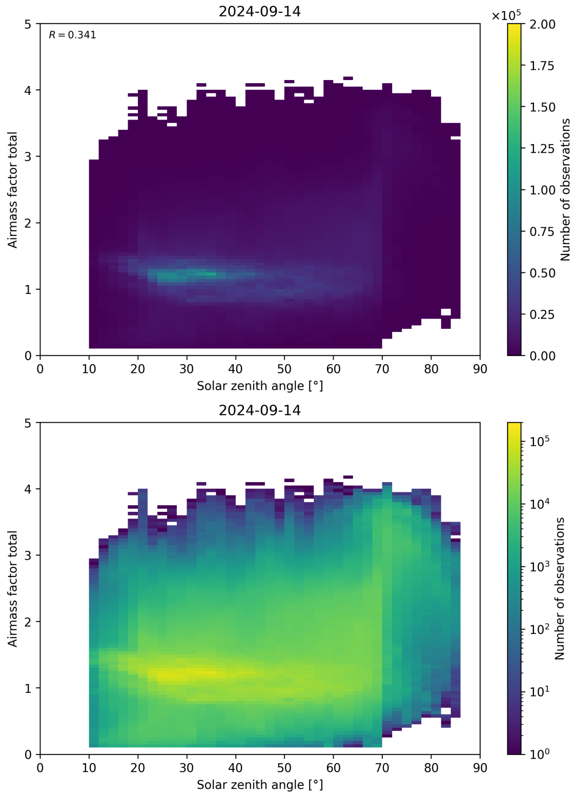
Figure 175: Scatter density plot of “Solar zenith angle” against “Airmass factor total” for 2024-09-13 to 2024-09-15.
