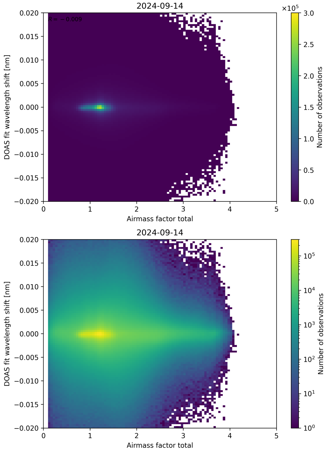
Figure 98: Scatter density plot of “Airmass factor total” against “DOAS fit wavelength shift” for 2024-09-13 to 2024-09-15.
