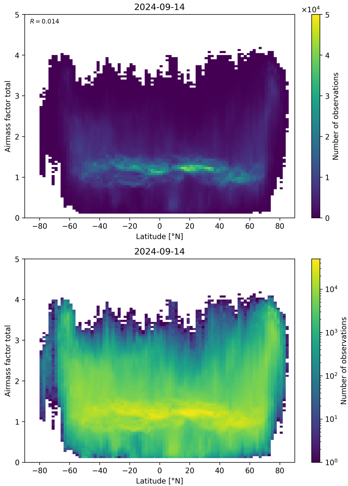
Figure 161: Scatter density plot of “Latitude” against “Airmass factor total” for 2024-09-13 to 2024-09-15.
