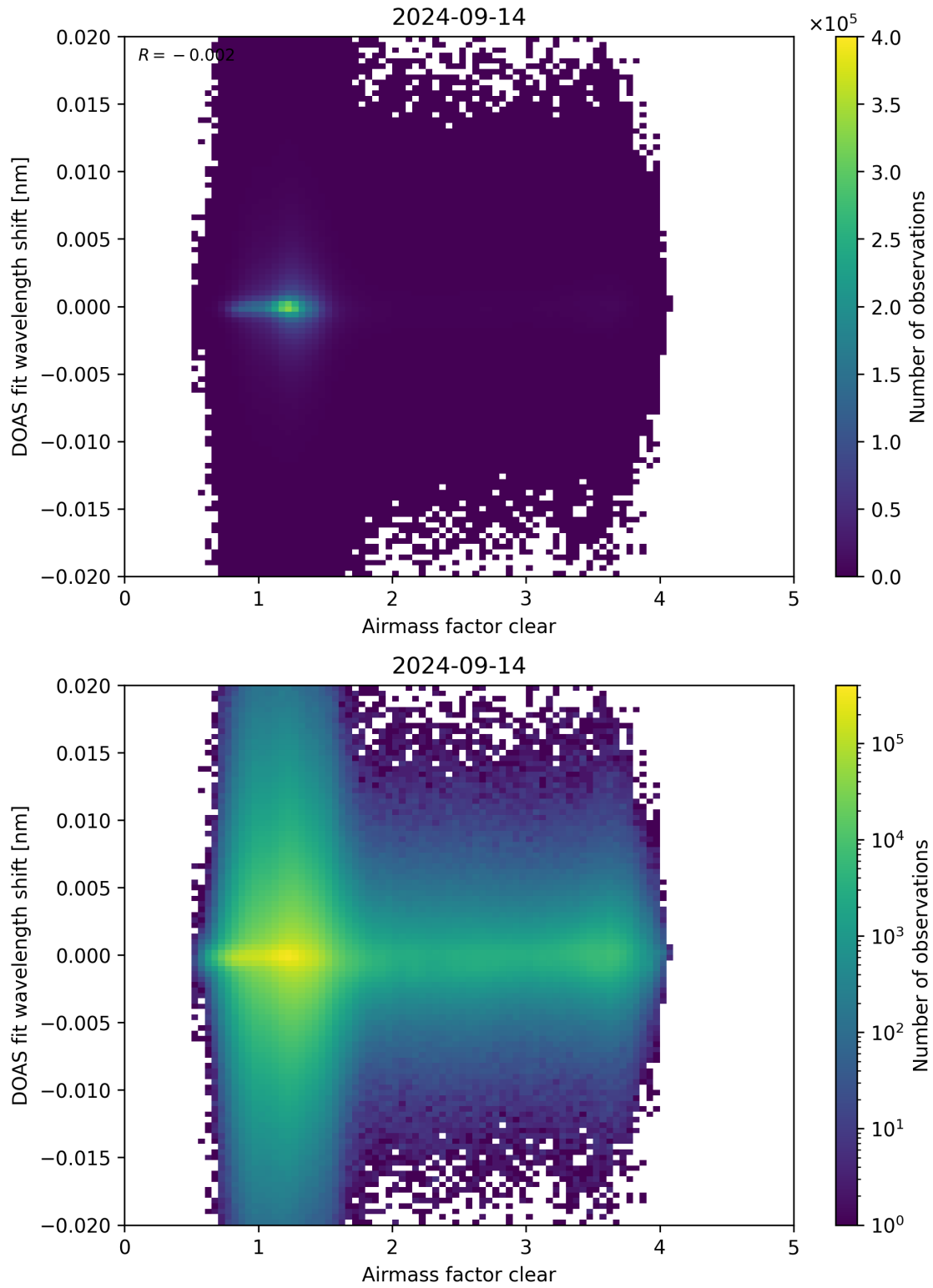
Figure 72: Scatter density plot of “Airmass factor clear” against “DOAS fit wavelength shift” for 2024-09-13 to 2024-09-15.
