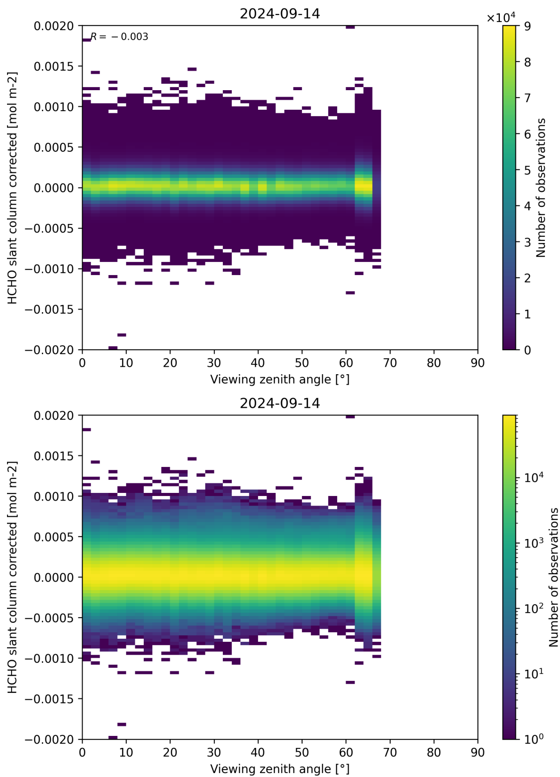
Figure 186: Scatter density plot of “Viewing zenith angle” against “HCHO slant column corrected” for 2024-09-13 to 2024-09-15.
