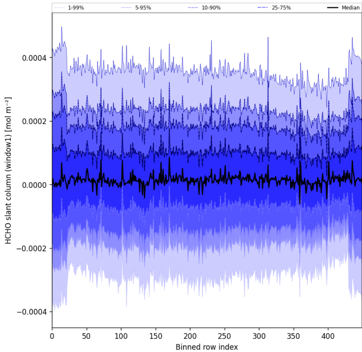
Figure 52: Along track statistics of “HCHO slant column (window1)” for 2024-09-13 to 2024-09-15
