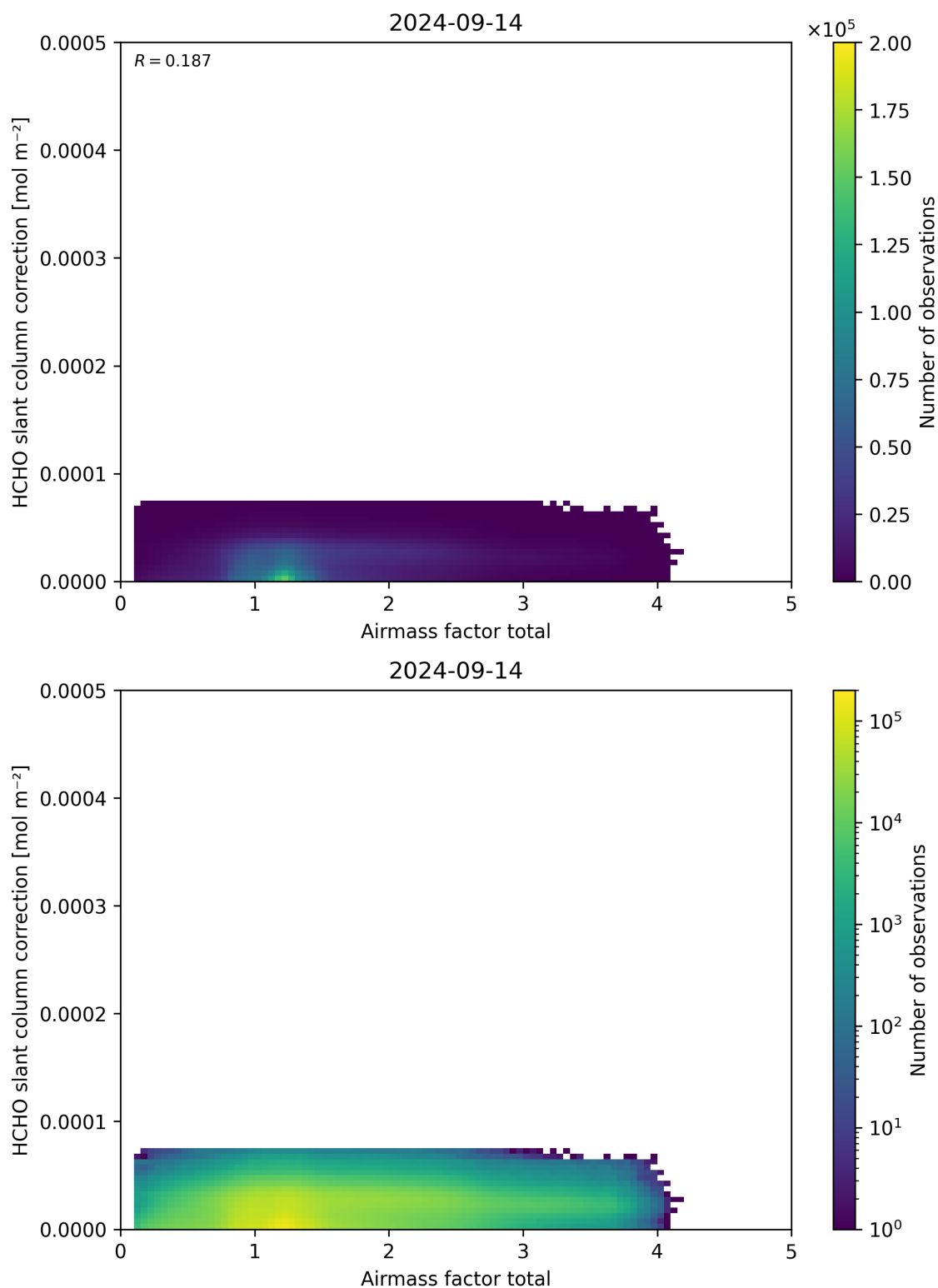
Figure 102: Scatter density plot of “Airmass factor total” against “HCHO slant column correction” for 2024-09-13 to 2024-09-15.
