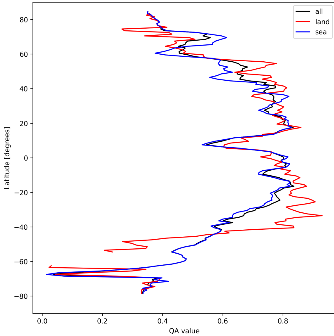
Figure 20: Zonal average of “QA value” for 2024-09-13 to 2024-09-15.
