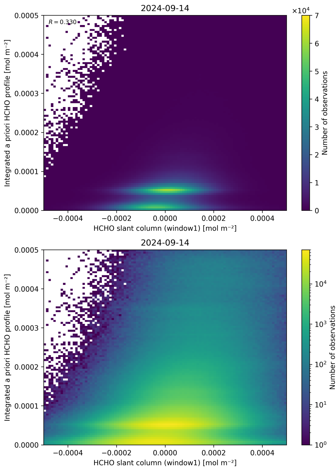
Figure 87: Scatter density plot of “HCHO slant column (window1)” against “Integrated a priori HCHO profile” for 2024-09-13 to 2024-09-15.
