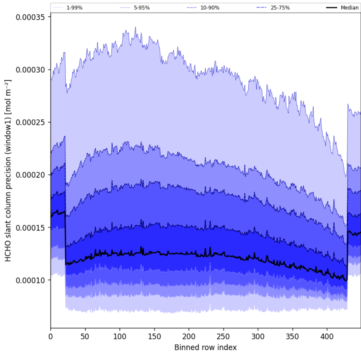
Figure 53: Along track statistics of “HCHO slant column precision (window1)” for 2024-09-13 to 2024-09-15
