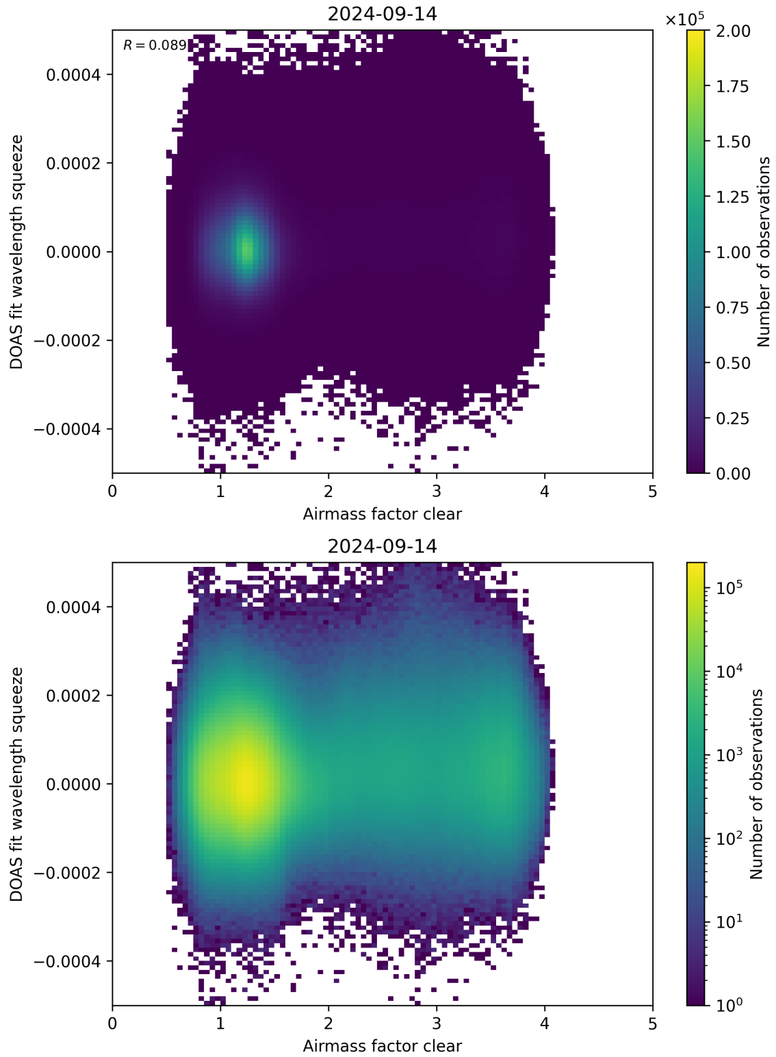
Figure 73: Scatter density plot of “Airmass factor clear” against “DOAS fit wavelength squeeze” for 2024-09-13 to 2024-09-15.
