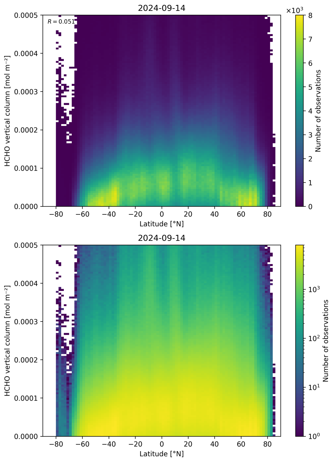
Figure 163: Scatter density plot of “Latitude” against “HCHO vertical column” for 2024-09-13 to 2024-09-15.
