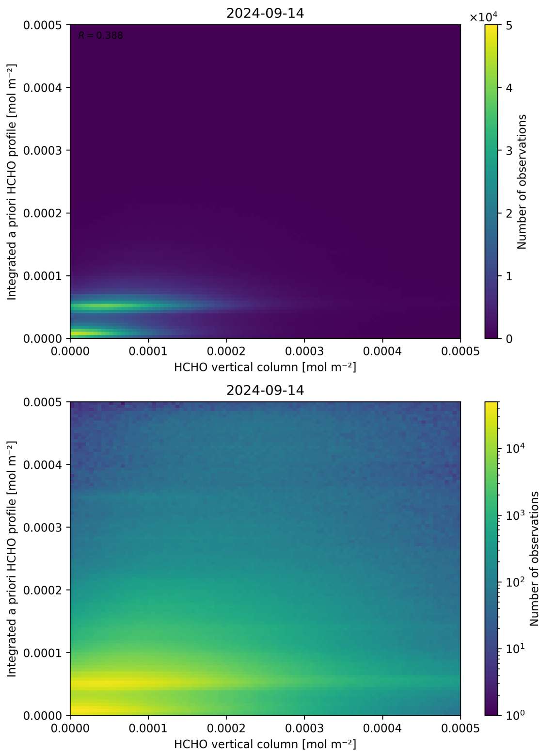
Figure 135: Scatter density plot of “HCHO vertical column” against “Integrated a priori HCHO profile” for 2024-09-13 to 2024-09-15.
