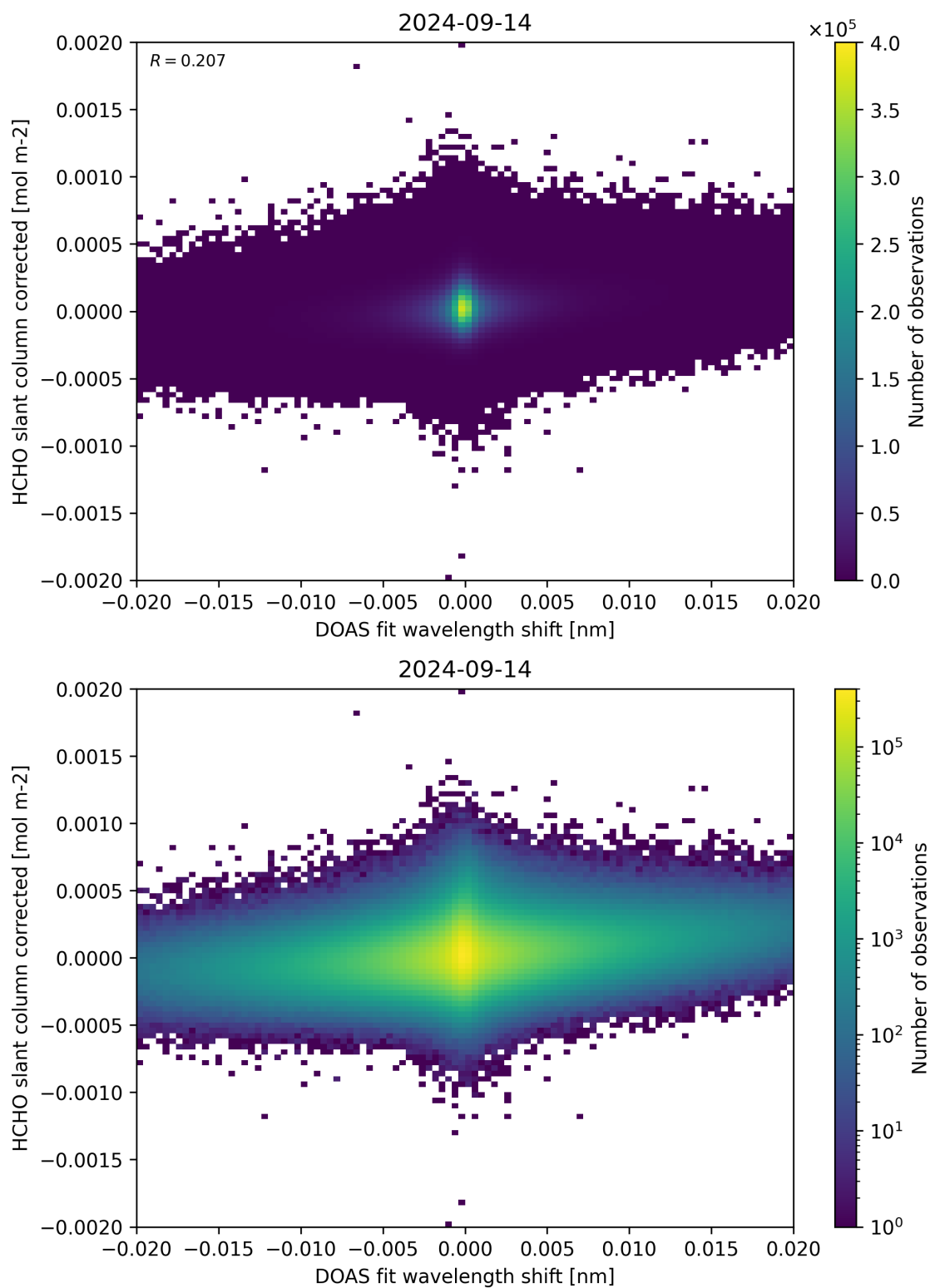
Figure 66: Scatter density plot of “DOAS fit wavelength shift” against “HCHO slant column corrected” for 2024-09-13 to 2024-09-15.
