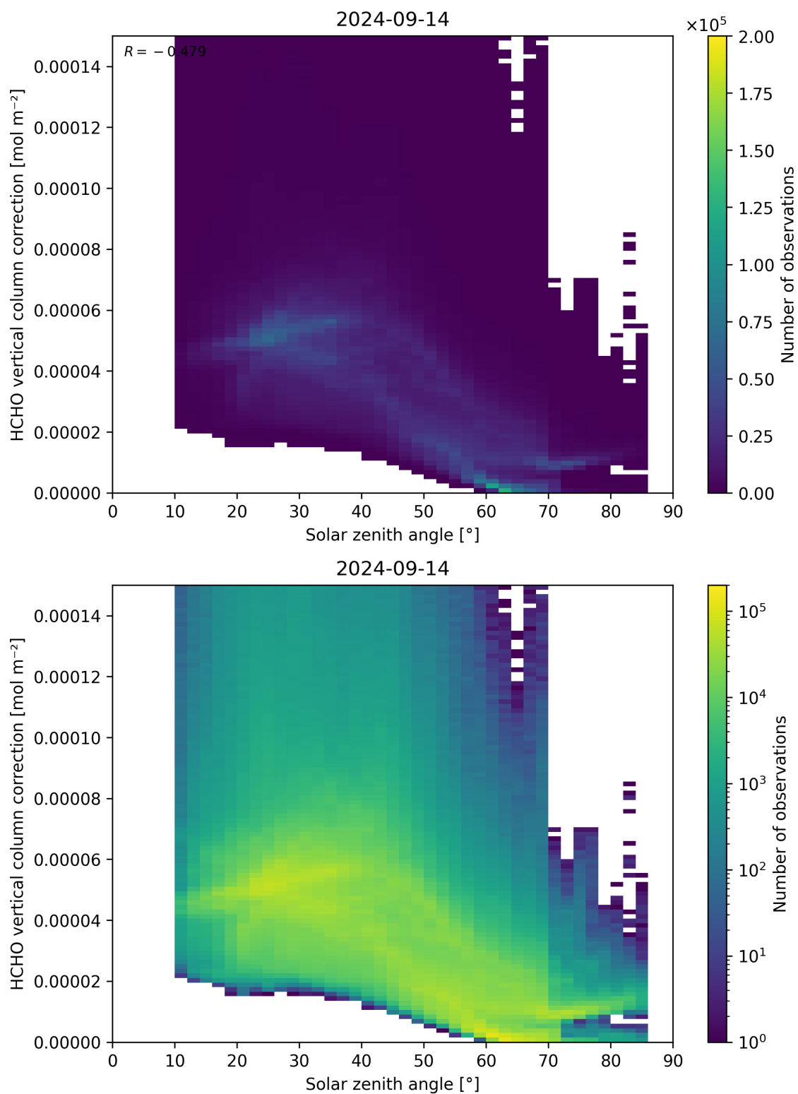
Figure 178: Scatter density plot of “Solar zenith angle” against “HCHO vertical column correction” for 2024-09-13 to 2024-09-15.
