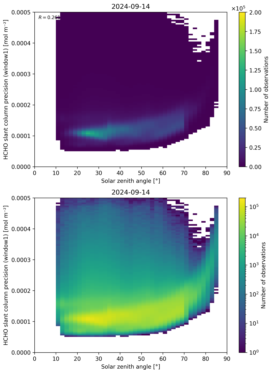
Figure 174: Scatter density plot of “Solar zenith angle” against “HCHO slant column precision (window1)” for 2024-09-13 to 2024-09-15.
