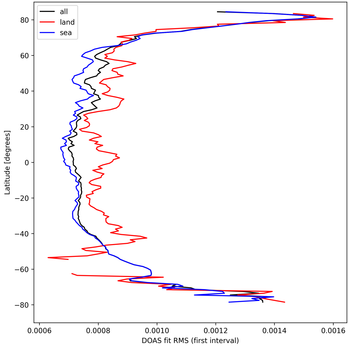
Figure 32: Zonal average of “DOAS fit RMS (first interval)” for 2024-09-13 to 2024-09-15.
