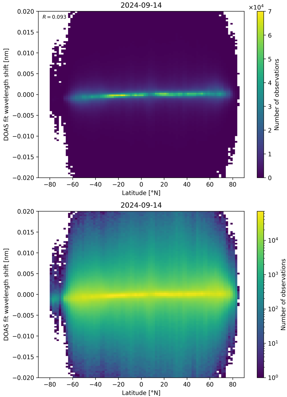
Figure 154: Scatter density plot of “Latitude” against “DOAS fit wavelength shift” for 2024-09-13 to 2024-09-15.
