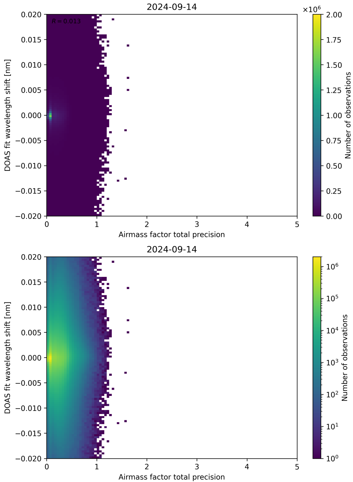
Figure 106: Scatter density plot of “Airmass factor total precision” against “DOAS fit wavelength shift” for 2024-09-13 to 2024-09-15.
