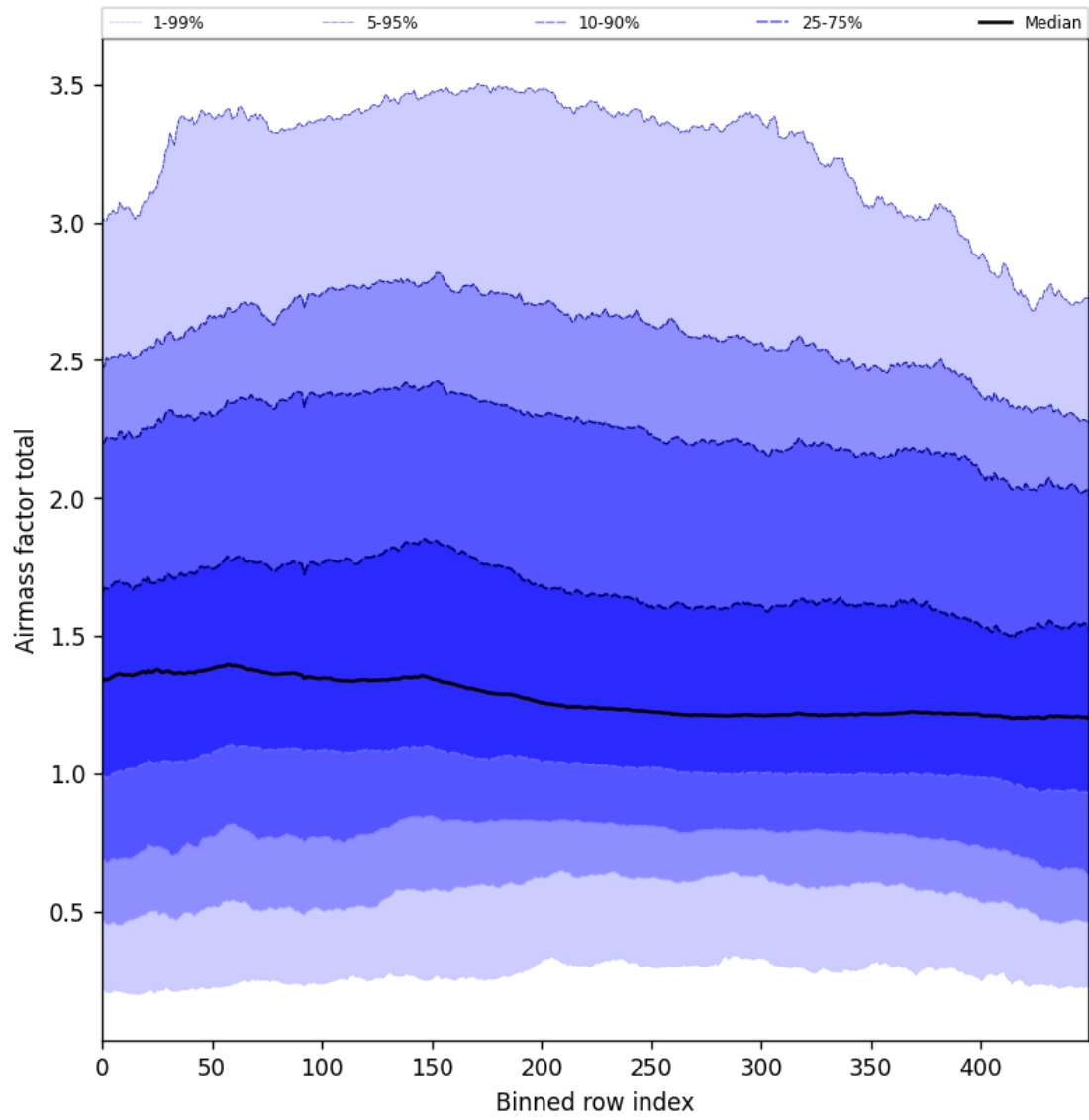
Figure 54: Along track statistics of “Airmass factor total” for 2024-09-13 to 2024-09-15
