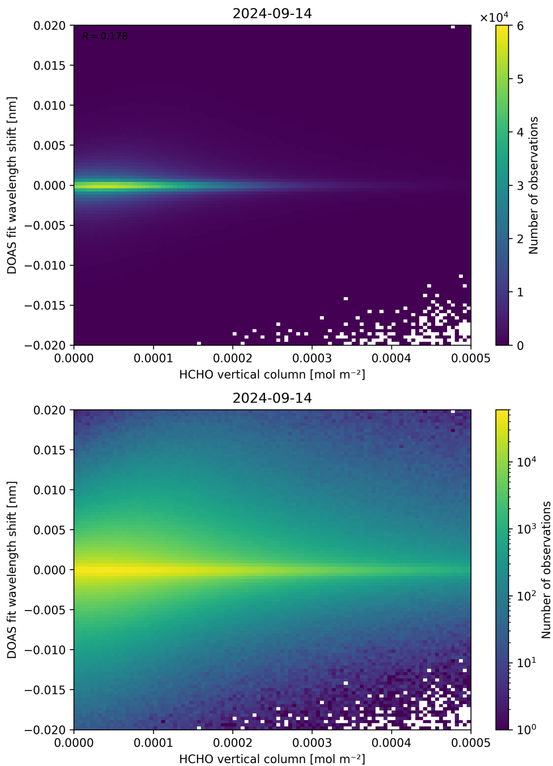
Figure 124: Scatter density plot of “HCHO vertical column” against “DOAS fit wavelength shift” for 2024-09-13 to 2024-09-15.
