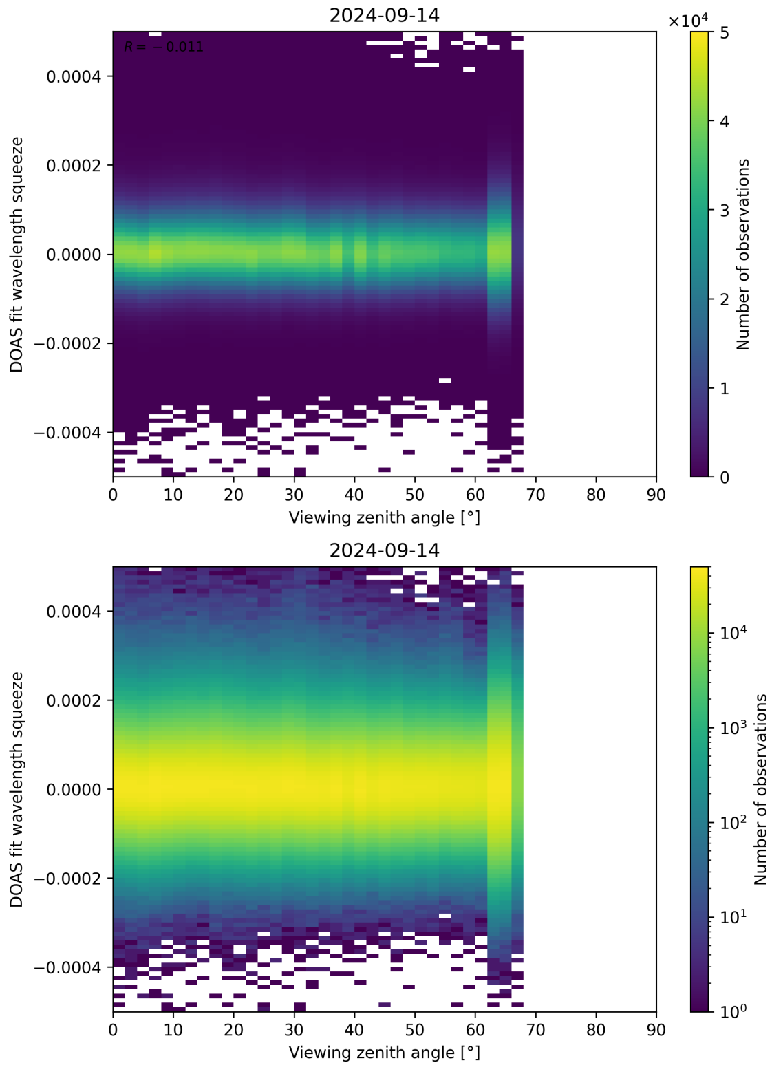
Figure 184: Scatter density plot of “Viewing zenith angle” against “DOAS fit wavelength squeeze” for 2024-09-13 to 2024-09-15.
