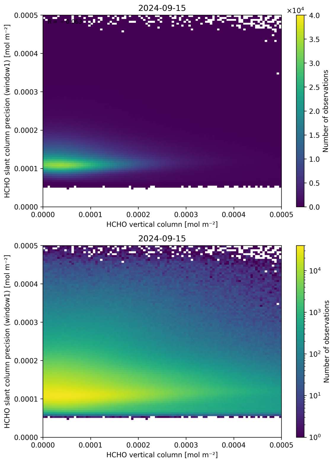
Figure 130: Scatter density plot of “HCHO vertical column” against “HCHO slant column precision (window1)” for 2024-09-14 to 2024-09-16.
