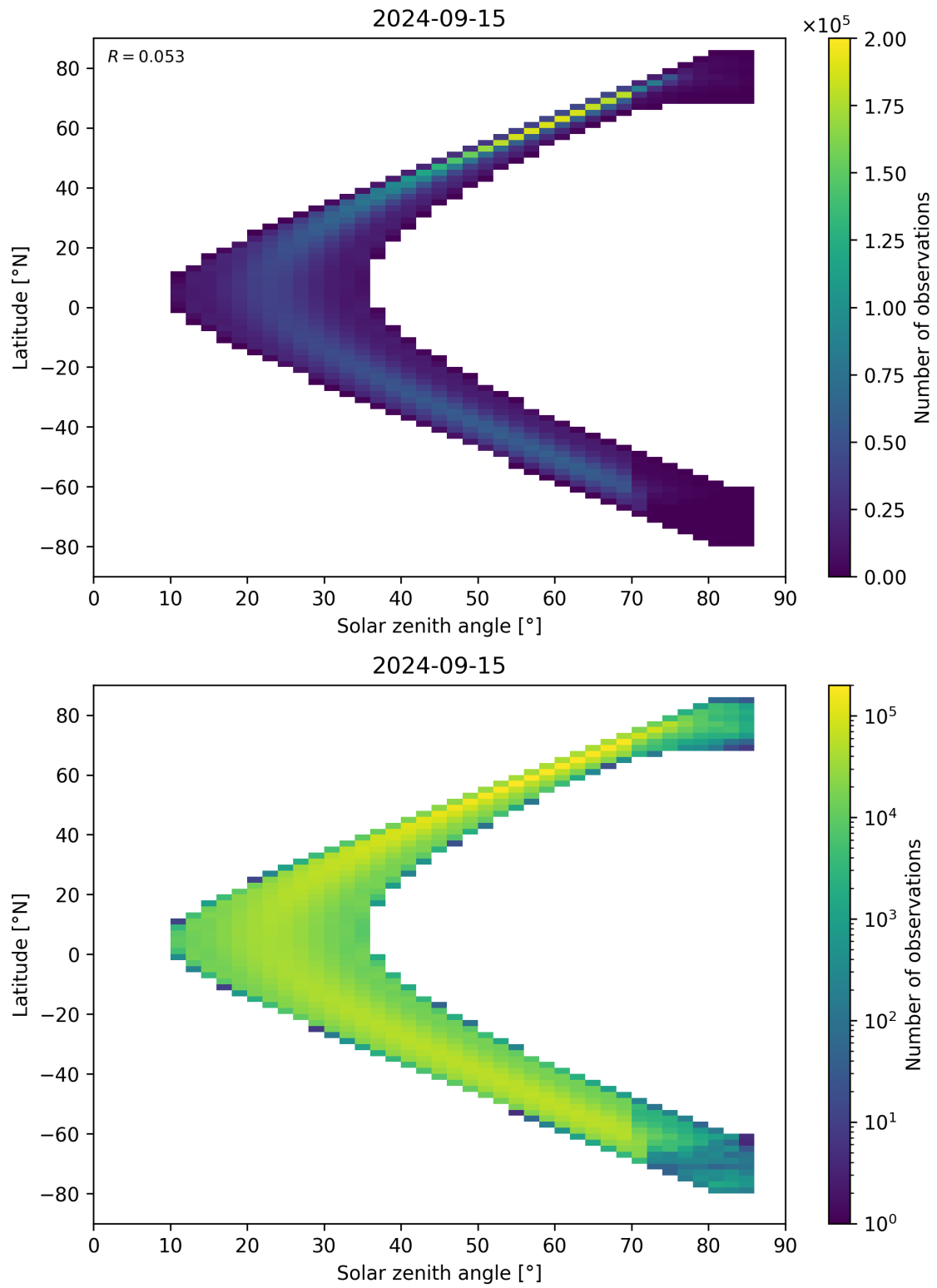
Figure 181: Scatter density plot of “Solar zenith angle” against “Latitude” for 2024-09-14 to 2024-09-16.
