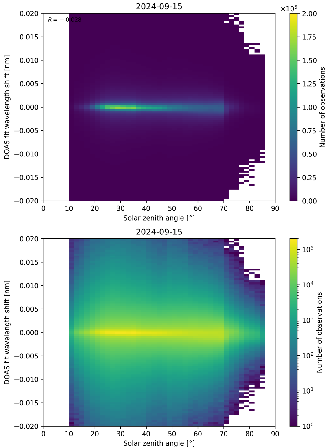
Figure 168: Scatter density plot of “Solar zenith angle” against “DOAS fit wavelength shift” for 2024-09-14 to 2024-09-16.
