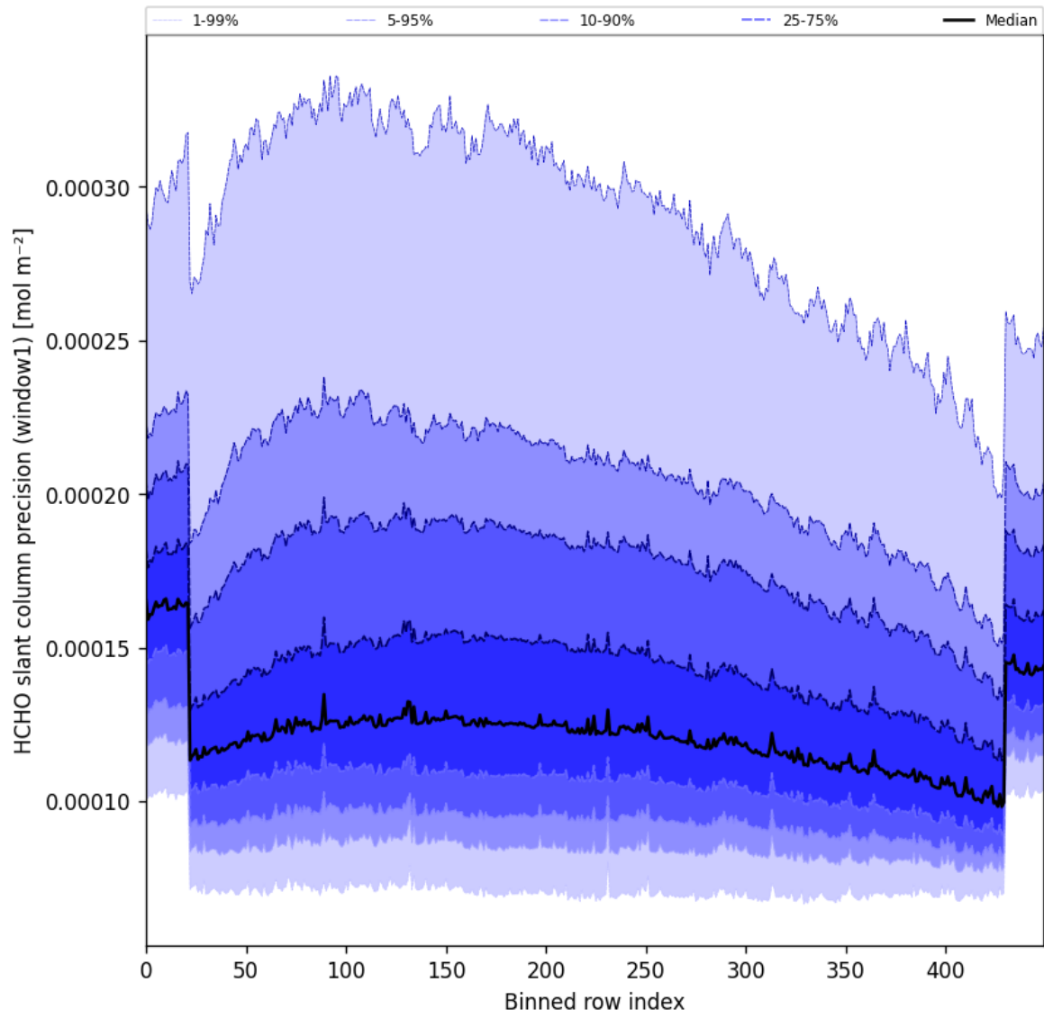
Figure 53: Along track statistics of “HCHO slant column precision (window1)” for 2024-09-14 to 2024-09-16
