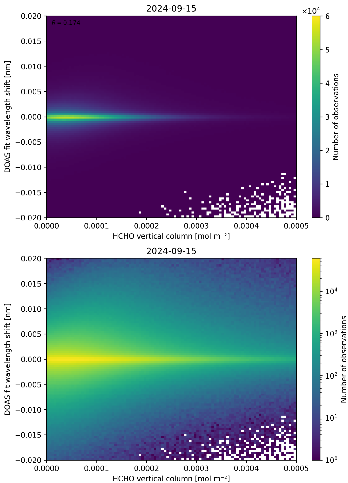
Figure 124: Scatter density plot of “HCHO vertical column” against “DOAS fit wavelength shift” for 2024-09-14 to 2024-09-16.
