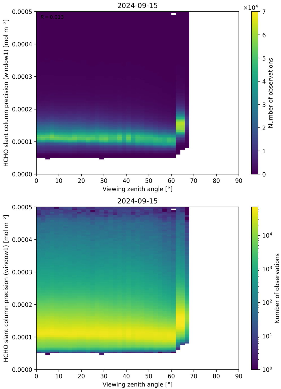
Figure 189: Scatter density plot of “Viewing zenith angle” against “HCHO slant column precision (window1)” for 2024-09-14 to 2024-09-16.
