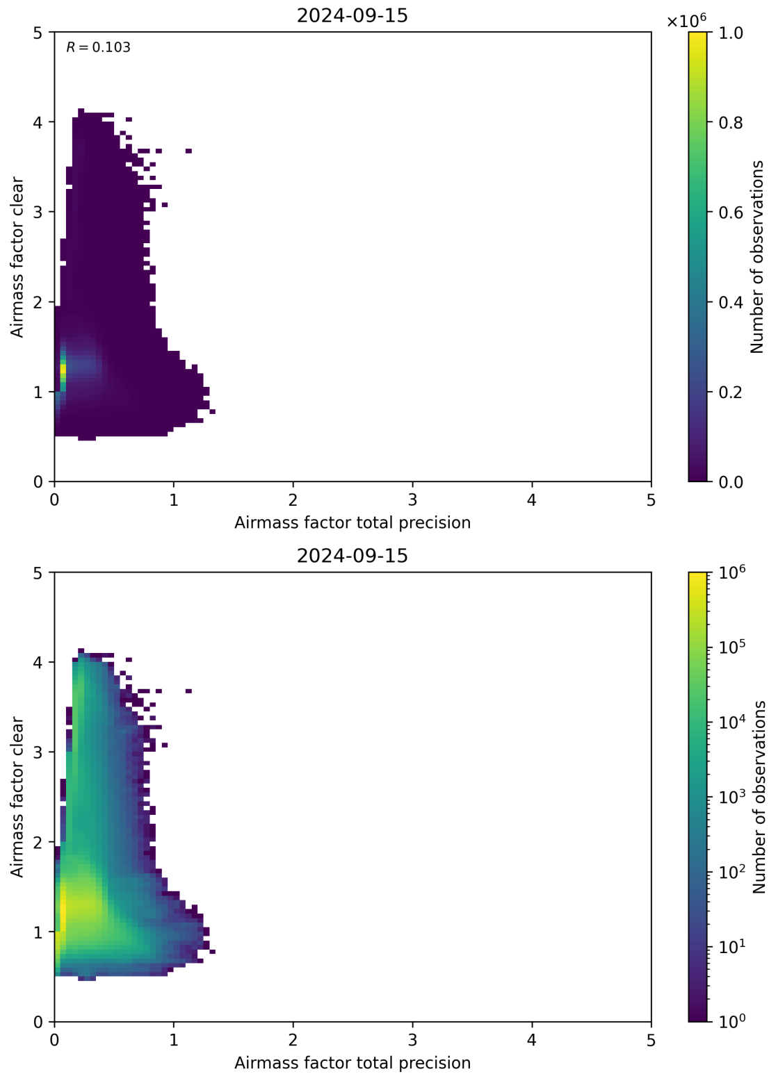
Figure 108: Scatter density plot of “Airmass factor total precision” against “Airmass factor clear” for 2024-09-14 to 2024-09-16.
