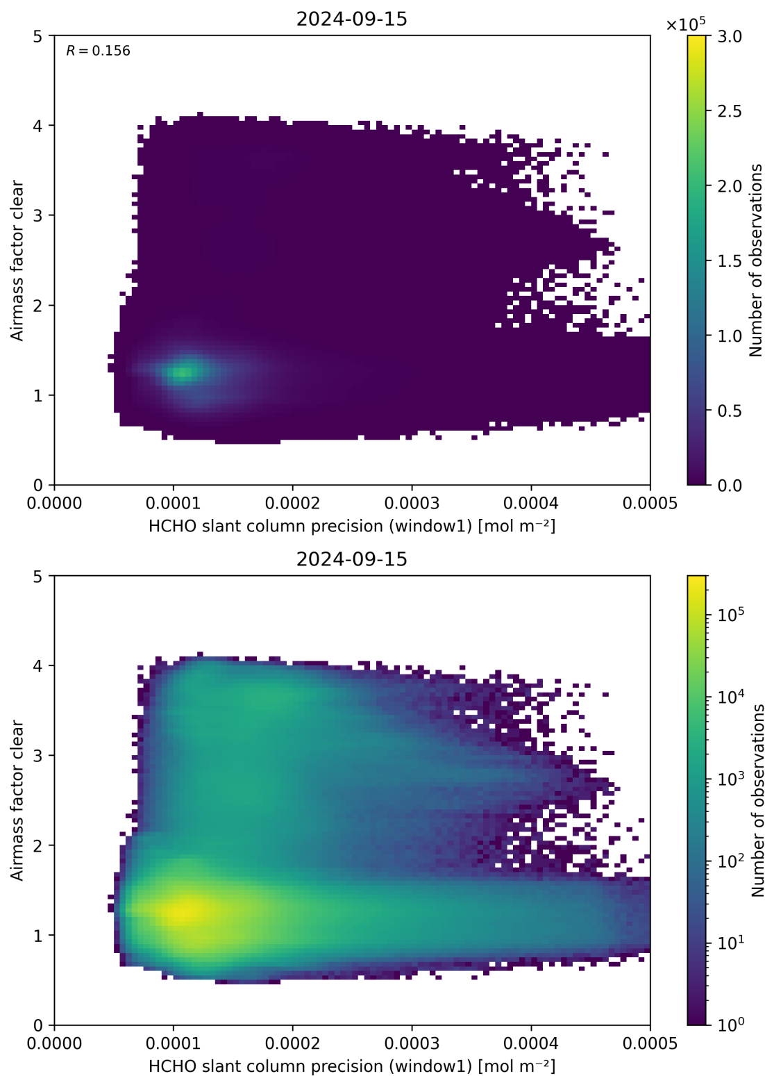
Figure 91: Scatter density plot of “HCHO slant column precision (window1)” against “Airmass factor clear” for 2024-09-14 to 2024-09-16.
