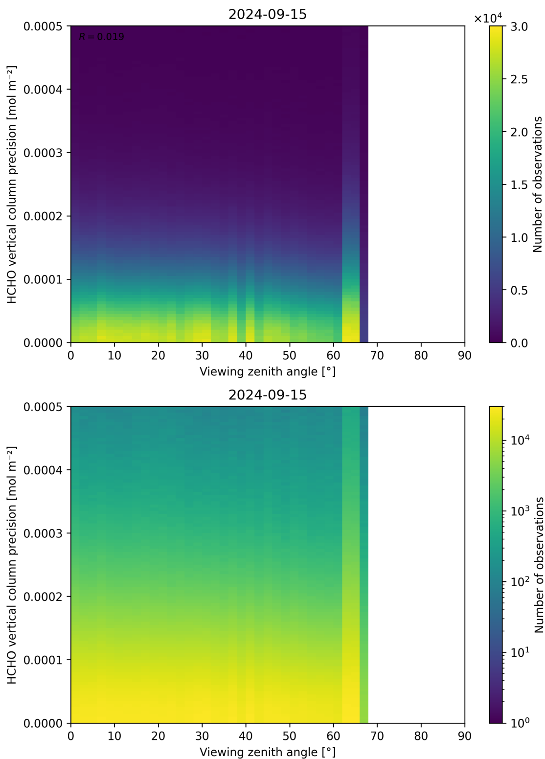
Figure 194: Scatter density plot of “Viewing zenith angle” against “HCHO vertical column precision” for 2024-09-14 to 2024-09-16.
