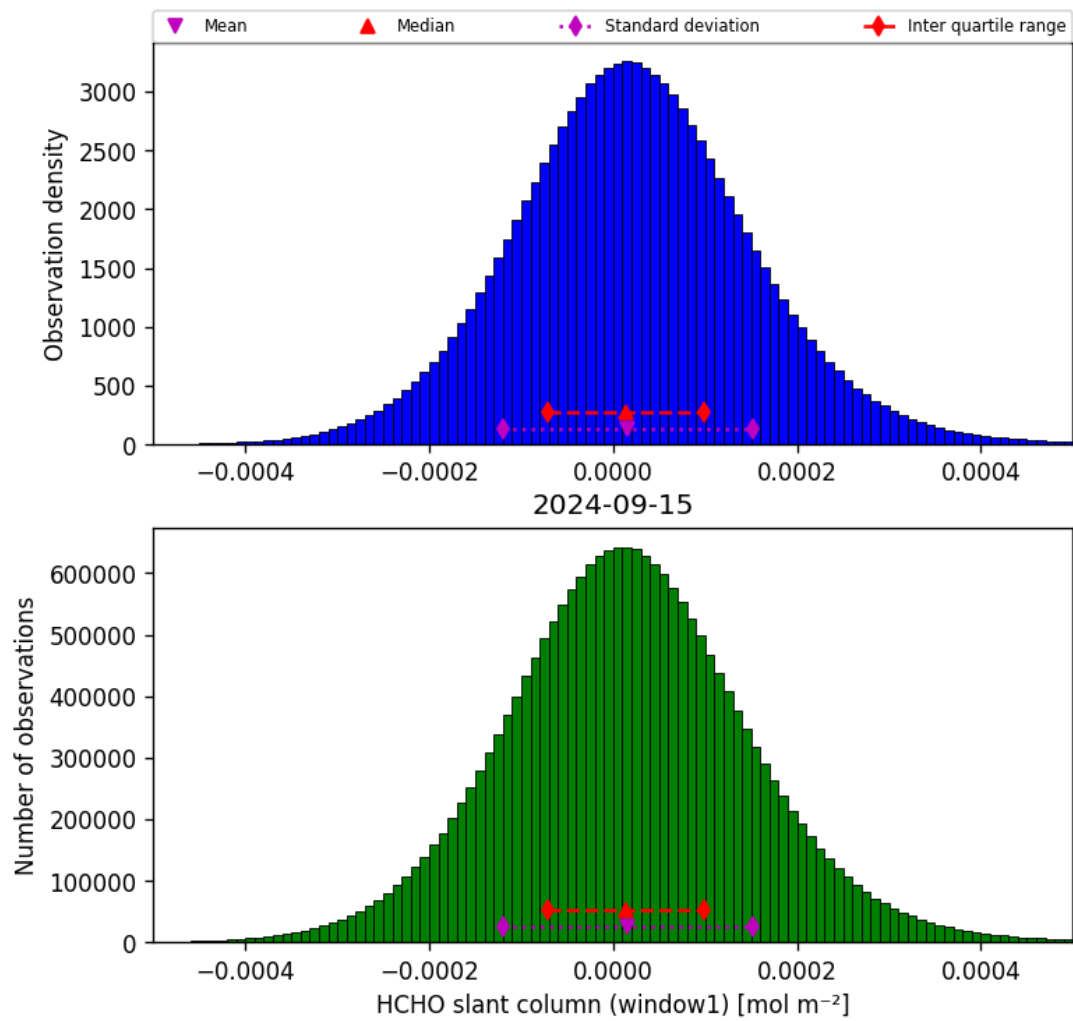
Figure 38: Histogram of “HCHO slant column (window1)” for 2024-09-14 to 2024-09-16
