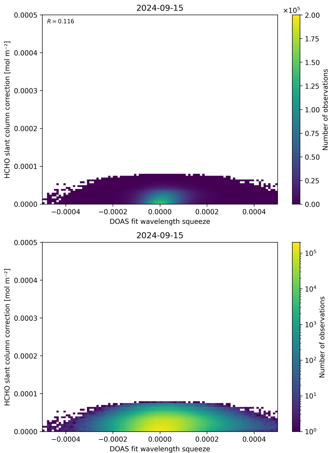
Figure 70: Scatter density plot of “DOAS fit wavelength squeeze” against “HCHO slant column correction” for 2024-09-14 to 2024-09-16.
