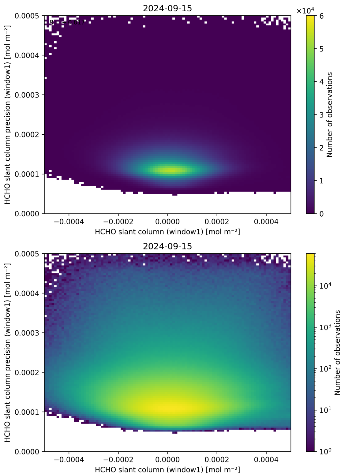
Figure 84: Scatter density plot of “HCHO slant column (window1)” against “HCHO slant column precision (window1)” for 2024-09-14 to 2024-09-16.
