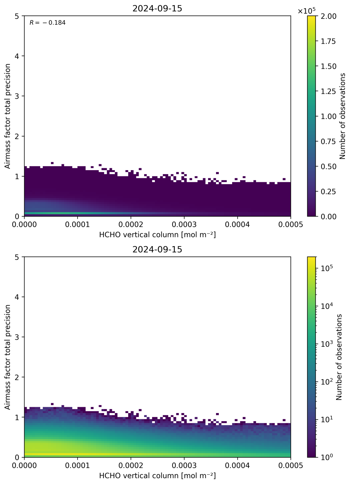
Figure 132: Scatter density plot of “HCHO vertical column” against “Airmass factor total precision” for 2024-09-14 to 2024-09-16.
