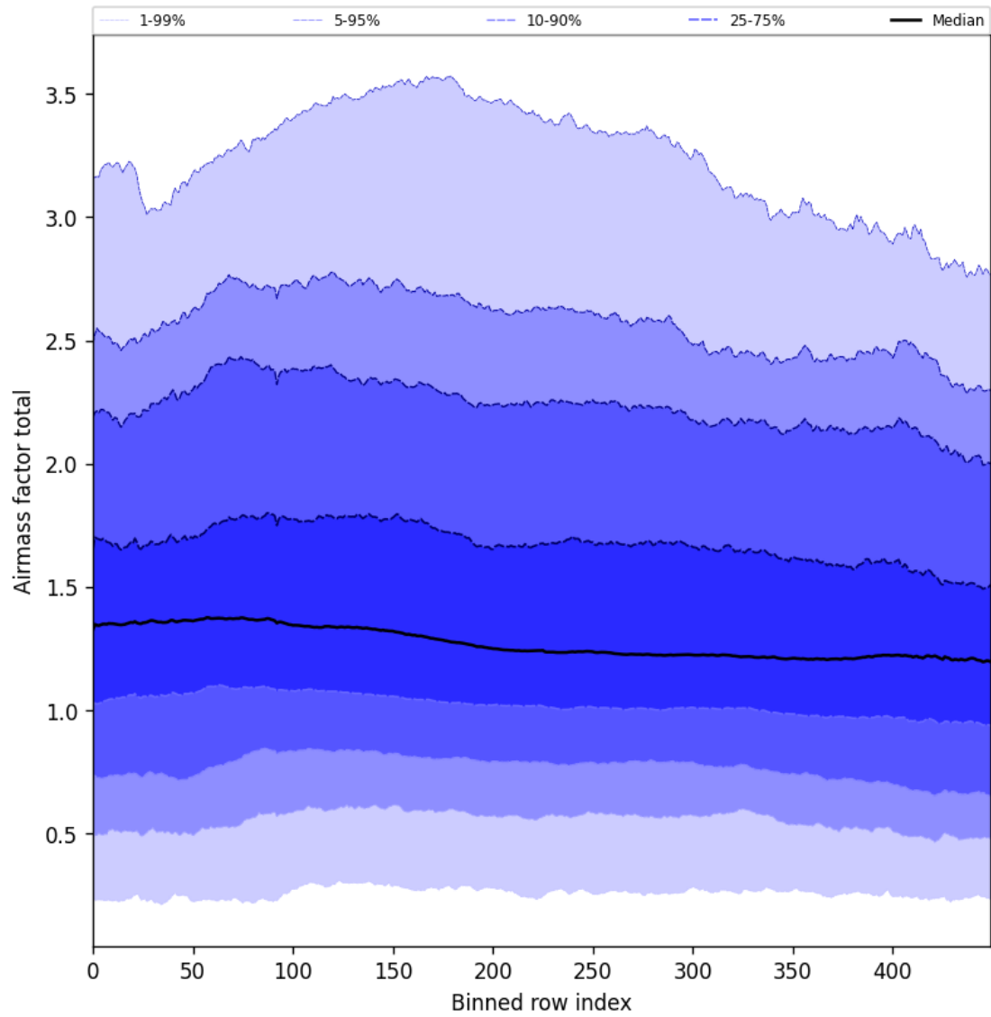
Figure 54: Along track statistics of “Airmass factor total” for 2024-09-14 to 2024-09-16
