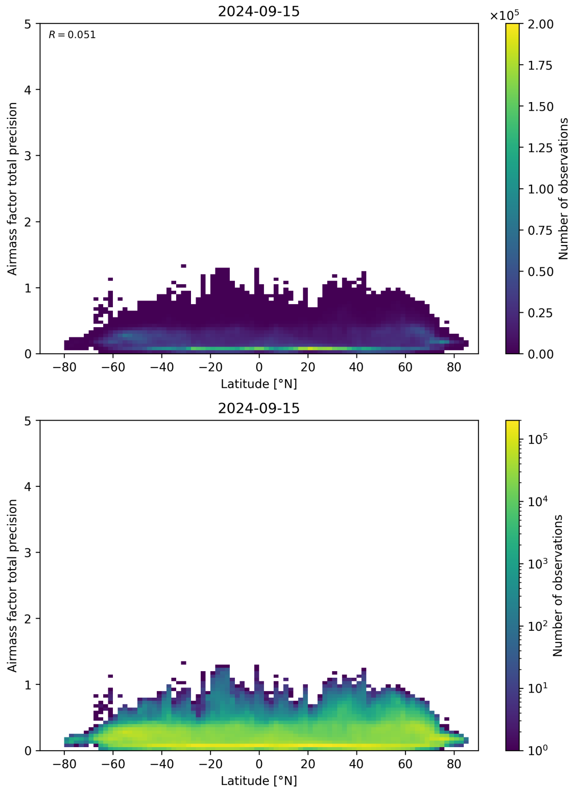
Figure 162: Scatter density plot of “Latitude” against “Airmass factor total precision” for 2024-09-14 to 2024-09-16.
