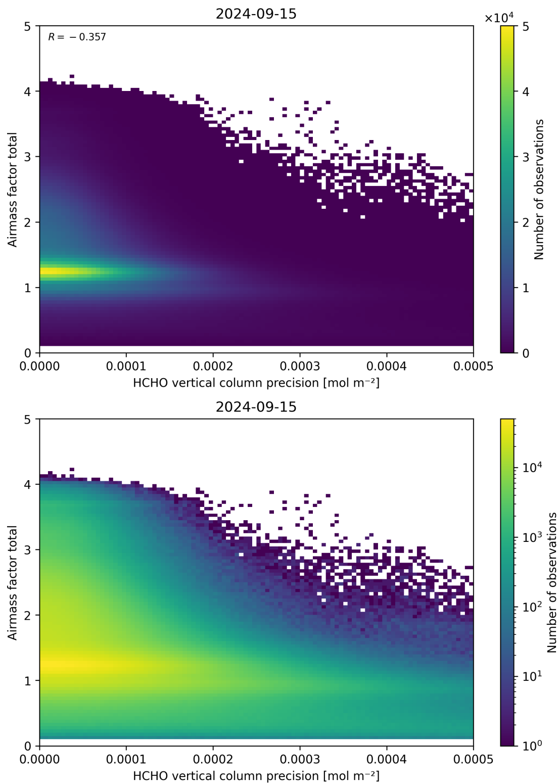
Figure 144: Scatter density plot of “HCHO vertical column precision” against “Airmass factor total” for 2024-09-14 to 2024-09-16.
