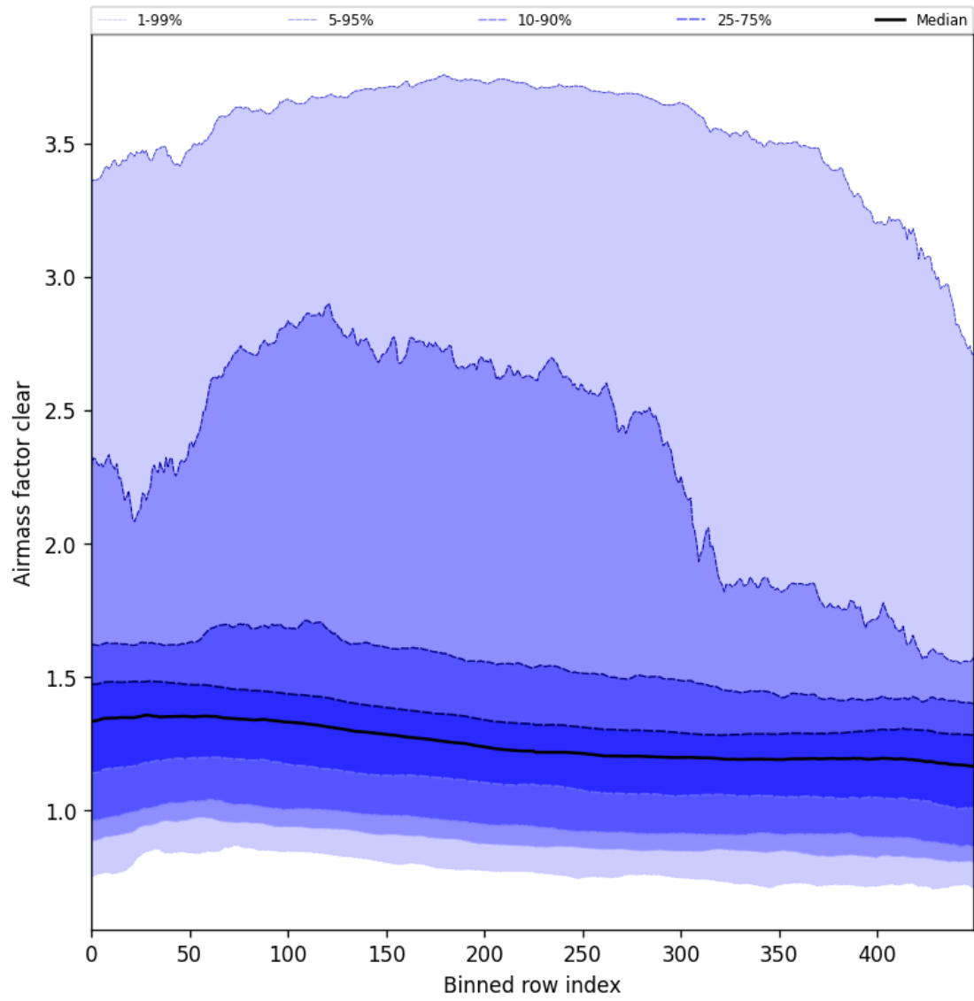
Figure 56: Along track statistics of “Airmass factor clear” for 2024-09-14 to 2024-09-16
