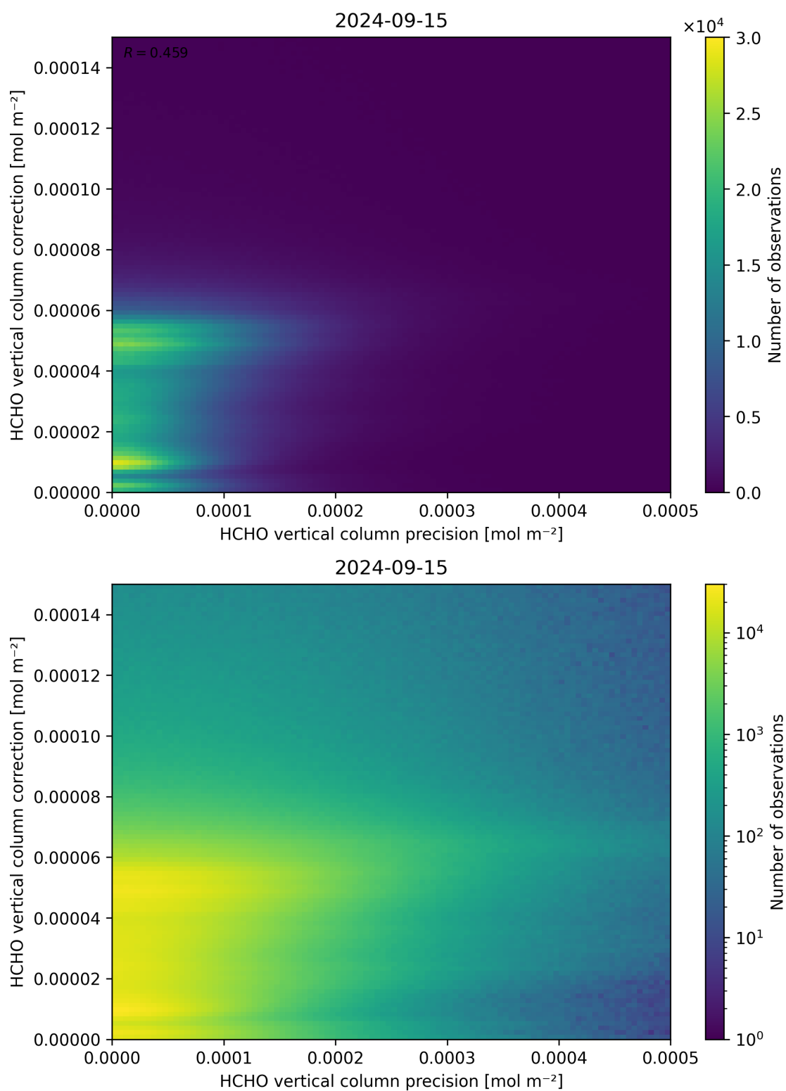
Figure 146: Scatter density plot of “HCHO vertical column precision” against “HCHO vertical column correction” for 2024-09-14 to 2024-09-16.
