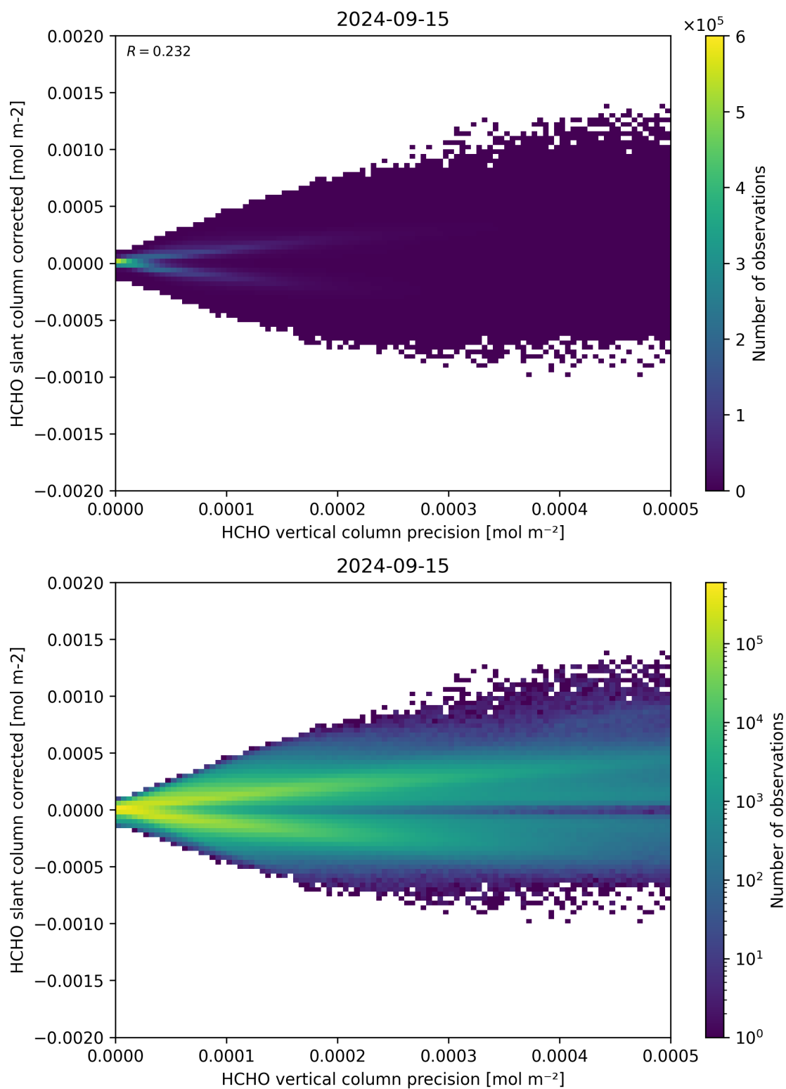
Figure 140: Scatter density plot of “HCHO vertical column precision” against “HCHO slant column corrected” for 2024-09-14 to 2024-09-16.
