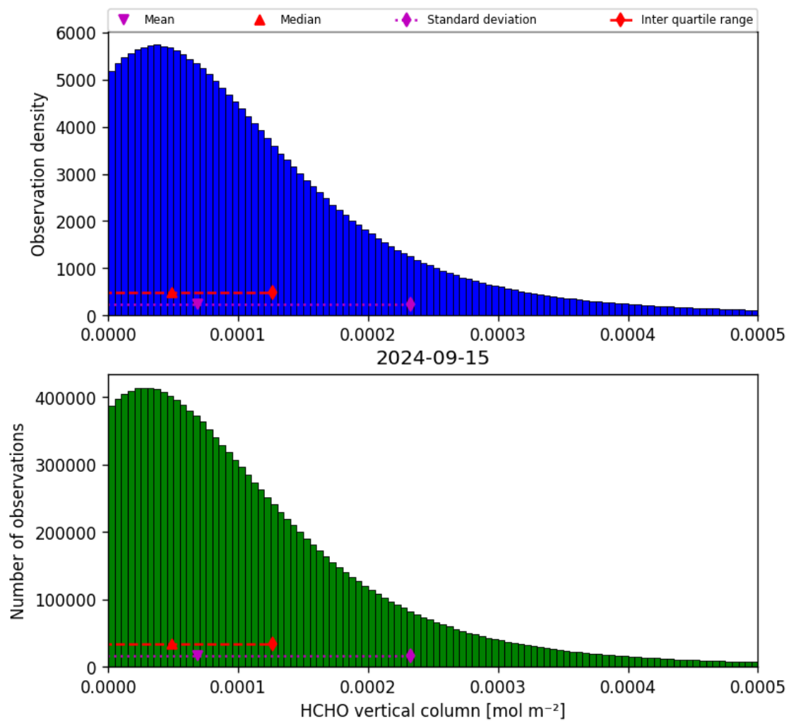
Figure 35: Histogram of “HCHO vertical column” for 2024-09-14 to 2024-09-16
