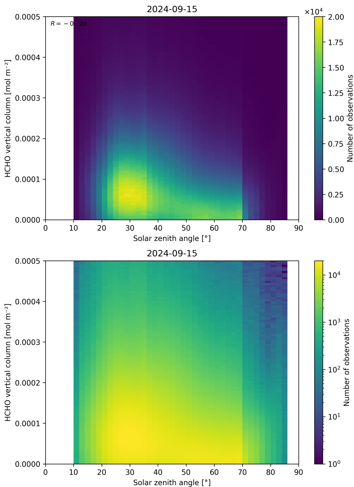
Figure 177: Scatter density plot of “Solar zenith angle” against “HCHO vertical column” for 2024-09-14 to 2024-09-16.
