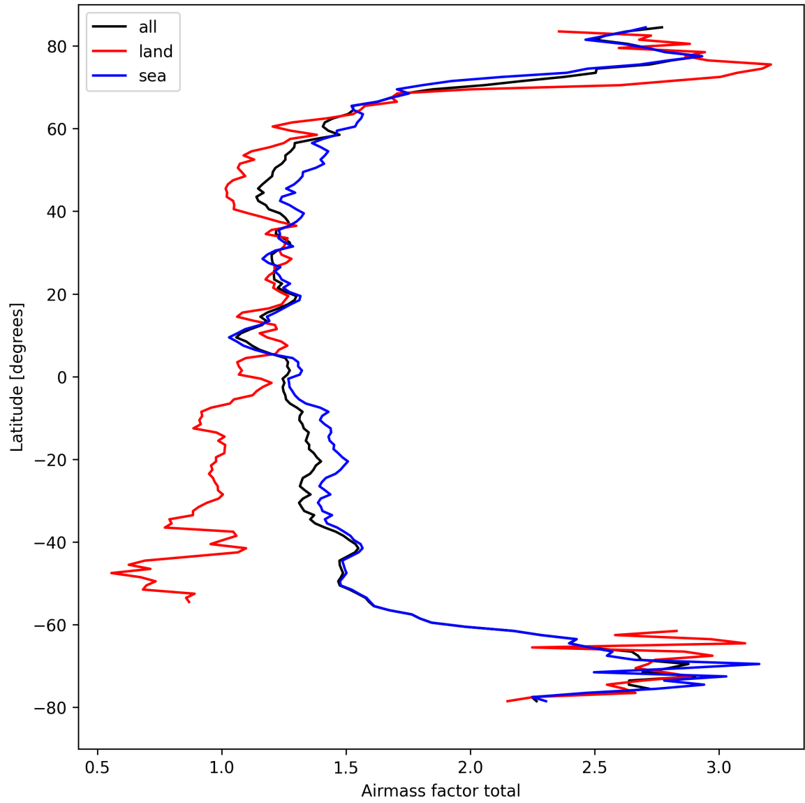
Figure 26: Zonal average of “Airmass factor total” for 2024-09-14 to 2024-09-16.
