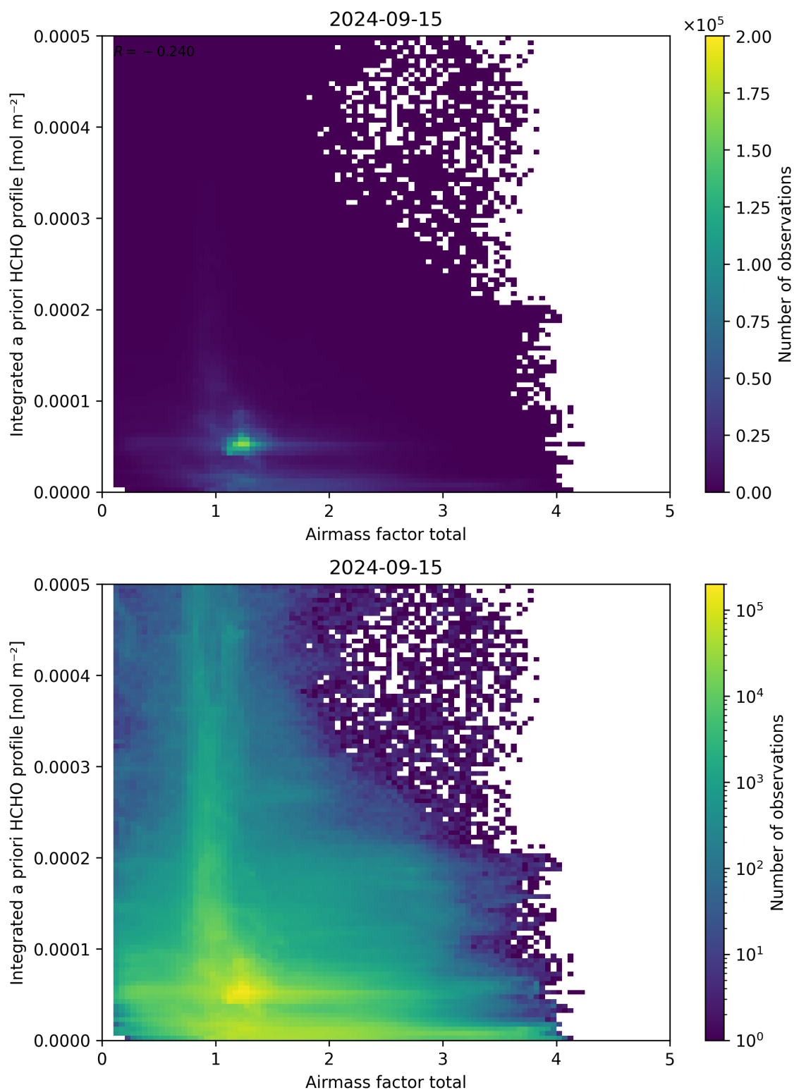
Figure 104: Scatter density plot of “Airmass factor total” against “Integrated a priori HCHO profile” for 2024-09-14 to 2024-09-16.
