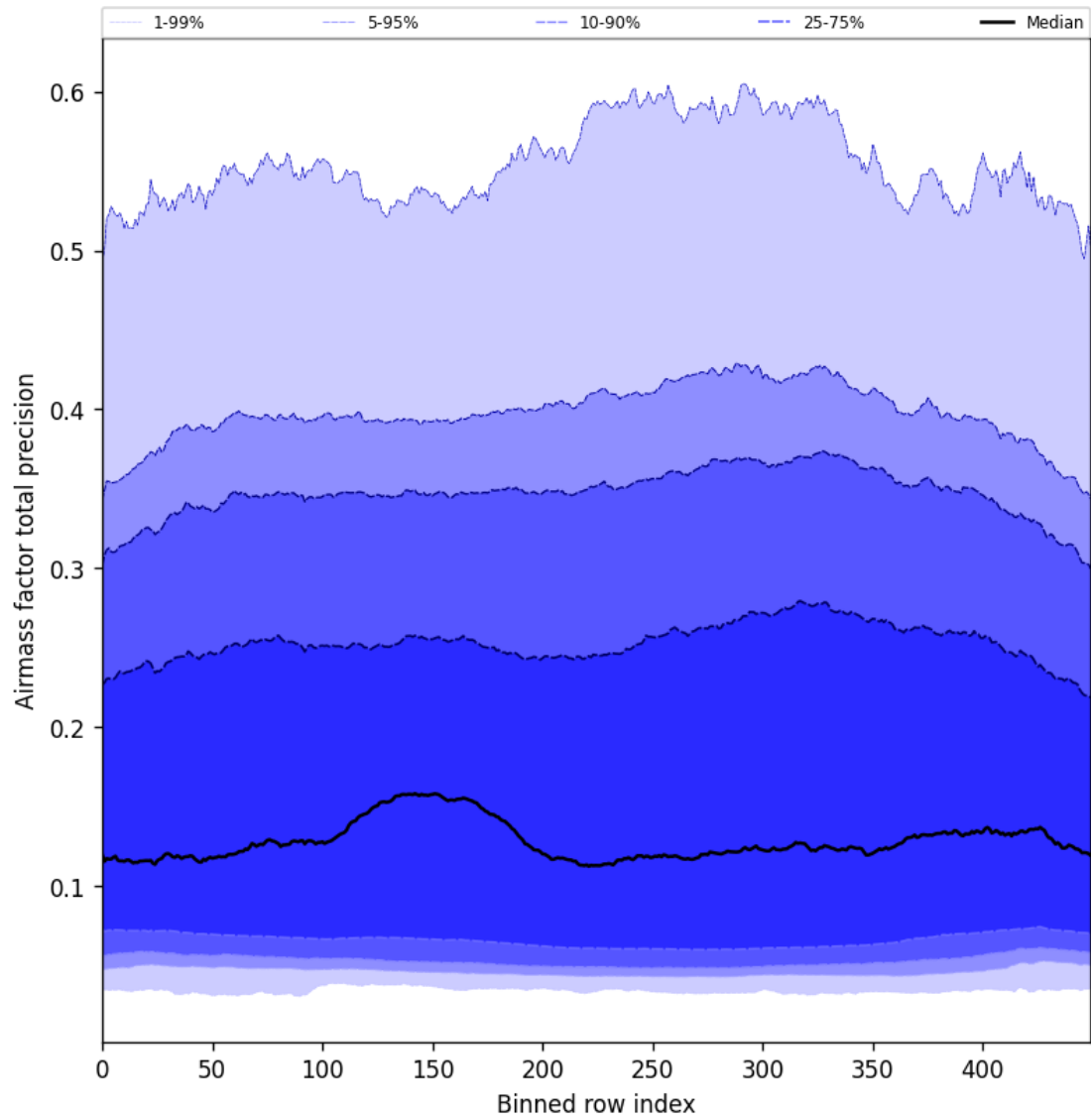
Figure 55: Along track statistics of “Airmass factor total precision” for 2024-09-14 to 2024-09-16
