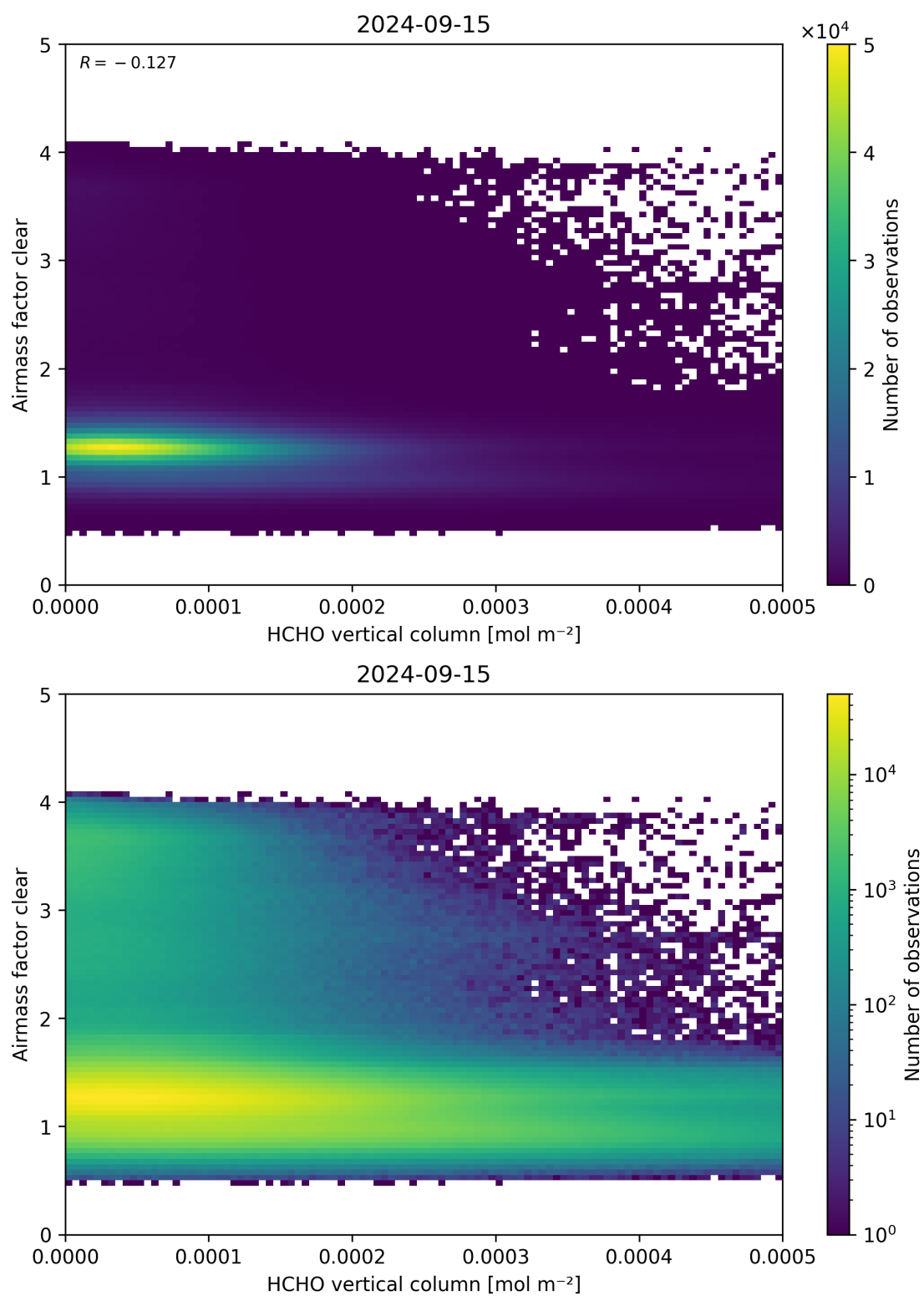
Figure 126: Scatter density plot of “HCHO vertical column” against “Airmass factor clear” for 2024-09-14 to 2024-09-16.
