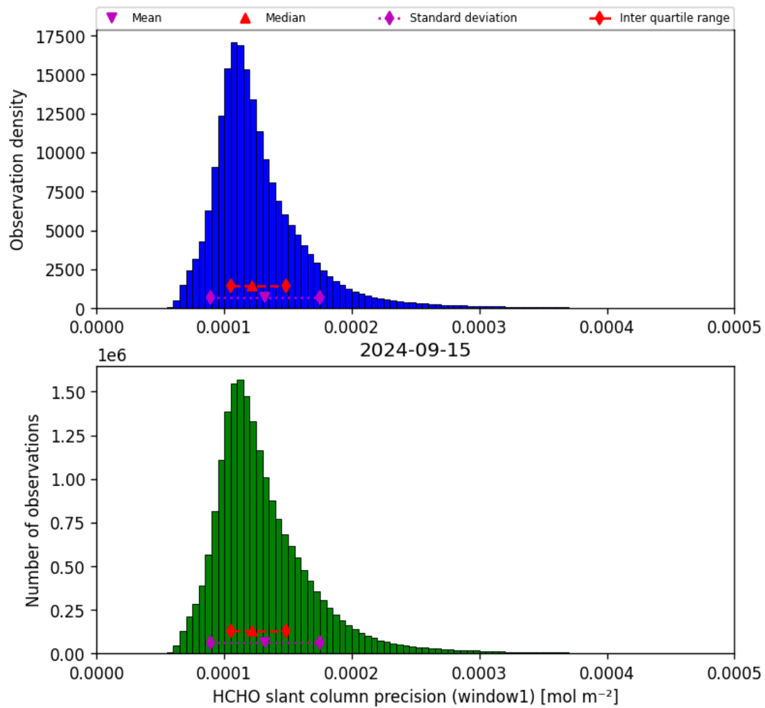
Figure 39: Histogram of “HCHO slant column precision (window1)” for 2024-09-14 to 2024-09-16
