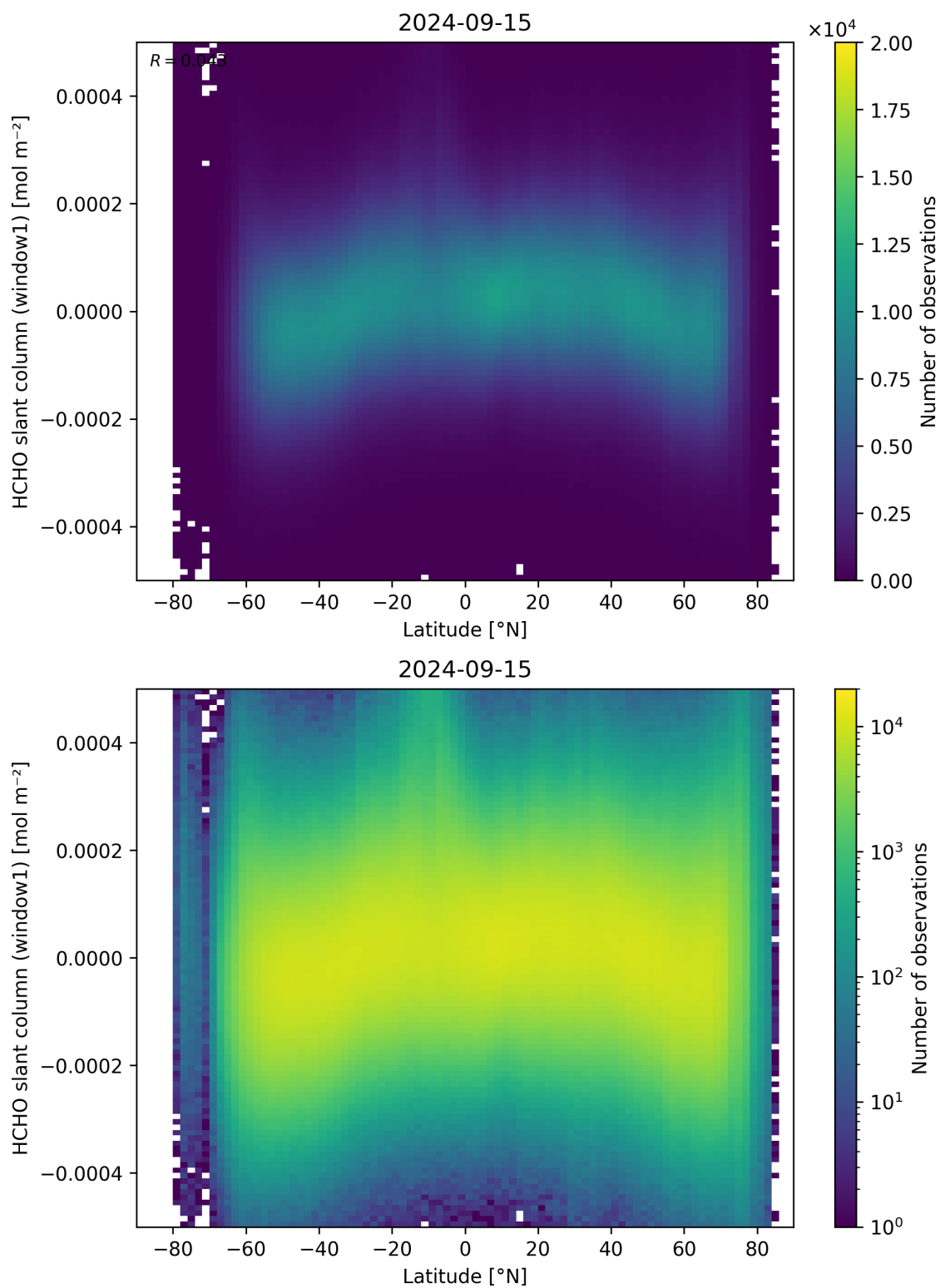
Figure 159: Scatter density plot of “Latitude” against “HCHO slant column (window1)” for 2024-09-14 to 2024-09-16.
