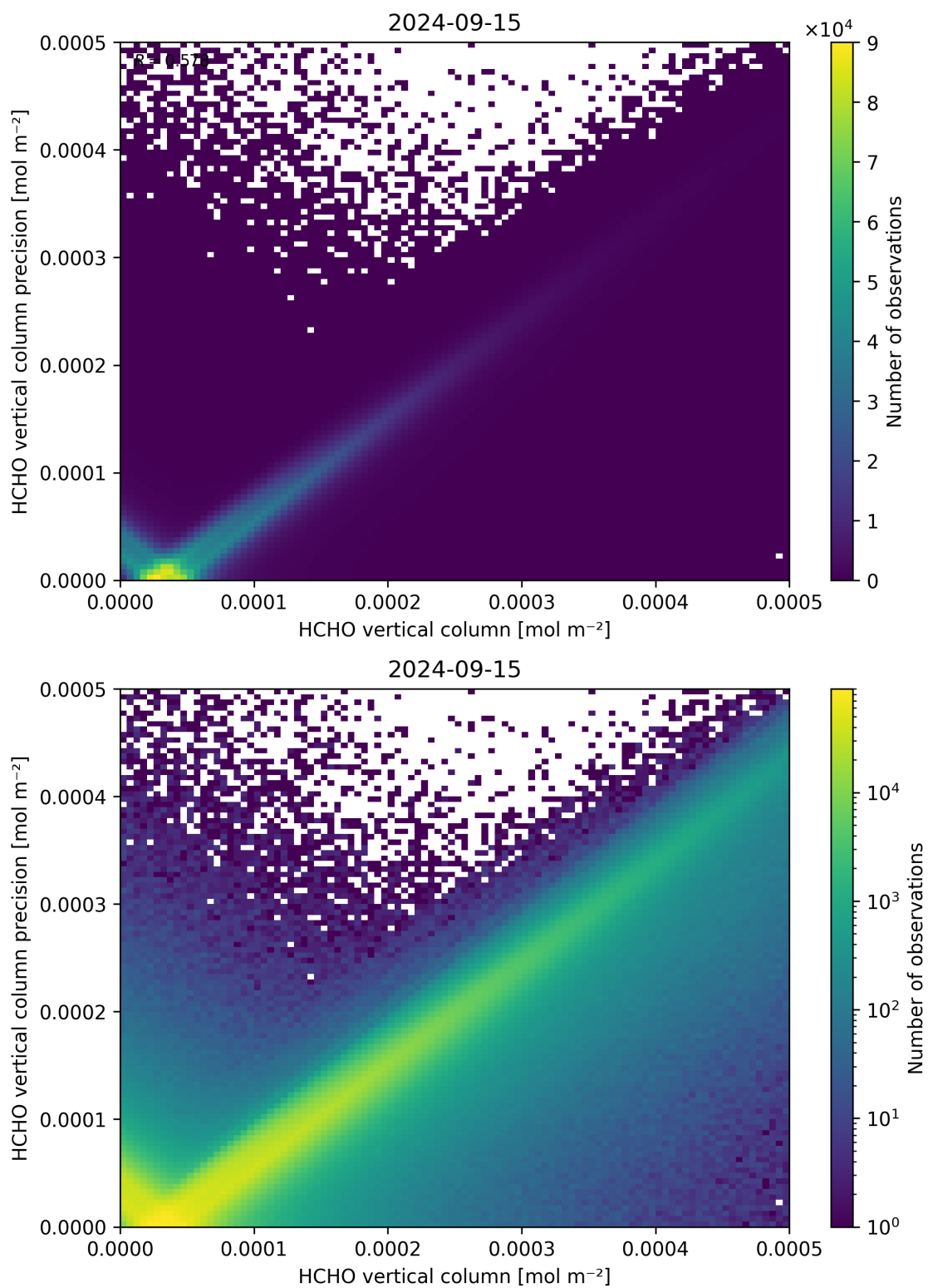
Figure 134: Scatter density plot of “HCHO vertical column” against “HCHO vertical column precision” for 2024-09-14 to 2024-09-16.
