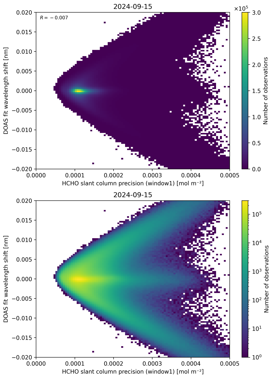
Figure 89: Scatter density plot of “HCHO slant column precision (window1)” against “DOAS fit wavelength shift” for 2024-09-14 to 2024-09-16.
