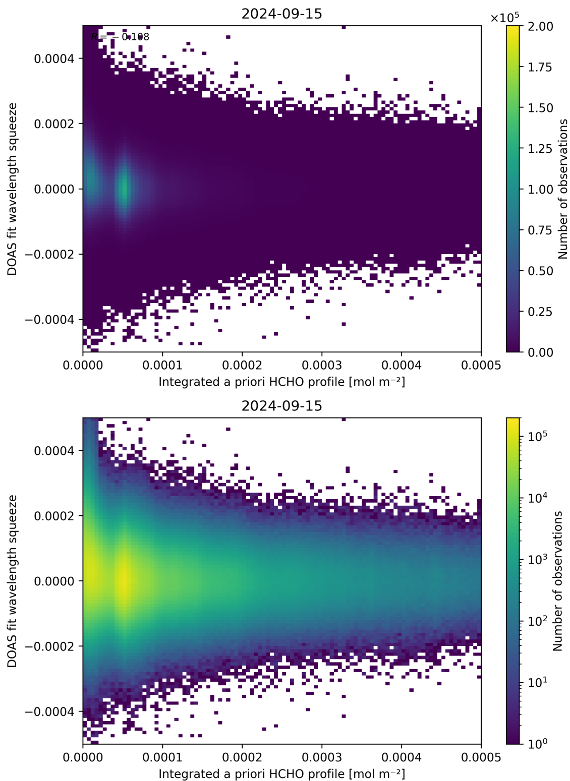
Figure 150: Scatter density plot of “Integrated a priori HCHO profile” against “DOAS fit wavelength squeeze” for 2024-09-14 to 2024-09-16.
