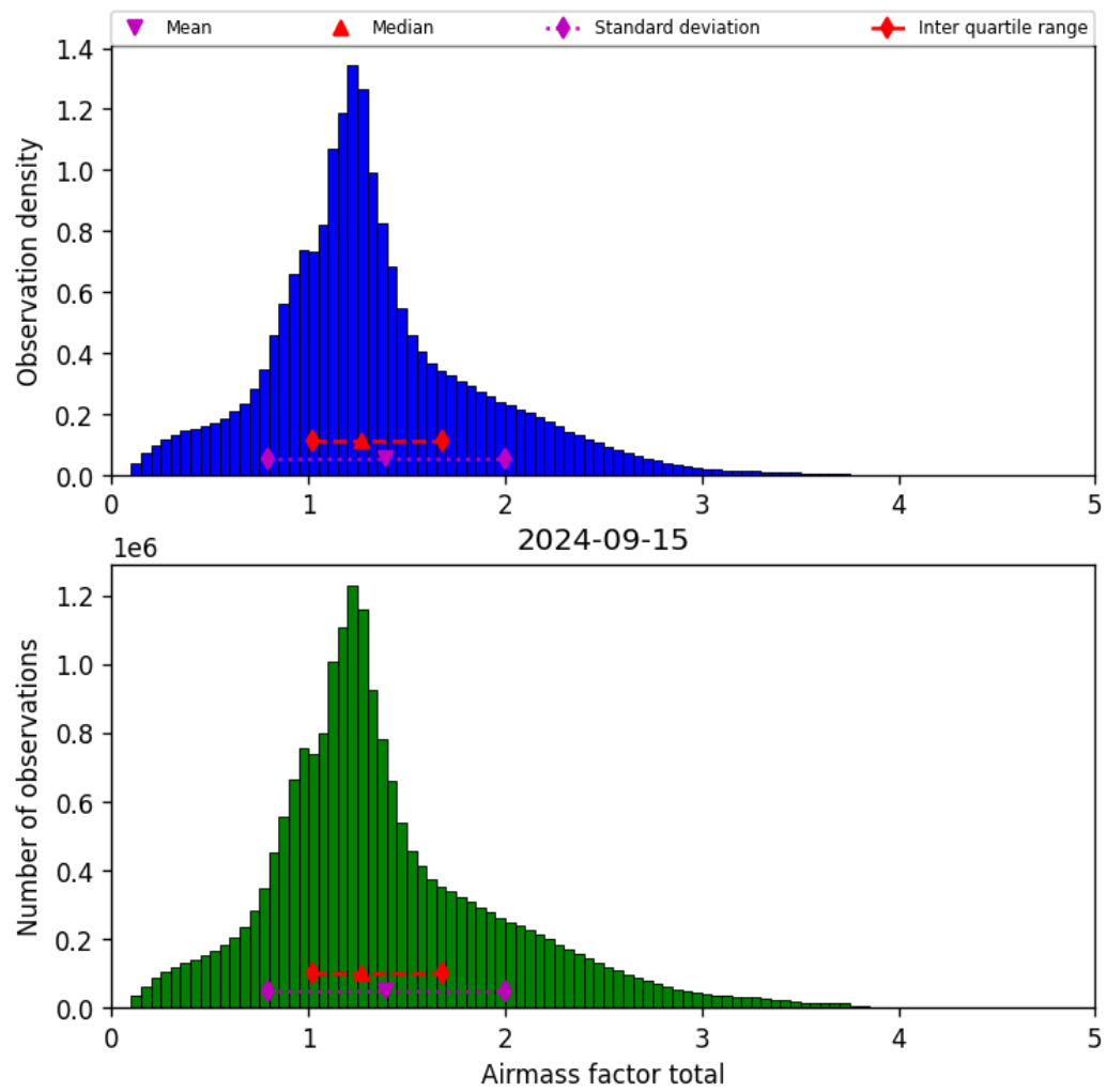
Figure 40: Histogram of “Airmass factor total” for 2024-09-14 to 2024-09-16
