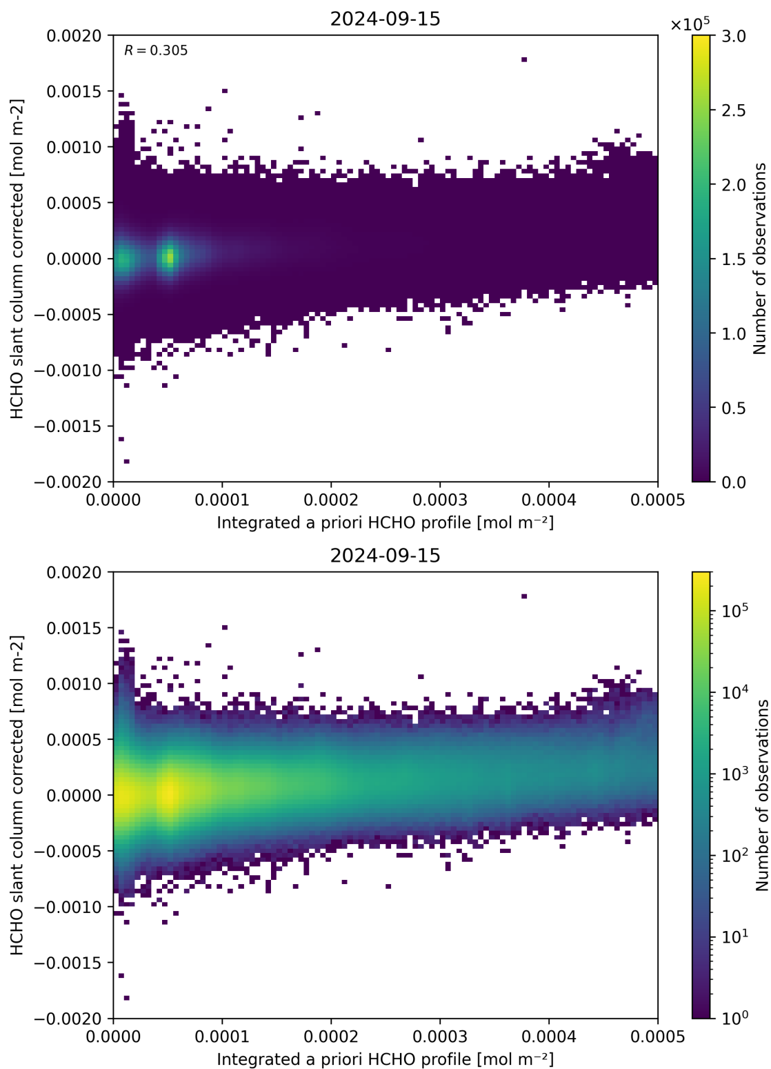
Figure 151: Scatter density plot of “Integrated a priori HCHO profile” against “HCHO slant column corrected” for 2024-09-14 to 2024-09-16.
