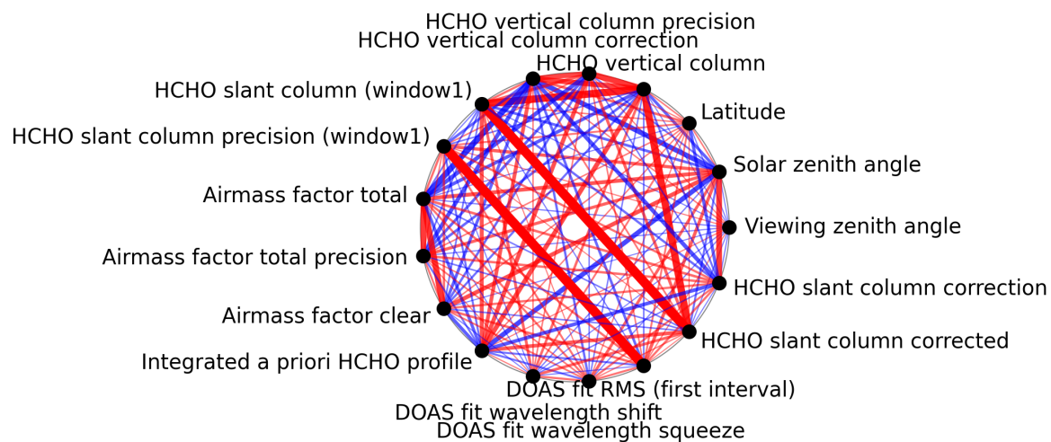
Figure 1: Map of correlation graph for 2024-09-14 to 2024-09-16.
