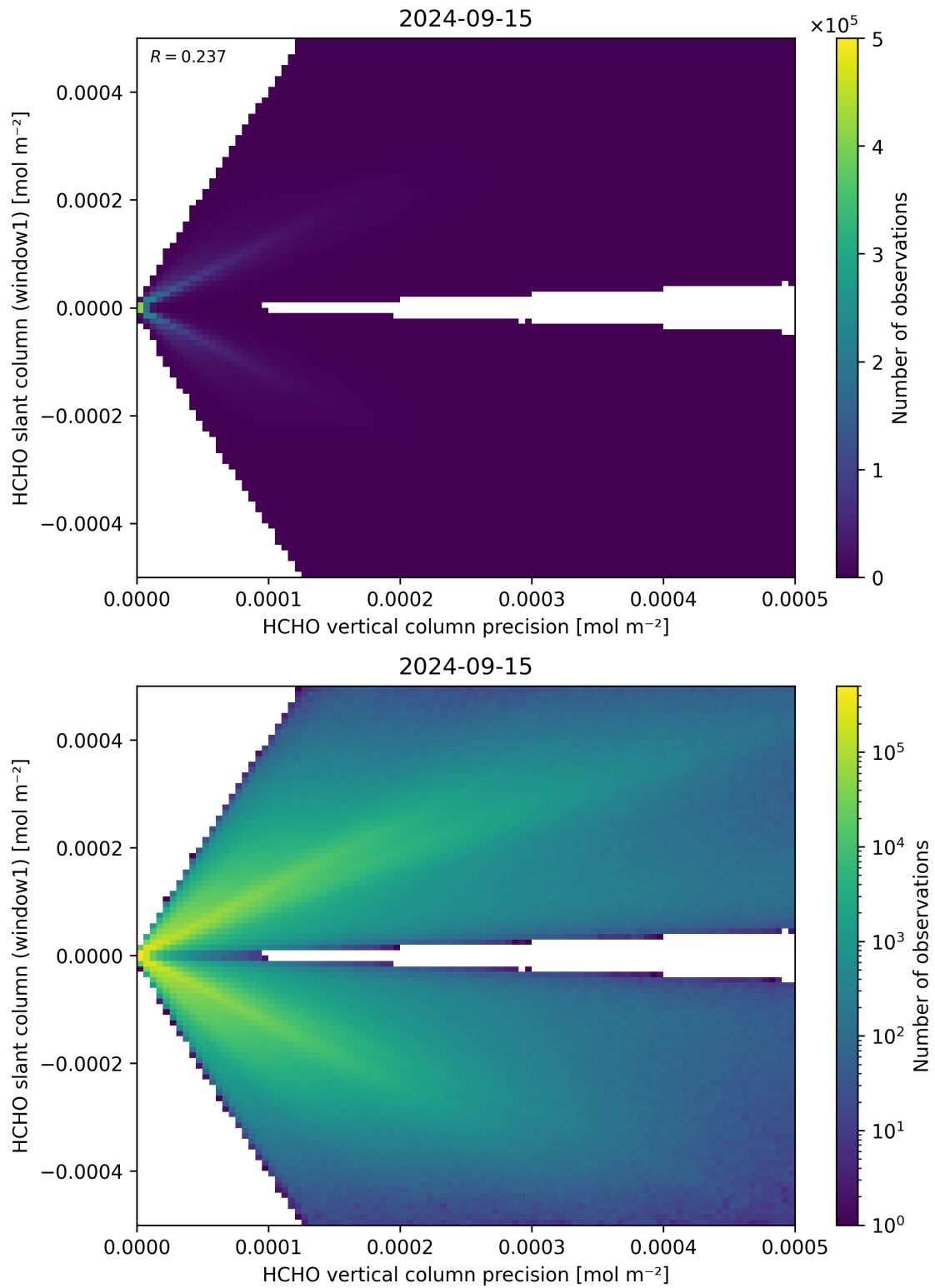
Figure 142: Scatter density plot of “HCHO vertical column precision” against “HCHO slant column (window1)” for 2024-09-14 to 2024-09-16.
