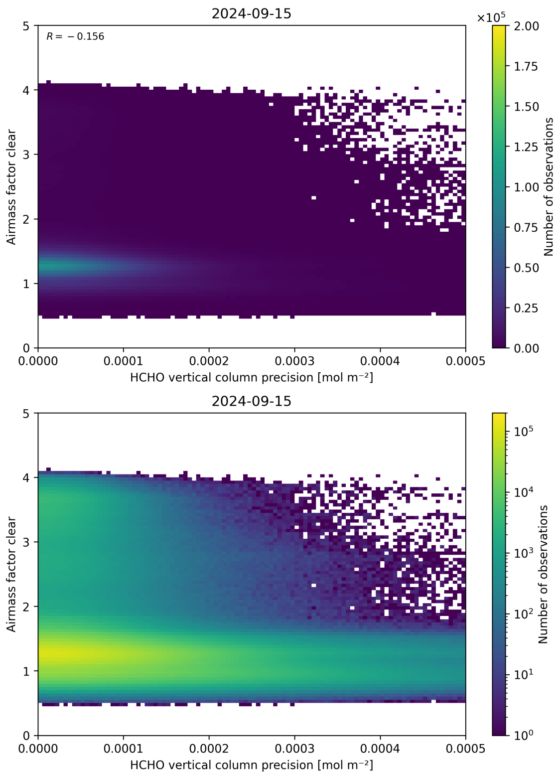
Figure 139: Scatter density plot of “HCHO vertical column precision” against “Airmass factor clear” for 2024-09-14 to 2024-09-16.
