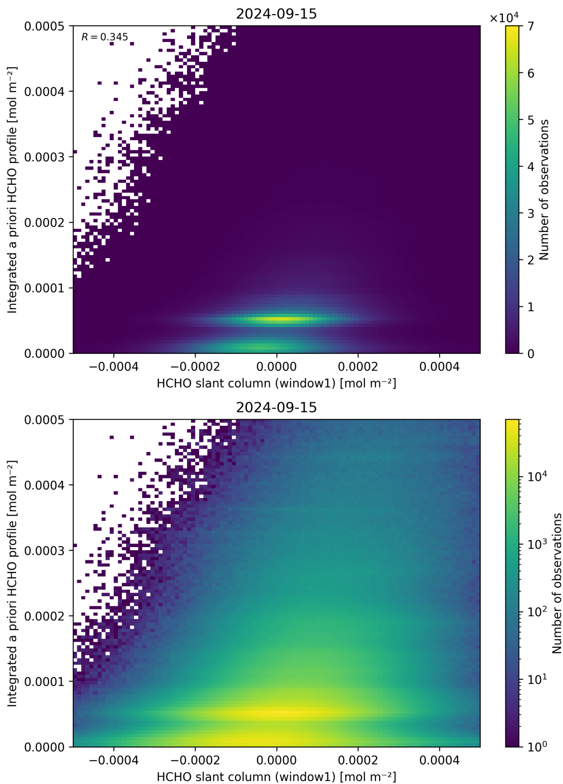
Figure 87: Scatter density plot of “HCHO slant column (window1)” against “Integrated a priori HCHO profile” for 2024-09-14 to 2024-09-16.
