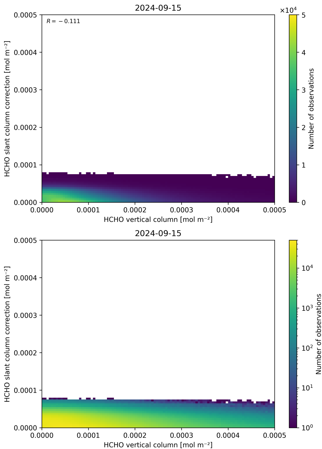
Figure 128: Scatter density plot of “HCHO vertical column” against “HCHO slant column correction” for 2024-09-14 to 2024-09-16.
