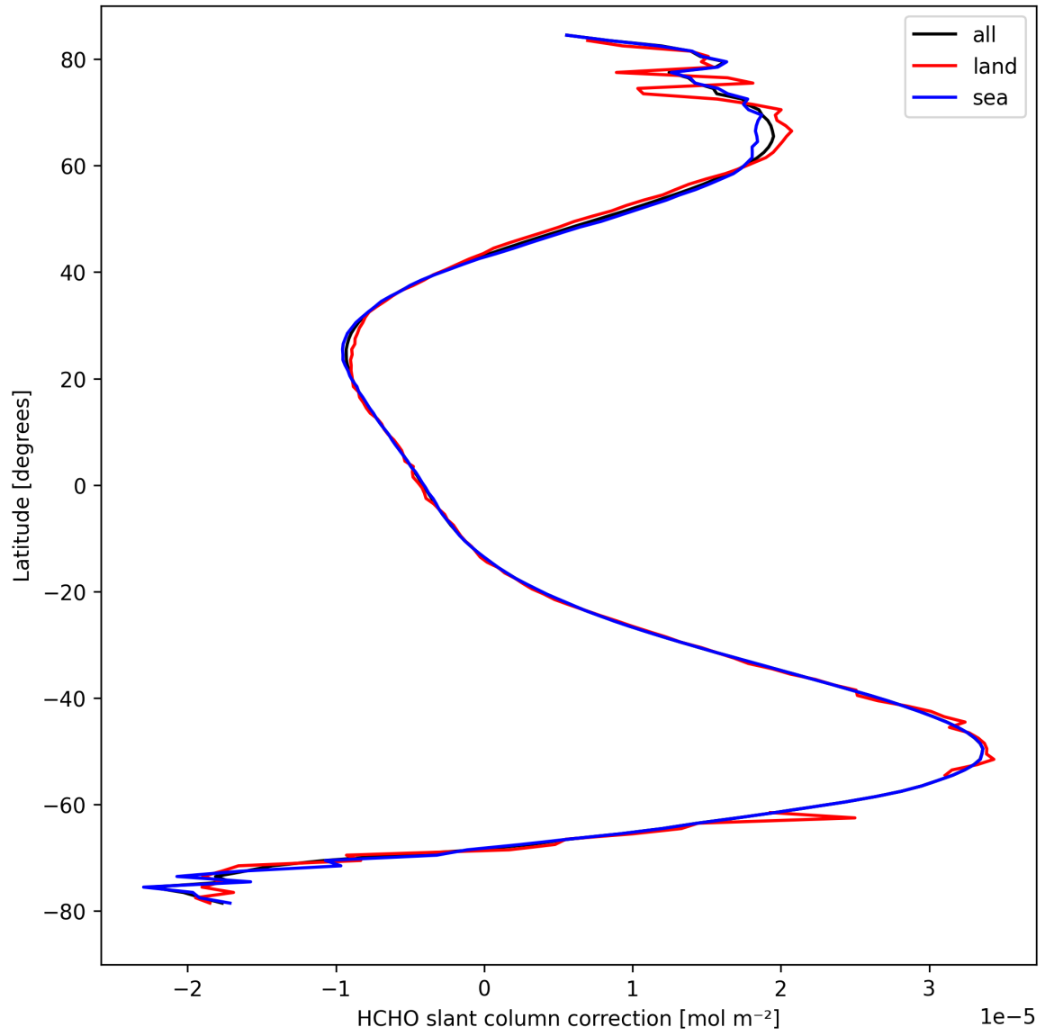
Figure 33: Zonal average of "HCHO slant column correction" for 2024-09-14 to 2024-09-16.
