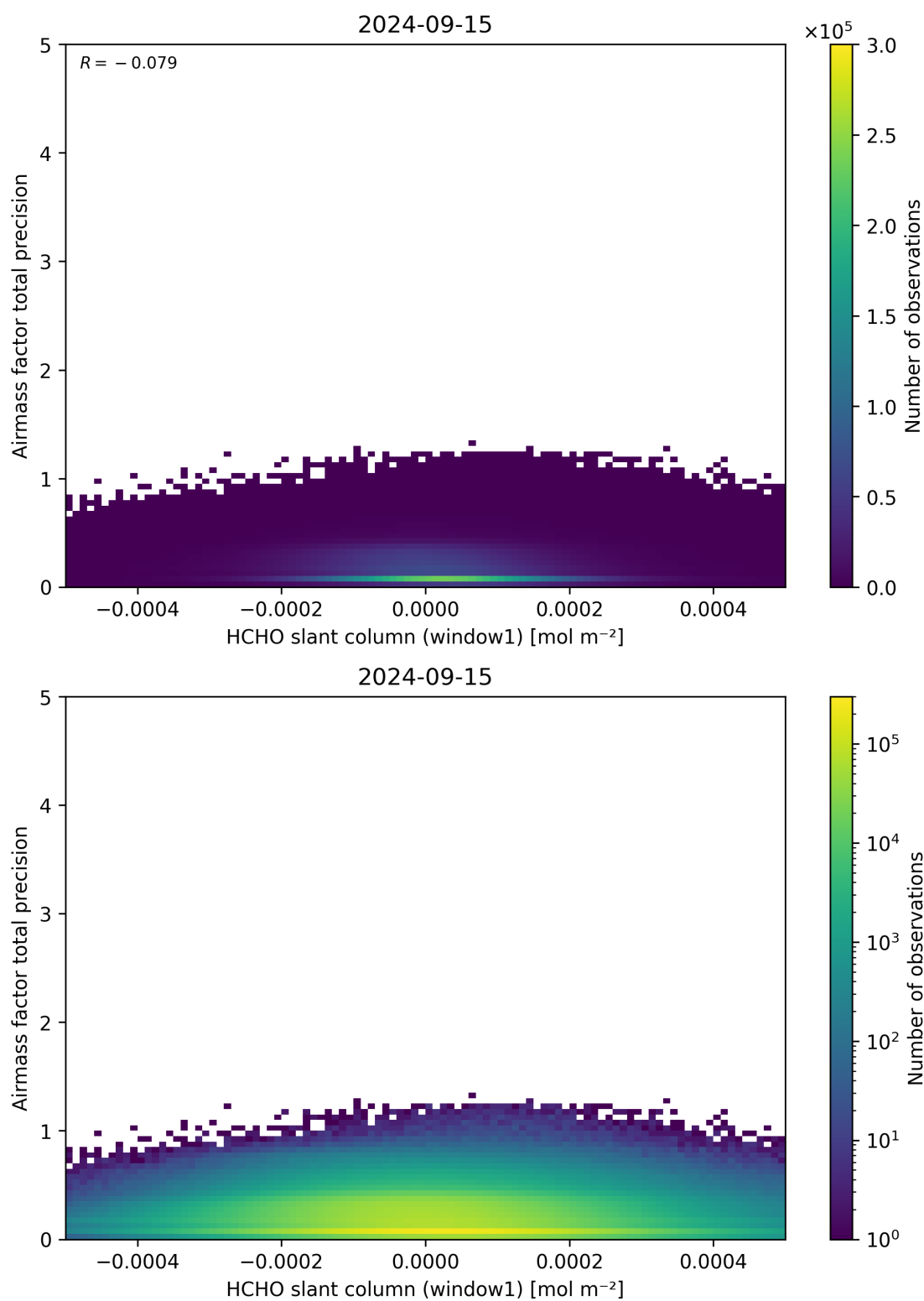
Figure 86: Scatter density plot of “HCHO slant column (window1)” against “Airmass factor total precision” for 2024-09-14 to 2024-09-16.
