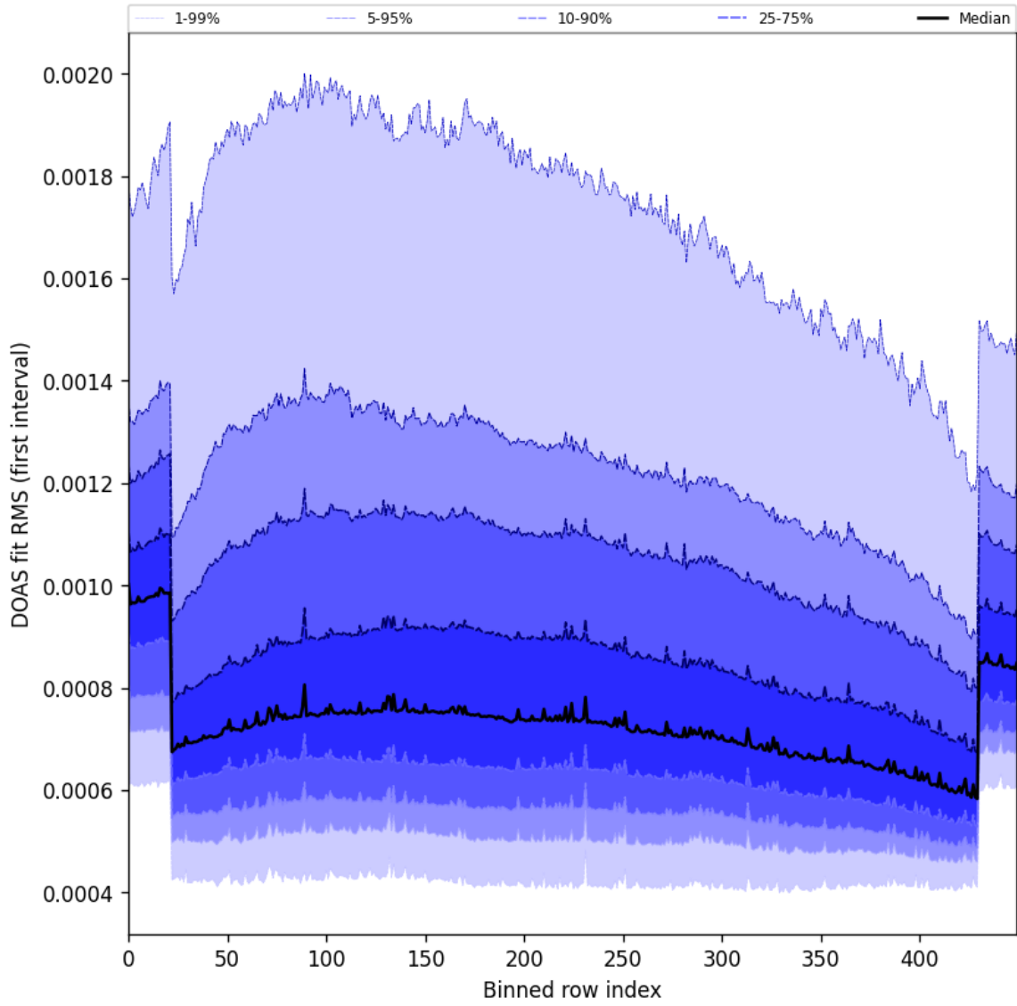
Figure 60: Along track statistics of “DOAS fit RMS (first interval)” for 2024-09-14 to 2024-09-16
