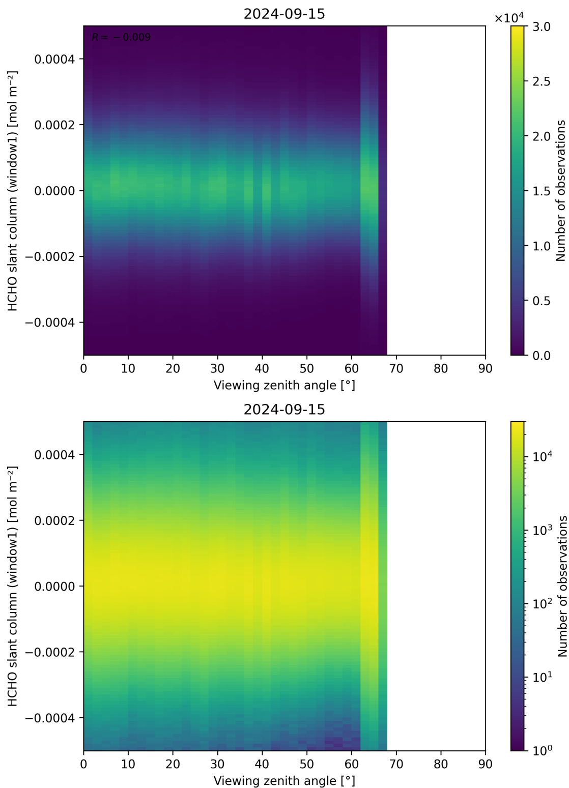
Figure 188: Scatter density plot of “Viewing zenith angle” against “HCHO slant column (window1)” for 2024-09-14 to 2024-09-16.
