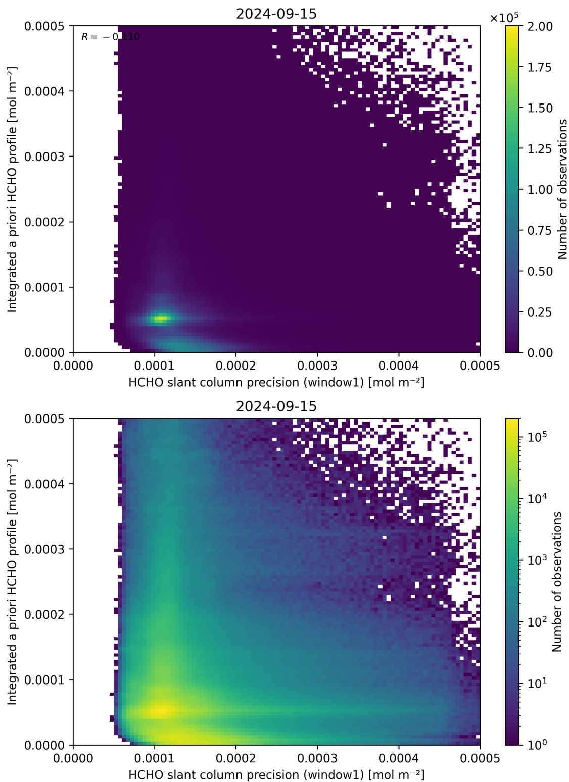
Figure 96: Scatter density plot of “HCHO slant column precision (window1)” against “Integrated a priori HCHO profile” for 2024-09-14 to 2024-09-16.
