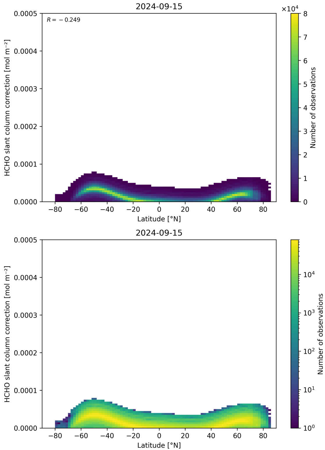
Figure 158: Scatter density plot of “Latitude” against “HCHO slant column correction” for 2024-09-14 to 2024-09-16.
