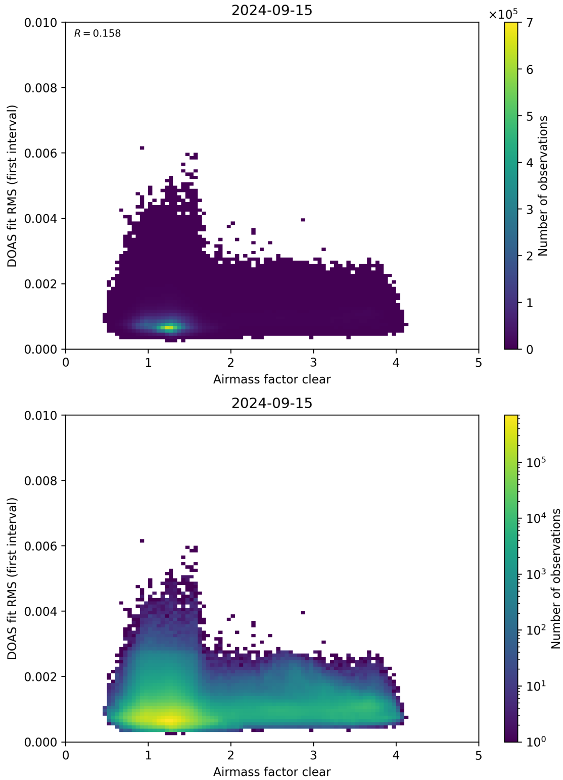
Figure 71: Scatter density plot of “Airmass factor clear” against “DOAS fit RMS (first interval)” for 2024-09-14 to 2024-09-16.
