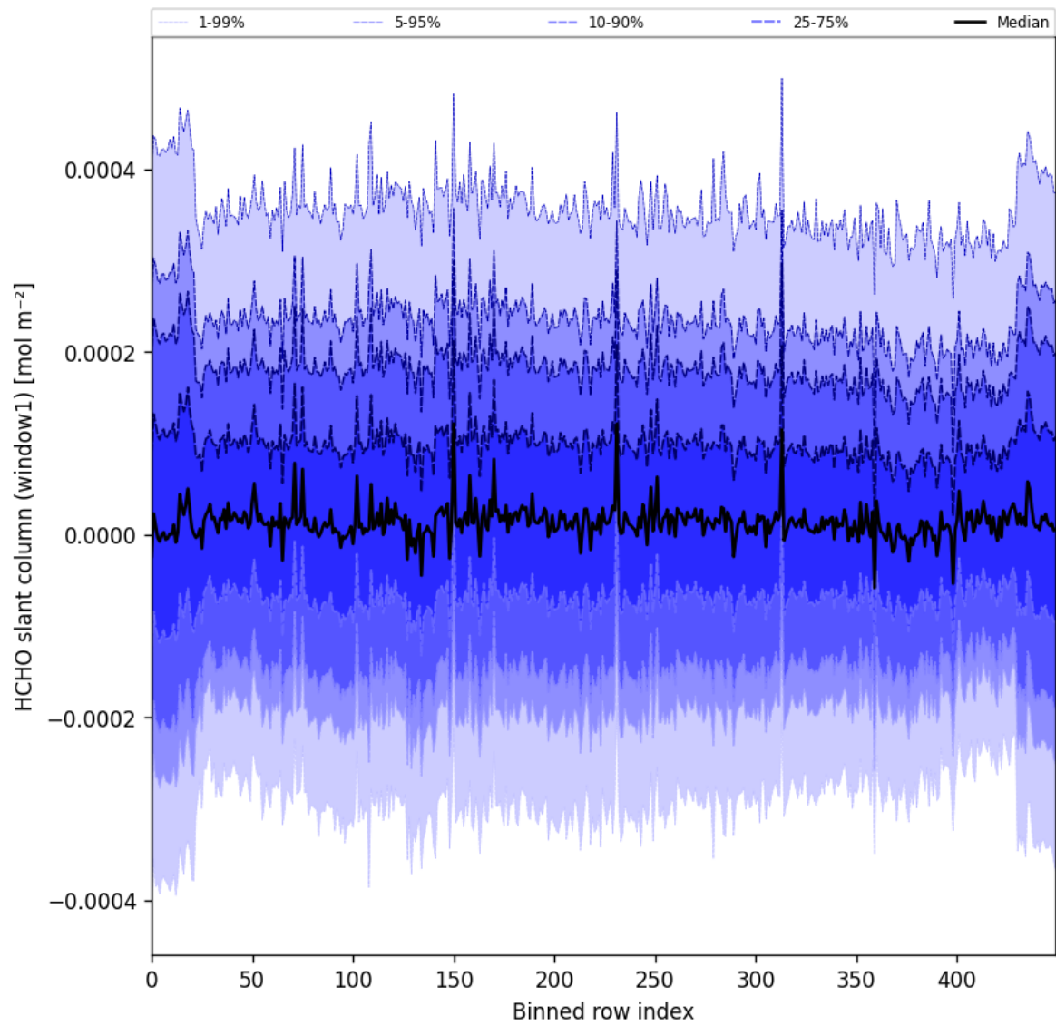
Figure 52: Along track statistics of “HCHO slant column (window1)” for 2024-09-14 to 2024-09-16
