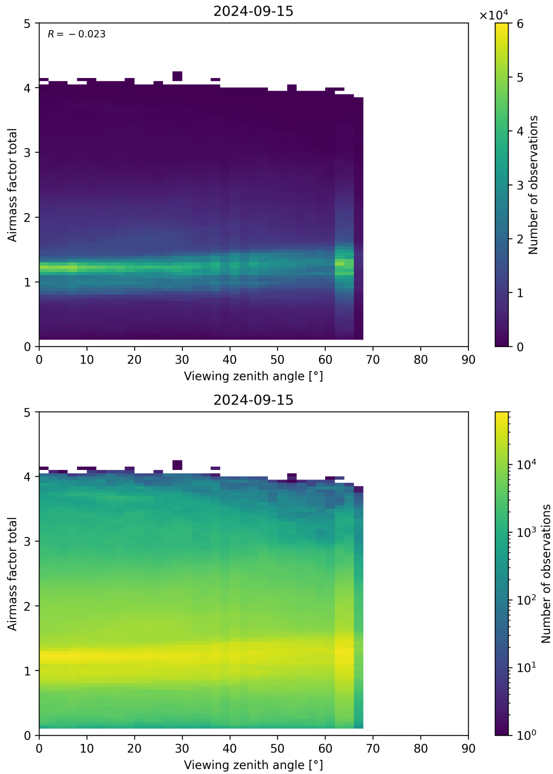
Figure 190: Scatter density plot of “Viewing zenith angle” against “Airmass factor total” for 2024-09-14 to 2024-09-16.
