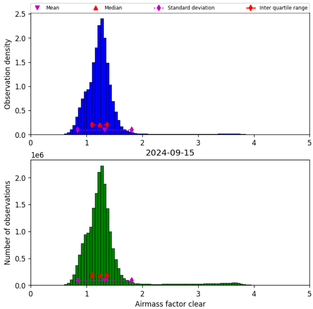
Figure 42: Histogram of “Airmass factor clear” for 2024-09-14 to 2024-09-16
