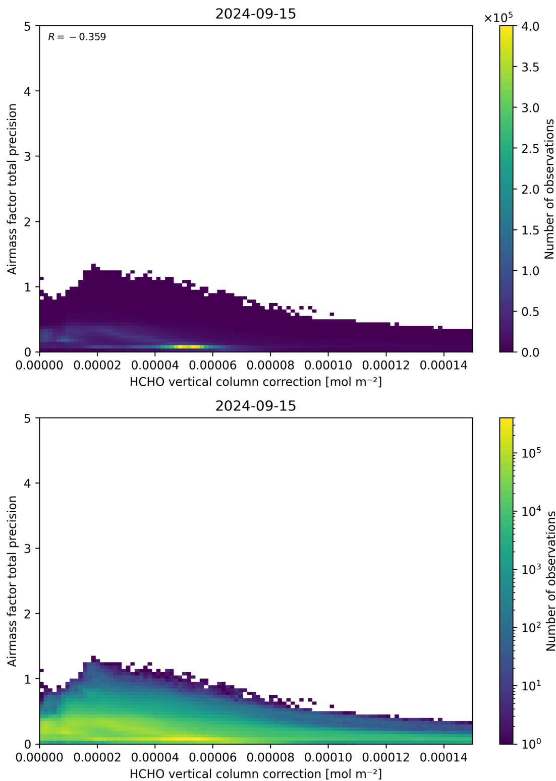
Figure 121: Scatter density plot of “HCHO vertical column correction” against “Airmass factor total precision” for 2024-09-14 to 2024-09-16.
