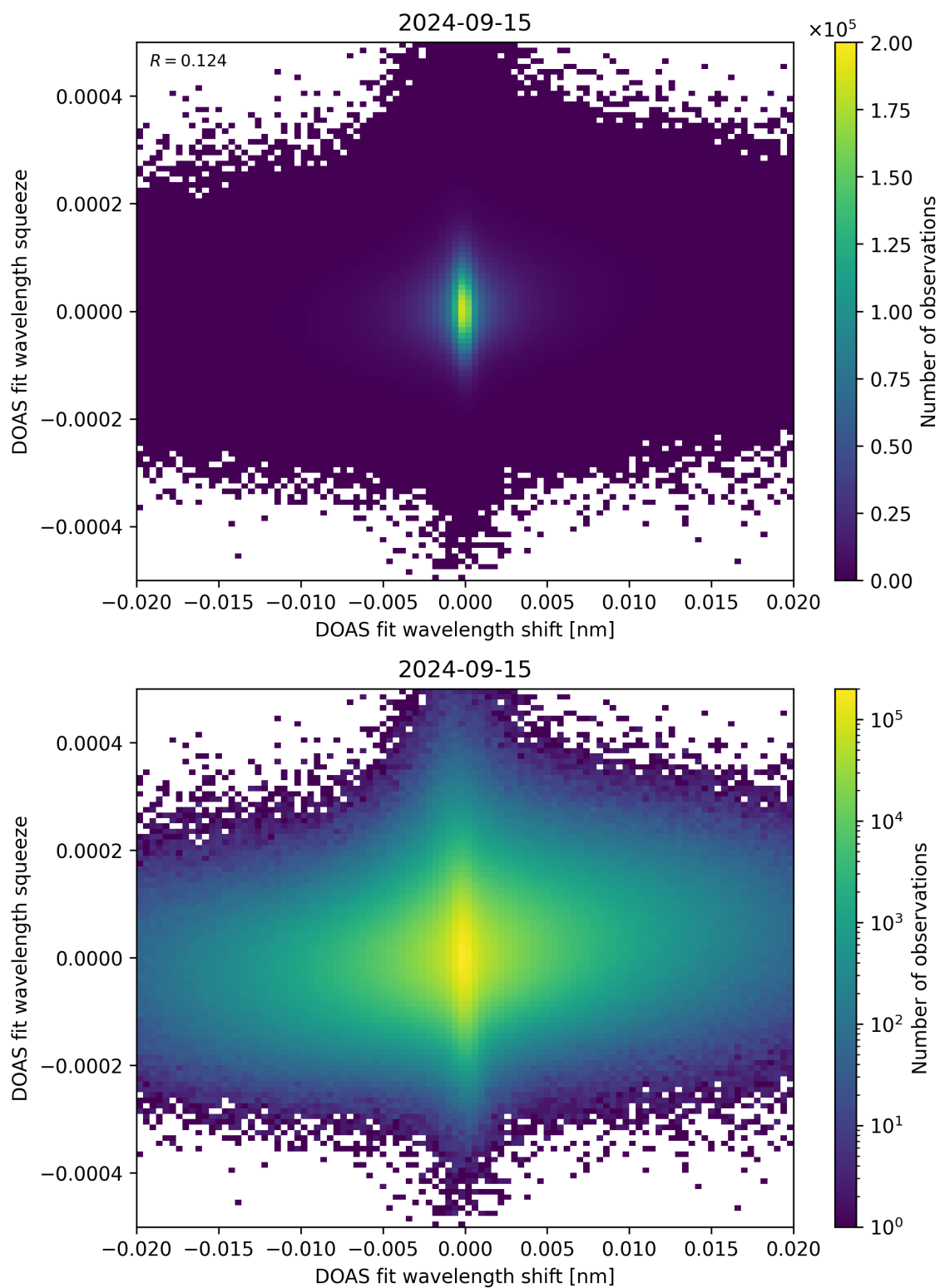
Figure 65: Scatter density plot of “DOAS fit wavelength shift” against “DOAS fit wavelength squeeze” for 2024-09-14 to 2024-09-16.
