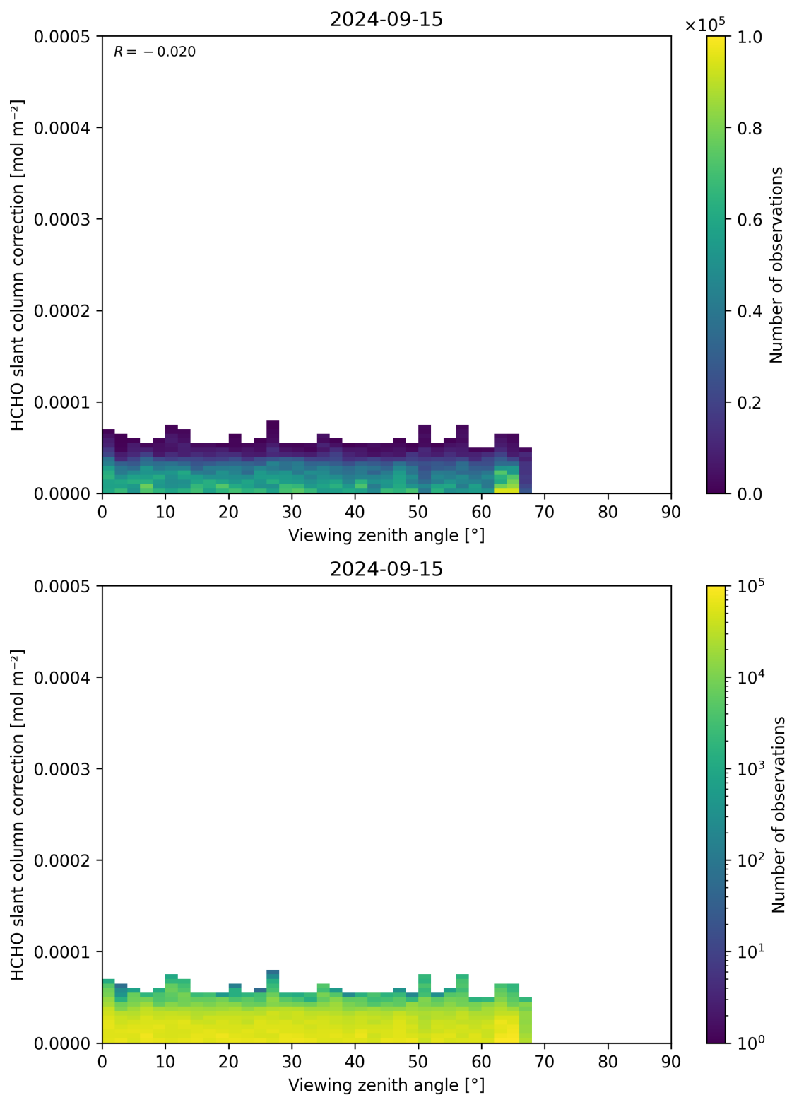
Figure 187: Scatter density plot of “Viewing zenith angle” against “HCHO slant column correction” for 2024-09-14 to 2024-09-16.
