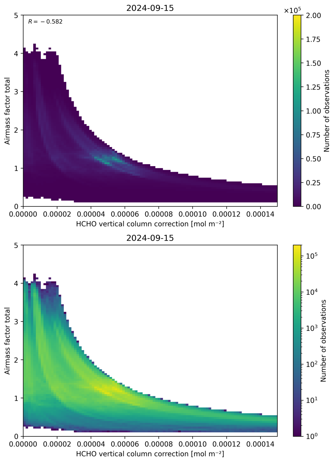
Figure 120: Scatter density plot of “HCHO vertical column correction” against “Airmass factor total” for 2024-09-14 to 2024-09-16.
