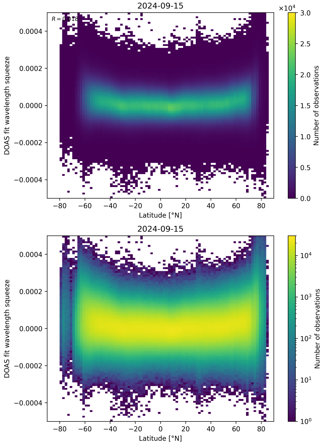
Figure 155: Scatter density plot of “Latitude” against “DOAS fit wavelength squeeze” for 2024-09-14 to 2024-09-16.
