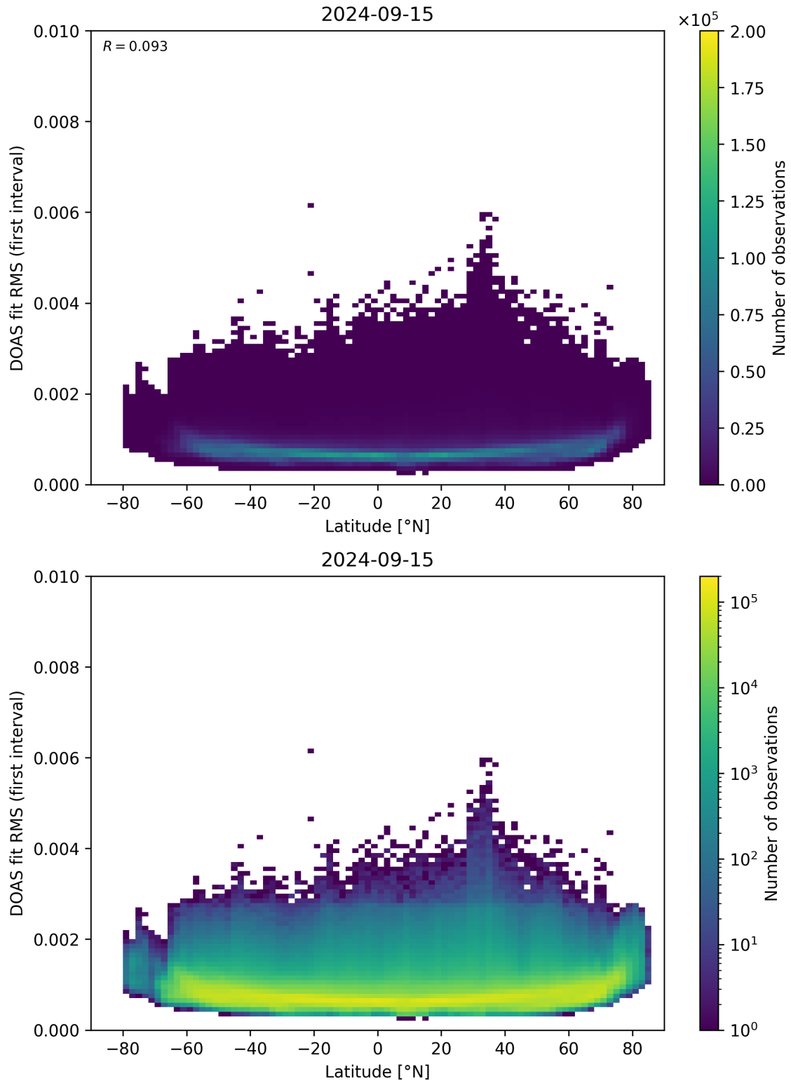
Figure 153: Scatter density plot of “Latitude” against “DOAS fit RMS (first interval)” for 2024-09-14 to 2024-09-16.
