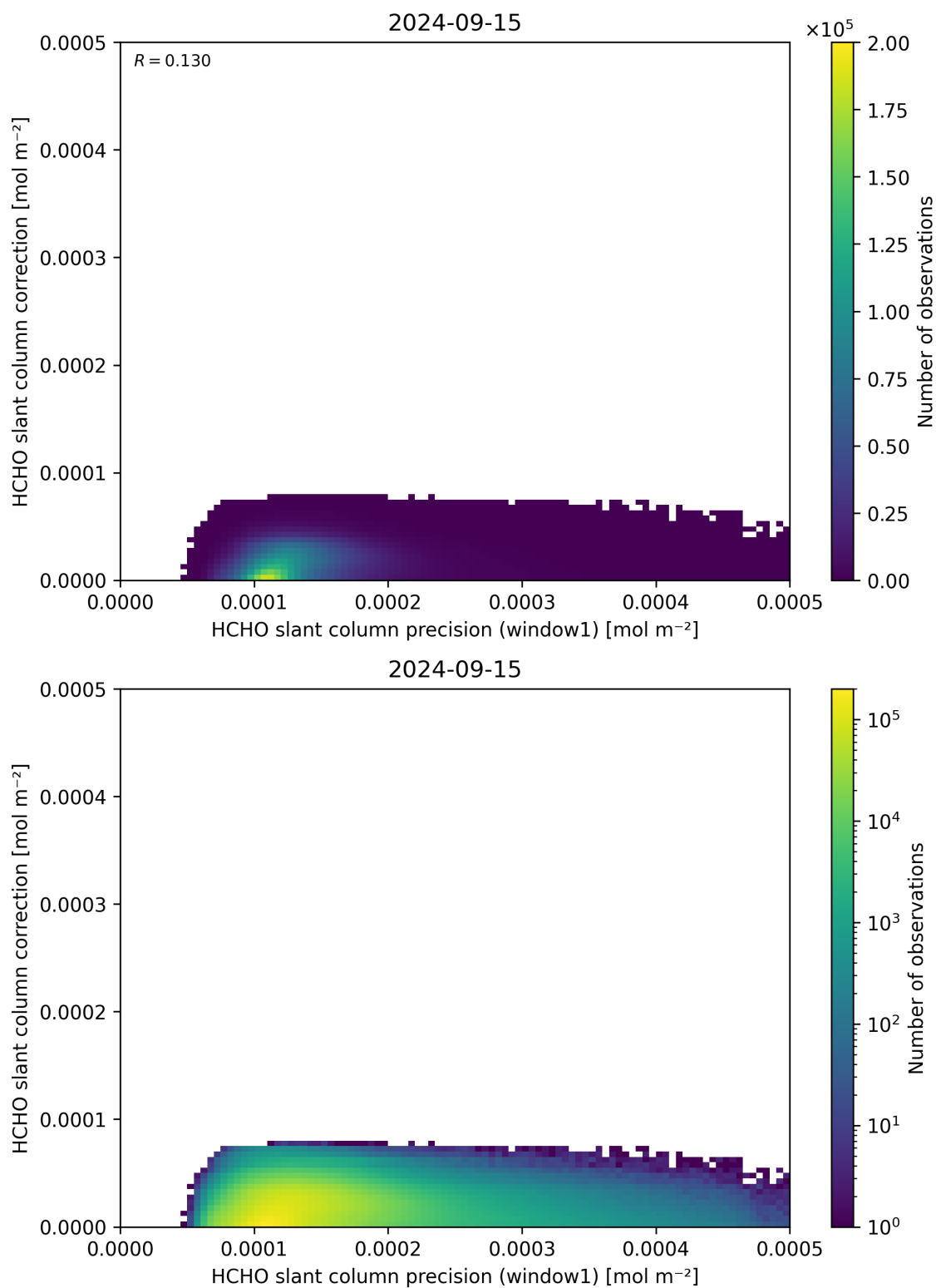
Figure 93: Scatter density plot of “HCHO slant column precision (window1)” against “HCHO slant column correction” for 2024-09-14 to 2024-09-16.
