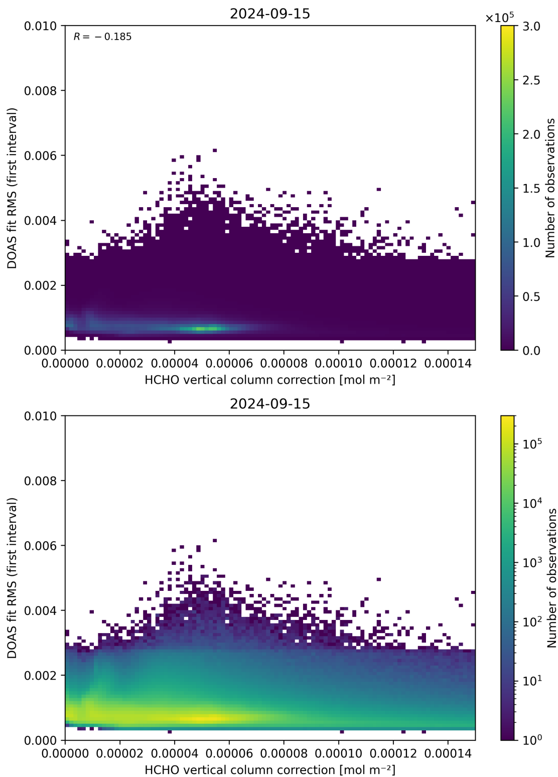
Figure 112: Scatter density plot of “HCHO vertical column correction” against “DOAS fit RMS (first interval)” for 2024-09-14 to 2024-09-16.
