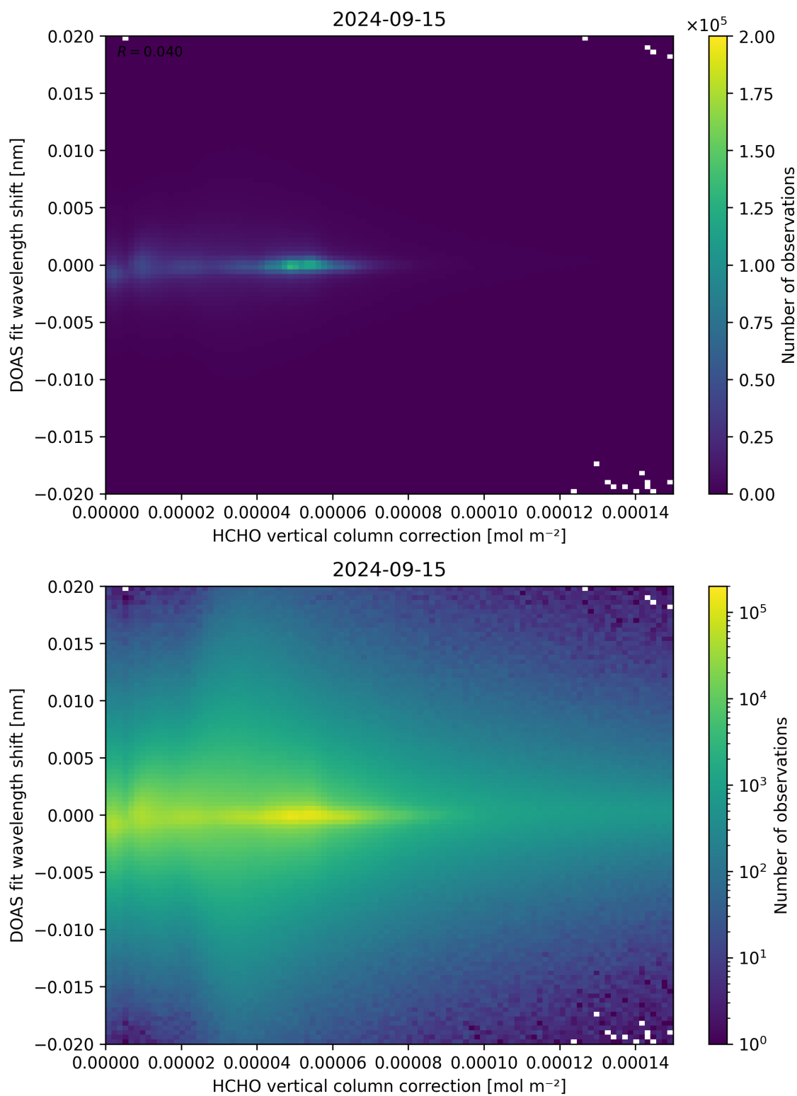
Figure 113: Scatter density plot of “HCHO vertical column correction” against “DOAS fit wavelength shift” for 2024-09-14 to 2024-09-16.
