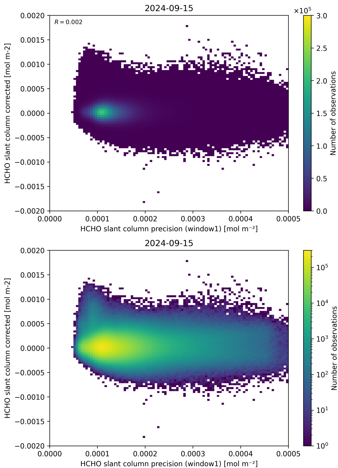
Figure 92: Scatter density plot of “HCHO slant column precision (window1)” against “HCHO slant column corrected” for 2024-09-14 to 2024-09-16.
