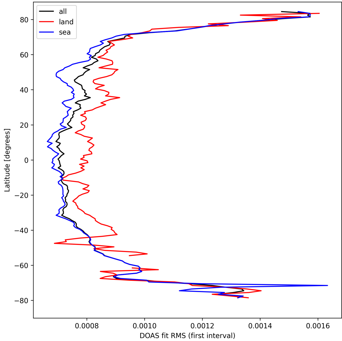
Figure 32: Zonal average of "DOAS fit RMS (first interval)" for 2024-09-14 to 2024-09-16.
