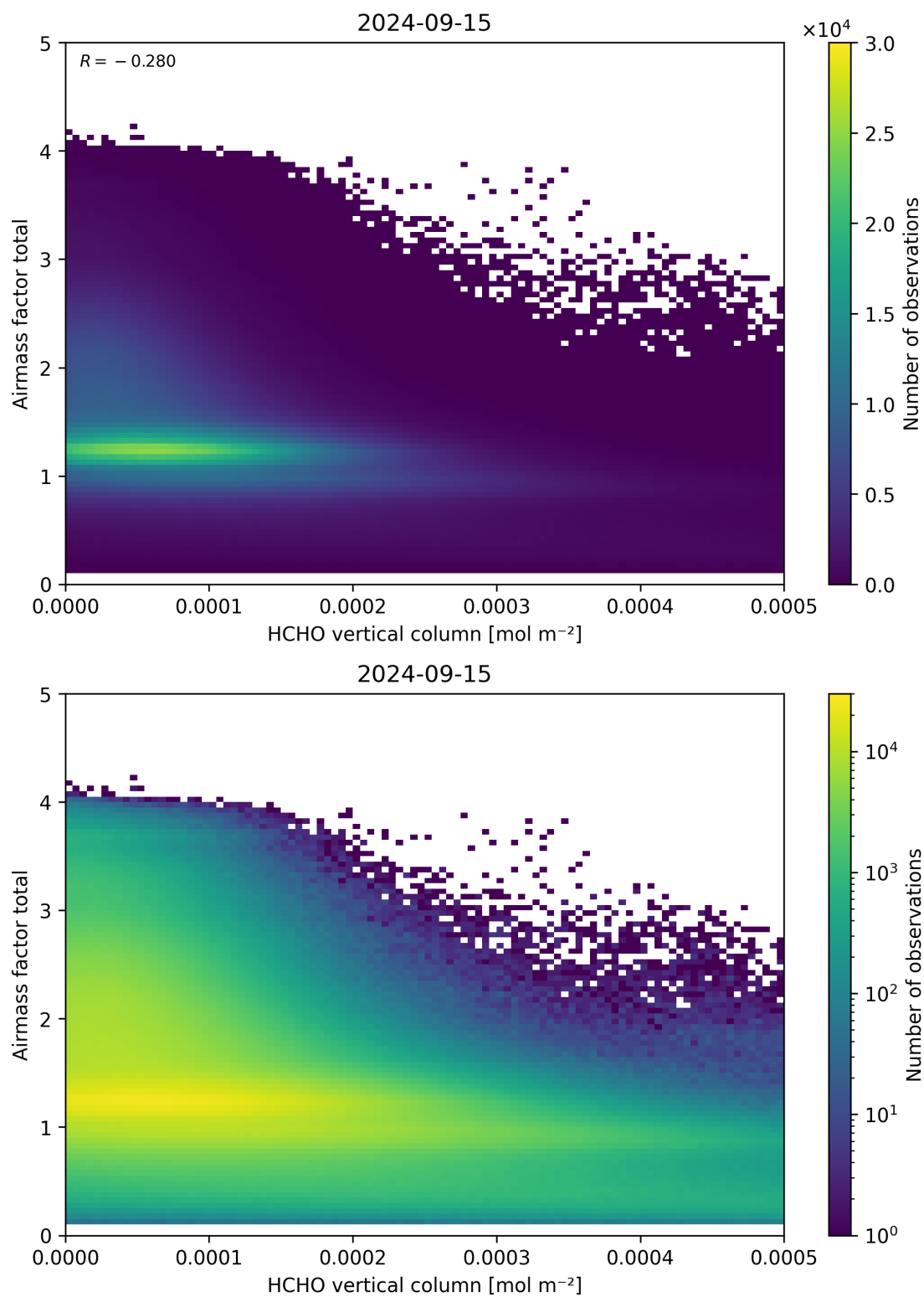
Figure 131: Scatter density plot of “HCHO vertical column” against “Airmass factor total” for 2024-09-14 to 2024-09-16.
