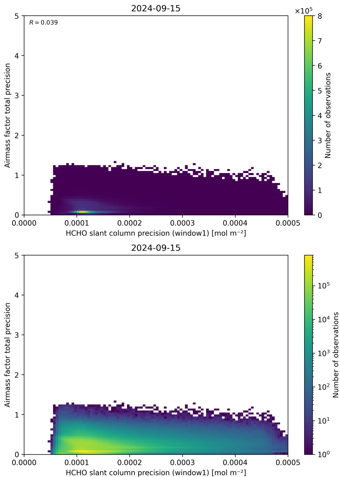
Figure 95: Scatter density plot of “HCHO slant column precision (window1)” against “Airmass factor total precision” for 2024-09-14 to 2024-09-16.
