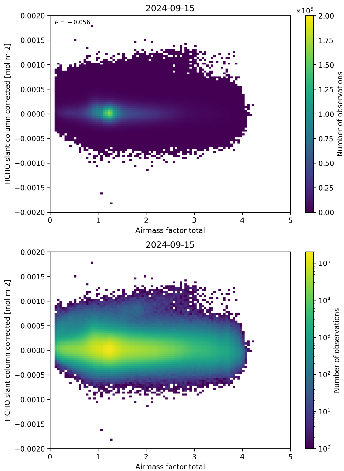
Figure 101: Scatter density plot of “Airmass factor total” against “HCHO slant column corrected” for 2024-09-14 to 2024-09-16.
