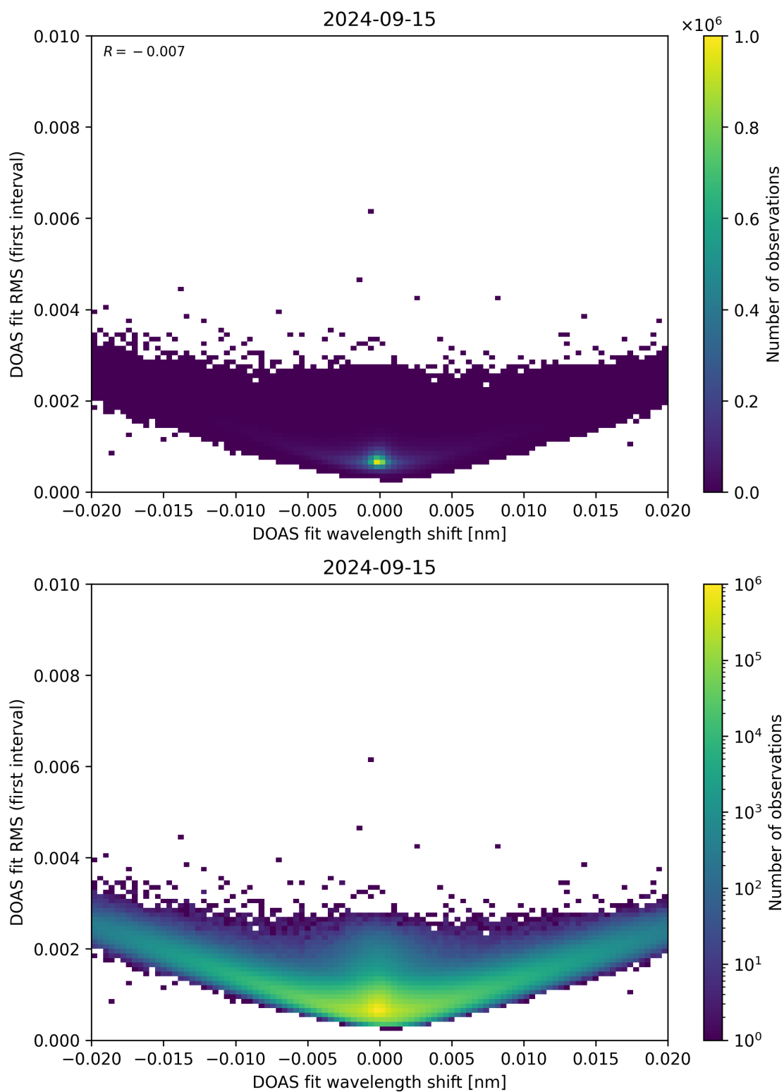
Figure 64: Scatter density plot of “DOAS fit wavelength shift” against “DOAS fit RMS (first interval)” for 2024-09-14 to 2024-09-16.
