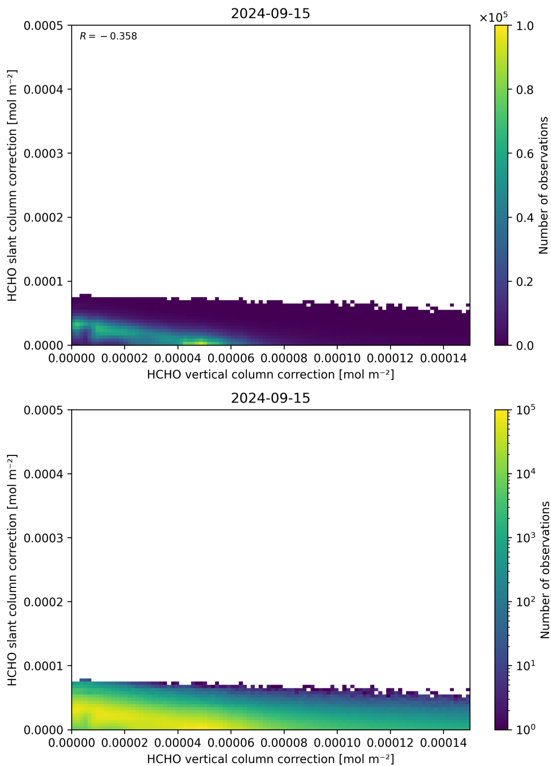
Figure 117: Scatter density plot of “HCHO vertical column correction” against “HCHO slant column correction” for 2024-09-14 to 2024-09-16.
