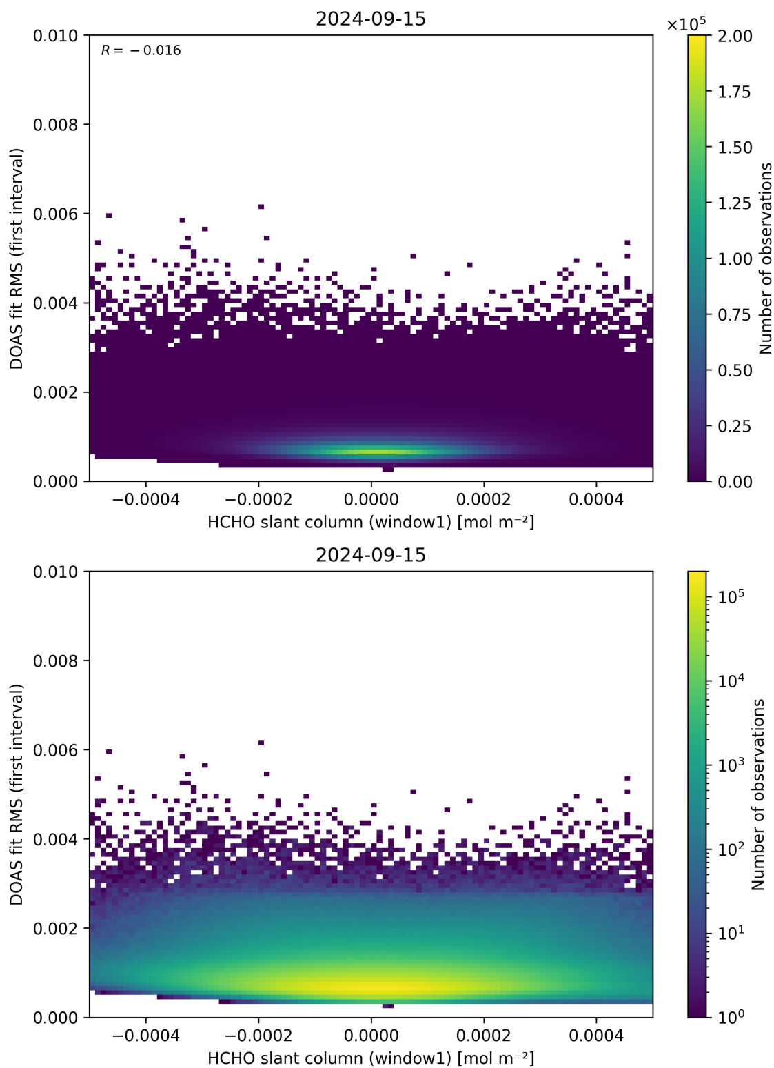
Figure 78: Scatter density plot of “HCHO slant column (window1)” against “DOAS fit RMS (first interval)” for 2024-09-14 to 2024-09-16.
