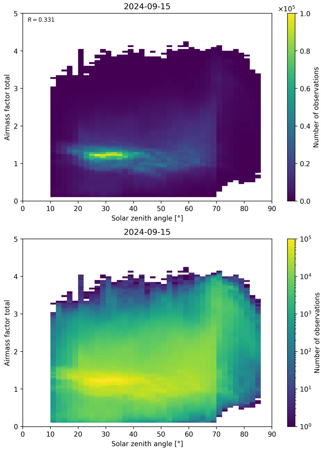
Figure 175: Scatter density plot of “Solar zenith angle” against “Airmass factor total” for 2024-09-14 to 2024-09-16.
