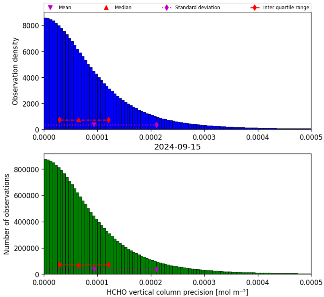
Figure 36: Histogram of “HCHO vertical column precision” for 2024-09-14 to 2024-09-16
