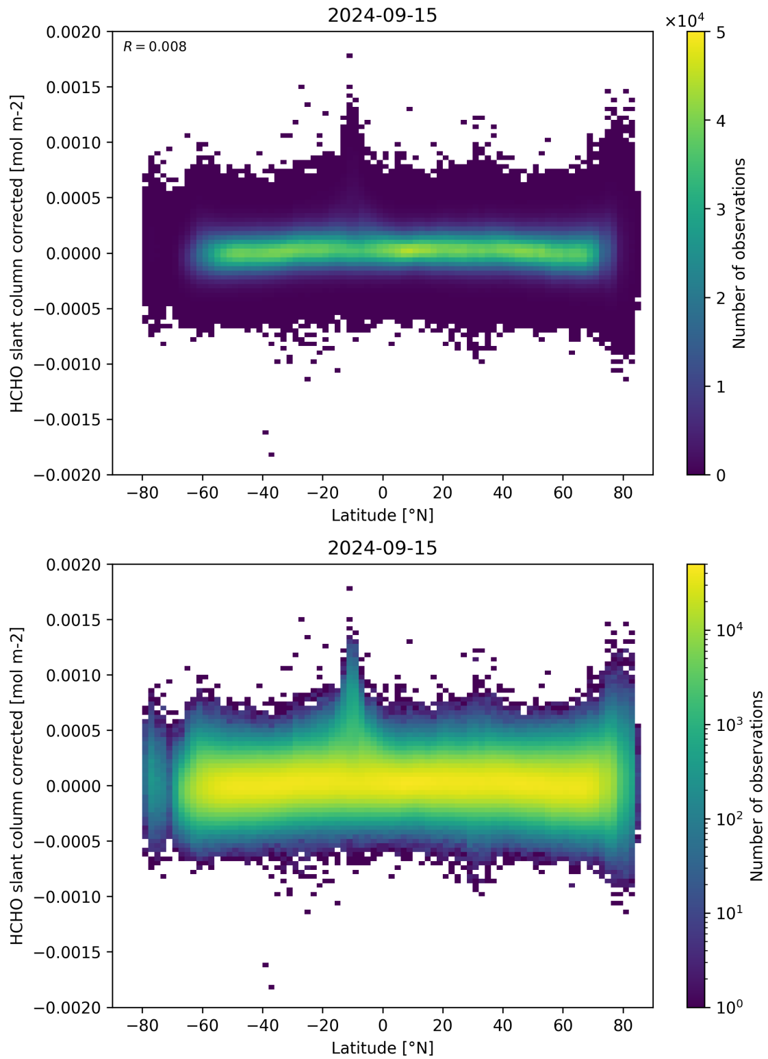
Figure 157: Scatter density plot of “Latitude” against “HCHO slant column corrected” for 2024-09-14 to 2024-09-16.
