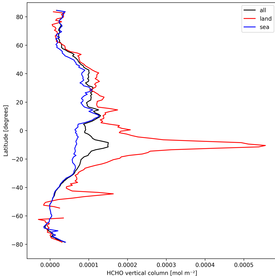
Figure 21: Zonal average of “HCHO vertical column” for 2024-09-14 to 2024-09-16.
