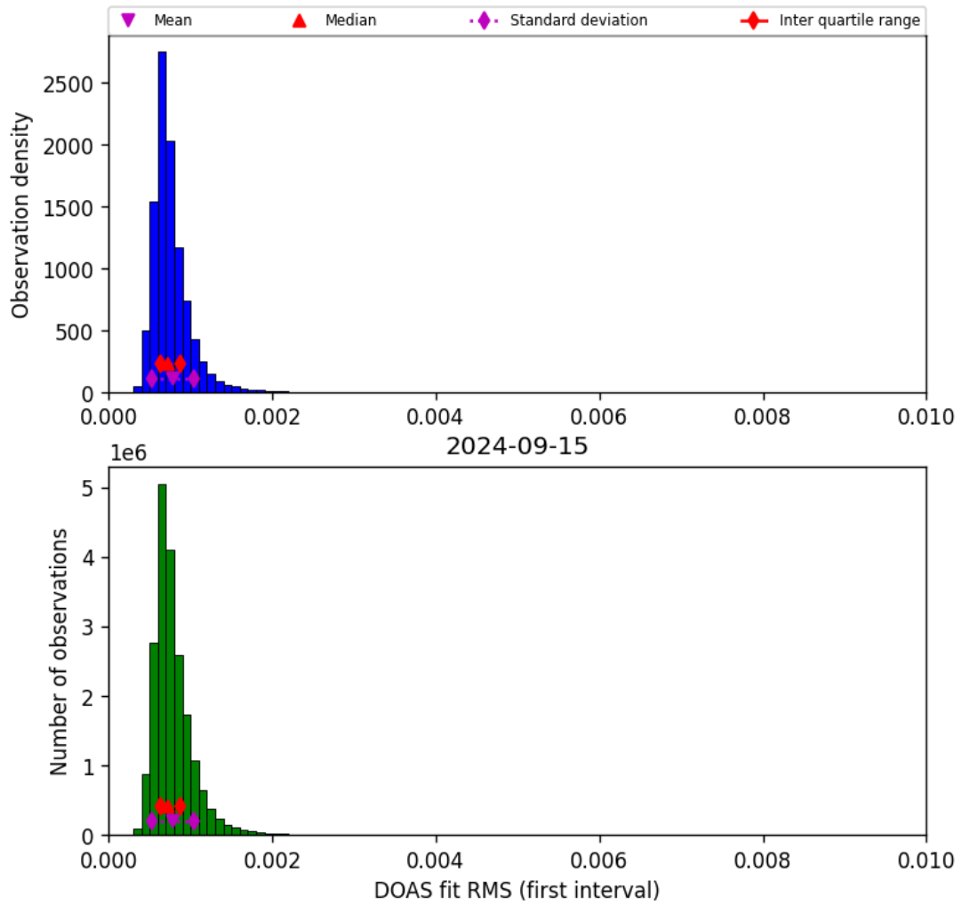
Figure 46: Histogram of “DOAS fit RMS (first interval)” for 2024-09-14 to 2024-09-16
