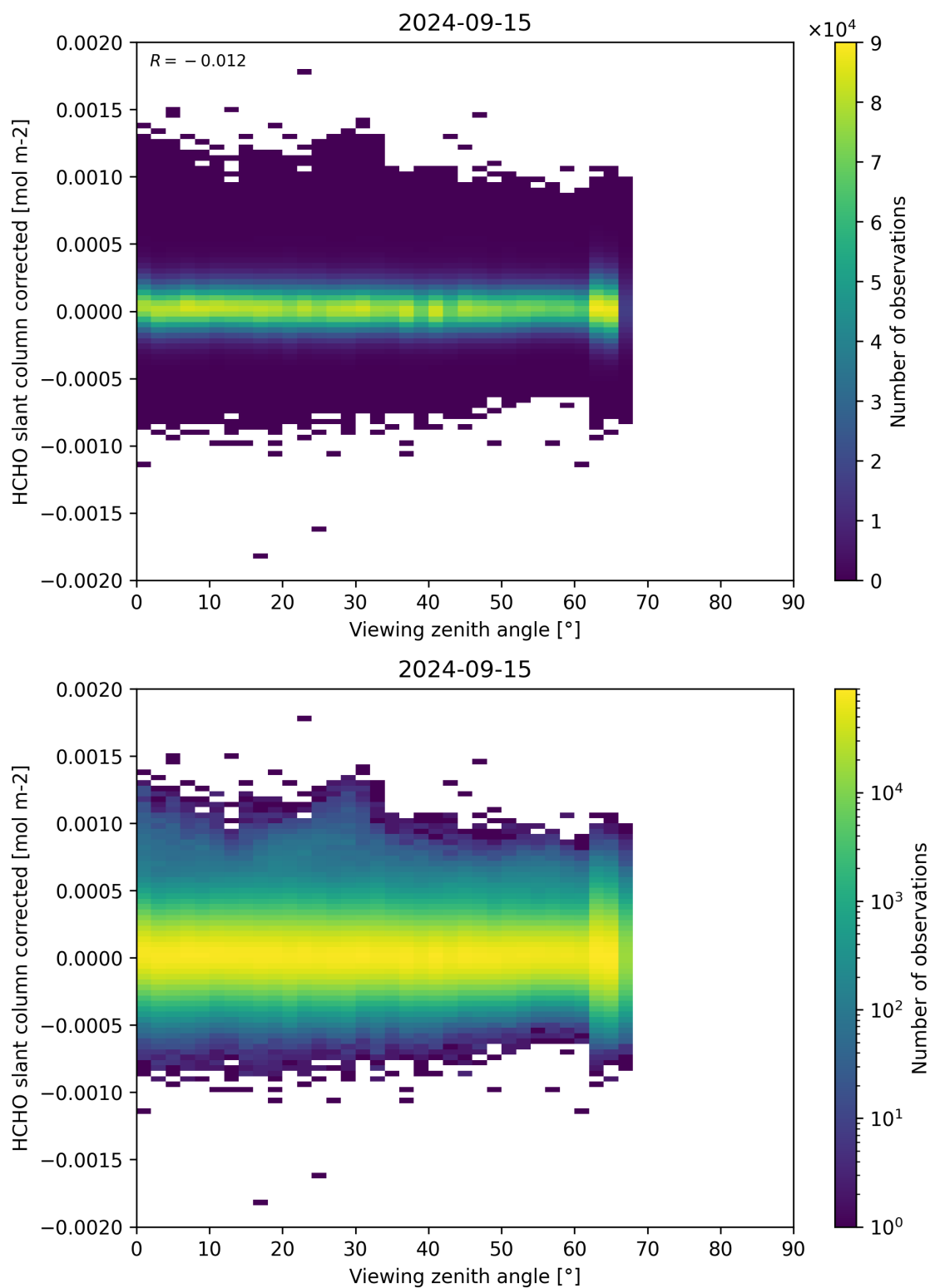
Figure 186: Scatter density plot of “Viewing zenith angle” against “HCHO slant column corrected” for 2024-09-14 to 2024-09-16.
