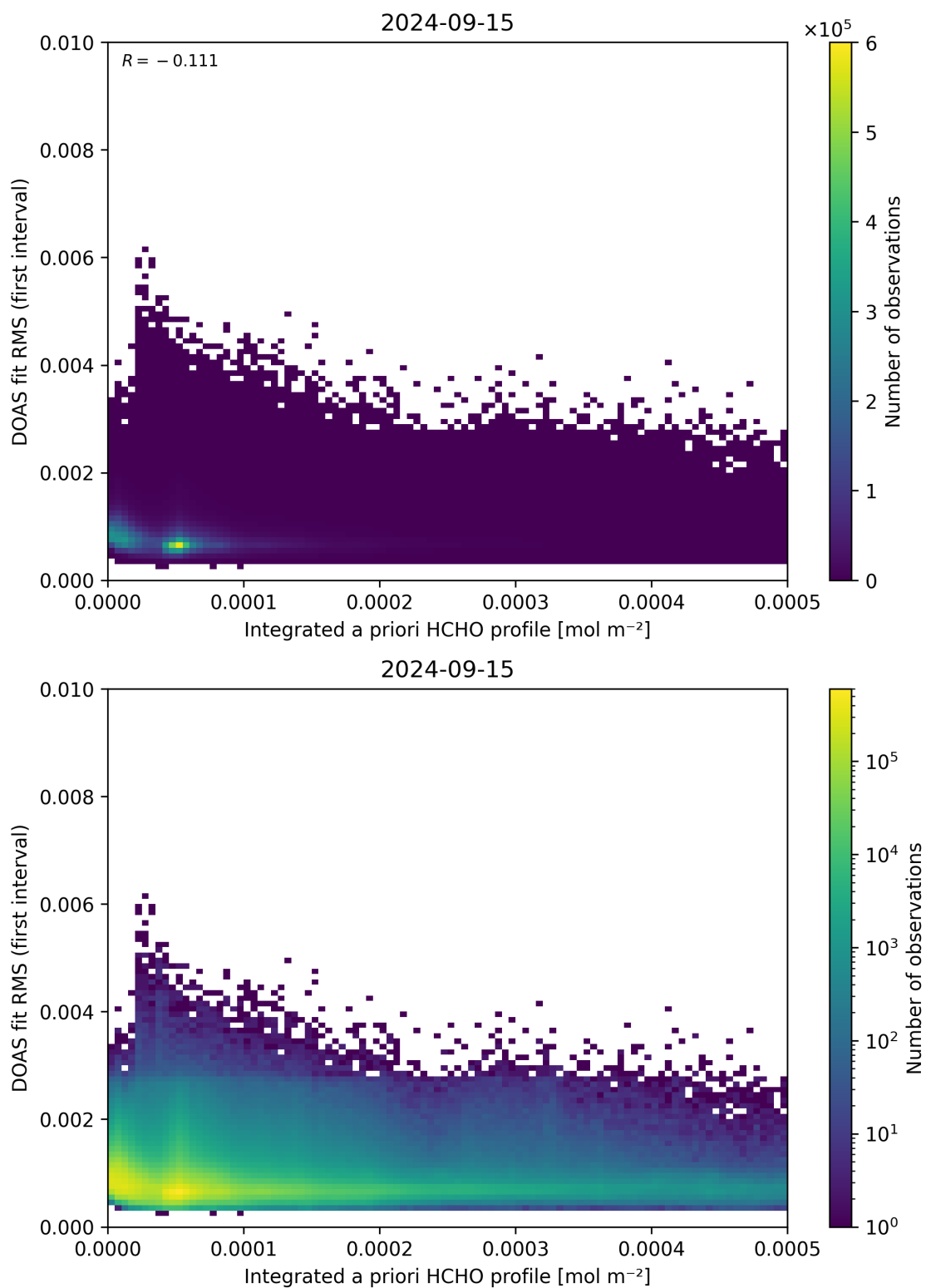
Figure 148: Scatter density plot of “Integrated a priori HCHO profile” against “DOAS fit RMS (first interval)” for 2024-09-14 to 2024-09-16.
