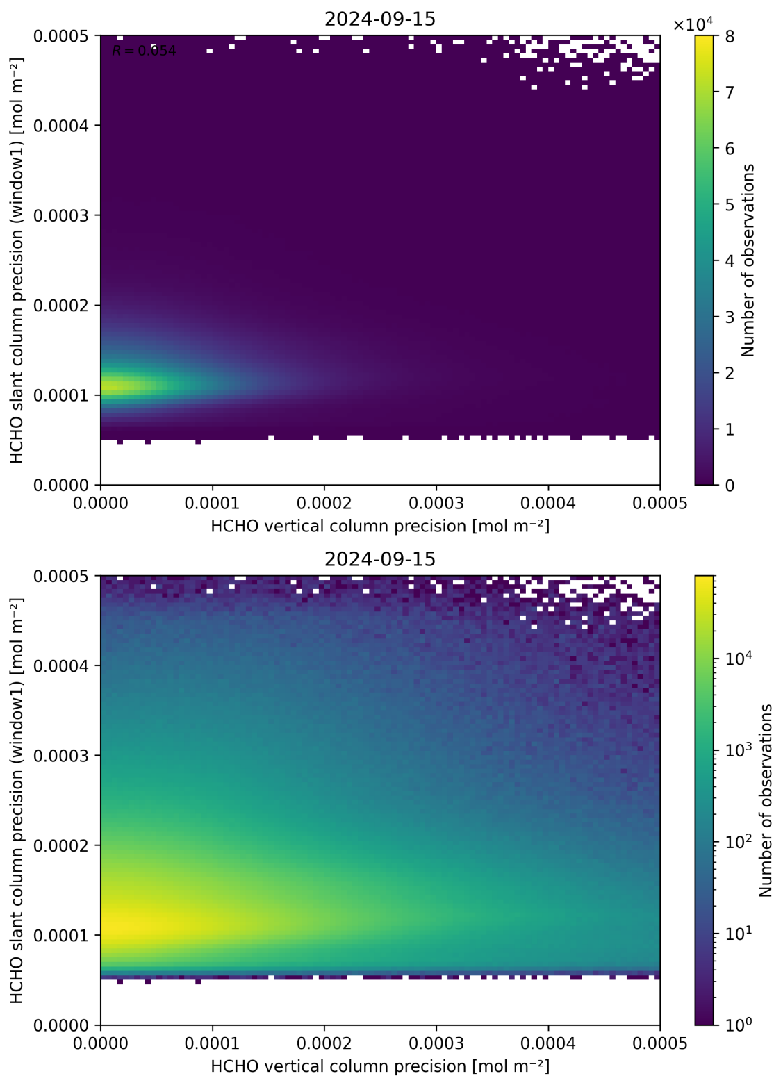
Figure 143: Scatter density plot of “HCHO vertical column precision” against “HCHO slant column precision (window1)” for 2024-09-14 to 2024-09-16.
