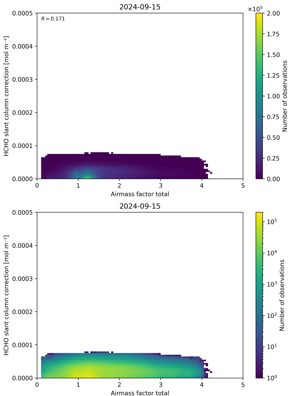
Figure 102: Scatter density plot of “Airmass factor total” against “HCHO slant column correction” for 2024-09-14 to 2024-09-16.
