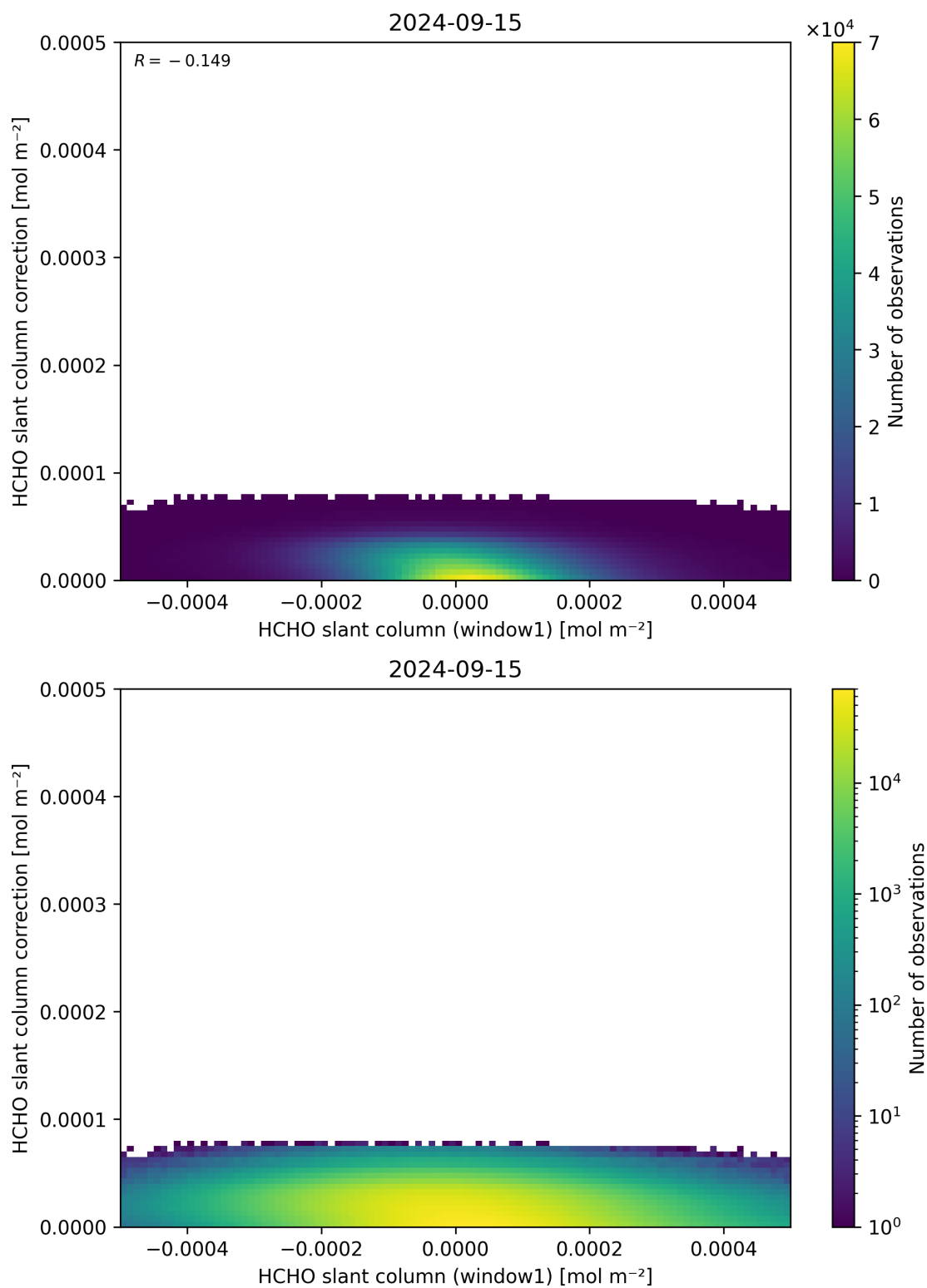
Figure 83: Scatter density plot of “HCHO slant column (window1)” against “HCHO slant column correction” for 2024-09-14 to 2024-09-16.
