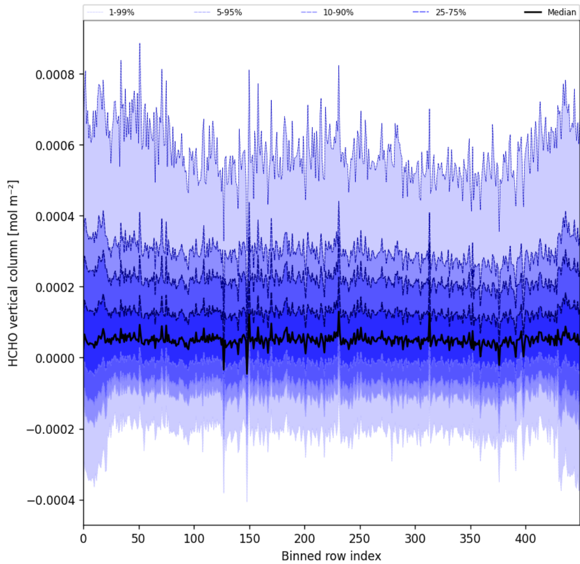
Figure 49: Along track statistics of “HCHO vertical column” for 2024-09-14 to 2024-09-16
