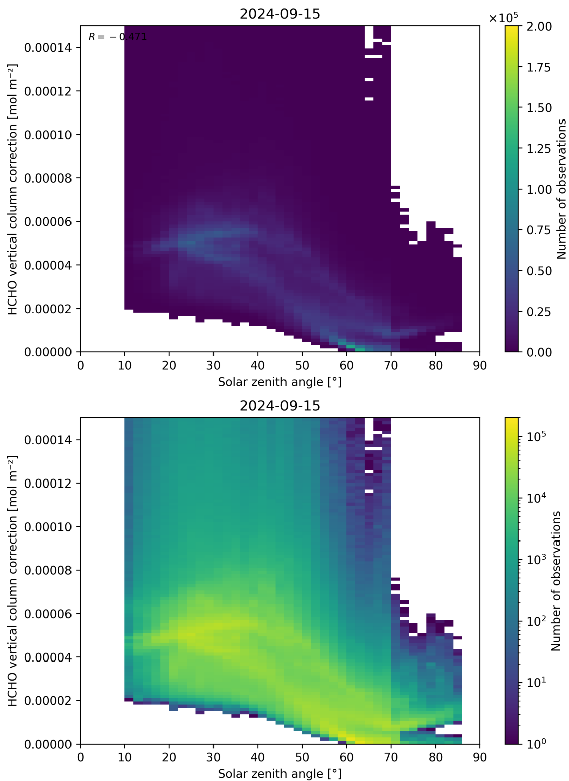
Figure 178: Scatter density plot of “Solar zenith angle” against “HCHO vertical column correction” for 2024-09-14 to 2024-09-16.
