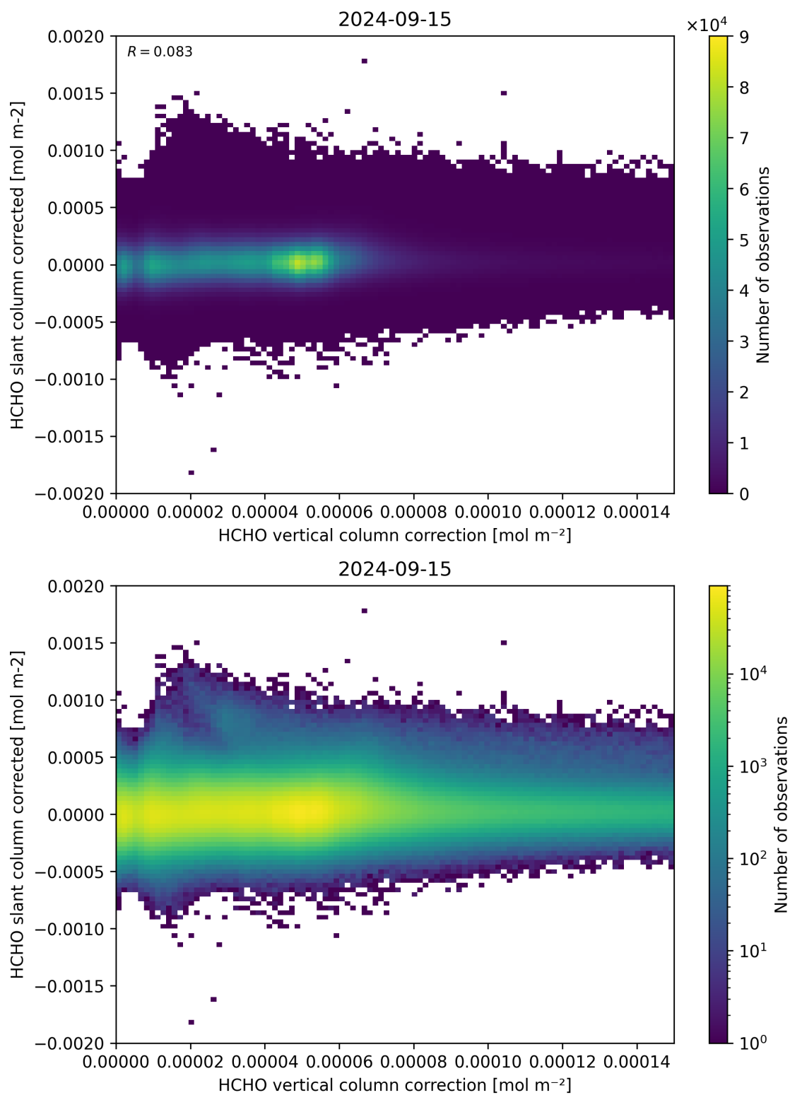
Figure 116: Scatter density plot of “HCHO vertical column correction” against “HCHO slant column corrected” for 2024-09-14 to 2024-09-16.
