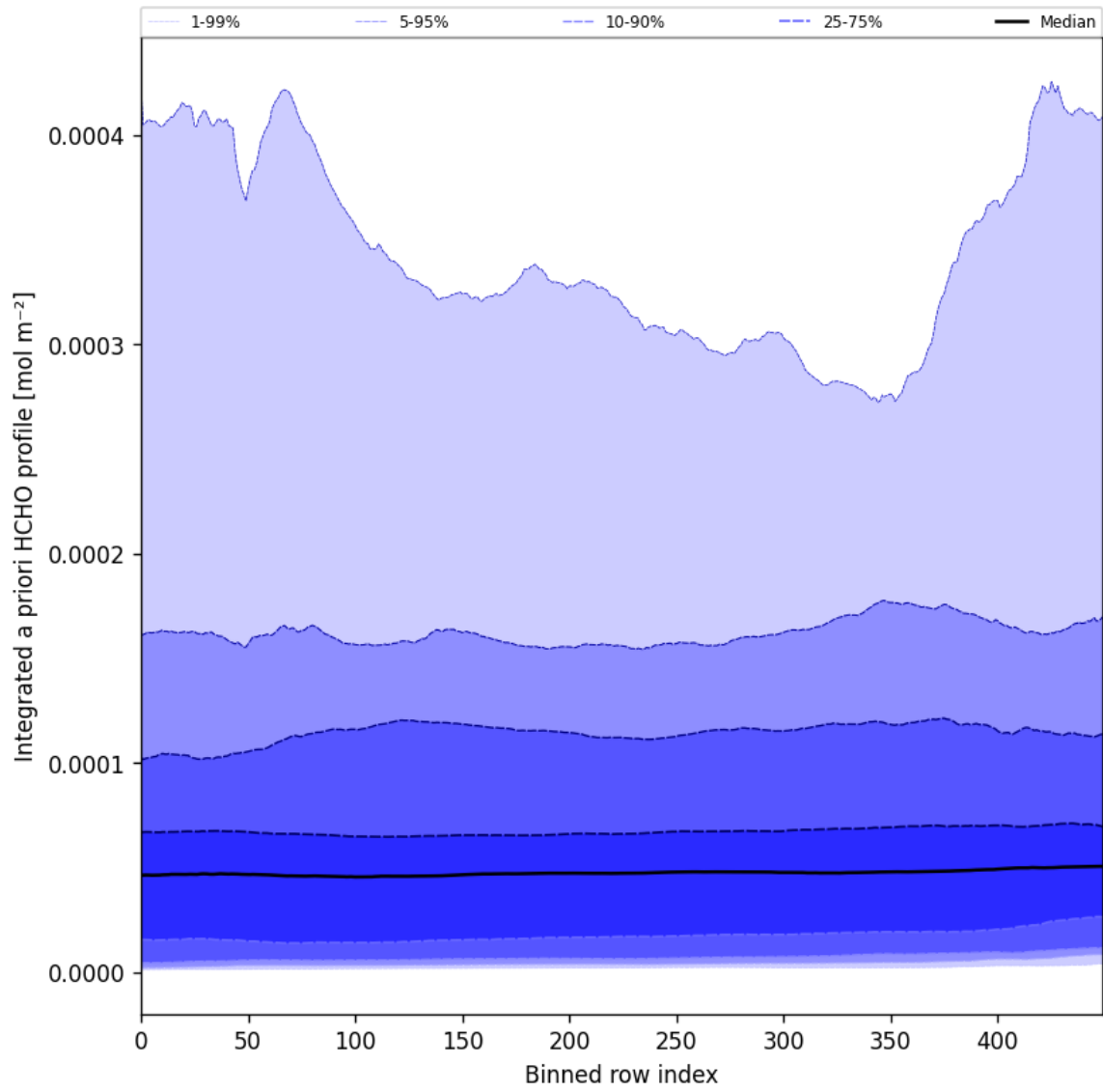
Figure 57: Along track statistics of "Integrated a priori HCHO profile" for 2024-09-14 to 2024-09-16
