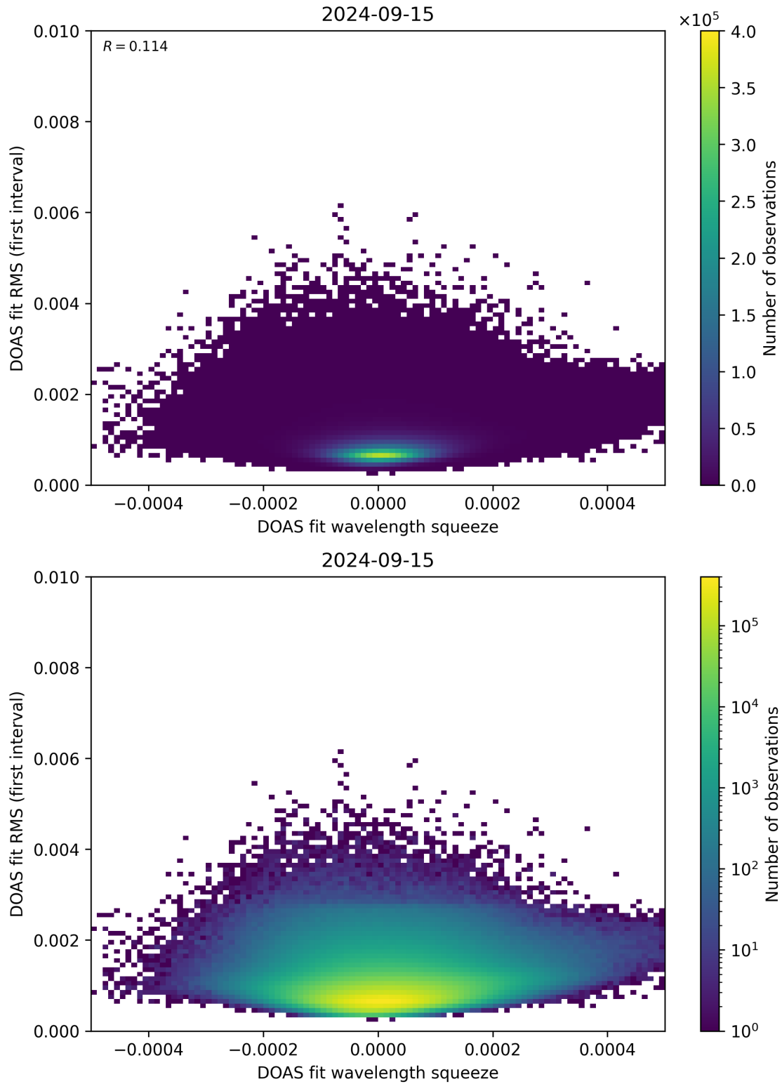
Figure 68: Scatter density plot of “DOAS fit wavelength squeeze” against “DOAS fit RMS (first interval)” for 2024-09-14 to 2024-09-16.
