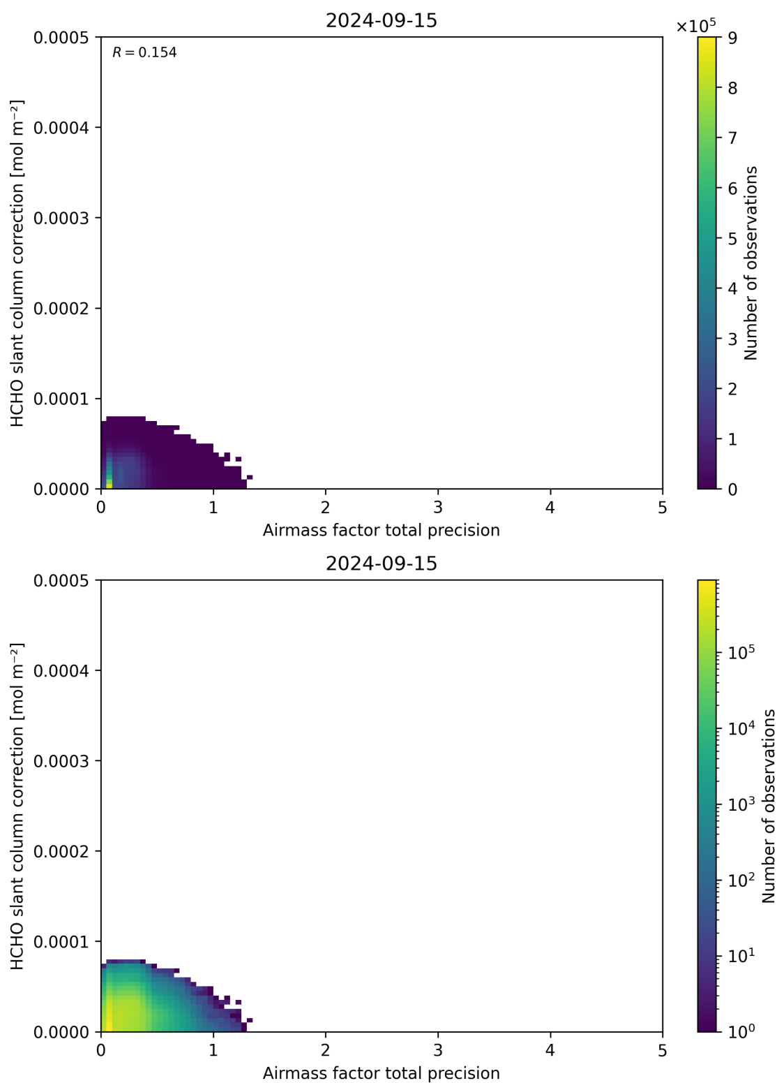
Figure 110: Scatter density plot of “Airmass factor total precision” against “HCHO slant column correction” for 2024-09-14 to 2024-09-16.
