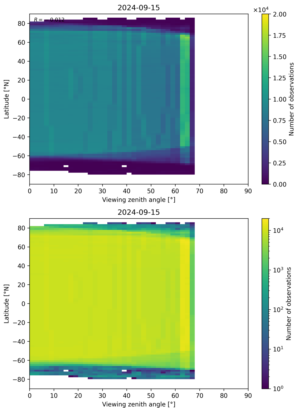
Figure 196: Scatter density plot of “Viewing zenith angle” against “Latitude” for 2024-09-14 to 2024-09-16.
