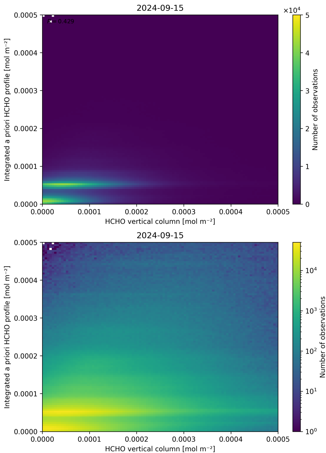
Figure 135: Scatter density plot of “HCHO vertical column” against “Integrated a priori HCHO profile” for 2024-09-14 to 2024-09-16.
