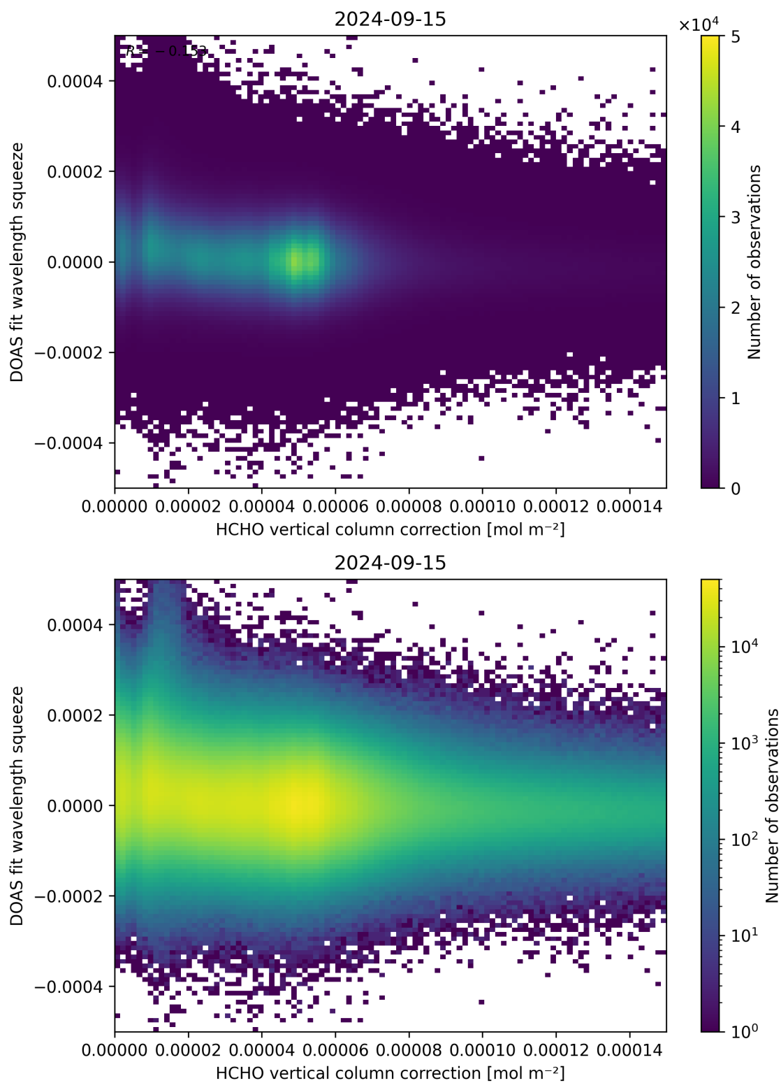
Figure 114: Scatter density plot of “HCHO vertical column correction” against “DOAS fit wavelength squeeze” for 2024-09-14 to 2024-09-16.
