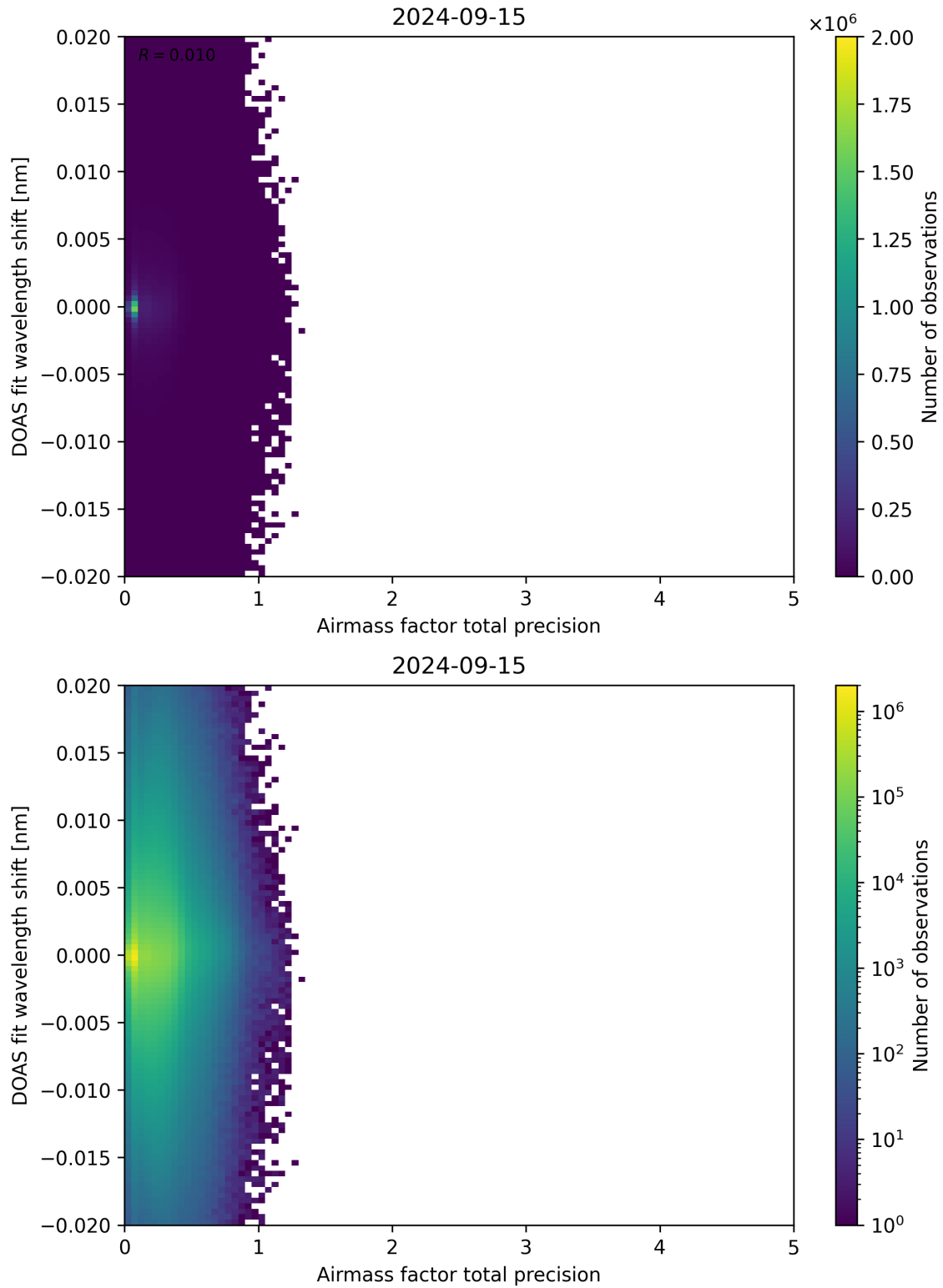
Figure 106: Scatter density plot of “Airmass factor total precision” against “DOAS fit wavelength shift” for 2024-09-14 to 2024-09-16.
