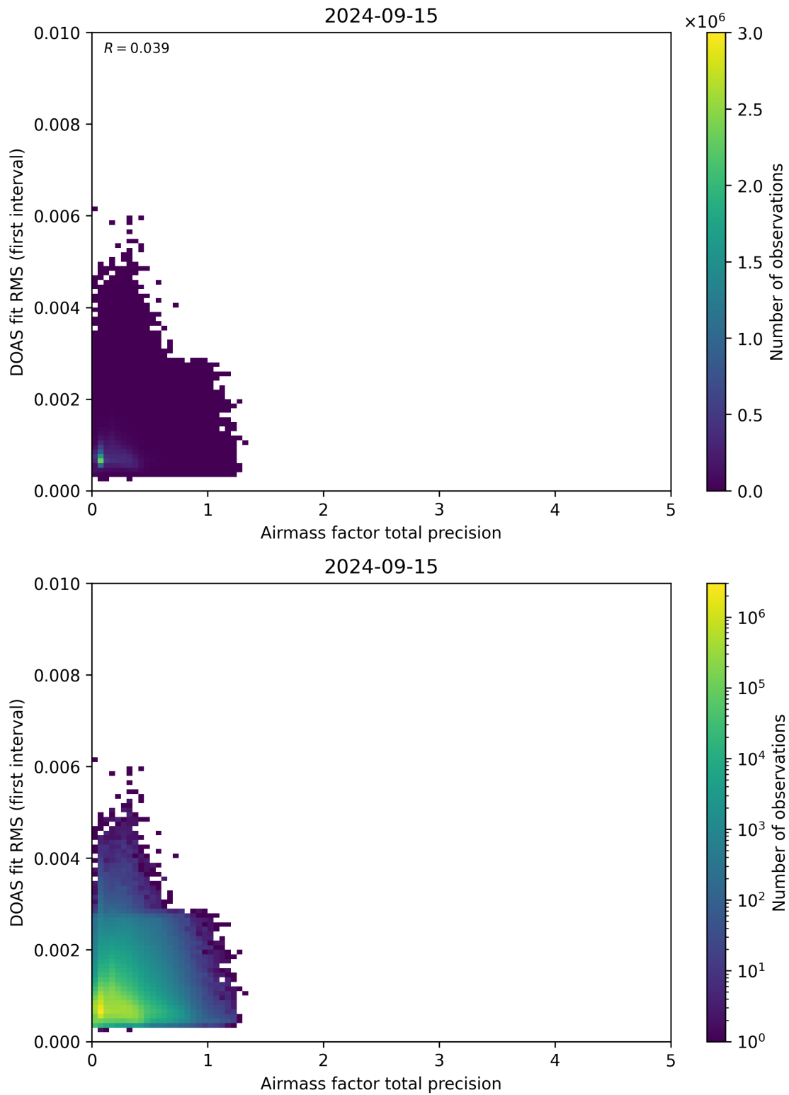
Figure 105: Scatter density plot of “Airmass factor total precision” against “DOAS fit RMS (first interval)” for 2024-09-14 to 2024-09-16.
