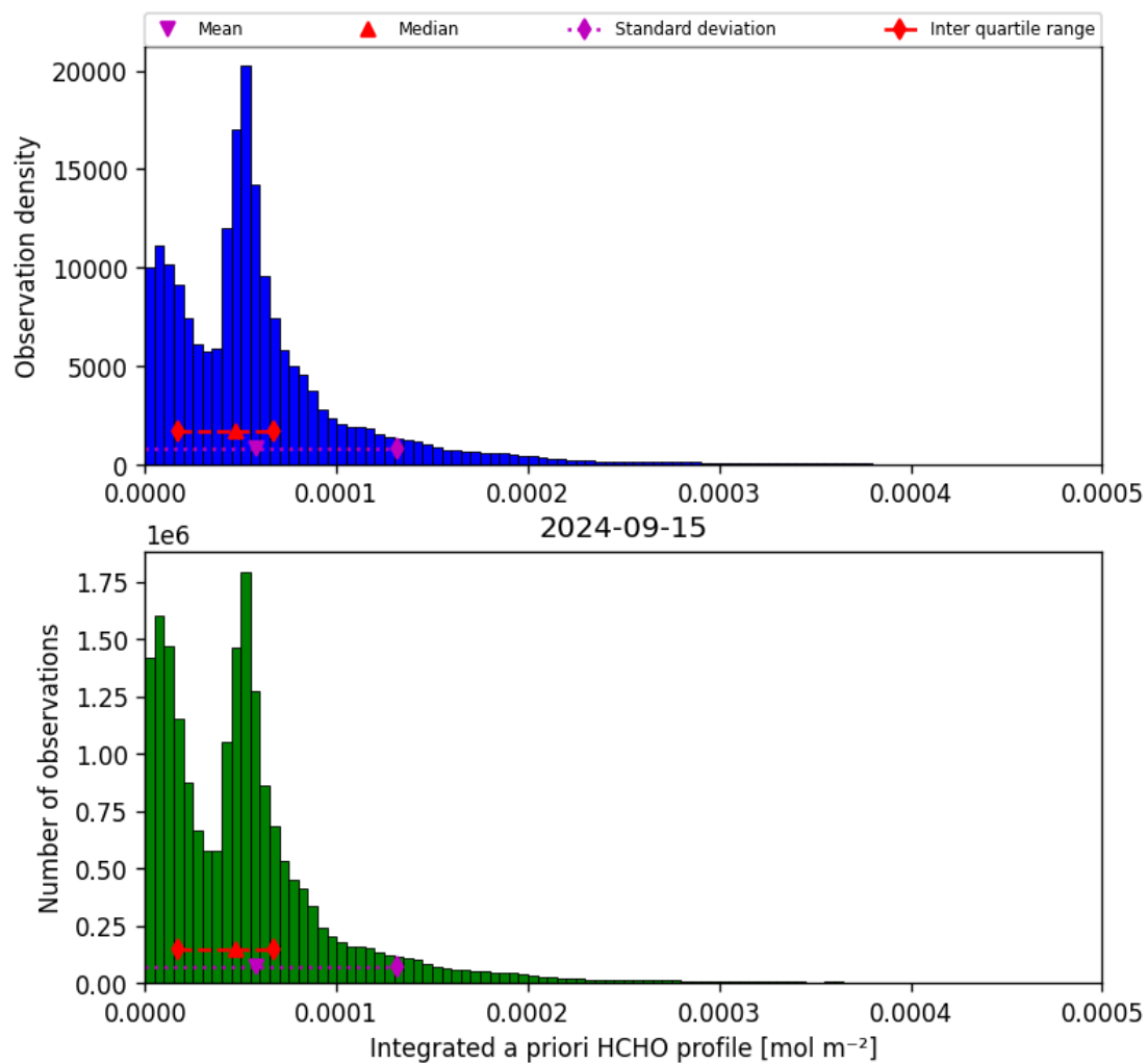
Figure 43: Histogram of “Integrated a priori HCHO profile” for 2024-09-14 to 2024-09-16
