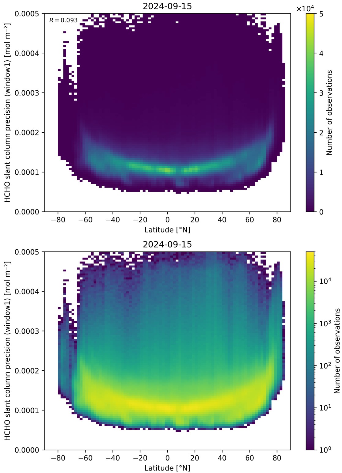
Figure 160: Scatter density plot of “Latitude” against “HCHO slant column precision (window1)” for 2024-09-14 to 2024-09-16.
