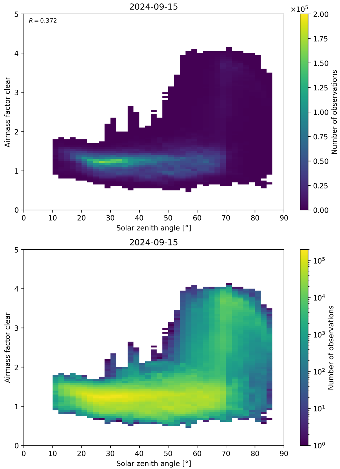
Figure 170: Scatter density plot of “Solar zenith angle” against “Airmass factor clear” for 2024-09-14 to 2024-09-16.
