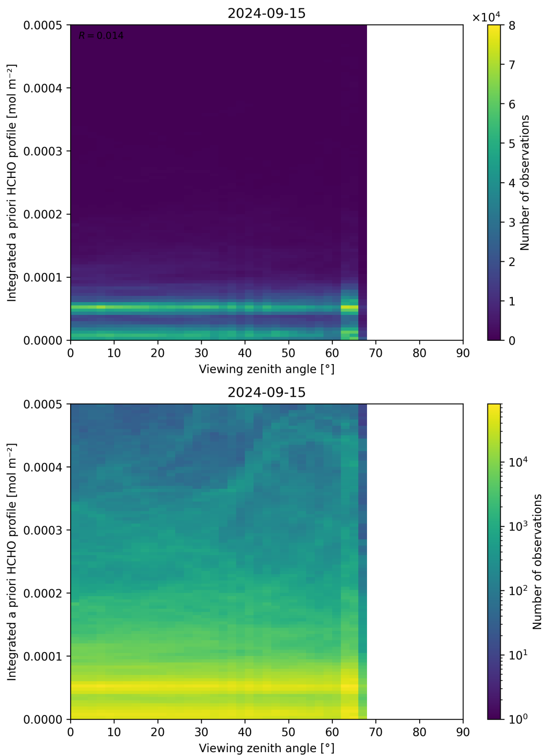
Figure 195: Scatter density plot of “Viewing zenith angle” against “Integrated a priori HCHO profile” for 2024-09-14 to 2024-09-16.
