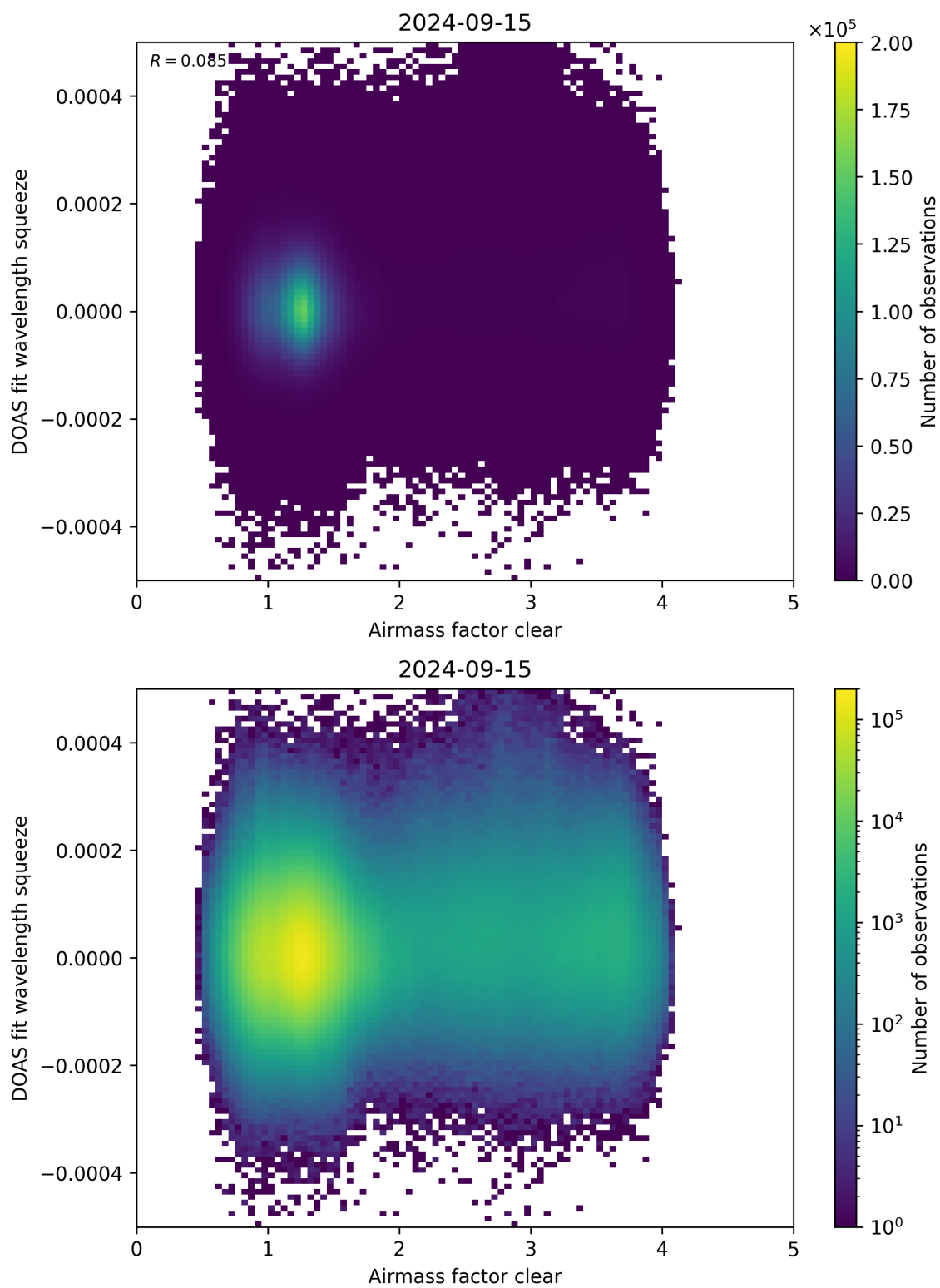
Figure 73: Scatter density plot of “Airmass factor clear” against “DOAS fit wavelength squeeze” for 2024-09-14 to 2024-09-16.
