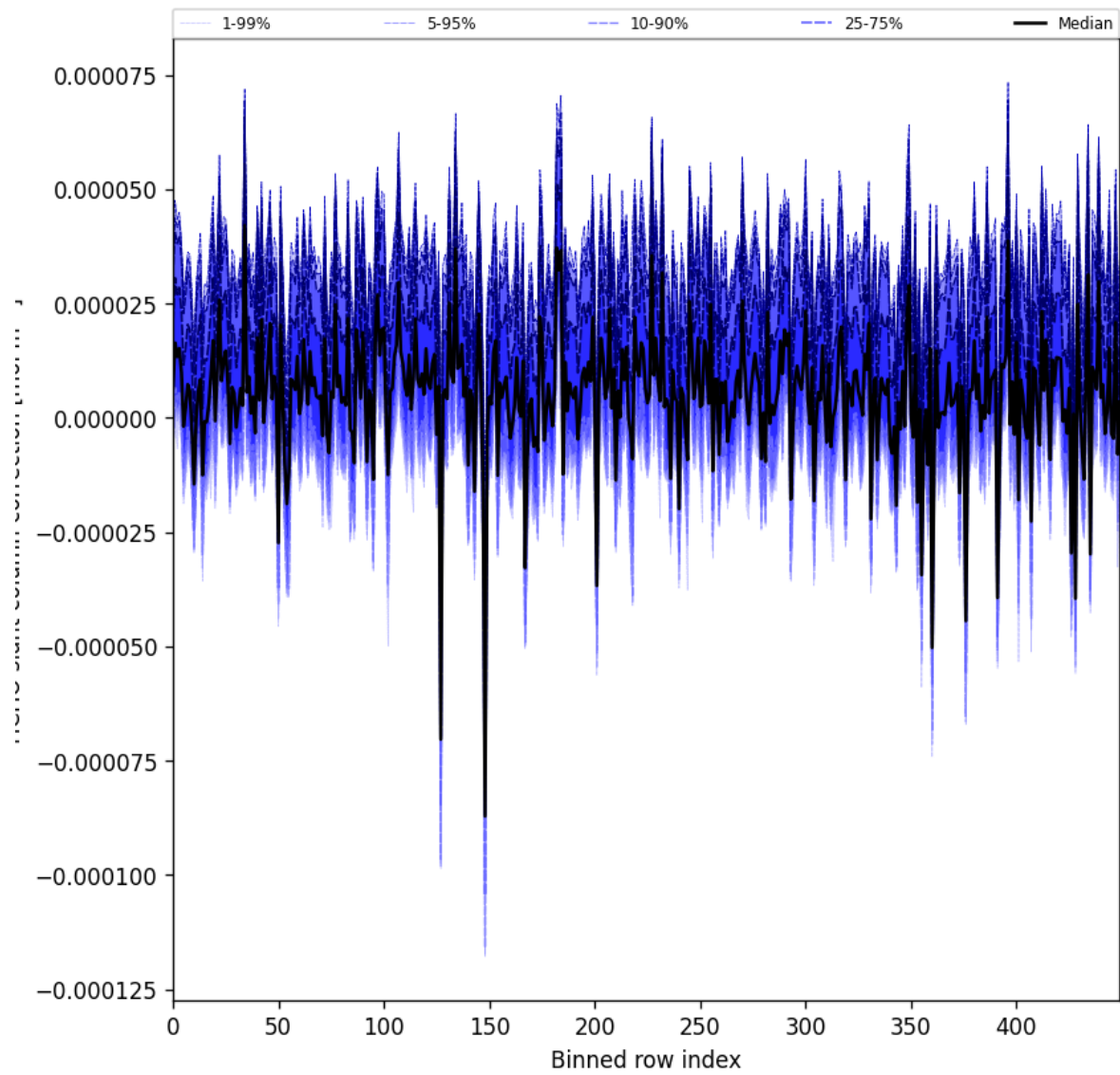
Figure 61: Along track statistics of “HCHO slant column correction” for 2024-09-14 to 2024-09-16
