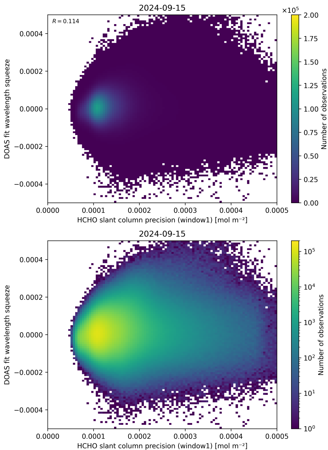
Figure 90: Scatter density plot of “HCHO slant column precision (window1)” against “DOAS fit wavelength squeeze” for 2024-09-14 to 2024-09-16.
