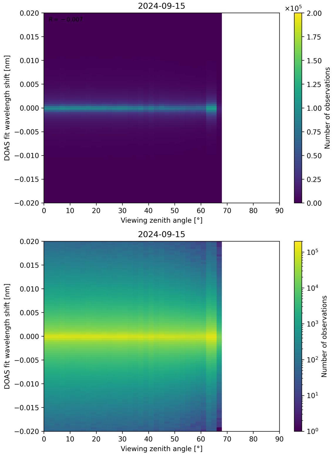
Figure 183: Scatter density plot of “Viewing zenith angle” against “DOAS fit wavelength shift” for 2024-09-14 to 2024-09-16.
