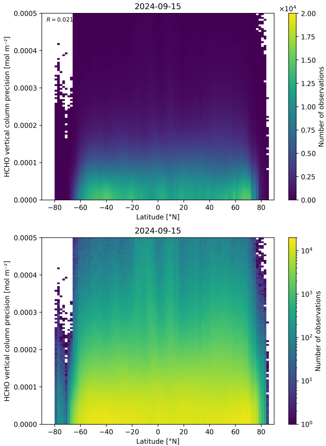
Figure 165: Scatter density plot of “Latitude” against “HCHO vertical column precision” for 2024-09-14 to 2024-09-16.
