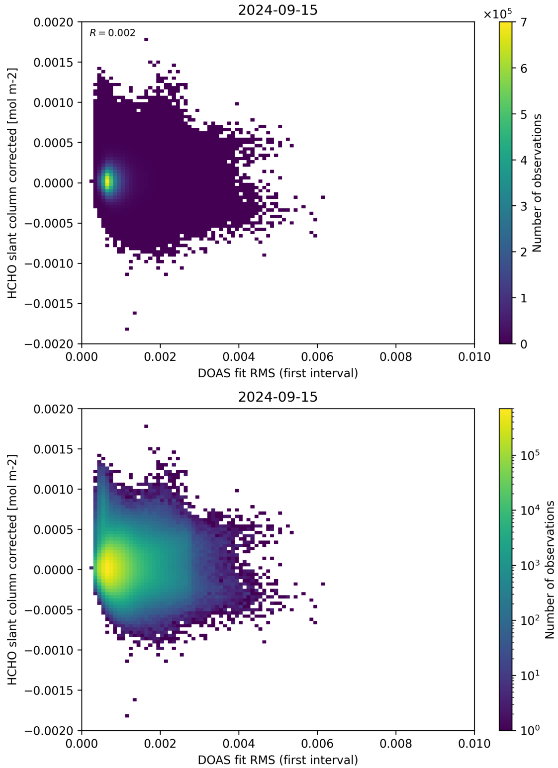
Figure 62: Scatter density plot of “DOAS fit RMS (first interval)” against “HCHO slant column corrected” for 2024-09-14 to 2024-09-16.
