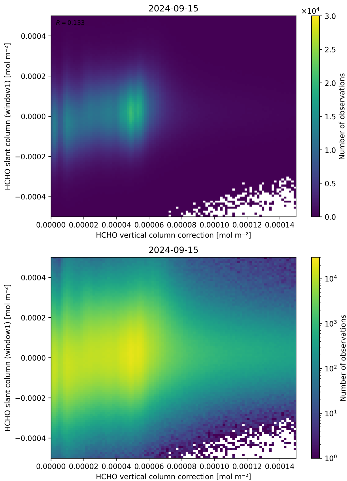
Figure 118: Scatter density plot of “HCHO vertical column correction” against “HCHO slant column (window1)” for 2024-09-14 to 2024-09-16.
