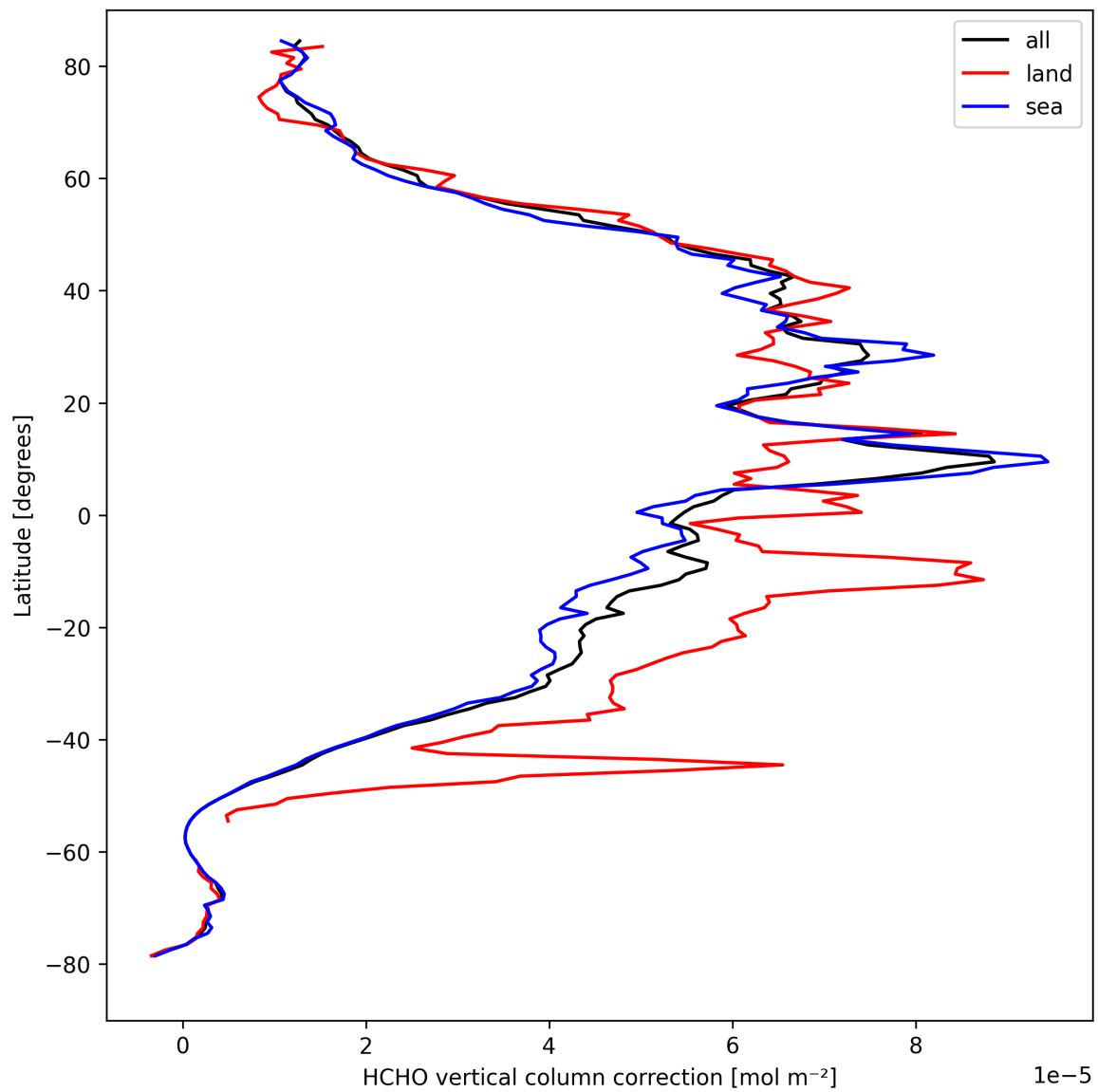
Figure 23: Zonal average of “HCHO vertical column correction” for 2024-09-14 to 2024-09-16.
