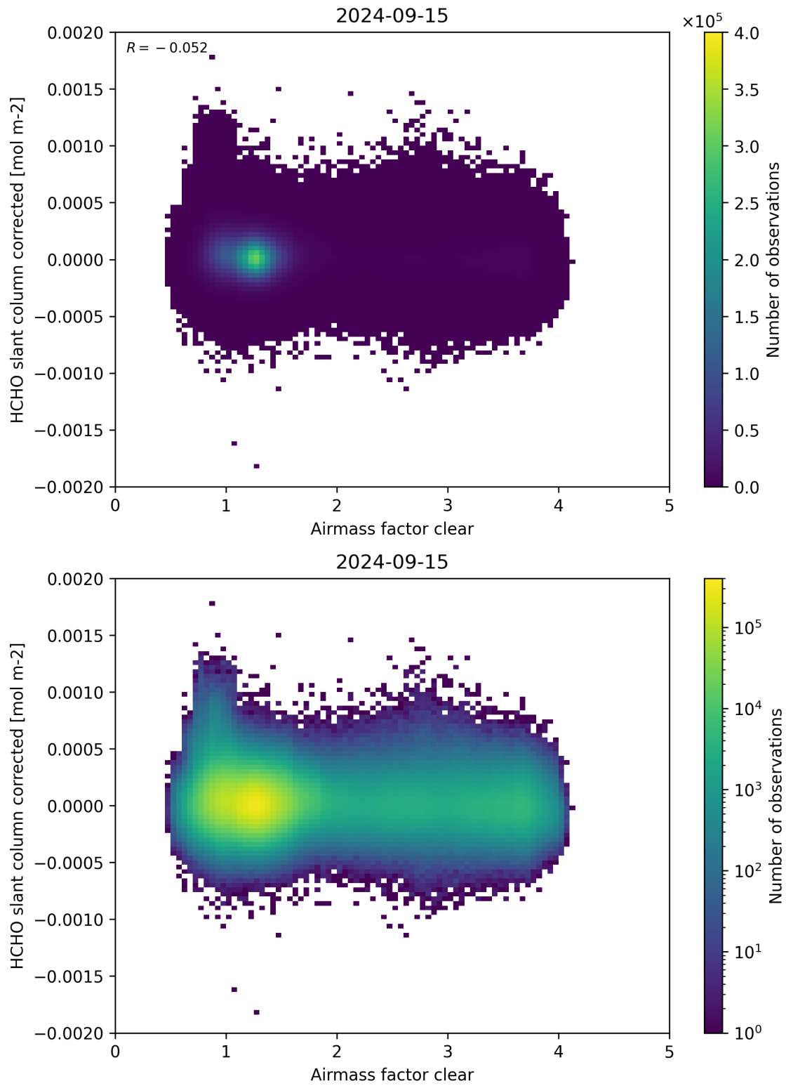
Figure 74: Scatter density plot of “Airmass factor clear” against “HCHO slant column corrected” for 2024-09-14 to 2024-09-16.
