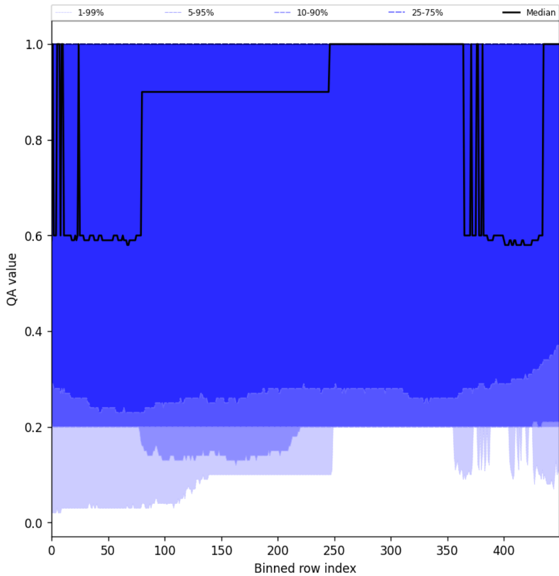
Figure 48: Along track statistics of “QA value” for 2024-09-14 to 2024-09-16
