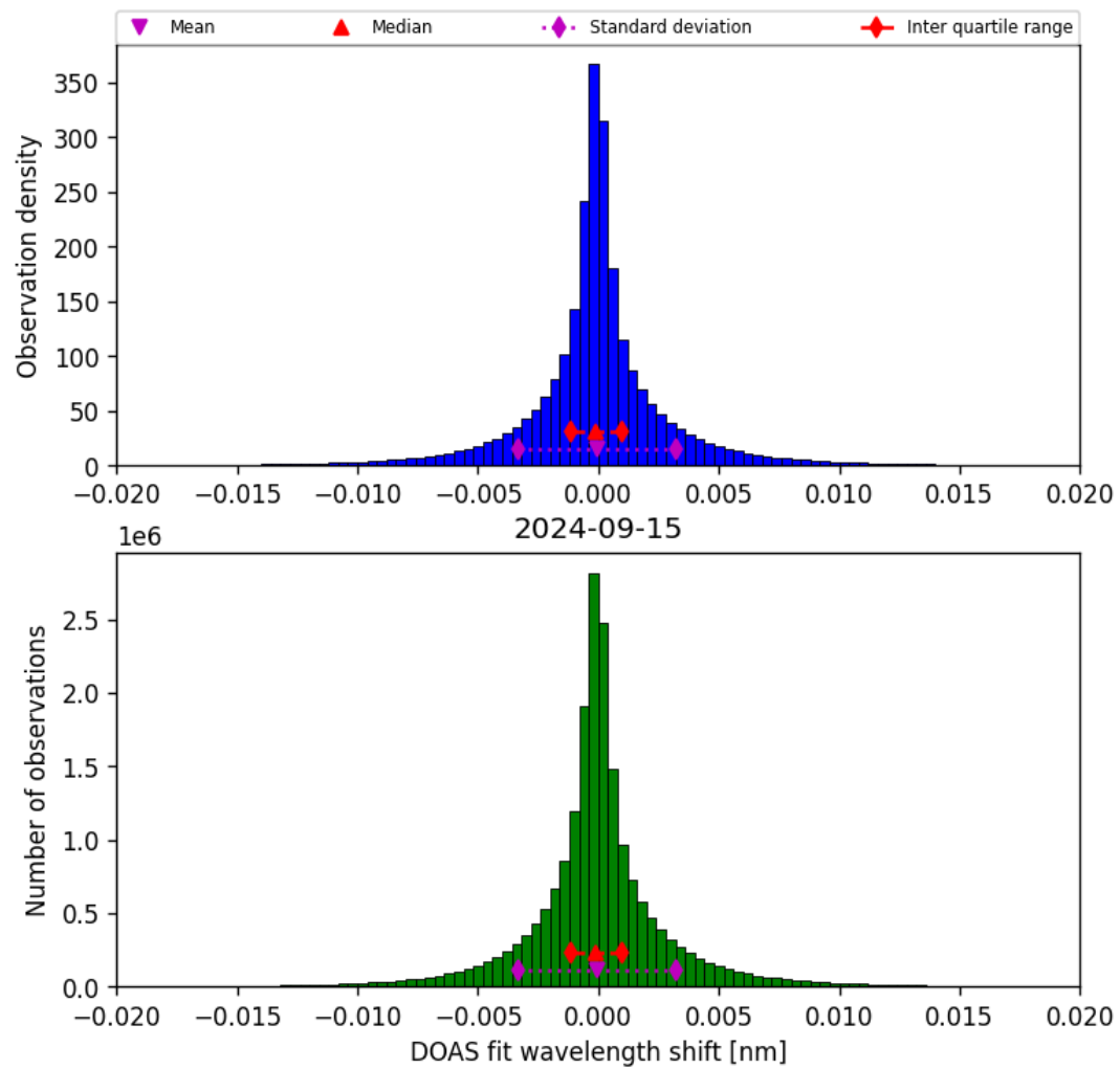
Figure 44: Histogram of “DOAS fit wavelength shift” for 2024-09-14 to 2024-09-16
