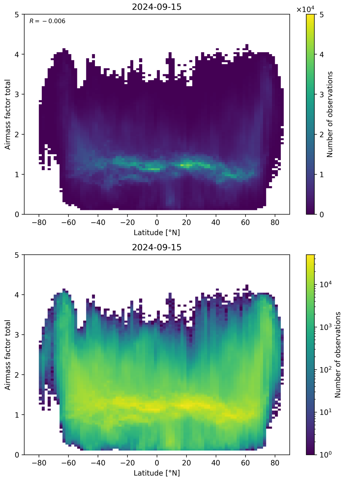
Figure 161: Scatter density plot of “Latitude” against “Airmass factor total” for 2024-09-14 to 2024-09-16.
