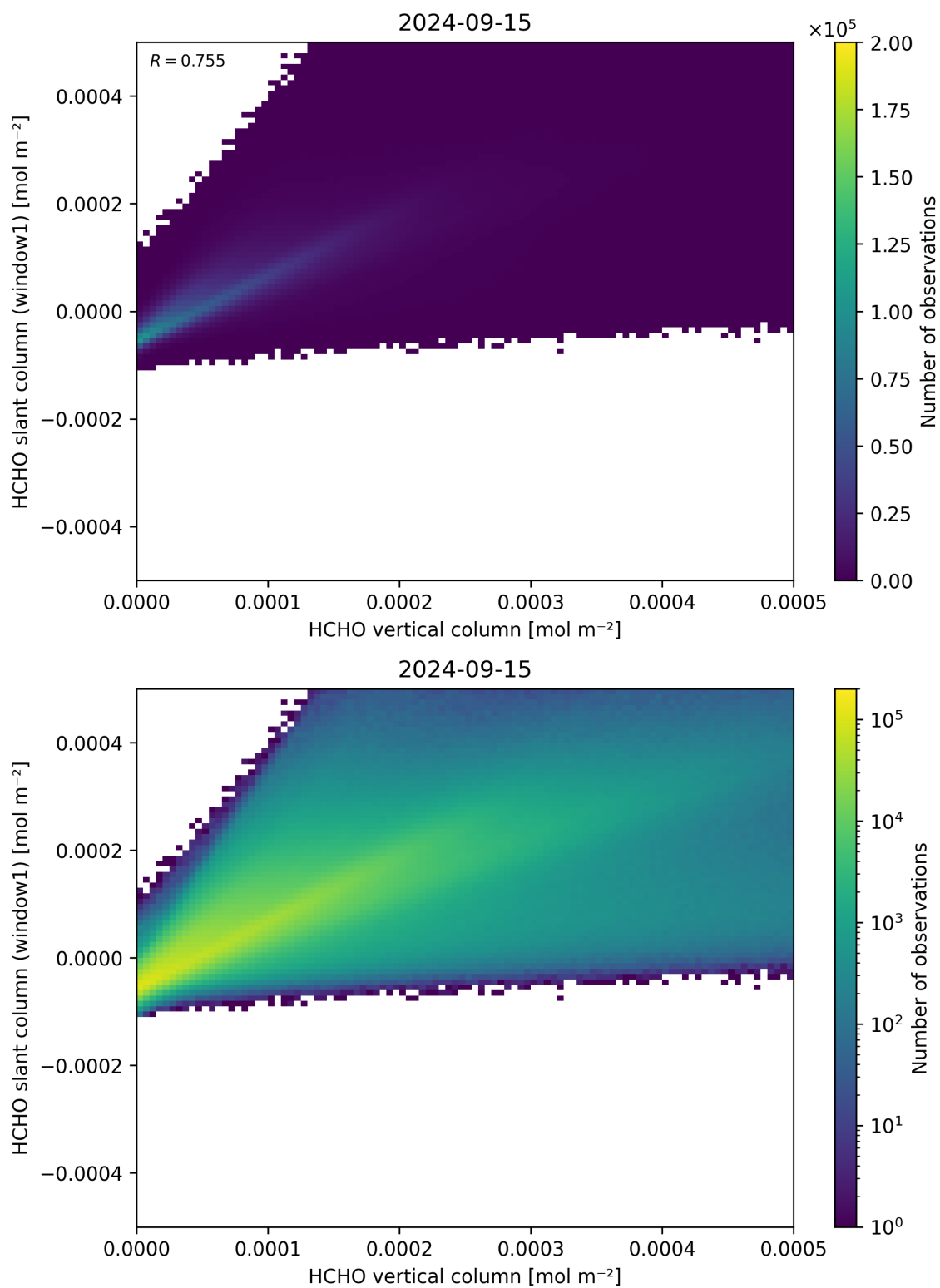
Figure 129: Scatter density plot of “HCHO vertical column” against “HCHO slant column (window1)” for 2024-09-14 to 2024-09-16.
