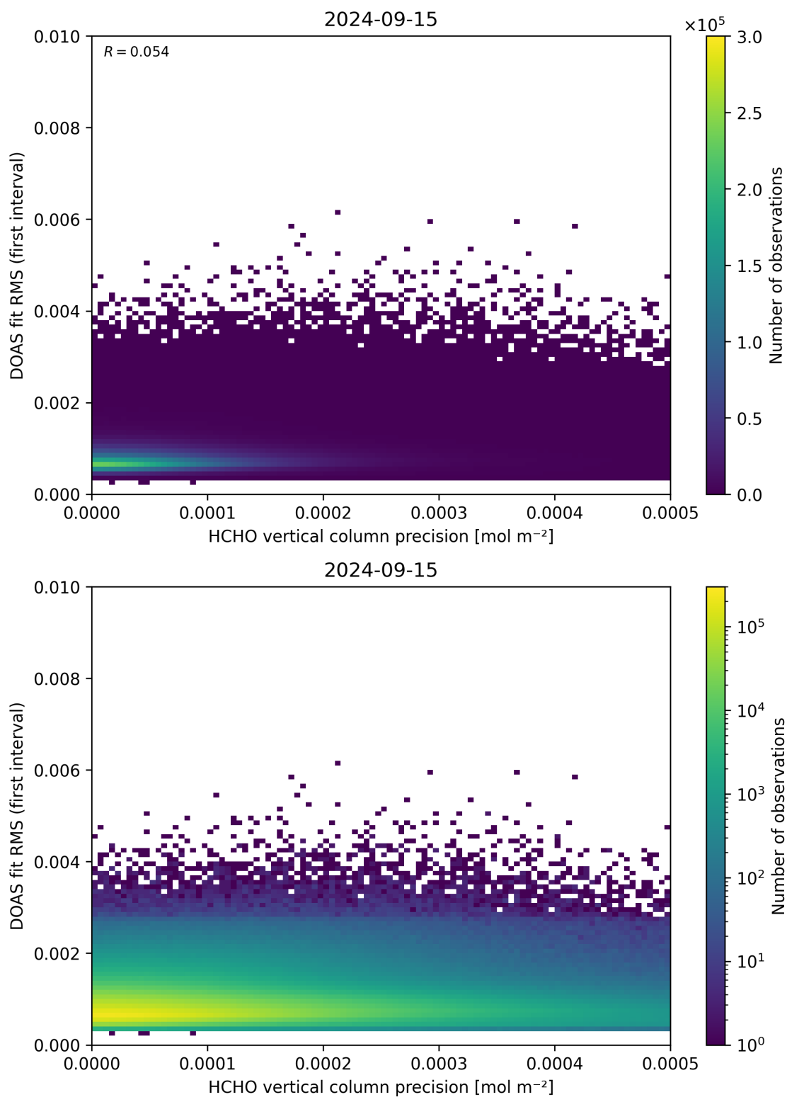
Figure 136: Scatter density plot of “HCHO vertical column precision” against “DOAS fit RMS (first interval)” for 2024-09-14 to 2024-09-16.
