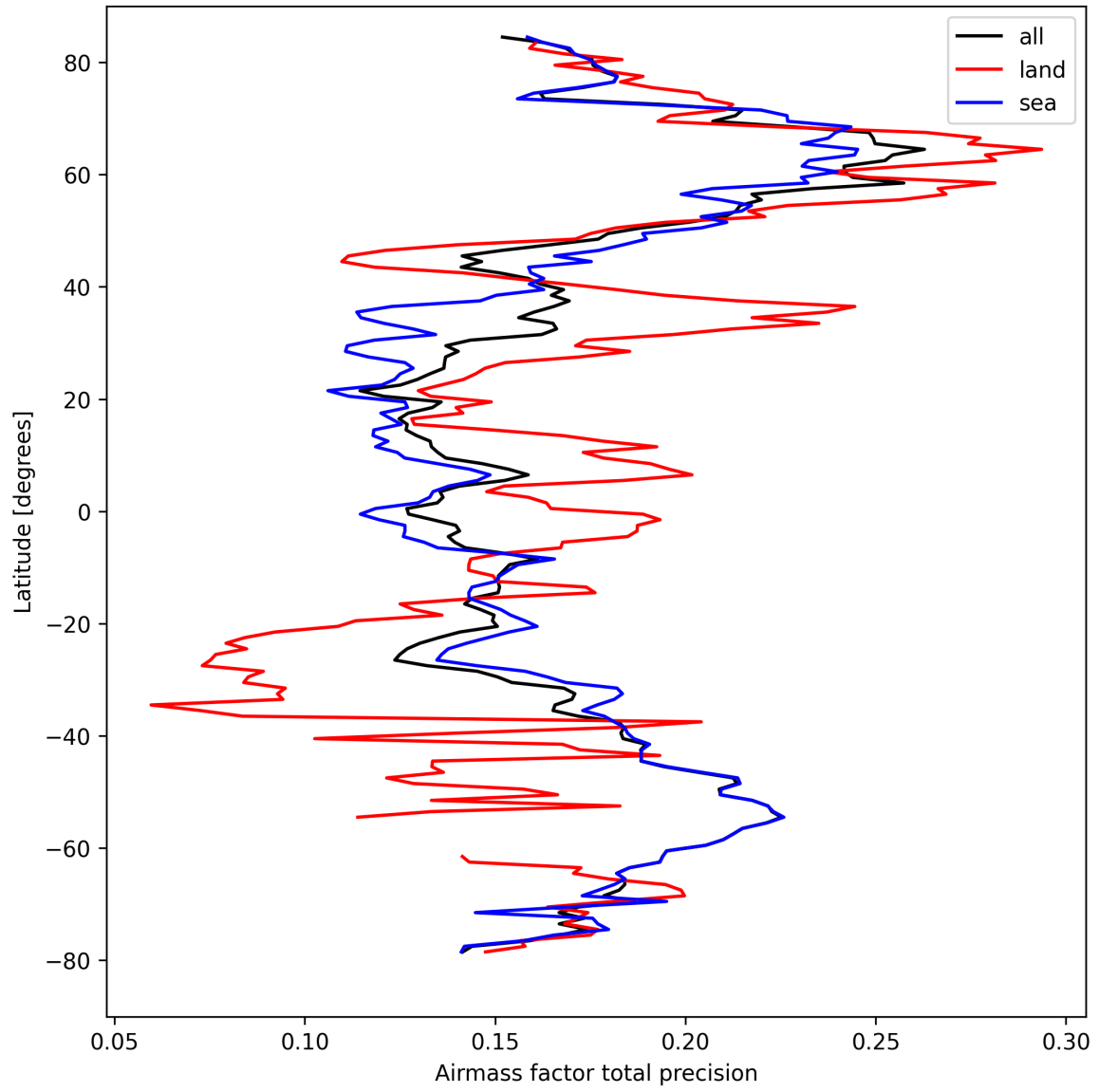
Figure 27: Zonal average of “Airmass factor total precision” for 2024-09-14 to 2024-09-16.
