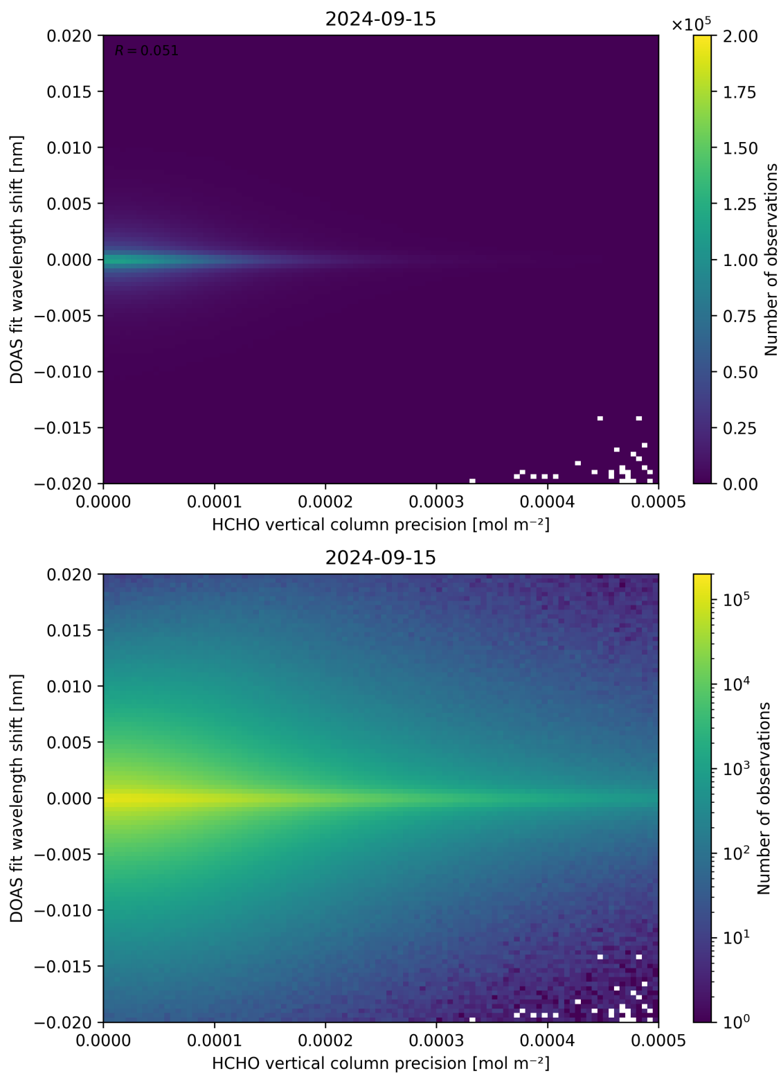
Figure 137: Scatter density plot of “HCHO vertical column precision” against “DOAS fit wavelength shift” for 2024-09-14 to 2024-09-16.
