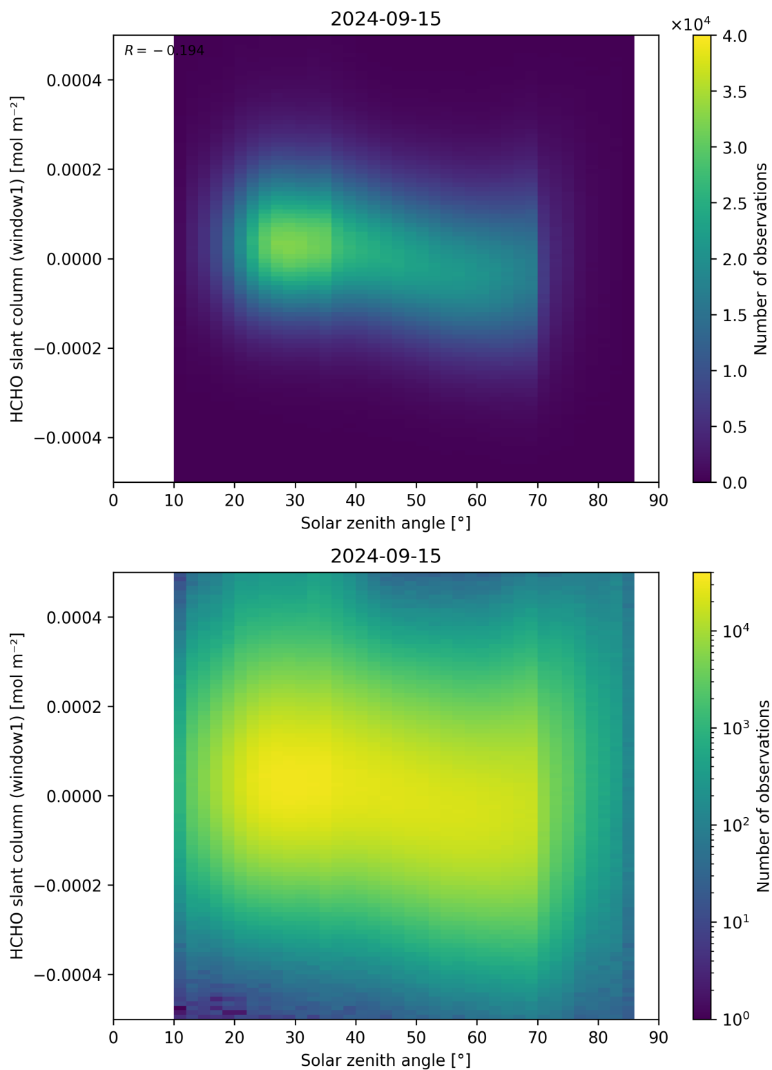
Figure 173: Scatter density plot of “Solar zenith angle” against “HCHO slant column (window1)” for 2024-09-14 to 2024-09-16.
