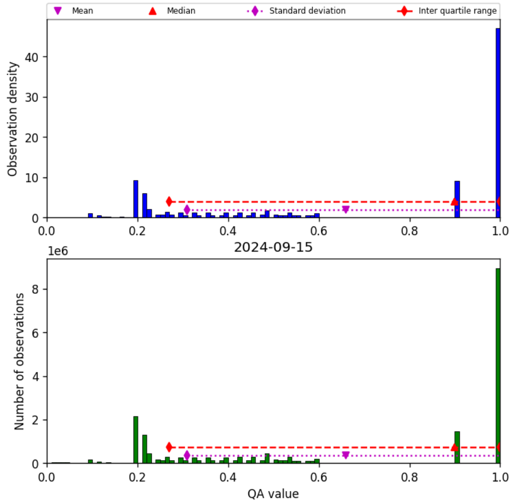
Figure 34: Histogram of “QA value” for 2024-09-14 to 2024-09-16
