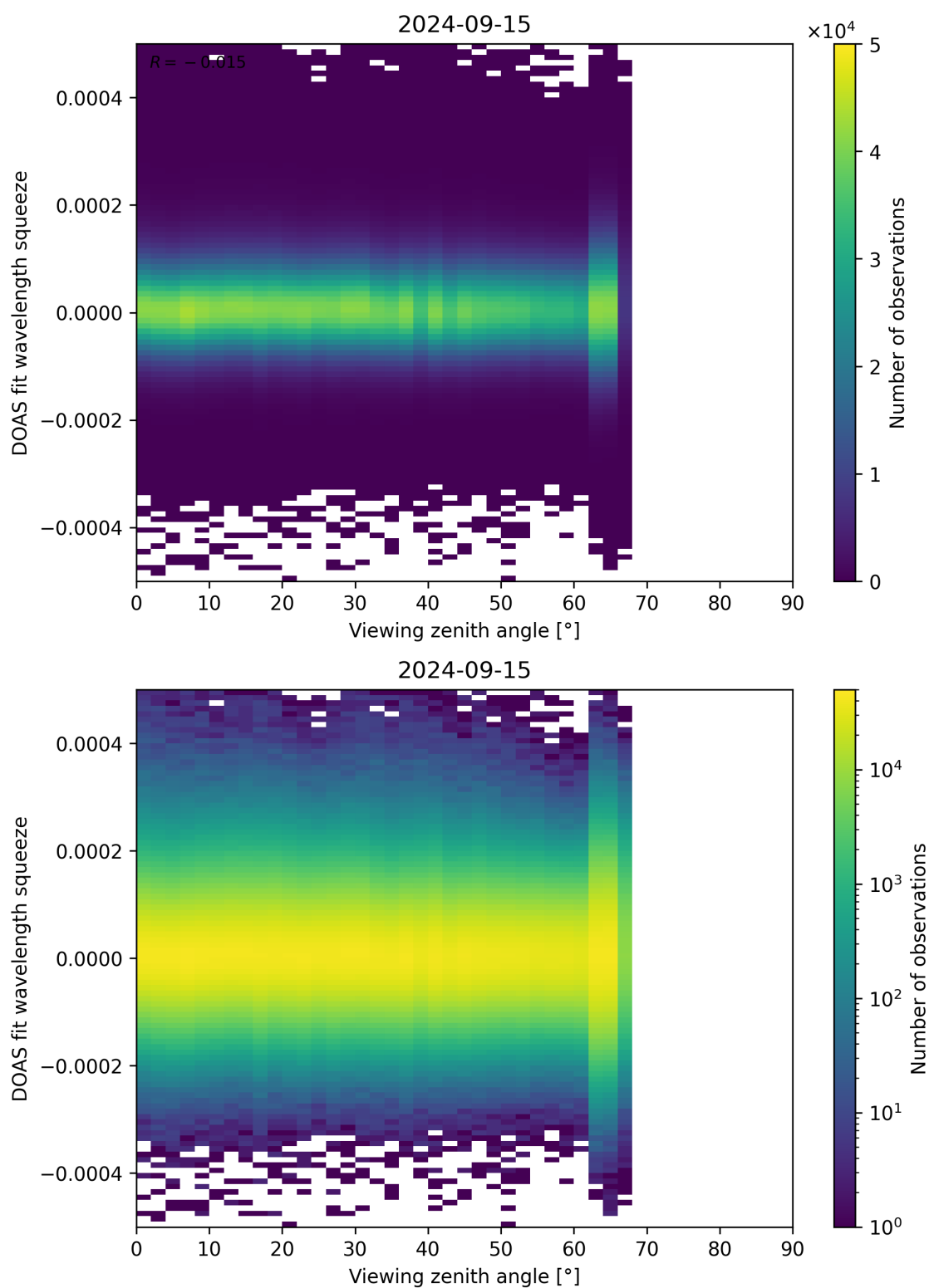
Figure 184: Scatter density plot of “Viewing zenith angle” against “DOAS fit wavelength squeeze” for 2024-09-14 to 2024-09-16.
