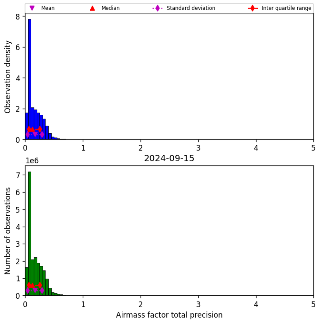
Figure 41: Histogram of “Airmass factor total precision” for 2024-09-14 to 2024-09-16
