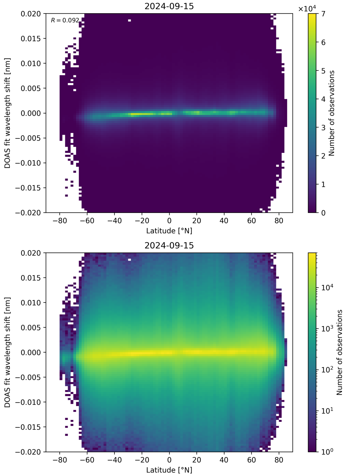
Figure 154: Scatter density plot of “Latitude” against “DOAS fit wavelength shift” for 2024-09-14 to 2024-09-16.
