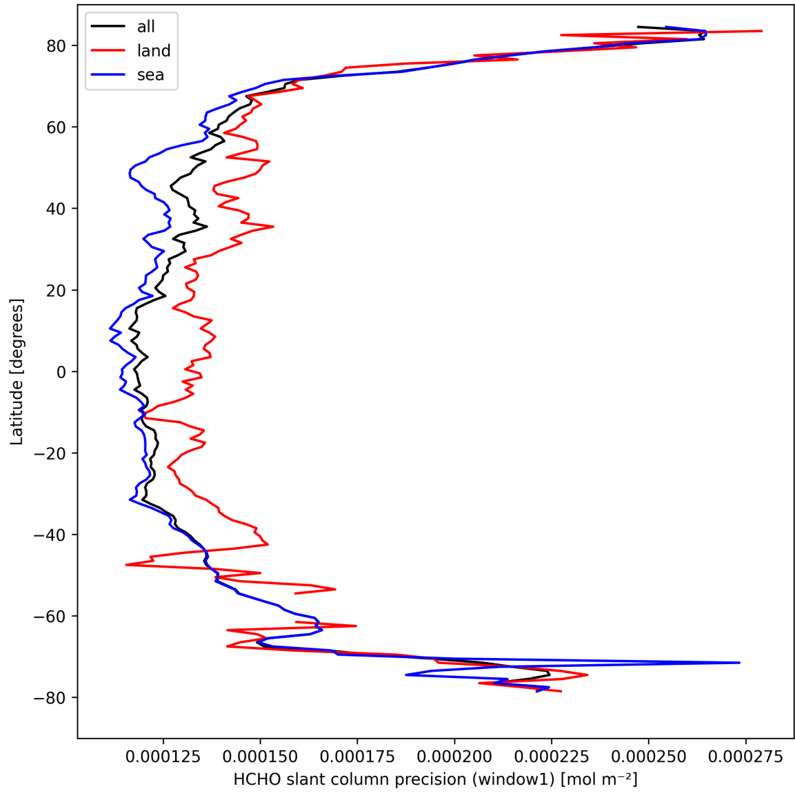
Figure 25: Zonal average of “HCHO slant column precision (window1)” for 2024-09-14 to 2024-09-16.
