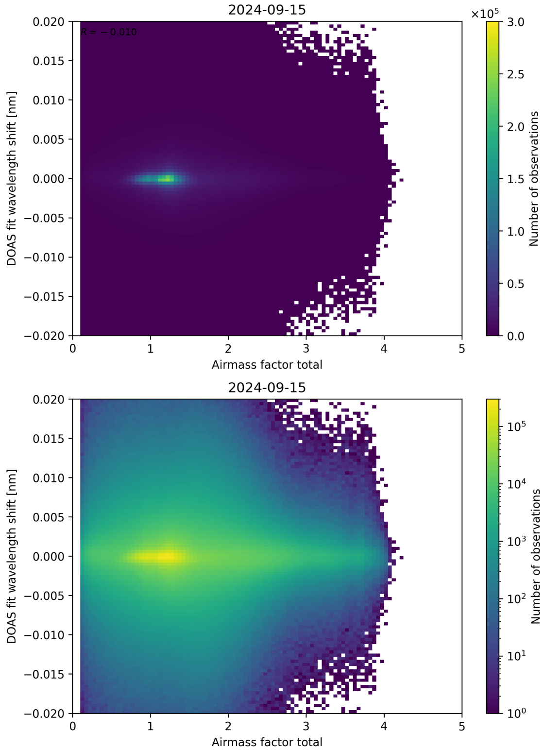
Figure 98: Scatter density plot of “Airmass factor total” against “DOAS fit wavelength shift” for 2024-09-14 to 2024-09-16.
