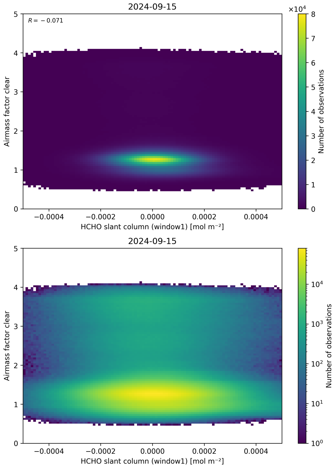
Figure 81: Scatter density plot of “HCHO slant column (window1)” against “Airmass factor clear” for 2024-09-14 to 2024-09-16.
