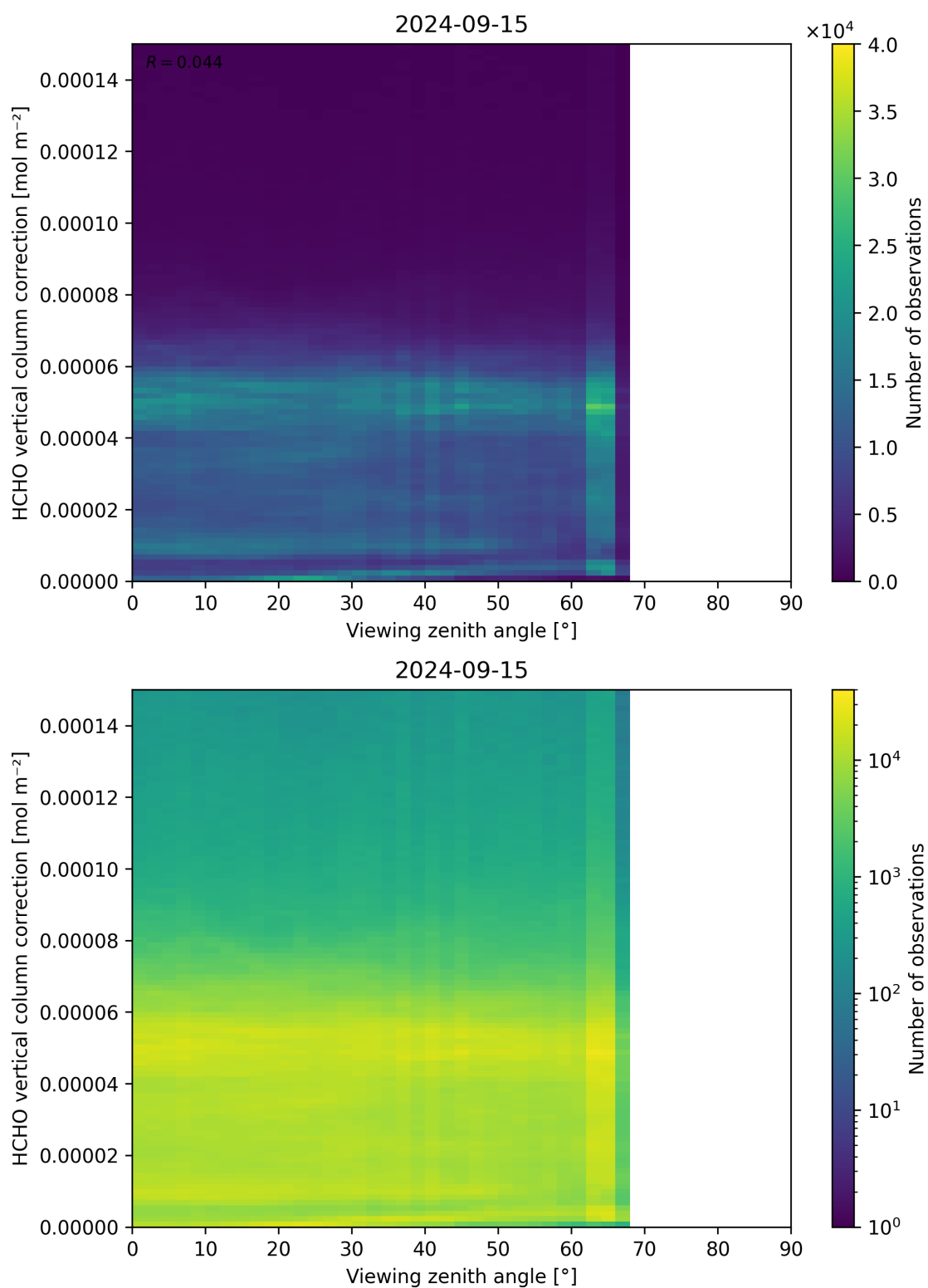
Figure 193: Scatter density plot of “Viewing zenith angle” against “HCHO vertical column correction” for 2024-09-14 to 2024-09-16.
