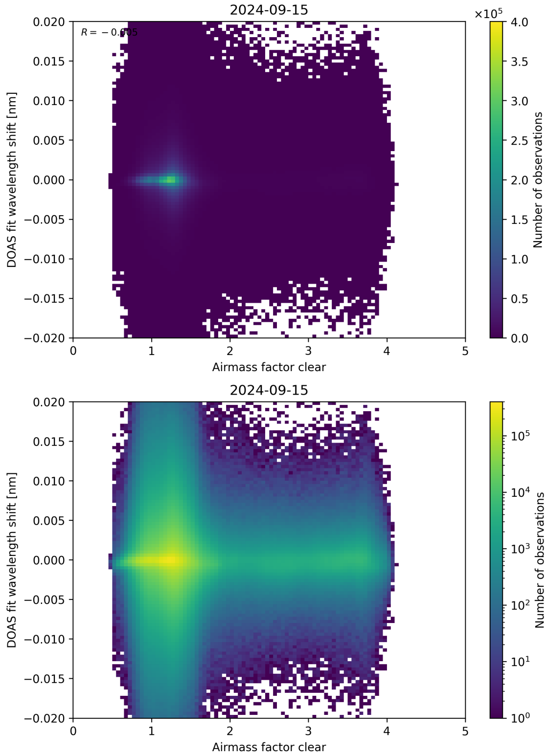
Figure 72: Scatter density plot of “Airmass factor clear” against “DOAS fit wavelength shift” for 2024-09-14 to 2024-09-16.
