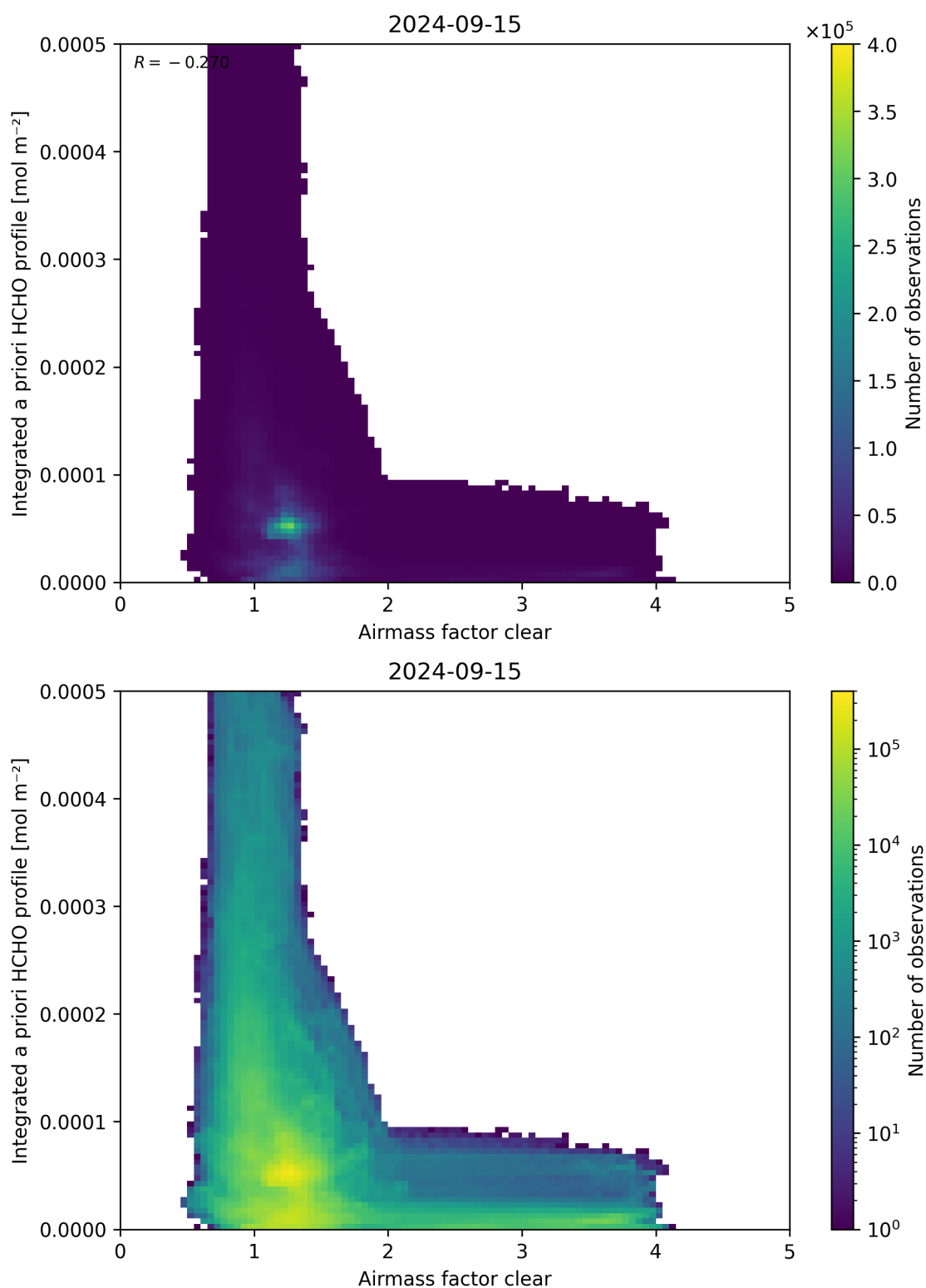
Figure 76: Scatter density plot of “Airmass factor clear” against “Integrated a priori HCHO profile” for 2024-09-14 to 2024-09-16.
