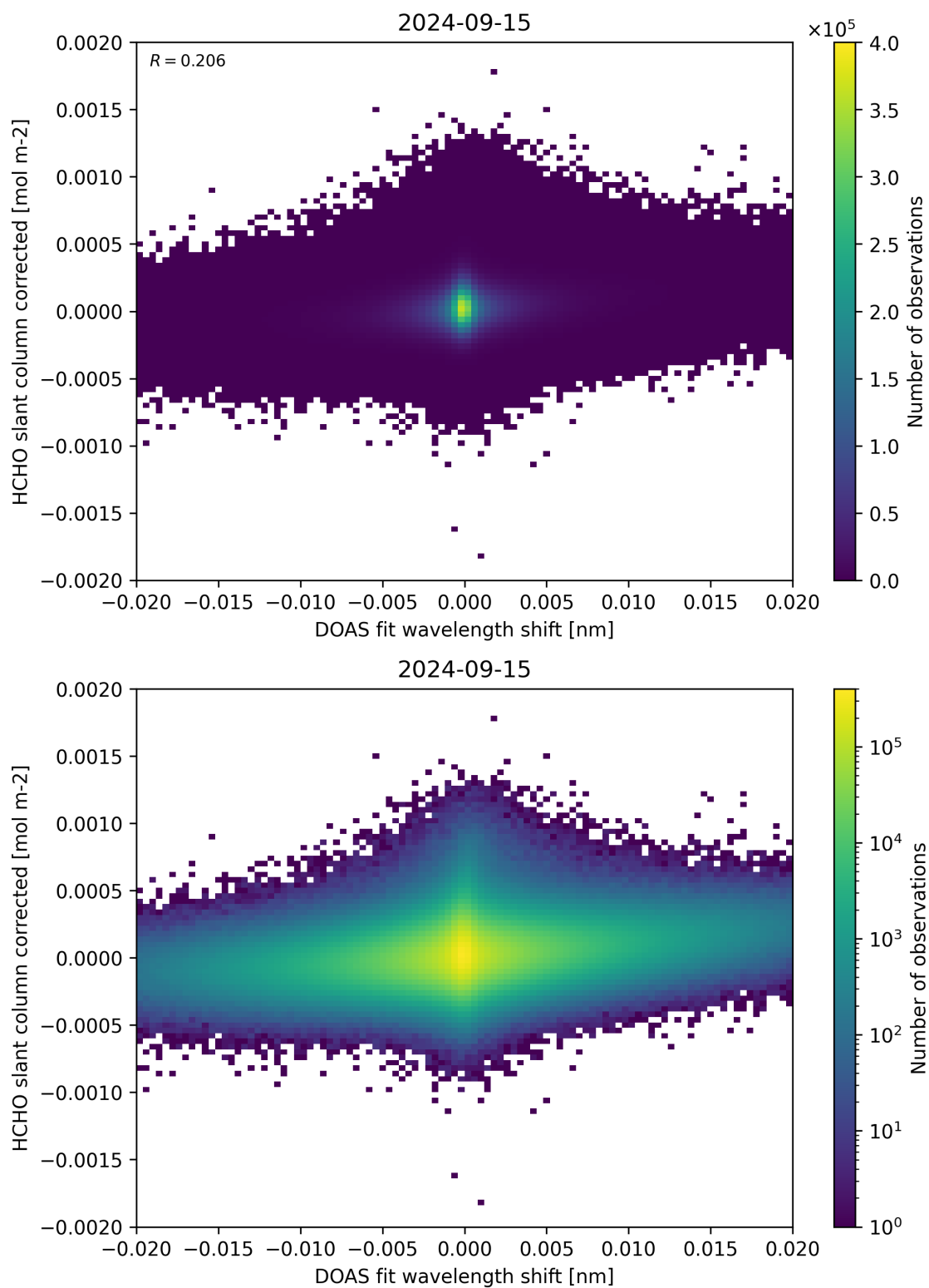
Figure 66: Scatter density plot of “DOAS fit wavelength shift” against “HCHO slant column corrected” for 2024-09-14 to 2024-09-16.
