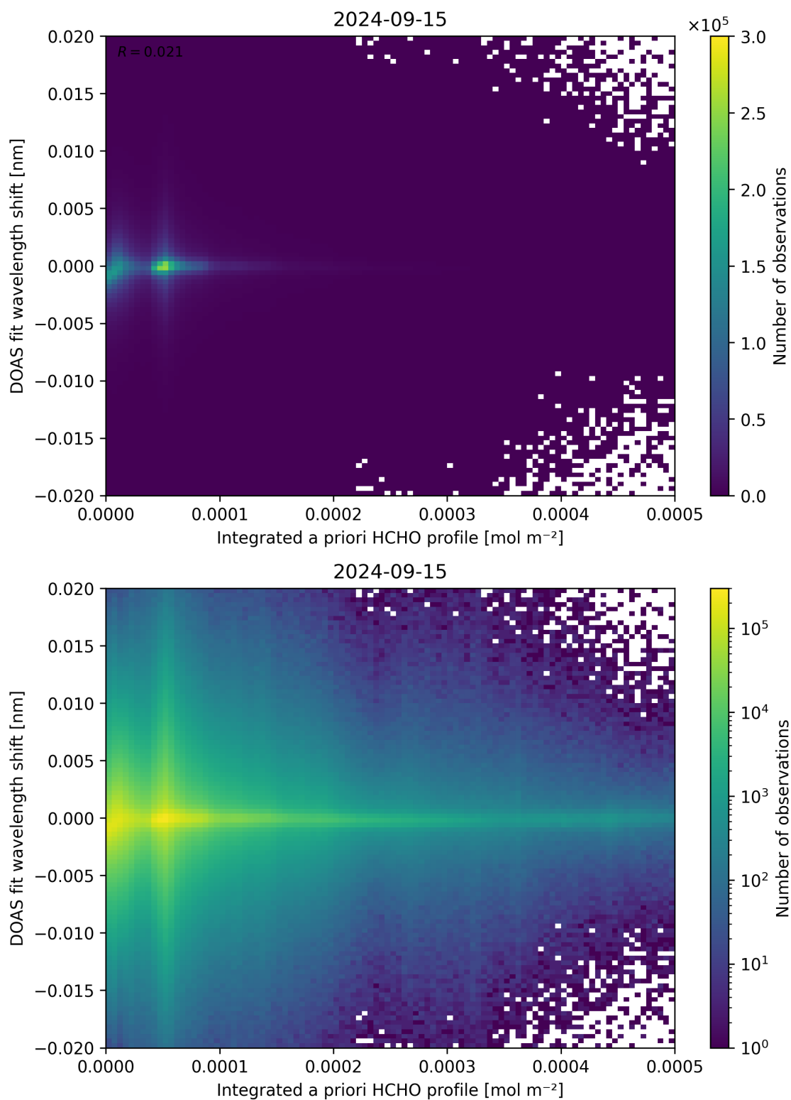
Figure 149: Scatter density plot of “Integrated a priori HCHO profile” against “DOAS fit wavelength shift” for 2024-09-14 to 2024-09-16.
