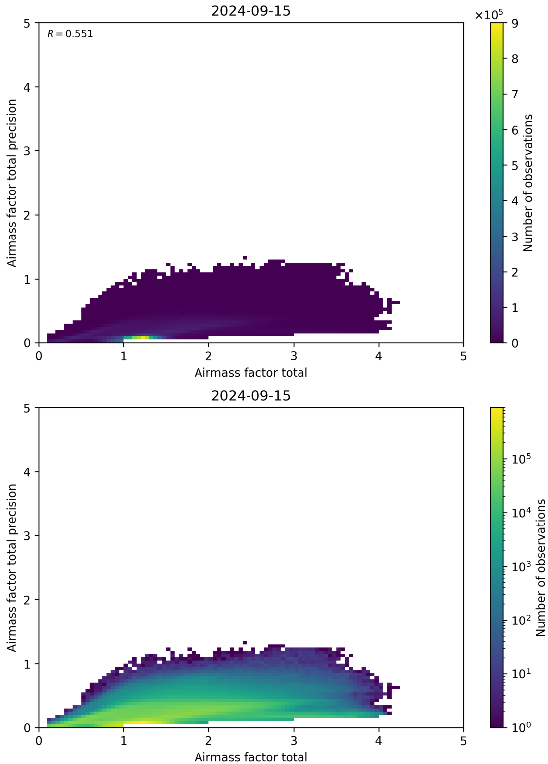
Figure 103: Scatter density plot of “Airmass factor total” against “Airmass factor total precision” for 2024-09-14 to 2024-09-16.
