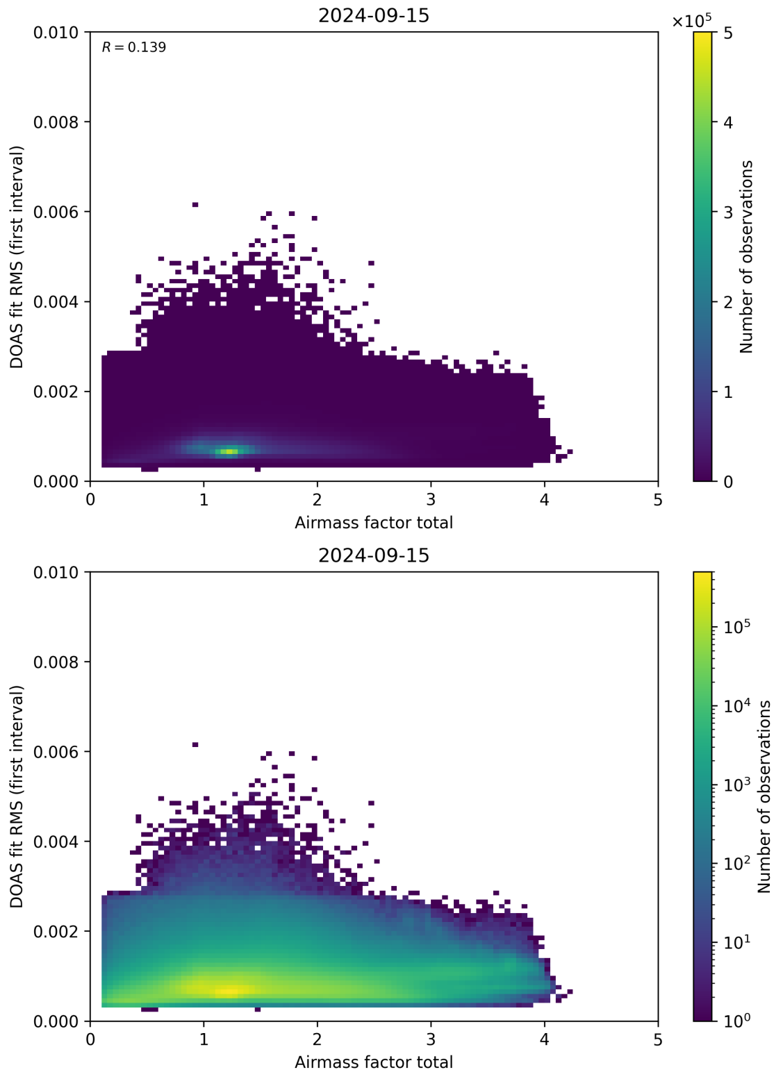
Figure 97: Scatter density plot of “Airmass factor total” against “DOAS fit RMS (first interval)” for 2024-09-14 to 2024-09-16.
