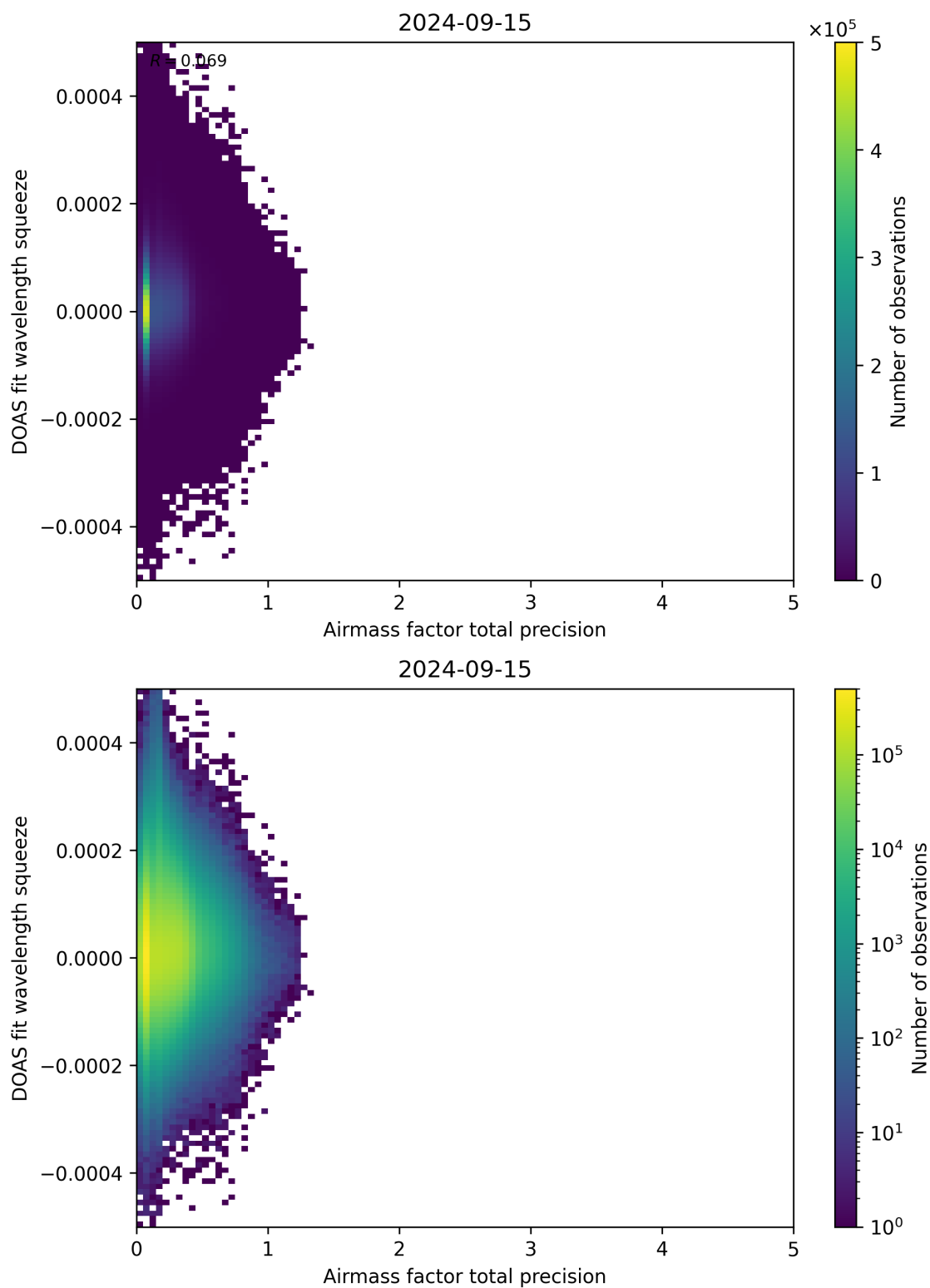
Figure 107: Scatter density plot of “Airmass factor total precision” against “DOAS fit wavelength squeeze” for 2024-09-14 to 2024-09-16.
