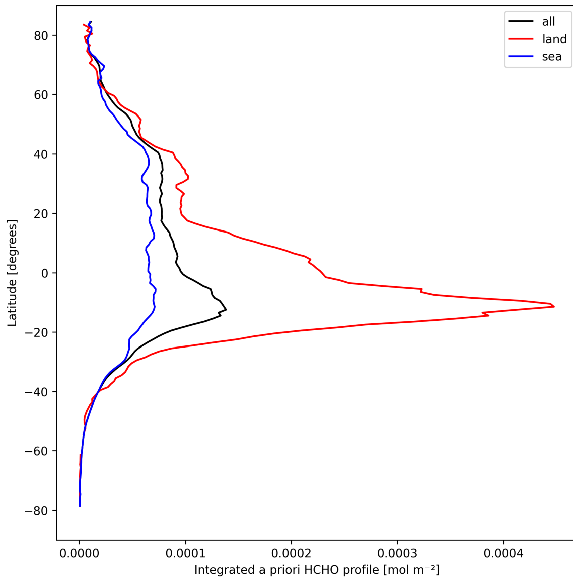
Figure 29: Zonal average of “Integrated a priori HCHO profile” for 2024-09-14 to 2024-09-16.
