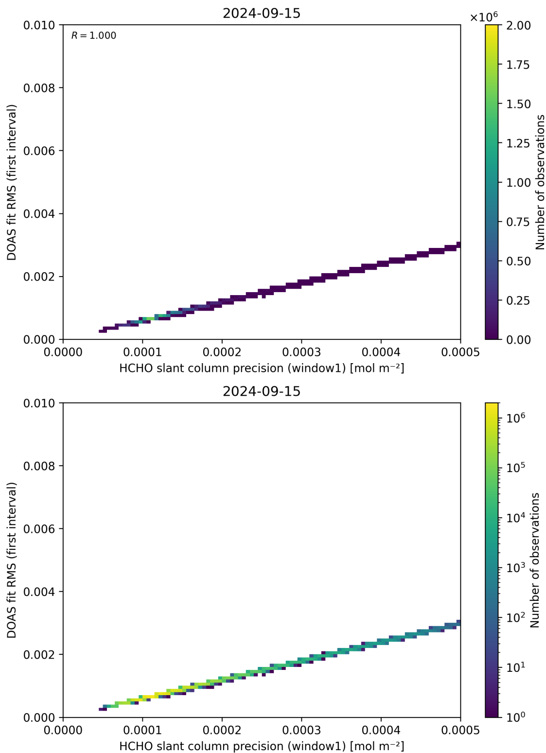
Figure 88: Scatter density plot of “HCHO slant column precision (window1)” against “DOAS fit RMS (first interval)” for 2024-09-14 to 2024-09-16.
