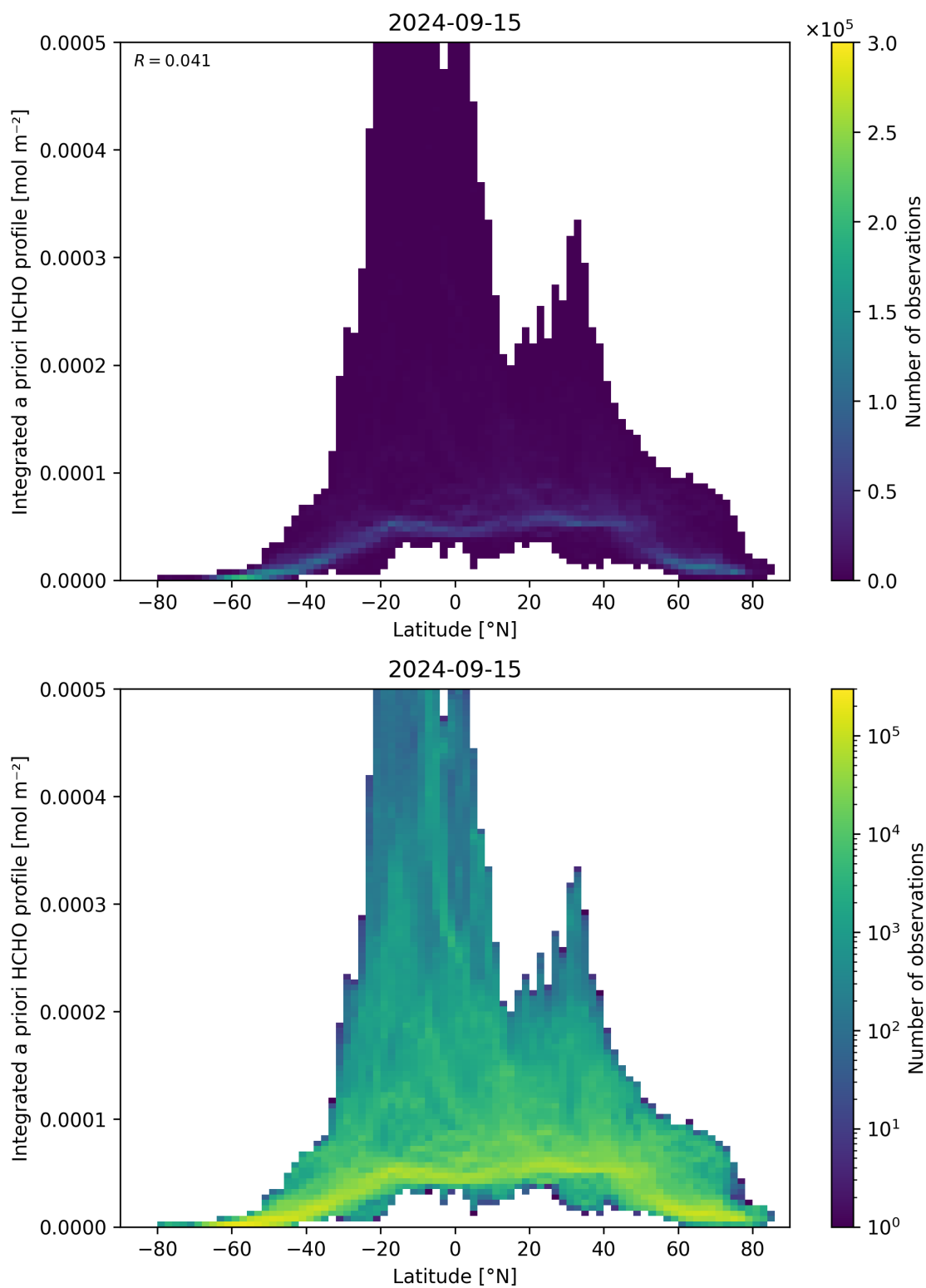
Figure 166: Scatter density plot of “Latitude” against “Integrated a priori HCHO profile” for 2024-09-14 to 2024-09-16.
