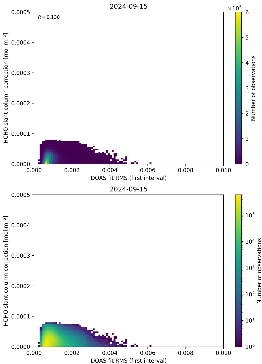
Figure 63: Scatter density plot of “DOAS fit RMS (first interval)” against “HCHO slant column correction” for 2024-09-14 to 2024-09-16.
