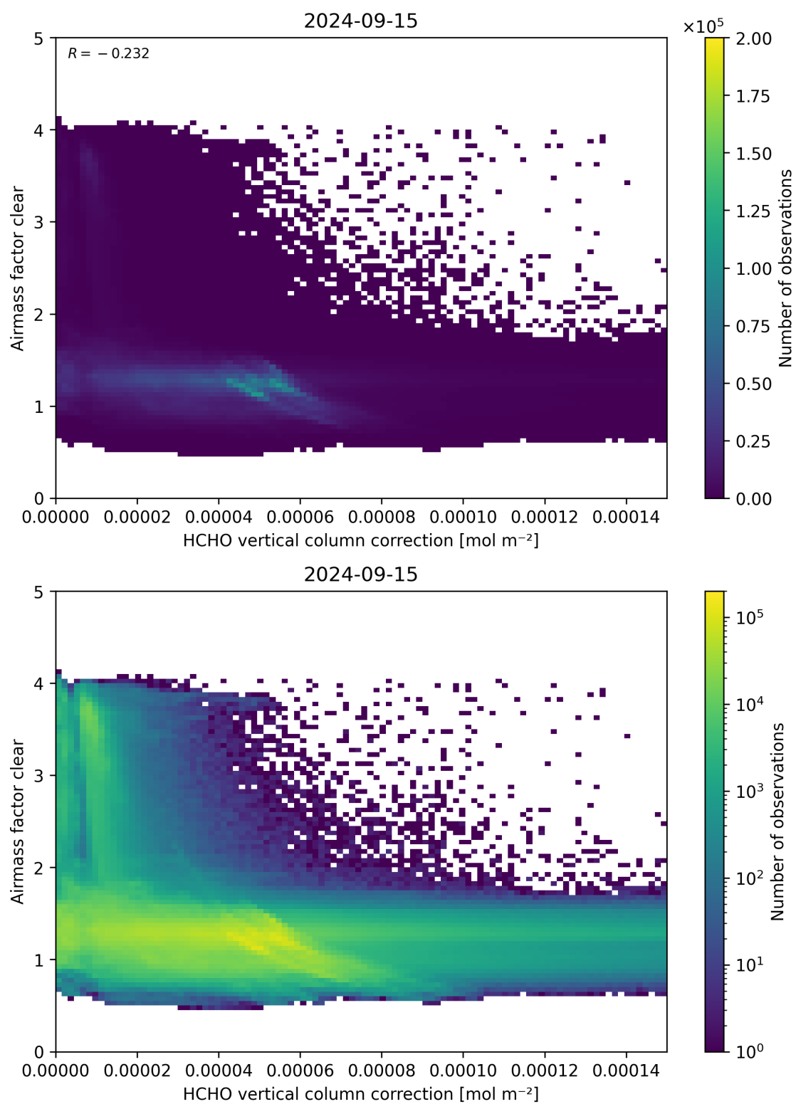
Figure 115: Scatter density plot of “HCHO vertical column correction” against “Airmass factor clear” for 2024-09-14 to 2024-09-16.
