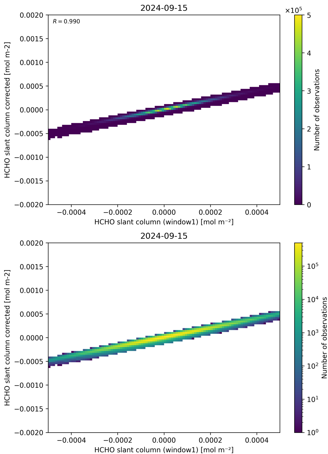
Figure 82: Scatter density plot of “HCHO slant column (window1)” against “HCHO slant column corrected” for 2024-09-14 to 2024-09-16.
