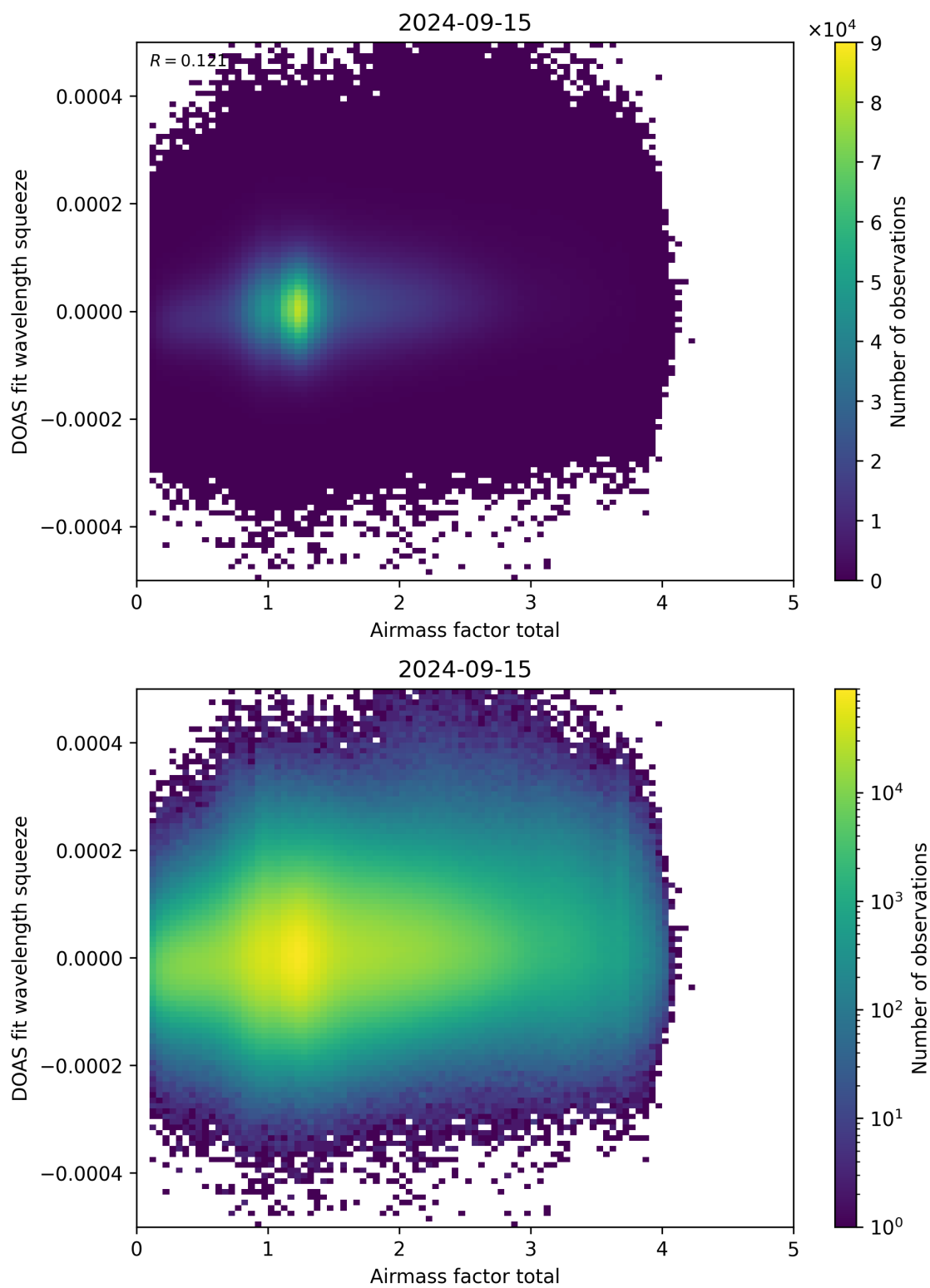
Figure 99: Scatter density plot of “Airmass factor total” against “DOAS fit wavelength squeeze” for 2024-09-14 to 2024-09-16.
