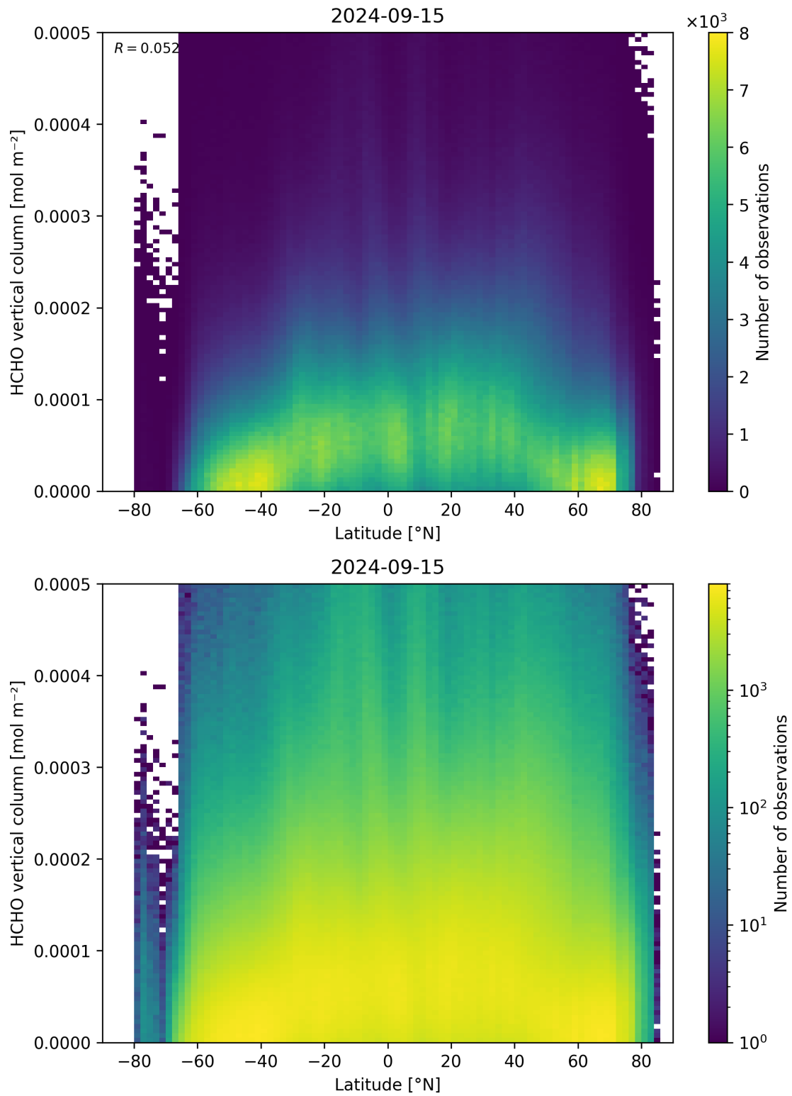
Figure 163: Scatter density plot of “Latitude” against “HCHO vertical column” for 2024-09-14 to 2024-09-16.
