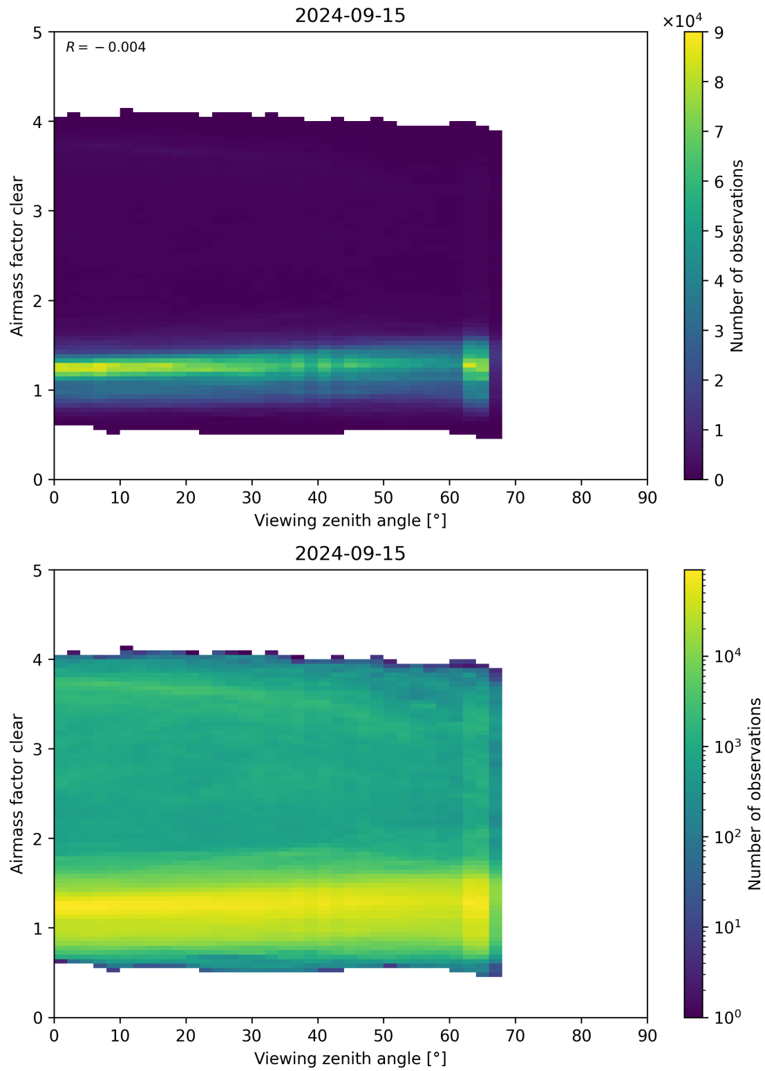
Figure 185: Scatter density plot of “Viewing zenith angle” against “Airmass factor clear” for 2024-09-14 to 2024-09-16.
