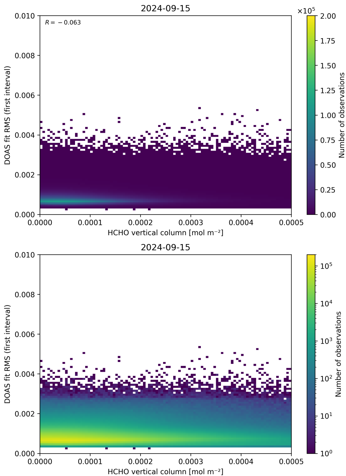
Figure 123: Scatter density plot of “HCHO vertical column” against “DOAS fit RMS (first interval)” for 2024-09-14 to 2024-09-16.
