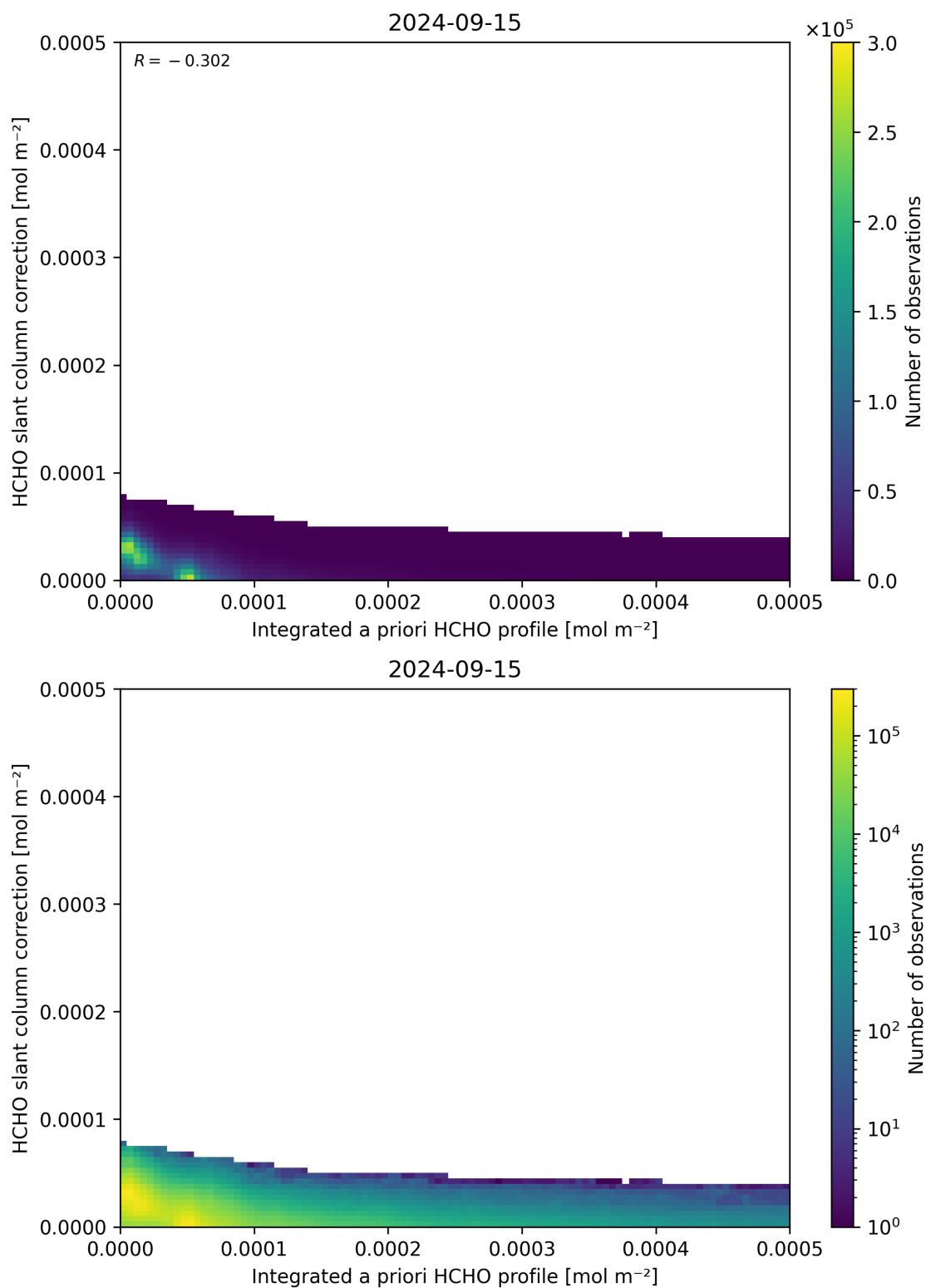
Figure 152: Scatter density plot of “Integrated a priori HCHO profile” against “HCHO slant column correction” for 2024-09-14 to 2024-09-16.
