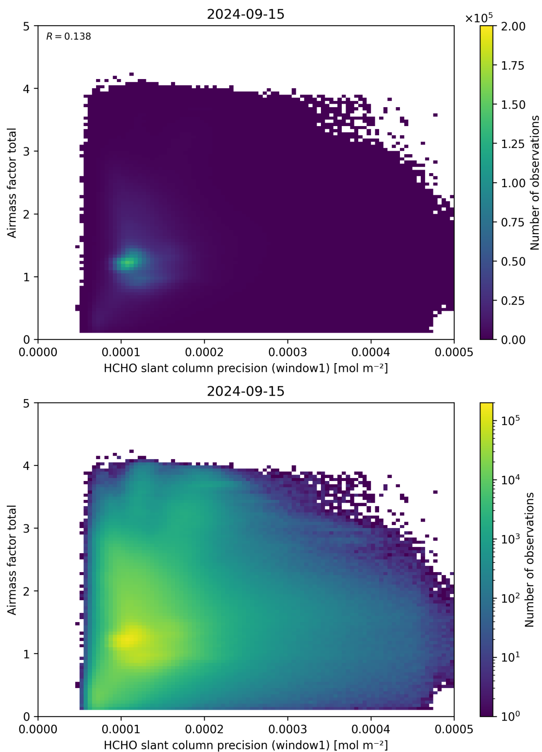
Figure 94: Scatter density plot of “HCHO slant column precision (window1)” against “Airmass factor total” for 2024-09-14 to 2024-09-16.
