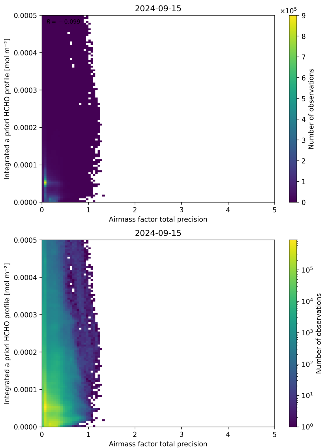
Figure 111: Scatter density plot of “Airmass factor total precision” against “Integrated a priori HCHO profile” for 2024-09-14 to 2024-09-16.
