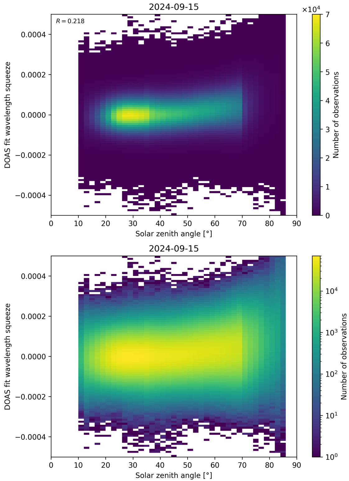
Figure 169: Scatter density plot of “Solar zenith angle” against “DOAS fit wavelength squeeze” for 2024-09-14 to 2024-09-16.
