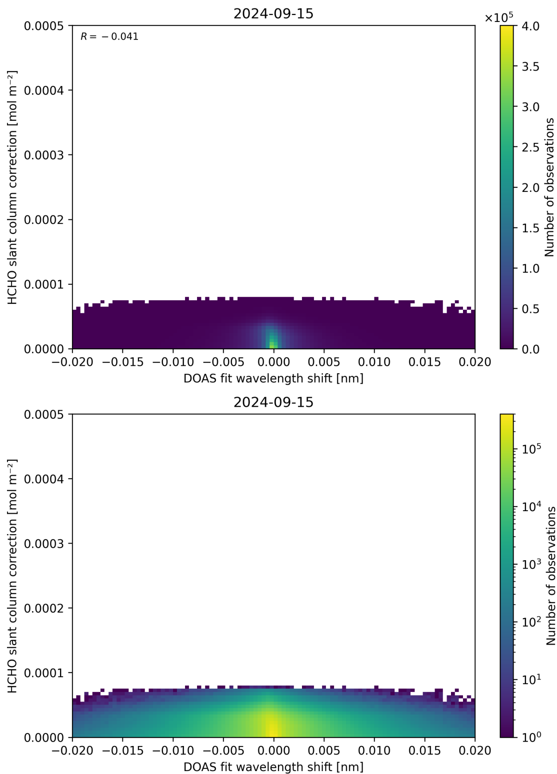
Figure 67: Scatter density plot of “DOAS fit wavelength shift” against “HCHO slant column correction” for 2024-09-14 to 2024-09-16.
