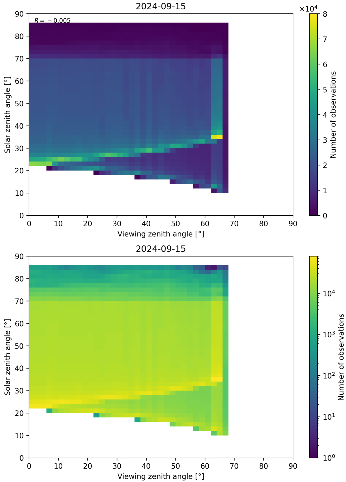
Figure 197: Scatter density plot of “Viewing zenith angle” against “Solar zenith angle” for 2024-09-14 to 2024-09-16.
