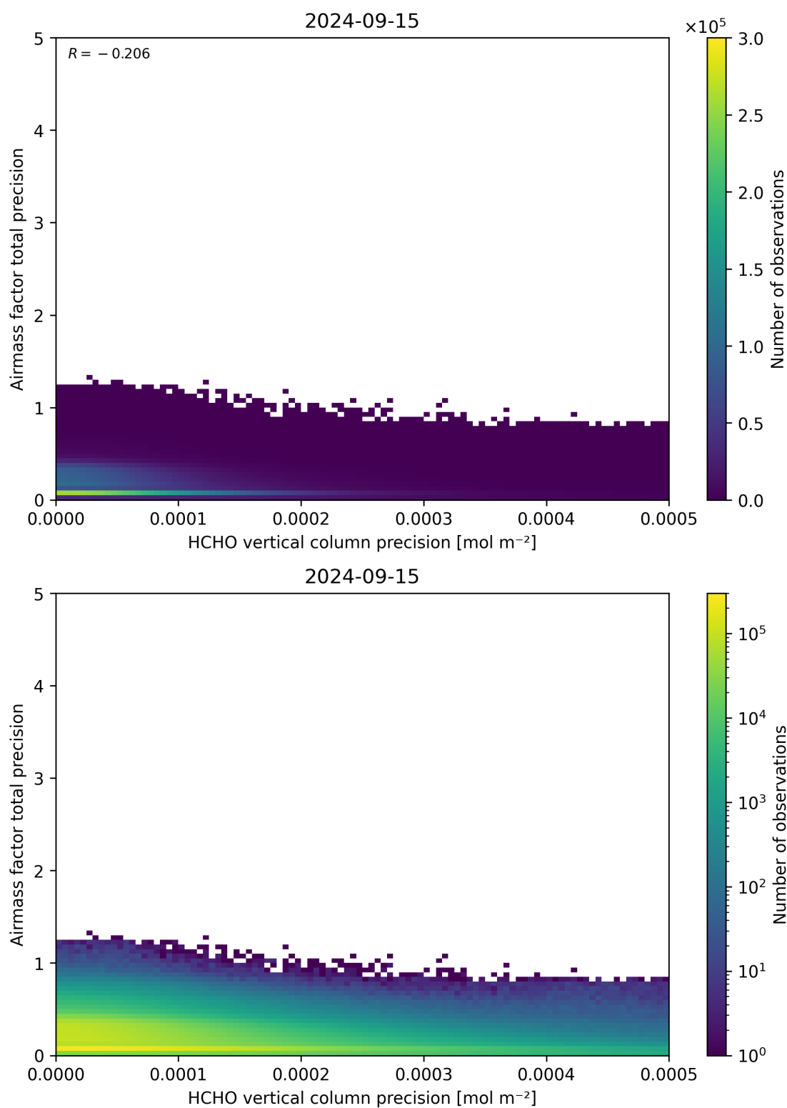
Figure 145: Scatter density plot of “HCHO vertical column precision” against “Airmass factor total precision” for 2024-09-14 to 2024-09-16.
