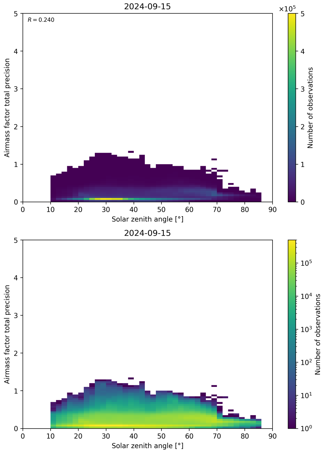
Figure 176: Scatter density plot of “Solar zenith angle” against “Airmass factor total precision” for 2024-09-14 to 2024-09-16.
