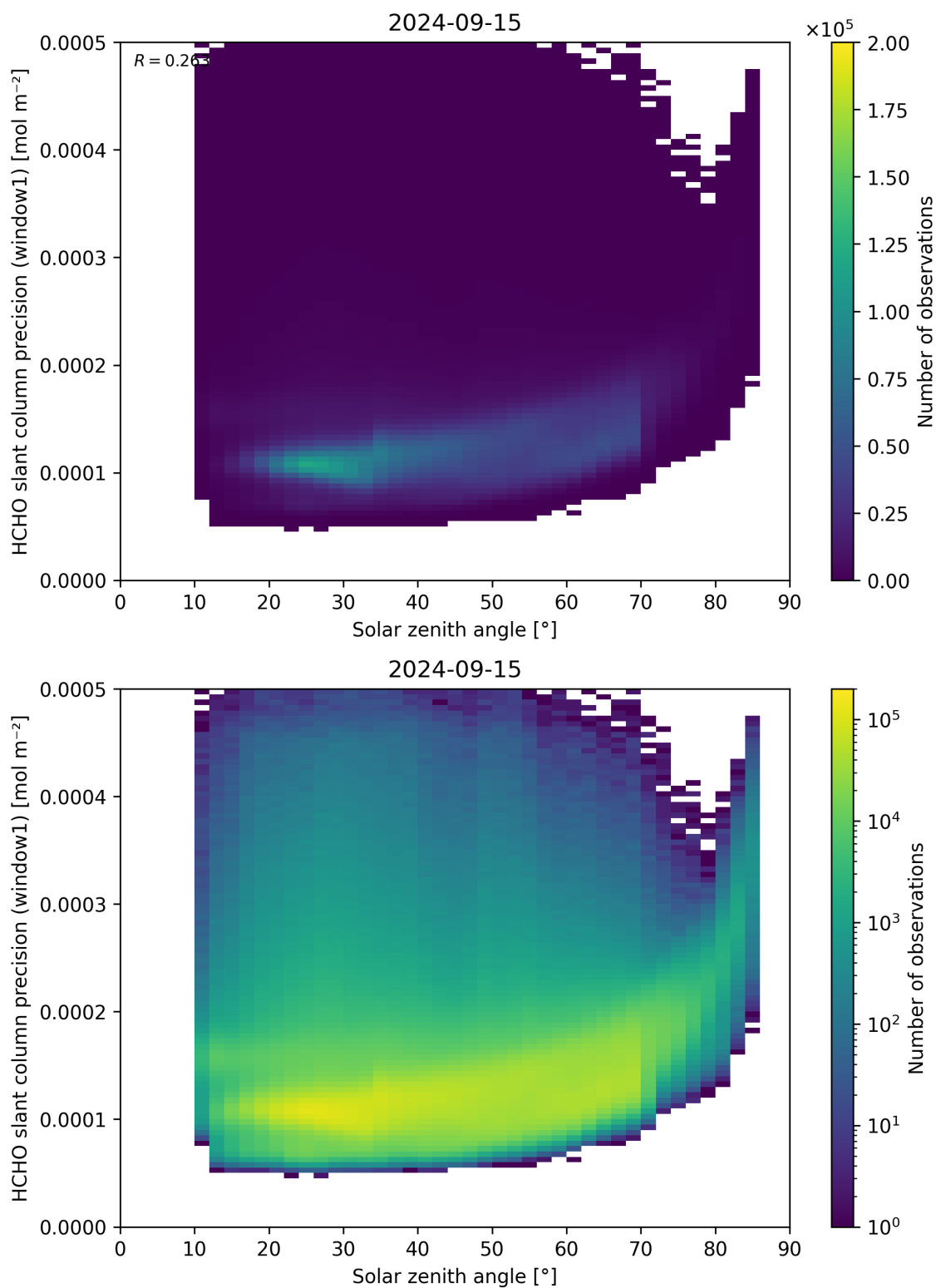
Figure 174: Scatter density plot of “Solar zenith angle” against “HCHO slant column precision (window1)” for 2024-09-14 to 2024-09-16.
