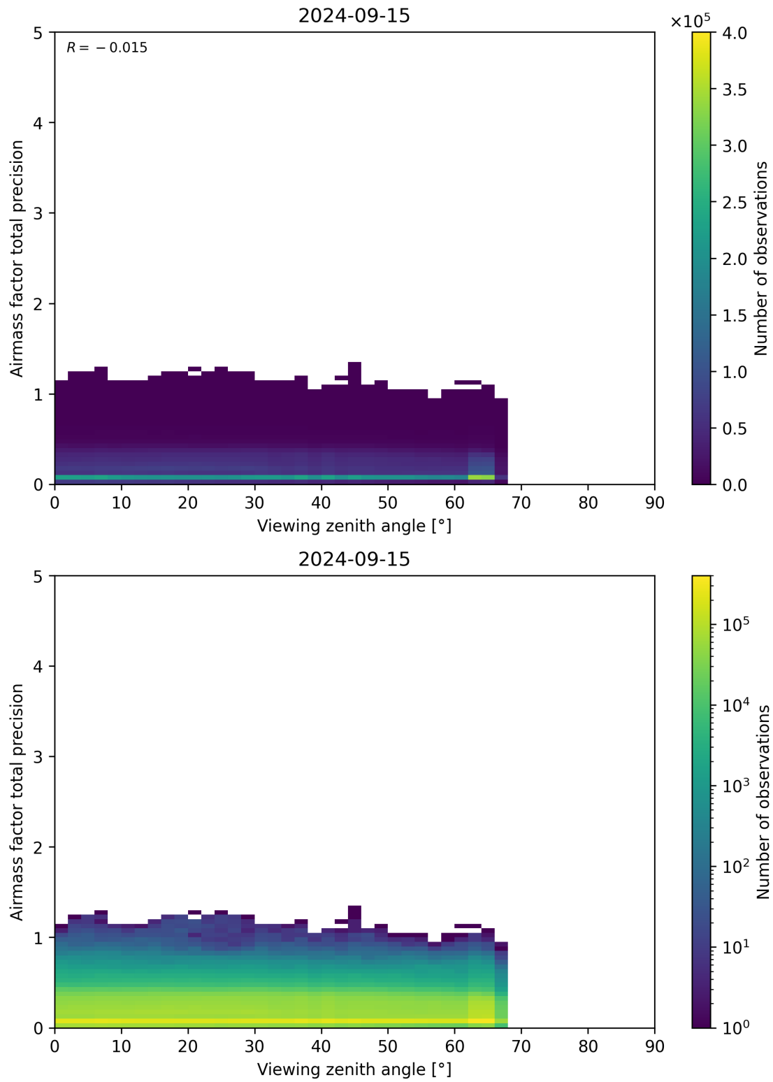
Figure 191: Scatter density plot of “Viewing zenith angle” against “Airmass factor total precision” for 2024-09-14 to 2024-09-16.
