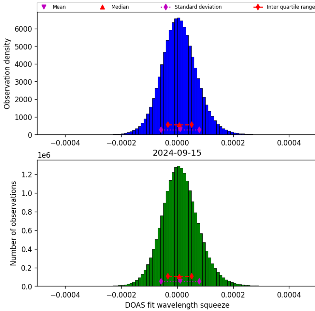
Figure 45: Histogram of “DOAS fit wavelength squeeze” for 2024-09-14 to 2024-09-16
