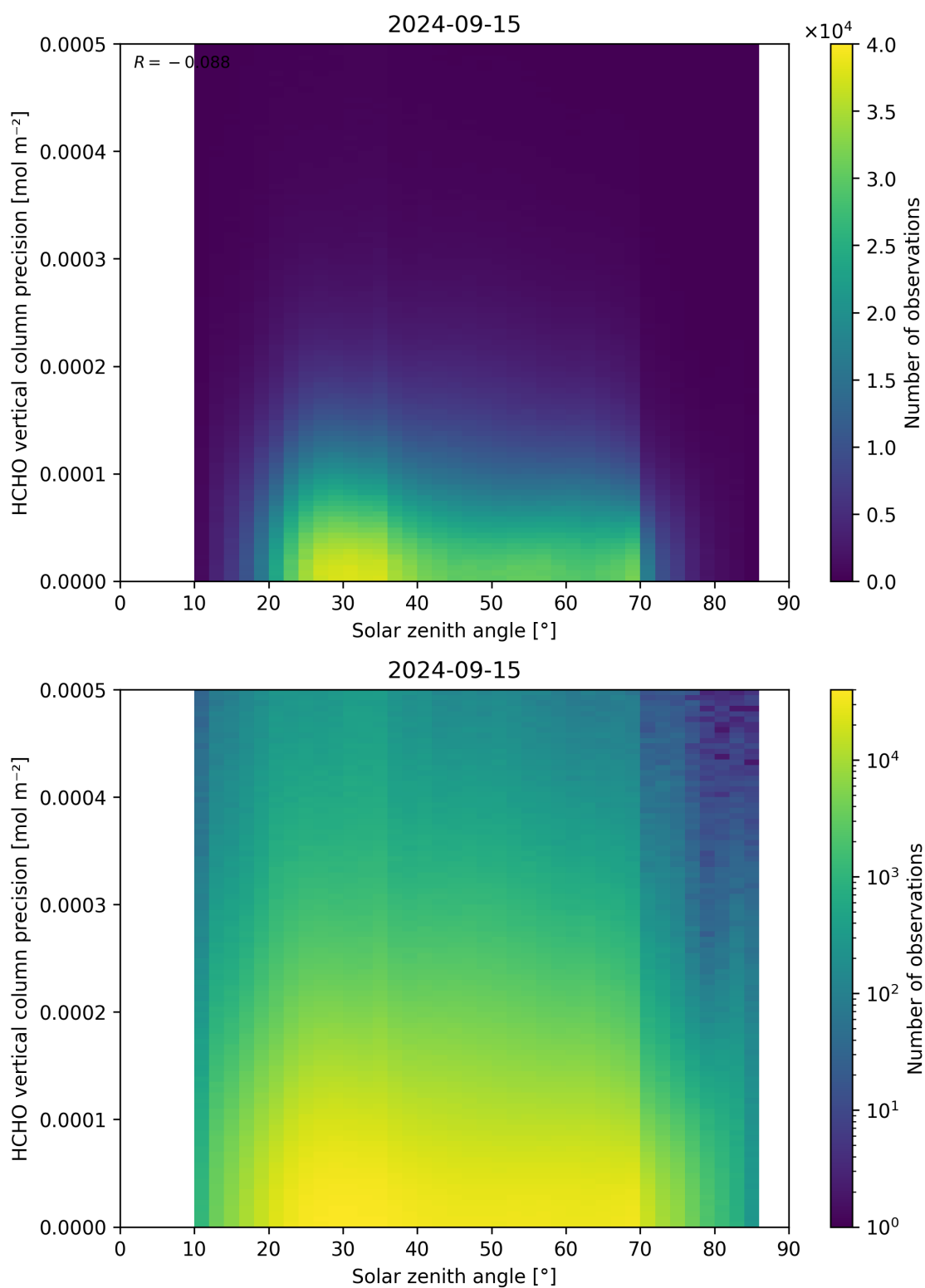
Figure 179: Scatter density plot of “Solar zenith angle” against “HCHO vertical column precision” for 2024-09-14 to 2024-09-16.
