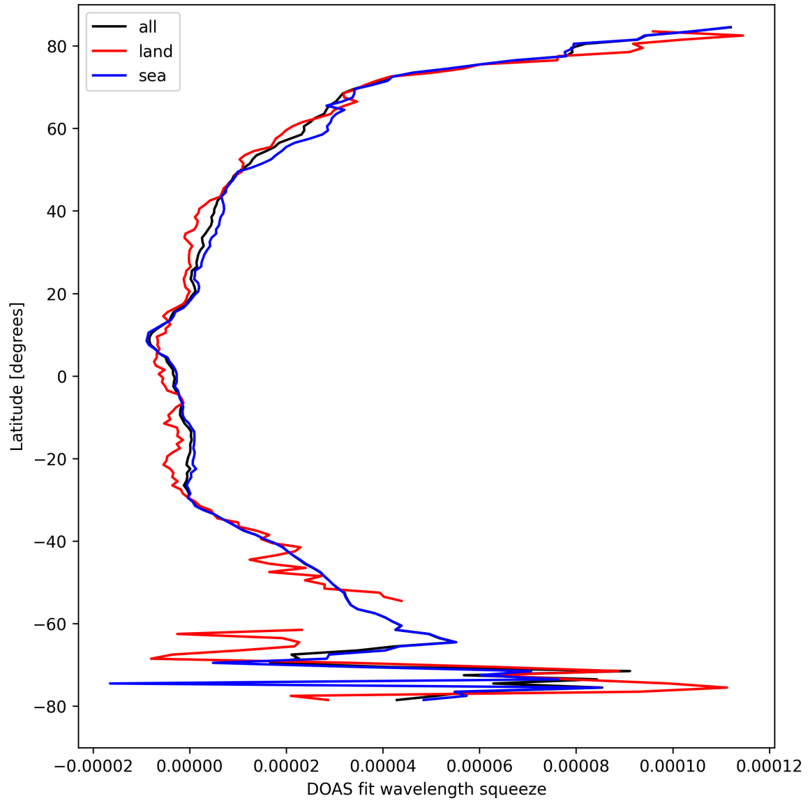
Figure 31: Zonal average of “DOAS fit wavelength squeeze” for 2024-09-14 to 2024-09-16.
