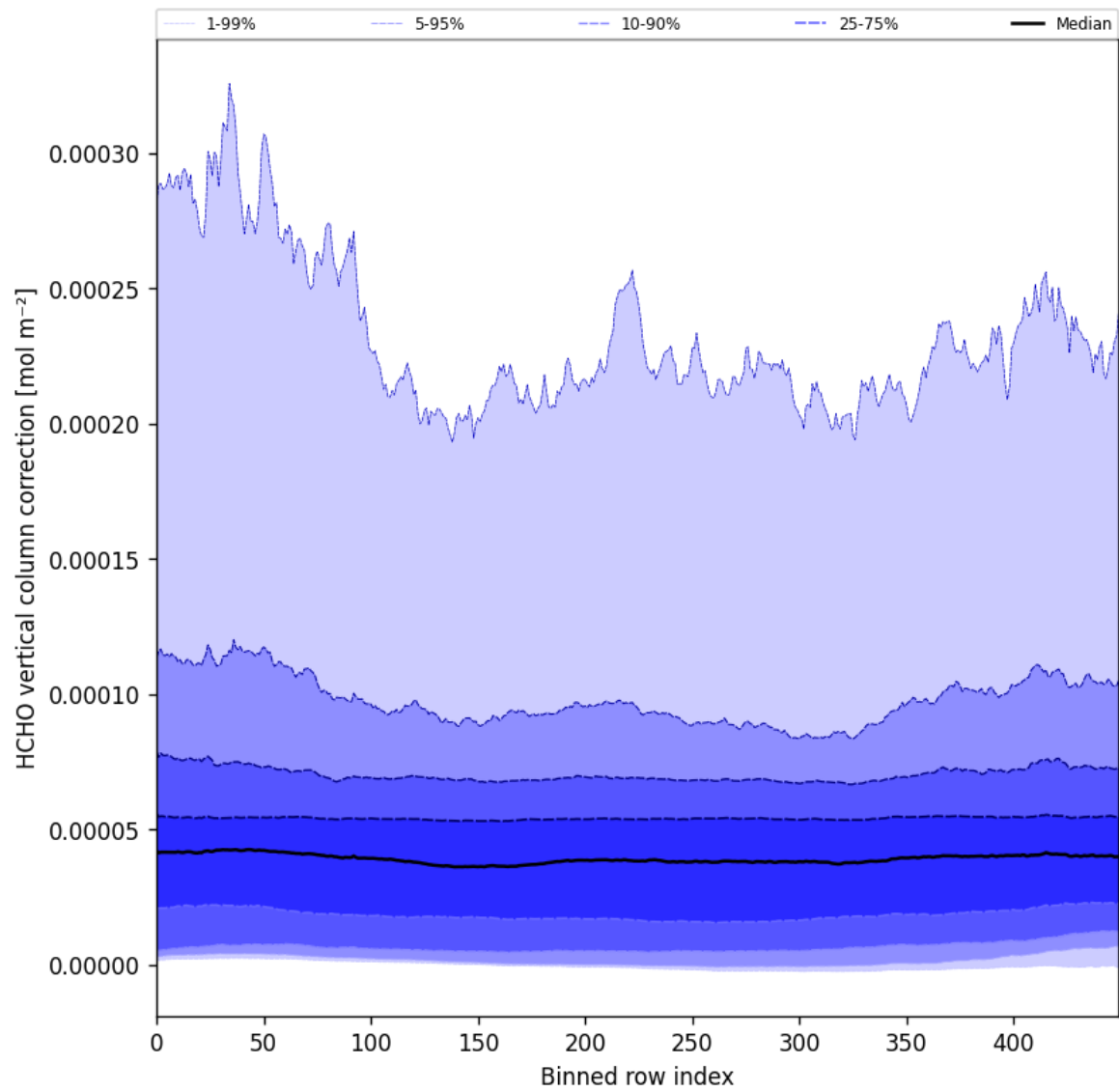
Figure 51: Along track statistics of “HCHO vertical column correction” for 2024-09-14 to 2024-09-16
