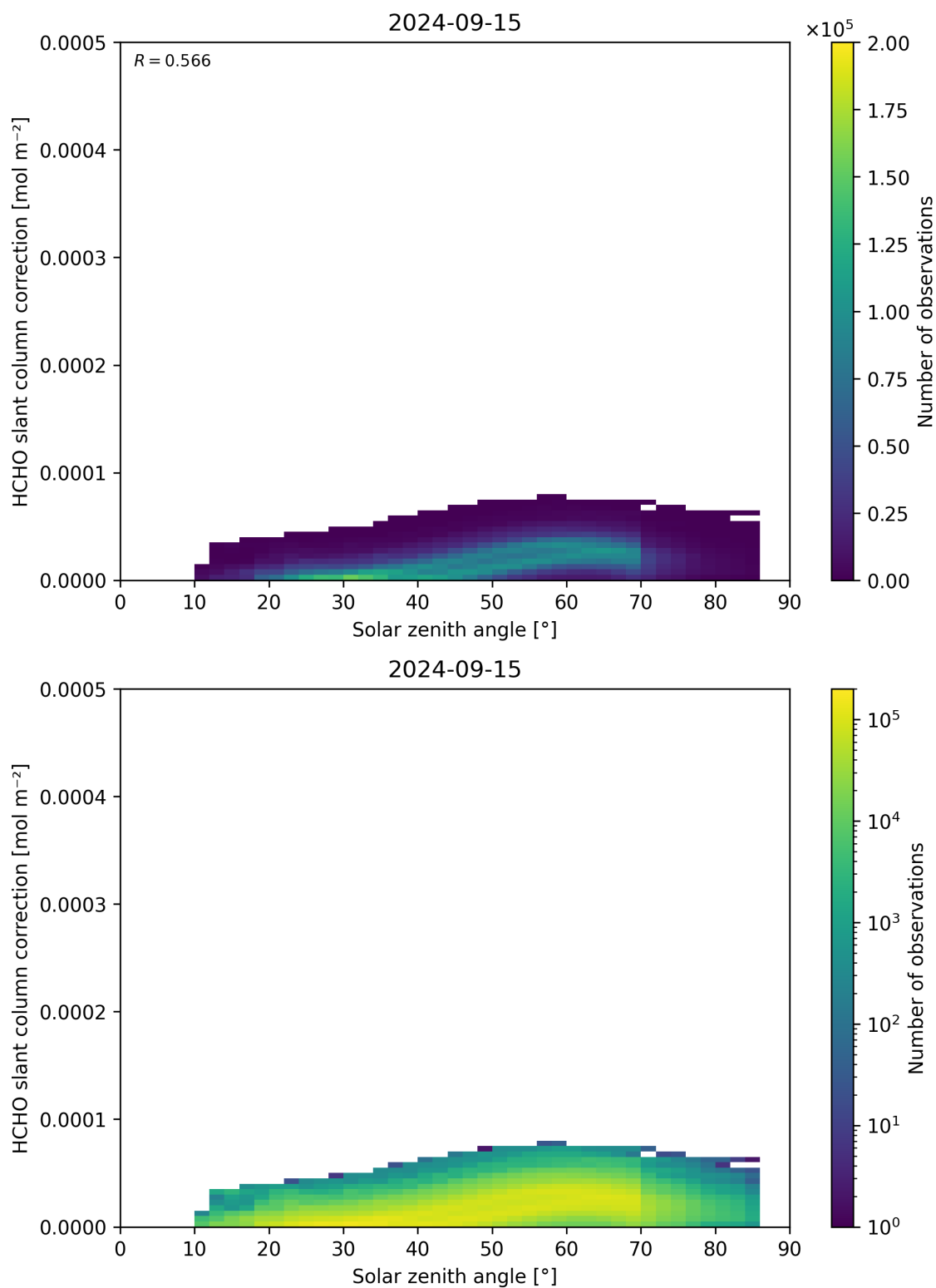
Figure 172: Scatter density plot of “Solar zenith angle” against “HCHO slant column correction” for 2024-09-14 to 2024-09-16.
