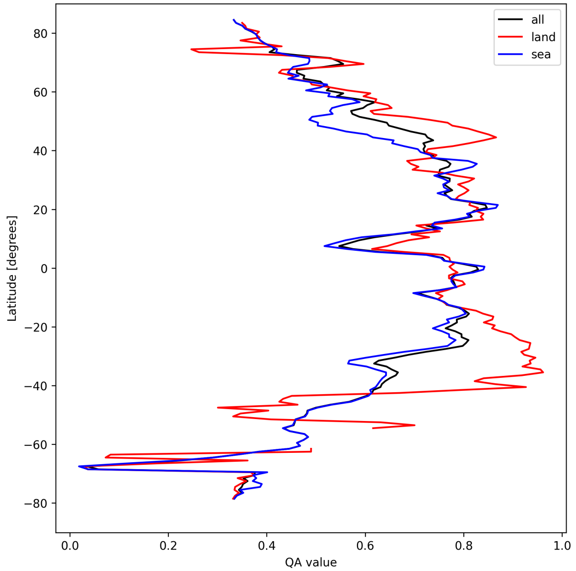
Figure 20: Zonal average of “QA value” for 2024-09-14 to 2024-09-16.
