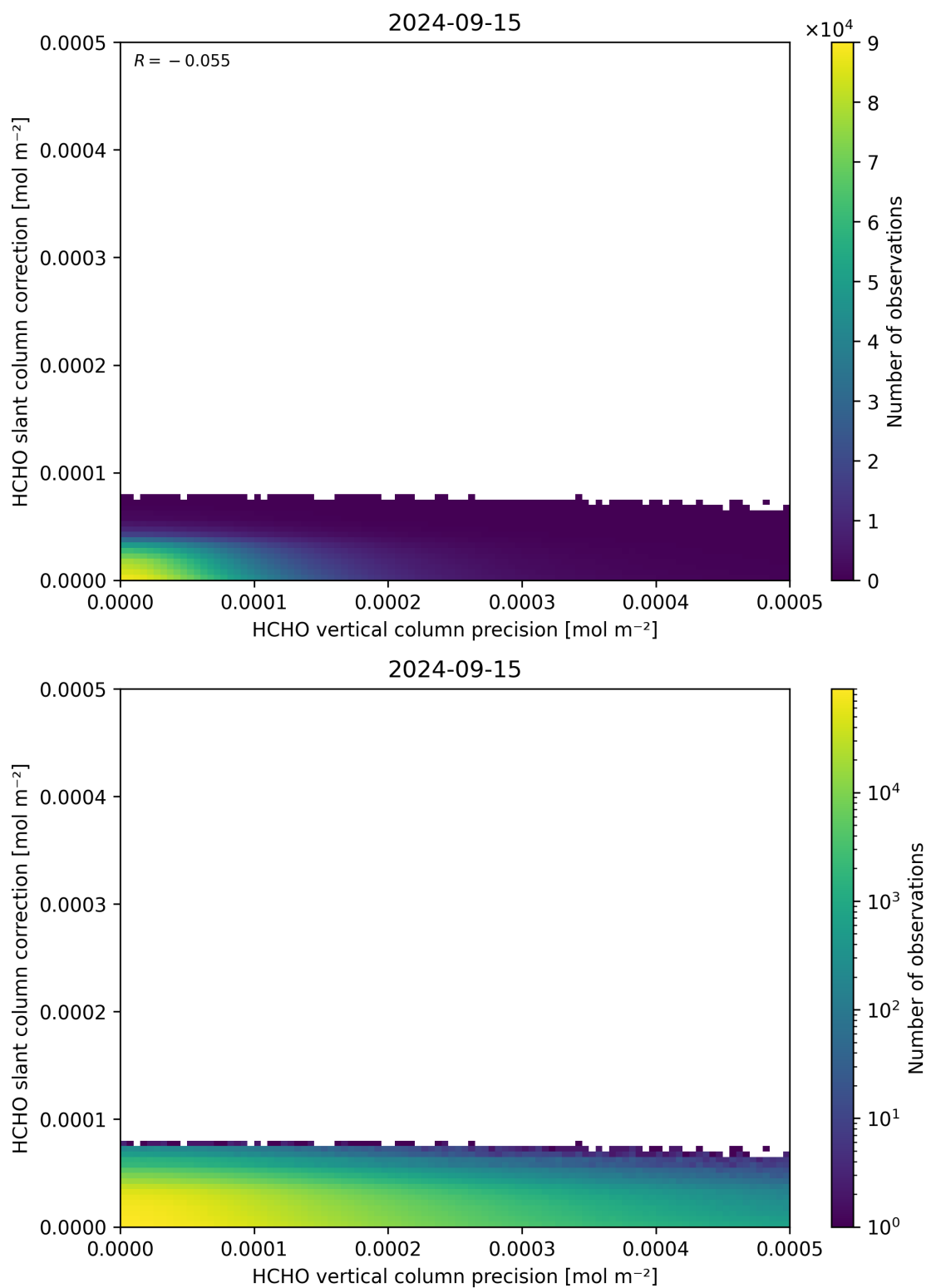
Figure 141: Scatter density plot of “HCHO vertical column precision” against “HCHO slant column correction” for 2024-09-14 to 2024-09-16.
