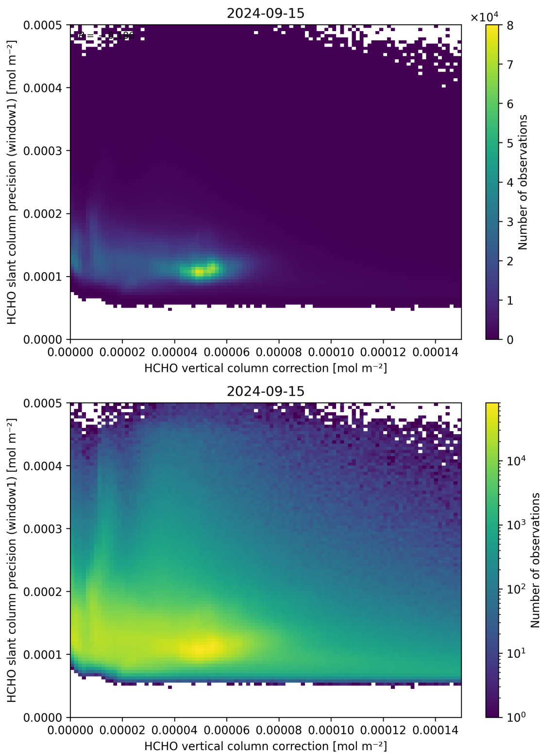
Figure 119: Scatter density plot of “HCHO vertical column correction” against “HCHO slant column precision (window1)” for 2024-09-14 to 2024-09-16.
