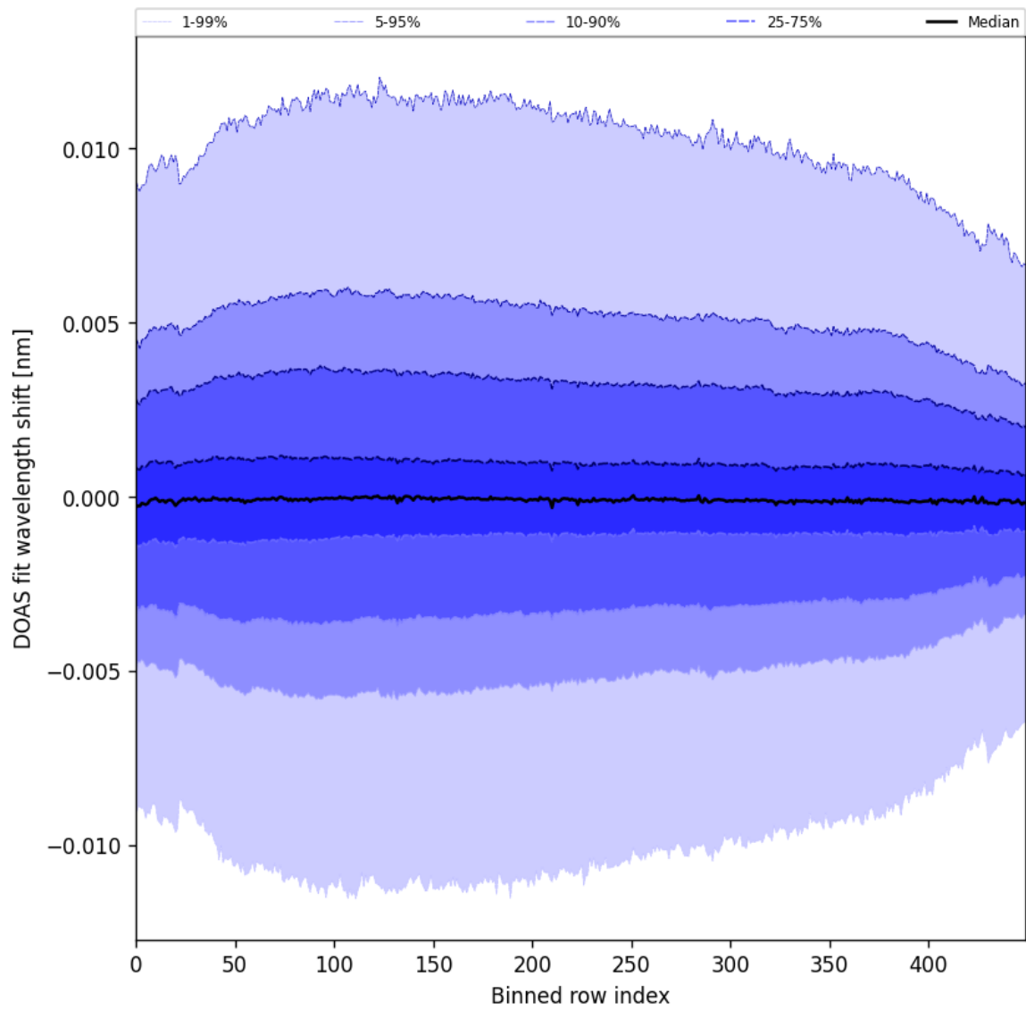
Figure 58: Along track statistics of “DOAS fit wavelength shift” for 2024-09-14 to 2024-09-16
