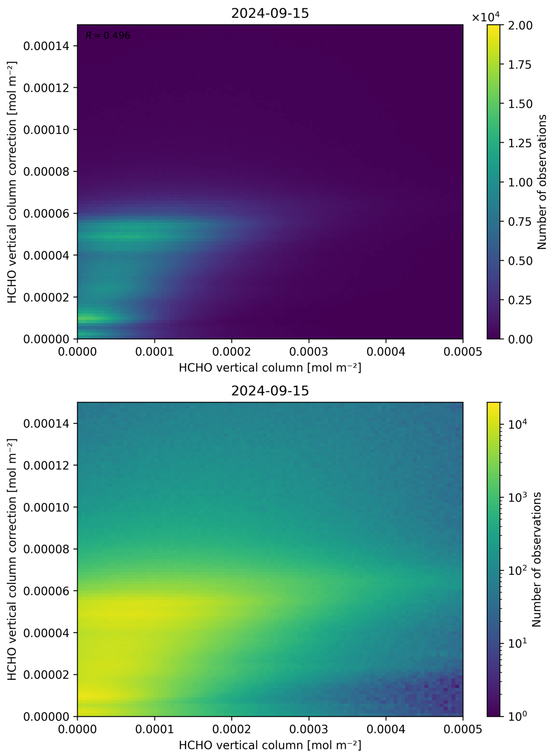
Figure 133: Scatter density plot of “HCHO vertical column” against “HCHO vertical column correction” for 2024-09-14 to 2024-09-16.
