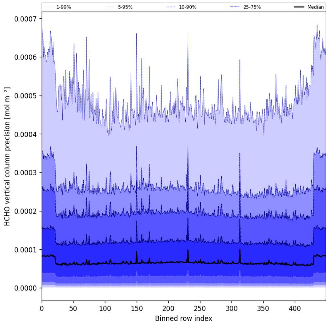
Figure 50: Along track statistics of “HCHO vertical column precision” for 2024-09-14 to 2024-09-16
