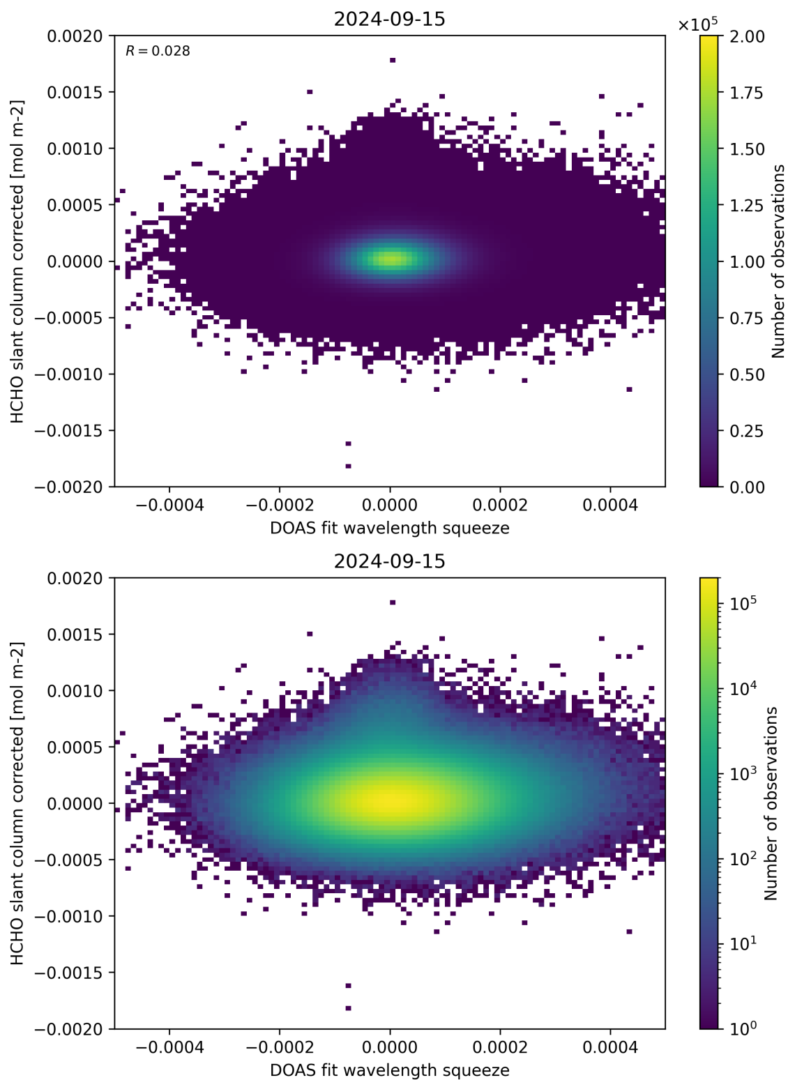
Figure 69: Scatter density plot of “DOAS fit wavelength squeeze” against “HCHO slant column corrected” for 2024-09-14 to 2024-09-16.
