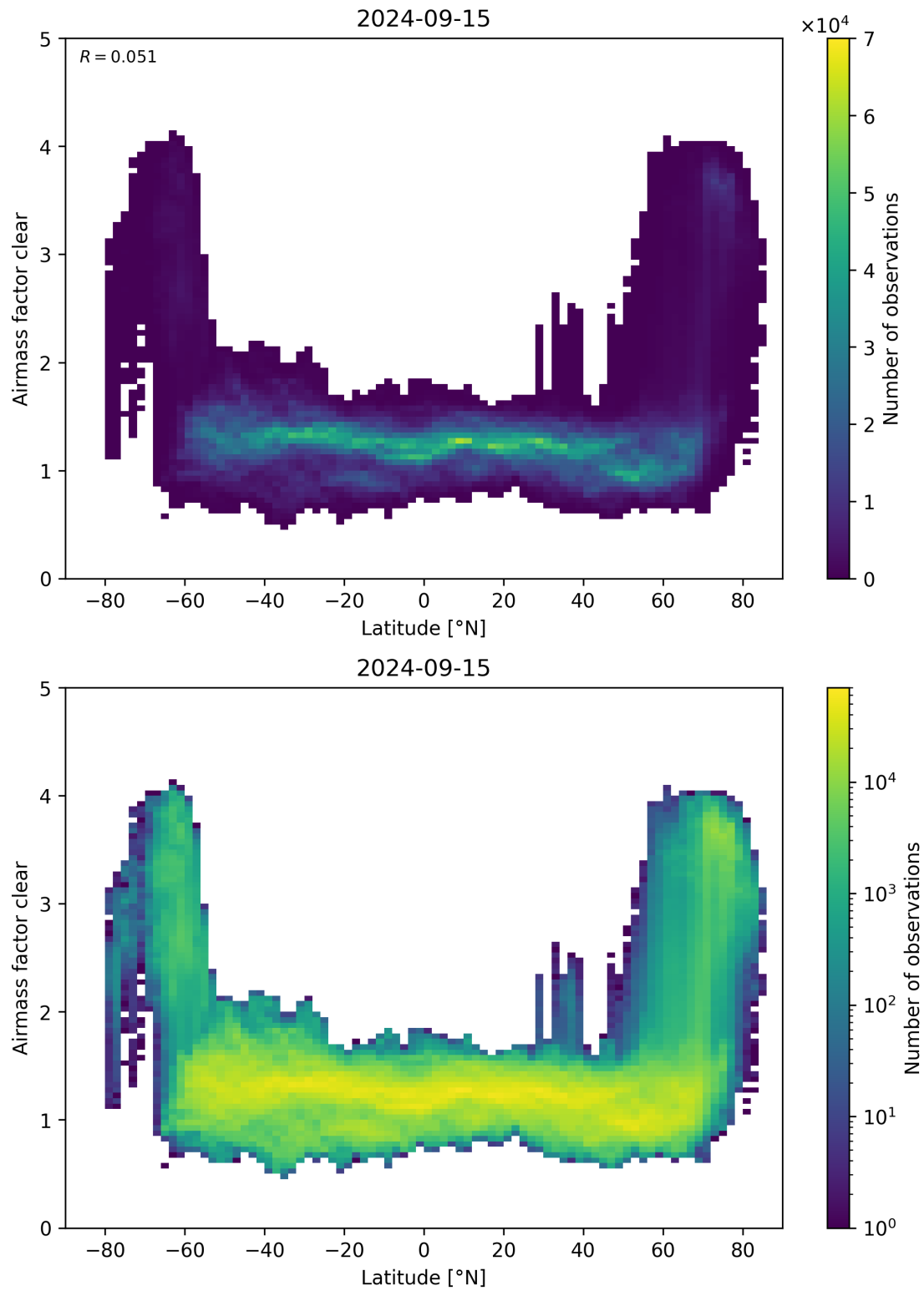
Figure 156: Scatter density plot of “Latitude” against “Airmass factor clear” for 2024-09-14 to 2024-09-16.
