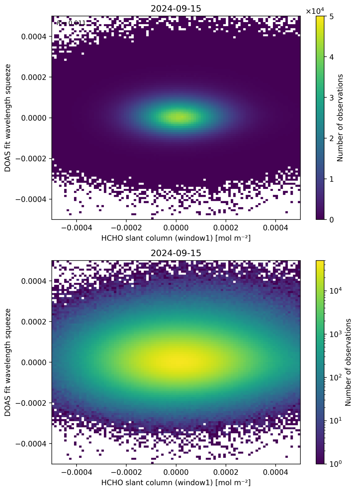
Figure 80: Scatter density plot of “HCHO slant column (window1)” against “DOAS fit wavelength squeeze” for 2024-09-14 to 2024-09-16.
