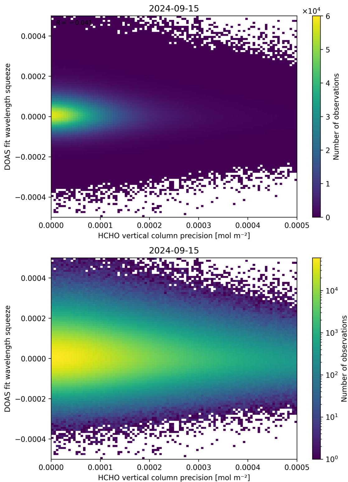
Figure 138: Scatter density plot of “HCHO vertical column precision” against “DOAS fit wavelength squeeze” for 2024-09-14 to 2024-09-16.
