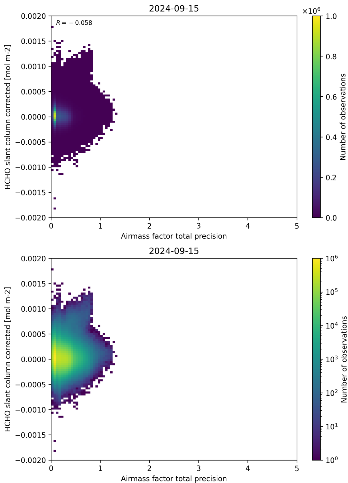
Figure 109: Scatter density plot of “Airmass factor total precision” against “HCHO slant column corrected” for 2024-09-14 to 2024-09-16.
