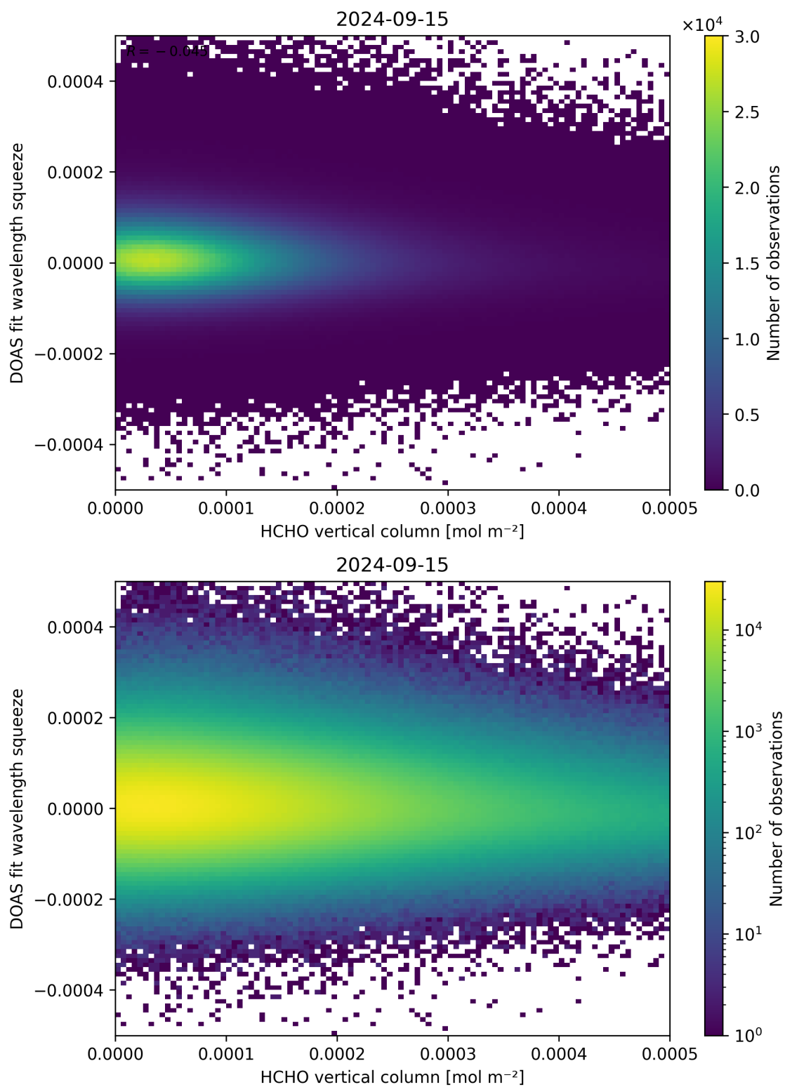
Figure 125: Scatter density plot of “HCHO vertical column” against “DOAS fit wavelength squeeze” for 2024-09-14 to 2024-09-16.
