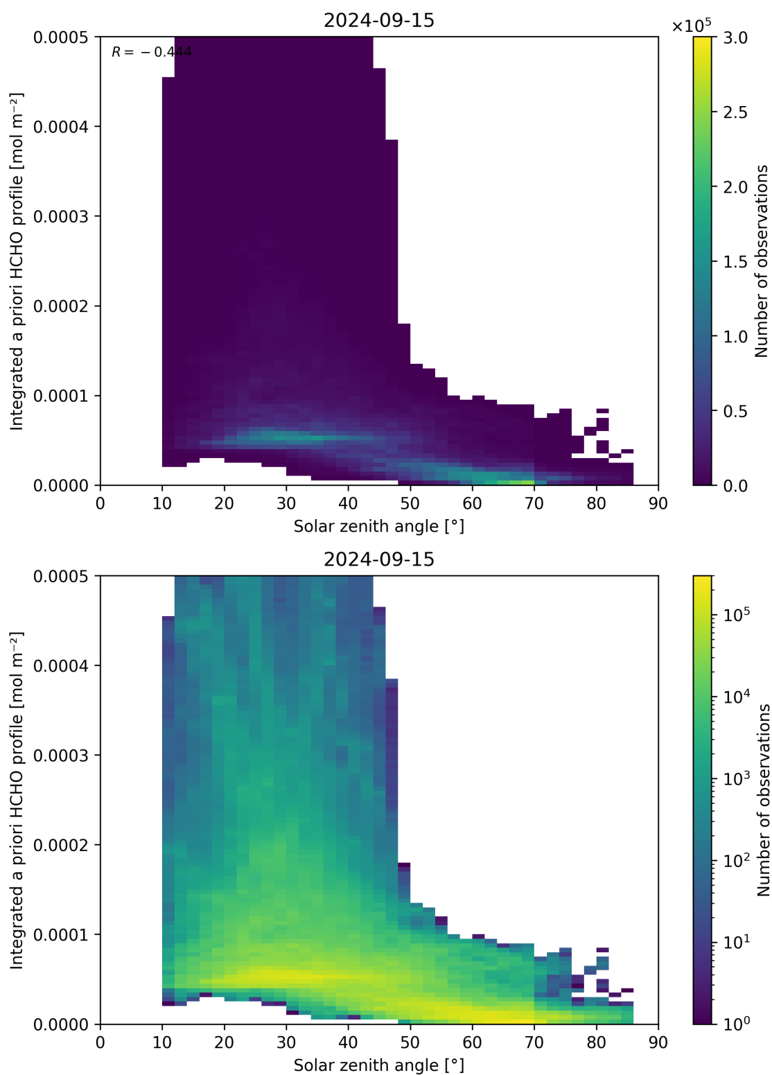
Figure 180: Scatter density plot of “Solar zenith angle” against “Integrated a priori HCHO profile” for 2024-09-14 to 2024-09-16.
