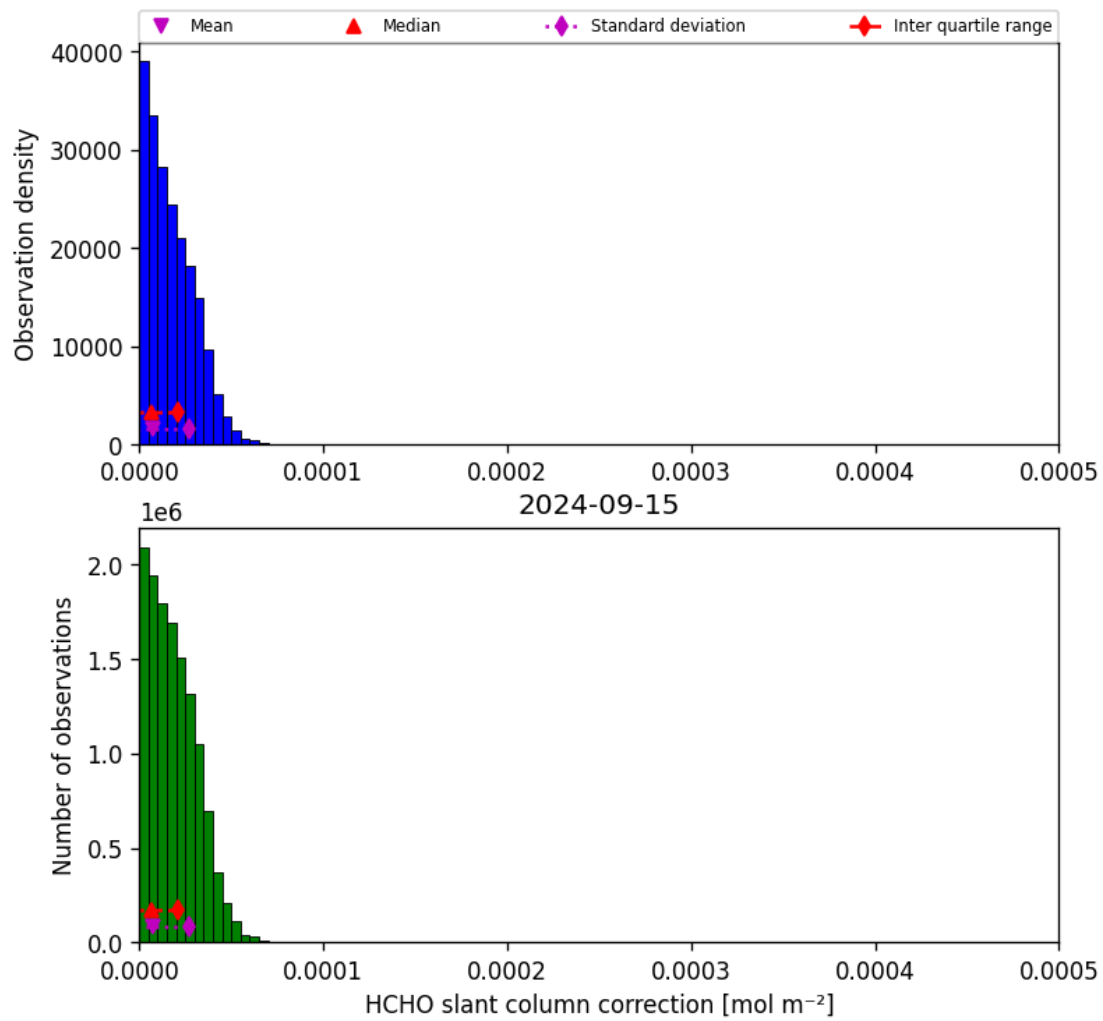
Figure 47: Histogram of “HCHO slant column correction” for 2024-09-14 to 2024-09-16
