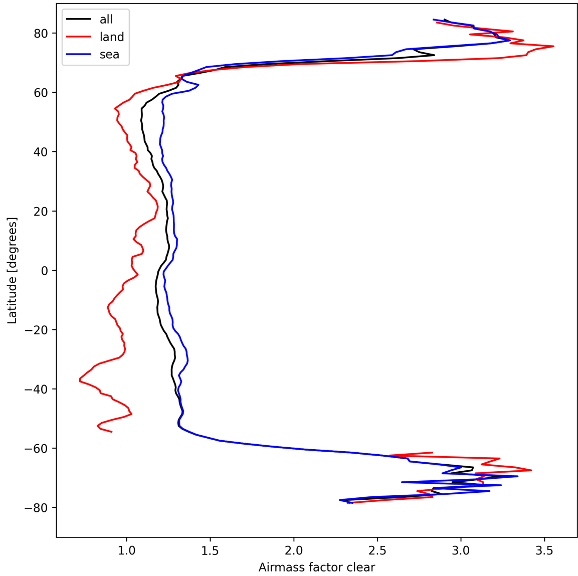
Figure 28: Zonal average of “Airmass factor clear” for 2024-09-14 to 2024-09-16.
