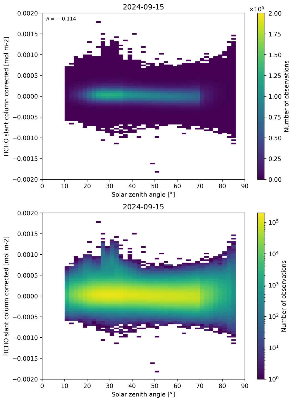
Figure 171: Scatter density plot of “Solar zenith angle” against “HCHO slant column corrected” for 2024-09-14 to 2024-09-16.
