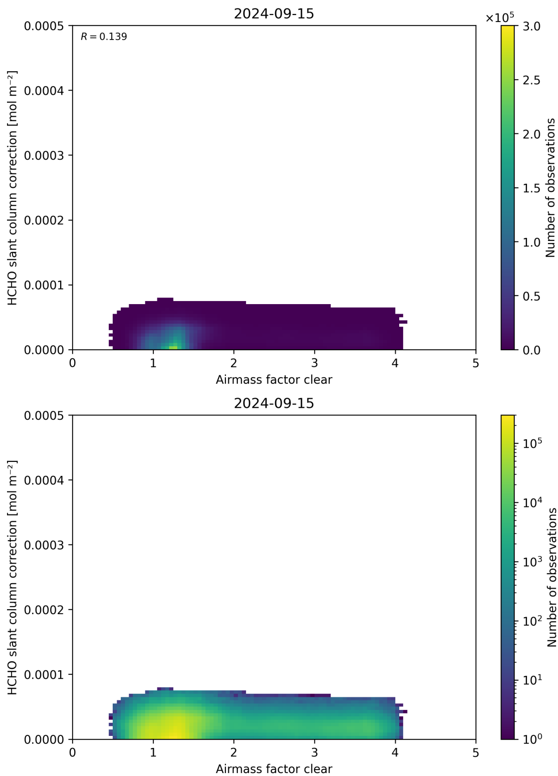
Figure 75: Scatter density plot of “Airmass factor clear” against “HCHO slant column correction” for 2024-09-14 to 2024-09-16.
