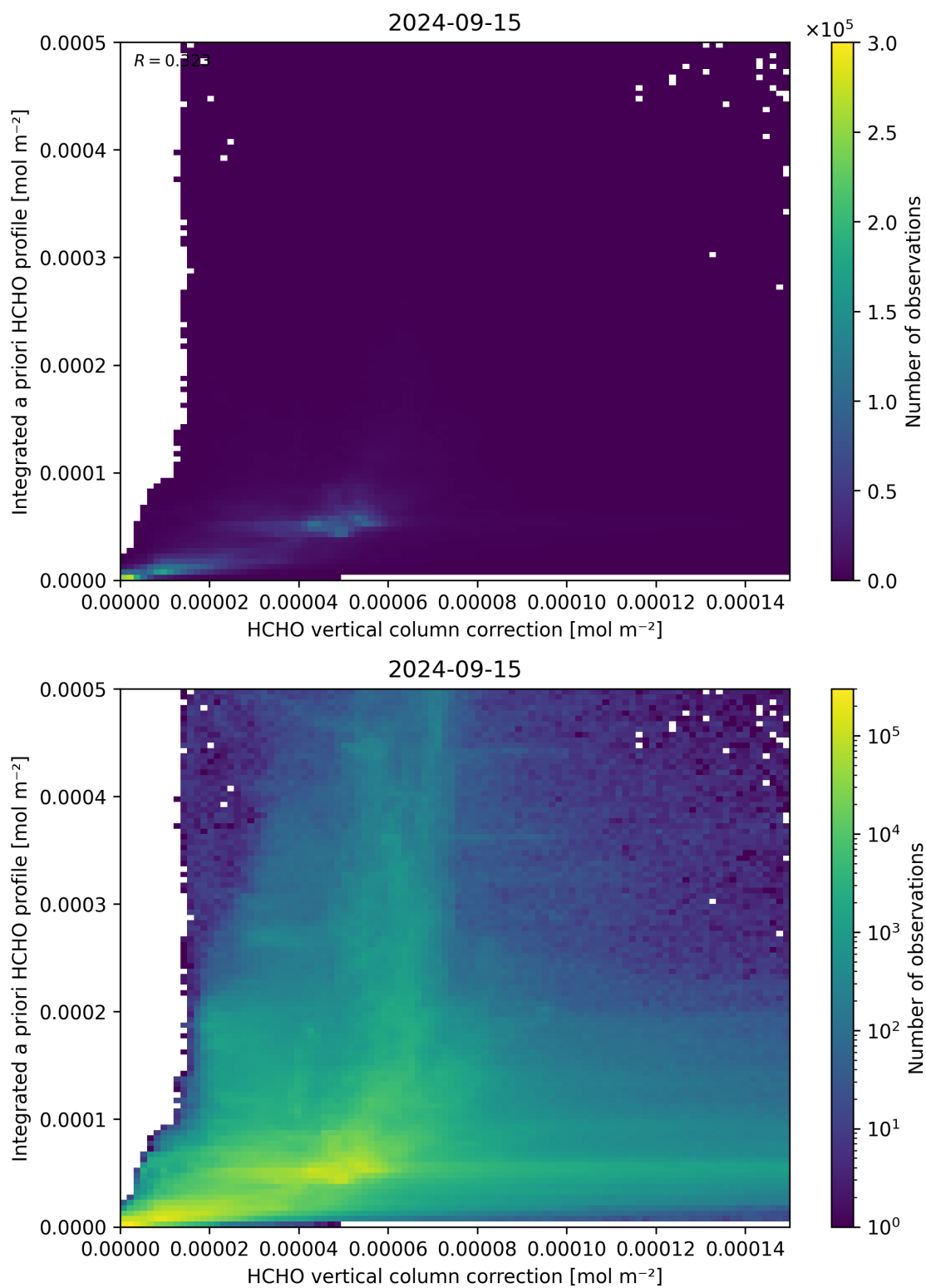
Figure 122: Scatter density plot of “HCHO vertical column correction” against “Integrated a priori HCHO profile” for 2024-09-14 to 2024-09-16.
