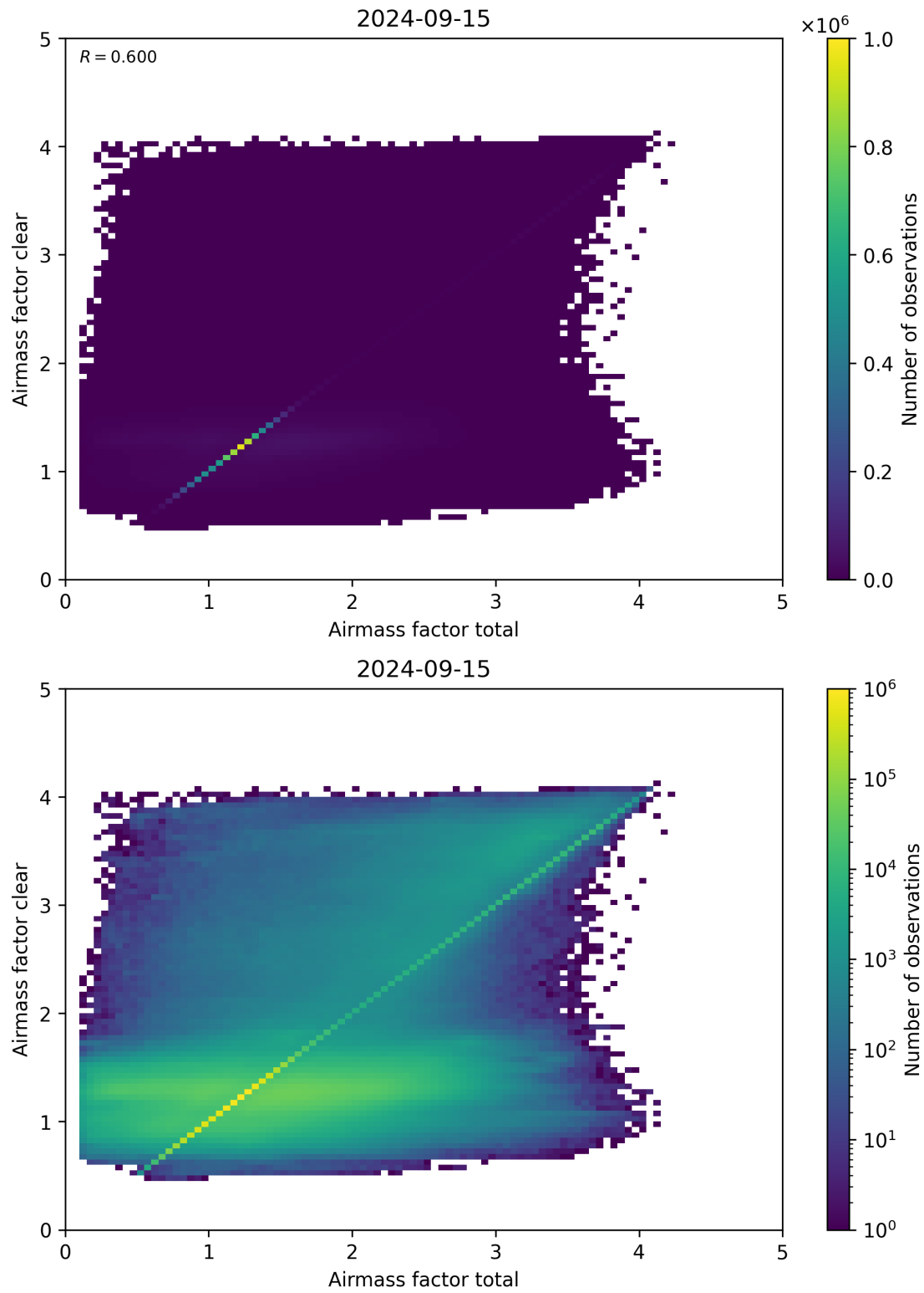
Figure 100: Scatter density plot of “Airmass factor total” against “Airmass factor clear” for 2024-09-14 to 2024-09-16.
