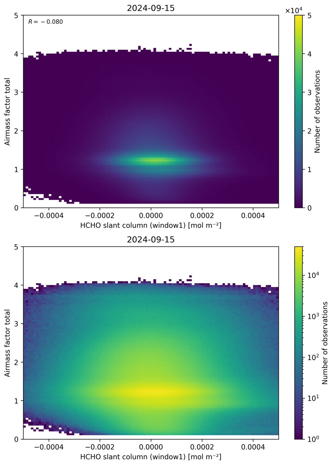
Figure 85: Scatter density plot of “HCHO slant column (window1)” against “Airmass factor total” for 2024-09-14 to 2024-09-16.
