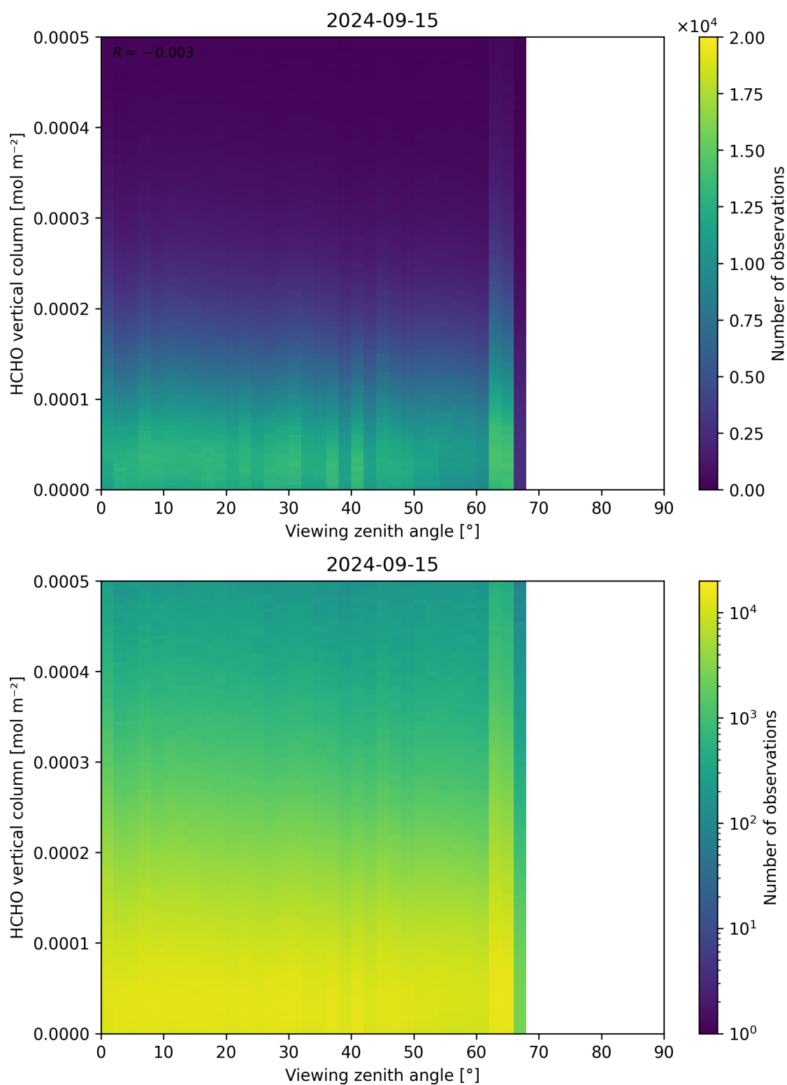
Figure 192: Scatter density plot of “Viewing zenith angle” against “HCHO vertical column” for 2024-09-14 to 2024-09-16.
