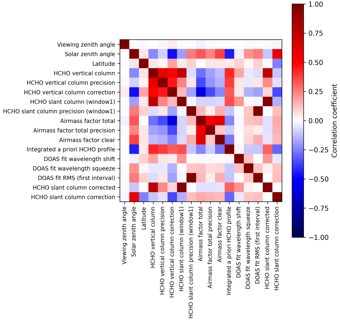
Figure 2: Map of correlation matrix for 2024-09-14 to 2024-09-16.
