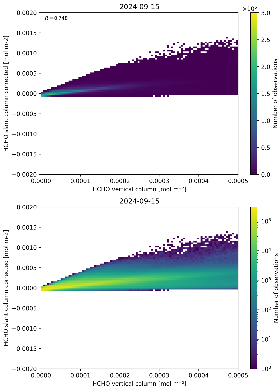
Figure 127: Scatter density plot of “HCHO vertical column” against “HCHO slant column corrected” for 2024-09-14 to 2024-09-16.
