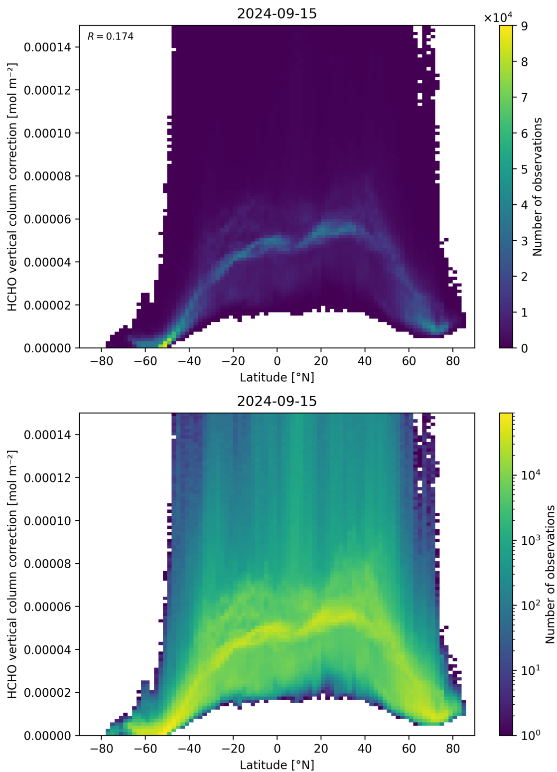
Figure 164: Scatter density plot of “Latitude” against “HCHO vertical column correction” for 2024-09-14 to 2024-09-16.
