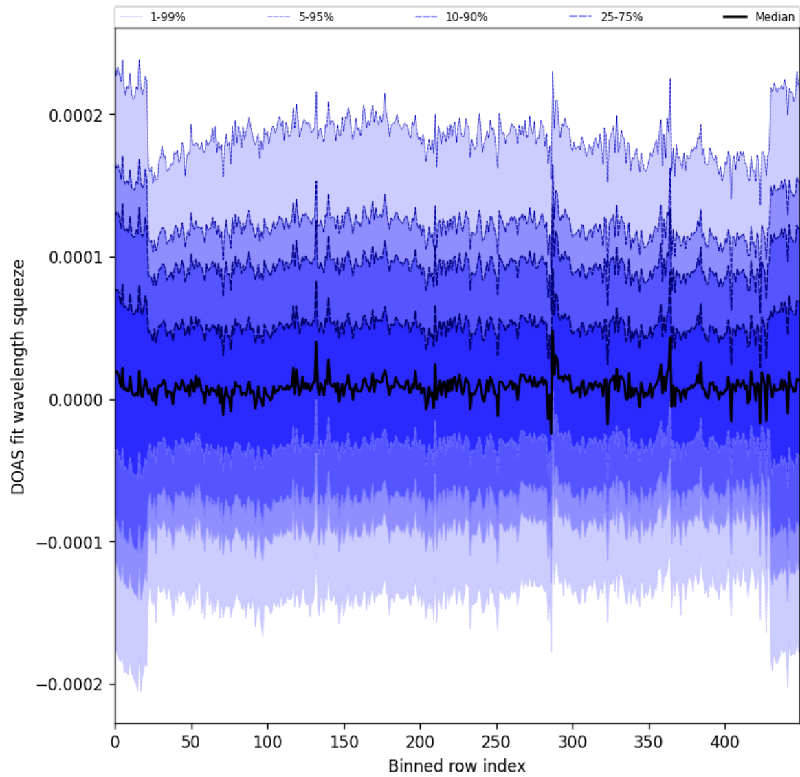
Figure 59: Along track statistics of “DOAS fit wavelength squeeze” for 2024-09-14 to 2024-09-16
