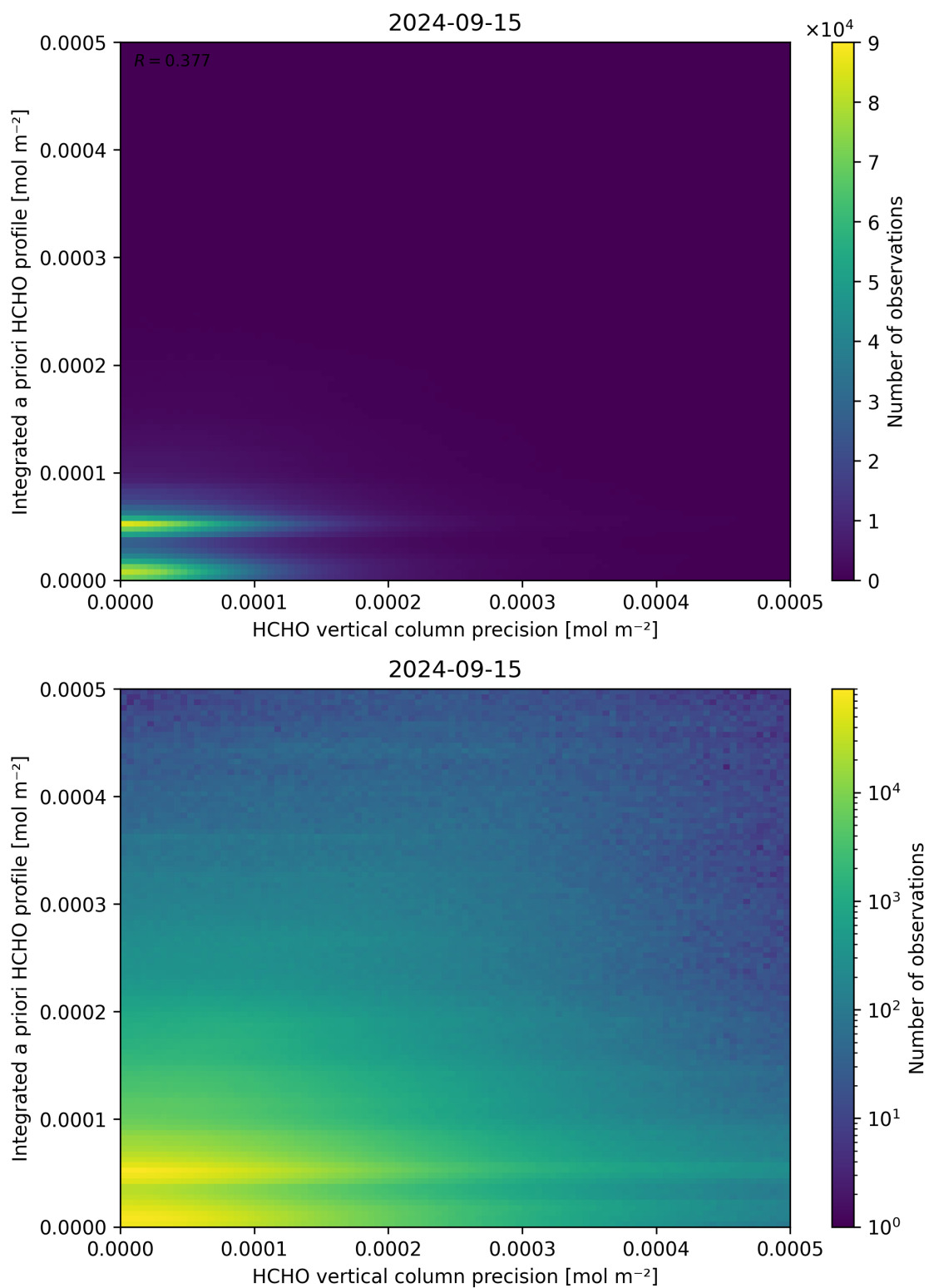
Figure 147: Scatter density plot of “HCHO vertical column precision” against “Integrated a priori HCHO profile” for 2024-09-14 to 2024-09-16.
