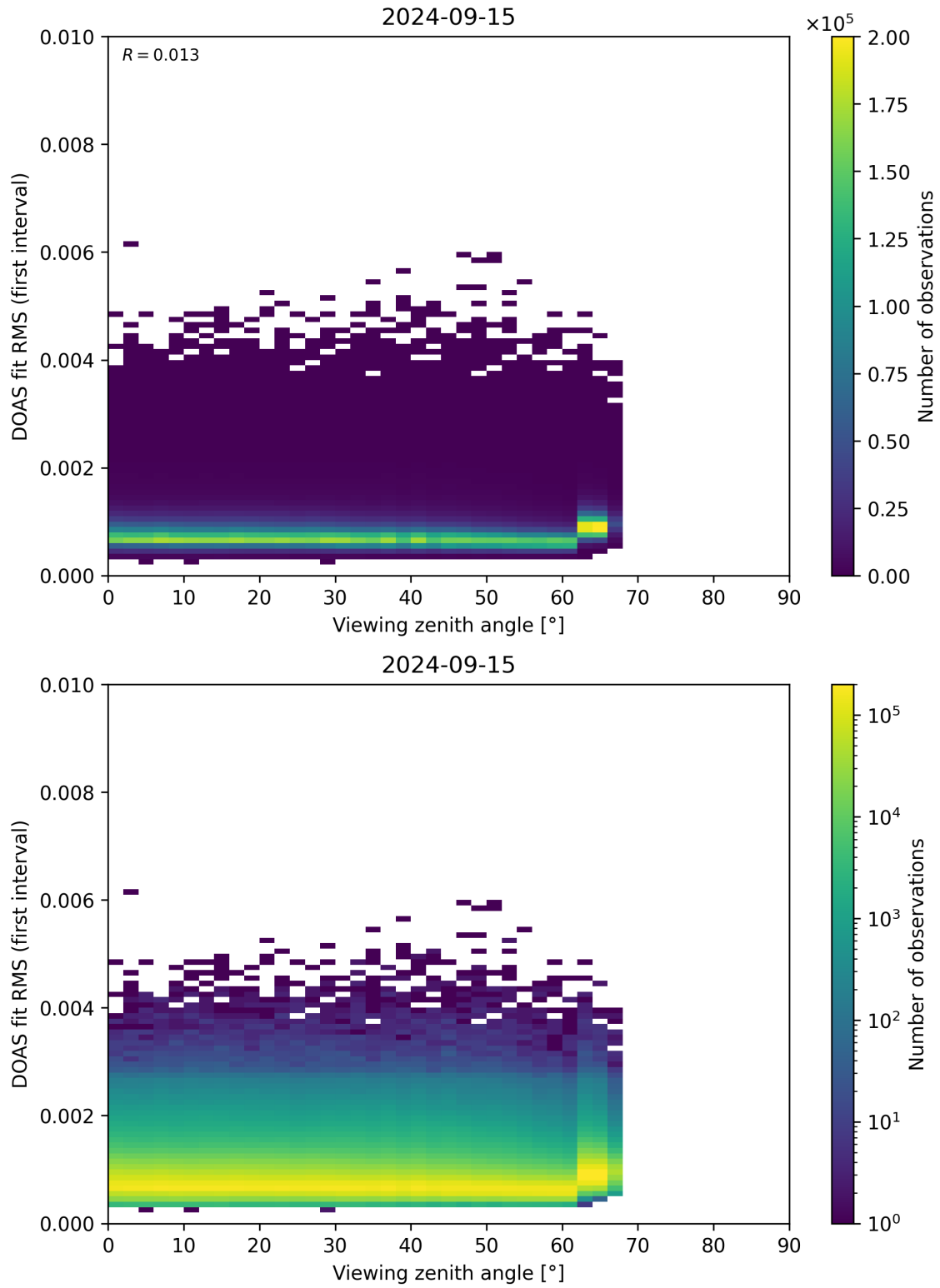
Figure 182: Scatter density plot of “Viewing zenith angle” against “DOAS fit RMS (first interval)” for 2024-09-14 to 2024-09-16.
