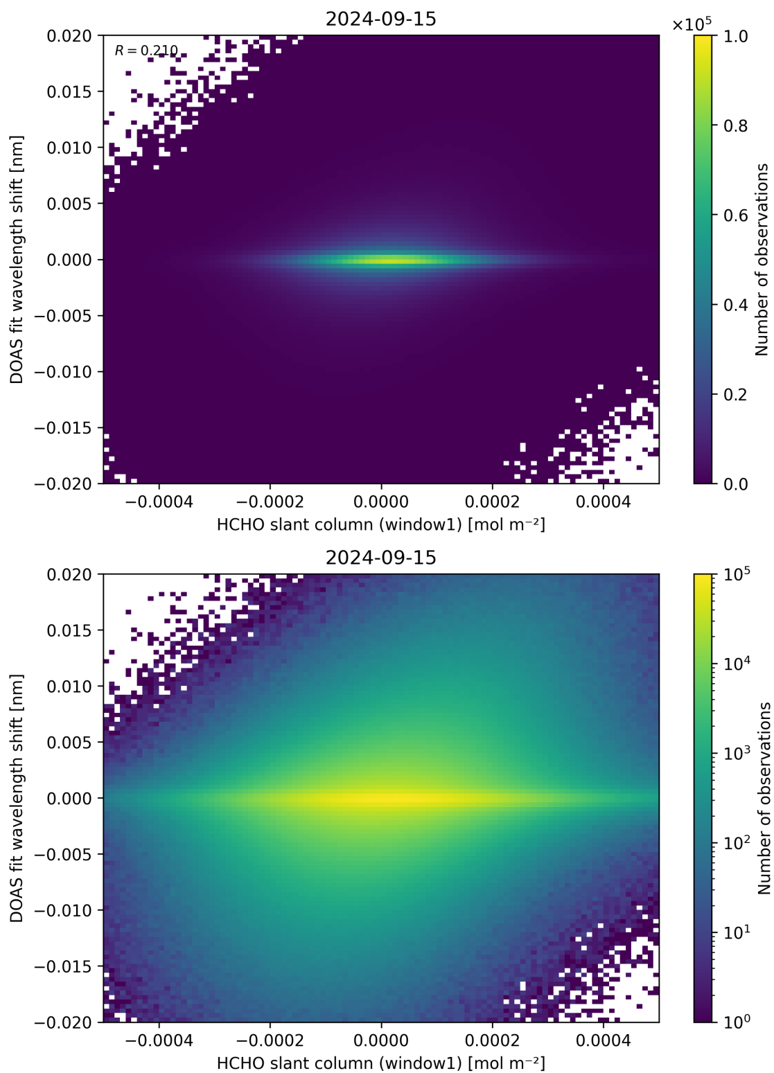
Figure 79: Scatter density plot of “HCHO slant column (window1)” against “DOAS fit wavelength shift” for 2024-09-14 to 2024-09-16.
