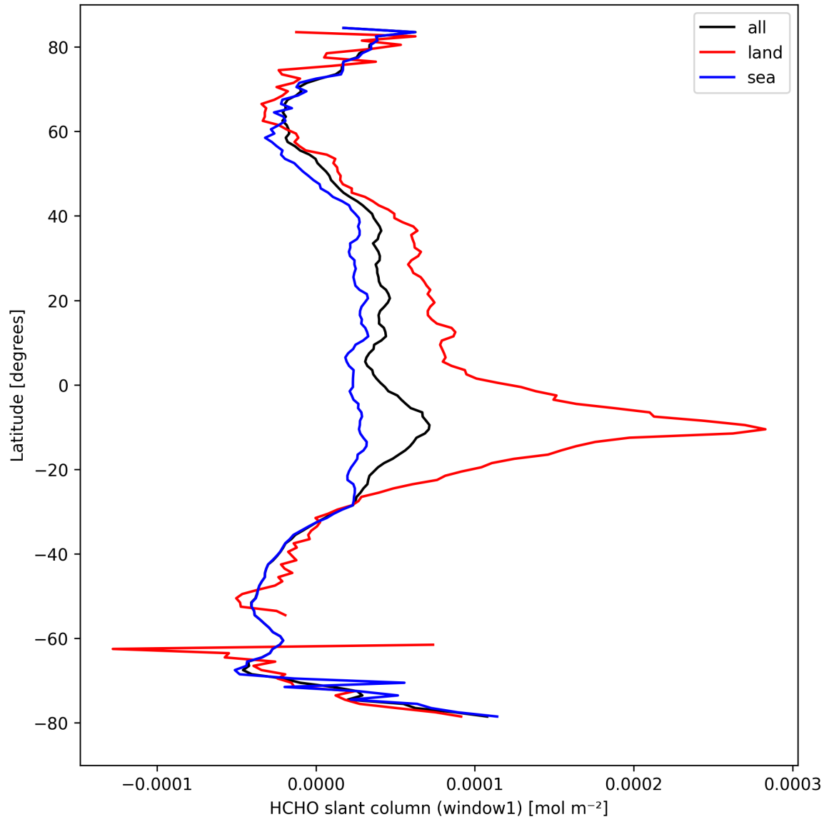
Figure 24: Zonal average of “HCHO slant column (window1)” for 2024-09-14 to 2024-09-16.
