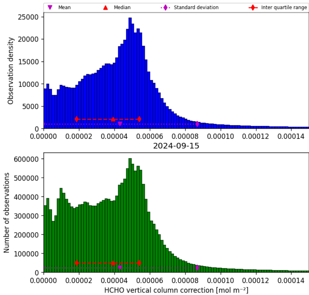
Figure 37: Histogram of “HCHO vertical column correction” for 2024-09-14 to 2024-09-16
