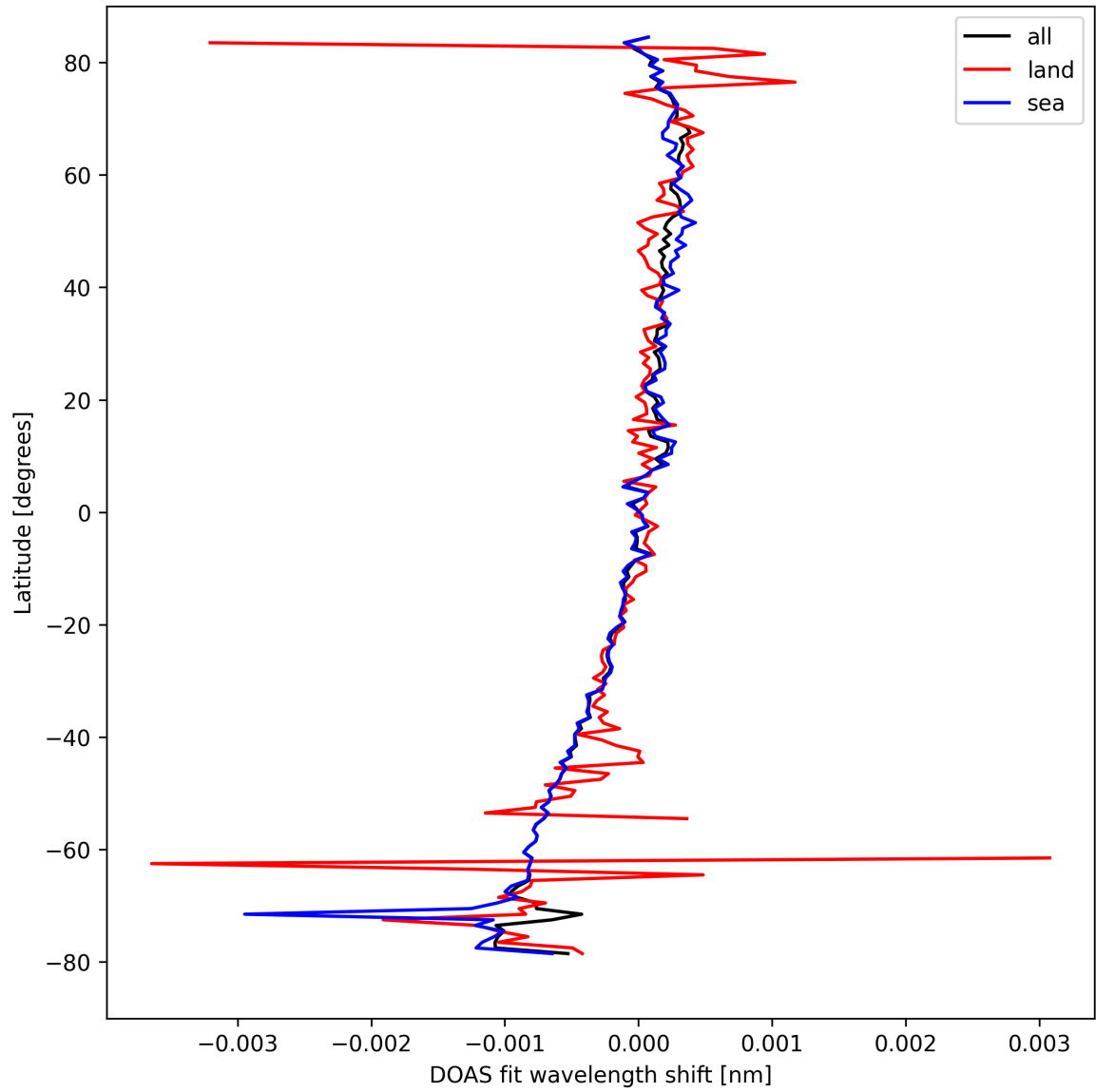
Figure 30: Zonal average of "DOAS fit wavelength shift" for 2024-09-14 to 2024-09-16.
