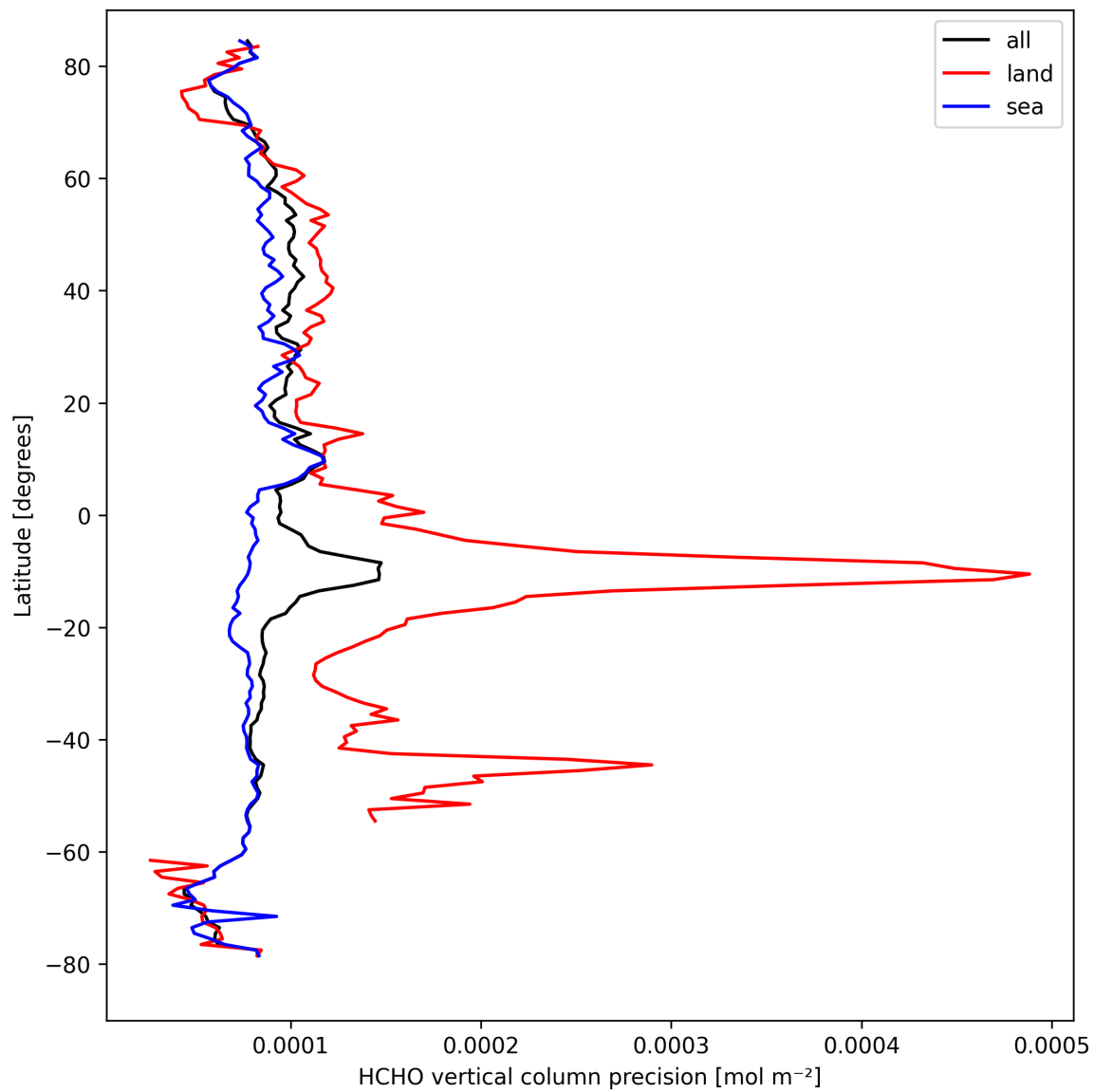
Figure 22: Zonal average of “HCHO vertical column precision” for 2024-09-14 to 2024-09-16.
