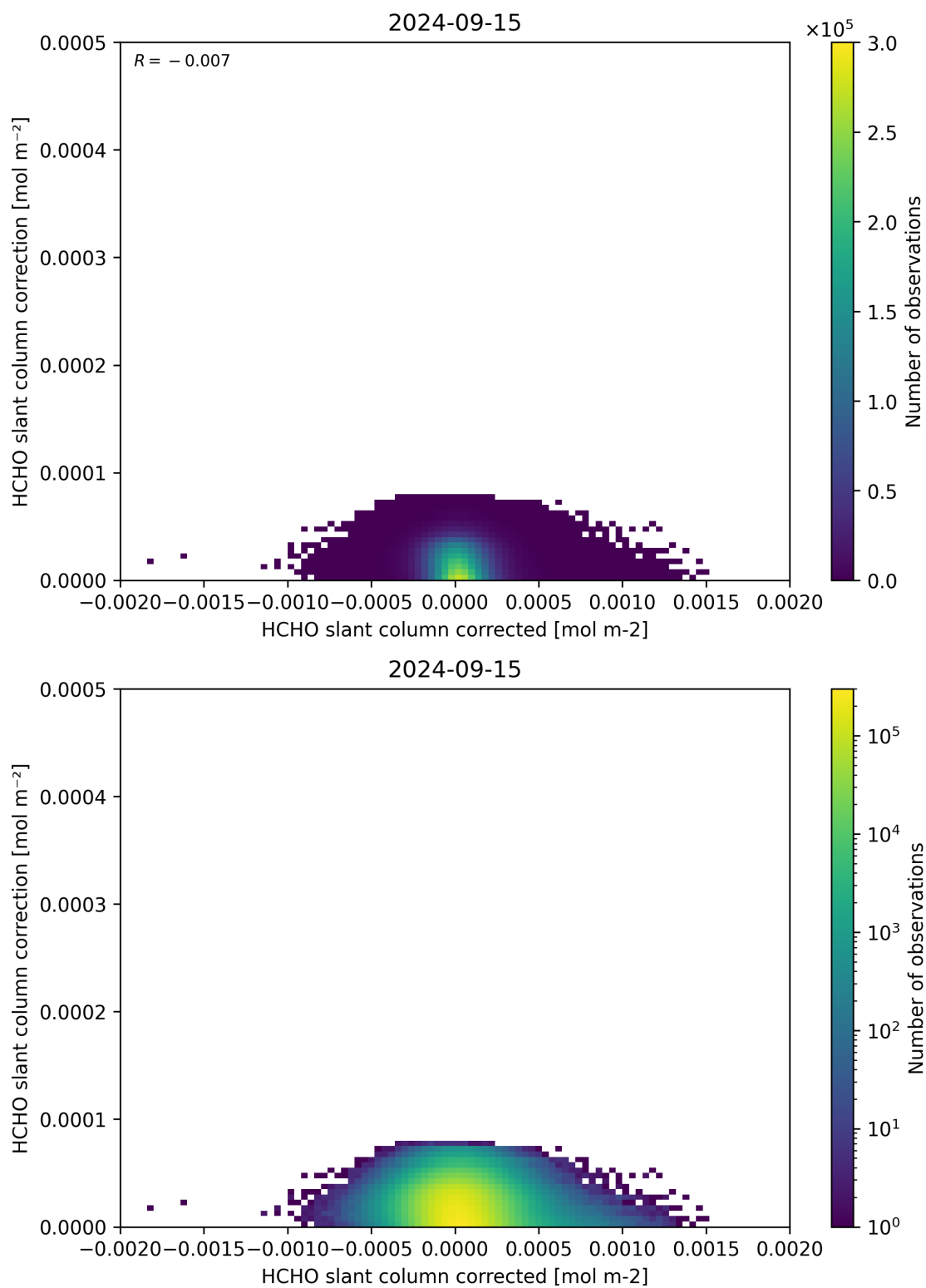
Figure 77: Scatter density plot of “HCHO slant column corrected” against “HCHO slant column correction” for 2024-09-14 to 2024-09-16.
