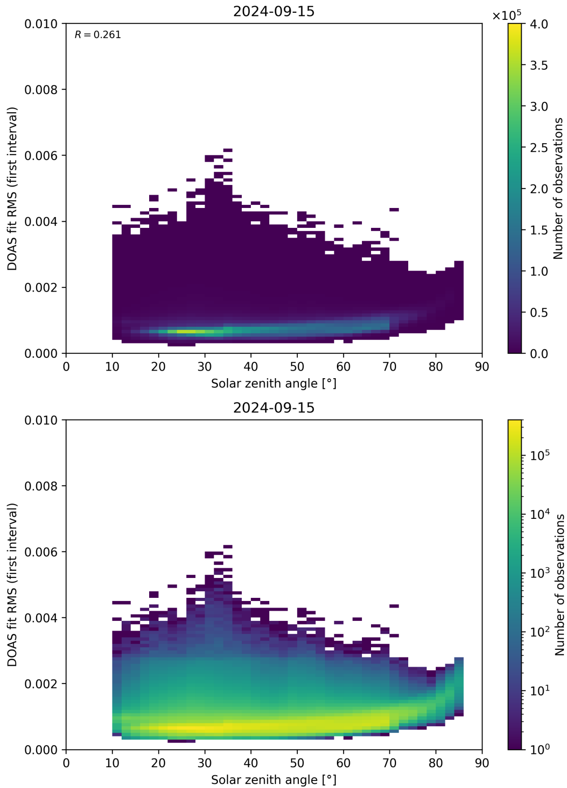
Figure 167: Scatter density plot of “Solar zenith angle” against “DOAS fit RMS (first interval)” for 2024-09-14 to 2024-09-16.
