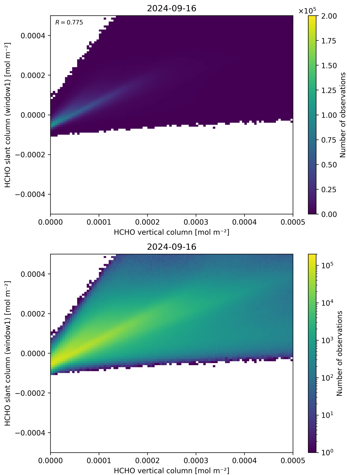
Figure 129: Scatter density plot of “HCHO vertical column” against “HCHO slant column (window1)” for 2024-09-15 to 2024-09-17.
