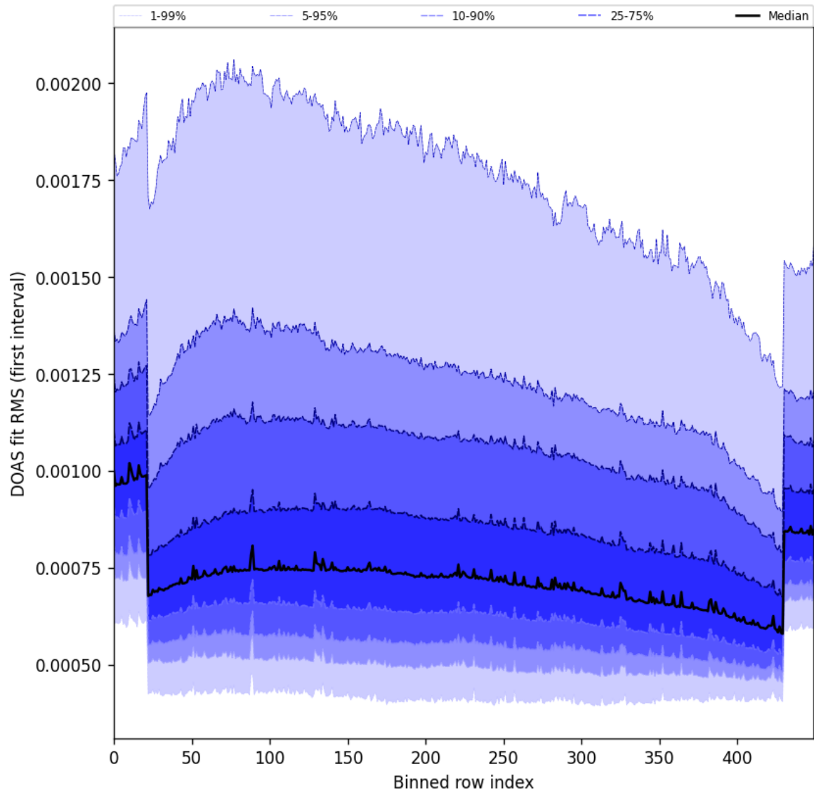
Figure 60: Along track statistics of “DOAS fit RMS (first interval)” for 2024-09-15 to 2024-09-17
