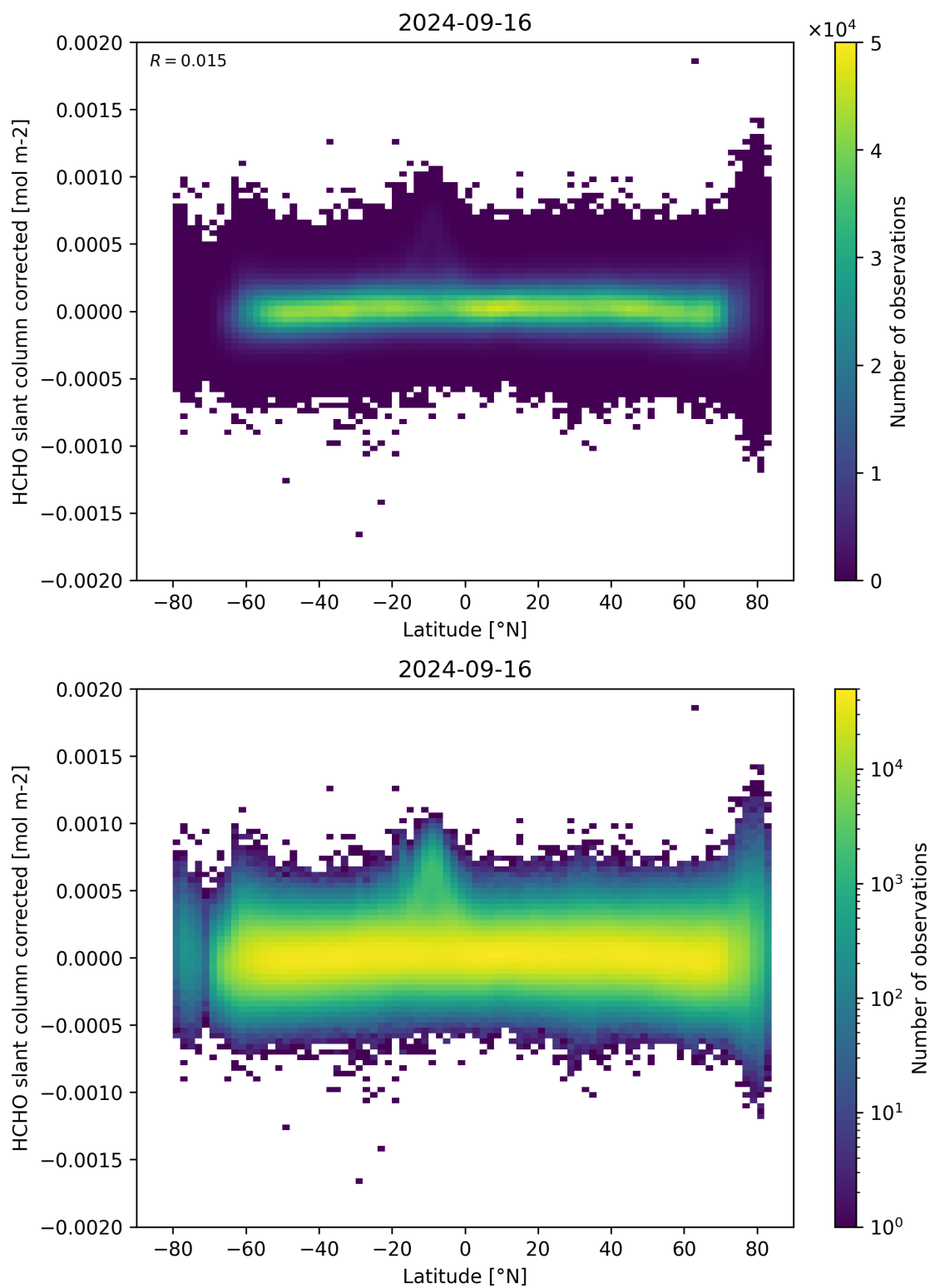
Figure 157: Scatter density plot of “Latitude” against “HCHO slant column corrected” for 2024-09-15 to 2024-09-17.
