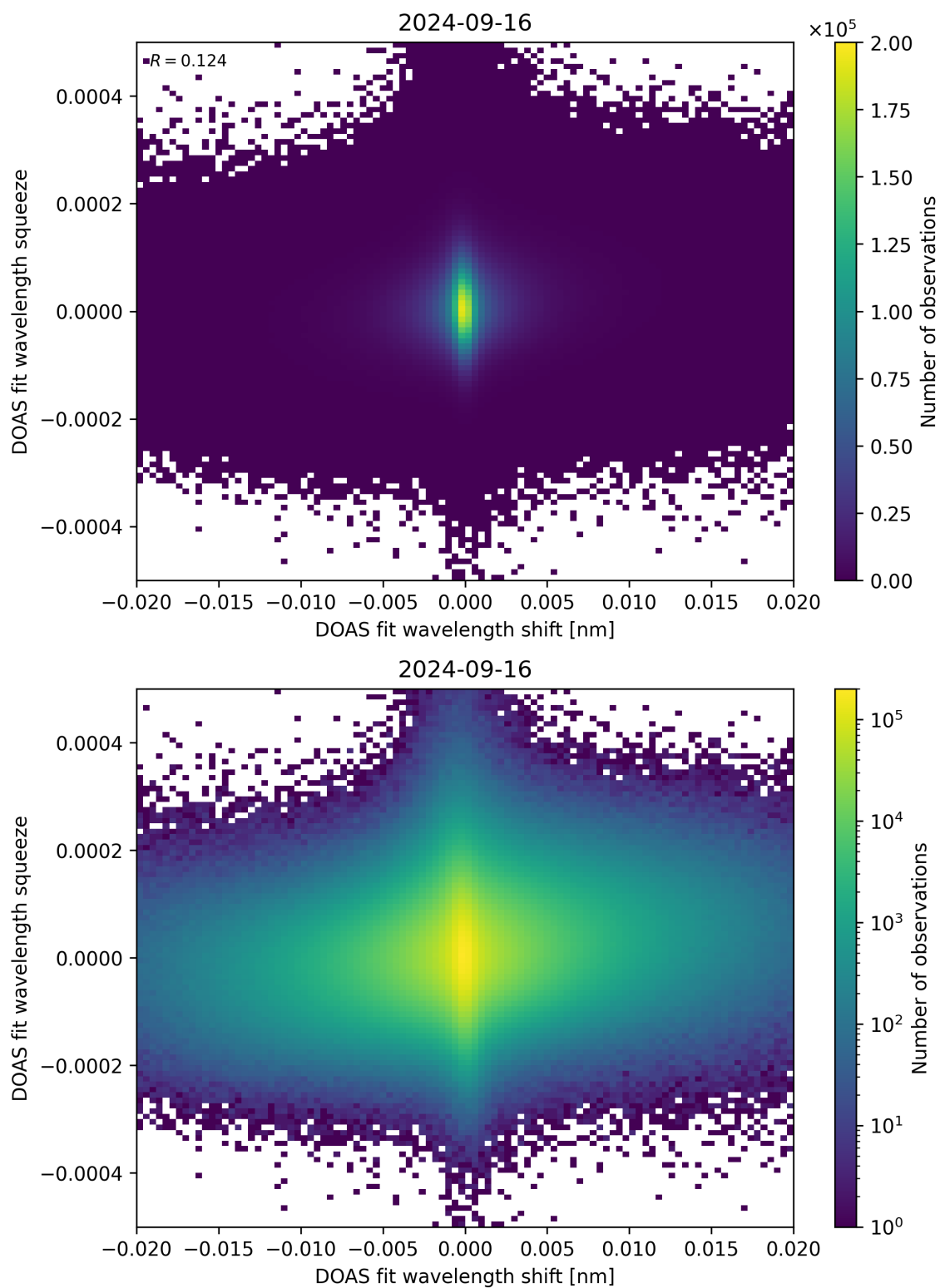
Figure 65: Scatter density plot of “DOAS fit wavelength shift” against “DOAS fit wavelength squeeze” for 2024-09-15 to 2024-09-17.
