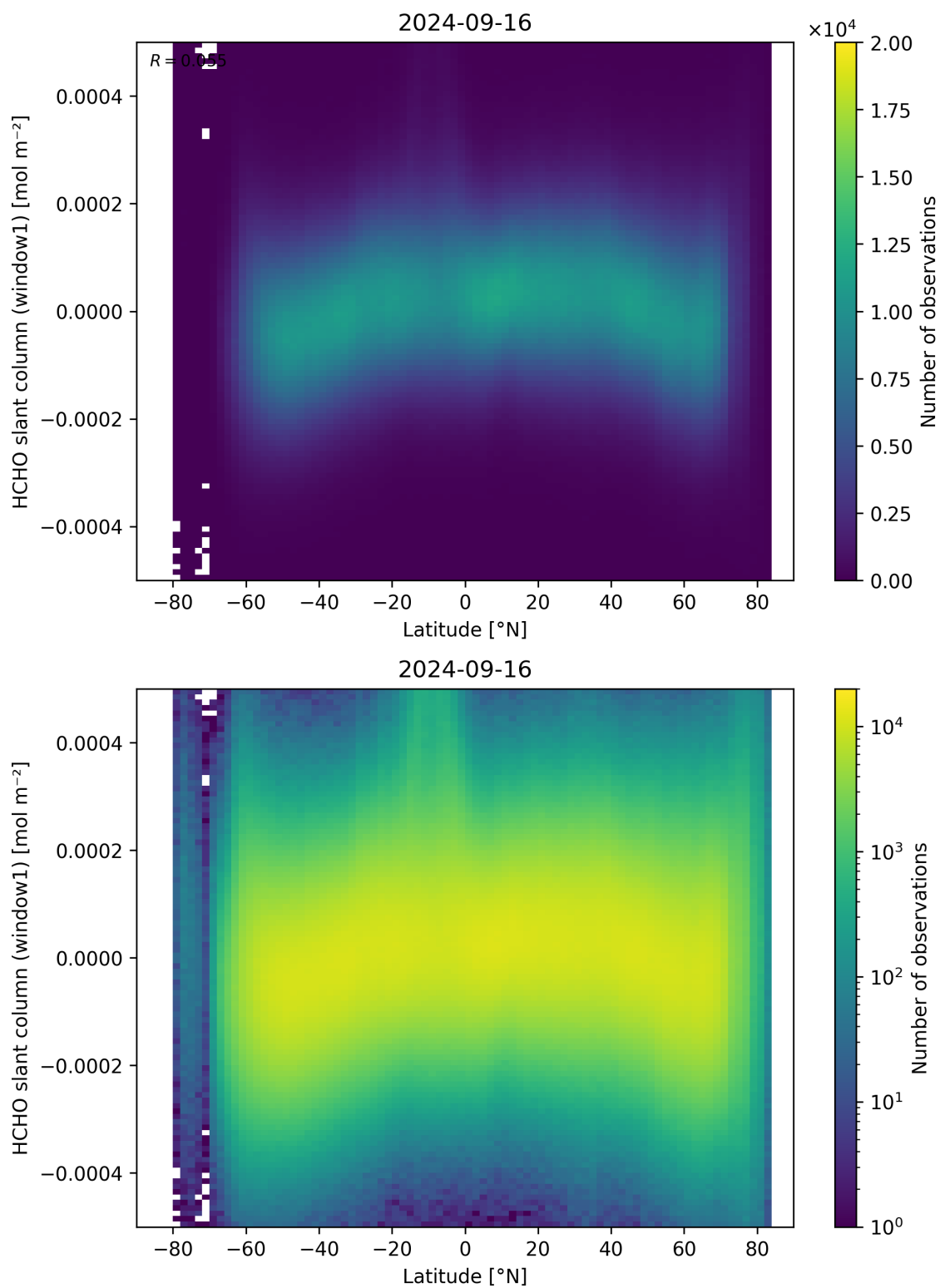
Figure 159: Scatter density plot of “Latitude” against “HCHO slant column (window1)” for 2024-09-15 to 2024-09-17.
