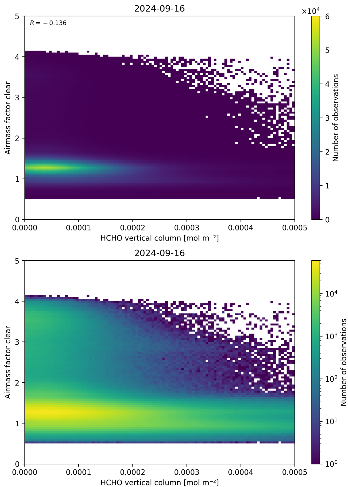
Figure 126: Scatter density plot of “HCHO vertical column” against “Airmass factor clear” for 2024-09-15 to 2024-09-17.
