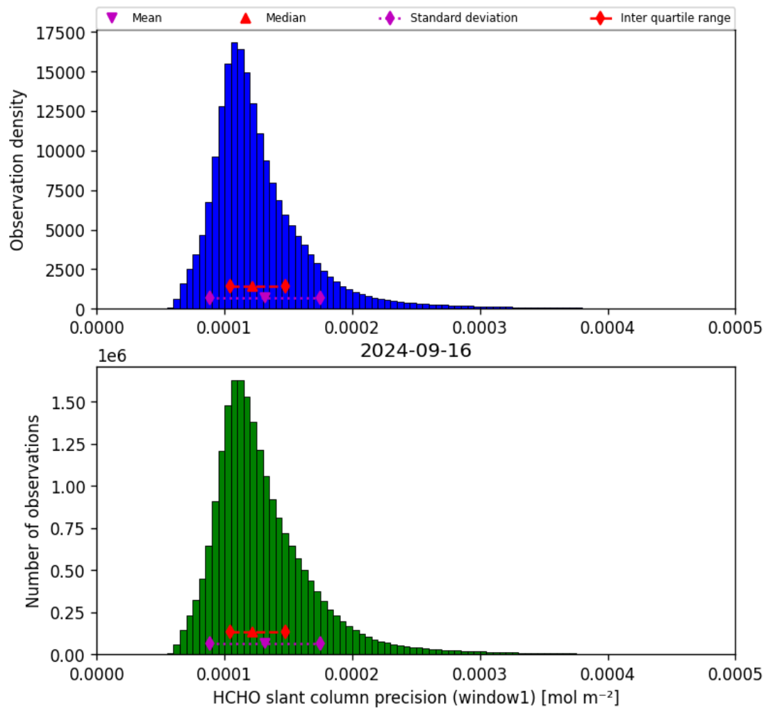
Figure 39: Histogram of “HCHO slant column precision (window1)” for 2024-09-15 to 2024-09-17
