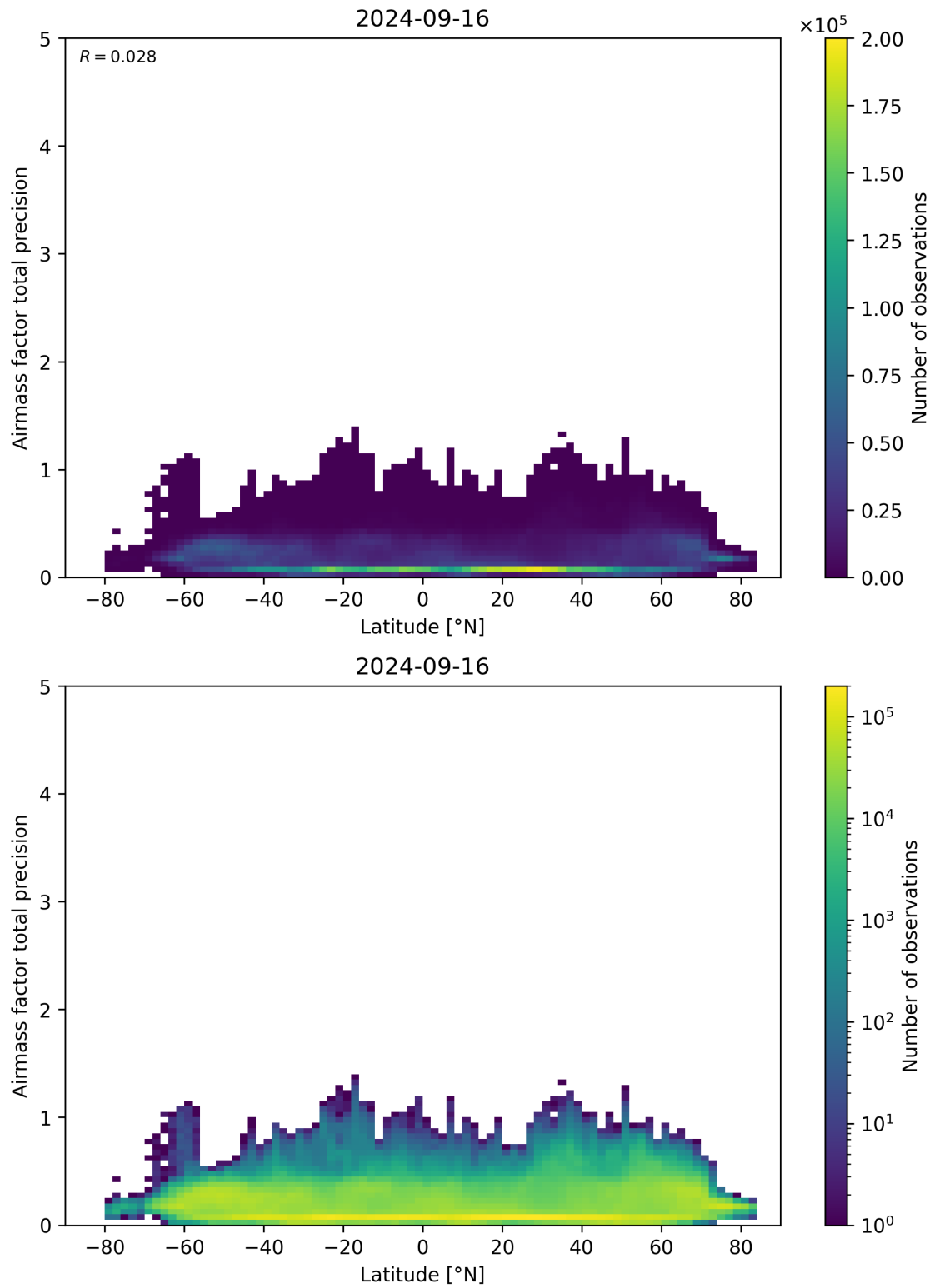
Figure 162: Scatter density plot of “Latitude” against “Airmass factor total precision” for 2024-09-15 to 2024-09-17.
