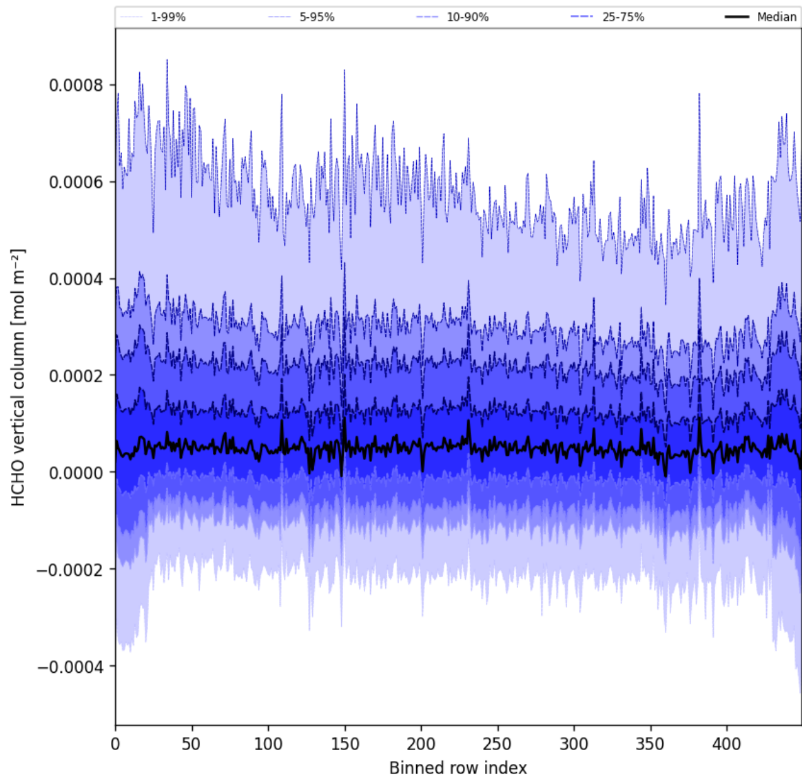
Figure 49: Along track statistics of “HCHO vertical column” for 2024-09-15 to 2024-09-17
