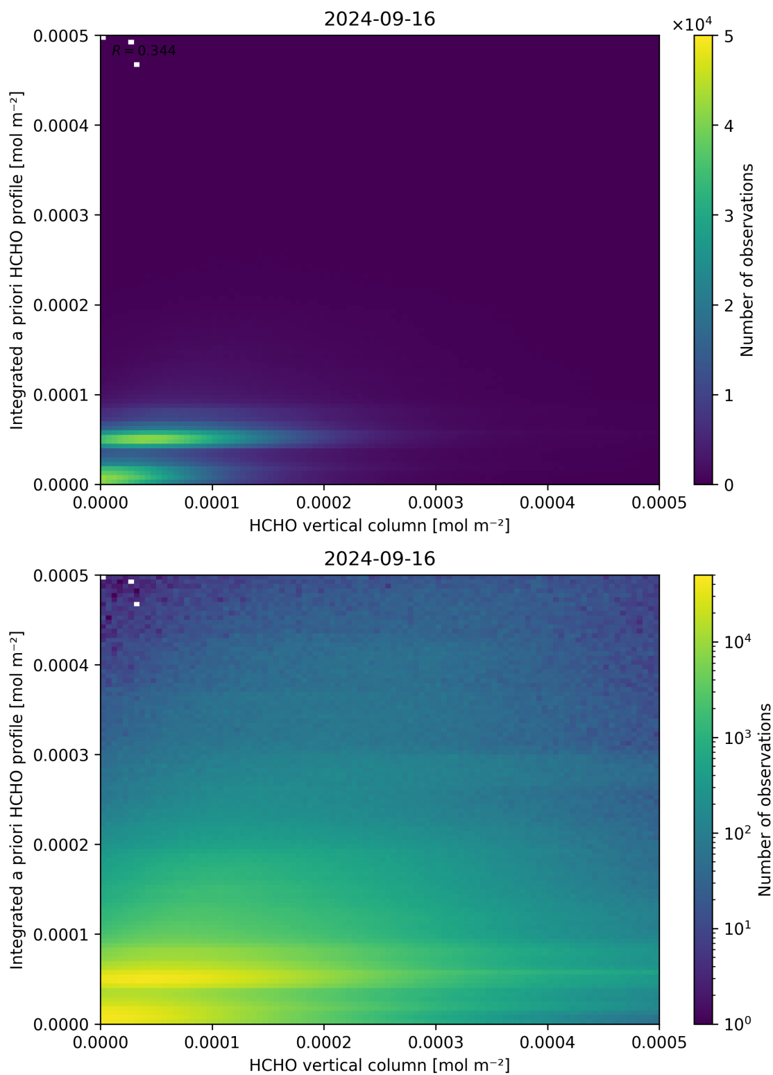
Figure 135: Scatter density plot of “HCHO vertical column” against “Integrated a priori HCHO profile” for 2024-09-15 to 2024-09-17.
