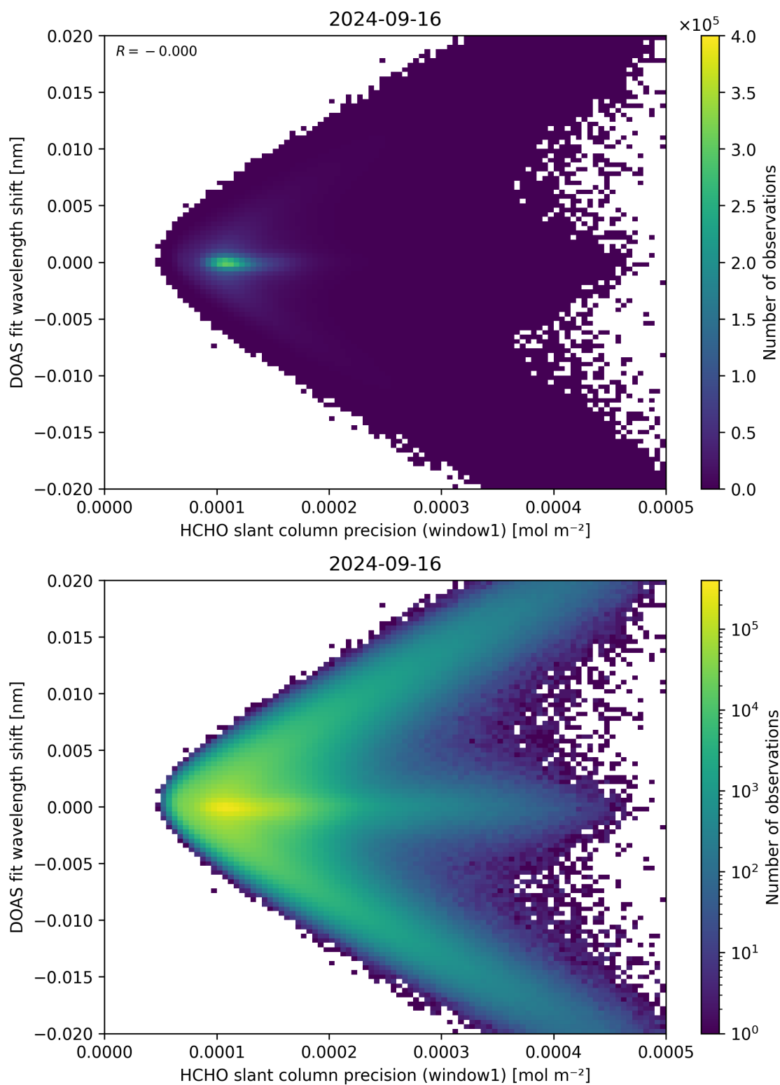
Figure 89: Scatter density plot of “HCHO slant column precision (window1)” against “DOAS fit wavelength shift” for 2024-09-15 to 2024-09-17.
