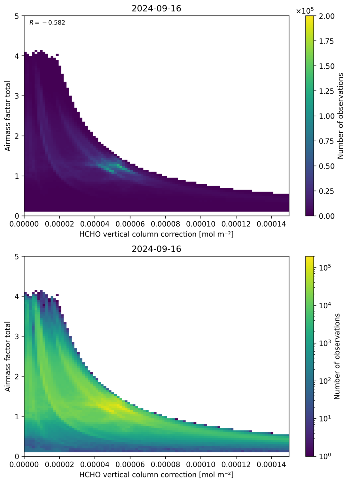
Figure 120: Scatter density plot of “HCHO vertical column correction” against “Airmass factor total” for 2024-09-15 to 2024-09-17.
