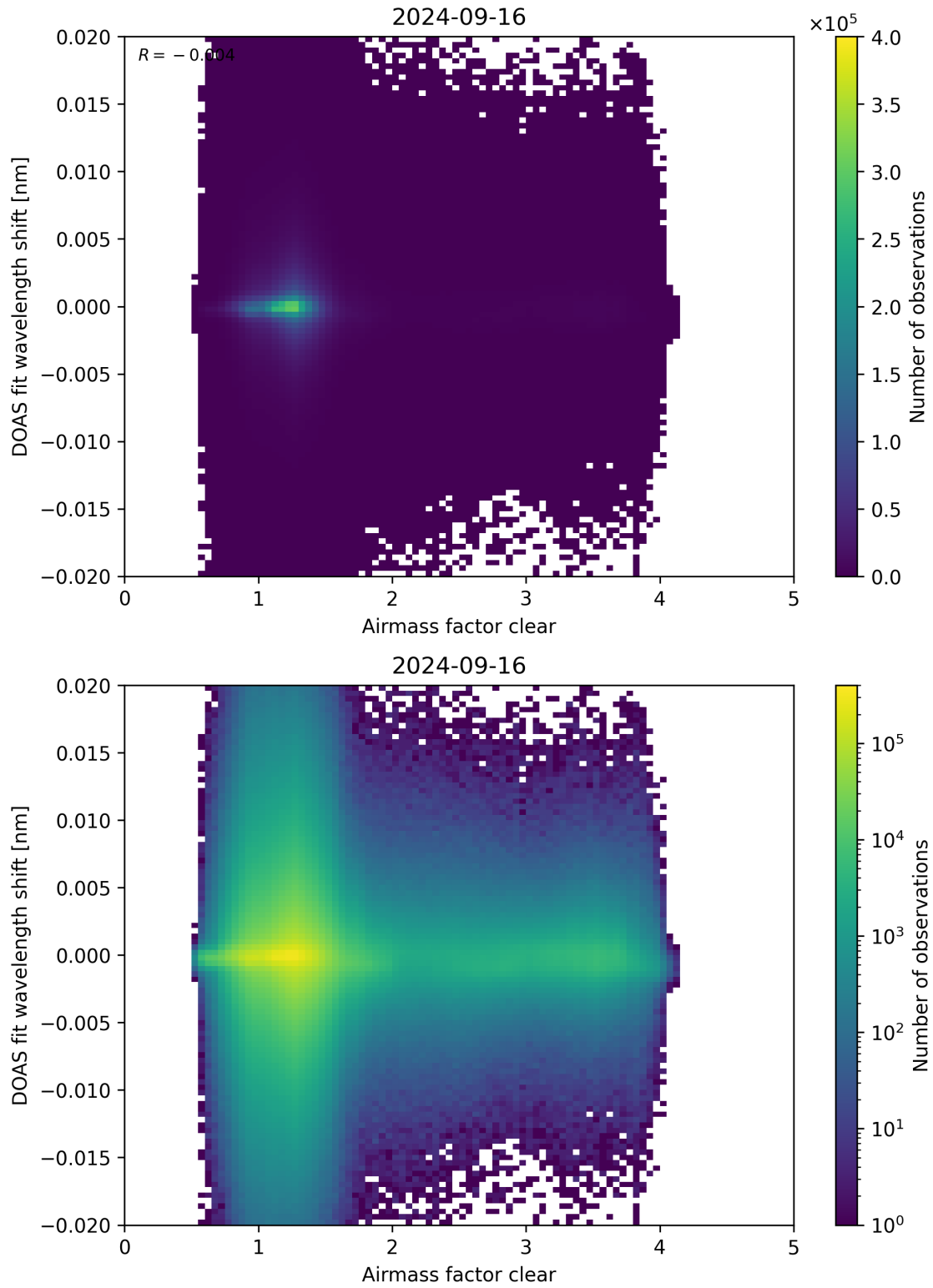
Figure 72: Scatter density plot of “Airmass factor clear” against “DOAS fit wavelength shift” for 2024-09-15 to 2024-09-17.
