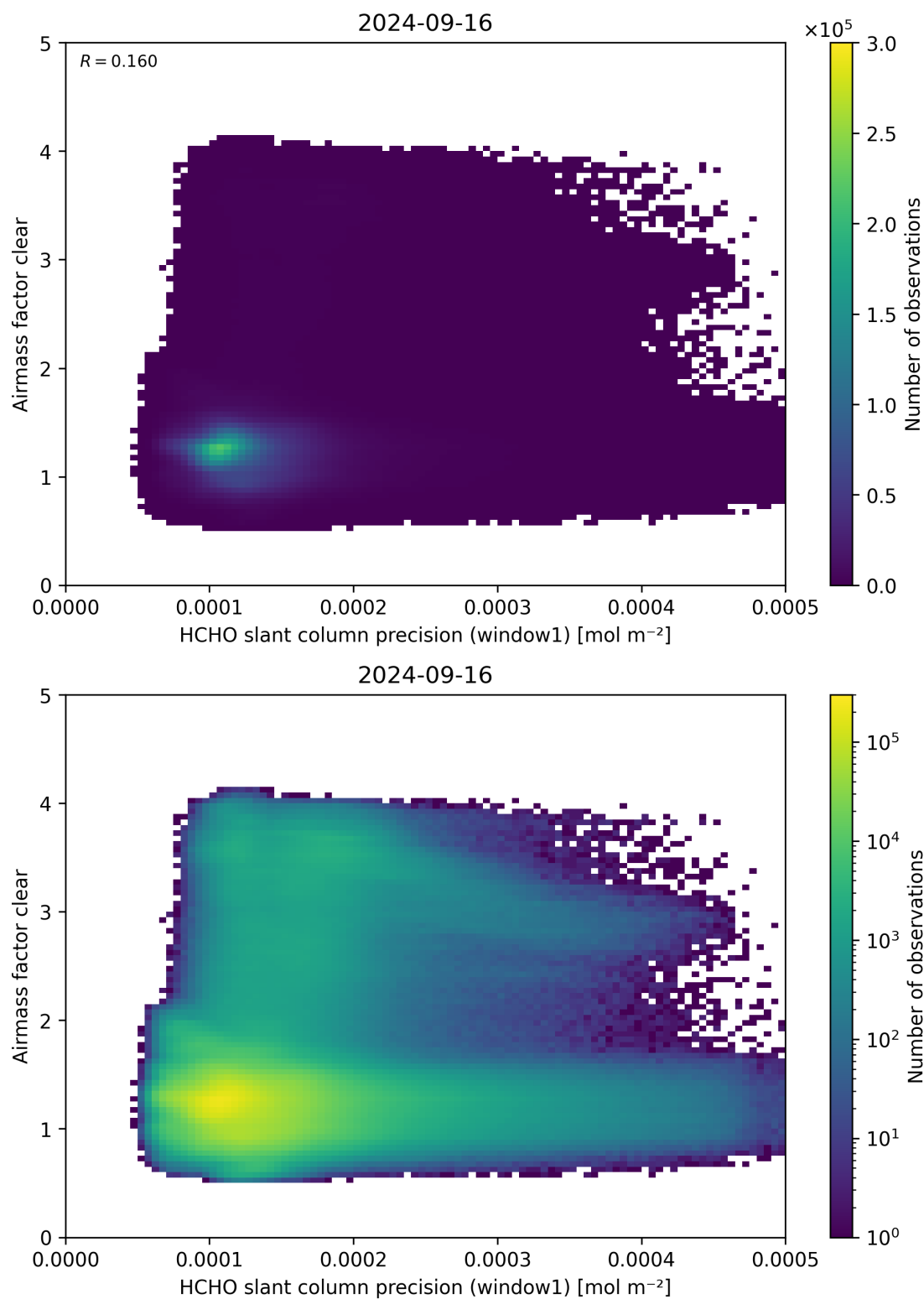
Figure 91: Scatter density plot of “HCHO slant column precision (window1)” against “Airmass factor clear” for 2024-09-15 to 2024-09-17.
