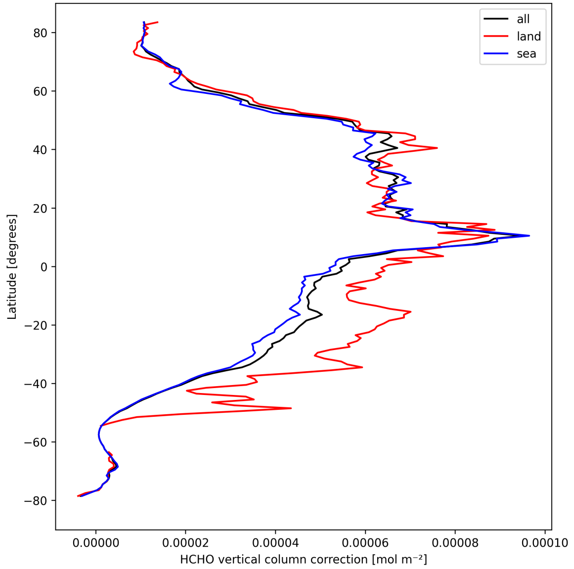
Figure 23: Zonal average of “HCHO vertical column correction” for 2024-09-15 to 2024-09-17.
