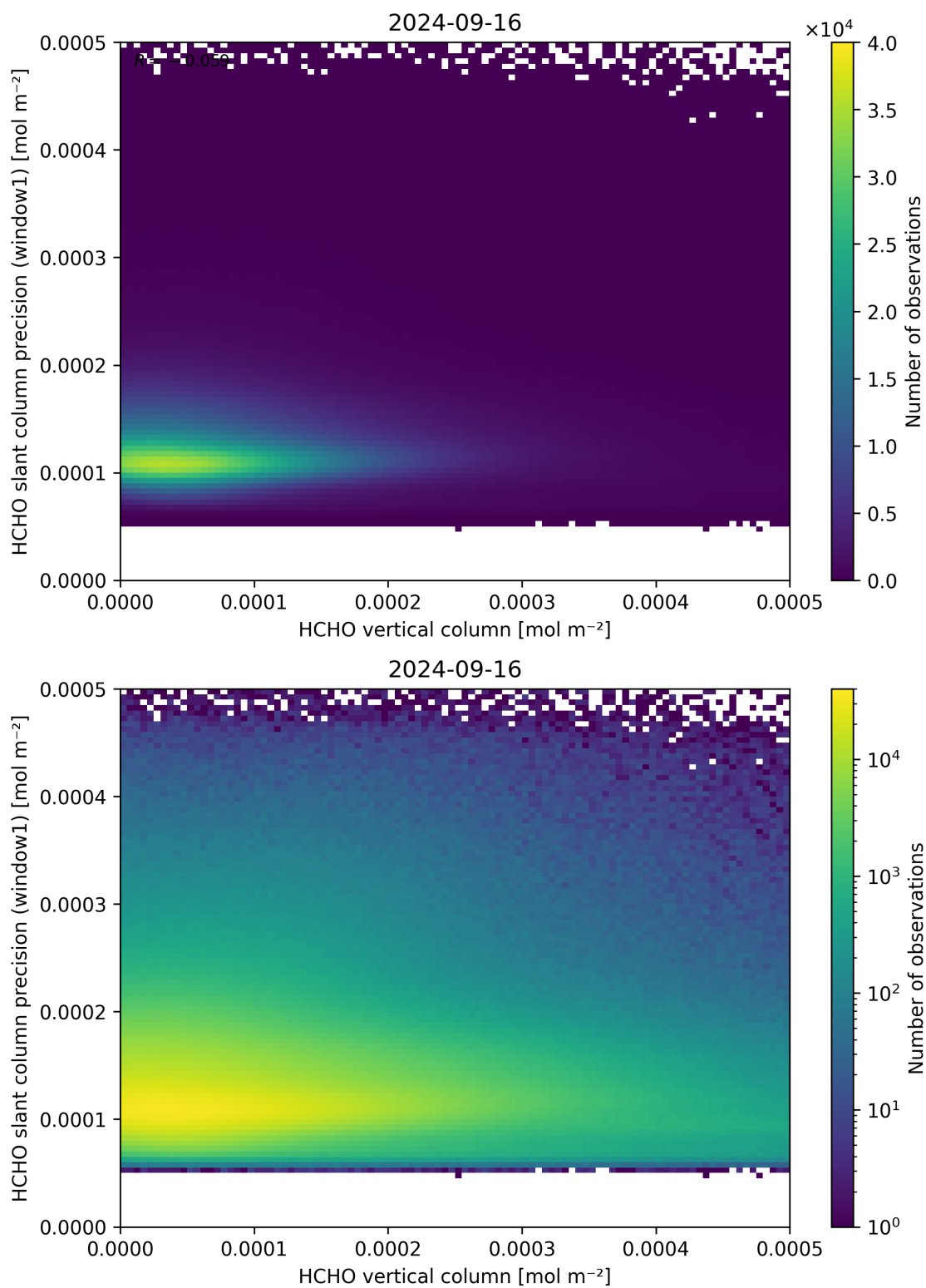
Figure 130: Scatter density plot of “HCHO vertical column” against “HCHO slant column precision (window1)” for 2024-09-15 to 2024-09-17.
