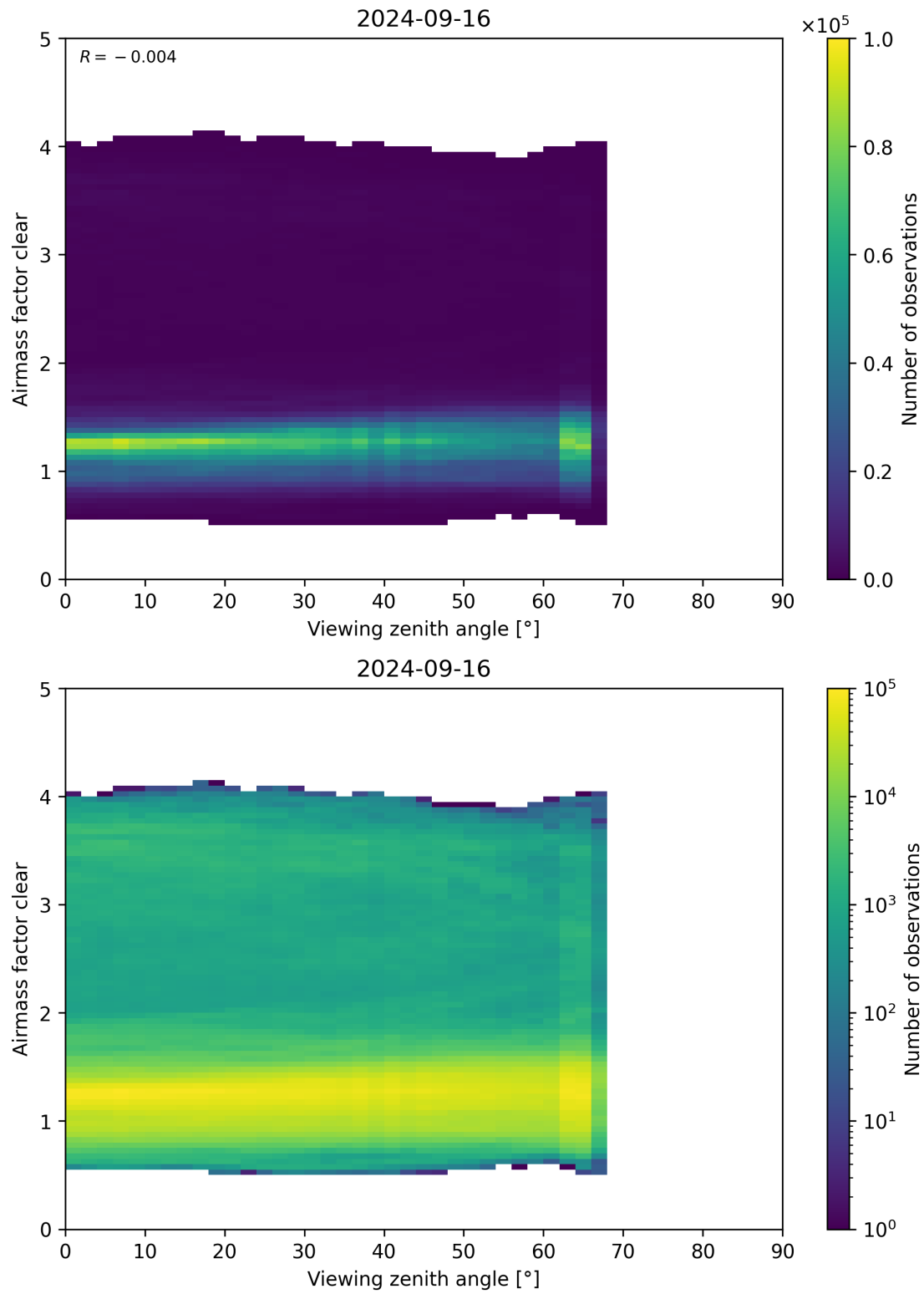
Figure 185: Scatter density plot of “Viewing zenith angle” against “Airmass factor clear” for 2024-09-15 to 2024-09-17.
