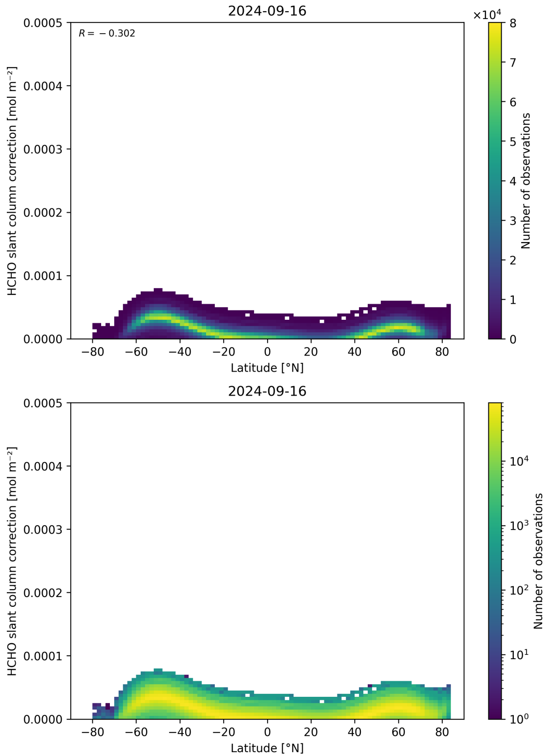
Figure 158: Scatter density plot of “Latitude” against “HCHO slant column correction” for 2024-09-15 to 2024-09-17.
