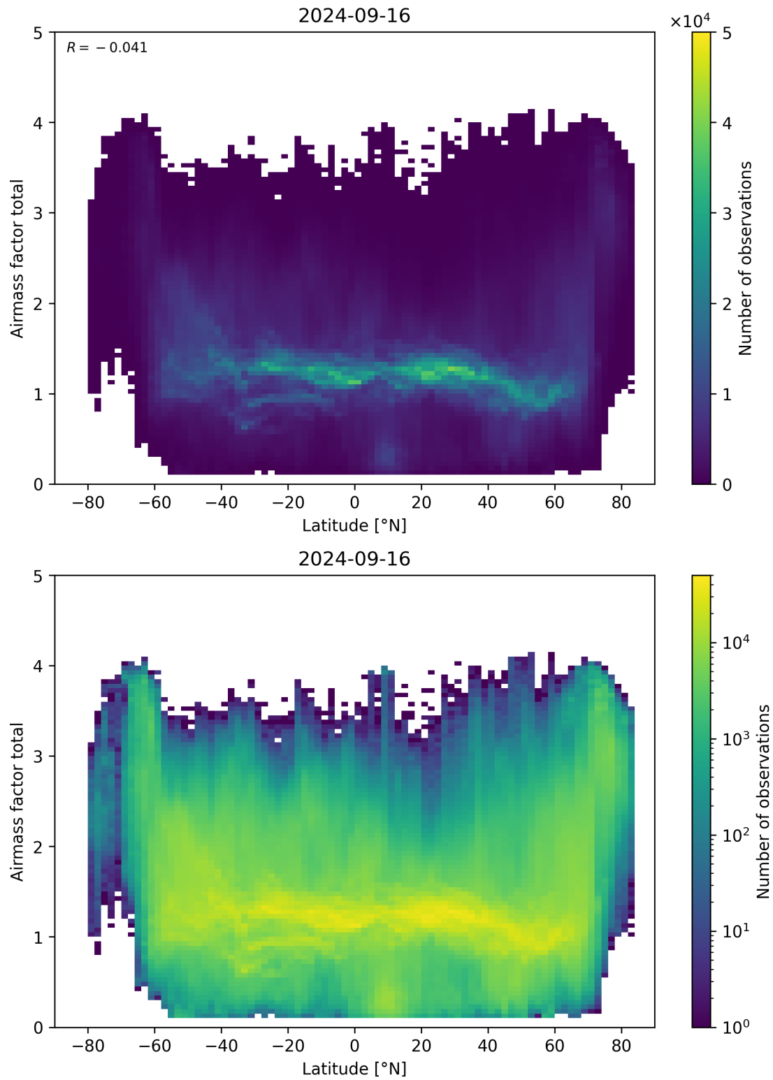
Figure 161: Scatter density plot of “Latitude” against “Airmass factor total” for 2024-09-15 to 2024-09-17.
