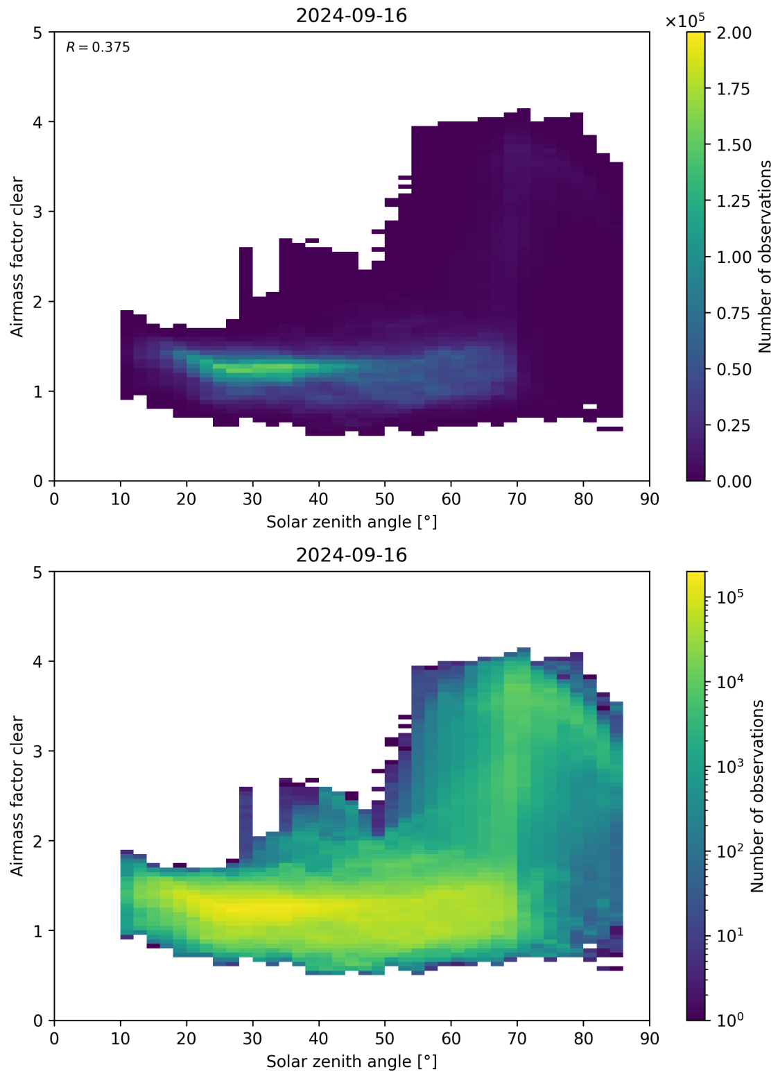
Figure 170: Scatter density plot of “Solar zenith angle” against “Airmass factor clear” for 2024-09-15 to 2024-09-17.
