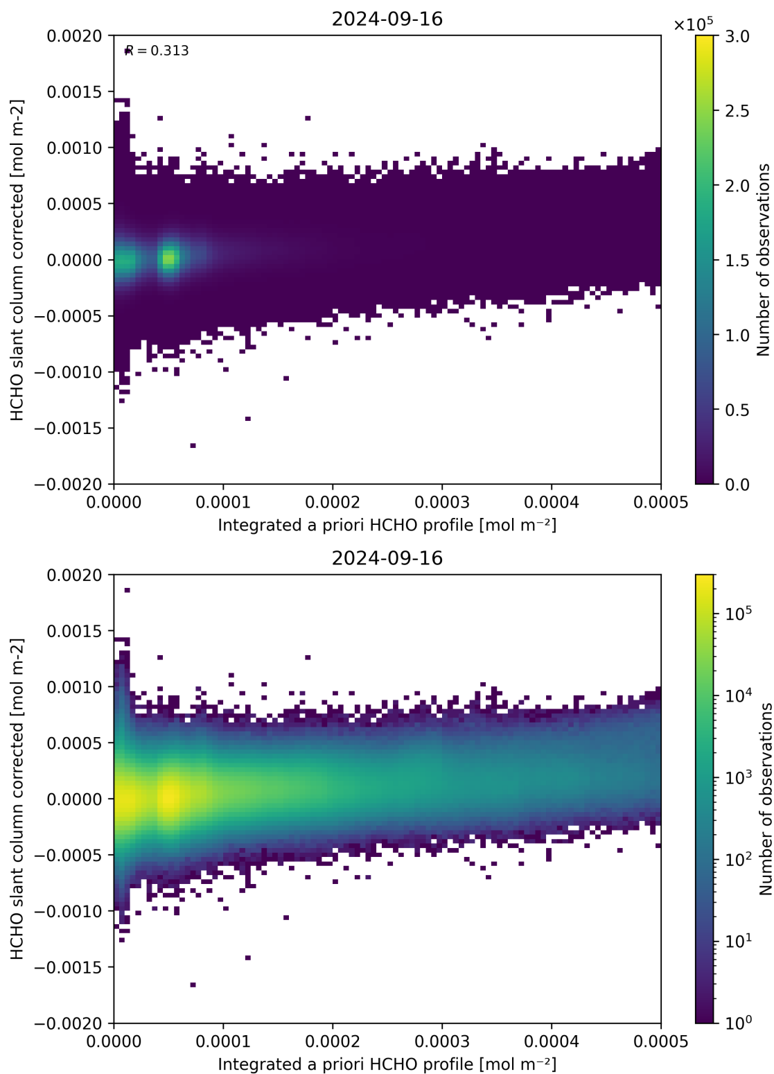
Figure 151: Scatter density plot of “Integrated a priori HCHO profile” against “HCHO slant column corrected” for 2024-09-15 to 2024-09-17.
