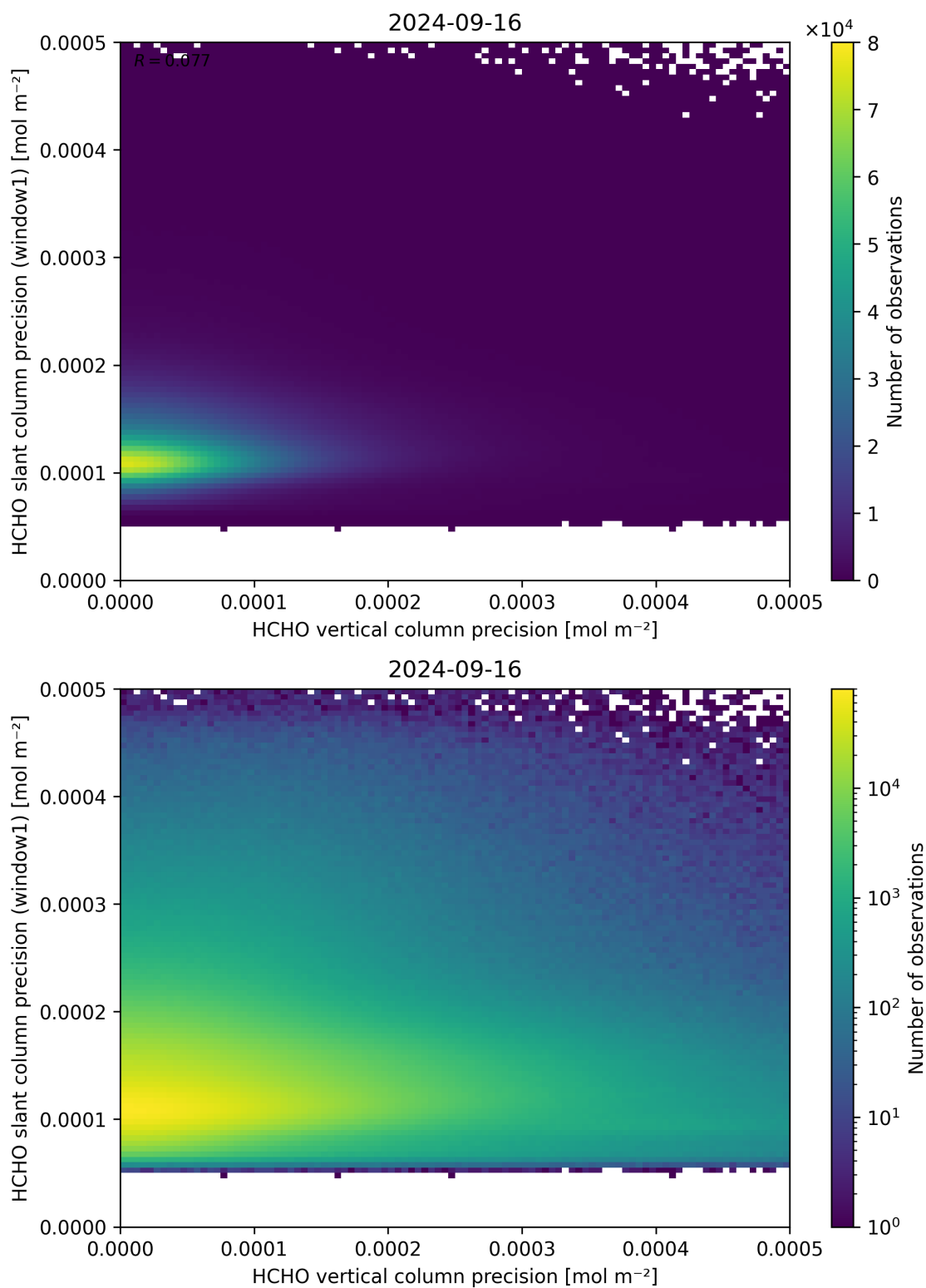
Figure 143: Scatter density plot of “HCHO vertical column precision” against “HCHO slant column precision (window1)” for 2024-09-15 to 2024-09-17.
