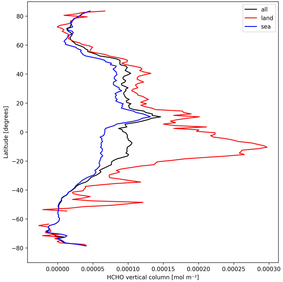
Figure 21: Zonal average of “HCHO vertical column” for 2024-09-15 to 2024-09-17.
