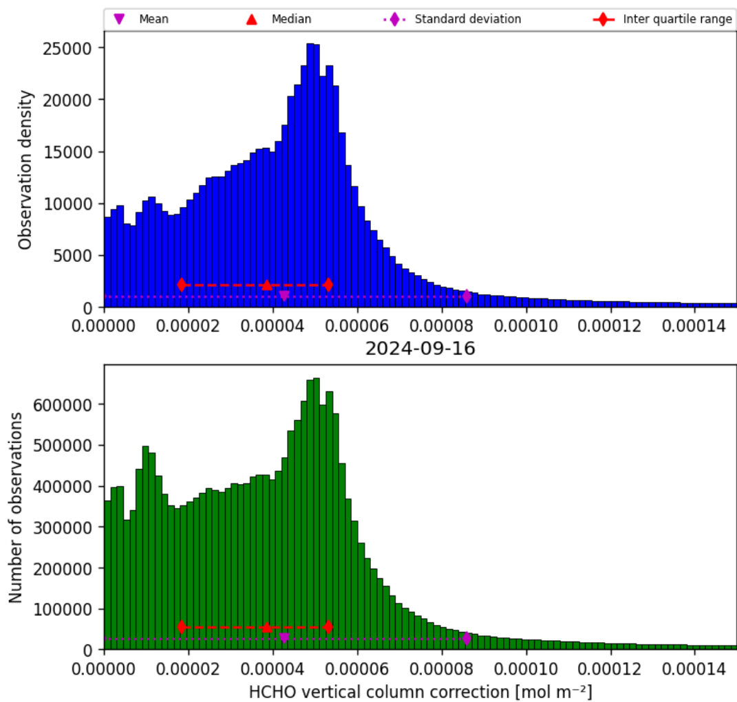
Figure 37: Histogram of “HCHO vertical column correction” for 2024-09-15 to 2024-09-17
