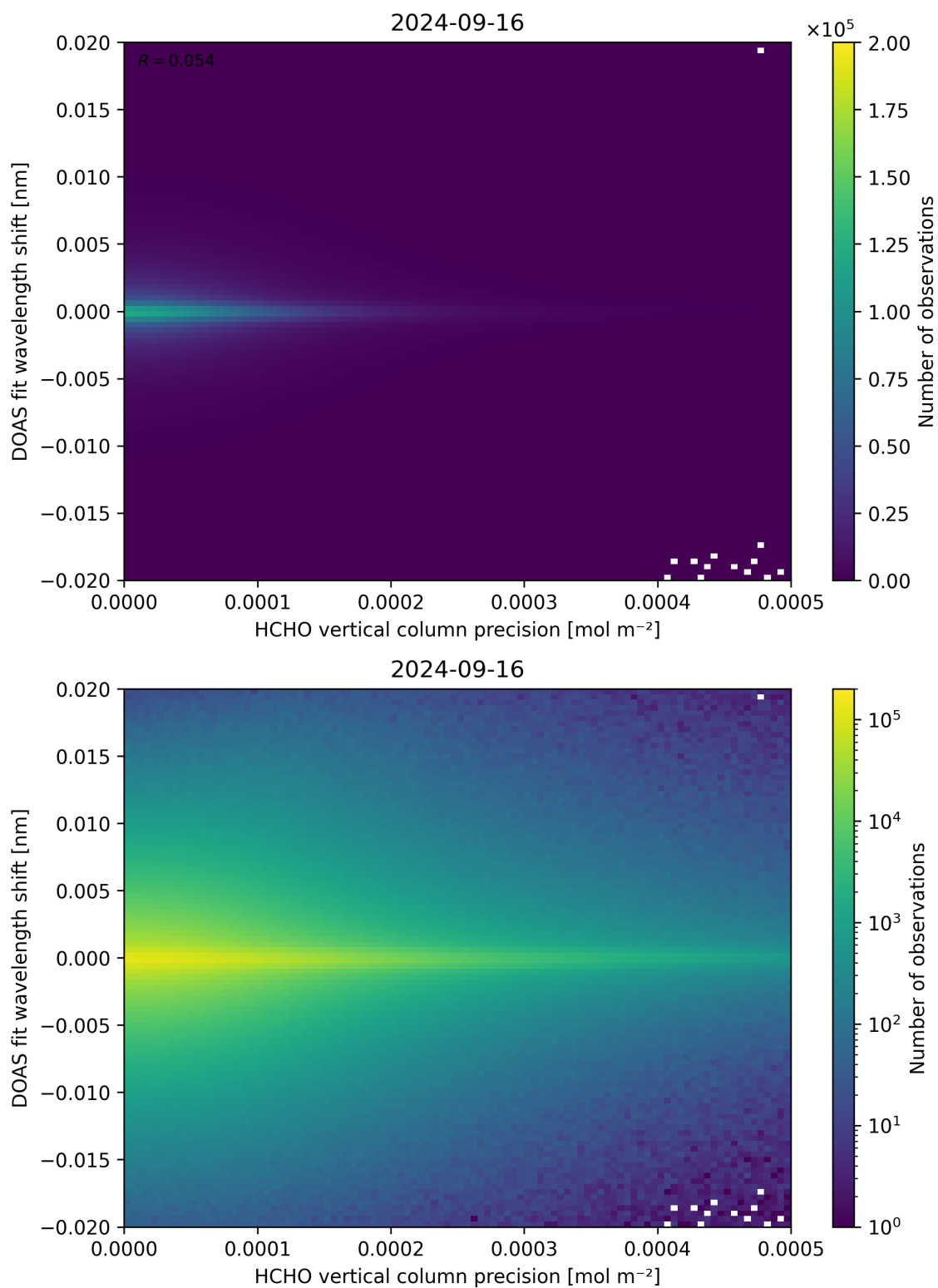
Figure 137: Scatter density plot of “HCHO vertical column precision” against “DOAS fit wavelength shift” for 2024-09-15 to 2024-09-17.
