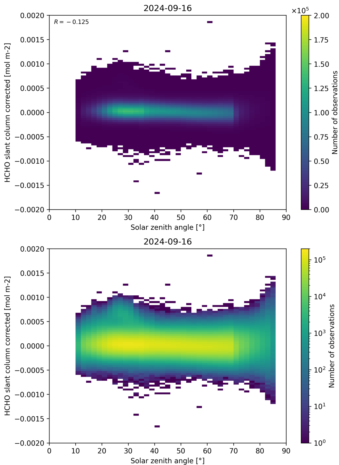
Figure 171: Scatter density plot of “Solar zenith angle” against “HCHO slant column corrected” for 2024-09-15 to 2024-09-17.
