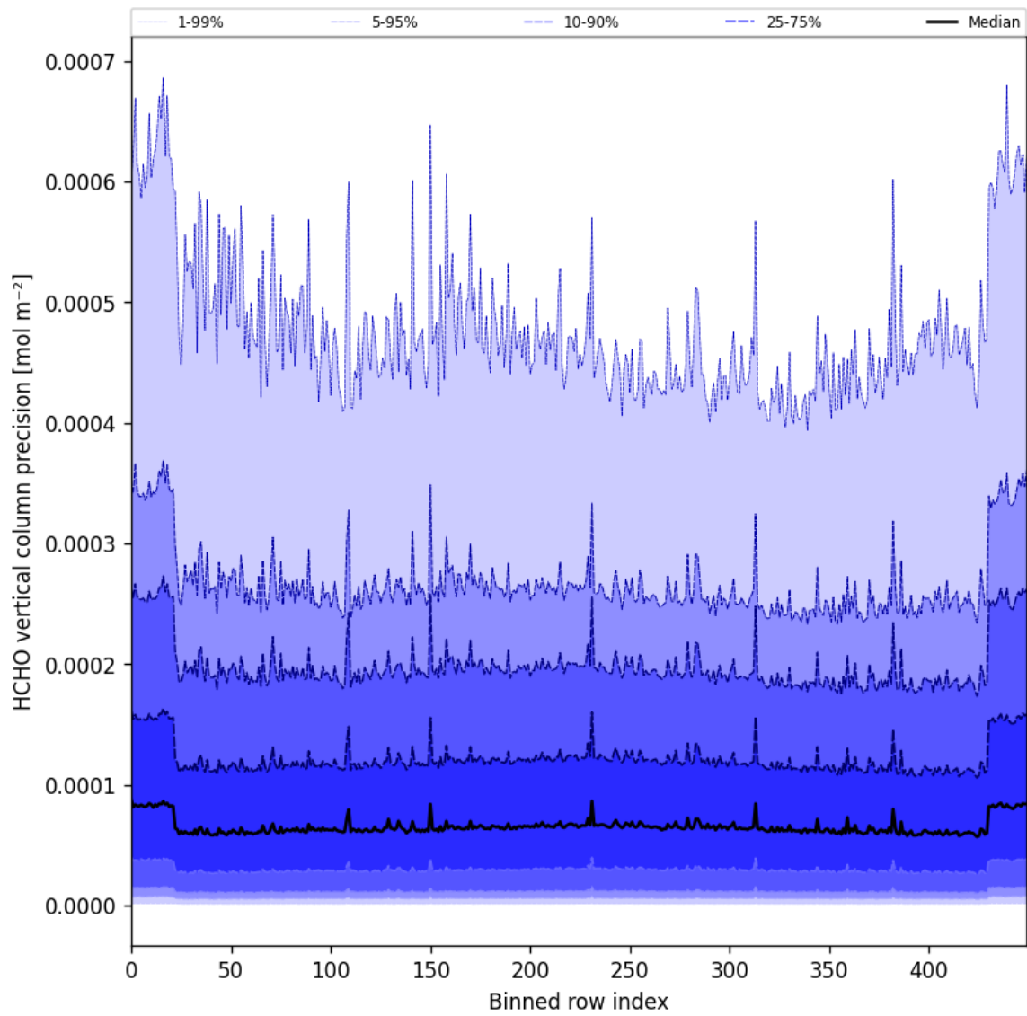
Figure 50: Along track statistics of “HCHO vertical column precision” for 2024-09-15 to 2024-09-17
