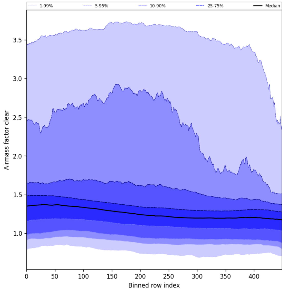
Figure 56: Along track statistics of “Airmass factor clear” for 2024-09-15 to 2024-09-17
