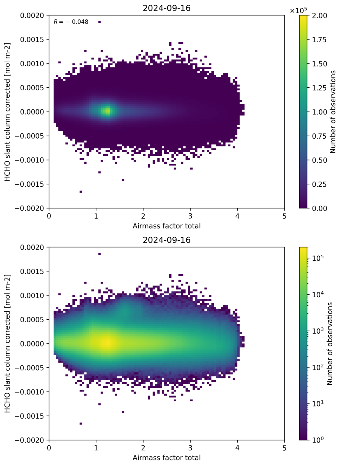
Figure 101: Scatter density plot of “Airmass factor total” against “HCHO slant column corrected” for 2024-09-15 to 2024-09-17.
