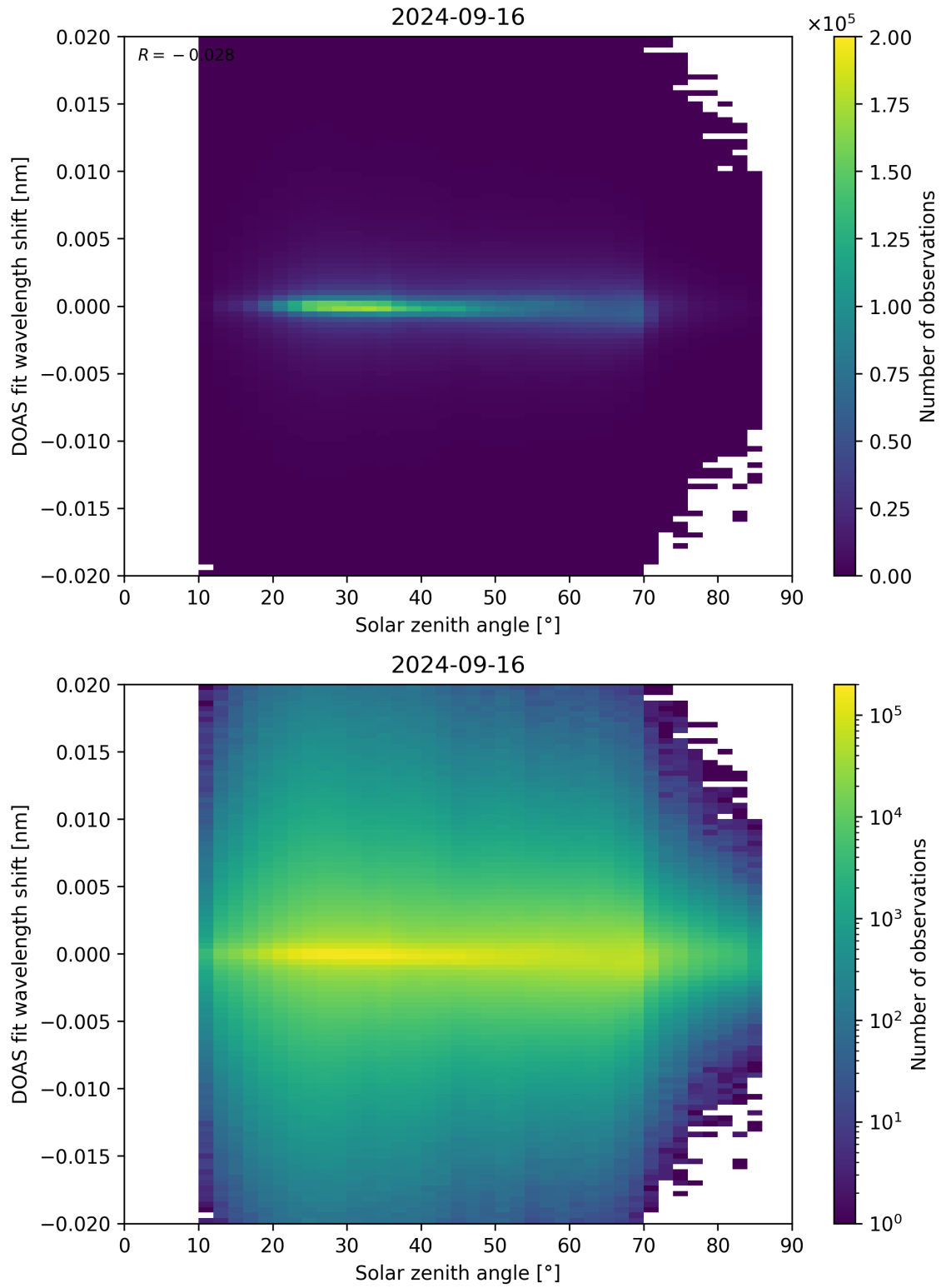
Figure 168: Scatter density plot of “Solar zenith angle” against “DOAS fit wavelength shift” for 2024-09-15 to 2024-09-17.
