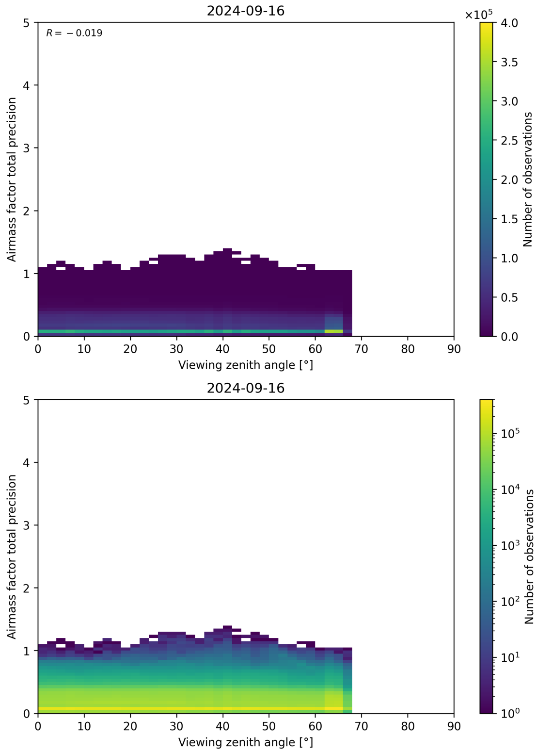
Figure 191: Scatter density plot of “Viewing zenith angle” against “Airmass factor total precision” for 2024-09-15 to 2024-09-17.
