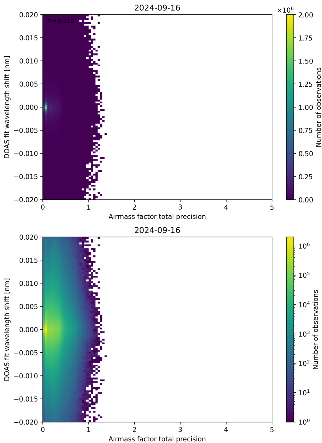
Figure 106: Scatter density plot of “Airmass factor total precision” against “DOAS fit wavelength shift” for 2024-09-15 to 2024-09-17.
