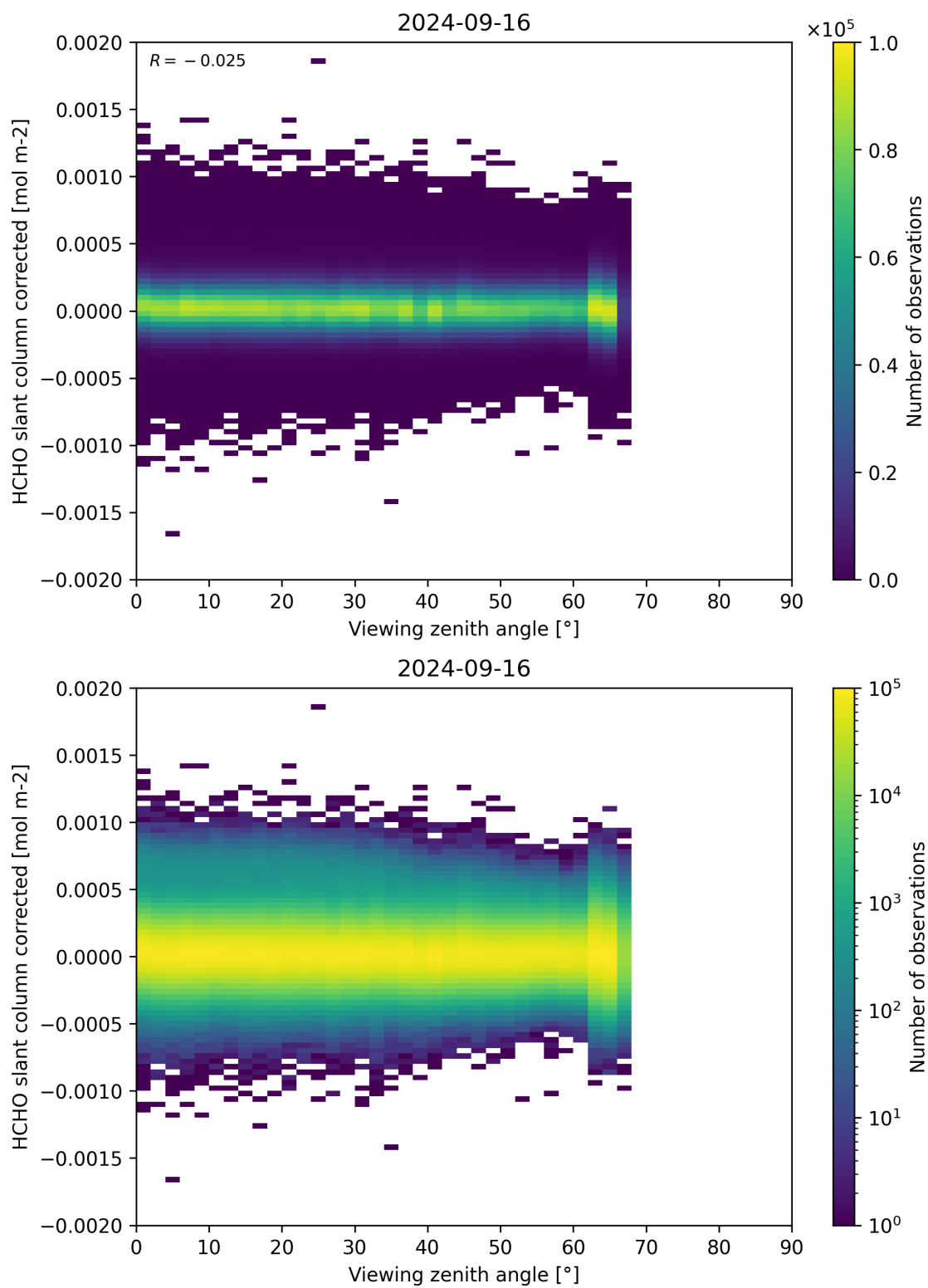
Figure 186: Scatter density plot of “Viewing zenith angle” against “HCHO slant column corrected” for 2024-09-15 to 2024-09-17.
