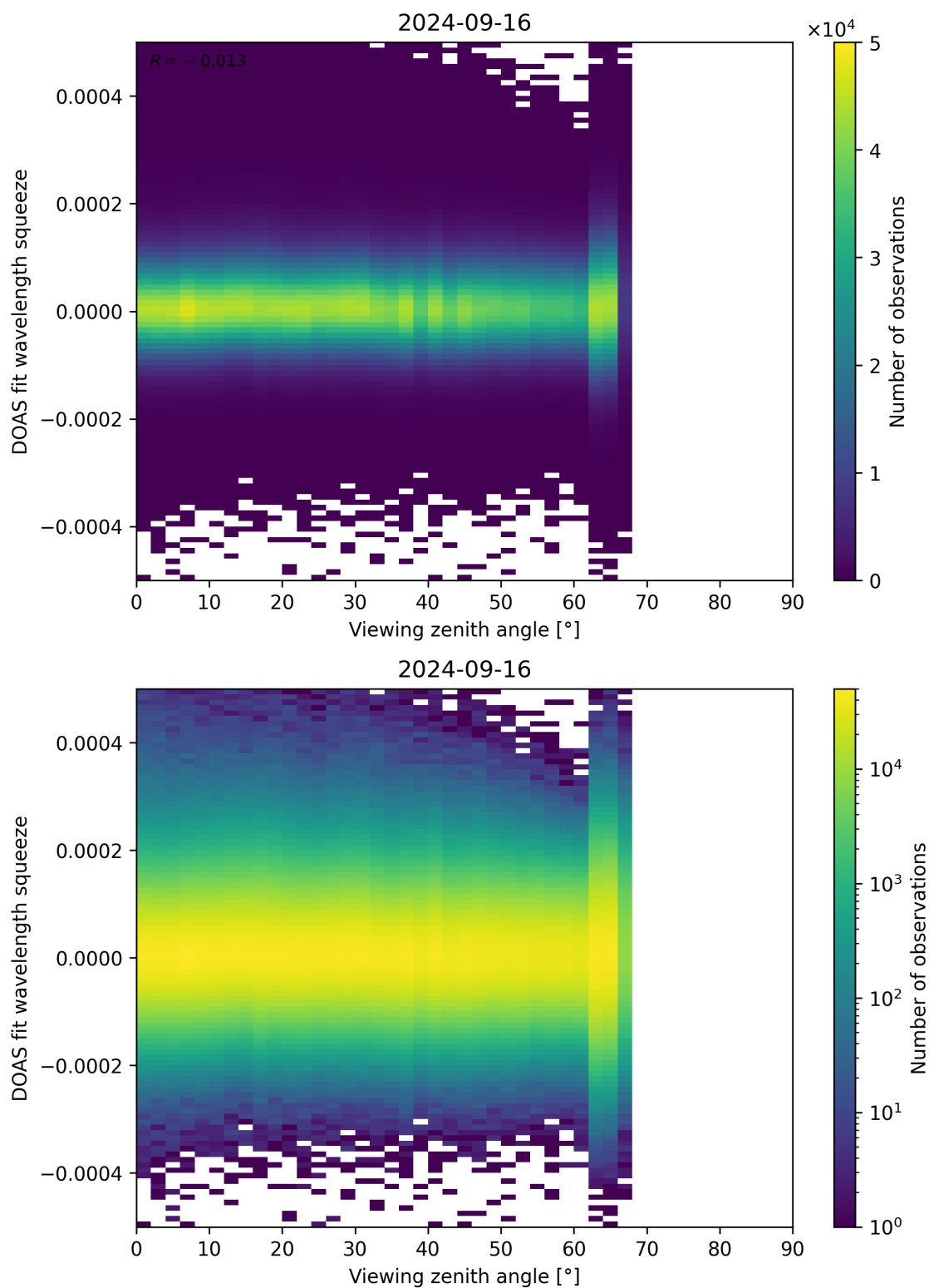
Figure 184: Scatter density plot of “Viewing zenith angle” against “DOAS fit wavelength squeeze” for 2024-09-15 to 2024-09-17.
