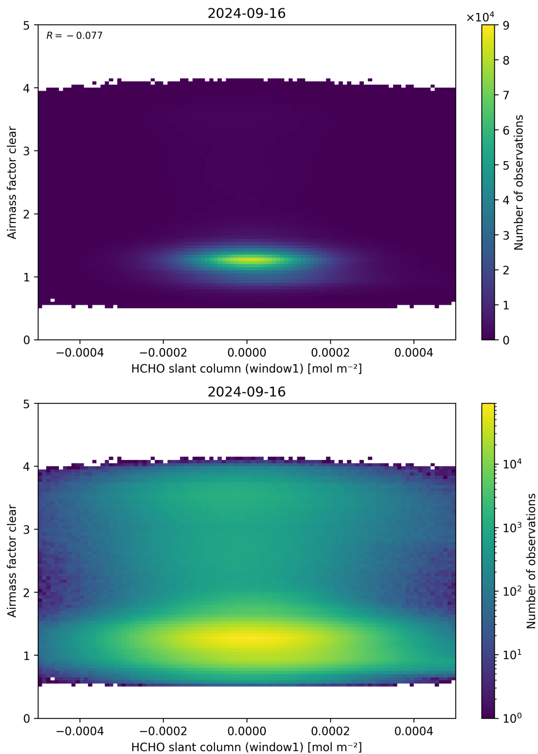
Figure 81: Scatter density plot of “HCHO slant column (window1)” against “Airmass factor clear” for 2024-09-15 to 2024-09-17.
