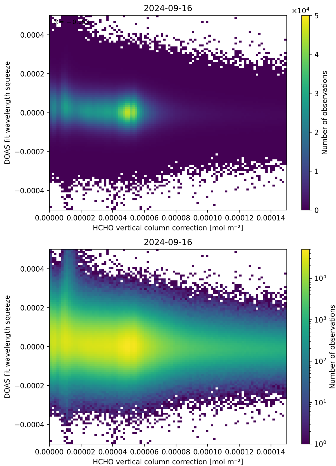
Figure 114: Scatter density plot of “HCHO vertical column correction” against “DOAS fit wavelength squeeze” for 2024-09-15 to 2024-09-17.
