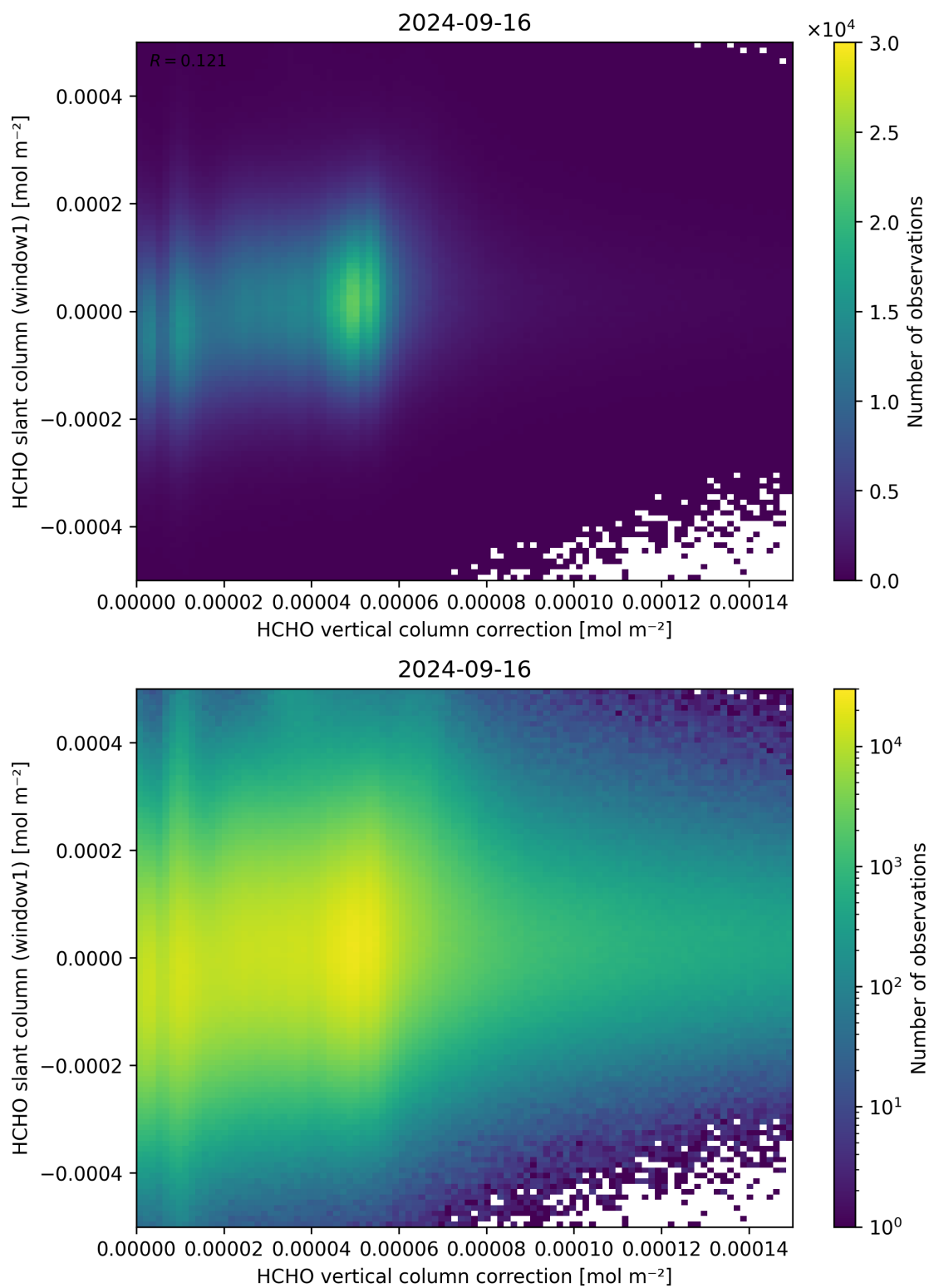
Figure 118: Scatter density plot of “HCHO vertical column correction” against “HCHO slant column (window1)” for 2024-09-15 to 2024-09-17.
