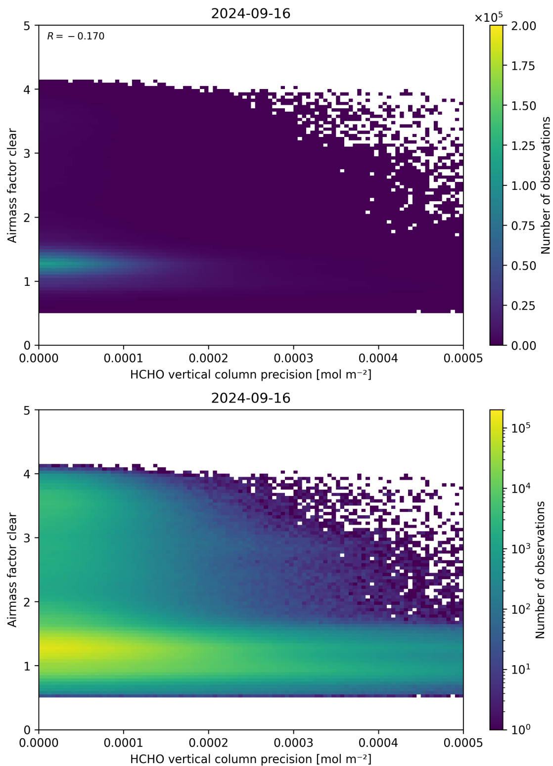
Figure 139: Scatter density plot of “HCHO vertical column precision” against “Airmass factor clear” for 2024-09-15 to 2024-09-17.
