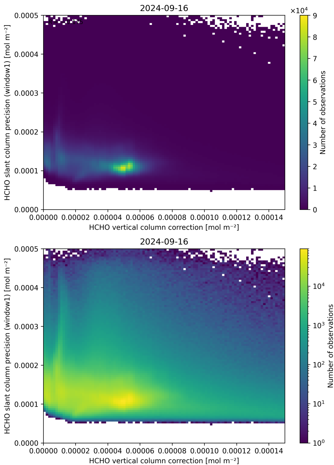
Figure 119: Scatter density plot of “HCHO vertical column correction” against “HCHO slant column precision (window1)” for 2024-09-15 to 2024-09-17.
