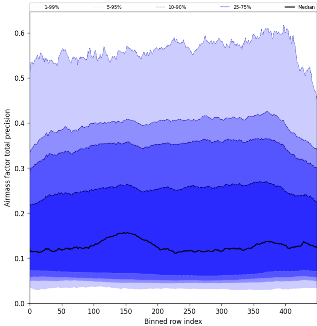
Figure 55: Along track statistics of “Airmass factor total precision” for 2024-09-15 to 2024-09-17
