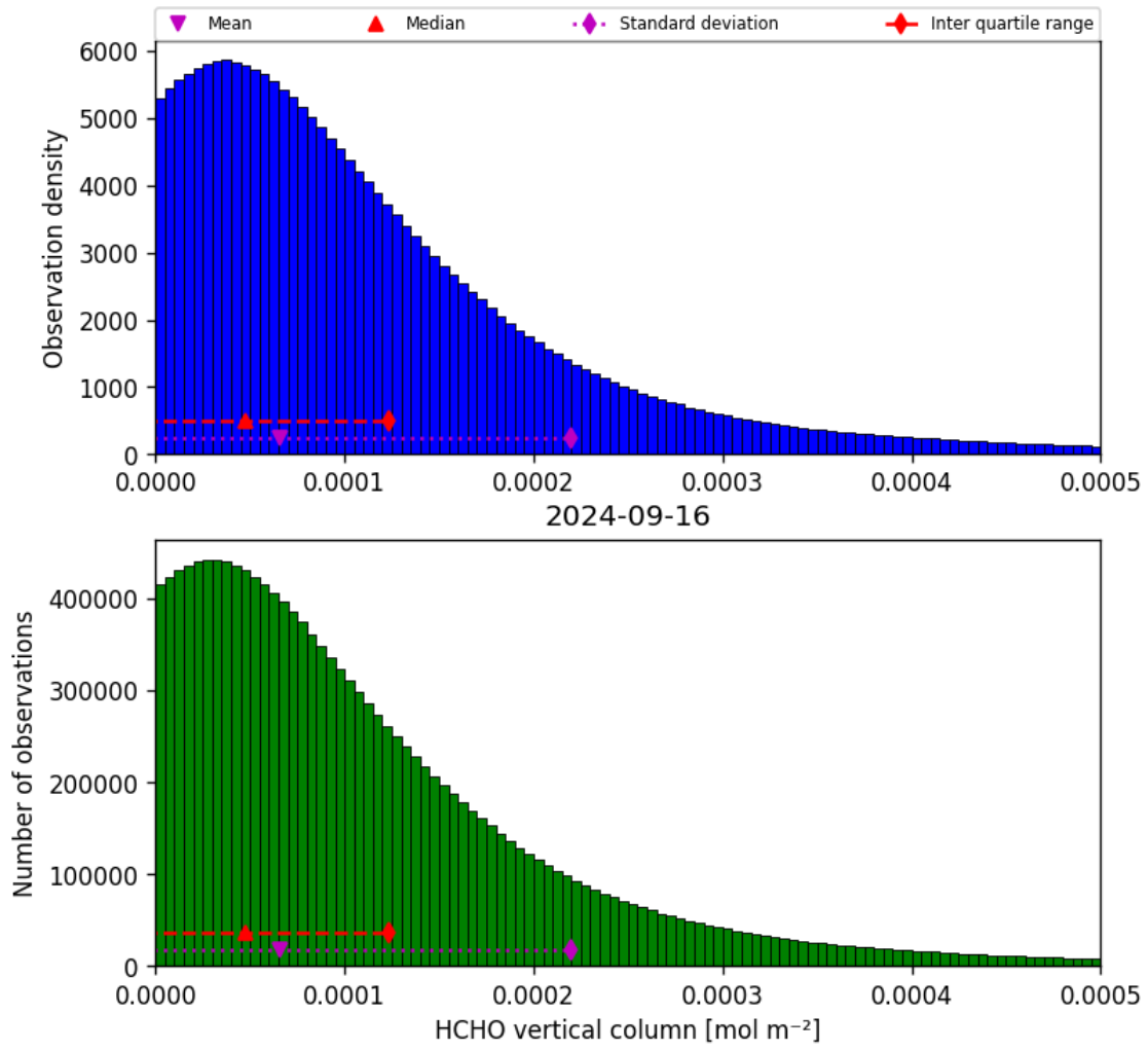
Figure 35: Histogram of “HCHO vertical column” for 2024-09-15 to 2024-09-17
