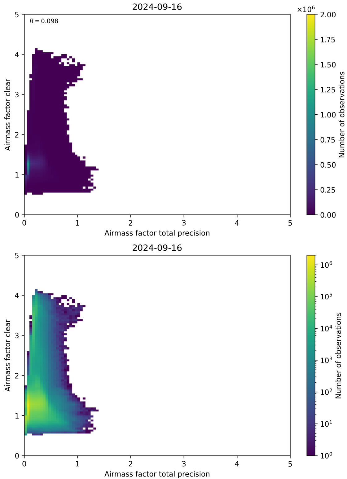
Figure 108: Scatter density plot of “Airmass factor total precision” against “Airmass factor clear” for 2024-09-15 to 2024-09-17.
