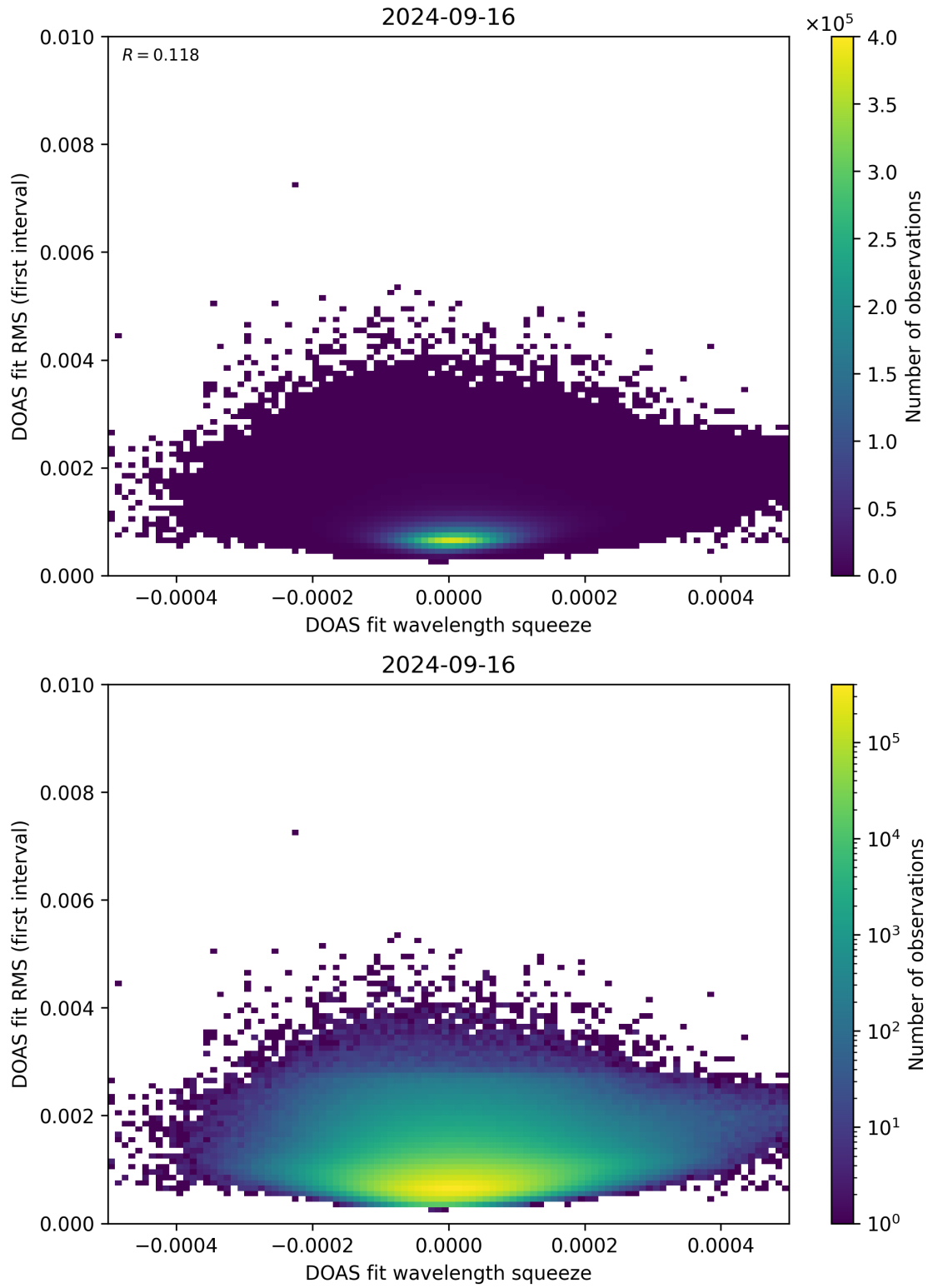
Figure 68: Scatter density plot of “DOAS fit wavelength squeeze” against “DOAS fit RMS (first interval)” for 2024-09-15 to 2024-09-17.
