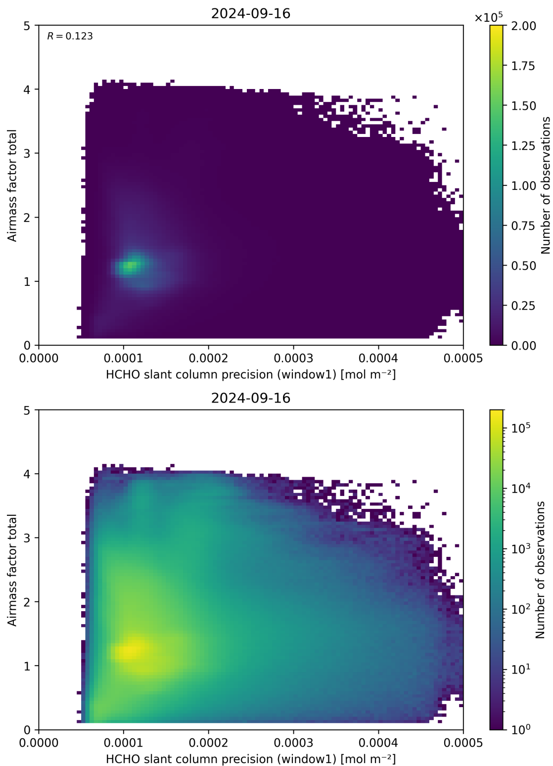
Figure 94: Scatter density plot of “HCHO slant column precision (window1)” against “Airmass factor total” for 2024-09-15 to 2024-09-17.
