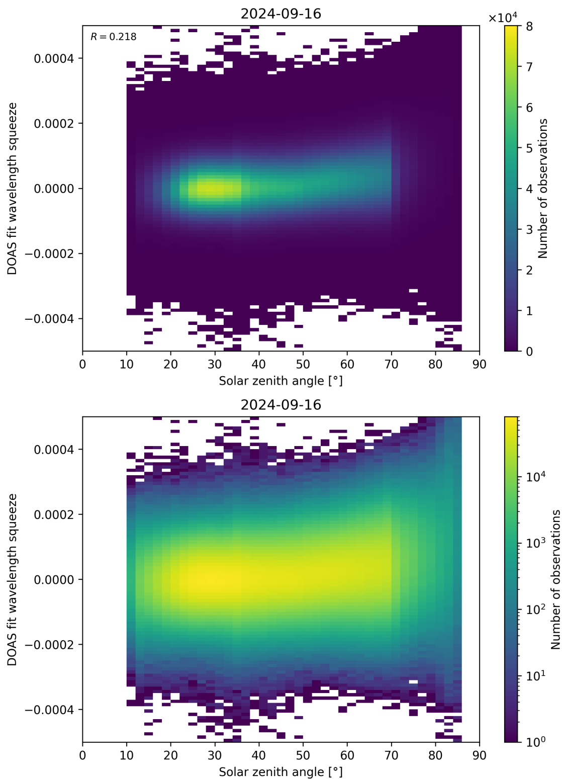
Figure 169: Scatter density plot of “Solar zenith angle” against “DOAS fit wavelength squeeze” for 2024-09-15 to 2024-09-17.
