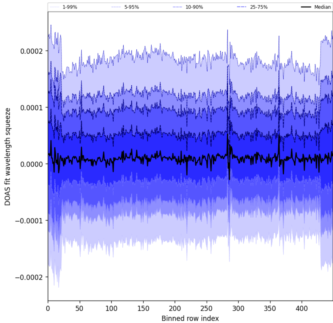
Figure 59: Along track statistics of “DOAS fit wavelength squeeze” for 2024-09-15 to 2024-09-17
