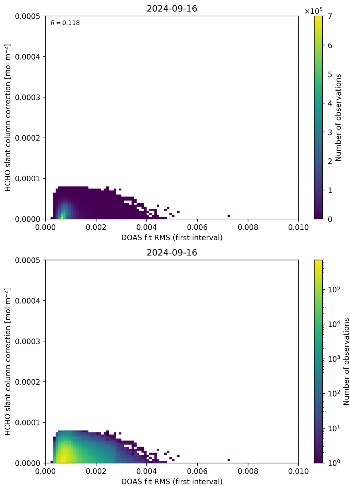
Figure 63: Scatter density plot of “DOAS fit RMS (first interval)” against “HCHO slant column correction” for 2024-09-15 to 2024-09-17.
