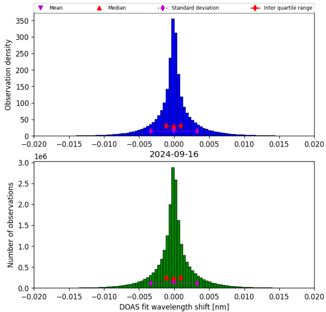
Figure 44: Histogram of “DOAS fit wavelength shift” for 2024-09-15 to 2024-09-17
