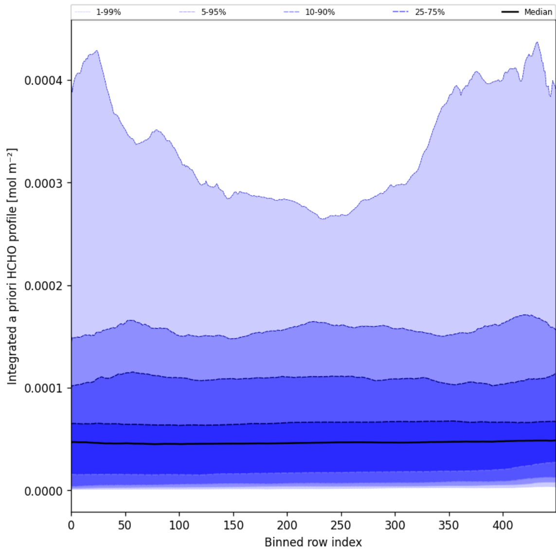
Figure 57: Along track statistics of “Integrated a priori HCHO profile” for 2024-09-15 to 2024-09-17
