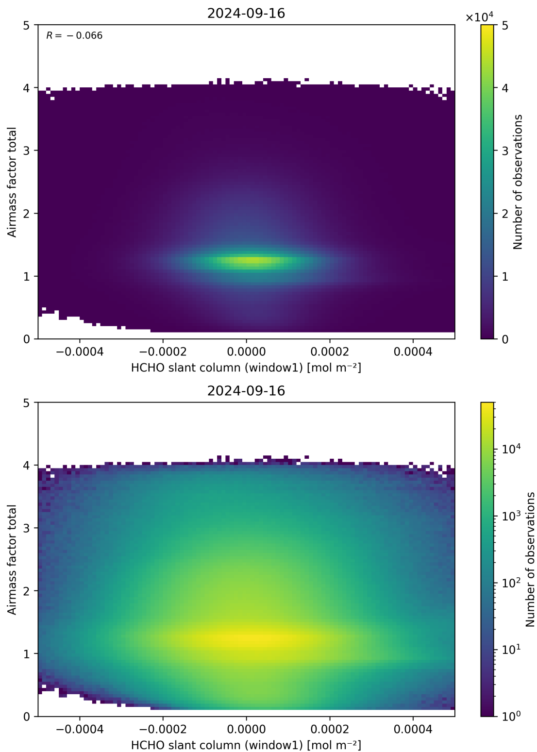
Figure 85: Scatter density plot of “HCHO slant column (window1)” against “Airmass factor total” for 2024-09-15 to 2024-09-17.
