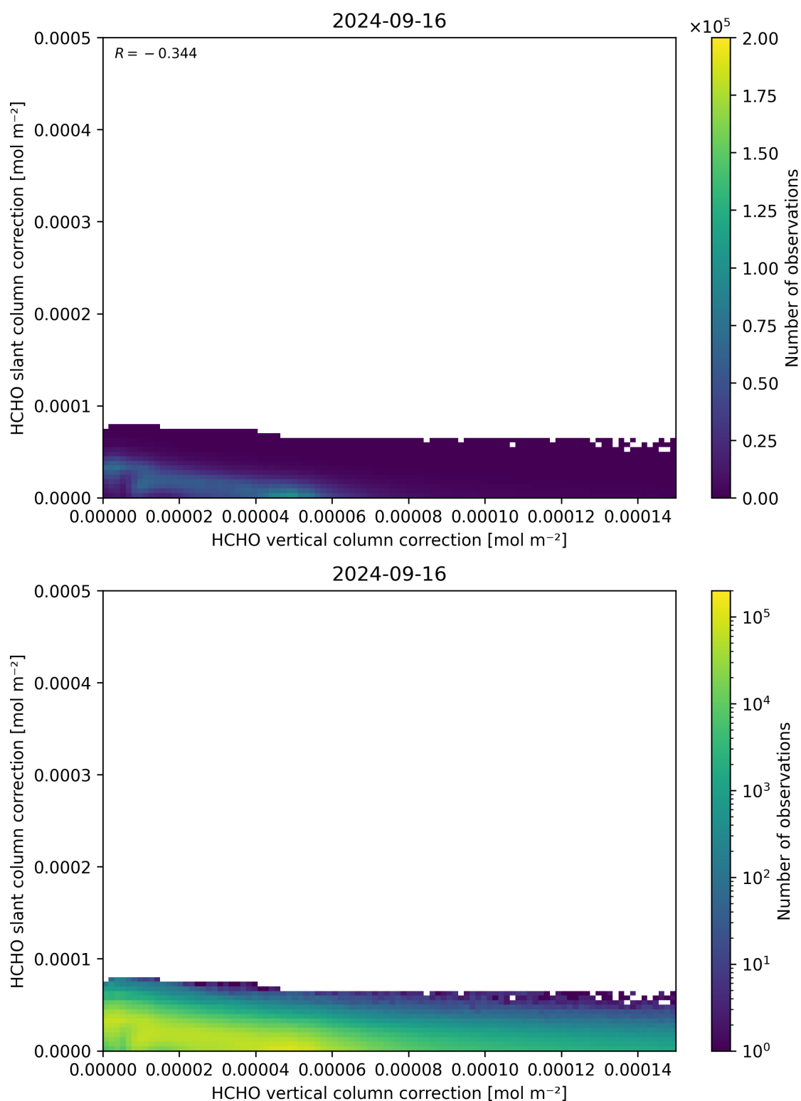
Figure 117: Scatter density plot of “HCHO vertical column correction” against “HCHO slant column correction” for 2024-09-15 to 2024-09-17.
