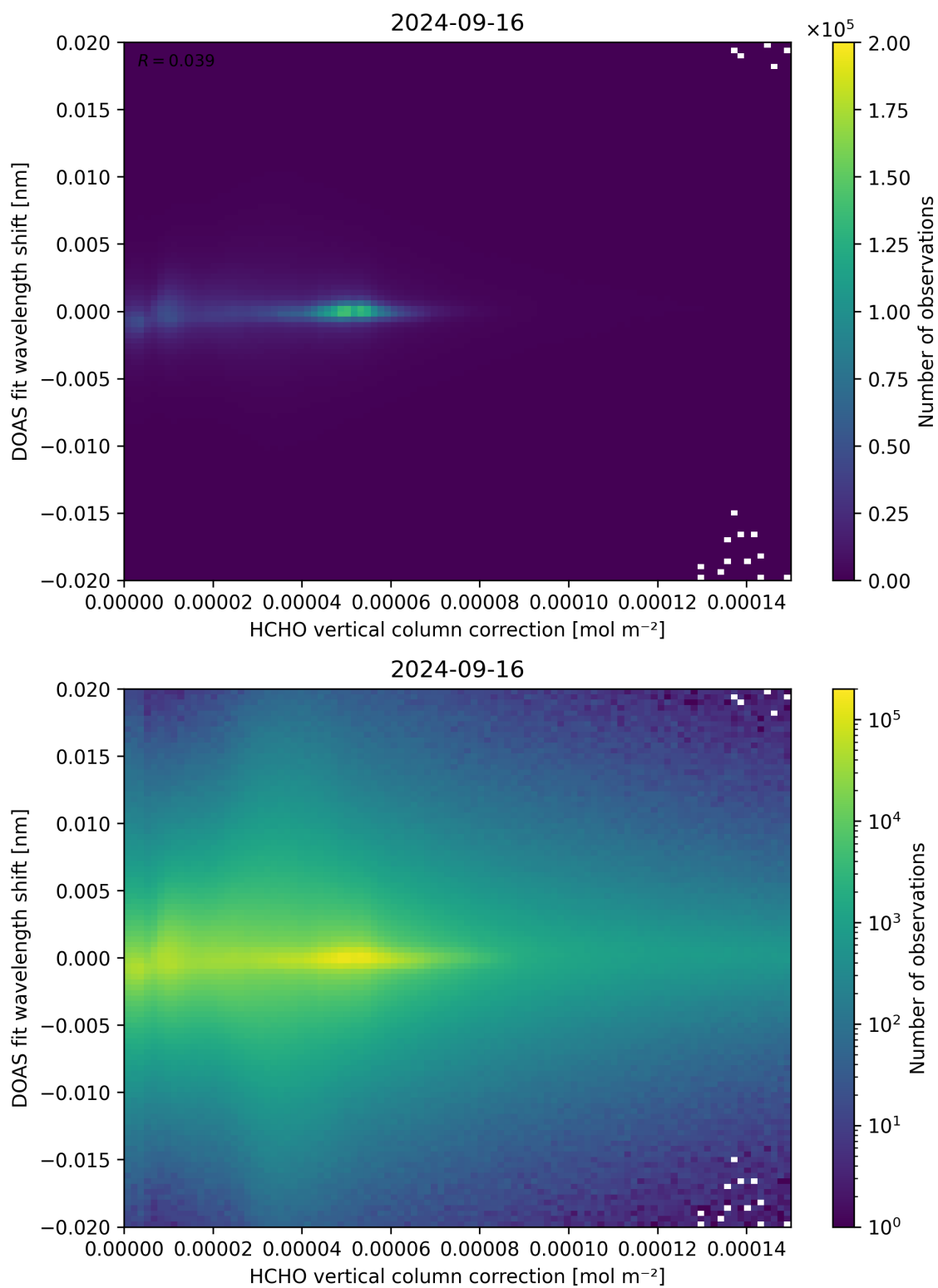
Figure 113: Scatter density plot of “HCHO vertical column correction” against “DOAS fit wavelength shift” for 2024-09-15 to 2024-09-17.
