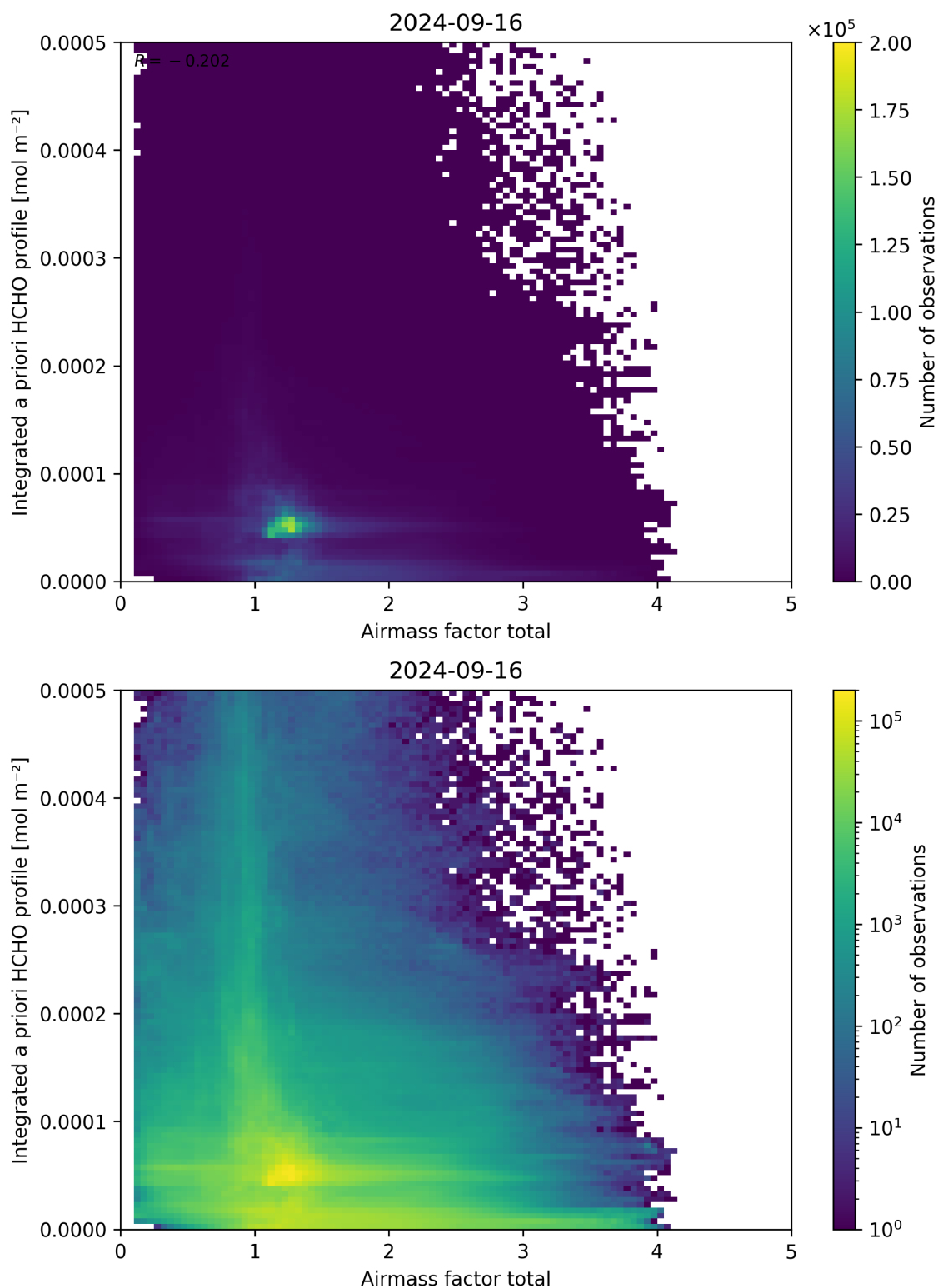
Figure 104: Scatter density plot of “Airmass factor total” against “Integrated a priori HCHO profile” for 2024-09-15 to 2024-09-17.
