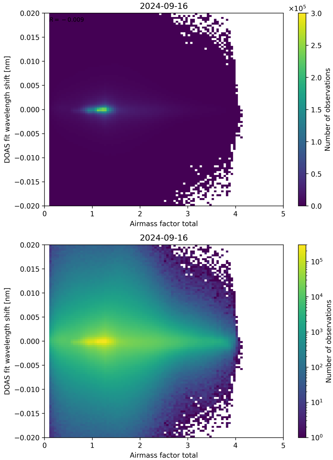
Figure 98: Scatter density plot of “Airmass factor total” against “DOAS fit wavelength shift” for 2024-09-15 to 2024-09-17.
