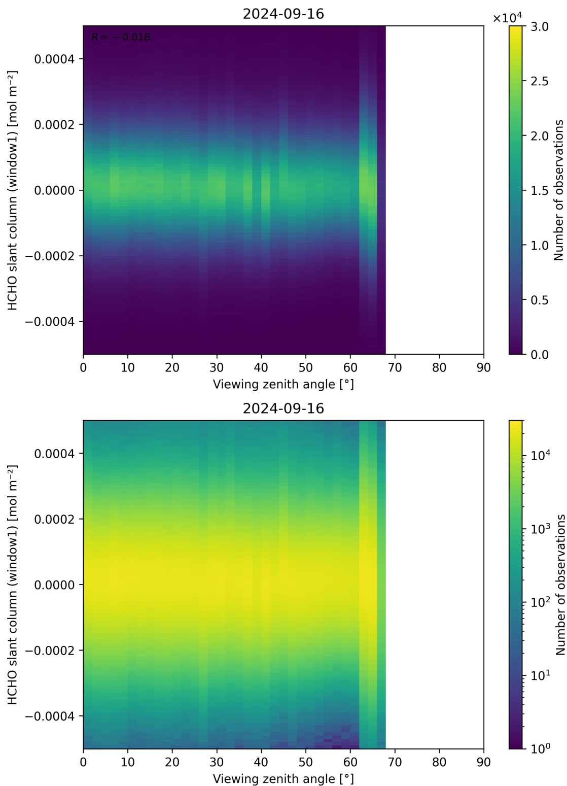
Figure 188: Scatter density plot of “Viewing zenith angle” against “HCHO slant column (window1)” for 2024-09-15 to 2024-09-17.
