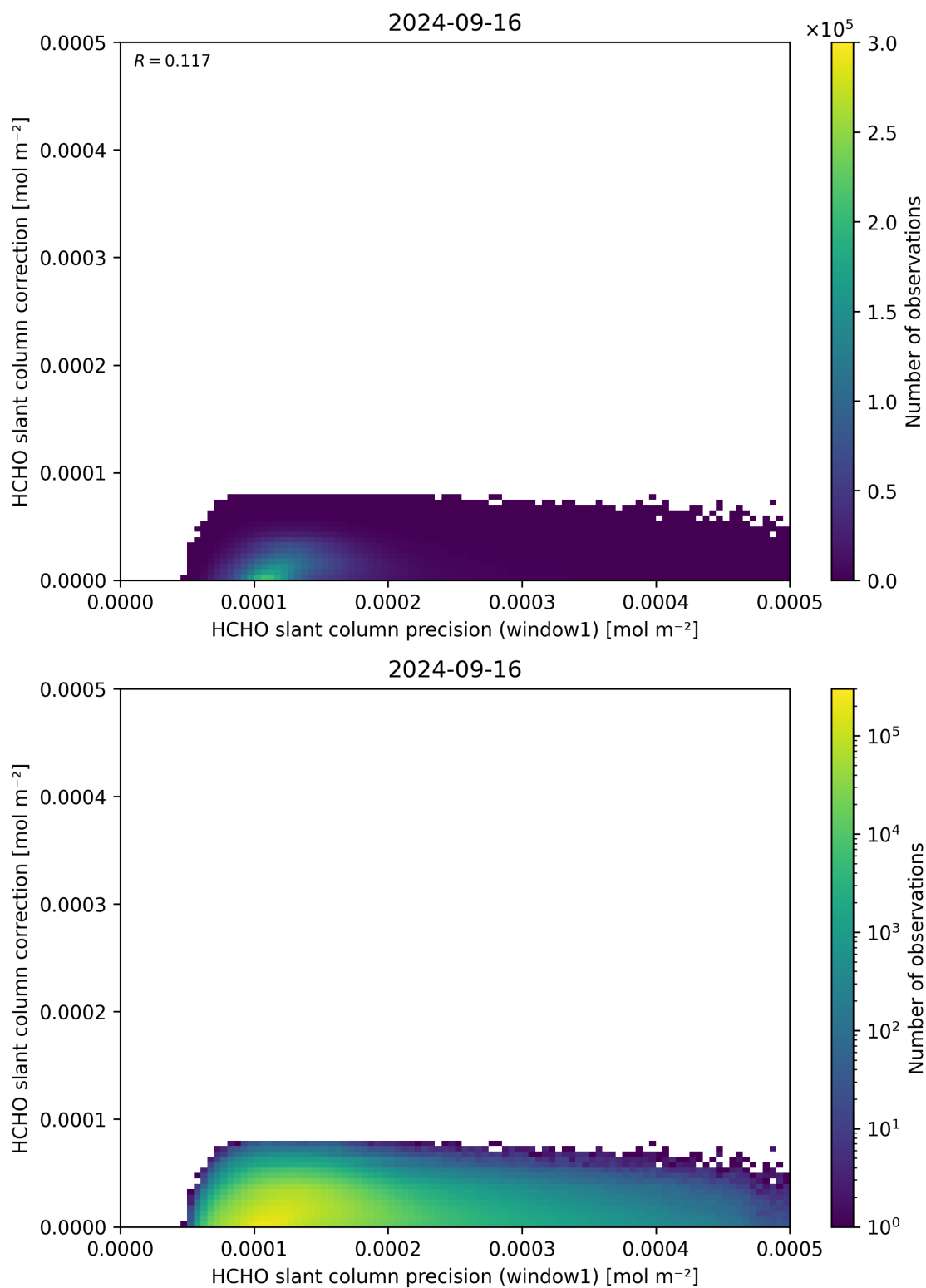
Figure 93: Scatter density plot of “HCHO slant column precision (window1)” against “HCHO slant column correction” for 2024-09-15 to 2024-09-17.
