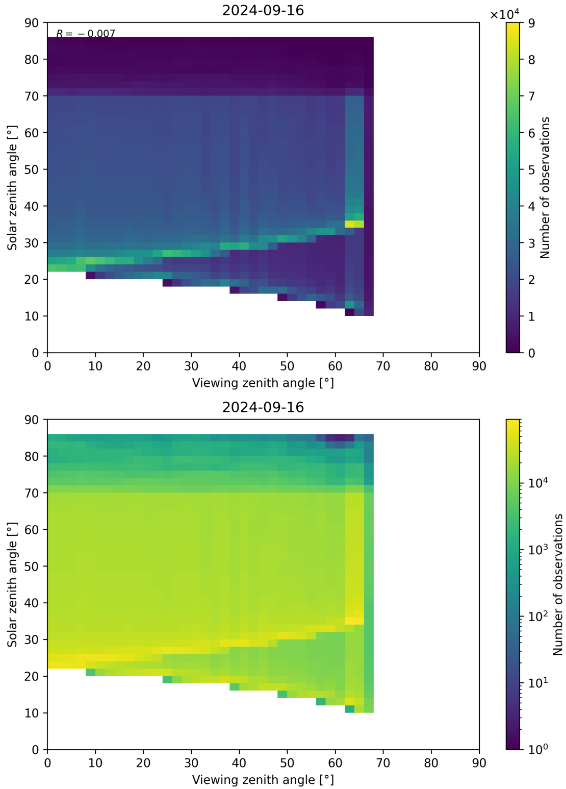
Figure 197: Scatter density plot of “Viewing zenith angle” against “Solar zenith angle” for 2024-09-15 to 2024-09-17.
