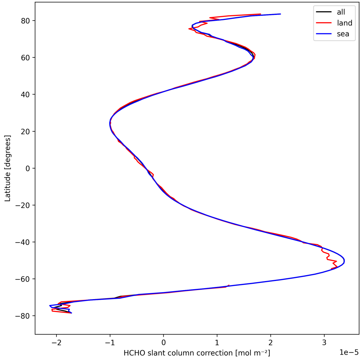
Figure 33: Zonal average of “HCHO slant column correction” for 2024-09-15 to 2024-09-17.
