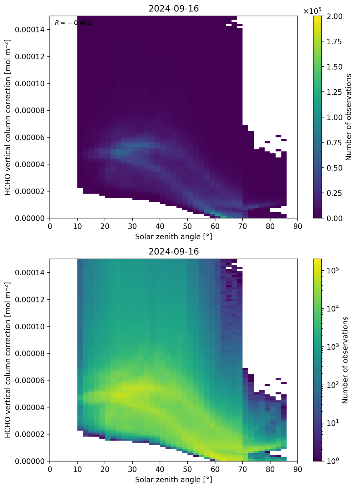
Figure 178: Scatter density plot of “Solar zenith angle” against “HCHO vertical column correction” for 2024-09-15 to 2024-09-17.
