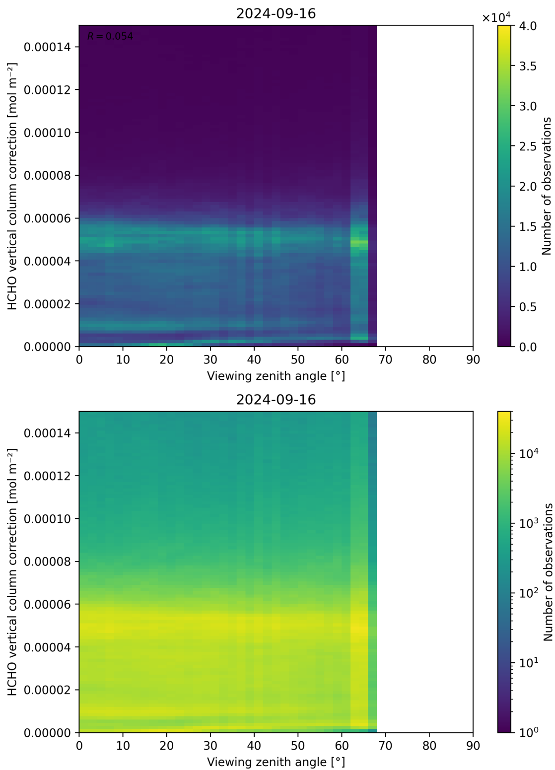
Figure 193: Scatter density plot of “Viewing zenith angle” against “HCHO vertical column correction” for 2024-09-15 to 2024-09-17.
