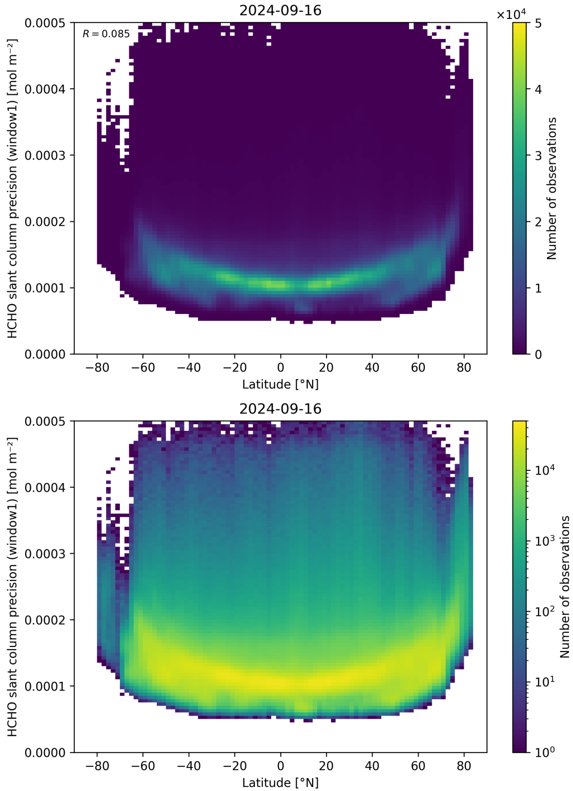
Figure 160: Scatter density plot of “Latitude” against “HCHO slant column precision (window1)” for 2024-09-15 to 2024-09-17.
