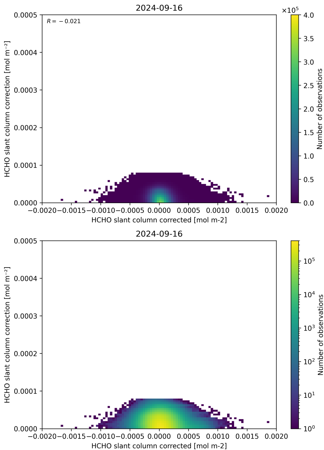
Figure 77: Scatter density plot of “HCHO slant column corrected” against “HCHO slant column correction” for 2024-09-15 to 2024-09-17.
