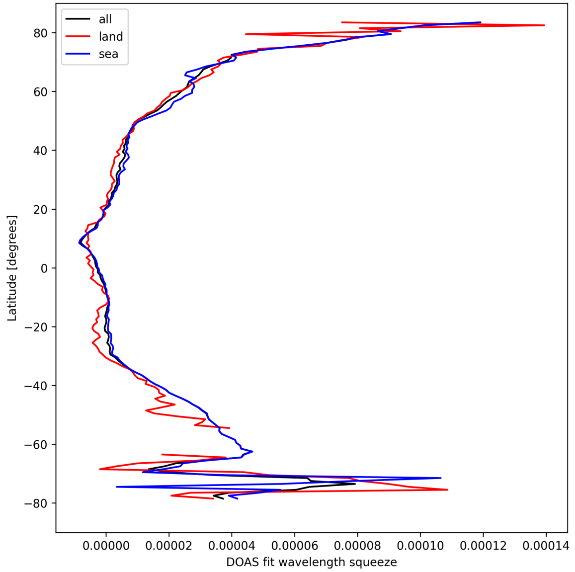
Figure 31: Zonal average of “DOAS fit wavelength squeeze” for 2024-09-15 to 2024-09-17.
