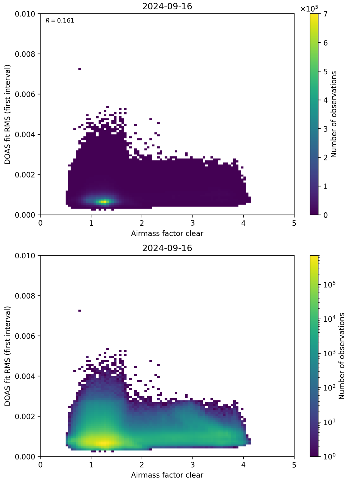
Figure 71: Scatter density plot of “Airmass factor clear” against “DOAS fit RMS (first interval)” for 2024-09-15 to 2024-09-17.
