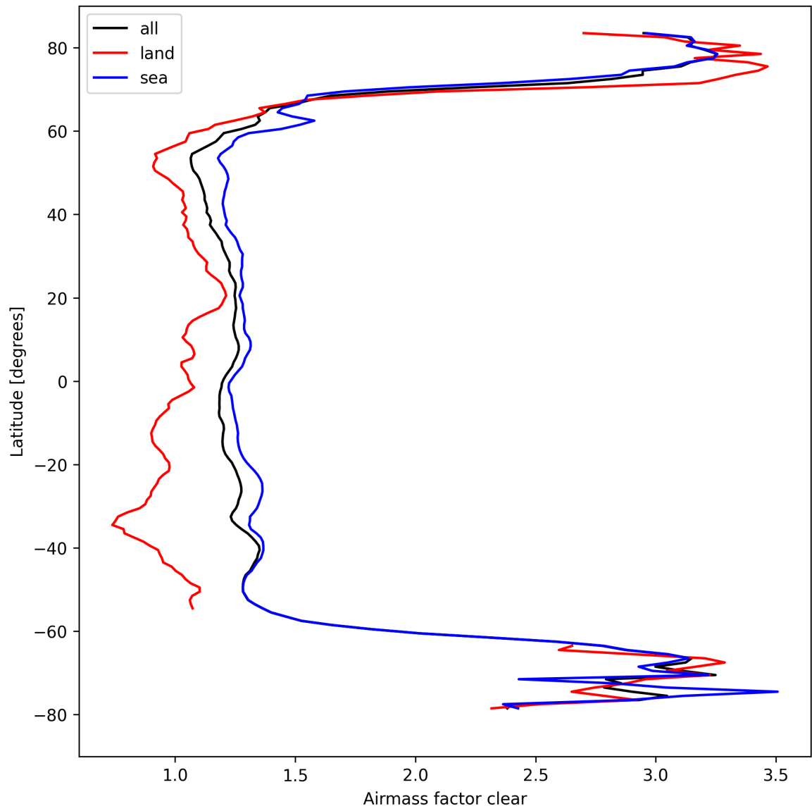
Figure 28: Zonal average of “Airmass factor clear” for 2024-09-15 to 2024-09-17.
