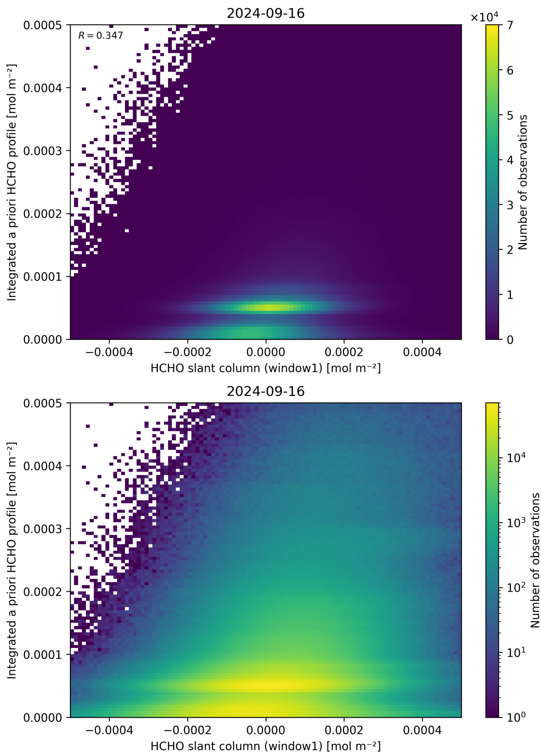
Figure 87: Scatter density plot of “HCHO slant column (window1)” against “Integrated a priori HCHO profile” for 2024-09-15 to 2024-09-17.
