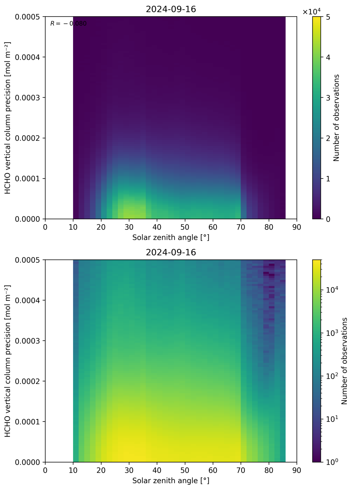
Figure 179: Scatter density plot of “Solar zenith angle” against “HCHO vertical column precision” for 2024-09-15 to 2024-09-17.
