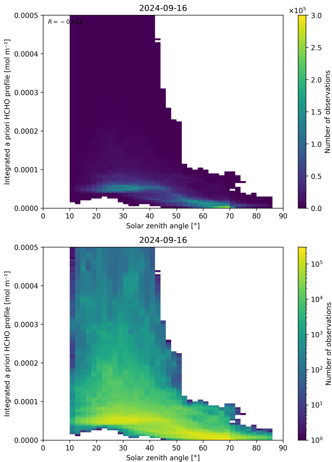
Figure 180: Scatter density plot of “Solar zenith angle” against “Integrated a priori HCHO profile” for 2024-09-15 to 2024-09-17.
