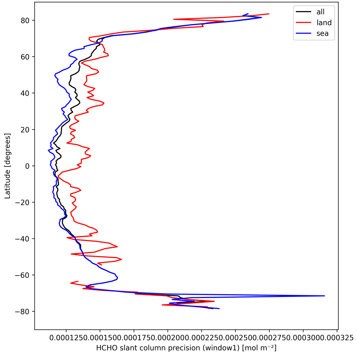
Figure 25: Zonal average of “HCHO slant column precision (window1)” for 2024-09-15 to 2024-09-17.
