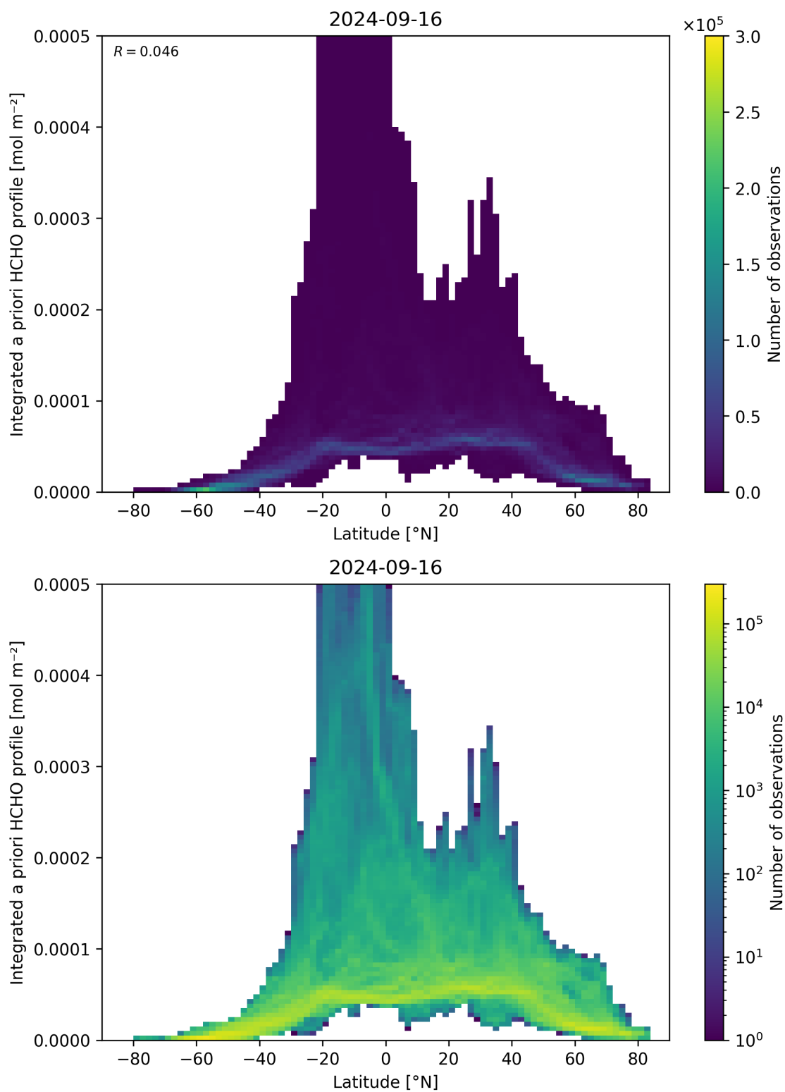
Figure 166: Scatter density plot of “Latitude” against “Integrated a priori HCHO profile” for 2024-09-15 to 2024-09-17.
