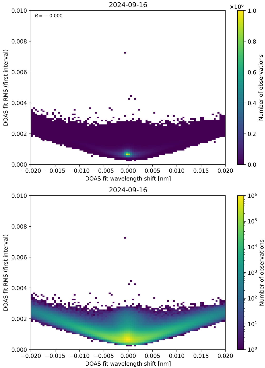
Figure 64: Scatter density plot of “DOAS fit wavelength shift” against “DOAS fit RMS (first interval)” for 2024-09-15 to 2024-09-17.
