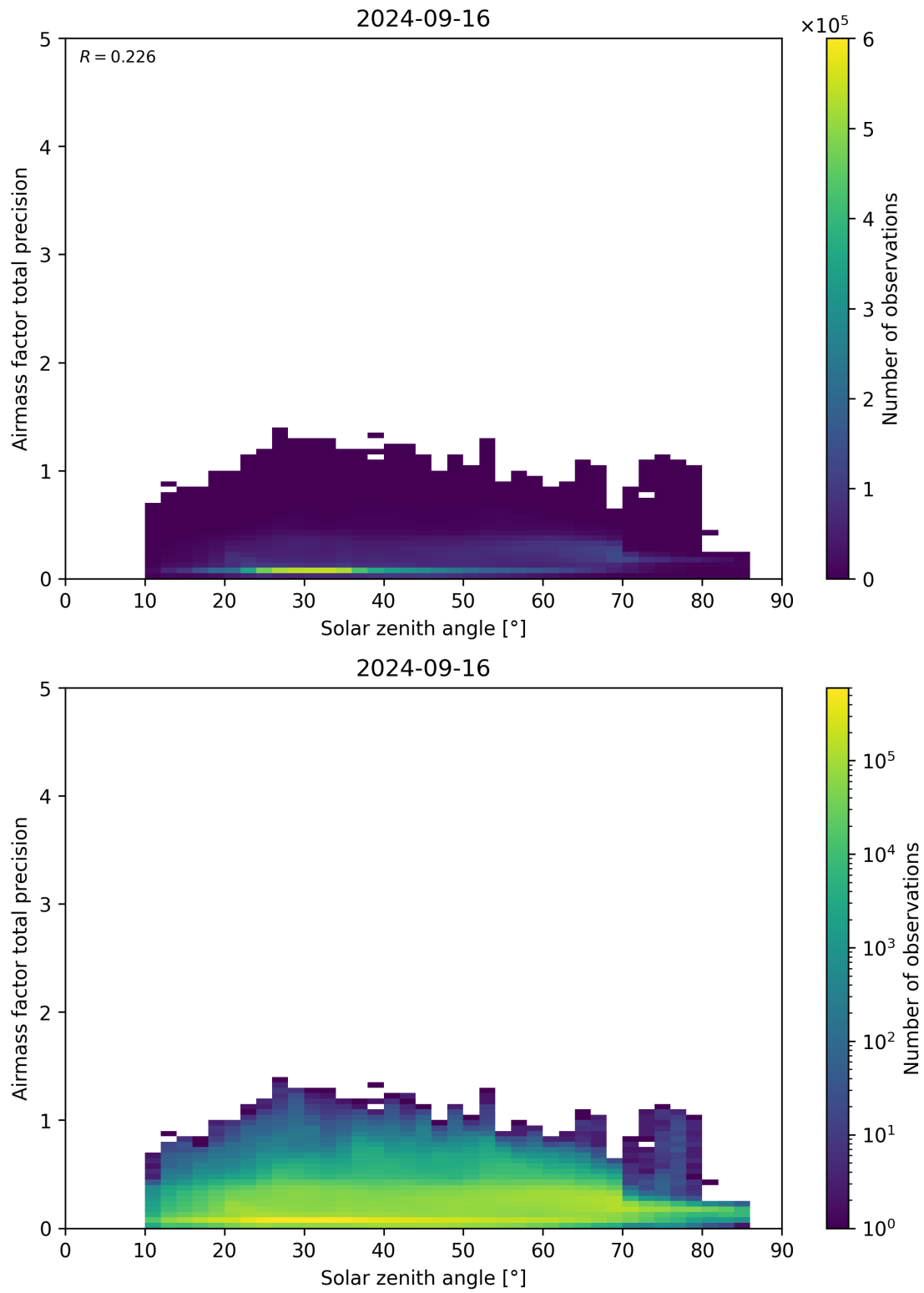
Figure 176: Scatter density plot of “Solar zenith angle” against “Airmass factor total precision” for 2024-09-15 to 2024-09-17.
