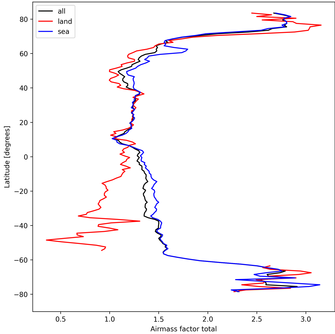
Figure 26: Zonal average of “Airmass factor total” for 2024-09-15 to 2024-09-17.
