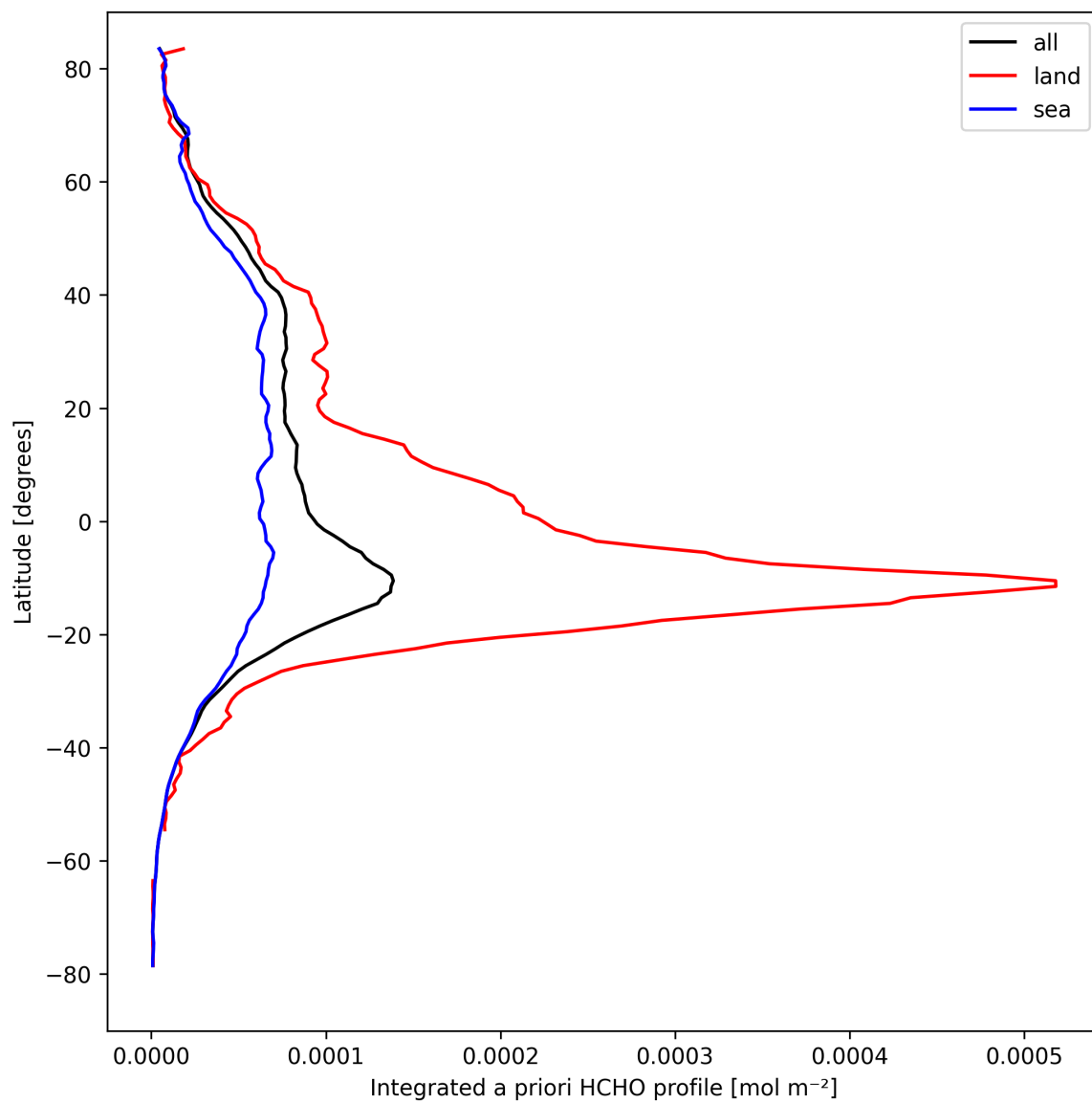
Figure 29: Zonal average of “Integrated a priori HCHO profile” for 2024-09-15 to 2024-09-17.
