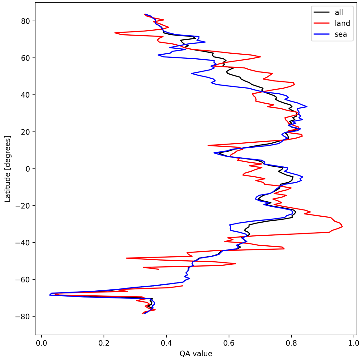
Figure 20: Zonal average of “QA value” for 2024-09-15 to 2024-09-17.
