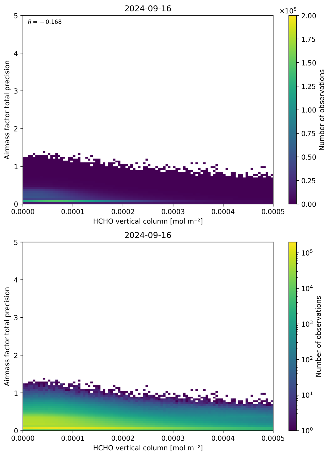
Figure 132: Scatter density plot of “HCHO vertical column” against “Airmass factor total precision” for 2024-09-15 to 2024-09-17.
