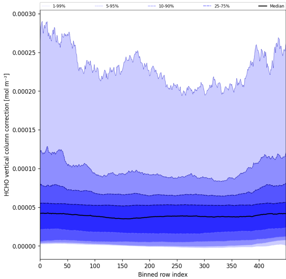
Figure 51: Along track statistics of "HCHO vertical column correction" for 2024-09-15 to 2024-09-17
