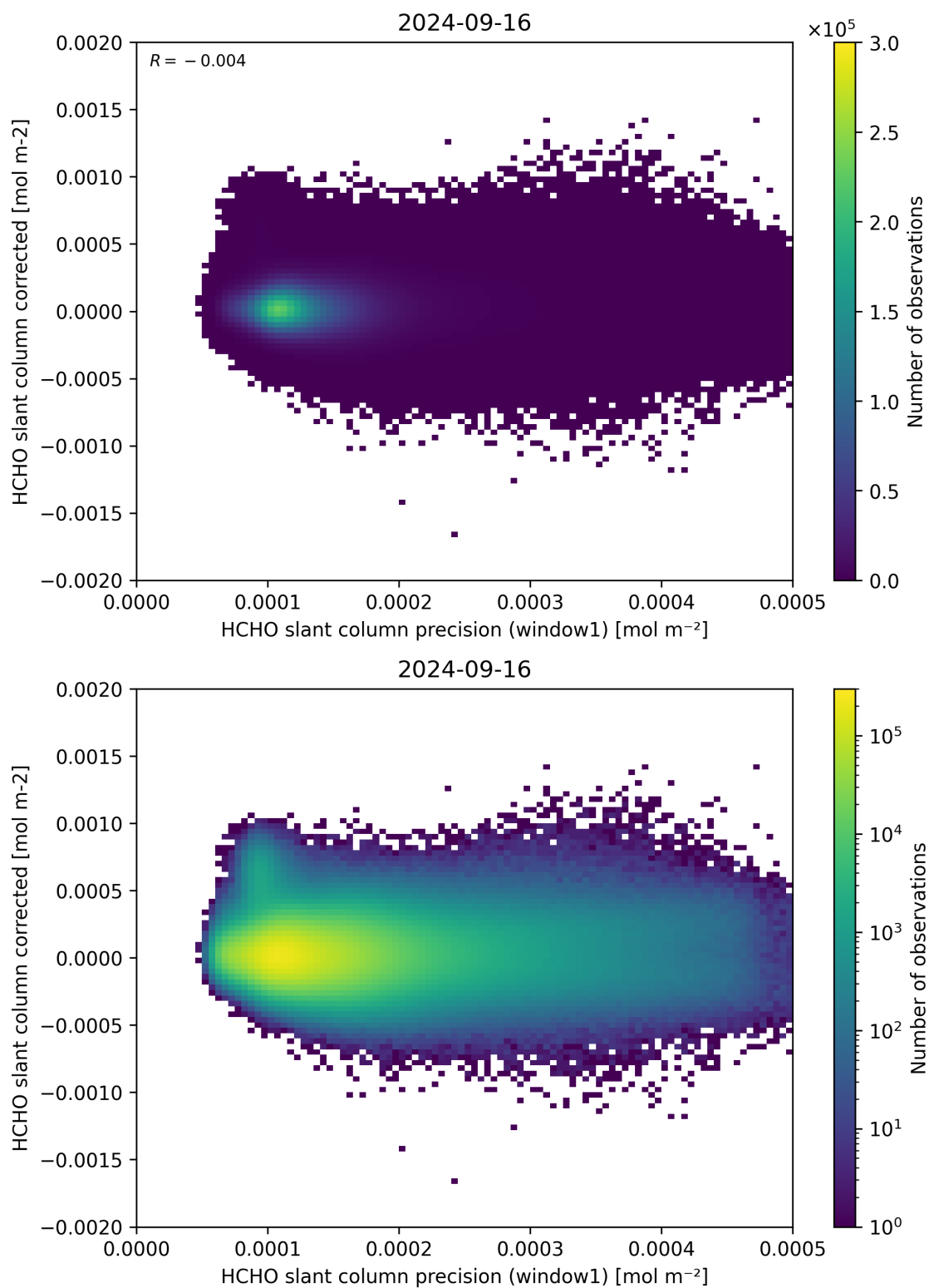
Figure 92: Scatter density plot of “HCHO slant column precision (window1)” against “HCHO slant column corrected” for 2024-09-15 to 2024-09-17.
