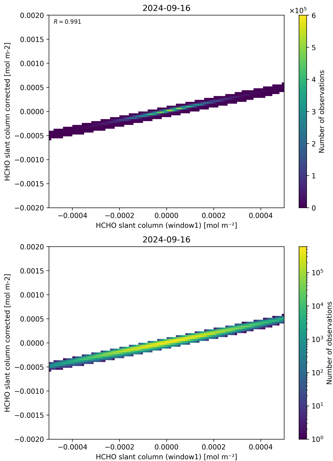
Figure 82: Scatter density plot of “HCHO slant column (window1)” against “HCHO slant column corrected” for 2024-09-15 to 2024-09-17.
