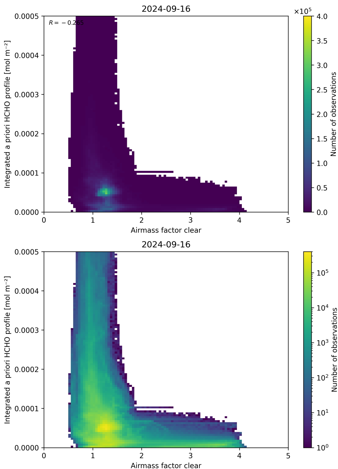
Figure 76: Scatter density plot of “Airmass factor clear” against “Integrated a priori HCHO profile” for 2024-09-15 to 2024-09-17.
