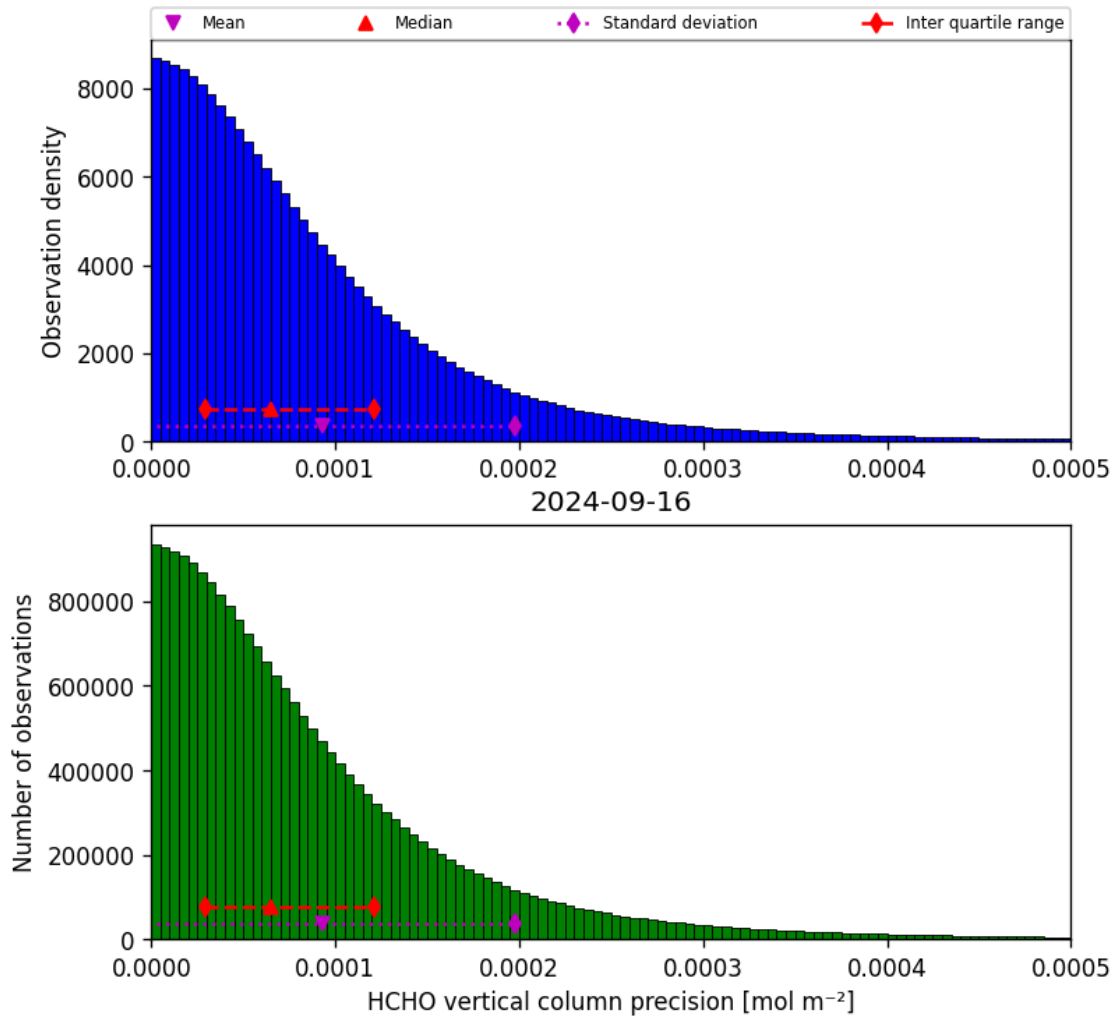
Figure 36: Histogram of “HCHO vertical column precision” for 2024-09-15 to 2024-09-17
