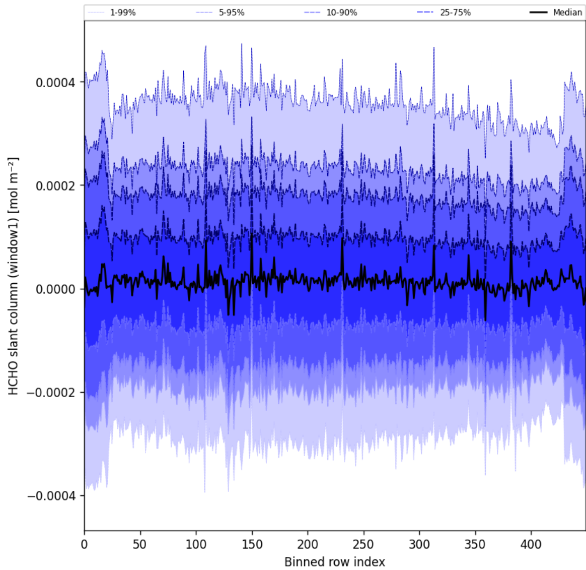
Figure 52: Along track statistics of “HCHO slant column (window1)” for 2024-09-15 to 2024-09-17
