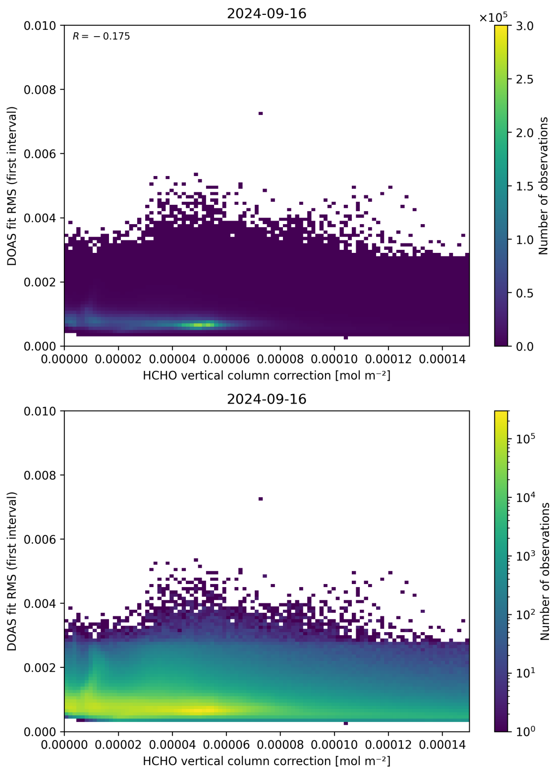
Figure 112: Scatter density plot of “HCHO vertical column correction” against “DOAS fit RMS (first interval)” for 2024-09-15 to 2024-09-17.
