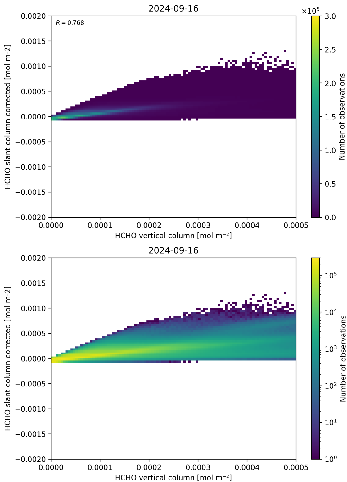
Figure 127: Scatter density plot of “HCHO vertical column” against “HCHO slant column corrected” for 2024-09-15 to 2024-09-17.
