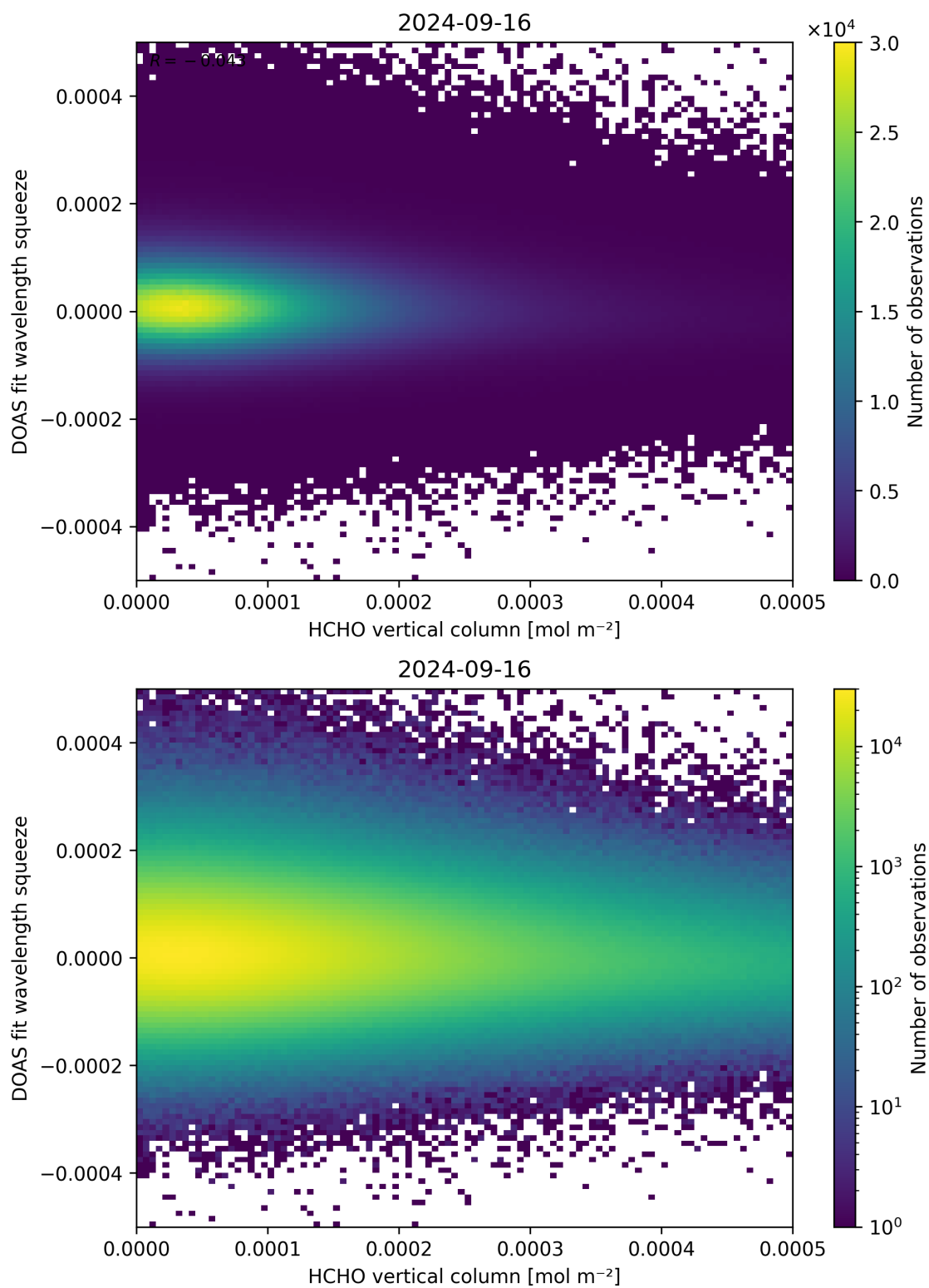
Figure 125: Scatter density plot of “HCHO vertical column” against “DOAS fit wavelength squeeze” for 2024-09-15 to 2024-09-17.
