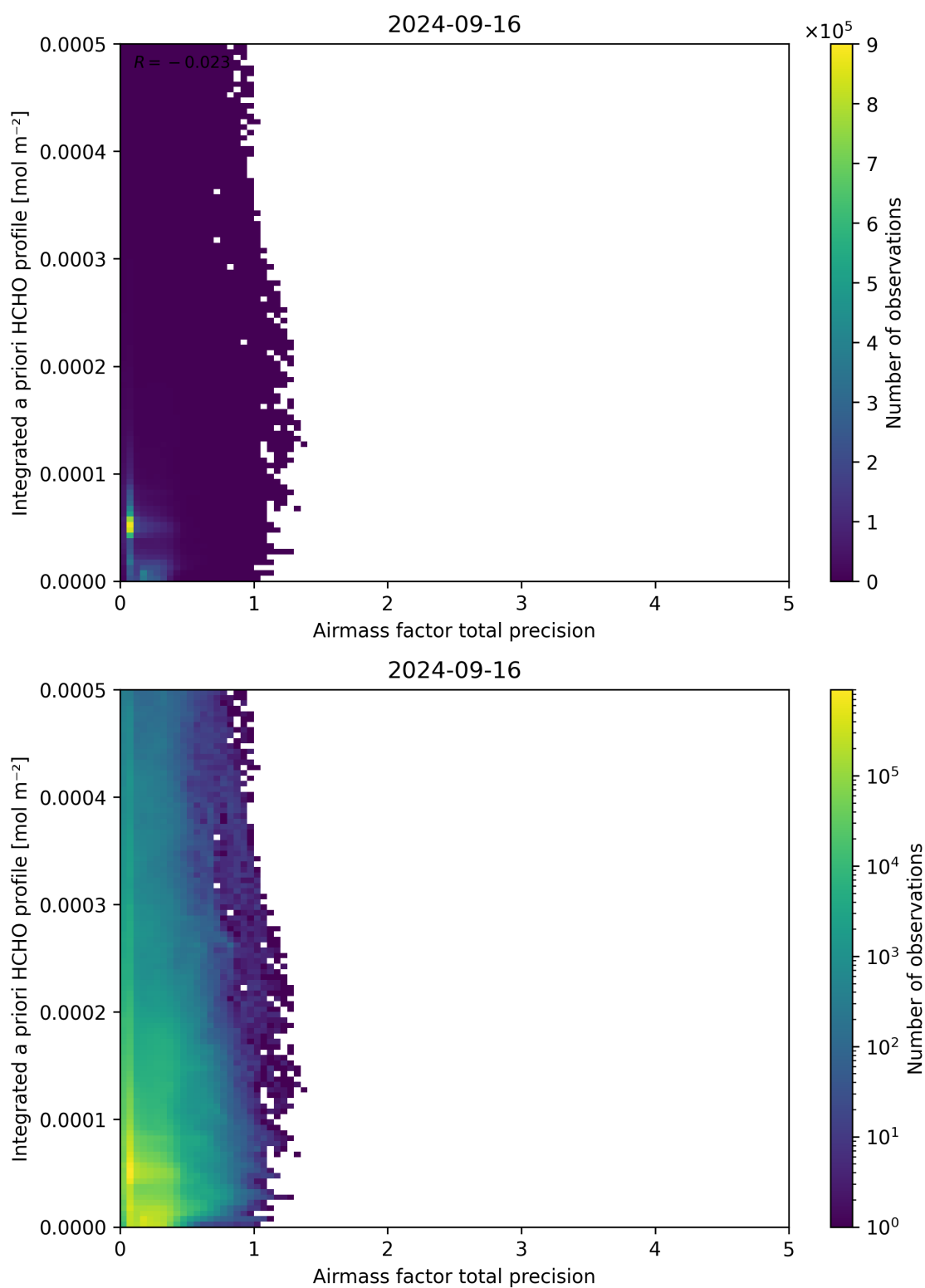
Figure 111: Scatter density plot of “Airmass factor total precision” against “Integrated a priori HCHO profile” for 2024-09-15 to 2024-09-17.
