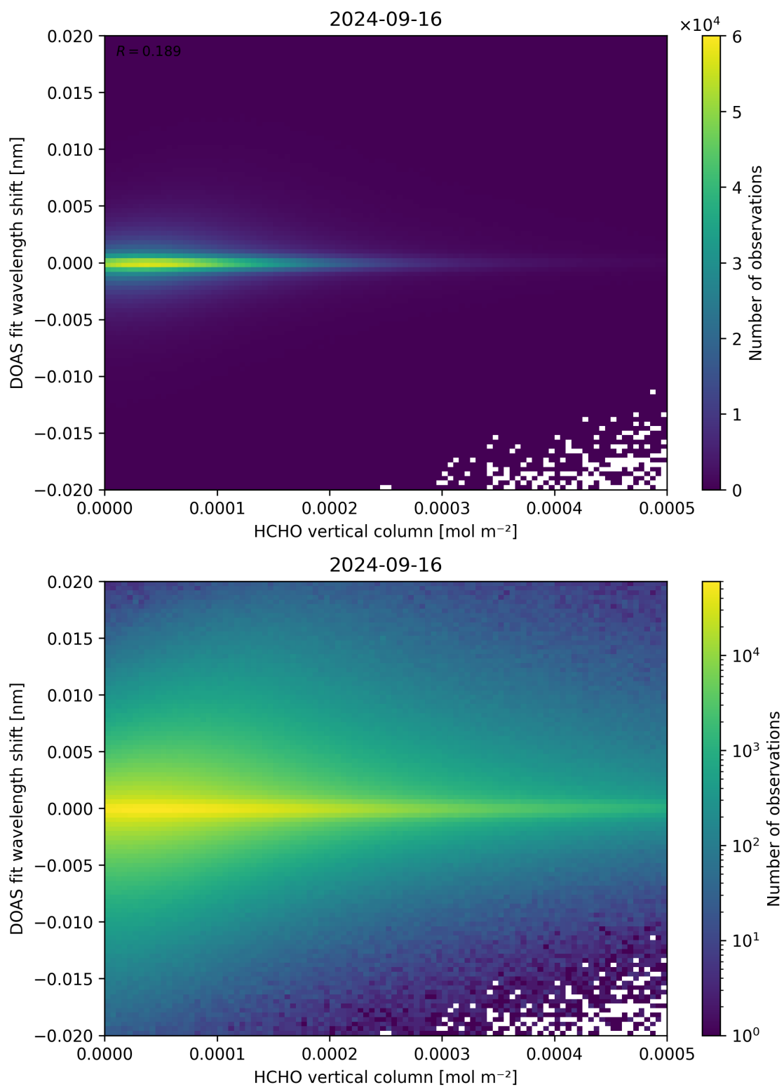
Figure 124: Scatter density plot of “HCHO vertical column” against “DOAS fit wavelength shift” for 2024-09-15 to 2024-09-17.
