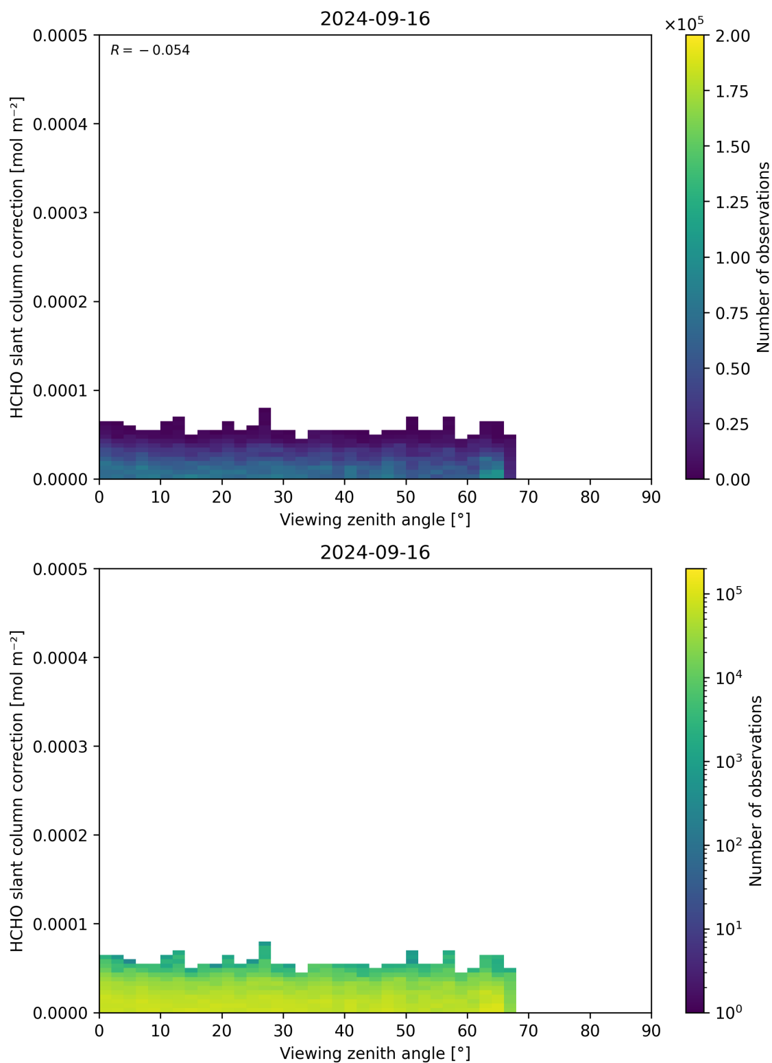
Figure 187: Scatter density plot of “Viewing zenith angle” against “HCHO slant column correction” for 2024-09-15 to 2024-09-17.
