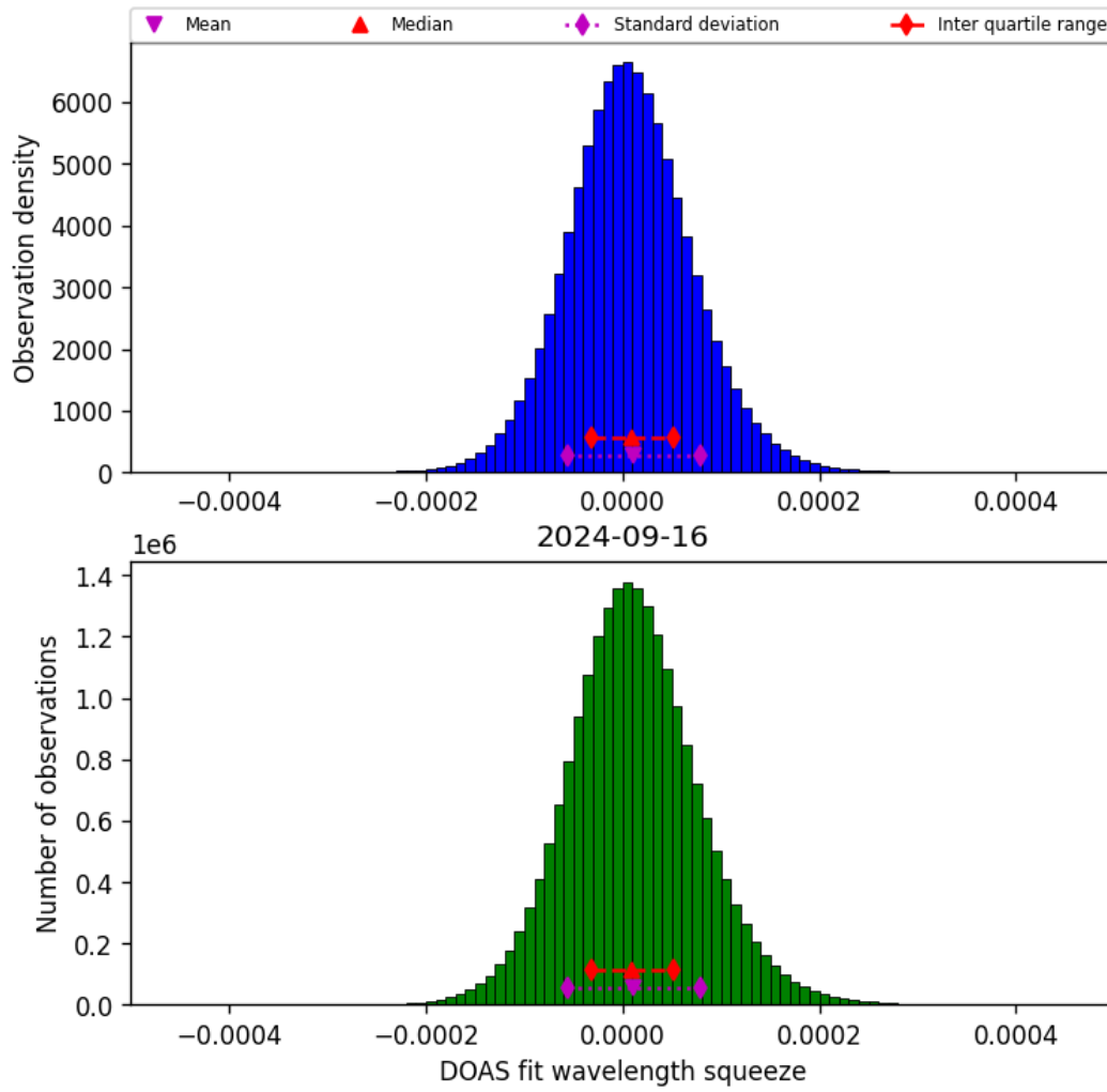
Figure 45: Histogram of “DOAS fit wavelength squeeze” for 2024-09-15 to 2024-09-17
