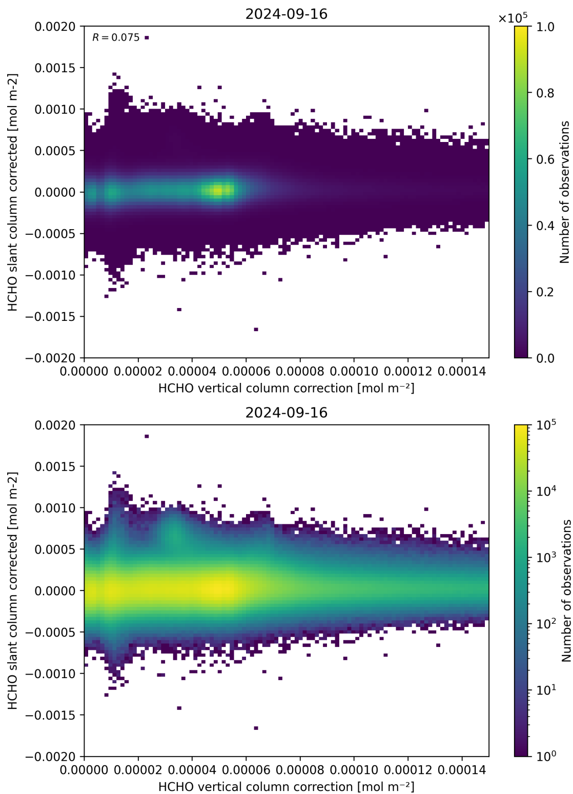
Figure 116: Scatter density plot of “HCHO vertical column correction” against “HCHO slant column corrected” for 2024-09-15 to 2024-09-17.
