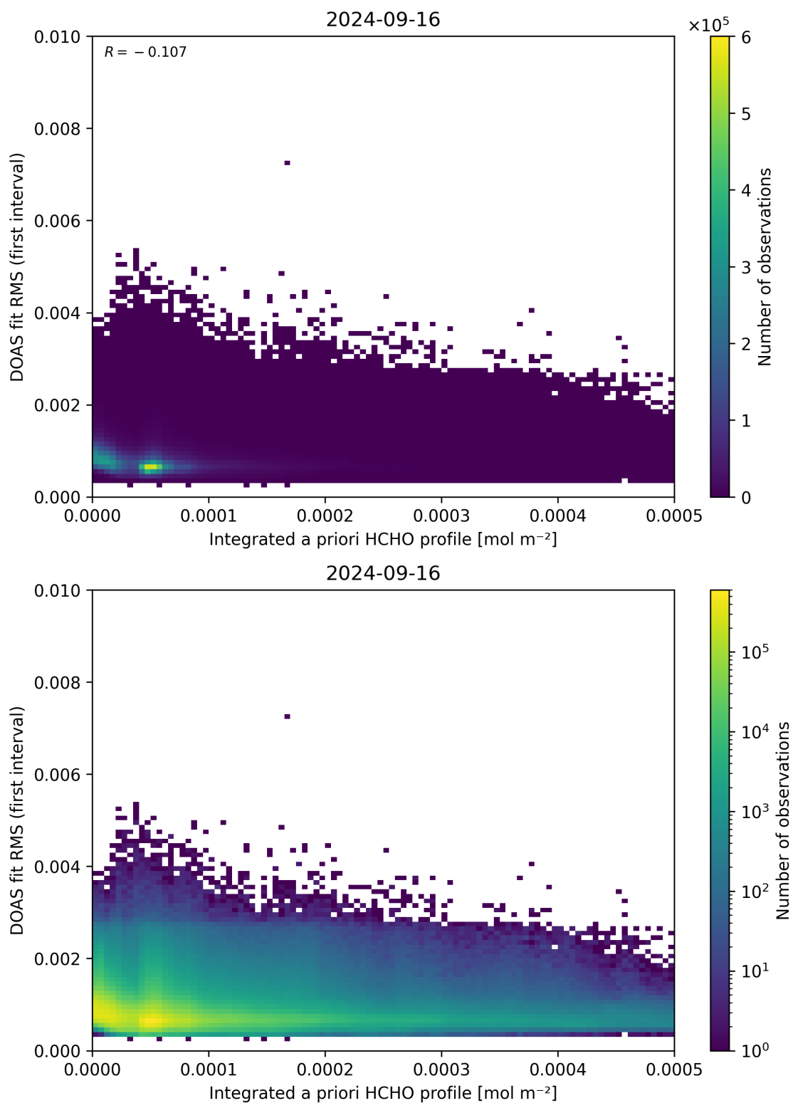
Figure 148: Scatter density plot of “Integrated a priori HCHO profile” against “DOAS fit RMS (first interval)” for 2024-09-15 to 2024-09-17.
