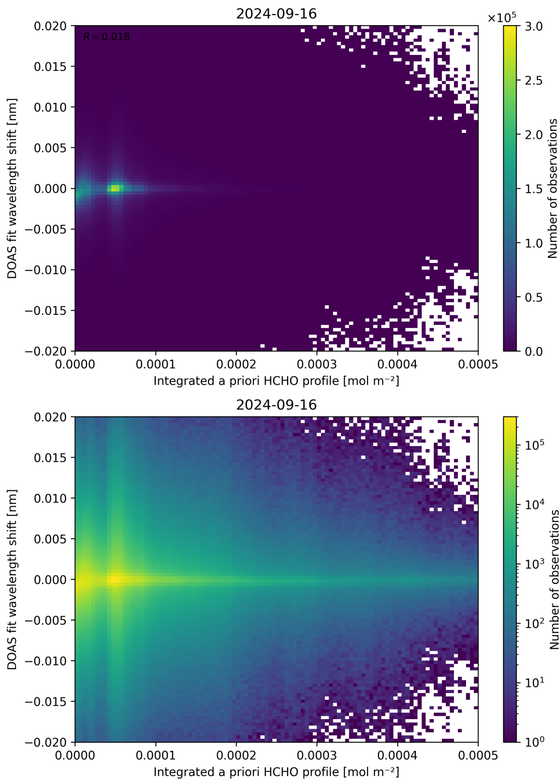
Figure 149: Scatter density plot of “Integrated a priori HCHO profile” against “DOAS fit wavelength shift” for 2024-09-15 to 2024-09-17.
