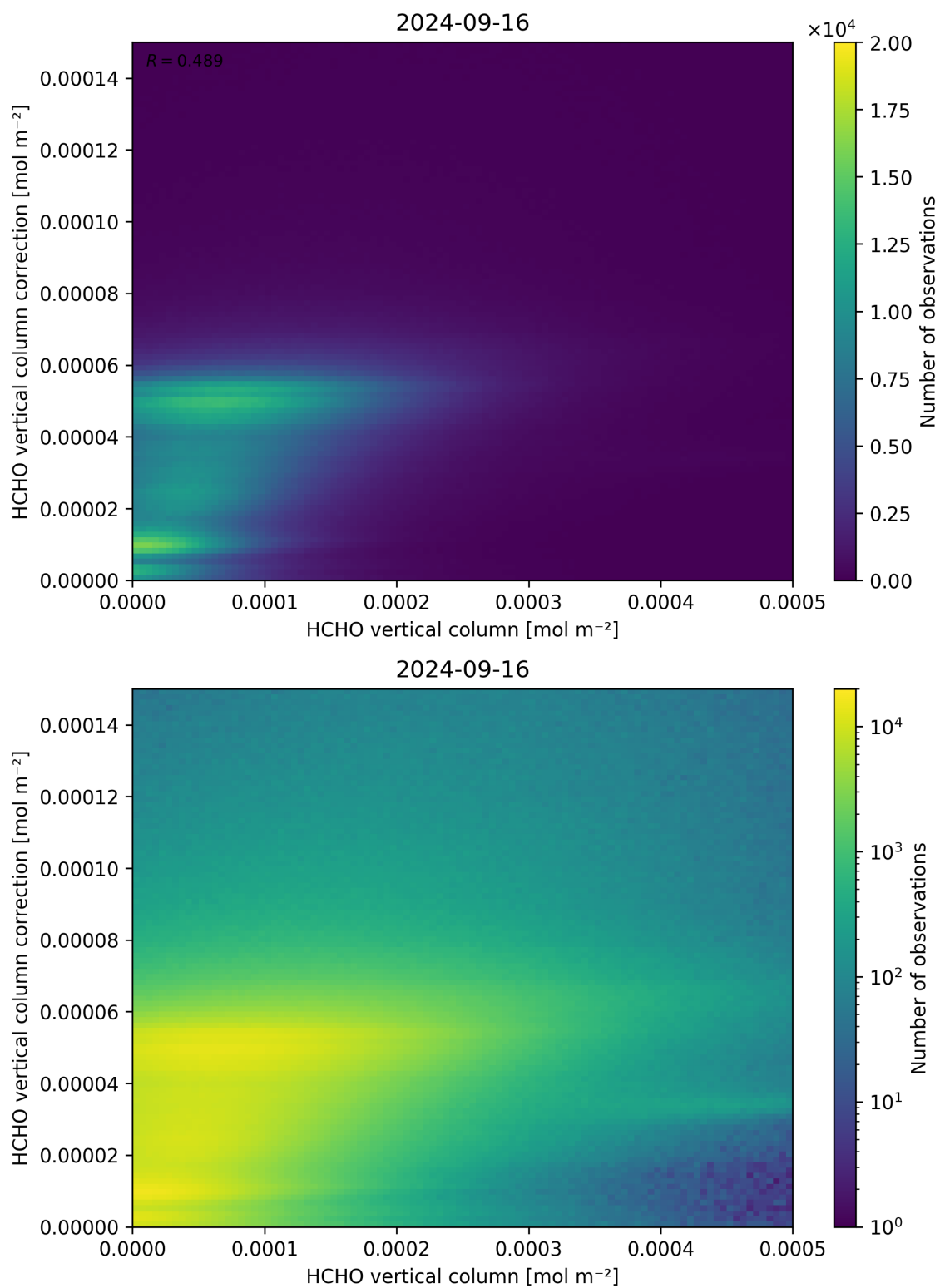
Figure 133: Scatter density plot of “HCHO vertical column” against “HCHO vertical column correction” for 2024-09-15 to 2024-09-17.
