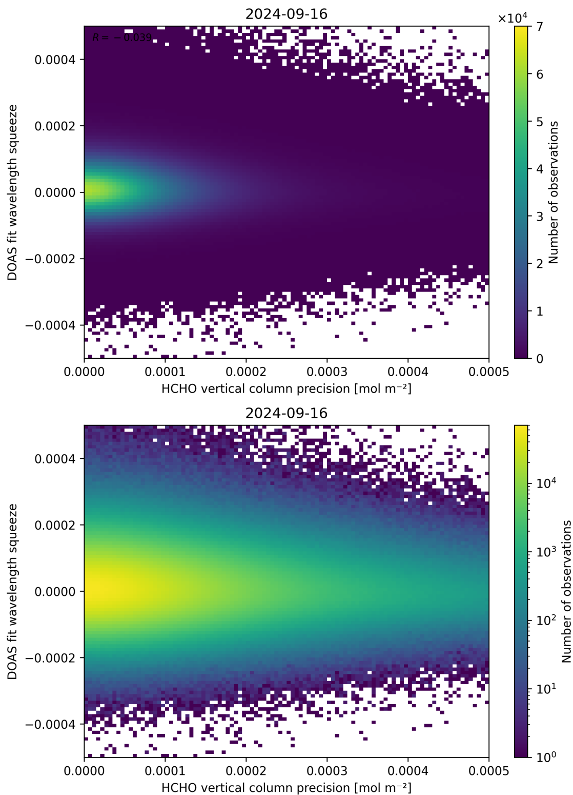
Figure 138: Scatter density plot of “HCHO vertical column precision” against “DOAS fit wavelength squeeze” for 2024-09-15 to 2024-09-17.
