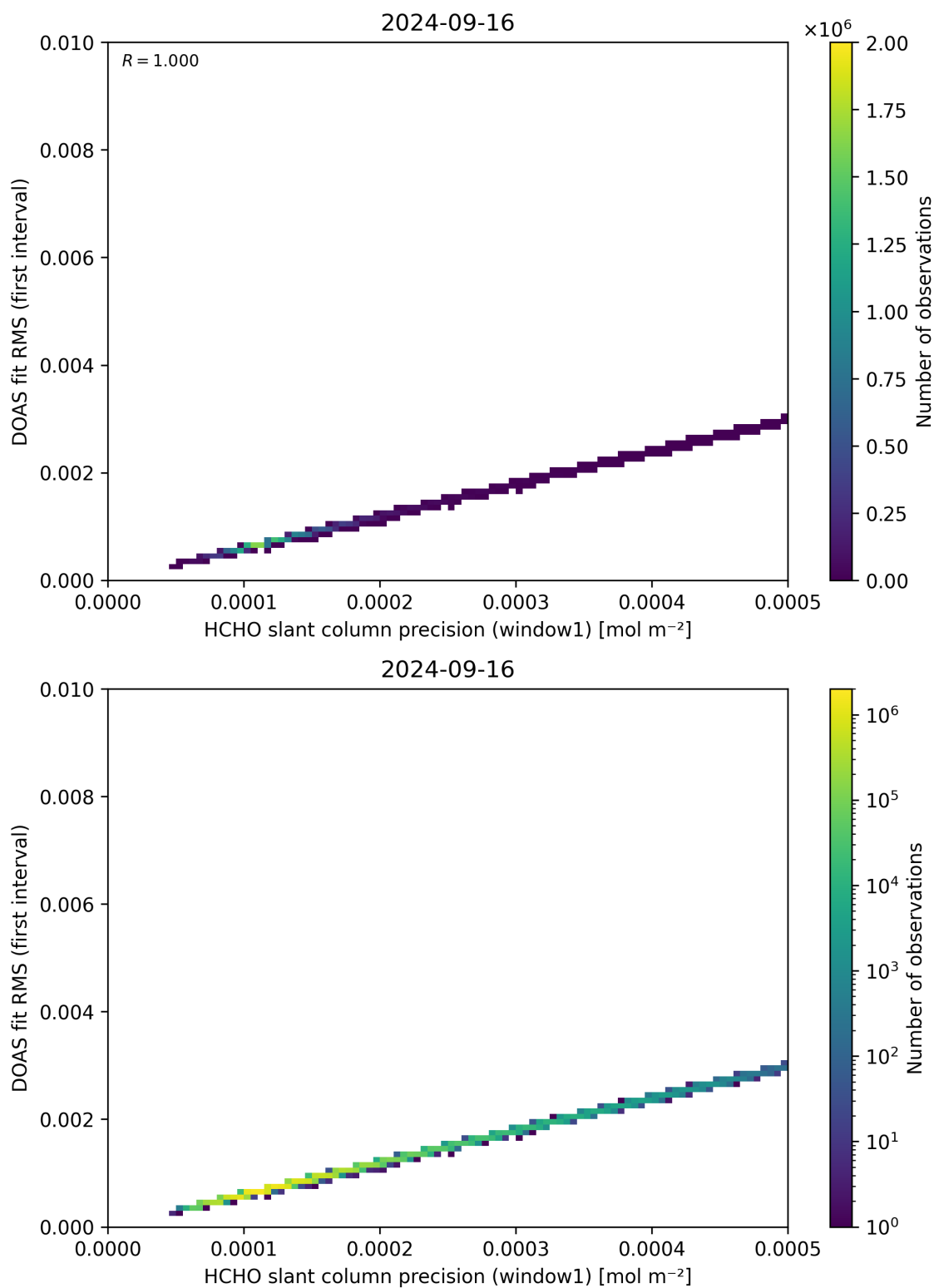
Figure 88: Scatter density plot of “HCHO slant column precision (window1)” against “DOAS fit RMS (first interval)” for 2024-09-15 to 2024-09-17.
