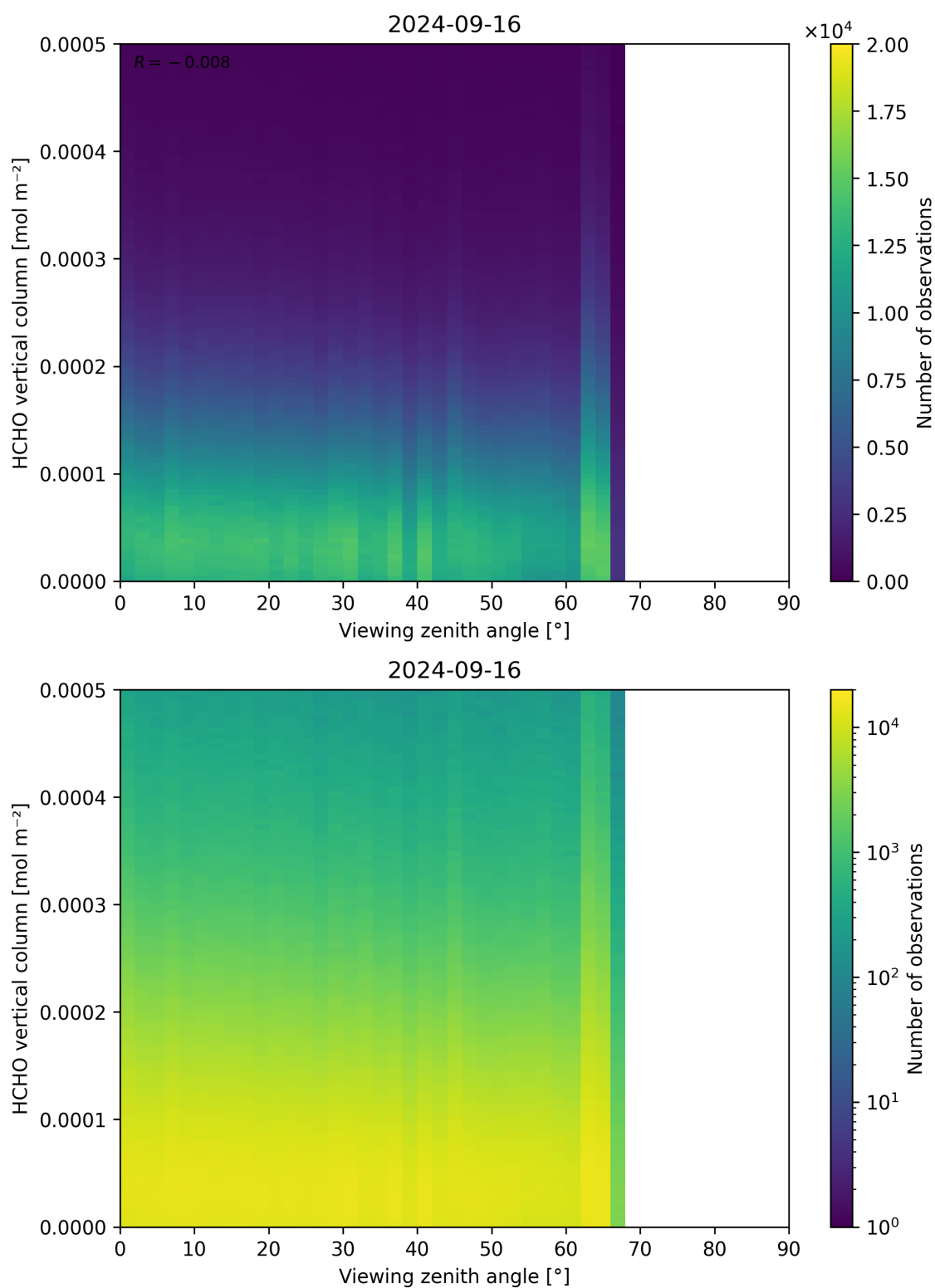
Figure 192: Scatter density plot of “Viewing zenith angle” against “HCHO vertical column” for 2024-09-15 to 2024-09-17.
