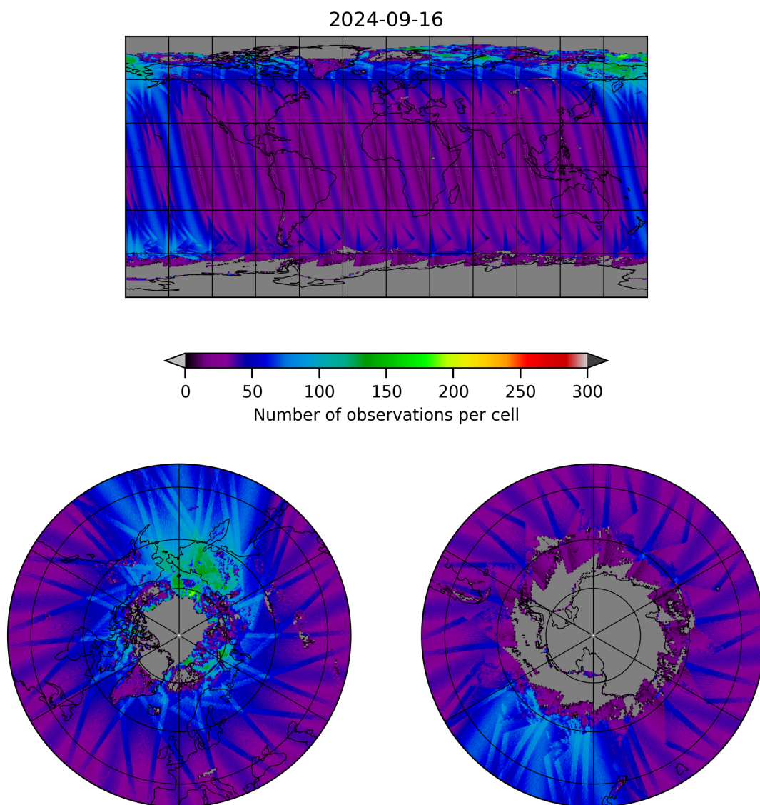
Figure 19: Map of the number of observations for 2024-09-15 to 2024-09-17
