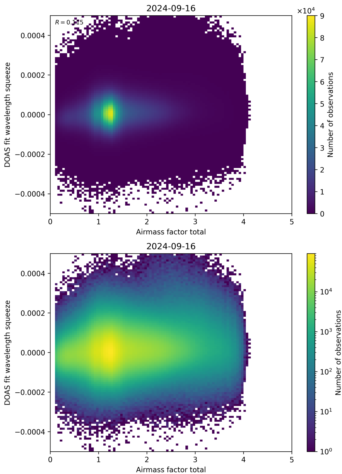
Figure 99: Scatter density plot of “Airmass factor total” against “DOAS fit wavelength squeeze” for 2024-09-15 to 2024-09-17.
