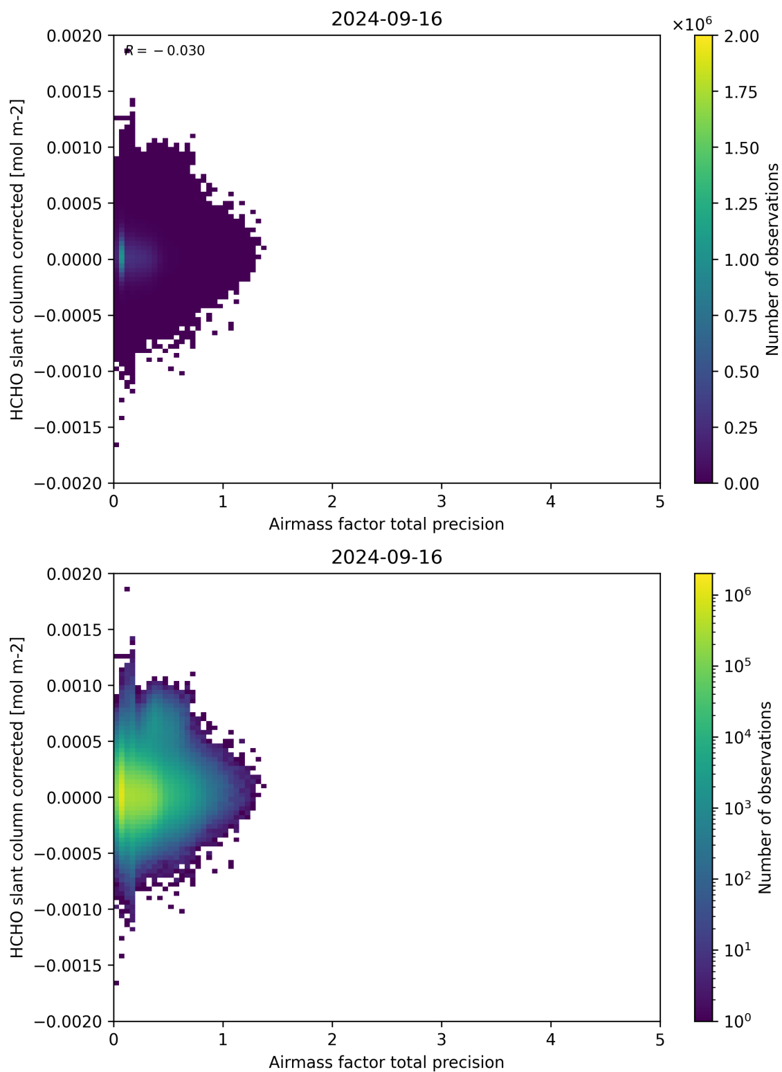
Figure 109: Scatter density plot of “Airmass factor total precision” against “HCHO slant column corrected” for 2024-09-15 to 2024-09-17.
