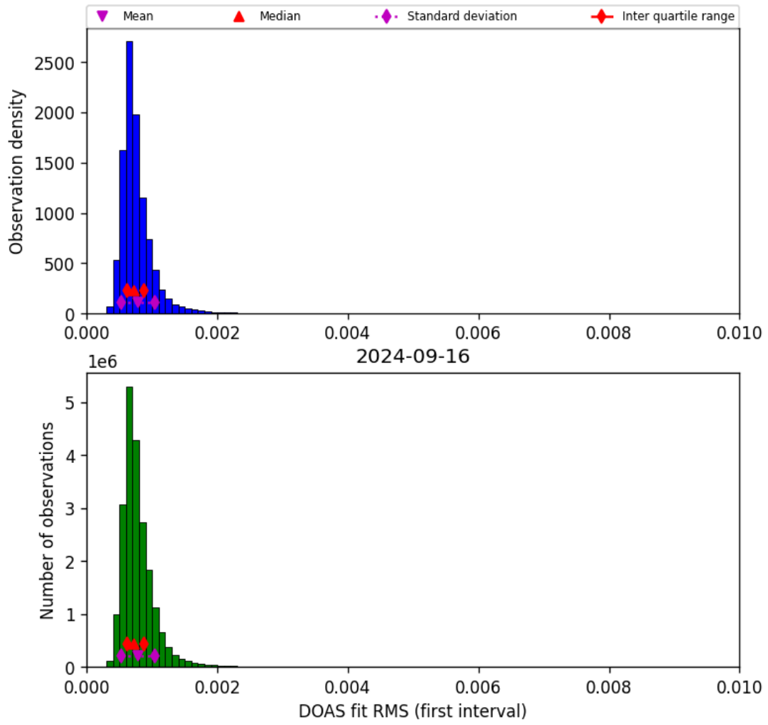
Figure 46: Histogram of “DOAS fit RMS (first interval)” for 2024-09-15 to 2024-09-17
