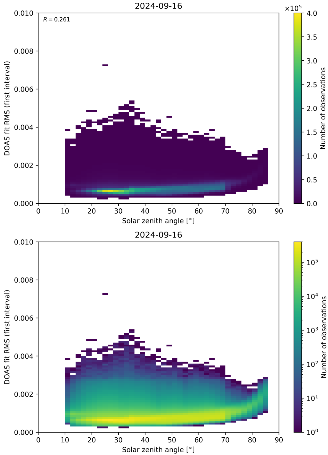
Figure 167: Scatter density plot of “Solar zenith angle” against “DOAS fit RMS (first interval)” for 2024-09-15 to 2024-09-17.
