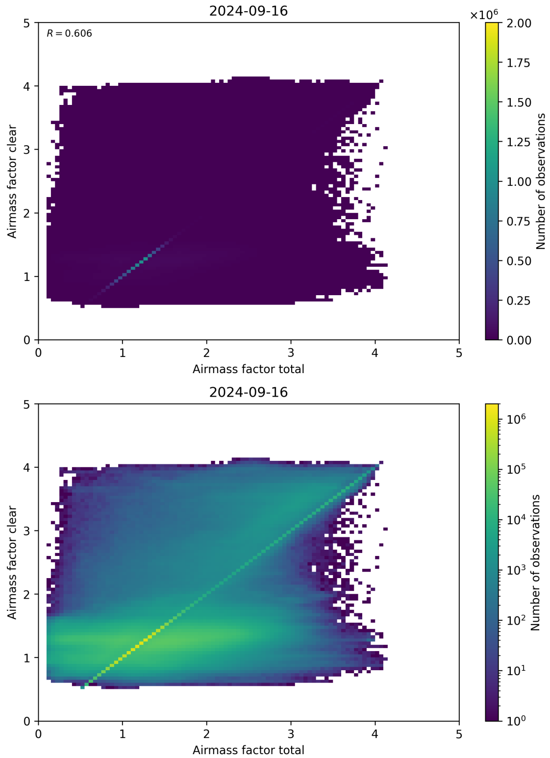
Figure 100: Scatter density plot of “Airmass factor total” against “Airmass factor clear” for 2024-09-15 to 2024-09-17.
