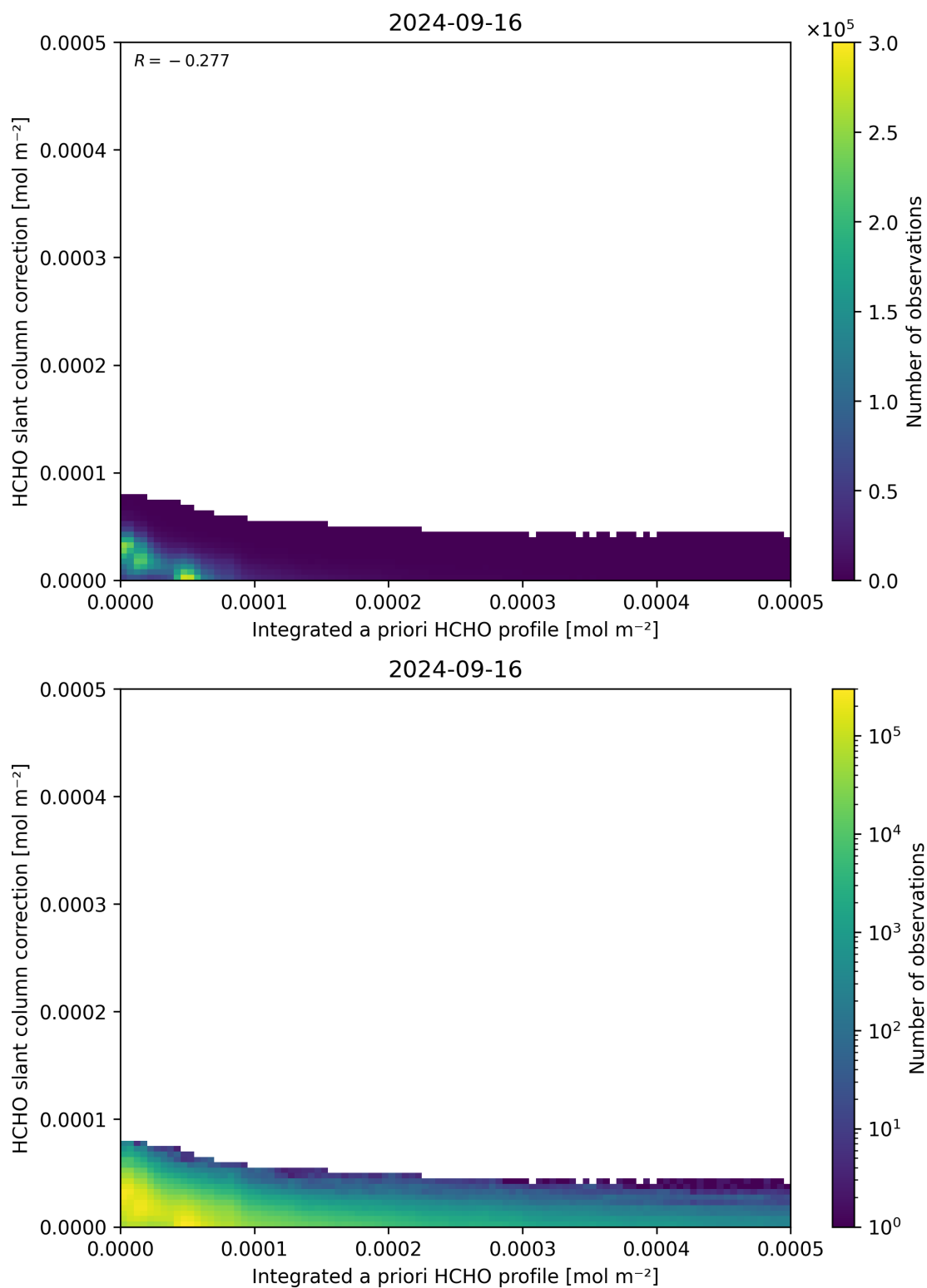
Figure 152: Scatter density plot of “Integrated a priori HCHO profile” against “HCHO slant column correction” for 2024-09-15 to 2024-09-17.
