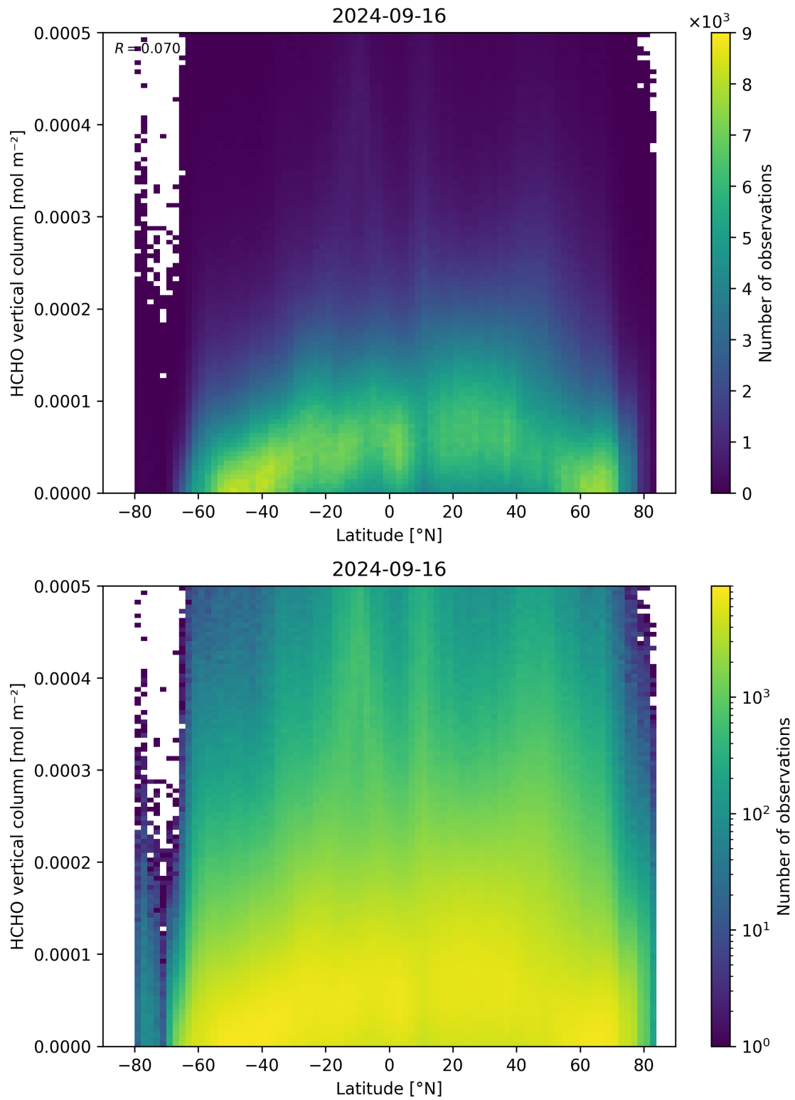
Figure 163: Scatter density plot of “Latitude” against “HCHO vertical column” for 2024-09-15 to 2024-09-17.
