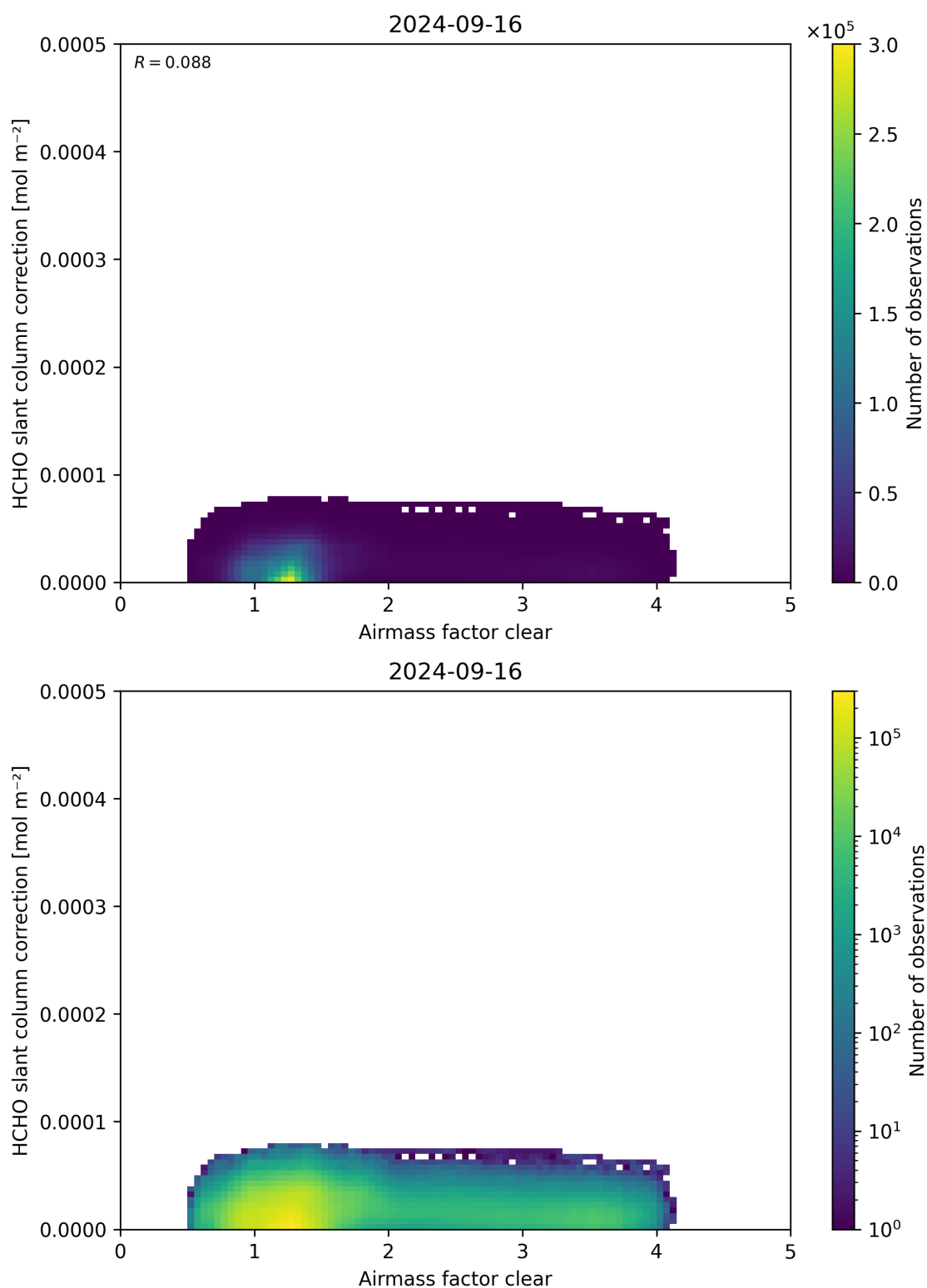
Figure 75: Scatter density plot of “Airmass factor clear” against “HCHO slant column correction” for 2024-09-15 to 2024-09-17.
