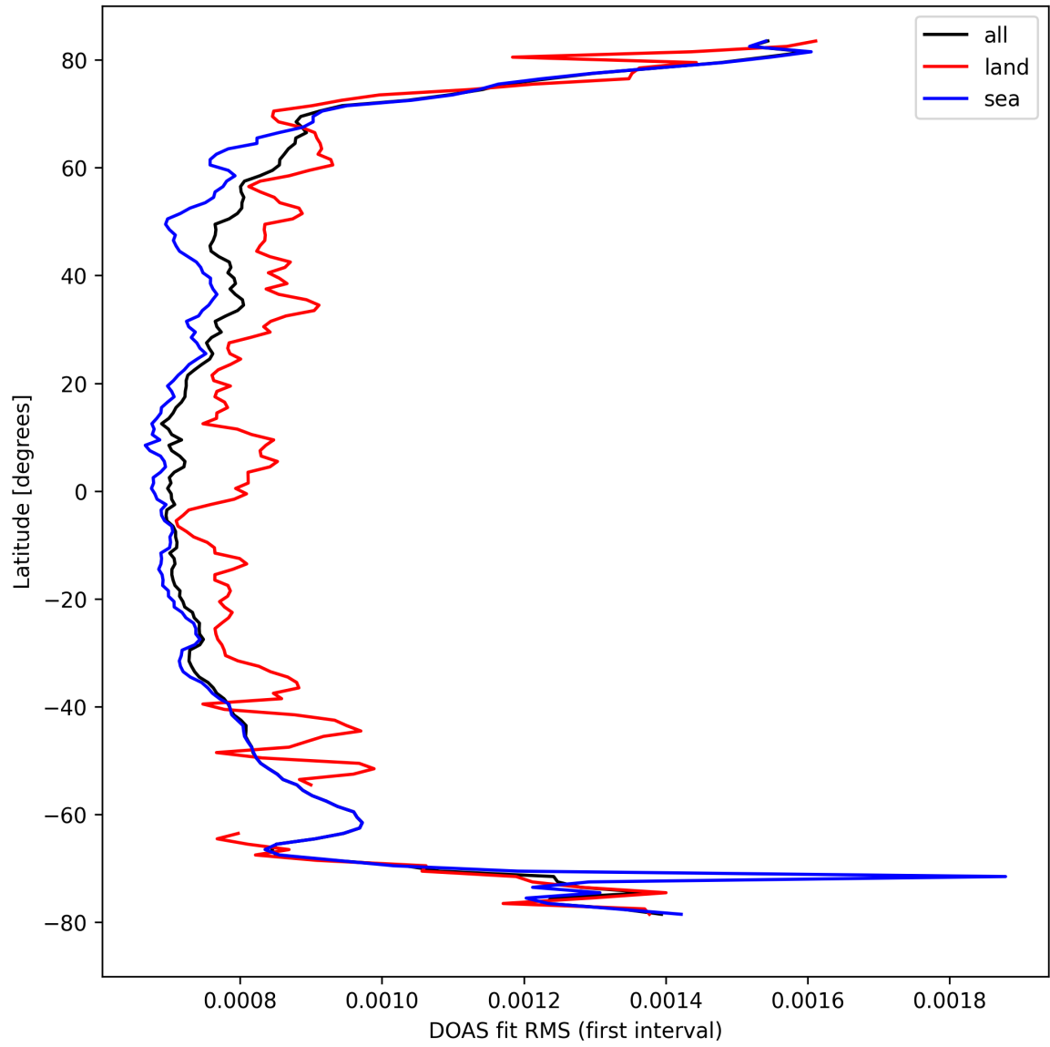
Figure 32: Zonal average of “DOAS fit RMS (first interval)” for 2024-09-15 to 2024-09-17.
