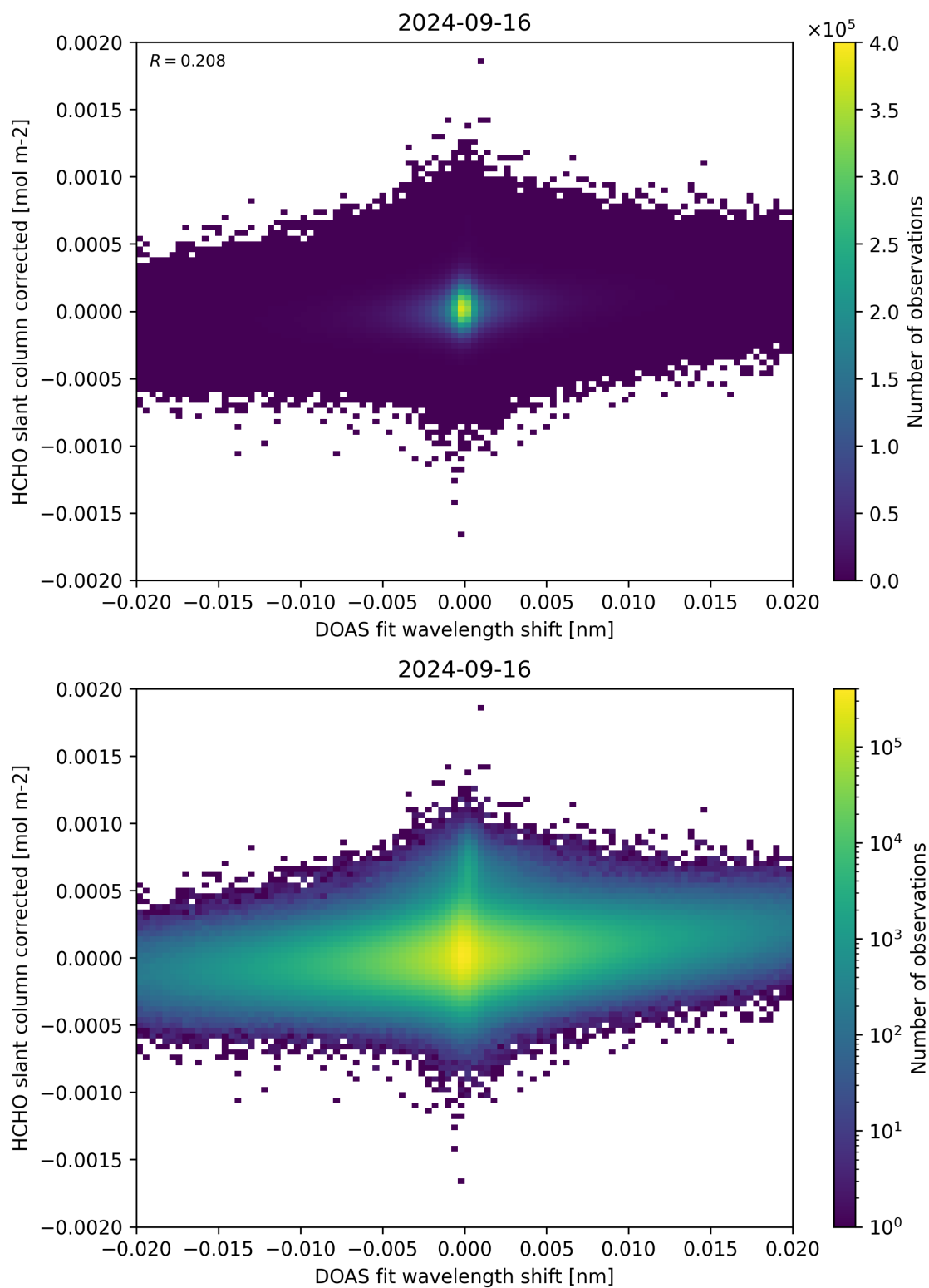
Figure 66: Scatter density plot of “DOAS fit wavelength shift” against “HCHO slant column corrected” for 2024-09-15 to 2024-09-17.
