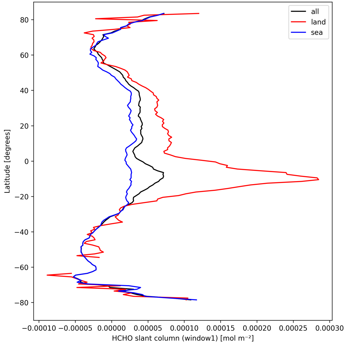
Figure 24: Zonal average of “HCHO slant column (window1)” for 2024-09-15 to 2024-09-17.
