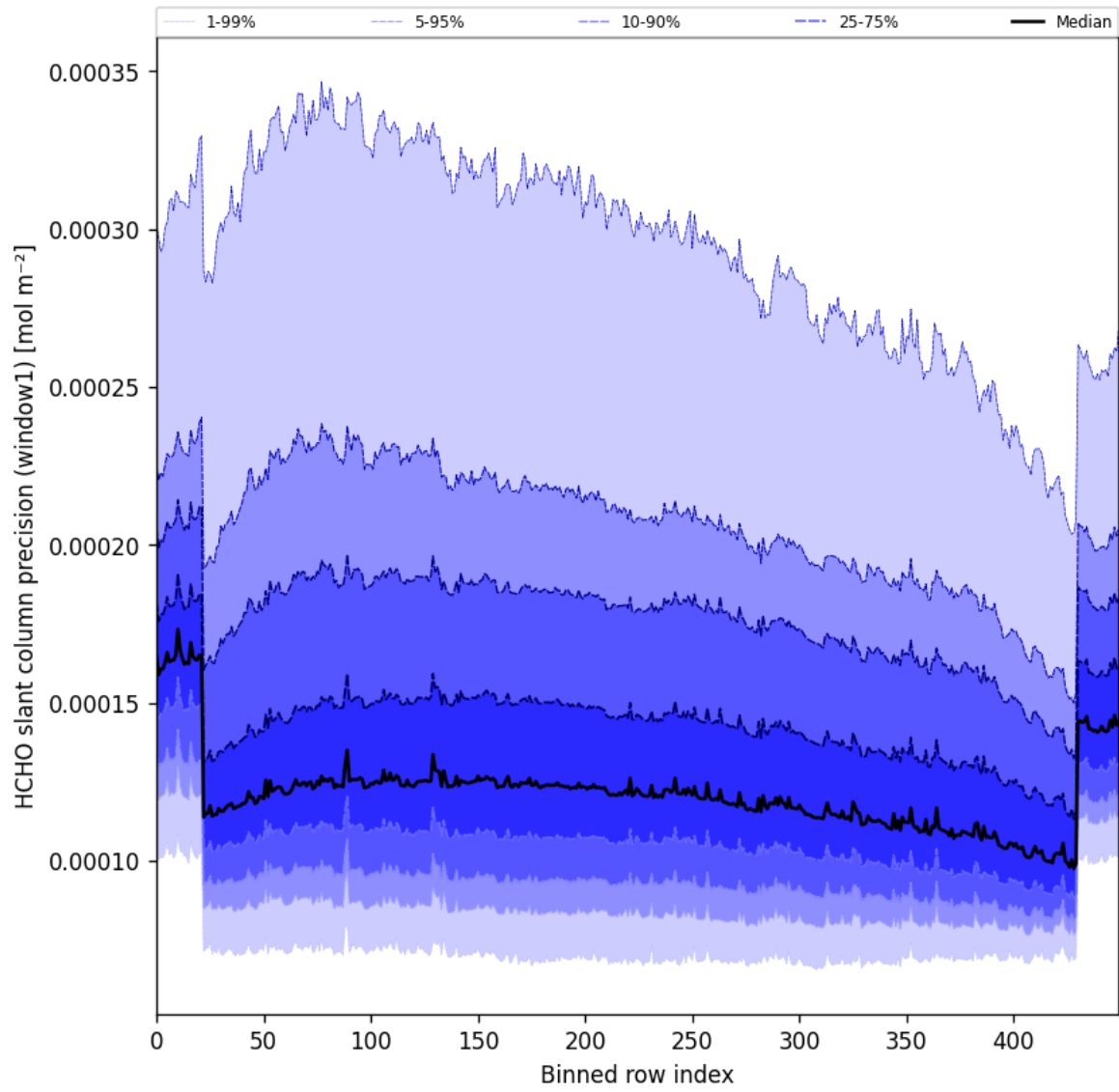
Figure 53: Along track statistics of “HCHO slant column precision (window1)” for 2024-09-15 to 2024-09-17
