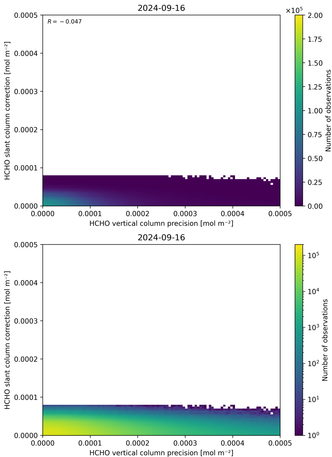
Figure 141: Scatter density plot of “HCHO vertical column precision” against “HCHO slant column correction” for 2024-09-15 to 2024-09-17.
