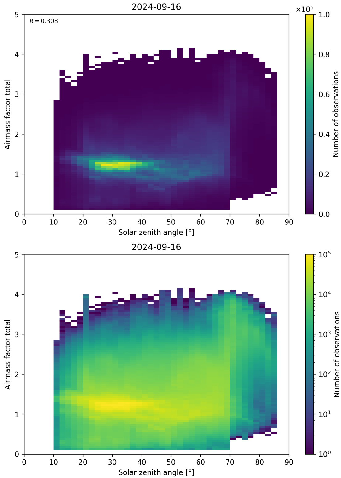
Figure 175: Scatter density plot of “Solar zenith angle” against “Airmass factor total” for 2024-09-15 to 2024-09-17.
