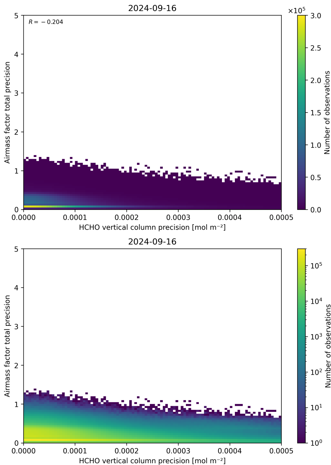
Figure 145: Scatter density plot of “HCHO vertical column precision” against “Airmass factor total precision” for 2024-09-15 to 2024-09-17.
