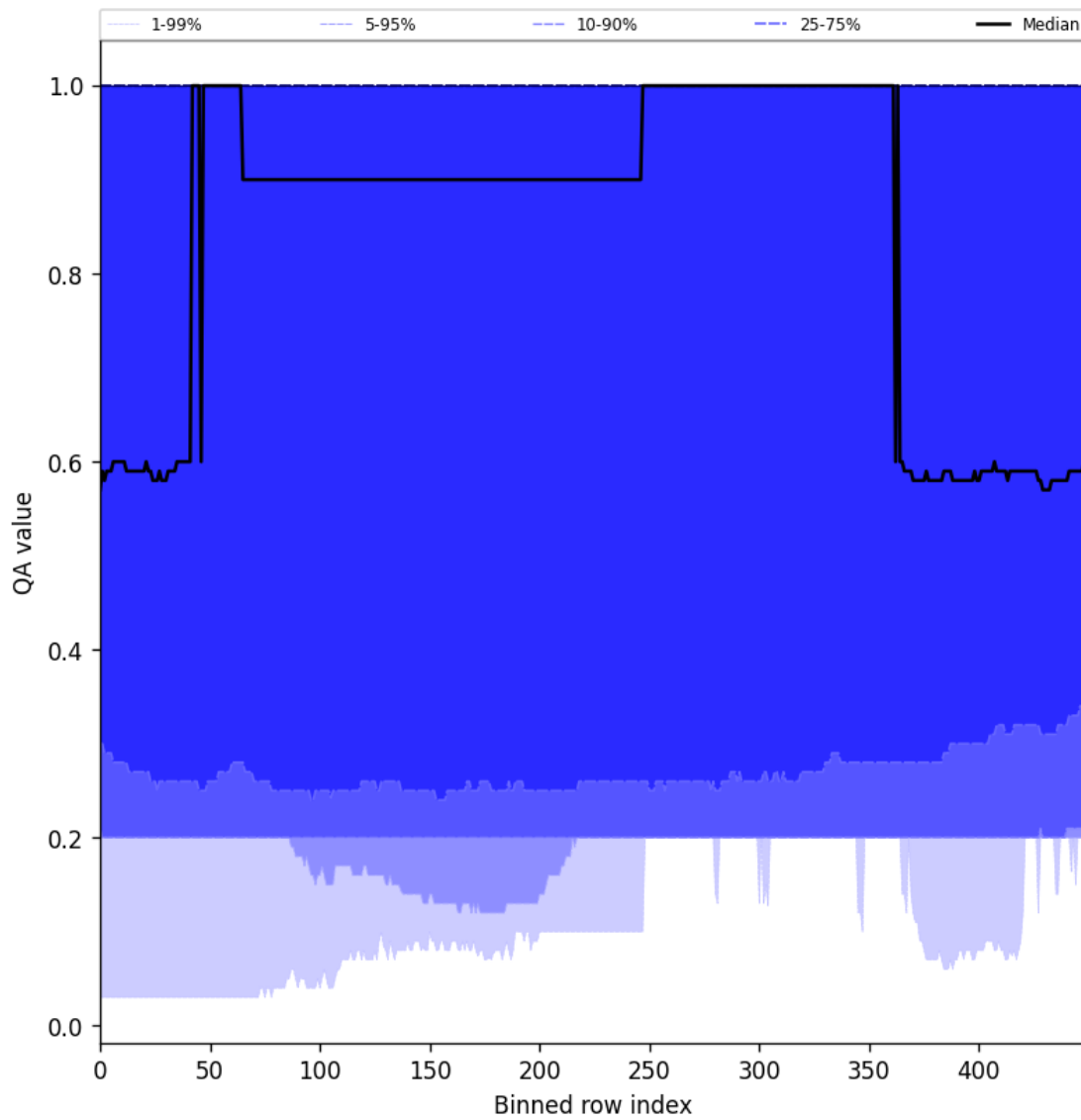
Figure 48: Along track statistics of “QA value” for 2024-09-15 to 2024-09-17
