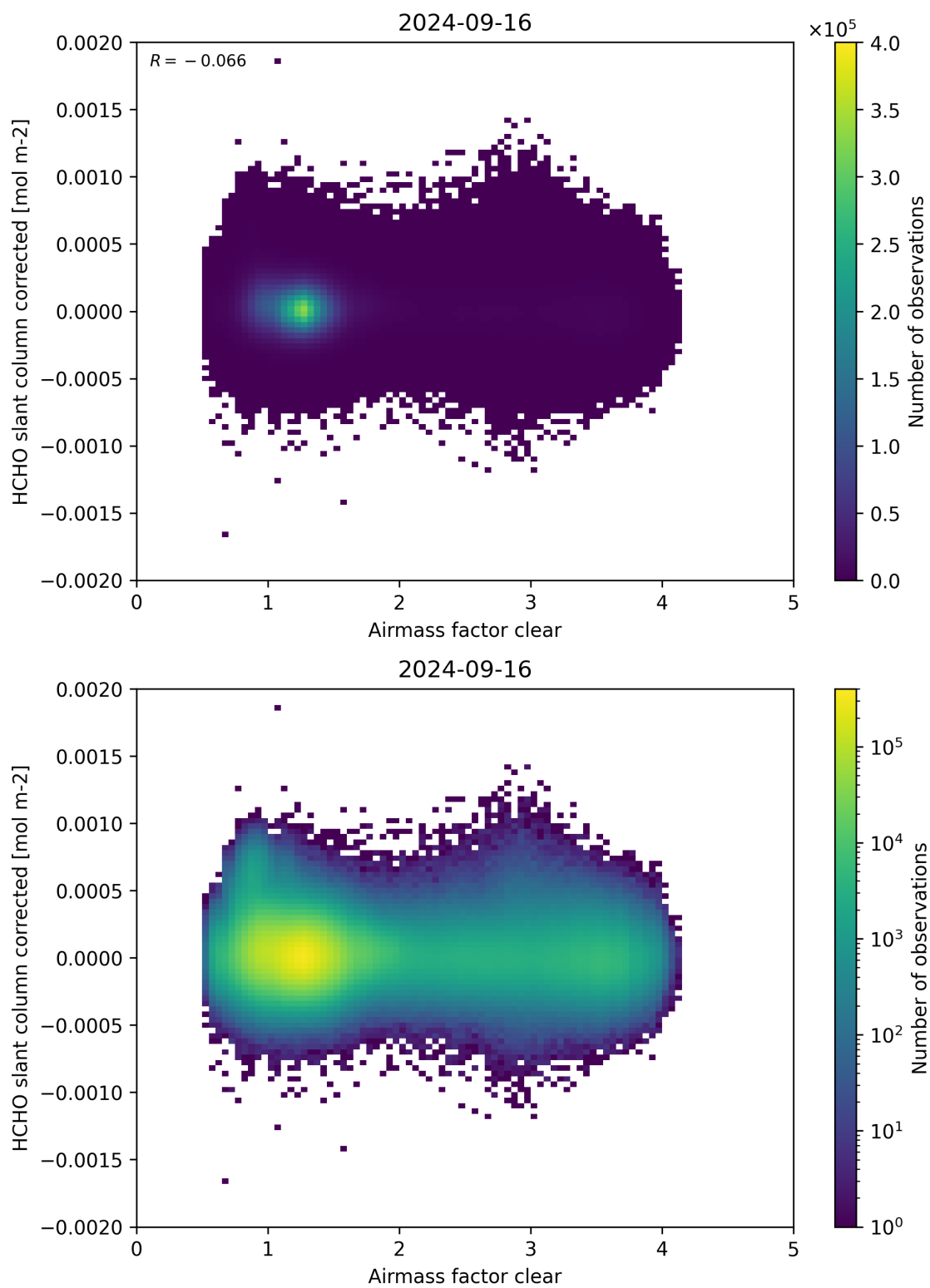
Figure 74: Scatter density plot of “Airmass factor clear” against “HCHO slant column corrected” for 2024-09-15 to 2024-09-17.
