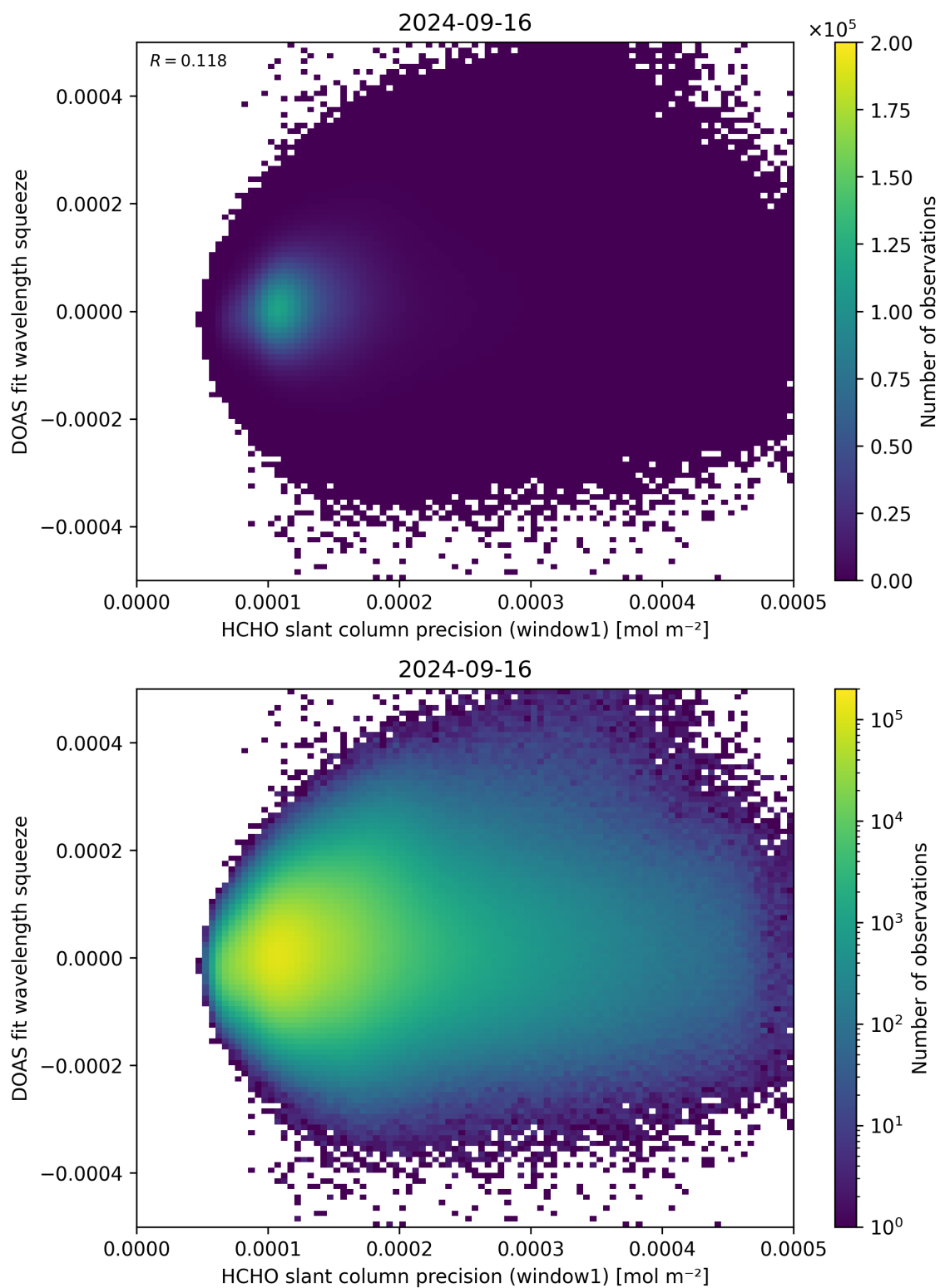
Figure 90: Scatter density plot of “HCHO slant column precision (window1)” against “DOAS fit wavelength squeeze” for 2024-09-15 to 2024-09-17.
