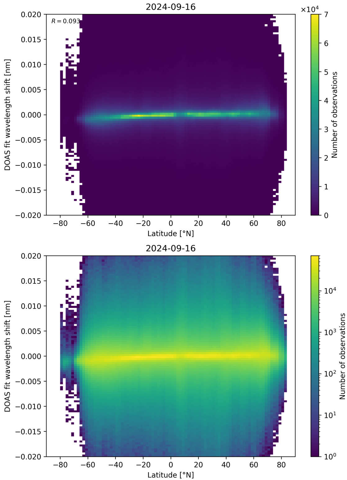
Figure 154: Scatter density plot of “Latitude” against “DOAS fit wavelength shift” for 2024-09-15 to 2024-09-17.
