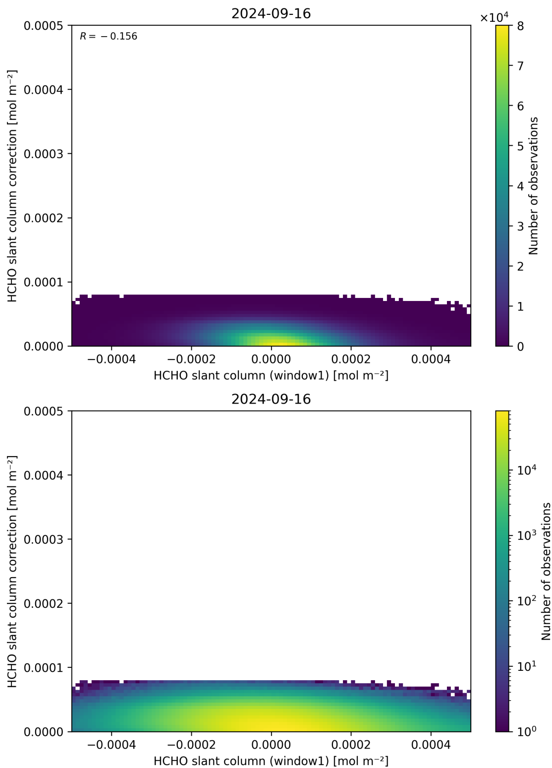
Figure 83: Scatter density plot of “HCHO slant column (window1)” against “HCHO slant column correction” for 2024-09-15 to 2024-09-17.
