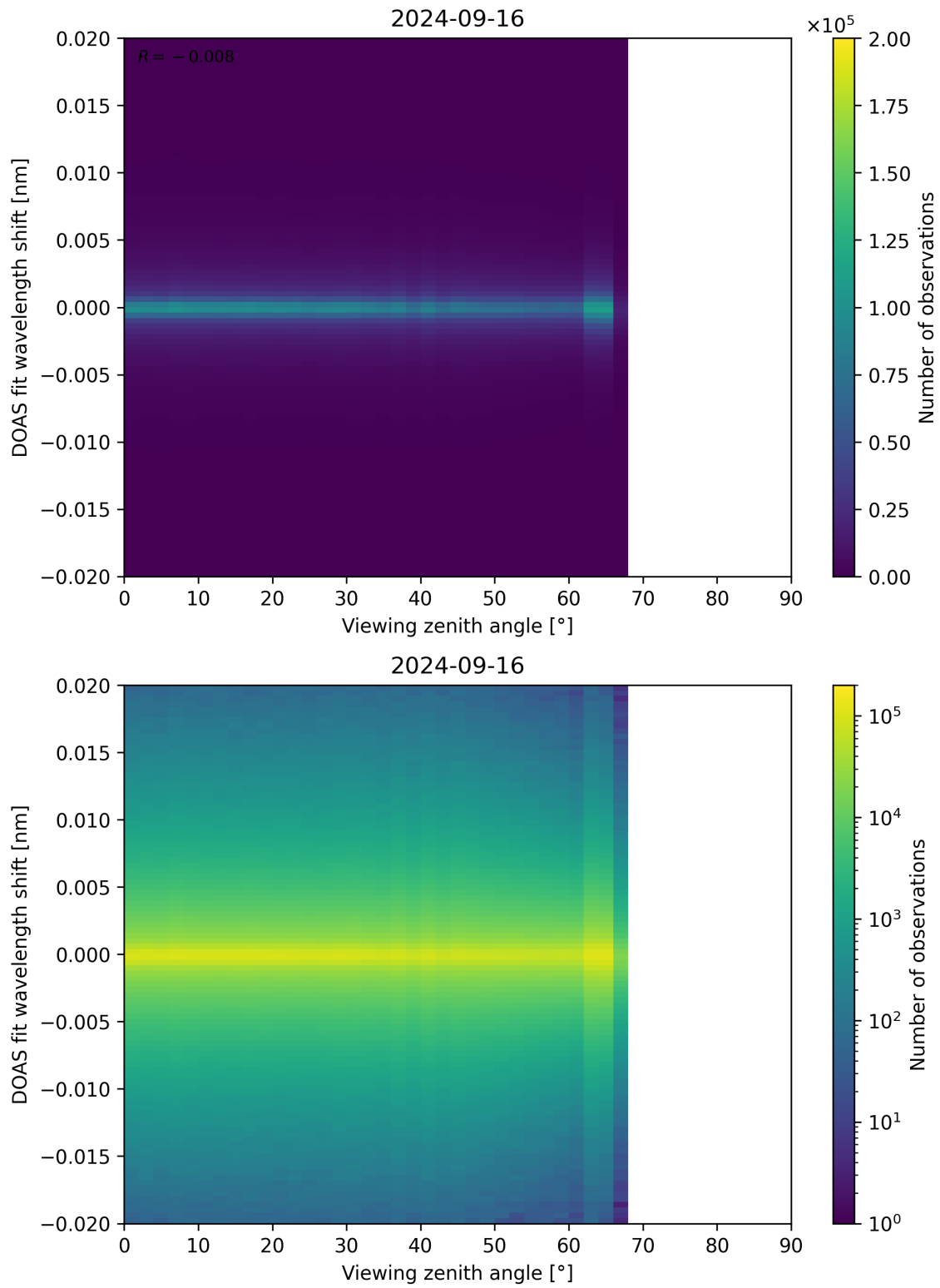
Figure 183: Scatter density plot of “Viewing zenith angle” against “DOAS fit wavelength shift” for 2024-09-15 to 2024-09-17.
