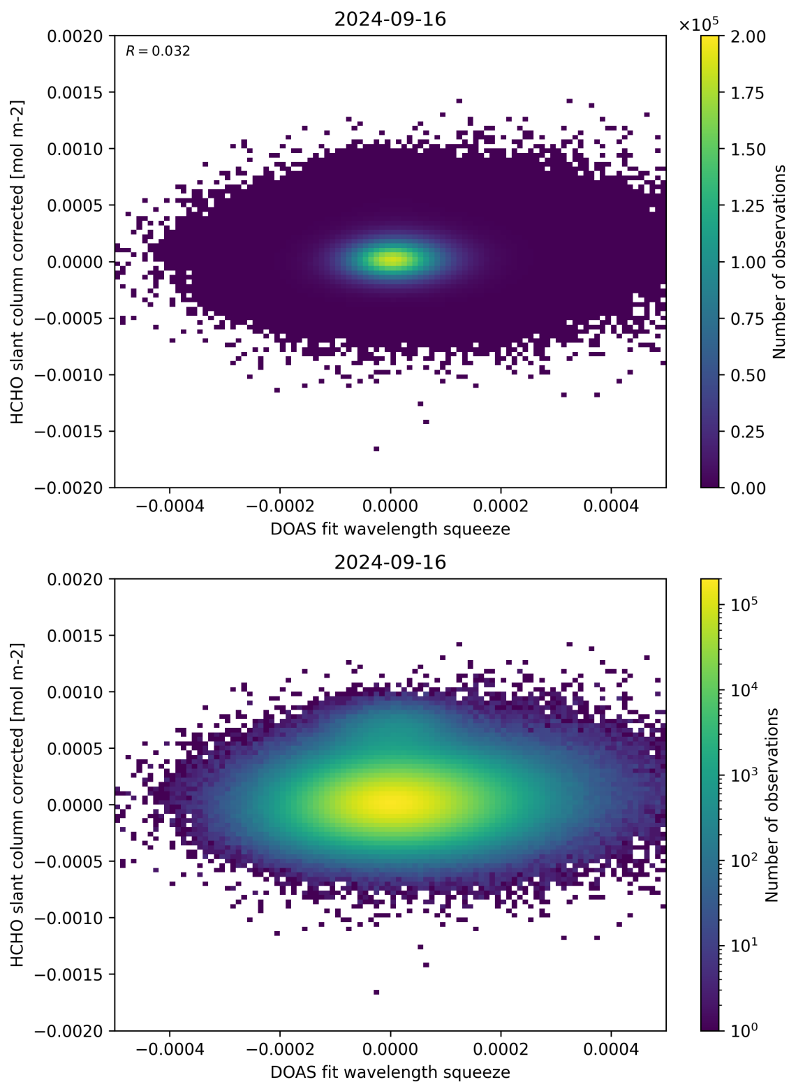
Figure 69: Scatter density plot of “DOAS fit wavelength squeeze” against “HCHO slant column corrected” for 2024-09-15 to 2024-09-17.
