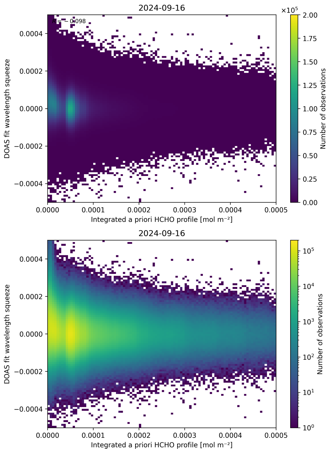
Figure 150: Scatter density plot of “Integrated a priori HCHO profile” against “DOAS fit wavelength squeeze” for 2024-09-15 to 2024-09-17.
