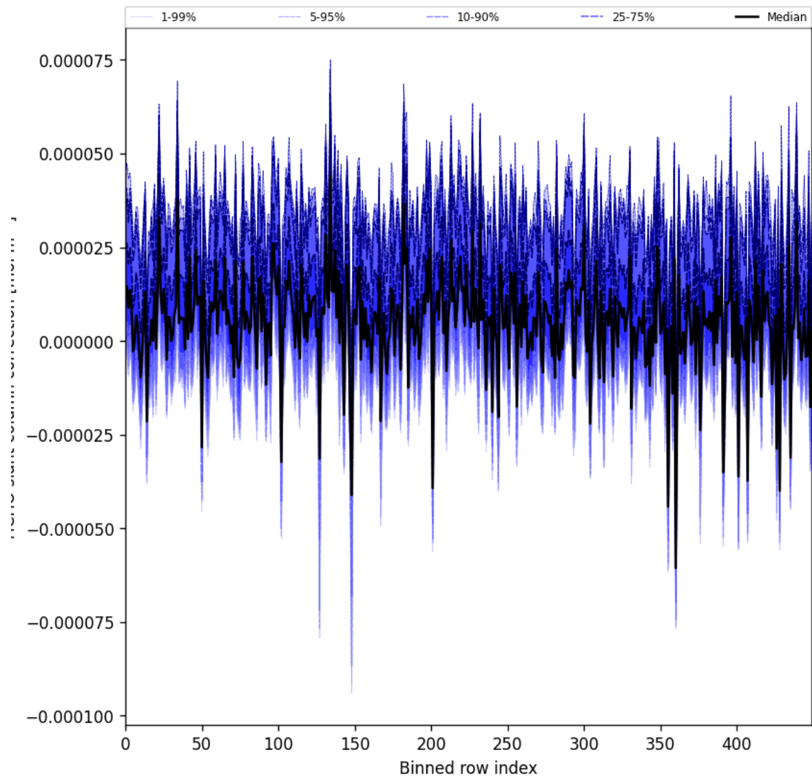
Figure 61: Along track statistics of “HCHO slant column correction” for 2024-09-15 to 2024-09-17
