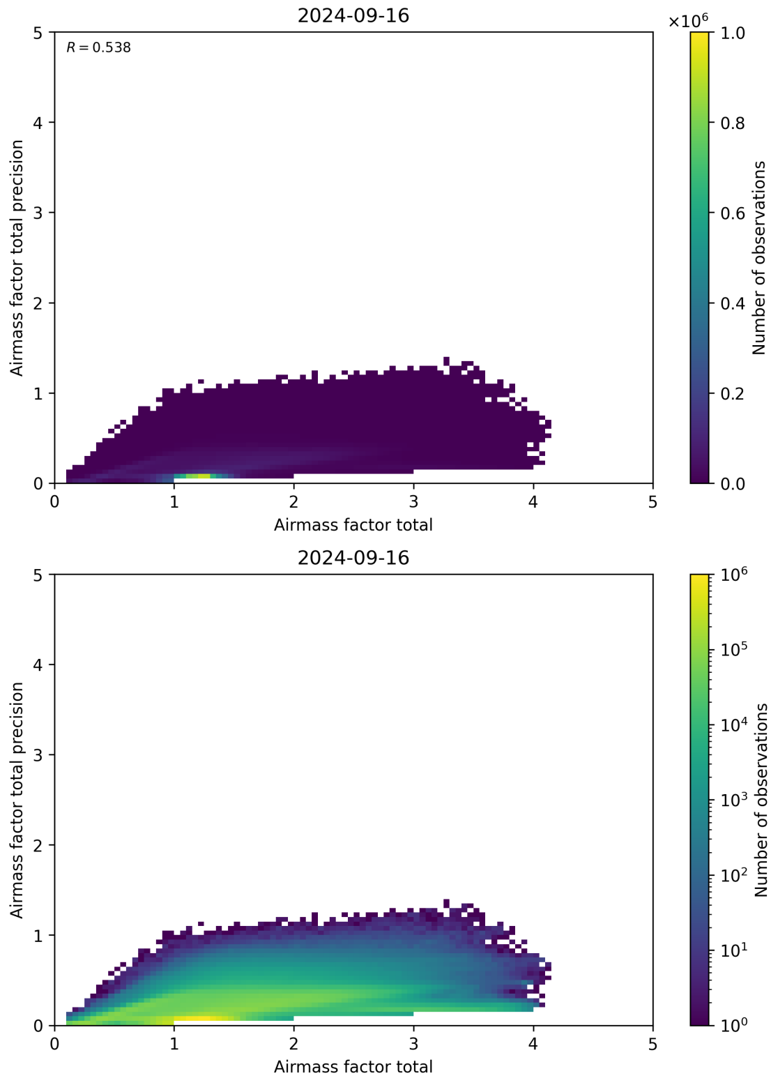
Figure 103: Scatter density plot of “Airmass factor total” against “Airmass factor total precision” for 2024-09-15 to 2024-09-17.
