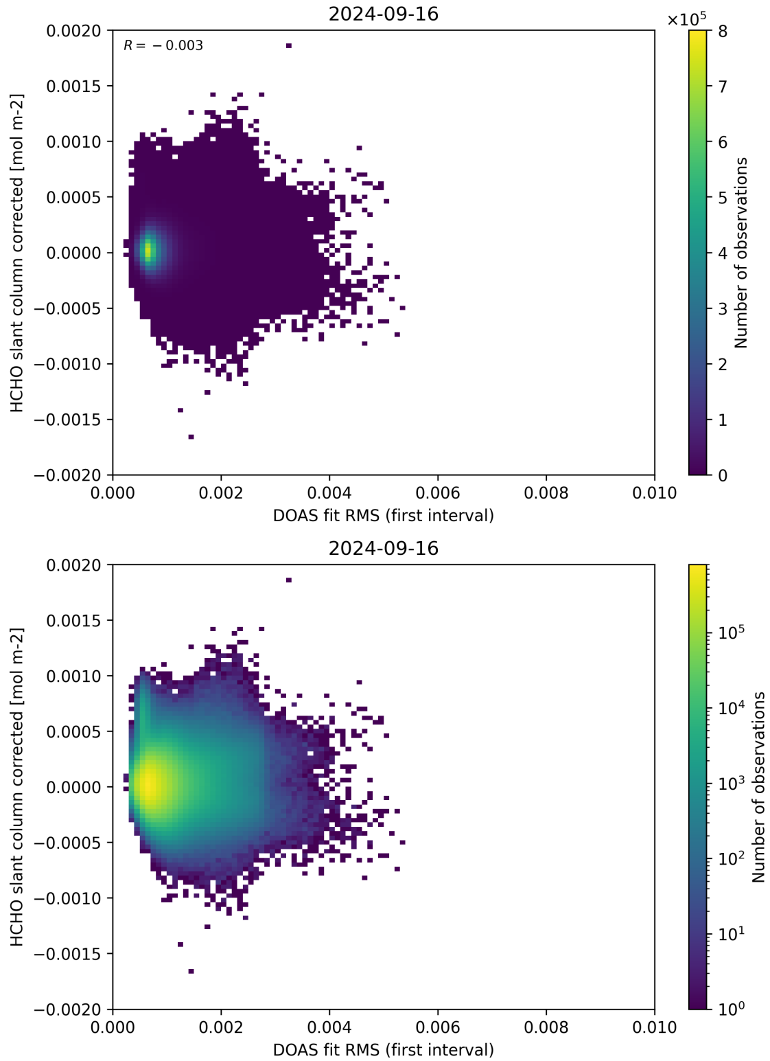
Figure 62: Scatter density plot of “DOAS fit RMS (first interval)” against “HCHO slant column corrected” for 2024-09-15 to 2024-09-17.
