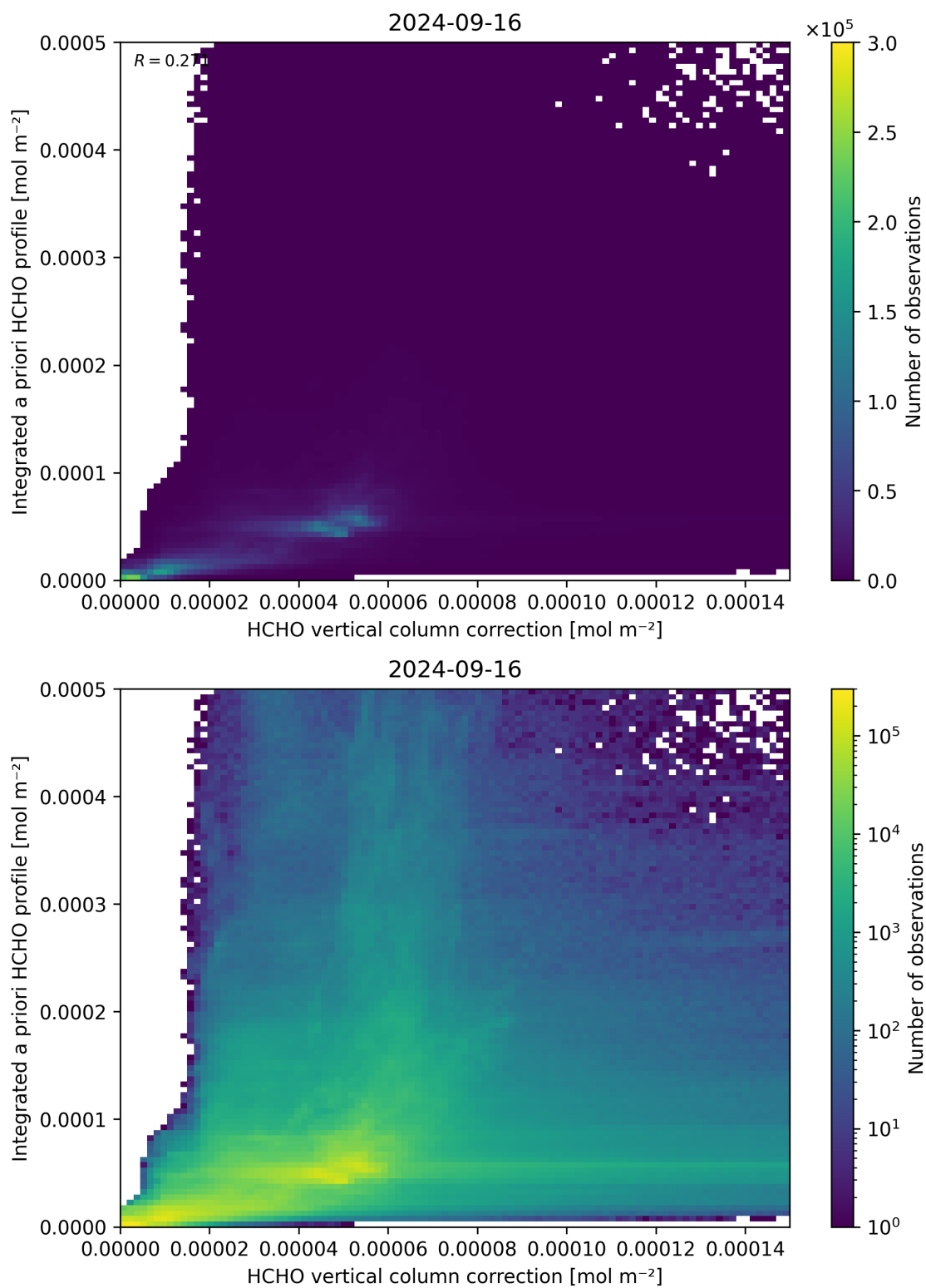
Figure 122: Scatter density plot of “HCHO vertical column correction” against “Integrated a priori HCHO profile” for 2024-09-15 to 2024-09-17.
