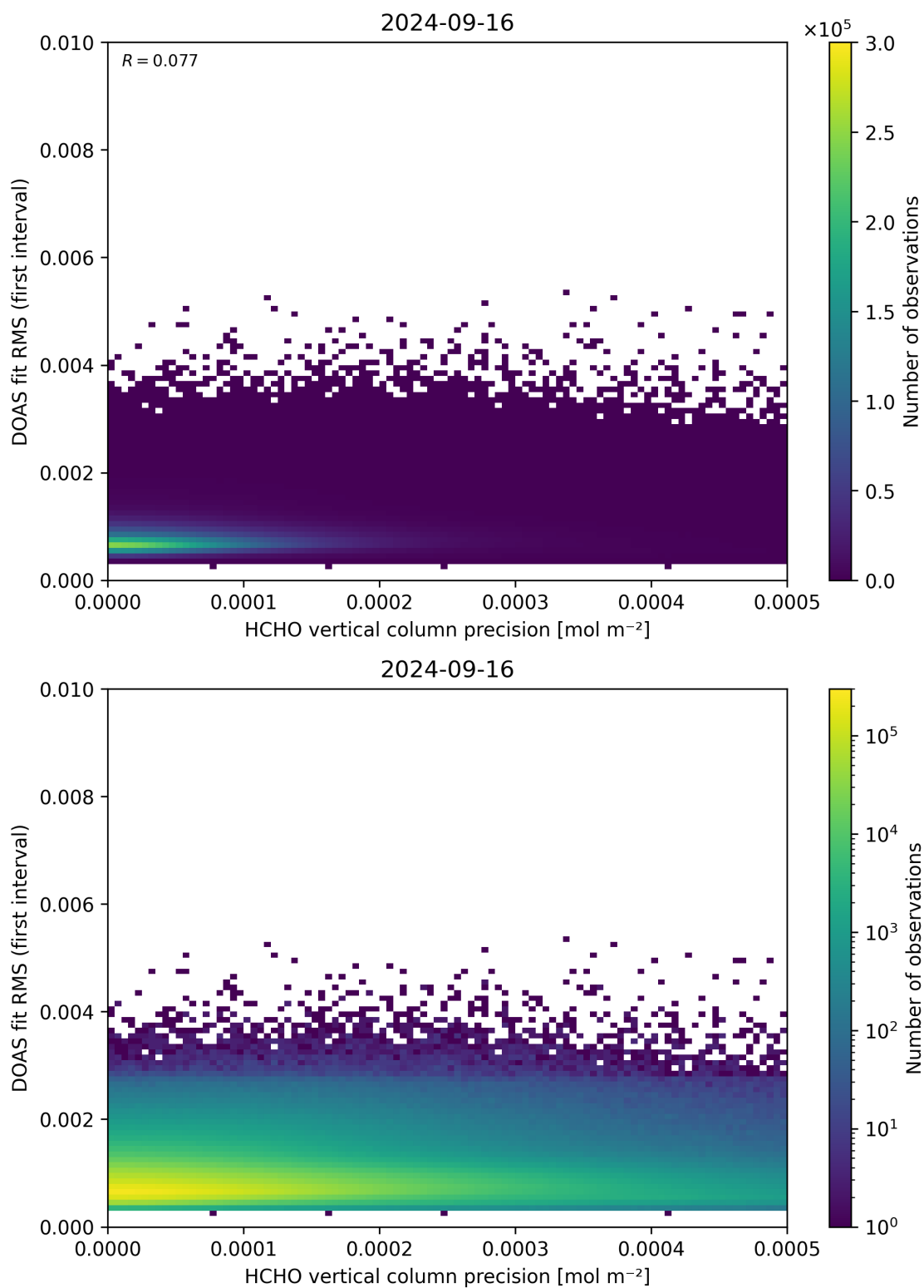
Figure 136: Scatter density plot of “HCHO vertical column precision” against “DOAS fit RMS (first interval)” for 2024-09-15 to 2024-09-17.
