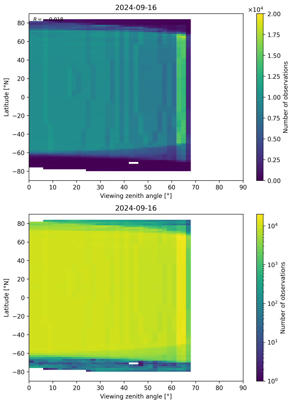
Figure 196: Scatter density plot of “Viewing zenith angle” against “Latitude” for 2024-09-15 to 2024-09-17.
