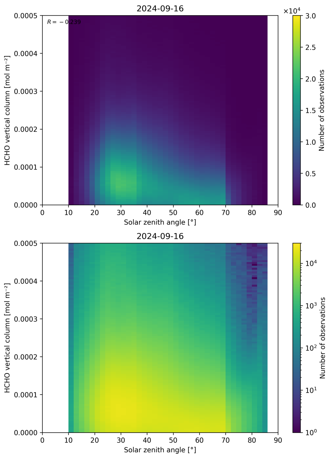
Figure 177: Scatter density plot of “Solar zenith angle” against “HCHO vertical column” for 2024-09-15 to 2024-09-17.
