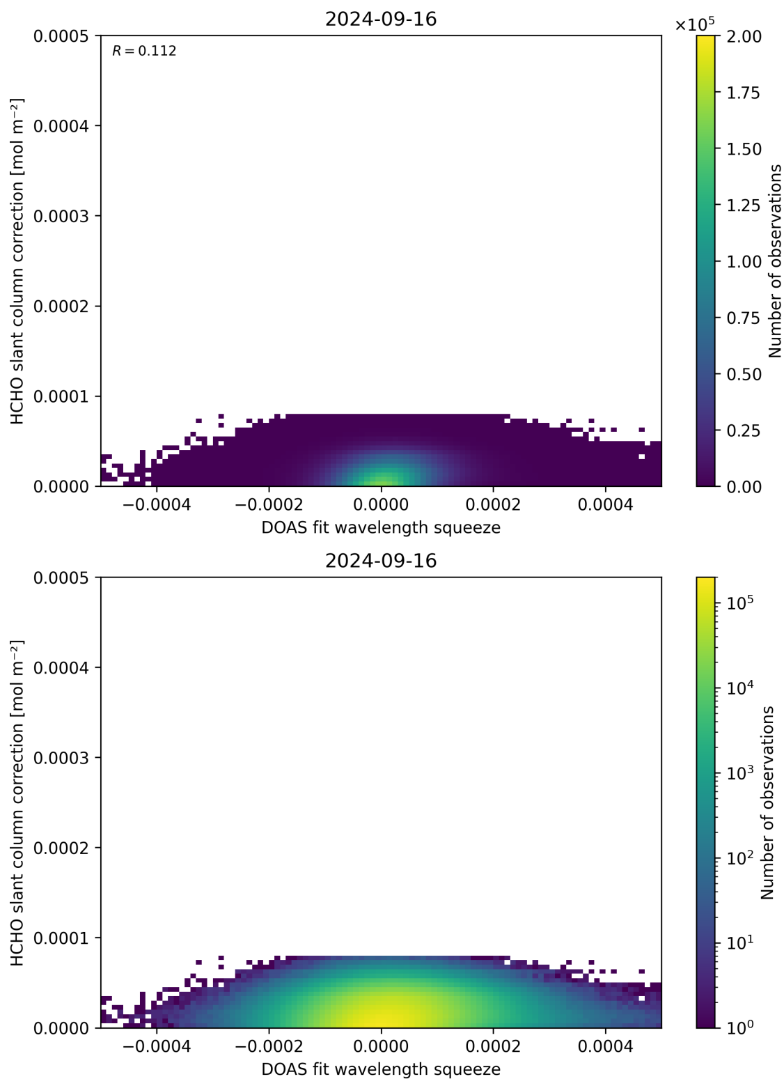
Figure 70: Scatter density plot of “DOAS fit wavelength squeeze” against “HCHO slant column correction” for 2024-09-15 to 2024-09-17.
