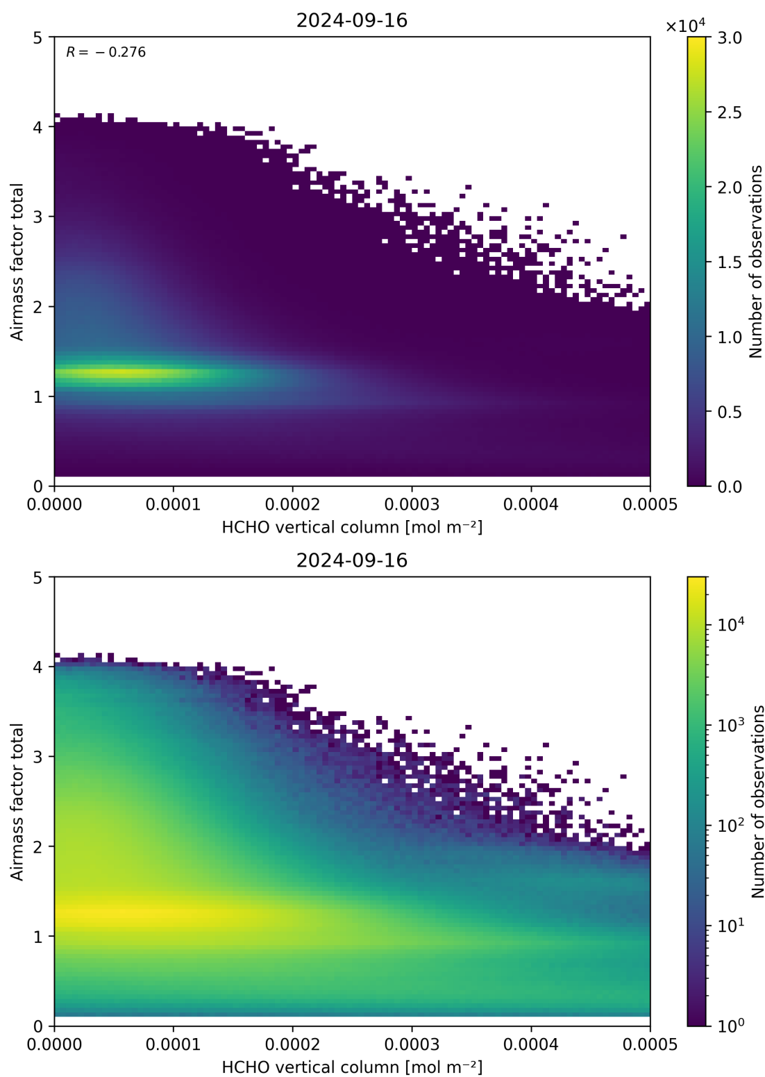
Figure 131: Scatter density plot of “HCHO vertical column” against “Airmass factor total” for 2024-09-15 to 2024-09-17.
