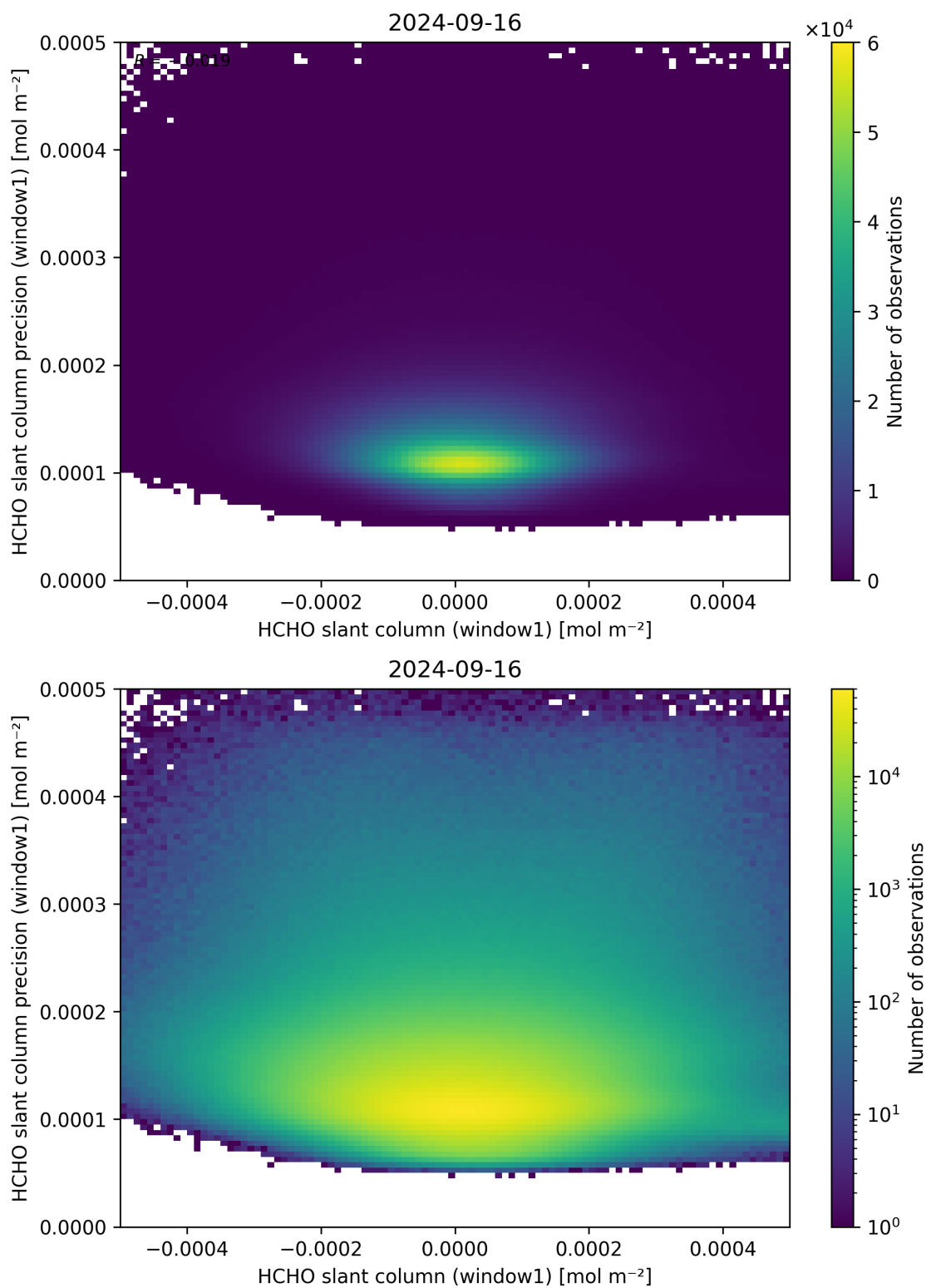
Figure 84: Scatter density plot of “HCHO slant column (window1)” against “HCHO slant column precision (window1)” for 2024-09-15 to 2024-09-17.
