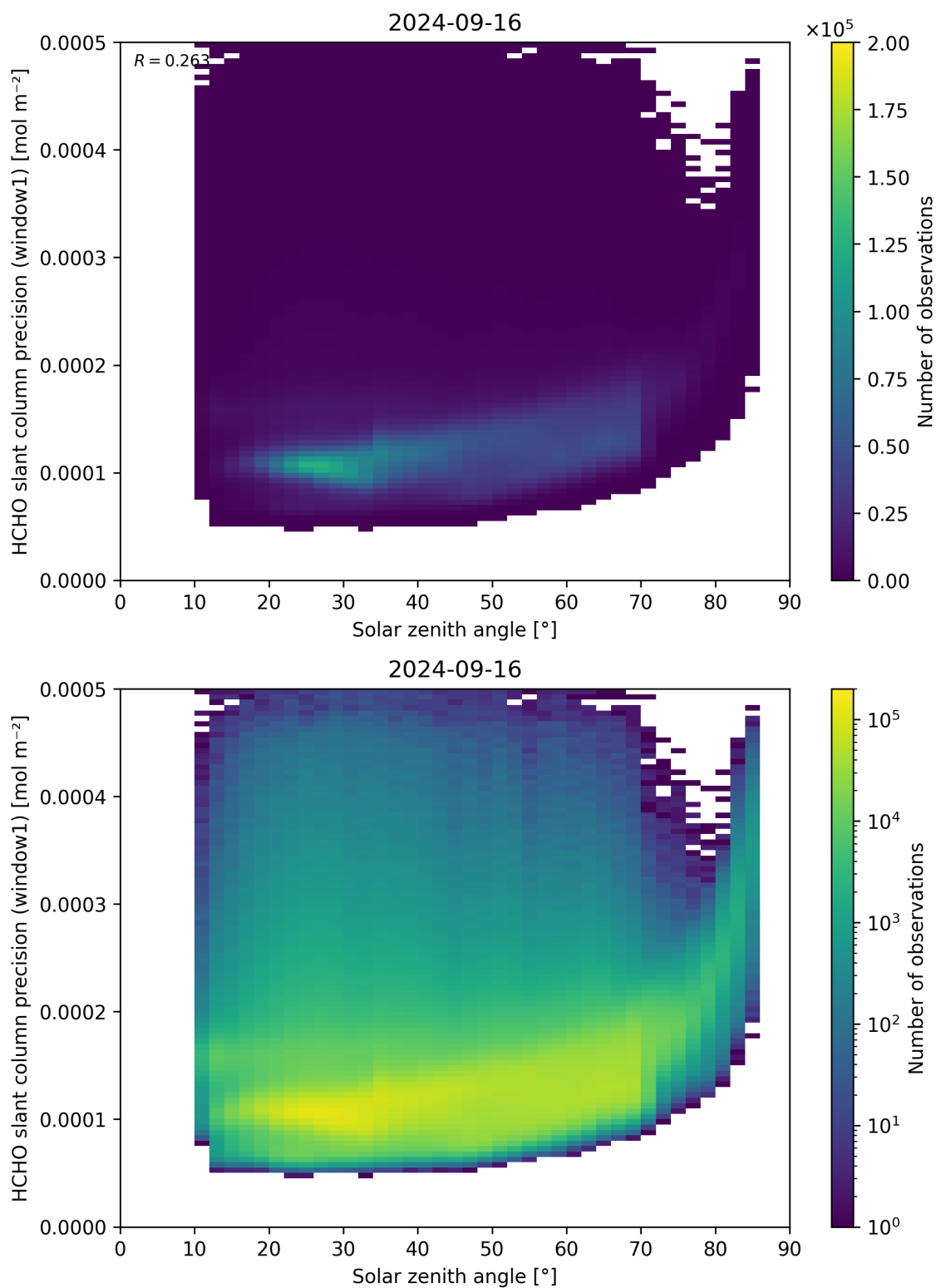
Figure 174: Scatter density plot of “Solar zenith angle” against “HCHO slant column precision (window1)” for 2024-09-15 to 2024-09-17.
