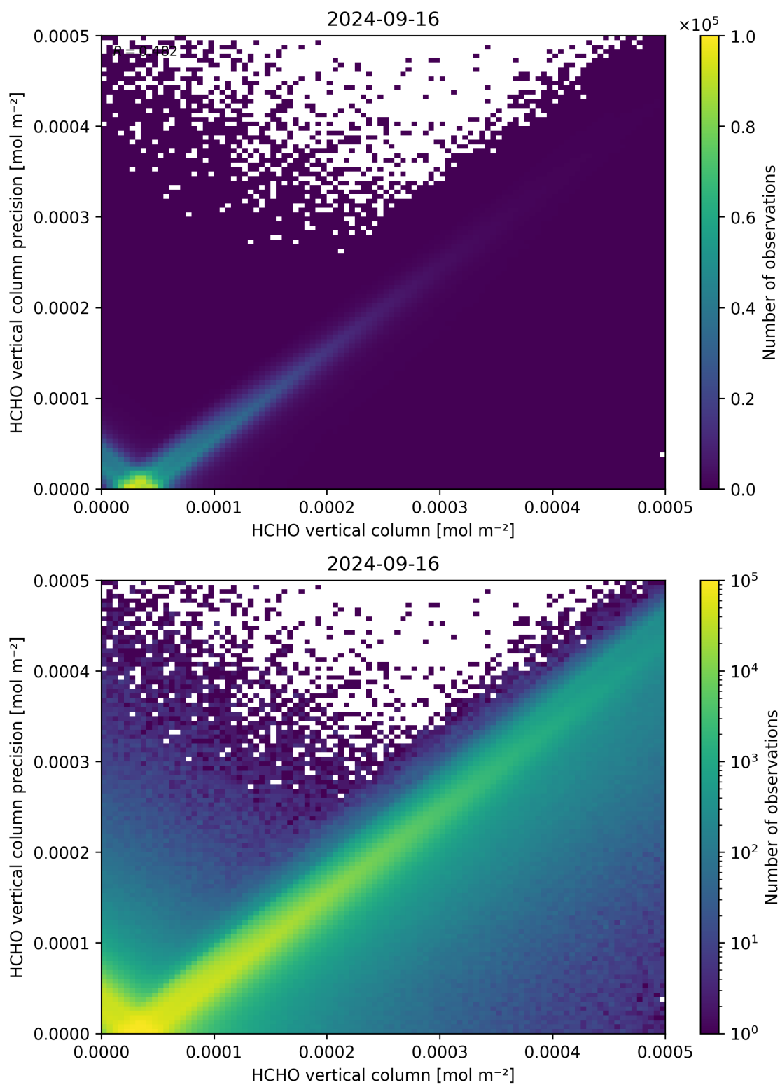
Figure 134: Scatter density plot of “HCHO vertical column” against “HCHO vertical column precision” for 2024-09-15 to 2024-09-17.
