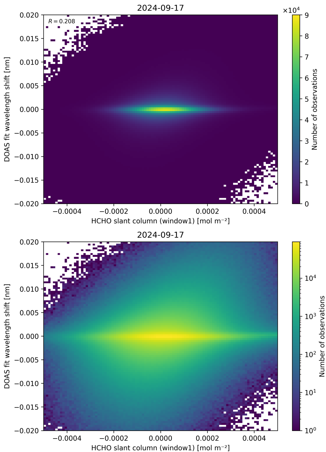
Figure 79: Scatter density plot of “HCHO slant column (window1)” against “DOAS fit wavelength shift” for 2024-09-17 to 2024-09-18.
