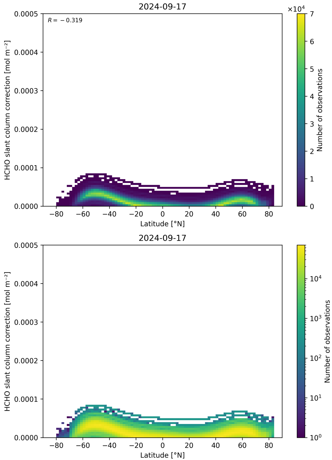
Figure 158: Scatter density plot of “Latitude” against “HCHO slant column correction” for 2024-09-17 to 2024-09-18.
