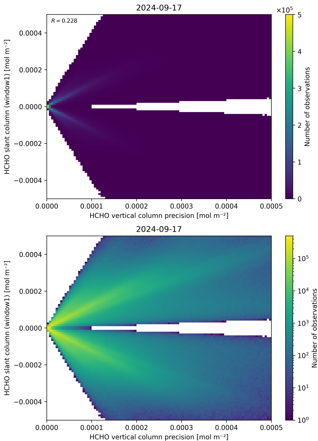
Figure 142: Scatter density plot of “HCHO vertical column precision” against “HCHO slant column (window1)” for 2024-09-17 to 2024-09-18.
