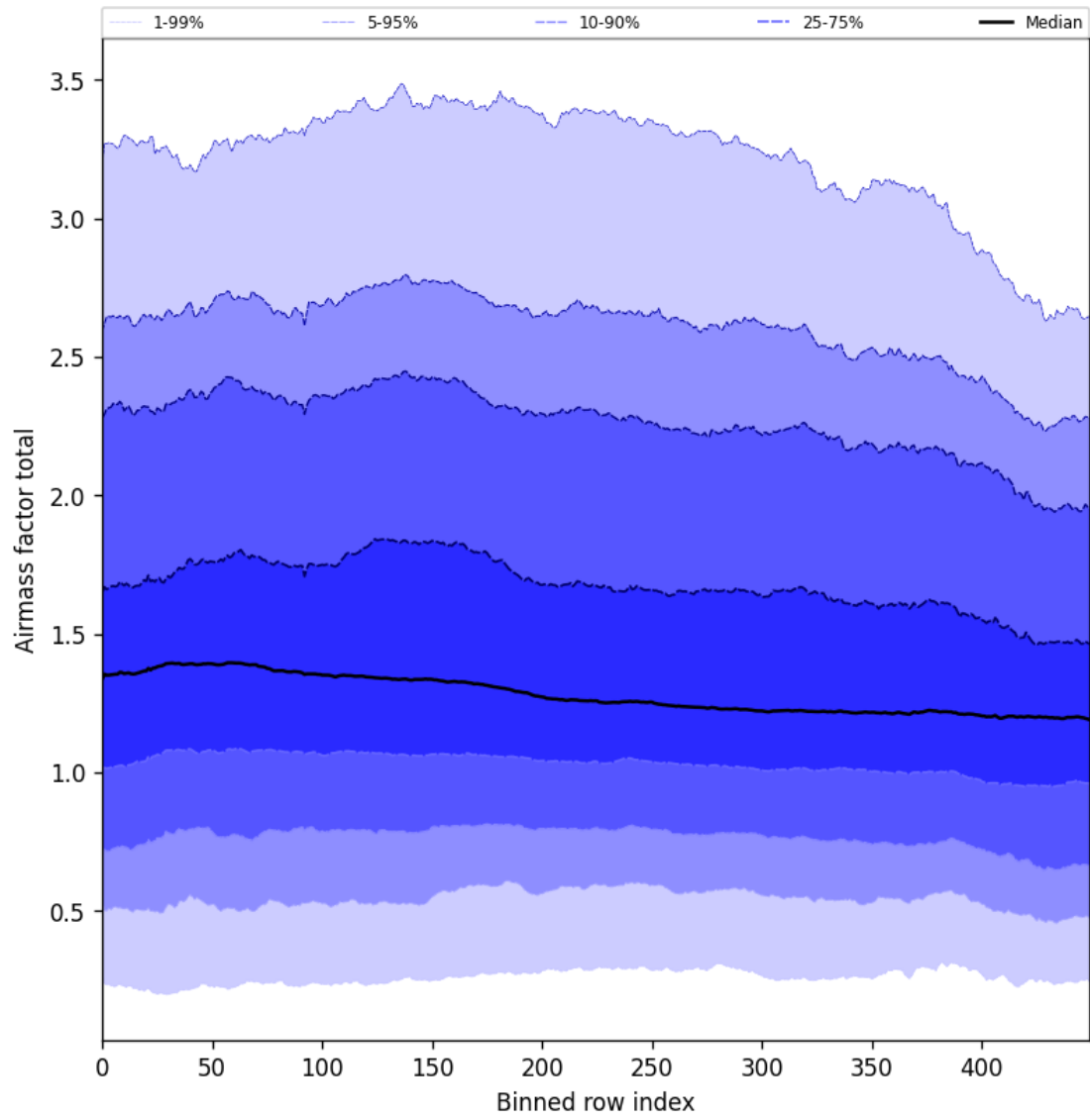
Figure 54: Along track statistics of “Airmass factor total” for 2024-09-17 to 2024-09-18
