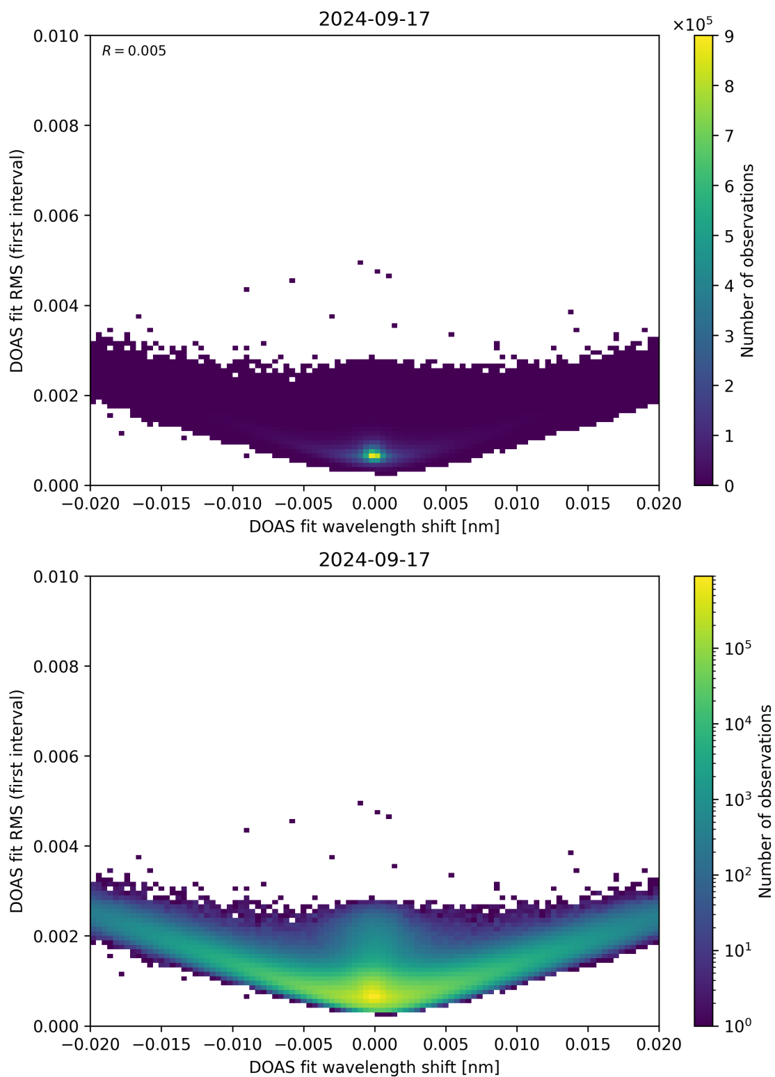
Figure 64: Scatter density plot of “DOAS fit wavelength shift” against “DOAS fit RMS (first interval)” for 2024-09-17 to 2024-09-18.
