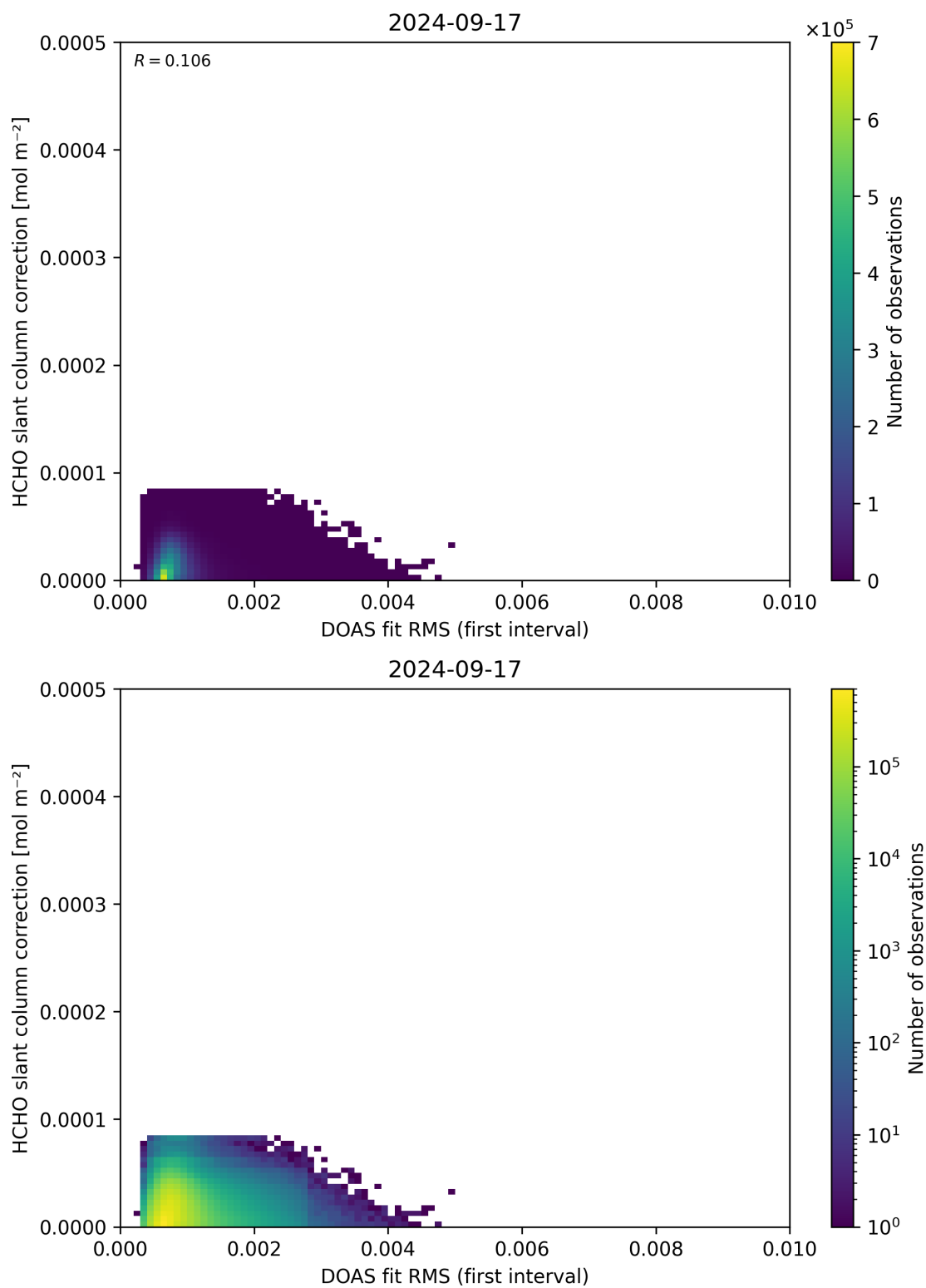
Figure 63: Scatter density plot of “DOAS fit RMS (first interval)” against “HCHO slant column correction” for 2024-09-17 to 2024-09-18.
