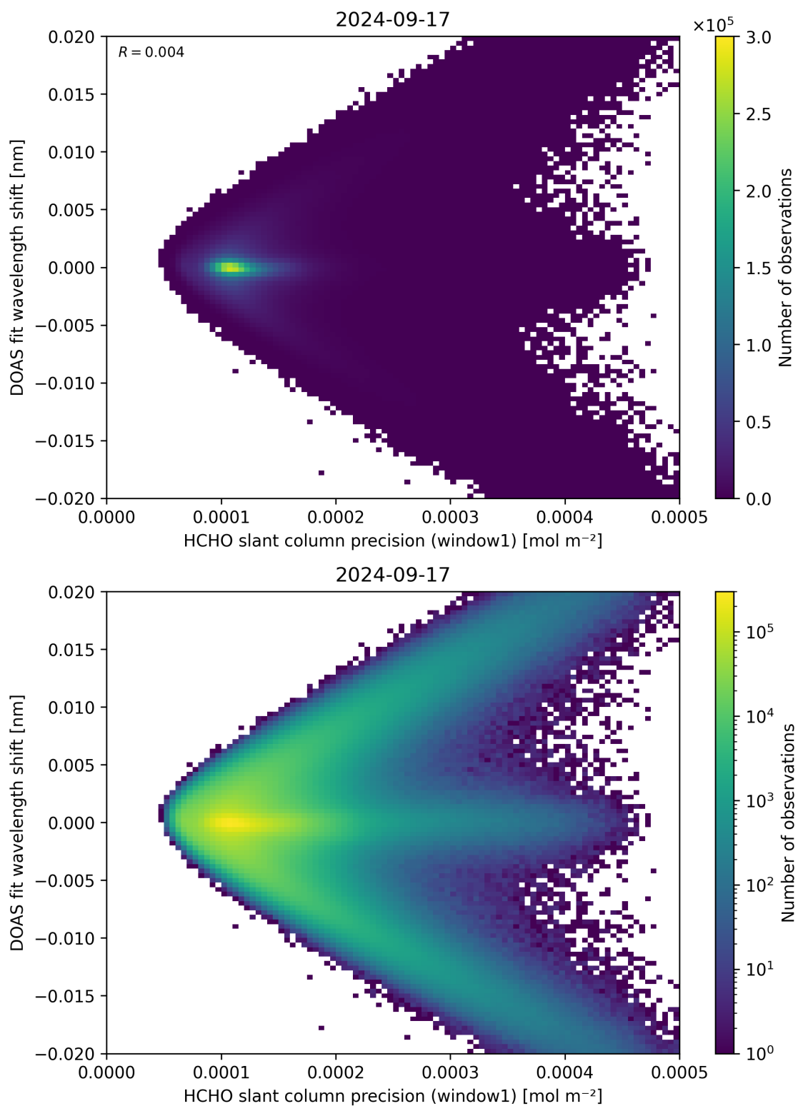
Figure 89: Scatter density plot of “HCHO slant column precision (window1)” against “DOAS fit wavelength shift” for 2024-09-17 to 2024-09-18.
