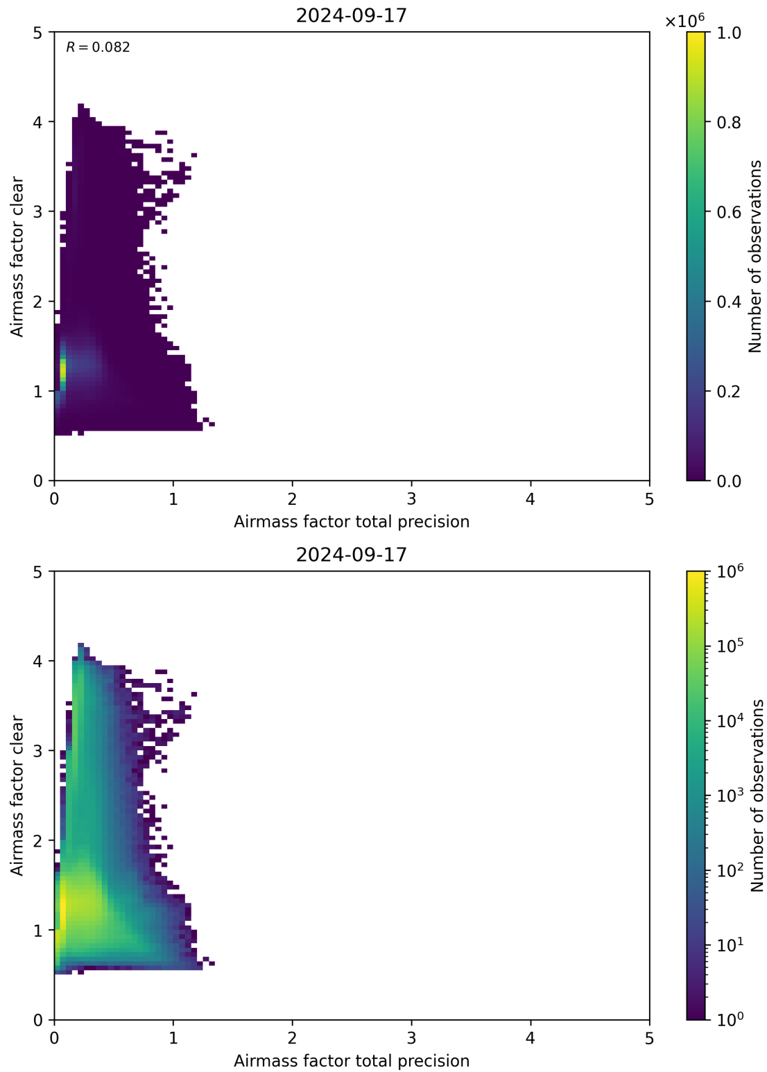
Figure 108: Scatter density plot of “Airmass factor total precision” against “Airmass factor clear” for 2024-09-17 to 2024-09-18.
