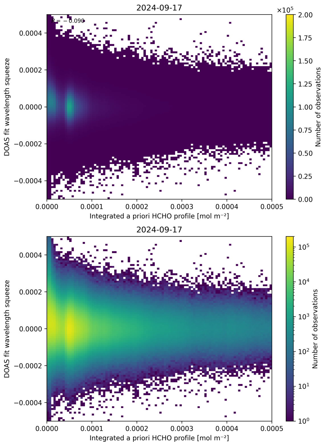
Figure 150: Scatter density plot of “Integrated a priori HCHO profile” against “DOAS fit wavelength squeeze” for 2024-09-17 to 2024-09-18.
