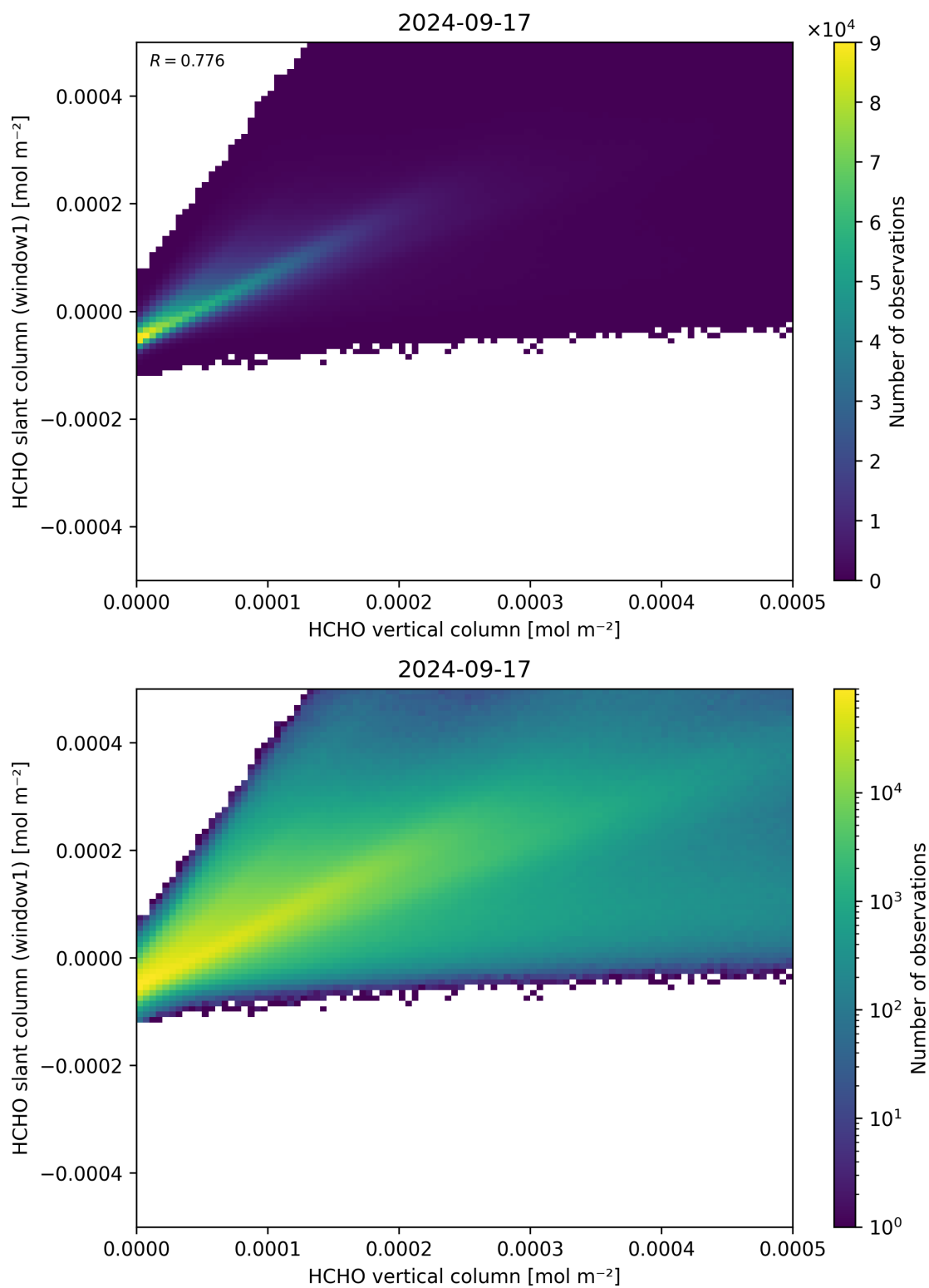
Figure 129: Scatter density plot of “HCHO vertical column” against “HCHO slant column (window1)” for 2024-09-17 to 2024-09-18.
