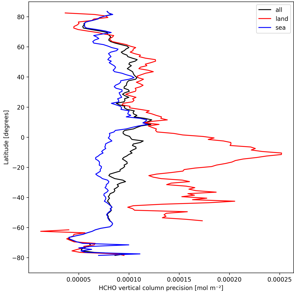
Figure 22: Zonal average of “HCHO vertical column precision” for 2024-09-17 to 2024-09-18.
