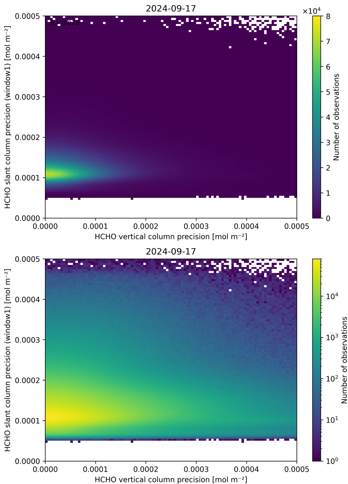
Figure 143: Scatter density plot of “HCHO vertical column precision” against “HCHO slant column precision (window1)” for 2024-09-17 to 2024-09-18.
