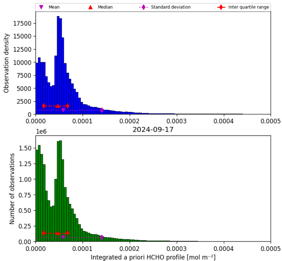
Figure 43: Histogram of “Integrated a priori HCHO profile” for 2024-09-17 to 2024-09-18
