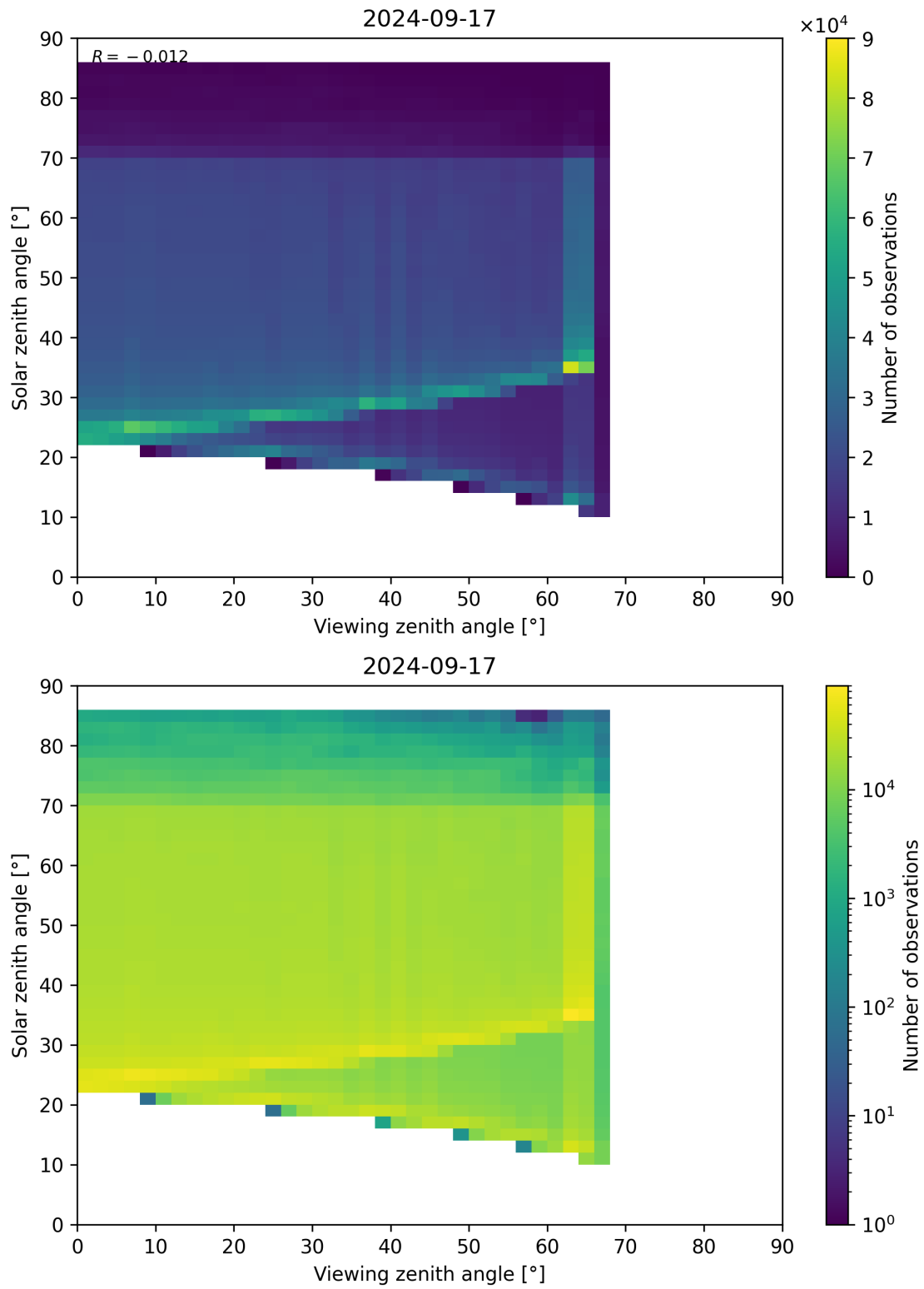
Figure 197: Scatter density plot of “Viewing zenith angle” against “Solar zenith angle” for 2024-09-17 to 2024-09-18.
