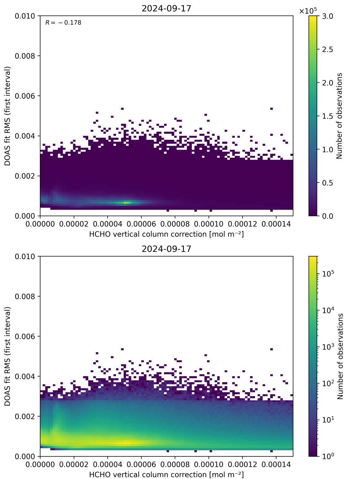
Figure 112: Scatter density plot of “HCHO vertical column correction” against “DOAS fit RMS (first interval)” for 2024-09-17 to 2024-09-18.
