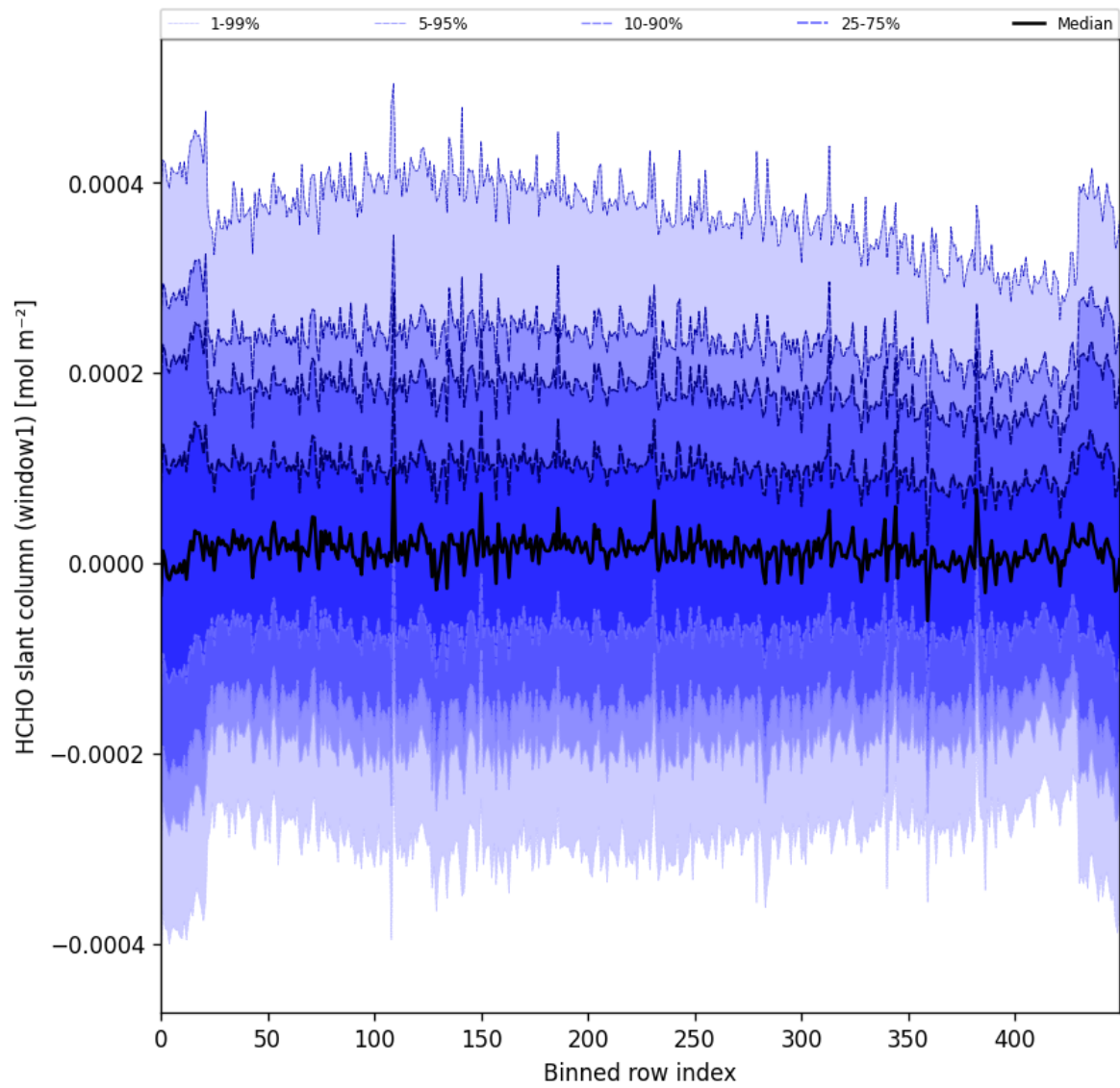
Figure 52: Along track statistics of “HCHO slant column (window1)” for 2024-09-17 to 2024-09-18
