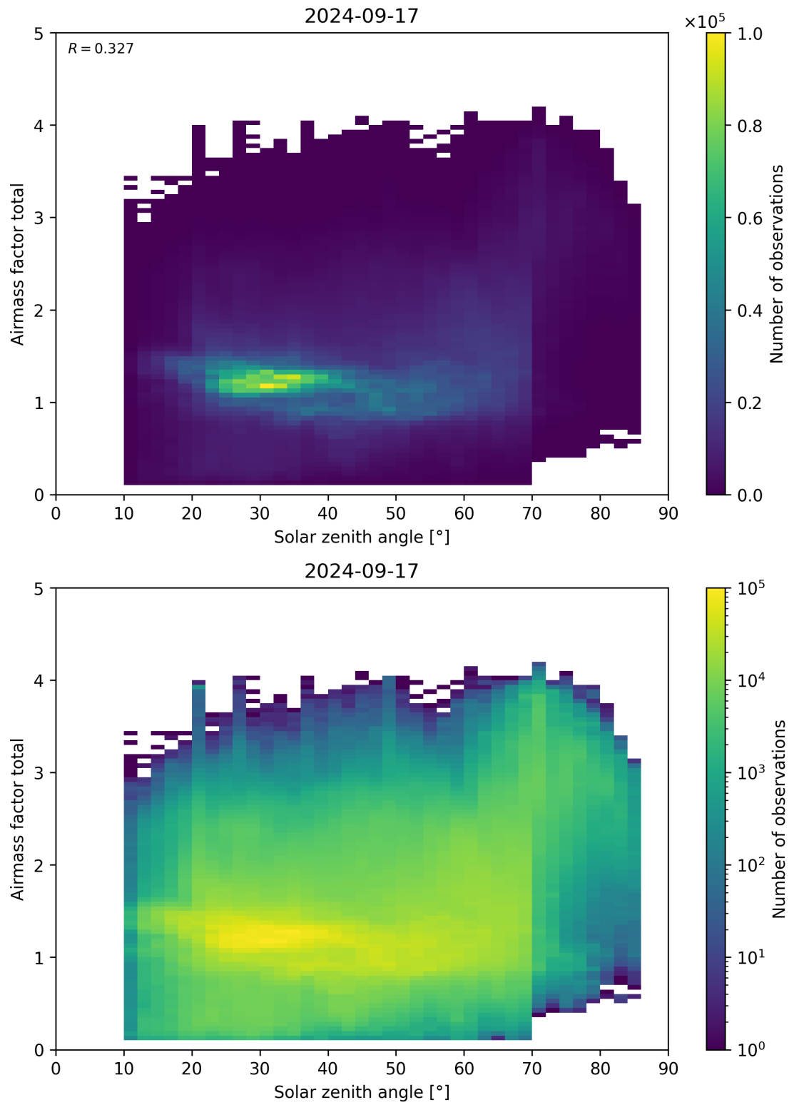
Figure 175: Scatter density plot of “Solar zenith angle” against “Airmass factor total” for 2024-09-17 to 2024-09-18.
