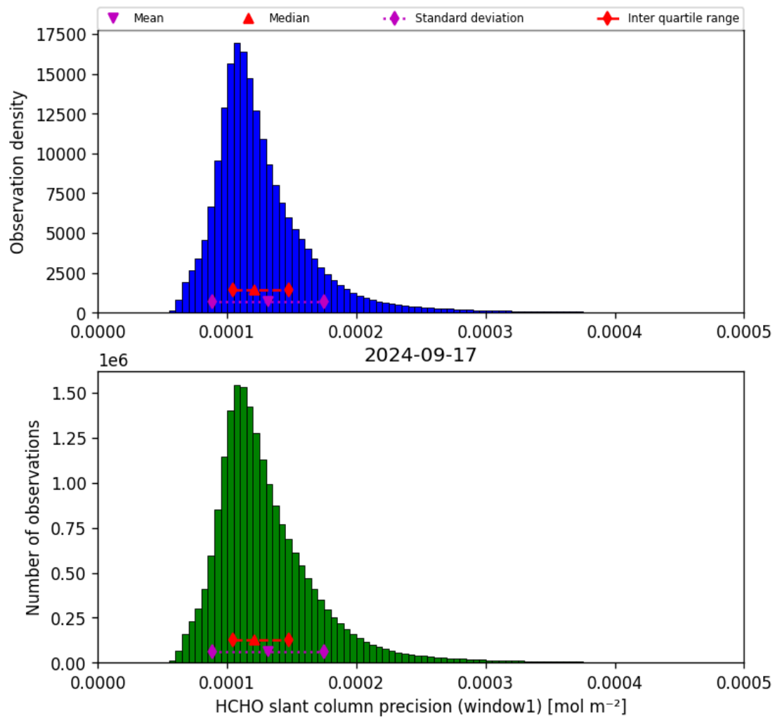
Figure 39: Histogram of “HCHO slant column precision (window1)” for 2024-09-17 to 2024-09-18
