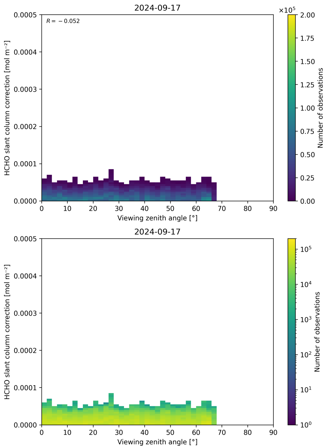
Figure 187: Scatter density plot of “Viewing zenith angle” against “HCHO slant column correction” for 2024-09-17 to 2024-09-18.
