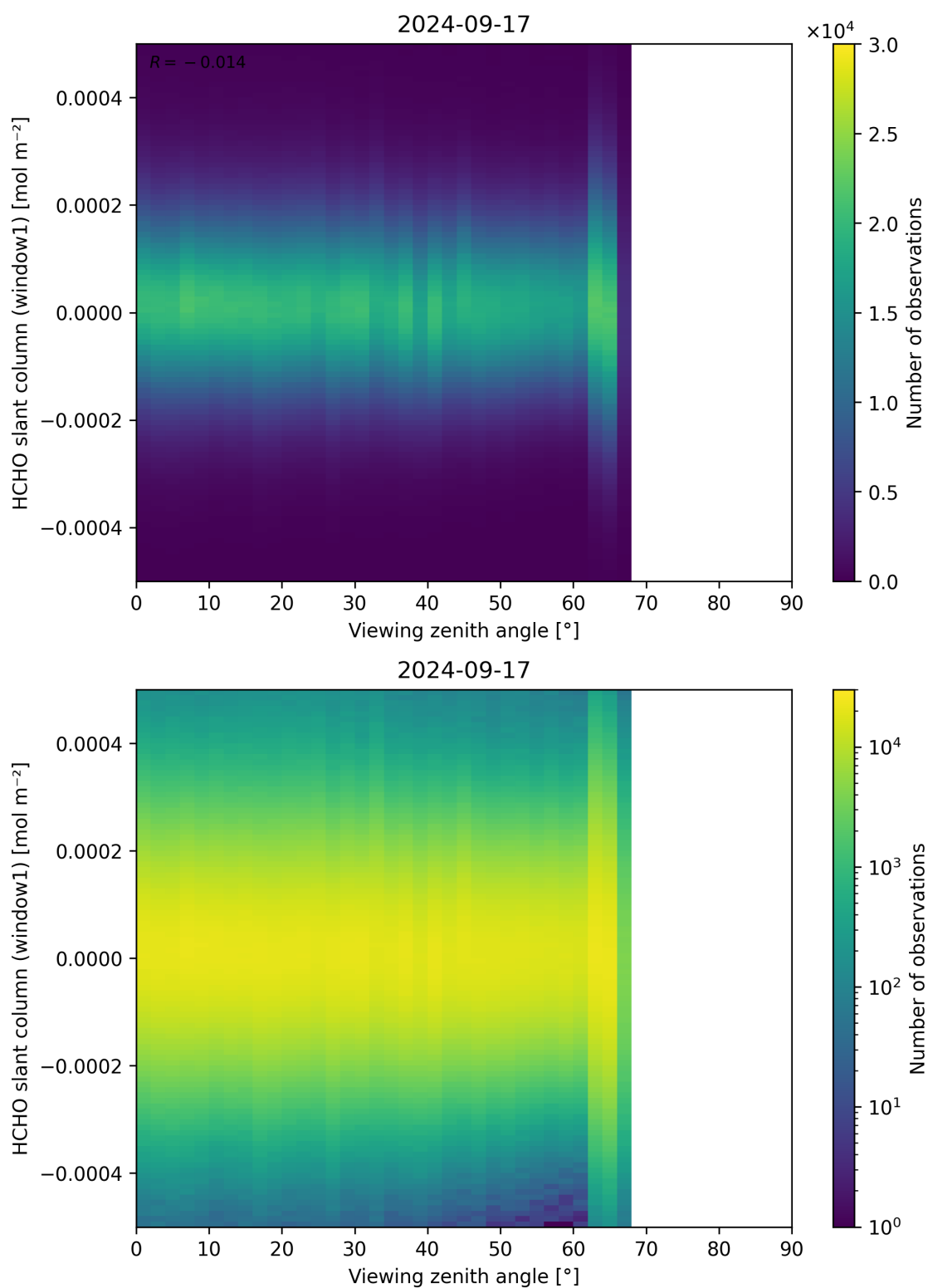
Figure 188: Scatter density plot of “Viewing zenith angle” against “HCHO slant column (window1)” for 2024-09-17 to 2024-09-18.
