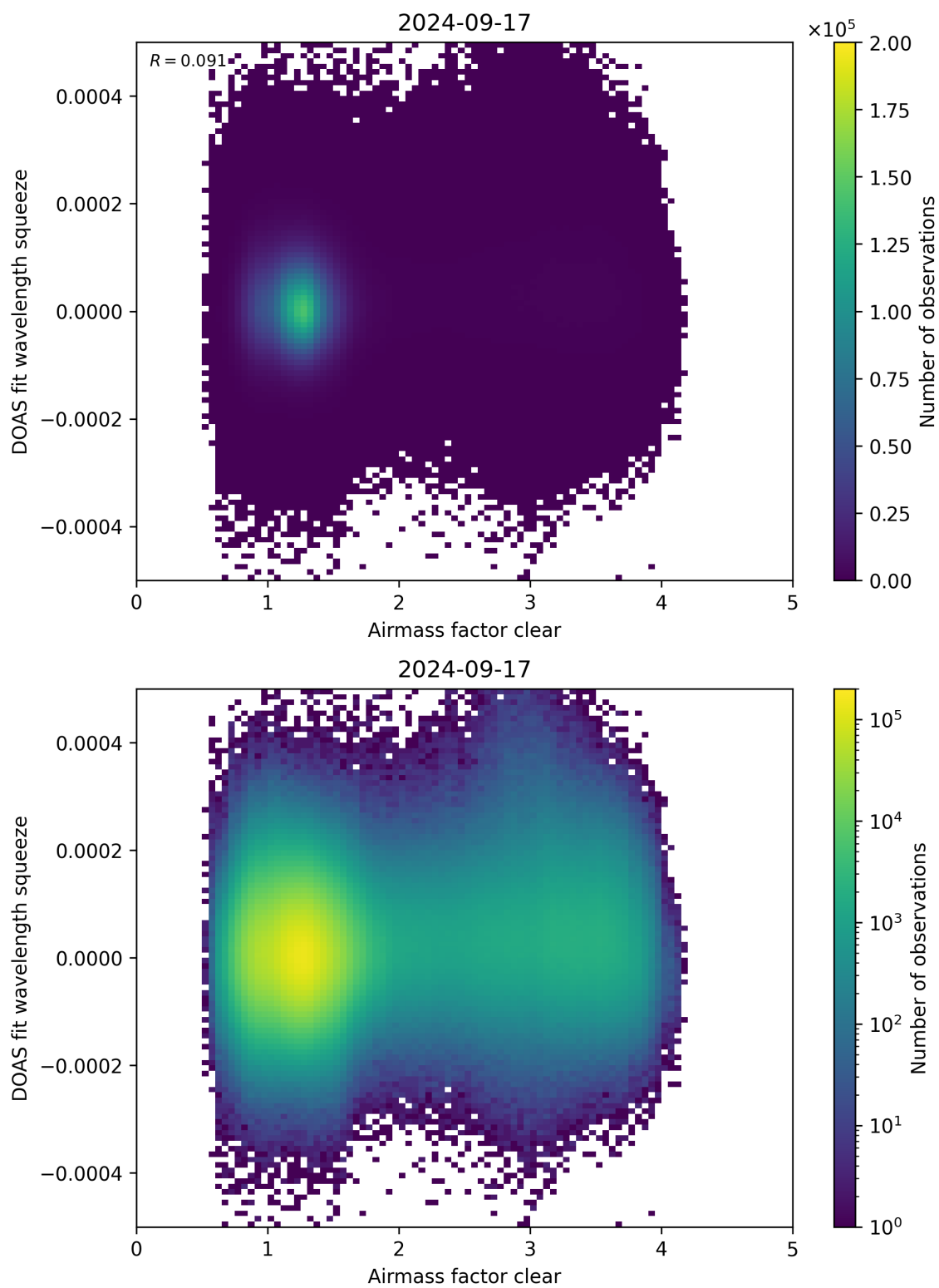
Figure 73: Scatter density plot of “Airmass factor clear” against “DOAS fit wavelength squeeze” for 2024-09-17 to 2024-09-18.
