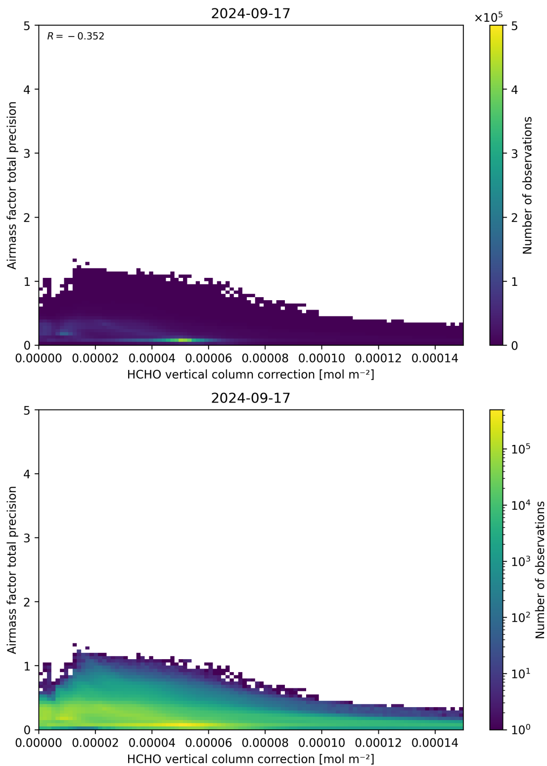
Figure 121: Scatter density plot of “HCHO vertical column correction” against “Airmass factor total precision” for 2024-09-17 to 2024-09-18.
