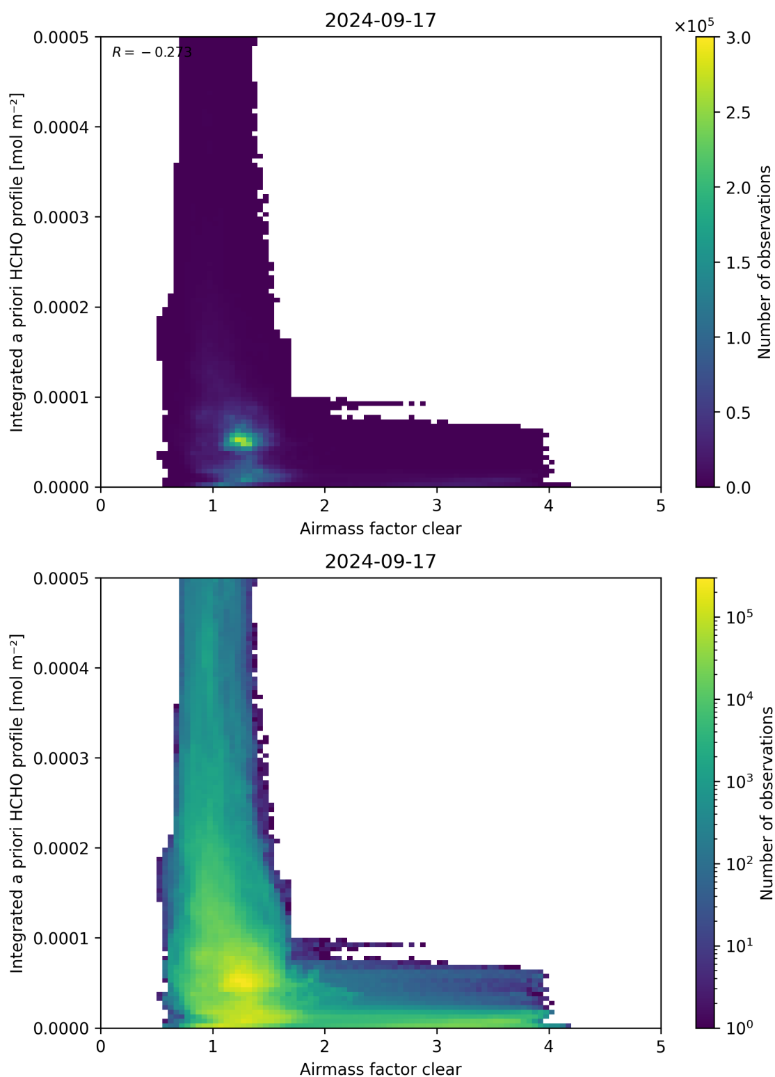
Figure 76: Scatter density plot of “Airmass factor clear” against “Integrated a priori HCHO profile” for 2024-09-17 to 2024-09-18.
