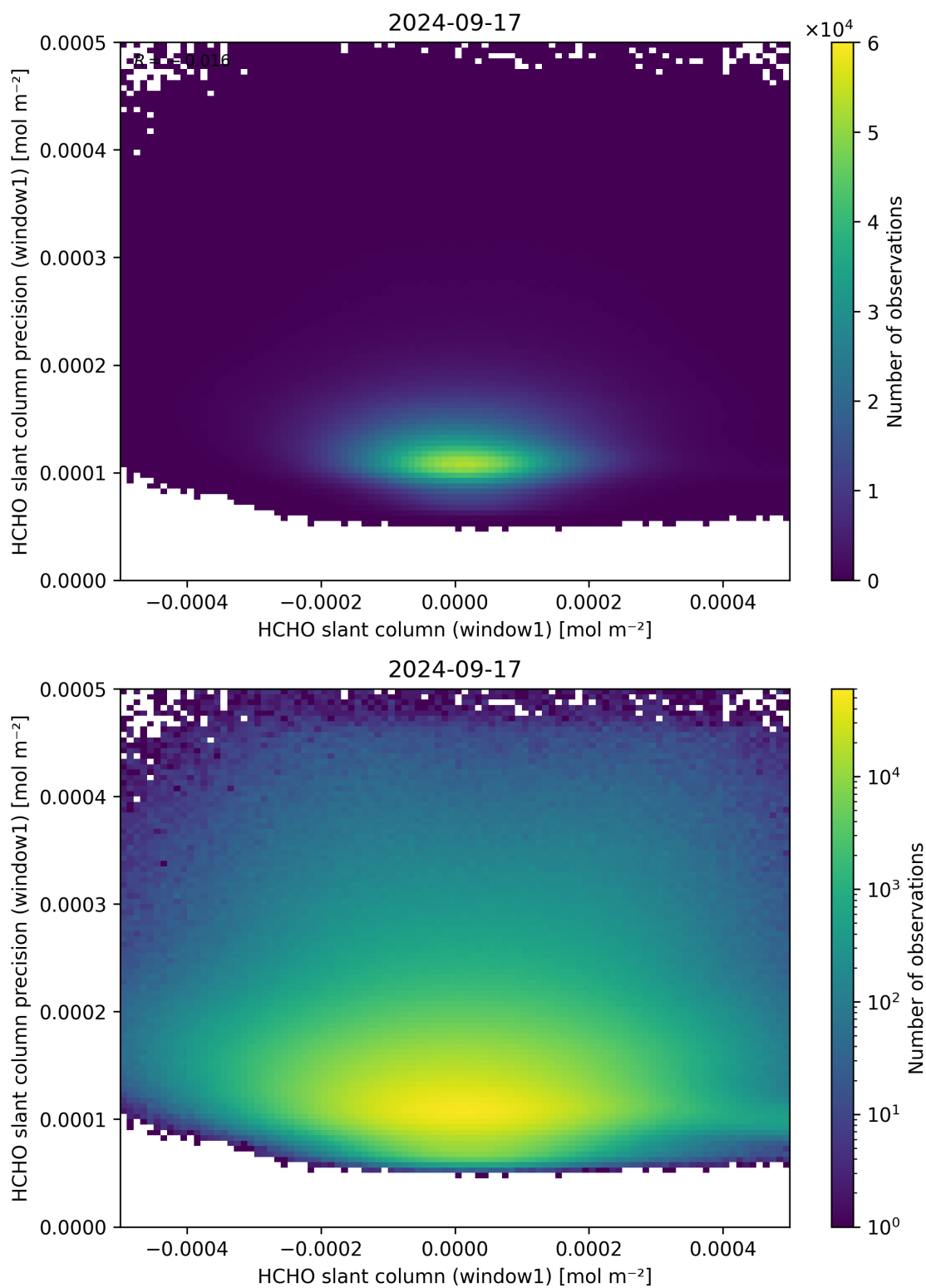
Figure 84: Scatter density plot of “HCHO slant column (window1)” against “HCHO slant column precision (window1)” for 2024-09-17 to 2024-09-18.
