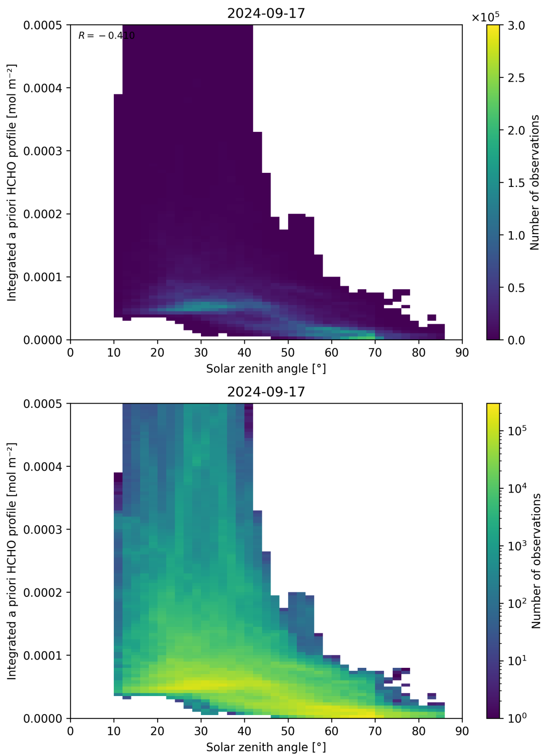
Figure 180: Scatter density plot of “Solar zenith angle” against “Integrated a priori HCHO profile” for 2024-09-17 to 2024-09-18.
