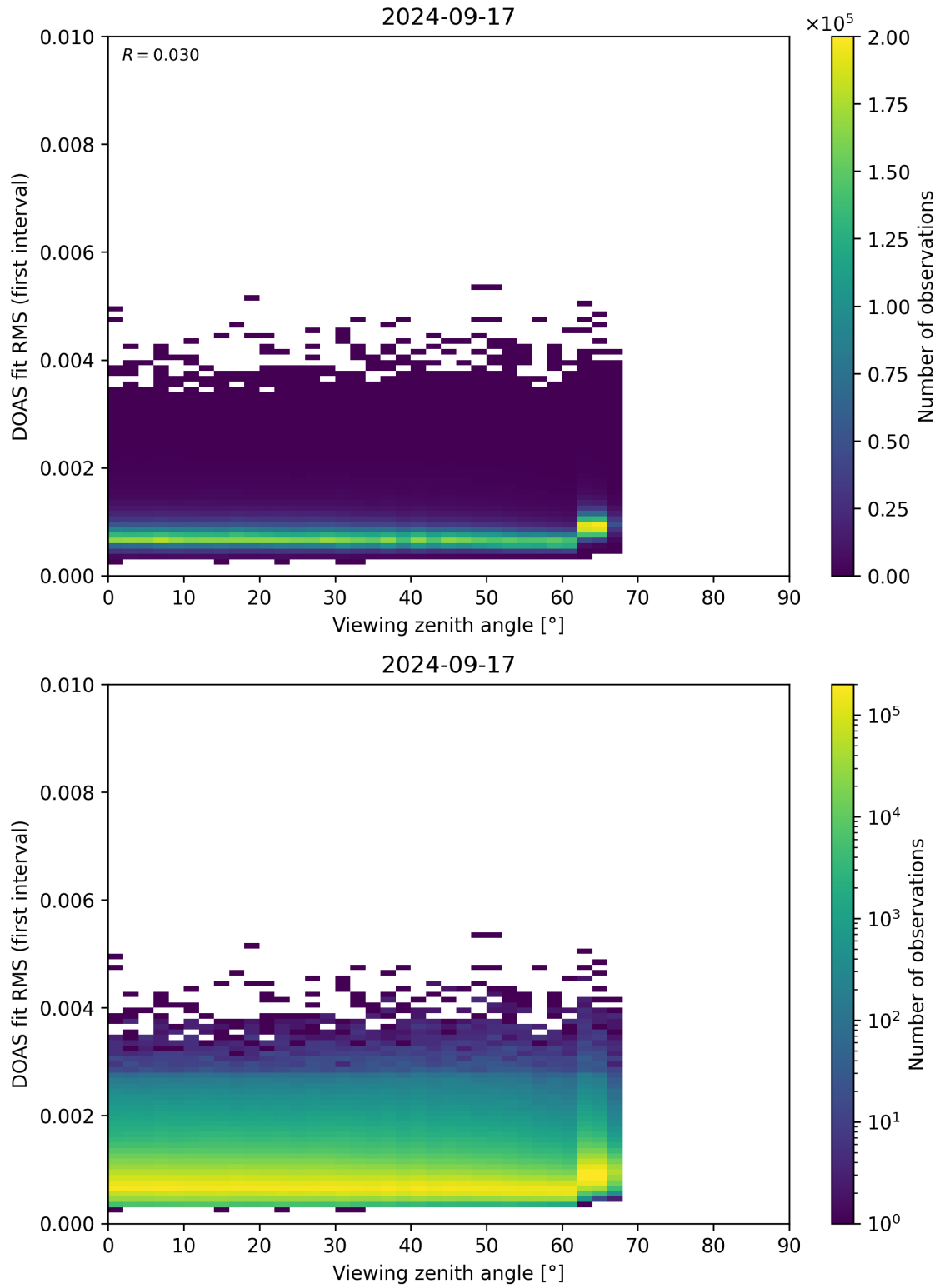
Figure 182: Scatter density plot of “Viewing zenith angle” against “DOAS fit RMS (first interval)” for 2024-09-17 to 2024-09-18.
