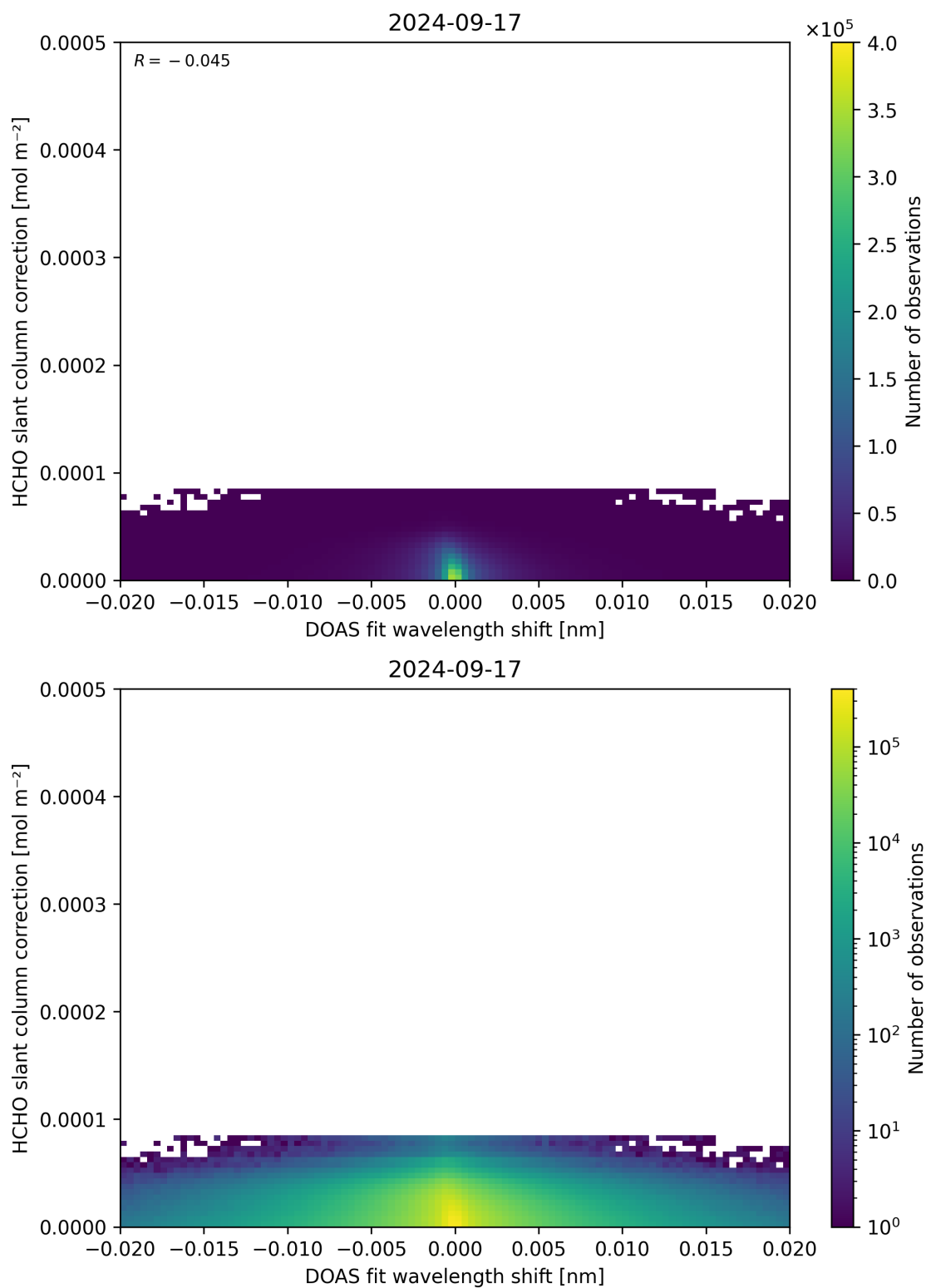
Figure 67: Scatter density plot of “DOAS fit wavelength shift” against “HCHO slant column correction” for 2024-09-17 to 2024-09-18.
