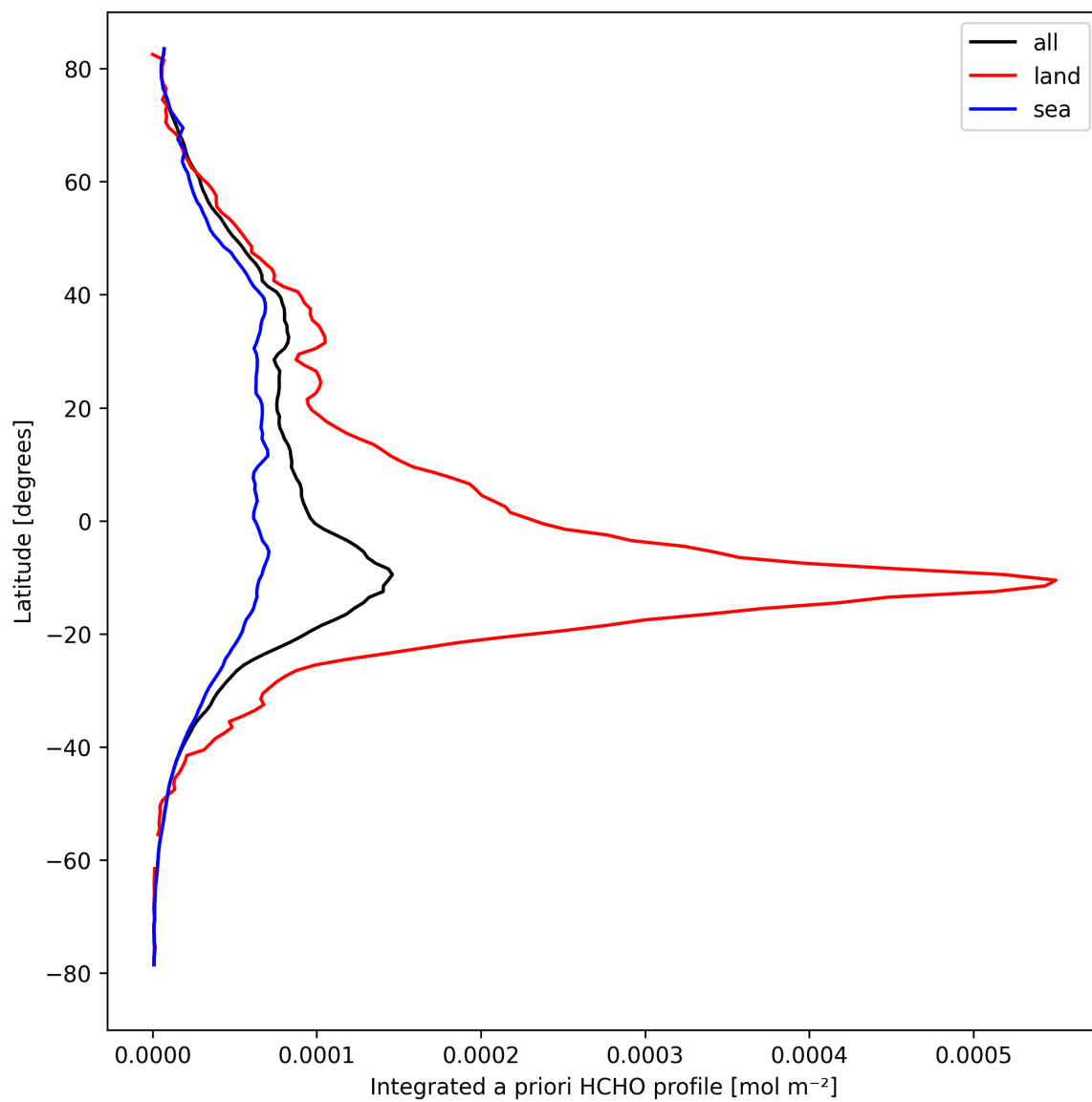
Figure 29: Zonal average of “Integrated a priori HCHO profile” for 2024-09-17 to 2024-09-18.
