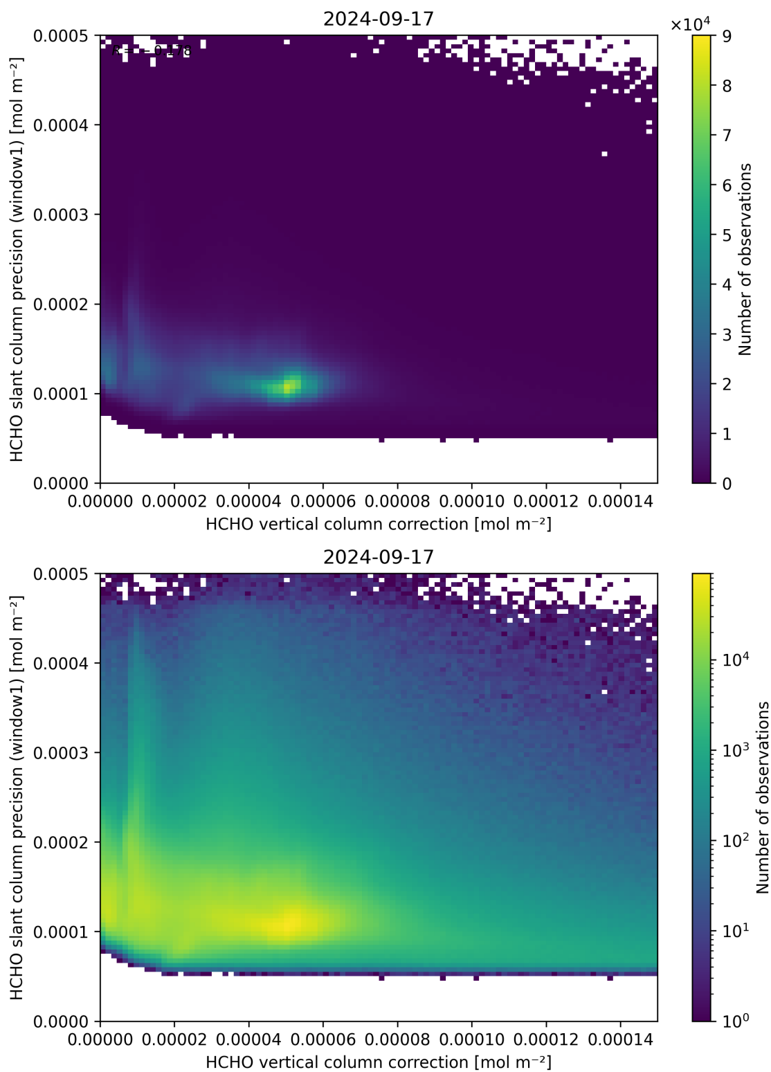
Figure 119: Scatter density plot of “HCHO vertical column correction” against “HCHO slant column precision (window1)” for 2024-09-17 to 2024-09-18.
