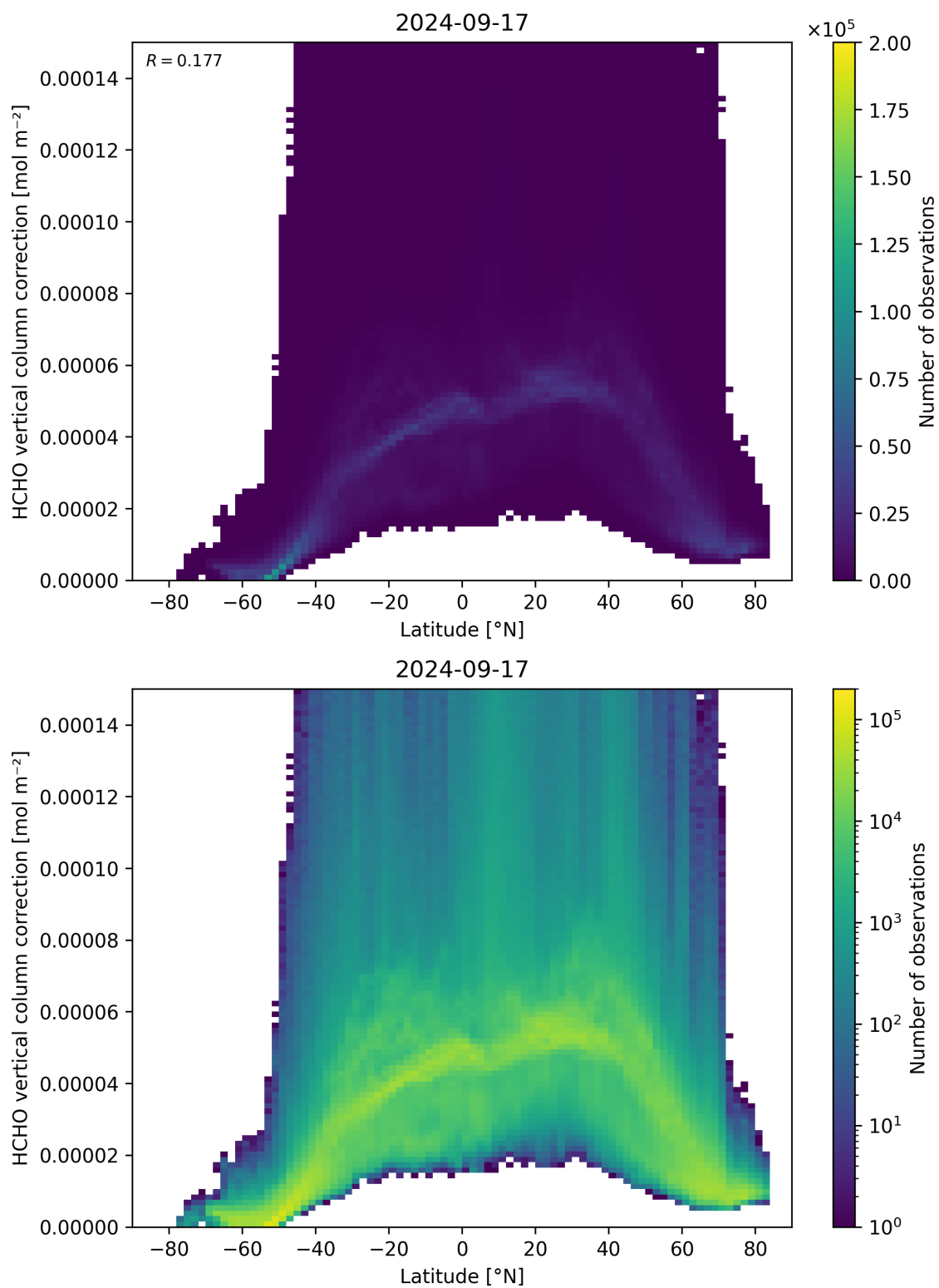
Figure 164: Scatter density plot of “Latitude” against “HCHO vertical column correction” for 2024-09-17 to 2024-09-18.
