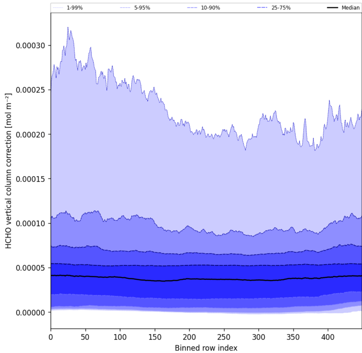
Figure 51: Along track statistics of “HCHO vertical column correction” for 2024-09-17 to 2024-09-18
