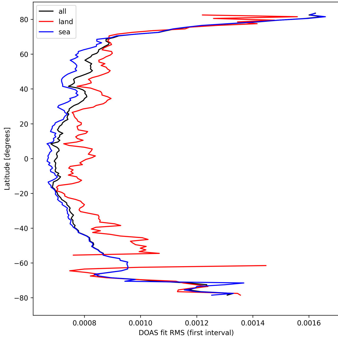
Figure 32: Zonal average of "DOAS fit RMS (first interval)" for 2024-09-17 to 2024-09-18.
