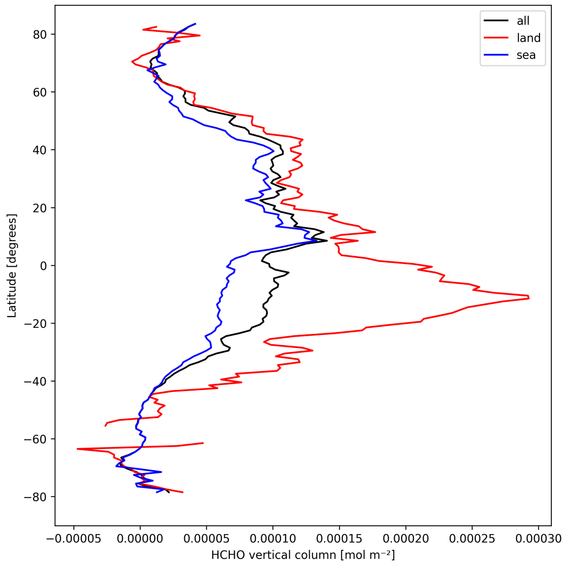
Figure 21: Zonal average of “HCHO vertical column” for 2024-09-17 to 2024-09-18.
