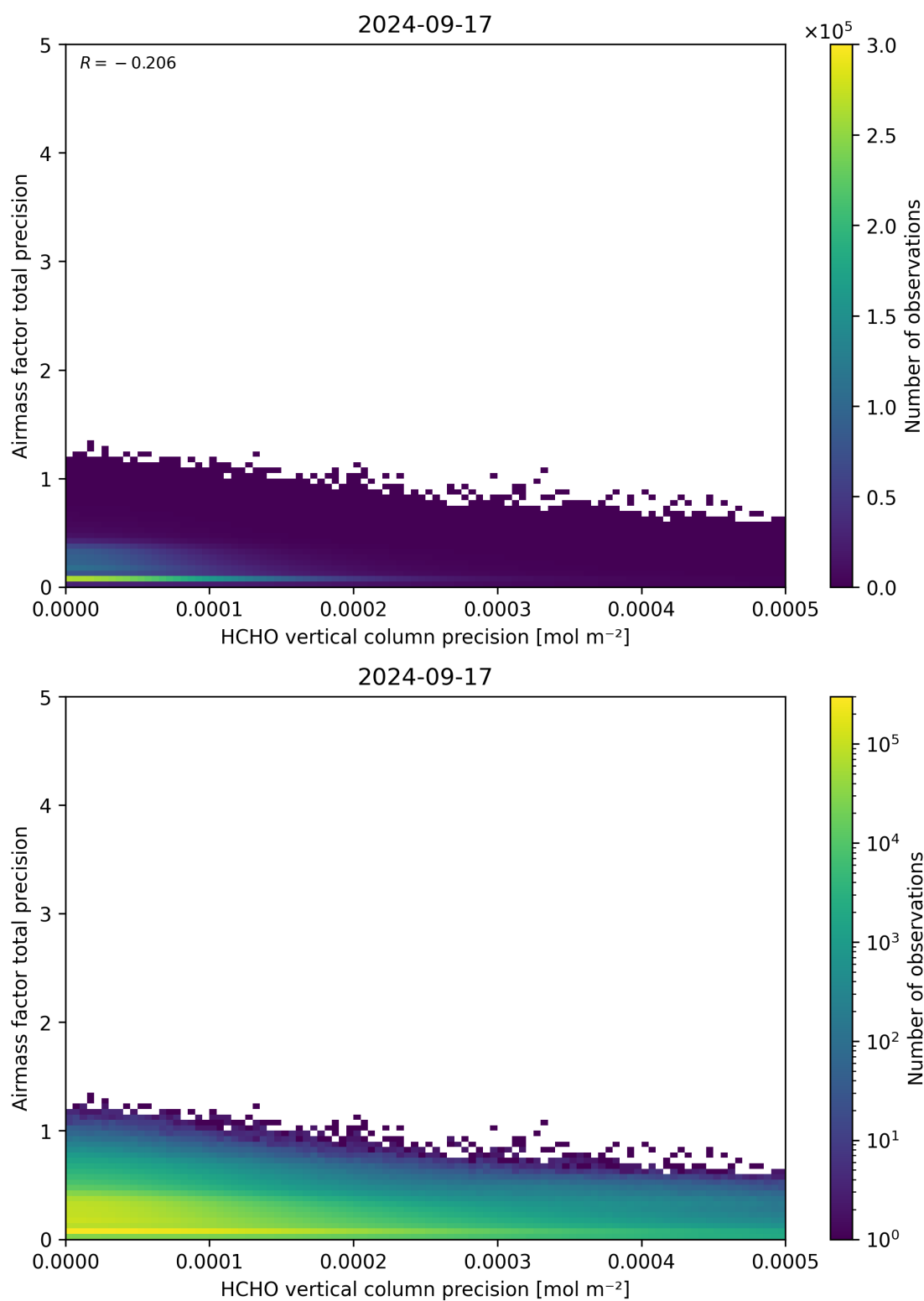
Figure 145: Scatter density plot of “HCHO vertical column precision” against “Airmass factor total precision” for 2024-09-17 to 2024-09-18.
