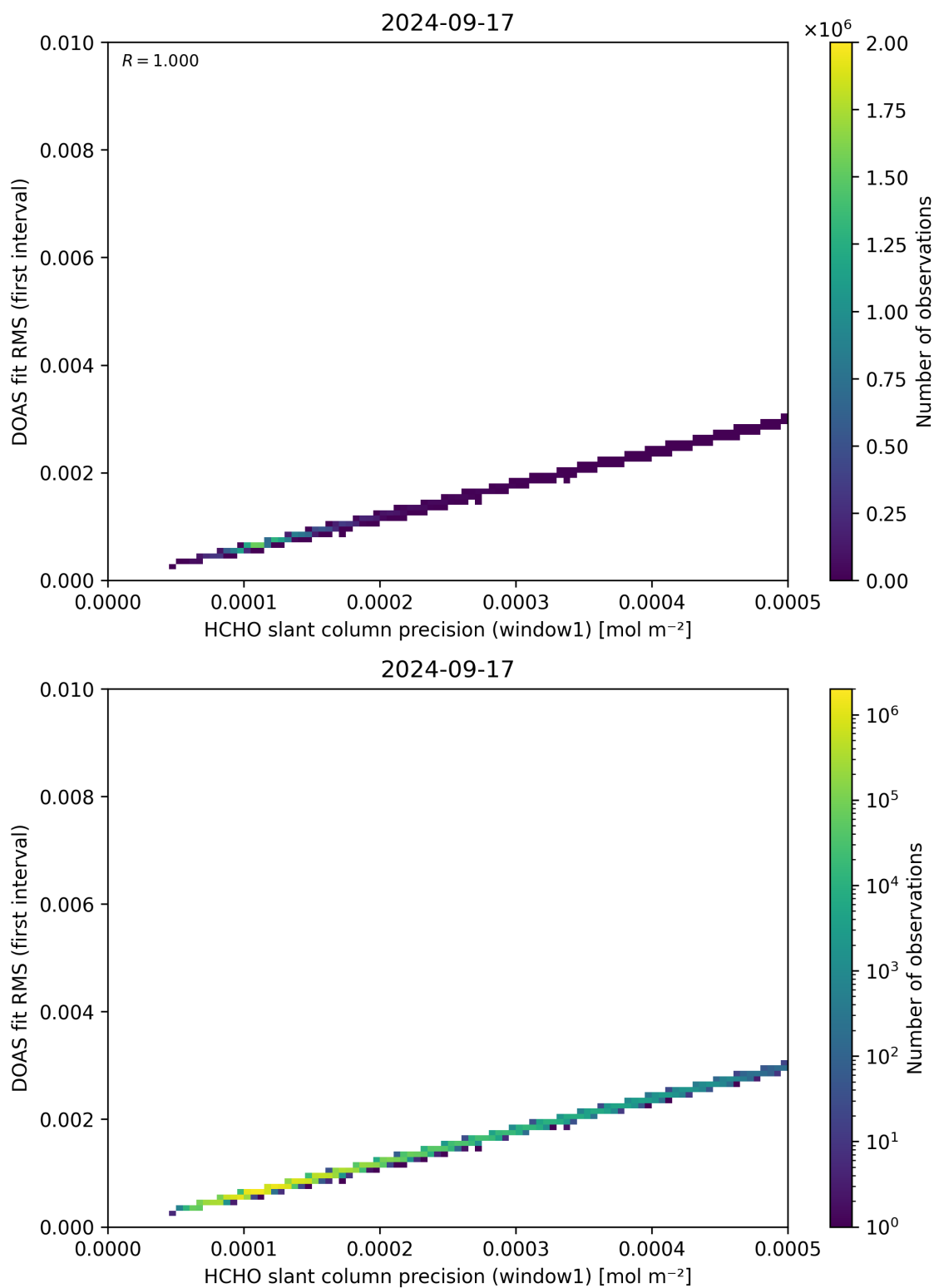
Figure 88: Scatter density plot of “HCHO slant column precision (window1)” against “DOAS fit RMS (first interval)” for 2024-09-17 to 2024-09-18.
