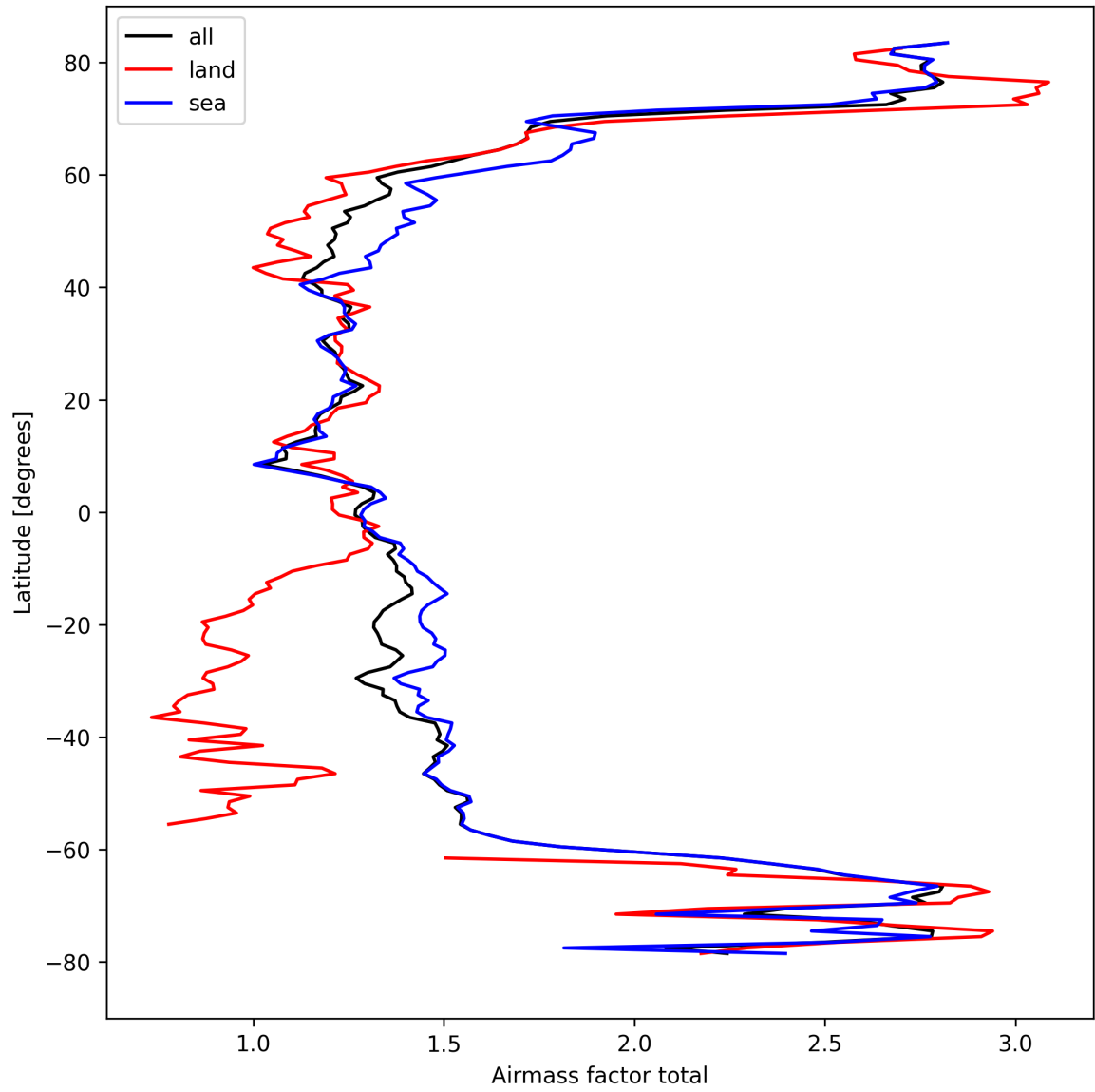
Figure 26: Zonal average of “Airmass factor total” for 2024-09-17 to 2024-09-18.
