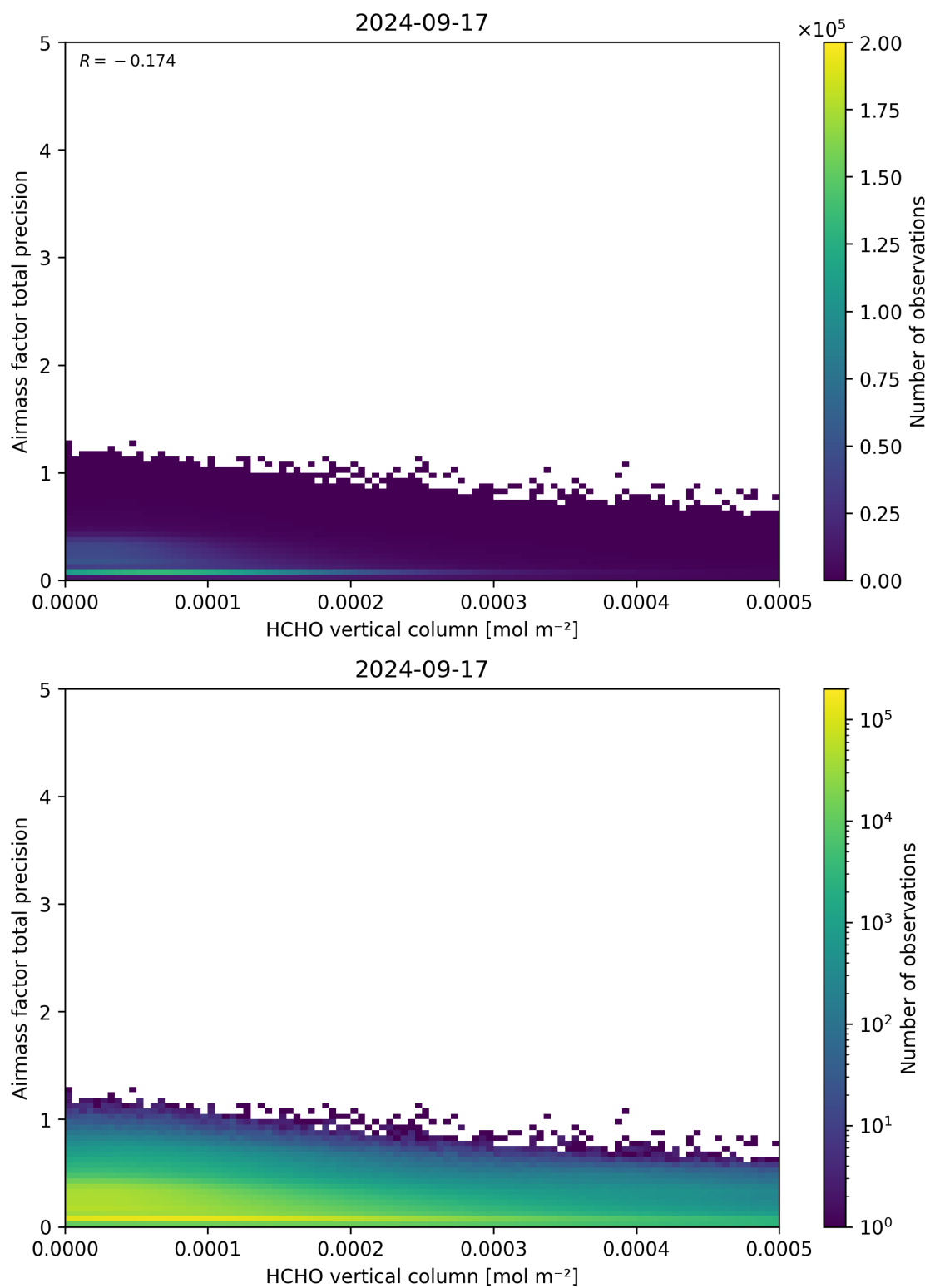
Figure 132: Scatter density plot of “HCHO vertical column” against “Airmass factor total precision” for 2024-09-17 to 2024-09-18.
