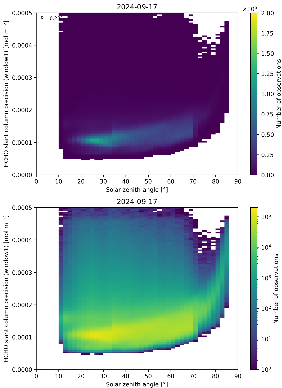
Figure 174: Scatter density plot of “Solar zenith angle” against “HCHO slant column precision (window1)” for 2024-09-17 to 2024-09-18.
