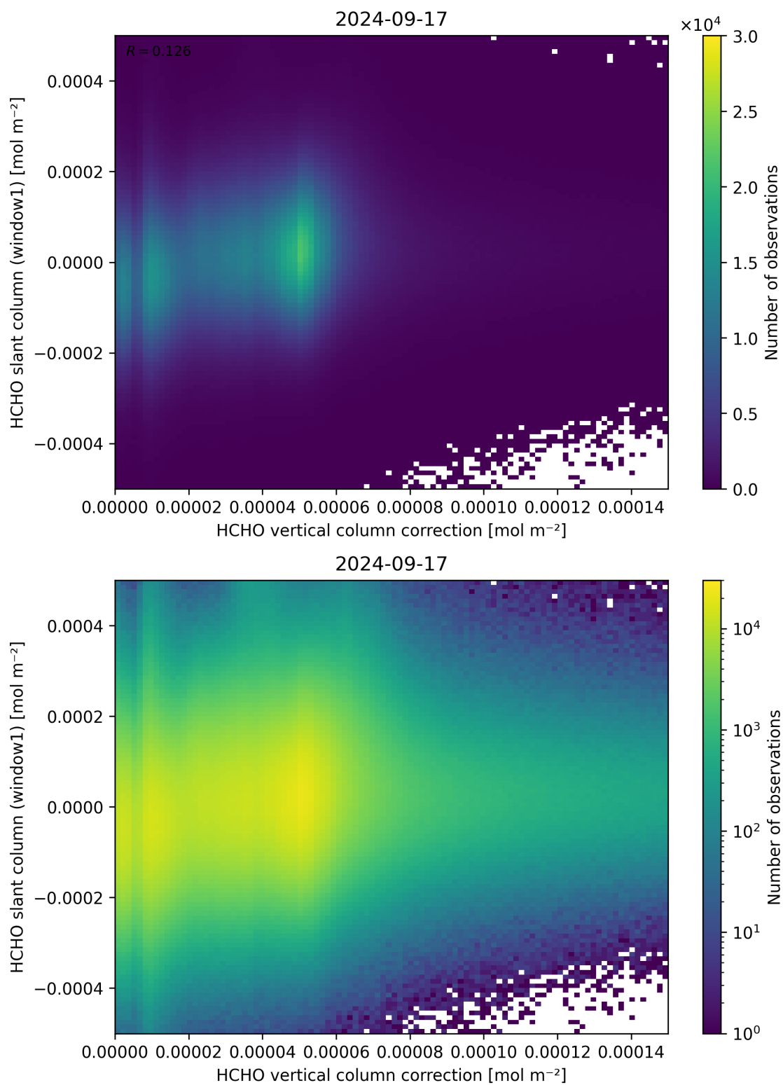
Figure 118: Scatter density plot of “HCHO vertical column correction” against “HCHO slant column (window1)” for 2024-09-17 to 2024-09-18.
