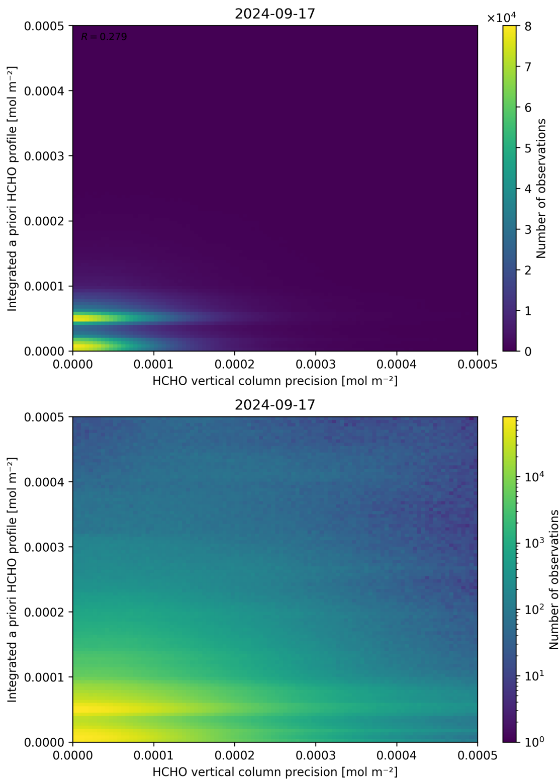
Figure 147: Scatter density plot of “HCHO vertical column precision” against “Integrated a priori HCHO profile” for 2024-09-17 to 2024-09-18.
