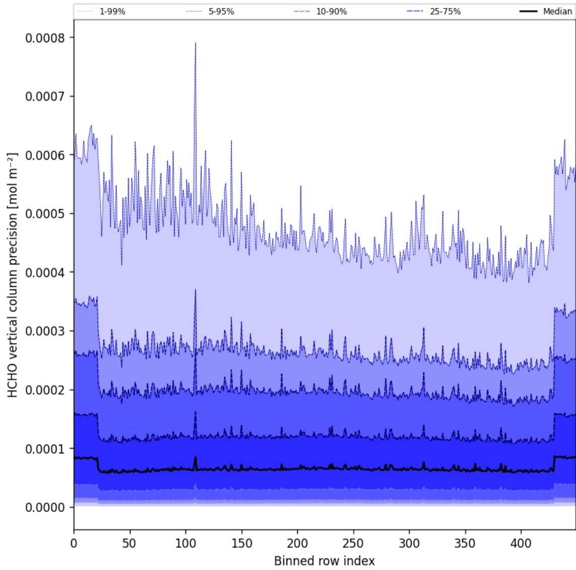
Figure 50: Along track statistics of “HCHO vertical column precision” for 2024-09-17 to 2024-09-18
