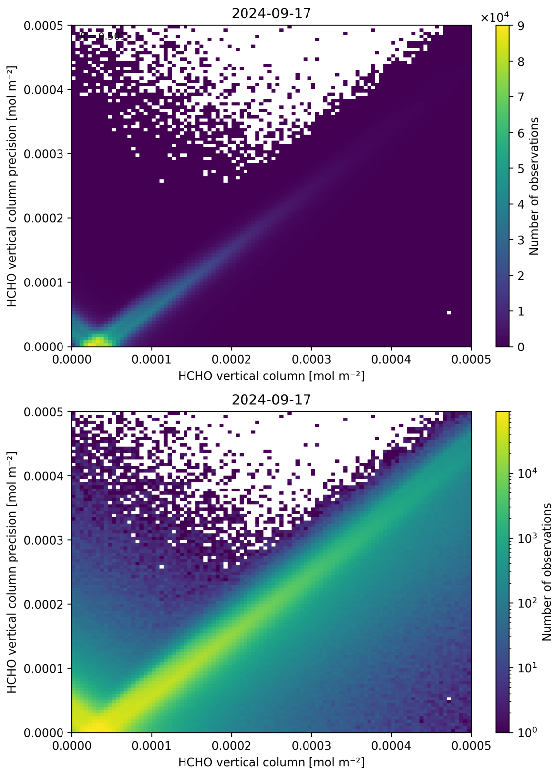
Figure 134: Scatter density plot of “HCHO vertical column” against “HCHO vertical column precision” for 2024-09-17 to 2024-09-18.
