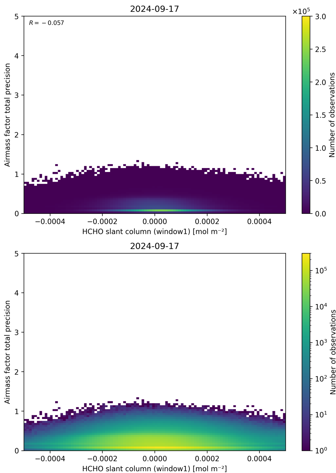
Figure 86: Scatter density plot of “HCHO slant column (window1)” against “Airmass factor total precision” for 2024-09-17 to 2024-09-18.
