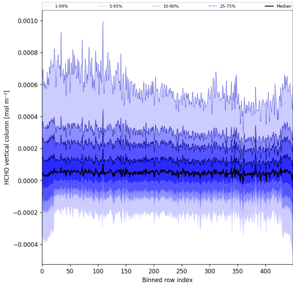
Figure 49: Along track statistics of “HCHO vertical column” for 2024-09-17 to 2024-09-18
