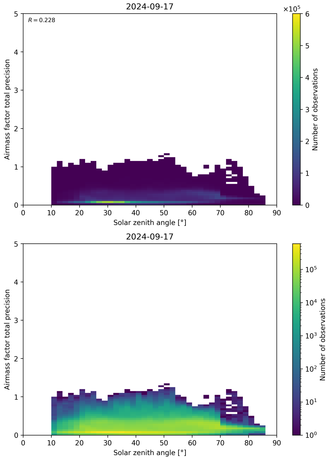
Figure 176: Scatter density plot of “Solar zenith angle” against “Airmass factor total precision” for 2024-09-17 to 2024-09-18.
