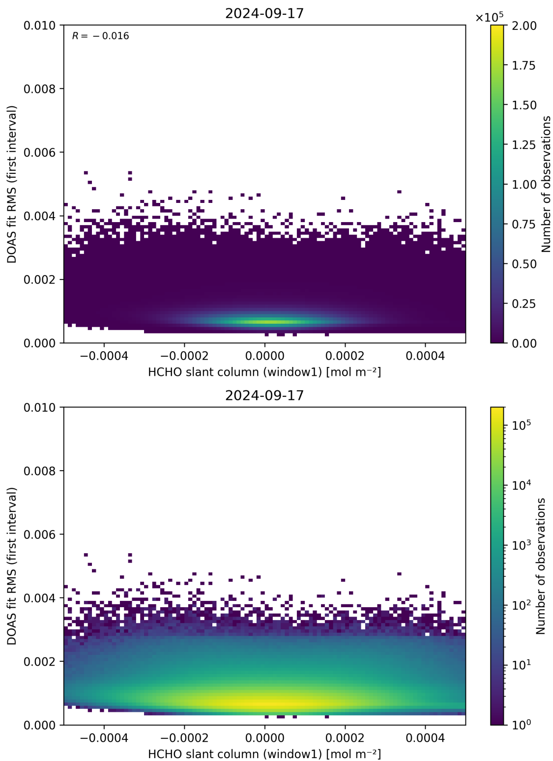
Figure 78: Scatter density plot of “HCHO slant column (window1)” against “DOAS fit RMS (first interval)” for 2024-09-17 to 2024-09-18.
