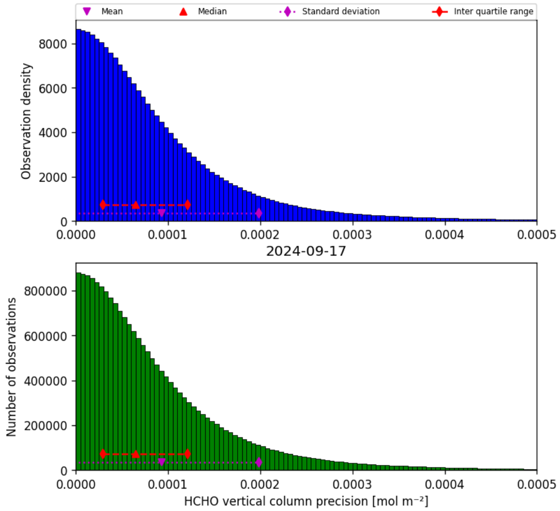
Figure 36: Histogram of “HCHO vertical column precision” for 2024-09-17 to 2024-09-18
