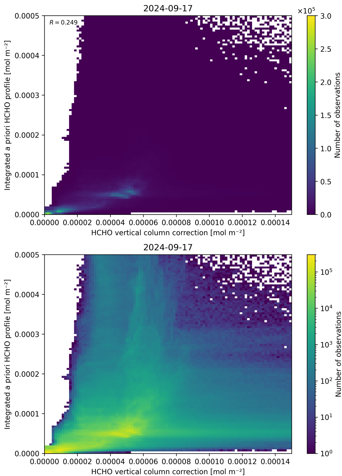
Figure 122: Scatter density plot of “HCHO vertical column correction” against “Integrated a priori HCHO profile” for 2024-09-17 to 2024-09-18.
