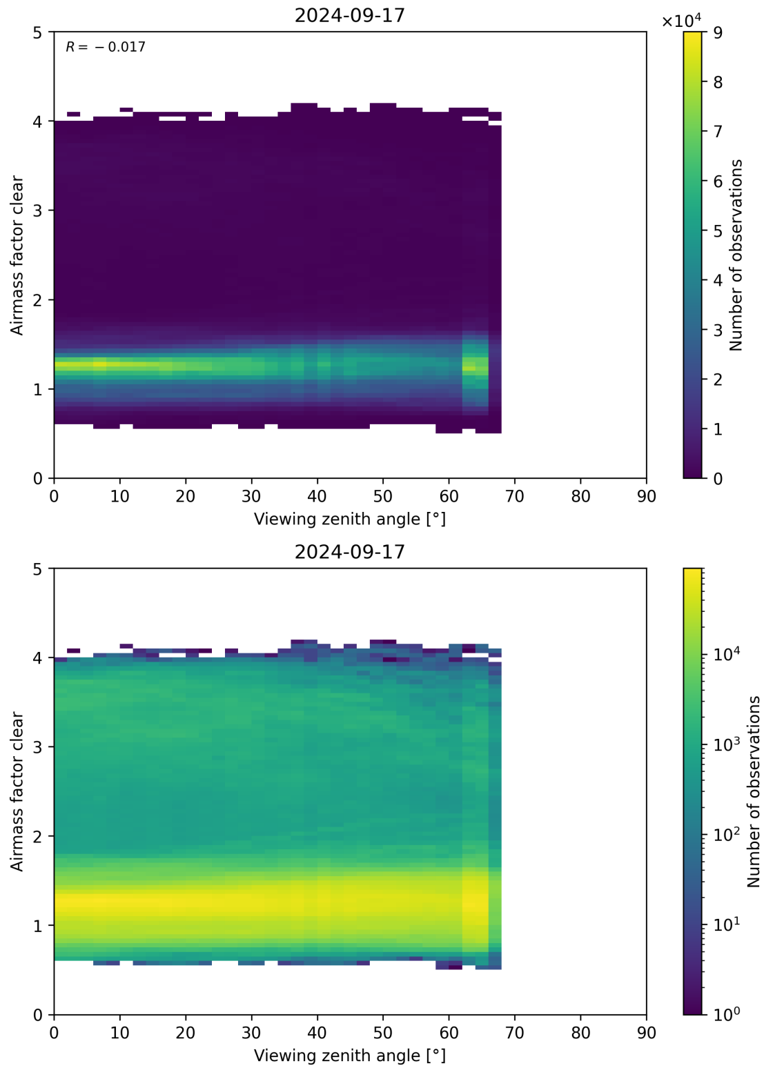
Figure 185: Scatter density plot of “Viewing zenith angle” against “Airmass factor clear” for 2024-09-17 to 2024-09-18.
