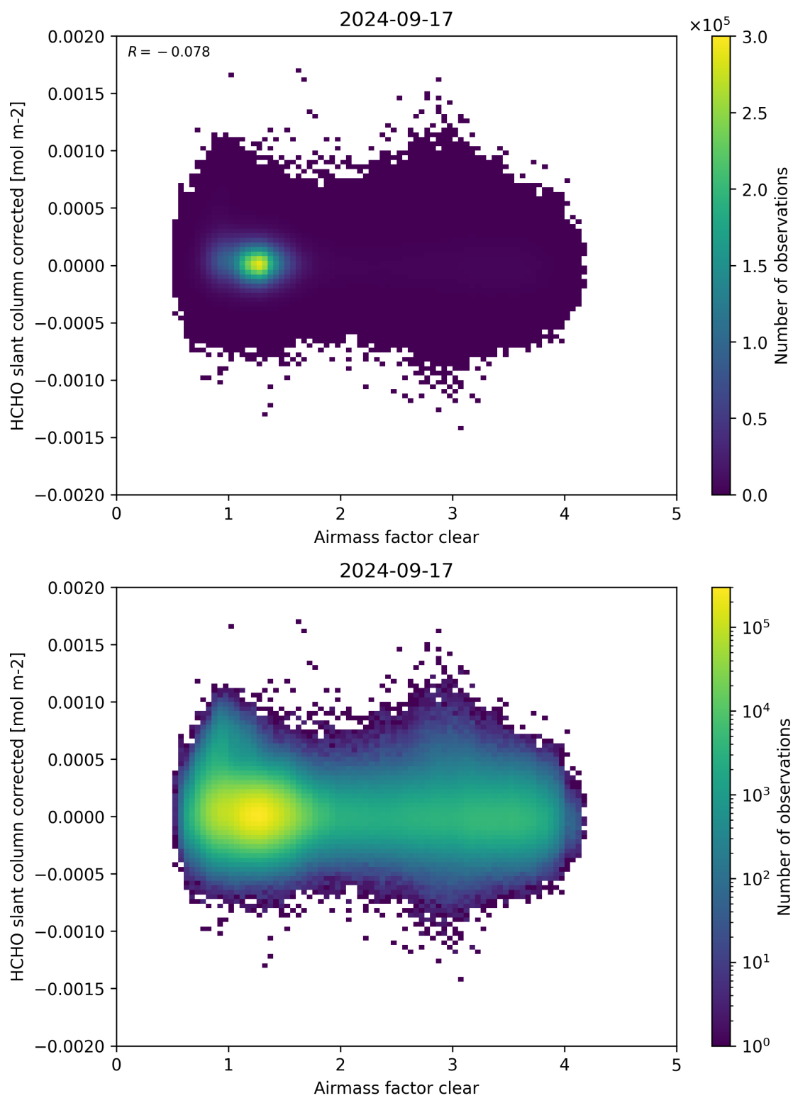
Figure 74: Scatter density plot of “Airmass factor clear” against “HCHO slant column corrected” for 2024-09-17 to 2024-09-18.
