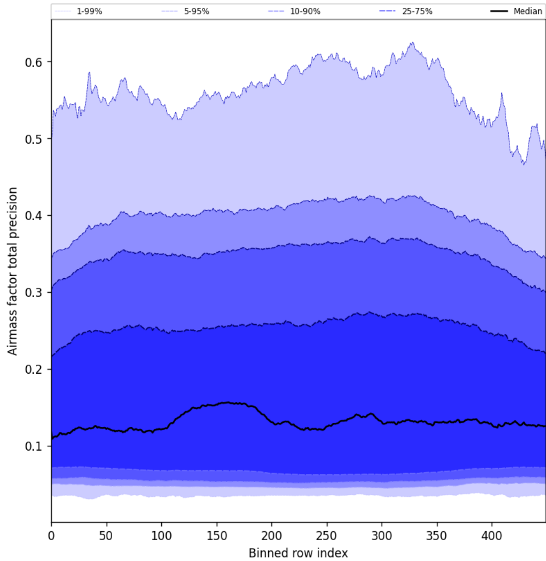
Figure 55: Along track statistics of “Airmass factor total precision” for 2024-09-17 to 2024-09-18
