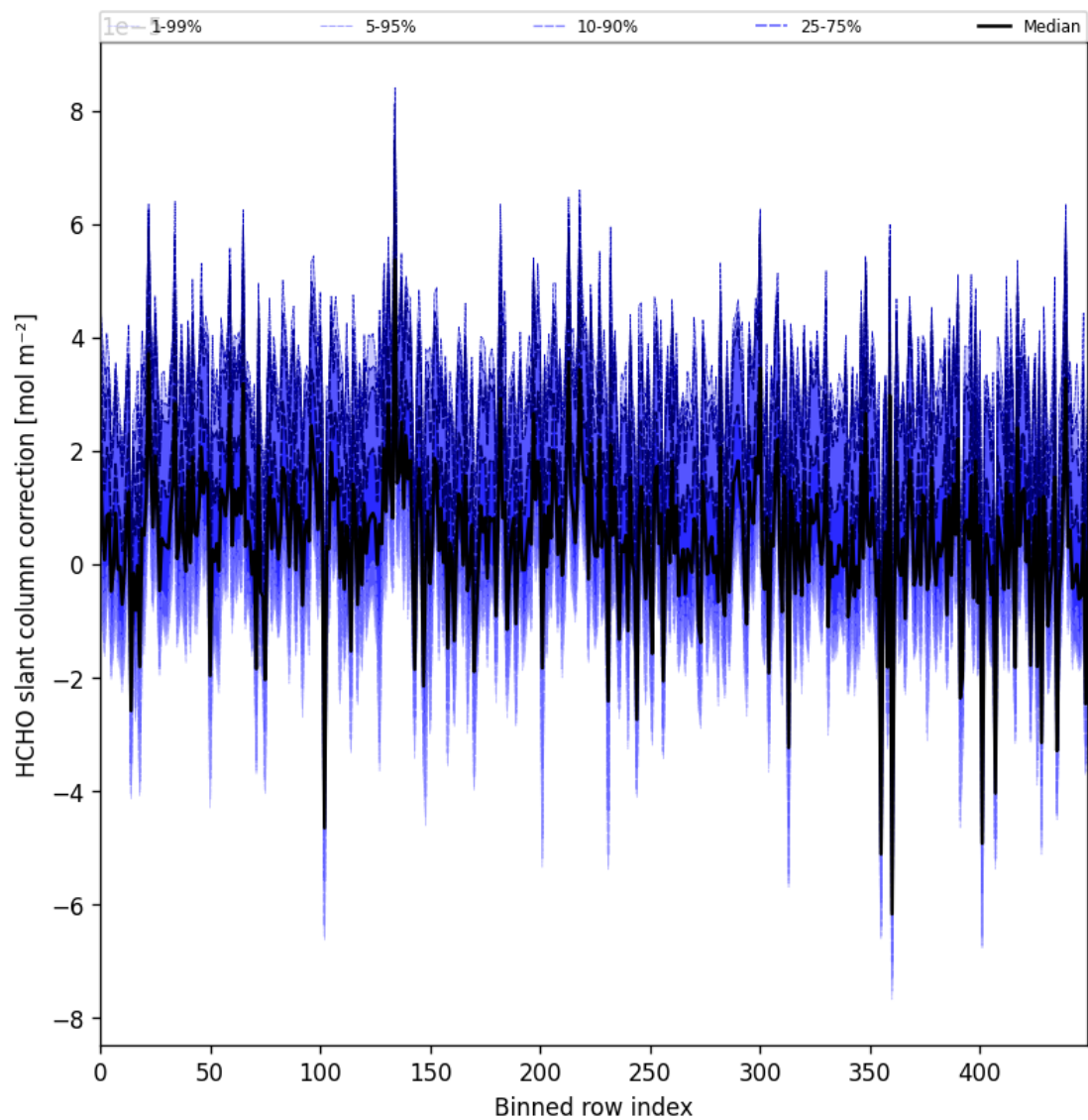
Figure 61: Along track statistics of “HCHO slant column correction” for 2024-09-17 to 2024-09-18
