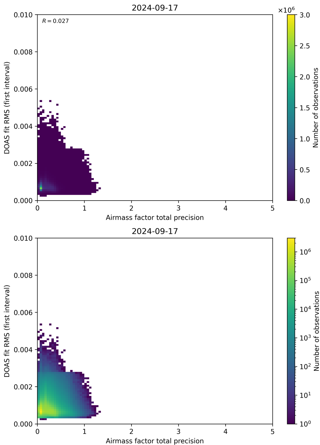
Figure 105: Scatter density plot of “Airmass factor total precision” against “DOAS fit RMS (first interval)” for 2024-09-17 to 2024-09-18.
