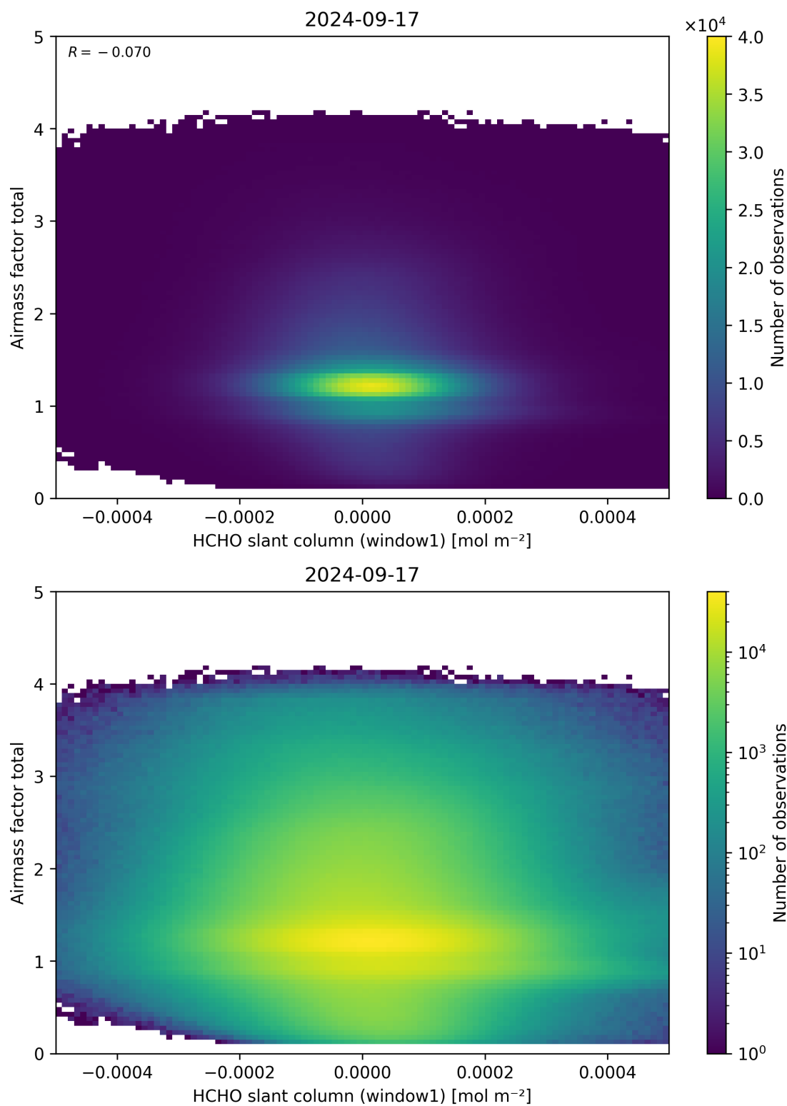
Figure 85: Scatter density plot of “HCHO slant column (window1)” against “Airmass factor total” for 2024-09-17 to 2024-09-18.
