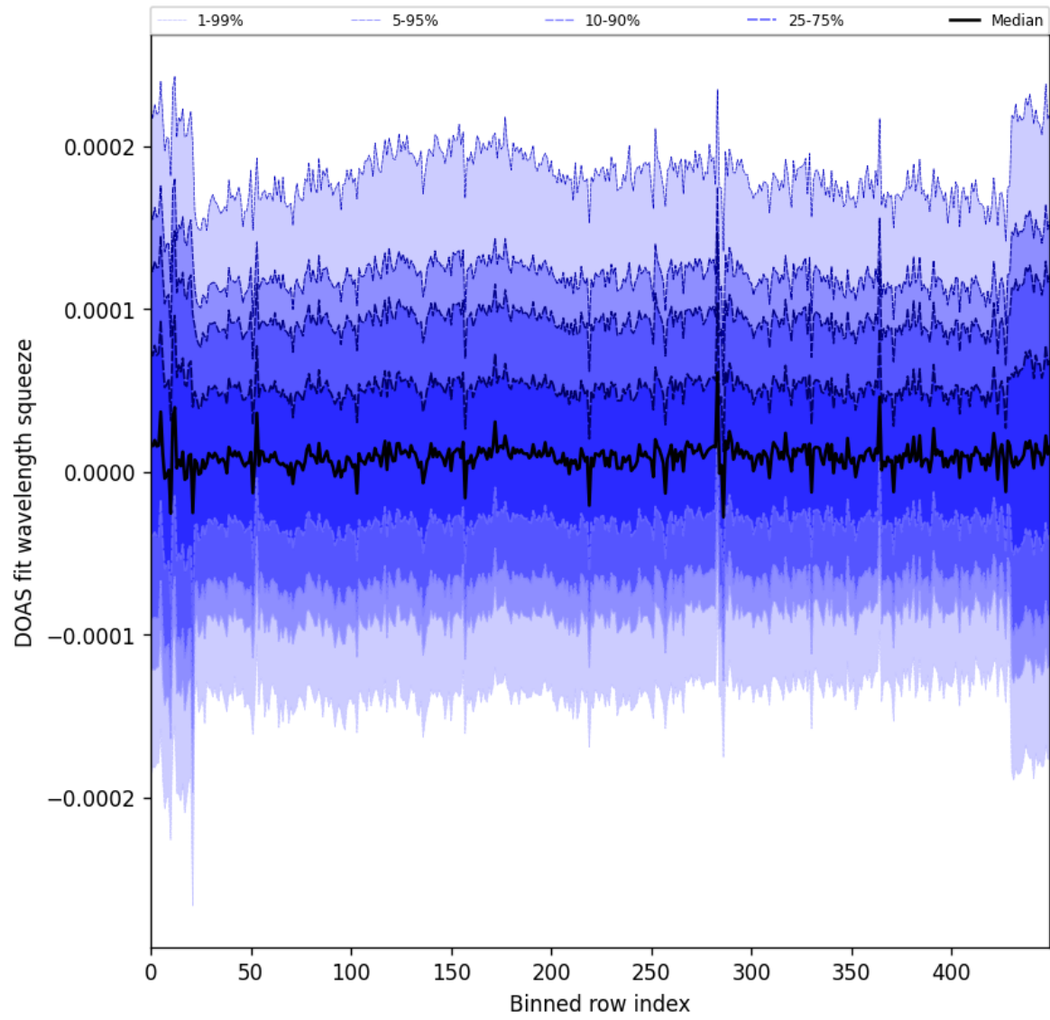
Figure 59: Along track statistics of “DOAS fit wavelength squeeze” for 2024-09-17 to 2024-09-18
