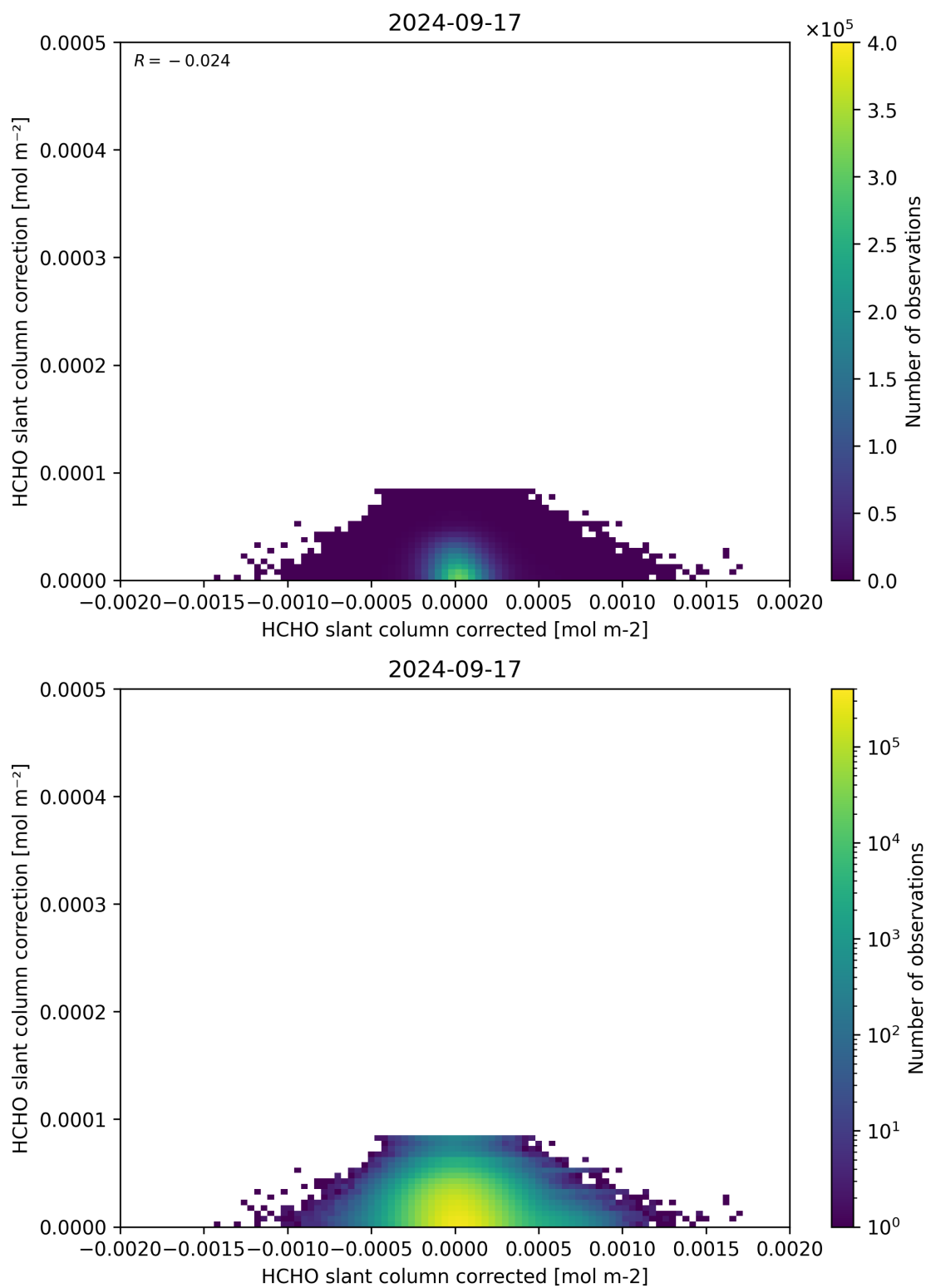
Figure 77: Scatter density plot of “HCHO slant column corrected” against “HCHO slant column correction” for 2024-09-17 to 2024-09-18.
