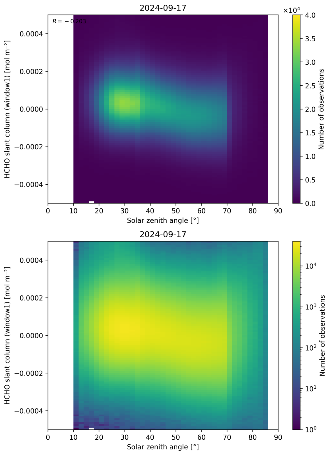
Figure 173: Scatter density plot of “Solar zenith angle” against “HCHO slant column (window1)” for 2024-09-17 to 2024-09-18.
