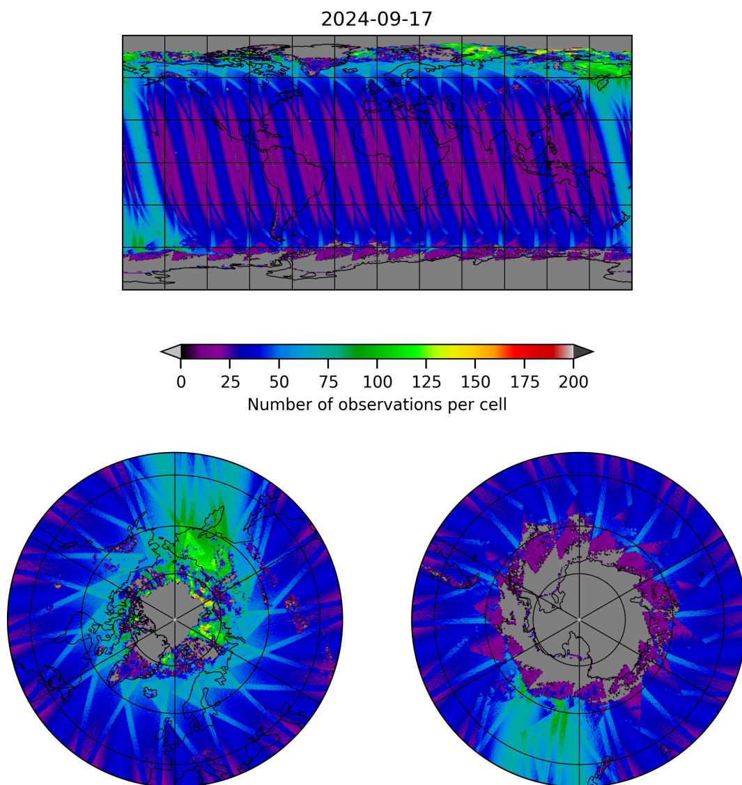
Figure 19: Map of the number of observations for 2024-09-17 to 2024-09-18
