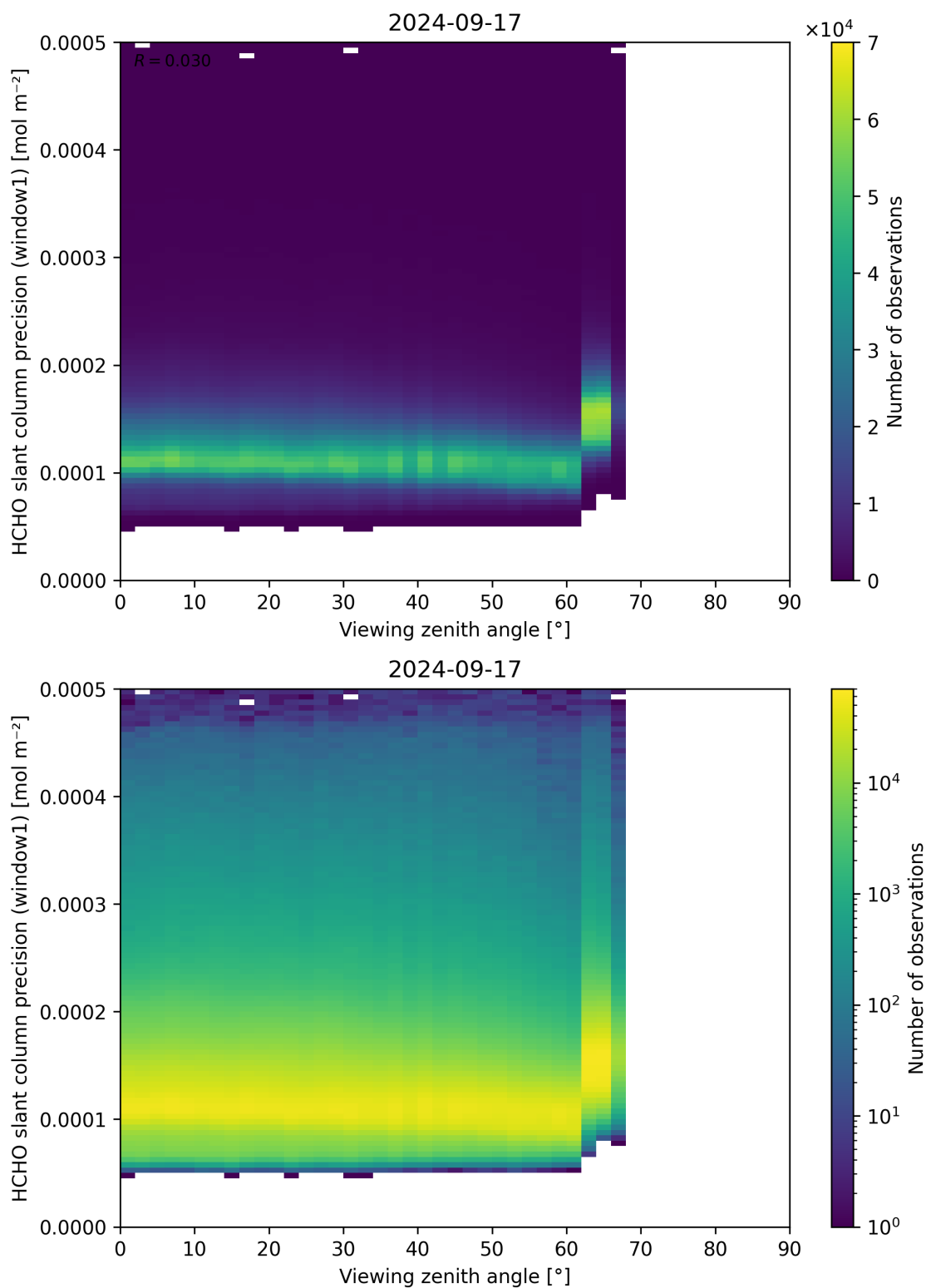
Figure 189: Scatter density plot of “Viewing zenith angle” against “HCHO slant column precision (window1)” for 2024-09-17 to 2024-09-18.
