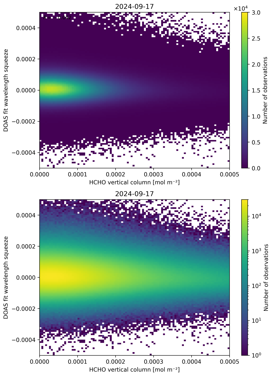
Figure 125: Scatter density plot of “HCHO vertical column” against “DOAS fit wavelength squeeze” for 2024-09-17 to 2024-09-18.
