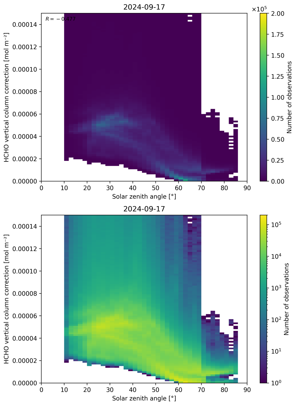
Figure 178: Scatter density plot of “Solar zenith angle” against “HCHO vertical column correction” for 2024-09-17 to 2024-09-18.
