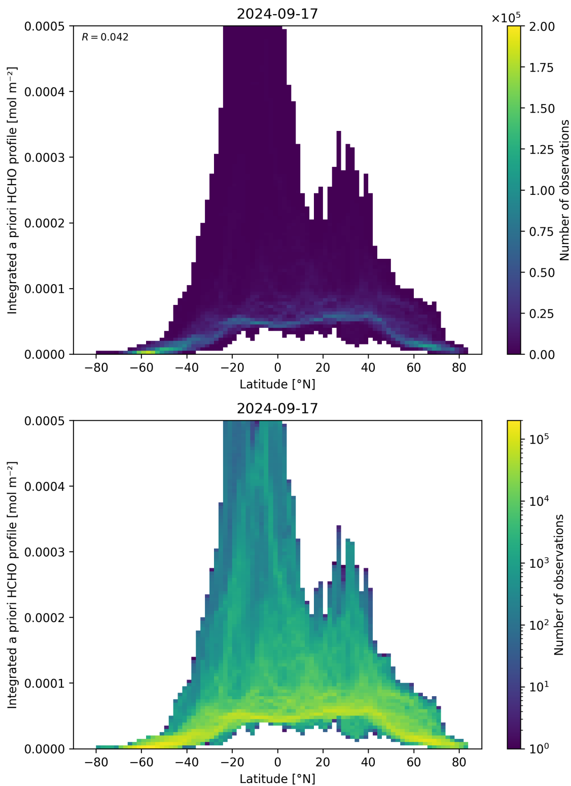
Figure 166: Scatter density plot of “Latitude” against “Integrated a priori HCHO profile” for 2024-09-17 to 2024-09-18.
