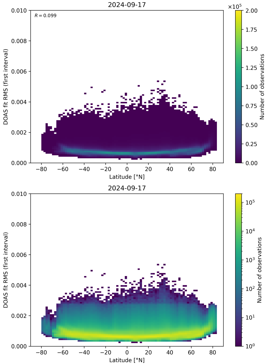
Figure 153: Scatter density plot of “Latitude” against “DOAS fit RMS (first interval)” for 2024-09-17 to 2024-09-18.
