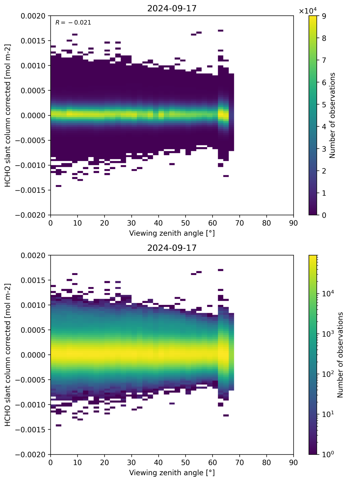
Figure 186: Scatter density plot of “Viewing zenith angle” against “HCHO slant column corrected” for 2024-09-17 to 2024-09-18.
