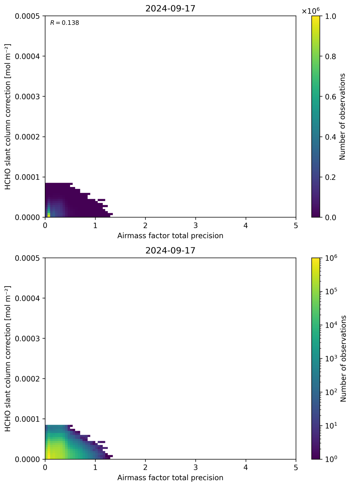
Figure 110: Scatter density plot of “Airmass factor total precision” against “HCHO slant column correction” for 2024-09-17 to 2024-09-18.
