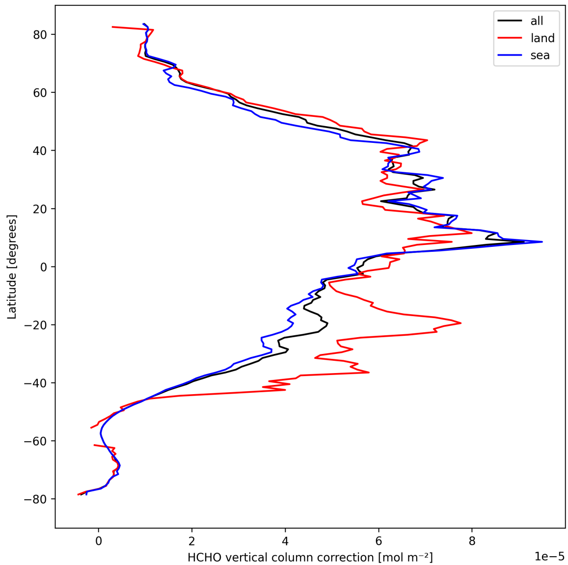
Figure 23: Zonal average of “HCHO vertical column correction” for 2024-09-17 to 2024-09-18.
