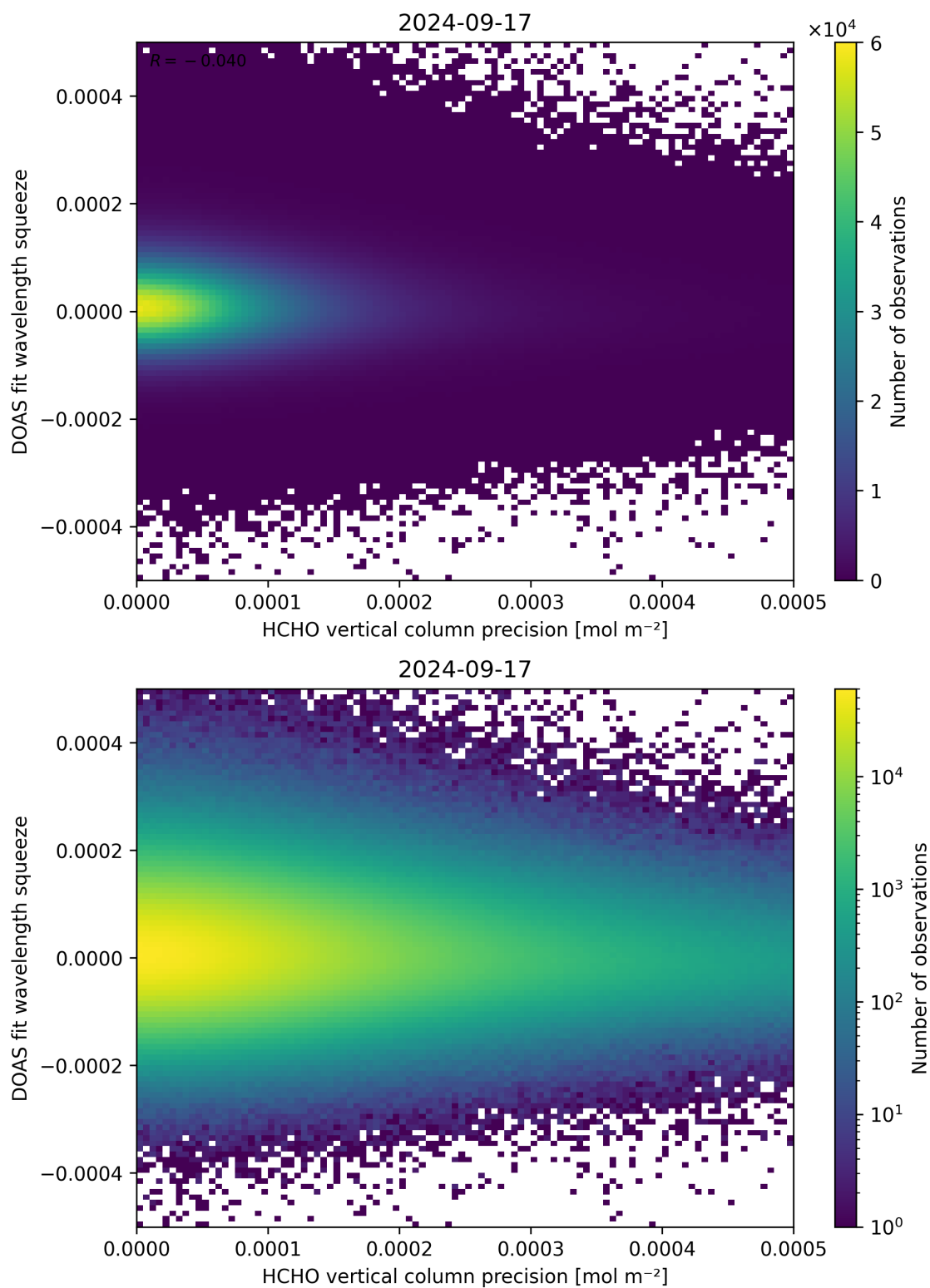
Figure 138: Scatter density plot of “HCHO vertical column precision” against “DOAS fit wavelength squeeze” for 2024-09-17 to 2024-09-18.
