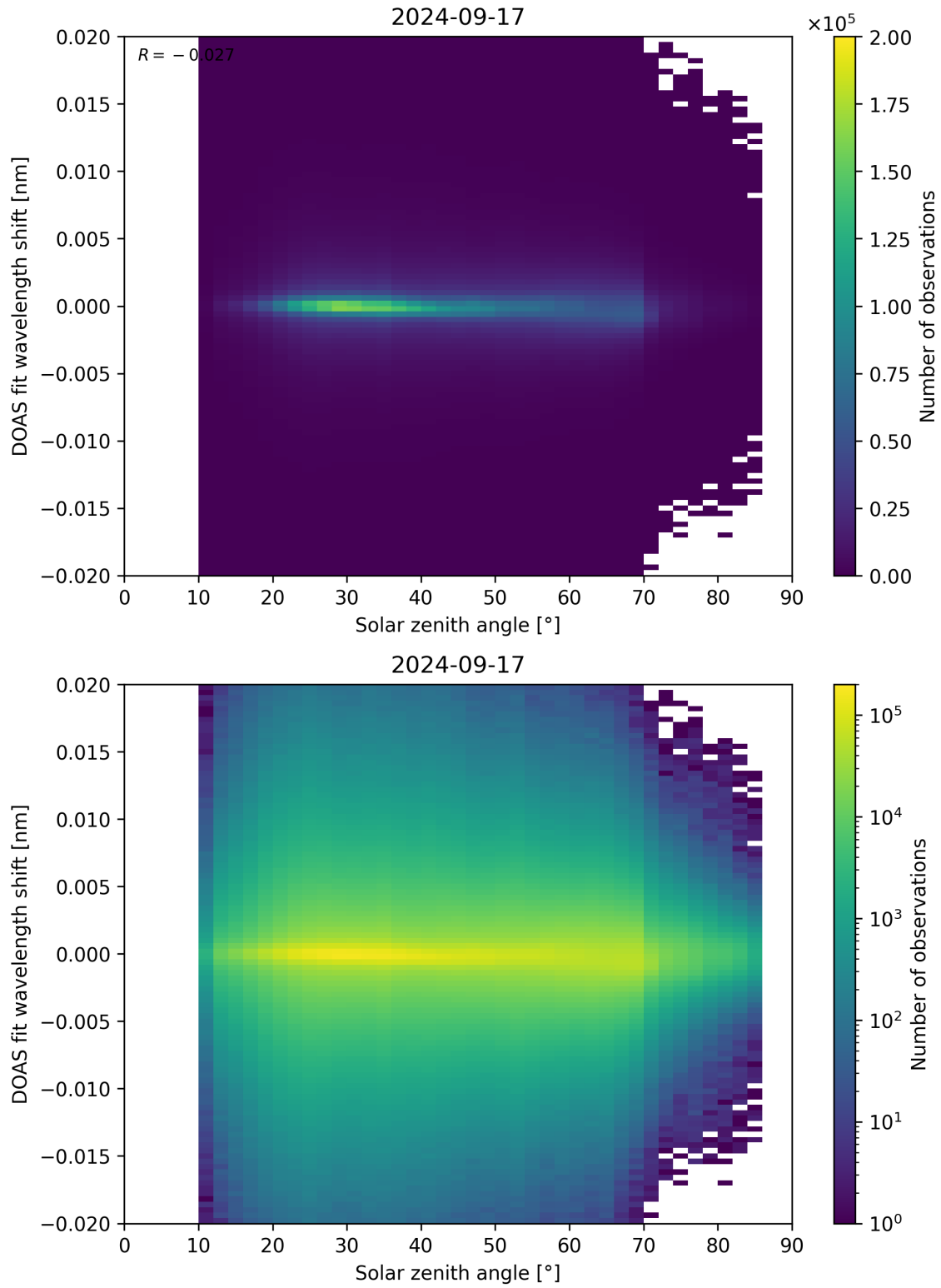
Figure 168: Scatter density plot of “Solar zenith angle” against “DOAS fit wavelength shift” for 2024-09-17 to 2024-09-18.
