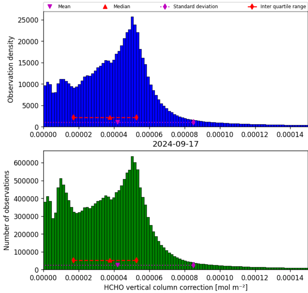
Figure 37: Histogram of “HCHO vertical column correction” for 2024-09-17 to 2024-09-18
