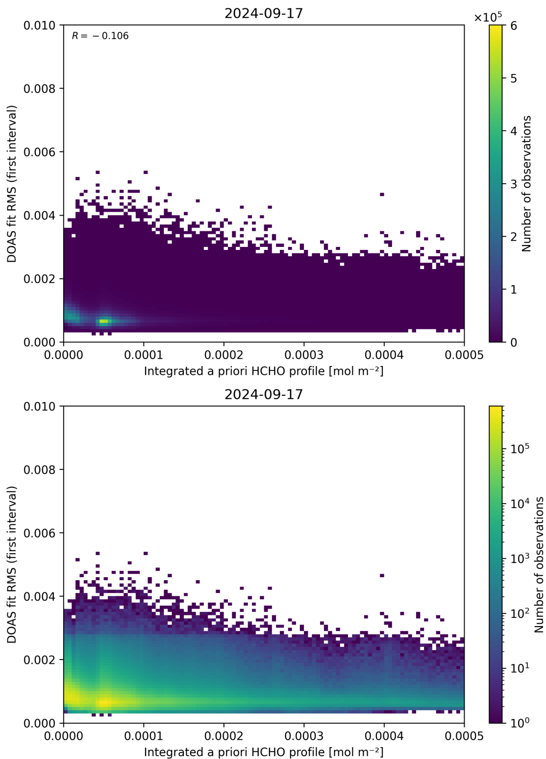
Figure 148: Scatter density plot of “Integrated a priori HCHO profile” against “DOAS fit RMS (first interval)” for 2024-09-17 to 2024-09-18.
