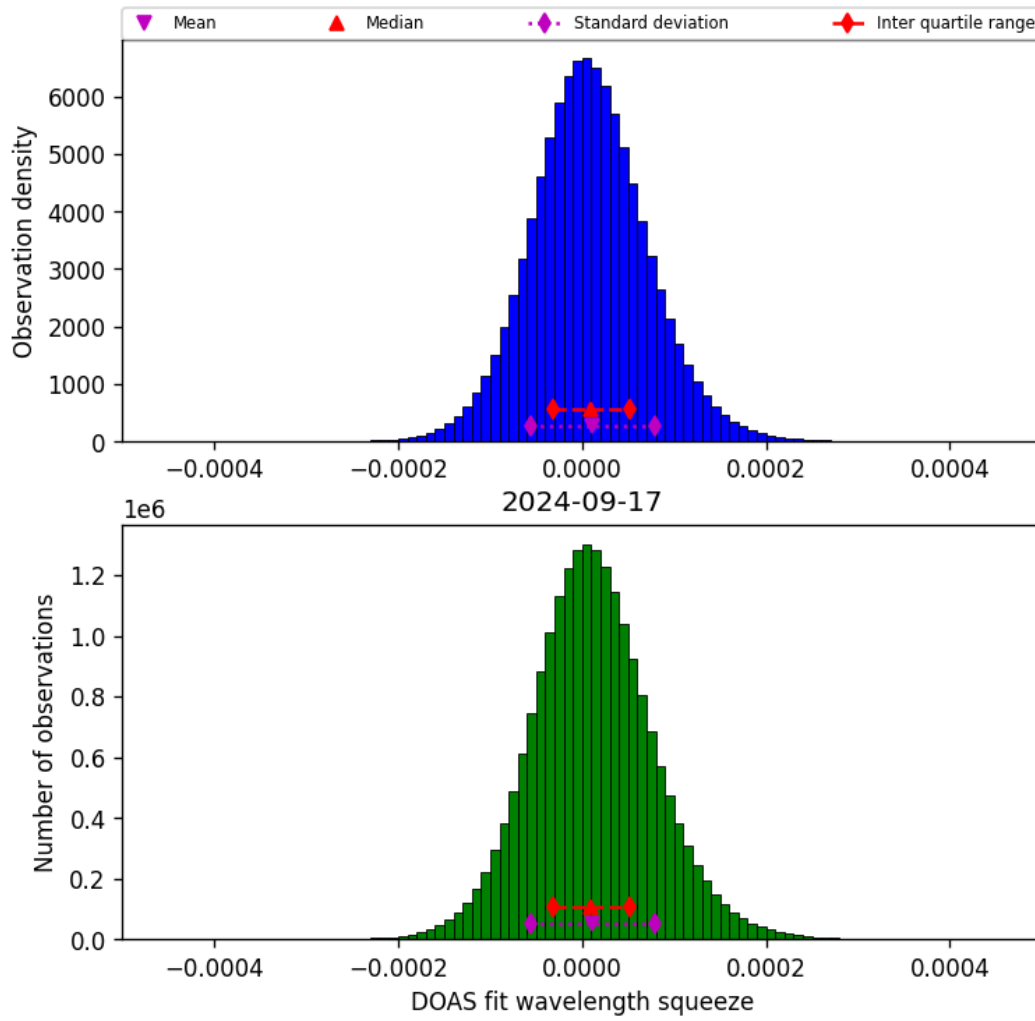
Figure 45: Histogram of “DOAS fit wavelength squeeze” for 2024-09-17 to 2024-09-18
