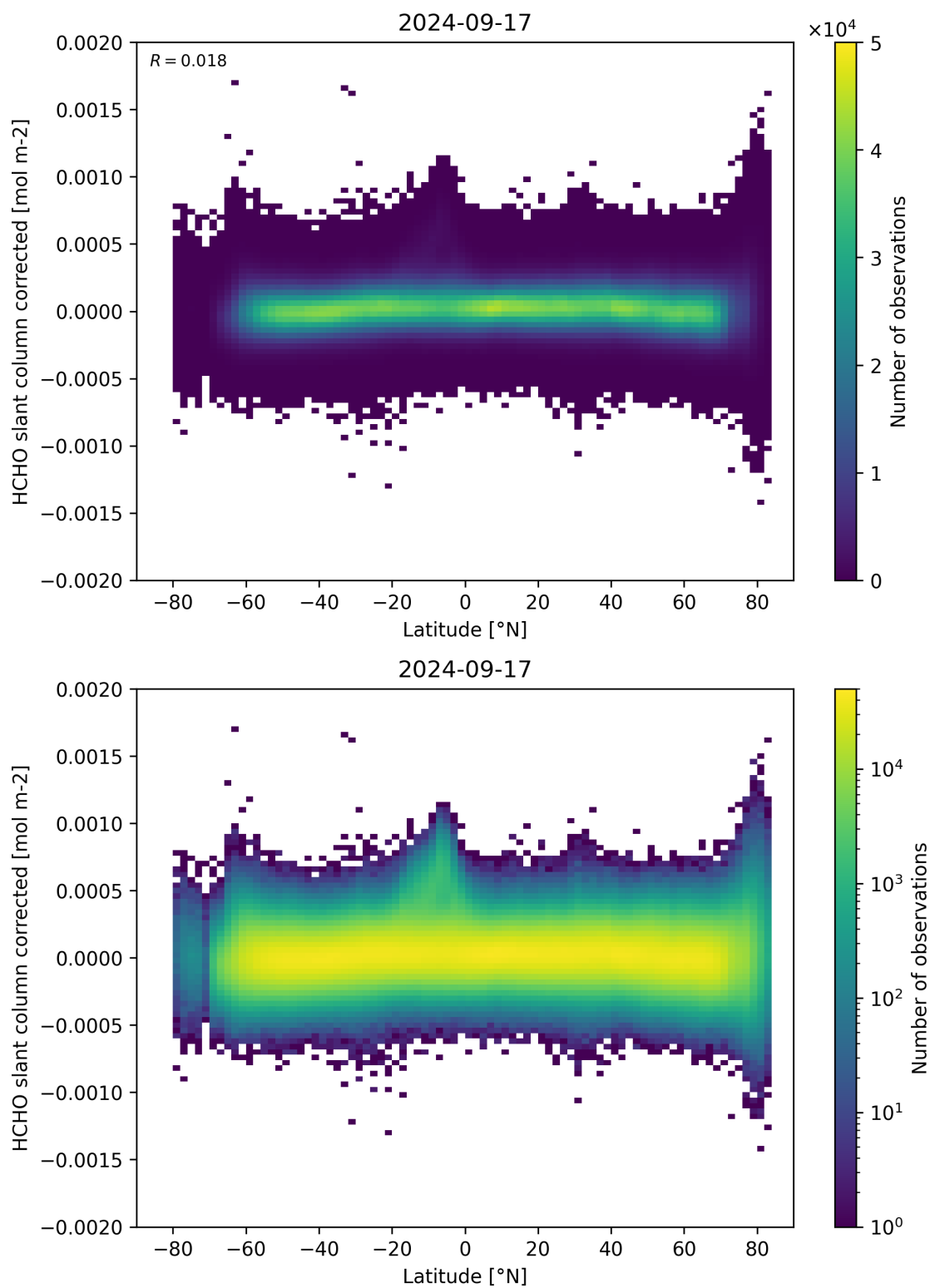
Figure 157: Scatter density plot of “Latitude” against “HCHO slant column corrected” for 2024-09-17 to 2024-09-18.
