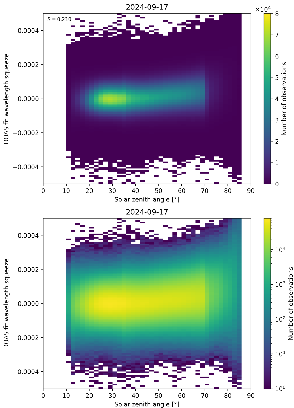
Figure 169: Scatter density plot of “Solar zenith angle” against “DOAS fit wavelength squeeze” for 2024-09-17 to 2024-09-18.
