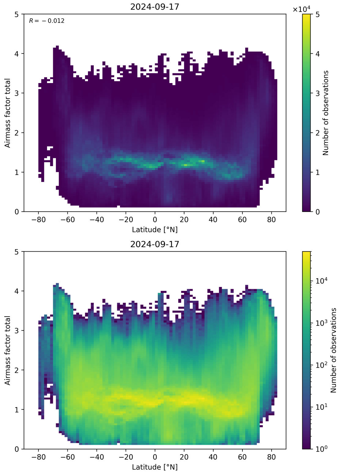
Figure 161: Scatter density plot of “Latitude” against “Airmass factor total” for 2024-09-17 to 2024-09-18.
