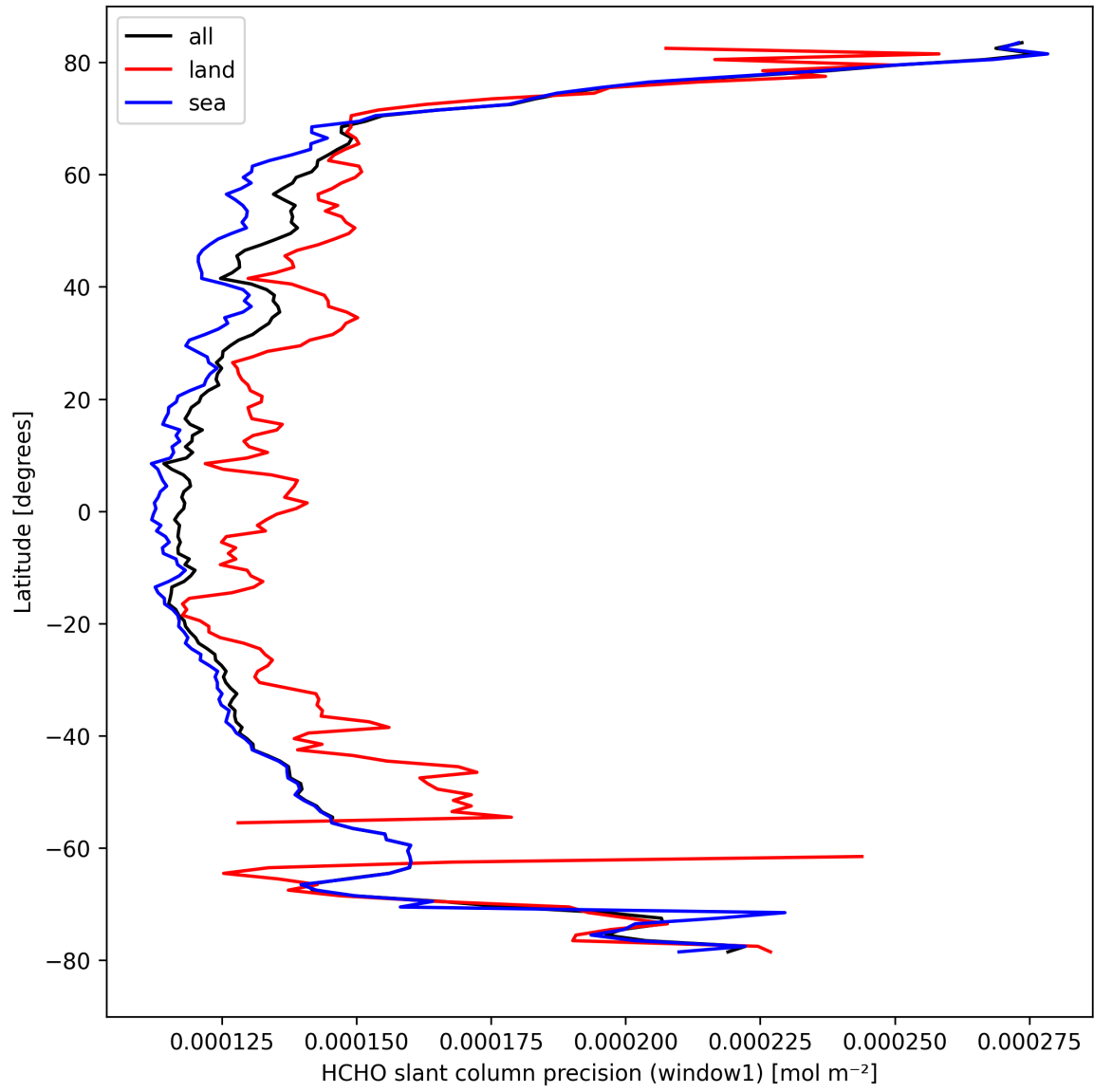
Figure 25: Zonal average of “HCHO slant column precision (window1)” for 2024-09-17 to 2024-09-18.
