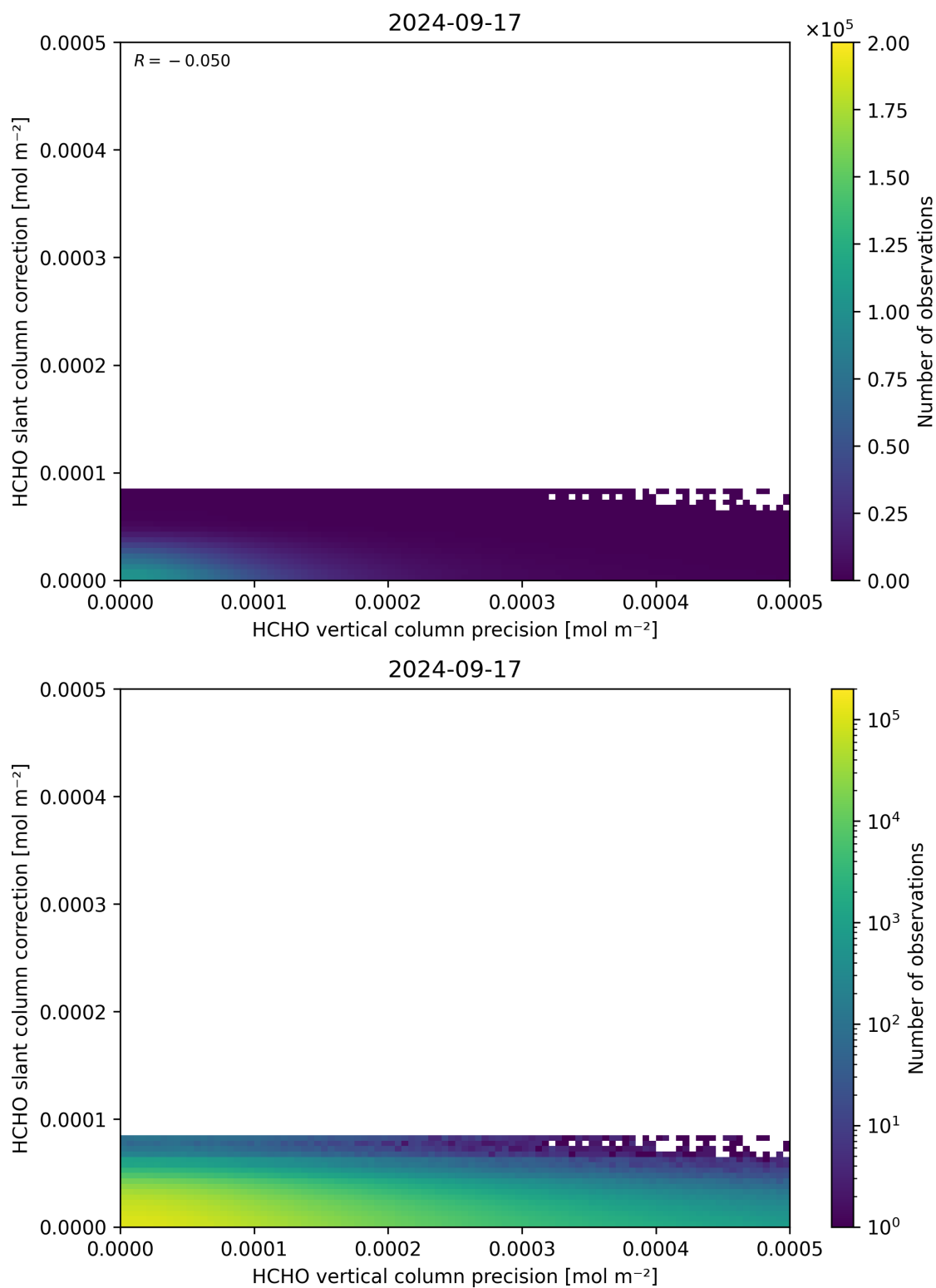
Figure 141: Scatter density plot of “HCHO vertical column precision” against “HCHO slant column correction” for 2024-09-17 to 2024-09-18.
