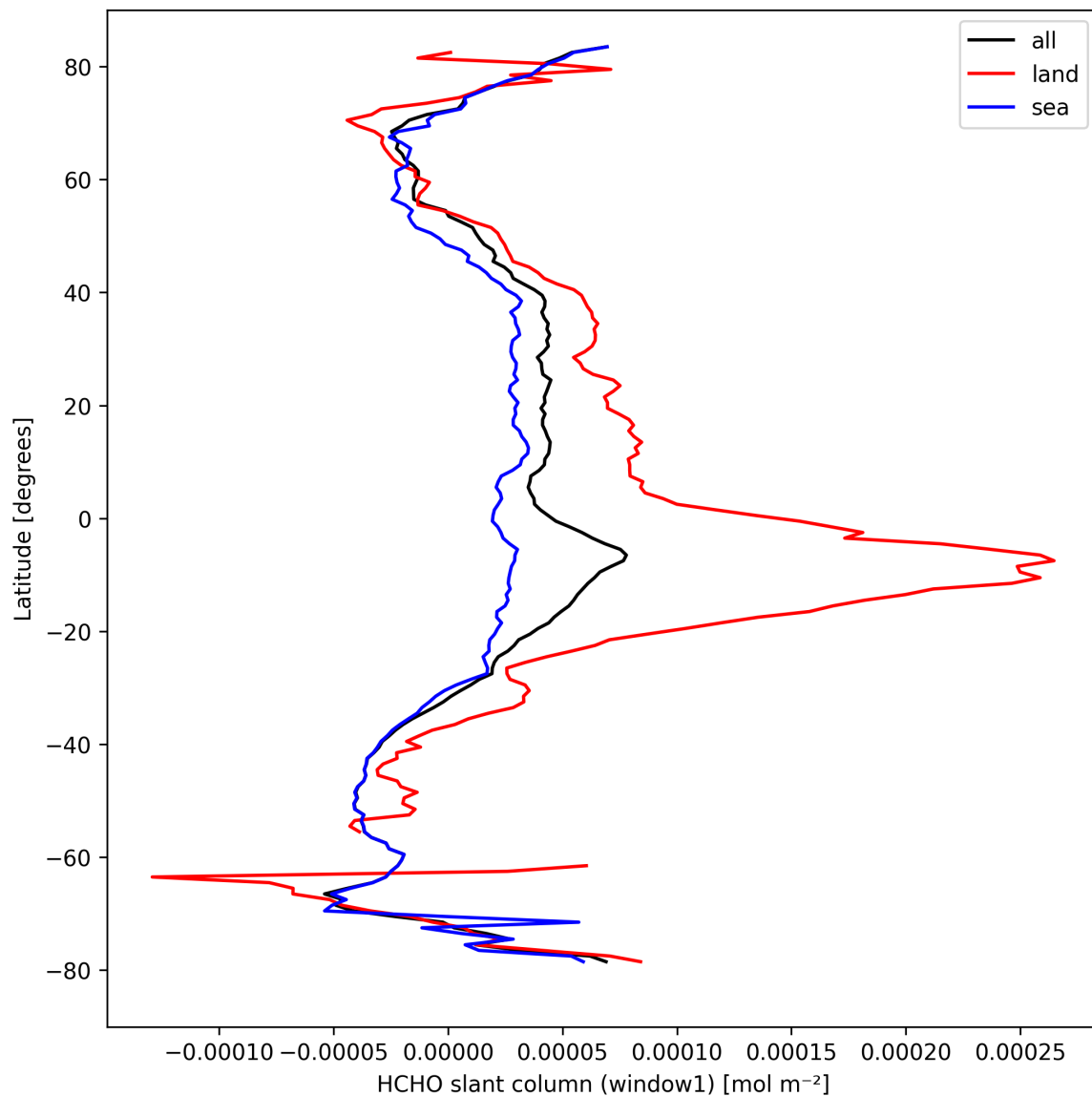
Figure 24: Zonal average of “HCHO slant column (window1)” for 2024-09-17 to 2024-09-18.
