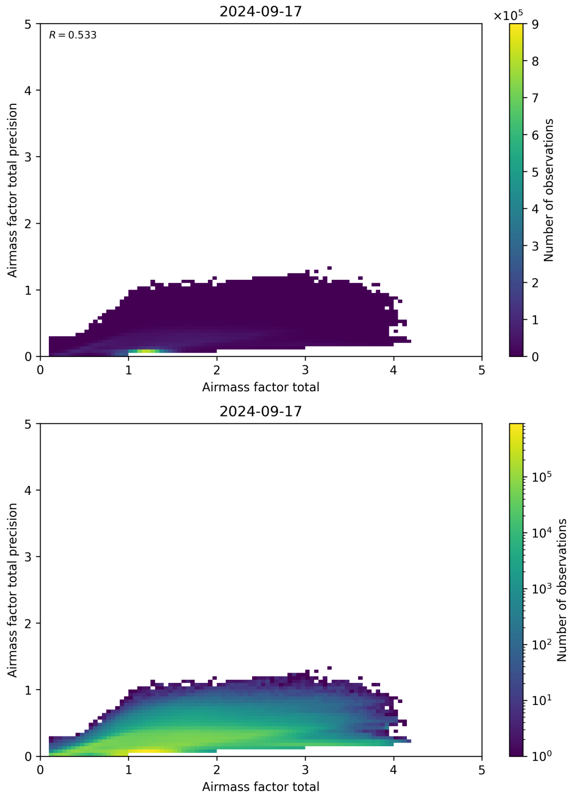
Figure 103: Scatter density plot of “Airmass factor total” against “Airmass factor total precision” for 2024-09-17 to 2024-09-18.
