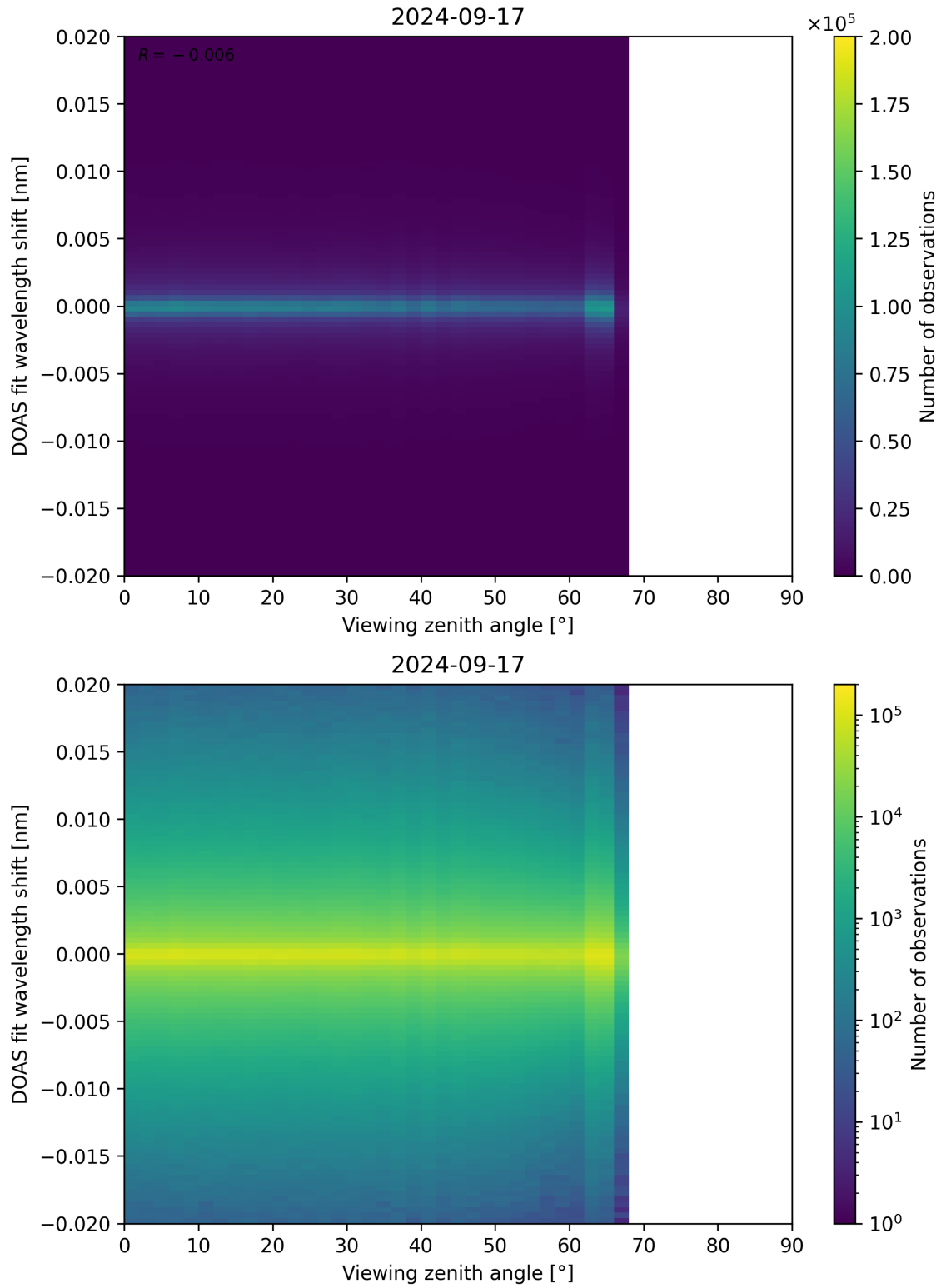
Figure 183: Scatter density plot of “Viewing zenith angle” against “DOAS fit wavelength shift” for 2024-09-17 to 2024-09-18.
