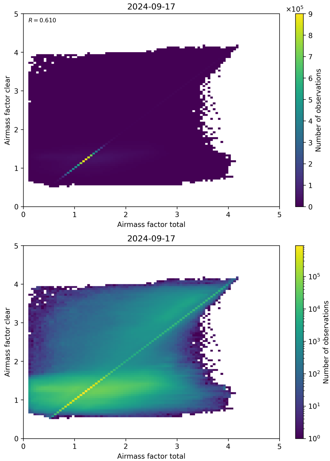
Figure 100: Scatter density plot of “Airmass factor total” against “Airmass factor clear” for 2024-09-17 to 2024-09-18.
