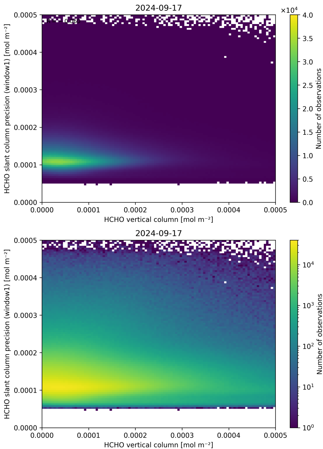
Figure 130: Scatter density plot of “HCHO vertical column” against “HCHO slant column precision (window1)” for 2024-09-17 to 2024-09-18.
