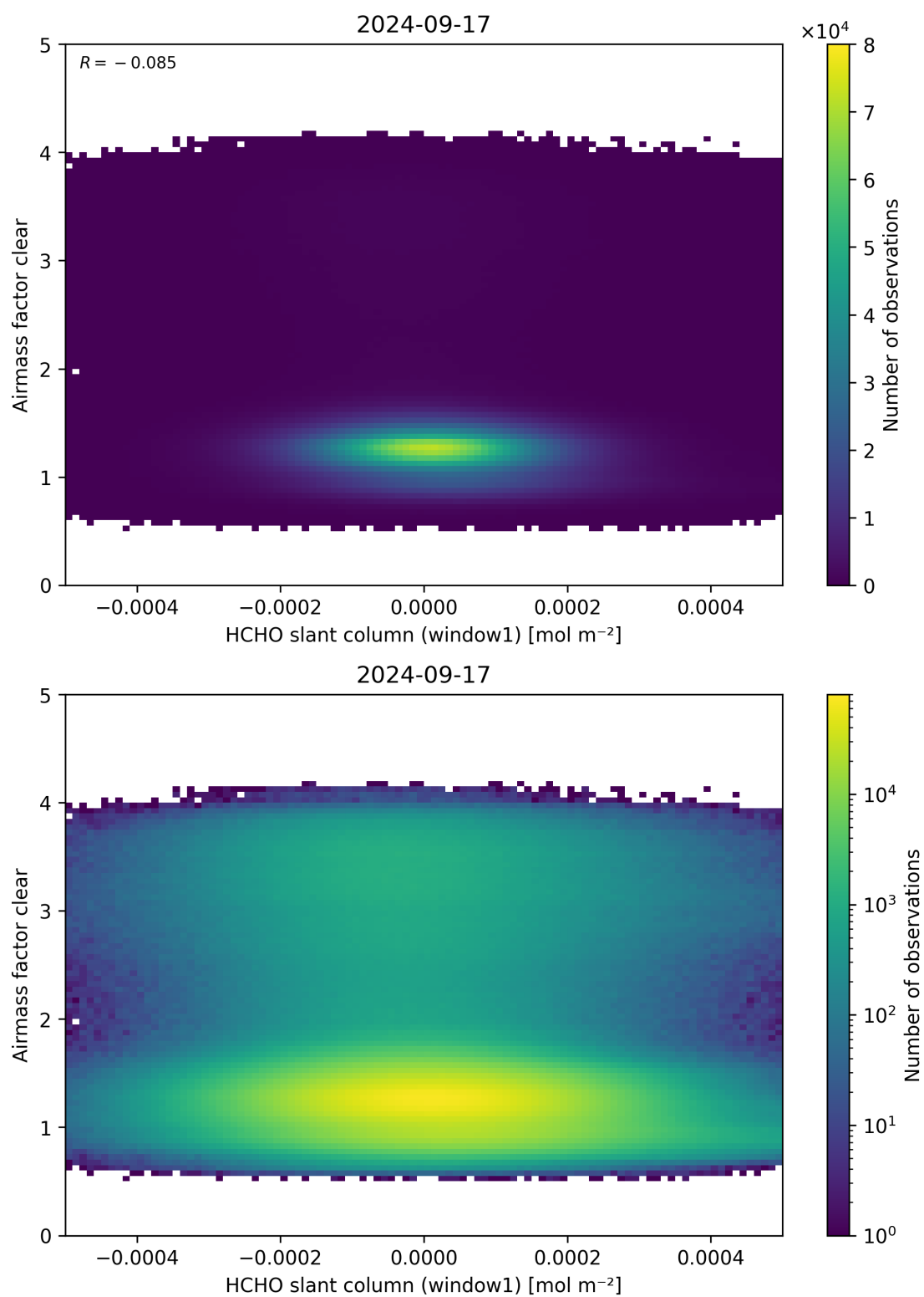
Figure 81: Scatter density plot of “HCHO slant column (window1)” against “Airmass factor clear” for 2024-09-17 to 2024-09-18.
