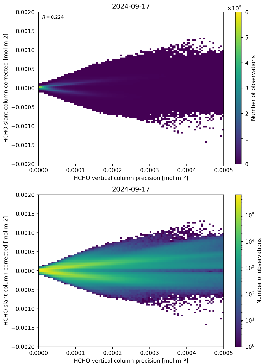
Figure 140: Scatter density plot of “HCHO vertical column precision” against “HCHO slant column corrected” for 2024-09-17 to 2024-09-18.
