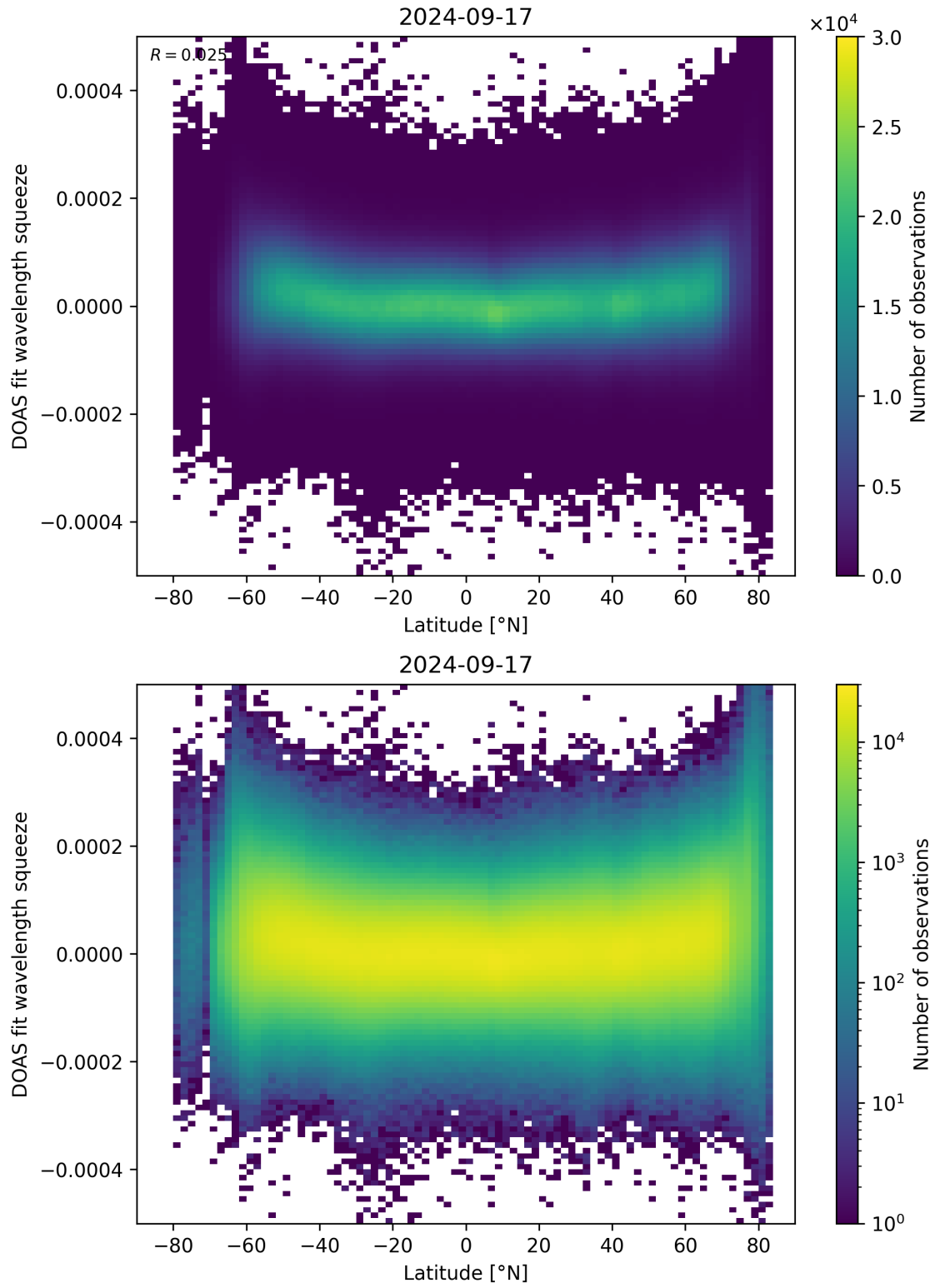
Figure 155: Scatter density plot of “Latitude” against “DOAS fit wavelength squeeze” for 2024-09-17 to 2024-09-18.
