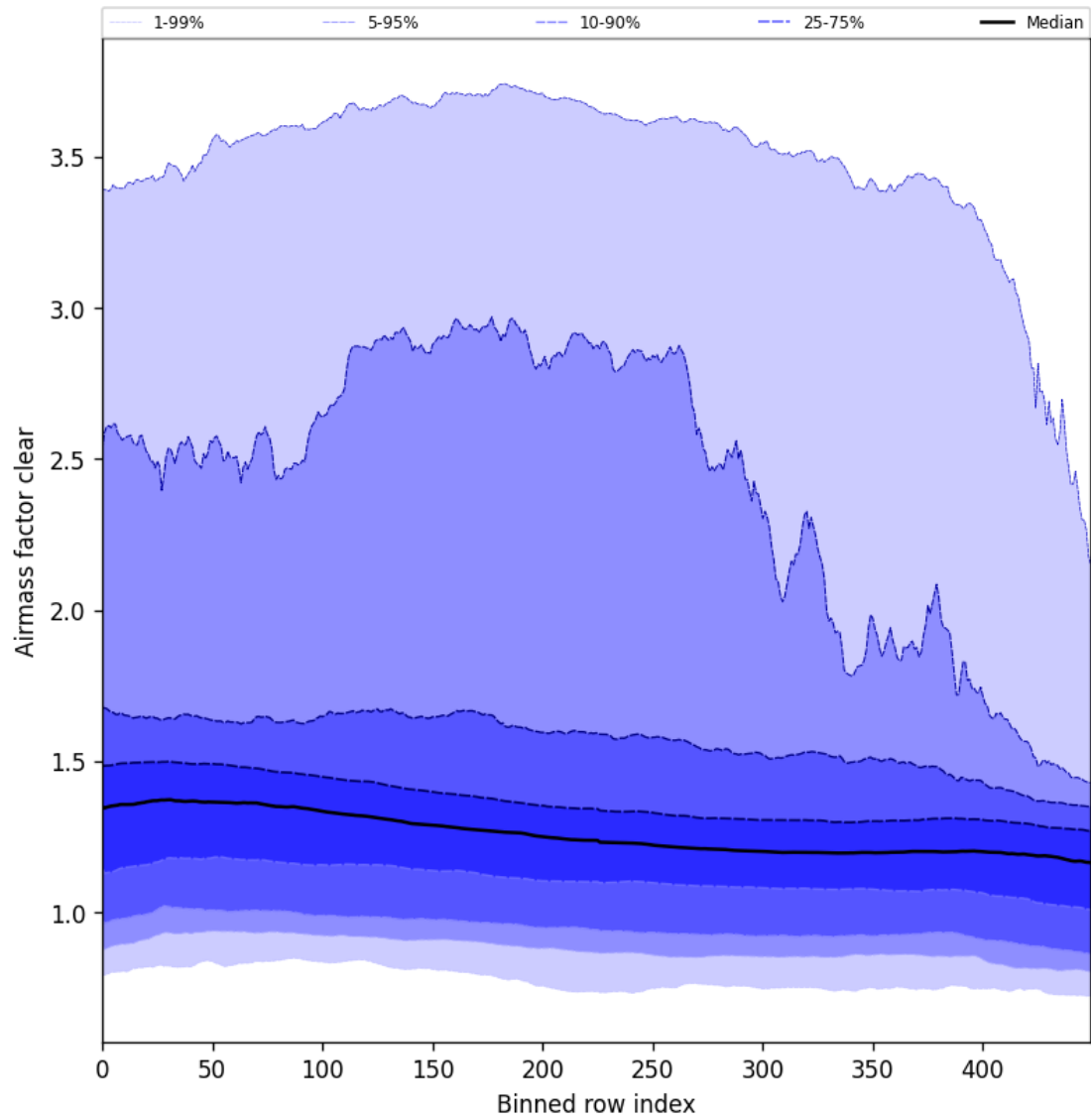
Figure 56: Along track statistics of “Airmass factor clear” for 2024-09-17 to 2024-09-18
