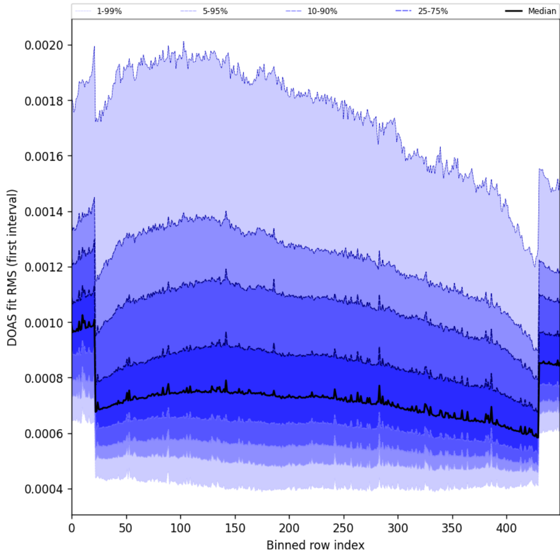
Figure 60: Along track statistics of “DOAS fit RMS (first interval)” for 2024-09-17 to 2024-09-18
