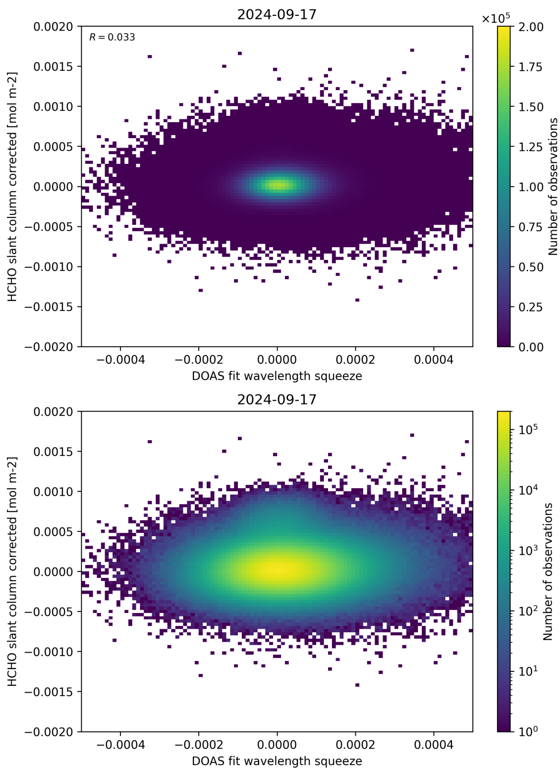
Figure 69: Scatter density plot of “DOAS fit wavelength squeeze” against “HCHO slant column corrected” for 2024-09-17 to 2024-09-18.
