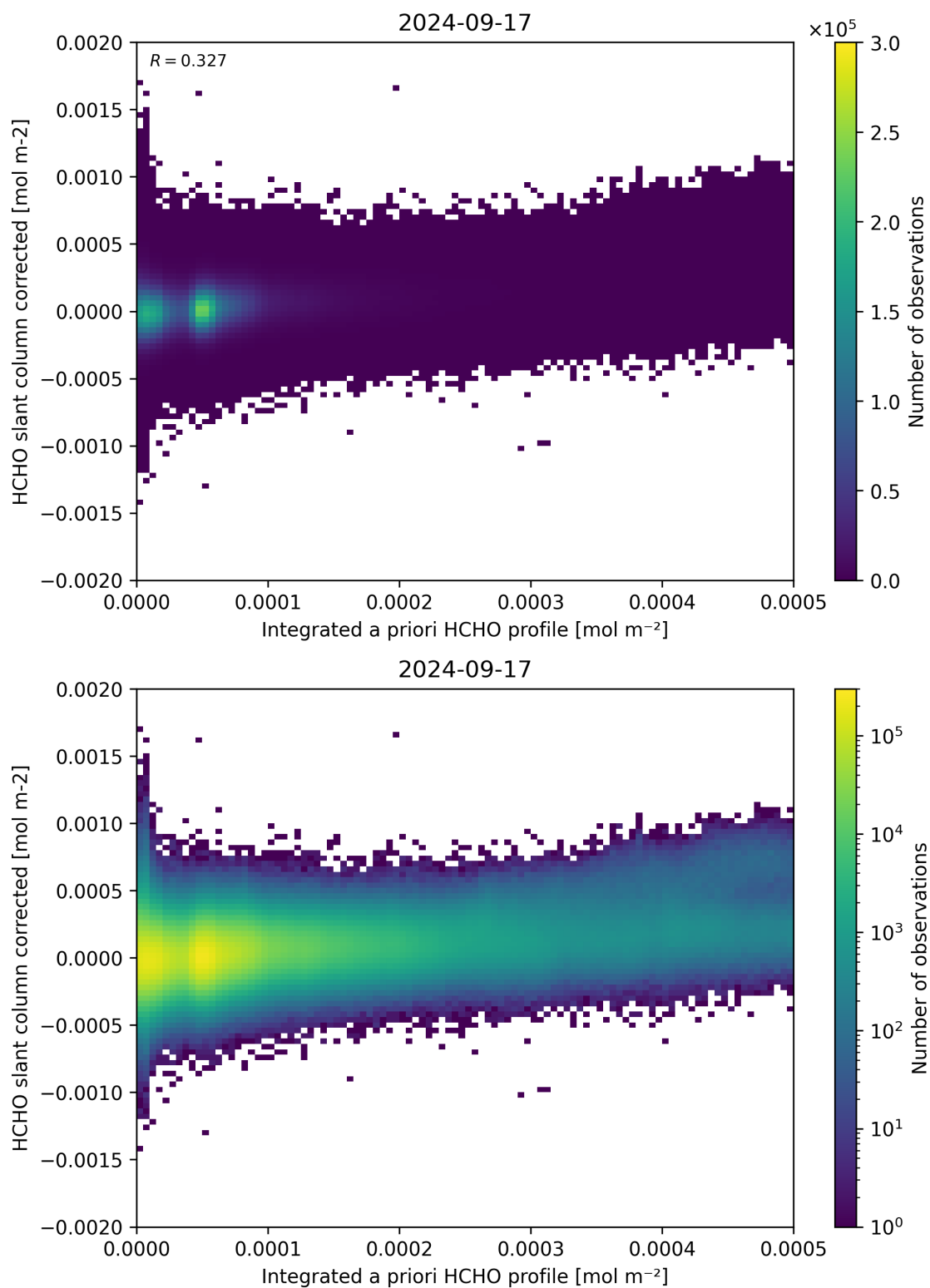
Figure 151: Scatter density plot of “Integrated a priori HCHO profile” against “HCHO slant column corrected” for 2024-09-17 to 2024-09-18.
