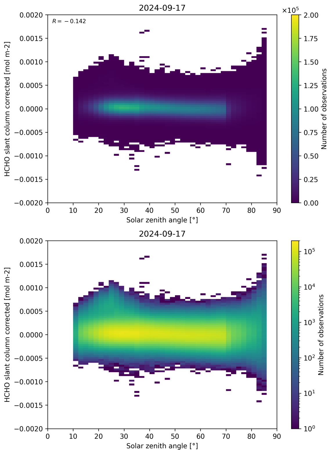
Figure 171: Scatter density plot of “Solar zenith angle” against “HCHO slant column corrected” for 2024-09-17 to 2024-09-18.
