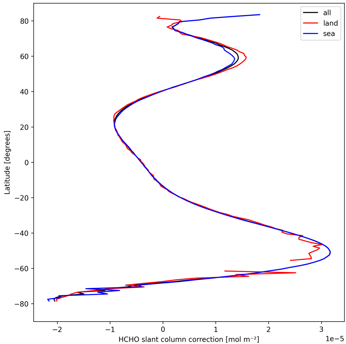
Figure 33: Zonal average of “HCHO slant column correction” for 2024-09-17 to 2024-09-18.
