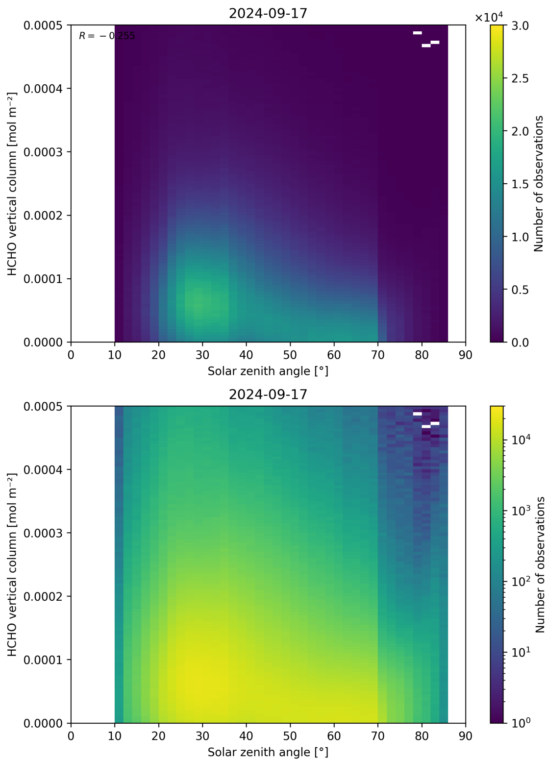
Figure 177: Scatter density plot of “Solar zenith angle” against “HCHO vertical column” for 2024-09-17 to 2024-09-18.
