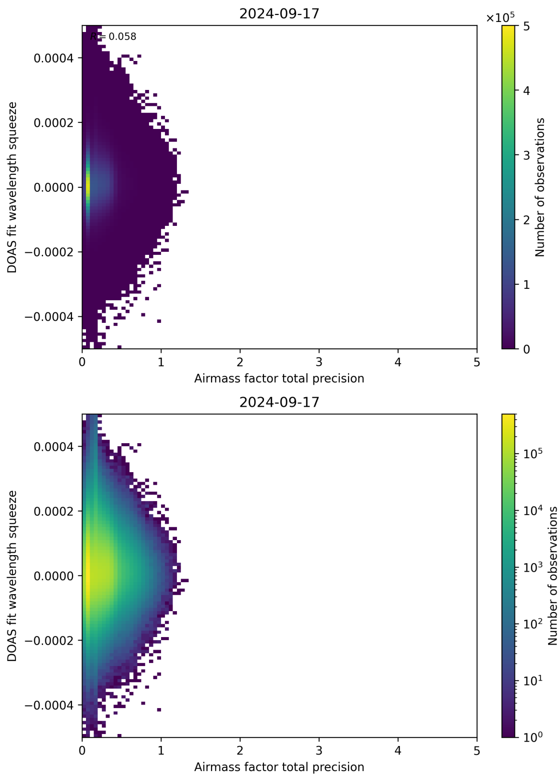
Figure 107: Scatter density plot of “Airmass factor total precision” against “DOAS fit wavelength squeeze” for 2024-09-17 to 2024-09-18.
