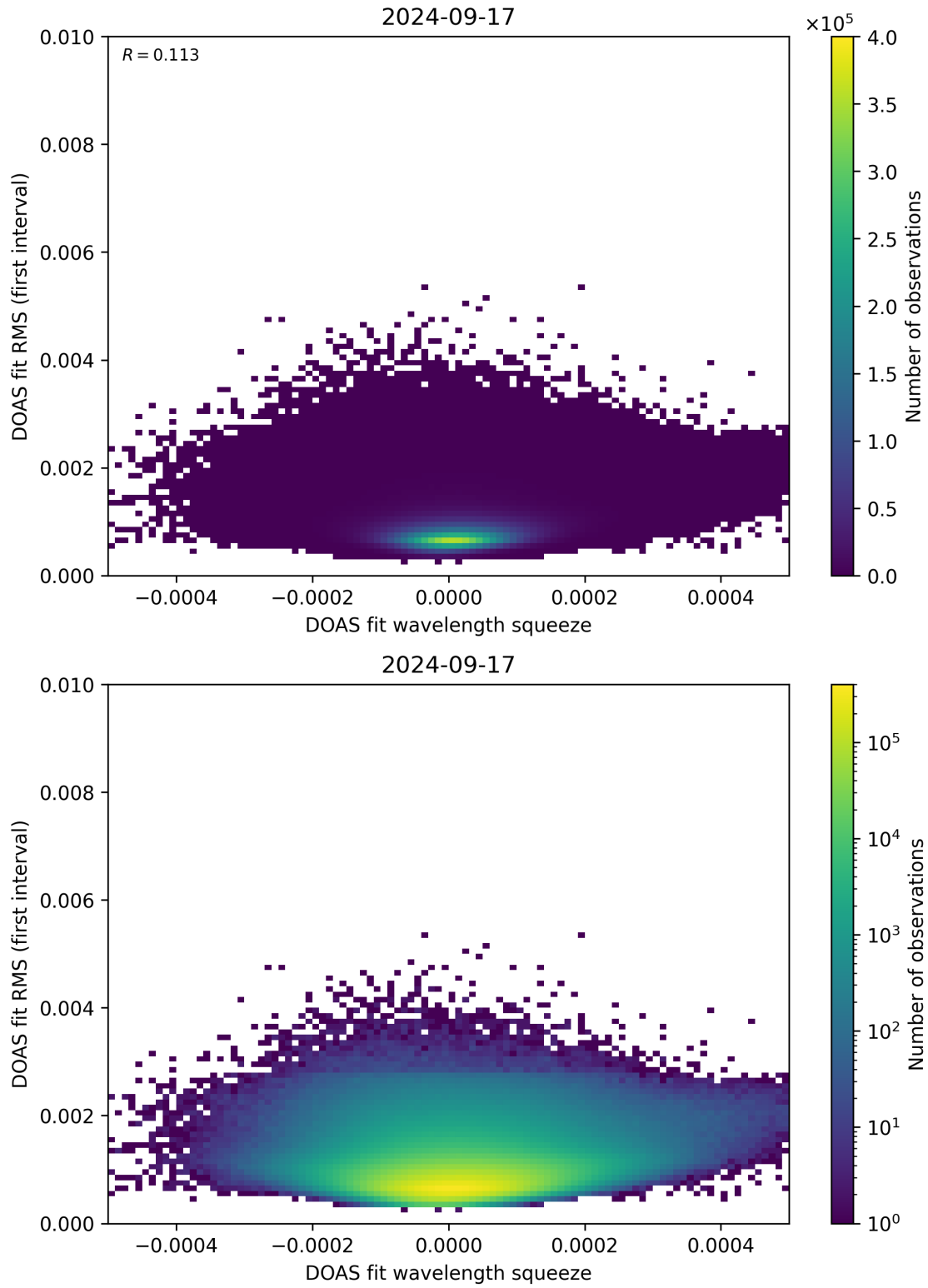
Figure 68: Scatter density plot of “DOAS fit wavelength squeeze” against “DOAS fit RMS (first interval)” for 2024-09-17 to 2024-09-18.
