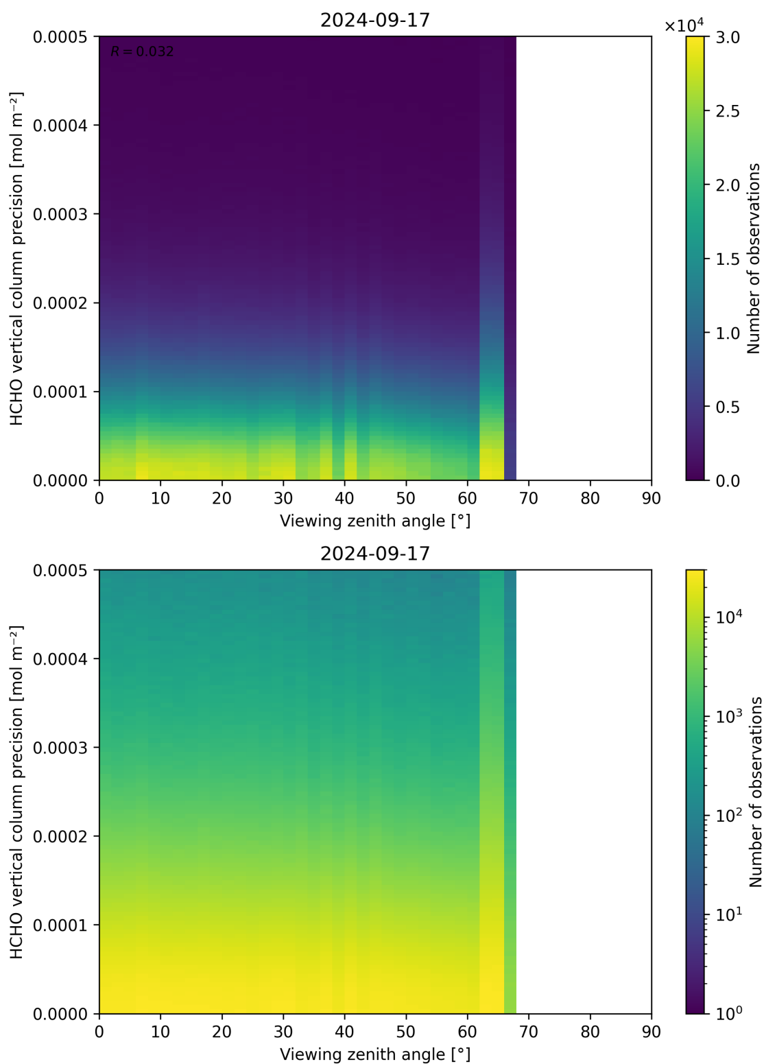
Figure 194: Scatter density plot of “Viewing zenith angle” against “HCHO vertical column precision” for 2024-09-17 to 2024-09-18.
