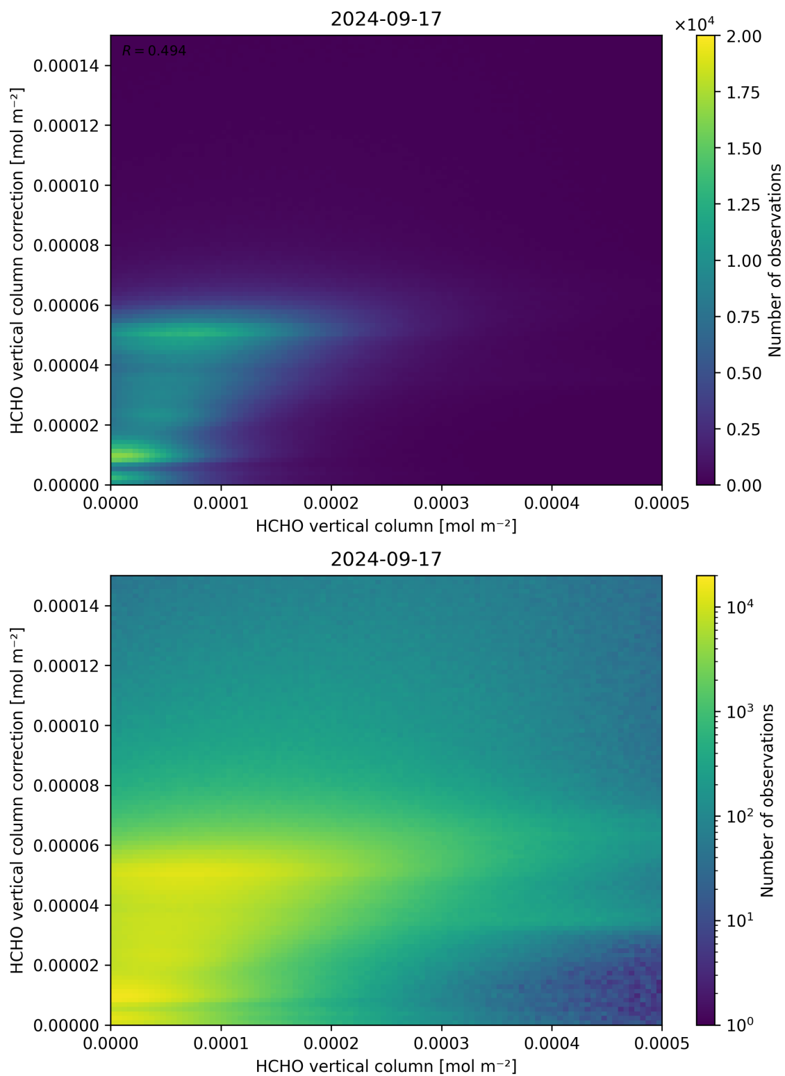
Figure 133: Scatter density plot of “HCHO vertical column” against “HCHO vertical column correction” for 2024-09-17 to 2024-09-18.
