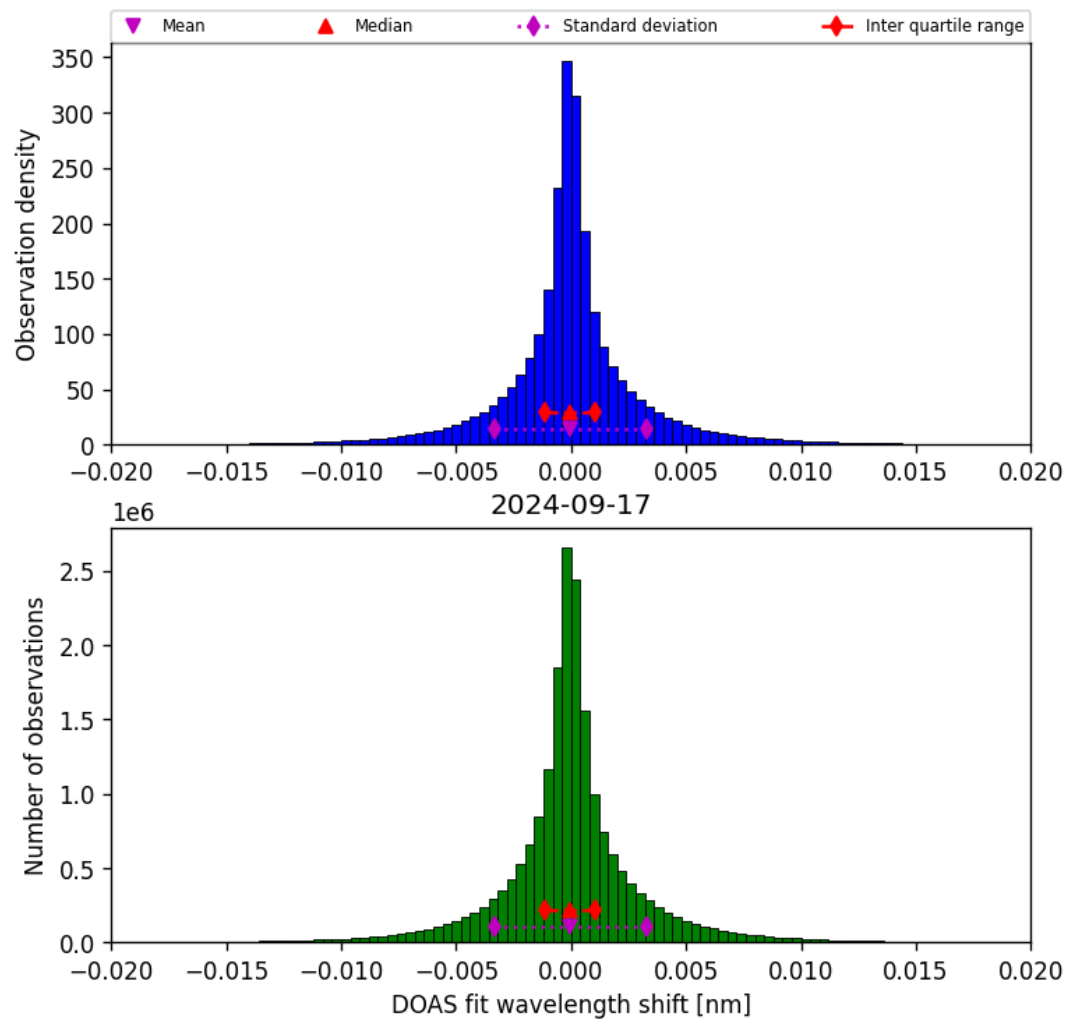
Figure 44: Histogram of “DOAS fit wavelength shift” for 2024-09-17 to 2024-09-18
