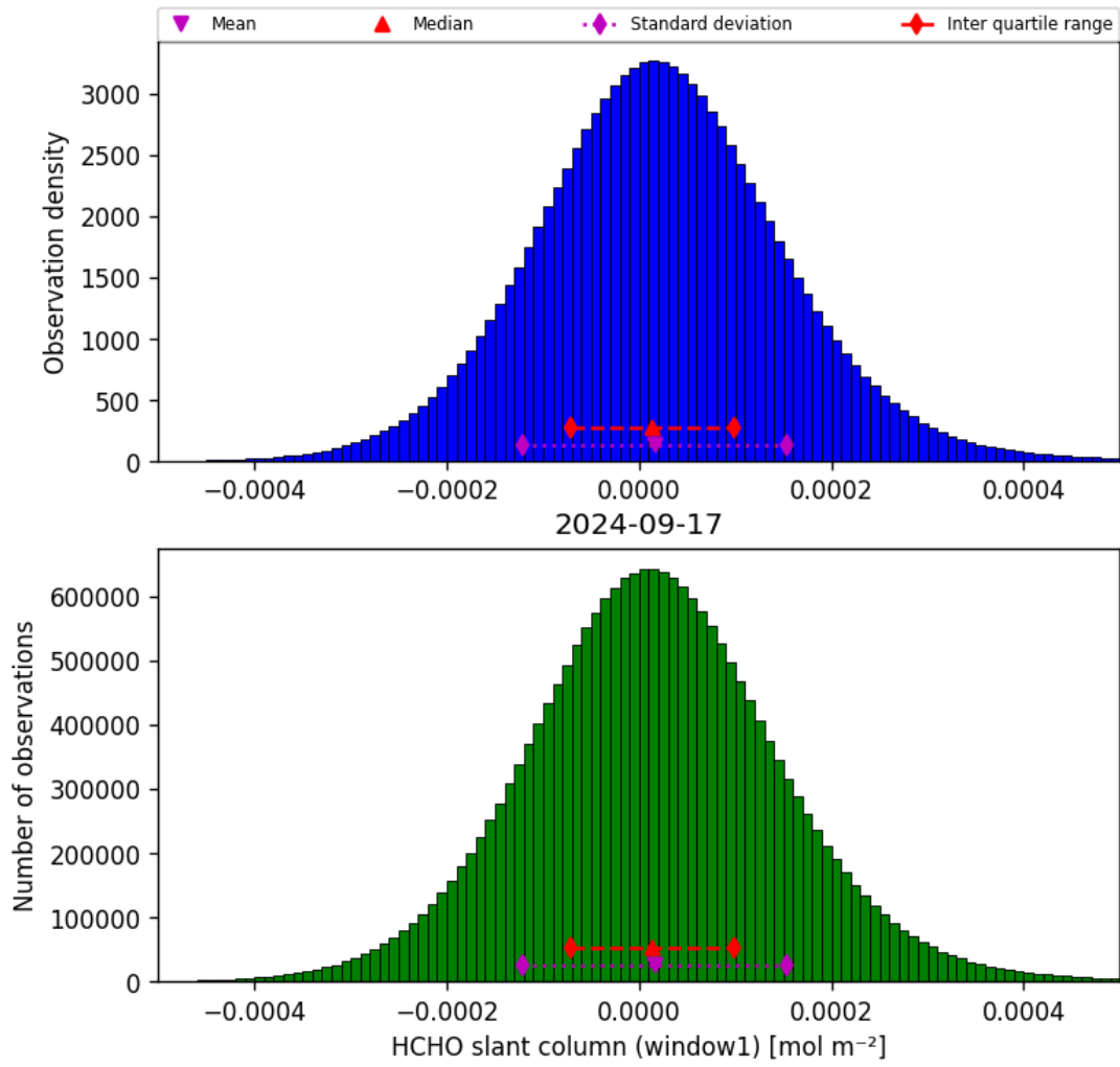
Figure 38: Histogram of “HCHO slant column (window1)” for 2024-09-17 to 2024-09-18
