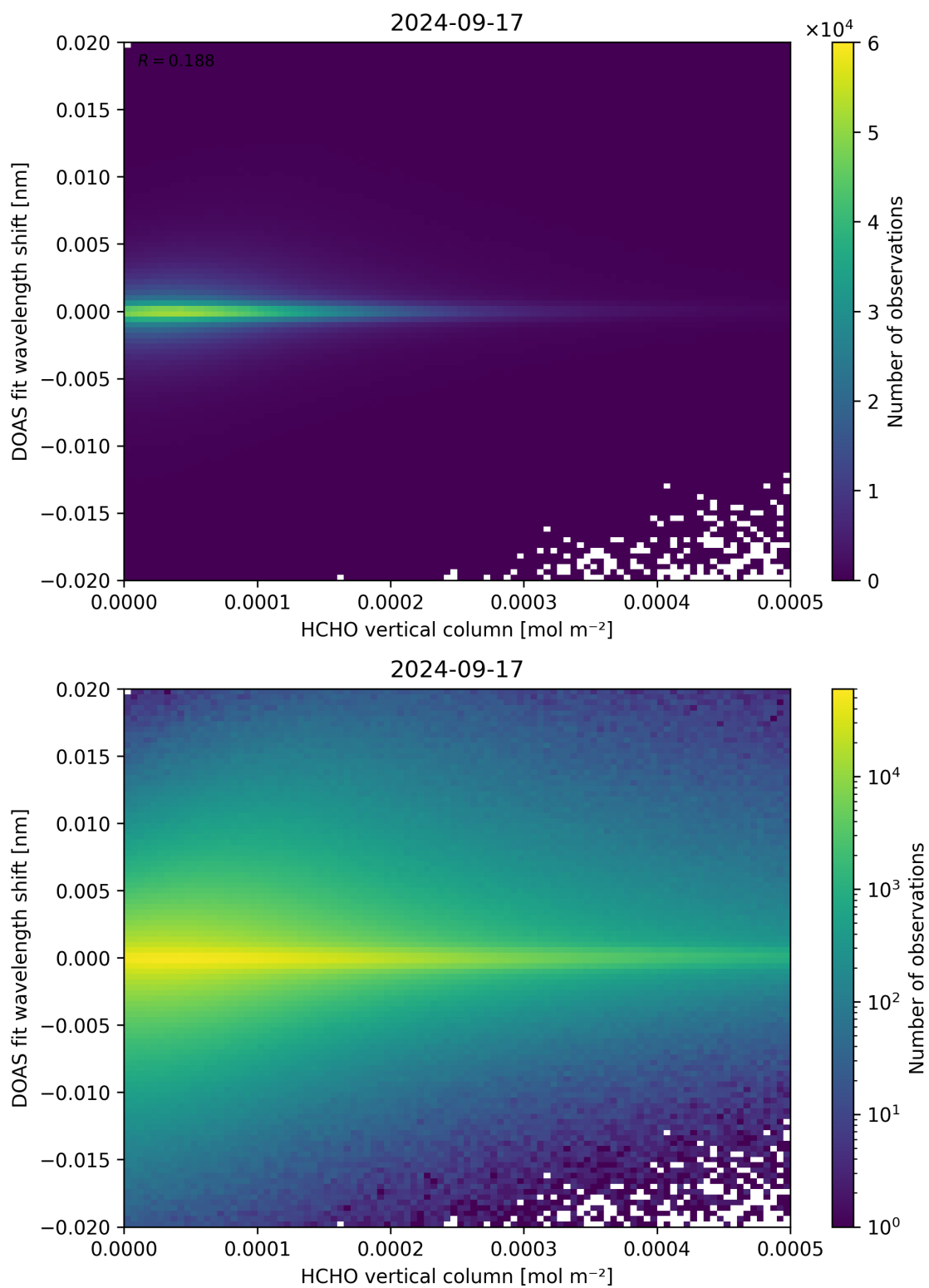
Figure 124: Scatter density plot of “HCHO vertical column” against “DOAS fit wavelength shift” for 2024-09-17 to 2024-09-18.
