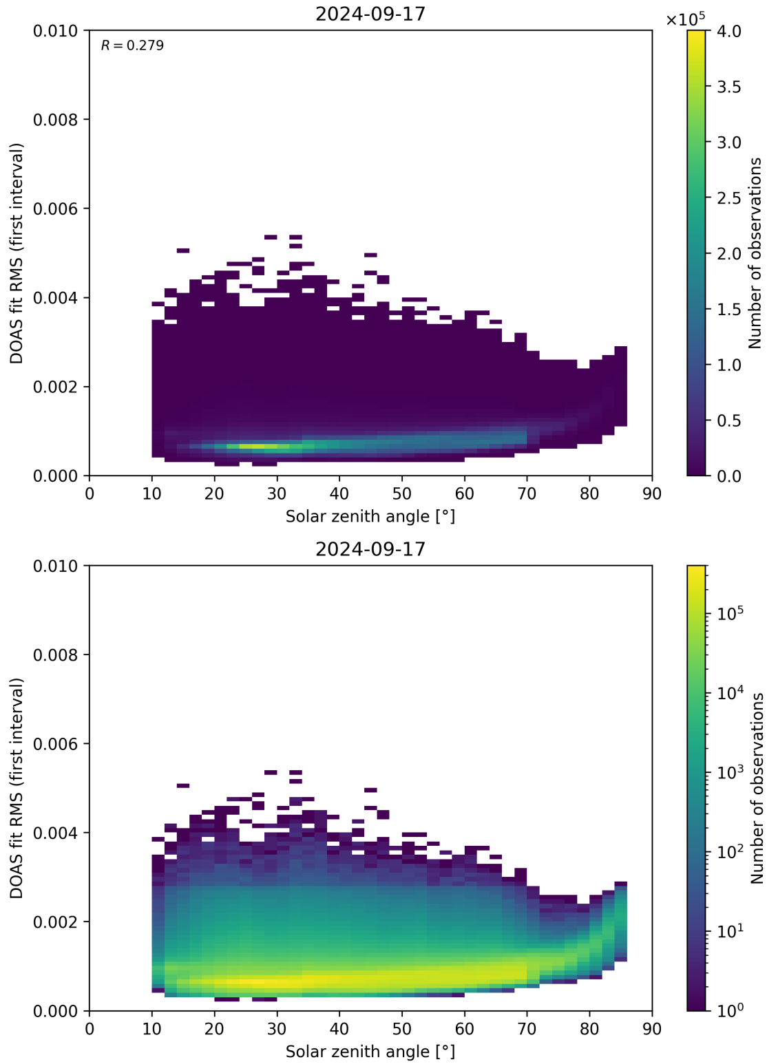
Figure 167: Scatter density plot of “Solar zenith angle” against “DOAS fit RMS (first interval)” for 2024-09-17 to 2024-09-18.
