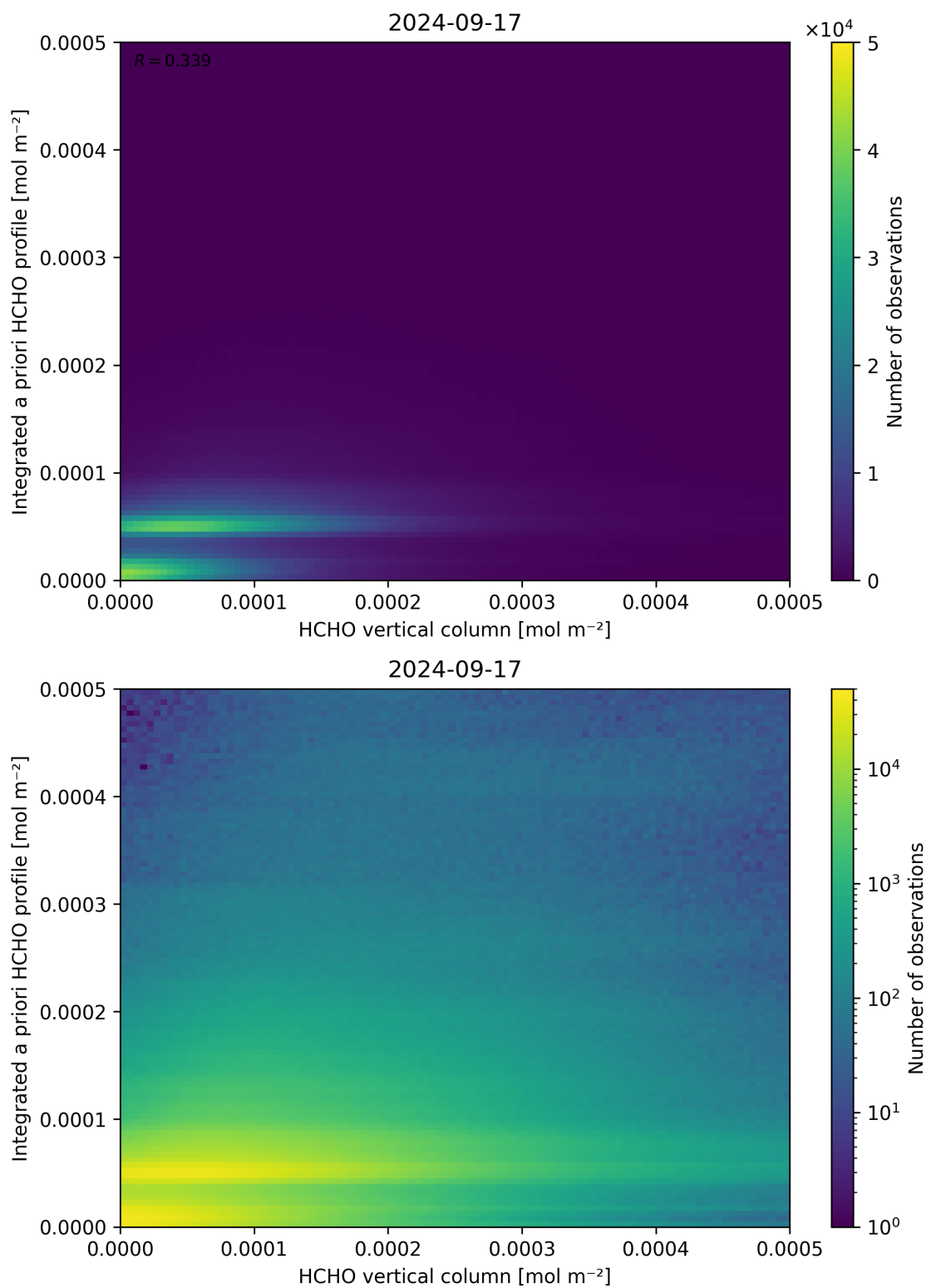
Figure 135: Scatter density plot of “HCHO vertical column” against “Integrated a priori HCHO profile” for 2024-09-17 to 2024-09-18.
