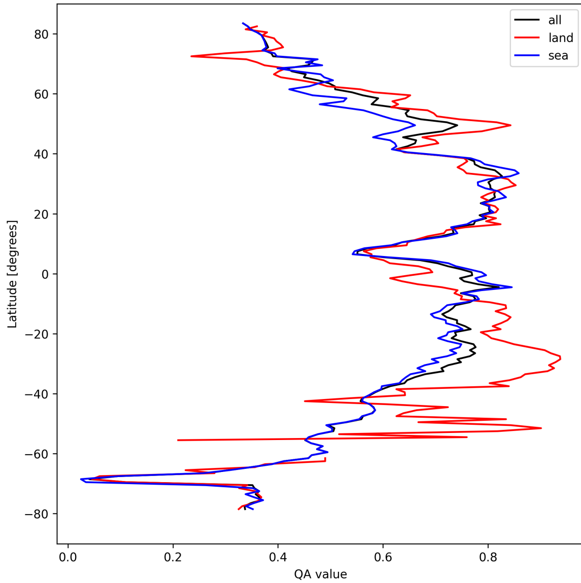
Figure 20: Zonal average of “QA value” for 2024-09-17 to 2024-09-18.
