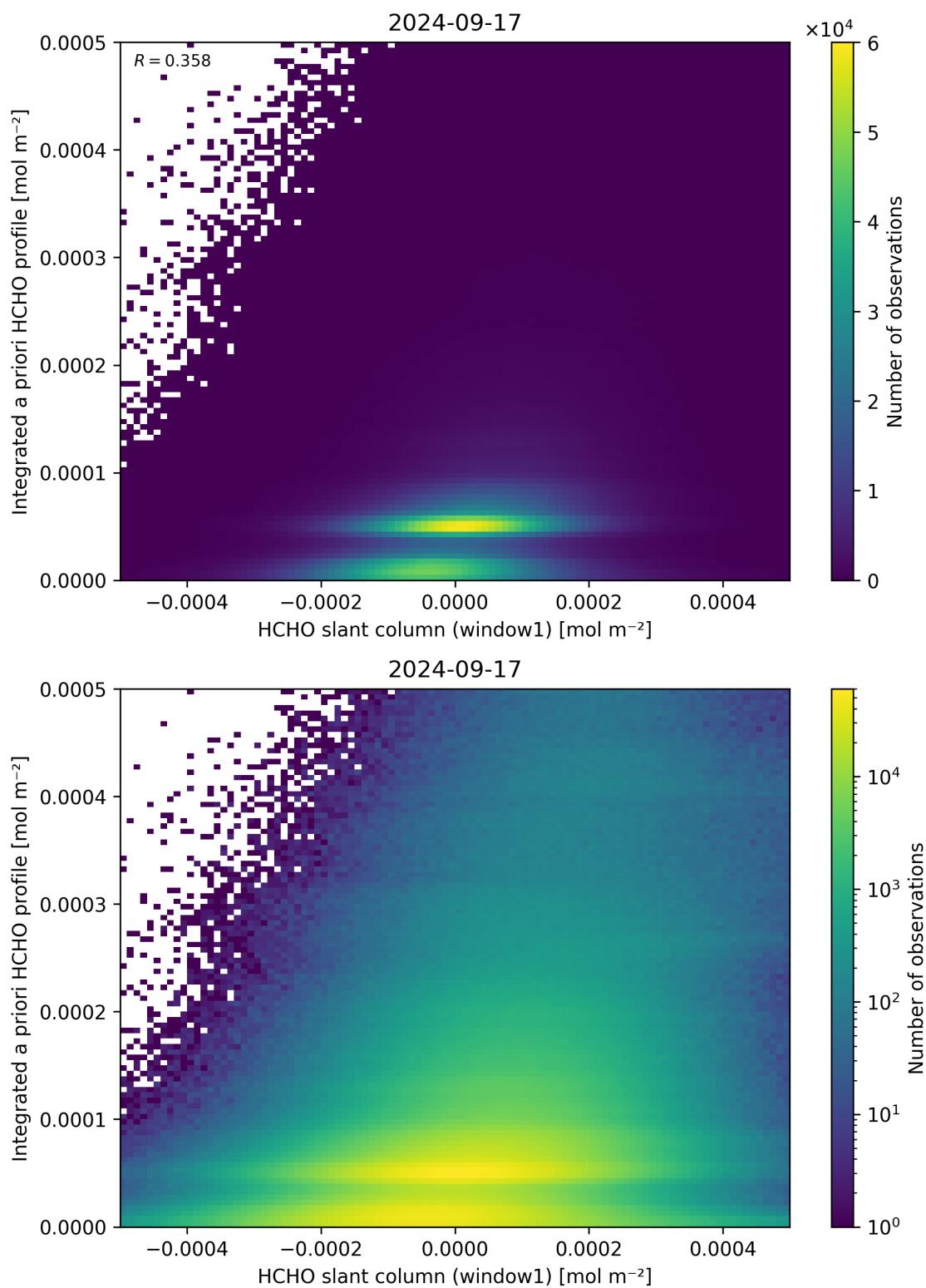
Figure 87: Scatter density plot of “HCHO slant column (window1)” against “Integrated a priori HCHO profile” for 2024-09-17 to 2024-09-18.
