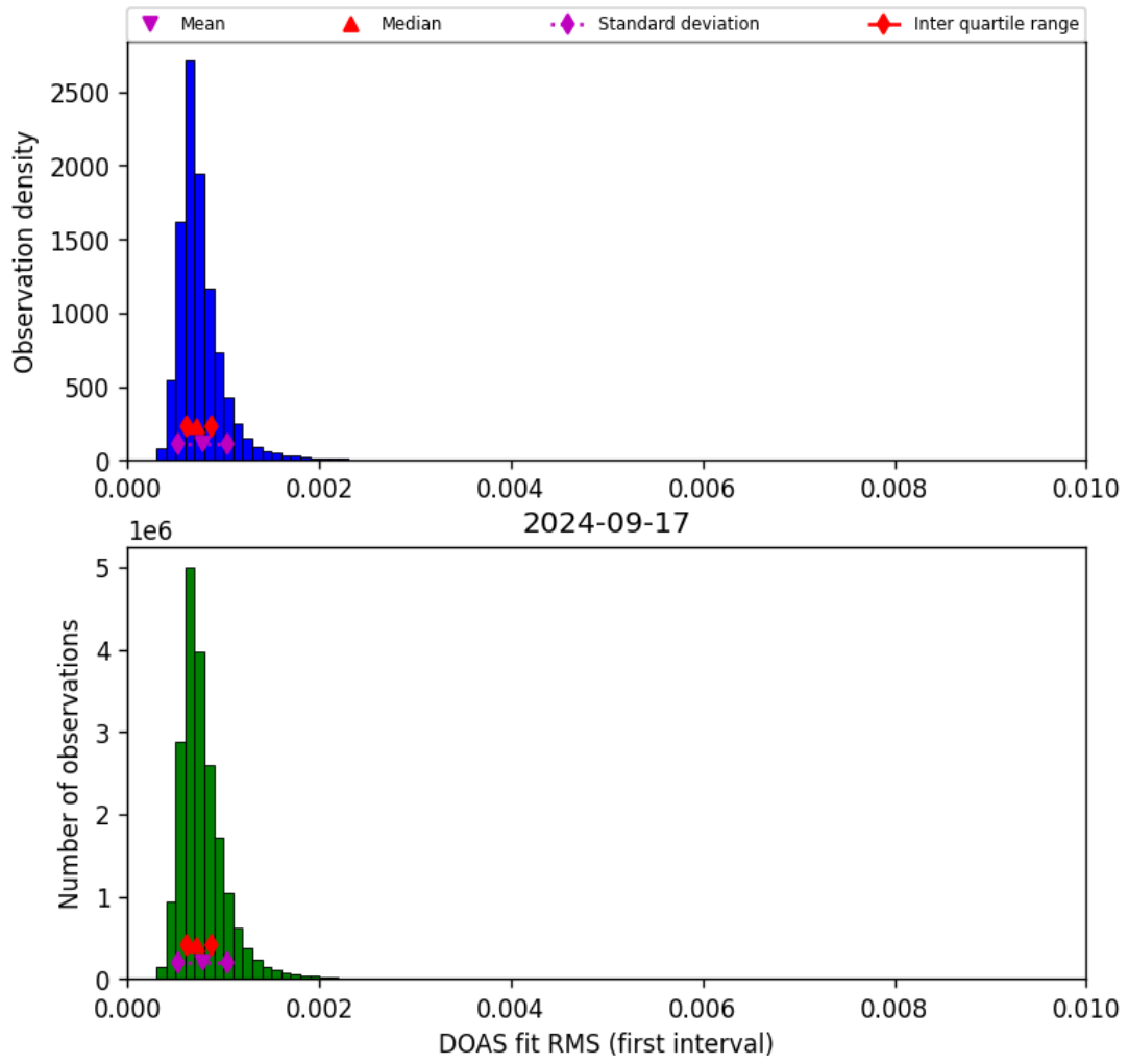
Figure 46: Histogram of “DOAS fit RMS (first interval)” for 2024-09-17 to 2024-09-18
