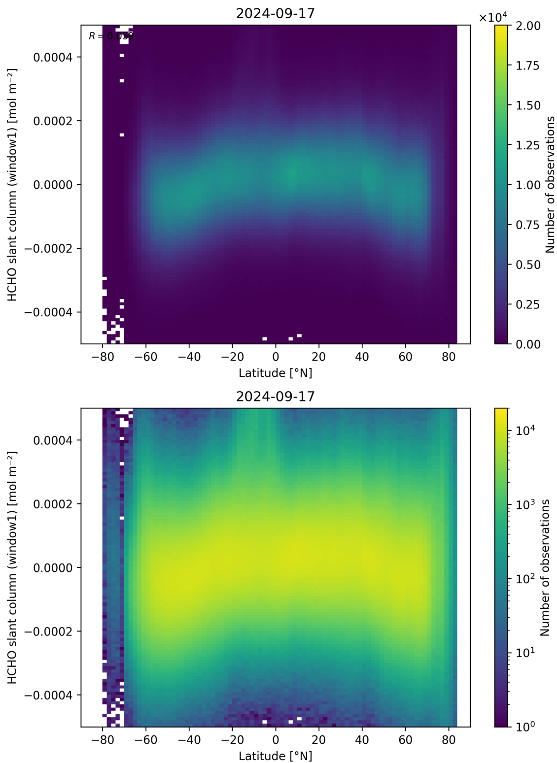
Figure 159: Scatter density plot of “Latitude” against “HCHO slant column (window1)” for 2024-09-17 to 2024-09-18.
