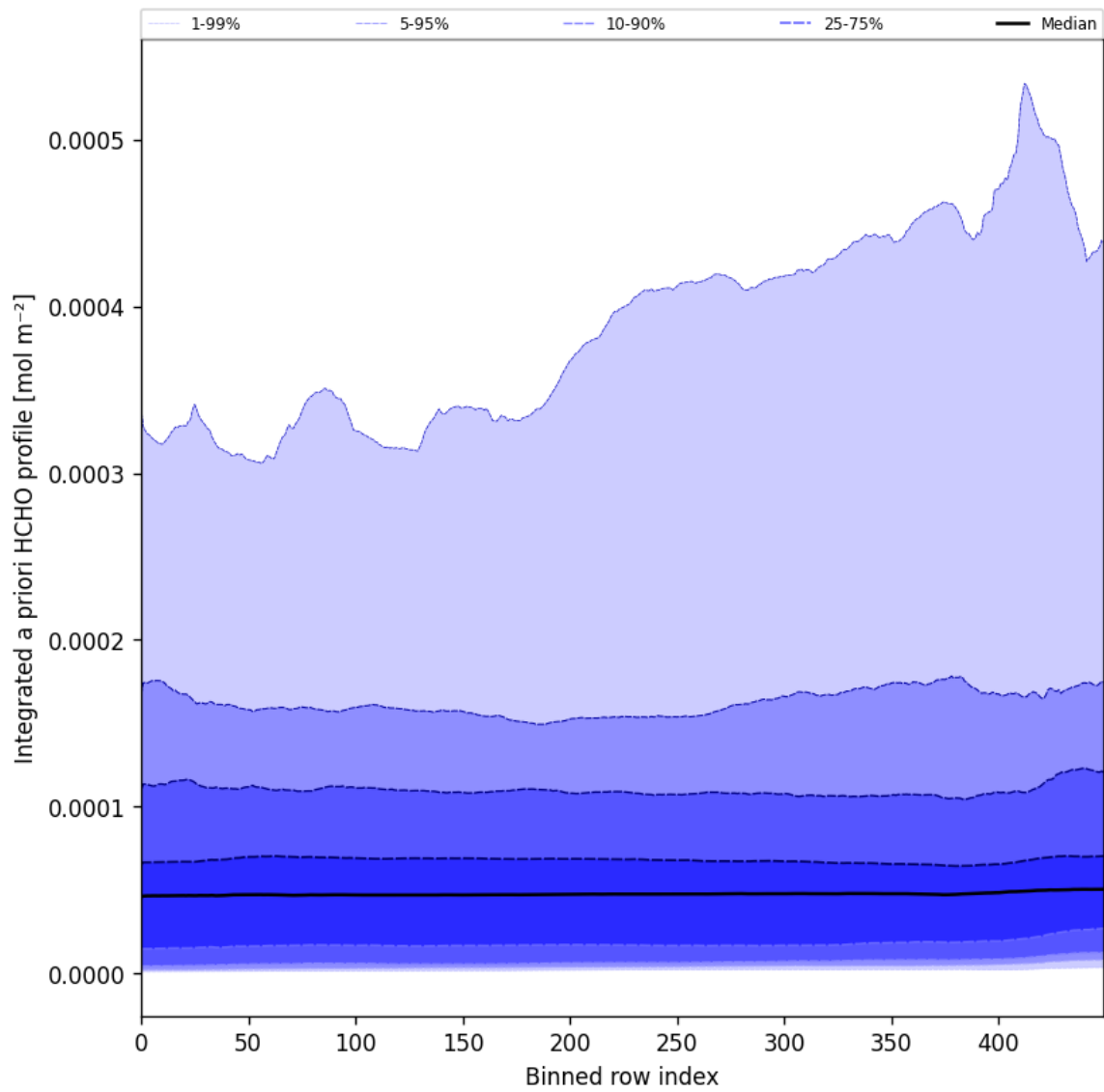
Figure 57: Along track statistics of “Integrated a priori HCHO profile” for 2024-09-17 to 2024-09-18
