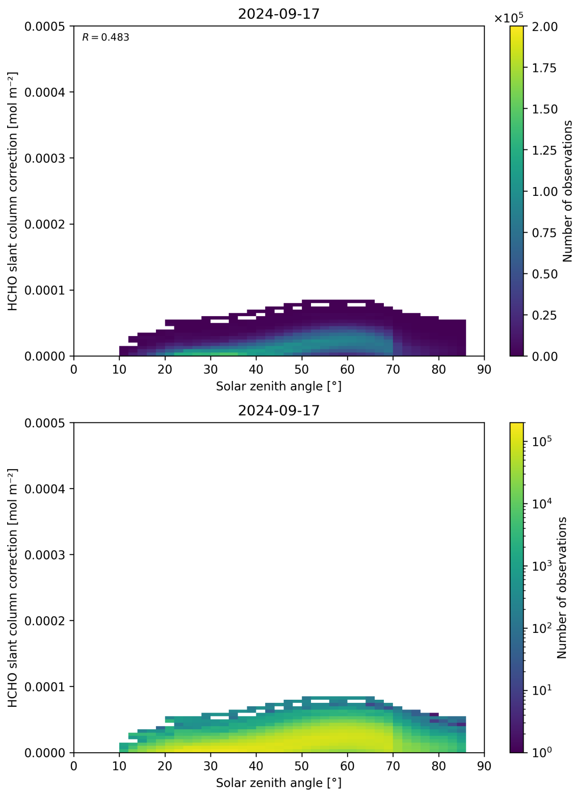
Figure 172: Scatter density plot of “Solar zenith angle” against “HCHO slant column correction” for 2024-09-17 to 2024-09-18.
