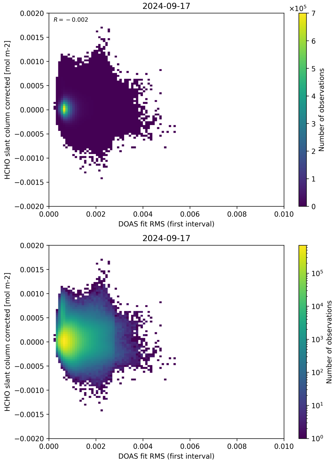
Figure 62: Scatter density plot of “DOAS fit RMS (first interval)” against “HCHO slant column corrected” for 2024-09-17 to 2024-09-18.
