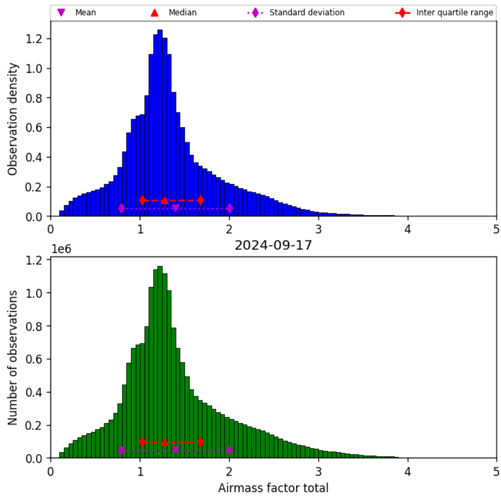
Figure 40: Histogram of “Airmass factor total” for 2024-09-17 to 2024-09-18
