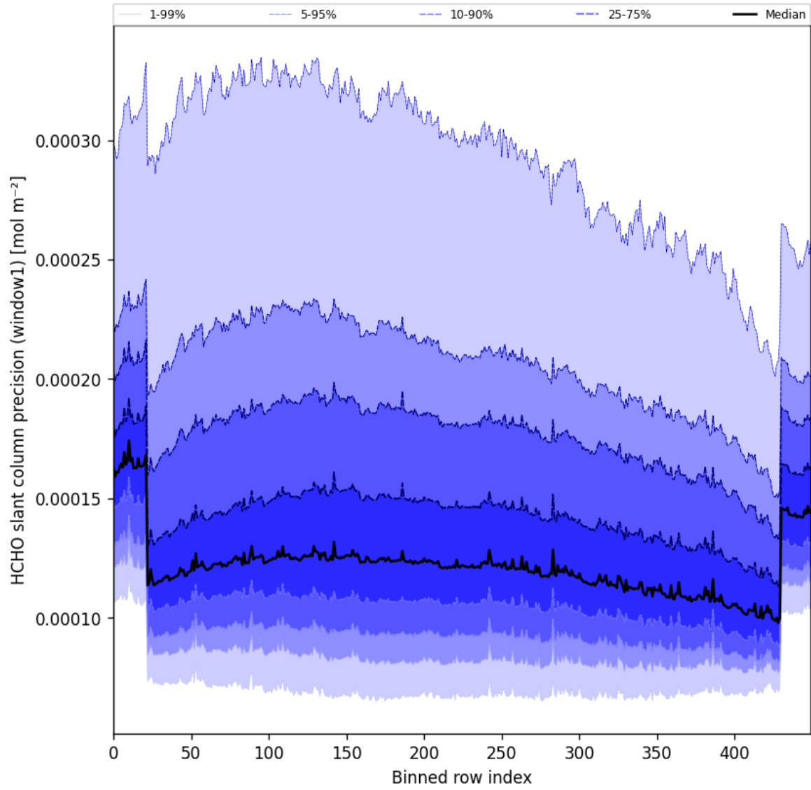
Figure 53: Along track statistics of “HCHO slant column precision (window1)” for 2024-09-17 to 2024-09-18
