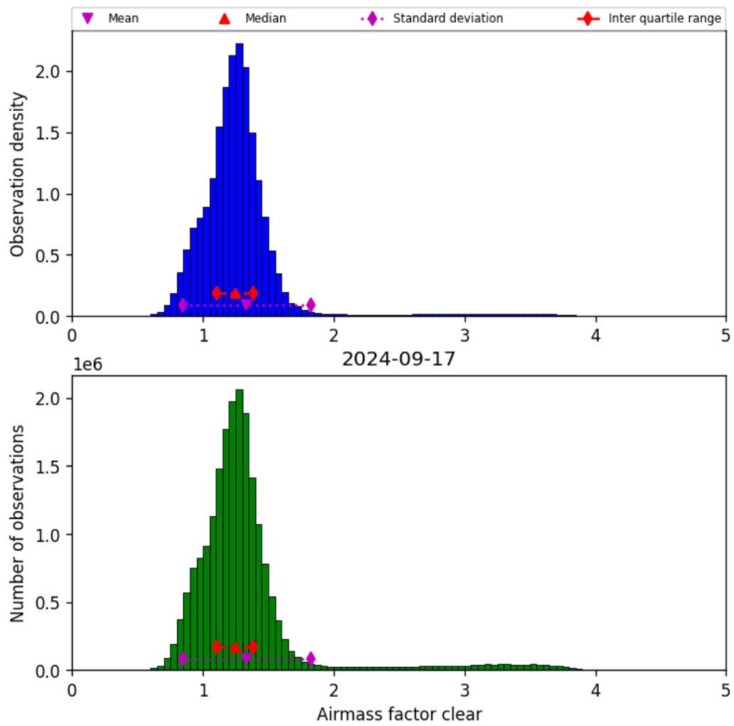
Figure 42: Histogram of “Airmass factor clear” for 2024-09-17 to 2024-09-18
