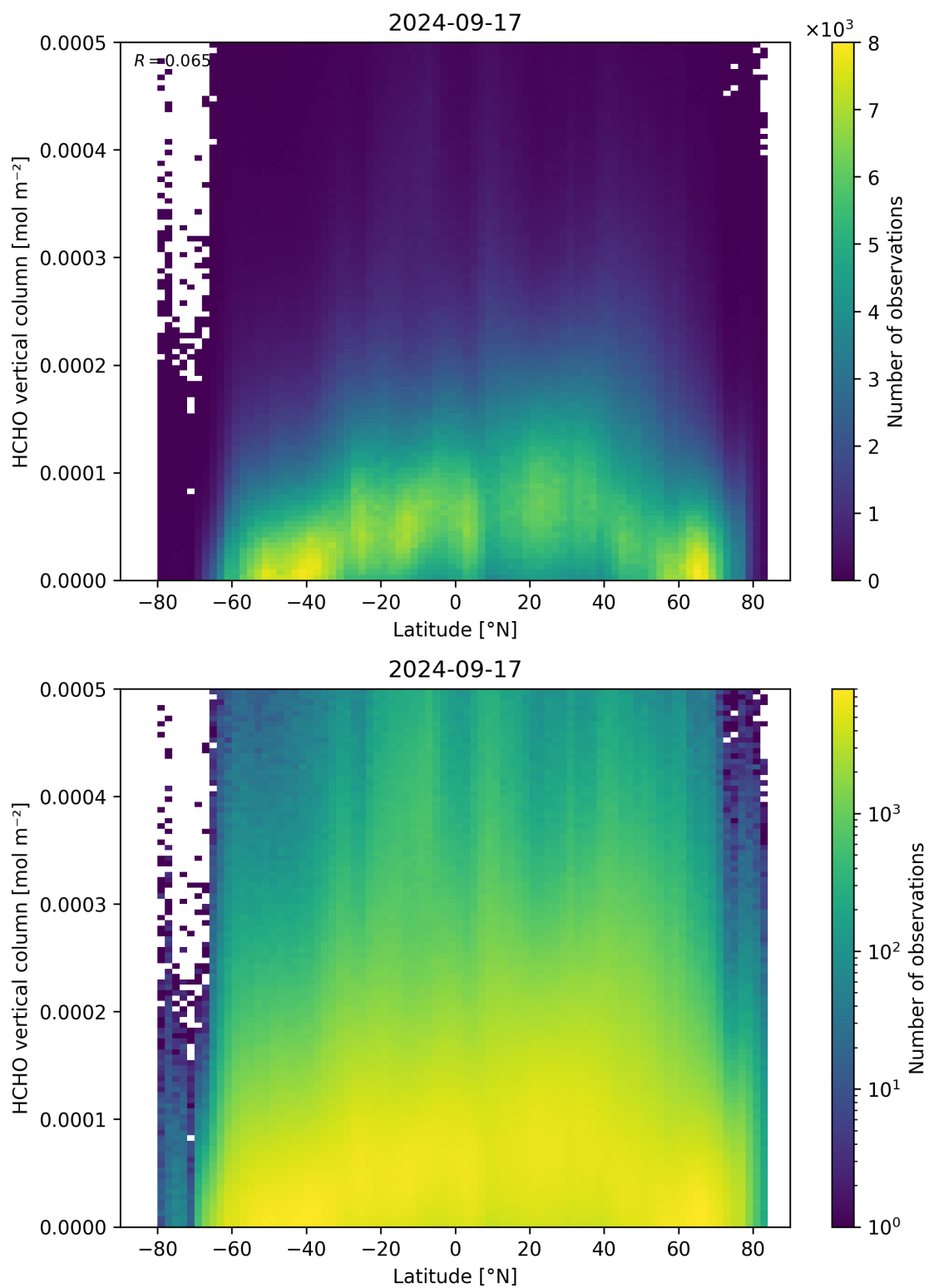
Figure 163: Scatter density plot of “Latitude” against “HCHO vertical column” for 2024-09-17 to 2024-09-18.
