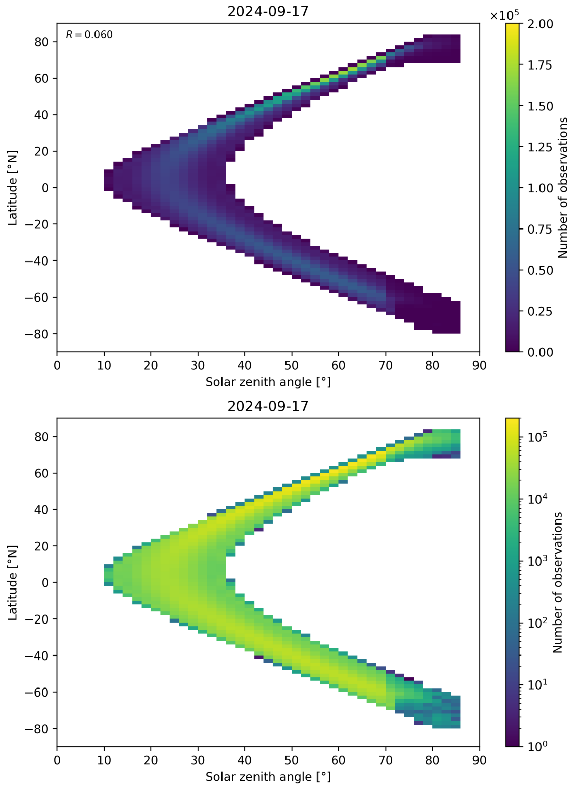
Figure 181: Scatter density plot of “Solar zenith angle” against “Latitude” for 2024-09-17 to 2024-09-18.
