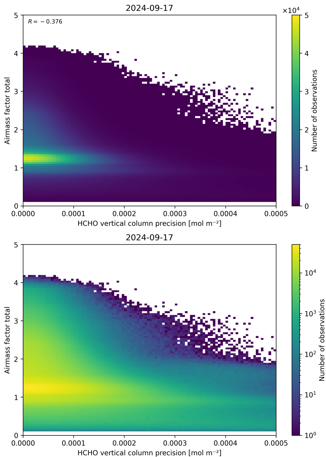
Figure 144: Scatter density plot of “HCHO vertical column precision” against “Airmass factor total” for 2024-09-17 to 2024-09-18.
