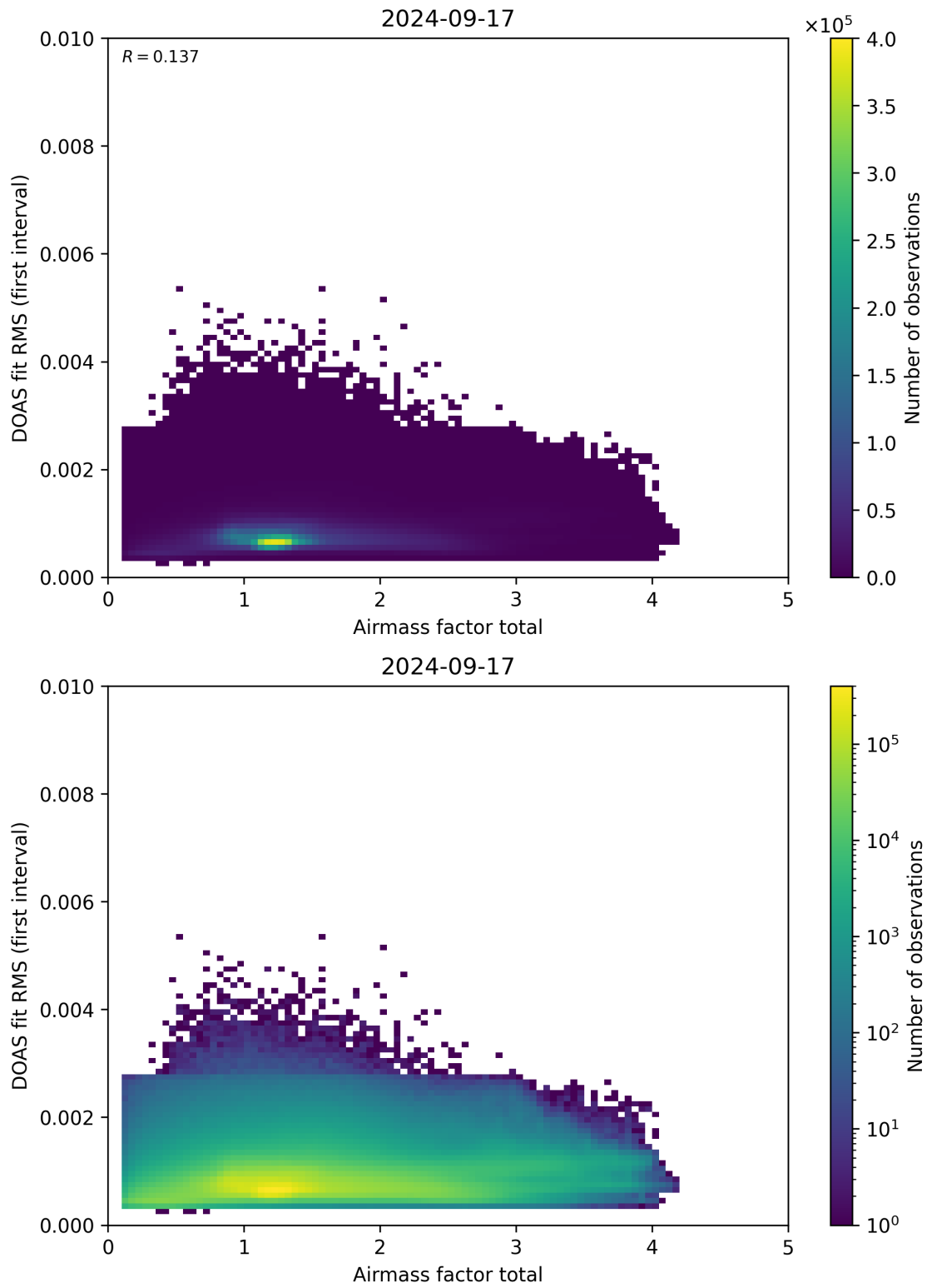
Figure 97: Scatter density plot of “Airmass factor total” against “DOAS fit RMS (first interval)” for 2024-09-17 to 2024-09-18.
