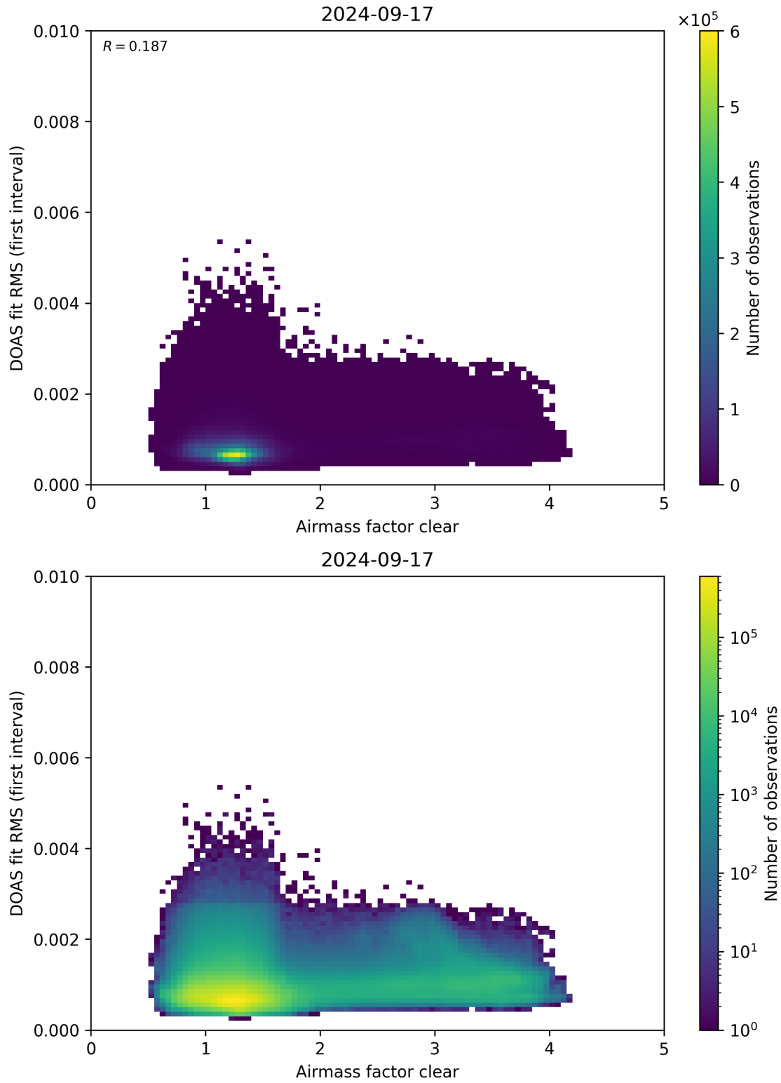
Figure 71: Scatter density plot of “Airmass factor clear” against “DOAS fit RMS (first interval)” for 2024-09-17 to 2024-09-18.
