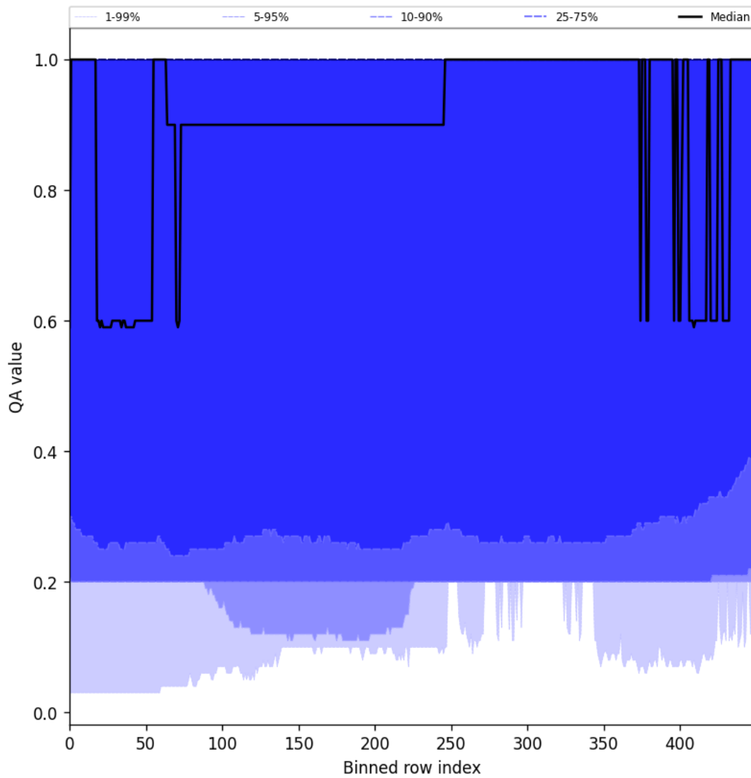
Figure 48: Along track statistics of “QA value” for 2024-09-17 to 2024-09-18
