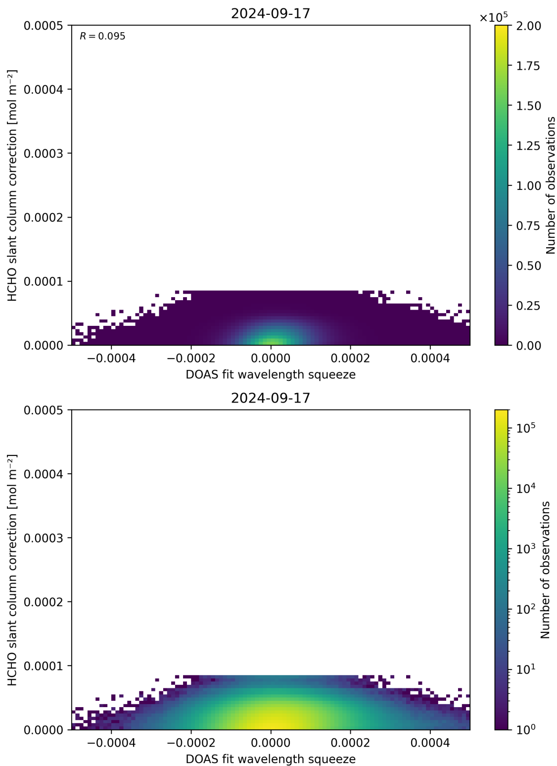
Figure 70: Scatter density plot of “DOAS fit wavelength squeeze” against “HCHO slant column correction” for 2024-09-17 to 2024-09-18.
