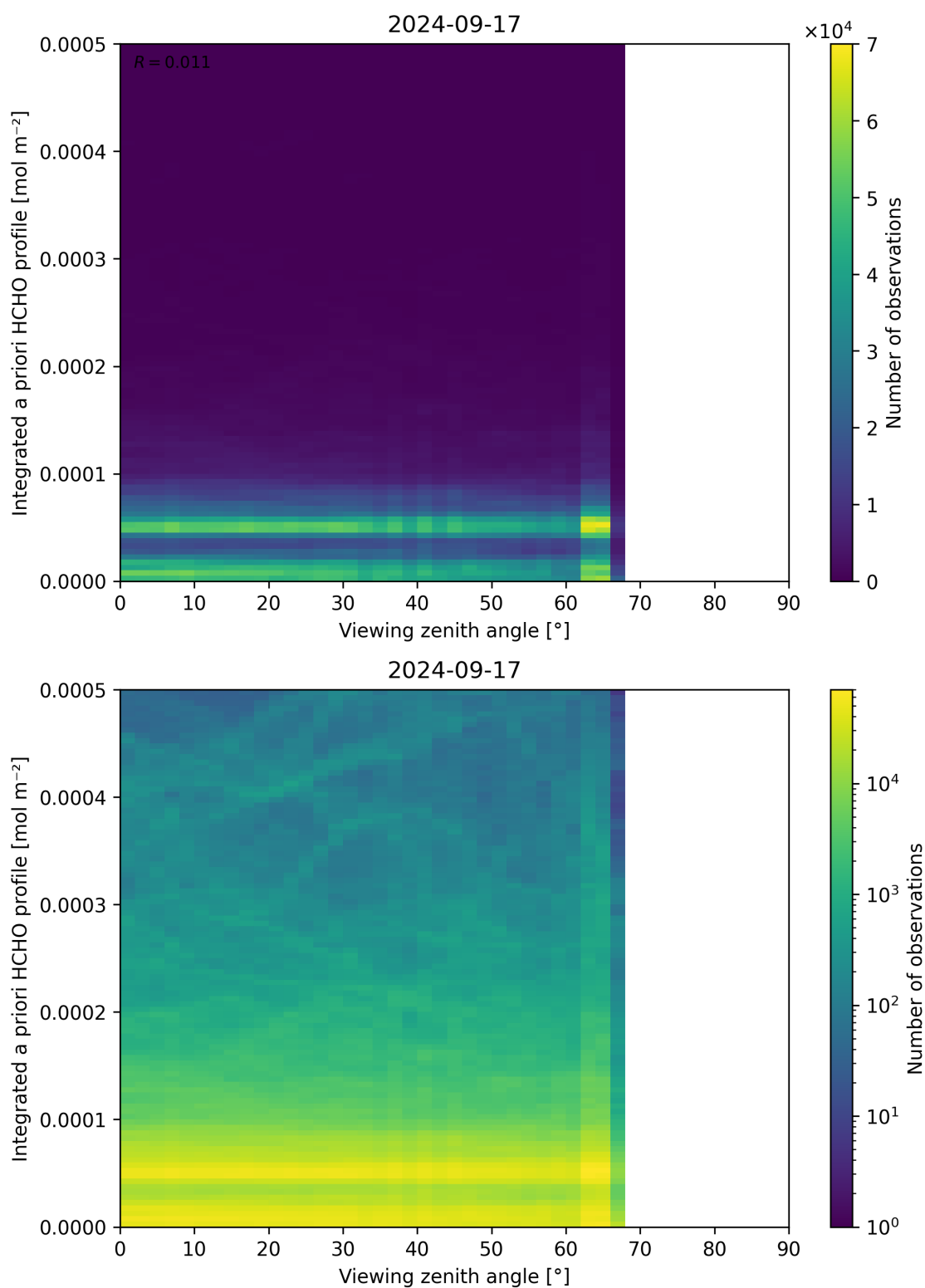
Figure 195: Scatter density plot of “Viewing zenith angle” against “Integrated a priori HCHO profile” for 2024-09-17 to 2024-09-18.
