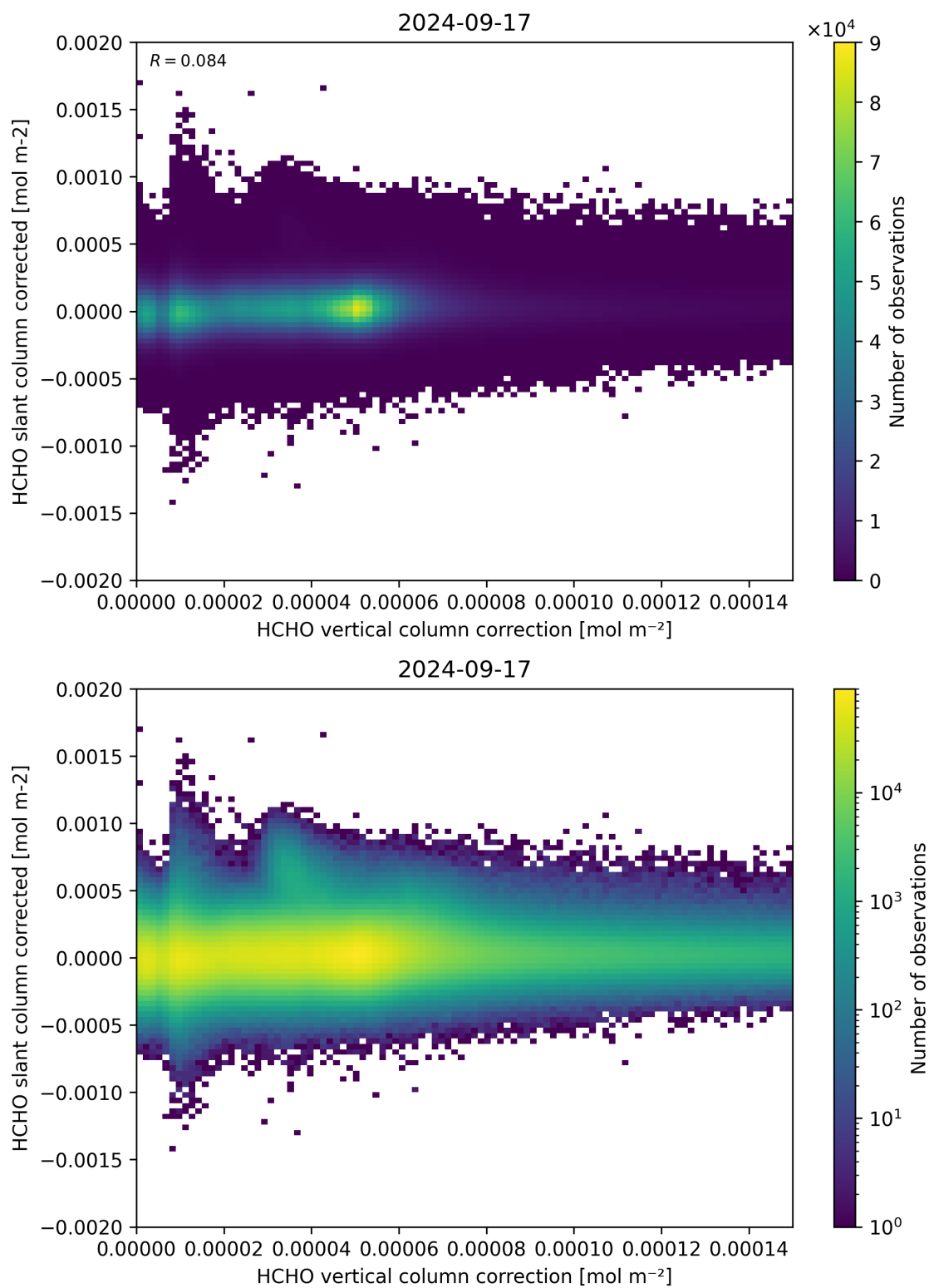
Figure 116: Scatter density plot of “HCHO vertical column correction” against “HCHO slant column corrected” for 2024-09-17 to 2024-09-18.
