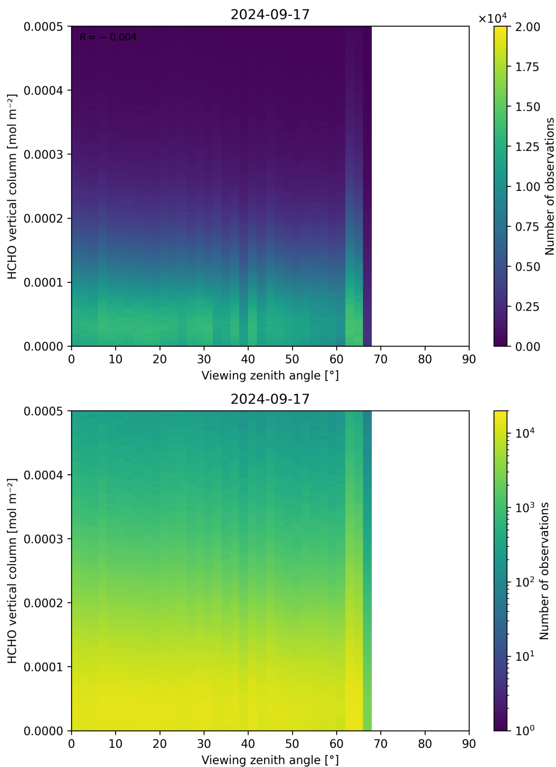
Figure 192: Scatter density plot of “Viewing zenith angle” against “HCHO vertical column” for 2024-09-17 to 2024-09-18.
