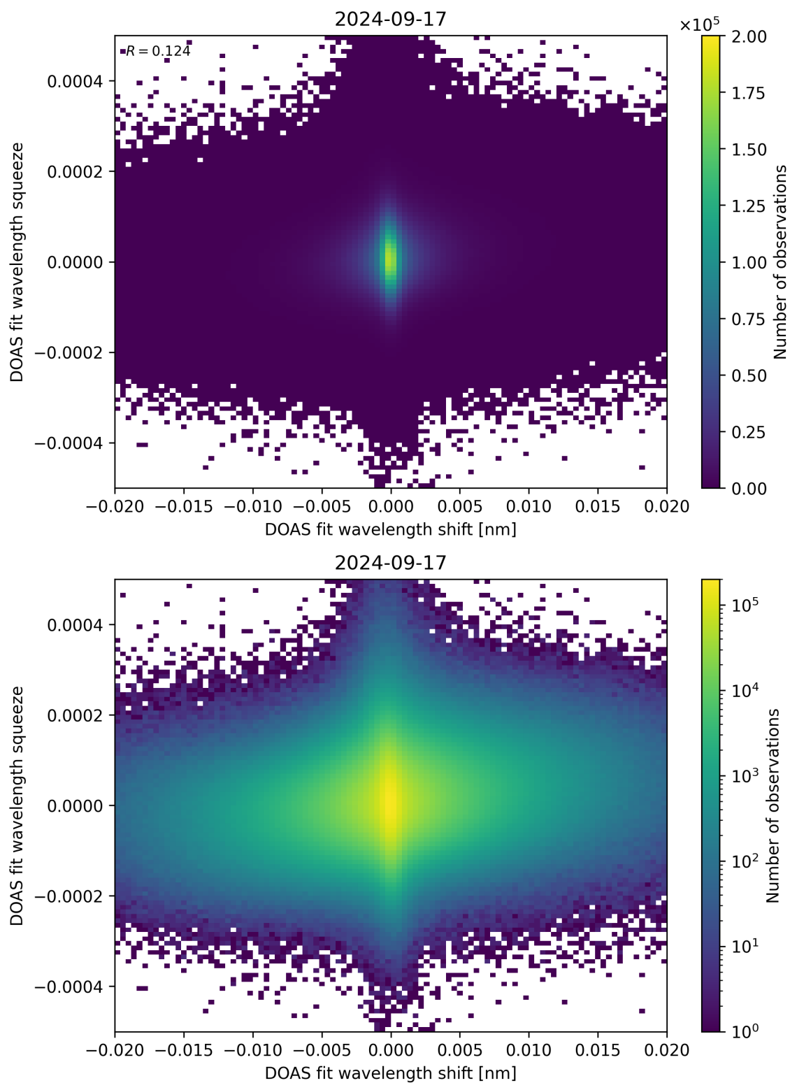
Figure 65: Scatter density plot of “DOAS fit wavelength shift” against “DOAS fit wavelength squeeze” for 2024-09-17 to 2024-09-18.
