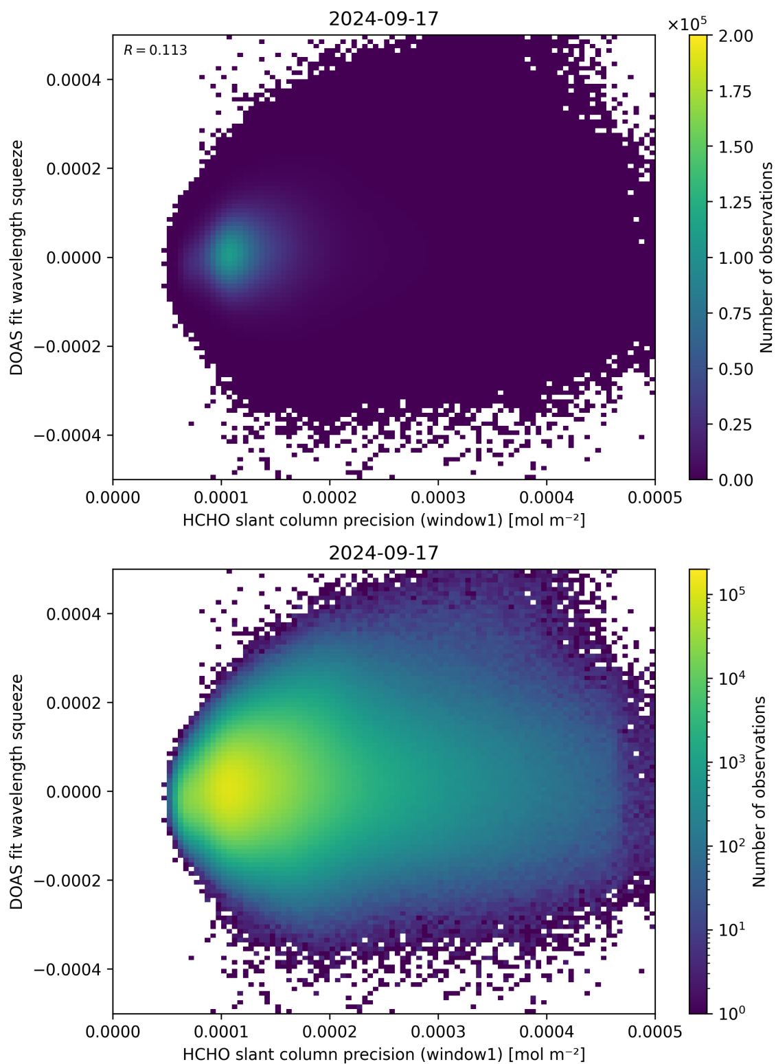
Figure 90: Scatter density plot of “HCHO slant column precision (window1)” against “DOAS fit wavelength squeeze” for 2024-09-17 to 2024-09-18.
