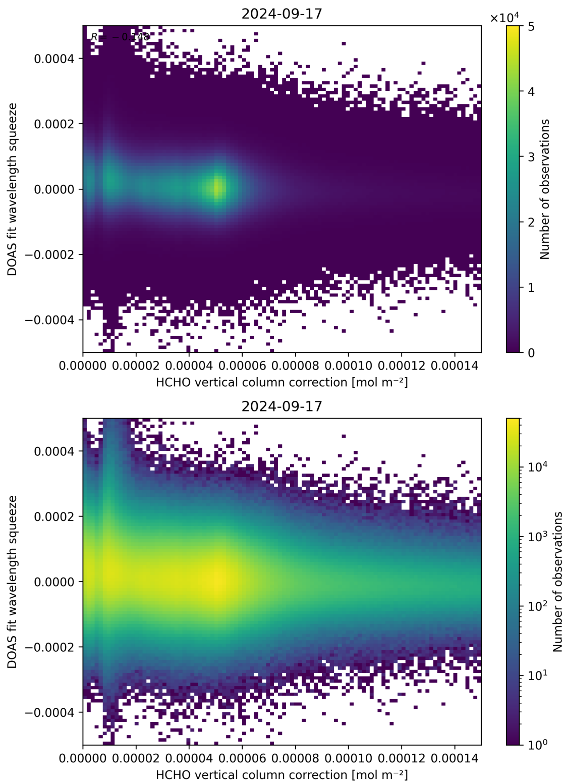
Figure 114: Scatter density plot of “HCHO vertical column correction” against “DOAS fit wavelength squeeze” for 2024-09-17 to 2024-09-18.
