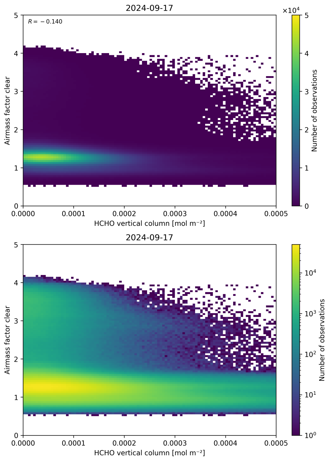
Figure 126: Scatter density plot of “HCHO vertical column” against “Airmass factor clear” for 2024-09-17 to 2024-09-18.
