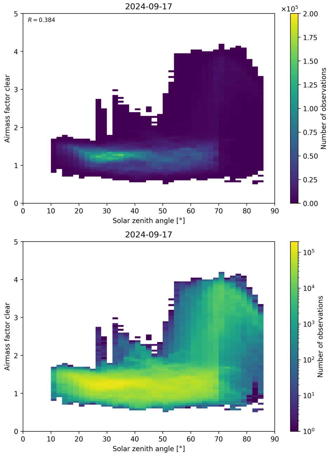
Figure 170: Scatter density plot of “Solar zenith angle” against “Airmass factor clear” for 2024-09-17 to 2024-09-18.
