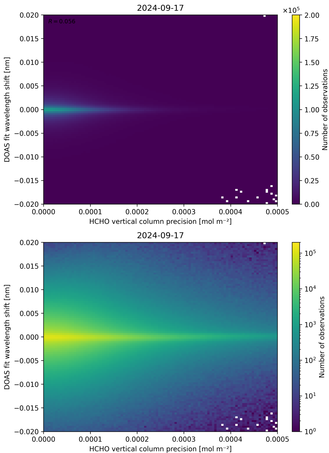
Figure 137: Scatter density plot of “HCHO vertical column precision” against “DOAS fit wavelength shift” for 2024-09-17 to 2024-09-18.
