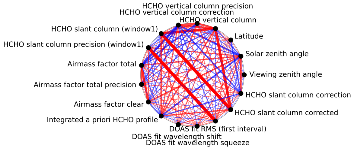
Figure 1: Map of correlation graph for 2024-09-17 to 2024-09-18.
