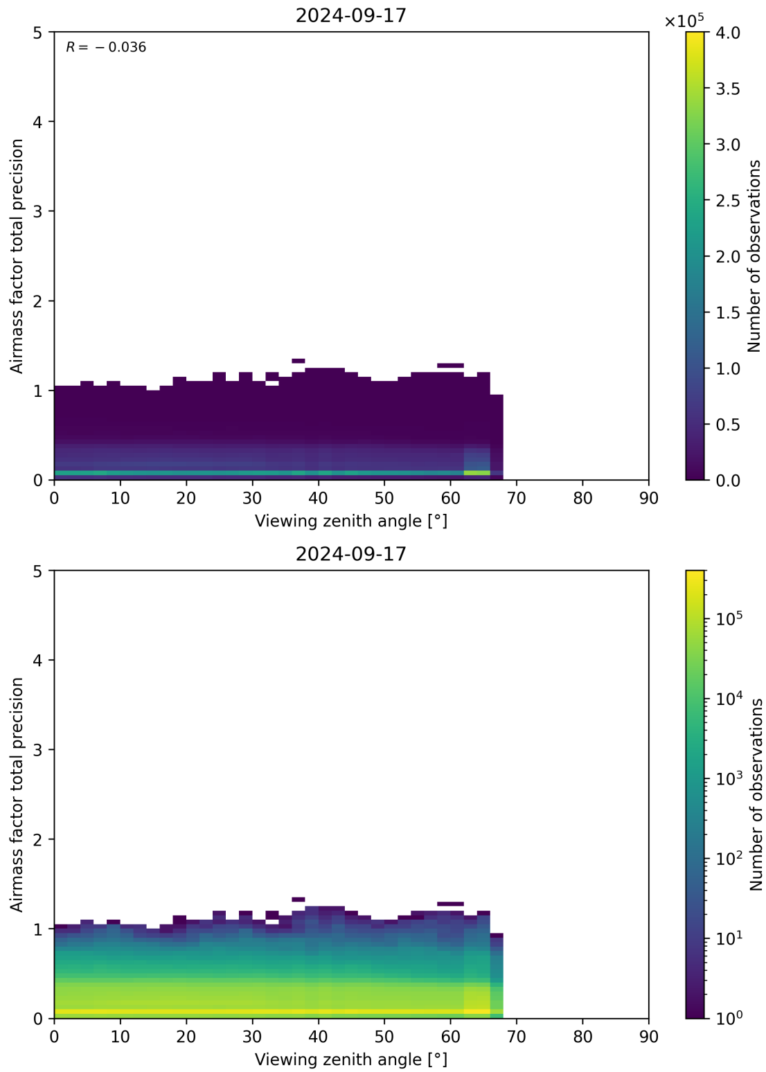
Figure 191: Scatter density plot of “Viewing zenith angle” against “Airmass factor total precision” for 2024-09-17 to 2024-09-18.
