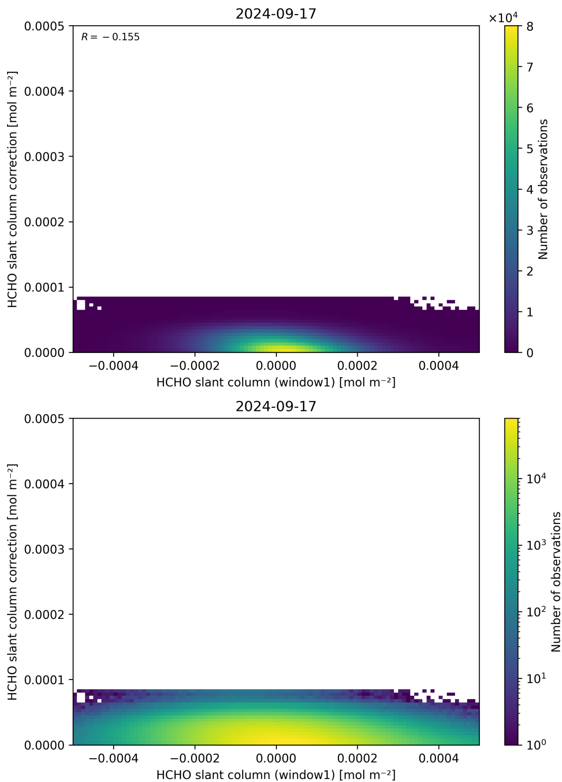
Figure 83: Scatter density plot of “HCHO slant column (window1)” against “HCHO slant column correction” for 2024-09-17 to 2024-09-18.
