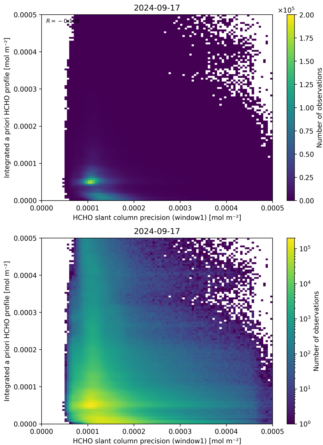
Figure 96: Scatter density plot of “HCHO slant column precision (window1)” against “Integrated a priori HCHO profile” for 2024-09-17 to 2024-09-18.
