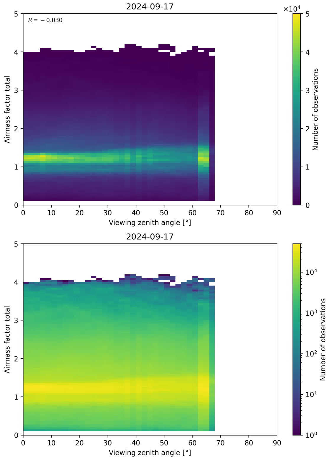
Figure 190: Scatter density plot of “Viewing zenith angle” against “Airmass factor total” for 2024-09-17 to 2024-09-18.
