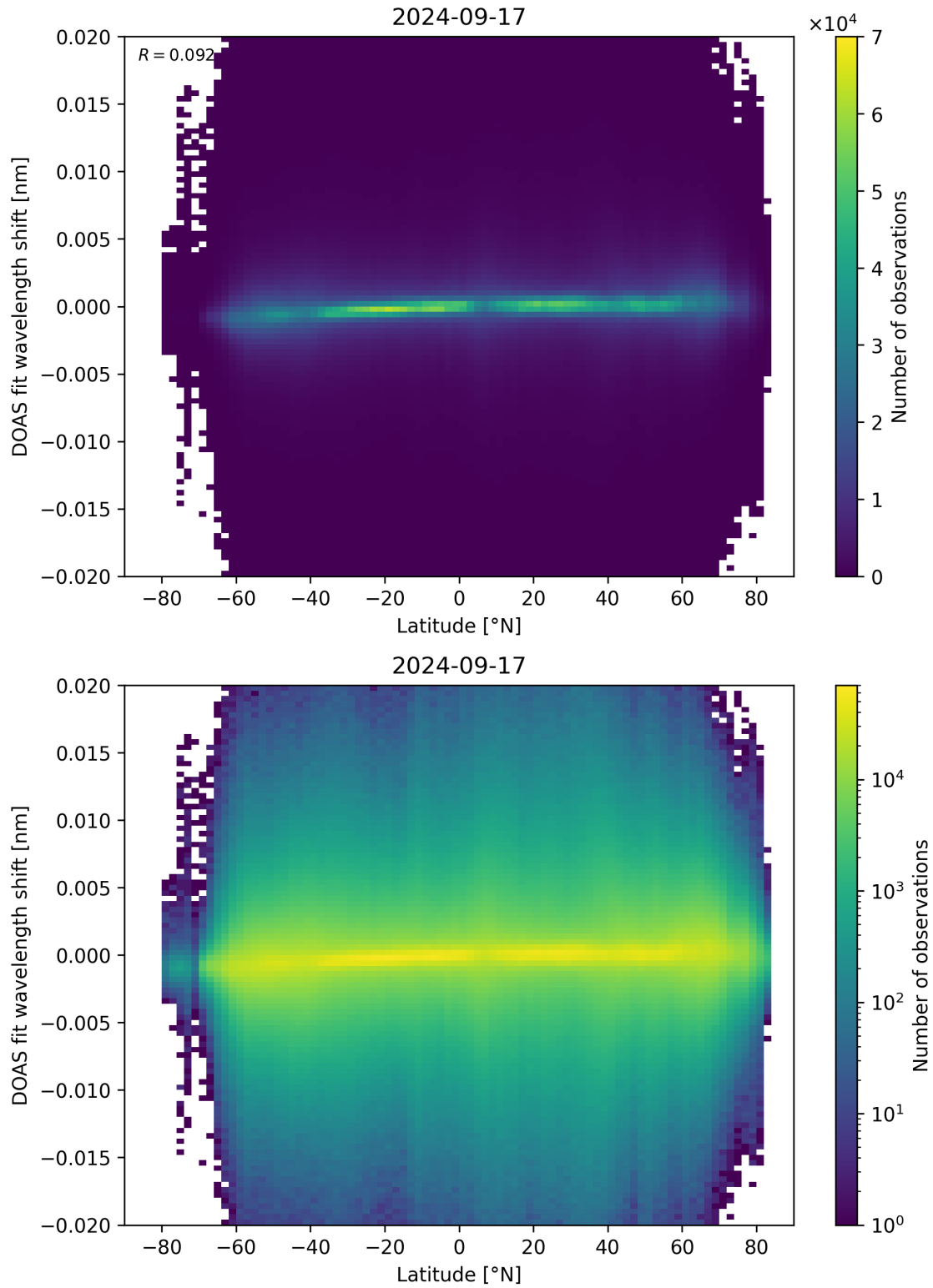
Figure 154: Scatter density plot of “Latitude” against “DOAS fit wavelength shift” for 2024-09-17 to 2024-09-18.
