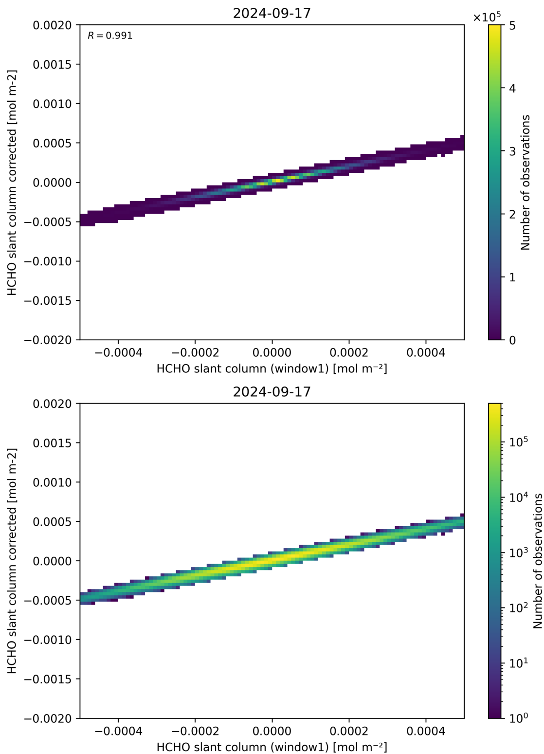
Figure 82: Scatter density plot of “HCHO slant column (window1)” against “HCHO slant column corrected” for 2024-09-17 to 2024-09-18.
