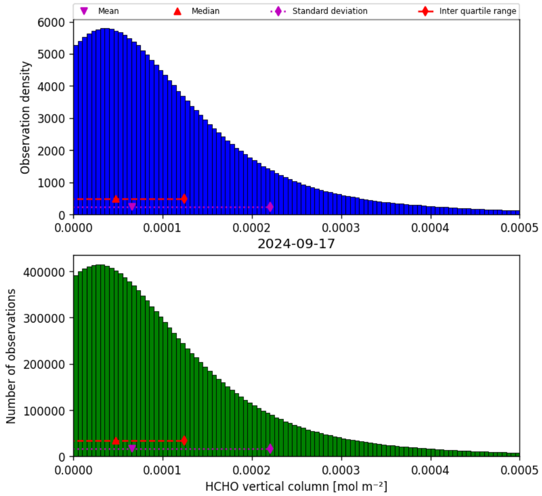
Figure 35: Histogram of “HCHO vertical column” for 2024-09-17 to 2024-09-18
