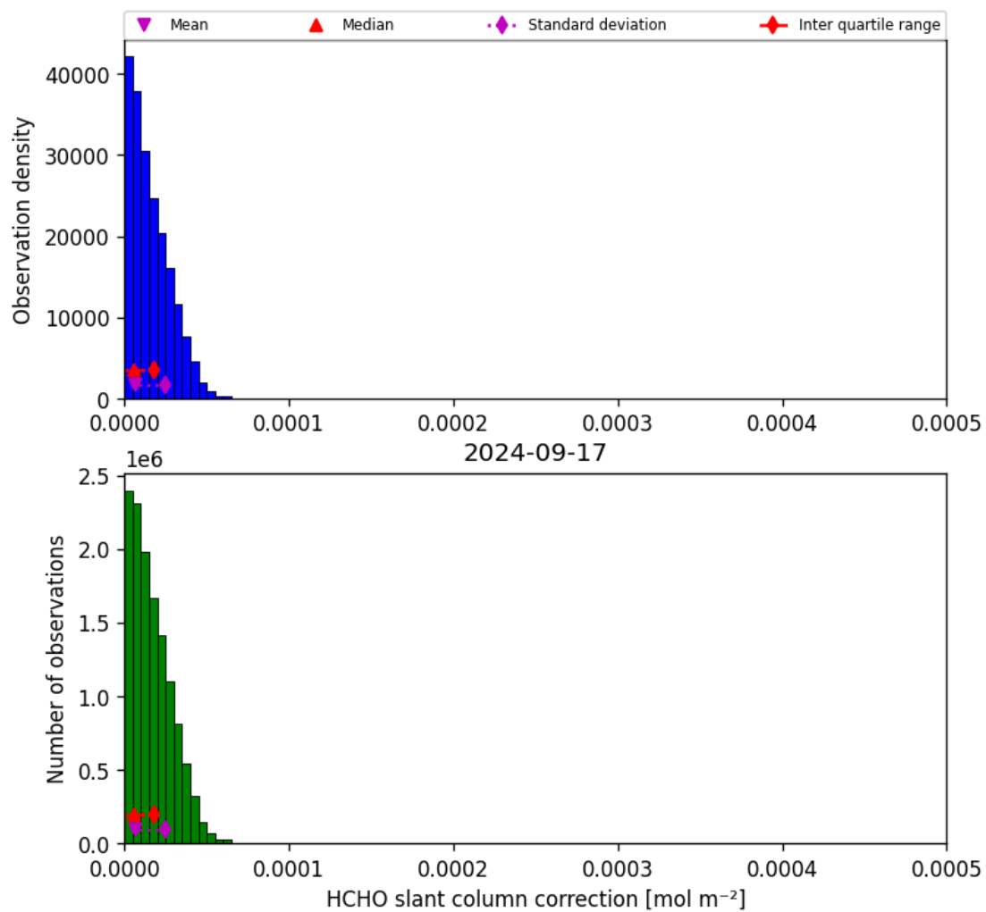
Figure 47: Histogram of “HCHO slant column correction” for 2024-09-17 to 2024-09-18
