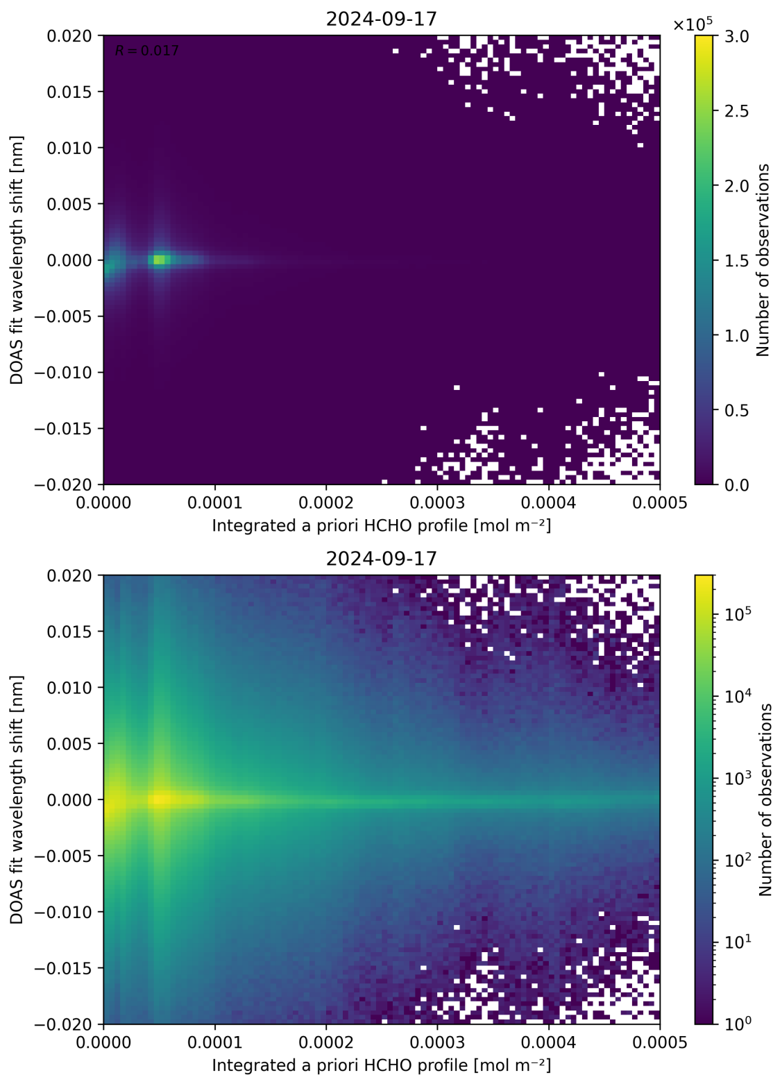
Figure 149: Scatter density plot of “Integrated a priori HCHO profile” against “DOAS fit wavelength shift” for 2024-09-17 to 2024-09-18.
