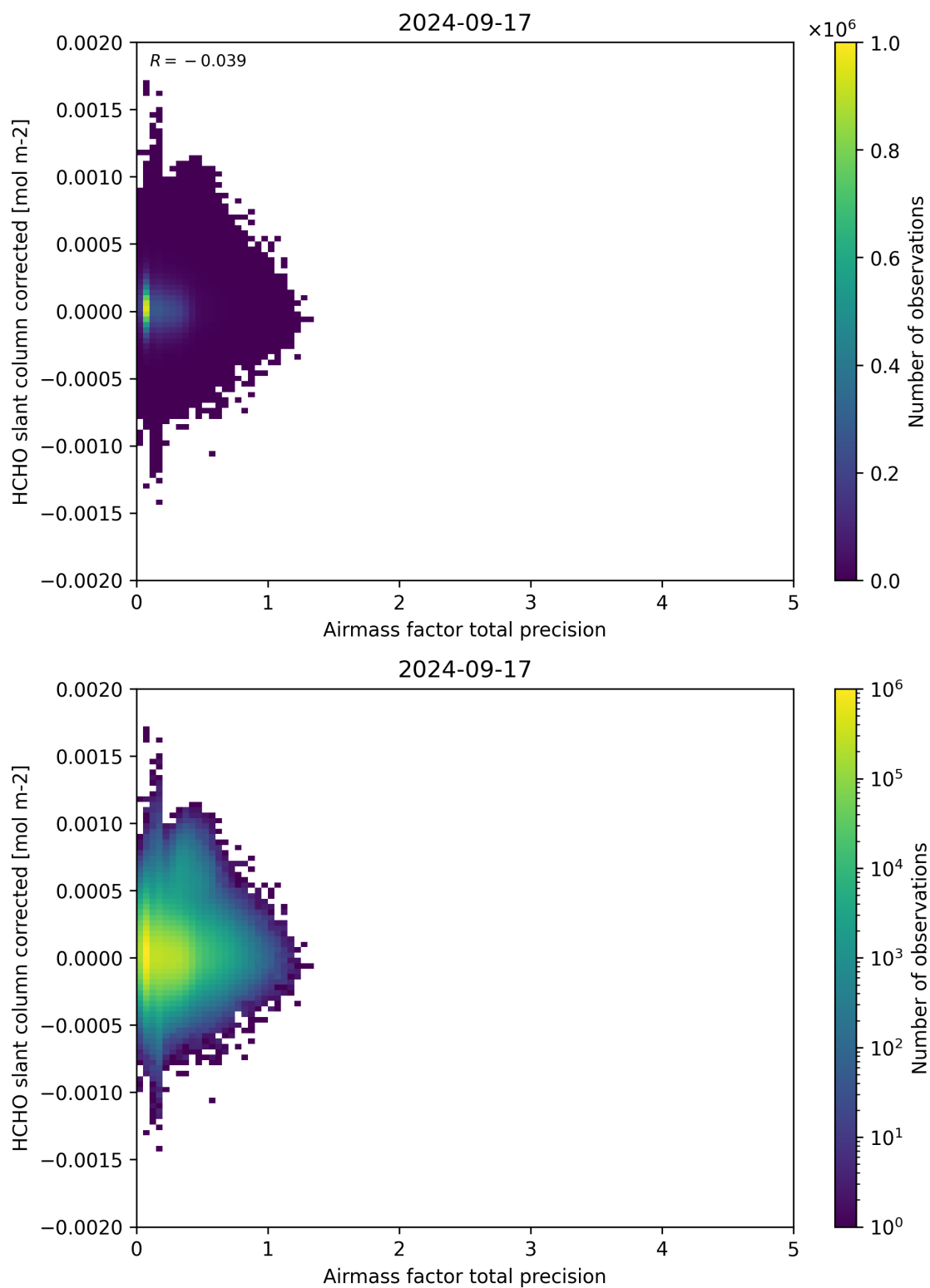
Figure 109: Scatter density plot of “Airmass factor total precision” against “HCHO slant column corrected” for 2024-09-17 to 2024-09-18.
