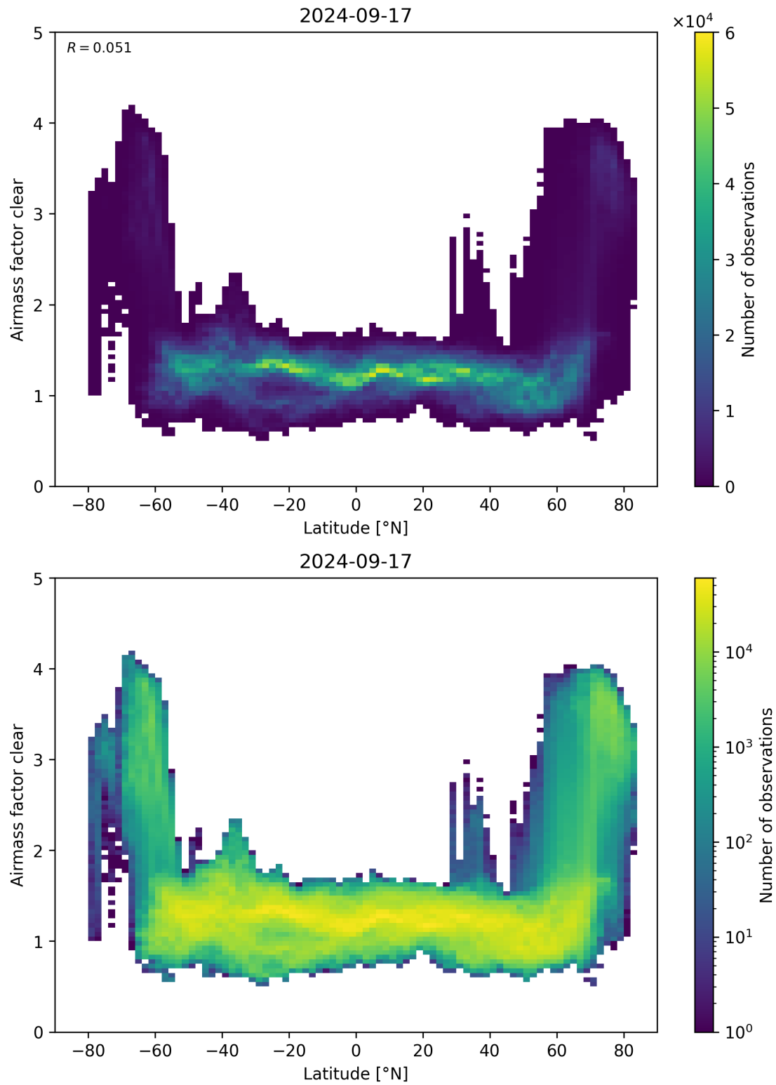
Figure 156: Scatter density plot of “Latitude” against “Airmass factor clear” for 2024-09-17 to 2024-09-18.
