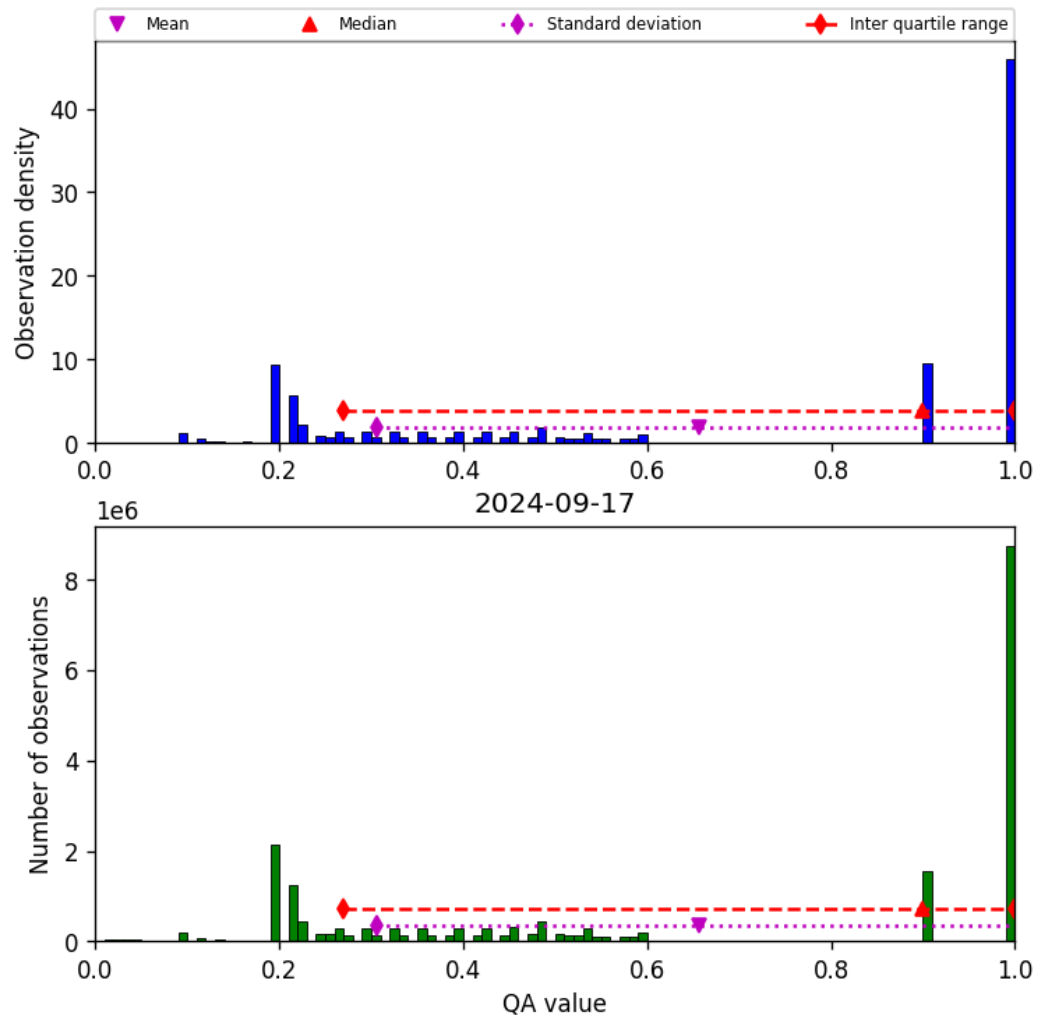
Figure 34: Histogram of “QA value” for 2024-09-17 to 2024-09-18
