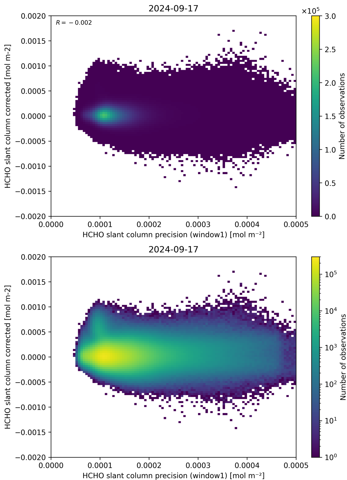
Figure 92: Scatter density plot of “HCHO slant column precision (window1)” against “HCHO slant column corrected” for 2024-09-17 to 2024-09-18.
