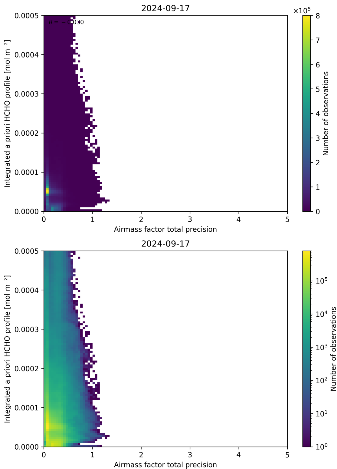
Figure 111: Scatter density plot of “Airmass factor total precision” against “Integrated a priori HCHO profile” for 2024-09-17 to 2024-09-18.
