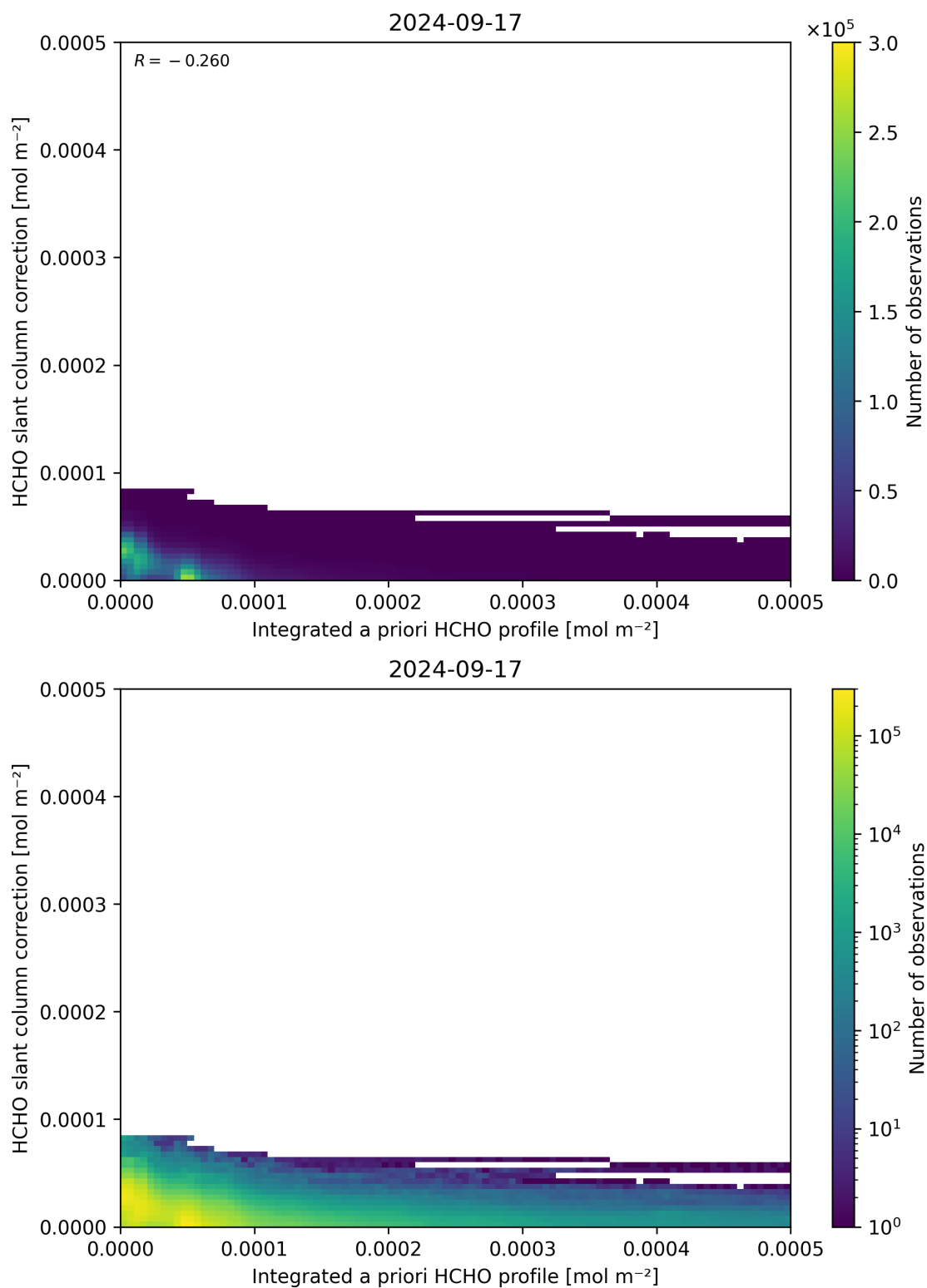
Figure 152: Scatter density plot of “Integrated a priori HCHO profile” against “HCHO slant column correction” for 2024-09-17 to 2024-09-18.
