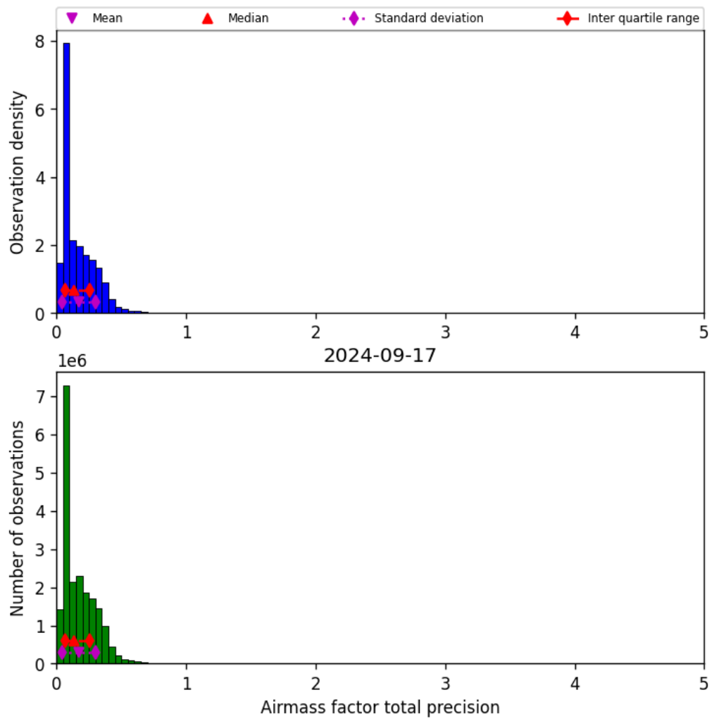
Figure 41: Histogram of “Airmass factor total precision” for 2024-09-17 to 2024-09-18
