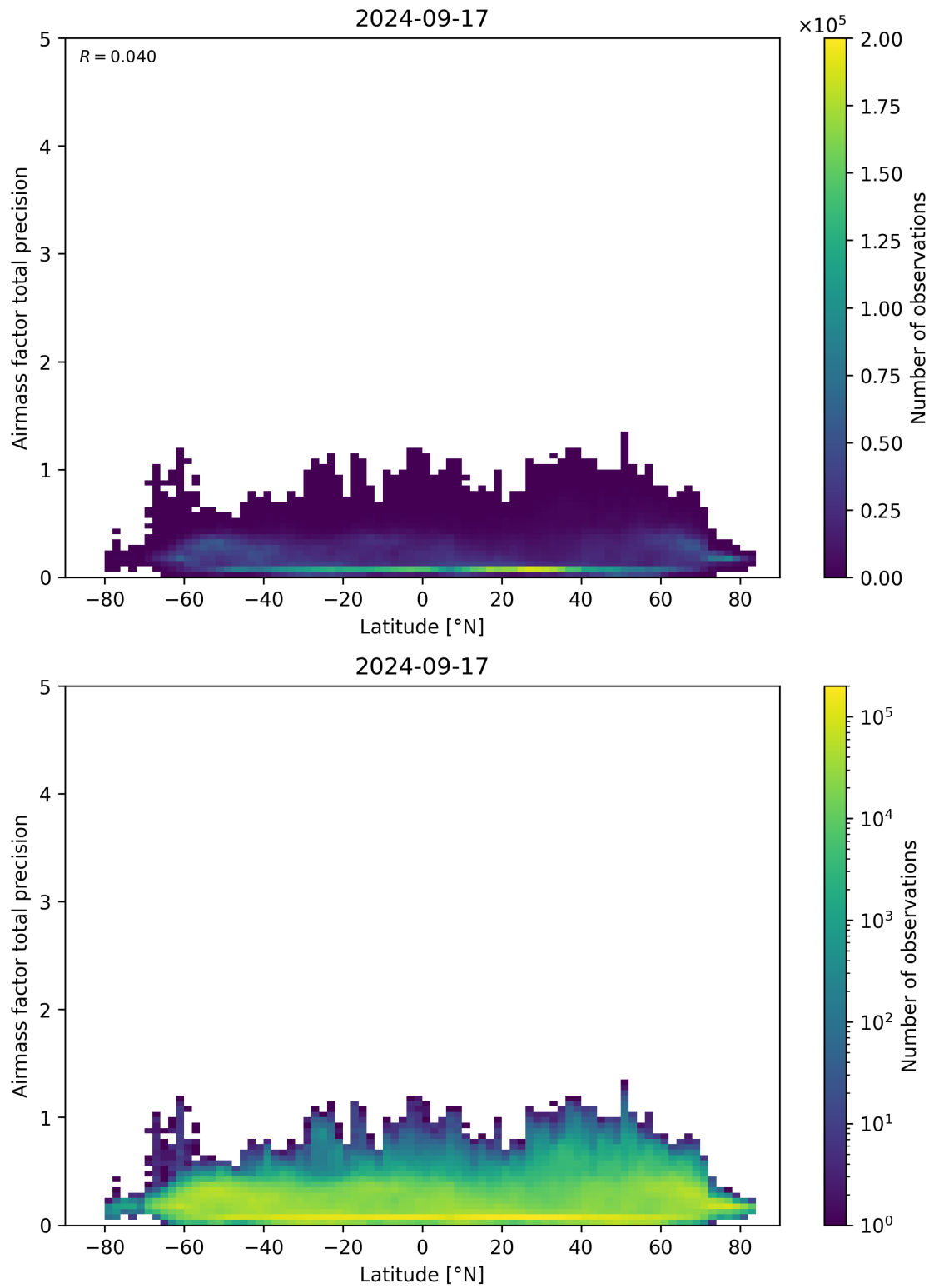
Figure 162: Scatter density plot of “Latitude” against “Airmass factor total precision” for 2024-09-17 to 2024-09-18.
