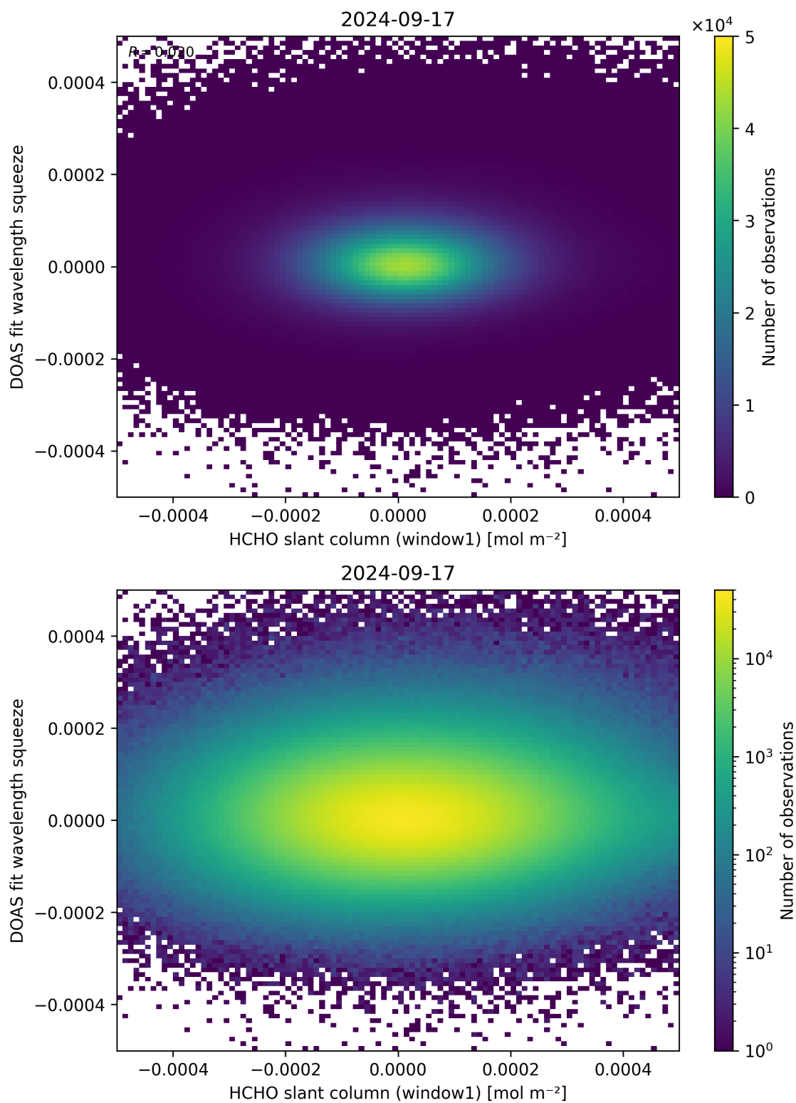
Figure 80: Scatter density plot of “HCHO slant column (window1)” against “DOAS fit wavelength squeeze” for 2024-09-17 to 2024-09-18.
