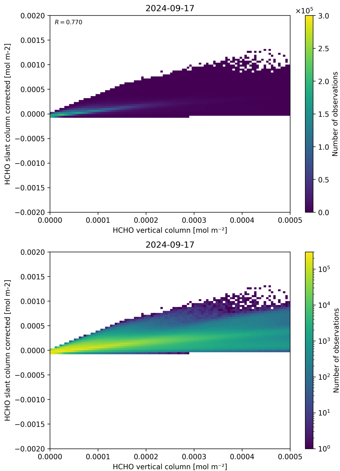
Figure 127: Scatter density plot of “HCHO vertical column” against “HCHO slant column corrected” for 2024-09-17 to 2024-09-18.
