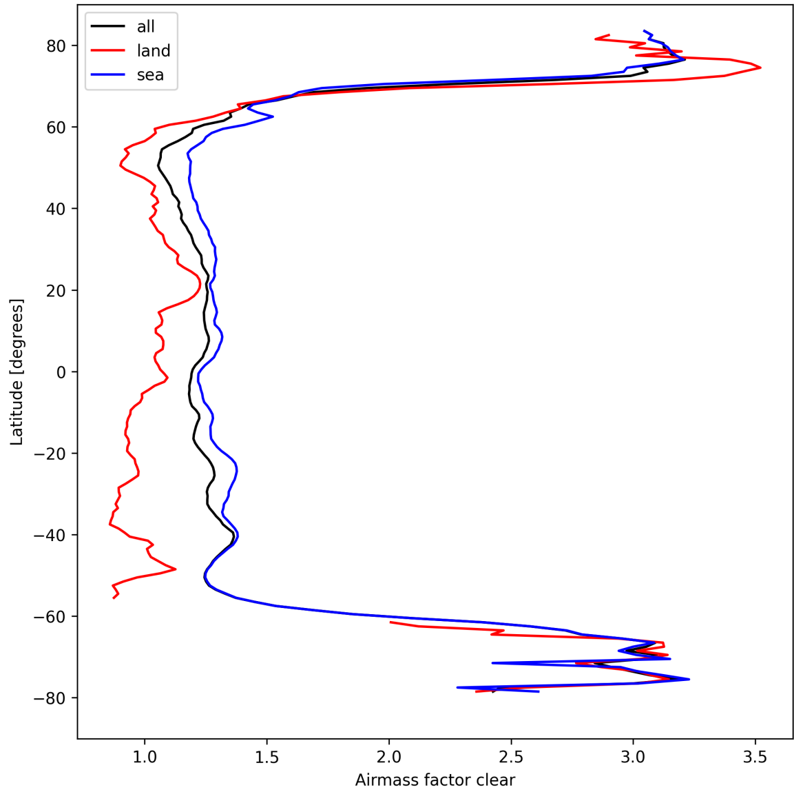
Figure 28: Zonal average of “Airmass factor clear” for 2024-09-17 to 2024-09-18.
