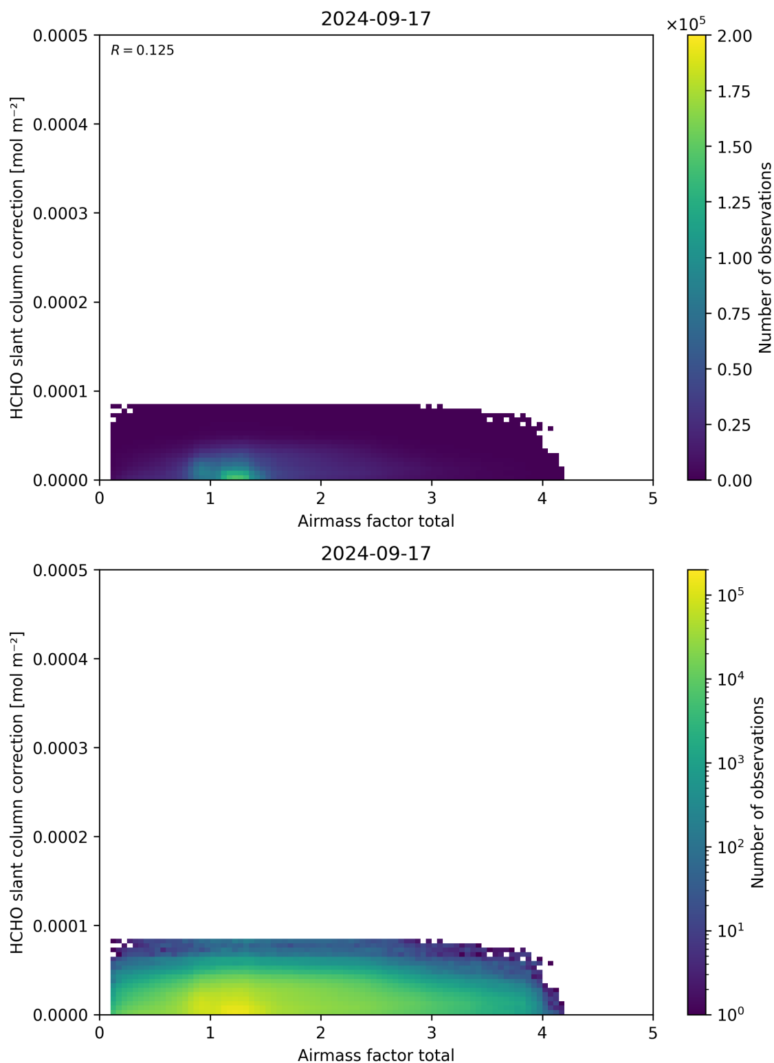
Figure 102: Scatter density plot of “Airmass factor total” against “HCHO slant column correction” for 2024-09-17 to 2024-09-18.
