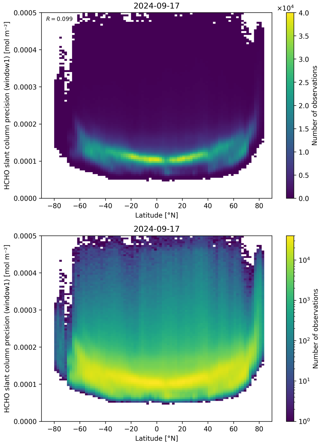
Figure 160: Scatter density plot of “Latitude” against “HCHO slant column precision (window1)” for 2024-09-17 to 2024-09-18.
