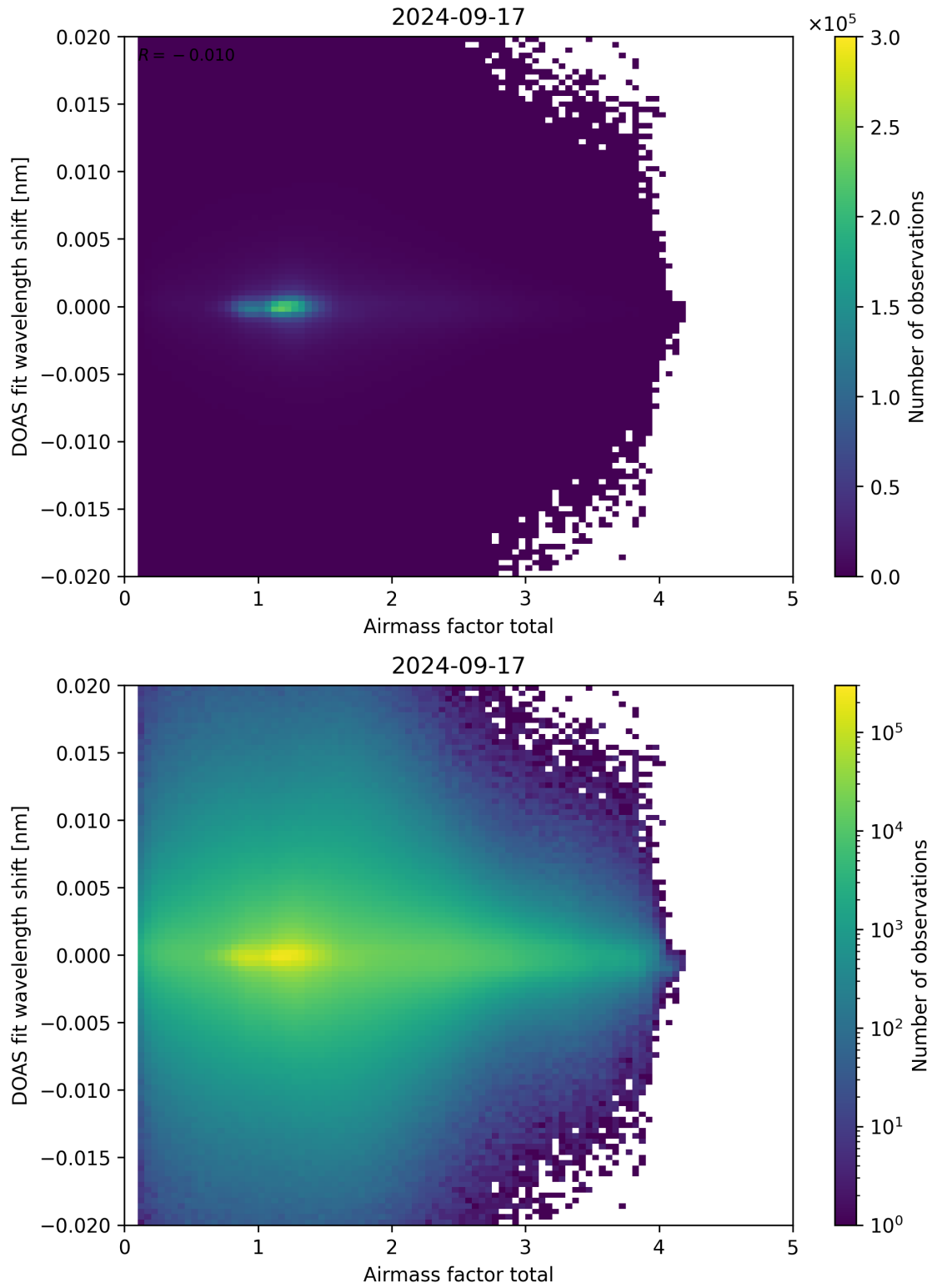
Figure 98: Scatter density plot of “Airmass factor total” against “DOAS fit wavelength shift” for 2024-09-17 to 2024-09-18.
