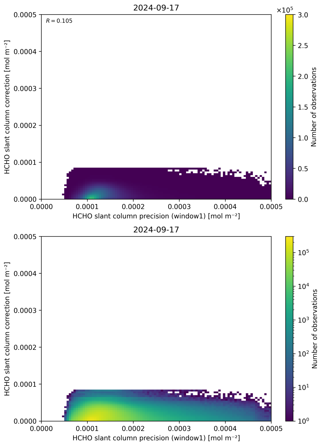
Figure 93: Scatter density plot of “HCHO slant column precision (window1)” against “HCHO slant column correction” for 2024-09-17 to 2024-09-18.
