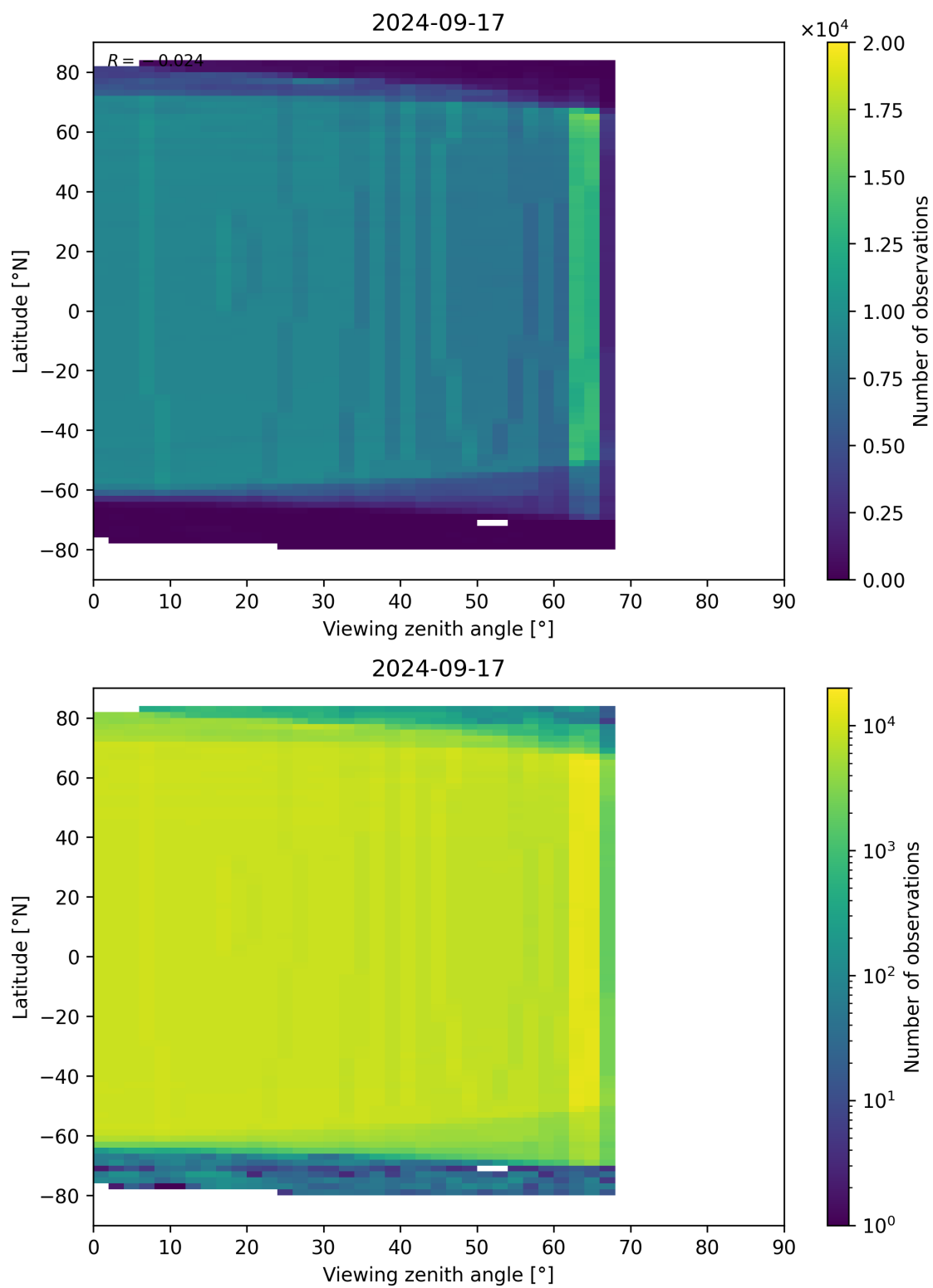
Figure 196: Scatter density plot of “Viewing zenith angle” against “Latitude” for 2024-09-17 to 2024-09-18.
