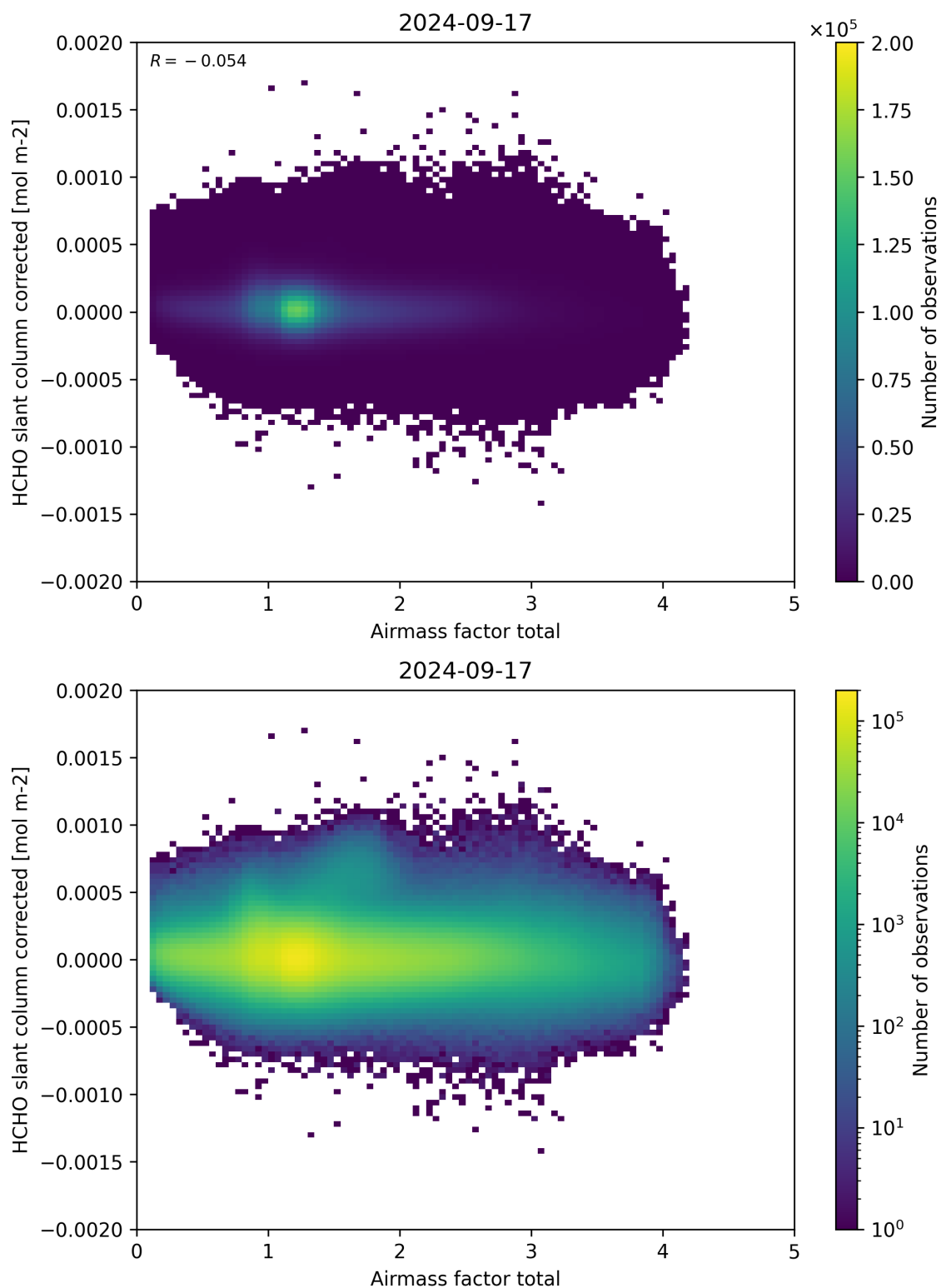
Figure 101: Scatter density plot of “Airmass factor total” against “HCHO slant column corrected” for 2024-09-17 to 2024-09-18.
