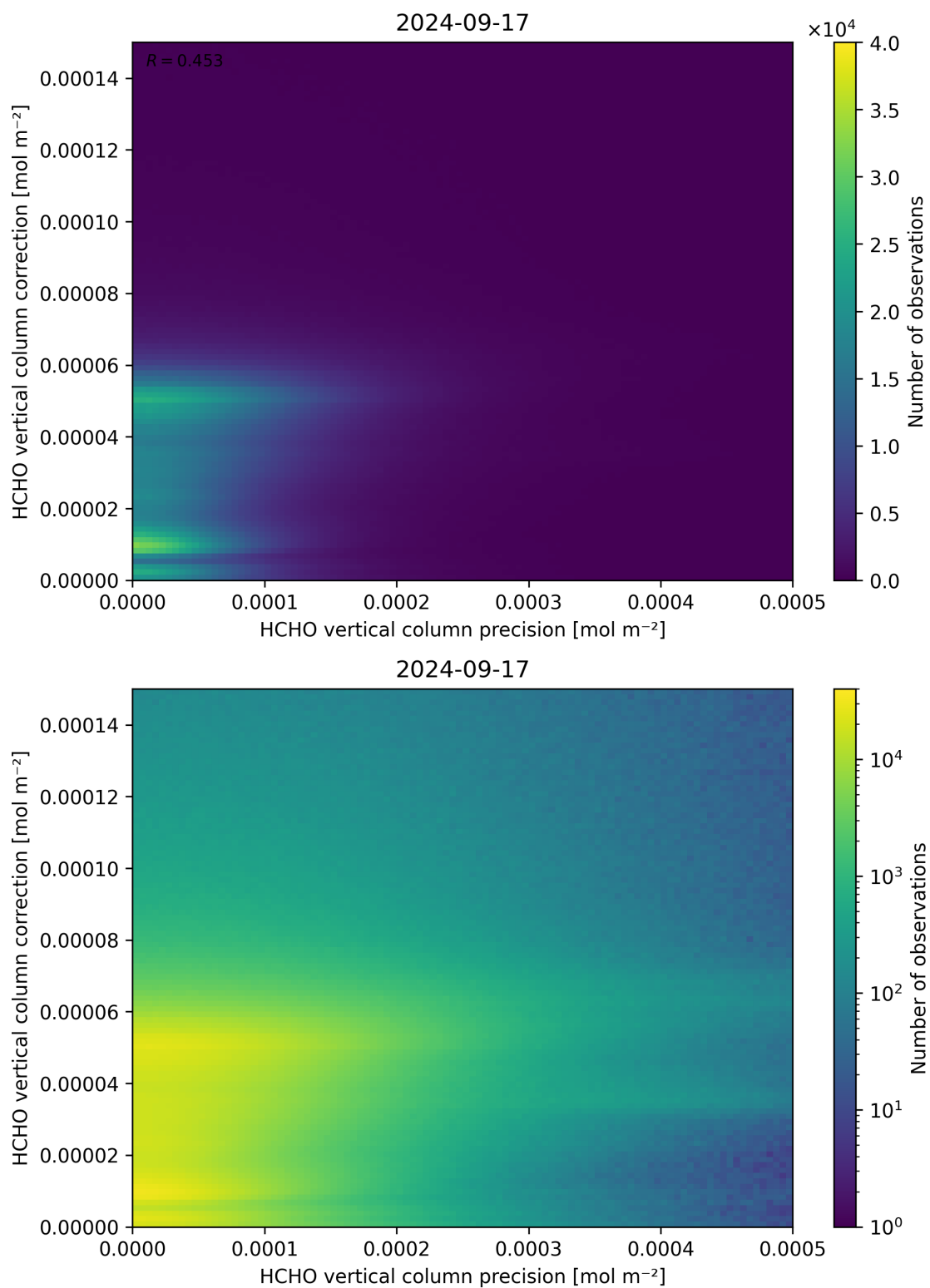
Figure 146: Scatter density plot of “HCHO vertical column precision” against “HCHO vertical column correction” for 2024-09-17 to 2024-09-18.
