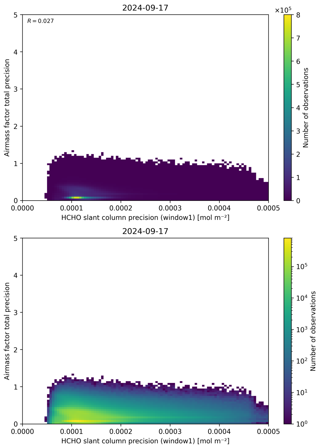
Figure 95: Scatter density plot of “HCHO slant column precision (window1)” against “Airmass factor total precision” for 2024-09-17 to 2024-09-18.
