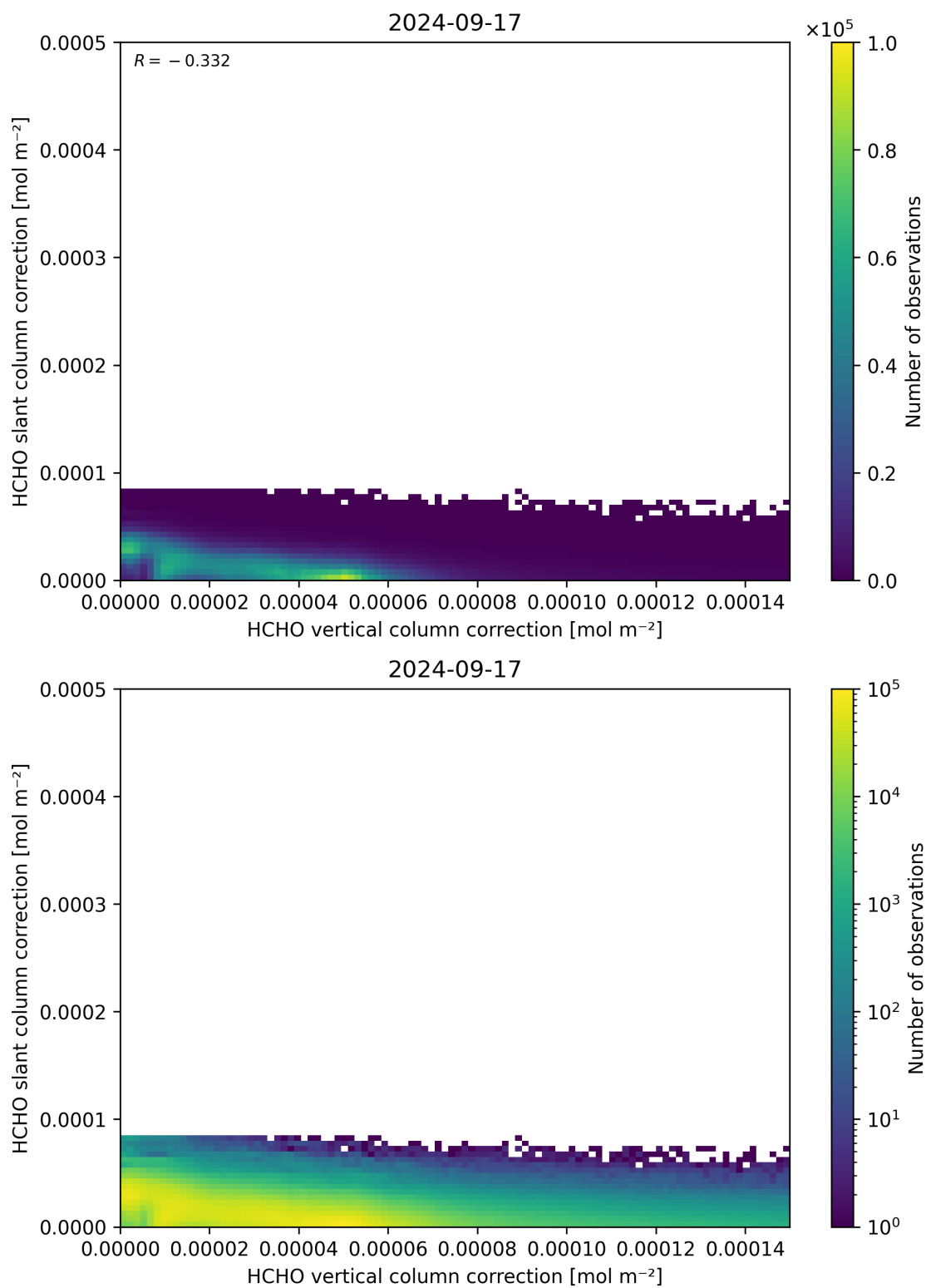
Figure 117: Scatter density plot of “HCHO vertical column correction” against “HCHO slant column correction” for 2024-09-17 to 2024-09-18.
