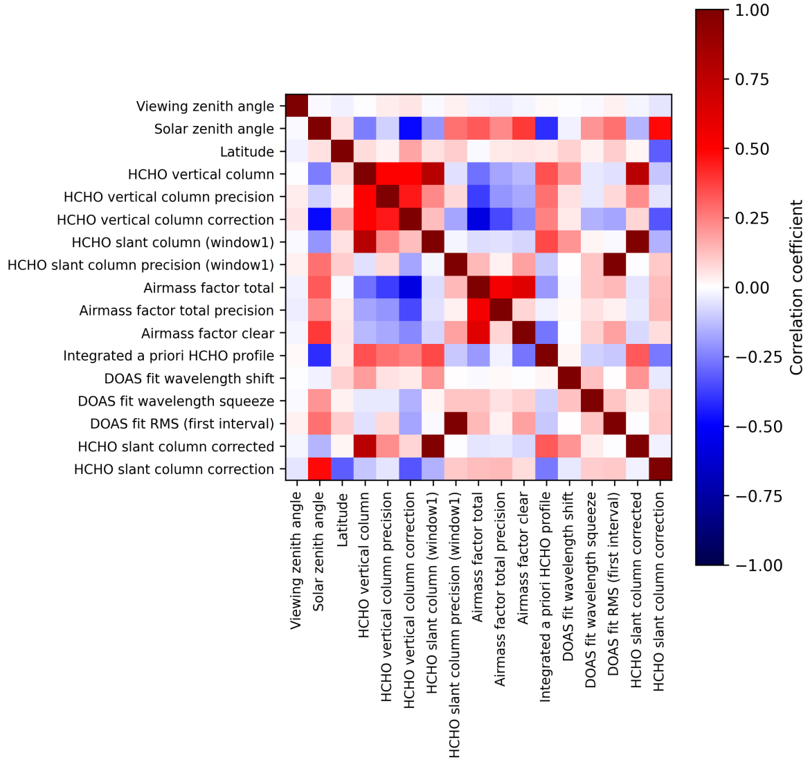
Figure 2: Map of correlation matrix for 2024-09-17 to 2024-09-18.
