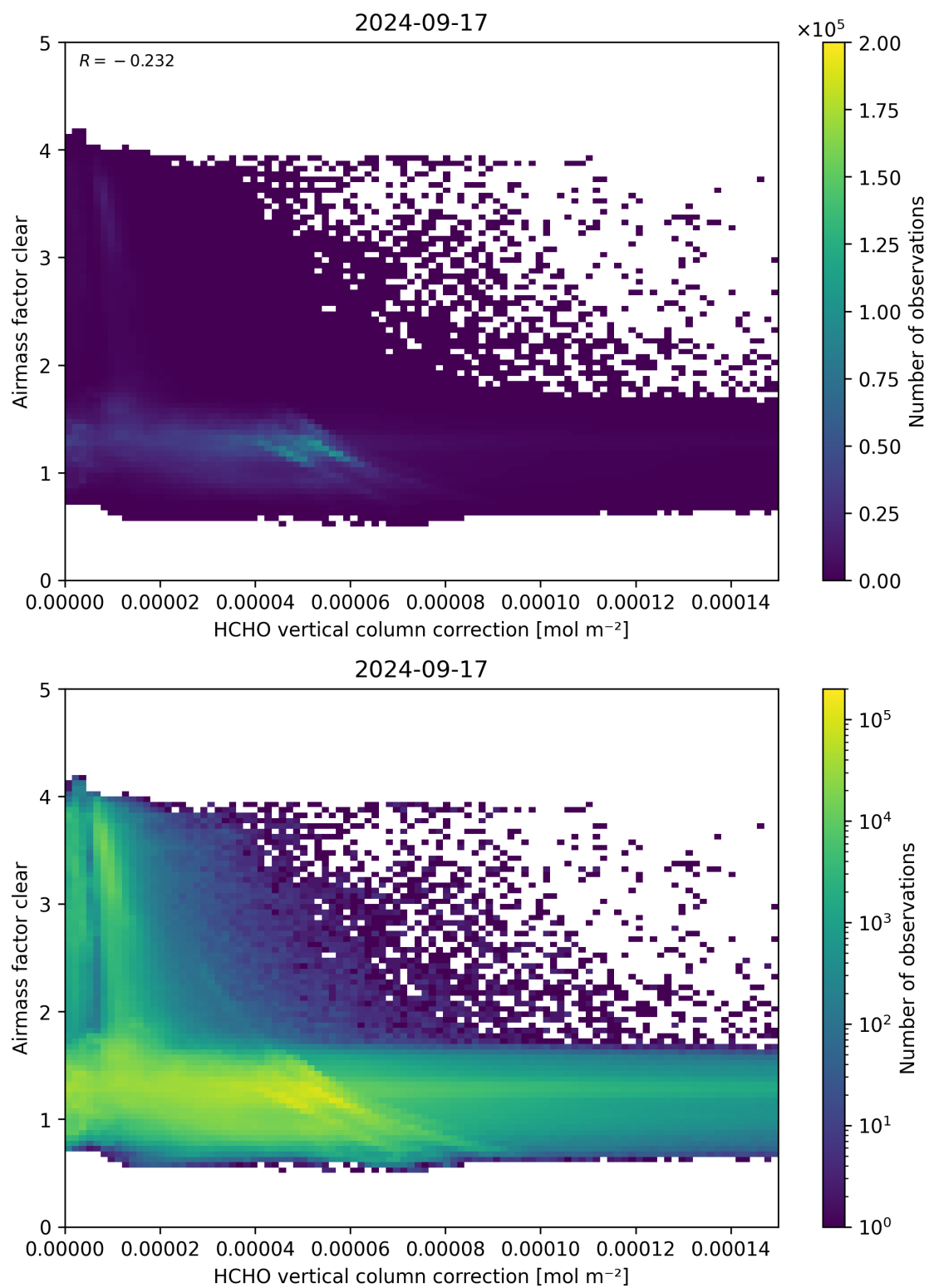
Figure 115: Scatter density plot of “HCHO vertical column correction” against “Airmass factor clear” for 2024-09-17 to 2024-09-18.
