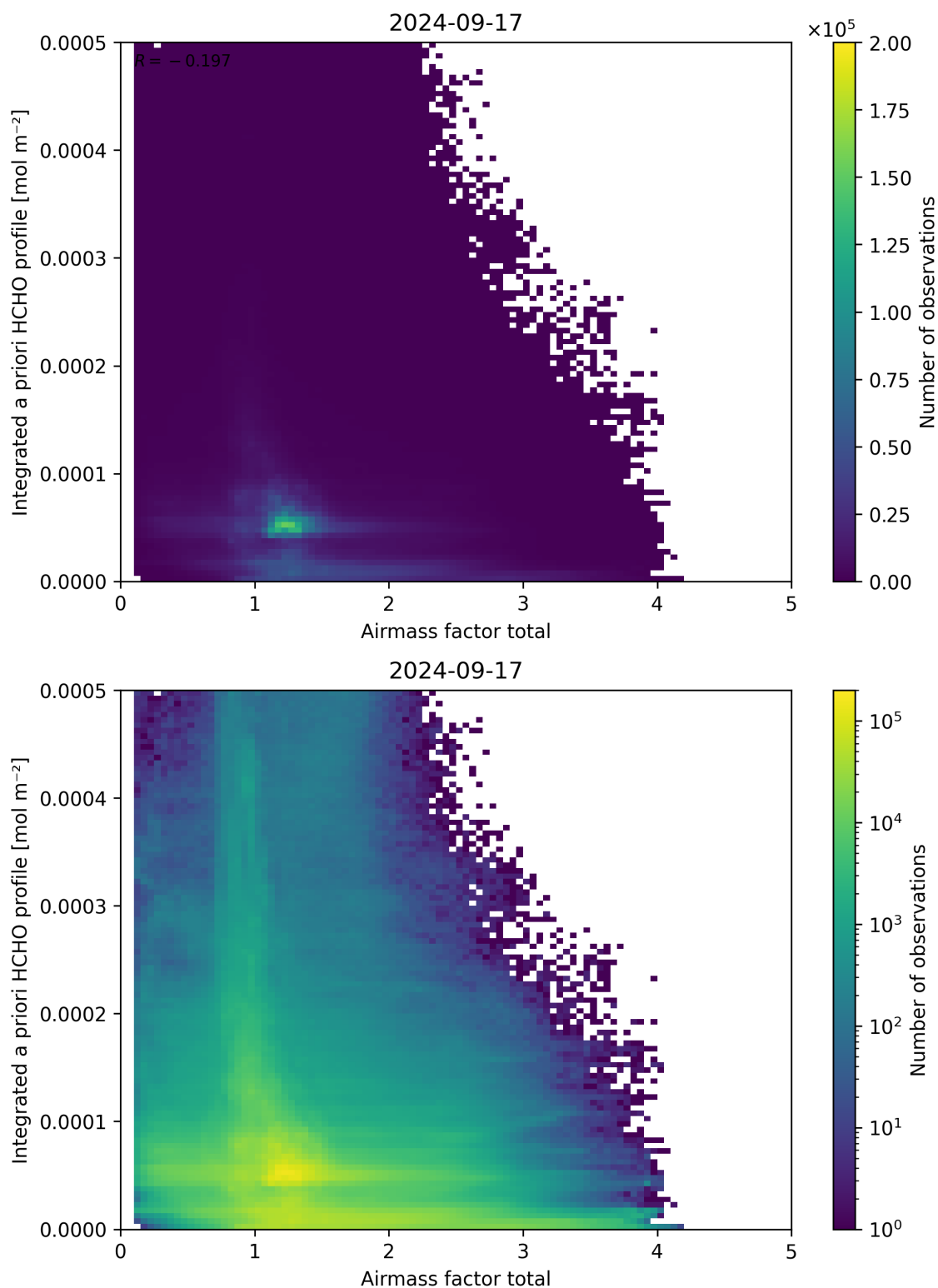
Figure 104: Scatter density plot of “Airmass factor total” against “Integrated a priori HCHO profile” for 2024-09-17 to 2024-09-18.
