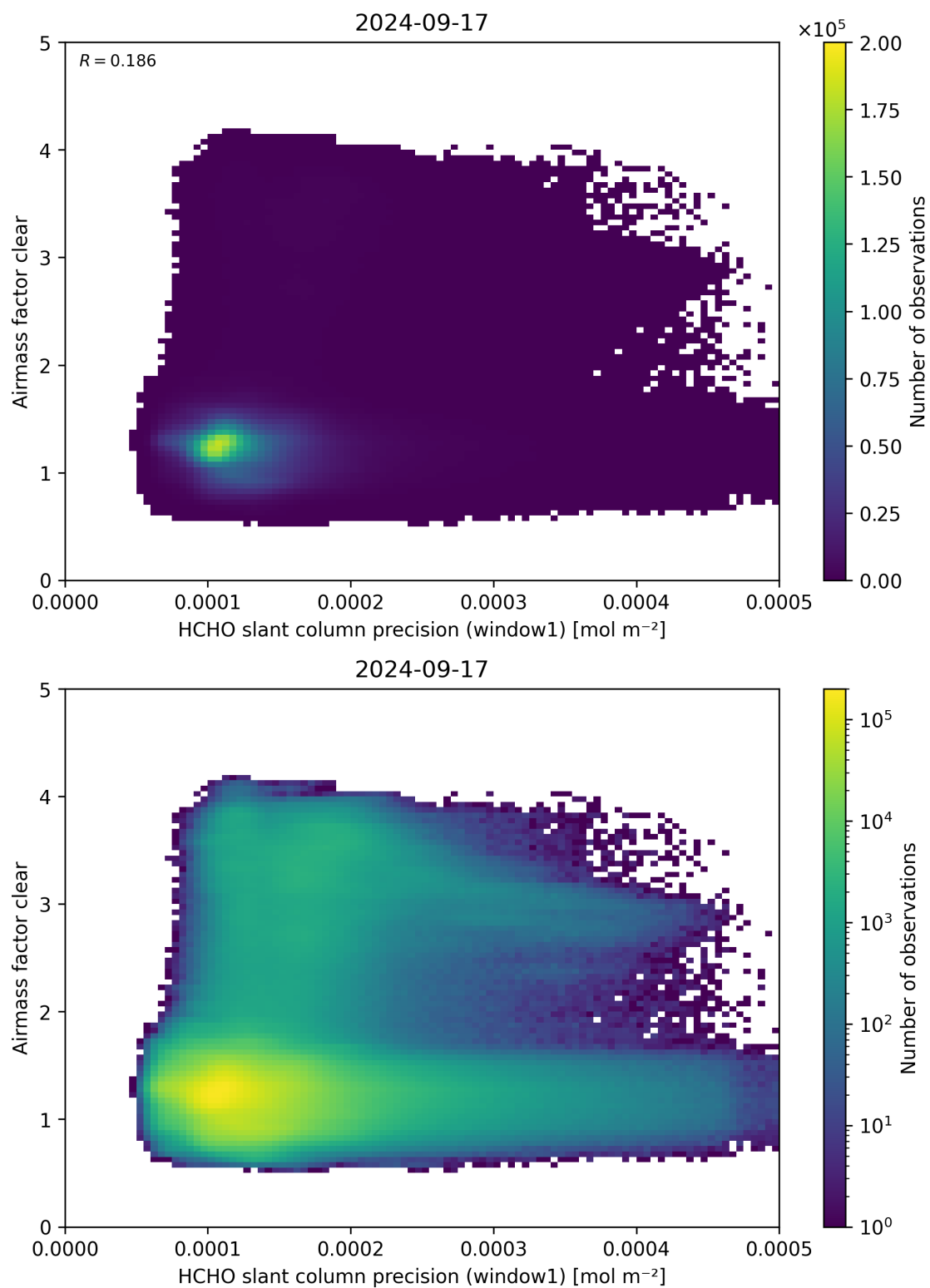
Figure 91: Scatter density plot of “HCHO slant column precision (window1)” against “Airmass factor clear” for 2024-09-17 to 2024-09-18.
