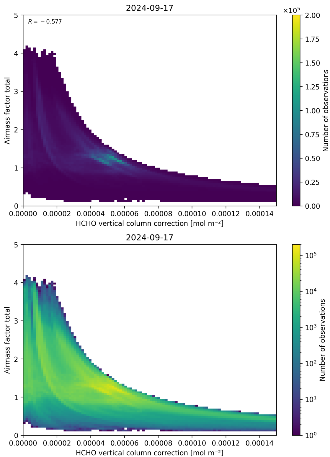
Figure 120: Scatter density plot of “HCHO vertical column correction” against “Airmass factor total” for 2024-09-17 to 2024-09-18.
