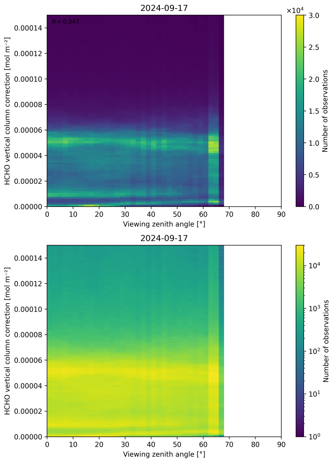
Figure 193: Scatter density plot of “Viewing zenith angle” against “HCHO vertical column correction” for 2024-09-17 to 2024-09-18.
