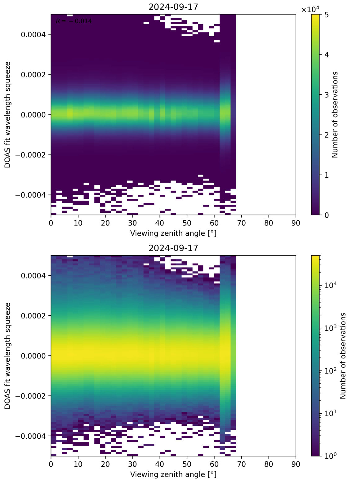
Figure 184: Scatter density plot of “Viewing zenith angle” against “DOAS fit wavelength squeeze” for 2024-09-17 to 2024-09-18.
