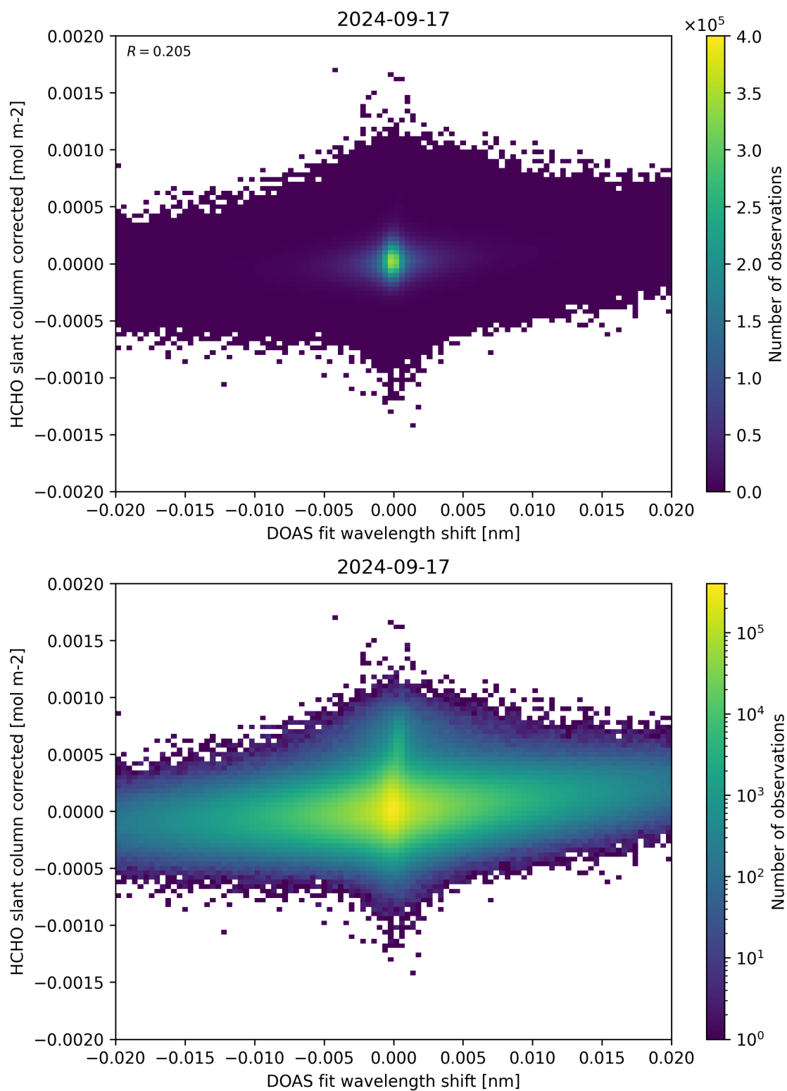
Figure 66: Scatter density plot of “DOAS fit wavelength shift” against “HCHO slant column corrected” for 2024-09-17 to 2024-09-18.
