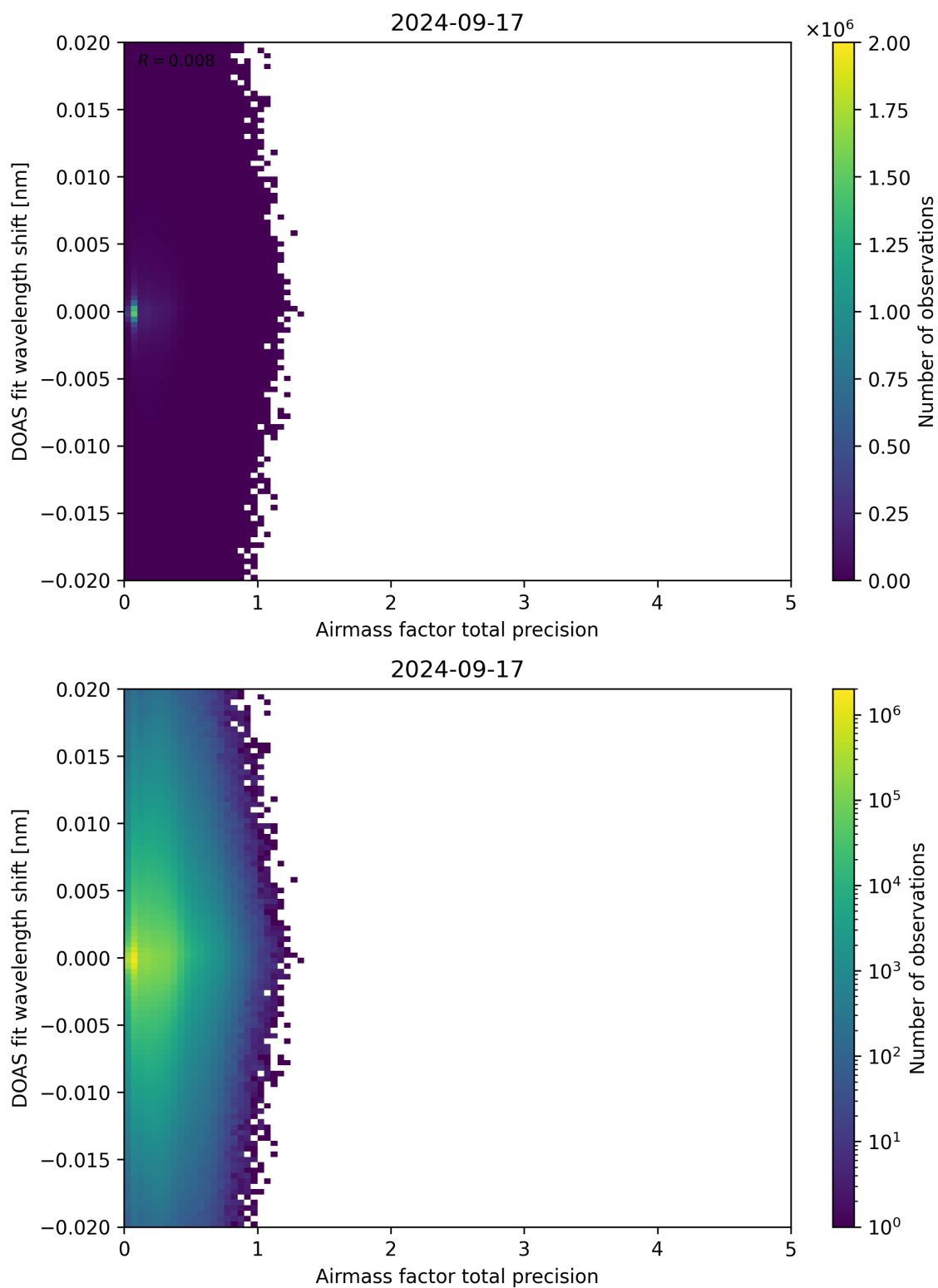
Figure 106: Scatter density plot of “Airmass factor total precision” against “DOAS fit wavelength shift” for 2024-09-17 to 2024-09-18.
