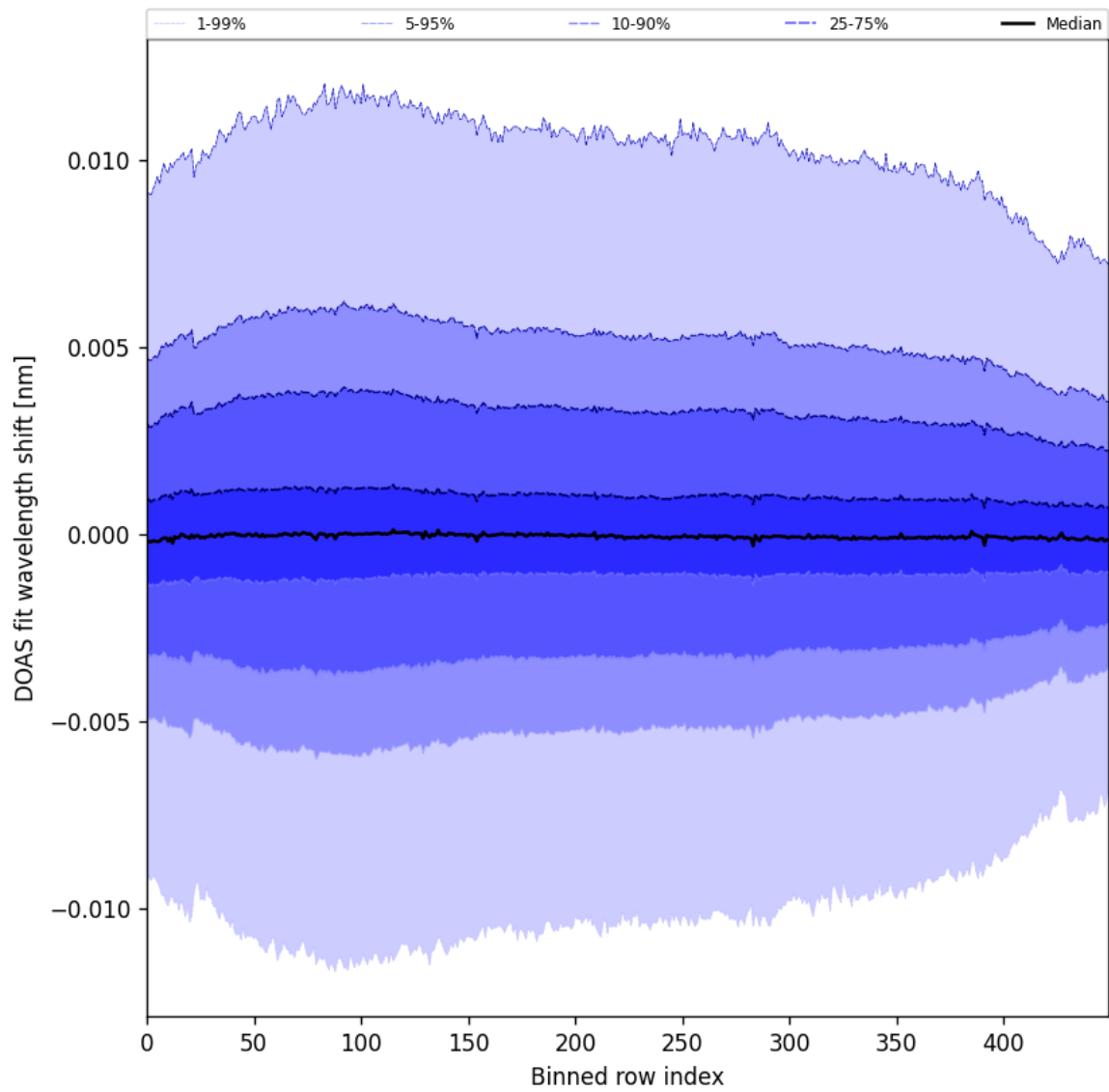
Figure 58: Along track statistics of “DOAS fit wavelength shift” for 2024-09-17 to 2024-09-18
