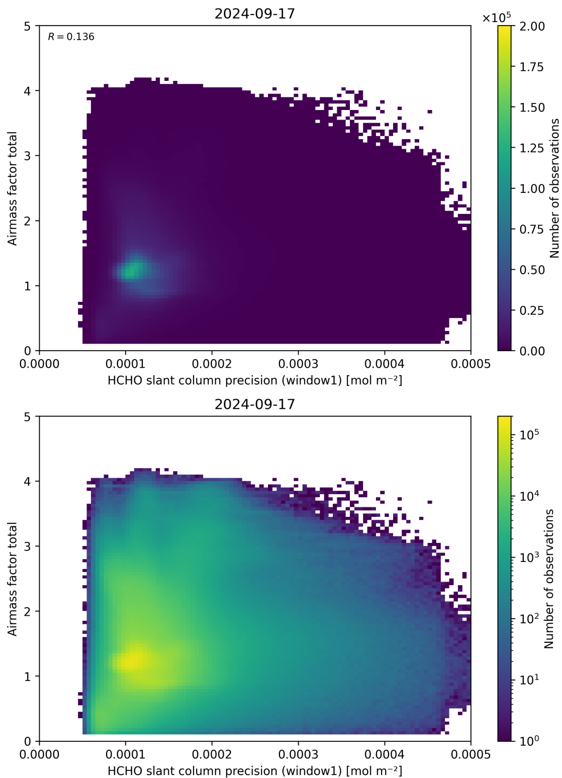
Figure 94: Scatter density plot of “HCHO slant column precision (window1)” against “Airmass factor total” for 2024-09-17 to 2024-09-18.
