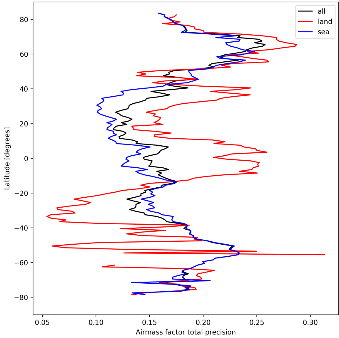
Figure 27: Zonal average of “Airmass factor total precision” for 2024-09-17 to 2024-09-18.
