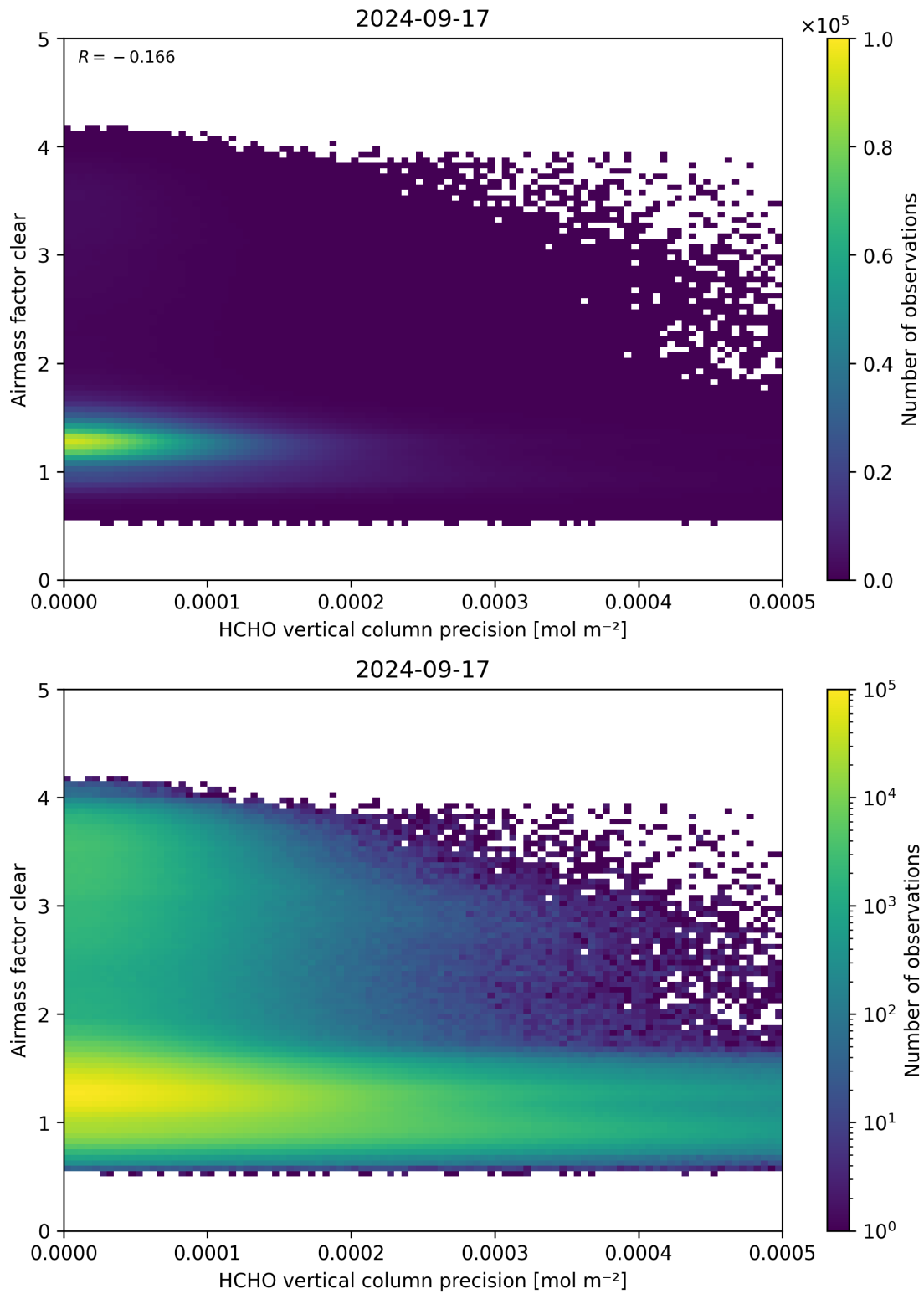
Figure 139: Scatter density plot of “HCHO vertical column precision” against “Airmass factor clear” for 2024-09-17 to 2024-09-18.
