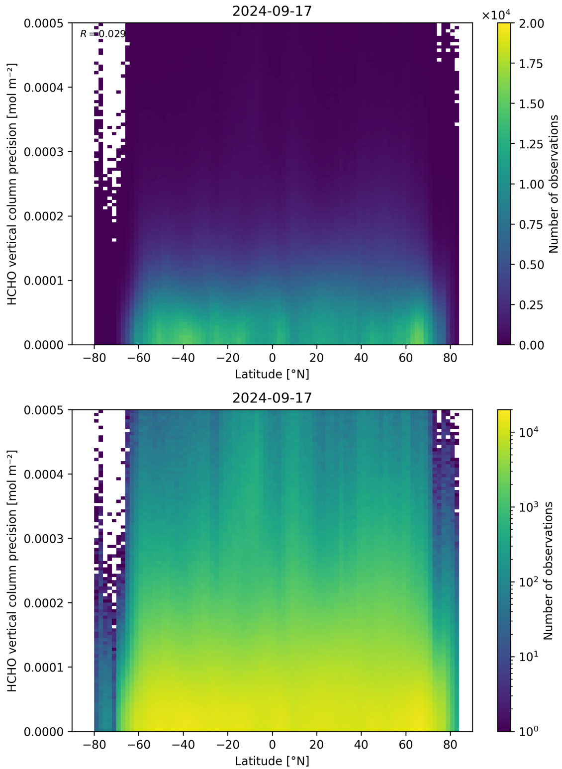
Figure 165: Scatter density plot of “Latitude” against “HCHO vertical column precision” for 2024-09-17 to 2024-09-18.
