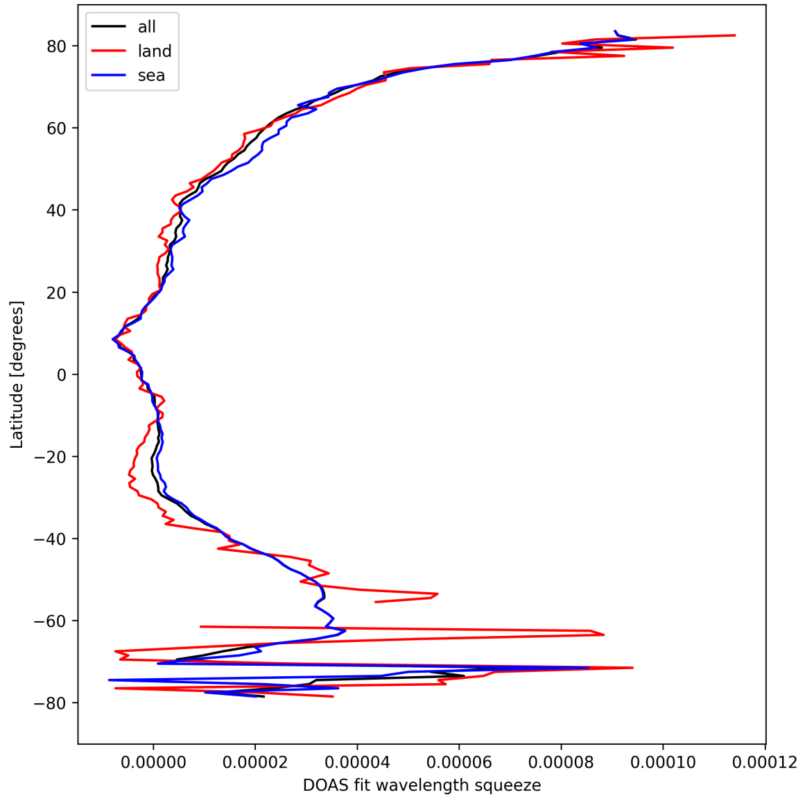
Figure 31: Zonal average of “DOAS fit wavelength squeeze” for 2024-09-17 to 2024-09-18.
