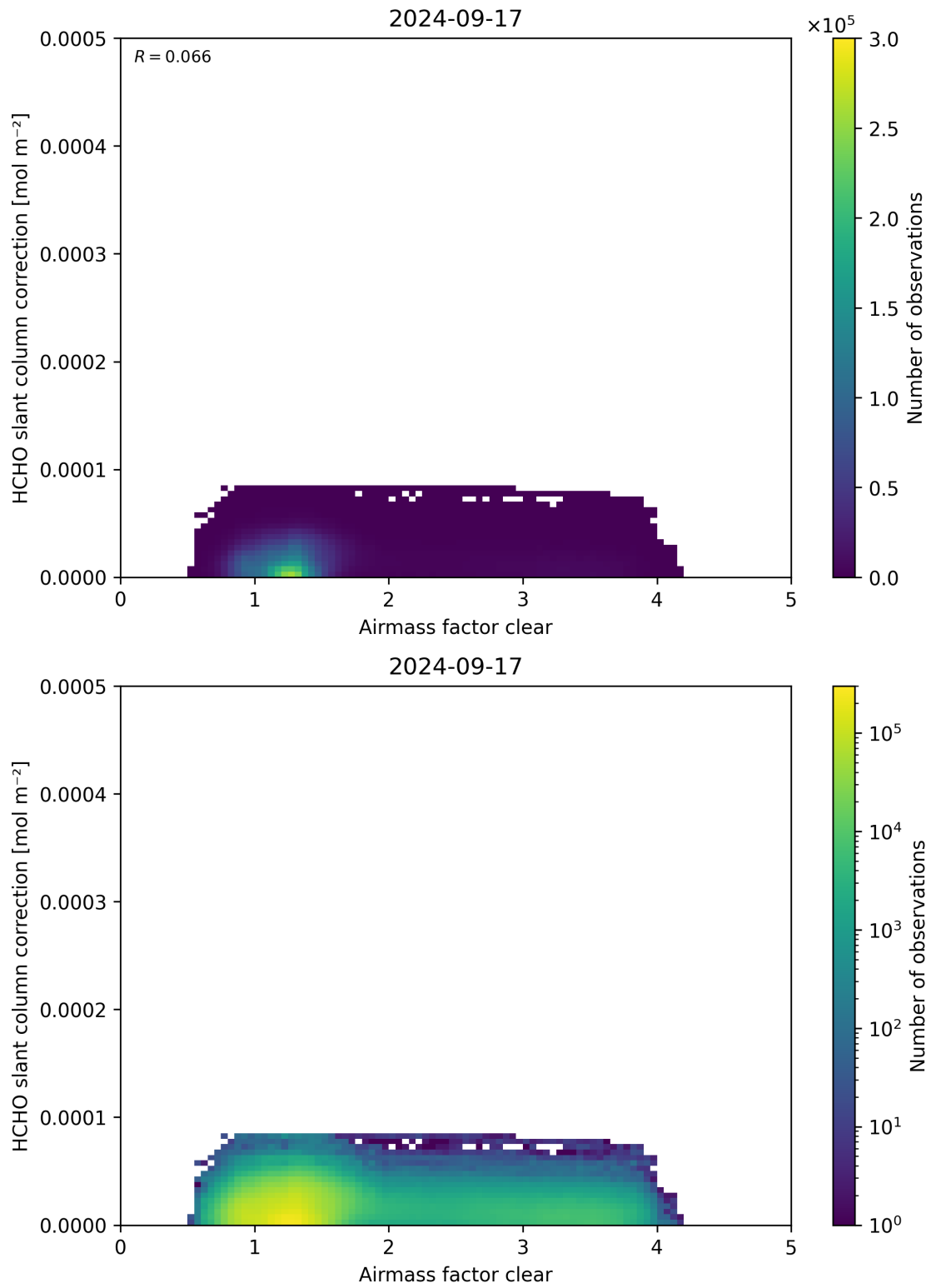
Figure 75: Scatter density plot of “Airmass factor clear” against “HCHO slant column correction” for 2024-09-17 to 2024-09-18.
