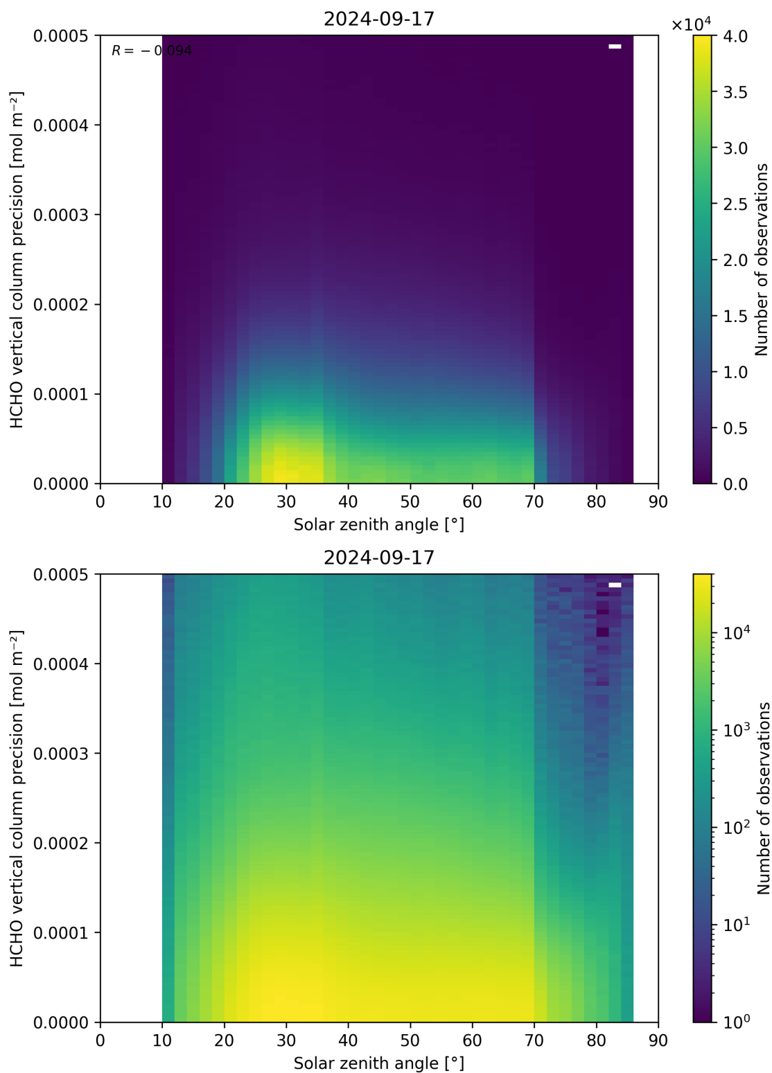
Figure 179: Scatter density plot of “Solar zenith angle” against “HCHO vertical column precision” for 2024-09-17 to 2024-09-18.
