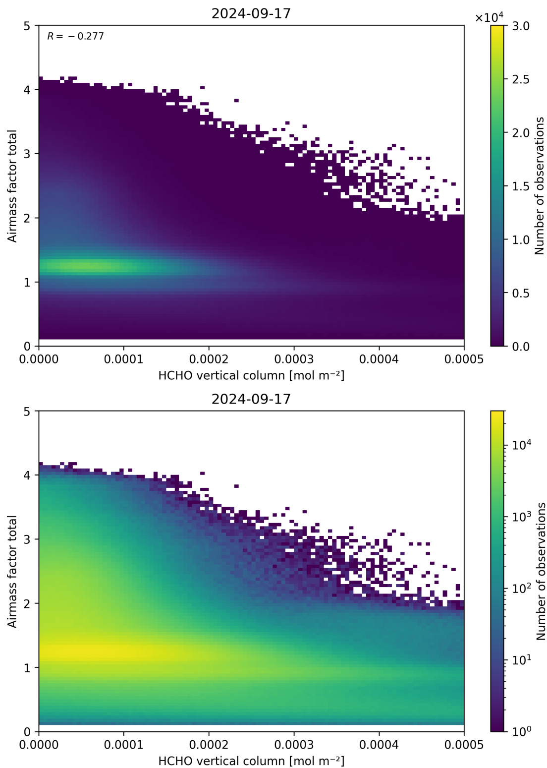
Figure 131: Scatter density plot of “HCHO vertical column” against “Airmass factor total” for 2024-09-17 to 2024-09-18.
