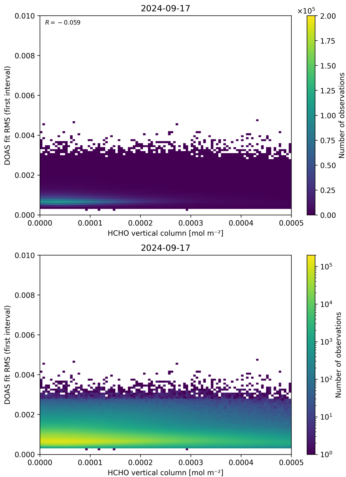
Figure 123: Scatter density plot of “HCHO vertical column” against “DOAS fit RMS (first interval)” for 2024-09-17 to 2024-09-18.
