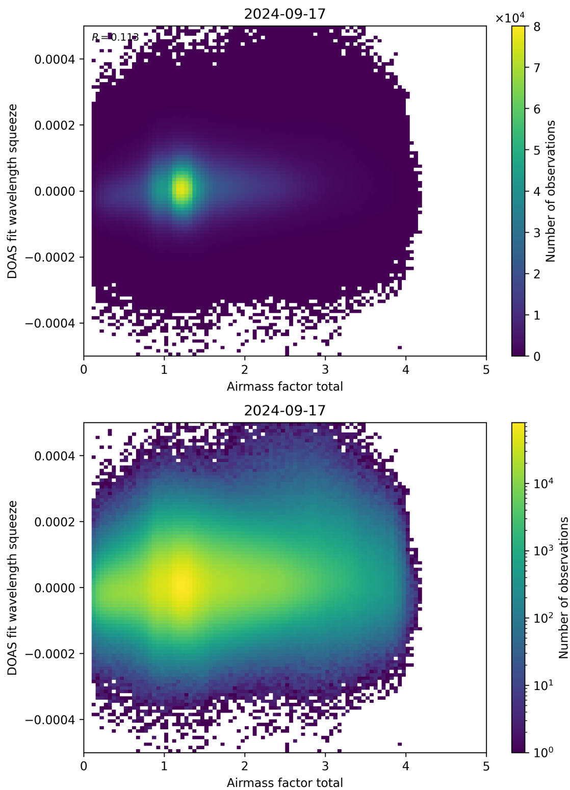
Figure 99: Scatter density plot of “Airmass factor total” against “DOAS fit wavelength squeeze” for 2024-09-17 to 2024-09-18.
