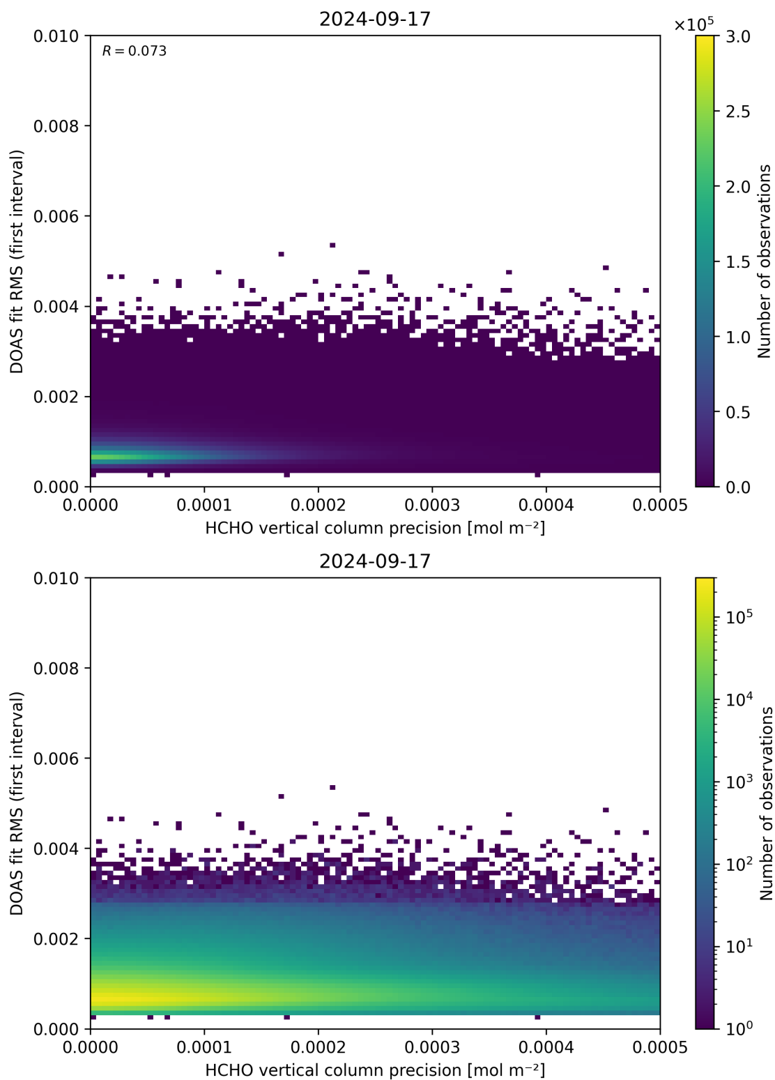
Figure 136: Scatter density plot of “HCHO vertical column precision” against “DOAS fit RMS (first interval)” for 2024-09-17 to 2024-09-18.
