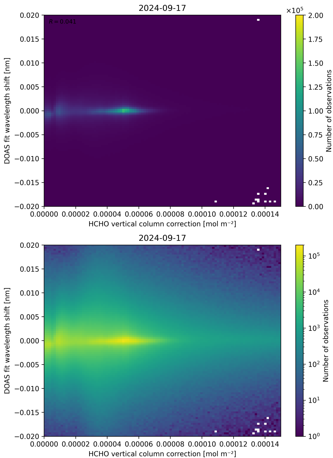
Figure 113: Scatter density plot of “HCHO vertical column correction” against “DOAS fit wavelength shift” for 2024-09-17 to 2024-09-18.
