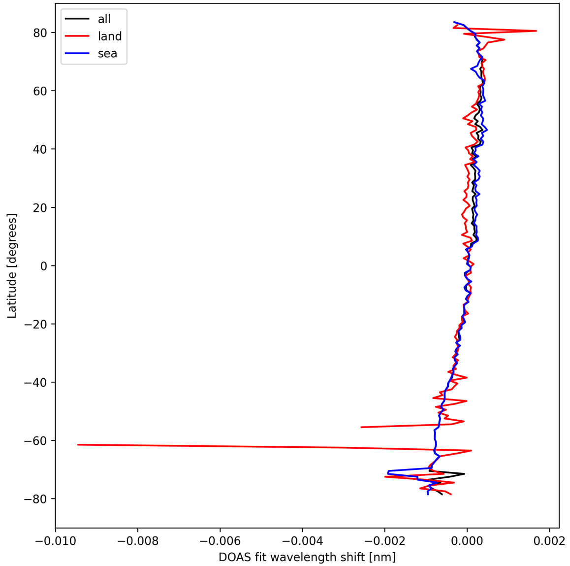
Figure 30: Zonal average of “DOAS fit wavelength shift” for 2024-09-17 to 2024-09-18.
