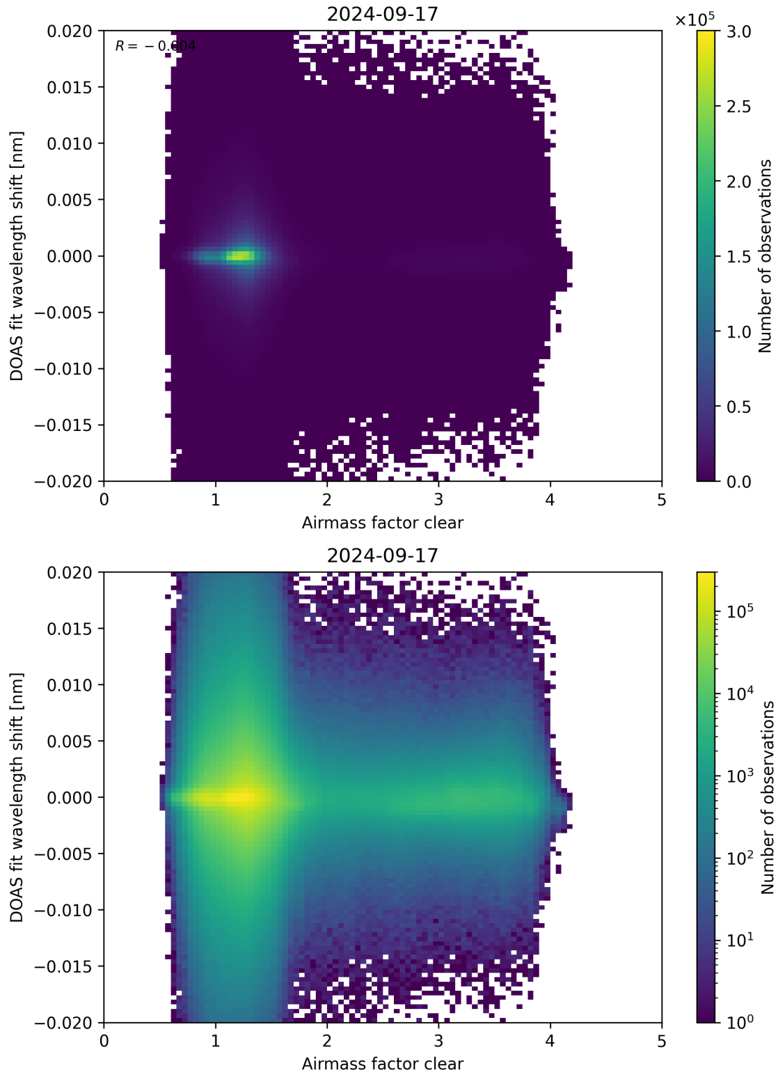
Figure 72: Scatter density plot of “Airmass factor clear” against “DOAS fit wavelength shift” for 2024-09-17 to 2024-09-18.
