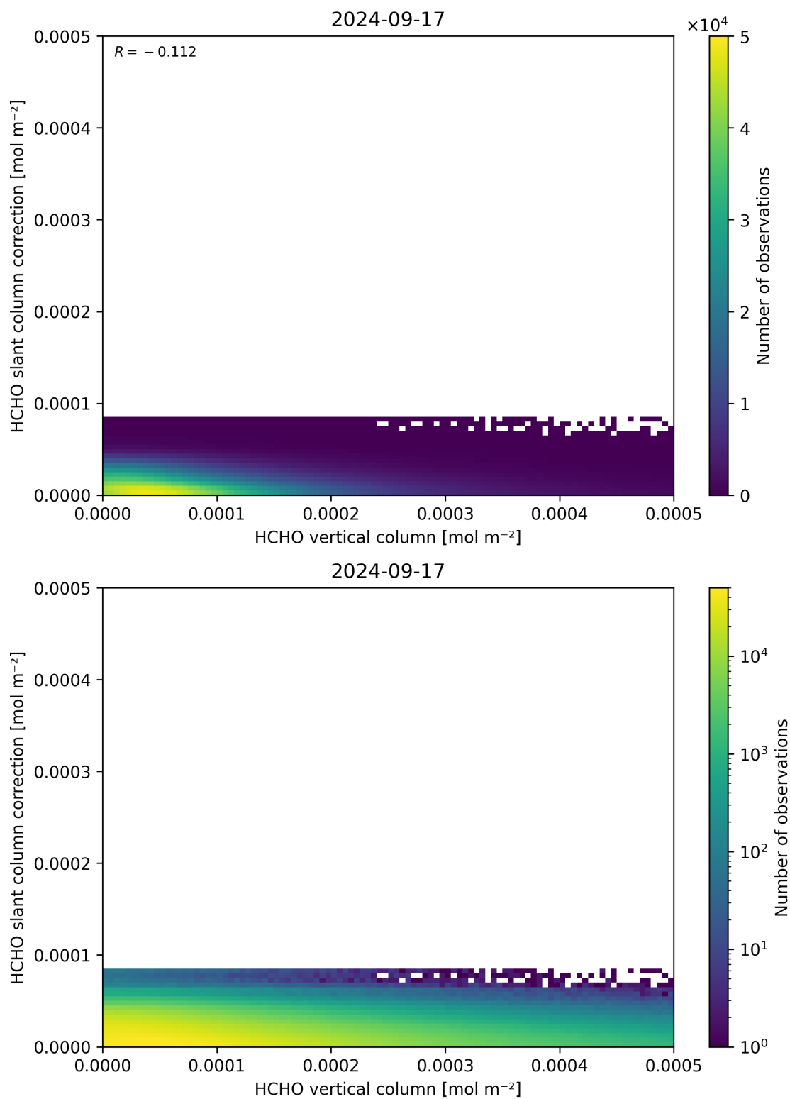
Figure 128: Scatter density plot of “HCHO vertical column” against “HCHO slant column correction” for 2024-09-17 to 2024-09-18.
