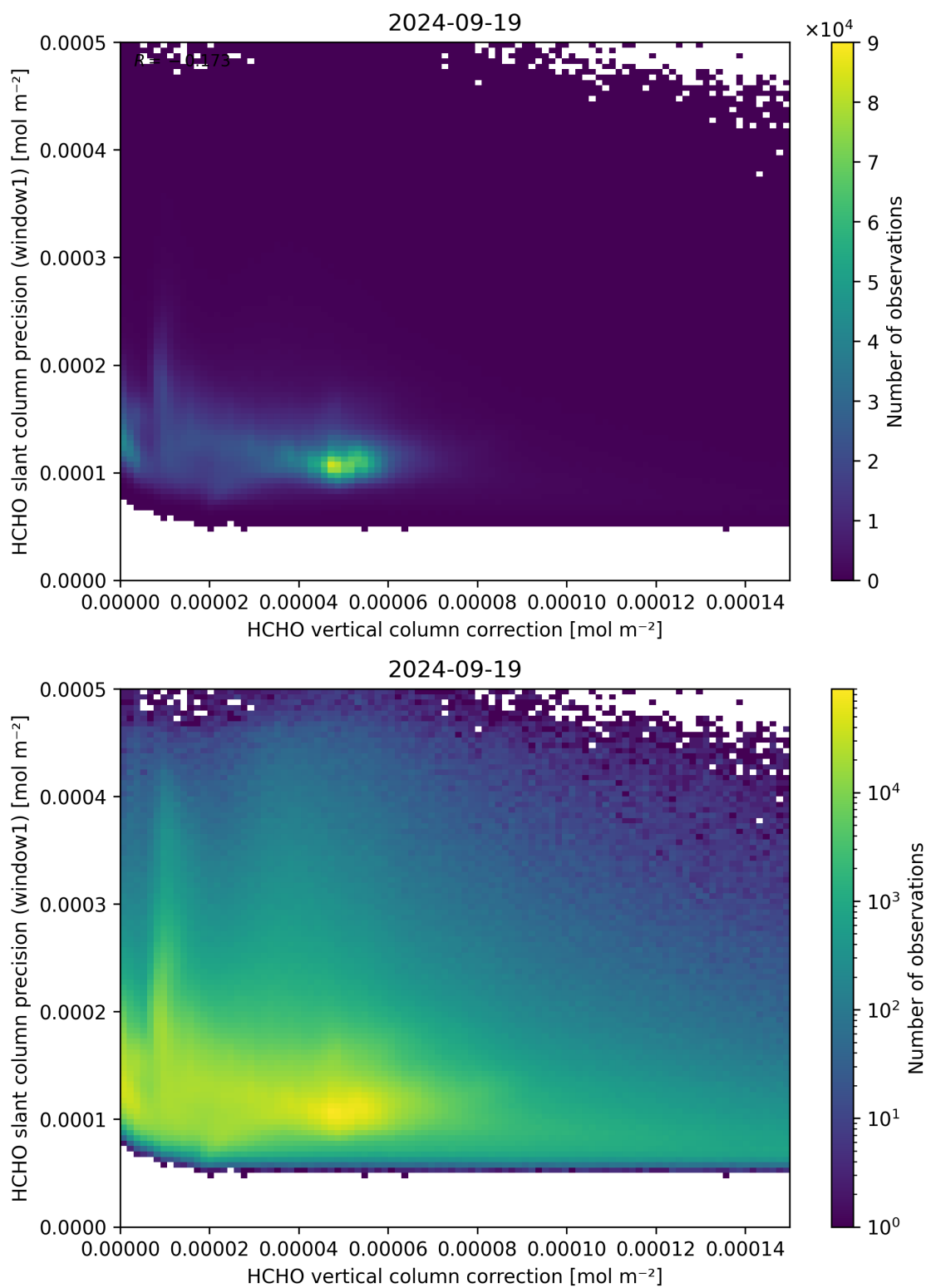
Figure 119: Scatter density plot of “HCHO vertical column correction” against “HCHO slant column precision (window1)” for 2024-09-18 to 2024-09-20.
