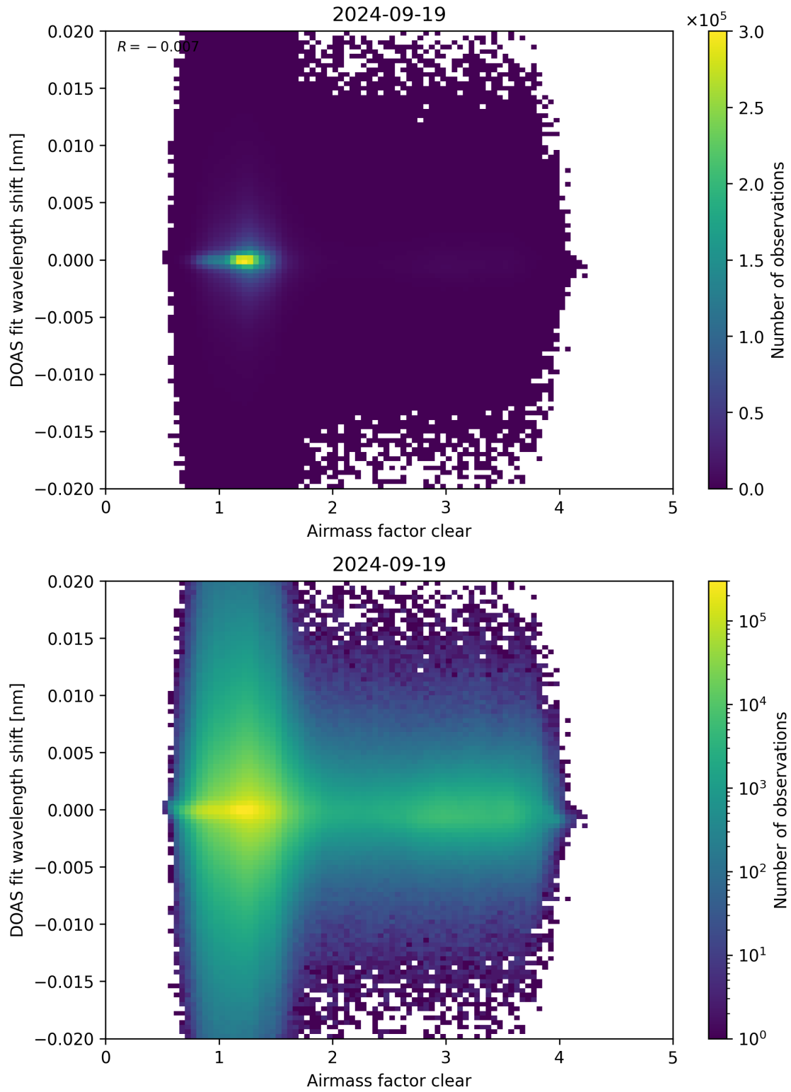
Figure 72: Scatter density plot of “Airmass factor clear” against “DOAS fit wavelength shift” for 2024-09-18 to 2024-09-20.
