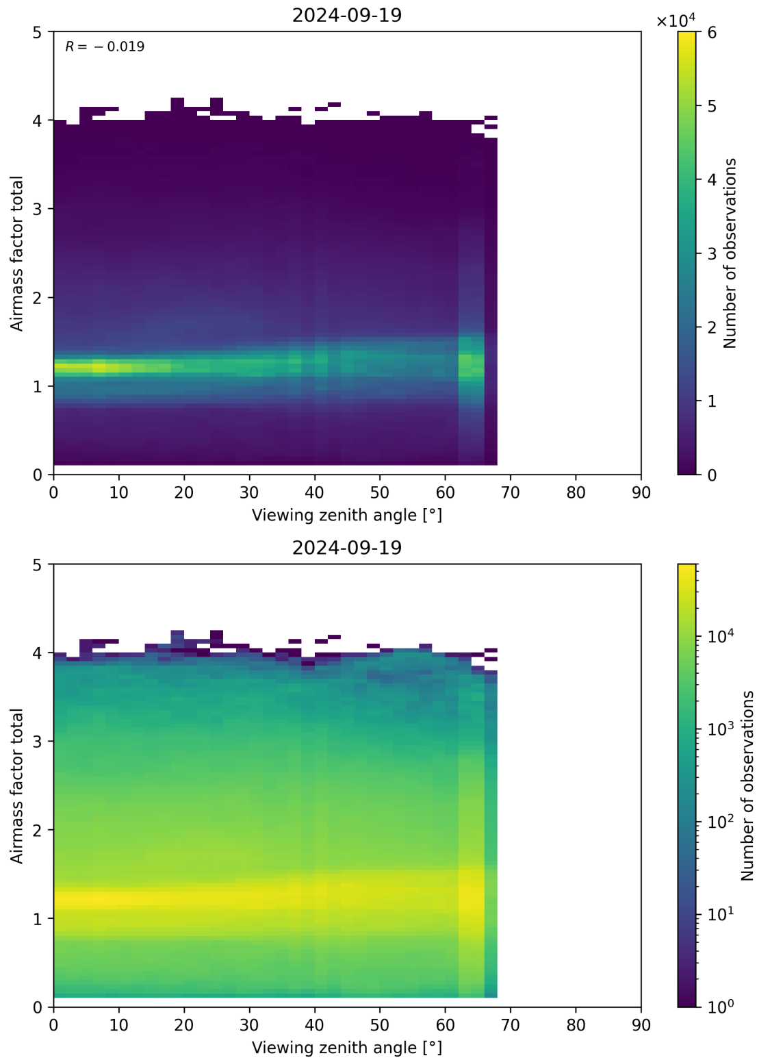
Figure 190: Scatter density plot of “Viewing zenith angle” against “Airmass factor total” for 2024-09-18 to 2024-09-20.
