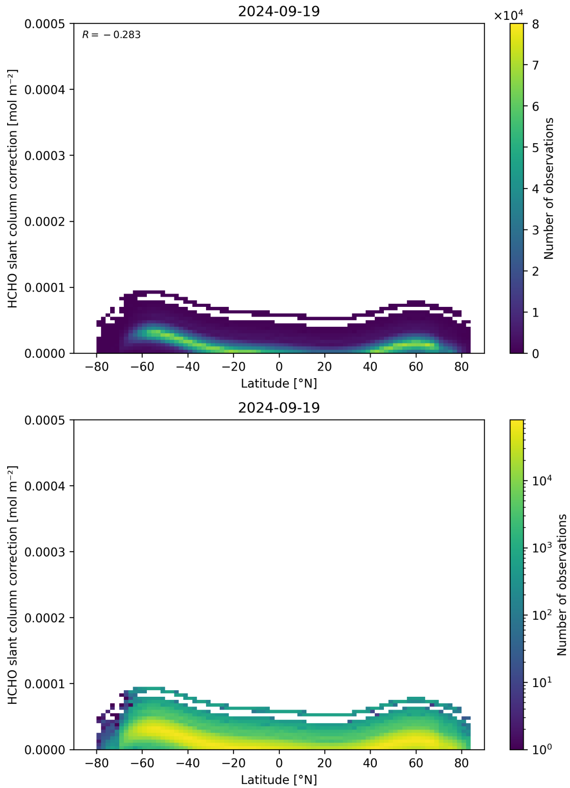
Figure 158: Scatter density plot of “Latitude” against “HCHO slant column correction” for 2024-09-18 to 2024-09-20.
