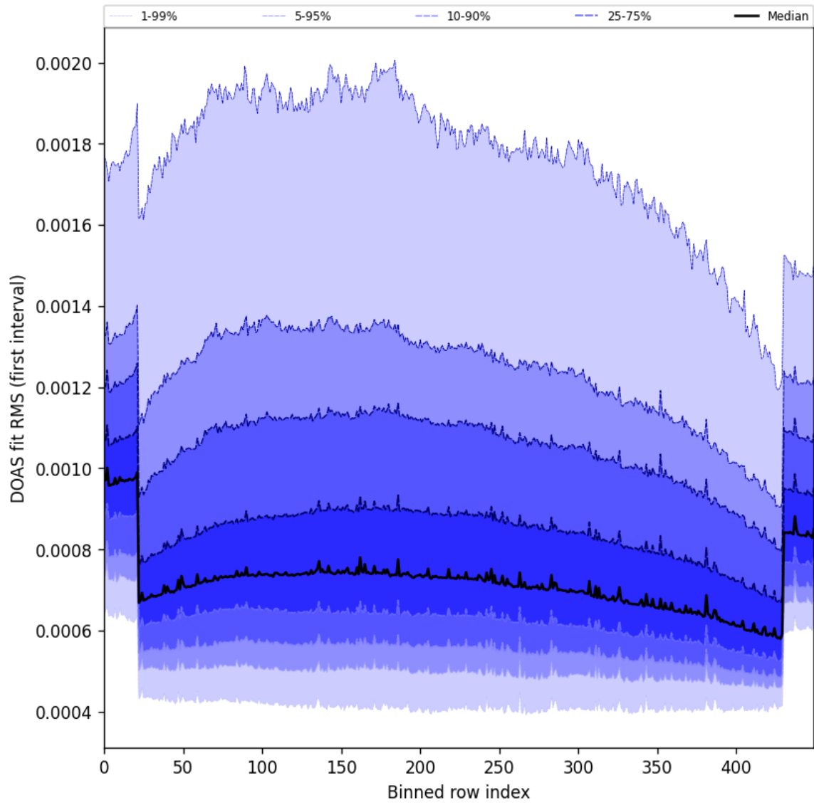
Figure 60: Along track statistics of “DOAS fit RMS (first interval)” for 2024-09-18 to 2024-09-20
