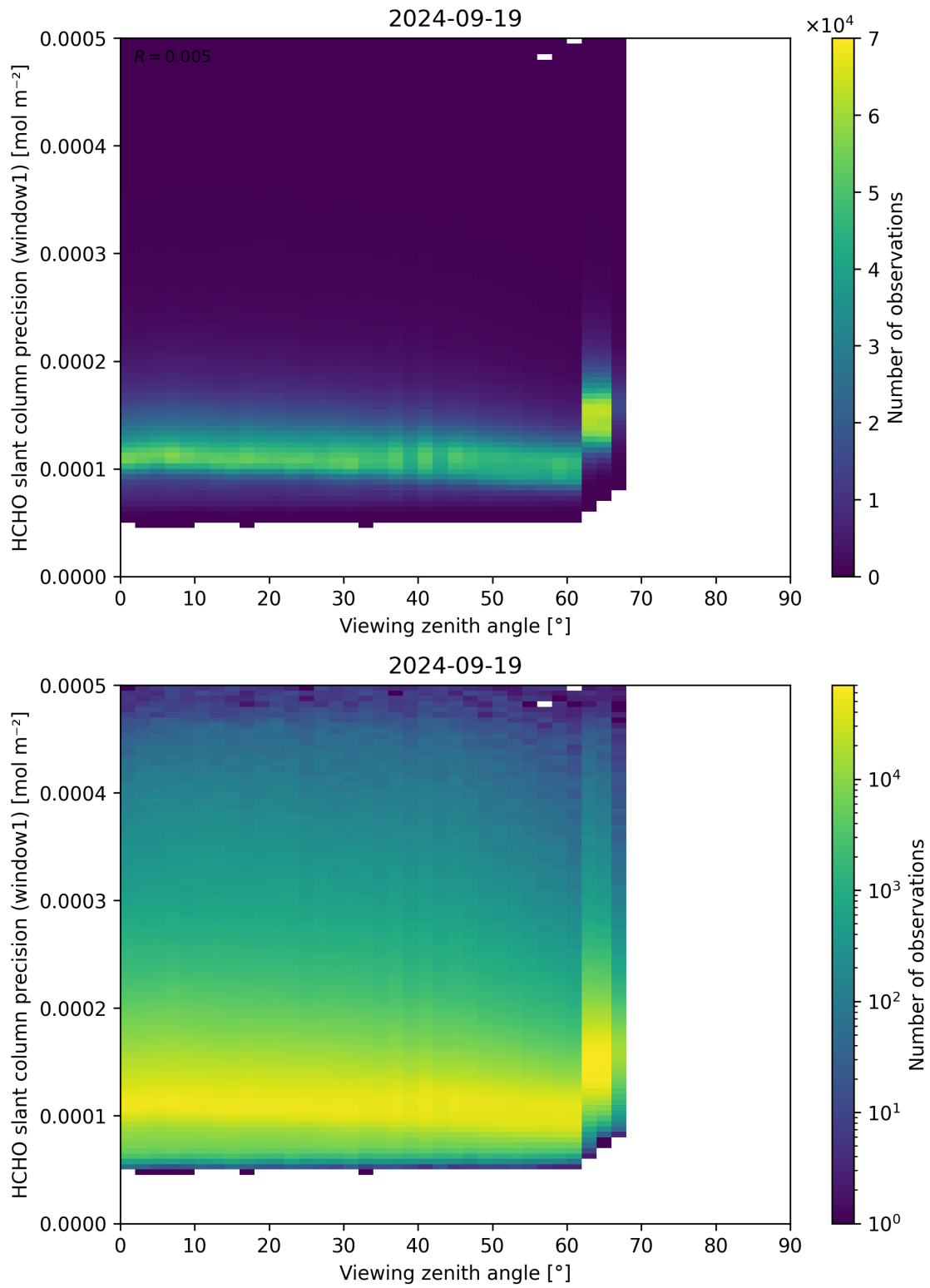
Figure 189: Scatter density plot of “Viewing zenith angle” against “HCHO slant column precision (window1)” for 2024-09-18 to 2024-09-20.
