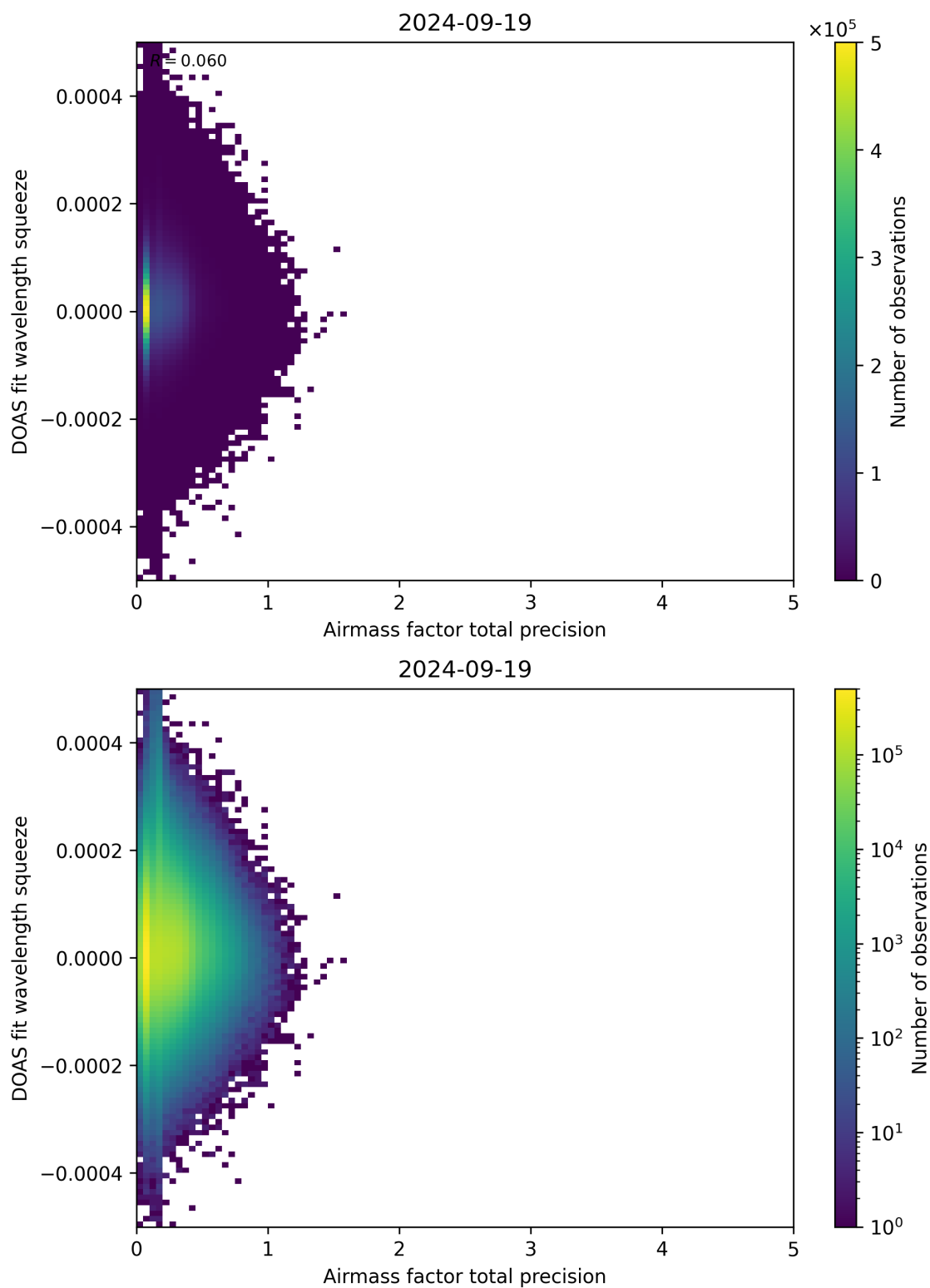
Figure 107: Scatter density plot of “Airmass factor total precision” against “DOAS fit wavelength squeeze” for 2024-09-18 to 2024-09-20.
