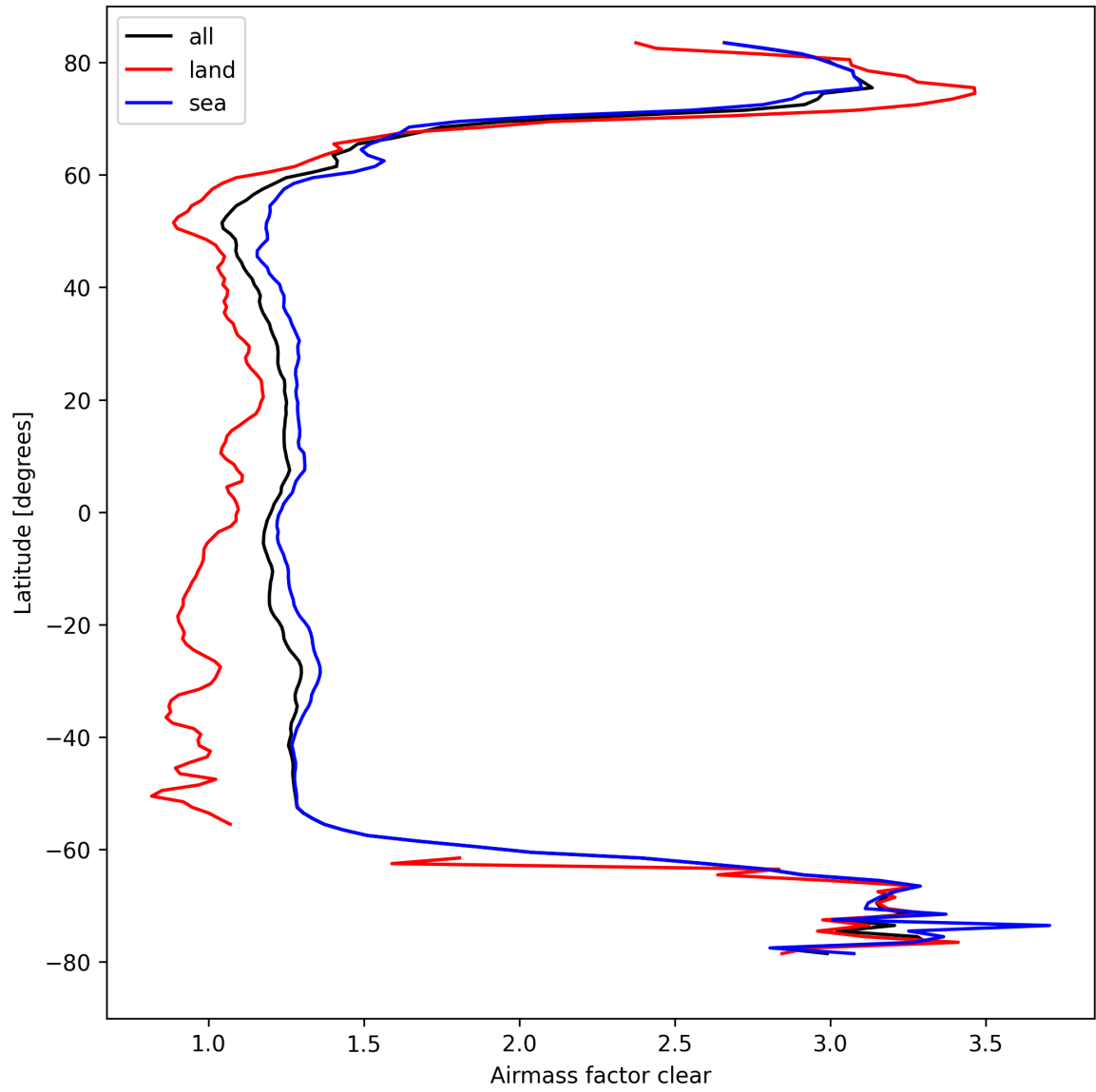
Figure 28: Zonal average of “Airmass factor clear” for 2024-09-18 to 2024-09-20.
