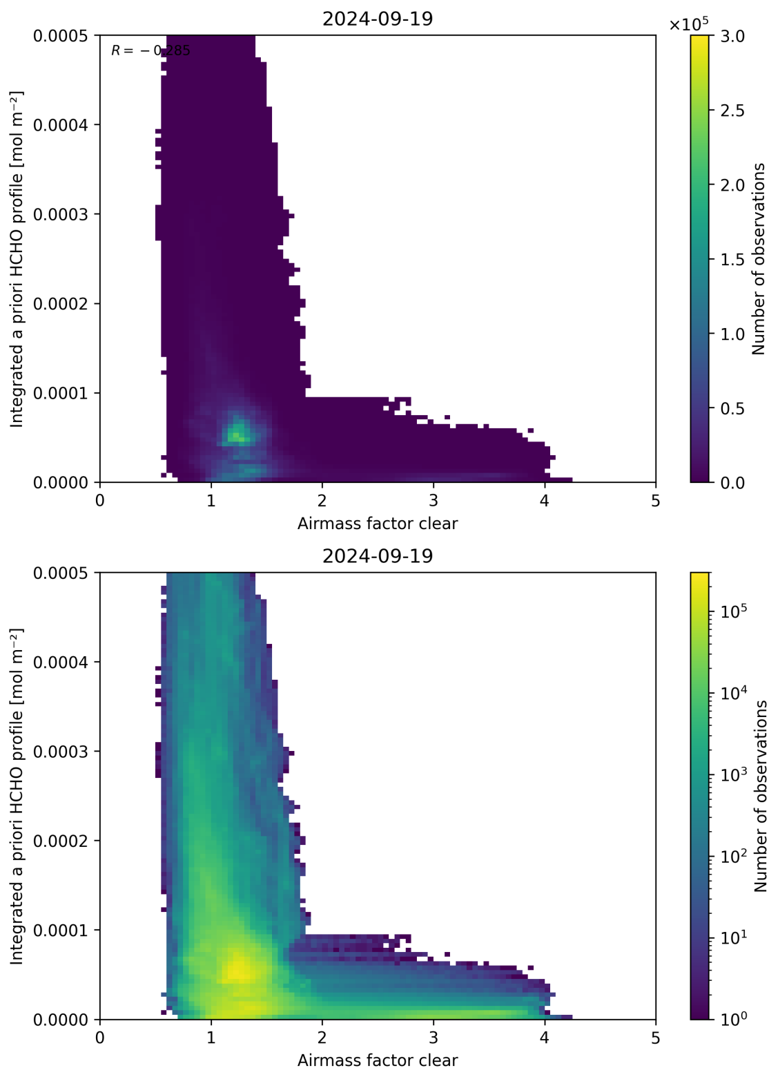
Figure 76: Scatter density plot of “Airmass factor clear” against “Integrated a priori HCHO profile” for 2024-09-18 to 2024-09-20.
