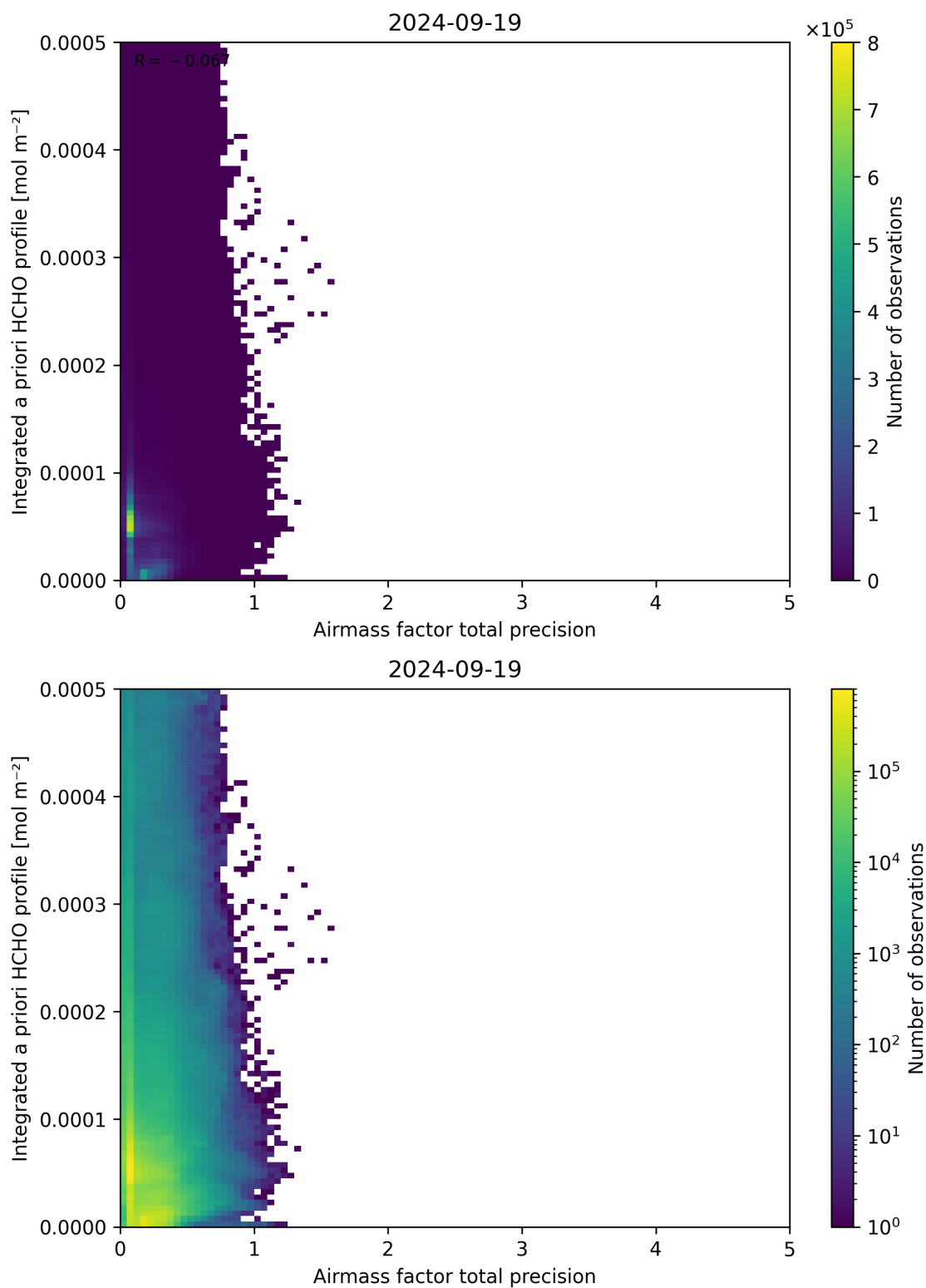
Figure 111: Scatter density plot of “Airmass factor total precision” against “Integrated a priori HCHO profile” for 2024-09-18 to 2024-09-20.
