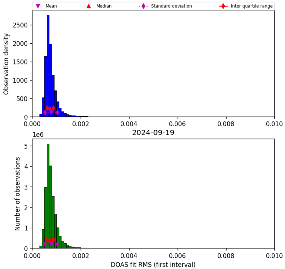
Figure 46: Histogram of “DOAS fit RMS (first interval)” for 2024-09-18 to 2024-09-20
