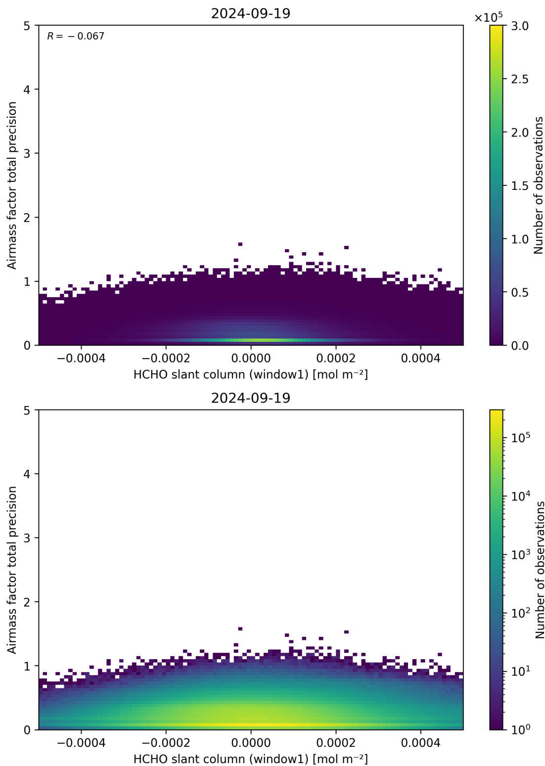
Figure 86: Scatter density plot of “HCHO slant column (window1)” against “Airmass factor total precision” for 2024-09-18 to 2024-09-20.
