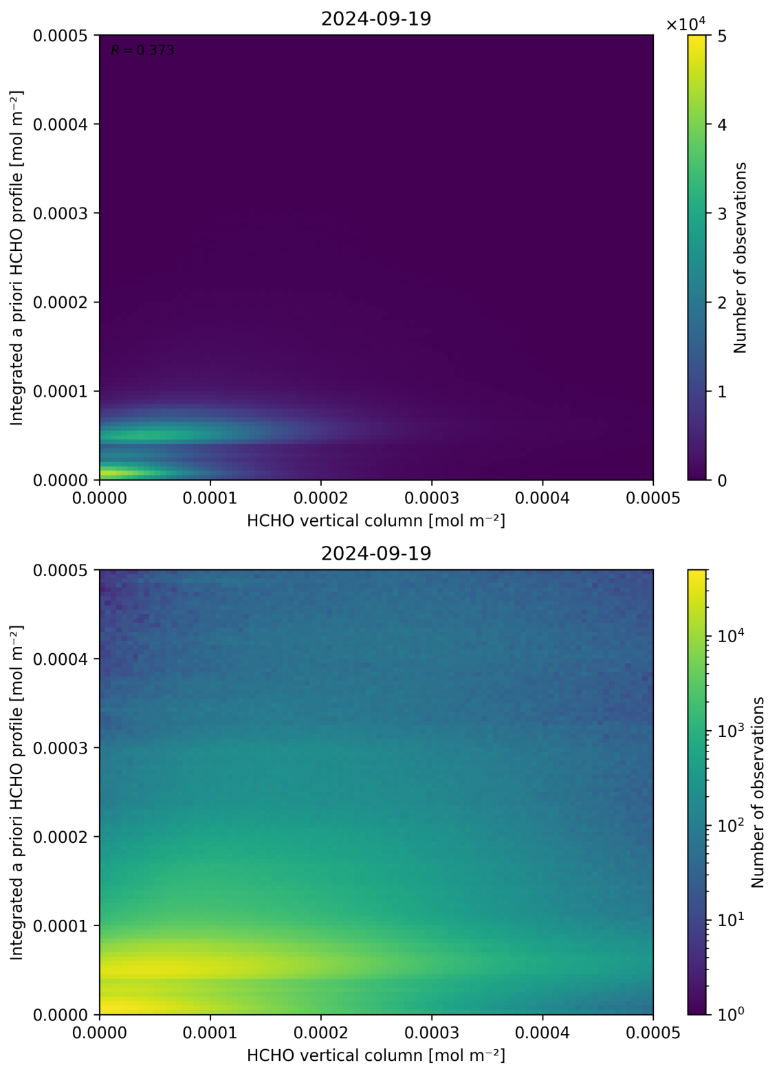
Figure 135: Scatter density plot of “HCHO vertical column” against “Integrated a priori HCHO profile” for 2024-09-18 to 2024-09-20.
