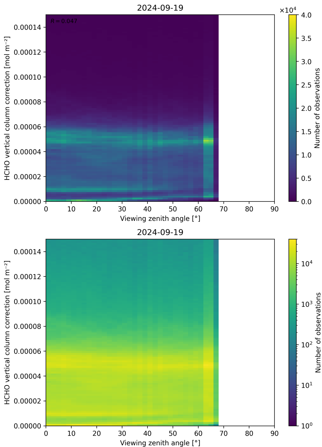
Figure 193: Scatter density plot of “Viewing zenith angle” against “HCHO vertical column correction” for 2024-09-18 to 2024-09-20.
