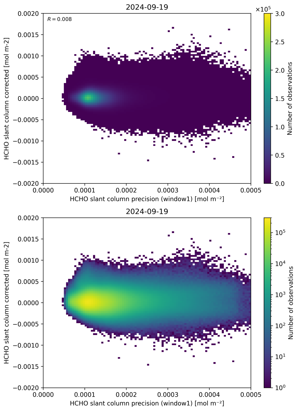
Figure 92: Scatter density plot of “HCHO slant column precision (window1)” against “HCHO slant column corrected” for 2024-09-18 to 2024-09-20.
