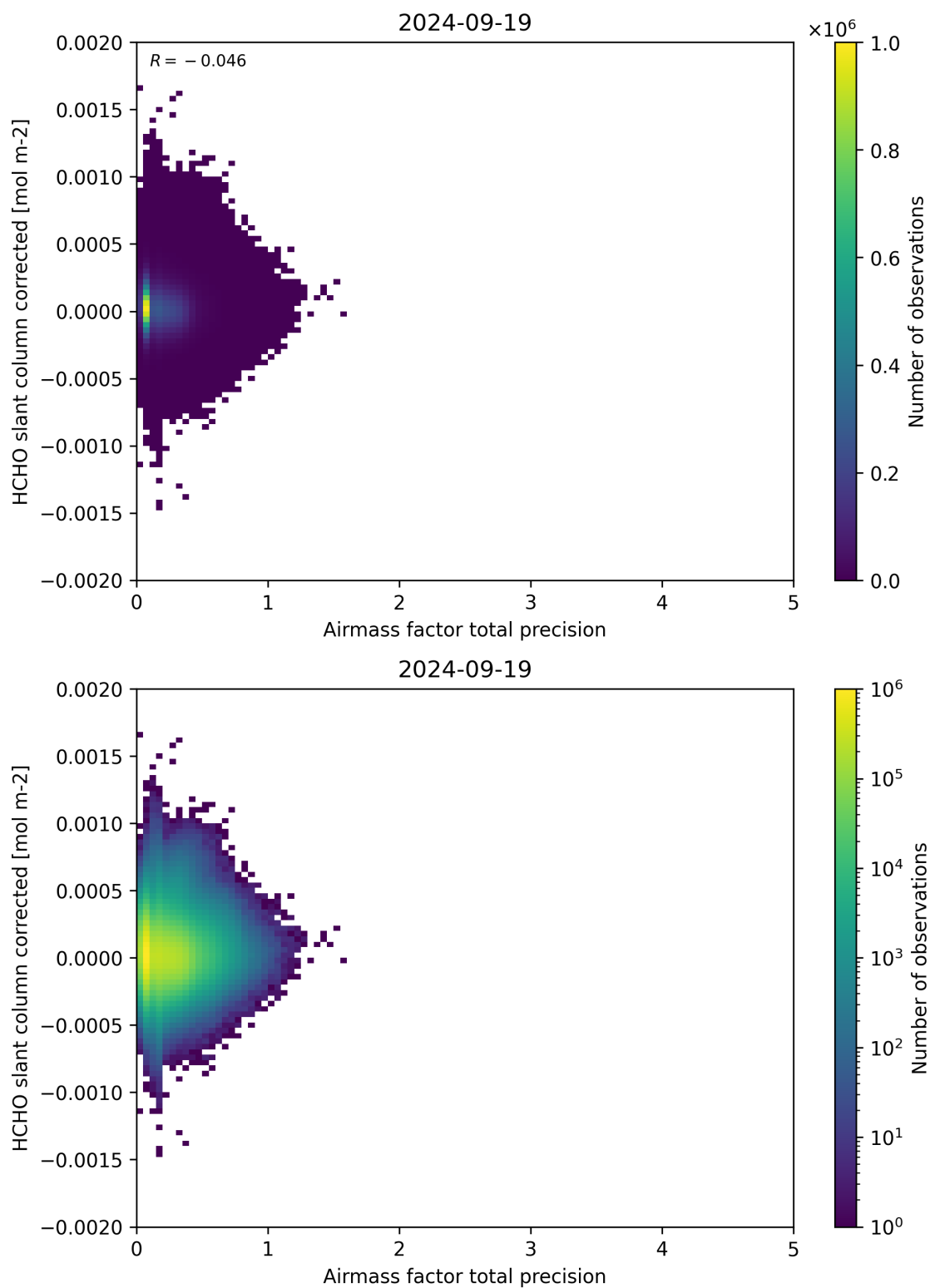
Figure 109: Scatter density plot of “Airmass factor total precision” against “HCHO slant column corrected” for 2024-09-18 to 2024-09-20.
