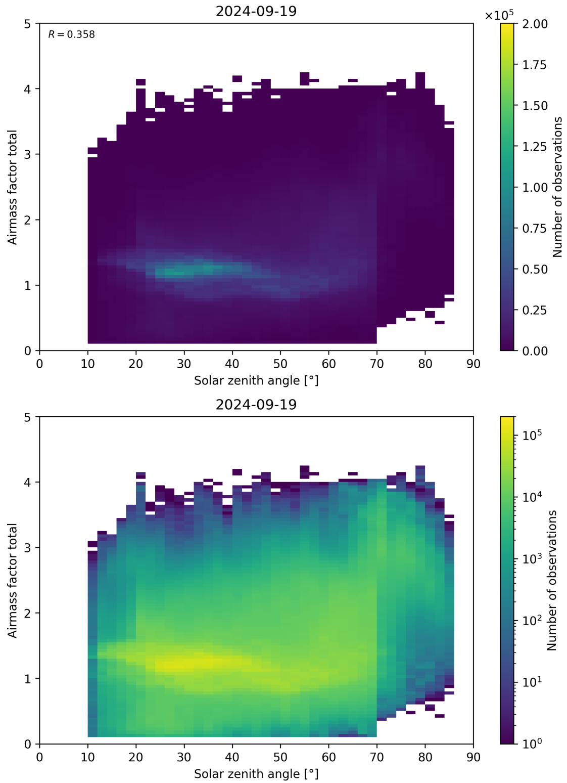
Figure 175: Scatter density plot of “Solar zenith angle” against “Airmass factor total” for 2024-09-18 to 2024-09-20.
