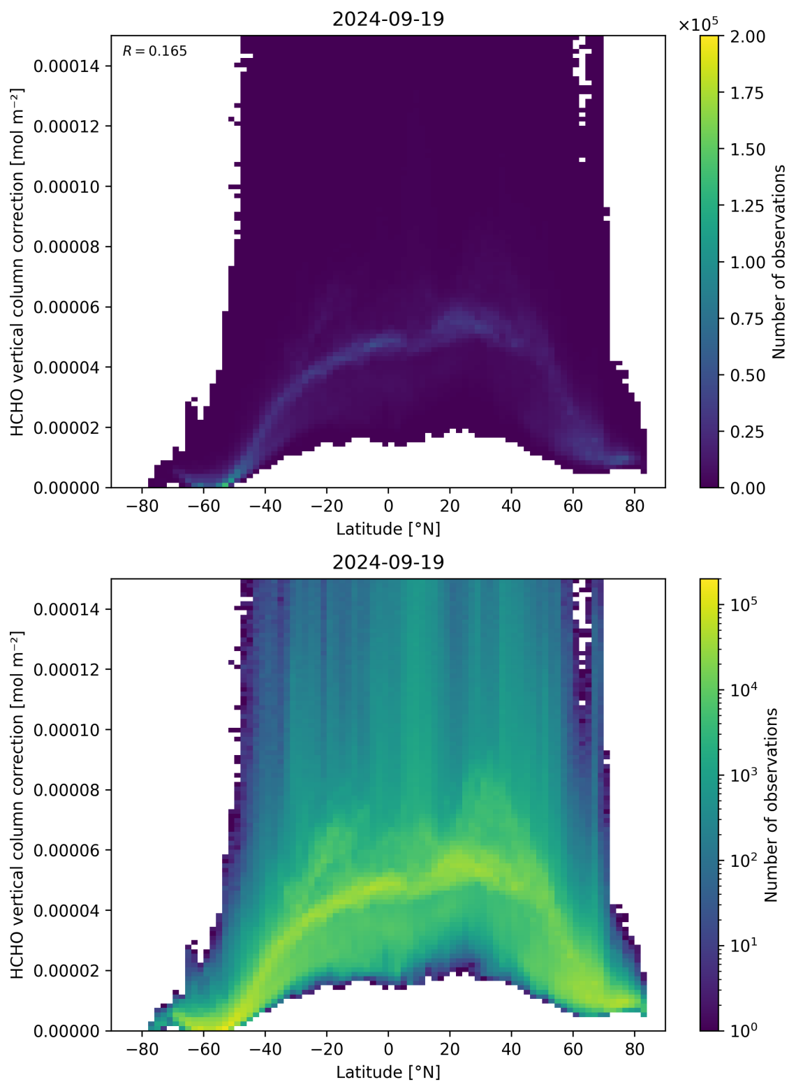
Figure 164: Scatter density plot of “Latitude” against “HCHO vertical column correction” for 2024-09-18 to 2024-09-20.
