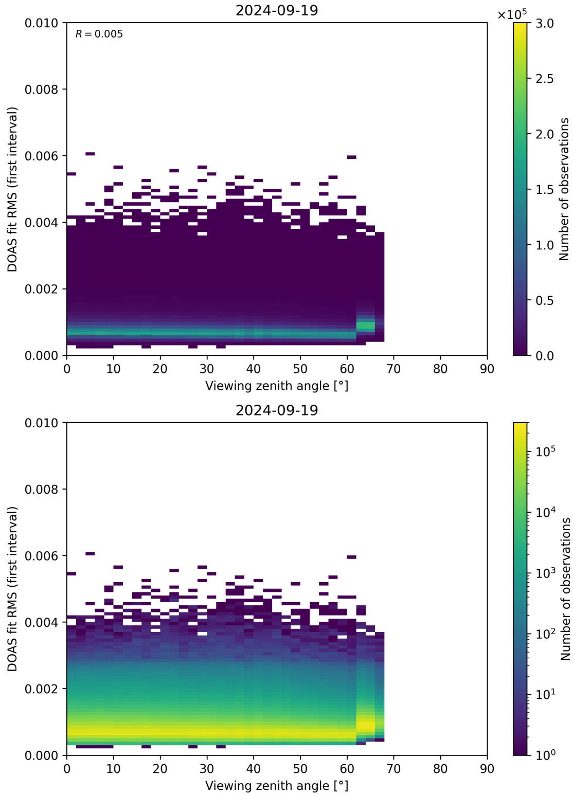
Figure 182: Scatter density plot of “Viewing zenith angle” against “DOAS fit RMS (first interval)” for 2024-09-18 to 2024-09-20.
