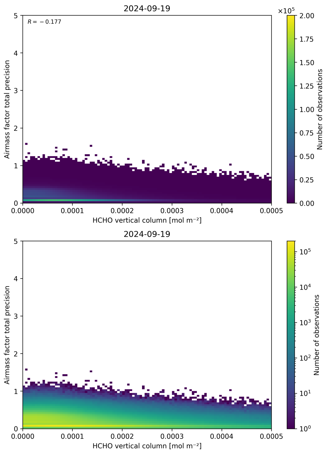
Figure 132: Scatter density plot of “HCHO vertical column” against “Airmass factor total precision” for 2024-09-18 to 2024-09-20.
