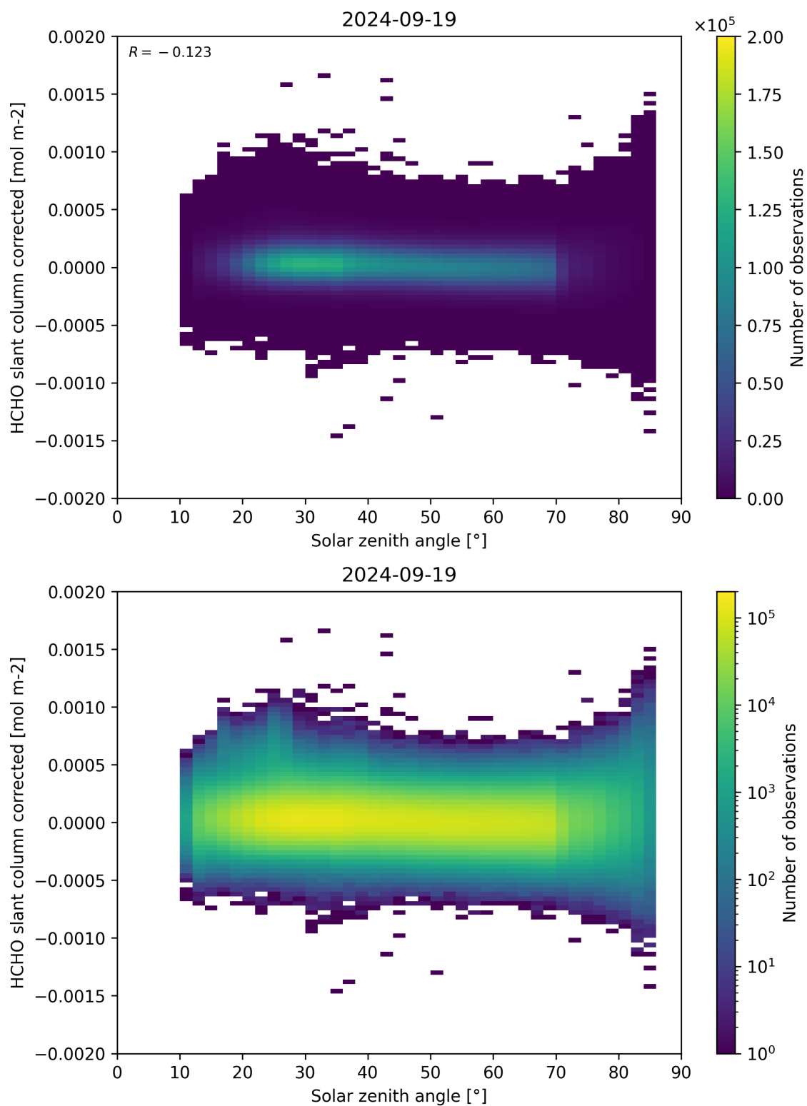
Figure 171: Scatter density plot of “Solar zenith angle” against “HCHO slant column corrected” for 2024-09-18 to 2024-09-20.
