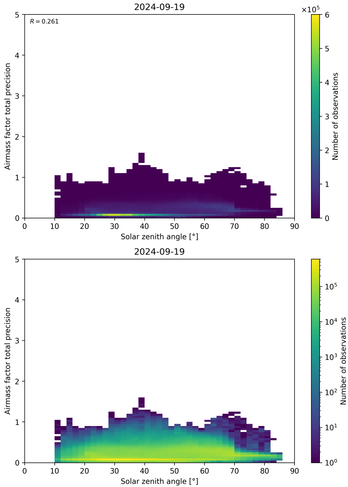
Figure 176: Scatter density plot of “Solar zenith angle” against “Airmass factor total precision” for 2024-09-18 to 2024-09-20.
