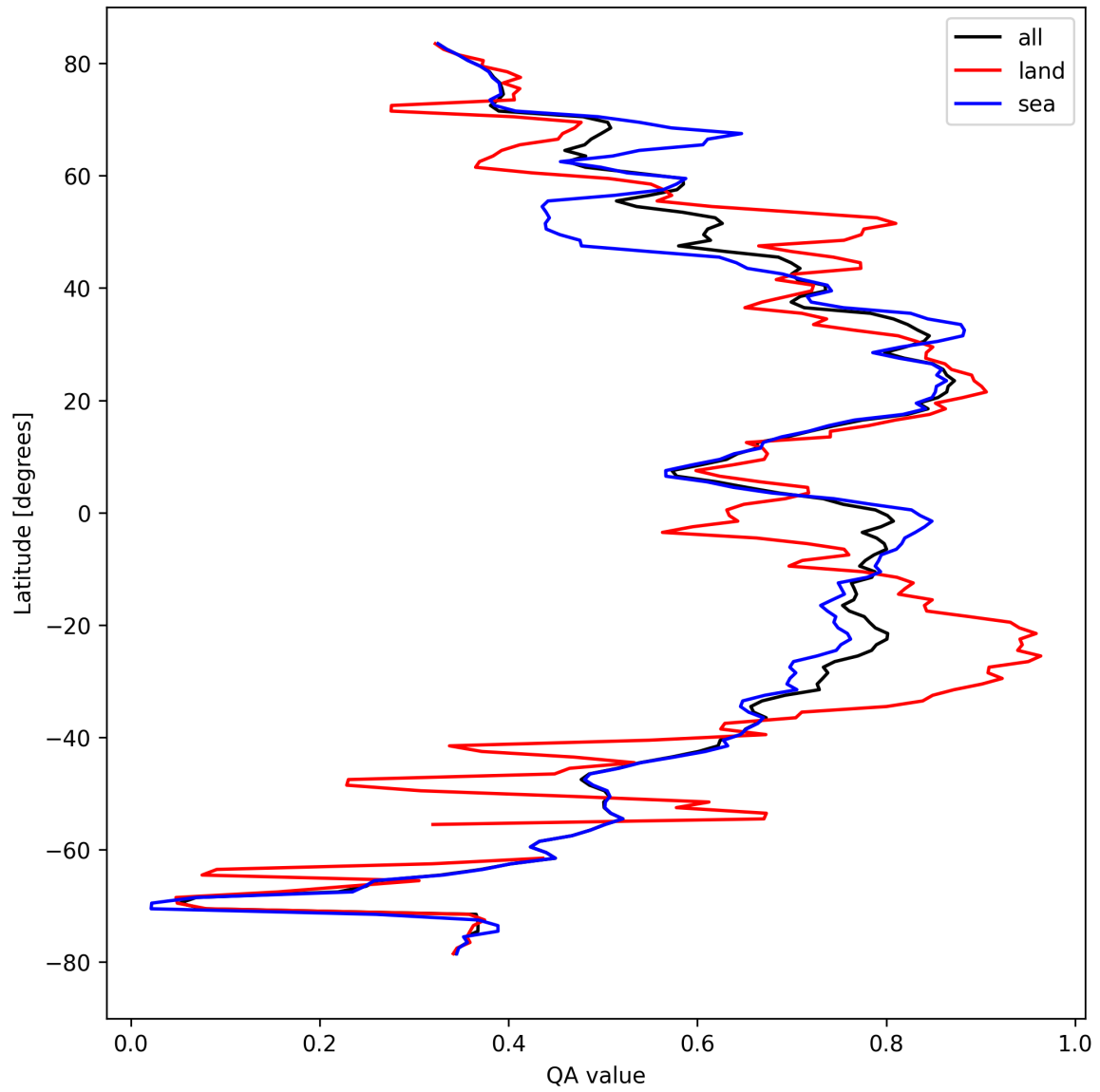
Figure 20: Zonal average of “QA value” for 2024-09-18 to 2024-09-20.
