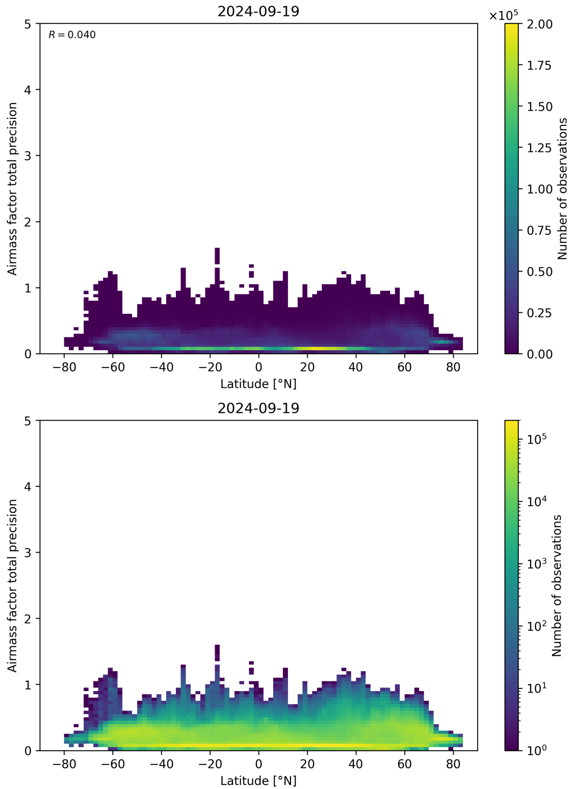
Figure 162: Scatter density plot of “Latitude” against “Airmass factor total precision” for 2024-09-18 to 2024-09-20.
