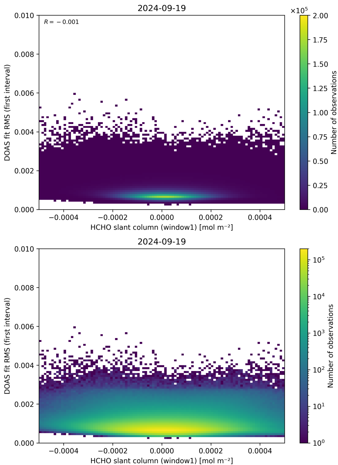
Figure 78: Scatter density plot of “HCHO slant column (window1)” against “DOAS fit RMS (first interval)” for 2024-09-18 to 2024-09-20.
