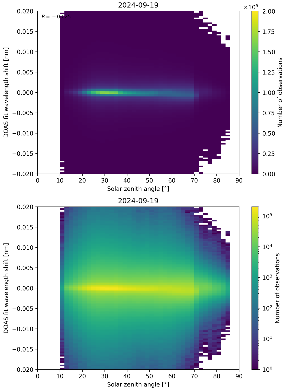
Figure 168: Scatter density plot of “Solar zenith angle” against “DOAS fit wavelength shift” for 2024-09-18 to 2024-09-20.
