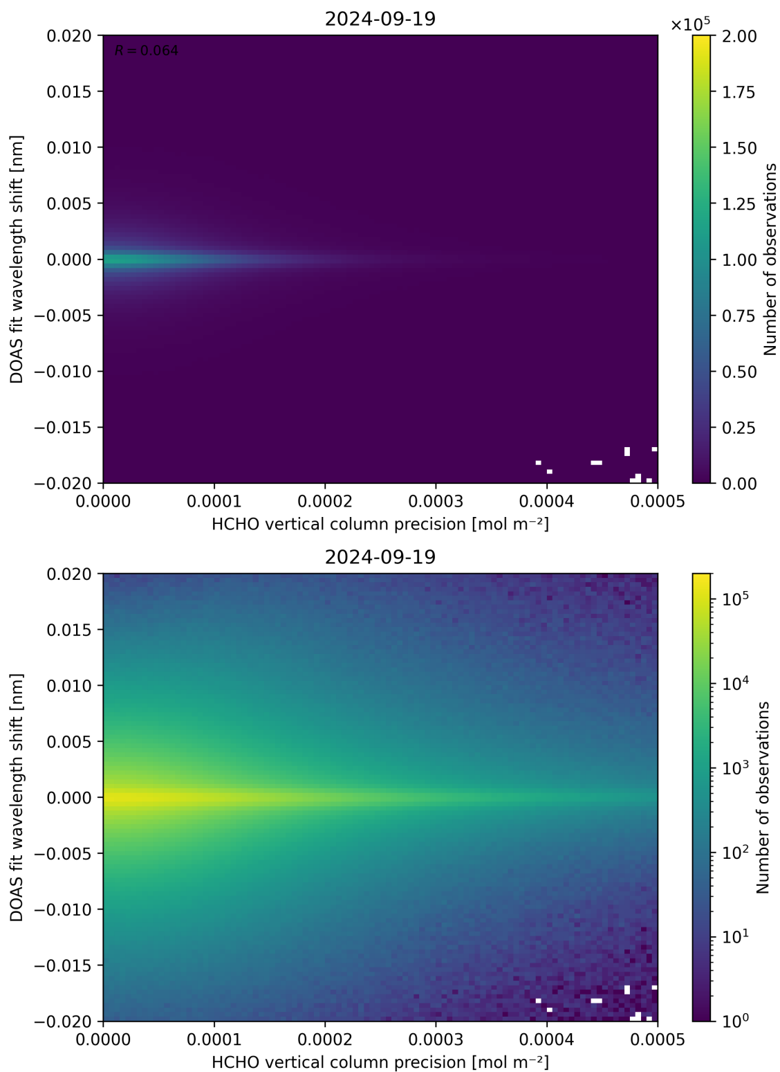
Figure 137: Scatter density plot of “HCHO vertical column precision” against “DOAS fit wavelength shift” for 2024-09-18 to 2024-09-20.
