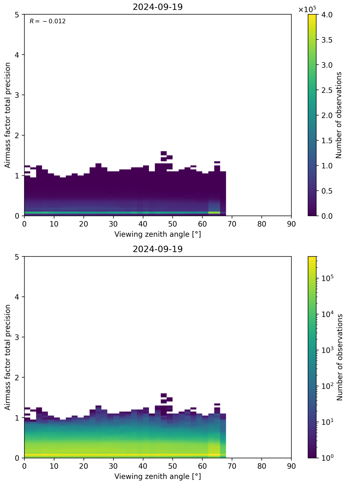
Figure 191: Scatter density plot of “Viewing zenith angle” against “Airmass factor total precision” for 2024-09-18 to 2024-09-20.
