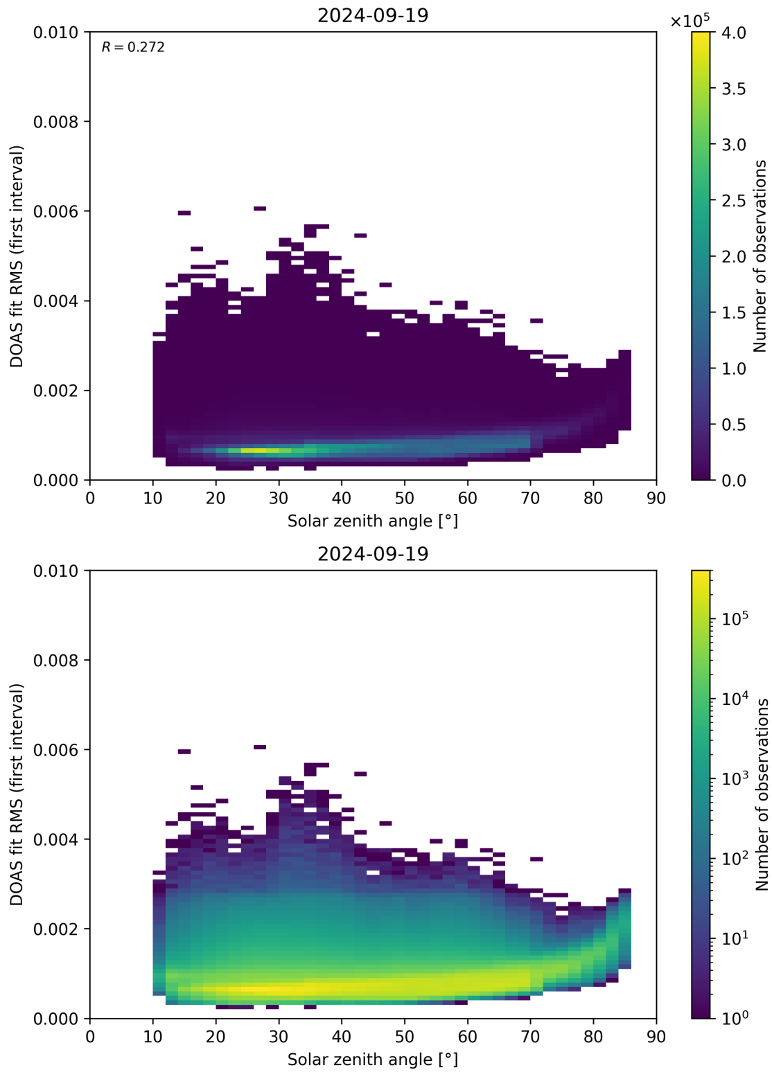
Figure 167: Scatter density plot of “Solar zenith angle” against “DOAS fit RMS (first interval)” for 2024-09-18 to 2024-09-20.
