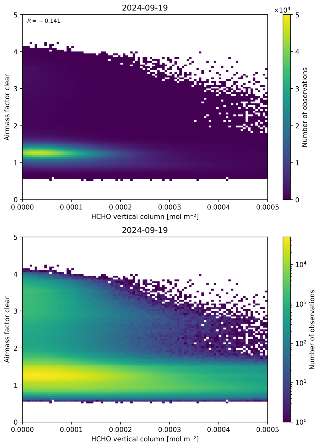
Figure 126: Scatter density plot of “HCHO vertical column” against “Airmass factor clear” for 2024-09-18 to 2024-09-20.
