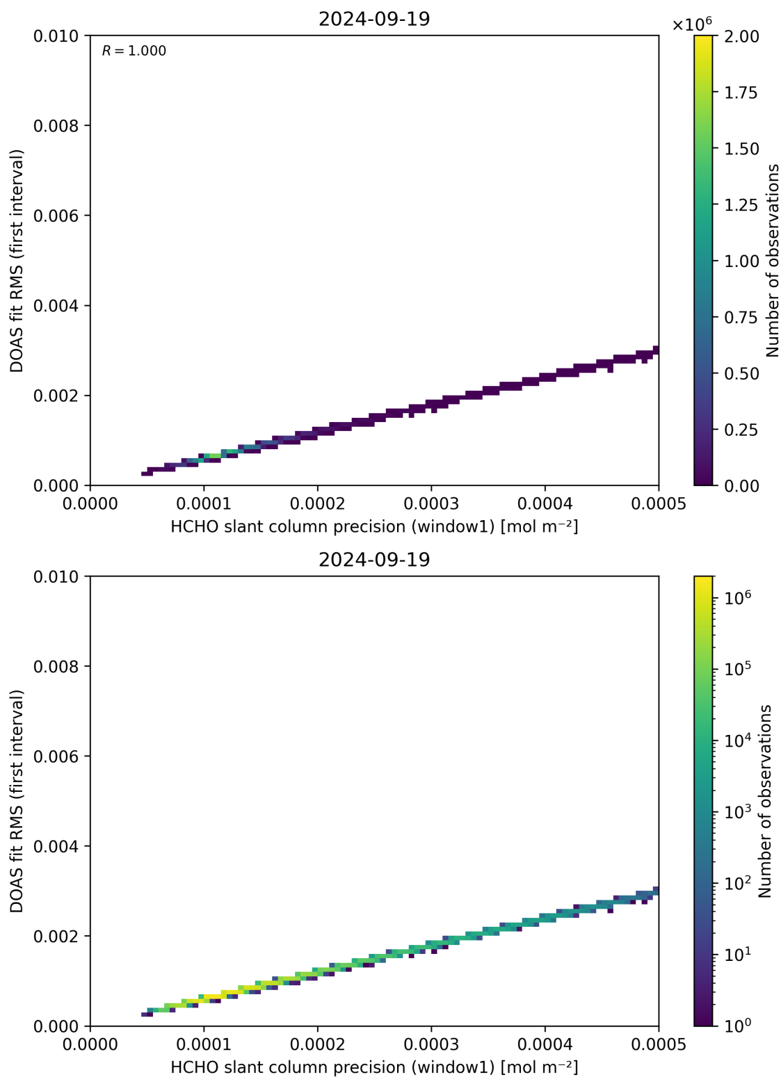
Figure 88: Scatter density plot of “HCHO slant column precision (window1)” against “DOAS fit RMS (first interval)” for 2024-09-18 to 2024-09-20.
