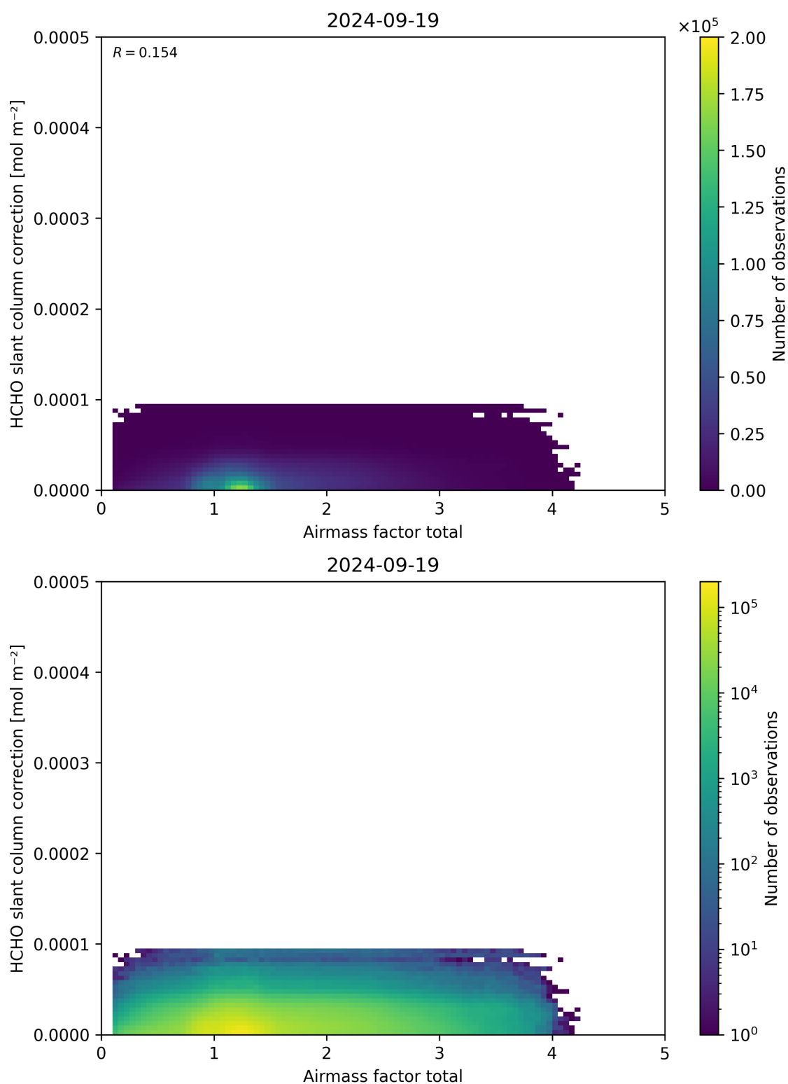
Figure 102: Scatter density plot of “Airmass factor total” against “HCHO slant column correction” for 2024-09-18 to 2024-09-20.
