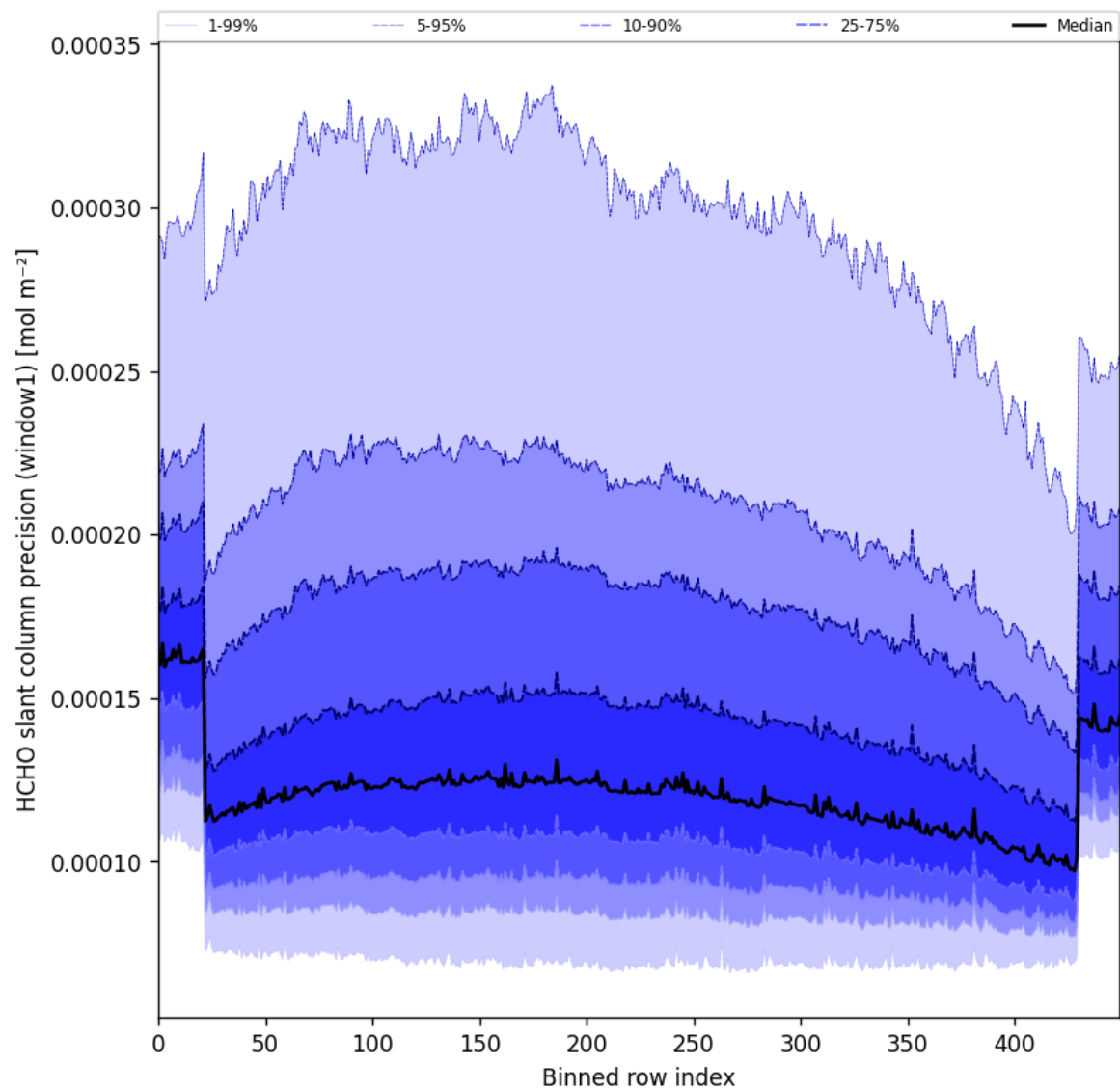
Figure 53: Along track statistics of “HCHO slant column precision (window1)” for 2024-09-18 to 2024-09-20
