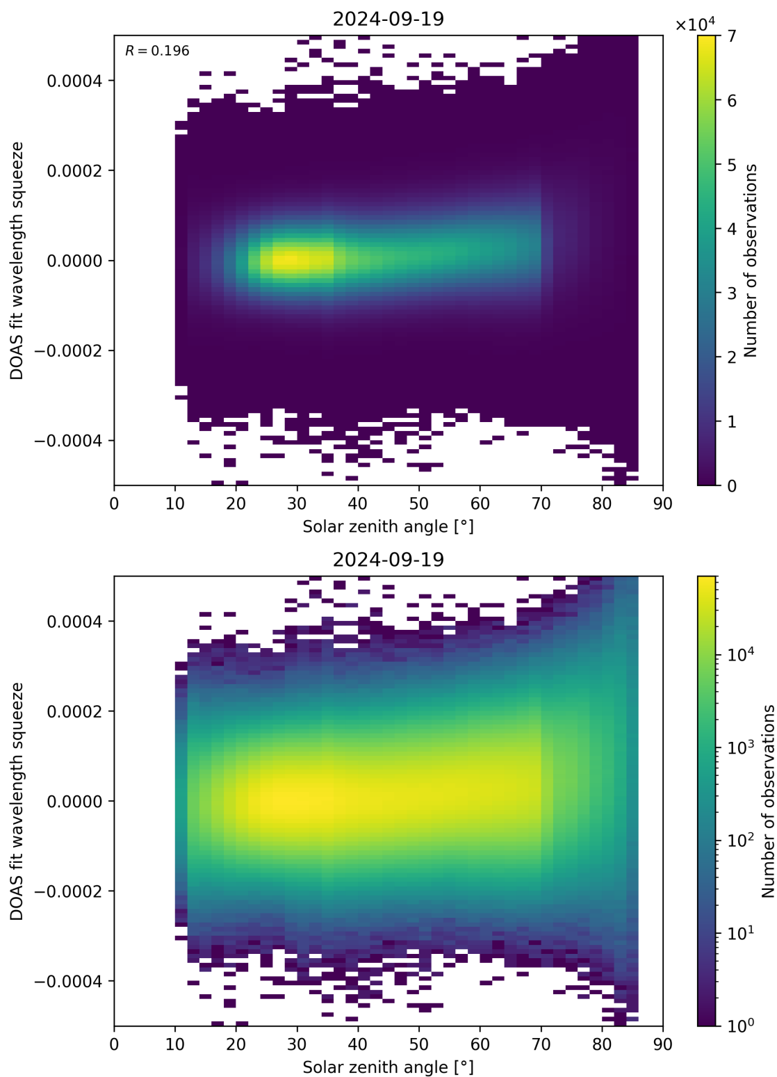
Figure 169: Scatter density plot of “Solar zenith angle” against “DOAS fit wavelength squeeze” for 2024-09-18 to 2024-09-20.
