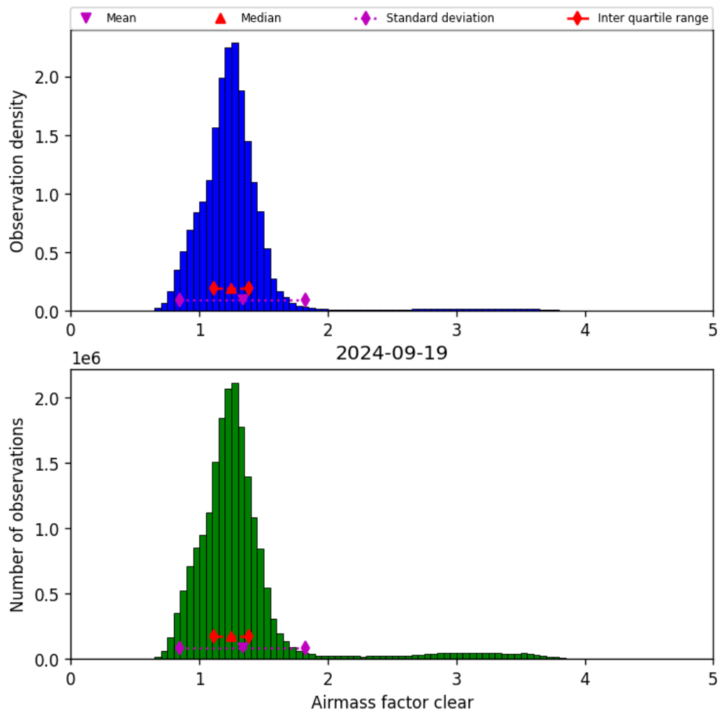
Figure 42: Histogram of “Airmass factor clear” for 2024-09-18 to 2024-09-20
