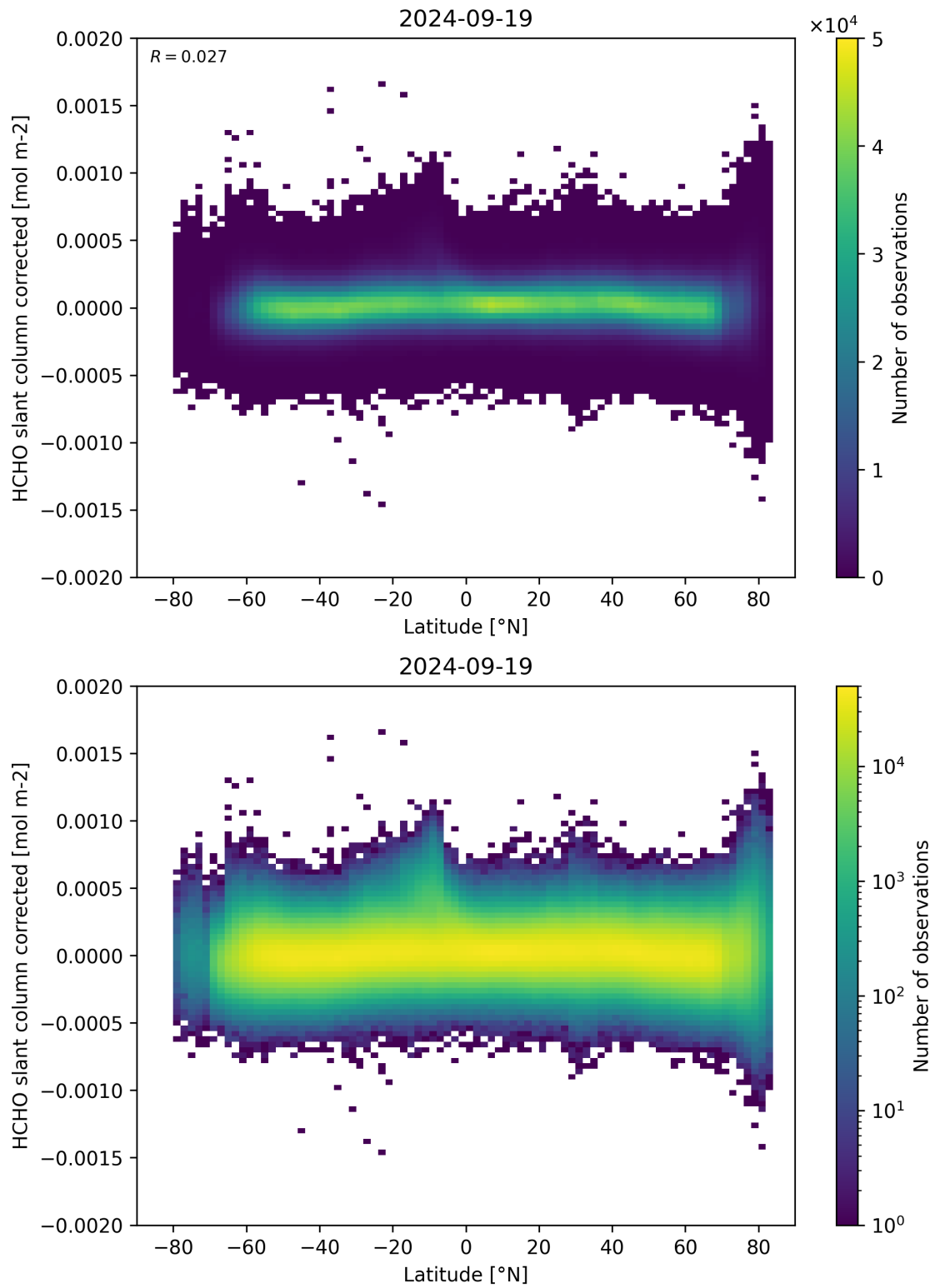
Figure 157: Scatter density plot of “Latitude” against “HCHO slant column corrected” for 2024-09-18 to 2024-09-20.
