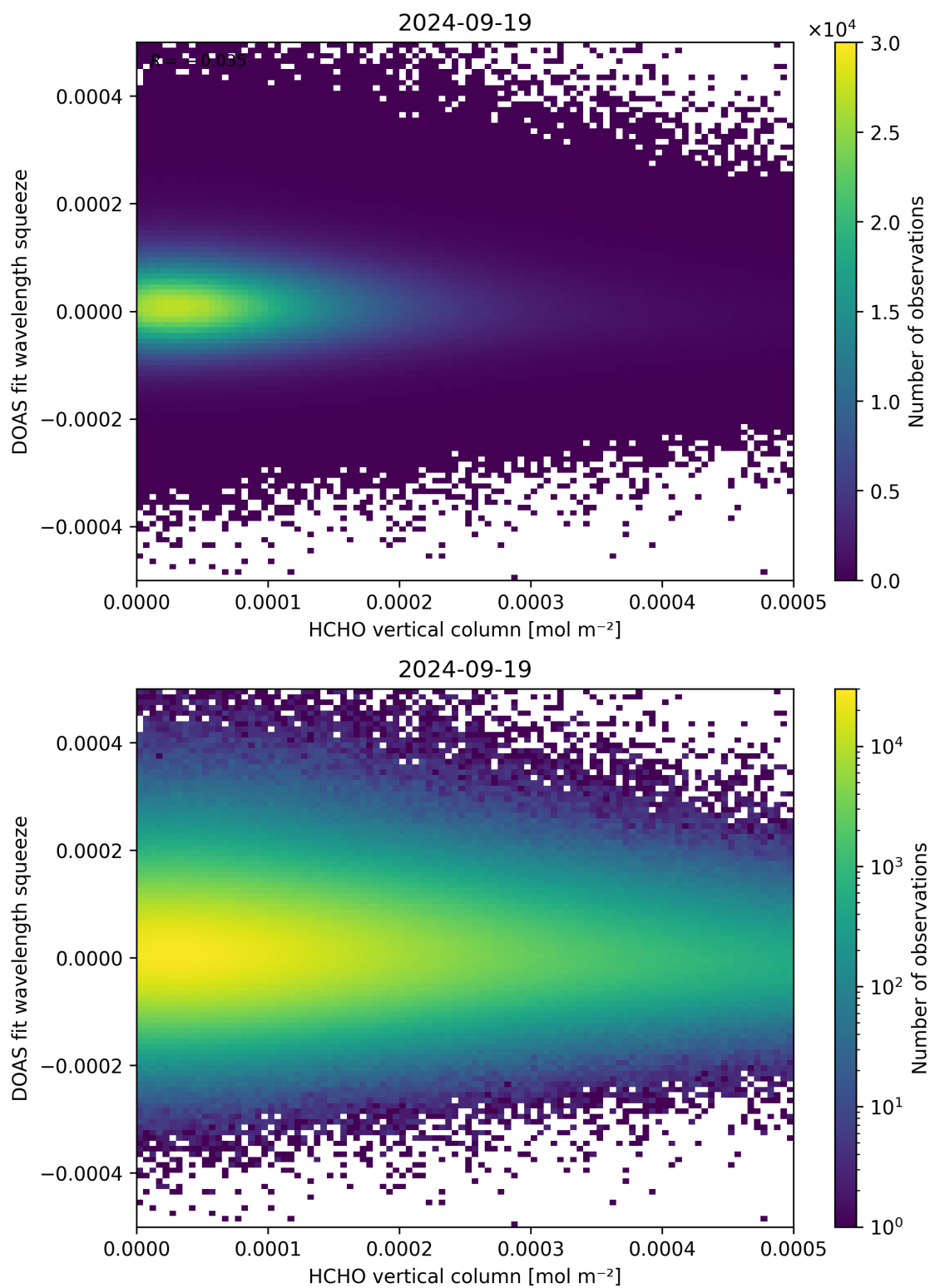
Figure 125: Scatter density plot of “HCHO vertical column” against “DOAS fit wavelength squeeze” for 2024-09-18 to 2024-09-20.
