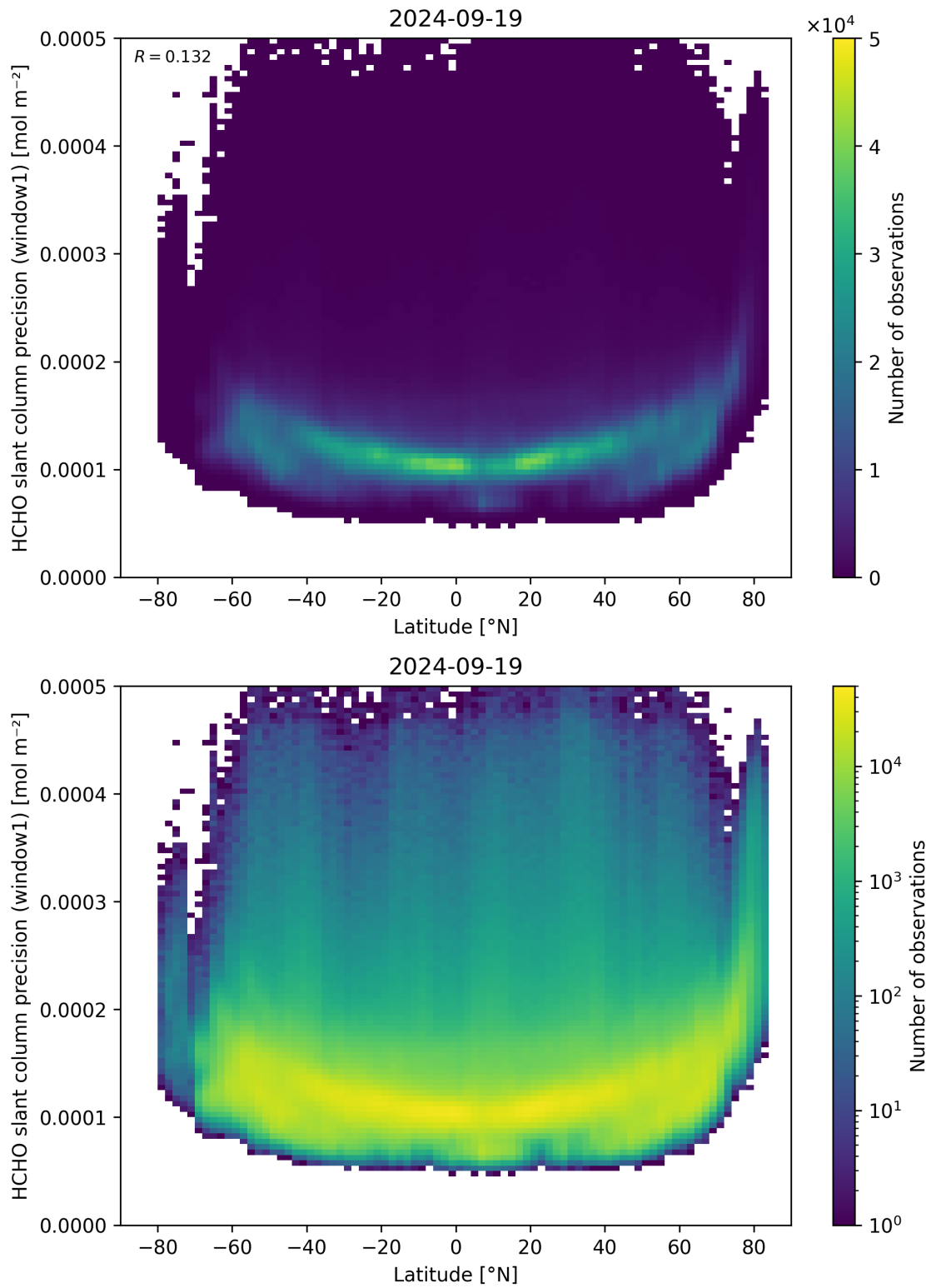
Figure 160: Scatter density plot of “Latitude” against “HCHO slant column precision (window1)” for 2024-09-18 to 2024-09-20.
