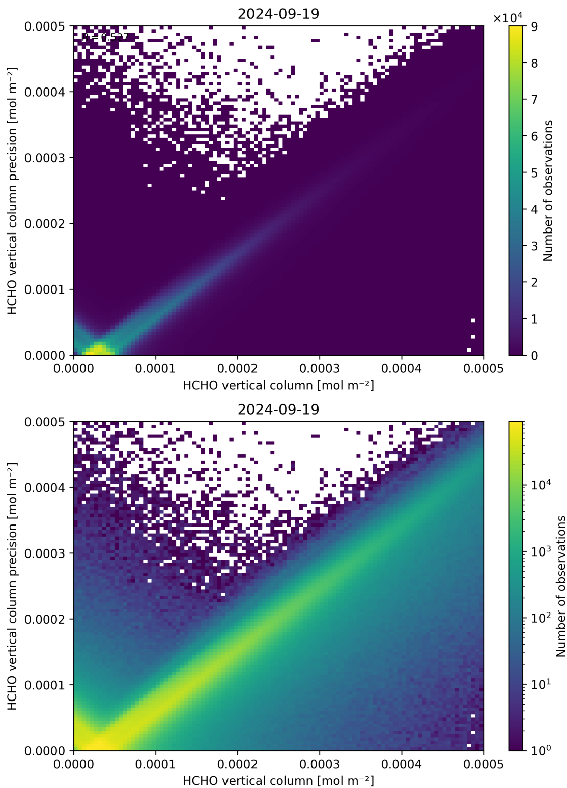
Figure 134: Scatter density plot of “HCHO vertical column” against “HCHO vertical column precision” for 2024-09-18 to 2024-09-20.
