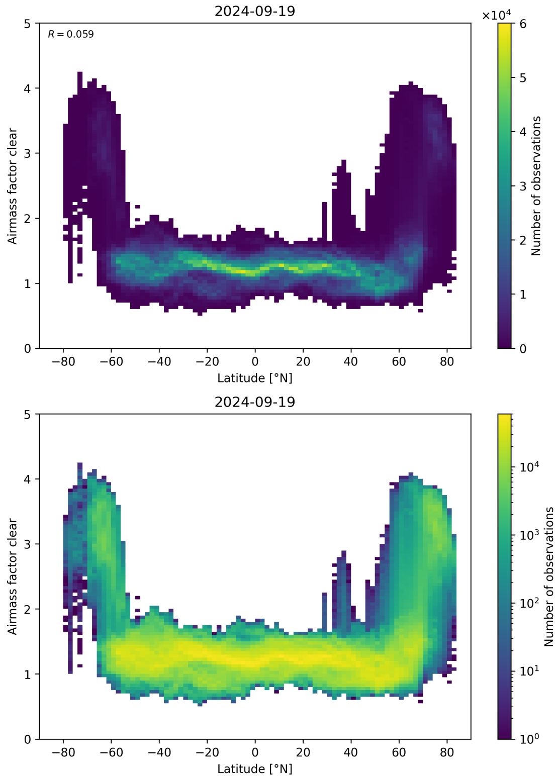
Figure 156: Scatter density plot of “Latitude” against “Airmass factor clear” for 2024-09-18 to 2024-09-20.
