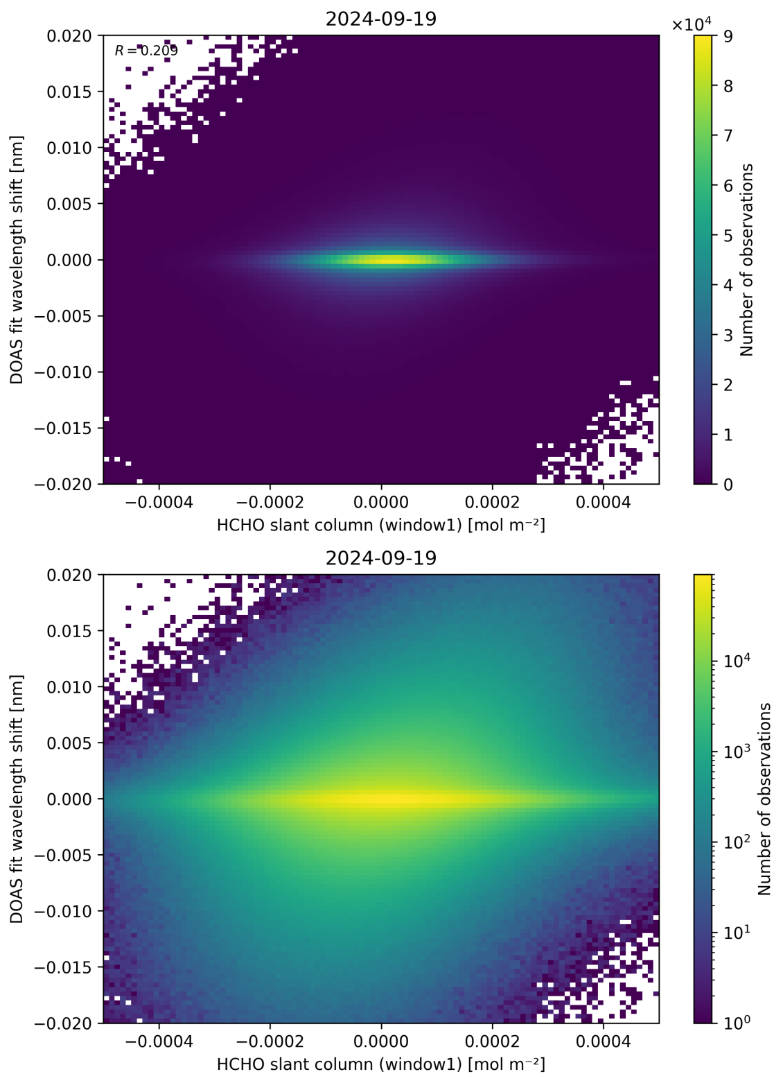
Figure 79: Scatter density plot of “HCHO slant column (window1)” against “DOAS fit wavelength shift” for 2024-09-18 to 2024-09-20.
