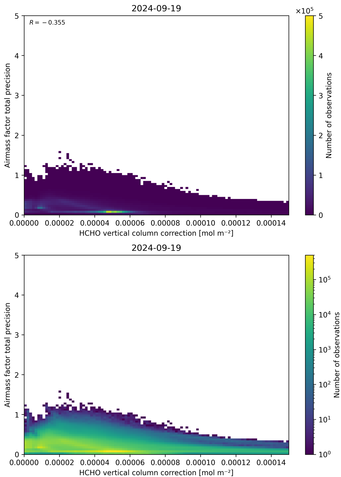
Figure 121: Scatter density plot of “HCHO vertical column correction” against “Airmass factor total precision” for 2024-09-18 to 2024-09-20.
