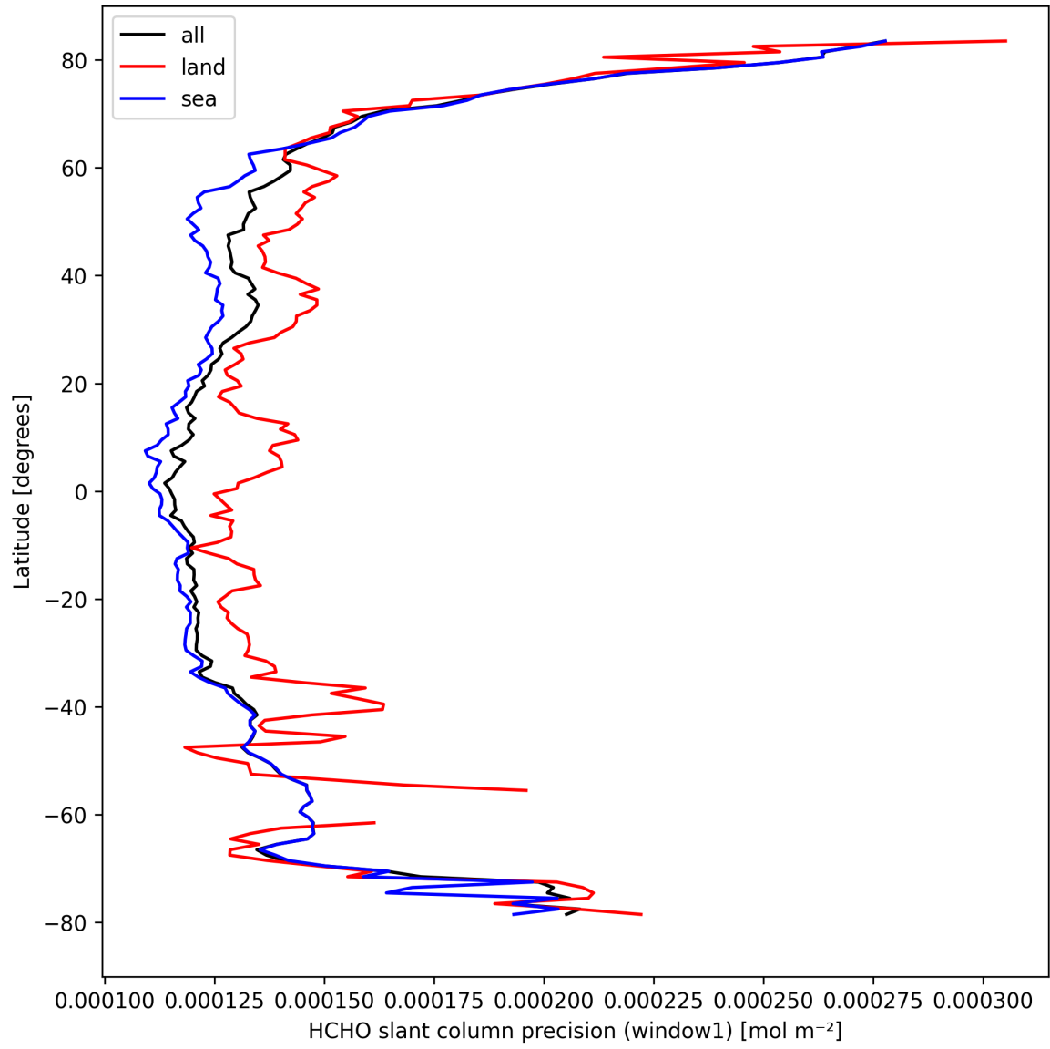
Figure 25: Zonal average of “HCHO slant column precision (window1)” for 2024-09-18 to 2024-09-20.
