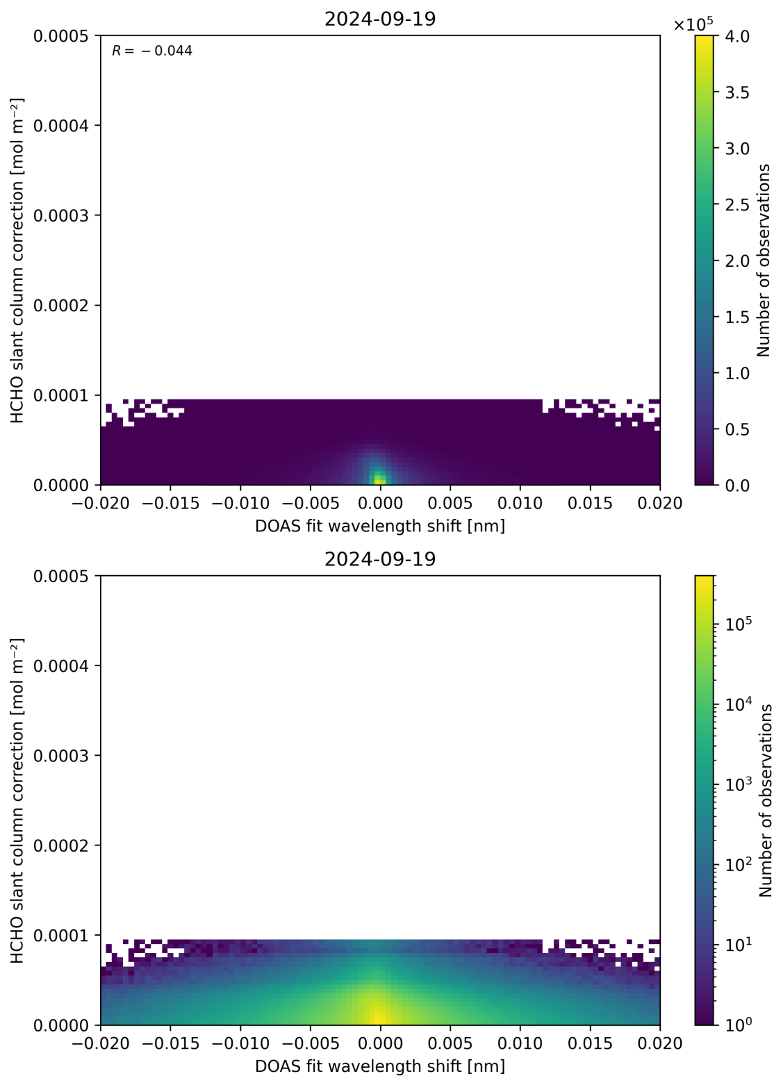
Figure 67: Scatter density plot of “DOAS fit wavelength shift” against “HCHO slant column correction” for 2024-09-18 to 2024-09-20.
