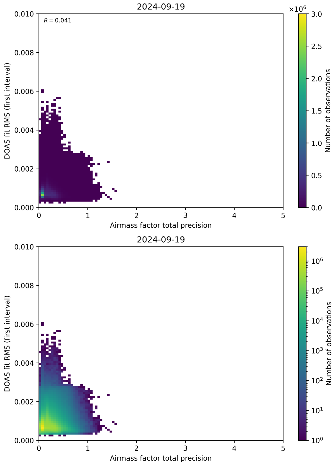
Figure 105: Scatter density plot of “Airmass factor total precision” against “DOAS fit RMS (first interval)” for 2024-09-18 to 2024-09-20.
