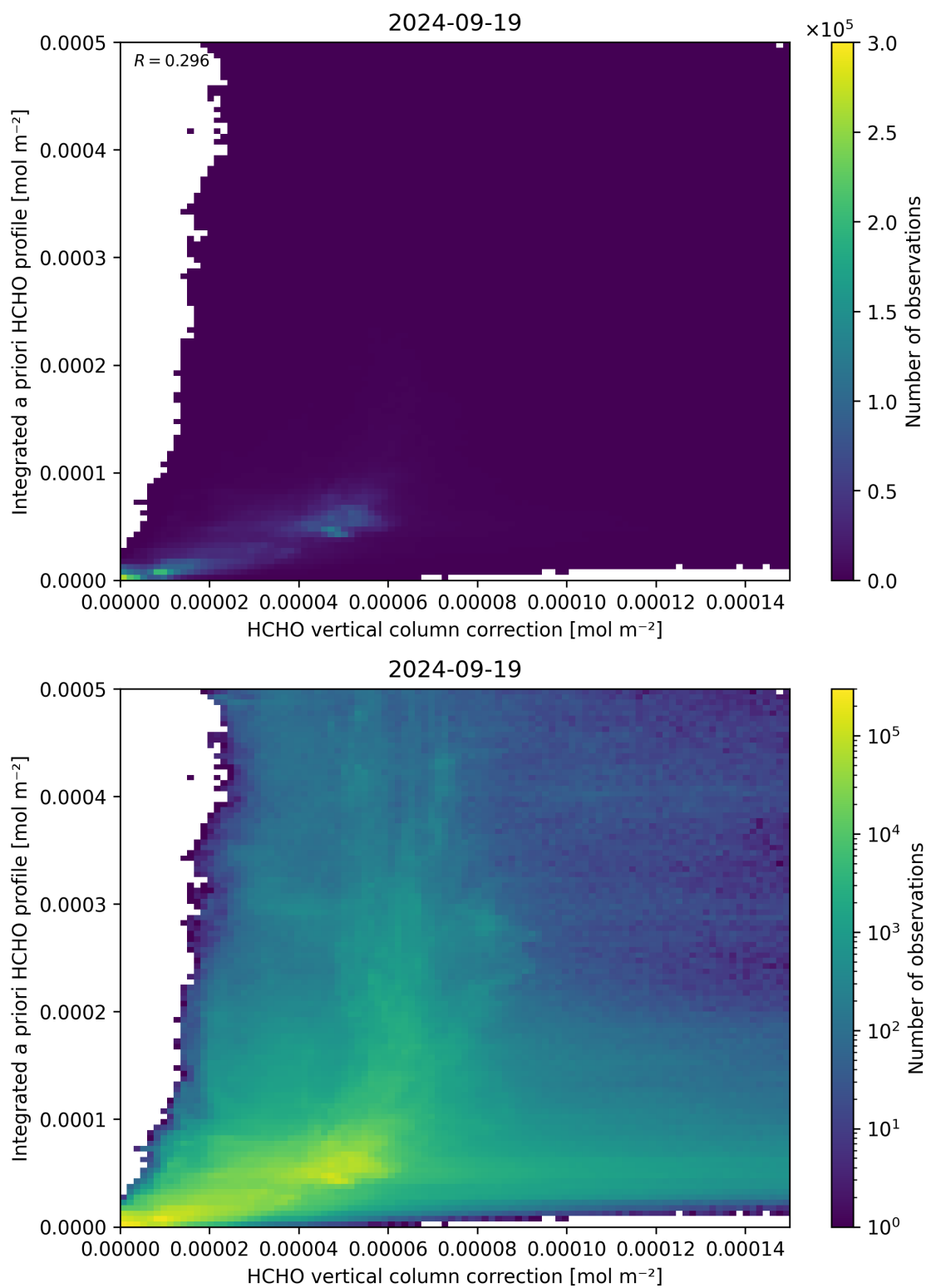
Figure 122: Scatter density plot of “HCHO vertical column correction” against “Integrated a priori HCHO profile” for 2024-09-18 to 2024-09-20.
