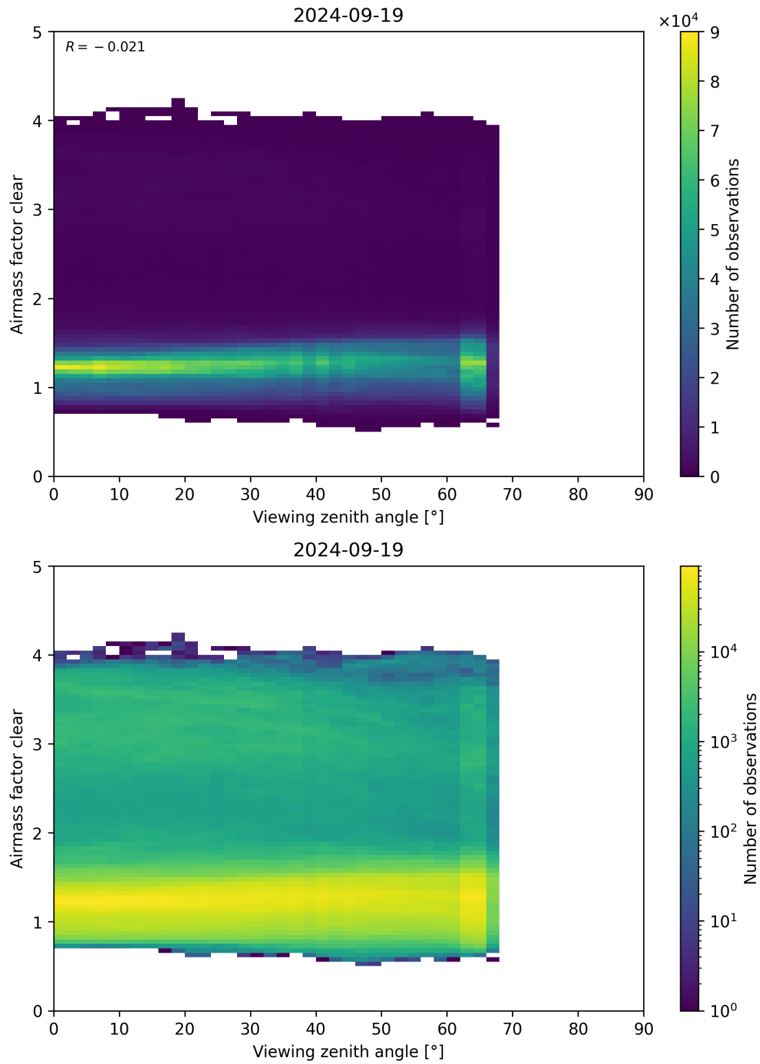
Figure 185: Scatter density plot of “Viewing zenith angle” against “Airmass factor clear” for 2024-09-18 to 2024-09-20.
