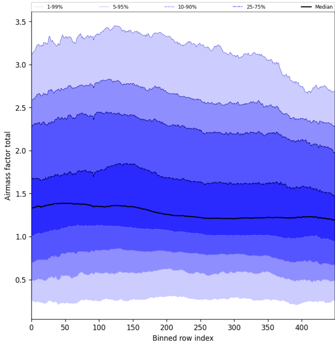
Figure 54: Along track statistics of “Airmass factor total” for 2024-09-18 to 2024-09-20
