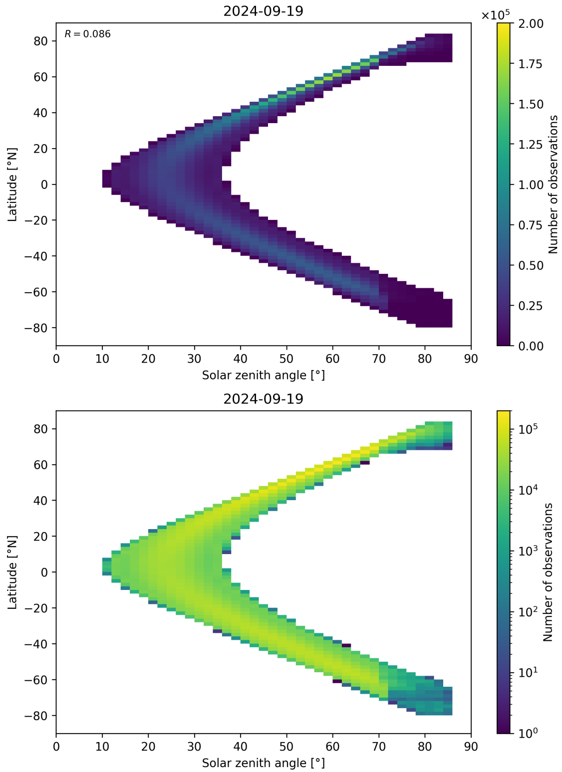
Figure 181: Scatter density plot of “Solar zenith angle” against “Latitude” for 2024-09-18 to 2024-09-20.
