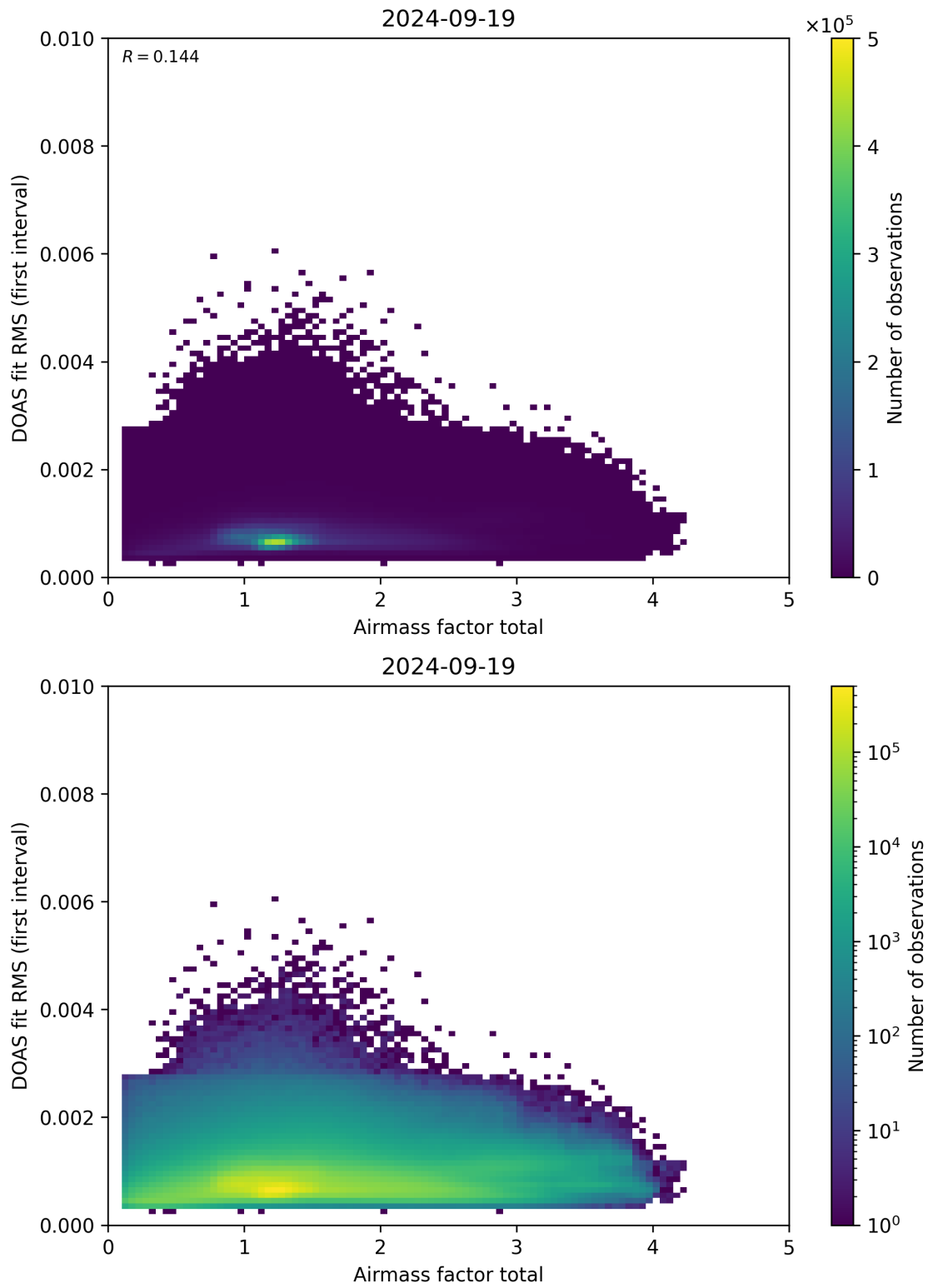
Figure 97: Scatter density plot of “Airmass factor total” against “DOAS fit RMS (first interval)” for 2024-09-18 to 2024-09-20.
