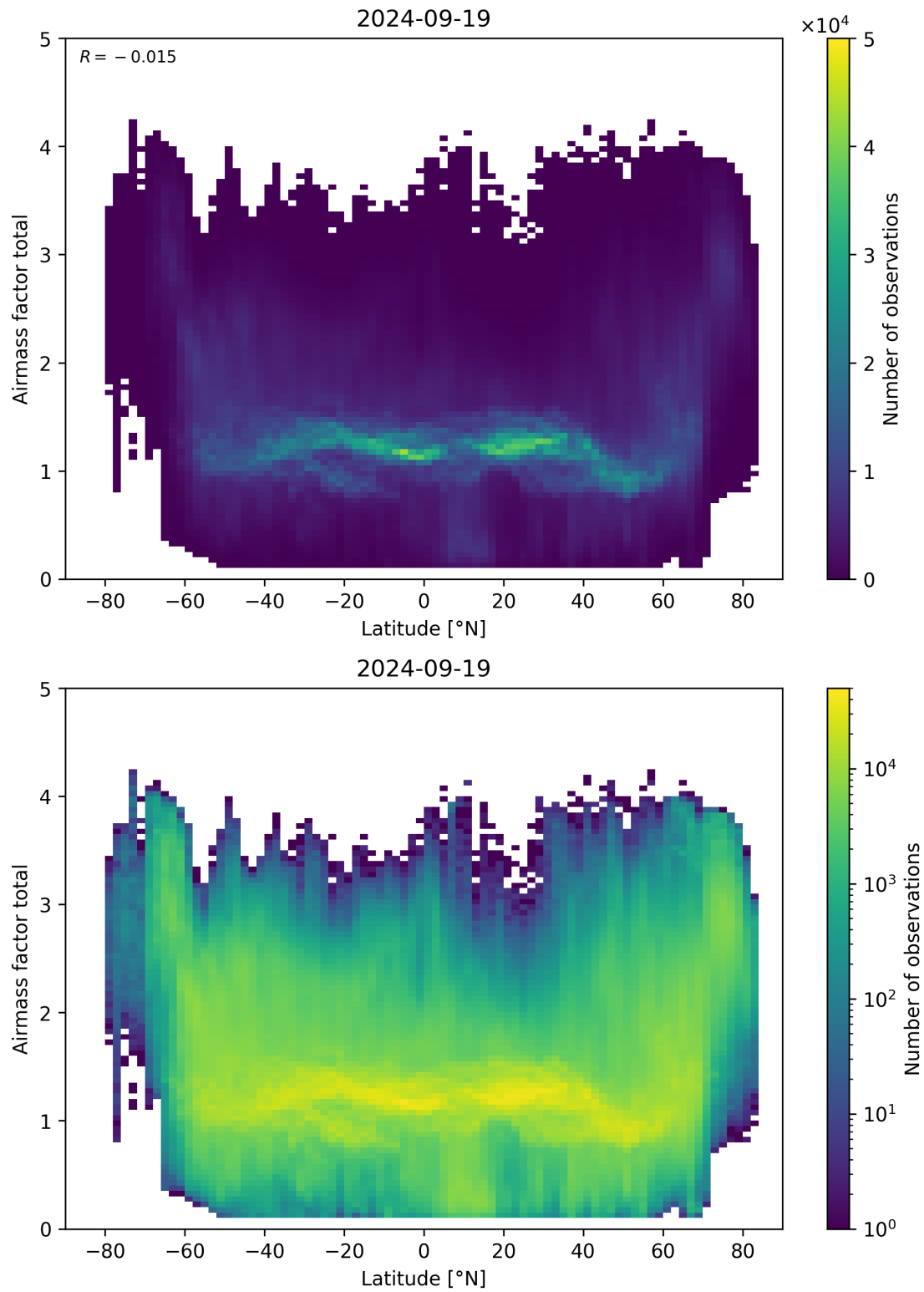
Figure 161: Scatter density plot of “Latitude” against “Airmass factor total” for 2024-09-18 to 2024-09-20.
