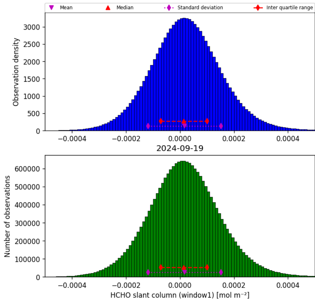
Figure 38: Histogram of “HCHO slant column (window1)” for 2024-09-18 to 2024-09-20
