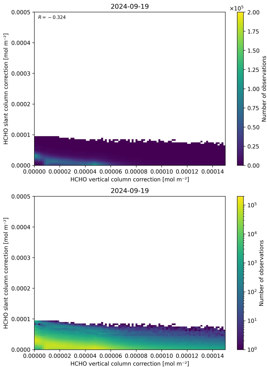
Figure 117: Scatter density plot of “HCHO vertical column correction” against “HCHO slant column correction” for 2024-09-18 to 2024-09-20.
