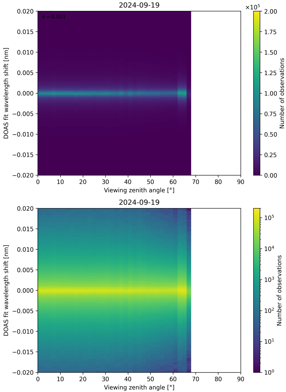
Figure 183: Scatter density plot of “Viewing zenith angle” against “DOAS fit wavelength shift” for 2024-09-18 to 2024-09-20.
