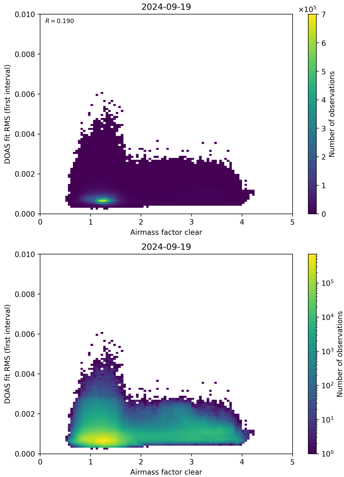
Figure 71: Scatter density plot of “Airmass factor clear” against “DOAS fit RMS (first interval)” for 2024-09-18 to 2024-09-20.
