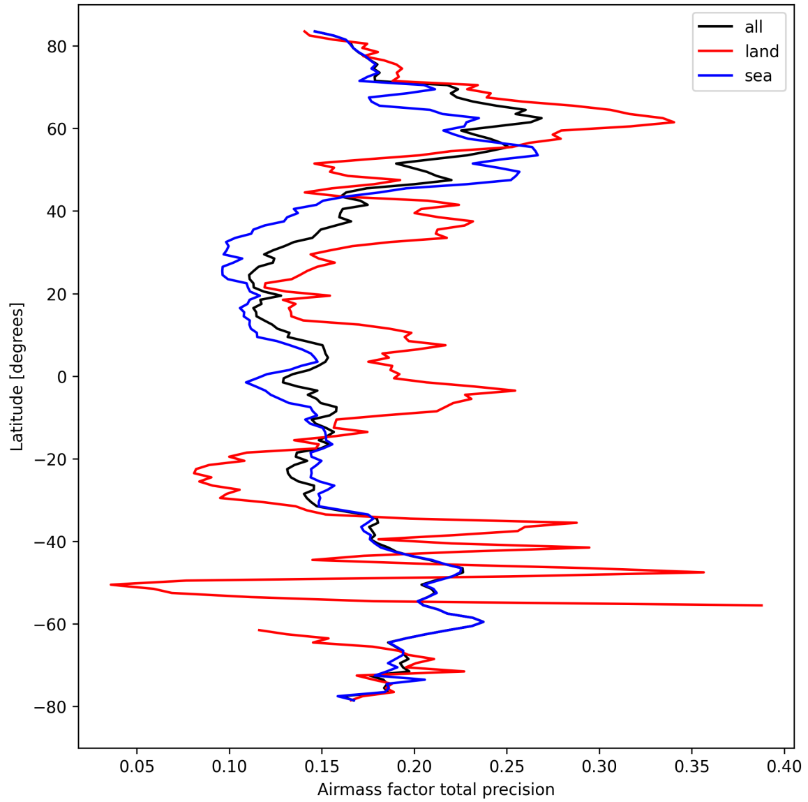
Figure 27: Zonal average of “Airmass factor total precision” for 2024-09-18 to 2024-09-20.
