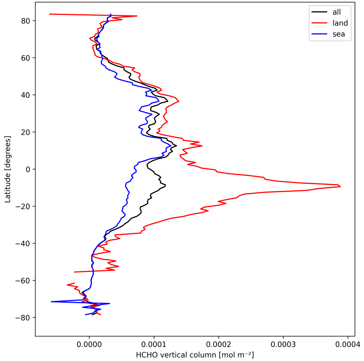
Figure 21: Zonal average of “HCHO vertical column” for 2024-09-18 to 2024-09-20.
