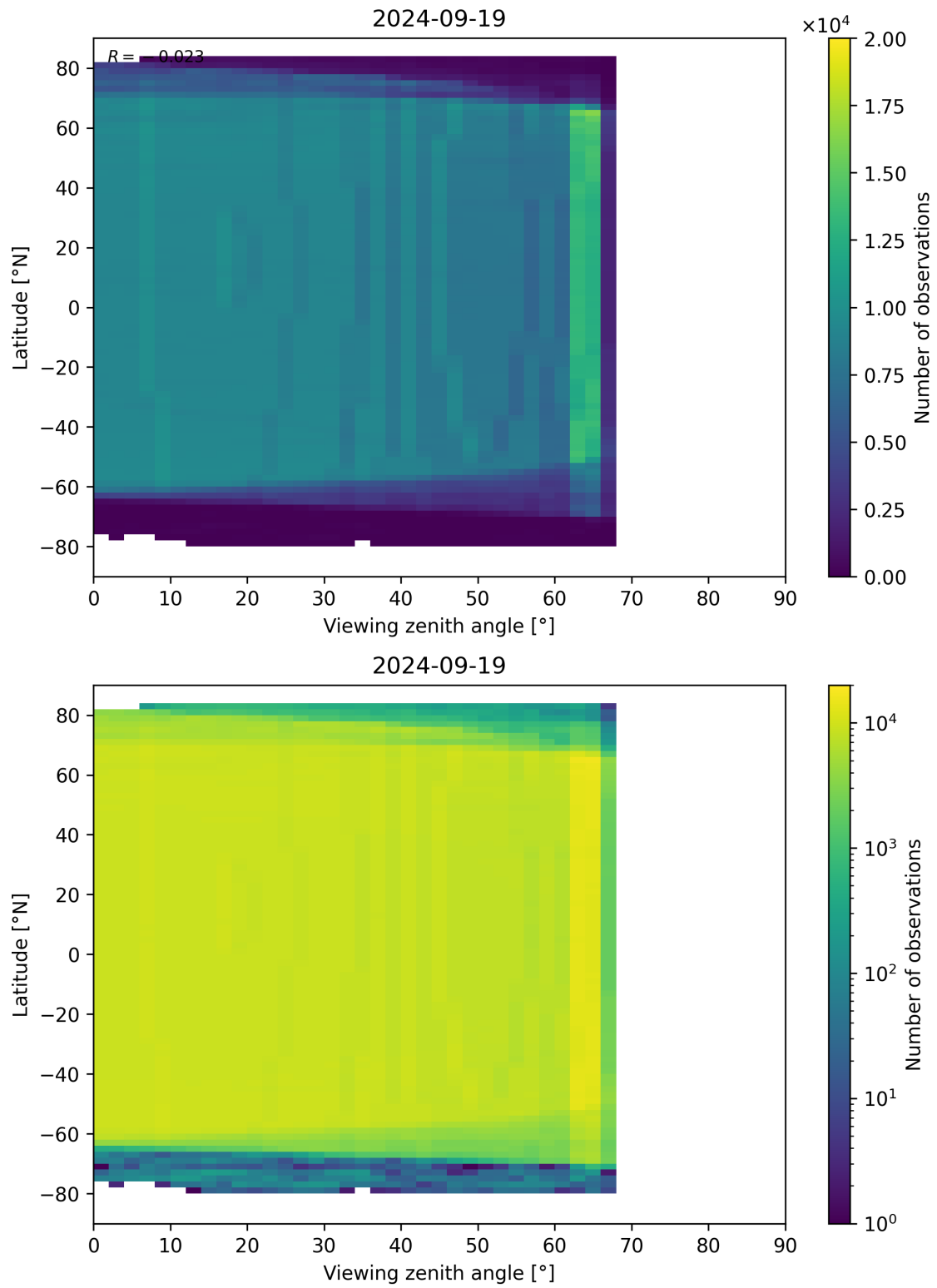
Figure 196: Scatter density plot of “Viewing zenith angle” against “Latitude” for 2024-09-18 to 2024-09-20.
