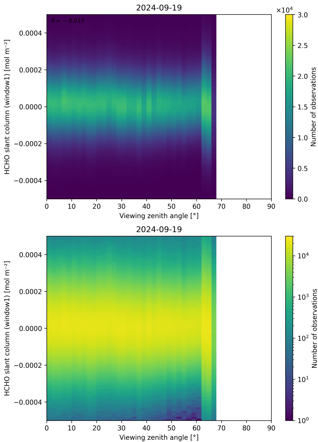
Figure 188: Scatter density plot of “Viewing zenith angle” against “HCHO slant column (window1)” for 2024-09-18 to 2024-09-20.
