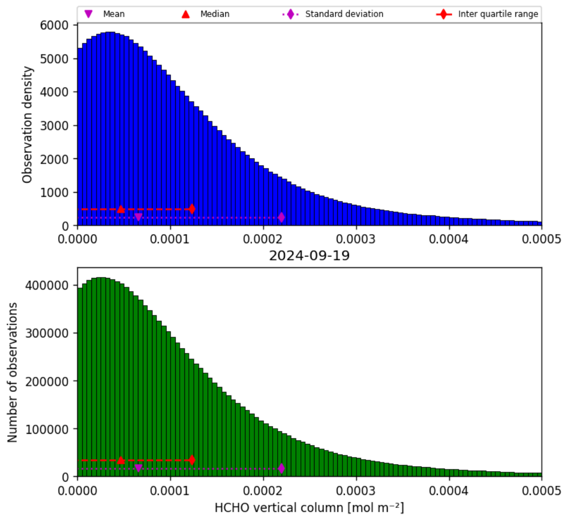
Figure 35: Histogram of “HCHO vertical column” for 2024-09-18 to 2024-09-20
