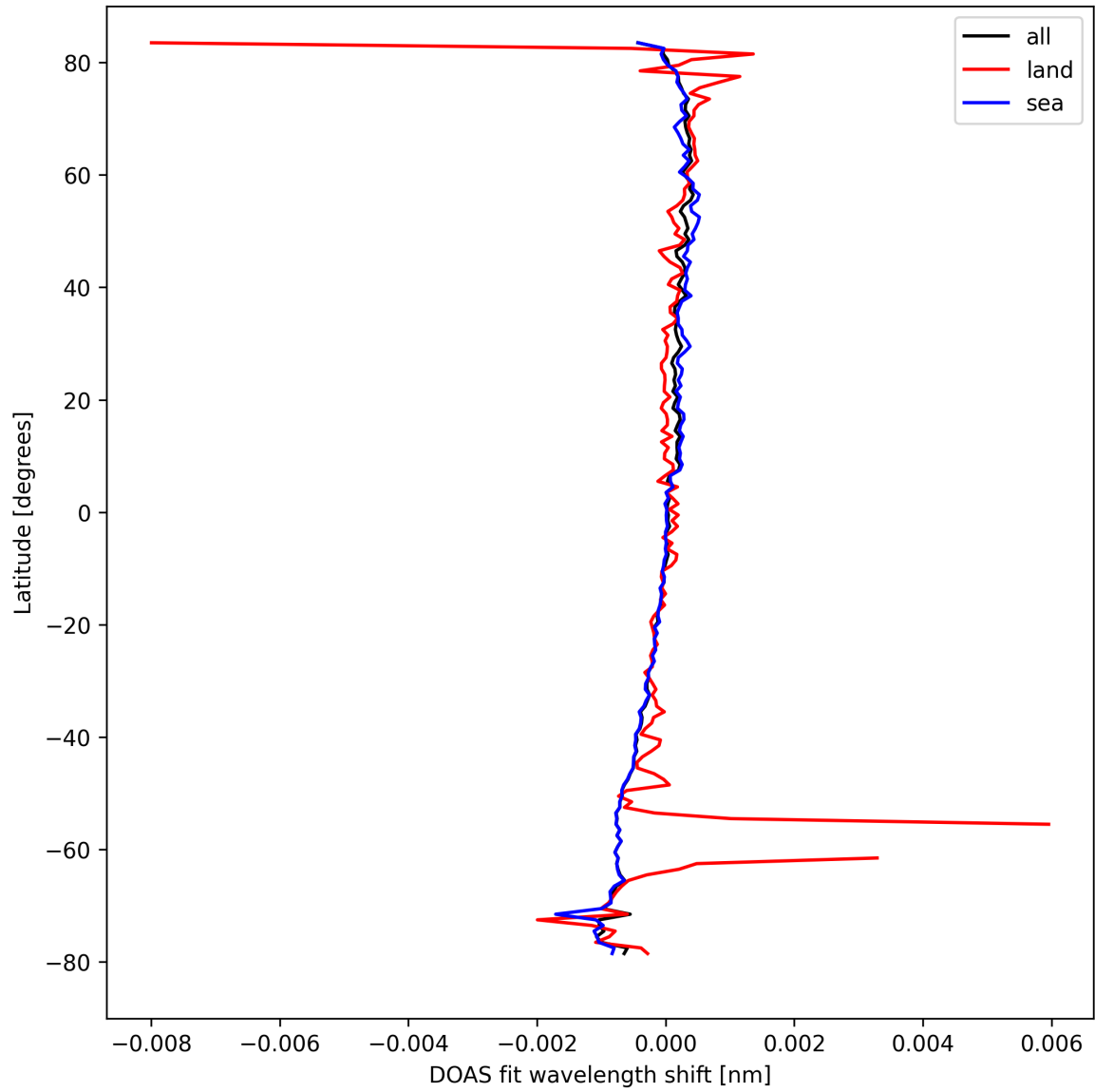
Figure 30: Zonal average of “DOAS fit wavelength shift” for 2024-09-18 to 2024-09-20.
