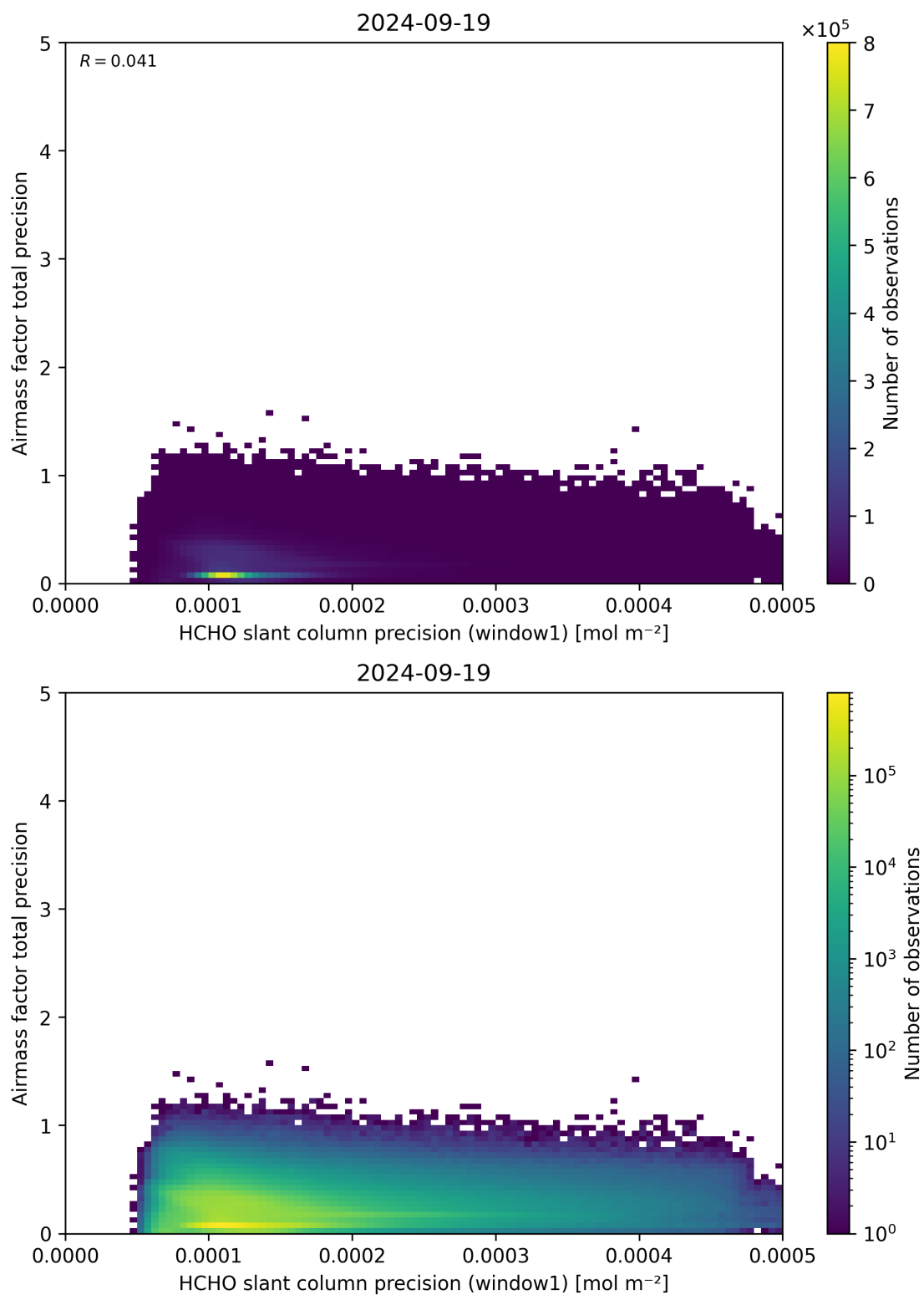
Figure 95: Scatter density plot of “HCHO slant column precision (window1)” against “Airmass factor total precision” for 2024-09-18 to 2024-09-20.
