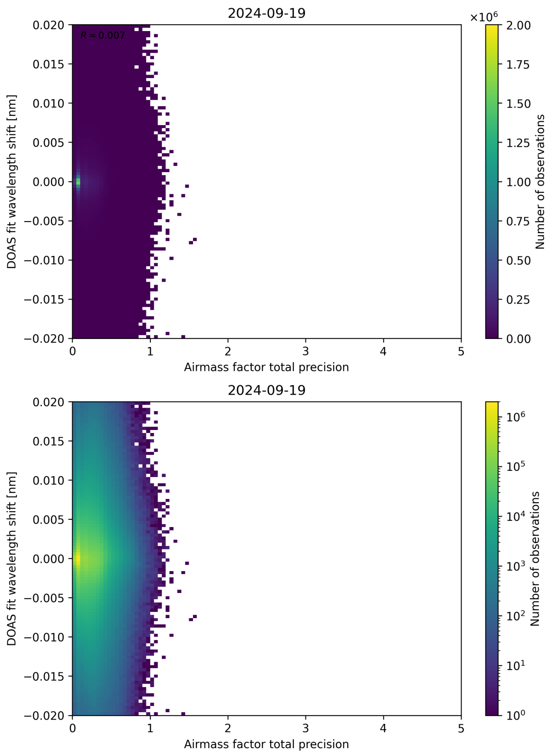
Figure 106: Scatter density plot of “Airmass factor total precision” against “DOAS fit wavelength shift” for 2024-09-18 to 2024-09-20.
