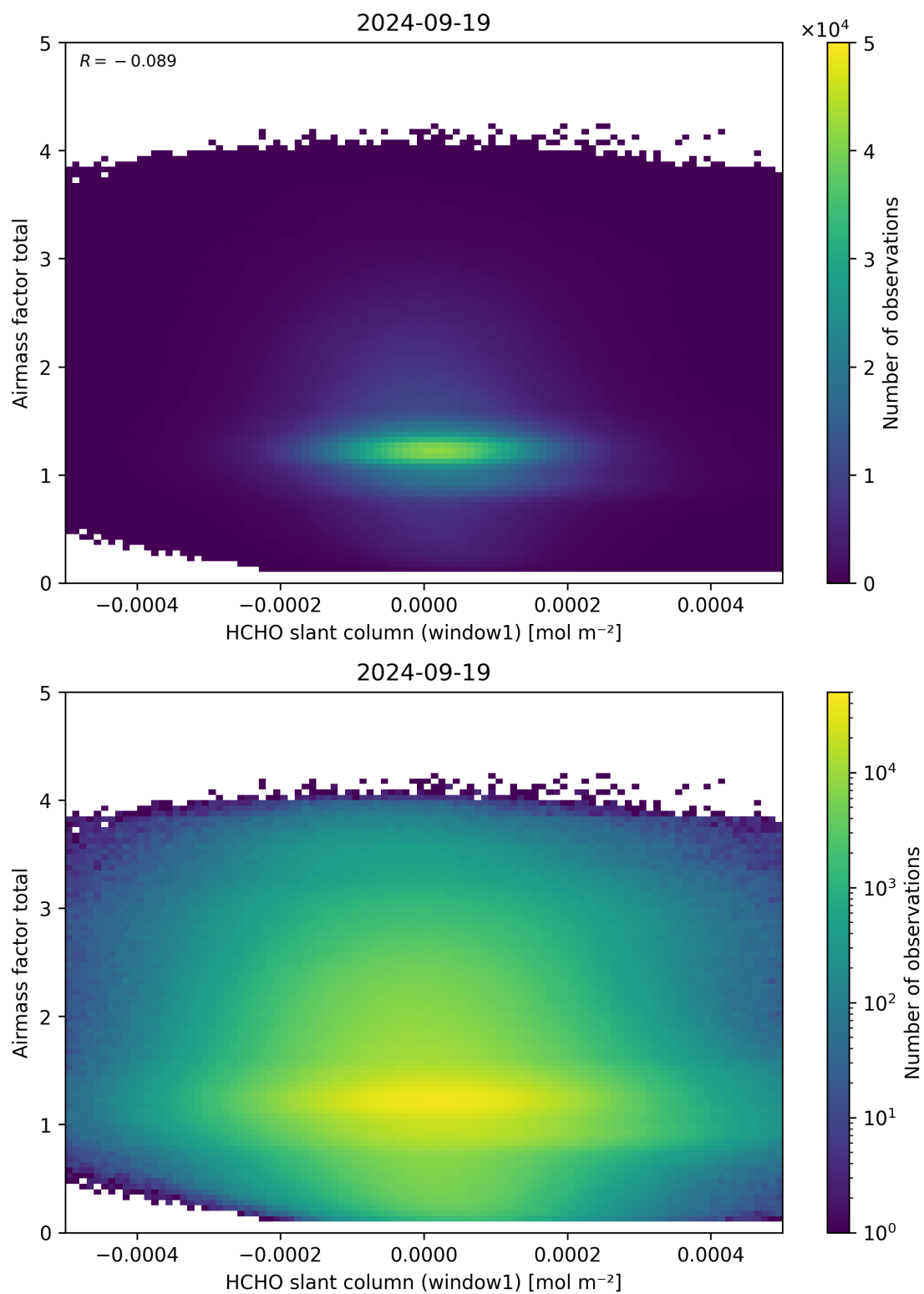
Figure 85: Scatter density plot of “HCHO slant column (window1)” against “Airmass factor total” for 2024-09-18 to 2024-09-20.
