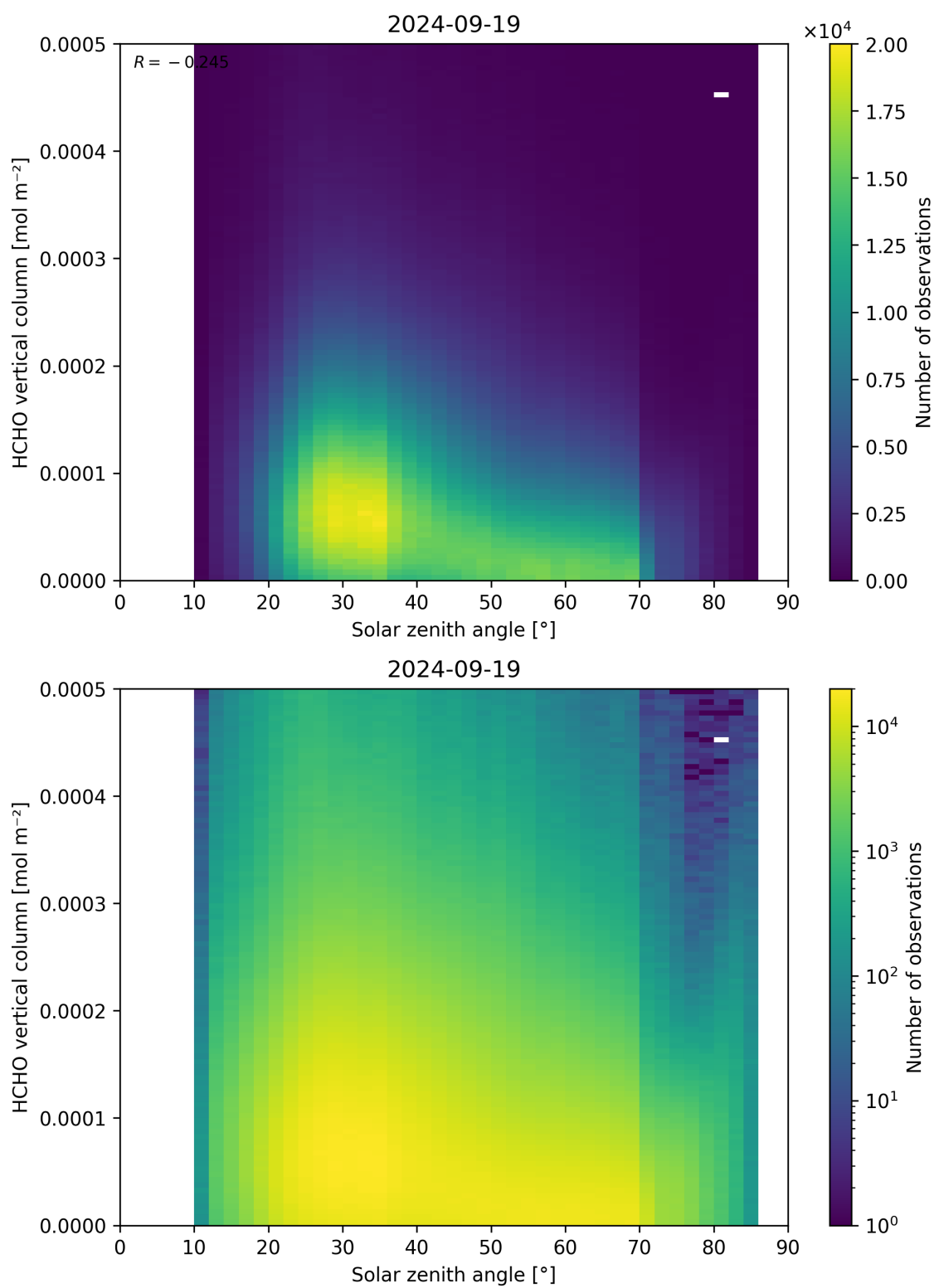
Figure 177: Scatter density plot of “Solar zenith angle” against “HCHO vertical column” for 2024-09-18 to 2024-09-20.
