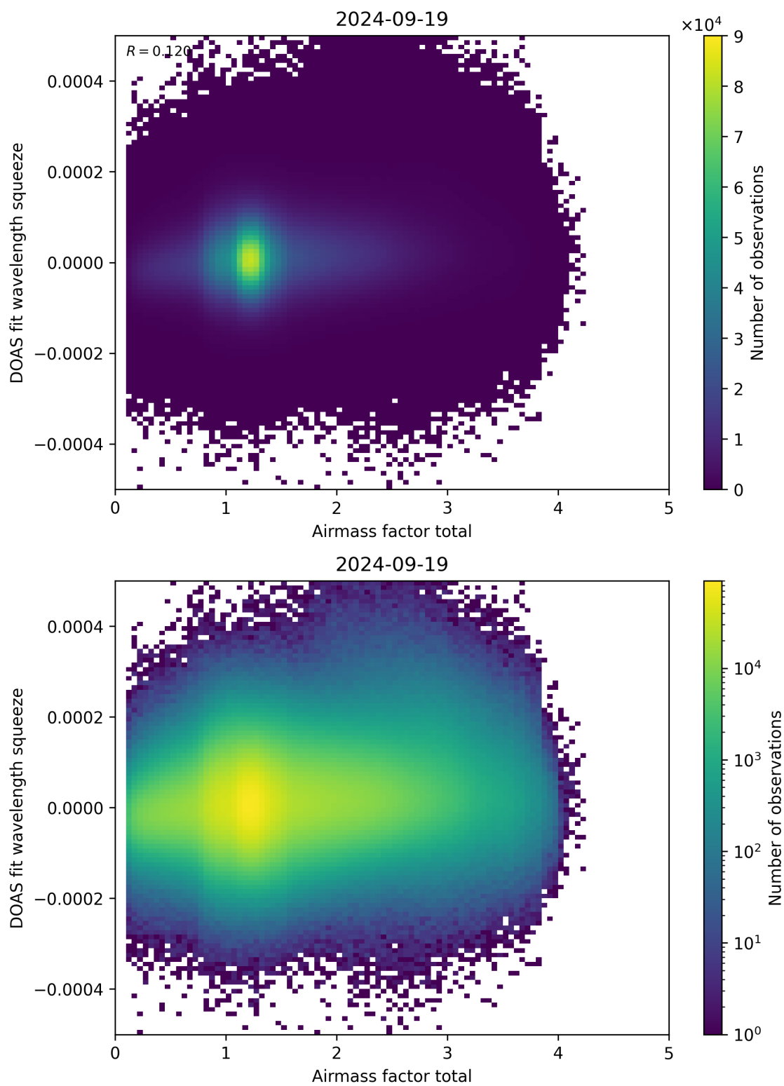
Figure 99: Scatter density plot of “Airmass factor total” against “DOAS fit wavelength squeeze” for 2024-09-18 to 2024-09-20.
