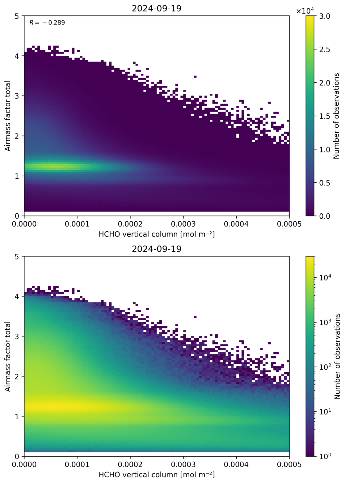
Figure 131: Scatter density plot of “HCHO vertical column” against “Airmass factor total” for 2024-09-18 to 2024-09-20.
