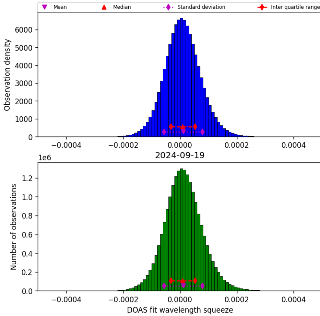
Figure 45: Histogram of “DOAS fit wavelength squeeze” for 2024-09-18 to 2024-09-20
