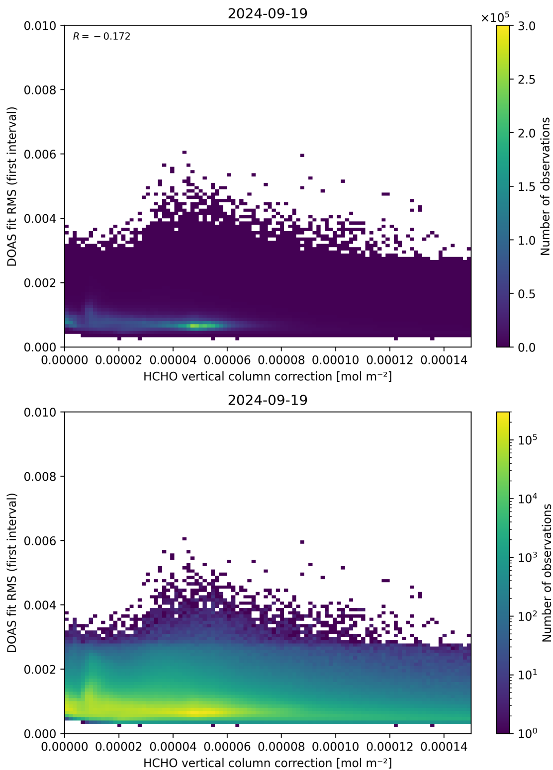
Figure 112: Scatter density plot of “HCHO vertical column correction” against “DOAS fit RMS (first interval)” for 2024-09-18 to 2024-09-20.
