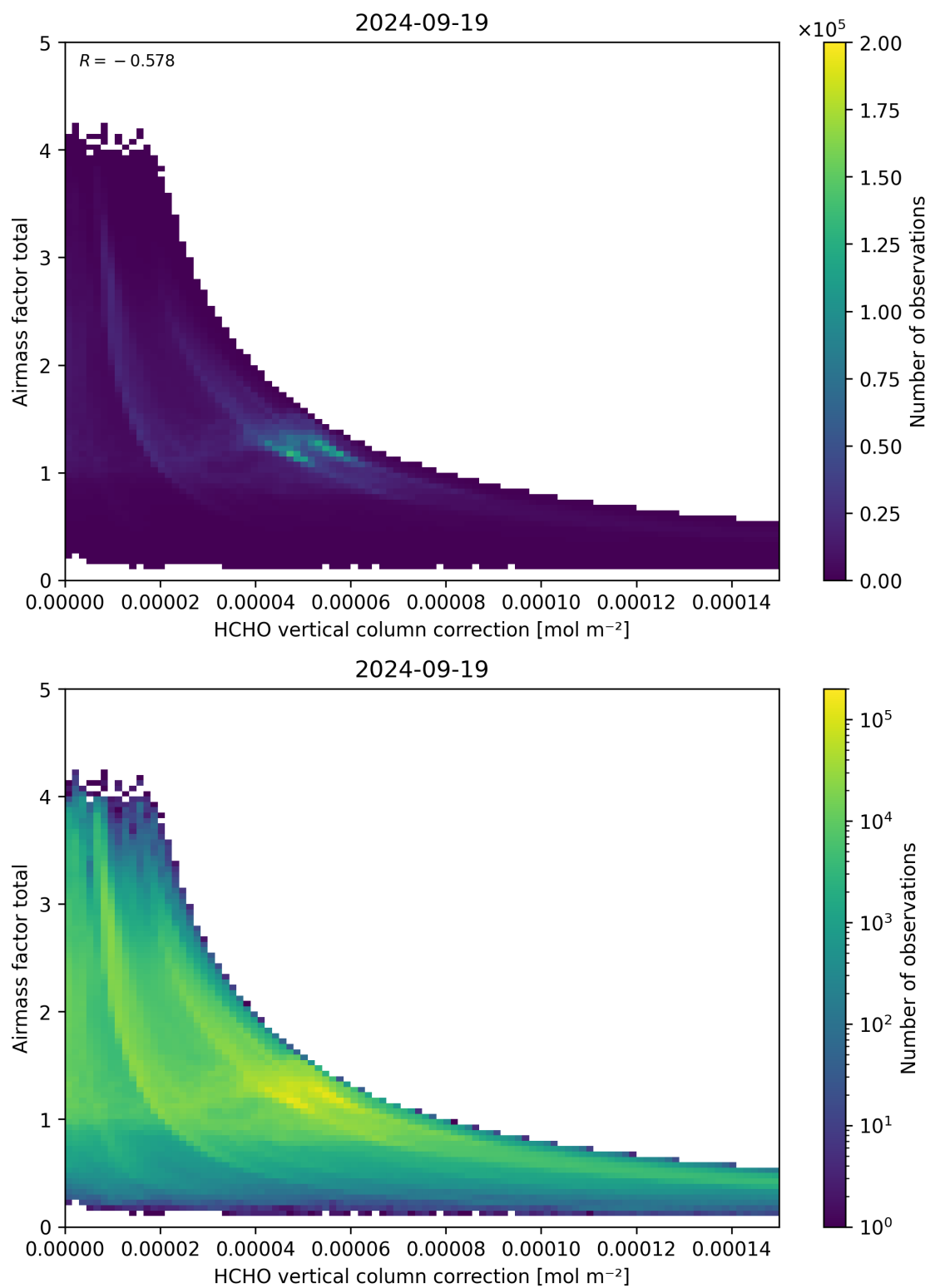
Figure 120: Scatter density plot of “HCHO vertical column correction” against “Airmass factor total” for 2024-09-18 to 2024-09-20.
