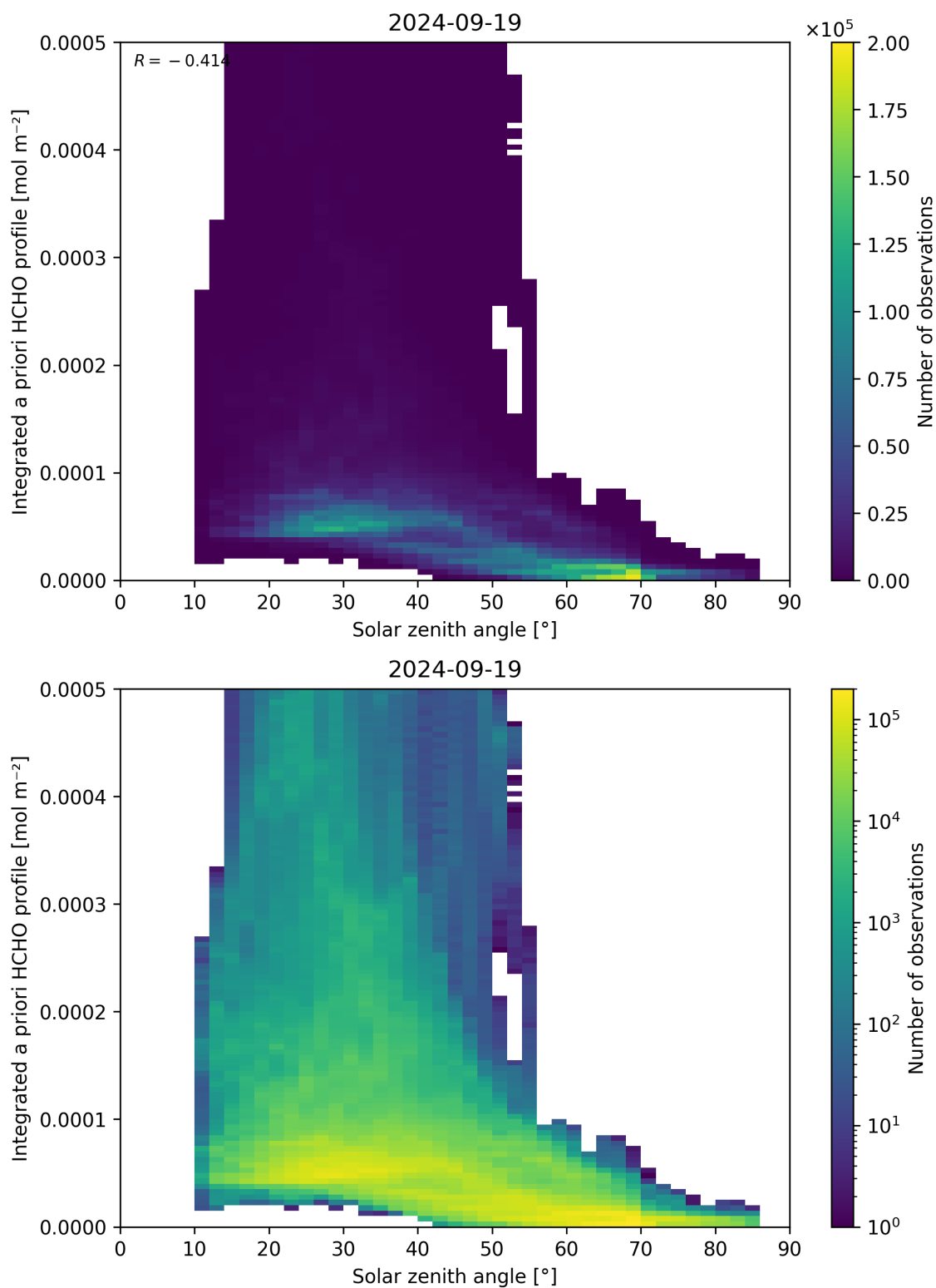
Figure 180: Scatter density plot of “Solar zenith angle” against “Integrated a priori HCHO profile” for 2024-09-18 to 2024-09-20.
