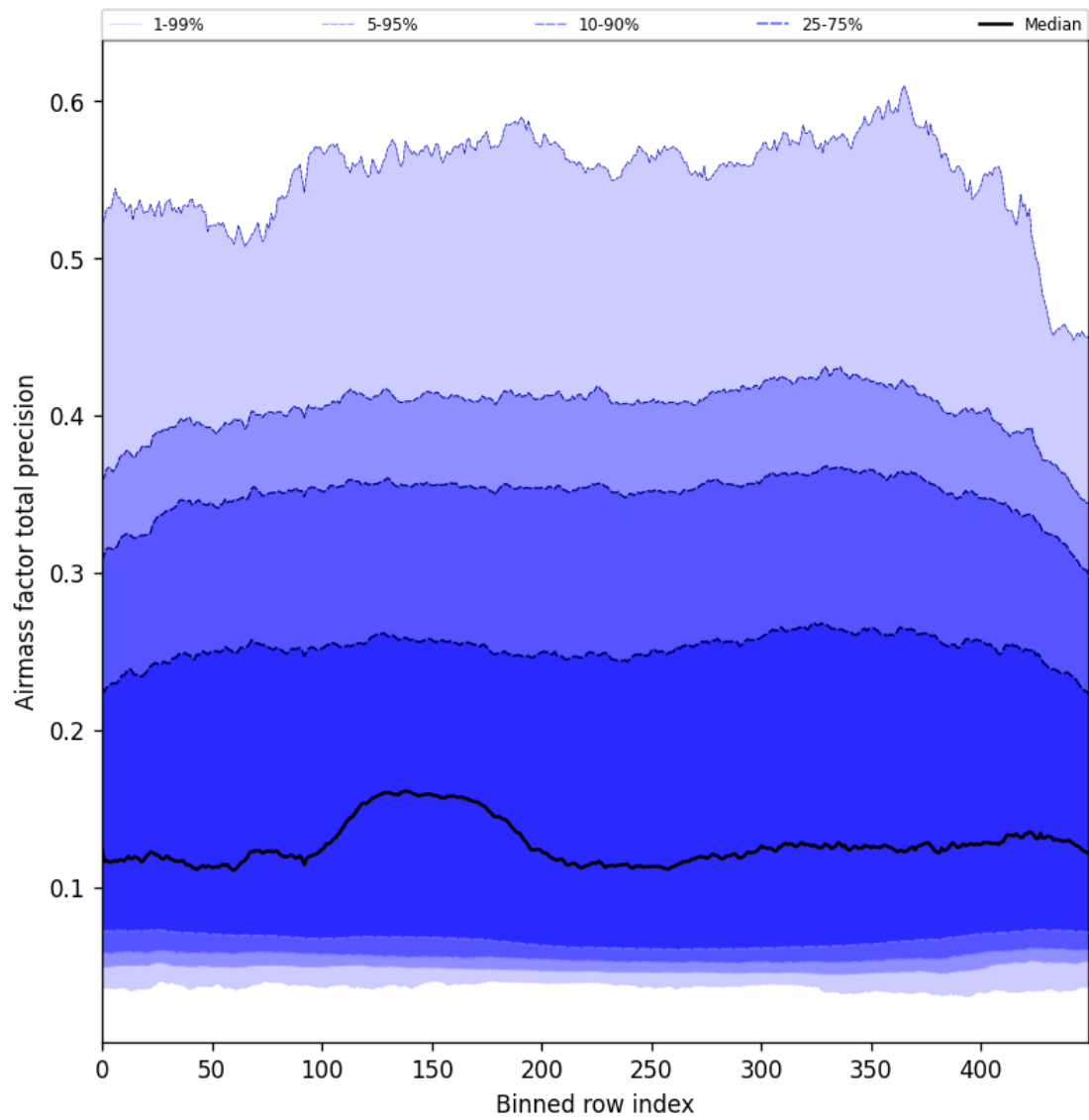
Figure 55: Along track statistics of “Airmass factor total precision” for 2024-09-18 to 2024-09-20
