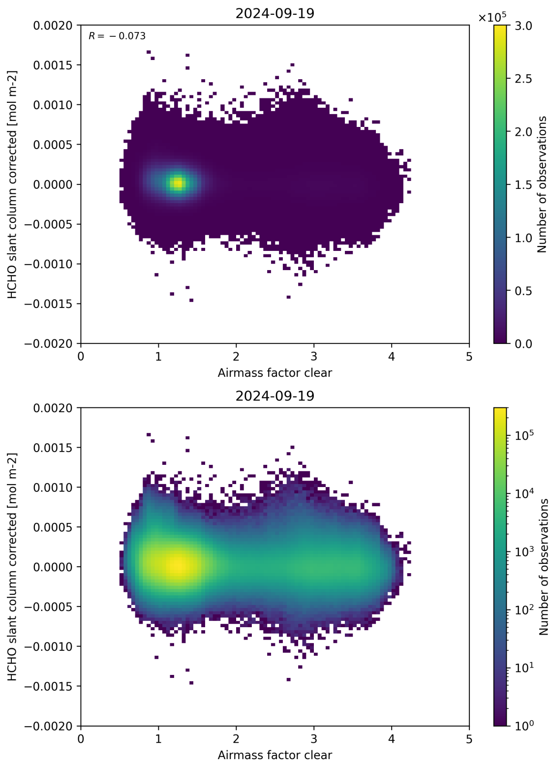
Figure 74: Scatter density plot of “Airmass factor clear” against “HCHO slant column corrected” for 2024-09-18 to 2024-09-20.
