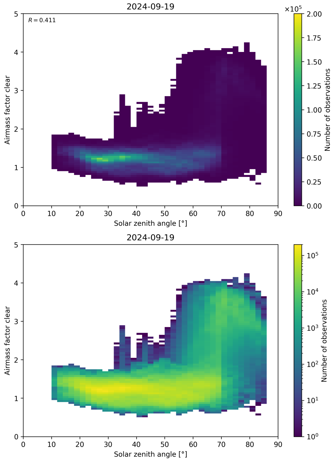
Figure 170: Scatter density plot of “Solar zenith angle” against “Airmass factor clear” for 2024-09-18 to 2024-09-20.
