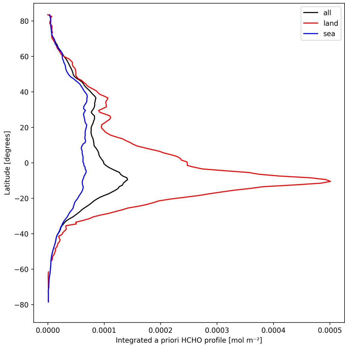
Figure 29: Zonal average of “Integrated a priori HCHO profile” for 2024-09-18 to 2024-09-20.
