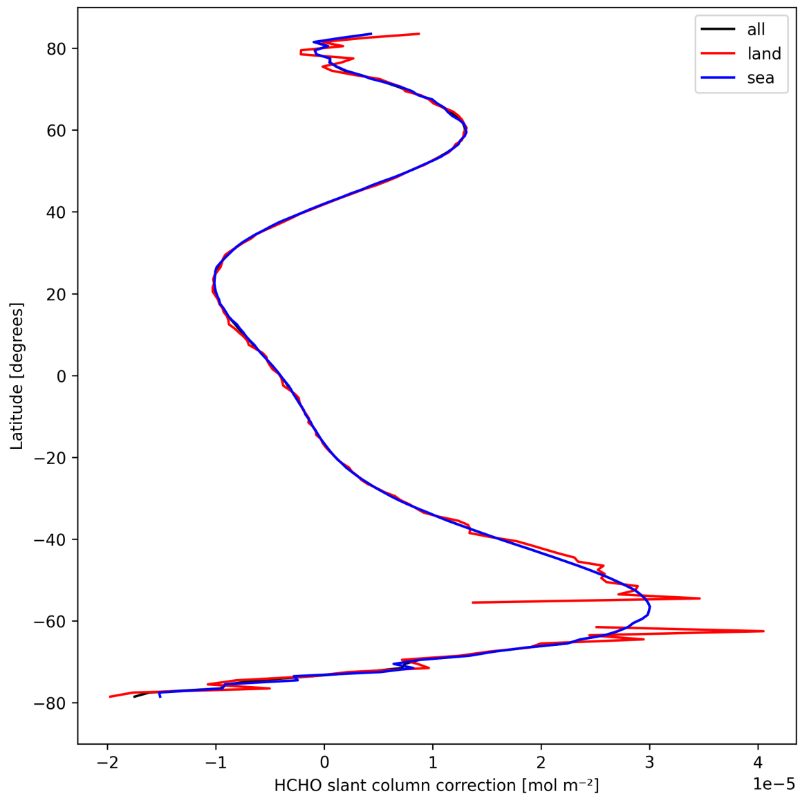
Figure 33: Zonal average of “HCHO slant column correction” for 2024-09-18 to 2024-09-20.
