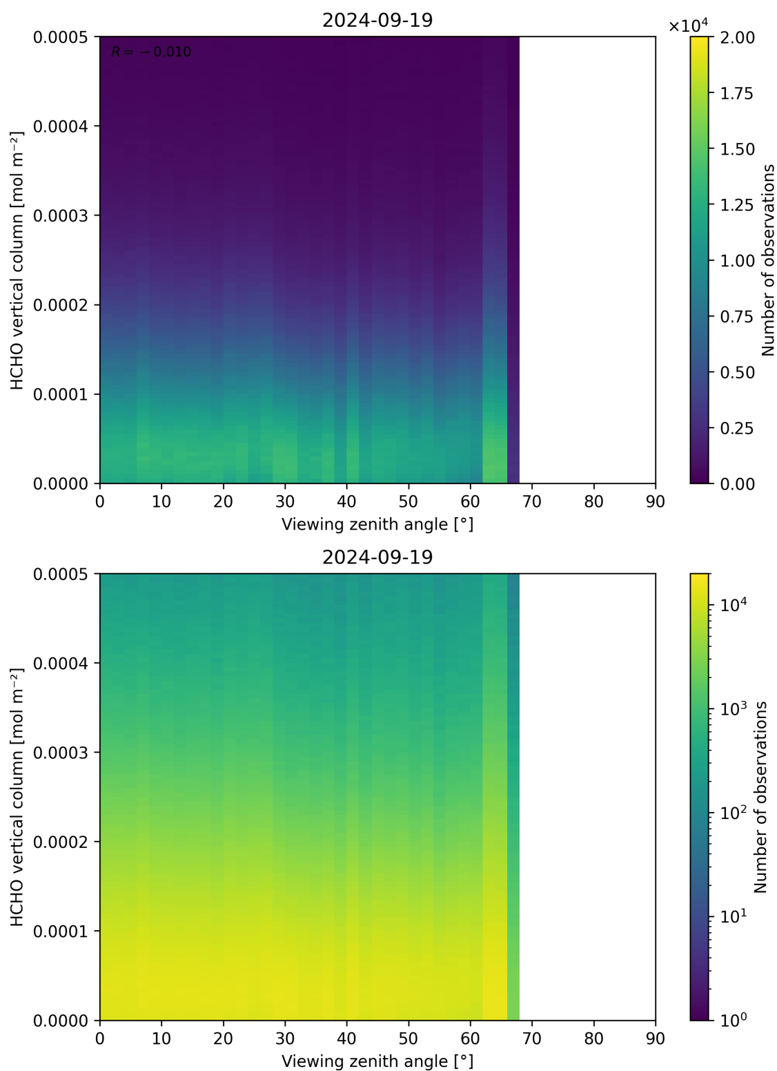
Figure 192: Scatter density plot of “Viewing zenith angle” against “HCHO vertical column” for 2024-09-18 to 2024-09-20.
