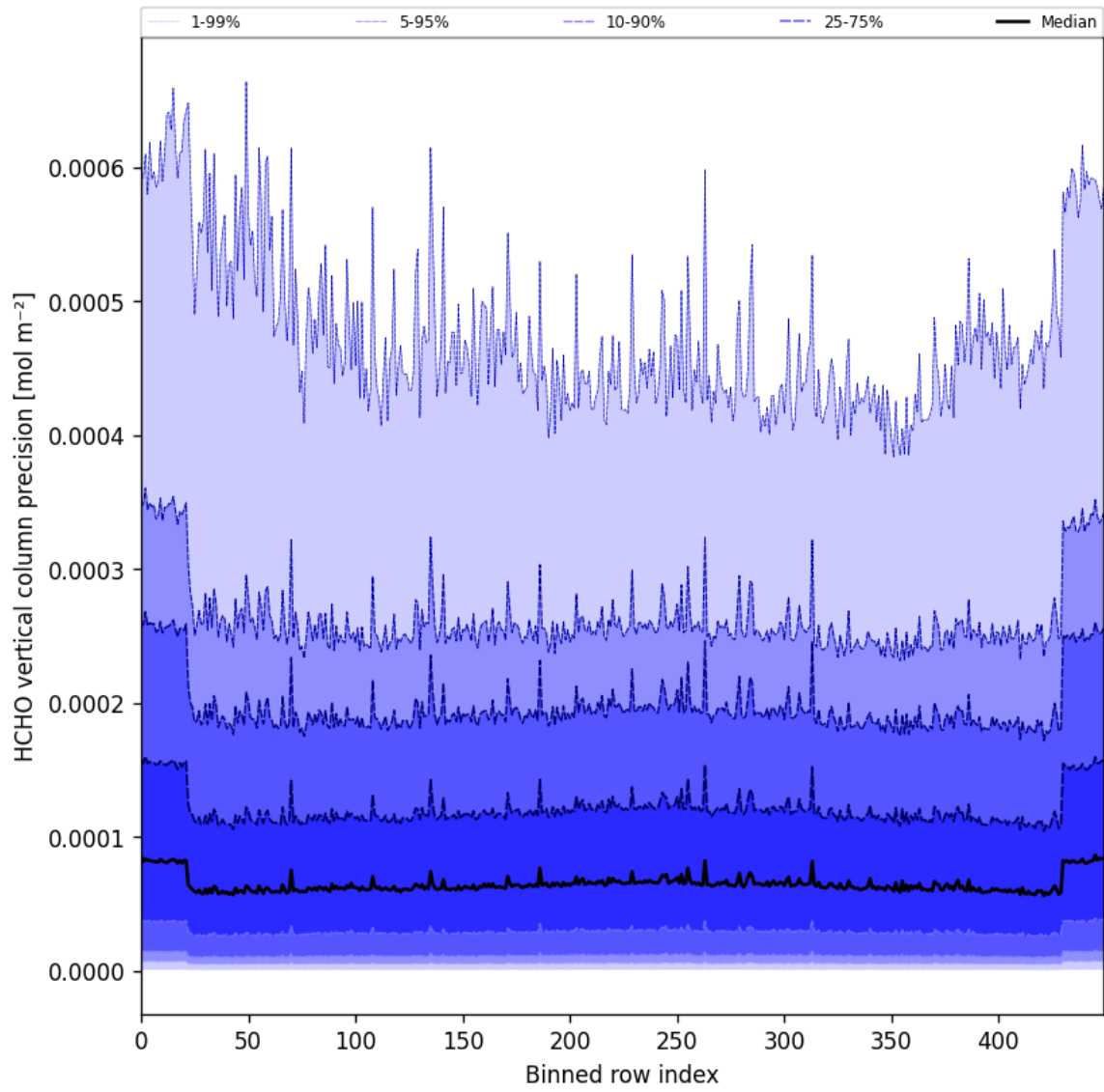
Figure 50: Along track statistics of “HCHO vertical column precision” for 2024-09-18 to 2024-09-20
