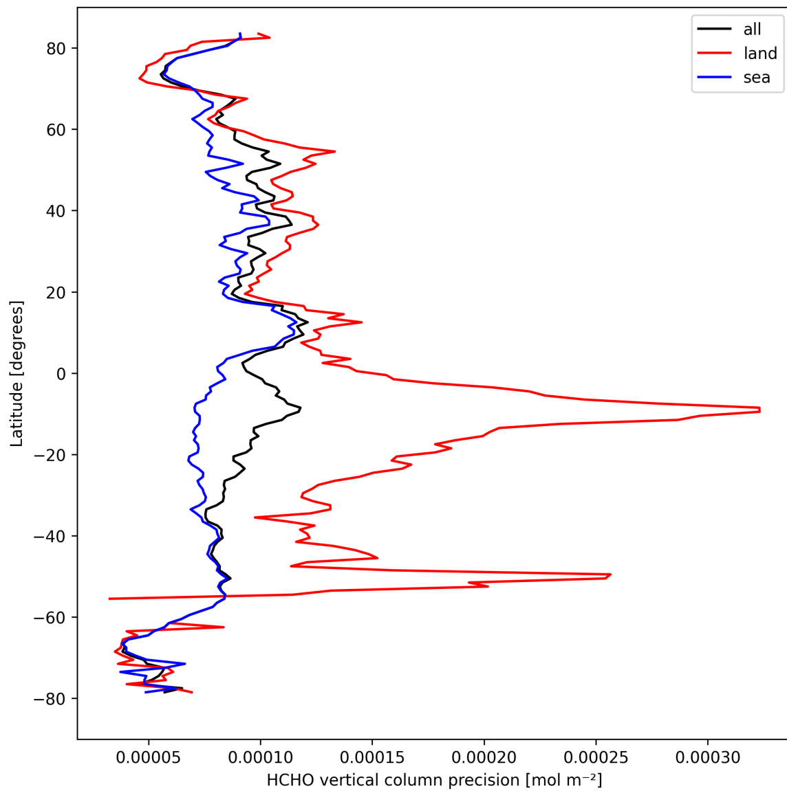
Figure 22: Zonal average of “HCHO vertical column precision” for 2024-09-18 to 2024-09-20.
