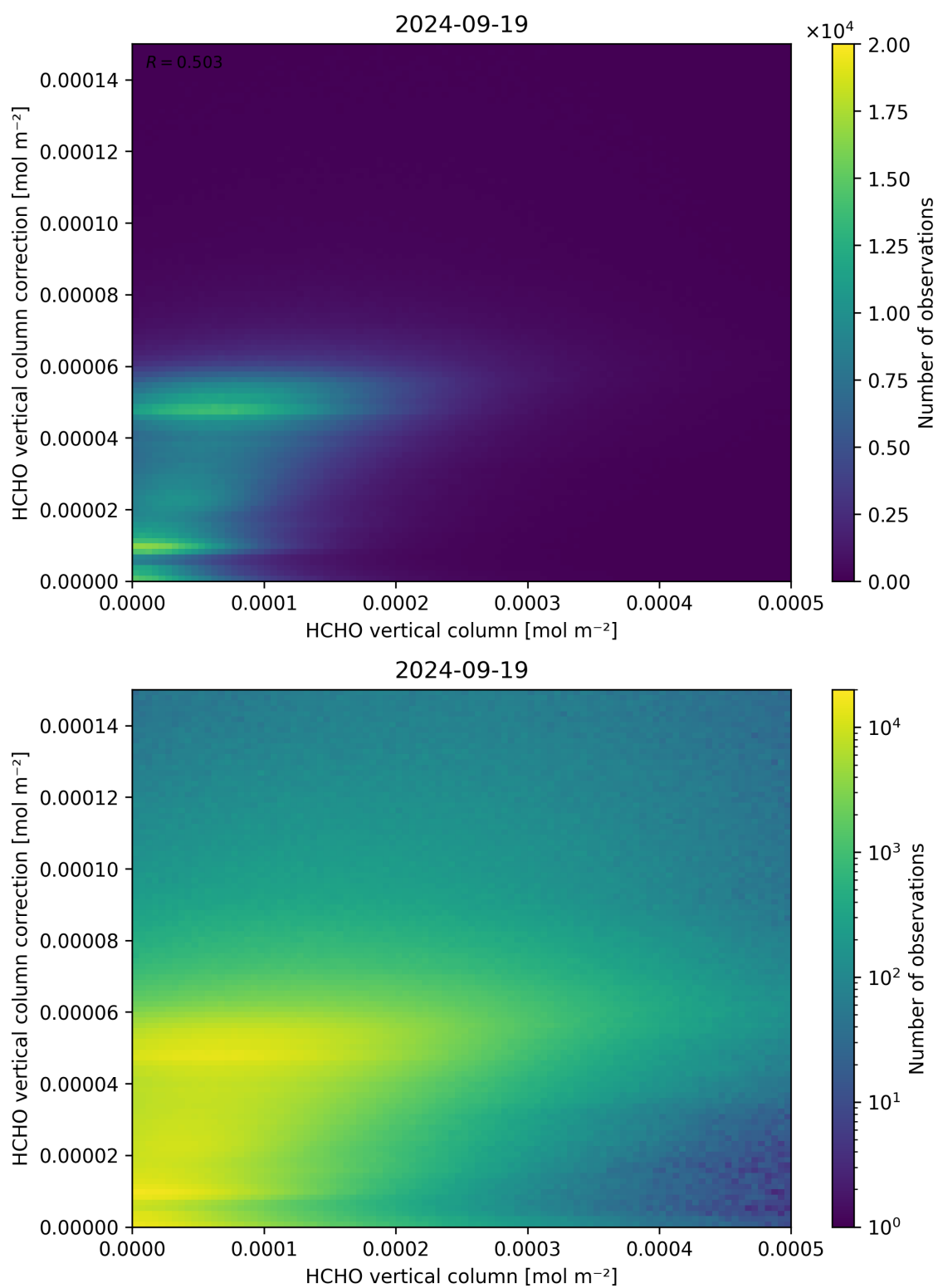
Figure 133: Scatter density plot of “HCHO vertical column” against “HCHO vertical column correction” for 2024-09-18 to 2024-09-20.
