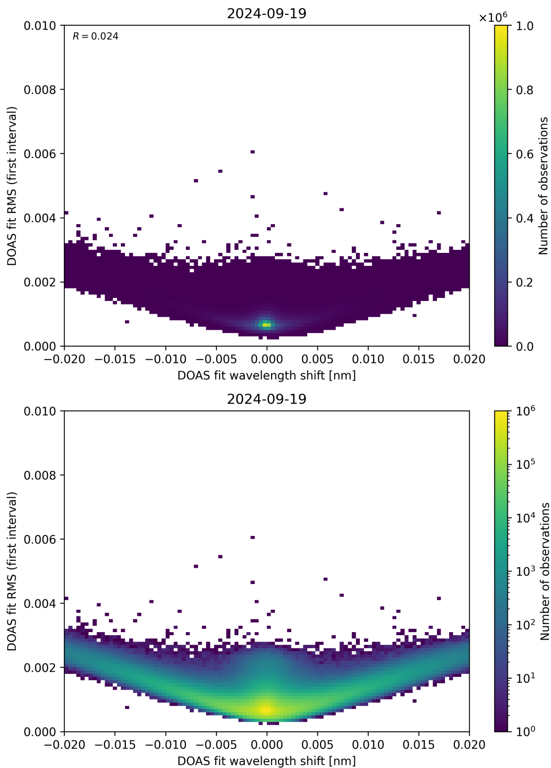
Figure 64: Scatter density plot of “DOAS fit wavelength shift” against “DOAS fit RMS (first interval)” for 2024-09-18 to 2024-09-20.
