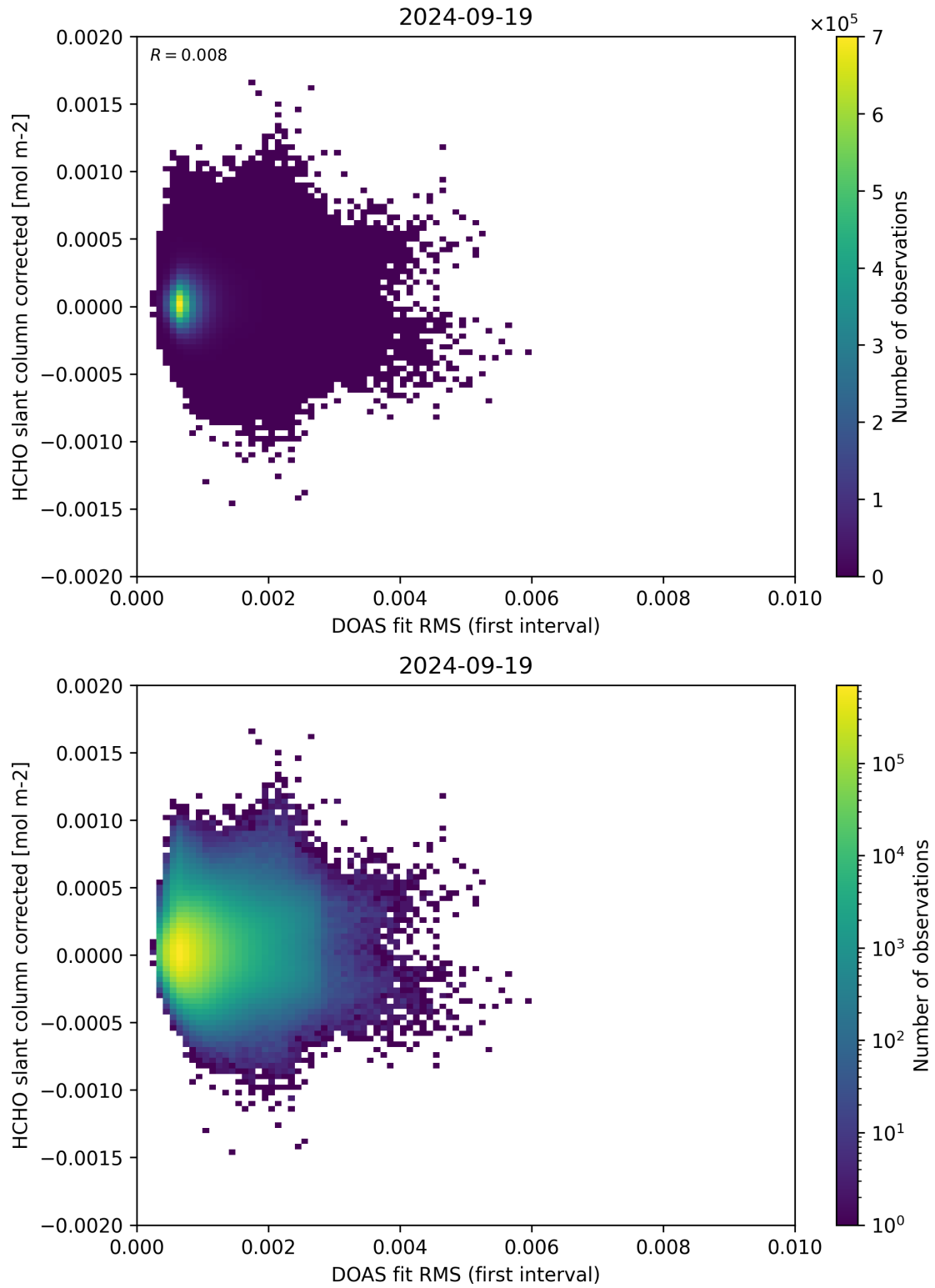
Figure 62: Scatter density plot of “DOAS fit RMS (first interval)” against “HCHO slant column corrected” for 2024-09-18 to 2024-09-20.
