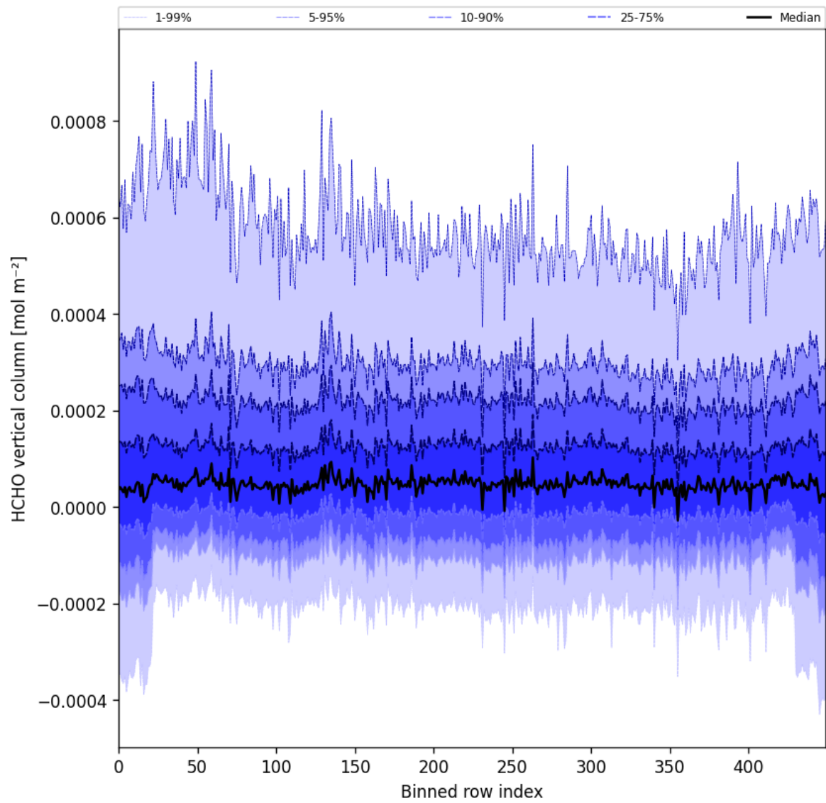
Figure 49: Along track statistics of “HCHO vertical column” for 2024-09-18 to 2024-09-20
