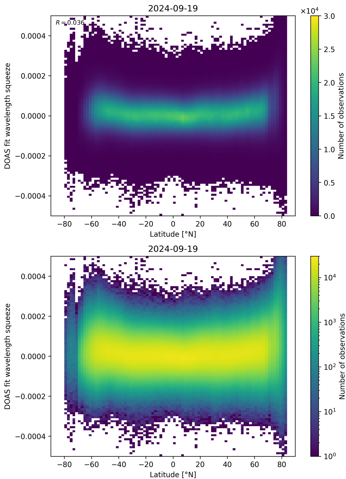
Figure 155: Scatter density plot of “Latitude” against “DOAS fit wavelength squeeze” for 2024-09-18 to 2024-09-20.
