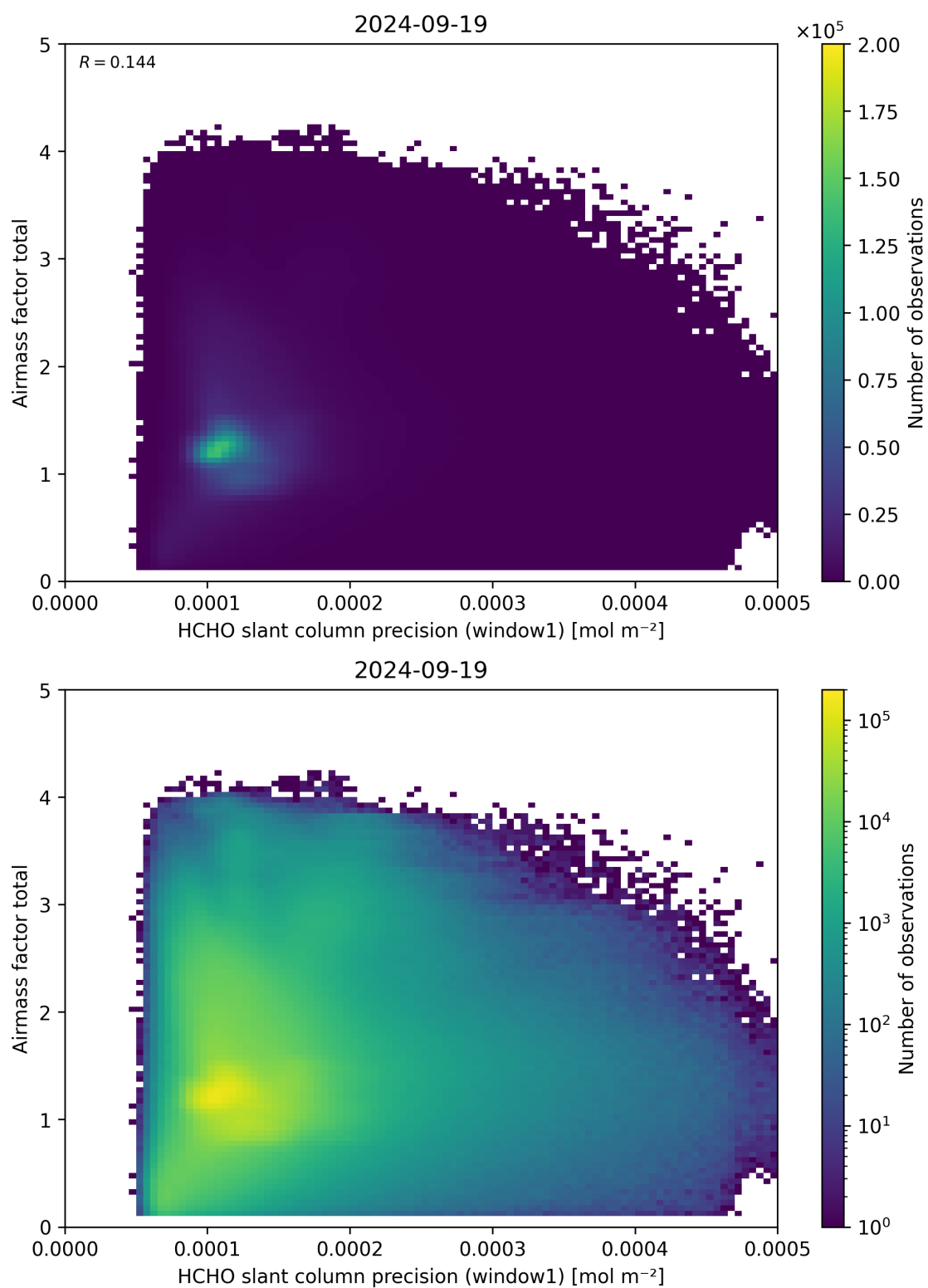
Figure 94: Scatter density plot of “HCHO slant column precision (window1)” against “Airmass factor total” for 2024-09-18 to 2024-09-20.
