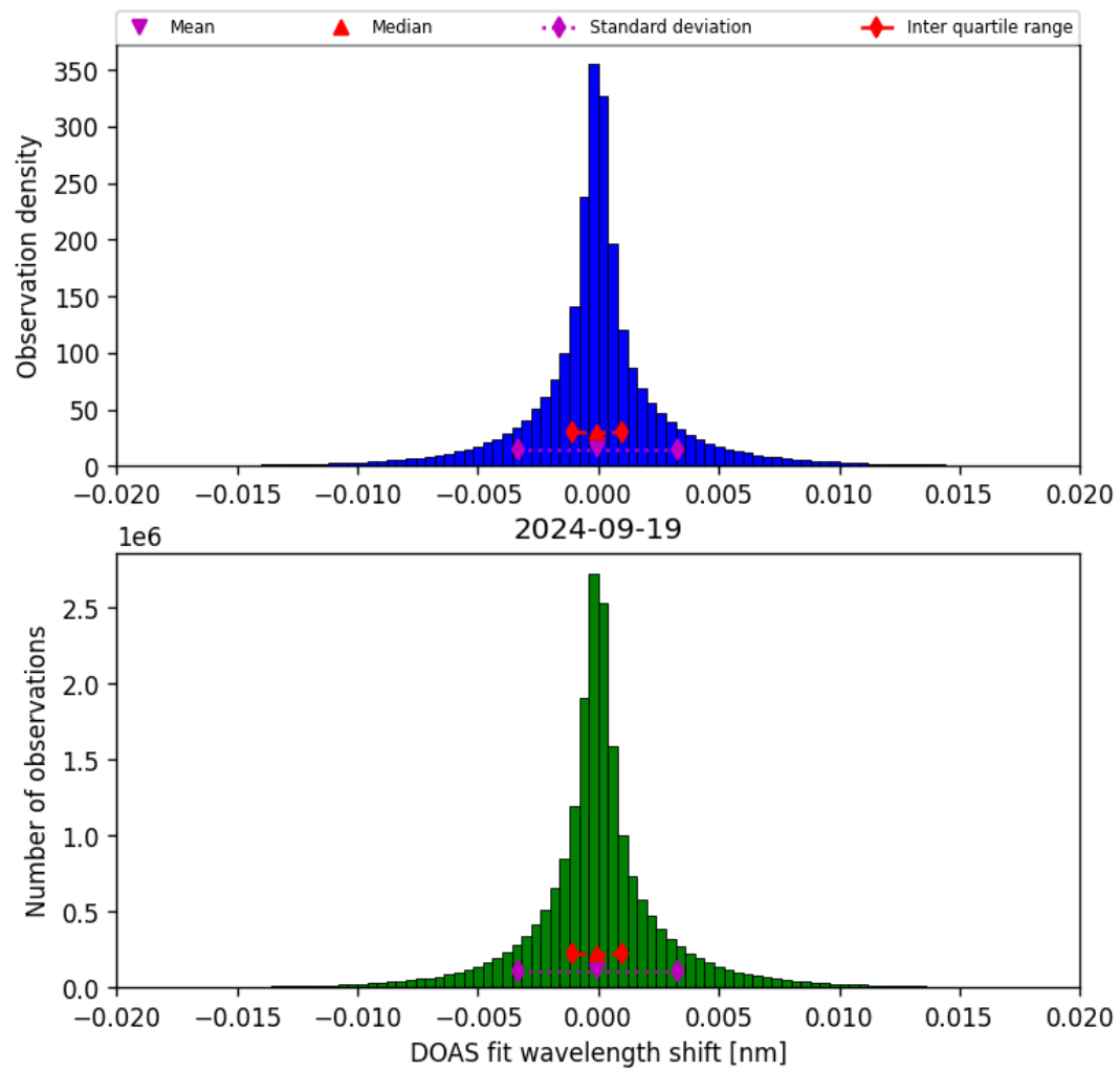
Figure 44: Histogram of “DOAS fit wavelength shift” for 2024-09-18 to 2024-09-20
