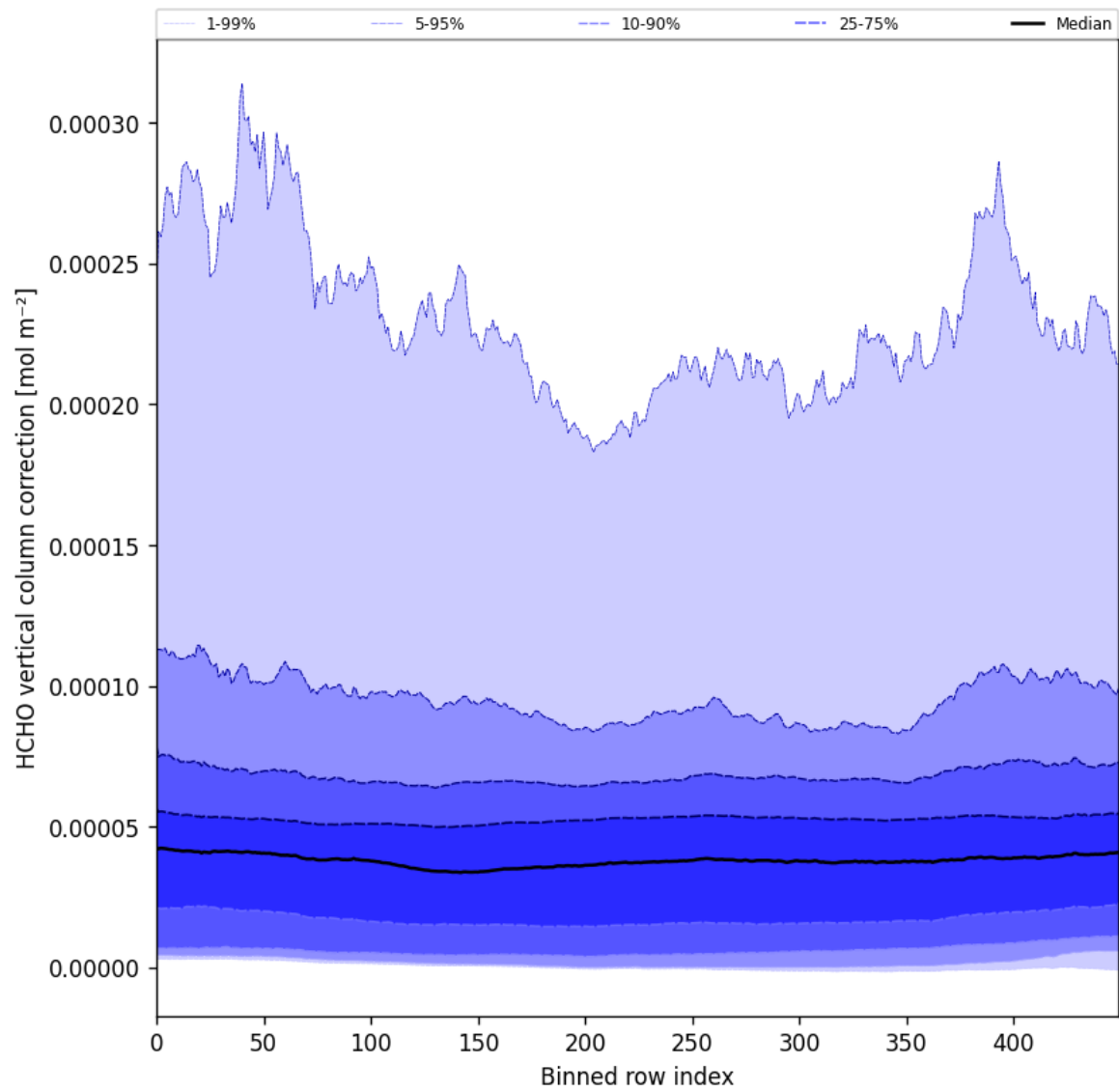
Figure 51: Along track statistics of “HCHO vertical column correction” for 2024-09-18 to 2024-09-20
