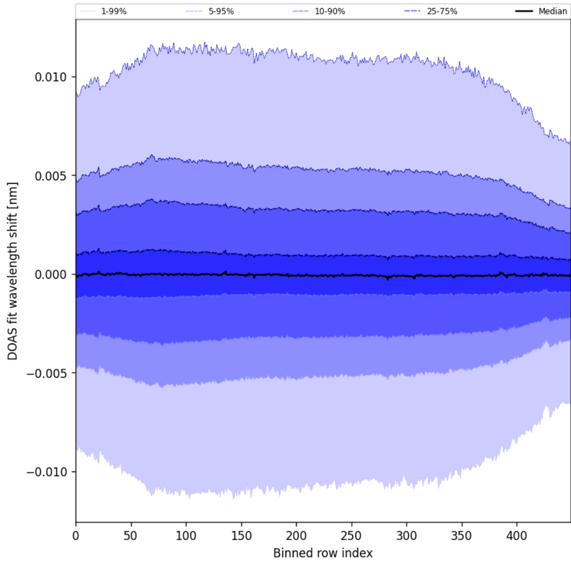
Figure 58: Along track statistics of “DOAS fit wavelength shift” for 2024-09-18 to 2024-09-20
