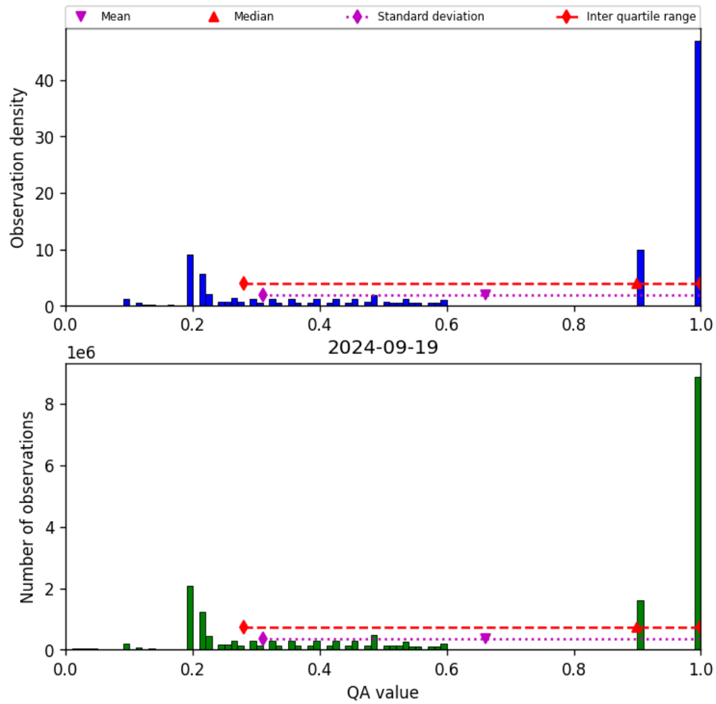
Figure 34: Histogram of “QA value” for 2024-09-18 to 2024-09-20
