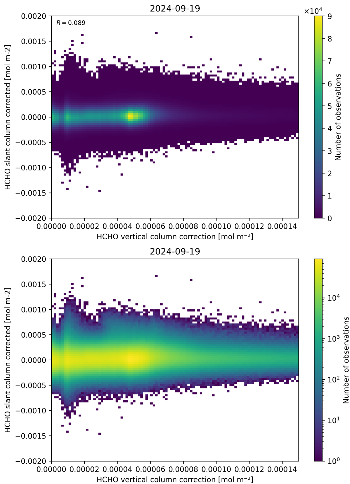
Figure 116: Scatter density plot of “HCHO vertical column correction” against “HCHO slant column corrected” for 2024-09-18 to 2024-09-20.
