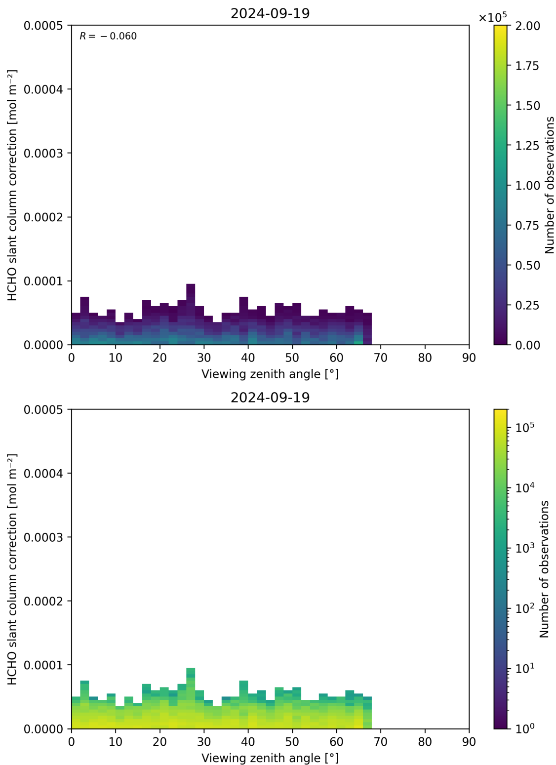
Figure 187: Scatter density plot of “Viewing zenith angle” against “HCHO slant column correction” for 2024-09-18 to 2024-09-20.
