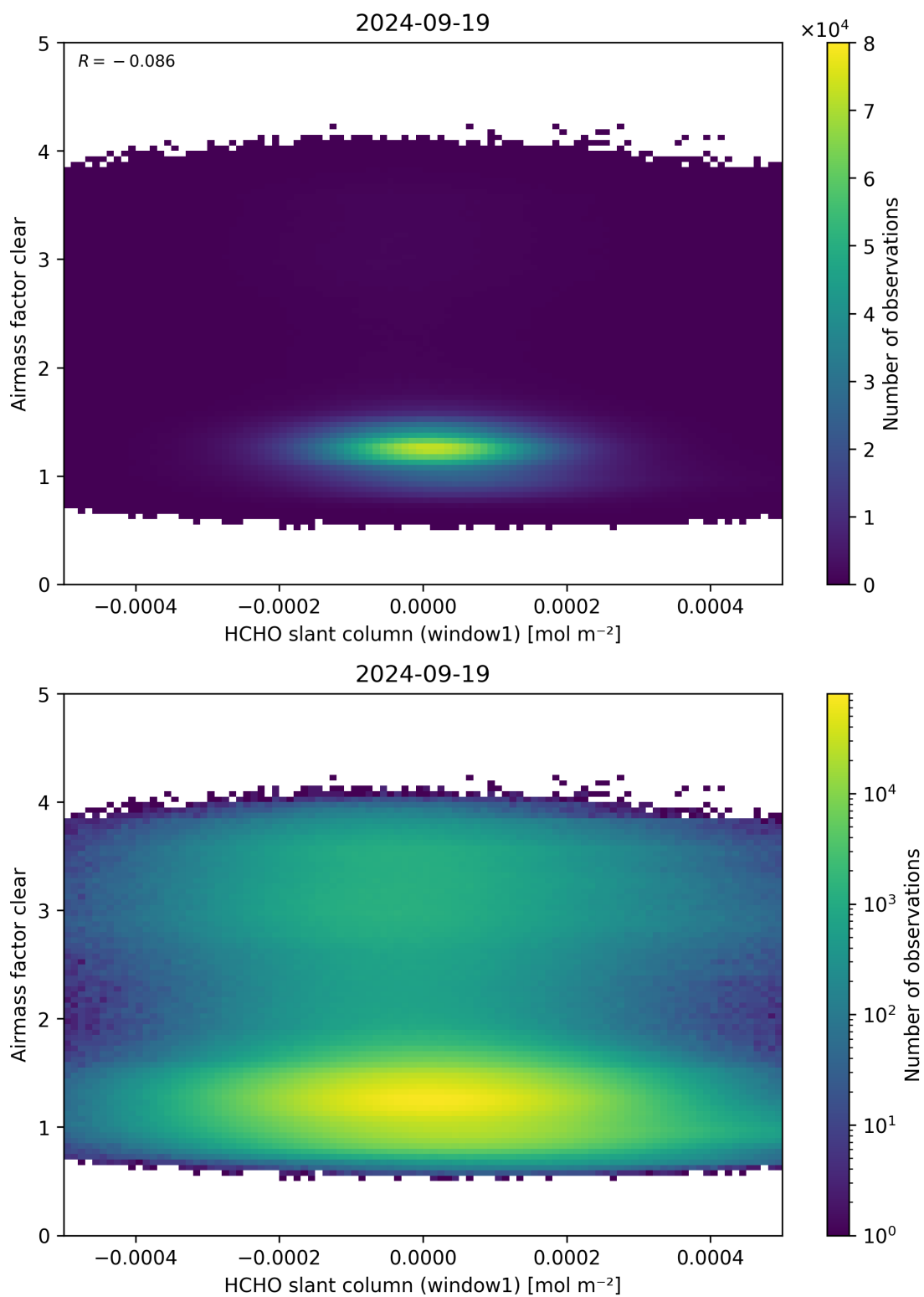
Figure 81: Scatter density plot of “HCHO slant column (window1)” against “Airmass factor clear” for 2024-09-18 to 2024-09-20.
