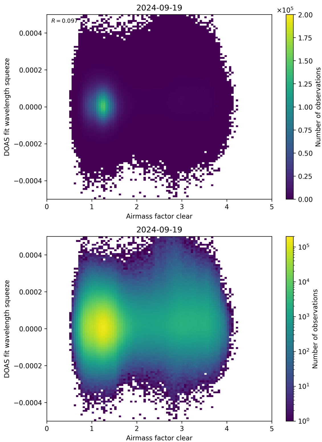
Figure 73: Scatter density plot of “Airmass factor clear” against “DOAS fit wavelength squeeze” for 2024-09-18 to 2024-09-20.
