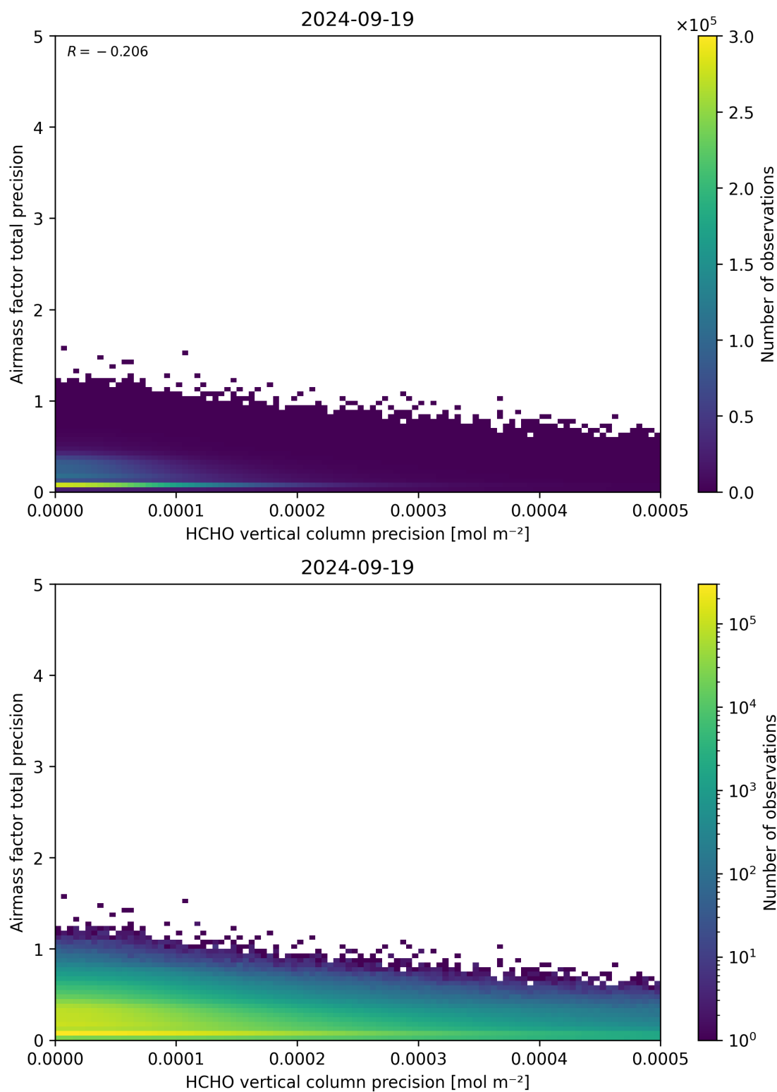
Figure 145: Scatter density plot of “HCHO vertical column precision” against “Airmass factor total precision” for 2024-09-18 to 2024-09-20.
