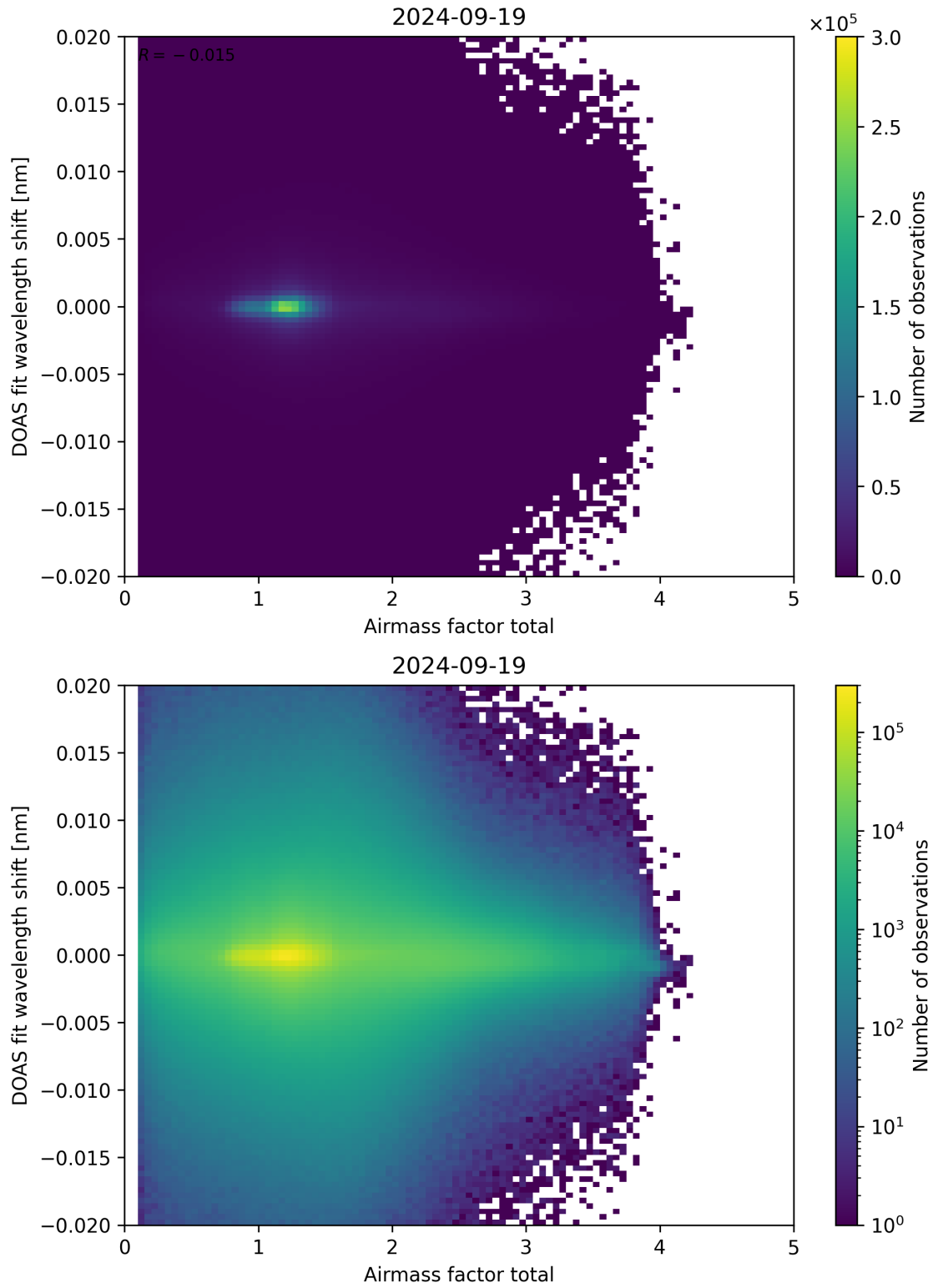
Figure 98: Scatter density plot of “Airmass factor total” against “DOAS fit wavelength shift” for 2024-09-18 to 2024-09-20.
