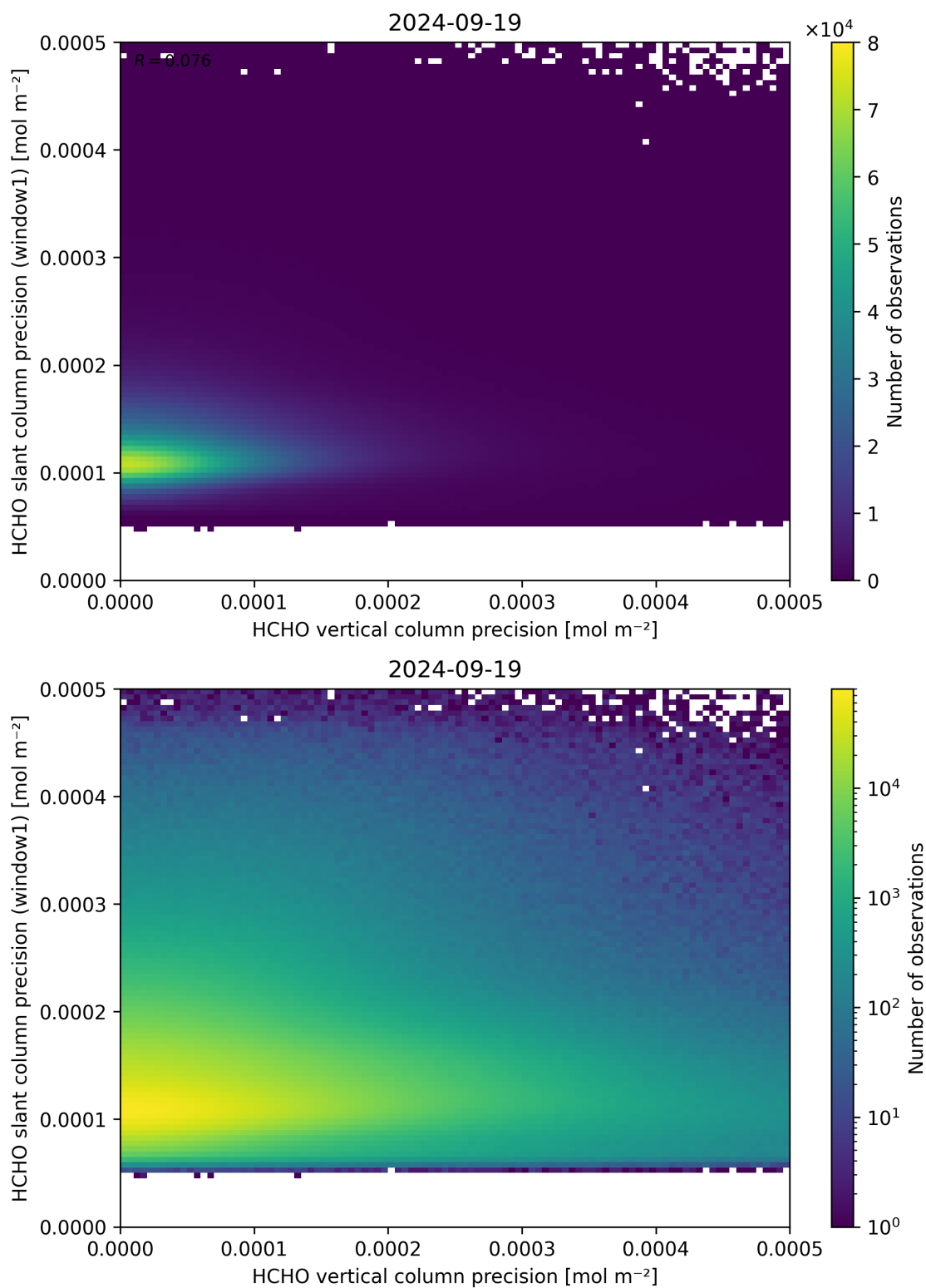
Figure 143: Scatter density plot of “HCHO vertical column precision” against “HCHO slant column precision (window1)” for 2024-09-18 to 2024-09-20.
