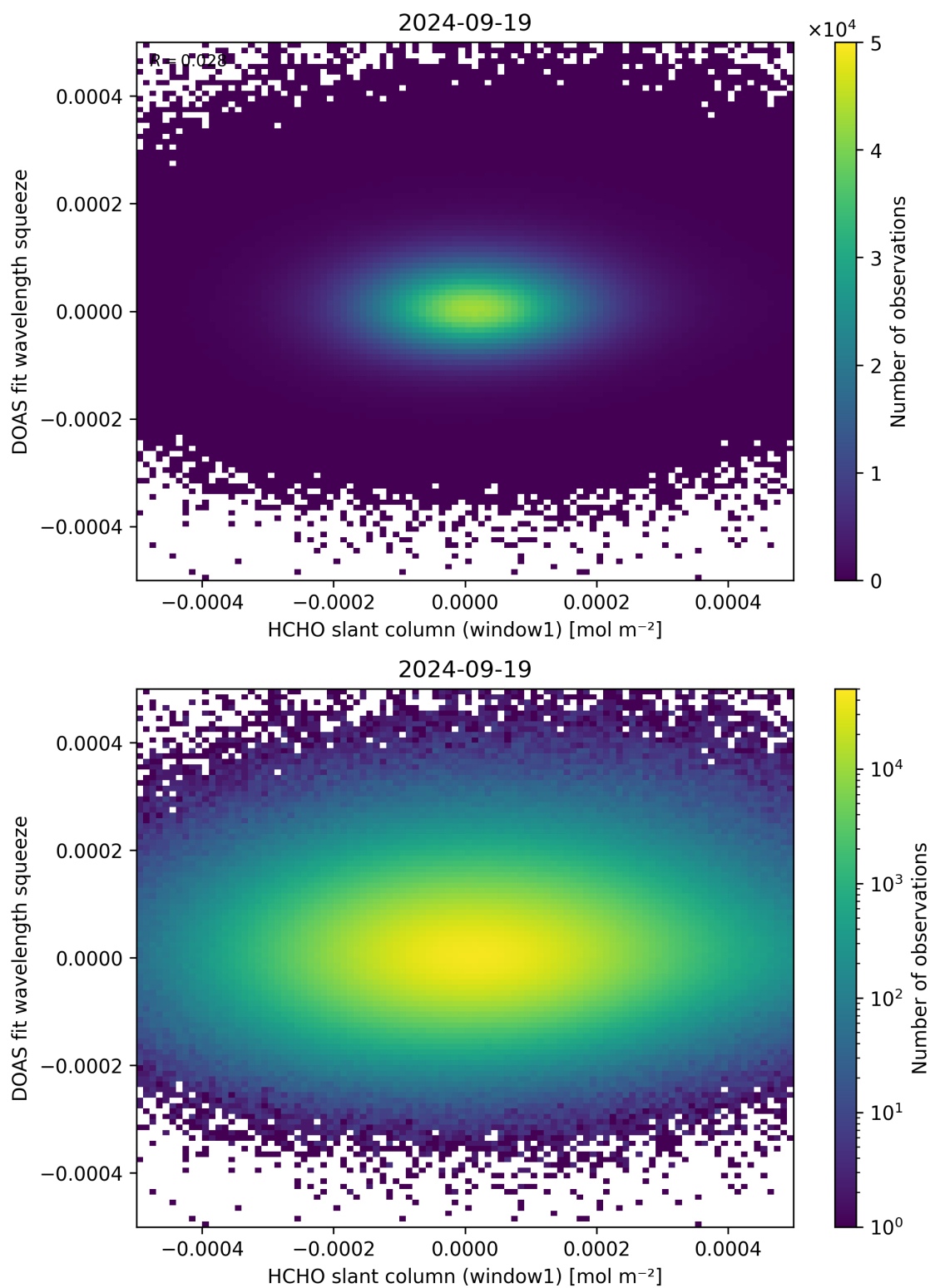
Figure 80: Scatter density plot of “HCHO slant column (window1)” against “DOAS fit wavelength squeeze” for 2024-09-18 to 2024-09-20.
