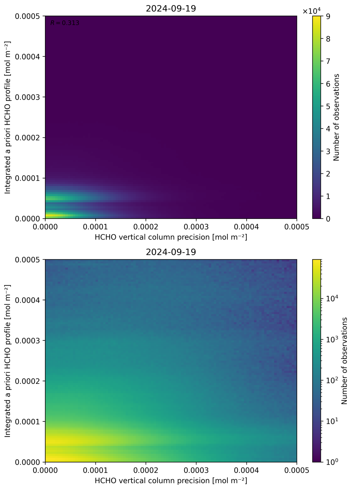
Figure 147: Scatter density plot of “HCHO vertical column precision” against “Integrated a priori HCHO profile” for 2024-09-18 to 2024-09-20.
