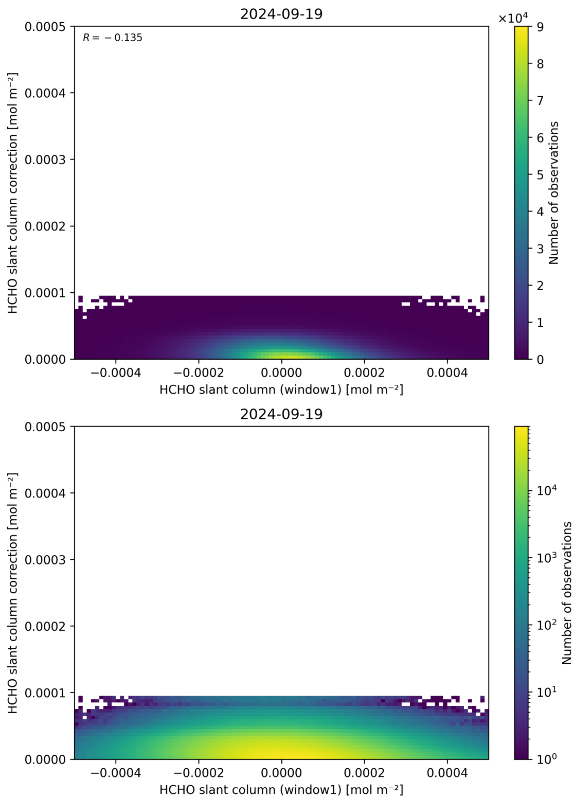
Figure 83: Scatter density plot of “HCHO slant column (window1)” against “HCHO slant column correction” for 2024-09-18 to 2024-09-20.
