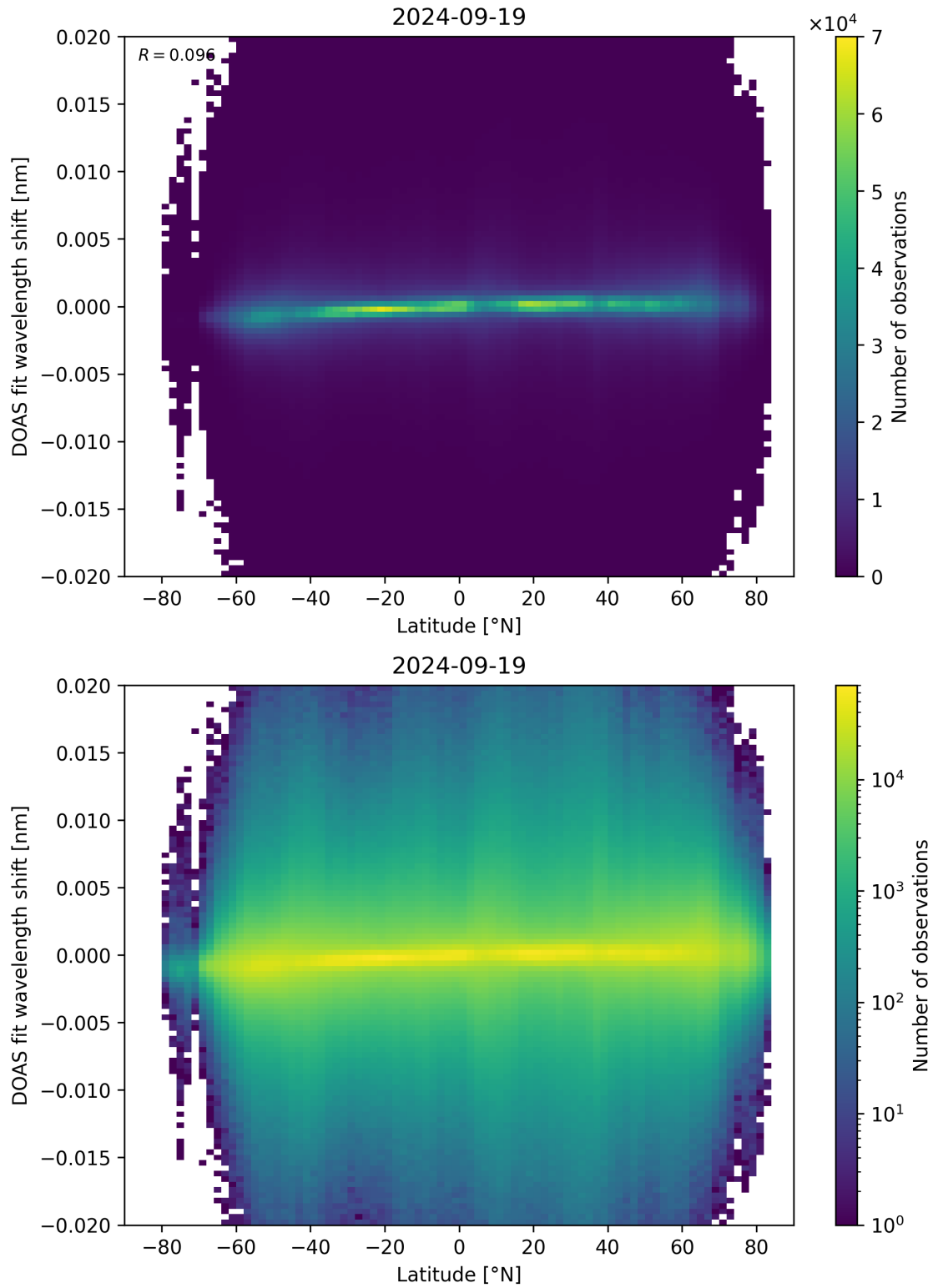
Figure 154: Scatter density plot of “Latitude” against “DOAS fit wavelength shift” for 2024-09-18 to 2024-09-20.
