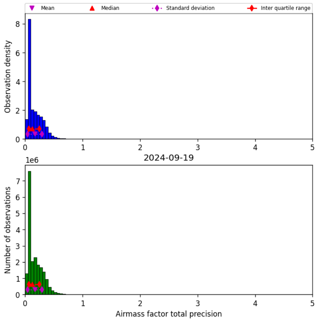
Figure 41: Histogram of “Airmass factor total precision” for 2024-09-18 to 2024-09-20
