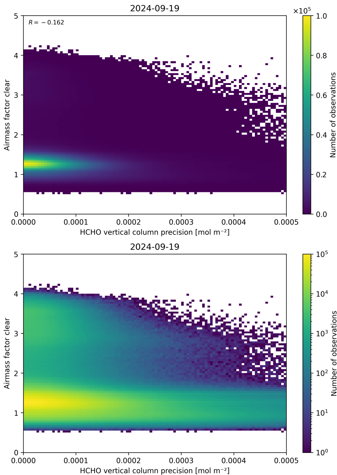
Figure 139: Scatter density plot of “HCHO vertical column precision” against “Airmass factor clear” for 2024-09-18 to 2024-09-20.
