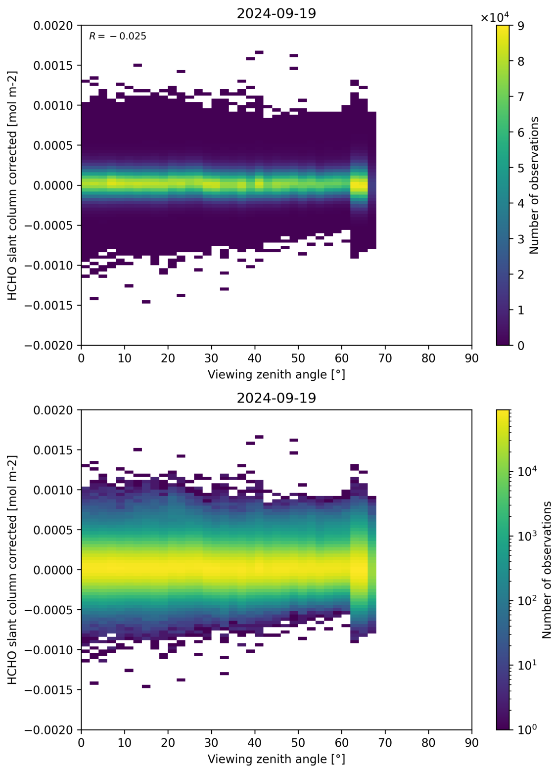
Figure 186: Scatter density plot of “Viewing zenith angle” against “HCHO slant column corrected” for 2024-09-18 to 2024-09-20.
