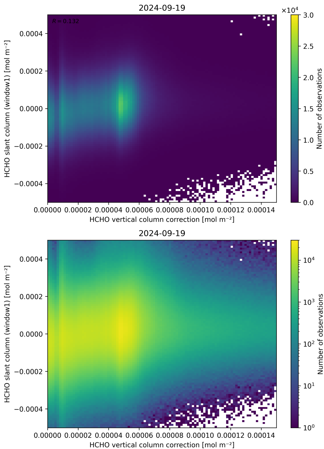
Figure 118: Scatter density plot of “HCHO vertical column correction” against “HCHO slant column (window1)” for 2024-09-18 to 2024-09-20.
