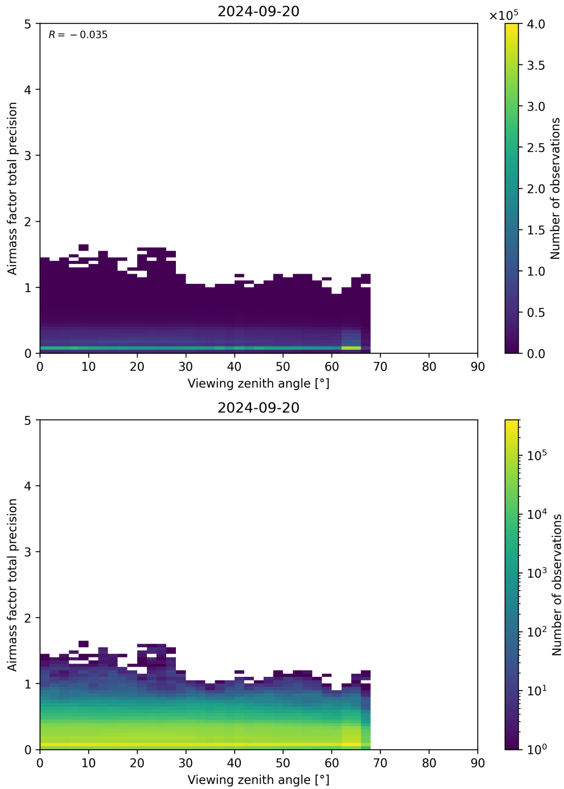
Figure 191: Scatter density plot of “Viewing zenith angle” against “Airmass factor total precision” for 2024-09-19 to 2024-09-21.
