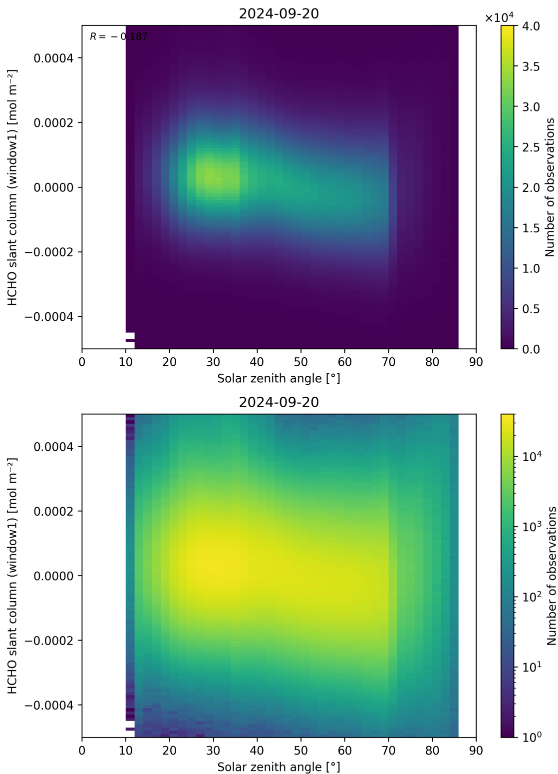
Figure 173: Scatter density plot of “Solar zenith angle” against “HCHO slant column (window1)” for 2024-09-19 to 2024-09-21.
