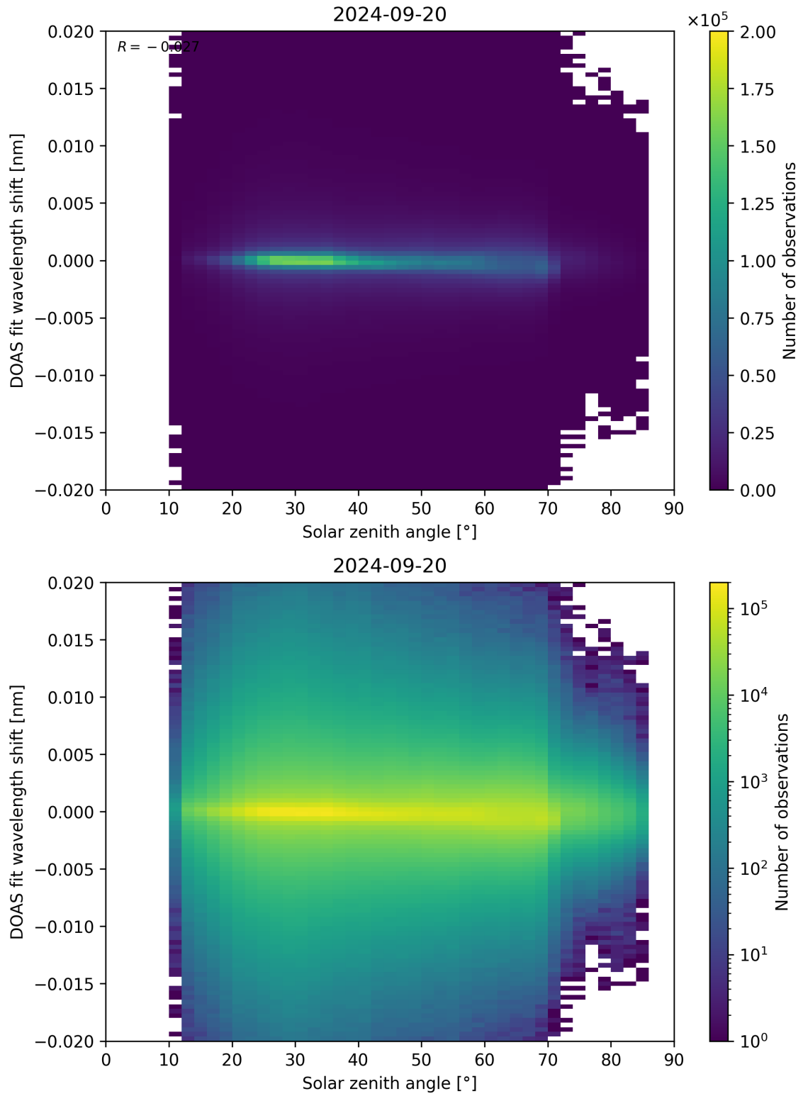
Figure 168: Scatter density plot of “Solar zenith angle” against “DOAS fit wavelength shift” for 2024-09-19 to 2024-09-21.
