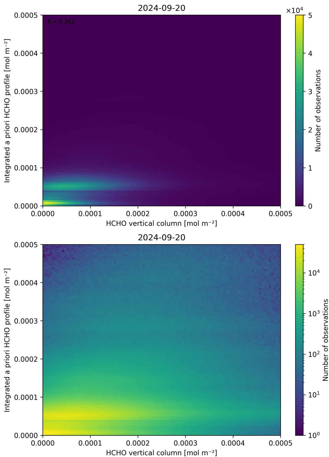
Figure 135: Scatter density plot of “HCHO vertical column” against “Integrated a priori HCHO profile” for 2024-09-19 to 2024-09-21.
