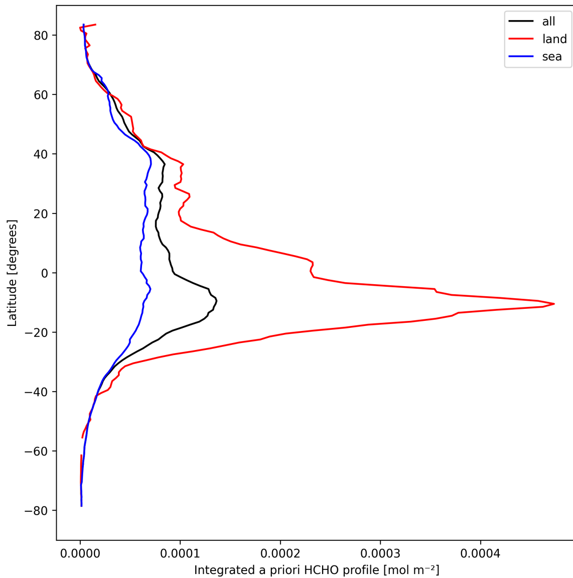
Figure 29: Zonal average of “Integrated a priori HCHO profile” for 2024-09-19 to 2024-09-21.
