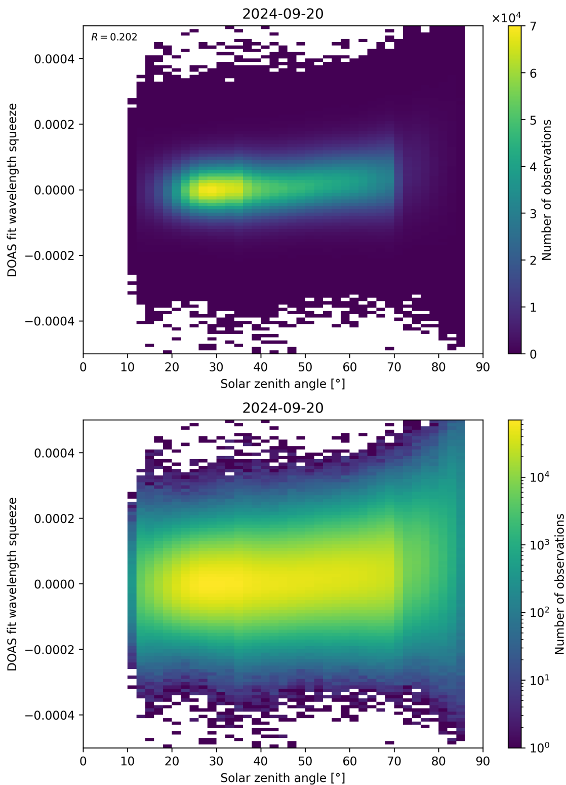
Figure 169: Scatter density plot of “Solar zenith angle” against “DOAS fit wavelength squeeze” for 2024-09-19 to 2024-09-21.
