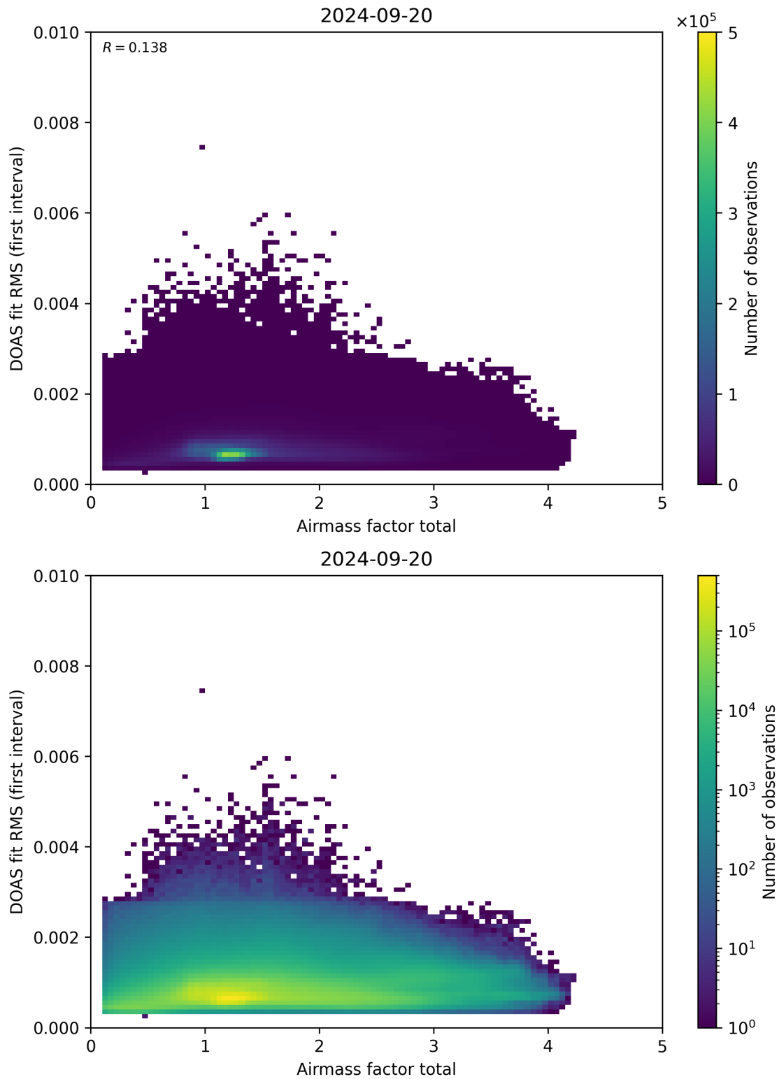
Figure 97: Scatter density plot of “Airmass factor total” against “DOAS fit RMS (first interval)” for 2024-09-19 to 2024-09-21.
