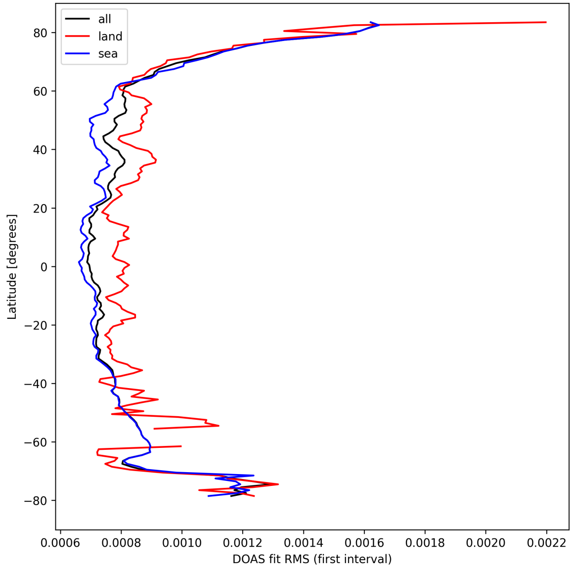
Figure 32: Zonal average of “DOAS fit RMS (first interval)” for 2024-09-19 to 2024-09-21.
