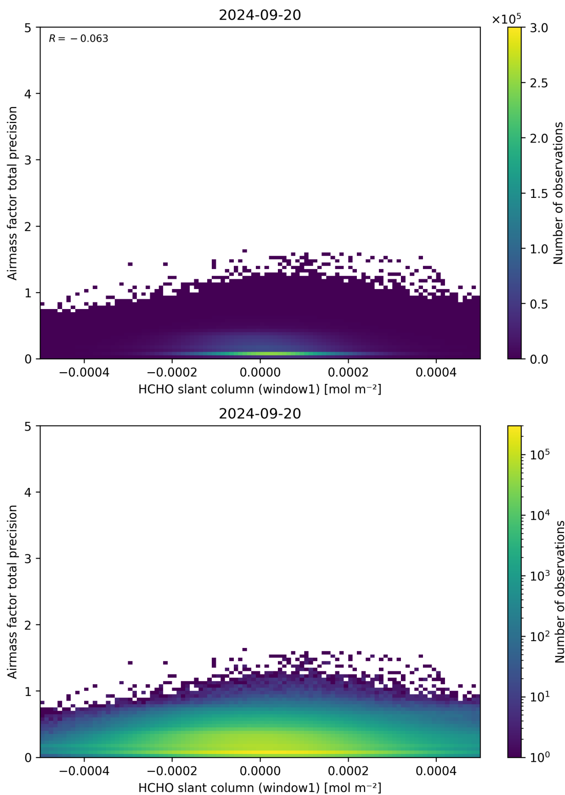
Figure 86: Scatter density plot of “HCHO slant column (window1)” against “Airmass factor total precision” for 2024-09-19 to 2024-09-21.
