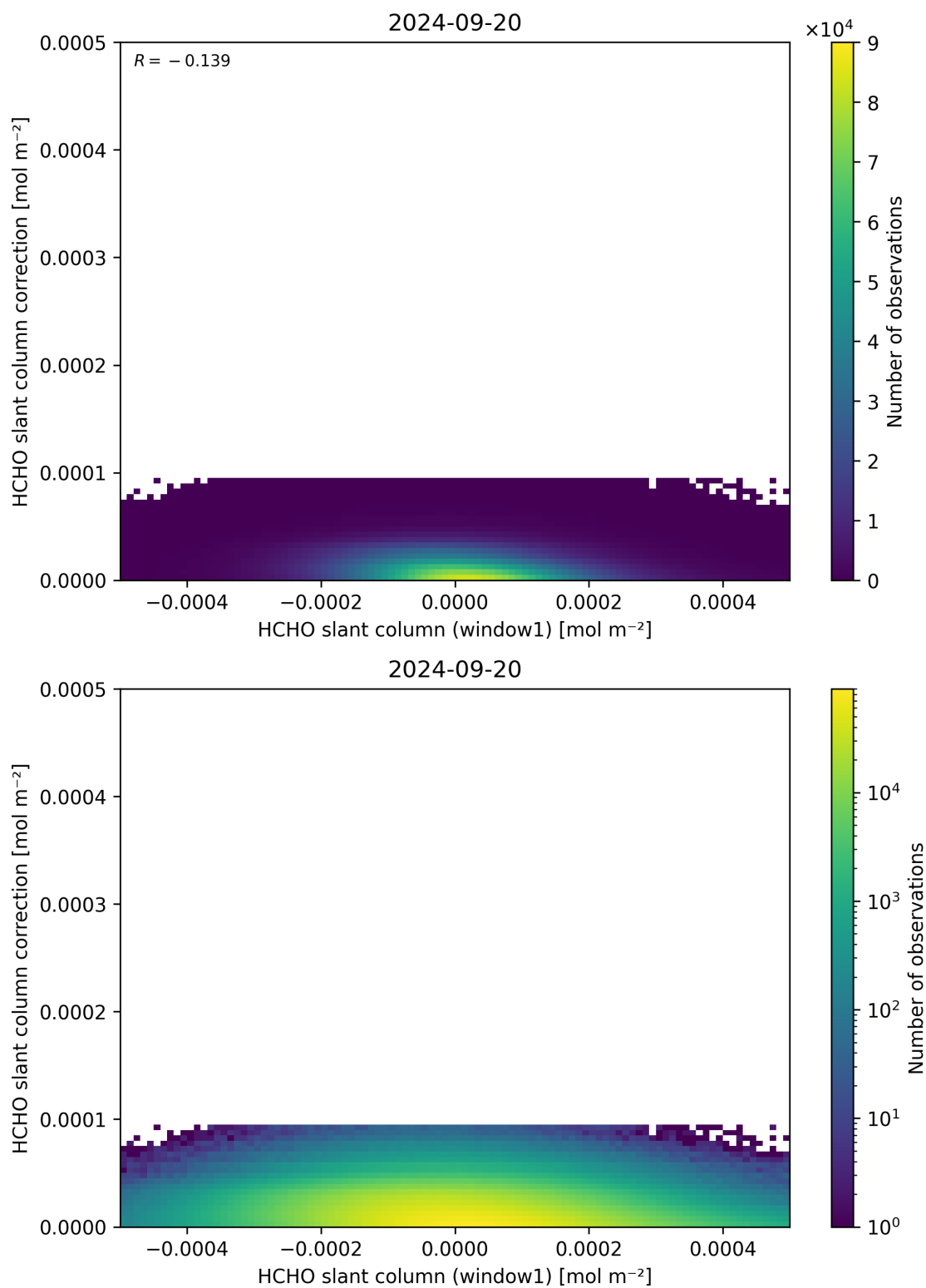
Figure 83: Scatter density plot of “HCHO slant column (window1)” against “HCHO slant column correction” for 2024-09-19 to 2024-09-21.
