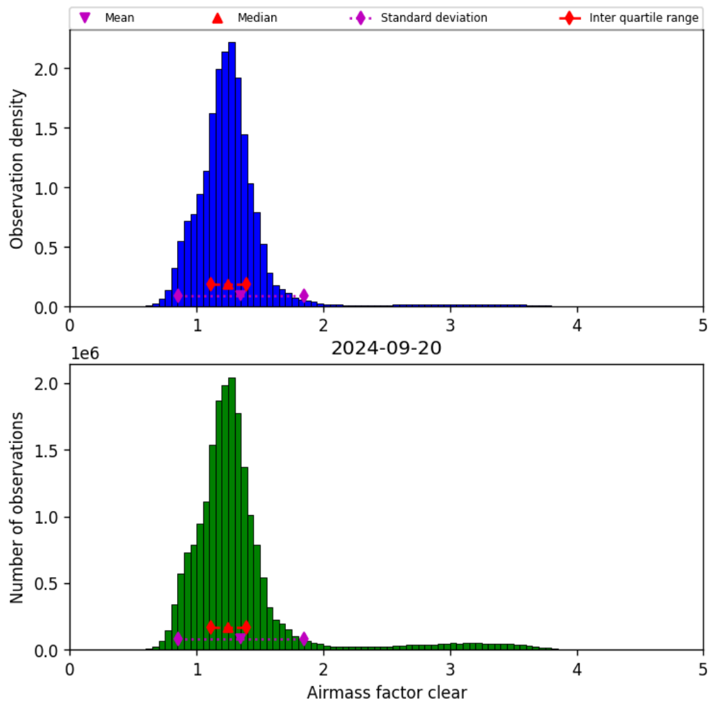
Figure 42: Histogram of “Airmass factor clear” for 2024-09-19 to 2024-09-21
