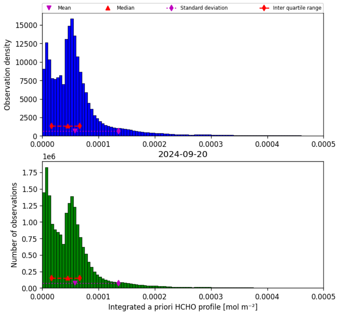
Figure 43: Histogram of “Integrated a priori HCHO profile” for 2024-09-19 to 2024-09-21
