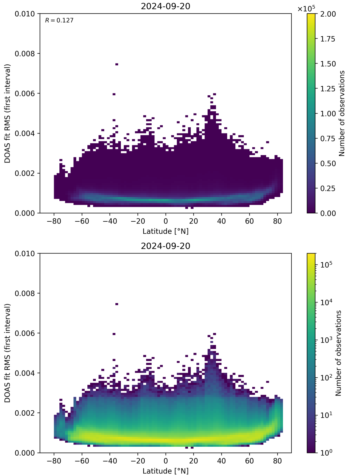
Figure 153: Scatter density plot of “Latitude” against “DOAS fit RMS (first interval)” for 2024-09-19 to 2024-09-21.
