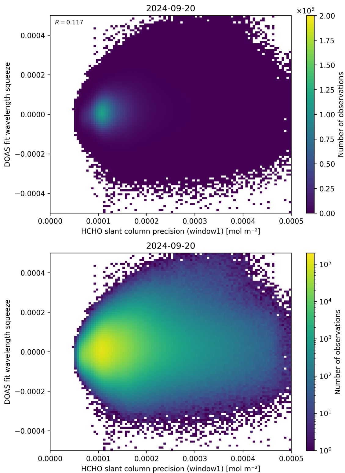
Figure 90: Scatter density plot of “HCHO slant column precision (window1)” against “DOAS fit wavelength squeeze” for 2024-09-19 to 2024-09-21.
