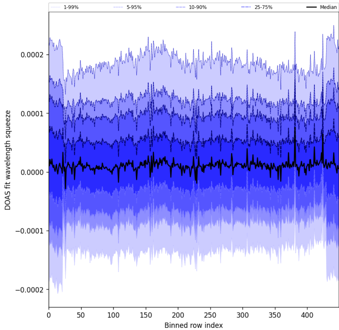
Figure 59: Along track statistics of “DOAS fit wavelength squeeze” for 2024-09-19 to 2024-09-21
