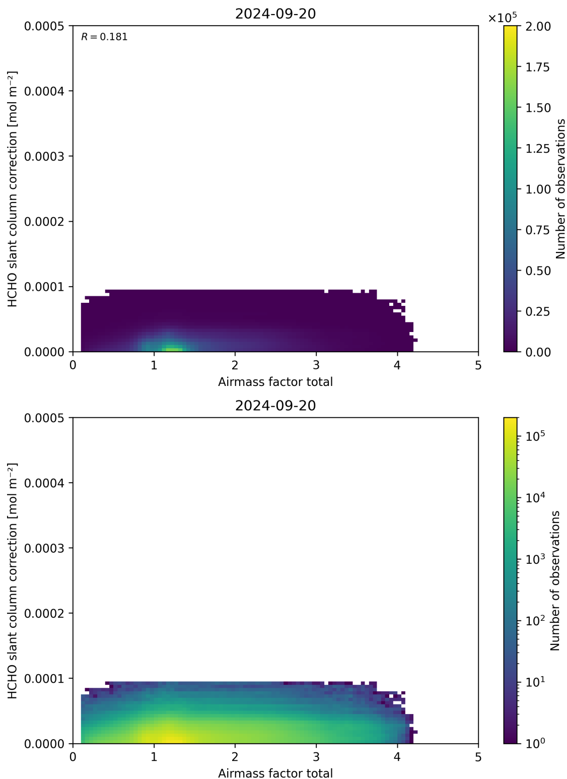
Figure 102: Scatter density plot of “Airmass factor total” against “HCHO slant column correction” for 2024-09-19 to 2024-09-21.
