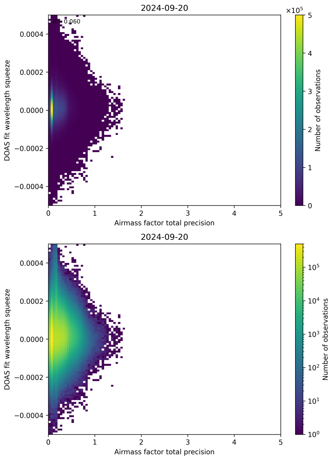
Figure 107: Scatter density plot of “Airmass factor total precision” against “DOAS fit wavelength squeeze” for 2024-09-19 to 2024-09-21.
