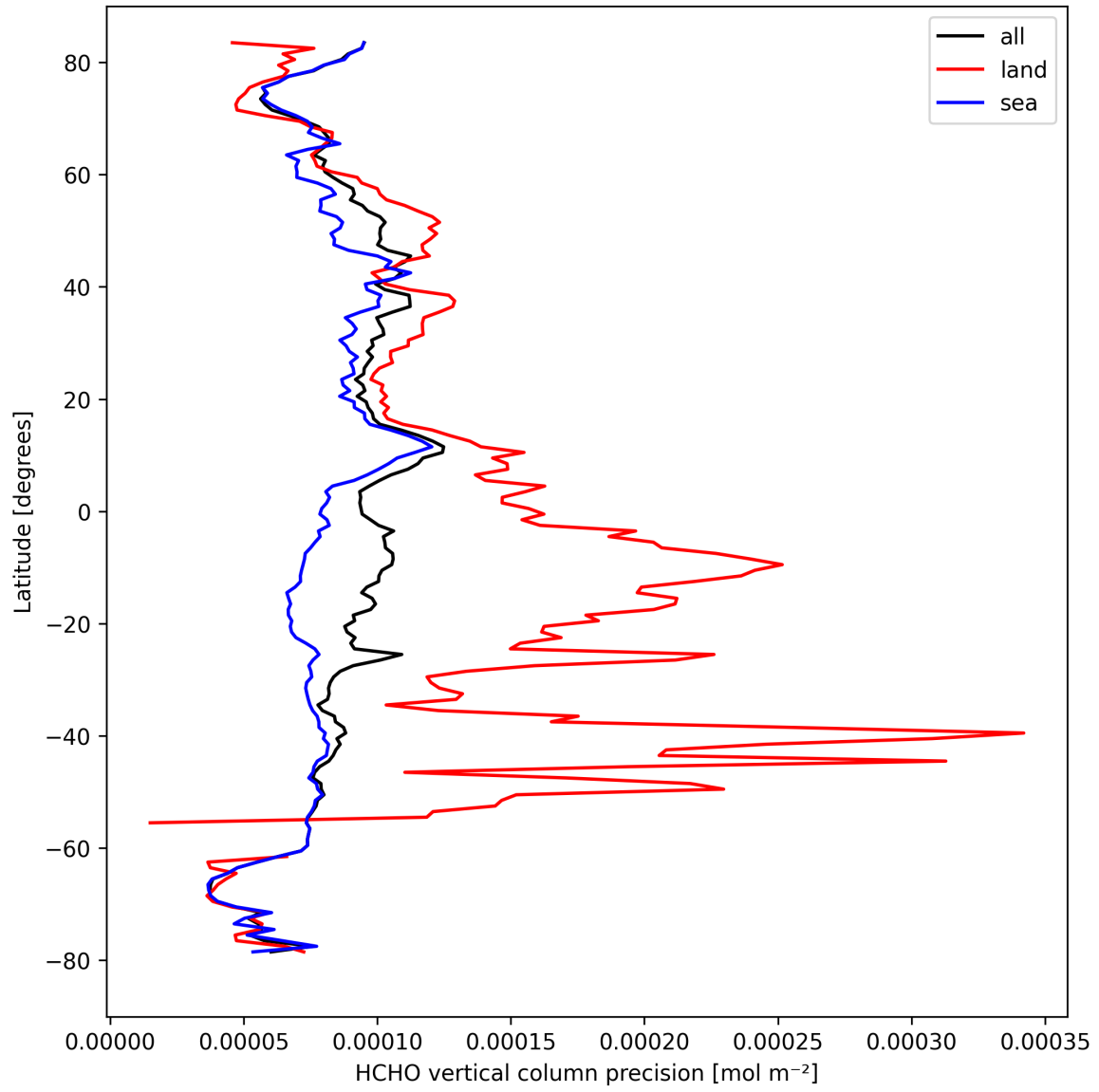
Figure 22: Zonal average of “HCHO vertical column precision” for 2024-09-19 to 2024-09-21.
