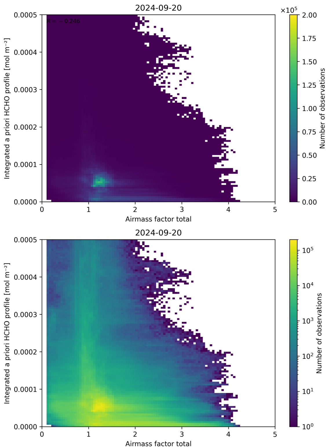
Figure 104: Scatter density plot of “Airmass factor total” against “Integrated a priori HCHO profile” for 2024-09-19 to 2024-09-21.
