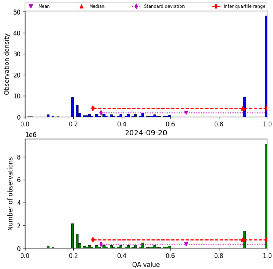
Figure 34: Histogram of “QA value” for 2024-09-19 to 2024-09-21
