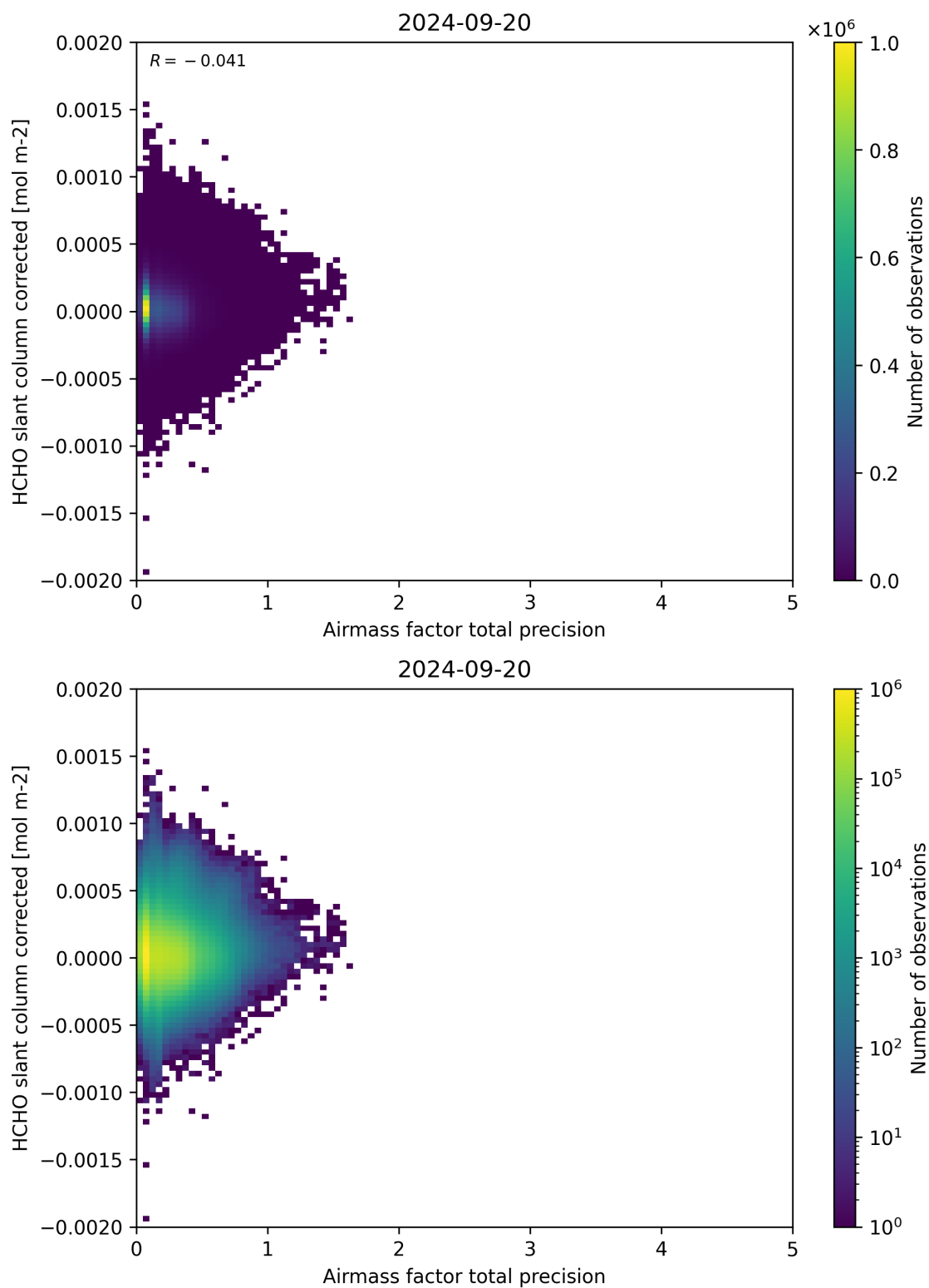
Figure 109: Scatter density plot of “Airmass factor total precision” against “HCHO slant column corrected” for 2024-09-19 to 2024-09-21.
