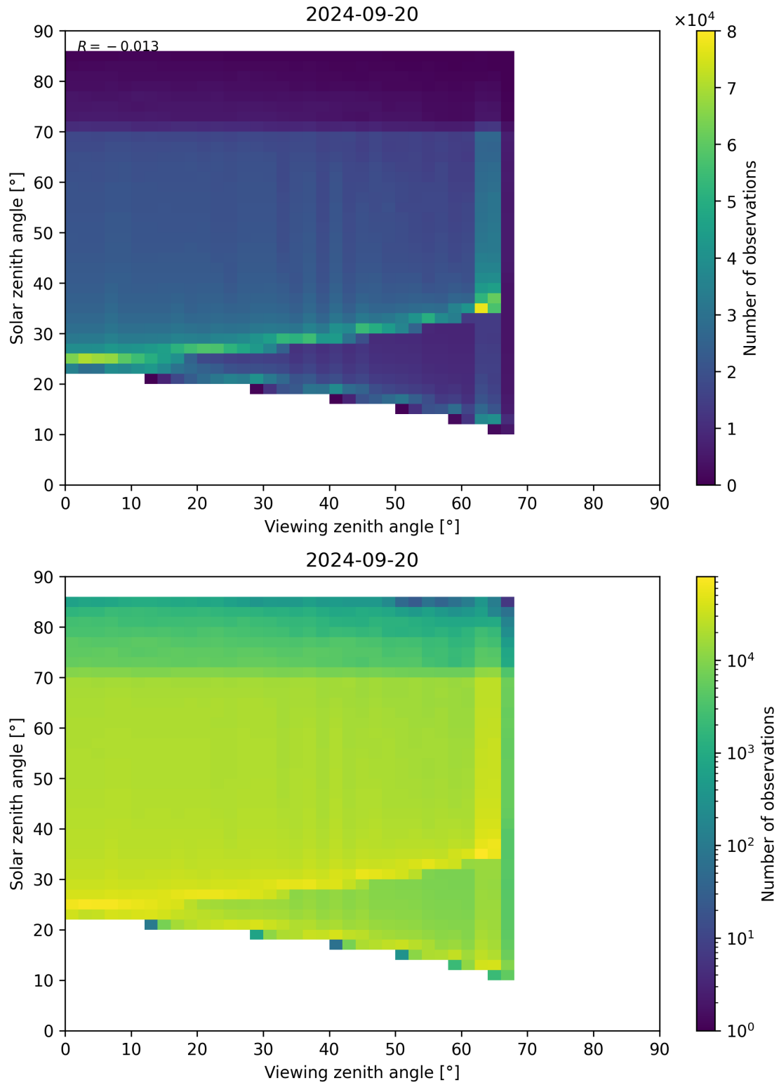
Figure 197: Scatter density plot of “Viewing zenith angle” against “Solar zenith angle” for 2024-09-19 to 2024-09-21.
