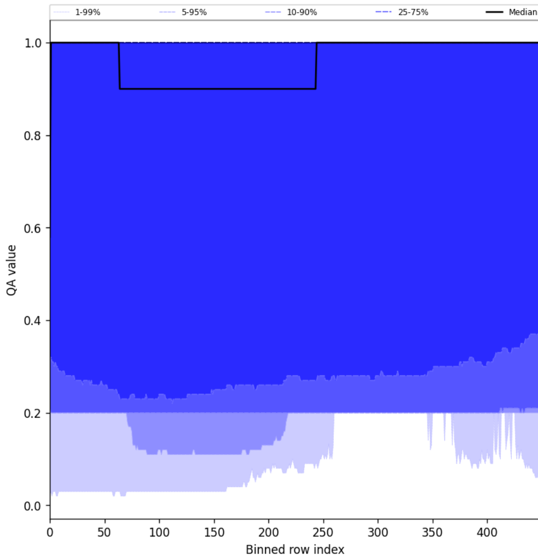
Figure 48: Along track statistics of “QA value” for 2024-09-19 to 2024-09-21
