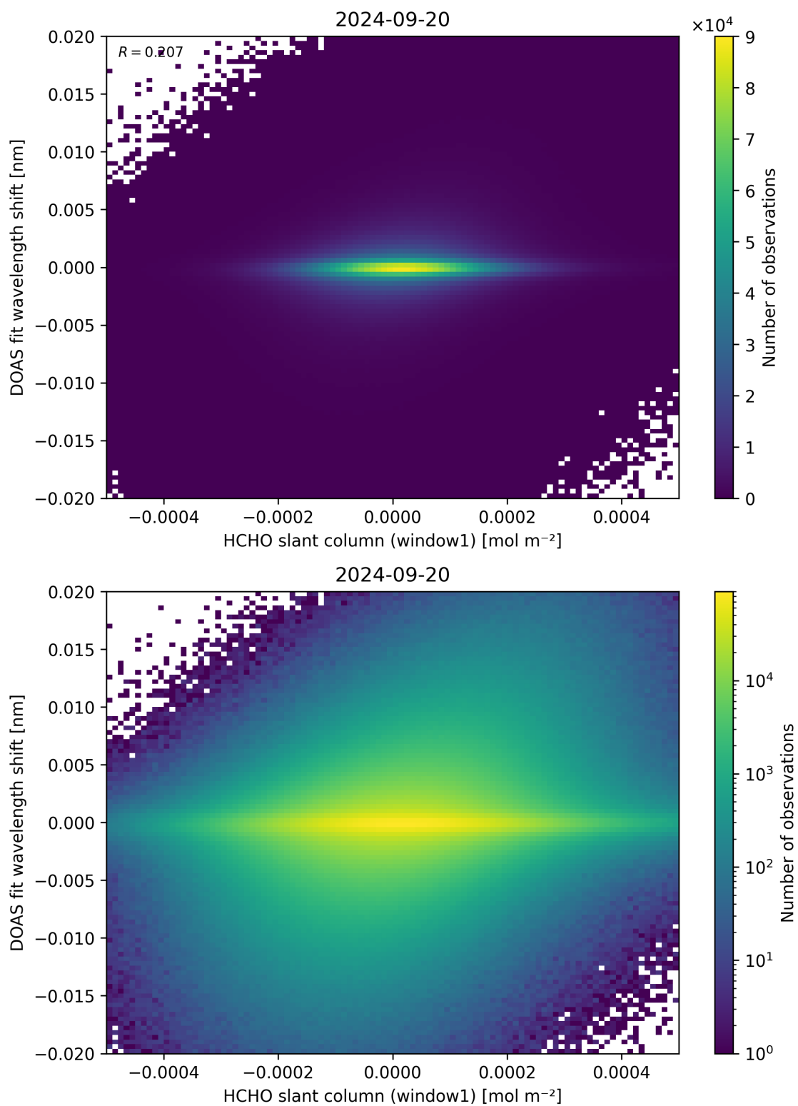
Figure 79: Scatter density plot of “HCHO slant column (window1)” against “DOAS fit wavelength shift” for 2024-09-19 to 2024-09-21.
