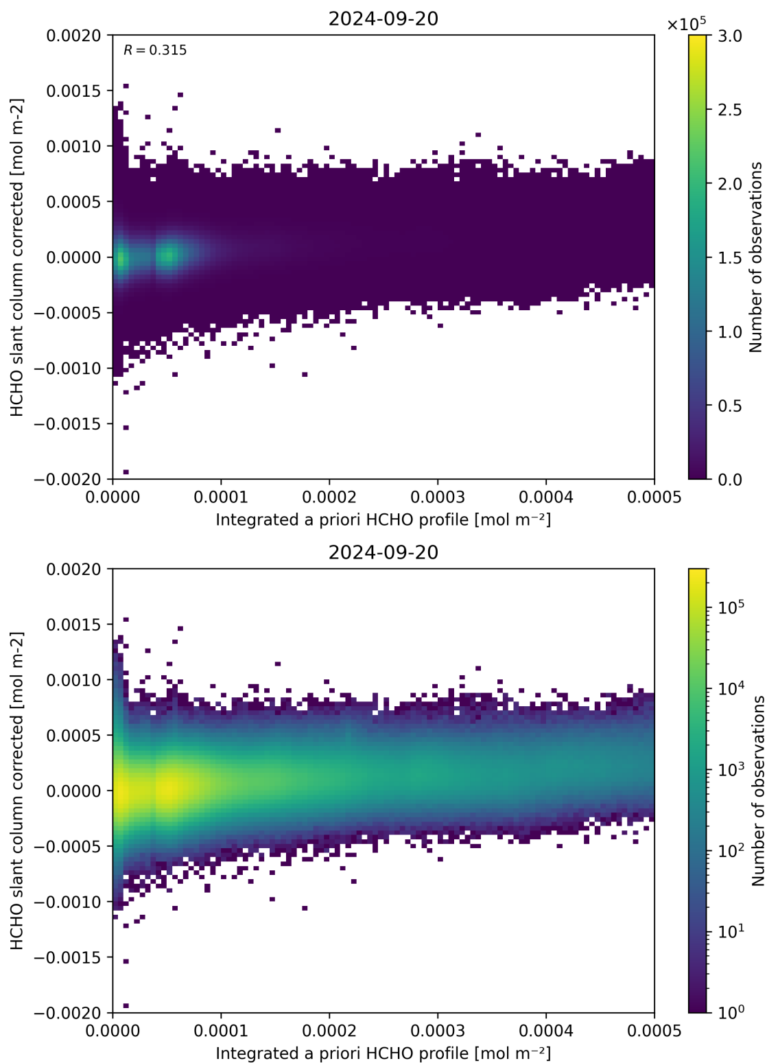
Figure 151: Scatter density plot of “Integrated a priori HCHO profile” against “HCHO slant column corrected” for 2024-09-19 to 2024-09-21.
