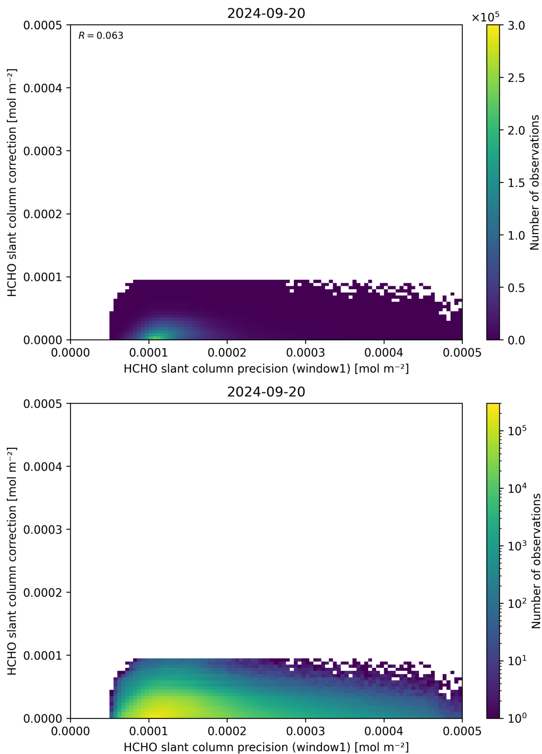
Figure 93: Scatter density plot of “HCHO slant column precision (window1)” against “HCHO slant column correction” for 2024-09-19 to 2024-09-21.
