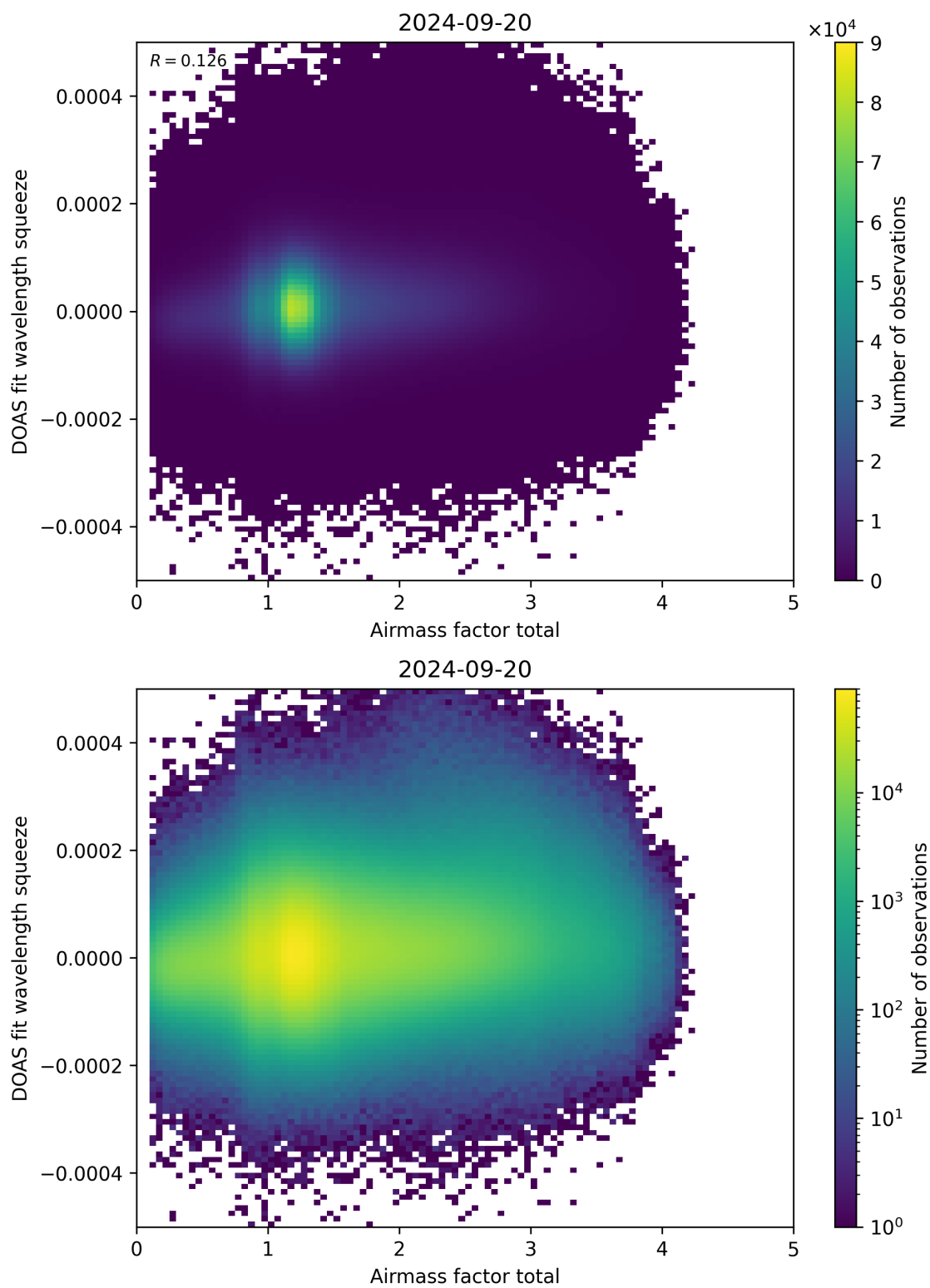
Figure 99: Scatter density plot of “Airmass factor total” against “DOAS fit wavelength squeeze” for 2024-09-19 to 2024-09-21.
