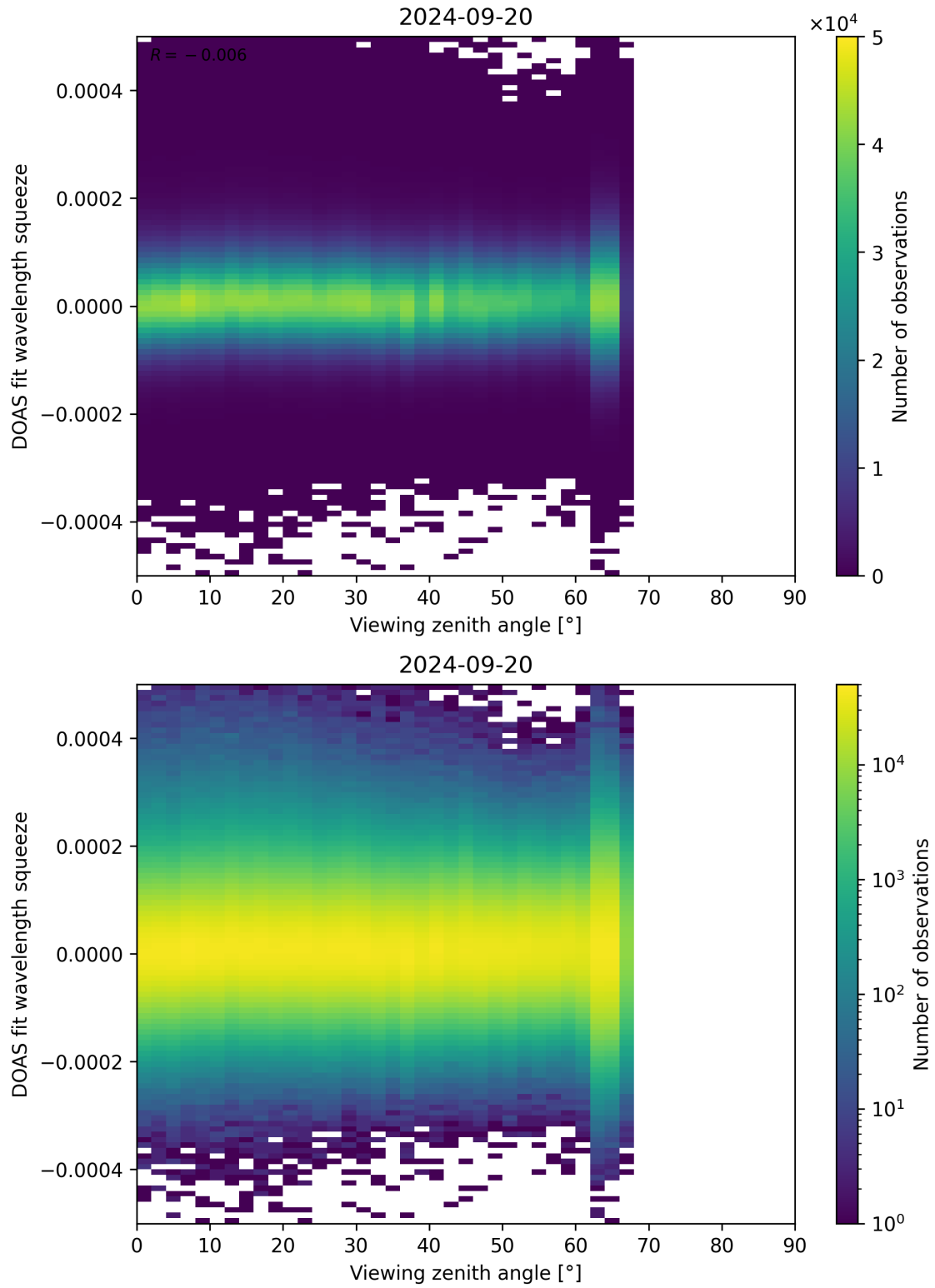
Figure 184: Scatter density plot of “Viewing zenith angle” against “DOAS fit wavelength squeeze” for 2024-09-19 to 2024-09-21.
