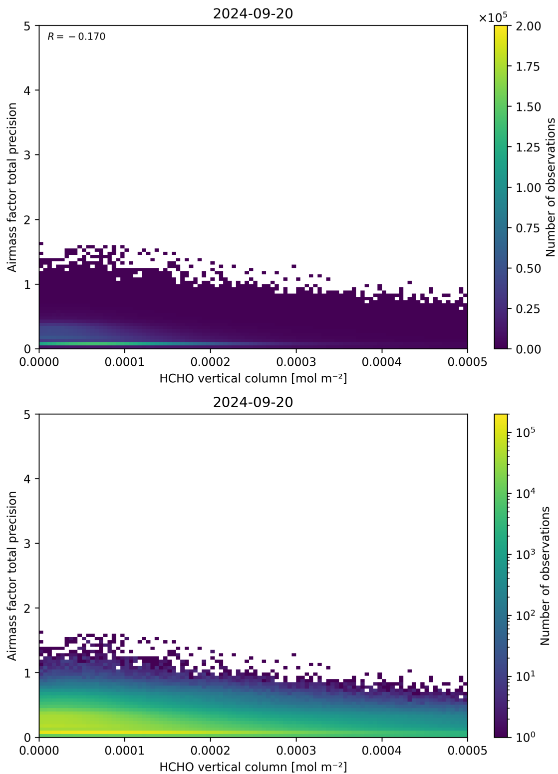
Figure 132: Scatter density plot of “HCHO vertical column” against “Airmass factor total precision” for 2024-09-19 to 2024-09-21.
