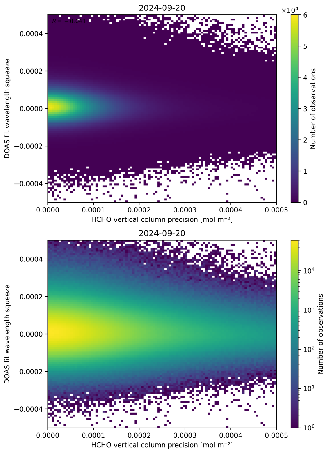
Figure 138: Scatter density plot of “HCHO vertical column precision” against “DOAS fit wavelength squeeze” for 2024-09-19 to 2024-09-21.
