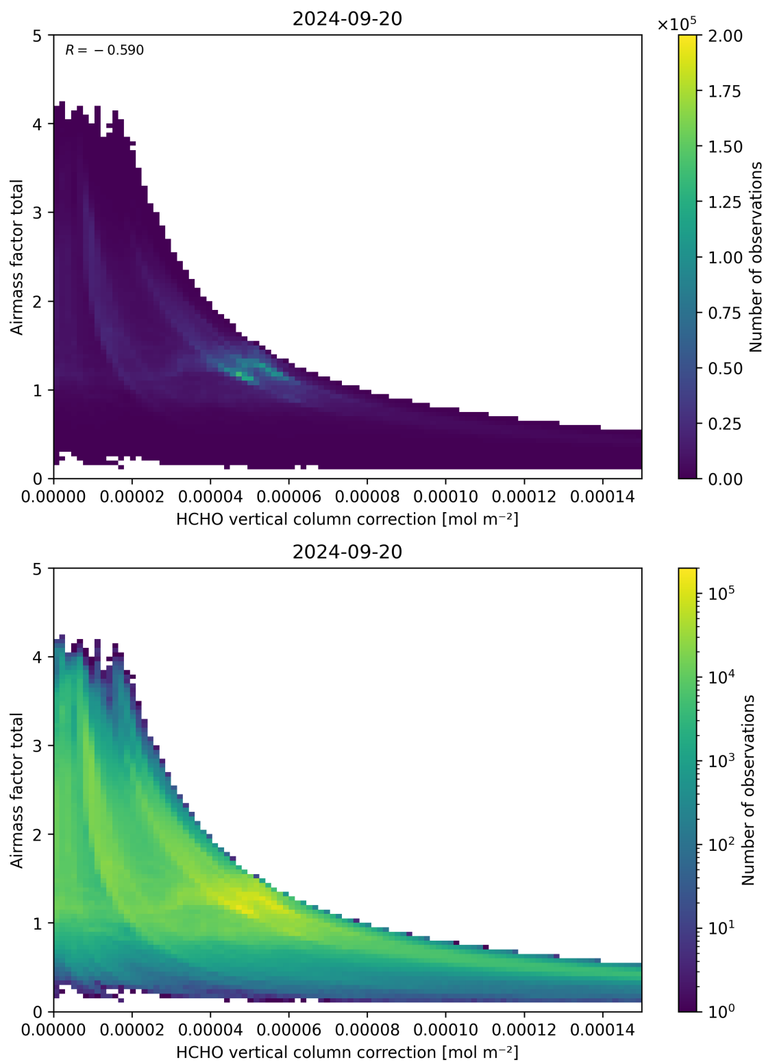
Figure 120: Scatter density plot of “HCHO vertical column correction” against “Airmass factor total” for 2024-09-19 to 2024-09-21.
