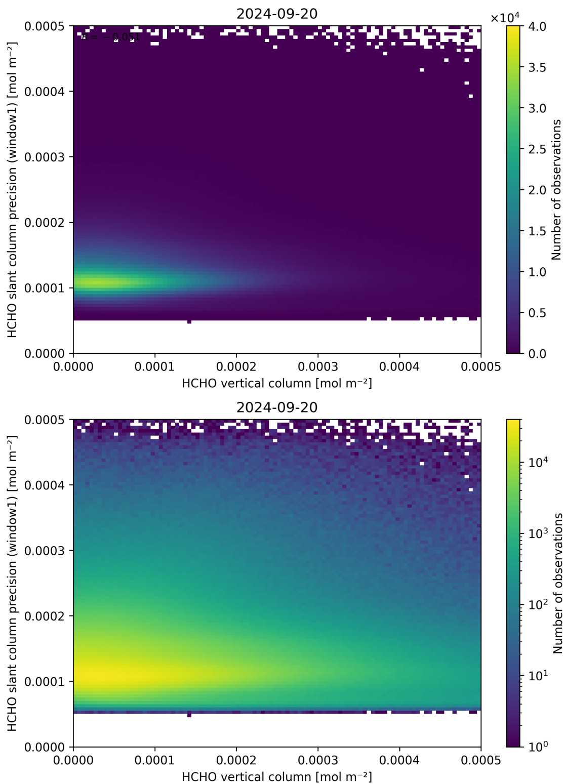
Figure 130: Scatter density plot of “HCHO vertical column” against “HCHO slant column precision (window1)” for 2024-09-19 to 2024-09-21.
