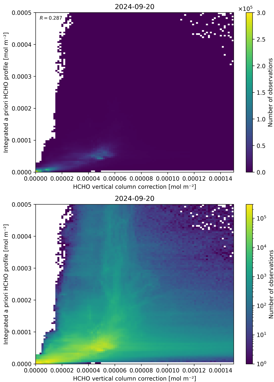
Figure 122: Scatter density plot of “HCHO vertical column correction” against “Integrated a priori HCHO profile” for 2024-09-19 to 2024-09-21.
