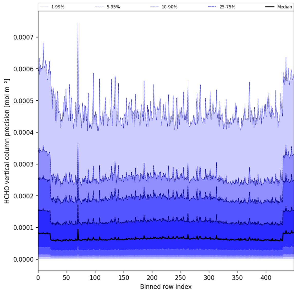
Figure 50: Along track statistics of “HCHO vertical column precision” for 2024-09-19 to 2024-09-21
