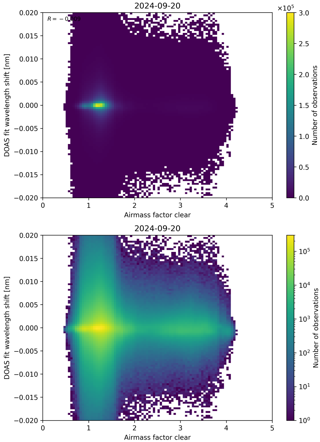
Figure 72: Scatter density plot of “Airmass factor clear” against “DOAS fit wavelength shift” for 2024-09-19 to 2024-09-21.
