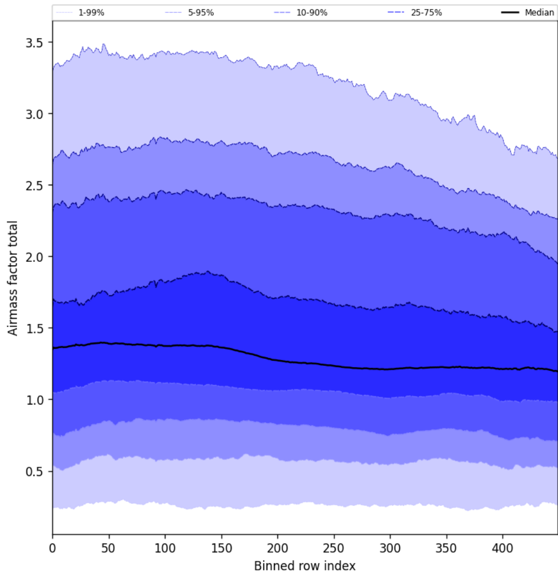
Figure 54: Along track statistics of “Airmass factor total” for 2024-09-19 to 2024-09-21
