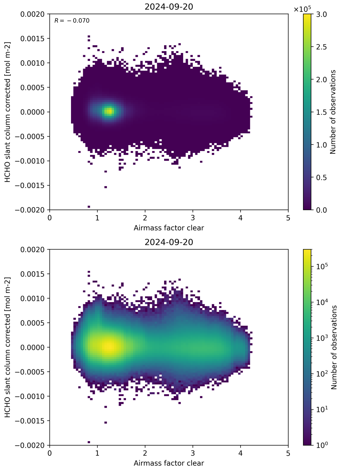
Figure 74: Scatter density plot of “Airmass factor clear” against “HCHO slant column corrected” for 2024-09-19 to 2024-09-21.
