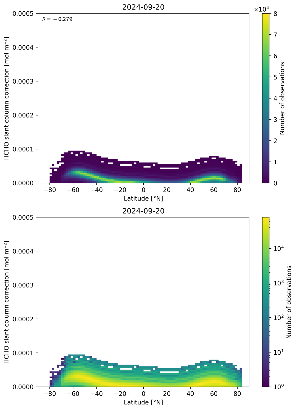
Figure 158: Scatter density plot of “Latitude” against “HCHO slant column correction” for 2024-09-19 to 2024-09-21.
