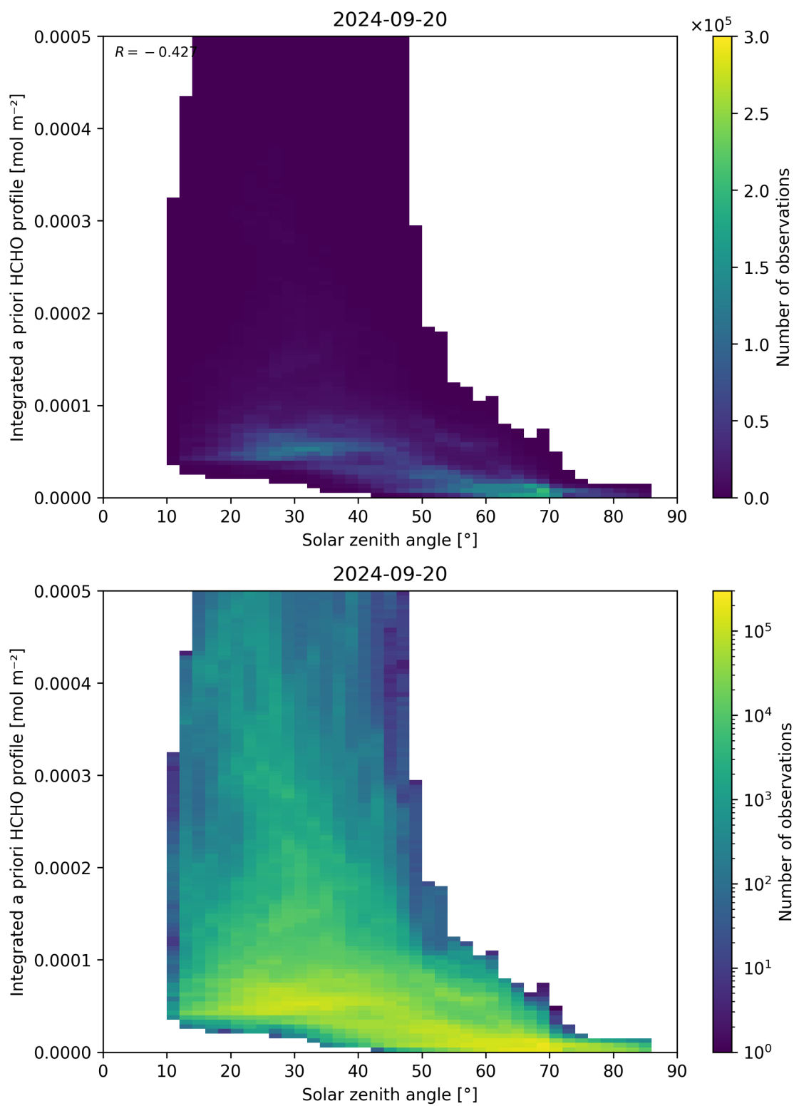
Figure 180: Scatter density plot of “Solar zenith angle” against “Integrated a priori HCHO profile” for 2024-09-19 to 2024-09-21.
