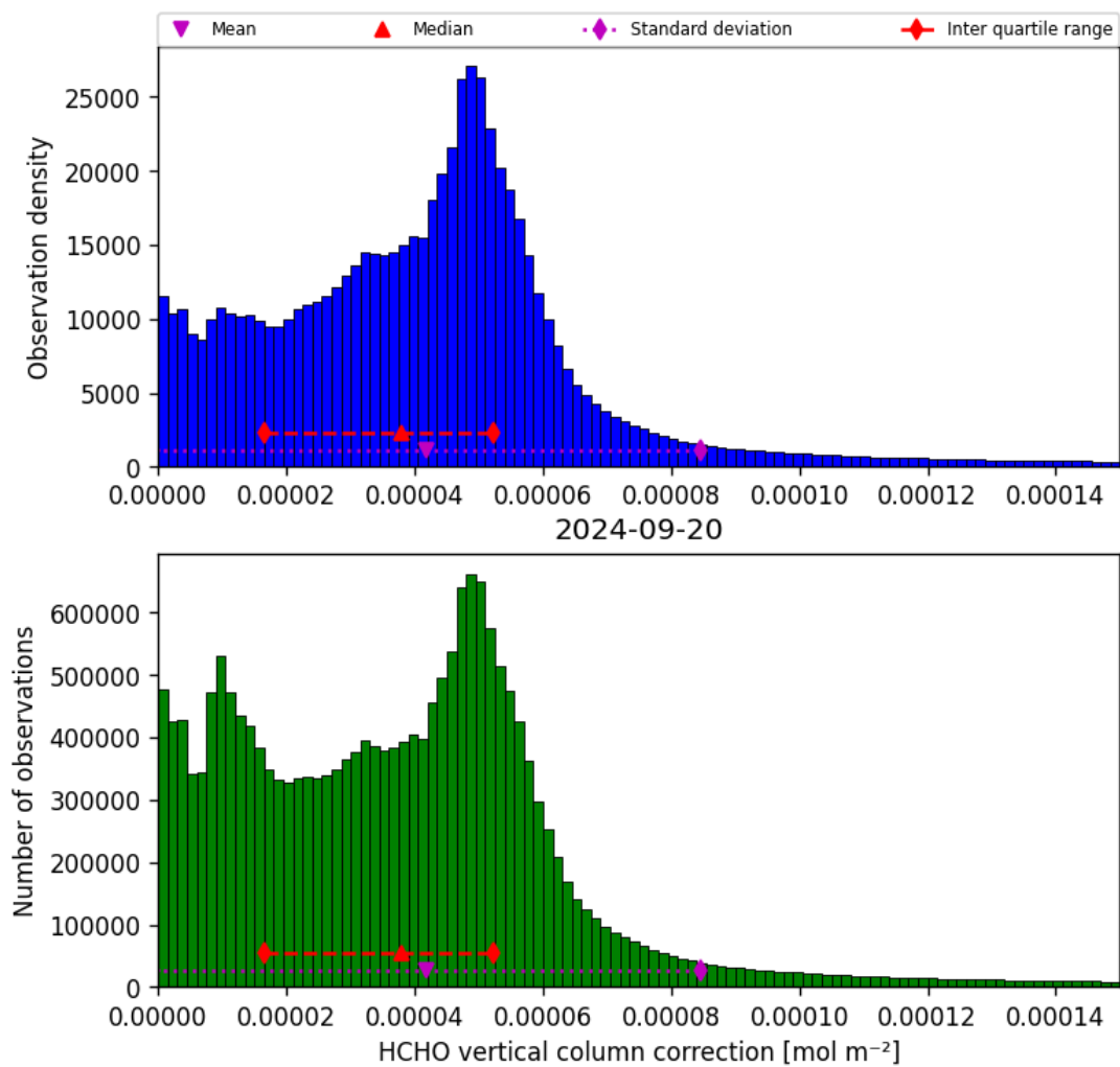
Figure 37: Histogram of “HCHO vertical column correction” for 2024-09-19 to 2024-09-21
