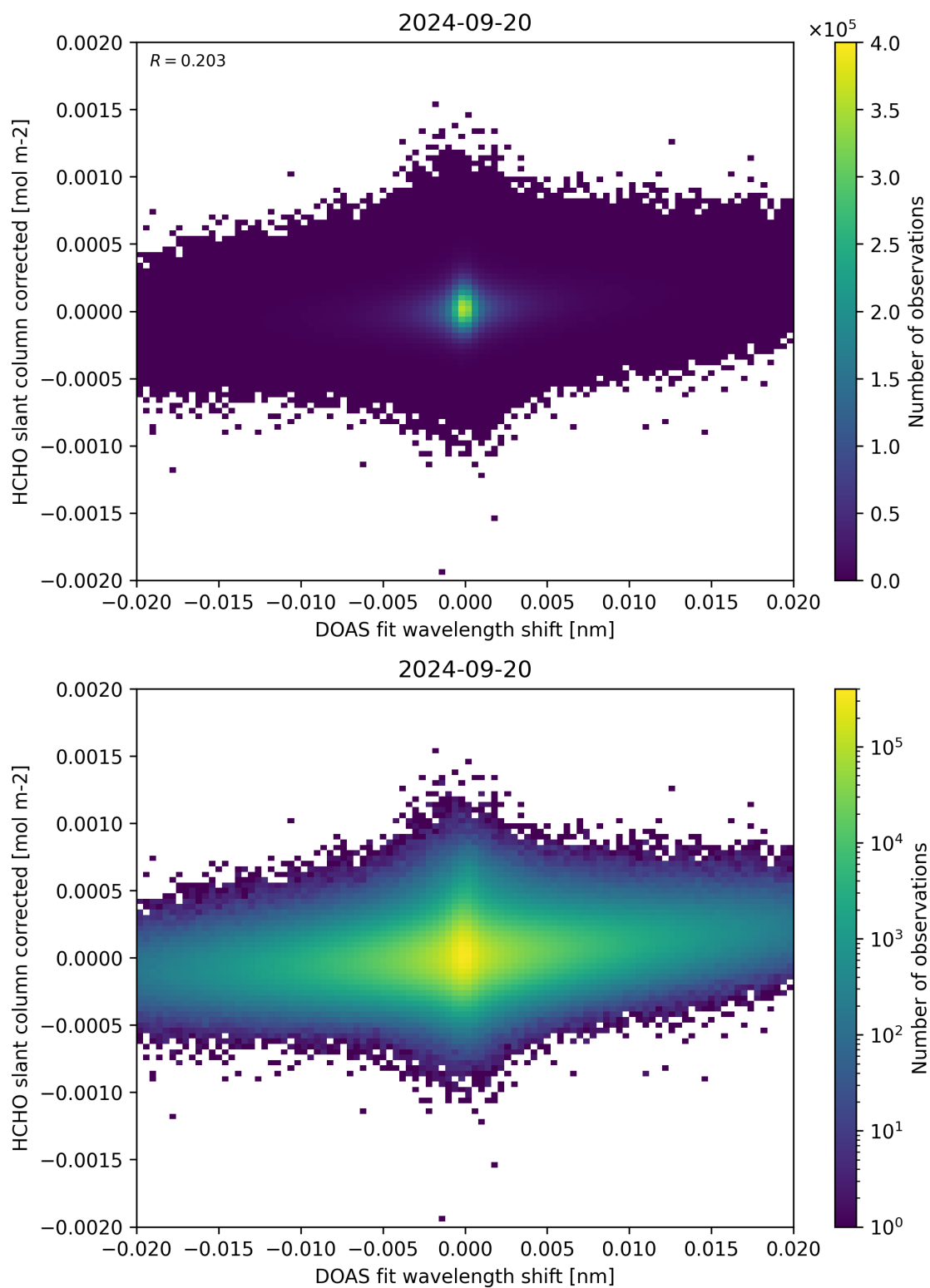
Figure 66: Scatter density plot of “DOAS fit wavelength shift” against “HCHO slant column corrected” for 2024-09-19 to 2024-09-21.
