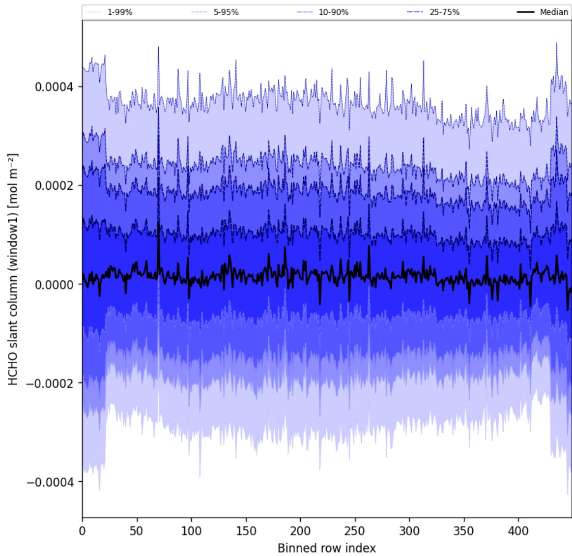
Figure 52: Along track statistics of “HCHO slant column (window1)” for 2024-09-19 to 2024-09-21
