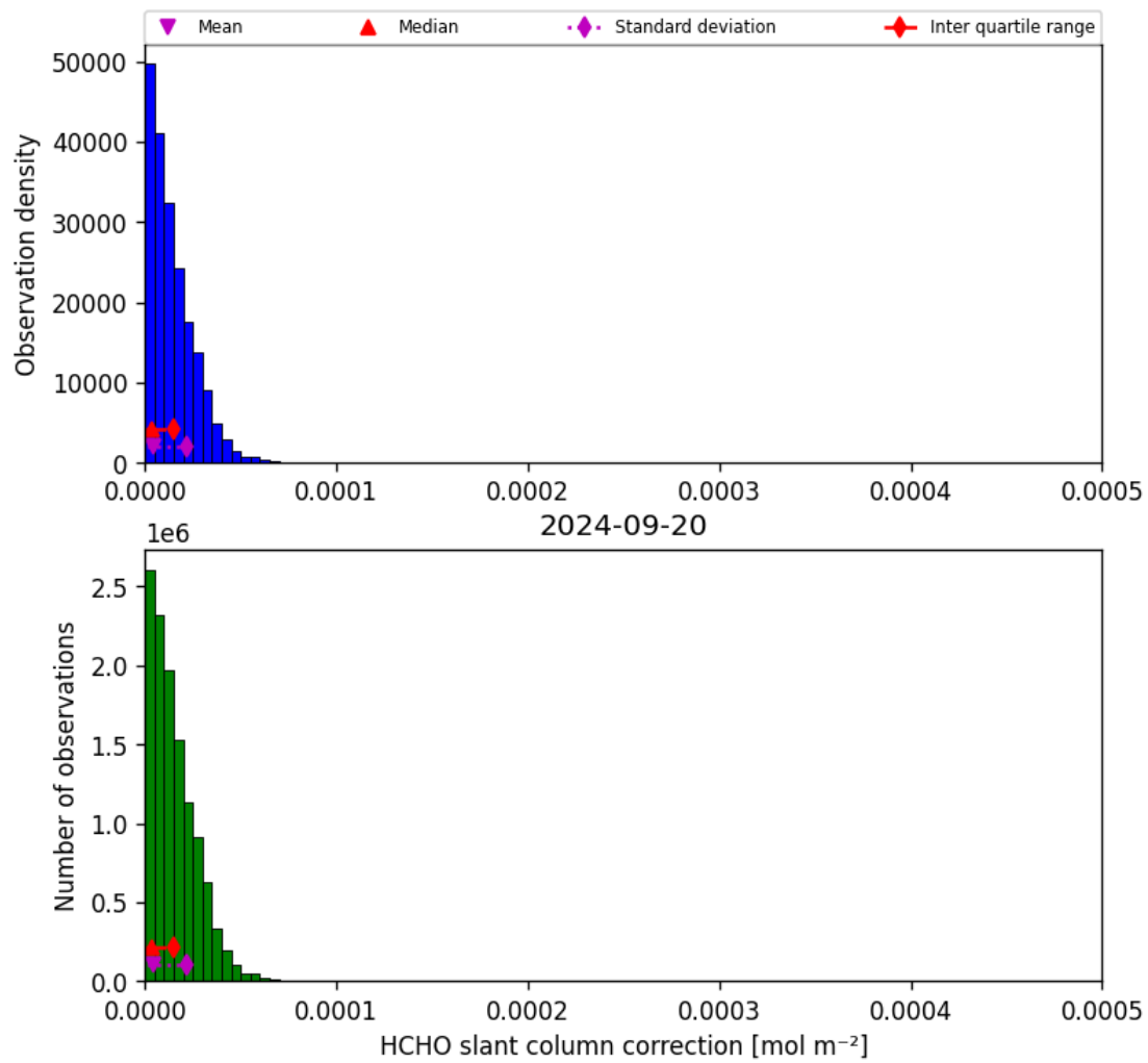
Figure 47: Histogram of “HCHO slant column correction” for 2024-09-19 to 2024-09-21
