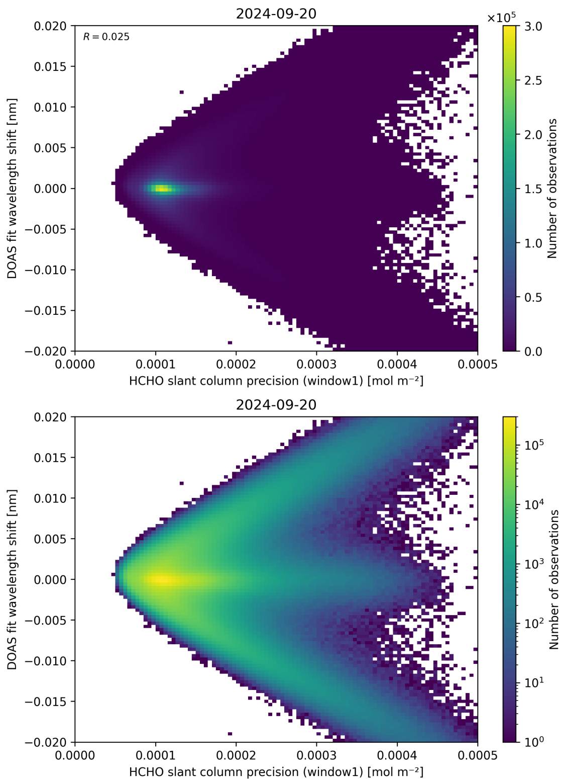
Figure 89: Scatter density plot of “HCHO slant column precision (window1)” against “DOAS fit wavelength shift” for 2024-09-19 to 2024-09-21.
