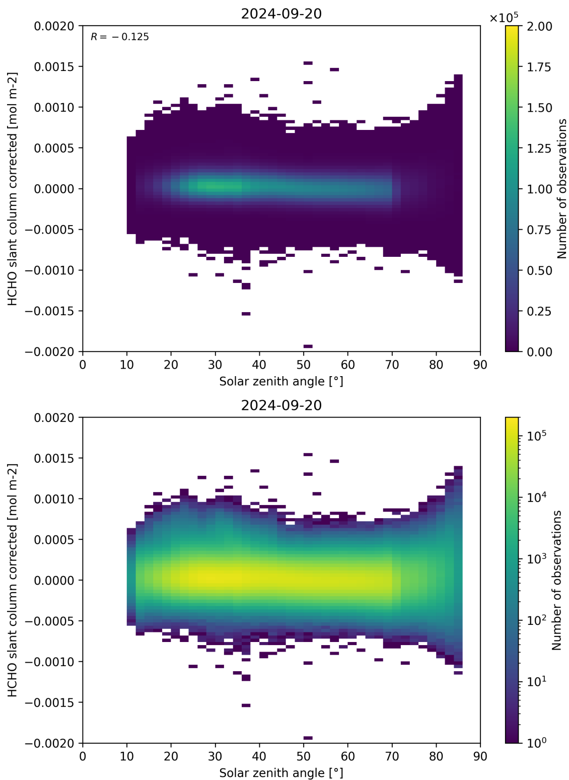
Figure 171: Scatter density plot of “Solar zenith angle” against “HCHO slant column corrected” for 2024-09-19 to 2024-09-21.
