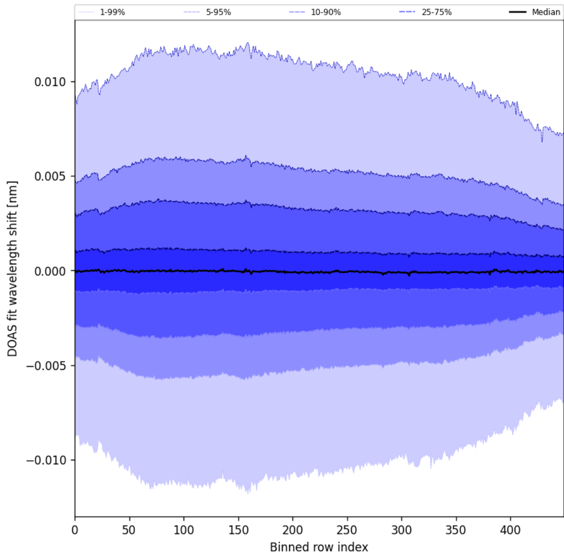
Figure 58: Along track statistics of “DOAS fit wavelength shift” for 2024-09-19 to 2024-09-21
