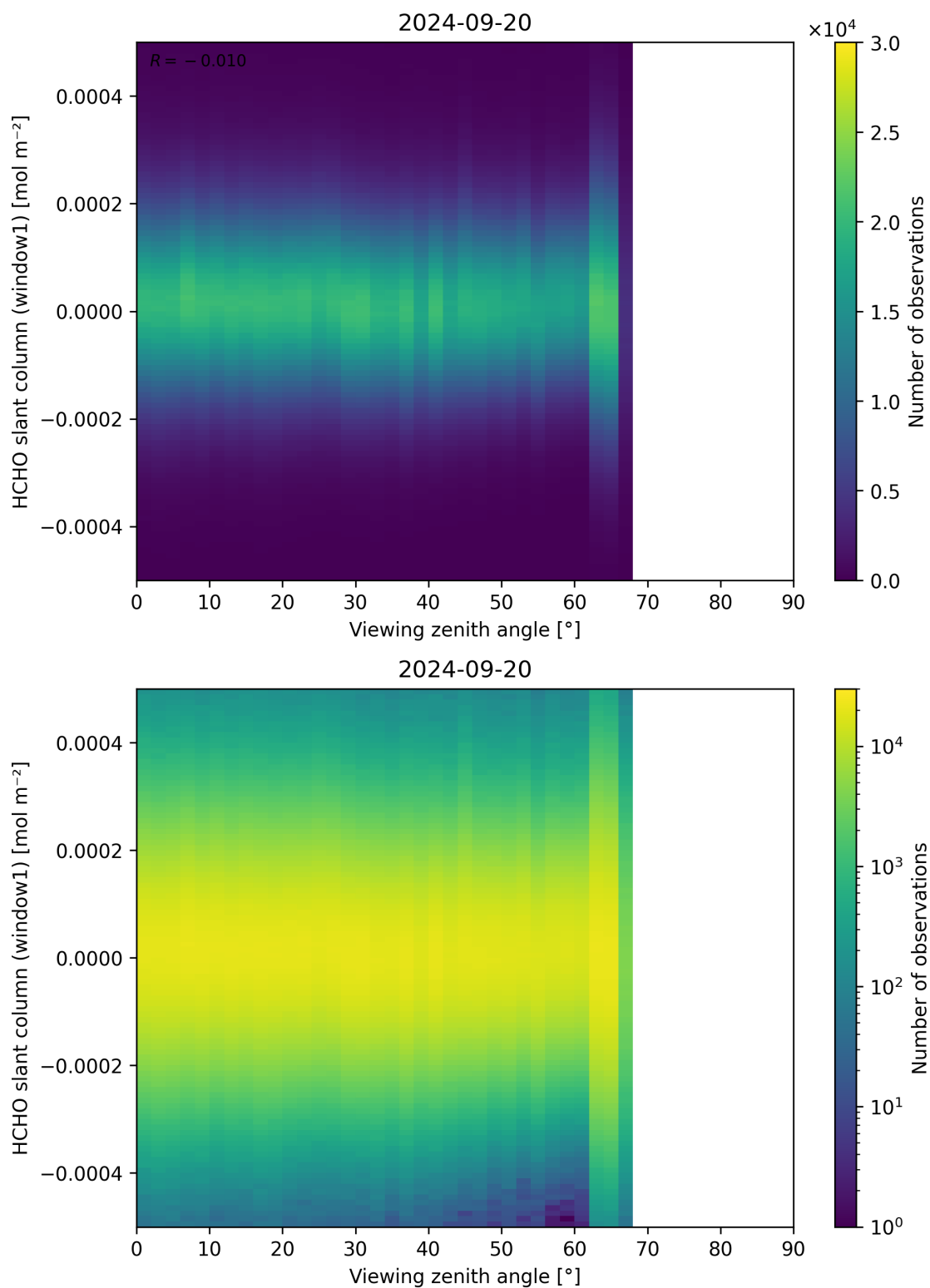
Figure 188: Scatter density plot of “Viewing zenith angle” against “HCHO slant column (window1)” for 2024-09-19 to 2024-09-21.
