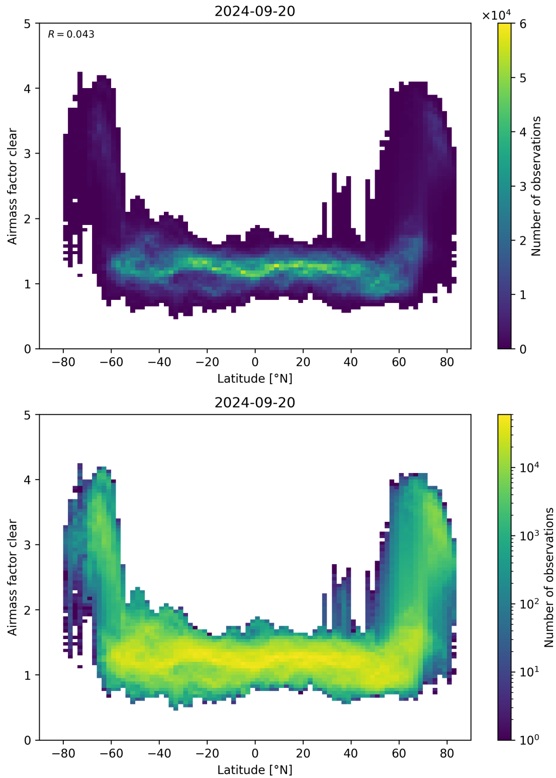
Figure 156: Scatter density plot of “Latitude” against “Airmass factor clear” for 2024-09-19 to 2024-09-21.
