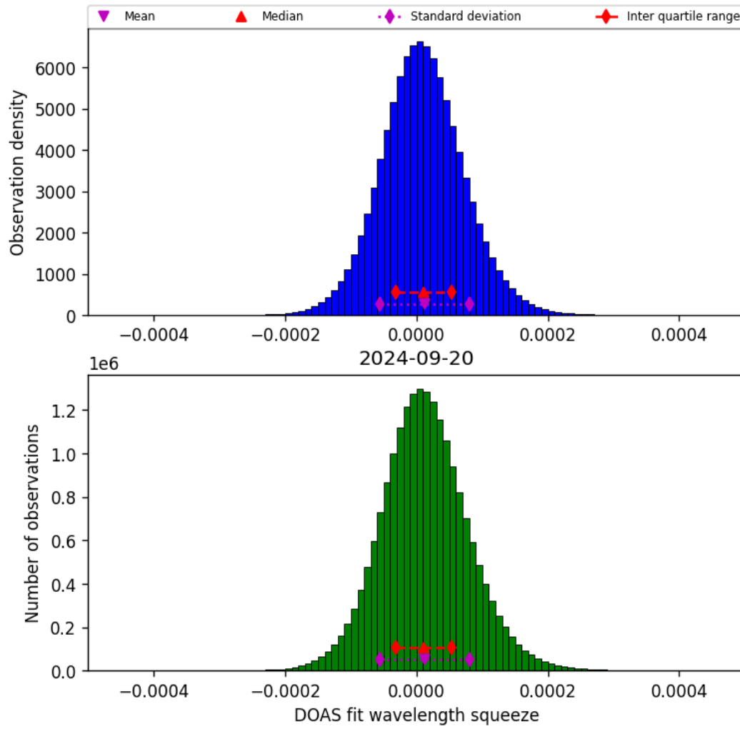
Figure 45: Histogram of “DOAS fit wavelength squeeze” for 2024-09-19 to 2024-09-21
