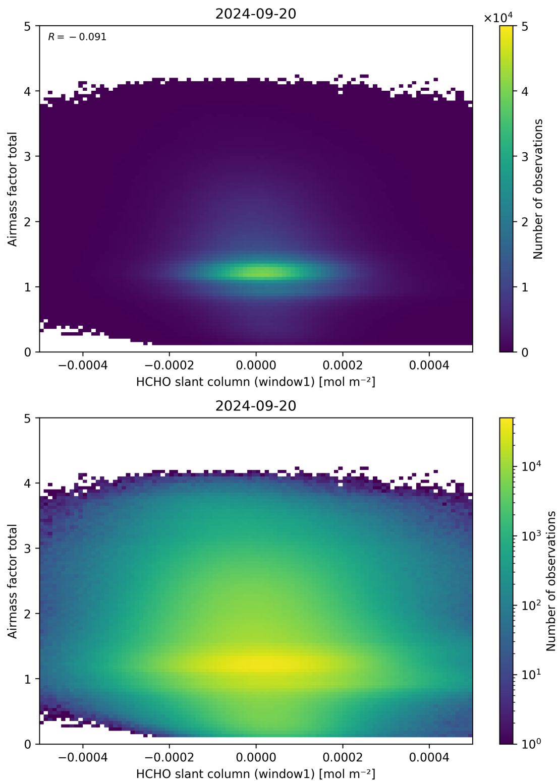
Figure 85: Scatter density plot of “HCHO slant column (window1)” against “Airmass factor total” for 2024-09-19 to 2024-09-21.
