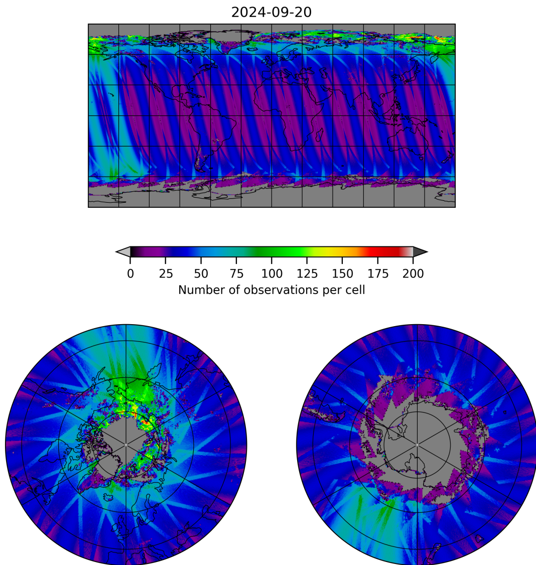
Figure 19: Map of the number of observations for 2024-09-19 to 2024-09-21
