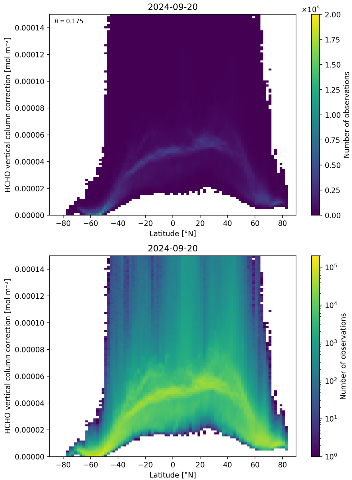
Figure 164: Scatter density plot of “Latitude” against “HCHO vertical column correction” for 2024-09-19 to 2024-09-21.
