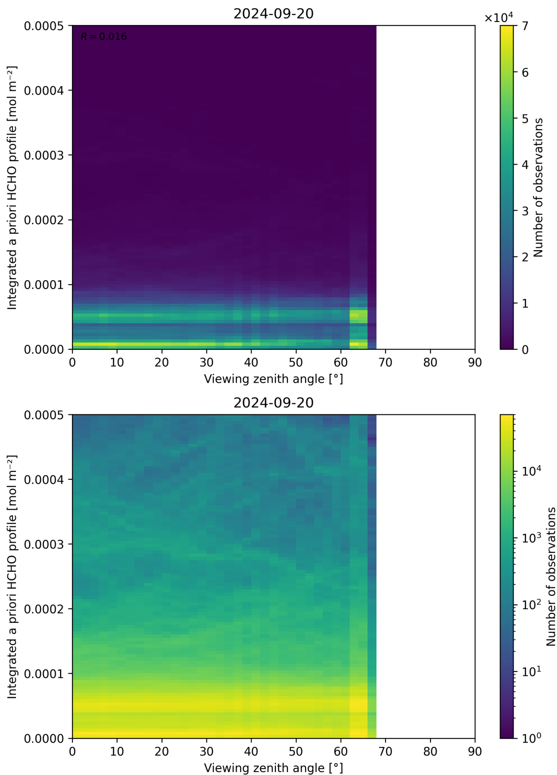
Figure 195: Scatter density plot of “Viewing zenith angle” against “Integrated a priori HCHO profile” for 2024-09-19 to 2024-09-21.
