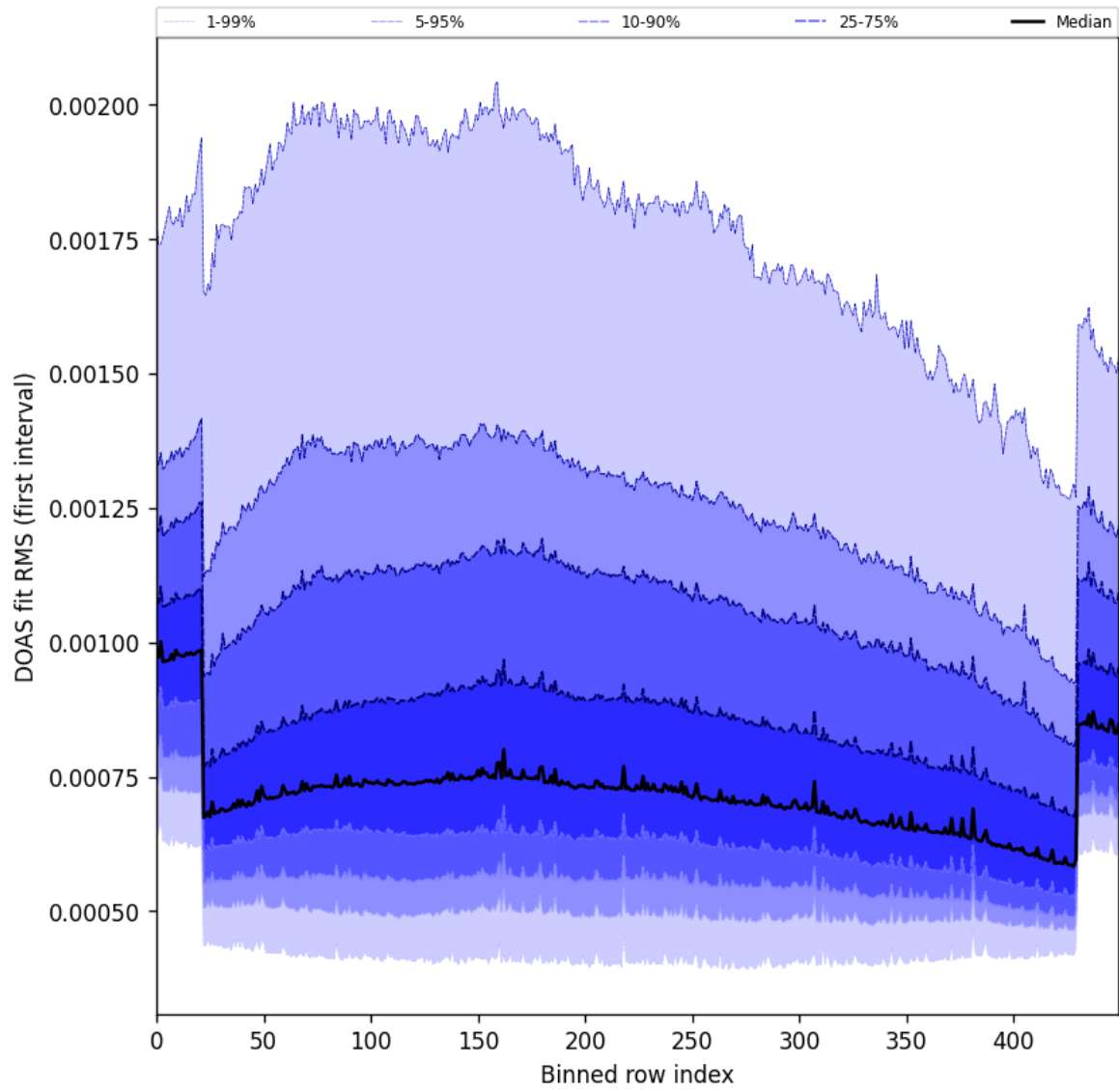
Figure 60: Along track statistics of “DOAS fit RMS (first interval)” for 2024-09-19 to 2024-09-21
