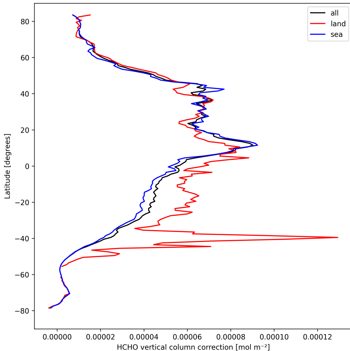
Figure 23: Zonal average of “HCHO vertical column correction” for 2024-09-19 to 2024-09-21.
