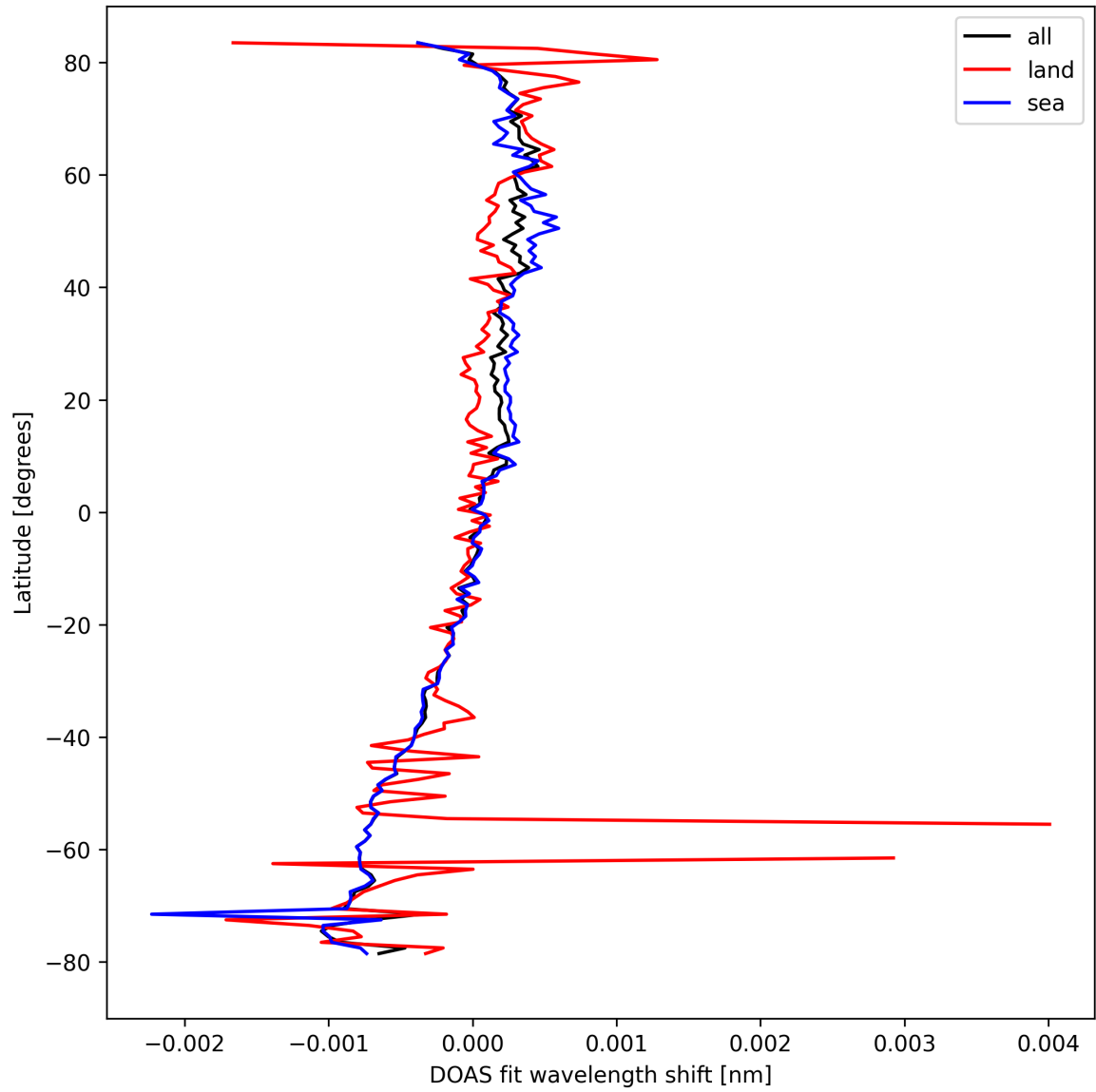
Figure 30: Zonal average of “DOAS fit wavelength shift” for 2024-09-19 to 2024-09-21.
