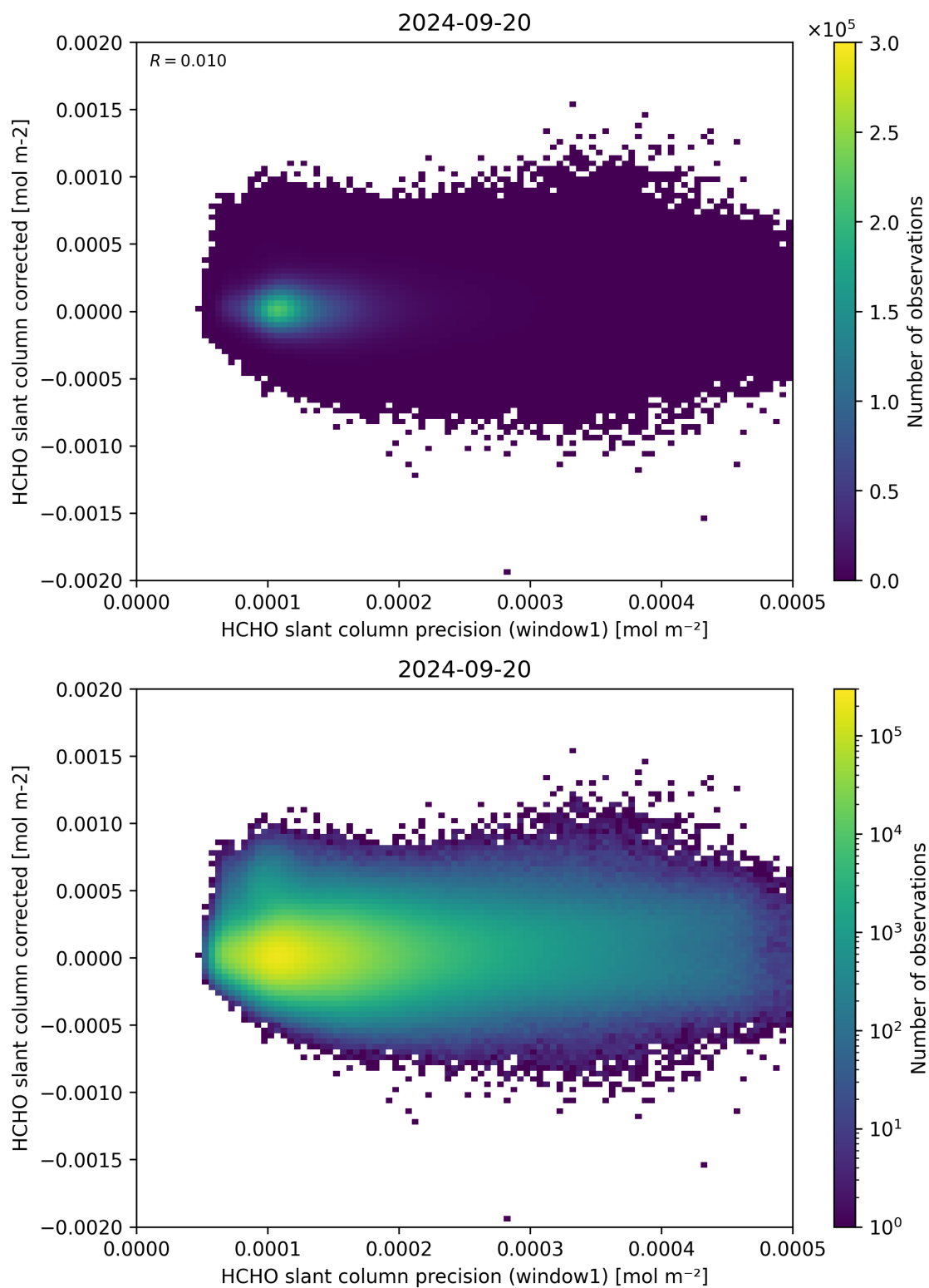
Figure 92: Scatter density plot of “HCHO slant column precision (window1)” against “HCHO slant column corrected” for 2024-09-19 to 2024-09-21.
