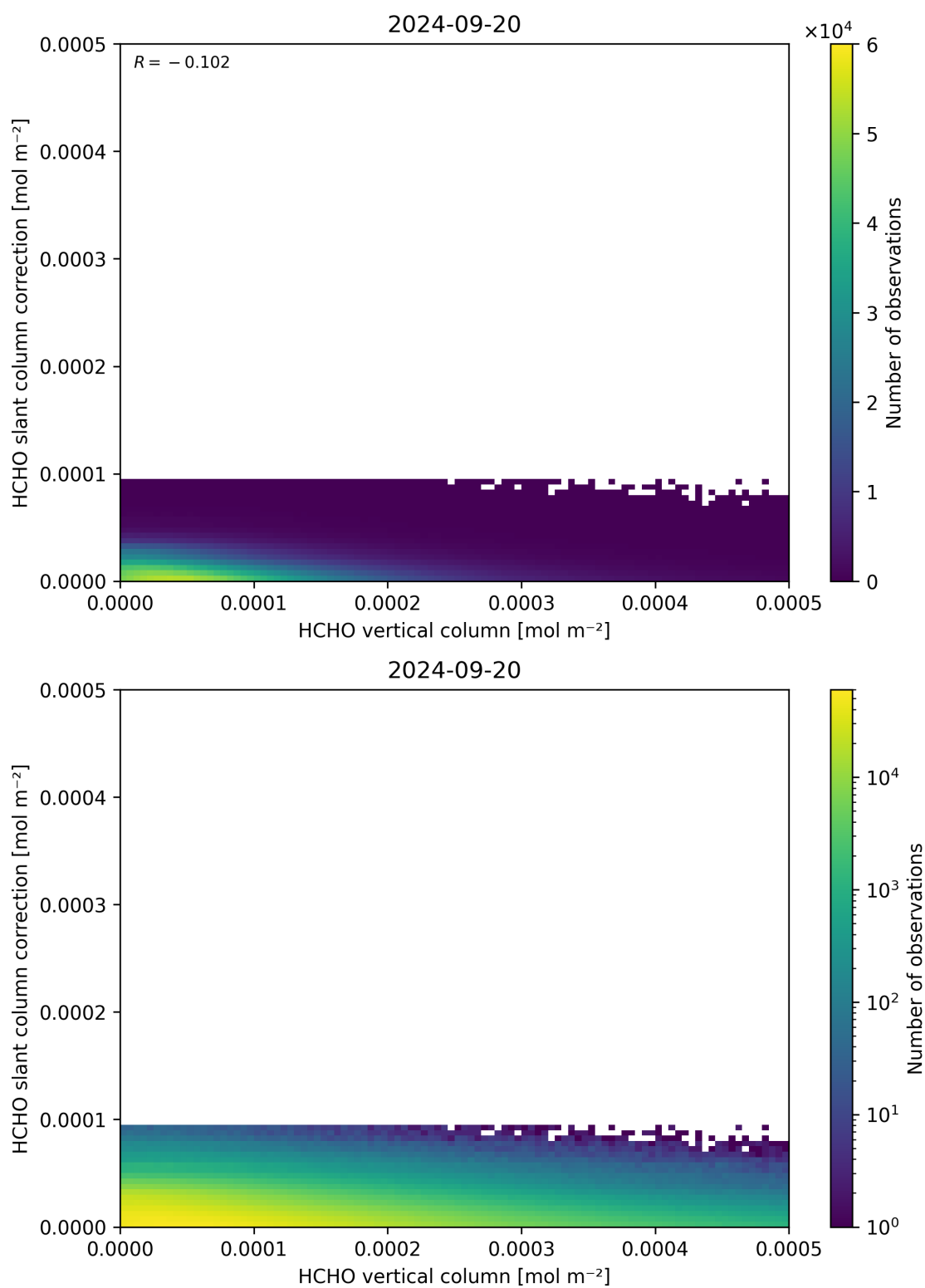
Figure 128: Scatter density plot of “HCHO vertical column” against “HCHO slant column correction” for 2024-09-19 to 2024-09-21.
