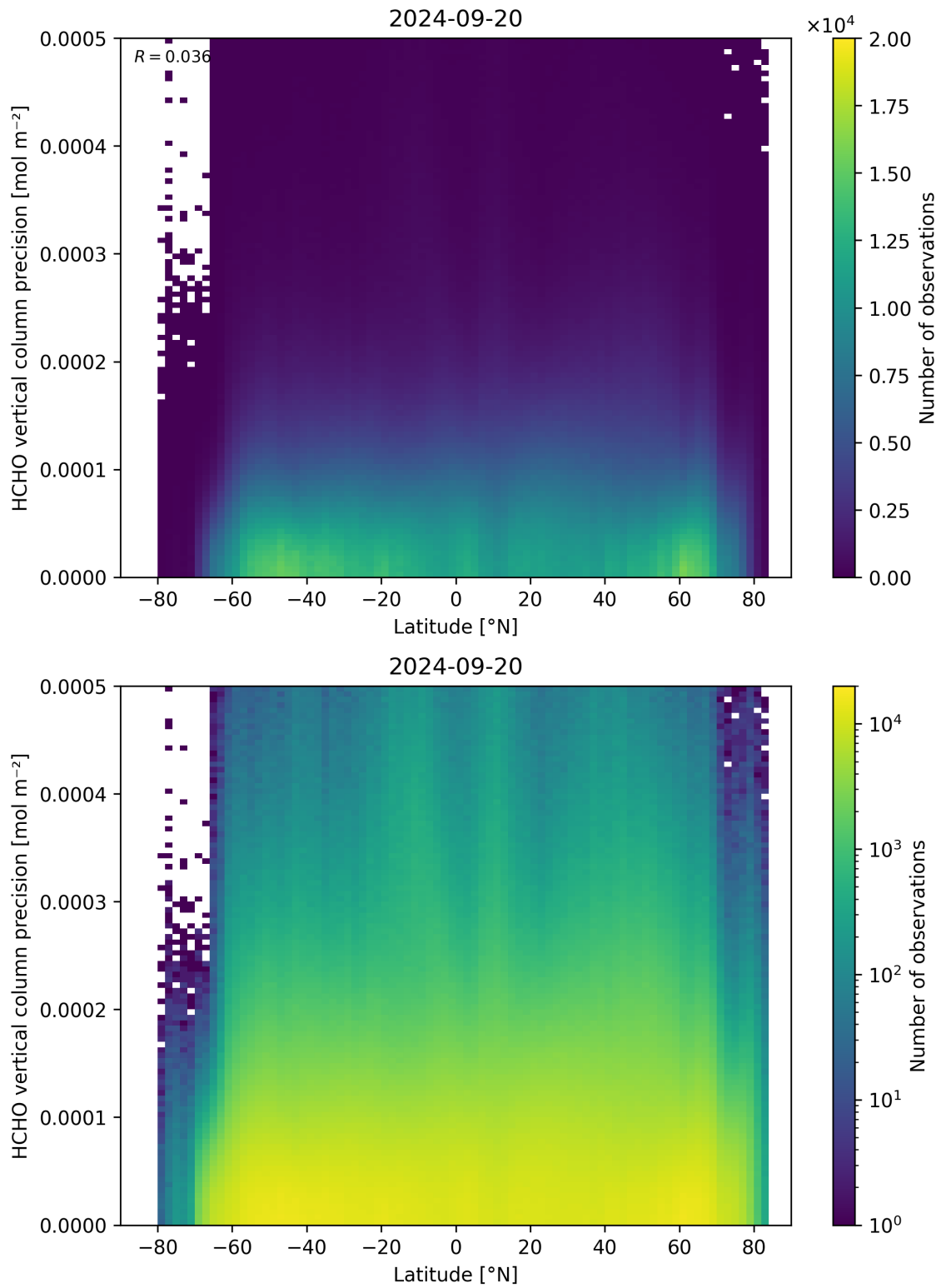
Figure 165: Scatter density plot of “Latitude” against “HCHO vertical column precision” for 2024-09-19 to 2024-09-21.
