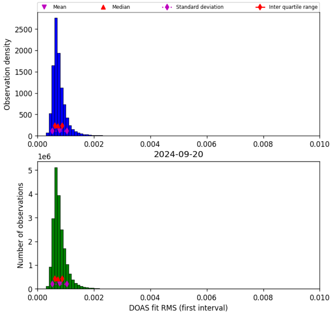
Figure 46: Histogram of “DOAS fit RMS (first interval)” for 2024-09-19 to 2024-09-21
