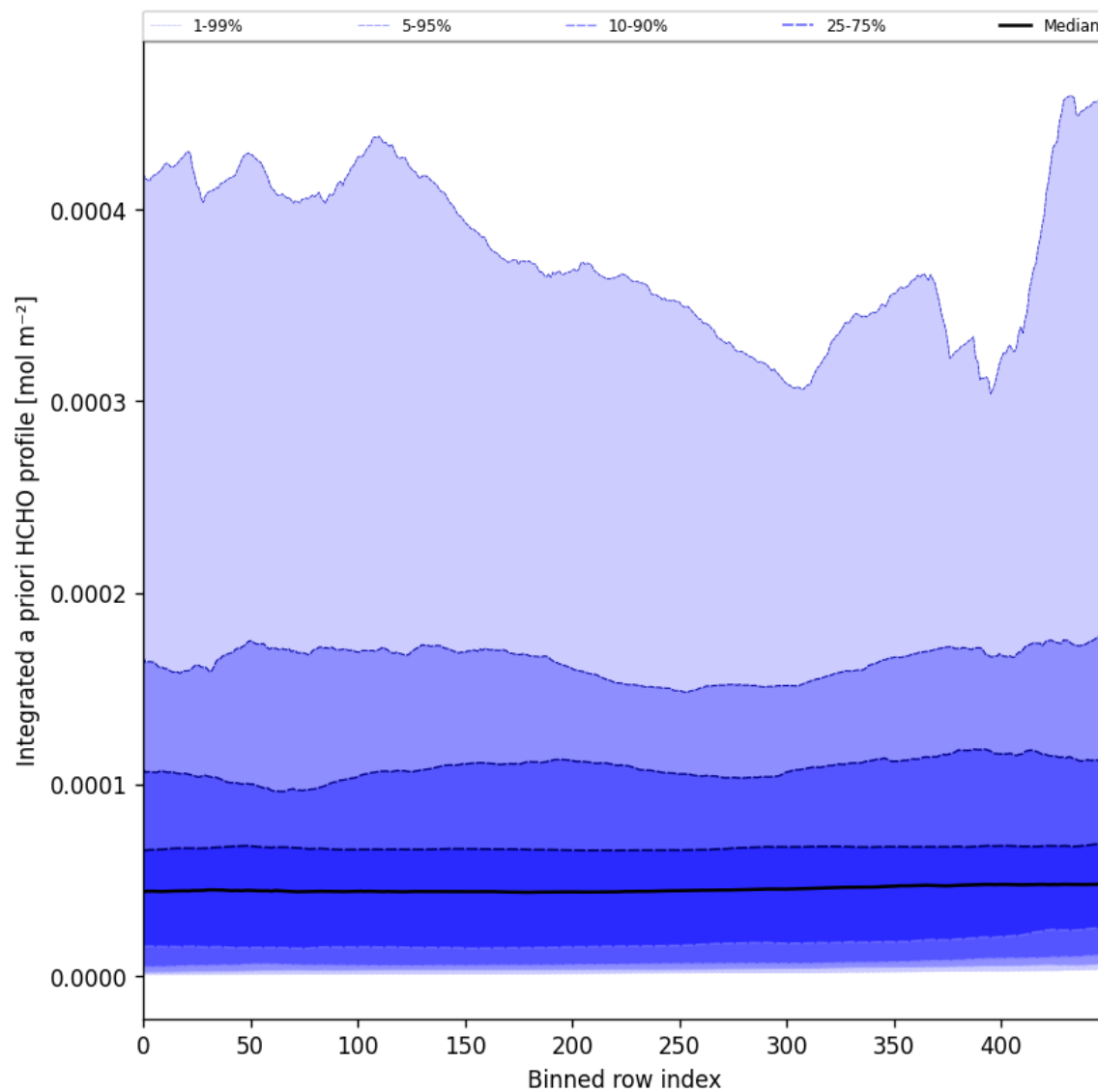
Figure 57: Along track statistics of "Integrated a priori HCHO profile" for 2024-09-19 to 2024-09-21
