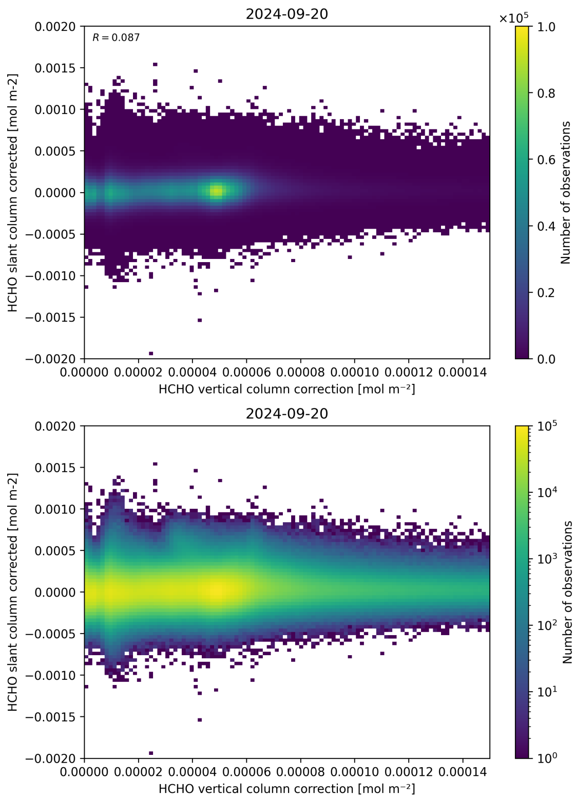
Figure 116: Scatter density plot of “HCHO vertical column correction” against “HCHO slant column corrected” for 2024-09-19 to 2024-09-21.
