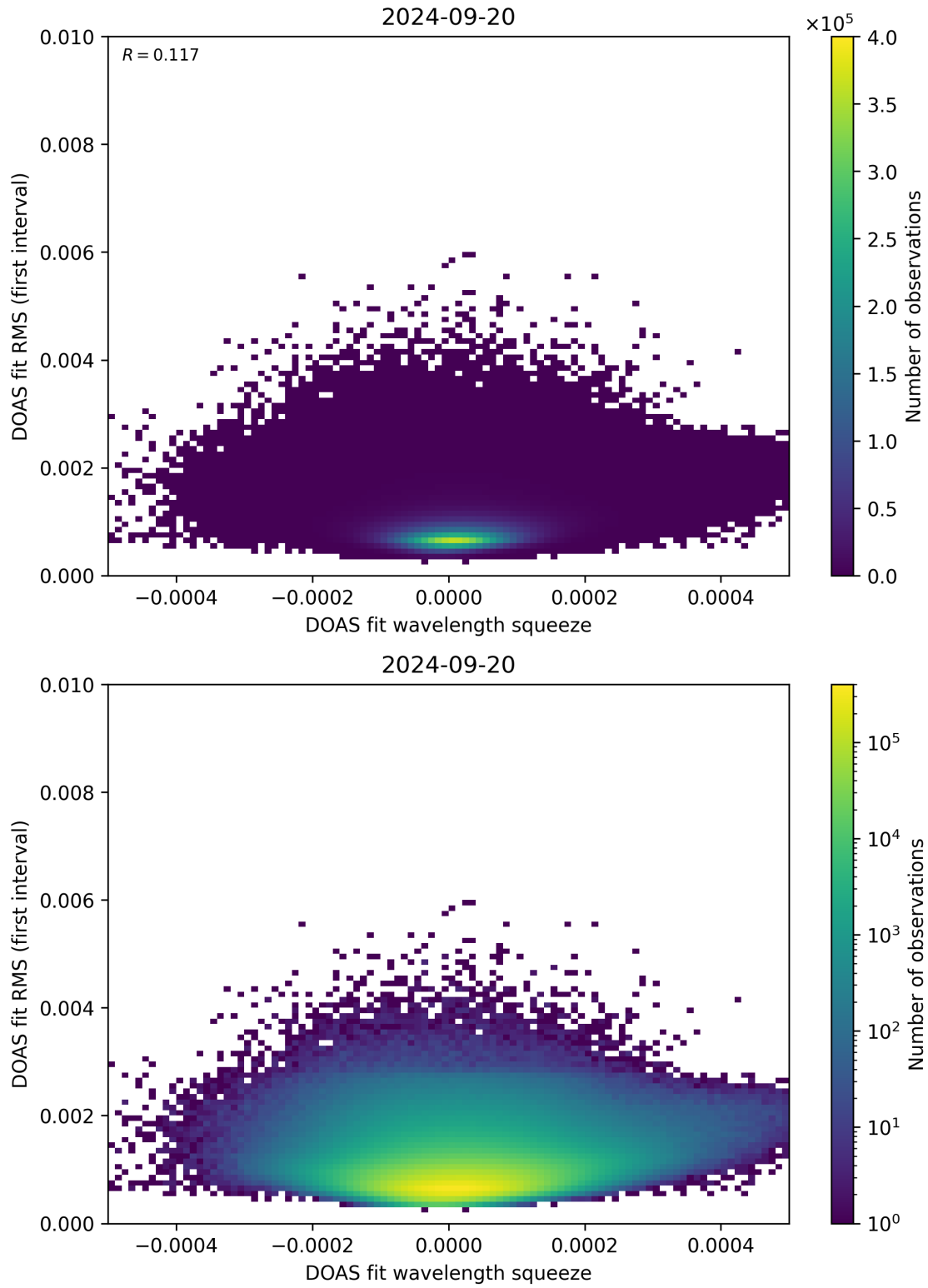
Figure 68: Scatter density plot of “DOAS fit wavelength squeeze” against “DOAS fit RMS (first interval)” for 2024-09-19 to 2024-09-21.
