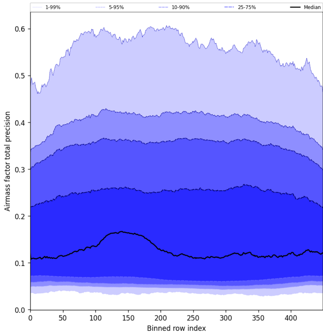
Figure 55: Along track statistics of “Airmass factor total precision” for 2024-09-19 to 2024-09-21
