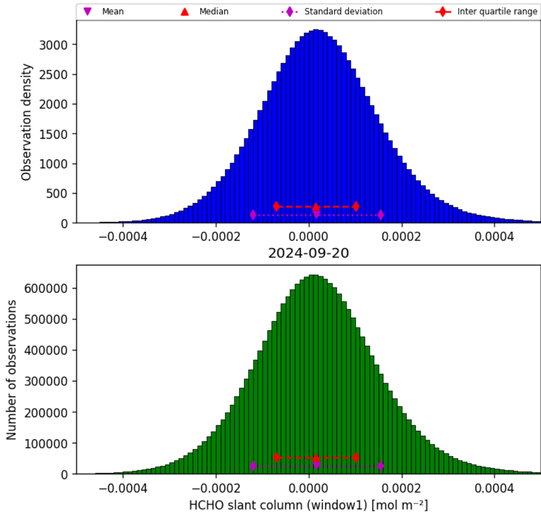
Figure 38: Histogram of “HCHO slant column (window1)” for 2024-09-19 to 2024-09-21
