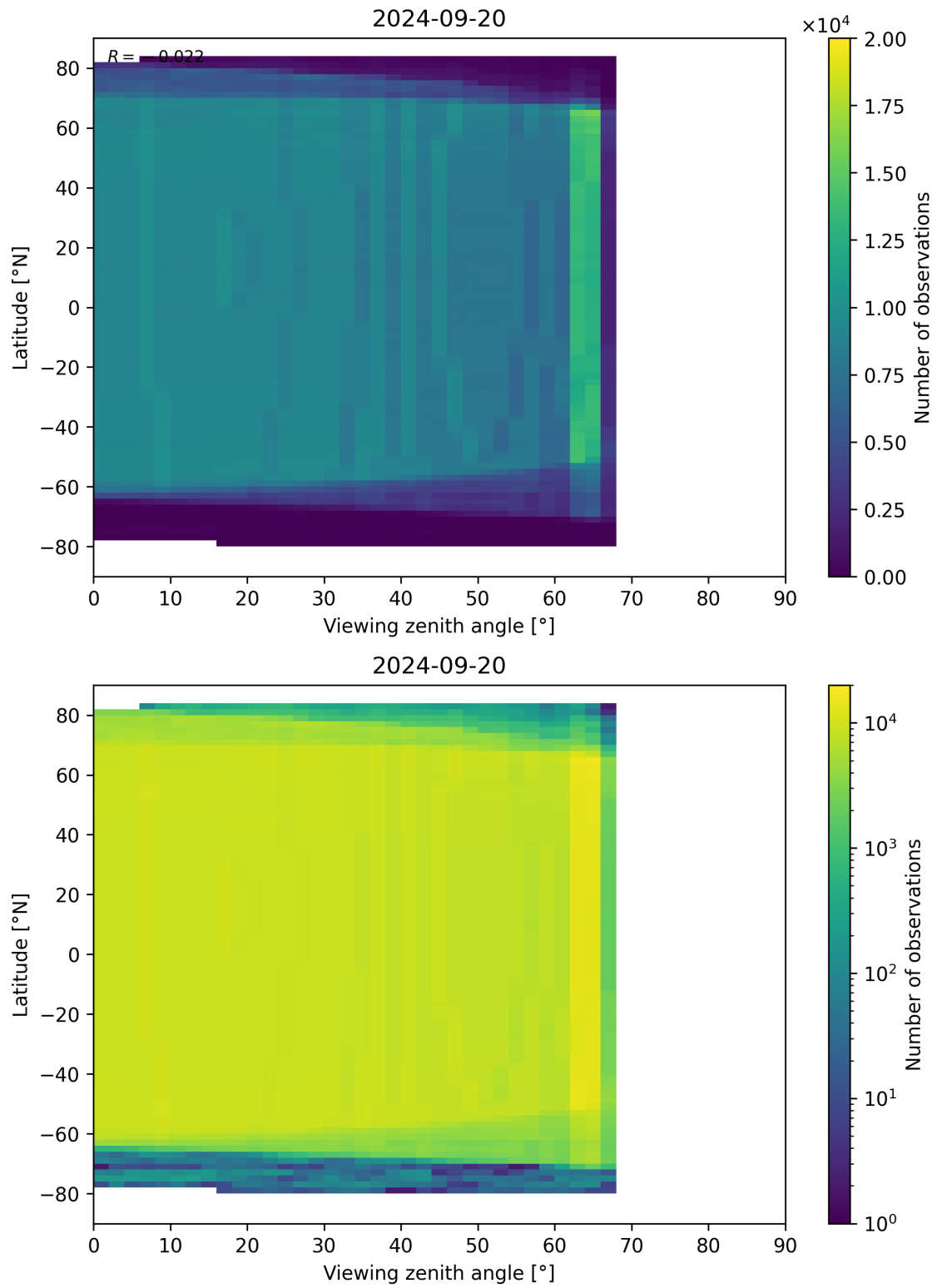
Figure 196: Scatter density plot of “Viewing zenith angle” against “Latitude” for 2024-09-19 to 2024-09-21.
