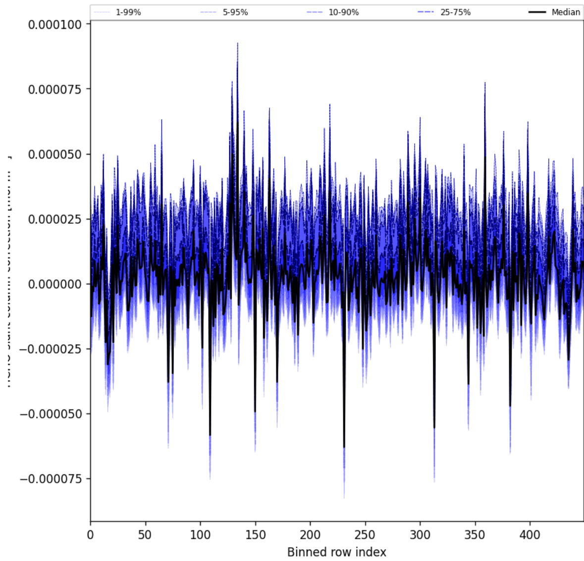
Figure 61: Along track statistics of “HCHO slant column correction” for 2024-09-19 to 2024-09-21
