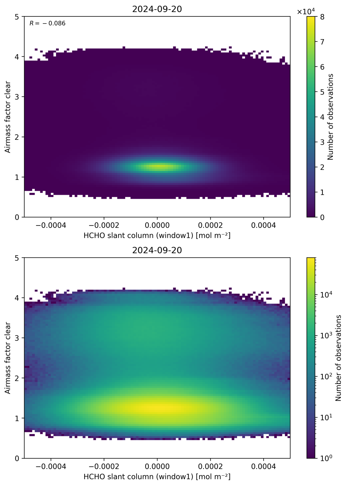
Figure 81: Scatter density plot of “HCHO slant column (window1)” against “Airmass factor clear” for 2024-09-19 to 2024-09-21.
