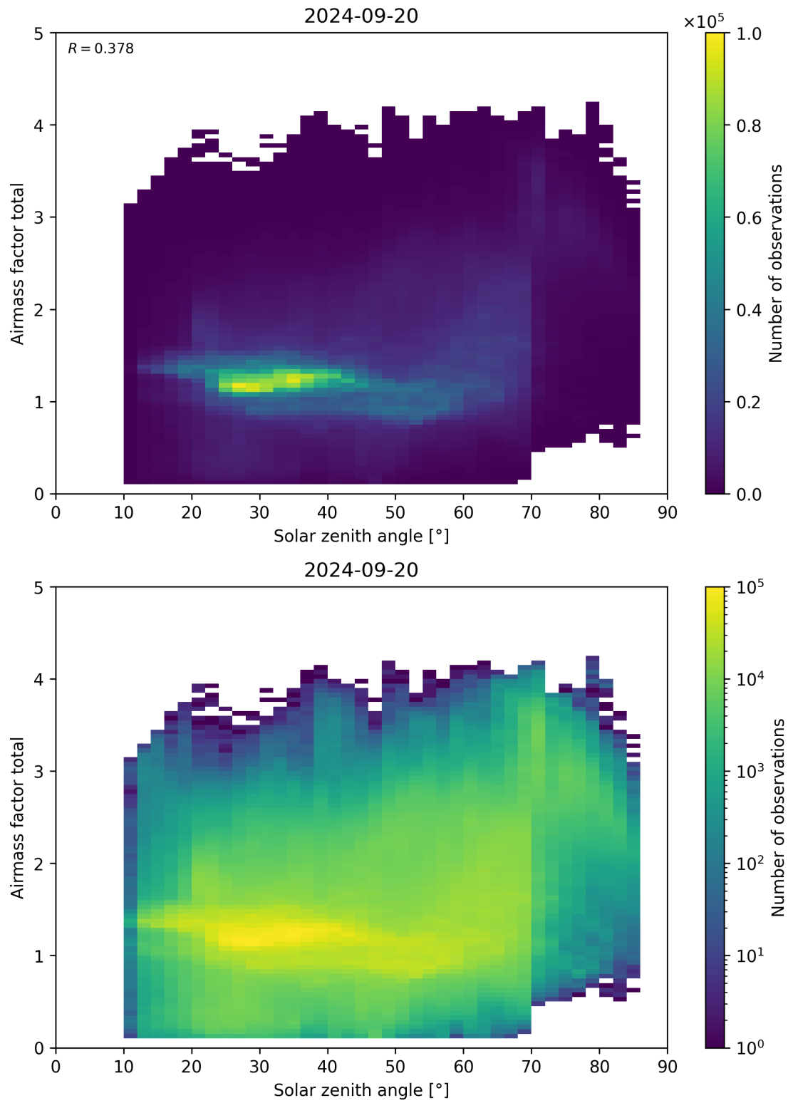
Figure 175: Scatter density plot of “Solar zenith angle” against “Airmass factor total” for 2024-09-19 to 2024-09-21.
