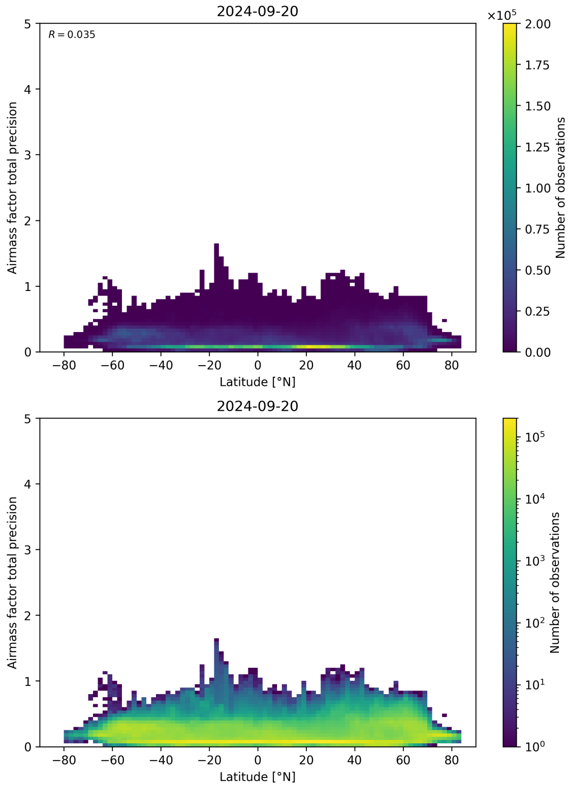
Figure 162: Scatter density plot of “Latitude” against “Airmass factor total precision” for 2024-09-19 to 2024-09-21.
