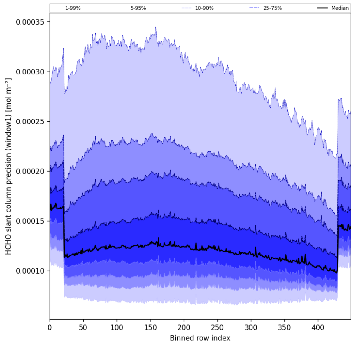
Figure 53: Along track statistics of “HCHO slant column precision (window1)” for 2024-09-19 to 2024-09-21
