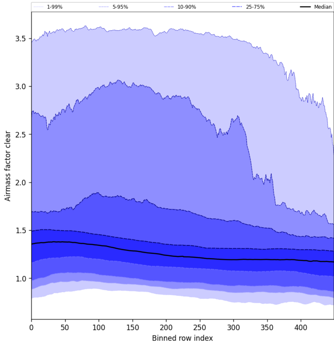
Figure 56: Along track statistics of “Airmass factor clear” for 2024-09-19 to 2024-09-21
