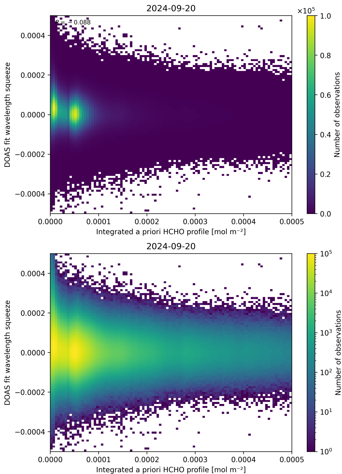
Figure 150: Scatter density plot of “Integrated a priori HCHO profile” against “DOAS fit wavelength squeeze” for 2024-09-19 to 2024-09-21.
