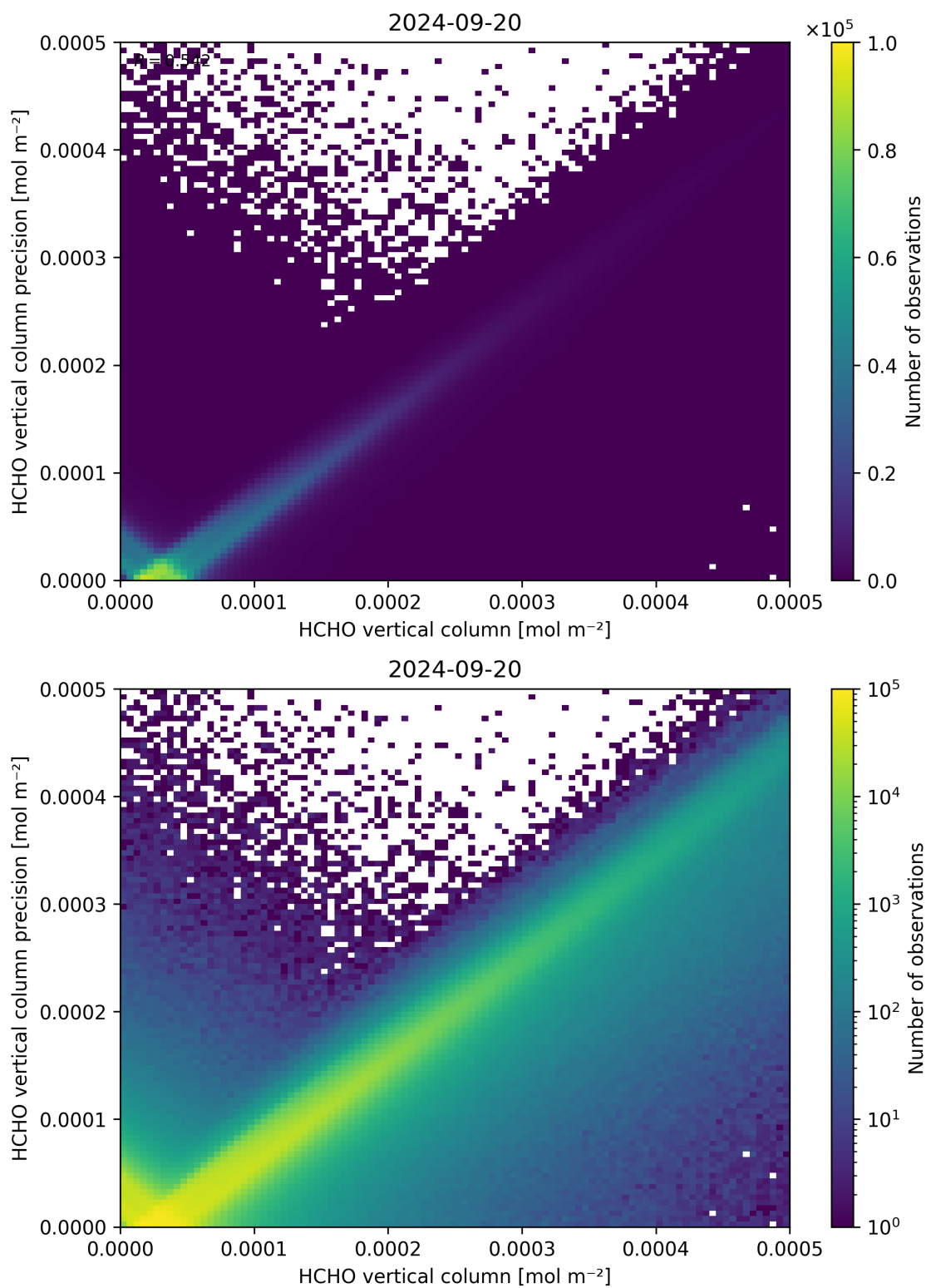
Figure 134: Scatter density plot of “HCHO vertical column” against “HCHO vertical column precision” for 2024-09-19 to 2024-09-21.
