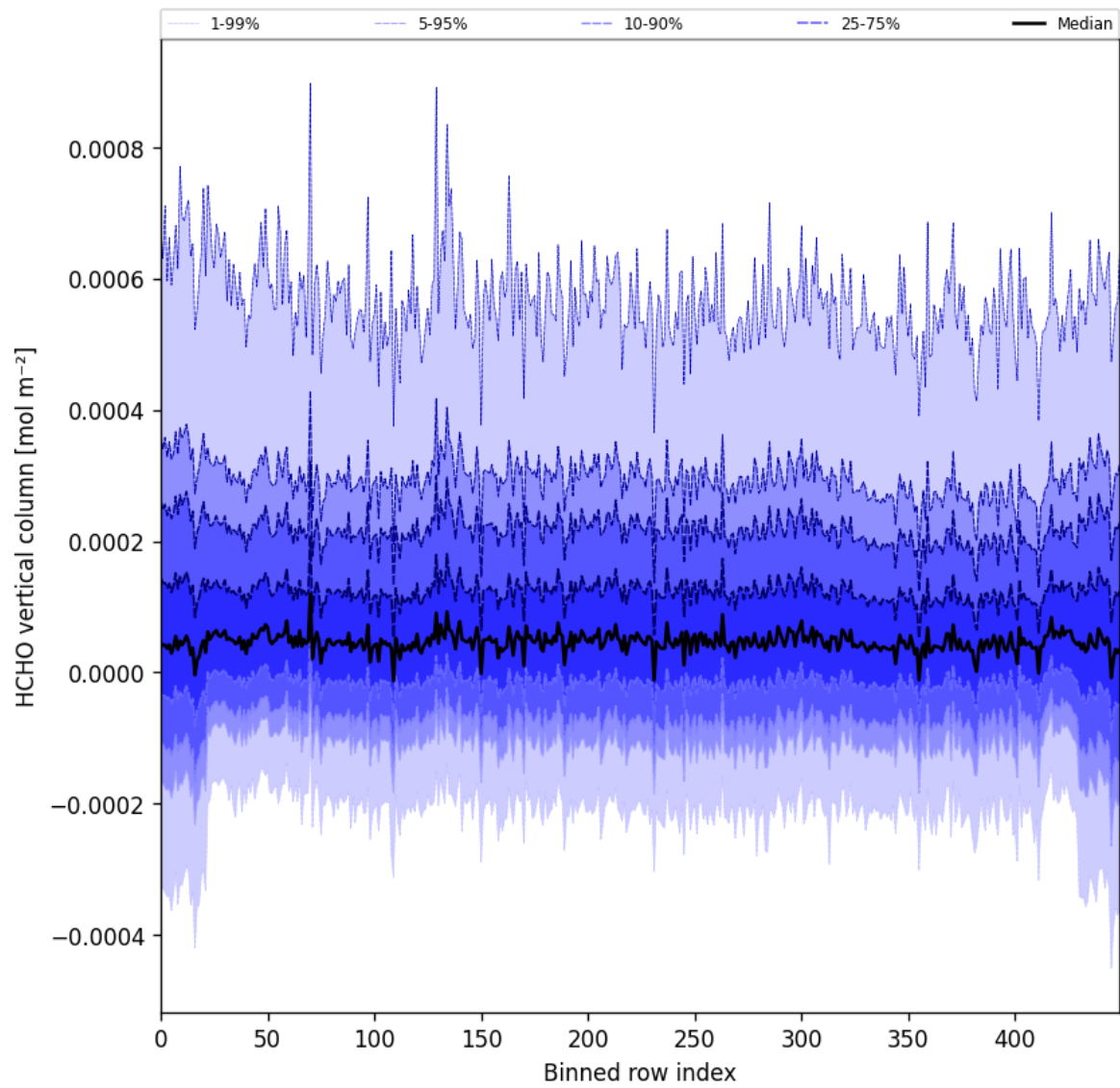
Figure 49: Along track statistics of “HCHO vertical column” for 2024-09-19 to 2024-09-21
