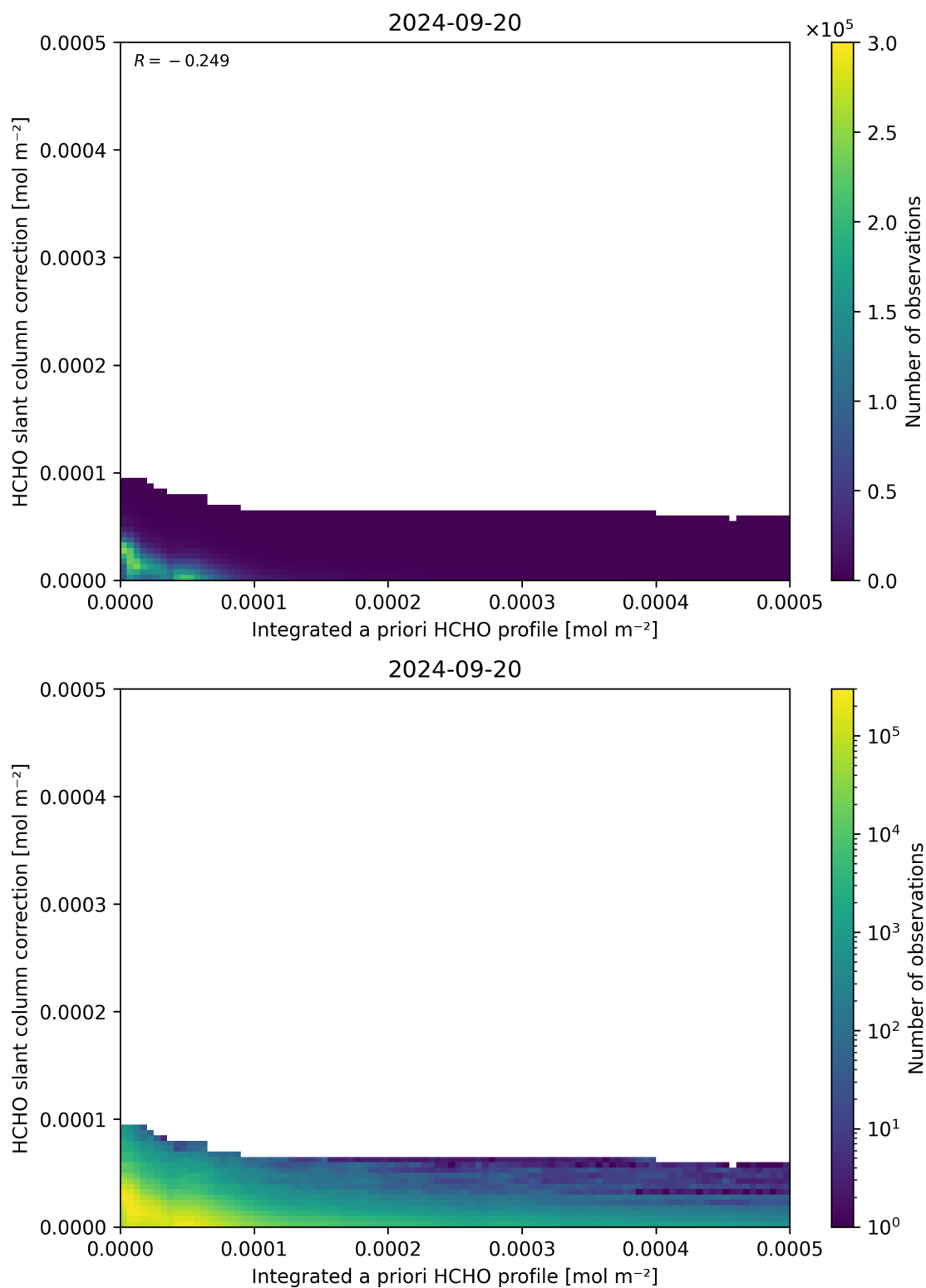
Figure 152: Scatter density plot of “Integrated a priori HCHO profile” against “HCHO slant column correction” for 2024-09-19 to 2024-09-21.
