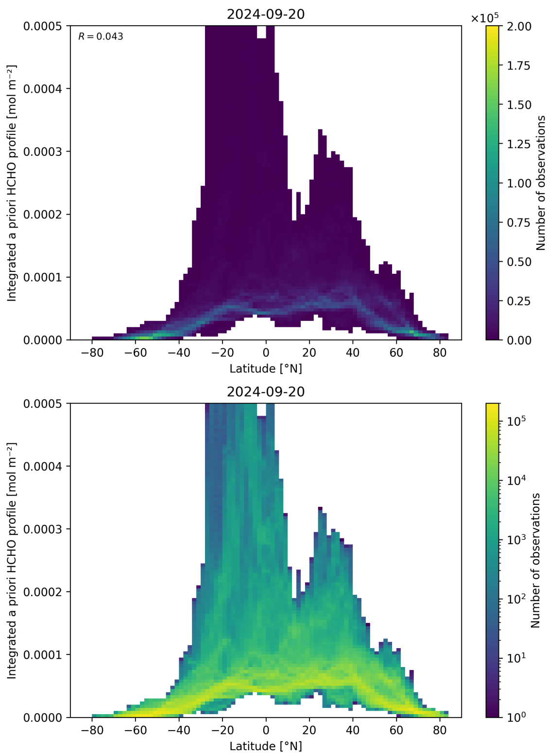
Figure 166: Scatter density plot of “Latitude” against “Integrated a priori HCHO profile” for 2024-09-19 to 2024-09-21.
