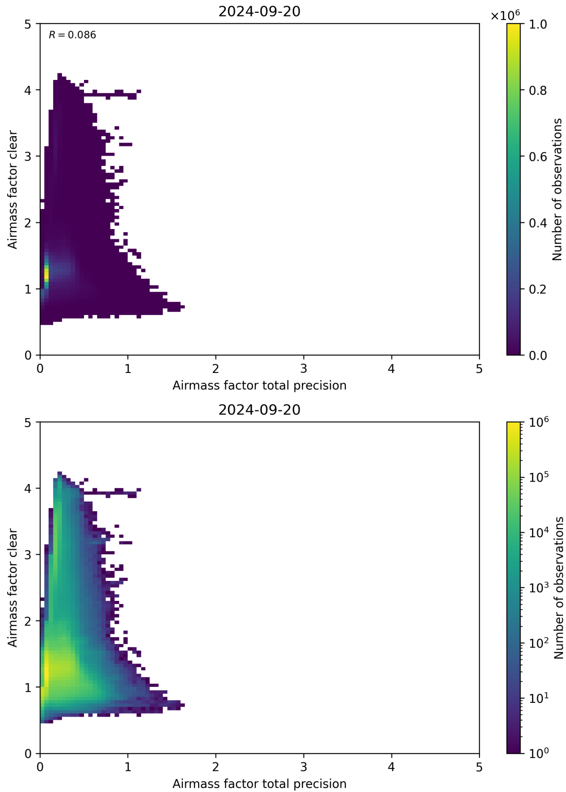
Figure 108: Scatter density plot of “Airmass factor total precision” against “Airmass factor clear” for 2024-09-19 to 2024-09-21.
