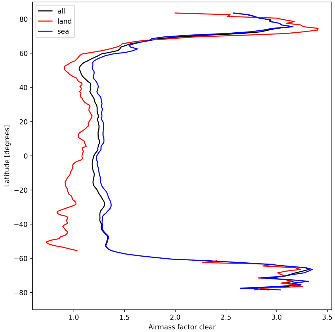
Figure 28: Zonal average of “Airmass factor clear” for 2024-09-19 to 2024-09-21.
