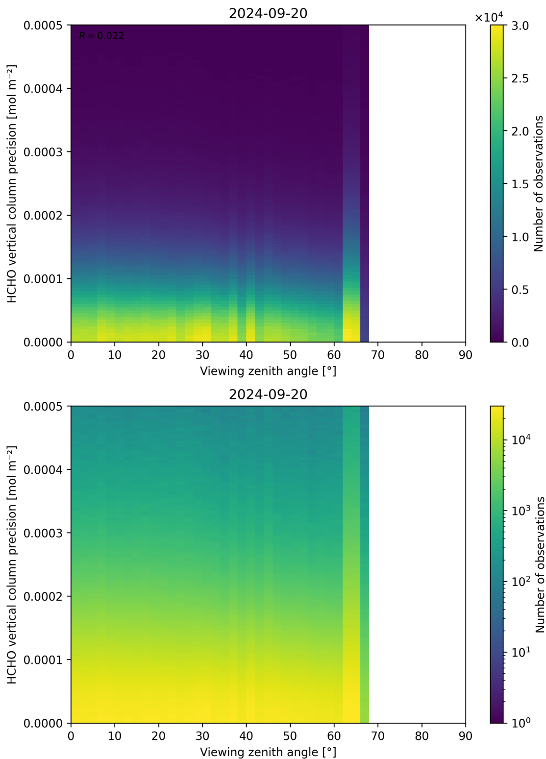
Figure 194: Scatter density plot of “Viewing zenith angle” against “HCHO vertical column precision” for 2024-09-19 to 2024-09-21.
