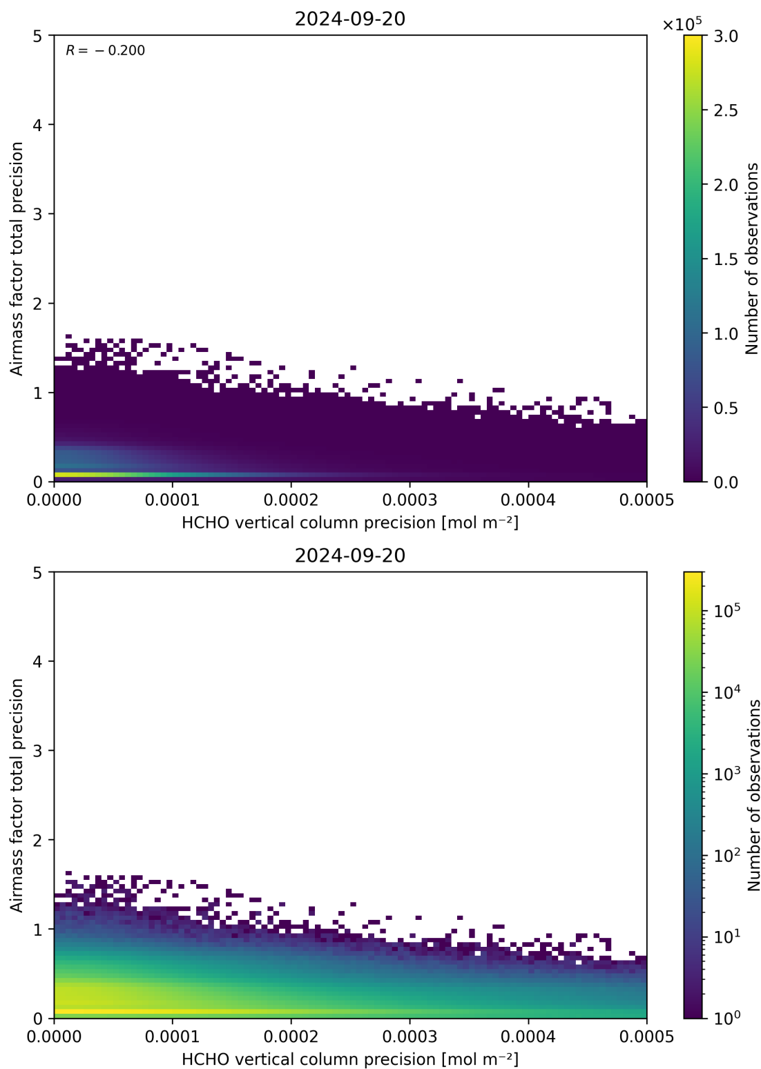
Figure 145: Scatter density plot of “HCHO vertical column precision” against “Airmass factor total precision” for 2024-09-19 to 2024-09-21.
