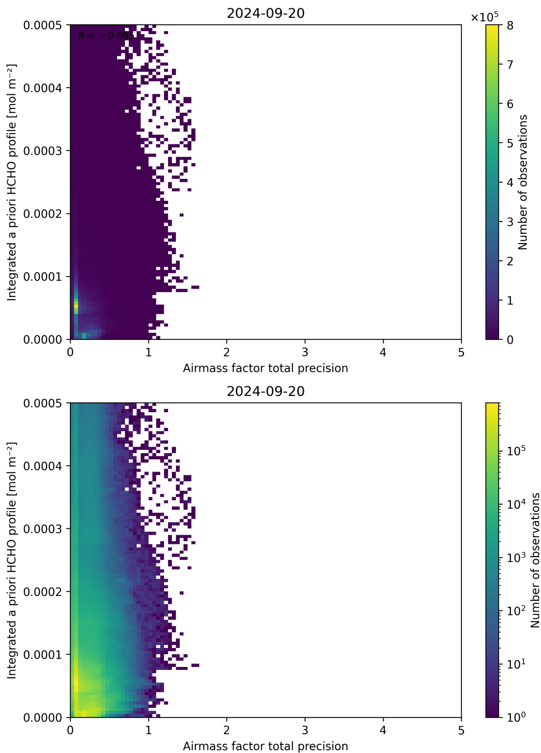
Figure 111: Scatter density plot of “Airmass factor total precision” against “Integrated a priori HCHO profile” for 2024-09-19 to 2024-09-21.
