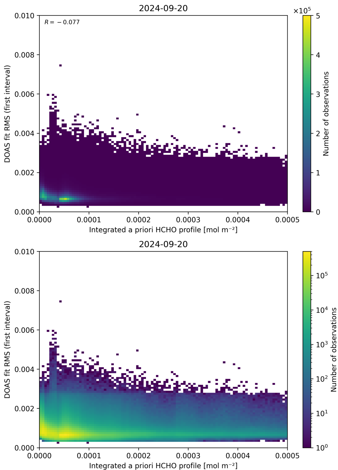
Figure 148: Scatter density plot of “Integrated a priori HCHO profile” against “DOAS fit RMS (first interval)” for 2024-09-19 to 2024-09-21.
