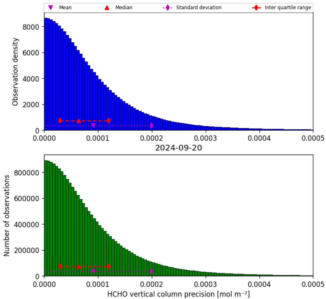
Figure 36: Histogram of “HCHO vertical column precision” for 2024-09-19 to 2024-09-21
