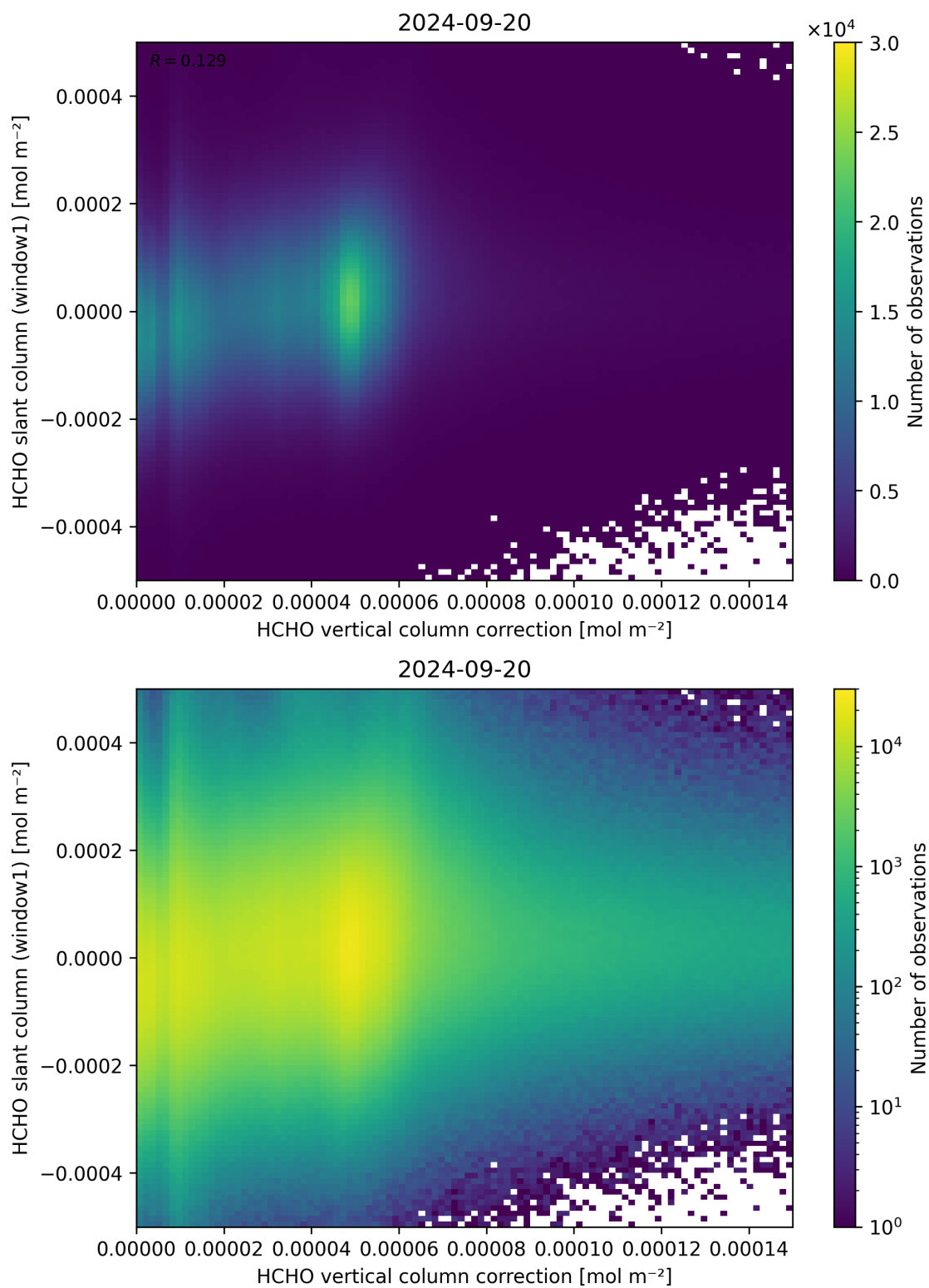
Figure 118: Scatter density plot of “HCHO vertical column correction” against “HCHO slant column (window1)” for 2024-09-19 to 2024-09-21.
