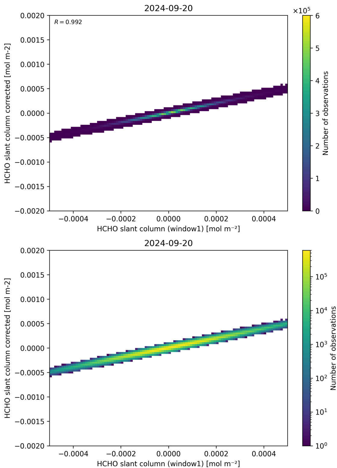
Figure 82: Scatter density plot of “HCHO slant column (window1)” against “HCHO slant column corrected” for 2024-09-19 to 2024-09-21.
