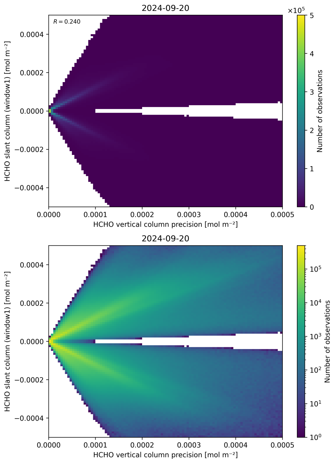
Figure 142: Scatter density plot of “HCHO vertical column precision” against “HCHO slant column (window1)” for 2024-09-19 to 2024-09-21.
