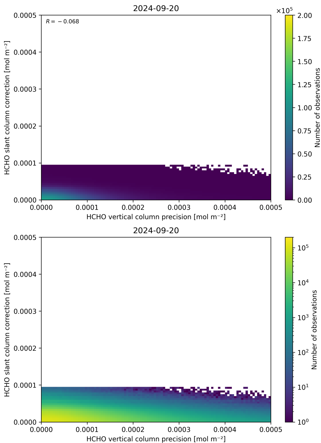
Figure 141: Scatter density plot of “HCHO vertical column precision” against “HCHO slant column correction” for 2024-09-19 to 2024-09-21.
