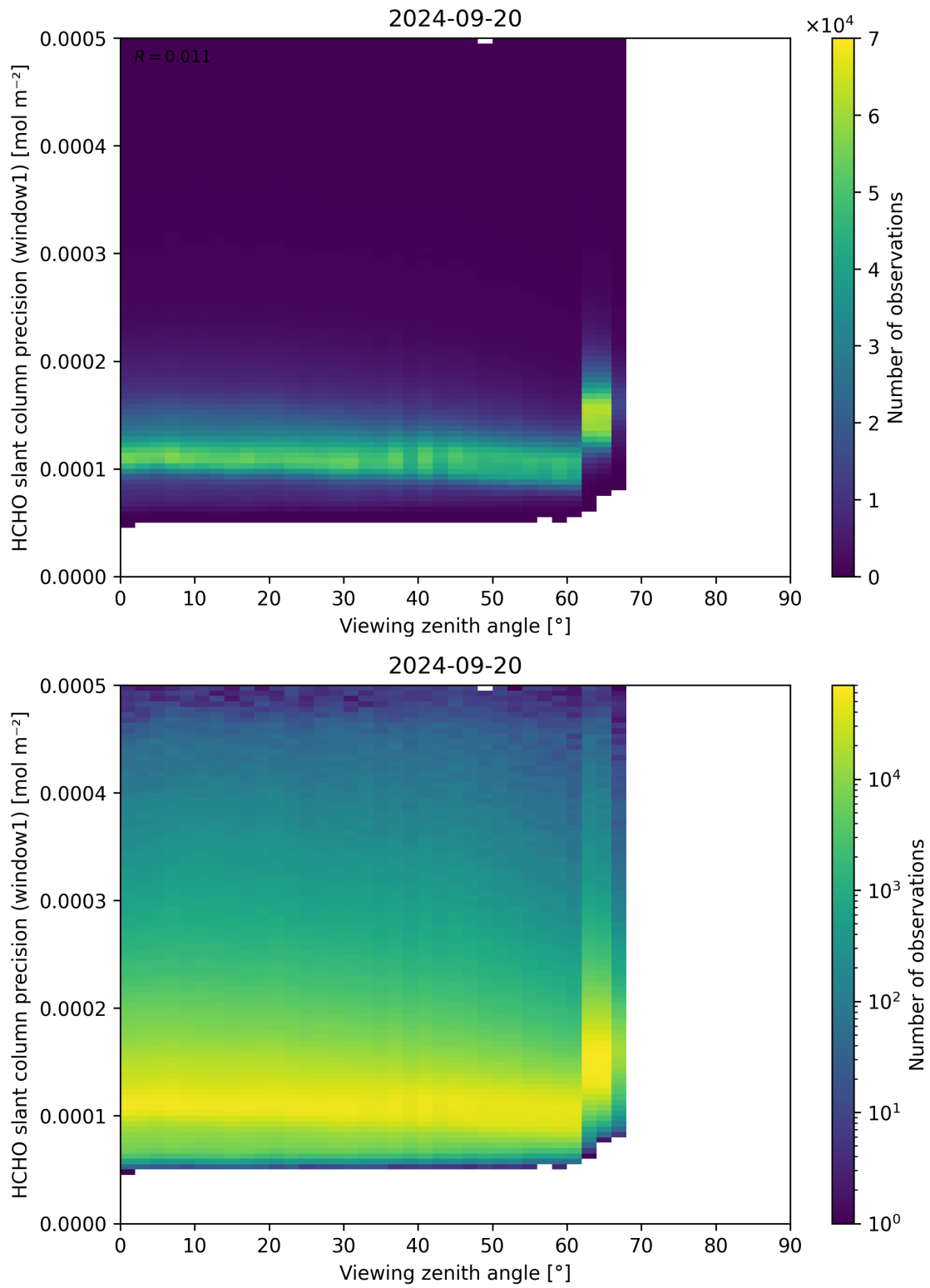
Figure 189: Scatter density plot of “Viewing zenith angle” against “HCHO slant column precision (window1)” for 2024-09-19 to 2024-09-21.
