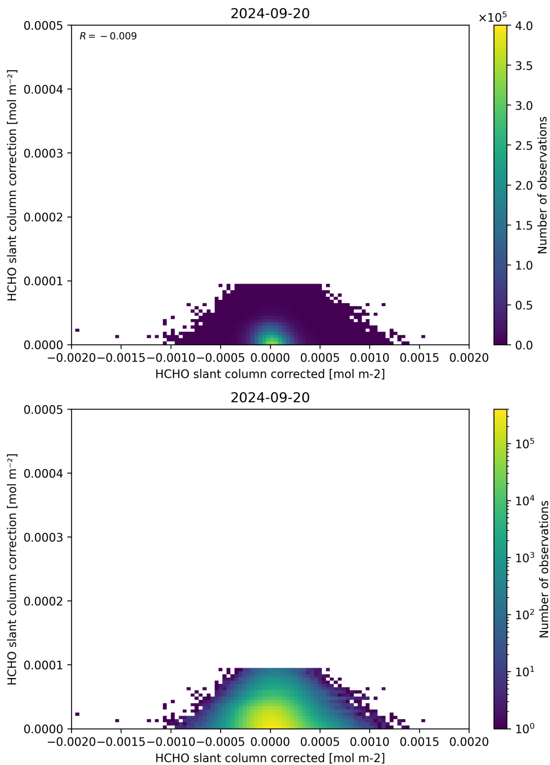
Figure 77: Scatter density plot of “HCHO slant column corrected” against “HCHO slant column correction” for 2024-09-19 to 2024-09-21.
