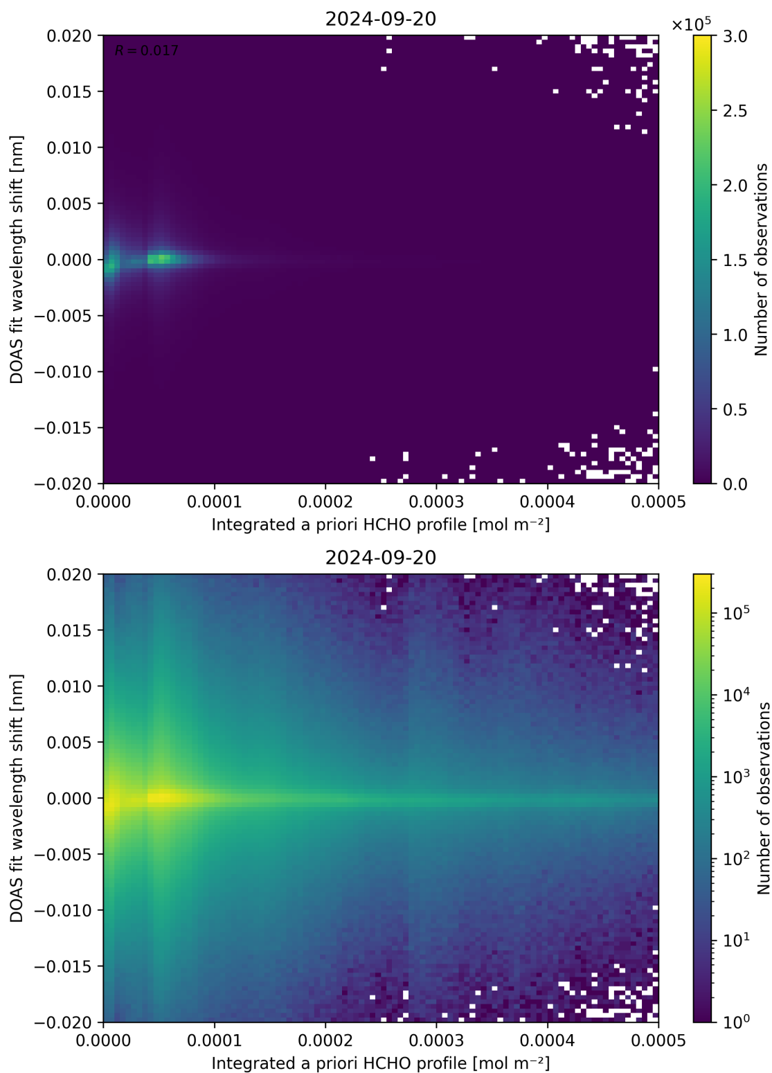
Figure 149: Scatter density plot of “Integrated a priori HCHO profile” against “DOAS fit wavelength shift” for 2024-09-19 to 2024-09-21.
