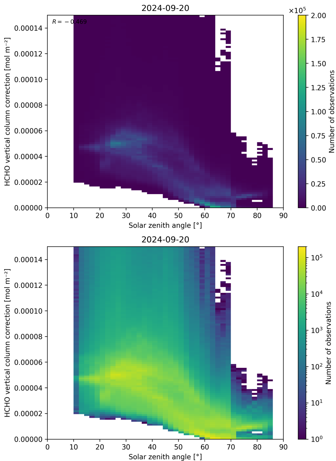
Figure 178: Scatter density plot of “Solar zenith angle” against “HCHO vertical column correction” for 2024-09-19 to 2024-09-21.
