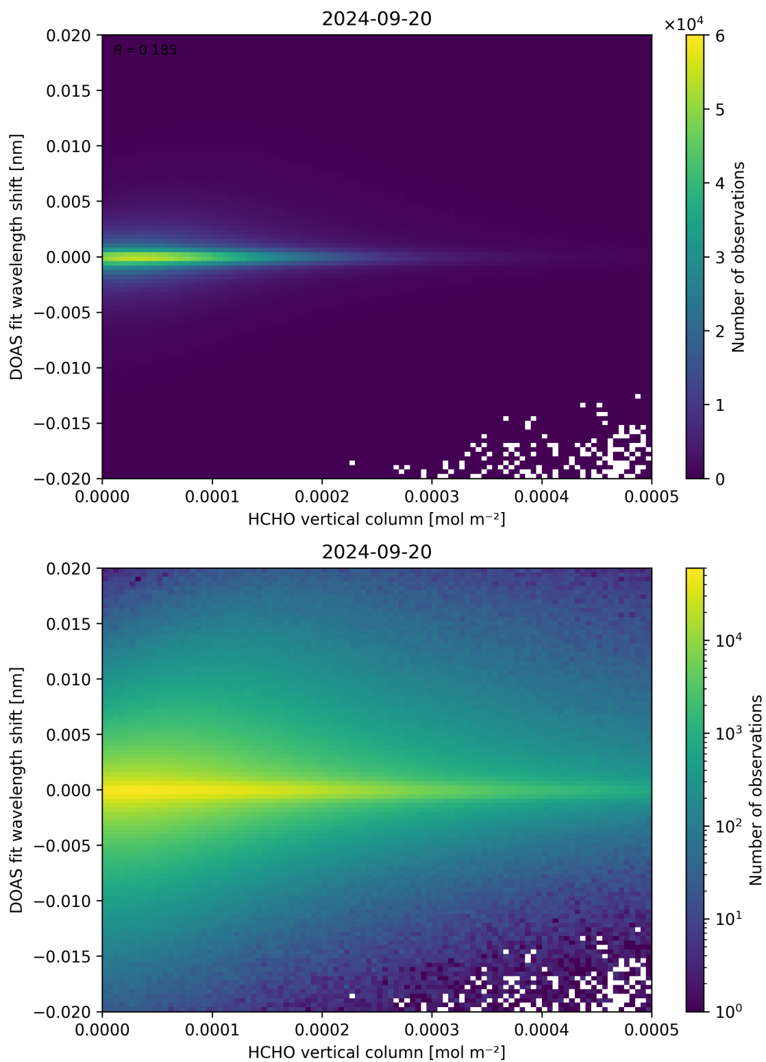
Figure 124: Scatter density plot of “HCHO vertical column” against “DOAS fit wavelength shift” for 2024-09-19 to 2024-09-21.
