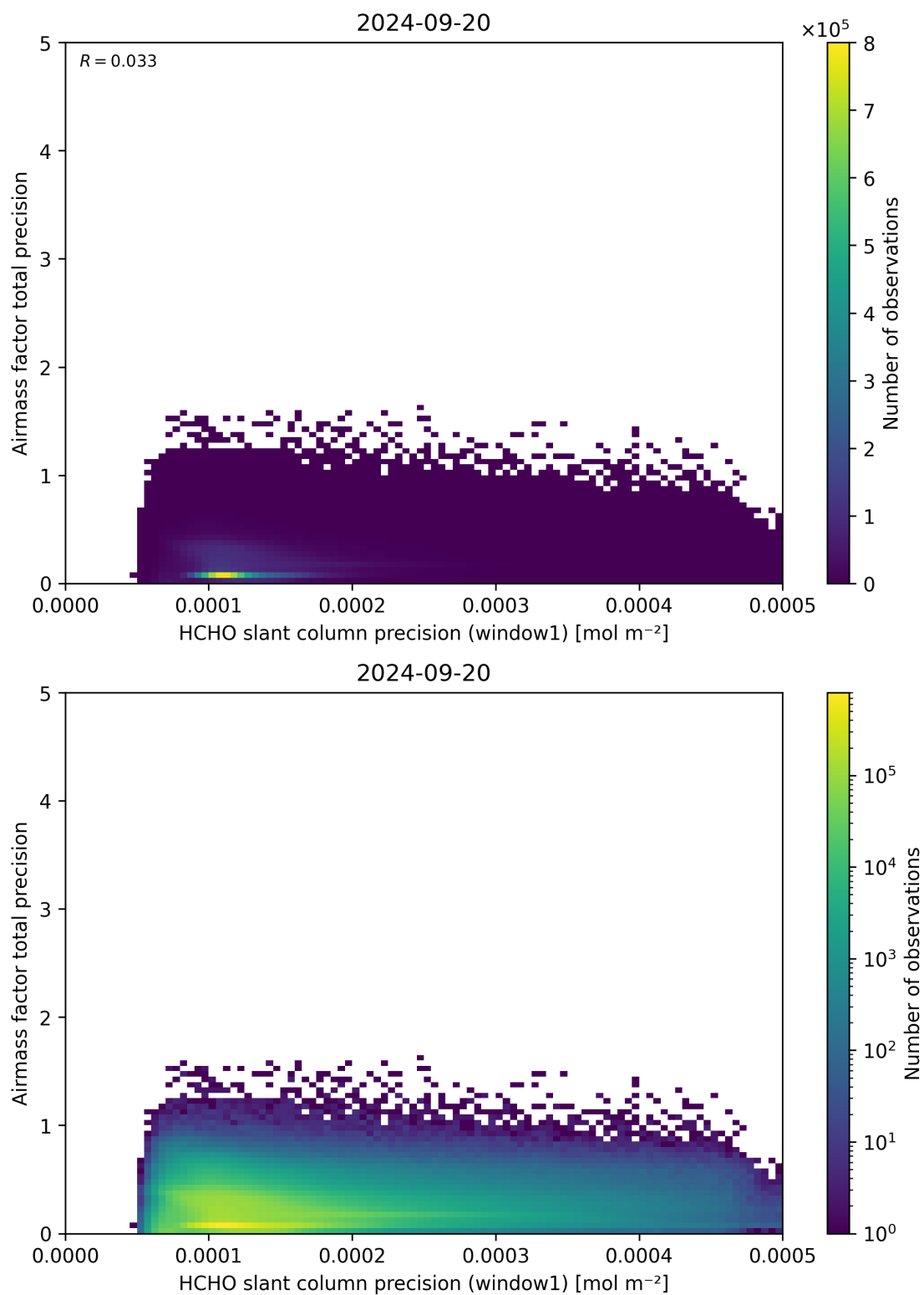
Figure 95: Scatter density plot of “HCHO slant column precision (window1)” against “Airmass factor total precision” for 2024-09-19 to 2024-09-21.
