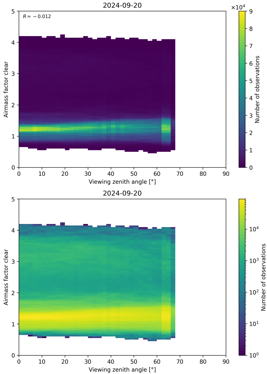
Figure 185: Scatter density plot of “Viewing zenith angle” against “Airmass factor clear” for 2024-09-19 to 2024-09-21.
