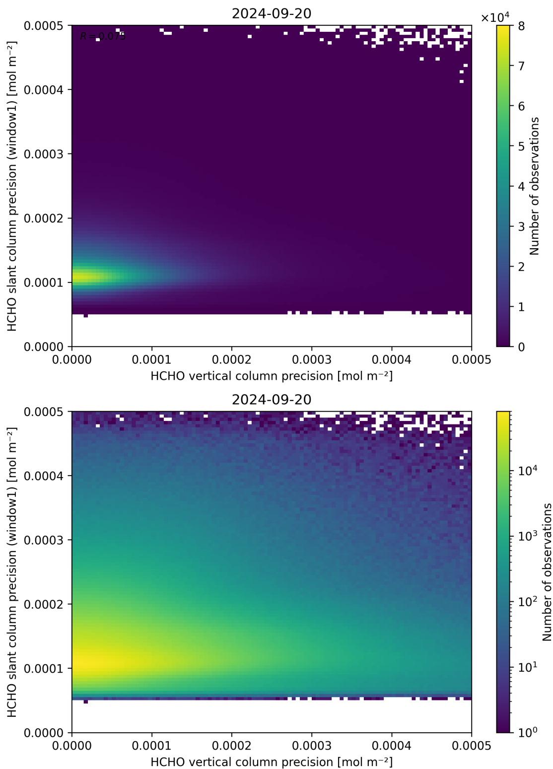
Figure 143: Scatter density plot of “HCHO vertical column precision” against “HCHO slant column precision (window1)” for 2024-09-19 to 2024-09-21.
