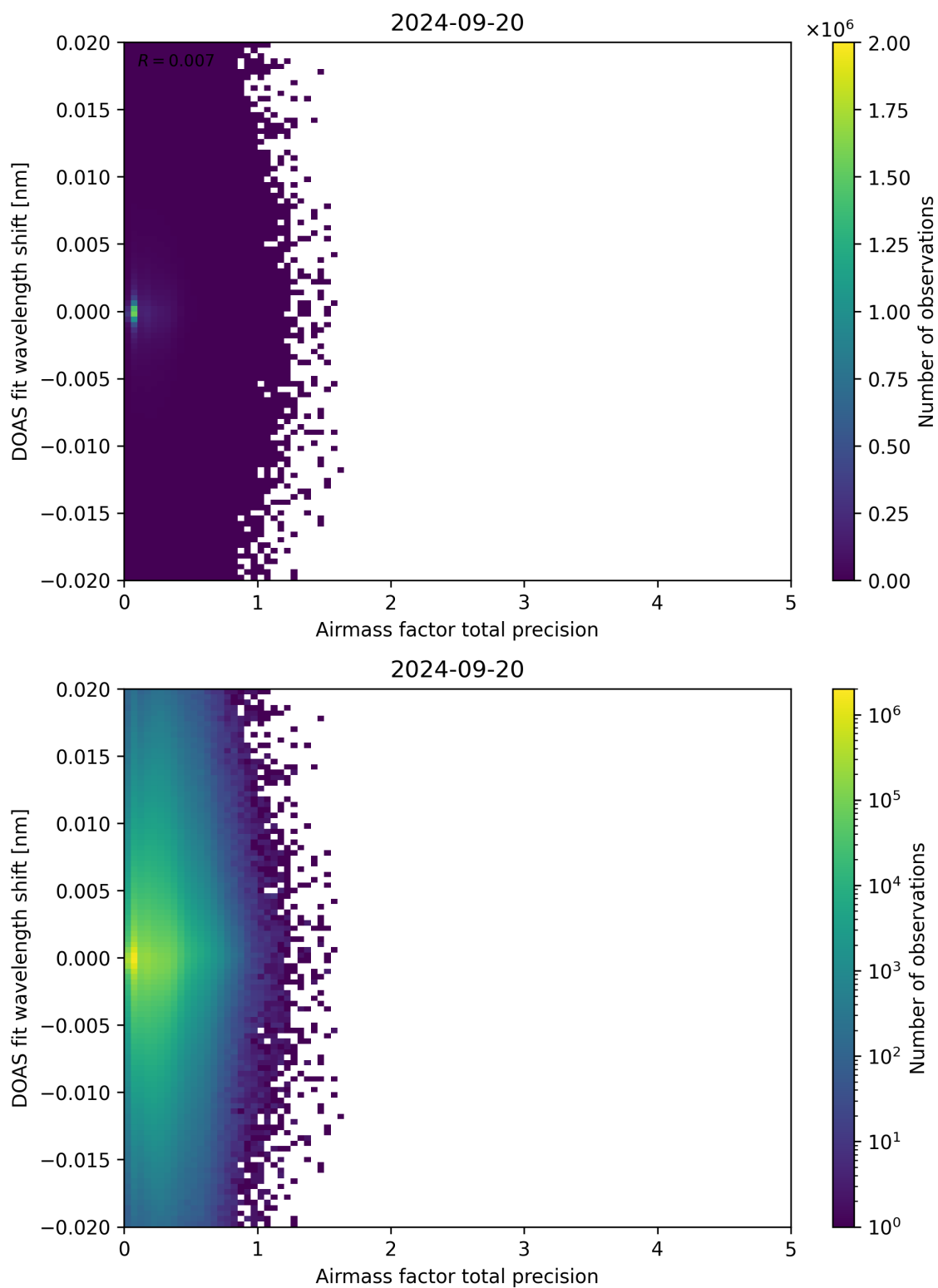
Figure 106: Scatter density plot of “Airmass factor total precision” against “DOAS fit wavelength shift” for 2024-09-19 to 2024-09-21.
