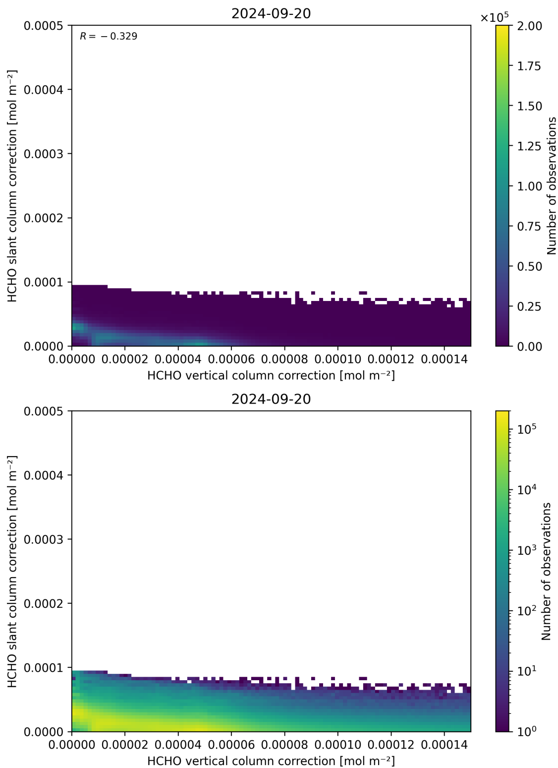
Figure 117: Scatter density plot of “HCHO vertical column correction” against “HCHO slant column correction” for 2024-09-19 to 2024-09-21.
