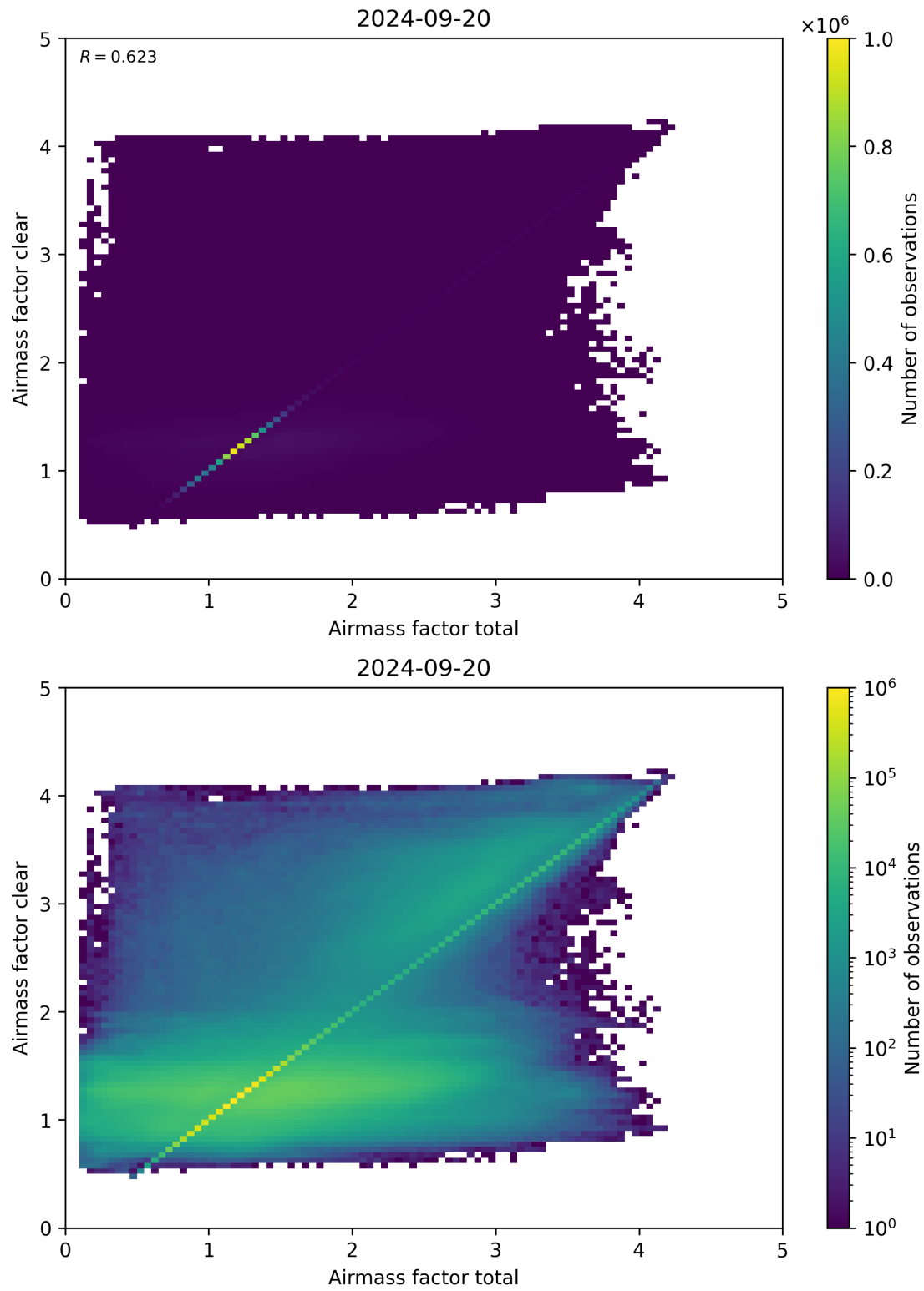
Figure 100: Scatter density plot of “Airmass factor total” against “Airmass factor clear” for 2024-09-19 to 2024-09-21.
