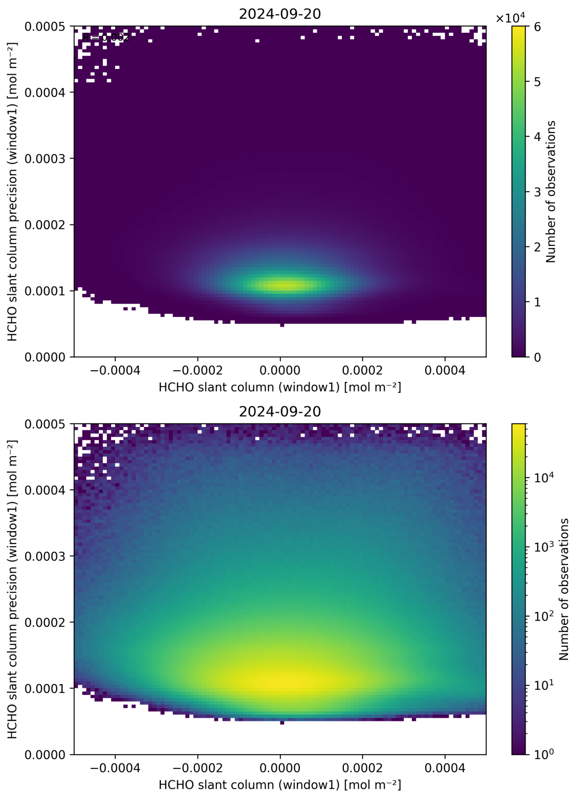
Figure 84: Scatter density plot of “HCHO slant column (window1)” against “HCHO slant column precision (window1)” for 2024-09-19 to 2024-09-21.
