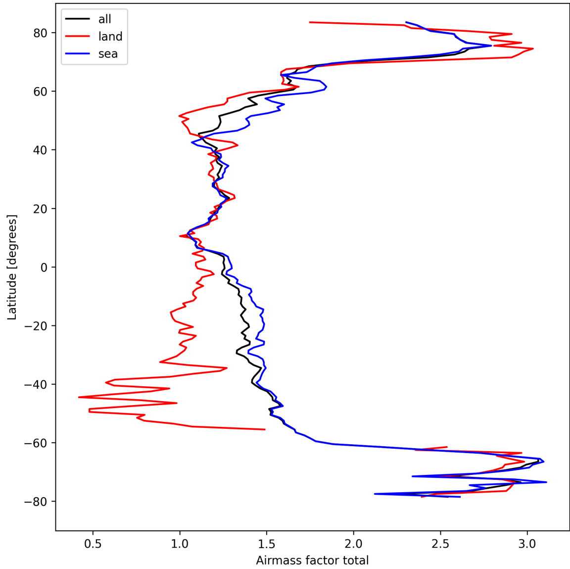
Figure 26: Zonal average of “Airmass factor total” for 2024-09-19 to 2024-09-21.
