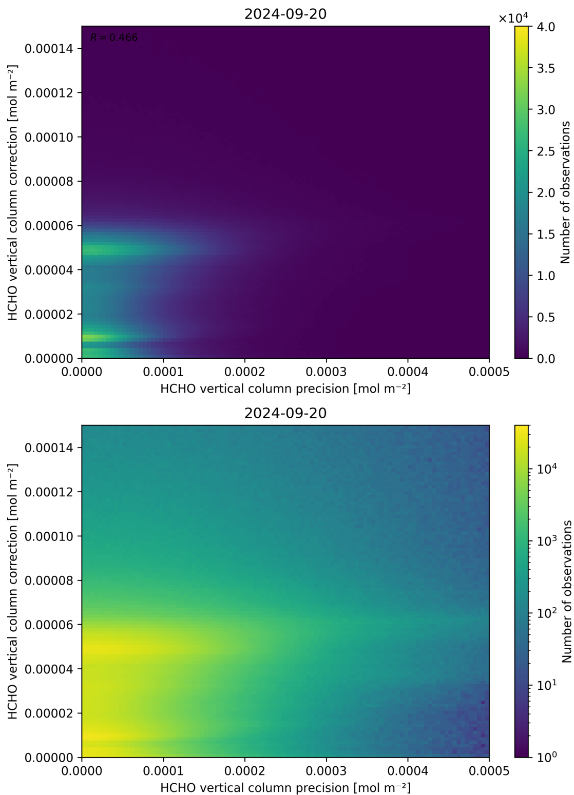
Figure 146: Scatter density plot of “HCHO vertical column precision” against “HCHO vertical column correction” for 2024-09-19 to 2024-09-21.
