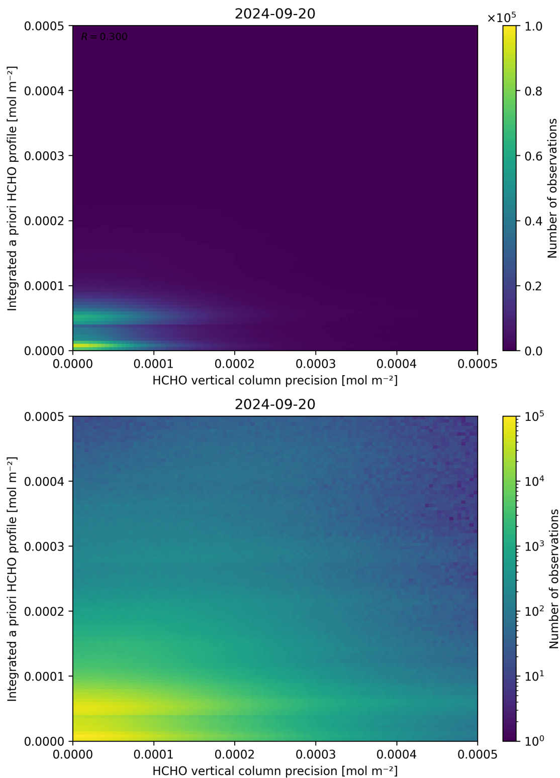
Figure 147: Scatter density plot of “HCHO vertical column precision” against “Integrated a priori HCHO profile” for 2024-09-19 to 2024-09-21.
