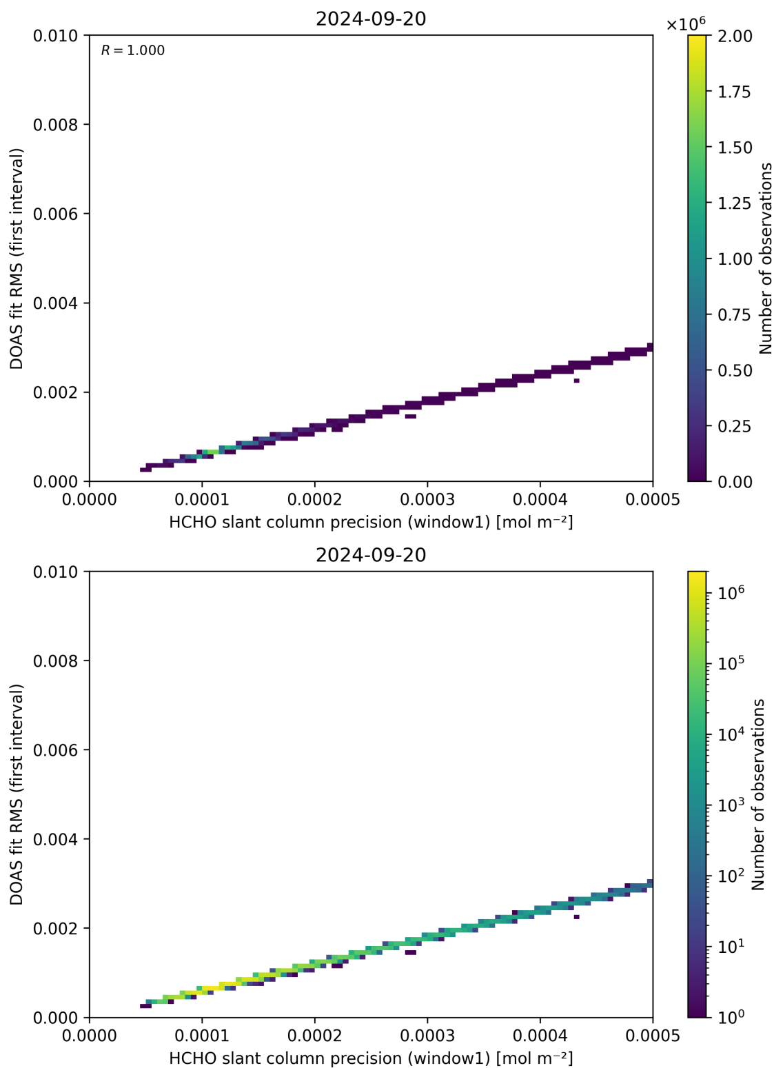
Figure 88: Scatter density plot of “HCHO slant column precision (window1)” against “DOAS fit RMS (first interval)” for 2024-09-19 to 2024-09-21.
