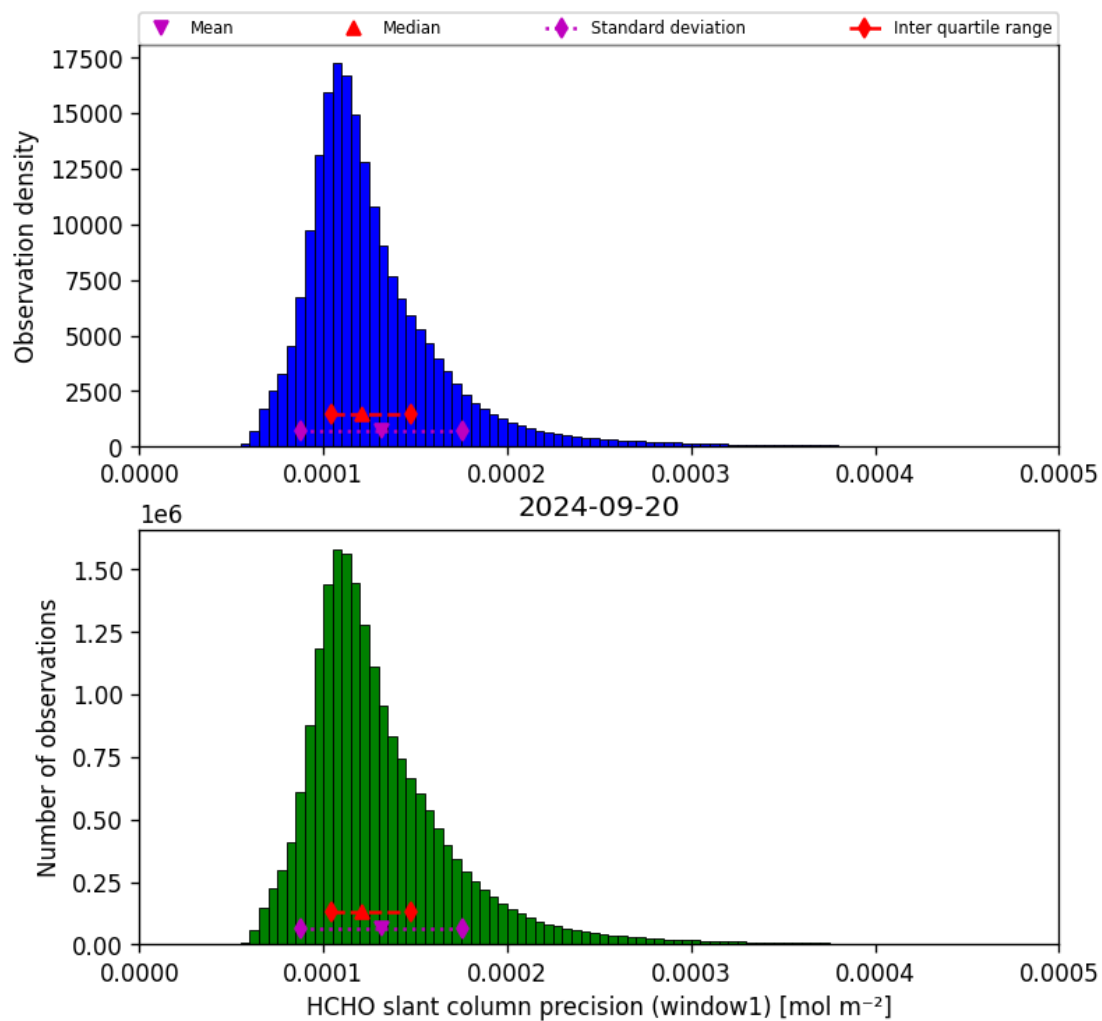
Figure 39: Histogram of “HCHO slant column precision (window1)” for 2024-09-19 to 2024-09-21
