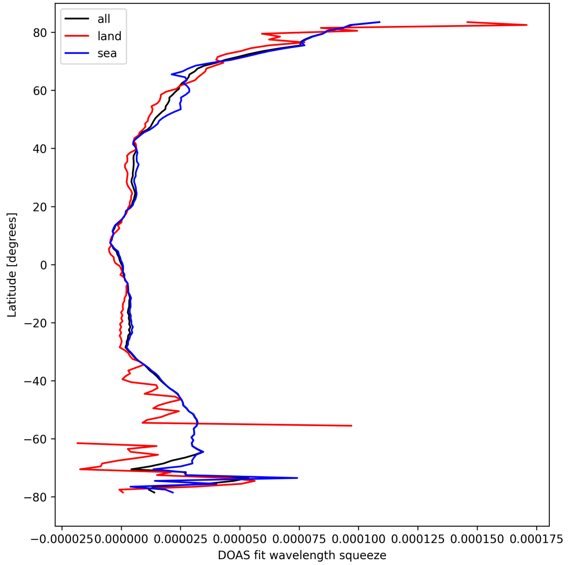
Figure 31: Zonal average of “DOAS fit wavelength squeeze” for 2024-09-19 to 2024-09-21.
