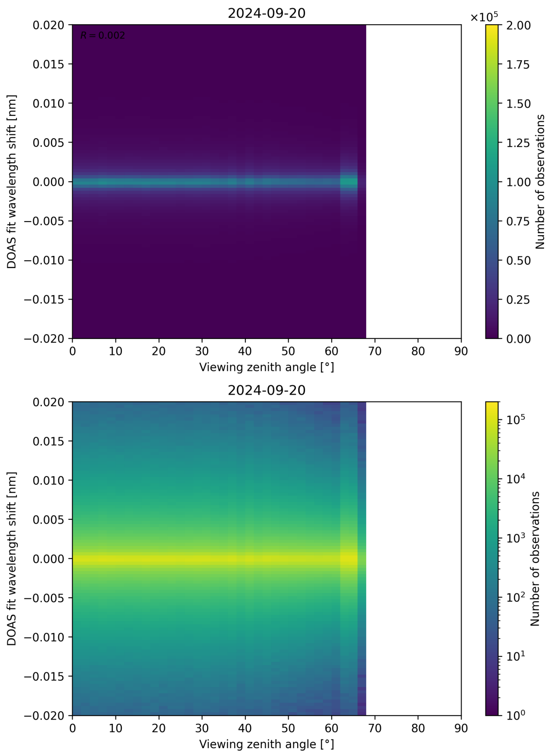
Figure 183: Scatter density plot of “Viewing zenith angle” against “DOAS fit wavelength shift” for 2024-09-19 to 2024-09-21.
