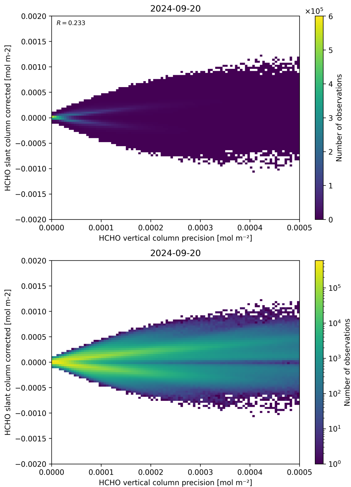
Figure 140: Scatter density plot of “HCHO vertical column precision” against “HCHO slant column corrected” for 2024-09-19 to 2024-09-21.
