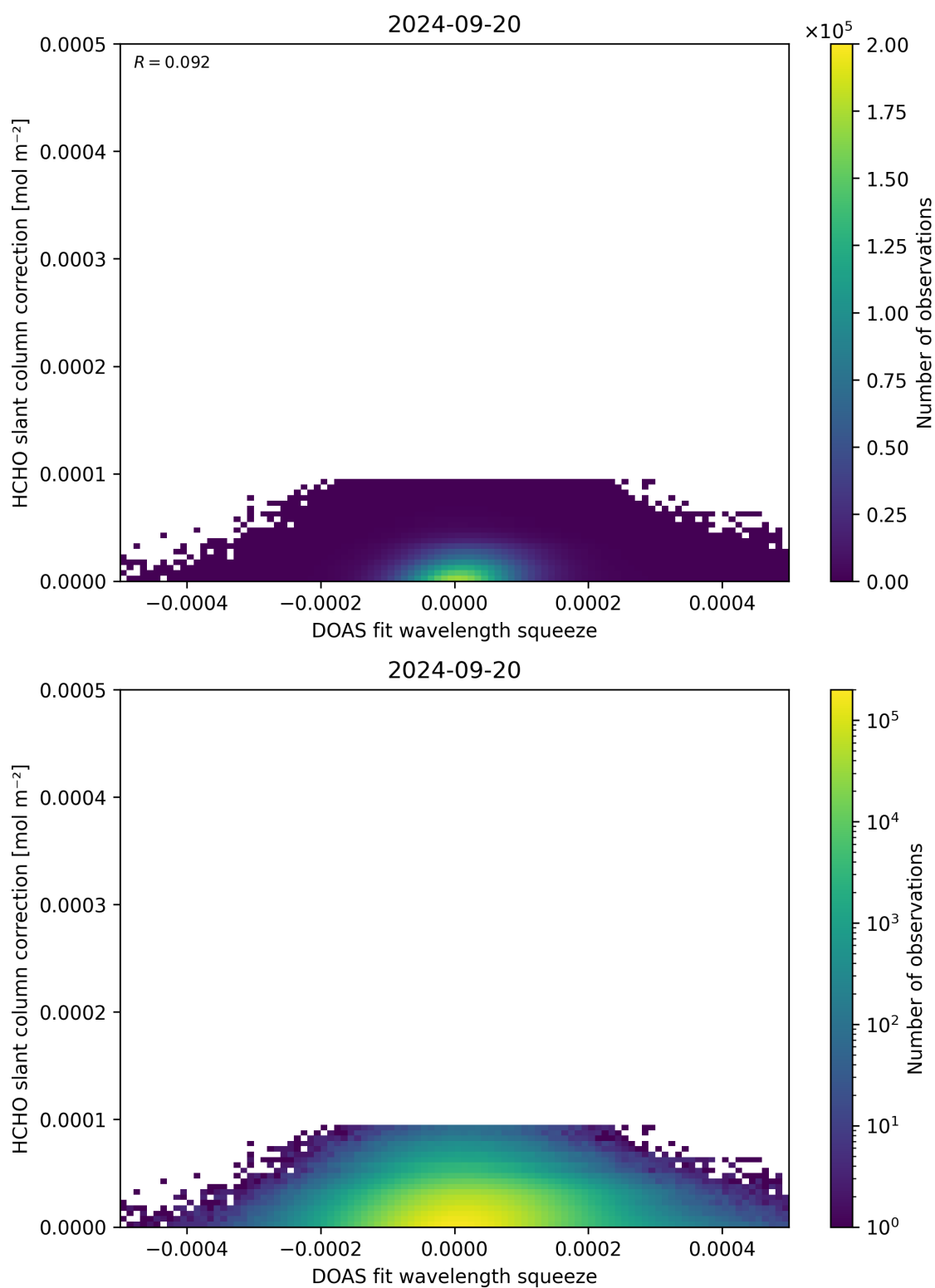
Figure 70: Scatter density plot of “DOAS fit wavelength squeeze” against “HCHO slant column correction” for 2024-09-19 to 2024-09-21.
