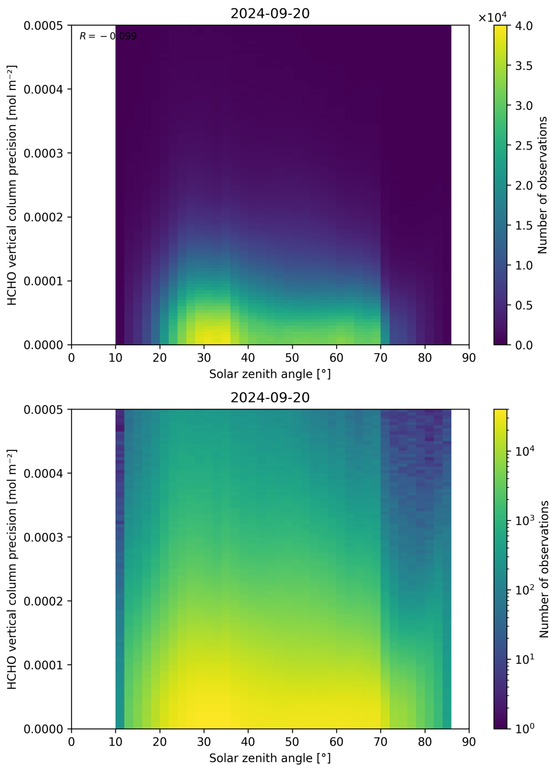
Figure 179: Scatter density plot of “Solar zenith angle” against “HCHO vertical column precision” for 2024-09-19 to 2024-09-21.
