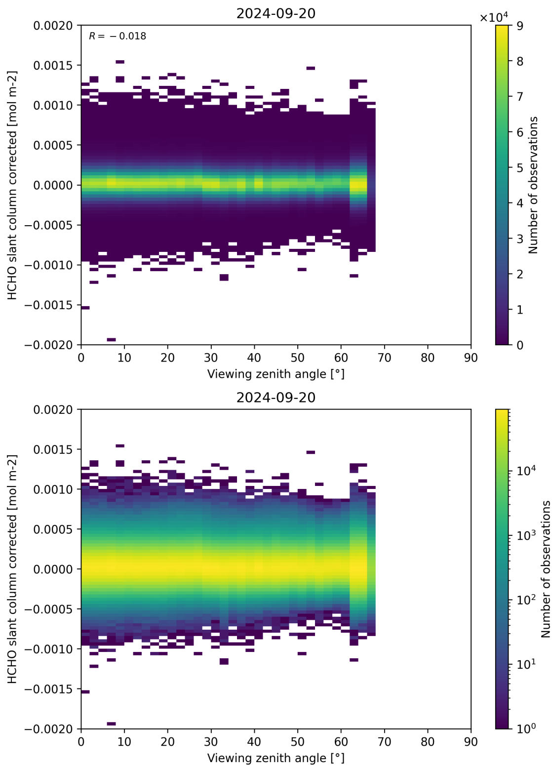
Figure 186: Scatter density plot of “Viewing zenith angle” against “HCHO slant column corrected” for 2024-09-19 to 2024-09-21.
