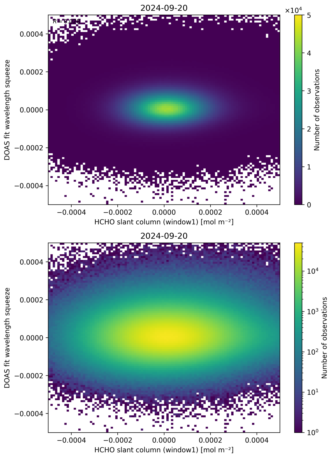
Figure 80: Scatter density plot of “HCHO slant column (window1)” against “DOAS fit wavelength squeeze” for 2024-09-19 to 2024-09-21.
