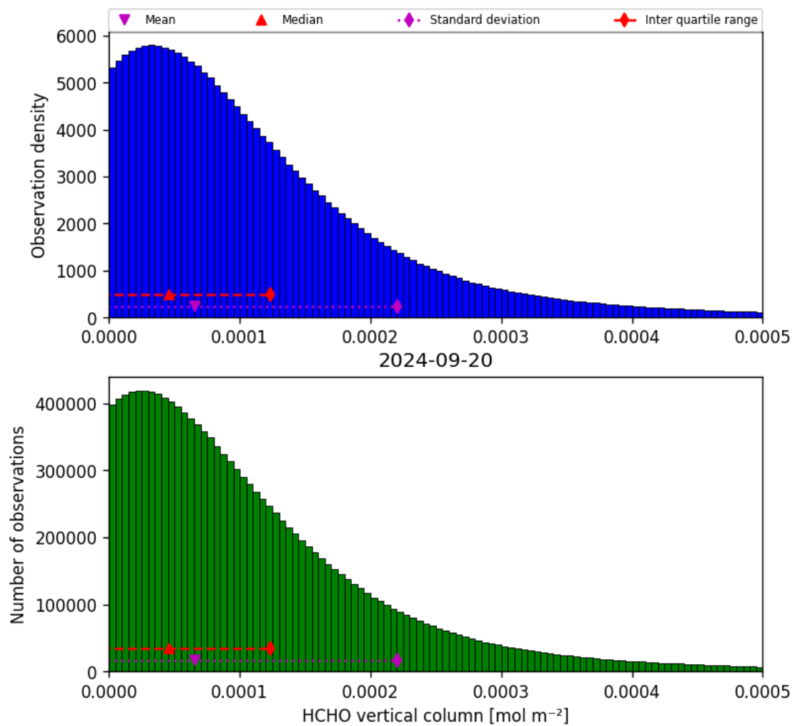
Figure 35: Histogram of “HCHO vertical column” for 2024-09-19 to 2024-09-21
