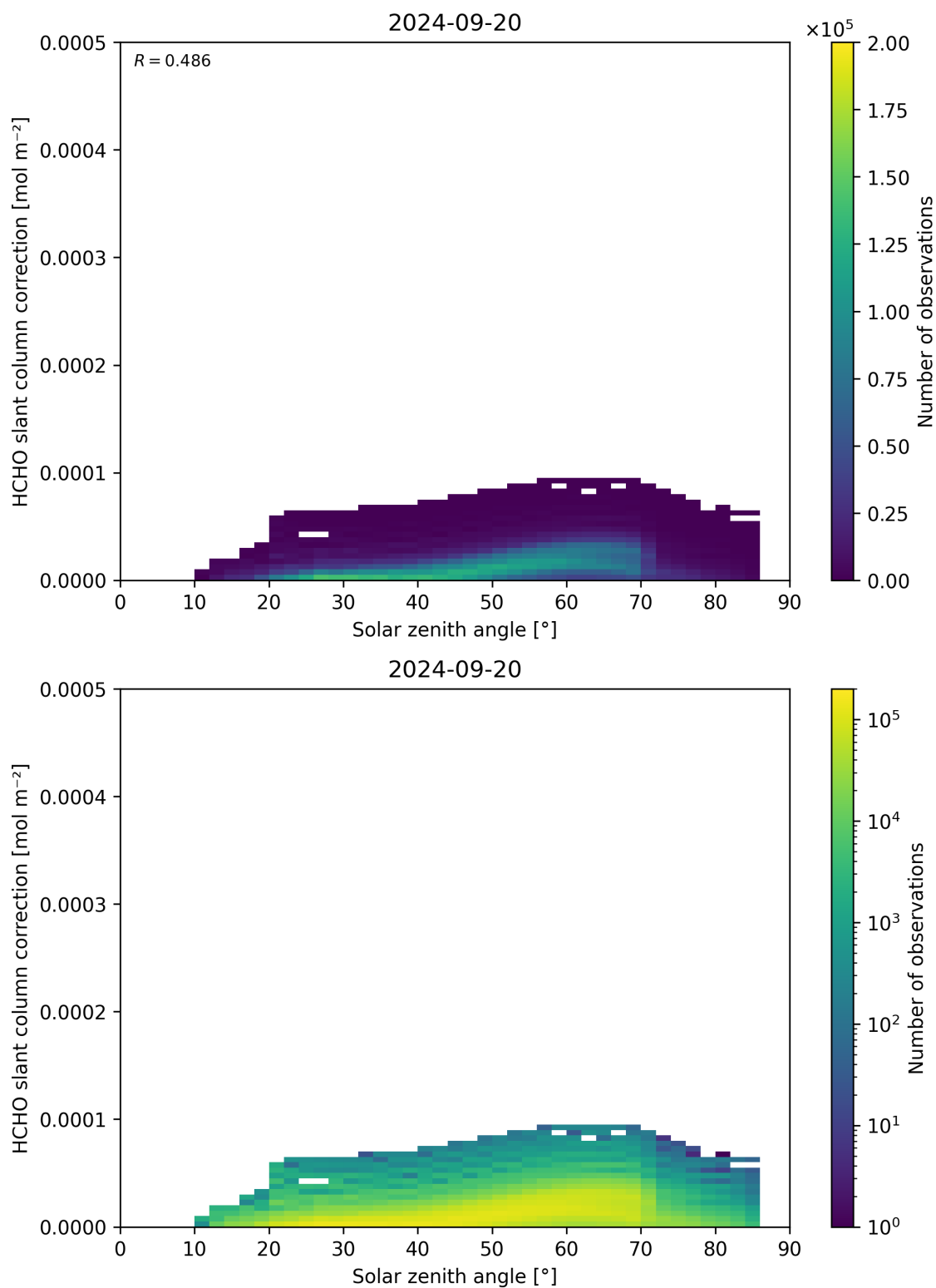
Figure 172: Scatter density plot of “Solar zenith angle” against “HCHO slant column correction” for 2024-09-19 to 2024-09-21.
