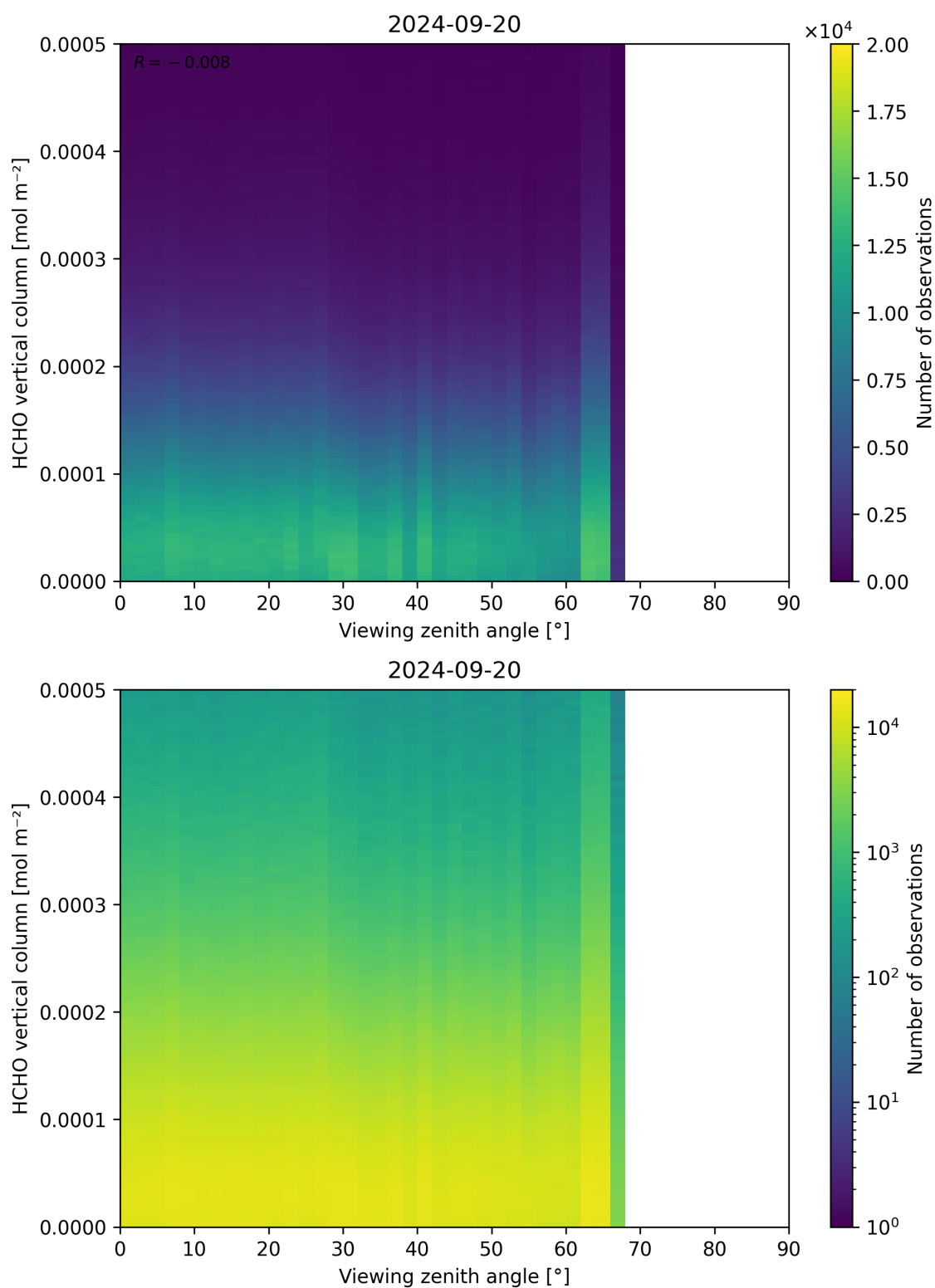
Figure 192: Scatter density plot of “Viewing zenith angle” against “HCHO vertical column” for 2024-09-19 to 2024-09-21.
