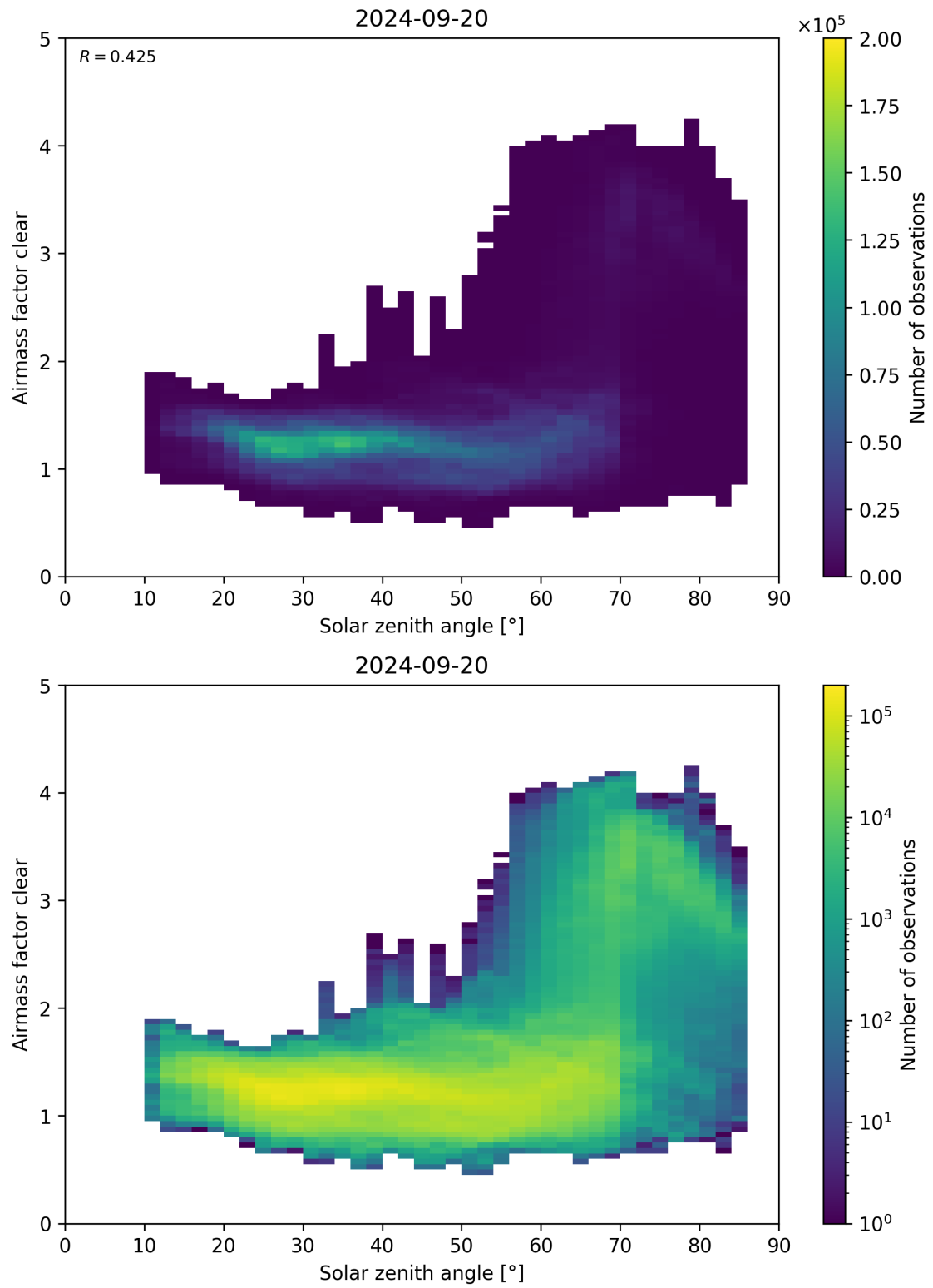
Figure 170: Scatter density plot of “Solar zenith angle” against “Airmass factor clear” for 2024-09-19 to 2024-09-21.
