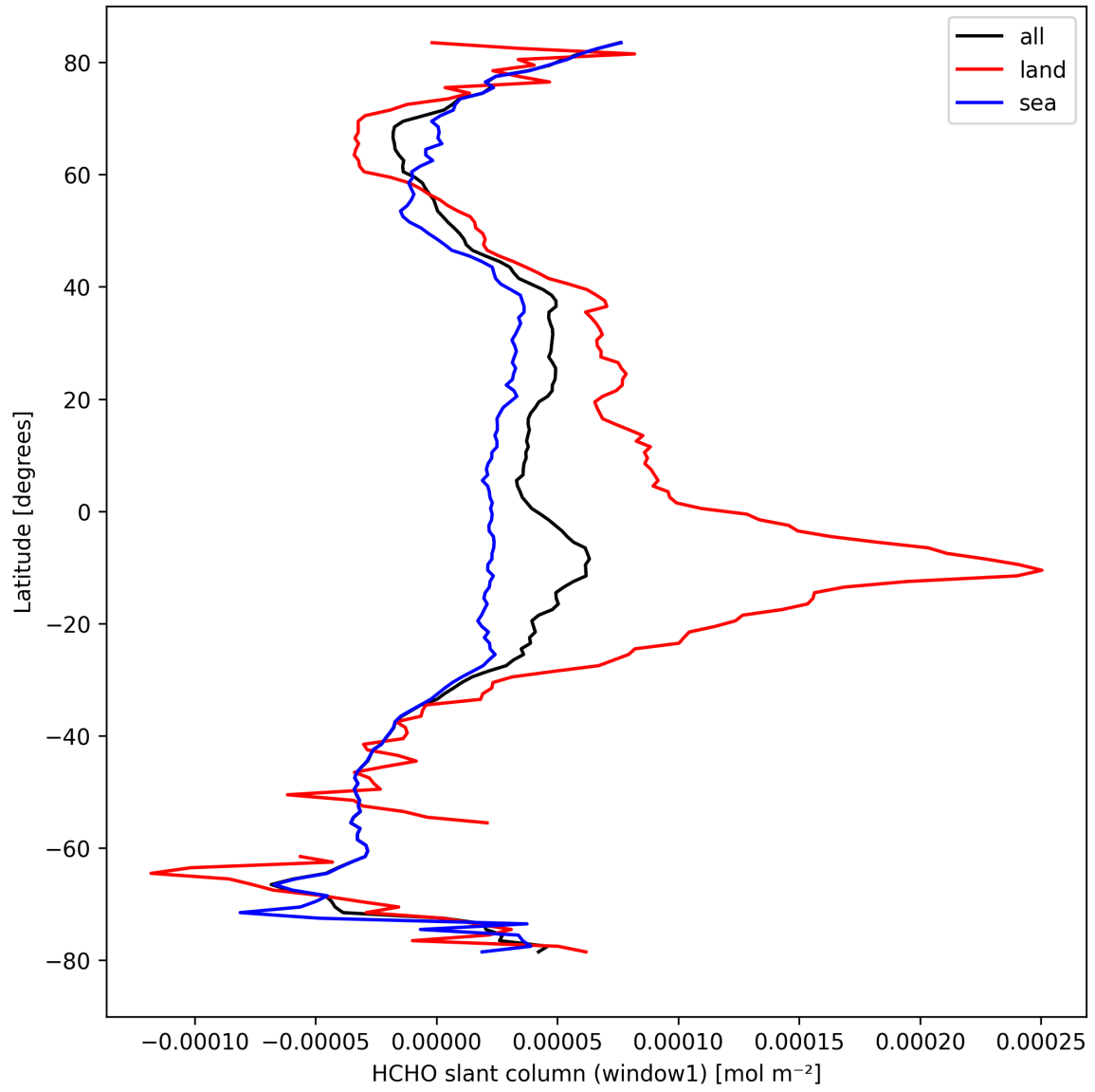
Figure 24: Zonal average of “HCHO slant column (window1)” for 2024-09-19 to 2024-09-21.
