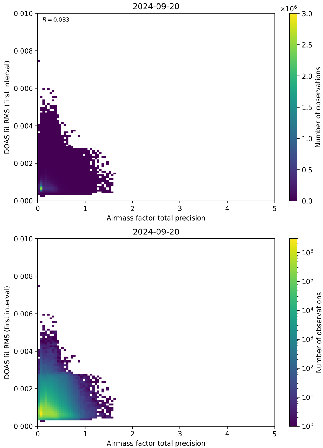
Figure 105: Scatter density plot of “Airmass factor total precision” against “DOAS fit RMS (first interval)” for 2024-09-19 to 2024-09-21.
