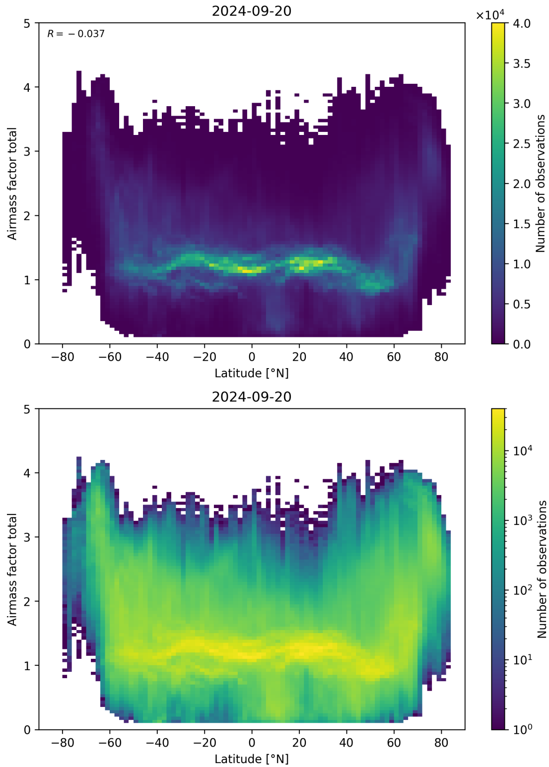
Figure 161: Scatter density plot of “Latitude” against “Airmass factor total” for 2024-09-19 to 2024-09-21.
