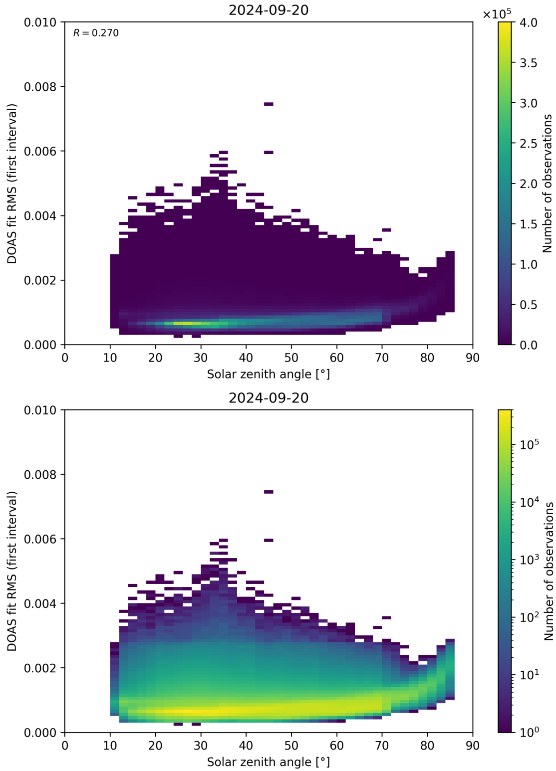
Figure 167: Scatter density plot of “Solar zenith angle” against “DOAS fit RMS (first interval)” for 2024-09-19 to 2024-09-21.
