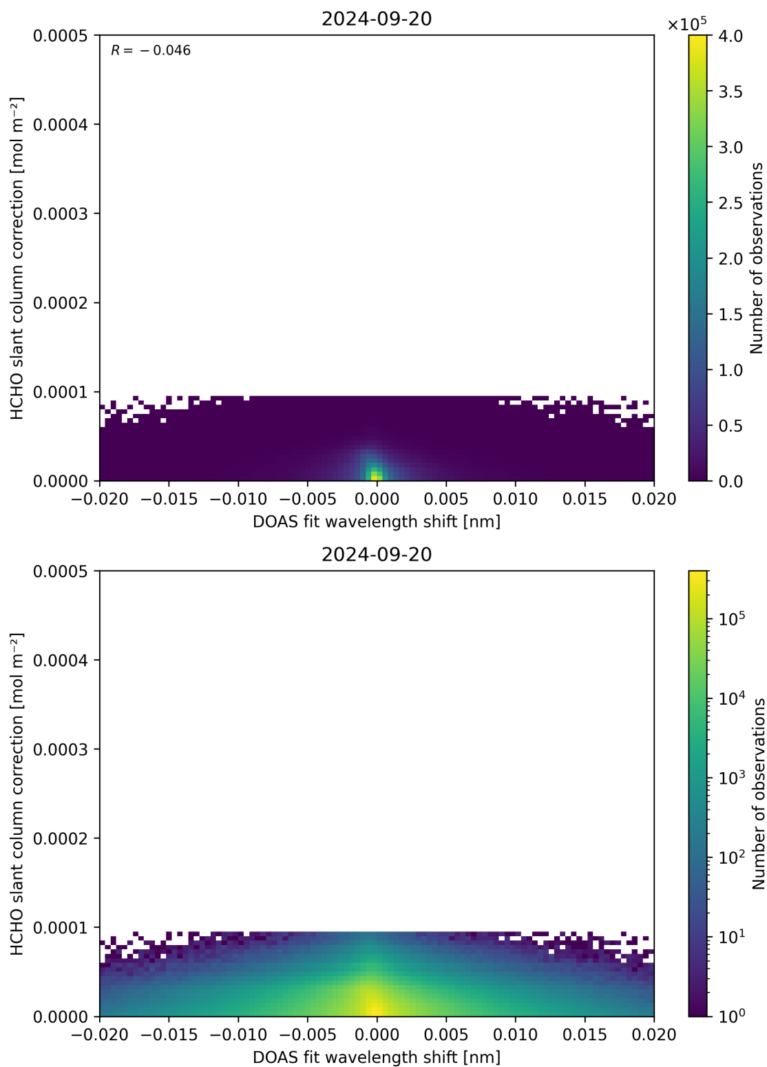
Figure 67: Scatter density plot of “DOAS fit wavelength shift” against “HCHO slant column correction” for 2024-09-19 to 2024-09-21.
