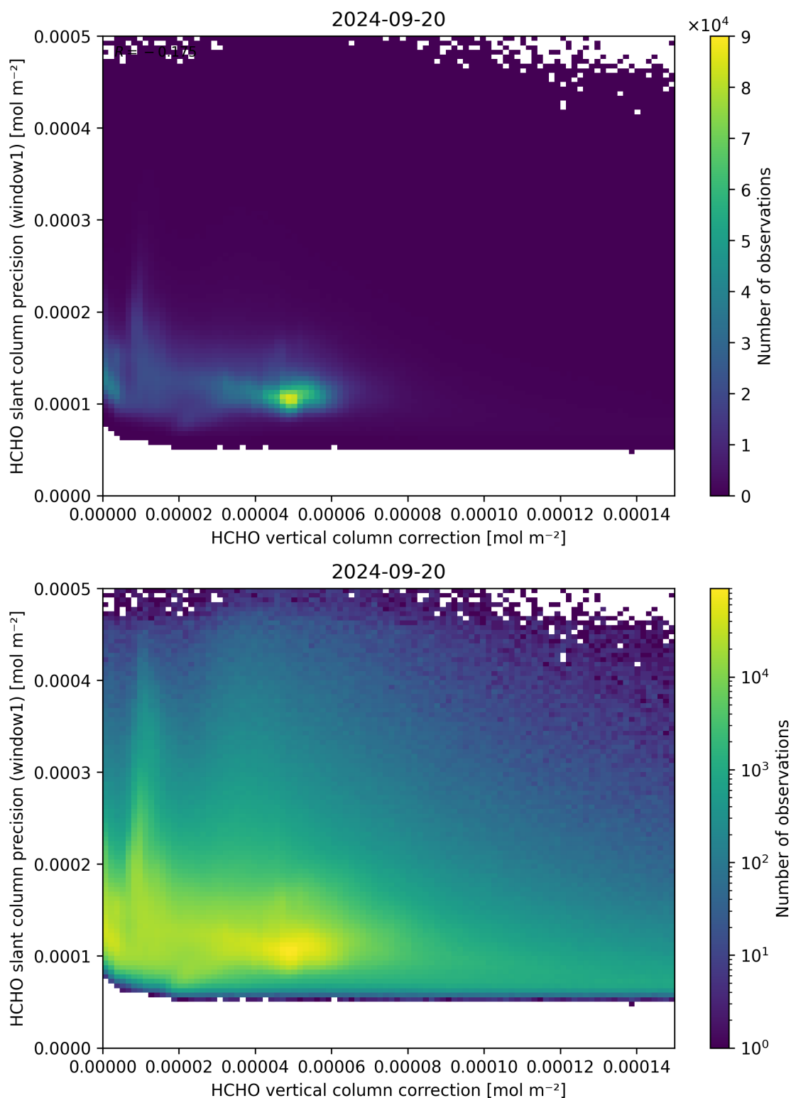
Figure 119: Scatter density plot of “HCHO vertical column correction” against “HCHO slant column precision (window1)” for 2024-09-19 to 2024-09-21.
