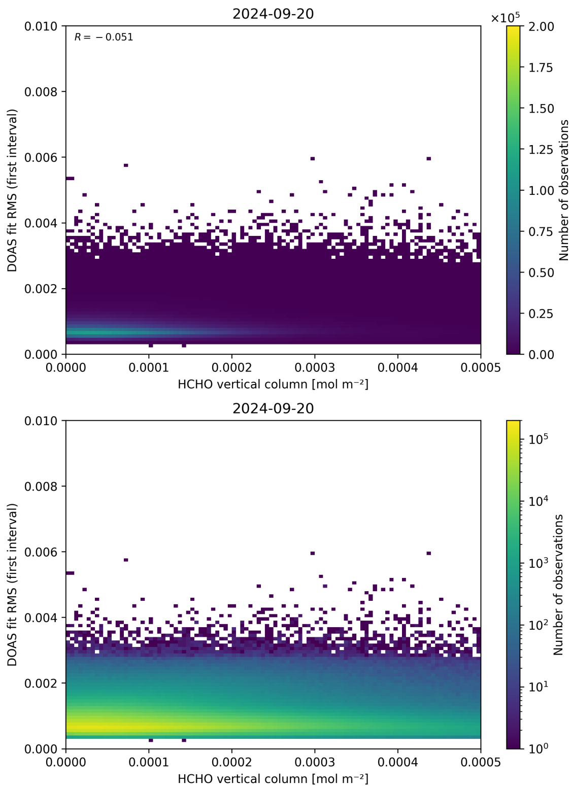
Figure 123: Scatter density plot of “HCHO vertical column” against “DOAS fit RMS (first interval)” for 2024-09-19 to 2024-09-21.
