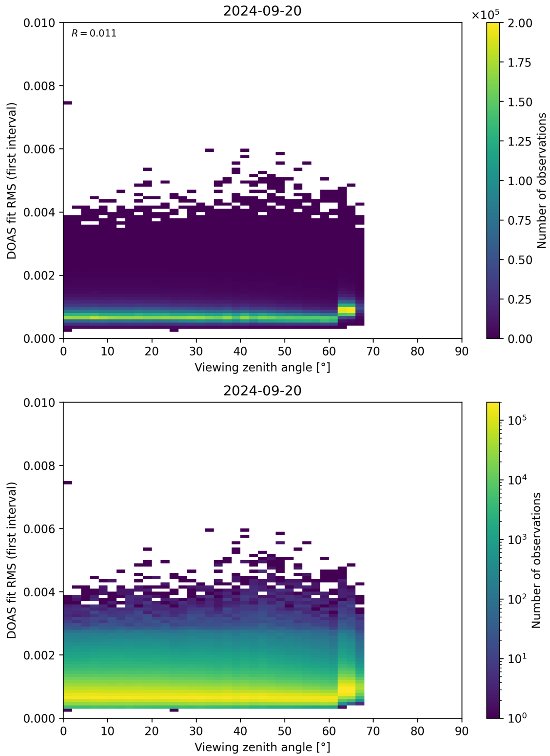
Figure 182: Scatter density plot of “Viewing zenith angle” against “DOAS fit RMS (first interval)” for 2024-09-19 to 2024-09-21.
