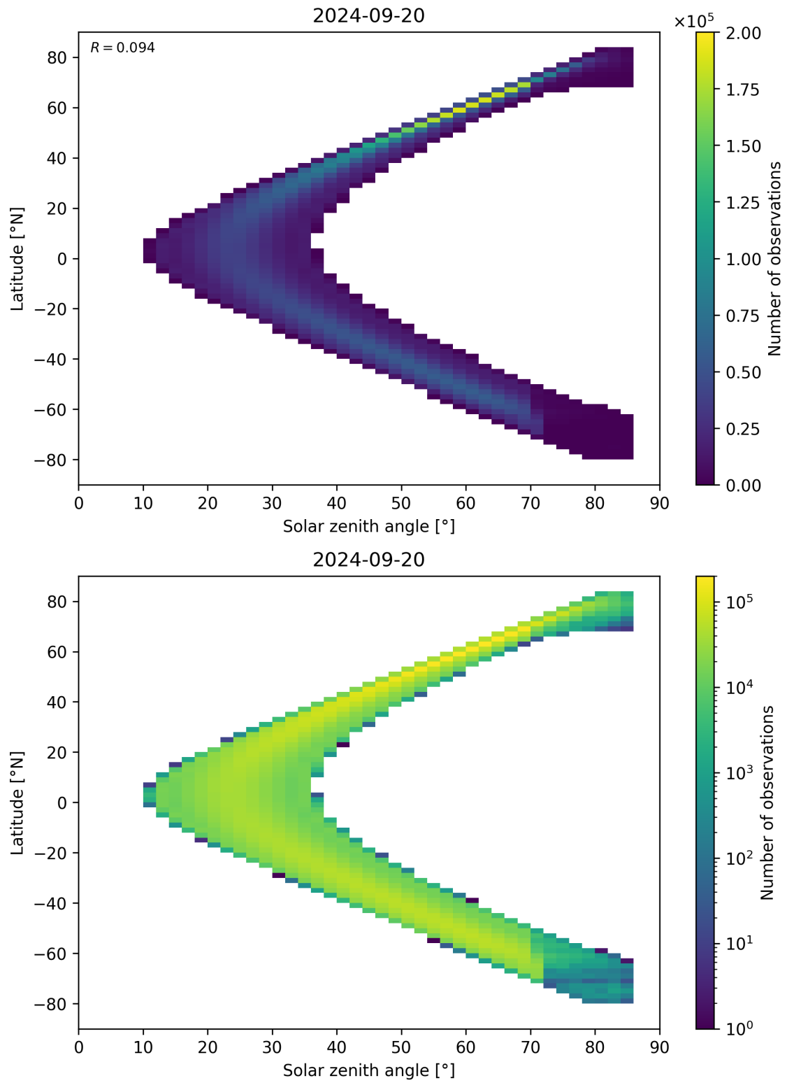
Figure 181: Scatter density plot of “Solar zenith angle” against “Latitude” for 2024-09-19 to 2024-09-21.
