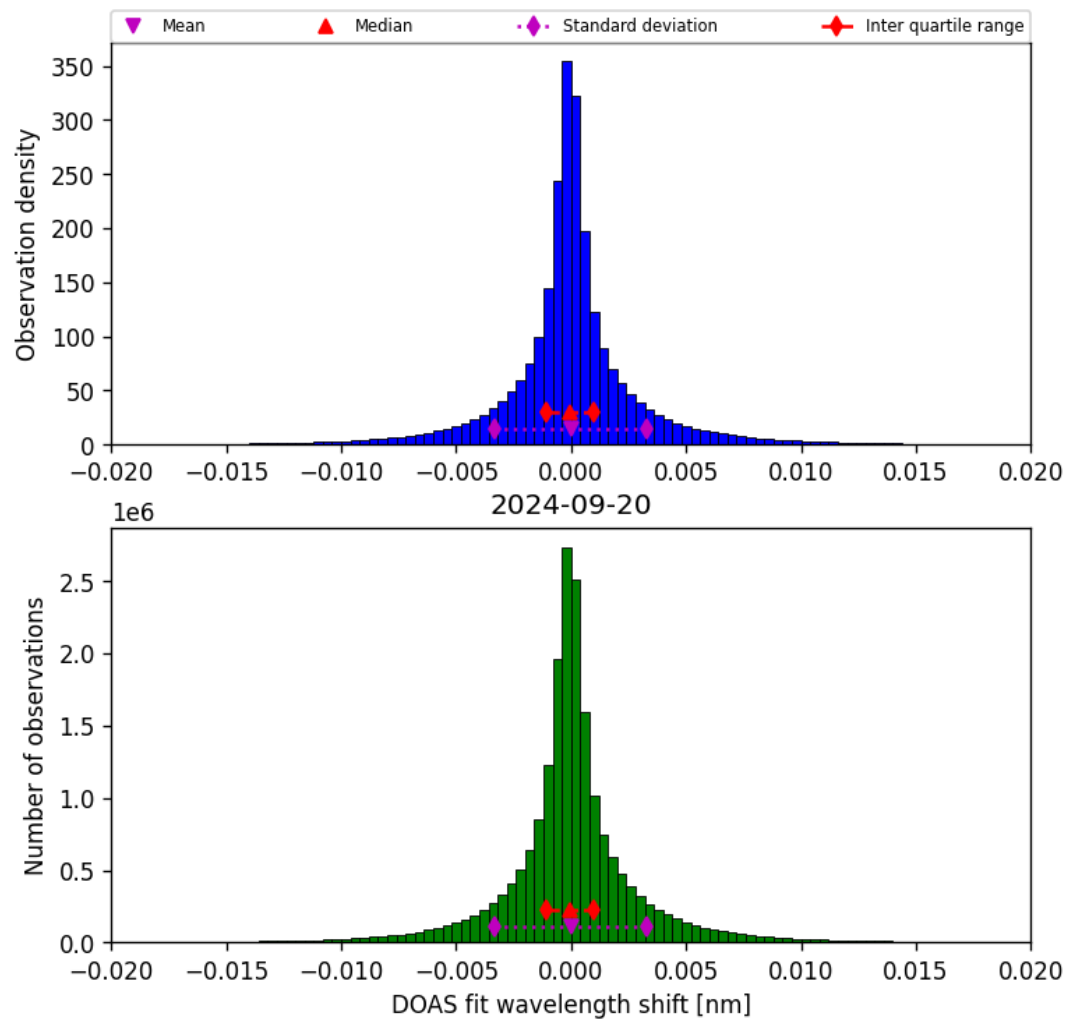
Figure 44: Histogram of “DOAS fit wavelength shift” for 2024-09-19 to 2024-09-21
