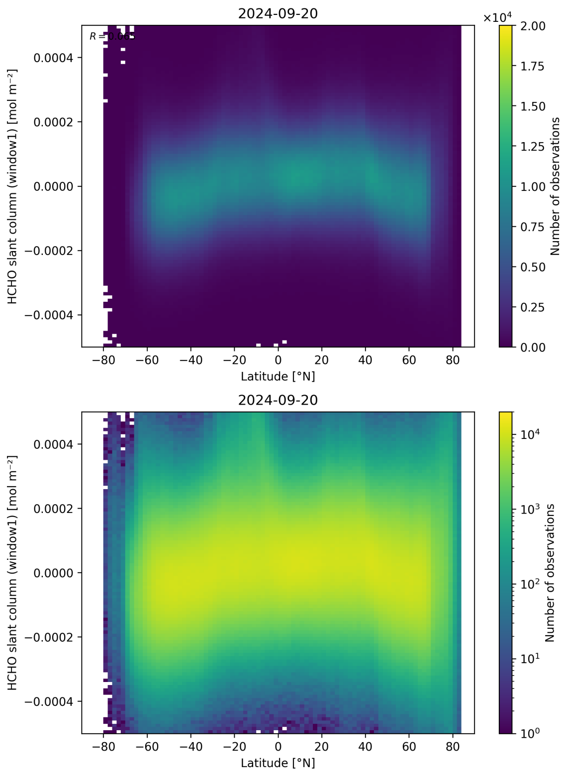
Figure 159: Scatter density plot of “Latitude” against “HCHO slant column (window1)” for 2024-09-19 to 2024-09-21.
