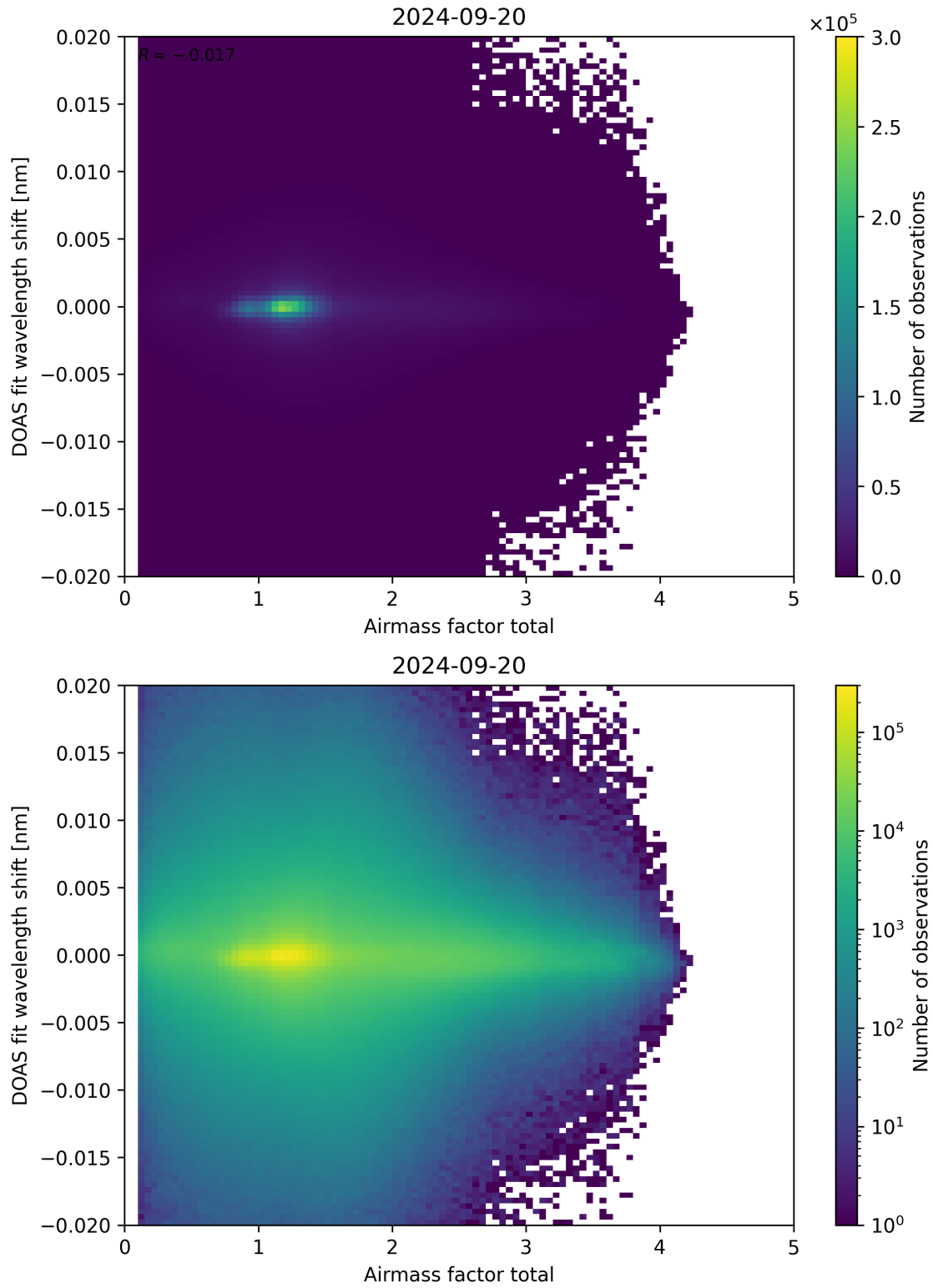
Figure 98: Scatter density plot of “Airmass factor total” against “DOAS fit wavelength shift” for 2024-09-19 to 2024-09-21.
