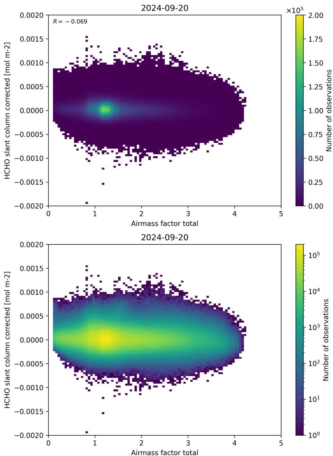
Figure 101: Scatter density plot of “Airmass factor total” against “HCHO slant column corrected” for 2024-09-19 to 2024-09-21.
