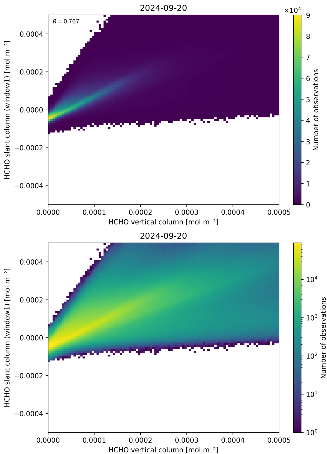
Figure 129: Scatter density plot of “HCHO vertical column” against “HCHO slant column (window1)” for 2024-09-19 to 2024-09-21.
