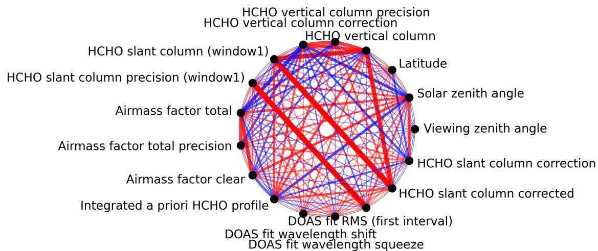
Figure 1: Map of correlation graph for 2024-09-19 to 2024-09-21.
