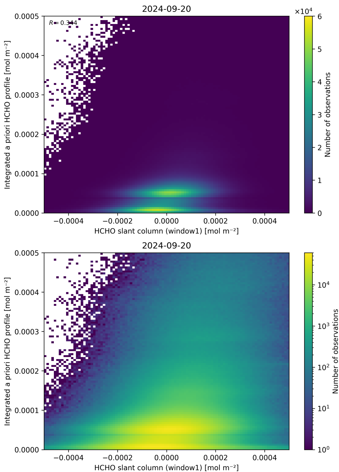
Figure 87: Scatter density plot of “HCHO slant column (window1)” against “Integrated a priori HCHO profile” for 2024-09-19 to 2024-09-21.
