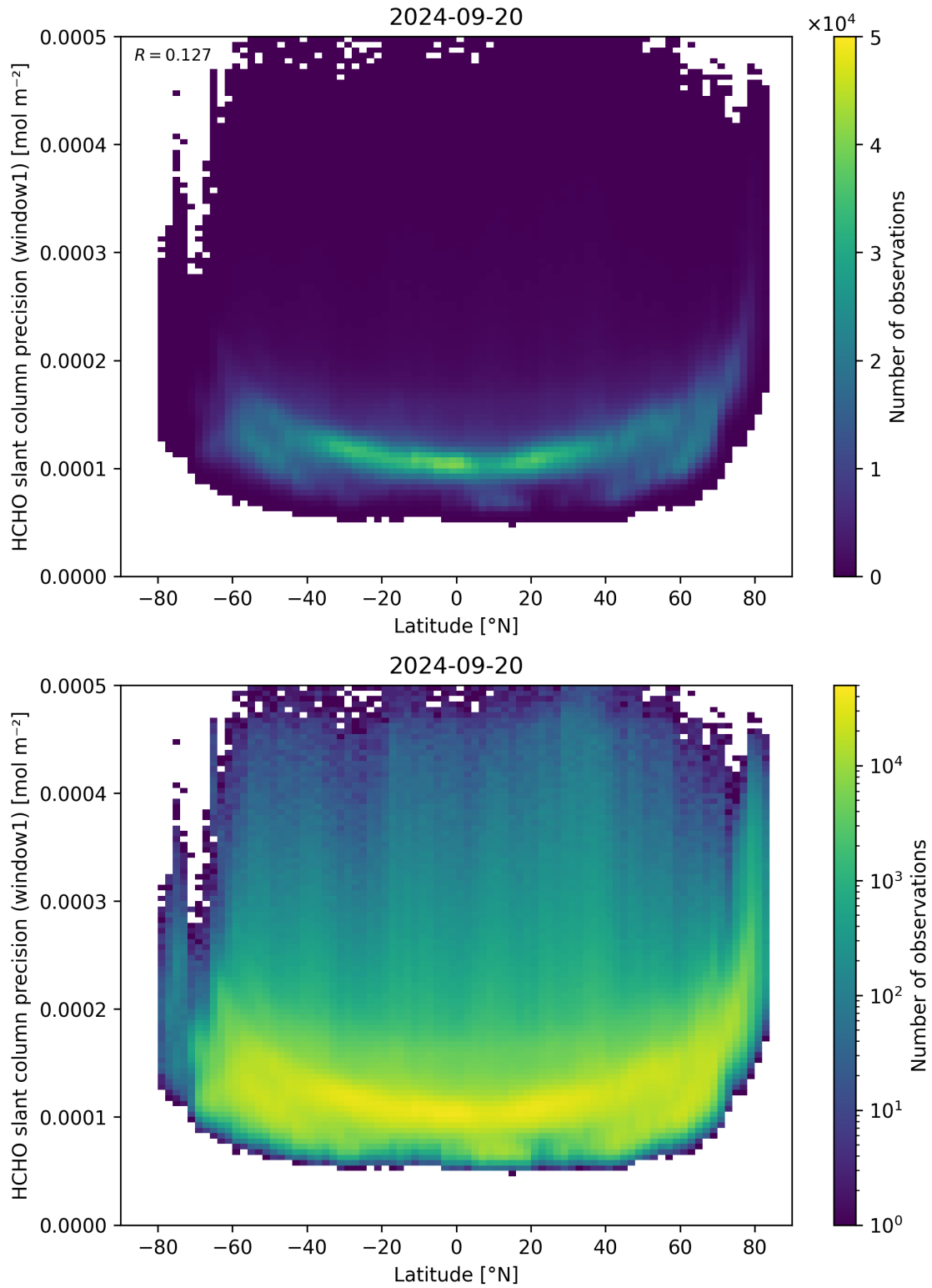
Figure 160: Scatter density plot of “Latitude” against “HCHO slant column precision (window1)” for 2024-09-19 to 2024-09-21.
