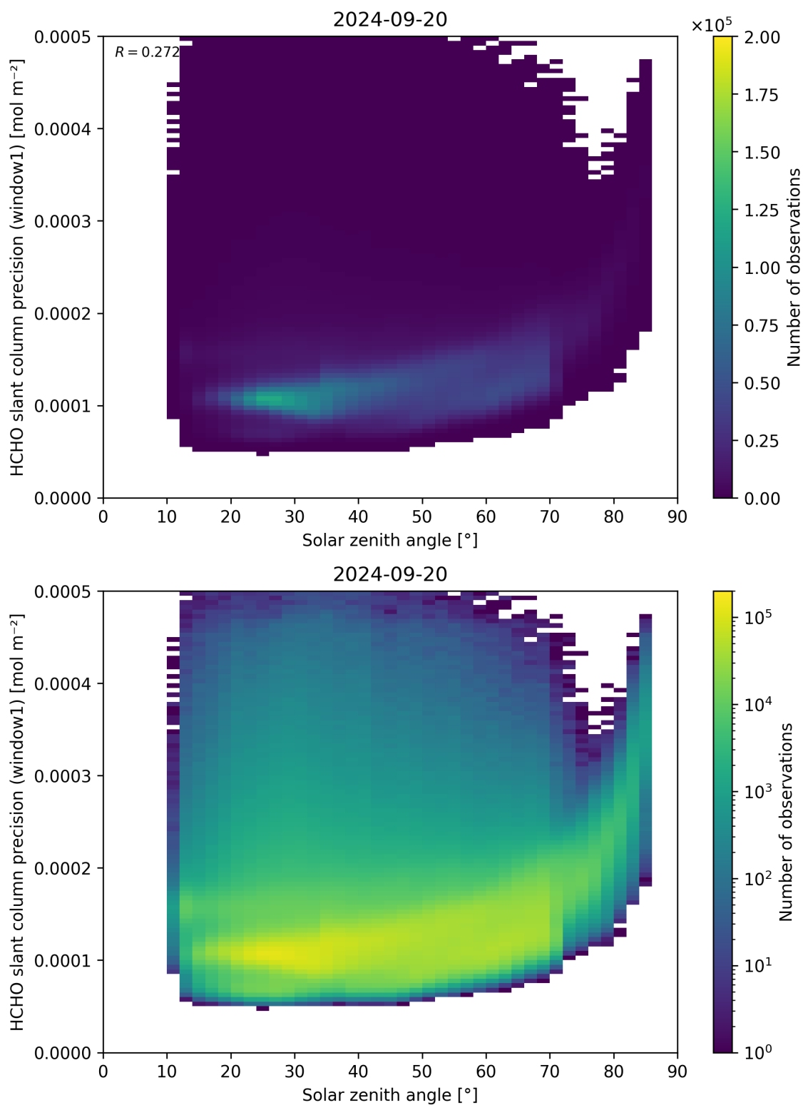
Figure 174: Scatter density plot of “Solar zenith angle” against “HCHO slant column precision (window1)” for 2024-09-19 to 2024-09-21.
