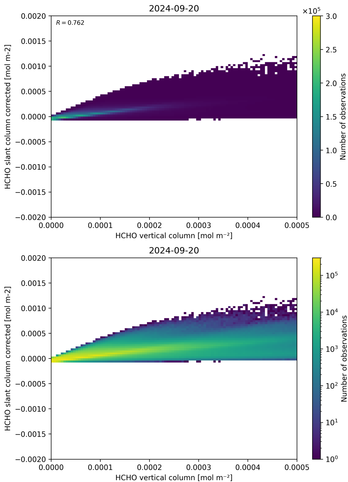
Figure 127: Scatter density plot of “HCHO vertical column” against “HCHO slant column corrected” for 2024-09-19 to 2024-09-21.
