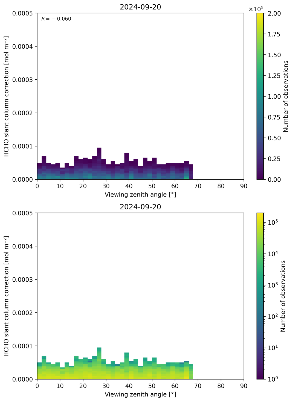
Figure 187: Scatter density plot of “Viewing zenith angle” against “HCHO slant column correction” for 2024-09-19 to 2024-09-21.
