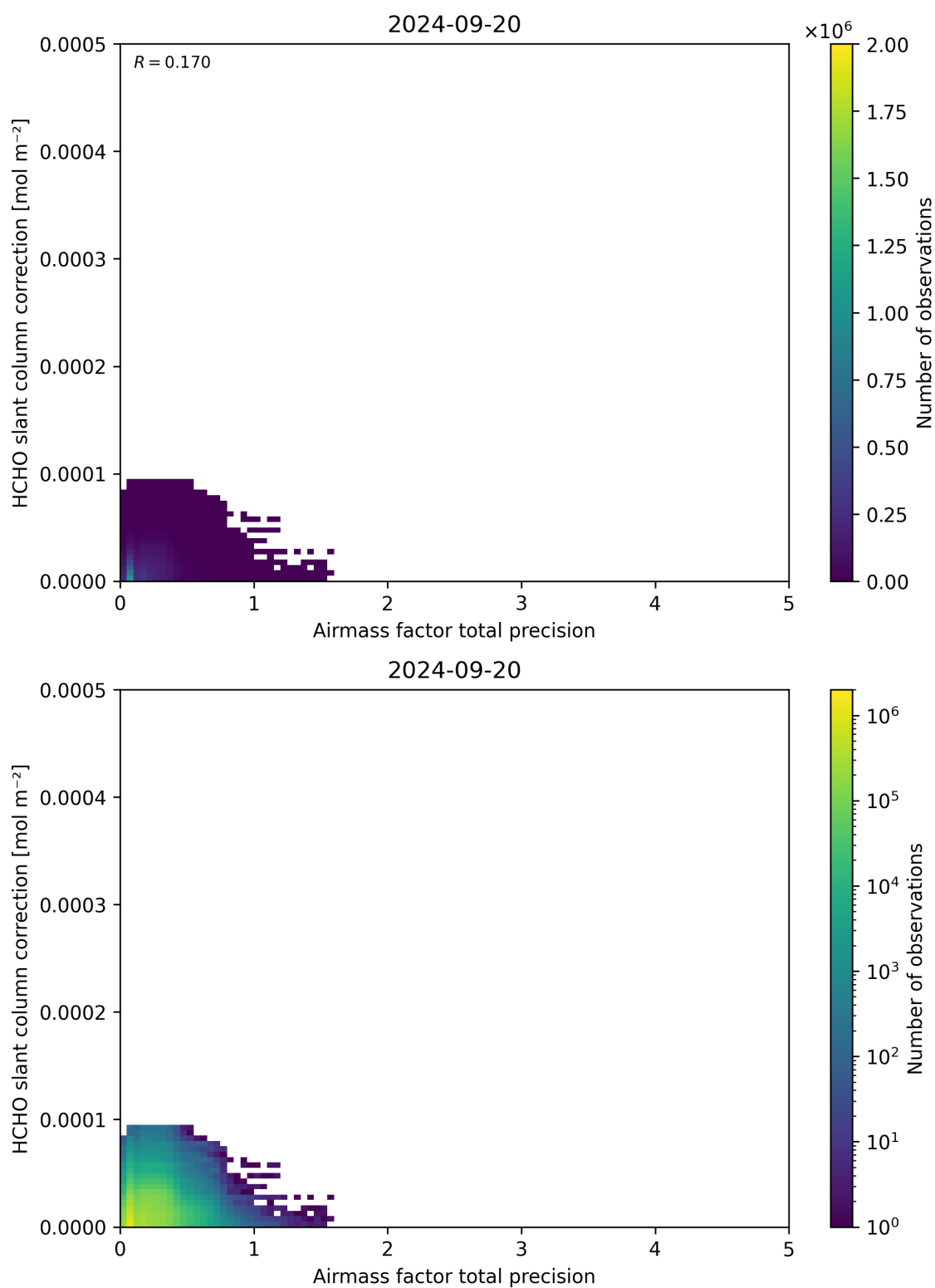
Figure 110: Scatter density plot of “Airmass factor total precision” against “HCHO slant column correction” for 2024-09-19 to 2024-09-21.
