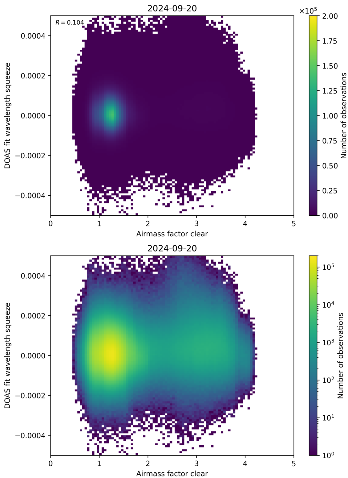
Figure 73: Scatter density plot of “Airmass factor clear” against “DOAS fit wavelength squeeze” for 2024-09-19 to 2024-09-21.
