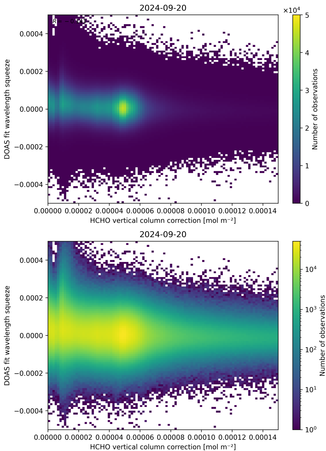
Figure 114: Scatter density plot of “HCHO vertical column correction” against “DOAS fit wavelength squeeze” for 2024-09-19 to 2024-09-21.
