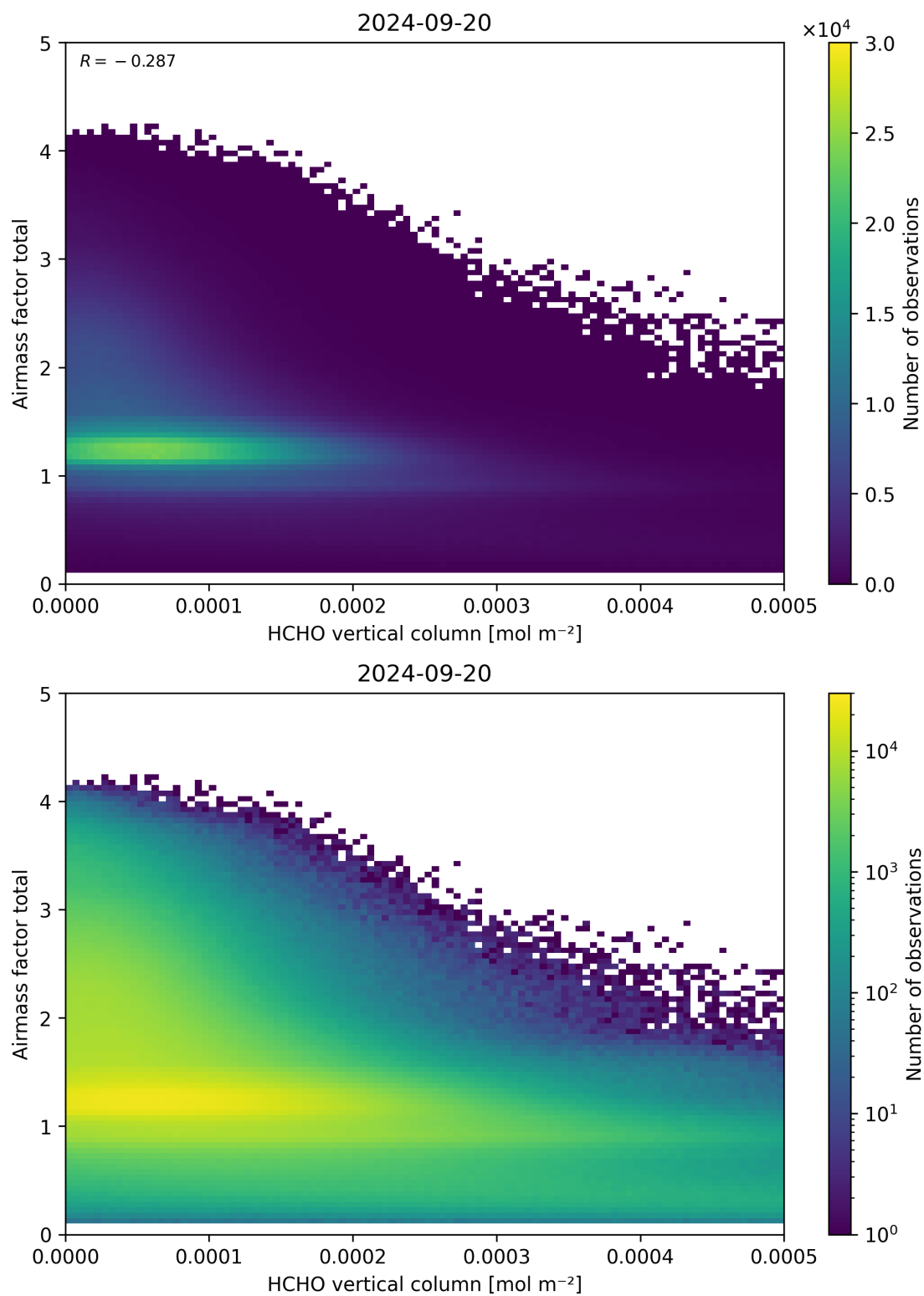
Figure 131: Scatter density plot of “HCHO vertical column” against “Airmass factor total” for 2024-09-19 to 2024-09-21.
