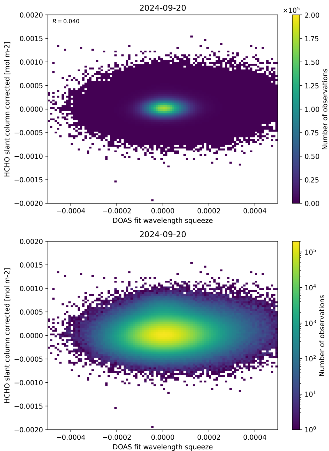
Figure 69: Scatter density plot of “DOAS fit wavelength squeeze” against “HCHO slant column corrected” for 2024-09-19 to 2024-09-21.
