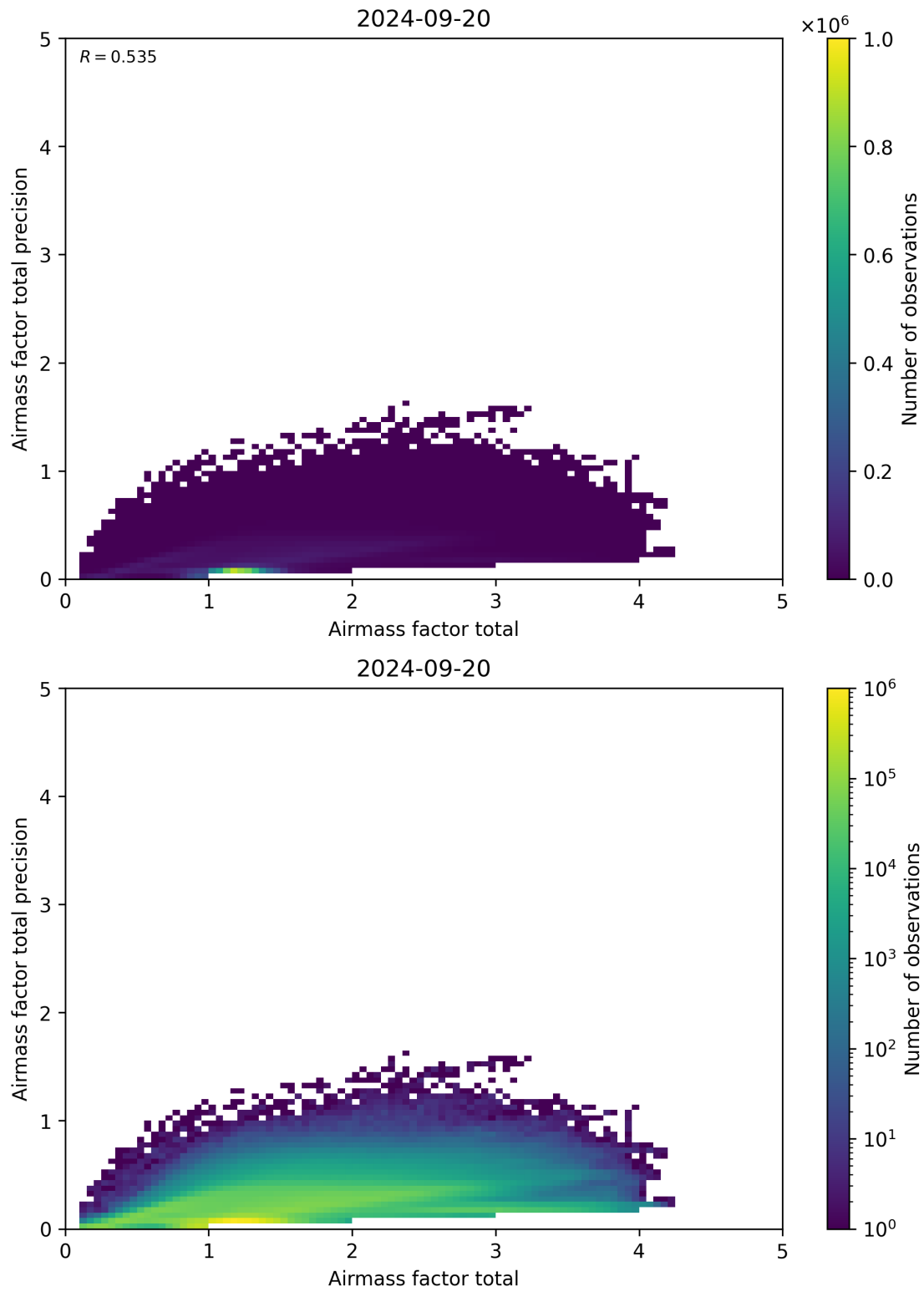
Figure 103: Scatter density plot of “Airmass factor total” against “Airmass factor total precision” for 2024-09-19 to 2024-09-21.
