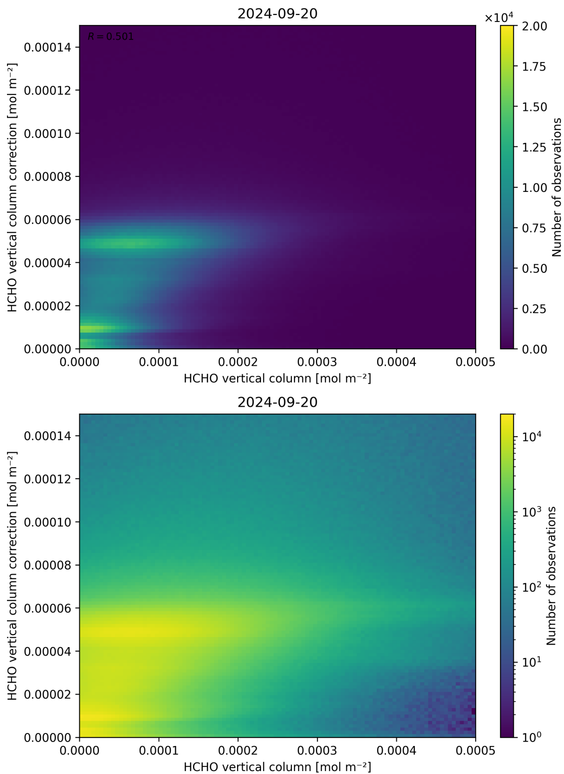
Figure 133: Scatter density plot of “HCHO vertical column” against “HCHO vertical column correction” for 2024-09-19 to 2024-09-21.
