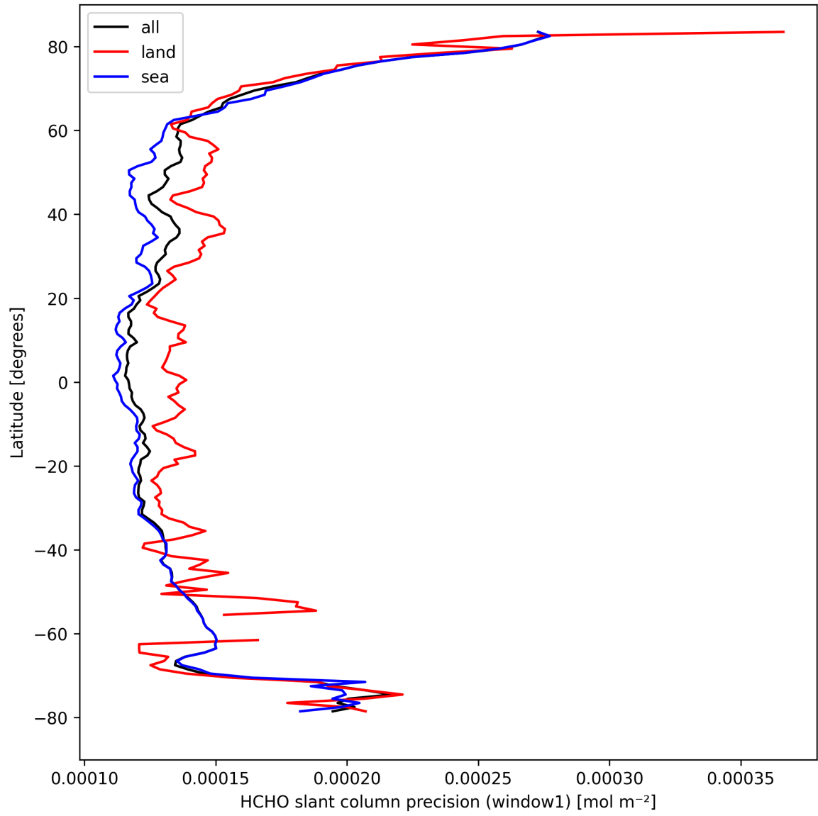
Figure 25: Zonal average of “HCHO slant column precision (window1)” for 2024-09-19 to 2024-09-21.
