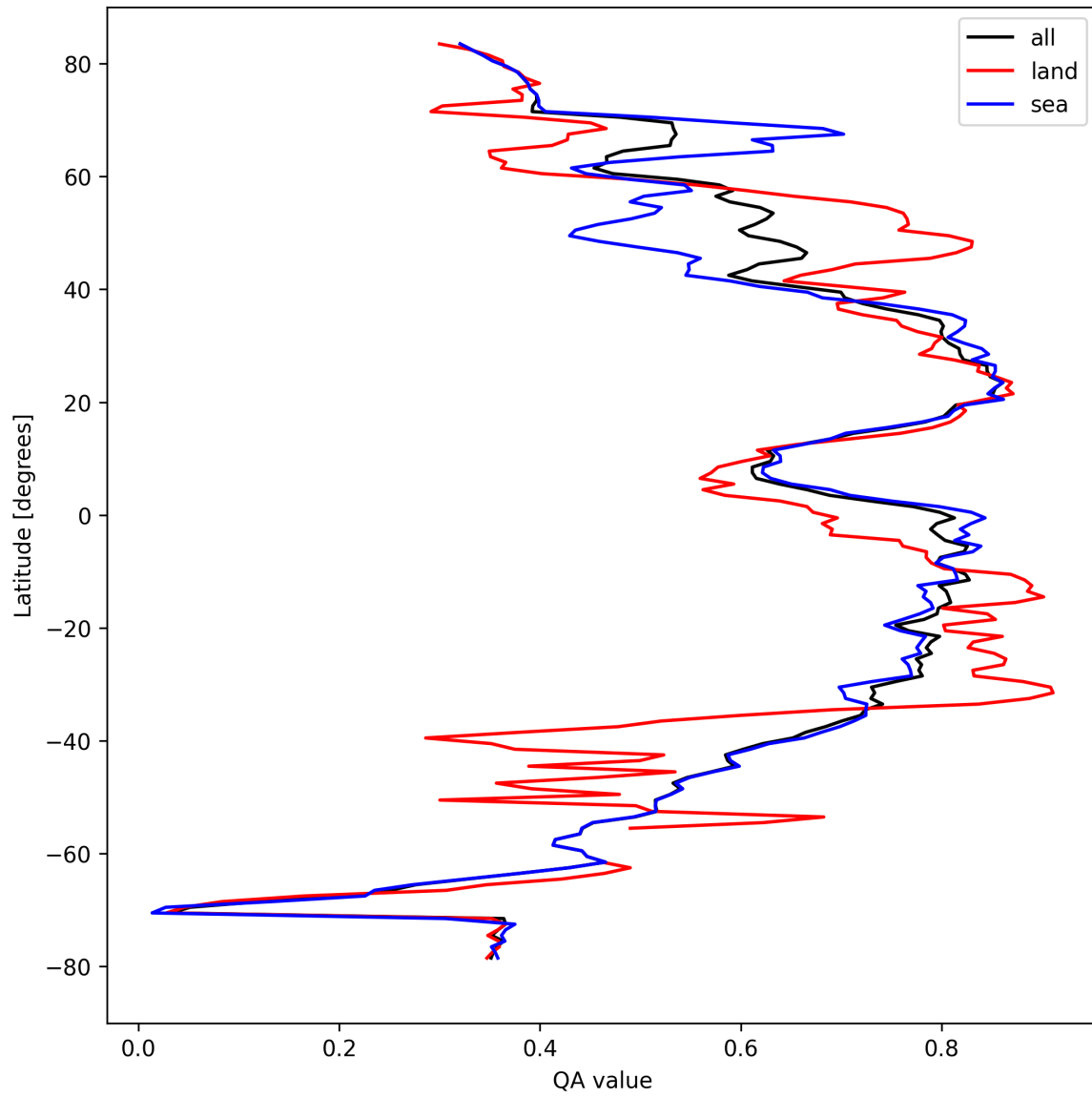
Figure 20: Zonal average of “QA value” for 2024-09-19 to 2024-09-21.
