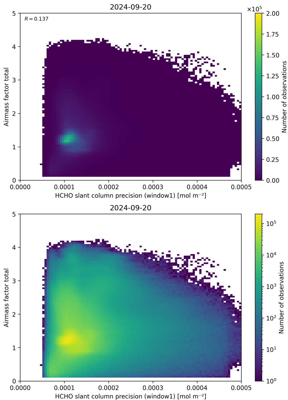
Figure 94: Scatter density plot of “HCHO slant column precision (window1)” against “Airmass factor total” for 2024-09-19 to 2024-09-21.
