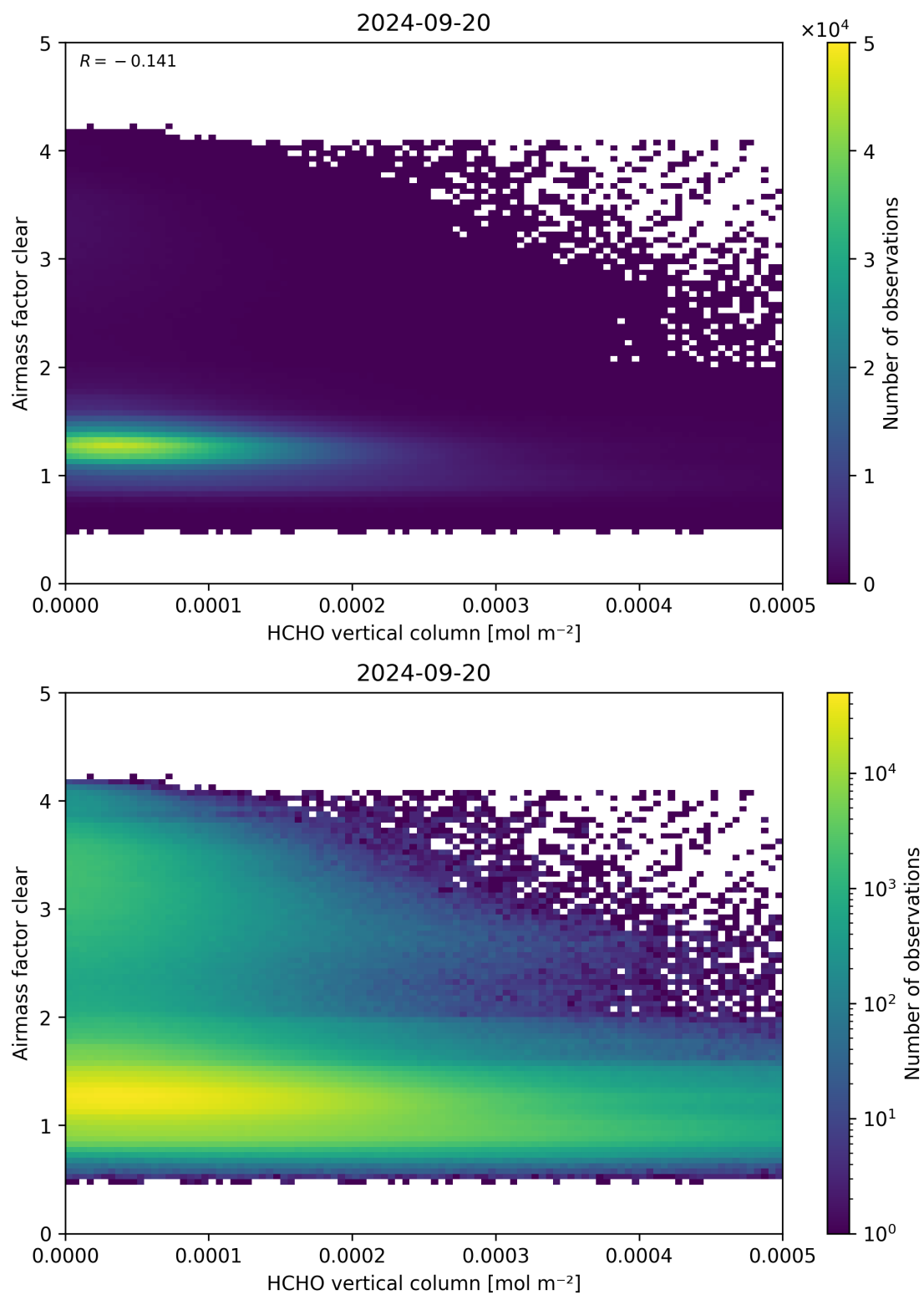
Figure 126: Scatter density plot of “HCHO vertical column” against “Airmass factor clear” for 2024-09-19 to 2024-09-21.
