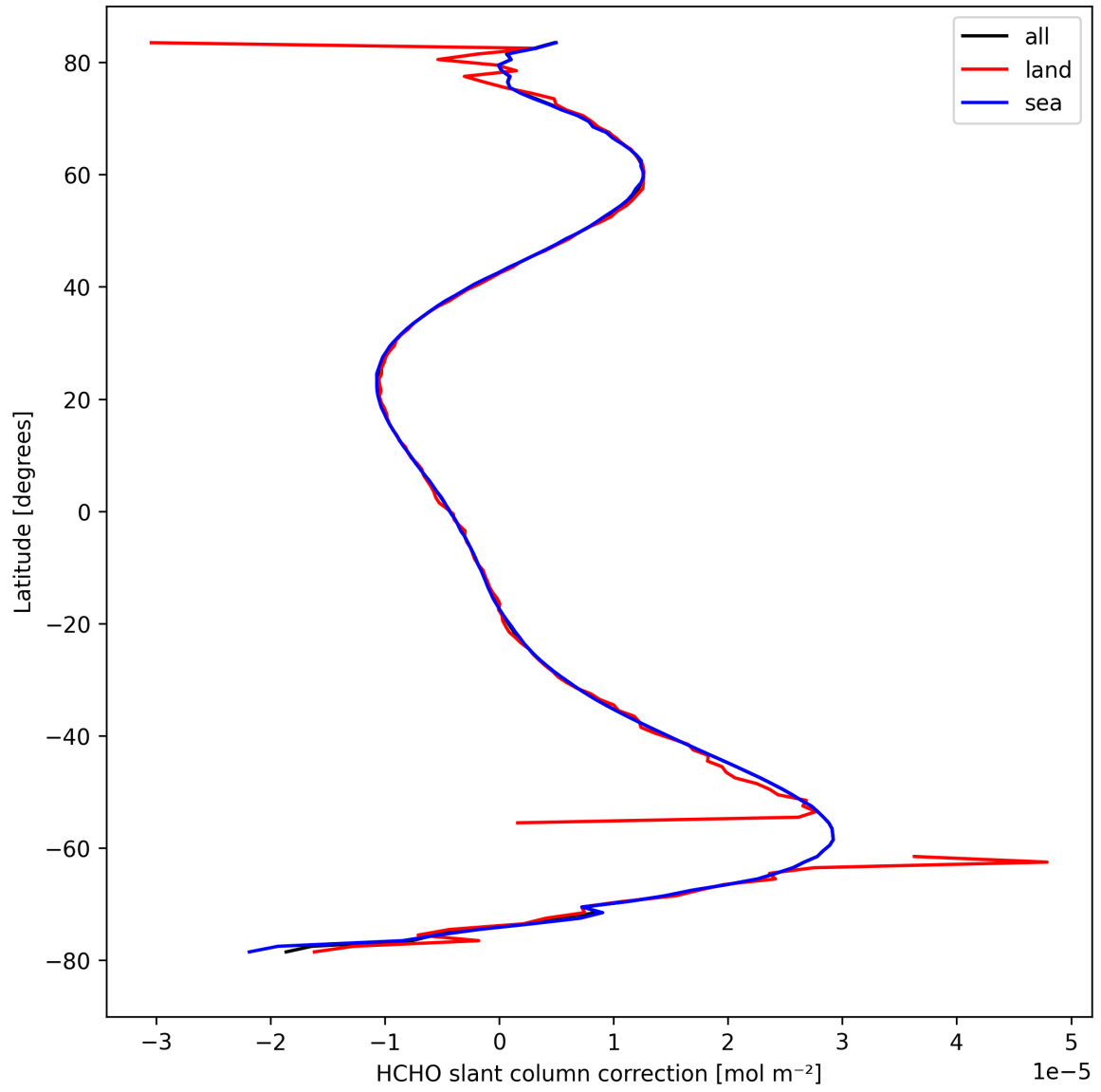
Figure 33: Zonal average of “HCHO slant column correction” for 2024-09-19 to 2024-09-21.
