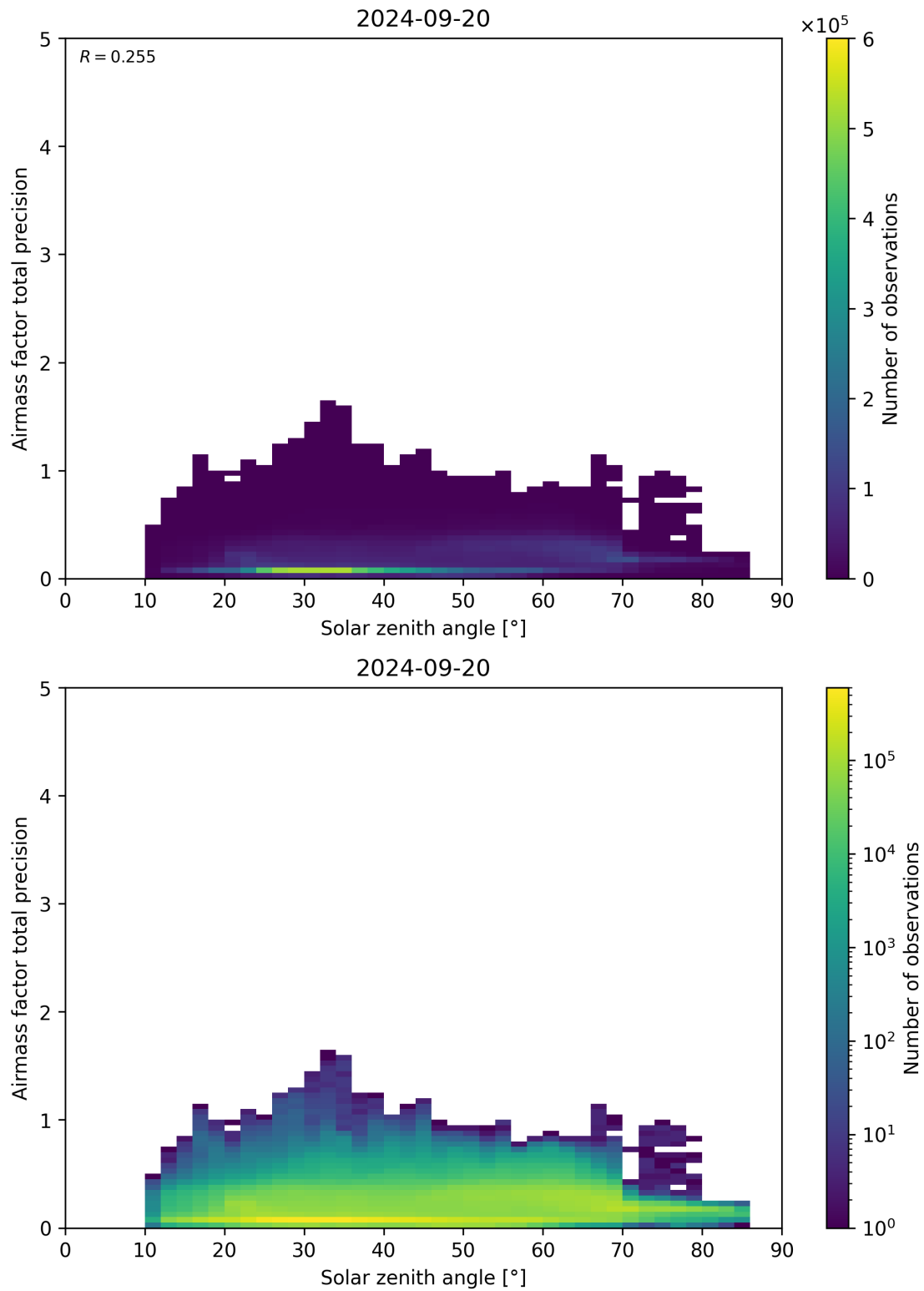
Figure 176: Scatter density plot of “Solar zenith angle” against “Airmass factor total precision” for 2024-09-19 to 2024-09-21.
