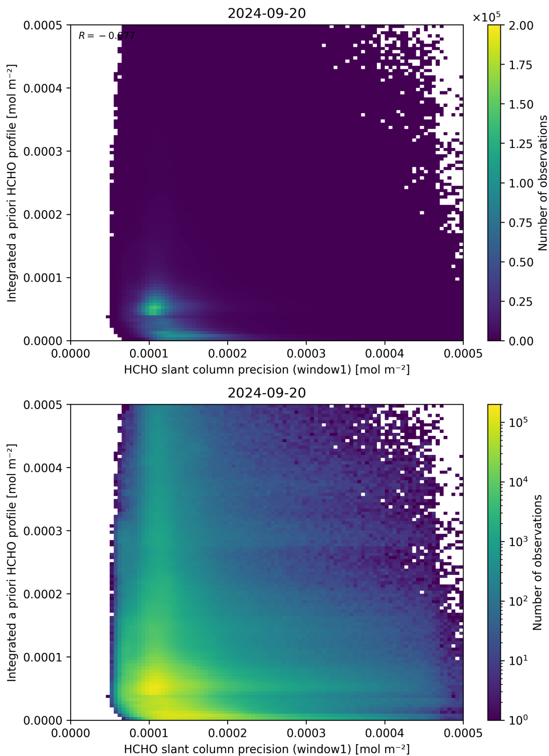
Figure 96: Scatter density plot of “HCHO slant column precision (window1)” against “Integrated a priori HCHO profile” for 2024-09-19 to 2024-09-21.
