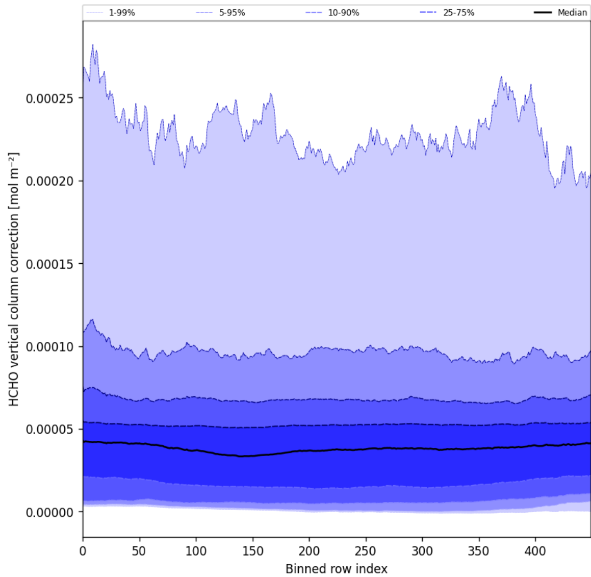
Figure 51: Along track statistics of “HCHO vertical column correction” for 2024-09-19 to 2024-09-21
