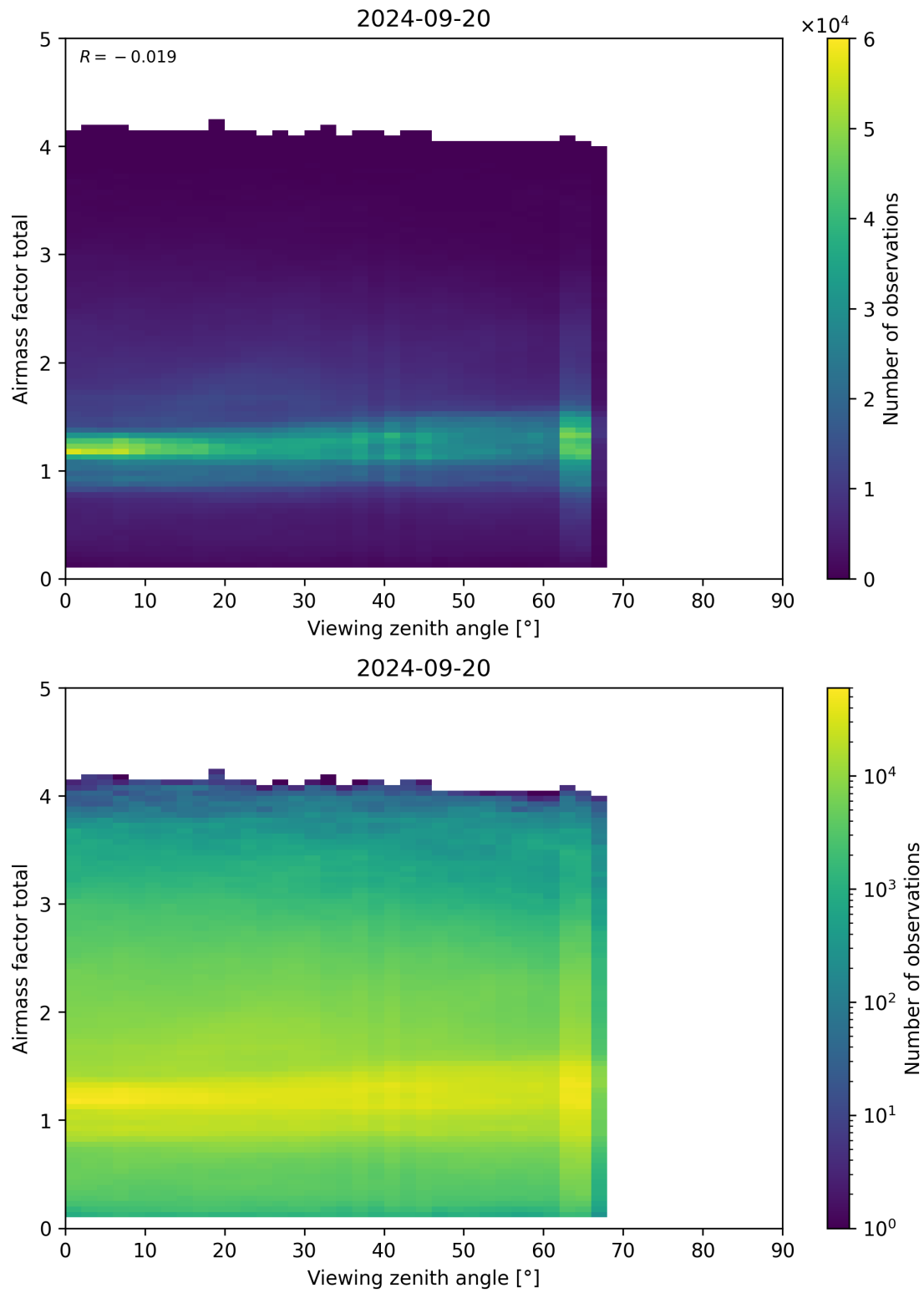
Figure 190: Scatter density plot of “Viewing zenith angle” against “Airmass factor total” for 2024-09-19 to 2024-09-21.
