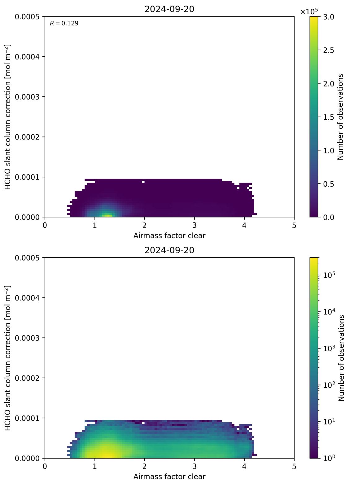
Figure 75: Scatter density plot of “Airmass factor clear” against “HCHO slant column correction” for 2024-09-19 to 2024-09-21.
