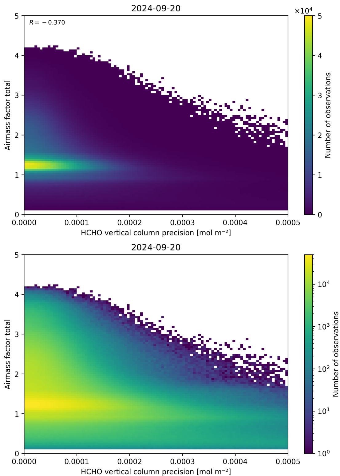
Figure 144: Scatter density plot of “HCHO vertical column precision” against “Airmass factor total” for 2024-09-19 to 2024-09-21.
