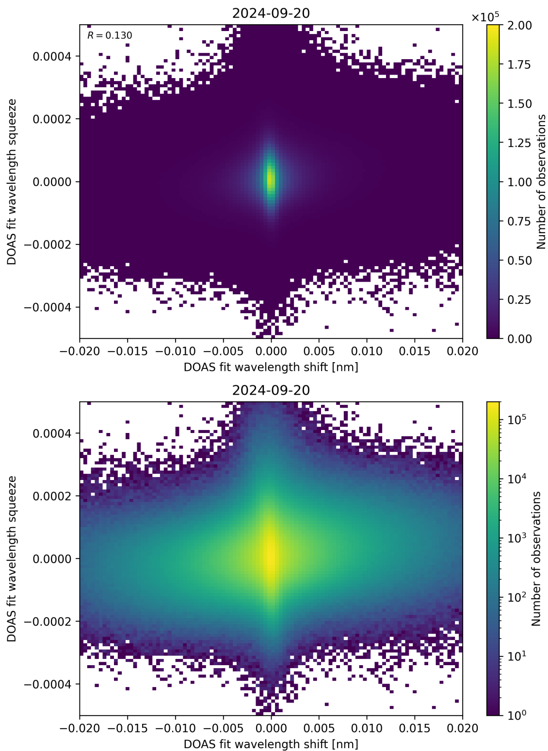
Figure 65: Scatter density plot of “DOAS fit wavelength shift” against “DOAS fit wavelength squeeze” for 2024-09-19 to 2024-09-21.
