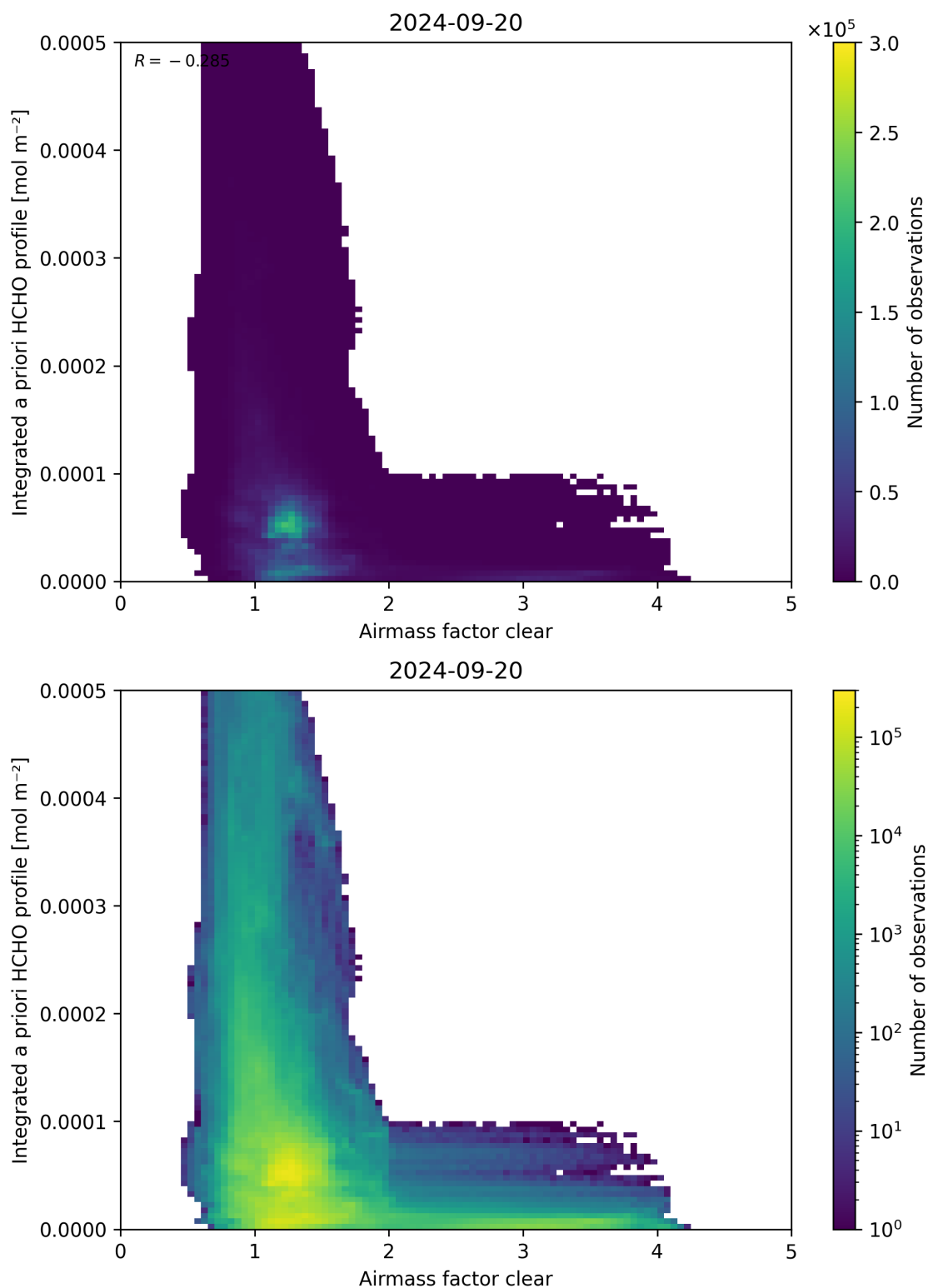
Figure 76: Scatter density plot of “Airmass factor clear” against “Integrated a priori HCHO profile” for 2024-09-19 to 2024-09-21.
