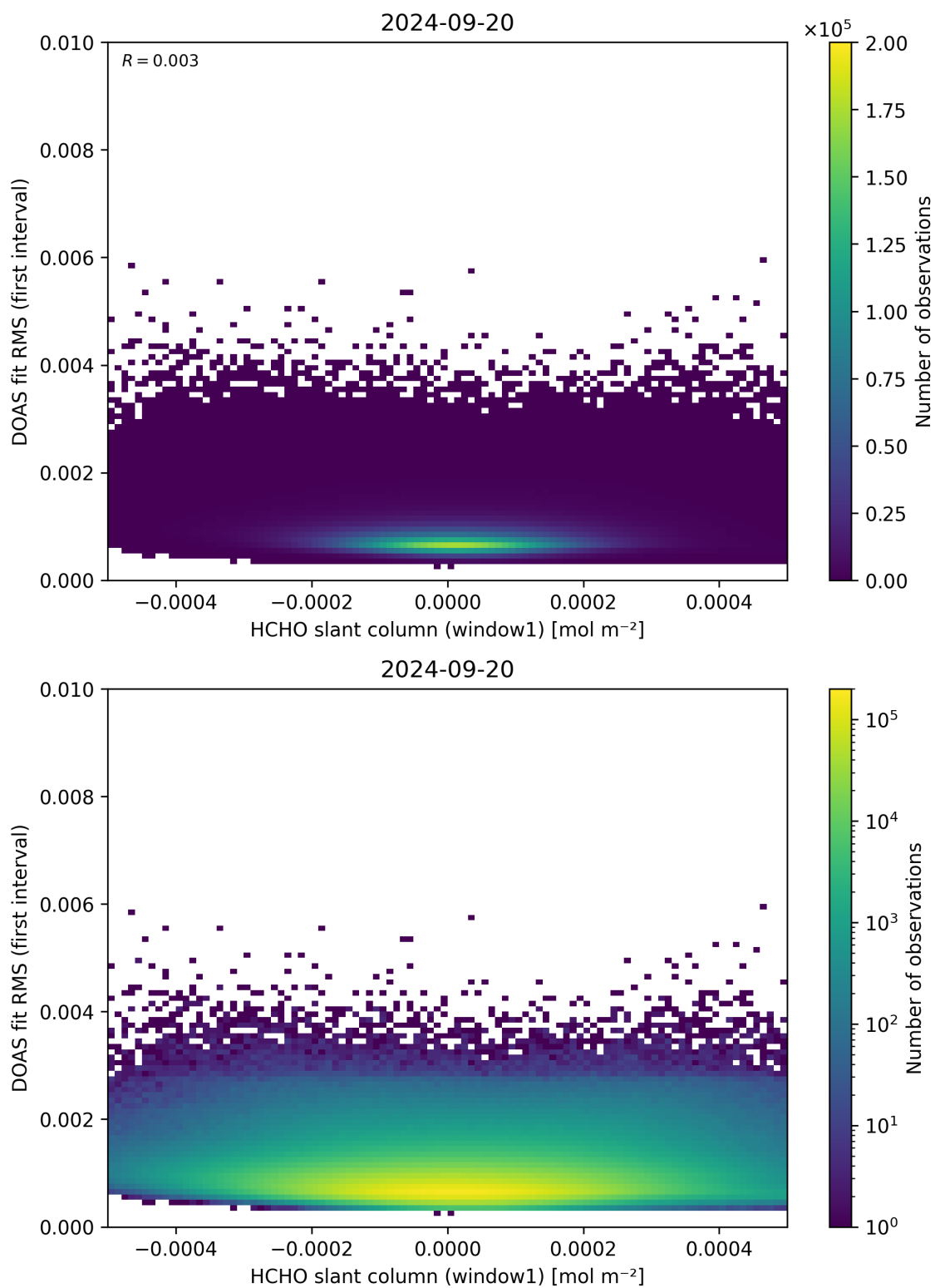
Figure 78: Scatter density plot of “HCHO slant column (window1)” against “DOAS fit RMS (first interval)” for 2024-09-19 to 2024-09-21.
