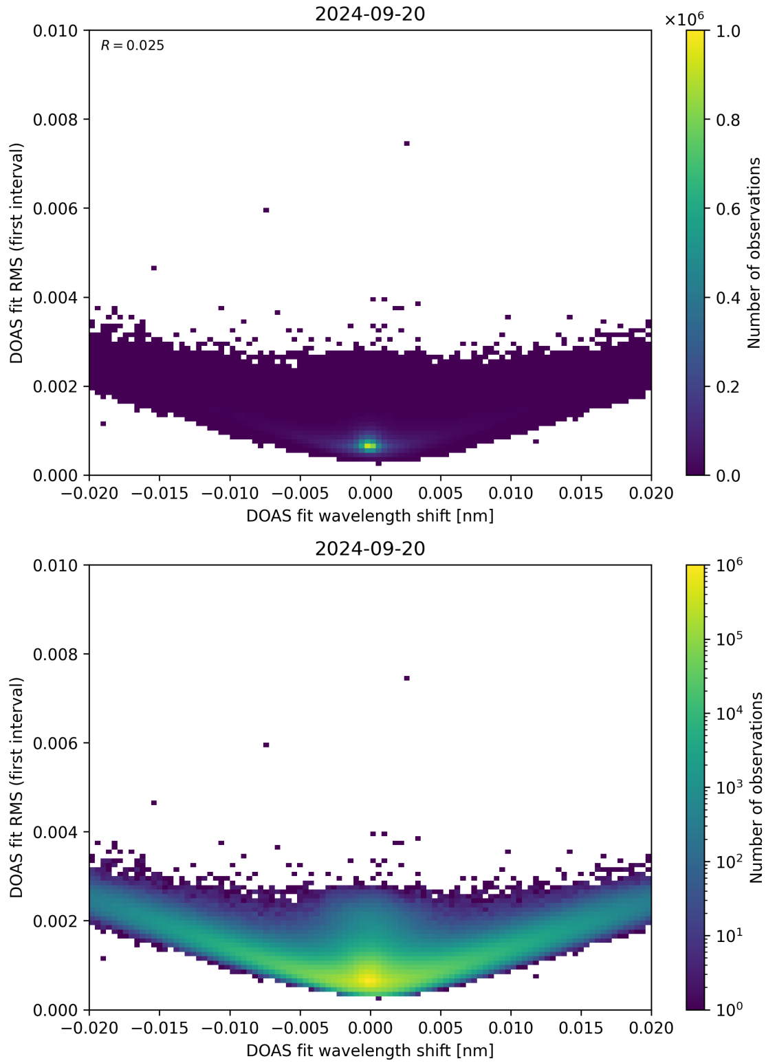
Figure 64: Scatter density plot of “DOAS fit wavelength shift” against “DOAS fit RMS (first interval)” for 2024-09-19 to 2024-09-21.
