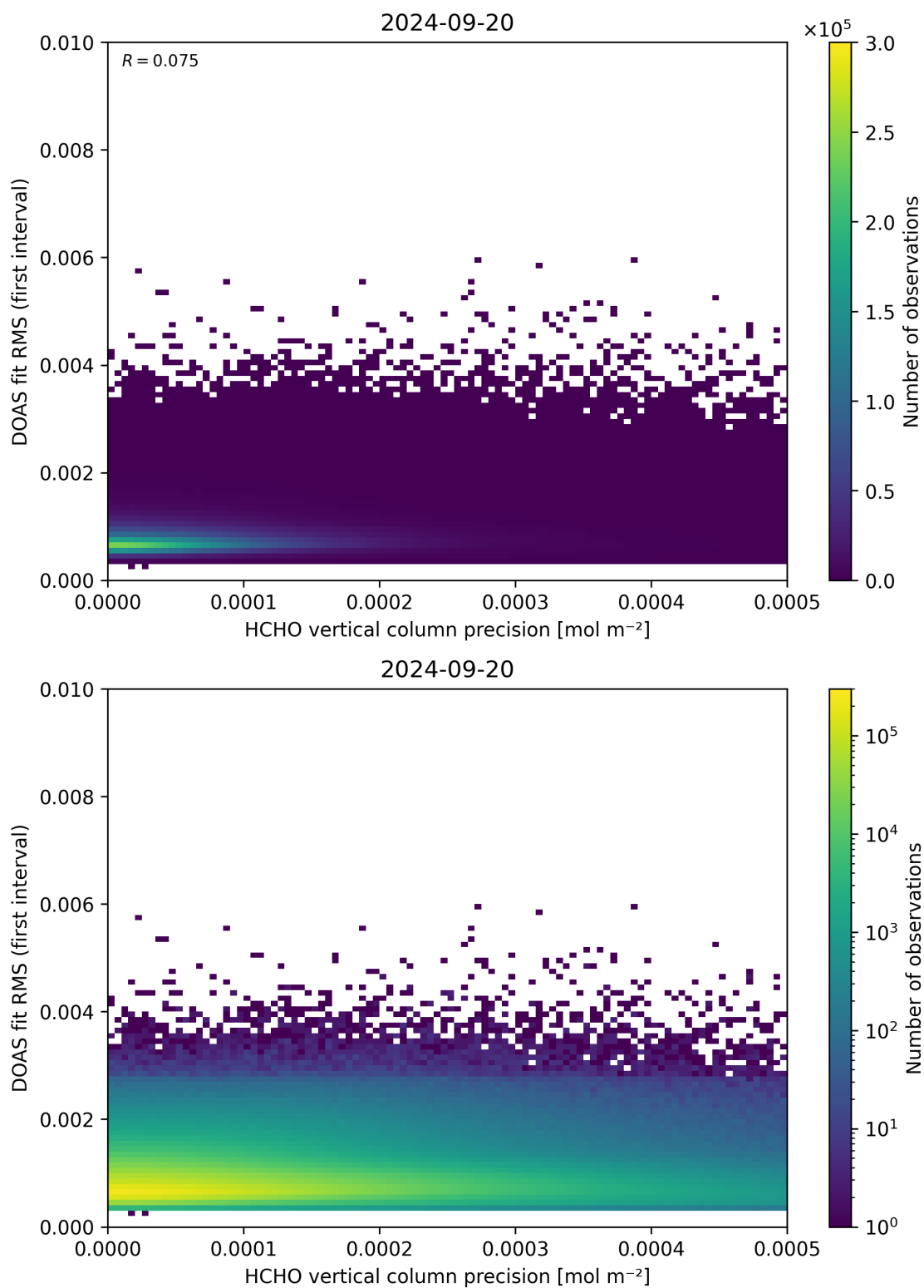
Figure 136: Scatter density plot of “HCHO vertical column precision” against “DOAS fit RMS (first interval)” for 2024-09-19 to 2024-09-21.
