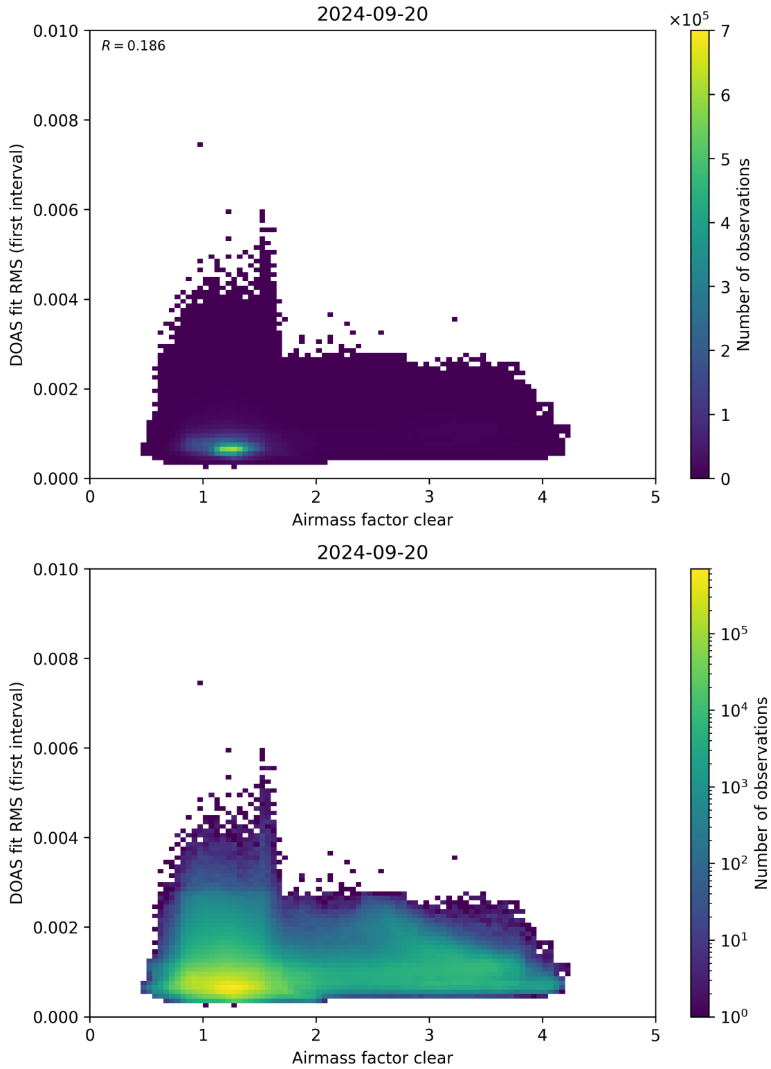
Figure 71: Scatter density plot of “Airmass factor clear” against “DOAS fit RMS (first interval)” for 2024-09-19 to 2024-09-21.
