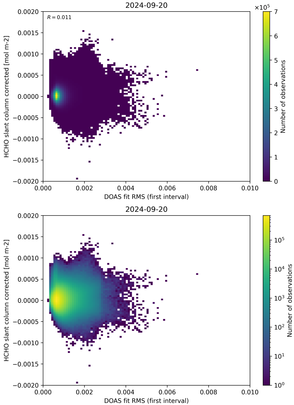
Figure 62: Scatter density plot of “DOAS fit RMS (first interval)” against “HCHO slant column corrected” for 2024-09-19 to 2024-09-21.
