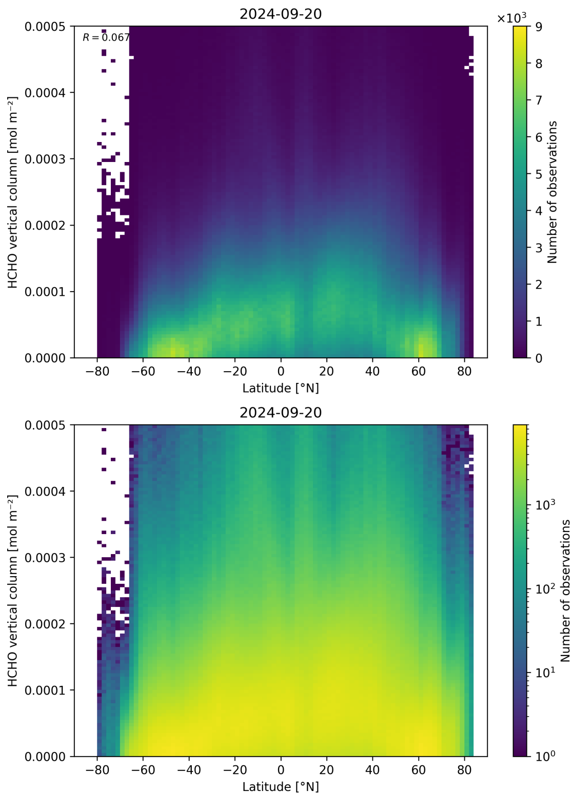
Figure 163: Scatter density plot of “Latitude” against “HCHO vertical column” for 2024-09-19 to 2024-09-21.
