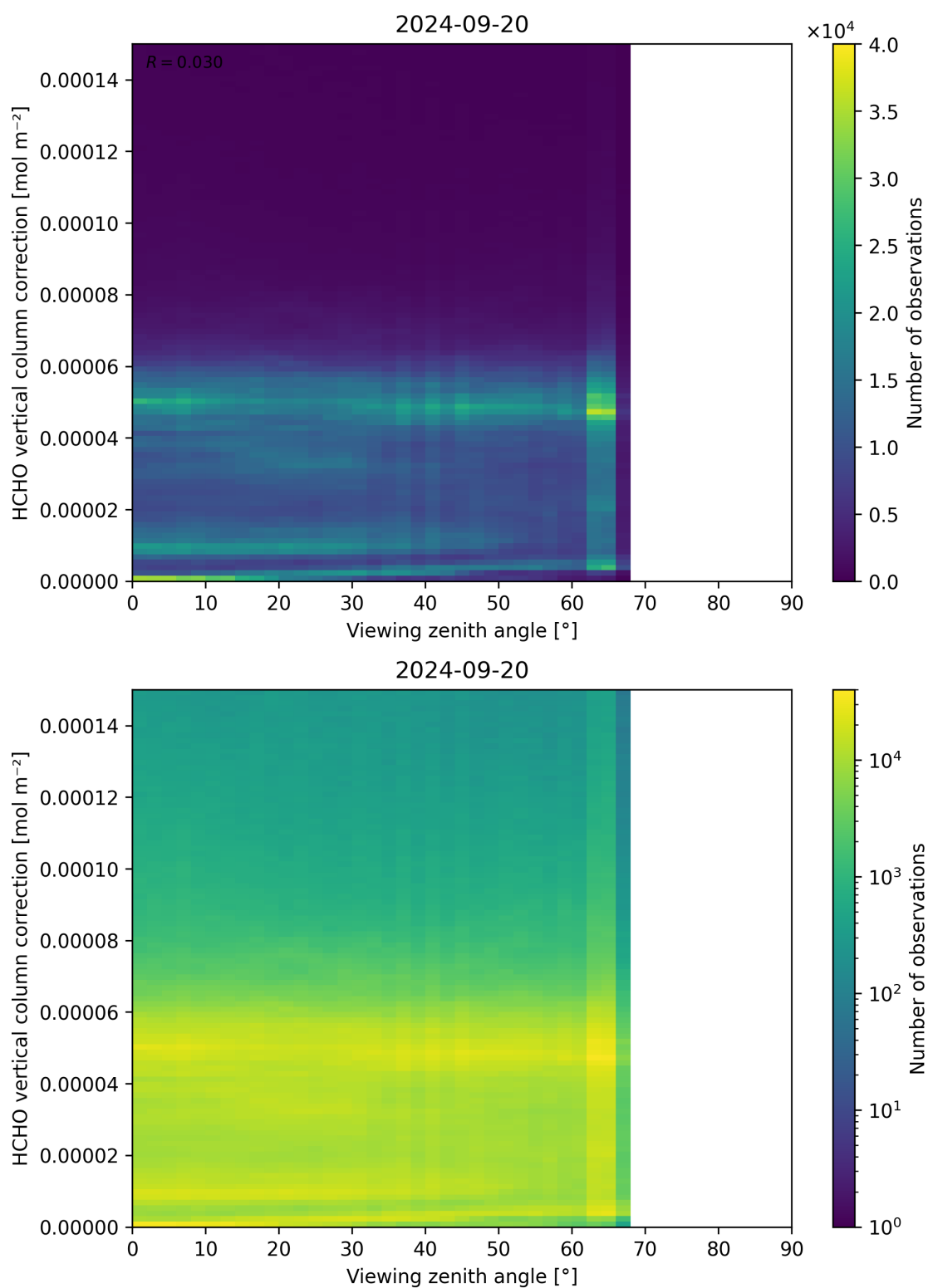
Figure 193: Scatter density plot of “Viewing zenith angle” against “HCHO vertical column correction” for 2024-09-19 to 2024-09-21.
