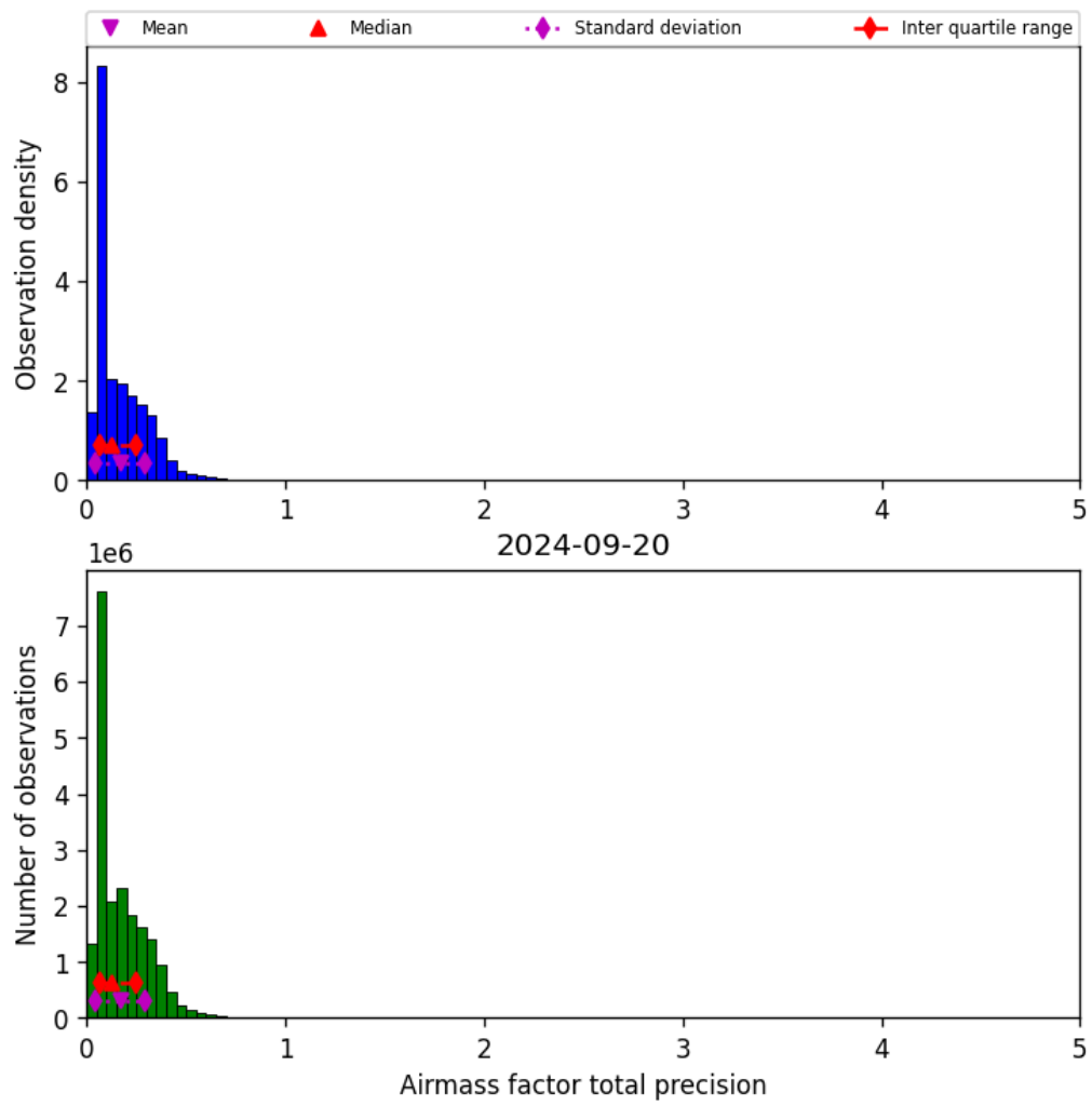
Figure 41: Histogram of “Airmass factor total precision” for 2024-09-19 to 2024-09-21
