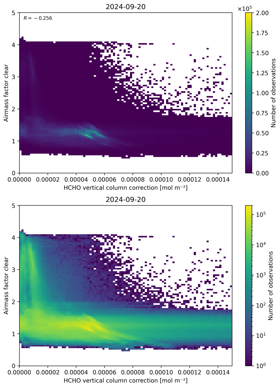
Figure 115: Scatter density plot of “HCHO vertical column correction” against “Airmass factor clear” for 2024-09-19 to 2024-09-21.
