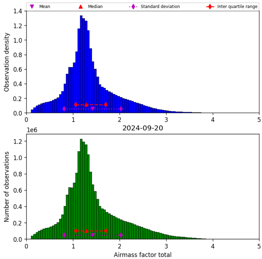
Figure 40: Histogram of “Airmass factor total” for 2024-09-19 to 2024-09-21
