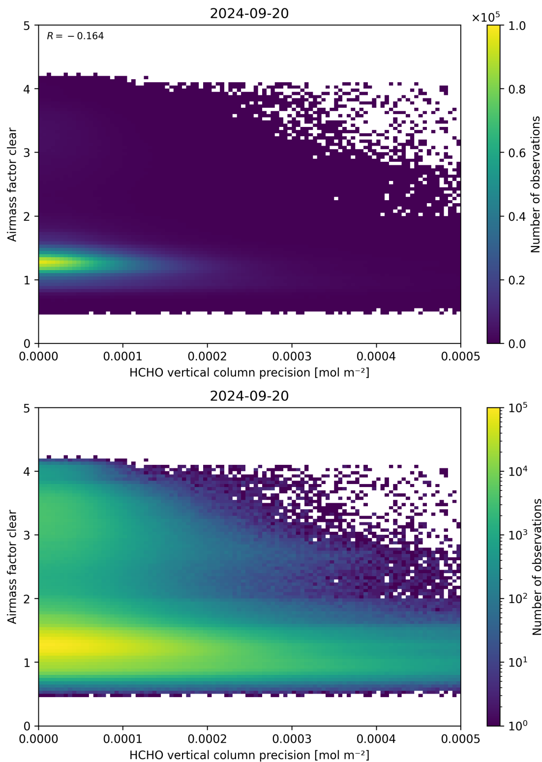
Figure 139: Scatter density plot of “HCHO vertical column precision” against “Airmass factor clear” for 2024-09-19 to 2024-09-21.
