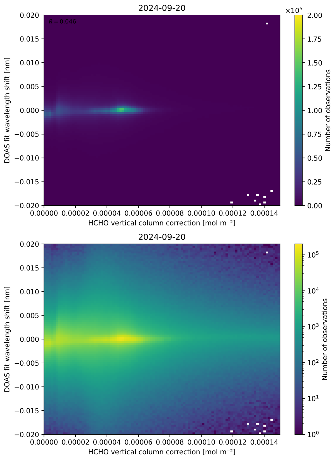
Figure 113: Scatter density plot of “HCHO vertical column correction” against “DOAS fit wavelength shift” for 2024-09-19 to 2024-09-21.
