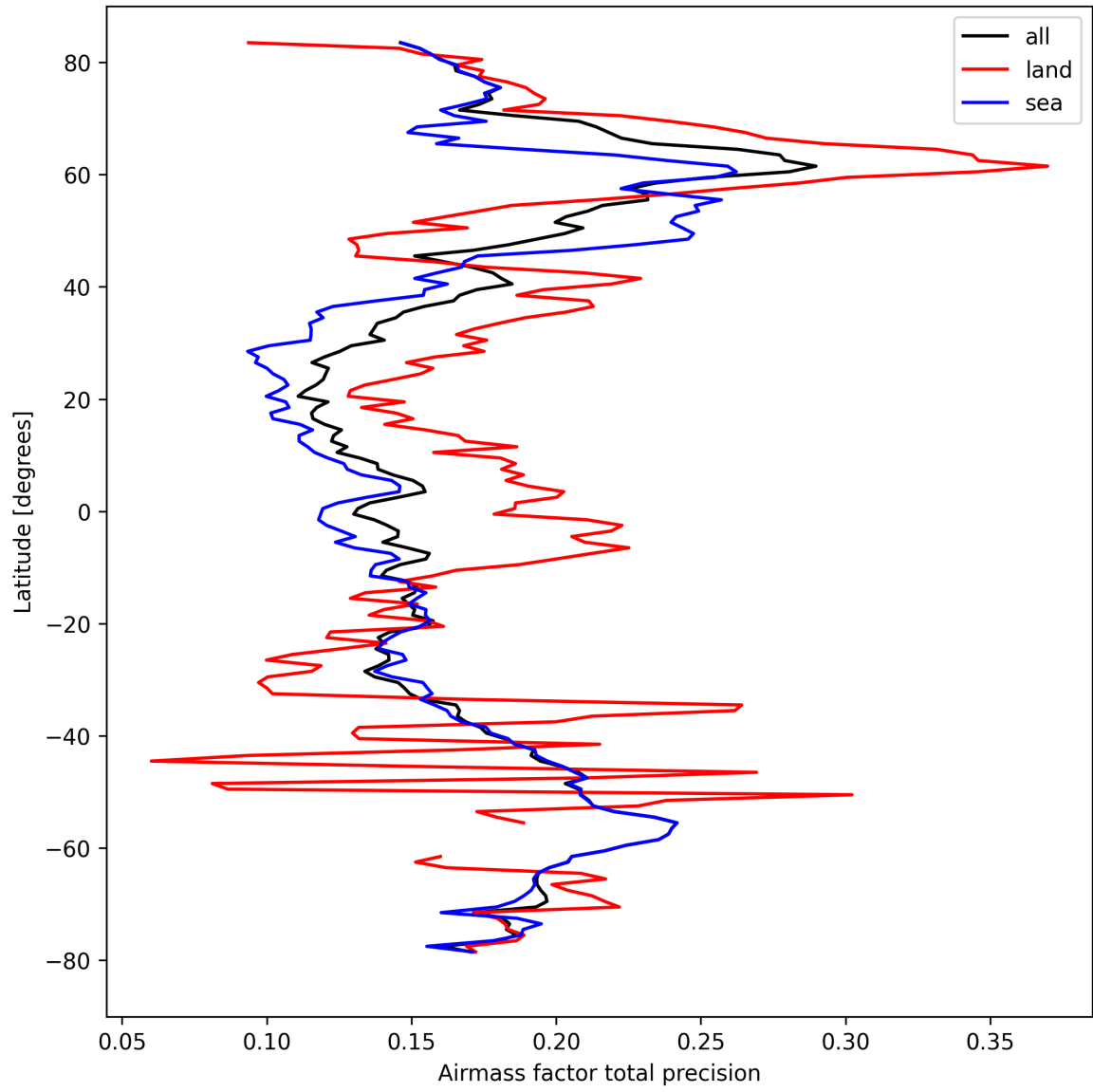
Figure 27: Zonal average of “Airmass factor total precision” for 2024-09-19 to 2024-09-21.
