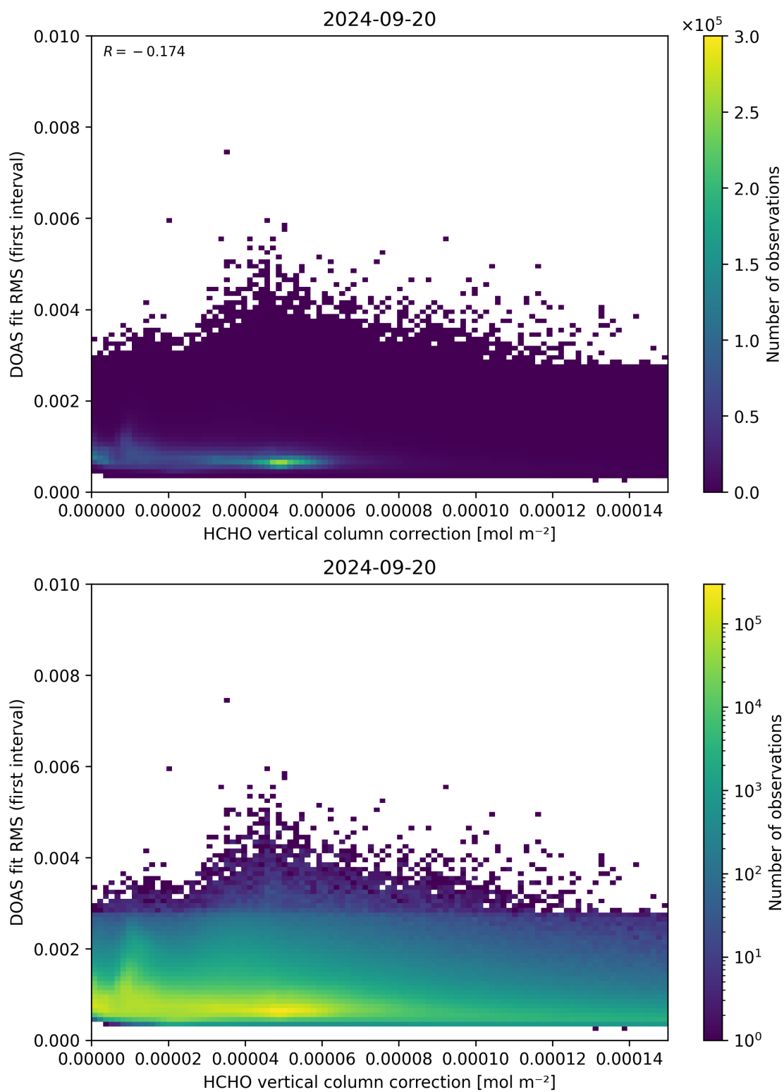
Figure 112: Scatter density plot of “HCHO vertical column correction” against “DOAS fit RMS (first interval)” for 2024-09-19 to 2024-09-21.
