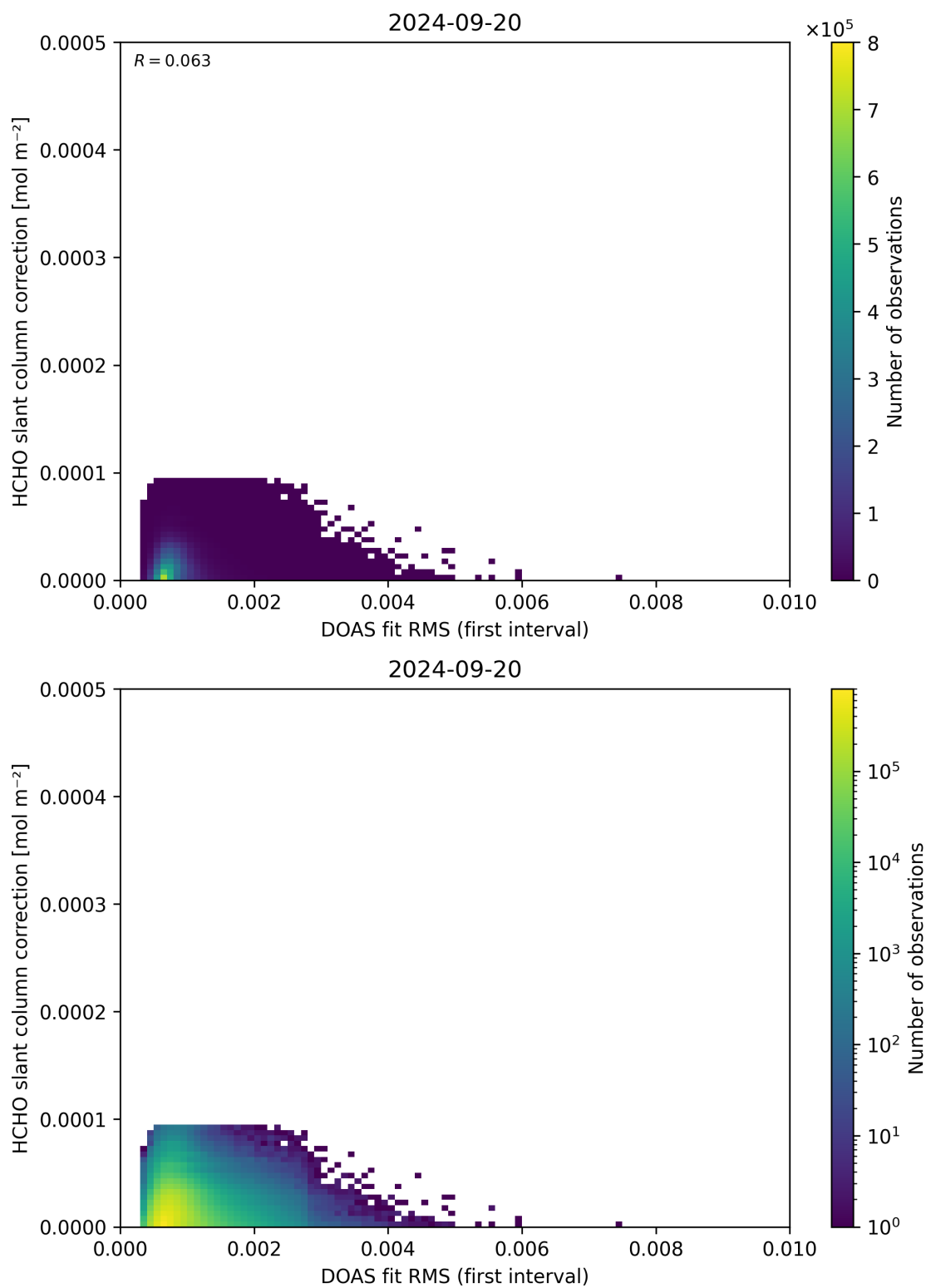
Figure 63: Scatter density plot of “DOAS fit RMS (first interval)” against “HCHO slant column correction” for 2024-09-19 to 2024-09-21.
