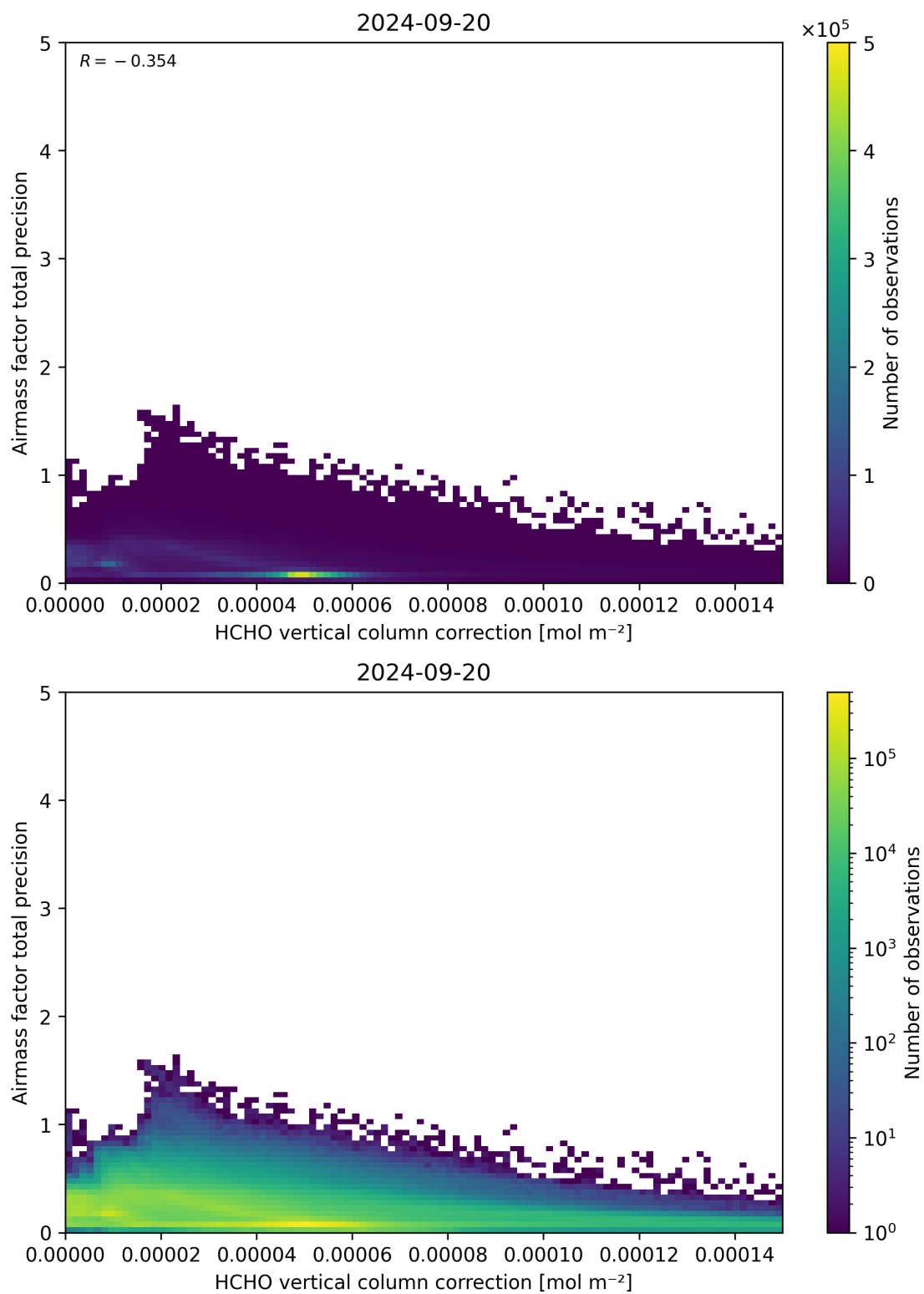
Figure 121: Scatter density plot of “HCHO vertical column correction” against “Airmass factor total precision” for 2024-09-19 to 2024-09-21.
