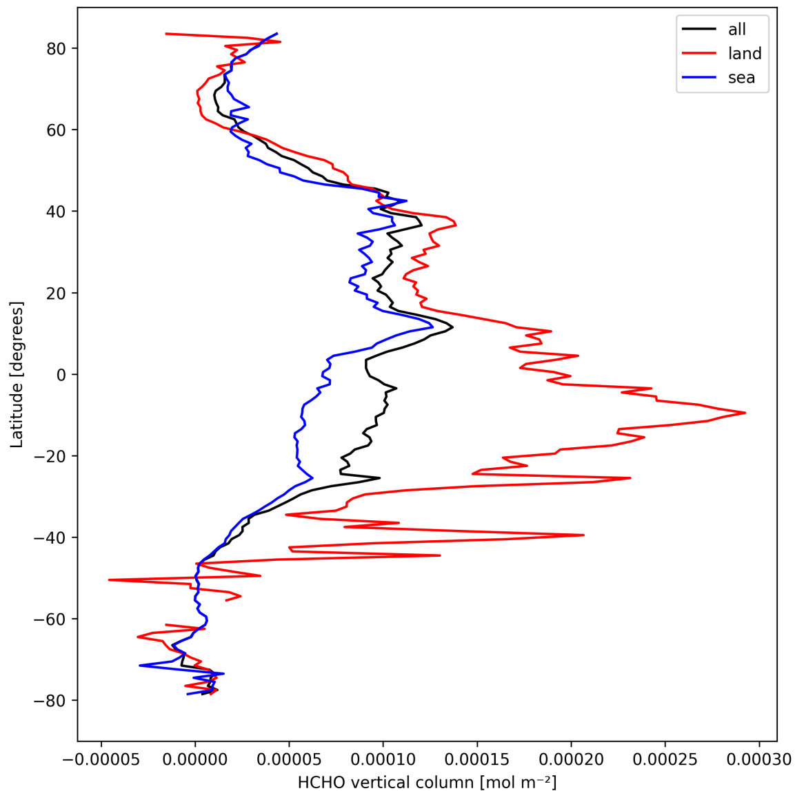
Figure 21: Zonal average of “HCHO vertical column” for 2024-09-19 to 2024-09-21.
