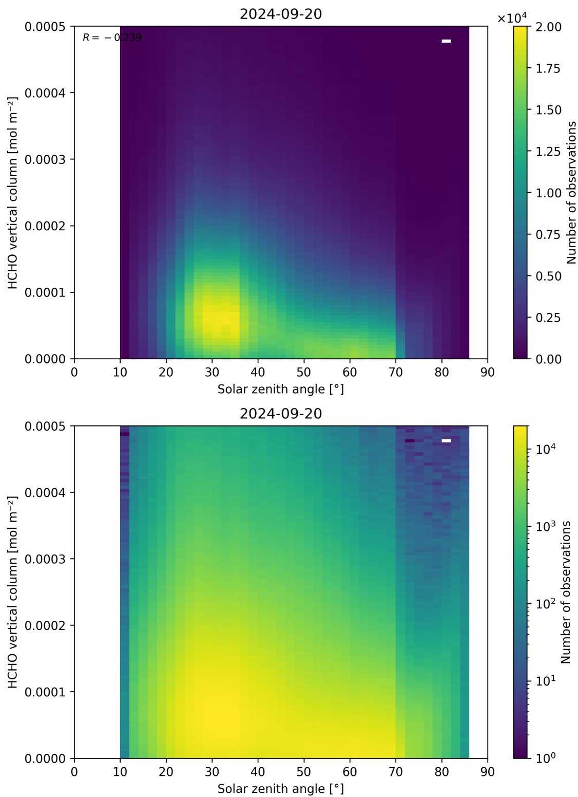
Figure 177: Scatter density plot of “Solar zenith angle” against “HCHO vertical column” for 2024-09-19 to 2024-09-21.
