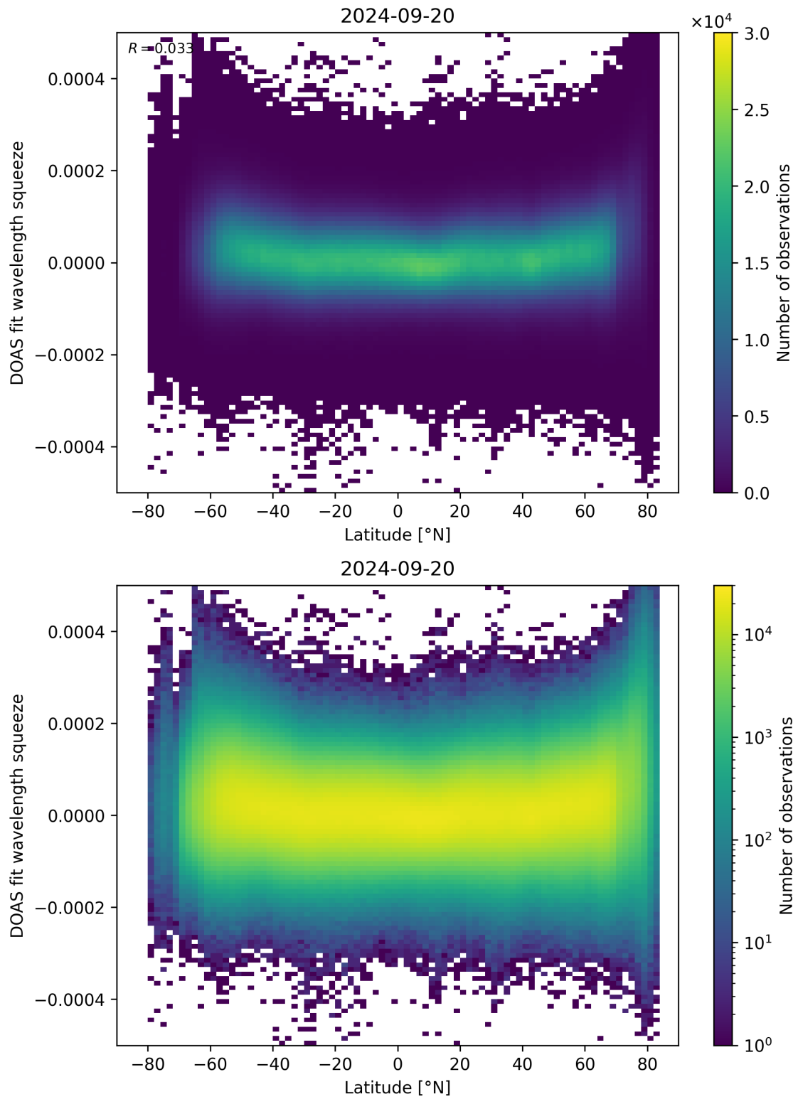
Figure 155: Scatter density plot of “Latitude” against “DOAS fit wavelength squeeze” for 2024-09-19 to 2024-09-21.
