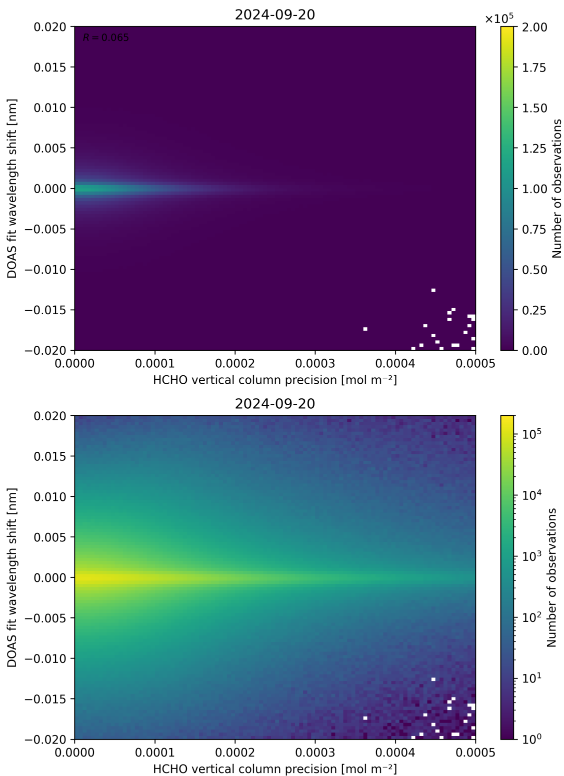
Figure 137: Scatter density plot of “HCHO vertical column precision” against “DOAS fit wavelength shift” for 2024-09-19 to 2024-09-21.
