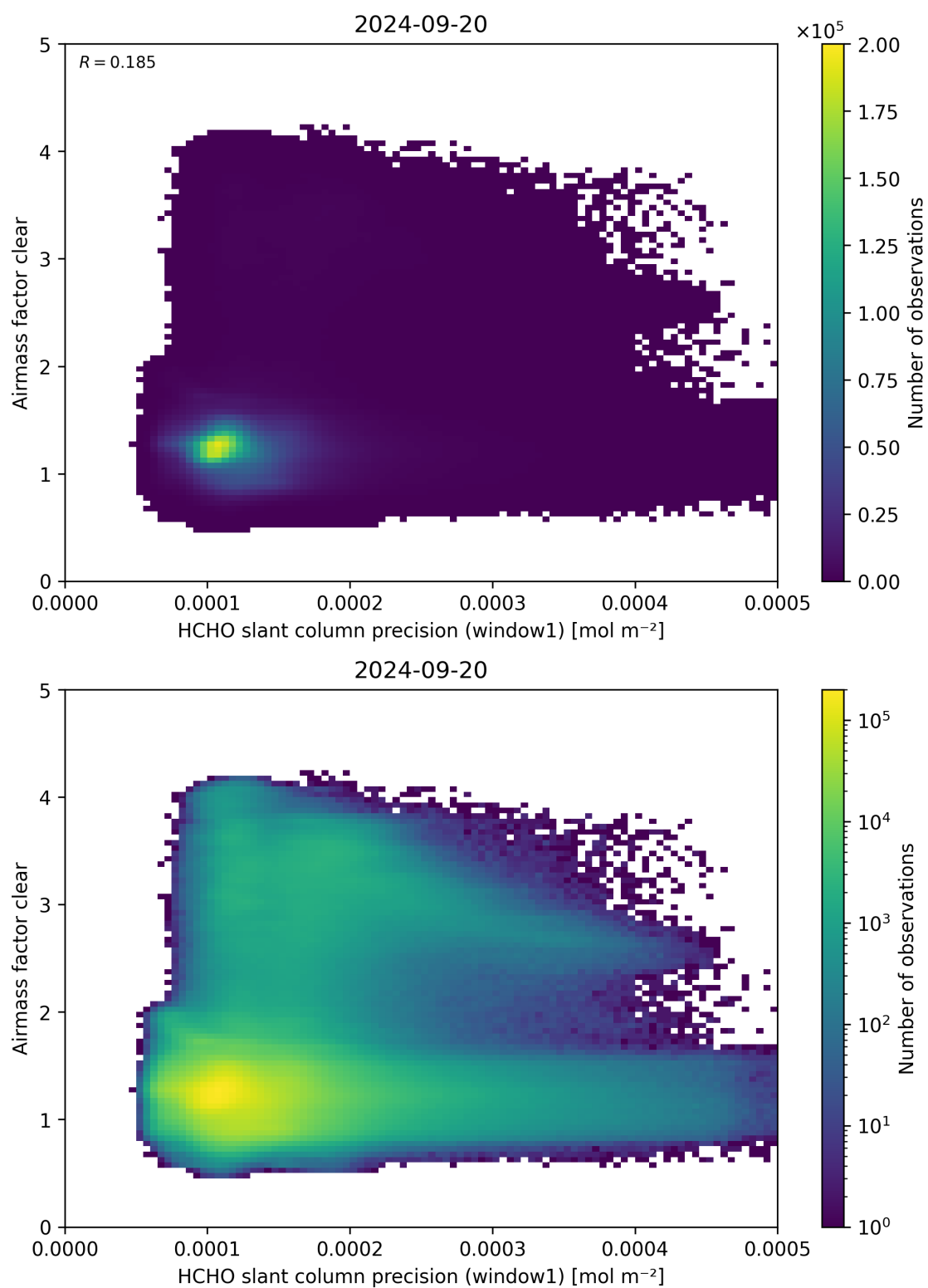
Figure 91: Scatter density plot of “HCHO slant column precision (window1)” against “Airmass factor clear” for 2024-09-19 to 2024-09-21.
