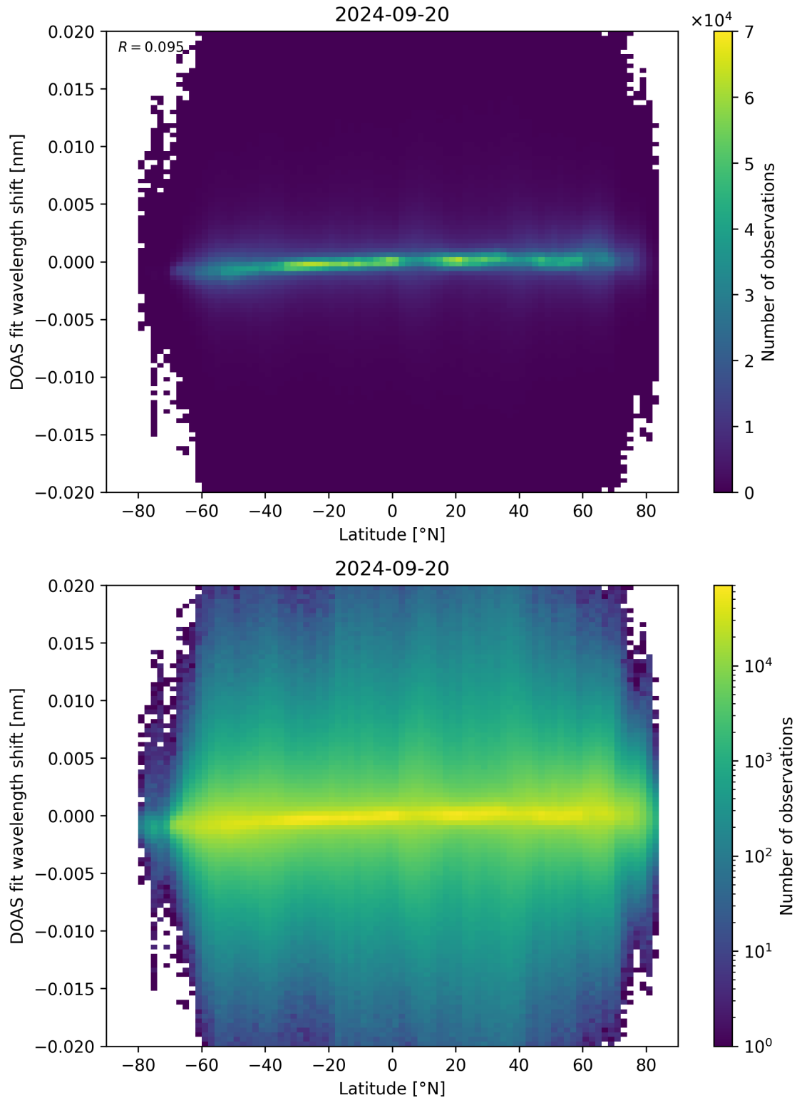
Figure 154: Scatter density plot of “Latitude” against “DOAS fit wavelength shift” for 2024-09-19 to 2024-09-21.
