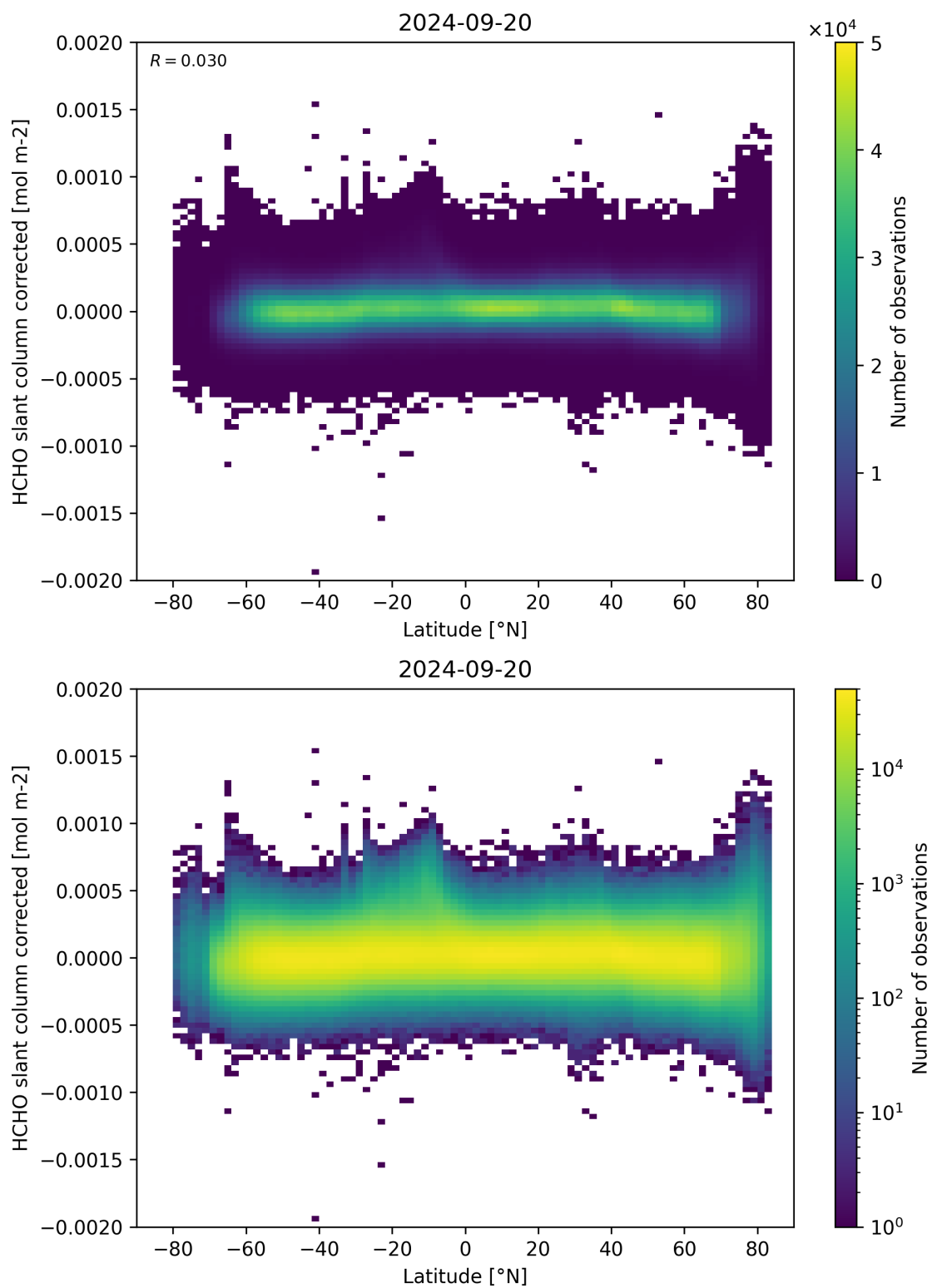
Figure 157: Scatter density plot of “Latitude” against “HCHO slant column corrected” for 2024-09-19 to 2024-09-21.
