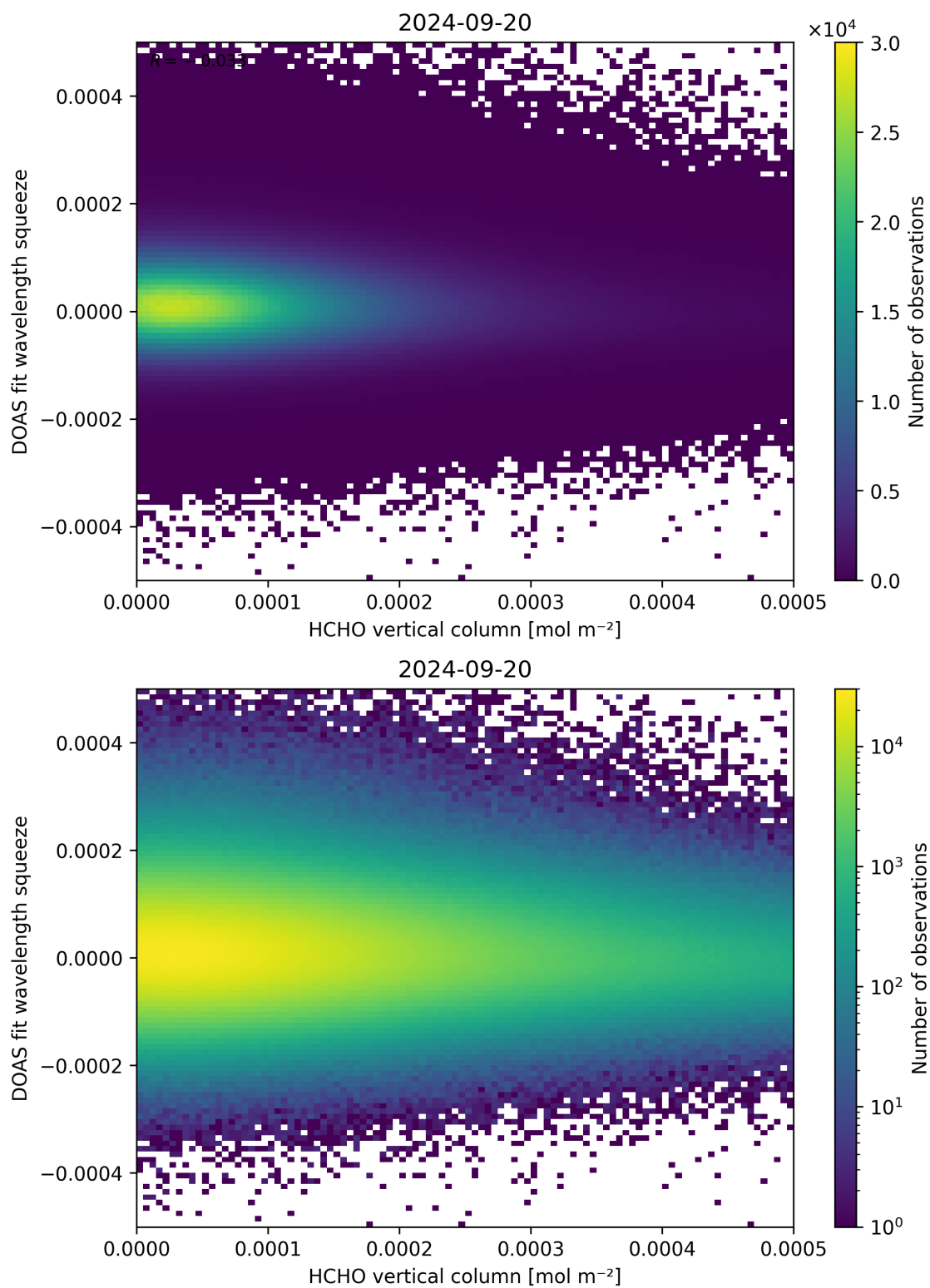
Figure 125: Scatter density plot of “HCHO vertical column” against “DOAS fit wavelength squeeze” for 2024-09-19 to 2024-09-21.
