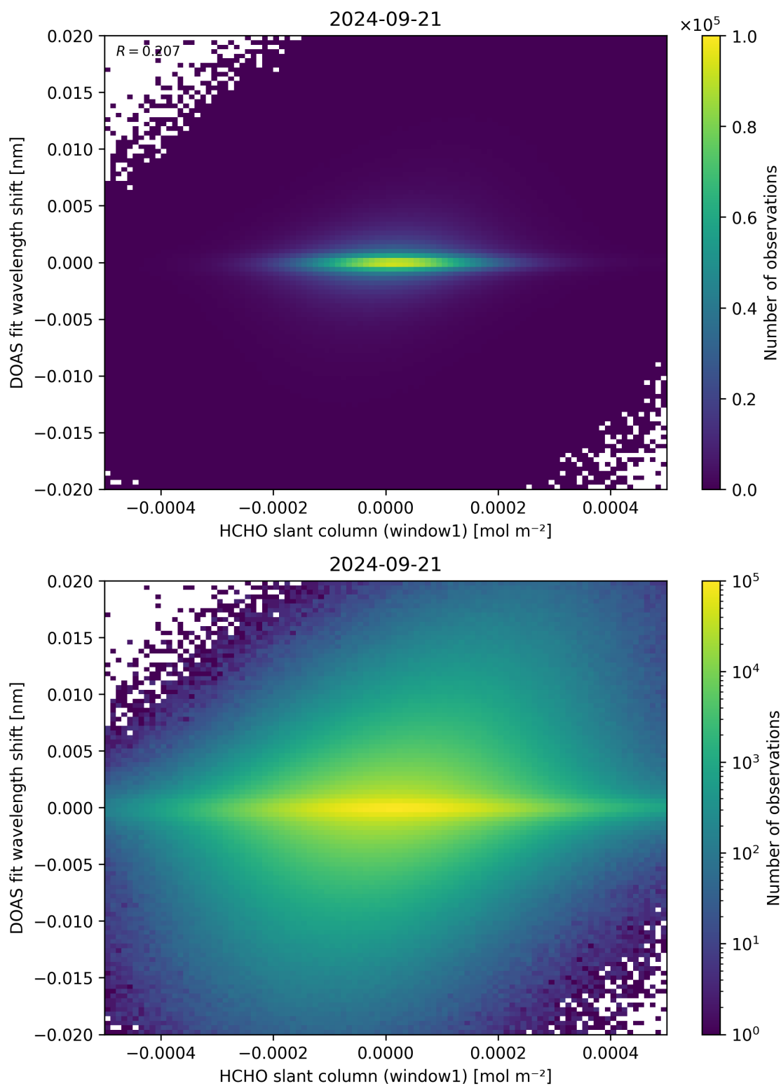
Figure 79: Scatter density plot of “HCHO slant column (window1)” against “DOAS fit wavelength shift” for 2024-09-20 to 2024-09-22.
