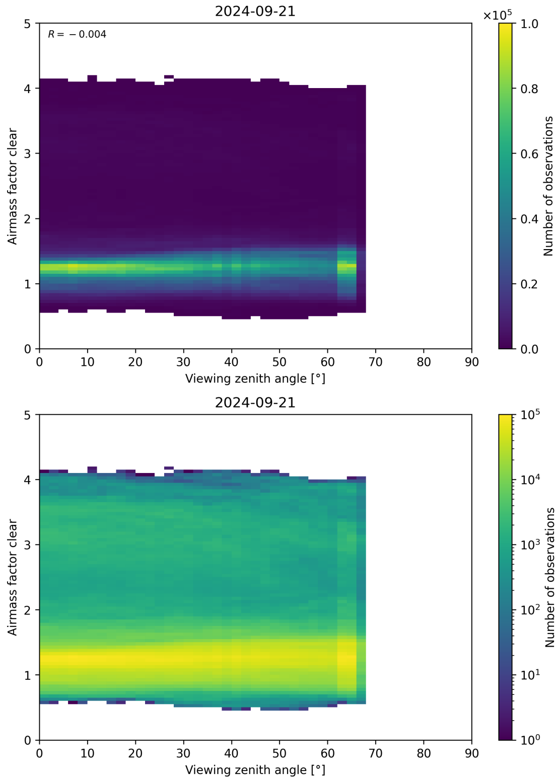
Figure 185: Scatter density plot of “Viewing zenith angle” against “Airmass factor clear” for 2024-09-20 to 2024-09-22.
