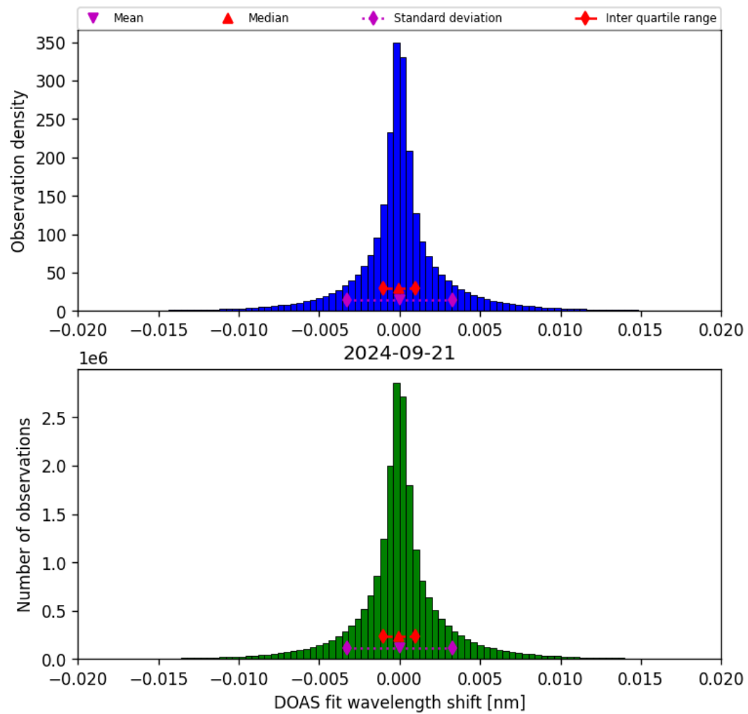
Figure 44: Histogram of “DOAS fit wavelength shift” for 2024-09-20 to 2024-09-22
