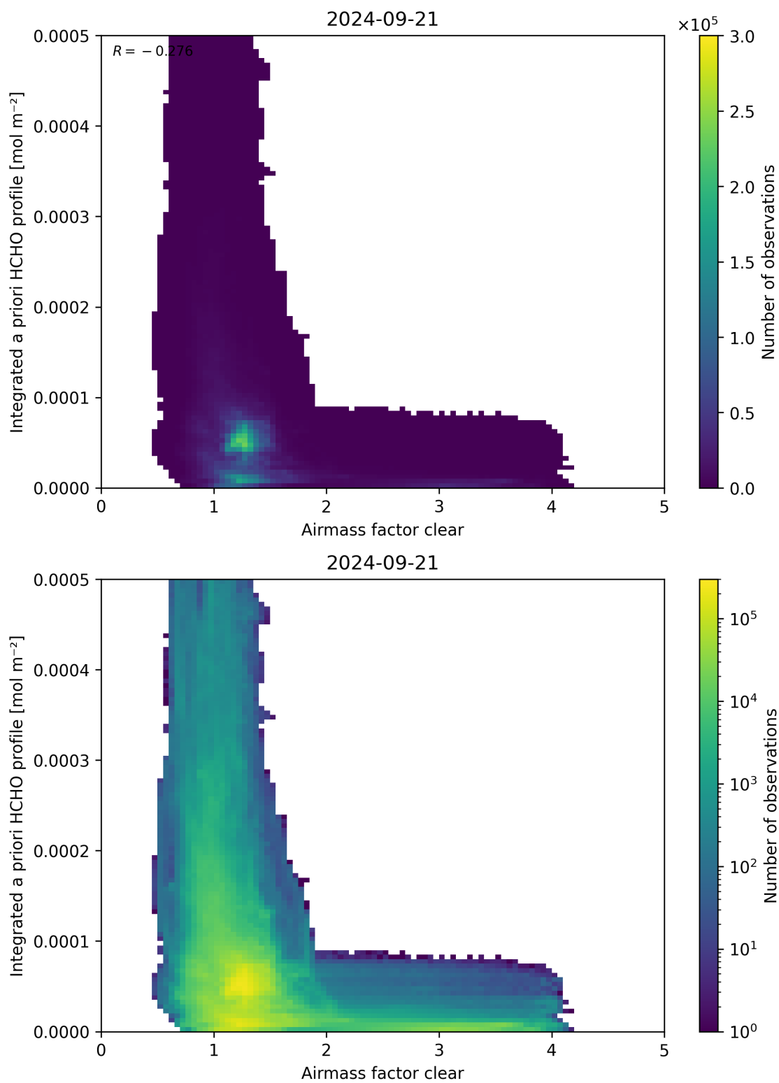
Figure 76: Scatter density plot of “Airmass factor clear” against “Integrated a priori HCHO profile” for 2024-09-20 to 2024-09-22.
