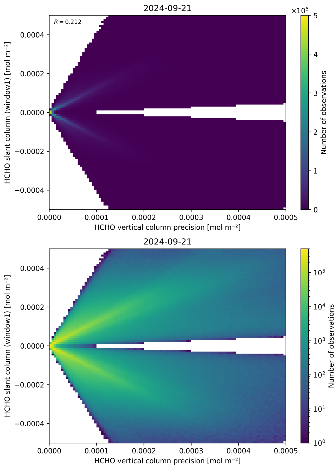
Figure 142: Scatter density plot of “HCHO vertical column precision” against “HCHO slant column (window1)” for 2024-09-20 to 2024-09-22.
