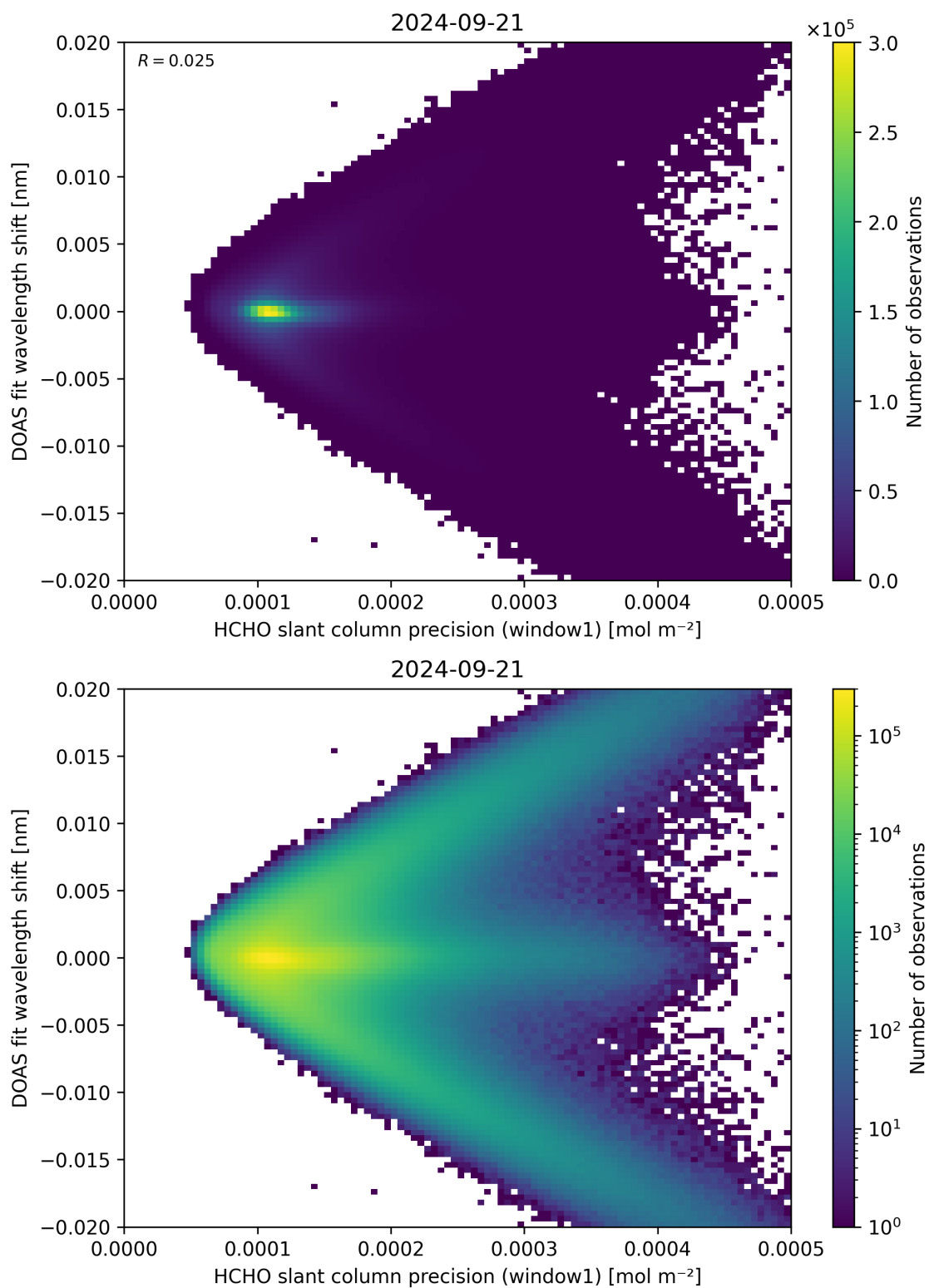
Figure 89: Scatter density plot of “HCHO slant column precision (window1)” against “DOAS fit wavelength shift” for 2024-09-20 to 2024-09-22.
