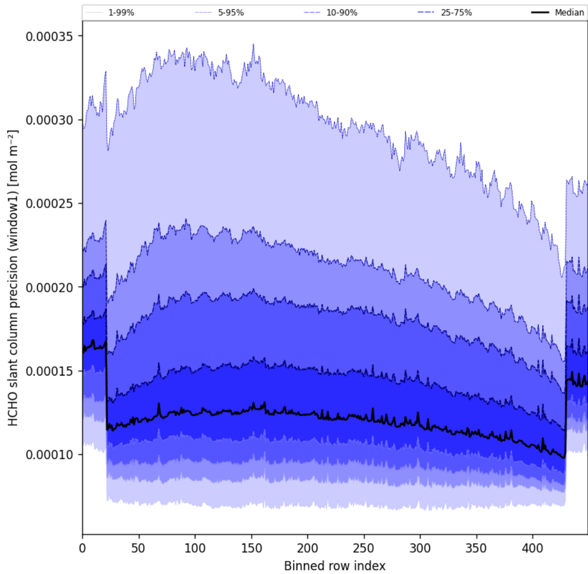
Figure 53: Along track statistics of “HCHO slant column precision (window1)” for 2024-09-20 to 2024-09-22
