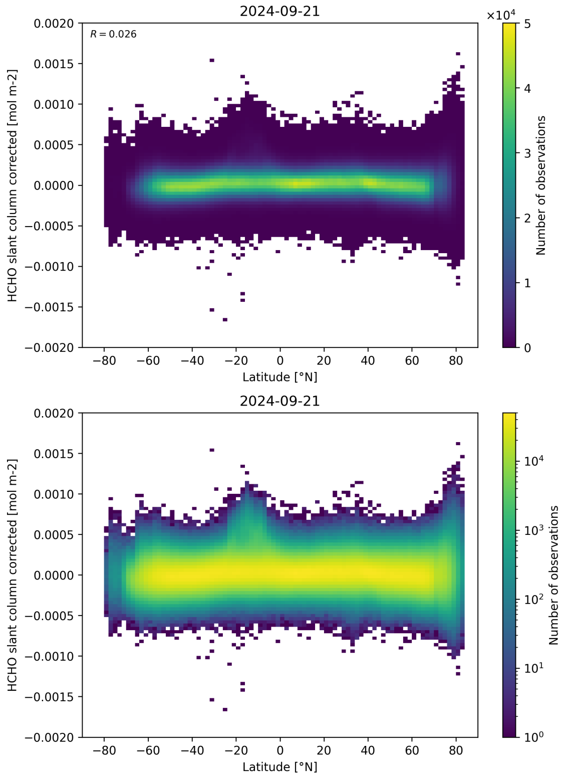
Figure 157: Scatter density plot of “Latitude” against “HCHO slant column corrected” for 2024-09-20 to 2024-09-22.
