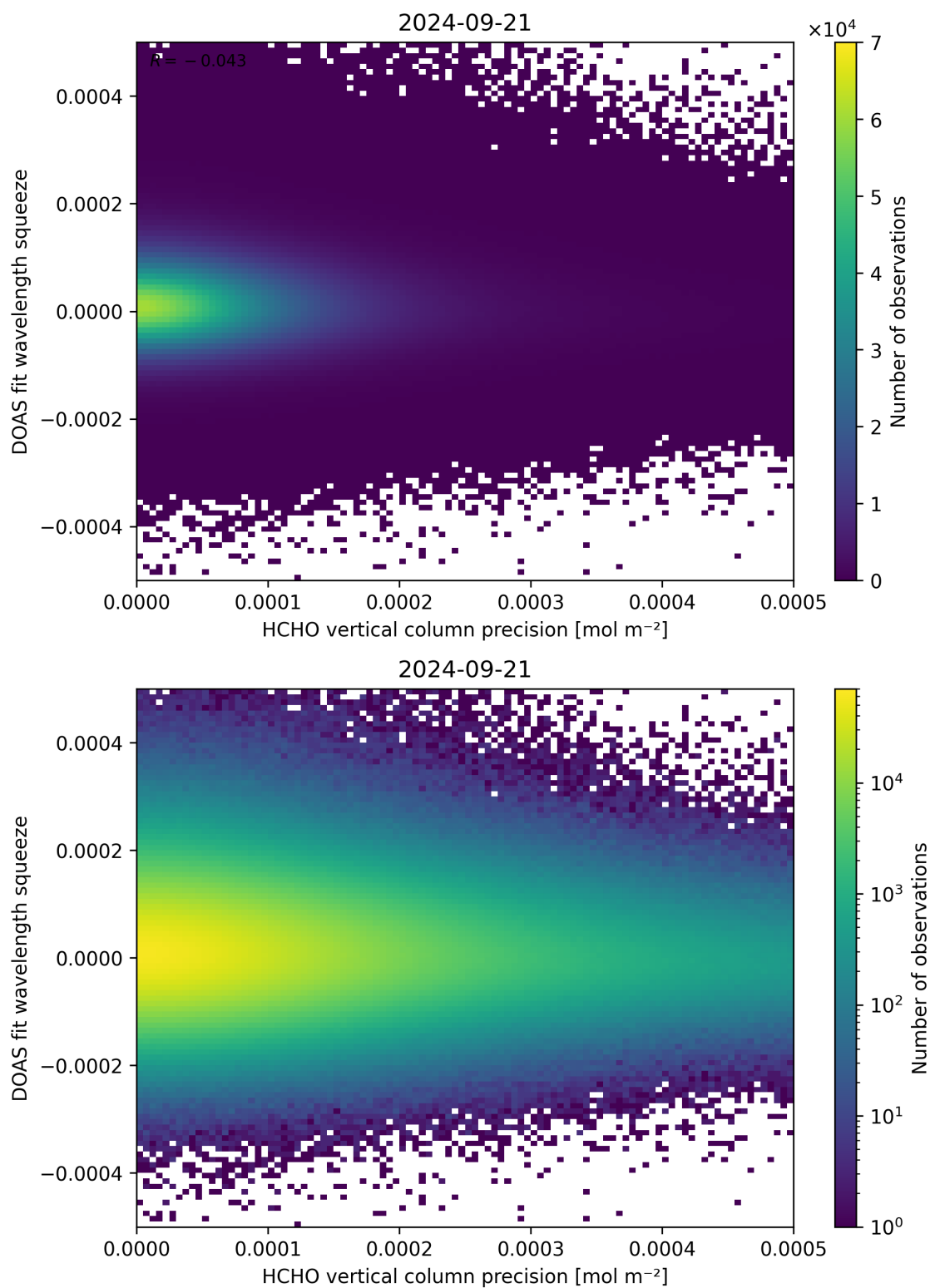
Figure 138: Scatter density plot of “HCHO vertical column precision” against “DOAS fit wavelength squeeze” for 2024-09-20 to 2024-09-22.
