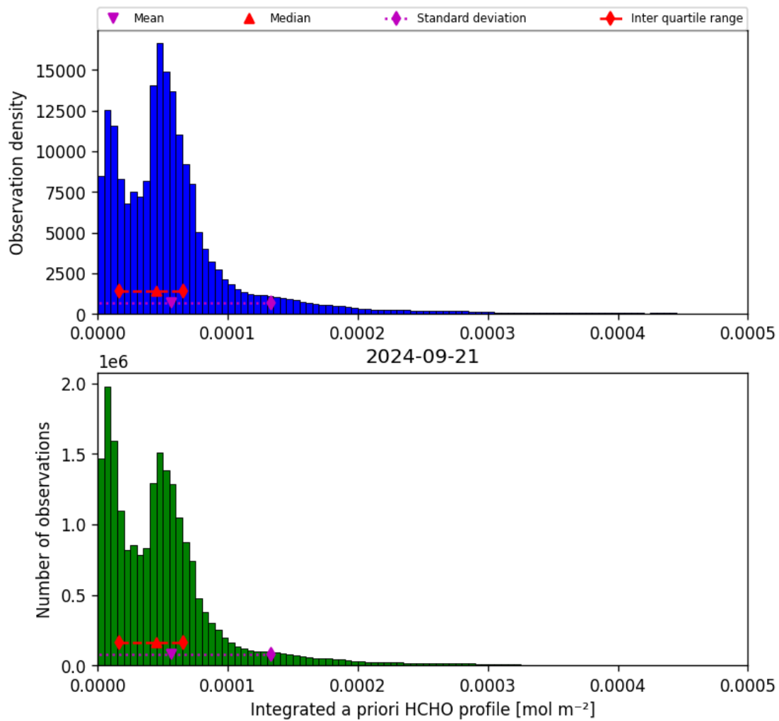
Figure 43: Histogram of “Integrated a priori HCHO profile” for 2024-09-20 to 2024-09-22
