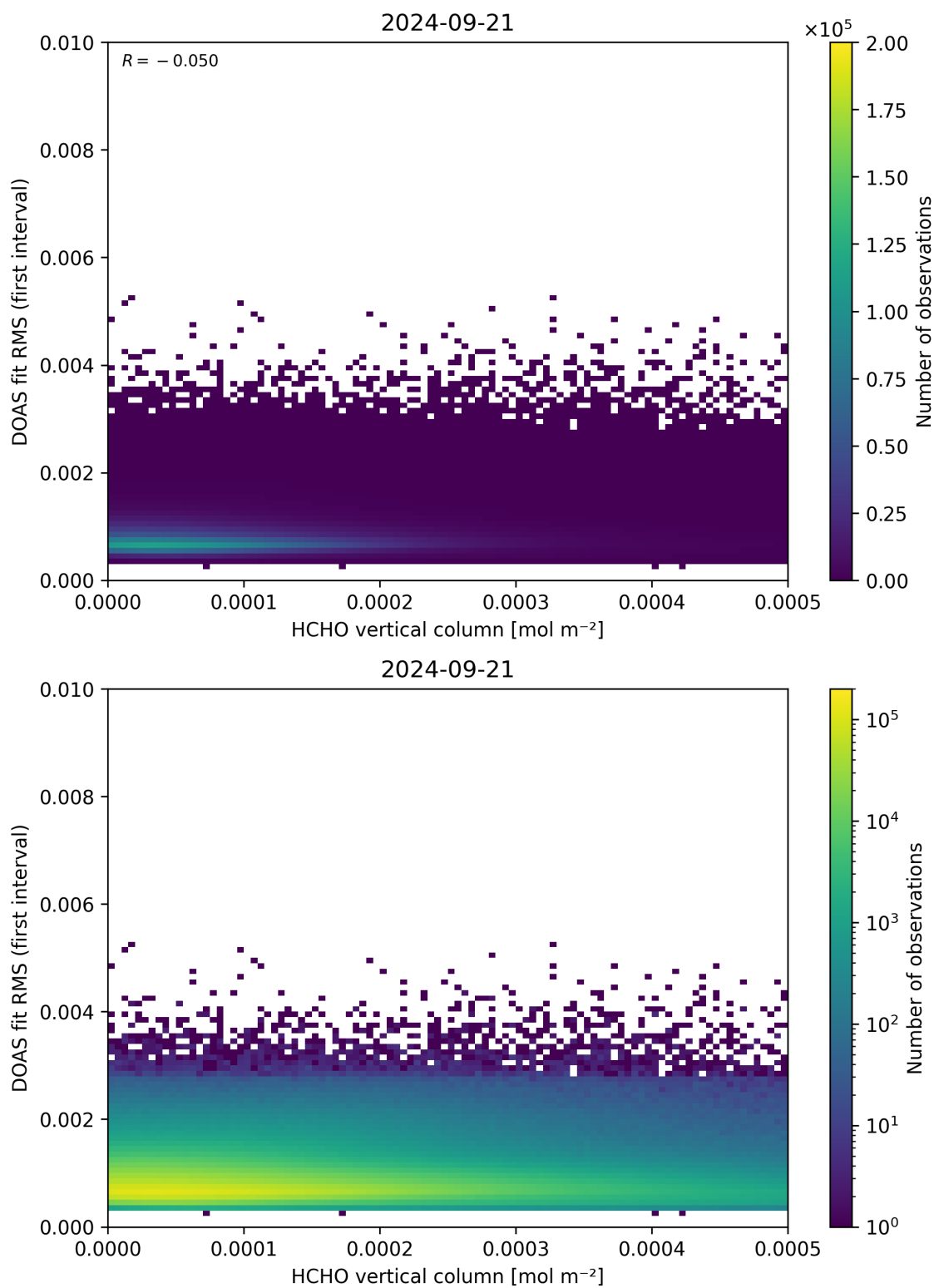
Figure 123: Scatter density plot of “HCHO vertical column” against “DOAS fit RMS (first interval)” for 2024-09-20 to 2024-09-22.
