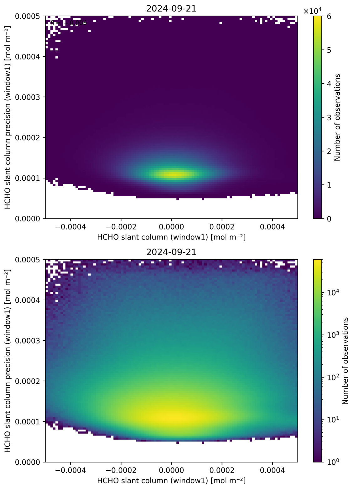
Figure 84: Scatter density plot of “HCHO slant column (window1)” against “HCHO slant column precision (window1)” for 2024-09-20 to 2024-09-22.
