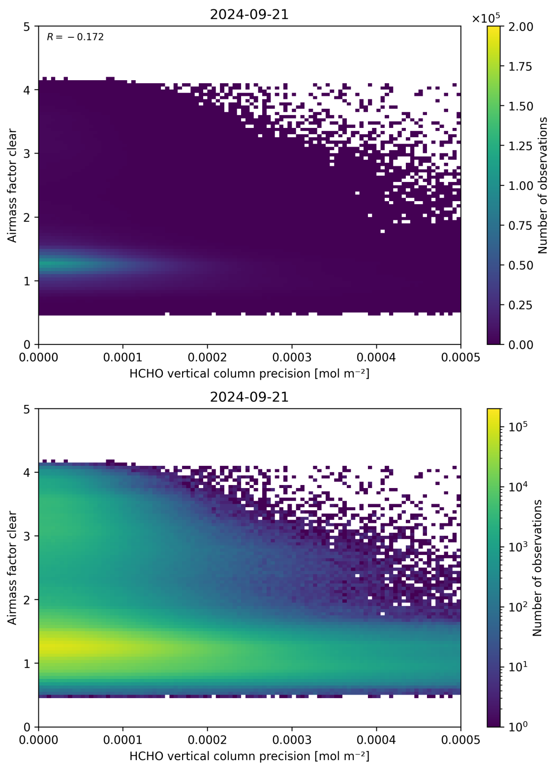
Figure 139: Scatter density plot of “HCHO vertical column precision” against “Airmass factor clear” for 2024-09-20 to 2024-09-22.
