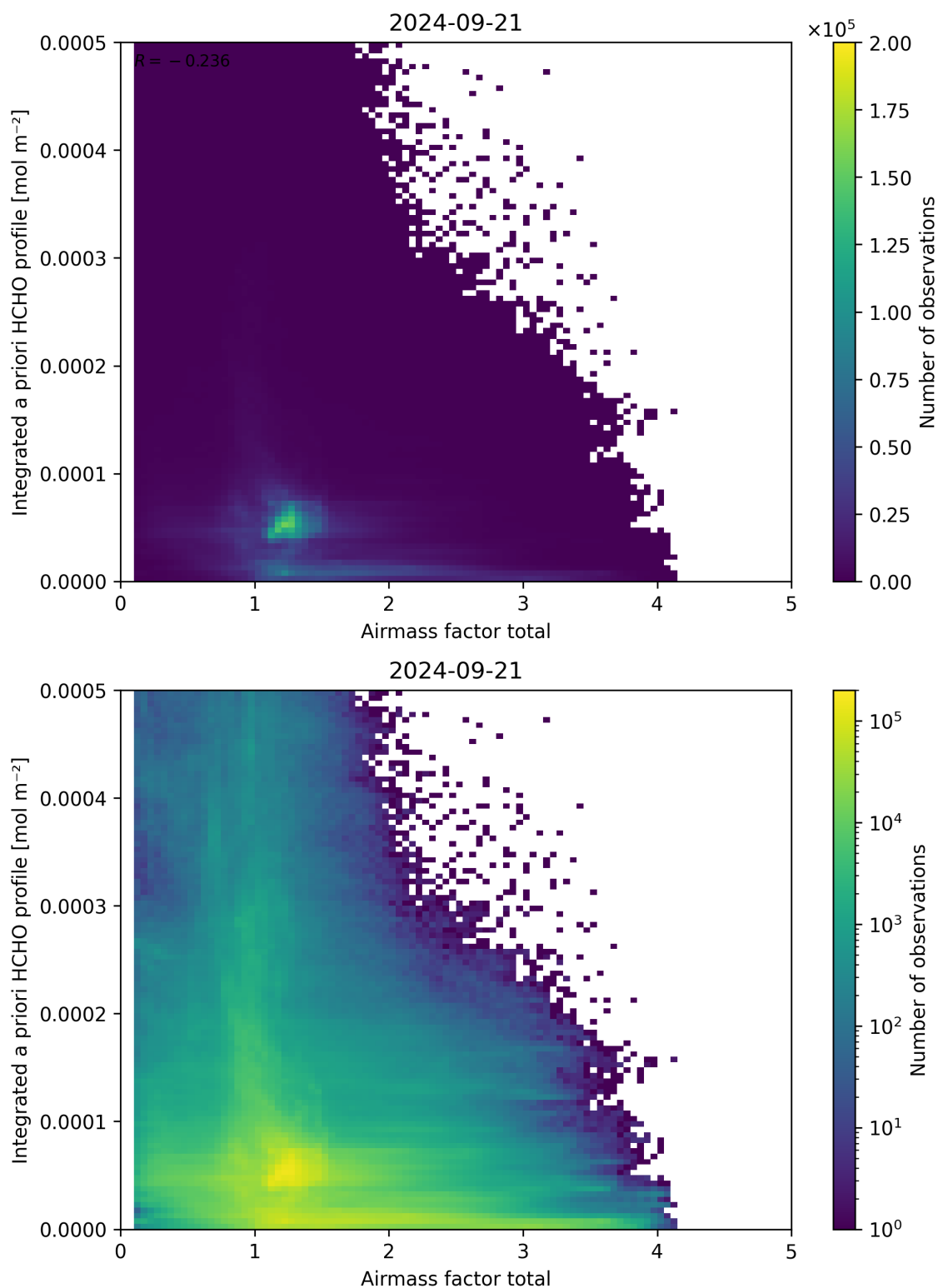
Figure 104: Scatter density plot of “Airmass factor total” against “Integrated a priori HCHO profile” for 2024-09-20 to 2024-09-22.
