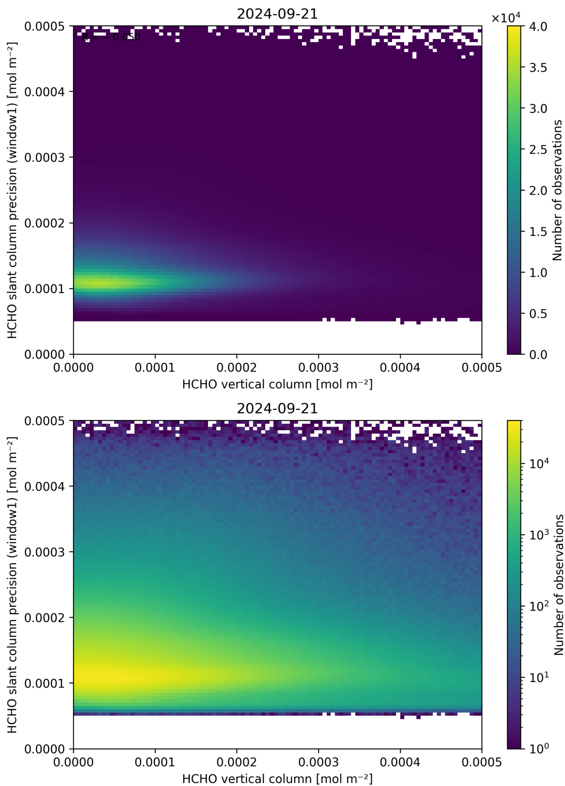
Figure 130: Scatter density plot of “HCHO vertical column” against “HCHO slant column precision (window1)” for 2024-09-20 to 2024-09-22.
