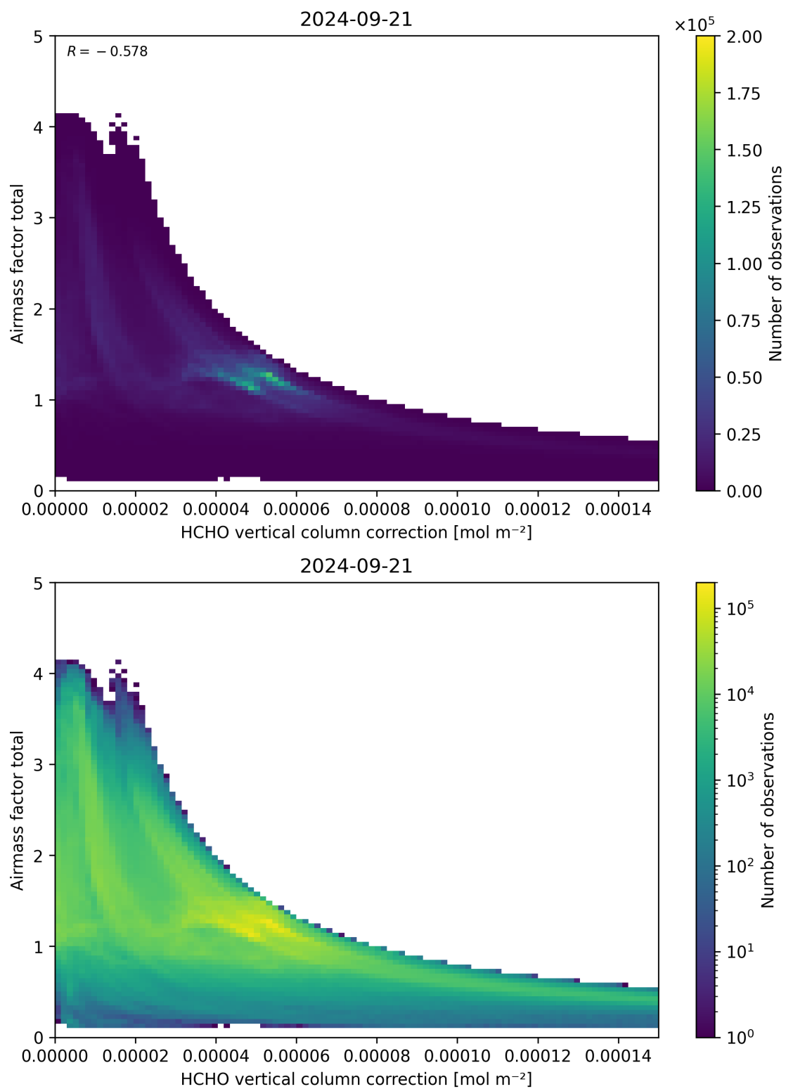
Figure 120: Scatter density plot of “HCHO vertical column correction” against “Airmass factor total” for 2024-09-20 to 2024-09-22.
