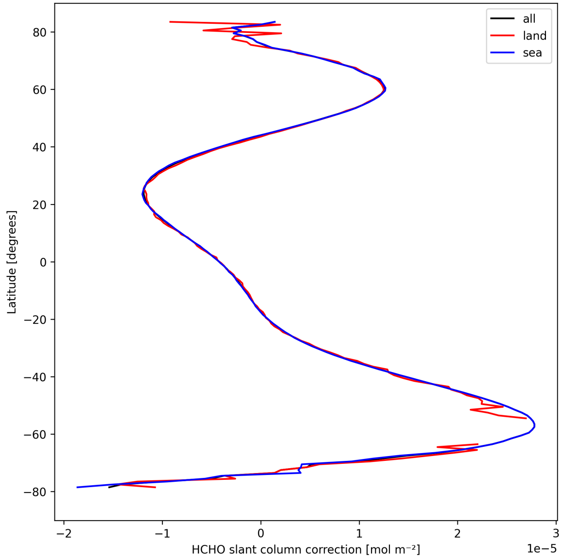
Figure 33: Zonal average of “HCHO slant column correction” for 2024-09-20 to 2024-09-22.
