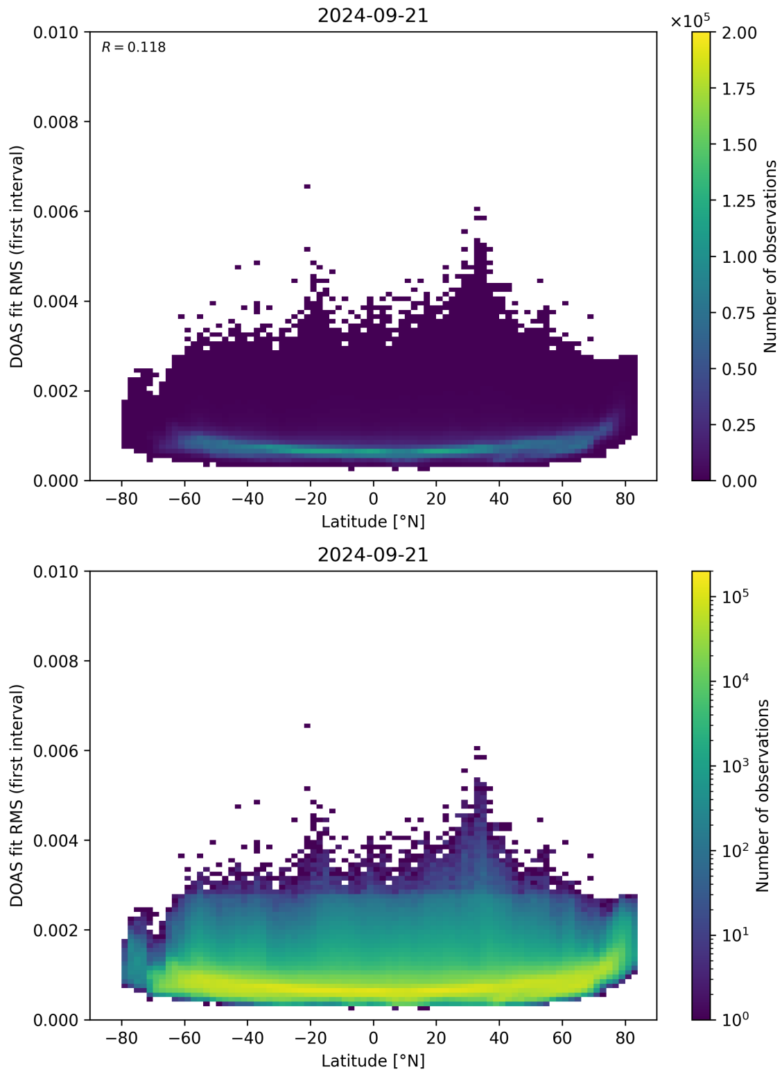
Figure 153: Scatter density plot of “Latitude” against “DOAS fit RMS (first interval)” for 2024-09-20 to 2024-09-22.
