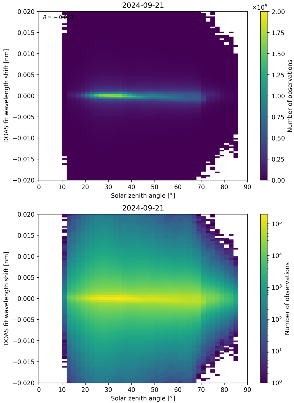
Figure 168: Scatter density plot of “Solar zenith angle” against “DOAS fit wavelength shift” for 2024-09-20 to 2024-09-22.
