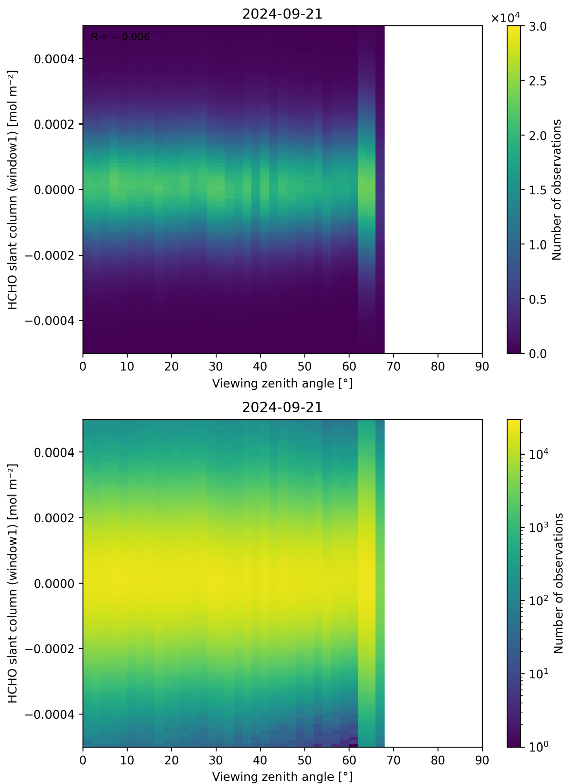
Figure 188: Scatter density plot of “Viewing zenith angle” against “HCHO slant column (window1)” for 2024-09-20 to 2024-09-22.
