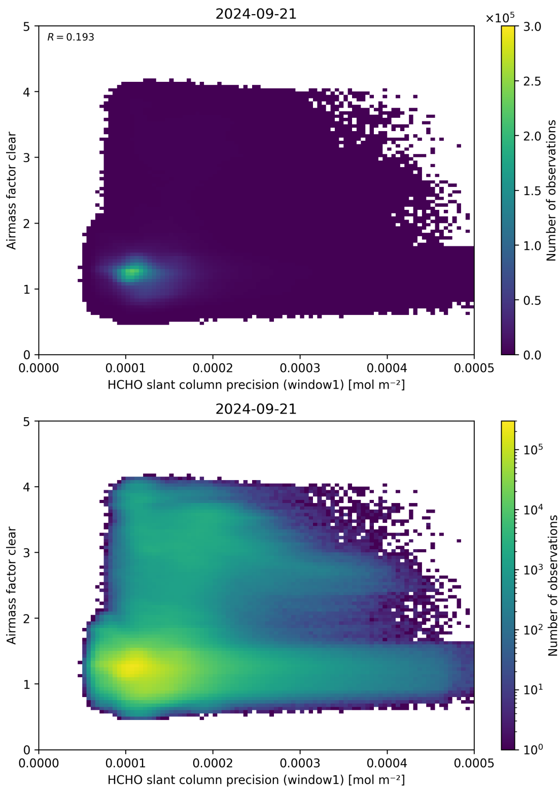
Figure 91: Scatter density plot of “HCHO slant column precision (window1)” against “Airmass factor clear” for 2024-09-20 to 2024-09-22.
