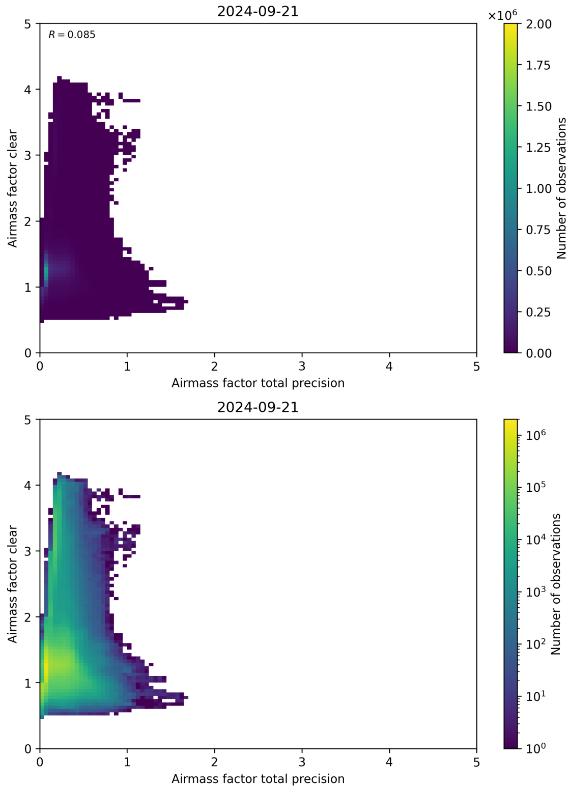
Figure 108: Scatter density plot of “Airmass factor total precision” against “Airmass factor clear” for 2024-09-20 to 2024-09-22.
