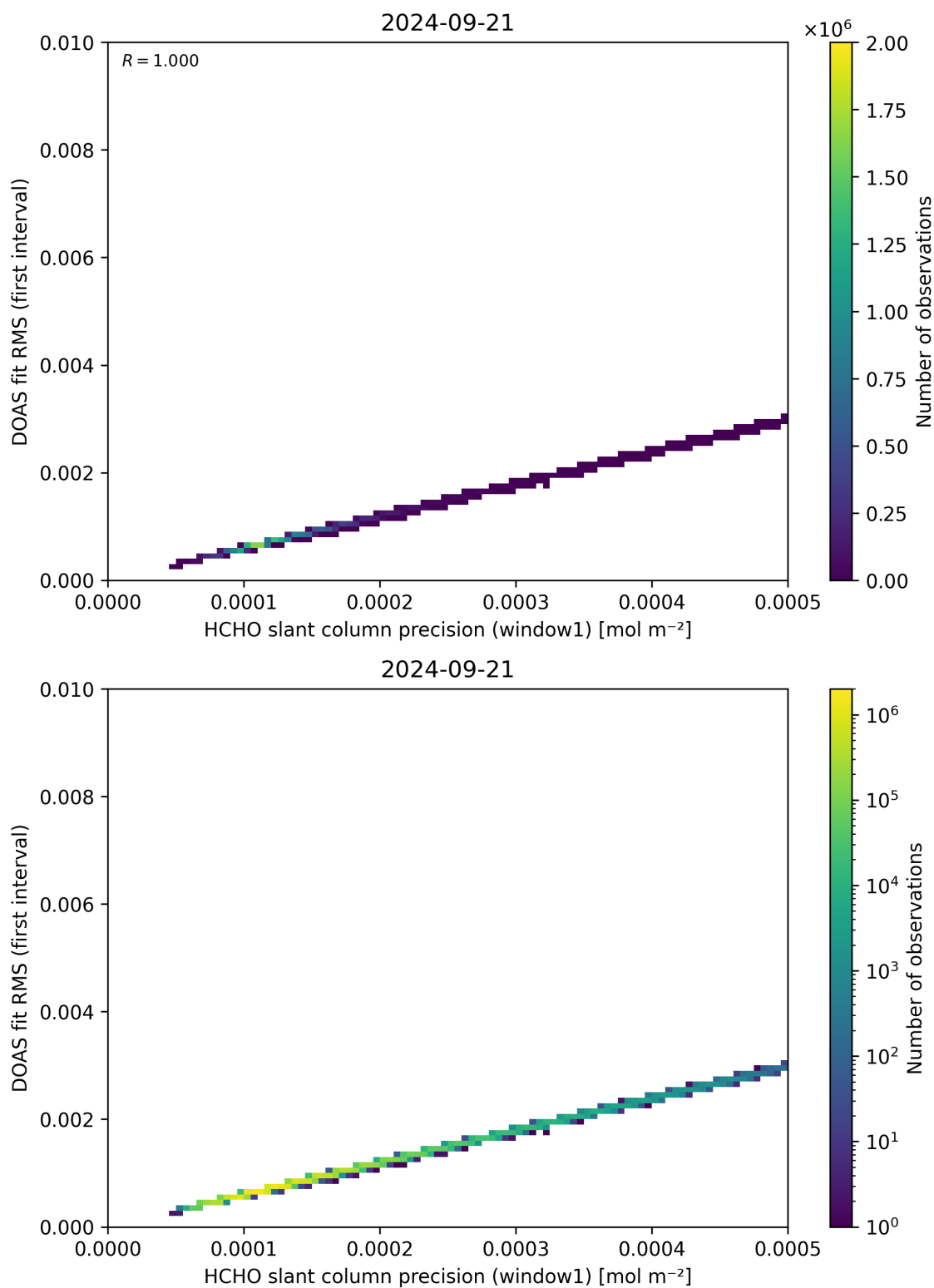
Figure 88: Scatter density plot of “HCHO slant column precision (window1)” against “DOAS fit RMS (first interval)” for 2024-09-20 to 2024-09-22.
