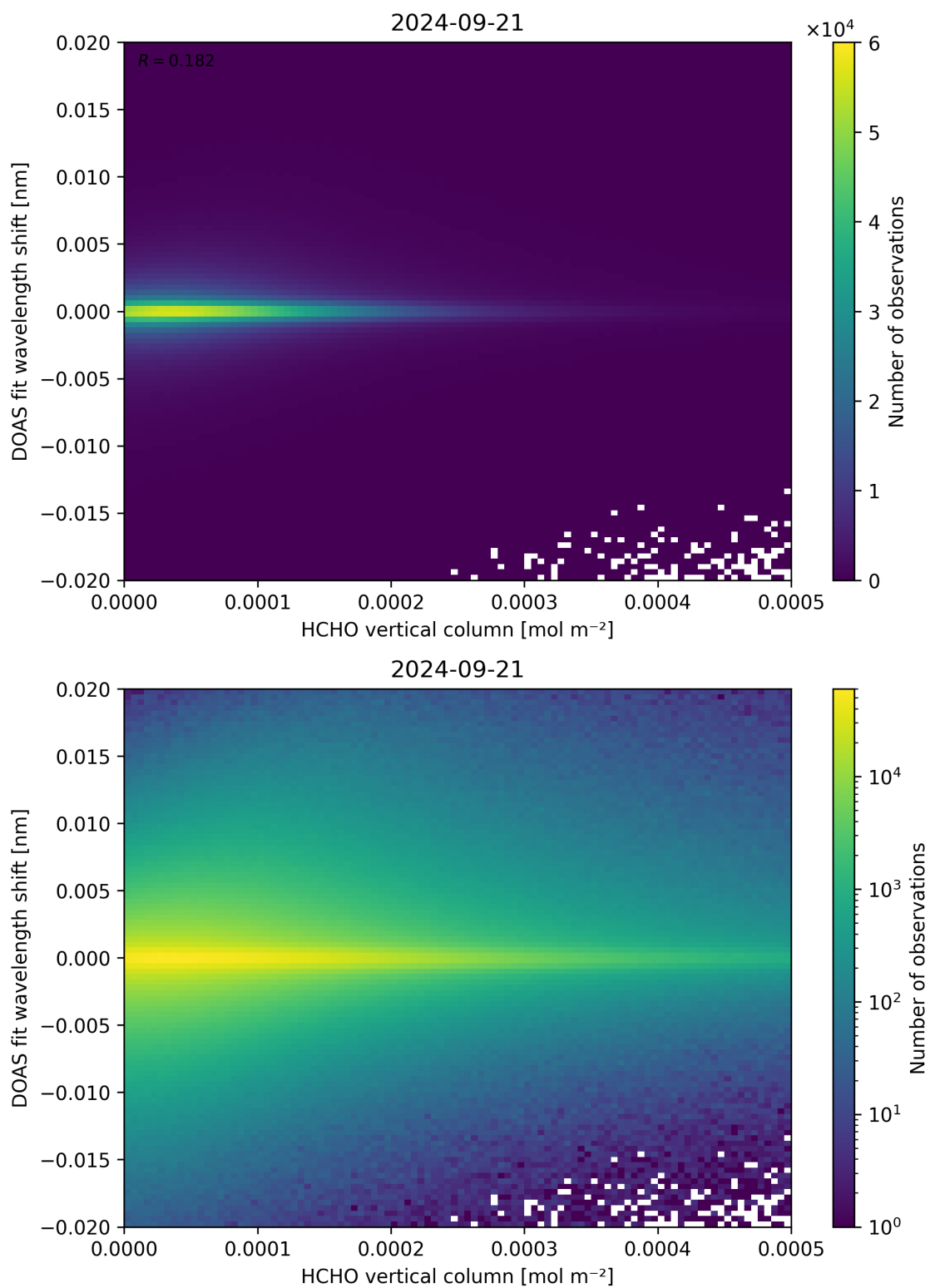
Figure 124: Scatter density plot of “HCHO vertical column” against “DOAS fit wavelength shift” for 2024-09-20 to 2024-09-22.
