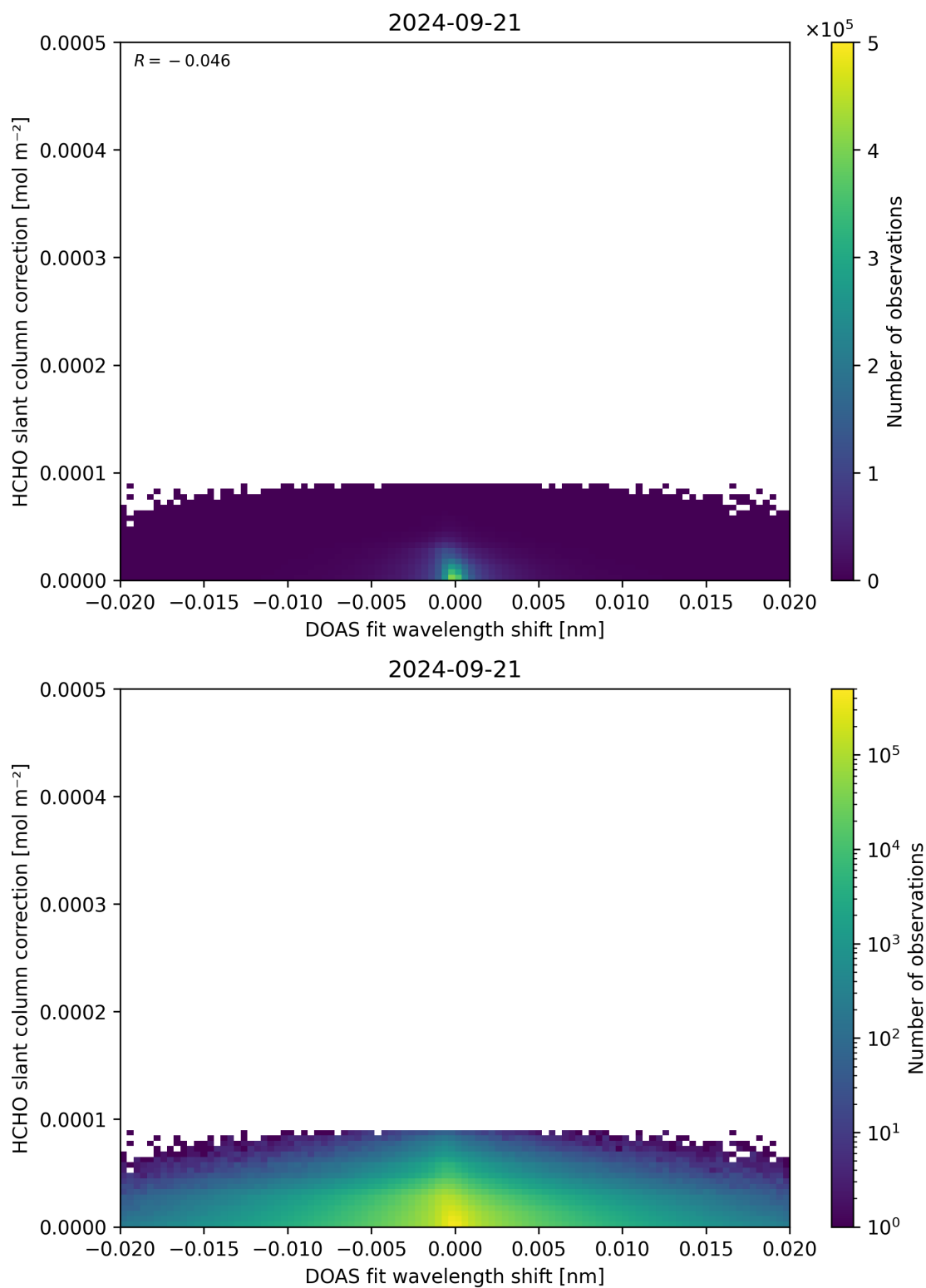
Figure 67: Scatter density plot of “DOAS fit wavelength shift” against “HCHO slant column correction” for 2024-09-20 to 2024-09-22.
