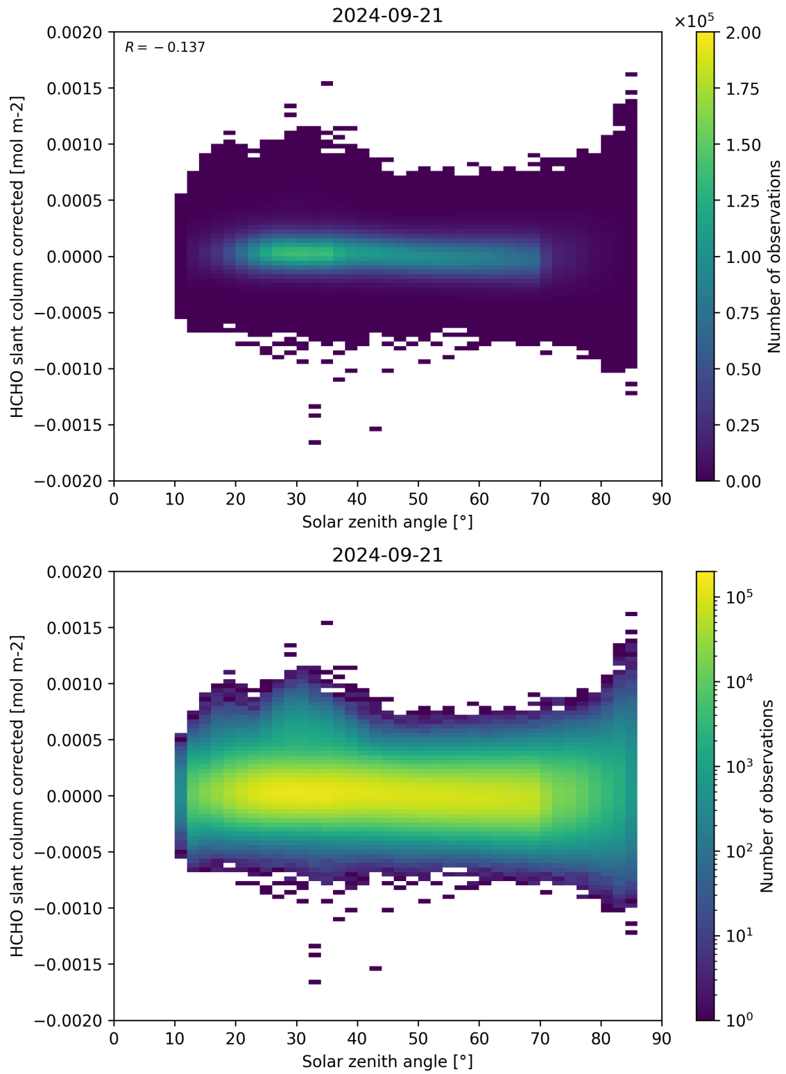
Figure 171: Scatter density plot of “Solar zenith angle” against “HCHO slant column corrected” for 2024-09-20 to 2024-09-22.
