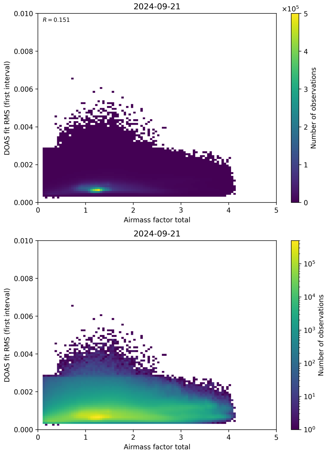
Figure 97: Scatter density plot of “Airmass factor total” against “DOAS fit RMS (first interval)” for 2024-09-20 to 2024-09-22.
