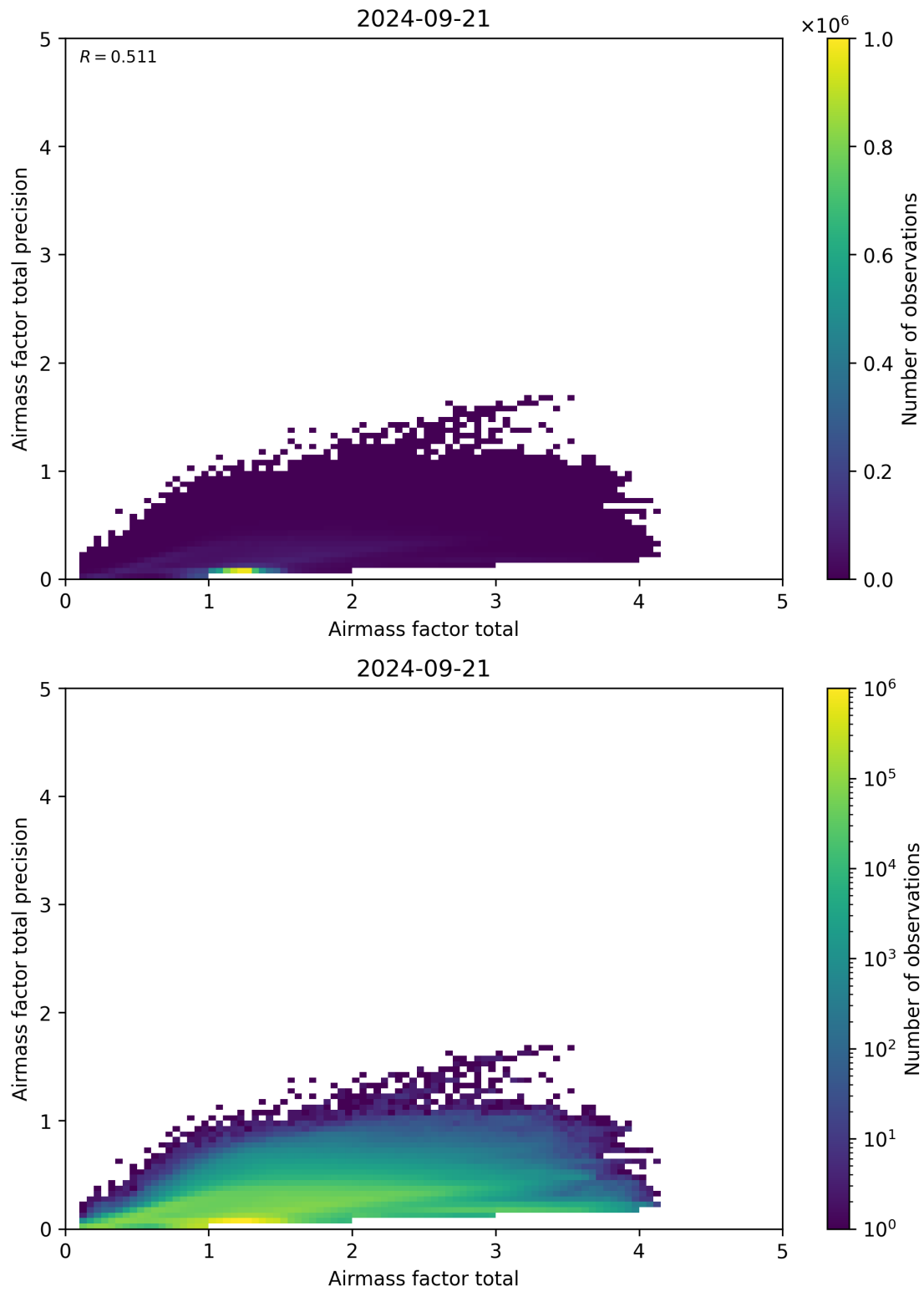
Figure 103: Scatter density plot of “Airmass factor total” against “Airmass factor total precision” for 2024-09-20 to 2024-09-22.
