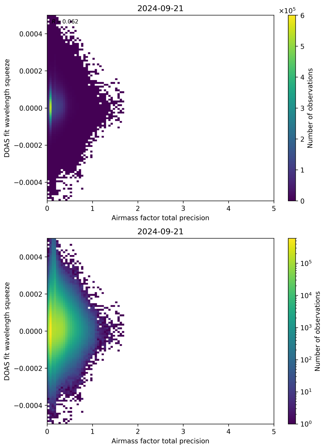
Figure 107: Scatter density plot of “Airmass factor total precision” against “DOAS fit wavelength squeeze” for 2024-09-20 to 2024-09-22.
