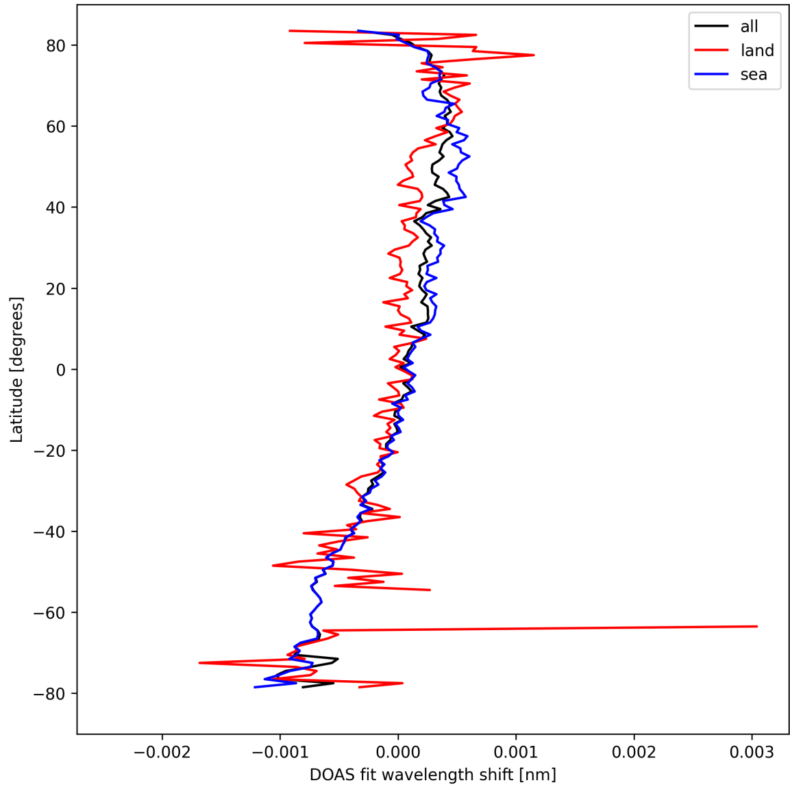
Figure 30: Zonal average of “DOAS fit wavelength shift” for 2024-09-20 to 2024-09-22.
