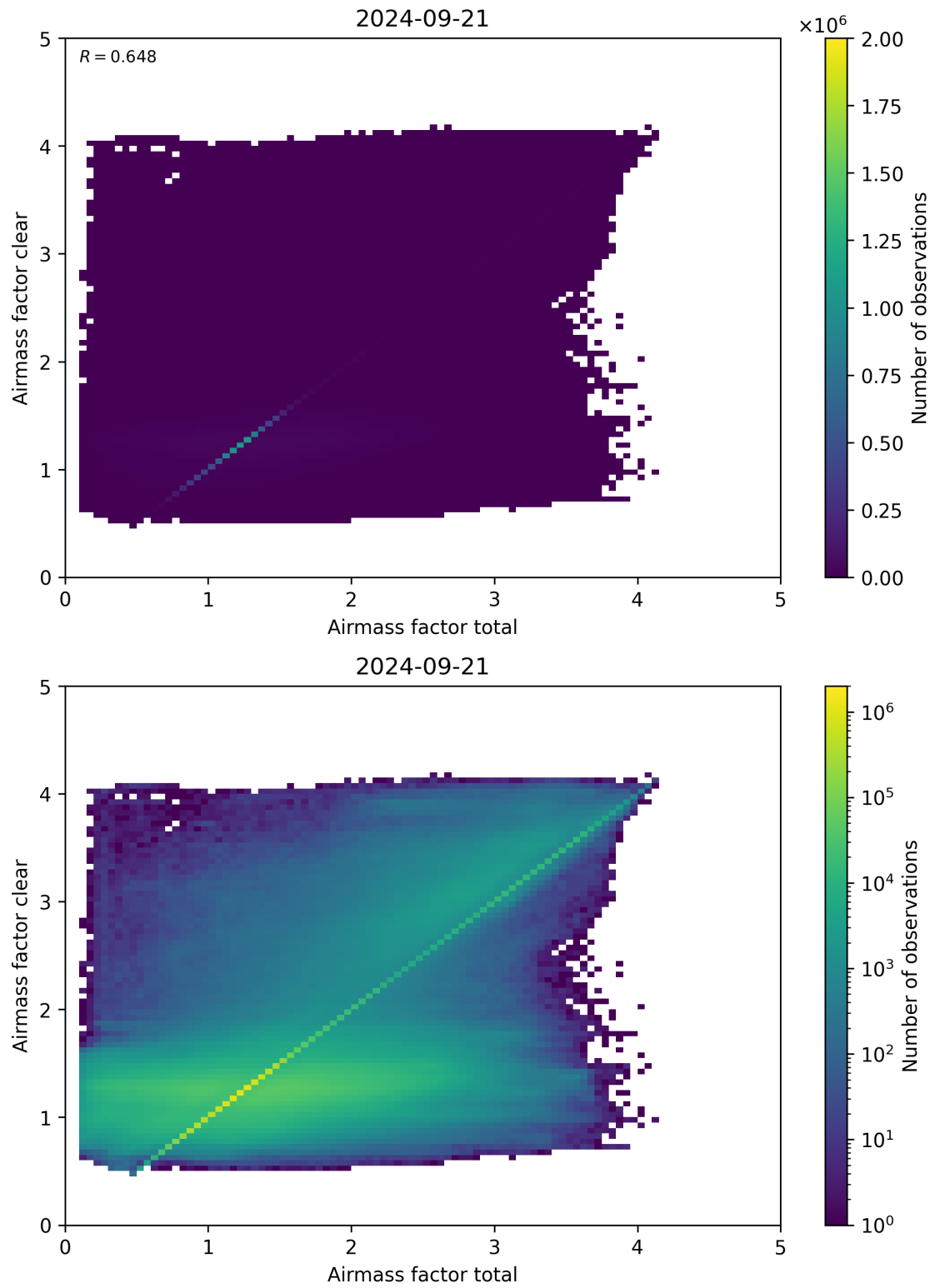
Figure 100: Scatter density plot of “Airmass factor total” against “Airmass factor clear” for 2024-09-20 to 2024-09-22.
