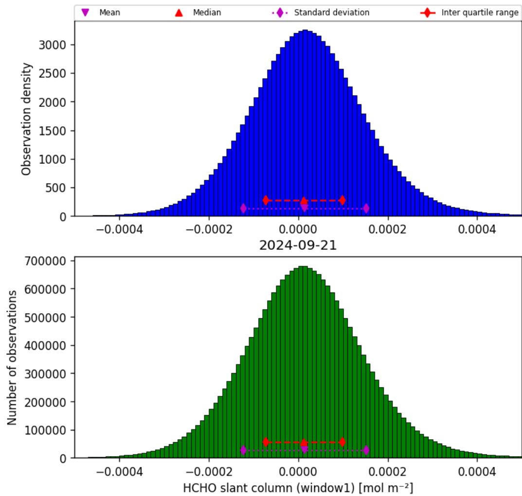
Figure 38: Histogram of “HCHO slant column (window1)” for 2024-09-20 to 2024-09-22
