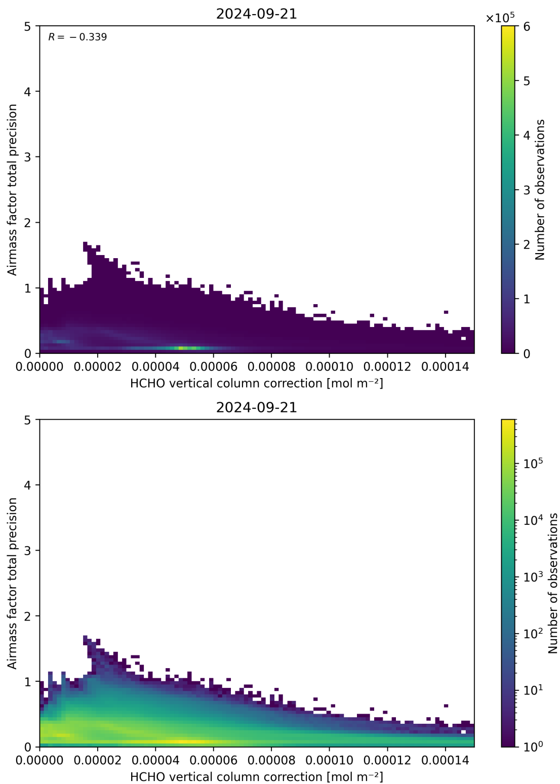
Figure 121: Scatter density plot of “HCHO vertical column correction” against “Airmass factor total precision” for 2024-09-20 to 2024-09-22.
