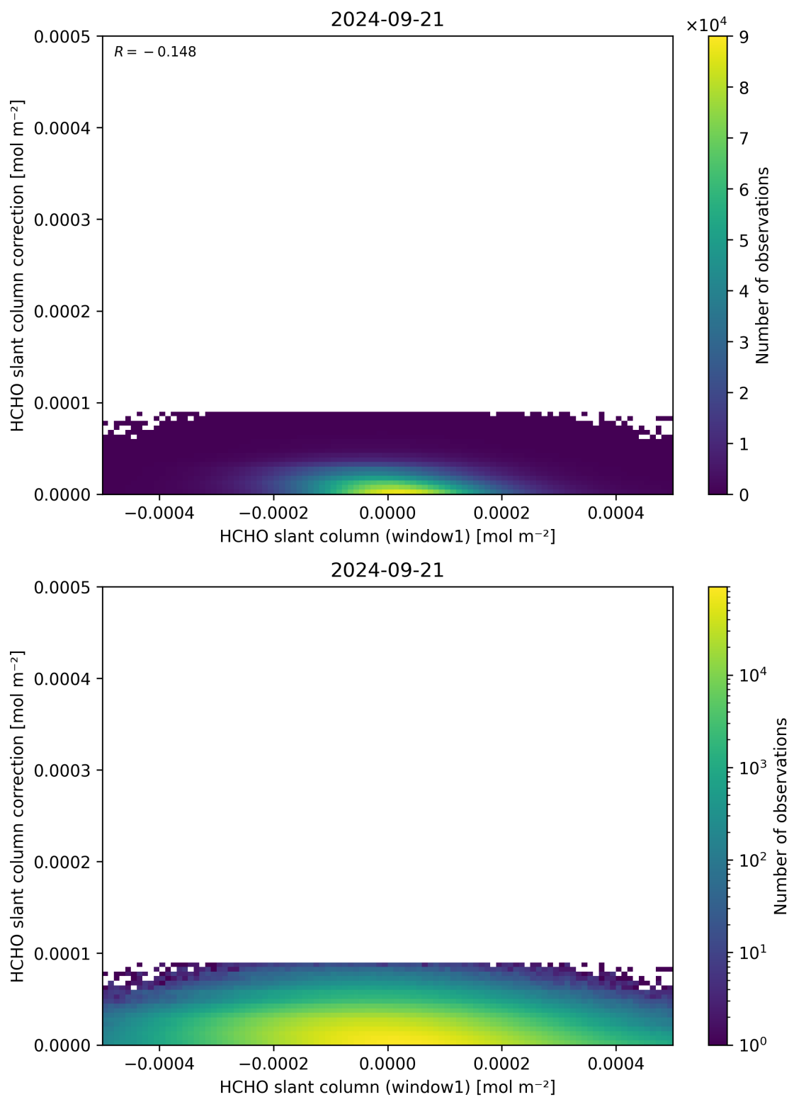
Figure 83: Scatter density plot of “HCHO slant column (window1)” against “HCHO slant column correction” for 2024-09-20 to 2024-09-22.
