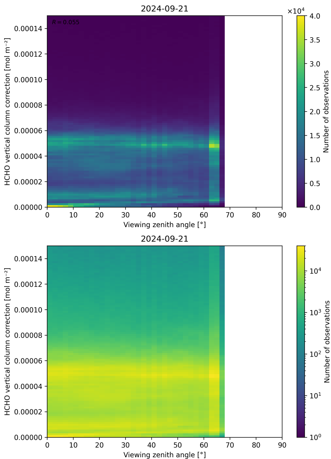
Figure 193: Scatter density plot of “Viewing zenith angle” against “HCHO vertical column correction” for 2024-09-20 to 2024-09-22.
