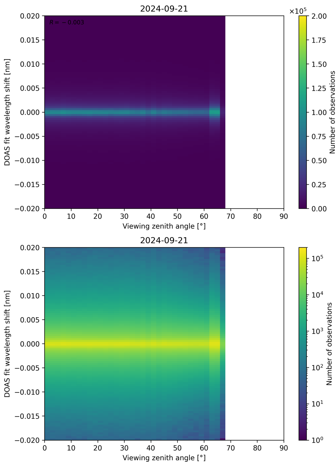
Figure 183: Scatter density plot of “Viewing zenith angle” against “DOAS fit wavelength shift” for 2024-09-20 to 2024-09-22.
