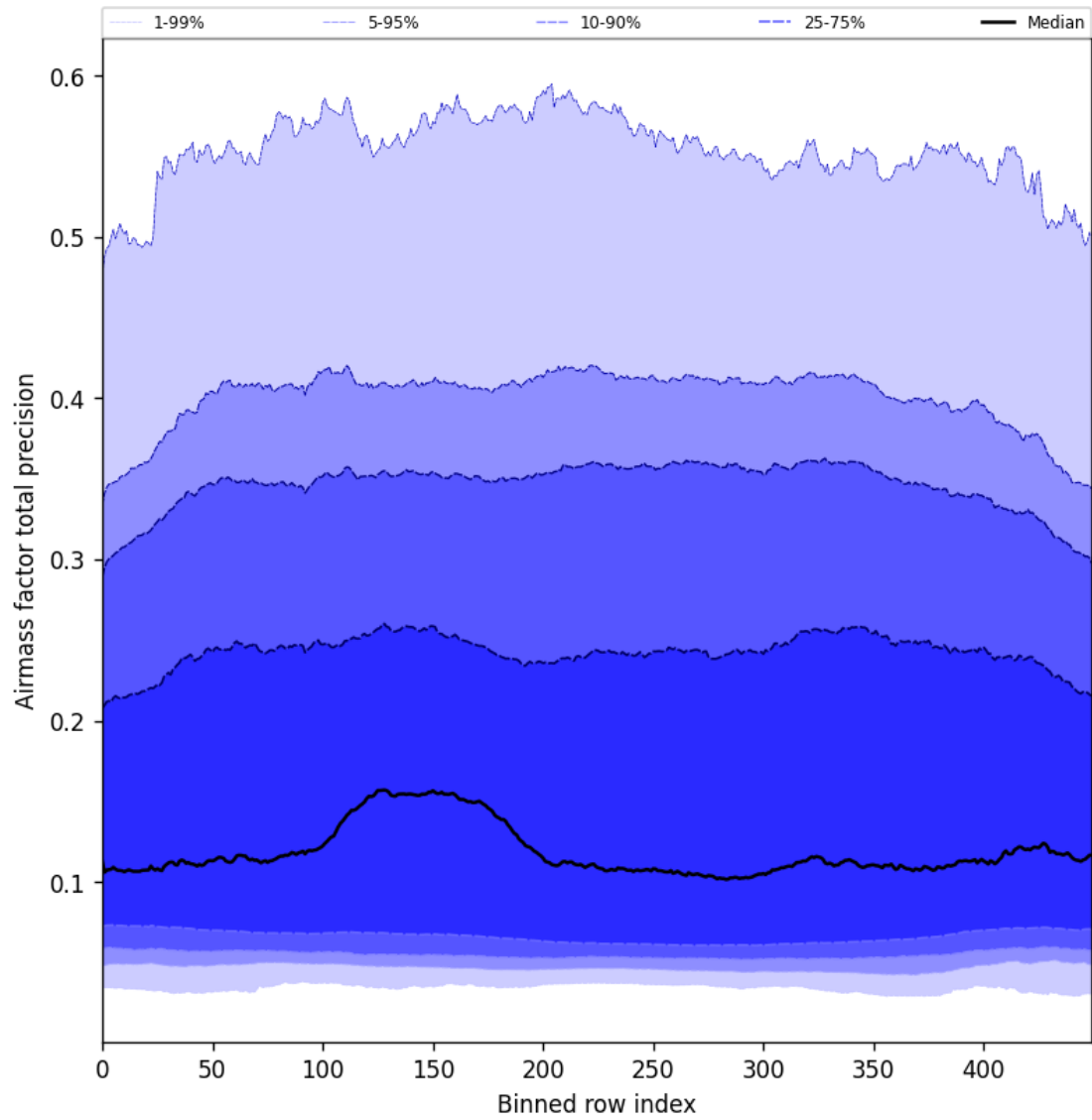
Figure 55: Along track statistics of “Airmass factor total precision” for 2024-09-20 to 2024-09-22
