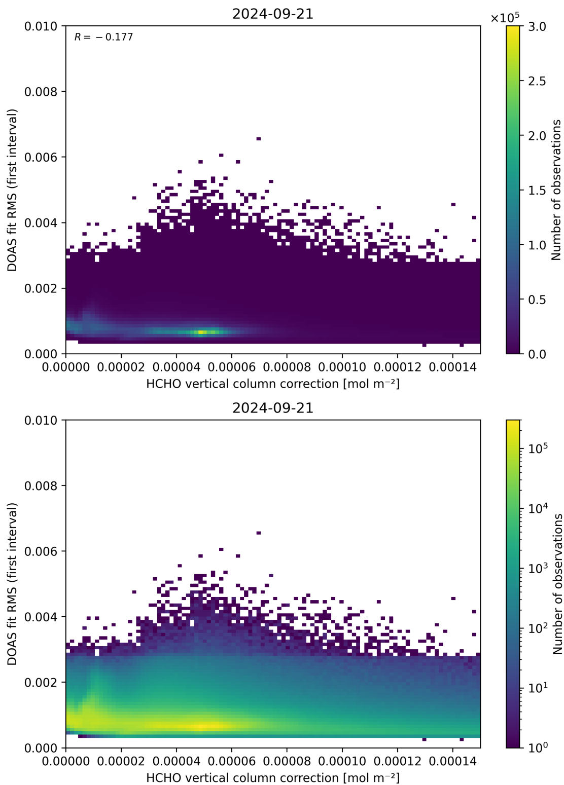
Figure 112: Scatter density plot of “HCHO vertical column correction” against “DOAS fit RMS (first interval)” for 2024-09-20 to 2024-09-22.
