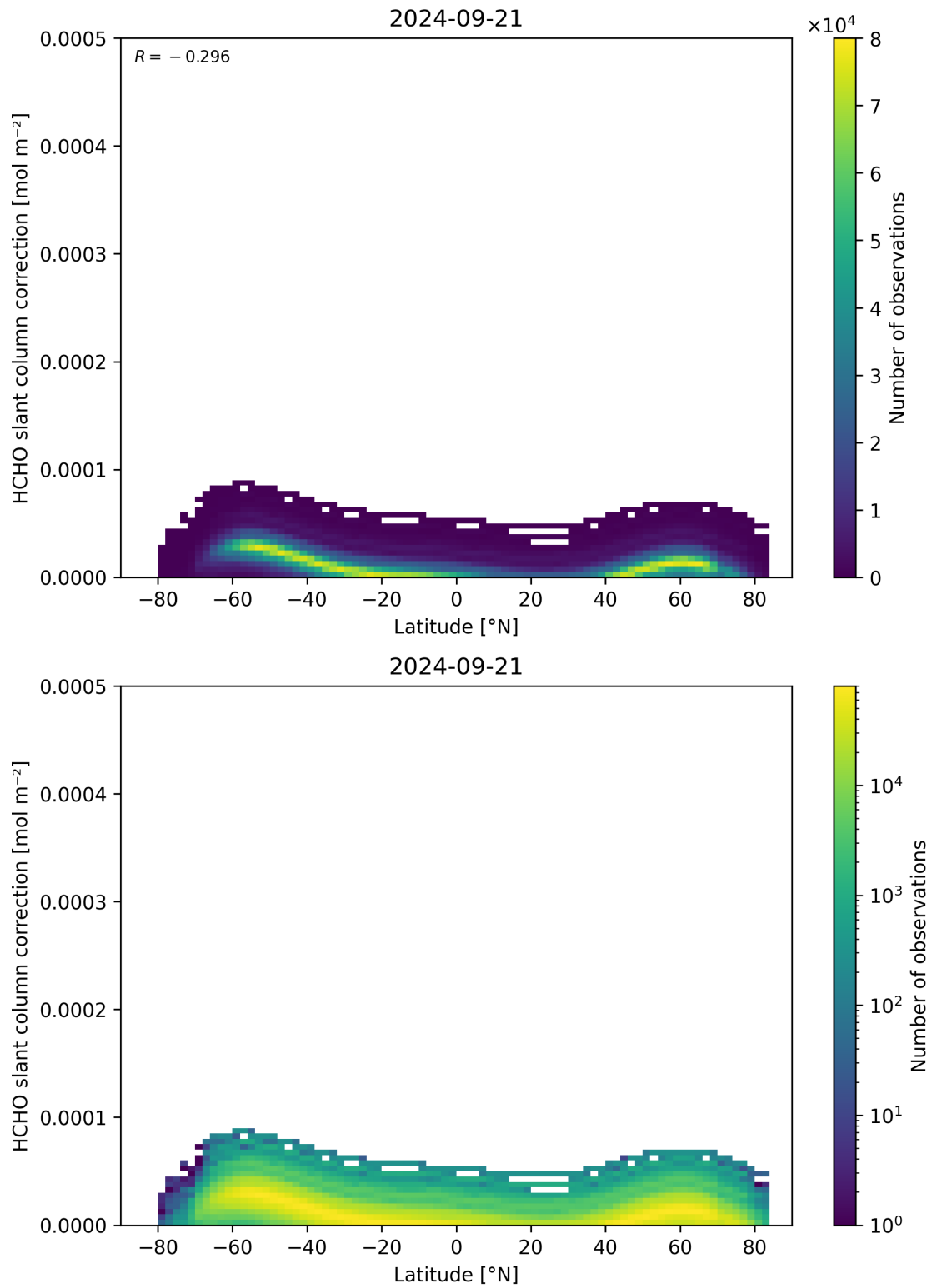
Figure 158: Scatter density plot of “Latitude” against “HCHO slant column correction” for 2024-09-20 to 2024-09-22.
