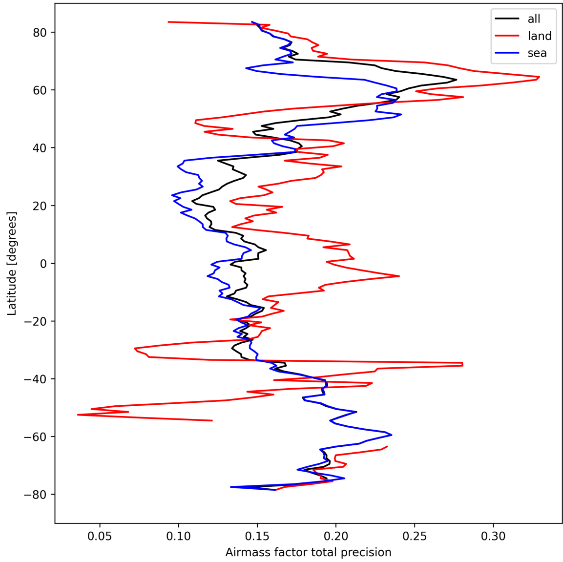
Figure 27: Zonal average of “Airmass factor total precision” for 2024-09-20 to 2024-09-22.
