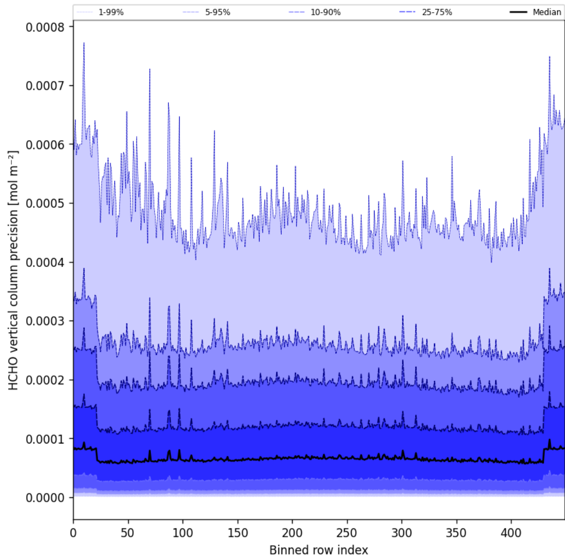
Figure 50: Along track statistics of “HCHO vertical column precision” for 2024-09-20 to 2024-09-22
