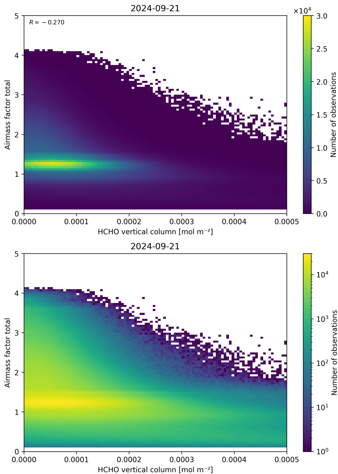
Figure 131: Scatter density plot of “HCHO vertical column” against “Airmass factor total” for 2024-09-20 to 2024-09-22.
