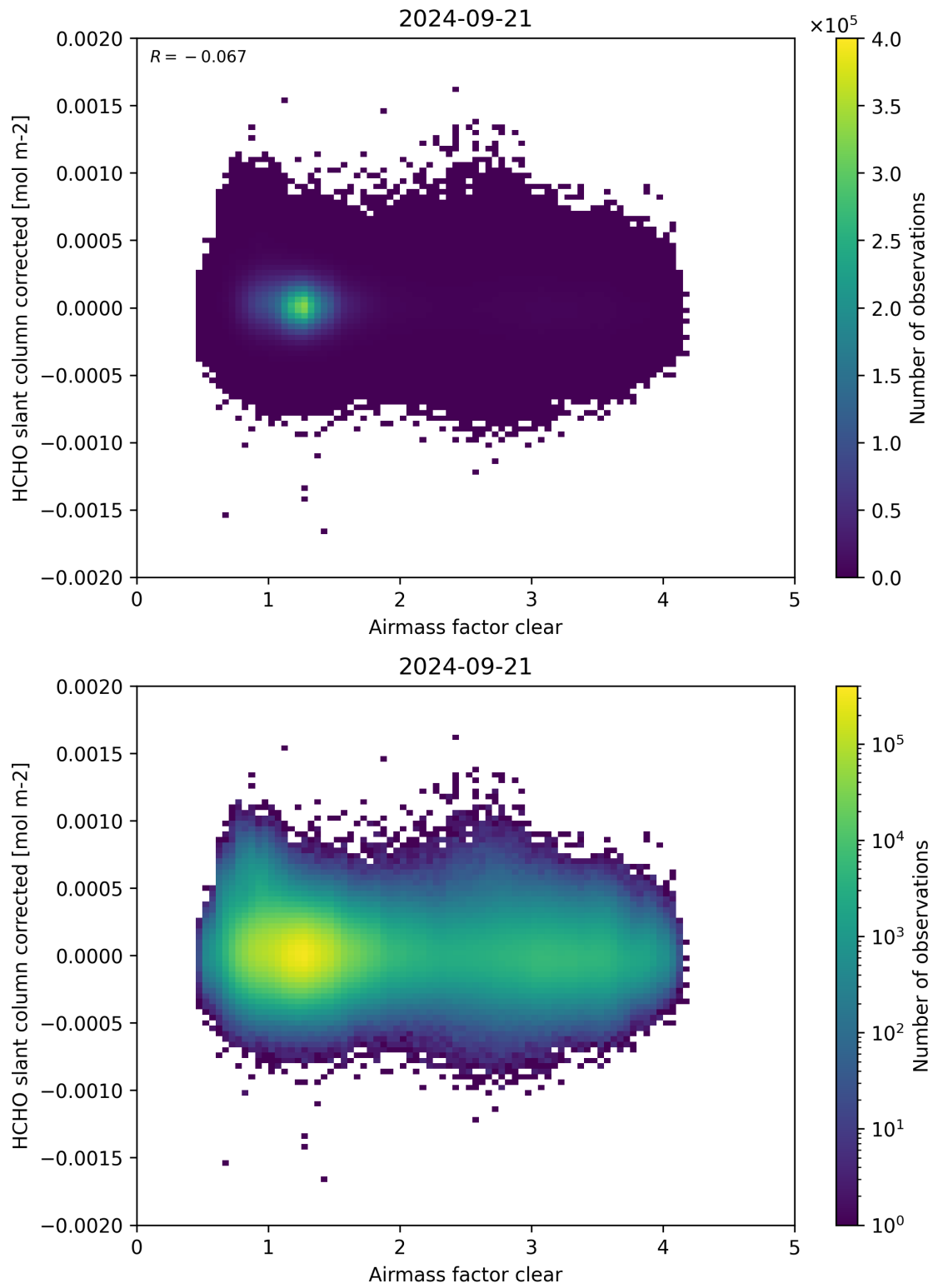
Figure 74: Scatter density plot of “Airmass factor clear” against “HCHO slant column corrected” for 2024-09-20 to 2024-09-22.
