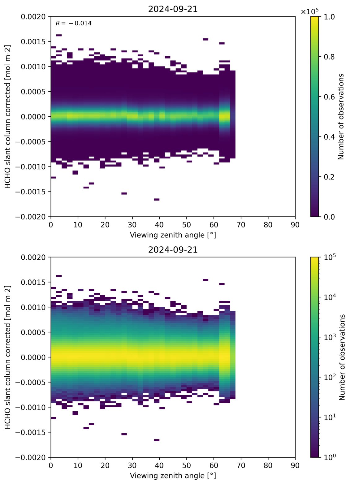
Figure 186: Scatter density plot of “Viewing zenith angle” against “HCHO slant column corrected” for 2024-09-20 to 2024-09-22.
