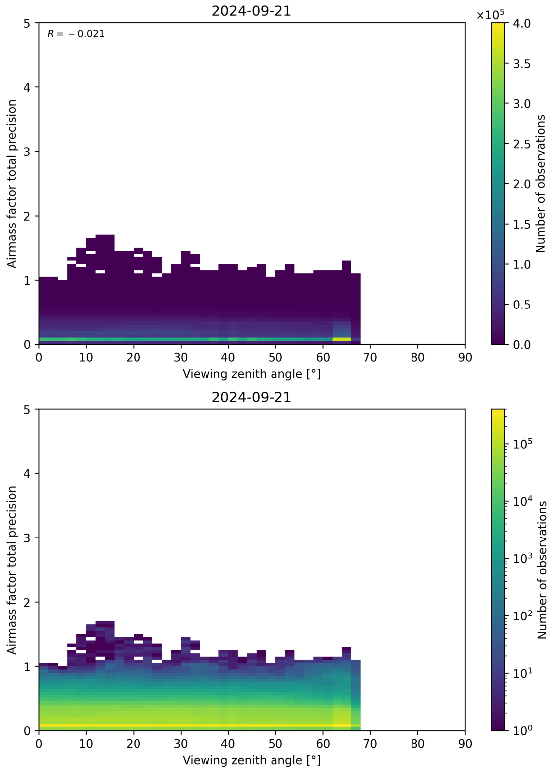
Figure 191: Scatter density plot of “Viewing zenith angle” against “Airmass factor total precision” for 2024-09-20 to 2024-09-22.
