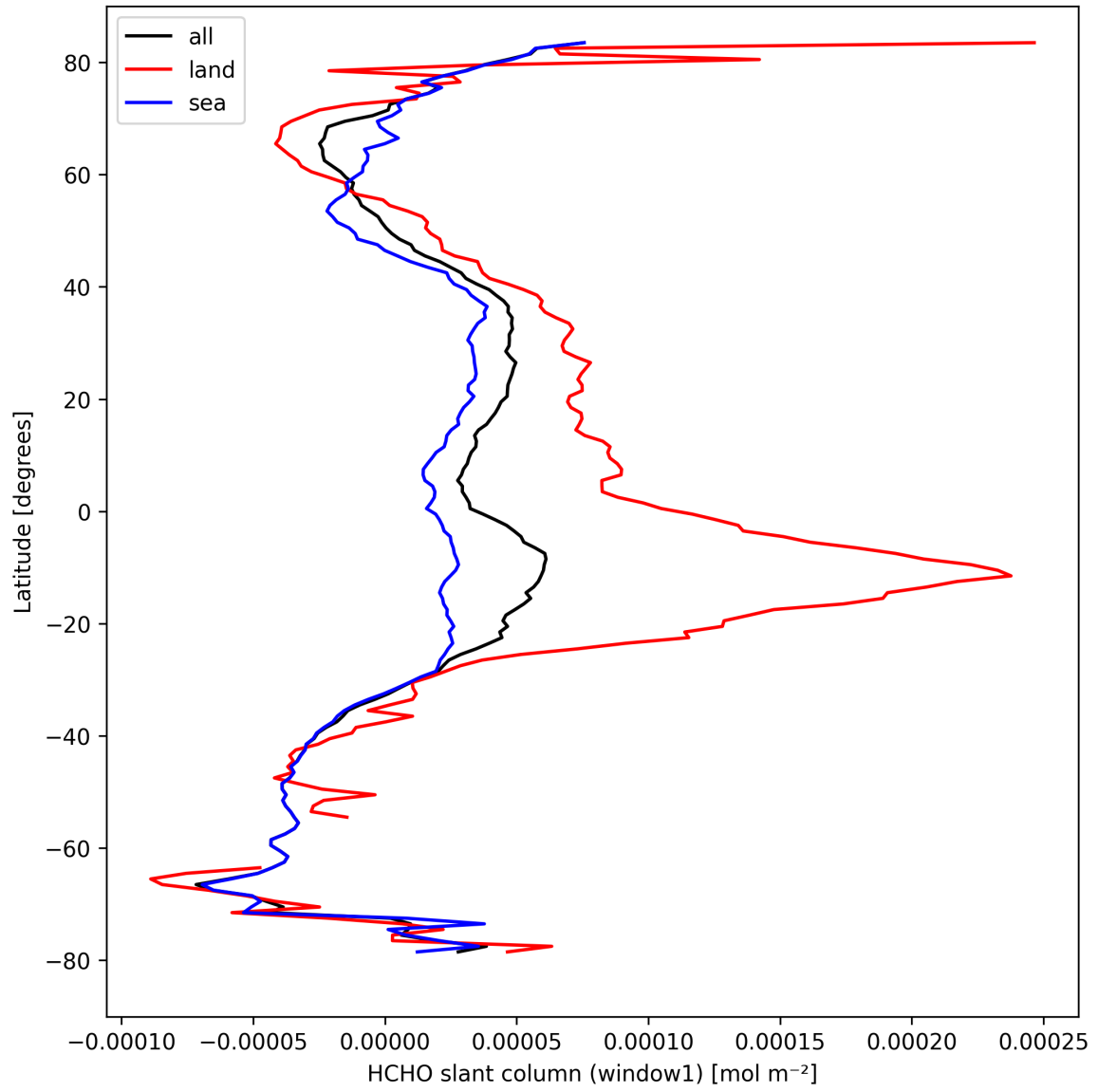
Figure 24: Zonal average of “HCHO slant column (window1)” for 2024-09-20 to 2024-09-22.
