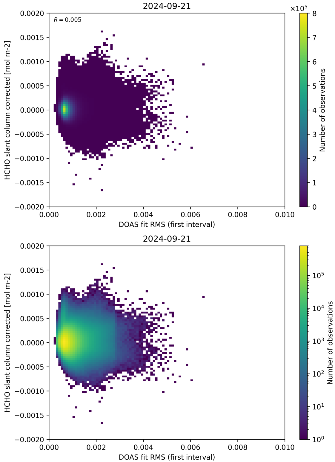
Figure 62: Scatter density plot of “DOAS fit RMS (first interval)” against “HCHO slant column corrected” for 2024-09-20 to 2024-09-22.
