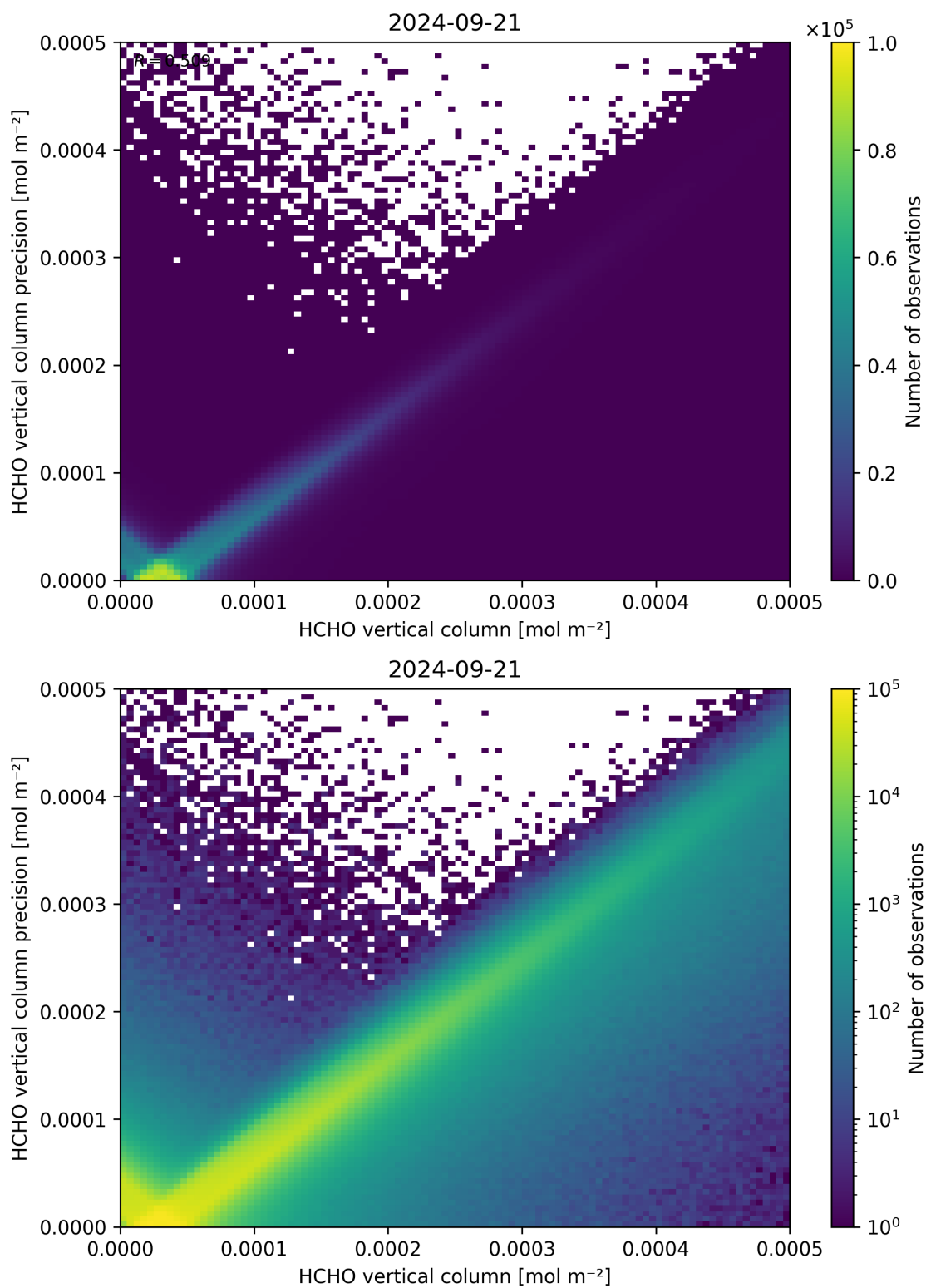
Figure 134: Scatter density plot of “HCHO vertical column” against “HCHO vertical column precision” for 2024-09-20 to 2024-09-22.
