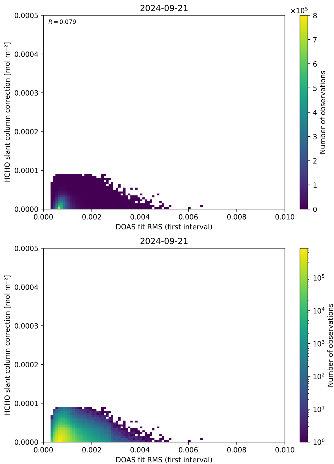
Figure 63: Scatter density plot of “DOAS fit RMS (first interval)” against “HCHO slant column correction” for 2024-09-20 to 2024-09-22.
