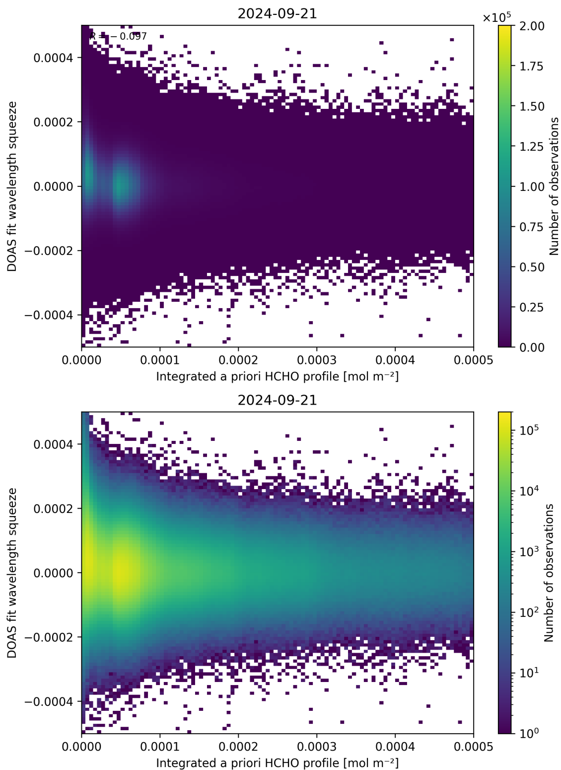
Figure 150: Scatter density plot of “Integrated a priori HCHO profile” against “DOAS fit wavelength squeeze” for 2024-09-20 to 2024-09-22.
