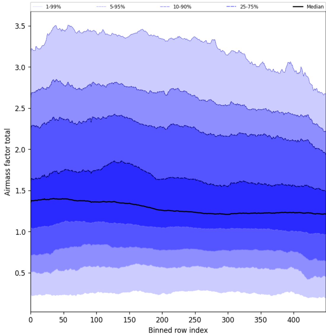
Figure 54: Along track statistics of “Airmass factor total” for 2024-09-20 to 2024-09-22
