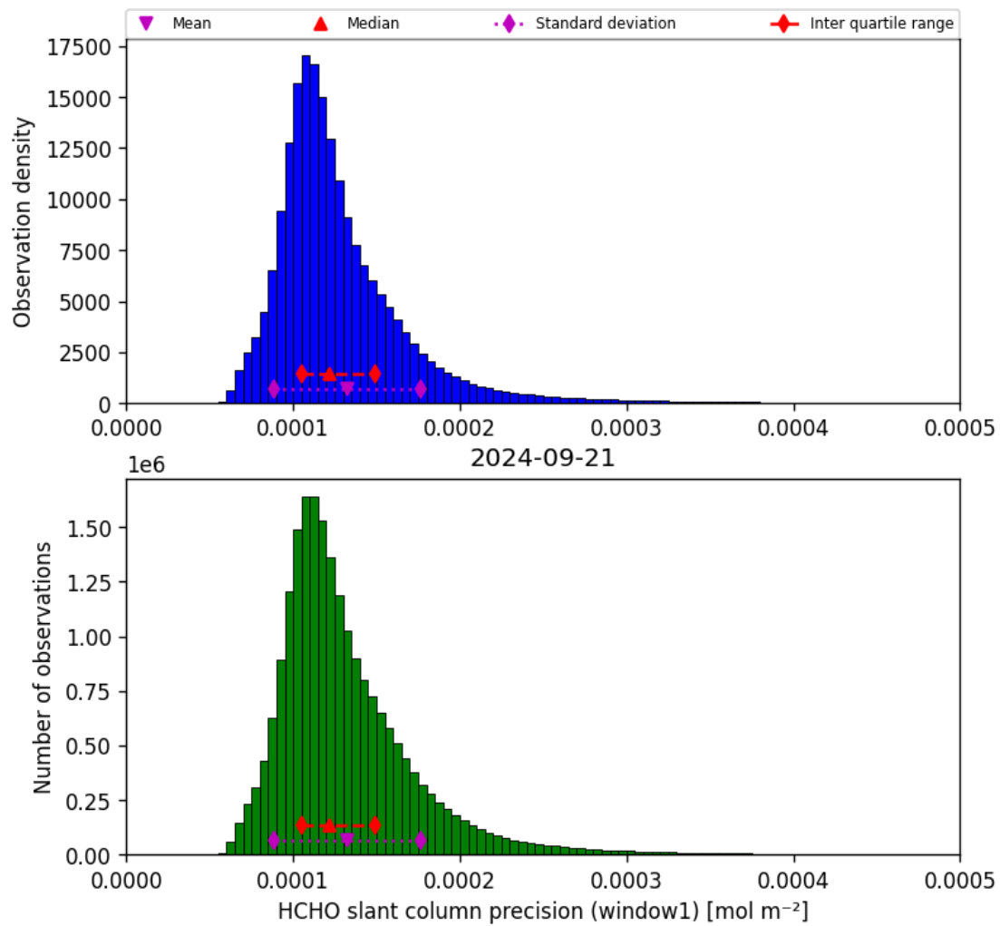
Figure 39: Histogram of “HCHO slant column precision (window1)” for 2024-09-20 to 2024-09-22
