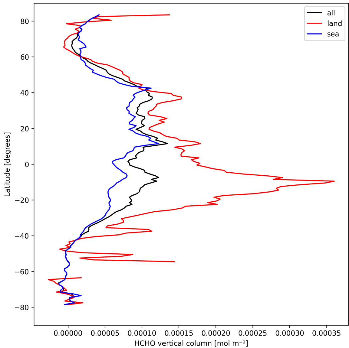
Figure 21: Zonal average of “HCHO vertical column” for 2024-09-20 to 2024-09-22.
