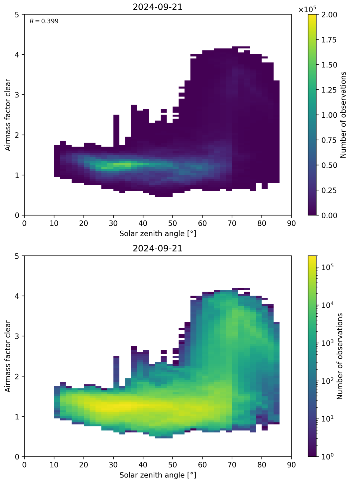
Figure 170: Scatter density plot of “Solar zenith angle” against “Airmass factor clear” for 2024-09-20 to 2024-09-22.
