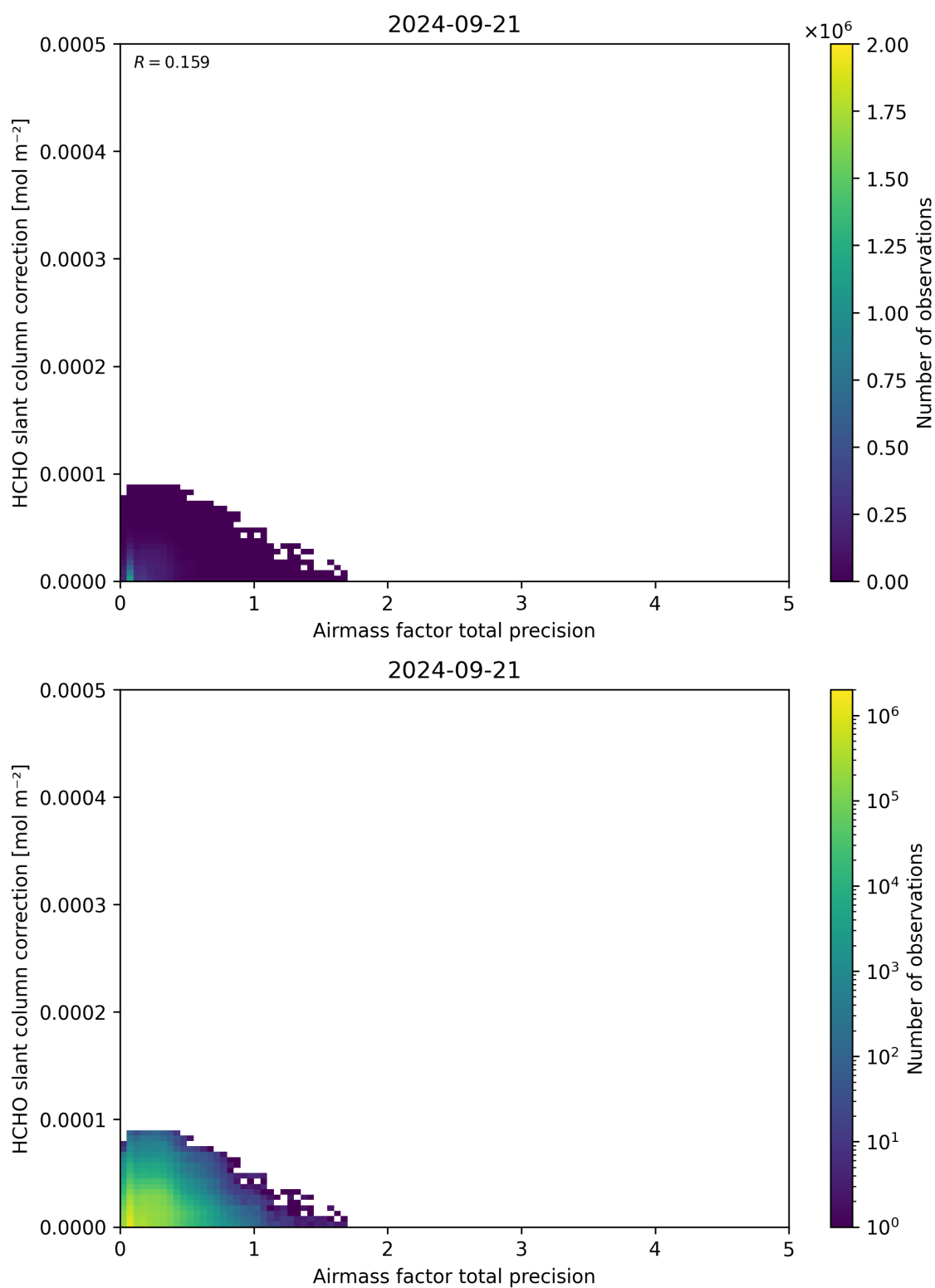
Figure 110: Scatter density plot of “Airmass factor total precision” against “HCHO slant column correction” for 2024-09-20 to 2024-09-22.
