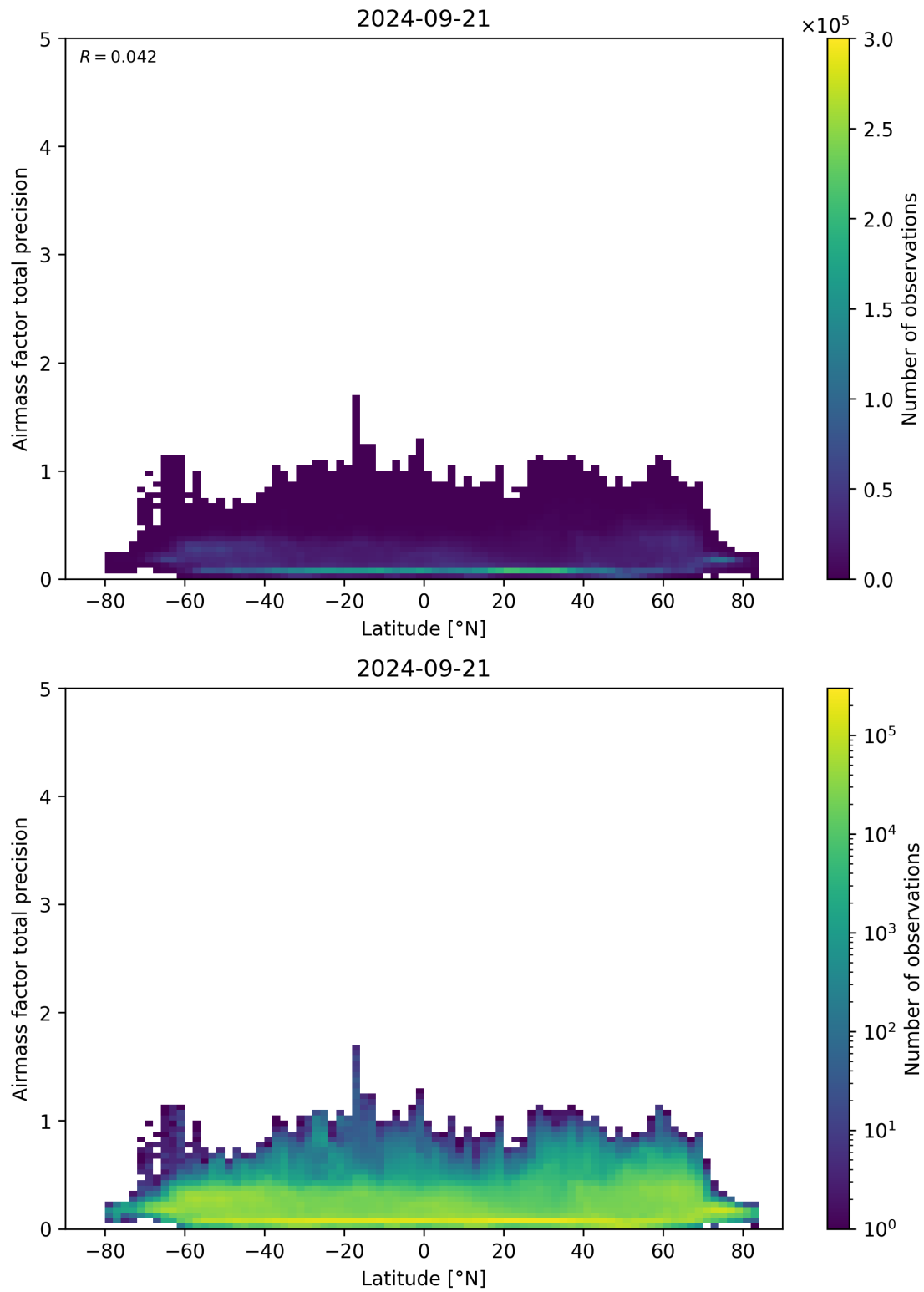
Figure 162: Scatter density plot of “Latitude” against “Airmass factor total precision” for 2024-09-20 to 2024-09-22.
