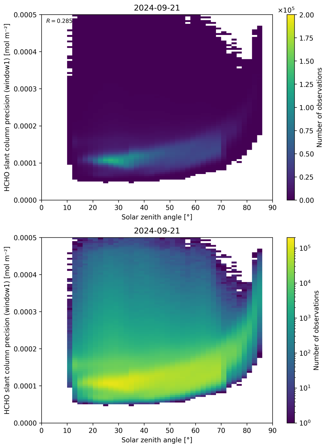
Figure 174: Scatter density plot of “Solar zenith angle” against “HCHO slant column precision (window1)” for 2024-09-20 to 2024-09-22.
