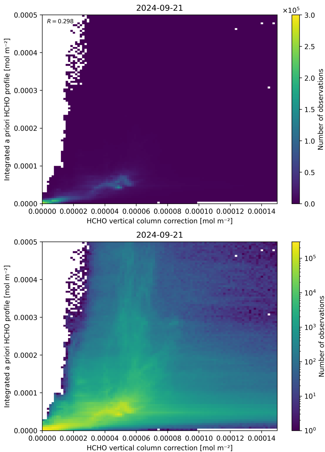
Figure 122: Scatter density plot of “HCHO vertical column correction” against “Integrated a priori HCHO profile” for 2024-09-20 to 2024-09-22.
