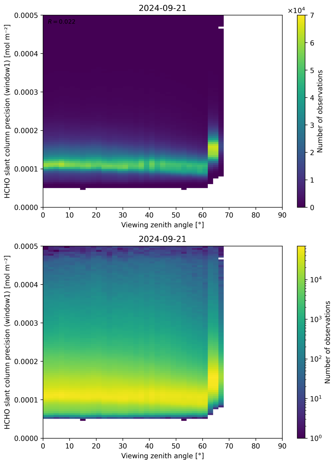
Figure 189: Scatter density plot of “Viewing zenith angle” against “HCHO slant column precision (window1)” for 2024-09-20 to 2024-09-22.
