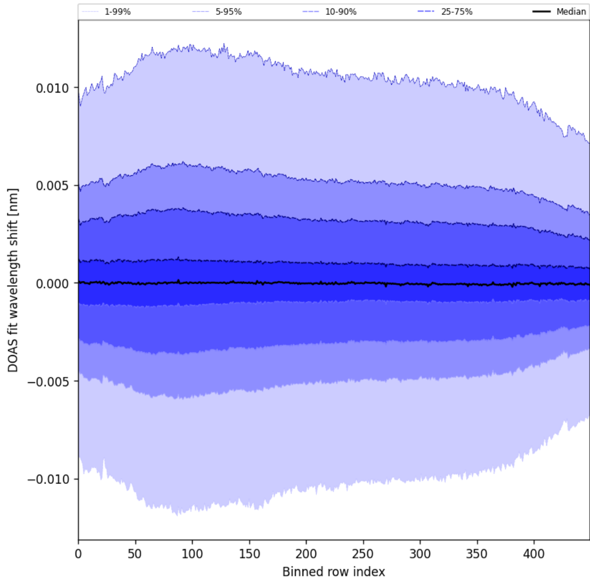
Figure 58: Along track statistics of “DOAS fit wavelength shift” for 2024-09-20 to 2024-09-22
