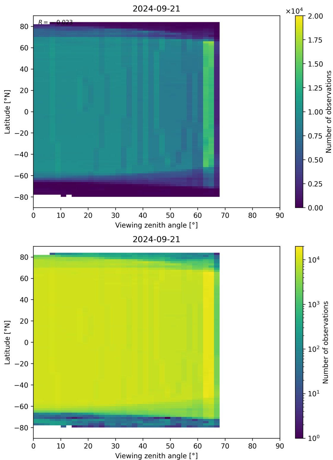
Figure 196: Scatter density plot of “Viewing zenith angle” against “Latitude” for 2024-09-20 to 2024-09-22.
