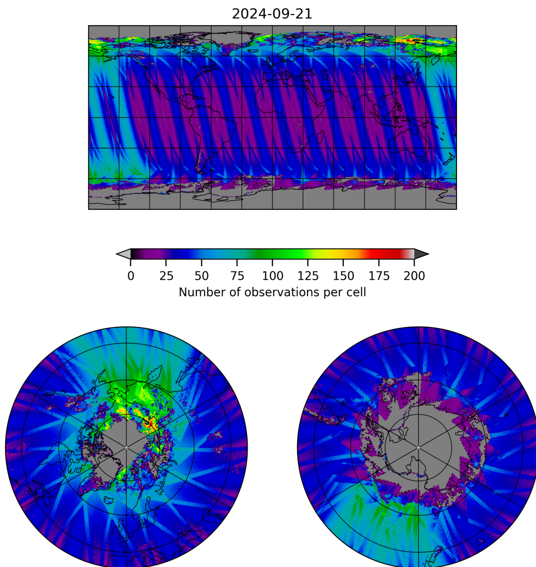
Figure 19: Map of the number of observations for 2024-09-20 to 2024-09-22
