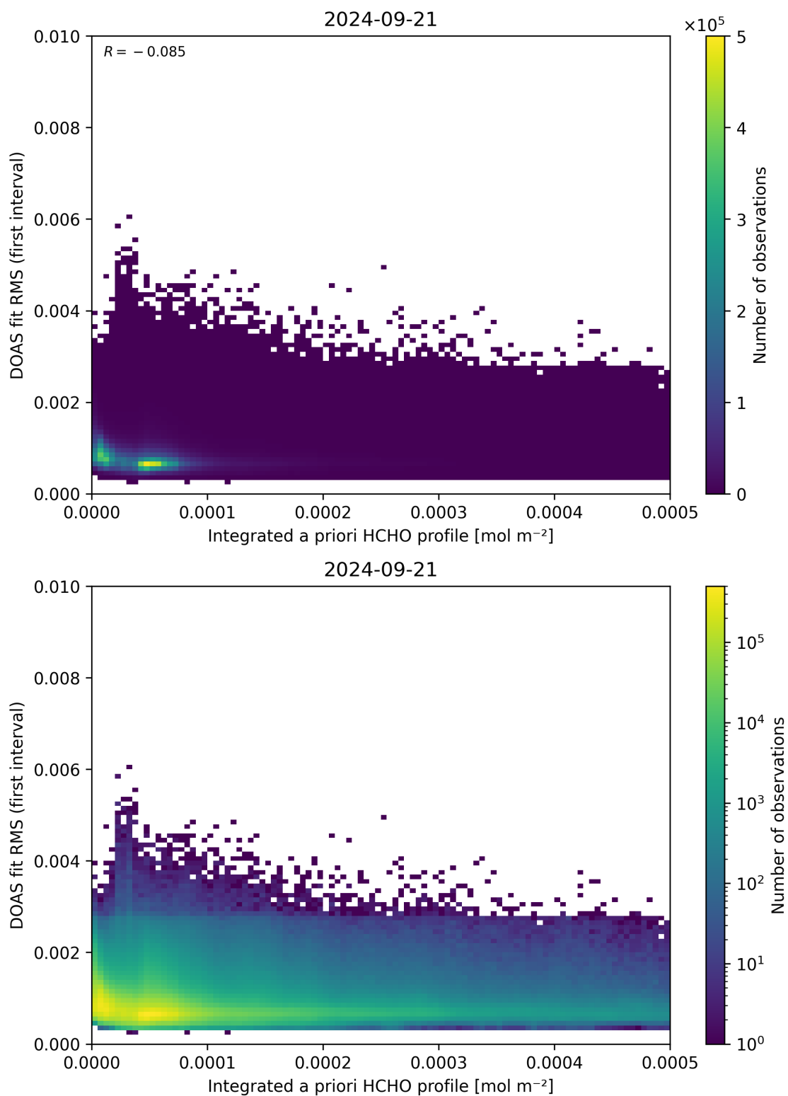
Figure 148: Scatter density plot of “Integrated a priori HCHO profile” against “DOAS fit RMS (first interval)” for 2024-09-20 to 2024-09-22.
