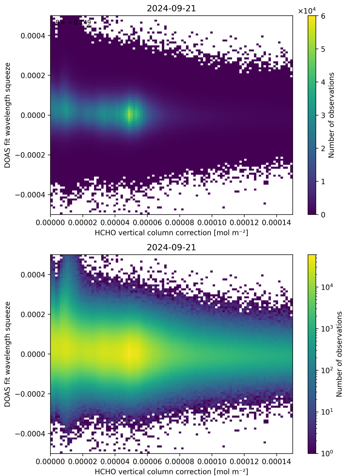
Figure 114: Scatter density plot of “HCHO vertical column correction” against “DOAS fit wavelength squeeze” for 2024-09-20 to 2024-09-22.
