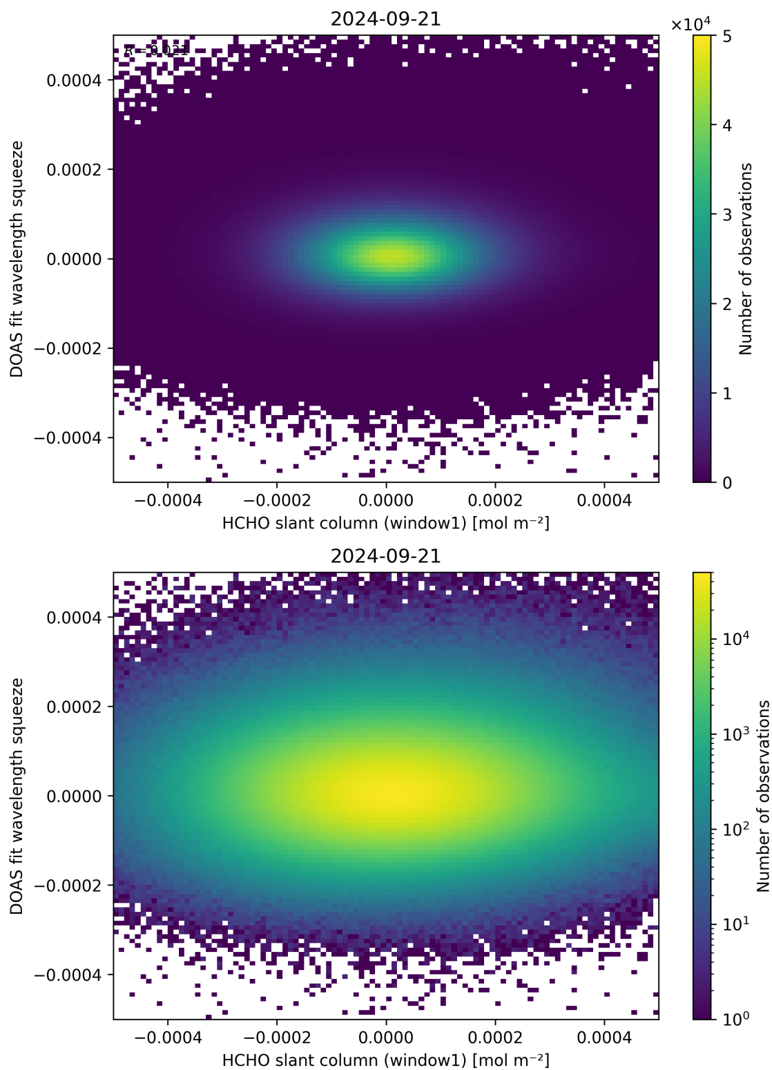
Figure 80: Scatter density plot of “HCHO slant column (window1)” against “DOAS fit wavelength squeeze” for 2024-09-20 to 2024-09-22.
