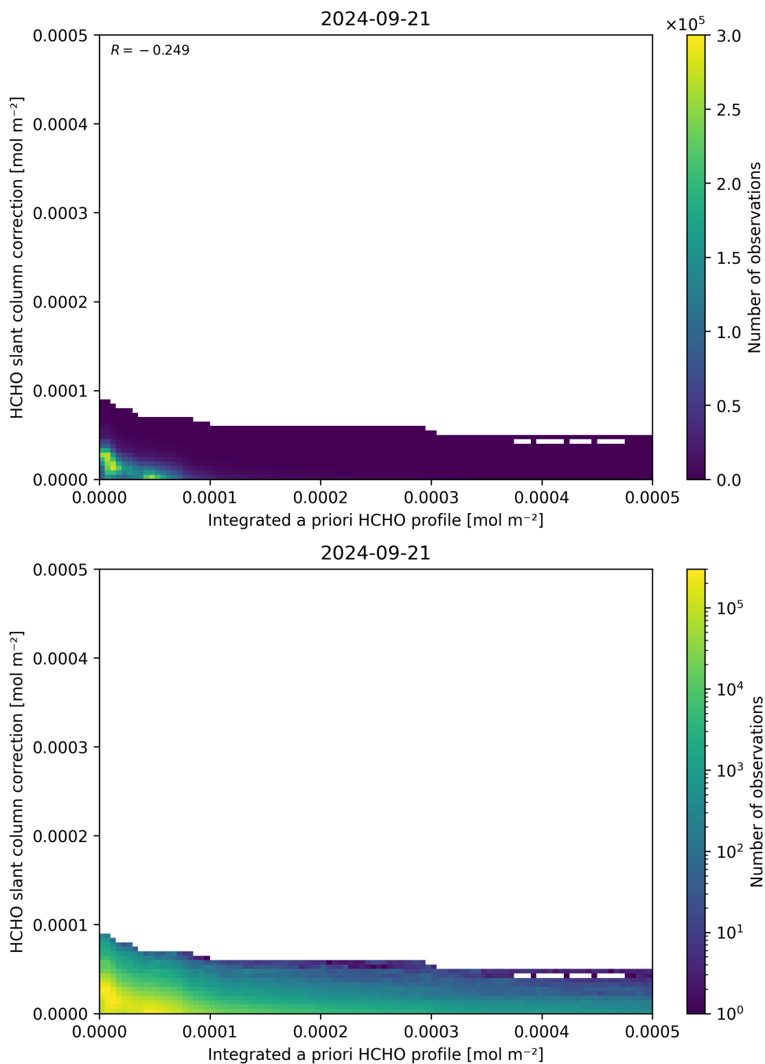
Figure 152: Scatter density plot of “Integrated a priori HCHO profile” against “HCHO slant column correction” for 2024-09-20 to 2024-09-22.
