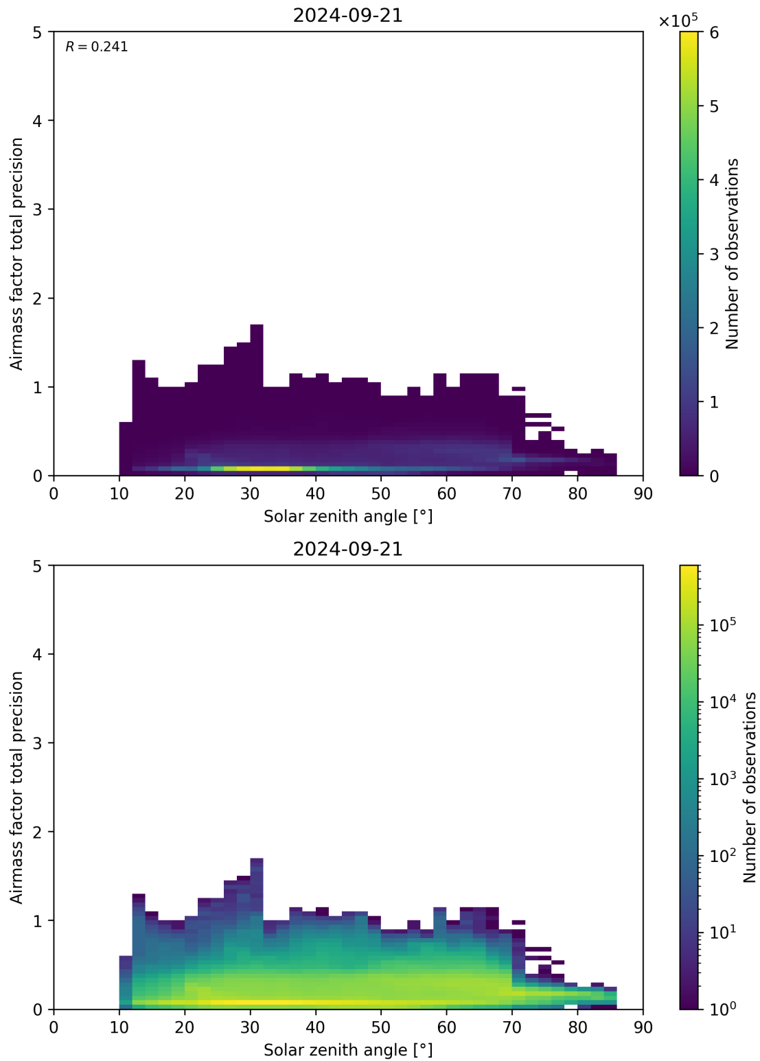
Figure 176: Scatter density plot of “Solar zenith angle” against “Airmass factor total precision” for 2024-09-20 to 2024-09-22.
