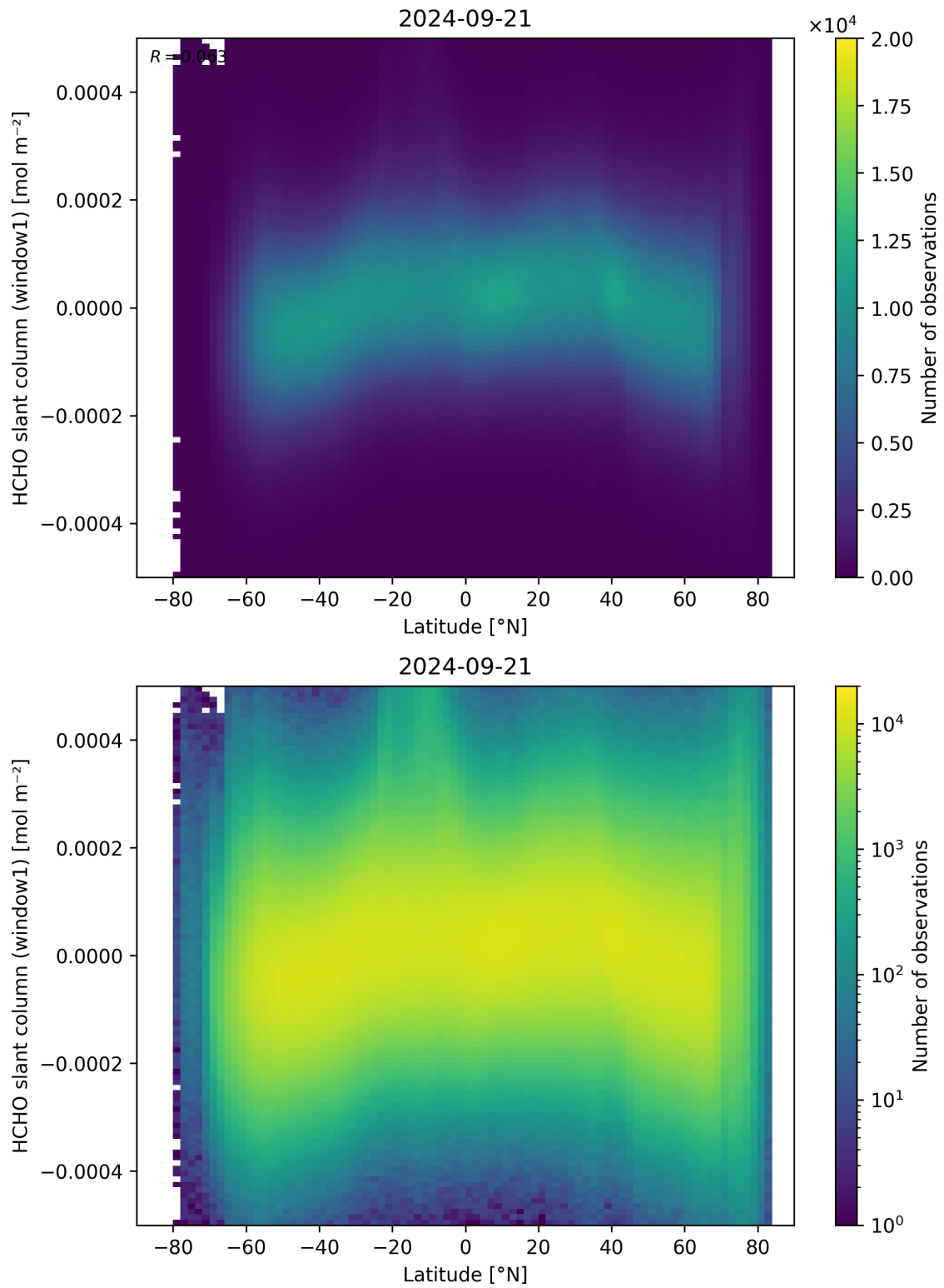
Figure 159: Scatter density plot of “Latitude” against “HCHO slant column (window1)” for 2024-09-20 to 2024-09-22.
