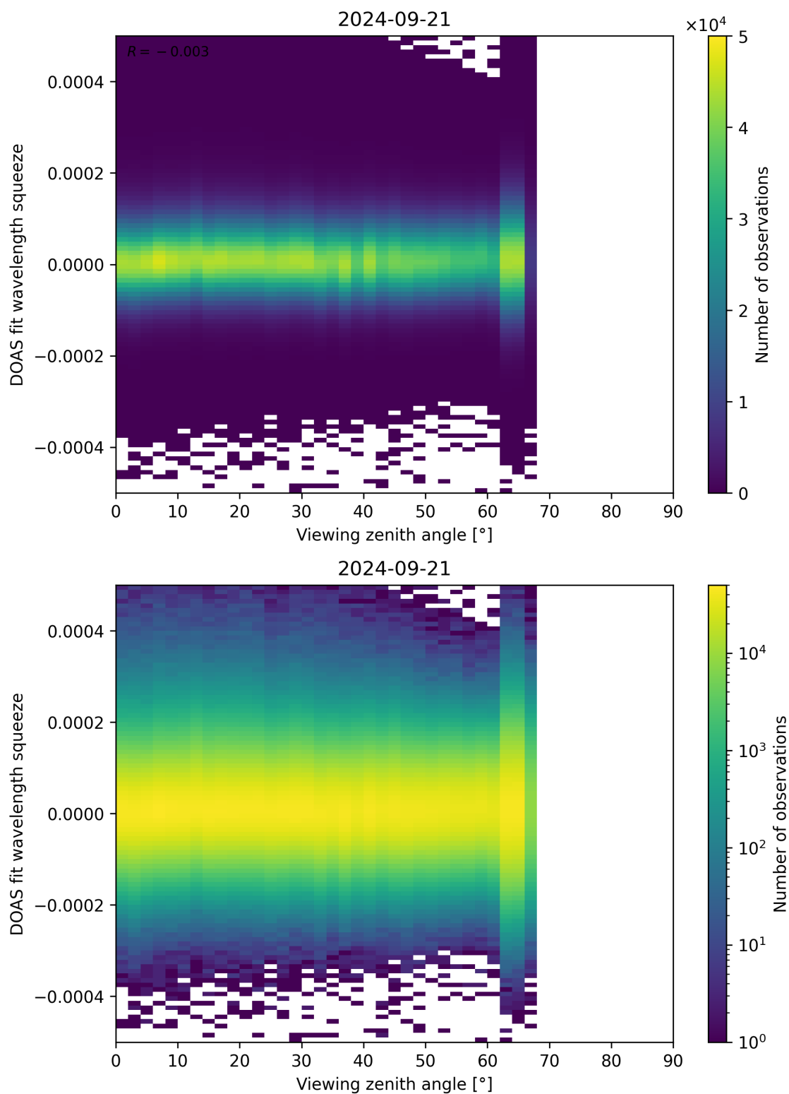
Figure 184: Scatter density plot of “Viewing zenith angle” against “DOAS fit wavelength squeeze” for 2024-09-20 to 2024-09-22.
