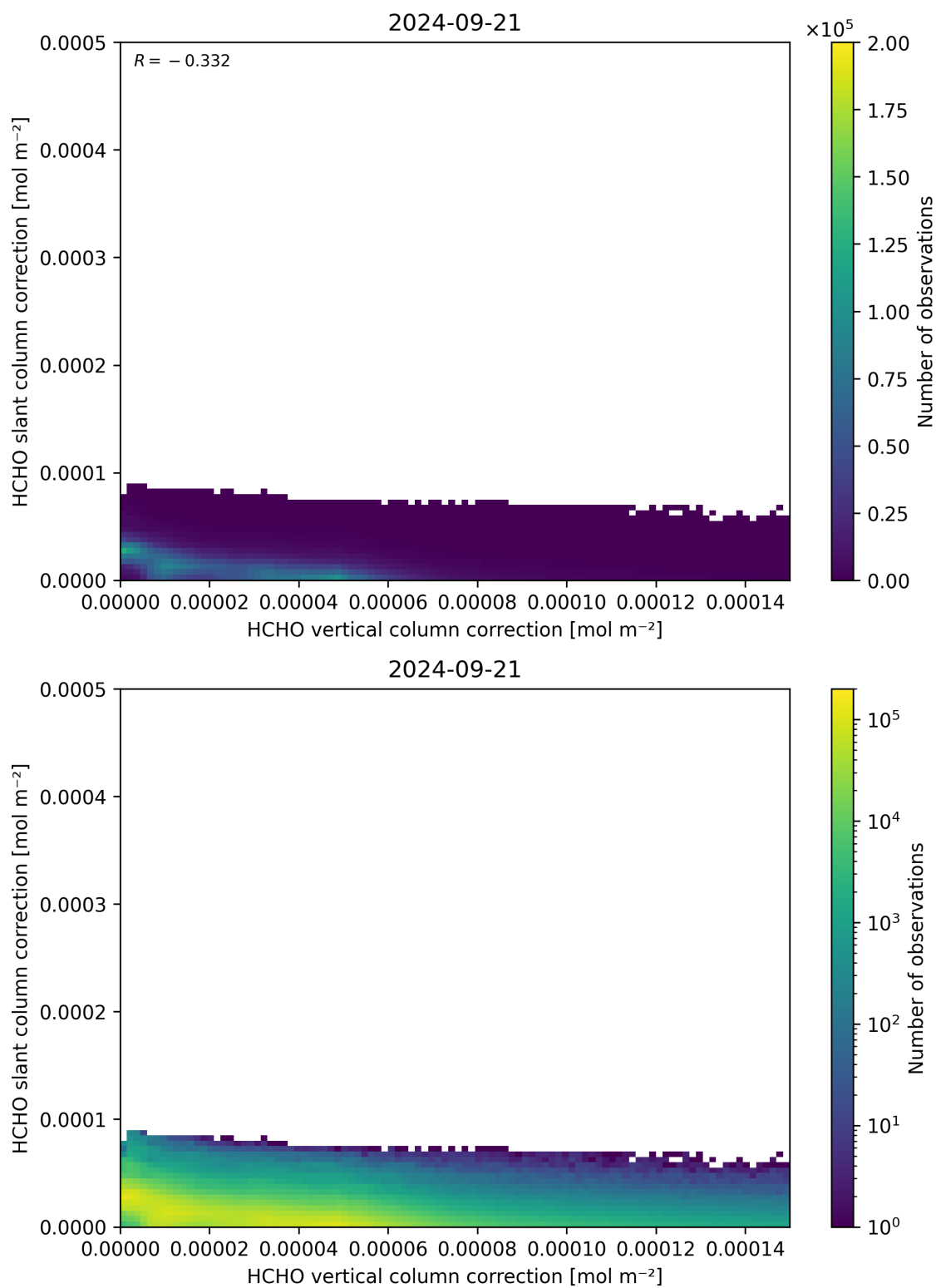
Figure 117: Scatter density plot of “HCHO vertical column correction” against “HCHO slant column correction” for 2024-09-20 to 2024-09-22.
