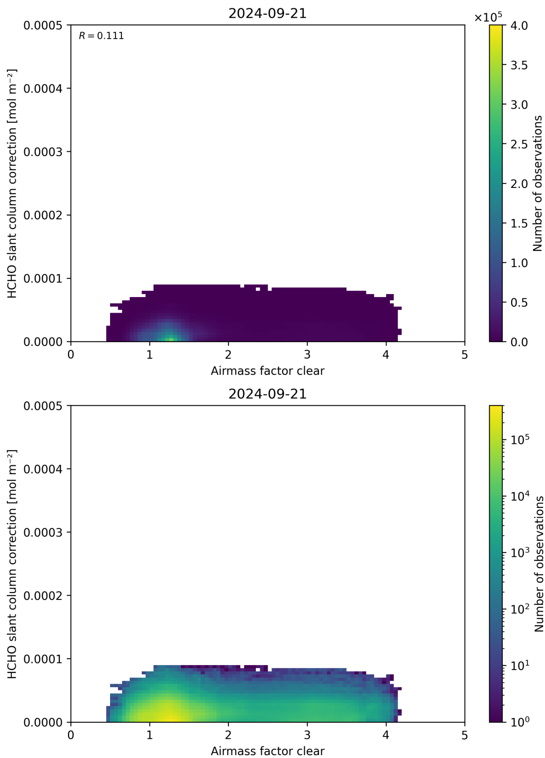
Figure 75: Scatter density plot of “Airmass factor clear” against “HCHO slant column correction” for 2024-09-20 to 2024-09-22.
