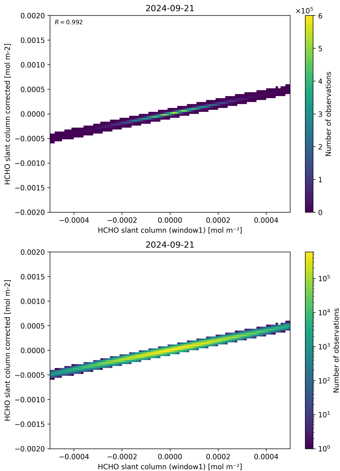
Figure 82: Scatter density plot of “HCHO slant column (window1)” against “HCHO slant column corrected” for 2024-09-20 to 2024-09-22.
