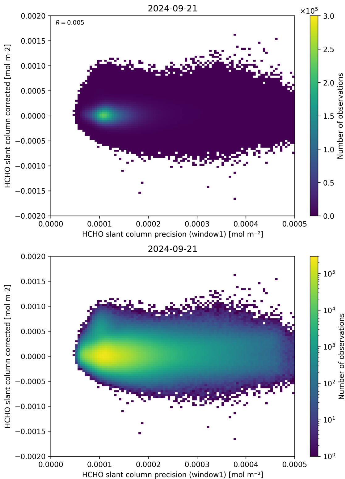
Figure 92: Scatter density plot of “HCHO slant column precision (window1)” against “HCHO slant column corrected” for 2024-09-20 to 2024-09-22.
