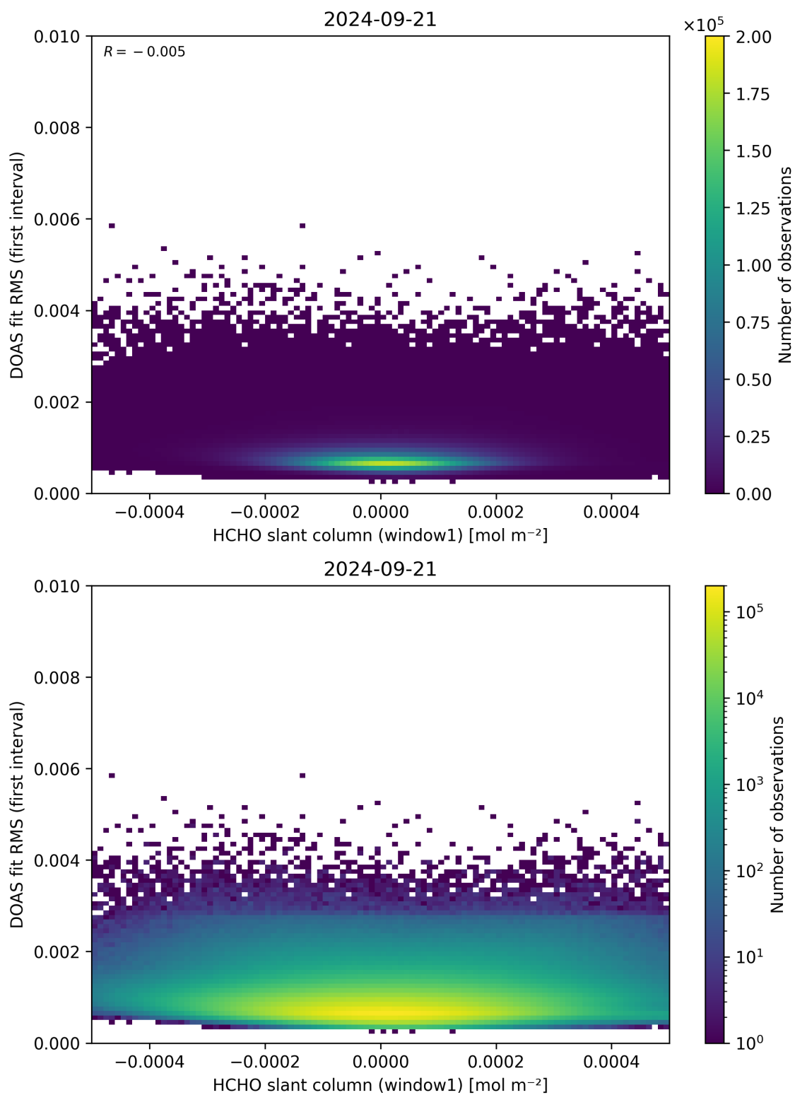
Figure 78: Scatter density plot of “HCHO slant column (window1)” against “DOAS fit RMS (first interval)” for 2024-09-20 to 2024-09-22.
