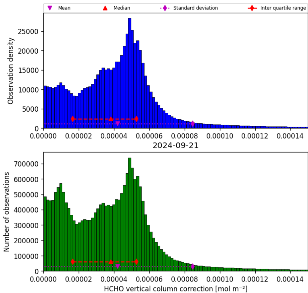
Figure 37: Histogram of “HCHO vertical column correction” for 2024-09-20 to 2024-09-22
