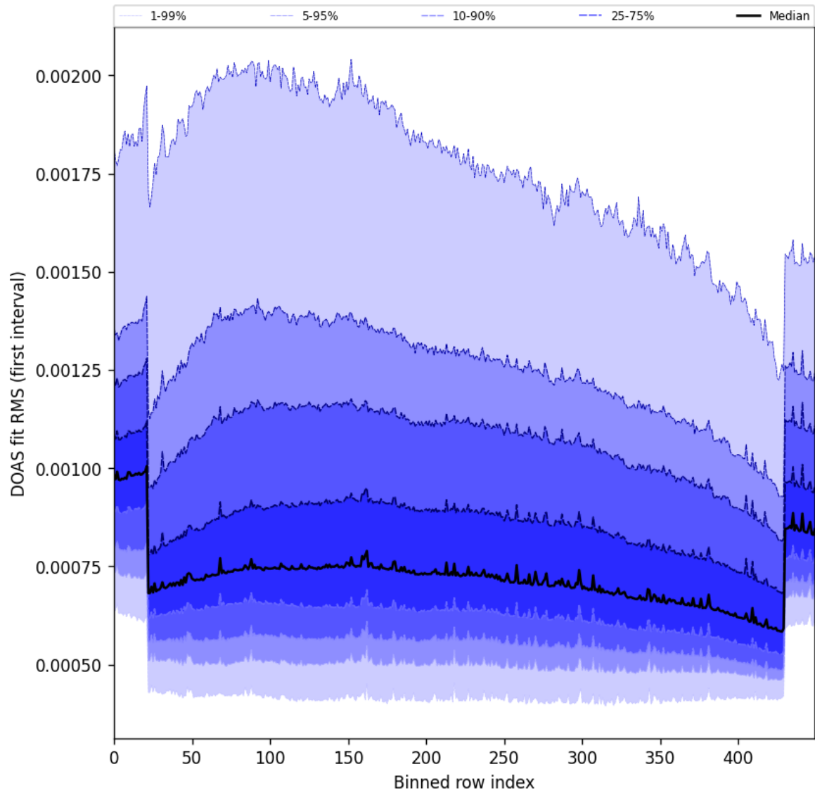
Figure 60: Along track statistics of “DOAS fit RMS (first interval)” for 2024-09-20 to 2024-09-22
