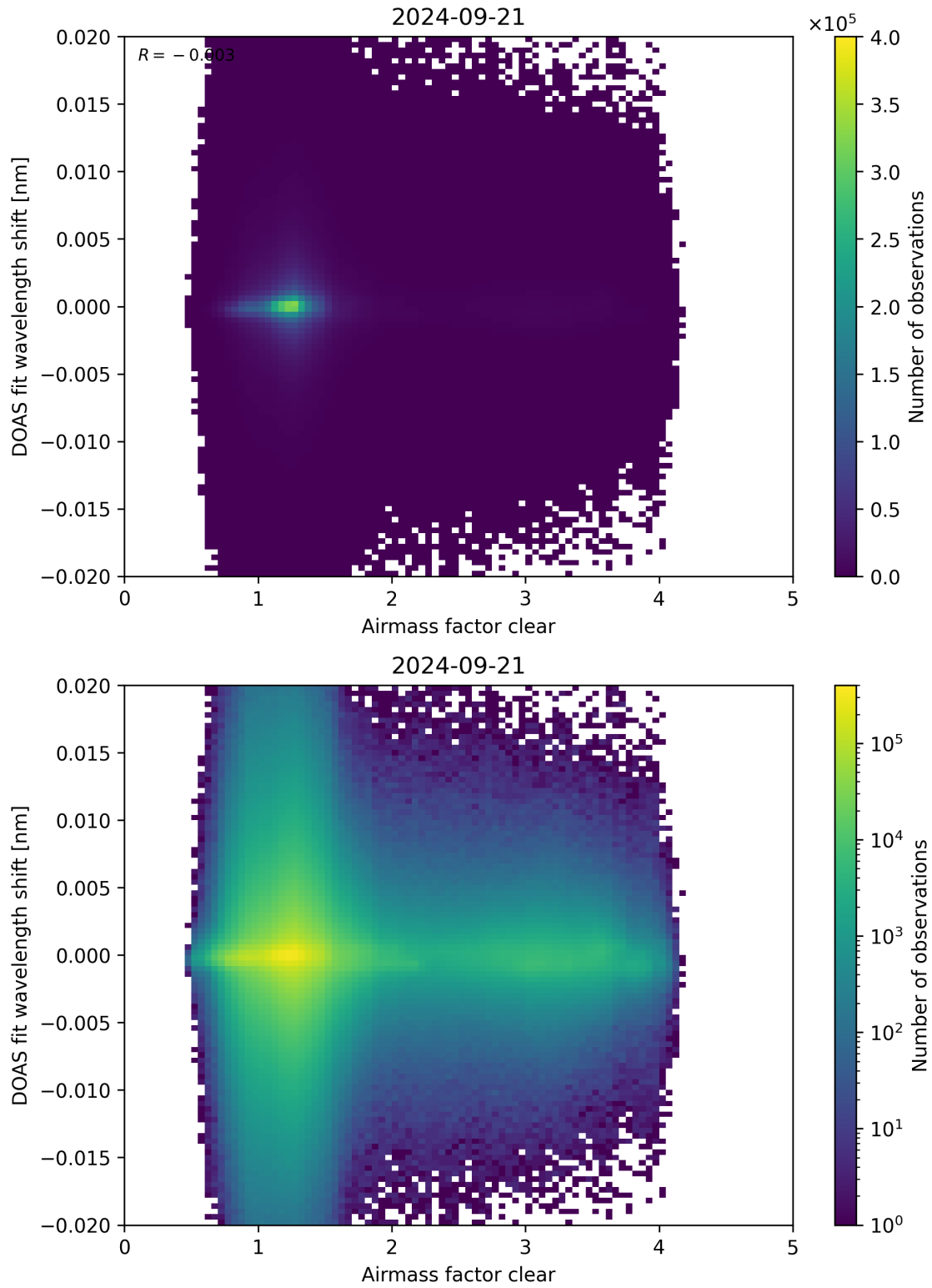
Figure 72: Scatter density plot of “Airmass factor clear” against “DOAS fit wavelength shift” for 2024-09-20 to 2024-09-22.
