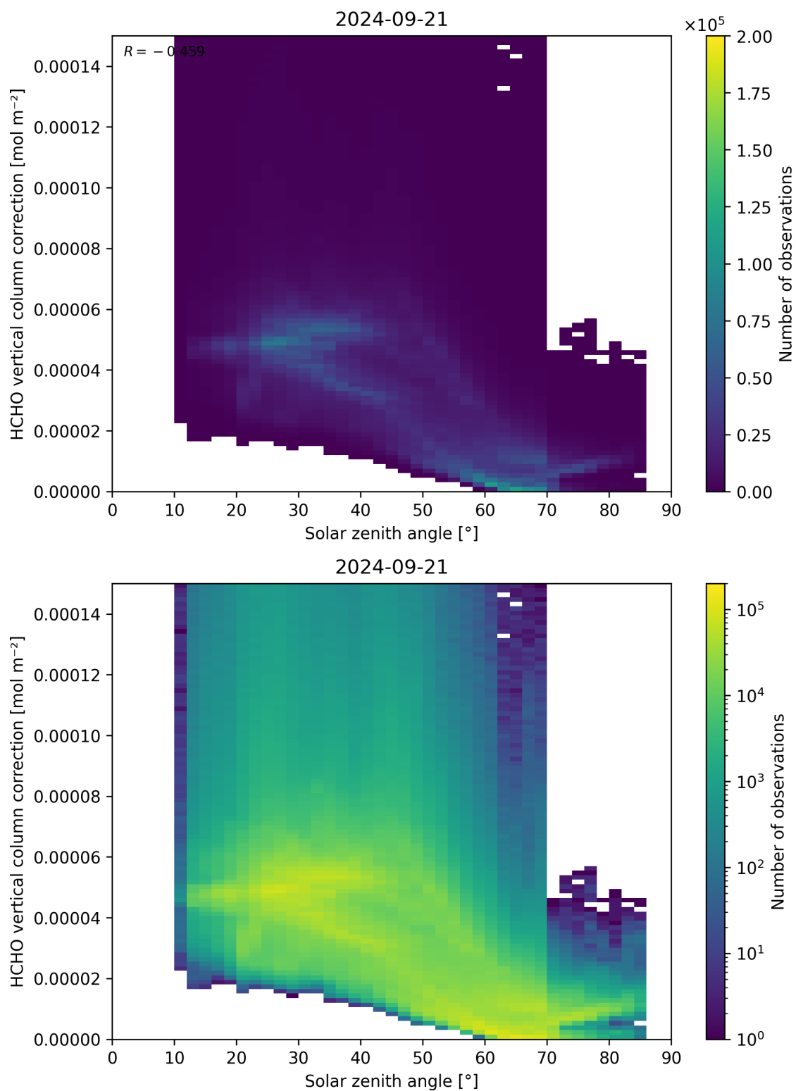
Figure 178: Scatter density plot of “Solar zenith angle” against “HCHO vertical column correction” for 2024-09-20 to 2024-09-22.
