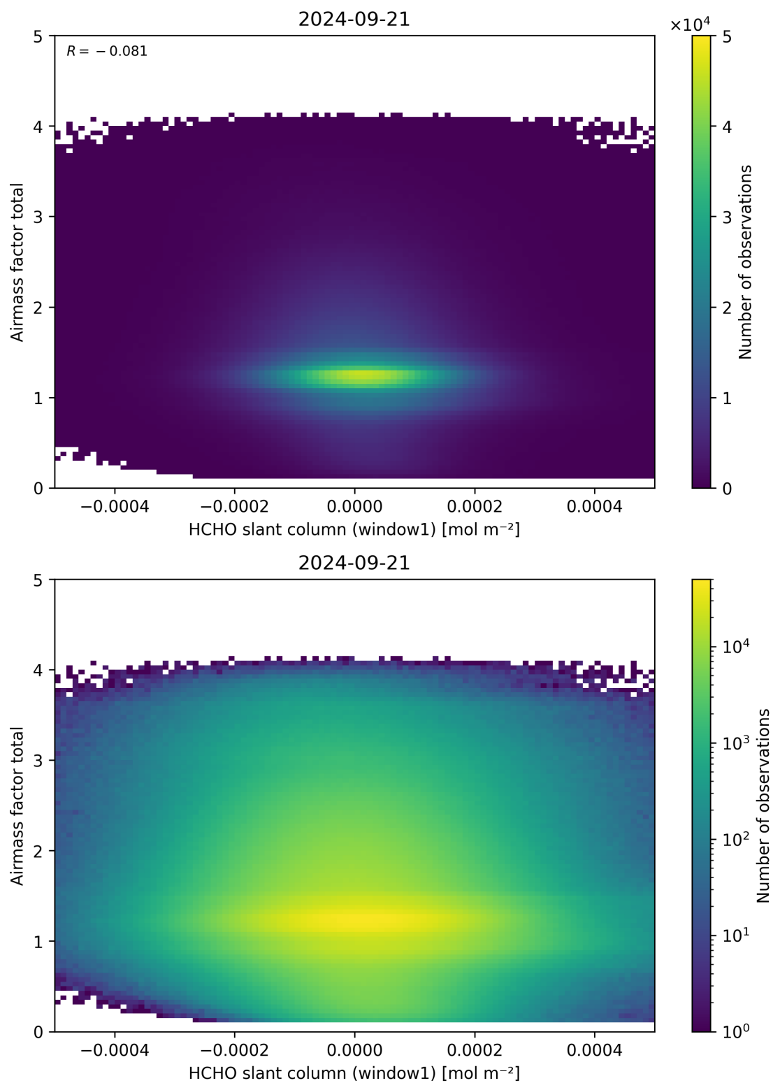
Figure 85: Scatter density plot of “HCHO slant column (window1)” against “Airmass factor total” for 2024-09-20 to 2024-09-22.
