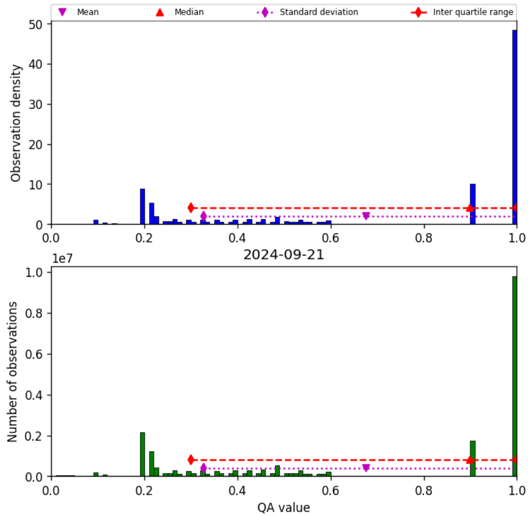
Figure 34: Histogram of “QA value” for 2024-09-20 to 2024-09-22
