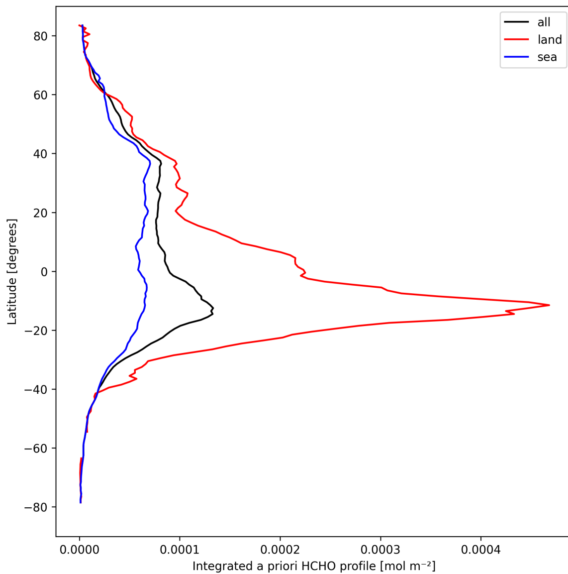
Figure 29: Zonal average of “Integrated a priori HCHO profile” for 2024-09-20 to 2024-09-22.
