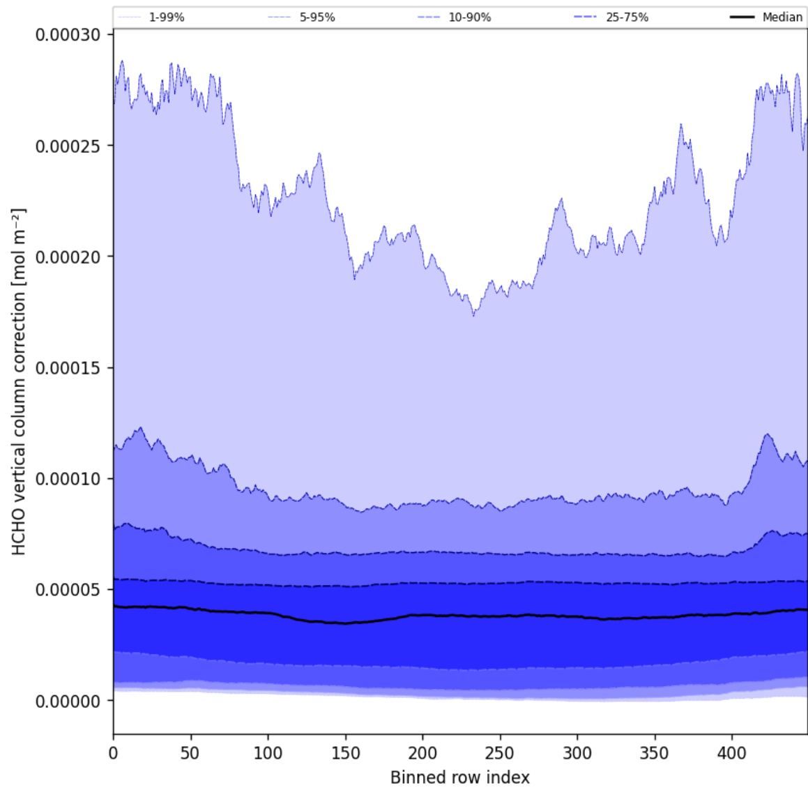
Figure 51: Along track statistics of “HCHO vertical column correction” for 2024-09-20 to 2024-09-22
