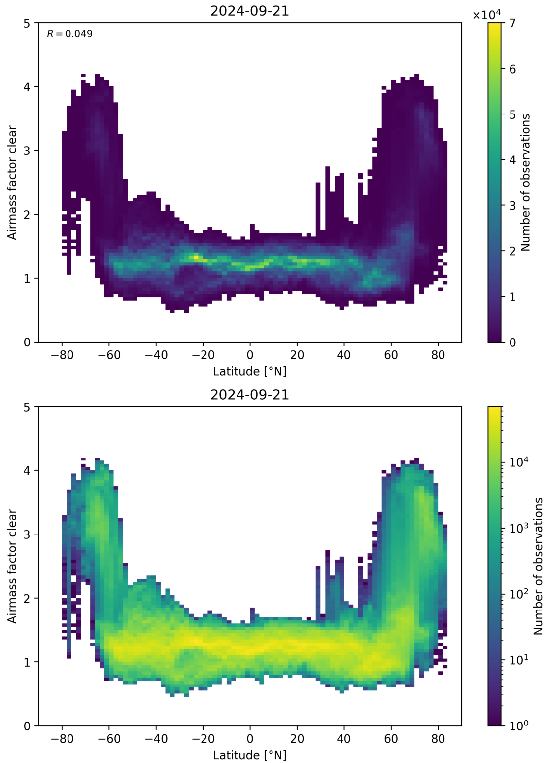
Figure 156: Scatter density plot of “Latitude” against “Airmass factor clear” for 2024-09-20 to 2024-09-22.
