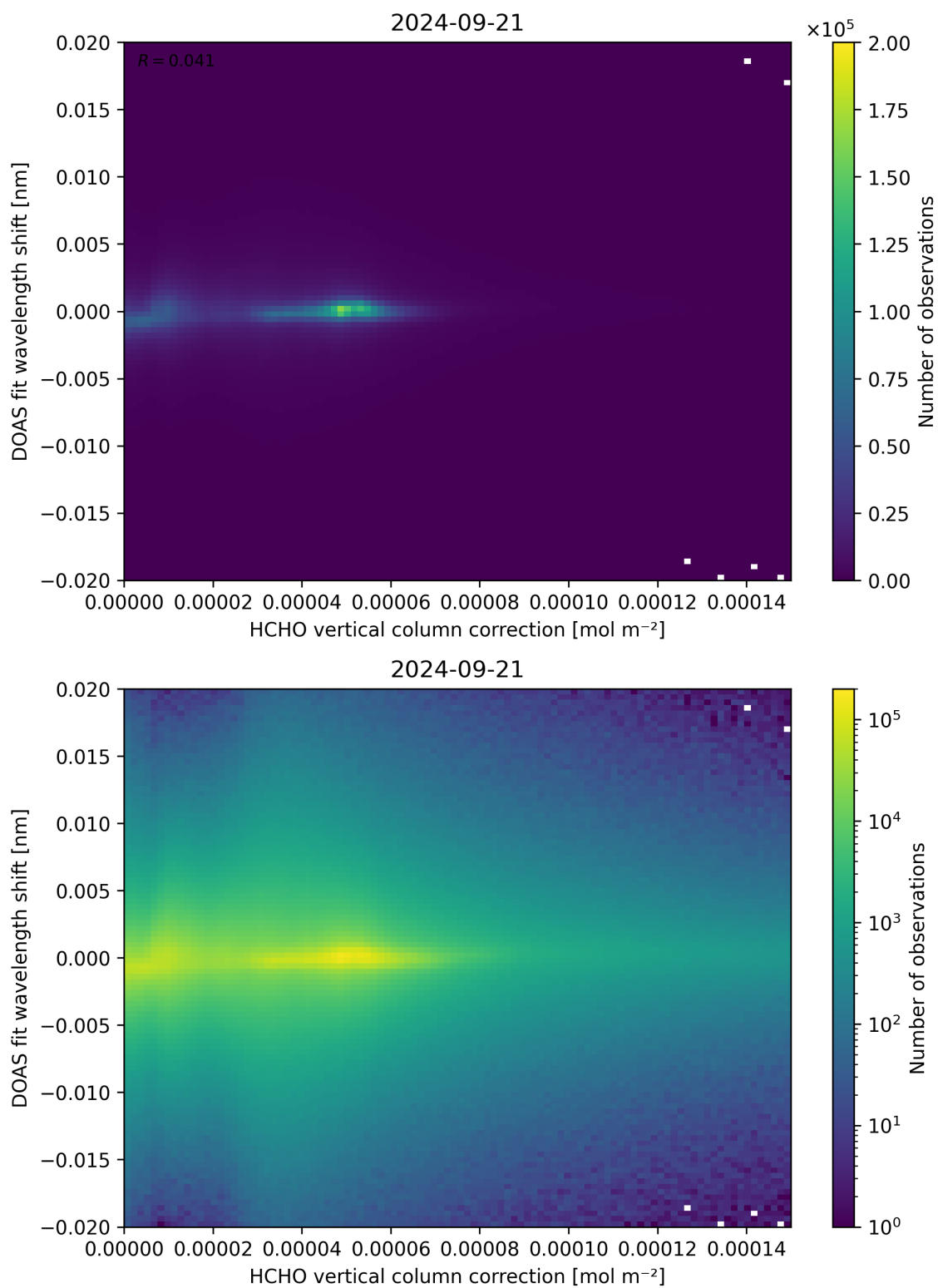
Figure 113: Scatter density plot of “HCHO vertical column correction” against “DOAS fit wavelength shift” for 2024-09-20 to 2024-09-22.
