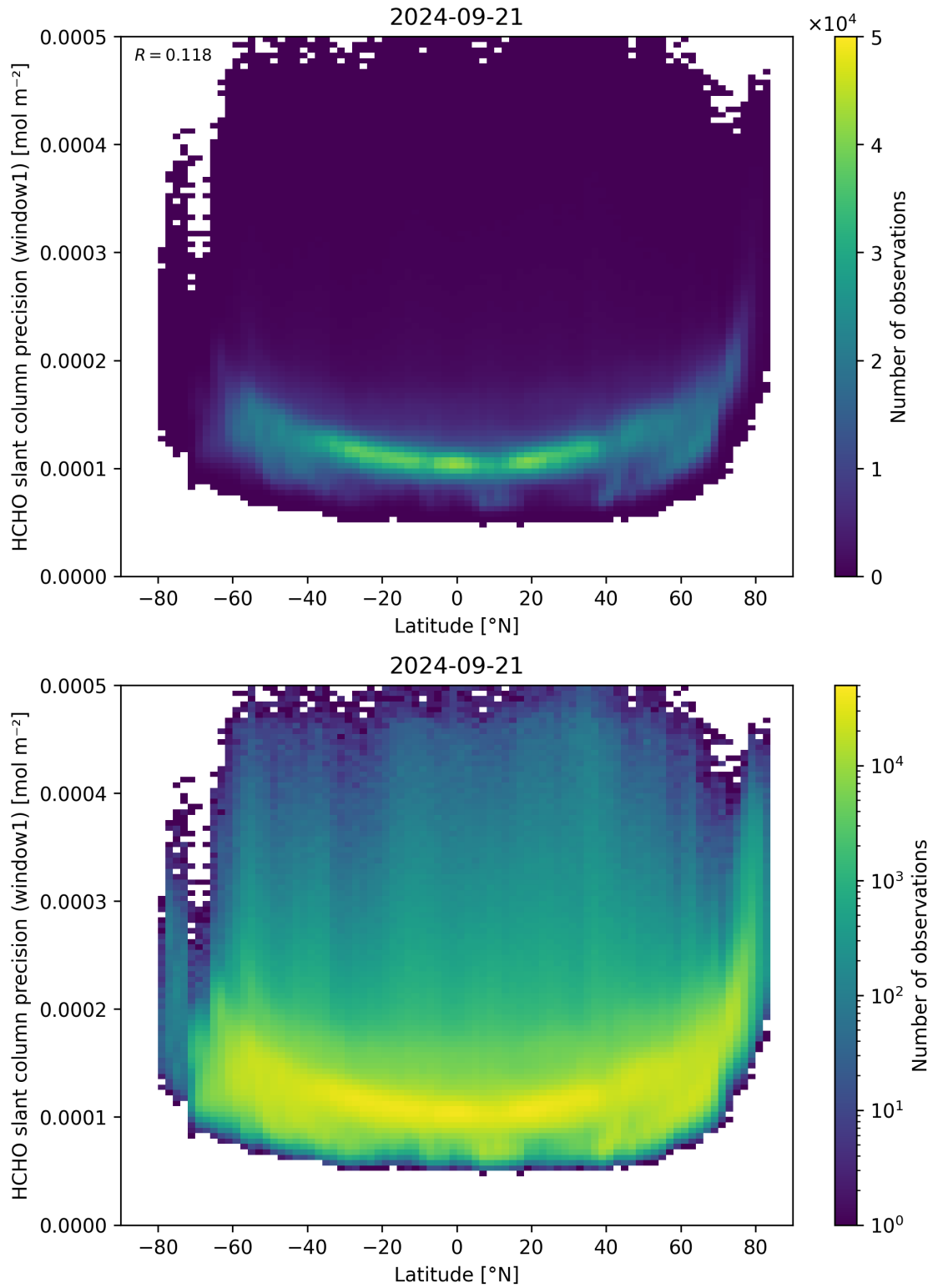
Figure 160: Scatter density plot of “Latitude” against “HCHO slant column precision (window1)” for 2024-09-20 to 2024-09-22.
