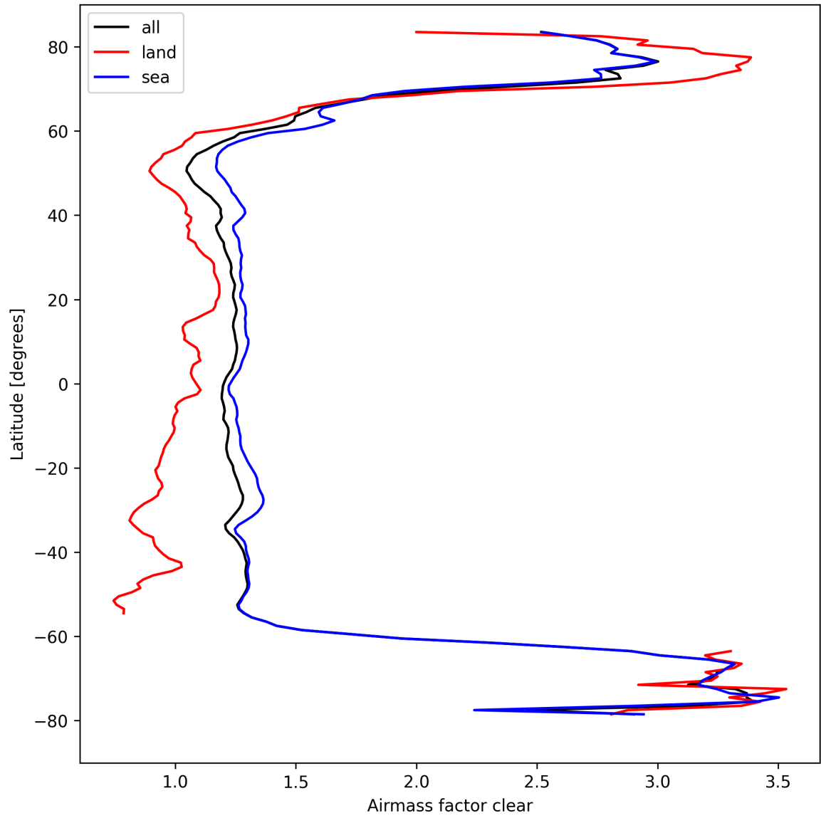
Figure 28: Zonal average of “Airmass factor clear” for 2024-09-20 to 2024-09-22.
