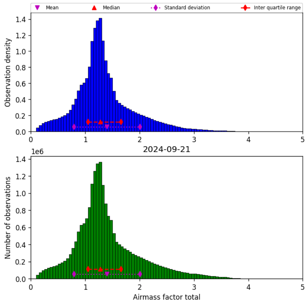
Figure 40: Histogram of “Airmass factor total” for 2024-09-20 to 2024-09-22
