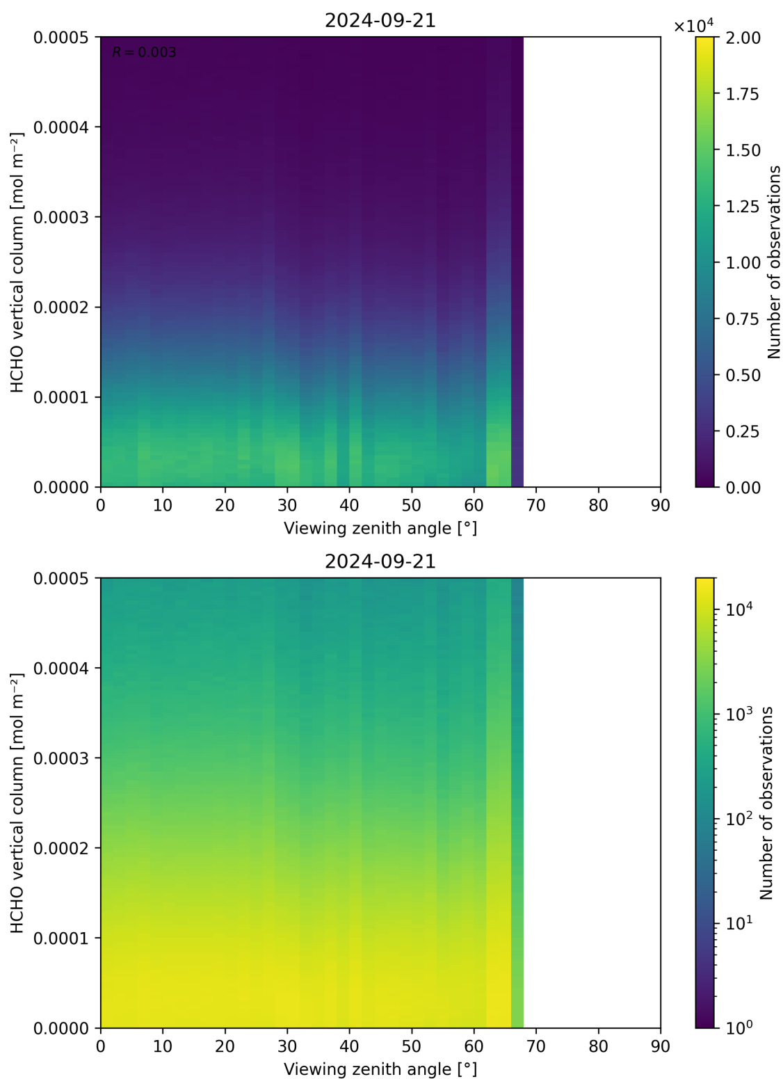
Figure 192: Scatter density plot of “Viewing zenith angle” against “HCHO vertical column” for 2024-09-20 to 2024-09-22.
