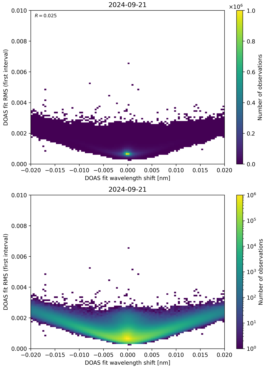
Figure 64: Scatter density plot of “DOAS fit wavelength shift” against “DOAS fit RMS (first interval)” for 2024-09-20 to 2024-09-22.
