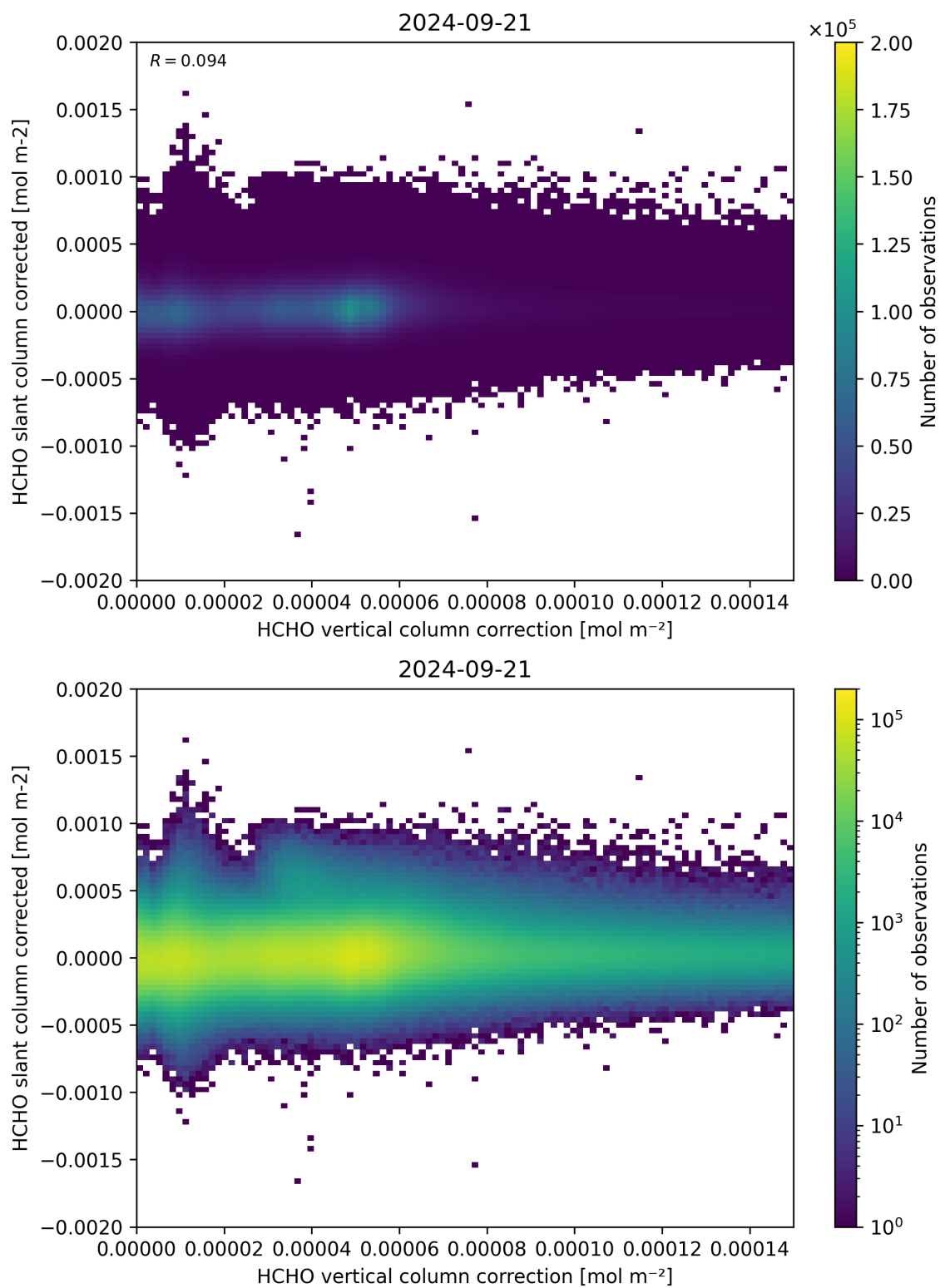
Figure 116: Scatter density plot of “HCHO vertical column correction” against “HCHO slant column corrected” for 2024-09-20 to 2024-09-22.
