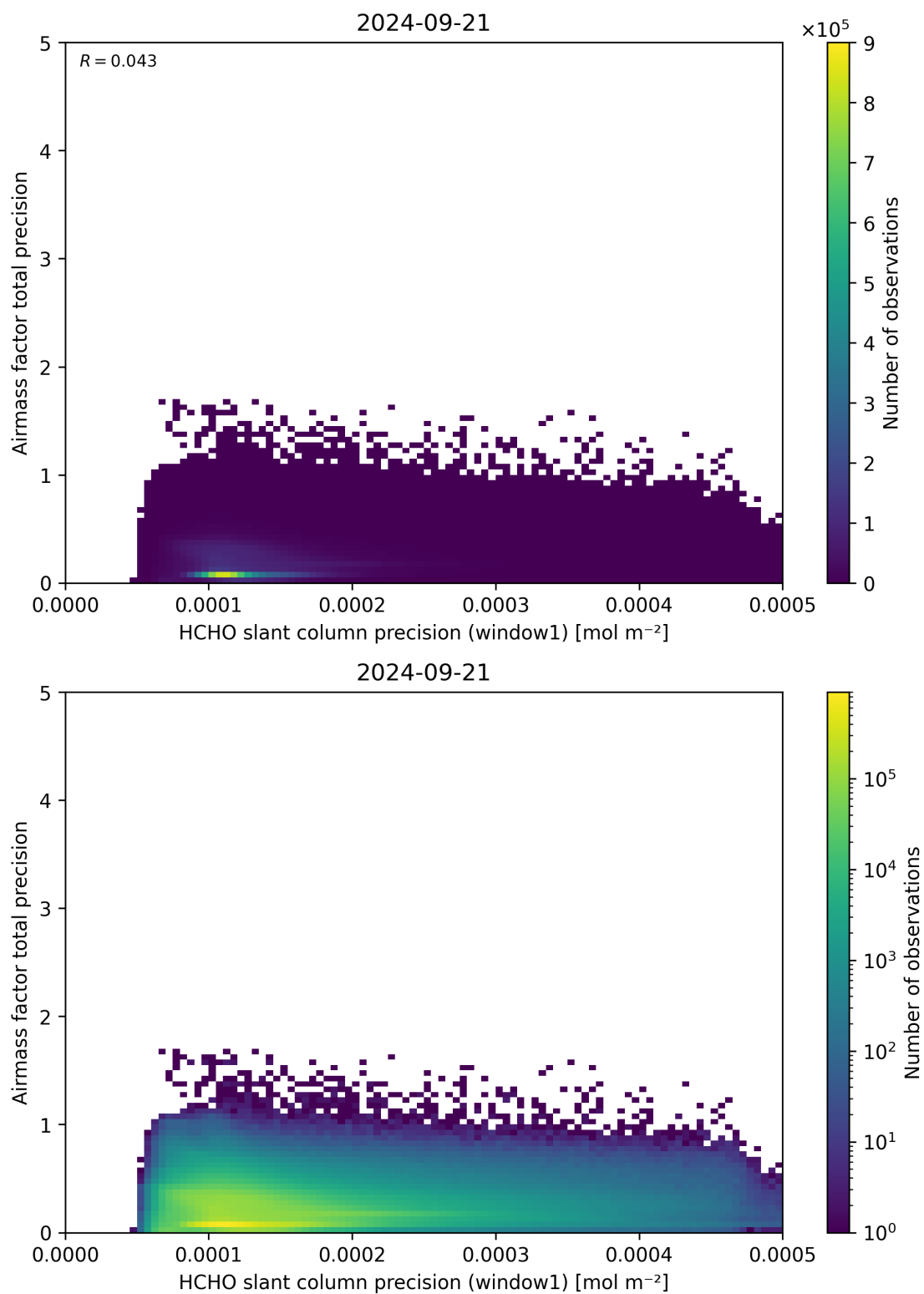
Figure 95: Scatter density plot of “HCHO slant column precision (window1)” against “Airmass factor total precision” for 2024-09-20 to 2024-09-22.
