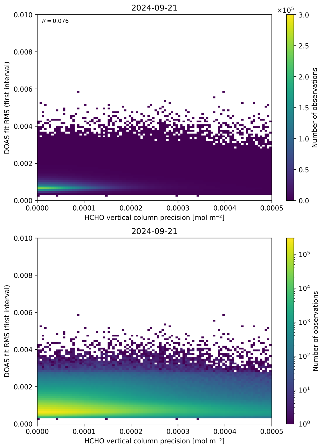
Figure 136: Scatter density plot of “HCHO vertical column precision” against “DOAS fit RMS (first interval)” for 2024-09-20 to 2024-09-22.
