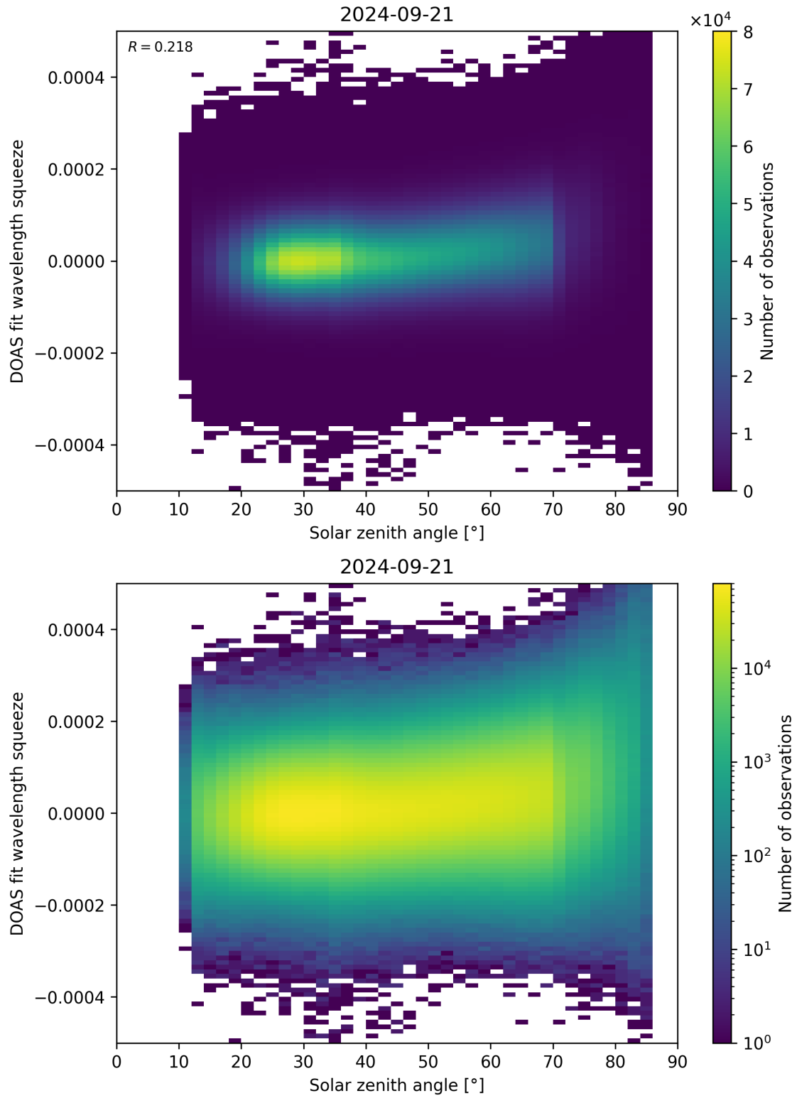
Figure 169: Scatter density plot of “Solar zenith angle” against “DOAS fit wavelength squeeze” for 2024-09-20 to 2024-09-22.
