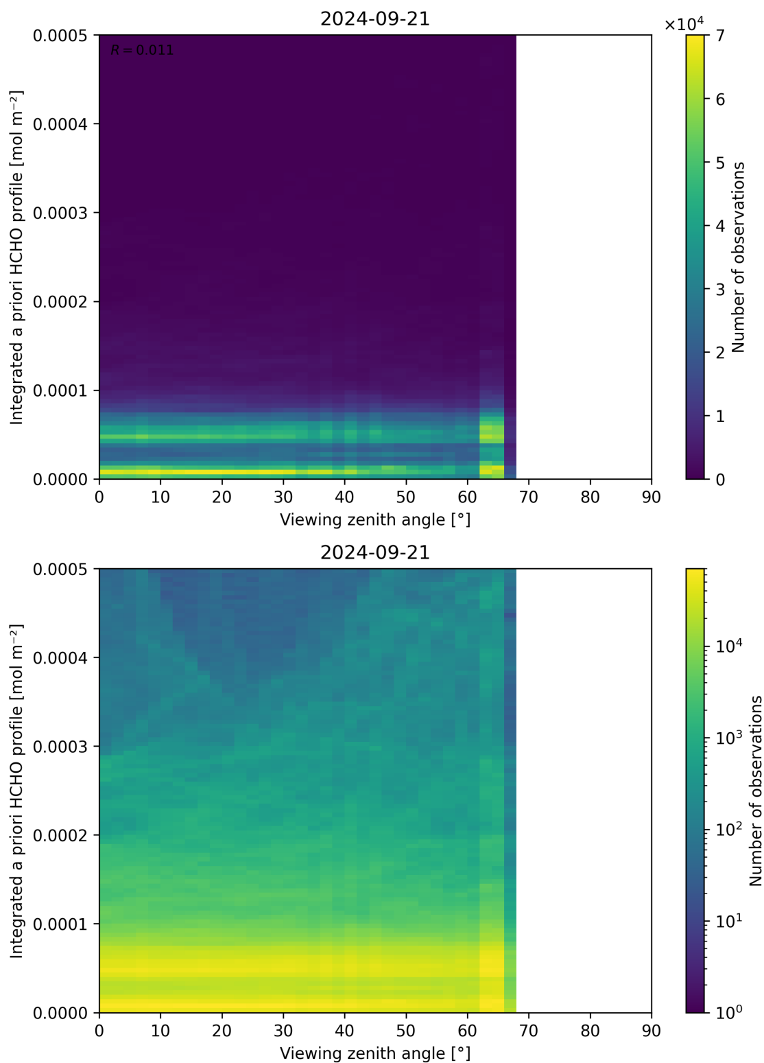
Figure 195: Scatter density plot of “Viewing zenith angle” against “Integrated a priori HCHO profile” for 2024-09-20 to 2024-09-22.
