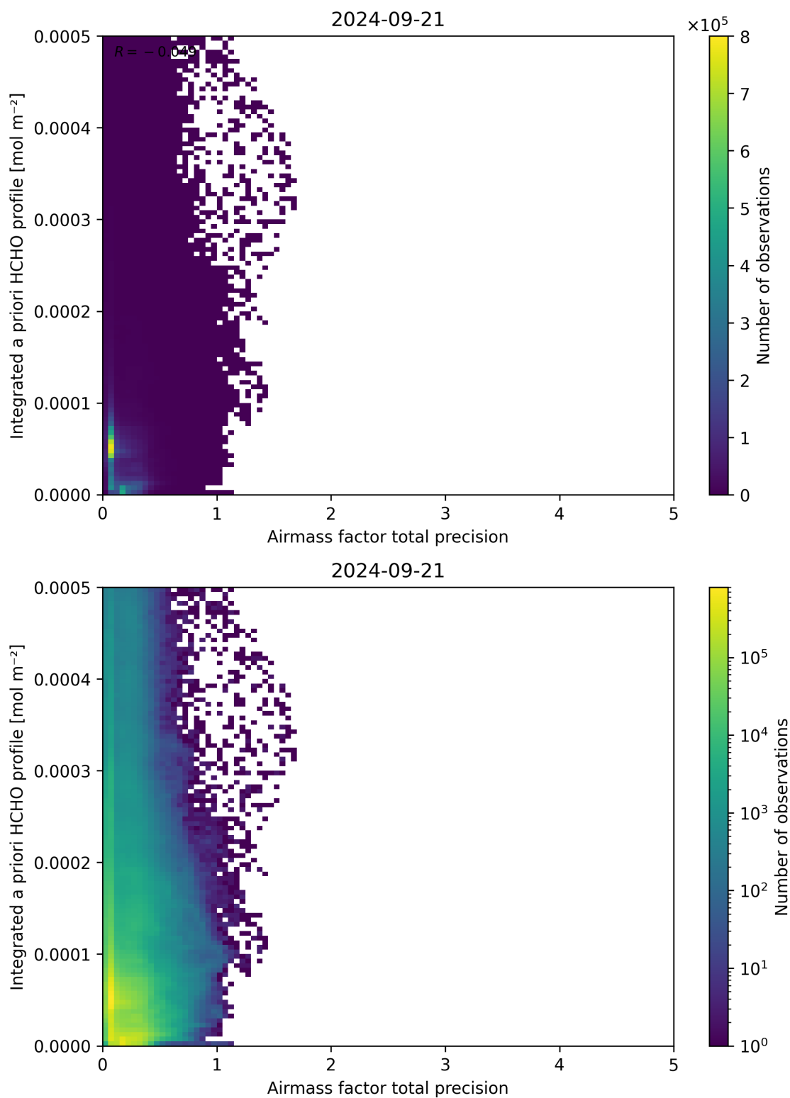
Figure 111: Scatter density plot of “Airmass factor total precision” against “Integrated a priori HCHO profile” for 2024-09-20 to 2024-09-22.
