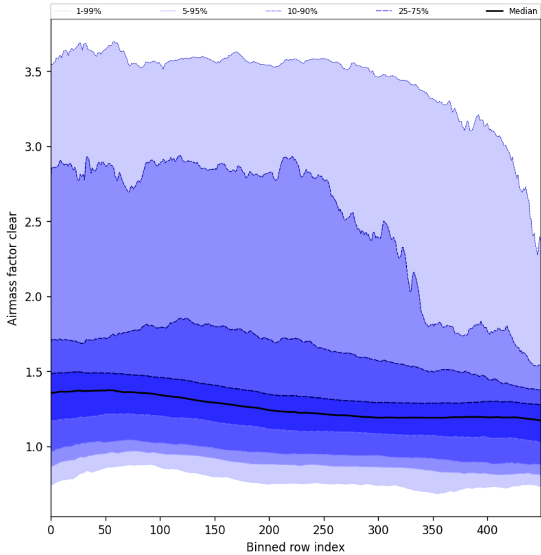
Figure 56: Along track statistics of “Airmass factor clear” for 2024-09-20 to 2024-09-22
