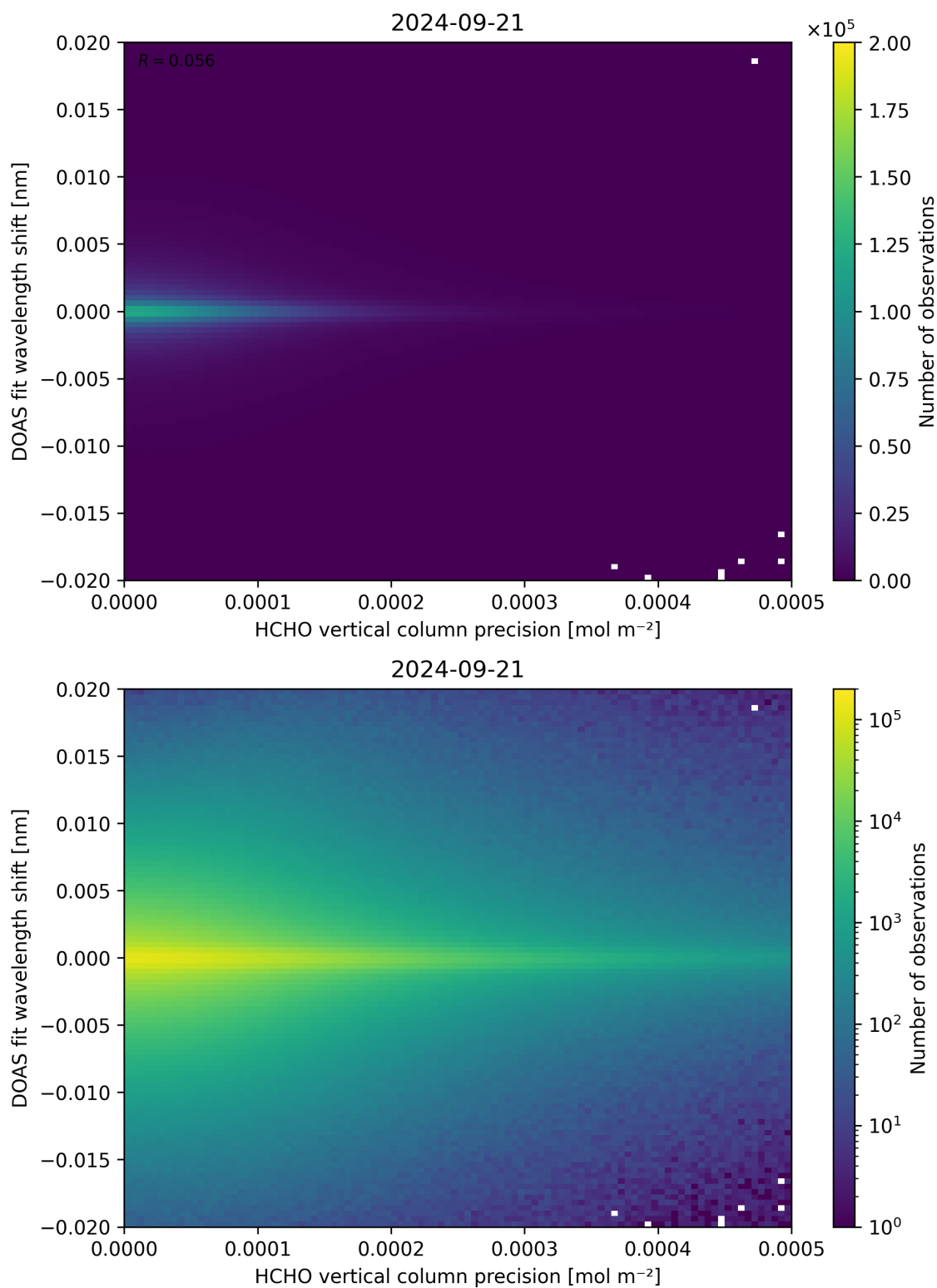
Figure 137: Scatter density plot of “HCHO vertical column precision” against “DOAS fit wavelength shift” for 2024-09-20 to 2024-09-22.
