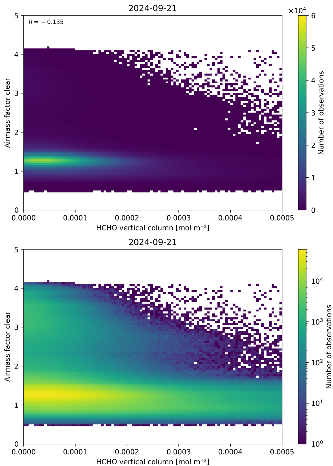
Figure 126: Scatter density plot of “HCHO vertical column” against “Airmass factor clear” for 2024-09-20 to 2024-09-22.
