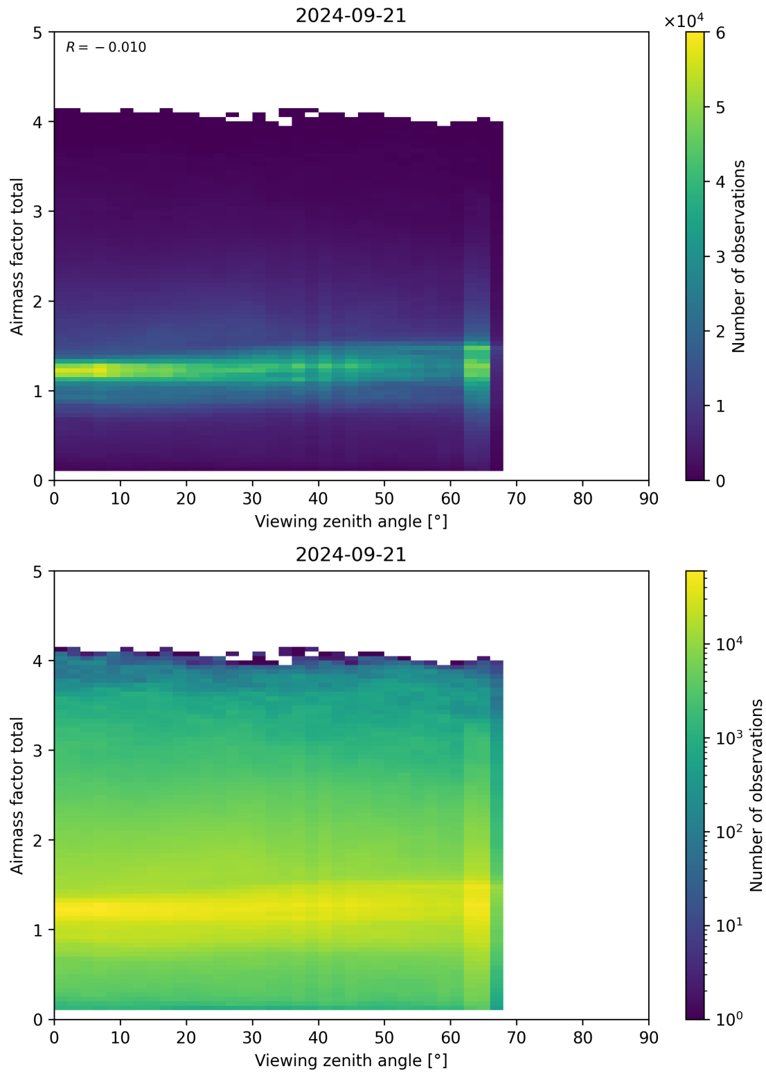
Figure 190: Scatter density plot of “Viewing zenith angle” against “Airmass factor total” for 2024-09-20 to 2024-09-22.
