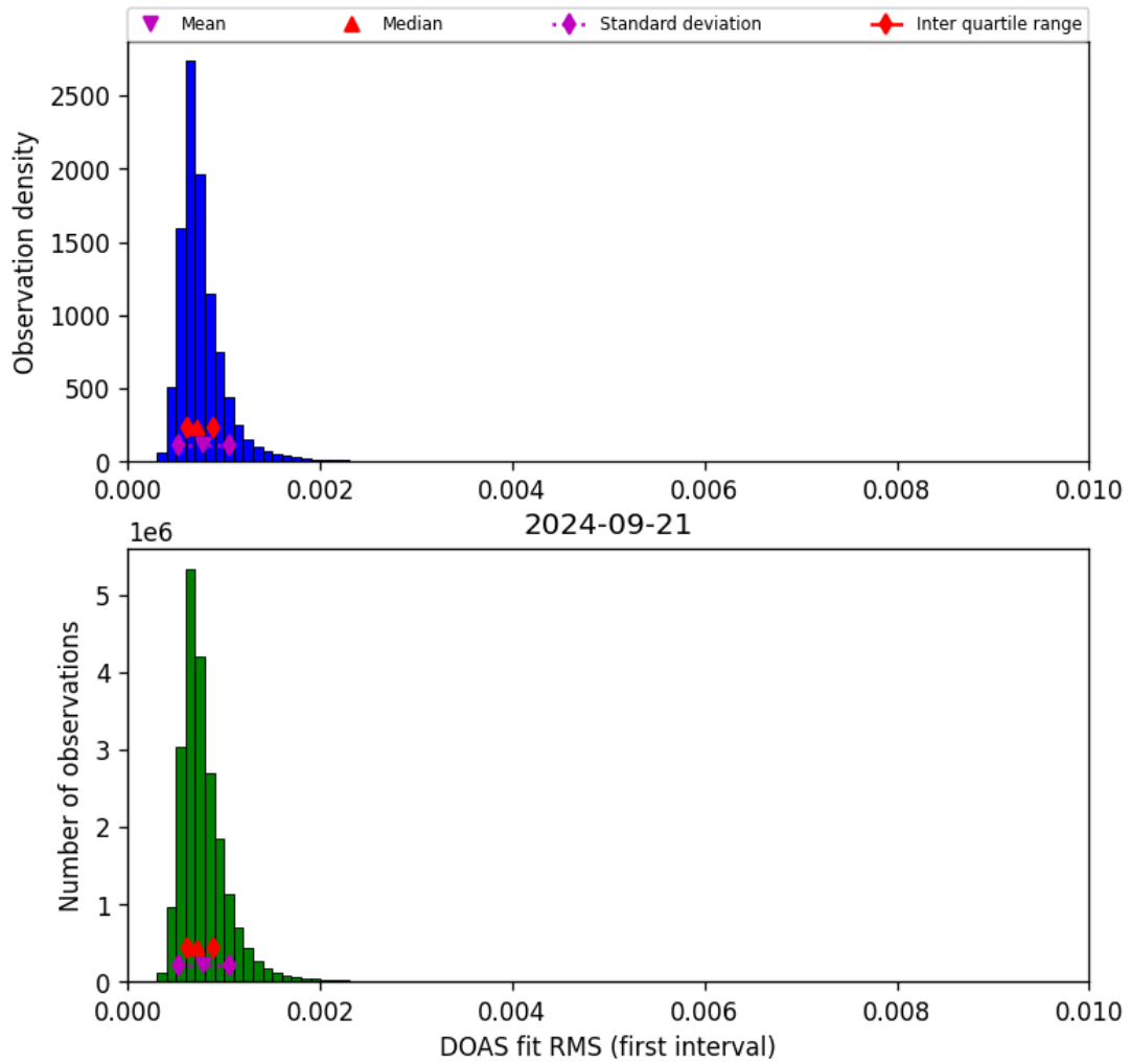
Figure 46: Histogram of “DOAS fit RMS (first interval)” for 2024-09-20 to 2024-09-22
