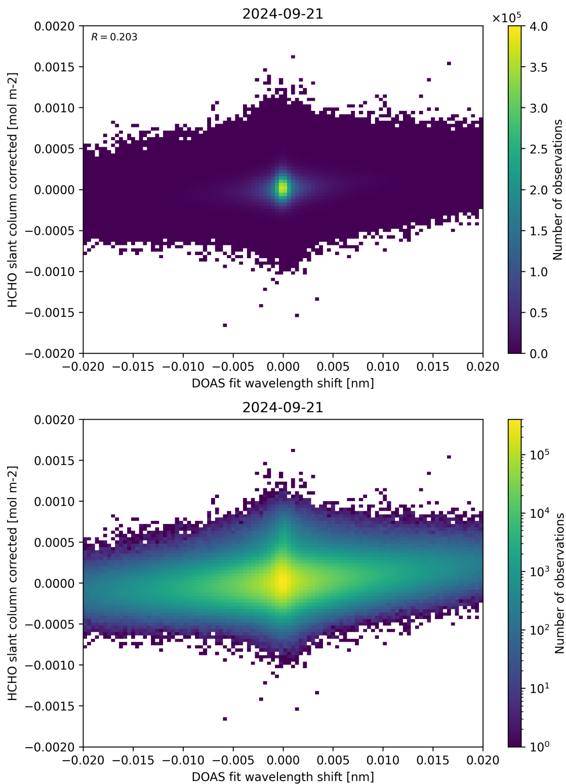
Figure 66: Scatter density plot of “DOAS fit wavelength shift” against “HCHO slant column corrected” for 2024-09-20 to 2024-09-22.
