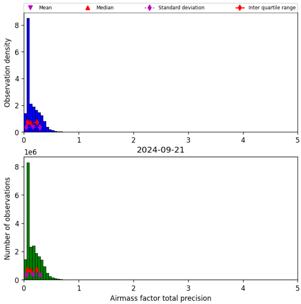
Figure 41: Histogram of “Airmass factor total precision” for 2024-09-20 to 2024-09-22
