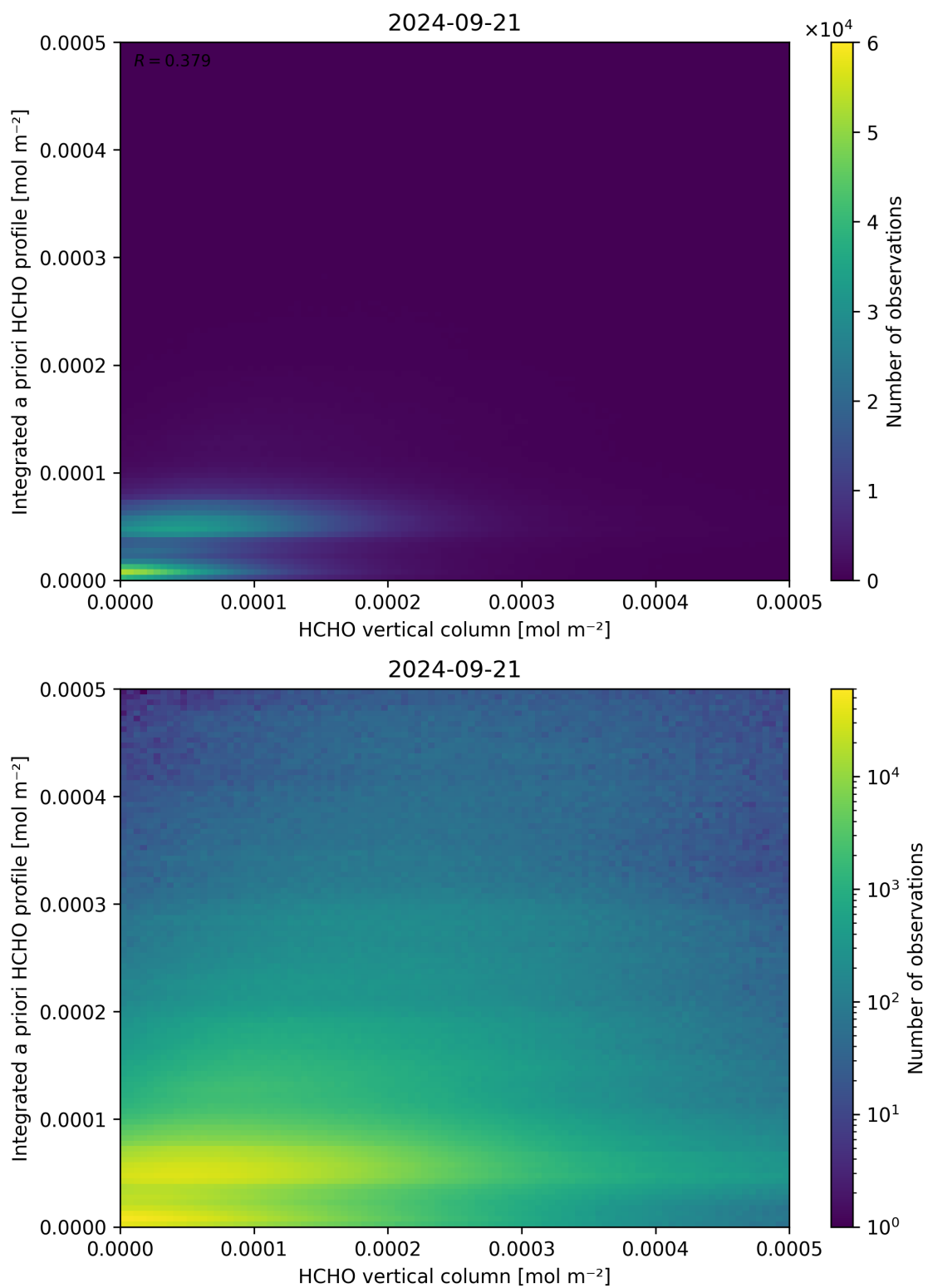
Figure 135: Scatter density plot of “HCHO vertical column” against “Integrated a priori HCHO profile” for 2024-09-20 to 2024-09-22.
