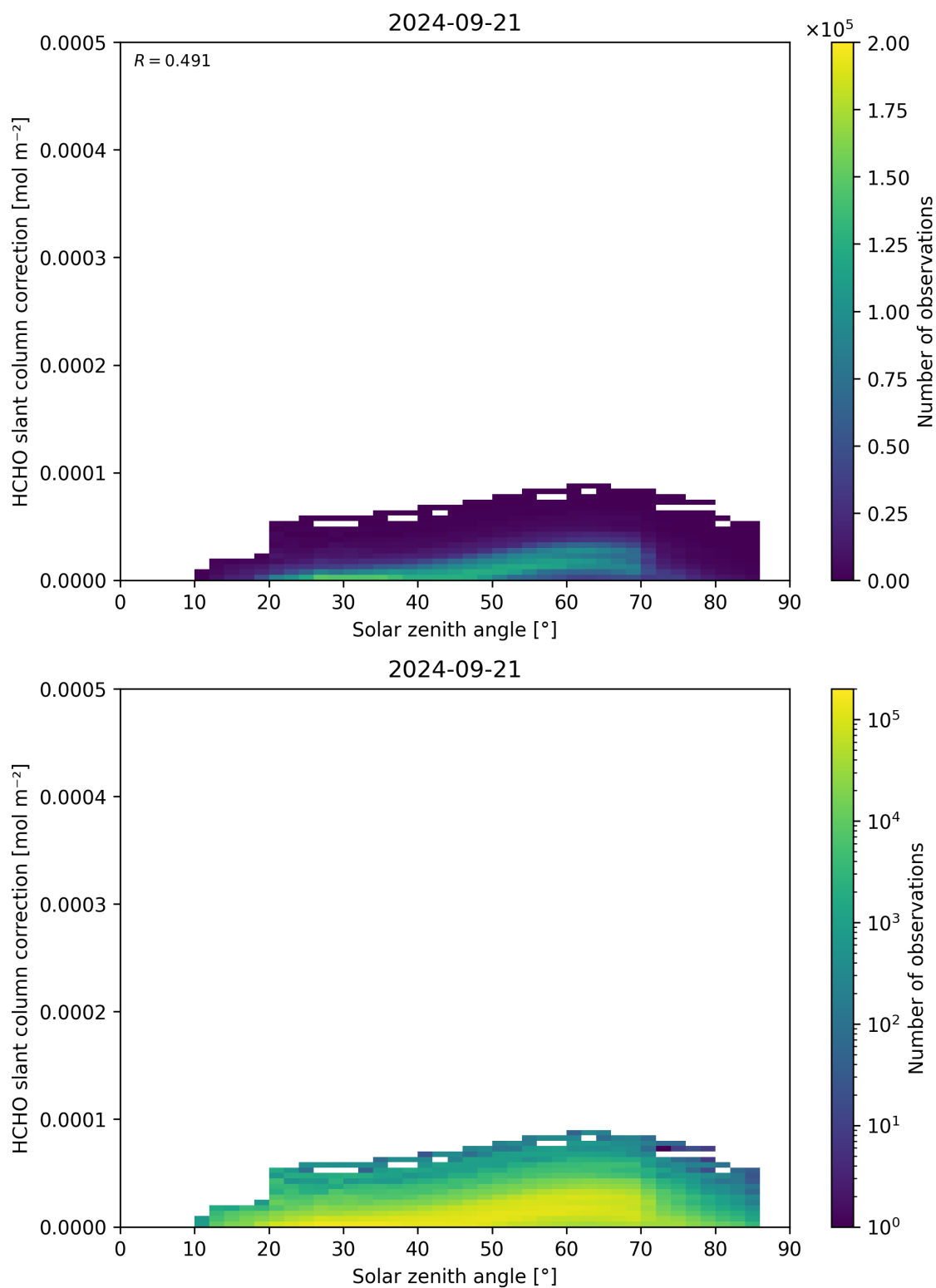
Figure 172: Scatter density plot of “Solar zenith angle” against “HCHO slant column correction” for 2024-09-20 to 2024-09-22.
