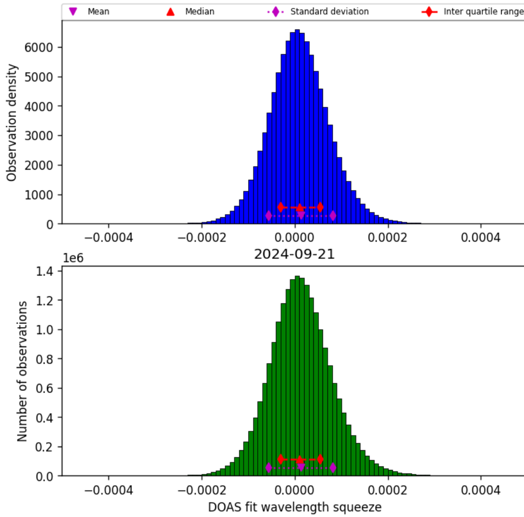
Figure 45: Histogram of “DOAS fit wavelength squeeze” for 2024-09-20 to 2024-09-22
