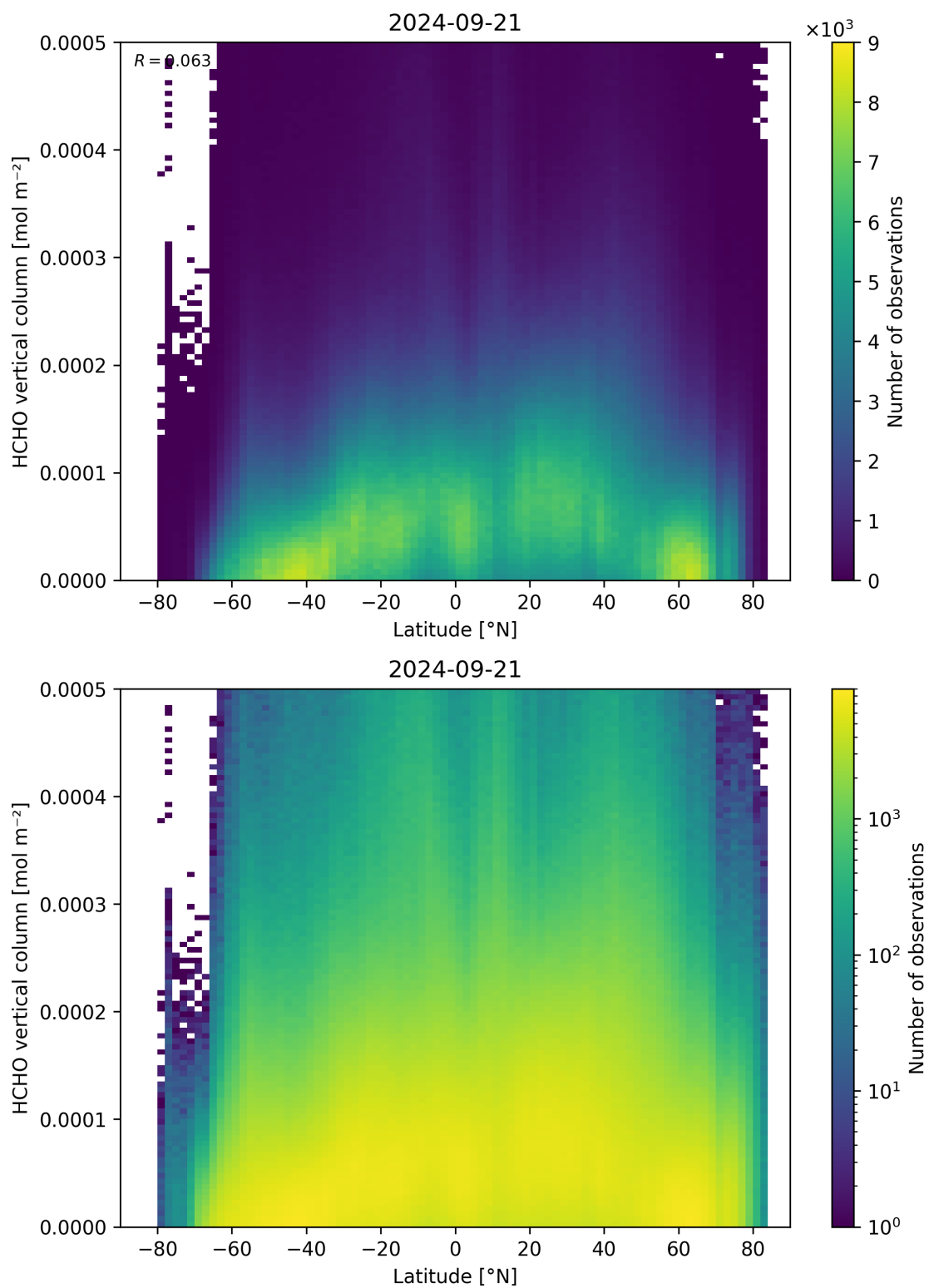
Figure 163: Scatter density plot of “Latitude” against “HCHO vertical column” for 2024-09-20 to 2024-09-22.
