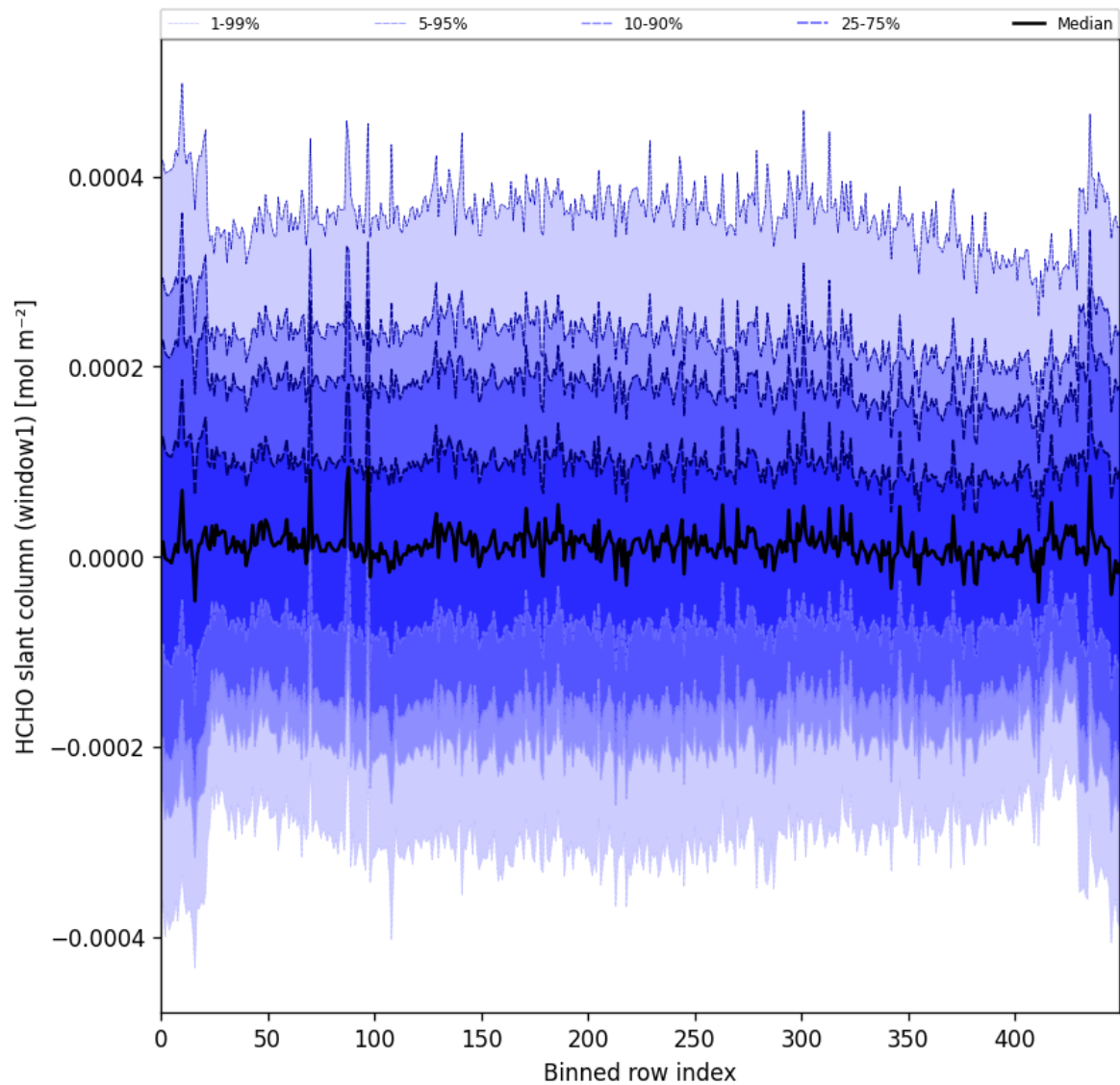
Figure 52: Along track statistics of “HCHO slant column (window1)” for 2024-09-20 to 2024-09-22
