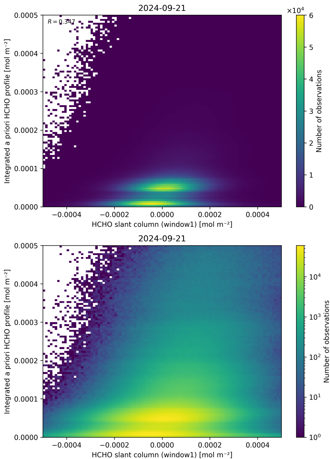
Figure 87: Scatter density plot of “HCHO slant column (window1)” against “Integrated a priori HCHO profile” for 2024-09-20 to 2024-09-22.
