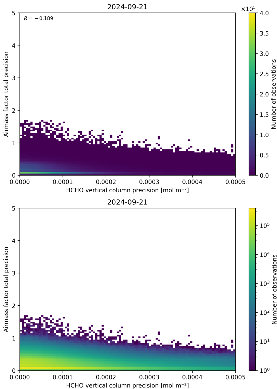
Figure 145: Scatter density plot of “HCHO vertical column precision” against “Airmass factor total precision” for 2024-09-20 to 2024-09-22.
