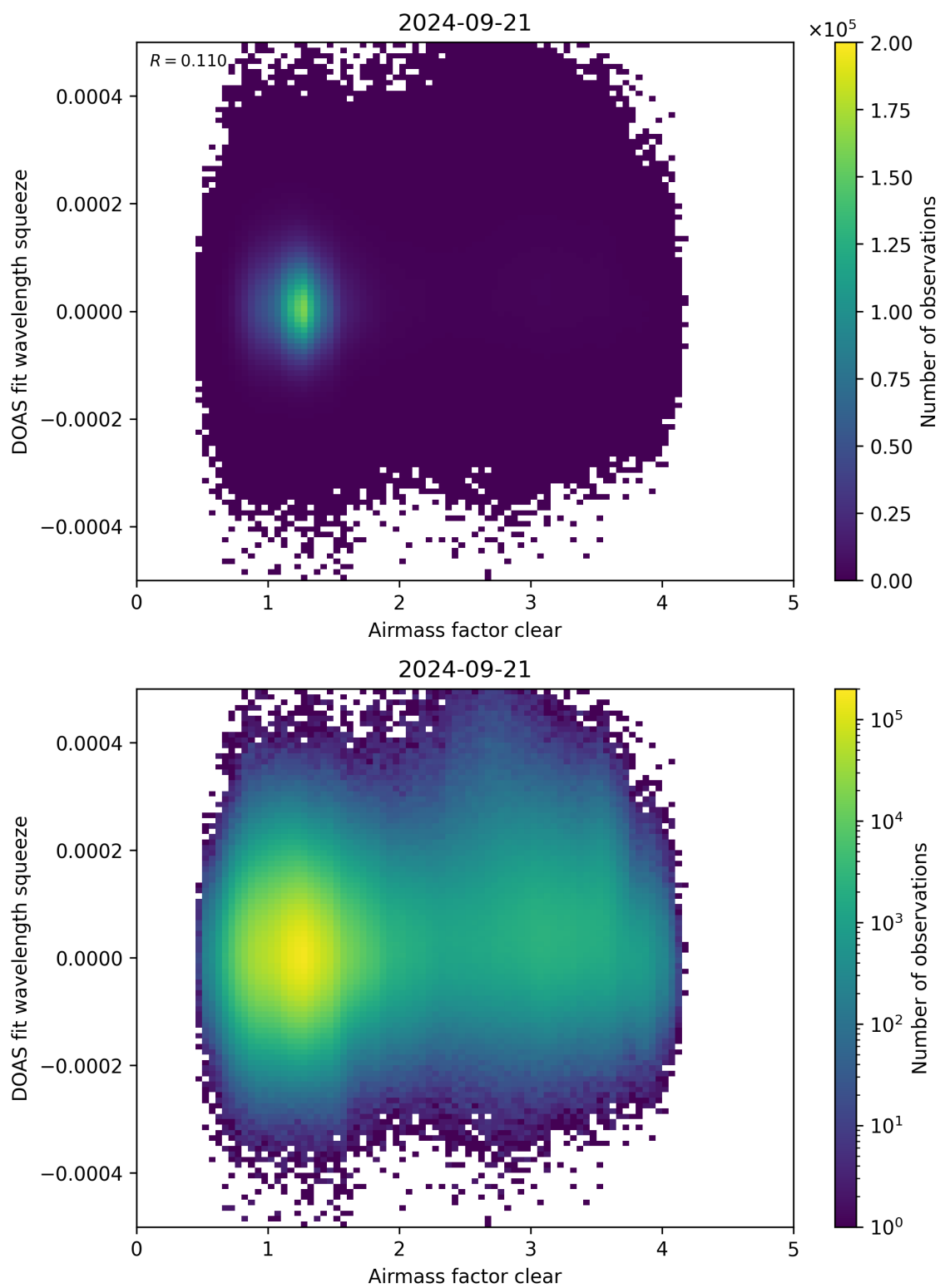
Figure 73: Scatter density plot of “Airmass factor clear” against “DOAS fit wavelength squeeze” for 2024-09-20 to 2024-09-22.
