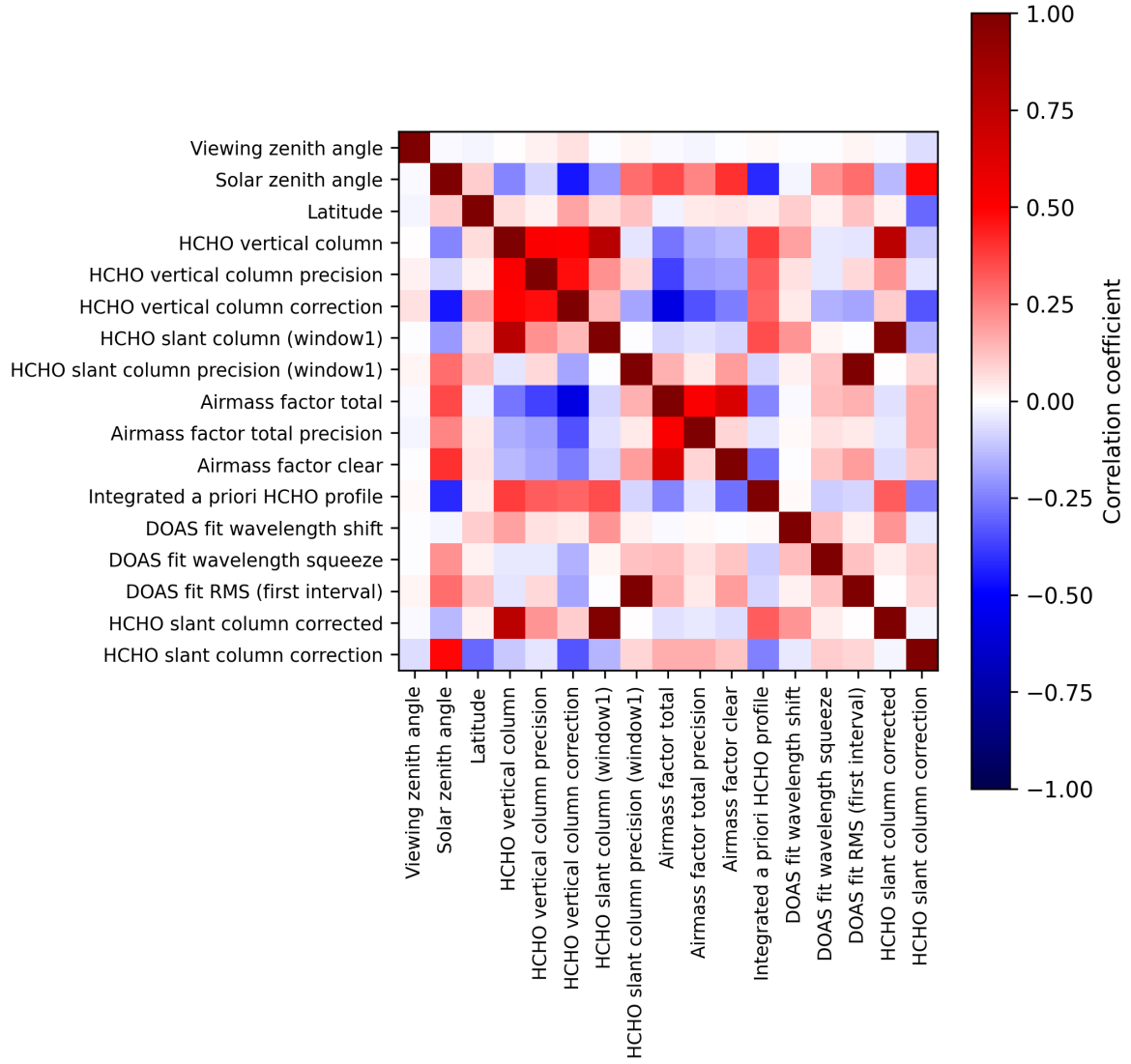
Figure 2: Map of correlation matrix for 2024-09-20 to 2024-09-22.
