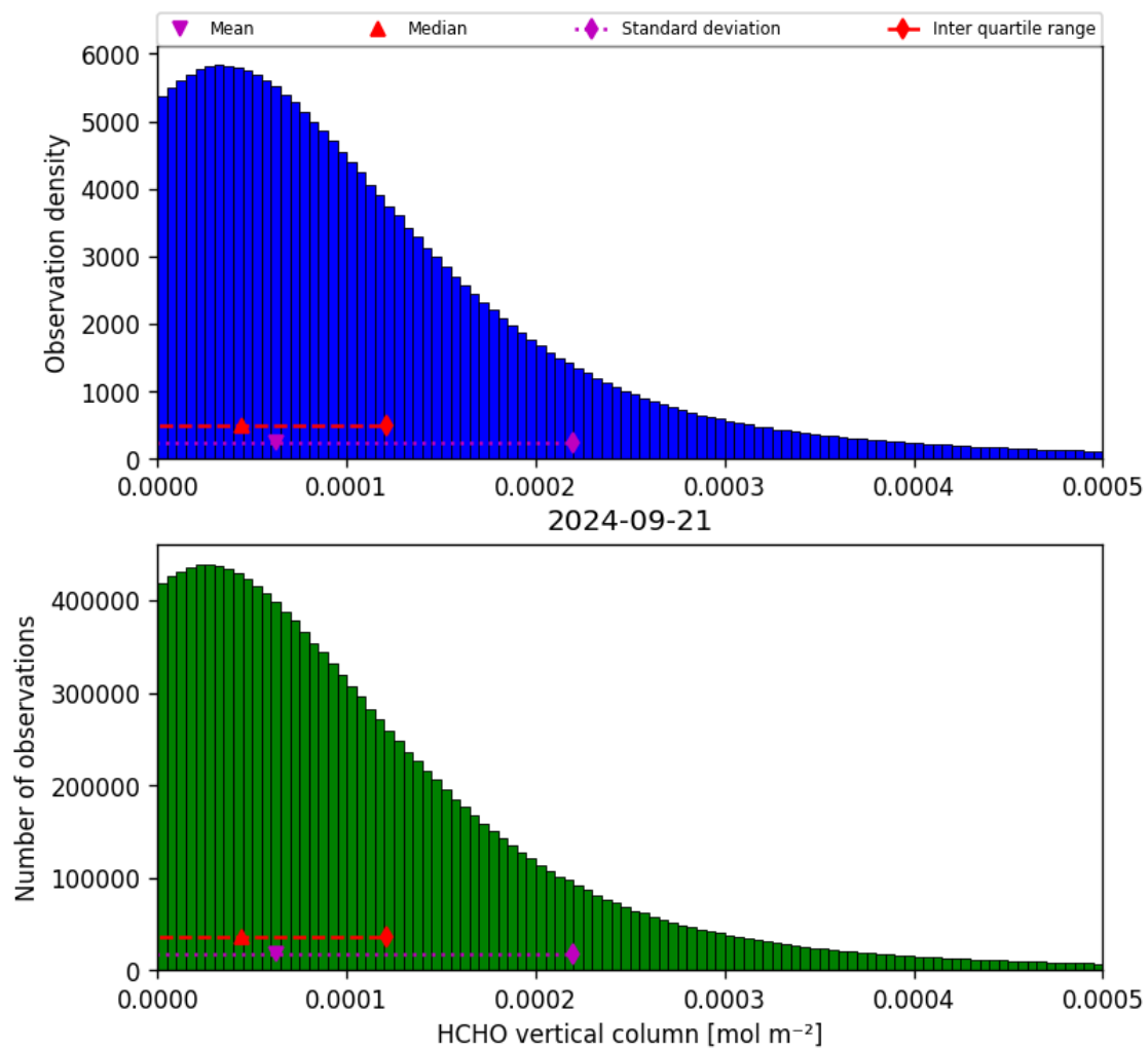
Figure 35: Histogram of “HCHO vertical column” for 2024-09-20 to 2024-09-22
