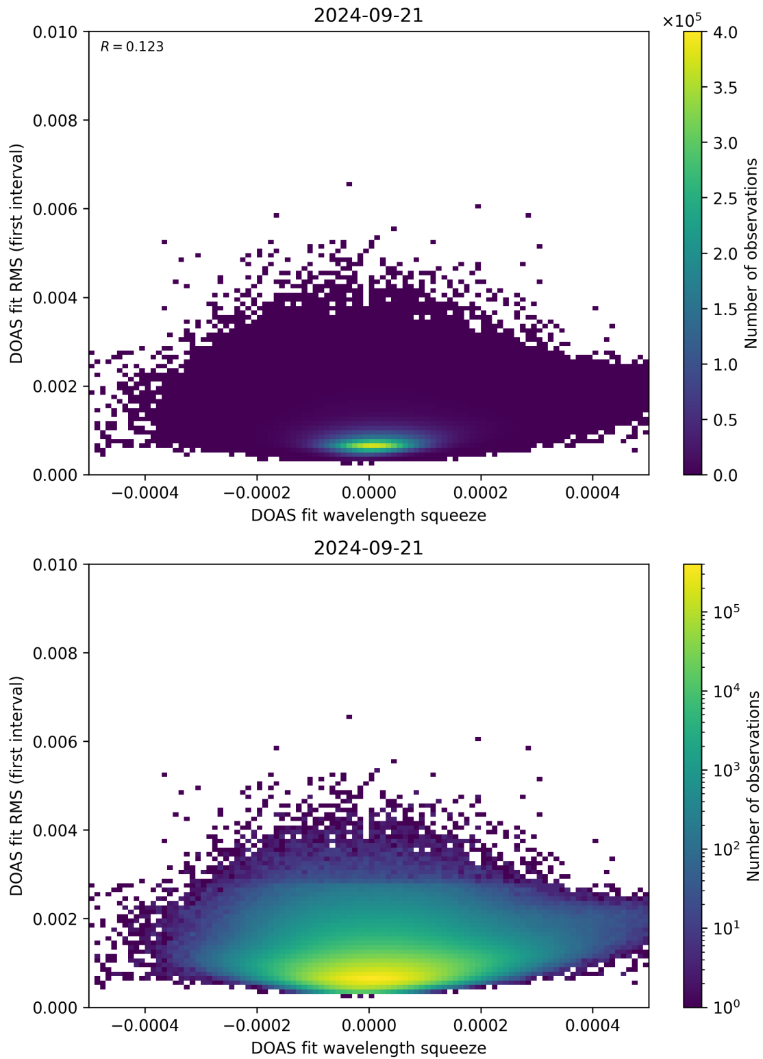
Figure 68: Scatter density plot of “DOAS fit wavelength squeeze” against “DOAS fit RMS (first interval)” for 2024-09-20 to 2024-09-22.
