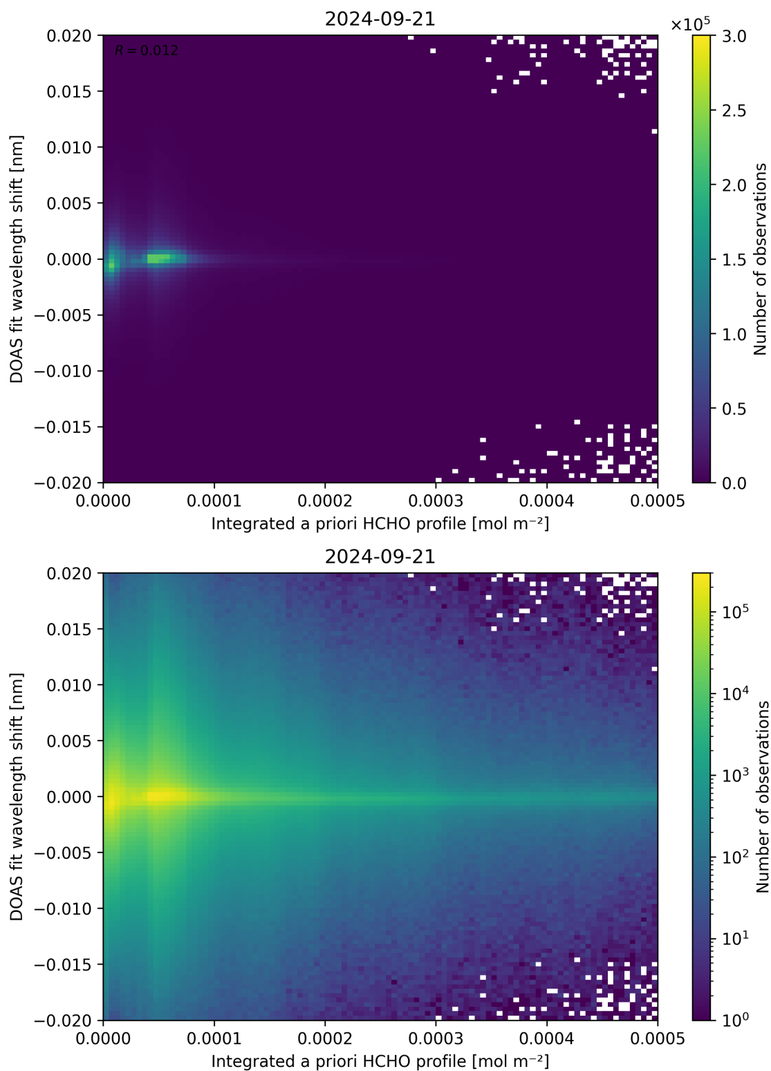
Figure 149: Scatter density plot of “Integrated a priori HCHO profile” against “DOAS fit wavelength shift” for 2024-09-20 to 2024-09-22.
