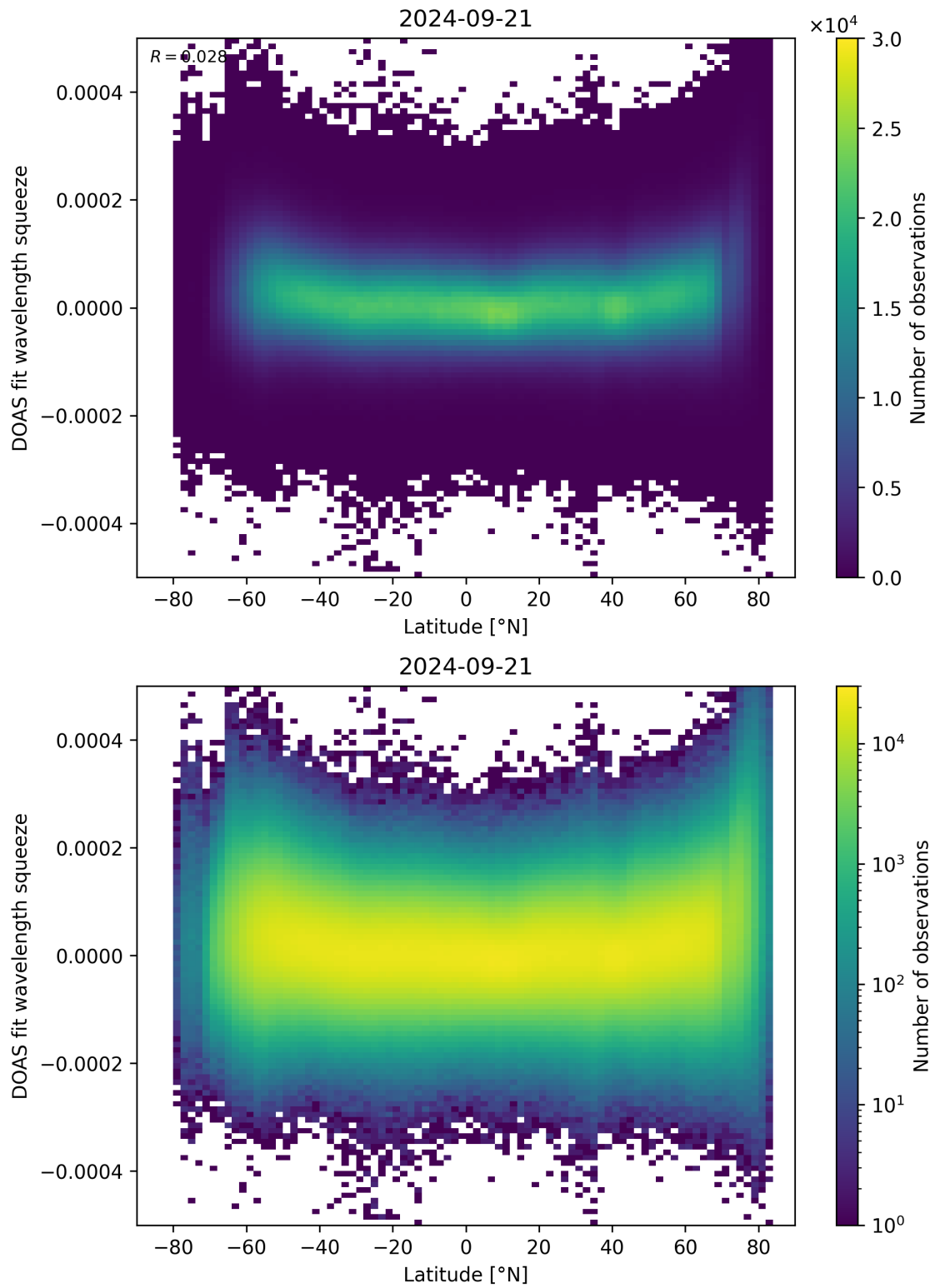
Figure 155: Scatter density plot of “Latitude” against “DOAS fit wavelength squeeze” for 2024-09-20 to 2024-09-22.
