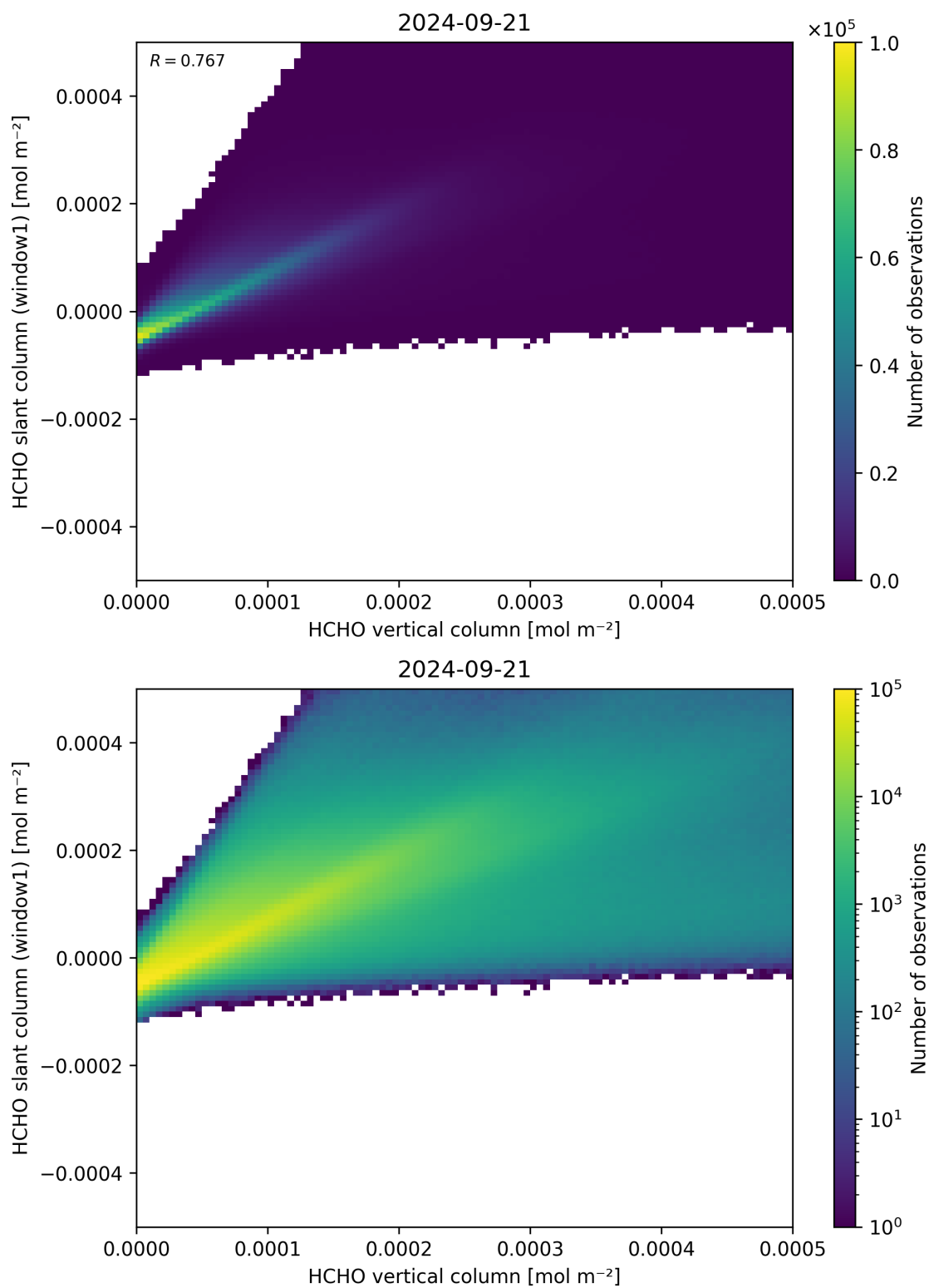
Figure 129: Scatter density plot of “HCHO vertical column” against “HCHO slant column (window1)” for 2024-09-20 to 2024-09-22.
