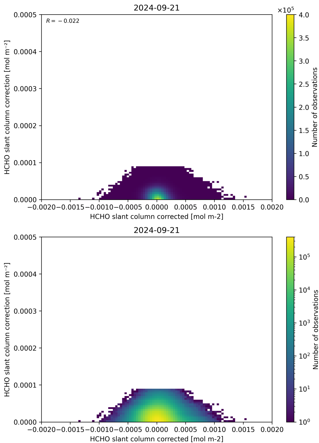
Figure 77: Scatter density plot of “HCHO slant column corrected” against “HCHO slant column correction” for 2024-09-20 to 2024-09-22.
