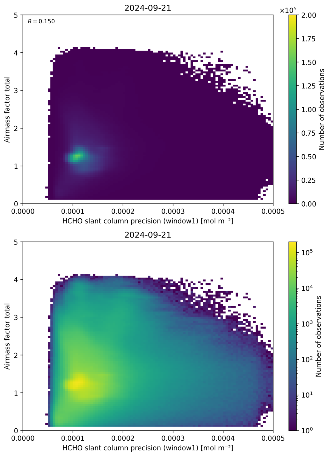
Figure 94: Scatter density plot of “HCHO slant column precision (window1)” against “Airmass factor total” for 2024-09-20 to 2024-09-22.
