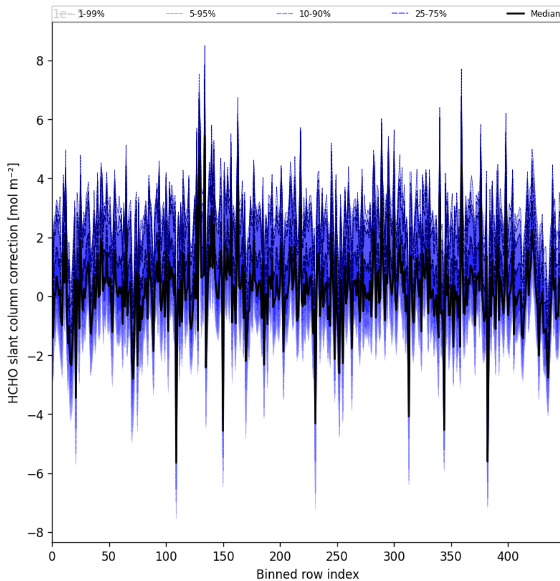
Figure 61: Along track statistics of “HCHO slant column correction” for 2024-09-20 to 2024-09-22
