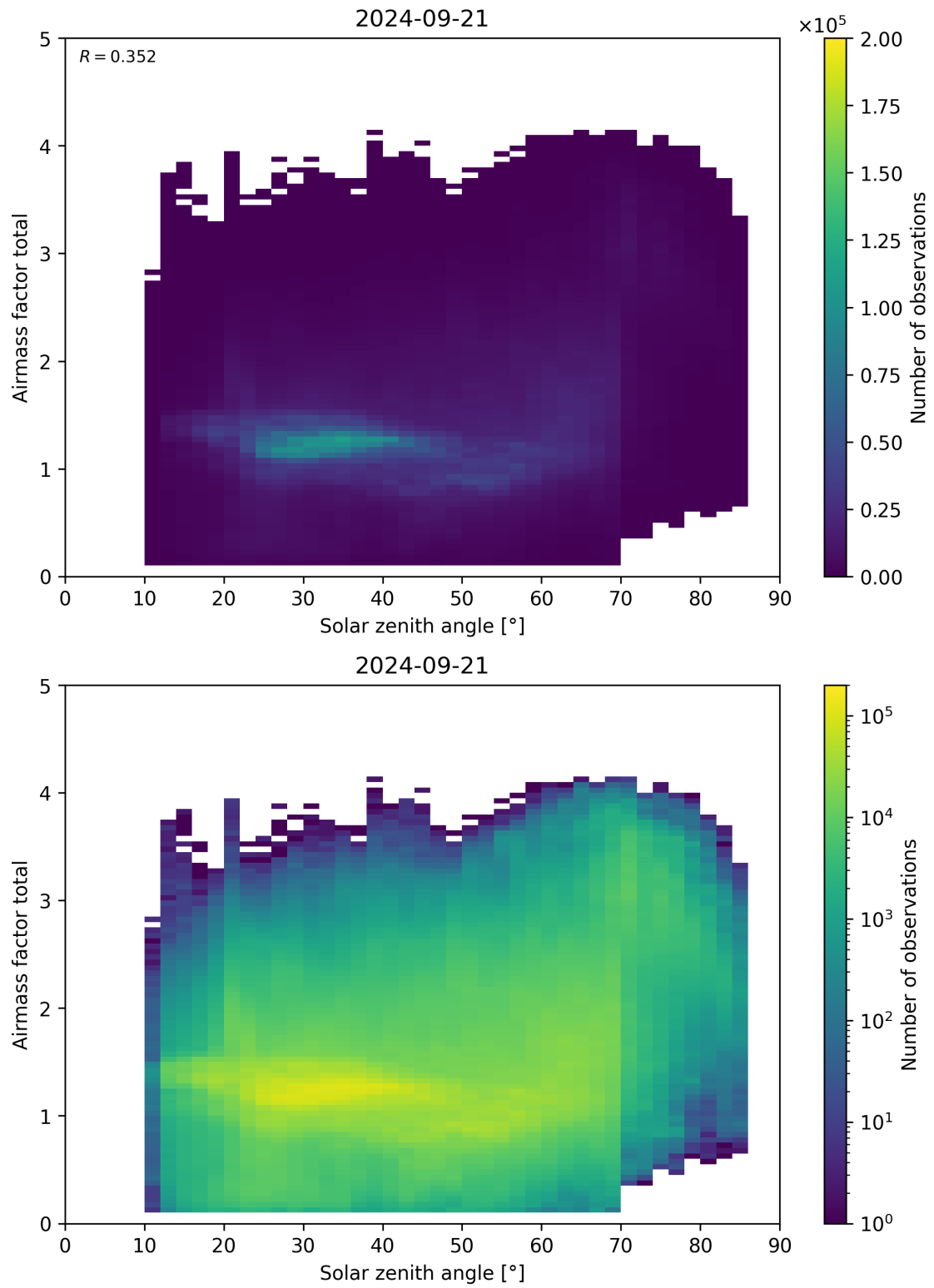
Figure 175: Scatter density plot of “Solar zenith angle” against “Airmass factor total” for 2024-09-20 to 2024-09-22.
