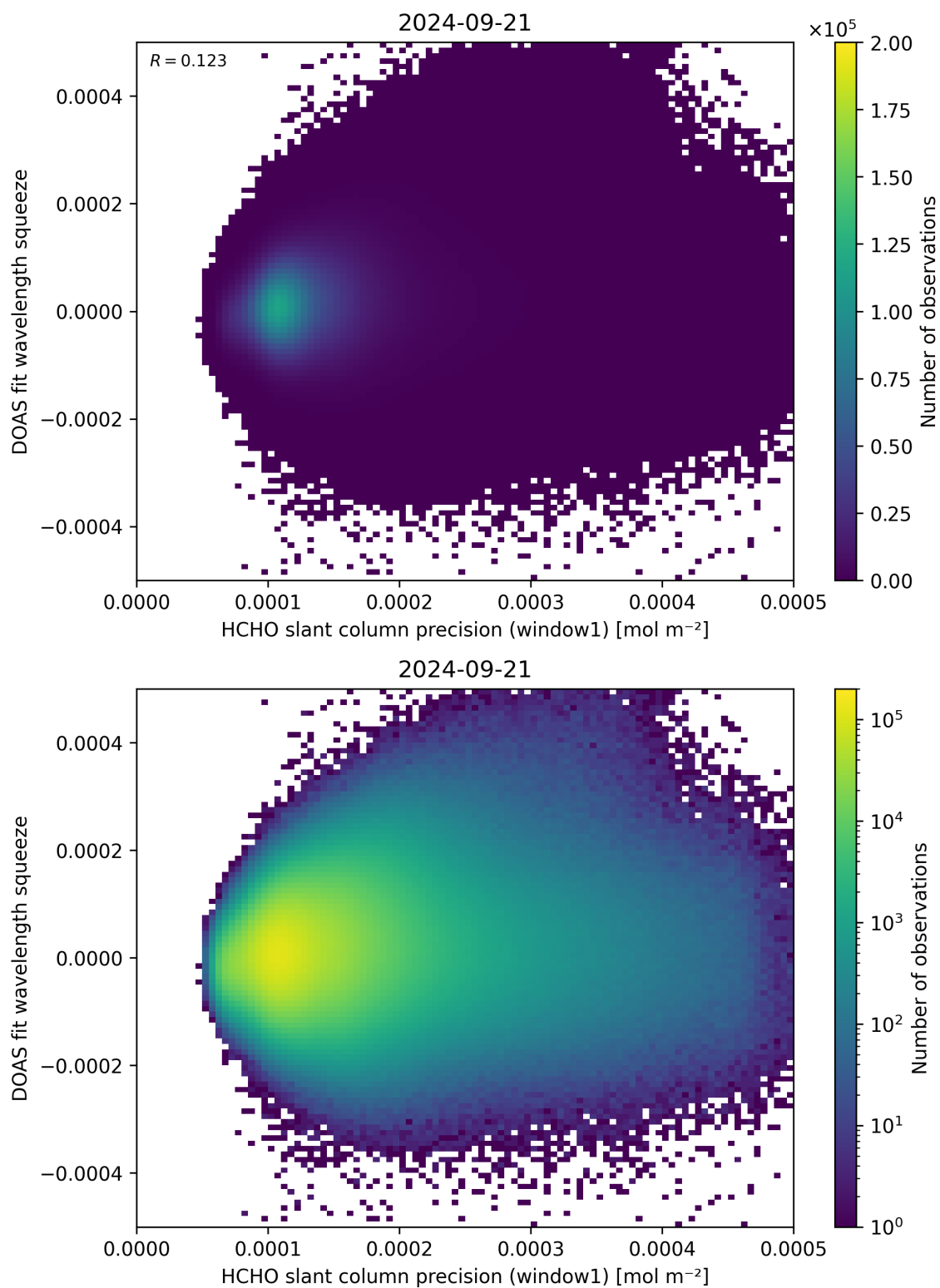
Figure 90: Scatter density plot of “HCHO slant column precision (window1)” against “DOAS fit wavelength squeeze” for 2024-09-20 to 2024-09-22.
