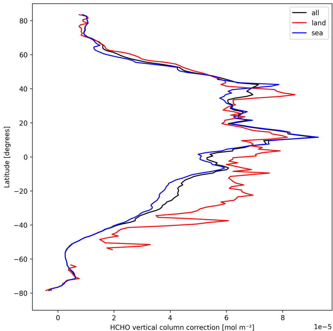
Figure 23: Zonal average of “HCHO vertical column correction” for 2024-09-20 to 2024-09-22.
