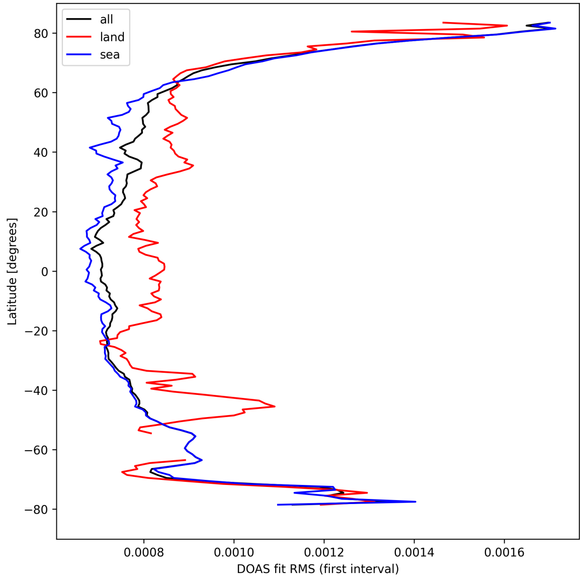
Figure 32: Zonal average of “DOAS fit RMS (first interval)” for 2024-09-20 to 2024-09-22.
