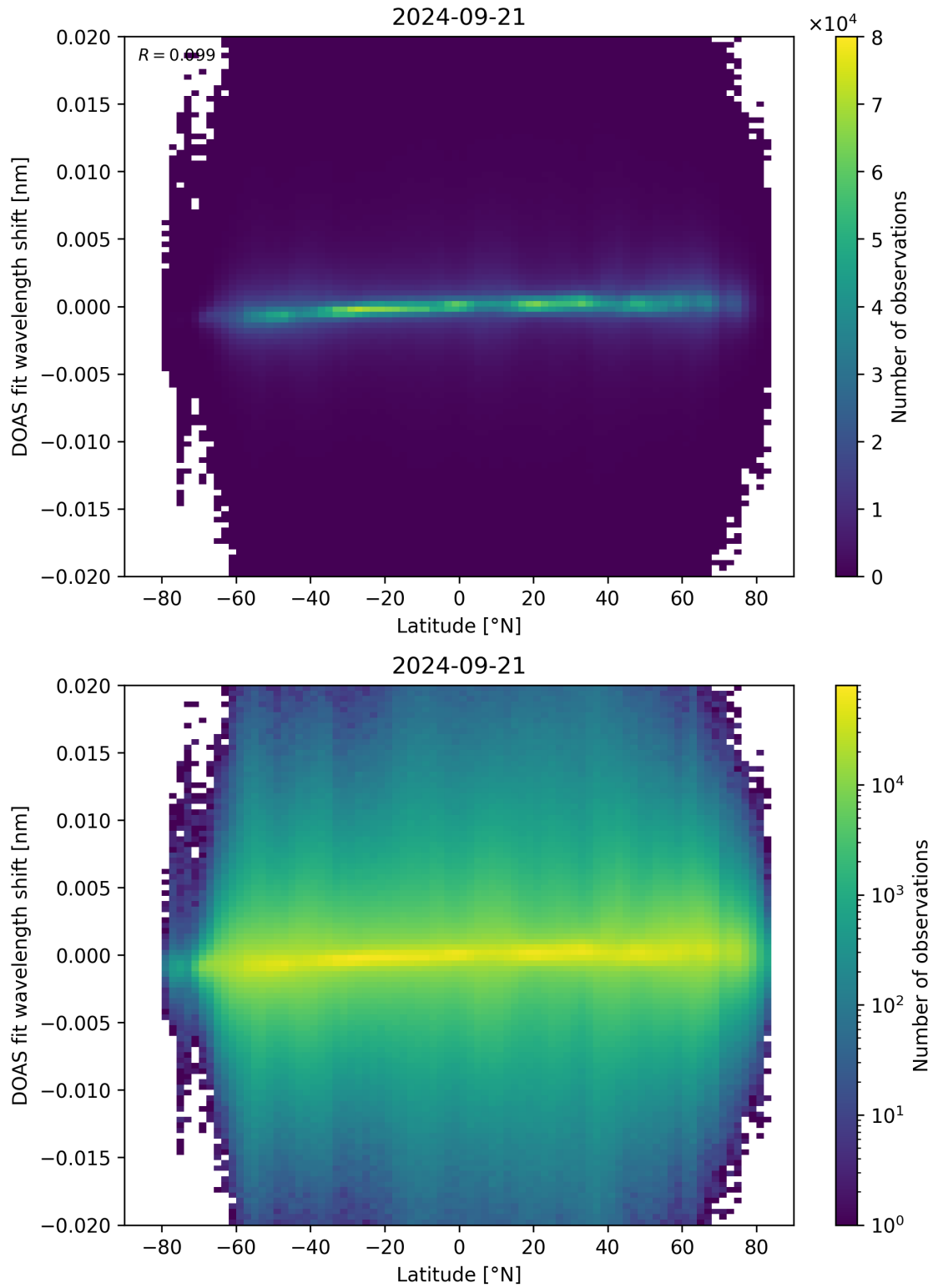
Figure 154: Scatter density plot of “Latitude” against “DOAS fit wavelength shift” for 2024-09-20 to 2024-09-22.
