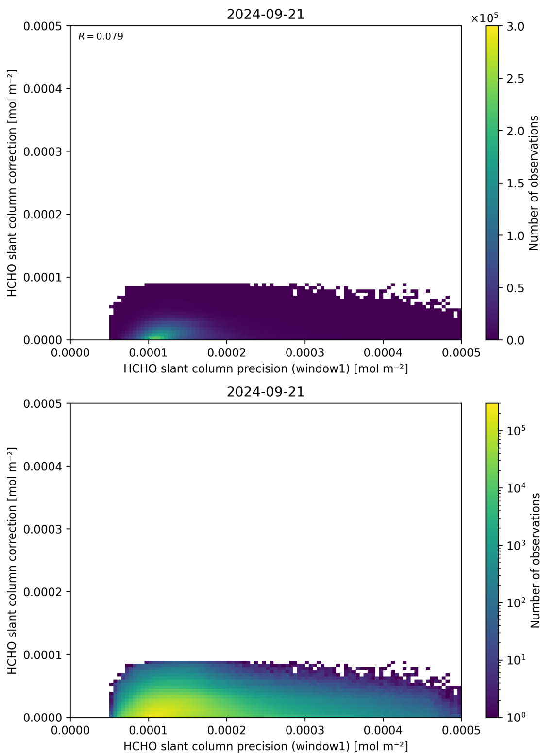
Figure 93: Scatter density plot of “HCHO slant column precision (window1)” against “HCHO slant column correction” for 2024-09-20 to 2024-09-22.
