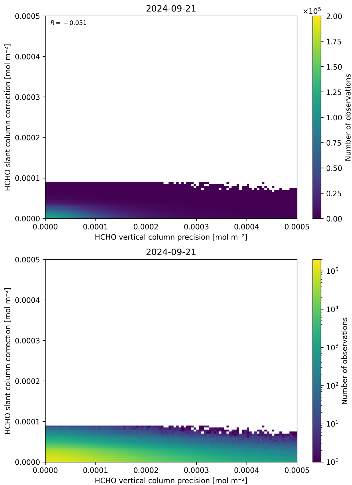
Figure 141: Scatter density plot of “HCHO vertical column precision” against “HCHO slant column correction” for 2024-09-20 to 2024-09-22.
