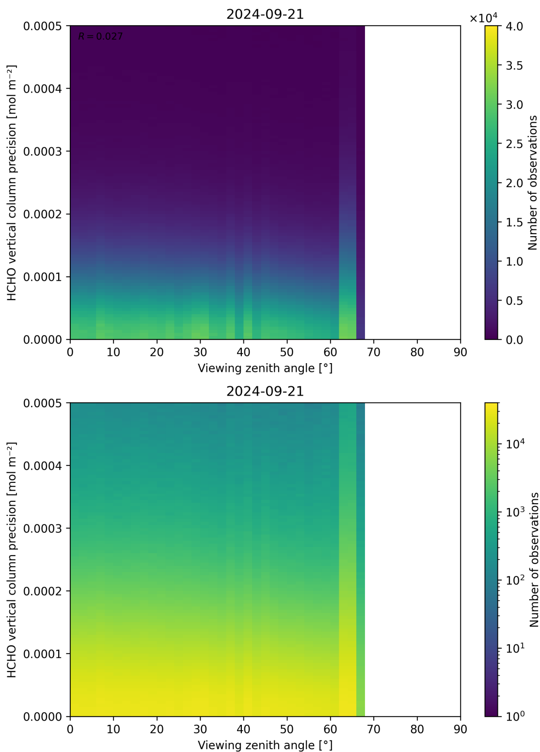
Figure 194: Scatter density plot of “Viewing zenith angle” against “HCHO vertical column precision” for 2024-09-20 to 2024-09-22.
