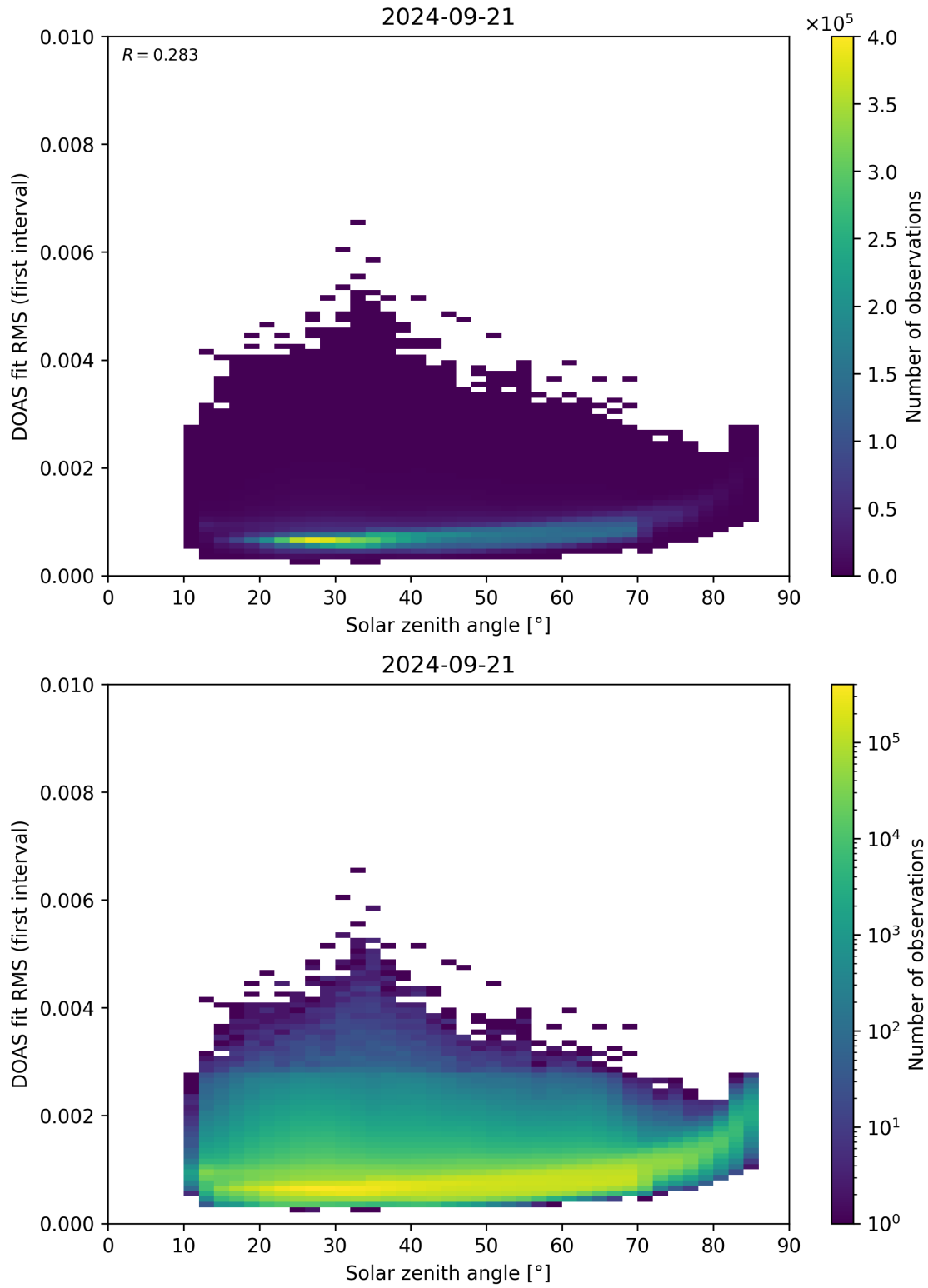
Figure 167: Scatter density plot of “Solar zenith angle” against “DOAS fit RMS (first interval)” for 2024-09-20 to 2024-09-22.
