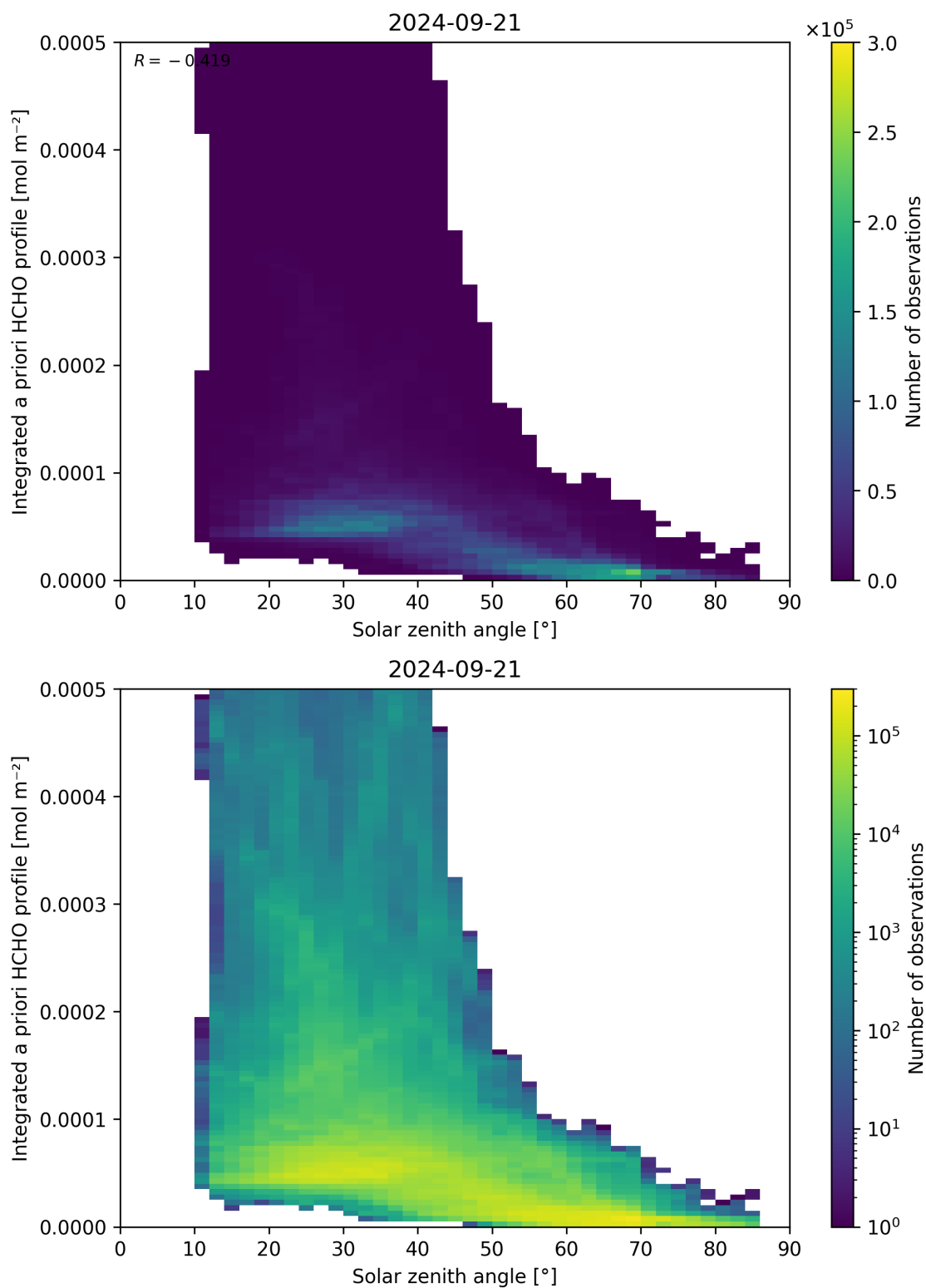
Figure 180: Scatter density plot of “Solar zenith angle” against “Integrated a priori HCHO profile” for 2024-09-20 to 2024-09-22.
