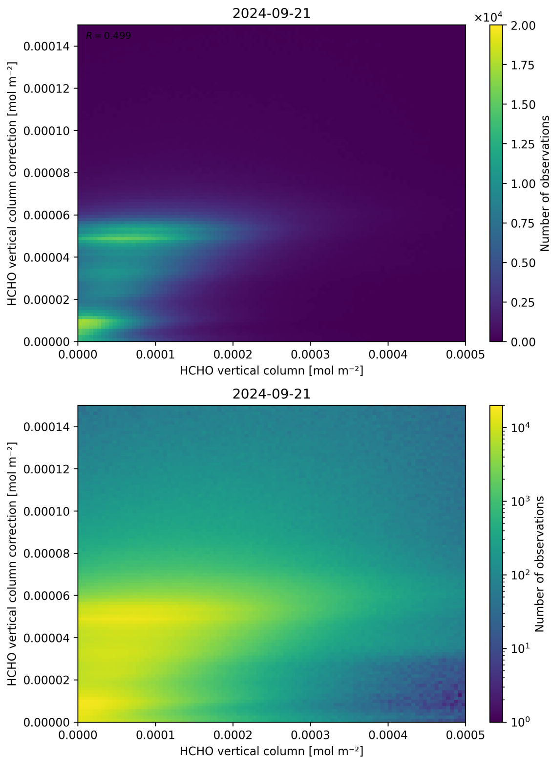
Figure 133: Scatter density plot of “HCHO vertical column” against “HCHO vertical column correction” for 2024-09-20 to 2024-09-22.
