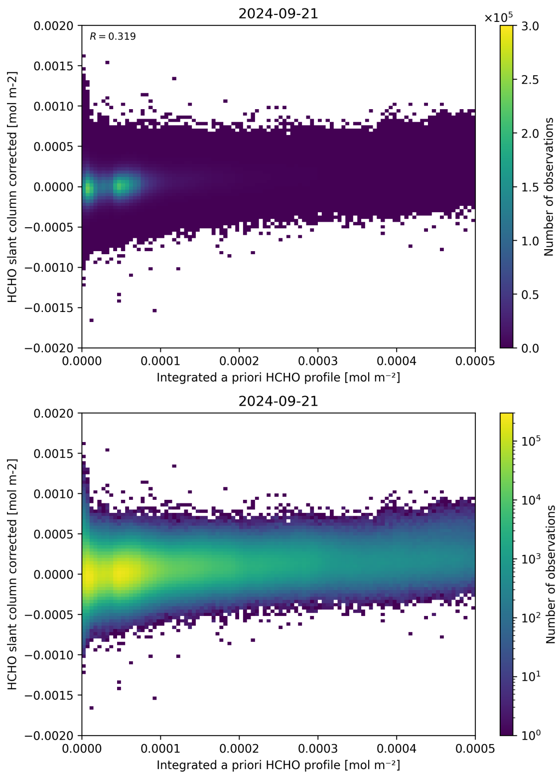
Figure 151: Scatter density plot of “Integrated a priori HCHO profile” against “HCHO slant column corrected” for 2024-09-20 to 2024-09-22.
