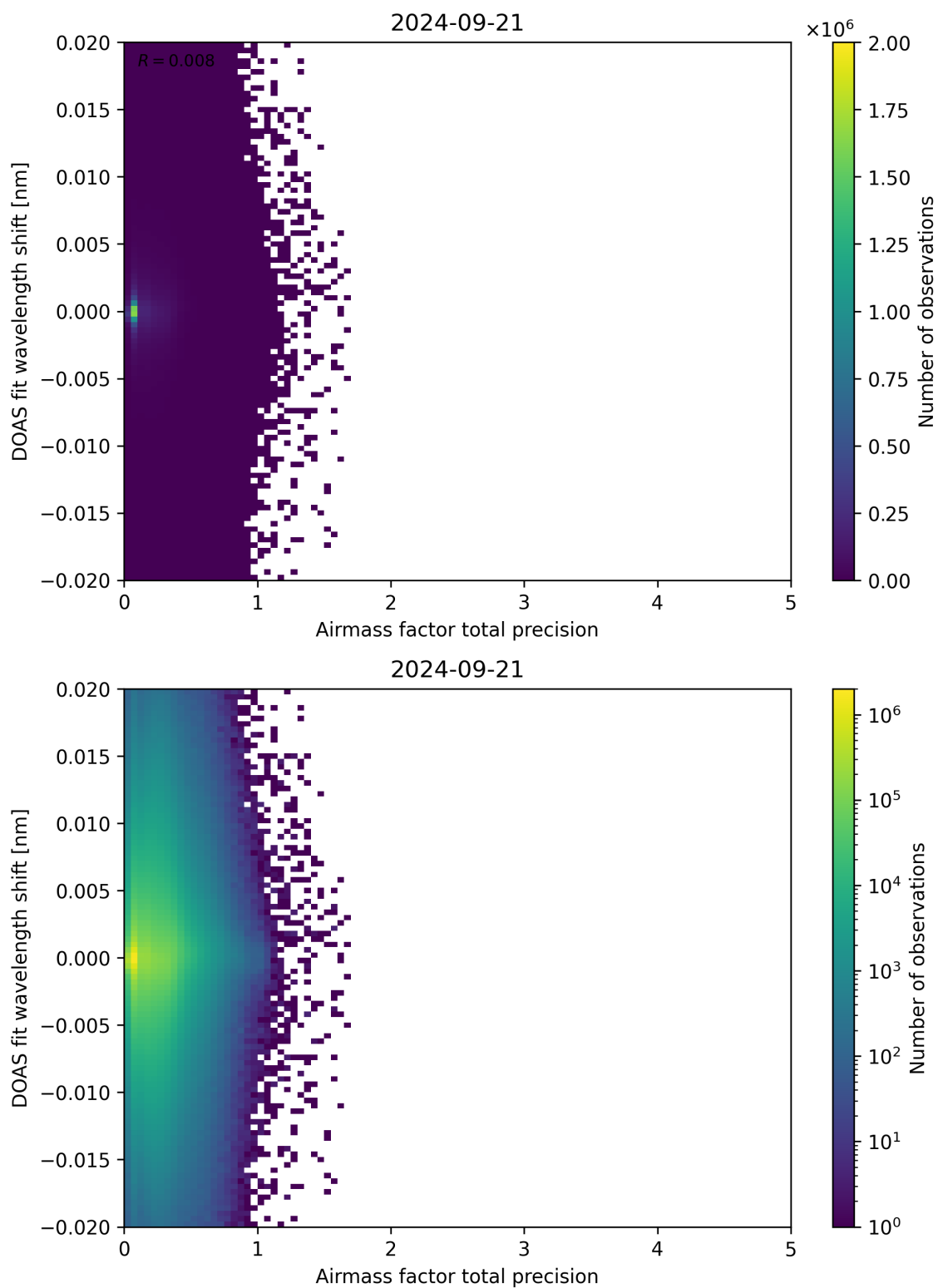
Figure 106: Scatter density plot of “Airmass factor total precision” against “DOAS fit wavelength shift” for 2024-09-20 to 2024-09-22.
