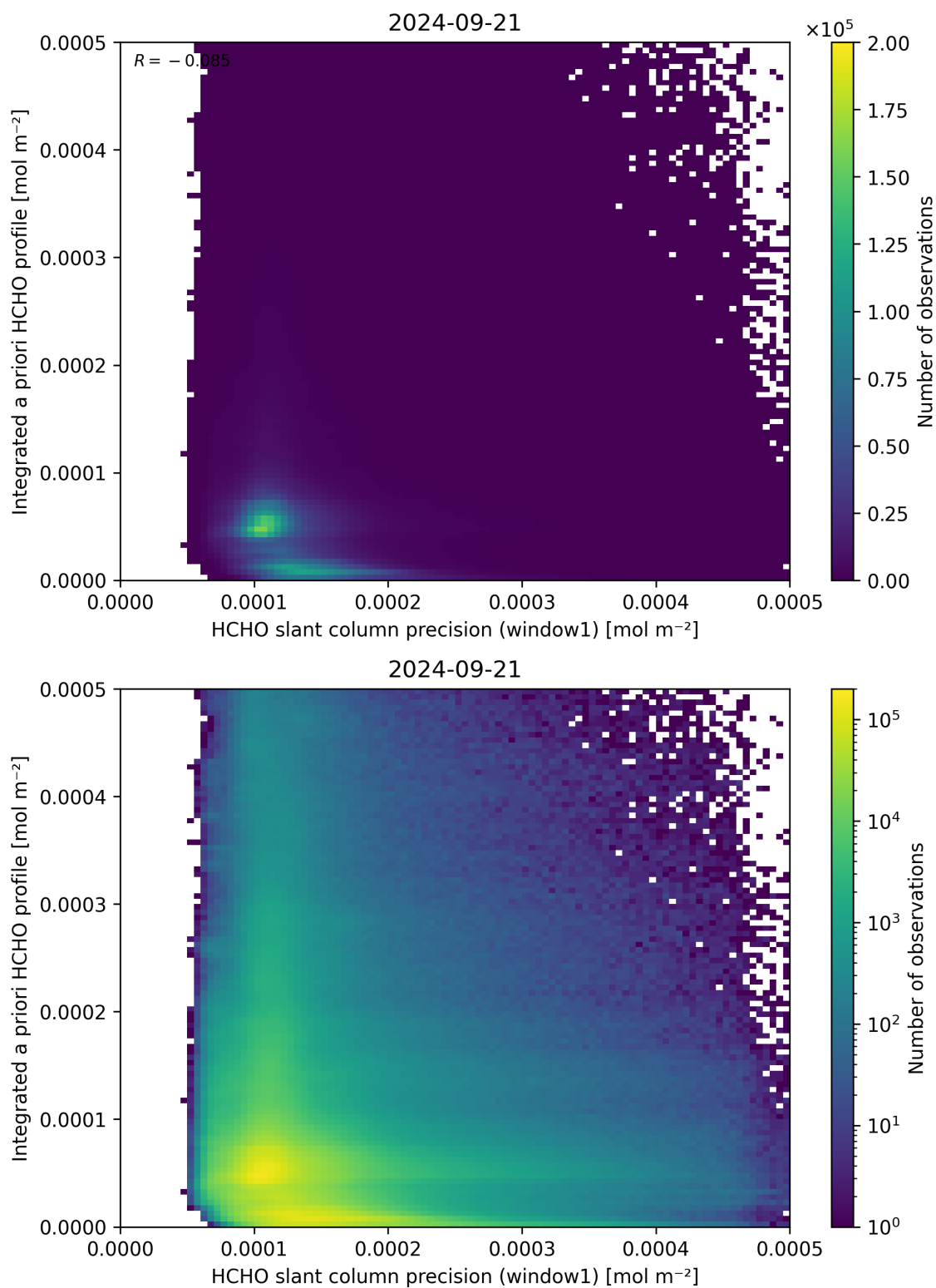
Figure 96: Scatter density plot of “HCHO slant column precision (window1)” against “Integrated a priori HCHO profile” for 2024-09-20 to 2024-09-22.
