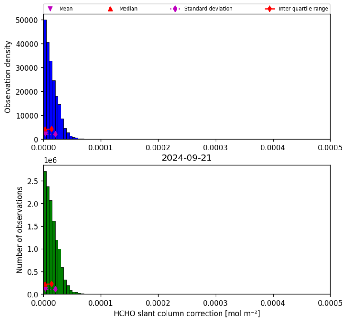
Figure 47: Histogram of “HCHO slant column correction” for 2024-09-20 to 2024-09-22
