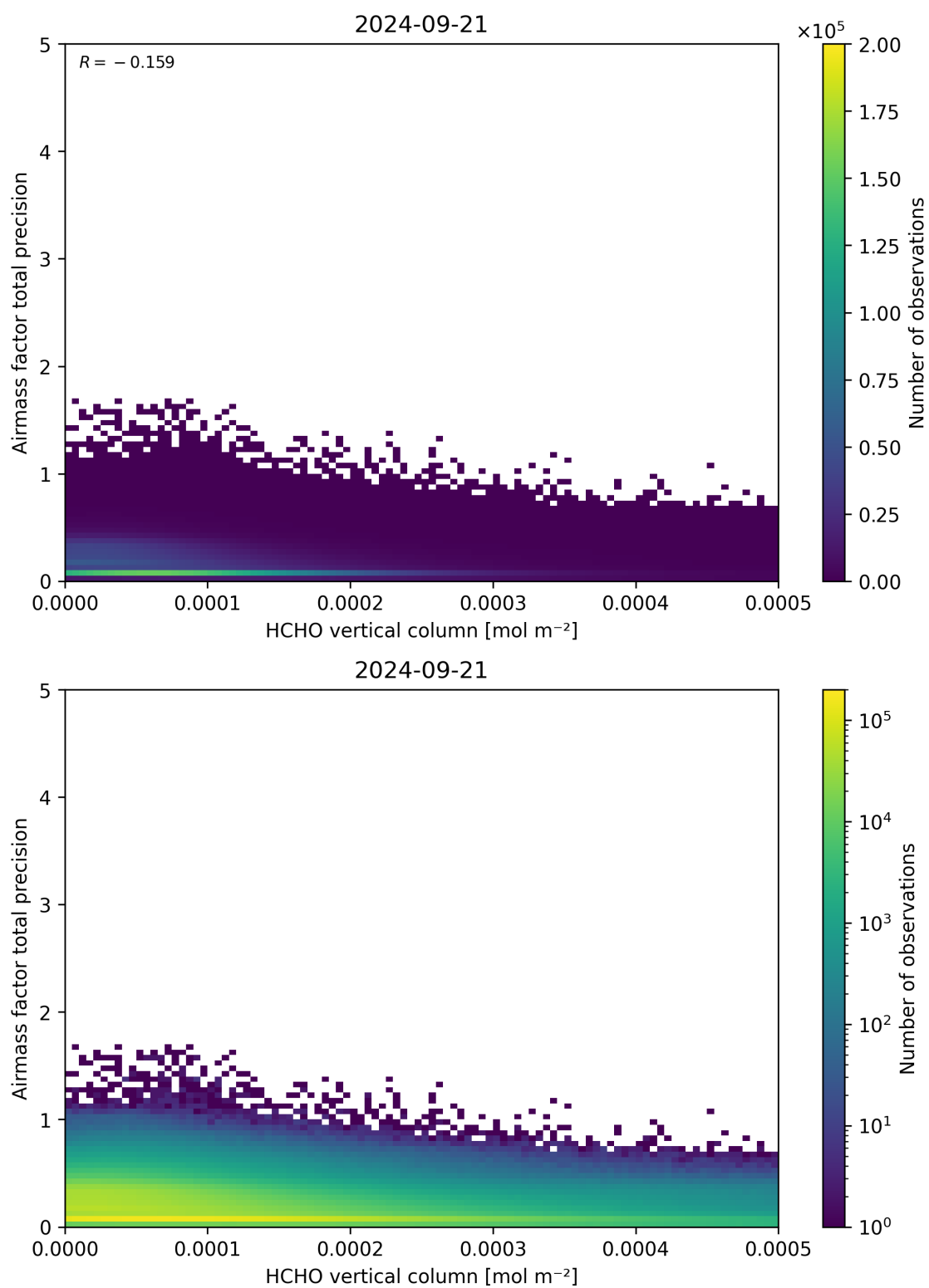
Figure 132: Scatter density plot of “HCHO vertical column” against “Airmass factor total precision” for 2024-09-20 to 2024-09-22.
