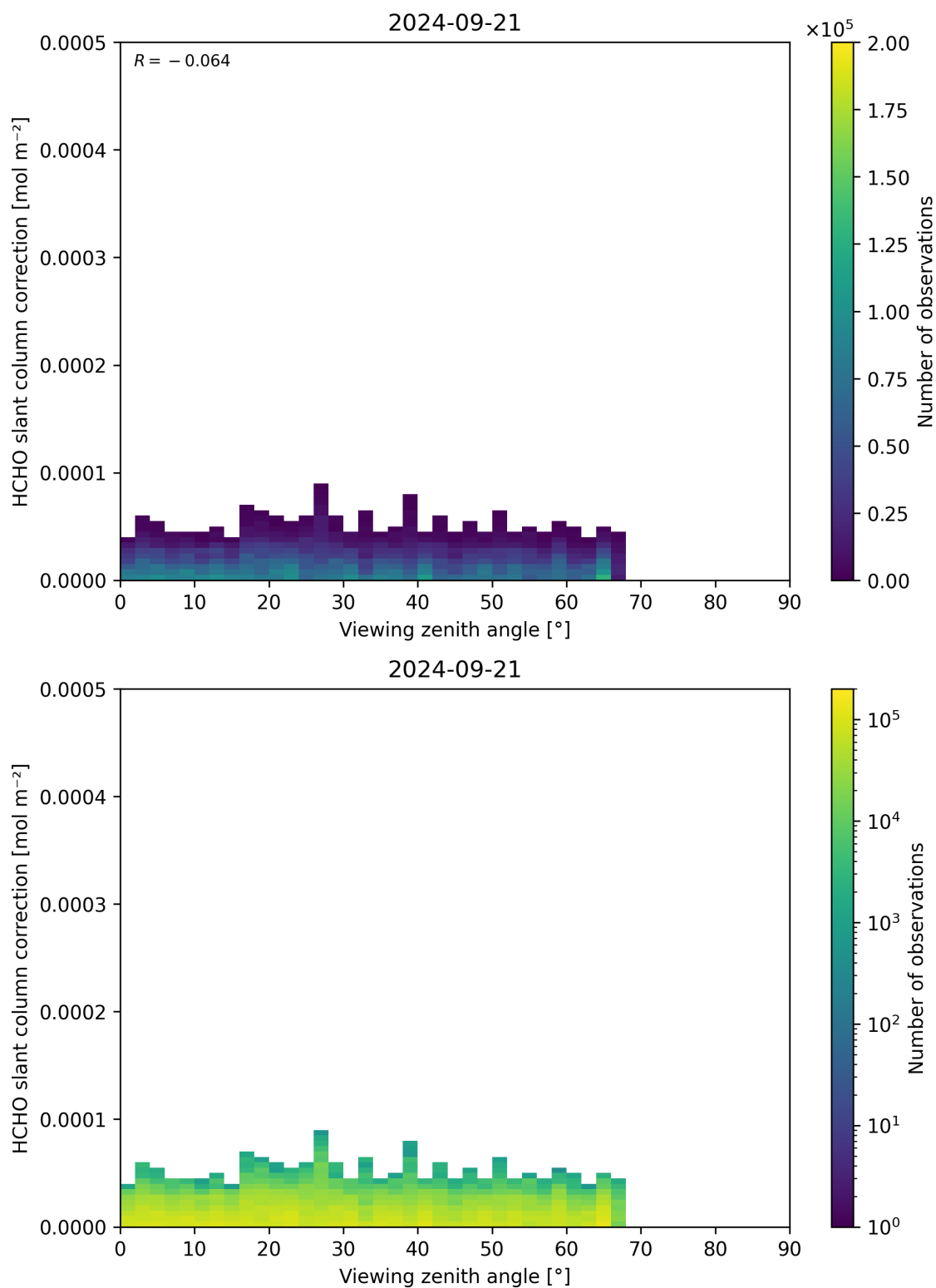
Figure 187: Scatter density plot of “Viewing zenith angle” against “HCHO slant column correction” for 2024-09-20 to 2024-09-22.
