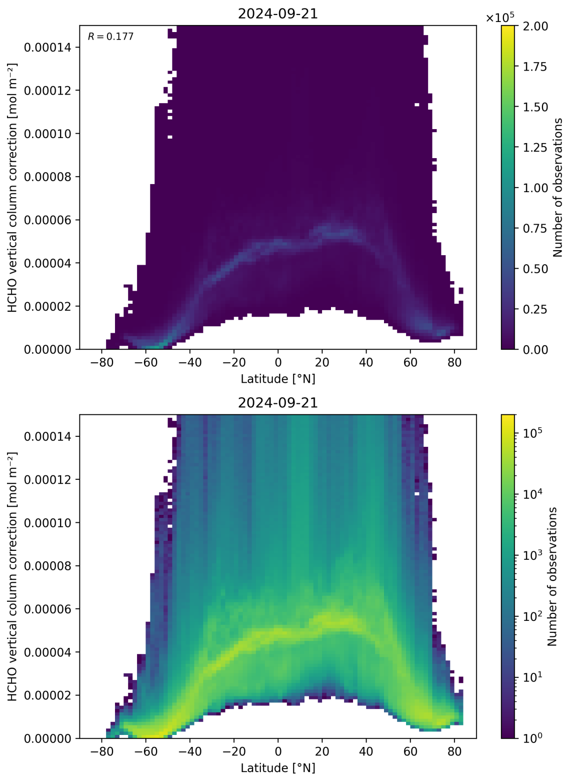
Figure 164: Scatter density plot of “Latitude” against “HCHO vertical column correction” for 2024-09-20 to 2024-09-22.
