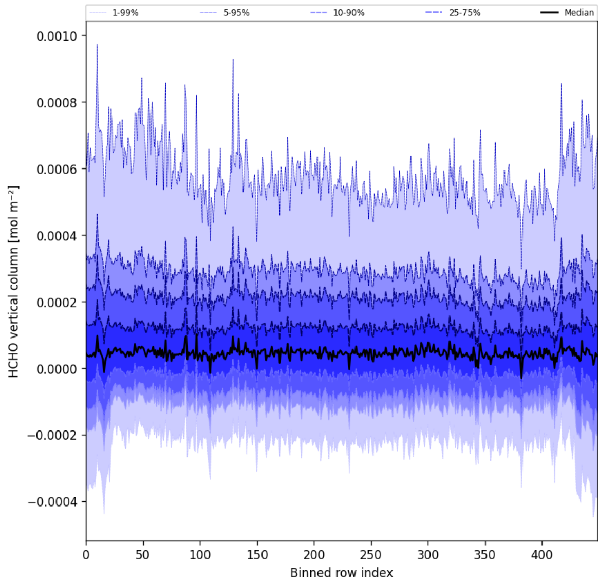
Figure 49: Along track statistics of “HCHO vertical column” for 2024-09-20 to 2024-09-22
