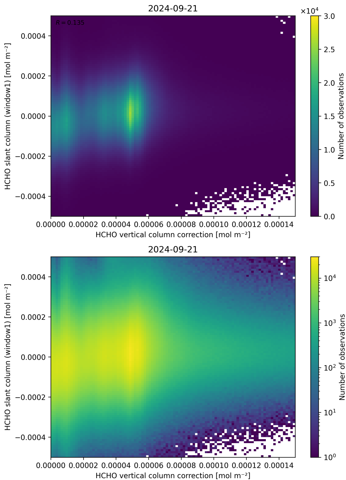
Figure 118: Scatter density plot of “HCHO vertical column correction” against “HCHO slant column (window1)” for 2024-09-20 to 2024-09-22.
