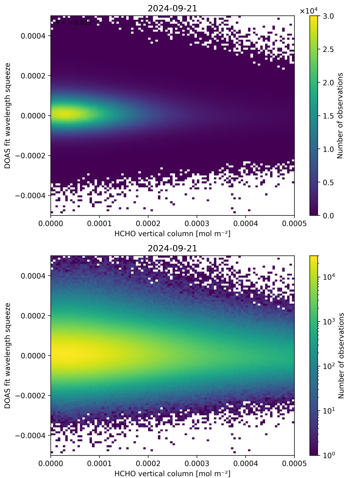
Figure 125: Scatter density plot of “HCHO vertical column” against “DOAS fit wavelength squeeze” for 2024-09-20 to 2024-09-22.
