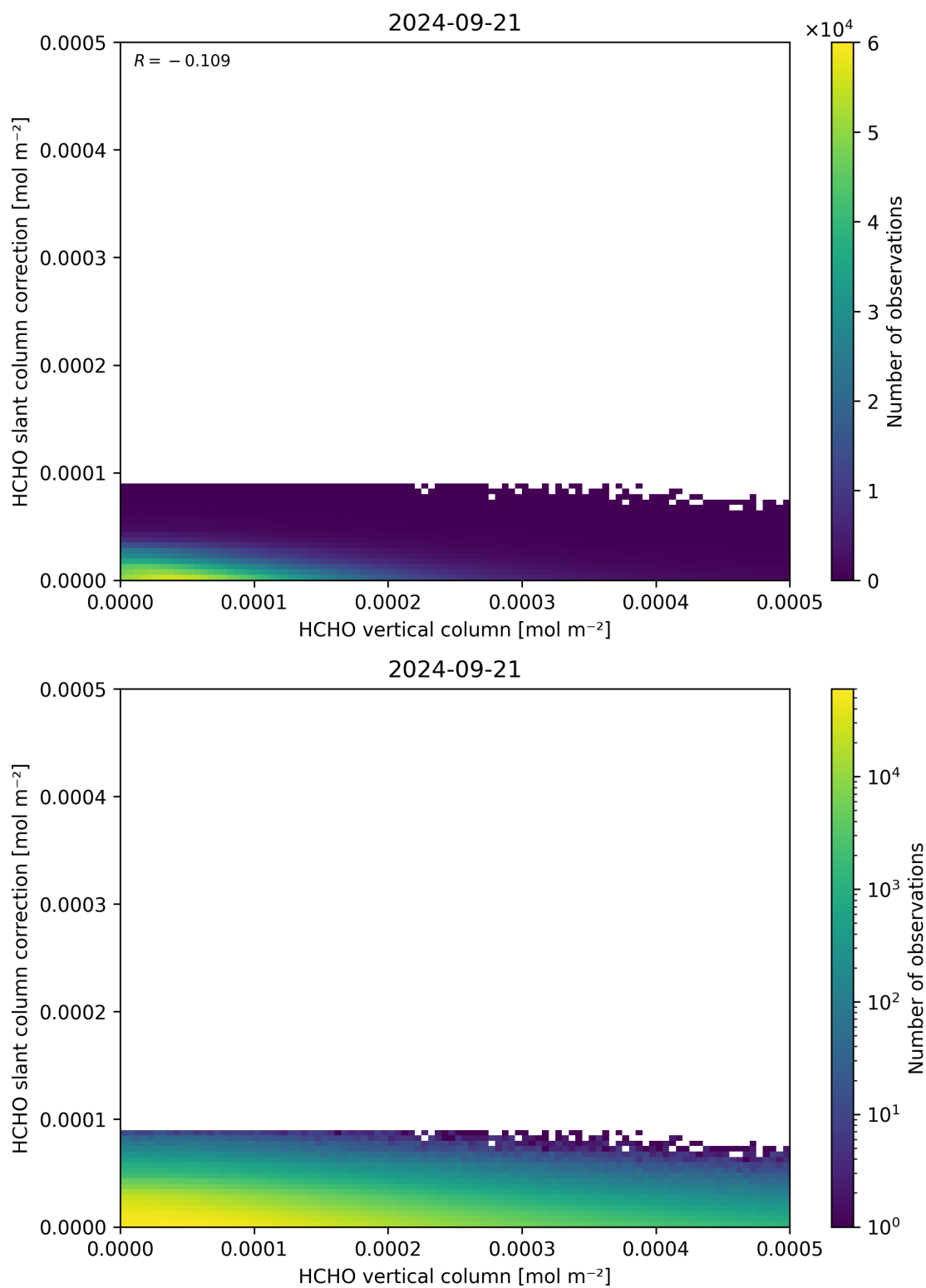
Figure 128: Scatter density plot of “HCHO vertical column” against “HCHO slant column correction” for 2024-09-20 to 2024-09-22.
