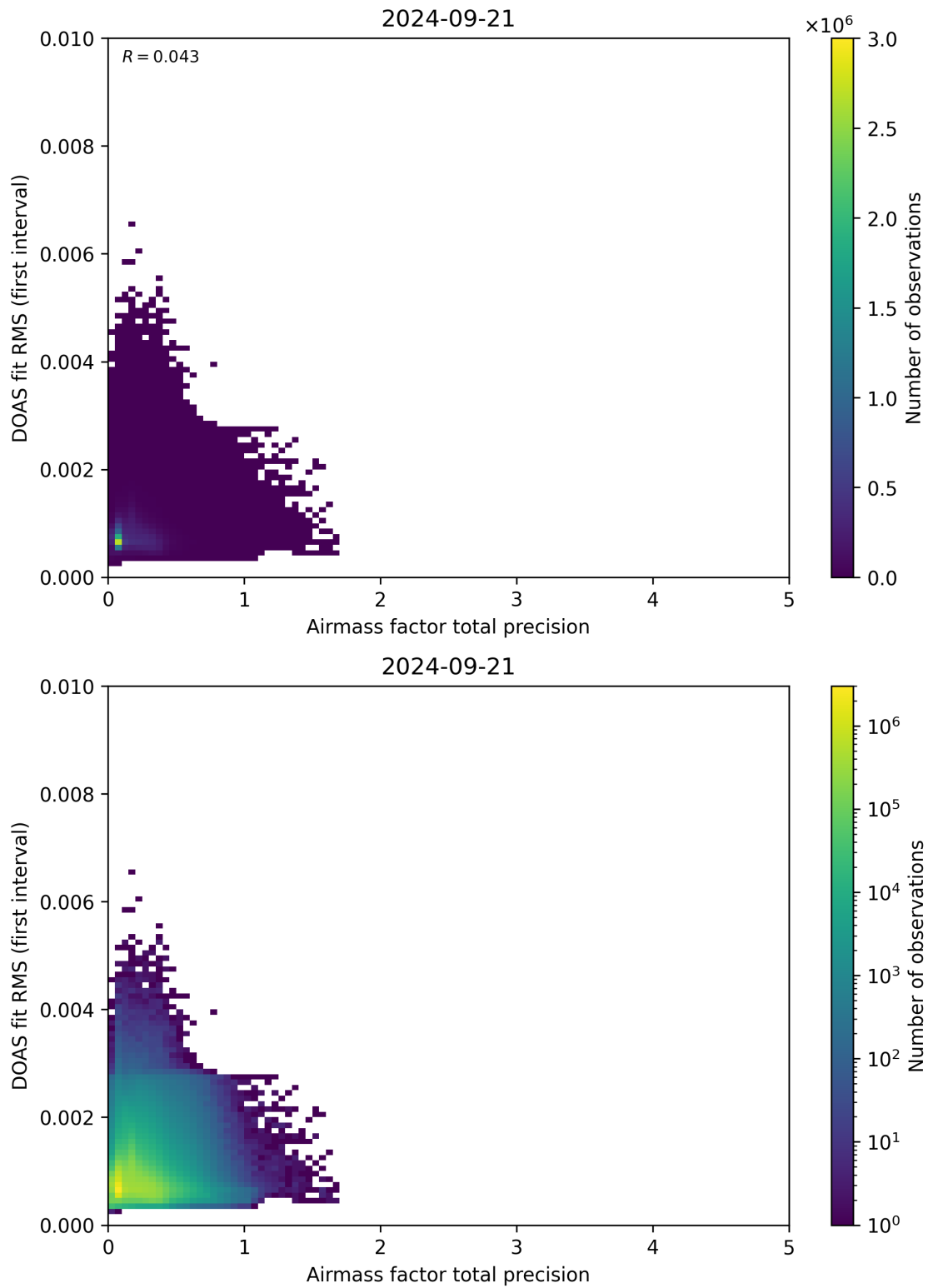
Figure 105: Scatter density plot of “Airmass factor total precision” against “DOAS fit RMS (first interval)” for 2024-09-20 to 2024-09-22.
