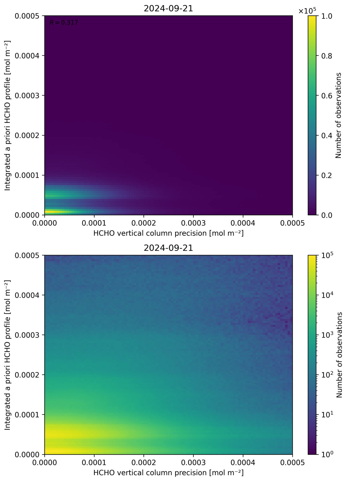
Figure 147: Scatter density plot of “HCHO vertical column precision” against “Integrated a priori HCHO profile” for 2024-09-20 to 2024-09-22.
