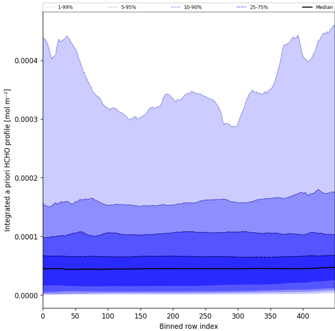
Figure 57: Along track statistics of “Integrated a priori HCHO profile” for 2024-09-20 to 2024-09-22
