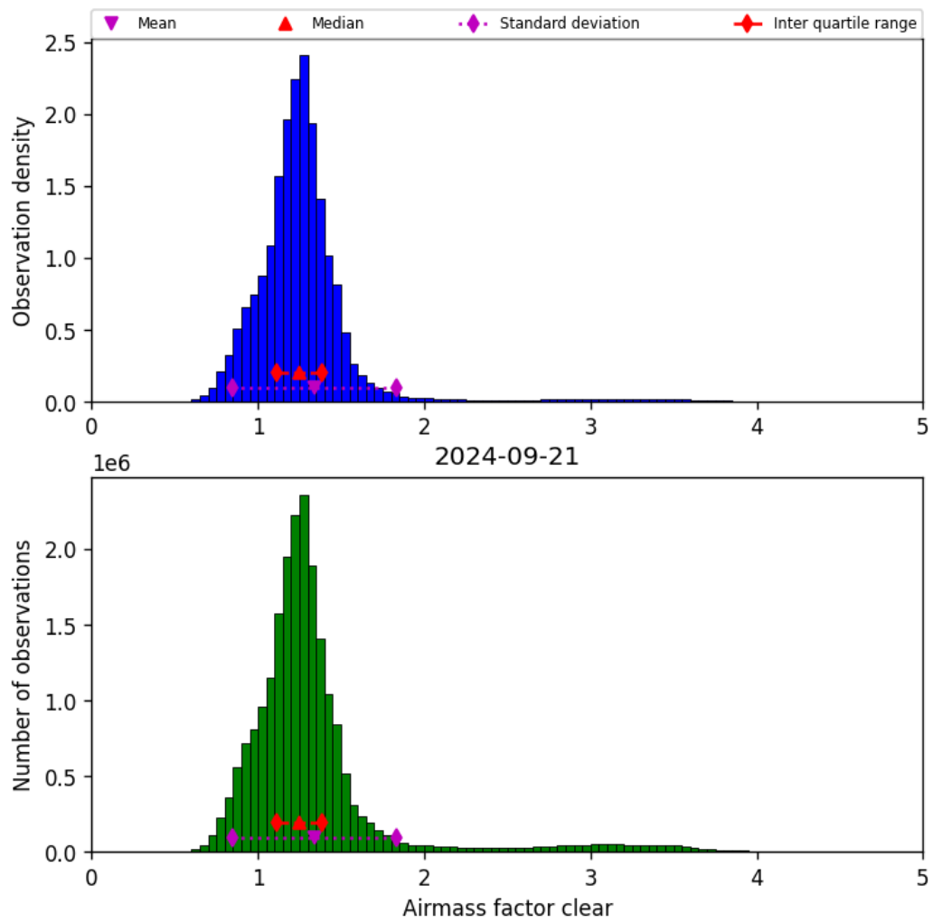
Figure 42: Histogram of “Airmass factor clear” for 2024-09-20 to 2024-09-22
