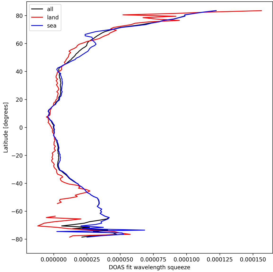
Figure 31: Zonal average of “DOAS fit wavelength squeeze” for 2024-09-20 to 2024-09-22.
