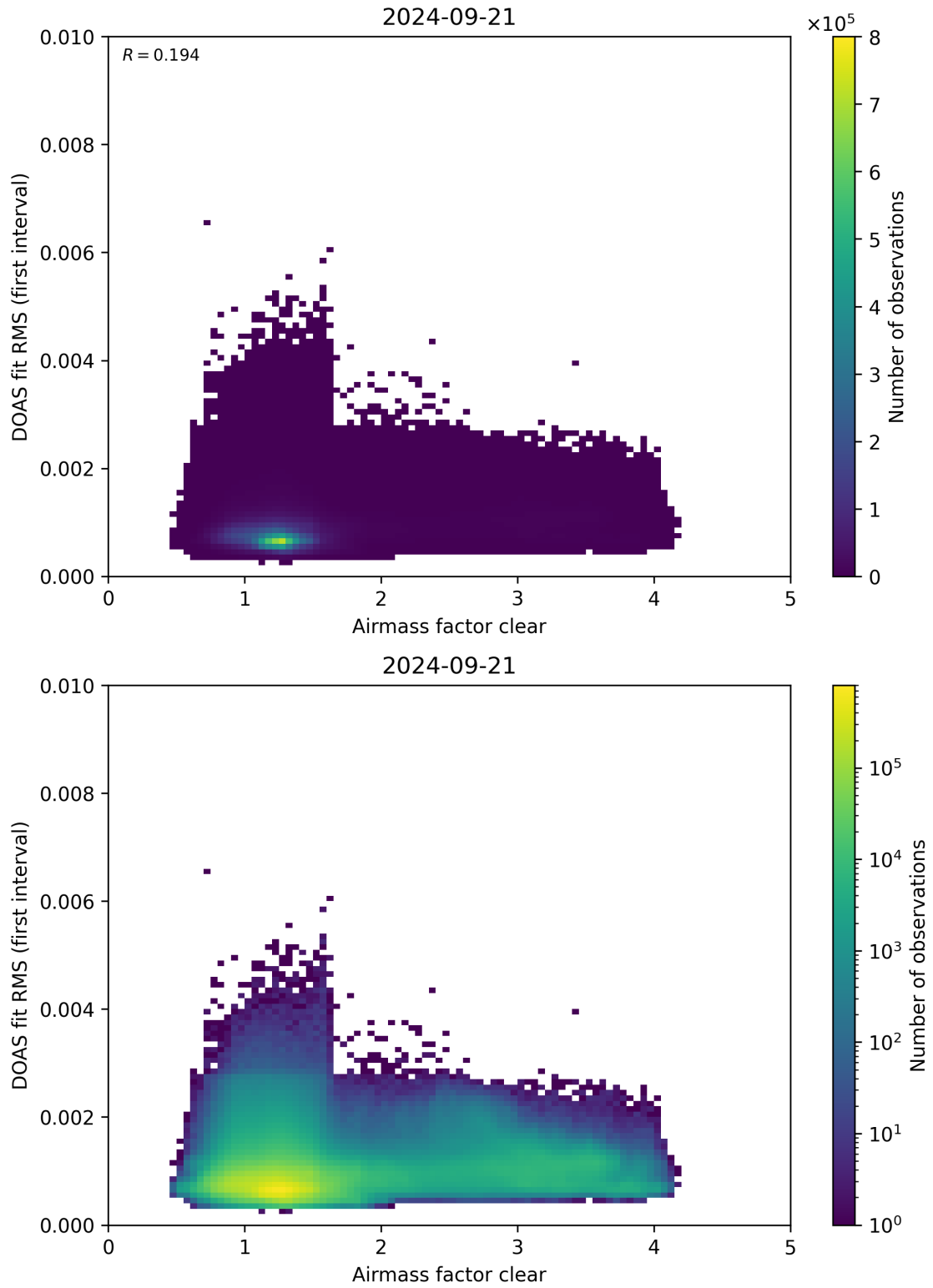
Figure 71: Scatter density plot of “Airmass factor clear” against “DOAS fit RMS (first interval)” for 2024-09-20 to 2024-09-22.
