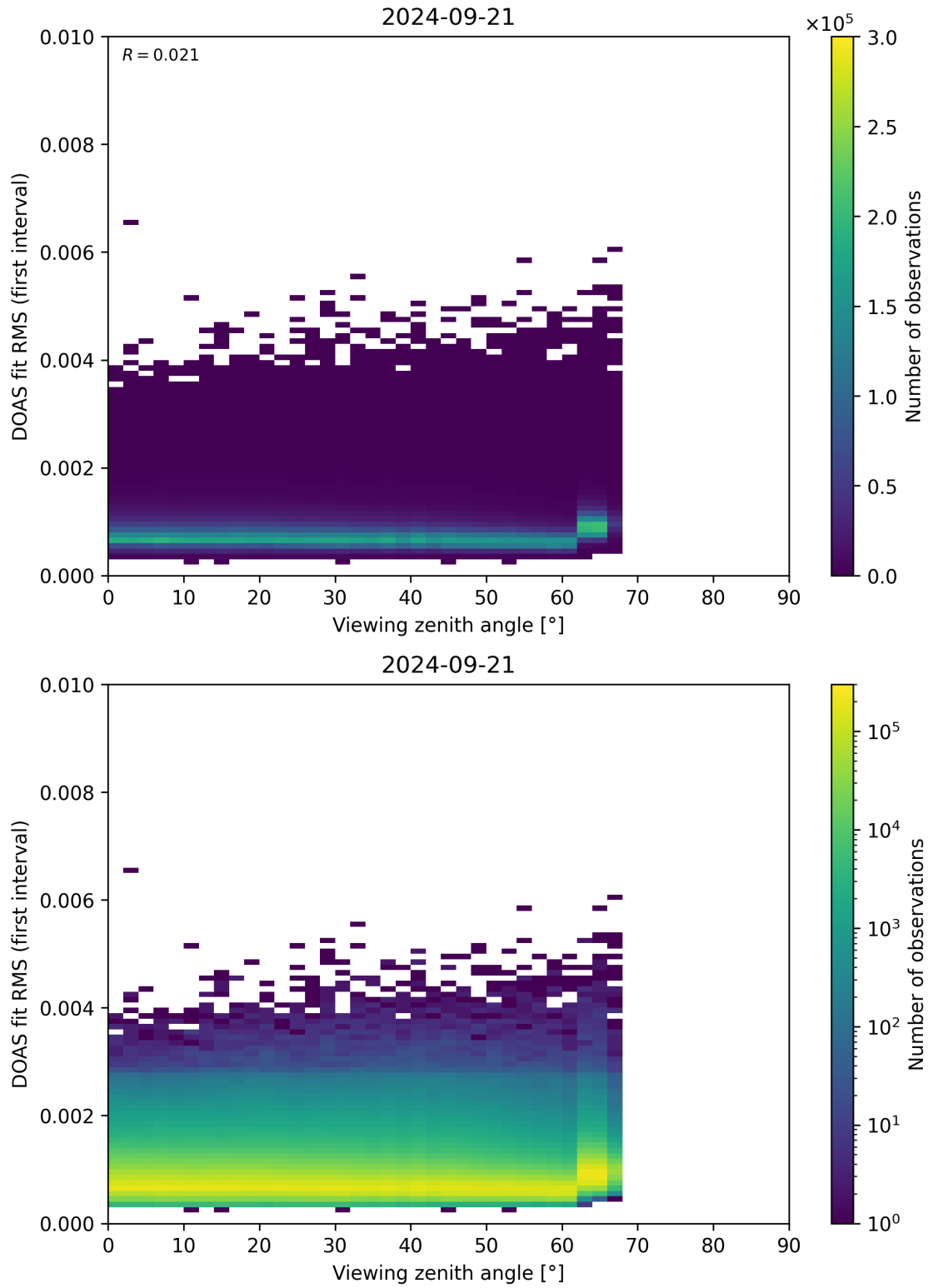
Figure 182: Scatter density plot of “Viewing zenith angle” against “DOAS fit RMS (first interval)” for 2024-09-20 to 2024-09-22.
