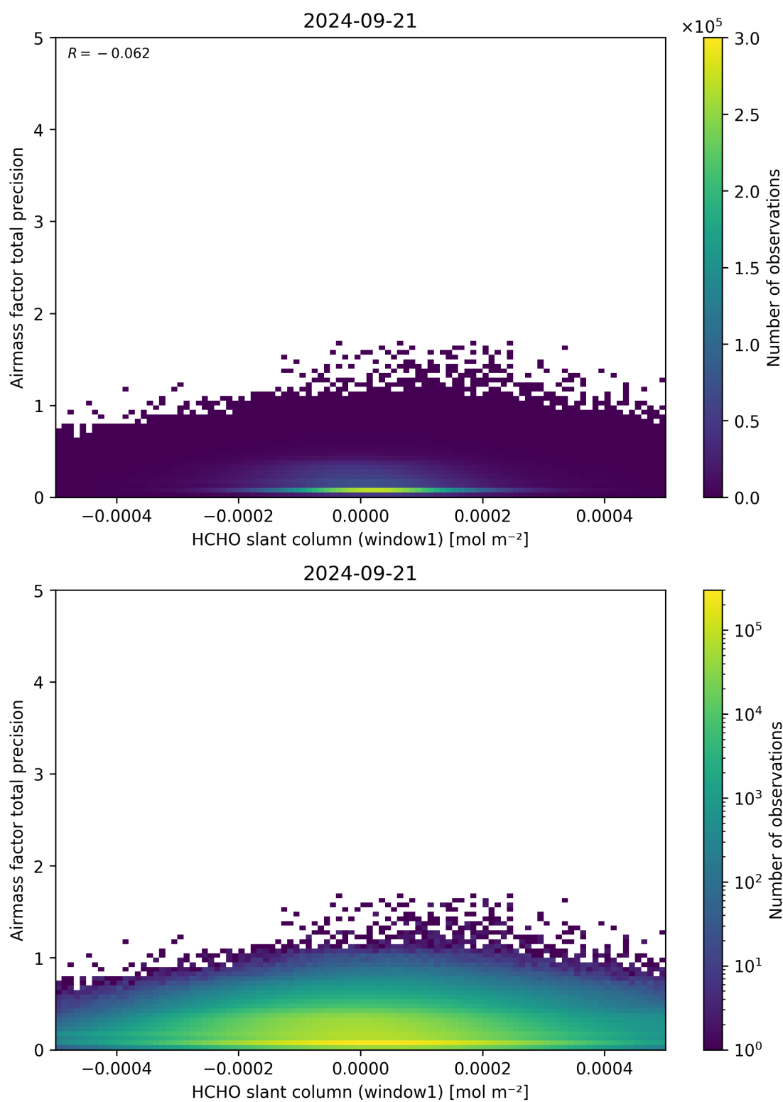
Figure 86: Scatter density plot of “HCHO slant column (window1)” against “Airmass factor total precision” for 2024-09-20 to 2024-09-22.
