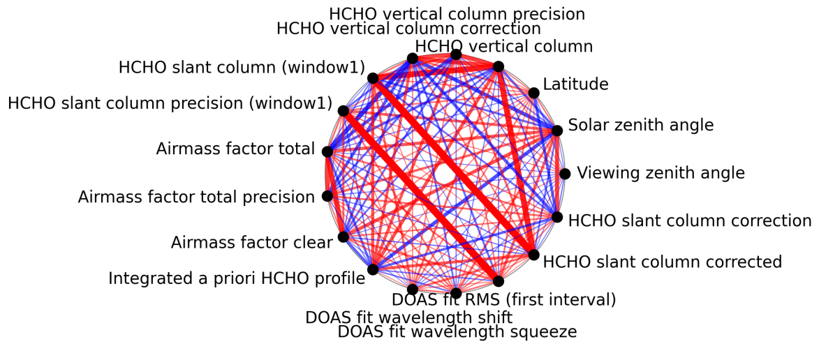
Figure 1: Map of correlation graph for 2024-09-20 to 2024-09-22.
