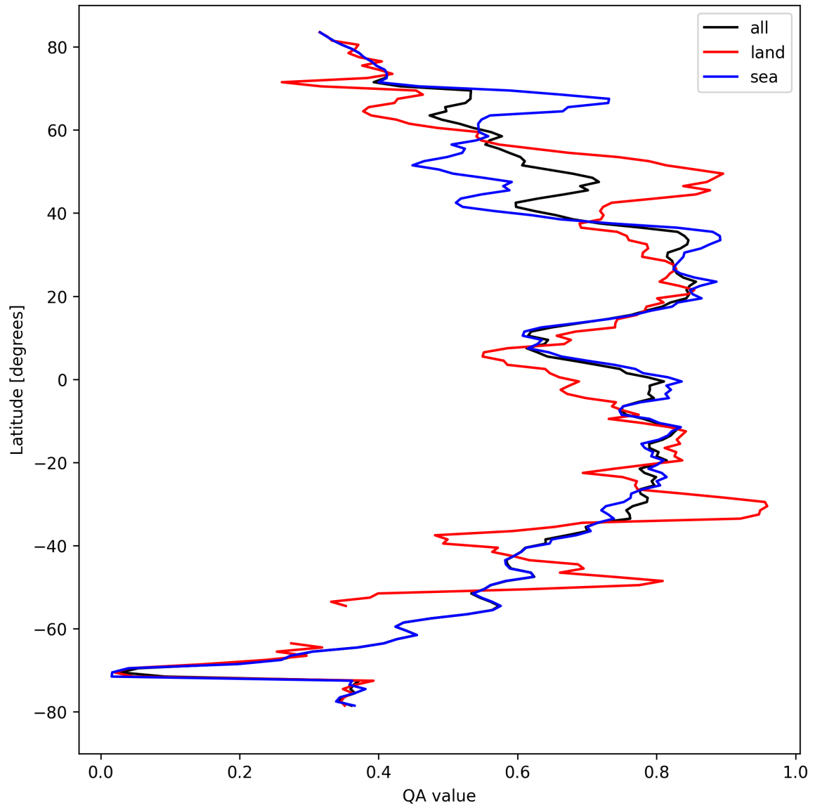
Figure 20: Zonal average of “QA value” for 2024-09-20 to 2024-09-22.
