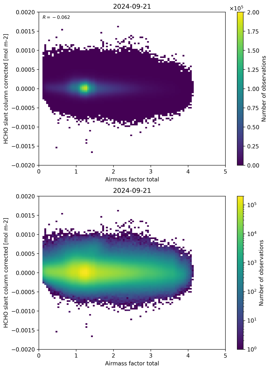
Figure 101: Scatter density plot of “Airmass factor total” against “HCHO slant column corrected” for 2024-09-20 to 2024-09-22.
