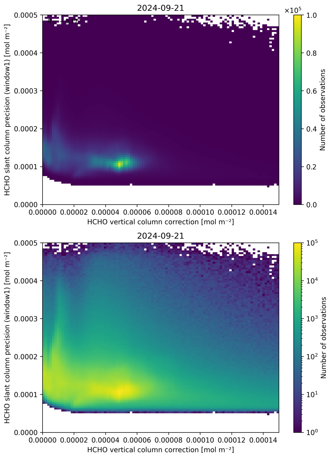
Figure 119: Scatter density plot of “HCHO vertical column correction” against “HCHO slant column precision (window1)” for 2024-09-20 to 2024-09-22.
