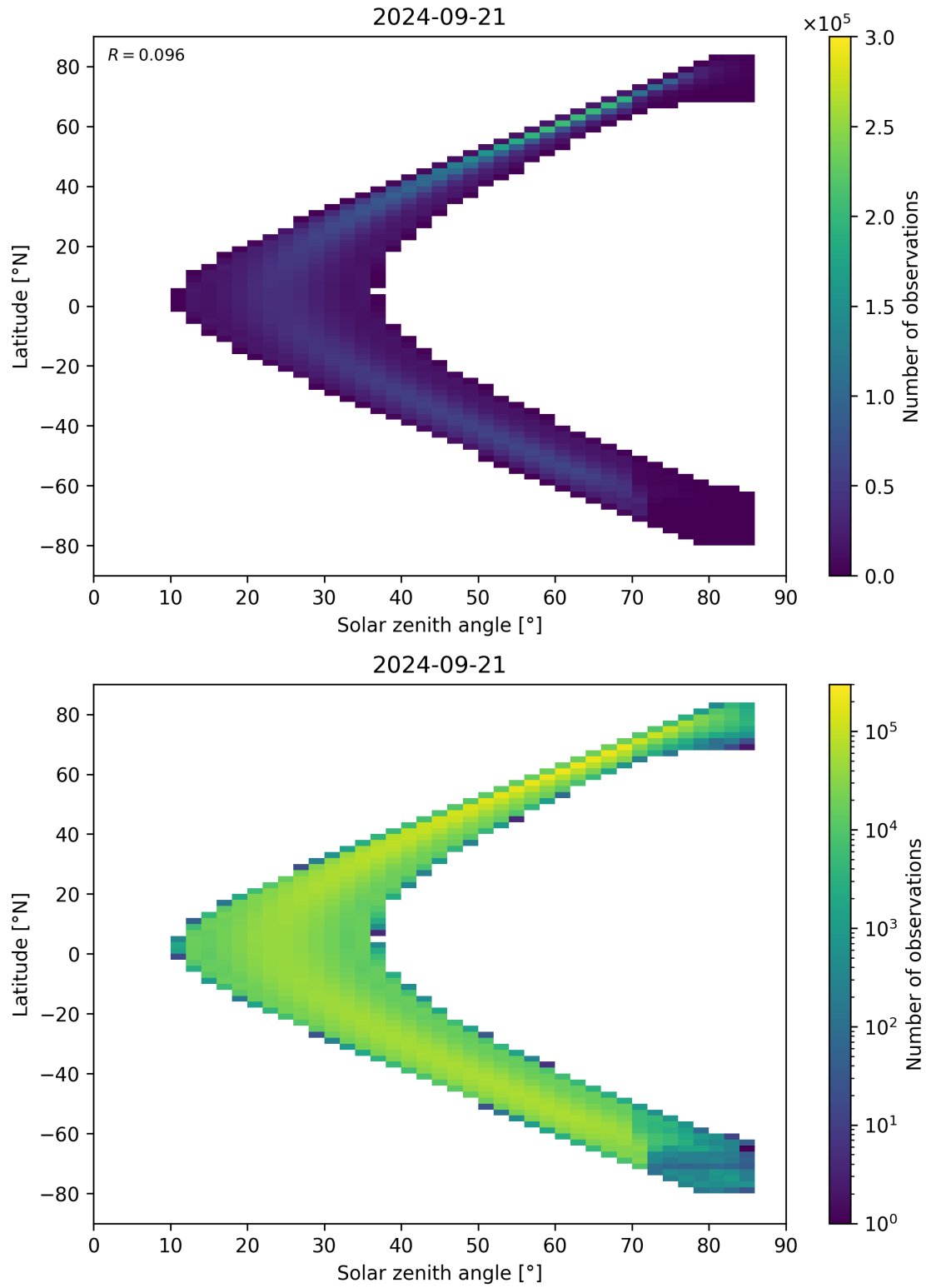
Figure 181: Scatter density plot of “Solar zenith angle” against “Latitude” for 2024-09-20 to 2024-09-22.
