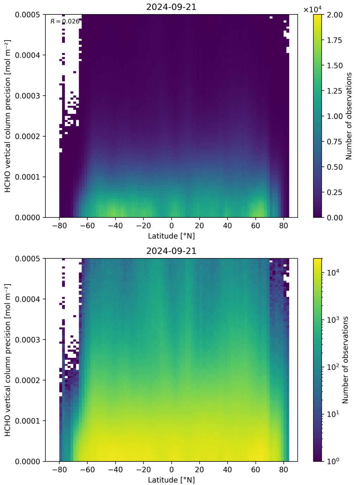
Figure 165: Scatter density plot of “Latitude” against “HCHO vertical column precision” for 2024-09-20 to 2024-09-22.
