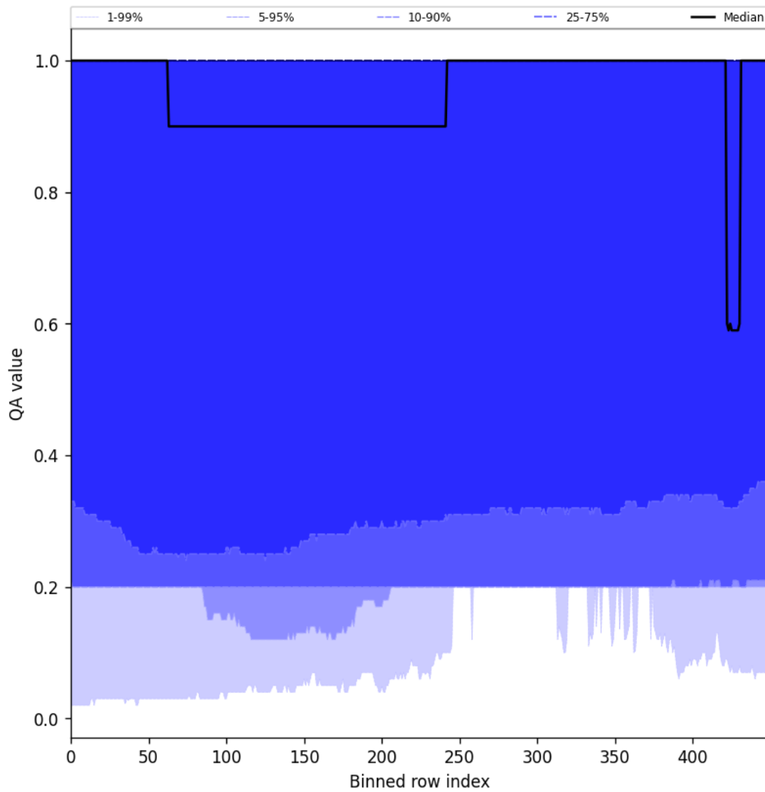
Figure 48: Along track statistics of “QA value” for 2024-09-20 to 2024-09-22
