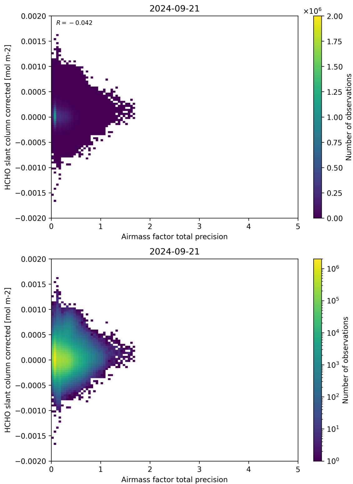
Figure 109: Scatter density plot of “Airmass factor total precision” against “HCHO slant column corrected” for 2024-09-20 to 2024-09-22.
