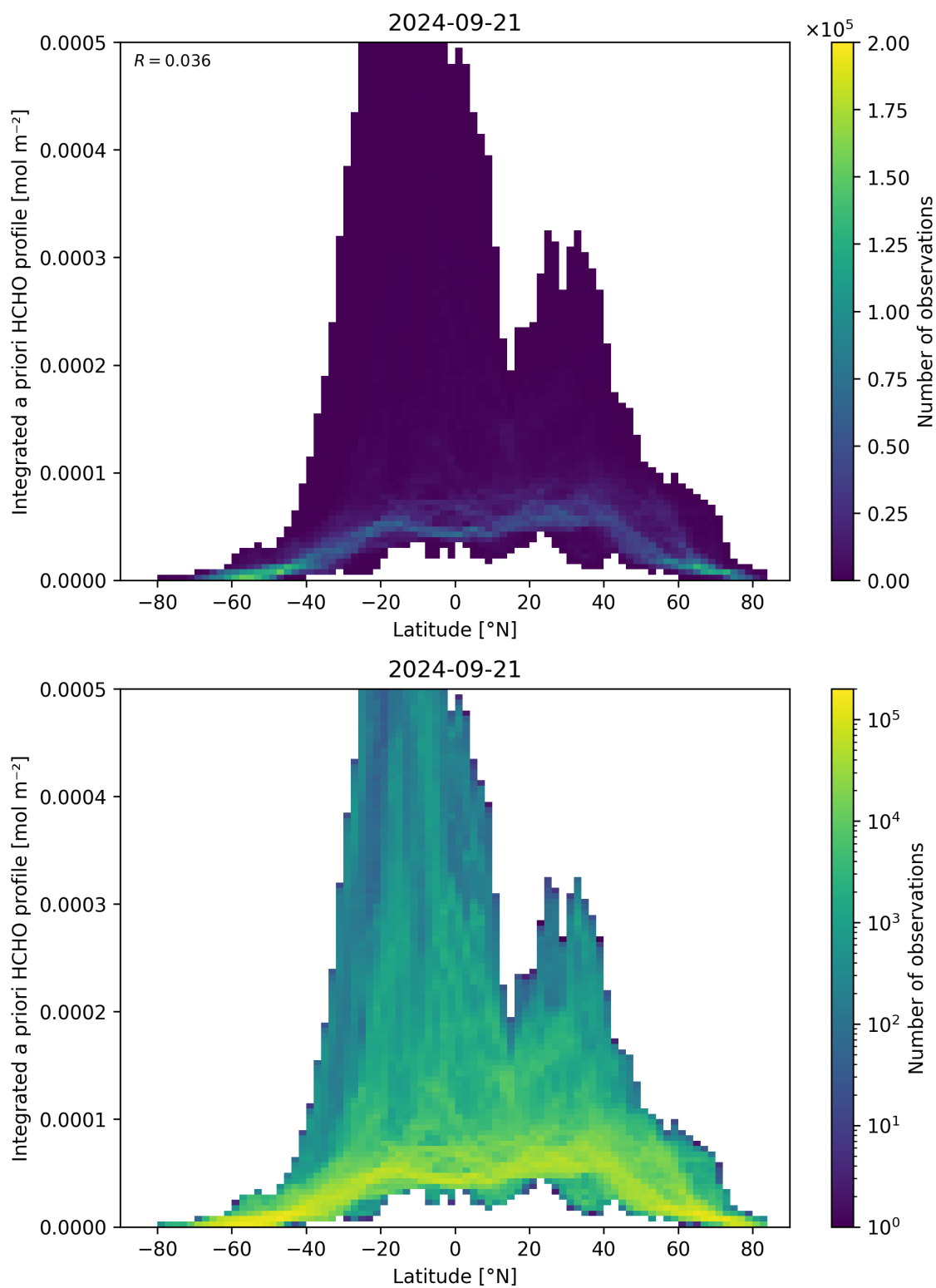
Figure 166: Scatter density plot of “Latitude” against “Integrated a priori HCHO profile” for 2024-09-20 to 2024-09-22.
