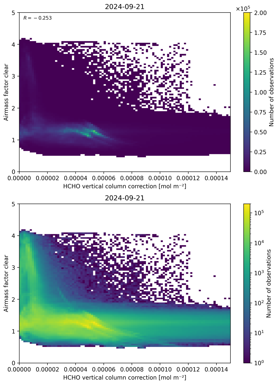
Figure 115: Scatter density plot of “HCHO vertical column correction” against “Airmass factor clear” for 2024-09-20 to 2024-09-22.
