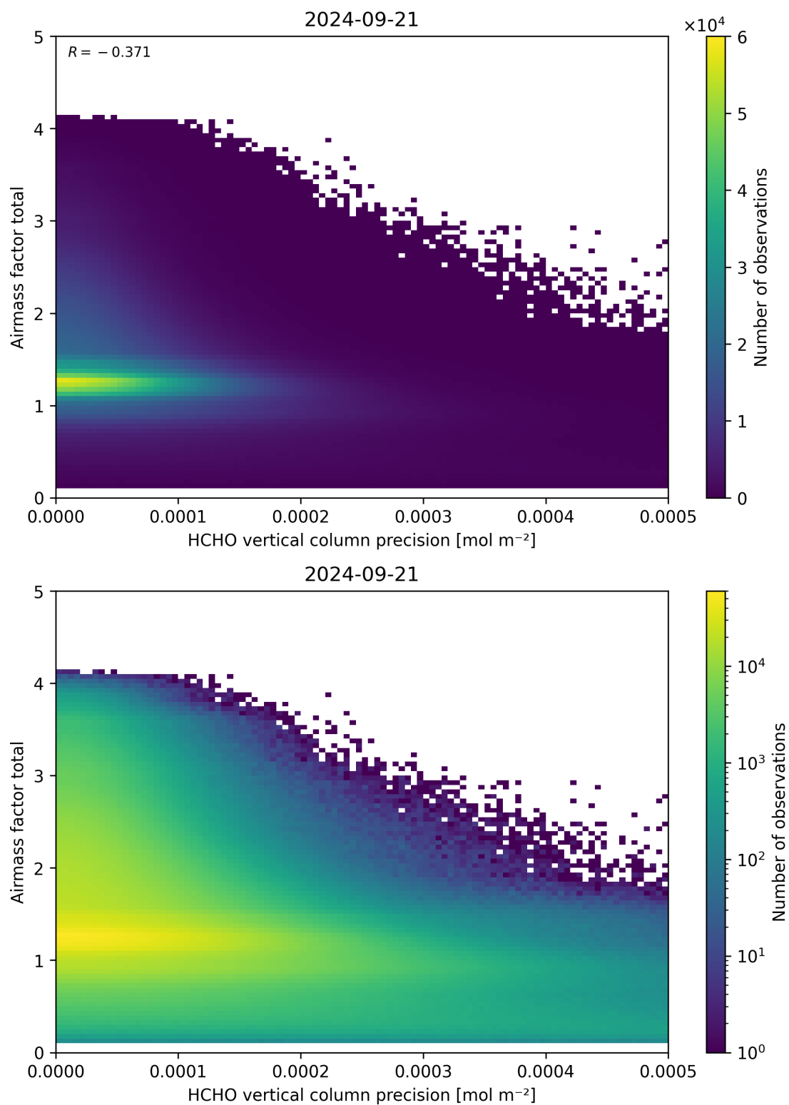
Figure 144: Scatter density plot of “HCHO vertical column precision” against “Airmass factor total” for 2024-09-20 to 2024-09-22.
