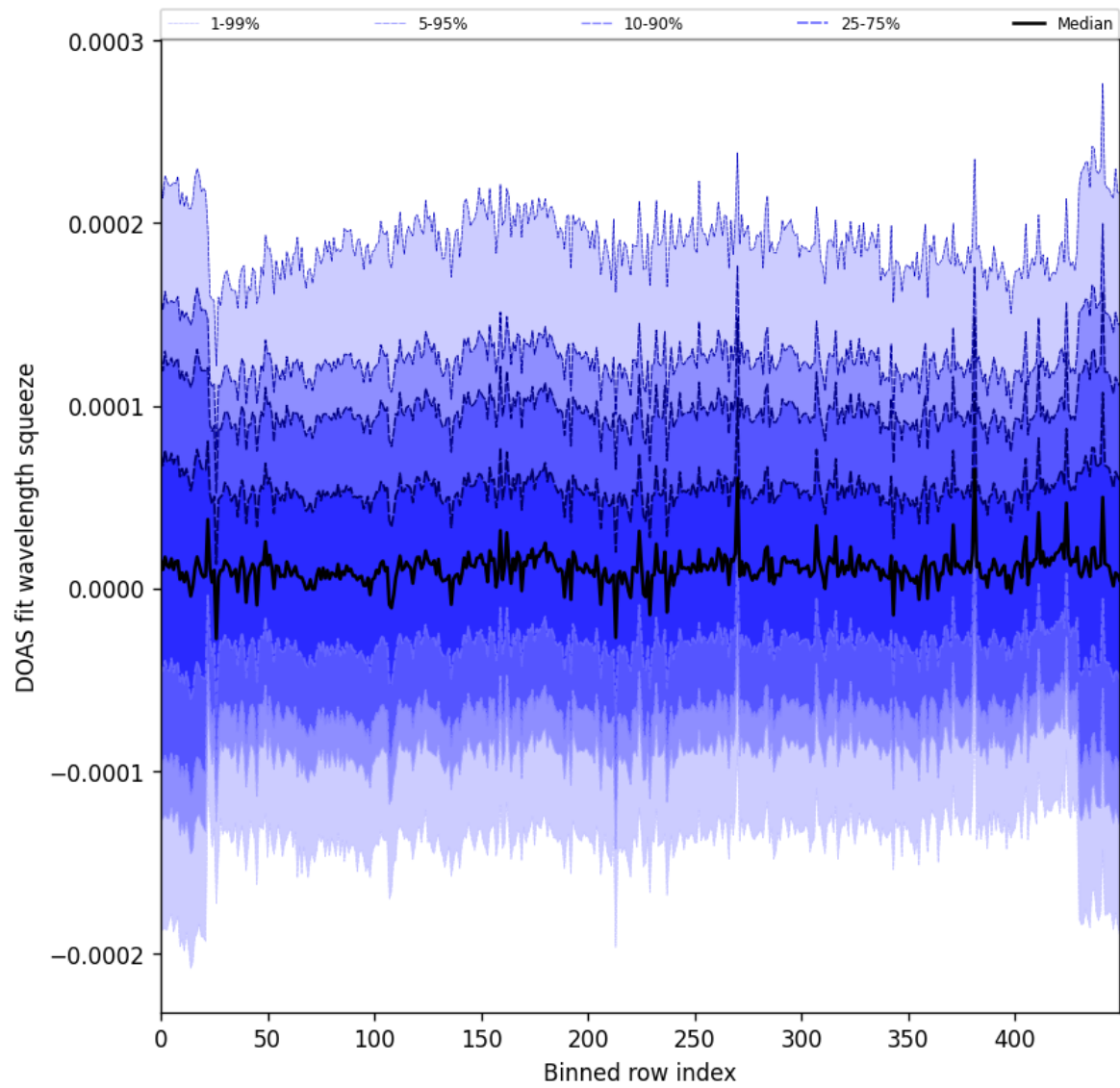
Figure 59: Along track statistics of “DOAS fit wavelength squeeze” for 2024-09-20 to 2024-09-22
