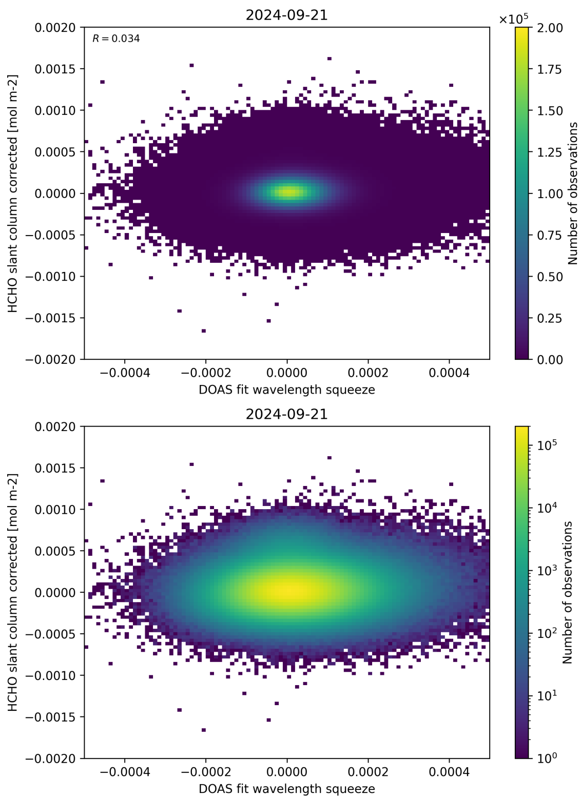
Figure 69: Scatter density plot of “DOAS fit wavelength squeeze” against “HCHO slant column corrected” for 2024-09-20 to 2024-09-22.
