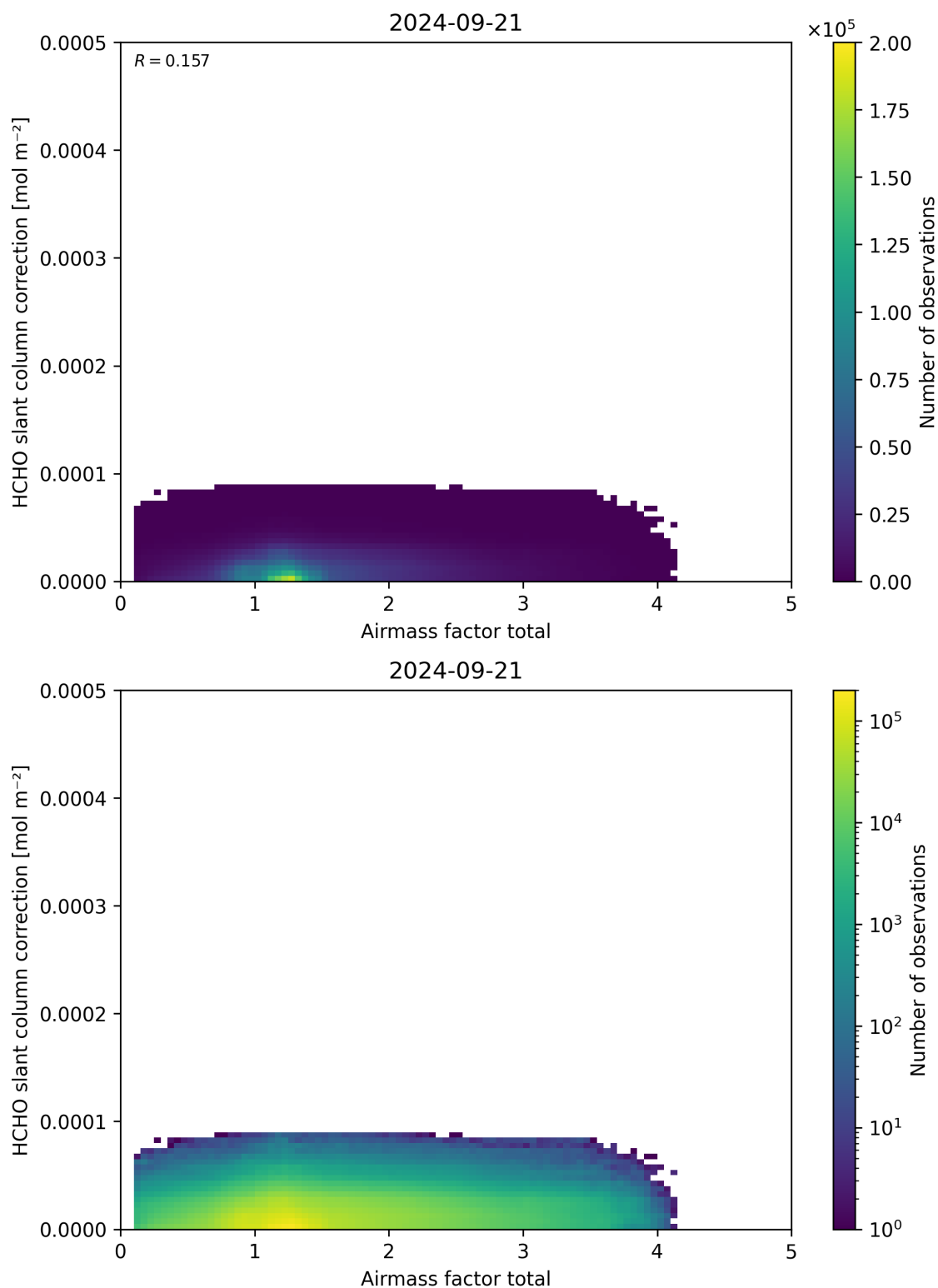
Figure 102: Scatter density plot of “Airmass factor total” against “HCHO slant column correction” for 2024-09-20 to 2024-09-22.
