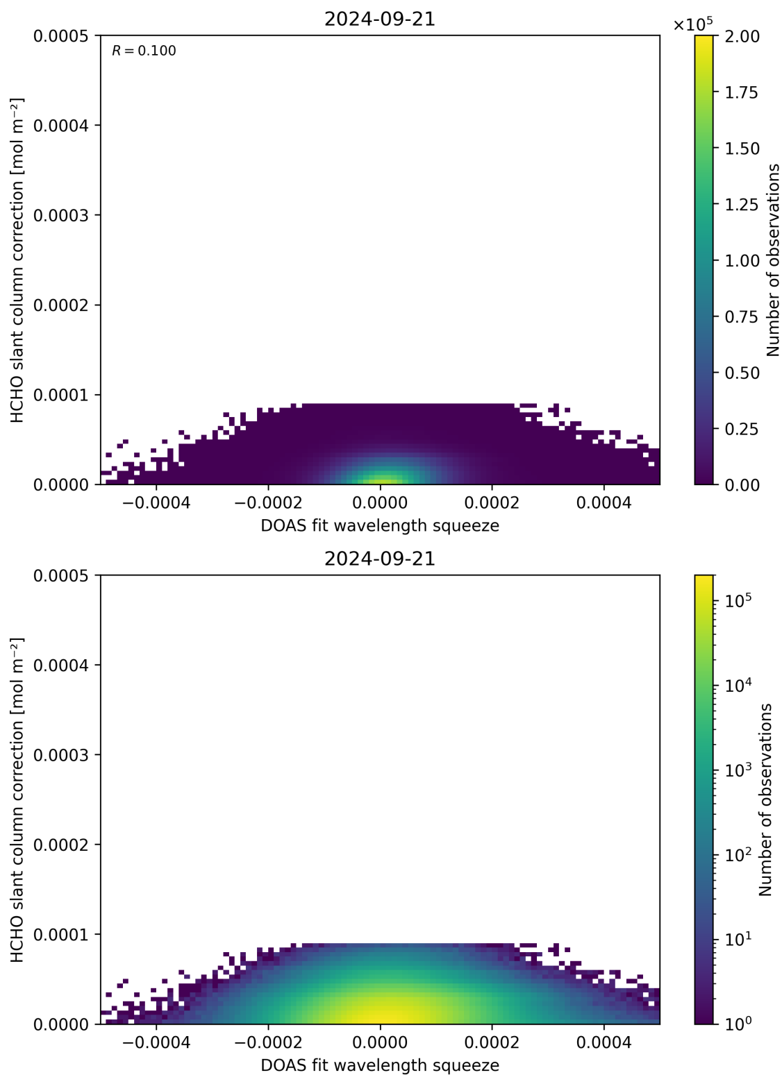
Figure 70: Scatter density plot of “DOAS fit wavelength squeeze” against “HCHO slant column correction” for 2024-09-20 to 2024-09-22.
