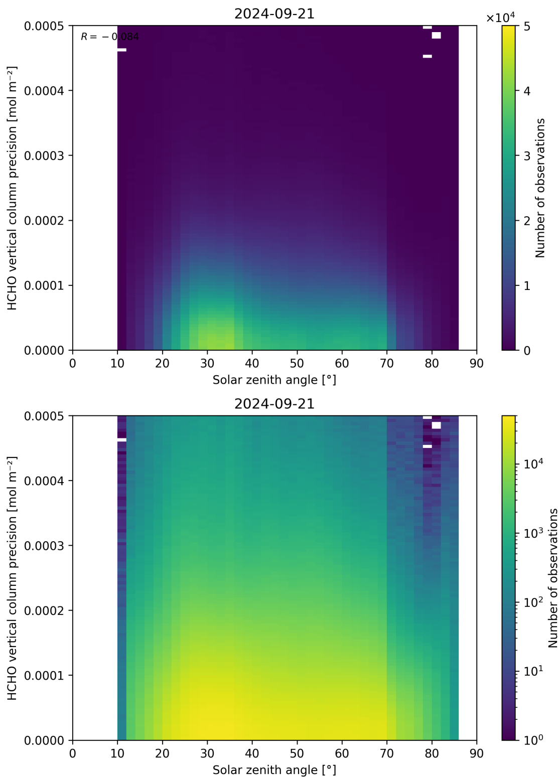
Figure 179: Scatter density plot of “Solar zenith angle” against “HCHO vertical column precision” for 2024-09-20 to 2024-09-22.
