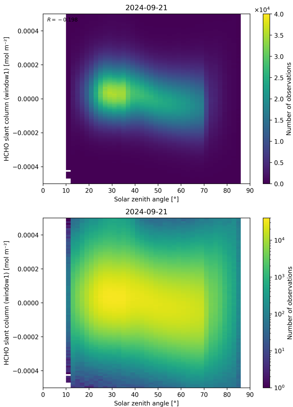
Figure 173: Scatter density plot of “Solar zenith angle” against “HCHO slant column (window1)” for 2024-09-20 to 2024-09-22.
