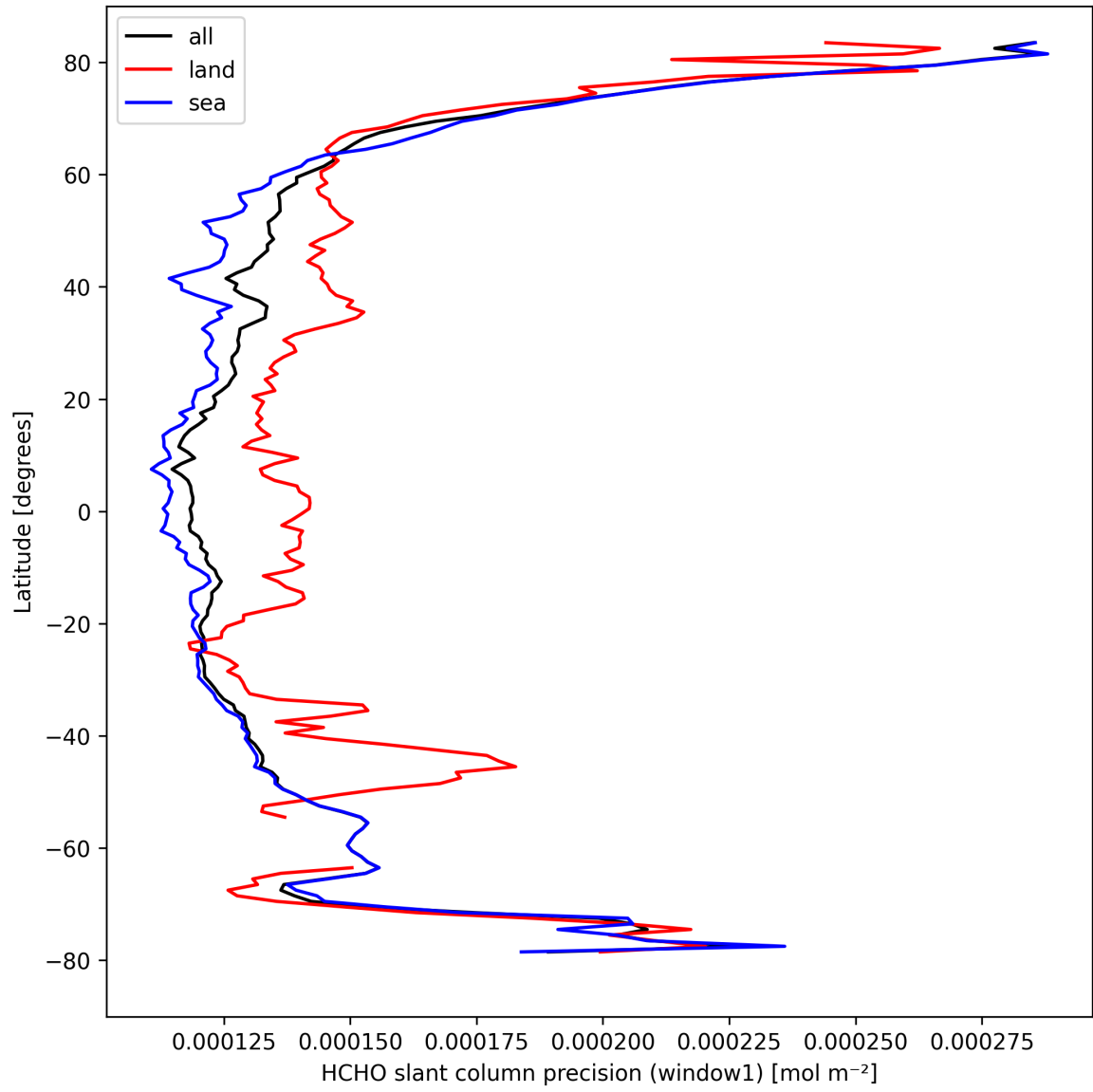
Figure 25: Zonal average of “HCHO slant column precision (window1)” for 2024-09-20 to 2024-09-22.
