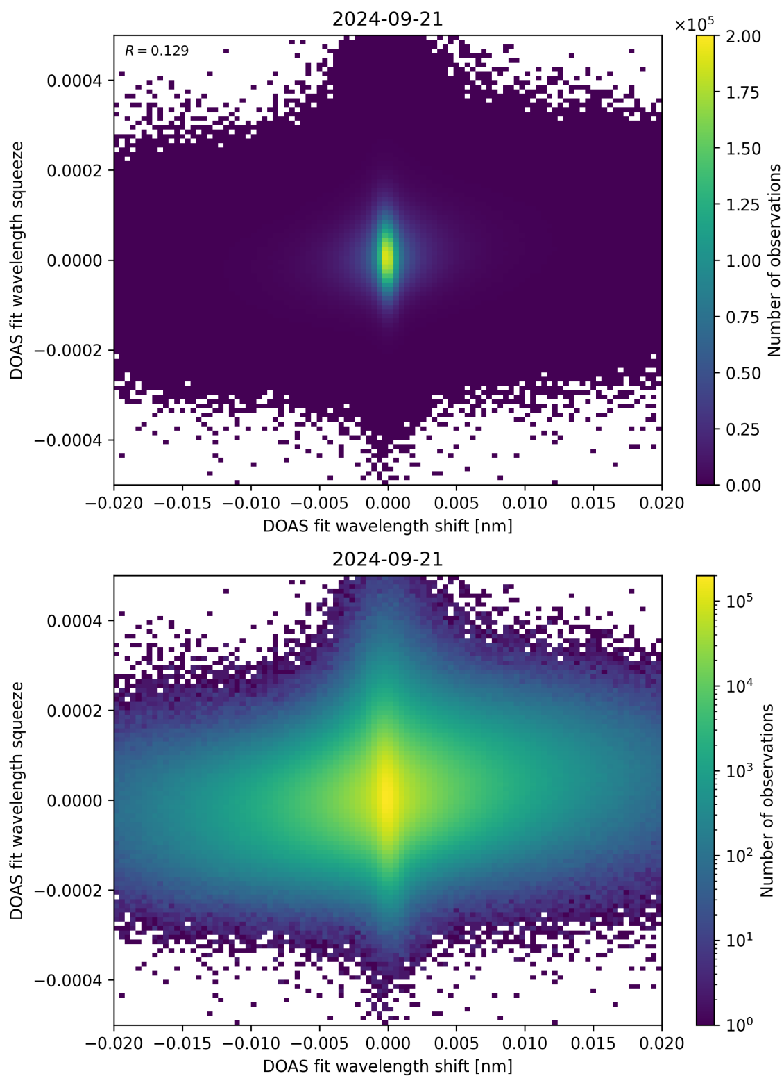
Figure 65: Scatter density plot of “DOAS fit wavelength shift” against “DOAS fit wavelength squeeze” for 2024-09-20 to 2024-09-22.
