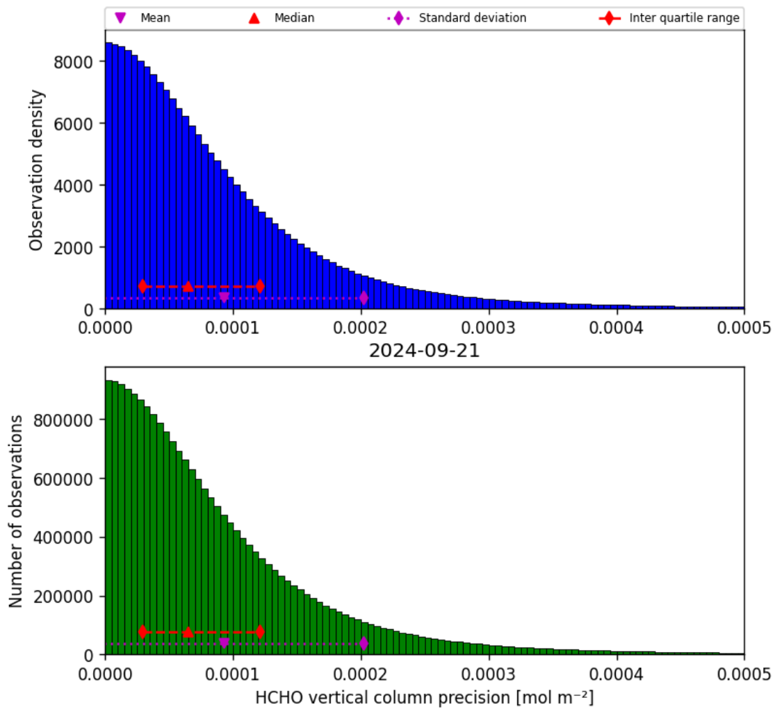
Figure 36: Histogram of “HCHO vertical column precision” for 2024-09-20 to 2024-09-22
