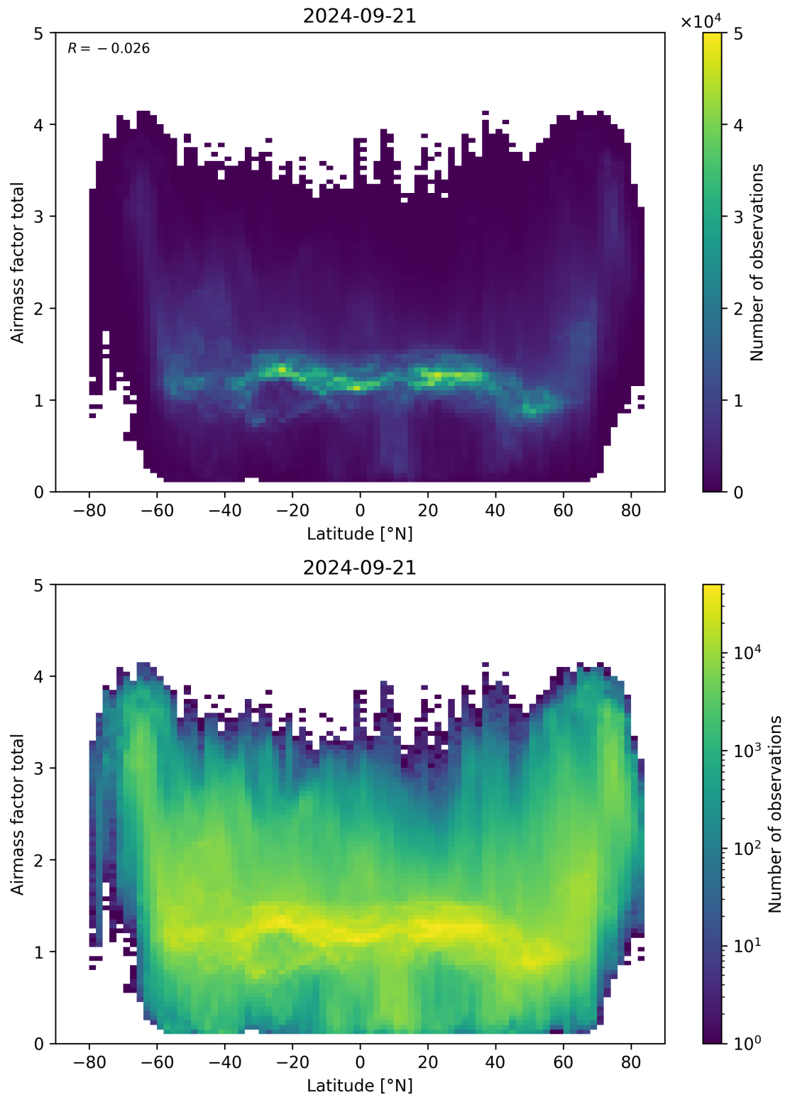
Figure 161: Scatter density plot of “Latitude” against “Airmass factor total” for 2024-09-20 to 2024-09-22.
