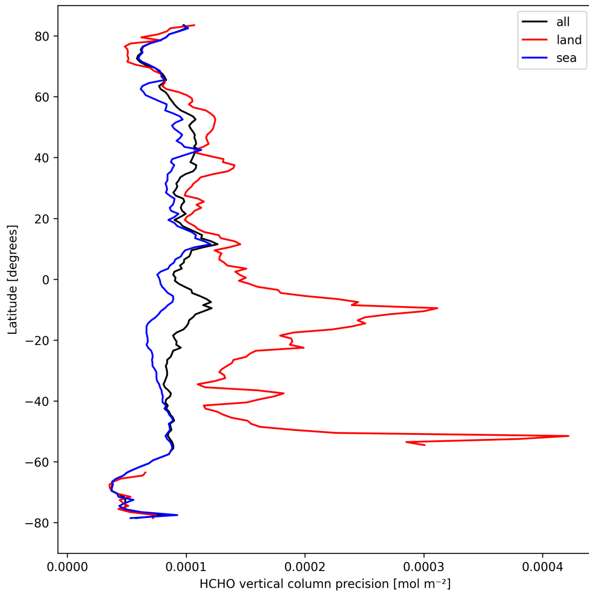
Figure 22: Zonal average of “HCHO vertical column precision” for 2024-09-20 to 2024-09-22.
