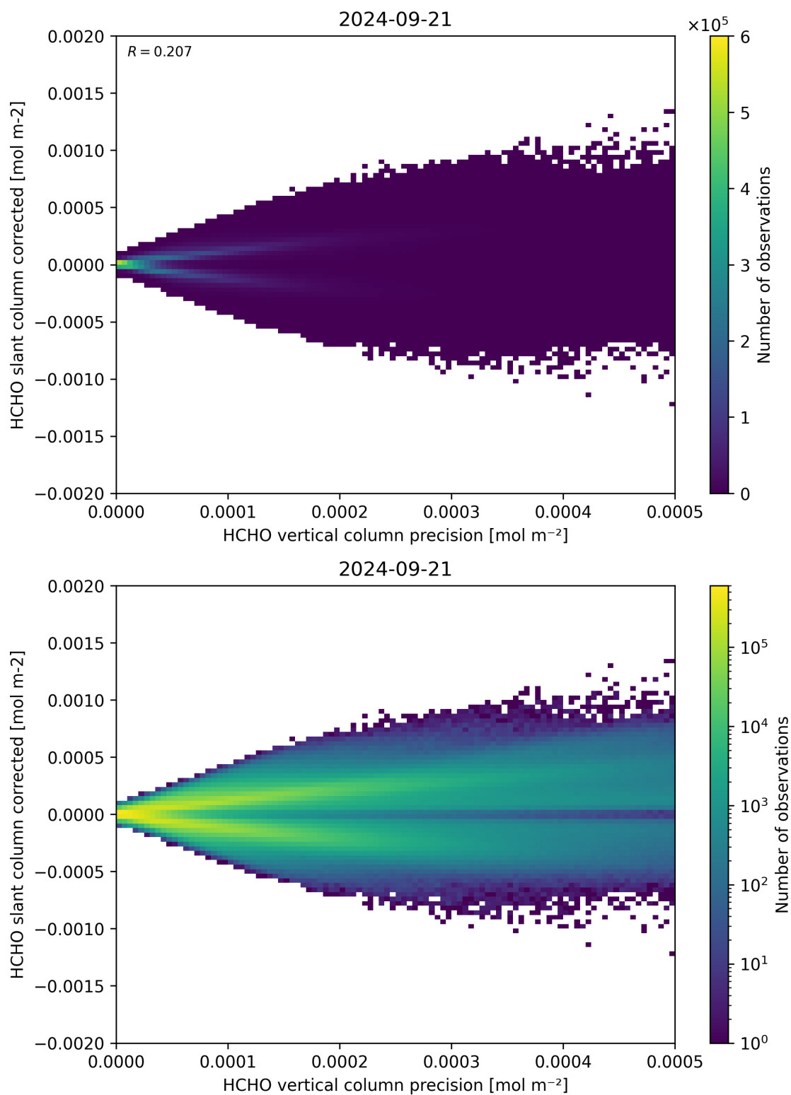
Figure 140: Scatter density plot of “HCHO vertical column precision” against “HCHO slant column corrected” for 2024-09-20 to 2024-09-22.
