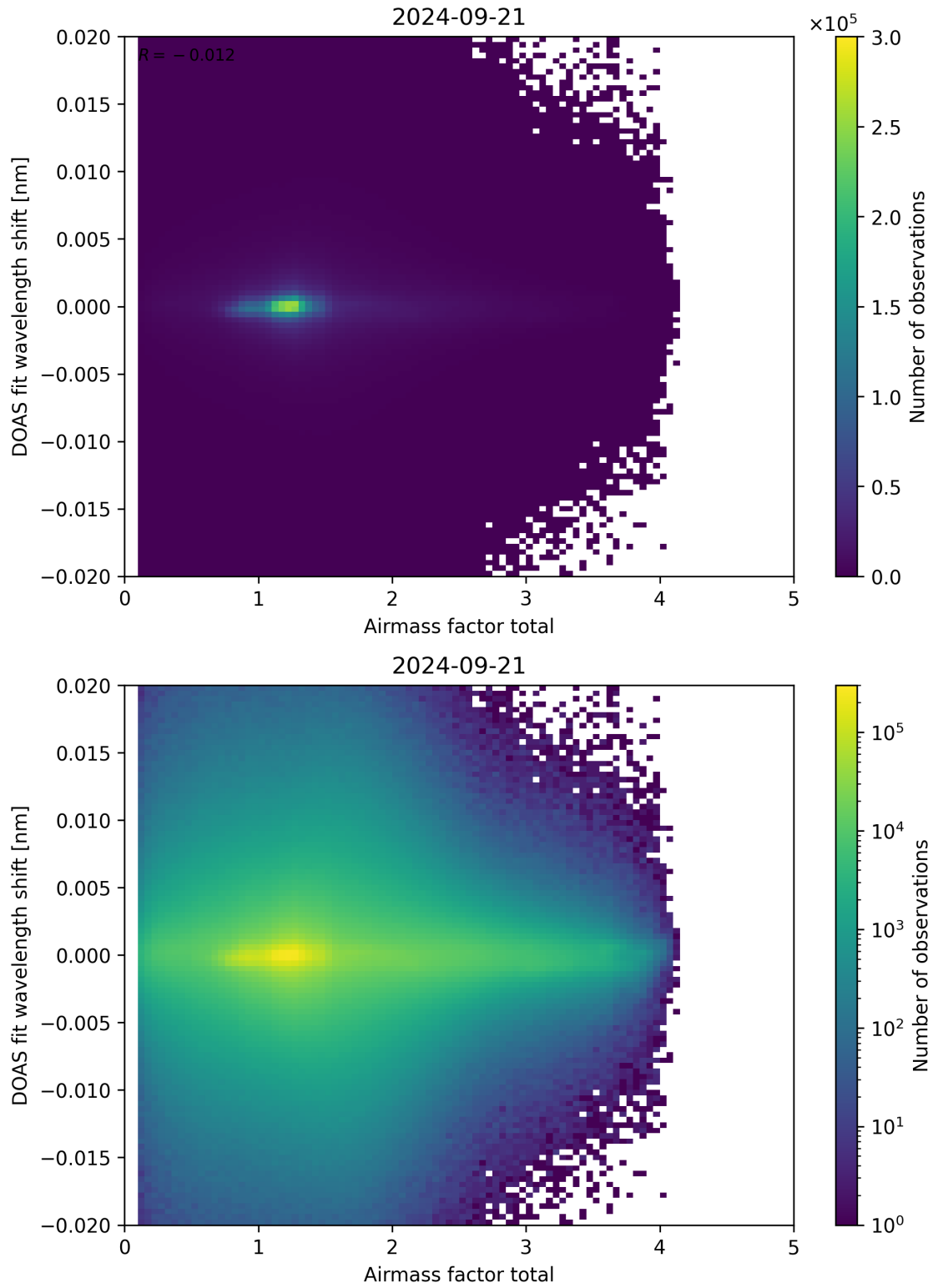
Figure 98: Scatter density plot of “Airmass factor total” against “DOAS fit wavelength shift” for 2024-09-20 to 2024-09-22.
