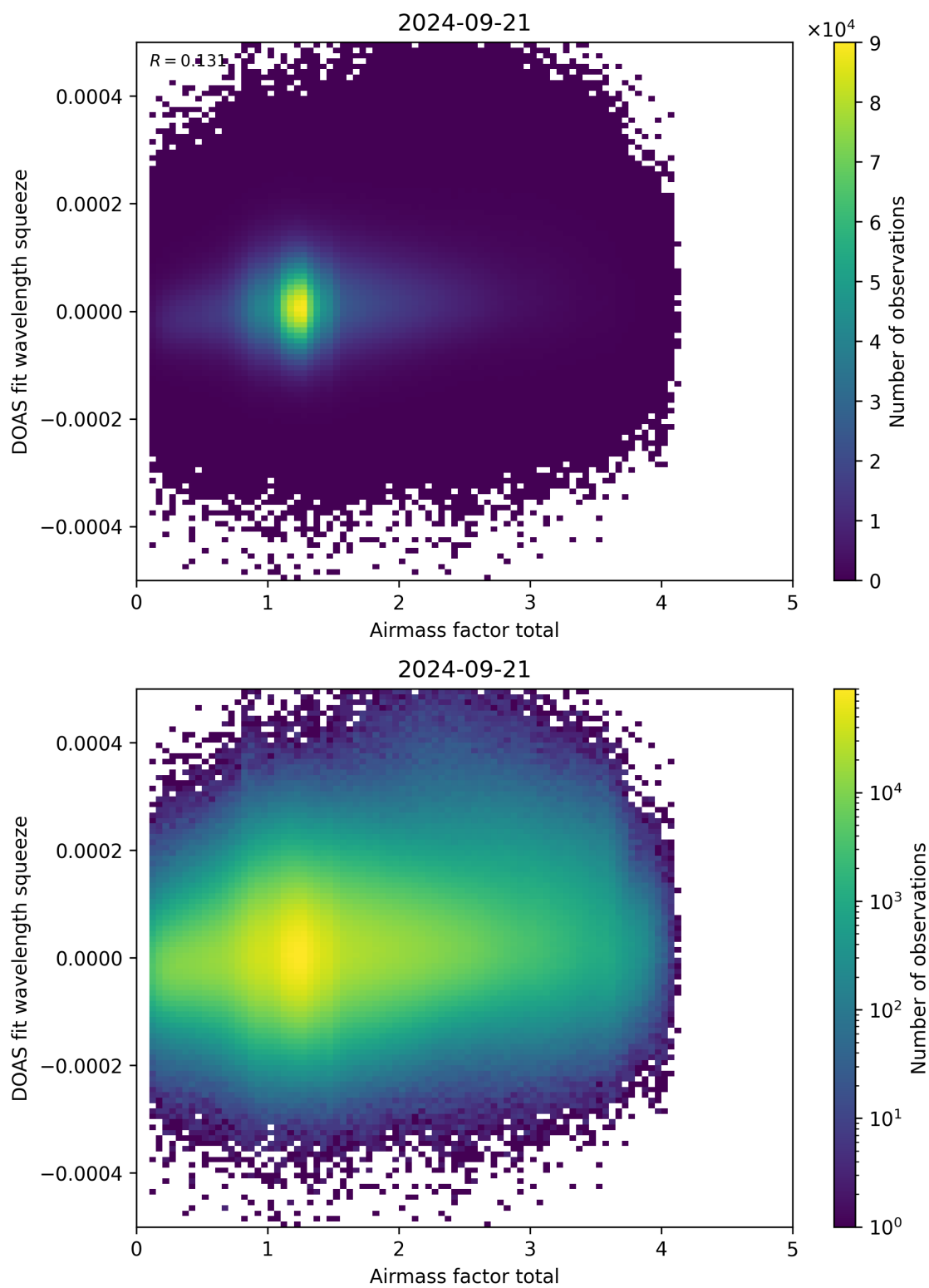
Figure 99: Scatter density plot of “Airmass factor total” against “DOAS fit wavelength squeeze” for 2024-09-20 to 2024-09-22.
