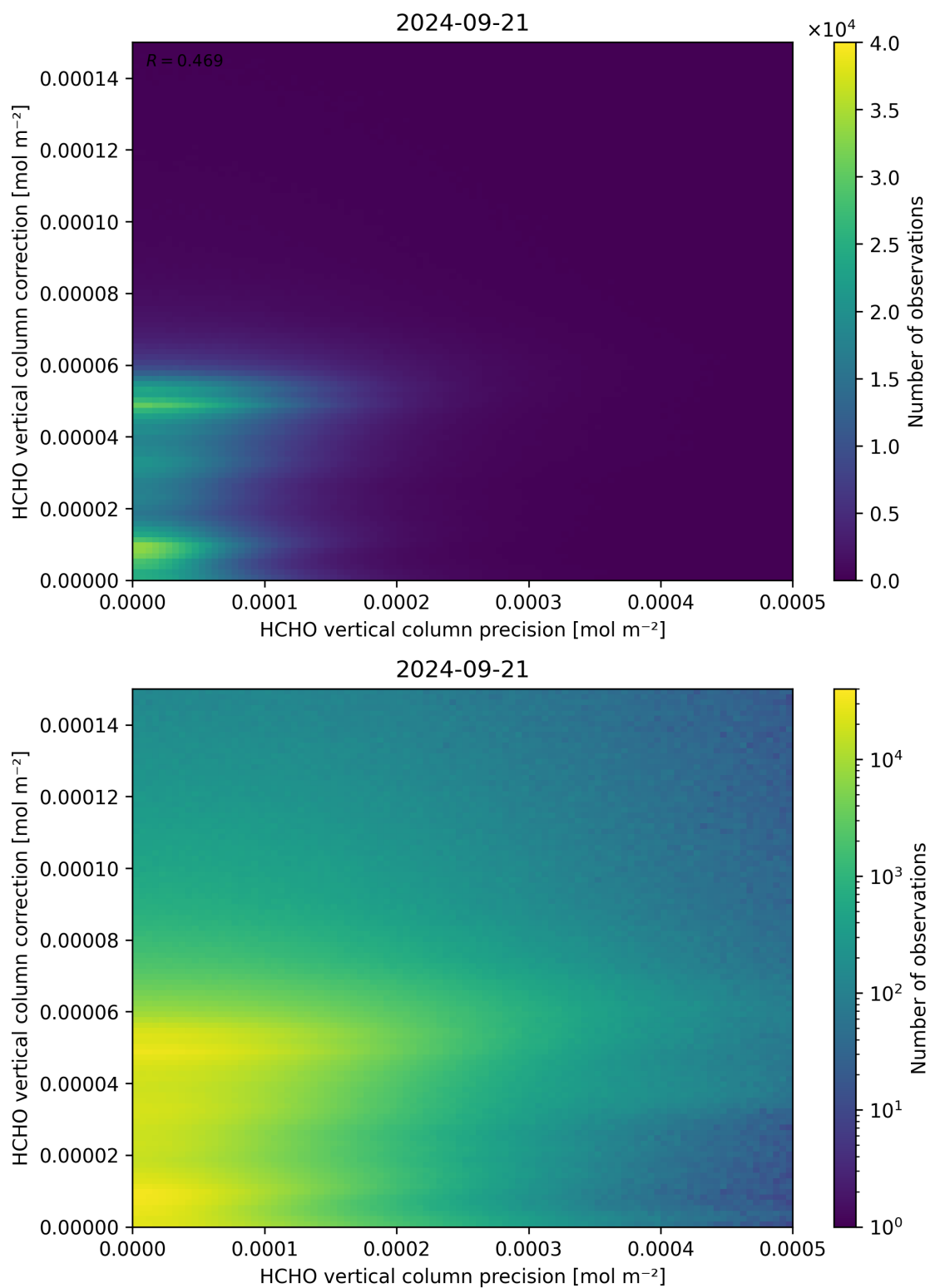
Figure 146: Scatter density plot of “HCHO vertical column precision” against “HCHO vertical column correction” for 2024-09-20 to 2024-09-22.
