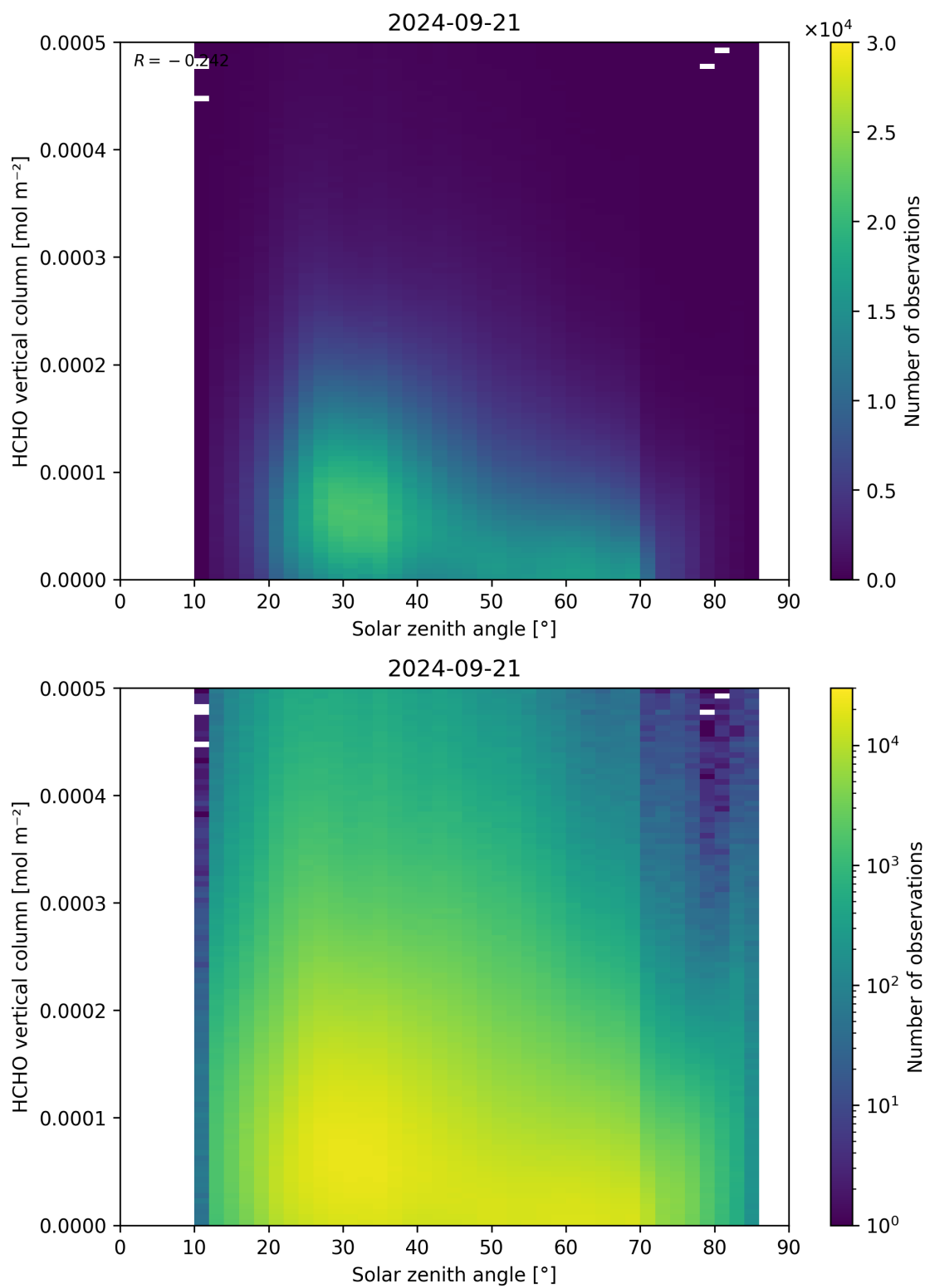
Figure 177: Scatter density plot of “Solar zenith angle” against “HCHO vertical column” for 2024-09-20 to 2024-09-22.
