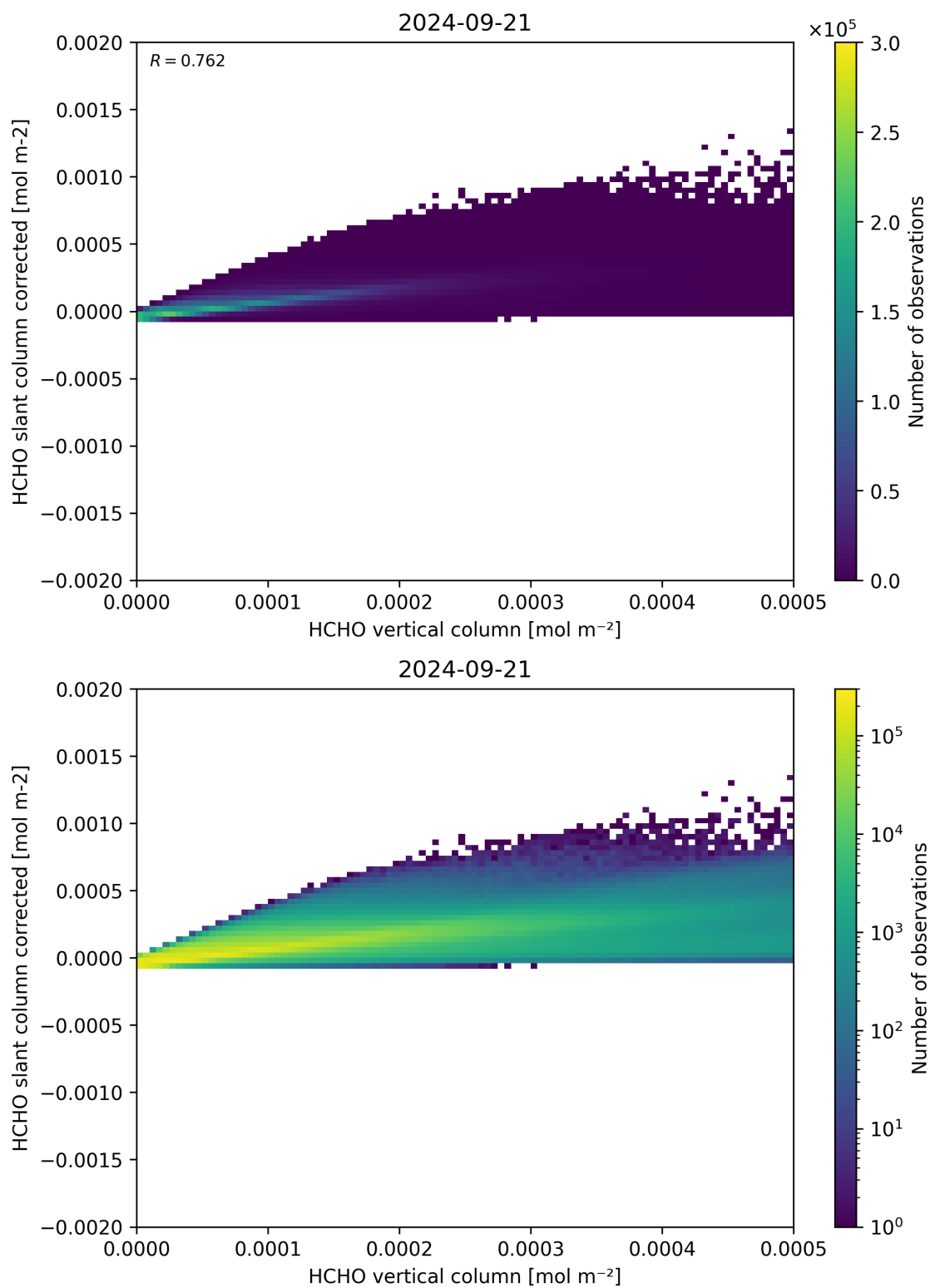
Figure 127: Scatter density plot of “HCHO vertical column” against “HCHO slant column corrected” for 2024-09-20 to 2024-09-22.
