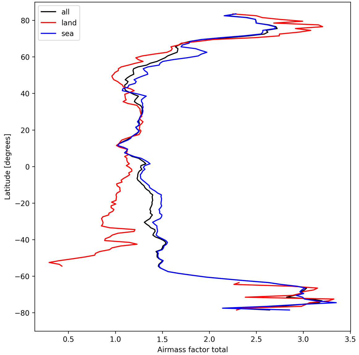
Figure 26: Zonal average of “Airmass factor total” for 2024-09-20 to 2024-09-22.
