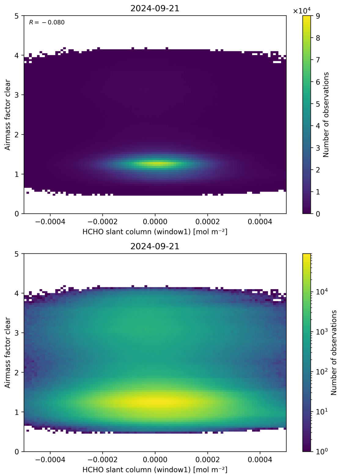
Figure 81: Scatter density plot of “HCHO slant column (window1)” against “Airmass factor clear” for 2024-09-20 to 2024-09-22.
