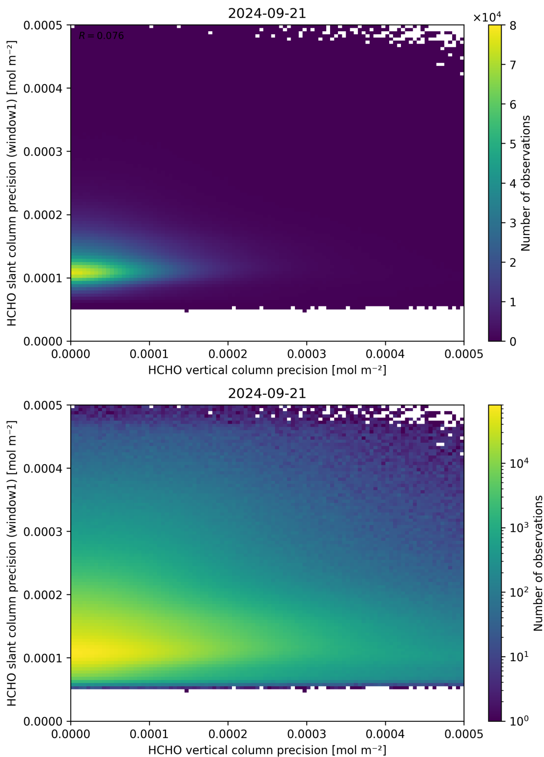
Figure 143: Scatter density plot of “HCHO vertical column precision” against “HCHO slant column precision (window1)” for 2024-09-20 to 2024-09-22.
