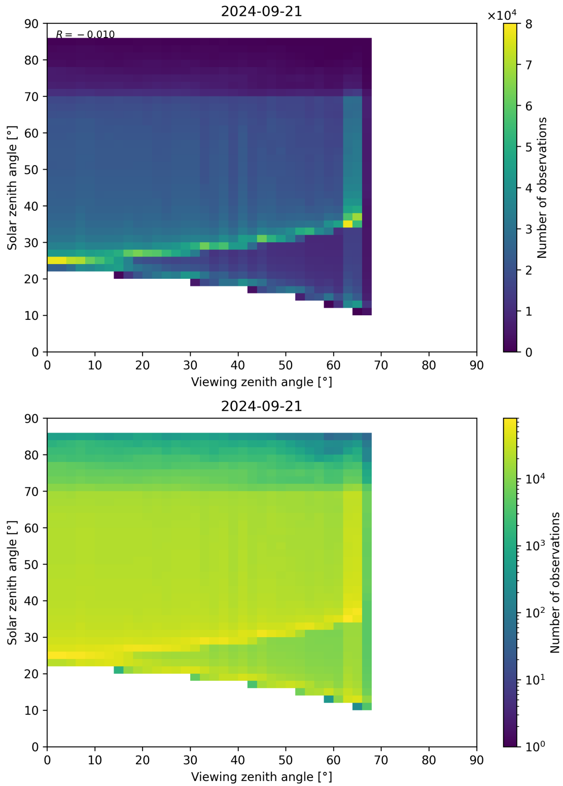
Figure 197: Scatter density plot of “Viewing zenith angle” against “Solar zenith angle” for 2024-09-20 to 2024-09-22.
