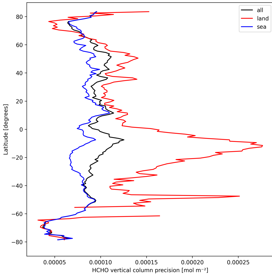
Figure 22: Zonal average of “HCHO vertical column precision” for 2024-09-22 to 2024-09-23.
