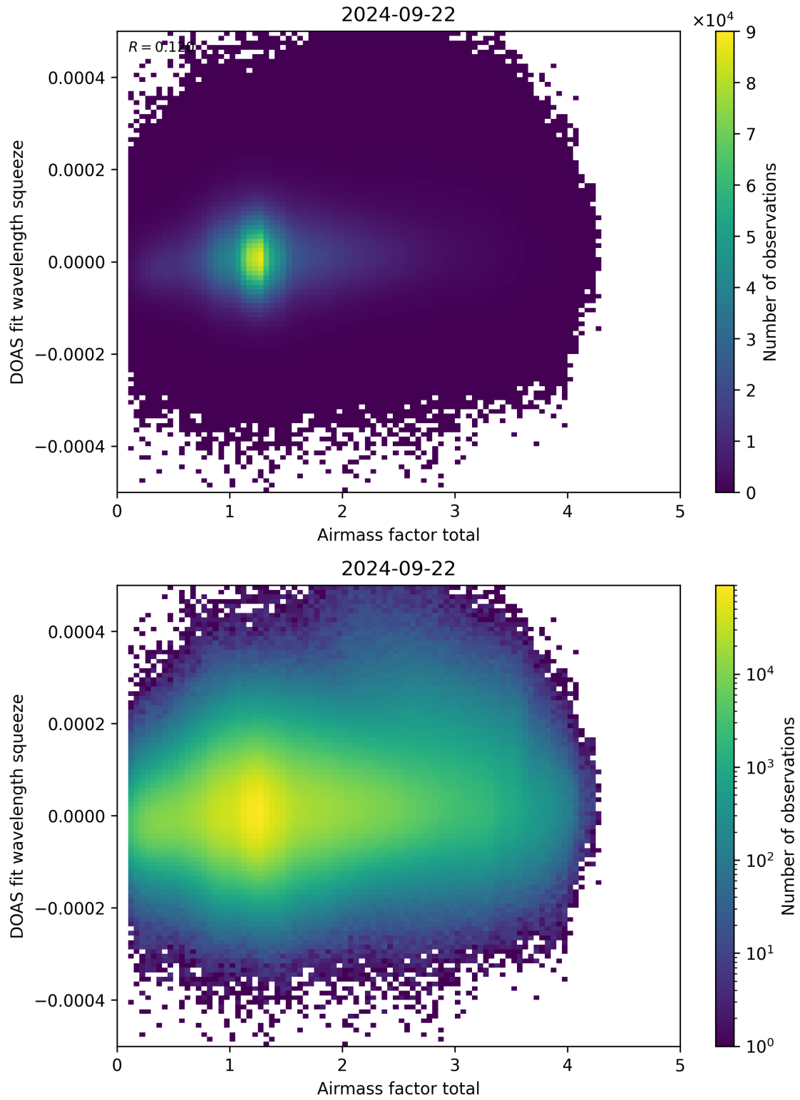
Figure 99: Scatter density plot of “Airmass factor total” against “DOAS fit wavelength squeeze” for 2024-09-22 to 2024-09-23.
