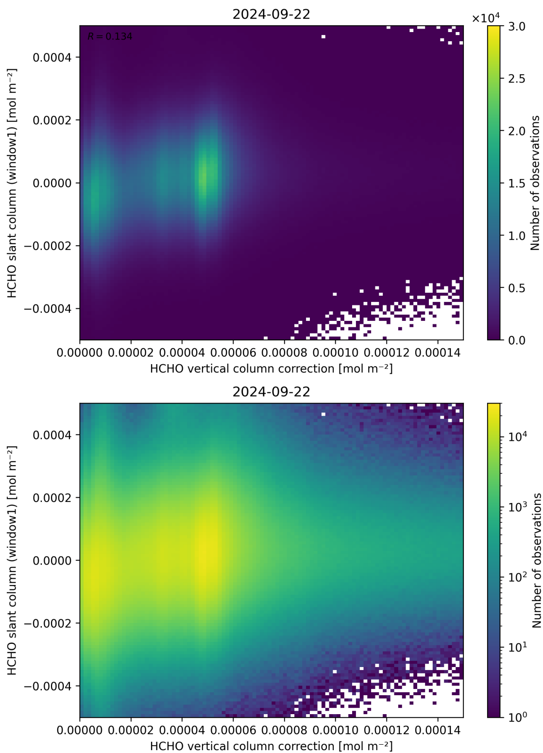
Figure 118: Scatter density plot of “HCHO vertical column correction” against “HCHO slant column (window1)” for 2024-09-22 to 2024-09-23.
