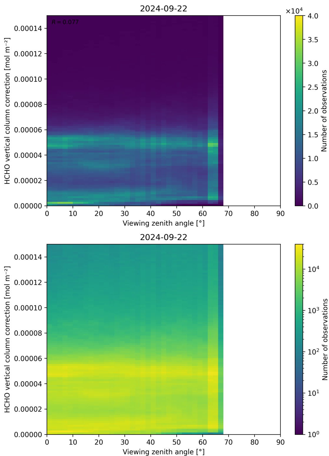
Figure 193: Scatter density plot of “Viewing zenith angle” against “HCHO vertical column correction” for 2024-09-22 to 2024-09-23.
