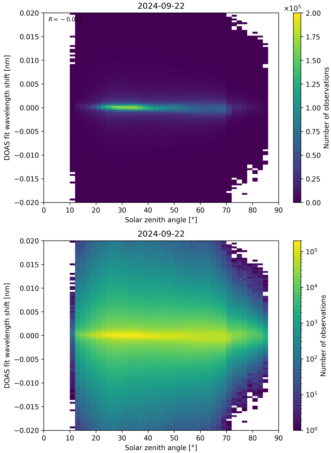
Figure 168: Scatter density plot of “Solar zenith angle” against “DOAS fit wavelength shift” for 2024-09-22 to 2024-09-23.
