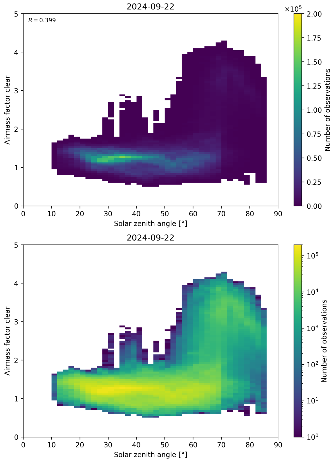
Figure 170: Scatter density plot of “Solar zenith angle” against “Airmass factor clear” for 2024-09-22 to 2024-09-23.
