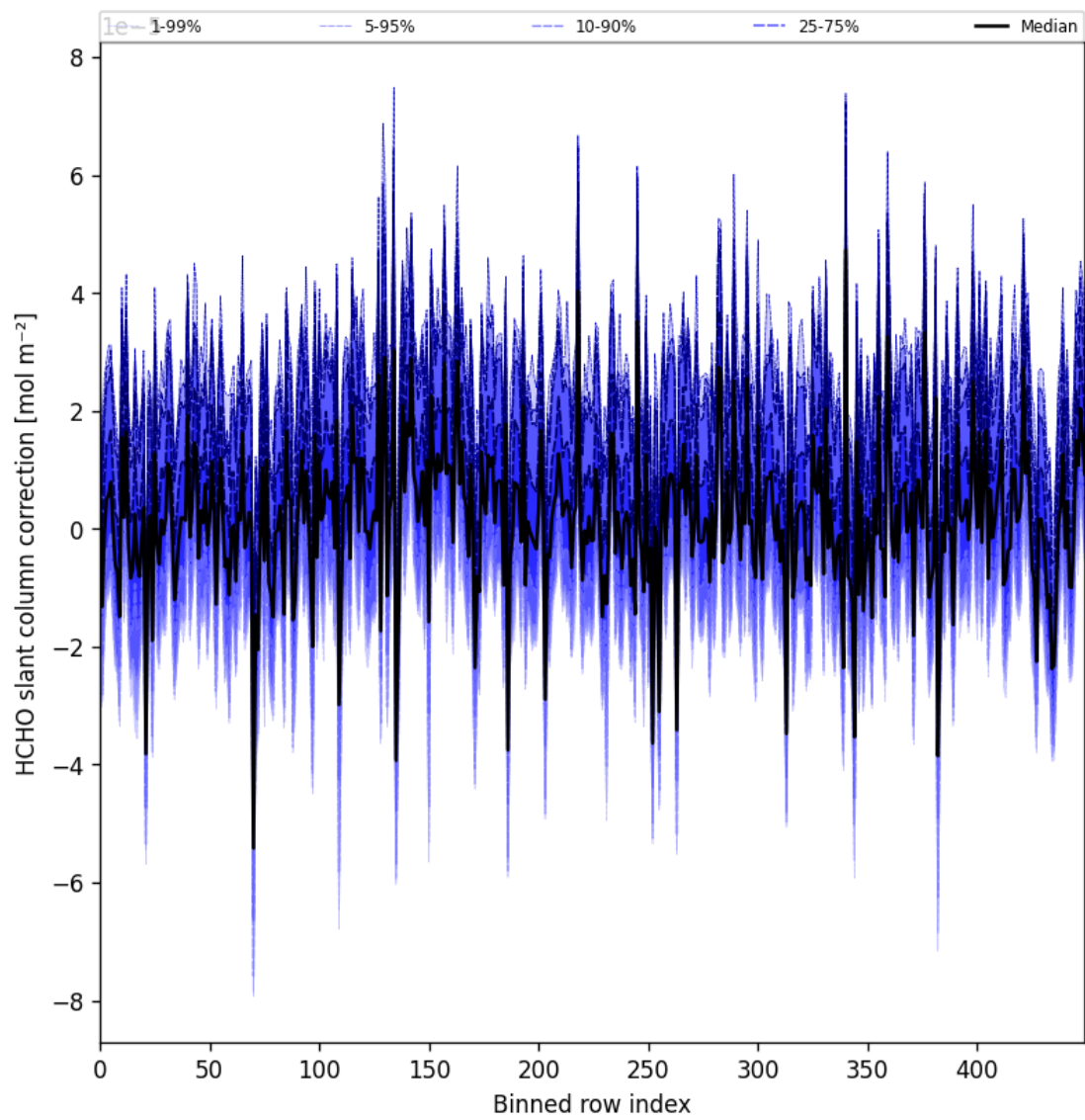
Figure 61: Along track statistics of “HCHO slant column correction” for 2024-09-22 to 2024-09-23
