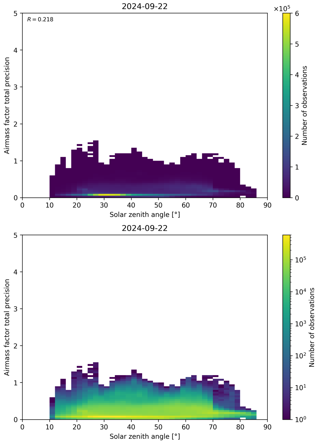
Figure 176: Scatter density plot of “Solar zenith angle” against “Airmass factor total precision” for 2024-09-22 to 2024-09-23.
