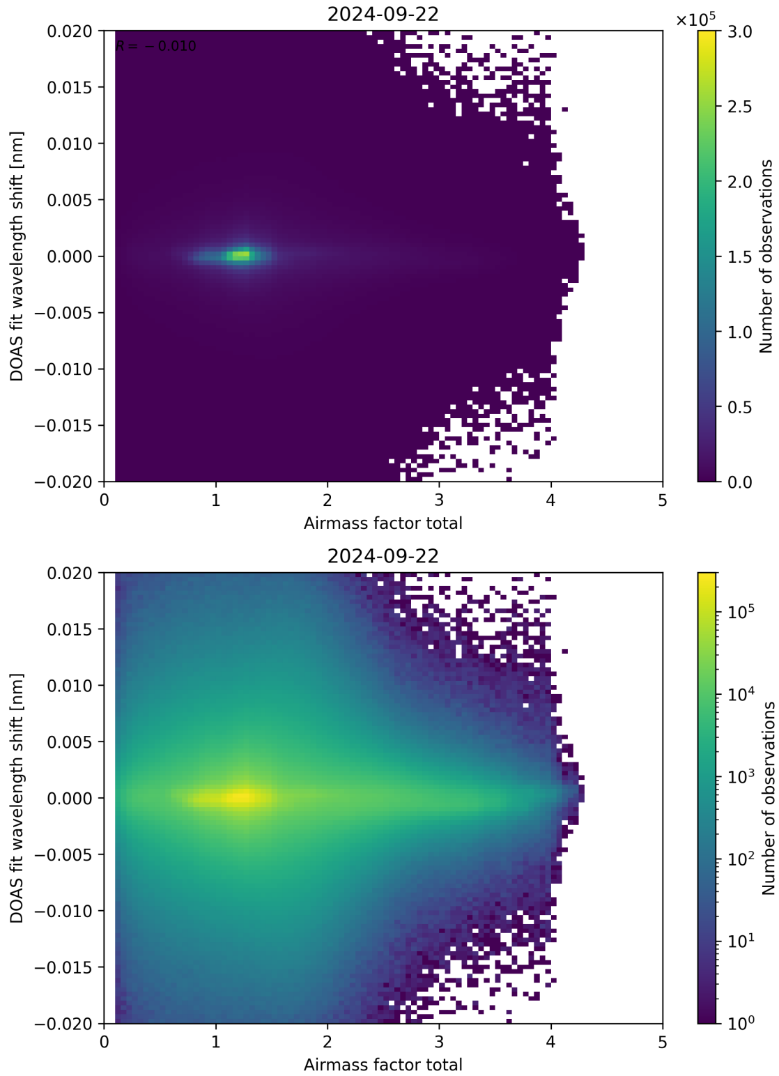
Figure 98: Scatter density plot of “Airmass factor total” against “DOAS fit wavelength shift” for 2024-09-22 to 2024-09-23.
