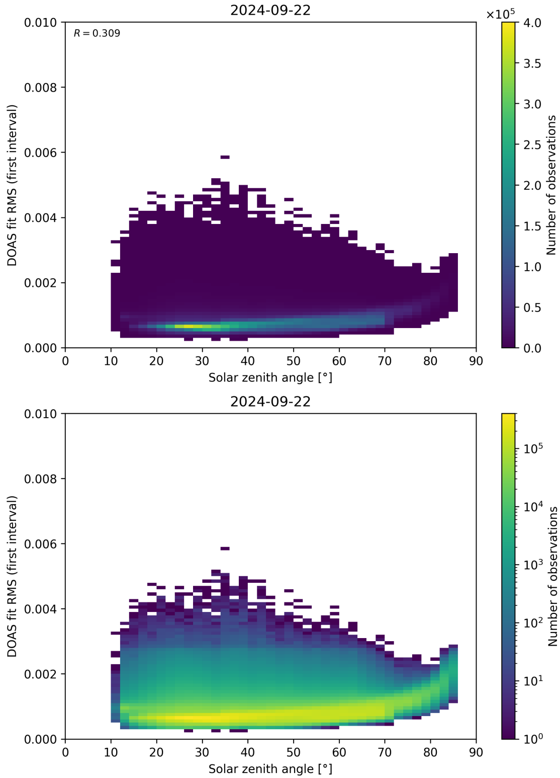
Figure 167: Scatter density plot of “Solar zenith angle” against “DOAS fit RMS (first interval)” for 2024-09-22 to 2024-09-23.
