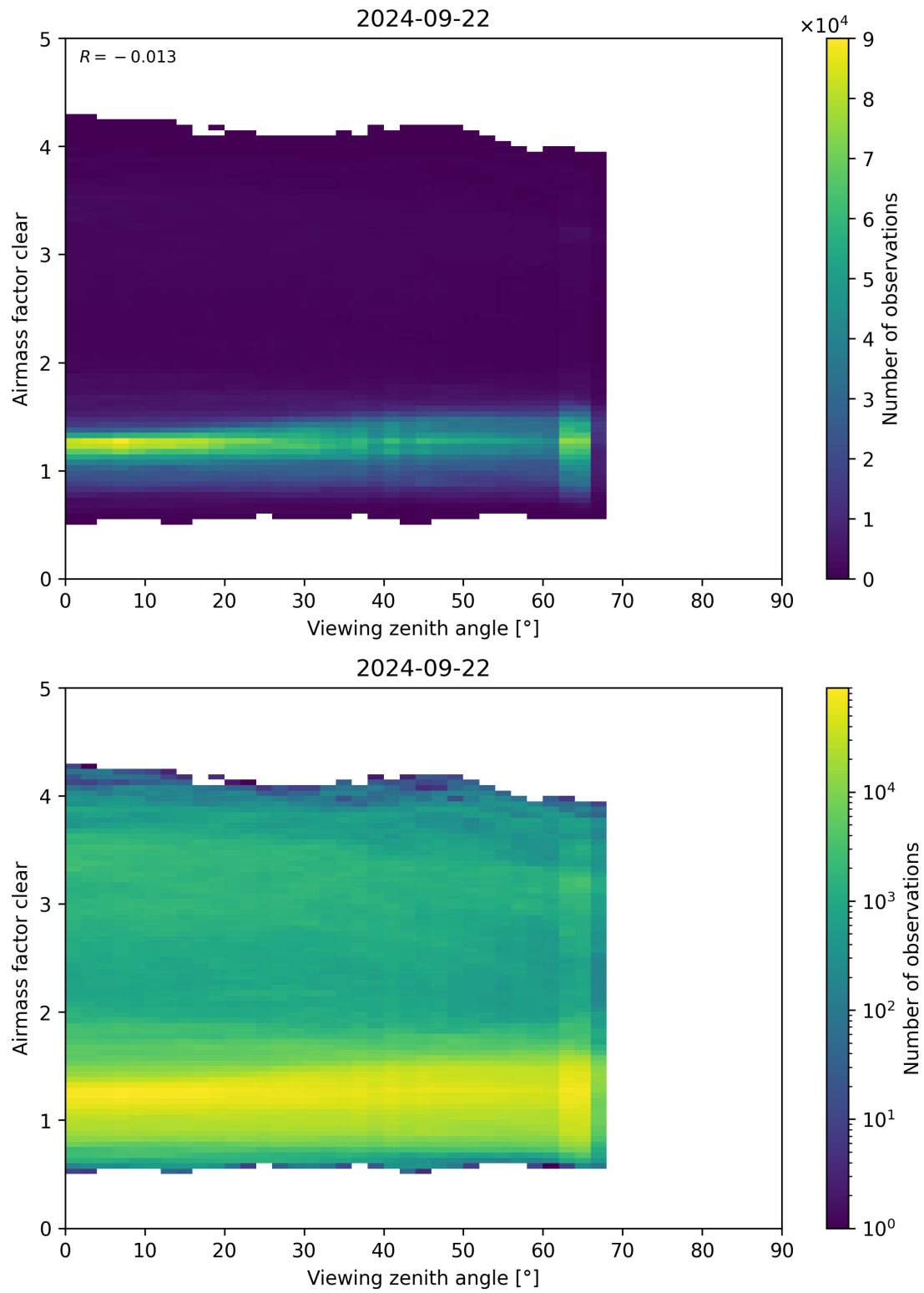
Figure 185: Scatter density plot of “Viewing zenith angle” against “Airmass factor clear” for 2024-09-22 to 2024-09-23.
