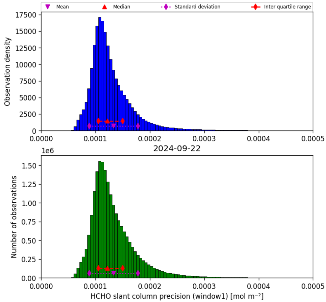
Figure 39: Histogram of “HCHO slant column precision (window1)” for 2024-09-22 to 2024-09-23
