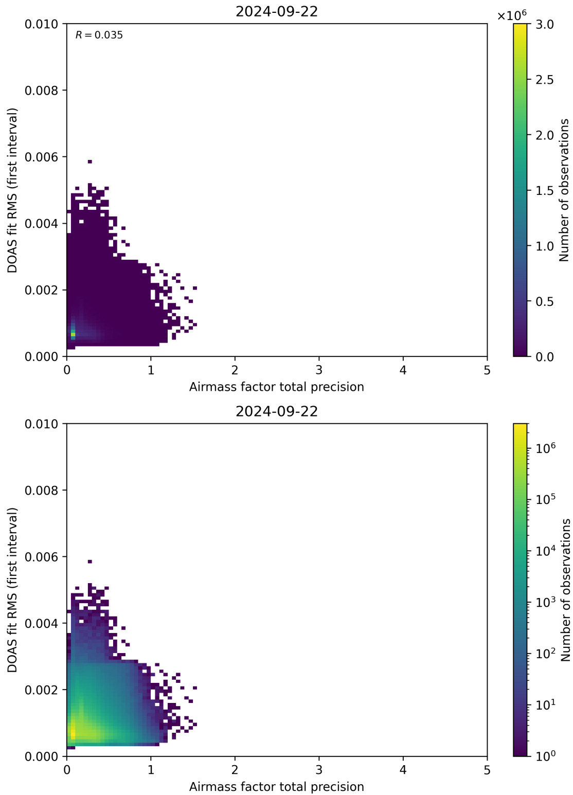
Figure 105: Scatter density plot of “Airmass factor total precision” against “DOAS fit RMS (first interval)” for 2024-09-22 to 2024-09-23.
