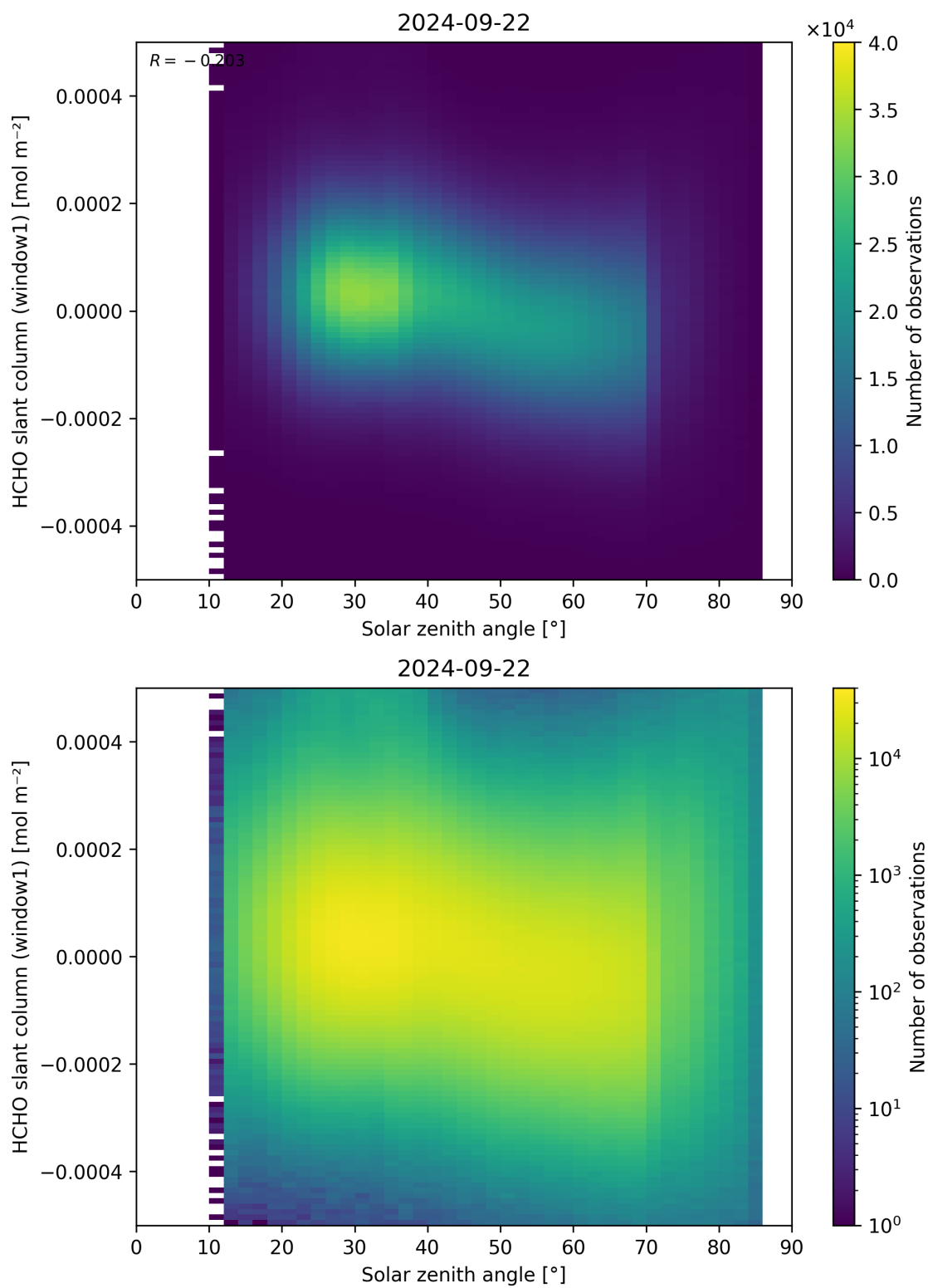
Figure 173: Scatter density plot of “Solar zenith angle” against “HCHO slant column (window1)” for 2024-09-22 to 2024-09-23.
