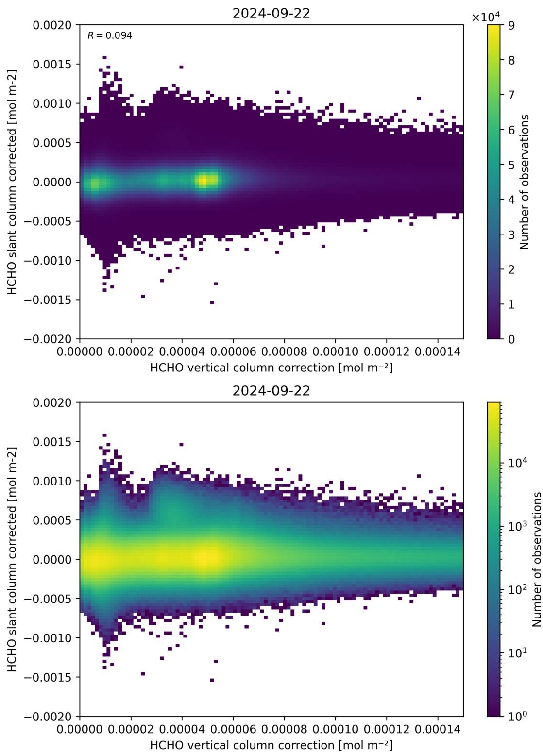
Figure 116: Scatter density plot of “HCHO vertical column correction” against “HCHO slant column corrected” for 2024-09-22 to 2024-09-23.
