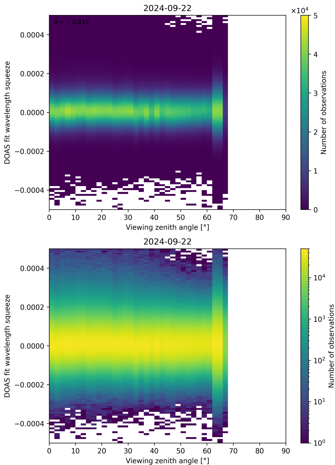
Figure 184: Scatter density plot of “Viewing zenith angle” against “DOAS fit wavelength squeeze” for 2024-09-22 to 2024-09-23.
