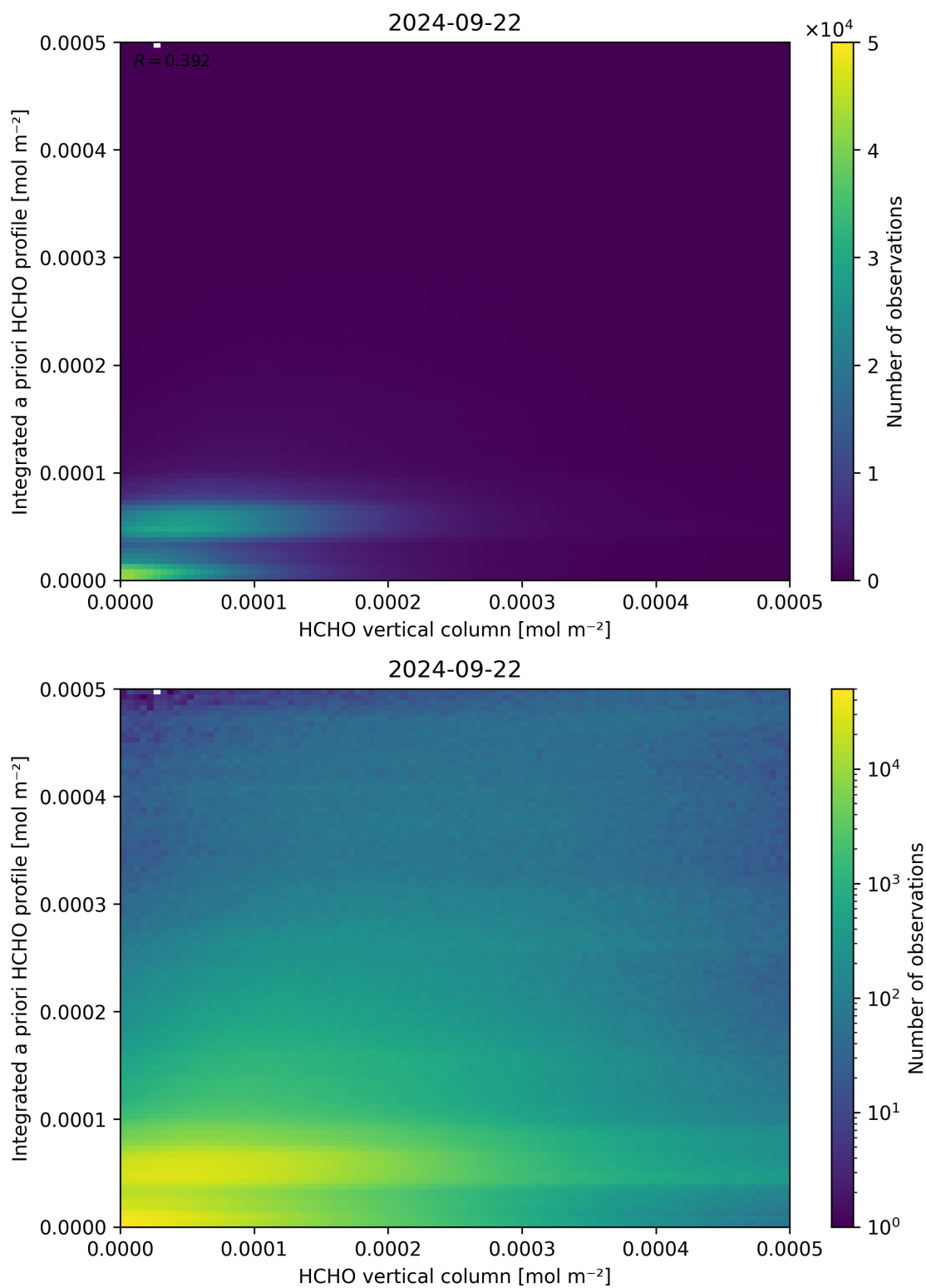
Figure 135: Scatter density plot of “HCHO vertical column” against “Integrated a priori HCHO profile” for 2024-09-22 to 2024-09-23.
