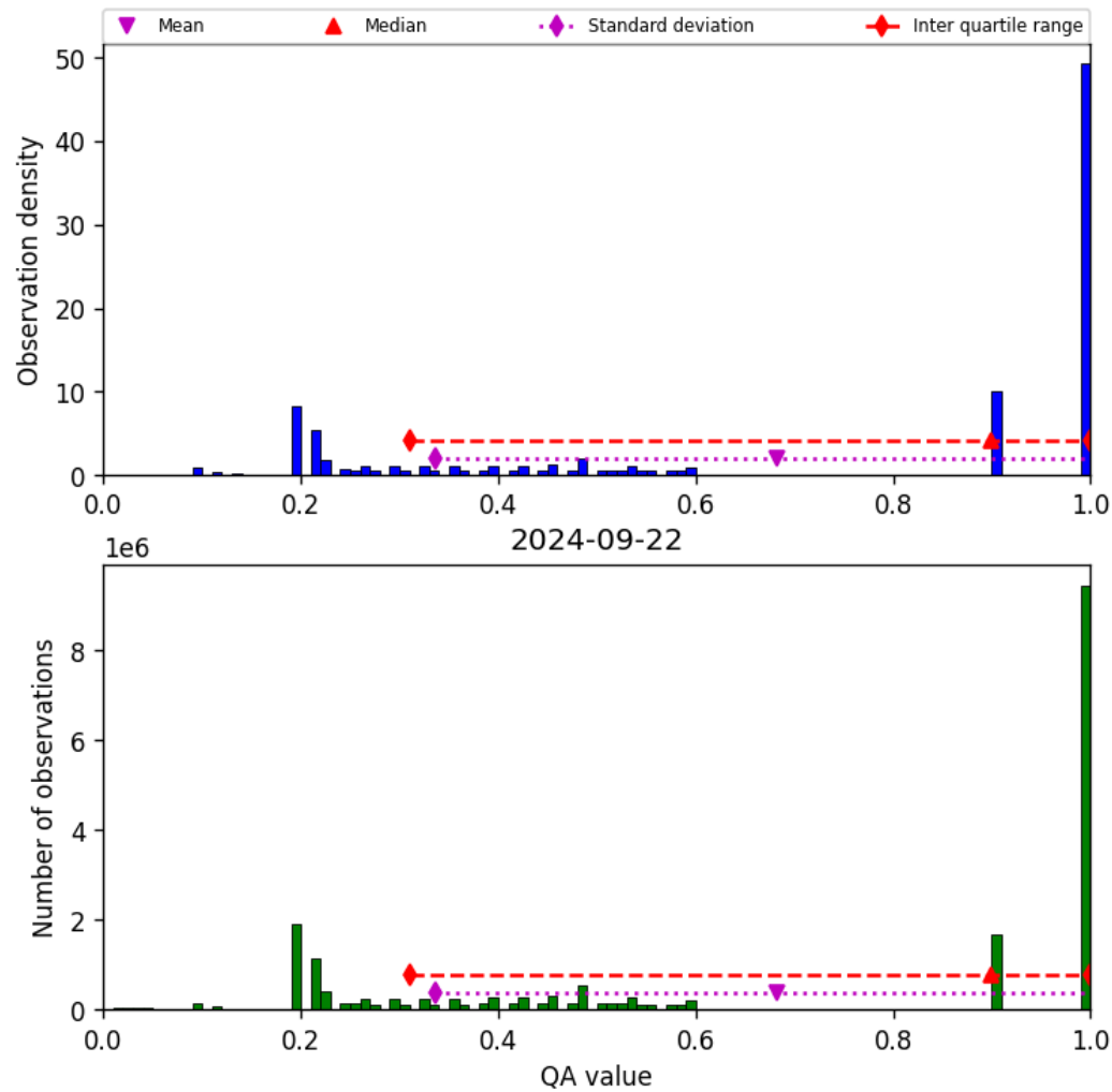
Figure 34: Histogram of “QA value” for 2024-09-22 to 2024-09-23
