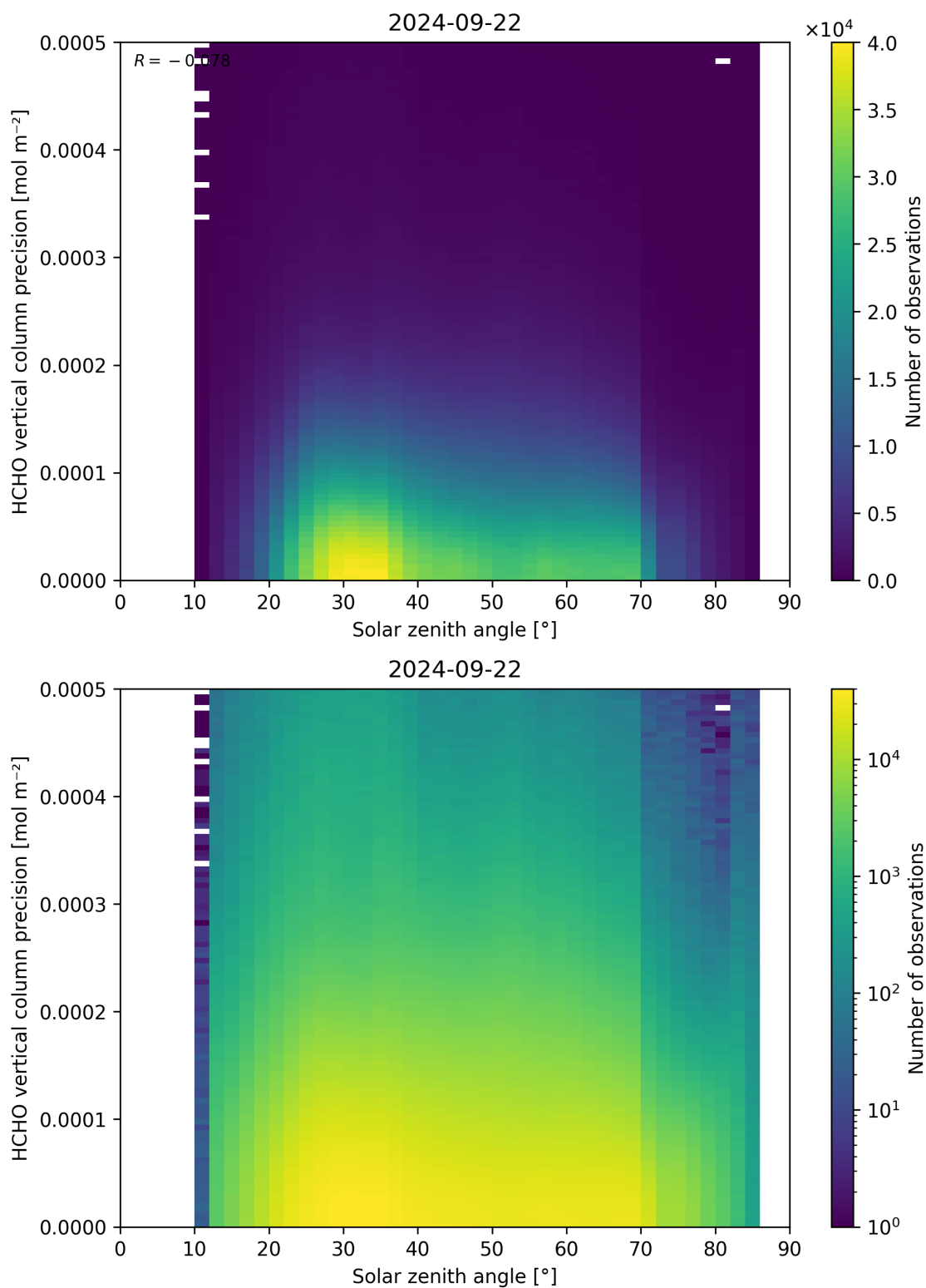
Figure 179: Scatter density plot of “Solar zenith angle” against “HCHO vertical column precision” for 2024-09-22 to 2024-09-23.
