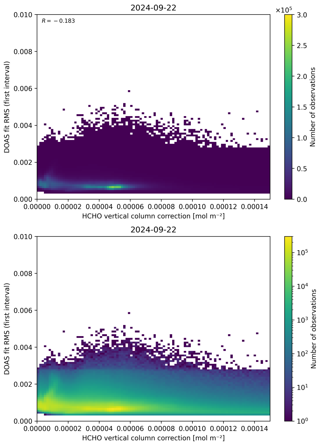
Figure 112: Scatter density plot of “HCHO vertical column correction” against “DOAS fit RMS (first interval)” for 2024-09-22 to 2024-09-23.
