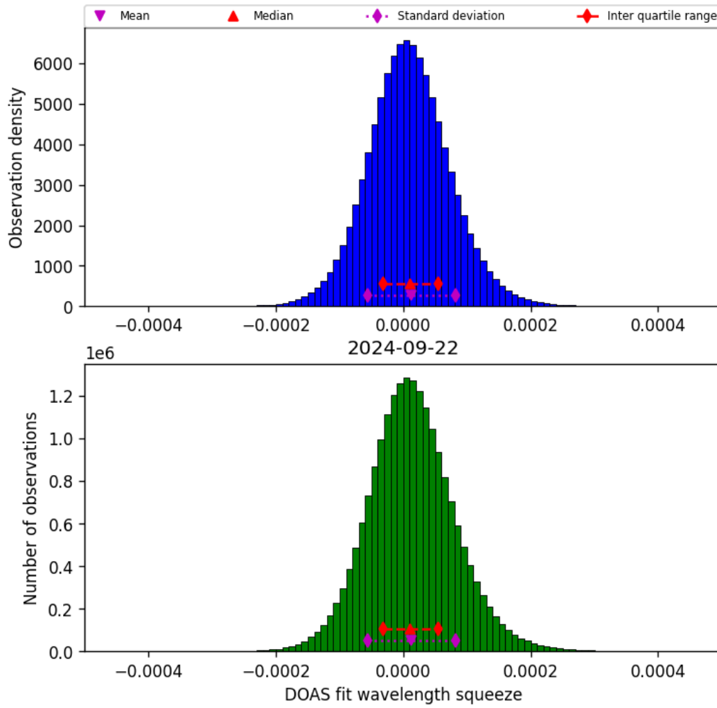
Figure 45: Histogram of “DOAS fit wavelength squeeze” for 2024-09-22 to 2024-09-23
