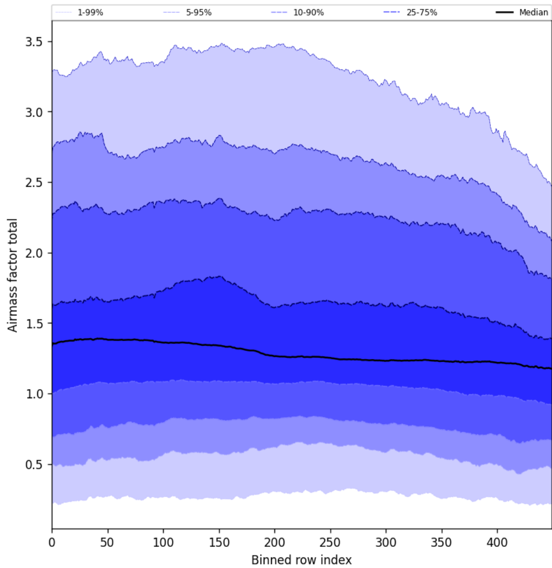
Figure 54: Along track statistics of “Airmass factor total” for 2024-09-22 to 2024-09-23
