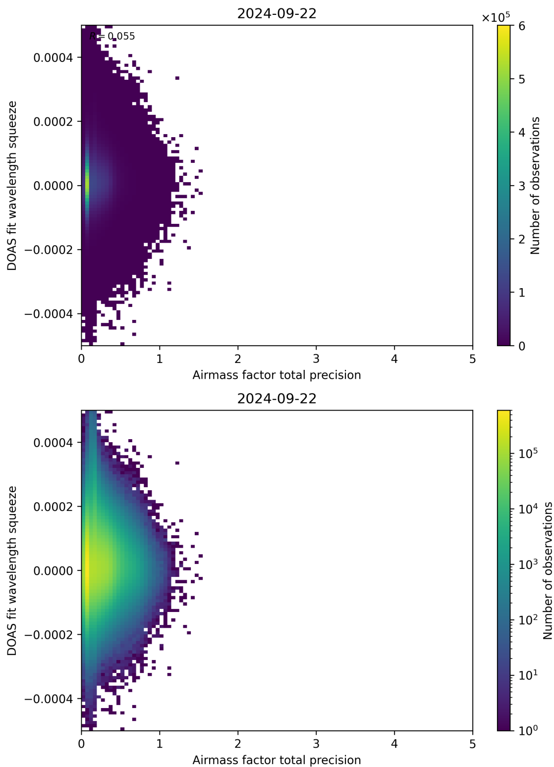
Figure 107: Scatter density plot of “Airmass factor total precision” against “DOAS fit wavelength squeeze” for 2024-09-22 to 2024-09-23.
