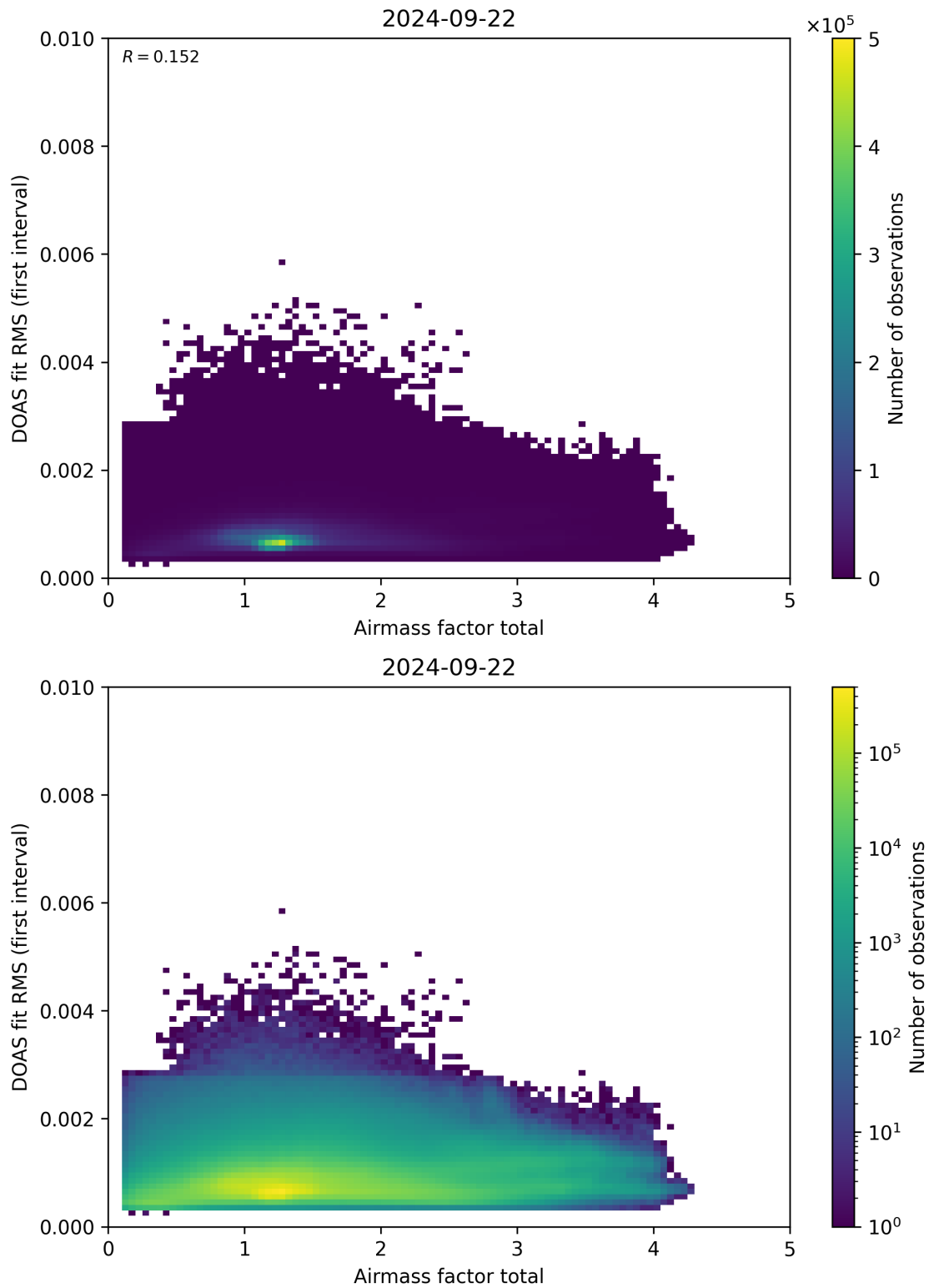
Figure 97: Scatter density plot of “Airmass factor total” against “DOAS fit RMS (first interval)” for 2024-09-22 to 2024-09-23.
