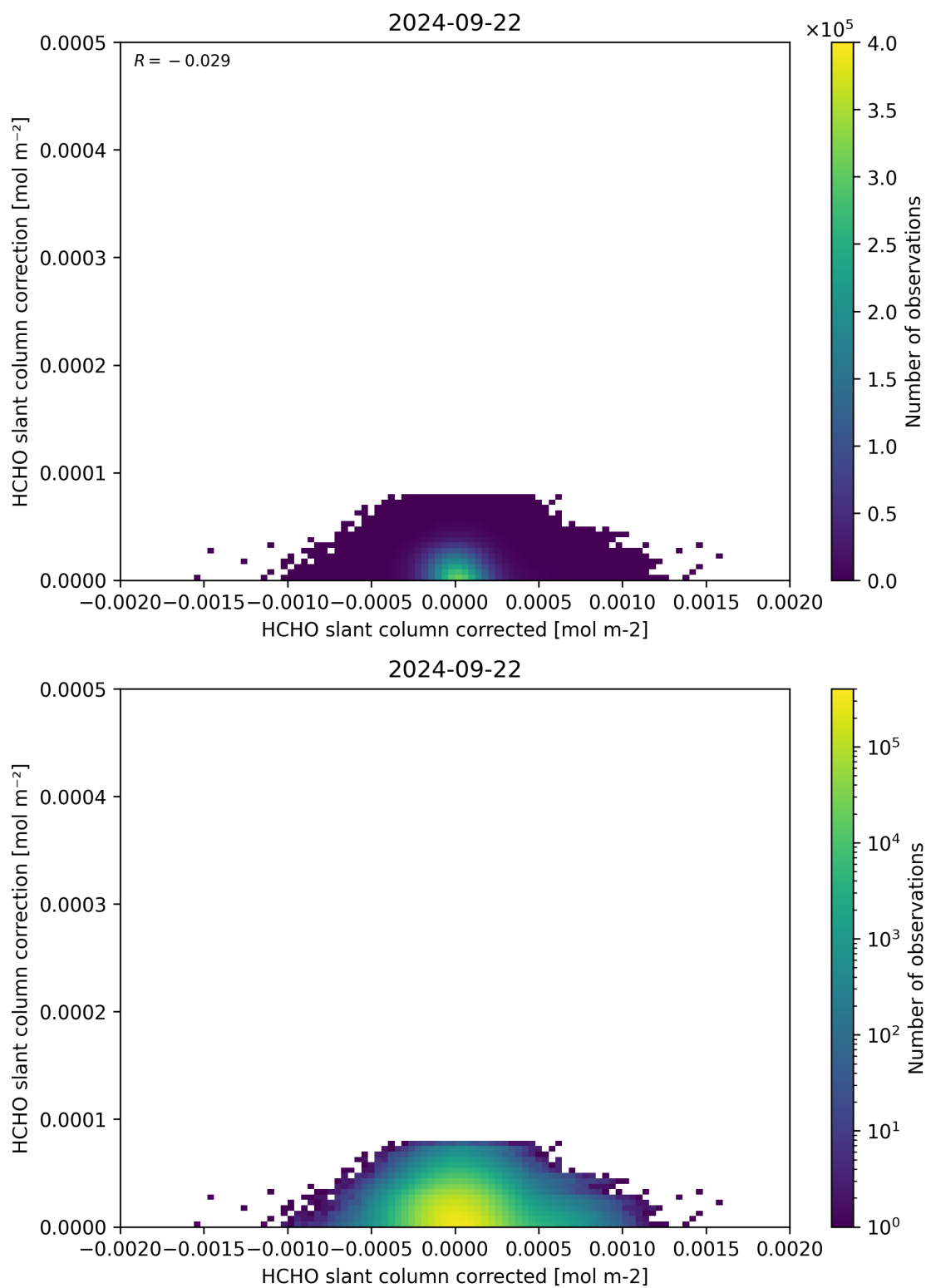
Figure 77: Scatter density plot of “HCHO slant column corrected” against “HCHO slant column correction” for 2024-09-22 to 2024-09-23.
