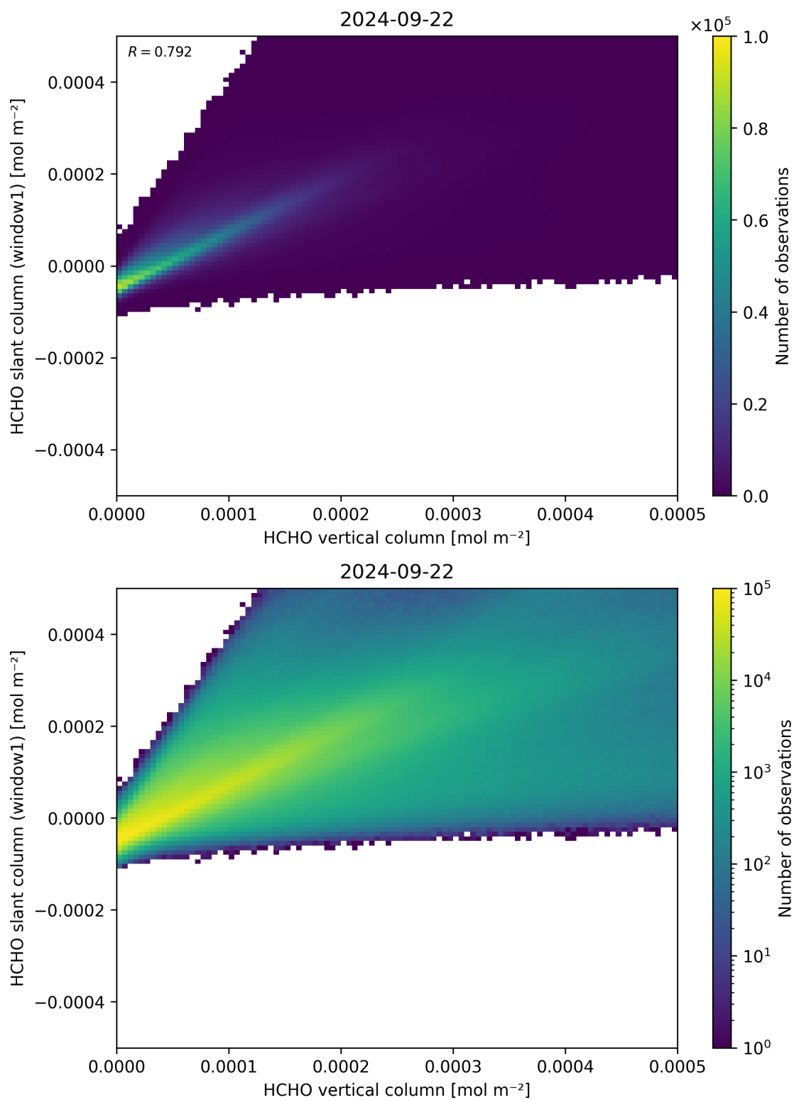
Figure 129: Scatter density plot of “HCHO vertical column” against “HCHO slant column (window1)” for 2024-09-22 to 2024-09-23.
