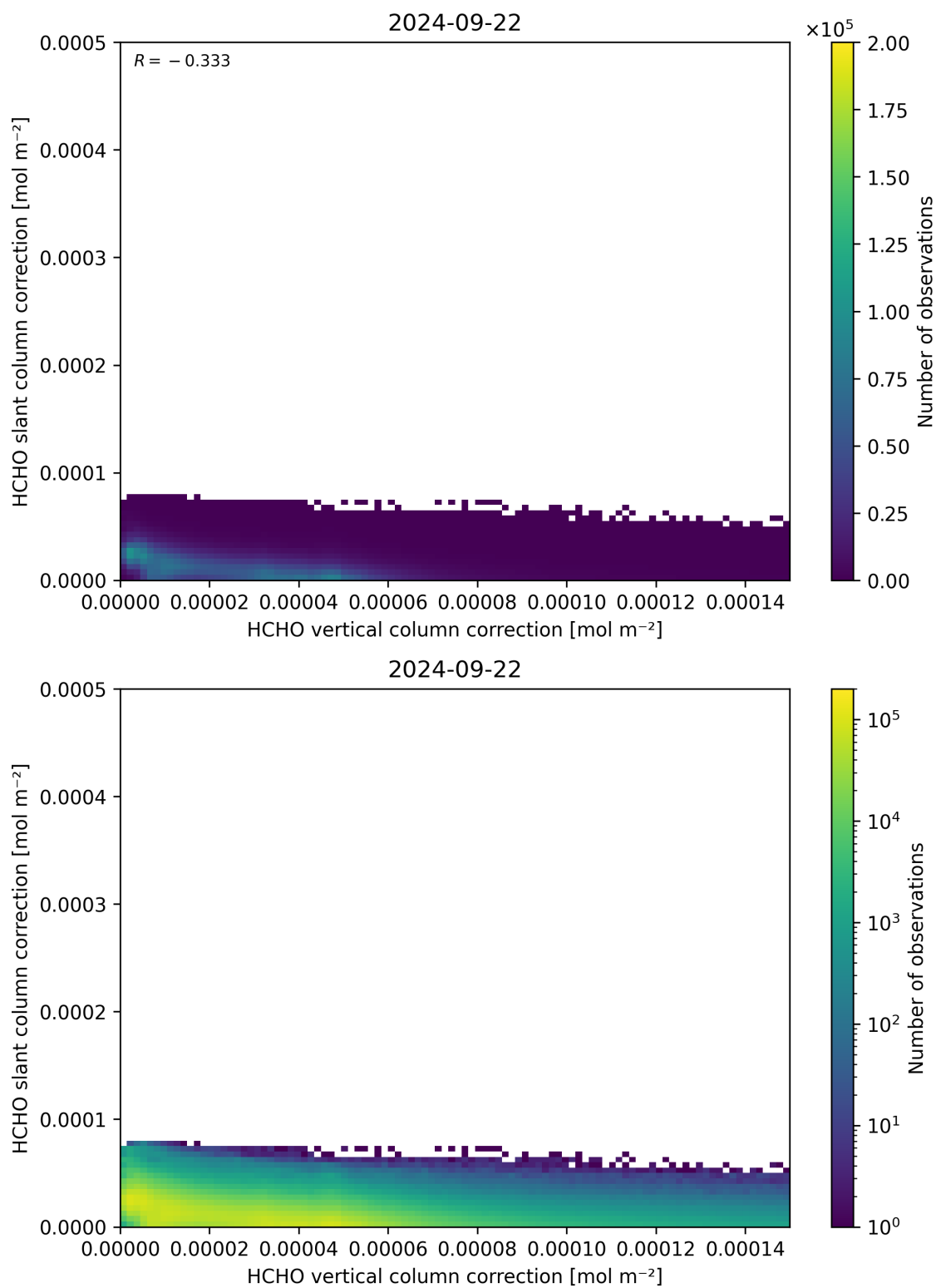
Figure 117: Scatter density plot of “HCHO vertical column correction” against “HCHO slant column correction” for 2024-09-22 to 2024-09-23.
