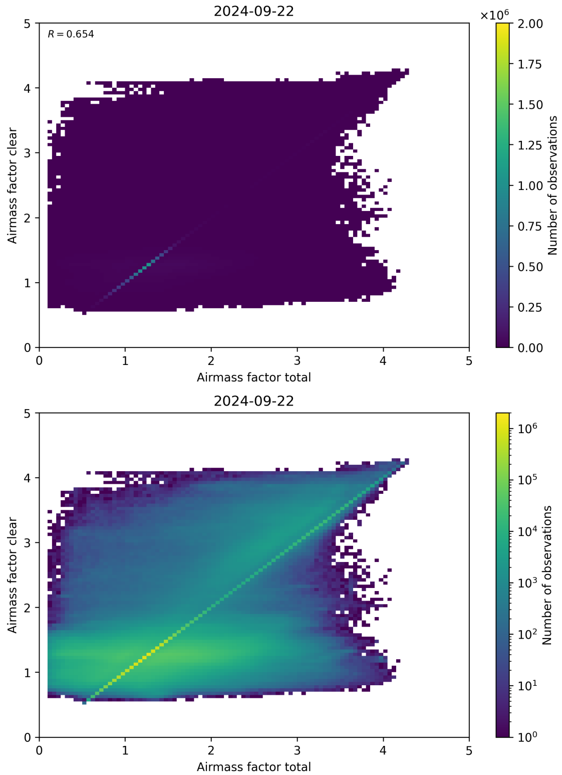
Figure 100: Scatter density plot of “Airmass factor total” against “Airmass factor clear” for 2024-09-22 to 2024-09-23.
