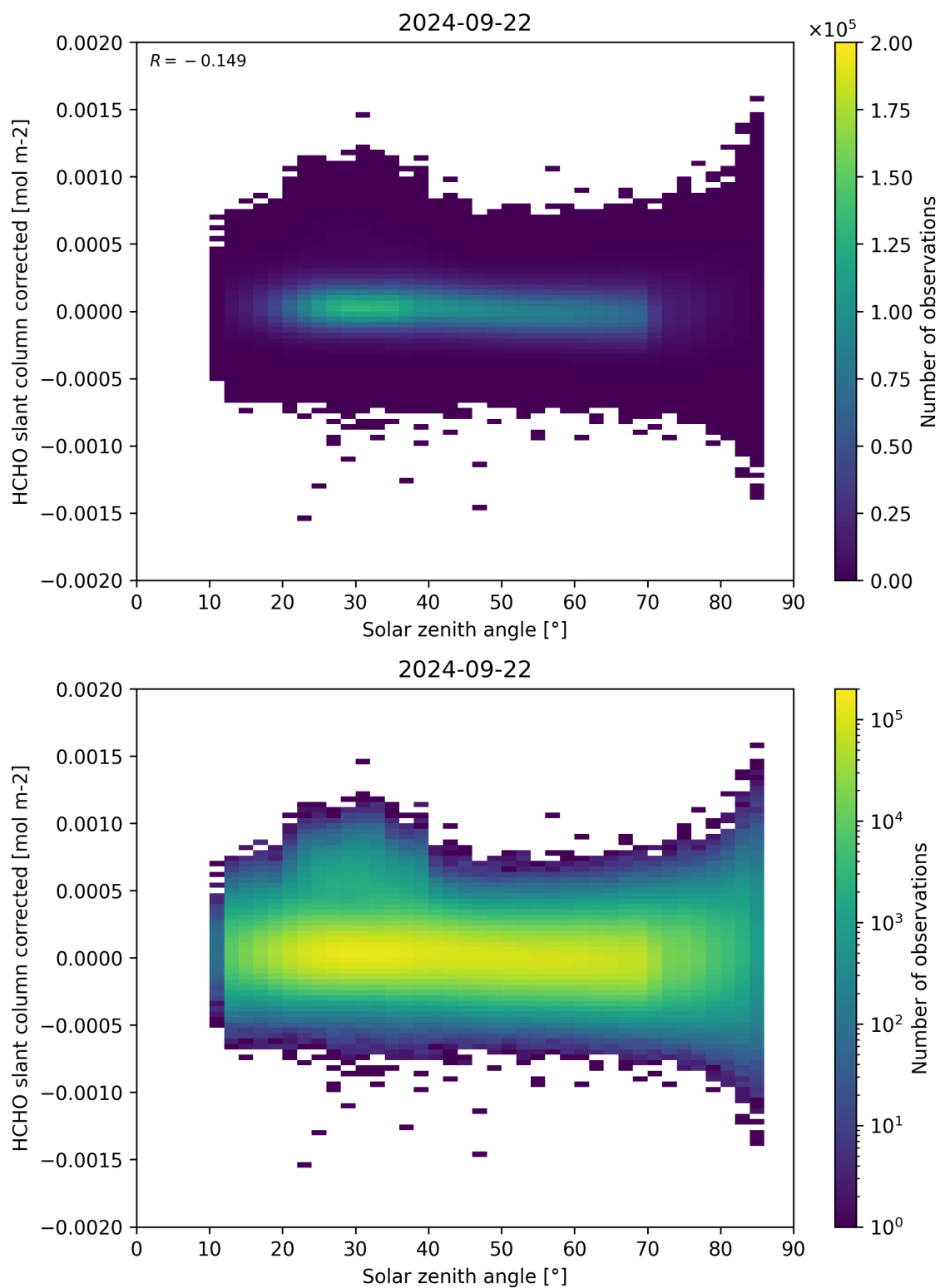
Figure 171: Scatter density plot of “Solar zenith angle” against “HCHO slant column corrected” for 2024-09-22 to 2024-09-23.
