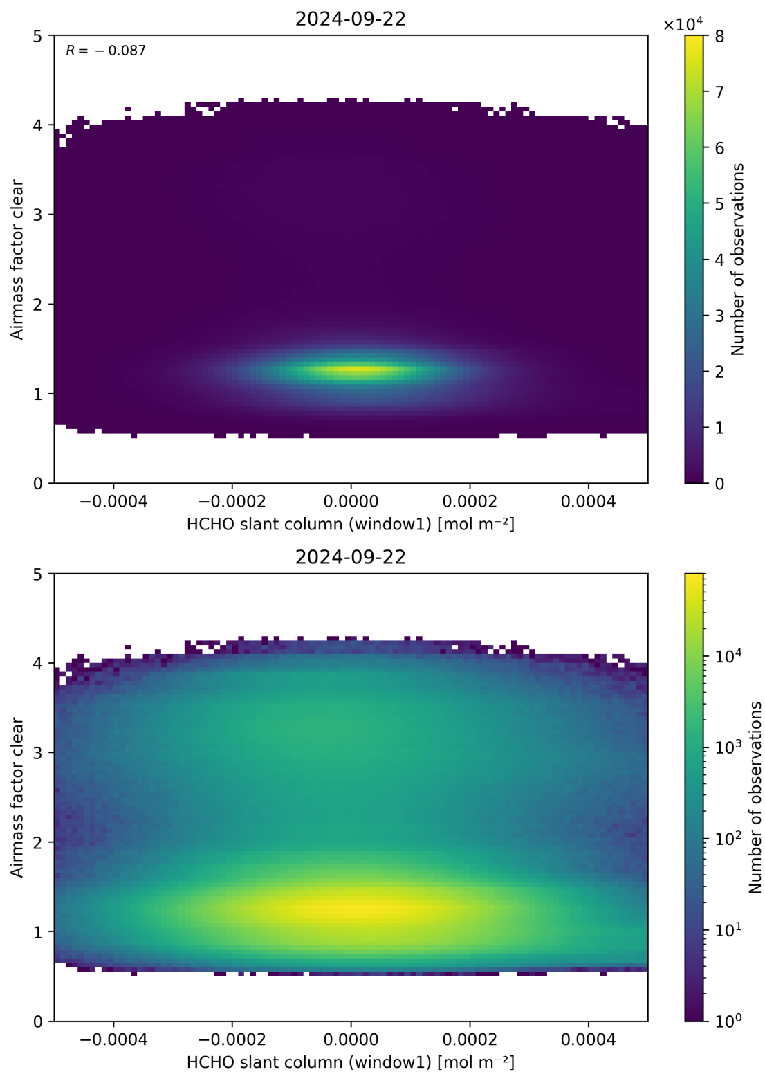
Figure 81: Scatter density plot of “HCHO slant column (window1)” against “Airmass factor clear” for 2024-09-22 to 2024-09-23.
