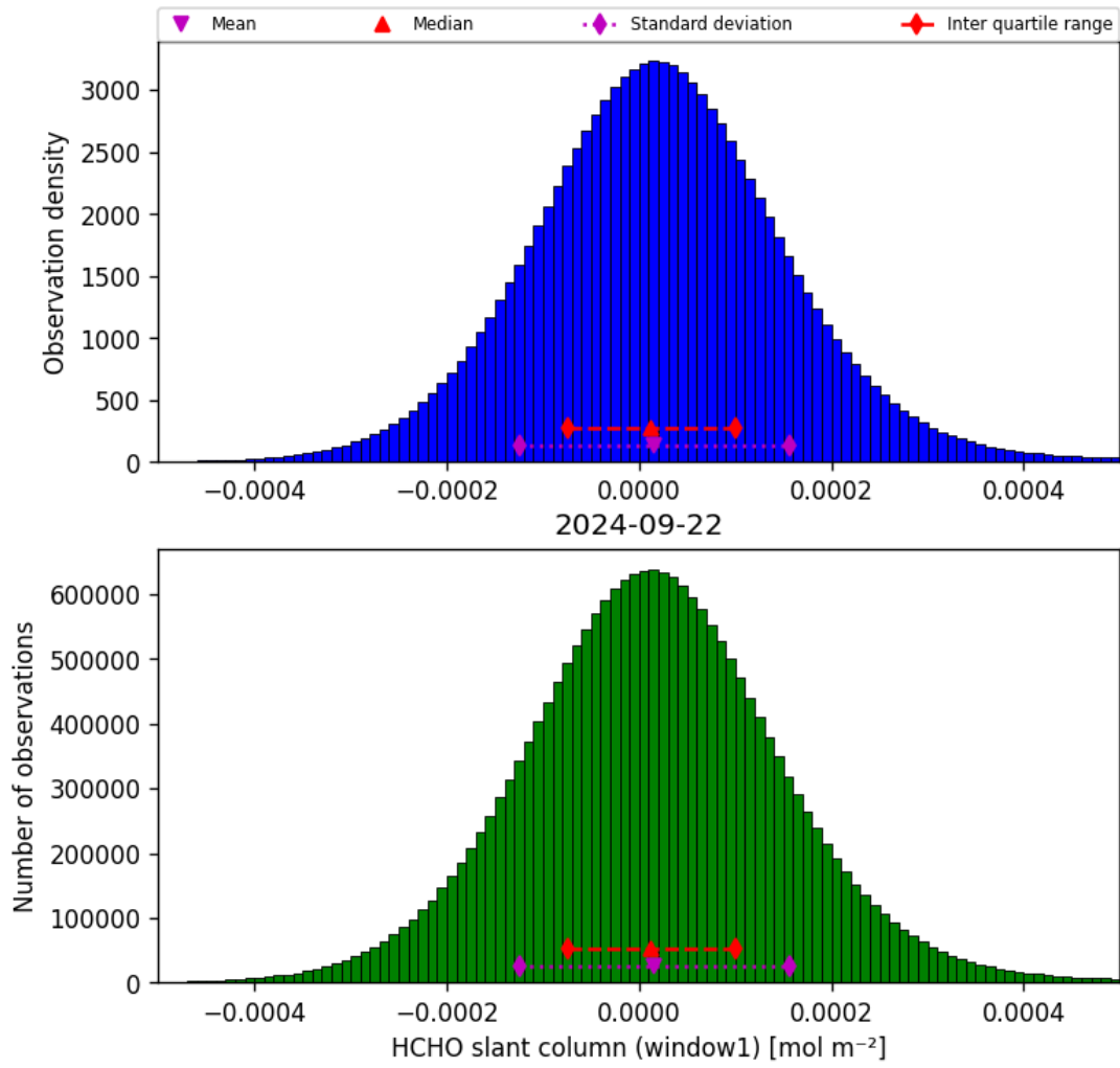
Figure 38: Histogram of “HCHO slant column (window1)” for 2024-09-22 to 2024-09-23
