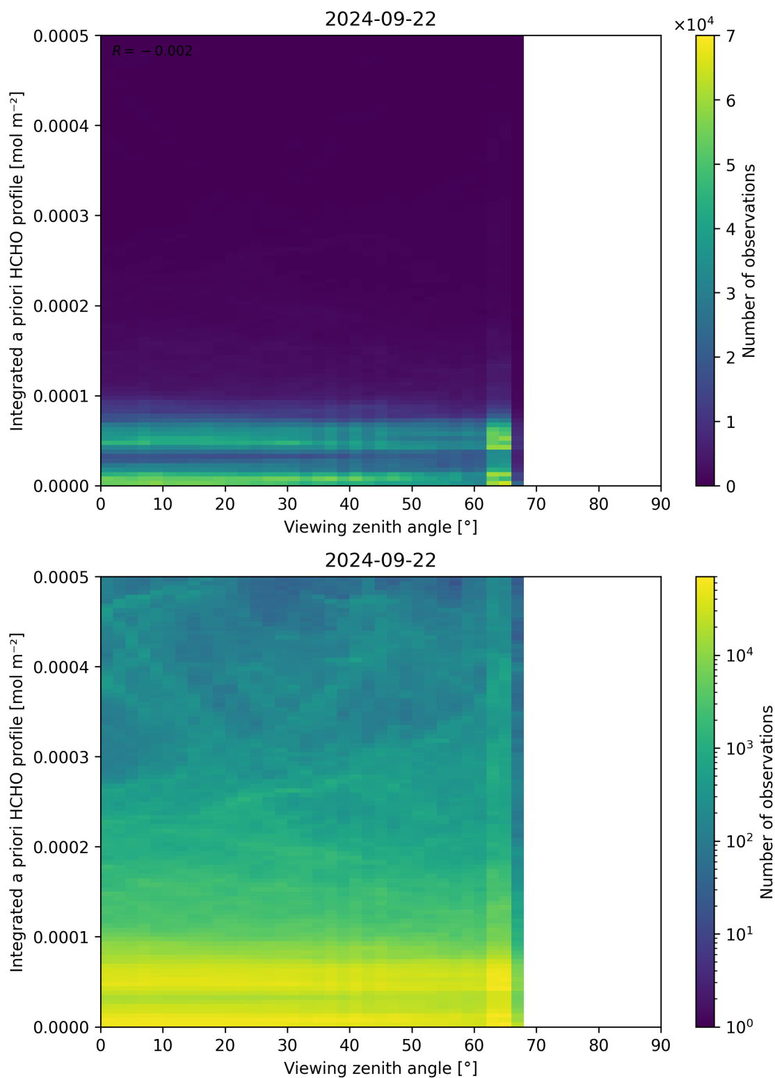
Figure 195: Scatter density plot of “Viewing zenith angle” against “Integrated a priori HCHO profile” for 2024-09-22 to 2024-09-23.
