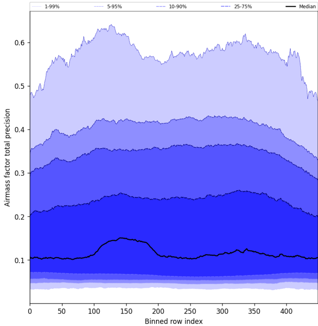
Figure 55: Along track statistics of “Airmass factor total precision” for 2024-09-22 to 2024-09-23
