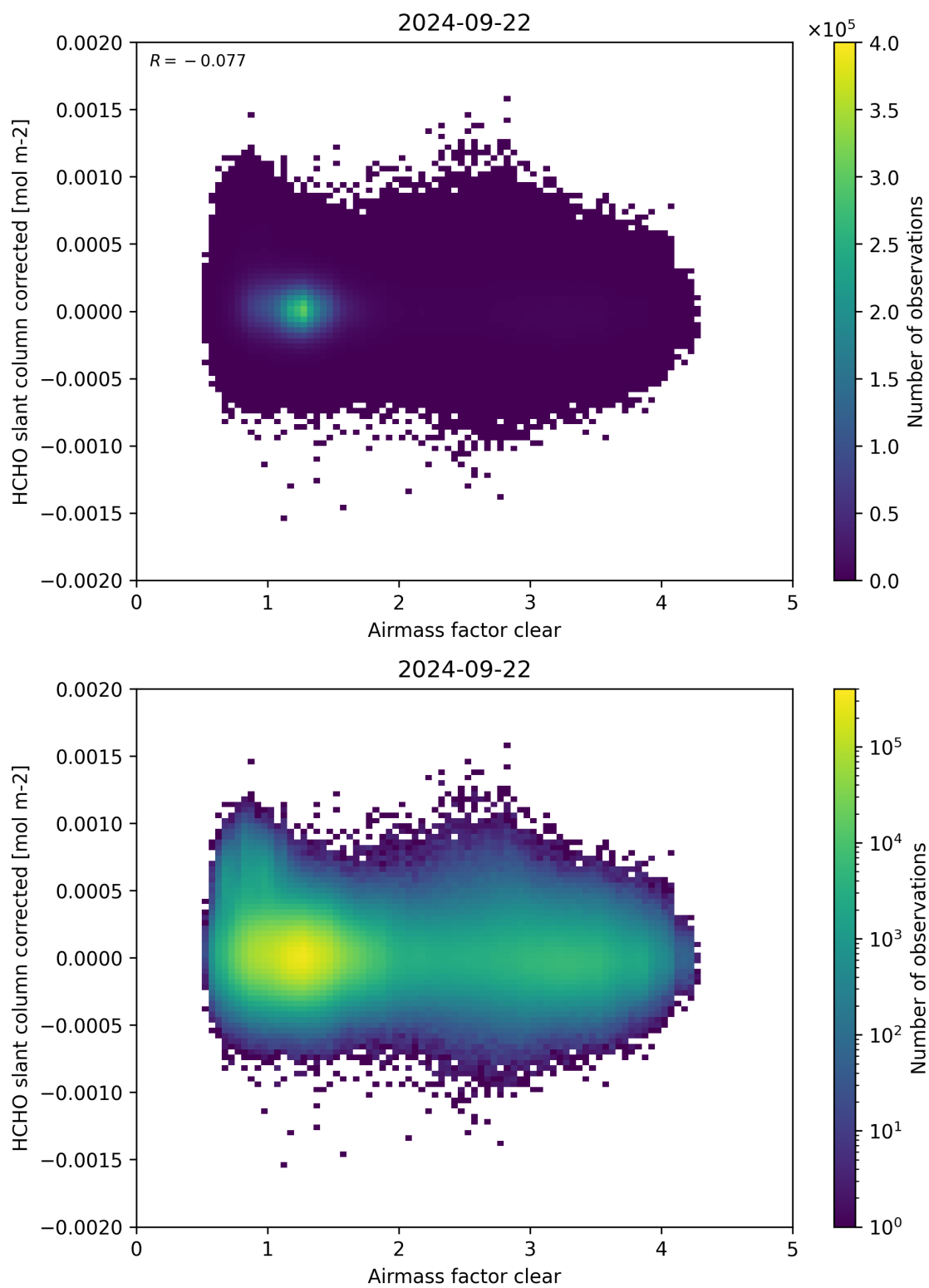
Figure 74: Scatter density plot of “Airmass factor clear” against “HCHO slant column corrected” for 2024-09-22 to 2024-09-23.
