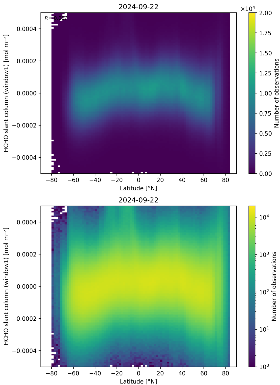
Figure 159: Scatter density plot of “Latitude” against “HCHO slant column (window1)” for 2024-09-22 to 2024-09-23.
