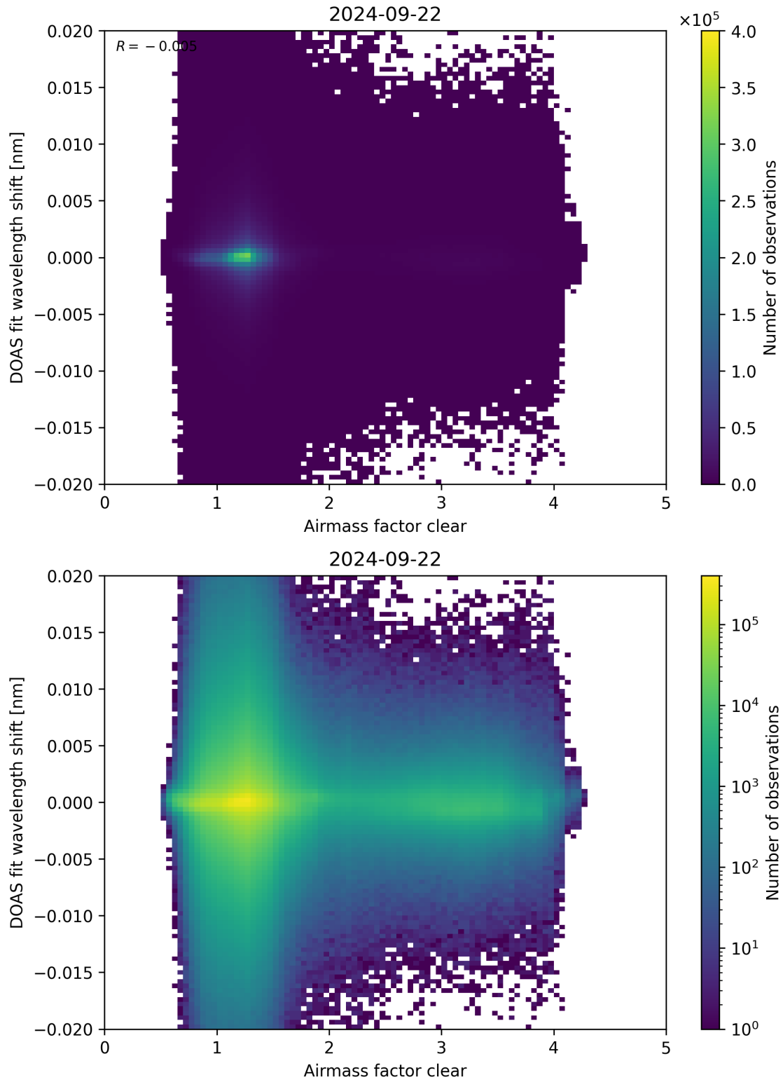
Figure 72: Scatter density plot of “Airmass factor clear” against “DOAS fit wavelength shift” for 2024-09-22 to 2024-09-23.
