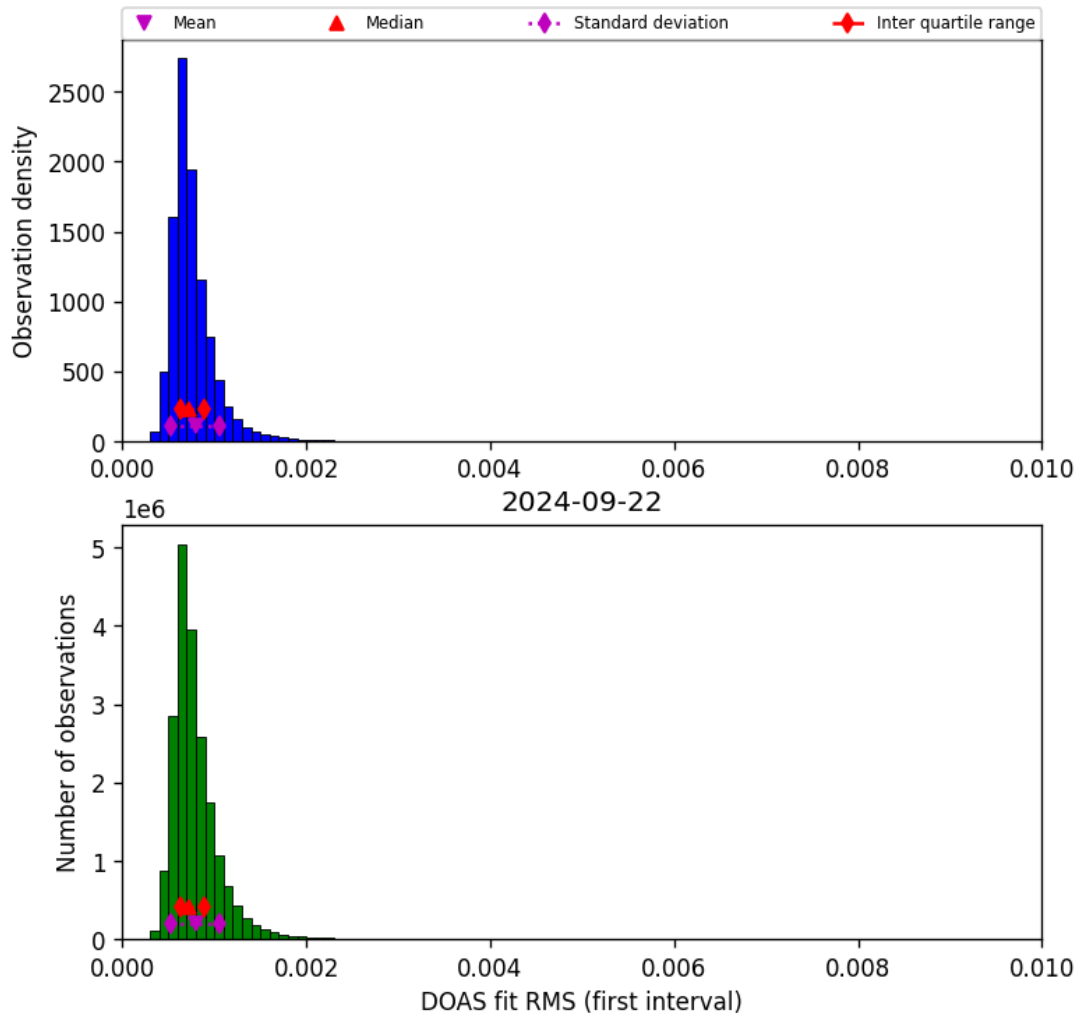
Figure 46: Histogram of “DOAS fit RMS (first interval)” for 2024-09-22 to 2024-09-23
