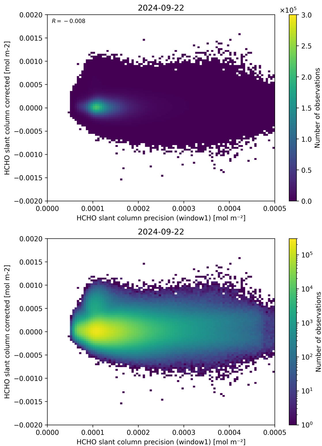
Figure 92: Scatter density plot of “HCHO slant column precision (window1)” against “HCHO slant column corrected” for 2024-09-22 to 2024-09-23.
