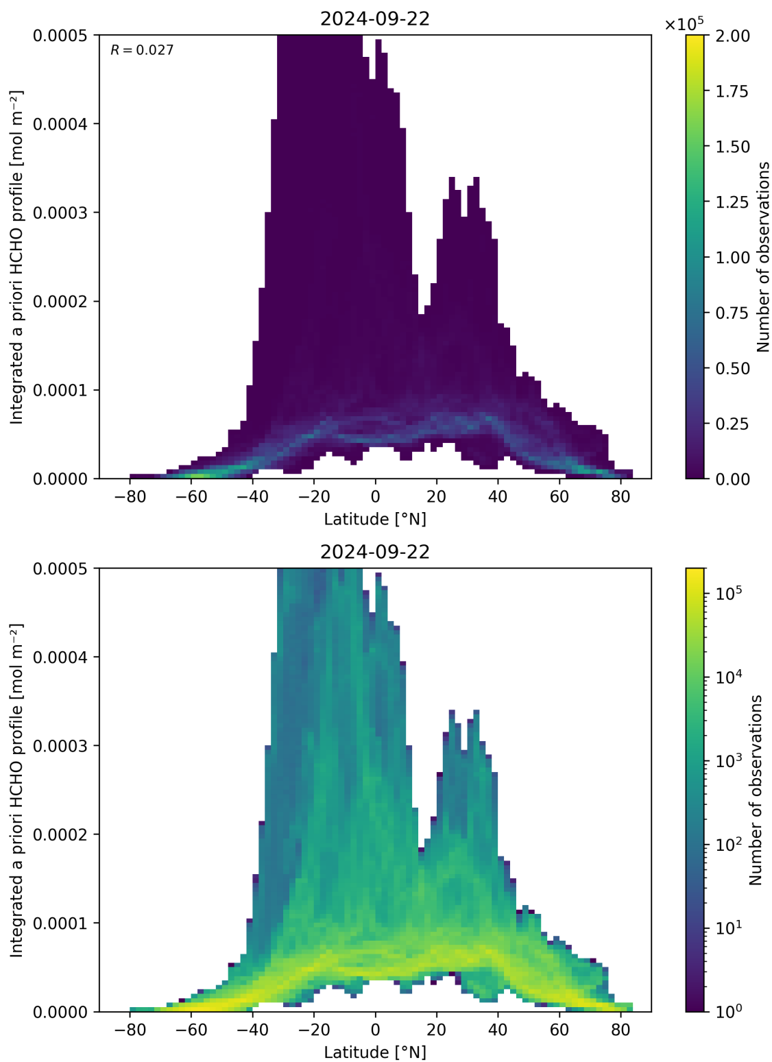
Figure 166: Scatter density plot of “Latitude” against “Integrated a priori HCHO profile” for 2024-09-22 to 2024-09-23.
