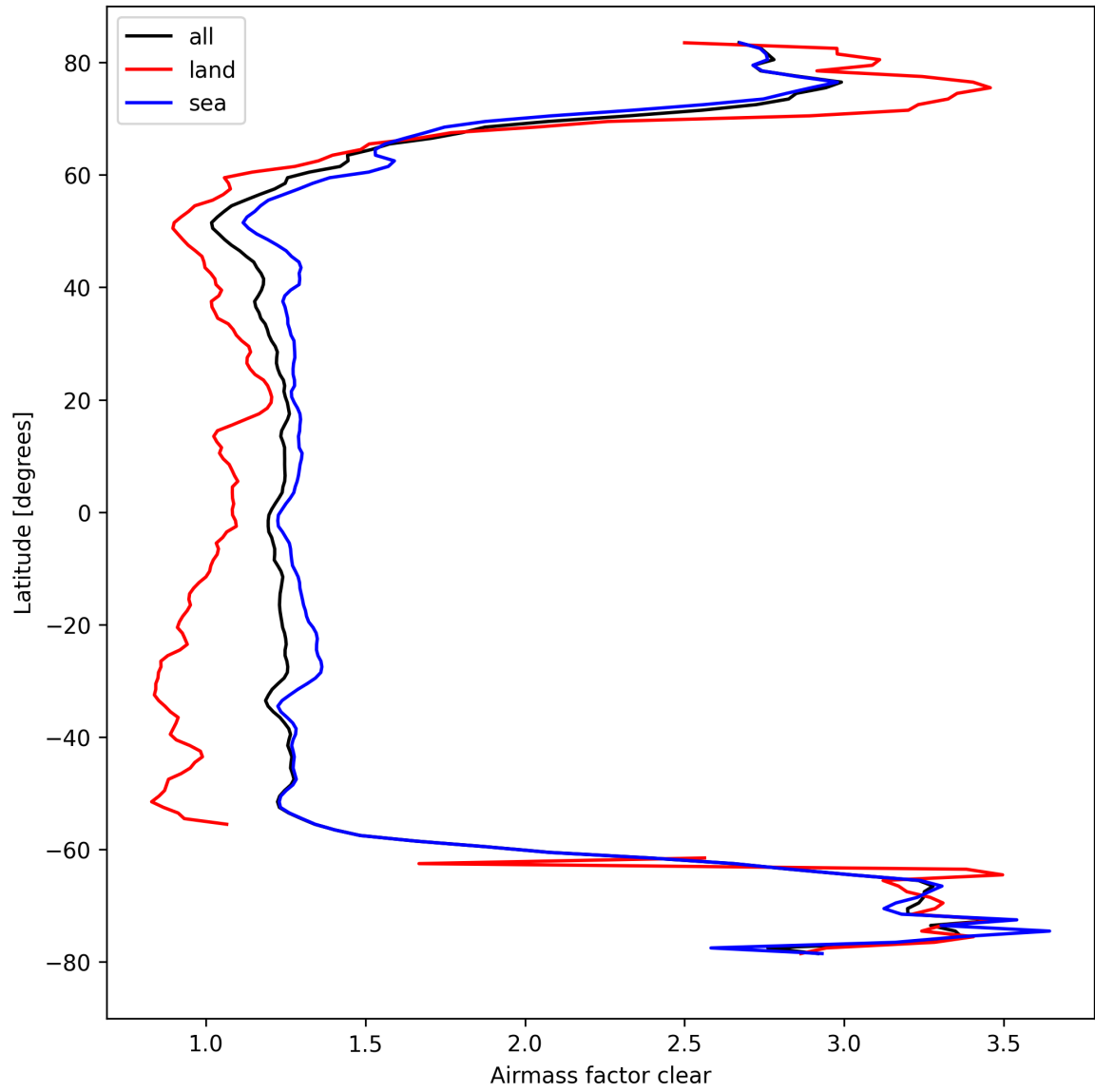
Figure 28: Zonal average of “Airmass factor clear” for 2024-09-22 to 2024-09-23.
