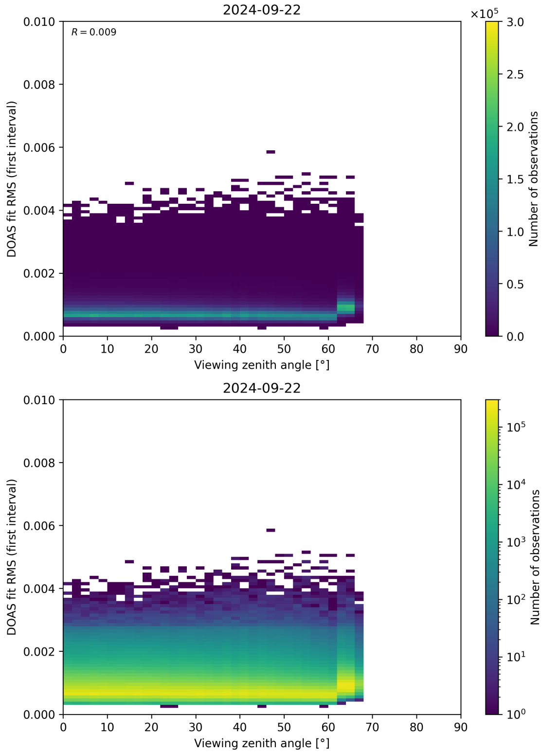
Figure 182: Scatter density plot of “Viewing zenith angle” against “DOAS fit RMS (first interval)” for 2024-09-22 to 2024-09-23.
