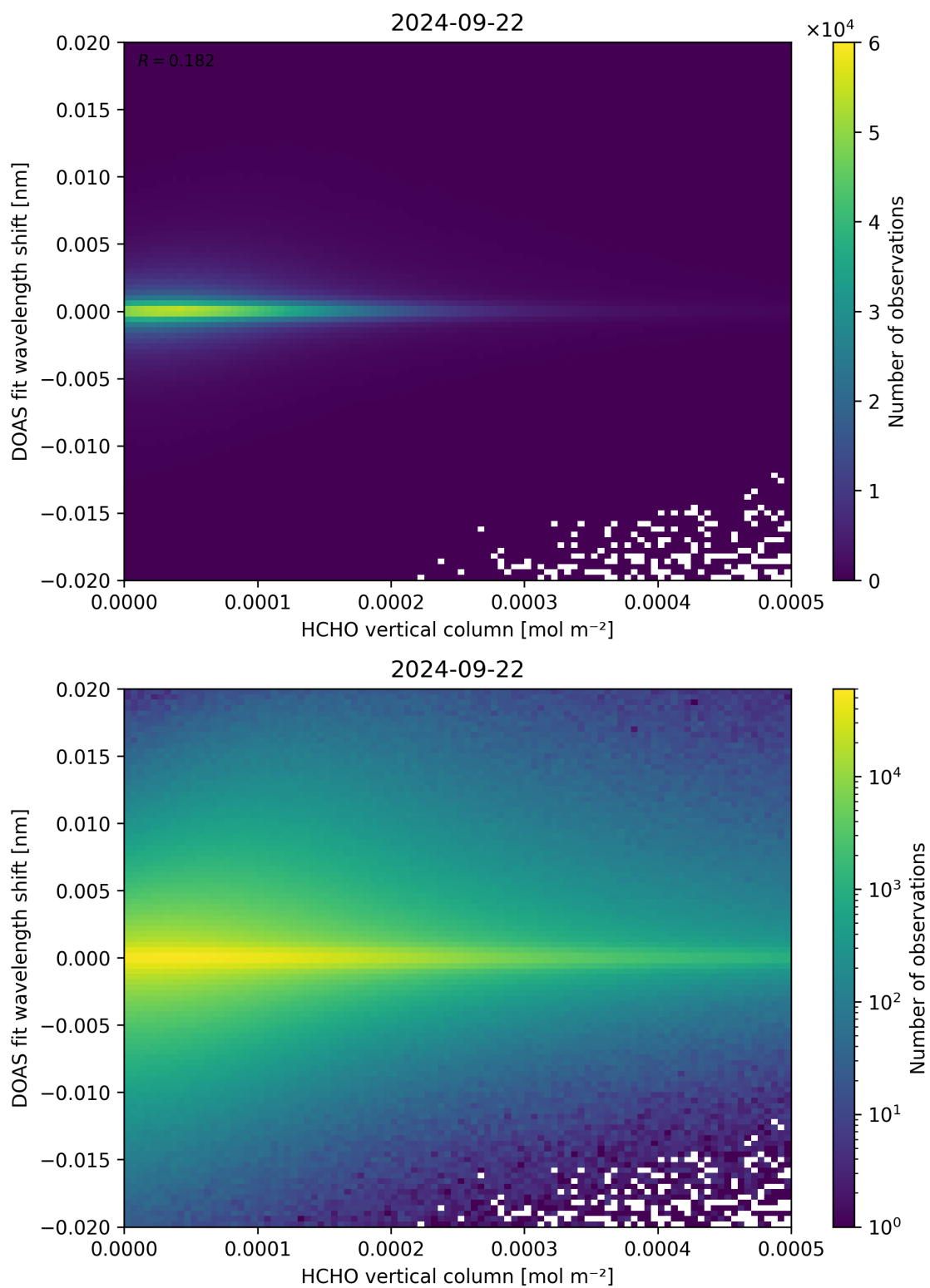
Figure 124: Scatter density plot of “HCHO vertical column” against “DOAS fit wavelength shift” for 2024-09-22 to 2024-09-23.
