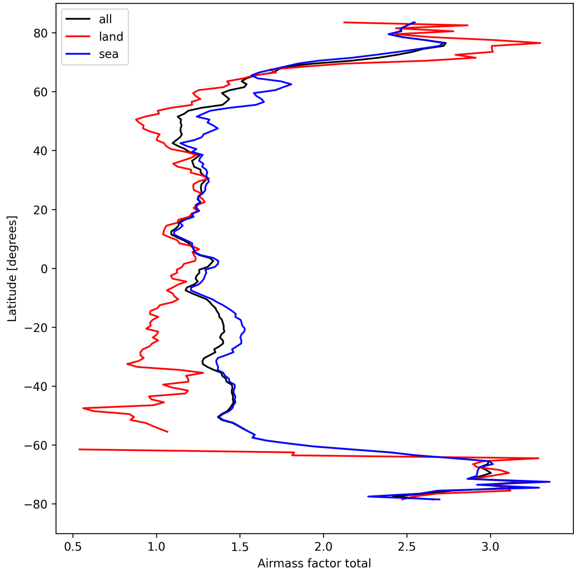
Figure 26: Zonal average of “Airmass factor total” for 2024-09-22 to 2024-09-23.
