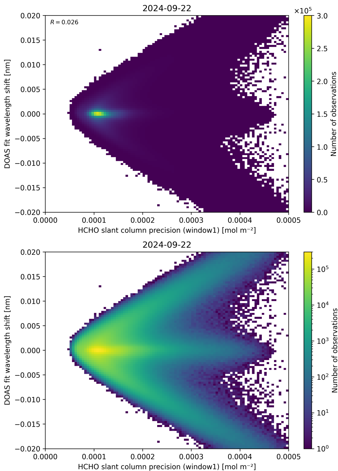
Figure 89: Scatter density plot of “HCHO slant column precision (window1)” against “DOAS fit wavelength shift” for 2024-09-22 to 2024-09-23.
