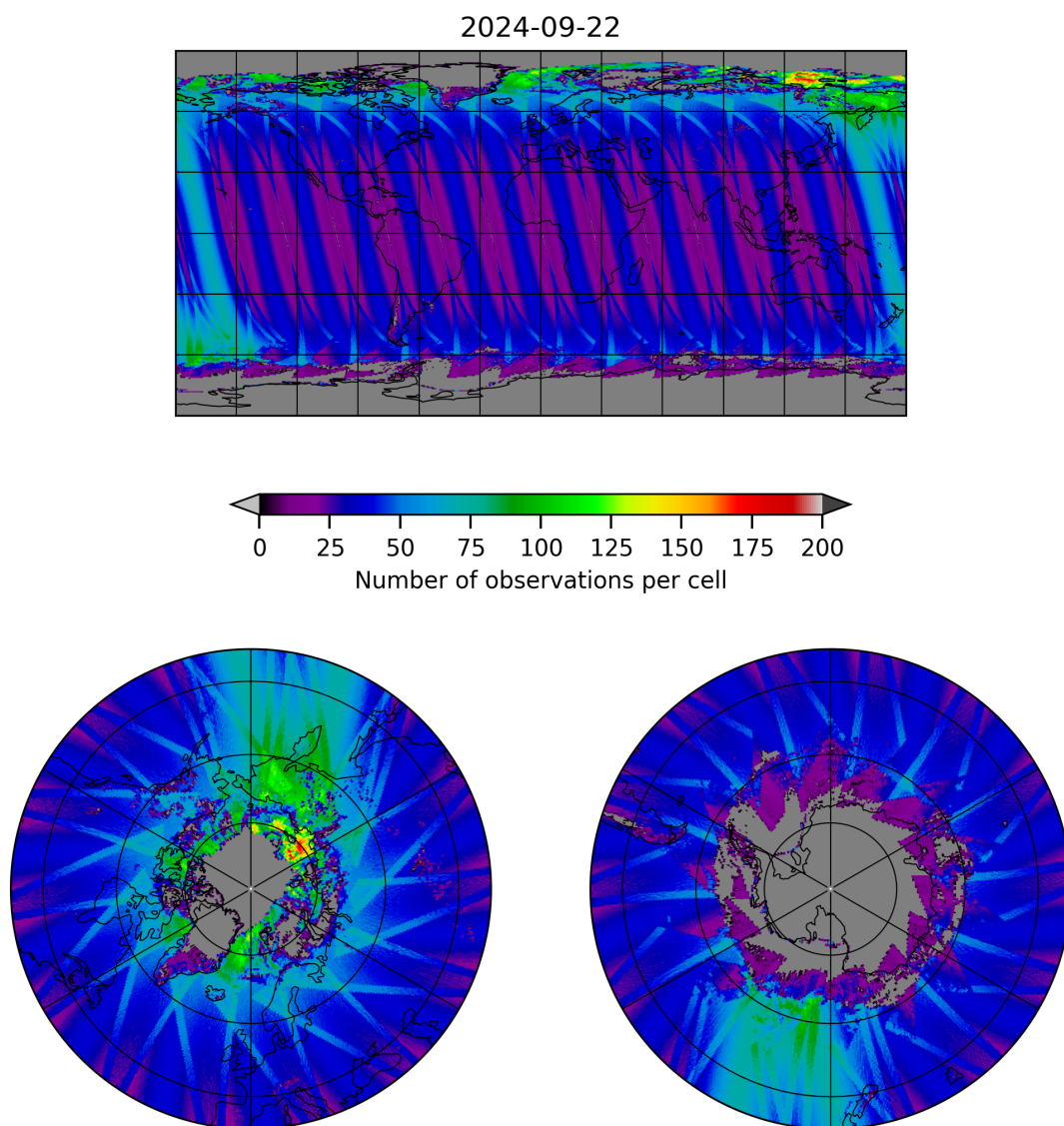
Figure 19: Map of the number of observations for 2024-09-22 to 2024-09-23
