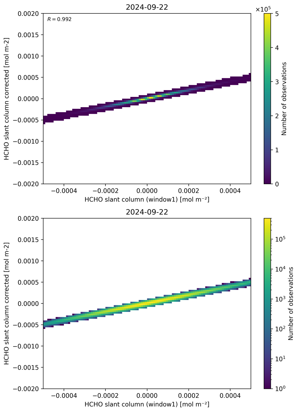
Figure 82: Scatter density plot of “HCHO slant column (window1)” against “HCHO slant column corrected” for 2024-09-22 to 2024-09-23.
