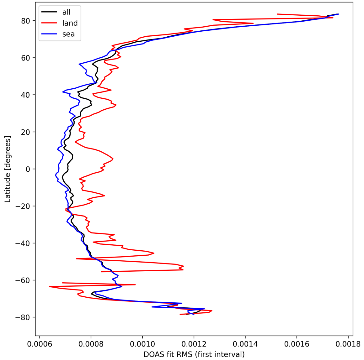
Figure 32: Zonal average of “DOAS fit RMS (first interval)” for 2024-09-22 to 2024-09-23.
