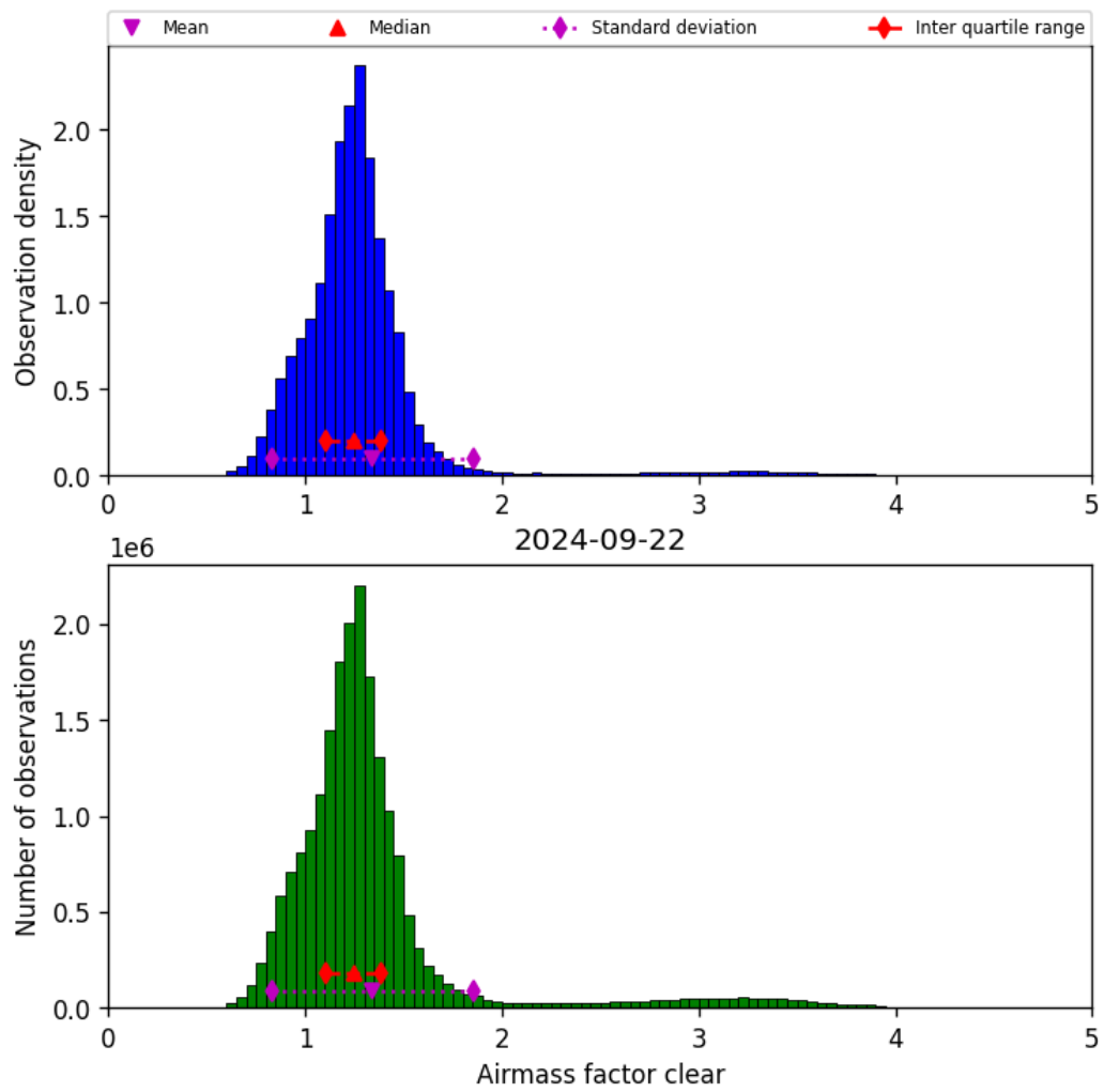
Figure 42: Histogram of “Airmass factor clear” for 2024-09-22 to 2024-09-23
