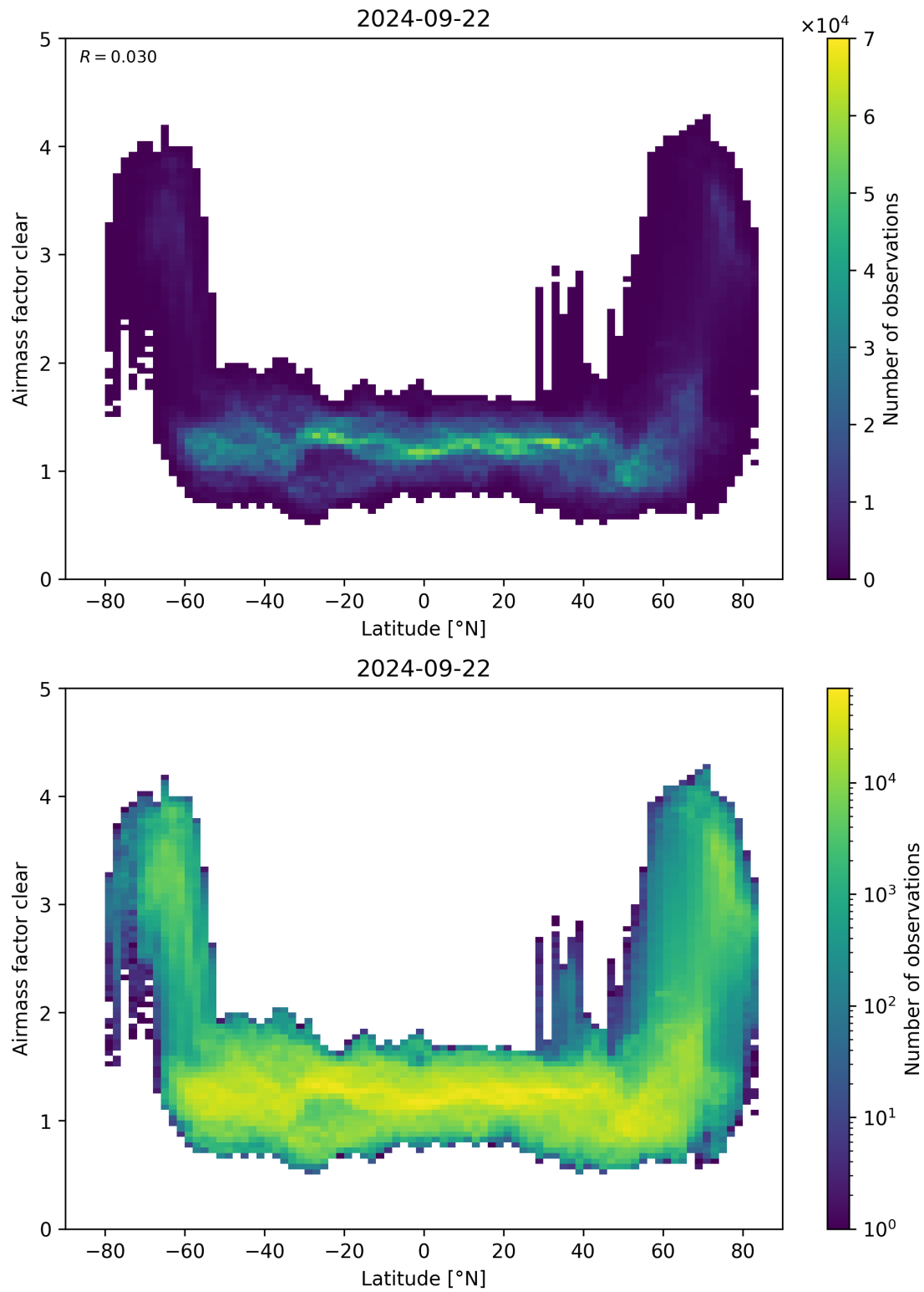
Figure 156: Scatter density plot of “Latitude” against “Airmass factor clear” for 2024-09-22 to 2024-09-23.
