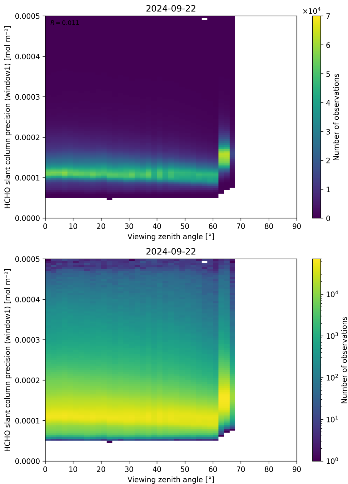
Figure 189: Scatter density plot of “Viewing zenith angle” against “HCHO slant column precision (window1)” for 2024-09-22 to 2024-09-23.
