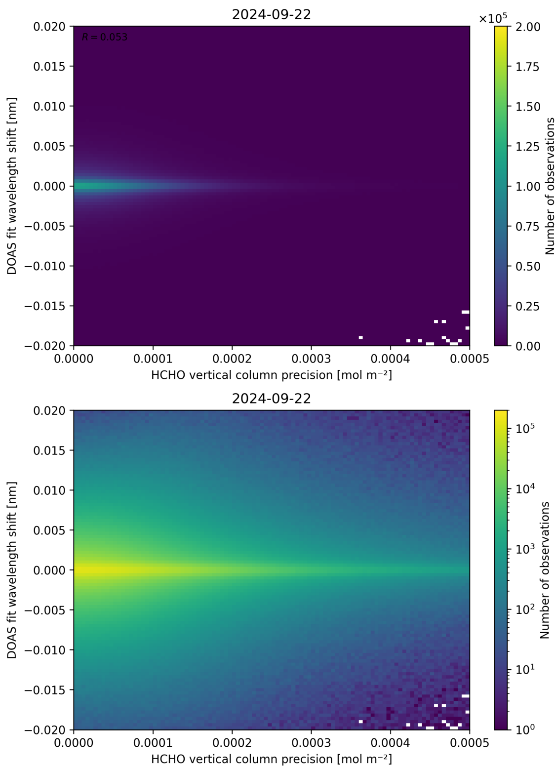
Figure 137: Scatter density plot of “HCHO vertical column precision” against “DOAS fit wavelength shift” for 2024-09-22 to 2024-09-23.
