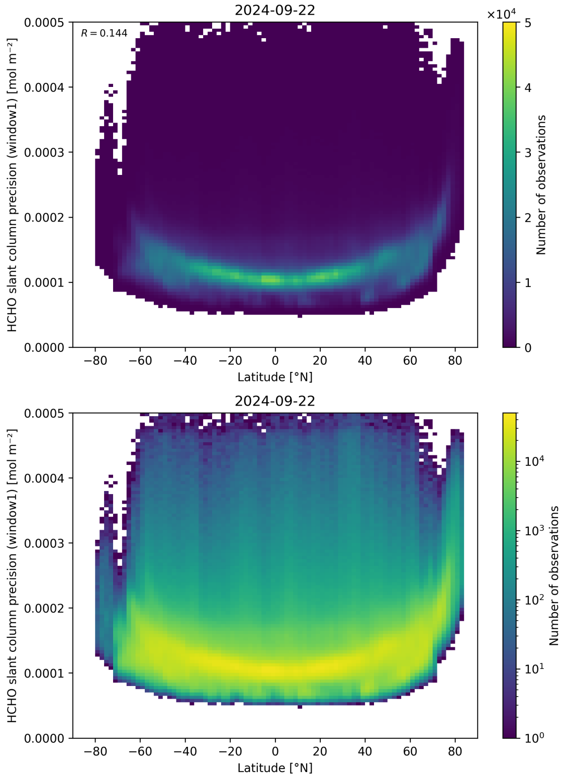
Figure 160: Scatter density plot of “Latitude” against “HCHO slant column precision (window1)” for 2024-09-22 to 2024-09-23.
