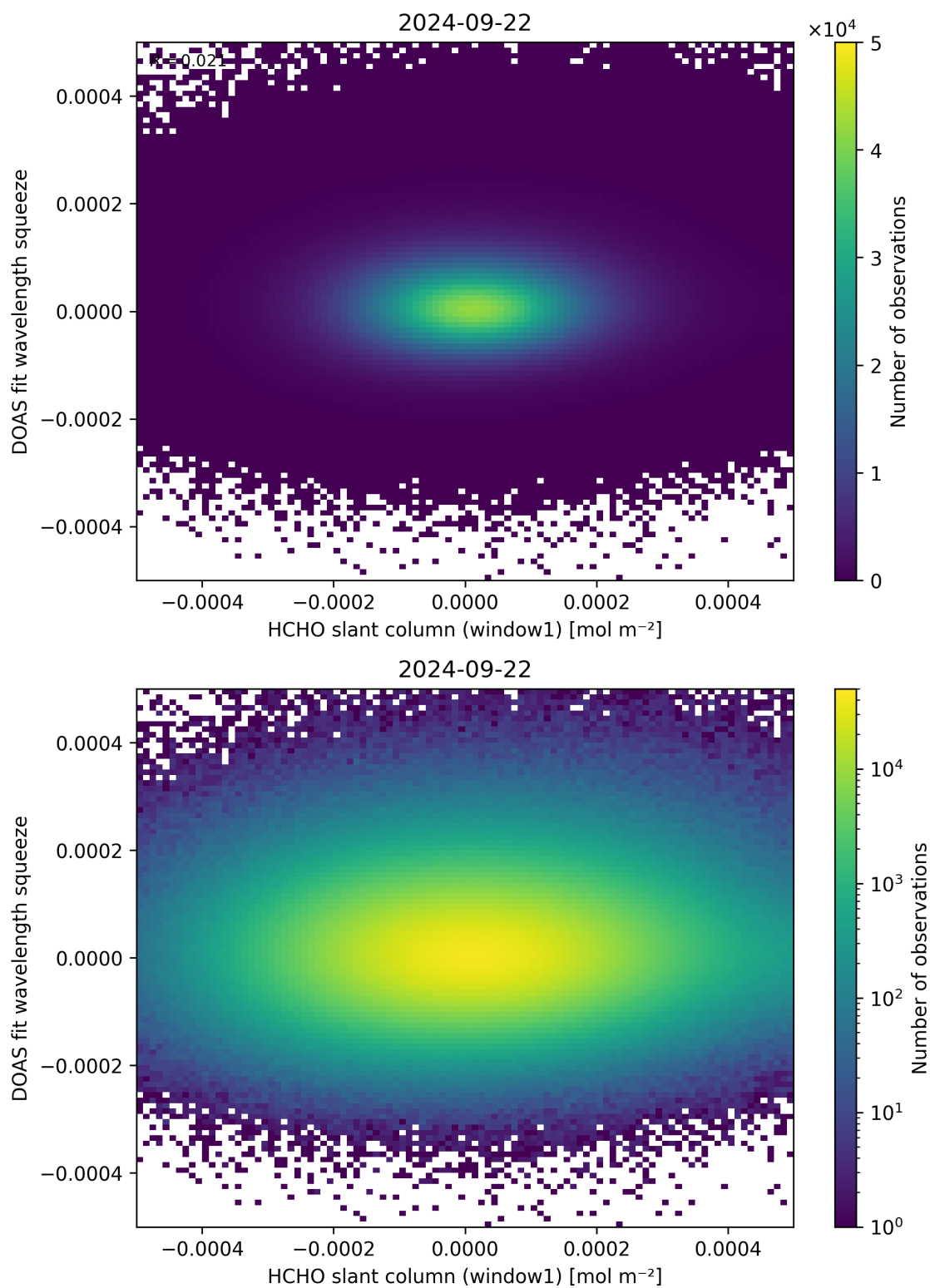
Figure 80: Scatter density plot of “HCHO slant column (window1)” against “DOAS fit wavelength squeeze” for 2024-09-22 to 2024-09-23.
