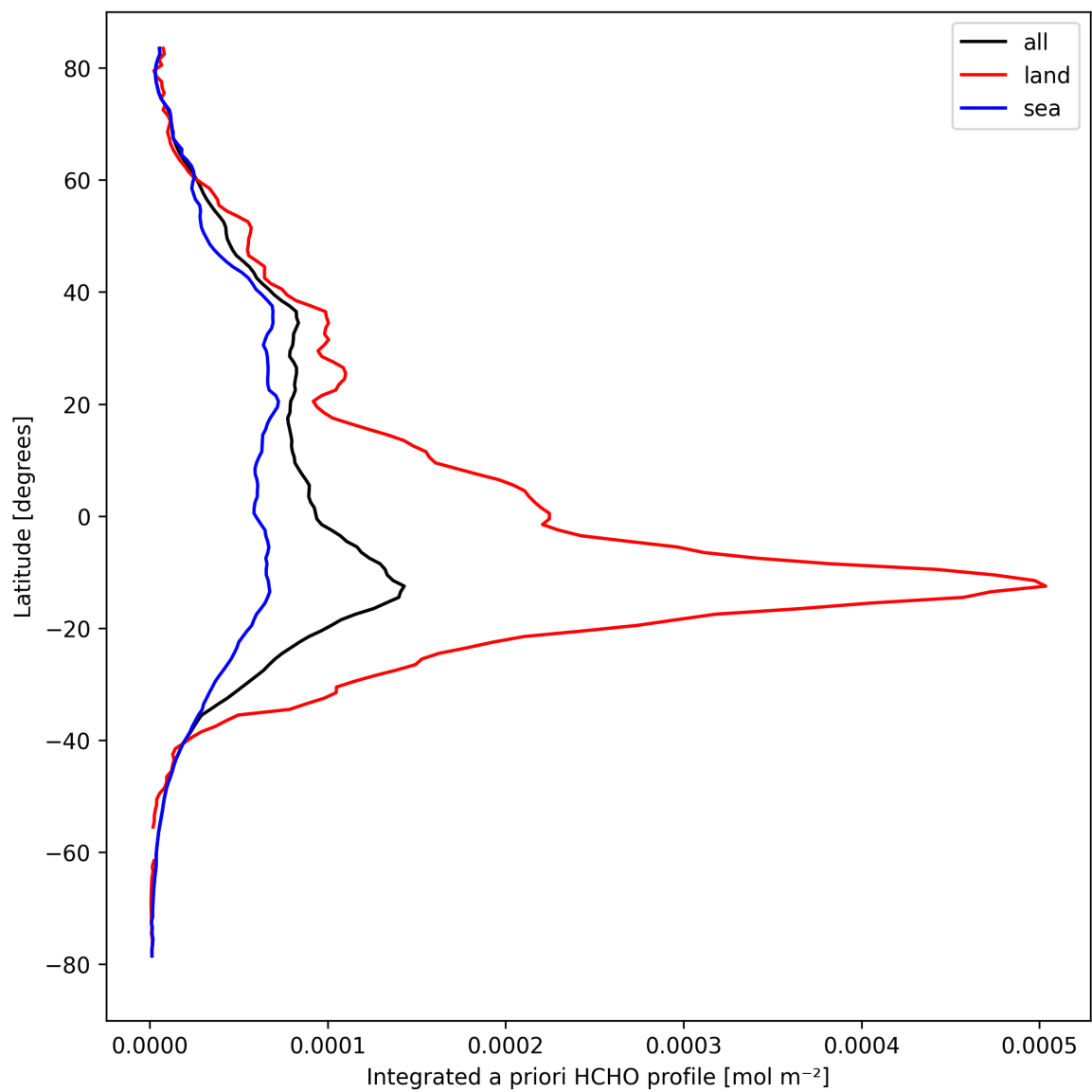
Figure 29: Zonal average of “Integrated a priori HCHO profile” for 2024-09-22 to 2024-09-23.
