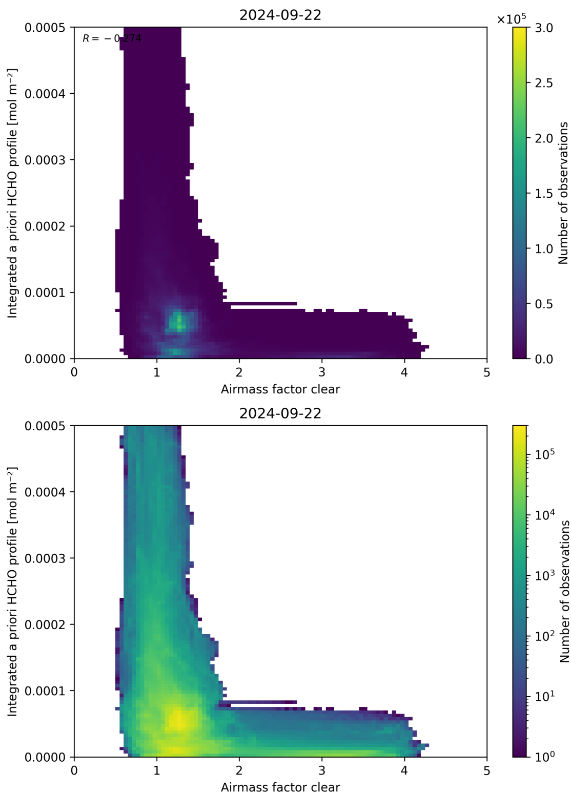
Figure 76: Scatter density plot of “Airmass factor clear” against “Integrated a priori HCHO profile” for 2024-09-22 to 2024-09-23.
