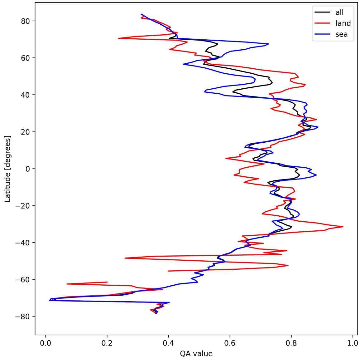
Figure 20: Zonal average of “QA value” for 2024-09-22 to 2024-09-23.
