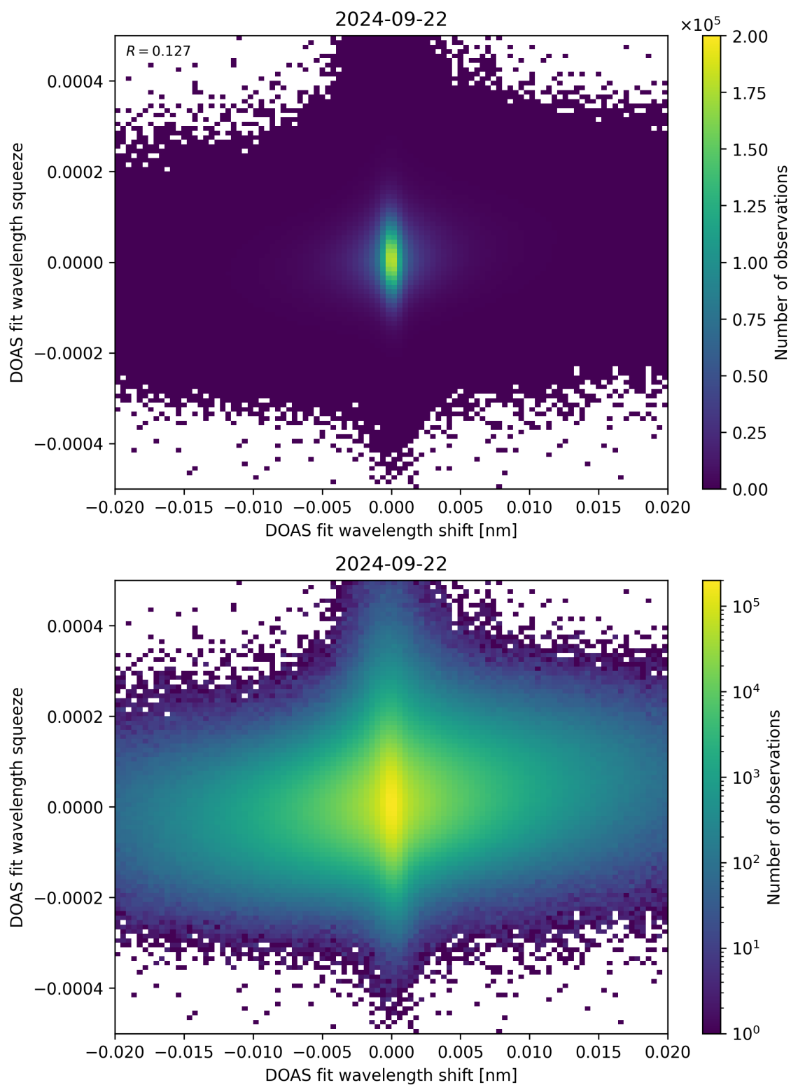
Figure 65: Scatter density plot of “DOAS fit wavelength shift” against “DOAS fit wavelength squeeze” for 2024-09-22 to 2024-09-23.
