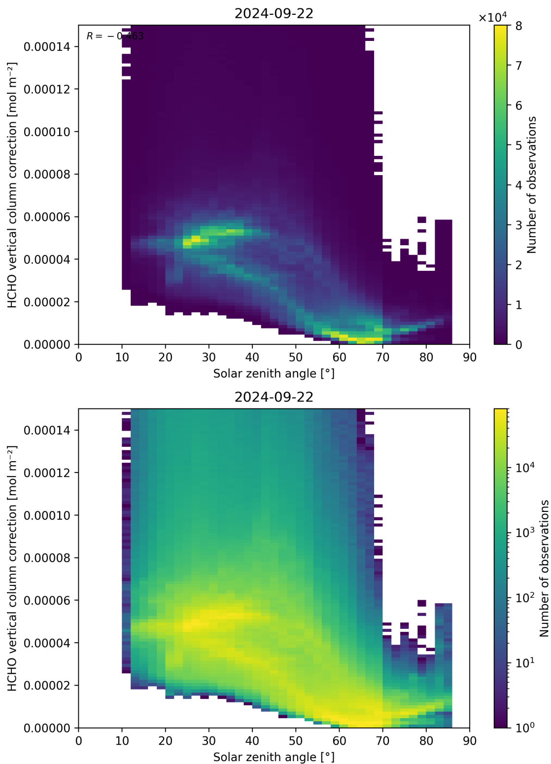
Figure 178: Scatter density plot of “Solar zenith angle” against “HCHO vertical column correction” for 2024-09-22 to 2024-09-23.
