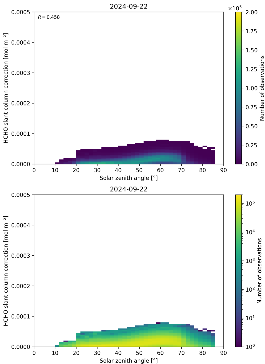
Figure 172: Scatter density plot of “Solar zenith angle” against “HCHO slant column correction” for 2024-09-22 to 2024-09-23.
