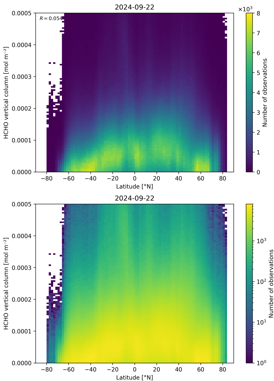
Figure 163: Scatter density plot of “Latitude” against “HCHO vertical column” for 2024-09-22 to 2024-09-23.
