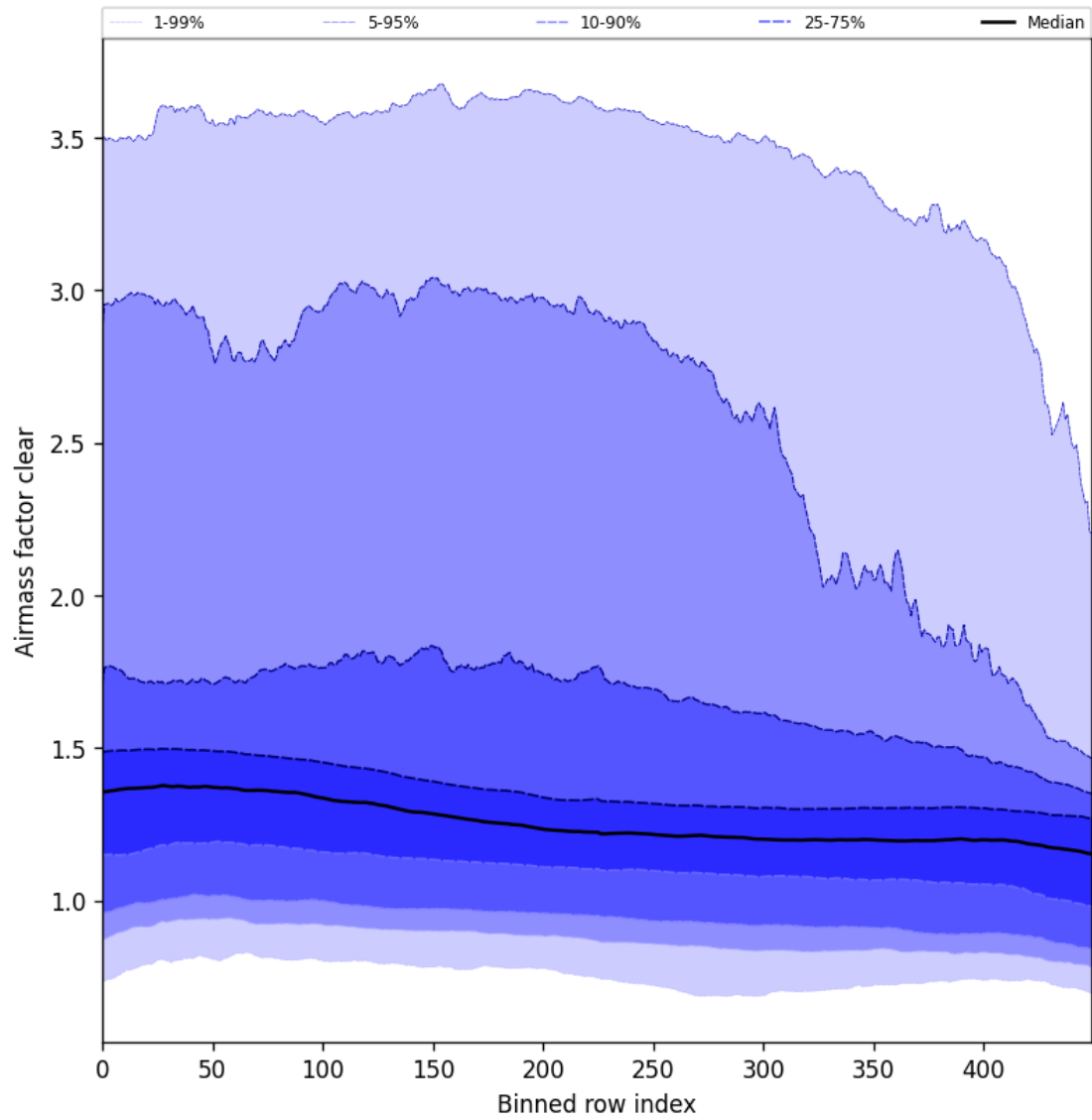
Figure 56: Along track statistics of “Airmass factor clear” for 2024-09-22 to 2024-09-23
