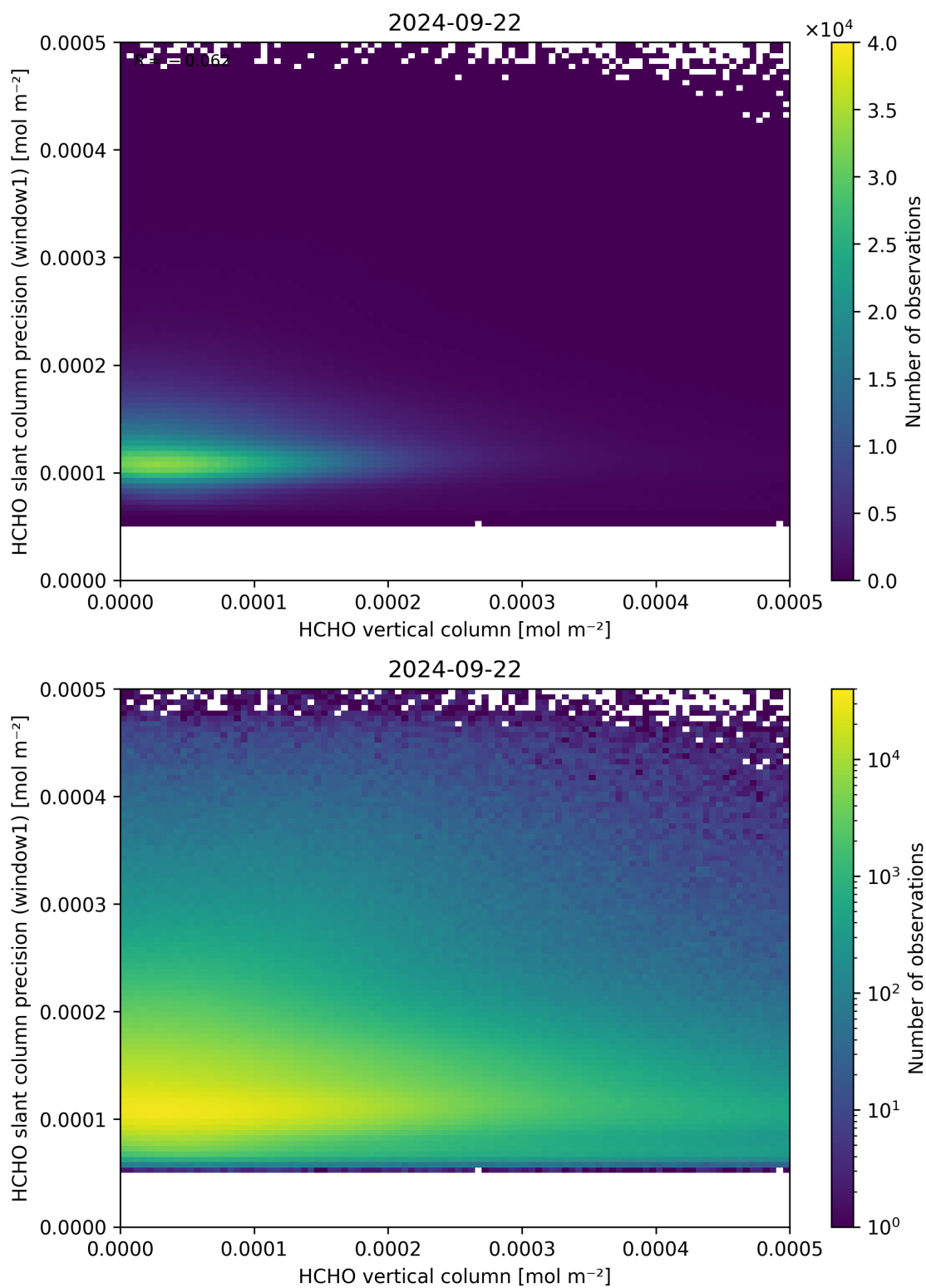
Figure 130: Scatter density plot of “HCHO vertical column” against “HCHO slant column precision (window1)” for 2024-09-22 to 2024-09-23.
