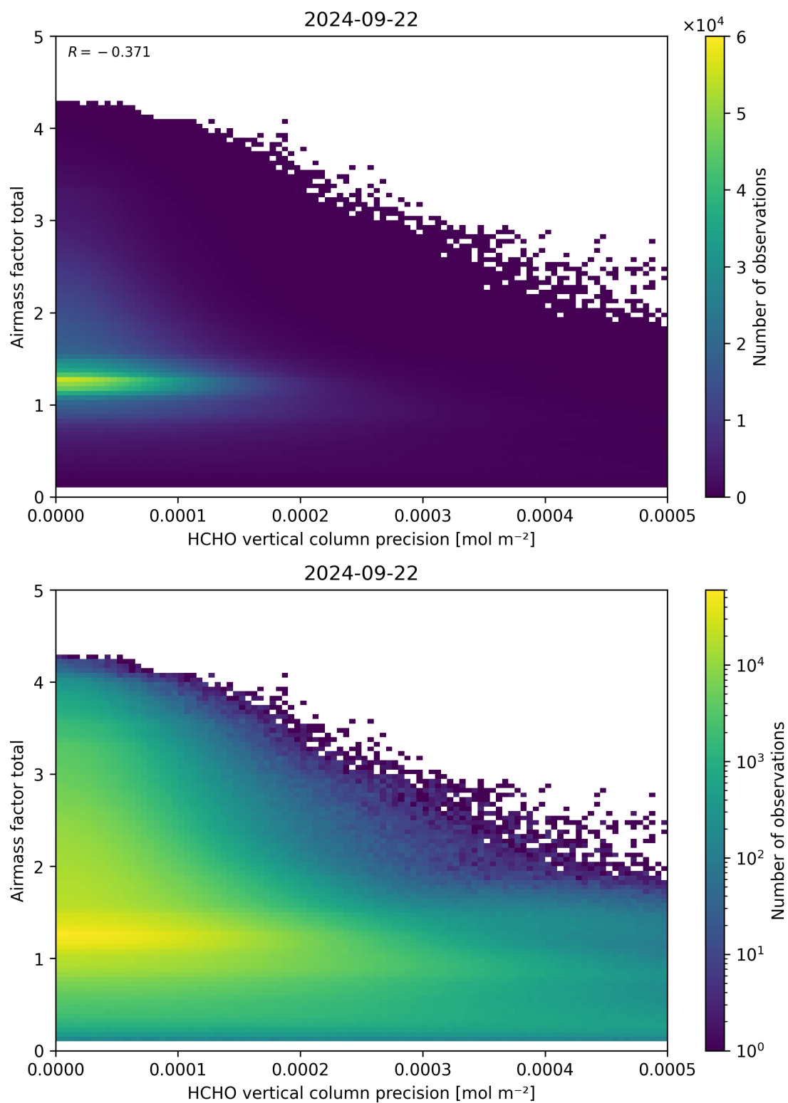
Figure 144: Scatter density plot of “HCHO vertical column precision” against “Airmass factor total” for 2024-09-22 to 2024-09-23.
