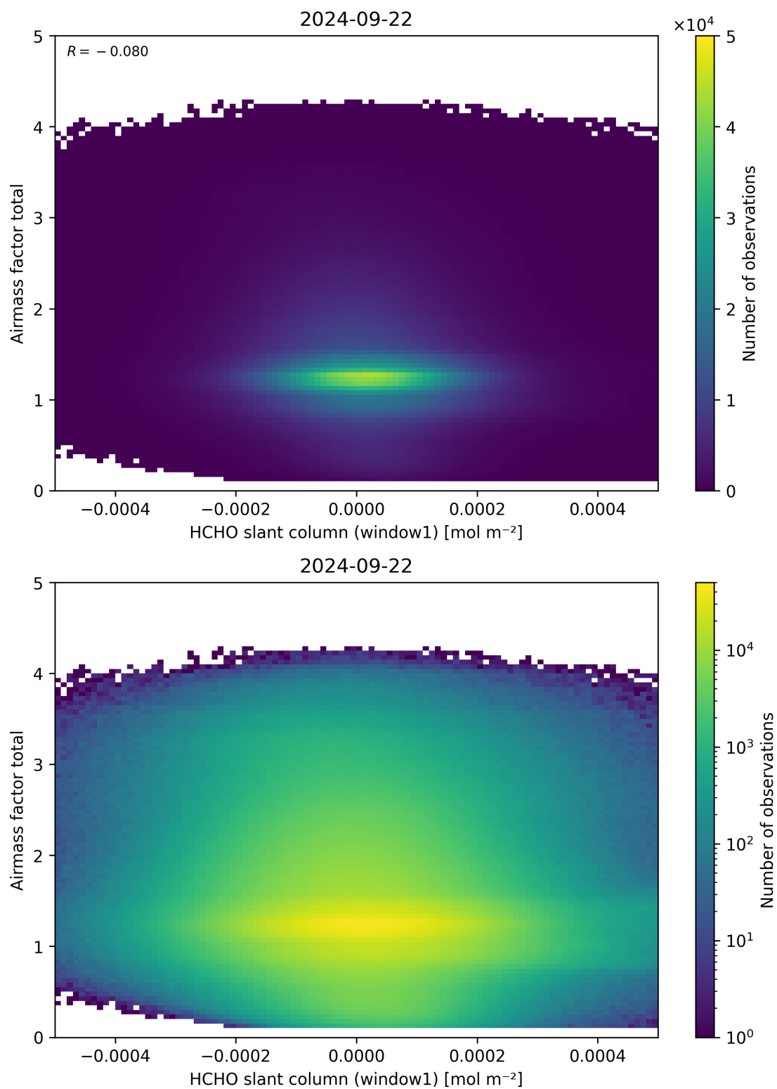
Figure 85: Scatter density plot of “HCHO slant column (window1)” against “Airmass factor total” for 2024-09-22 to 2024-09-23.
