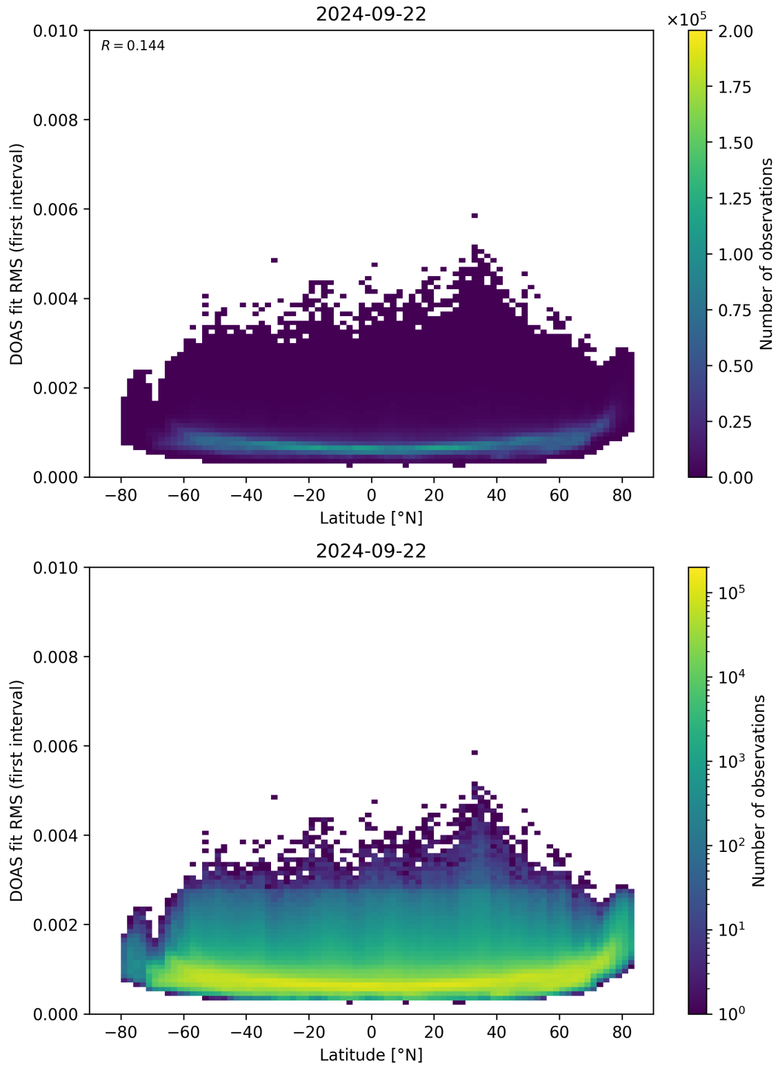
Figure 153: Scatter density plot of “Latitude” against “DOAS fit RMS (first interval)” for 2024-09-22 to 2024-09-23.
