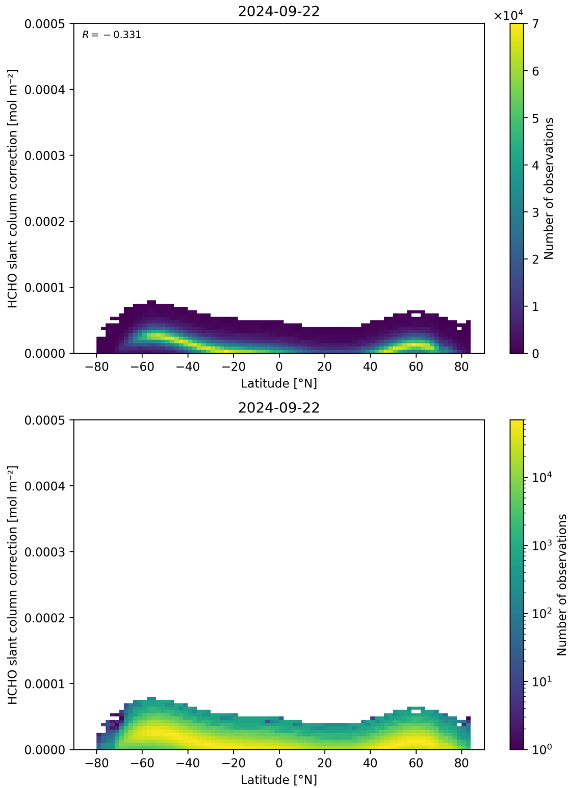
Figure 158: Scatter density plot of “Latitude” against “HCHO slant column correction” for 2024-09-22 to 2024-09-23.
