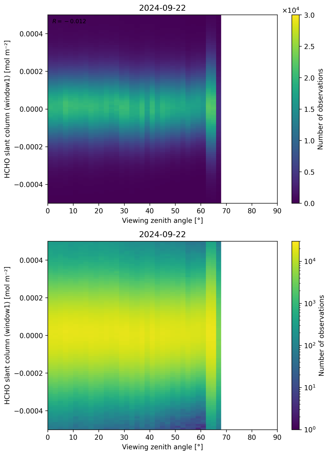
Figure 188: Scatter density plot of “Viewing zenith angle” against “HCHO slant column (window1)” for 2024-09-22 to 2024-09-23.
