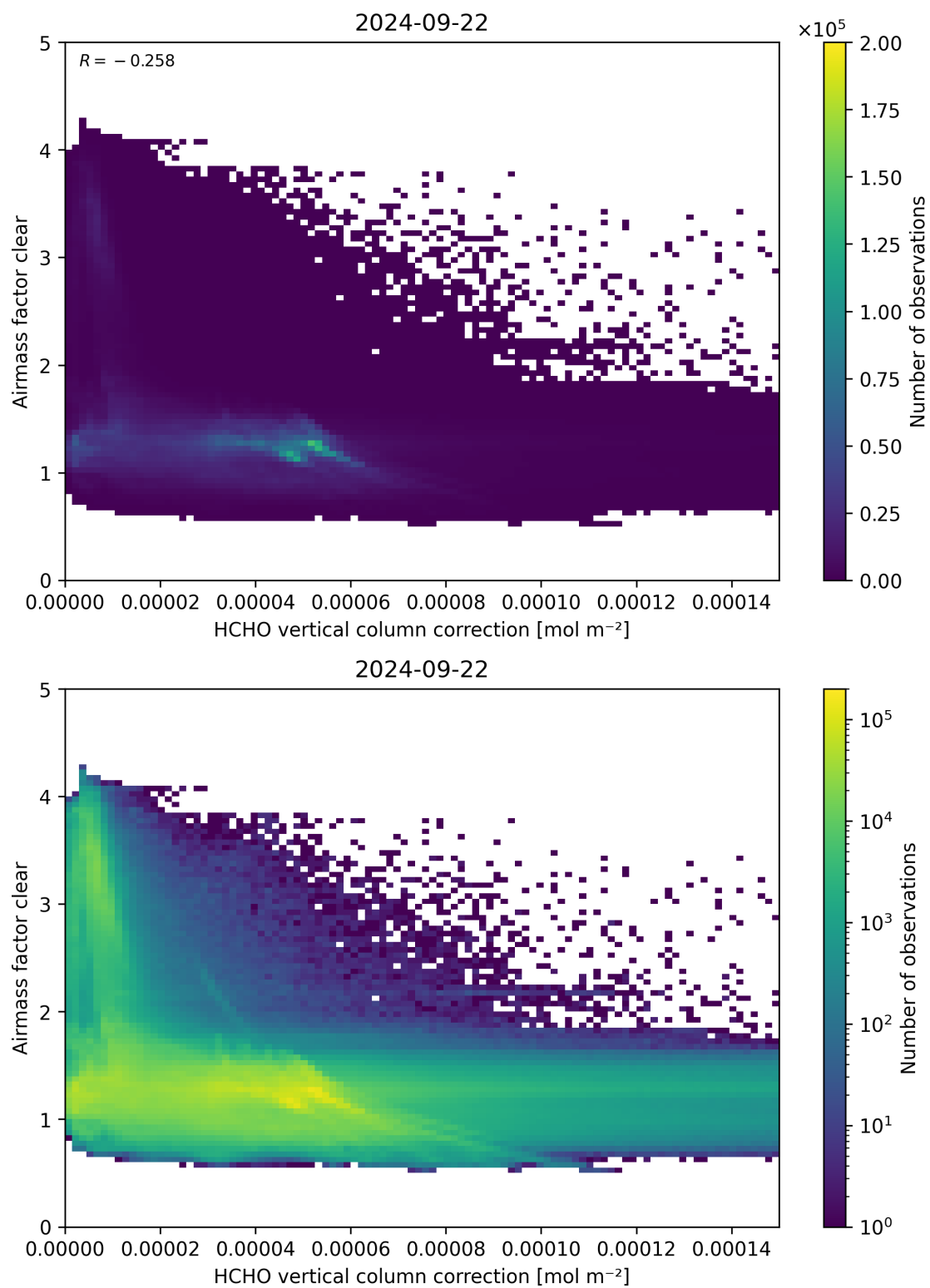
Figure 115: Scatter density plot of “HCHO vertical column correction” against “Airmass factor clear” for 2024-09-22 to 2024-09-23.
