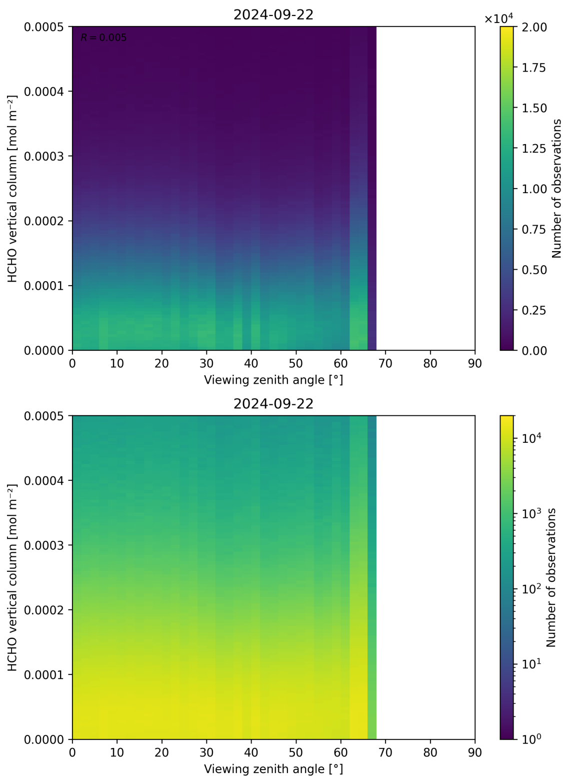
Figure 192: Scatter density plot of “Viewing zenith angle” against “HCHO vertical column” for 2024-09-22 to 2024-09-23.
