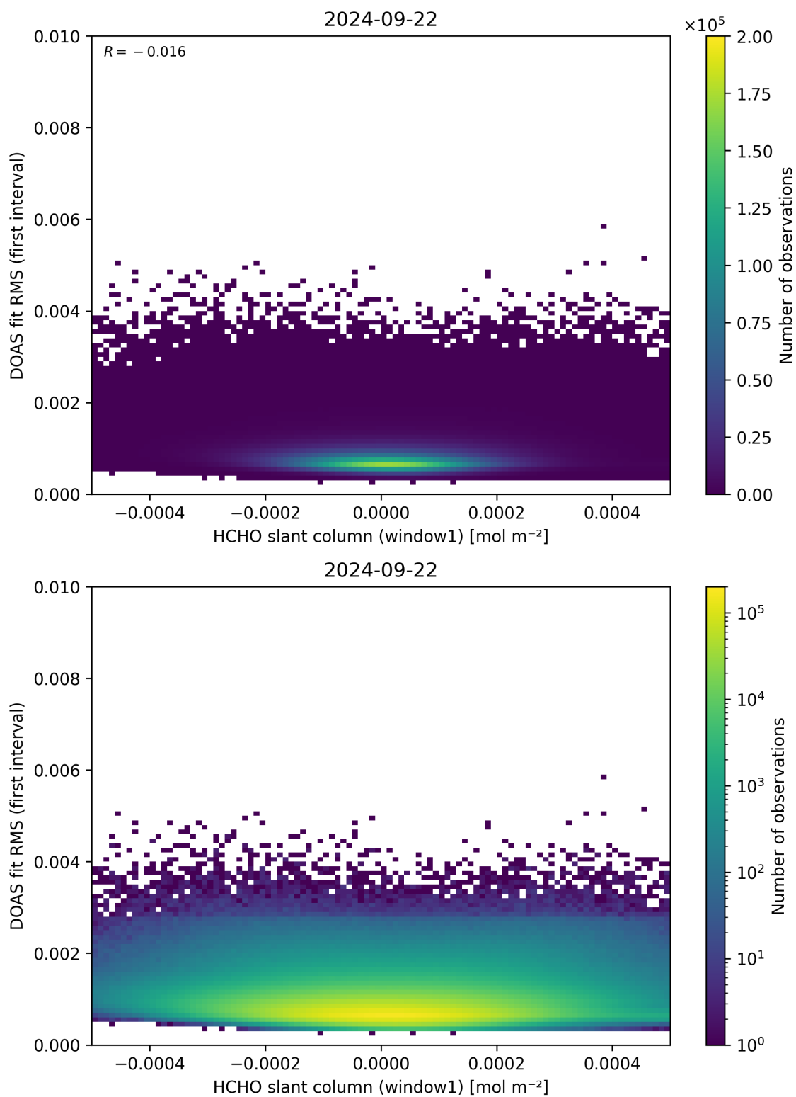
Figure 78: Scatter density plot of “HCHO slant column (window1)” against “DOAS fit RMS (first interval)” for 2024-09-22 to 2024-09-23.
