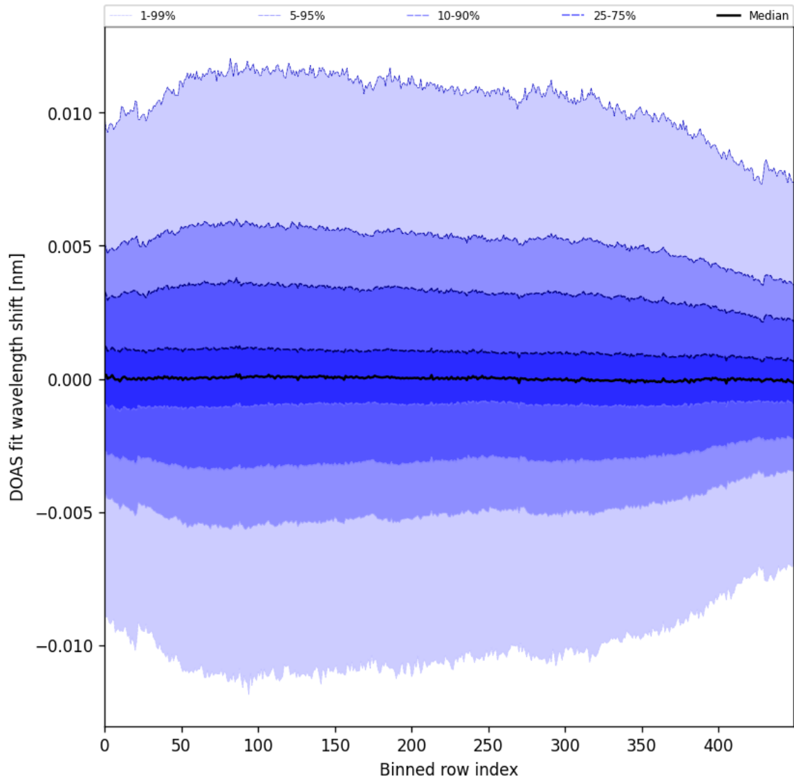
Figure 58: Along track statistics of “DOAS fit wavelength shift” for 2024-09-22 to 2024-09-23
