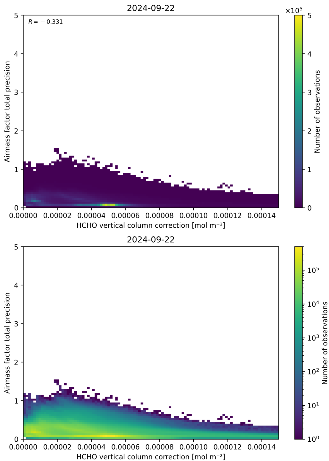
Figure 121: Scatter density plot of “HCHO vertical column correction” against “Airmass factor total precision” for 2024-09-22 to 2024-09-23.
