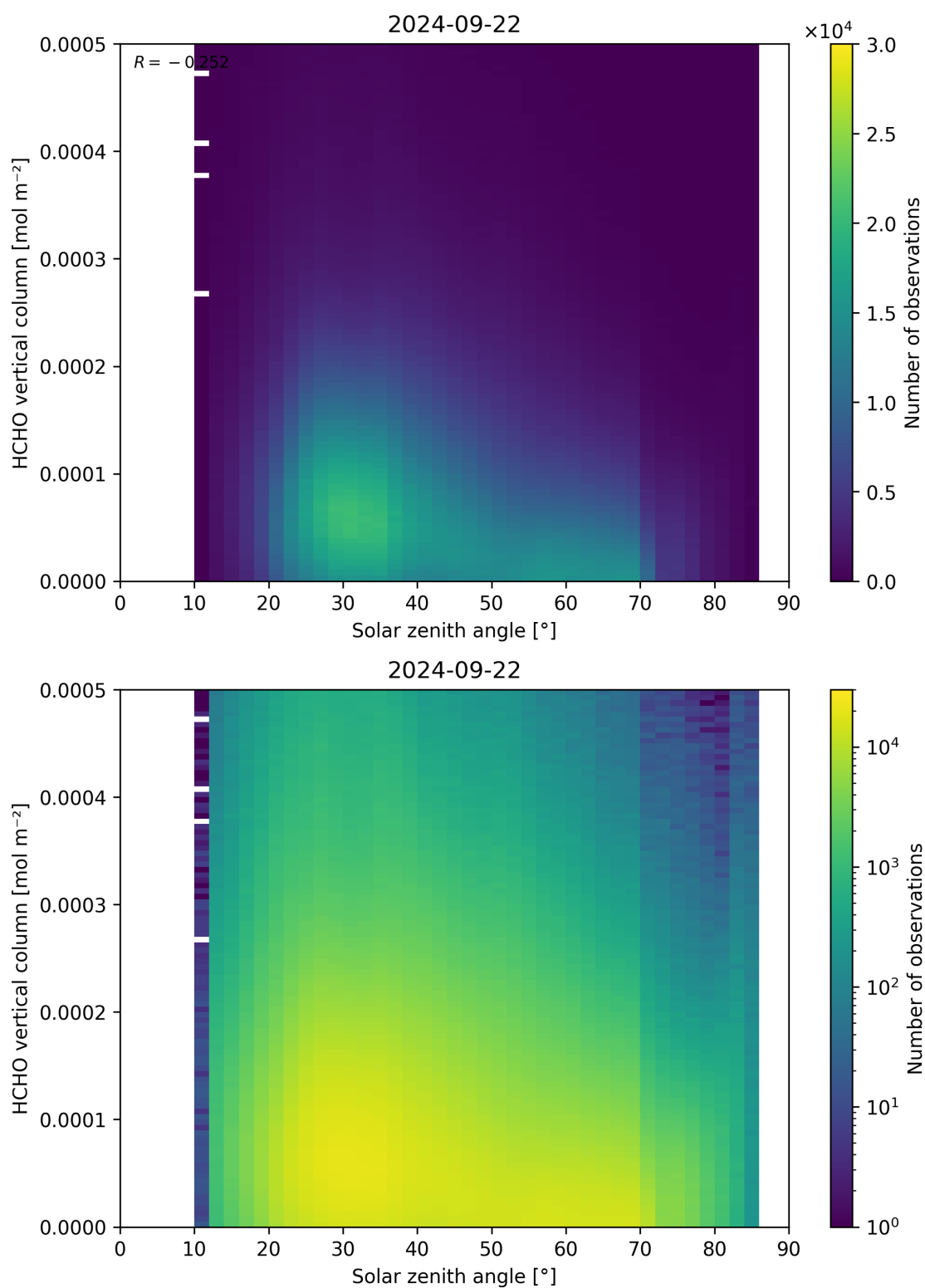
Figure 177: Scatter density plot of “Solar zenith angle” against “HCHO vertical column” for 2024-09-22 to 2024-09-23.
