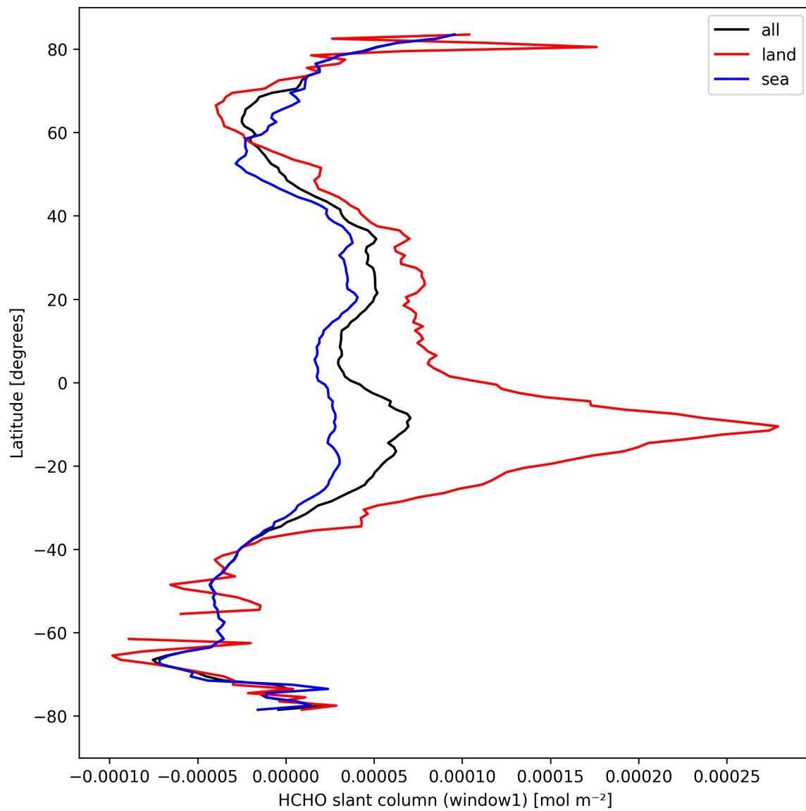
Figure 24: Zonal average of “HCHO slant column (window1)” for 2024-09-22 to 2024-09-23.
