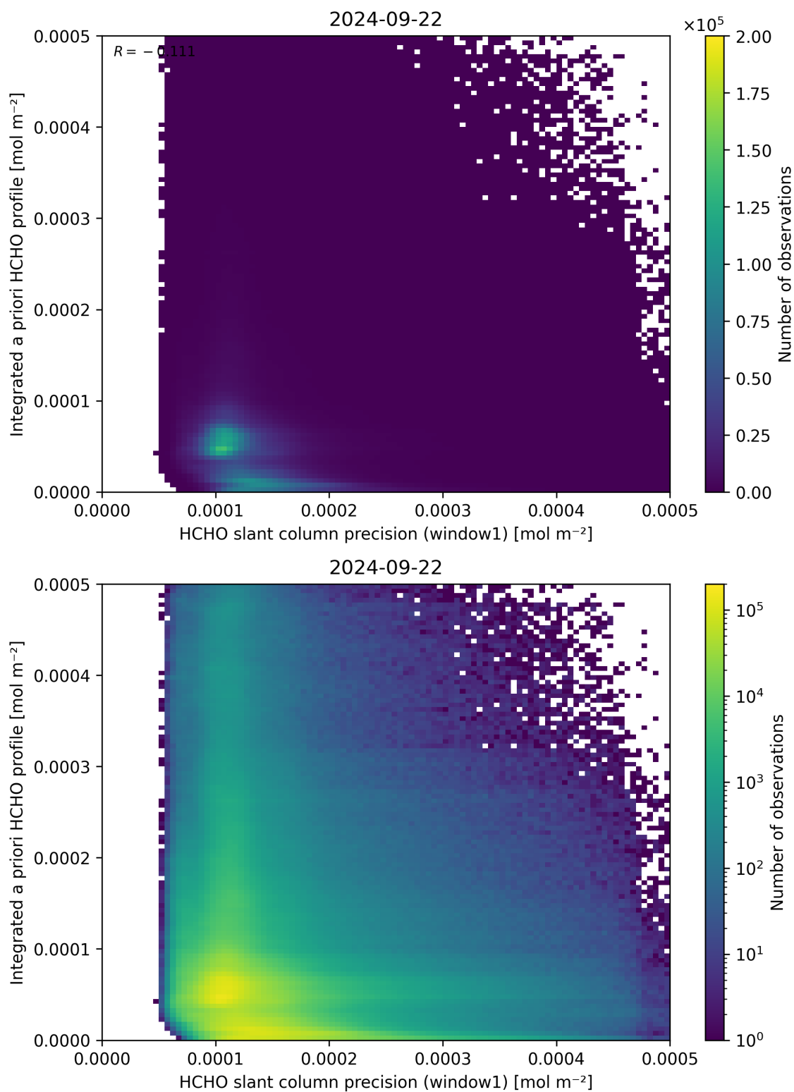
Figure 96: Scatter density plot of “HCHO slant column precision (window1)” against “Integrated a priori HCHO profile” for 2024-09-22 to 2024-09-23.
