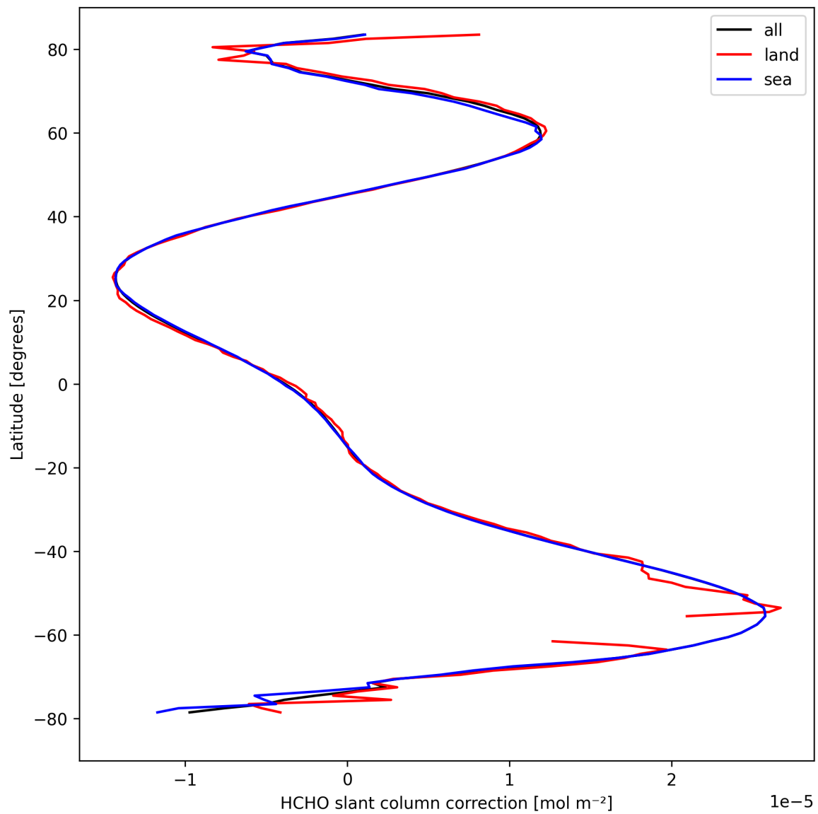
Figure 33: Zonal average of “HCHO slant column correction” for 2024-09-22 to 2024-09-23.
