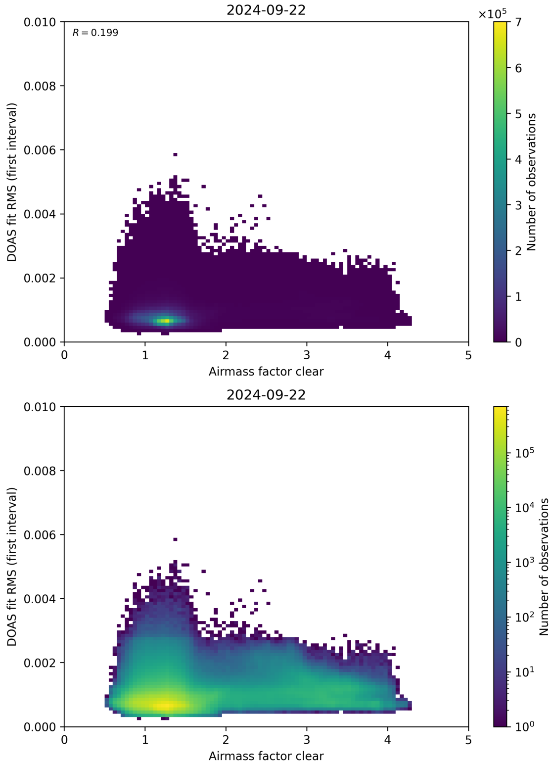
Figure 71: Scatter density plot of “Airmass factor clear” against “DOAS fit RMS (first interval)” for 2024-09-22 to 2024-09-23.
