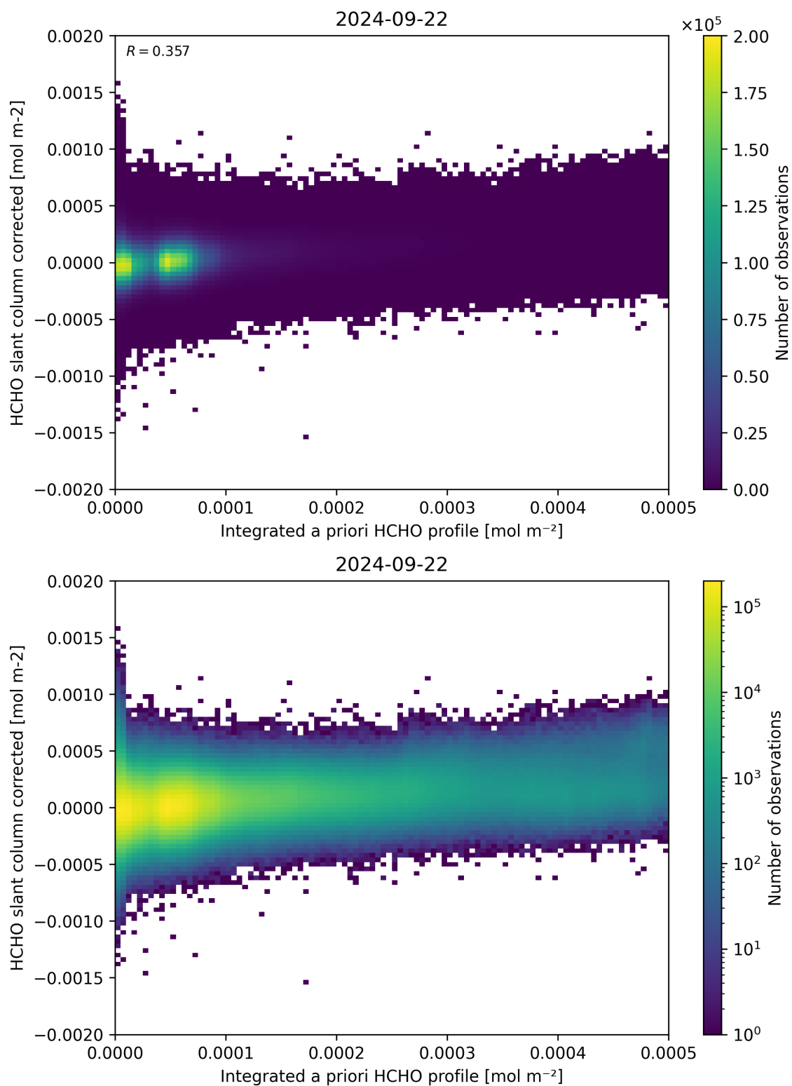
Figure 151: Scatter density plot of “Integrated a priori HCHO profile” against “HCHO slant column corrected” for 2024-09-22 to 2024-09-23.
