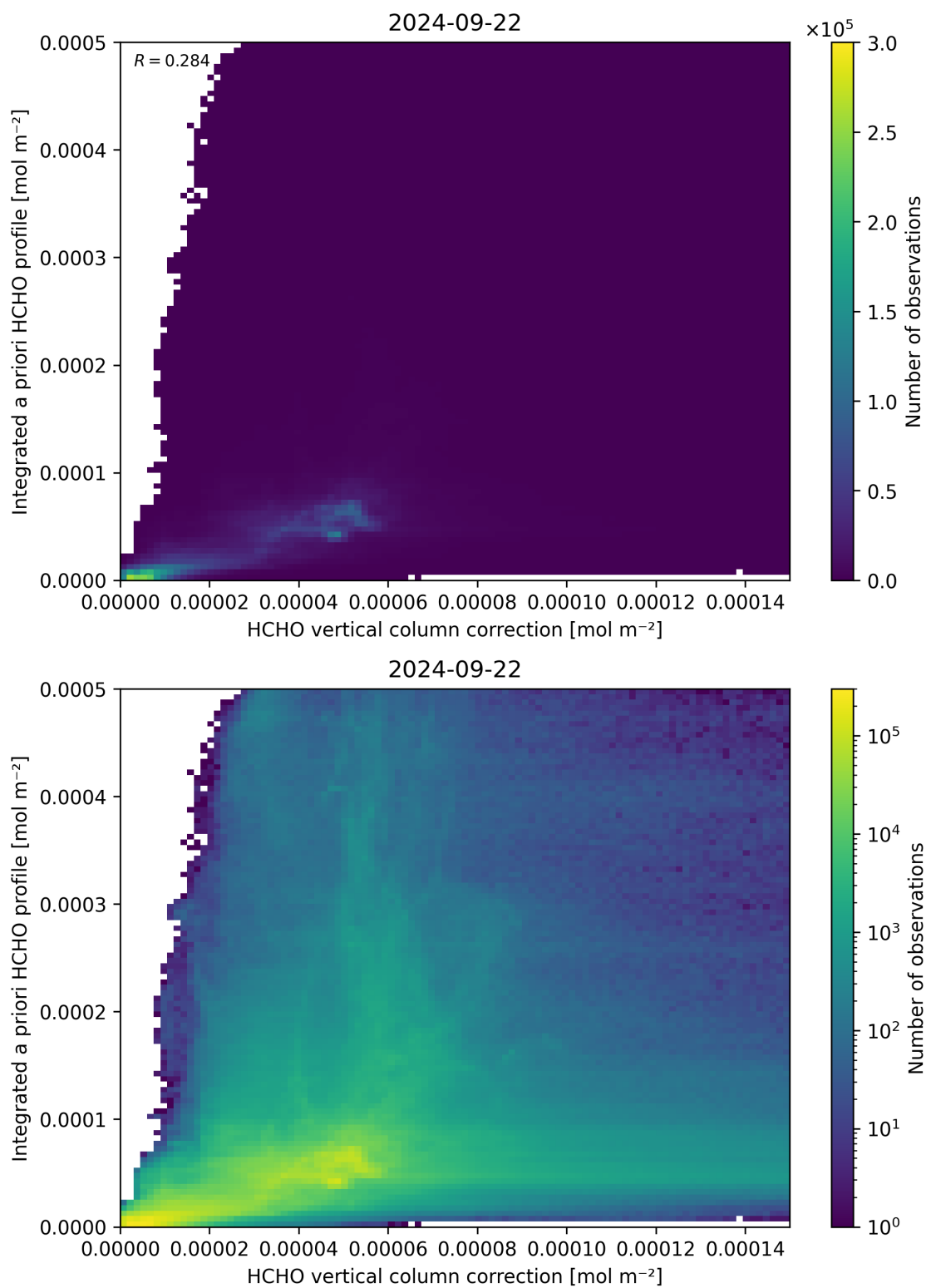
Figure 122: Scatter density plot of “HCHO vertical column correction” against “Integrated a priori HCHO profile” for 2024-09-22 to 2024-09-23.
