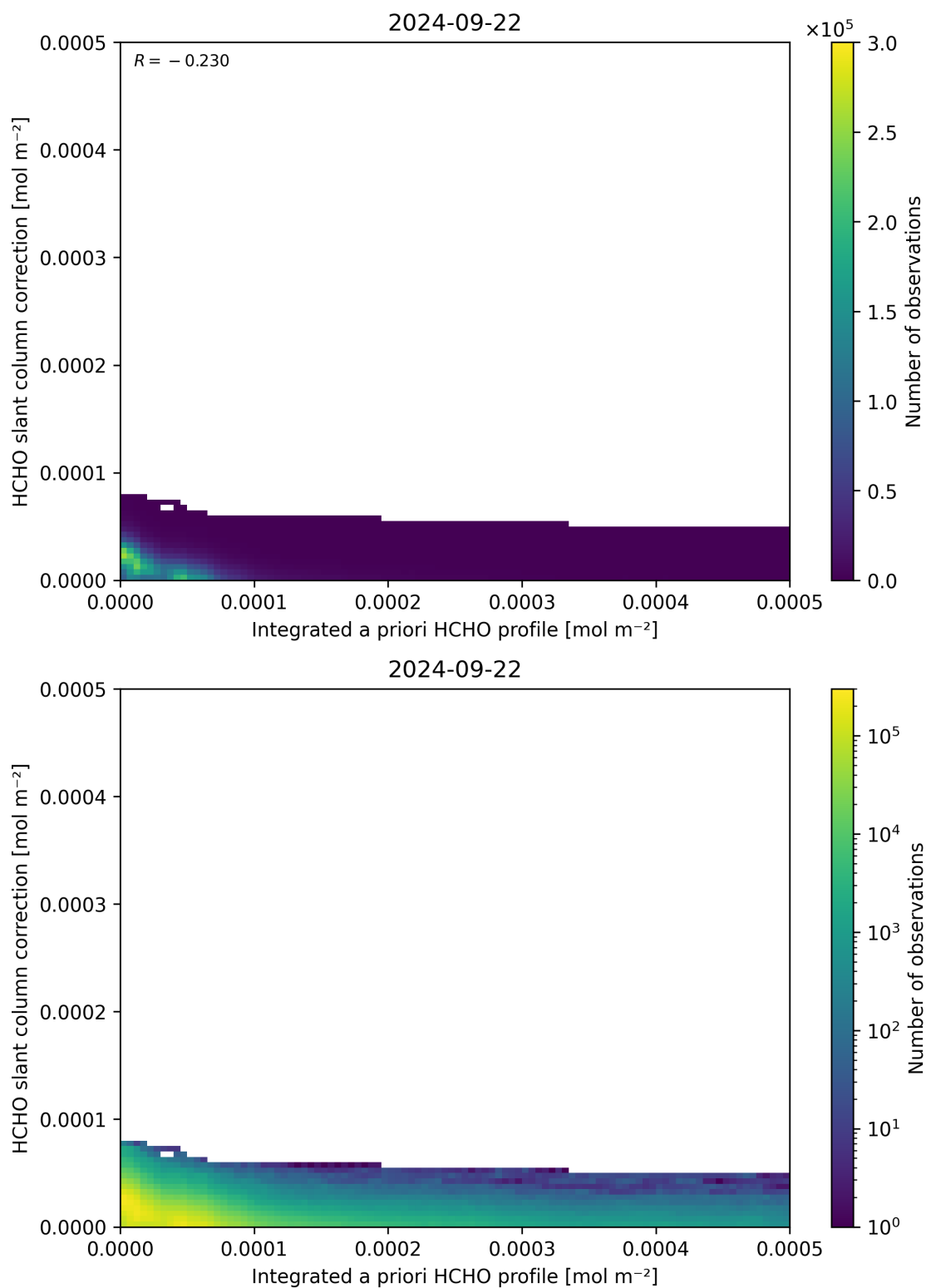
Figure 152: Scatter density plot of “Integrated a priori HCHO profile” against “HCHO slant column correction” for 2024-09-22 to 2024-09-23.
