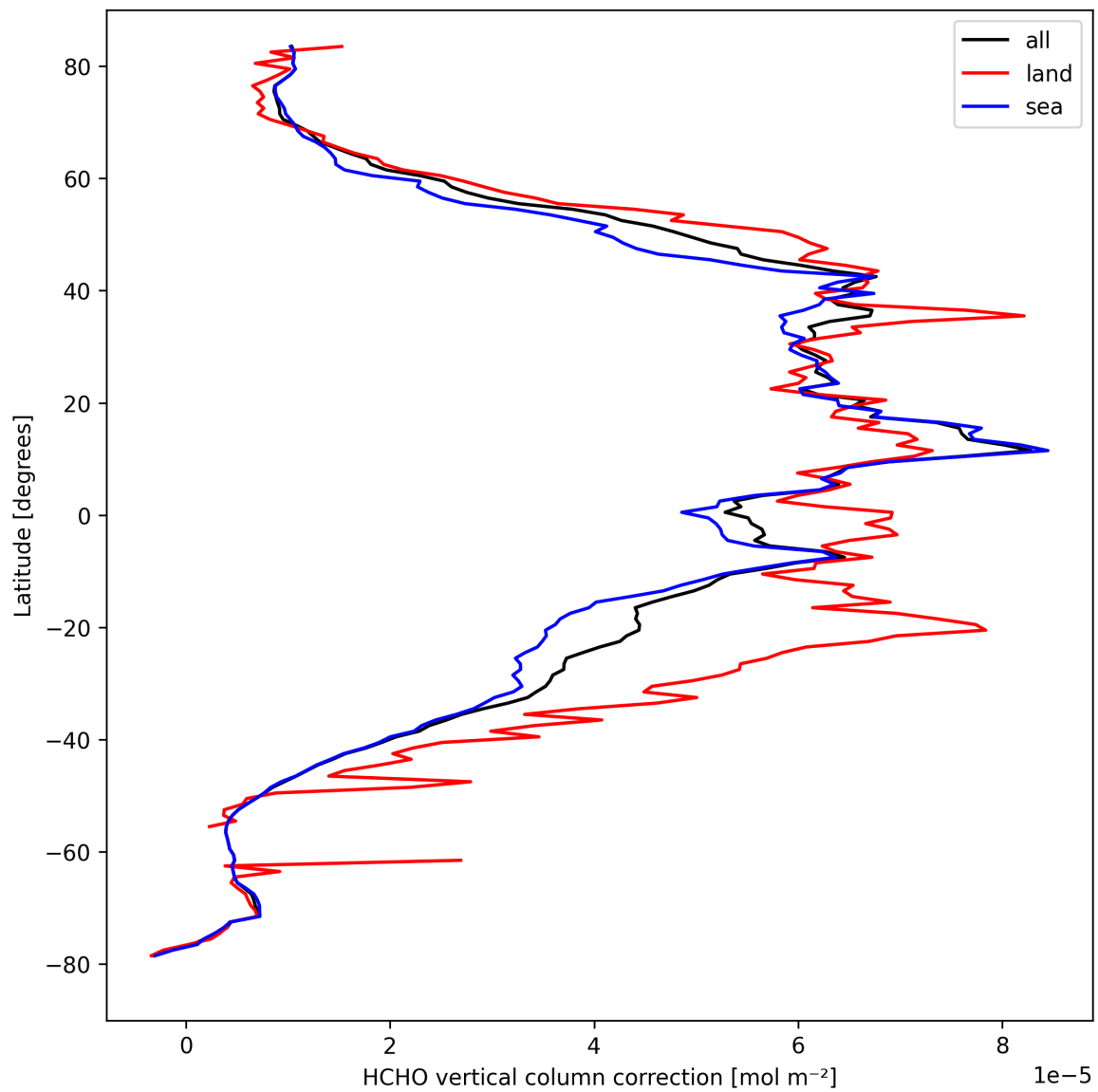
Figure 23: Zonal average of “HCHO vertical column correction” for 2024-09-22 to 2024-09-23.
