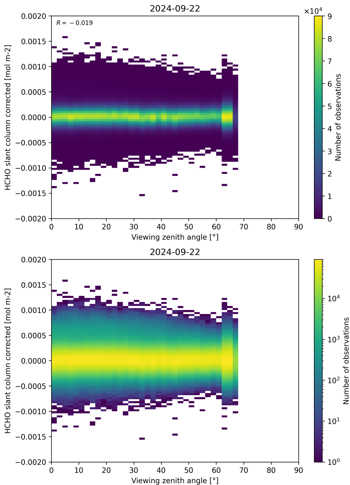
Figure 186: Scatter density plot of “Viewing zenith angle” against “HCHO slant column corrected” for 2024-09-22 to 2024-09-23.
