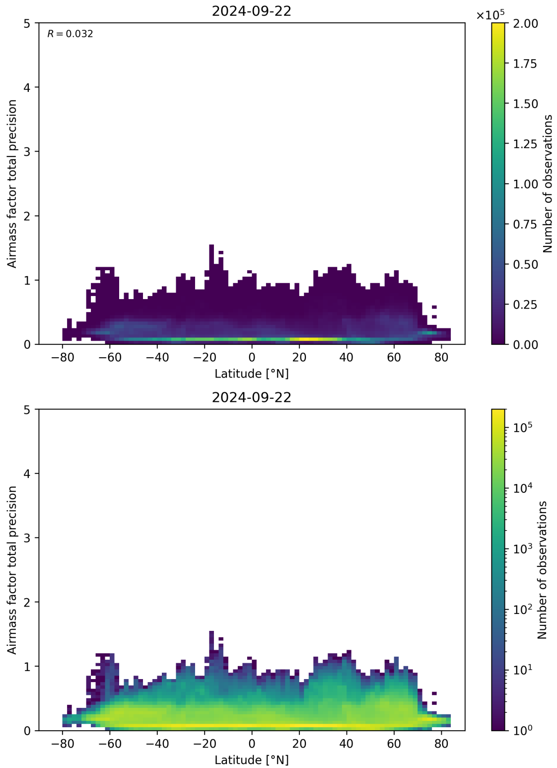
Figure 162: Scatter density plot of “Latitude” against “Airmass factor total precision” for 2024-09-22 to 2024-09-23.
