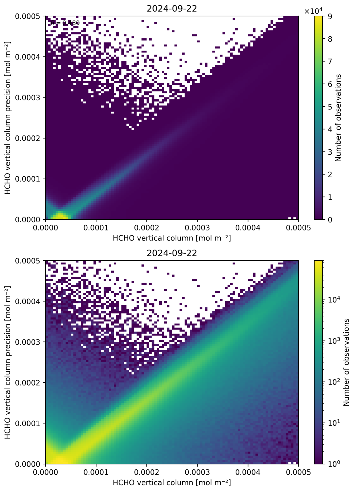
Figure 134: Scatter density plot of “HCHO vertical column” against “HCHO vertical column precision” for 2024-09-22 to 2024-09-23.
