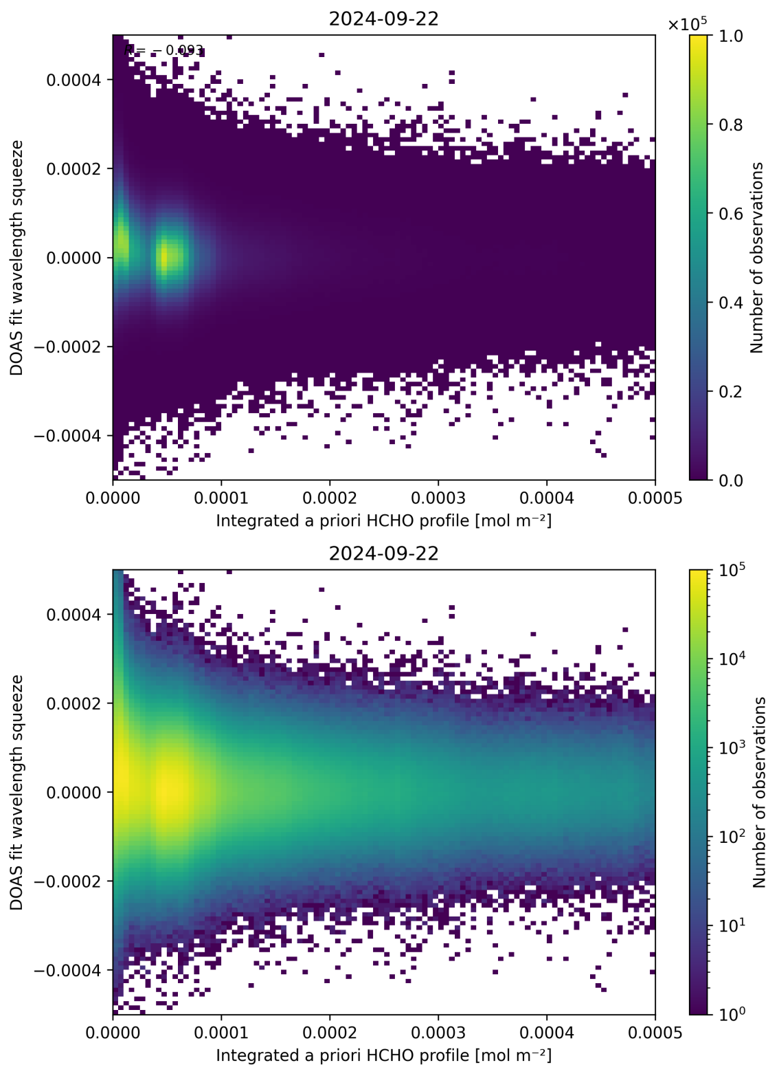
Figure 150: Scatter density plot of “Integrated a priori HCHO profile” against “DOAS fit wavelength squeeze” for 2024-09-22 to 2024-09-23.
