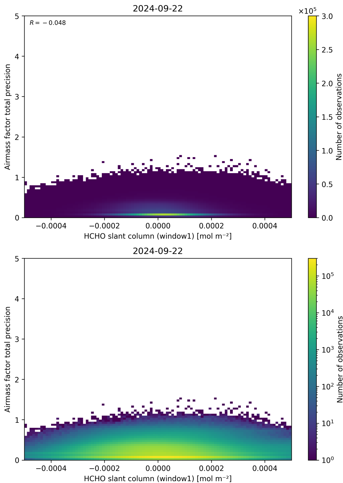
Figure 86: Scatter density plot of “HCHO slant column (window1)” against “Airmass factor total precision” for 2024-09-22 to 2024-09-23.
