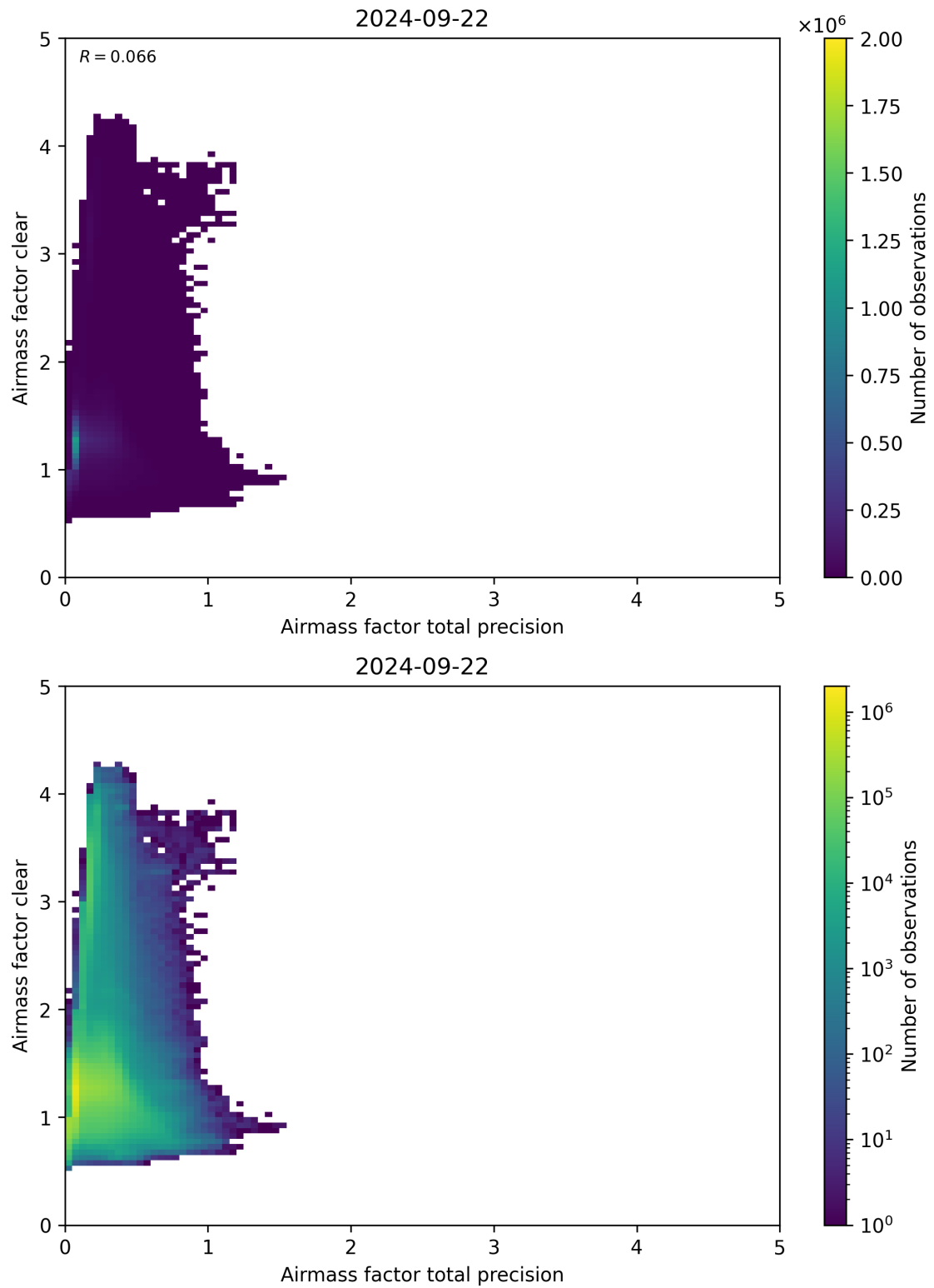
Figure 108: Scatter density plot of “Airmass factor total precision” against “Airmass factor clear” for 2024-09-22 to 2024-09-23.
