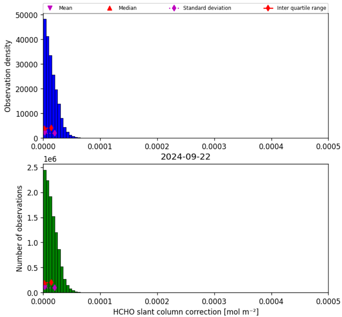
Figure 47: Histogram of “HCHO slant column correction” for 2024-09-22 to 2024-09-23
