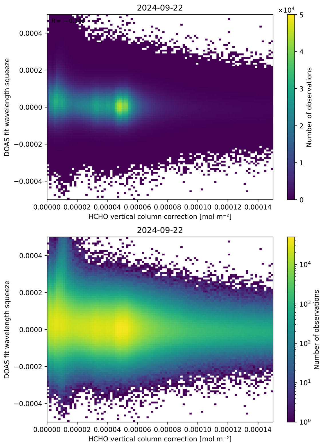
Figure 114: Scatter density plot of “HCHO vertical column correction” against “DOAS fit wavelength squeeze” for 2024-09-22 to 2024-09-23.
