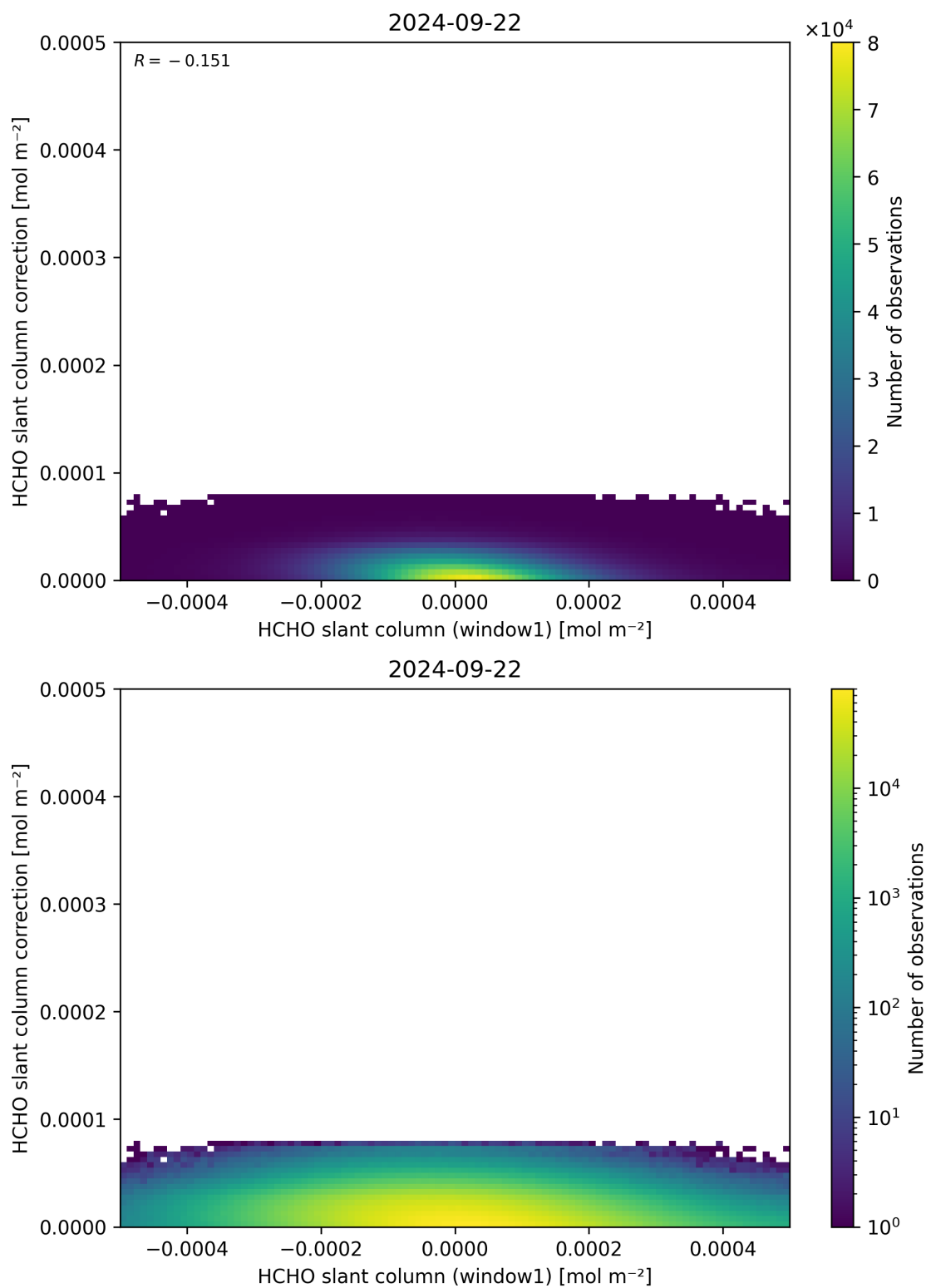
Figure 83: Scatter density plot of “HCHO slant column (window1)” against “HCHO slant column correction” for 2024-09-22 to 2024-09-23.
