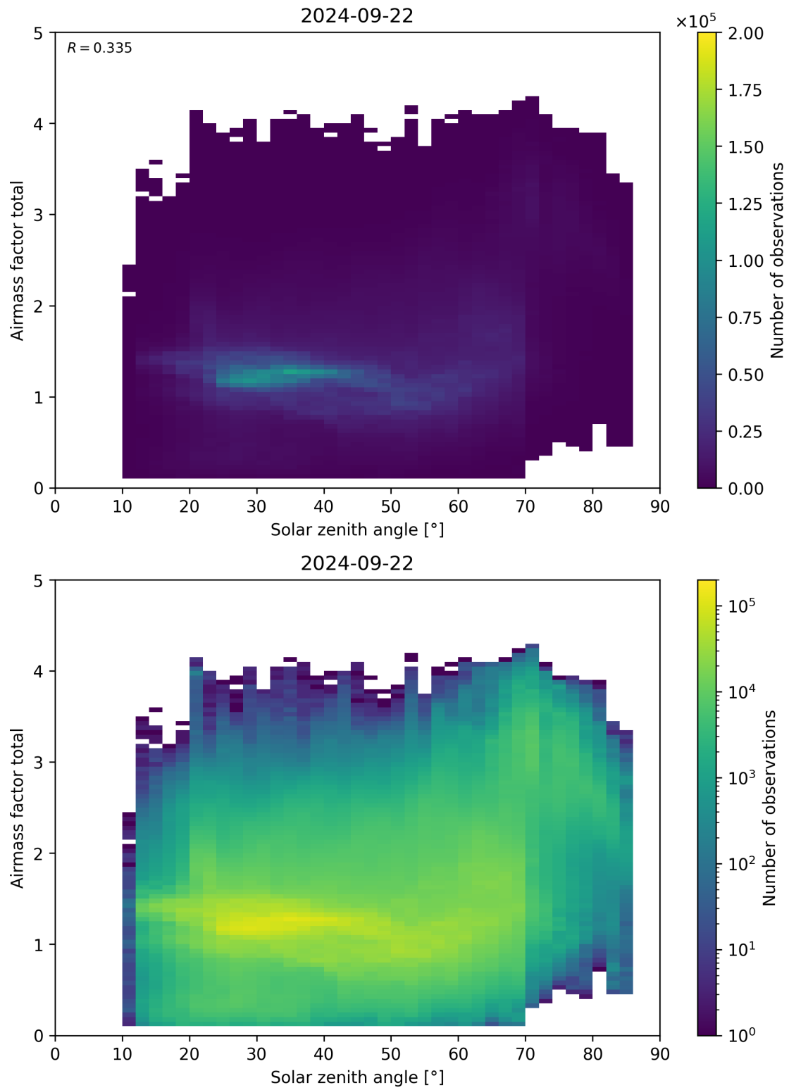
Figure 175: Scatter density plot of “Solar zenith angle” against “Airmass factor total” for 2024-09-22 to 2024-09-23.
