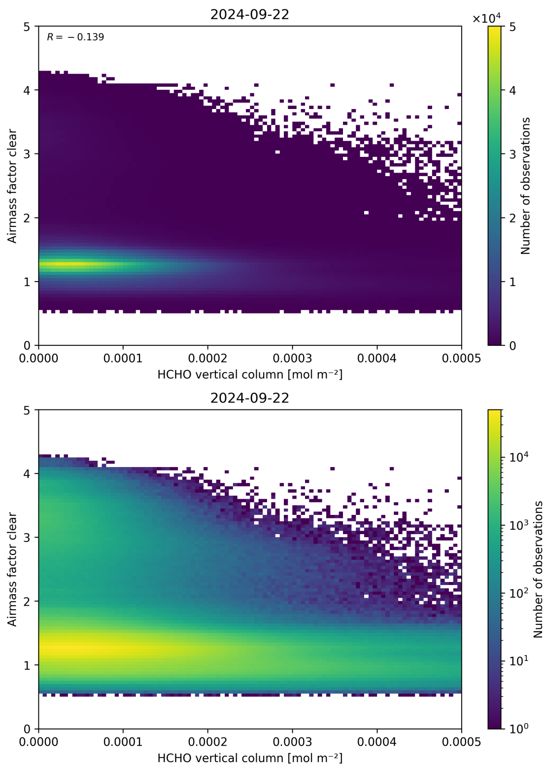
Figure 126: Scatter density plot of “HCHO vertical column” against “Airmass factor clear” for 2024-09-22 to 2024-09-23.
