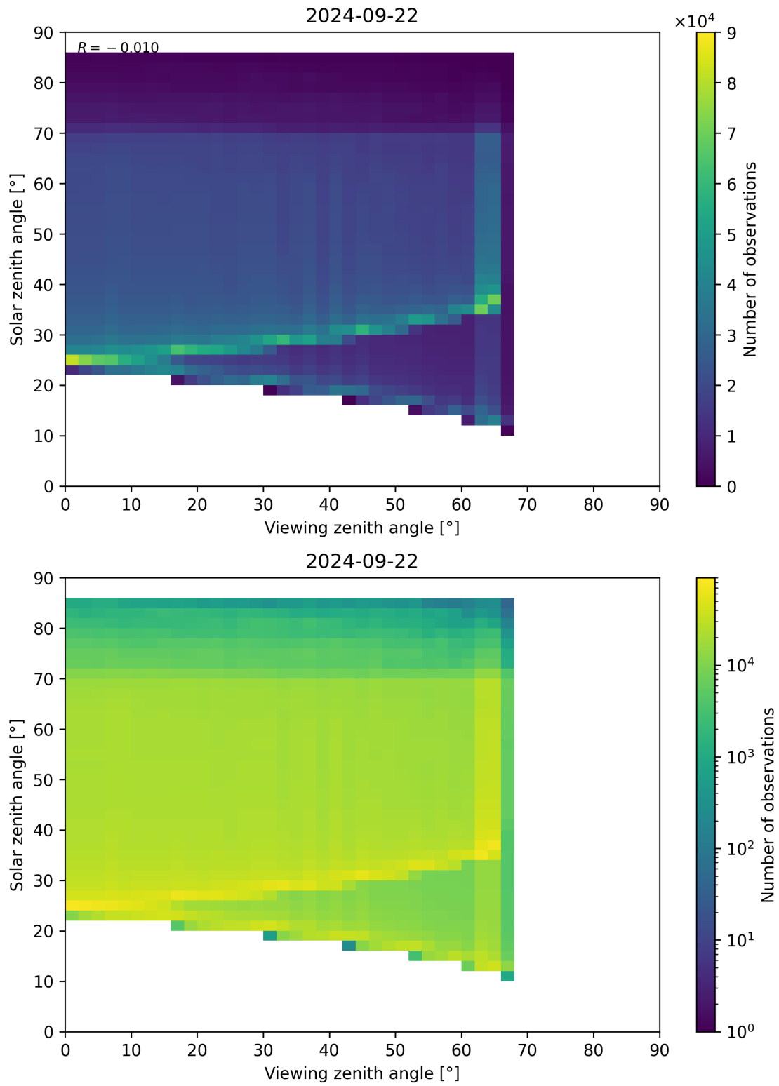
Figure 197: Scatter density plot of “Viewing zenith angle” against “Solar zenith angle” for 2024-09-22 to 2024-09-23.
