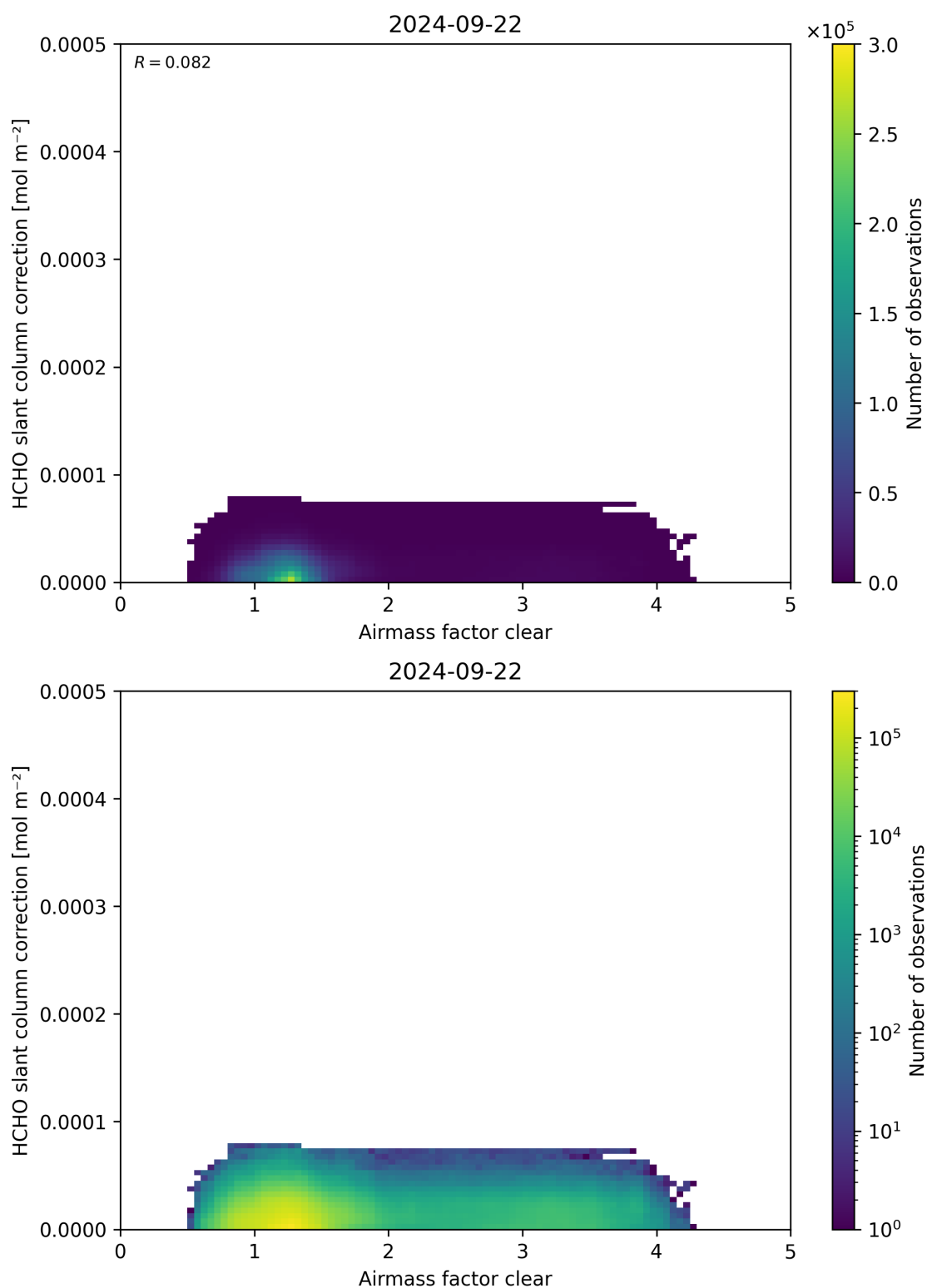
Figure 75: Scatter density plot of “Airmass factor clear” against “HCHO slant column correction” for 2024-09-22 to 2024-09-23.
