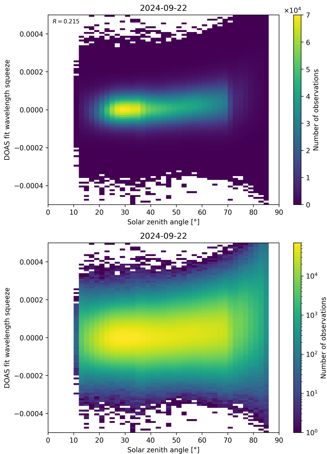
Figure 169: Scatter density plot of “Solar zenith angle” against “DOAS fit wavelength squeeze” for 2024-09-22 to 2024-09-23.
