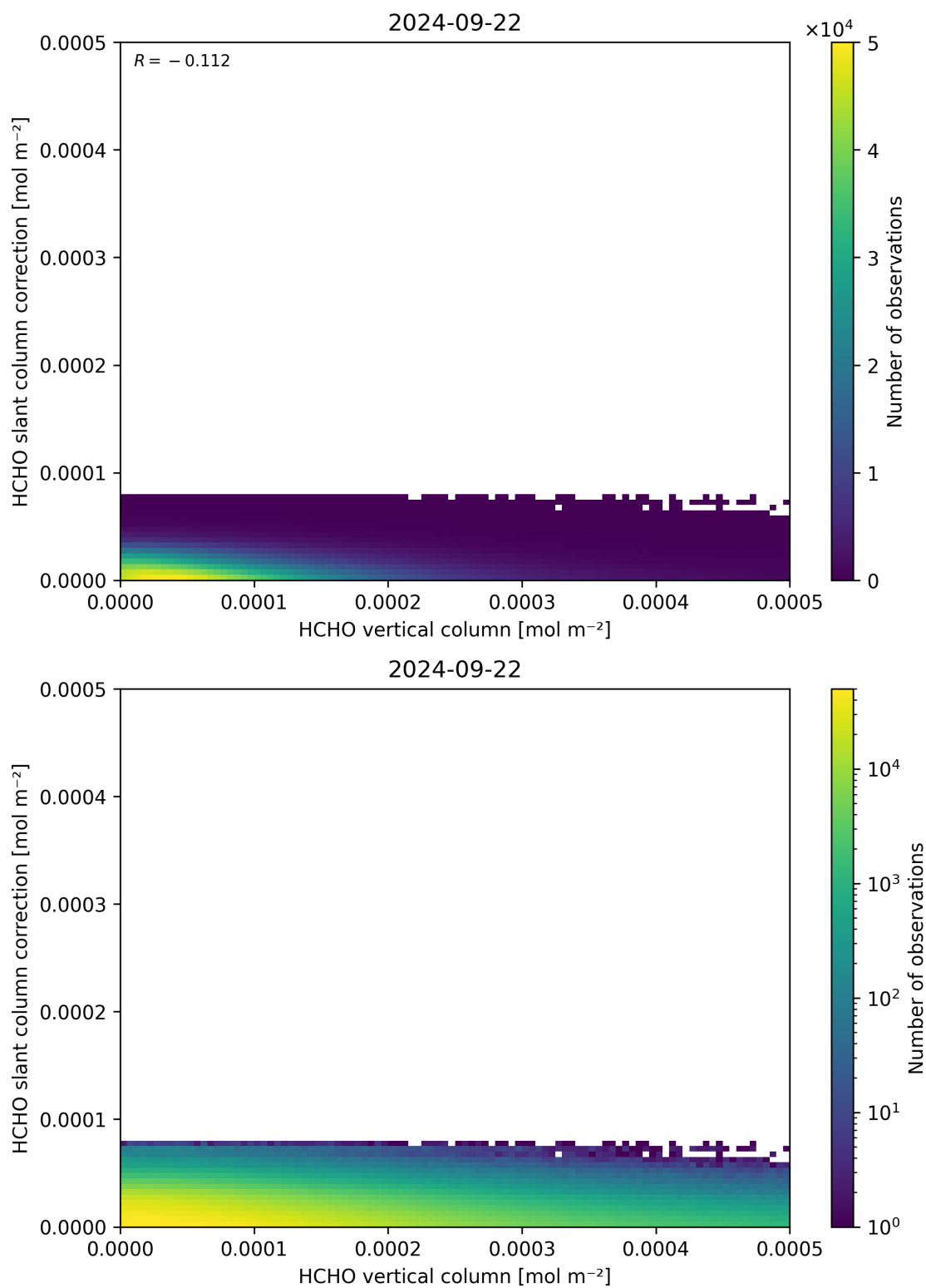
Figure 128: Scatter density plot of “HCHO vertical column” against “HCHO slant column correction” for 2024-09-22 to 2024-09-23.
