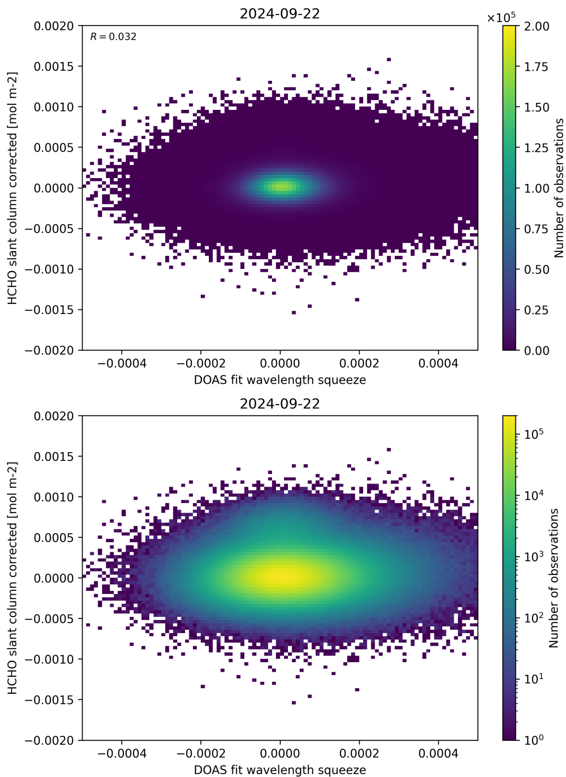
Figure 69: Scatter density plot of “DOAS fit wavelength squeeze” against “HCHO slant column corrected” for 2024-09-22 to 2024-09-23.
