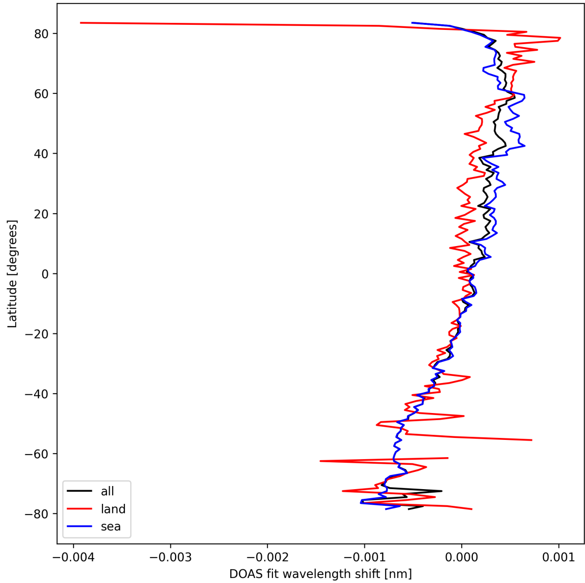
Figure 30: Zonal average of "DOAS fit wavelength shift" for 2024-09-22 to 2024-09-23.
