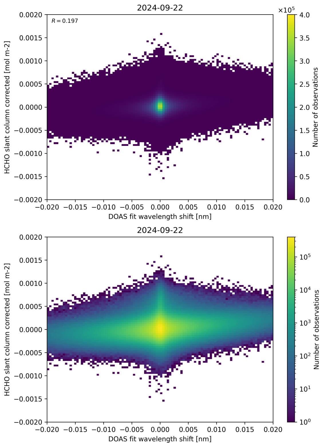
Figure 66: Scatter density plot of “DOAS fit wavelength shift” against “HCHO slant column corrected” for 2024-09-22 to 2024-09-23.
