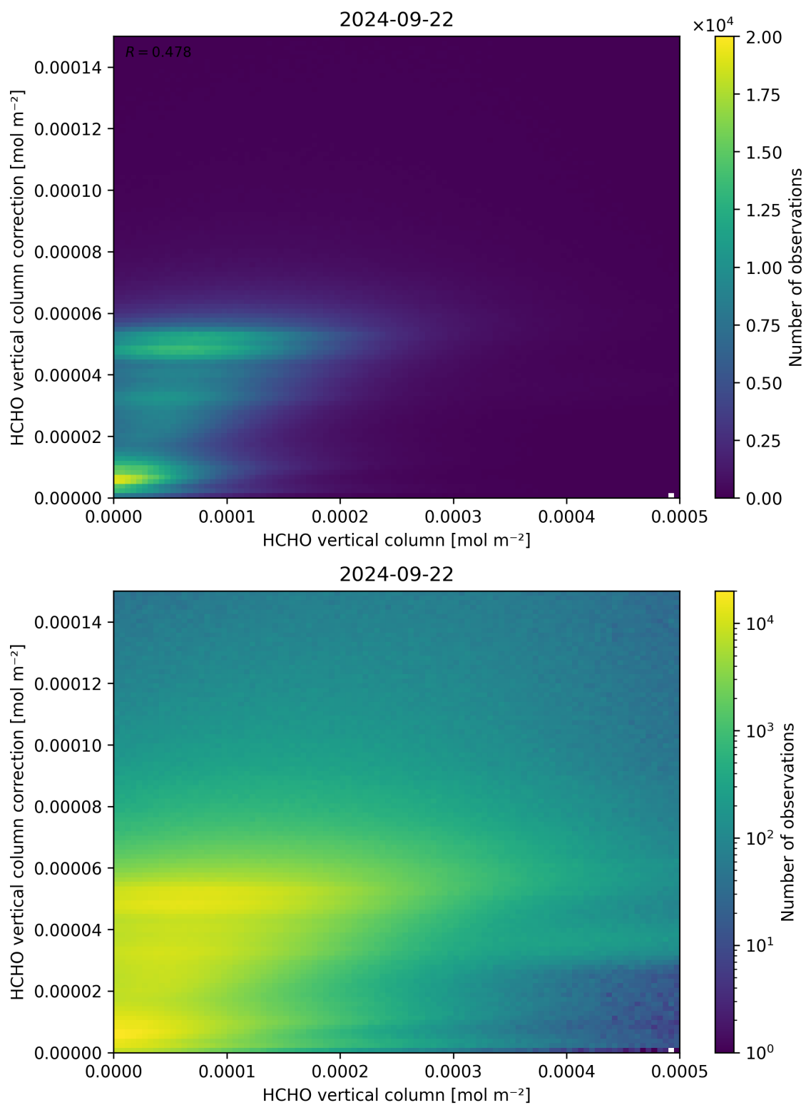
Figure 133: Scatter density plot of “HCHO vertical column” against “HCHO vertical column correction” for 2024-09-22 to 2024-09-23.
