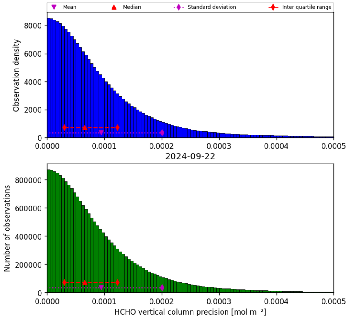
Figure 36: Histogram of “HCHO vertical column precision” for 2024-09-22 to 2024-09-23
