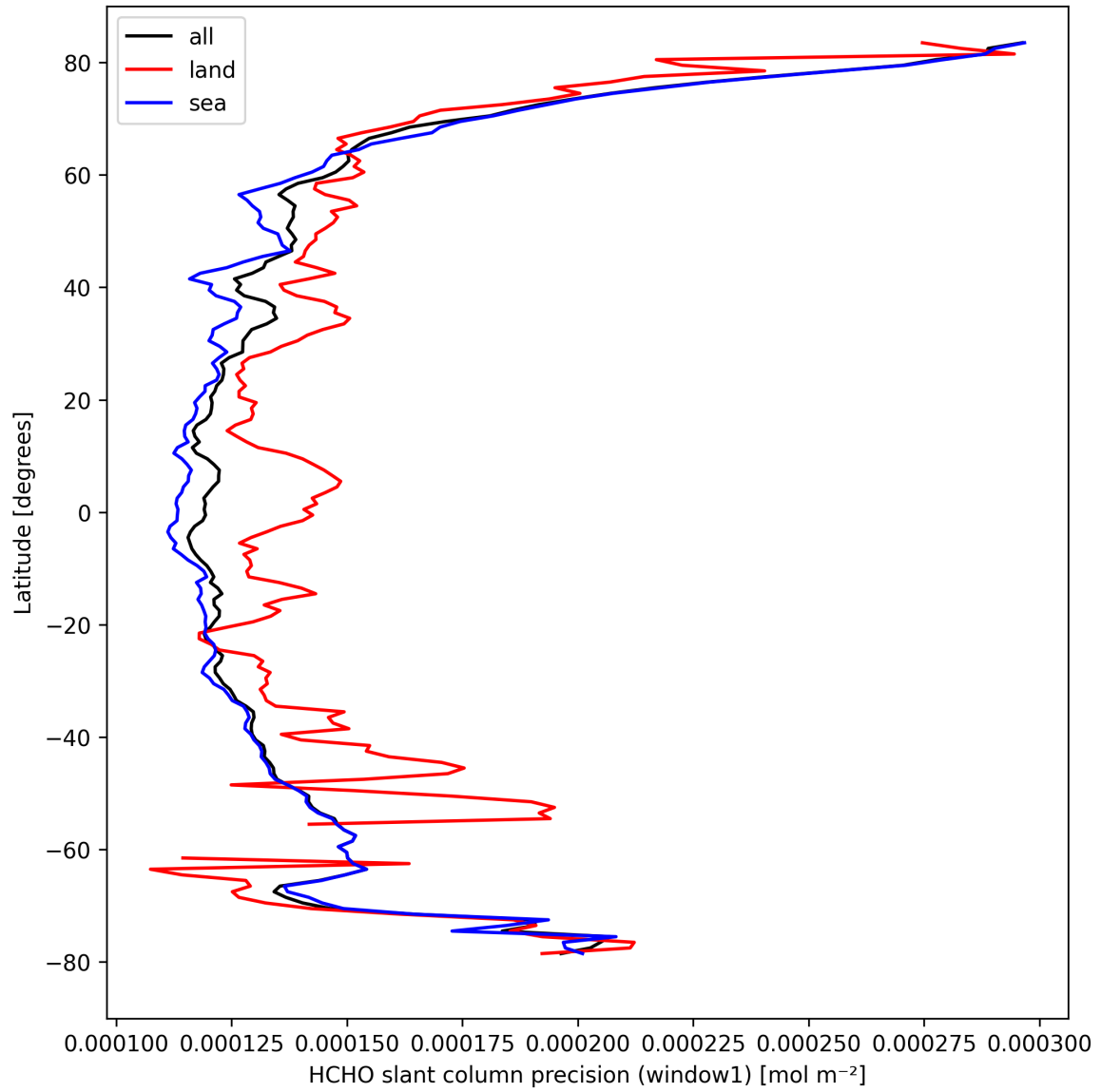
Figure 25: Zonal average of “HCHO slant column precision (window1)” for 2024-09-22 to 2024-09-23.
