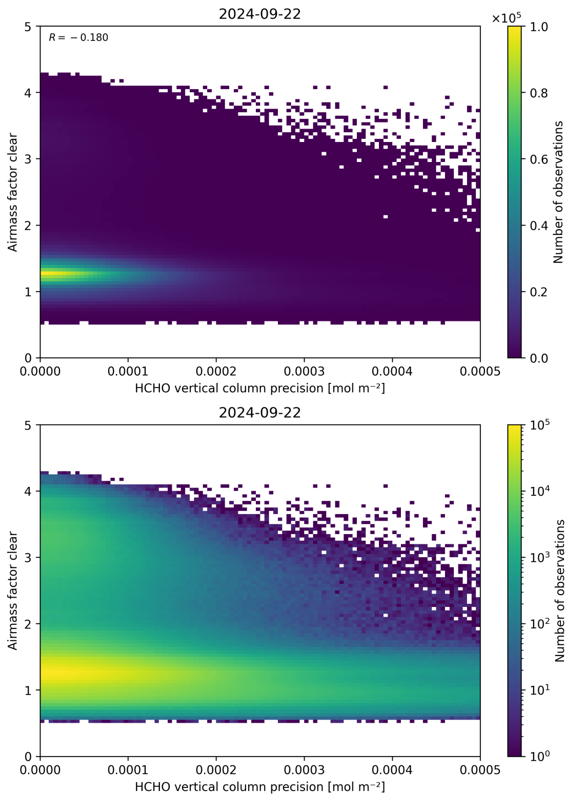
Figure 139: Scatter density plot of “HCHO vertical column precision” against “Airmass factor clear” for 2024-09-22 to 2024-09-23.
