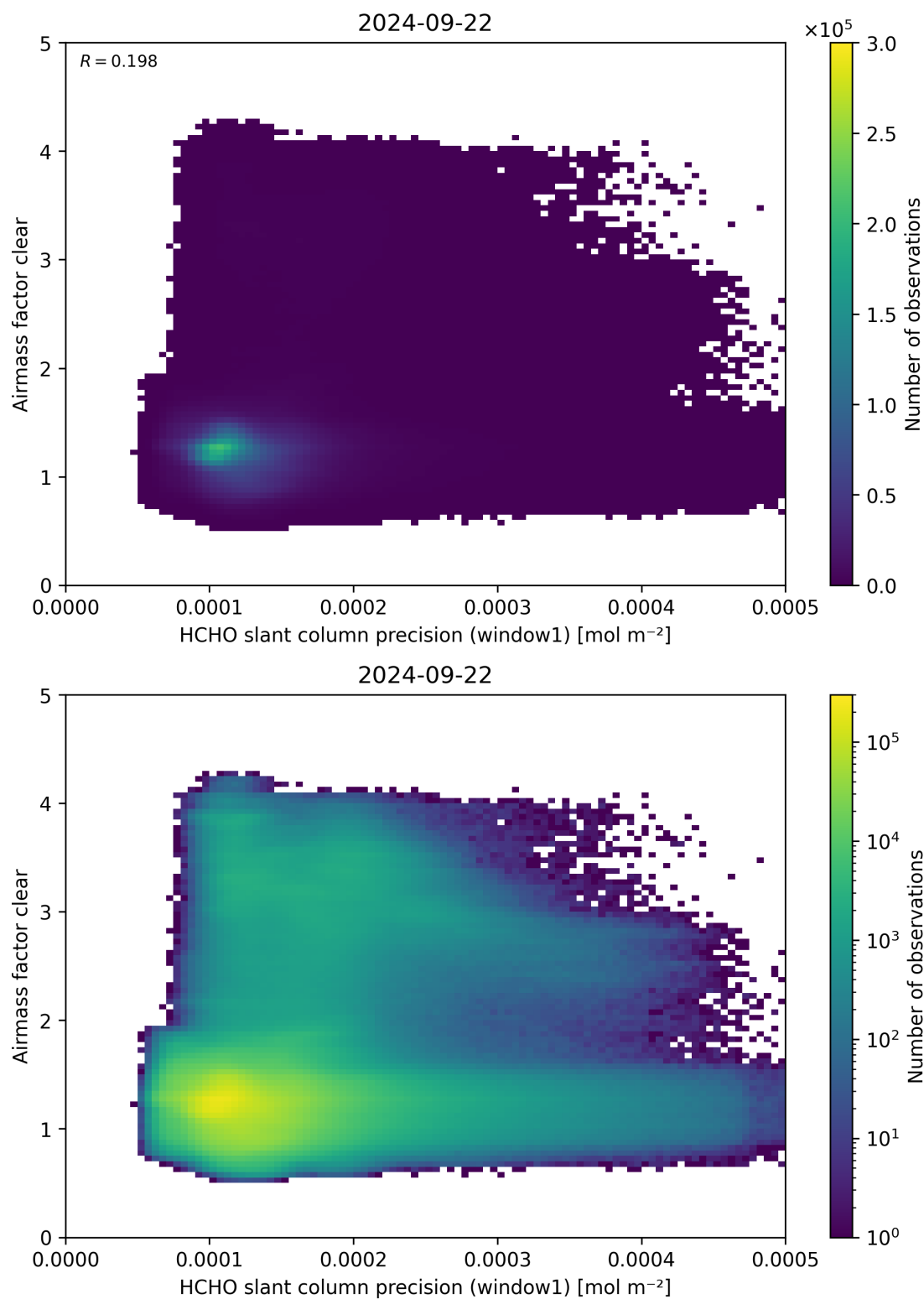
Figure 91: Scatter density plot of “HCHO slant column precision (window1)” against “Airmass factor clear” for 2024-09-22 to 2024-09-23.
