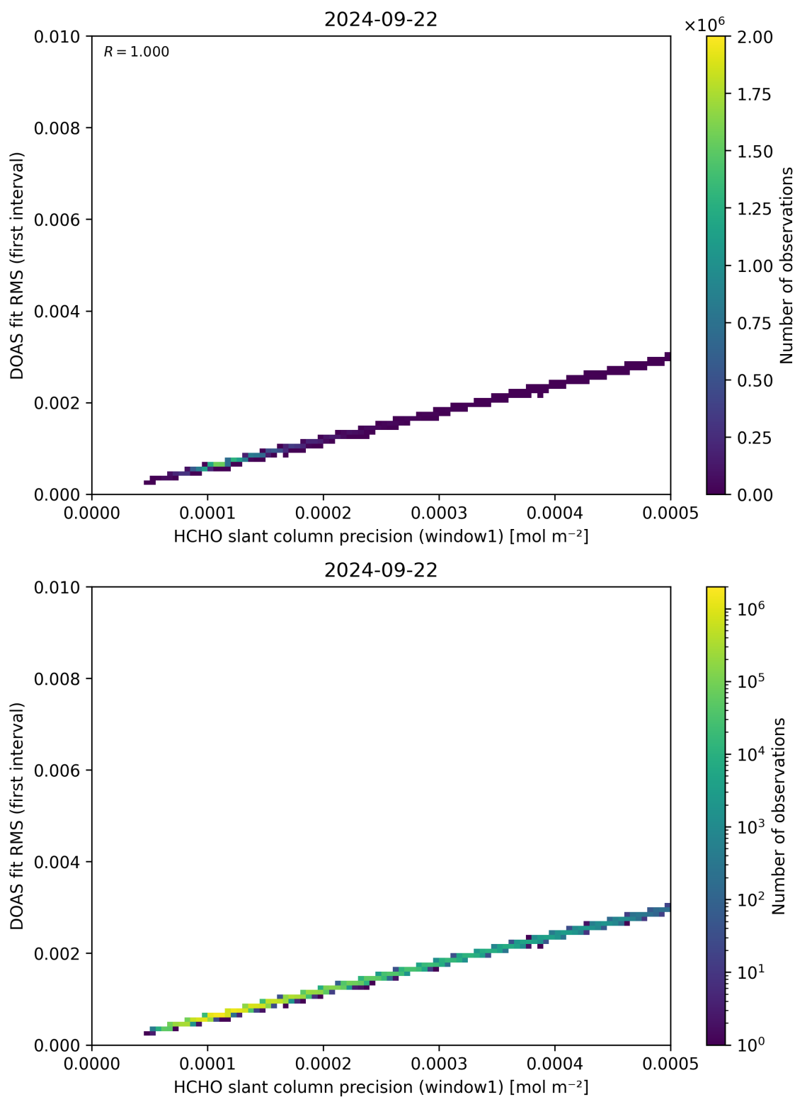
Figure 88: Scatter density plot of “HCHO slant column precision (window1)” against “DOAS fit RMS (first interval)” for 2024-09-22 to 2024-09-23.
