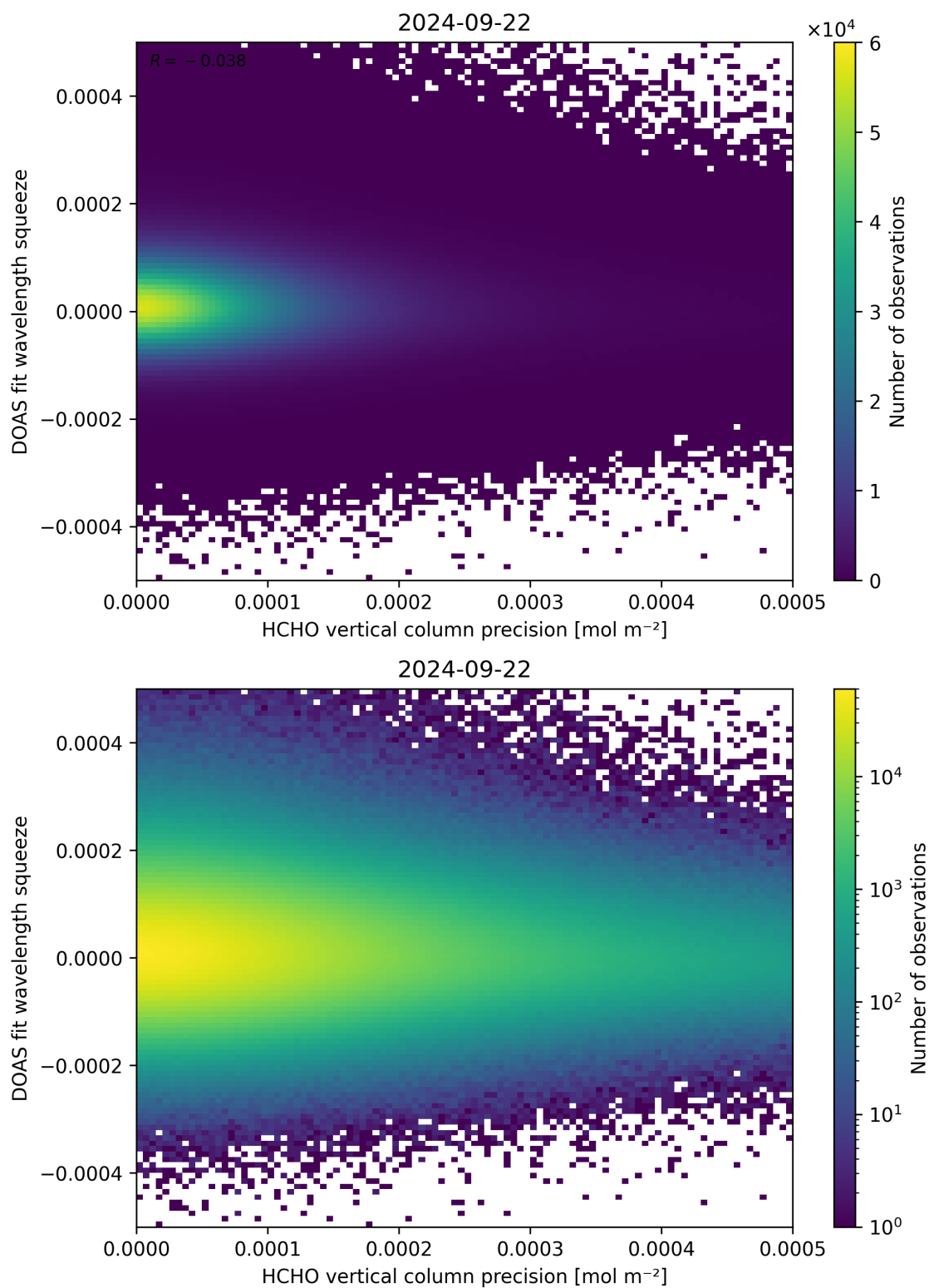
Figure 138: Scatter density plot of “HCHO vertical column precision” against “DOAS fit wavelength squeeze” for 2024-09-22 to 2024-09-23.
