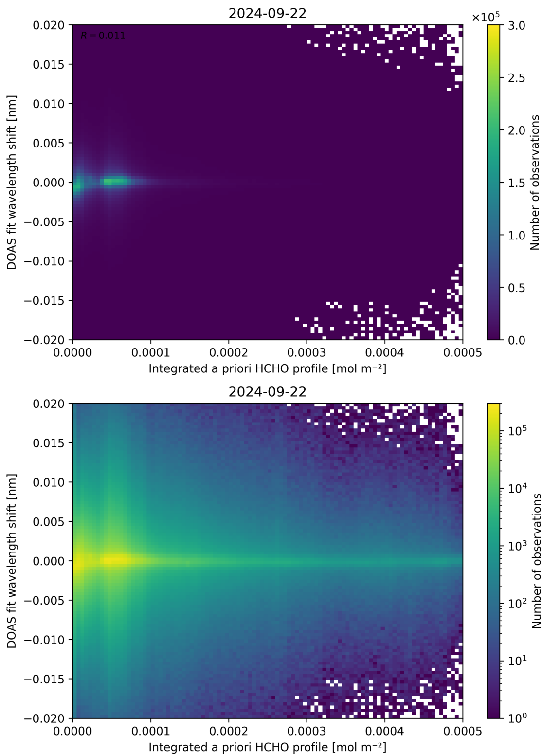
Figure 149: Scatter density plot of “Integrated a priori HCHO profile” against “DOAS fit wavelength shift” for 2024-09-22 to 2024-09-23.
