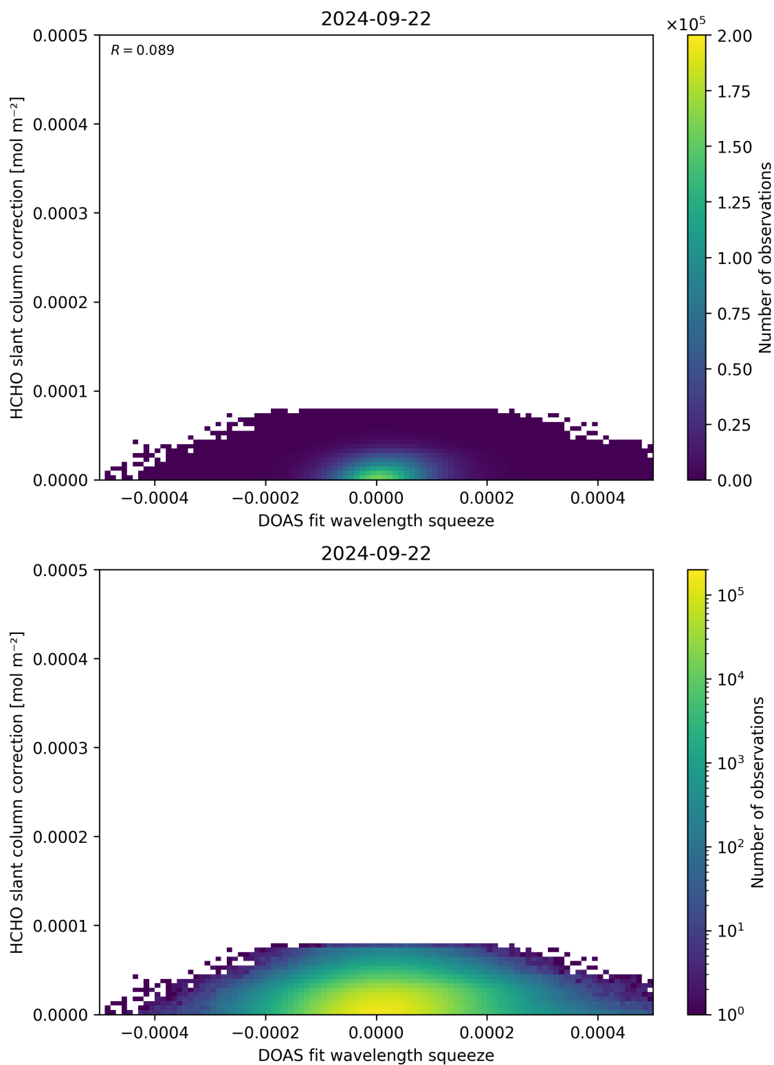
Figure 70: Scatter density plot of “DOAS fit wavelength squeeze” against “HCHO slant column correction” for 2024-09-22 to 2024-09-23.
