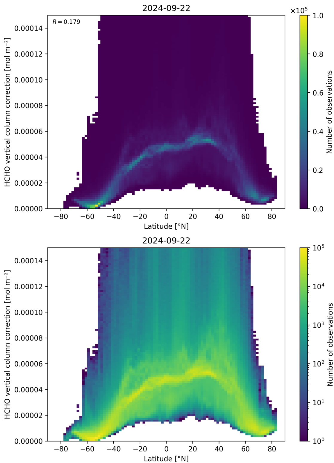
Figure 164: Scatter density plot of “Latitude” against “HCHO vertical column correction” for 2024-09-22 to 2024-09-23.
