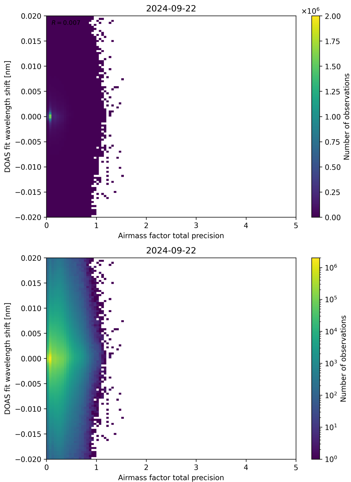
Figure 106: Scatter density plot of “Airmass factor total precision” against “DOAS fit wavelength shift” for 2024-09-22 to 2024-09-23.
