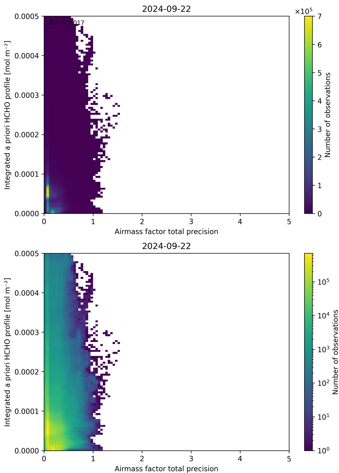
Figure 111: Scatter density plot of “Airmass factor total precision” against “Integrated a priori HCHO profile” for 2024-09-22 to 2024-09-23.
