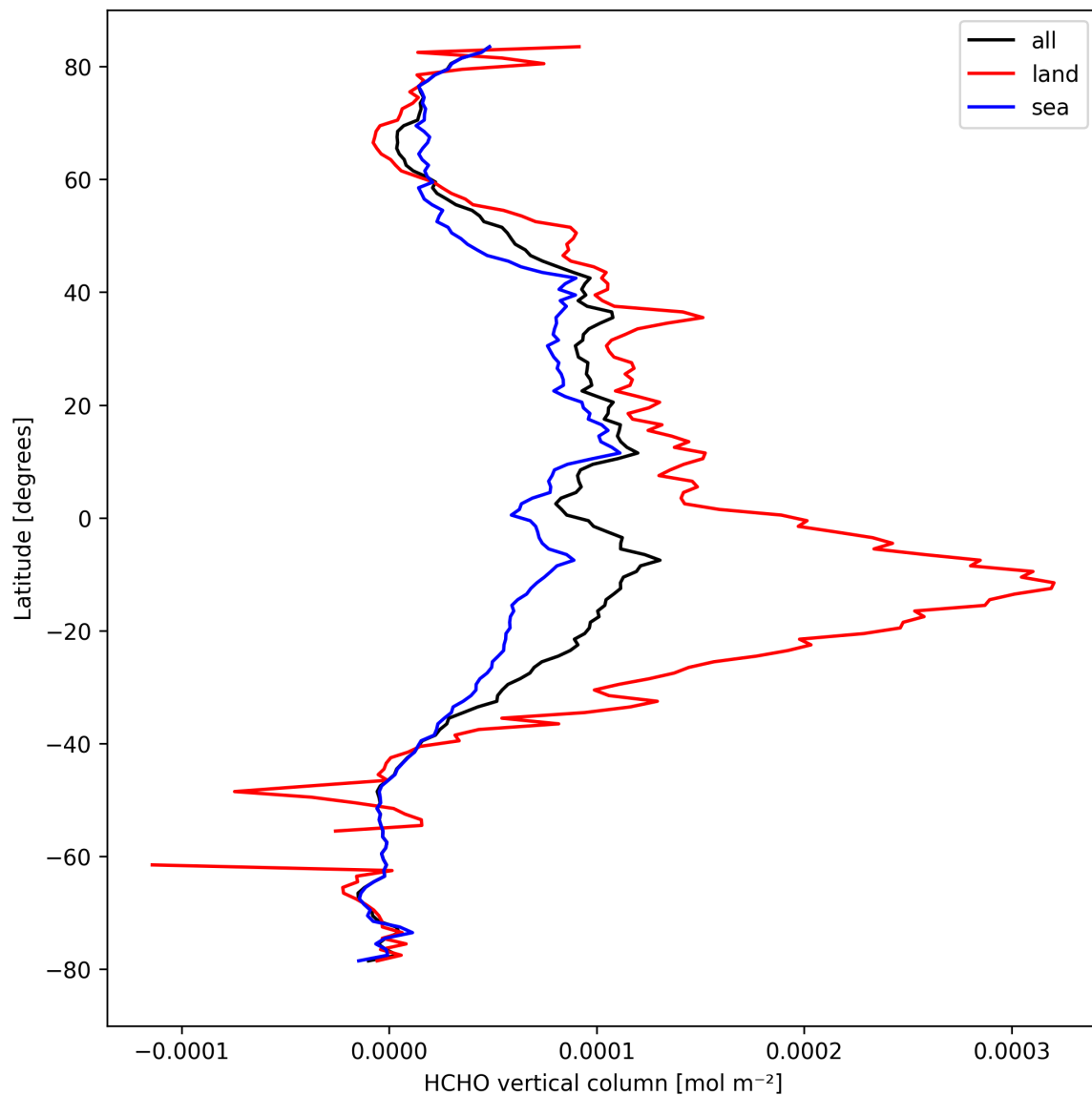
Figure 21: Zonal average of “HCHO vertical column” for 2024-09-22 to 2024-09-23.
