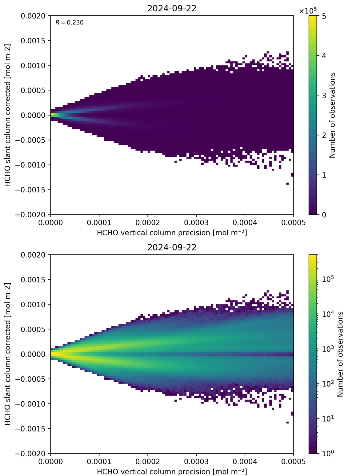
Figure 140: Scatter density plot of “HCHO vertical column precision” against “HCHO slant column corrected” for 2024-09-22 to 2024-09-23.
