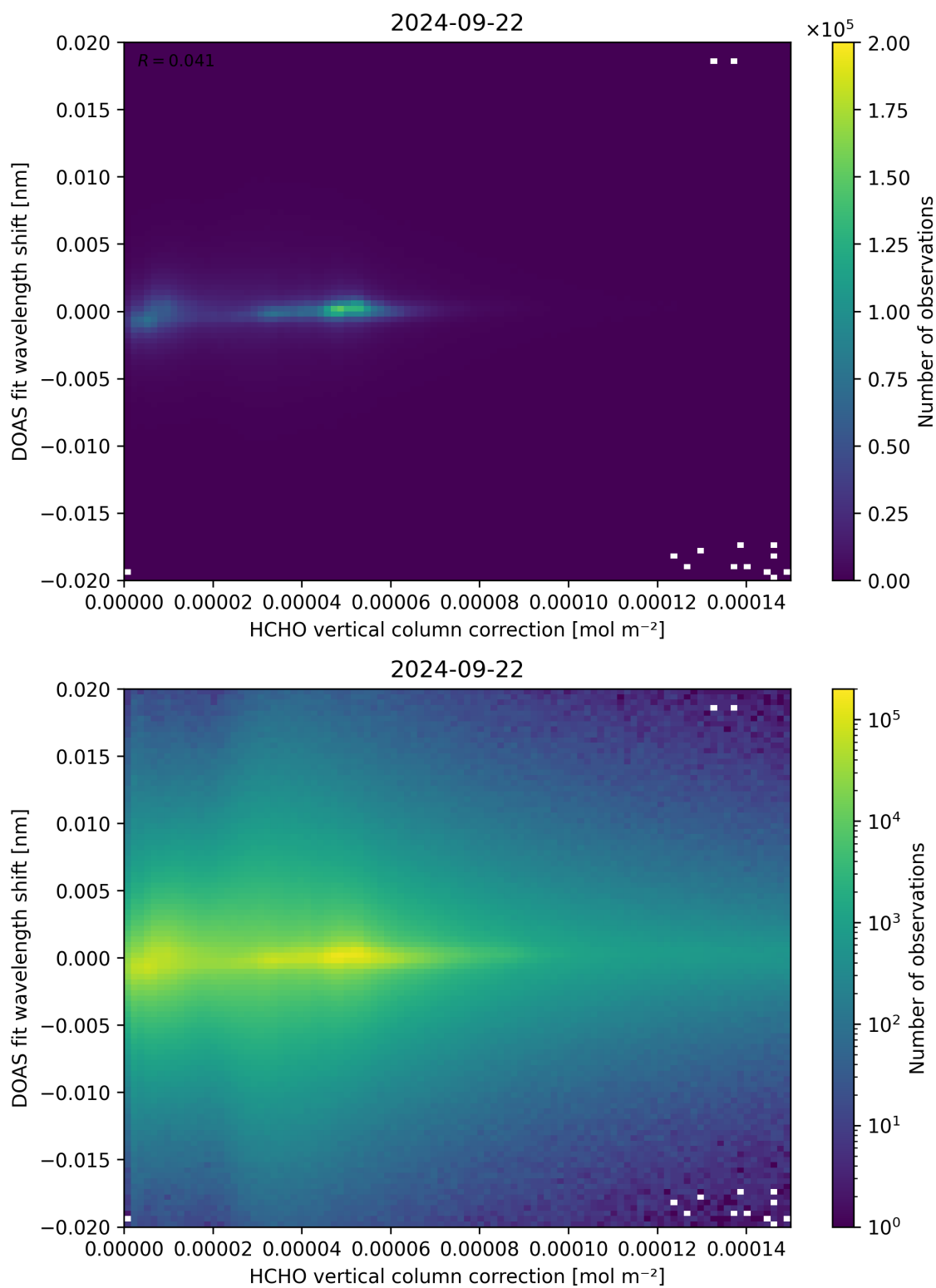
Figure 113: Scatter density plot of “HCHO vertical column correction” against “DOAS fit wavelength shift” for 2024-09-22 to 2024-09-23.
