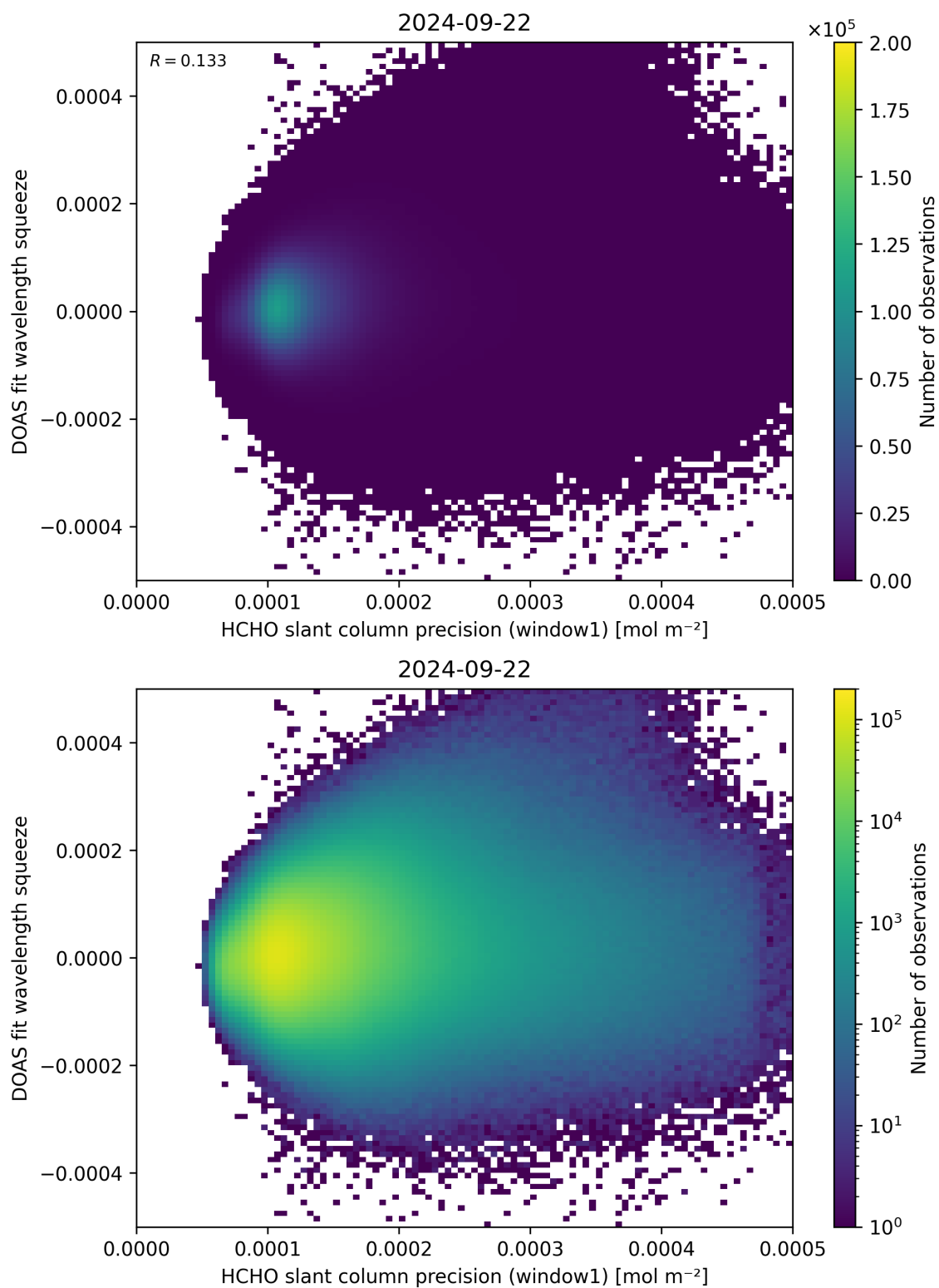
Figure 90: Scatter density plot of “HCHO slant column precision (window1)” against “DOAS fit wavelength squeeze” for 2024-09-22 to 2024-09-23.
