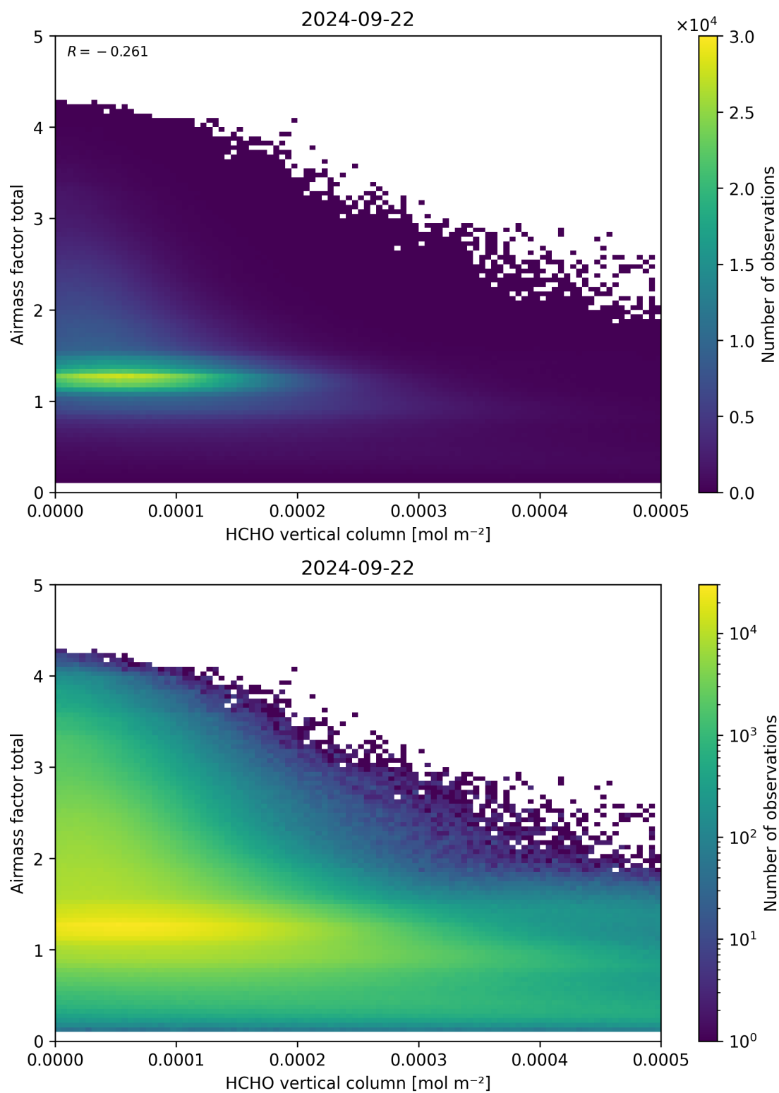
Figure 131: Scatter density plot of “HCHO vertical column” against “Airmass factor total” for 2024-09-22 to 2024-09-23.
