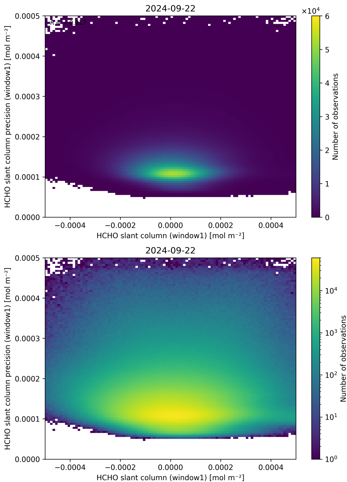
Figure 84: Scatter density plot of “HCHO slant column (window1)” against “HCHO slant column precision (window1)” for 2024-09-22 to 2024-09-23.
