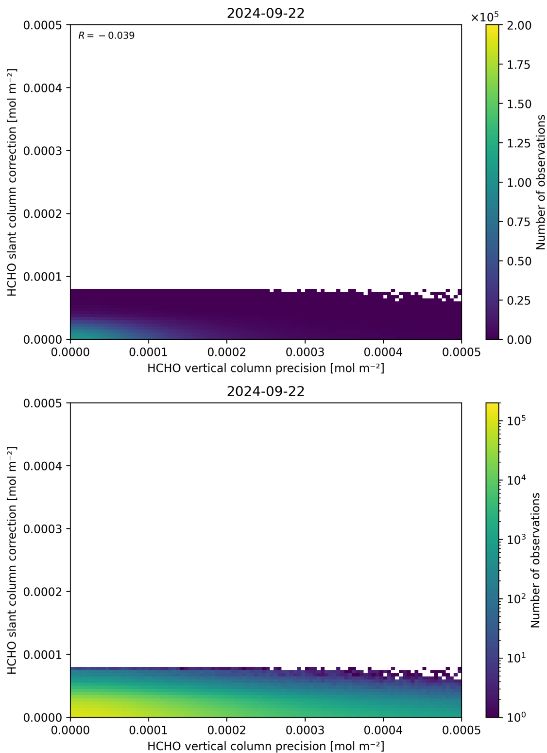
Figure 141: Scatter density plot of “HCHO vertical column precision” against “HCHO slant column correction” for 2024-09-22 to 2024-09-23.
