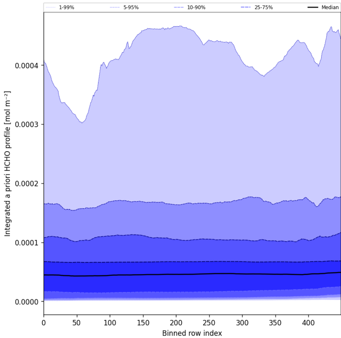
Figure 57: Along track statistics of “Integrated a priori HCHO profile” for 2024-09-22 to 2024-09-23
