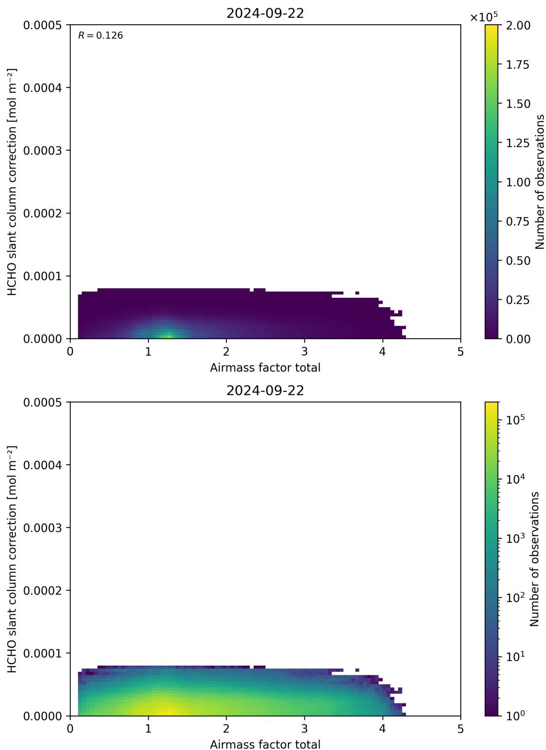
Figure 102: Scatter density plot of “Airmass factor total” against “HCHO slant column correction” for 2024-09-22 to 2024-09-23.
