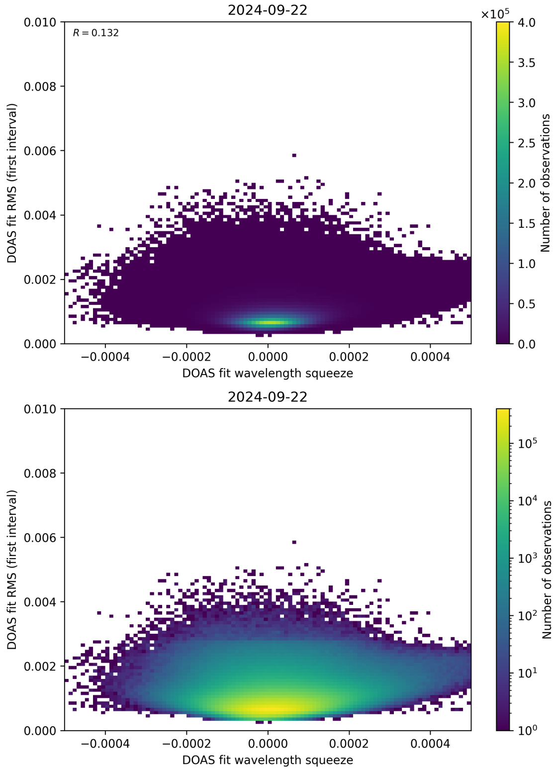
Figure 68: Scatter density plot of “DOAS fit wavelength squeeze” against “DOAS fit RMS (first interval)” for 2024-09-22 to 2024-09-23.
