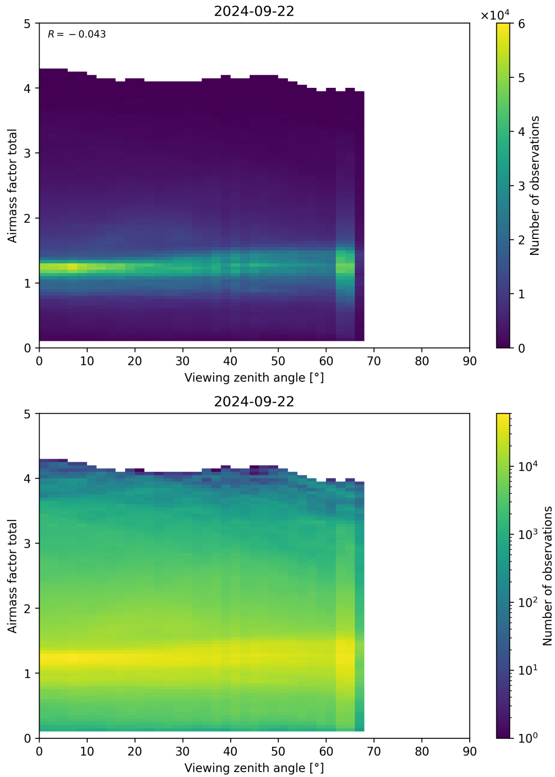
Figure 190: Scatter density plot of “Viewing zenith angle” against “Airmass factor total” for 2024-09-22 to 2024-09-23.
