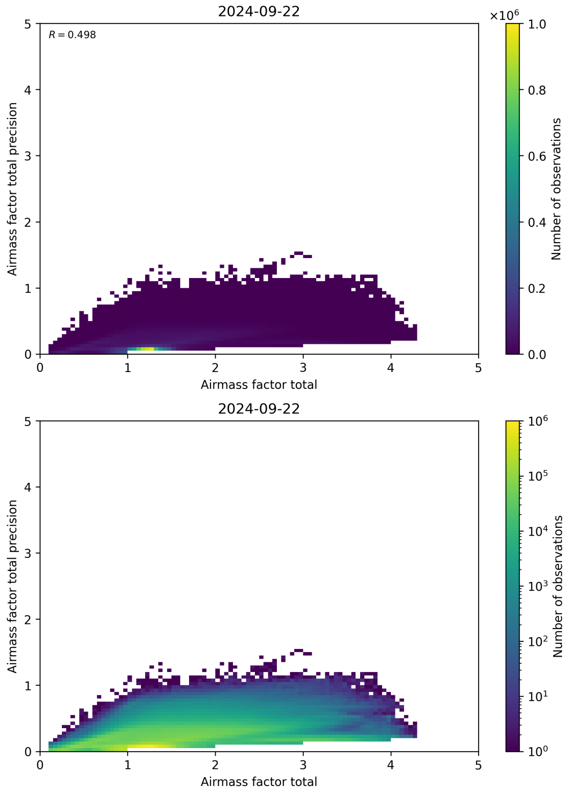
Figure 103: Scatter density plot of “Airmass factor total” against “Airmass factor total precision” for 2024-09-22 to 2024-09-23.
