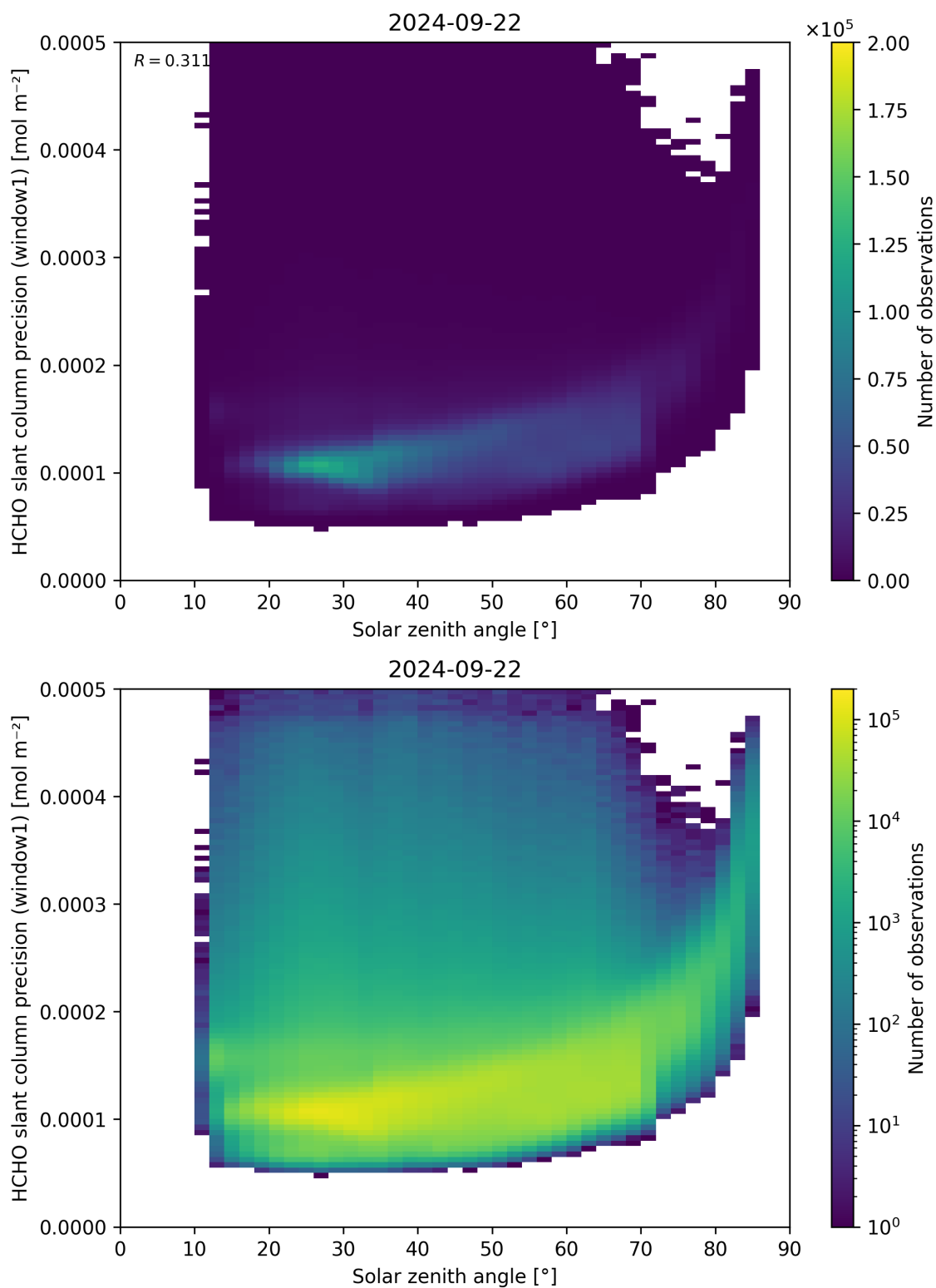
Figure 174: Scatter density plot of “Solar zenith angle” against “HCHO slant column precision (window1)” for 2024-09-22 to 2024-09-23.
