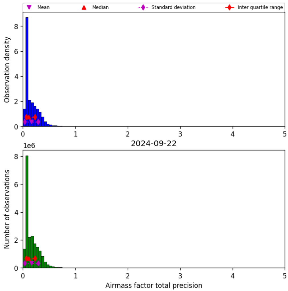
Figure 41: Histogram of “Airmass factor total precision” for 2024-09-22 to 2024-09-23
