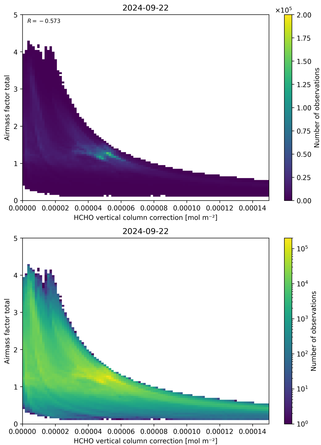
Figure 120: Scatter density plot of “HCHO vertical column correction” against “Airmass factor total” for 2024-09-22 to 2024-09-23.
