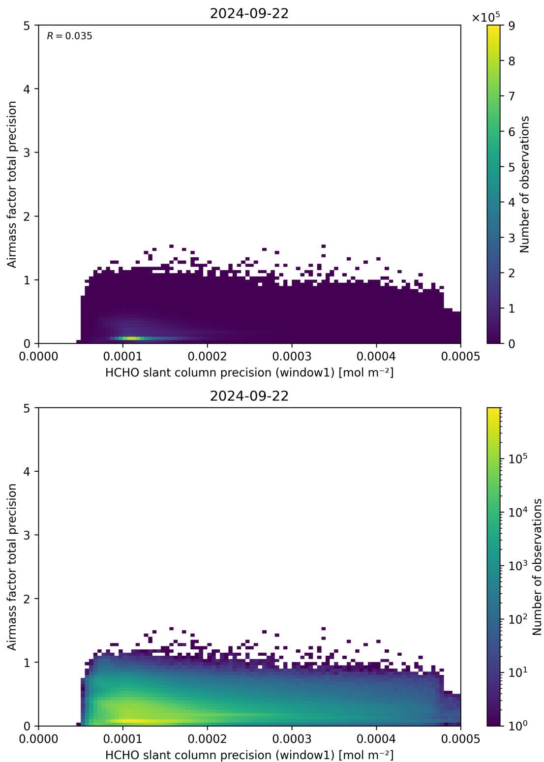
Figure 95: Scatter density plot of “HCHO slant column precision (window1)” against “Airmass factor total precision” for 2024-09-22 to 2024-09-23.
