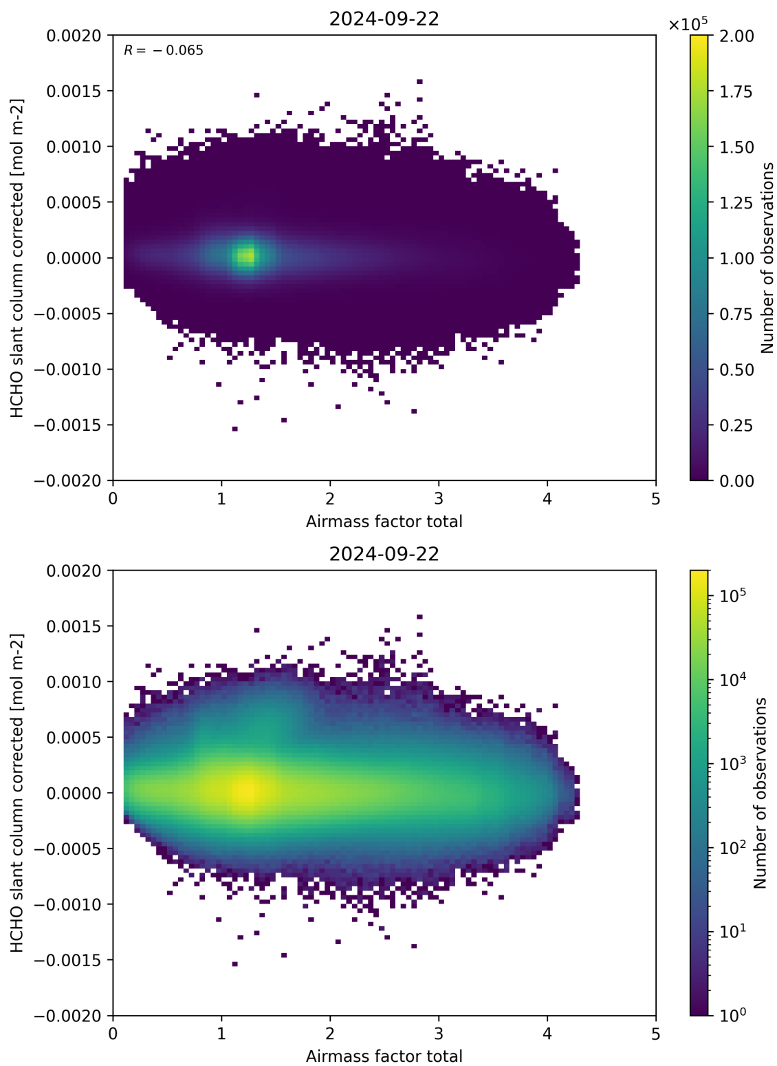
Figure 101: Scatter density plot of “Airmass factor total” against “HCHO slant column corrected” for 2024-09-22 to 2024-09-23.
