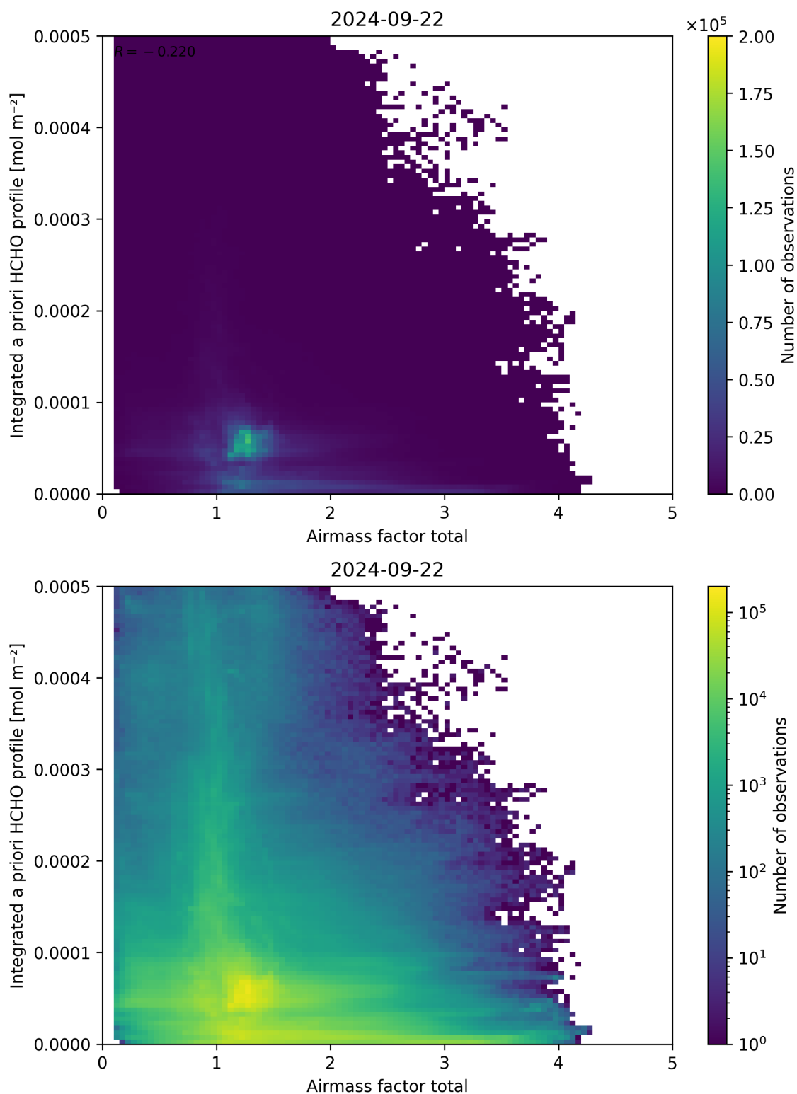
Figure 104: Scatter density plot of “Airmass factor total” against “Integrated a priori HCHO profile” for 2024-09-22 to 2024-09-23.
