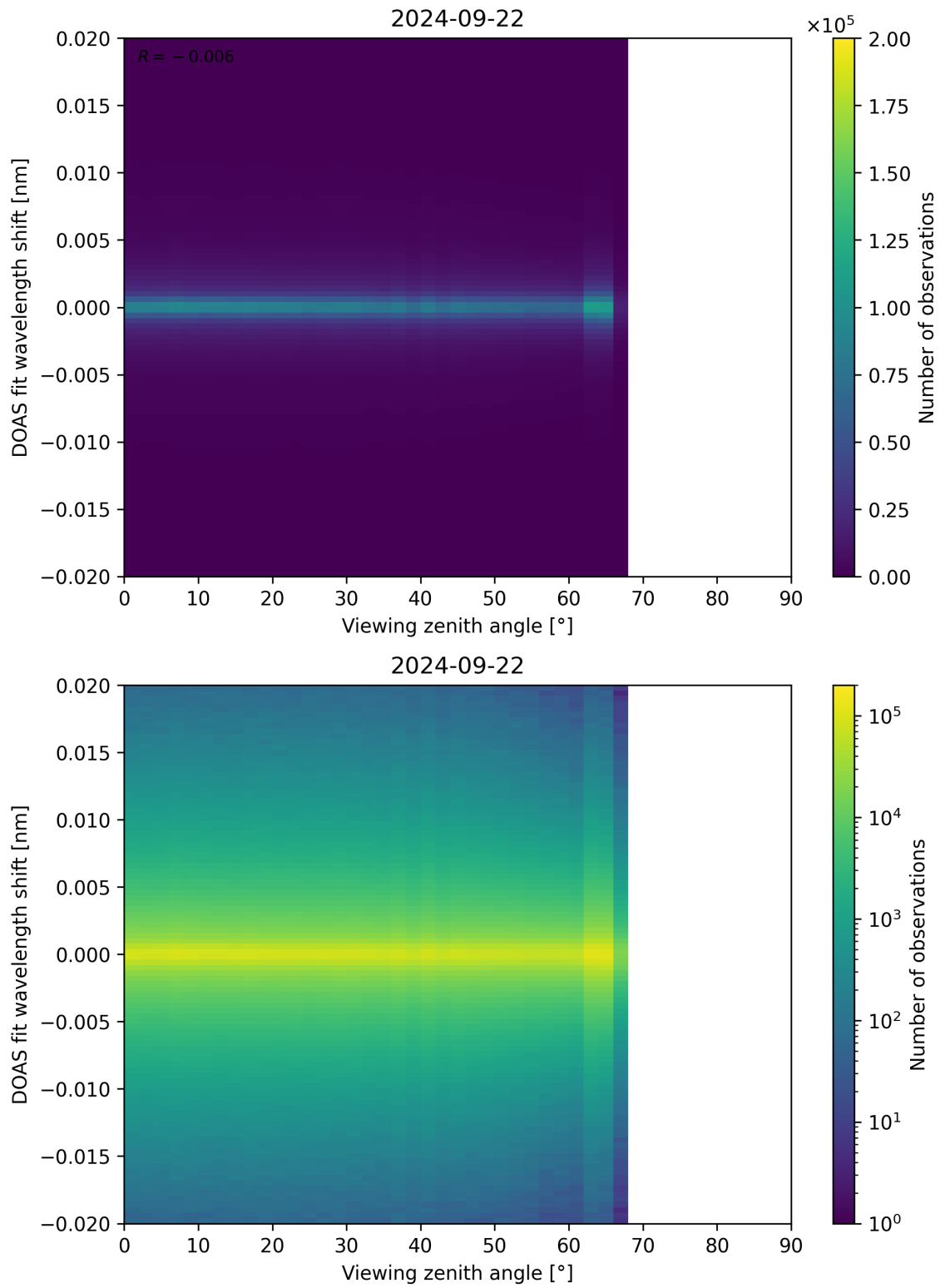
Figure 183: Scatter density plot of “Viewing zenith angle” against “DOAS fit wavelength shift” for 2024-09-22 to 2024-09-23.
