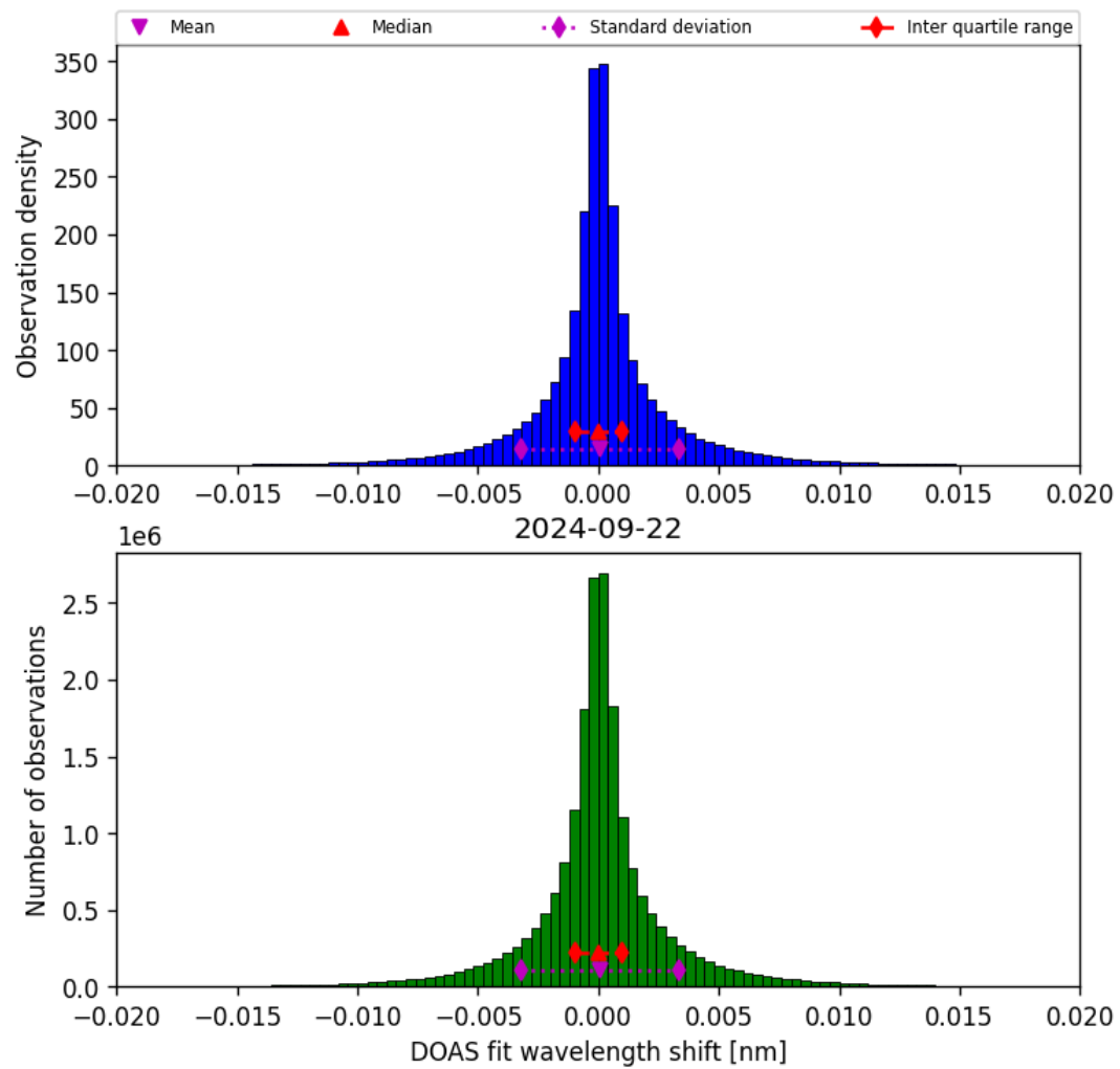
Figure 44: Histogram of “DOAS fit wavelength shift” for 2024-09-22 to 2024-09-23
