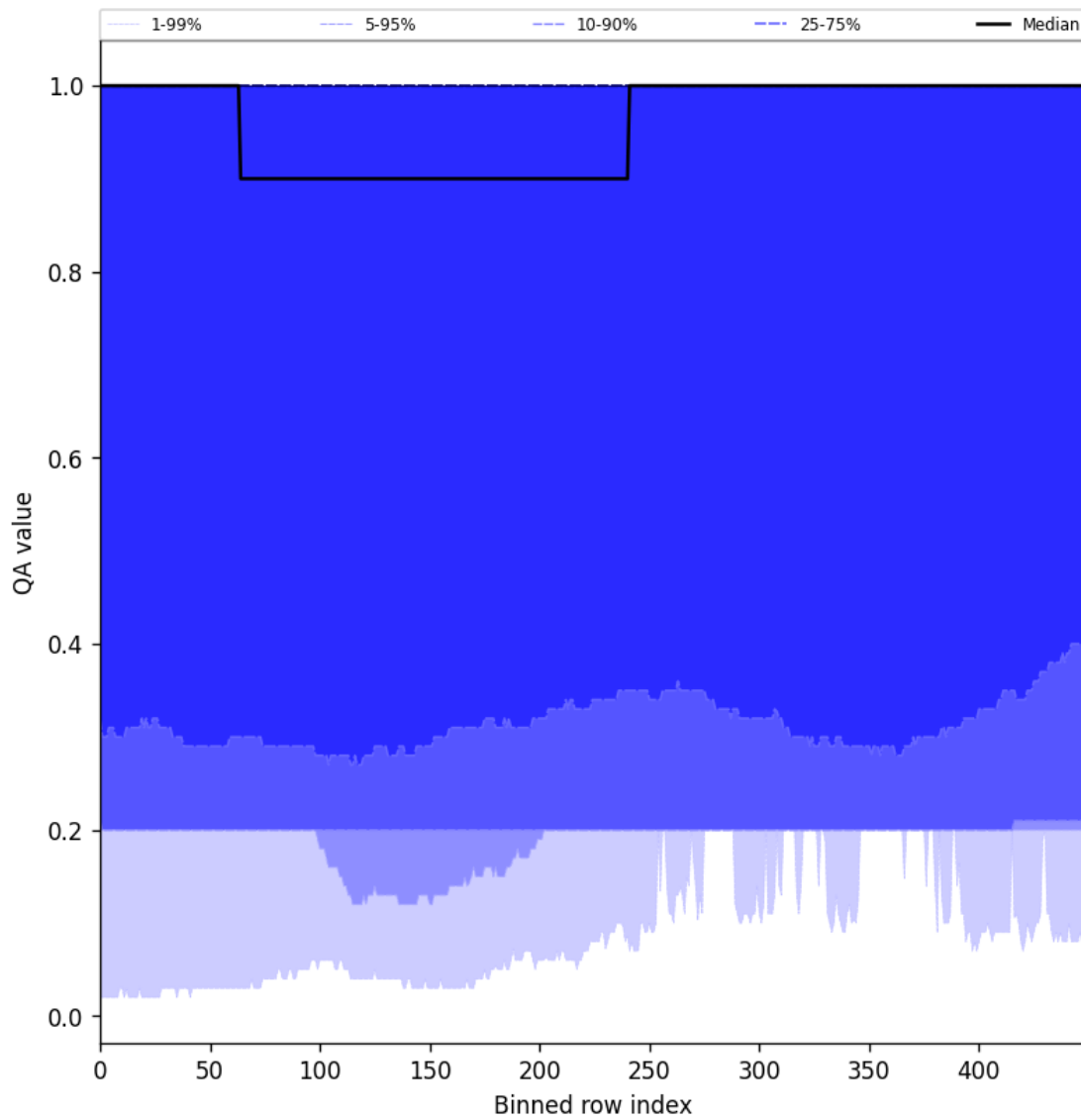
Figure 48: Along track statistics of “QA value” for 2024-09-22 to 2024-09-23
