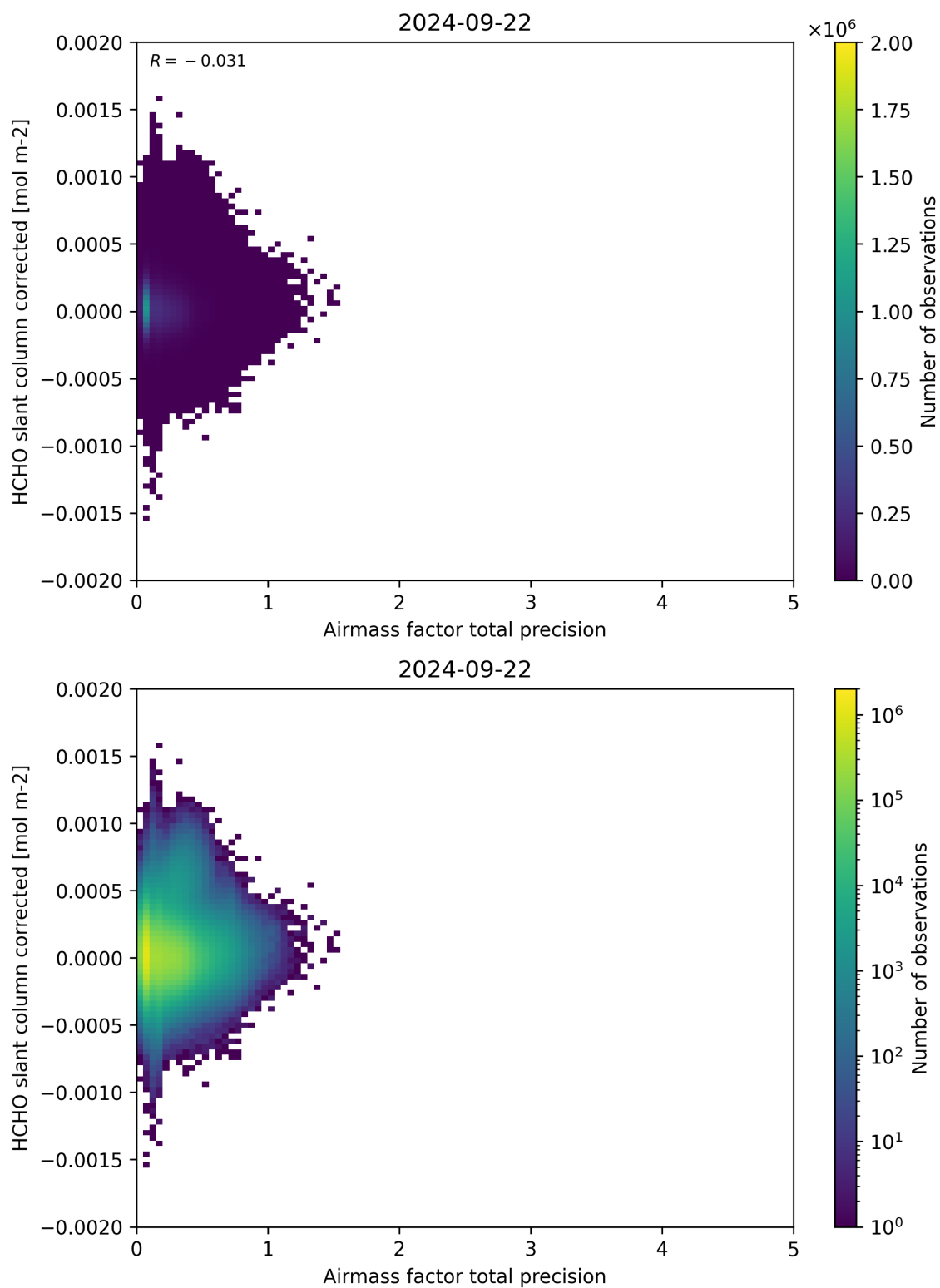
Figure 109: Scatter density plot of “Airmass factor total precision” against “HCHO slant column corrected” for 2024-09-22 to 2024-09-23.
