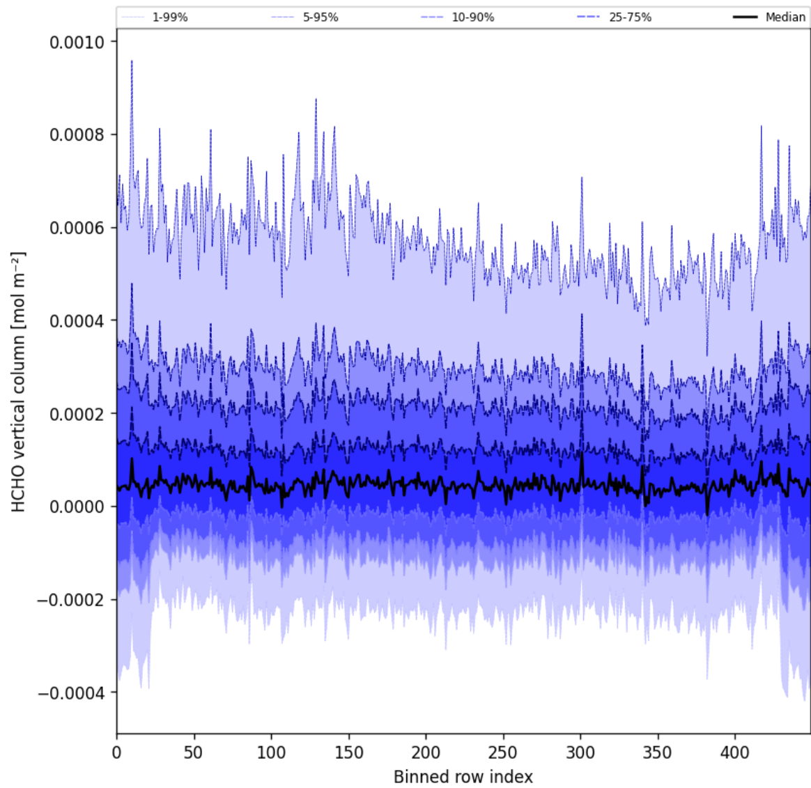
Figure 49: Along track statistics of “HCHO vertical column” for 2024-09-22 to 2024-09-23
