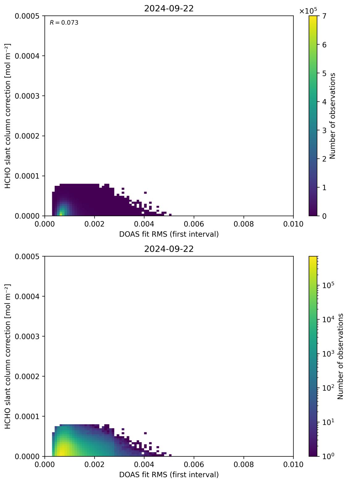
Figure 63: Scatter density plot of “DOAS fit RMS (first interval)” against “HCHO slant column correction” for 2024-09-22 to 2024-09-23.
