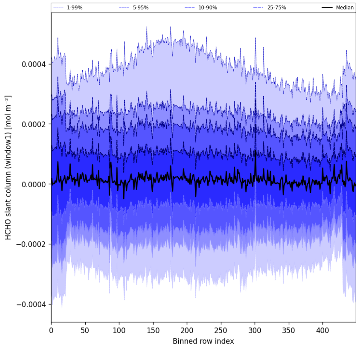
Figure 52: Along track statistics of “HCHO slant column (window1)” for 2024-09-22 to 2024-09-23
