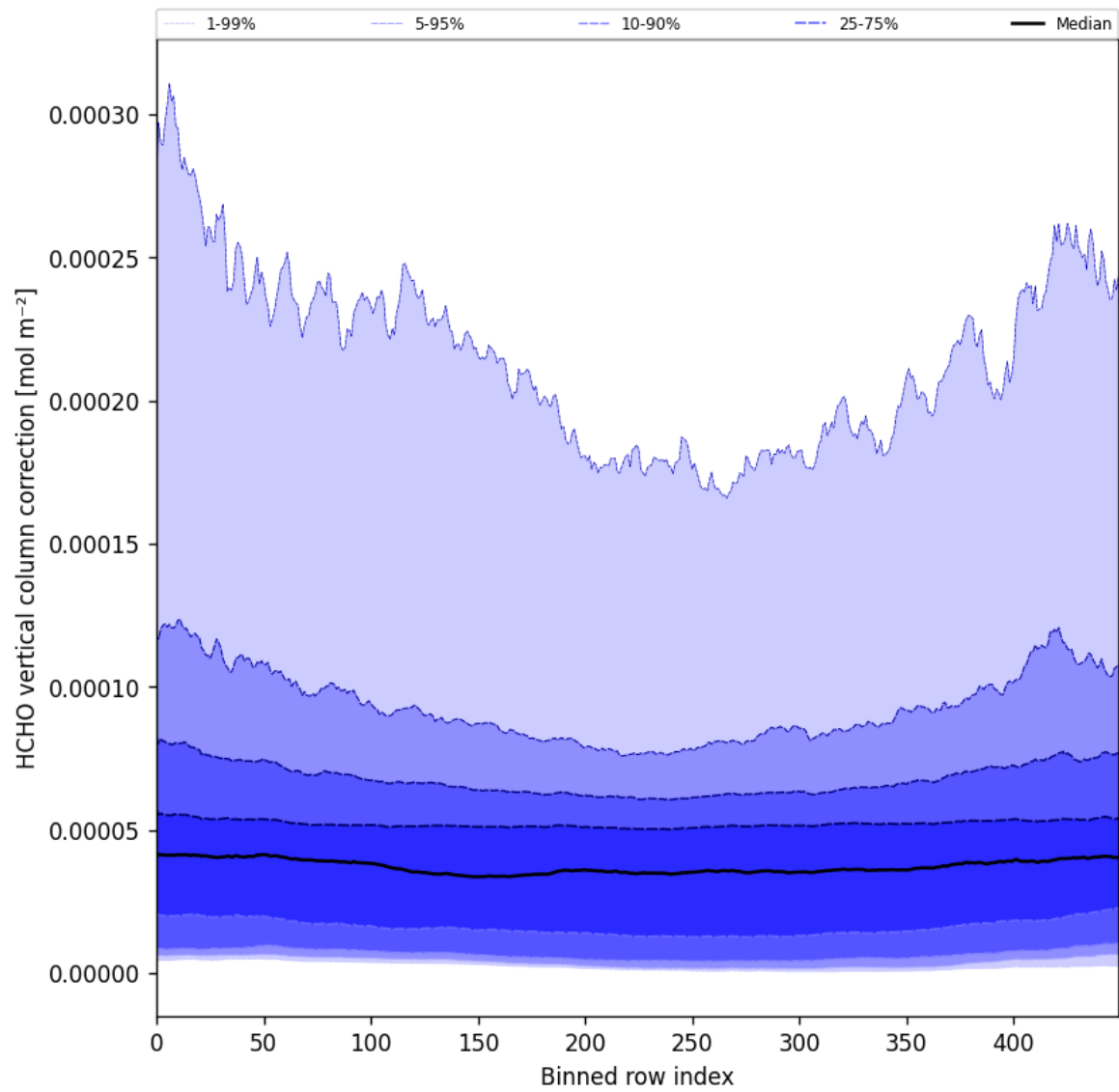
Figure 51: Along track statistics of “HCHO vertical column correction” for 2024-09-22 to 2024-09-23
