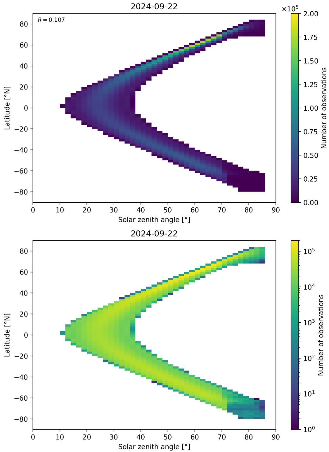
Figure 181: Scatter density plot of “Solar zenith angle” against “Latitude” for 2024-09-22 to 2024-09-23.
