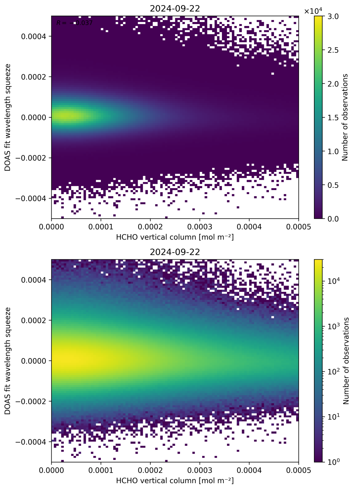
Figure 125: Scatter density plot of “HCHO vertical column” against “DOAS fit wavelength squeeze” for 2024-09-22 to 2024-09-23.
