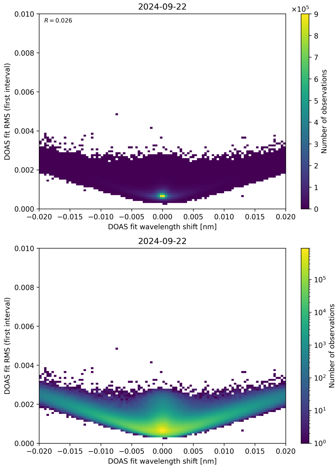
Figure 64: Scatter density plot of “DOAS fit wavelength shift” against “DOAS fit RMS (first interval)” for 2024-09-22 to 2024-09-23.
