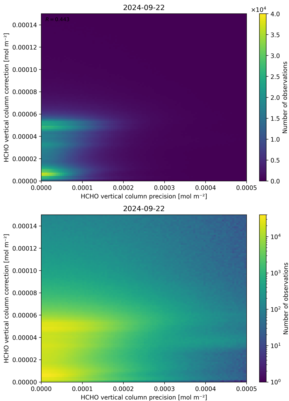
Figure 146: Scatter density plot of “HCHO vertical column precision” against “HCHO vertical column correction” for 2024-09-22 to 2024-09-23.
