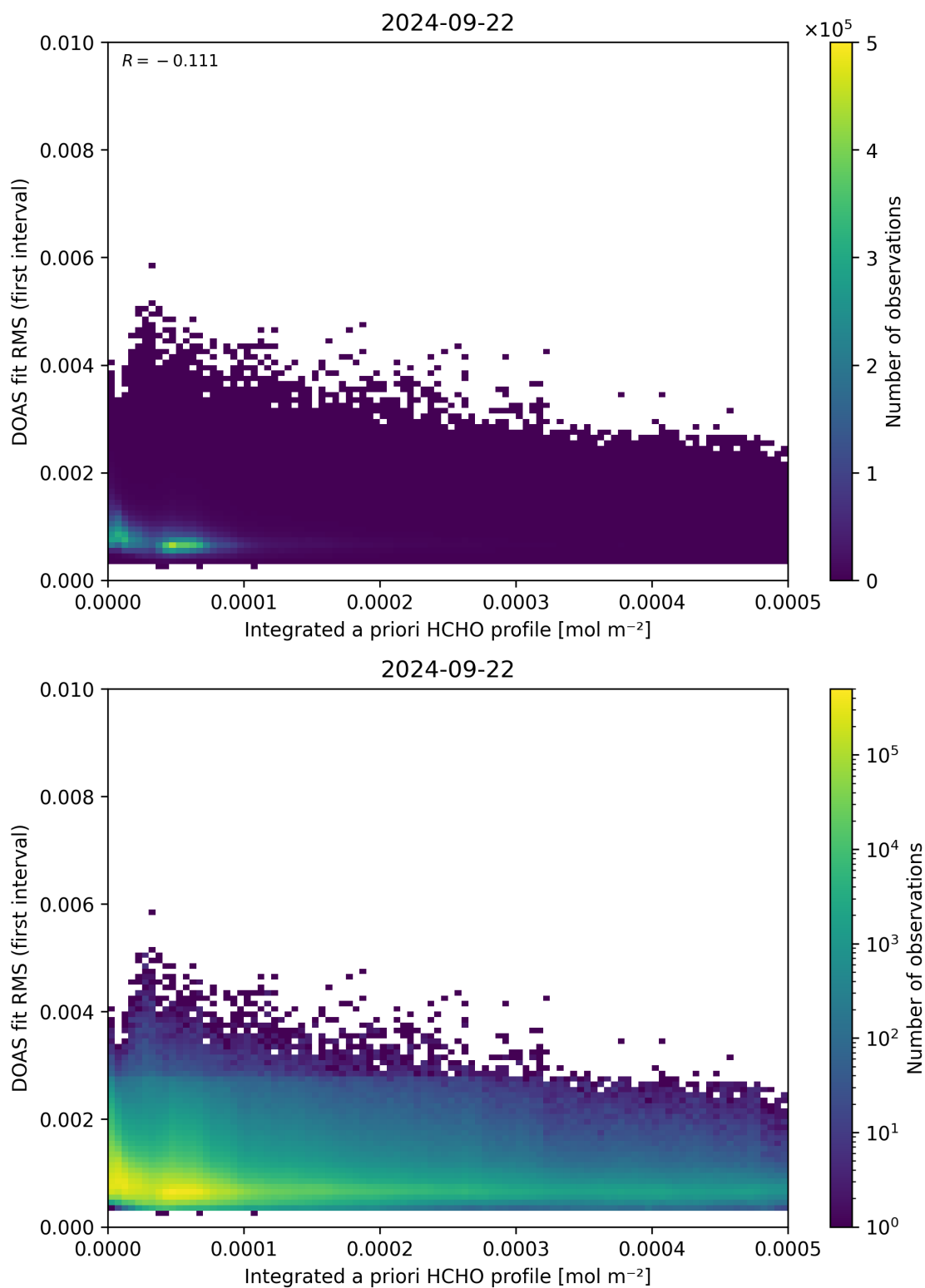
Figure 148: Scatter density plot of “Integrated a priori HCHO profile” against “DOAS fit RMS (first interval)” for 2024-09-22 to 2024-09-23.
