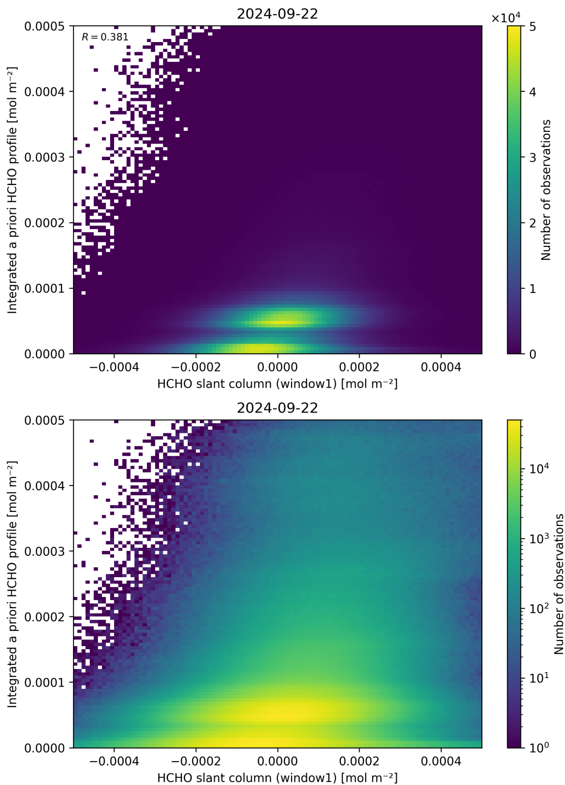
Figure 87: Scatter density plot of “HCHO slant column (window1)” against “Integrated a priori HCHO profile” for 2024-09-22 to 2024-09-23.
