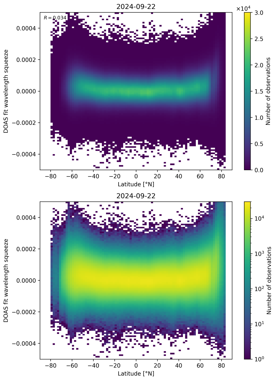
Figure 155: Scatter density plot of “Latitude” against “DOAS fit wavelength squeeze” for 2024-09-22 to 2024-09-23.
