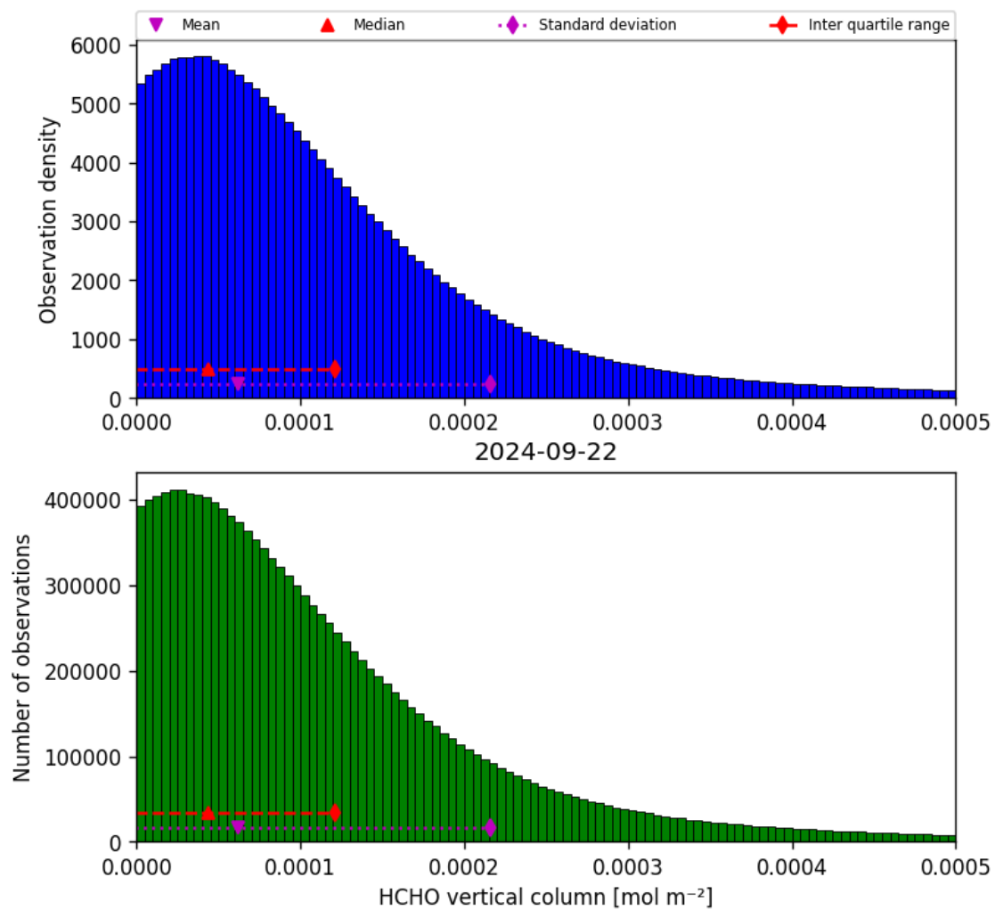
Figure 35: Histogram of “HCHO vertical column” for 2024-09-22 to 2024-09-23
