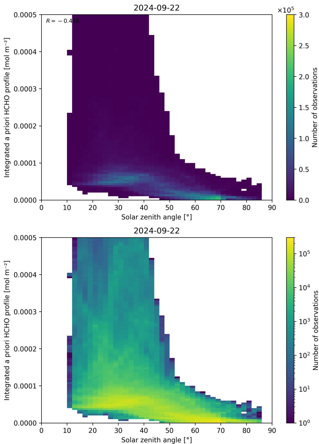
Figure 180: Scatter density plot of “Solar zenith angle” against “Integrated a priori HCHO profile” for 2024-09-22 to 2024-09-23.
