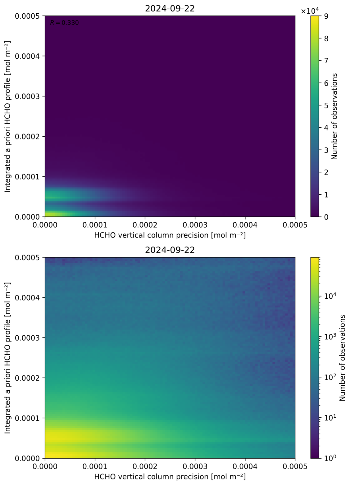
Figure 147: Scatter density plot of “HCHO vertical column precision” against “Integrated a priori HCHO profile” for 2024-09-22 to 2024-09-23.
