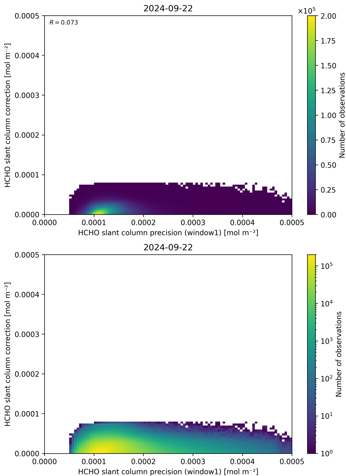
Figure 93: Scatter density plot of “HCHO slant column precision (window1)” against “HCHO slant column correction” for 2024-09-22 to 2024-09-23.
