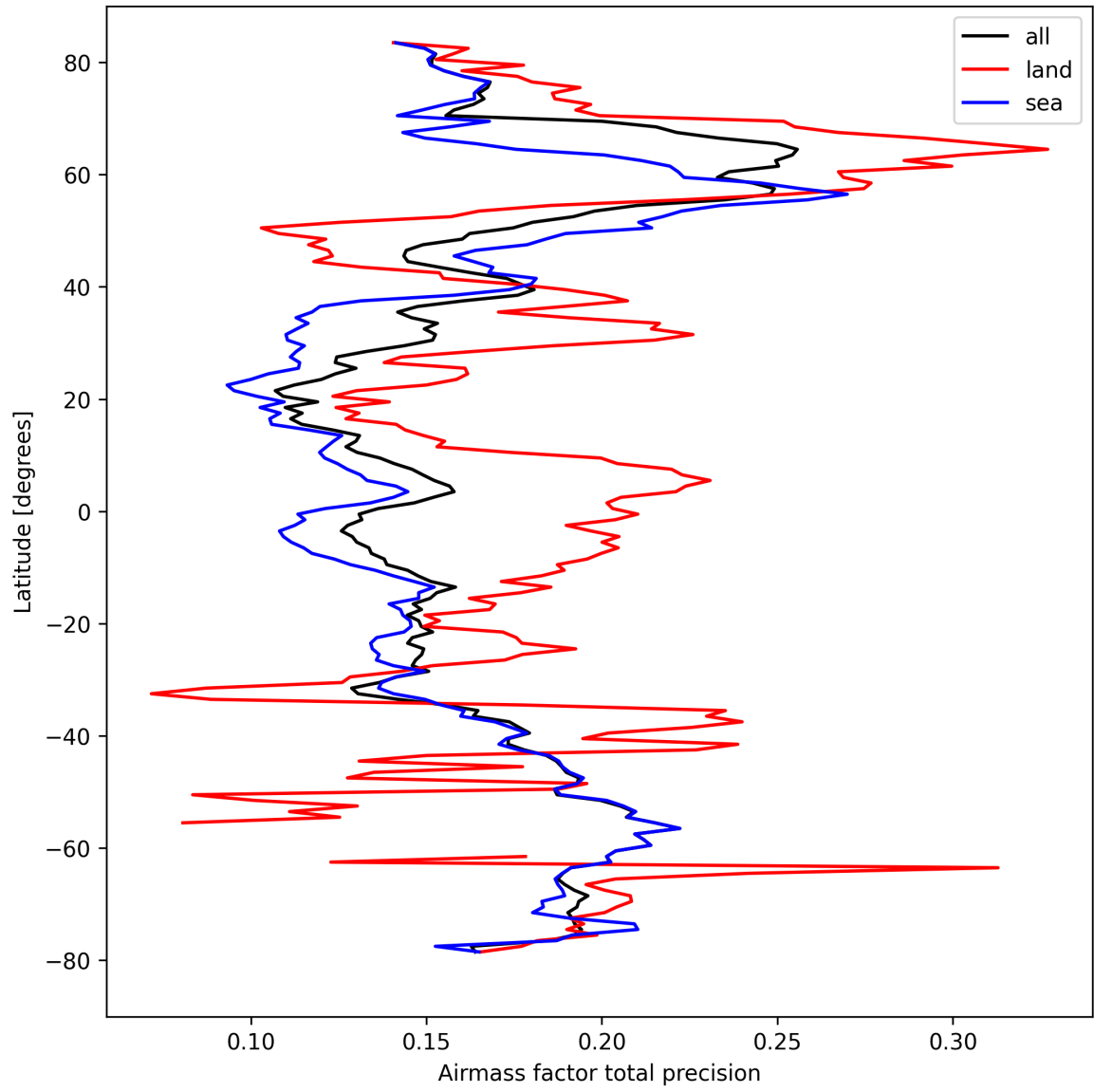
Figure 27: Zonal average of “Airmass factor total precision” for 2024-09-22 to 2024-09-23.
