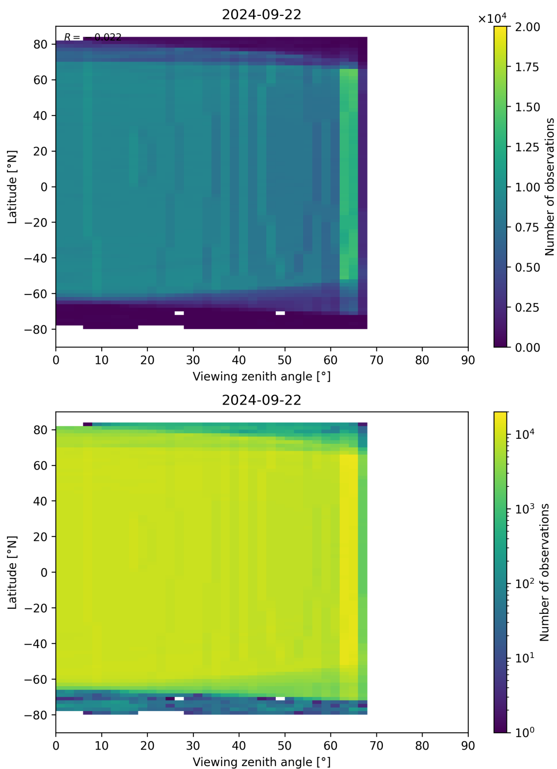
Figure 196: Scatter density plot of “Viewing zenith angle” against “Latitude” for 2024-09-22 to 2024-09-23.
