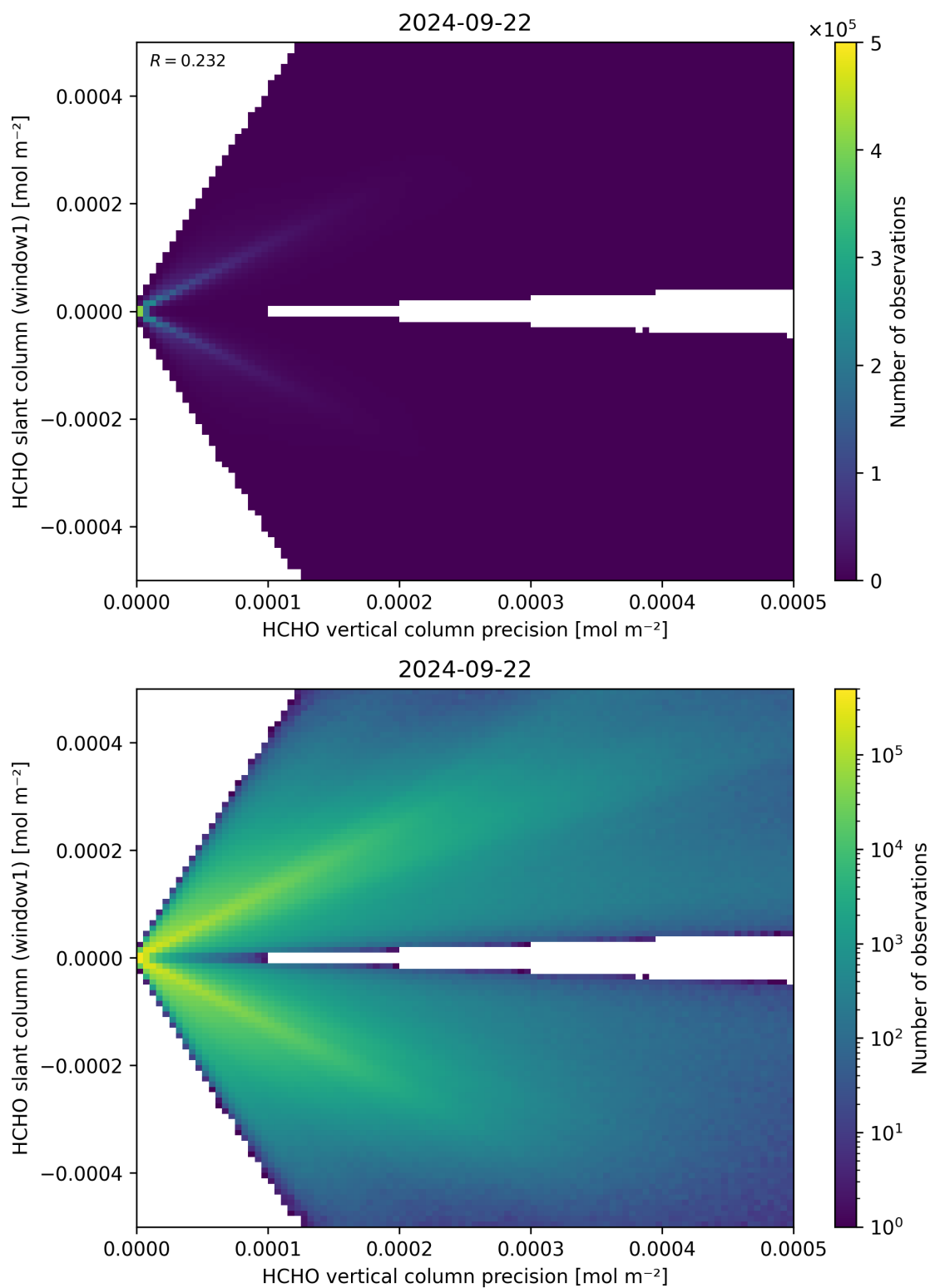
Figure 142: Scatter density plot of “HCHO vertical column precision” against “HCHO slant column (window1)” for 2024-09-22 to 2024-09-23.
