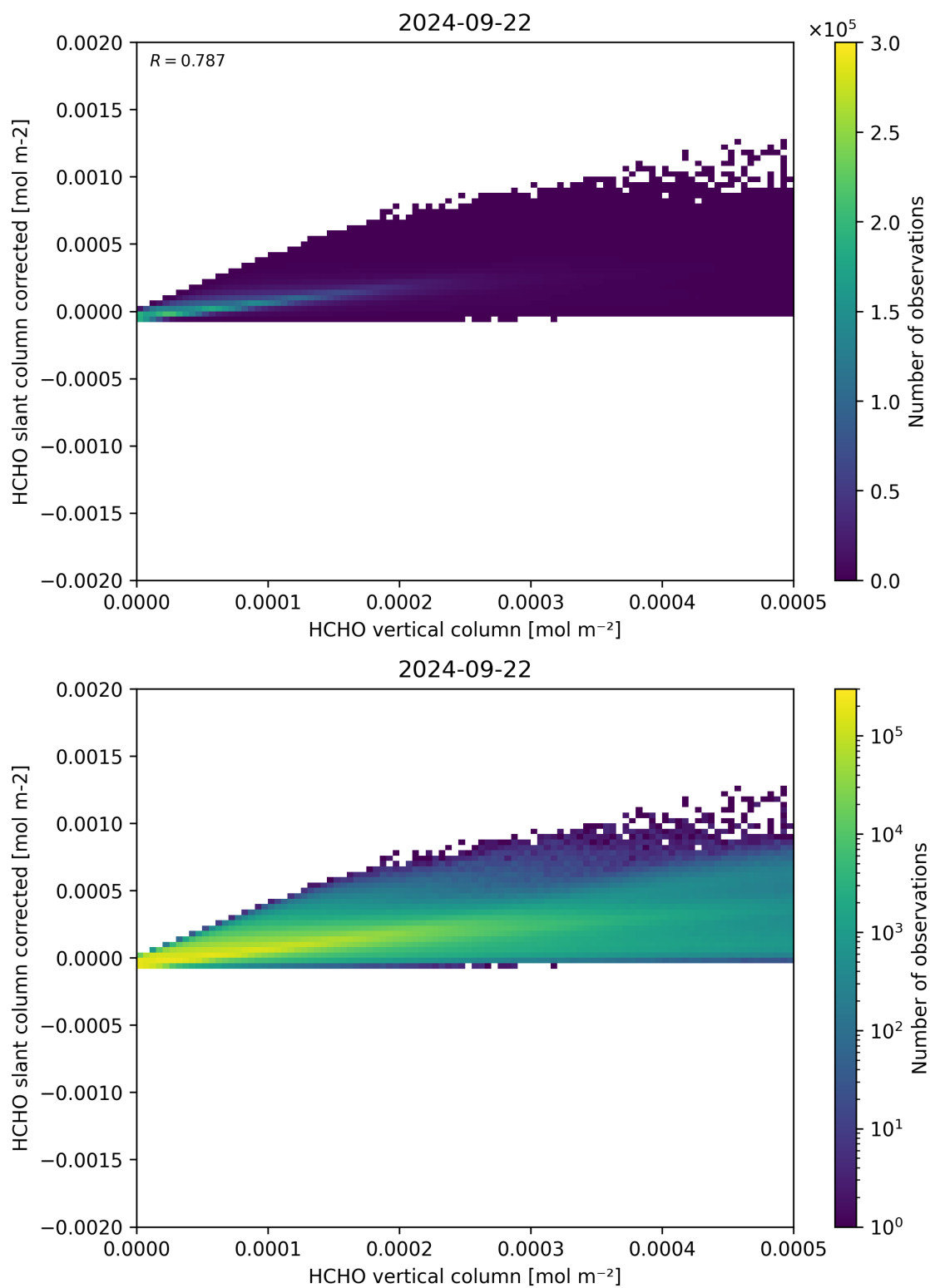
Figure 127: Scatter density plot of “HCHO vertical column” against “HCHO slant column corrected” for 2024-09-22 to 2024-09-23.
