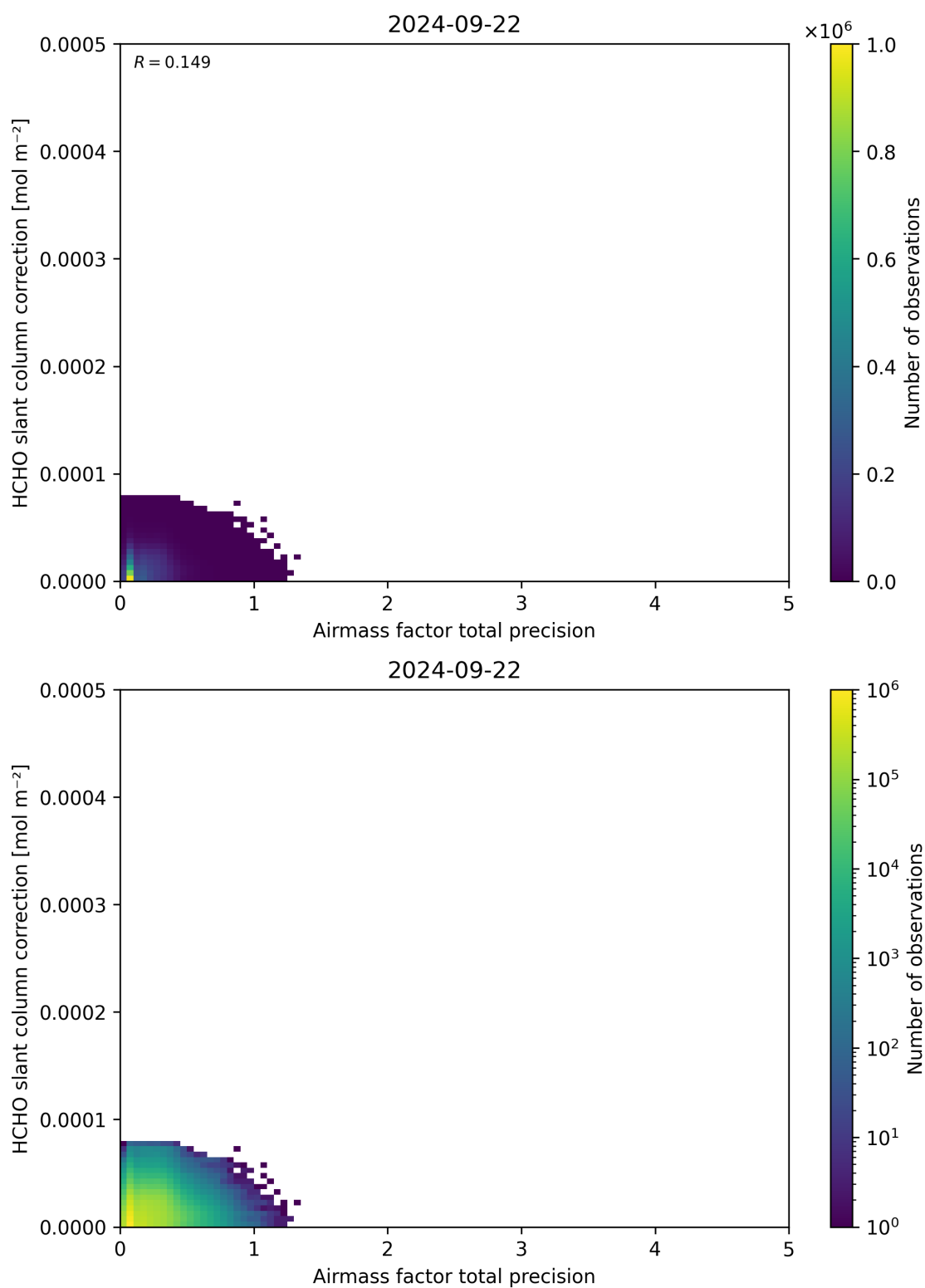
Figure 110: Scatter density plot of “Airmass factor total precision” against “HCHO slant column correction” for 2024-09-22 to 2024-09-23.
