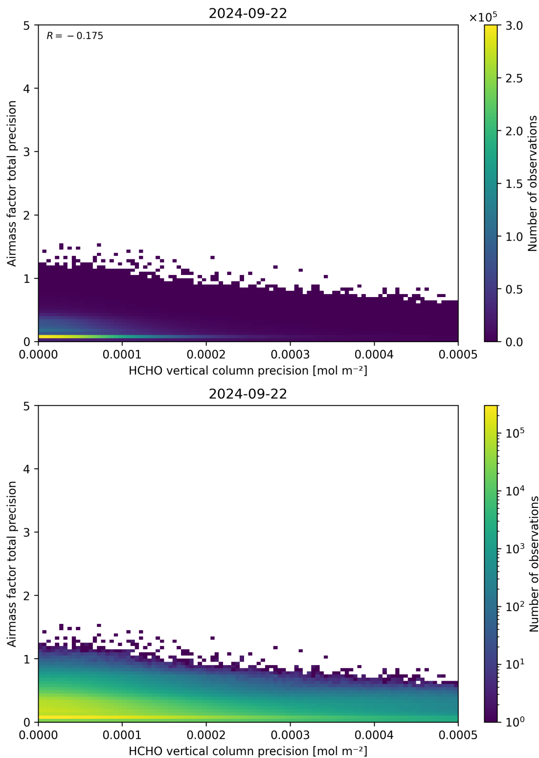
Figure 145: Scatter density plot of “HCHO vertical column precision” against “Airmass factor total precision” for 2024-09-22 to 2024-09-23.
