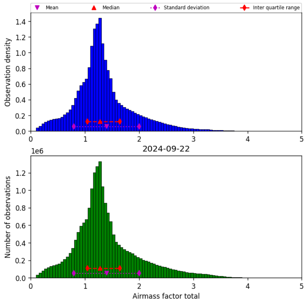
Figure 40: Histogram of “Airmass factor total” for 2024-09-22 to 2024-09-23
