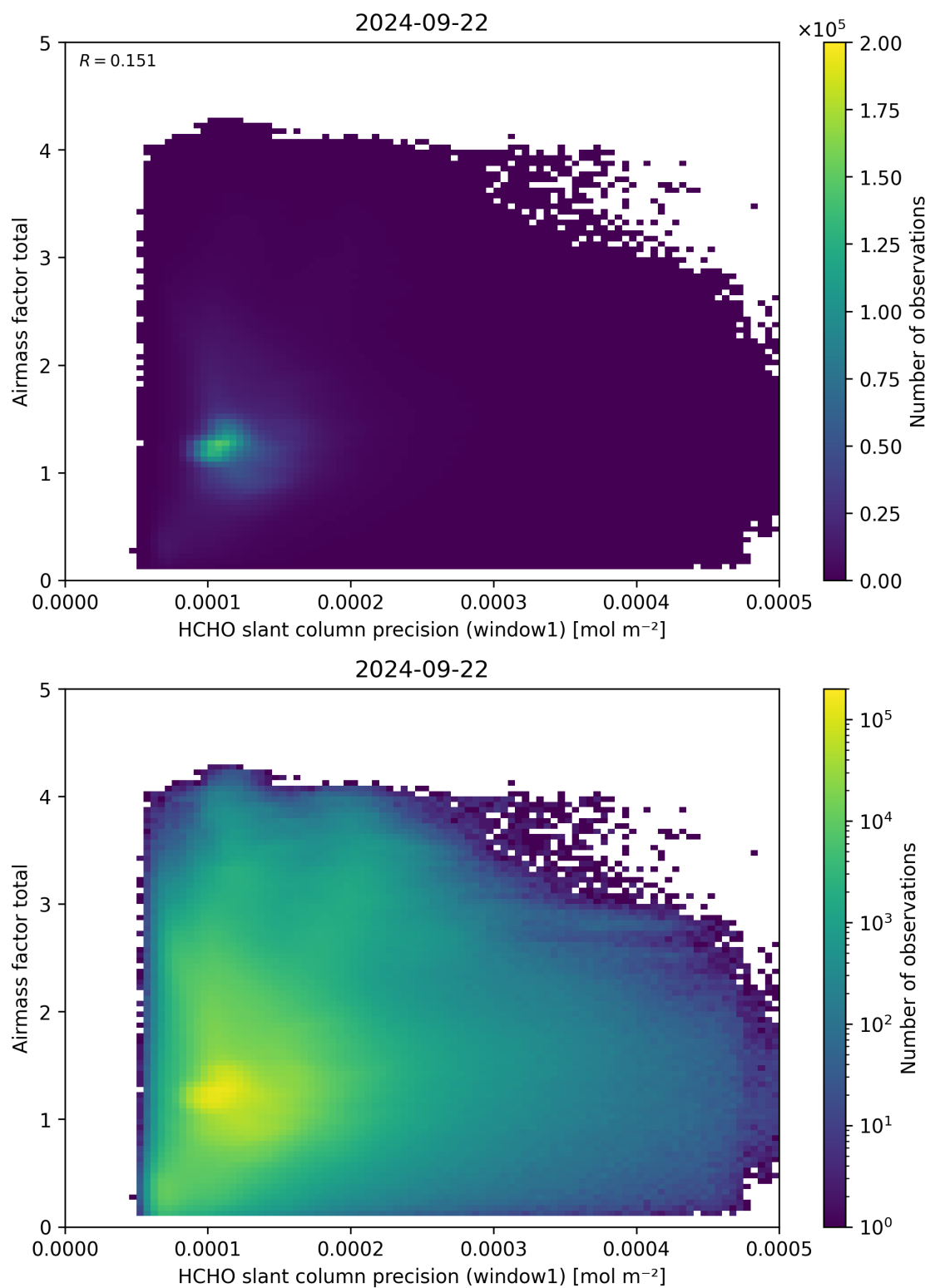
Figure 94: Scatter density plot of “HCHO slant column precision (window1)” against “Airmass factor total” for 2024-09-22 to 2024-09-23.
