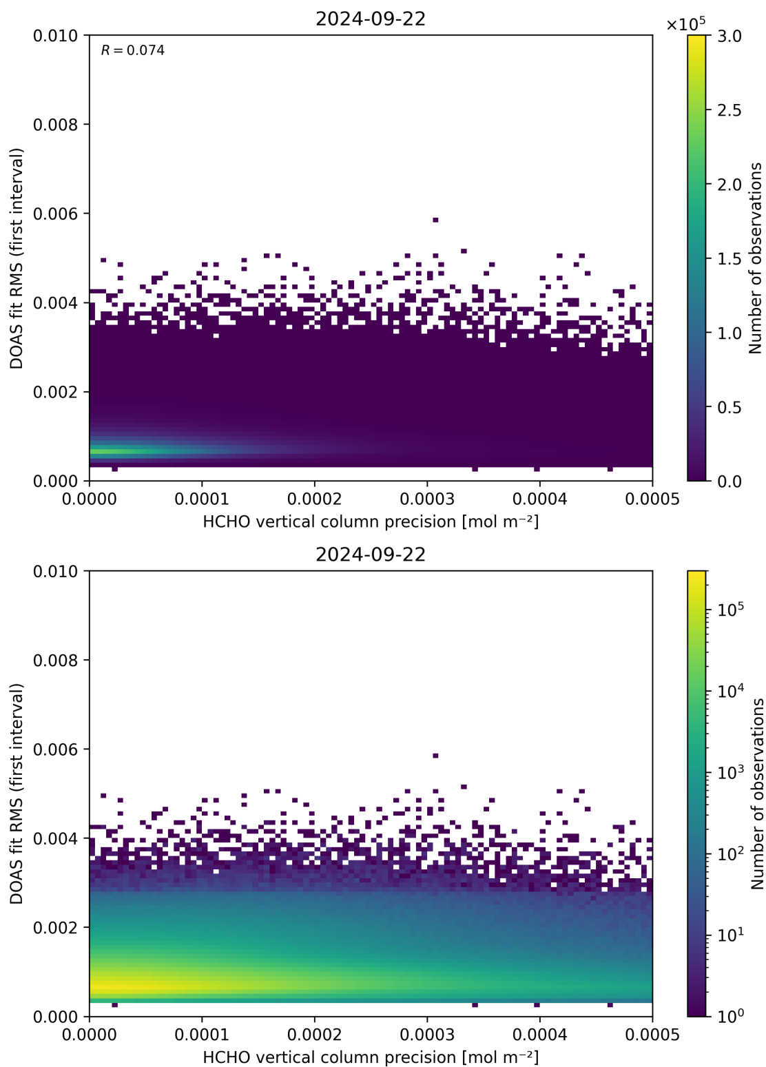
Figure 136: Scatter density plot of “HCHO vertical column precision” against “DOAS fit RMS (first interval)” for 2024-09-22 to 2024-09-23.
