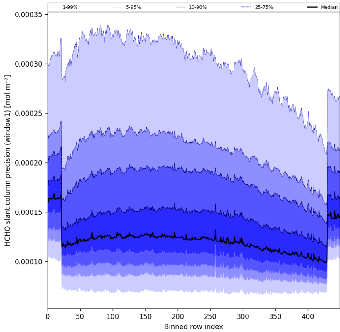
Figure 53: Along track statistics of “HCHO slant column precision (window1)” for 2024-09-22 to 2024-09-23
