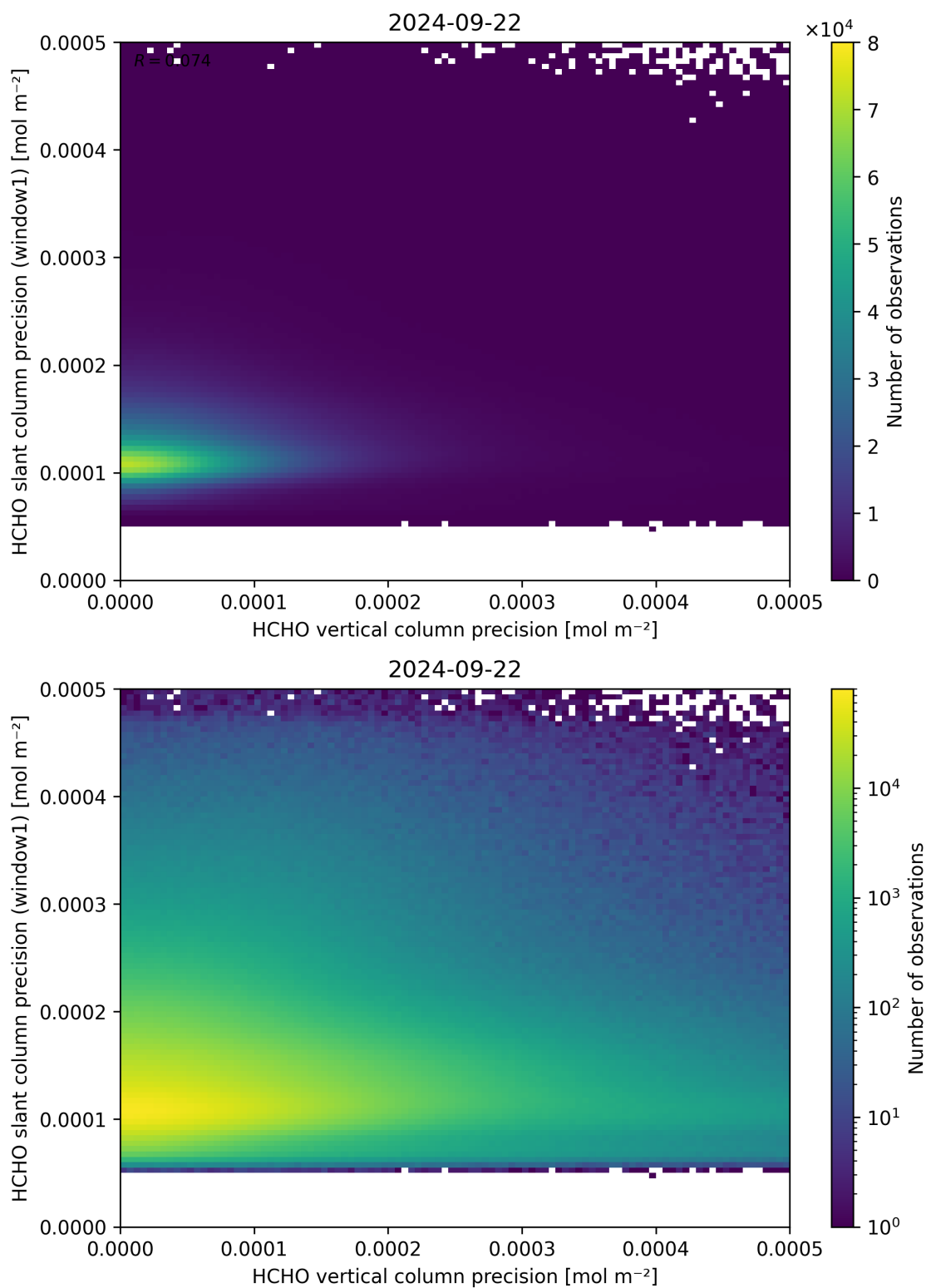
Figure 143: Scatter density plot of “HCHO vertical column precision” against “HCHO slant column precision (window1)” for 2024-09-22 to 2024-09-23.
