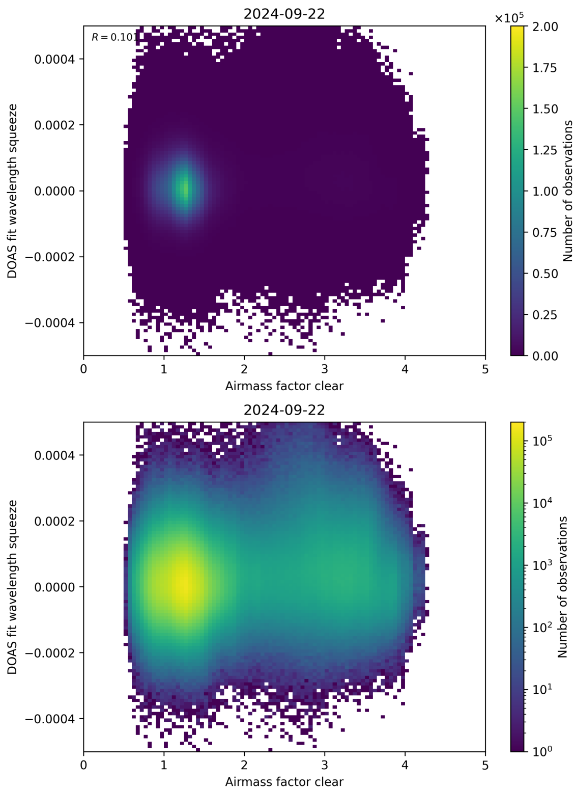
Figure 73: Scatter density plot of “Airmass factor clear” against “DOAS fit wavelength squeeze” for 2024-09-22 to 2024-09-23.
