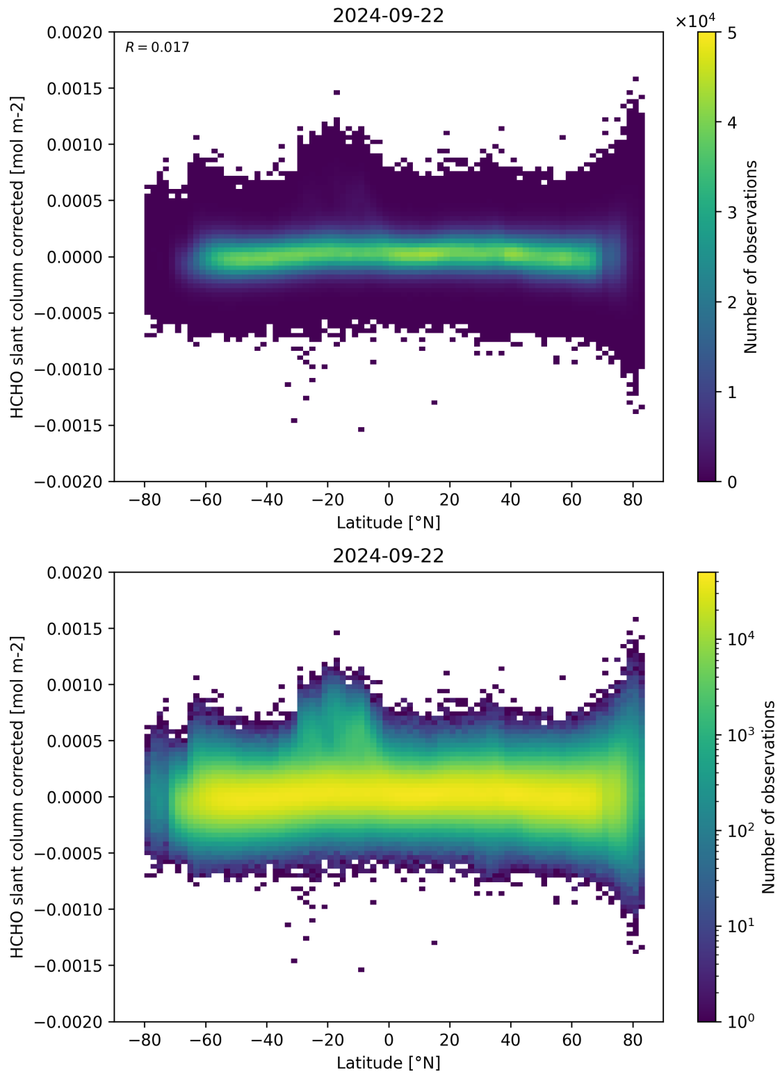
Figure 157: Scatter density plot of “Latitude” against “HCHO slant column corrected” for 2024-09-22 to 2024-09-23.
