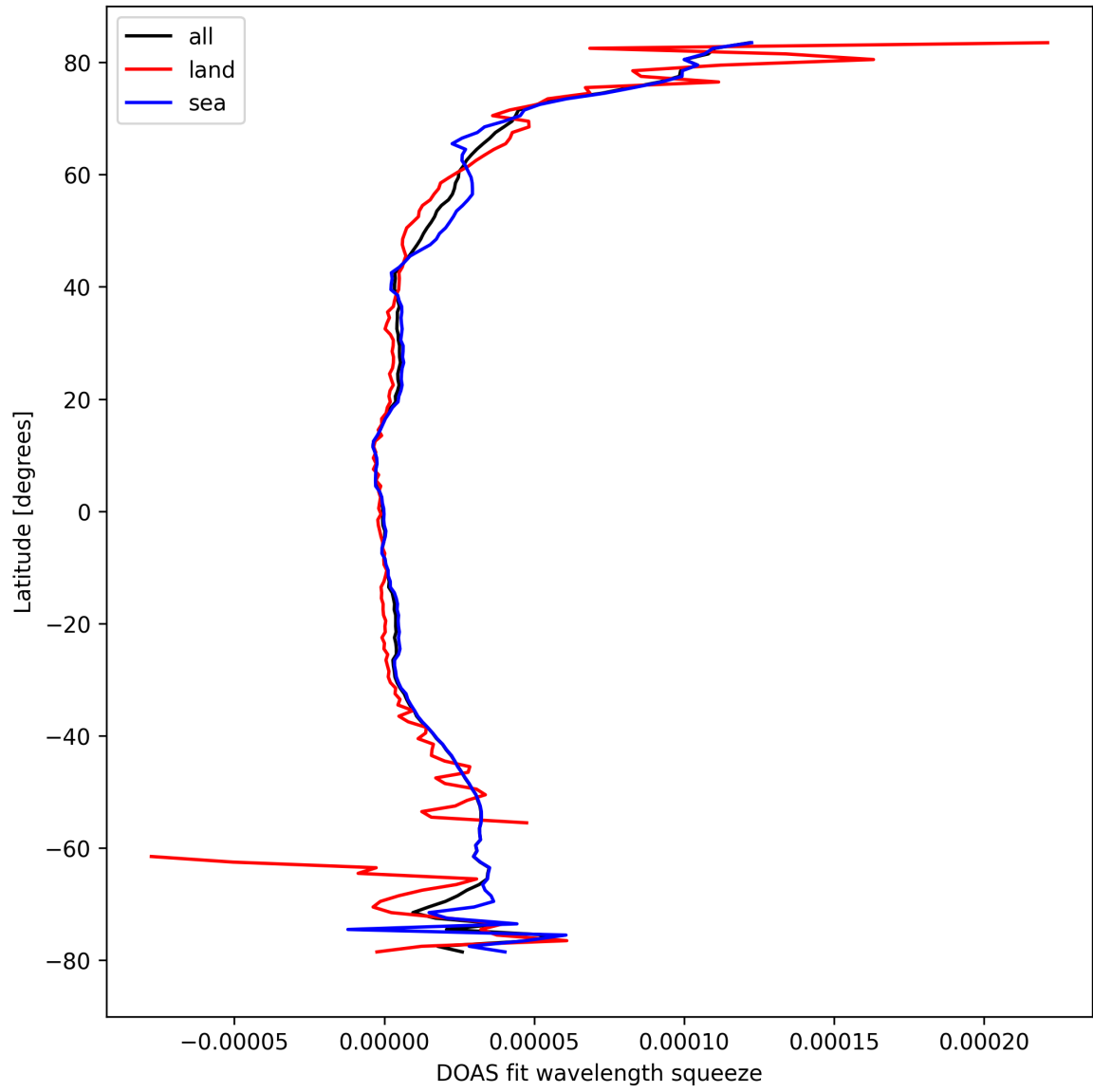
Figure 31: Zonal average of “DOAS fit wavelength squeeze” for 2024-09-22 to 2024-09-23.
