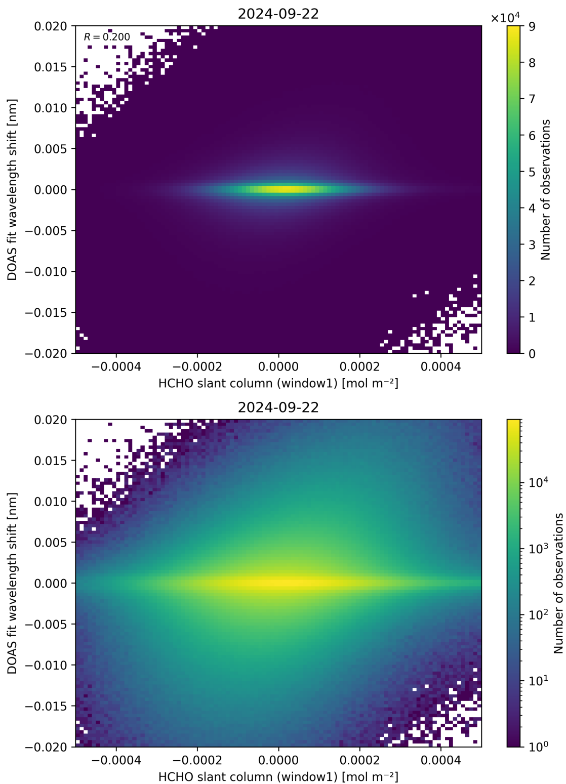
Figure 79: Scatter density plot of “HCHO slant column (window1)” against “DOAS fit wavelength shift” for 2024-09-22 to 2024-09-23.
