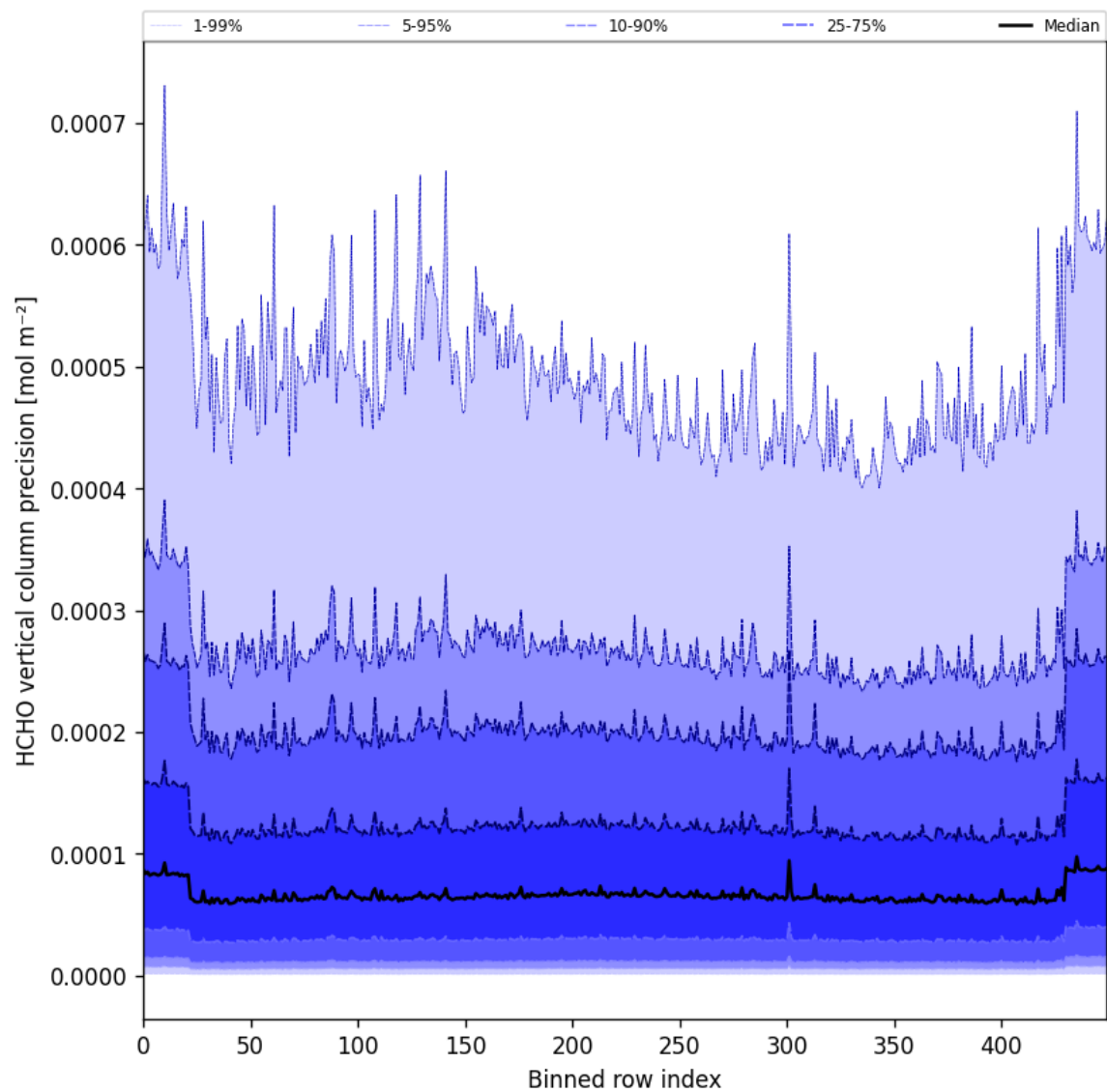
Figure 50: Along track statistics of “HCHO vertical column precision” for 2024-09-22 to 2024-09-23
