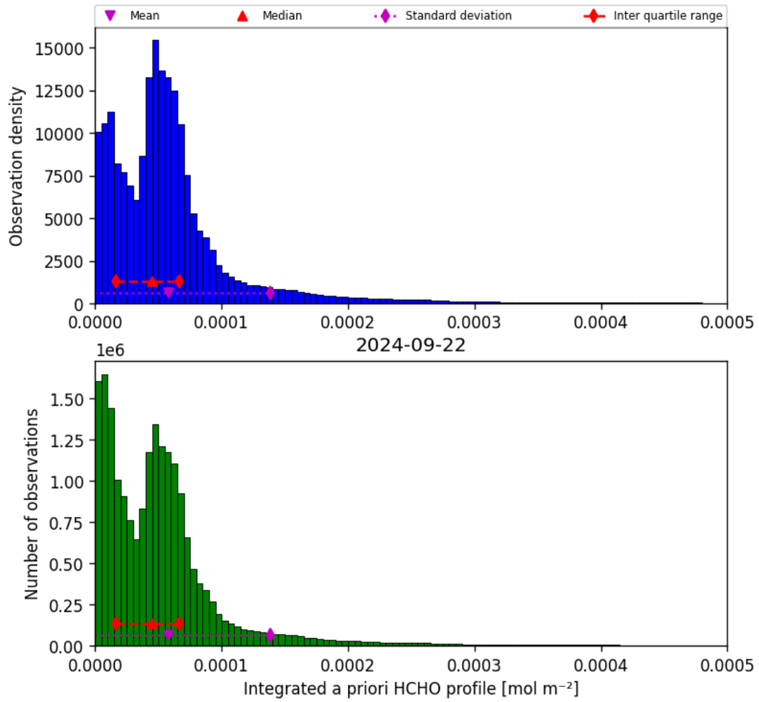
Figure 43: Histogram of “Integrated a priori HCHO profile” for 2024-09-22 to 2024-09-23
