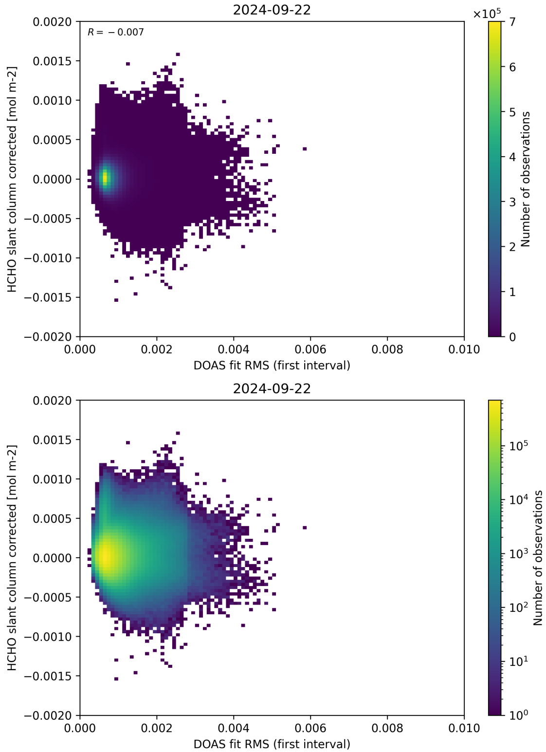
Figure 62: Scatter density plot of “DOAS fit RMS (first interval)” against “HCHO slant column corrected” for 2024-09-22 to 2024-09-23.
