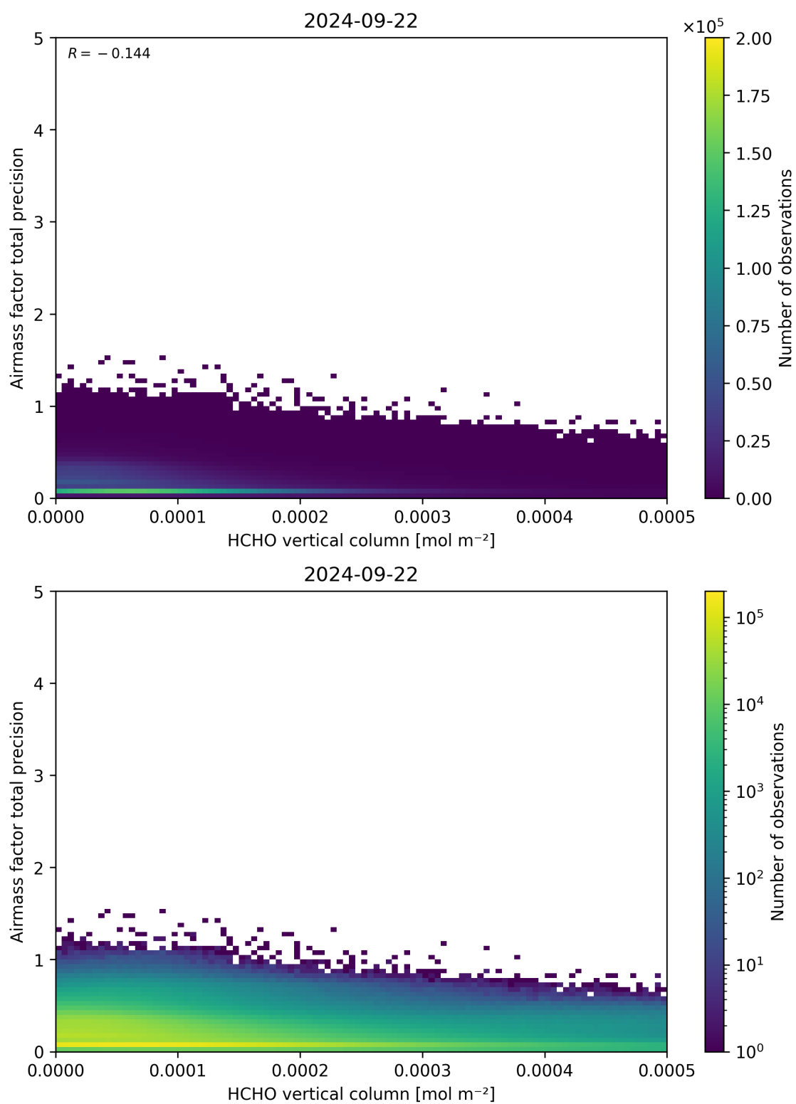
Figure 132: Scatter density plot of “HCHO vertical column” against “Airmass factor total precision” for 2024-09-22 to 2024-09-23.
