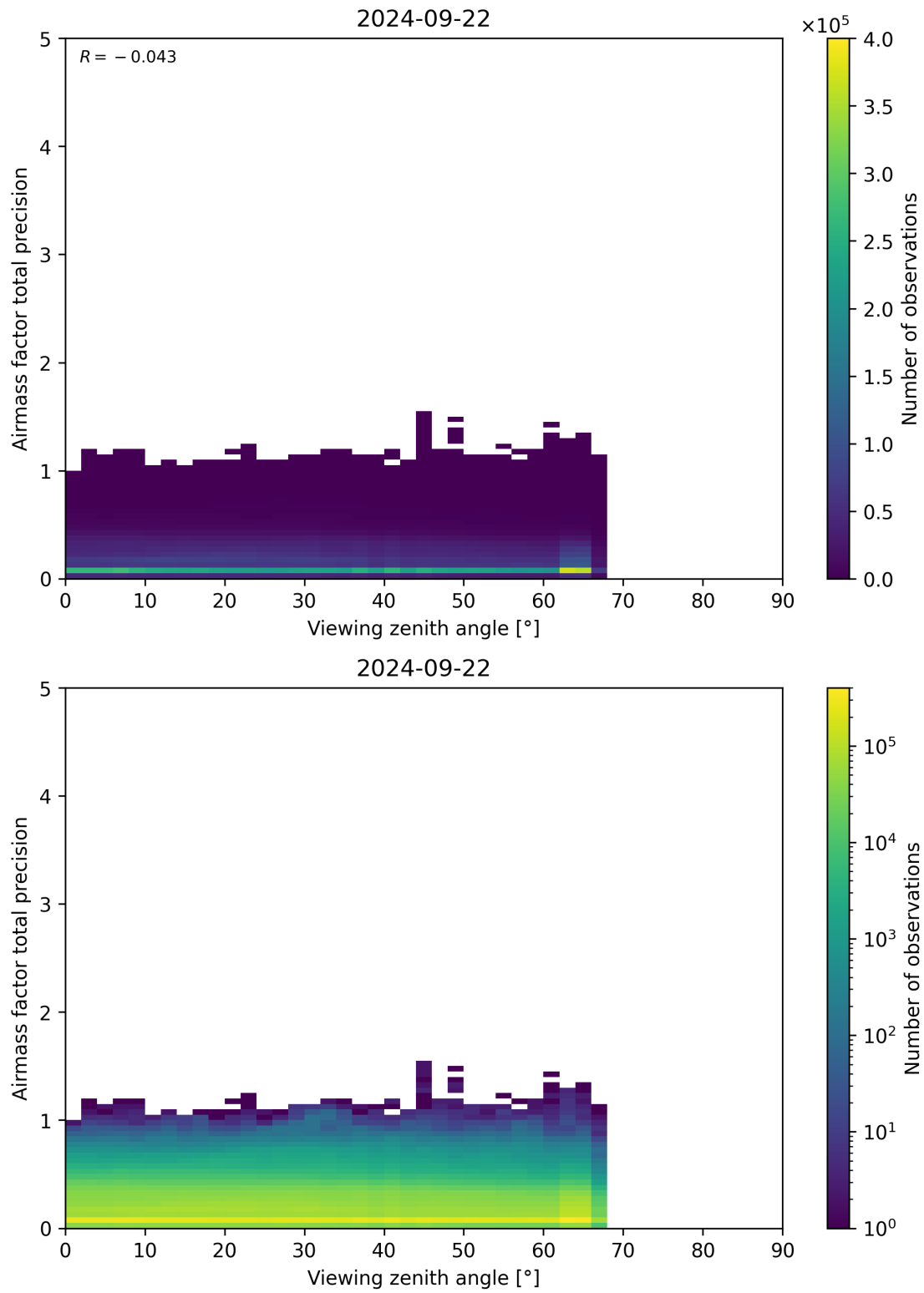
Figure 191: Scatter density plot of “Viewing zenith angle” against “Airmass factor total precision” for 2024-09-22 to 2024-09-23.
