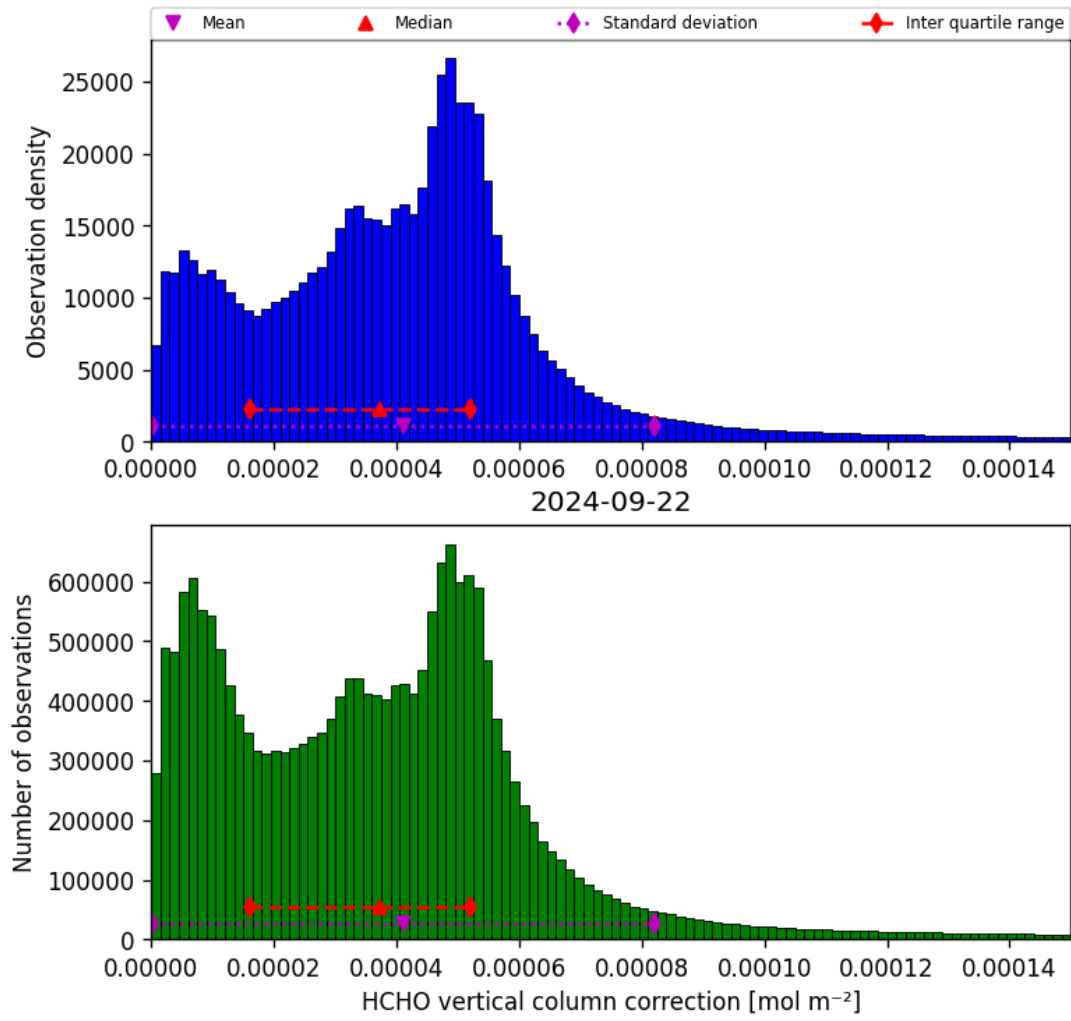
Figure 37: Histogram of “HCHO vertical column correction” for 2024-09-22 to 2024-09-23
