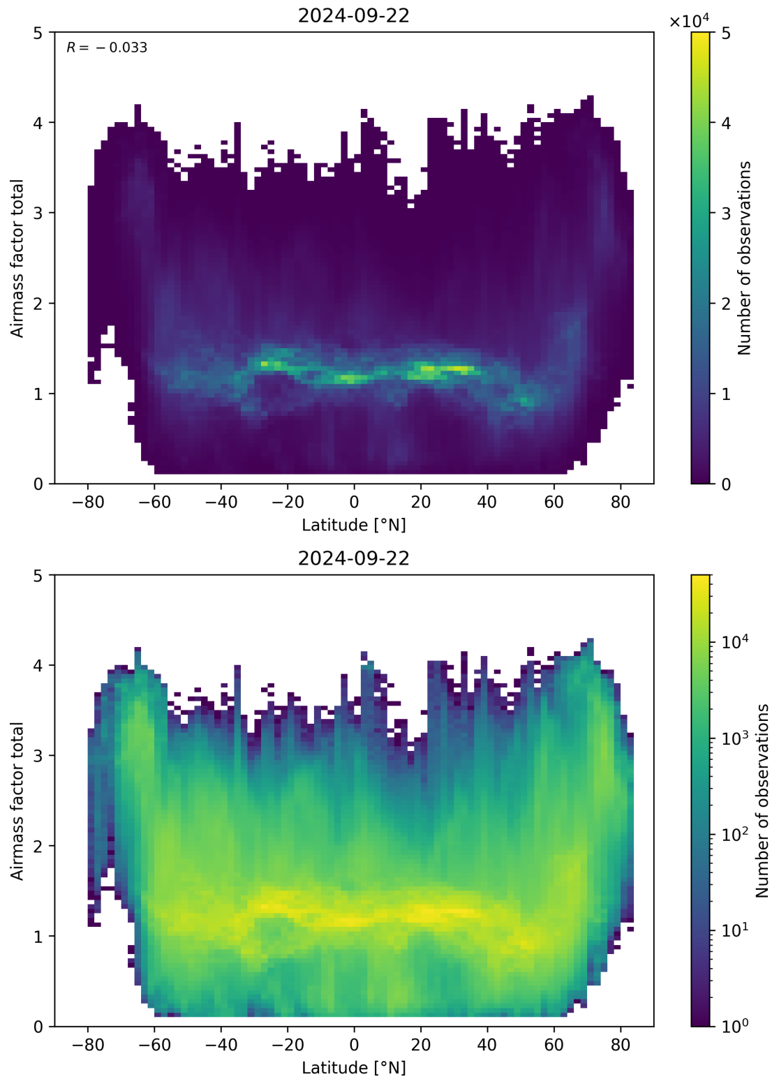
Figure 161: Scatter density plot of “Latitude” against “Airmass factor total” for 2024-09-22 to 2024-09-23.
