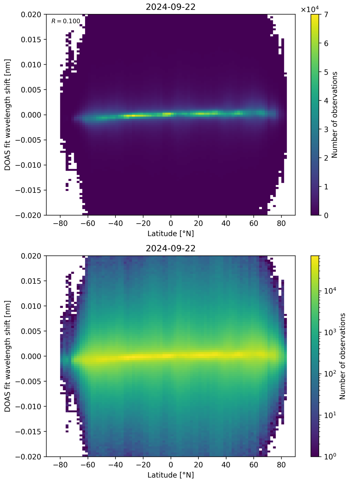
Figure 154: Scatter density plot of “Latitude” against “DOAS fit wavelength shift” for 2024-09-22 to 2024-09-23.
