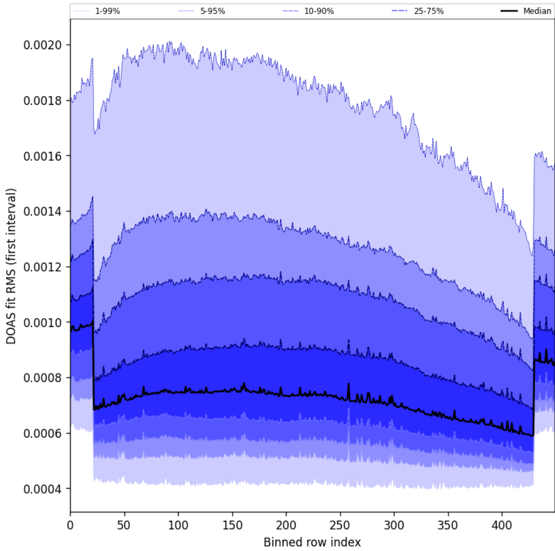
Figure 60: Along track statistics of “DOAS fit RMS (first interval)” for 2024-09-22 to 2024-09-23
