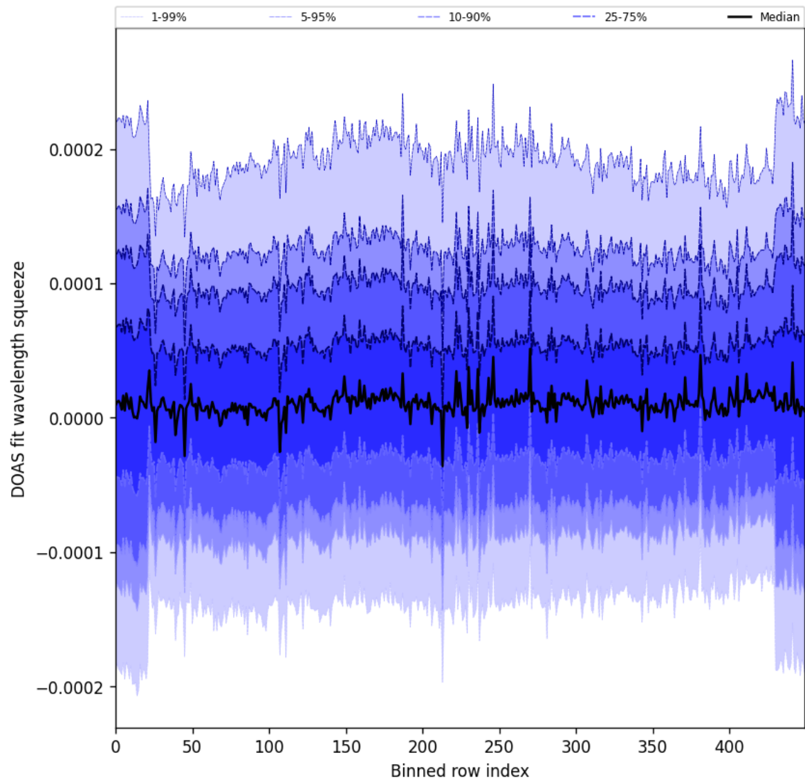
Figure 59: Along track statistics of “DOAS fit wavelength squeeze” for 2024-09-22 to 2024-09-23
