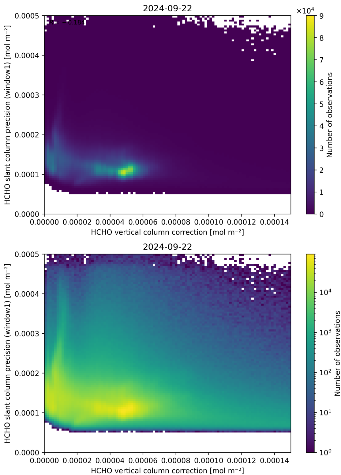
Figure 119: Scatter density plot of “HCHO vertical column correction” against “HCHO slant column precision (window1)” for 2024-09-22 to 2024-09-23.
