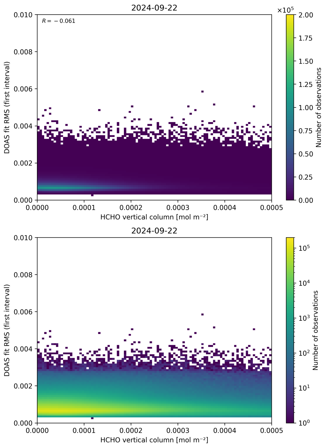
Figure 123: Scatter density plot of “HCHO vertical column” against “DOAS fit RMS (first interval)” for 2024-09-22 to 2024-09-23.
