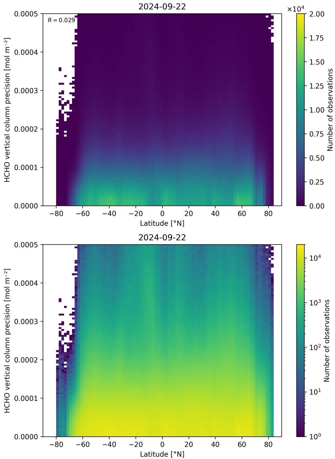
Figure 165: Scatter density plot of “Latitude” against “HCHO vertical column precision” for 2024-09-22 to 2024-09-23.
