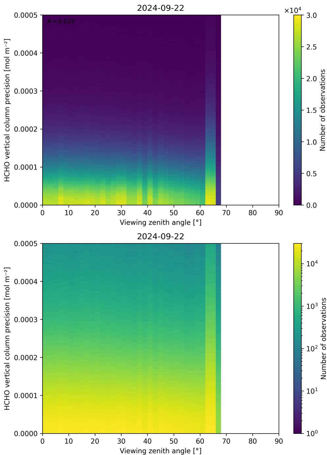
Figure 194: Scatter density plot of “Viewing zenith angle” against “HCHO vertical column precision” for 2024-09-22 to 2024-09-23.
