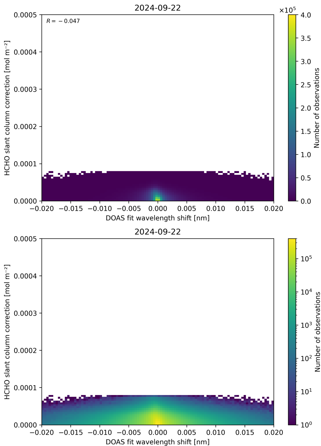
Figure 67: Scatter density plot of “DOAS fit wavelength shift” against “HCHO slant column correction” for 2024-09-22 to 2024-09-23.
