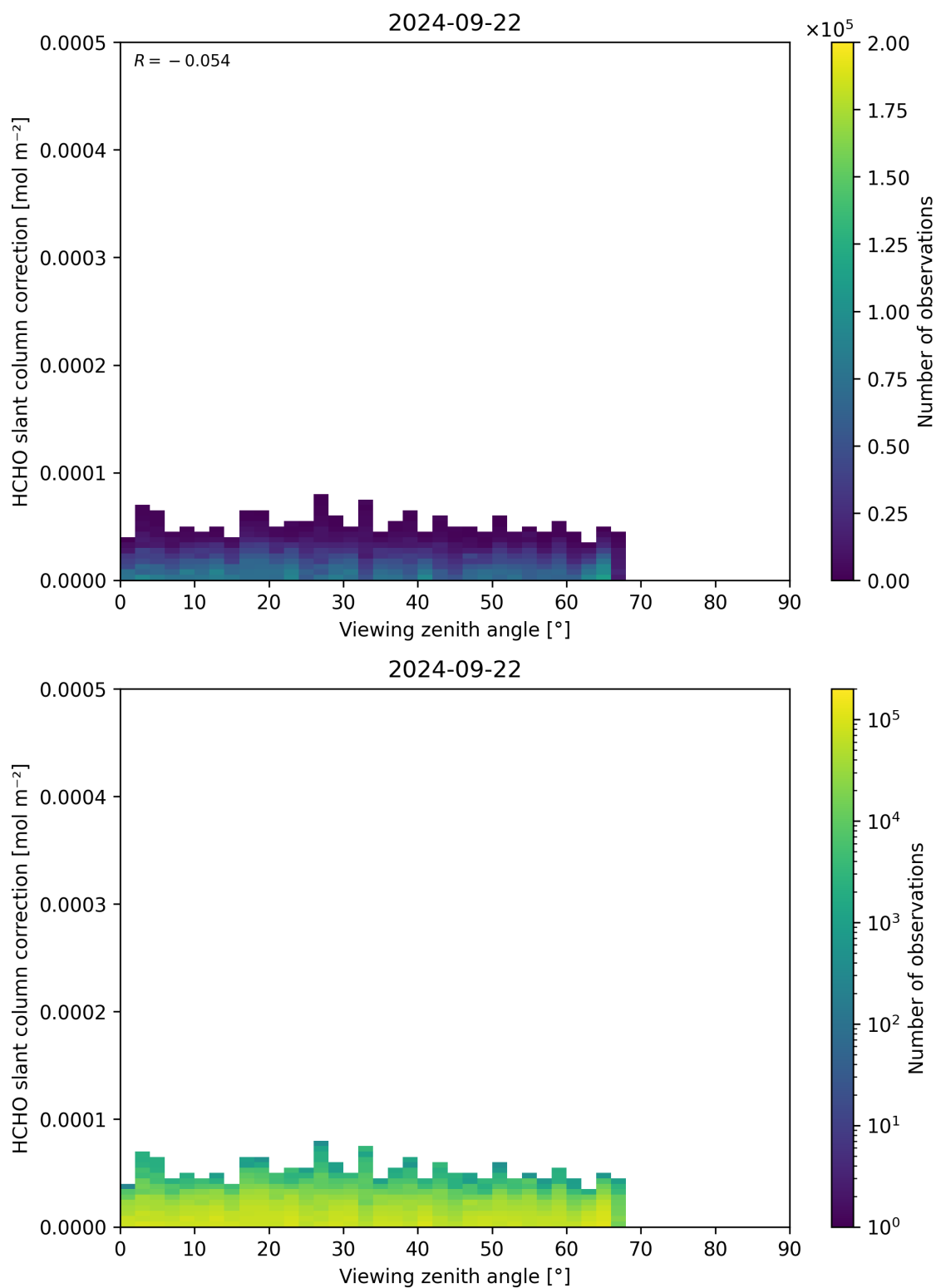
Figure 187: Scatter density plot of “Viewing zenith angle” against “HCHO slant column correction” for 2024-09-22 to 2024-09-23.
