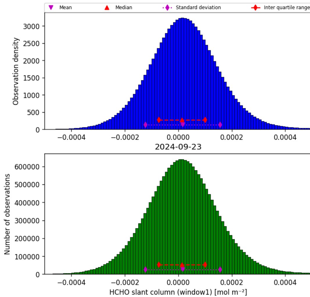
Figure 38: Histogram of “HCHO slant column (window1)” for 2024-09-22 to 2024-09-24
