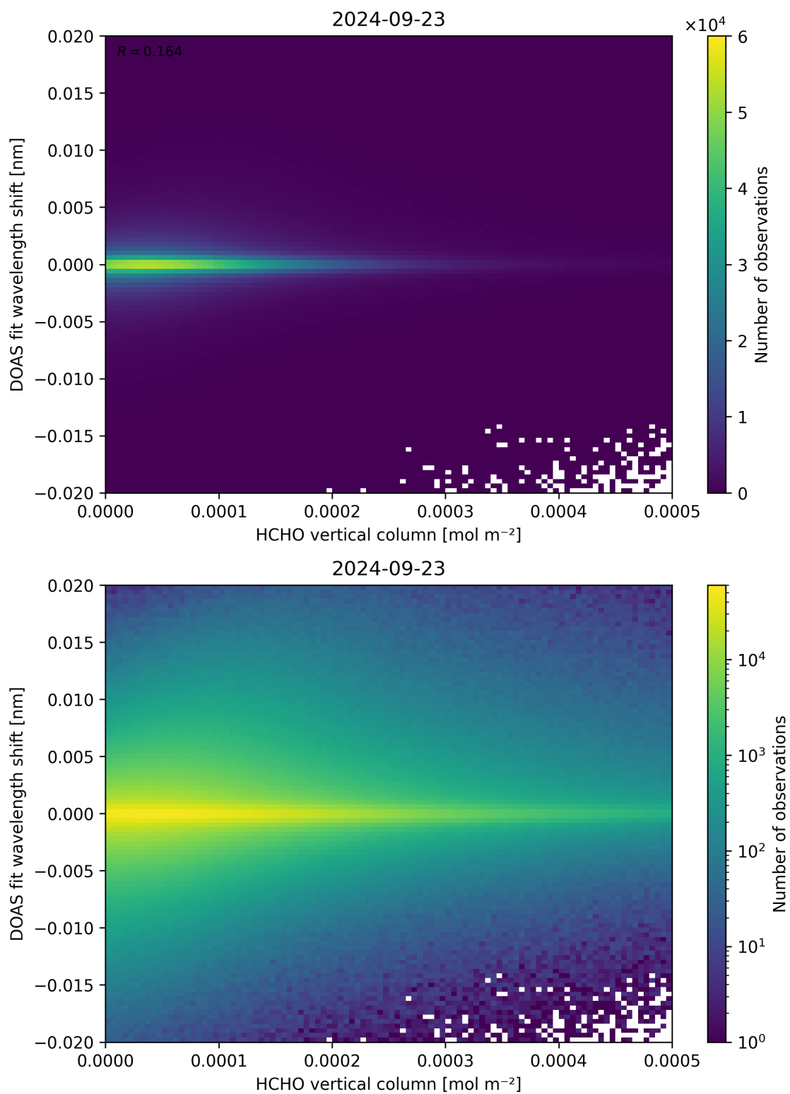
Figure 124: Scatter density plot of “HCHO vertical column” against “DOAS fit wavelength shift” for 2024-09-22 to 2024-09-24.
