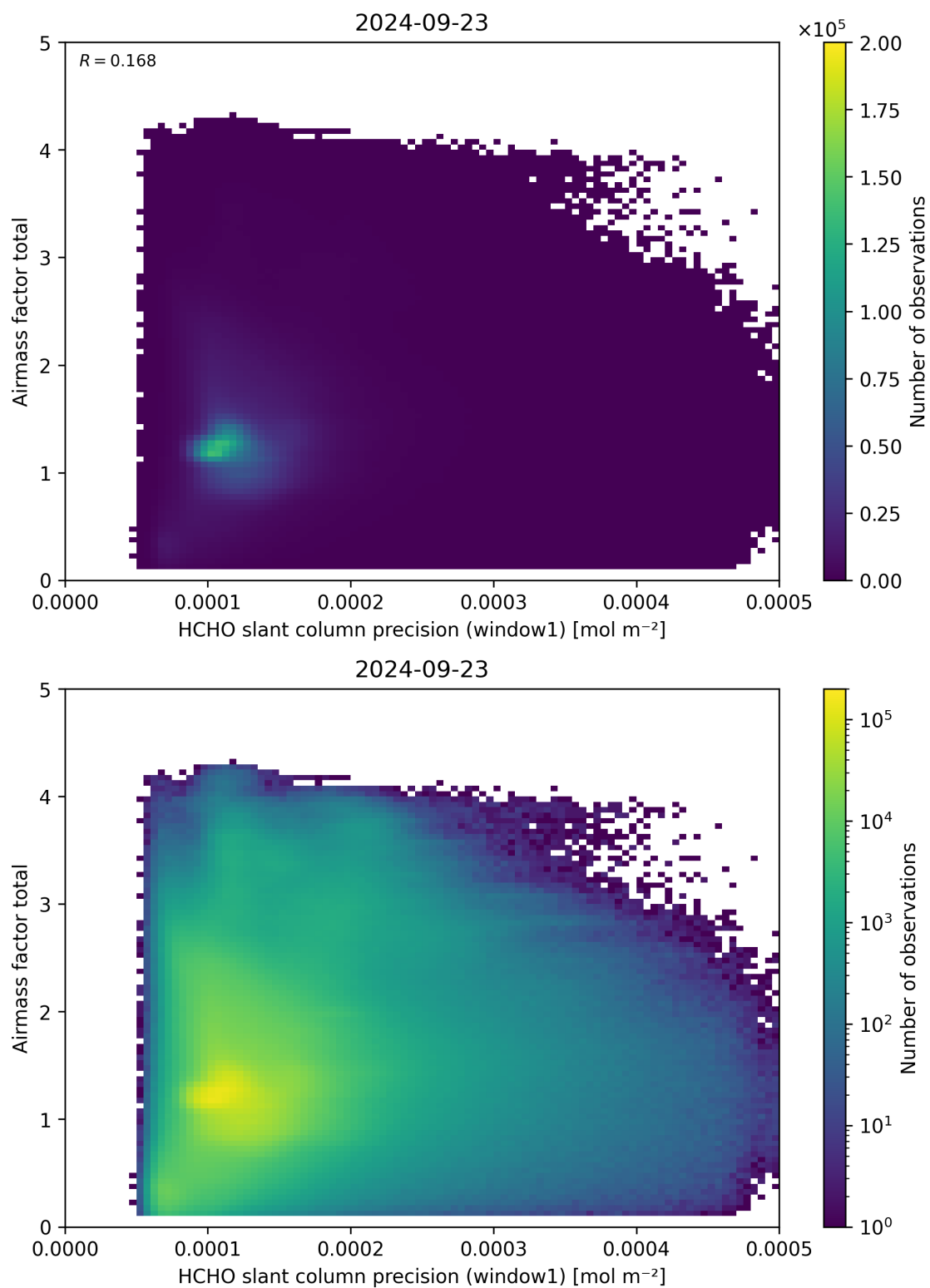
Figure 94: Scatter density plot of “HCHO slant column precision (window1)” against “Airmass factor total” for 2024-09-22 to 2024-09-24.
