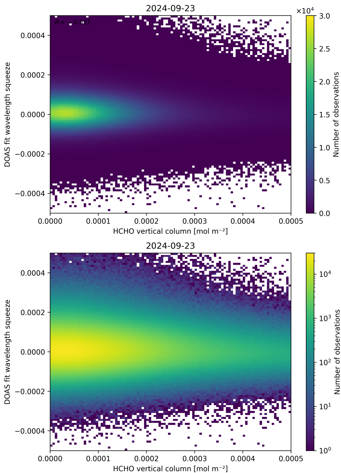
Figure 125: Scatter density plot of “HCHO vertical column” against “DOAS fit wavelength squeeze” for 2024-09-22 to 2024-09-24.
