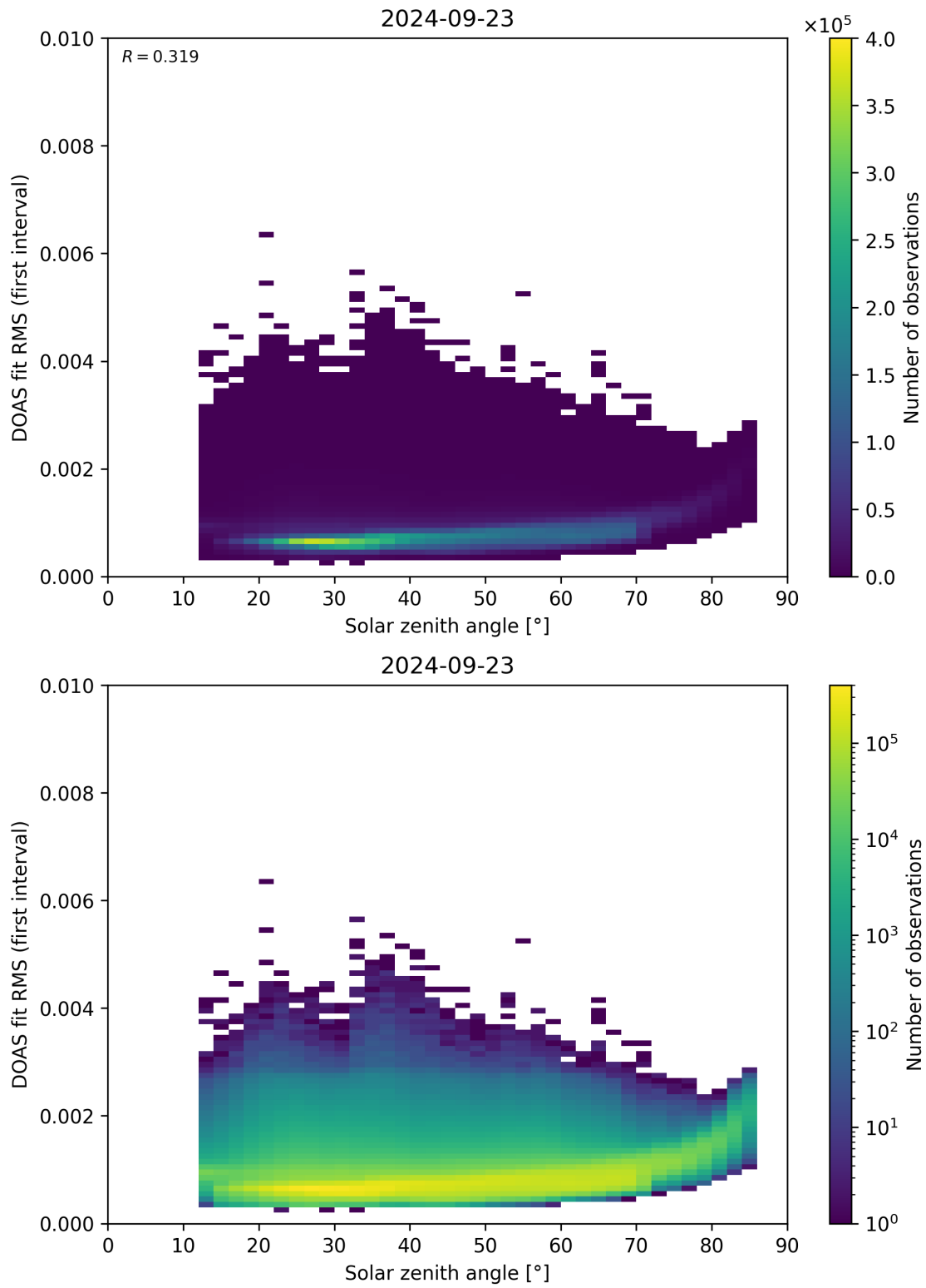
Figure 167: Scatter density plot of “Solar zenith angle” against “DOAS fit RMS (first interval)” for 2024-09-22 to 2024-09-24.
