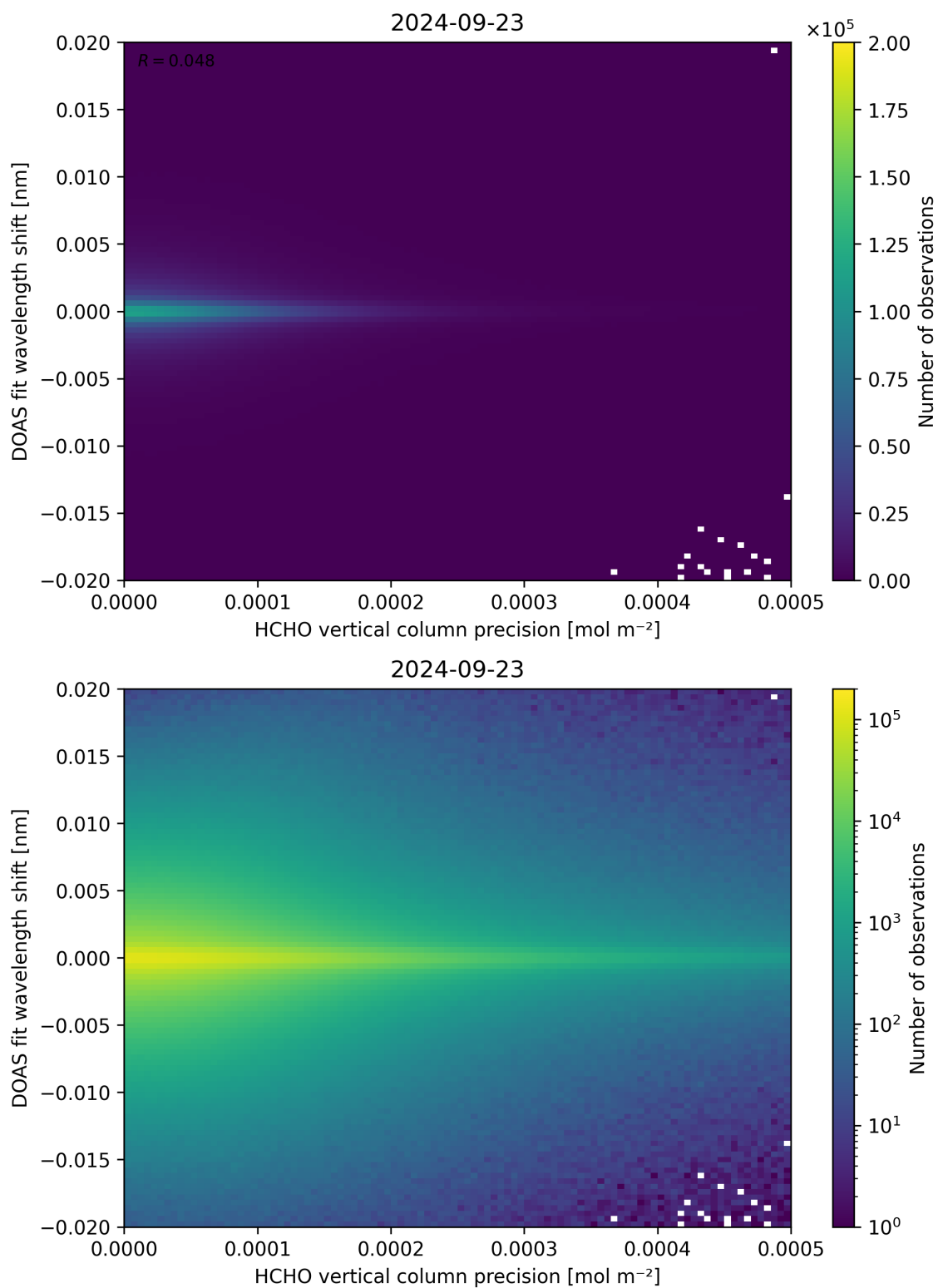
Figure 137: Scatter density plot of “HCHO vertical column precision” against “DOAS fit wavelength shift” for 2024-09-22 to 2024-09-24.
