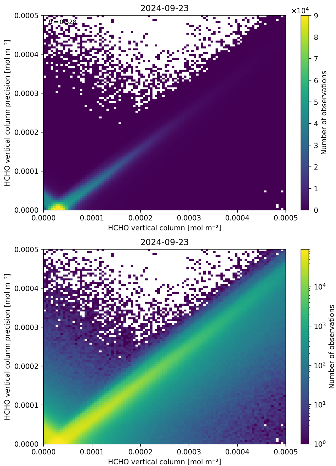
Figure 134: Scatter density plot of “HCHO vertical column” against “HCHO vertical column precision” for 2024-09-22 to 2024-09-24.
