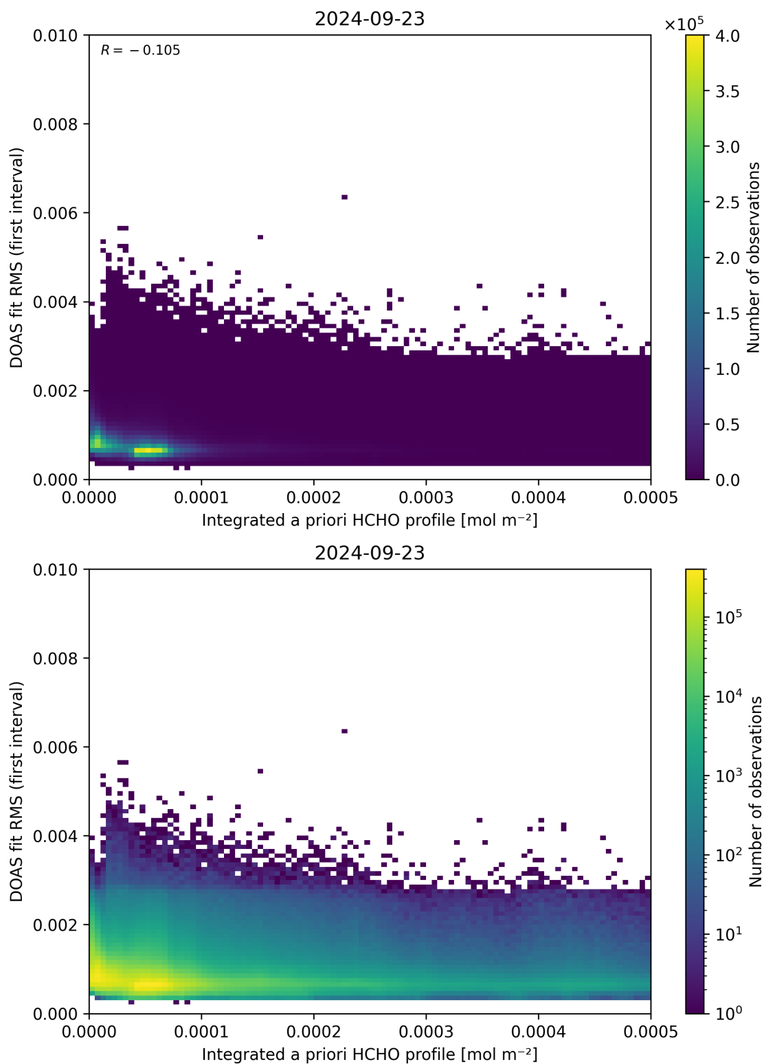
Figure 148: Scatter density plot of “Integrated a priori HCHO profile” against “DOAS fit RMS (first interval)” for 2024-09-22 to 2024-09-24.
