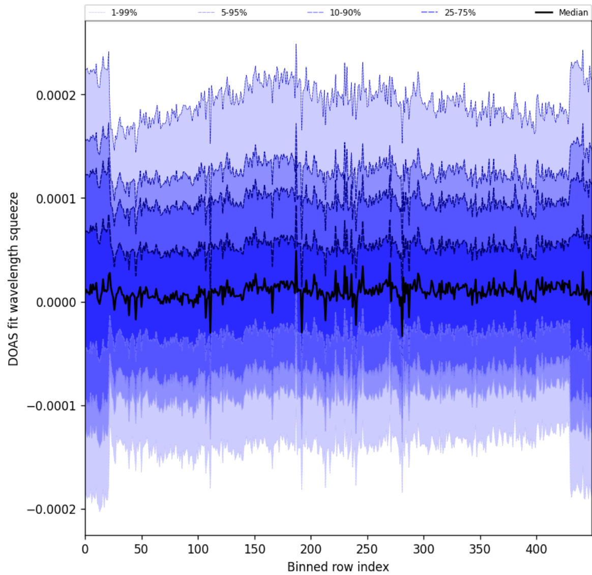
Figure 59: Along track statistics of “DOAS fit wavelength squeeze” for 2024-09-22 to 2024-09-24
