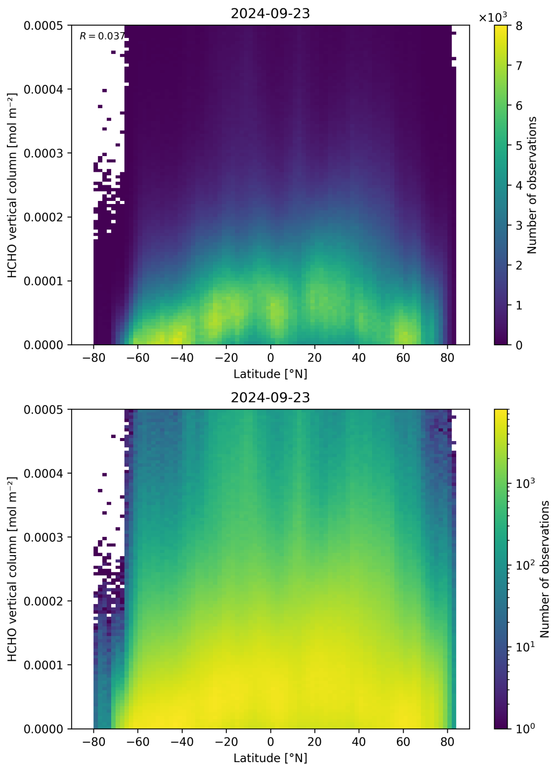
Figure 163: Scatter density plot of “Latitude” against “HCHO vertical column” for 2024-09-22 to 2024-09-24.
