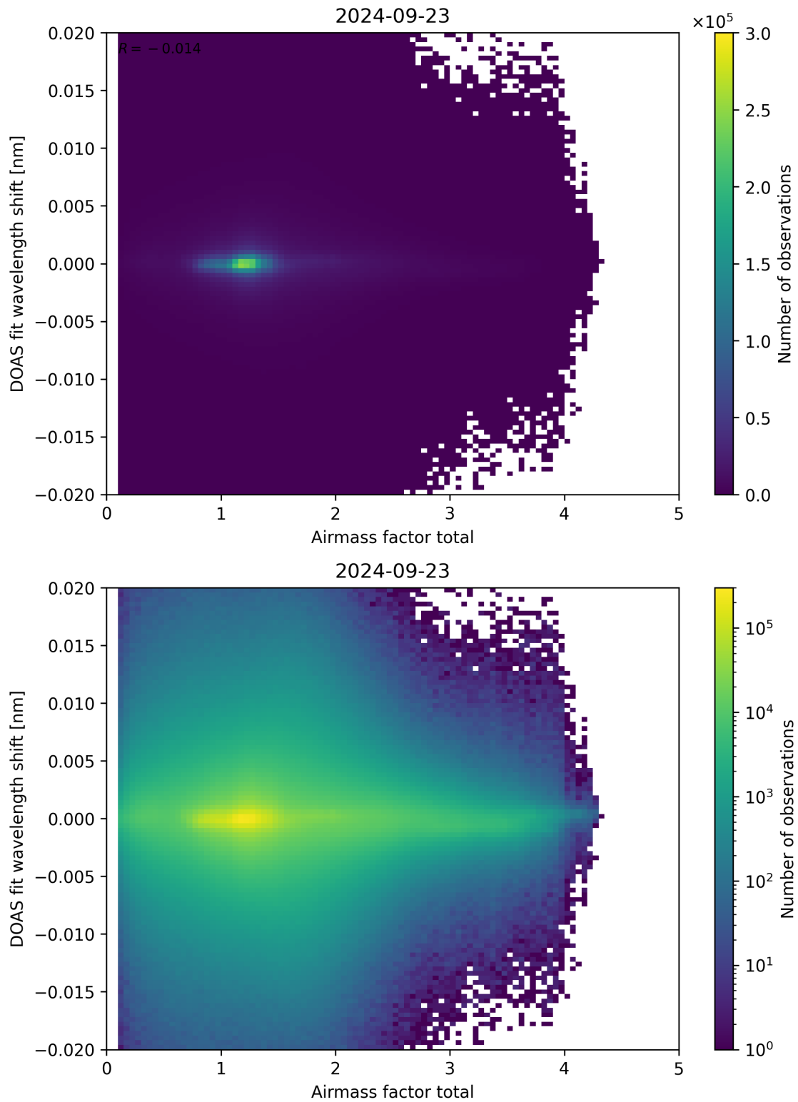
Figure 98: Scatter density plot of “Airmass factor total” against “DOAS fit wavelength shift” for 2024-09-22 to 2024-09-24.
