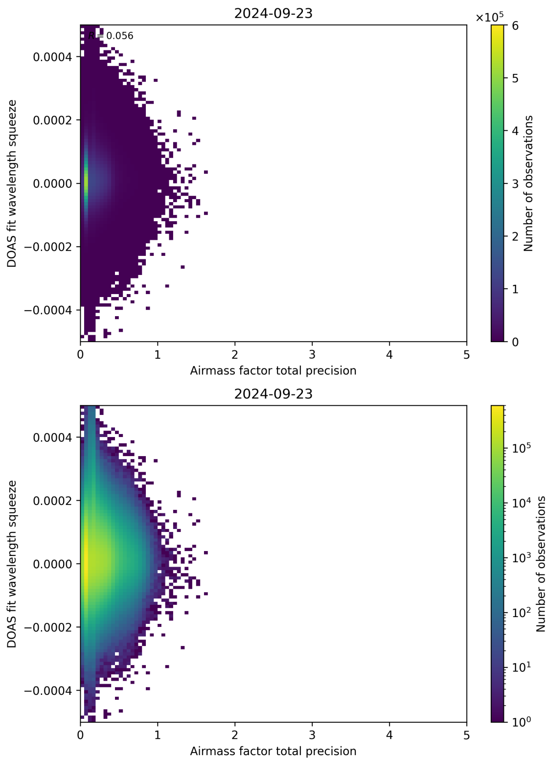
Figure 107: Scatter density plot of “Airmass factor total precision” against “DOAS fit wavelength squeeze” for 2024-09-22 to 2024-09-24.
