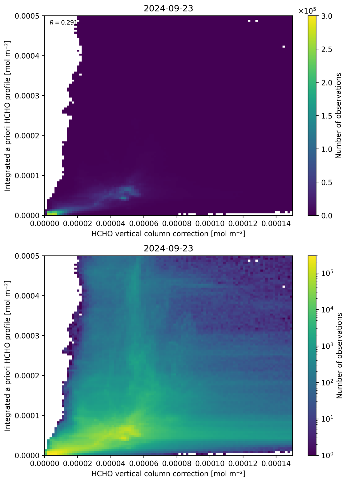
Figure 122: Scatter density plot of “HCHO vertical column correction” against “Integrated a priori HCHO profile” for 2024-09-22 to 2024-09-24.
