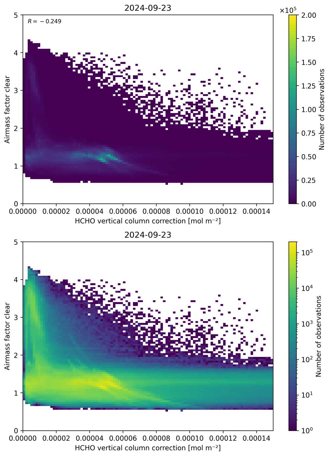
Figure 115: Scatter density plot of “HCHO vertical column correction” against “Airmass factor clear” for 2024-09-22 to 2024-09-24.
