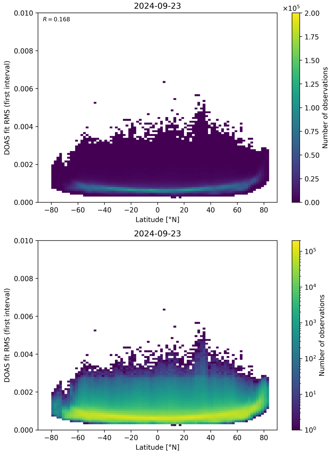
Figure 153: Scatter density plot of “Latitude” against “DOAS fit RMS (first interval)” for 2024-09-22 to 2024-09-24.
