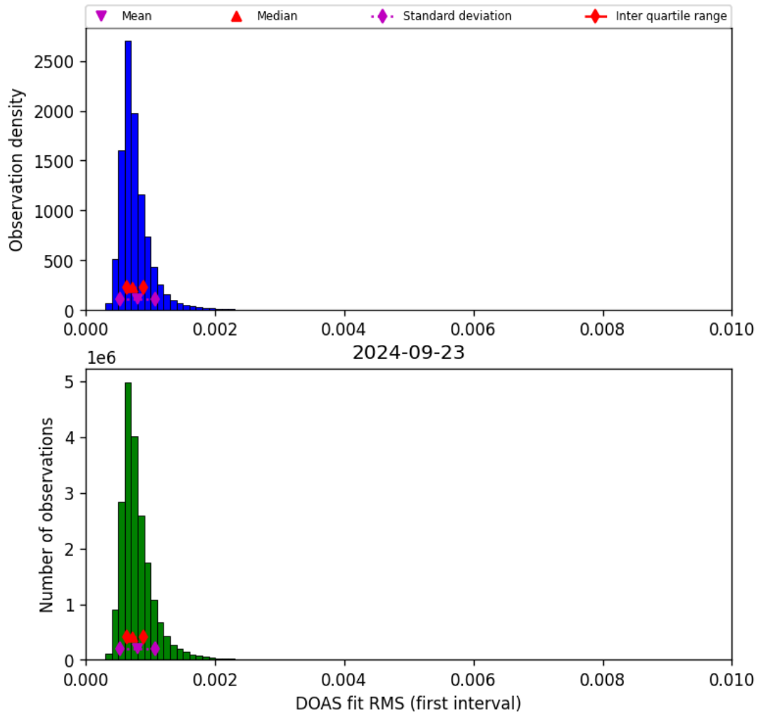
Figure 46: Histogram of “DOAS fit RMS (first interval)” for 2024-09-22 to 2024-09-24
