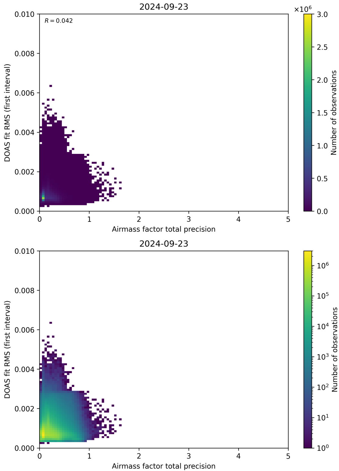
Figure 105: Scatter density plot of “Airmass factor total precision” against “DOAS fit RMS (first interval)” for 2024-09-22 to 2024-09-24.
