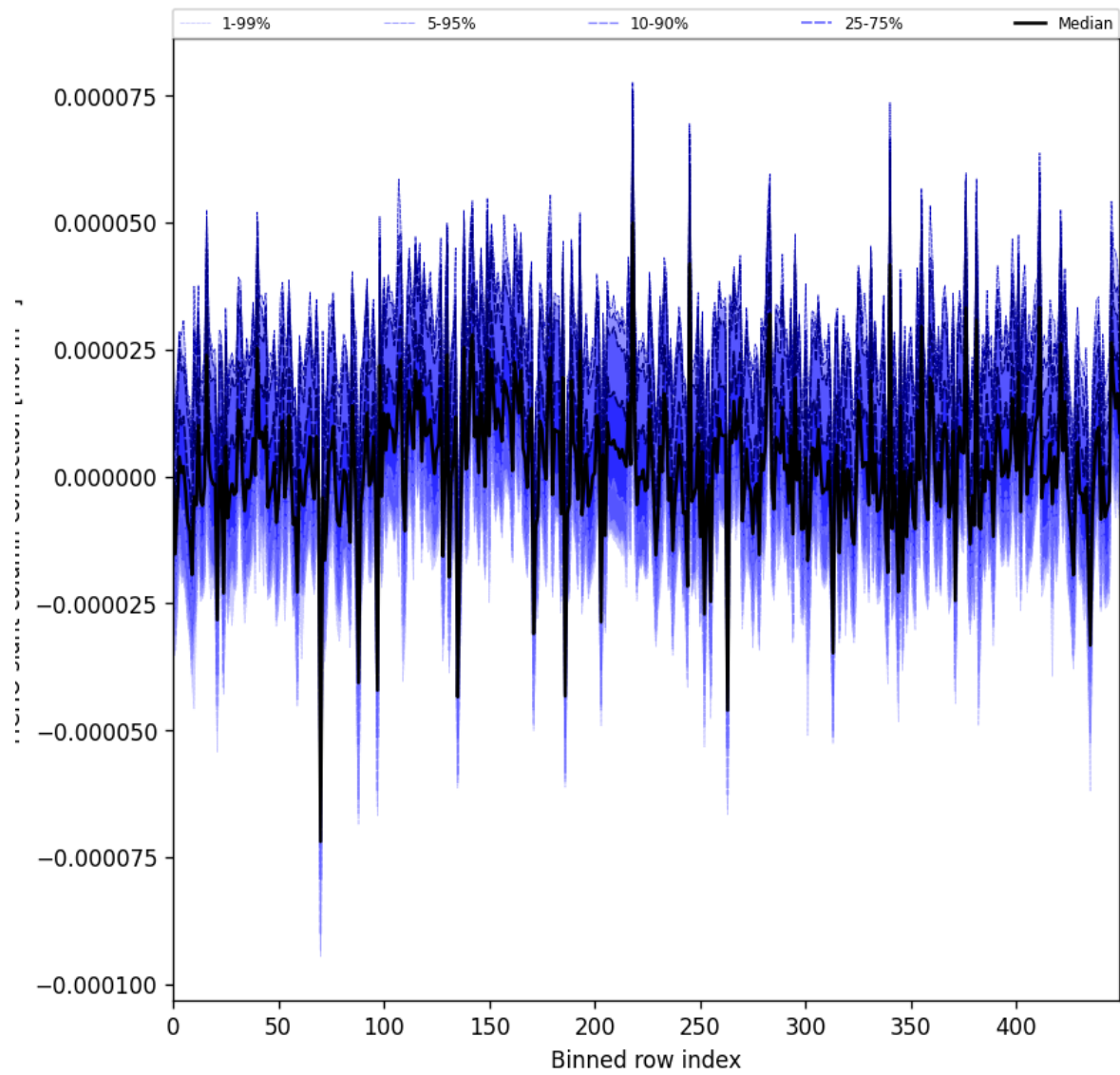
Figure 61: Along track statistics of “HCHO slant column correction” for 2024-09-22 to 2024-09-24
