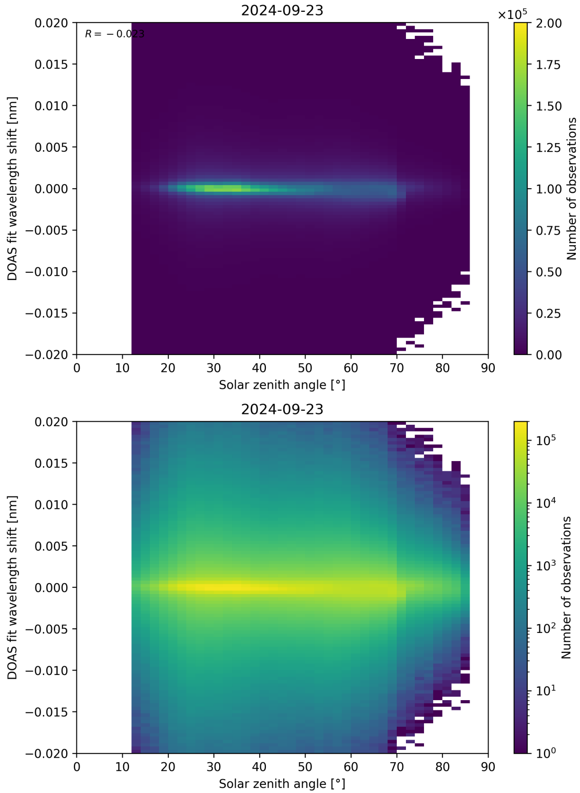
Figure 168: Scatter density plot of “Solar zenith angle” against “DOAS fit wavelength shift” for 2024-09-22 to 2024-09-24.
