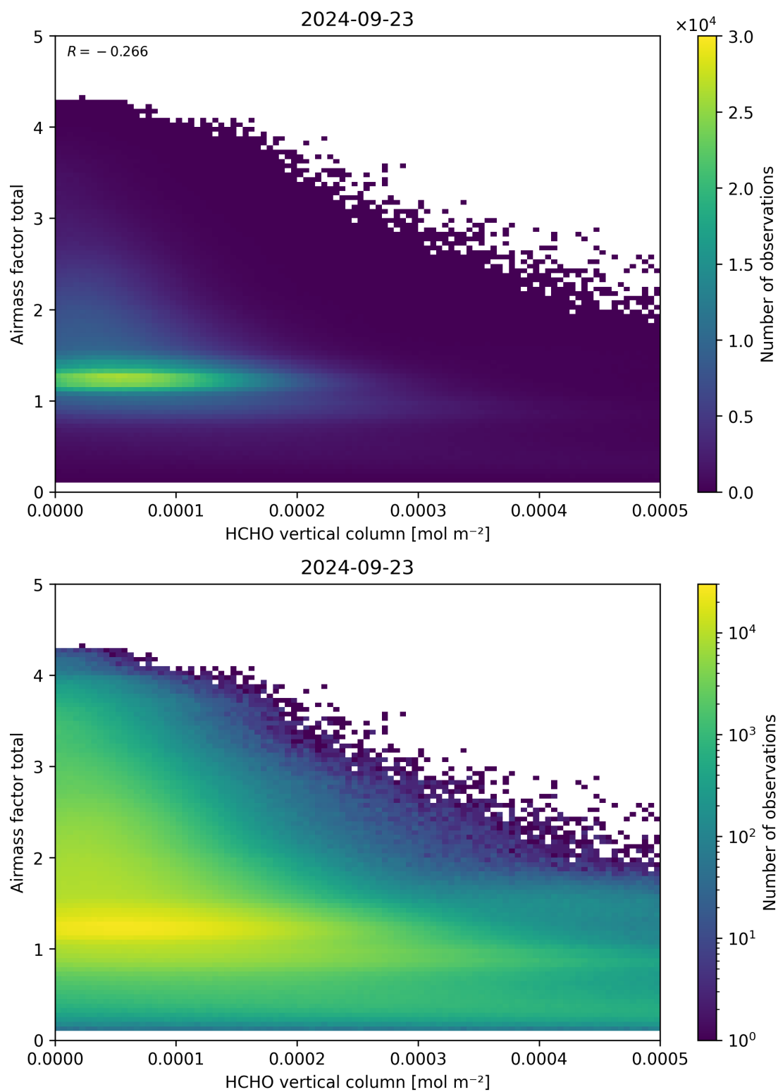
Figure 131: Scatter density plot of “HCHO vertical column” against “Airmass factor total” for 2024-09-22 to 2024-09-24.
