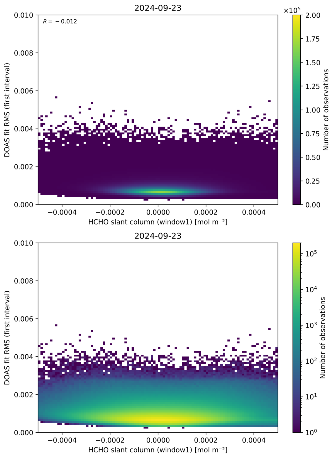
Figure 78: Scatter density plot of “HCHO slant column (window1)” against “DOAS fit RMS (first interval)” for 2024-09-22 to 2024-09-24.
