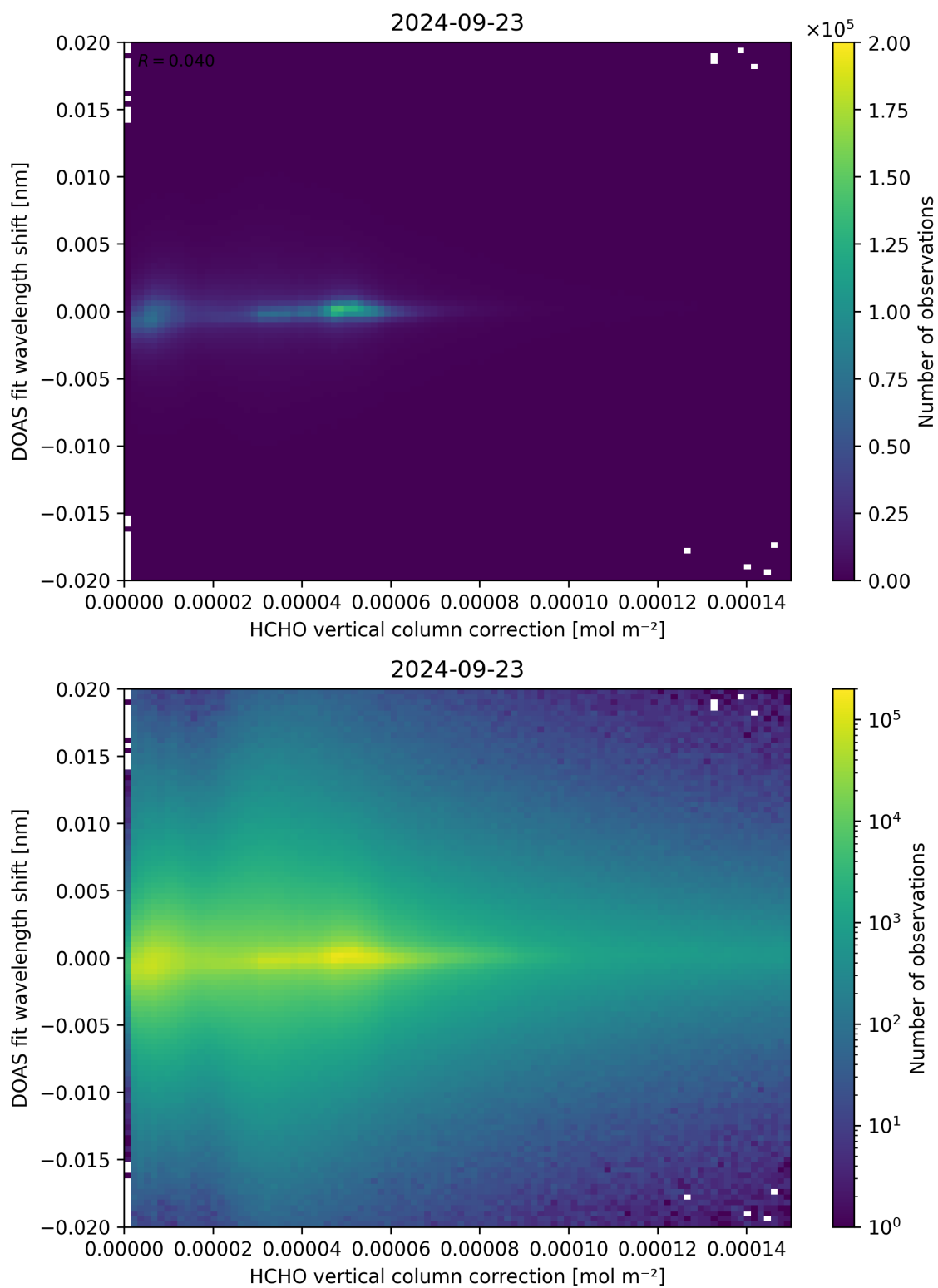
Figure 113: Scatter density plot of “HCHO vertical column correction” against “DOAS fit wavelength shift” for 2024-09-22 to 2024-09-24.
