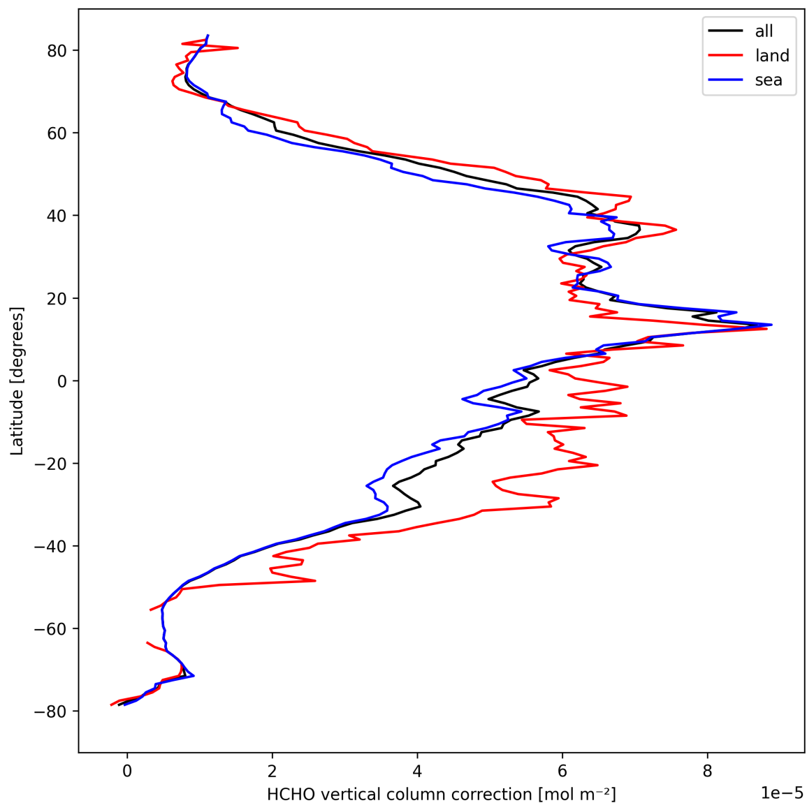
Figure 23: Zonal average of “HCHO vertical column correction” for 2024-09-22 to 2024-09-24.
