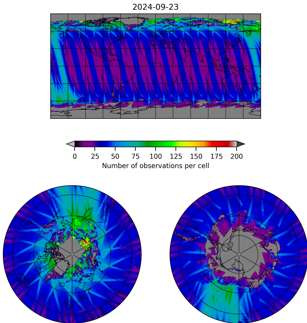
Figure 19: Map of the number of observations for 2024-09-22 to 2024-09-24
