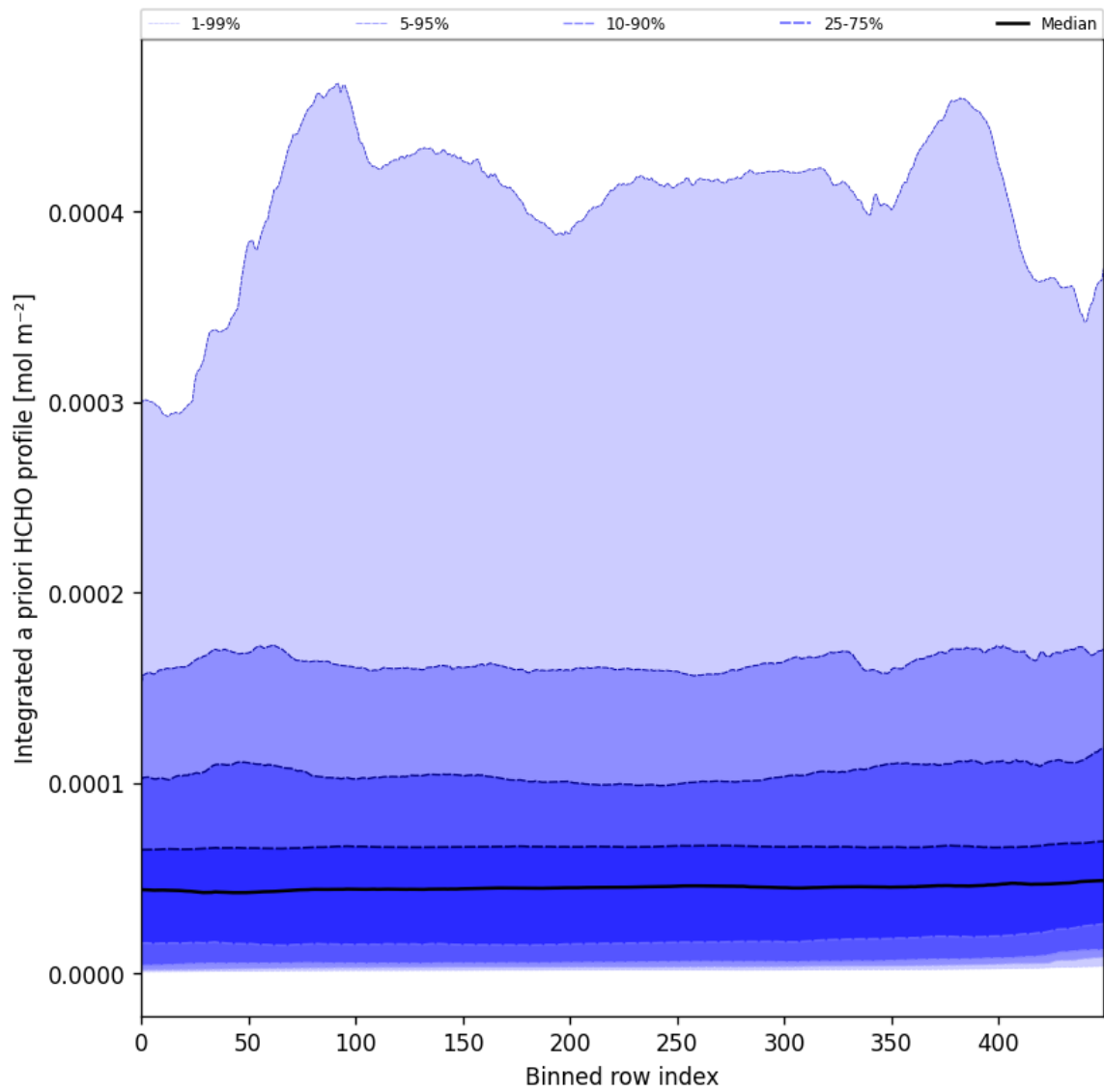
Figure 57: Along track statistics of “Integrated a priori HCHO profile” for 2024-09-22 to 2024-09-24
