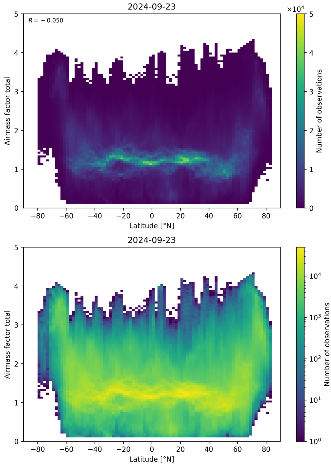
Figure 161: Scatter density plot of “Latitude” against “Airmass factor total” for 2024-09-22 to 2024-09-24.
