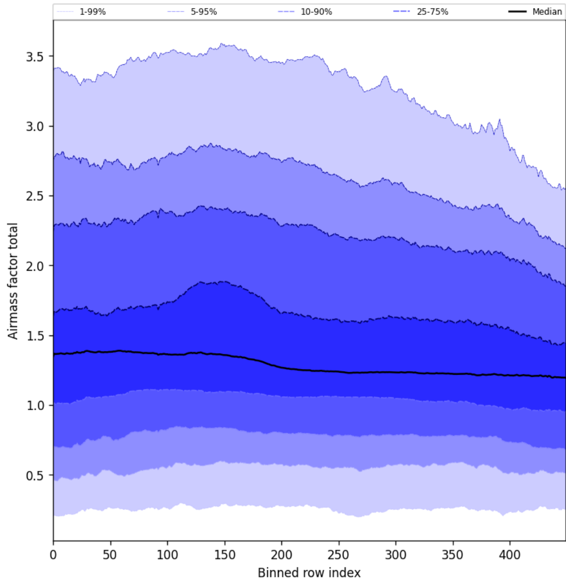
Figure 54: Along track statistics of “Airmass factor total” for 2024-09-22 to 2024-09-24
