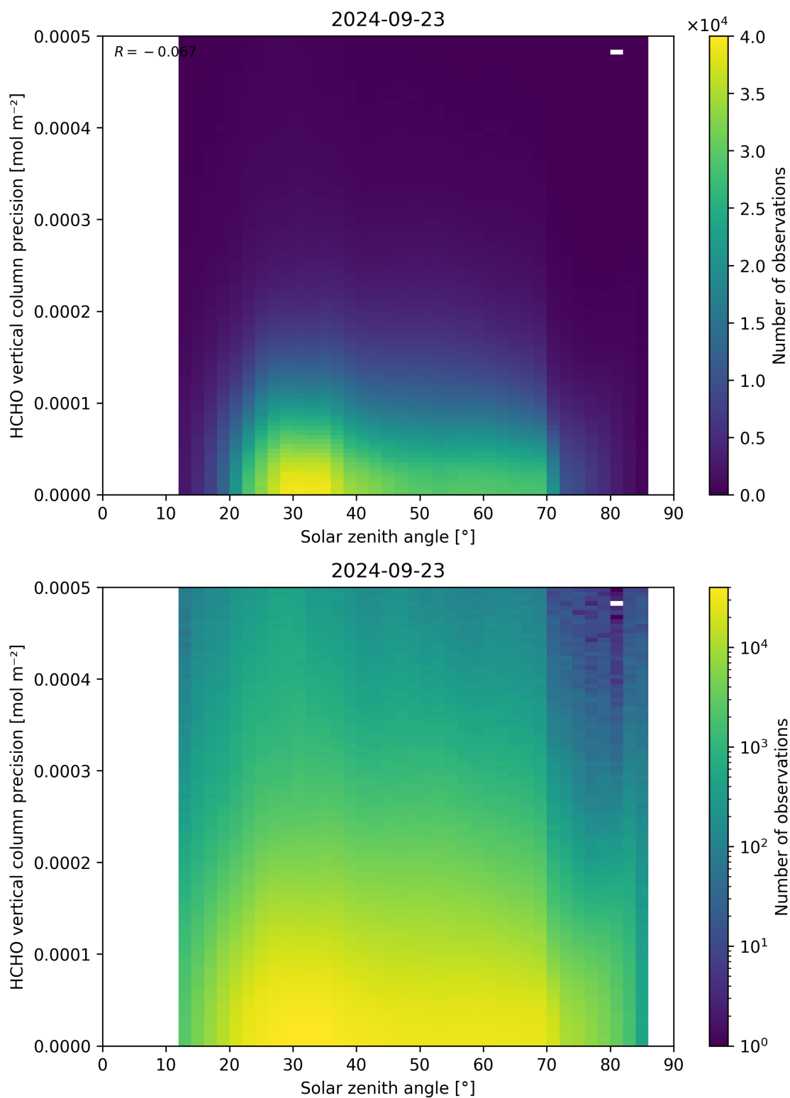
Figure 179: Scatter density plot of “Solar zenith angle” against “HCHO vertical column precision” for 2024-09-22 to 2024-09-24.
