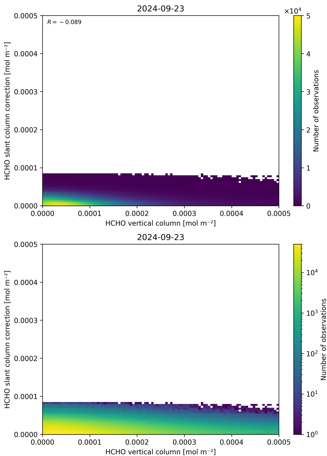
Figure 128: Scatter density plot of “HCHO vertical column” against “HCHO slant column correction” for 2024-09-22 to 2024-09-24.
