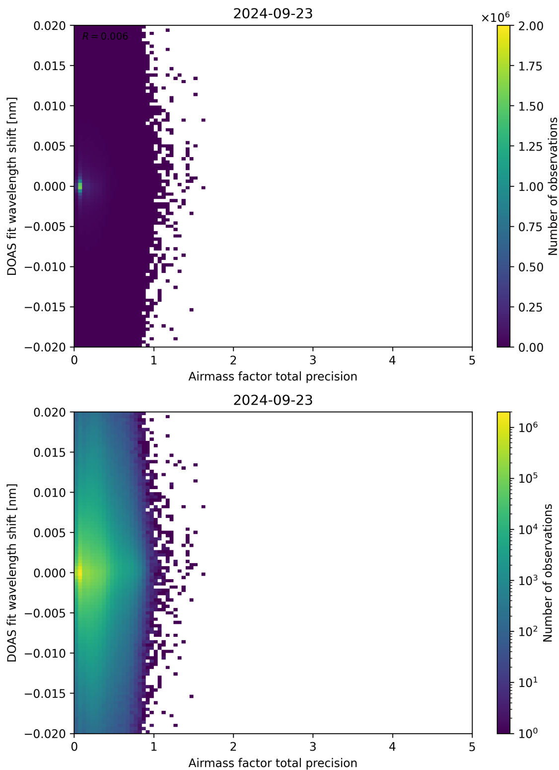
Figure 106: Scatter density plot of “Airmass factor total precision” against “DOAS fit wavelength shift” for 2024-09-22 to 2024-09-24.
