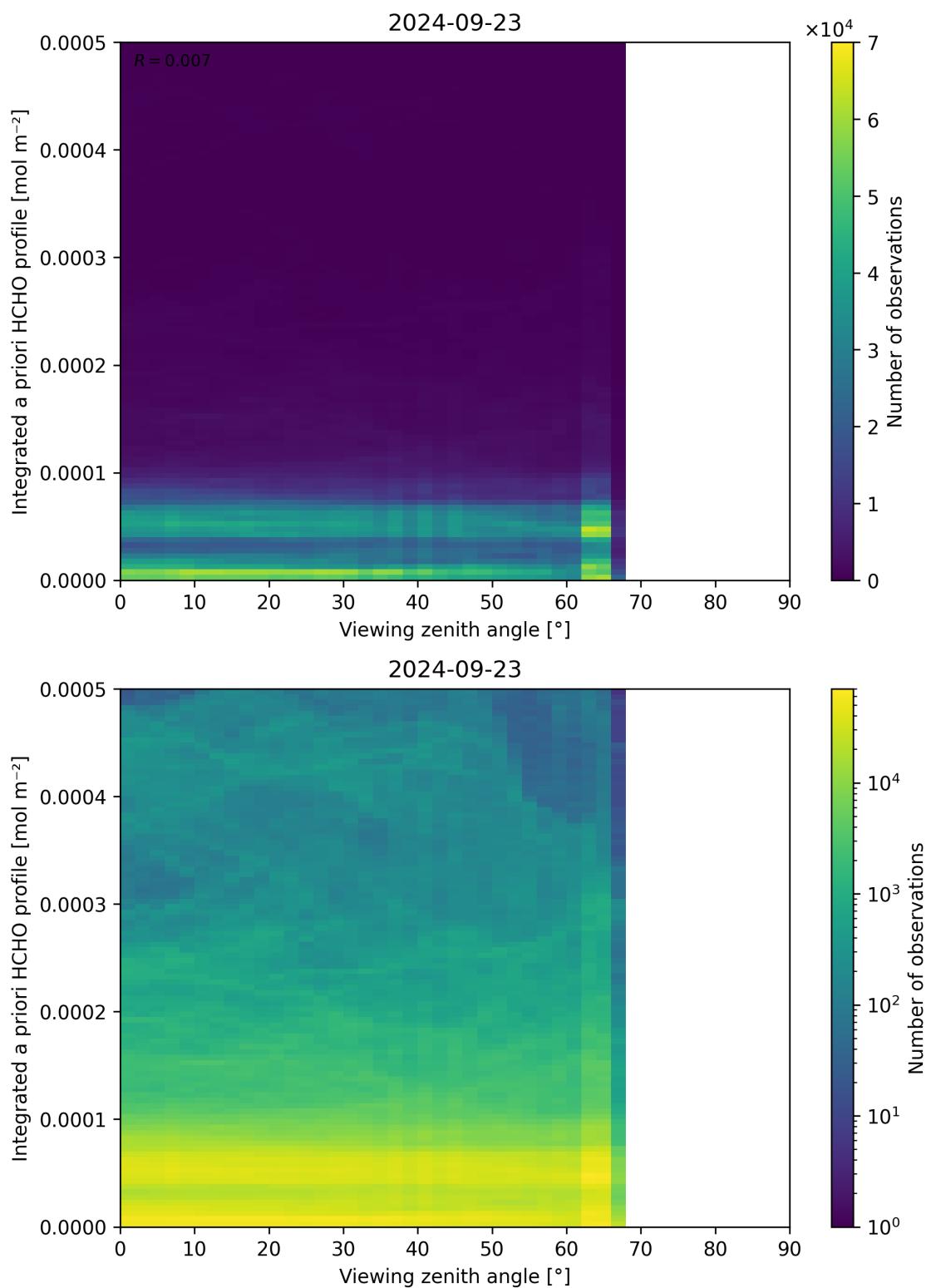
Figure 195: Scatter density plot of “Viewing zenith angle” against “Integrated a priori HCHO profile” for 2024-09-22 to 2024-09-24.
