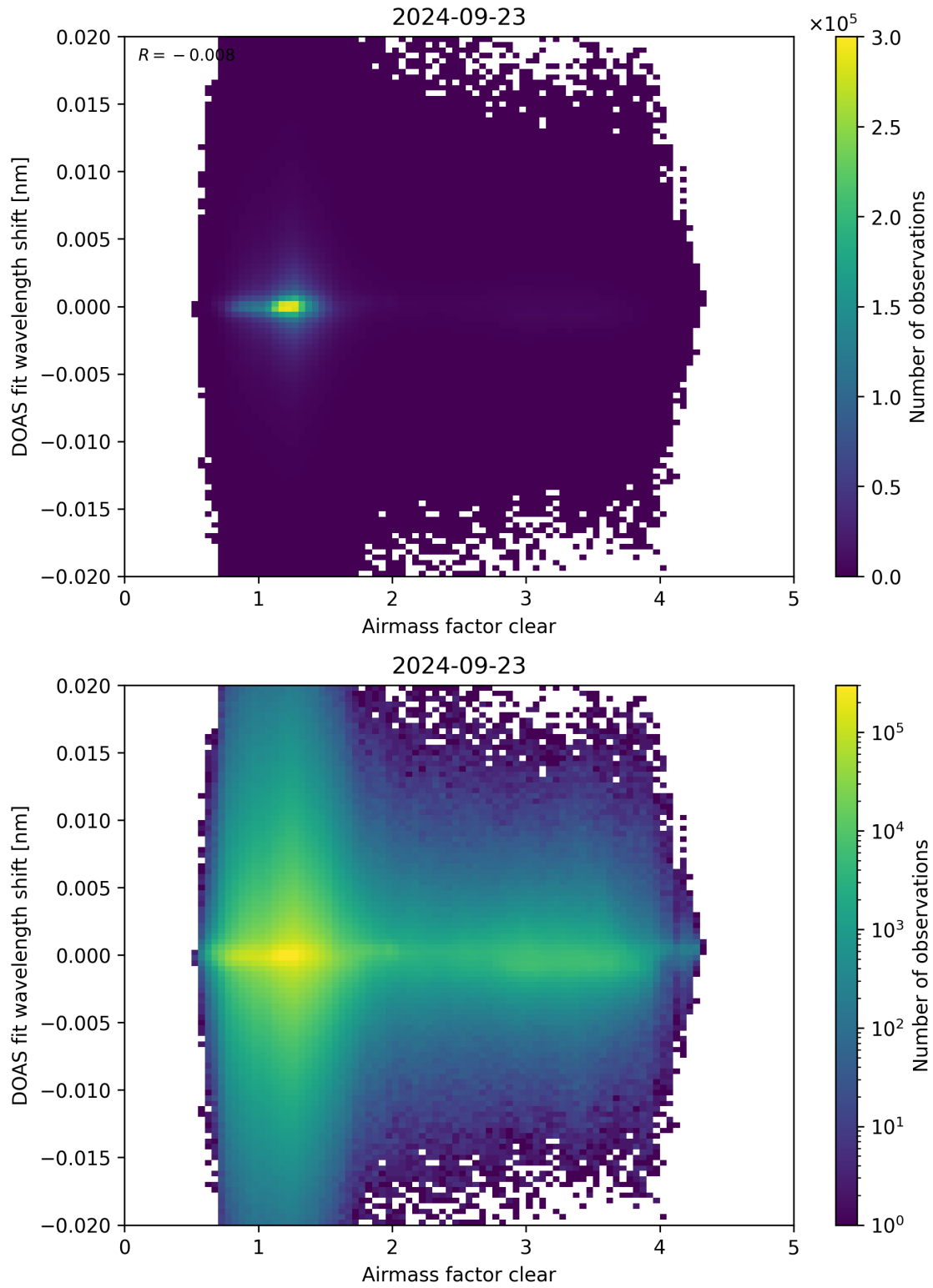
Figure 72: Scatter density plot of “Airmass factor clear” against “DOAS fit wavelength shift” for 2024-09-22 to 2024-09-24.
