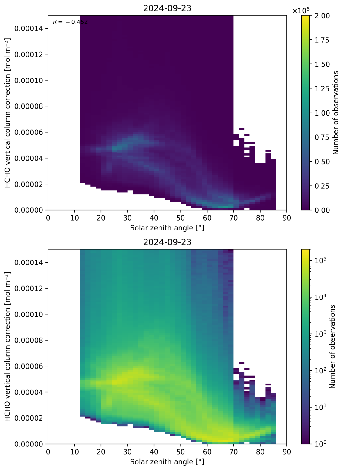
Figure 178: Scatter density plot of “Solar zenith angle” against “HCHO vertical column correction” for 2024-09-22 to 2024-09-24.
