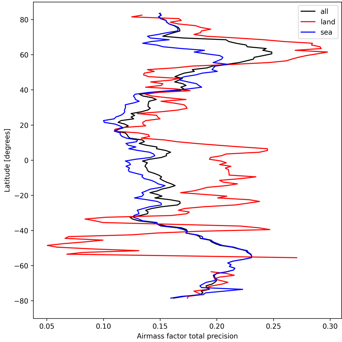
Figure 27: Zonal average of “Airmass factor total precision” for 2024-09-22 to 2024-09-24.
