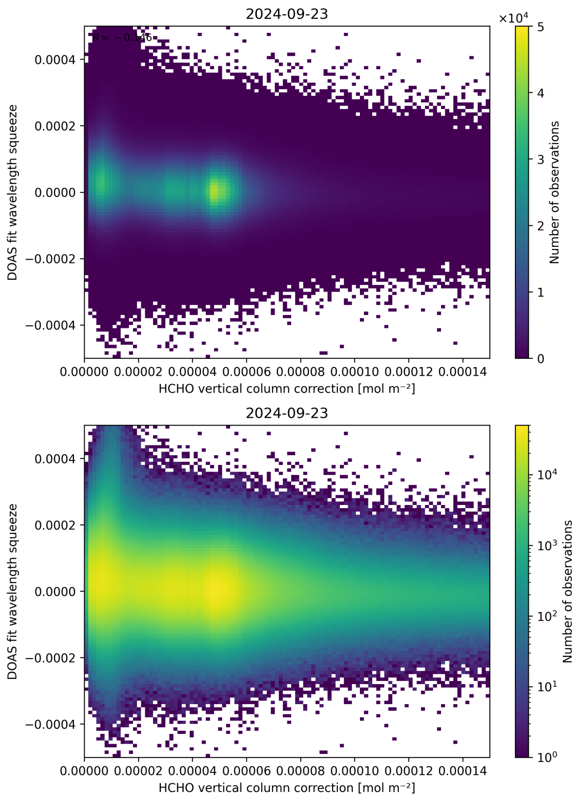
Figure 114: Scatter density plot of “HCHO vertical column correction” against “DOAS fit wavelength squeeze” for 2024-09-22 to 2024-09-24.
