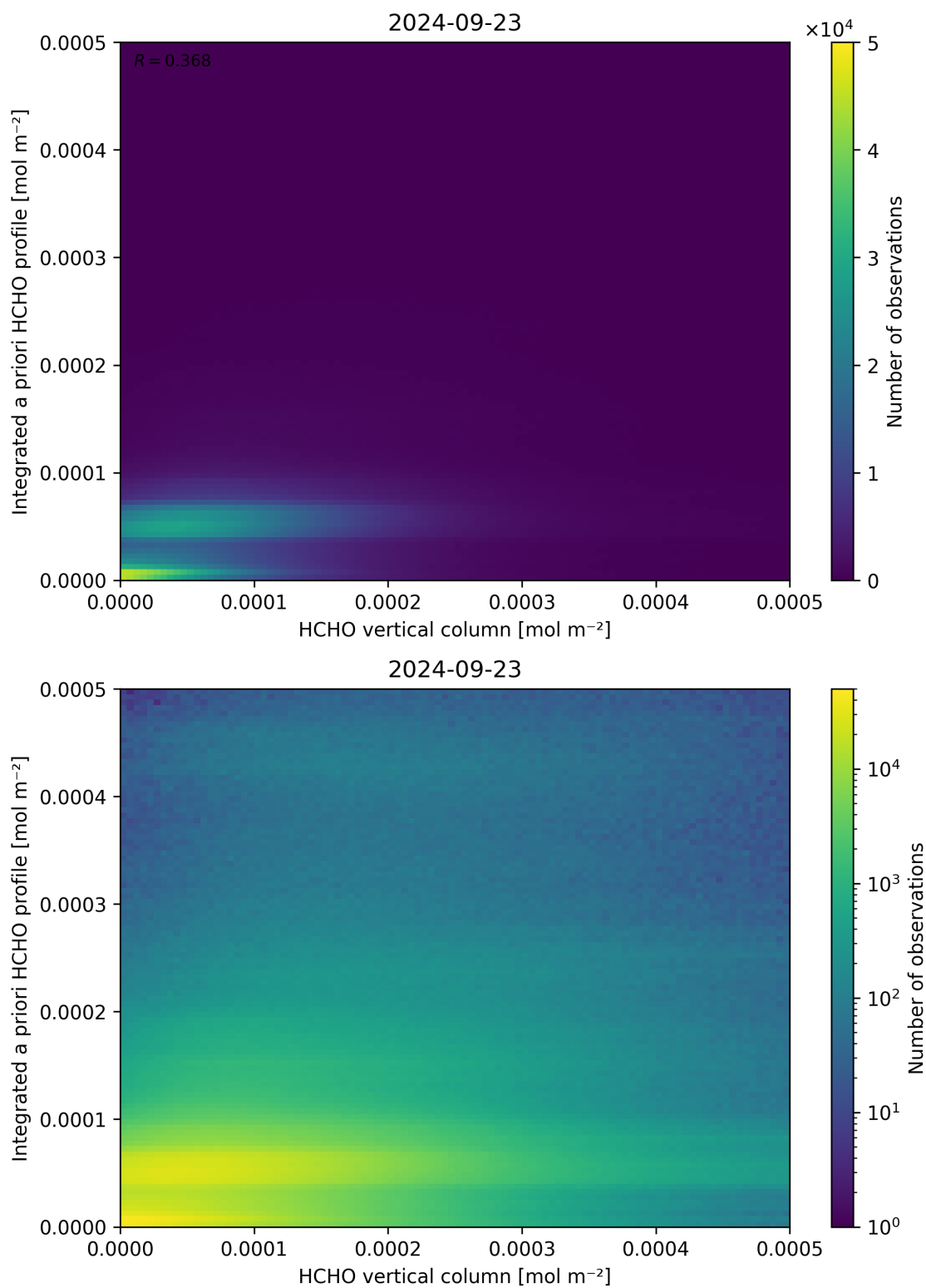
Figure 135: Scatter density plot of “HCHO vertical column” against “Integrated a priori HCHO profile” for 2024-09-22 to 2024-09-24.
