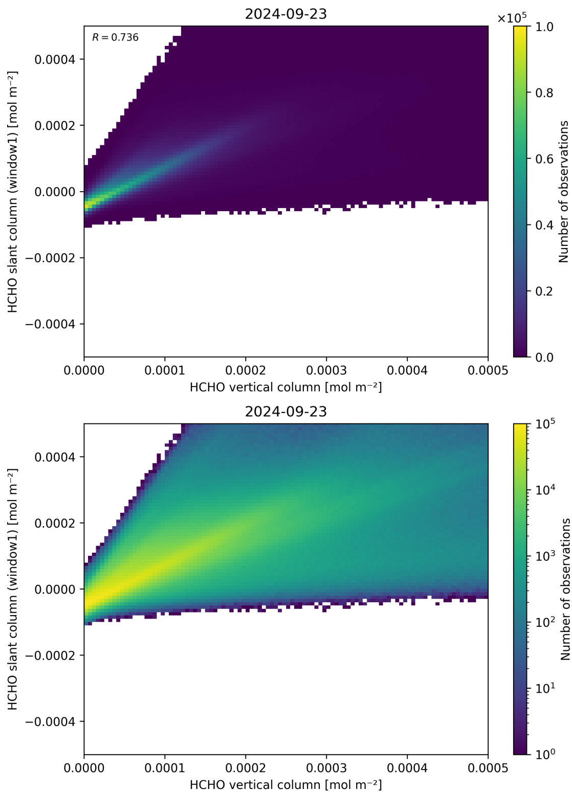
Figure 129: Scatter density plot of “HCHO vertical column” against “HCHO slant column (window1)” for 2024-09-22 to 2024-09-24.
