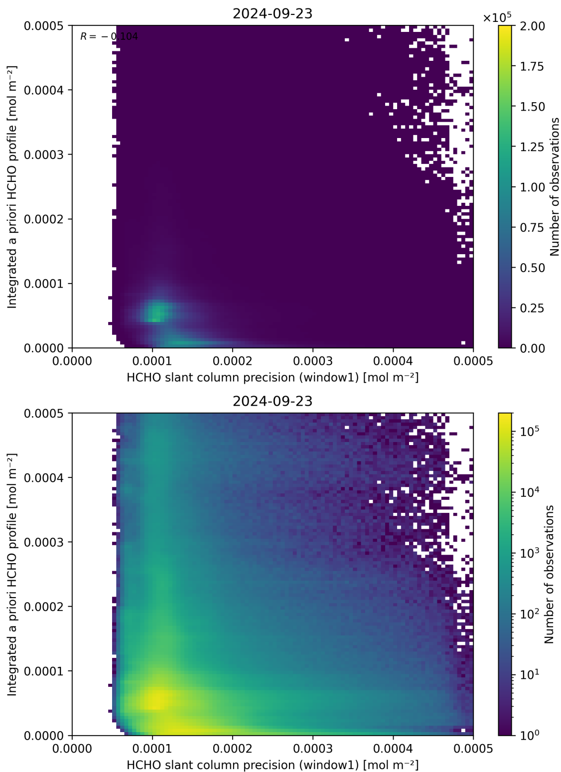
Figure 96: Scatter density plot of “HCHO slant column precision (window1)” against “Integrated a priori HCHO profile” for 2024-09-22 to 2024-09-24.
