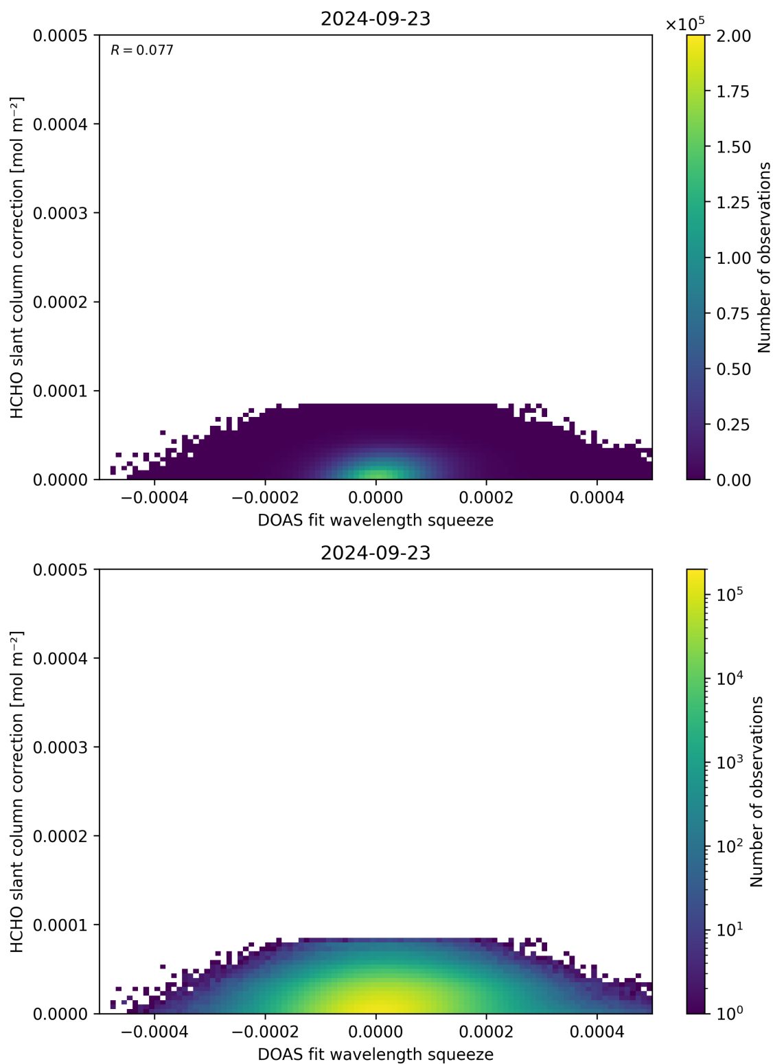
Figure 70: Scatter density plot of “DOAS fit wavelength squeeze” against “HCHO slant column correction” for 2024-09-22 to 2024-09-24.
