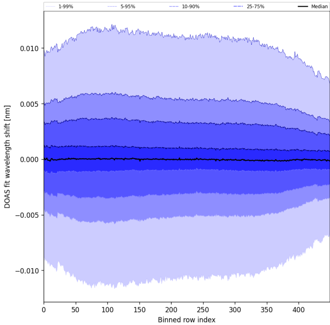
Figure 58: Along track statistics of “DOAS fit wavelength shift” for 2024-09-22 to 2024-09-24
