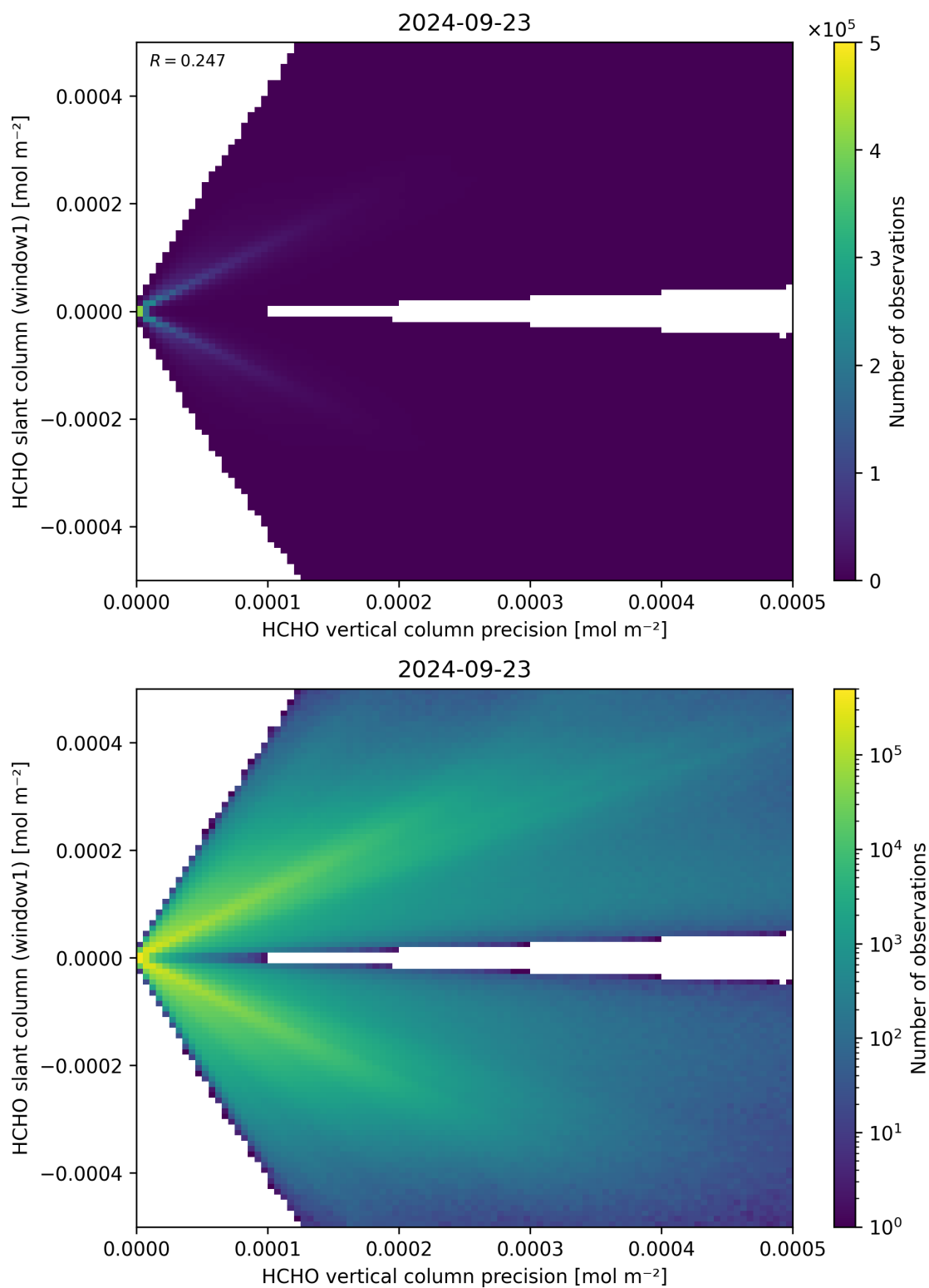
Figure 142: Scatter density plot of “HCHO vertical column precision” against “HCHO slant column (window1)” for 2024-09-22 to 2024-09-24.
