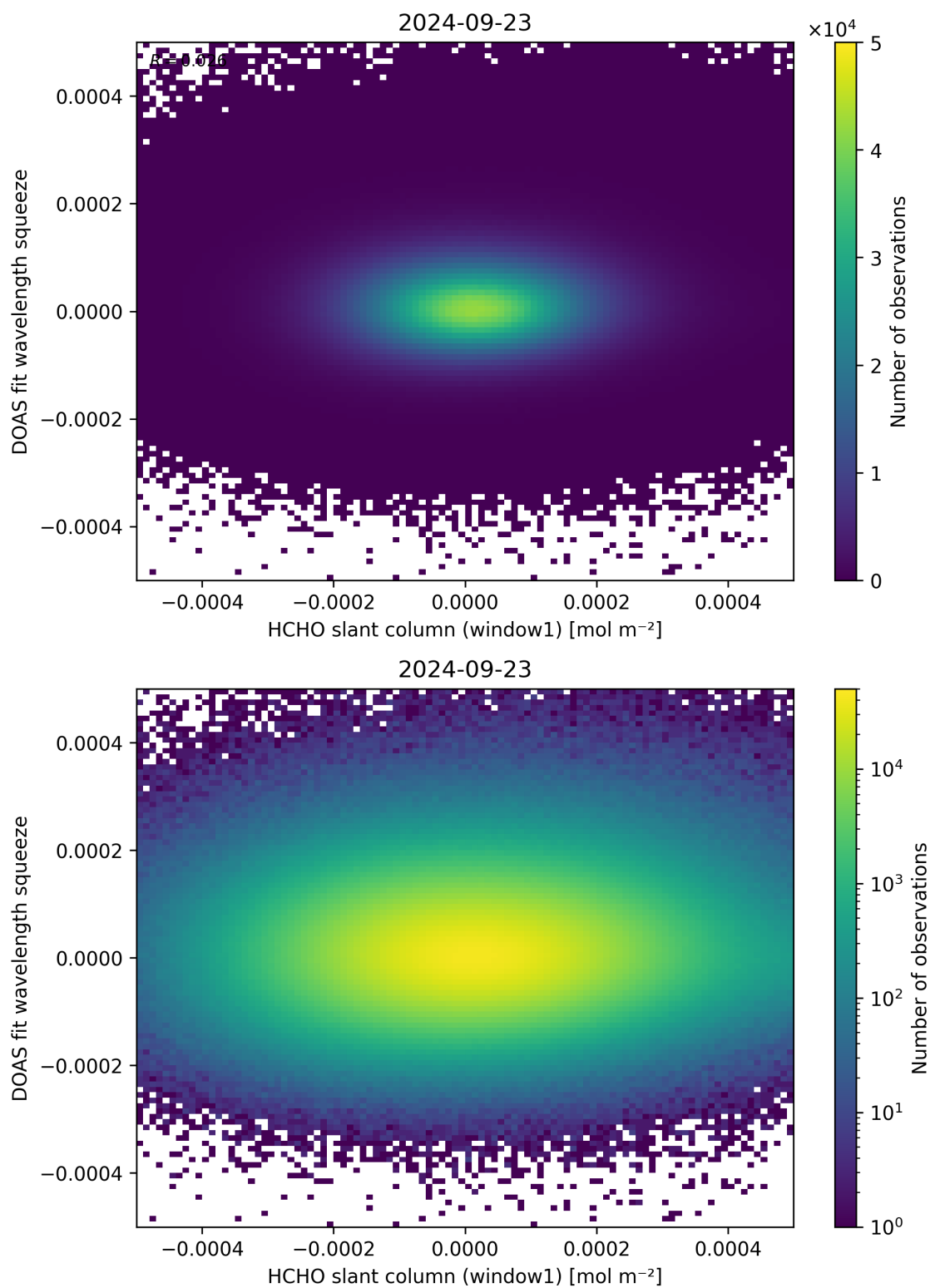
Figure 80: Scatter density plot of “HCHO slant column (window1)” against “DOAS fit wavelength squeeze” for 2024-09-22 to 2024-09-24.
