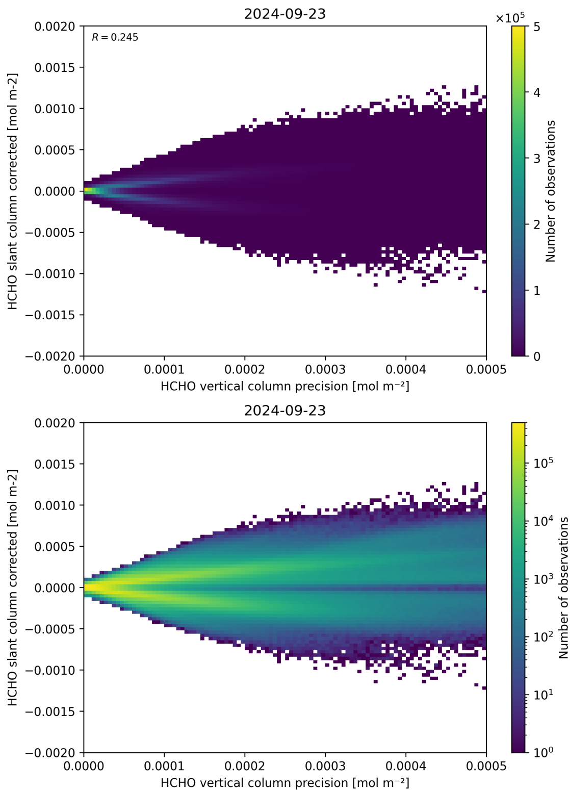
Figure 140: Scatter density plot of “HCHO vertical column precision” against “HCHO slant column corrected” for 2024-09-22 to 2024-09-24.
