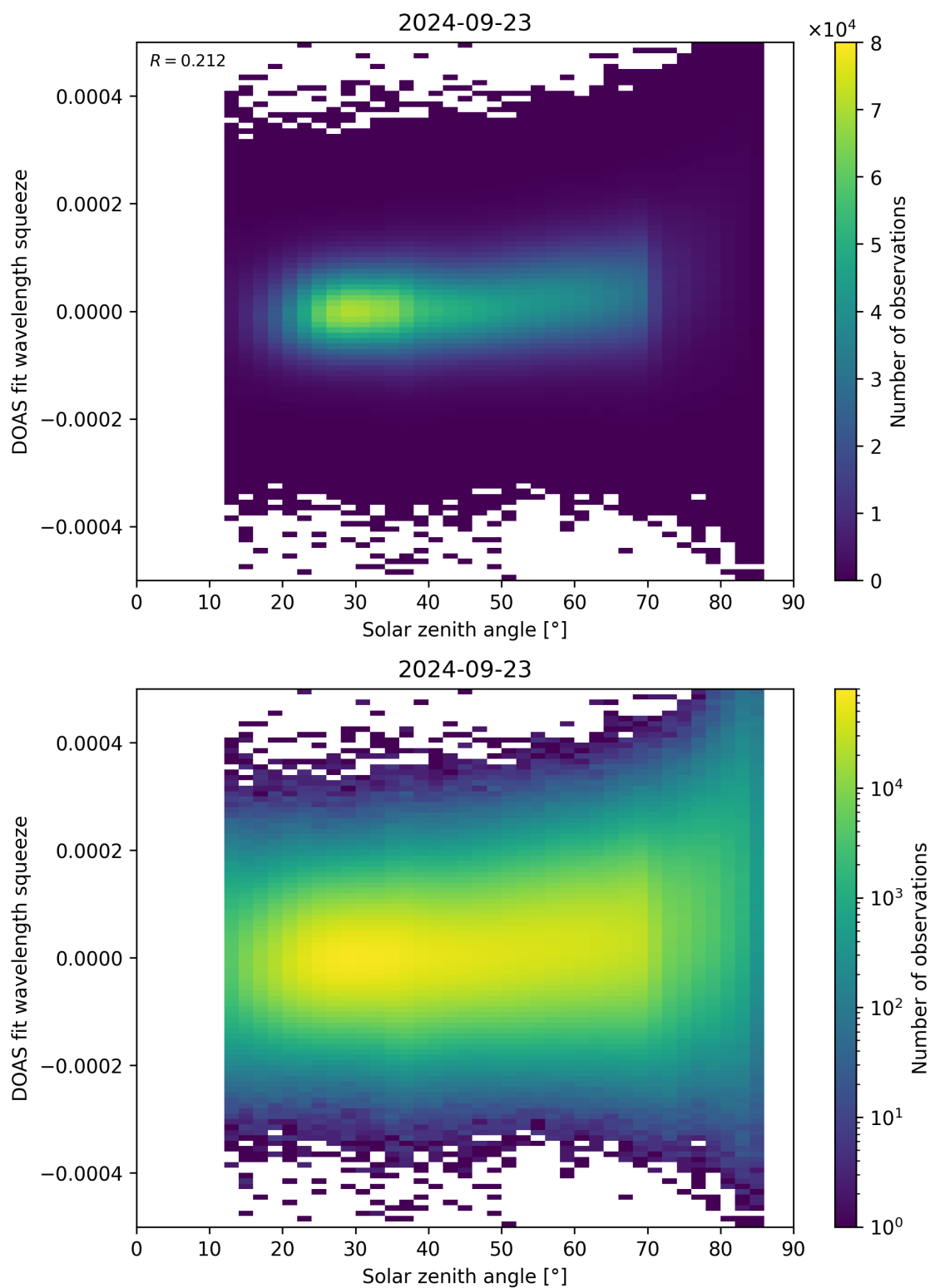
Figure 169: Scatter density plot of “Solar zenith angle” against “DOAS fit wavelength squeeze” for 2024-09-22 to 2024-09-24.
