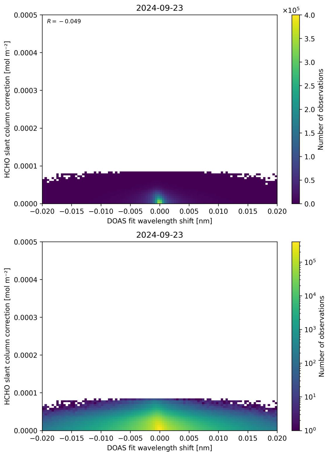
Figure 67: Scatter density plot of “DOAS fit wavelength shift” against “HCHO slant column correction” for 2024-09-22 to 2024-09-24.
