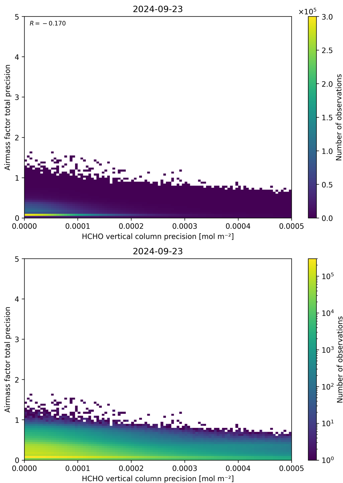
Figure 145: Scatter density plot of “HCHO vertical column precision” against “Airmass factor total precision” for 2024-09-22 to 2024-09-24.
