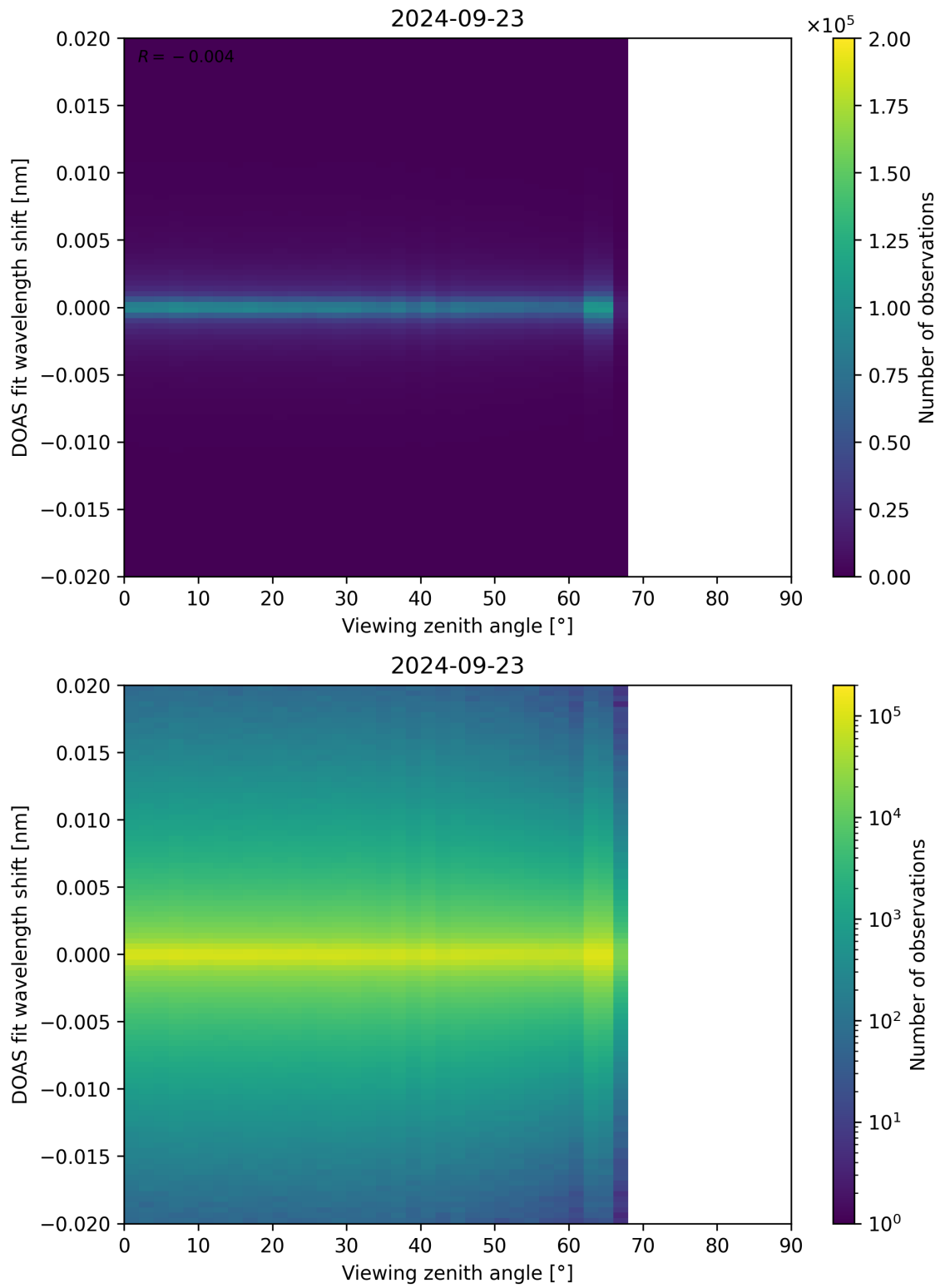
Figure 183: Scatter density plot of “Viewing zenith angle” against “DOAS fit wavelength shift” for 2024-09-22 to 2024-09-24.
