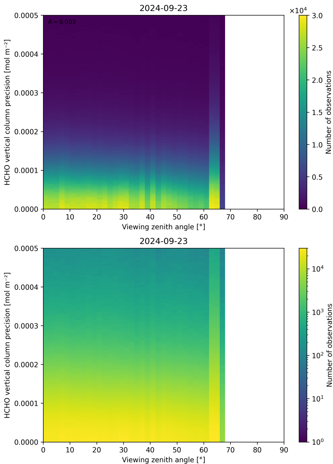
Figure 194: Scatter density plot of “Viewing zenith angle” against “HCHO vertical column precision” for 2024-09-22 to 2024-09-24.
