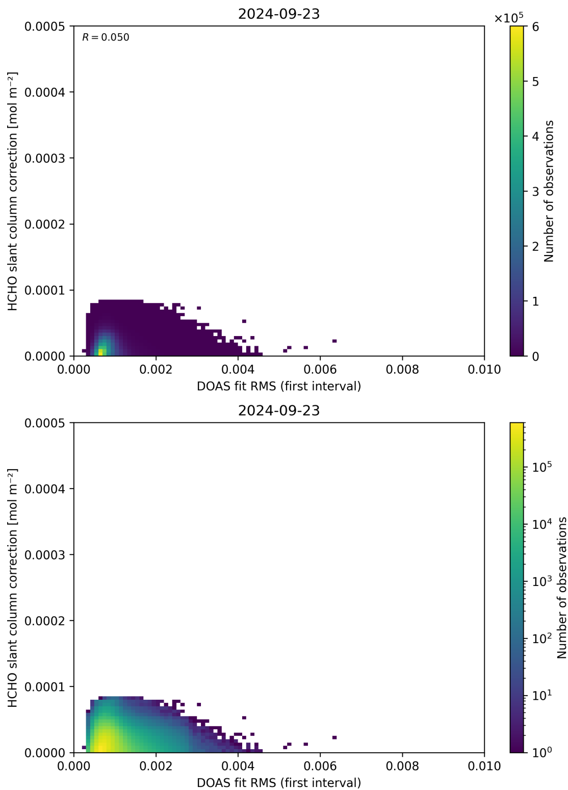
Figure 63: Scatter density plot of “DOAS fit RMS (first interval)” against “HCHO slant column correction” for 2024-09-22 to 2024-09-24.
