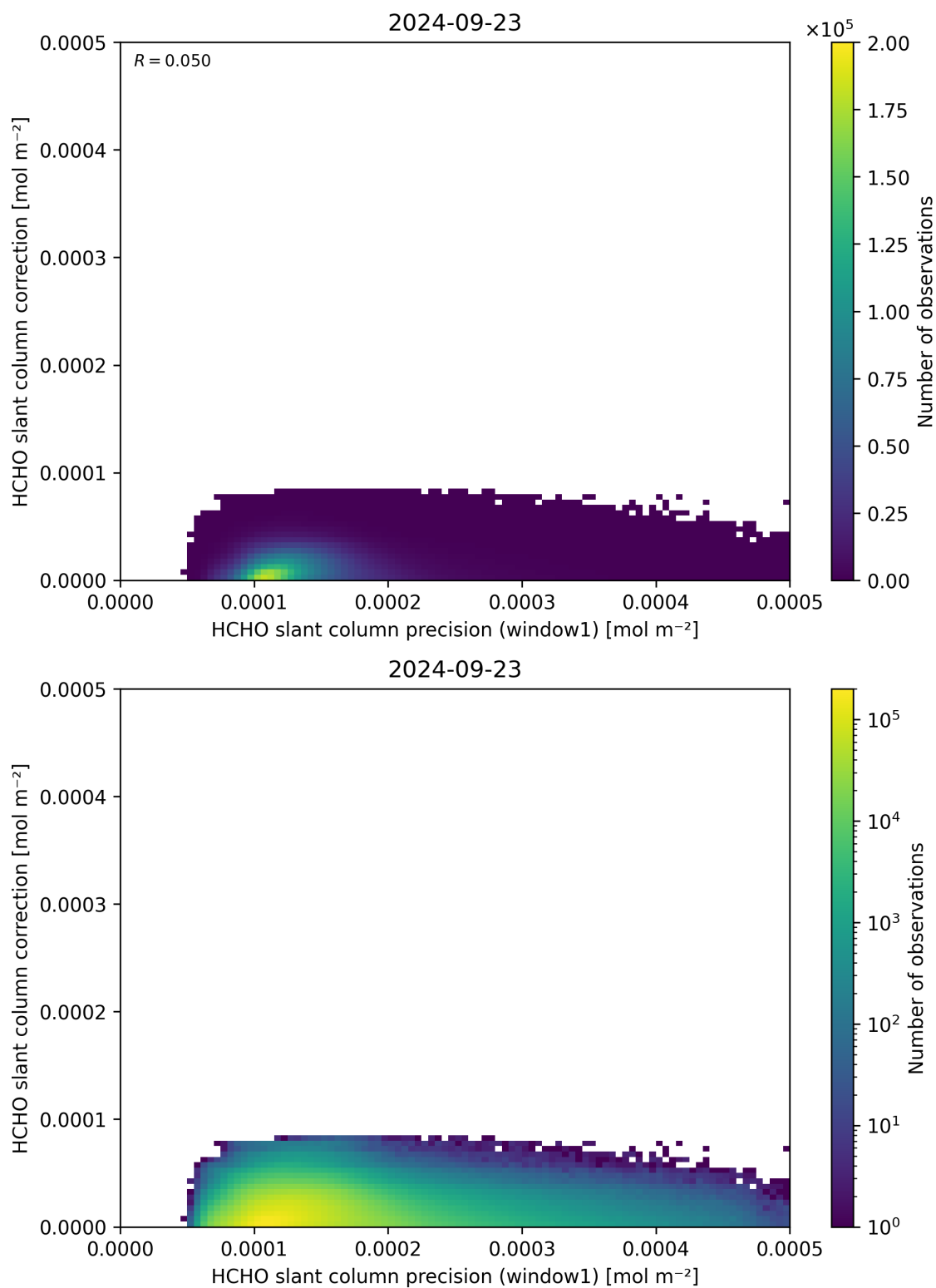
Figure 93: Scatter density plot of “HCHO slant column precision (window1)” against “HCHO slant column correction” for 2024-09-22 to 2024-09-24.
