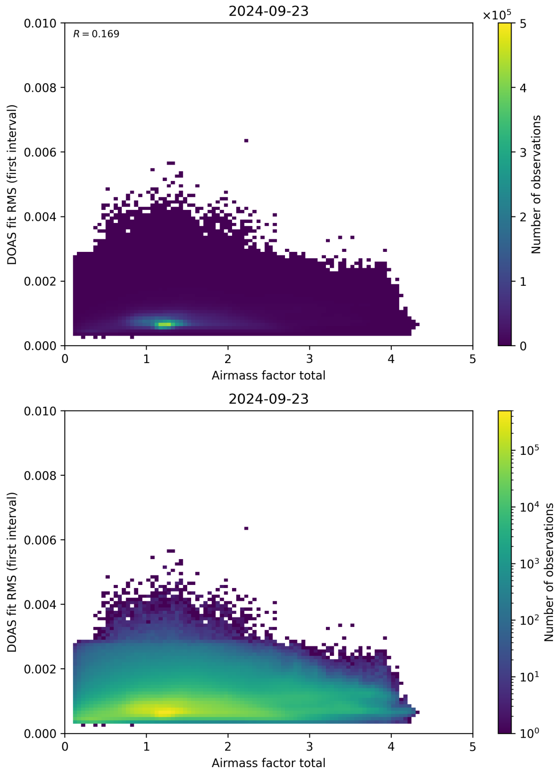
Figure 97: Scatter density plot of “Airmass factor total” against “DOAS fit RMS (first interval)” for 2024-09-22 to 2024-09-24.
