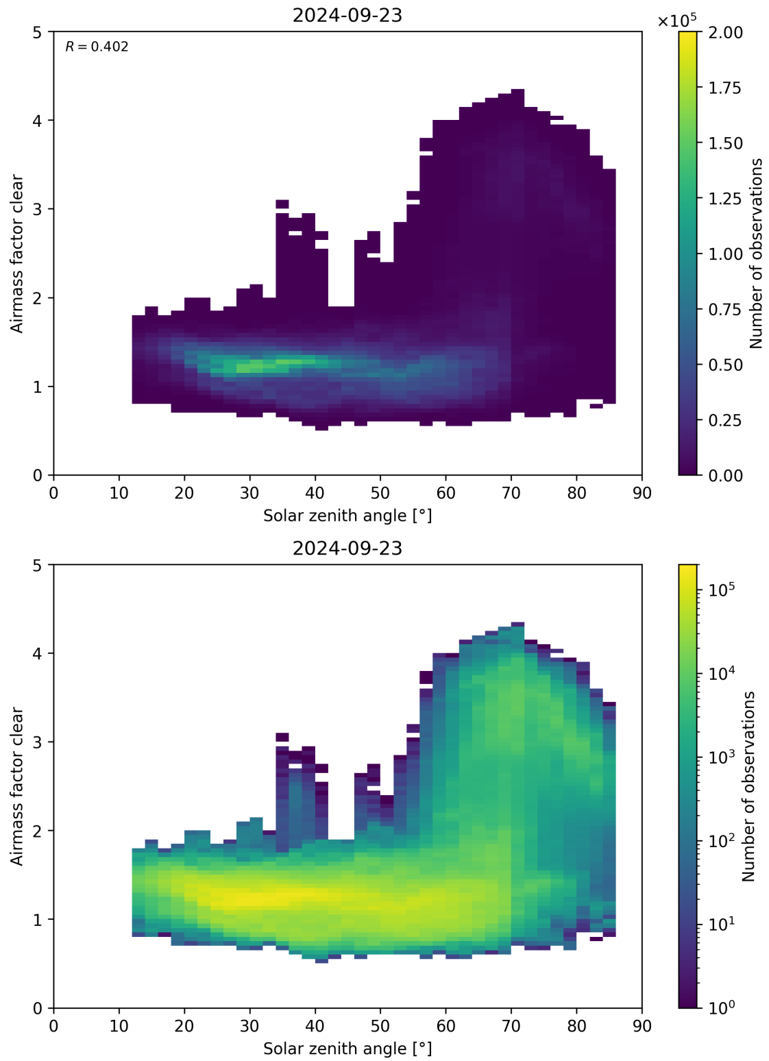
Figure 170: Scatter density plot of “Solar zenith angle” against “Airmass factor clear” for 2024-09-22 to 2024-09-24.
