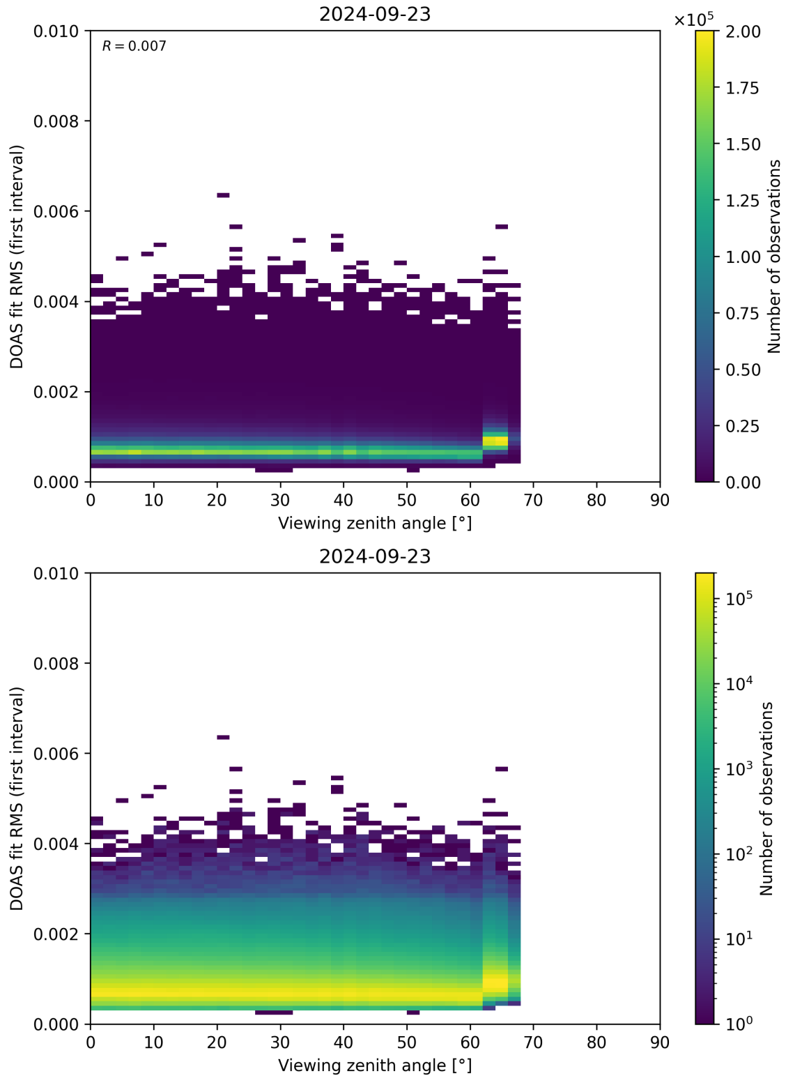
Figure 182: Scatter density plot of “Viewing zenith angle” against “DOAS fit RMS (first interval)” for 2024-09-22 to 2024-09-24.
