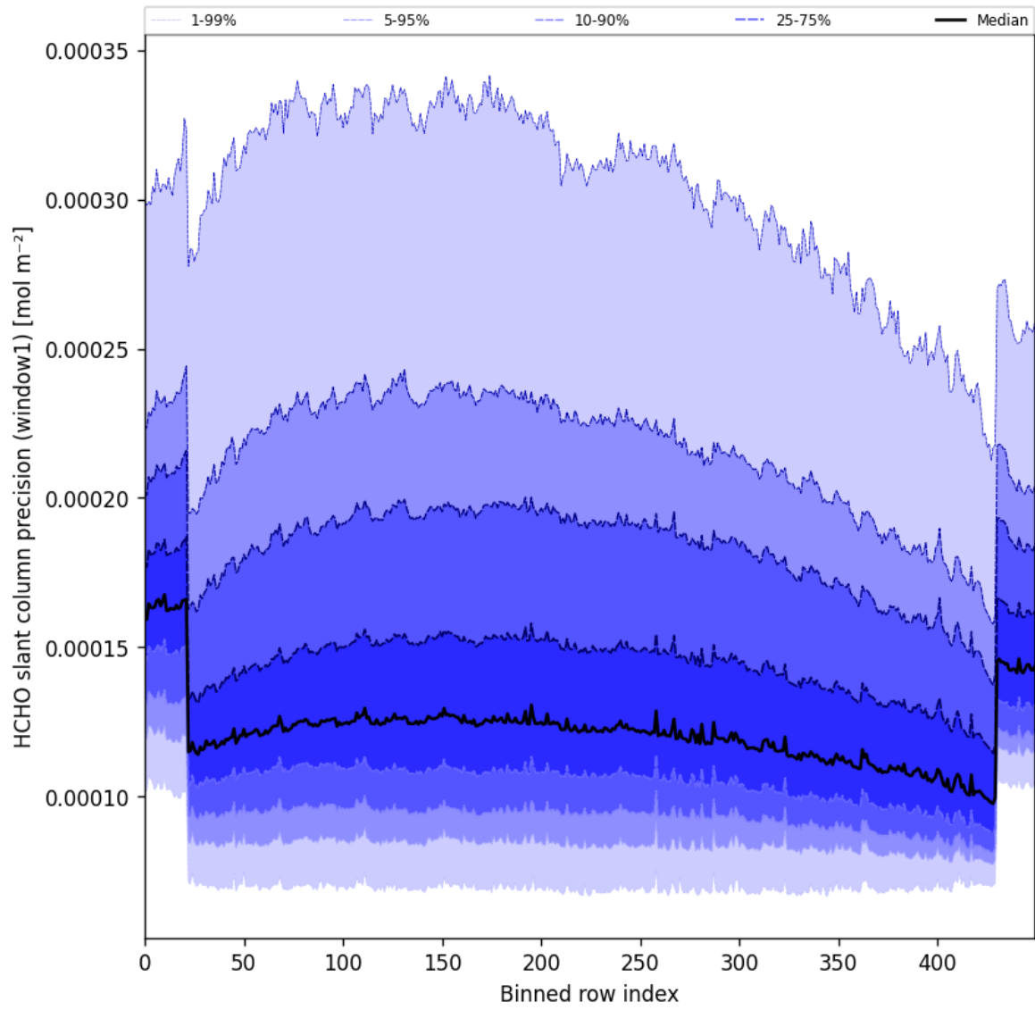
Figure 53: Along track statistics of “HCHO slant column precision (window1)” for 2024-09-22 to 2024-09-24
