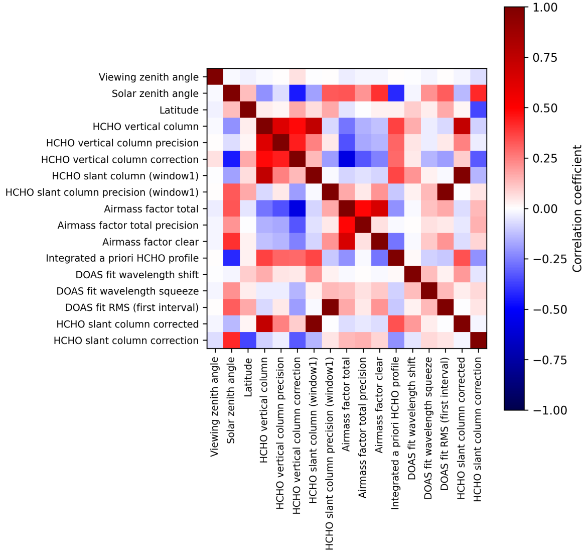
Figure 2: Map of correlation matrix for 2024-09-22 to 2024-09-24.
