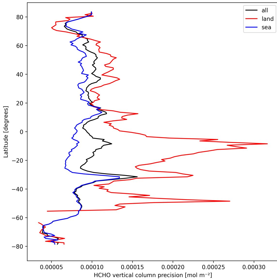
Figure 22: Zonal average of “HCHO vertical column precision” for 2024-09-22 to 2024-09-24.
