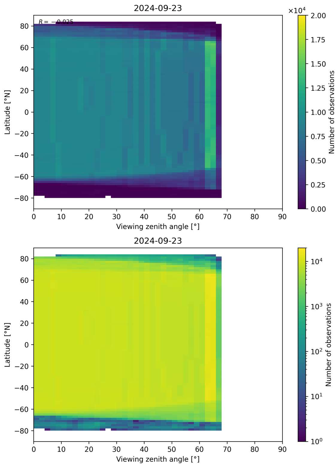
Figure 196: Scatter density plot of “Viewing zenith angle” against “Latitude” for 2024-09-22 to 2024-09-24.
