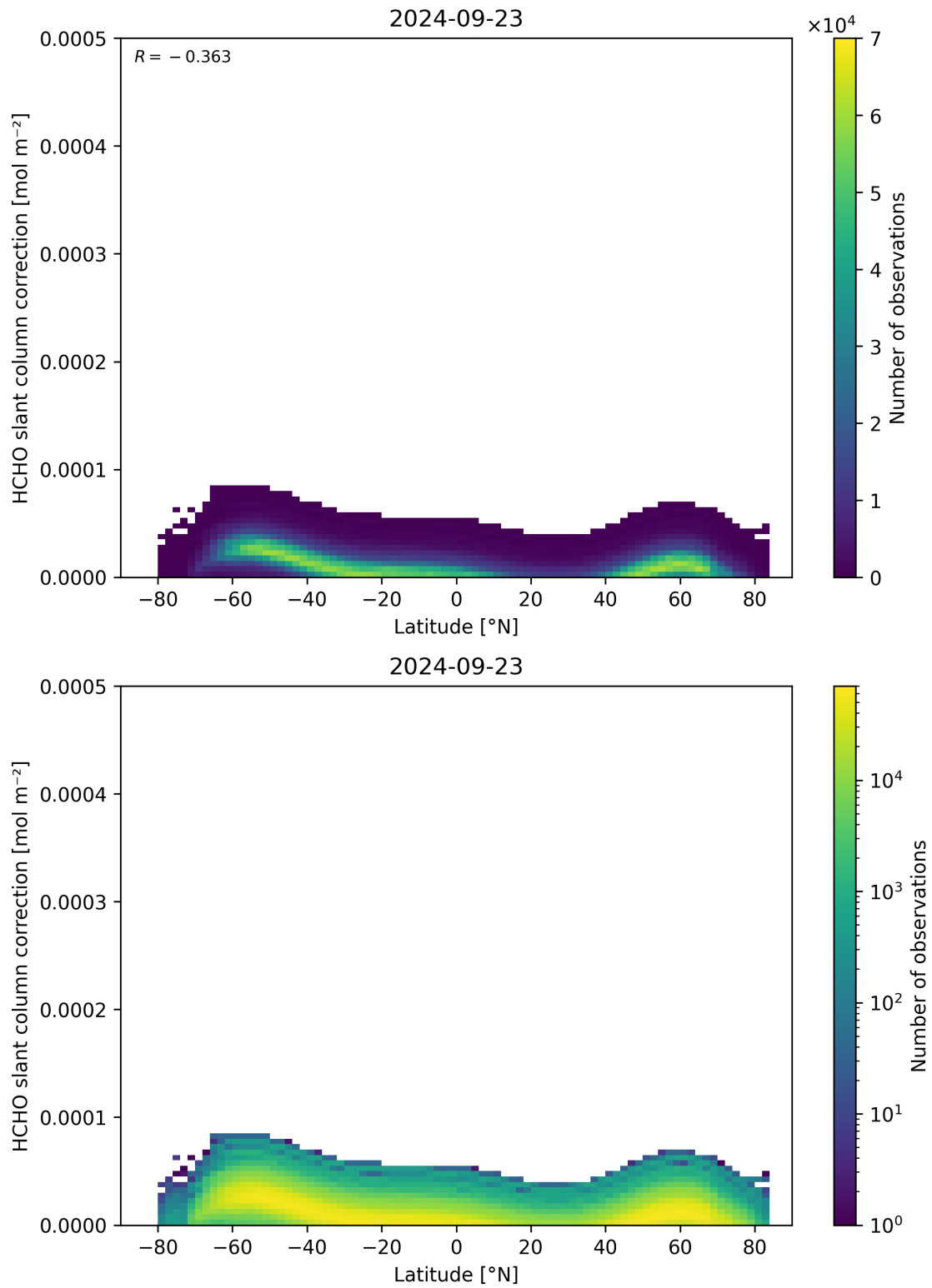
Figure 158: Scatter density plot of “Latitude” against “HCHO slant column correction” for 2024-09-22 to 2024-09-24.
