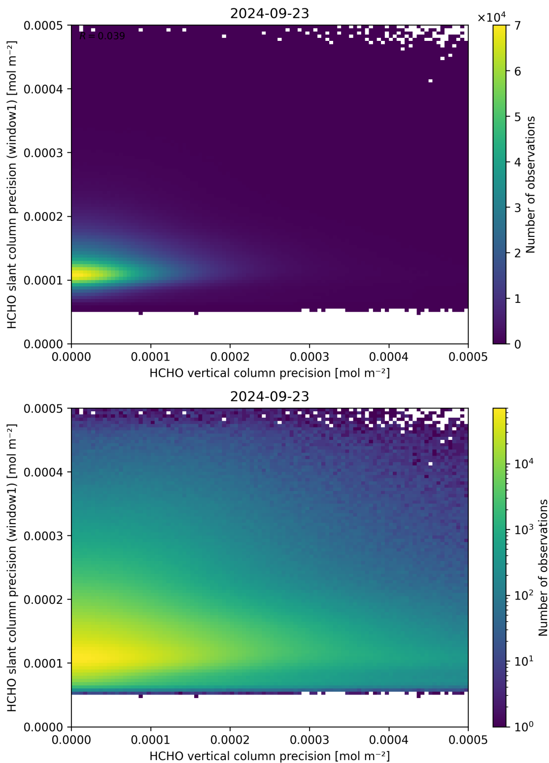
Figure 143: Scatter density plot of “HCHO vertical column precision” against “HCHO slant column precision (window1)” for 2024-09-22 to 2024-09-24.
