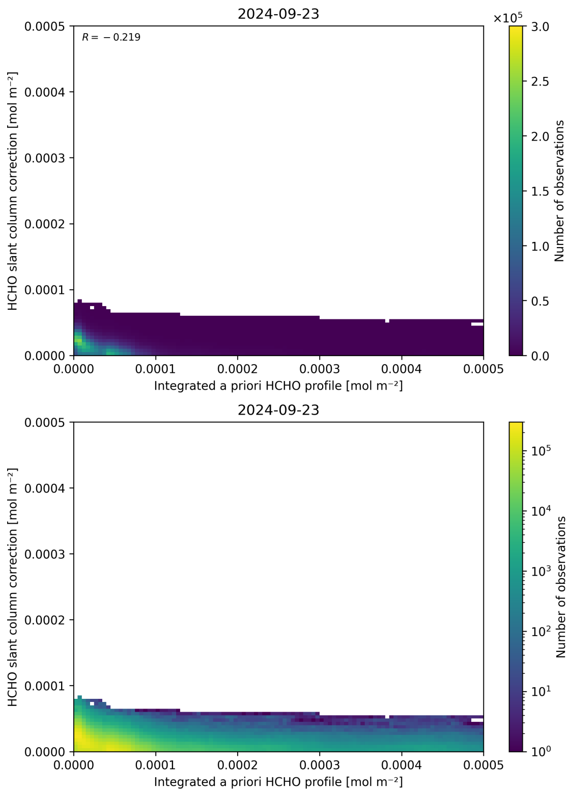
Figure 152: Scatter density plot of “Integrated a priori HCHO profile” against “HCHO slant column correction” for 2024-09-22 to 2024-09-24.
