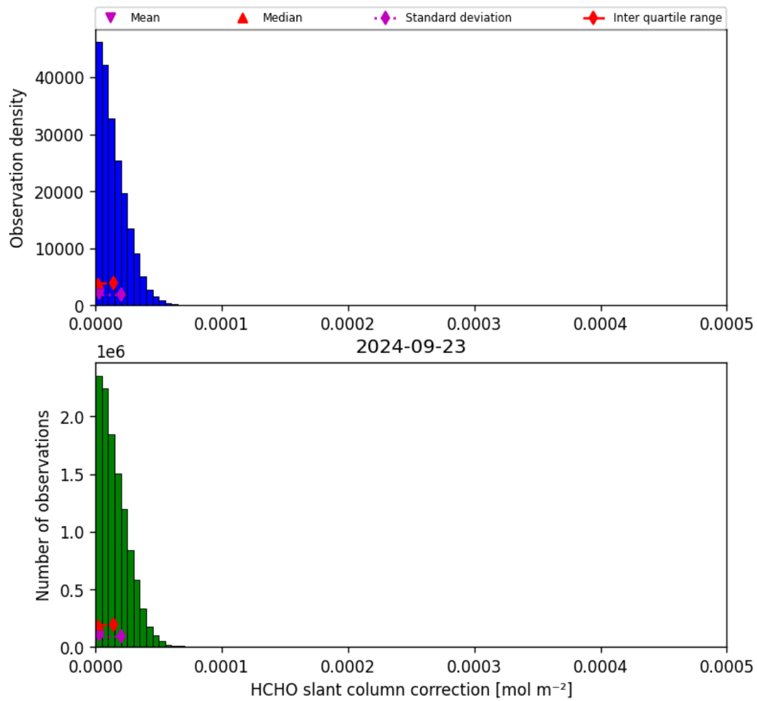
Figure 47: Histogram of “HCHO slant column correction” for 2024-09-22 to 2024-09-24
