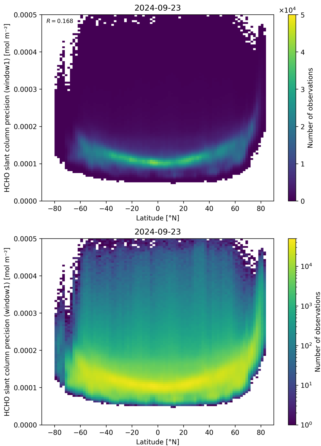
Figure 160: Scatter density plot of “Latitude” against “HCHO slant column precision (window1)” for 2024-09-22 to 2024-09-24.
