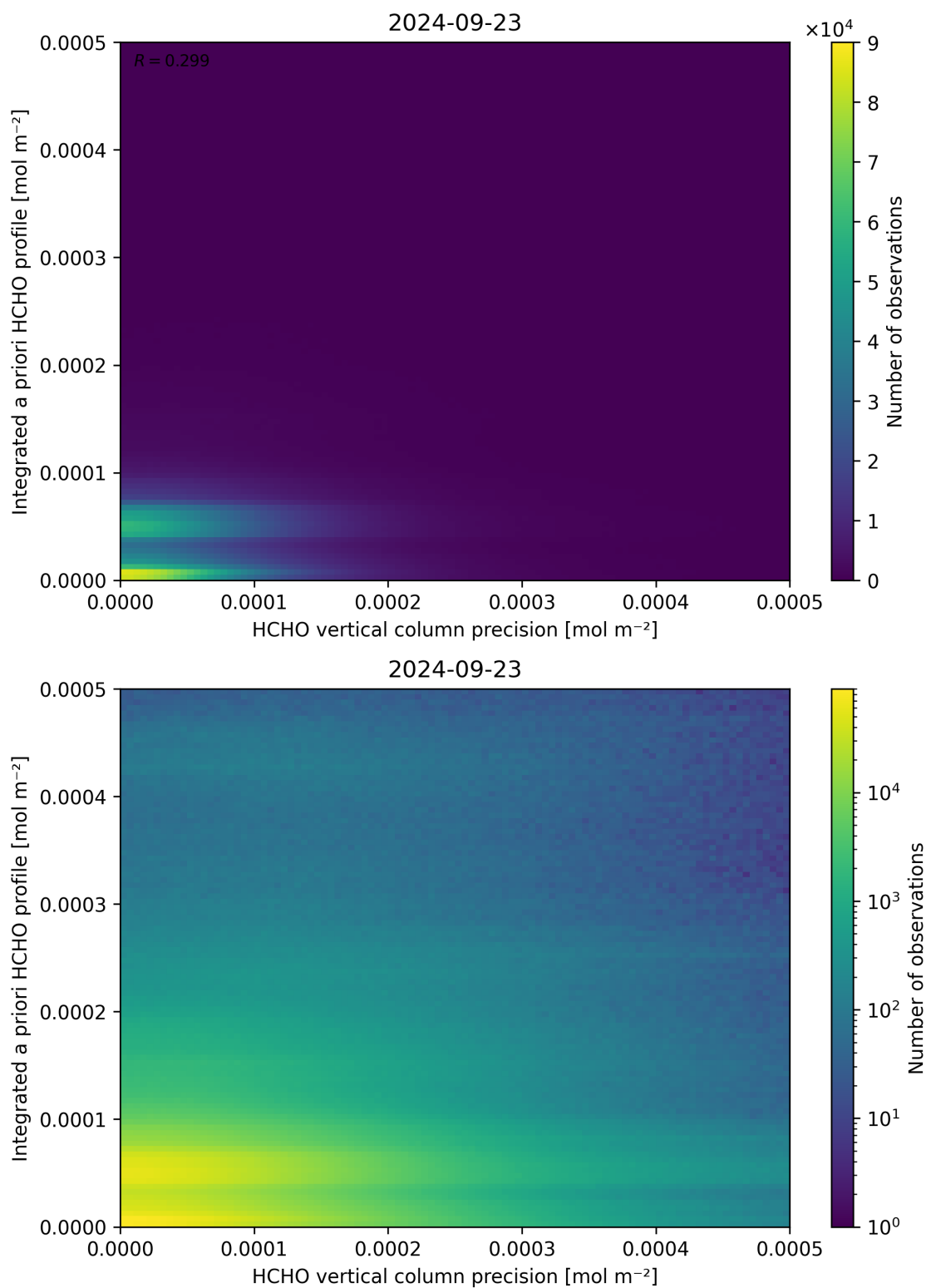
Figure 147: Scatter density plot of “HCHO vertical column precision” against “Integrated a priori HCHO profile” for 2024-09-22 to 2024-09-24.
