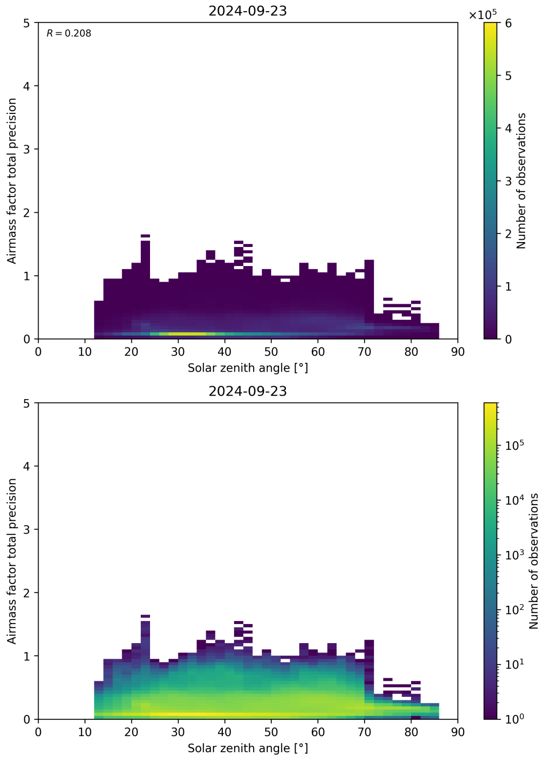
Figure 176: Scatter density plot of “Solar zenith angle” against “Airmass factor total precision” for 2024-09-22 to 2024-09-24.
