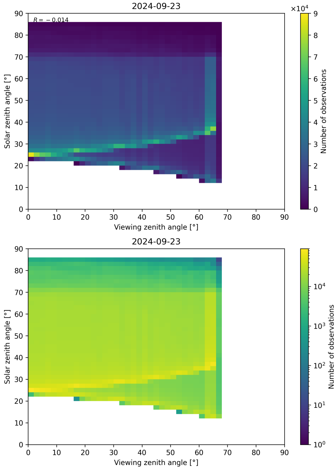
Figure 197: Scatter density plot of “Viewing zenith angle” against “Solar zenith angle” for 2024-09-22 to 2024-09-24.
