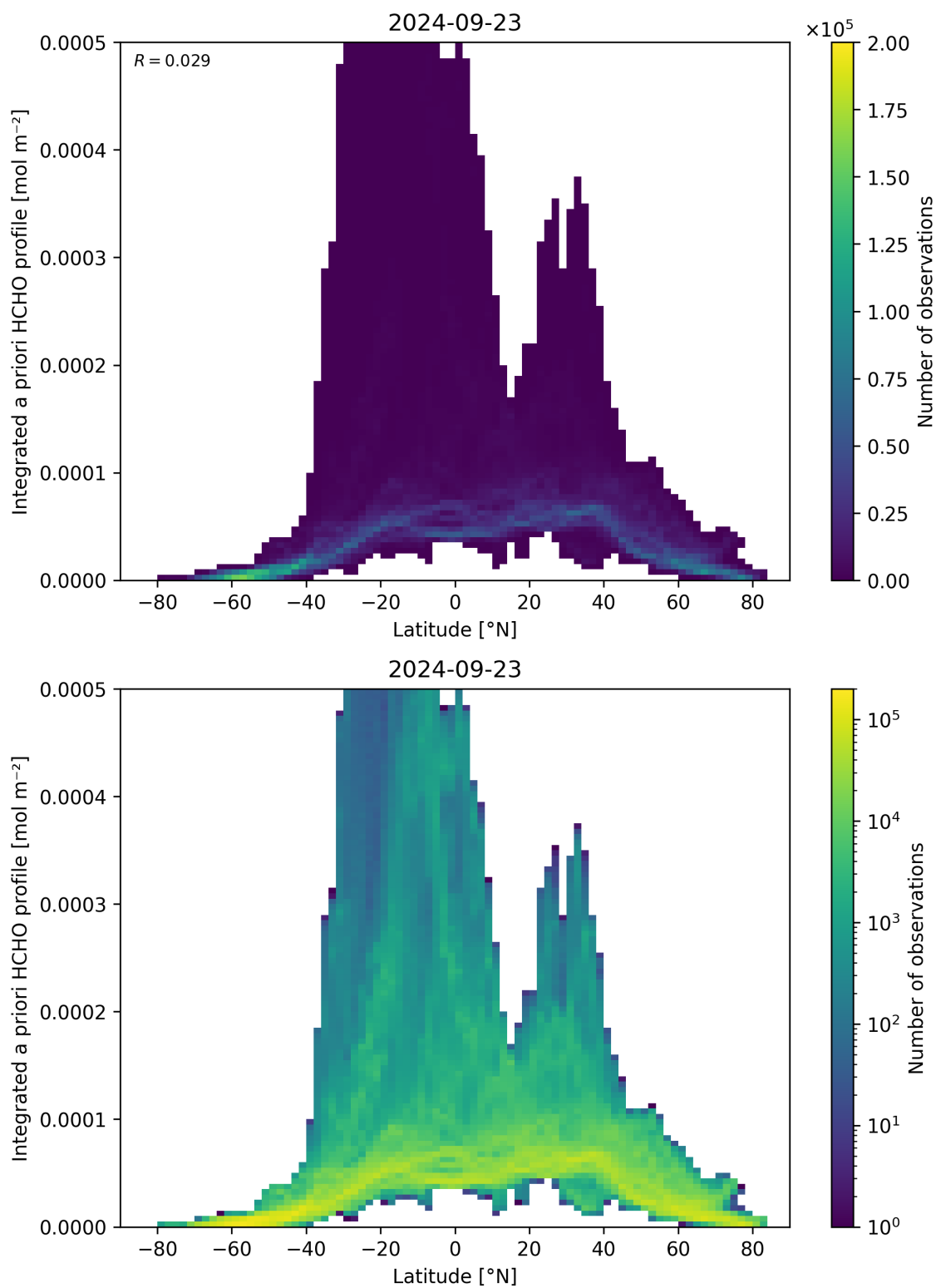
Figure 166: Scatter density plot of “Latitude” against “Integrated a priori HCHO profile” for 2024-09-22 to 2024-09-24.
