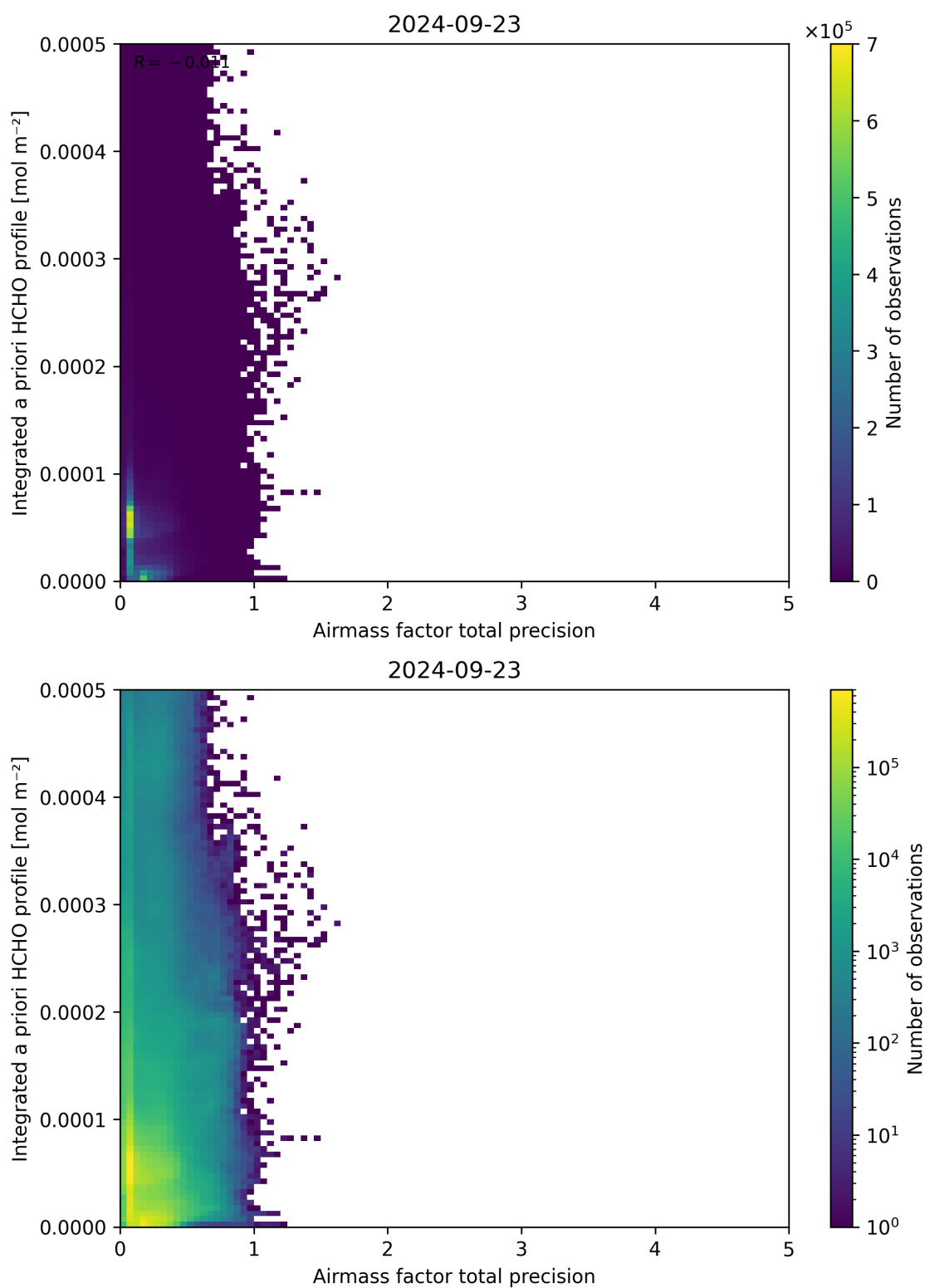
Figure 111: Scatter density plot of “Airmass factor total precision” against “Integrated a priori HCHO profile” for 2024-09-22 to 2024-09-24.
