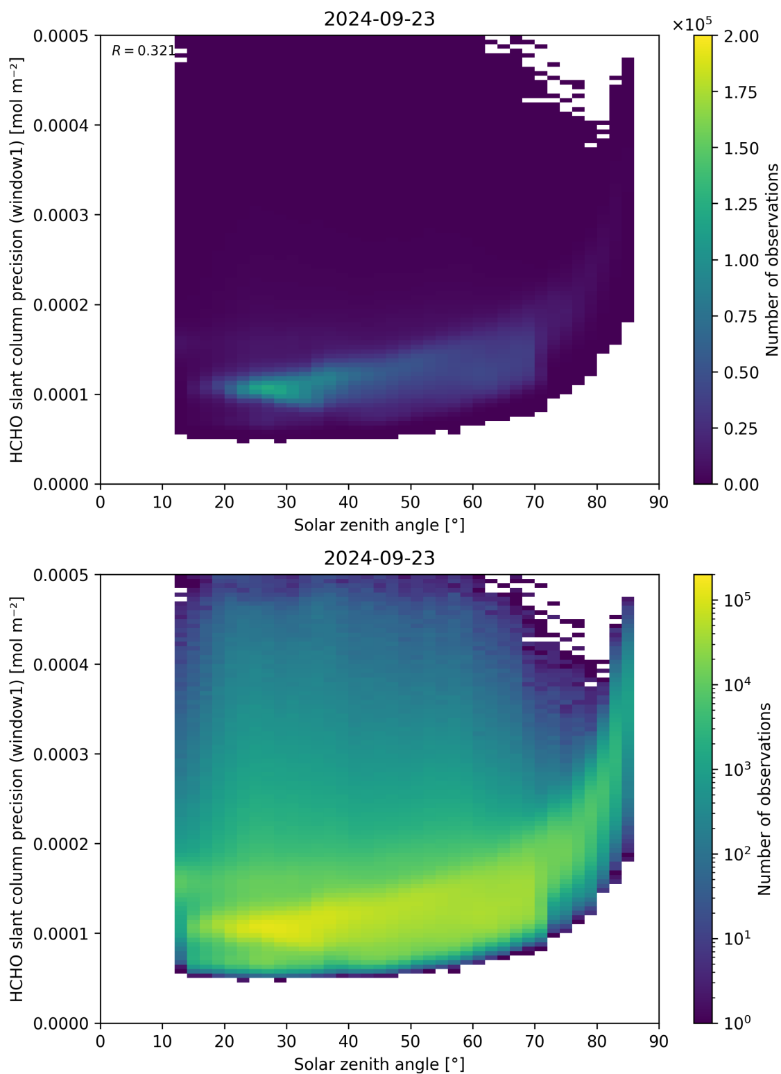
Figure 174: Scatter density plot of “Solar zenith angle” against “HCHO slant column precision (window1)” for 2024-09-22 to 2024-09-24.
