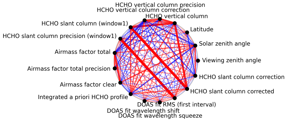
Figure 1: Map of correlation graph for 2024-09-22 to 2024-09-24.
