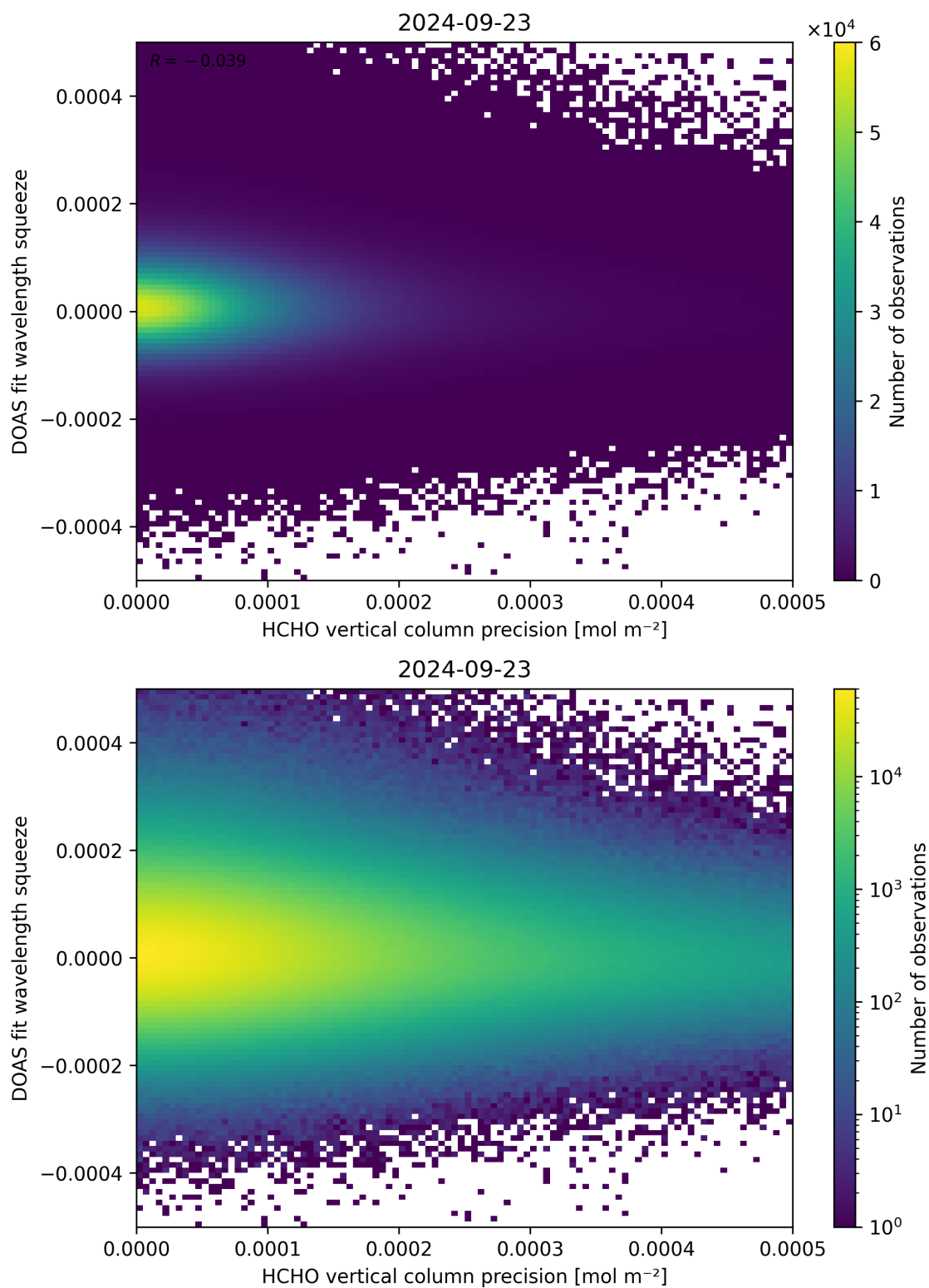
Figure 138: Scatter density plot of “HCHO vertical column precision” against “DOAS fit wavelength squeeze” for 2024-09-22 to 2024-09-24.
