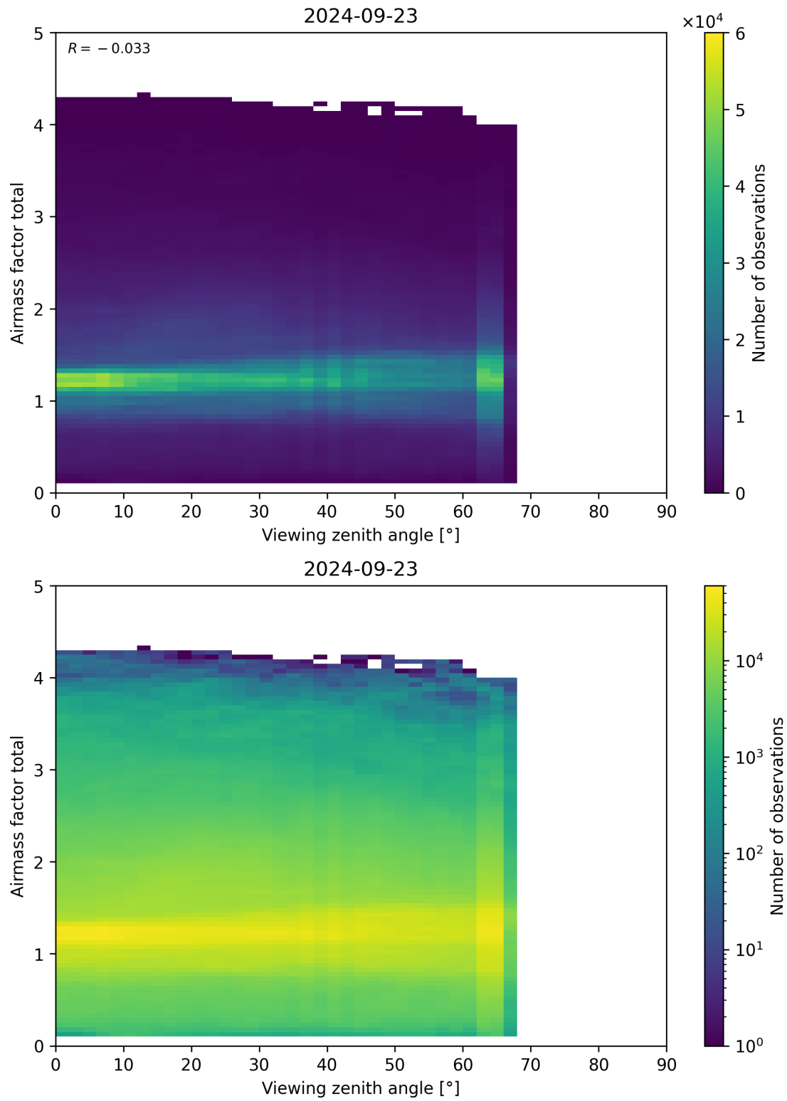
Figure 190: Scatter density plot of “Viewing zenith angle” against “Airmass factor total” for 2024-09-22 to 2024-09-24.
