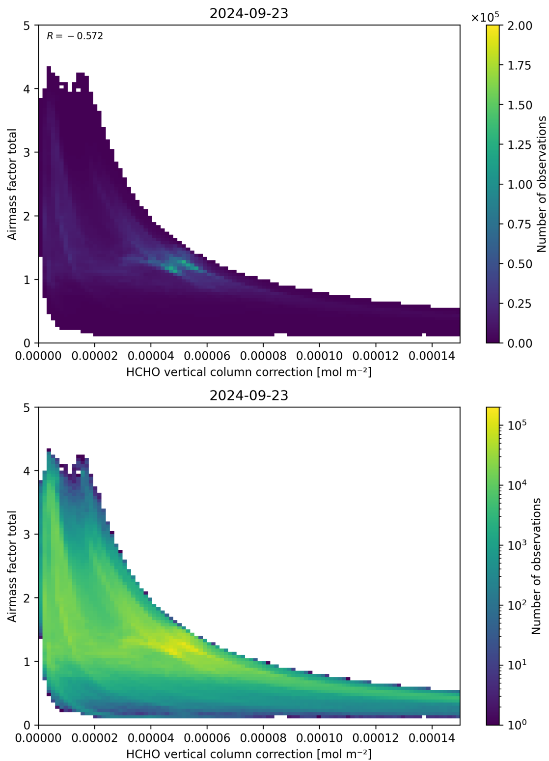
Figure 120: Scatter density plot of “HCHO vertical column correction” against “Airmass factor total” for 2024-09-22 to 2024-09-24.
