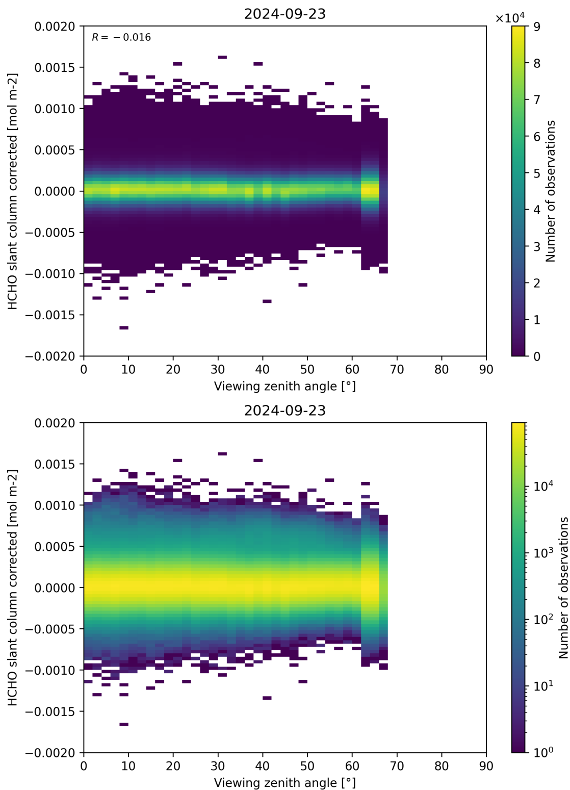
Figure 186: Scatter density plot of “Viewing zenith angle” against “HCHO slant column corrected” for 2024-09-22 to 2024-09-24.
