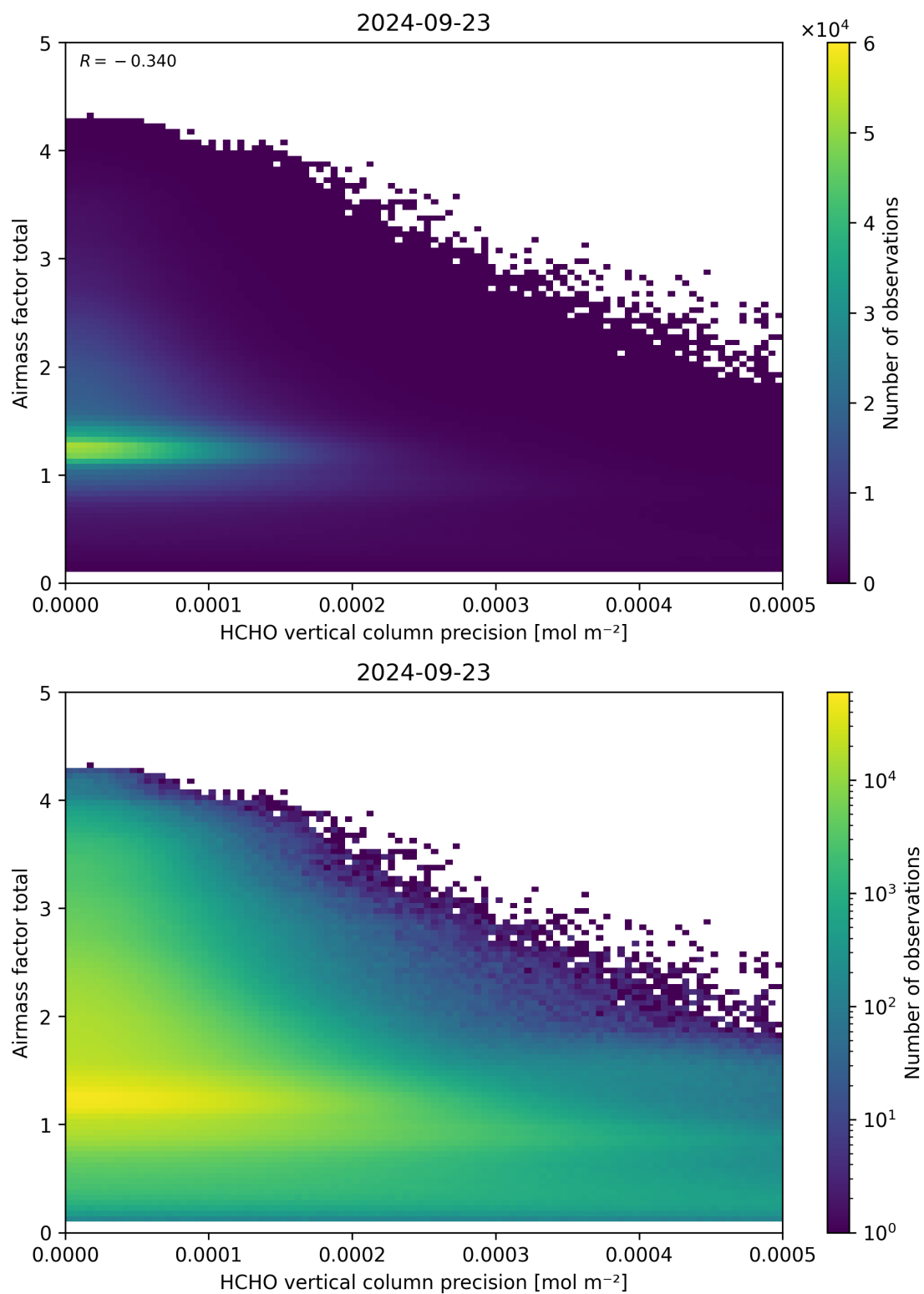
Figure 144: Scatter density plot of “HCHO vertical column precision” against “Airmass factor total” for 2024-09-22 to 2024-09-24.
