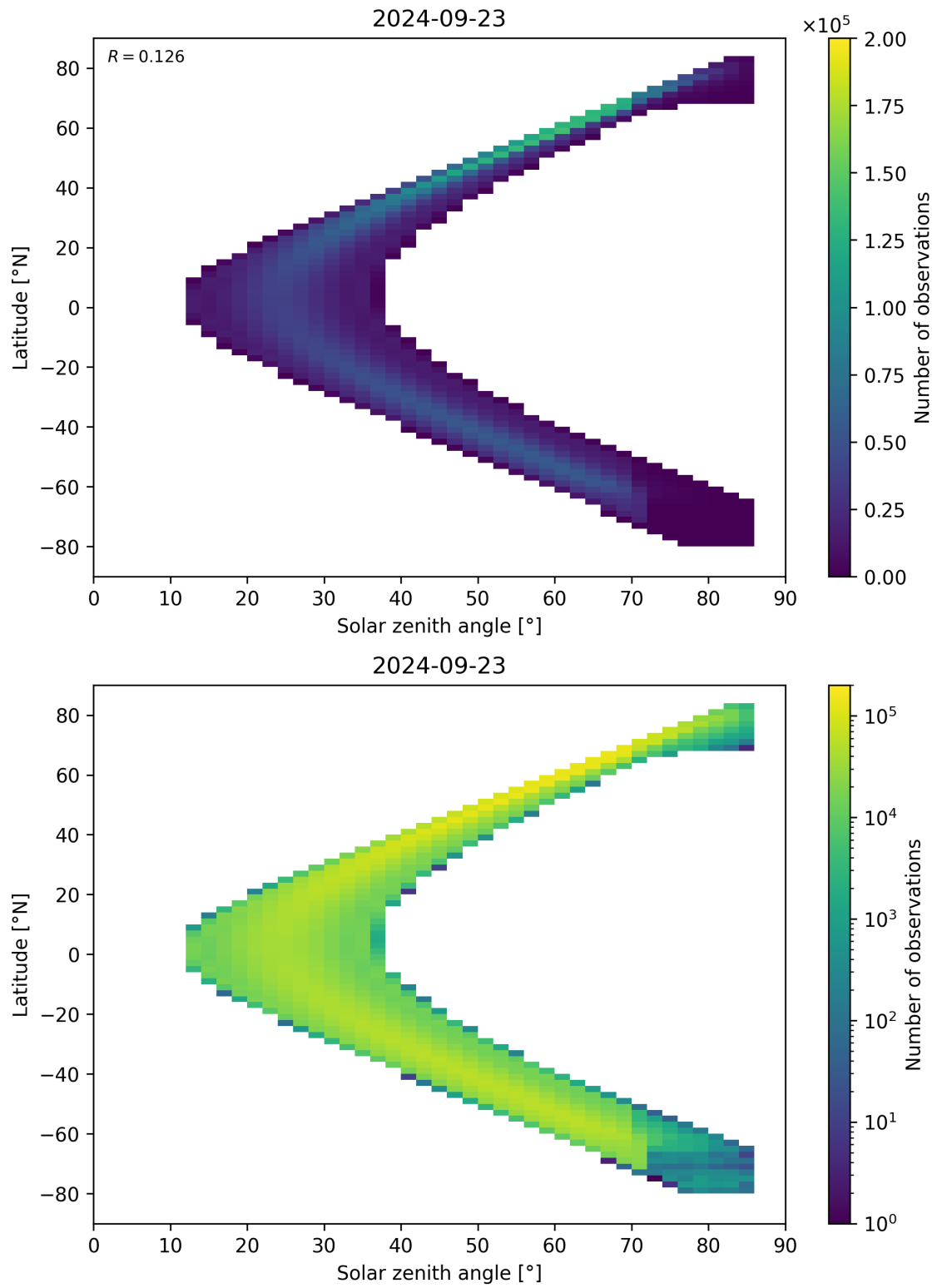
Figure 181: Scatter density plot of “Solar zenith angle” against “Latitude” for 2024-09-22 to 2024-09-24.
