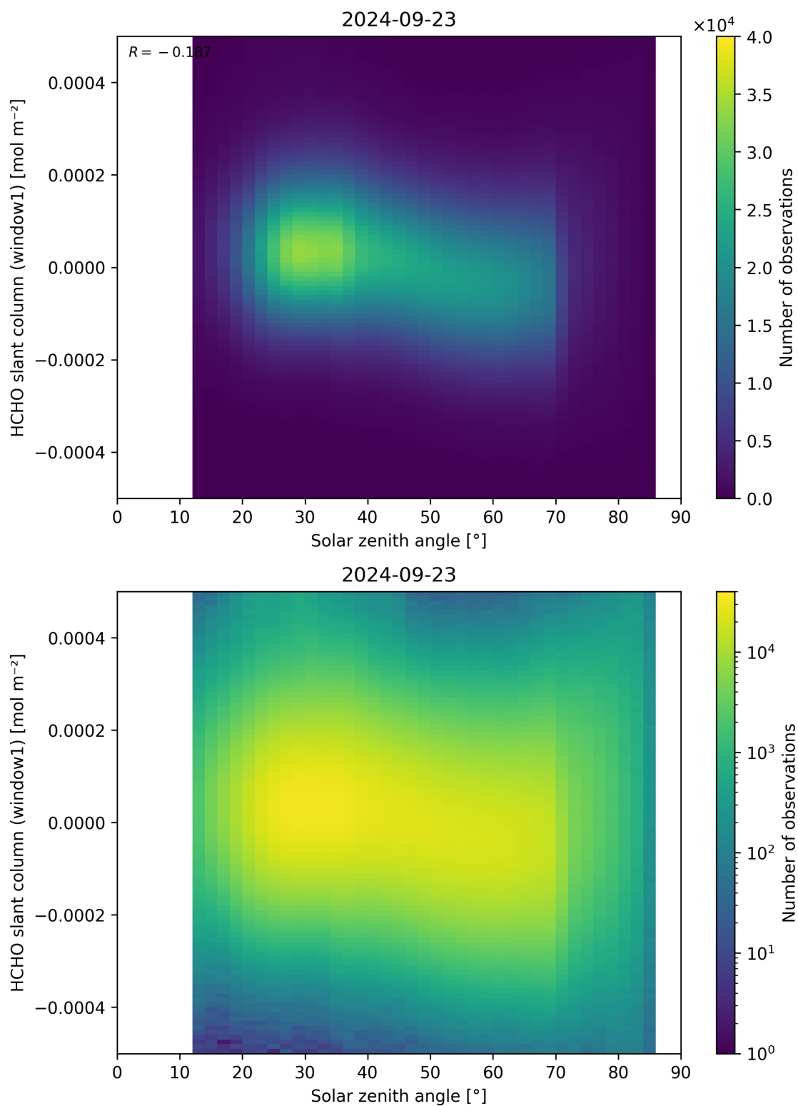
Figure 173: Scatter density plot of “Solar zenith angle” against “HCHO slant column (window1)” for 2024-09-22 to 2024-09-24.
