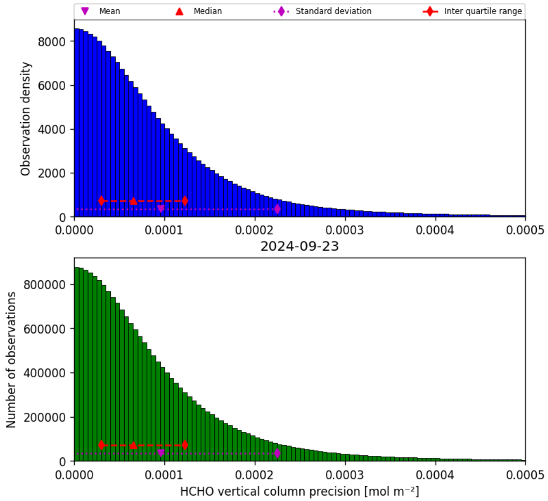
Figure 36: Histogram of “HCHO vertical column precision” for 2024-09-22 to 2024-09-24
