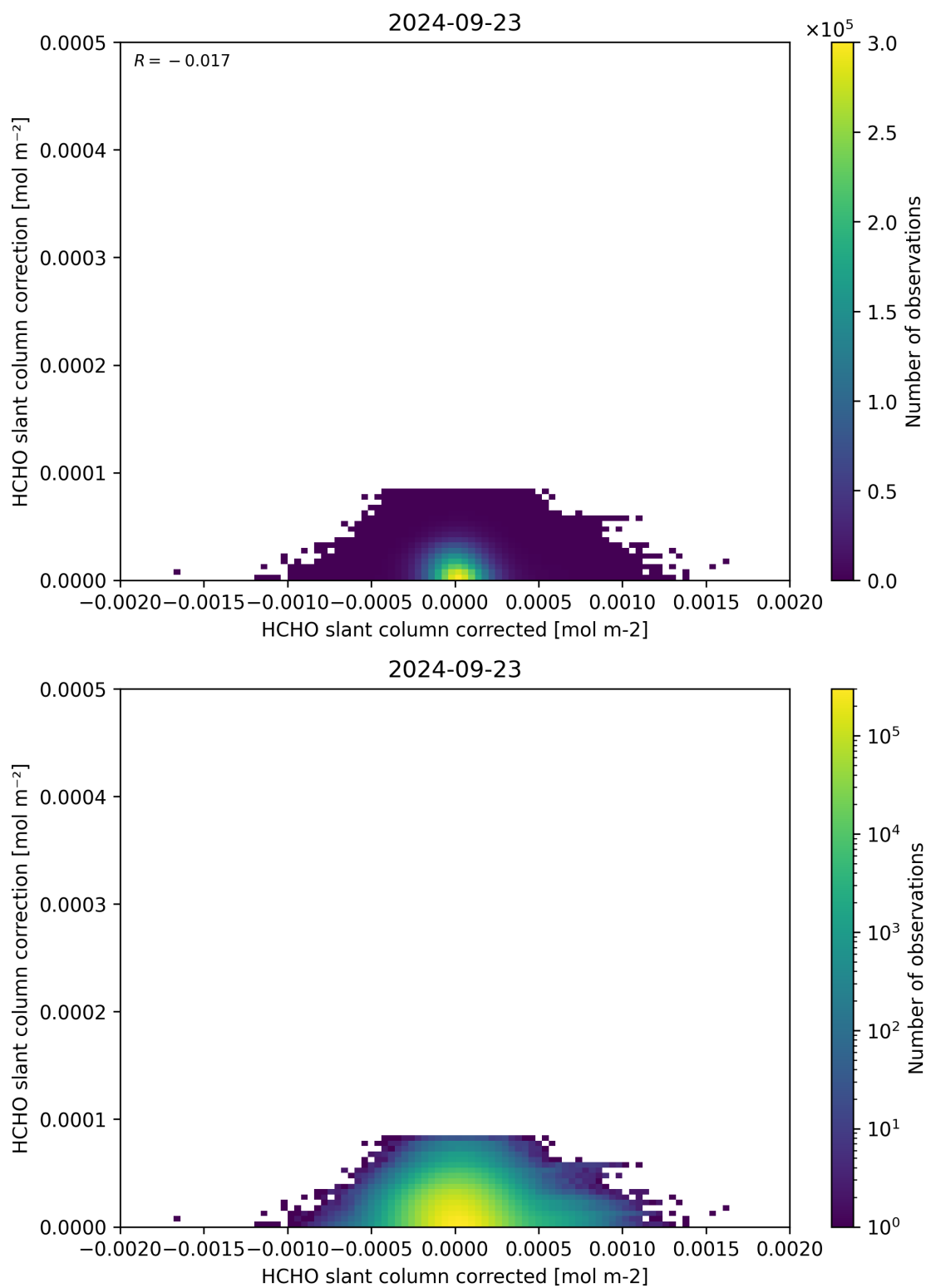
Figure 77: Scatter density plot of “HCHO slant column corrected” against “HCHO slant column correction” for 2024-09-22 to 2024-09-24.
