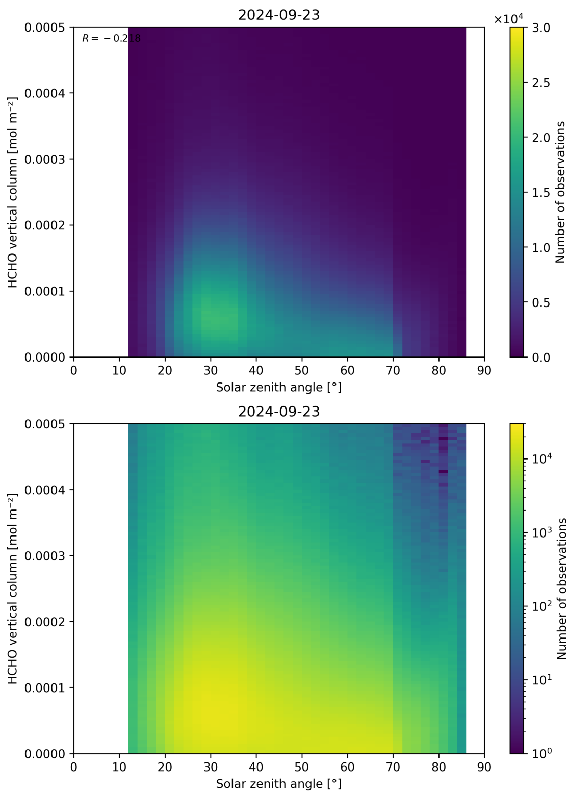
Figure 177: Scatter density plot of “Solar zenith angle” against “HCHO vertical column” for 2024-09-22 to 2024-09-24.
