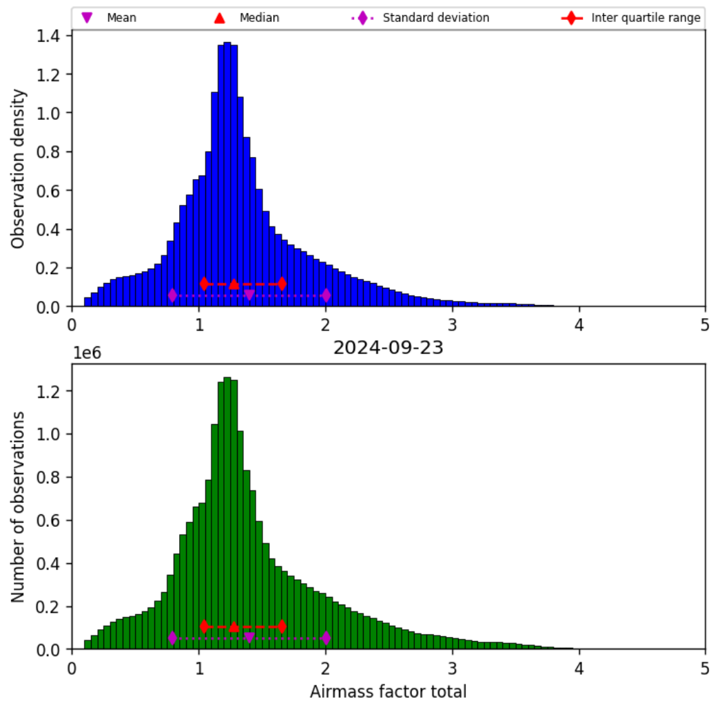
Figure 40: Histogram of “Airmass factor total” for 2024-09-22 to 2024-09-24
