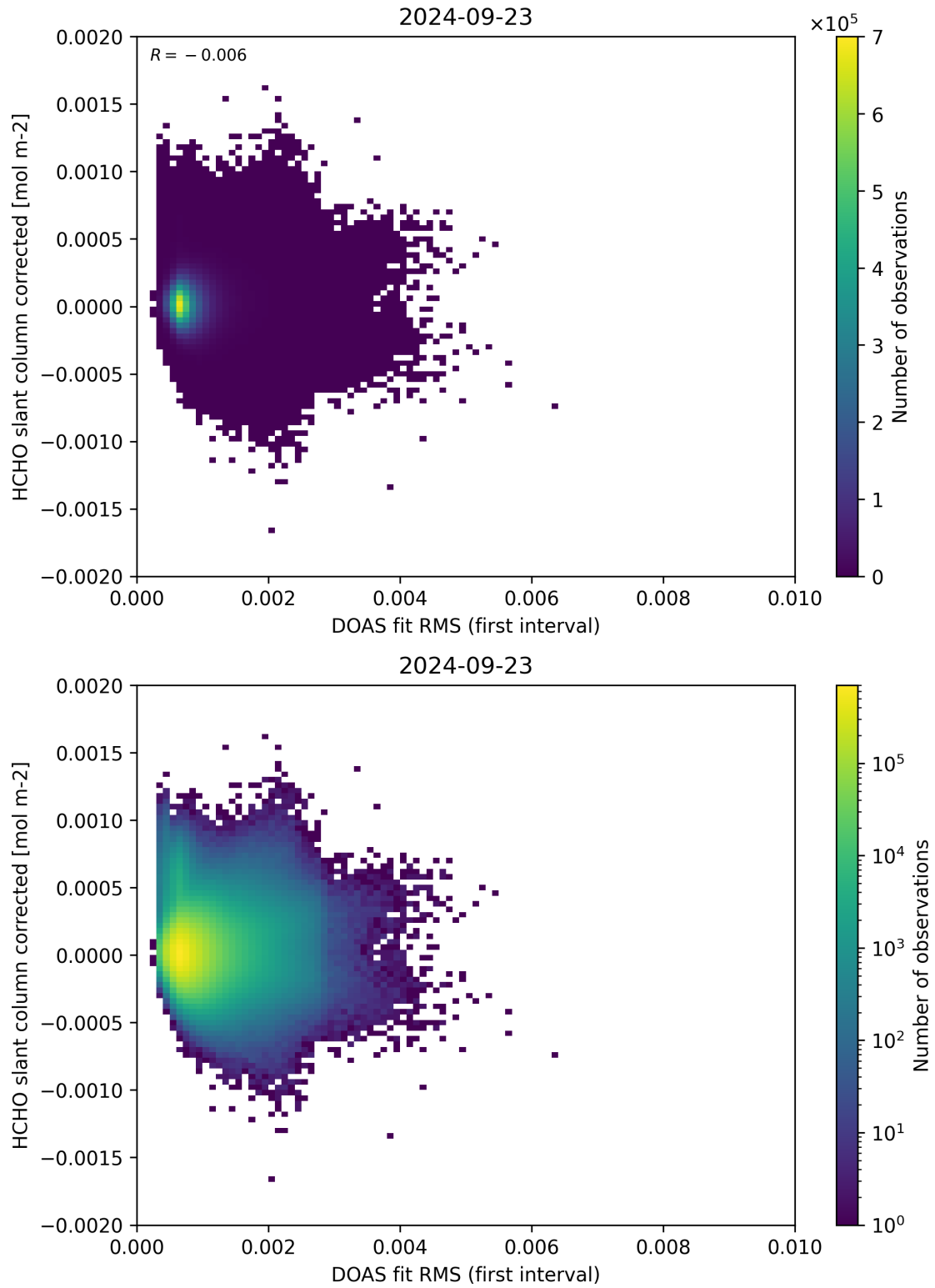
Figure 62: Scatter density plot of “DOAS fit RMS (first interval)” against “HCHO slant column corrected” for 2024-09-22 to 2024-09-24.
