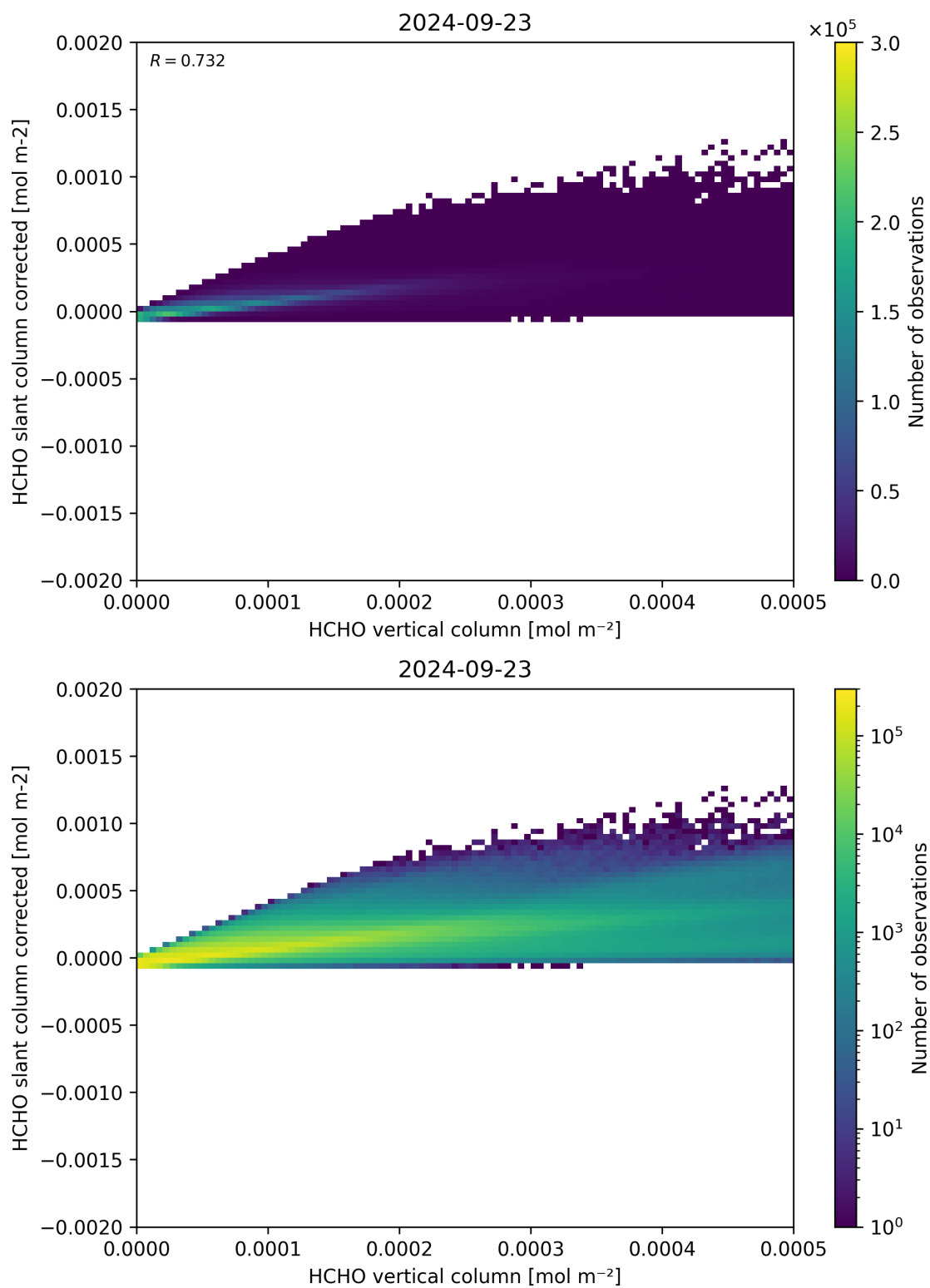
Figure 127: Scatter density plot of “HCHO vertical column” against “HCHO slant column corrected” for 2024-09-22 to 2024-09-24.
