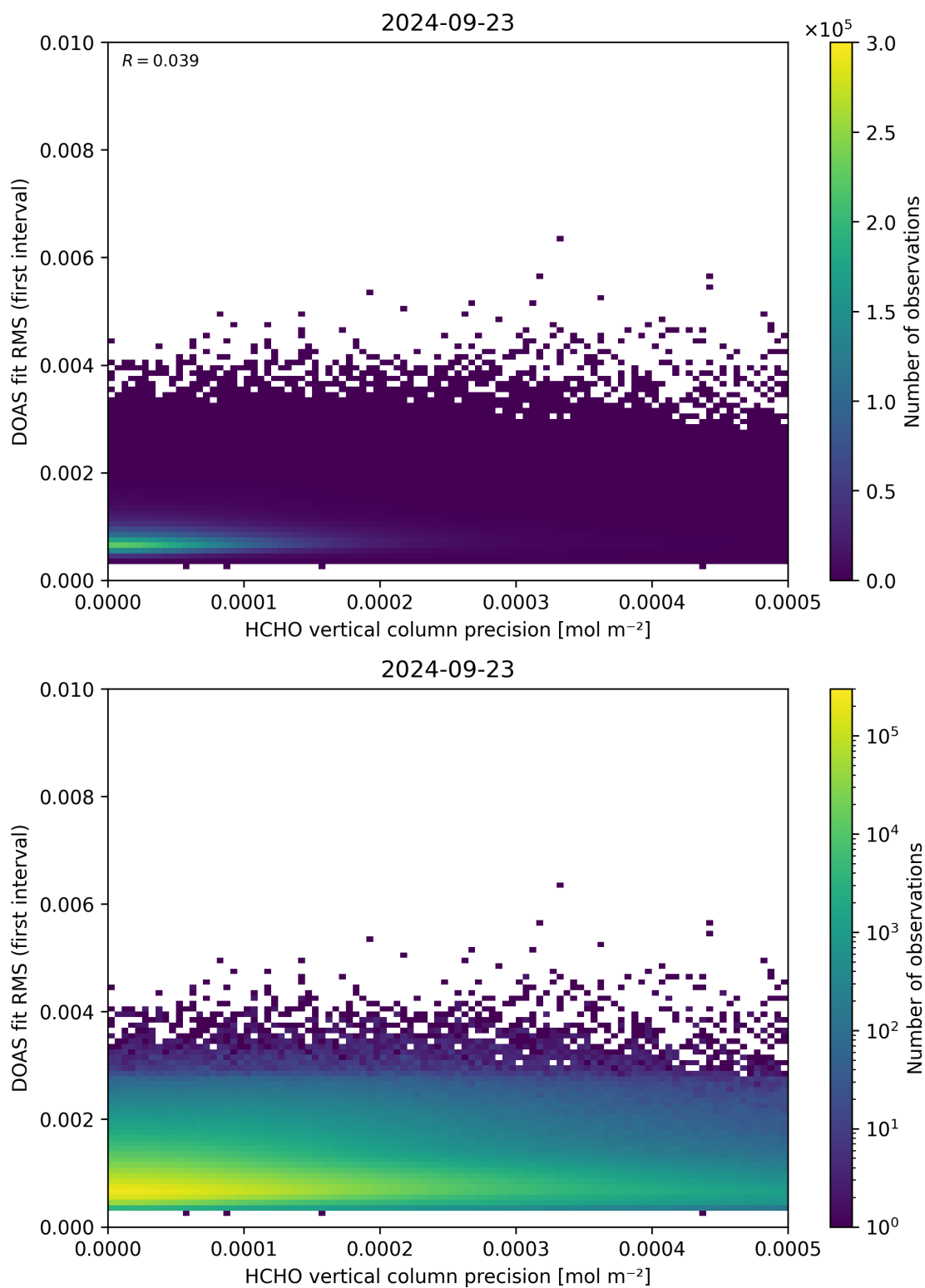
Figure 136: Scatter density plot of “HCHO vertical column precision” against “DOAS fit RMS (first interval)” for 2024-09-22 to 2024-09-24.
