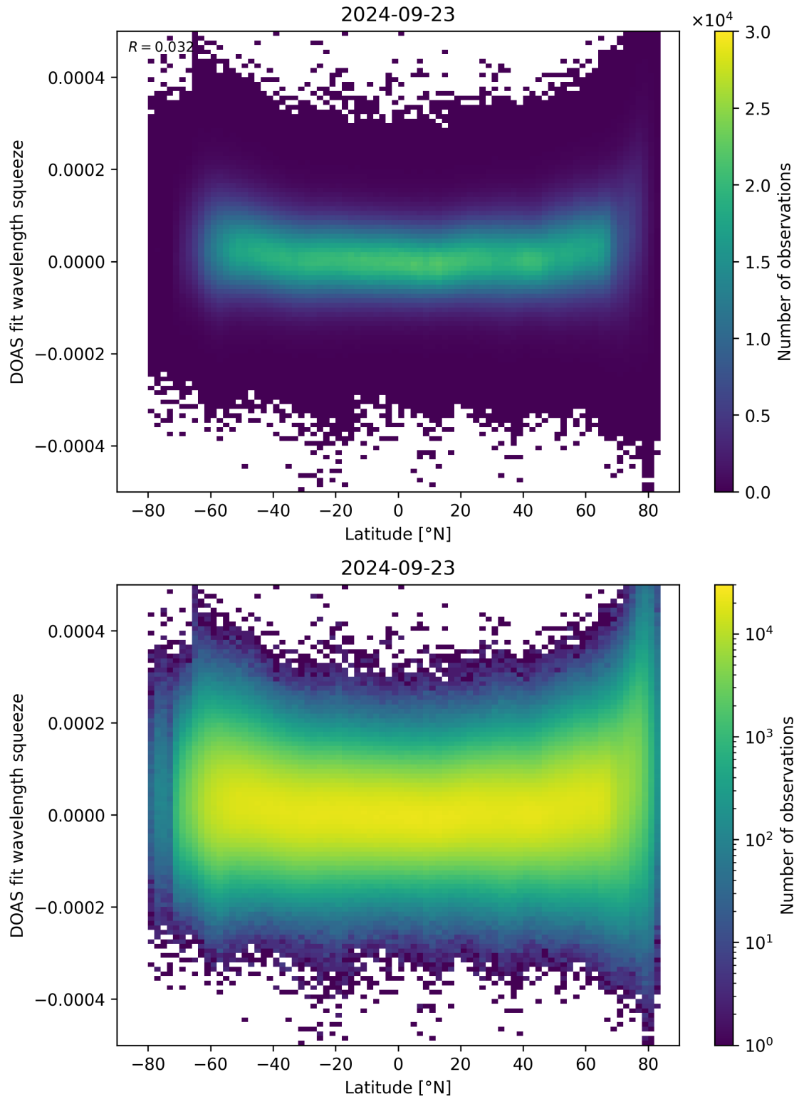
Figure 155: Scatter density plot of “Latitude” against “DOAS fit wavelength squeeze” for 2024-09-22 to 2024-09-24.
