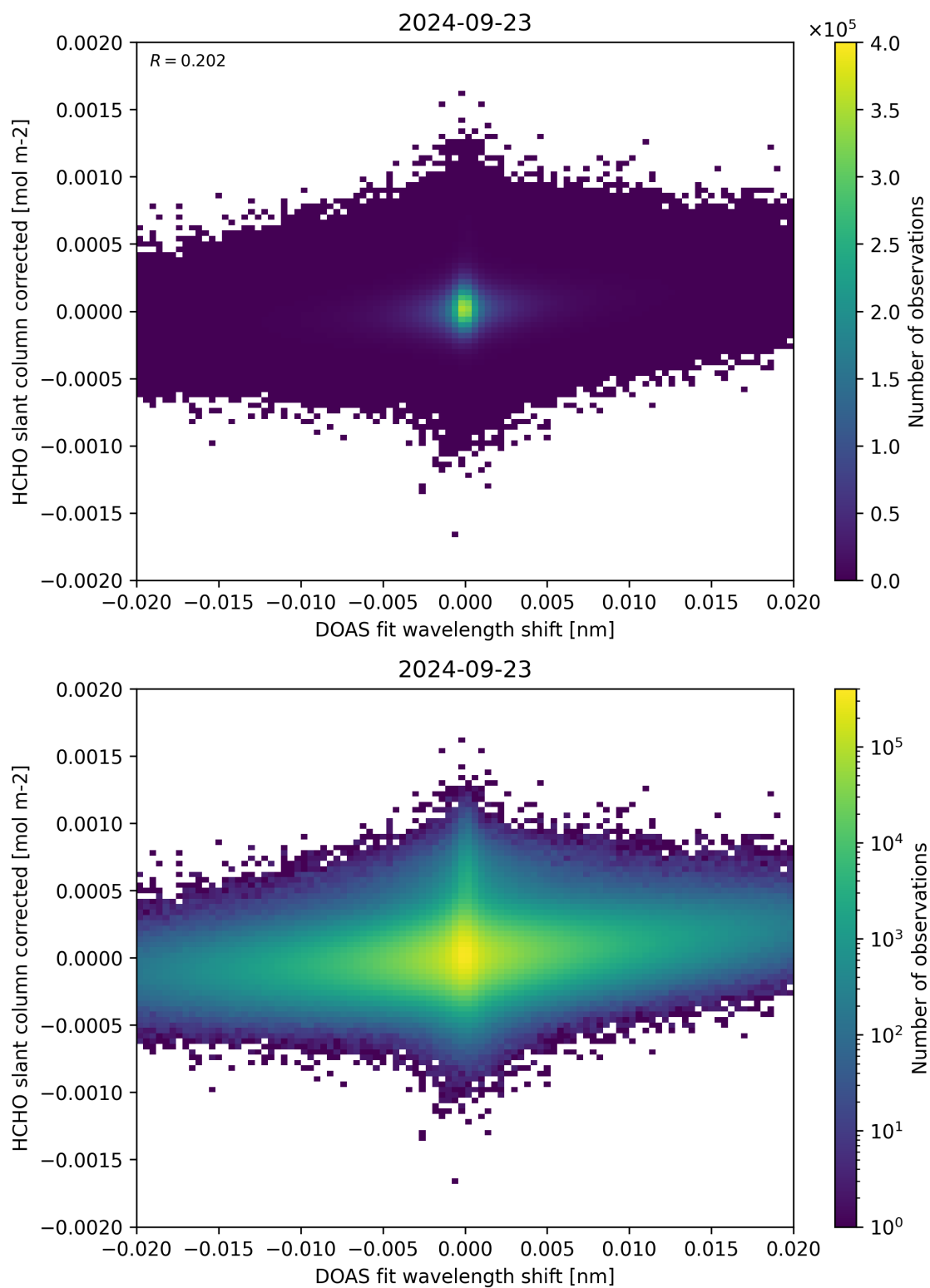
Figure 66: Scatter density plot of “DOAS fit wavelength shift” against “HCHO slant column corrected” for 2024-09-22 to 2024-09-24.
