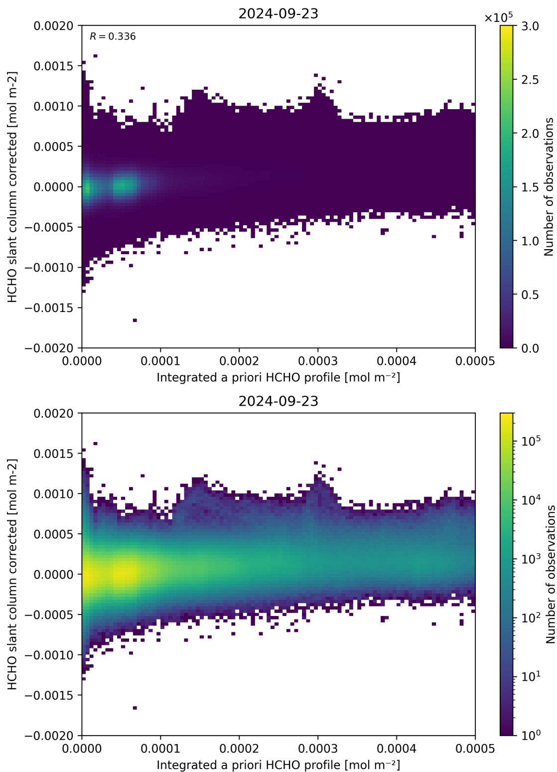
Figure 151: Scatter density plot of “Integrated a priori HCHO profile” against “HCHO slant column corrected” for 2024-09-22 to 2024-09-24.
