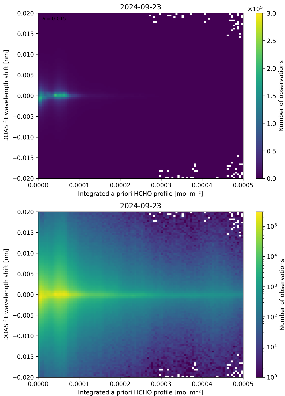
Figure 149: Scatter density plot of “Integrated a priori HCHO profile” against “DOAS fit wavelength shift” for 2024-09-22 to 2024-09-24.
