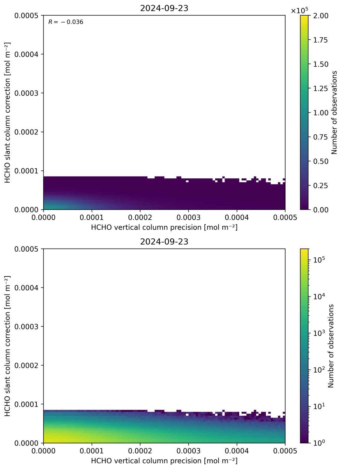
Figure 141: Scatter density plot of “HCHO vertical column precision” against “HCHO slant column correction” for 2024-09-22 to 2024-09-24.
