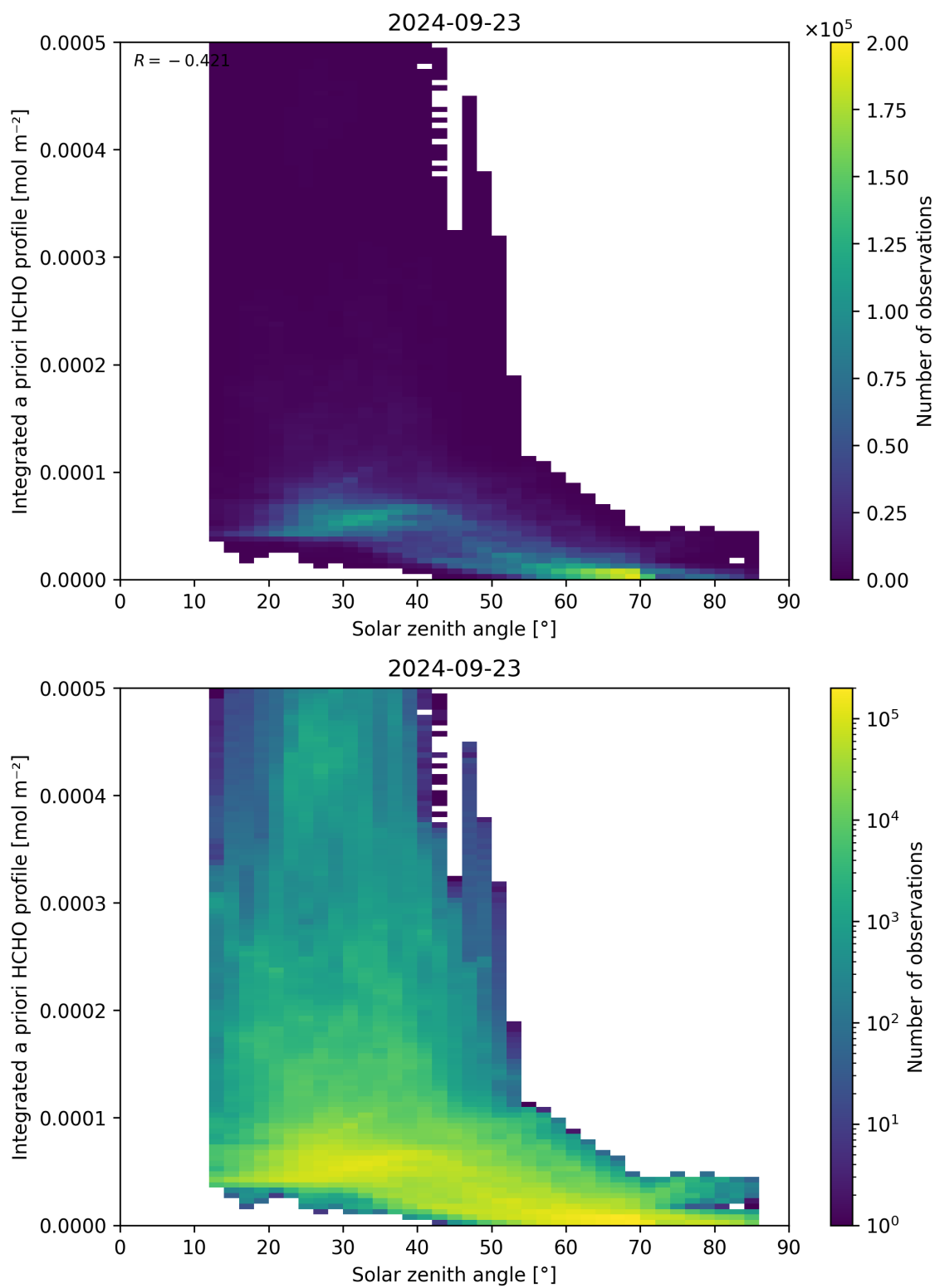
Figure 180: Scatter density plot of “Solar zenith angle” against “Integrated a priori HCHO profile” for 2024-09-22 to 2024-09-24.
