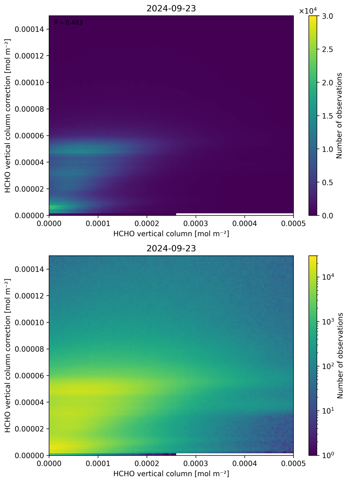
Figure 133: Scatter density plot of “HCHO vertical column” against “HCHO vertical column correction” for 2024-09-22 to 2024-09-24.
