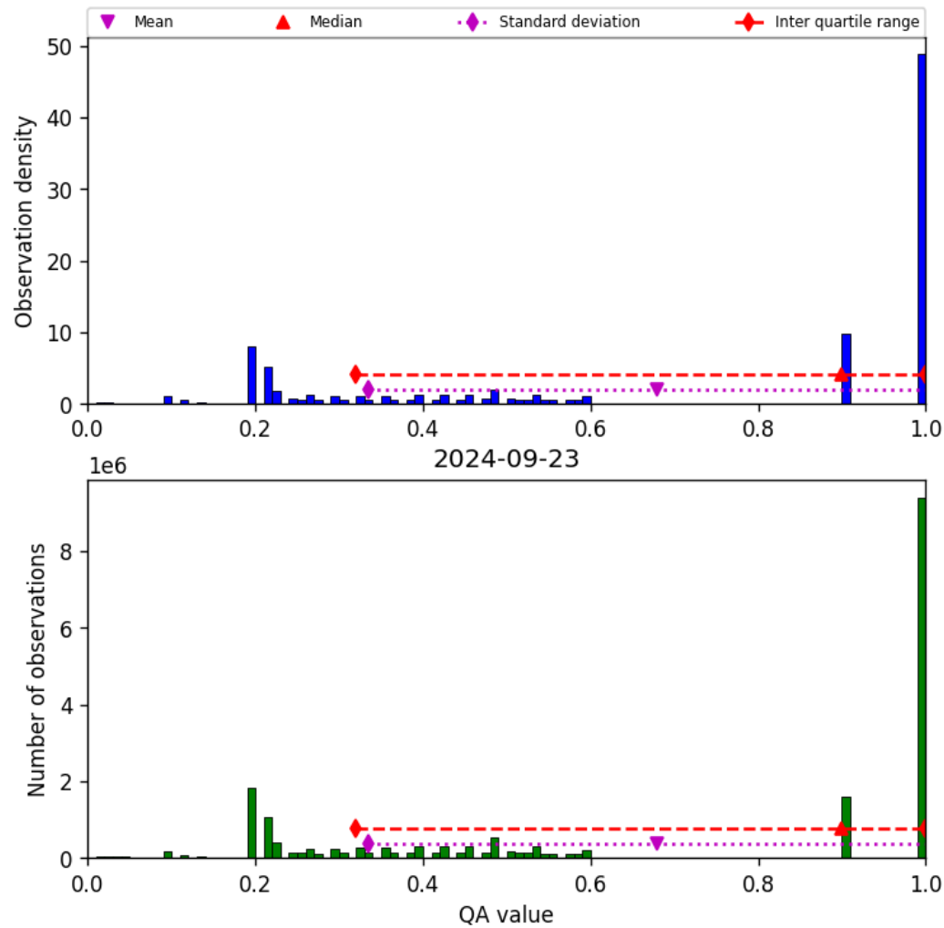
Figure 34: Histogram of “QA value” for 2024-09-22 to 2024-09-24
