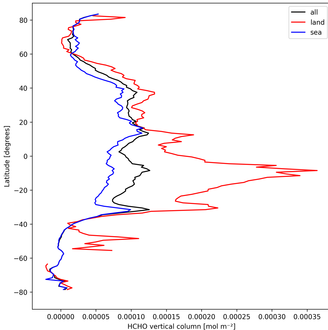
Figure 21: Zonal average of “HCHO vertical column” for 2024-09-22 to 2024-09-24.
