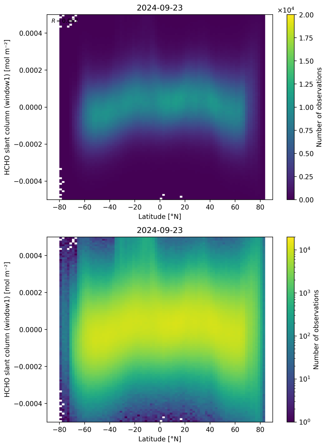
Figure 159: Scatter density plot of “Latitude” against “HCHO slant column (window1)” for 2024-09-22 to 2024-09-24.
