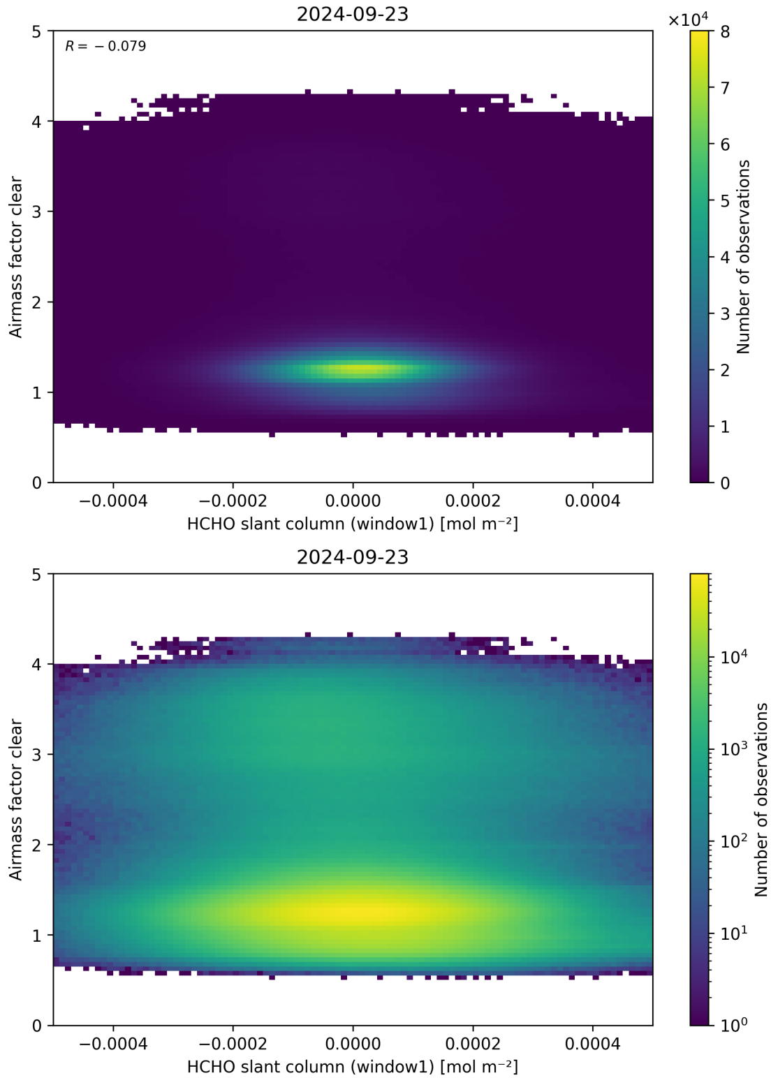
Figure 81: Scatter density plot of “HCHO slant column (window1)” against “Airmass factor clear” for 2024-09-22 to 2024-09-24.
