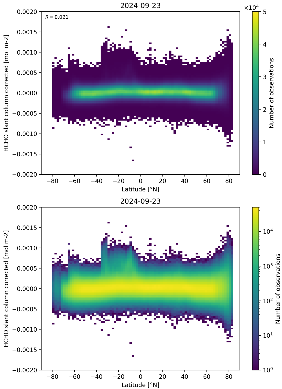
Figure 157: Scatter density plot of “Latitude” against “HCHO slant column corrected” for 2024-09-22 to 2024-09-24.
