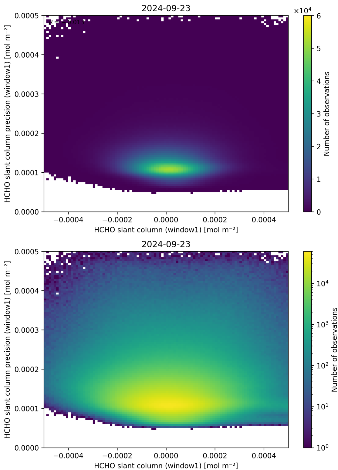
Figure 84: Scatter density plot of “HCHO slant column (window1)” against “HCHO slant column precision (window1)” for 2024-09-22 to 2024-09-24.
