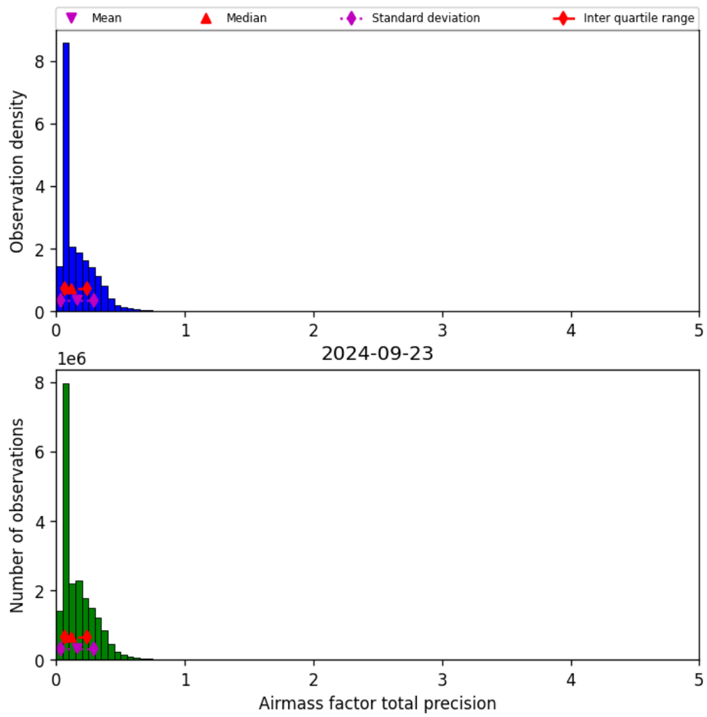
Figure 41: Histogram of “Airmass factor total precision” for 2024-09-22 to 2024-09-24
