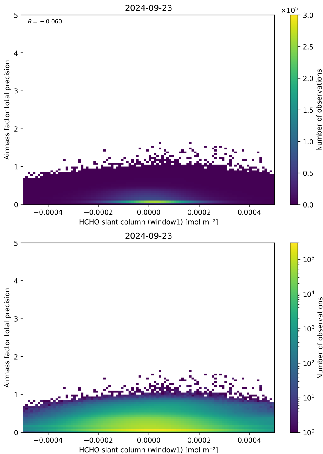
Figure 86: Scatter density plot of “HCHO slant column (window1)” against “Airmass factor total precision” for 2024-09-22 to 2024-09-24.
