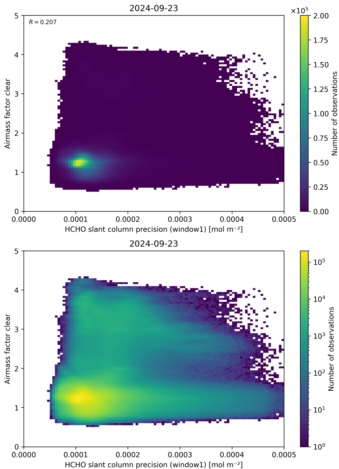
Figure 91: Scatter density plot of “HCHO slant column precision (window1)” against “Airmass factor clear” for 2024-09-22 to 2024-09-24.
