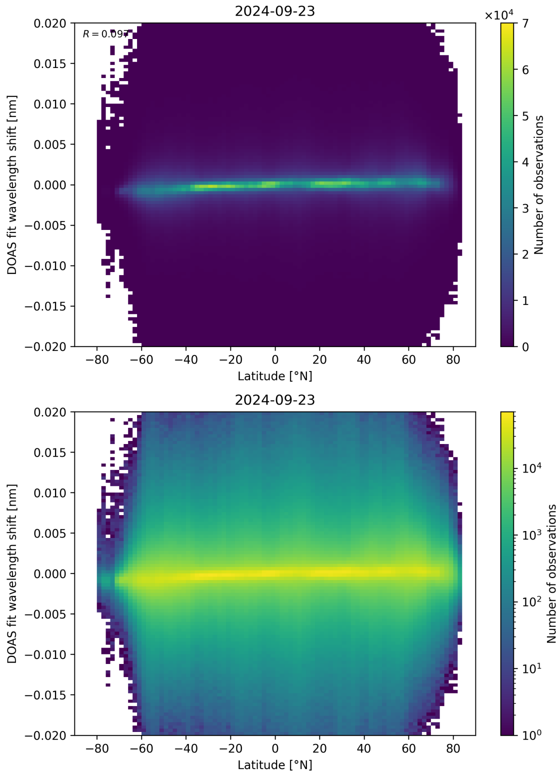
Figure 154: Scatter density plot of “Latitude” against “DOAS fit wavelength shift” for 2024-09-22 to 2024-09-24.
