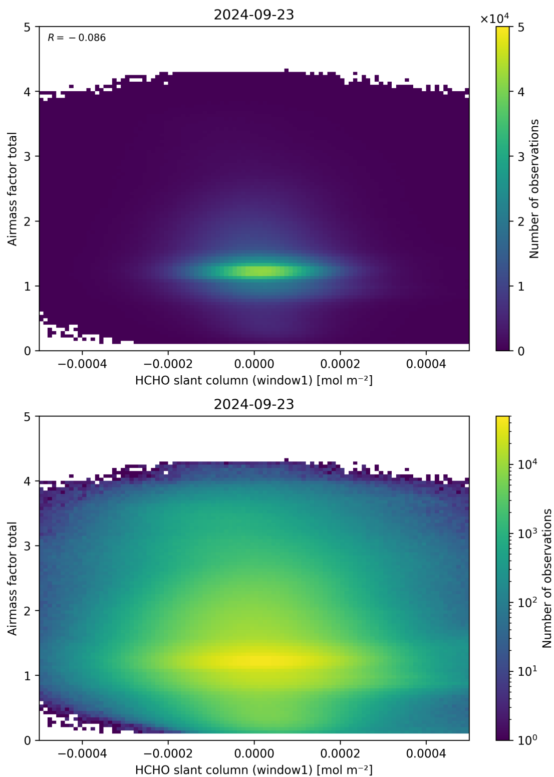
Figure 85: Scatter density plot of “HCHO slant column (window1)” against “Airmass factor total” for 2024-09-22 to 2024-09-24.
