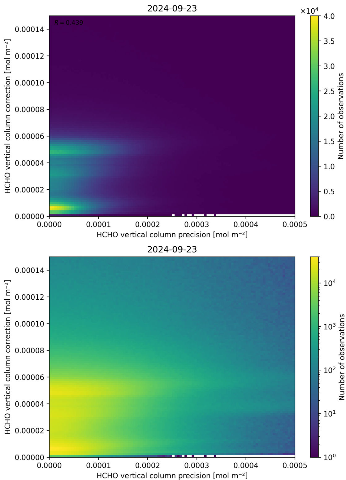
Figure 146: Scatter density plot of “HCHO vertical column precision” against “HCHO vertical column correction” for 2024-09-22 to 2024-09-24.
