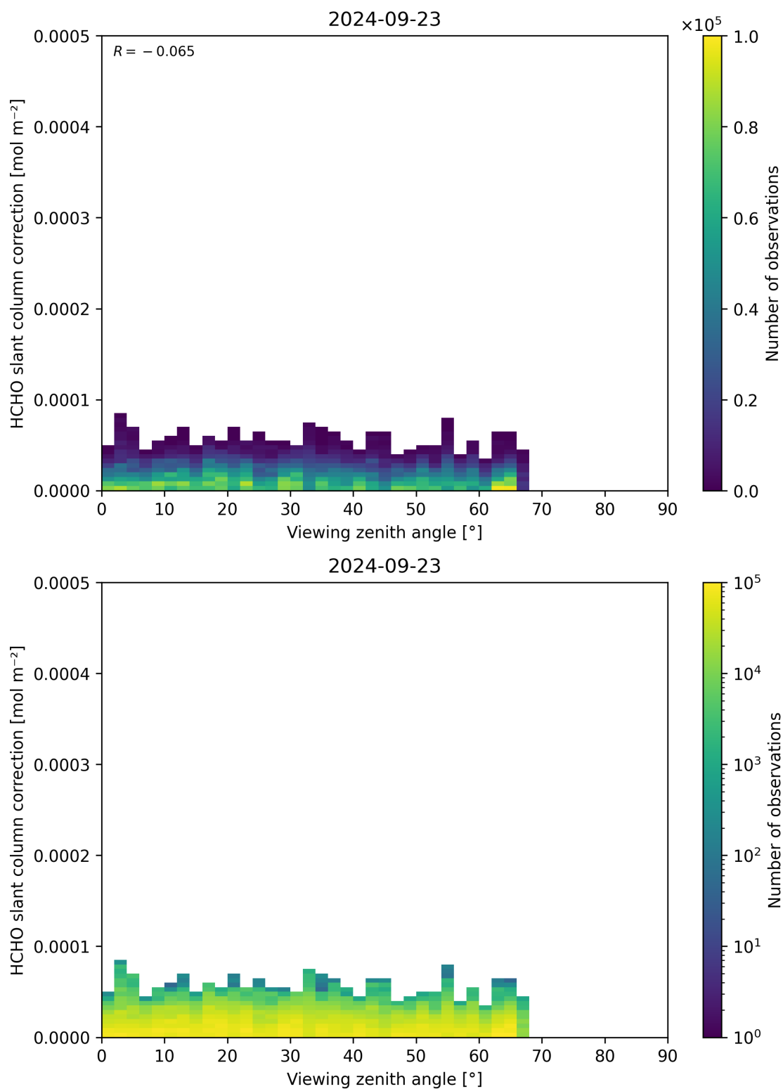
Figure 187: Scatter density plot of “Viewing zenith angle” against “HCHO slant column correction” for 2024-09-22 to 2024-09-24.
