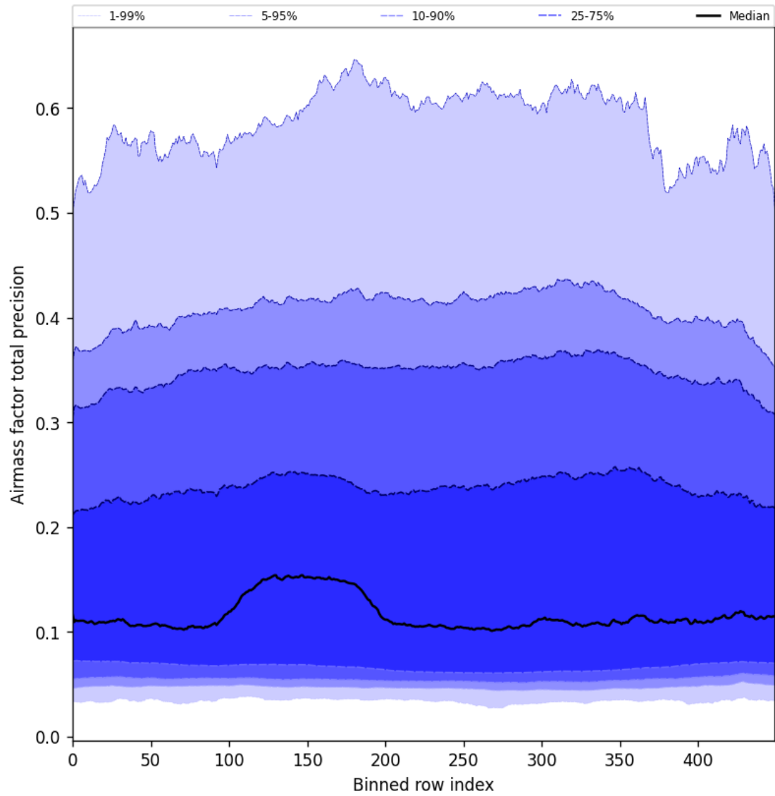
Figure 55: Along track statistics of “Airmass factor total precision” for 2024-09-22 to 2024-09-24
