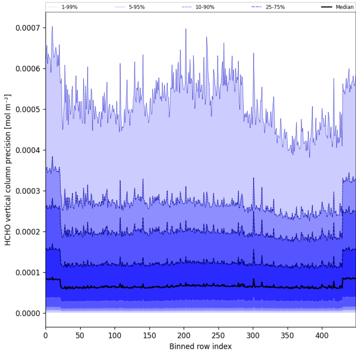
Figure 50: Along track statistics of “HCHO vertical column precision” for 2024-09-22 to 2024-09-24
