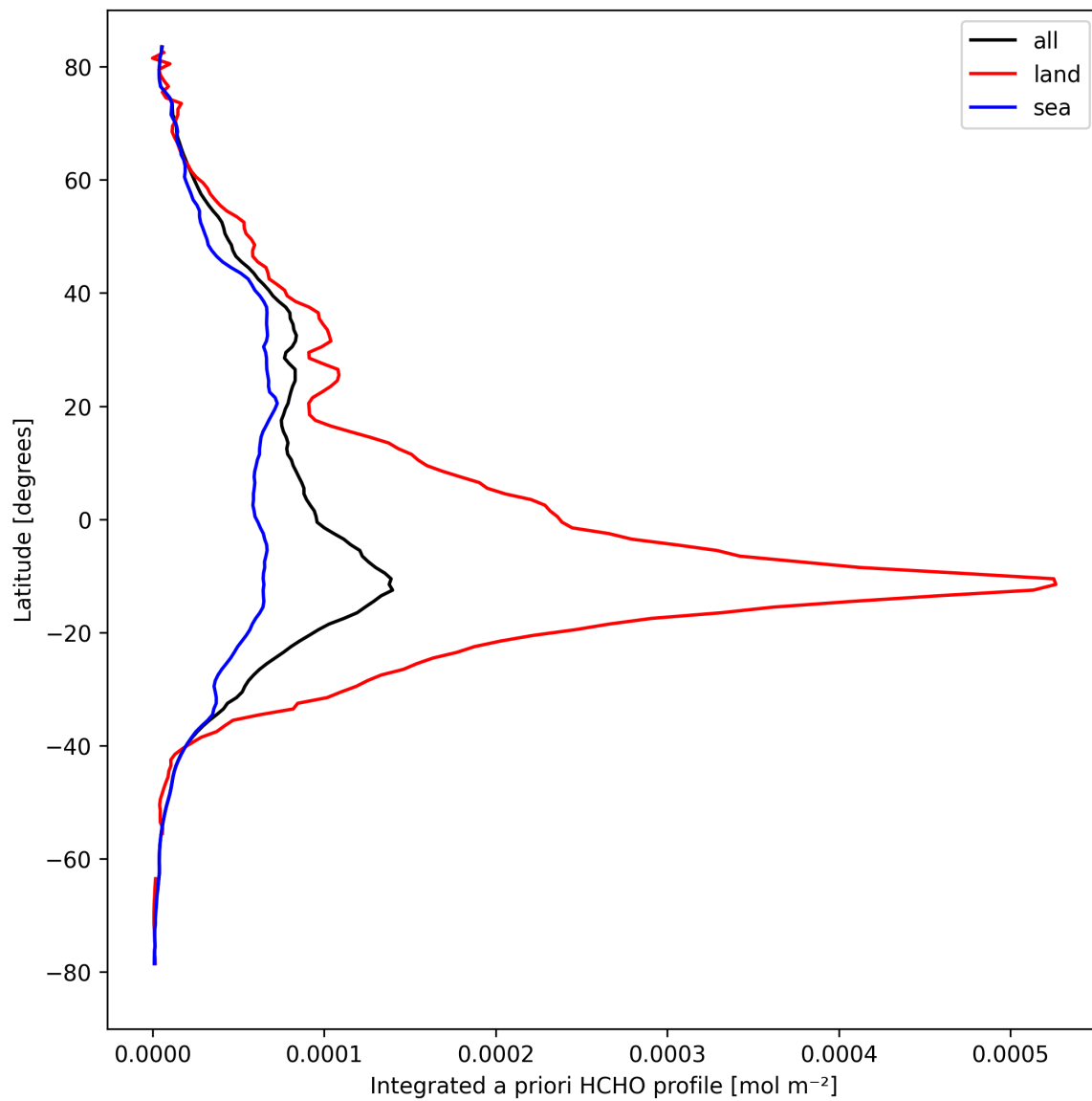
Figure 29: Zonal average of “Integrated a priori HCHO profile” for 2024-09-22 to 2024-09-24.
