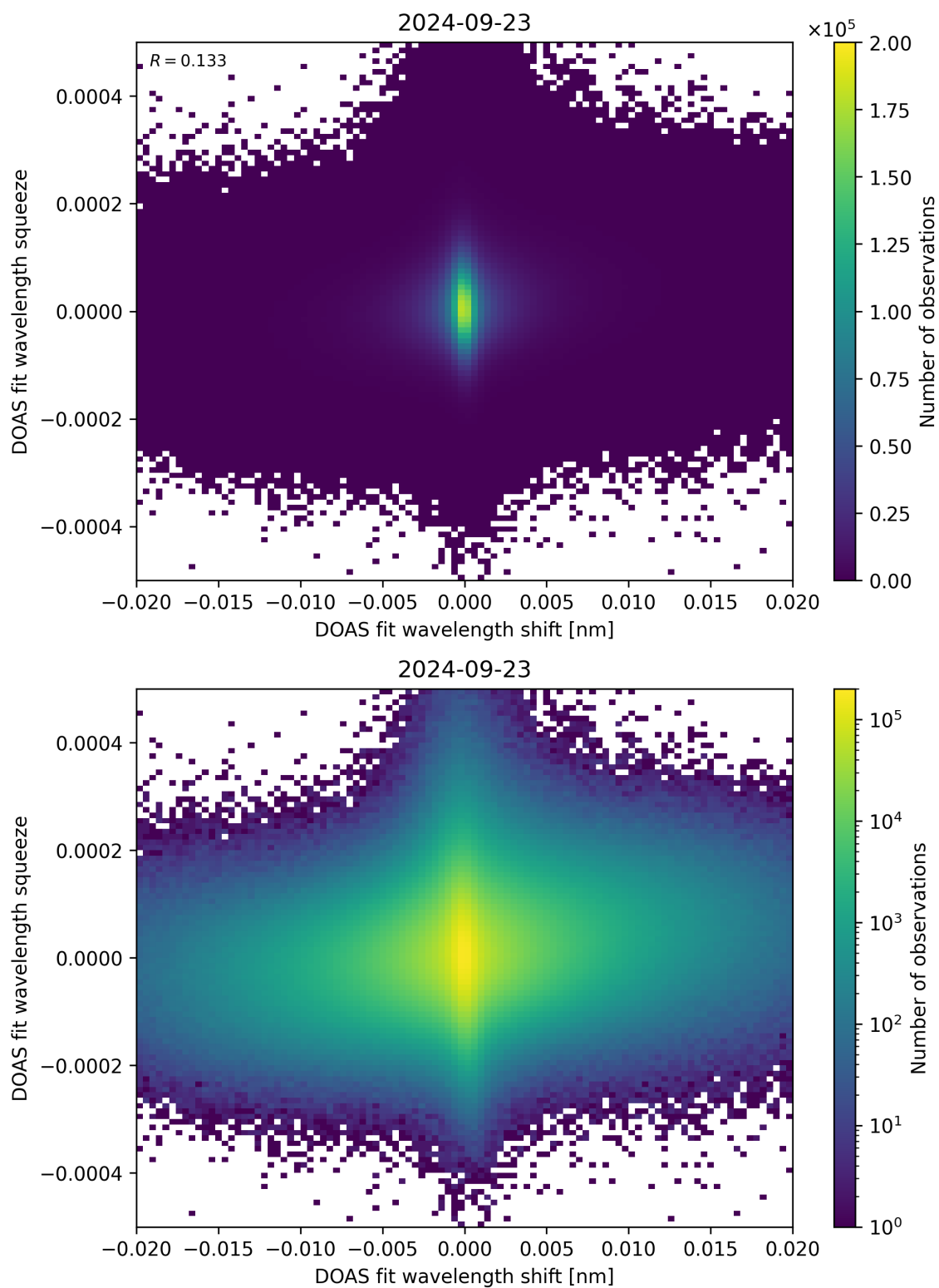
Figure 65: Scatter density plot of “DOAS fit wavelength shift” against “DOAS fit wavelength squeeze” for 2024-09-22 to 2024-09-24.
