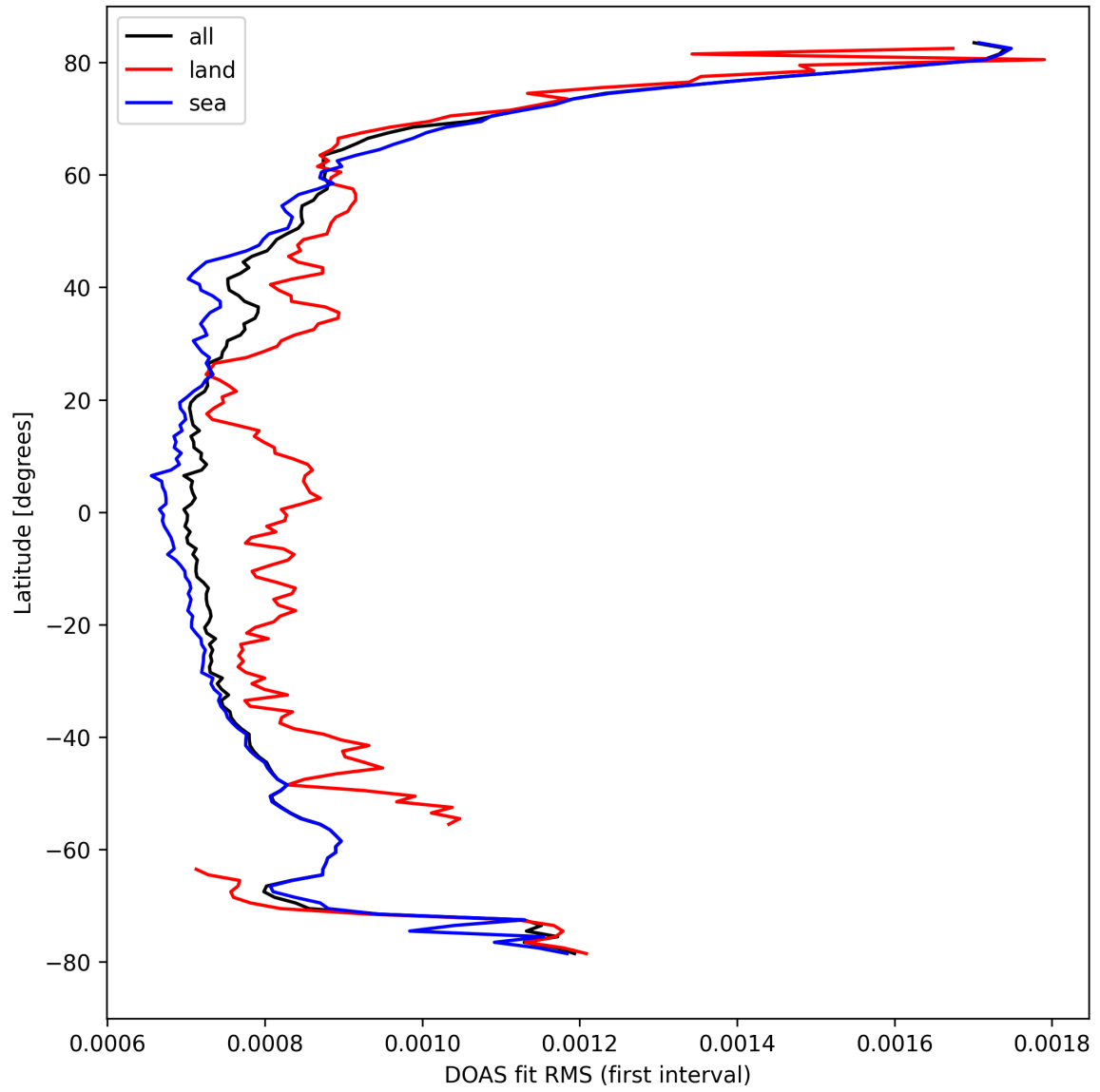
Figure 32: Zonal average of "DOAS fit RMS (first interval)" for 2024-09-22 to 2024-09-24.
