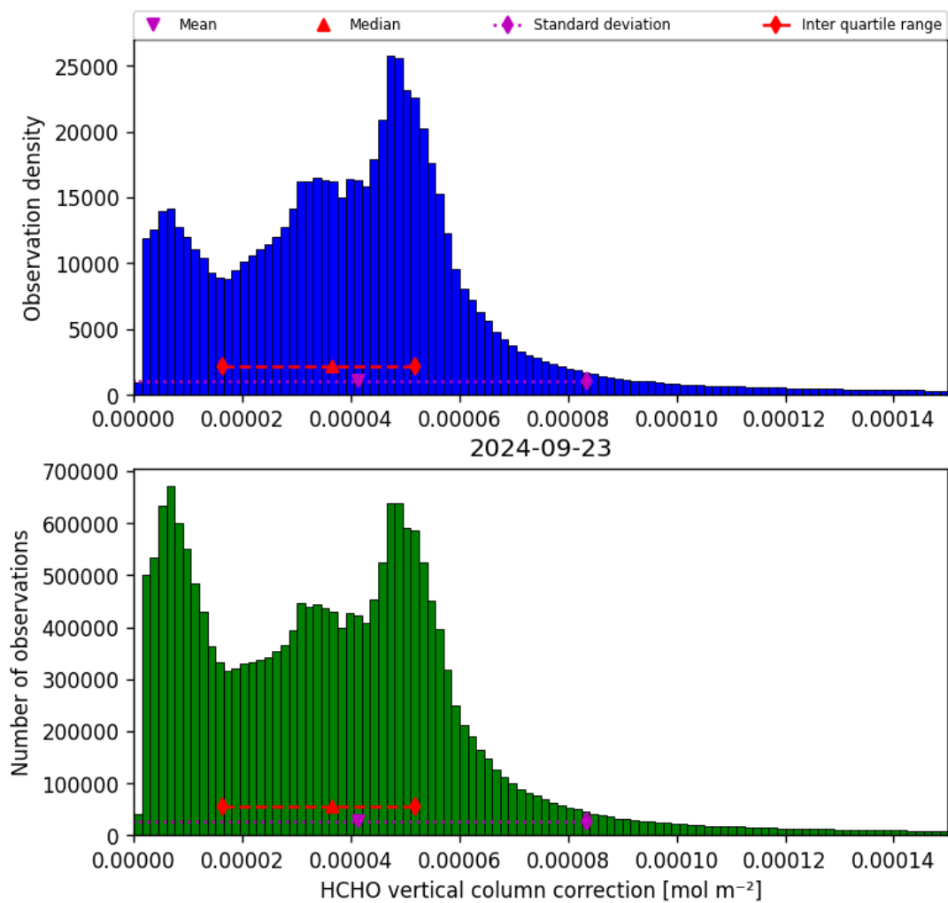
Figure 37: Histogram of “HCHO vertical column correction” for 2024-09-22 to 2024-09-24
