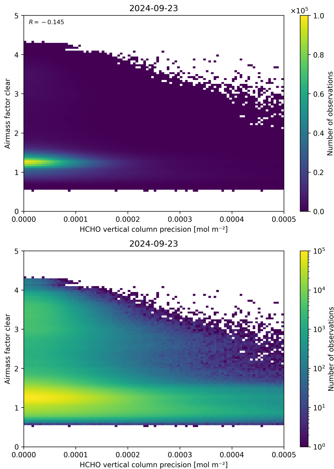
Figure 139: Scatter density plot of “HCHO vertical column precision” against “Airmass factor clear” for 2024-09-22 to 2024-09-24.
