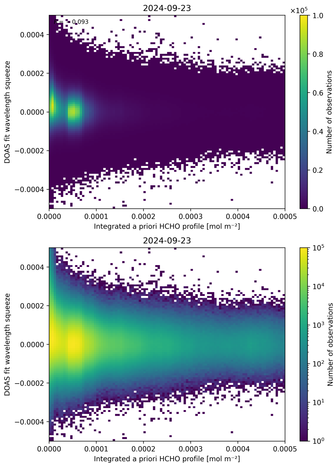
Figure 150: Scatter density plot of “Integrated a priori HCHO profile” against “DOAS fit wavelength squeeze” for 2024-09-22 to 2024-09-24.
