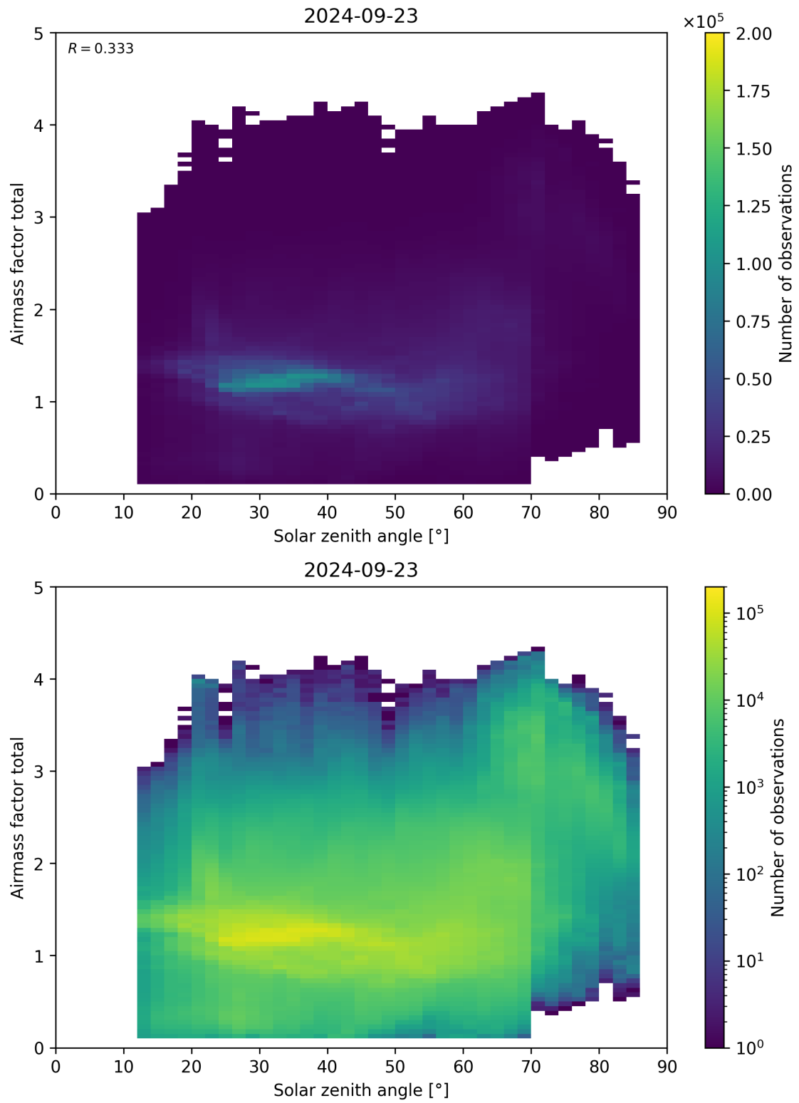
Figure 175: Scatter density plot of “Solar zenith angle” against “Airmass factor total” for 2024-09-22 to 2024-09-24.
