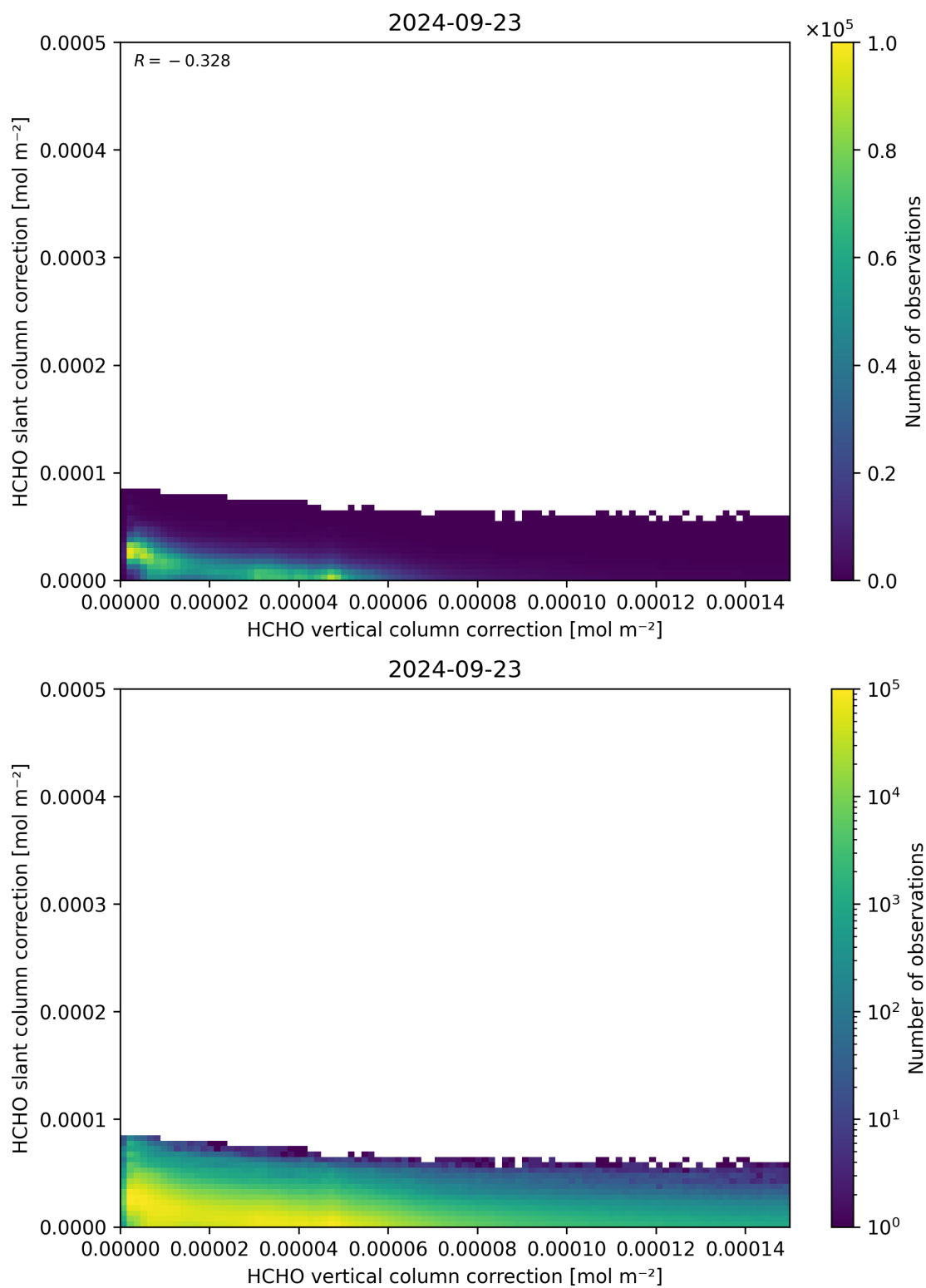
Figure 117: Scatter density plot of “HCHO vertical column correction” against “HCHO slant column correction” for 2024-09-22 to 2024-09-24.
