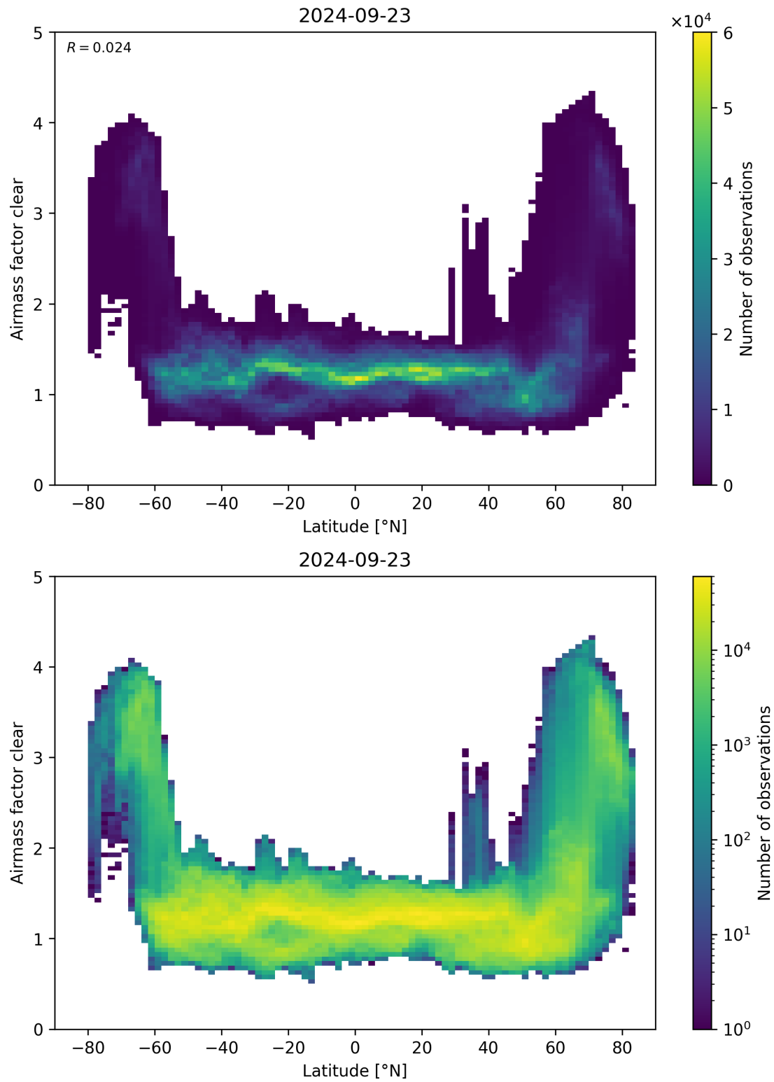
Figure 156: Scatter density plot of “Latitude” against “Airmass factor clear” for 2024-09-22 to 2024-09-24.
