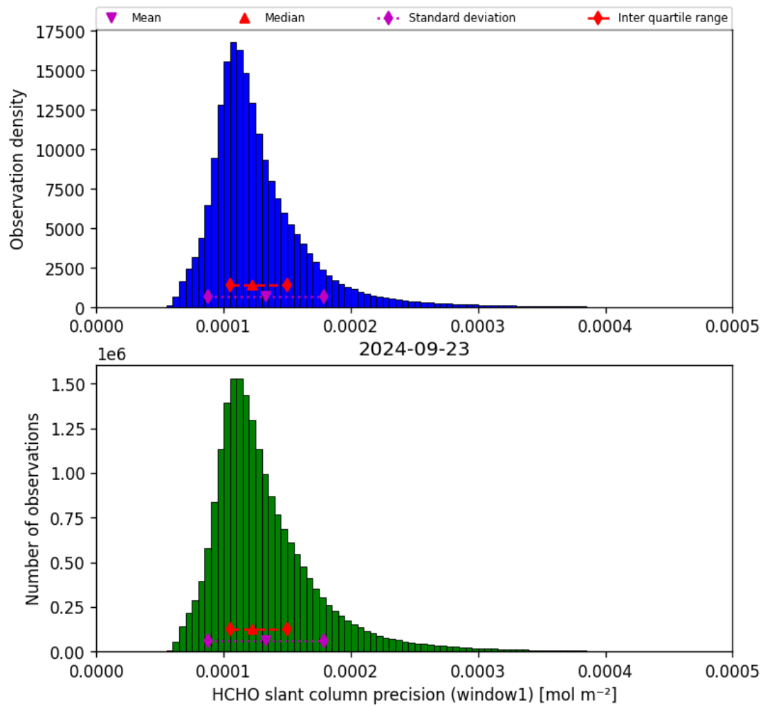
Figure 39: Histogram of “HCHO slant column precision (window1)” for 2024-09-22 to 2024-09-24
