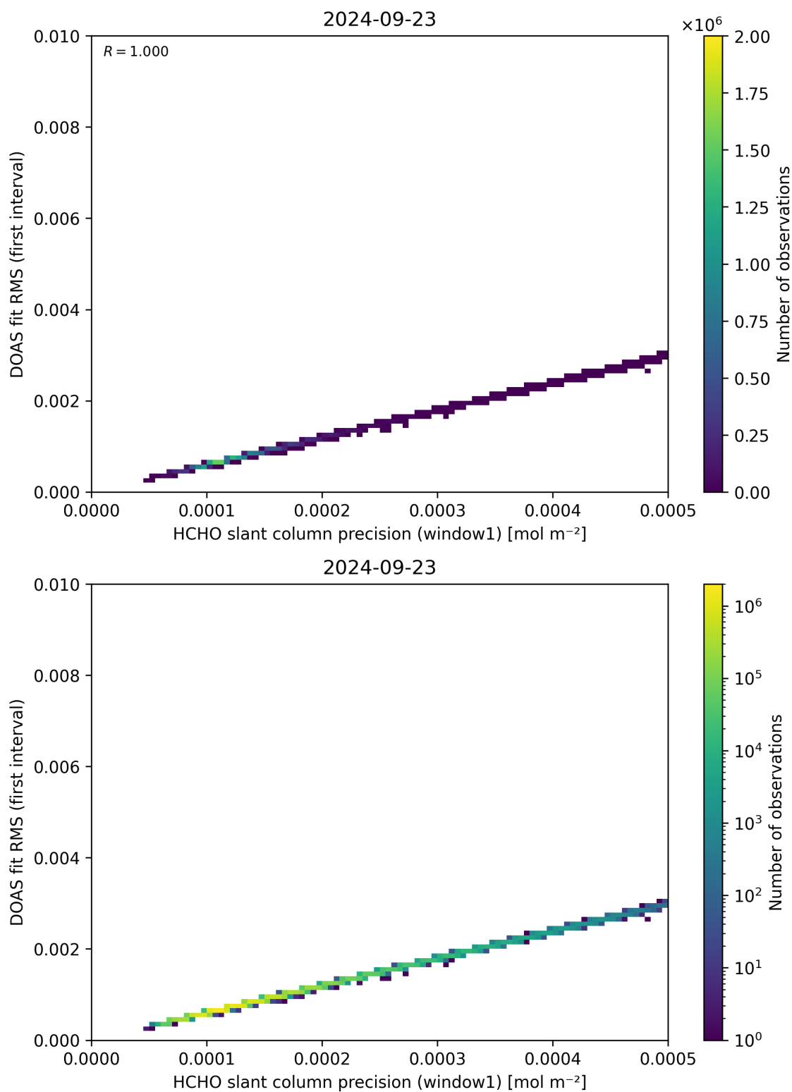
Figure 88: Scatter density plot of “HCHO slant column precision (window1)” against “DOAS fit RMS (first interval)” for 2024-09-22 to 2024-09-24.
