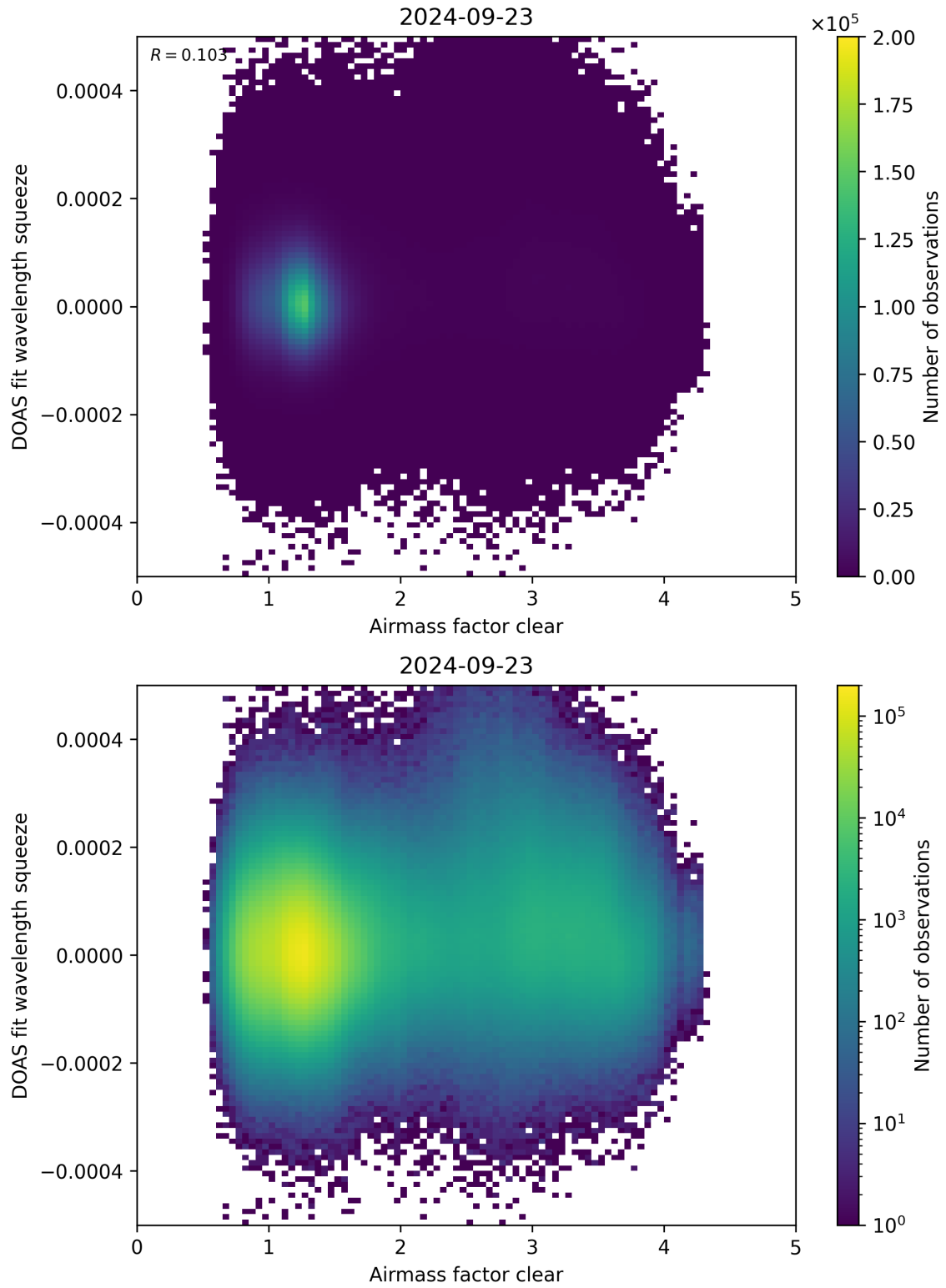
Figure 73: Scatter density plot of “Airmass factor clear” against “DOAS fit wavelength squeeze” for 2024-09-22 to 2024-09-24.
