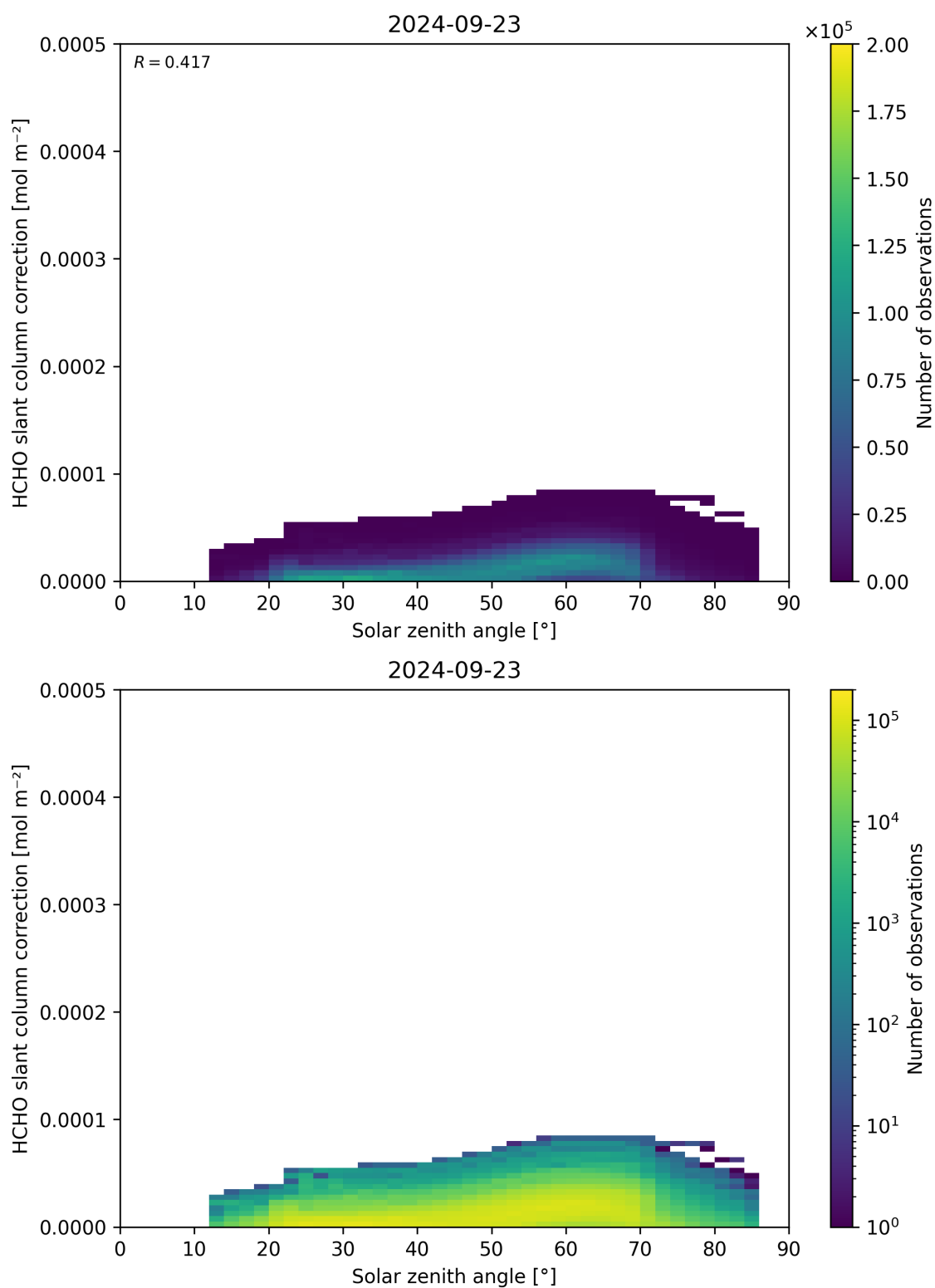
Figure 172: Scatter density plot of “Solar zenith angle” against “HCHO slant column correction” for 2024-09-22 to 2024-09-24.
