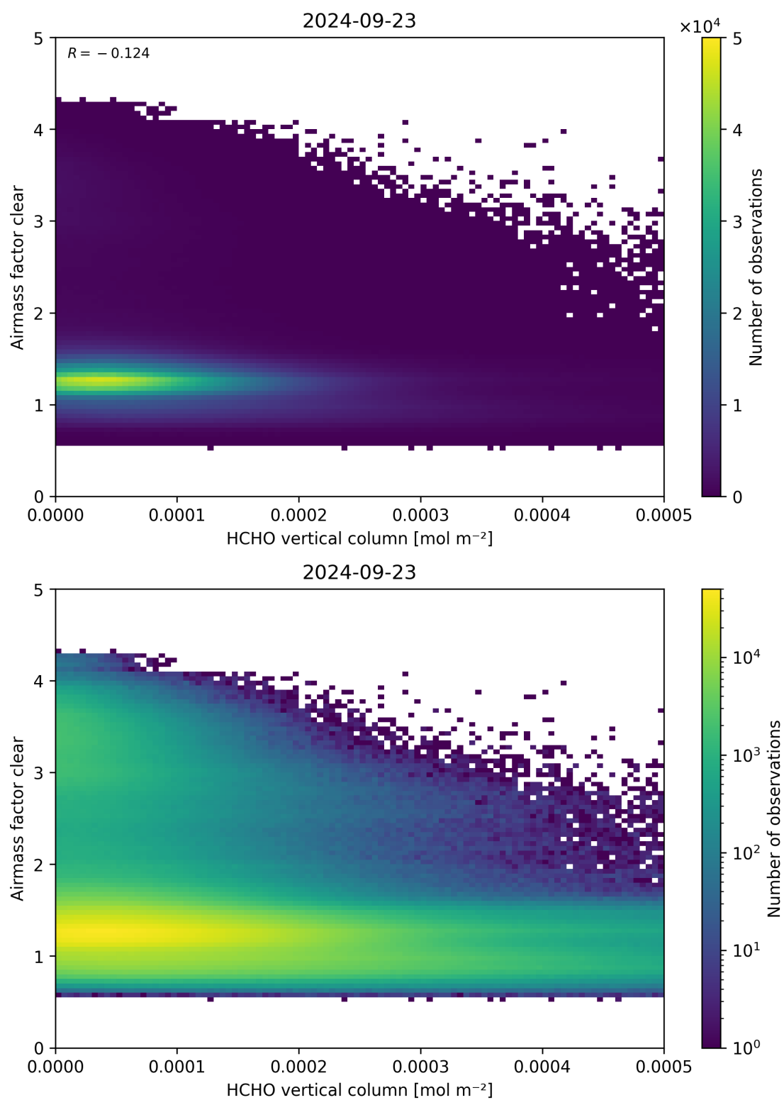
Figure 126: Scatter density plot of “HCHO vertical column” against “Airmass factor clear” for 2024-09-22 to 2024-09-24.
