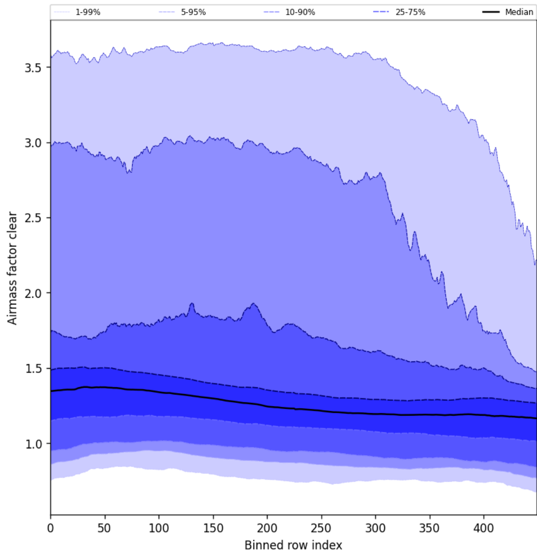
Figure 56: Along track statistics of “Airmass factor clear” for 2024-09-22 to 2024-09-24
