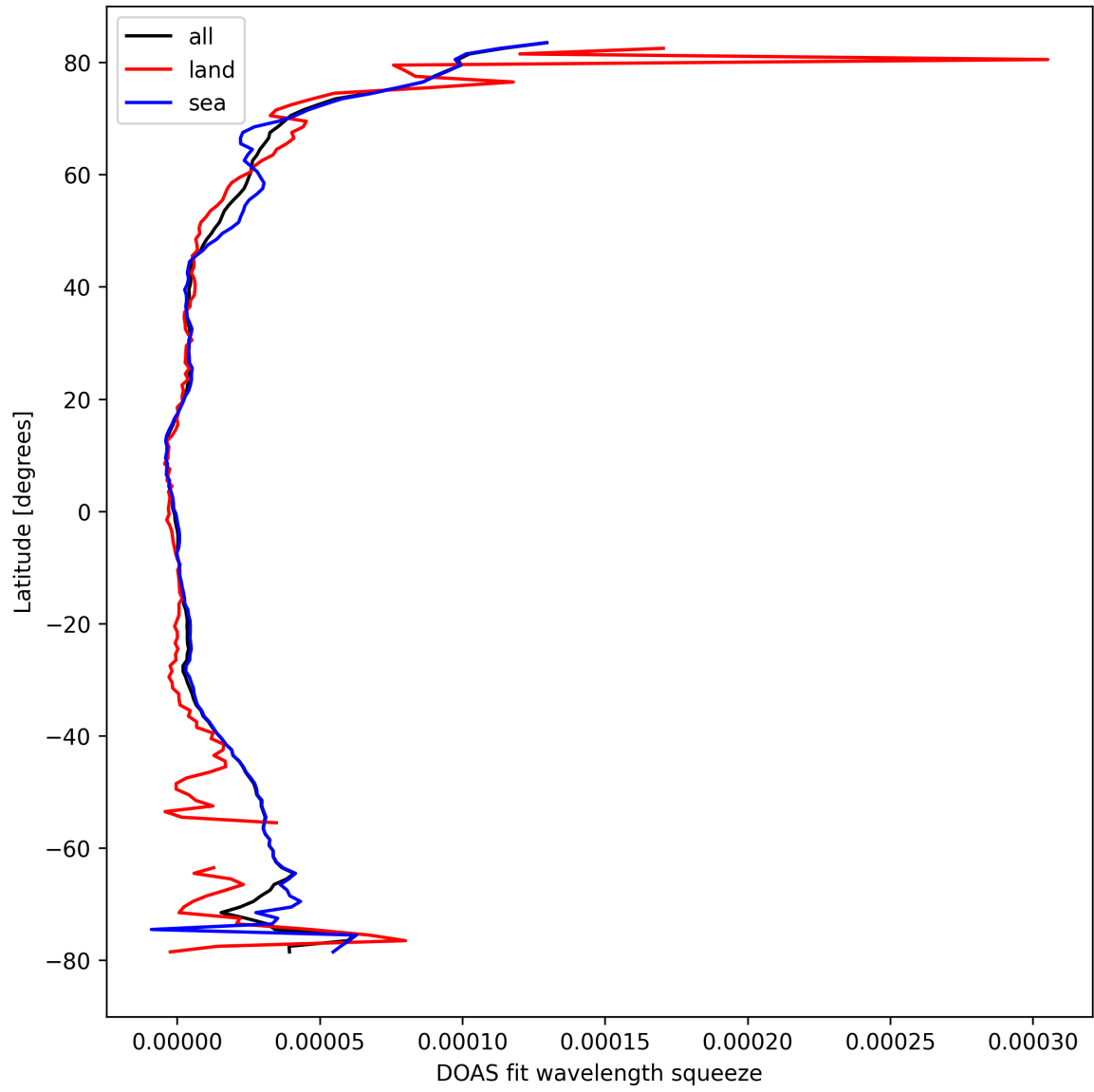
Figure 31: Zonal average of “DOAS fit wavelength squeeze” for 2024-09-22 to 2024-09-24.
