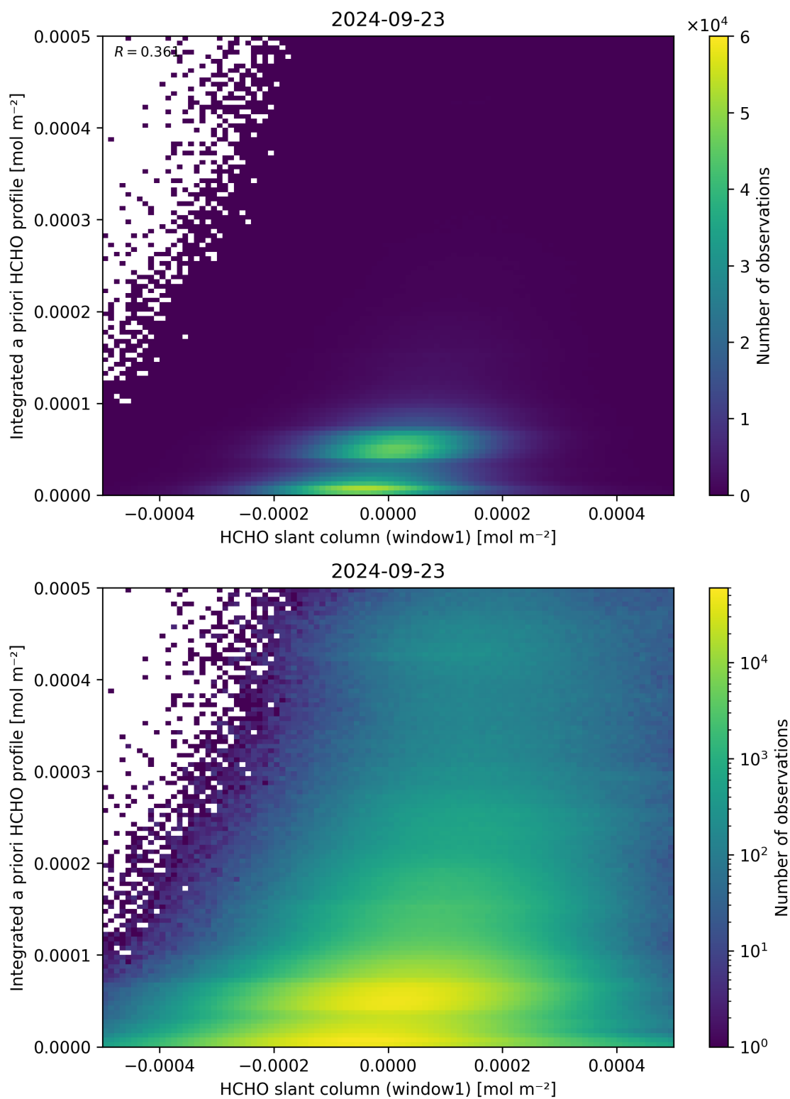
Figure 87: Scatter density plot of “HCHO slant column (window1)” against “Integrated a priori HCHO profile” for 2024-09-22 to 2024-09-24.
