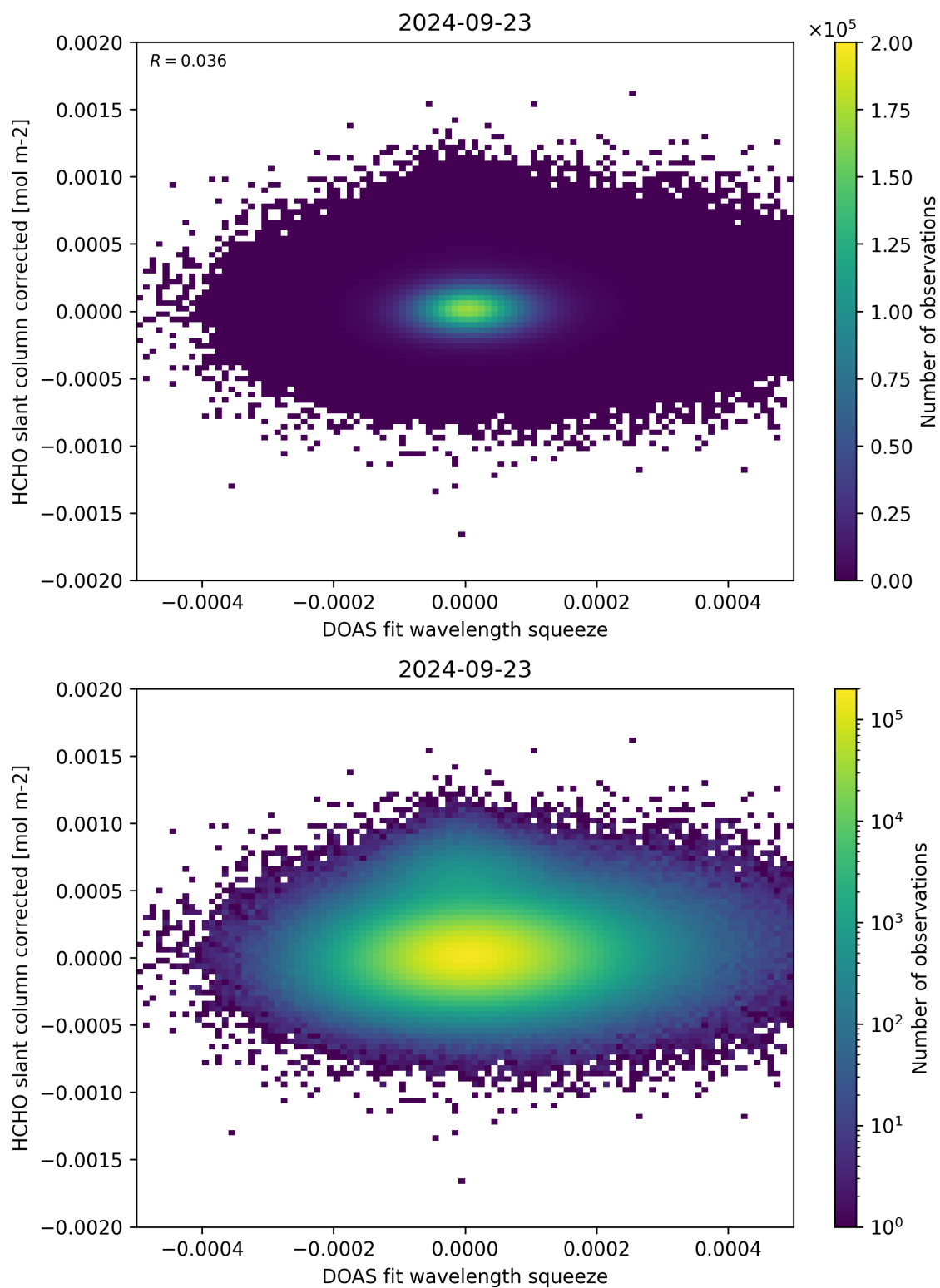
Figure 69: Scatter density plot of “DOAS fit wavelength squeeze” against “HCHO slant column corrected” for 2024-09-22 to 2024-09-24.
