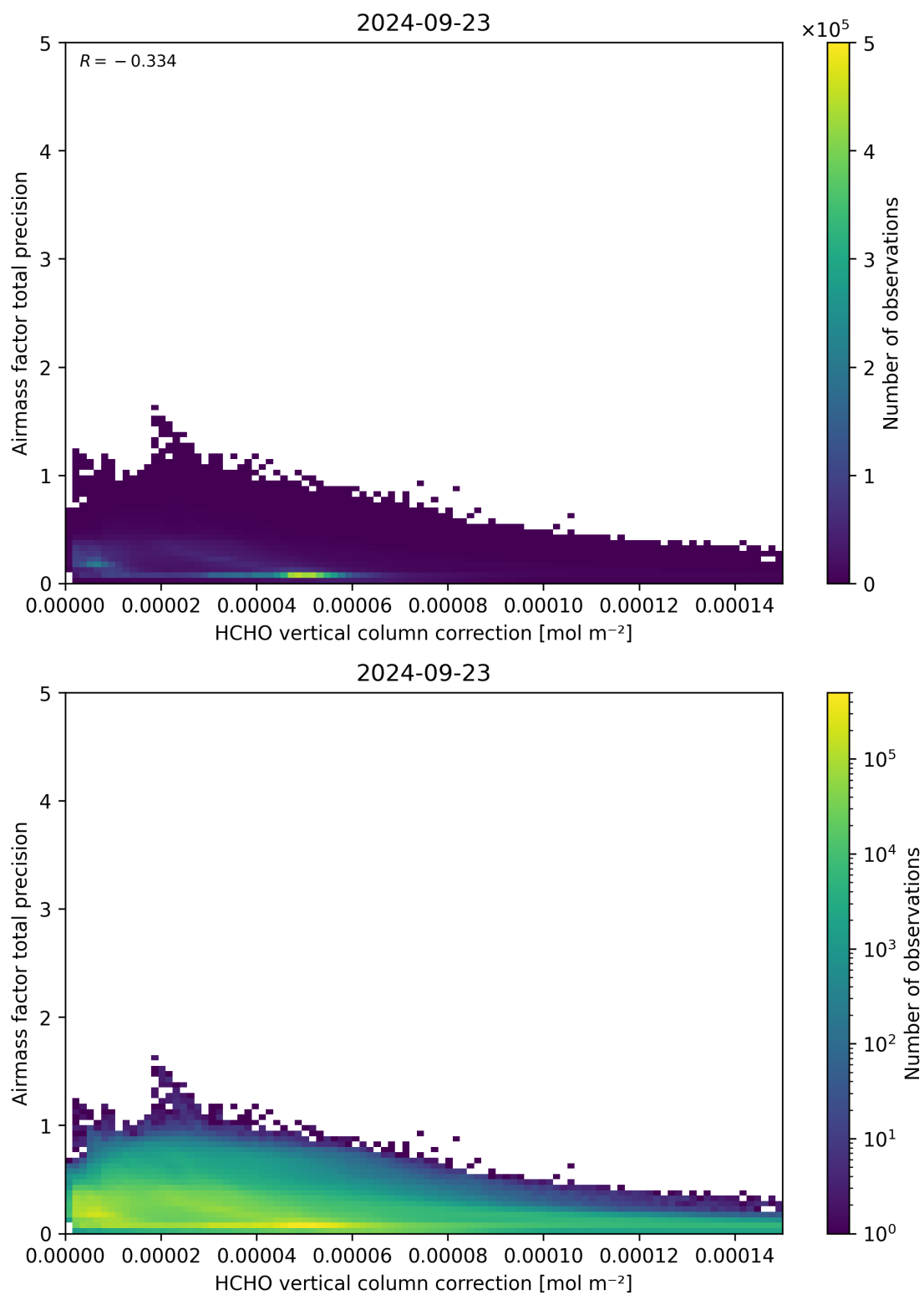
Figure 121: Scatter density plot of “HCHO vertical column correction” against “Airmass factor total precision” for 2024-09-22 to 2024-09-24.
