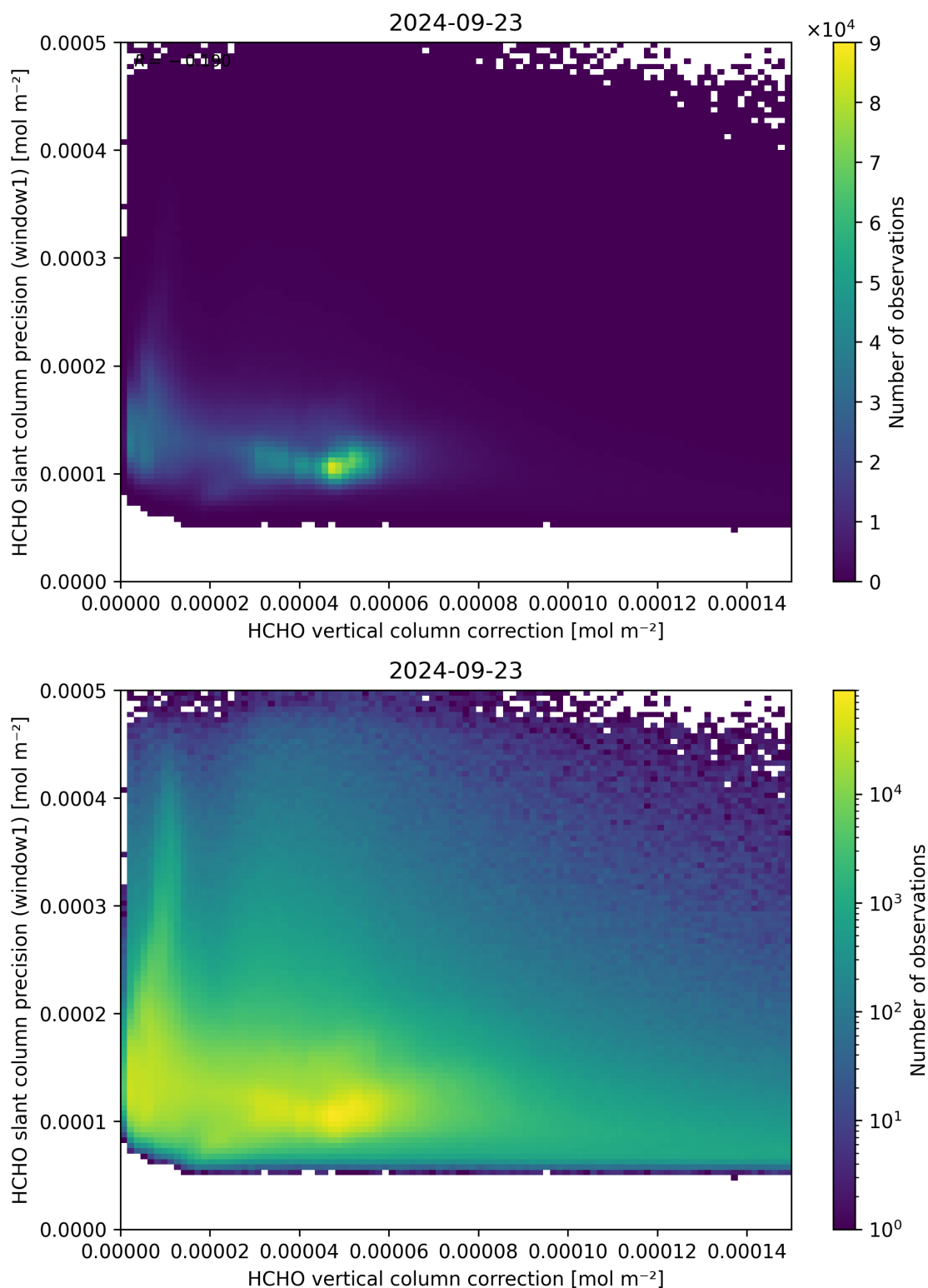
Figure 119: Scatter density plot of “HCHO vertical column correction” against “HCHO slant column precision (window1)” for 2024-09-22 to 2024-09-24.
