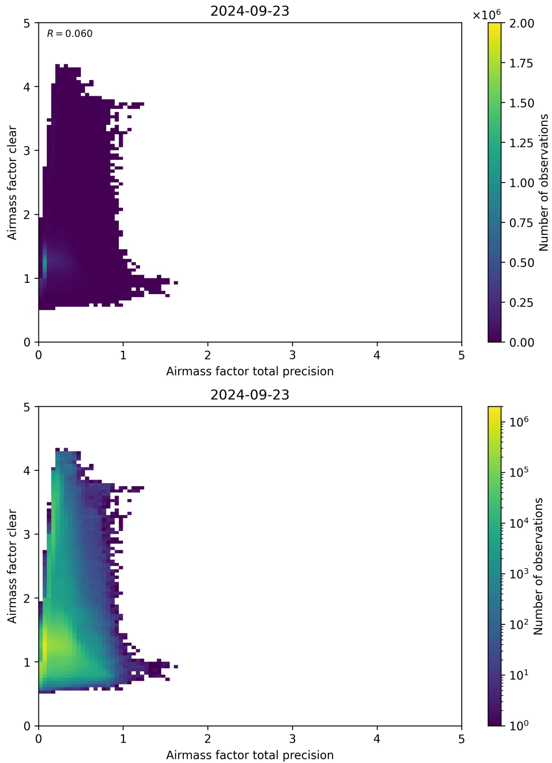
Figure 108: Scatter density plot of “Airmass factor total precision” against “Airmass factor clear” for 2024-09-22 to 2024-09-24.
