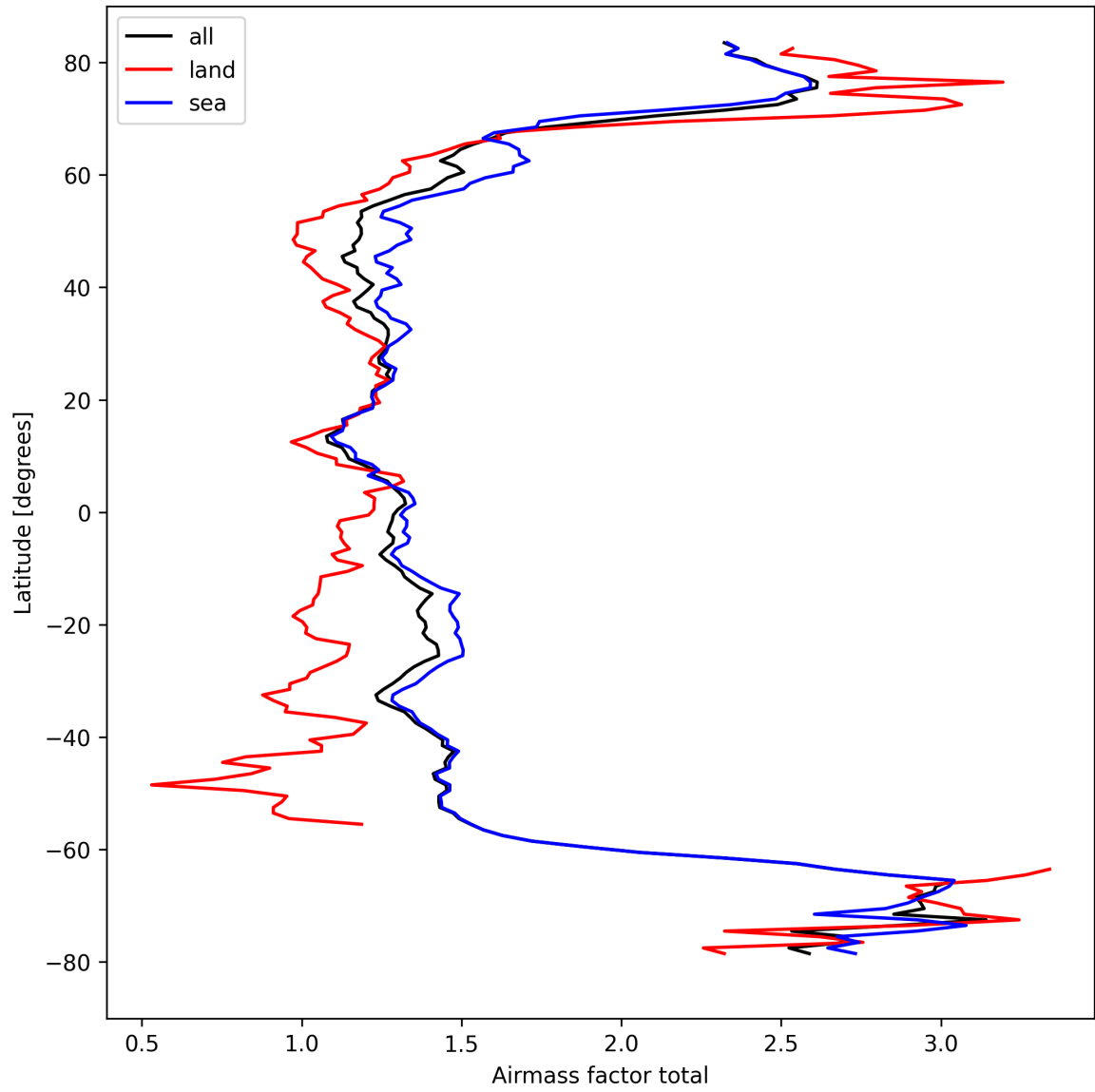
Figure 26: Zonal average of “Airmass factor total” for 2024-09-22 to 2024-09-24.
