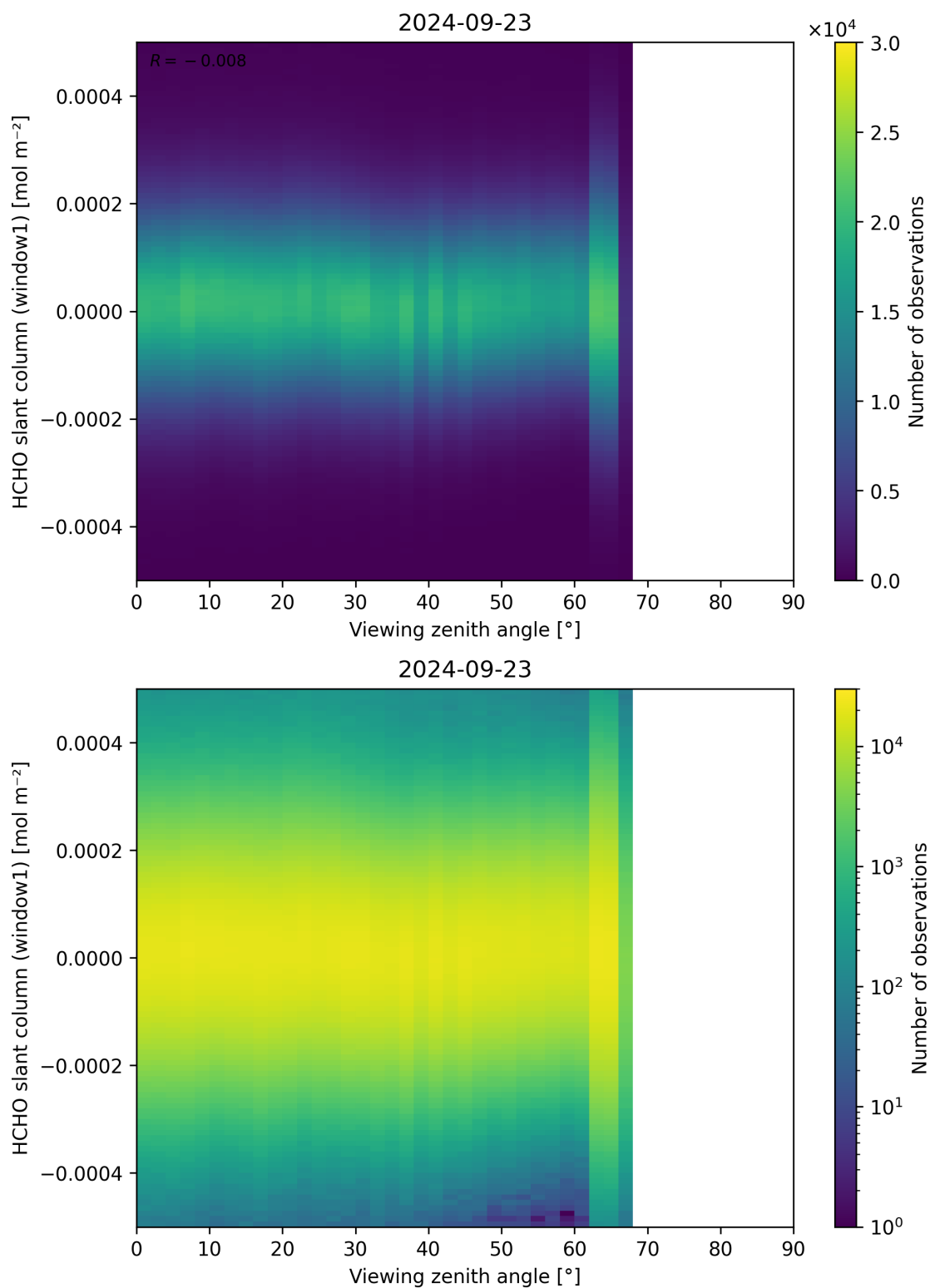
Figure 188: Scatter density plot of “Viewing zenith angle” against “HCHO slant column (window1)” for 2024-09-22 to 2024-09-24.
