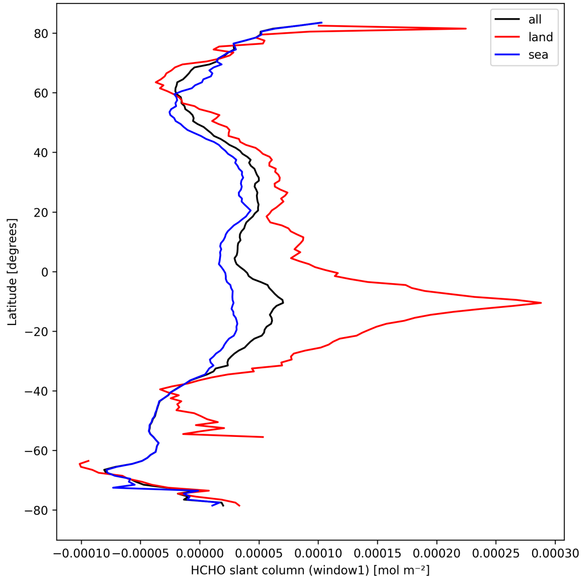
Figure 24: Zonal average of “HCHO slant column (window1)” for 2024-09-22 to 2024-09-24.
