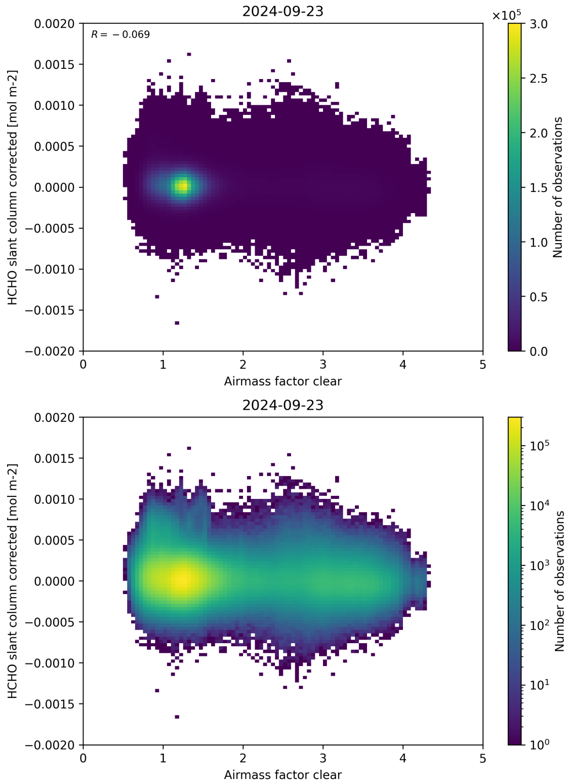
Figure 74: Scatter density plot of “Airmass factor clear” against “HCHO slant column corrected” for 2024-09-22 to 2024-09-24.
