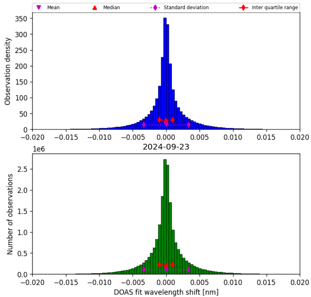
Figure 44: Histogram of “DOAS fit wavelength shift” for 2024-09-22 to 2024-09-24
