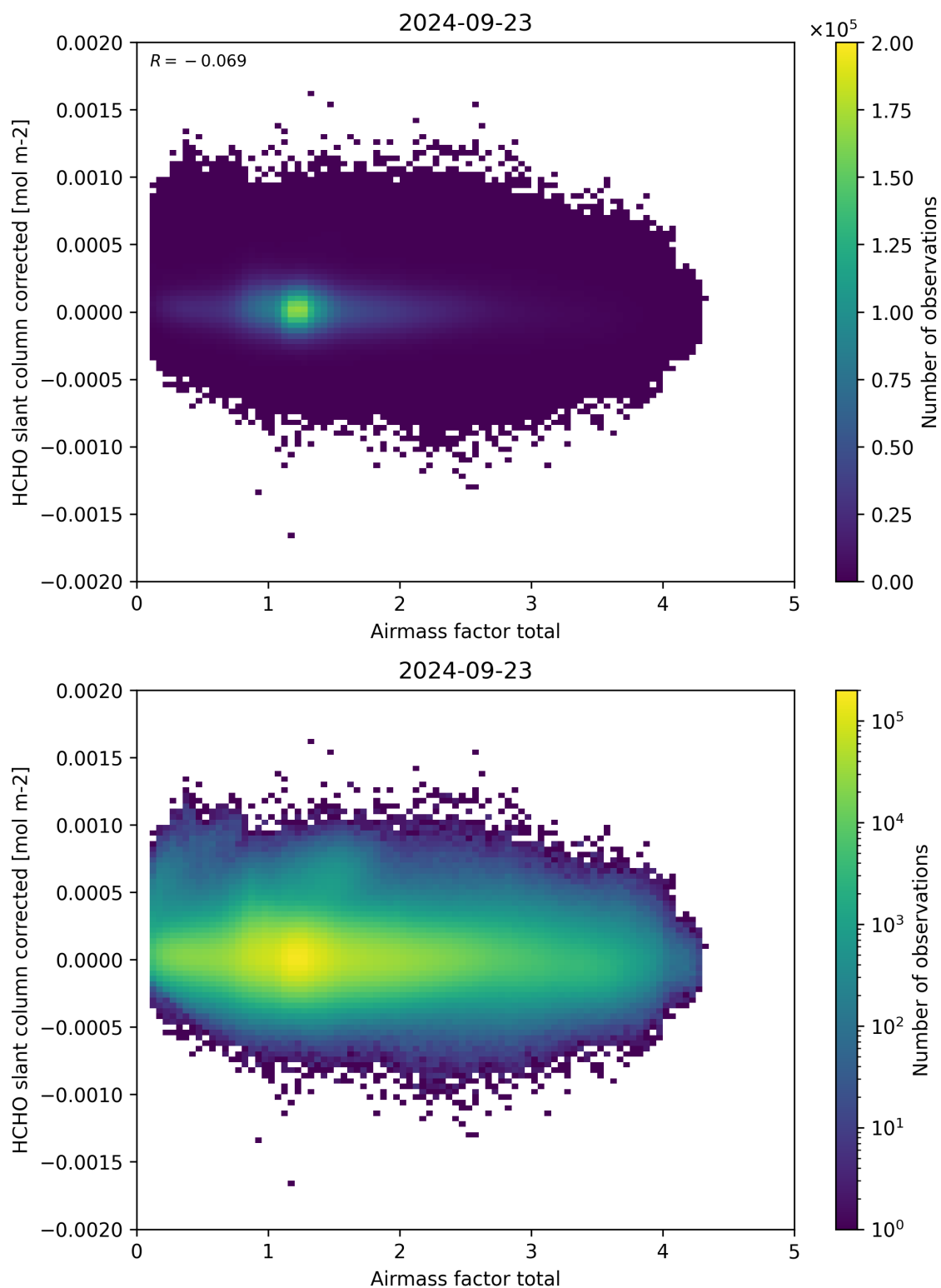
Figure 101: Scatter density plot of “Airmass factor total” against “HCHO slant column corrected” for 2024-09-22 to 2024-09-24.
