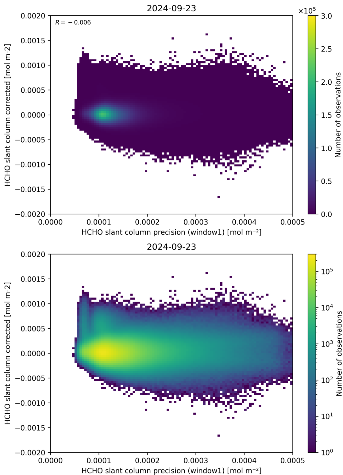
Figure 92: Scatter density plot of “HCHO slant column precision (window1)” against “HCHO slant column corrected” for 2024-09-22 to 2024-09-24.
