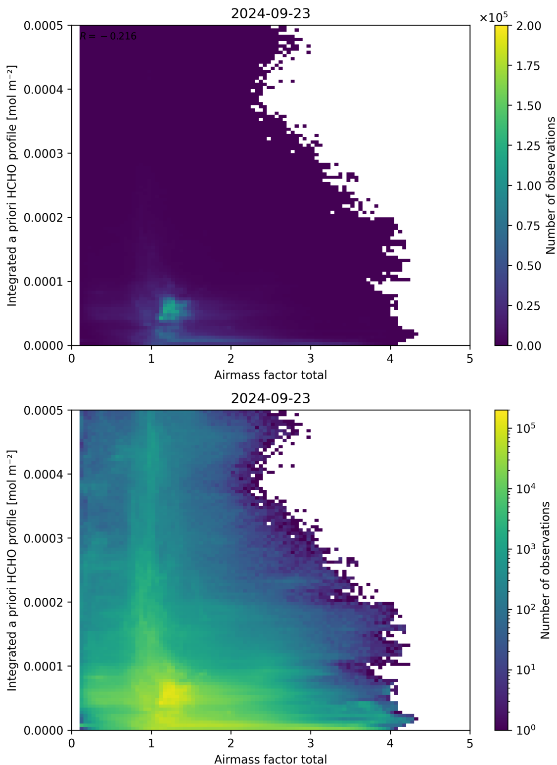
Figure 104: Scatter density plot of “Airmass factor total” against “Integrated a priori HCHO profile” for 2024-09-22 to 2024-09-24.
