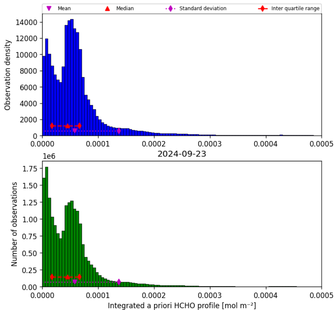
Figure 43: Histogram of “Integrated a priori HCHO profile” for 2024-09-22 to 2024-09-24
