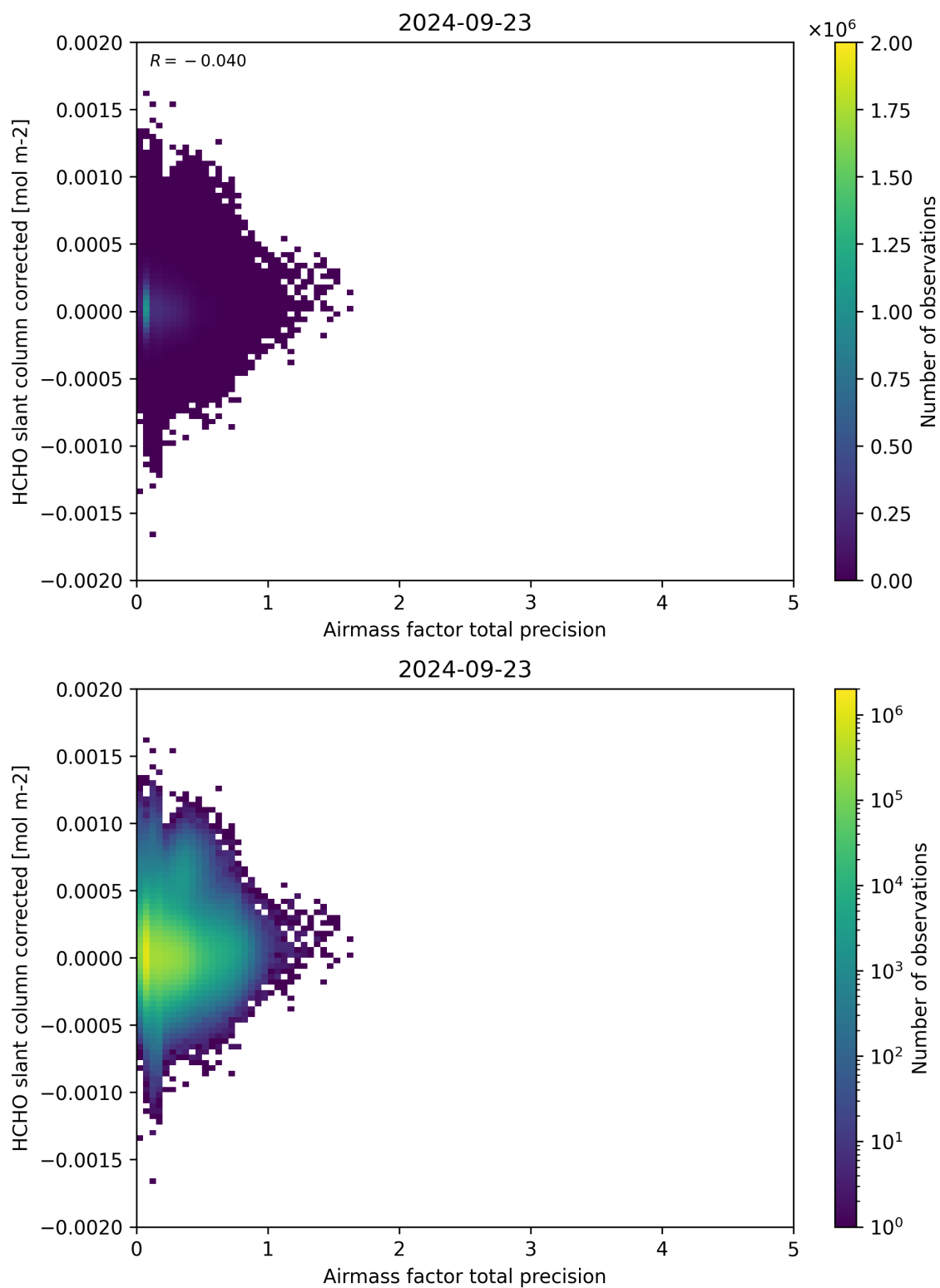
Figure 109: Scatter density plot of “Airmass factor total precision” against “HCHO slant column corrected” for 2024-09-22 to 2024-09-24.
