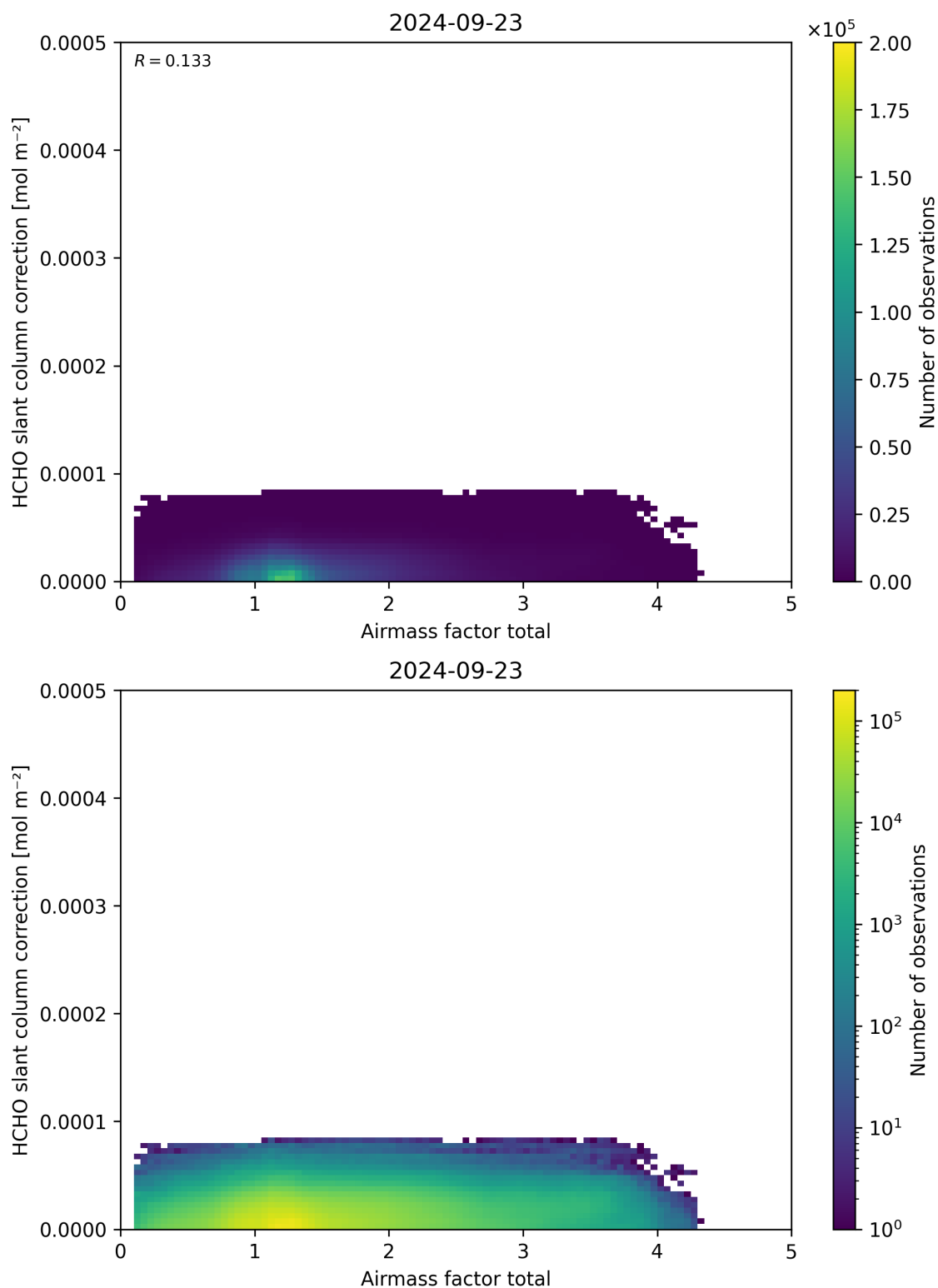
Figure 102: Scatter density plot of “Airmass factor total” against “HCHO slant column correction” for 2024-09-22 to 2024-09-24.
