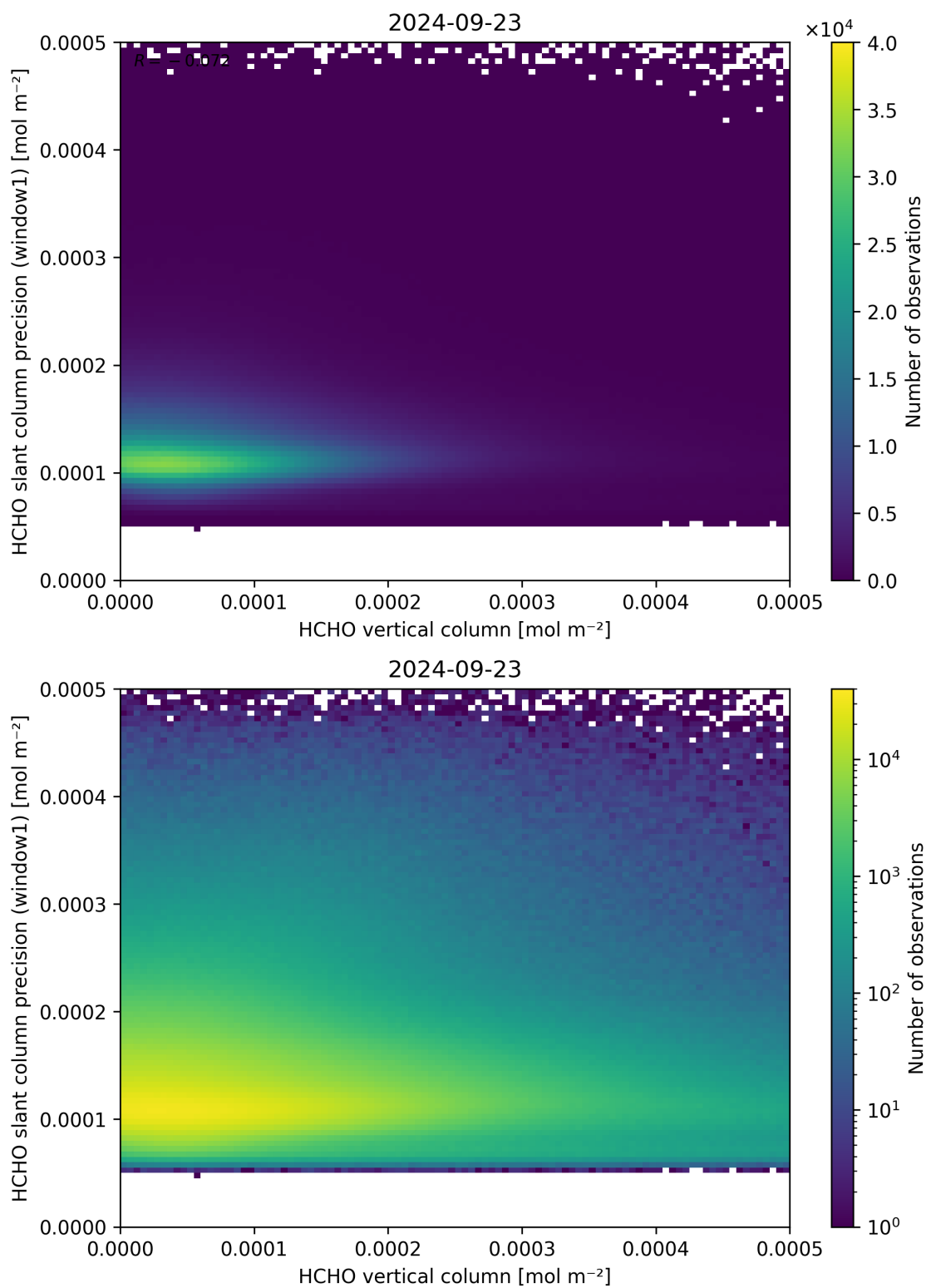
Figure 130: Scatter density plot of “HCHO vertical column” against “HCHO slant column precision (window1)” for 2024-09-22 to 2024-09-24.
