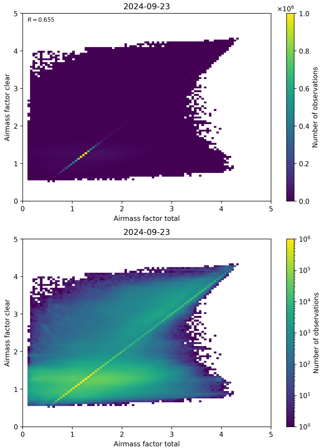
Figure 100: Scatter density plot of “Airmass factor total” against “Airmass factor clear” for 2024-09-22 to 2024-09-24.
