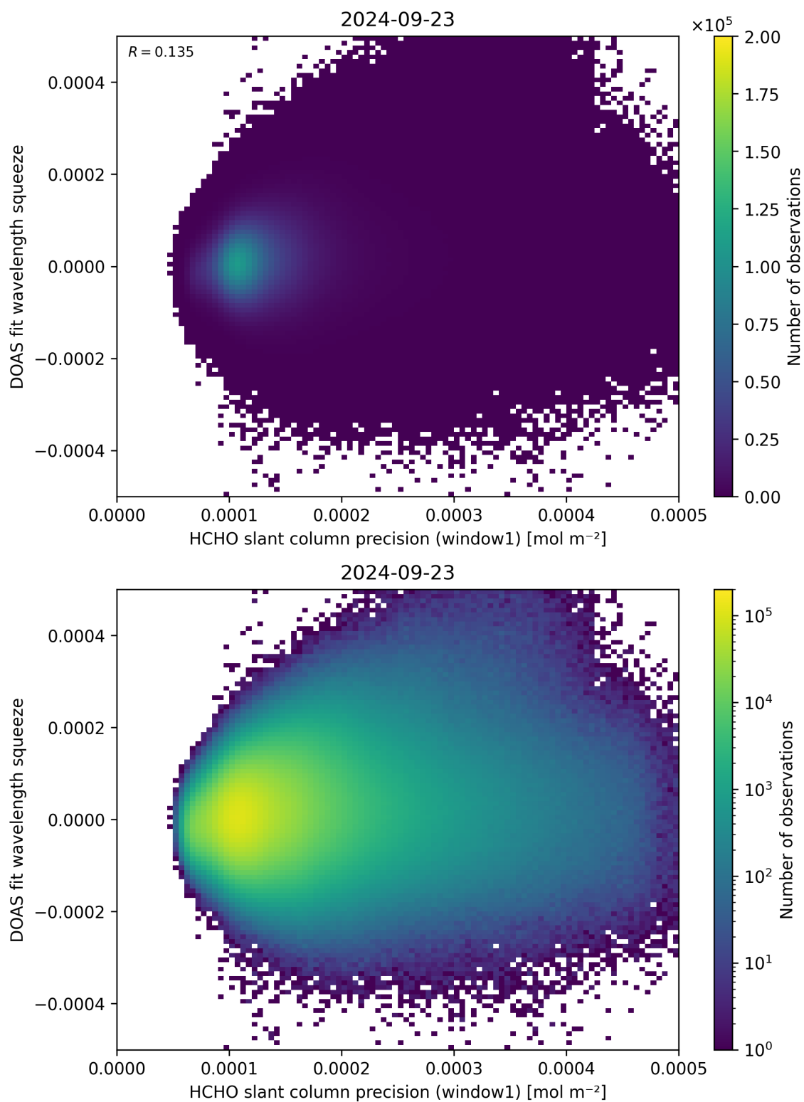
Figure 90: Scatter density plot of “HCHO slant column precision (window1)” against “DOAS fit wavelength squeeze” for 2024-09-22 to 2024-09-24.
