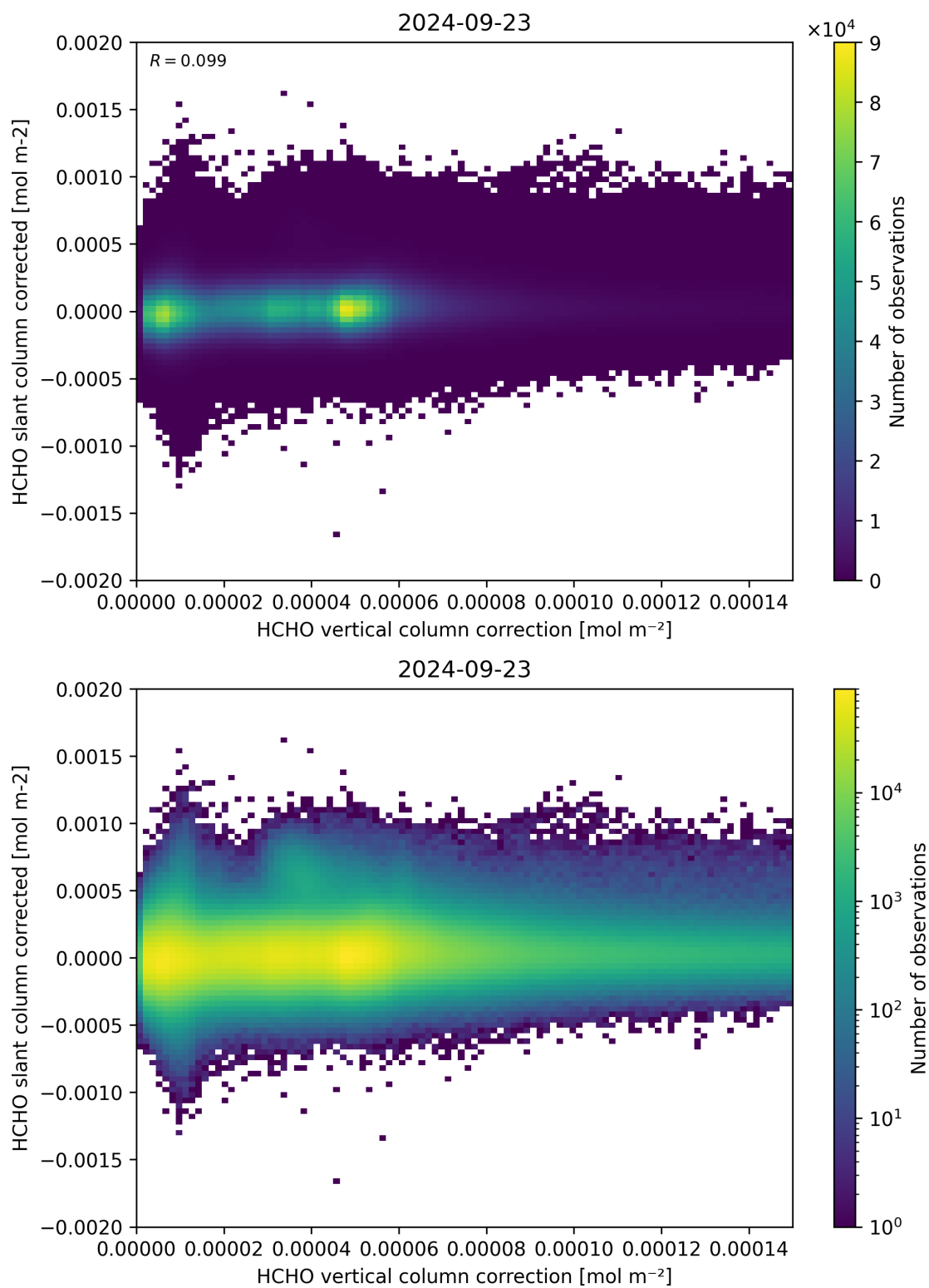
Figure 116: Scatter density plot of “HCHO vertical column correction” against “HCHO slant column corrected” for 2024-09-22 to 2024-09-24.
