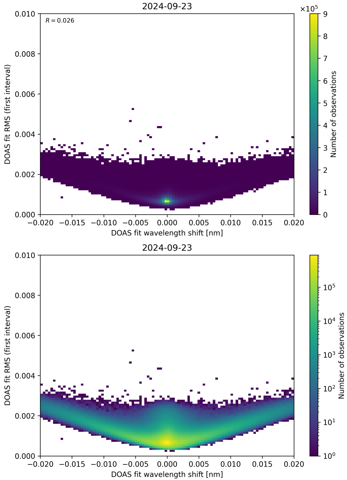
Figure 64: Scatter density plot of “DOAS fit wavelength shift” against “DOAS fit RMS (first interval)” for 2024-09-22 to 2024-09-24.
