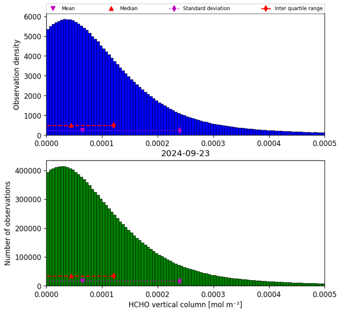
Figure 35: Histogram of “HCHO vertical column” for 2024-09-22 to 2024-09-24
