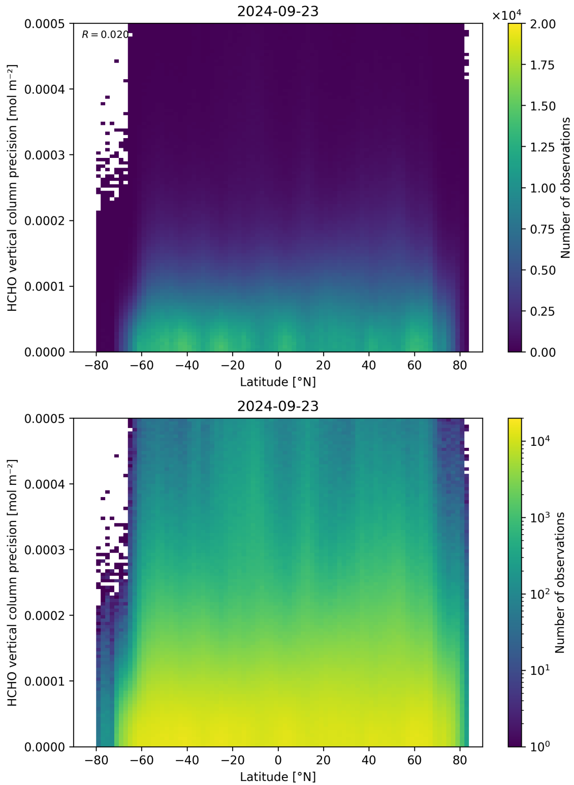
Figure 165: Scatter density plot of “Latitude” against “HCHO vertical column precision” for 2024-09-22 to 2024-09-24.
