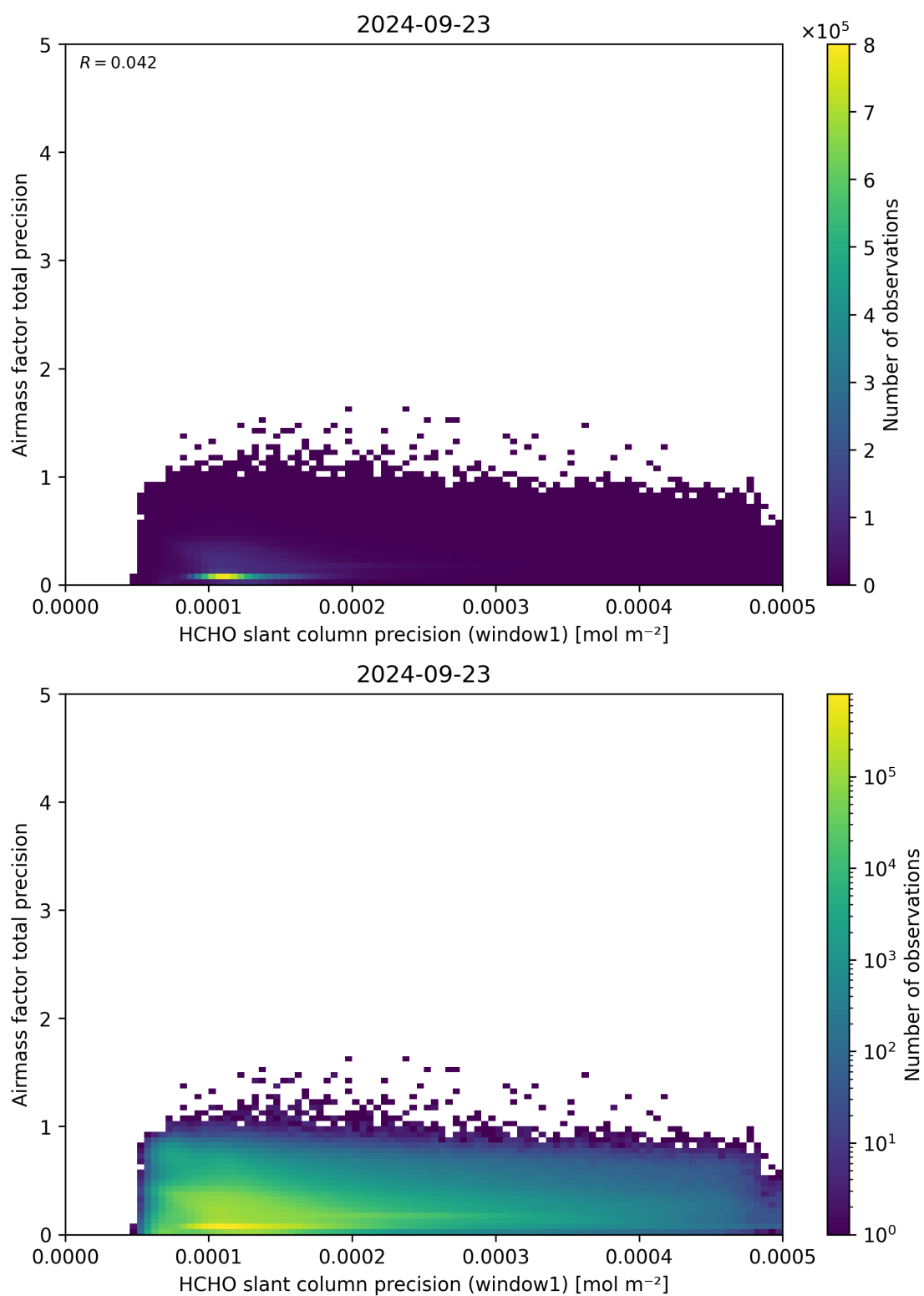
Figure 95: Scatter density plot of “HCHO slant column precision (window1)” against “Airmass factor total precision” for 2024-09-22 to 2024-09-24.
