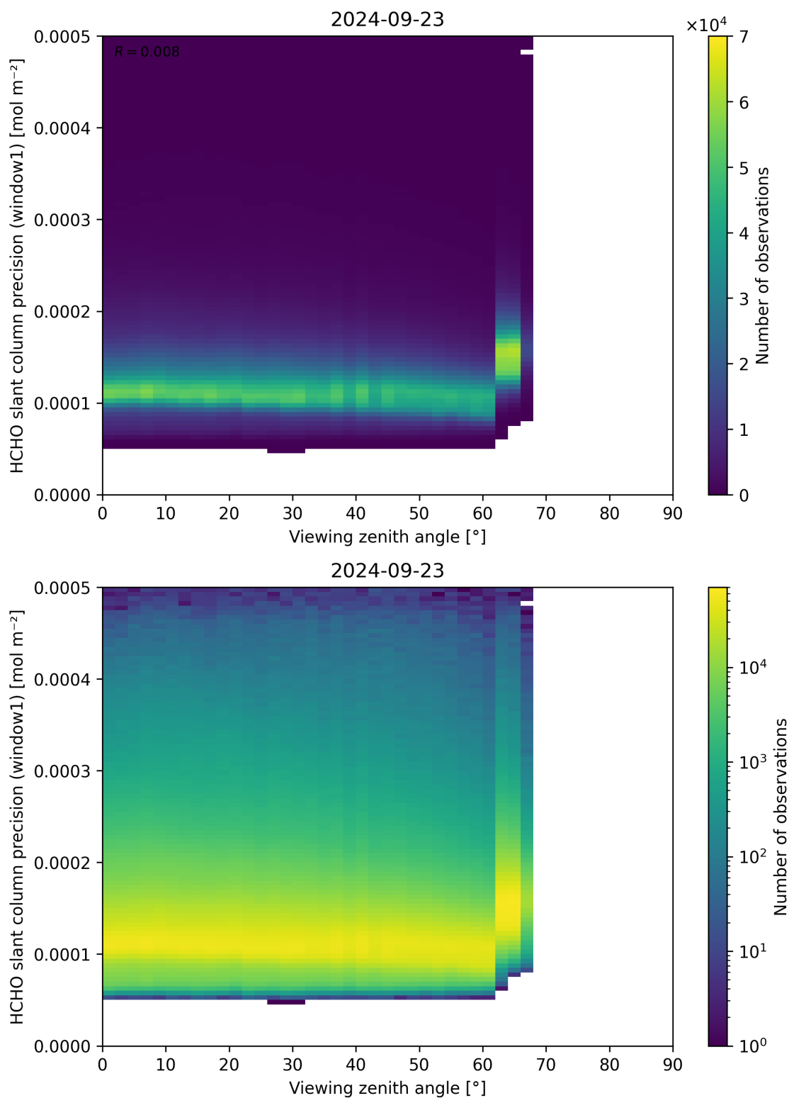
Figure 189: Scatter density plot of “Viewing zenith angle” against “HCHO slant column precision (window1)” for 2024-09-22 to 2024-09-24.
