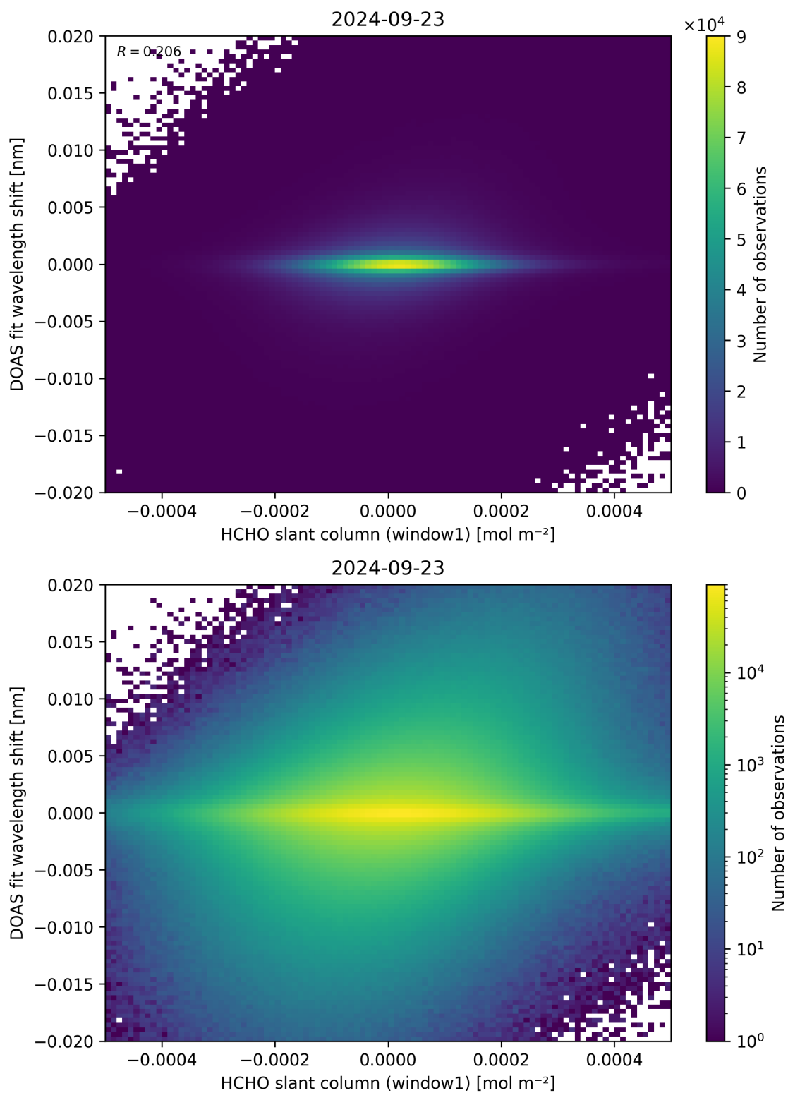
Figure 79: Scatter density plot of “HCHO slant column (window1)” against “DOAS fit wavelength shift” for 2024-09-22 to 2024-09-24.
