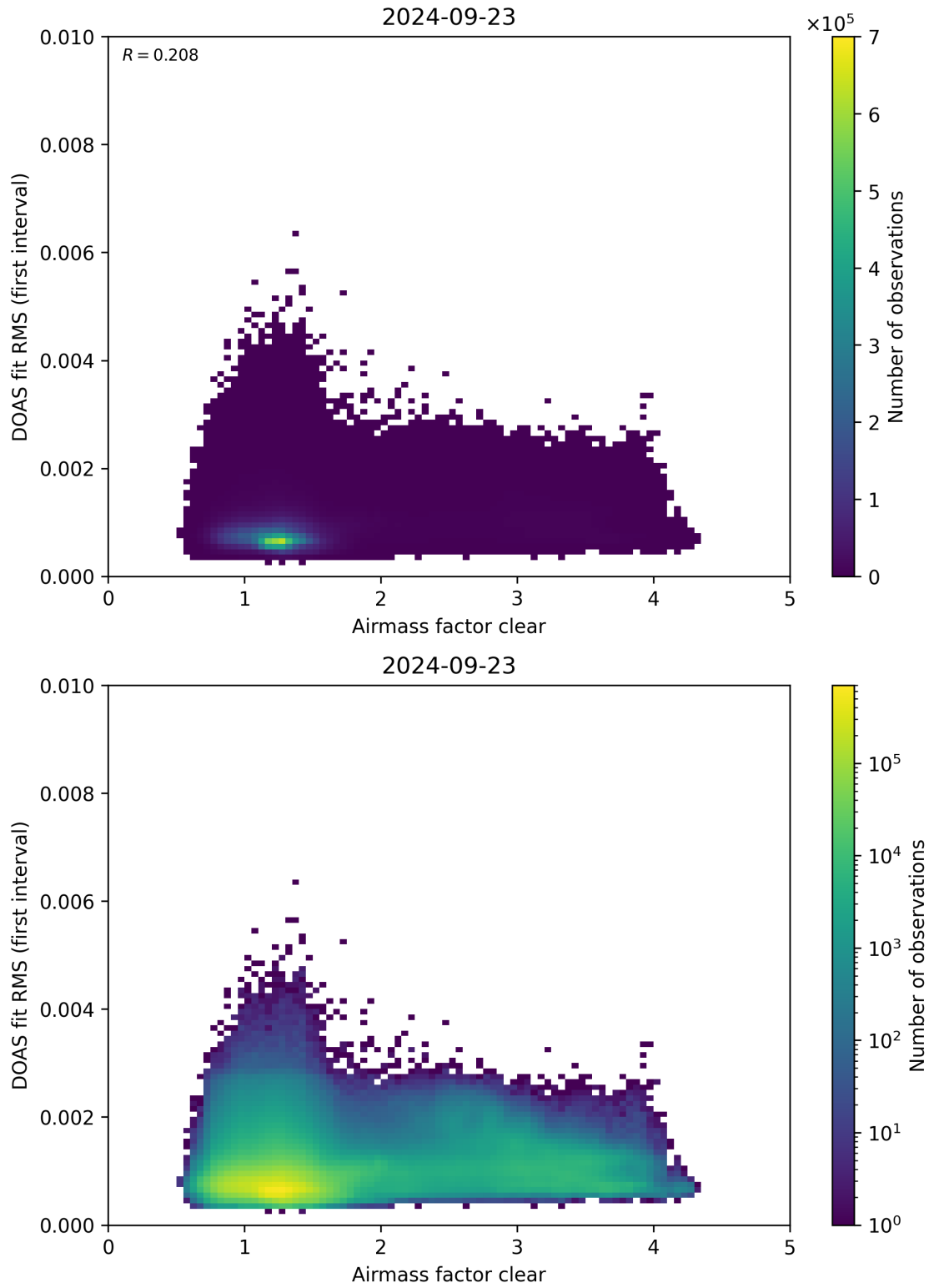
Figure 71: Scatter density plot of “Airmass factor clear” against “DOAS fit RMS (first interval)” for 2024-09-22 to 2024-09-24.
