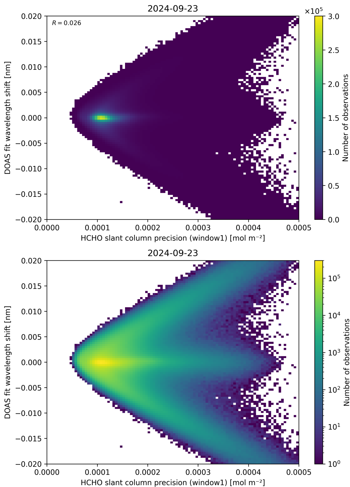
Figure 89: Scatter density plot of “HCHO slant column precision (window1)” against “DOAS fit wavelength shift” for 2024-09-22 to 2024-09-24.
