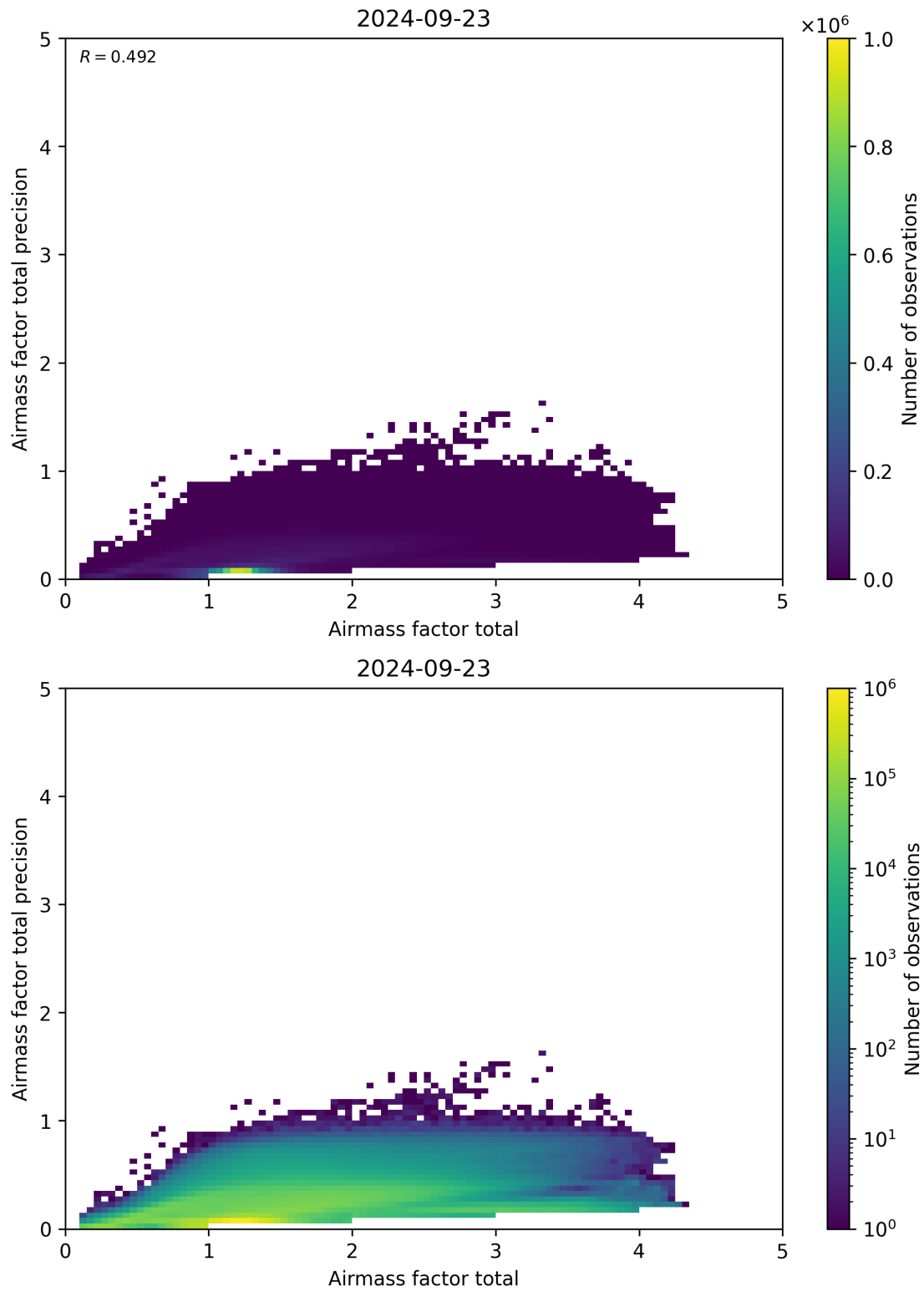
Figure 103: Scatter density plot of “Airmass factor total” against “Airmass factor total precision” for 2024-09-22 to 2024-09-24.
