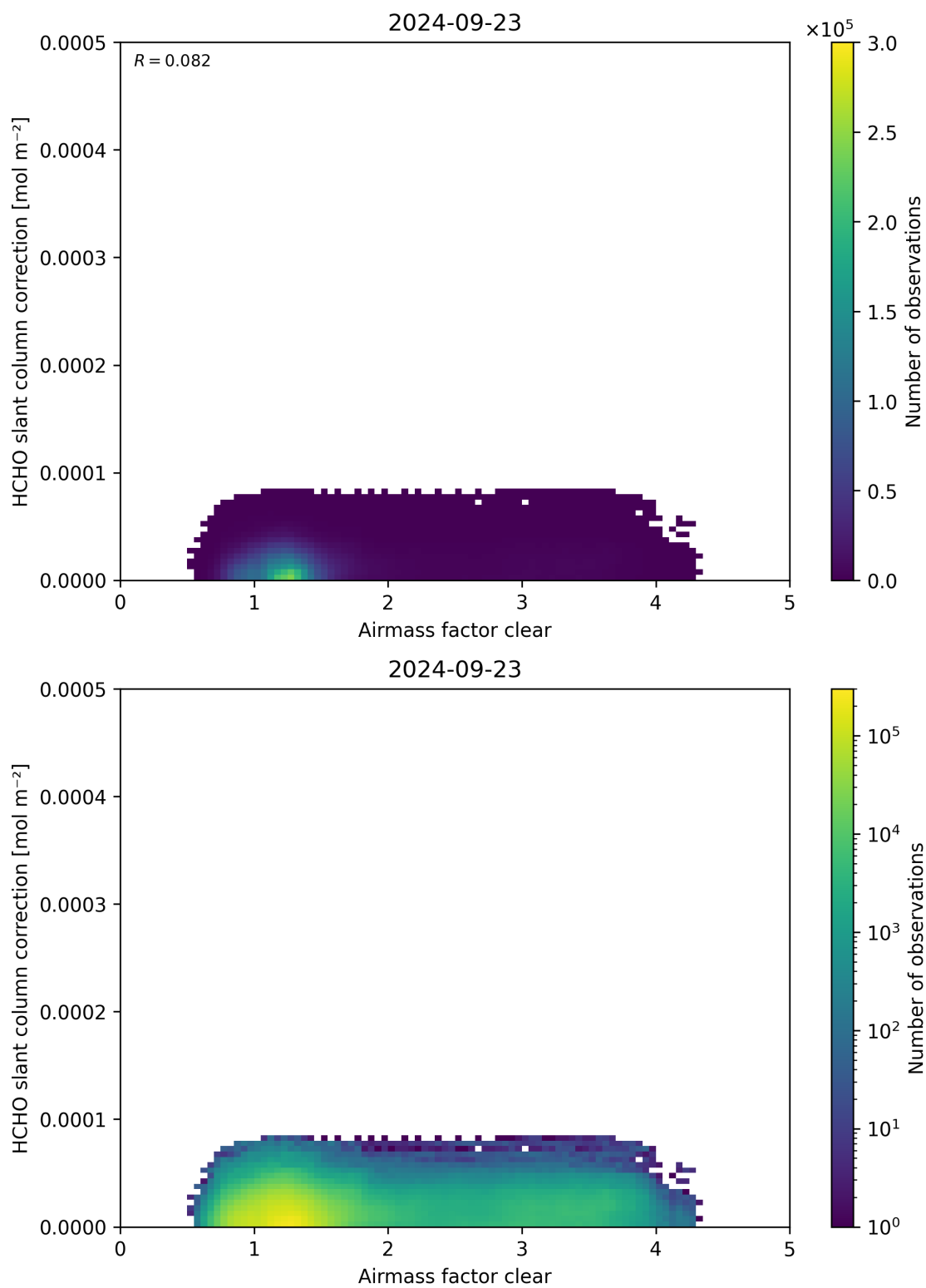
Figure 75: Scatter density plot of “Airmass factor clear” against “HCHO slant column correction” for 2024-09-22 to 2024-09-24.
