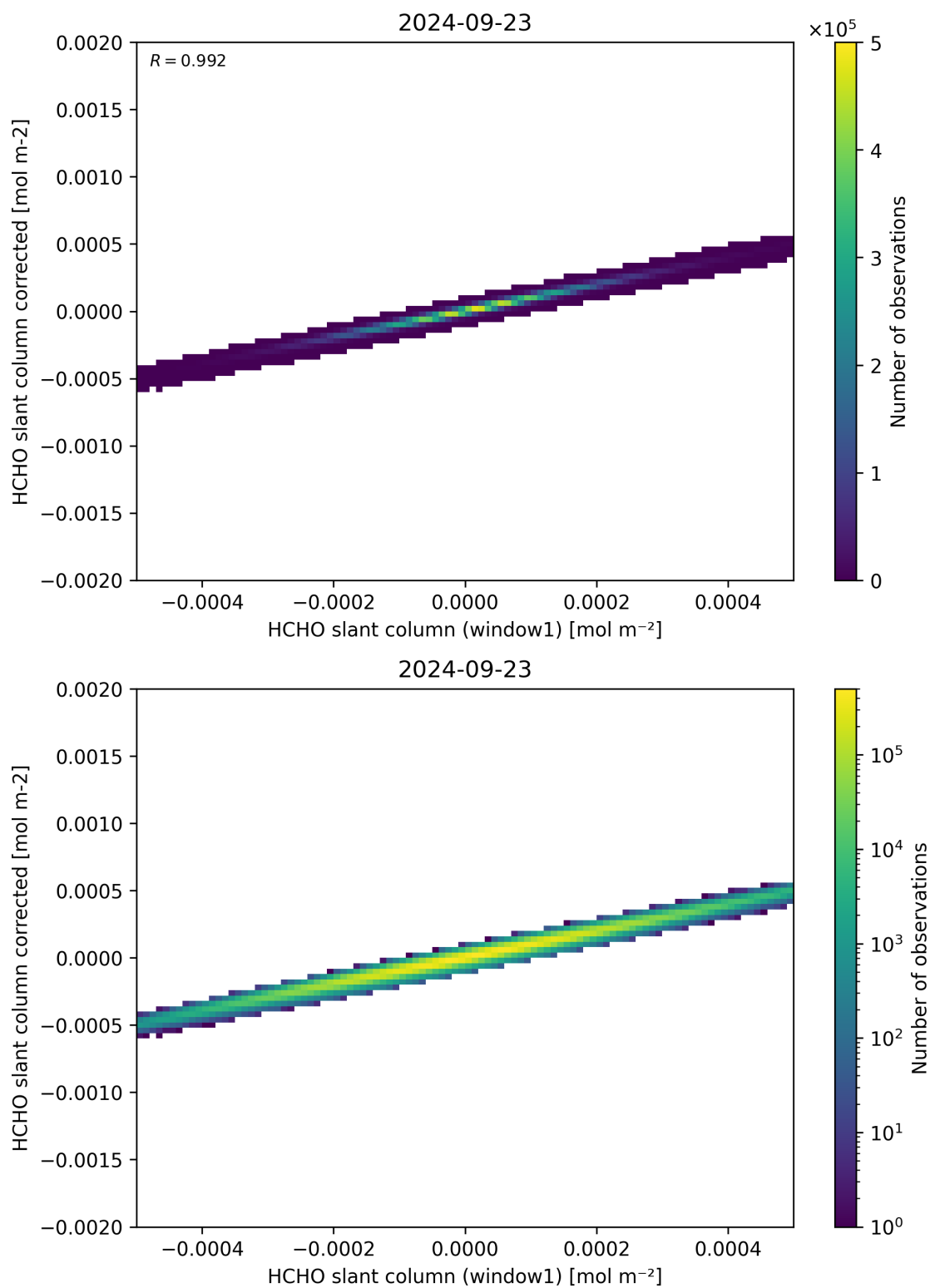
Figure 82: Scatter density plot of “HCHO slant column (window1)” against “HCHO slant column corrected” for 2024-09-22 to 2024-09-24.
