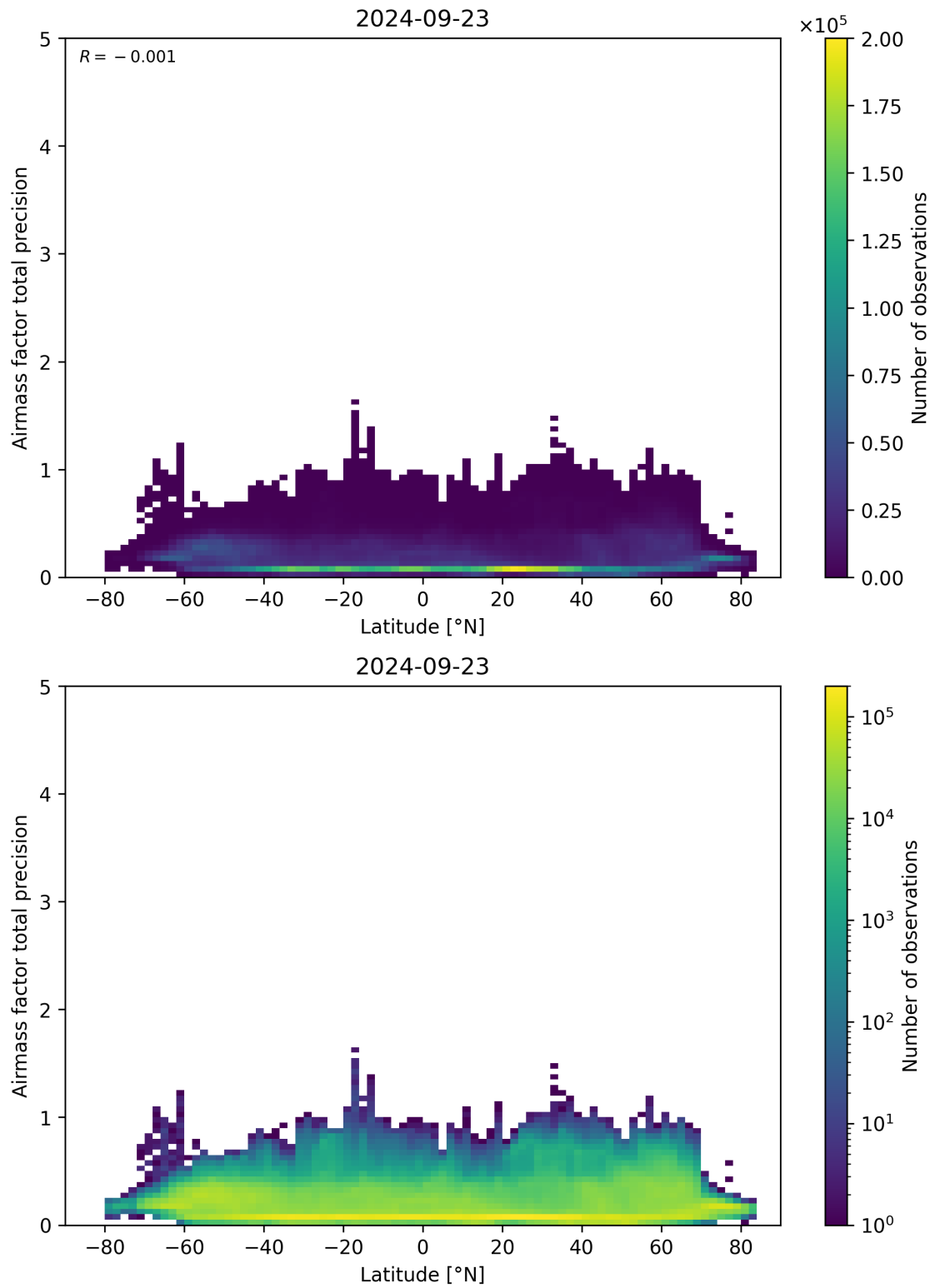
Figure 162: Scatter density plot of “Latitude” against “Airmass factor total precision” for 2024-09-22 to 2024-09-24.
