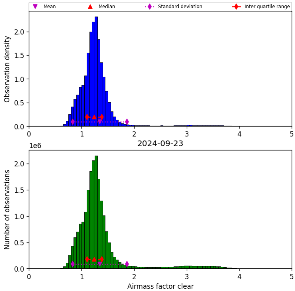
Figure 42: Histogram of “Airmass factor clear” for 2024-09-22 to 2024-09-24
