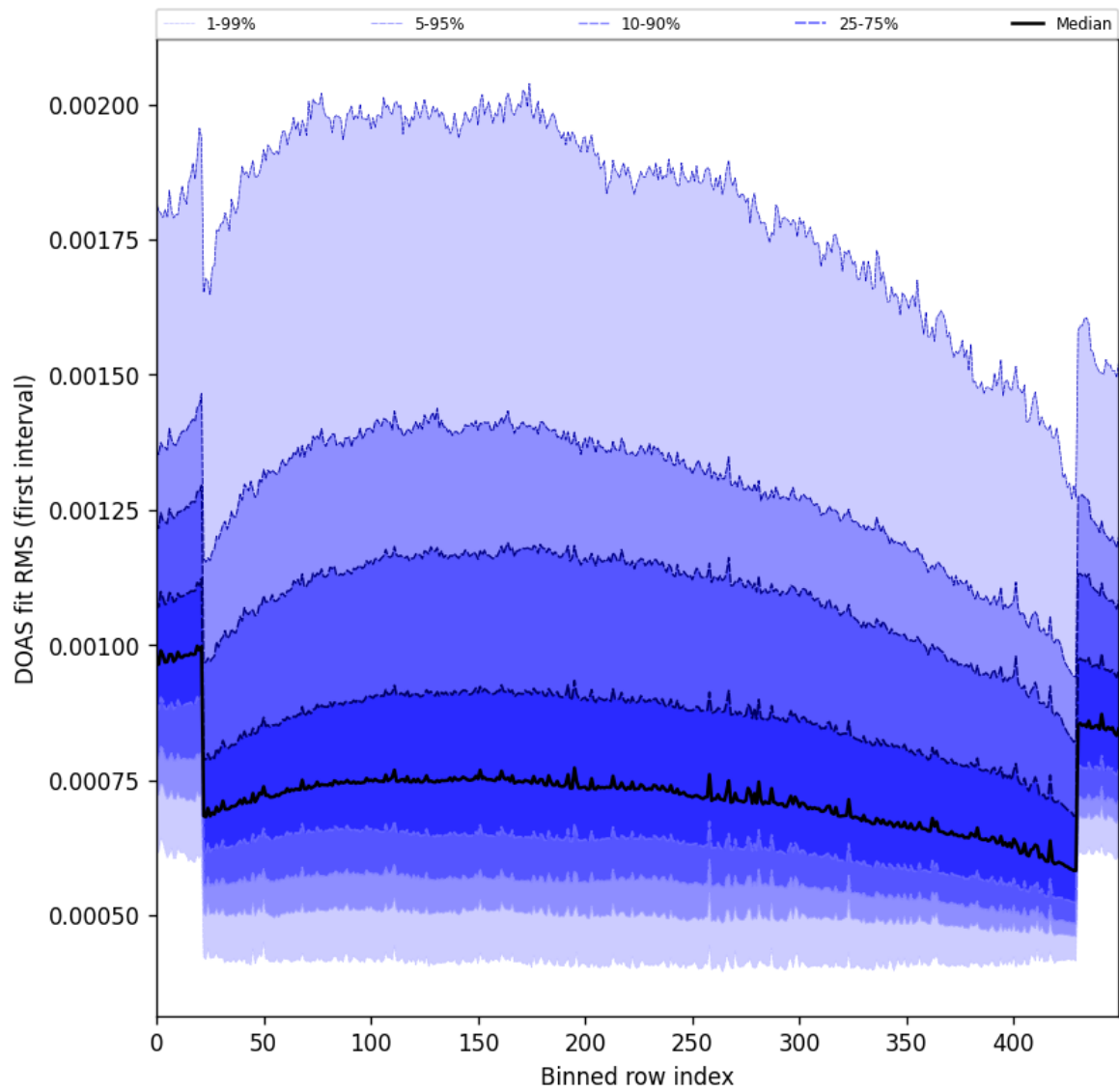
Figure 60: Along track statistics of “DOAS fit RMS (first interval)” for 2024-09-22 to 2024-09-24
