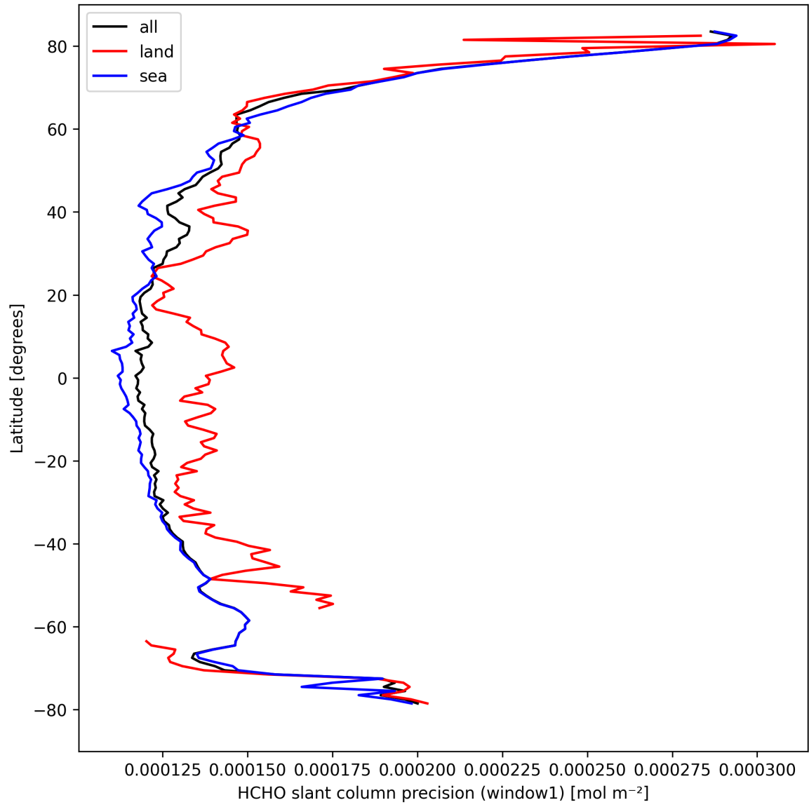
Figure 25: Zonal average of “HCHO slant column precision (window1)” for 2024-09-22 to 2024-09-24.
