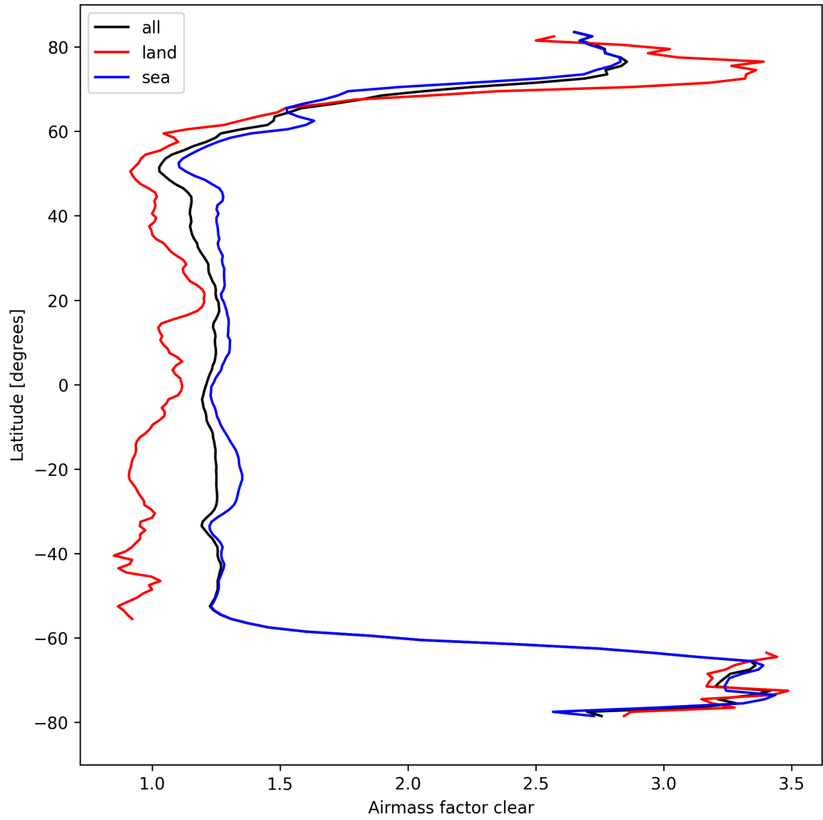
Figure 28: Zonal average of “Airmass factor clear” for 2024-09-22 to 2024-09-24.
