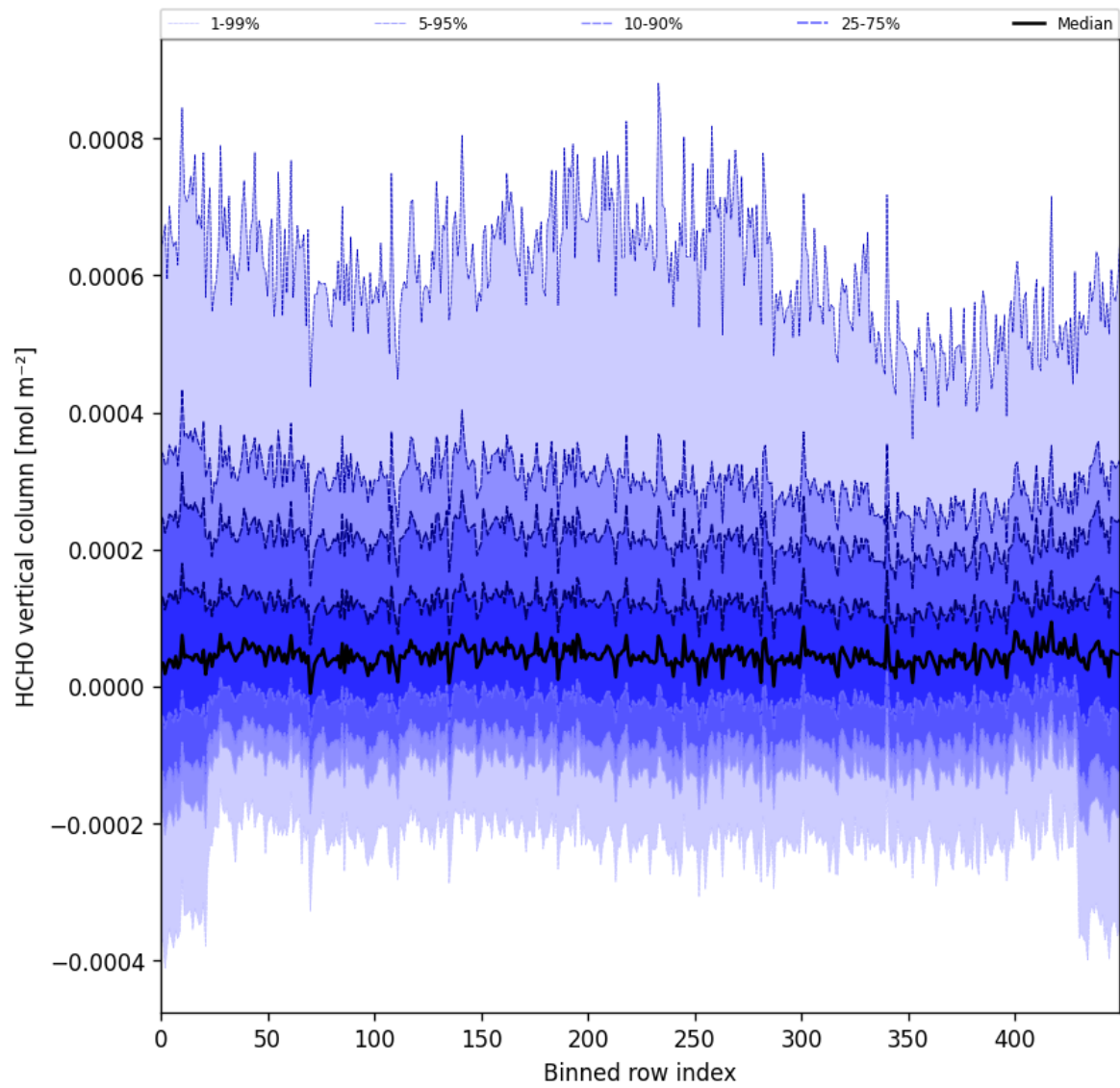
Figure 49: Along track statistics of “HCHO vertical column” for 2024-09-22 to 2024-09-24
