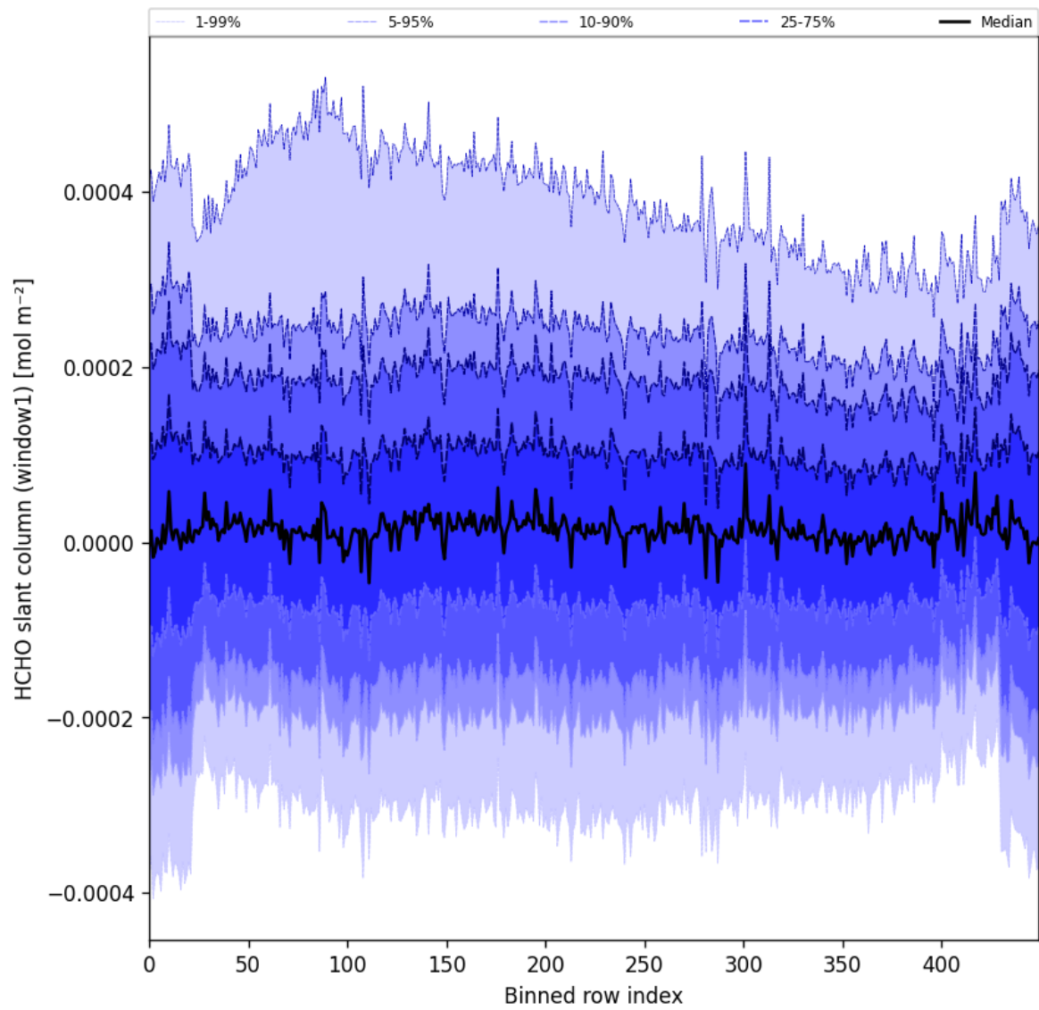
Figure 52: Along track statistics of “HCHO slant column (window1)” for 2024-09-22 to 2024-09-24
