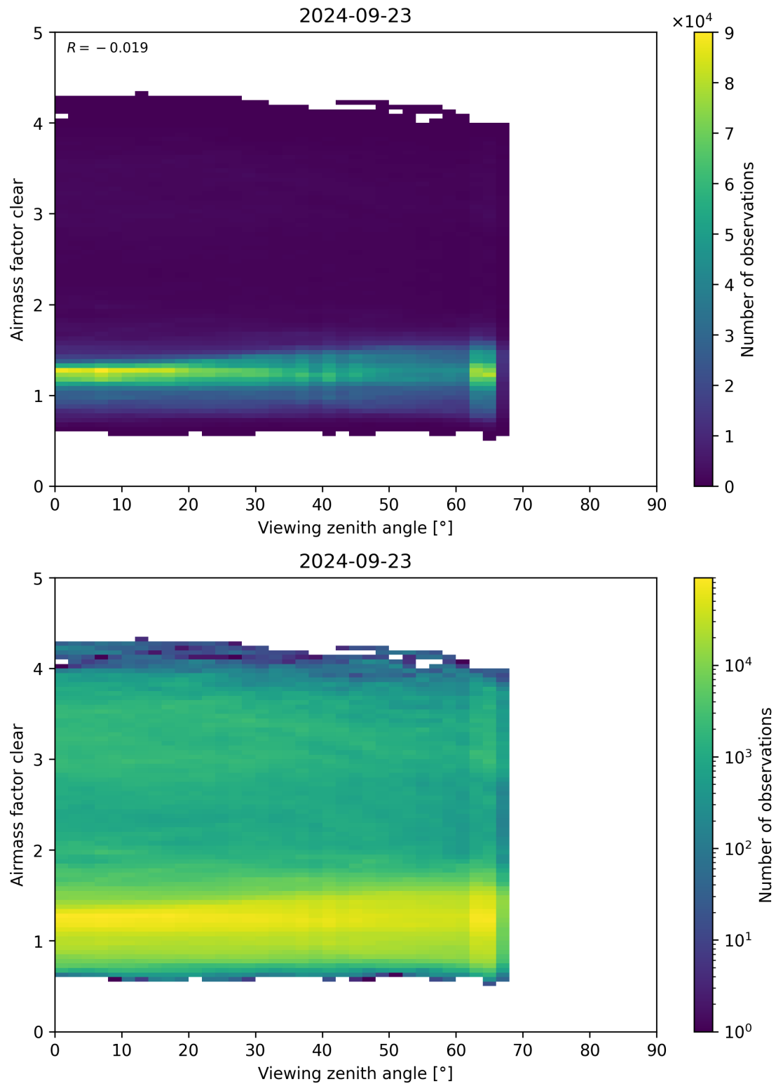
Figure 185: Scatter density plot of “Viewing zenith angle” against “Airmass factor clear” for 2024-09-22 to 2024-09-24.
