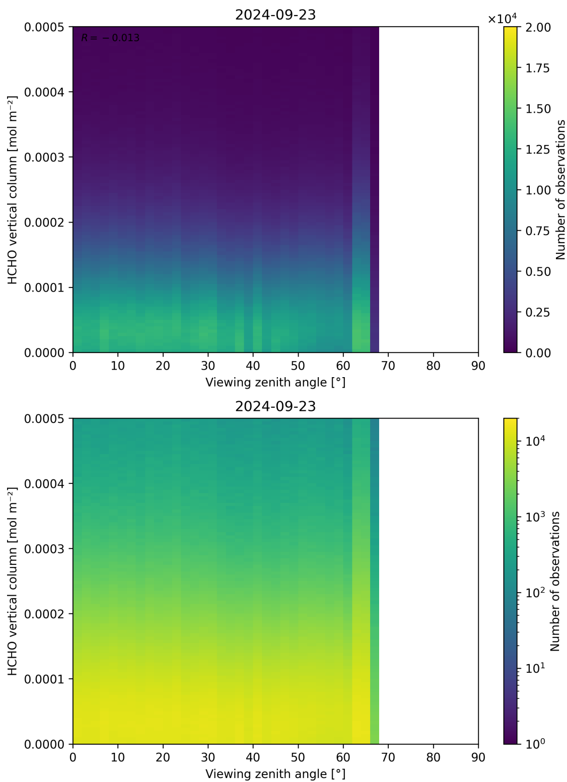
Figure 192: Scatter density plot of “Viewing zenith angle” against “HCHO vertical column” for 2024-09-22 to 2024-09-24.
