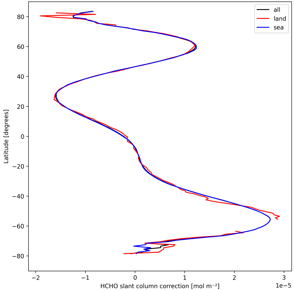
Figure 33: Zonal average of “HCHO slant column correction” for 2024-09-22 to 2024-09-24.
