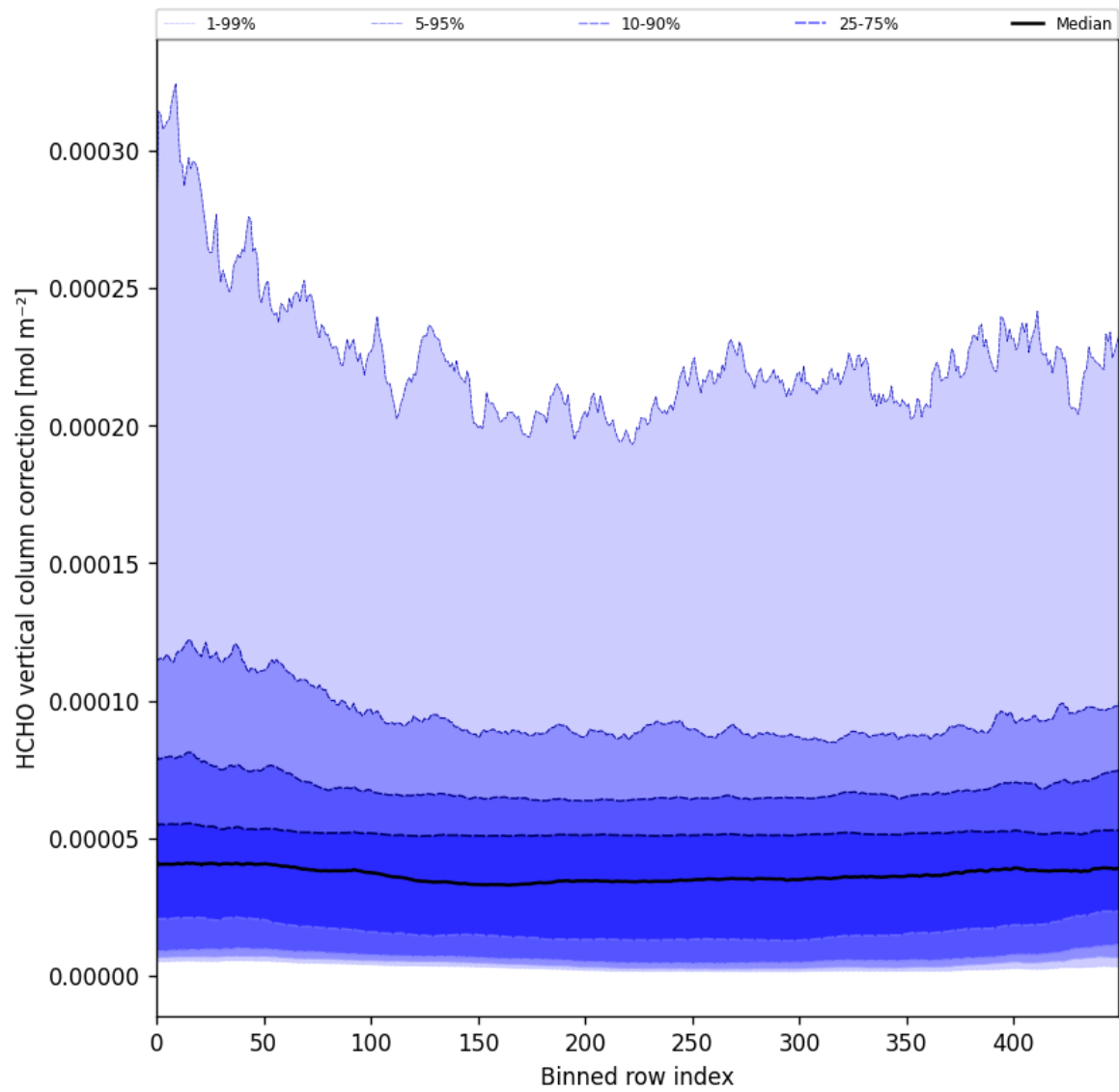
Figure 51: Along track statistics of “HCHO vertical column correction” for 2024-09-22 to 2024-09-24
