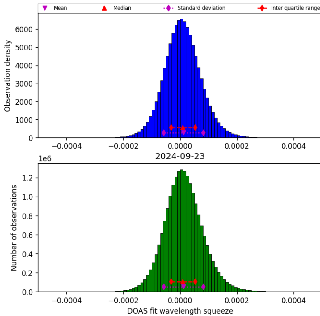
Figure 45: Histogram of “DOAS fit wavelength squeeze” for 2024-09-22 to 2024-09-24
