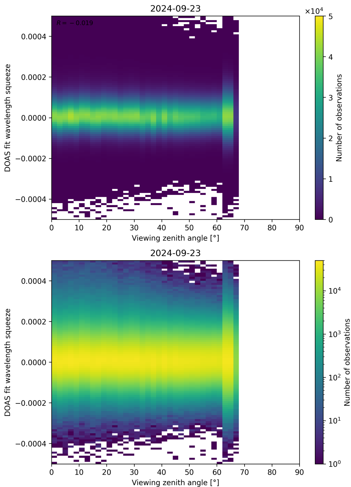
Figure 184: Scatter density plot of “Viewing zenith angle” against “DOAS fit wavelength squeeze” for 2024-09-22 to 2024-09-24.
