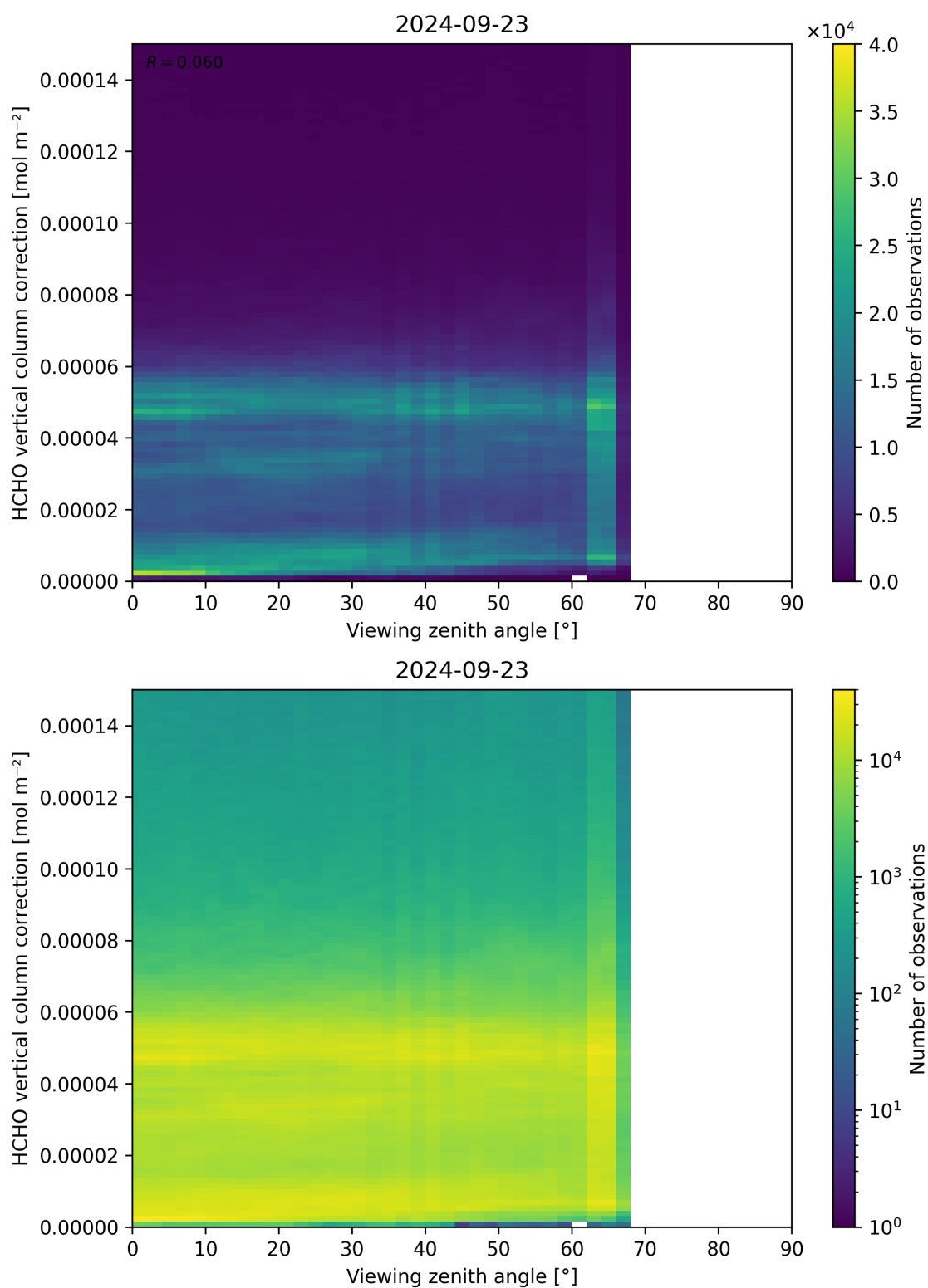
Figure 193: Scatter density plot of “Viewing zenith angle” against “HCHO vertical column correction” for 2024-09-22 to 2024-09-24.
