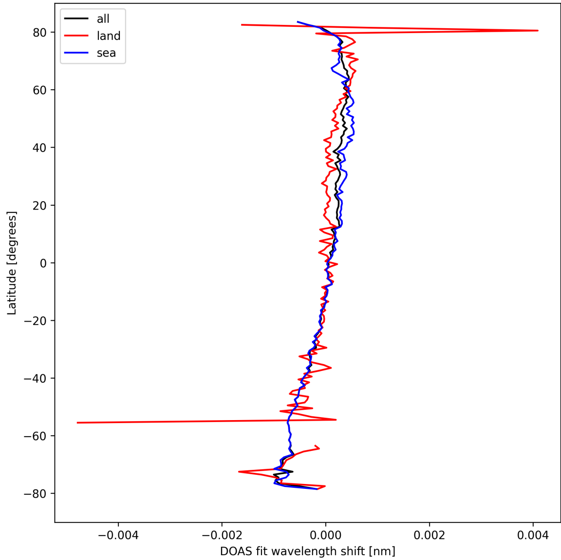
Figure 30: Zonal average of “DOAS fit wavelength shift” for 2024-09-22 to 2024-09-24.
