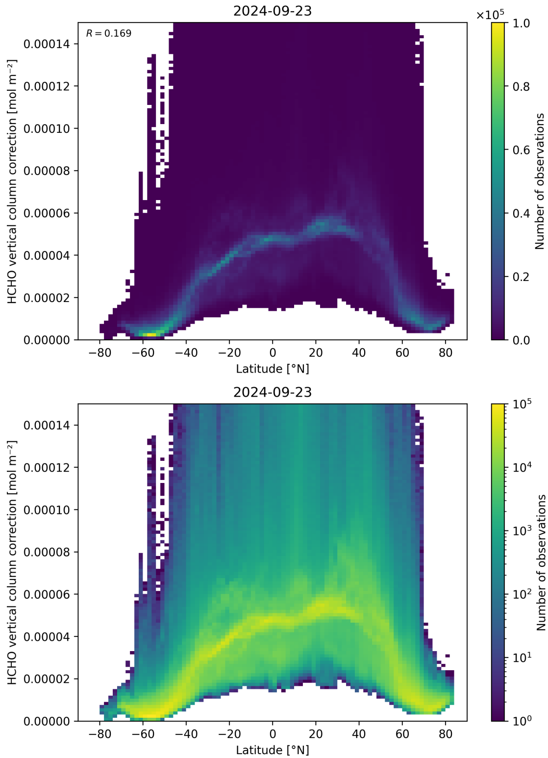
Figure 164: Scatter density plot of “Latitude” against “HCHO vertical column correction” for 2024-09-22 to 2024-09-24.
