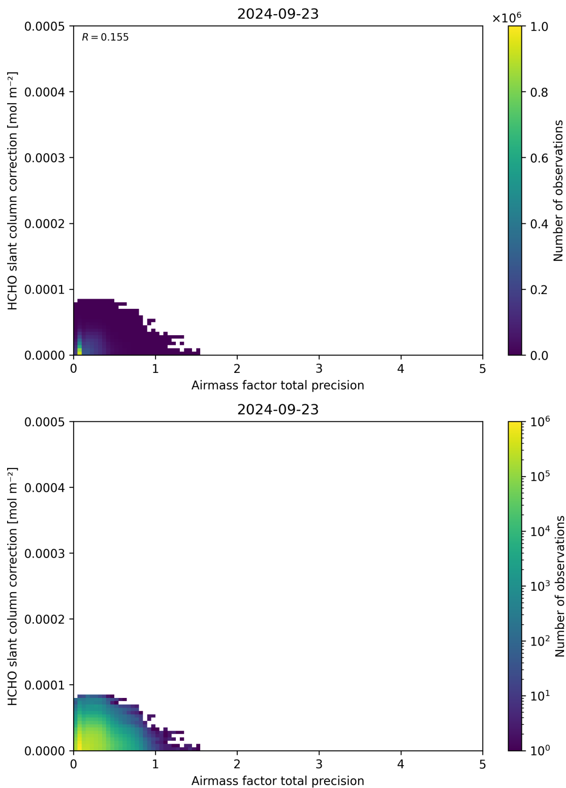
Figure 110: Scatter density plot of “Airmass factor total precision” against “HCHO slant column correction” for 2024-09-22 to 2024-09-24.
