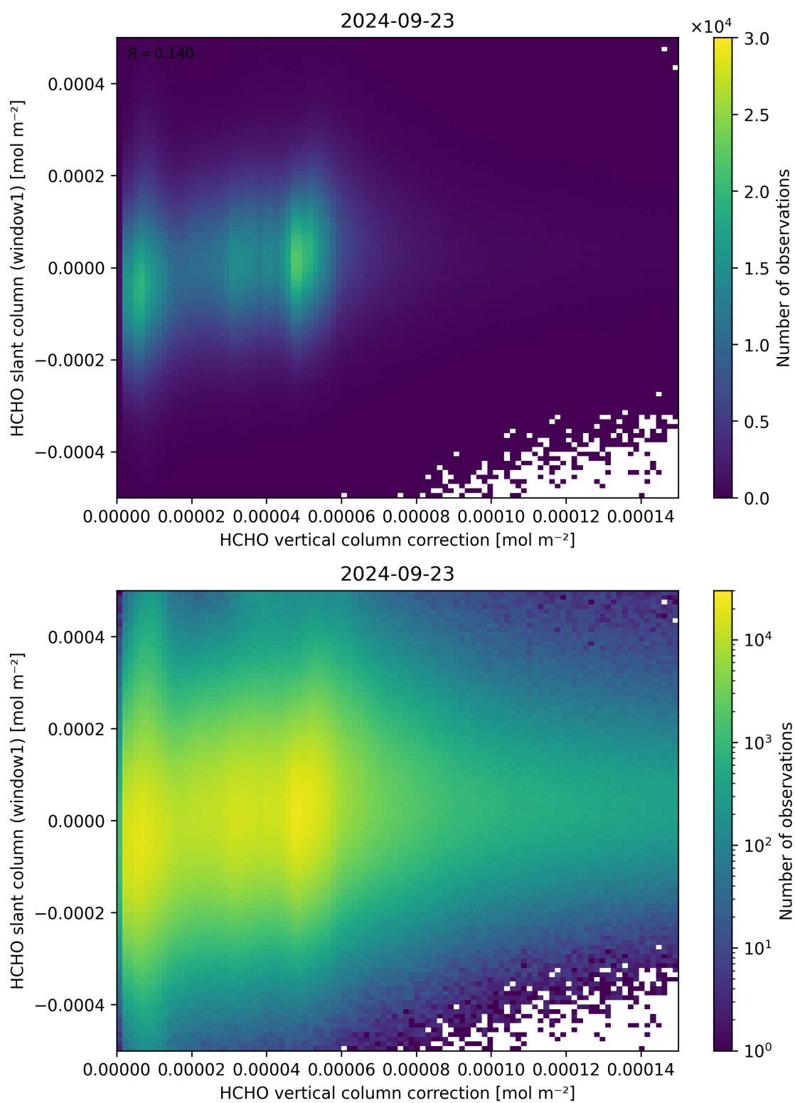
Figure 118: Scatter density plot of “HCHO vertical column correction” against “HCHO slant column (window1)” for 2024-09-22 to 2024-09-24.
