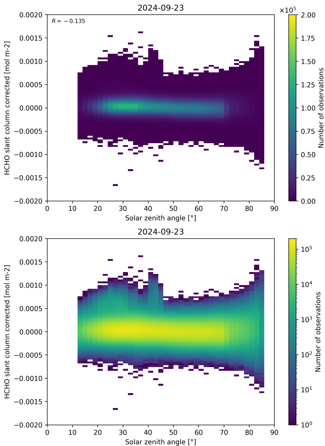
Figure 171: Scatter density plot of “Solar zenith angle” against “HCHO slant column corrected” for 2024-09-22 to 2024-09-24.
