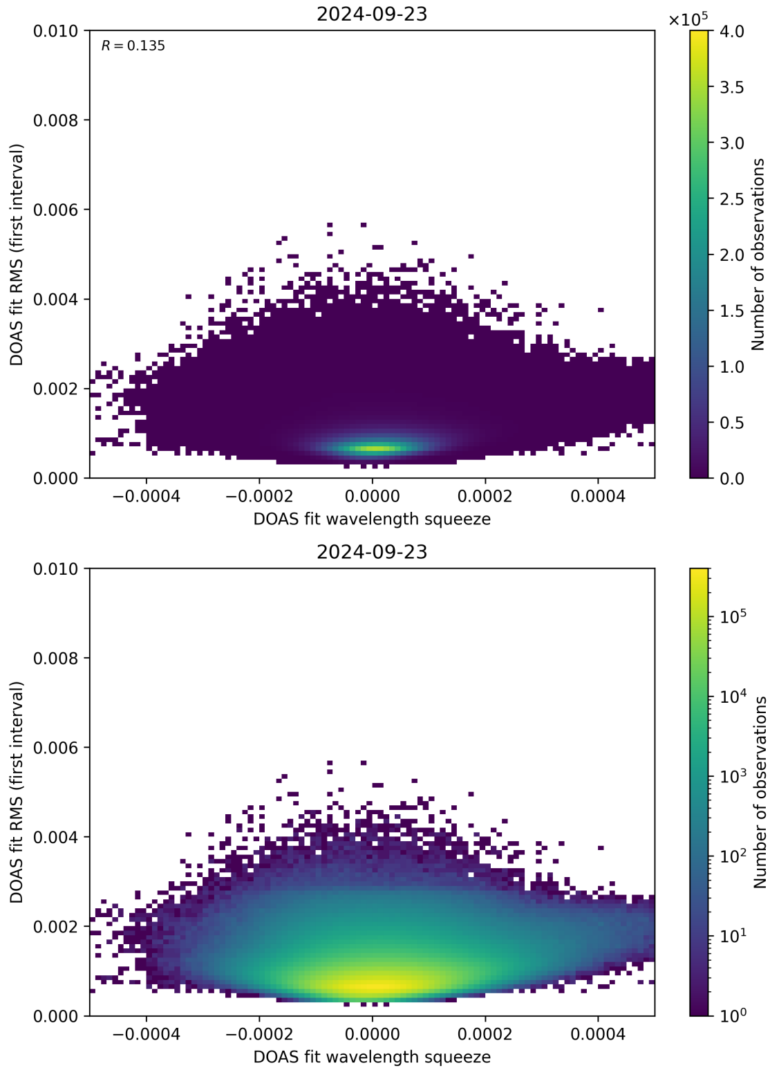
Figure 68: Scatter density plot of “DOAS fit wavelength squeeze” against “DOAS fit RMS (first interval)” for 2024-09-22 to 2024-09-24.
