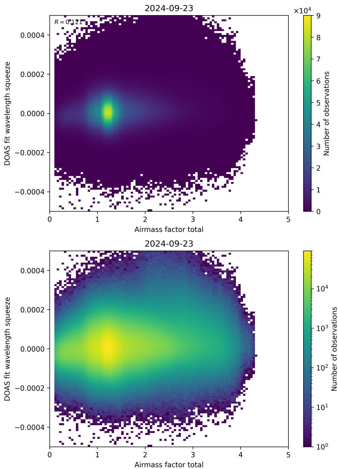
Figure 99: Scatter density plot of “Airmass factor total” against “DOAS fit wavelength squeeze” for 2024-09-22 to 2024-09-24.
