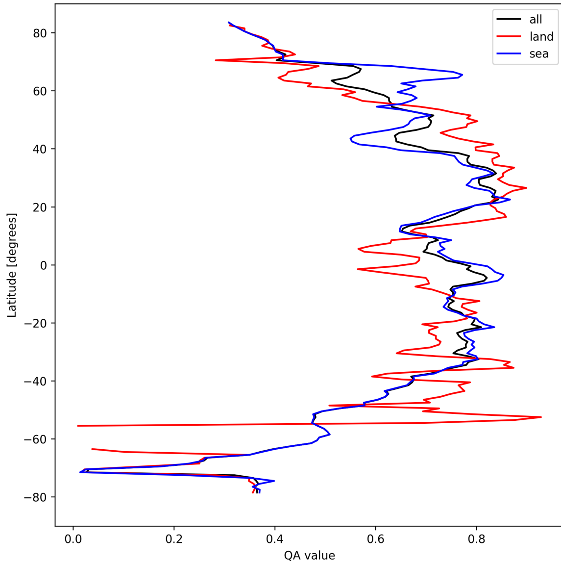
Figure 20: Zonal average of “QA value” for 2024-09-22 to 2024-09-24.
