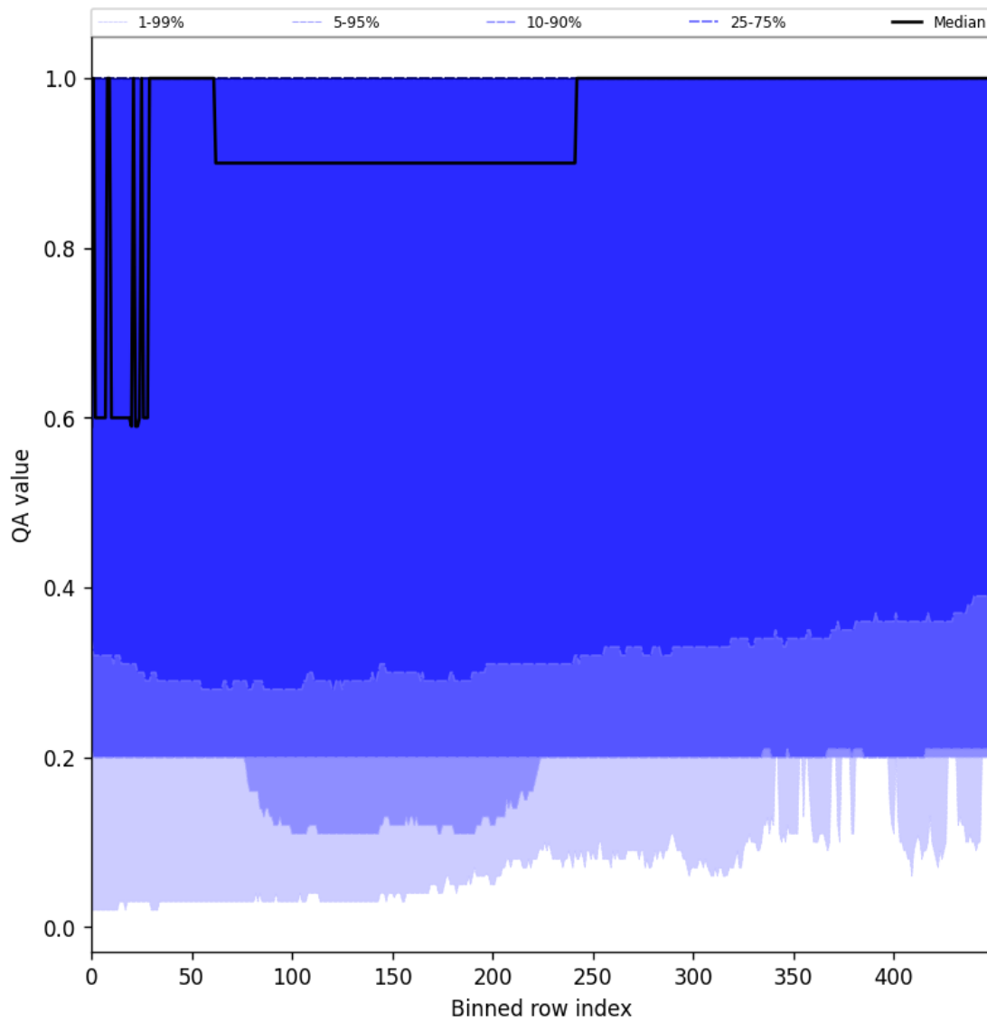
Figure 48: Along track statistics of “QA value” for 2024-09-22 to 2024-09-24
