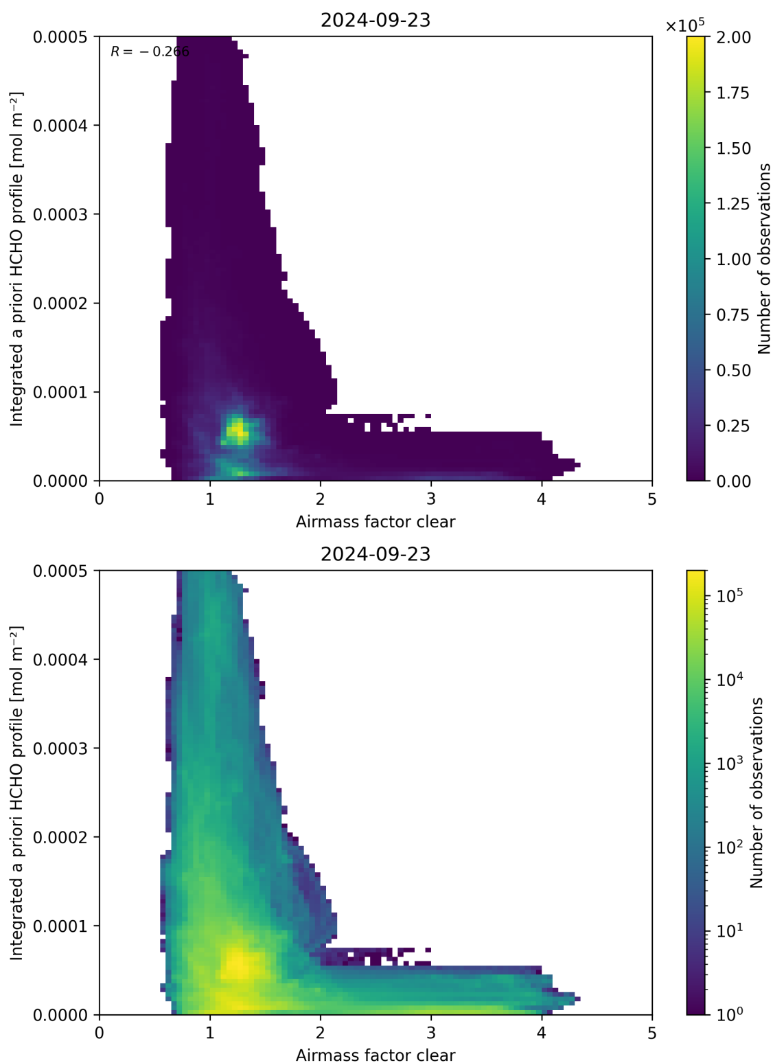
Figure 76: Scatter density plot of “Airmass factor clear” against “Integrated a priori HCHO profile” for 2024-09-22 to 2024-09-24.
