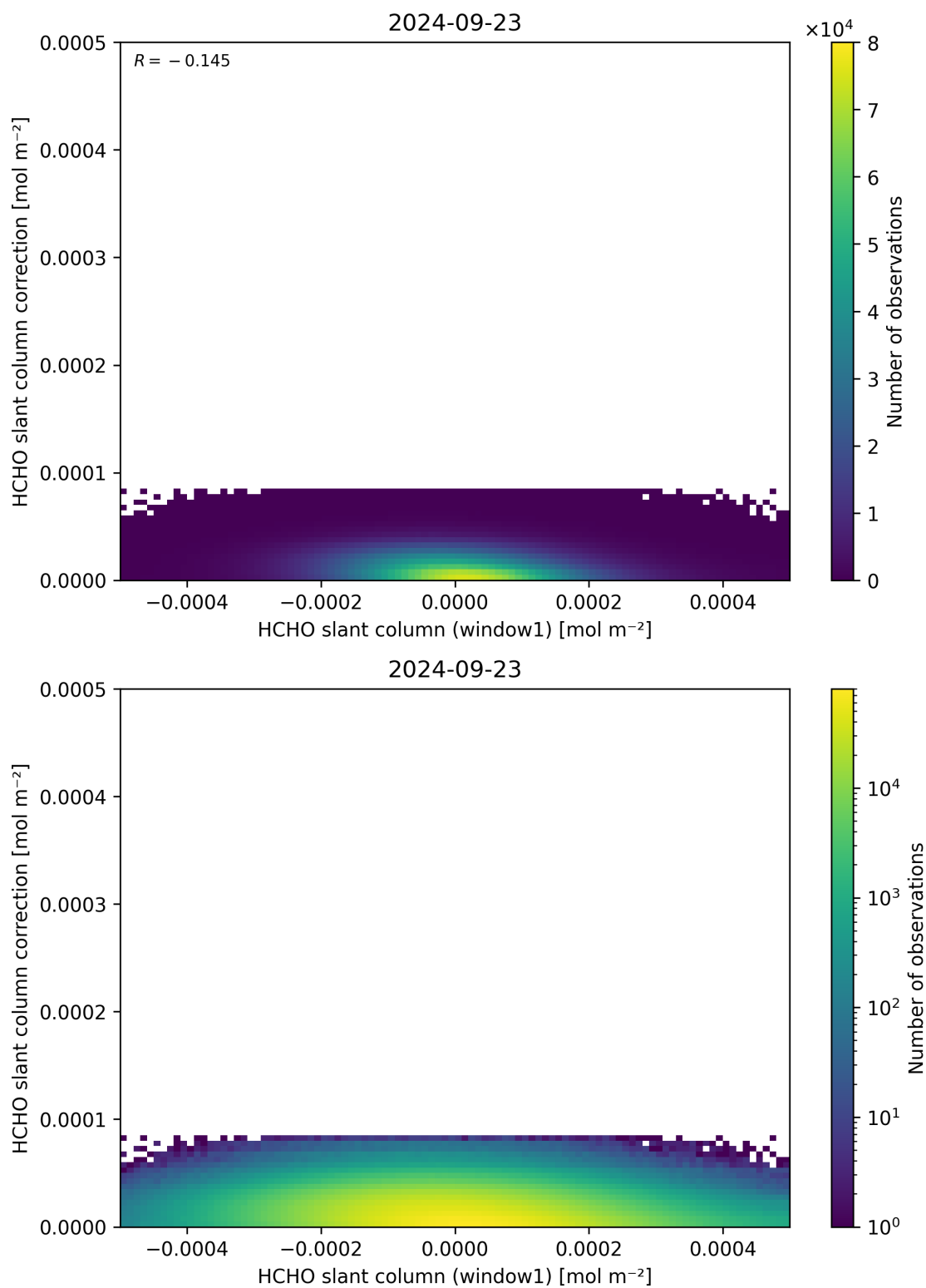
Figure 83: Scatter density plot of “HCHO slant column (window1)” against “HCHO slant column correction” for 2024-09-22 to 2024-09-24.
