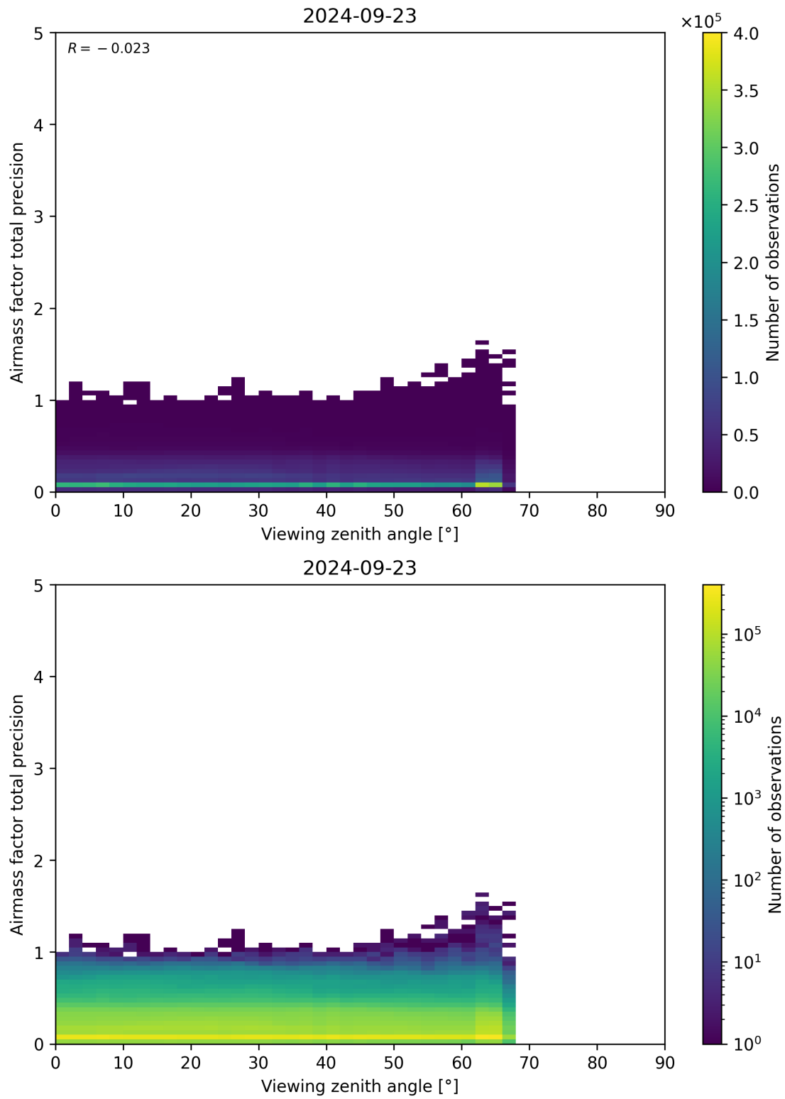
Figure 191: Scatter density plot of “Viewing zenith angle” against “Airmass factor total precision” for 2024-09-22 to 2024-09-24.
