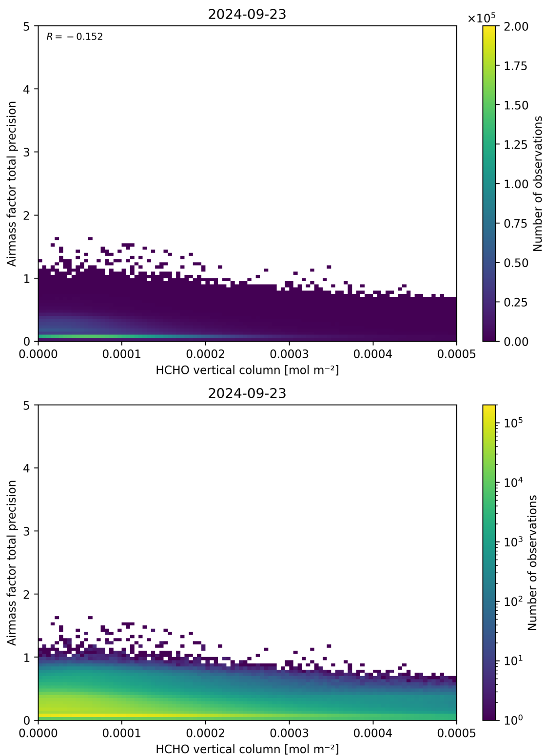
Figure 132: Scatter density plot of “HCHO vertical column” against “Airmass factor total precision” for 2024-09-22 to 2024-09-24.
