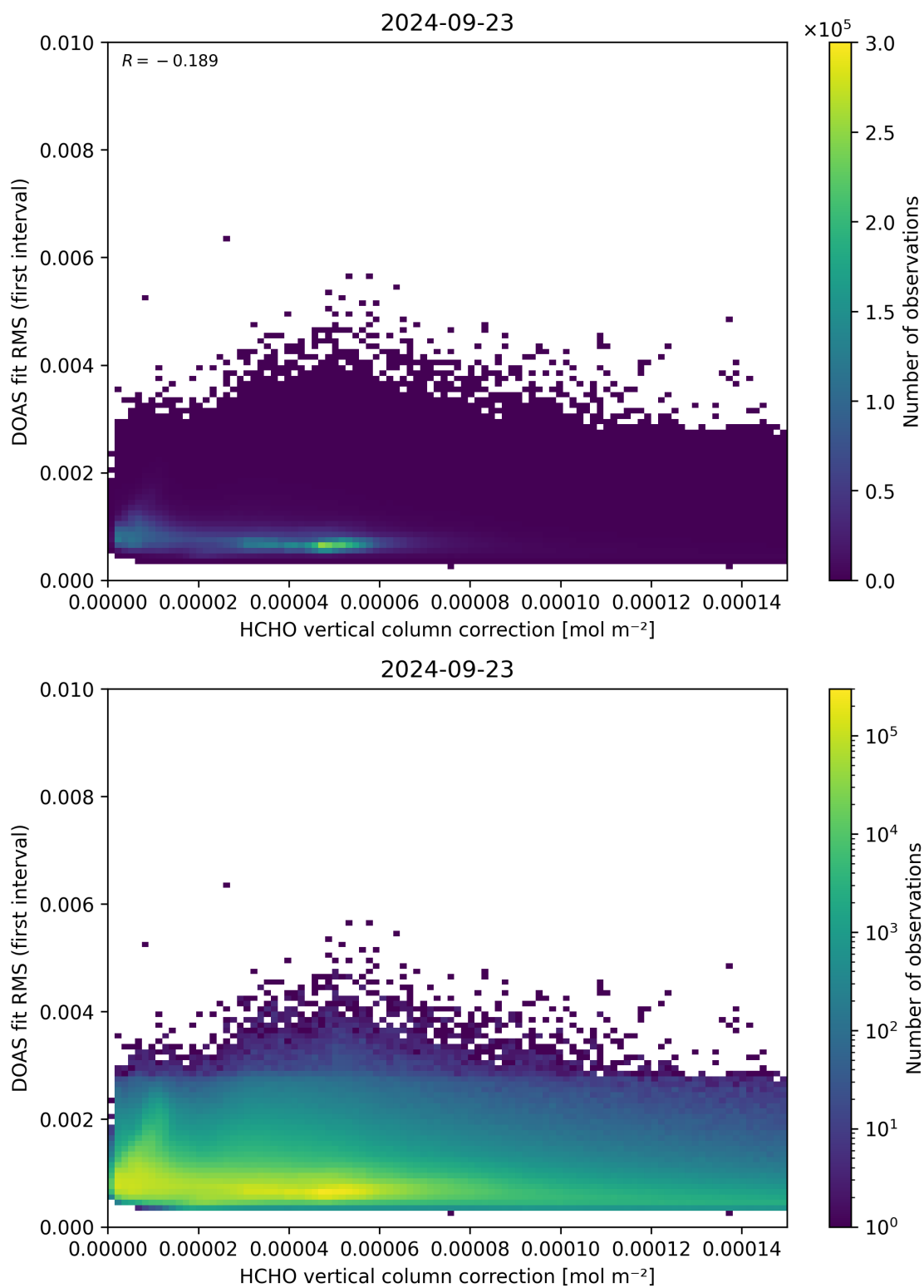
Figure 112: Scatter density plot of “HCHO vertical column correction” against “DOAS fit RMS (first interval)” for 2024-09-22 to 2024-09-24.
