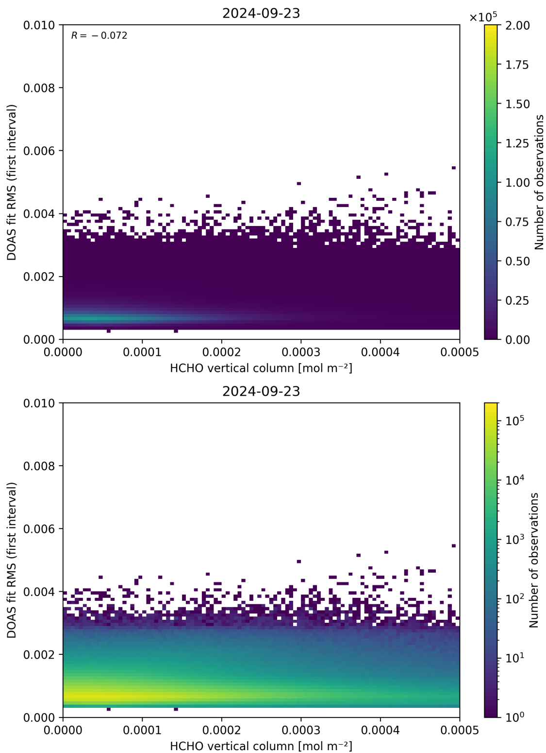
Figure 123: Scatter density plot of “HCHO vertical column” against “DOAS fit RMS (first interval)” for 2024-09-22 to 2024-09-24.
