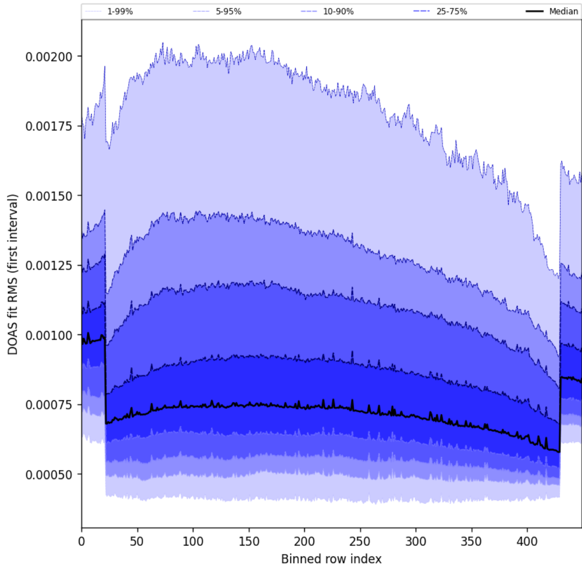
Figure 60: Along track statistics of “DOAS fit RMS (first interval)” for 2024-09-23 to 2024-09-25
