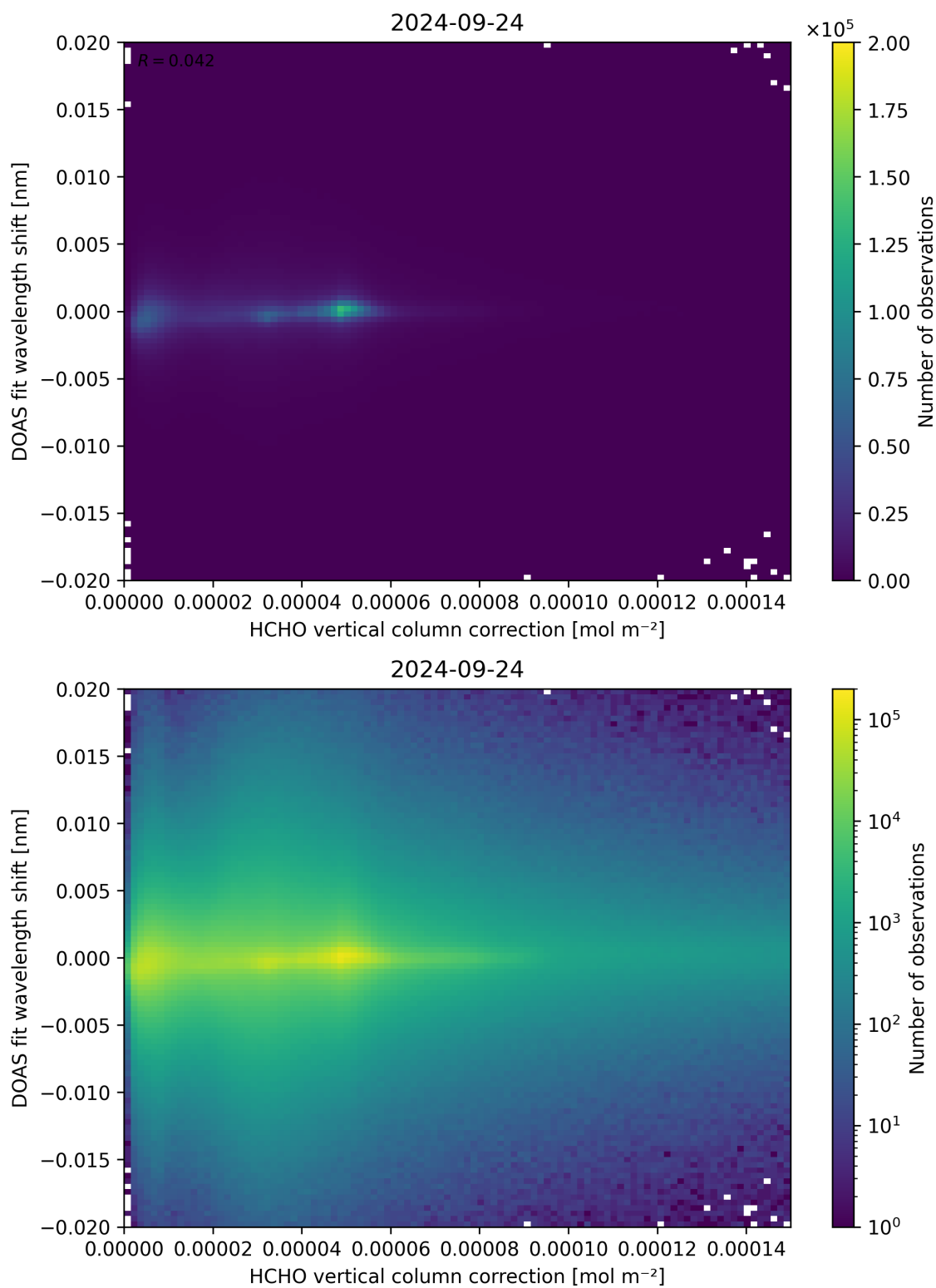
Figure 113: Scatter density plot of “HCHO vertical column correction” against “DOAS fit wavelength shift” for 2024-09-23 to 2024-09-25.
