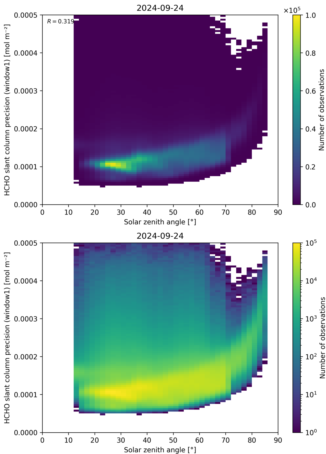
Figure 174: Scatter density plot of “Solar zenith angle” against “HCHO slant column precision (window1)” for 2024-09-23 to 2024-09-25.
