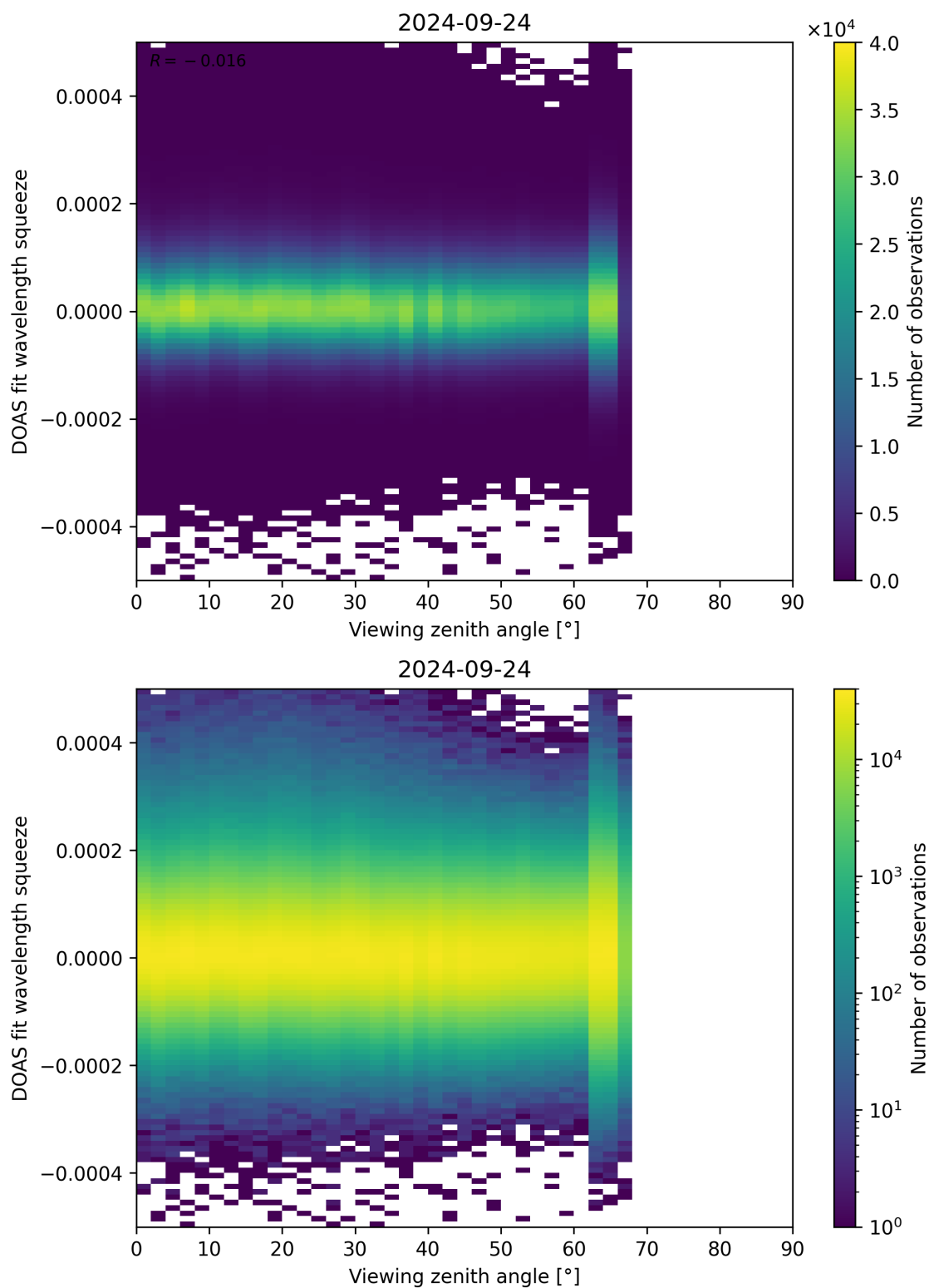
Figure 184: Scatter density plot of “Viewing zenith angle” against “DOAS fit wavelength squeeze” for 2024-09-23 to 2024-09-25.
