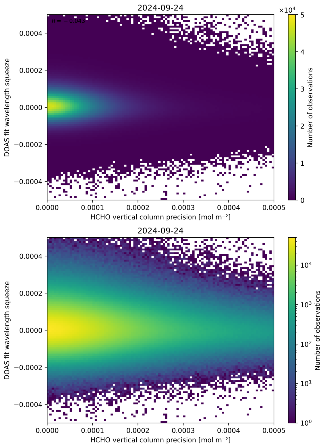
Figure 138: Scatter density plot of “HCHO vertical column precision” against “DOAS fit wavelength squeeze” for 2024-09-23 to 2024-09-25.
