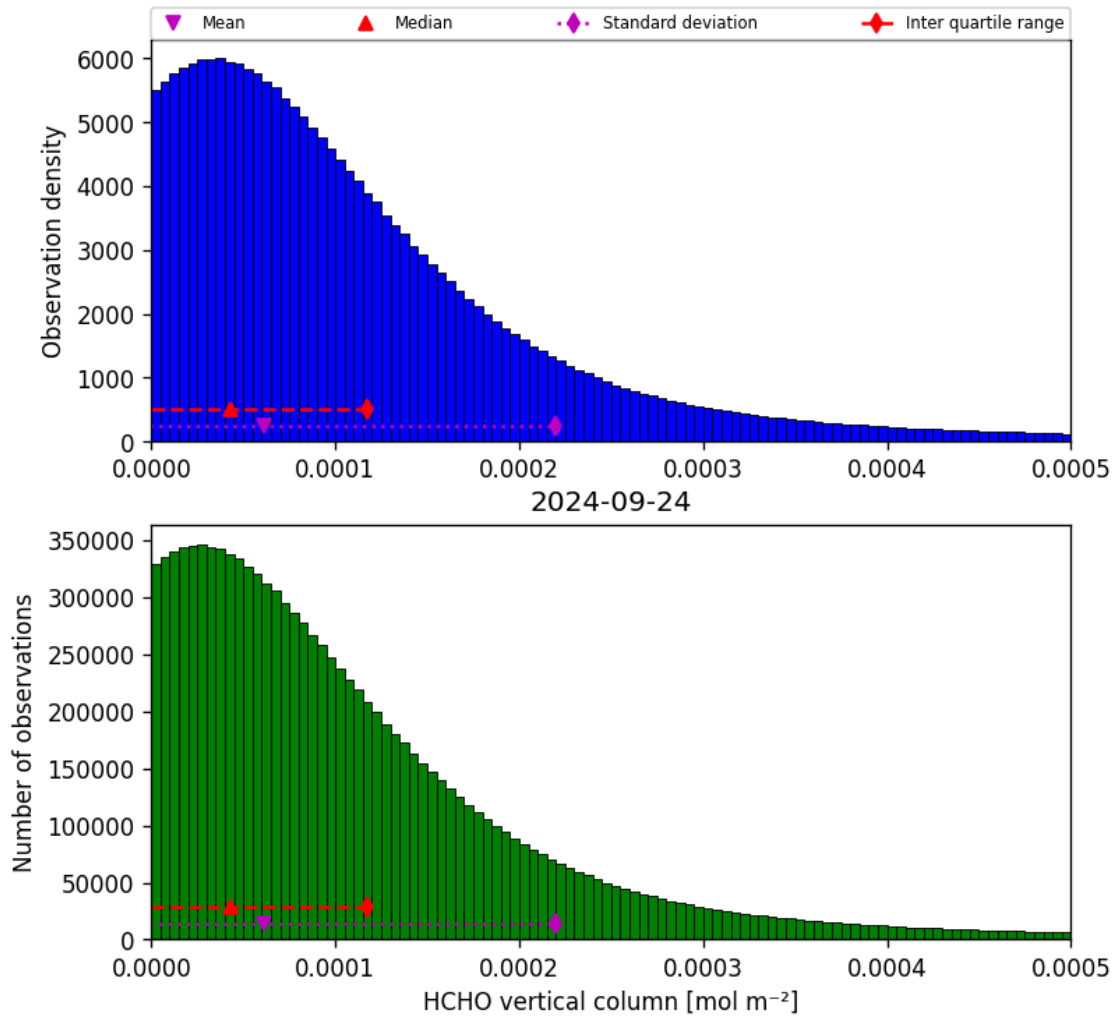
Figure 35: Histogram of “HCHO vertical column” for 2024-09-23 to 2024-09-25
