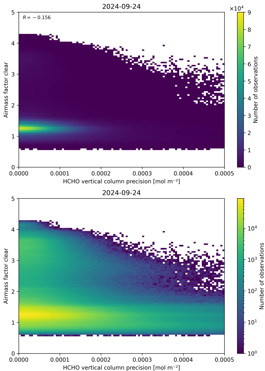
Figure 139: Scatter density plot of “HCHO vertical column precision” against “Airmass factor clear” for 2024-09-23 to 2024-09-25.
