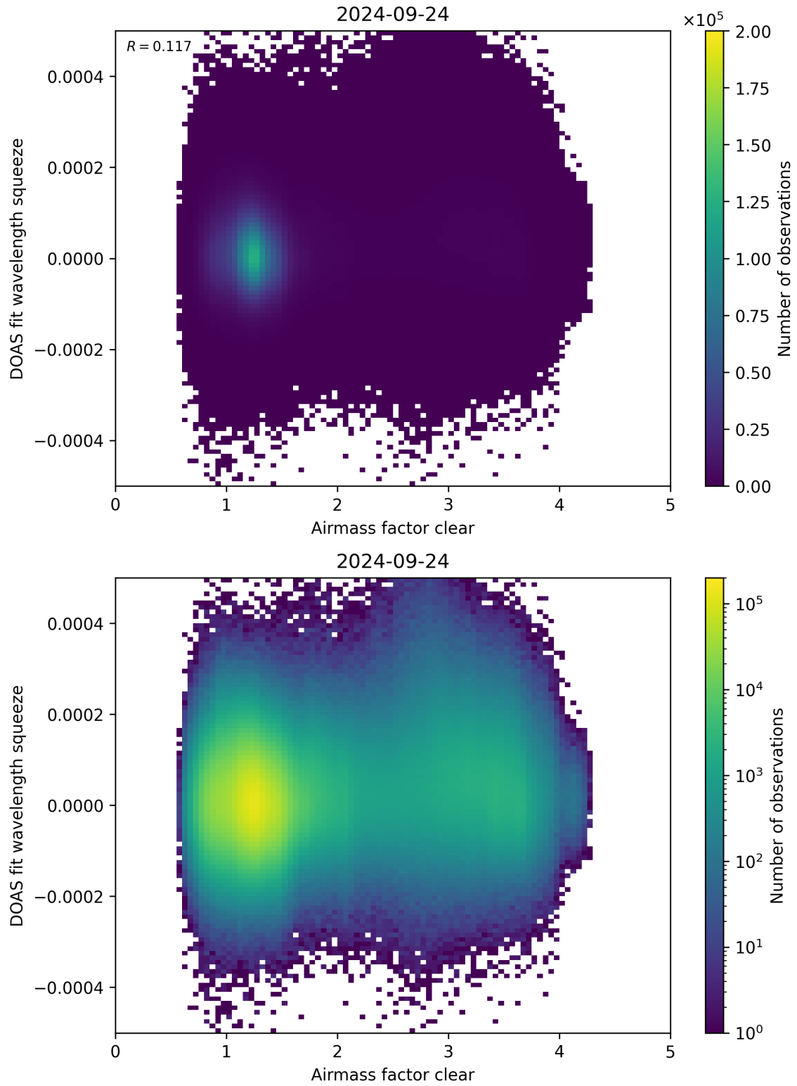
Figure 73: Scatter density plot of “Airmass factor clear” against “DOAS fit wavelength squeeze” for 2024-09-23 to 2024-09-25.
