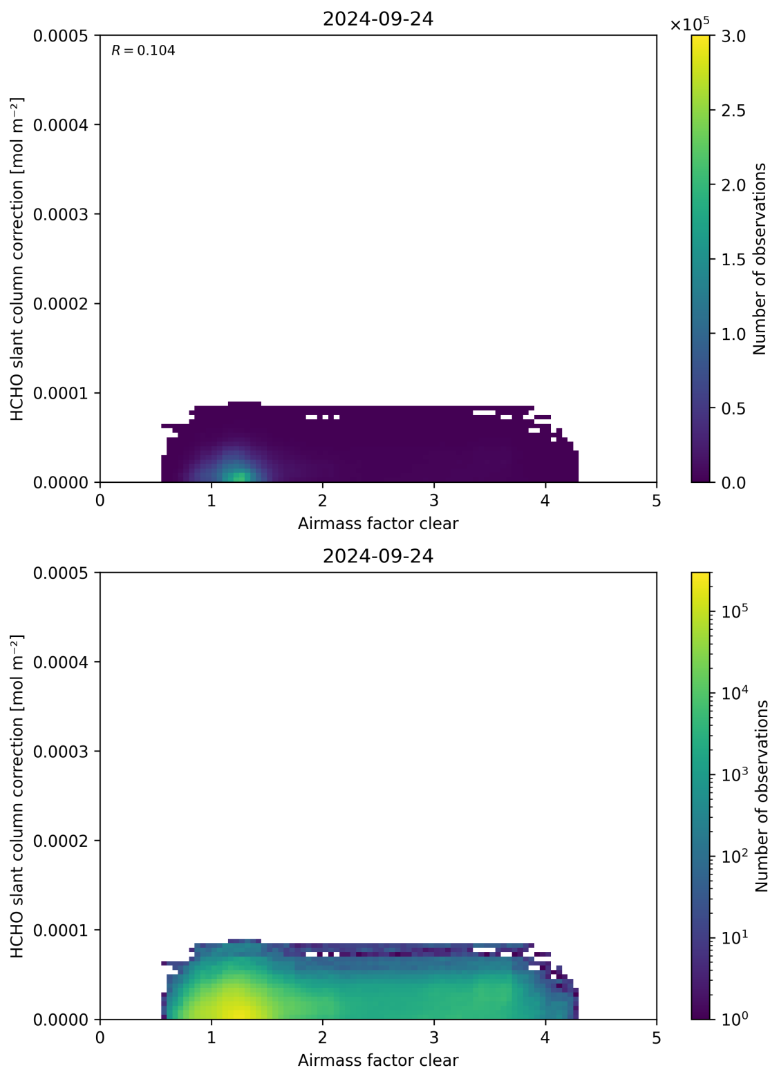
Figure 75: Scatter density plot of “Airmass factor clear” against “HCHO slant column correction” for 2024-09-23 to 2024-09-25.
