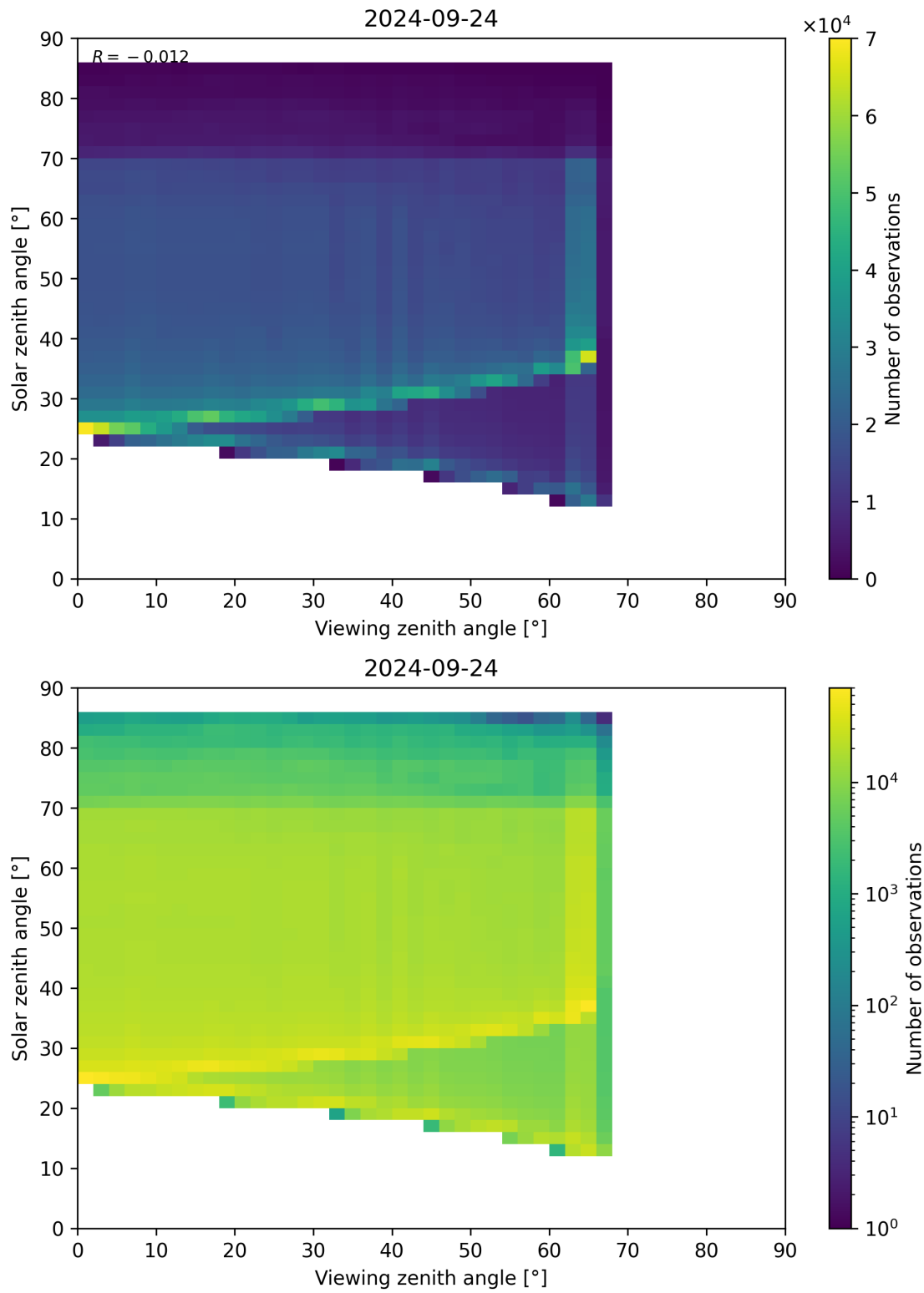
Figure 197: Scatter density plot of “Viewing zenith angle” against “Solar zenith angle” for 2024-09-23 to 2024-09-25.
