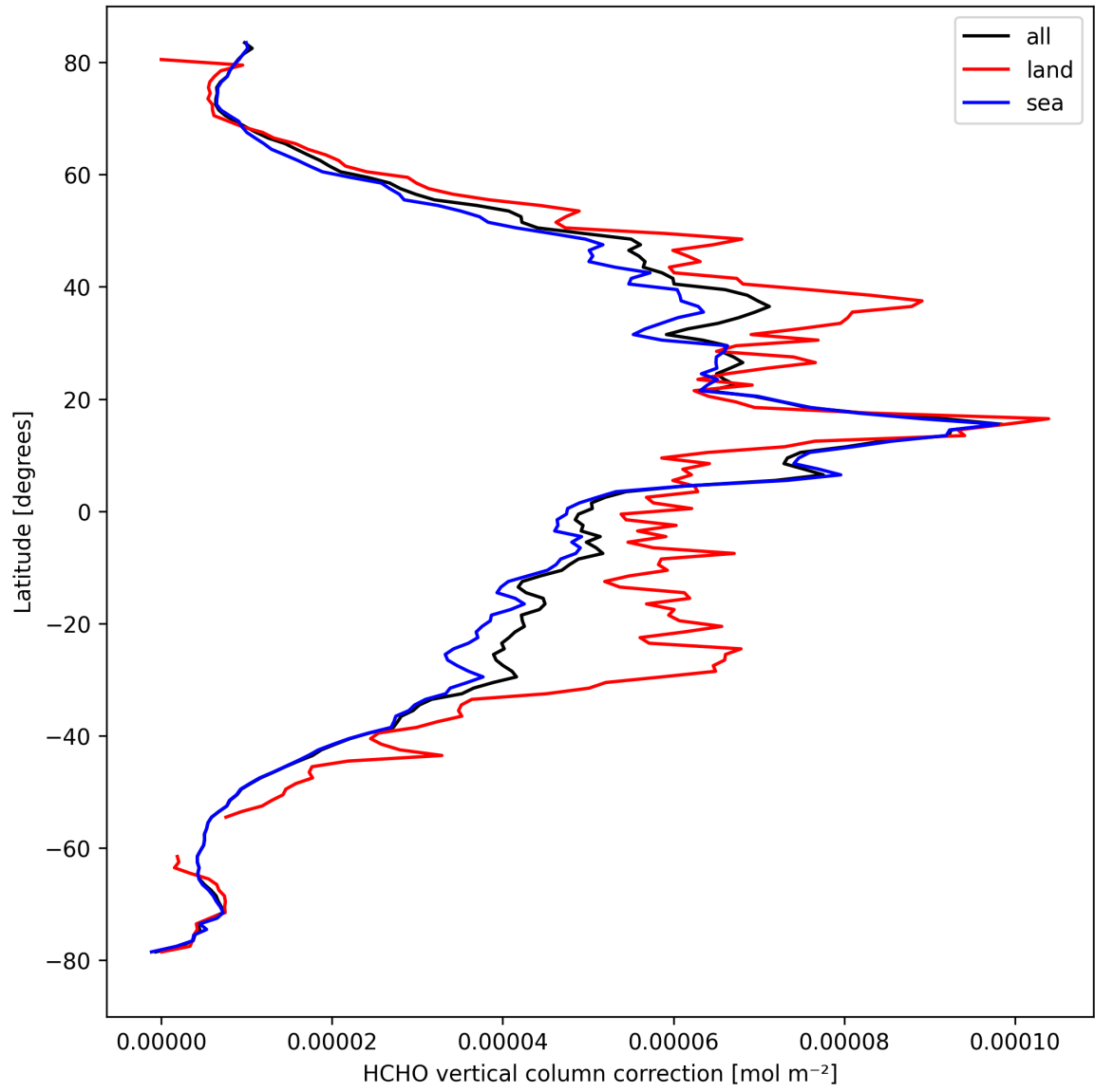
Figure 23: Zonal average of “HCHO vertical column correction” for 2024-09-23 to 2024-09-25.
