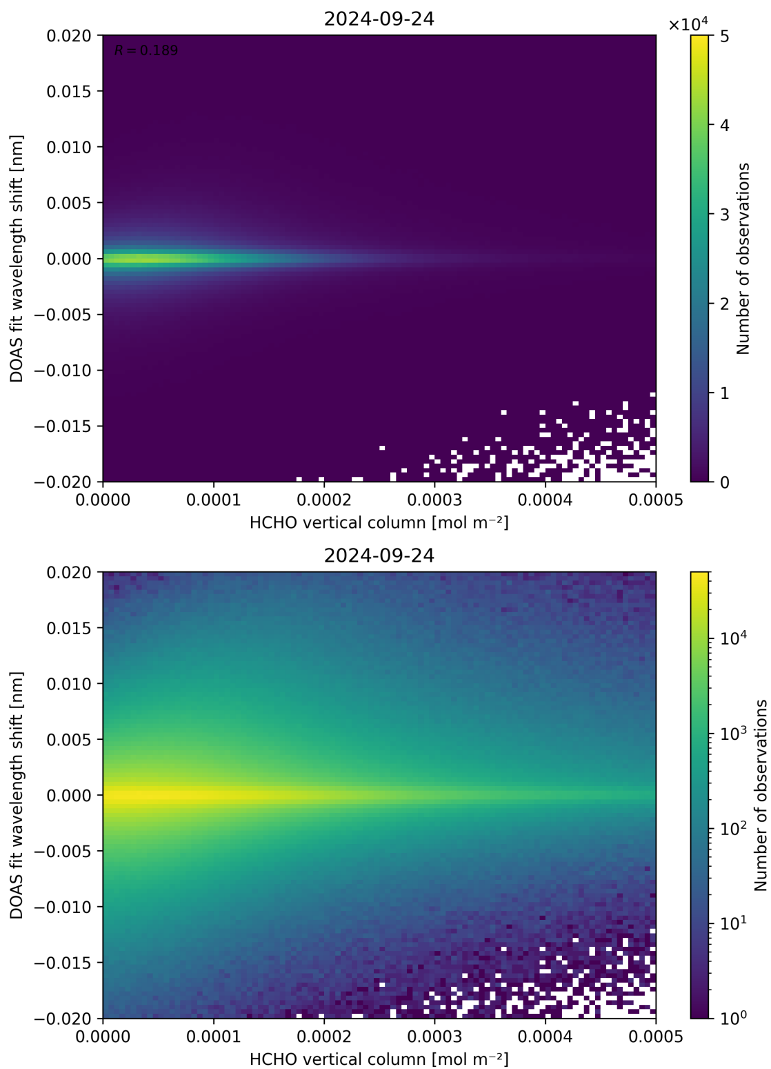
Figure 124: Scatter density plot of “HCHO vertical column” against “DOAS fit wavelength shift” for 2024-09-23 to 2024-09-25.
