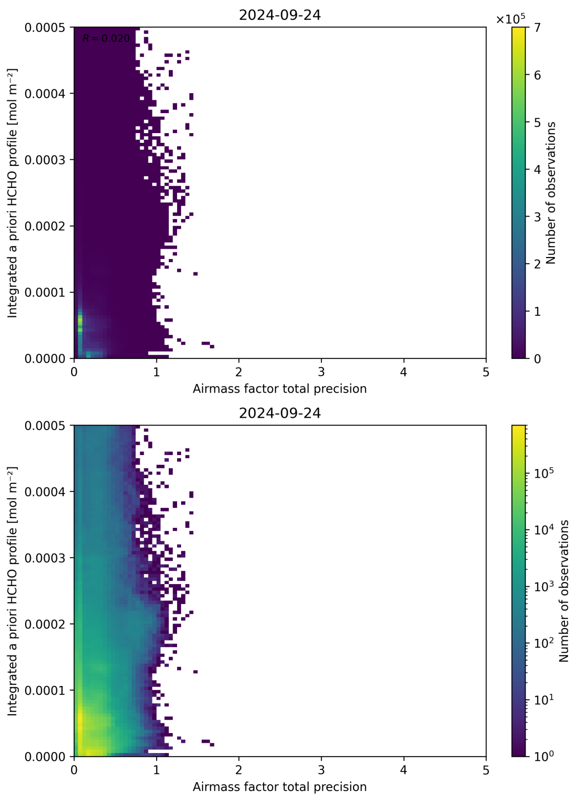
Figure 111: Scatter density plot of “Airmass factor total precision” against “Integrated a priori HCHO profile” for 2024-09-23 to 2024-09-25.
