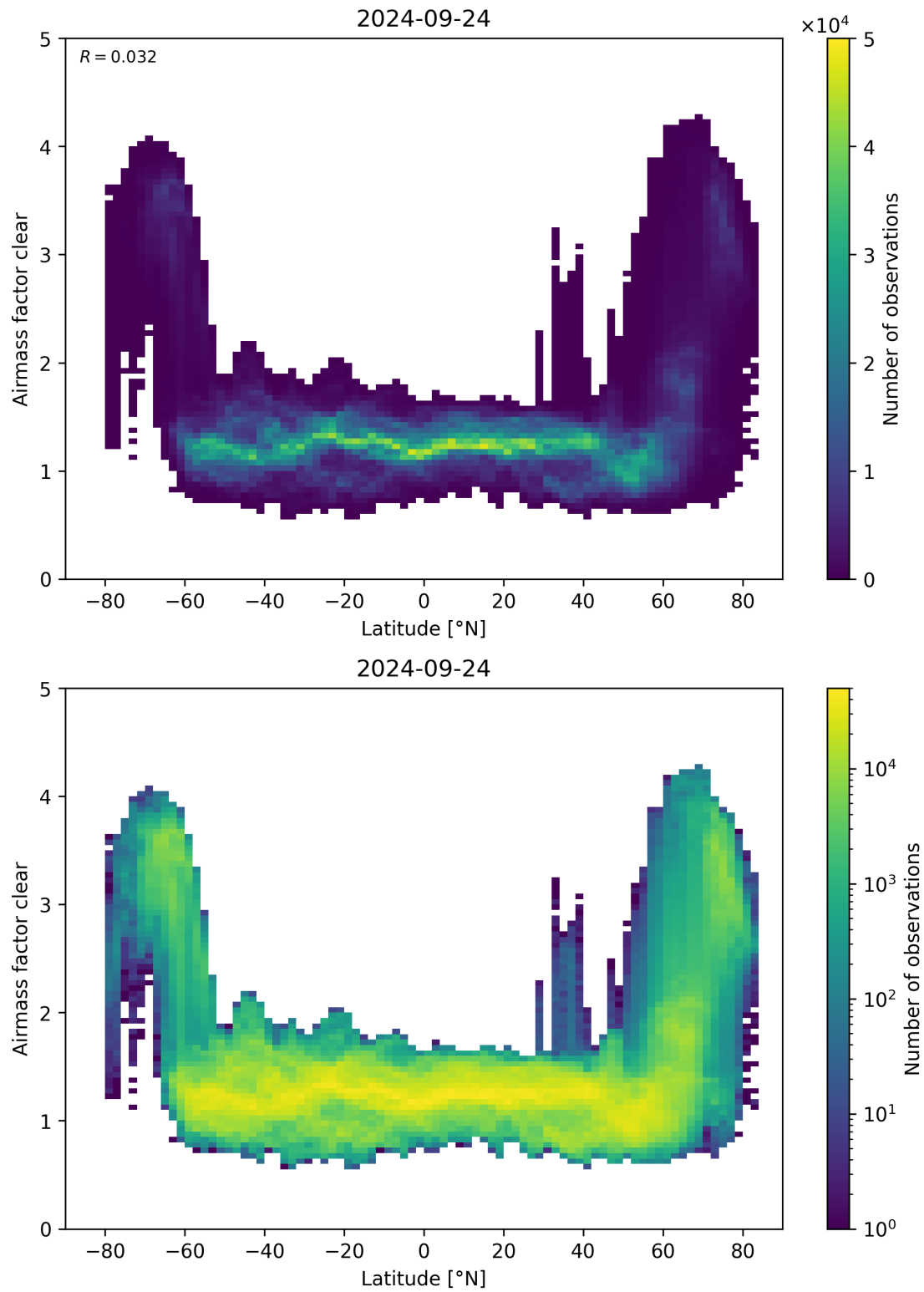
Figure 156: Scatter density plot of “Latitude” against “Airmass factor clear” for 2024-09-23 to 2024-09-25.
