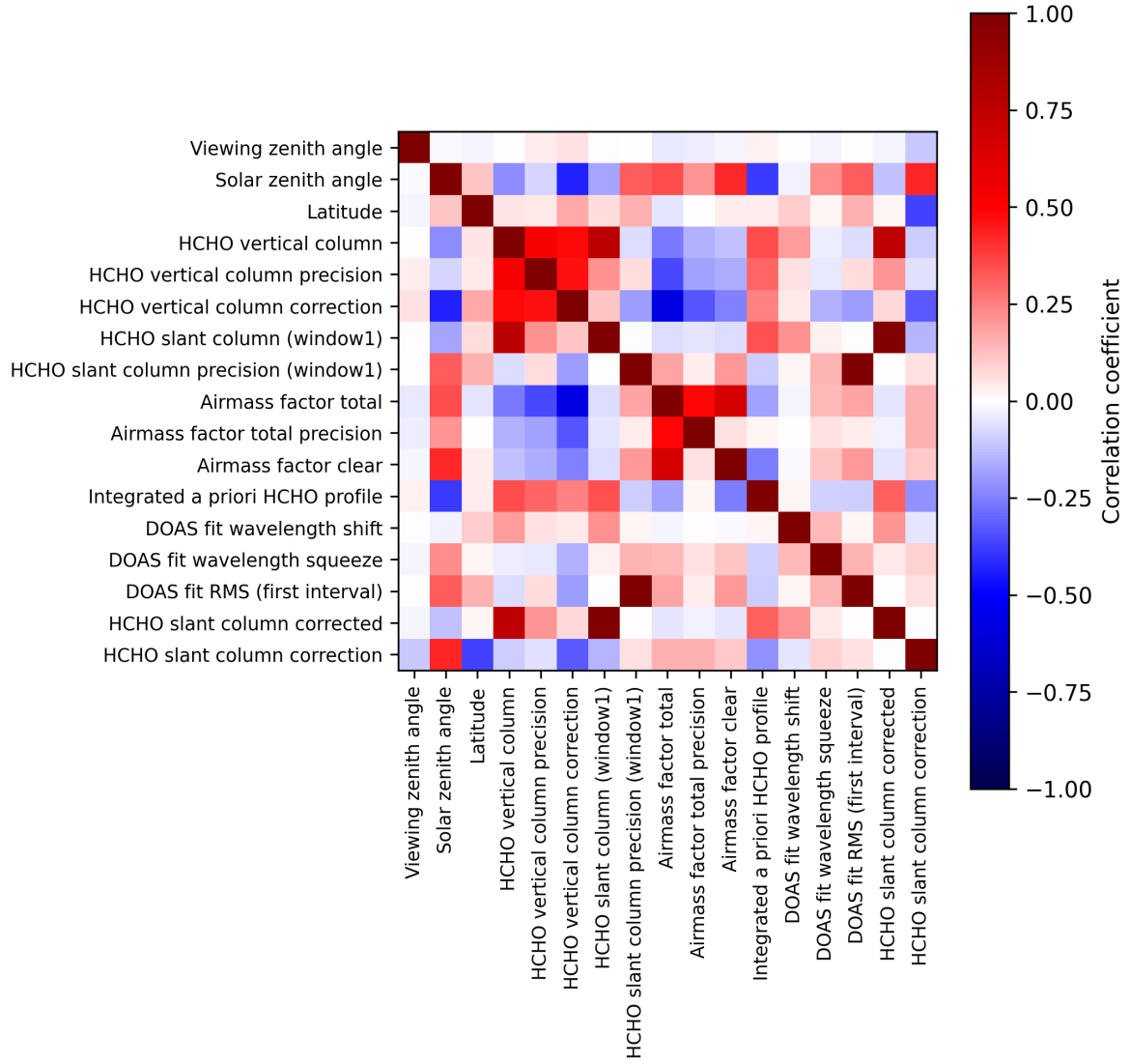
Figure 2: Map of correlation matrix for 2024-09-23 to 2024-09-25.
