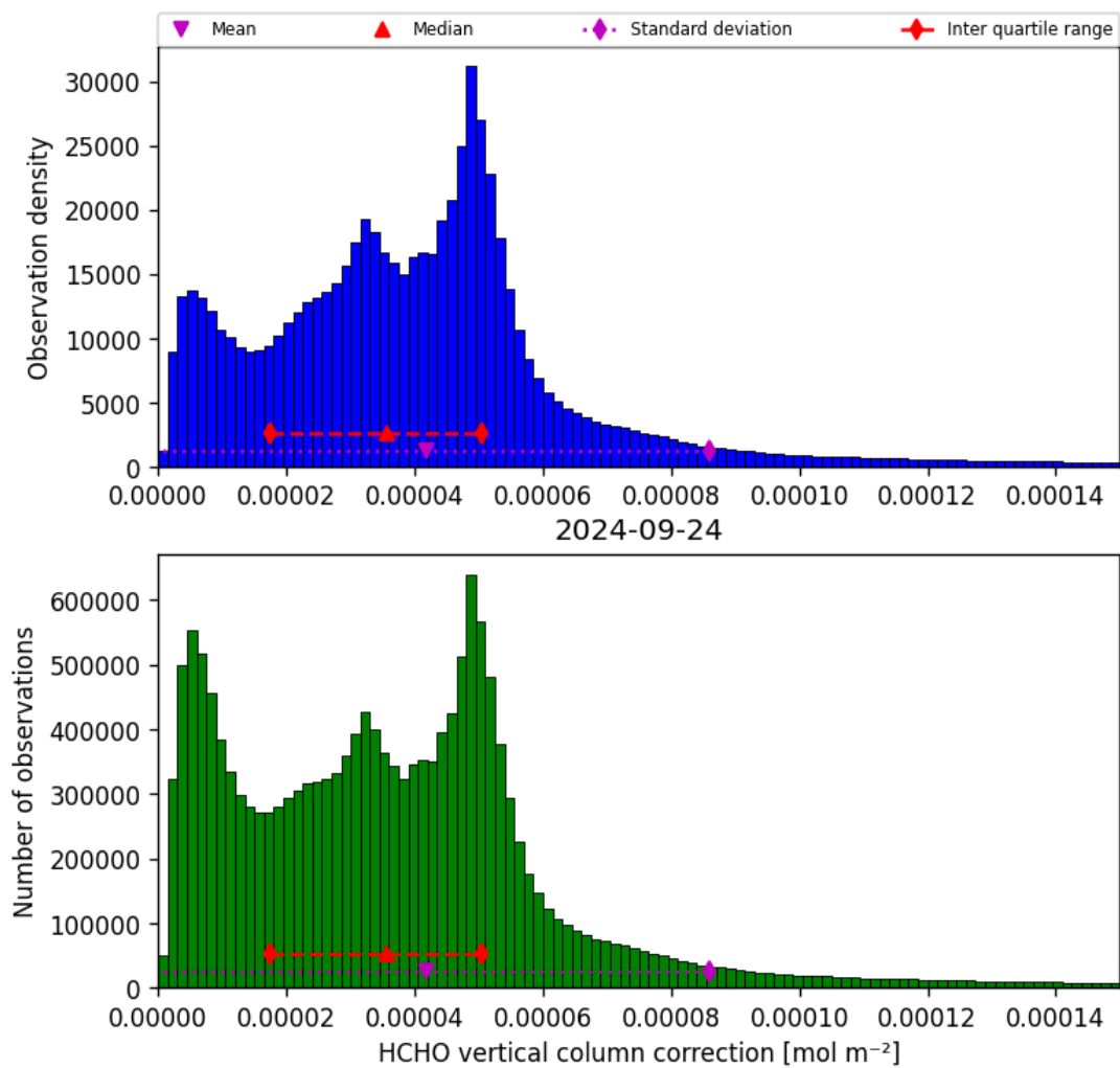
Figure 37: Histogram of “HCHO vertical column correction” for 2024-09-23 to 2024-09-25
