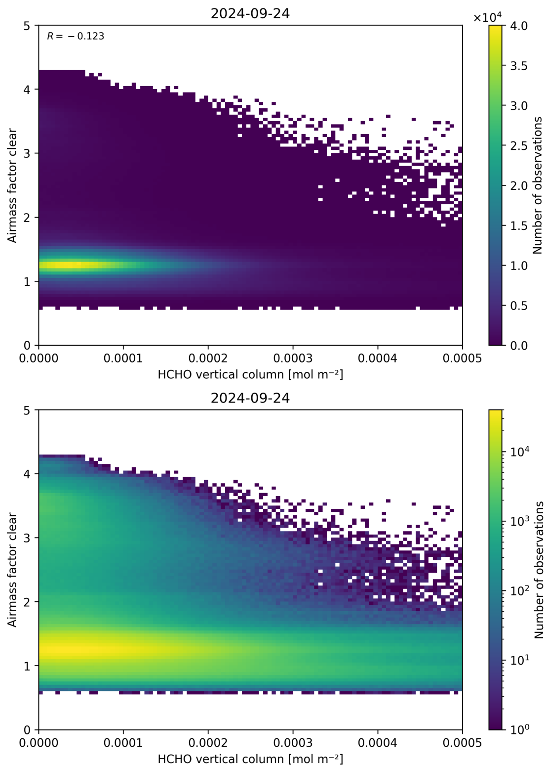
Figure 126: Scatter density plot of “HCHO vertical column” against “Airmass factor clear” for 2024-09-23 to 2024-09-25.
