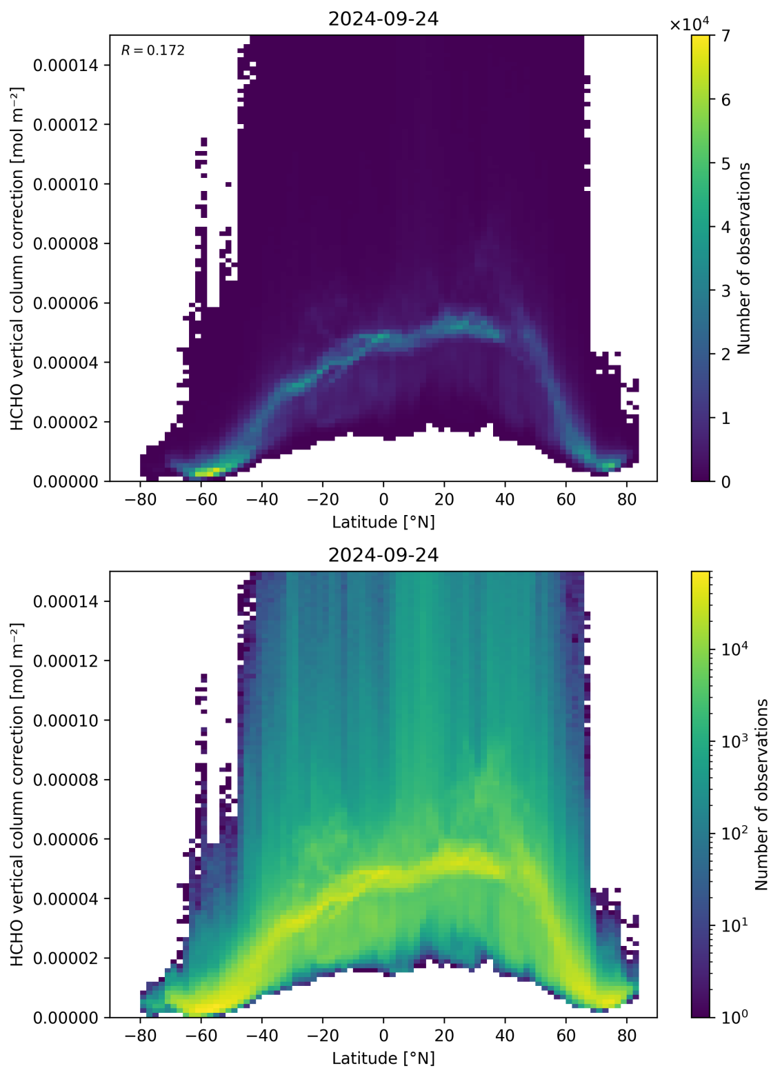
Figure 164: Scatter density plot of “Latitude” against “HCHO vertical column correction” for 2024-09-23 to 2024-09-25.
