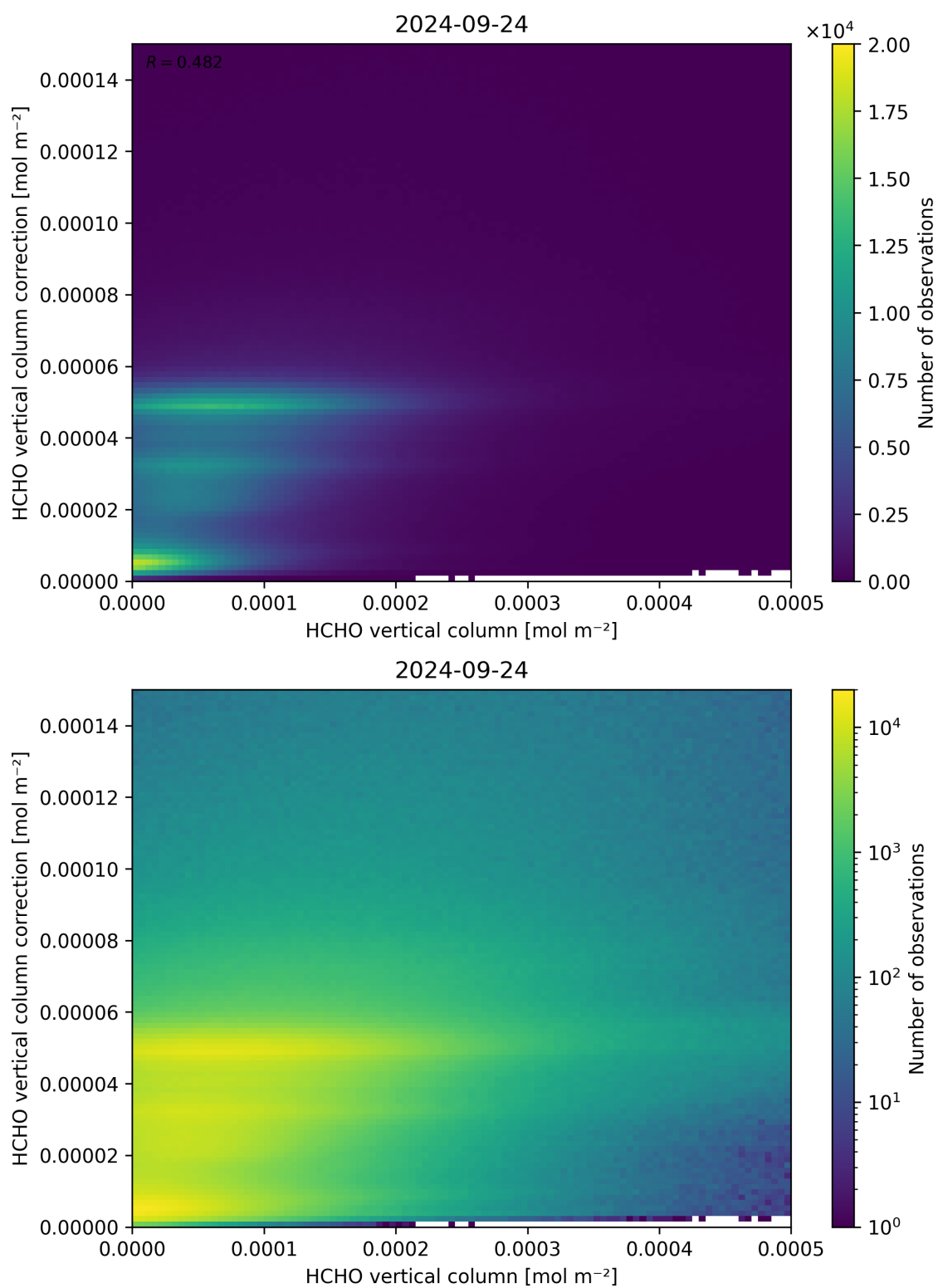
Figure 133: Scatter density plot of “HCHO vertical column” against “HCHO vertical column correction” for 2024-09-23 to 2024-09-25.
