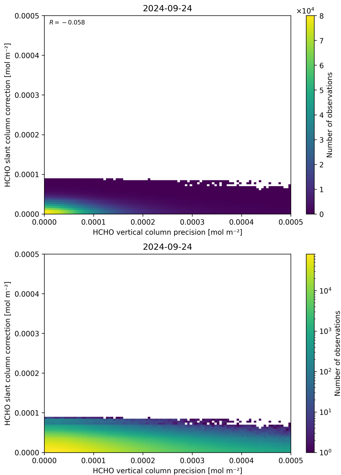
Figure 141: Scatter density plot of “HCHO vertical column precision” against “HCHO slant column correction” for 2024-09-23 to 2024-09-25.
