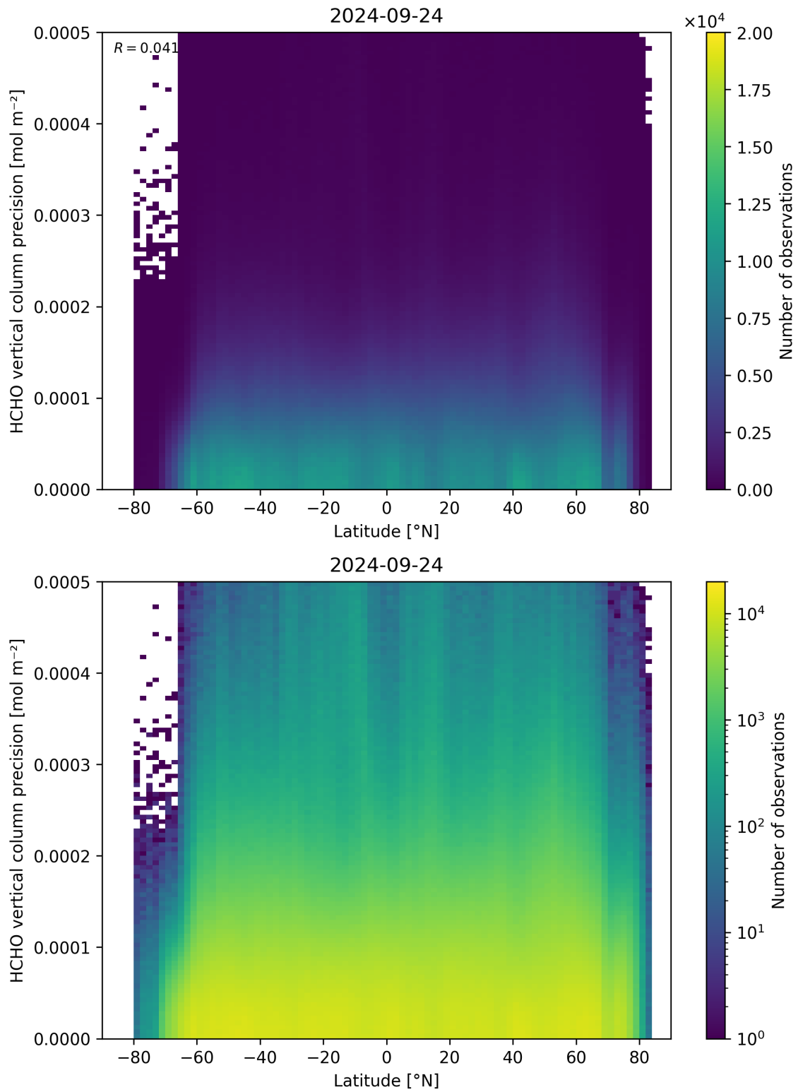
Figure 165: Scatter density plot of “Latitude” against “HCHO vertical column precision” for 2024-09-23 to 2024-09-25.
