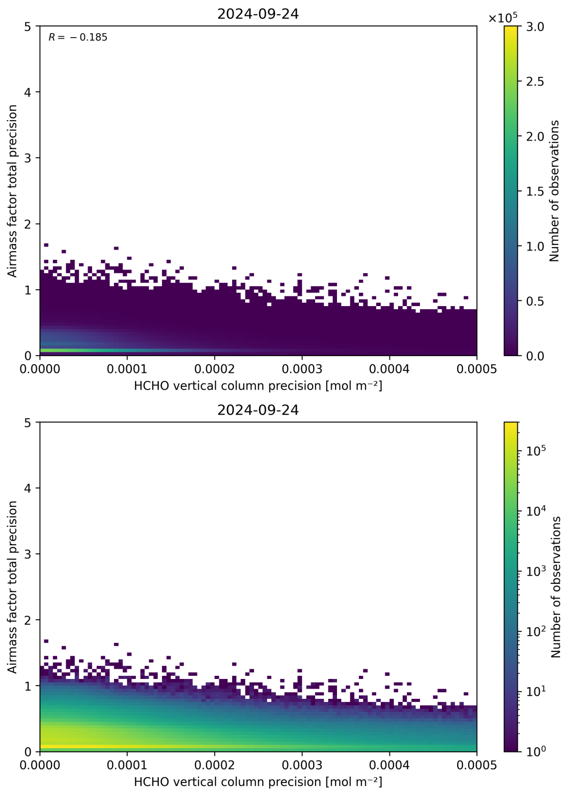
Figure 145: Scatter density plot of “HCHO vertical column precision” against “Airmass factor total precision” for 2024-09-23 to 2024-09-25.
