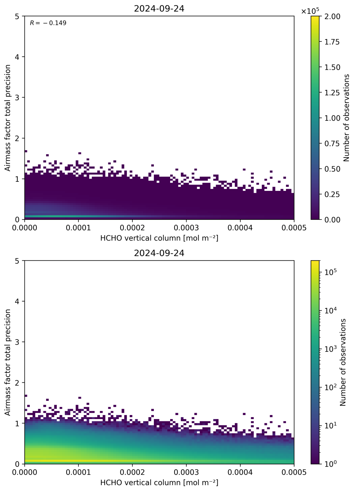
Figure 132: Scatter density plot of “HCHO vertical column” against “Airmass factor total precision” for 2024-09-23 to 2024-09-25.
