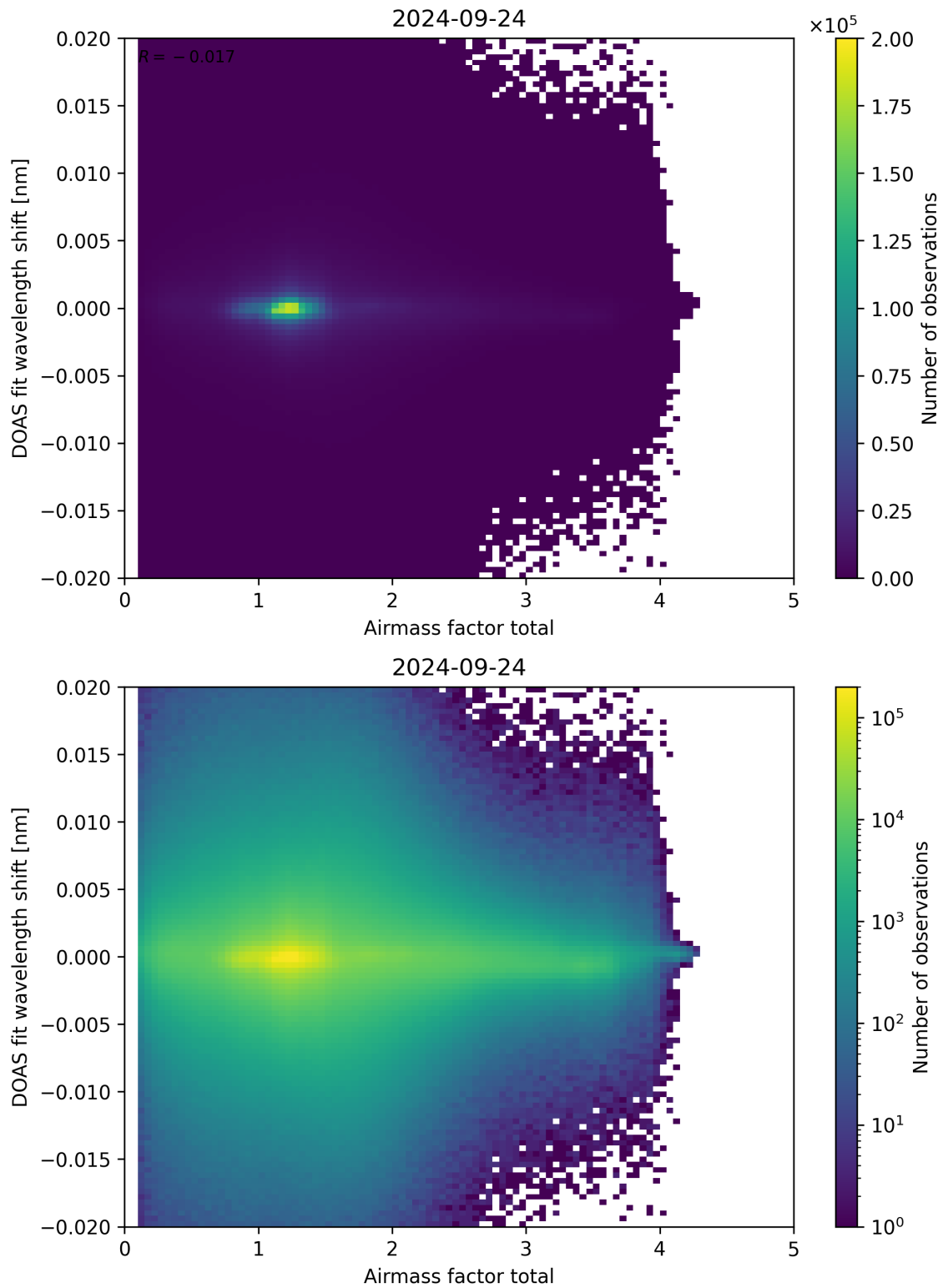
Figure 98: Scatter density plot of “Airmass factor total” against “DOAS fit wavelength shift” for 2024-09-23 to 2024-09-25.
