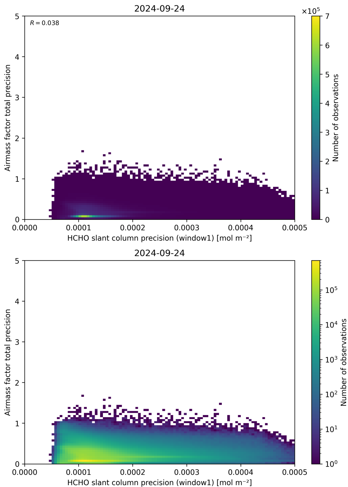
Figure 95: Scatter density plot of “HCHO slant column precision (window1)” against “Airmass factor total precision” for 2024-09-23 to 2024-09-25.
