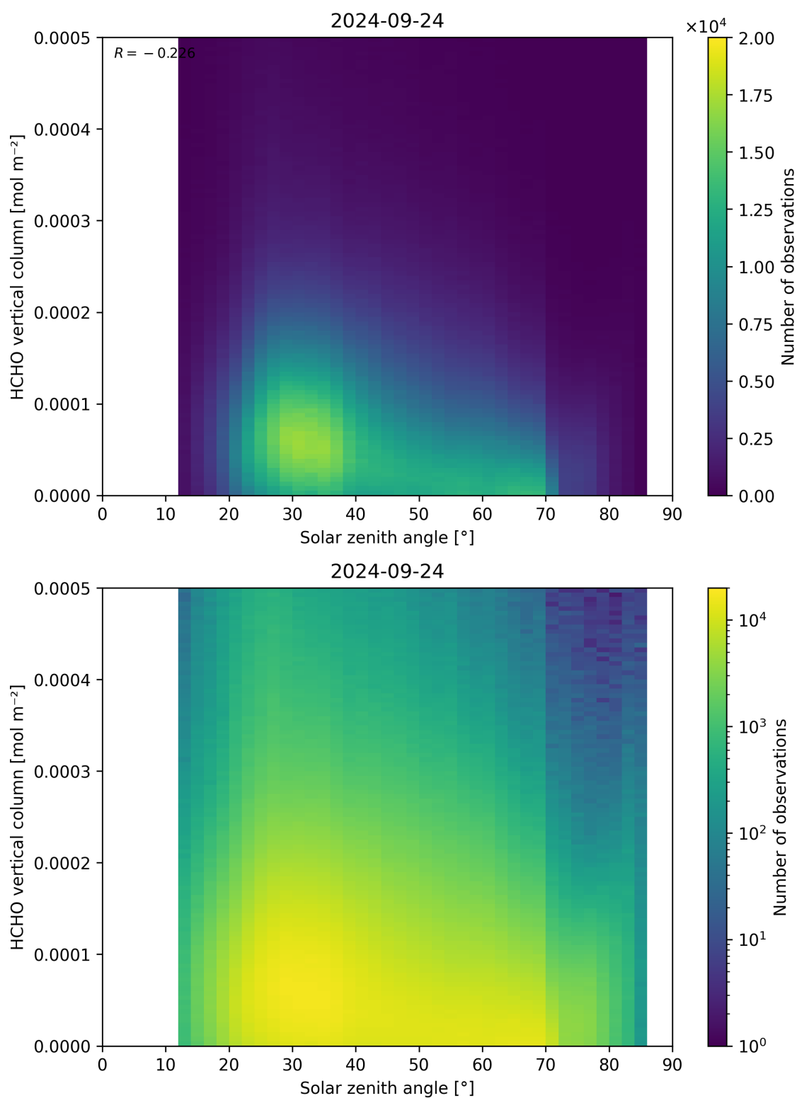
Figure 177: Scatter density plot of “Solar zenith angle” against “HCHO vertical column” for 2024-09-23 to 2024-09-25.
