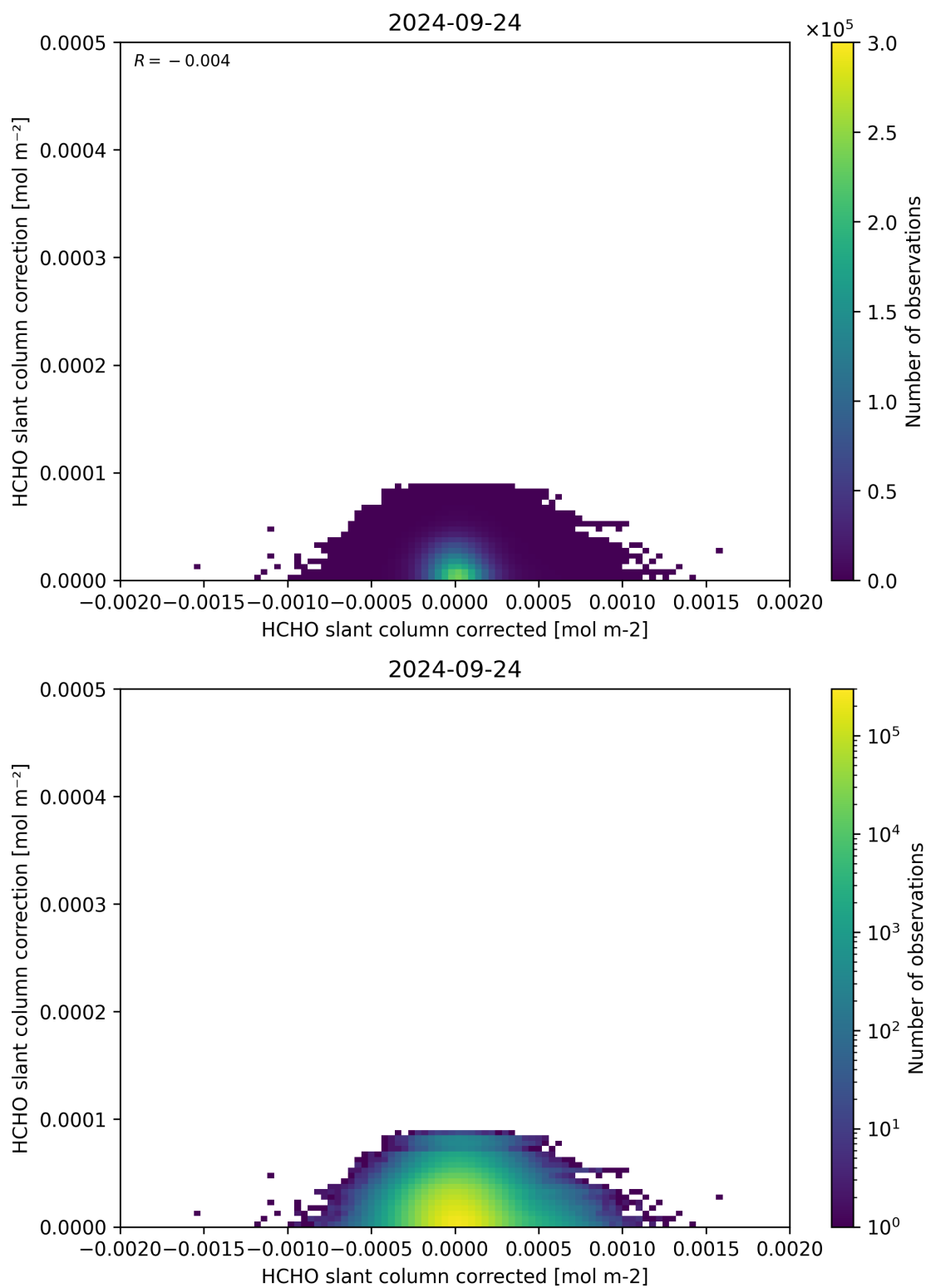
Figure 77: Scatter density plot of “HCHO slant column corrected” against “HCHO slant column correction” for 2024-09-23 to 2024-09-25.
