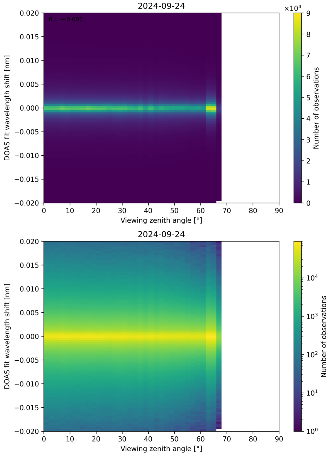
Figure 183: Scatter density plot of “Viewing zenith angle” against “DOAS fit wavelength shift” for 2024-09-23 to 2024-09-25.
