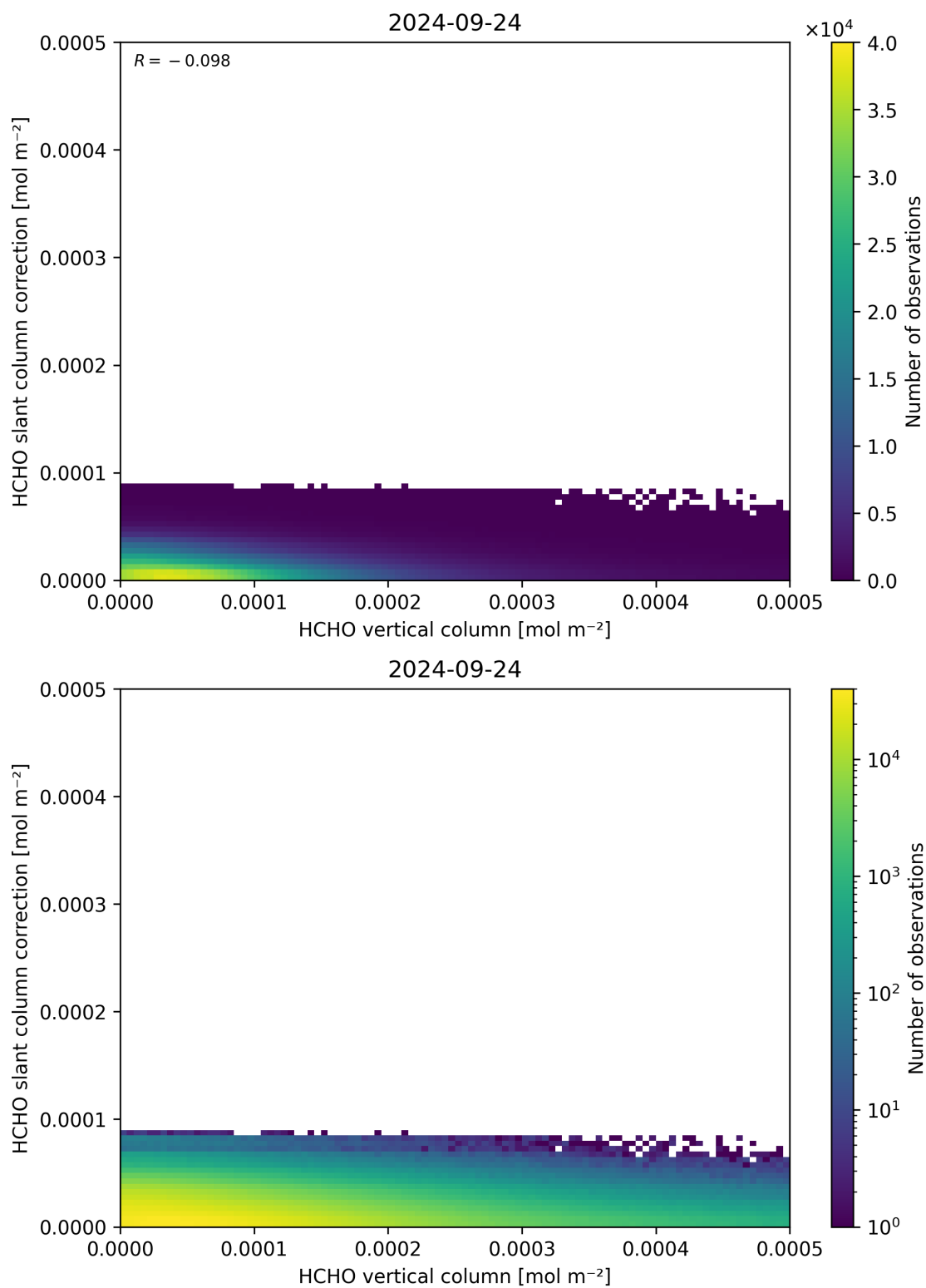
Figure 128: Scatter density plot of “HCHO vertical column” against “HCHO slant column correction” for 2024-09-23 to 2024-09-25.
