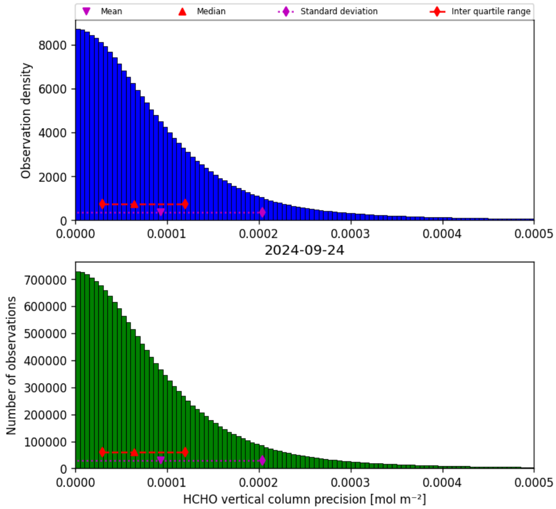
Figure 36: Histogram of “HCHO vertical column precision” for 2024-09-23 to 2024-09-25
