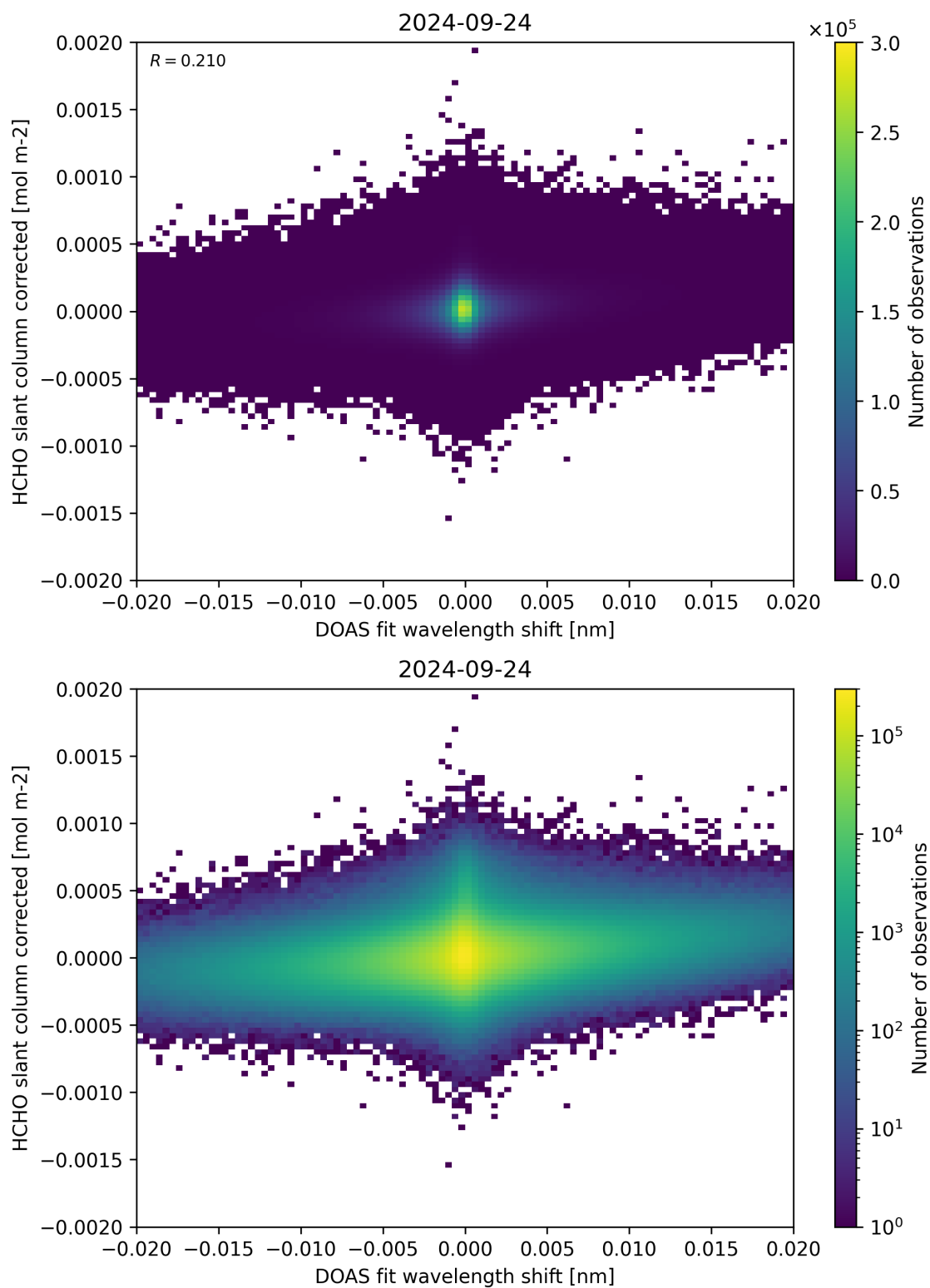
Figure 66: Scatter density plot of “DOAS fit wavelength shift” against “HCHO slant column corrected” for 2024-09-23 to 2024-09-25.
