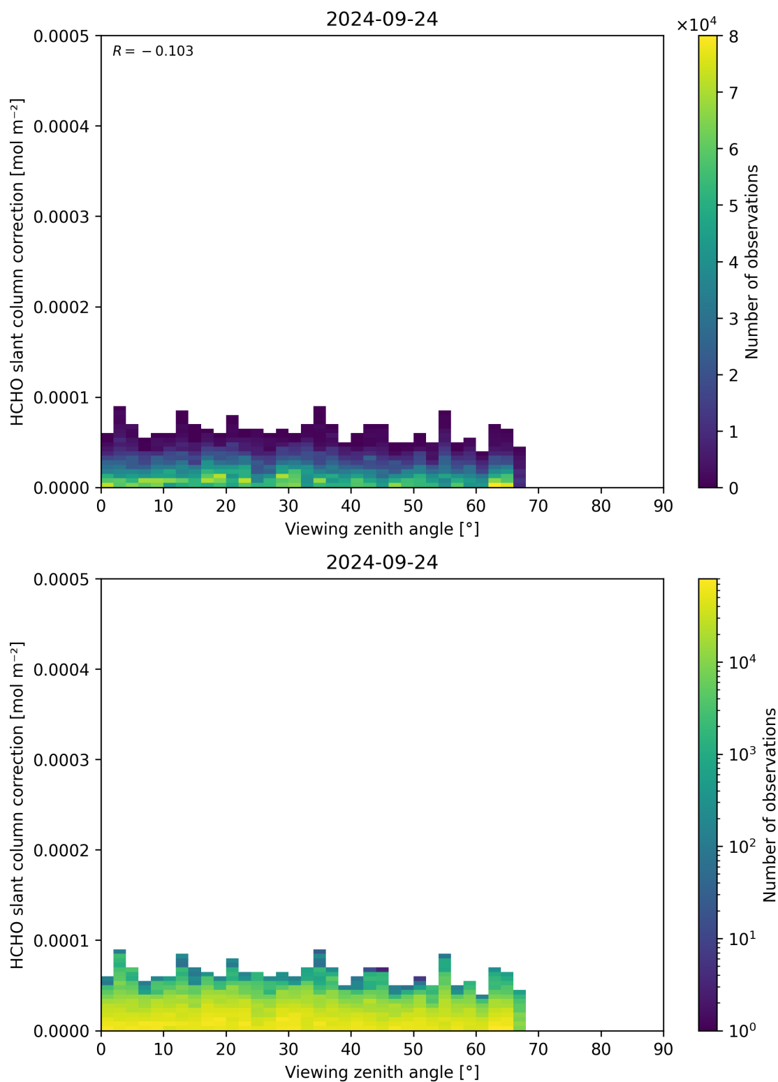
Figure 187: Scatter density plot of “Viewing zenith angle” against “HCHO slant column correction” for 2024-09-23 to 2024-09-25.
