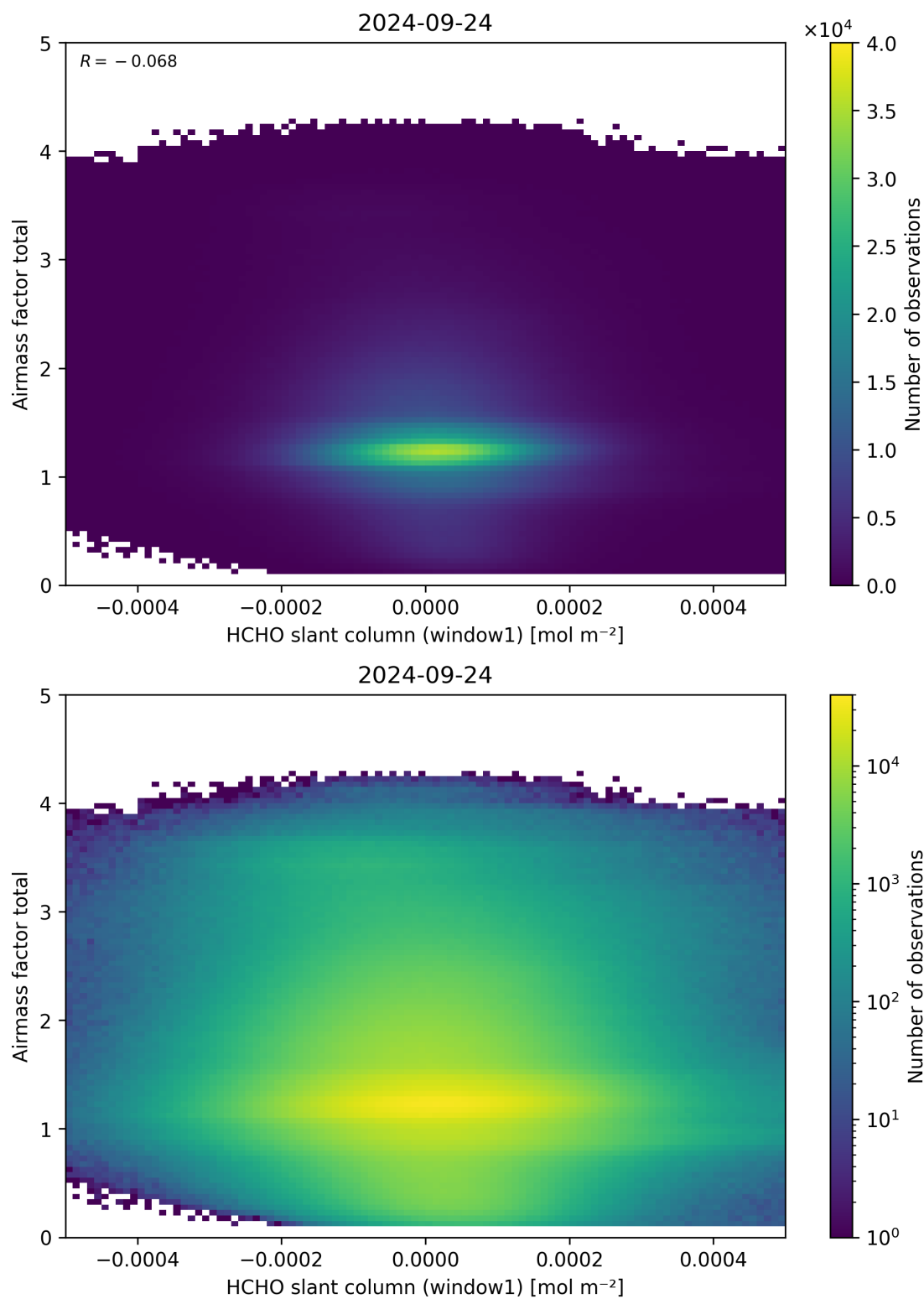
Figure 85: Scatter density plot of “HCHO slant column (window1)” against “Airmass factor total” for 2024-09-23 to 2024-09-25.
