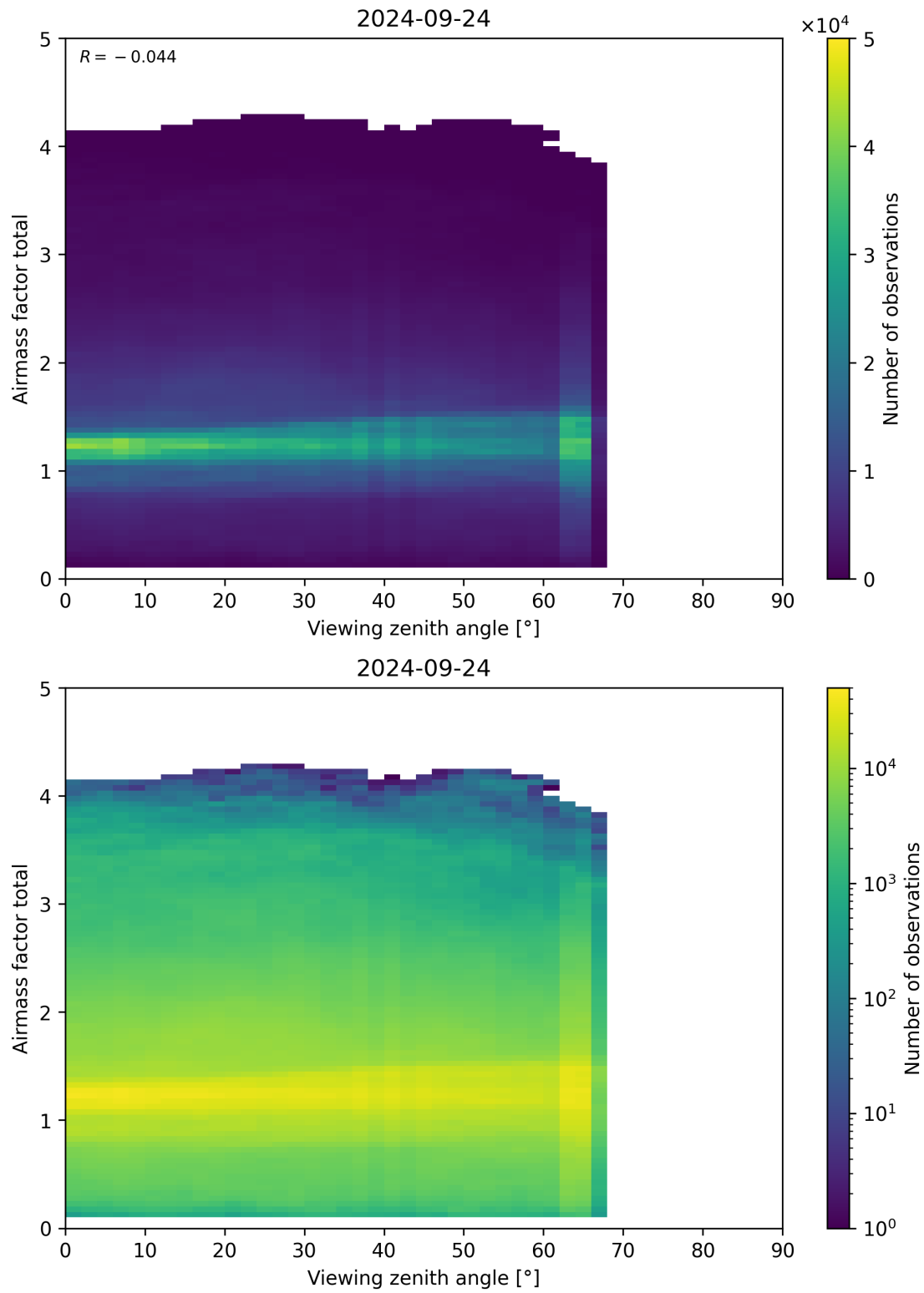
Figure 190: Scatter density plot of “Viewing zenith angle” against “Airmass factor total” for 2024-09-23 to 2024-09-25.
