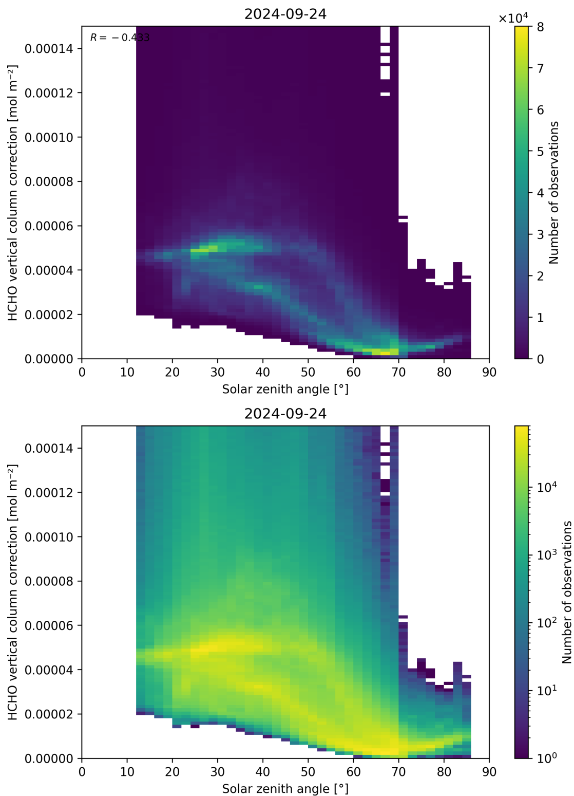
Figure 178: Scatter density plot of “Solar zenith angle” against “HCHO vertical column correction” for 2024-09-23 to 2024-09-25.
