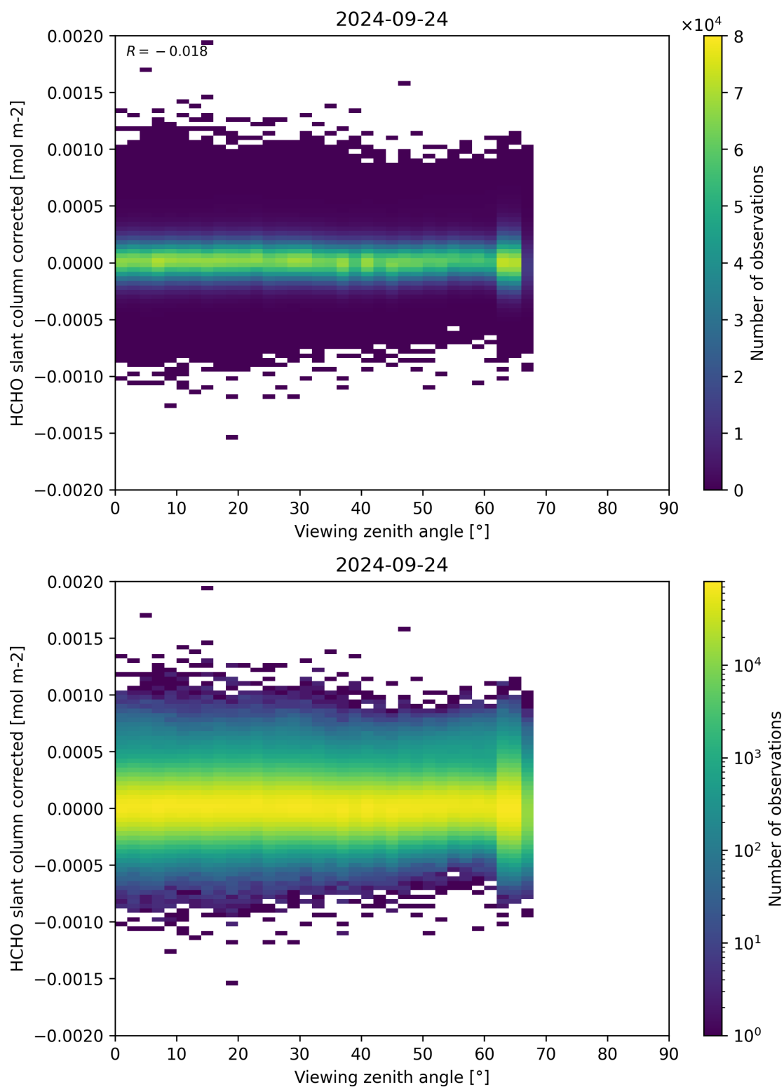
Figure 186: Scatter density plot of “Viewing zenith angle” against “HCHO slant column corrected” for 2024-09-23 to 2024-09-25.
