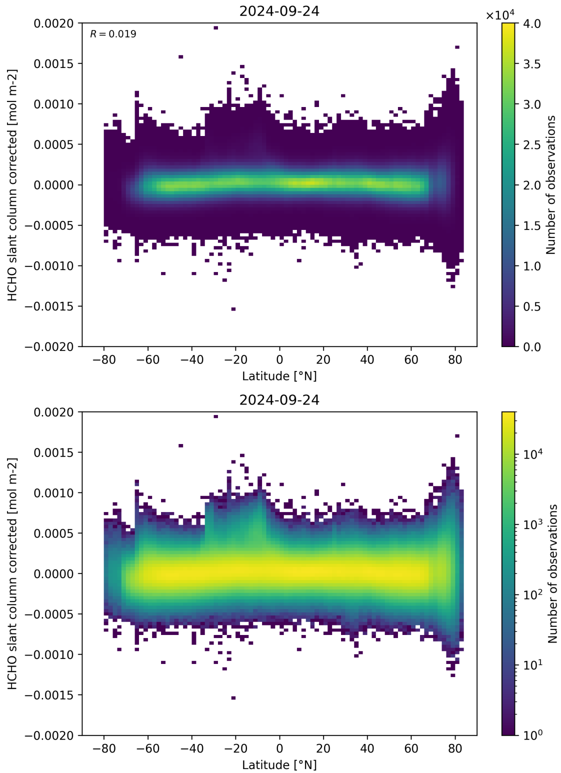
Figure 157: Scatter density plot of “Latitude” against “HCHO slant column corrected” for 2024-09-23 to 2024-09-25.
