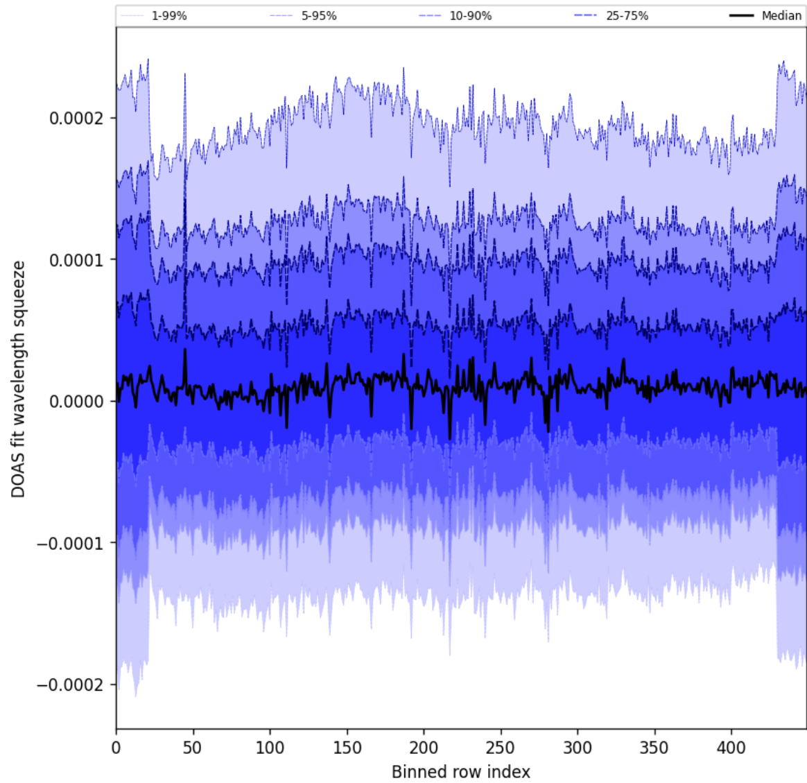
Figure 59: Along track statistics of “DOAS fit wavelength squeeze” for 2024-09-23 to 2024-09-25
