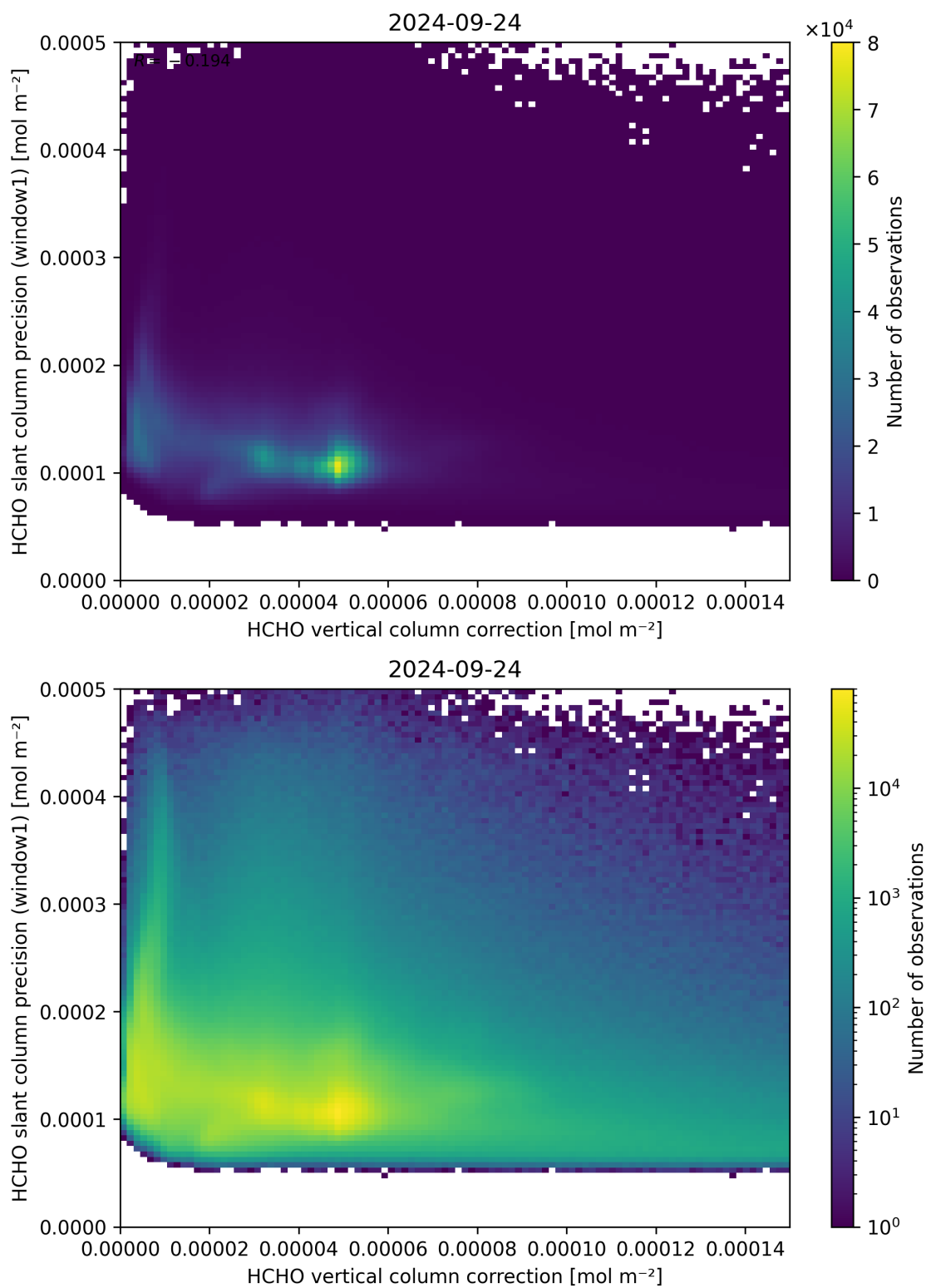
Figure 119: Scatter density plot of “HCHO vertical column correction” against “HCHO slant column precision (window1)” for 2024-09-23 to 2024-09-25.
