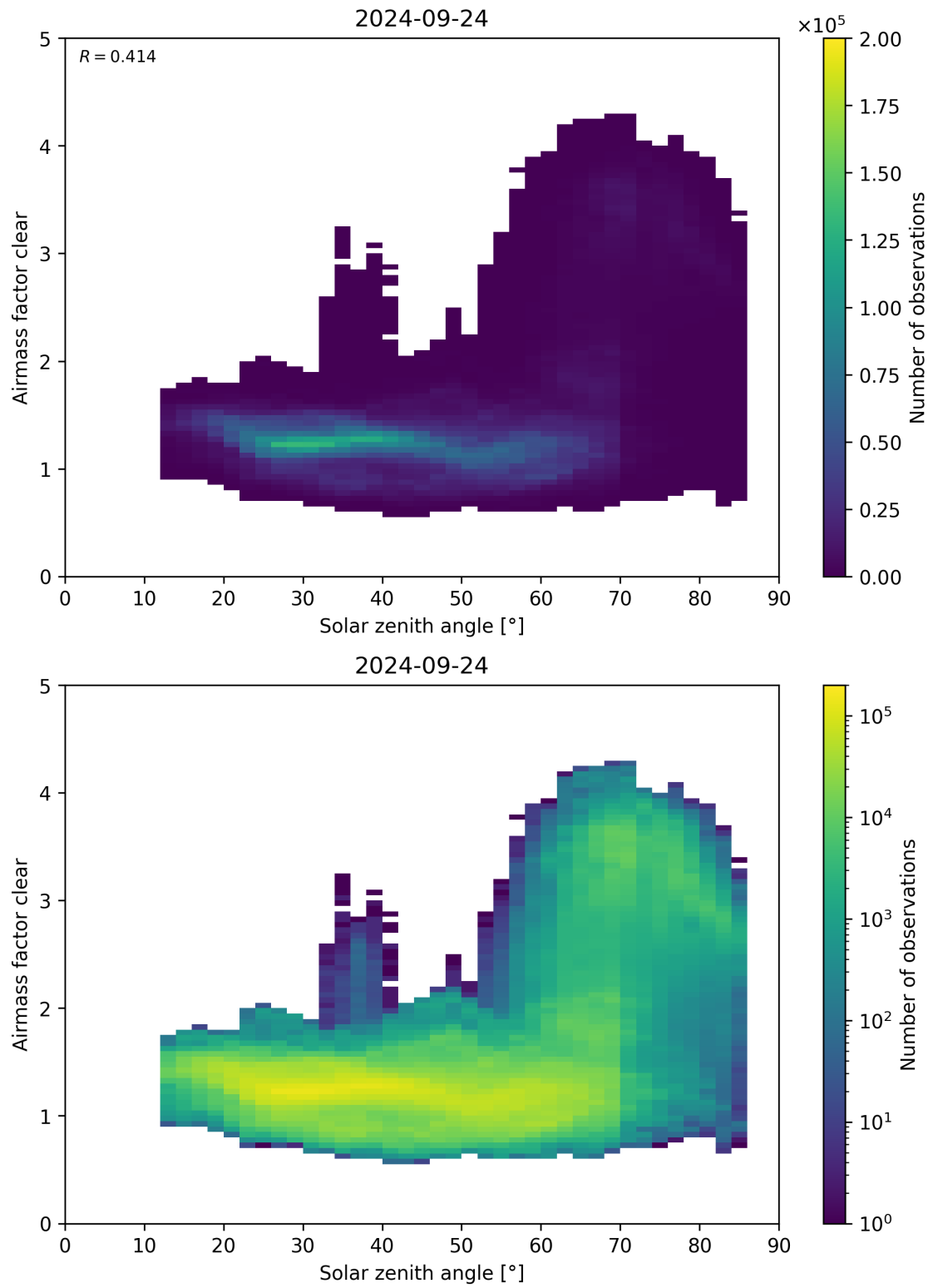
Figure 170: Scatter density plot of “Solar zenith angle” against “Airmass factor clear” for 2024-09-23 to 2024-09-25.
