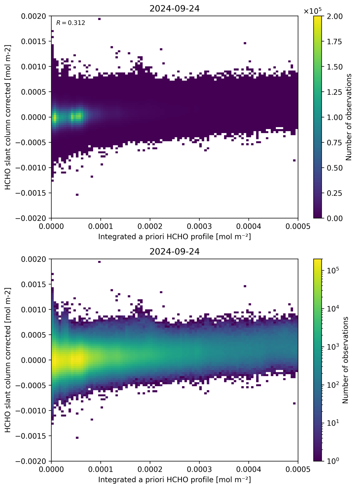
Figure 151: Scatter density plot of “Integrated a priori HCHO profile” against “HCHO slant column corrected” for 2024-09-23 to 2024-09-25.
