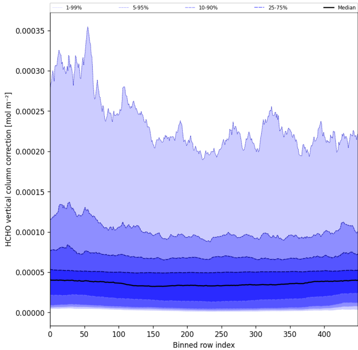
Figure 51: Along track statistics of “HCHO vertical column correction” for 2024-09-23 to 2024-09-25
