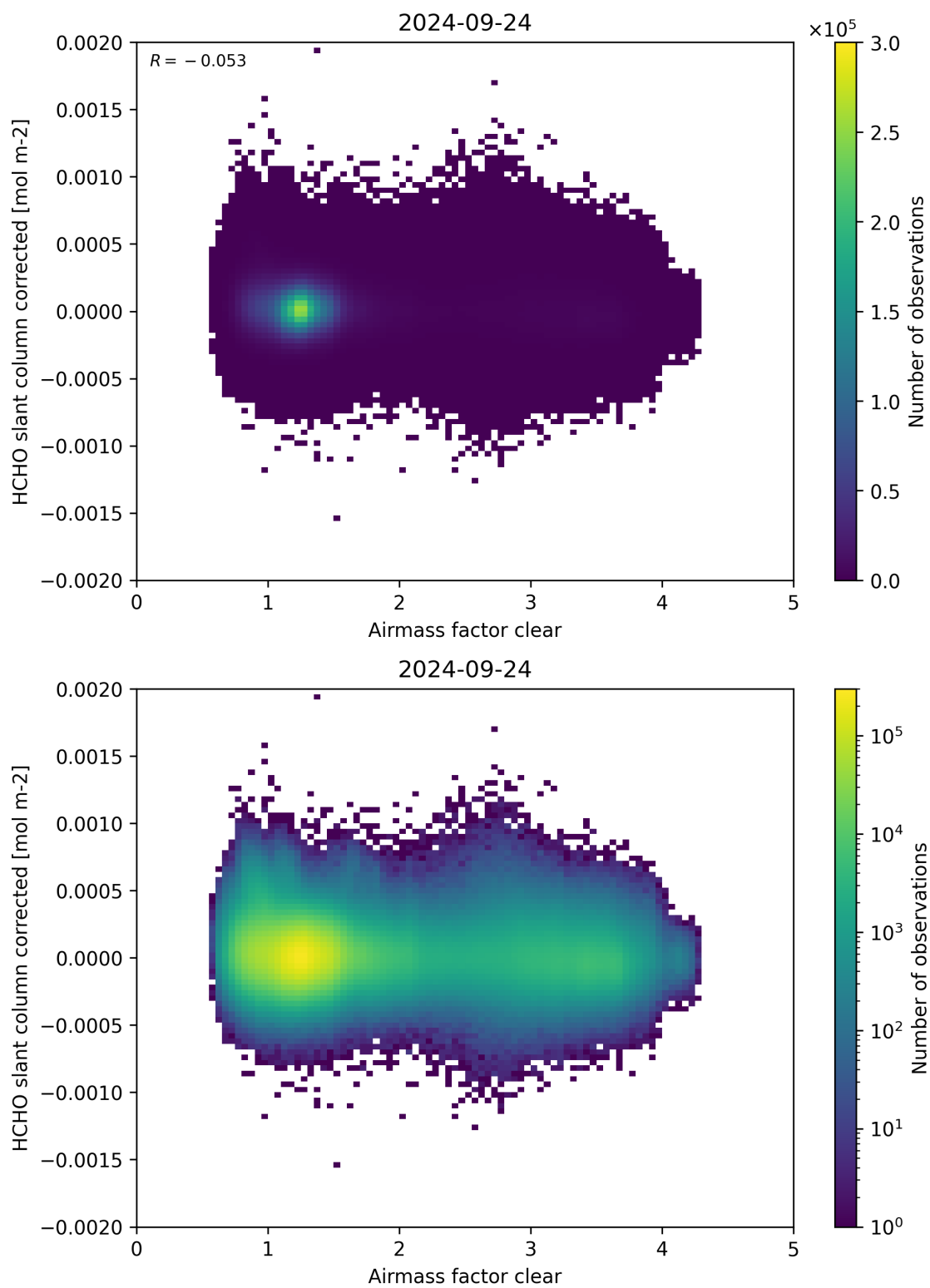
Figure 74: Scatter density plot of “Airmass factor clear” against “HCHO slant column corrected” for 2024-09-23 to 2024-09-25.
