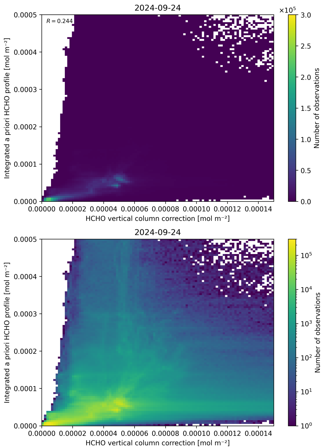
Figure 122: Scatter density plot of “HCHO vertical column correction” against “Integrated a priori HCHO profile” for 2024-09-23 to 2024-09-25.
