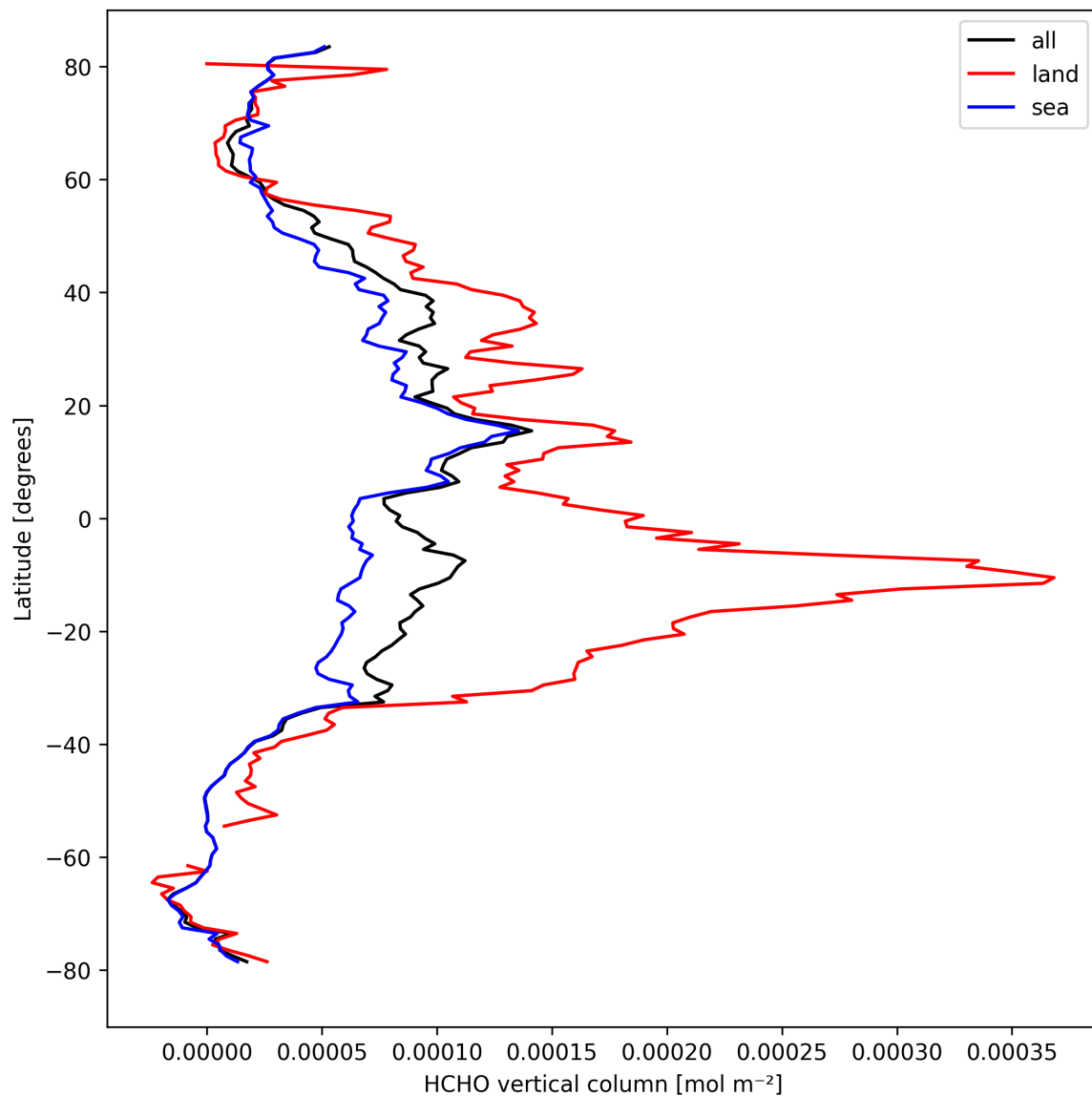
Figure 21: Zonal average of “HCHO vertical column” for 2024-09-23 to 2024-09-25.
