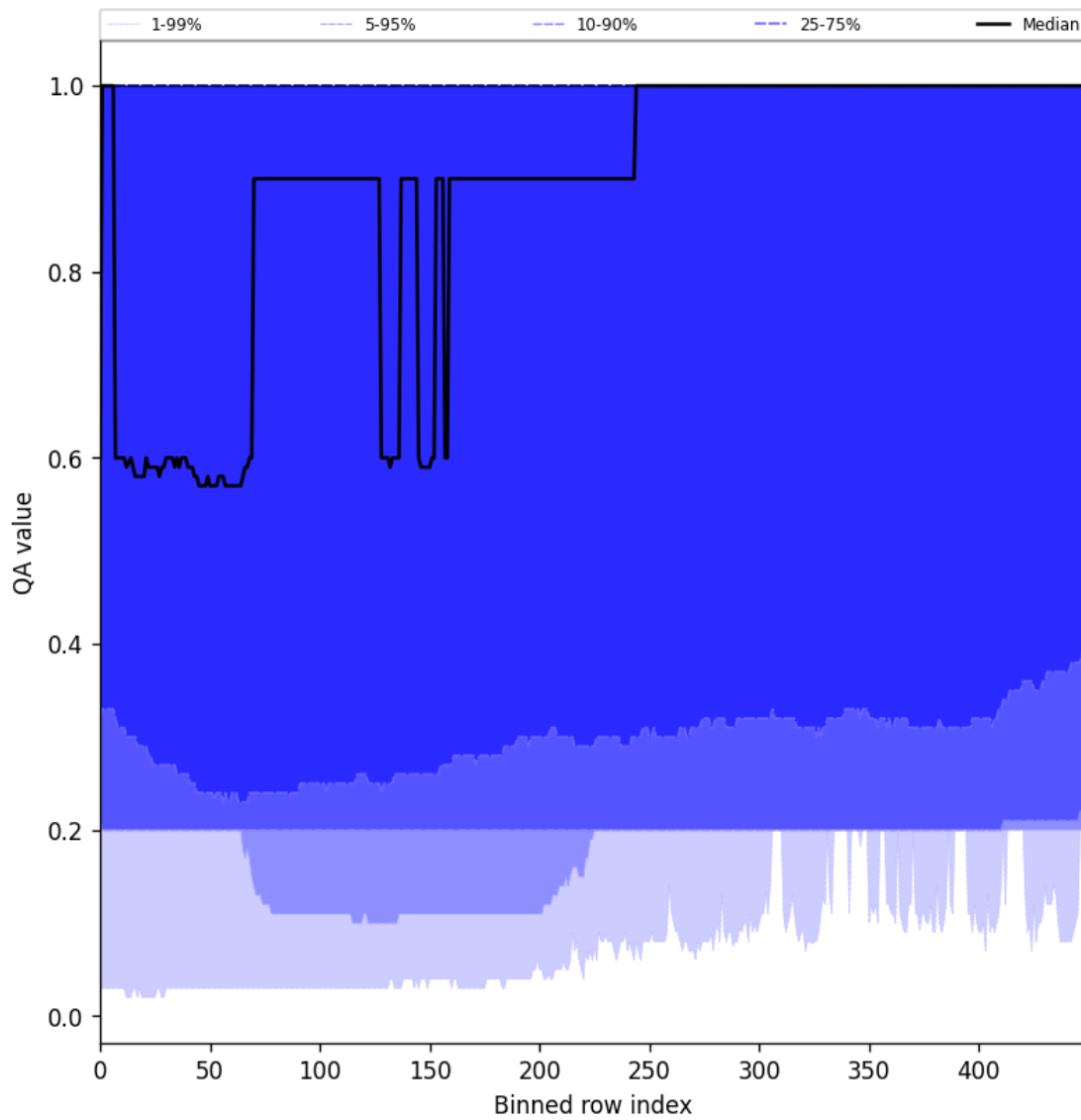
Figure 48: Along track statistics of “QA value” for 2024-09-23 to 2024-09-25
