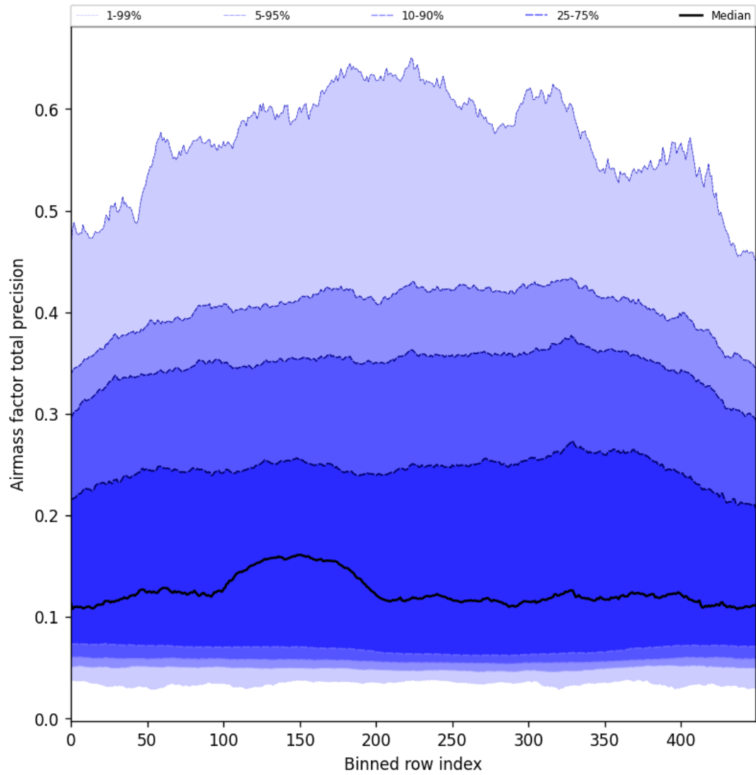
Figure 55: Along track statistics of “Airmass factor total precision” for 2024-09-23 to 2024-09-25
