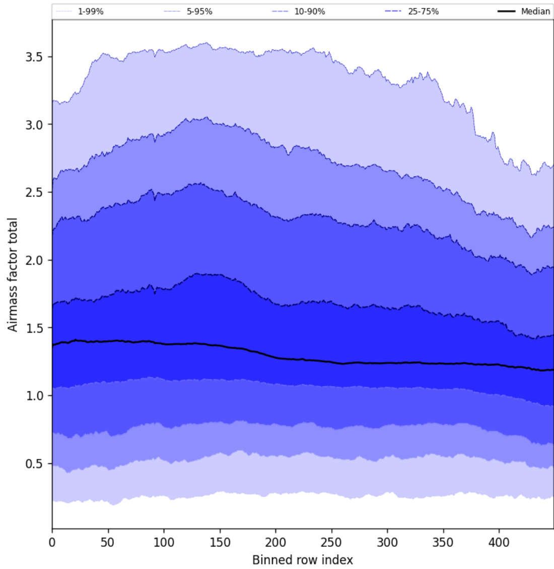
Figure 54: Along track statistics of “Airmass factor total” for 2024-09-23 to 2024-09-25
