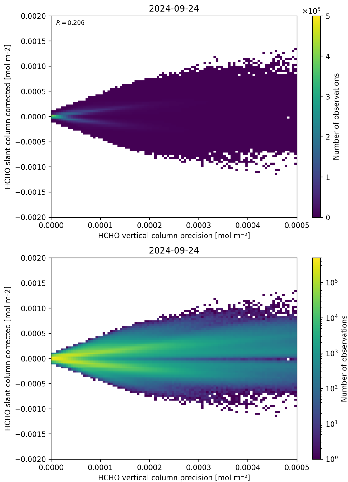
Figure 140: Scatter density plot of “HCHO vertical column precision” against “HCHO slant column corrected” for 2024-09-23 to 2024-09-25.
