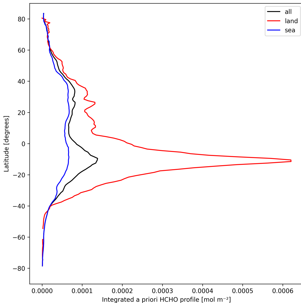
Figure 29: Zonal average of “Integrated a priori HCHO profile” for 2024-09-23 to 2024-09-25.
