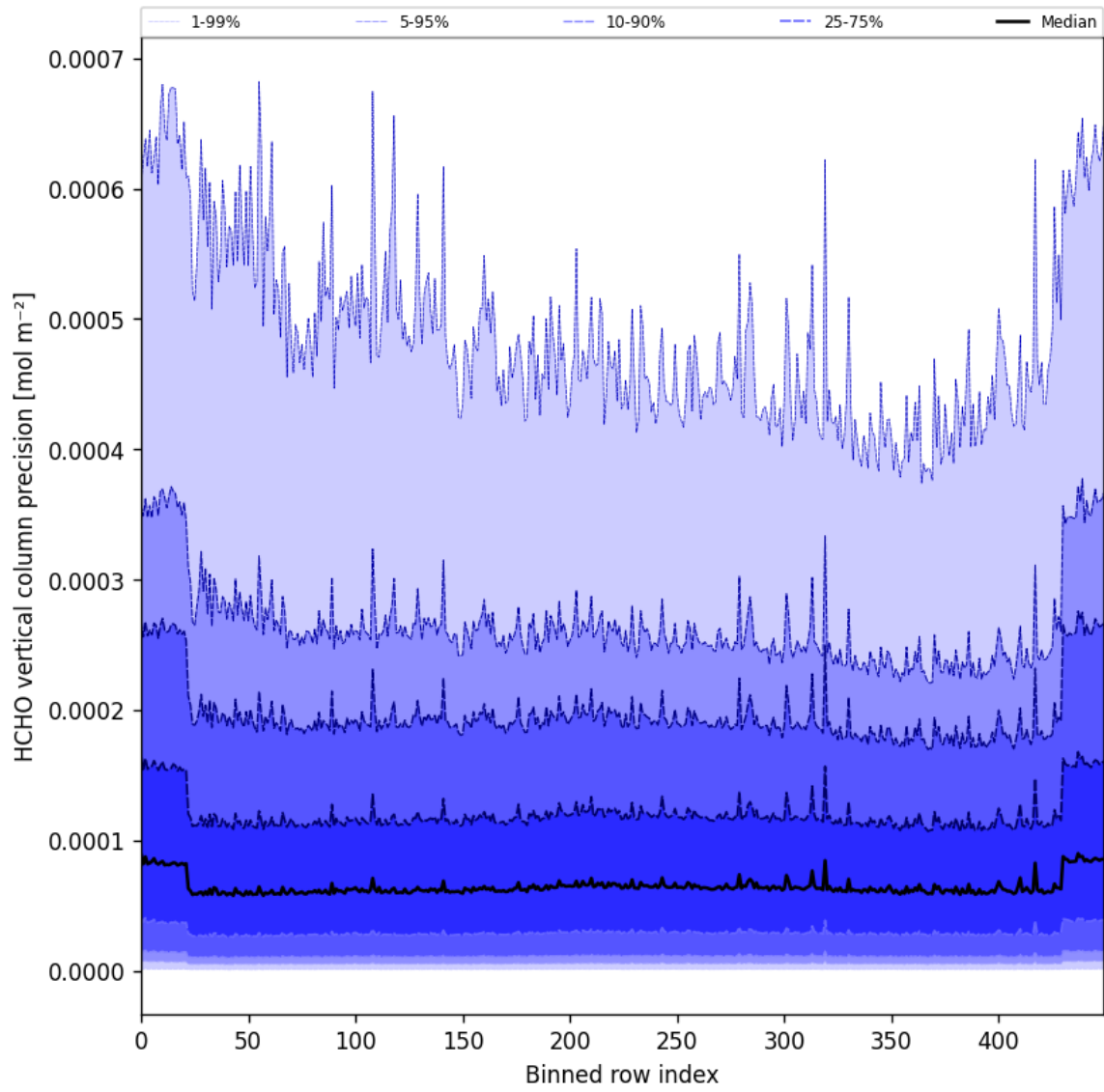
Figure 50: Along track statistics of “HCHO vertical column precision” for 2024-09-23 to 2024-09-25
