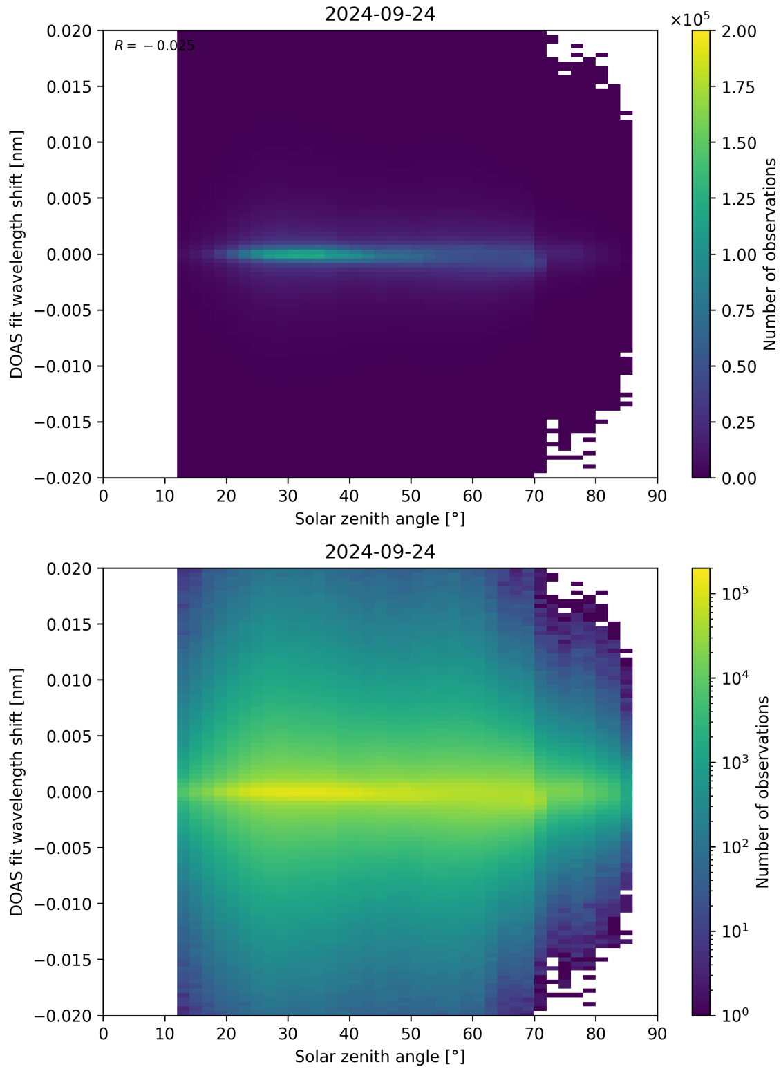
Figure 168: Scatter density plot of “Solar zenith angle” against “DOAS fit wavelength shift” for 2024-09-23 to 2024-09-25.
