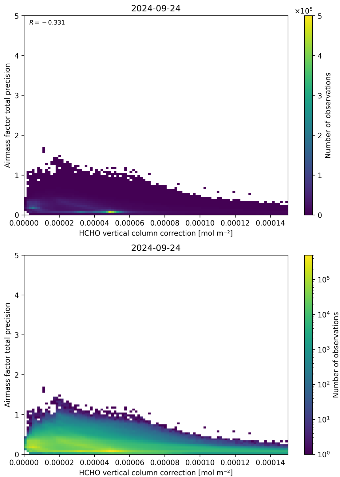
Figure 121: Scatter density plot of “HCHO vertical column correction” against “Airmass factor total precision” for 2024-09-23 to 2024-09-25.
