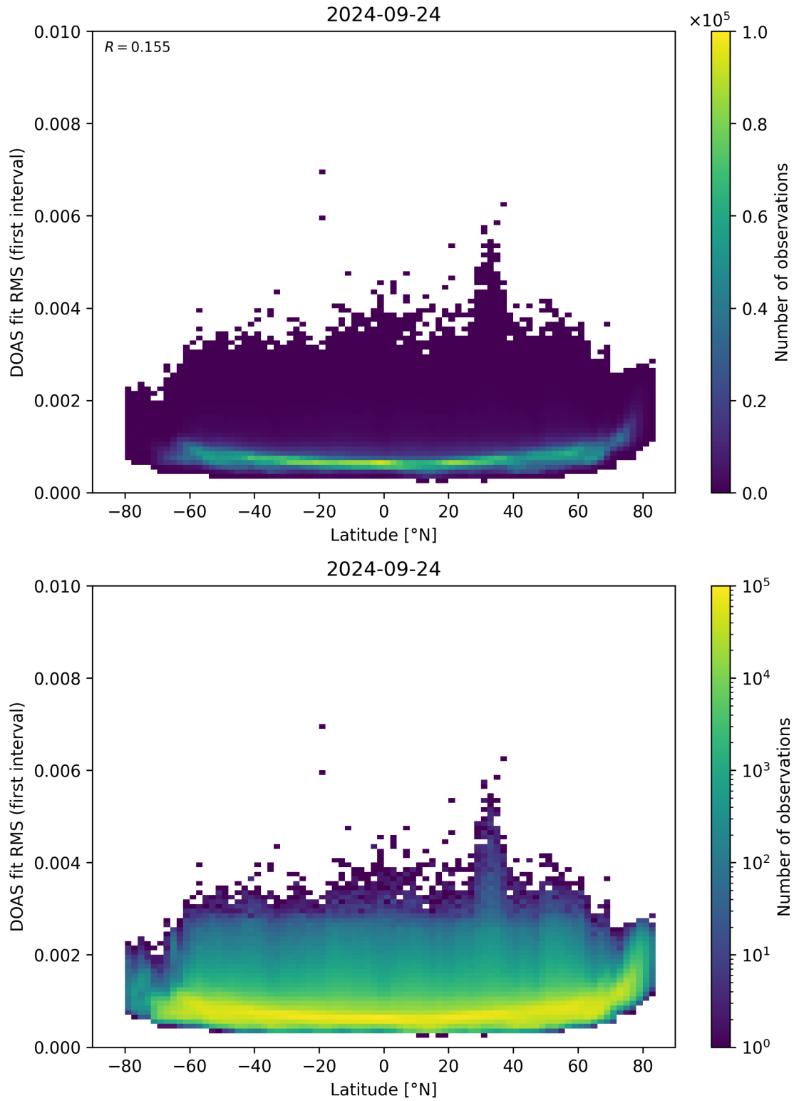
Figure 153: Scatter density plot of “Latitude” against “DOAS fit RMS (first interval)” for 2024-09-23 to 2024-09-25.
