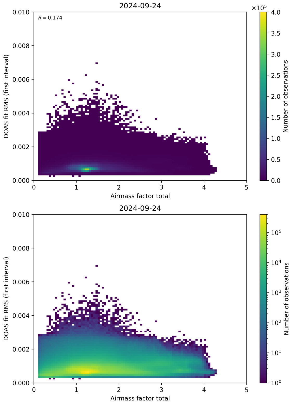
Figure 97: Scatter density plot of “Airmass factor total” against “DOAS fit RMS (first interval)” for 2024-09-23 to 2024-09-25.
