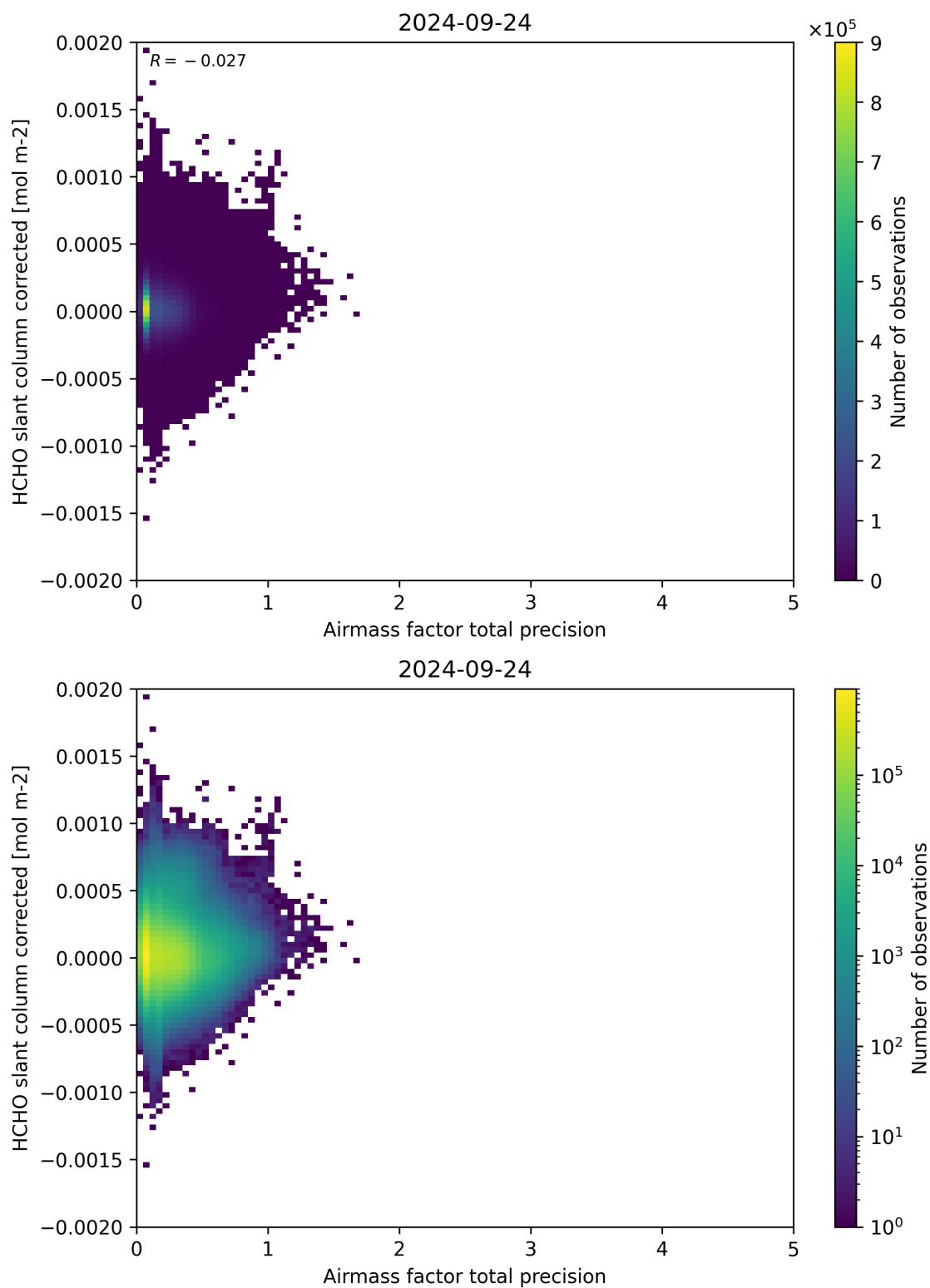
Figure 109: Scatter density plot of “Airmass factor total precision” against “HCHO slant column corrected” for 2024-09-23 to 2024-09-25.
