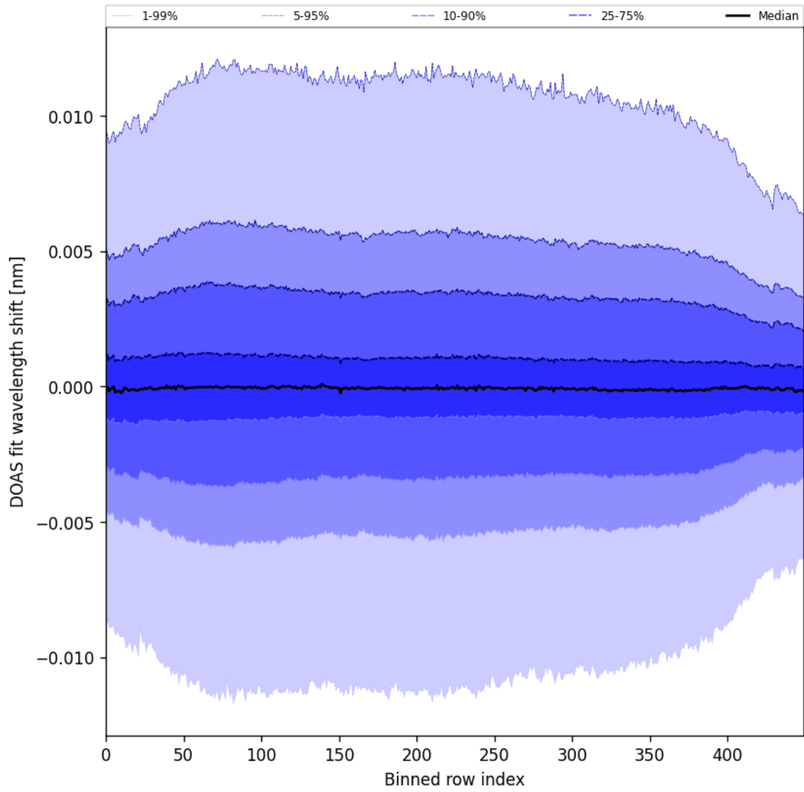
Figure 58: Along track statistics of “DOAS fit wavelength shift” for 2024-09-23 to 2024-09-25
