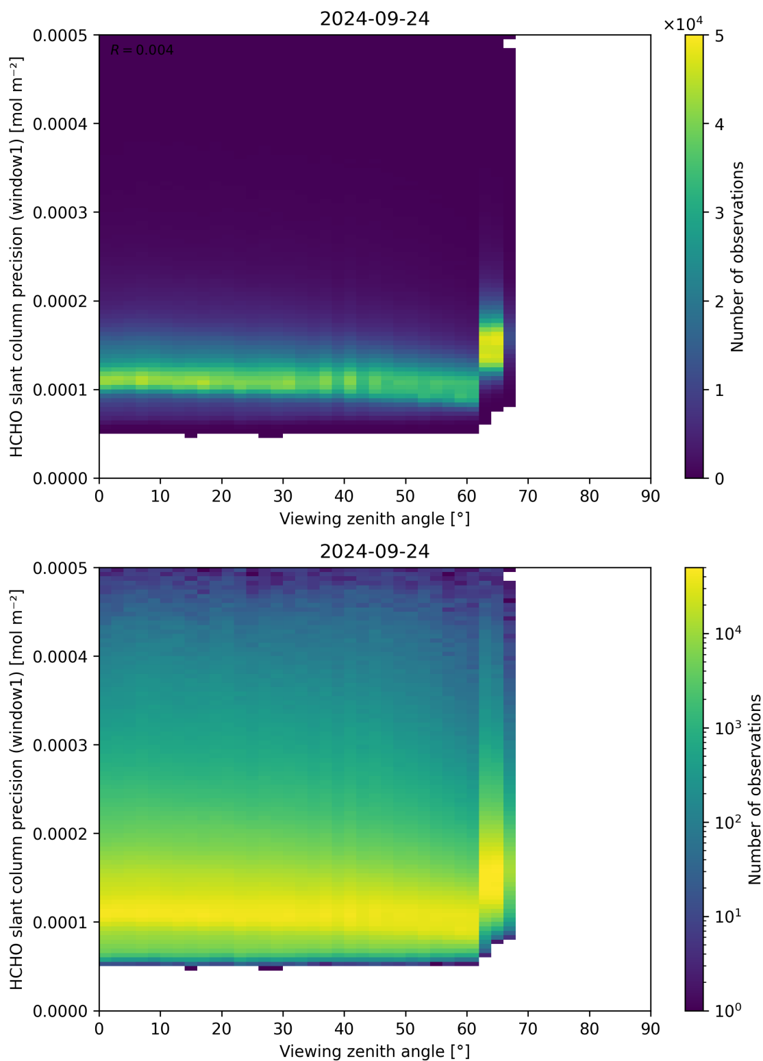
Figure 189: Scatter density plot of “Viewing zenith angle” against “HCHO slant column precision (window1)” for 2024-09-23 to 2024-09-25.
