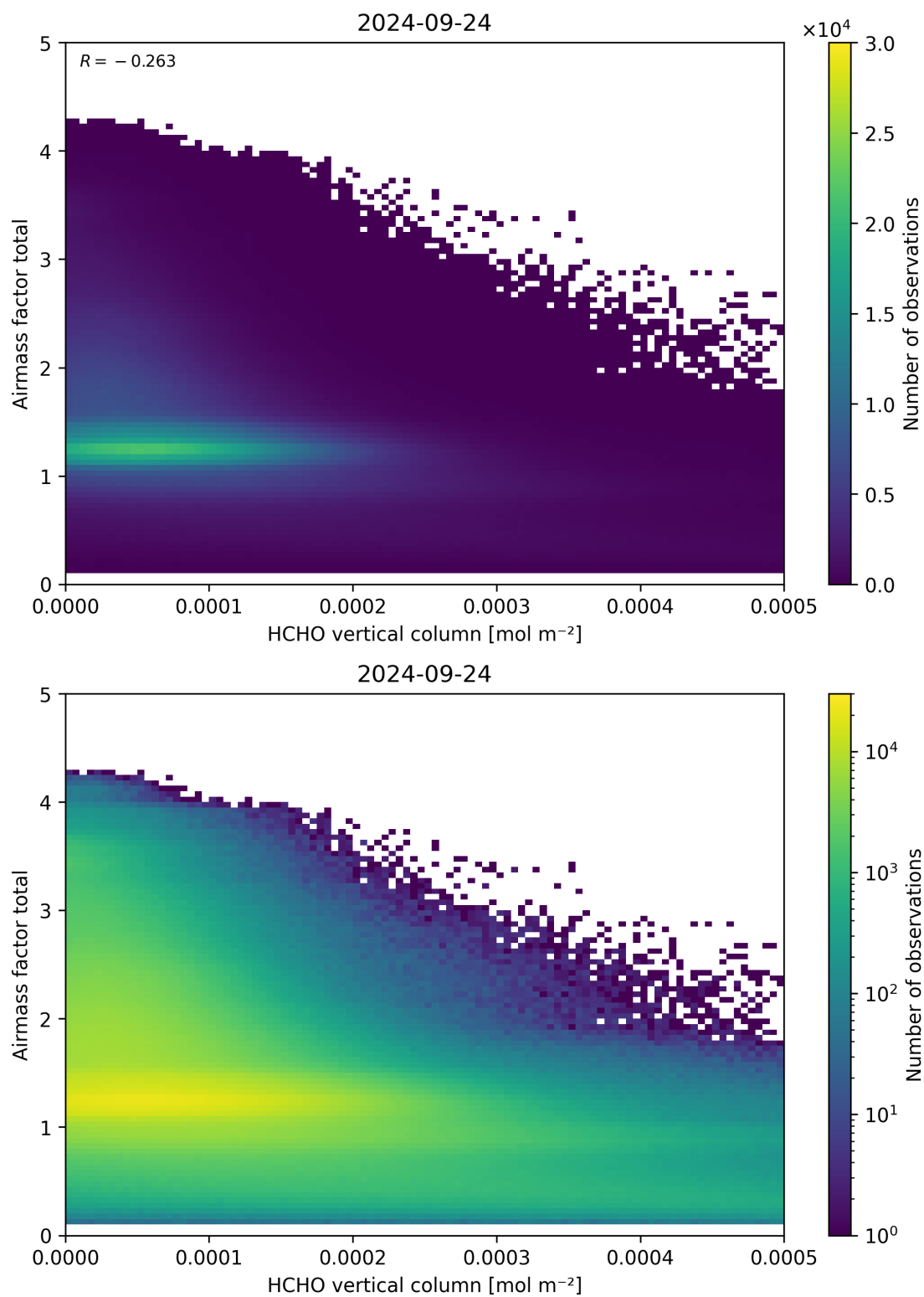
Figure 131: Scatter density plot of “HCHO vertical column” against “Airmass factor total” for 2024-09-23 to 2024-09-25.
