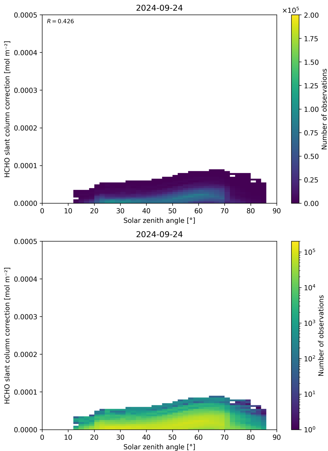
Figure 172: Scatter density plot of “Solar zenith angle” against “HCHO slant column correction” for 2024-09-23 to 2024-09-25.
