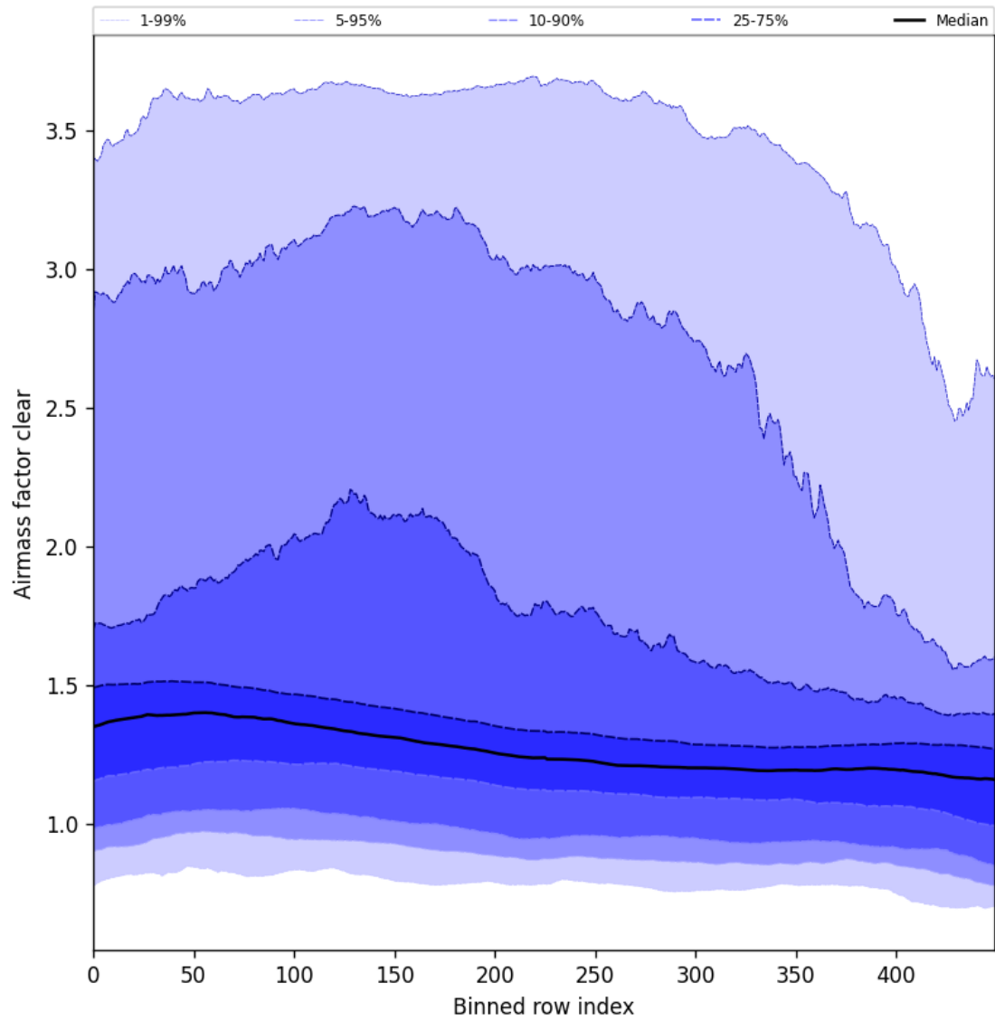
Figure 56: Along track statistics of “Airmass factor clear” for 2024-09-23 to 2024-09-25
