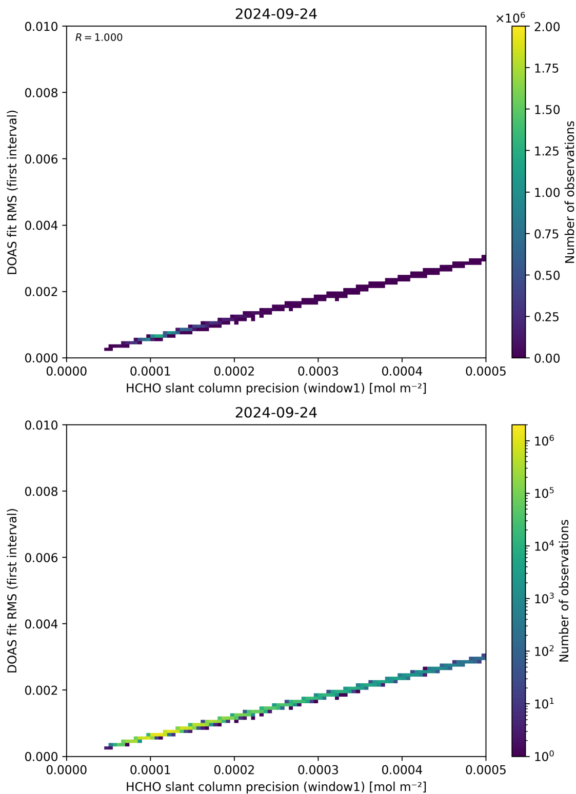
Figure 88: Scatter density plot of “HCHO slant column precision (window1)” against “DOAS fit RMS (first interval)” for 2024-09-23 to 2024-09-25.
