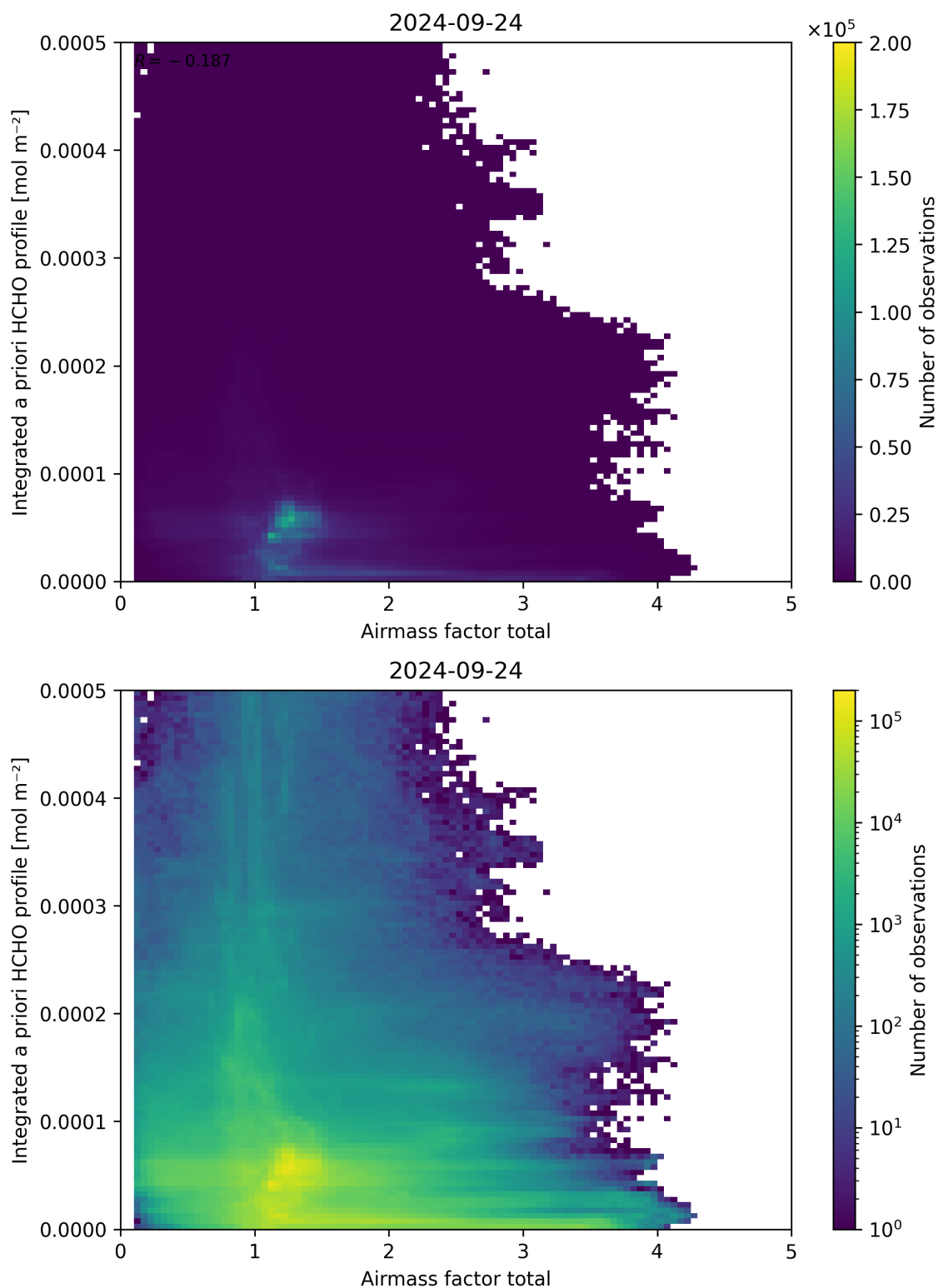
Figure 104: Scatter density plot of “Airmass factor total” against “Integrated a priori HCHO profile” for 2024-09-23 to 2024-09-25.
