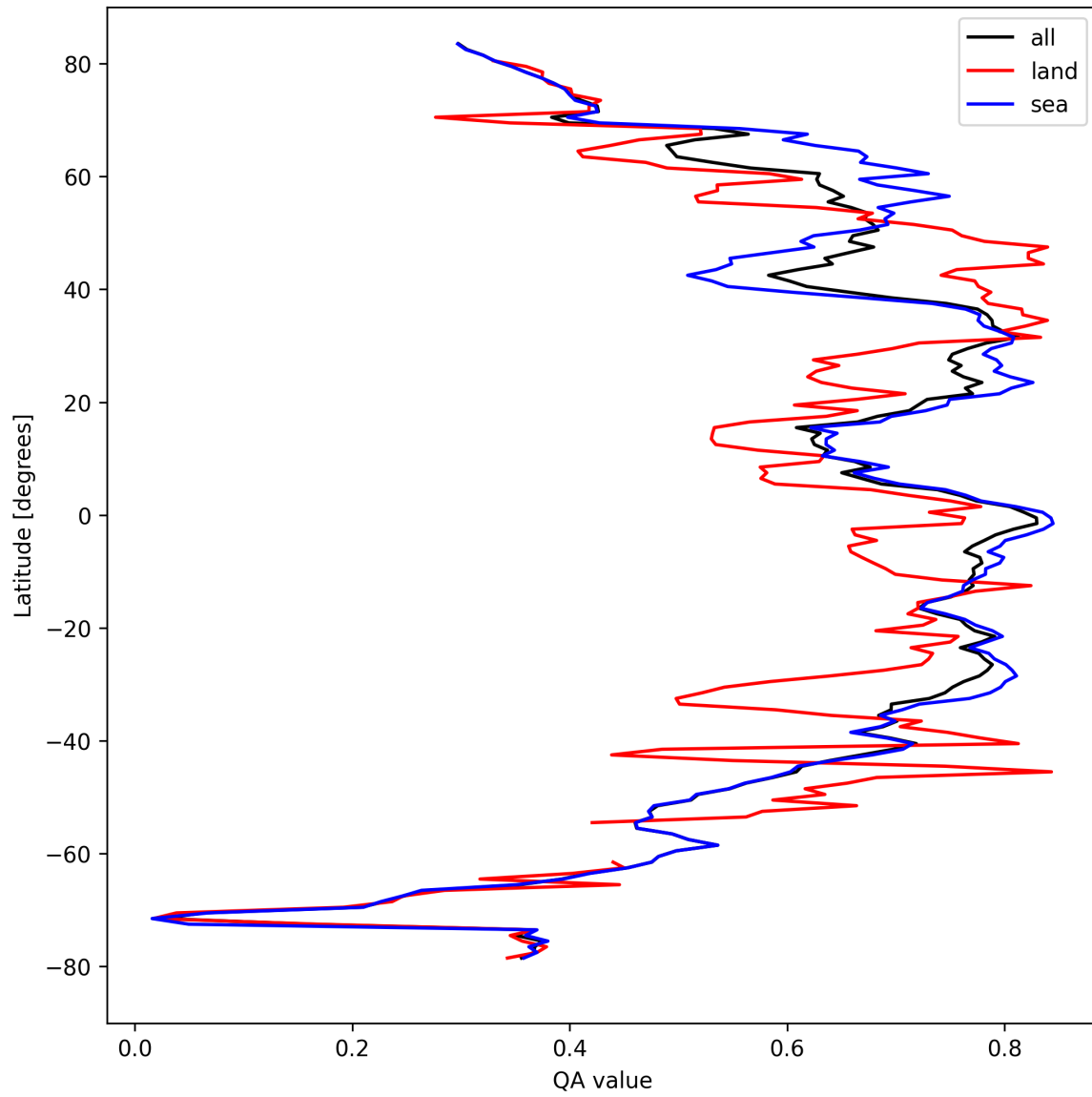
Figure 20: Zonal average of “QA value” for 2024-09-23 to 2024-09-25.
