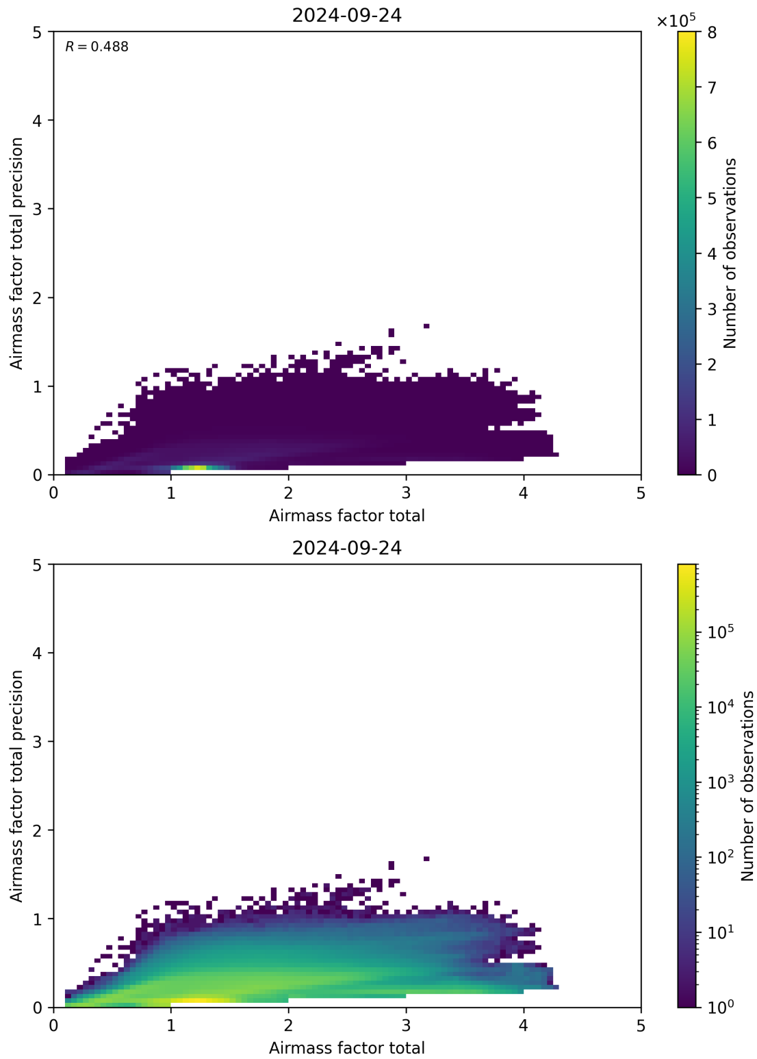
Figure 103: Scatter density plot of “Airmass factor total” against “Airmass factor total precision” for 2024-09-23 to 2024-09-25.
