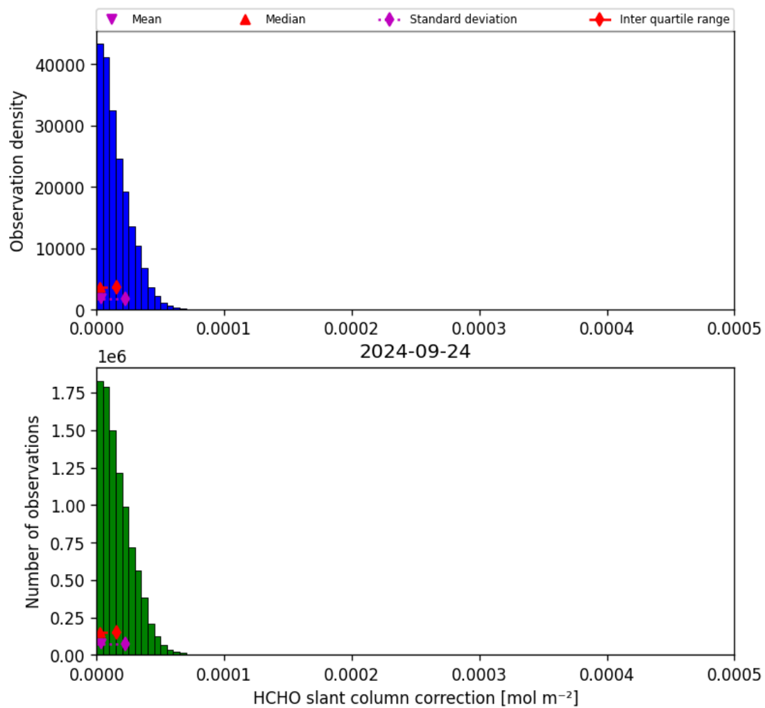
Figure 47: Histogram of “HCHO slant column correction” for 2024-09-23 to 2024-09-25
