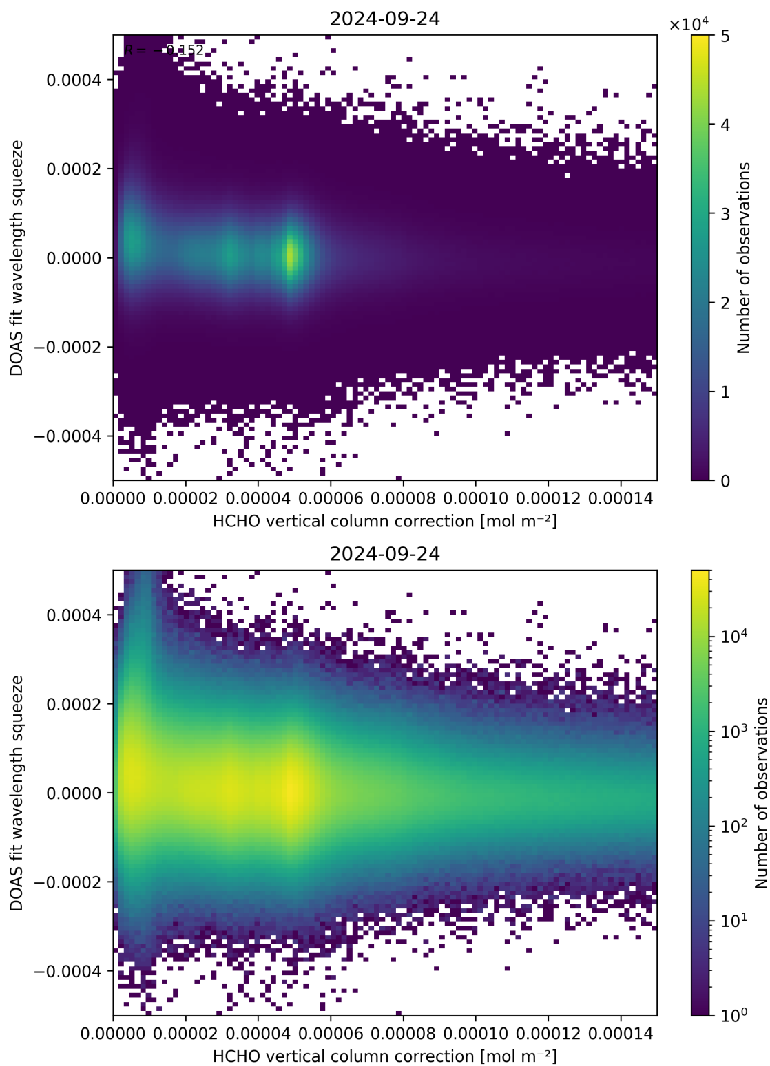
Figure 114: Scatter density plot of “HCHO vertical column correction” against “DOAS fit wavelength squeeze” for 2024-09-23 to 2024-09-25.
