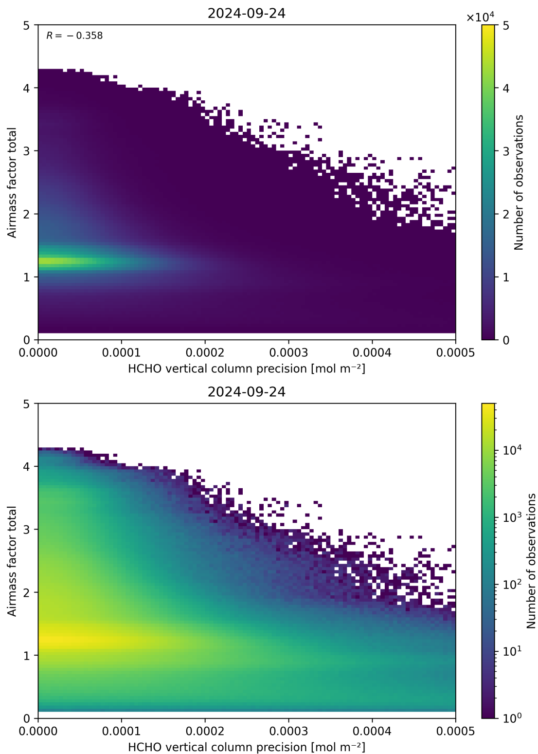
Figure 144: Scatter density plot of “HCHO vertical column precision” against “Airmass factor total” for 2024-09-23 to 2024-09-25.
