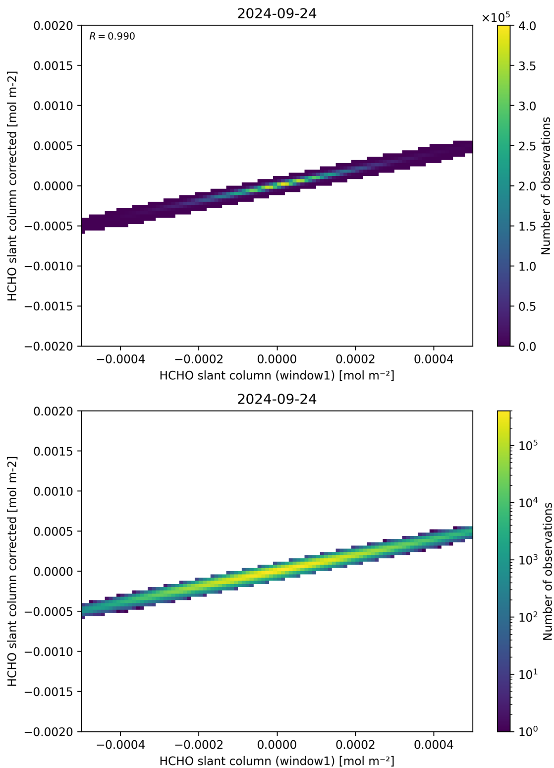
Figure 82: Scatter density plot of “HCHO slant column (window1)” against “HCHO slant column corrected” for 2024-09-23 to 2024-09-25.
