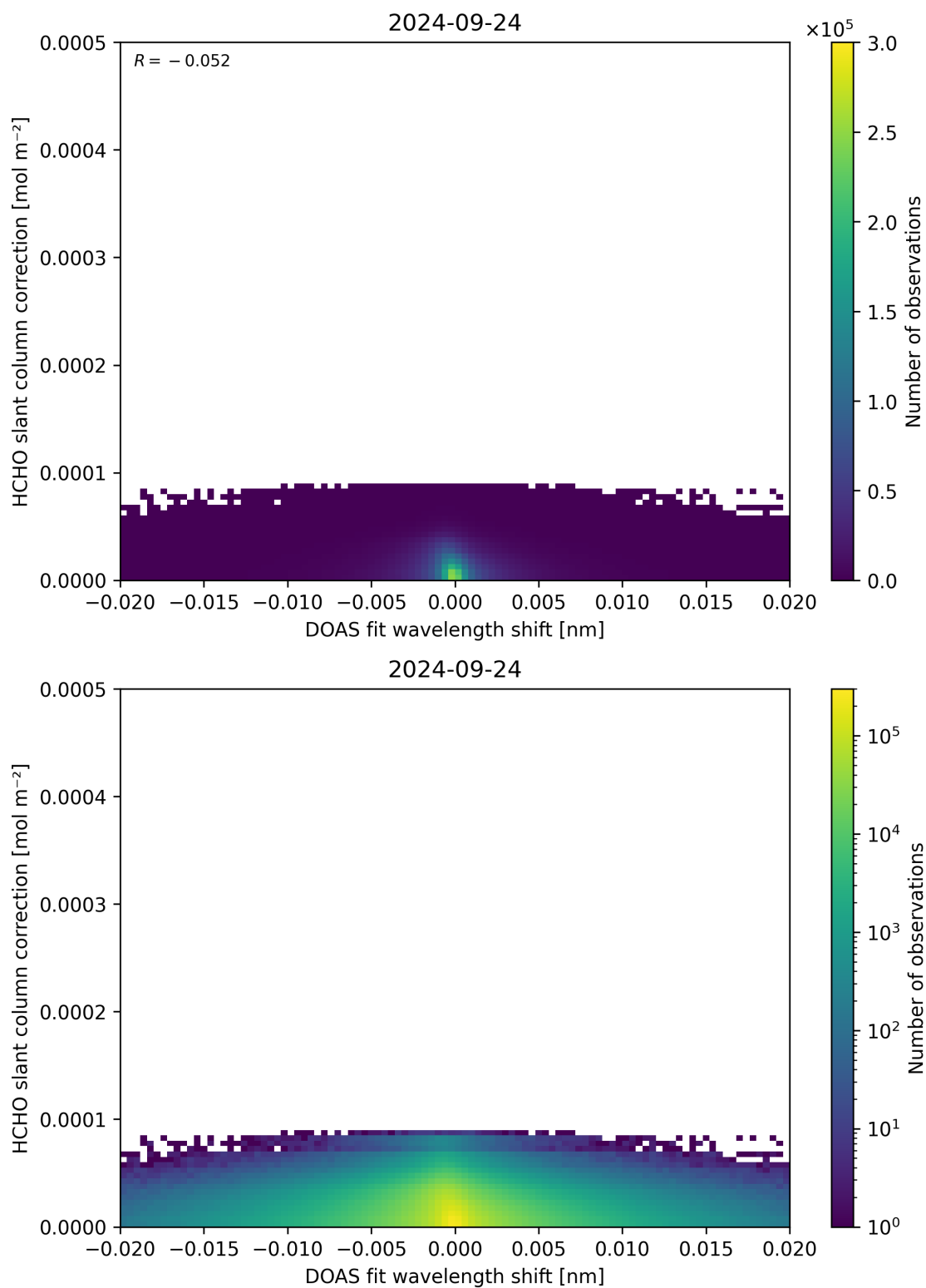
Figure 67: Scatter density plot of “DOAS fit wavelength shift” against “HCHO slant column correction” for 2024-09-23 to 2024-09-25.
