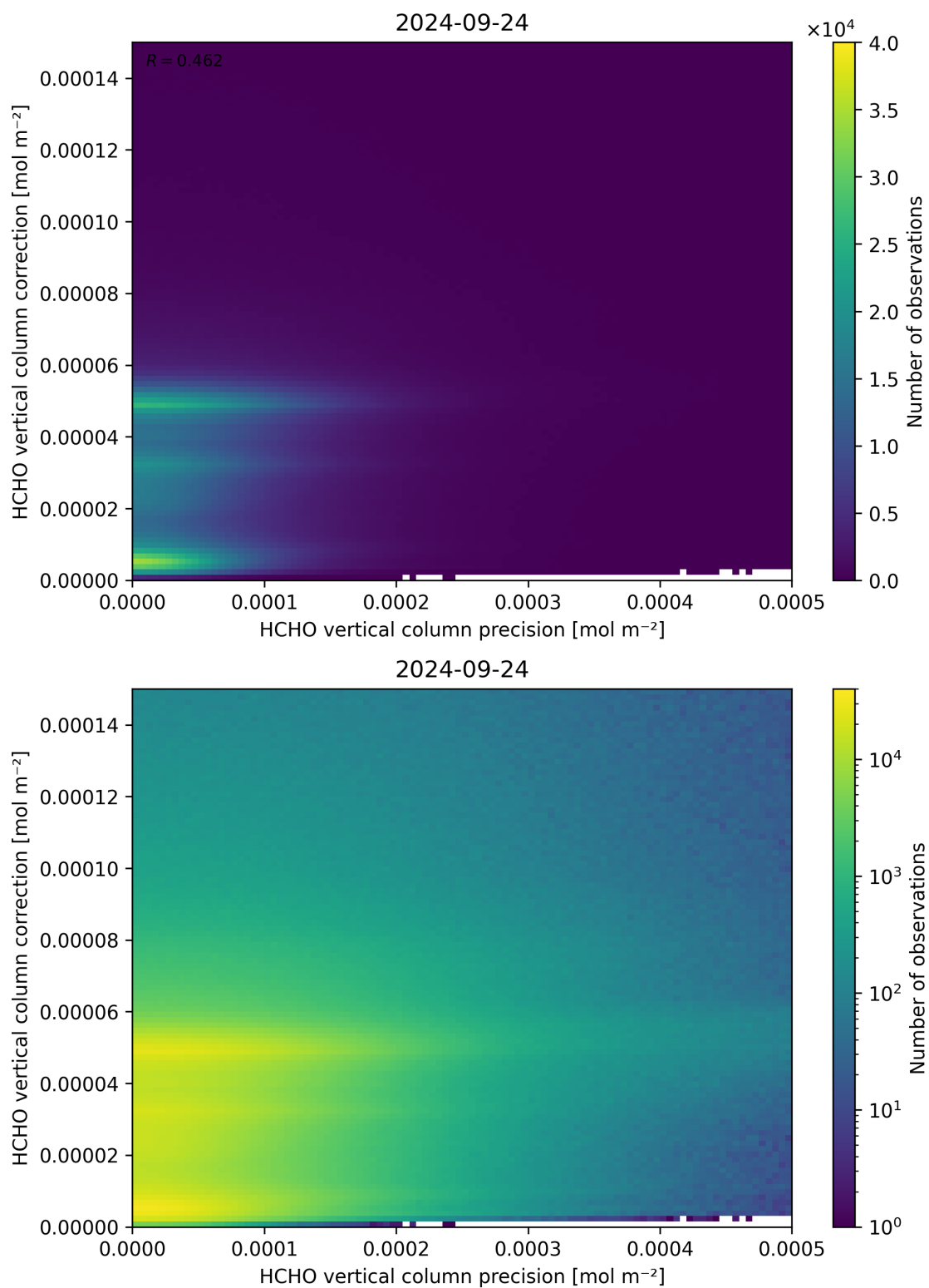
Figure 146: Scatter density plot of “HCHO vertical column precision” against “HCHO vertical column correction” for 2024-09-23 to 2024-09-25.
