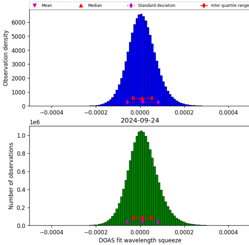
Figure 45: Histogram of “DOAS fit wavelength squeeze” for 2024-09-23 to 2024-09-25
