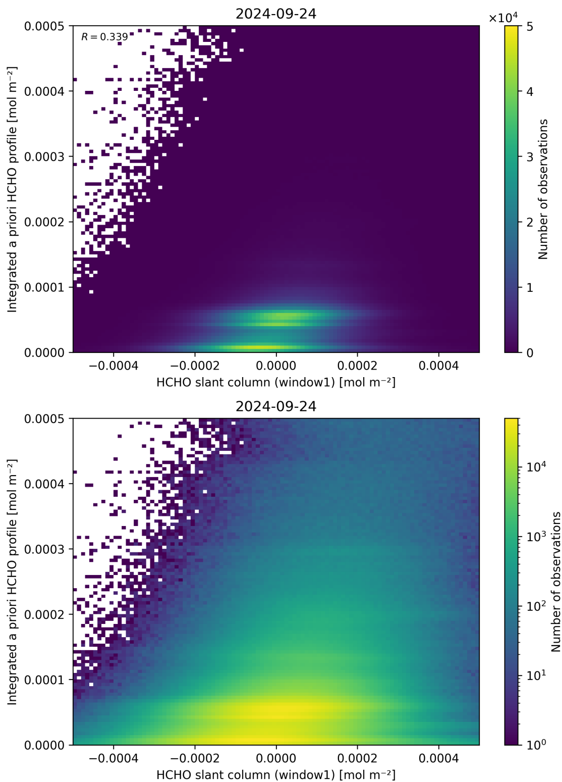
Figure 87: Scatter density plot of “HCHO slant column (window1)” against “Integrated a priori HCHO profile” for 2024-09-23 to 2024-09-25.
