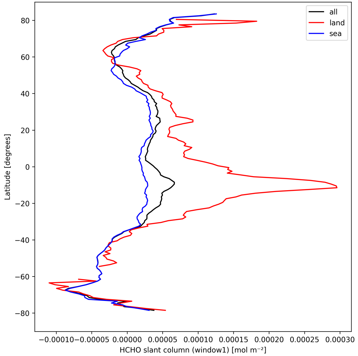
Figure 24: Zonal average of “HCHO slant column (window1)” for 2024-09-23 to 2024-09-25.
