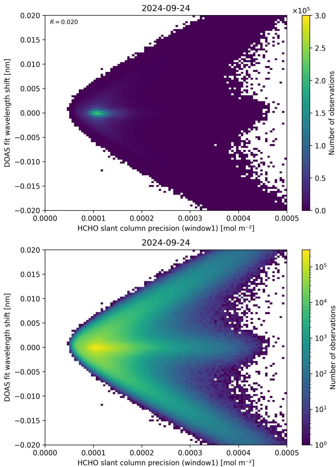
Figure 89: Scatter density plot of “HCHO slant column precision (window1)” against “DOAS fit wavelength shift” for 2024-09-23 to 2024-09-25.
