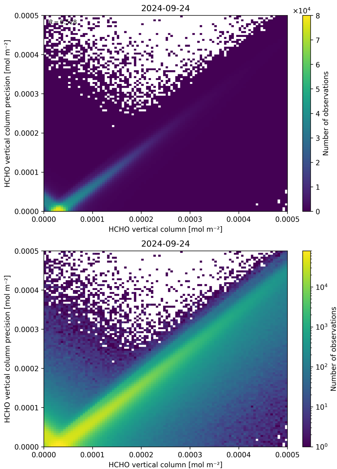
Figure 134: Scatter density plot of “HCHO vertical column” against “HCHO vertical column precision” for 2024-09-23 to 2024-09-25.
