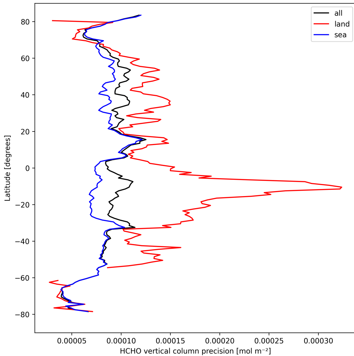
Figure 22: Zonal average of “HCHO vertical column precision” for 2024-09-23 to 2024-09-25.
