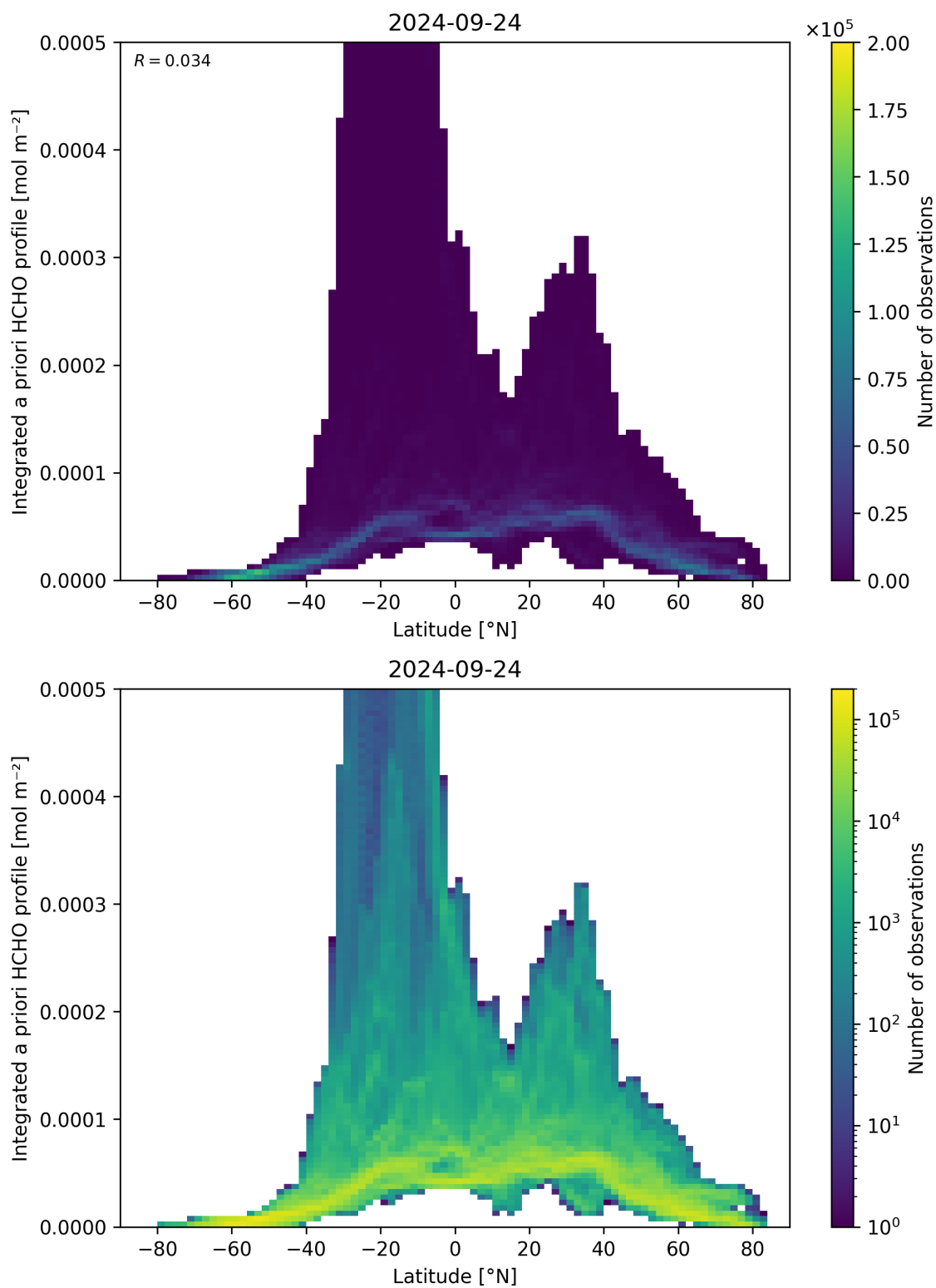
Figure 166: Scatter density plot of “Latitude” against “Integrated a priori HCHO profile” for 2024-09-23 to 2024-09-25.
