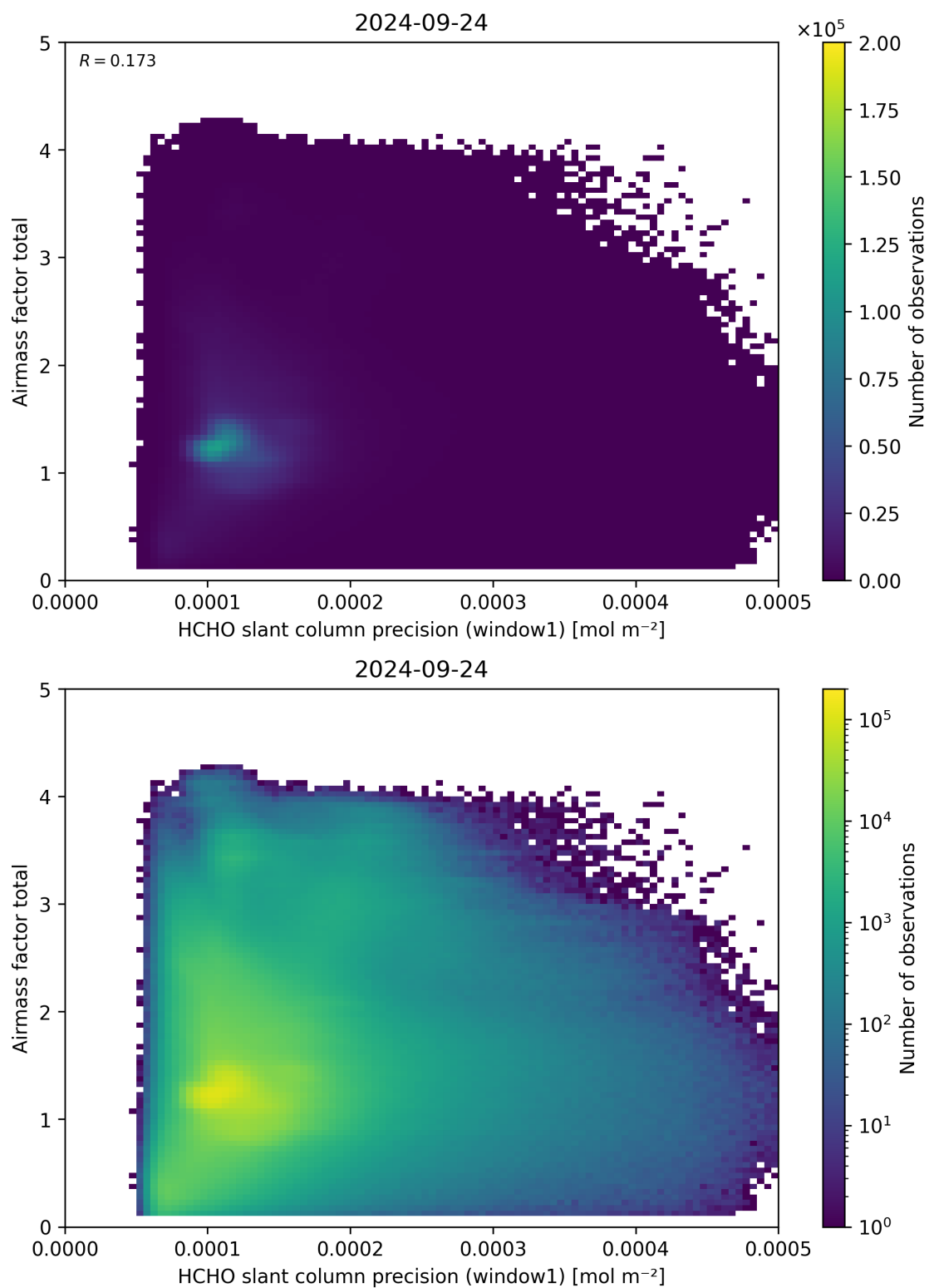
Figure 94: Scatter density plot of “HCHO slant column precision (window1)” against “Airmass factor total” for 2024-09-23 to 2024-09-25.
