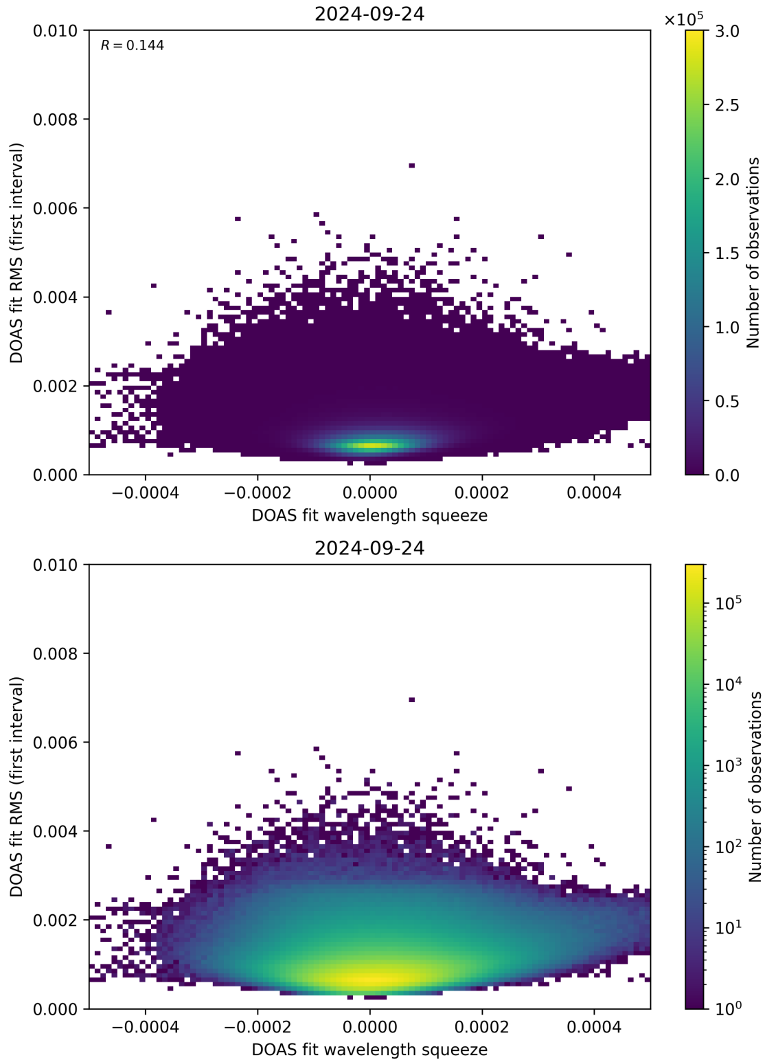
Figure 68: Scatter density plot of “DOAS fit wavelength squeeze” against “DOAS fit RMS (first interval)” for 2024-09-23 to 2024-09-25.
