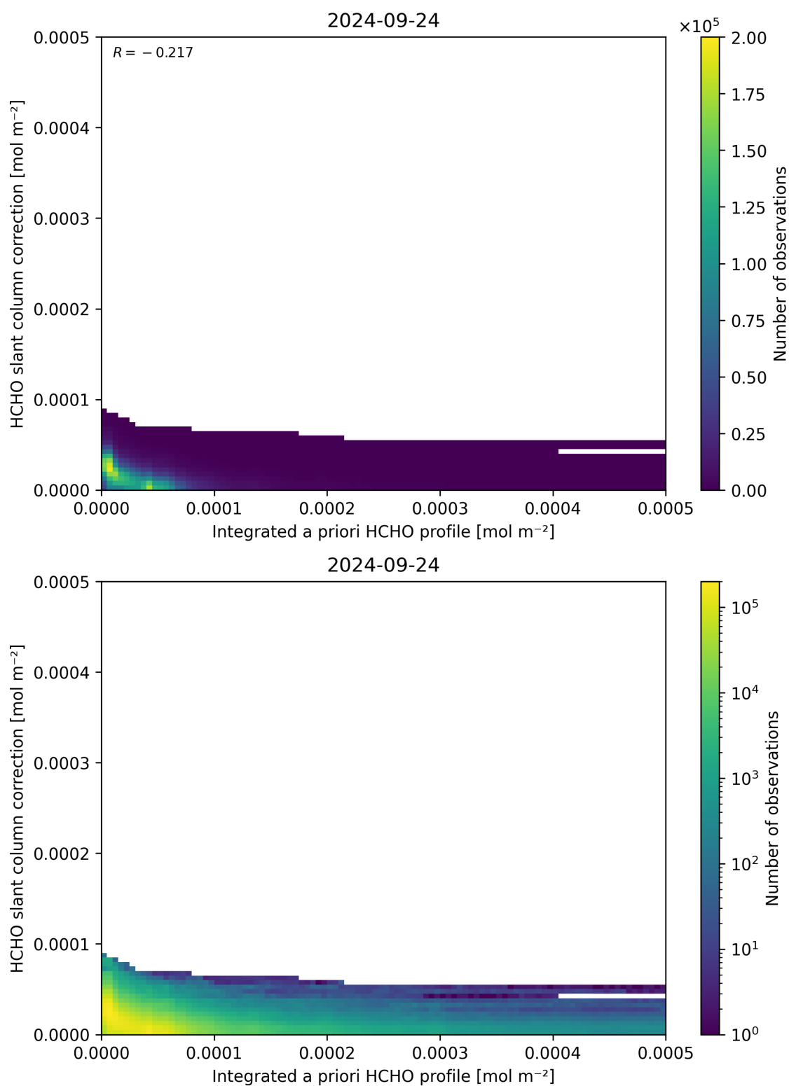
Figure 152: Scatter density plot of “Integrated a priori HCHO profile” against “HCHO slant column correction” for 2024-09-23 to 2024-09-25.
