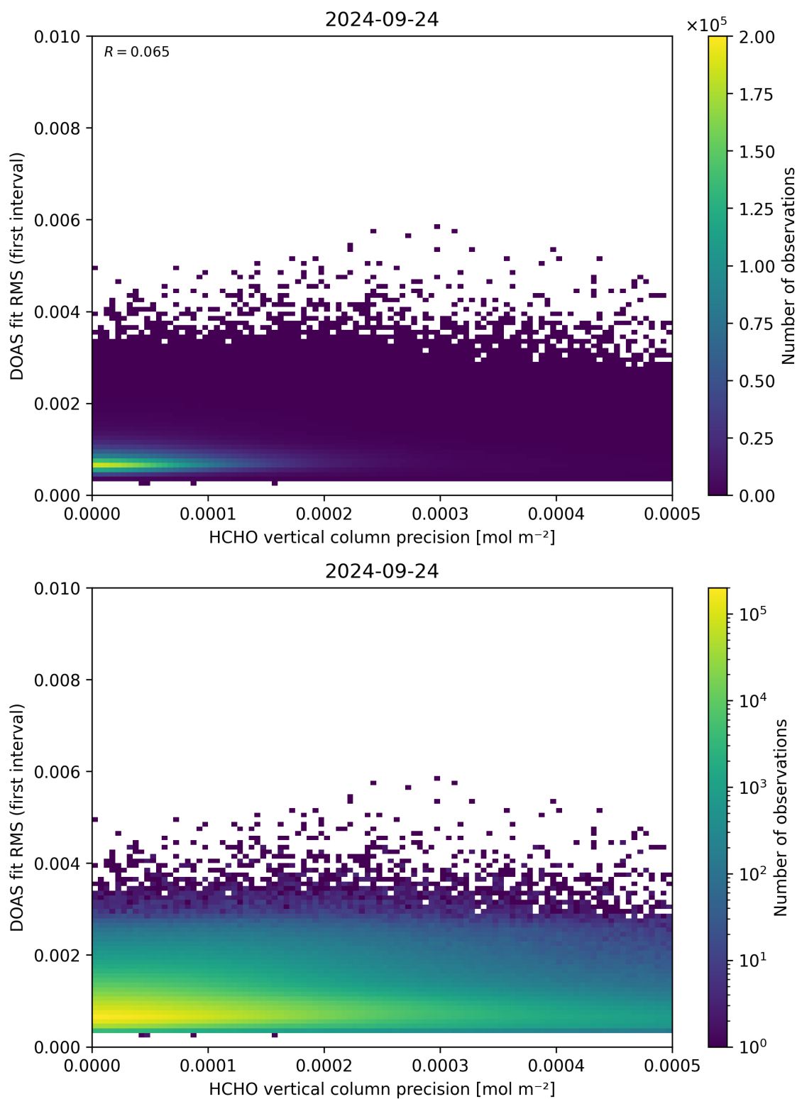
Figure 136: Scatter density plot of “HCHO vertical column precision” against “DOAS fit RMS (first interval)” for 2024-09-23 to 2024-09-25.
