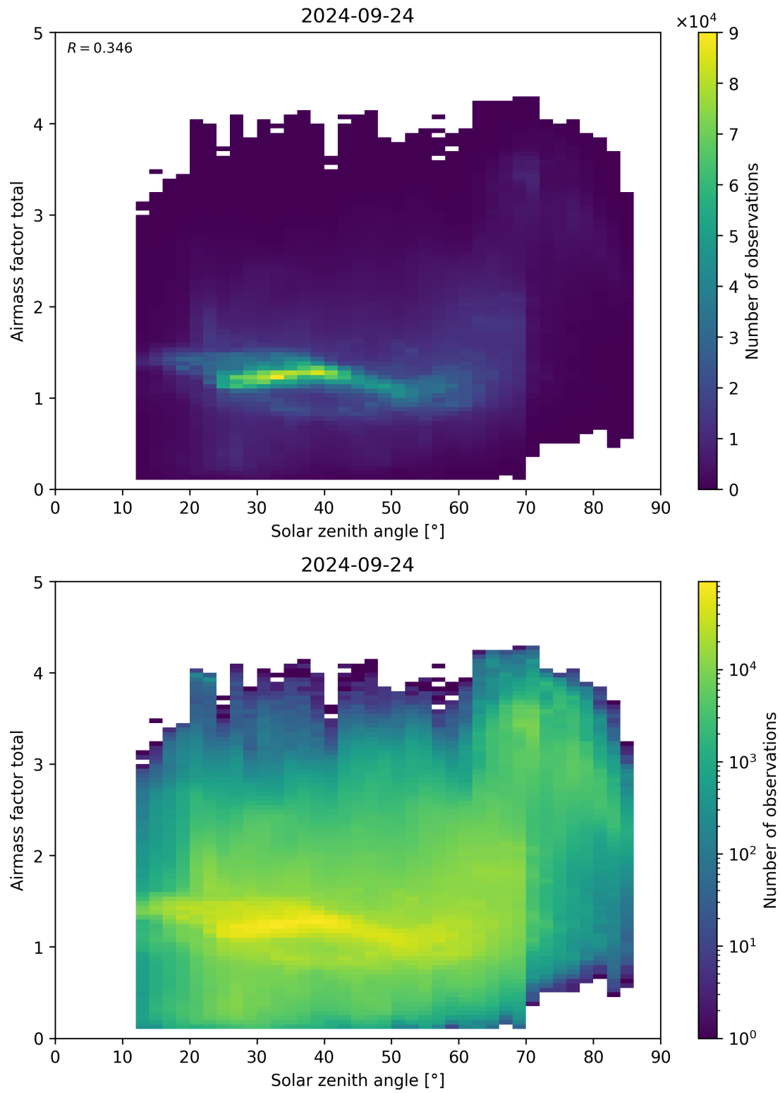
Figure 175: Scatter density plot of “Solar zenith angle” against “Airmass factor total” for 2024-09-23 to 2024-09-25.
