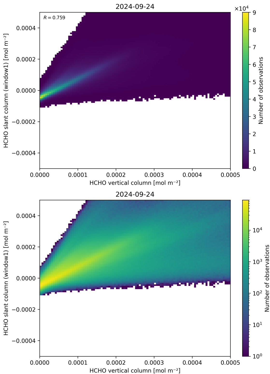
Figure 129: Scatter density plot of “HCHO vertical column” against “HCHO slant column (window1)” for 2024-09-23 to 2024-09-25.
