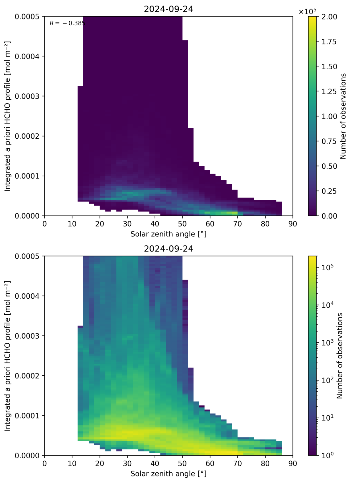
Figure 180: Scatter density plot of “Solar zenith angle” against “Integrated a priori HCHO profile” for 2024-09-23 to 2024-09-25.
