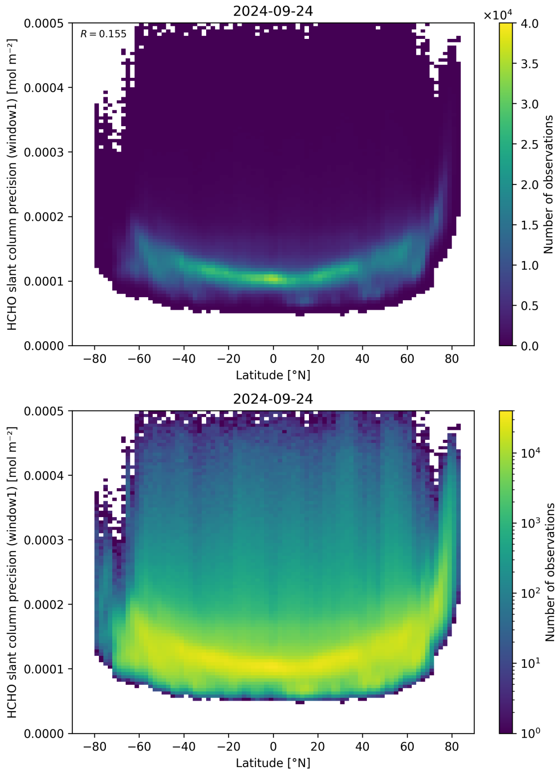
Figure 160: Scatter density plot of “Latitude” against “HCHO slant column precision (window1)” for 2024-09-23 to 2024-09-25.
