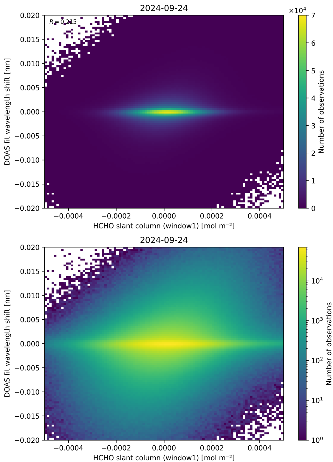
Figure 79: Scatter density plot of “HCHO slant column (window1)” against “DOAS fit wavelength shift” for 2024-09-23 to 2024-09-25.
