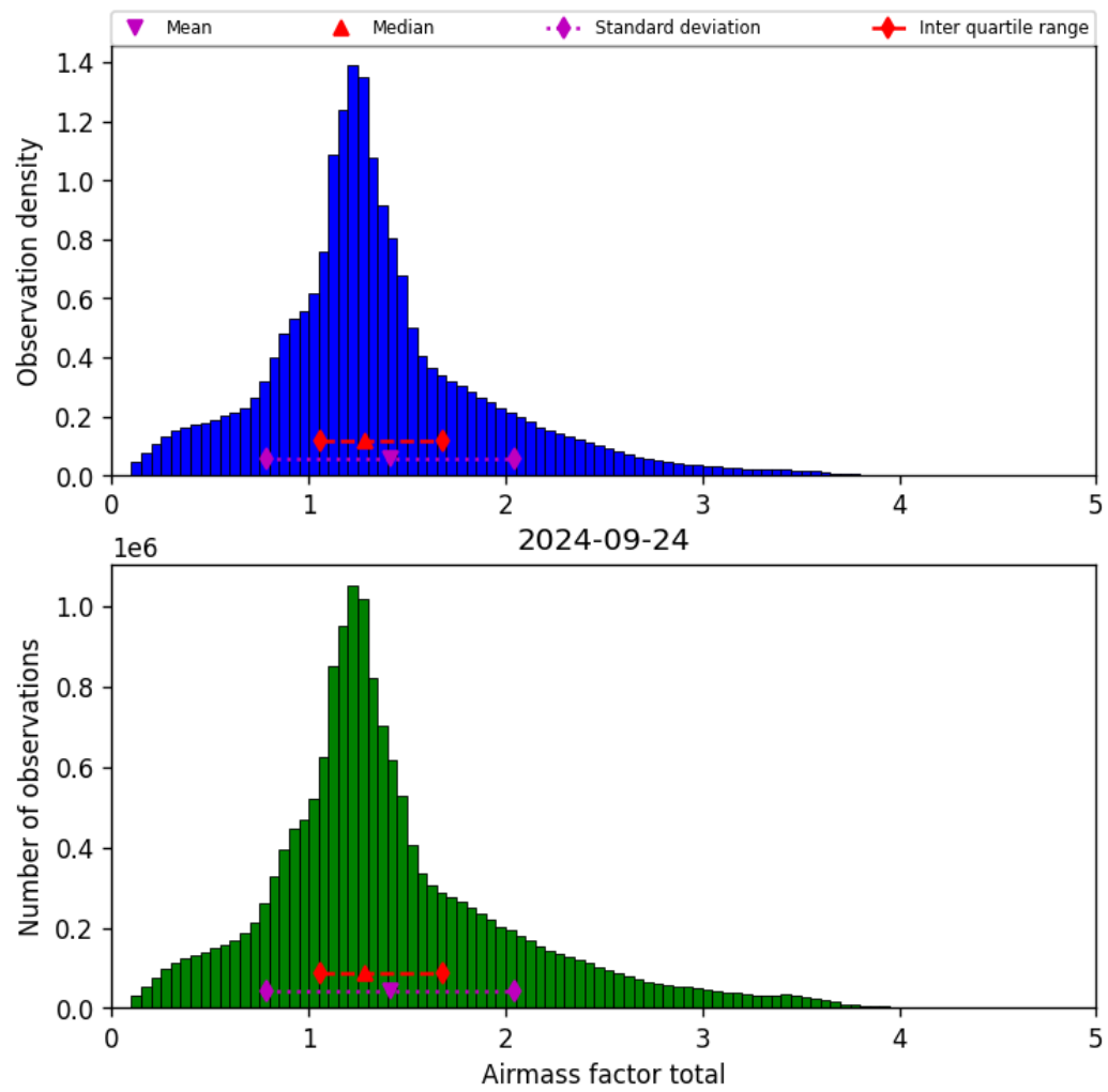
Figure 40: Histogram of “Airmass factor total” for 2024-09-23 to 2024-09-25
