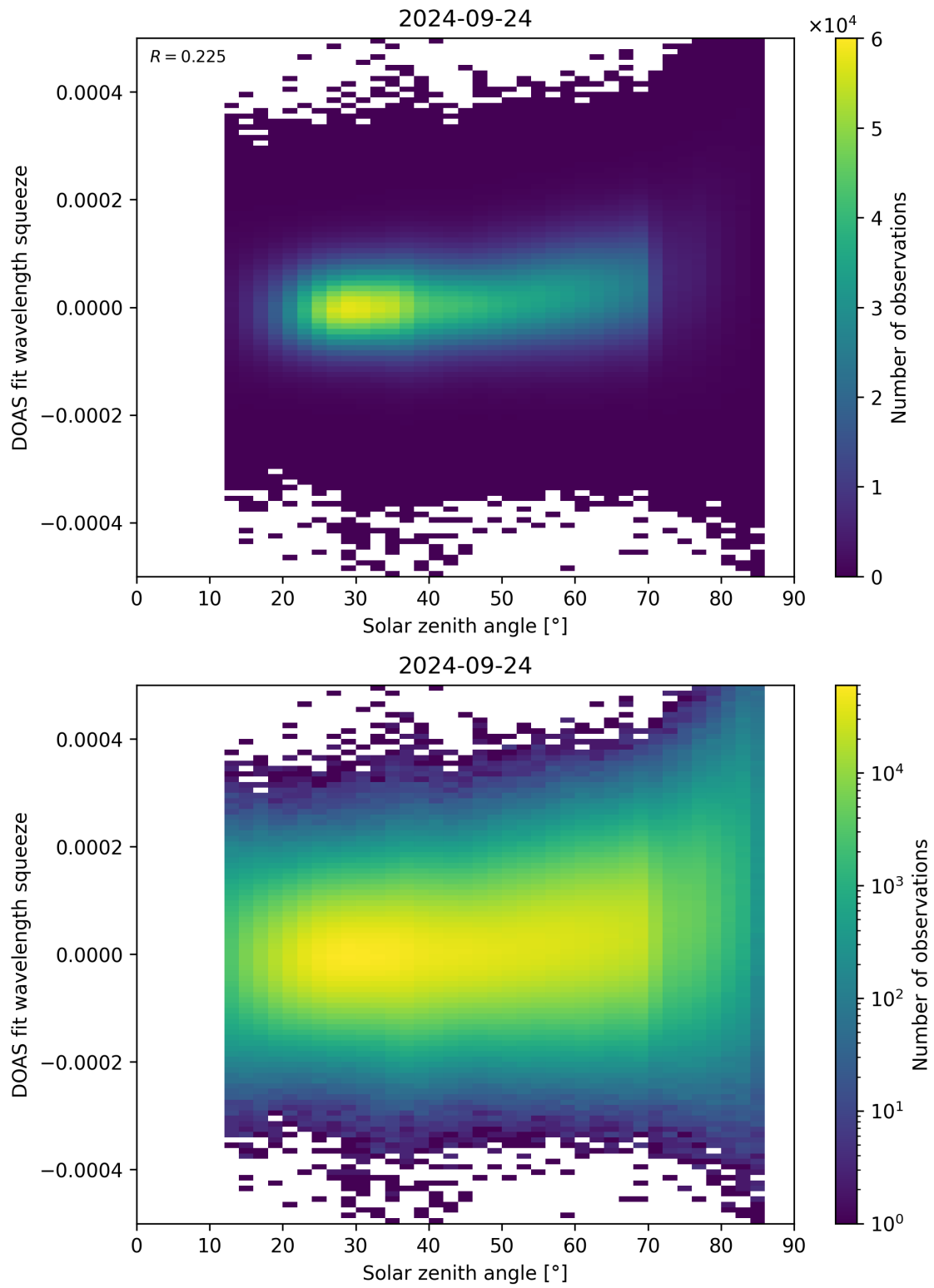
Figure 169: Scatter density plot of “Solar zenith angle” against “DOAS fit wavelength squeeze” for 2024-09-23 to 2024-09-25.
