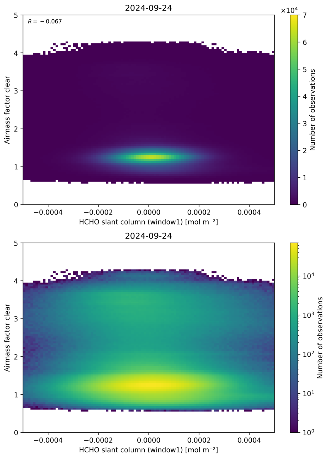
Figure 81: Scatter density plot of “HCHO slant column (window1)” against “Airmass factor clear” for 2024-09-23 to 2024-09-25.
