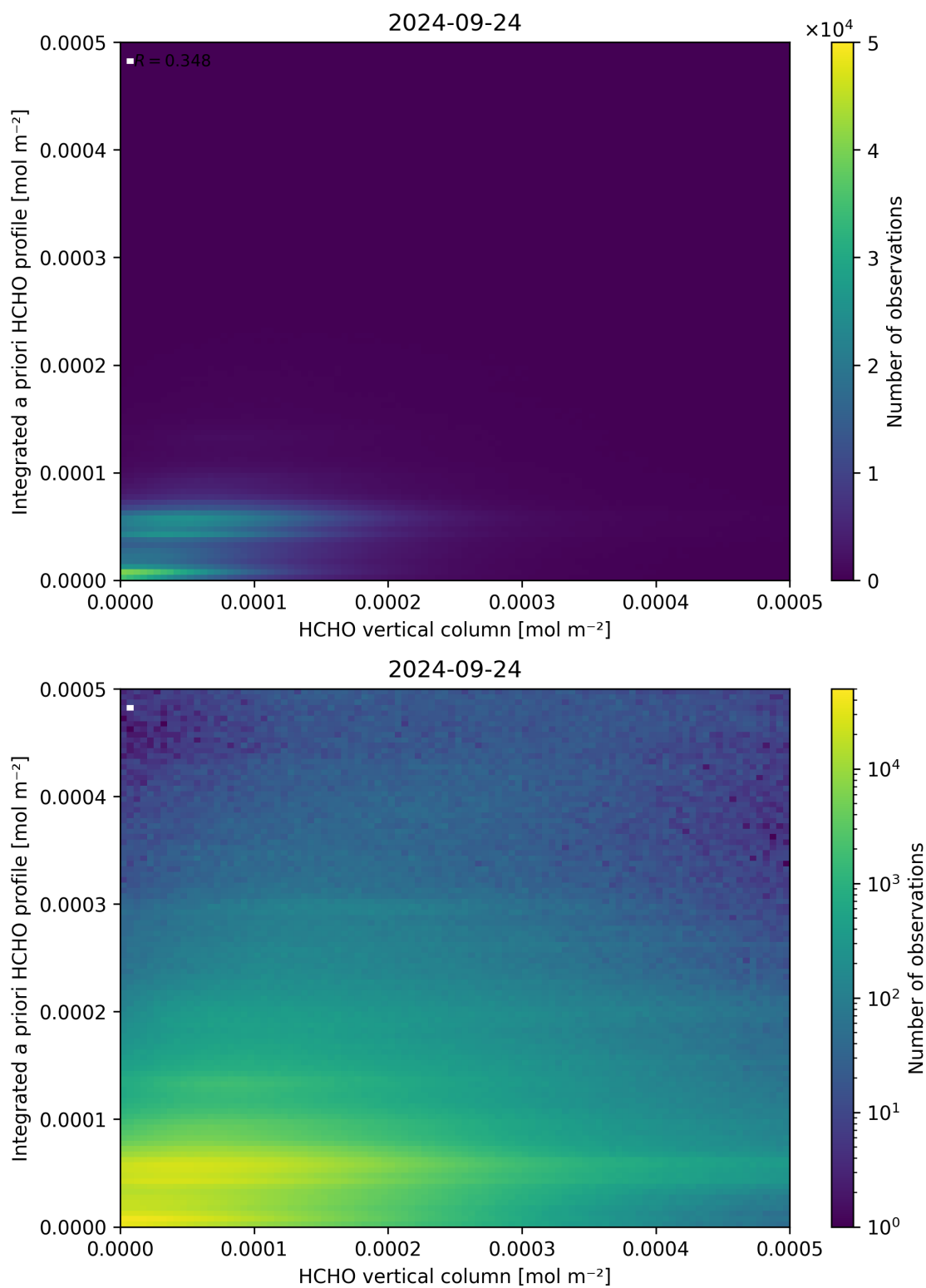
Figure 135: Scatter density plot of “HCHO vertical column” against “Integrated a priori HCHO profile” for 2024-09-23 to 2024-09-25.
