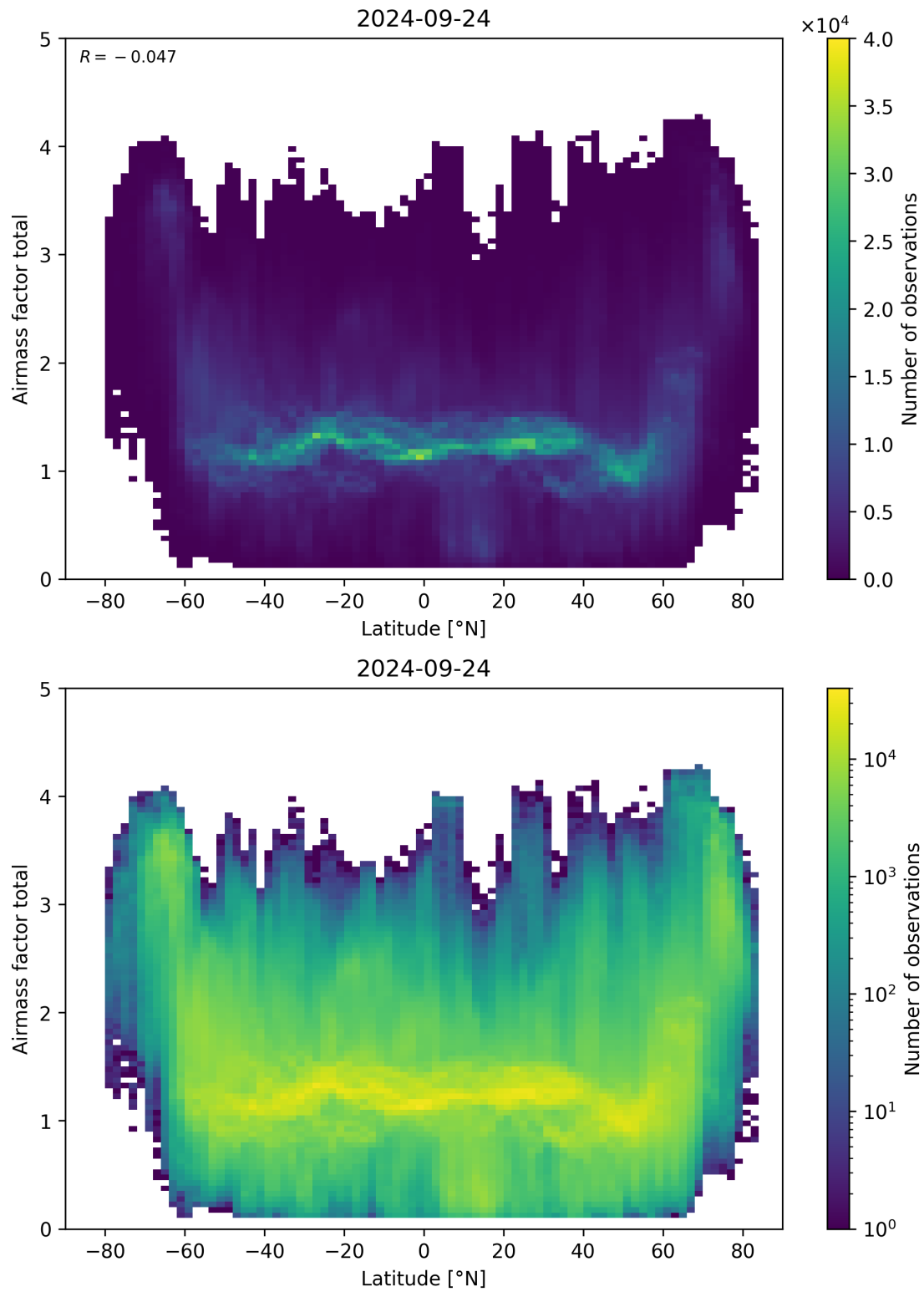
Figure 161: Scatter density plot of “Latitude” against “Airmass factor total” for 2024-09-23 to 2024-09-25.
