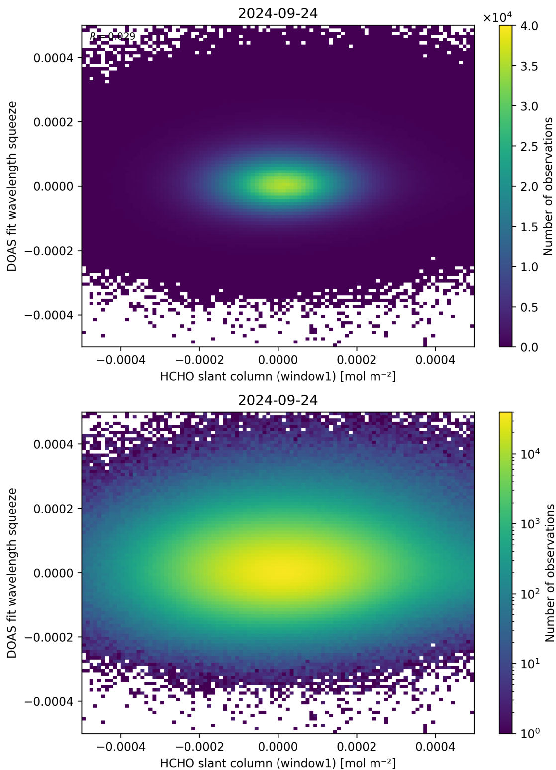
Figure 80: Scatter density plot of “HCHO slant column (window1)” against “DOAS fit wavelength squeeze” for 2024-09-23 to 2024-09-25.
