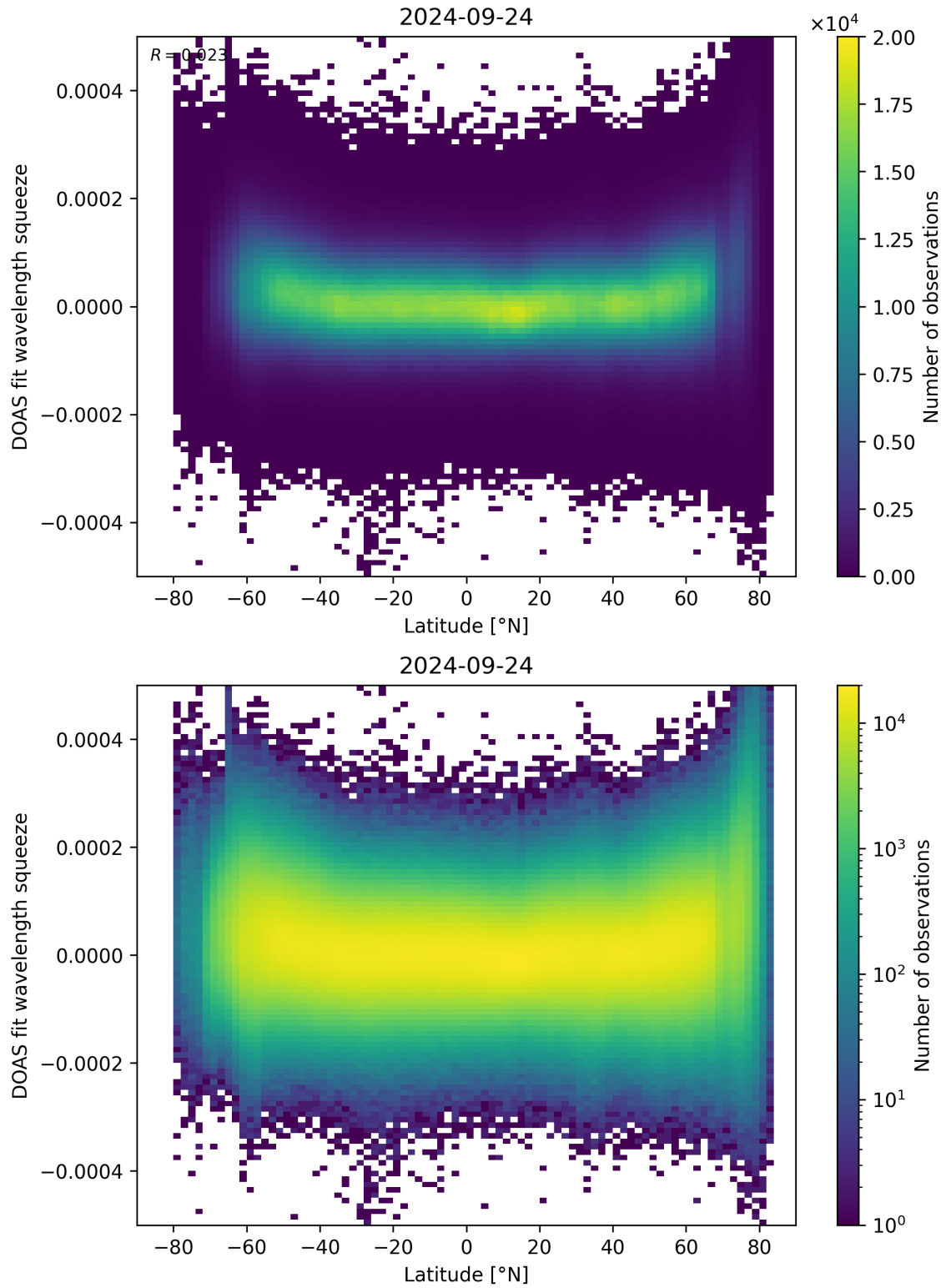
Figure 155: Scatter density plot of “Latitude” against “DOAS fit wavelength squeeze” for 2024-09-23 to 2024-09-25.
