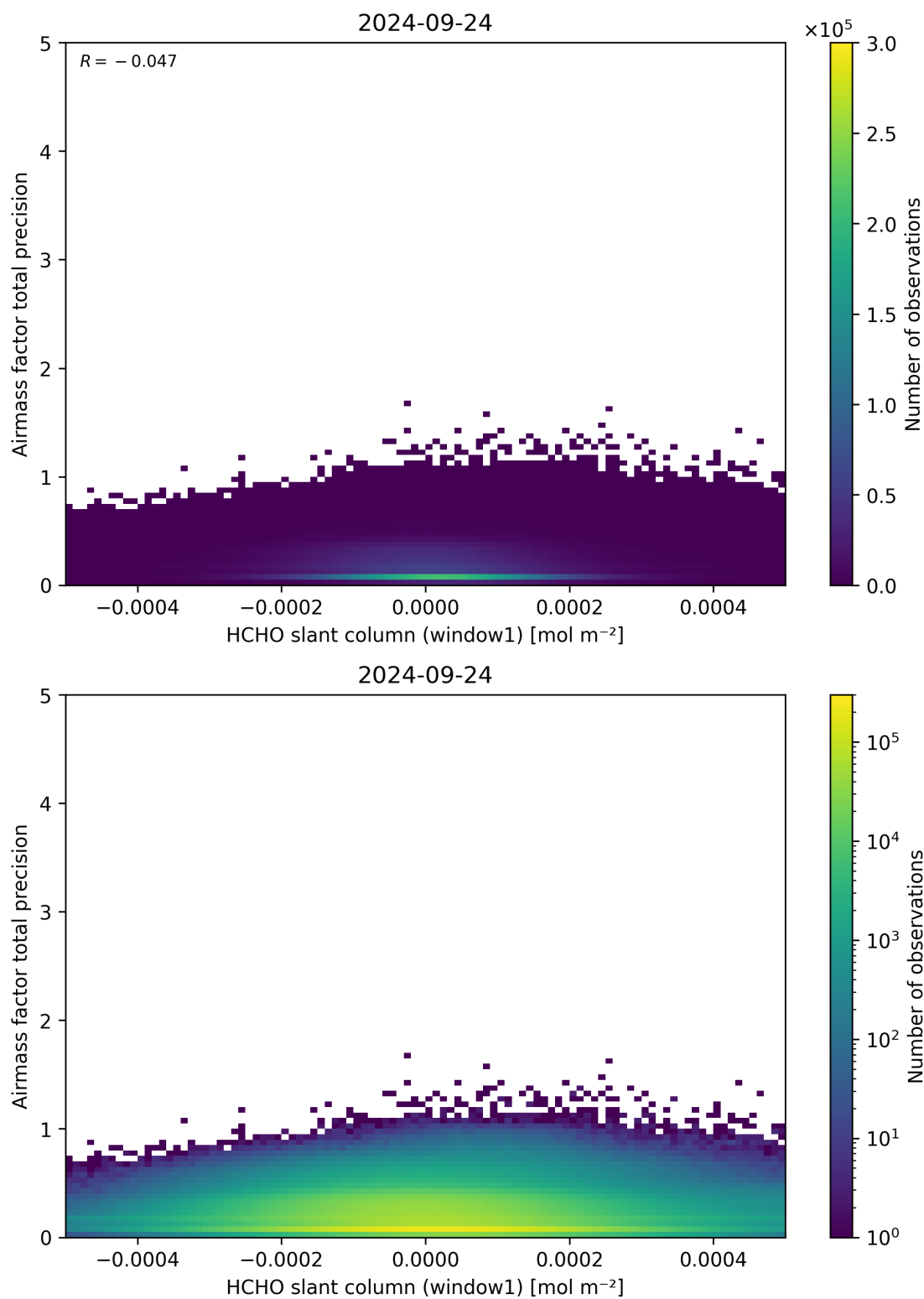
Figure 86: Scatter density plot of “HCHO slant column (window1)” against “Airmass factor total precision” for 2024-09-23 to 2024-09-25.
