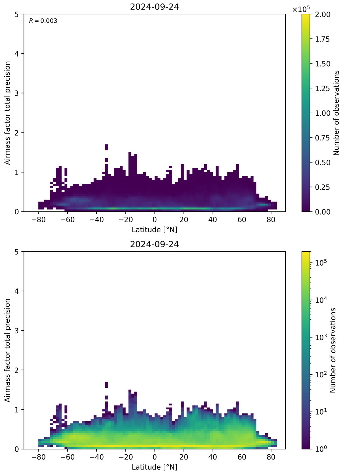
Figure 162: Scatter density plot of “Latitude” against “Airmass factor total precision” for 2024-09-23 to 2024-09-25.
