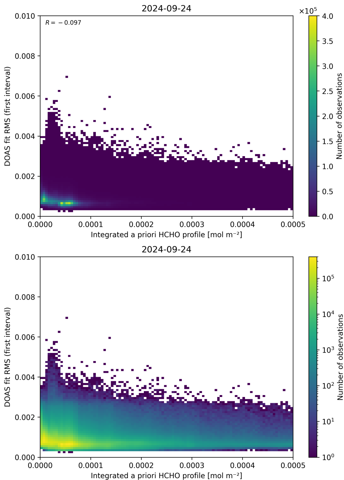
Figure 148: Scatter density plot of “Integrated a priori HCHO profile” against “DOAS fit RMS (first interval)” for 2024-09-23 to 2024-09-25.
