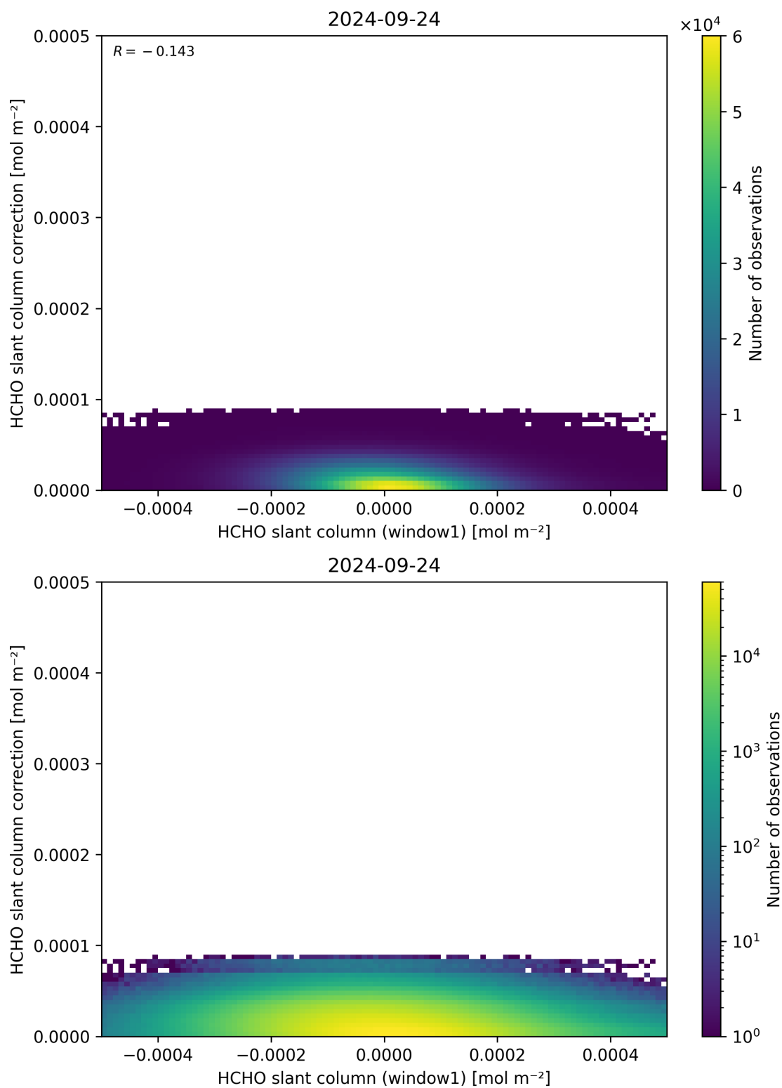
Figure 83: Scatter density plot of “HCHO slant column (window1)” against “HCHO slant column correction” for 2024-09-23 to 2024-09-25.
