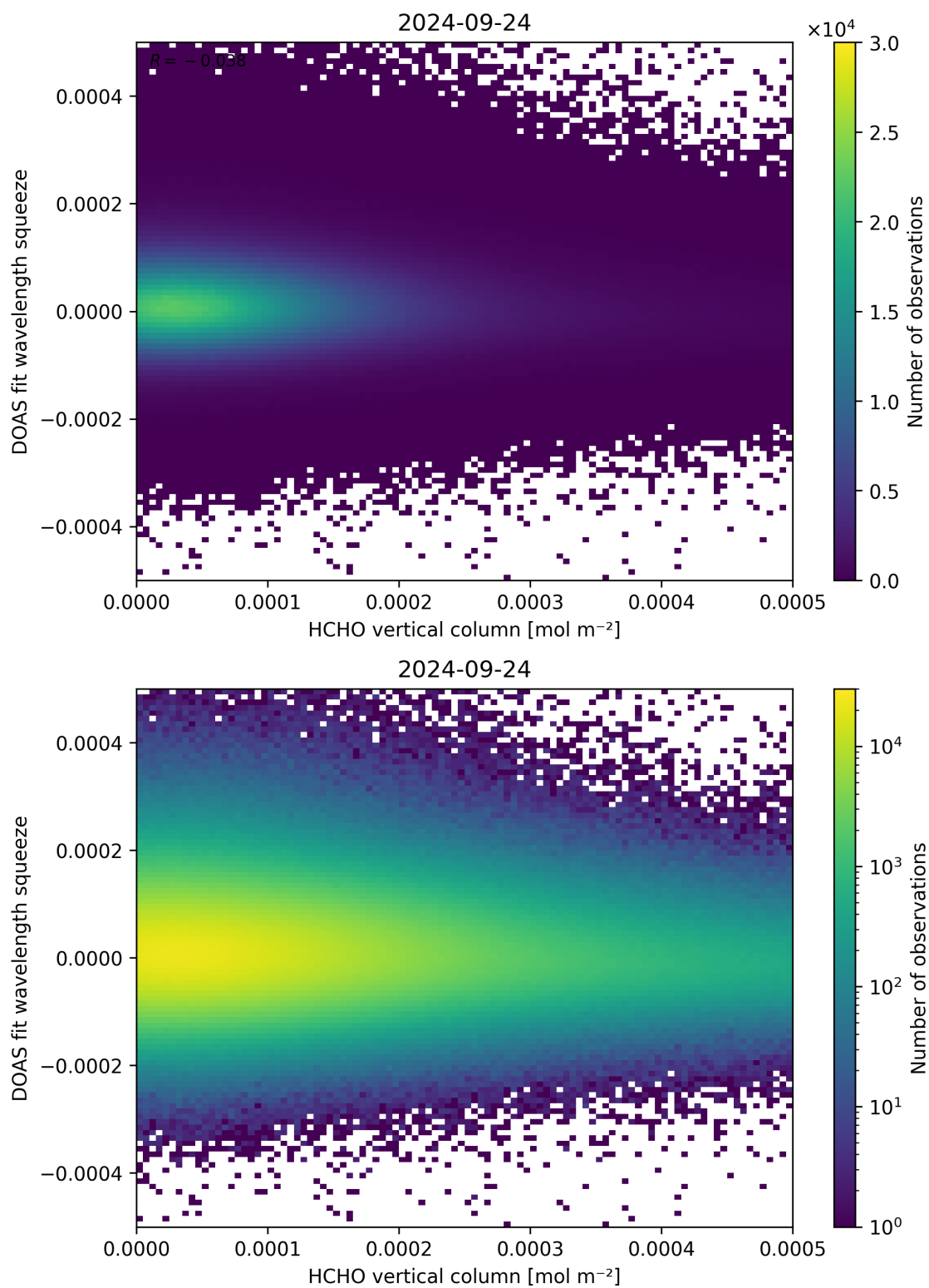
Figure 125: Scatter density plot of “HCHO vertical column” against “DOAS fit wavelength squeeze” for 2024-09-23 to 2024-09-25.
