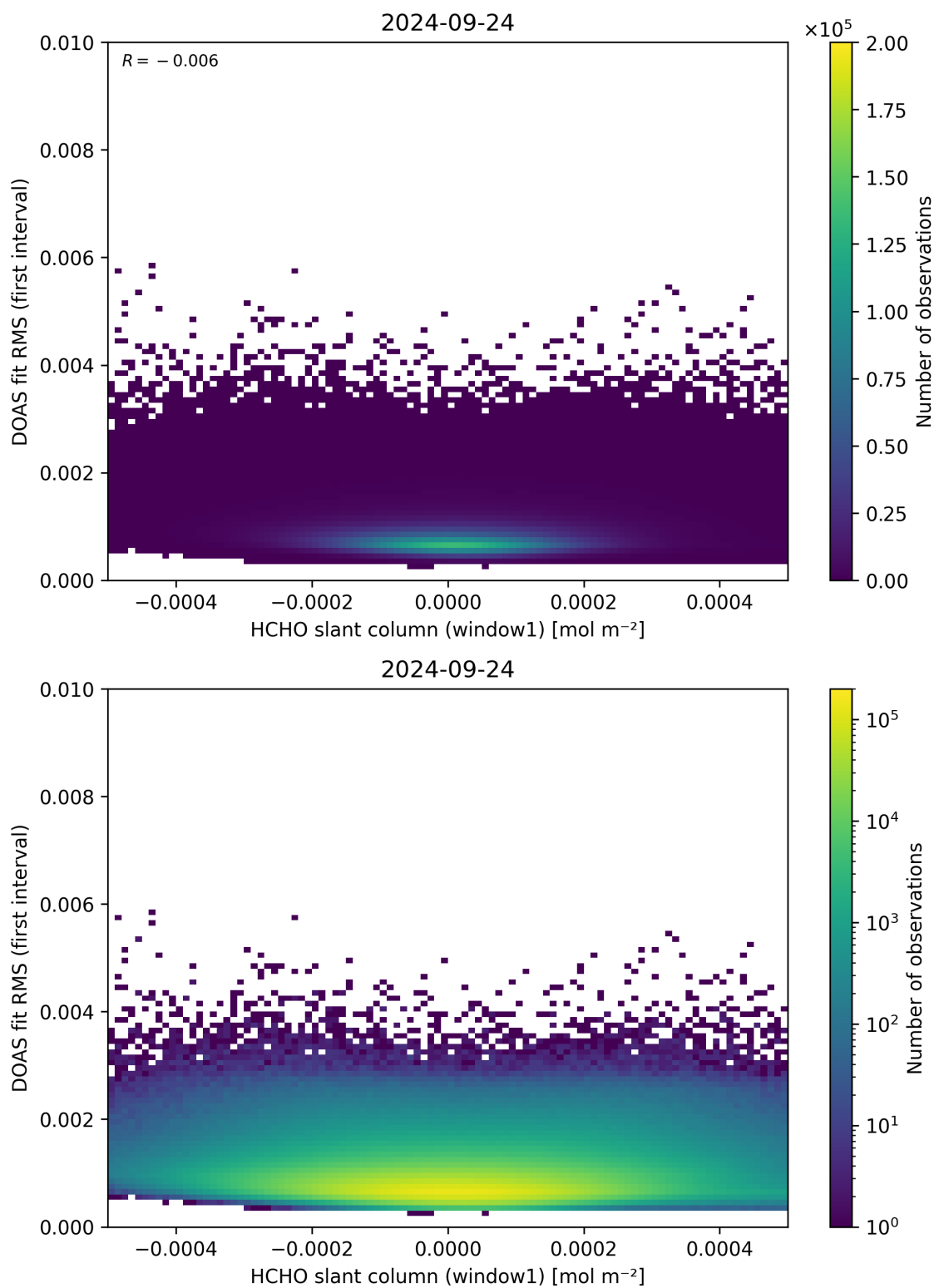
Figure 78: Scatter density plot of “HCHO slant column (window1)” against “DOAS fit RMS (first interval)” for 2024-09-23 to 2024-09-25.
