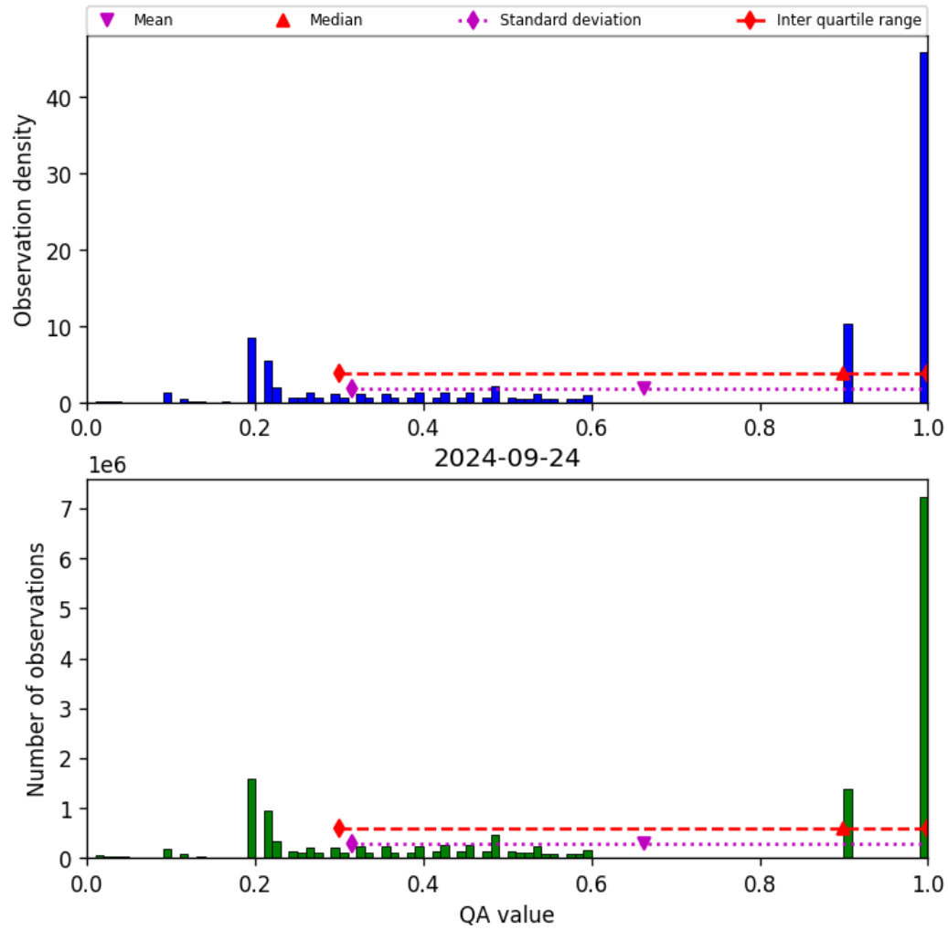
Figure 34: Histogram of “QA value” for 2024-09-23 to 2024-09-25
