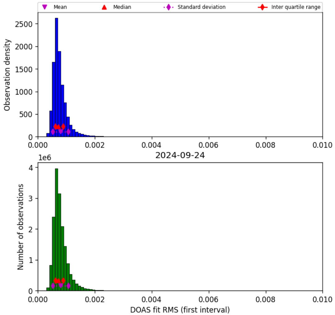
Figure 46: Histogram of “DOAS fit RMS (first interval)” for 2024-09-23 to 2024-09-25
