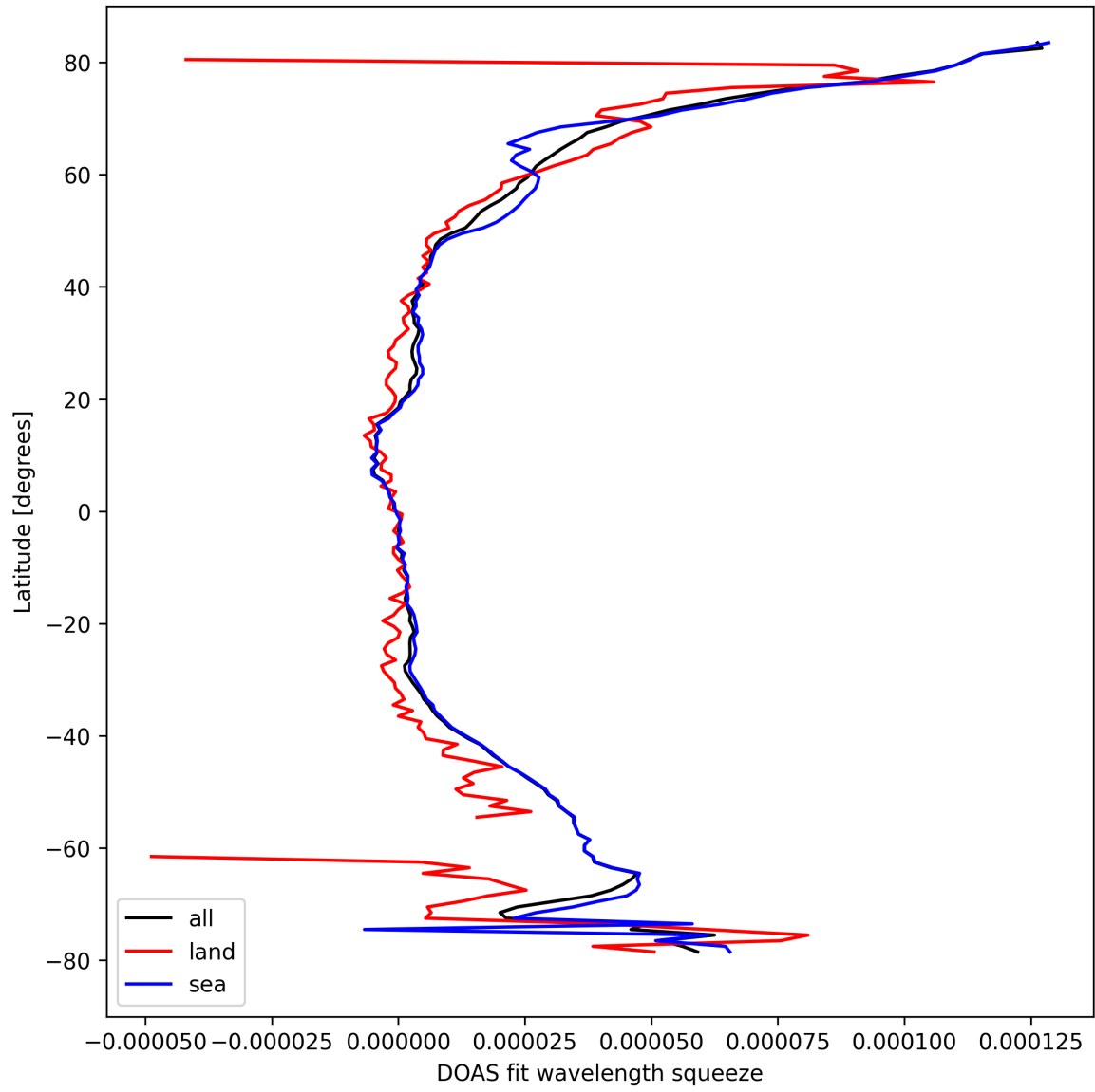
Figure 31: Zonal average of “DOAS fit wavelength squeeze” for 2024-09-23 to 2024-09-25.
