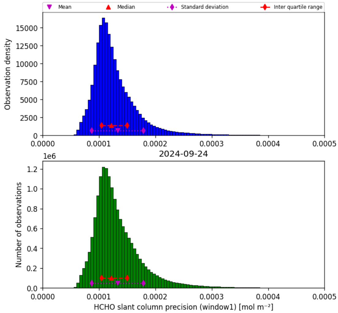
Figure 39: Histogram of “HCHO slant column precision (window1)” for 2024-09-23 to 2024-09-25
