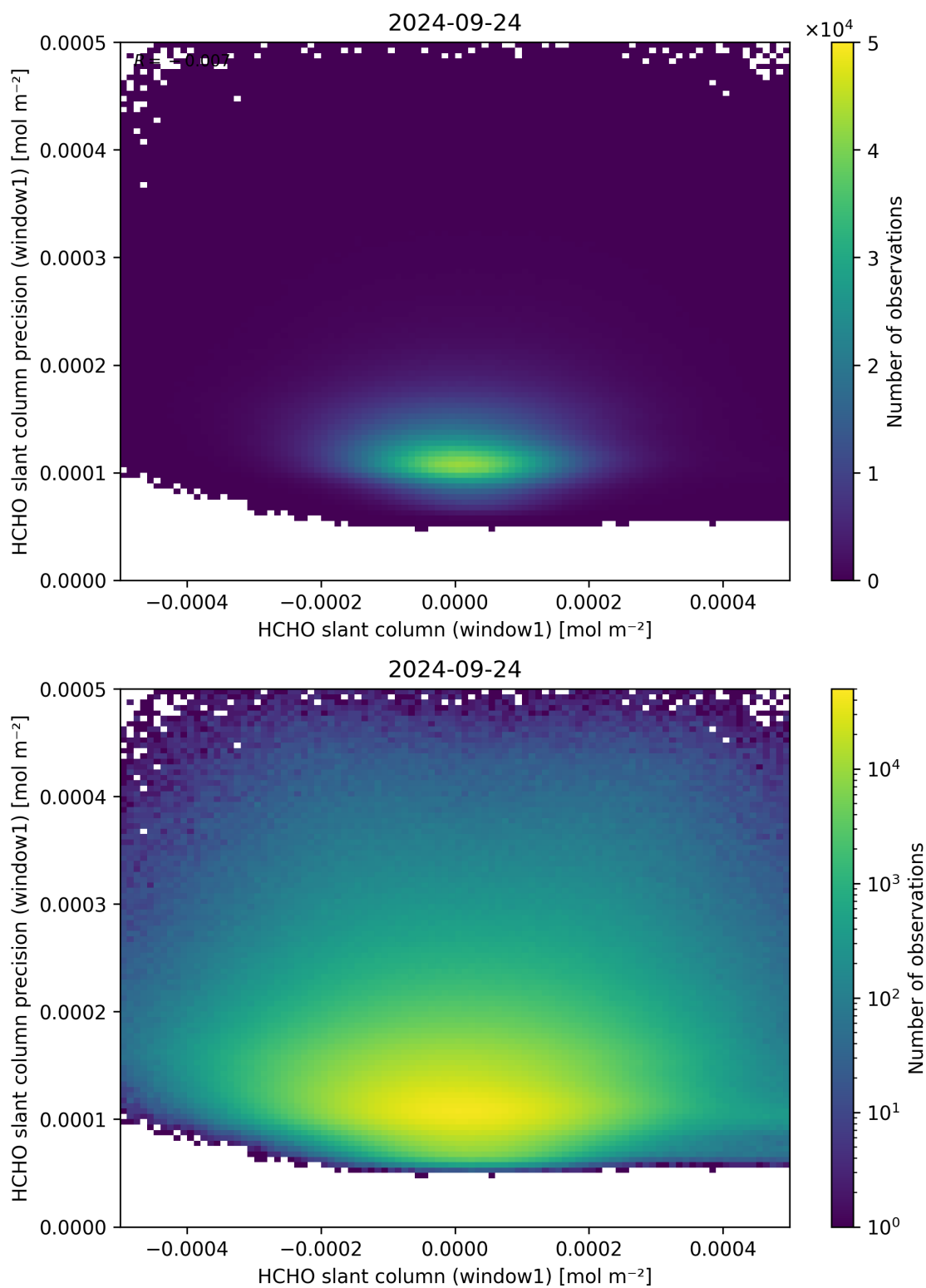
Figure 84: Scatter density plot of “HCHO slant column (window1)” against “HCHO slant column precision (window1)” for 2024-09-23 to 2024-09-25.
