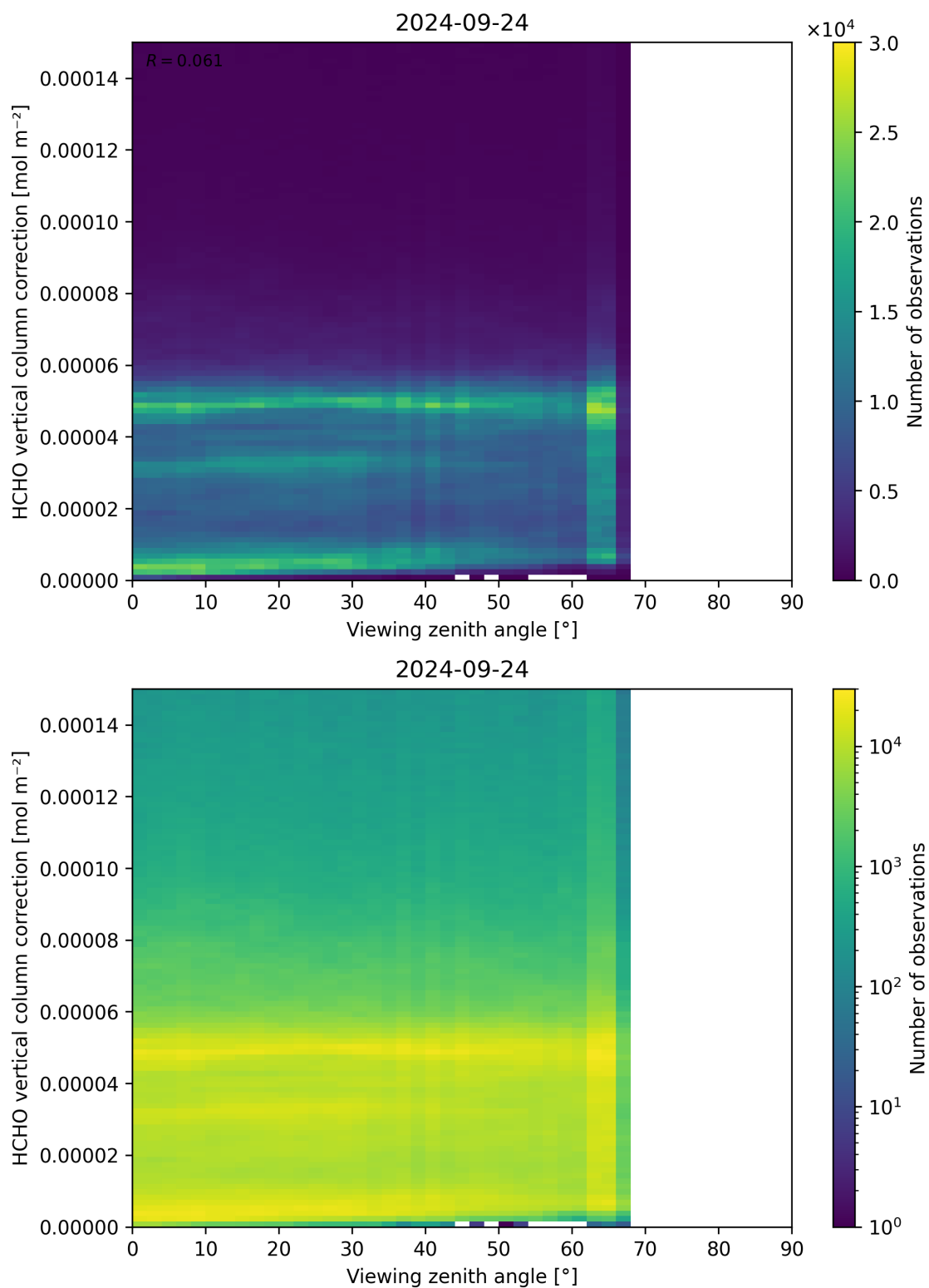
Figure 193: Scatter density plot of “Viewing zenith angle” against “HCHO vertical column correction” for 2024-09-23 to 2024-09-25.
