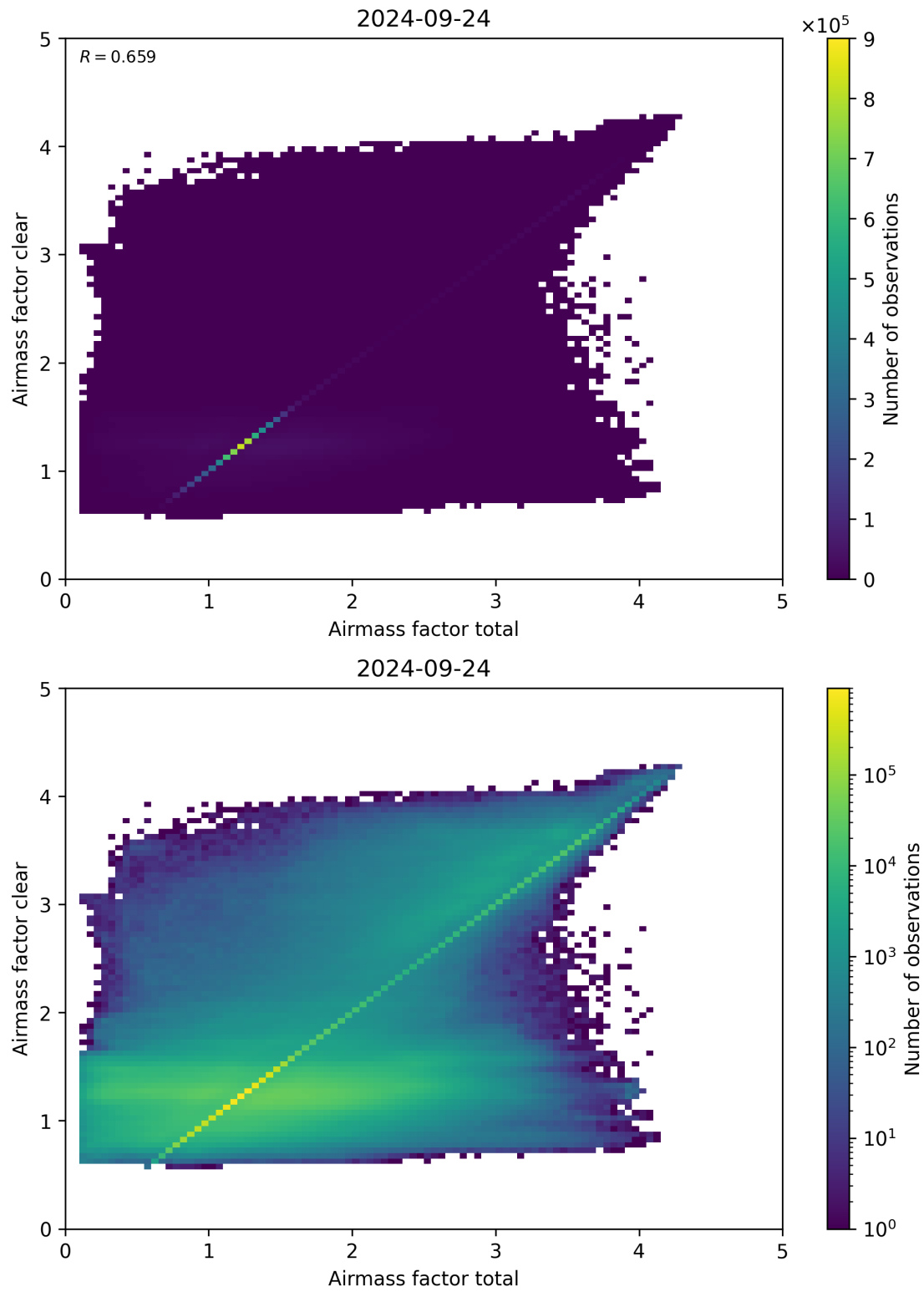
Figure 100: Scatter density plot of “Airmass factor total” against “Airmass factor clear” for 2024-09-23 to 2024-09-25.
