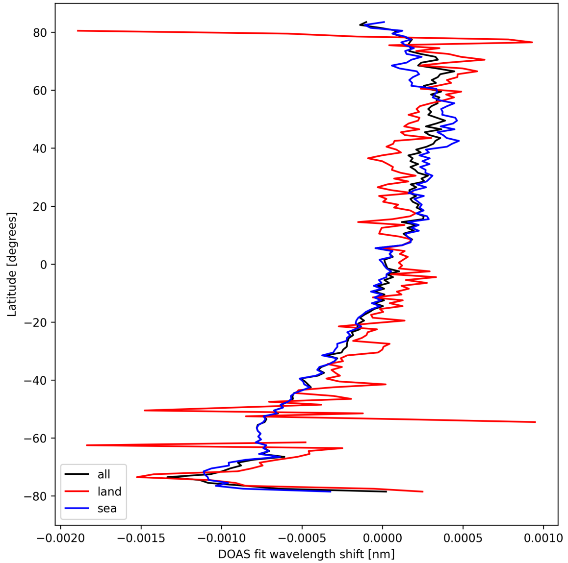
Figure 30: Zonal average of “DOAS fit wavelength shift” for 2024-09-23 to 2024-09-25.
