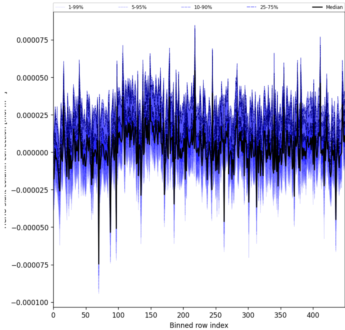
Figure 61: Along track statistics of “HCHO slant column correction” for 2024-09-23 to 2024-09-25
