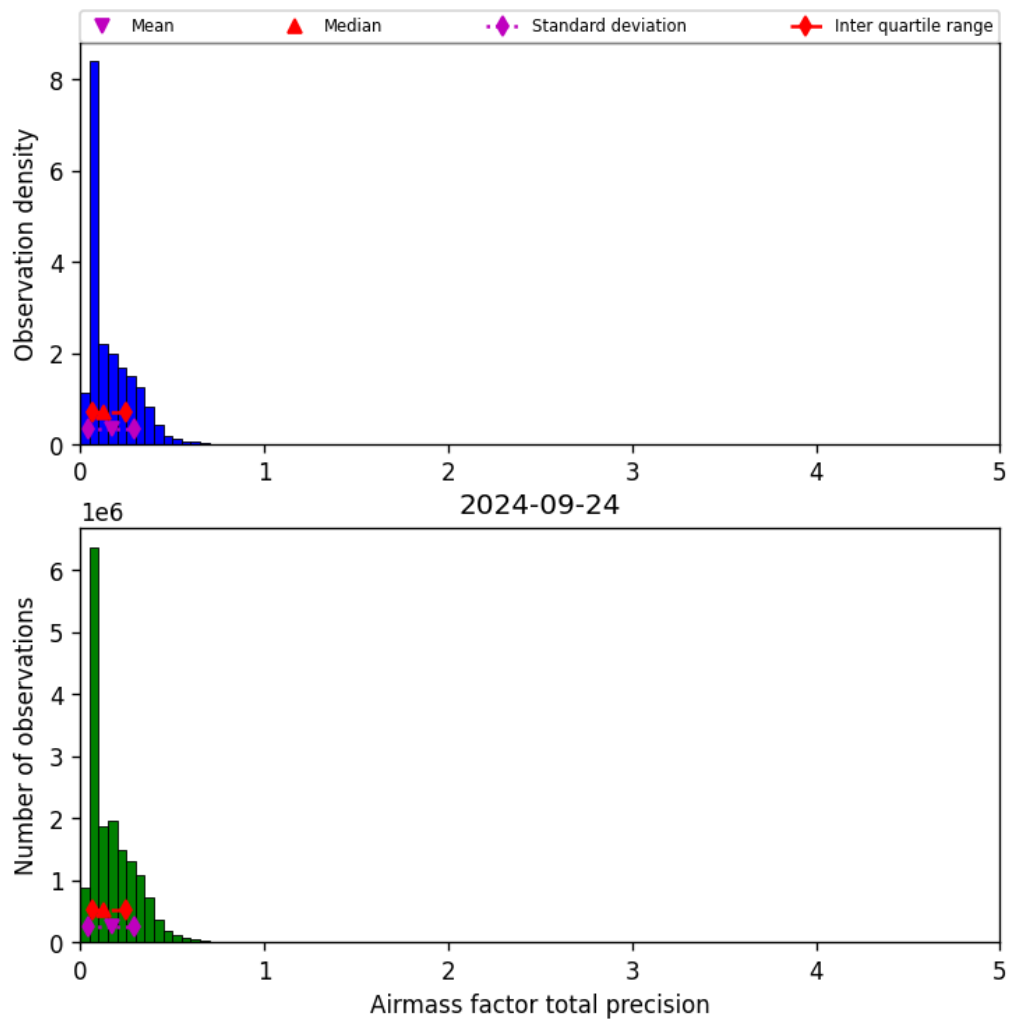
Figure 41: Histogram of “Airmass factor total precision” for 2024-09-23 to 2024-09-25
