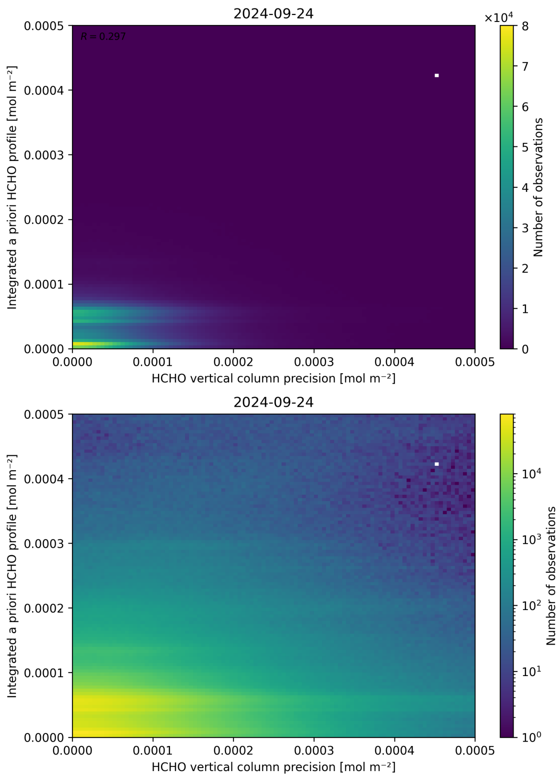
Figure 147: Scatter density plot of “HCHO vertical column precision” against “Integrated a priori HCHO profile” for 2024-09-23 to 2024-09-25.
