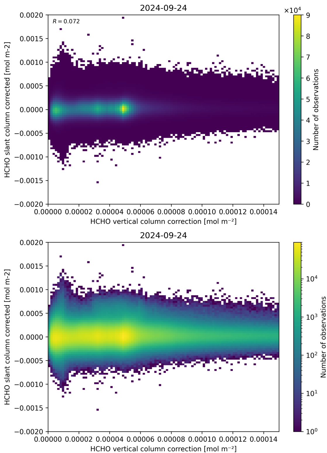
Figure 116: Scatter density plot of “HCHO vertical column correction” against “HCHO slant column corrected” for 2024-09-23 to 2024-09-25.
