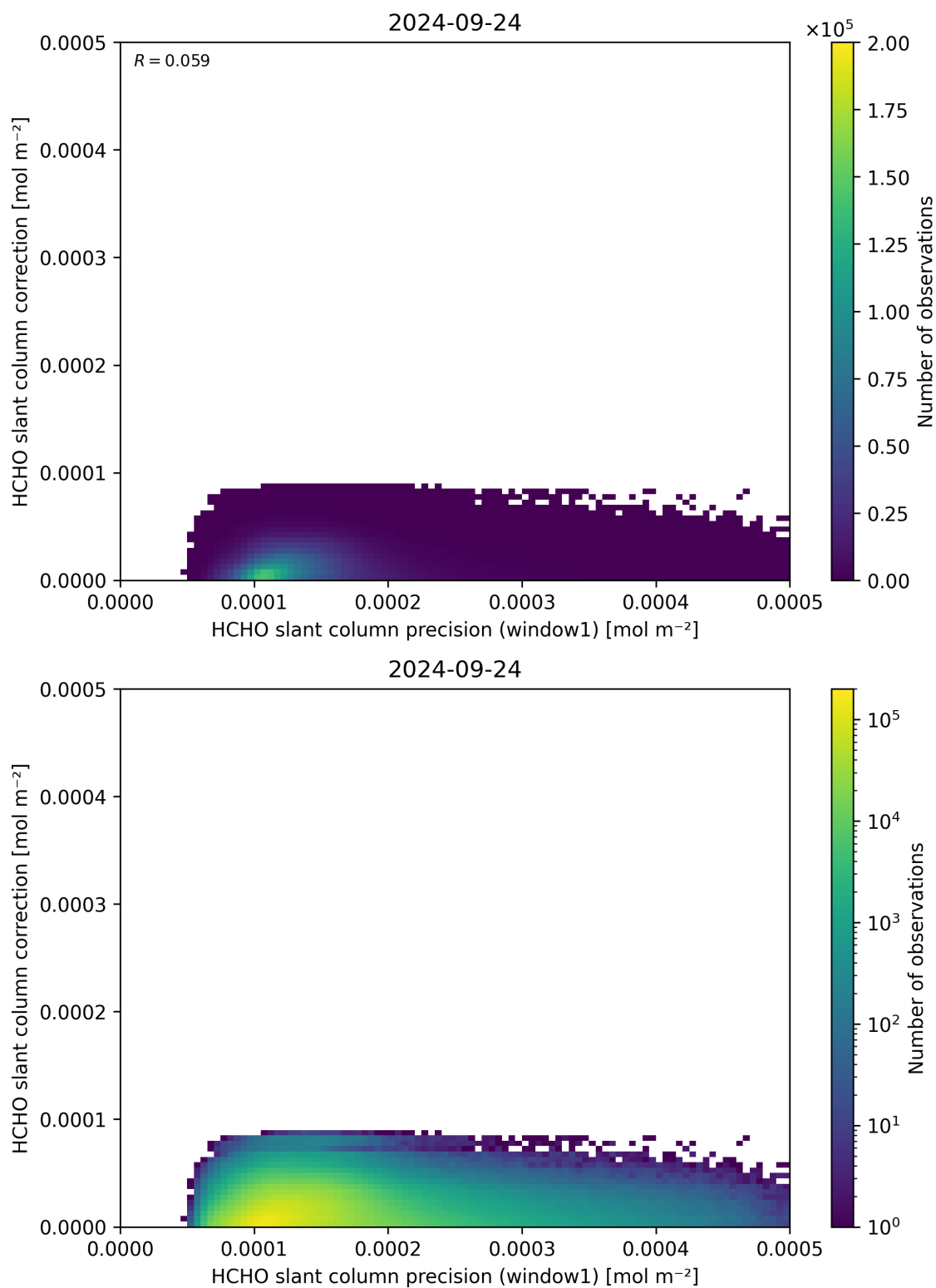
Figure 93: Scatter density plot of “HCHO slant column precision (window1)” against “HCHO slant column correction” for 2024-09-23 to 2024-09-25.
