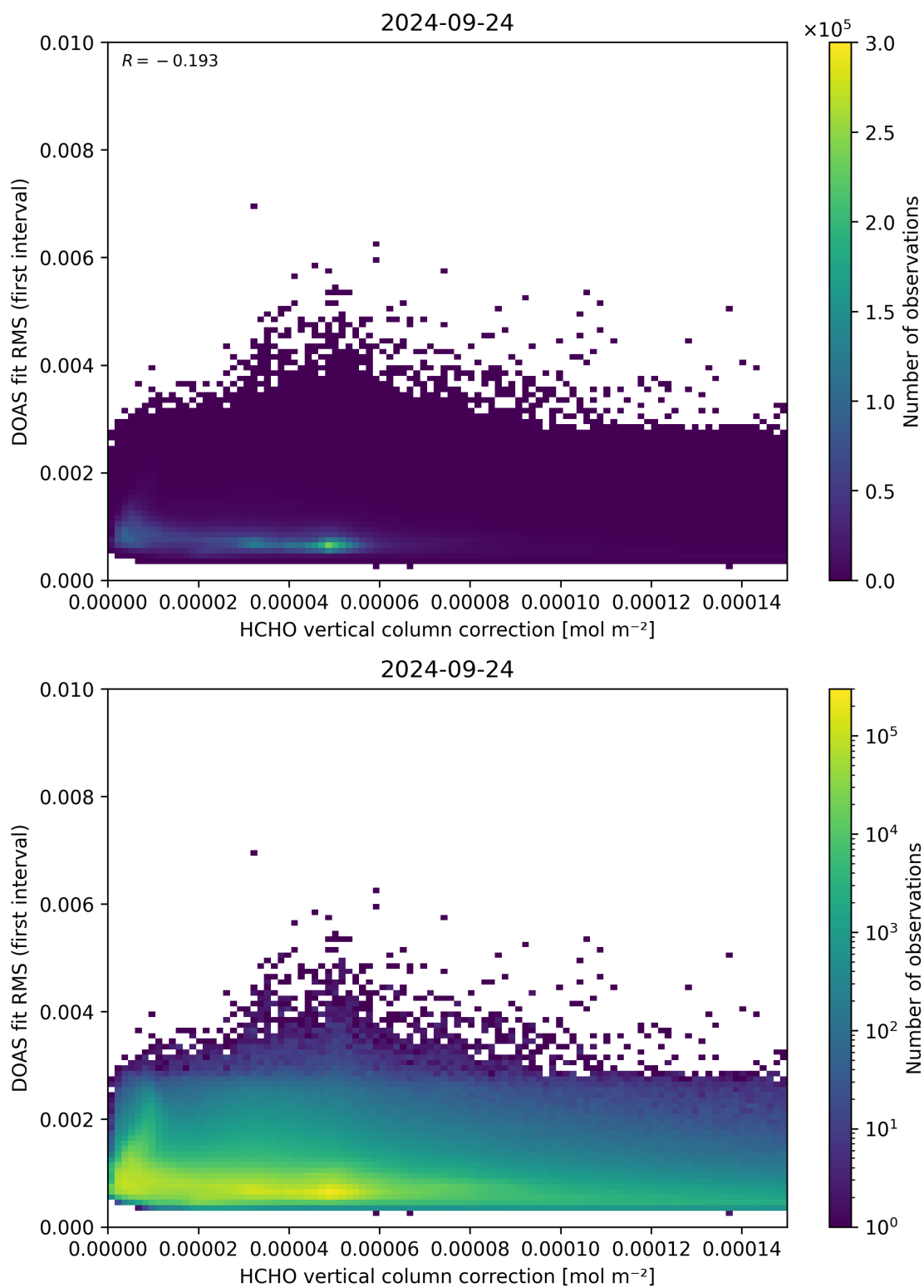
Figure 112: Scatter density plot of “HCHO vertical column correction” against “DOAS fit RMS (first interval)” for 2024-09-23 to 2024-09-25.
