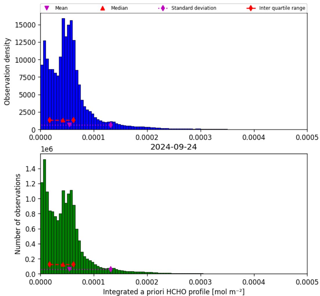
Figure 43: Histogram of “Integrated a priori HCHO profile” for 2024-09-23 to 2024-09-25
