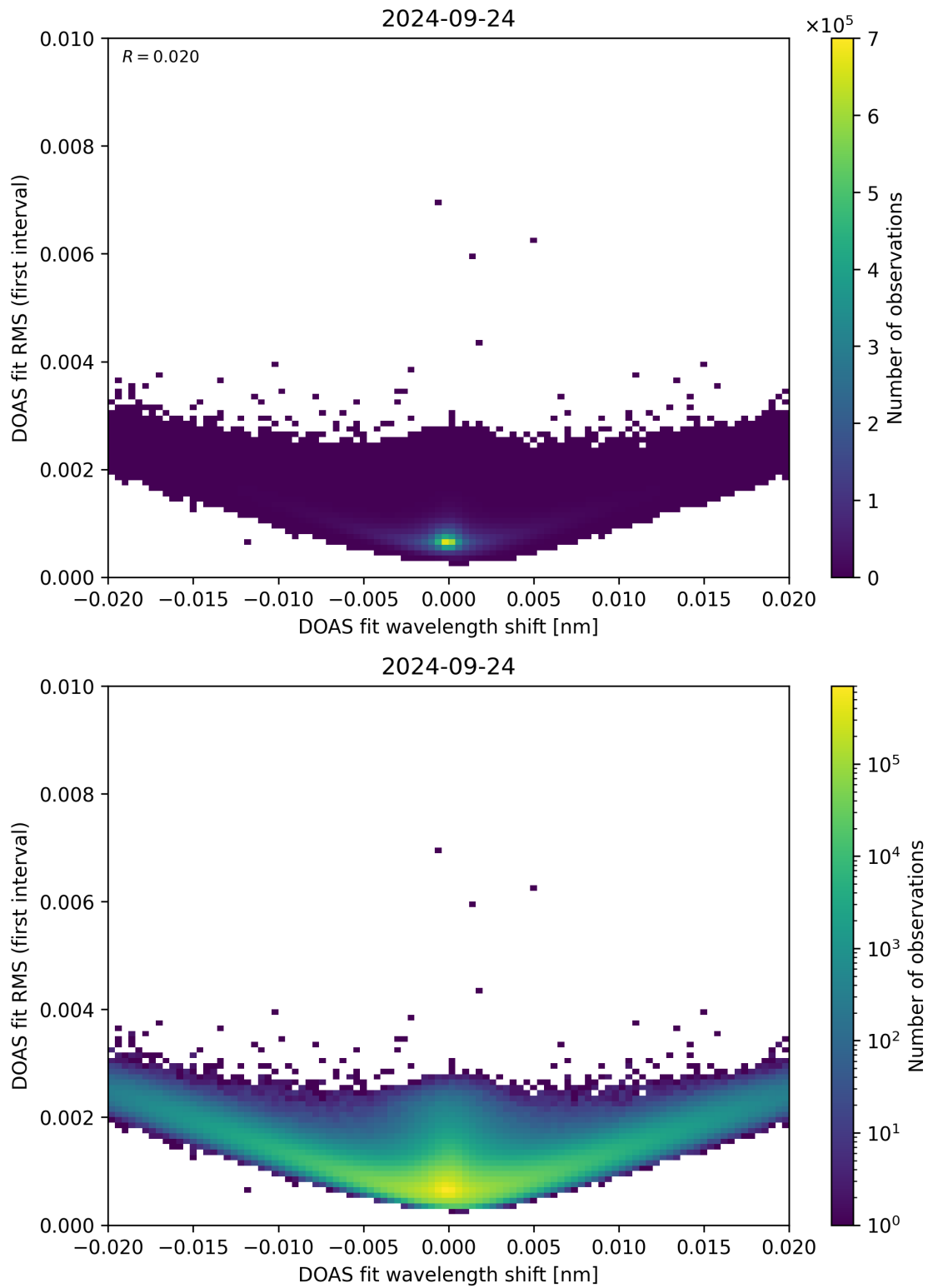
Figure 64: Scatter density plot of “DOAS fit wavelength shift” against “DOAS fit RMS (first interval)” for 2024-09-23 to 2024-09-25.
