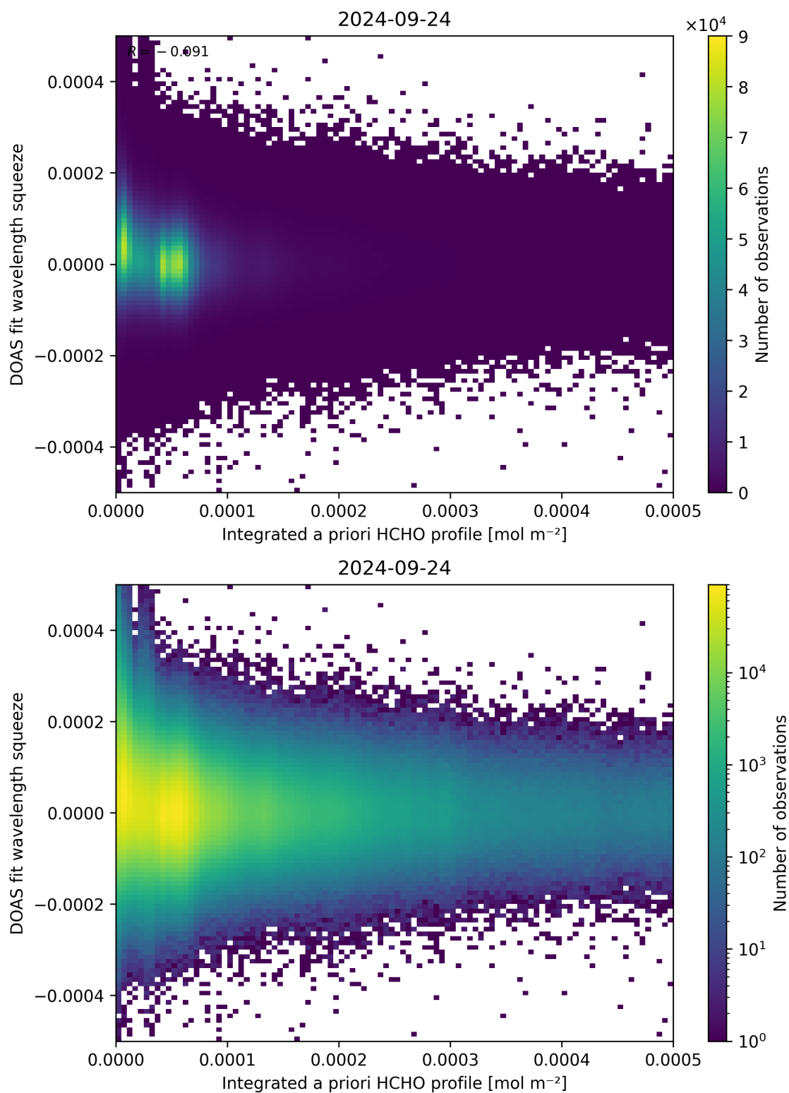
Figure 150: Scatter density plot of “Integrated a priori HCHO profile” against “DOAS fit wavelength squeeze” for 2024-09-23 to 2024-09-25.
