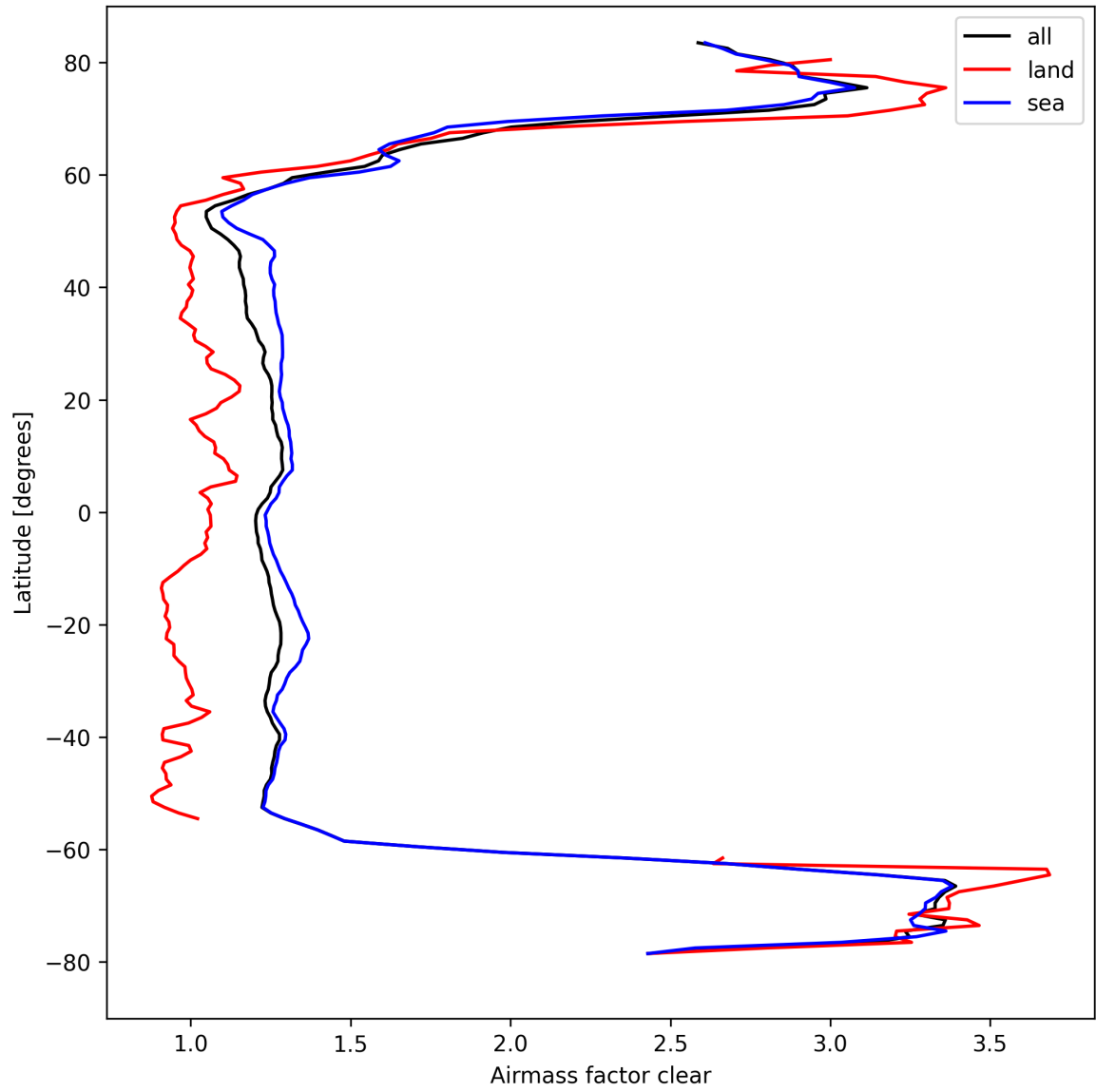
Figure 28: Zonal average of “Airmass factor clear” for 2024-09-23 to 2024-09-25.
