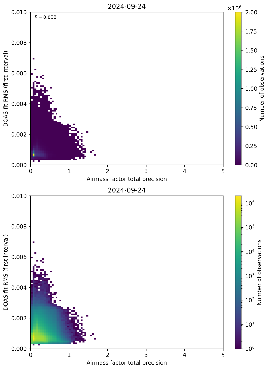
Figure 105: Scatter density plot of “Airmass factor total precision” against “DOAS fit RMS (first interval)” for 2024-09-23 to 2024-09-25.
