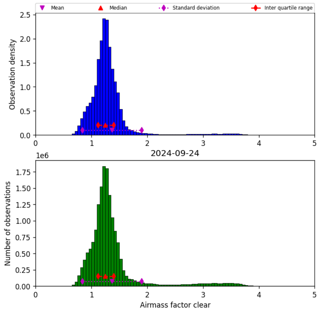
Figure 42: Histogram of “Airmass factor clear” for 2024-09-23 to 2024-09-25
