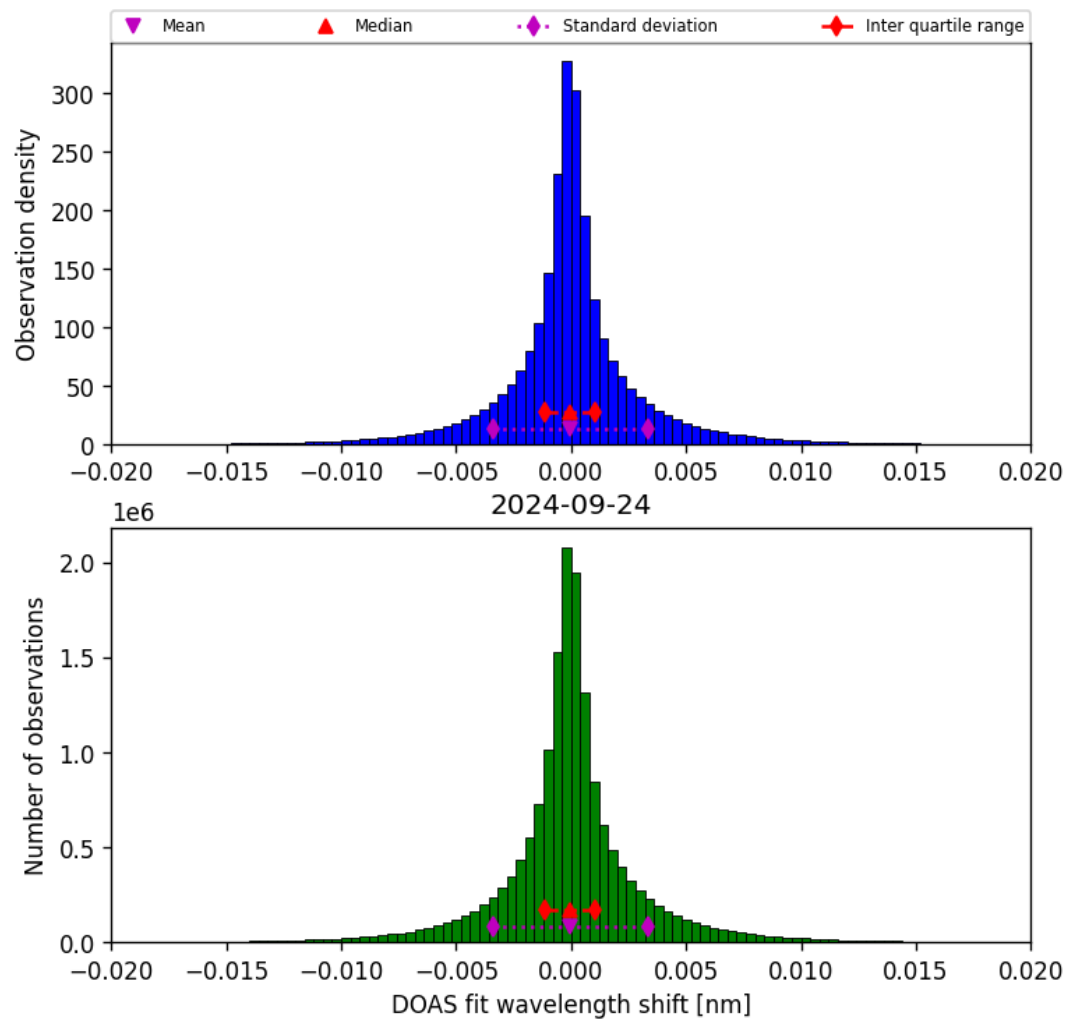
Figure 44: Histogram of “DOAS fit wavelength shift” for 2024-09-23 to 2024-09-25
