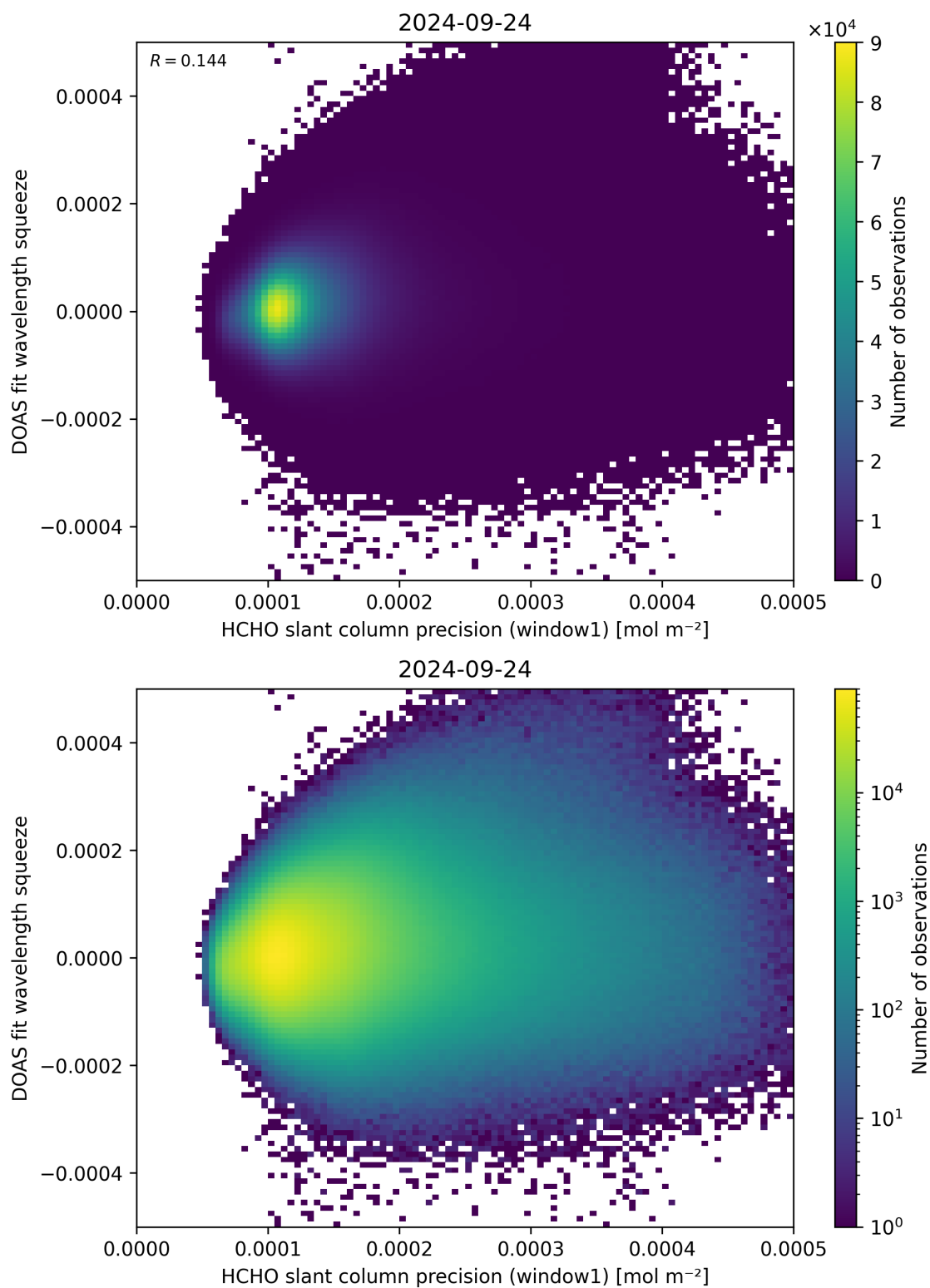
Figure 90: Scatter density plot of “HCHO slant column precision (window1)” against “DOAS fit wavelength squeeze” for 2024-09-23 to 2024-09-25.
