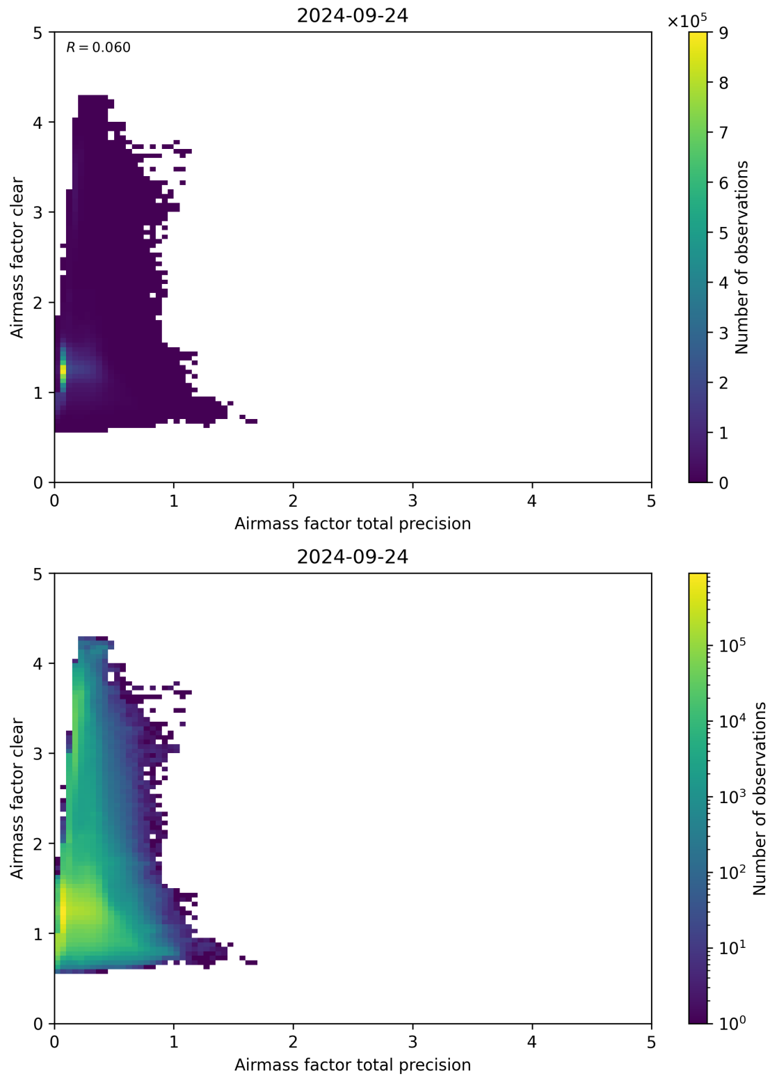
Figure 108: Scatter density plot of “Airmass factor total precision” against “Airmass factor clear” for 2024-09-23 to 2024-09-25.
