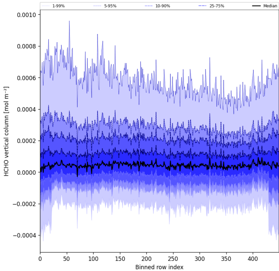
Figure 49: Along track statistics of “HCHO vertical column” for 2024-09-23 to 2024-09-25
