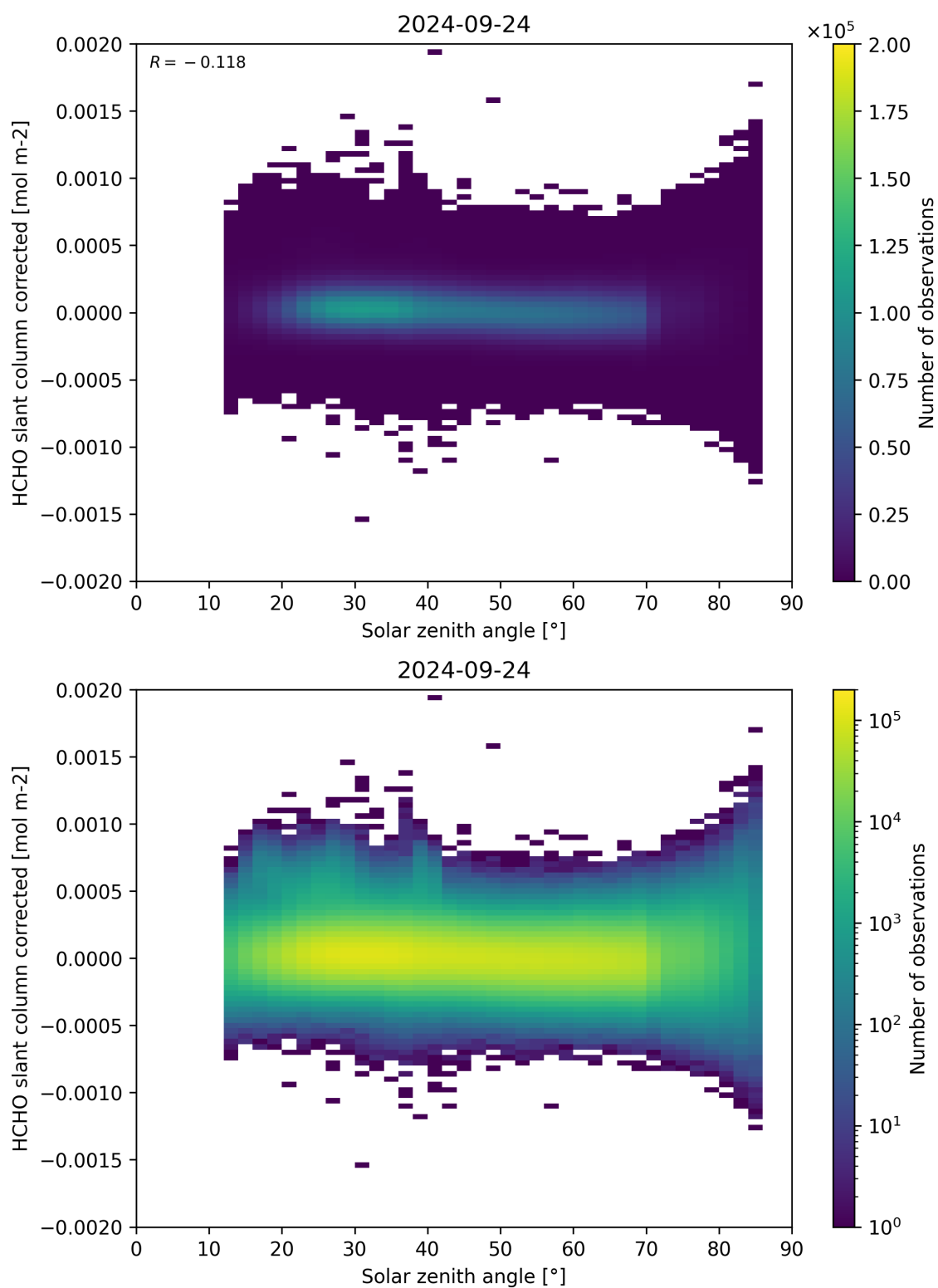
Figure 171: Scatter density plot of “Solar zenith angle” against “HCHO slant column corrected” for 2024-09-23 to 2024-09-25.
