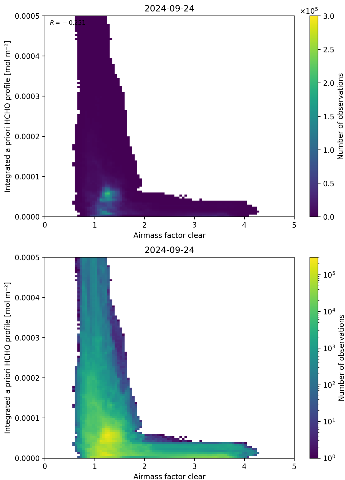
Figure 76: Scatter density plot of “Airmass factor clear” against “Integrated a priori HCHO profile” for 2024-09-23 to 2024-09-25.
