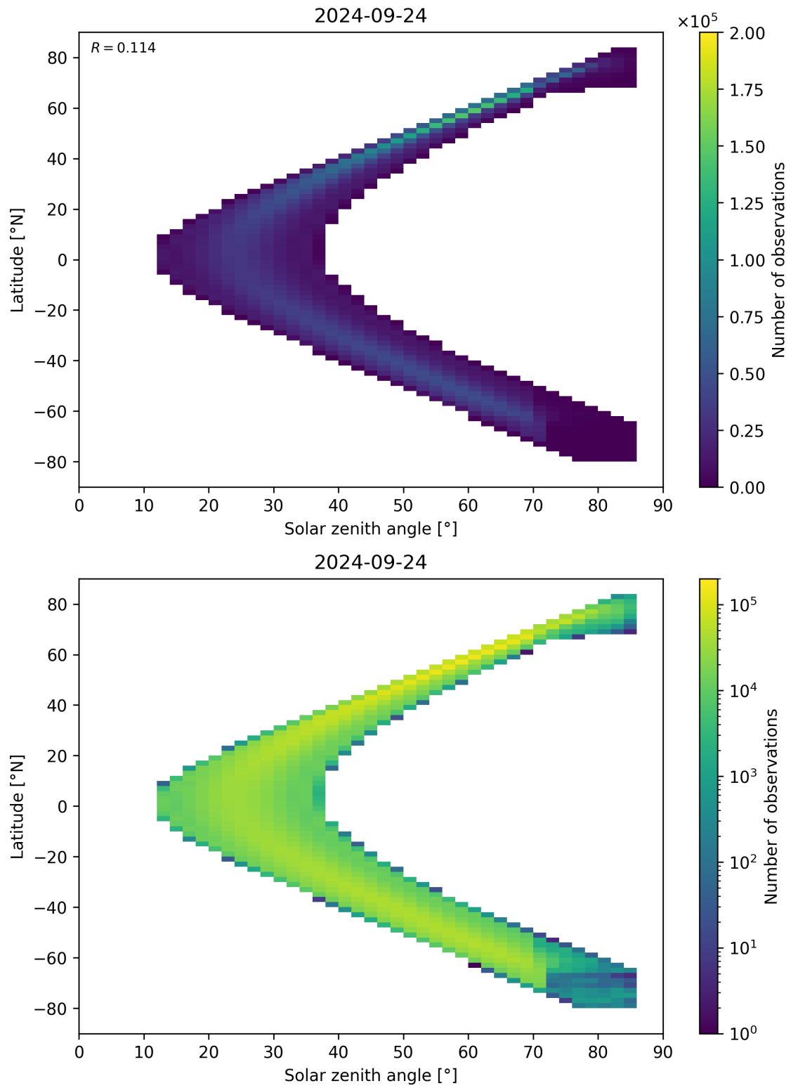
Figure 181: Scatter density plot of “Solar zenith angle” against “Latitude” for 2024-09-23 to 2024-09-25.
