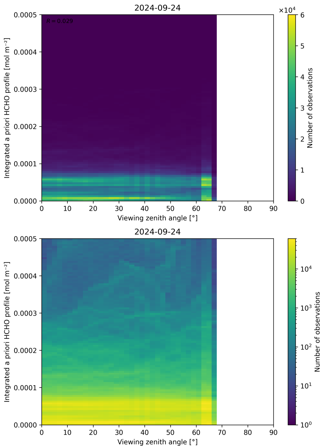
Figure 195: Scatter density plot of “Viewing zenith angle” against “Integrated a priori HCHO profile” for 2024-09-23 to 2024-09-25.
