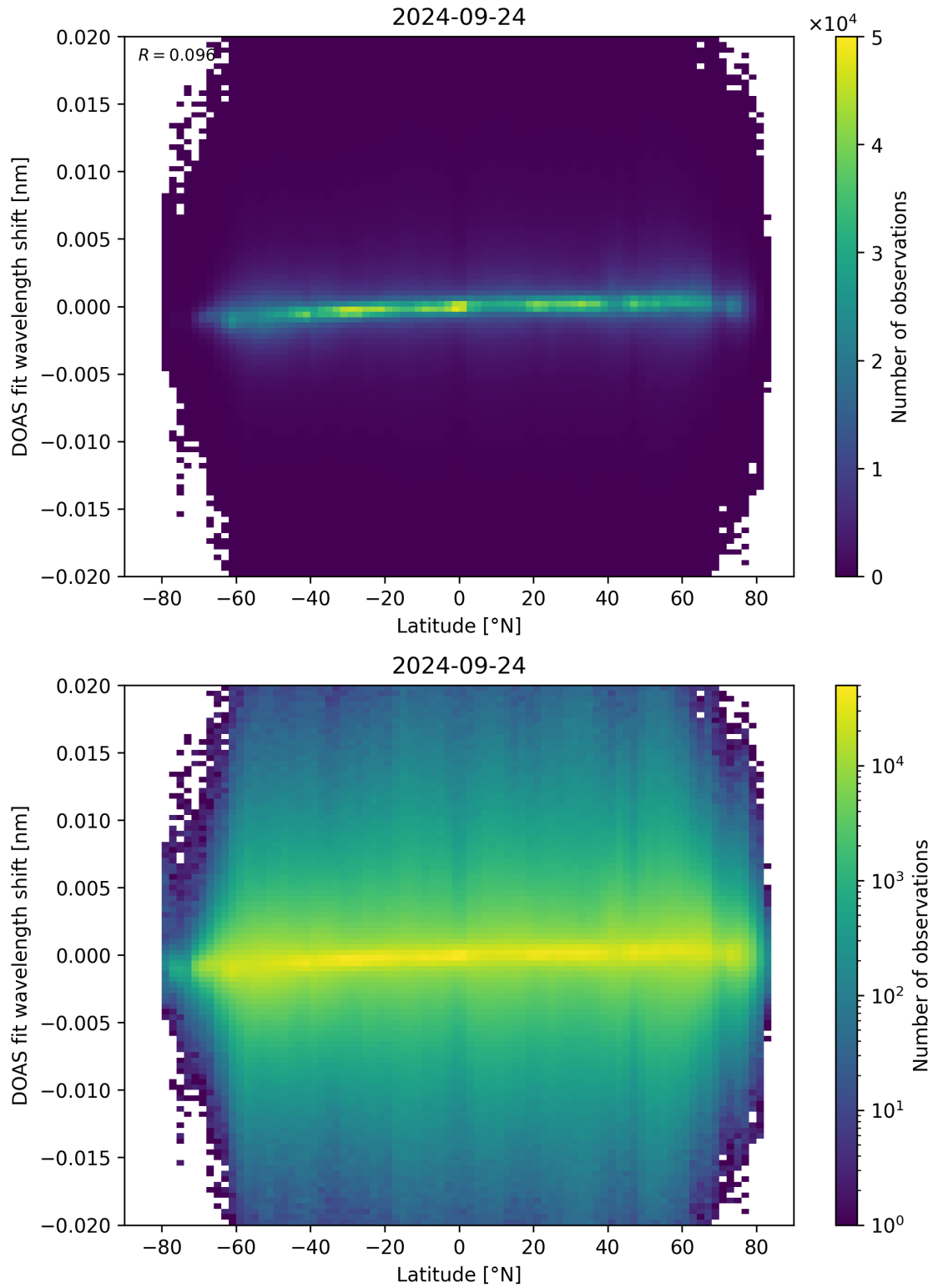
Figure 154: Scatter density plot of “Latitude” against “DOAS fit wavelength shift” for 2024-09-23 to 2024-09-25.
