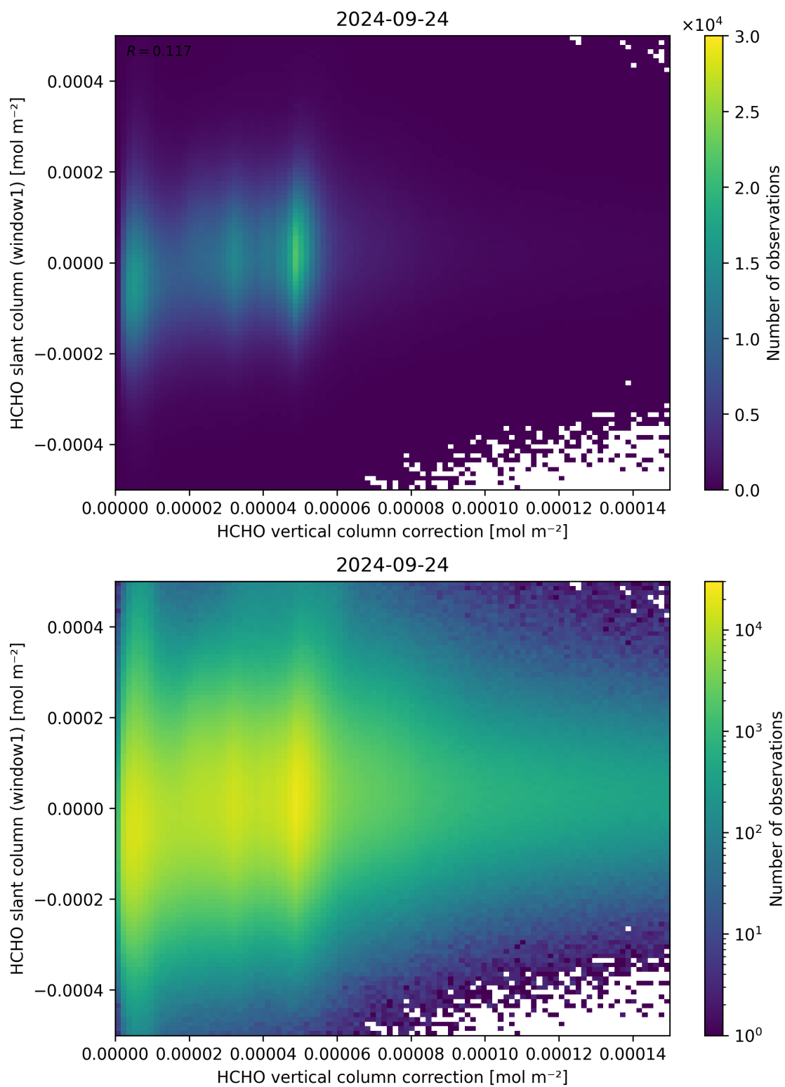
Figure 118: Scatter density plot of “HCHO vertical column correction” against “HCHO slant column (window1)” for 2024-09-23 to 2024-09-25.
