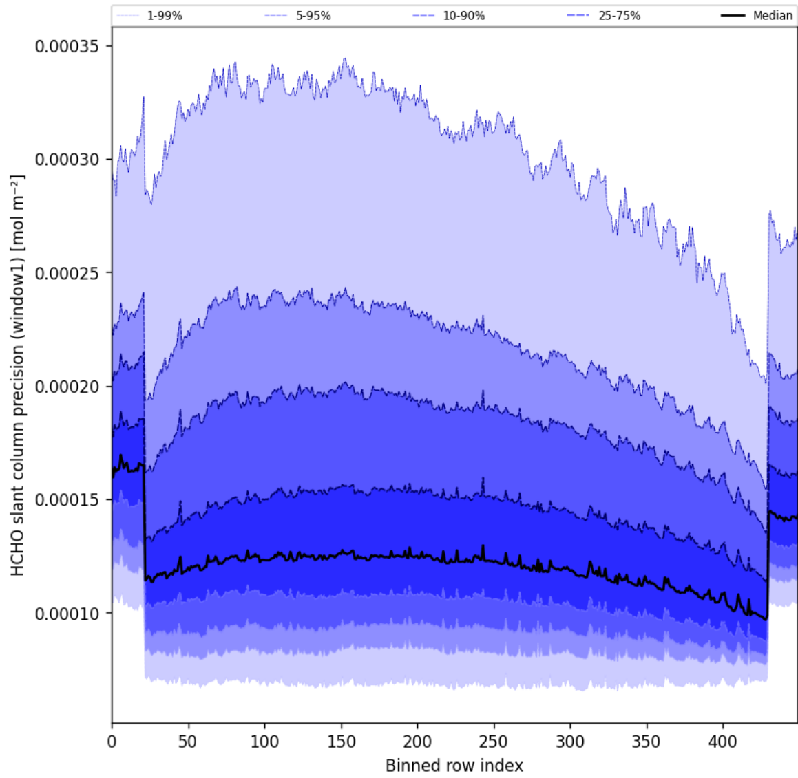
Figure 53: Along track statistics of “HCHO slant column precision (window1)” for 2024-09-23 to 2024-09-25
