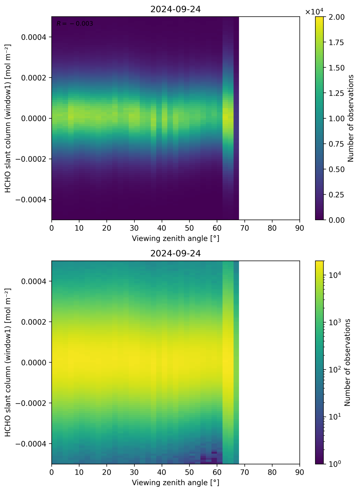
Figure 188: Scatter density plot of “Viewing zenith angle” against “HCHO slant column (window1)” for 2024-09-23 to 2024-09-25.
