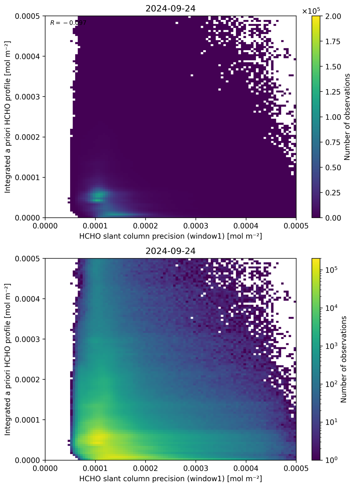
Figure 96: Scatter density plot of “HCHO slant column precision (window1)” against “Integrated a priori HCHO profile” for 2024-09-23 to 2024-09-25.
