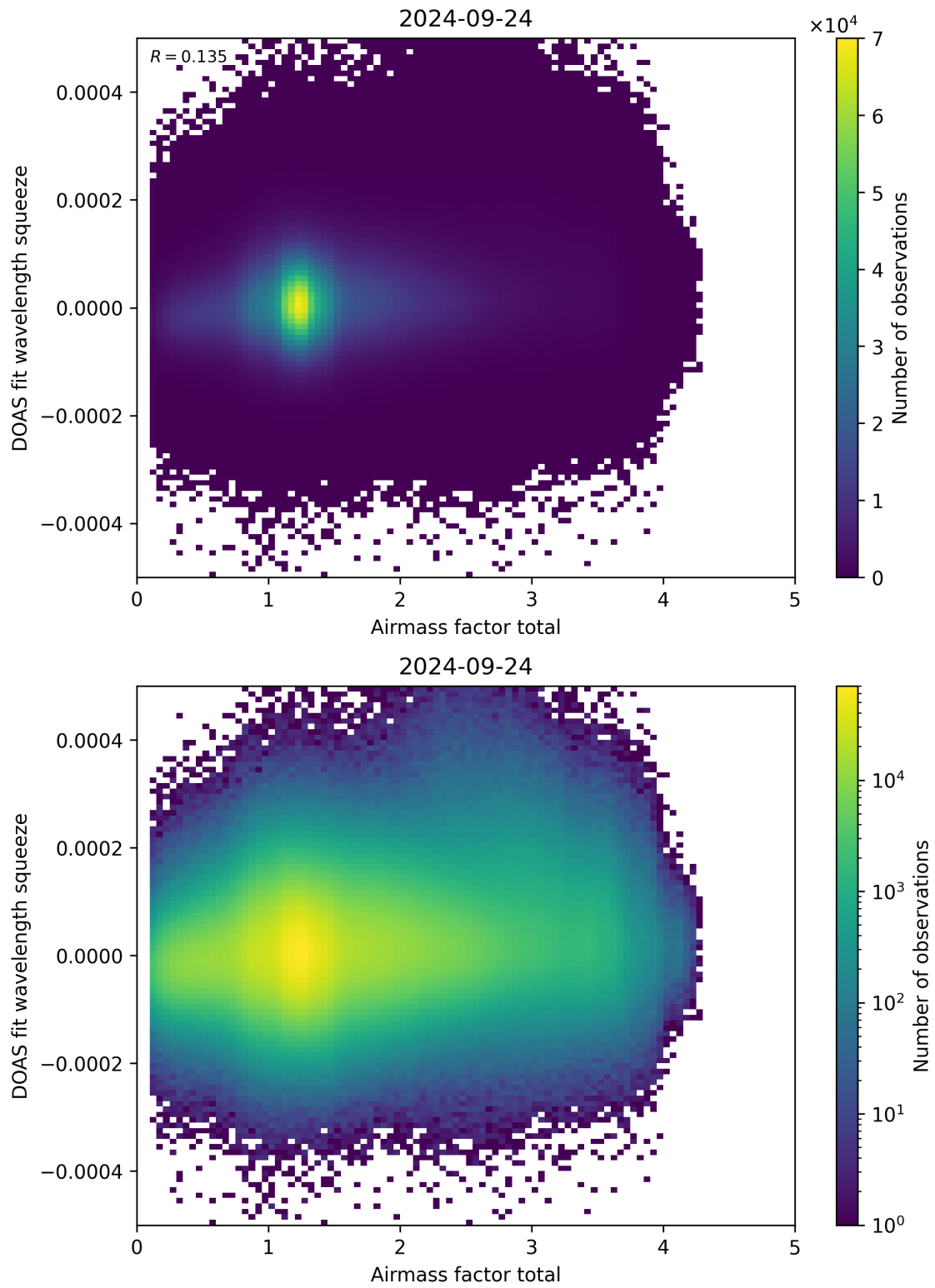
Figure 99: Scatter density plot of “Airmass factor total” against “DOAS fit wavelength squeeze” for 2024-09-23 to 2024-09-25.
