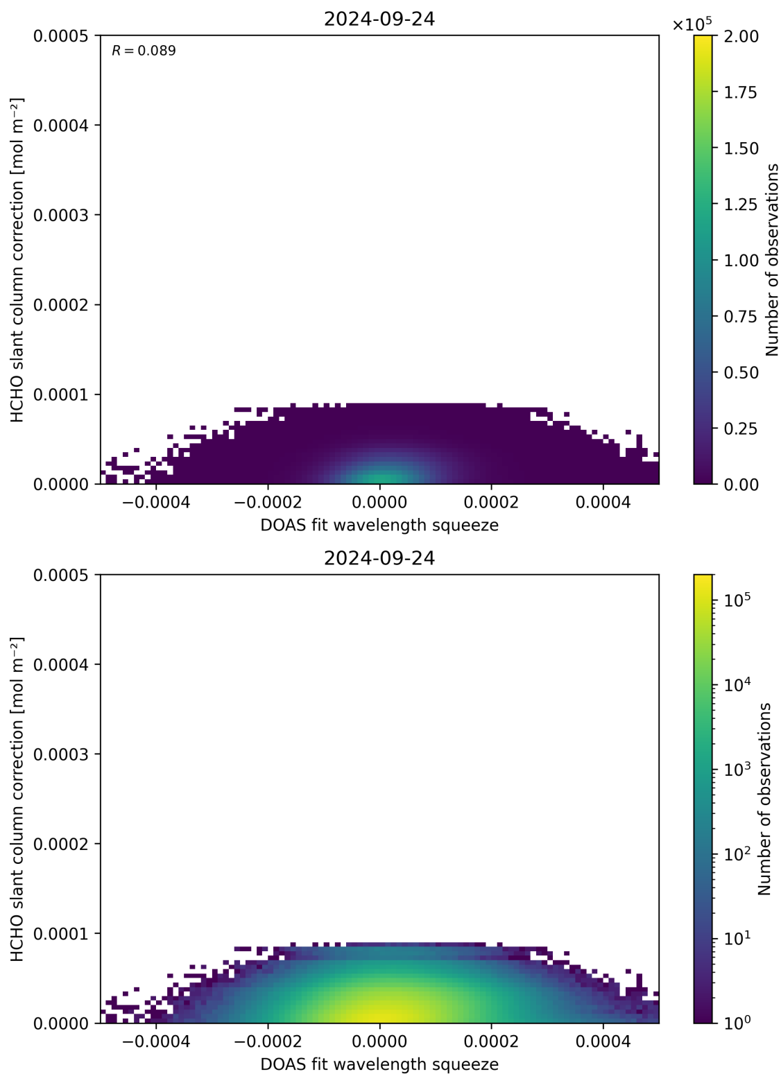
Figure 70: Scatter density plot of “DOAS fit wavelength squeeze” against “HCHO slant column correction” for 2024-09-23 to 2024-09-25.
