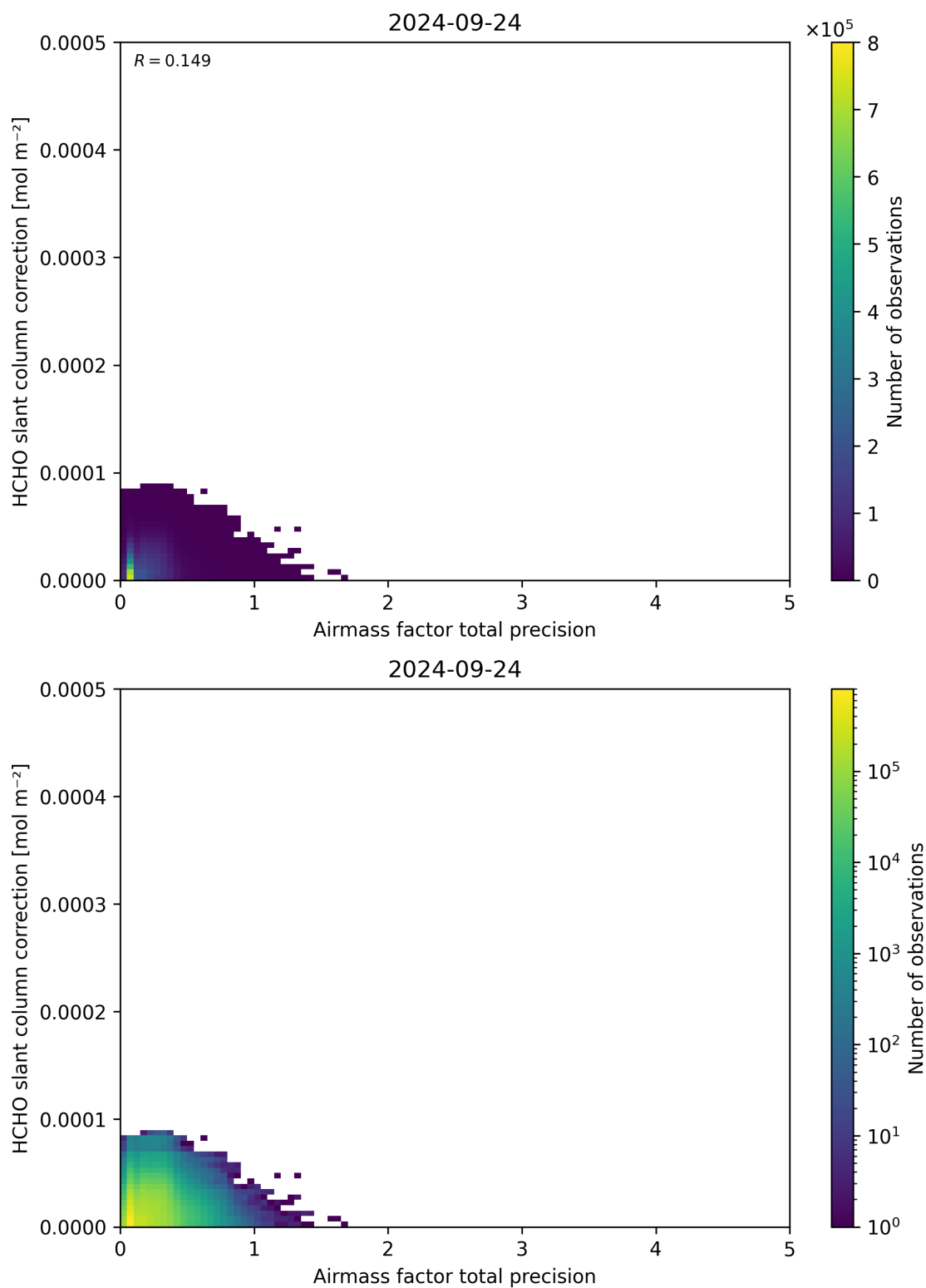
Figure 110: Scatter density plot of “Airmass factor total precision” against “HCHO slant column correction” for 2024-09-23 to 2024-09-25.
