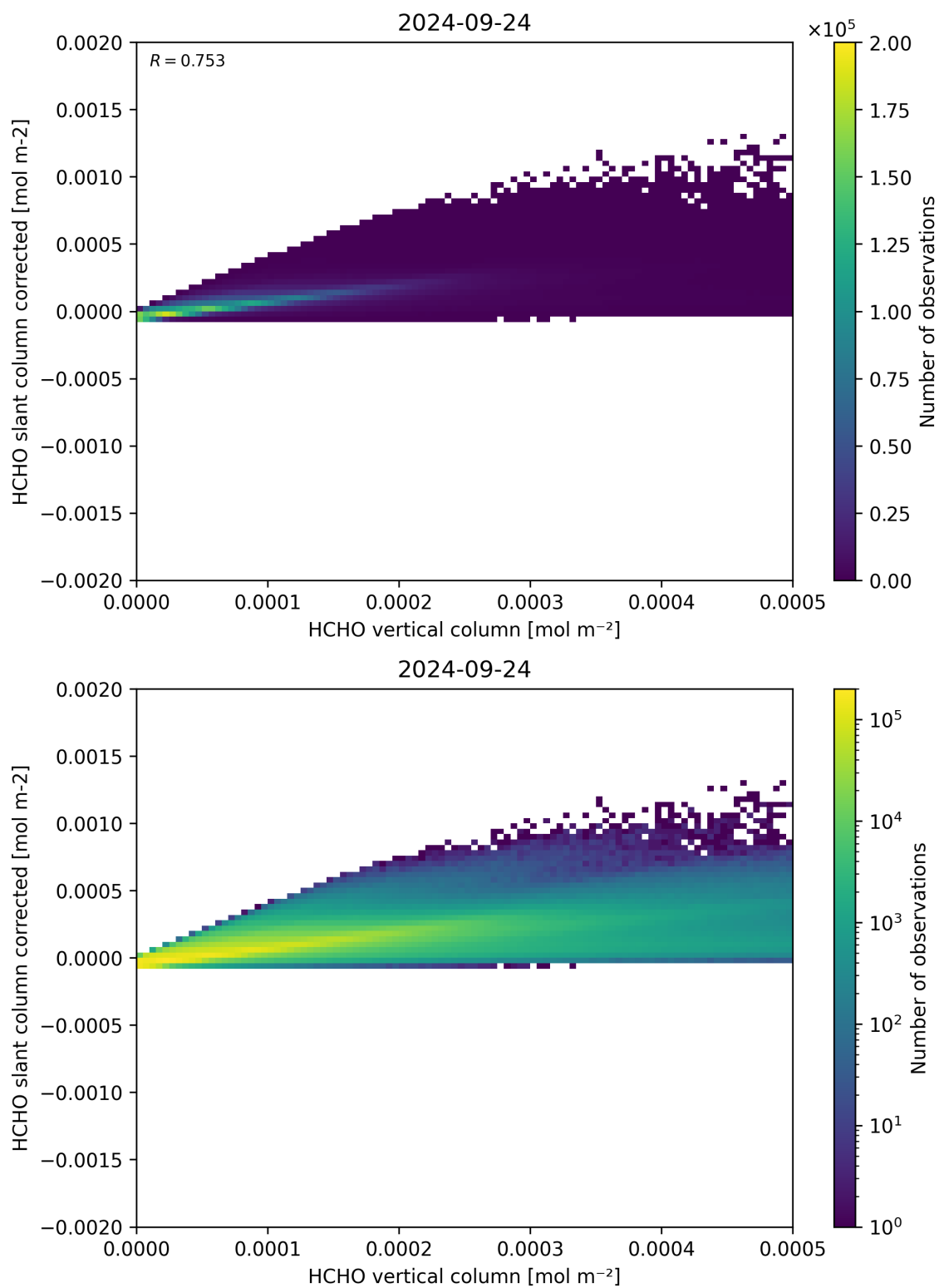
Figure 127: Scatter density plot of “HCHO vertical column” against “HCHO slant column corrected” for 2024-09-23 to 2024-09-25.
