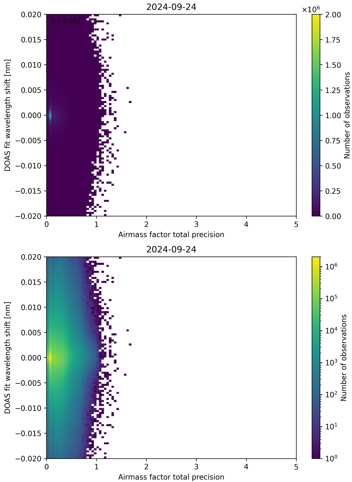
Figure 106: Scatter density plot of “Airmass factor total precision” against “DOAS fit wavelength shift” for 2024-09-23 to 2024-09-25.
