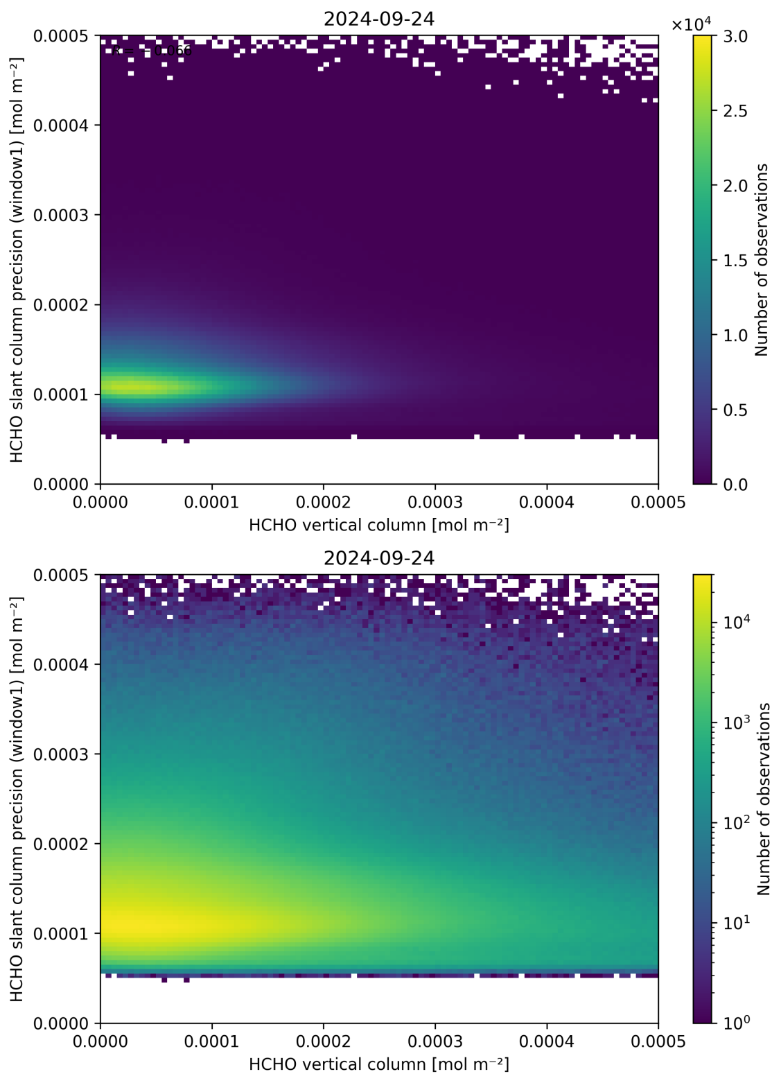
Figure 130: Scatter density plot of “HCHO vertical column” against “HCHO slant column precision (window1)” for 2024-09-23 to 2024-09-25.
