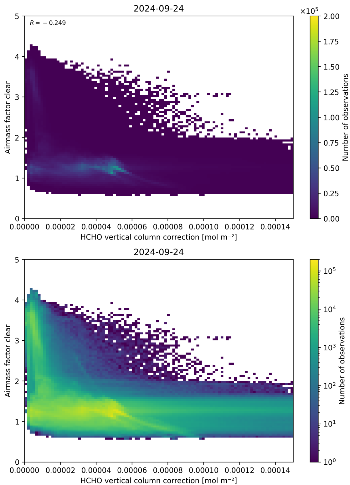
Figure 115: Scatter density plot of “HCHO vertical column correction” against “Airmass factor clear” for 2024-09-23 to 2024-09-25.
