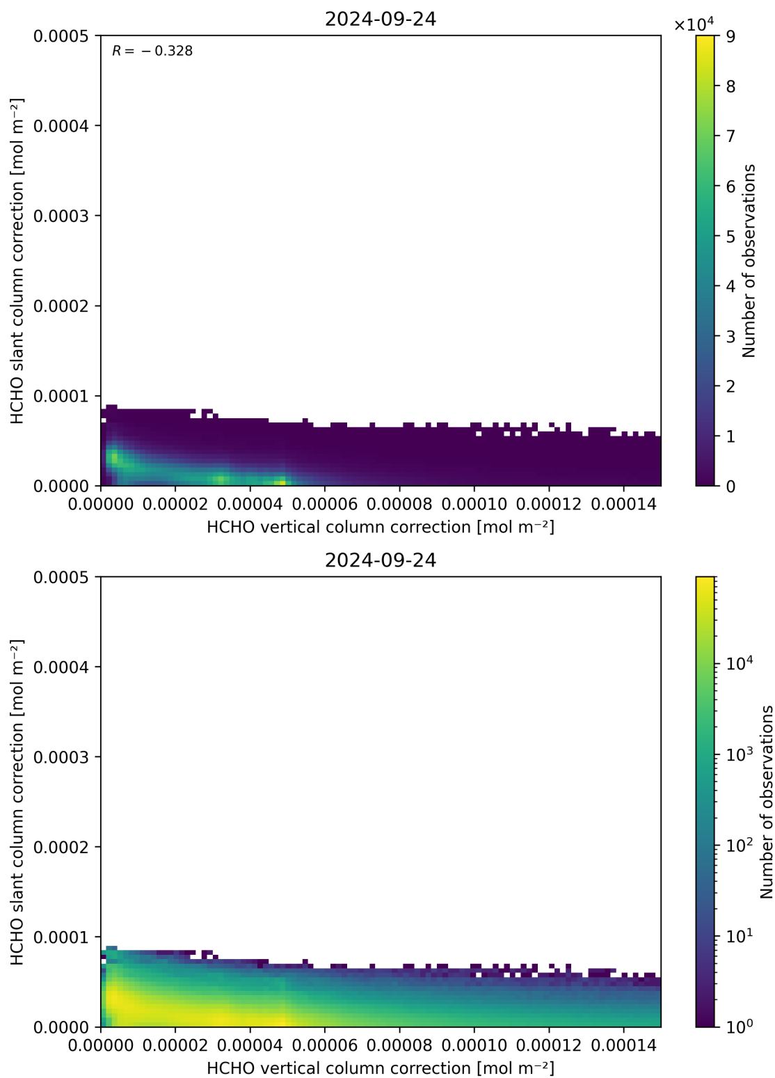
Figure 117: Scatter density plot of “HCHO vertical column correction” against “HCHO slant column correction” for 2024-09-23 to 2024-09-25.
