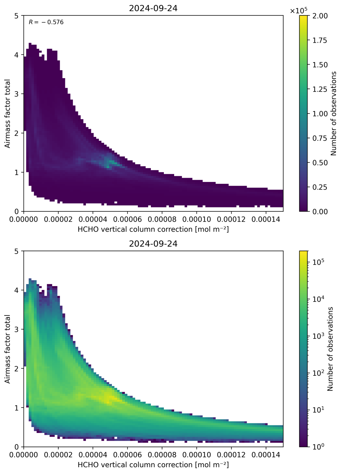
Figure 120: Scatter density plot of “HCHO vertical column correction” against “Airmass factor total” for 2024-09-23 to 2024-09-25.
