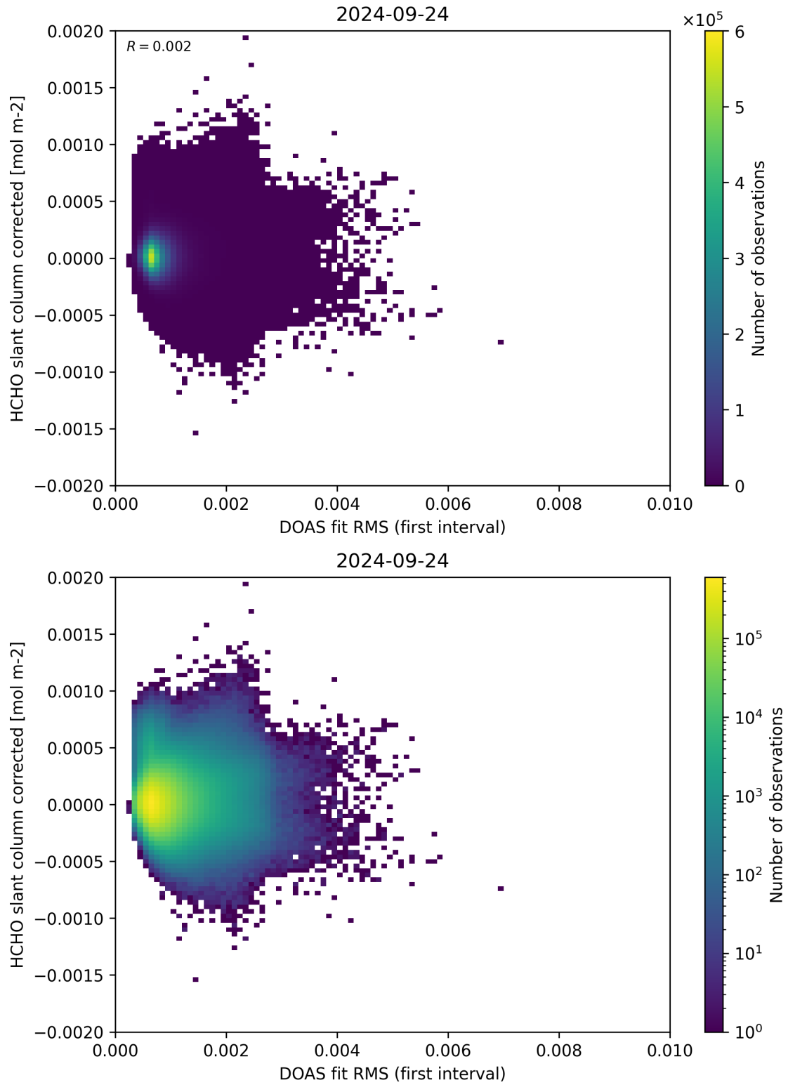
Figure 62: Scatter density plot of “DOAS fit RMS (first interval)” against “HCHO slant column corrected” for 2024-09-23 to 2024-09-25.
