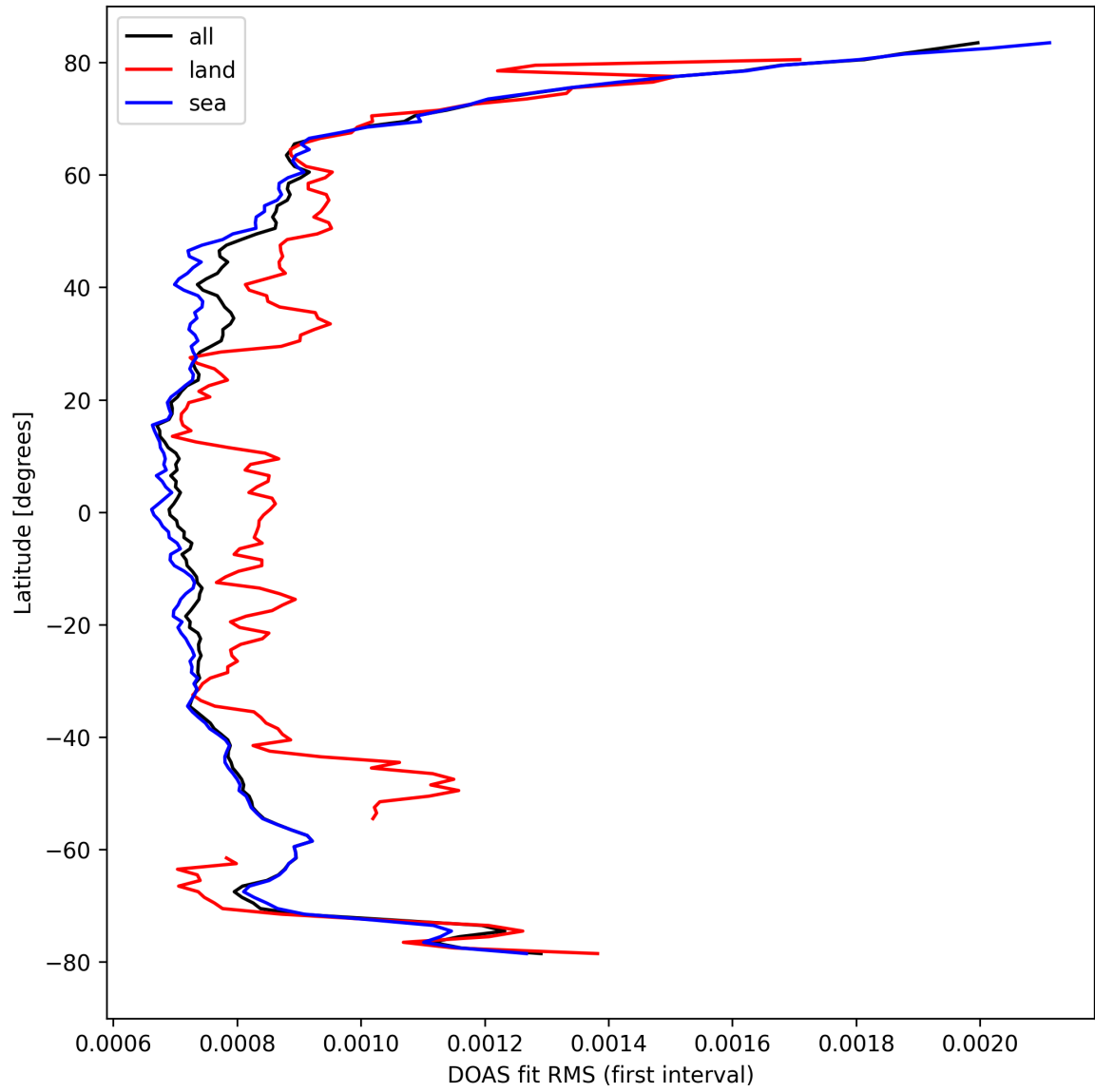
Figure 32: Zonal average of “DOAS fit RMS (first interval)” for 2024-09-23 to 2024-09-25.
