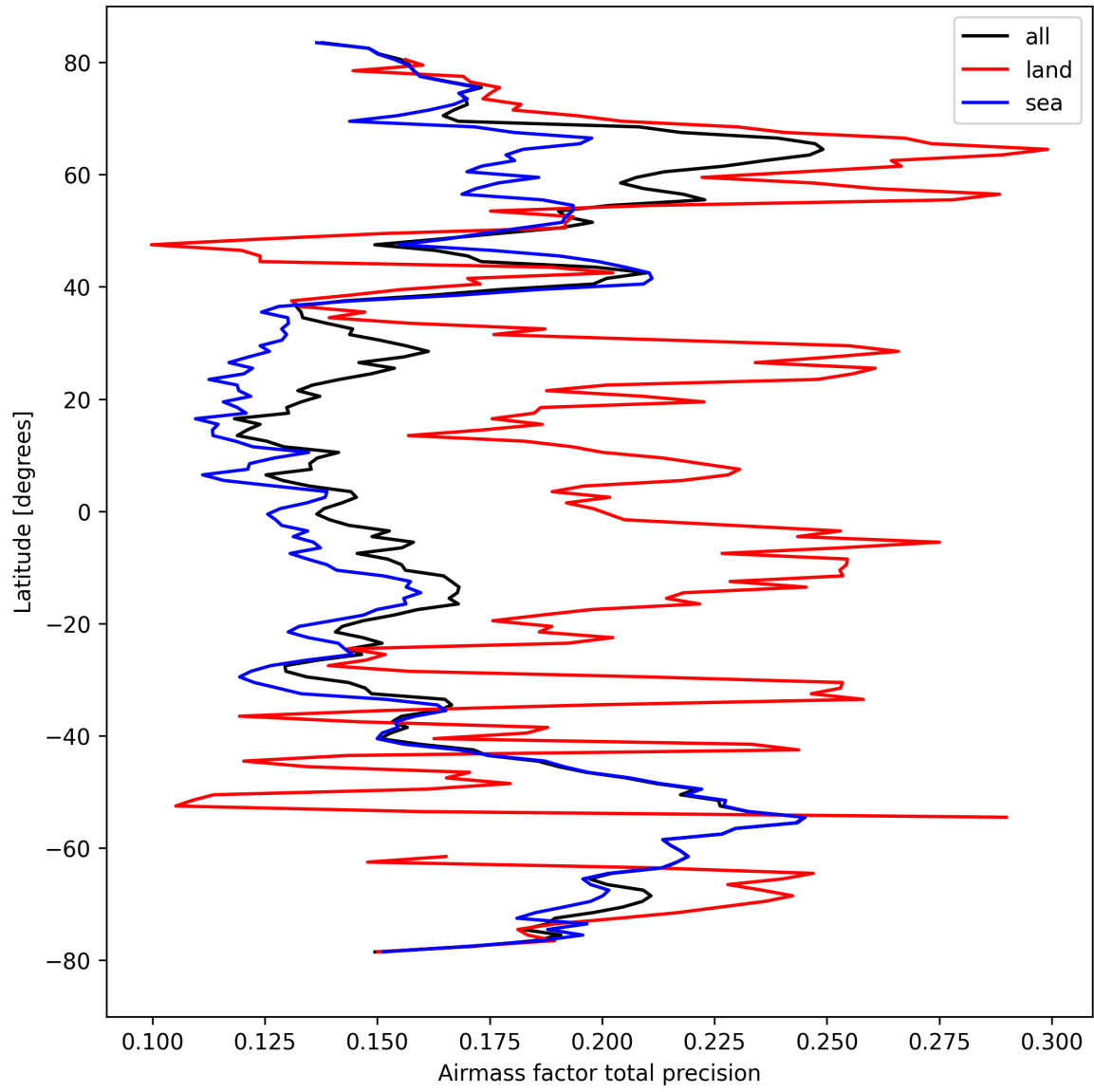
Figure 27: Zonal average of “Airmass factor total precision” for 2024-09-23 to 2024-09-25.
