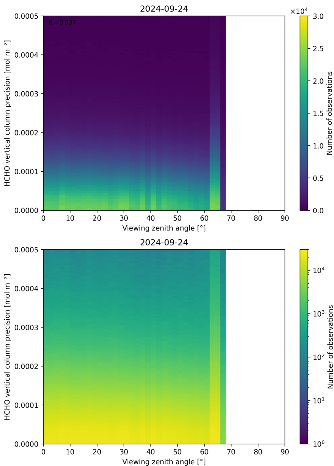
Figure 194: Scatter density plot of “Viewing zenith angle” against “HCHO vertical column precision” for 2024-09-23 to 2024-09-25.
