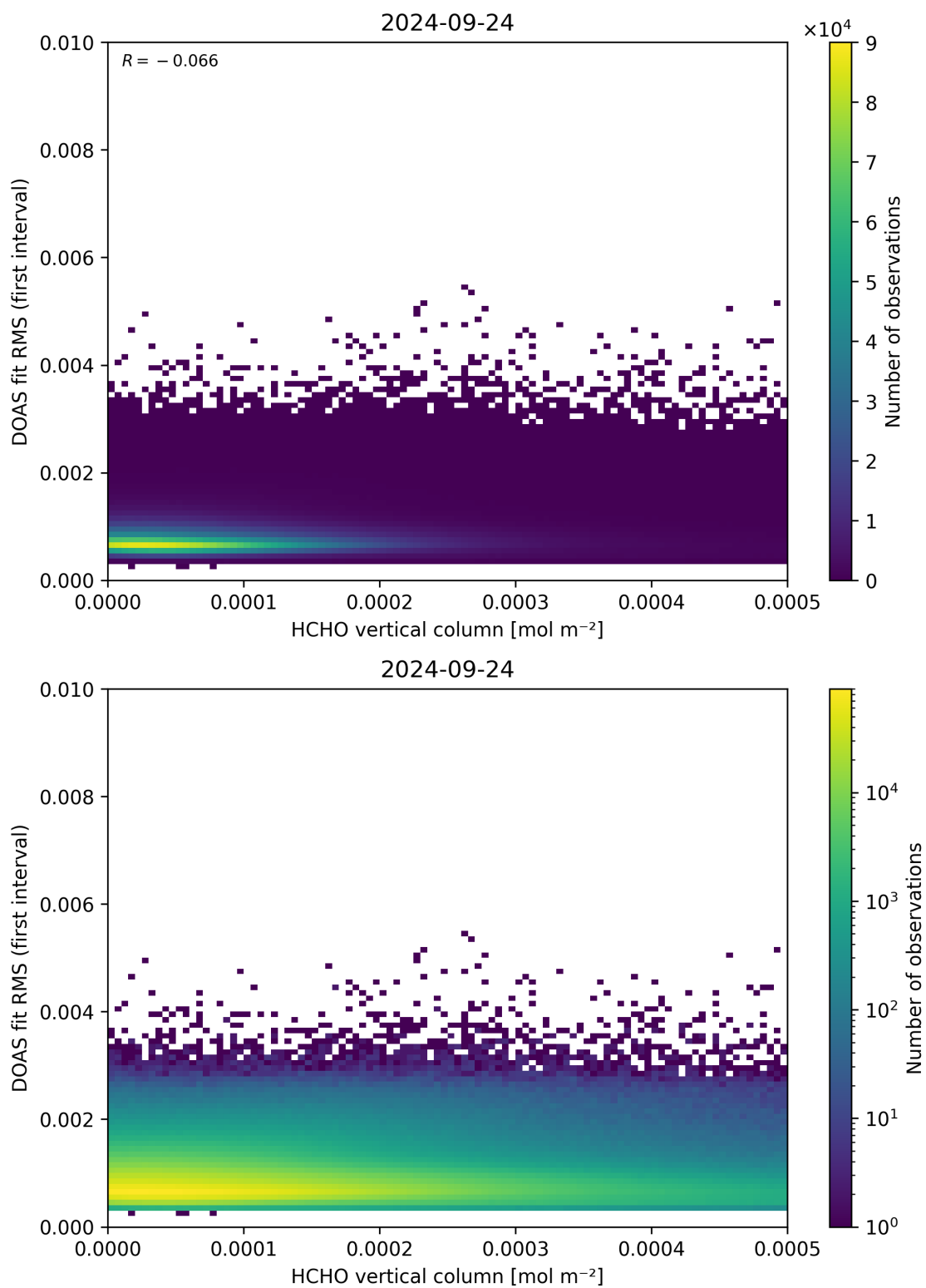
Figure 123: Scatter density plot of “HCHO vertical column” against “DOAS fit RMS (first interval)” for 2024-09-23 to 2024-09-25.
