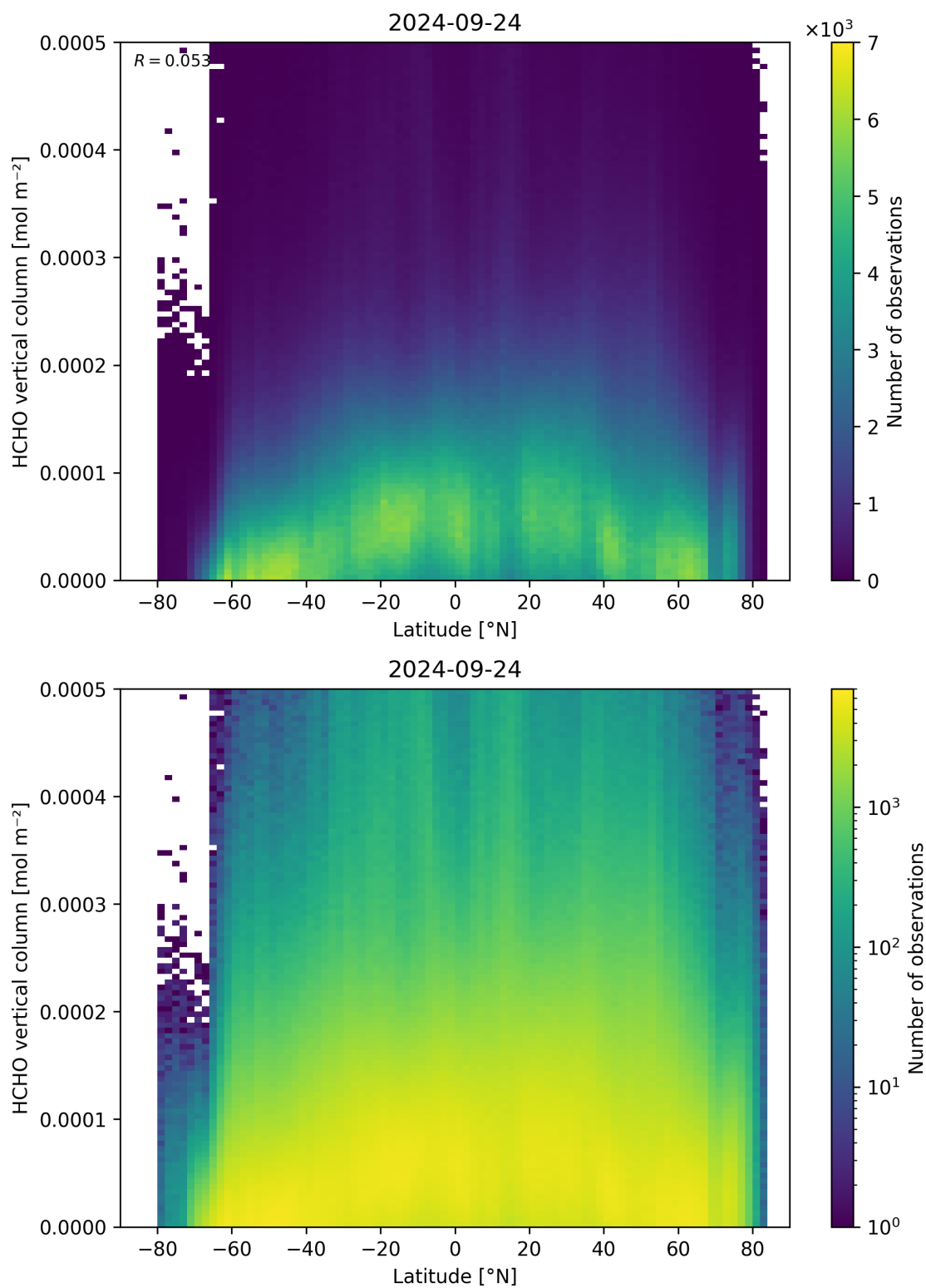
Figure 163: Scatter density plot of “Latitude” against “HCHO vertical column” for 2024-09-23 to 2024-09-25.
