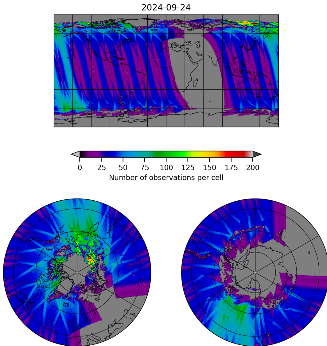
Figure 19: Map of the number of observations for 2024-09-23 to 2024-09-25
