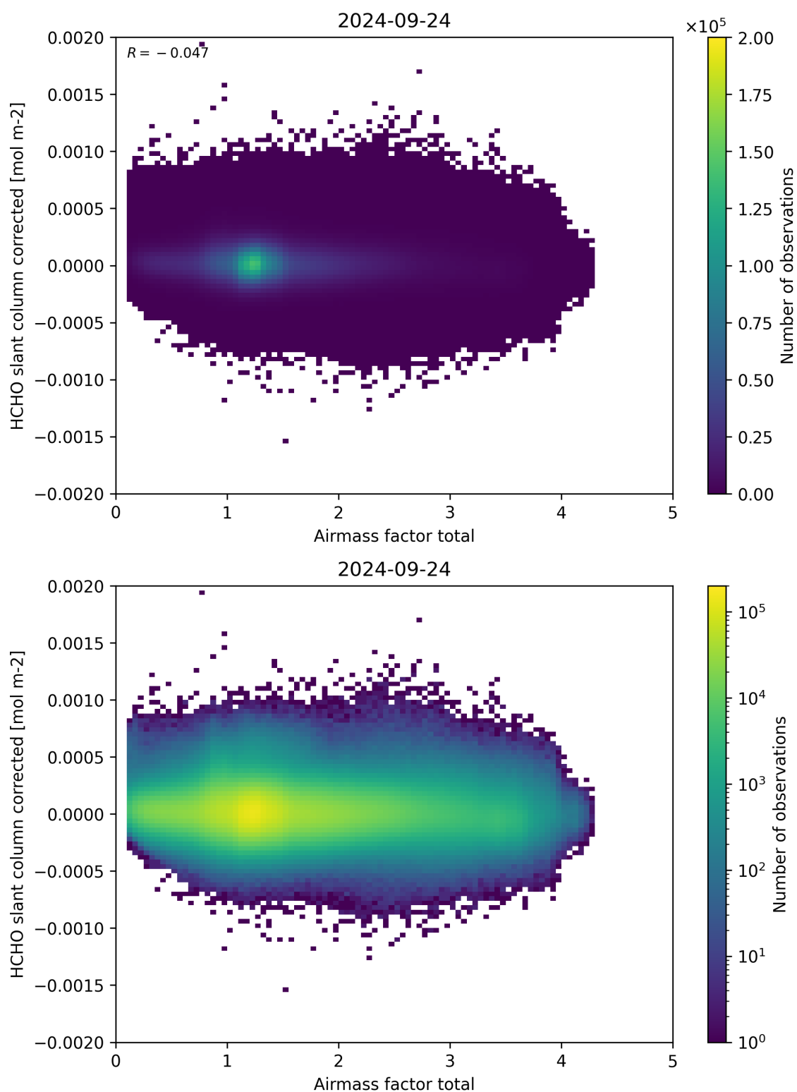
Figure 101: Scatter density plot of “Airmass factor total” against “HCHO slant column corrected” for 2024-09-23 to 2024-09-25.
