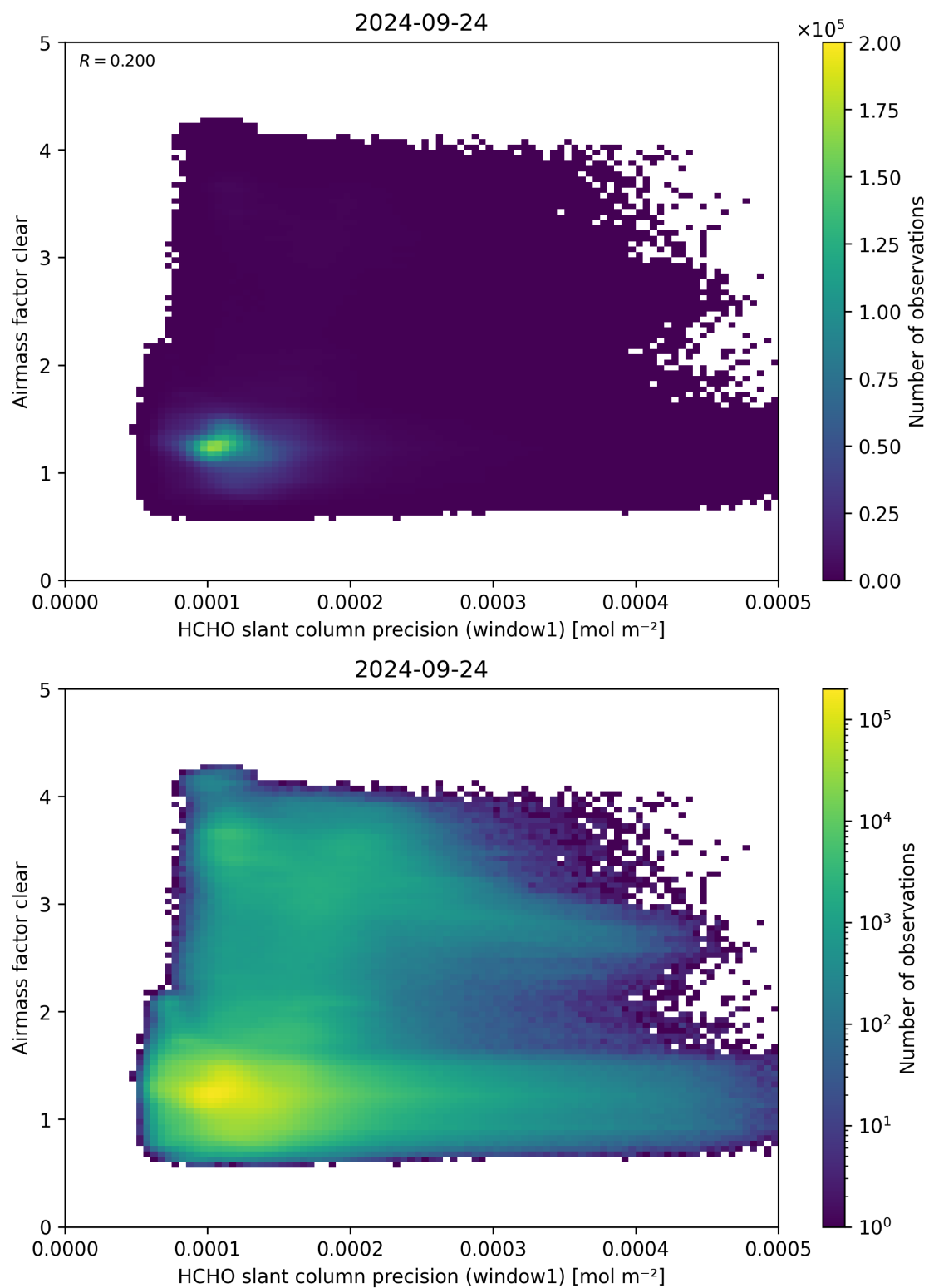
Figure 91: Scatter density plot of “HCHO slant column precision (window1)” against “Airmass factor clear” for 2024-09-23 to 2024-09-25.
