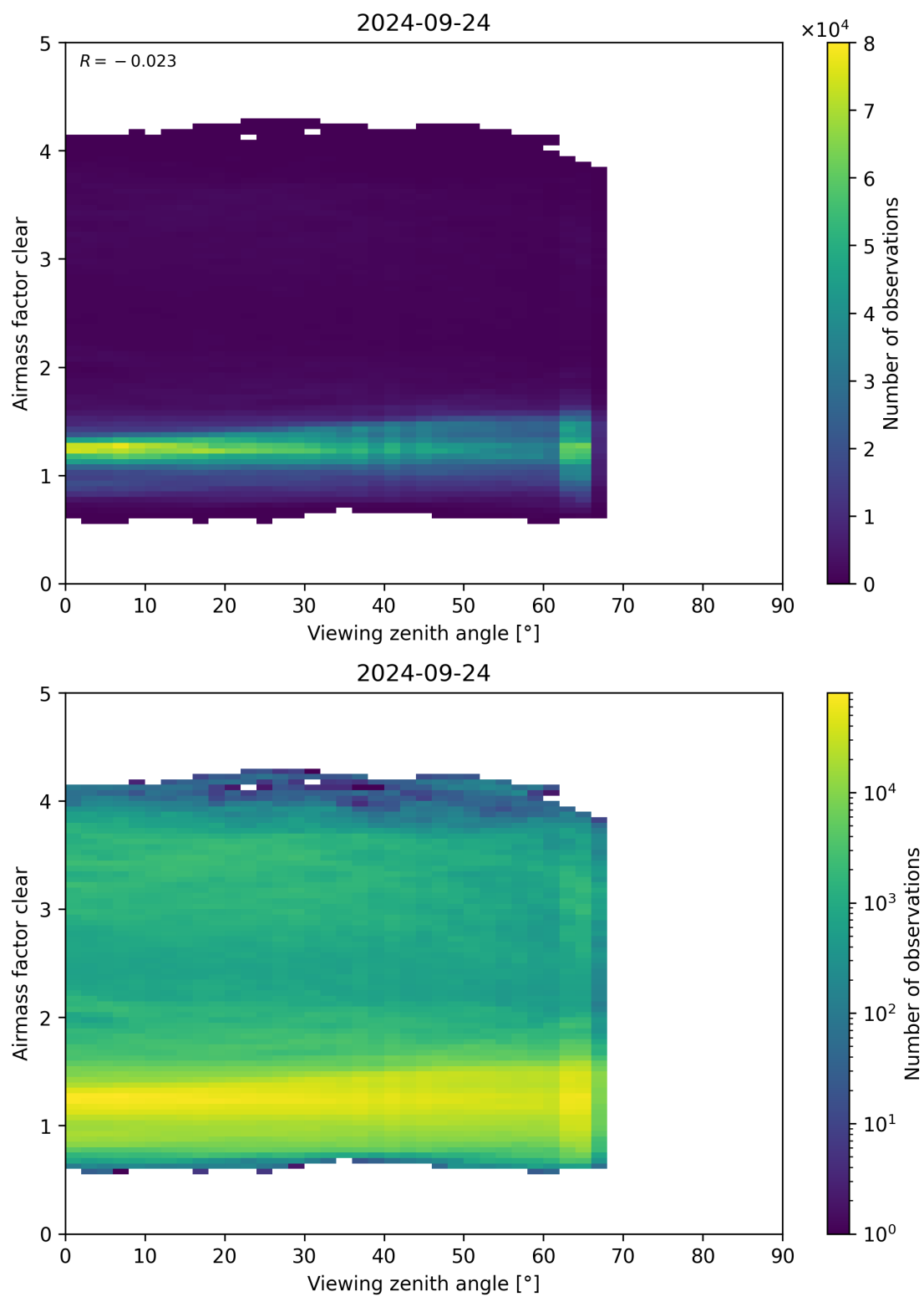
Figure 185: Scatter density plot of “Viewing zenith angle” against “Airmass factor clear” for 2024-09-23 to 2024-09-25.
