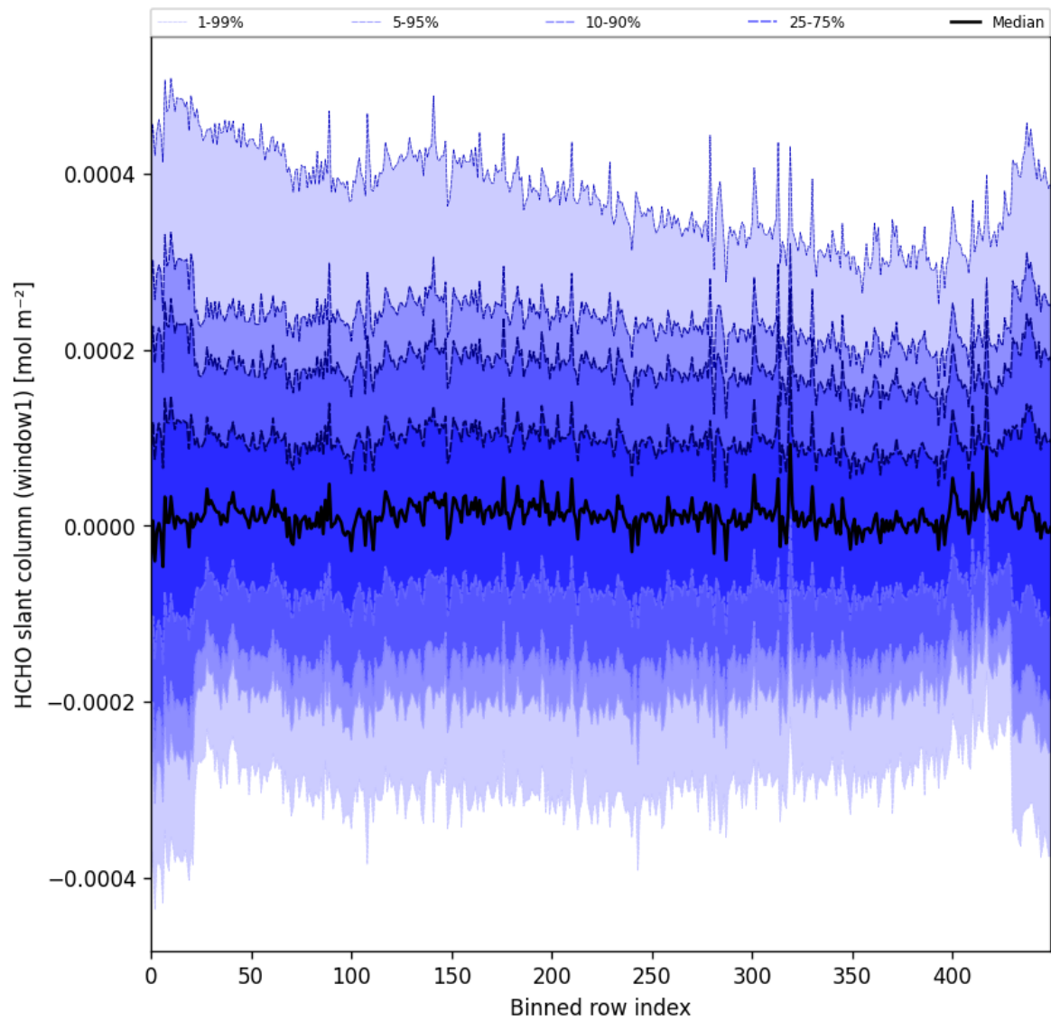
Figure 52: Along track statistics of “HCHO slant column (window1)” for 2024-09-23 to 2024-09-25
