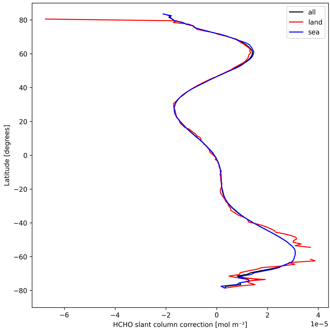
Figure 33: Zonal average of “HCHO slant column correction” for 2024-09-23 to 2024-09-25.
