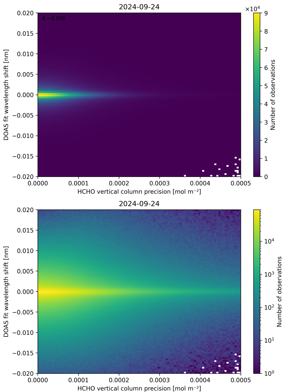
Figure 137: Scatter density plot of “HCHO vertical column precision” against “DOAS fit wavelength shift” for 2024-09-23 to 2024-09-25.
