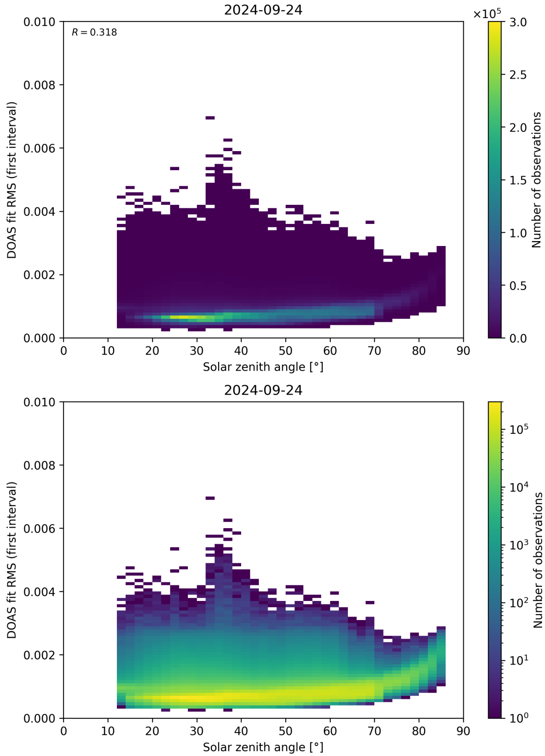
Figure 167: Scatter density plot of “Solar zenith angle” against “DOAS fit RMS (first interval)” for 2024-09-23 to 2024-09-25.
