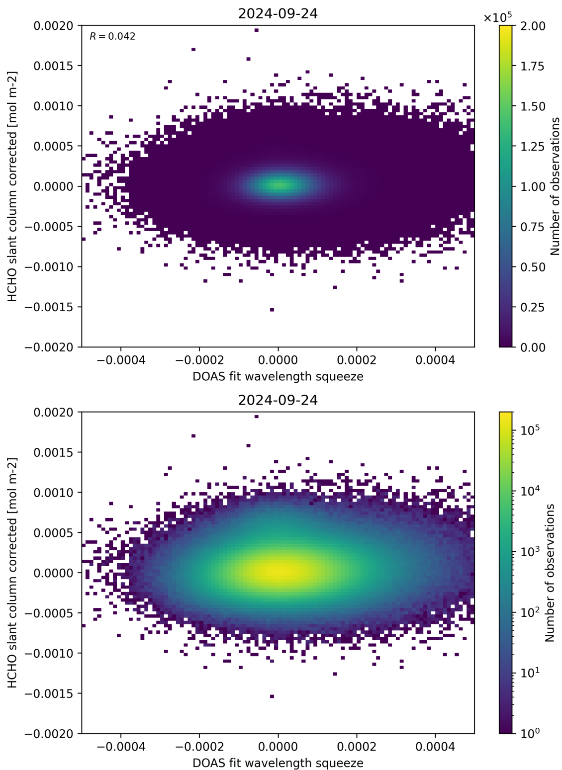
Figure 69: Scatter density plot of “DOAS fit wavelength squeeze” against “HCHO slant column corrected” for 2024-09-23 to 2024-09-25.
