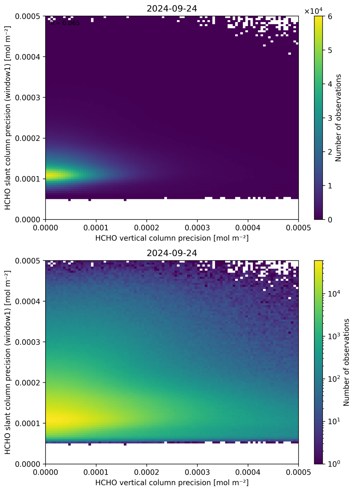
Figure 143: Scatter density plot of “HCHO vertical column precision” against “HCHO slant column precision (window1)” for 2024-09-23 to 2024-09-25.
