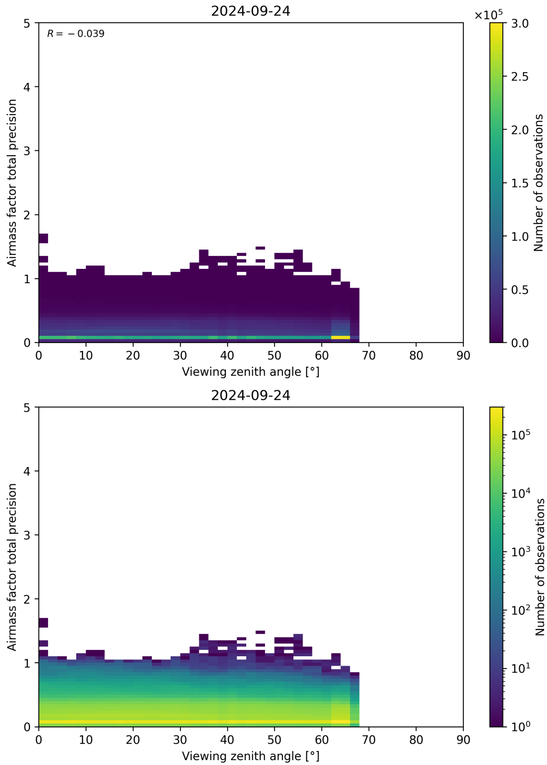
Figure 191: Scatter density plot of “Viewing zenith angle” against “Airmass factor total precision” for 2024-09-23 to 2024-09-25.
