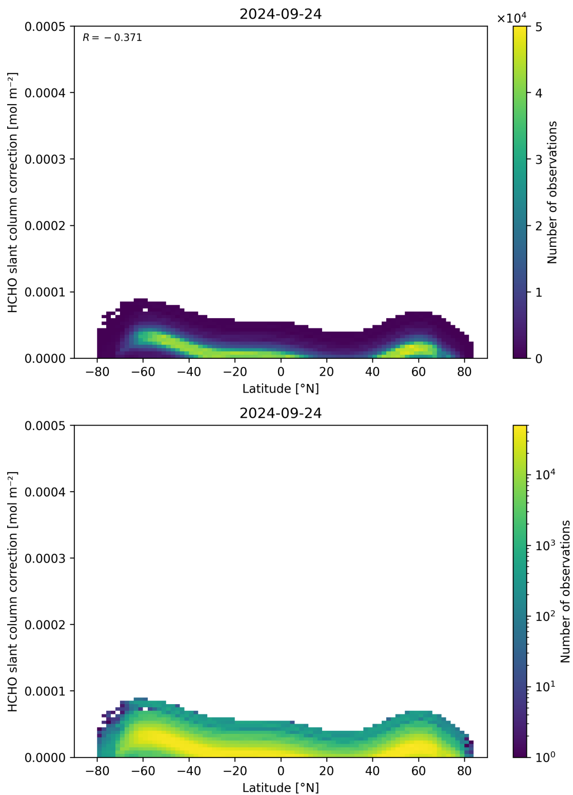
Figure 158: Scatter density plot of “Latitude” against “HCHO slant column correction” for 2024-09-23 to 2024-09-25.
