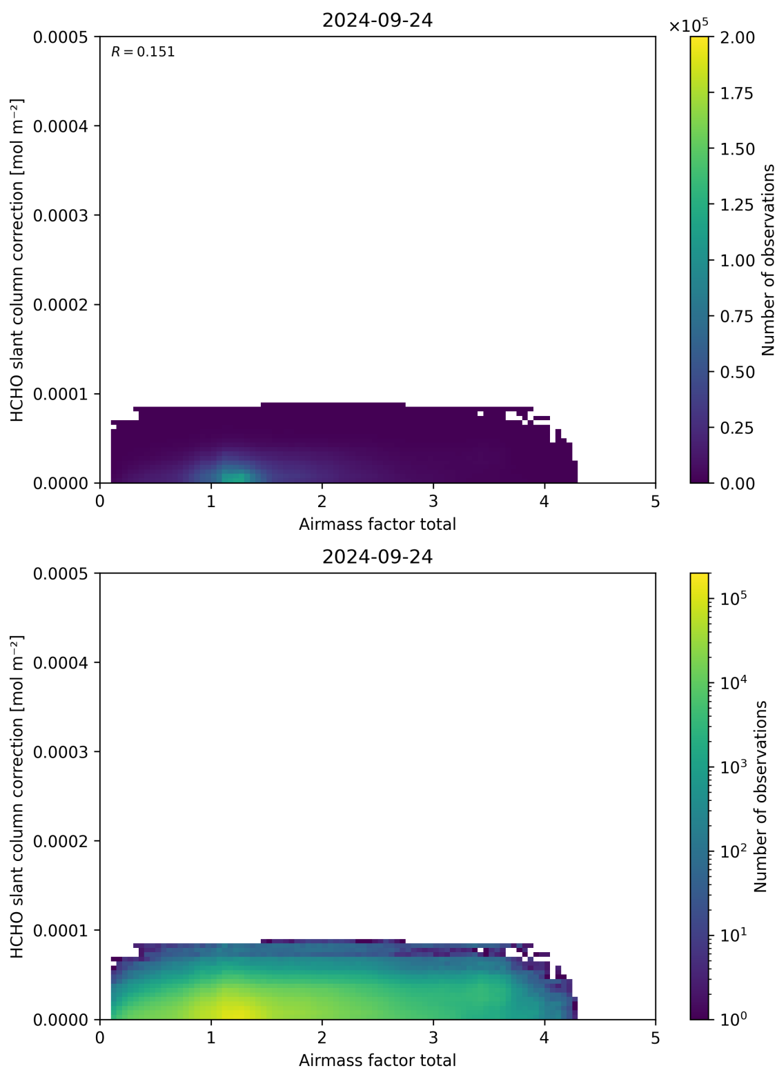
Figure 102: Scatter density plot of “Airmass factor total” against “HCHO slant column correction” for 2024-09-23 to 2024-09-25.
