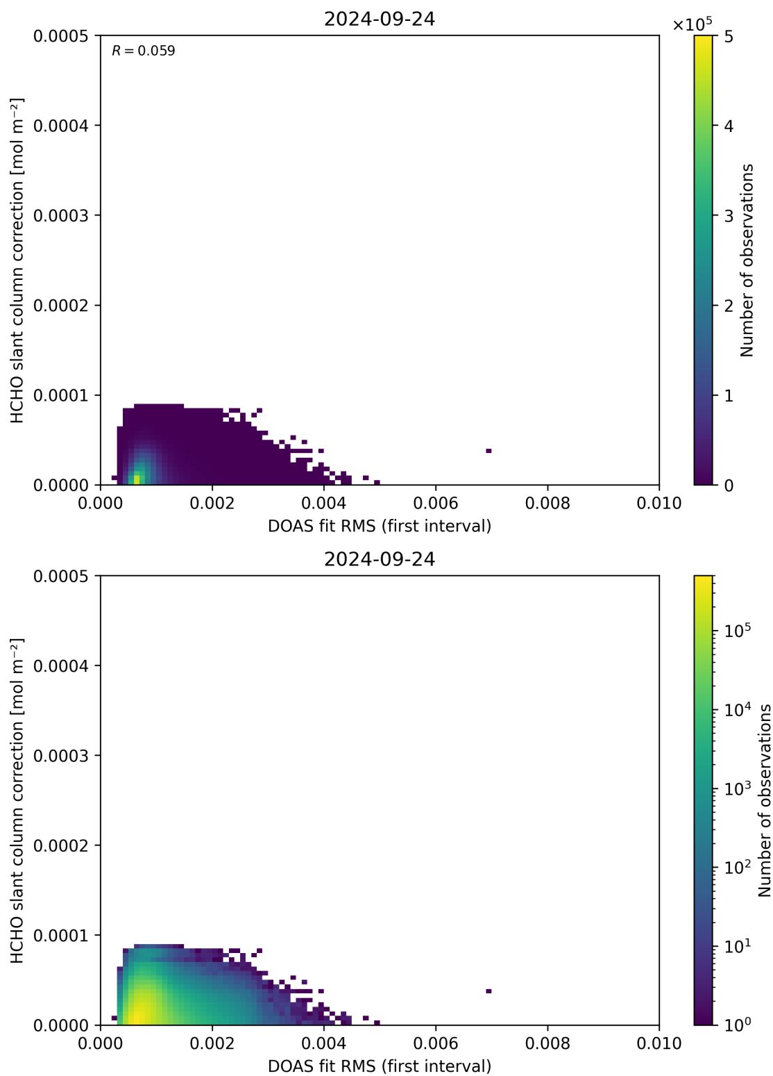
Figure 63: Scatter density plot of “DOAS fit RMS (first interval)” against “HCHO slant column correction” for 2024-09-23 to 2024-09-25.
