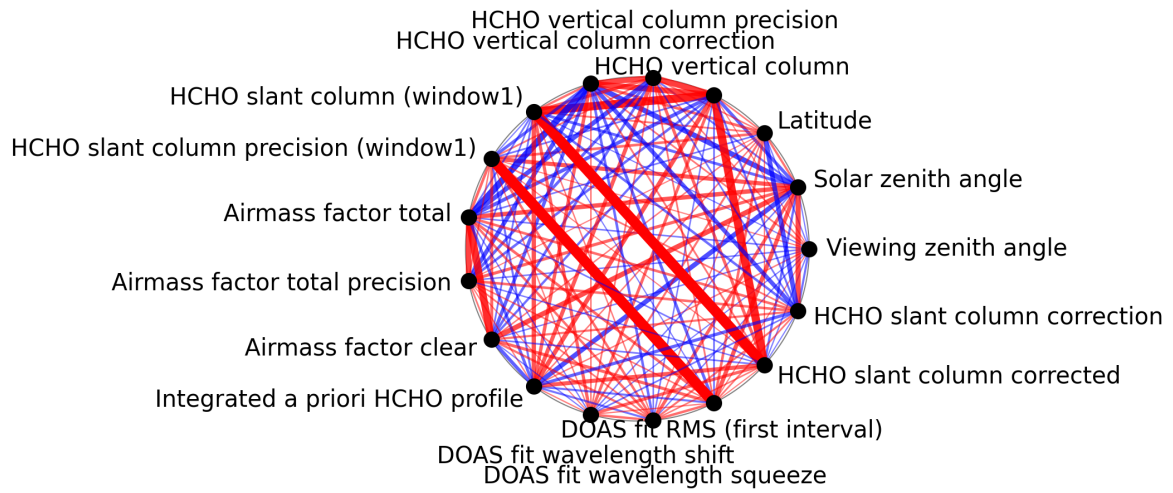
Figure 1: Map of correlation graph for 2024-09-23 to 2024-09-25.
