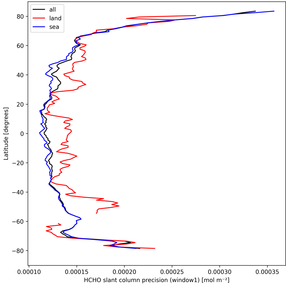
Figure 25: Zonal average of “HCHO slant column precision (window1)” for 2024-09-23 to 2024-09-25.
