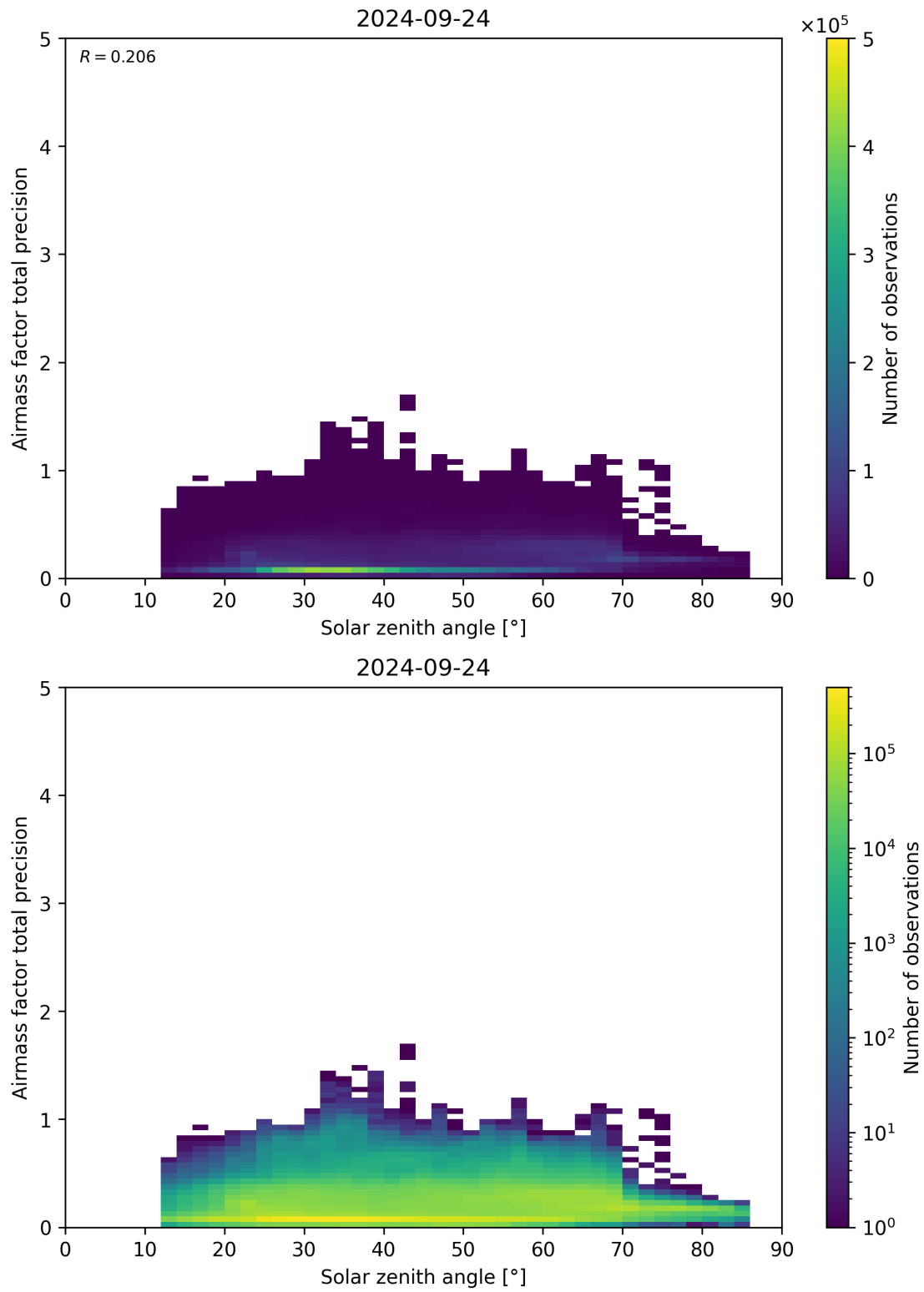
Figure 176: Scatter density plot of “Solar zenith angle” against “Airmass factor total precision” for 2024-09-23 to 2024-09-25.
