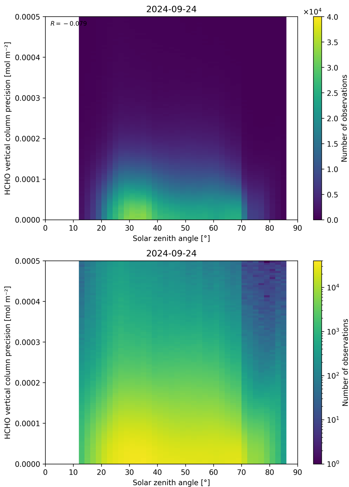
Figure 179: Scatter density plot of “Solar zenith angle” against “HCHO vertical column precision” for 2024-09-23 to 2024-09-25.
