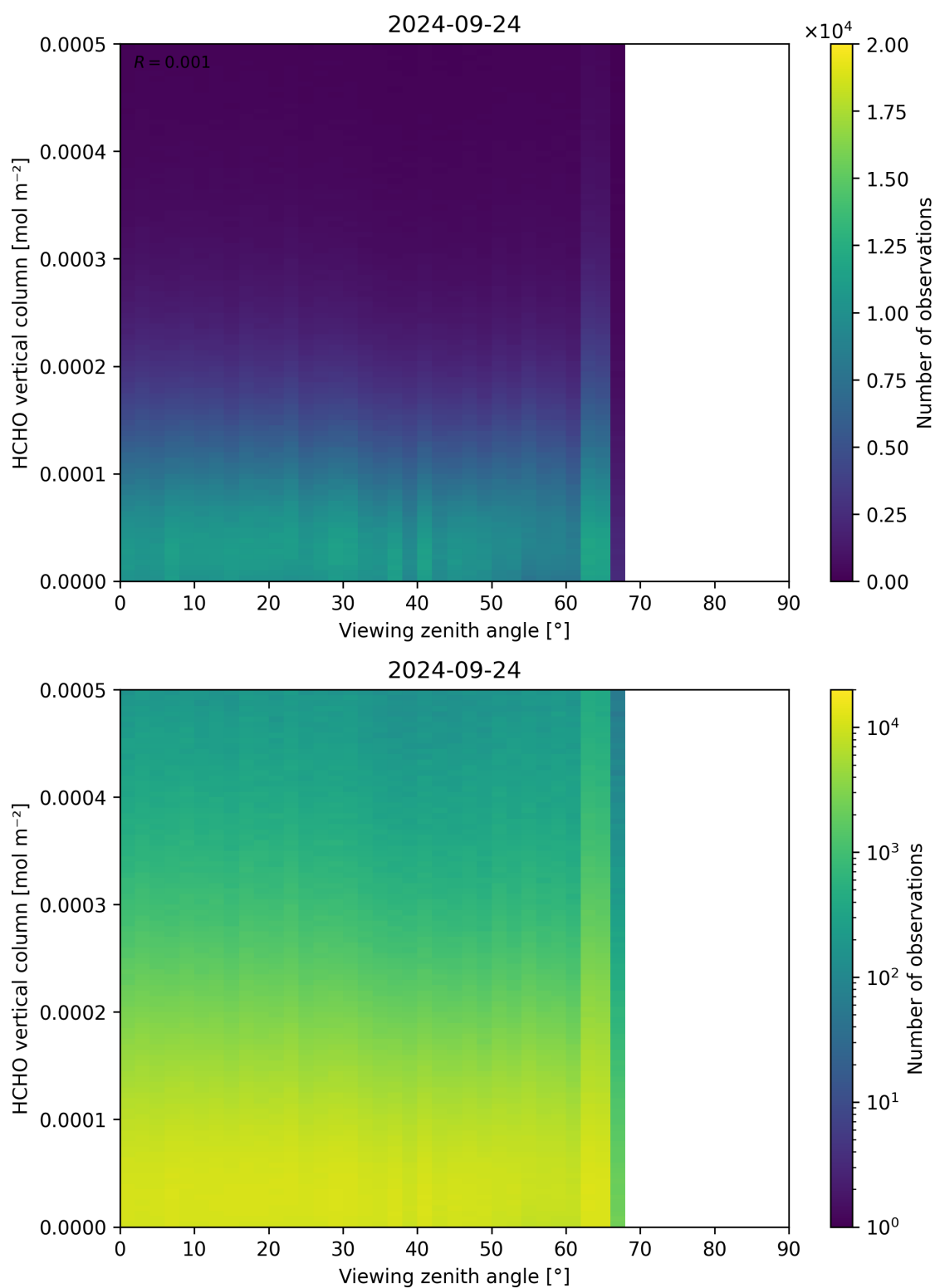
Figure 192: Scatter density plot of “Viewing zenith angle” against “HCHO vertical column” for 2024-09-23 to 2024-09-25.
