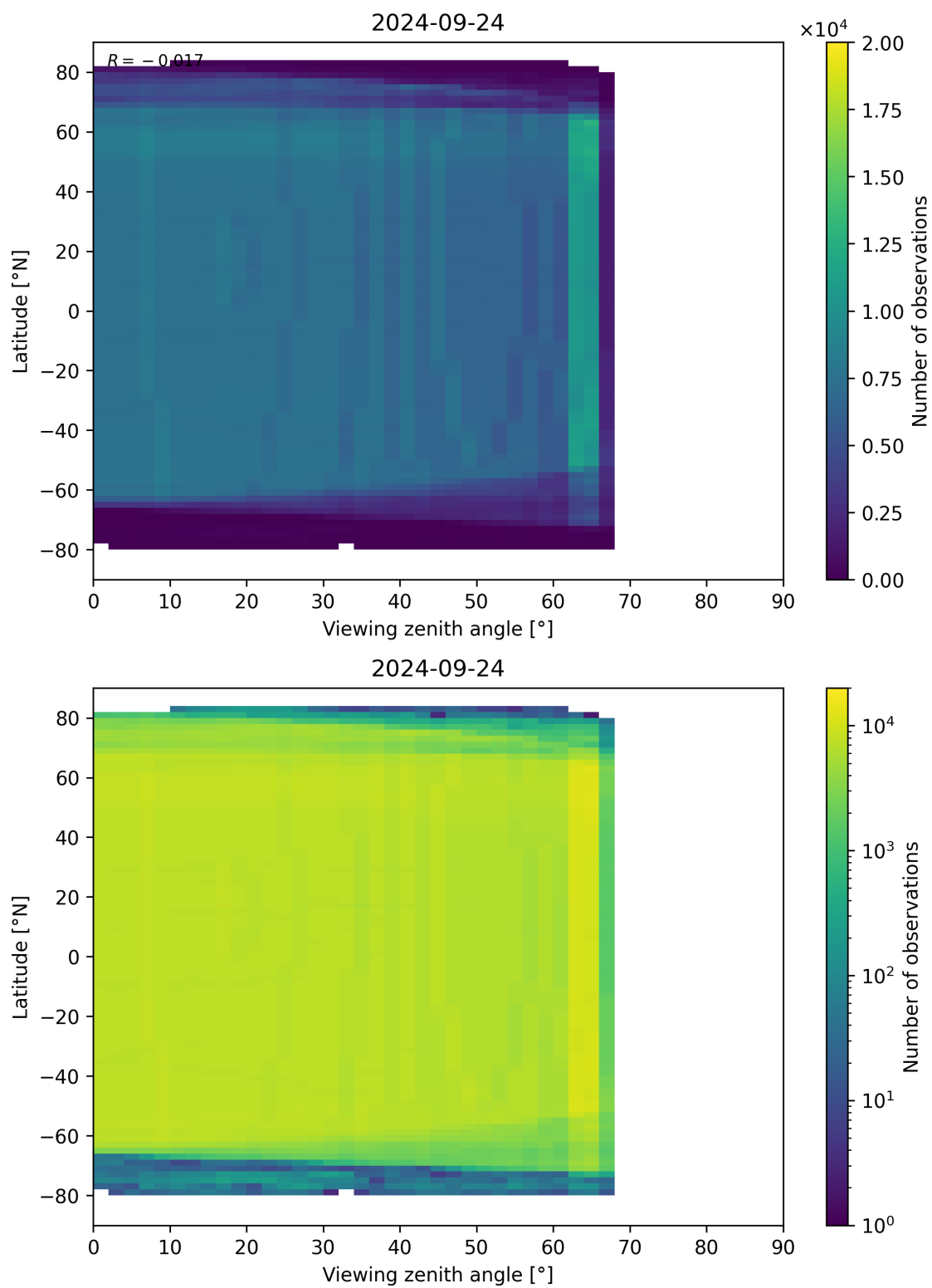
Figure 196: Scatter density plot of “Viewing zenith angle” against “Latitude” for 2024-09-23 to 2024-09-25.
