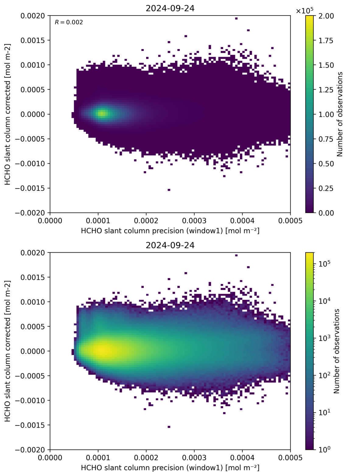
Figure 92: Scatter density plot of “HCHO slant column precision (window1)” against “HCHO slant column corrected” for 2024-09-23 to 2024-09-25.
