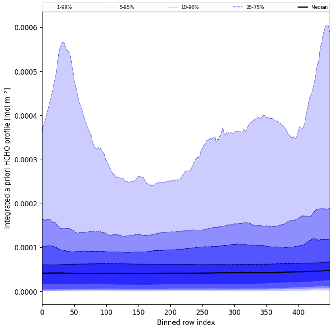
Figure 57: Along track statistics of “Integrated a priori HCHO profile” for 2024-09-23 to 2024-09-25
