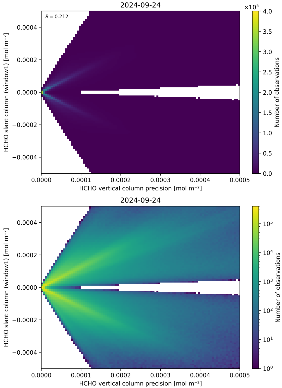
Figure 142: Scatter density plot of “HCHO vertical column precision” against “HCHO slant column (window1)” for 2024-09-23 to 2024-09-25.
