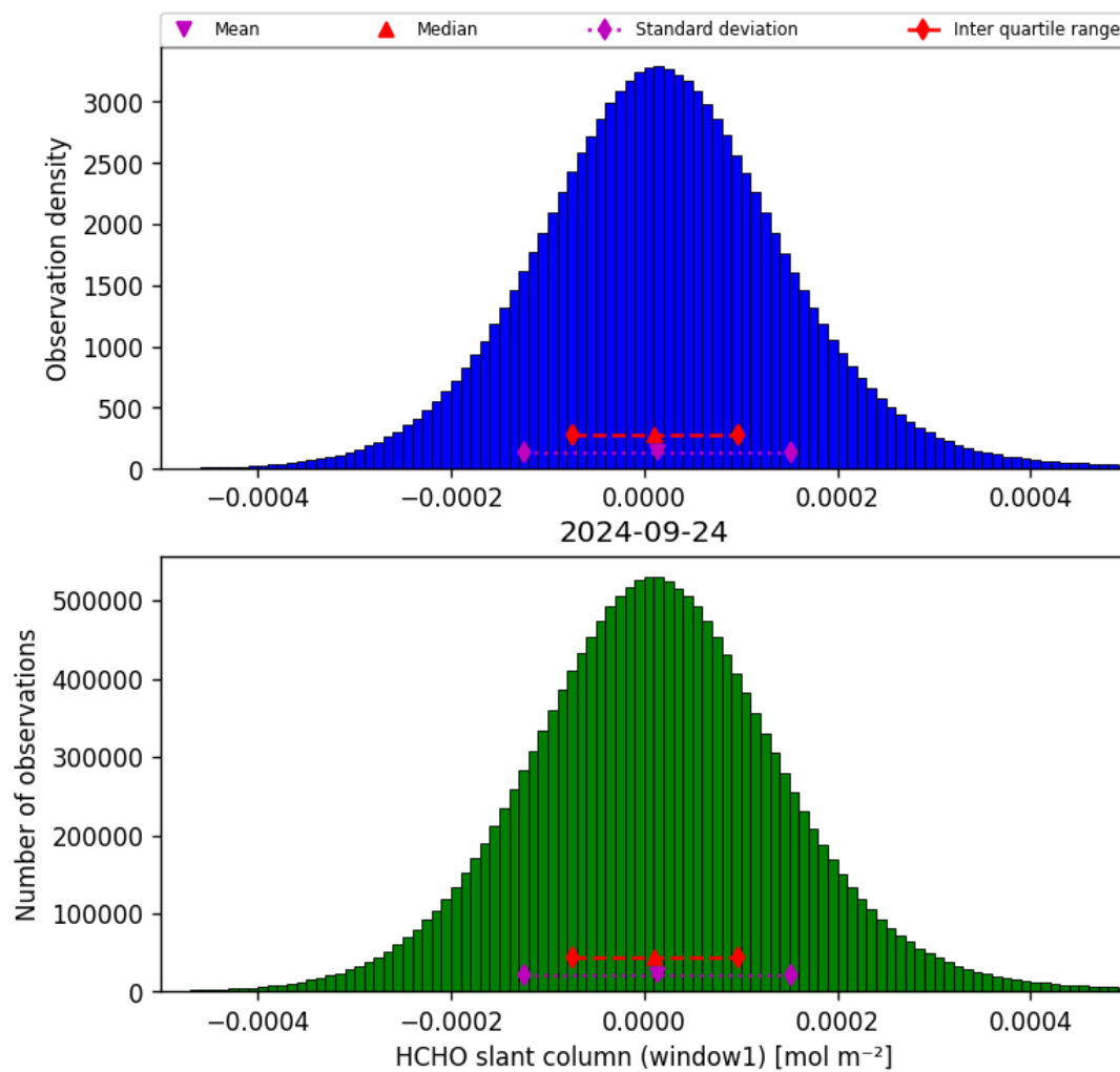
Figure 38: Histogram of “HCHO slant column (window1)” for 2024-09-23 to 2024-09-25
