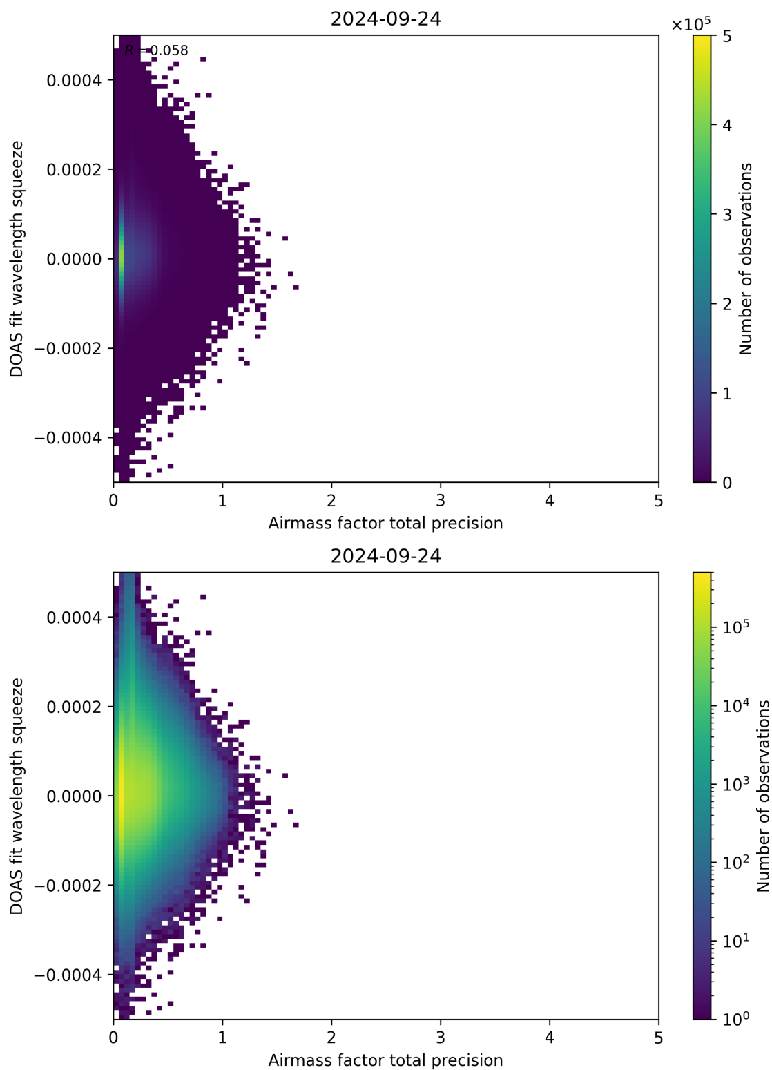
Figure 107: Scatter density plot of “Airmass factor total precision” against “DOAS fit wavelength squeeze” for 2024-09-23 to 2024-09-25.
