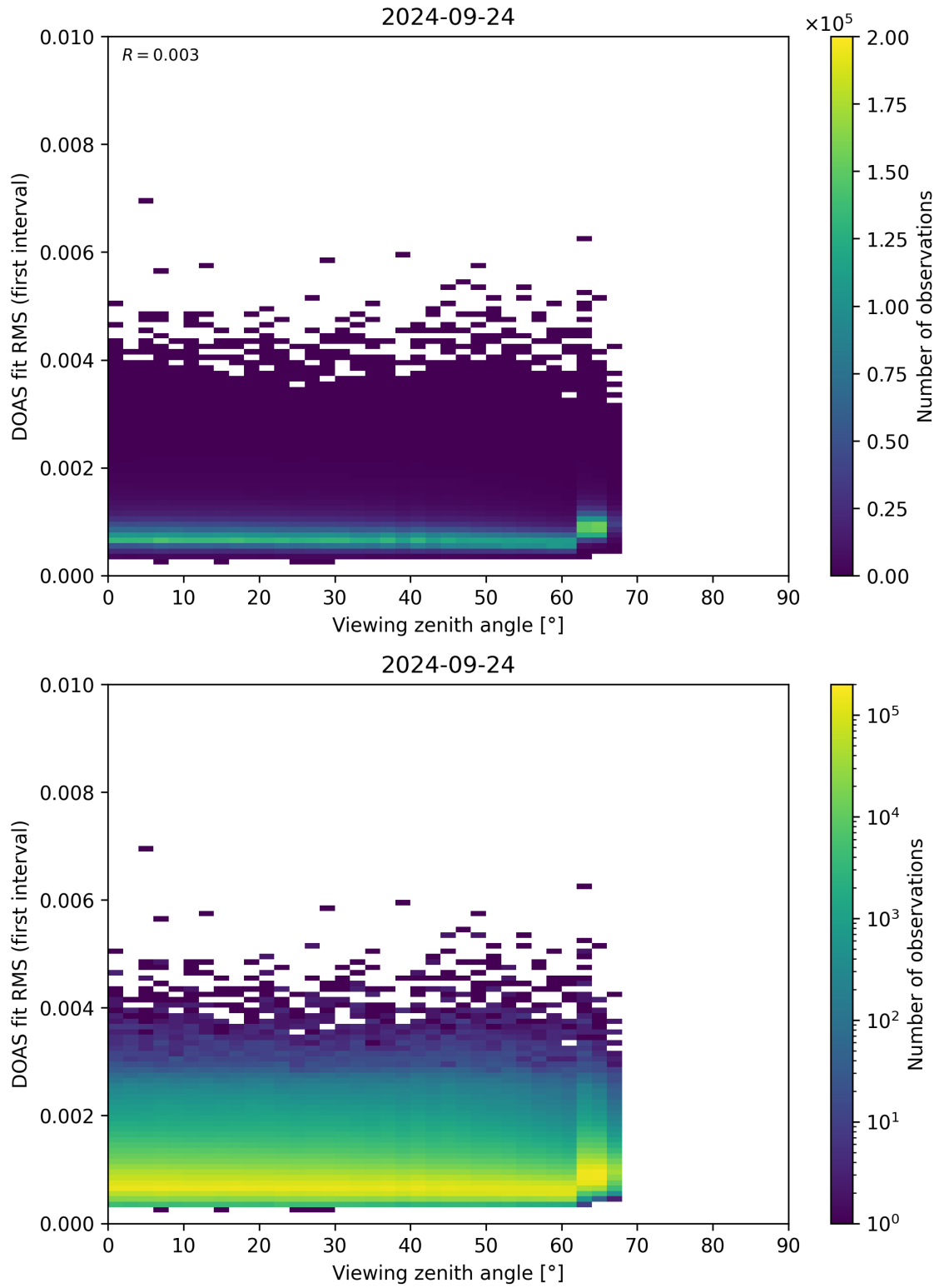
Figure 182: Scatter density plot of “Viewing zenith angle” against “DOAS fit RMS (first interval)” for 2024-09-23 to 2024-09-25.
