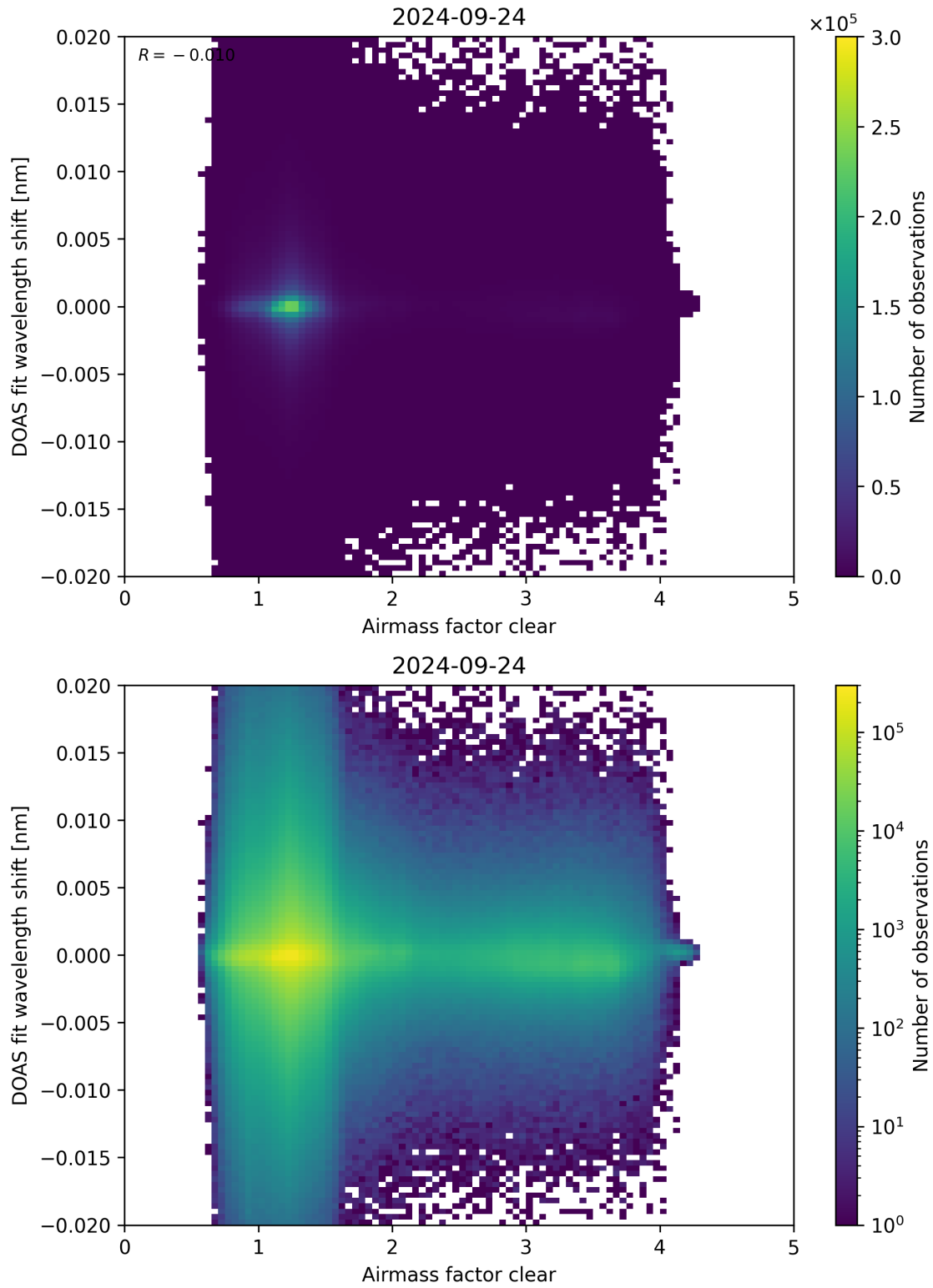
Figure 72: Scatter density plot of “Airmass factor clear” against “DOAS fit wavelength shift” for 2024-09-23 to 2024-09-25.
