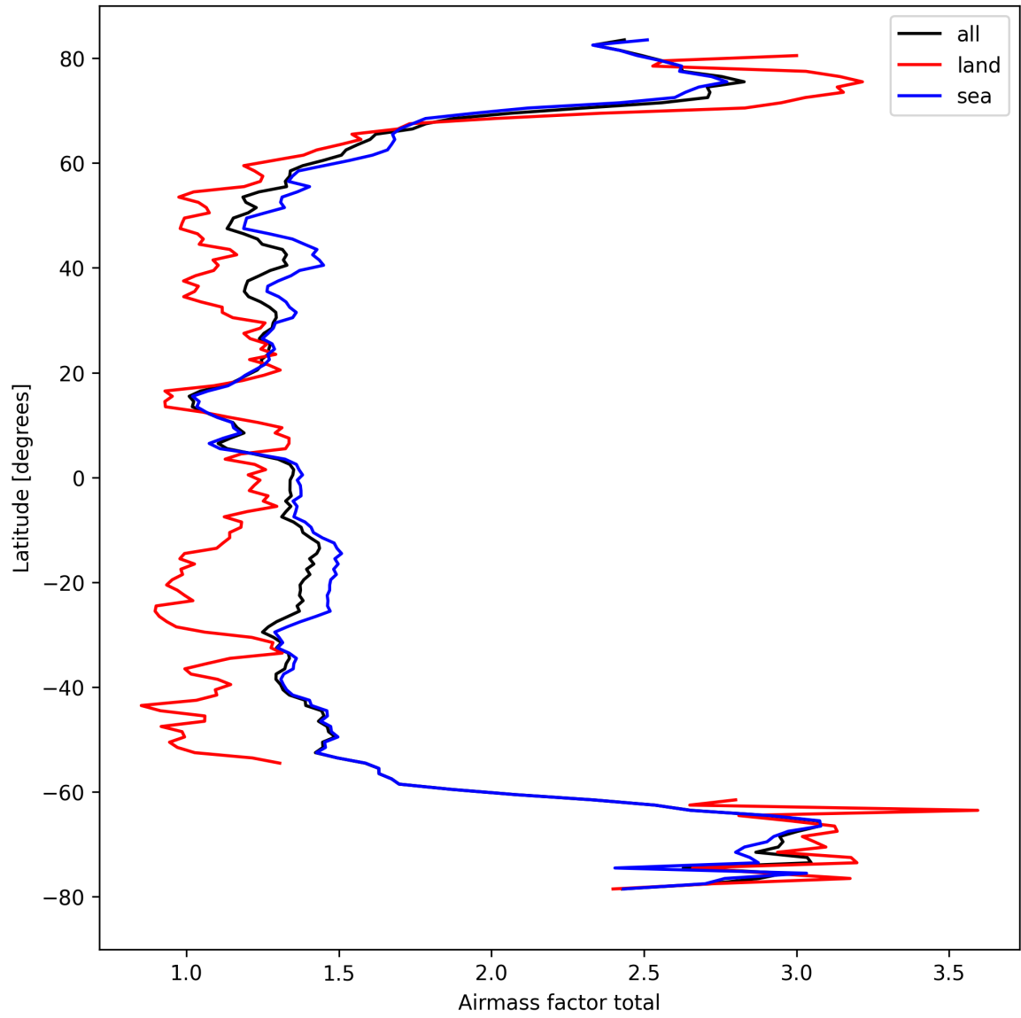
Figure 26: Zonal average of “Airmass factor total” for 2024-09-23 to 2024-09-25.
