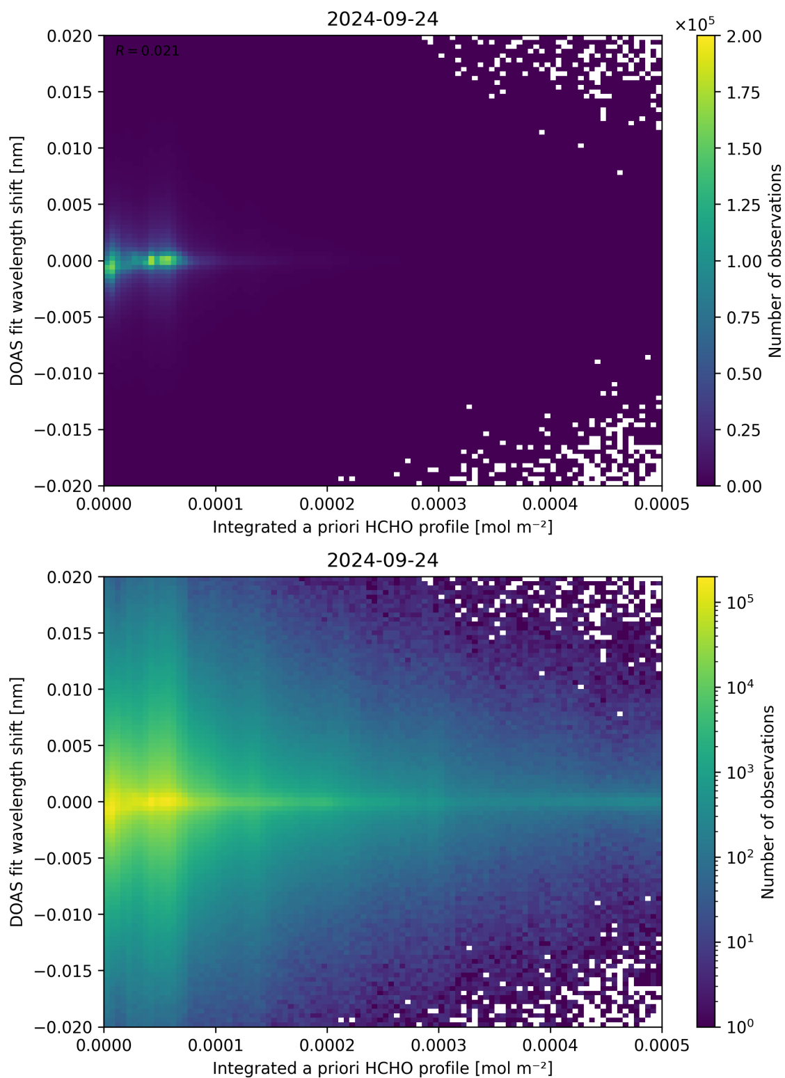
Figure 149: Scatter density plot of “Integrated a priori HCHO profile” against “DOAS fit wavelength shift” for 2024-09-23 to 2024-09-25.
