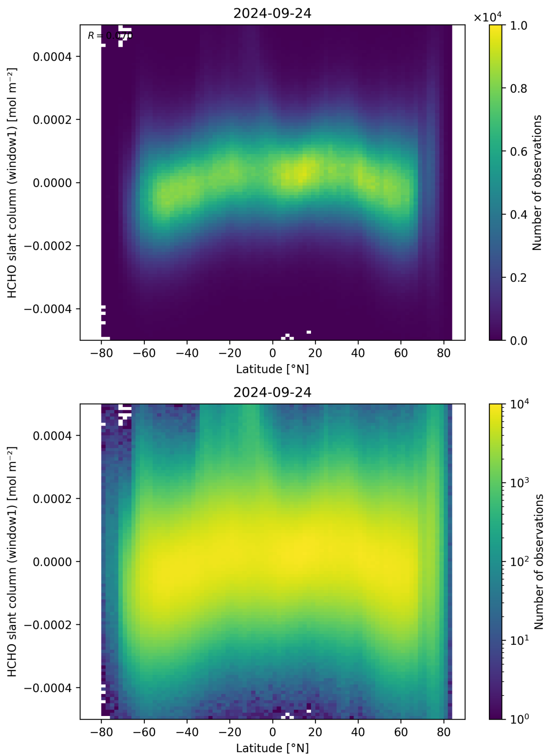
Figure 159: Scatter density plot of “Latitude” against “HCHO slant column (window1)” for 2024-09-23 to 2024-09-25.
