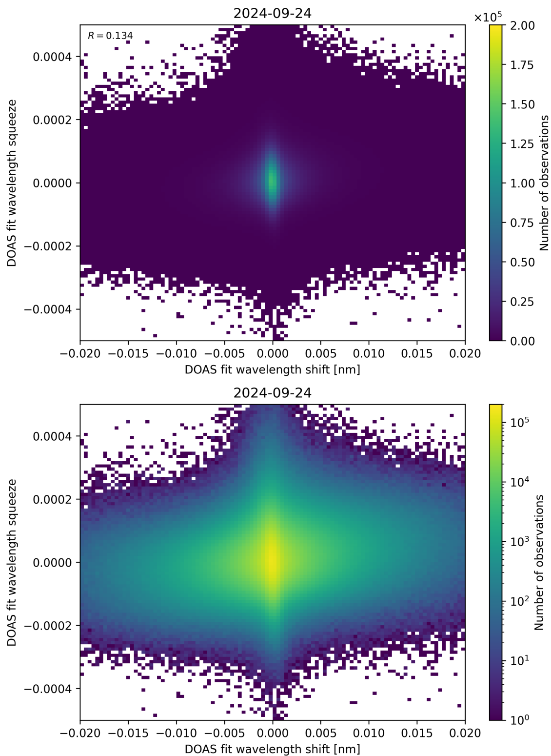
Figure 65: Scatter density plot of “DOAS fit wavelength shift” against “DOAS fit wavelength squeeze” for 2024-09-23 to 2024-09-25.
