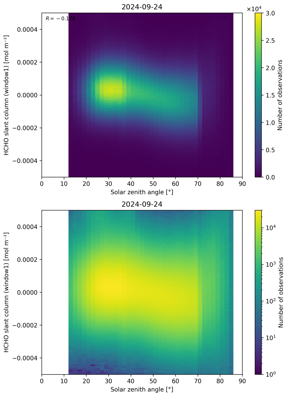
Figure 173: Scatter density plot of “Solar zenith angle” against “HCHO slant column (window1)” for 2024-09-23 to 2024-09-25.
