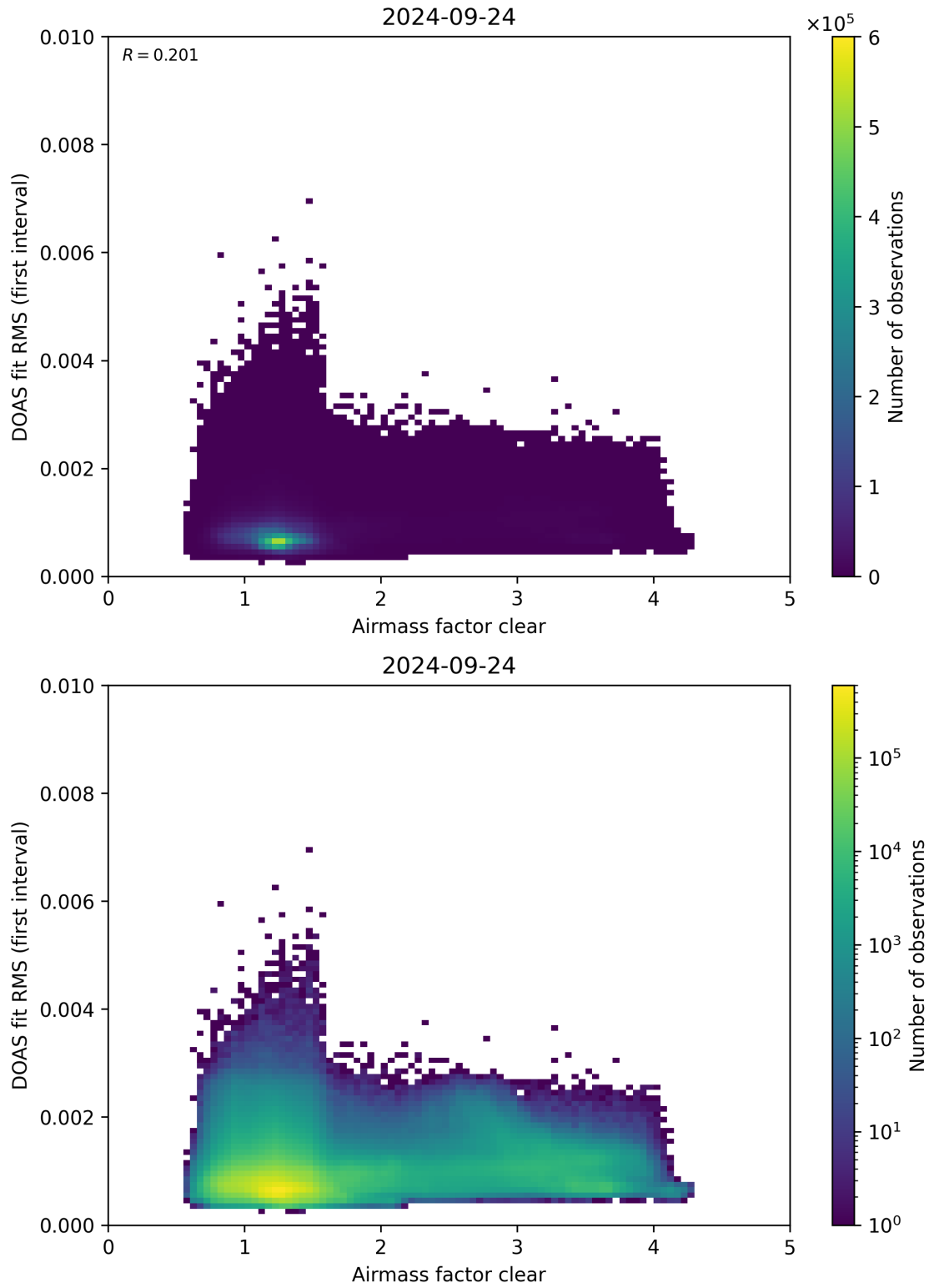
Figure 71: Scatter density plot of “Airmass factor clear” against “DOAS fit RMS (first interval)” for 2024-09-23 to 2024-09-25.
