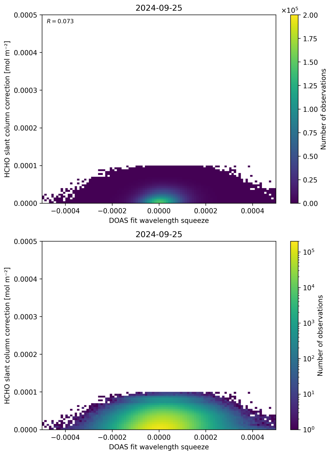
Figure 70: Scatter density plot of “DOAS fit wavelength squeeze” against “HCHO slant column correction” for 2024-09-24 to 2024-09-26.
