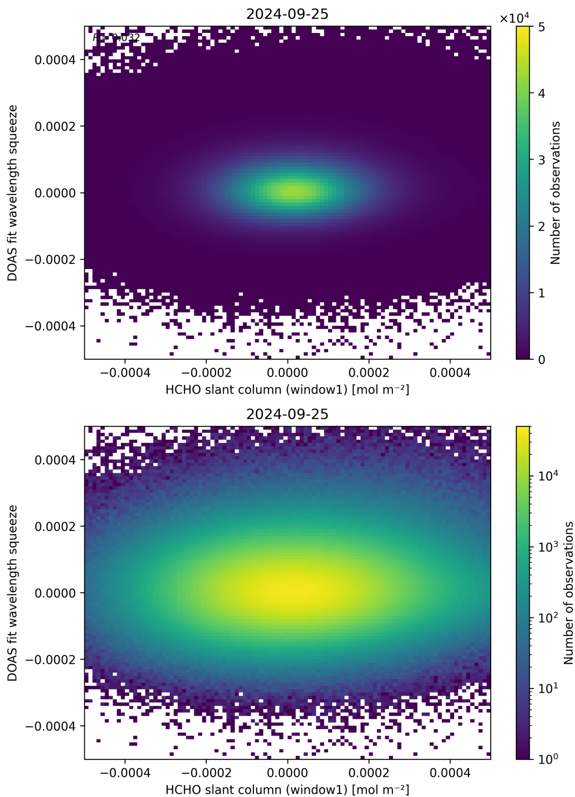
Figure 80: Scatter density plot of “HCHO slant column (window1)” against “DOAS fit wavelength squeeze” for 2024-09-24 to 2024-09-26.
