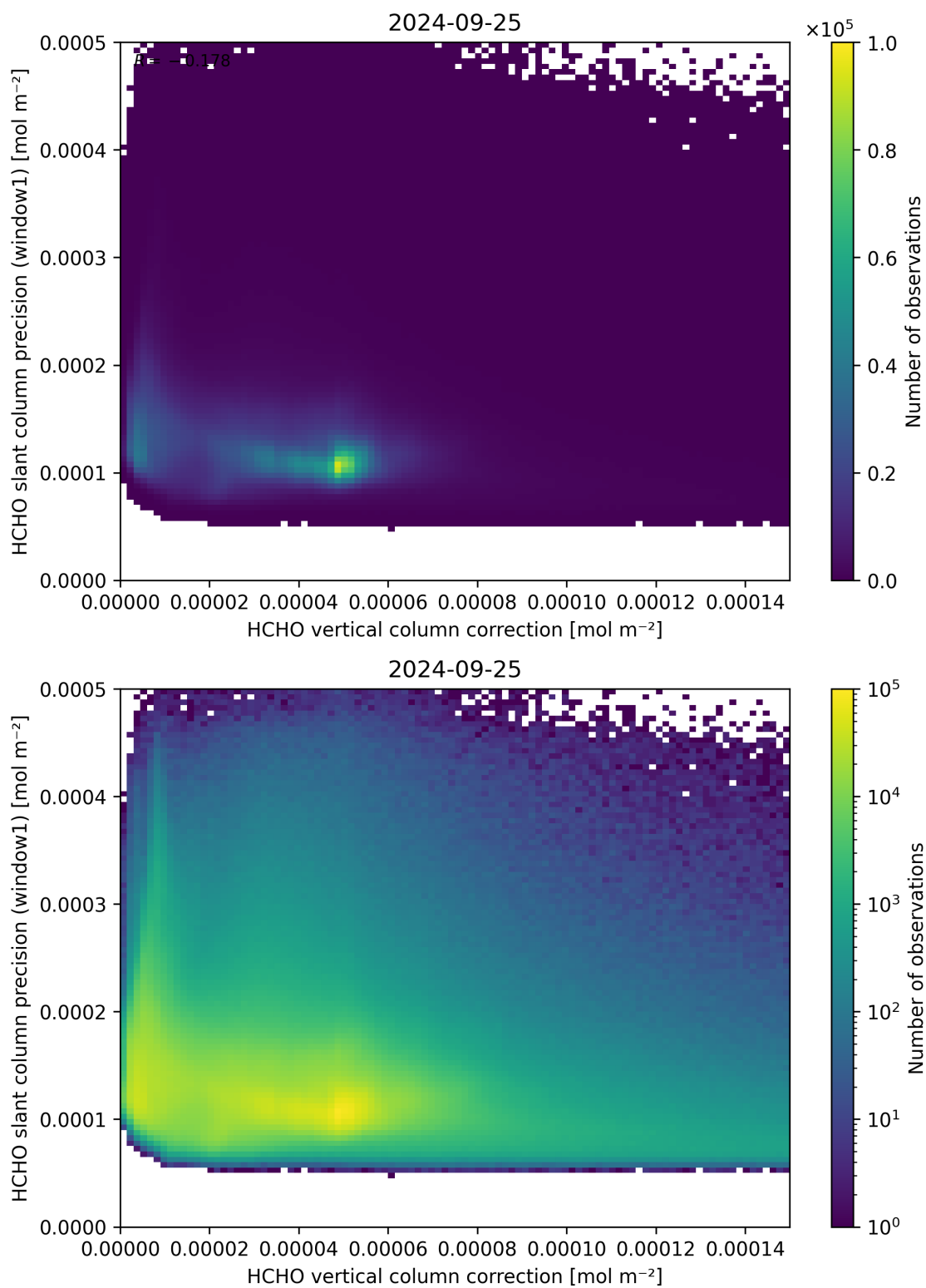
Figure 119: Scatter density plot of “HCHO vertical column correction” against “HCHO slant column precision (window1)” for 2024-09-24 to 2024-09-26.
