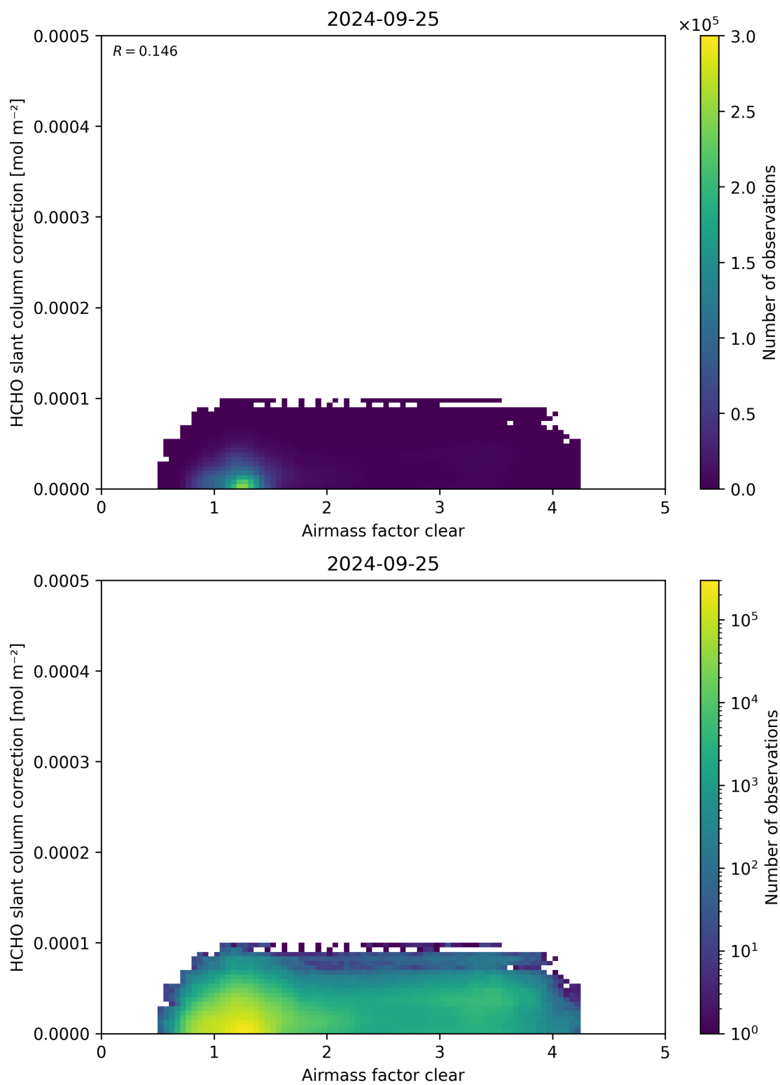
Figure 75: Scatter density plot of “Airmass factor clear” against “HCHO slant column correction” for 2024-09-24 to 2024-09-26.
