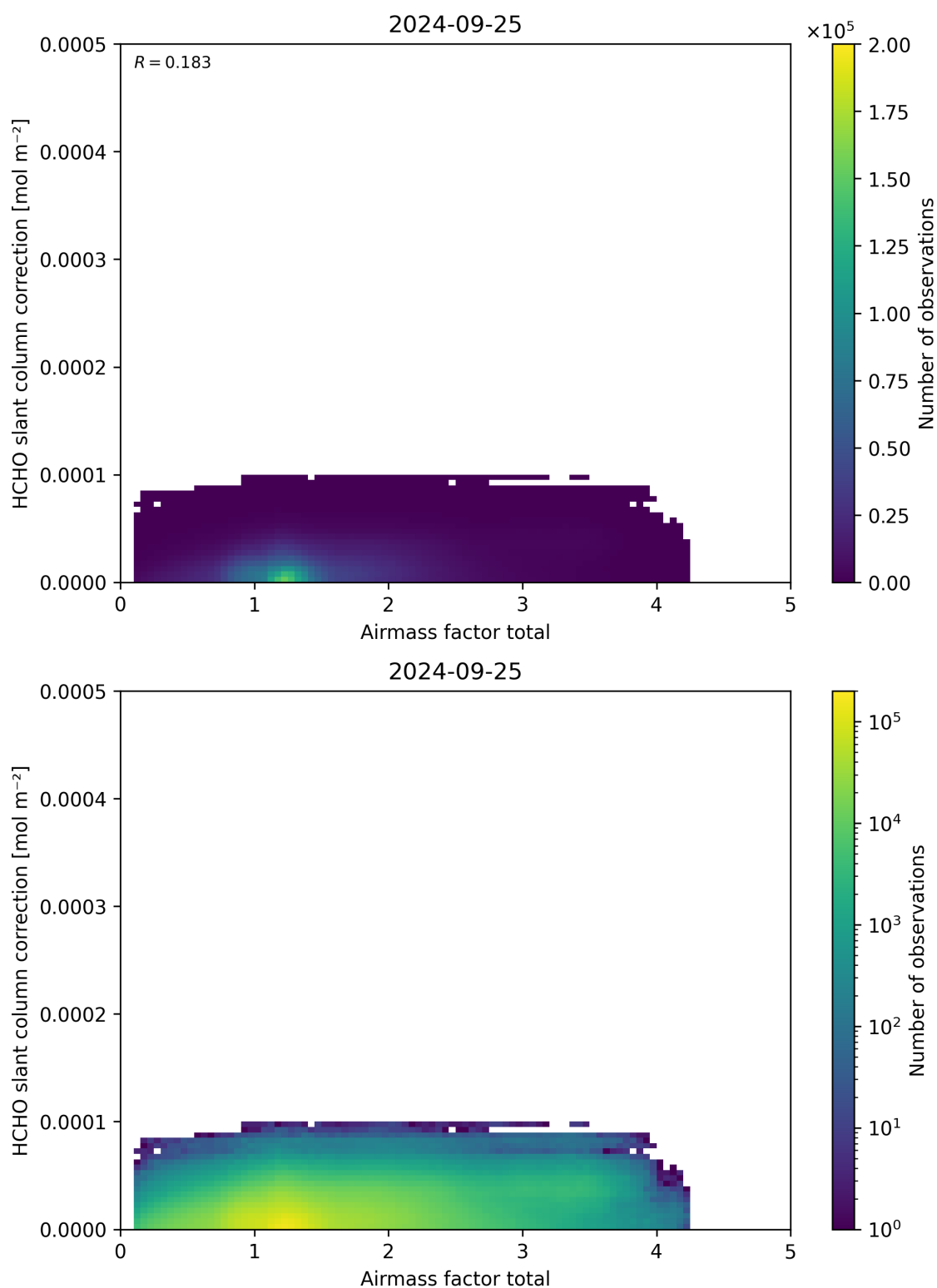
Figure 102: Scatter density plot of “Airmass factor total” against “HCHO slant column correction” for 2024-09-24 to 2024-09-26.
