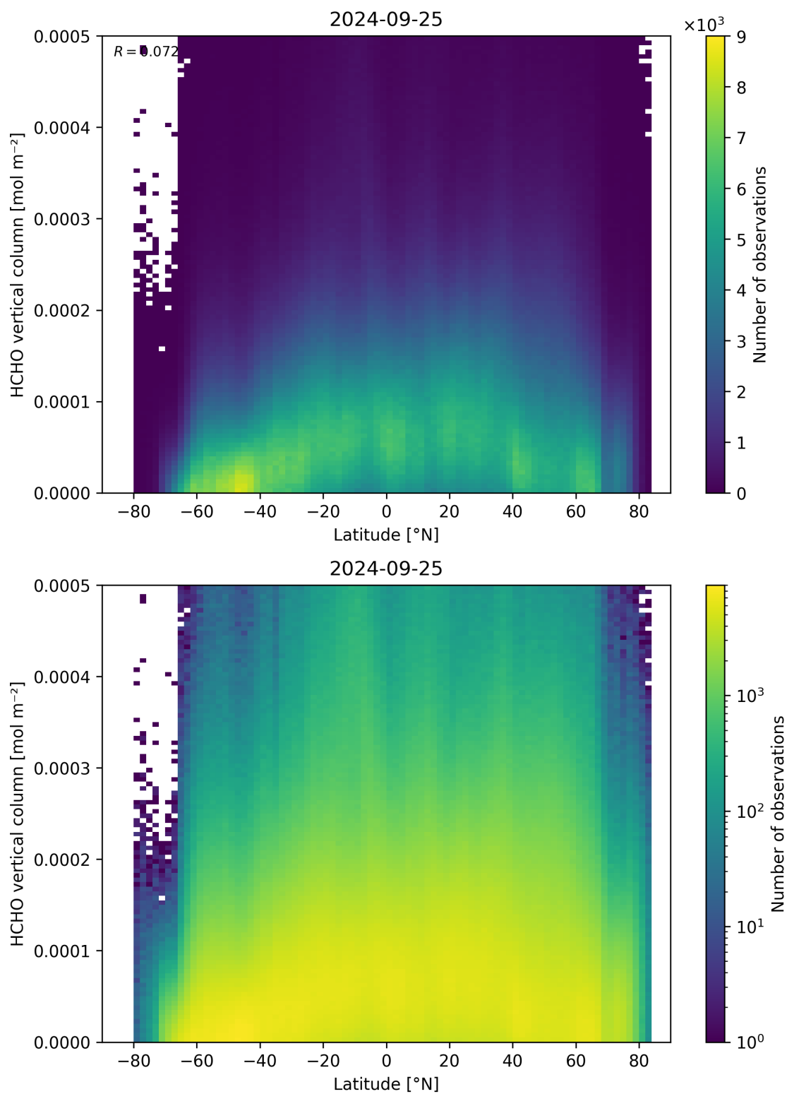
Figure 163: Scatter density plot of “Latitude” against “HCHO vertical column” for 2024-09-24 to 2024-09-26.
