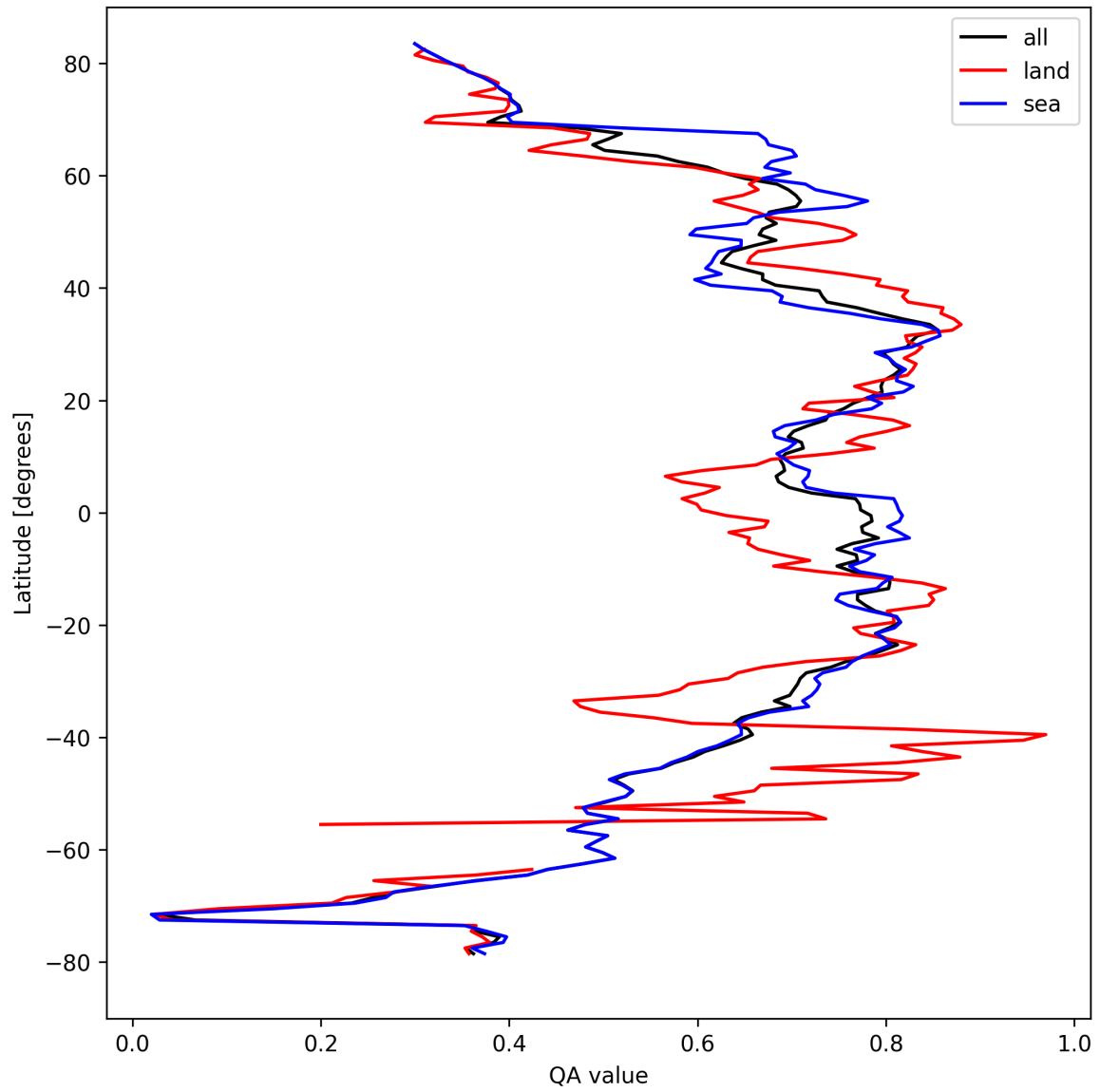
Figure 20: Zonal average of “QA value” for 2024-09-24 to 2024-09-26.
