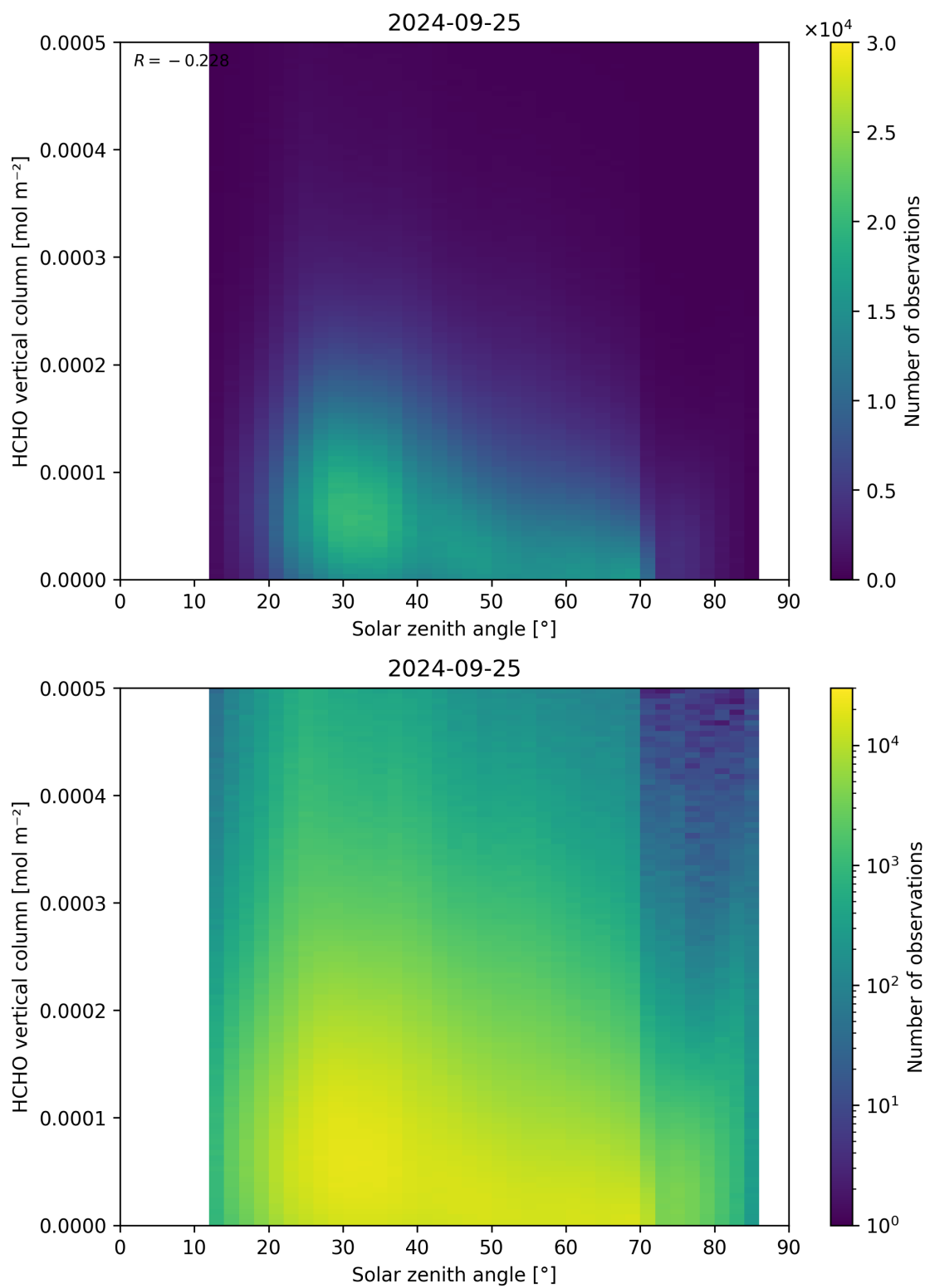
Figure 177: Scatter density plot of “Solar zenith angle” against “HCHO vertical column” for 2024-09-24 to 2024-09-26.
