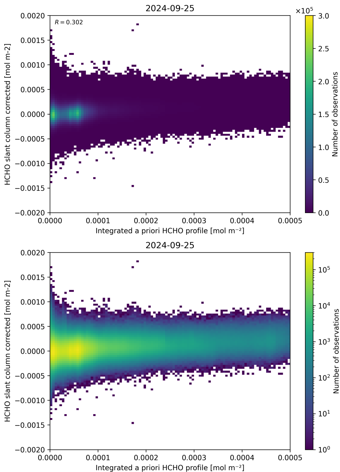
Figure 151: Scatter density plot of “Integrated a priori HCHO profile” against “HCHO slant column corrected” for 2024-09-24 to 2024-09-26.
