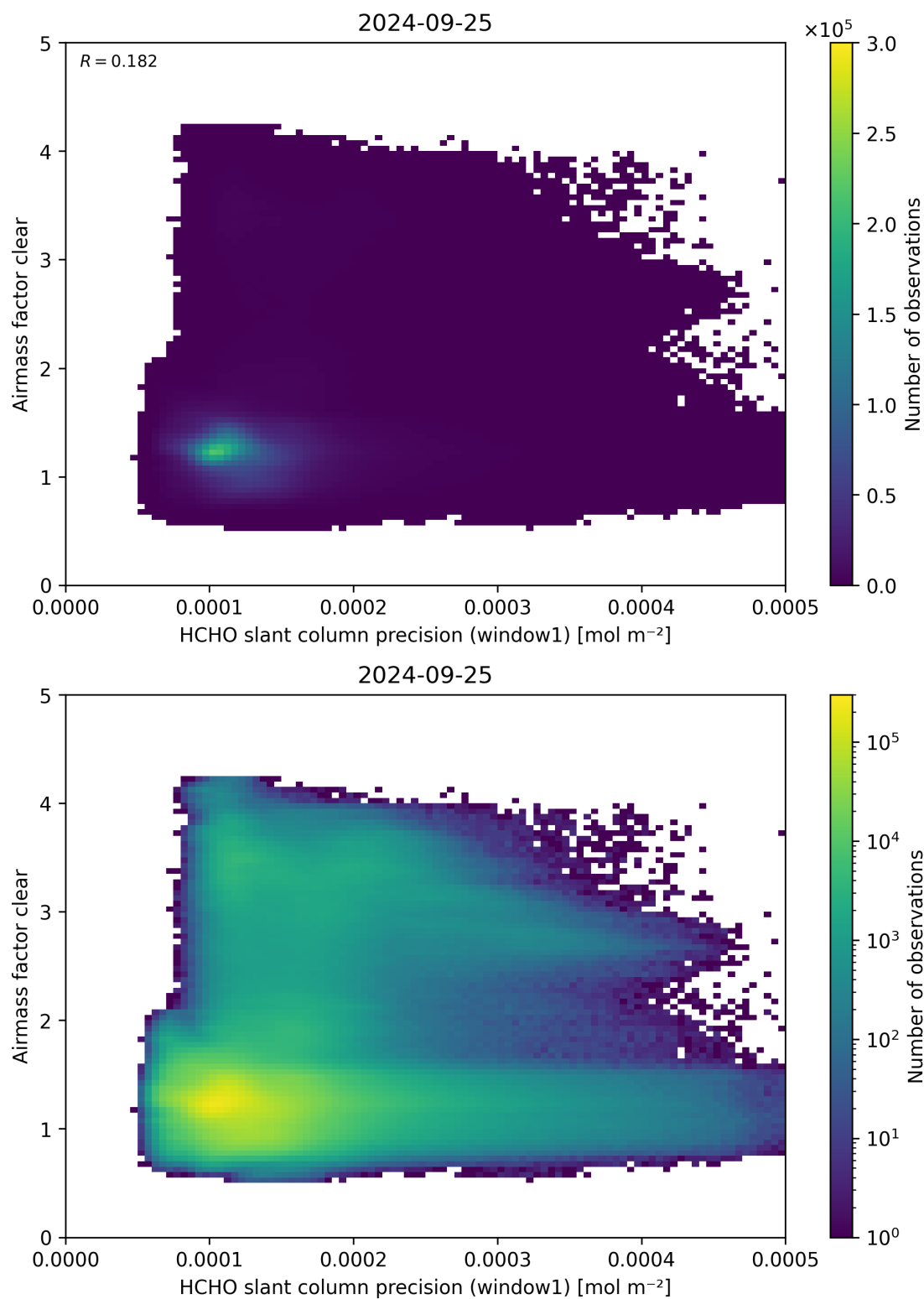
Figure 91: Scatter density plot of “HCHO slant column precision (window1)” against “Airmass factor clear” for 2024-09-24 to 2024-09-26.
