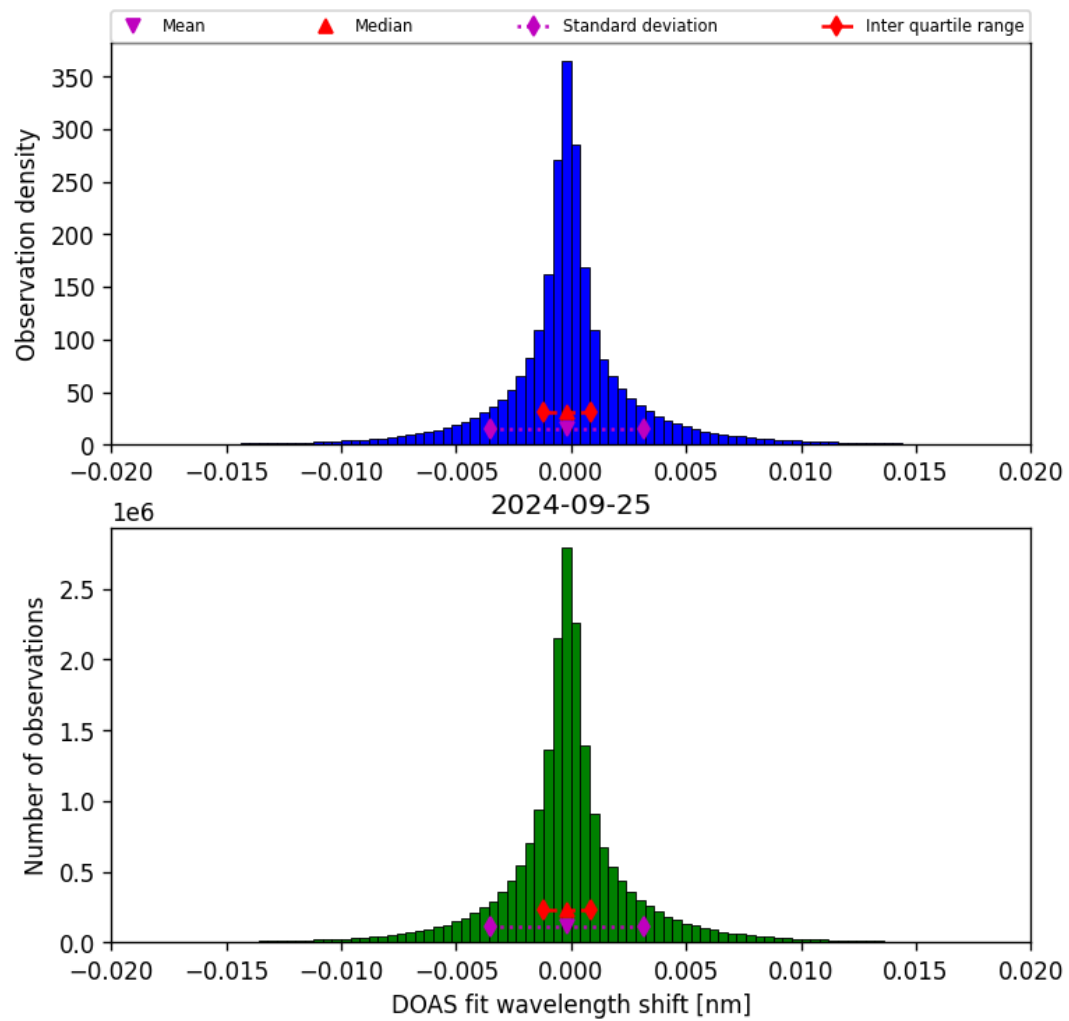
Figure 44: Histogram of “DOAS fit wavelength shift” for 2024-09-24 to 2024-09-26
