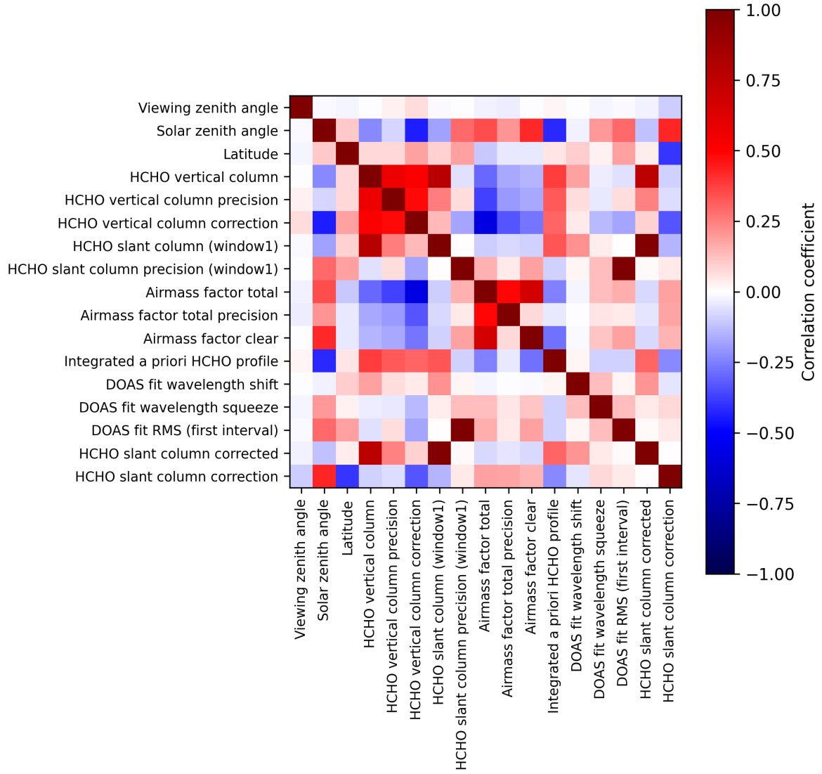
Figure 2: Map of correlation matrix for 2024-09-24 to 2024-09-26.
