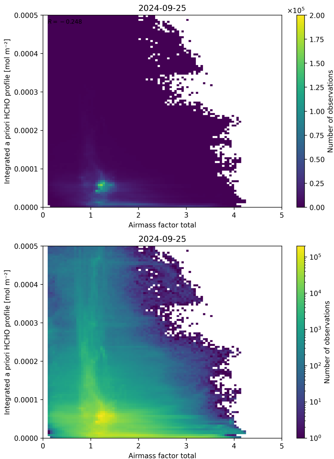
Figure 104: Scatter density plot of “Airmass factor total” against “Integrated a priori HCHO profile” for 2024-09-24 to 2024-09-26.
