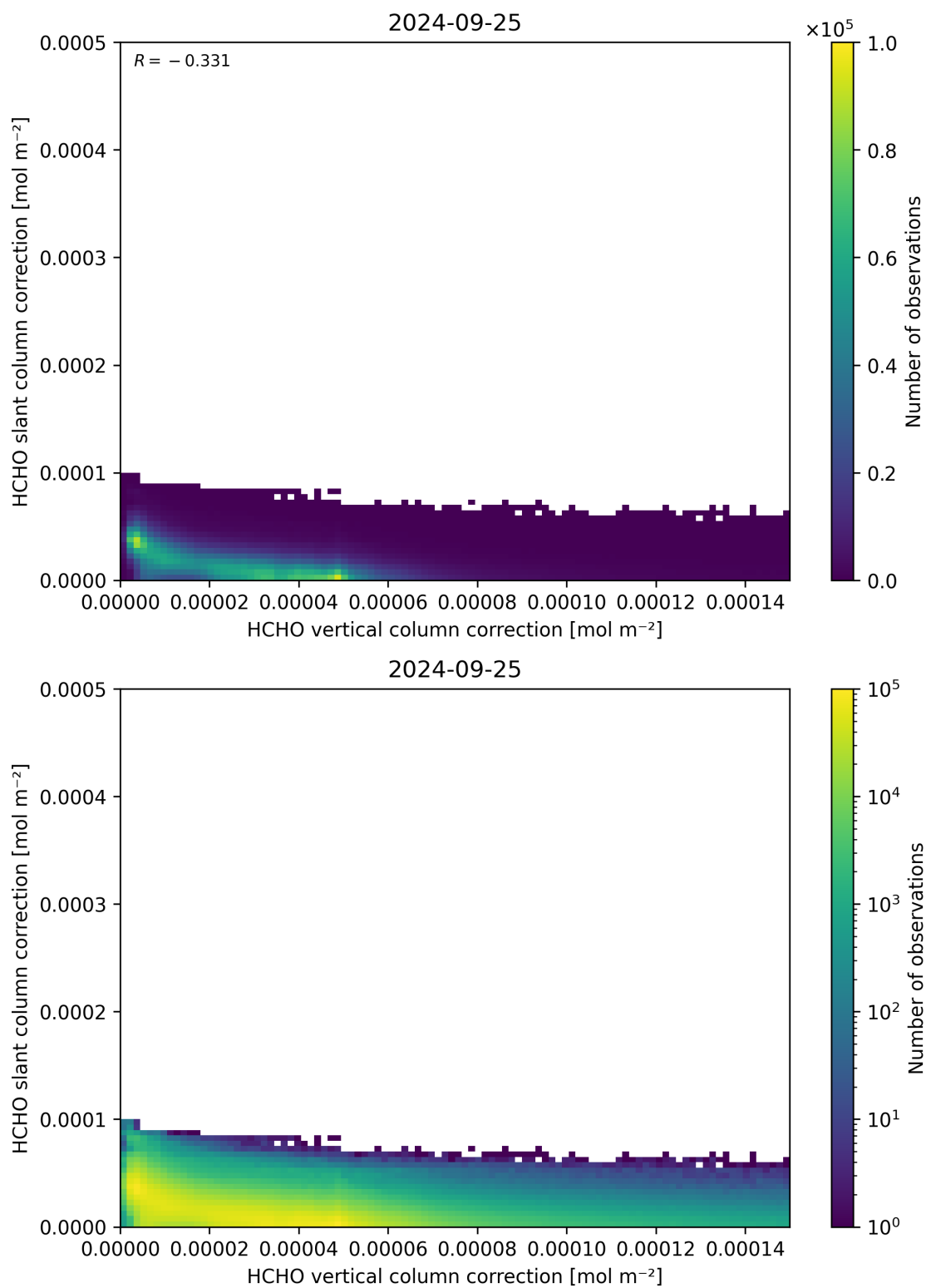
Figure 117: Scatter density plot of “HCHO vertical column correction” against “HCHO slant column correction” for 2024-09-24 to 2024-09-26.
