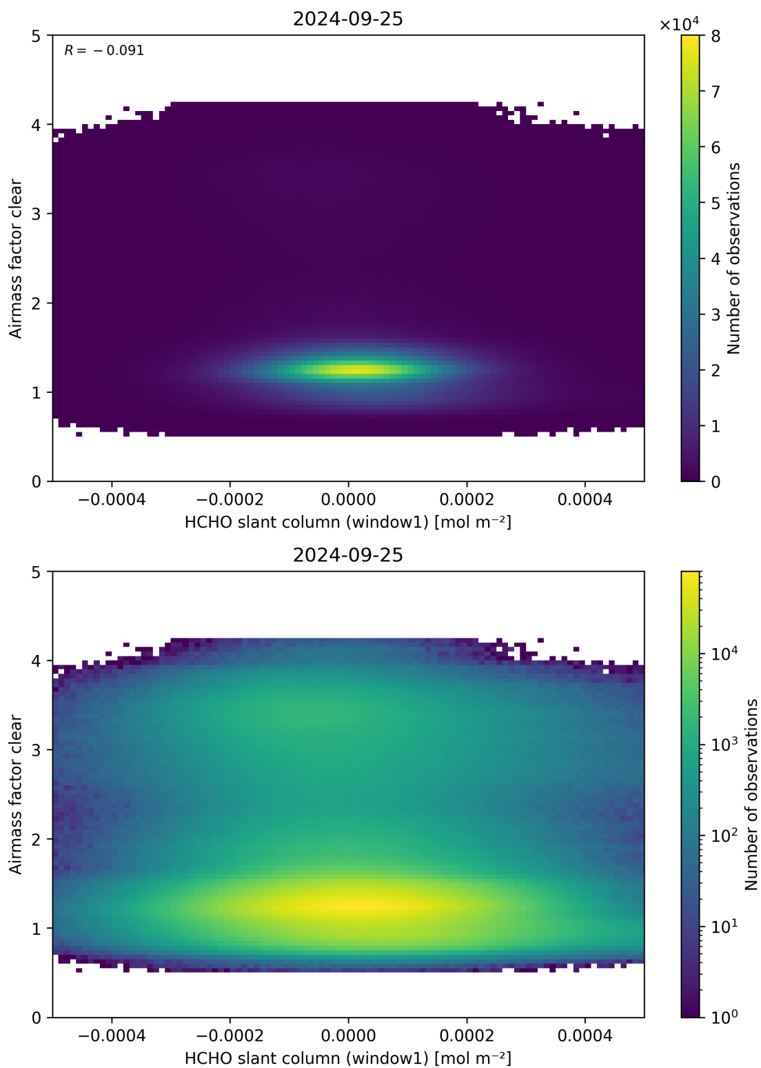
Figure 81: Scatter density plot of “HCHO slant column (window1)” against “Airmass factor clear” for 2024-09-24 to 2024-09-26.
