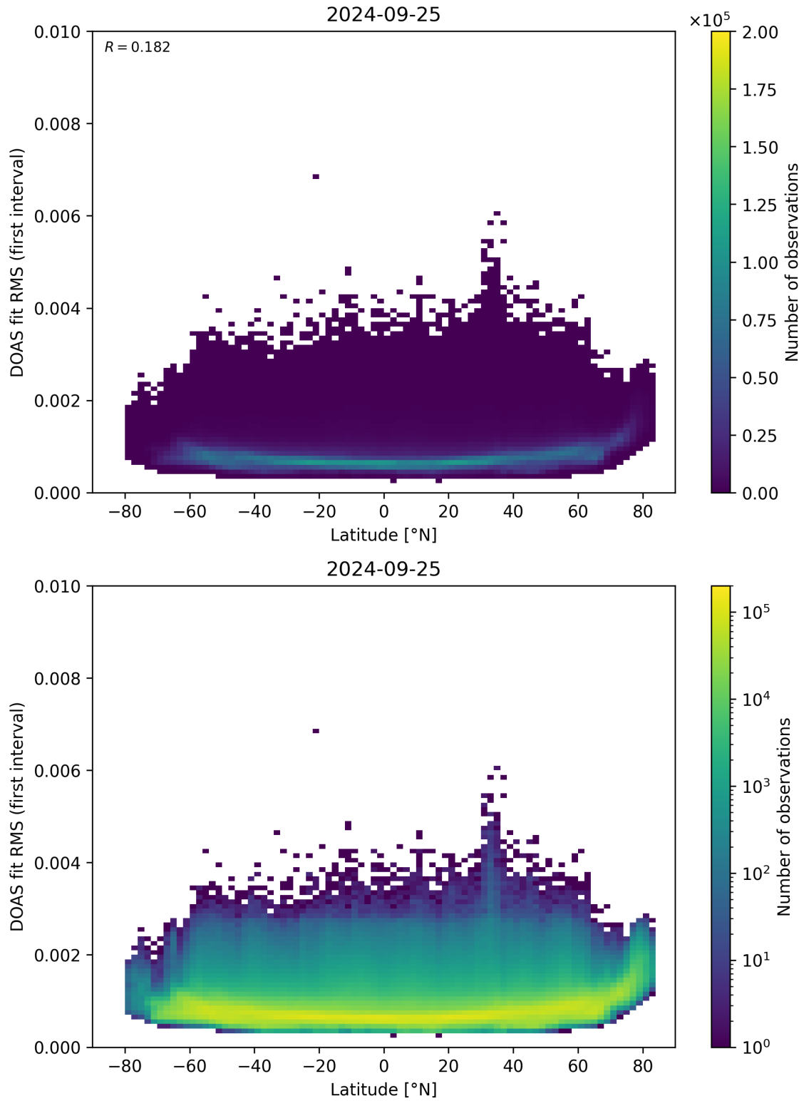
Figure 153: Scatter density plot of “Latitude” against “DOAS fit RMS (first interval)” for 2024-09-24 to 2024-09-26.
