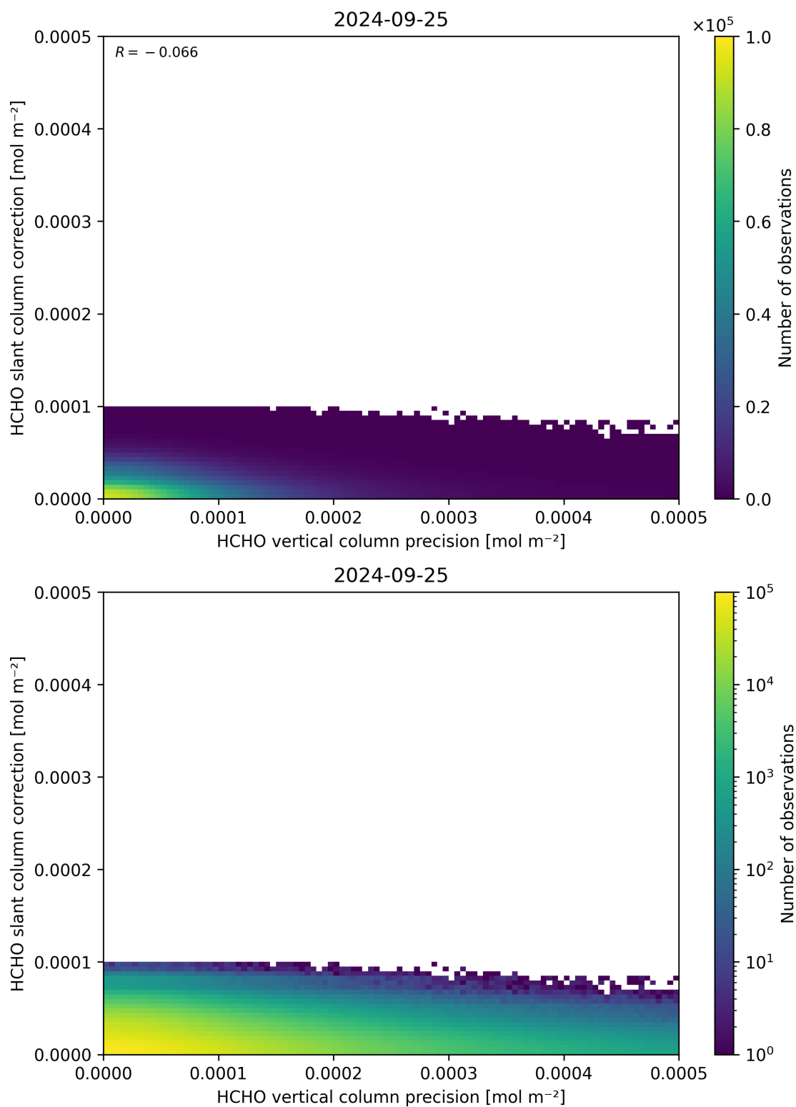
Figure 141: Scatter density plot of “HCHO vertical column precision” against “HCHO slant column correction” for 2024-09-24 to 2024-09-26.
