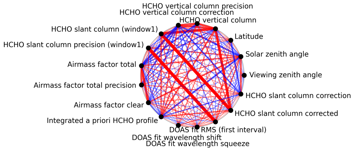
Figure 1: Map of correlation graph for 2024-09-24 to 2024-09-26.
