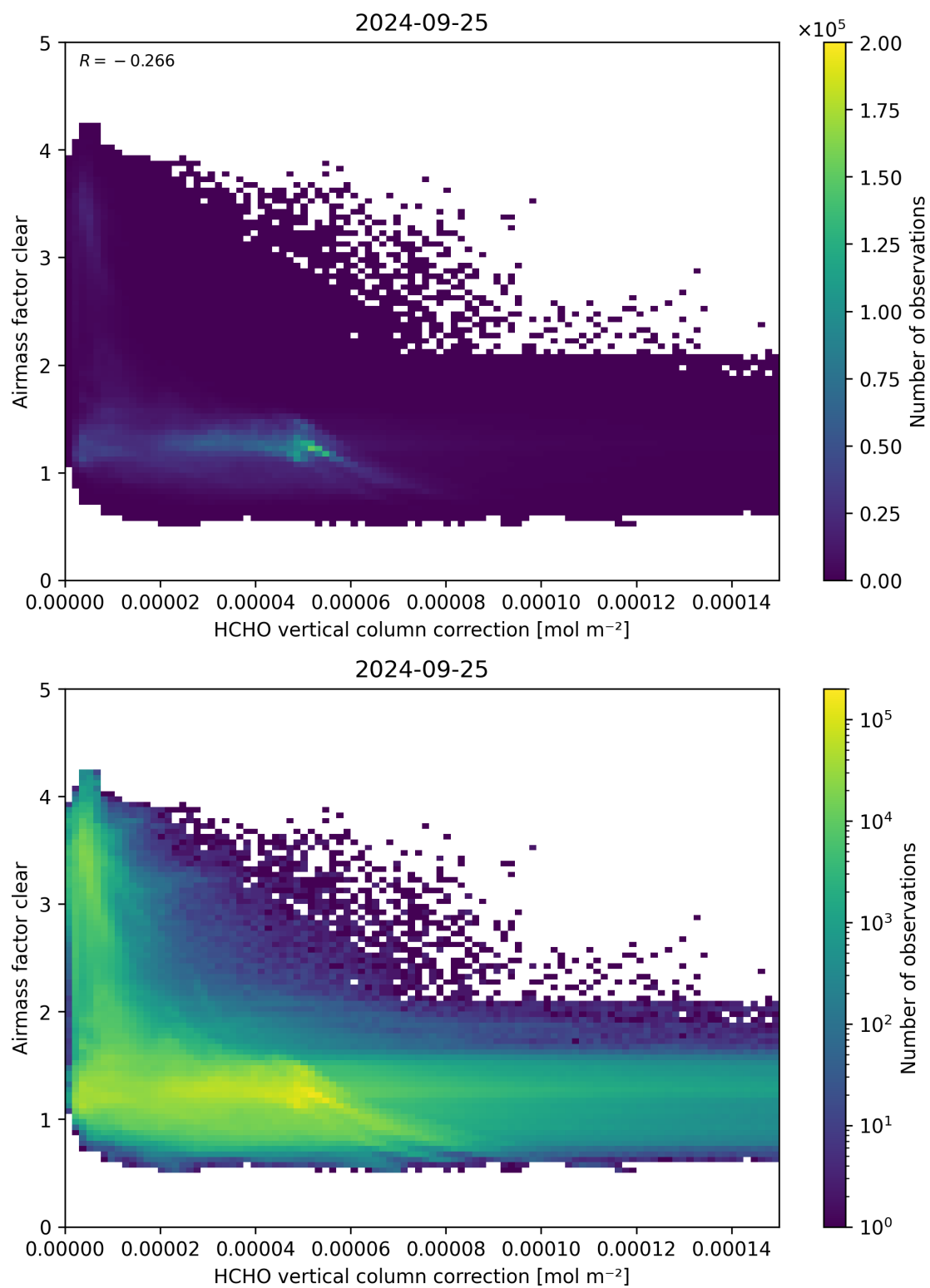
Figure 115: Scatter density plot of “HCHO vertical column correction” against “Airmass factor clear” for 2024-09-24 to 2024-09-26.
