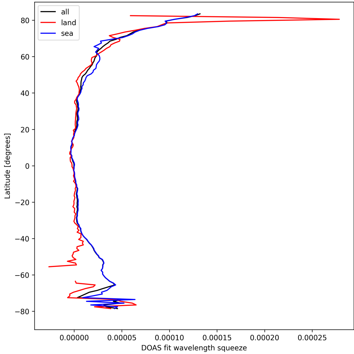
Figure 31: Zonal average of “DOAS fit wavelength squeeze” for 2024-09-24 to 2024-09-26.
