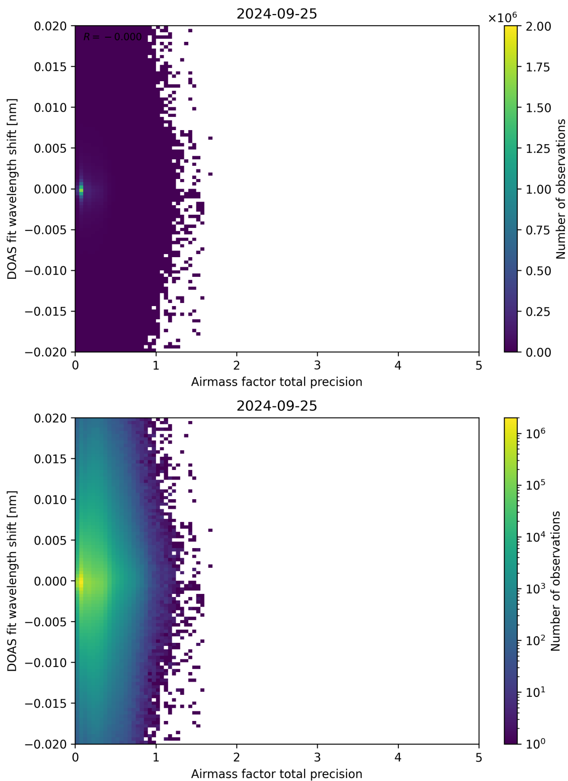
Figure 106: Scatter density plot of “Airmass factor total precision” against “DOAS fit wavelength shift” for 2024-09-24 to 2024-09-26.
