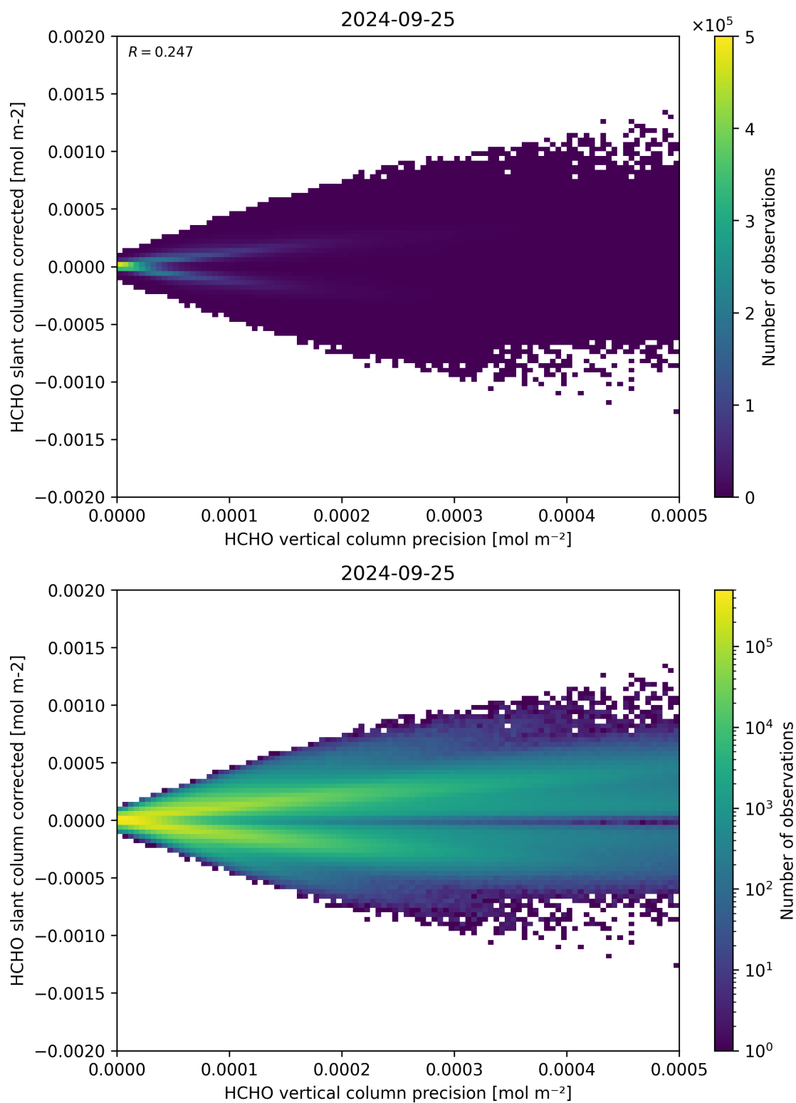
Figure 140: Scatter density plot of “HCHO vertical column precision” against “HCHO slant column corrected” for 2024-09-24 to 2024-09-26.
