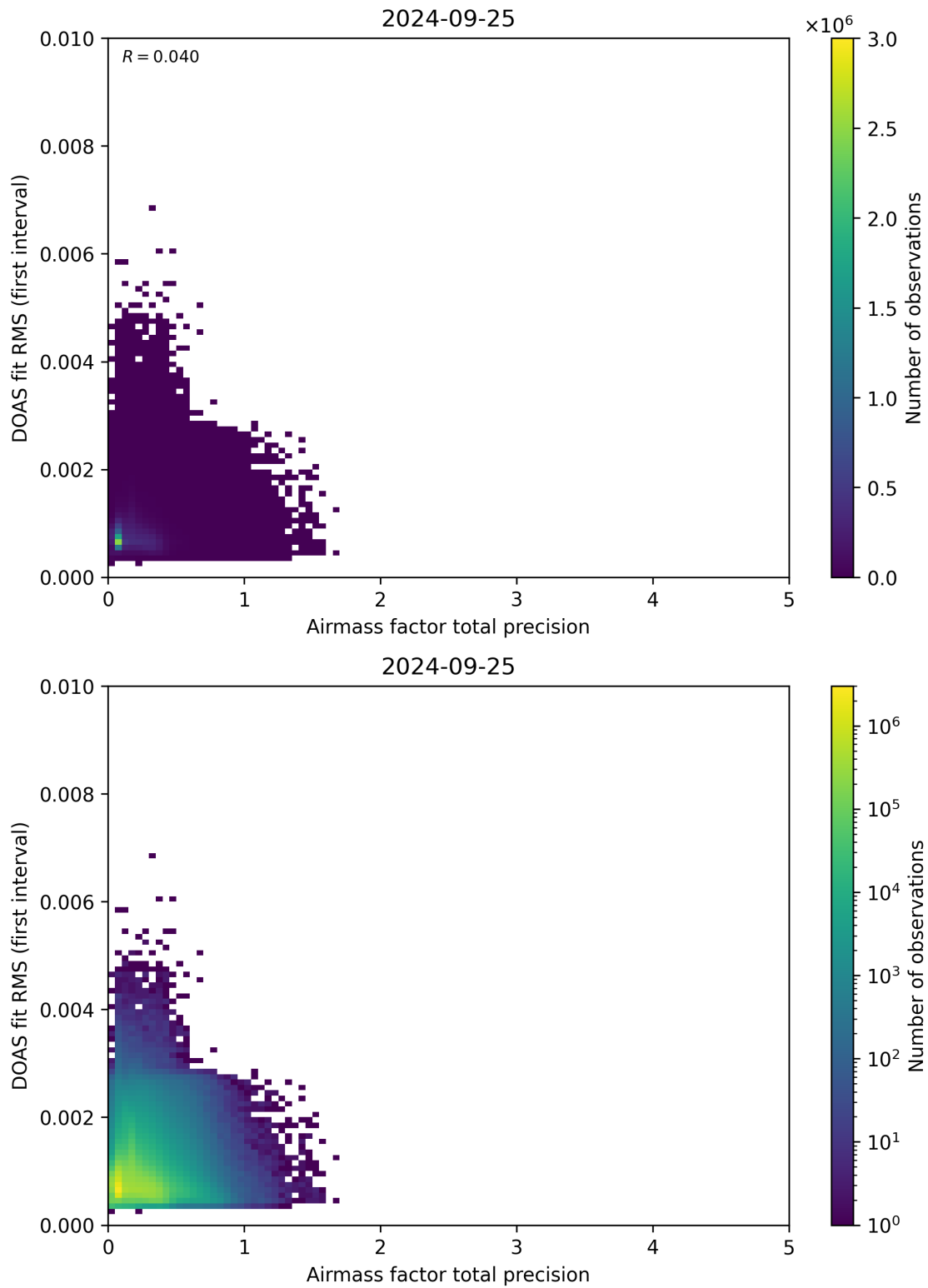
Figure 105: Scatter density plot of “Airmass factor total precision” against “DOAS fit RMS (first interval)” for 2024-09-24 to 2024-09-26.
