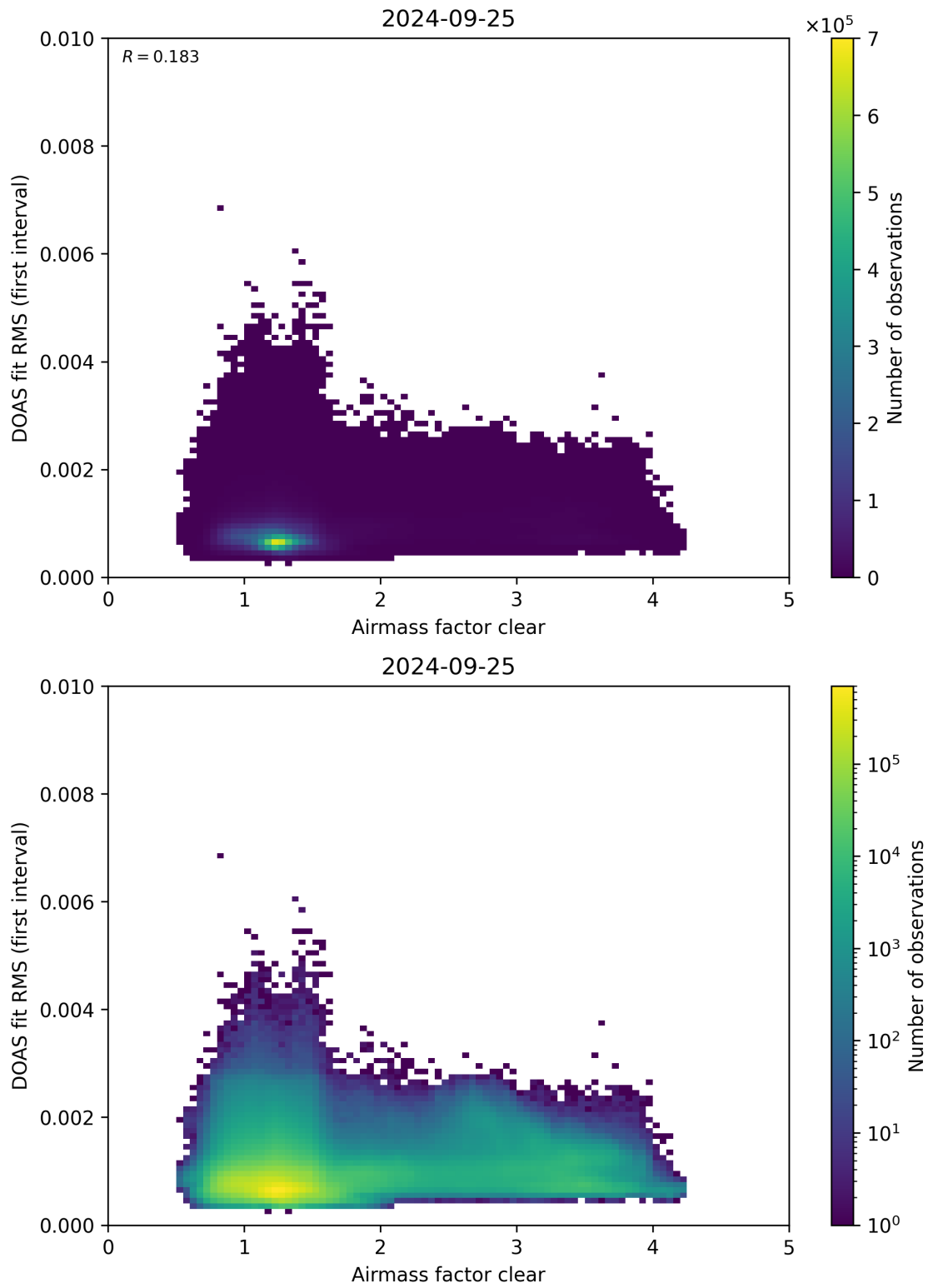
Figure 71: Scatter density plot of “Airmass factor clear” against “DOAS fit RMS (first interval)” for 2024-09-24 to 2024-09-26.
