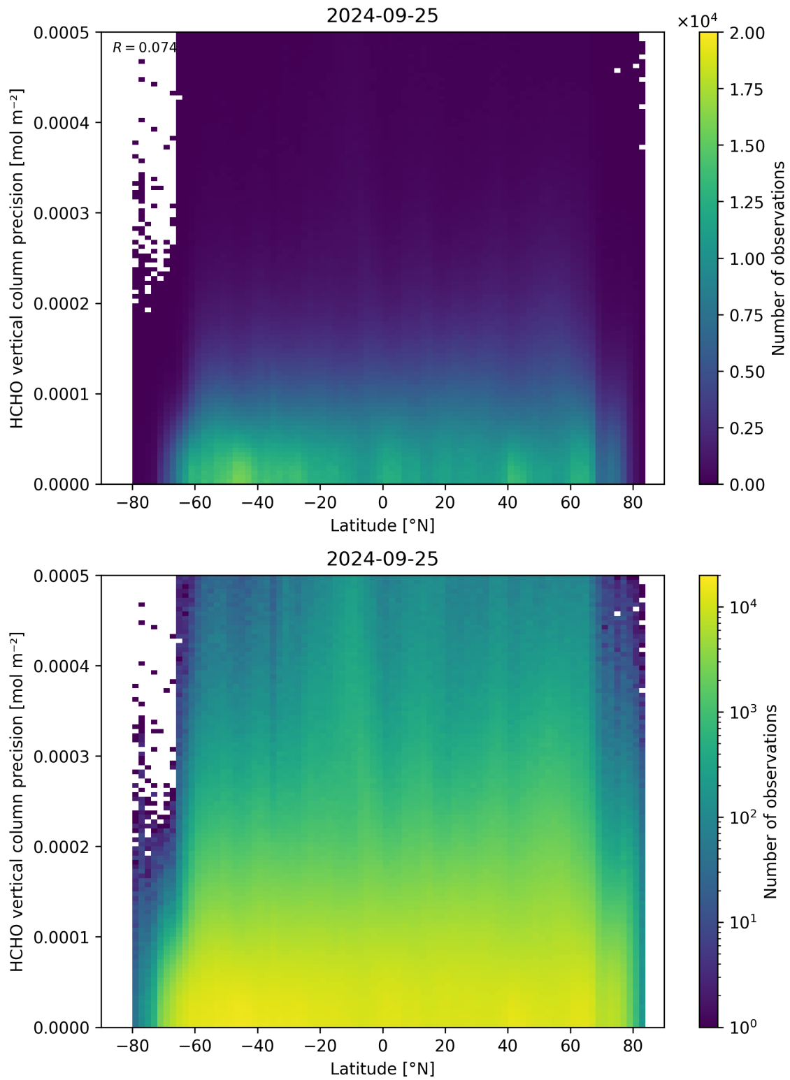
Figure 165: Scatter density plot of “Latitude” against “HCHO vertical column precision” for 2024-09-24 to 2024-09-26.
