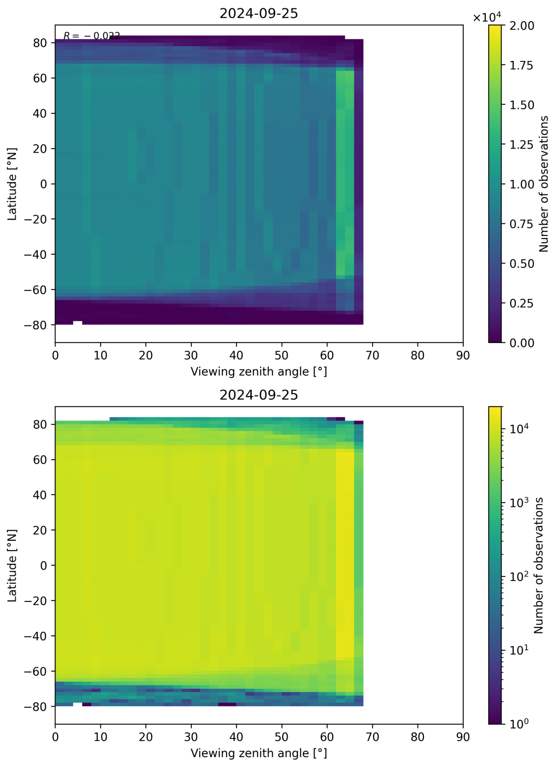
Figure 196: Scatter density plot of “Viewing zenith angle” against “Latitude” for 2024-09-24 to 2024-09-26.
