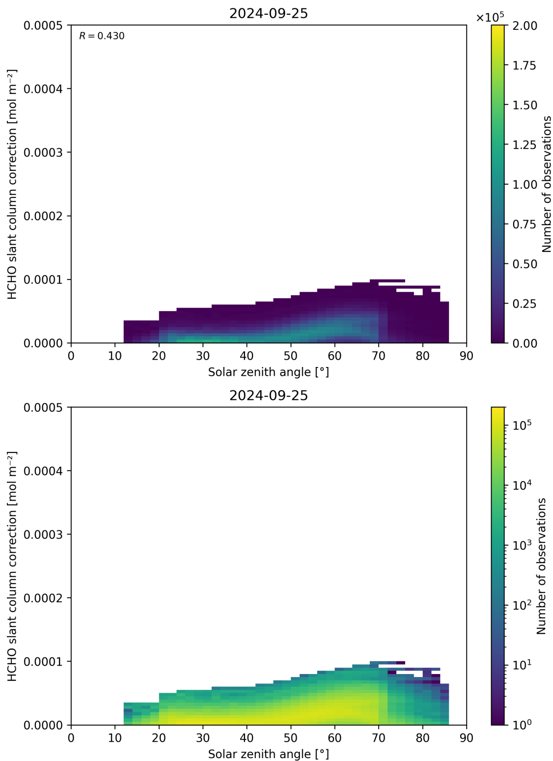
Figure 172: Scatter density plot of “Solar zenith angle” against “HCHO slant column correction” for 2024-09-24 to 2024-09-26.
