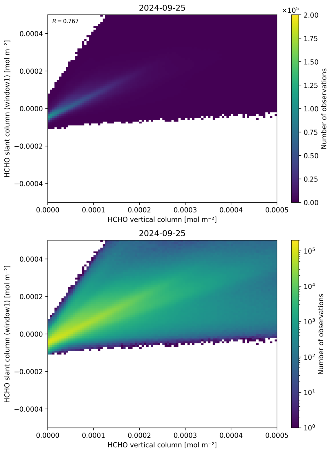
Figure 129: Scatter density plot of “HCHO vertical column” against “HCHO slant column (window1)” for 2024-09-24 to 2024-09-26.
