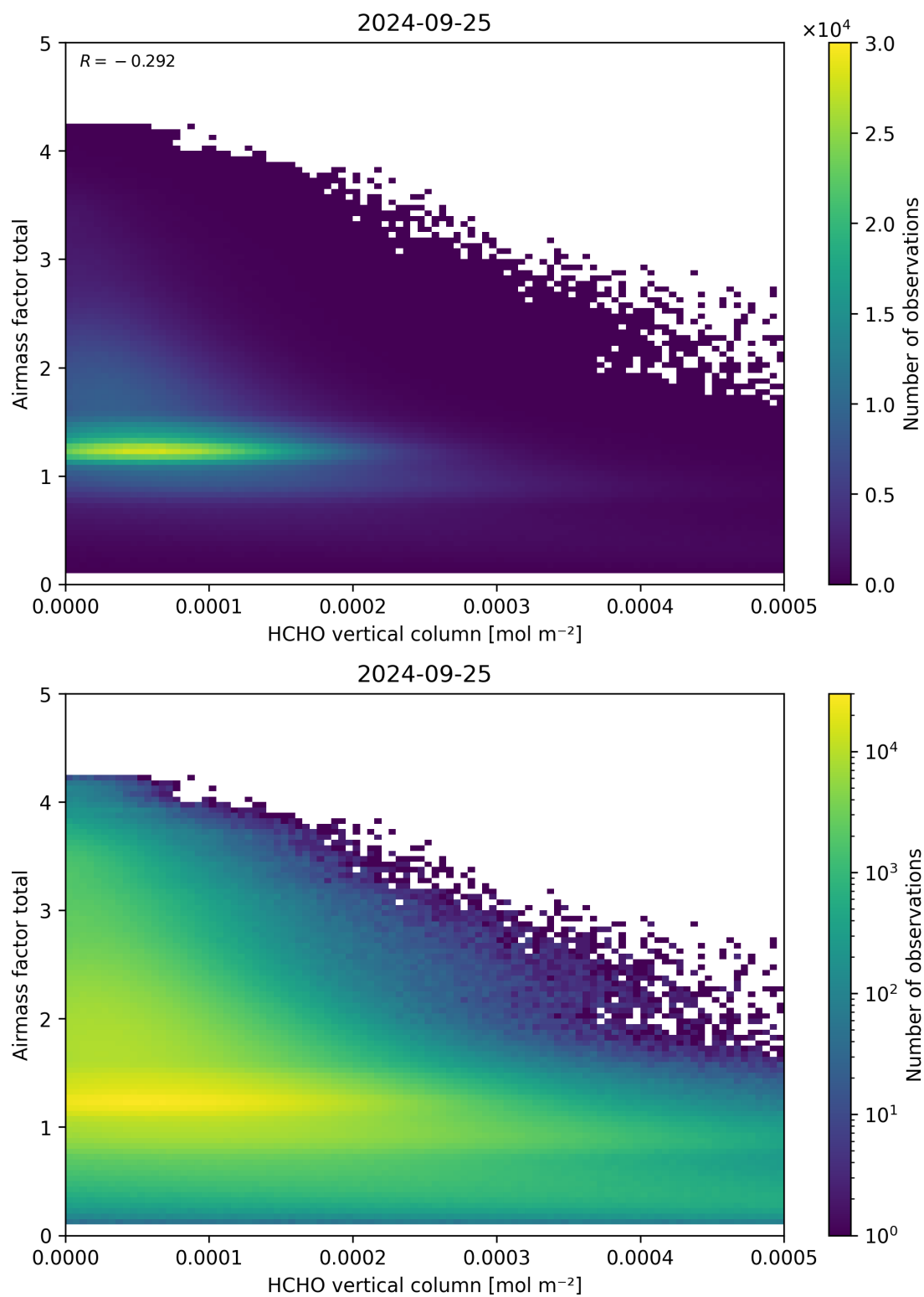
Figure 131: Scatter density plot of “HCHO vertical column” against “Airmass factor total” for 2024-09-24 to 2024-09-26.
