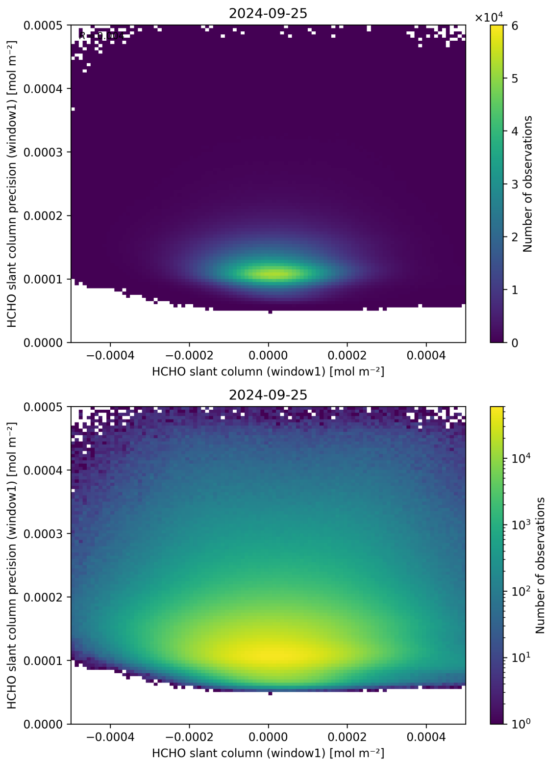
Figure 84: Scatter density plot of “HCHO slant column (window1)” against “HCHO slant column precision (window1)” for 2024-09-24 to 2024-09-26.
