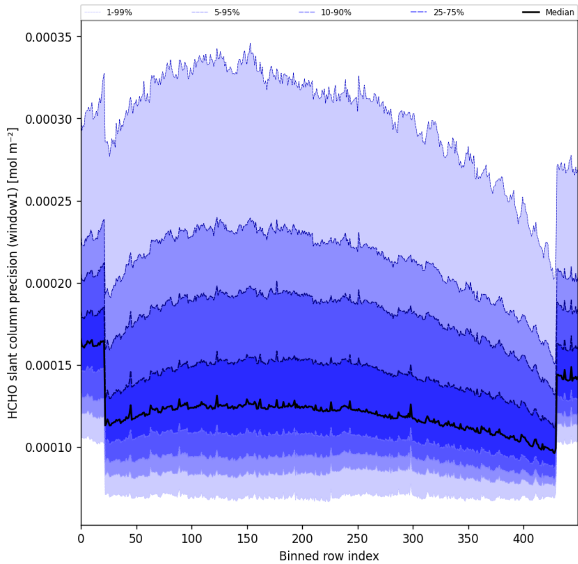
Figure 53: Along track statistics of “HCHO slant column precision (window1)” for 2024-09-24 to 2024-09-26
