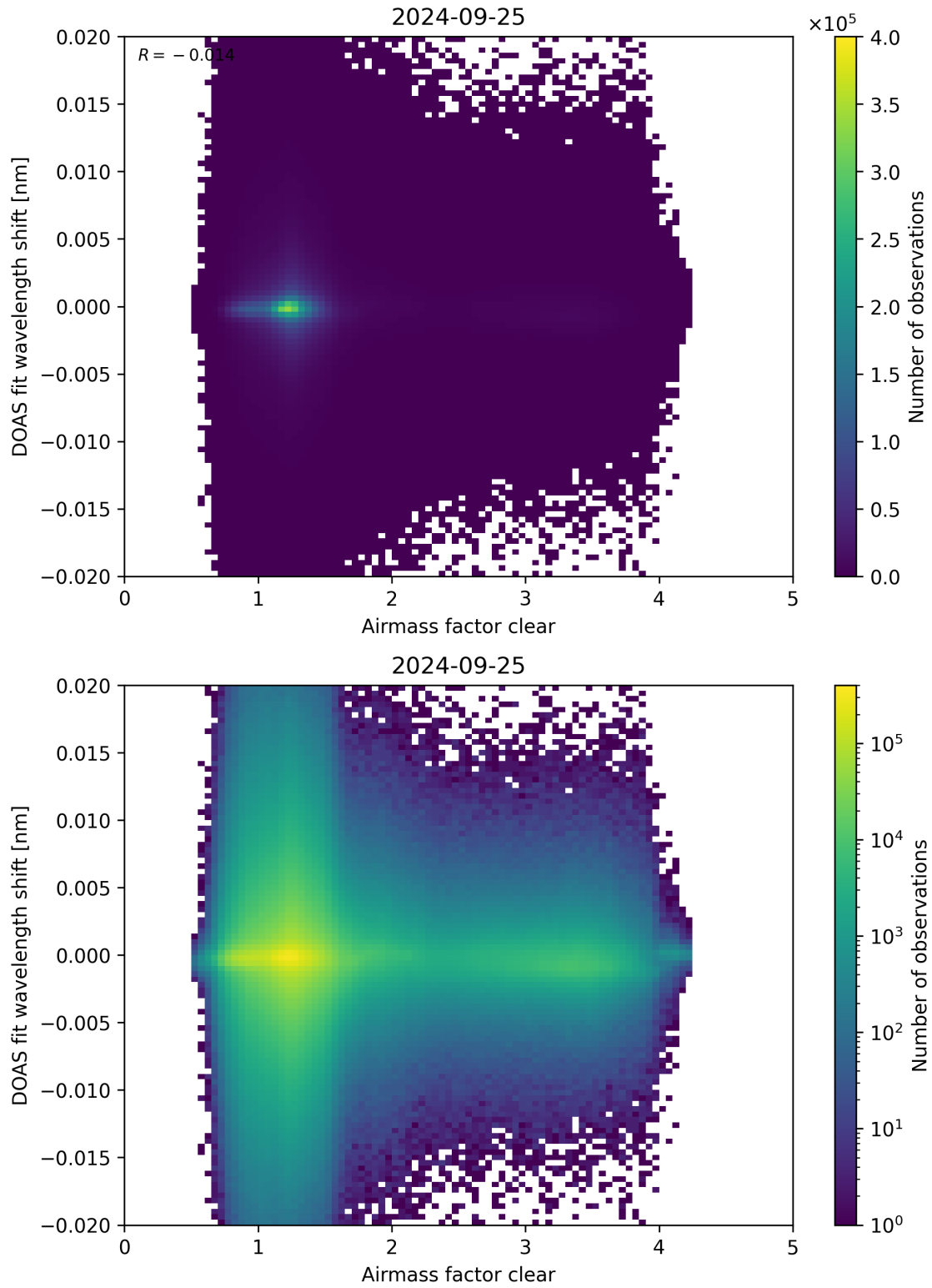
Figure 72: Scatter density plot of “Airmass factor clear” against “DOAS fit wavelength shift” for 2024-09-24 to 2024-09-26.
