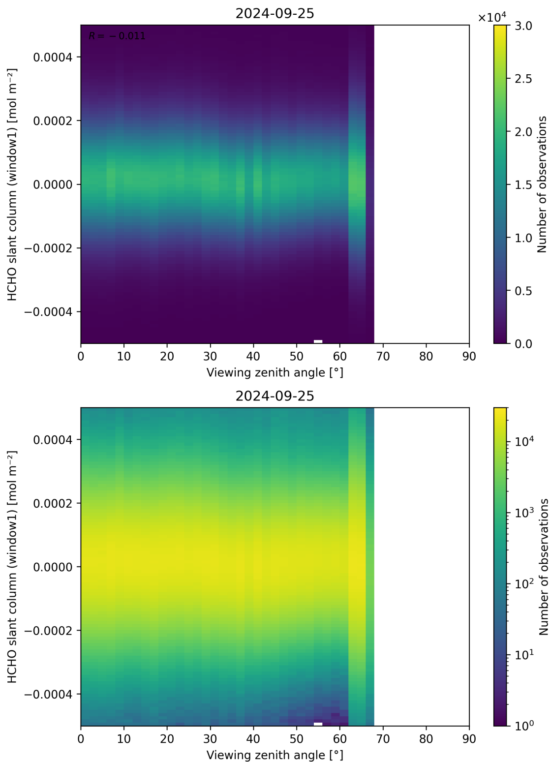
Figure 188: Scatter density plot of “Viewing zenith angle” against “HCHO slant column (window1)” for 2024-09-24 to 2024-09-26.
