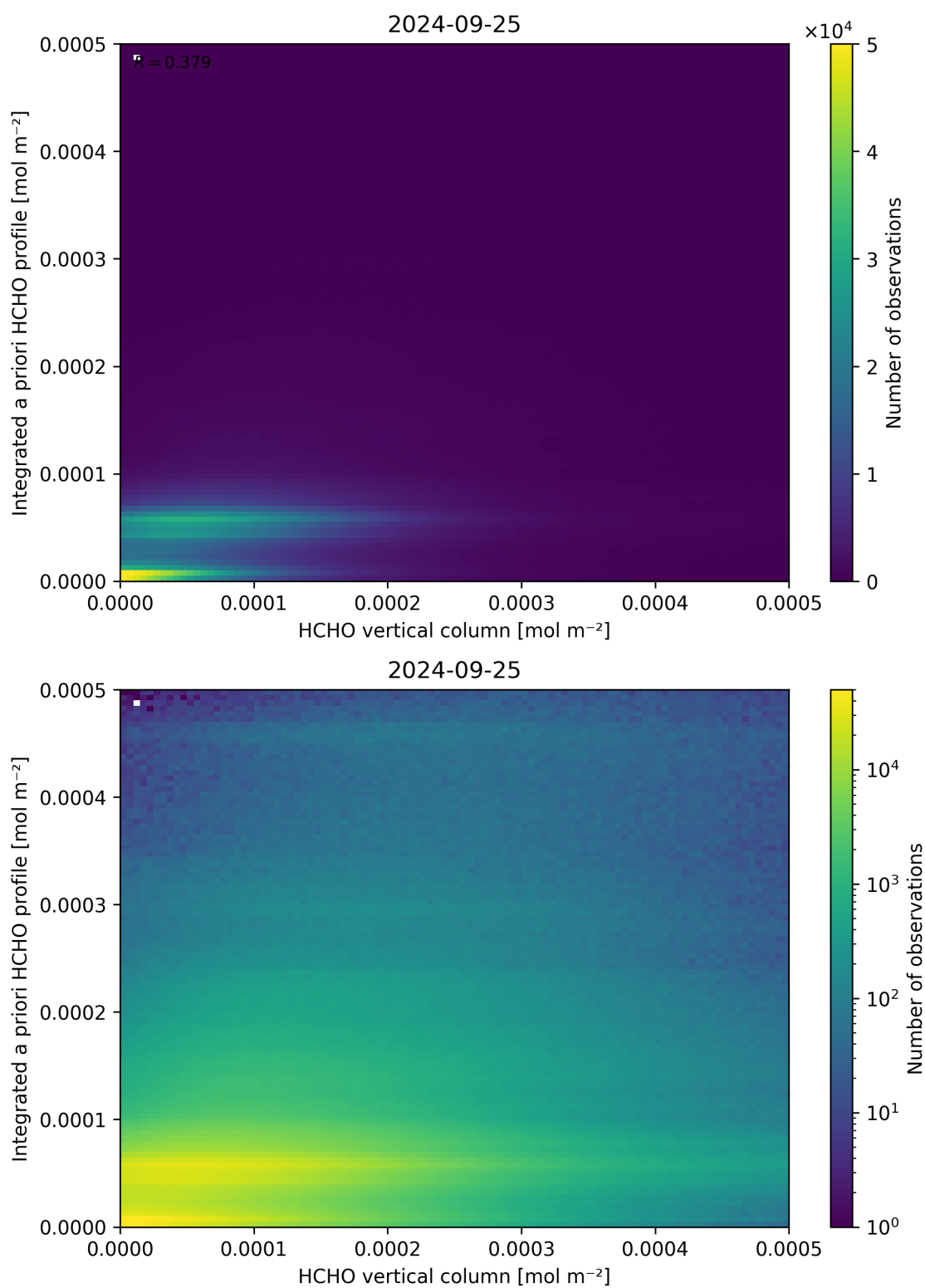
Figure 135: Scatter density plot of “HCHO vertical column” against “Integrated a priori HCHO profile” for 2024-09-24 to 2024-09-26.
