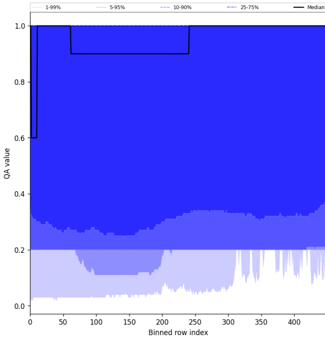
Figure 48: Along track statistics of “QA value” for 2024-09-24 to 2024-09-26
