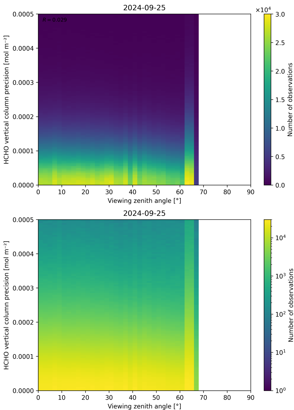
Figure 194: Scatter density plot of “Viewing zenith angle” against “HCHO vertical column precision” for 2024-09-24 to 2024-09-26.
