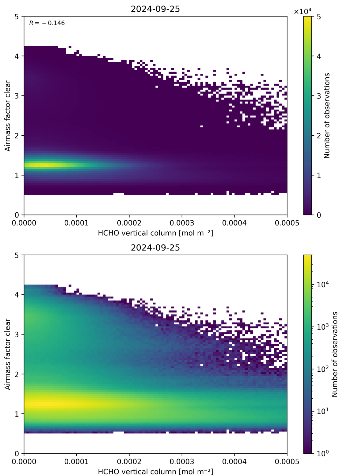
Figure 126: Scatter density plot of “HCHO vertical column” against “Airmass factor clear” for 2024-09-24 to 2024-09-26.
