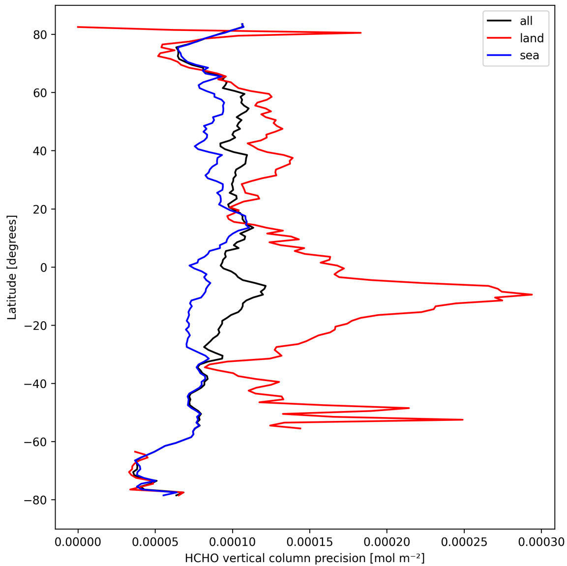
Figure 22: Zonal average of “HCHO vertical column precision” for 2024-09-24 to 2024-09-26.
