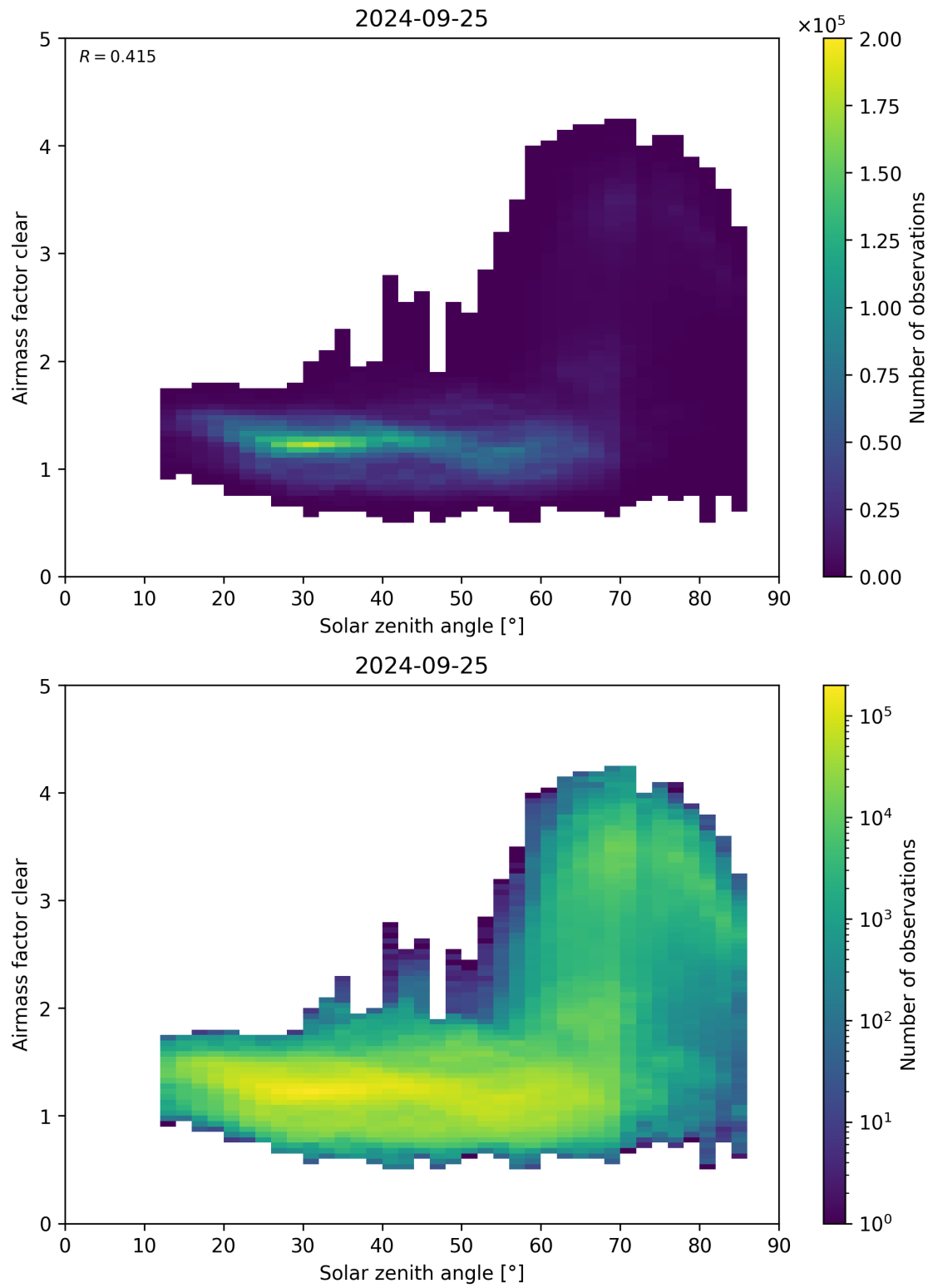
Figure 170: Scatter density plot of “Solar zenith angle” against “Airmass factor clear” for 2024-09-24 to 2024-09-26.
