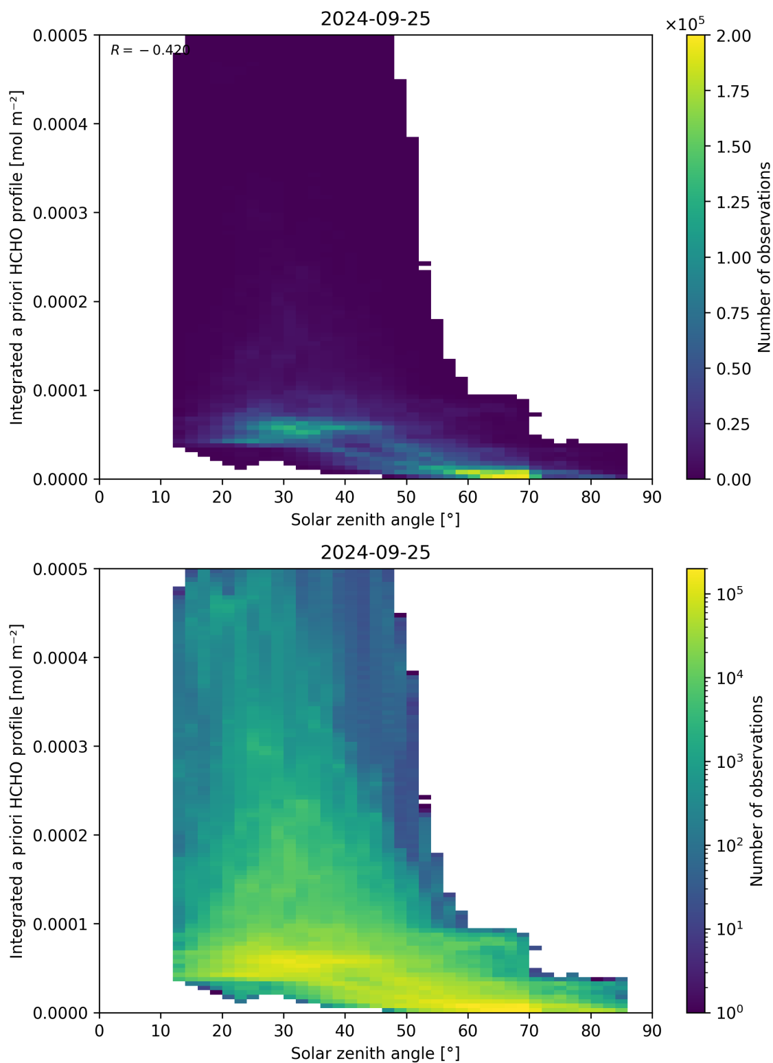
Figure 180: Scatter density plot of “Solar zenith angle” against “Integrated a priori HCHO profile” for 2024-09-24 to 2024-09-26.
