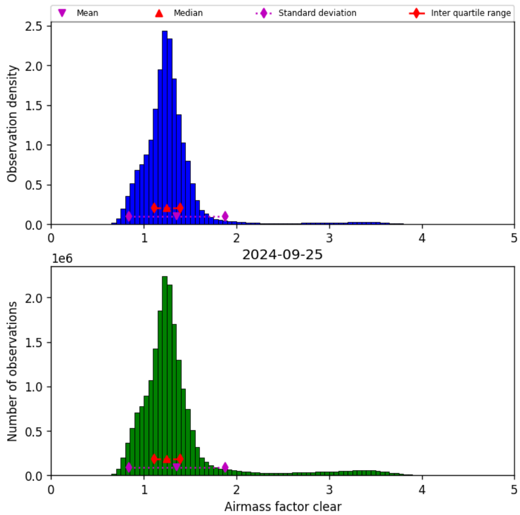
Figure 42: Histogram of “Airmass factor clear” for 2024-09-24 to 2024-09-26
