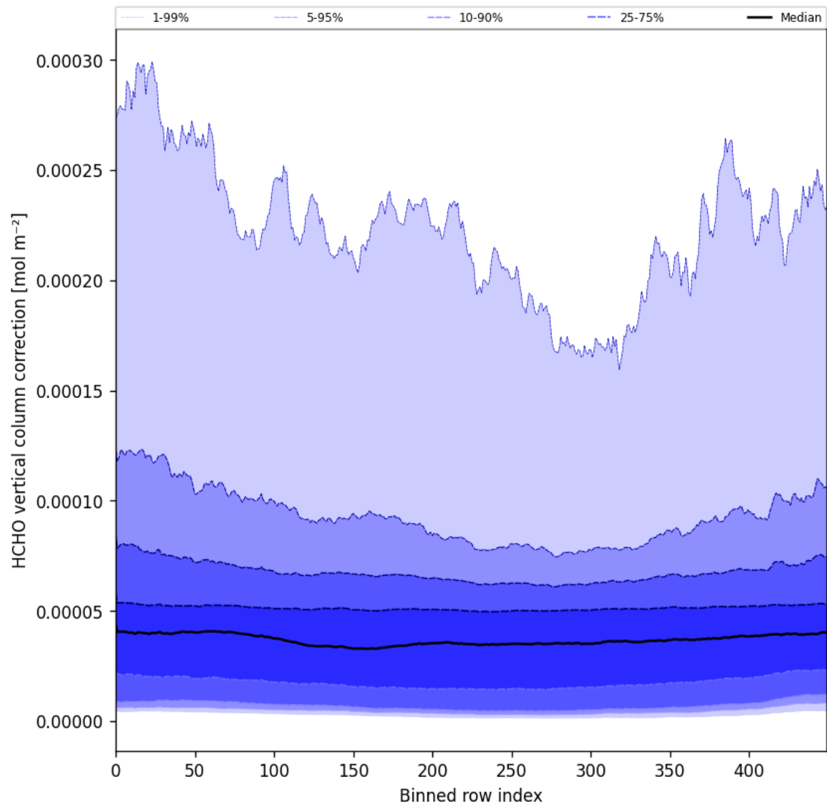
Figure 51: Along track statistics of "HCHO vertical column correction" for 2024-09-24 to 2024-09-26
