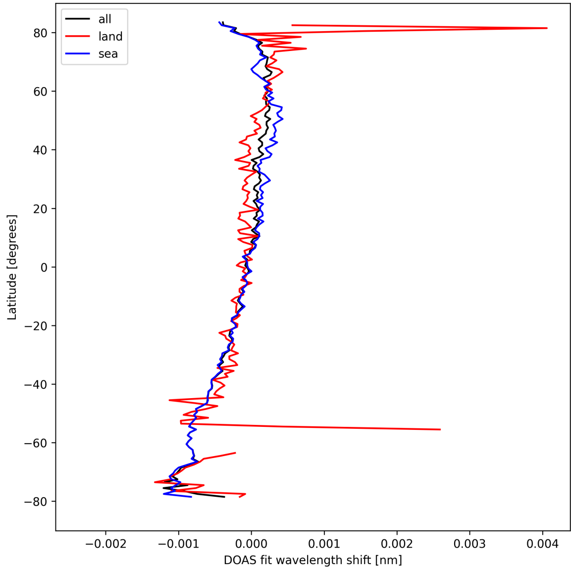
Figure 30: Zonal average of “DOAS fit wavelength shift” for 2024-09-24 to 2024-09-26.
