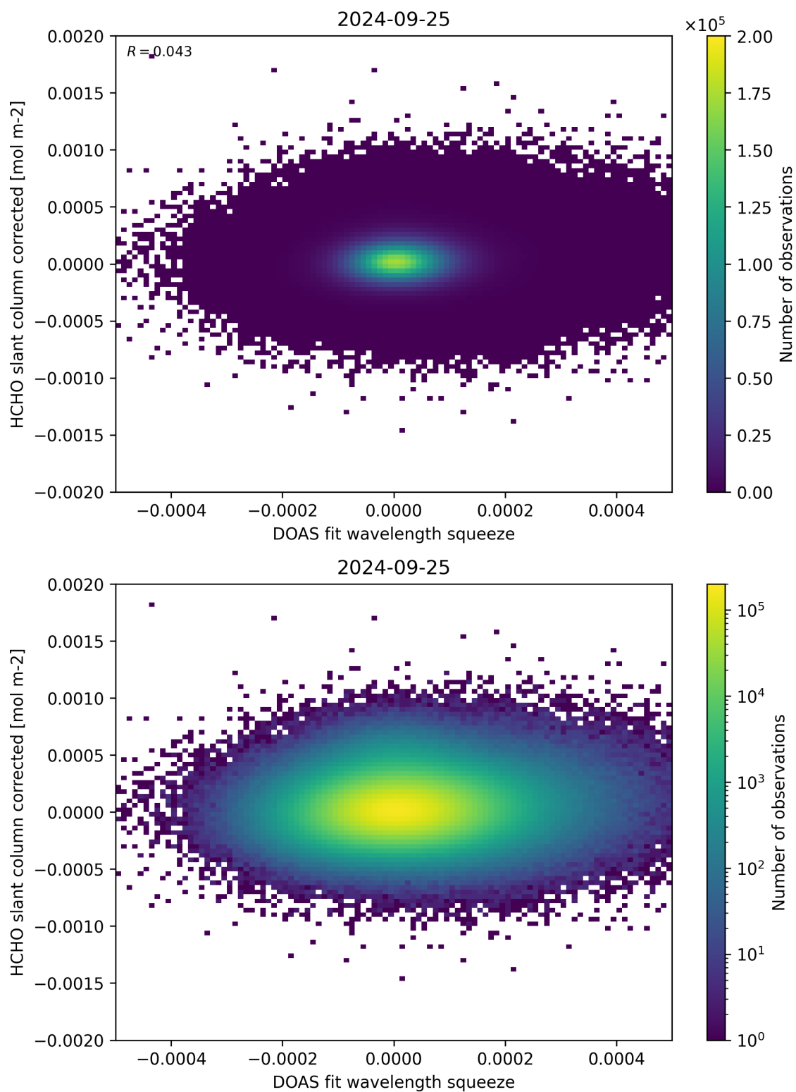
Figure 69: Scatter density plot of “DOAS fit wavelength squeeze” against “HCHO slant column corrected” for 2024-09-24 to 2024-09-26.
