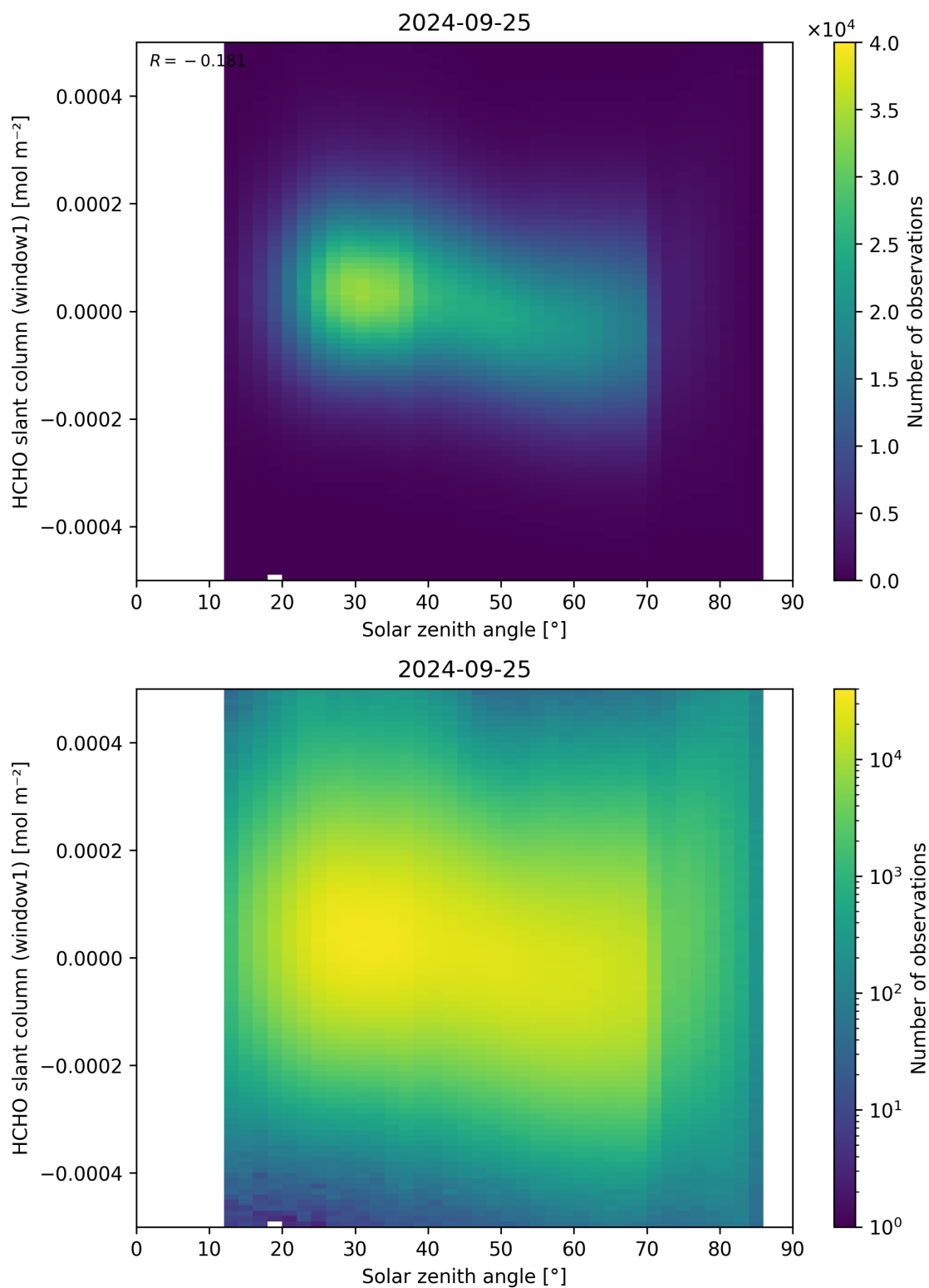
Figure 173: Scatter density plot of “Solar zenith angle” against “HCHO slant column (window1)” for 2024-09-24 to 2024-09-26.
