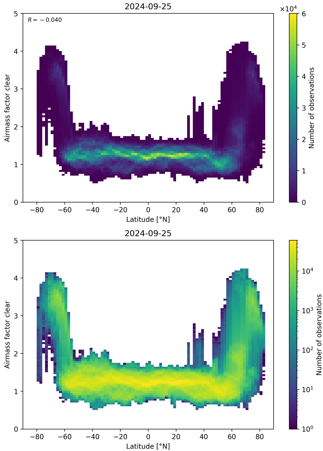
Figure 156: Scatter density plot of “Latitude” against “Airmass factor clear” for 2024-09-24 to 2024-09-26.
