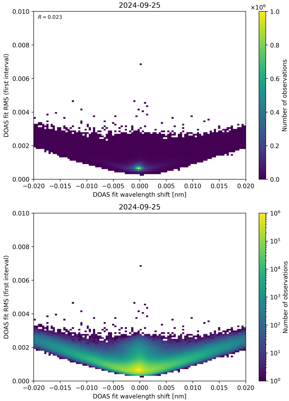
Figure 64: Scatter density plot of “DOAS fit wavelength shift” against “DOAS fit RMS (first interval)” for 2024-09-24 to 2024-09-26.
