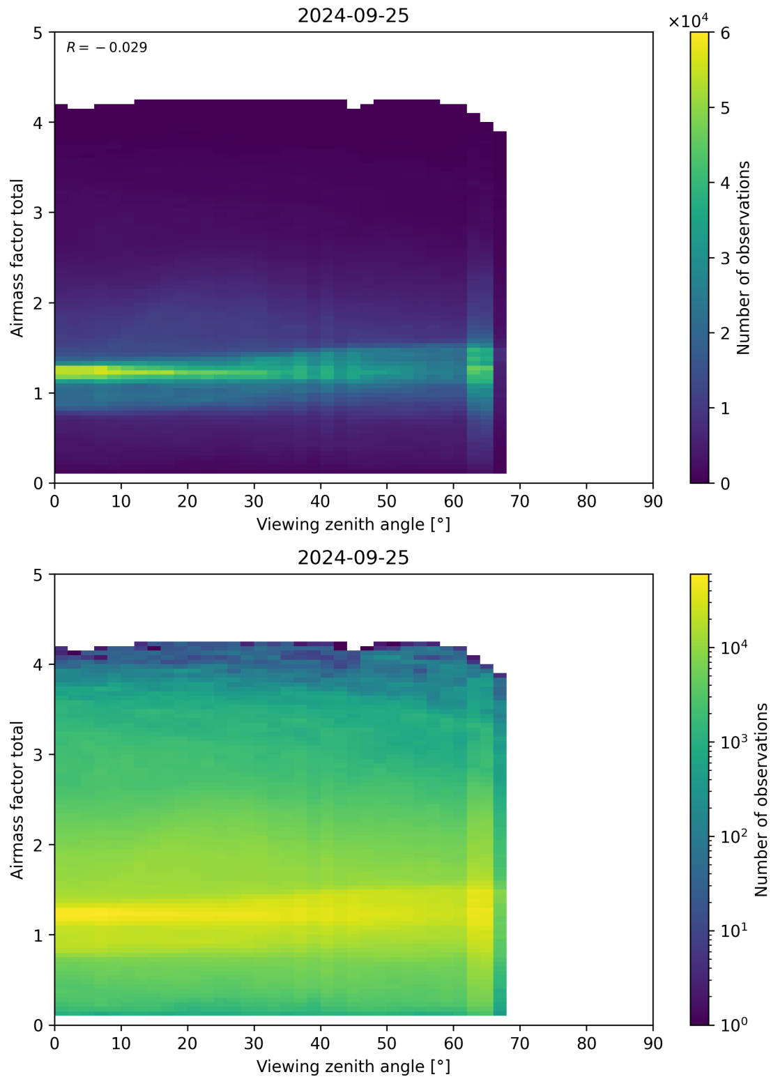
Figure 190: Scatter density plot of “Viewing zenith angle” against “Airmass factor total” for 2024-09-24 to 2024-09-26.
