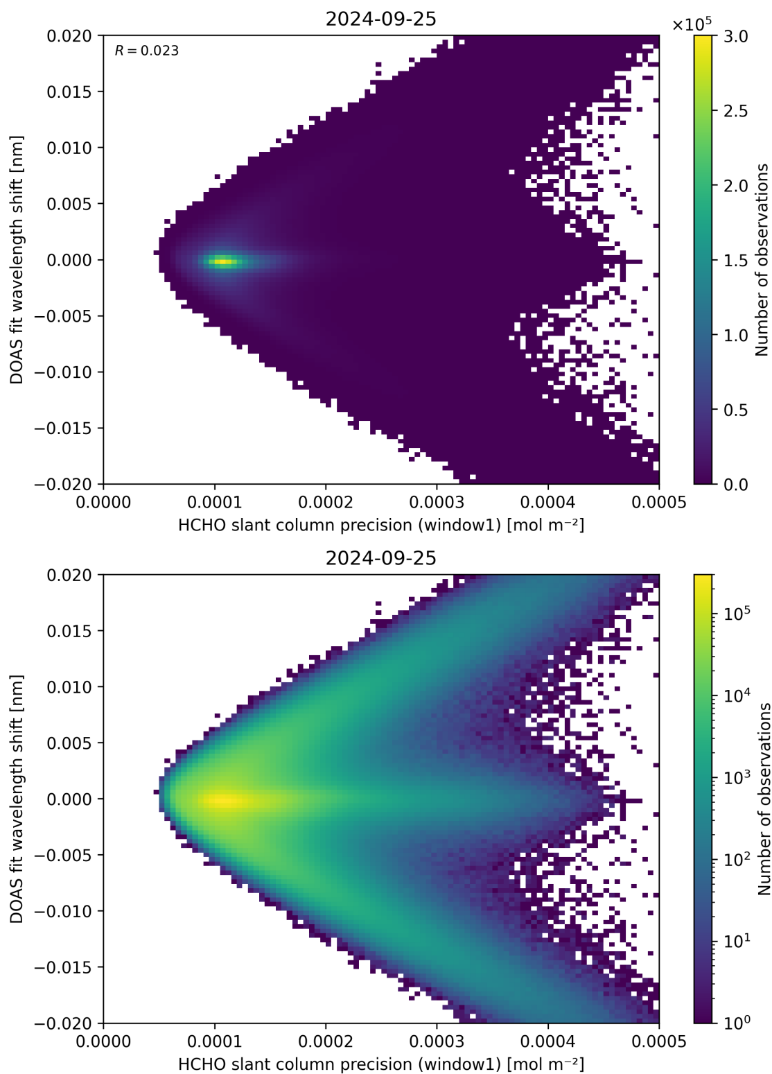
Figure 89: Scatter density plot of “HCHO slant column precision (window1)” against “DOAS fit wavelength shift” for 2024-09-24 to 2024-09-26.
