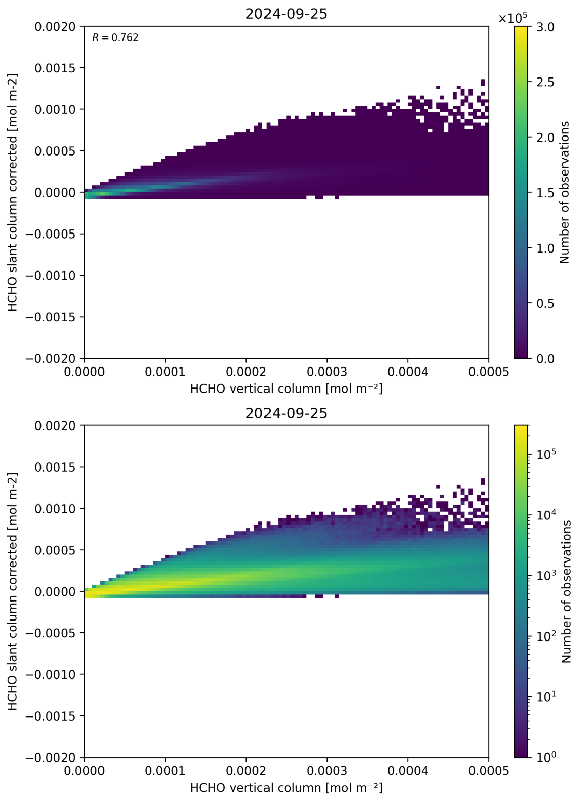
Figure 127: Scatter density plot of “HCHO vertical column” against “HCHO slant column corrected” for 2024-09-24 to 2024-09-26.
