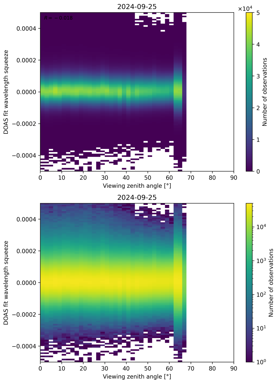
Figure 184: Scatter density plot of “Viewing zenith angle” against “DOAS fit wavelength squeeze” for 2024-09-24 to 2024-09-26.
