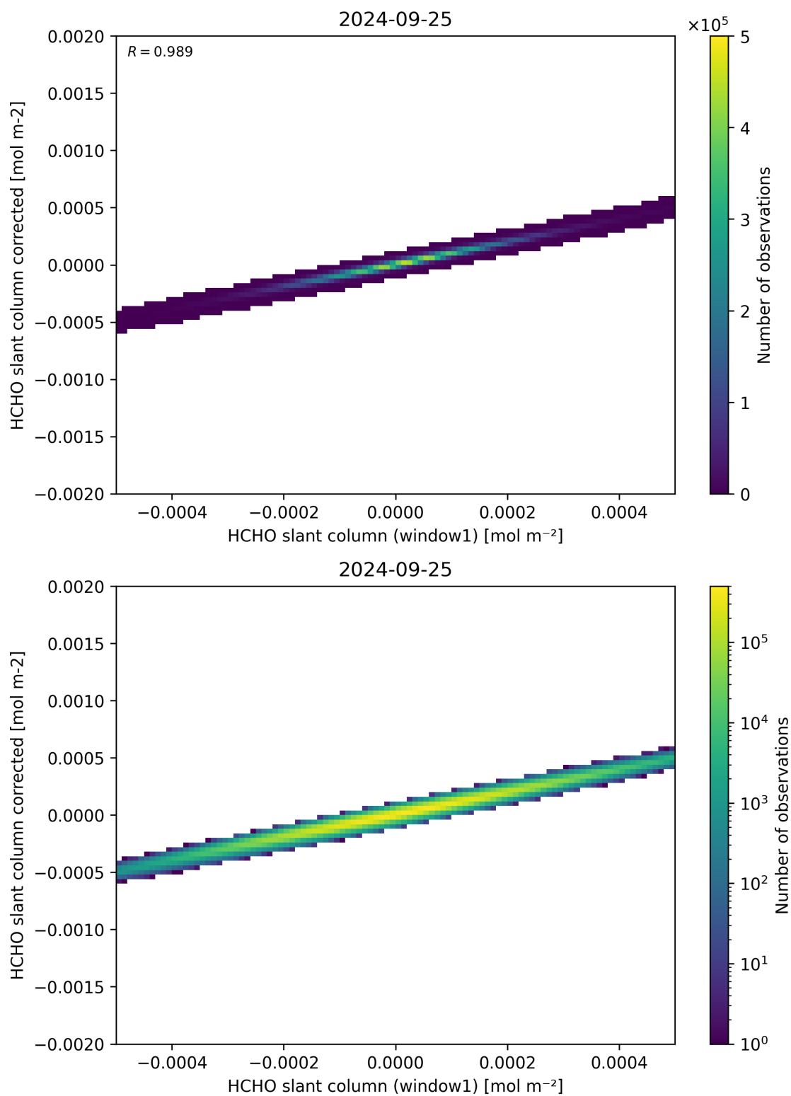
Figure 82: Scatter density plot of “HCHO slant column (window1)” against “HCHO slant column corrected” for 2024-09-24 to 2024-09-26.
