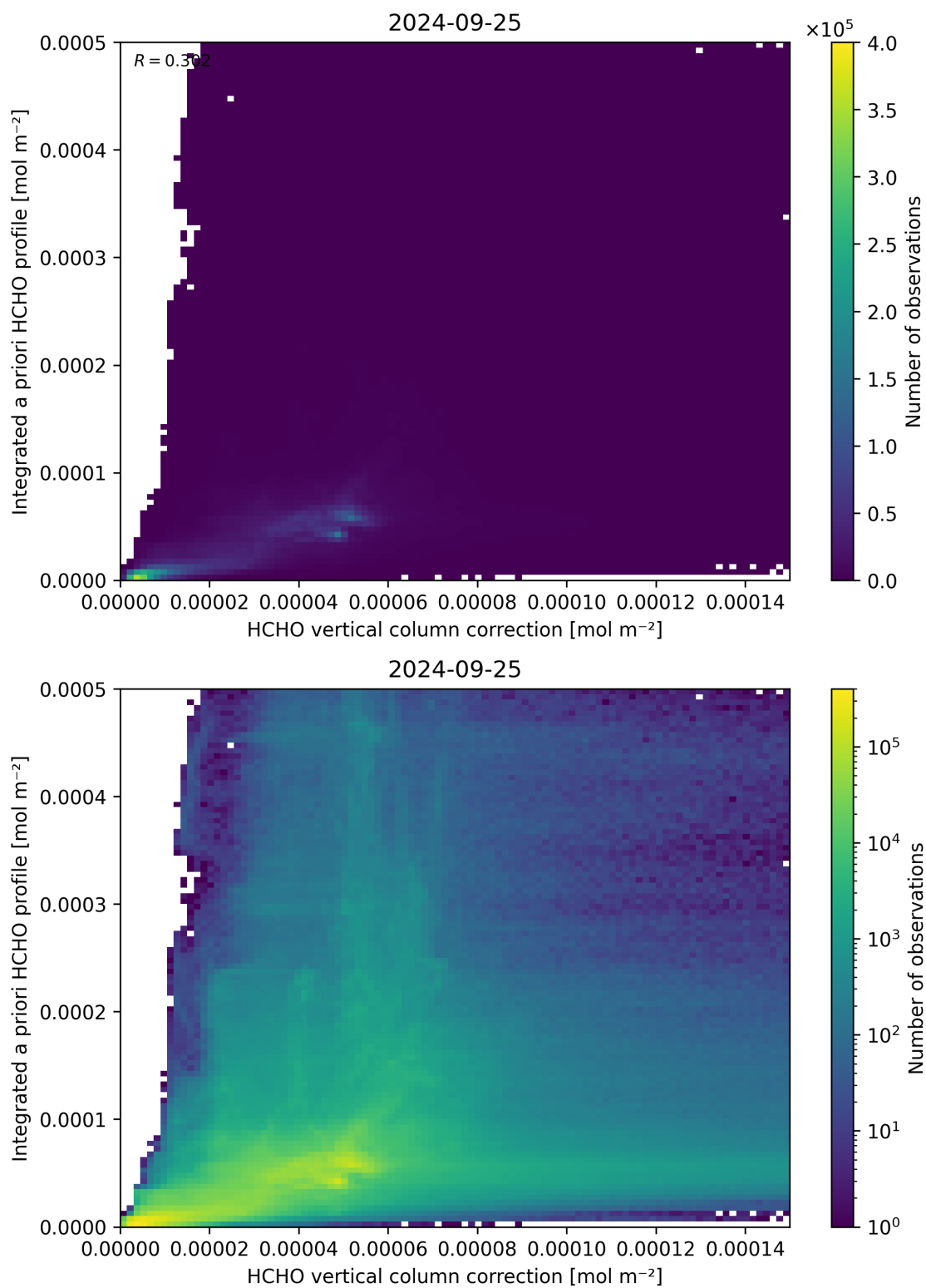
Figure 122: Scatter density plot of “HCHO vertical column correction” against “Integrated a priori HCHO profile” for 2024-09-24 to 2024-09-26.
