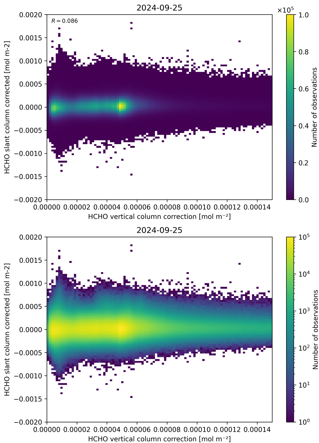
Figure 116: Scatter density plot of “HCHO vertical column correction” against “HCHO slant column corrected” for 2024-09-24 to 2024-09-26.
