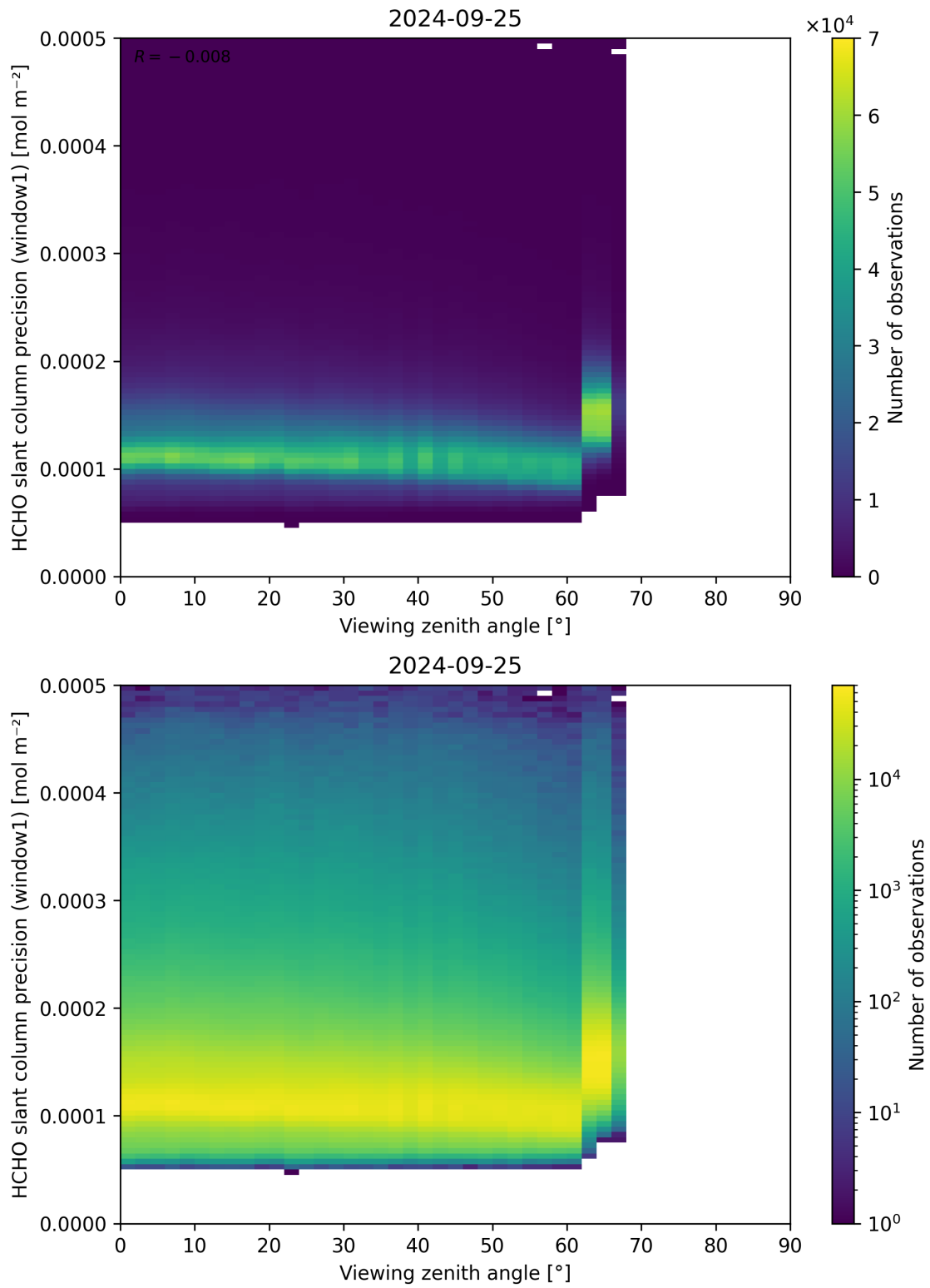
Figure 189: Scatter density plot of “Viewing zenith angle” against “HCHO slant column precision (window1)” for 2024-09-24 to 2024-09-26.
