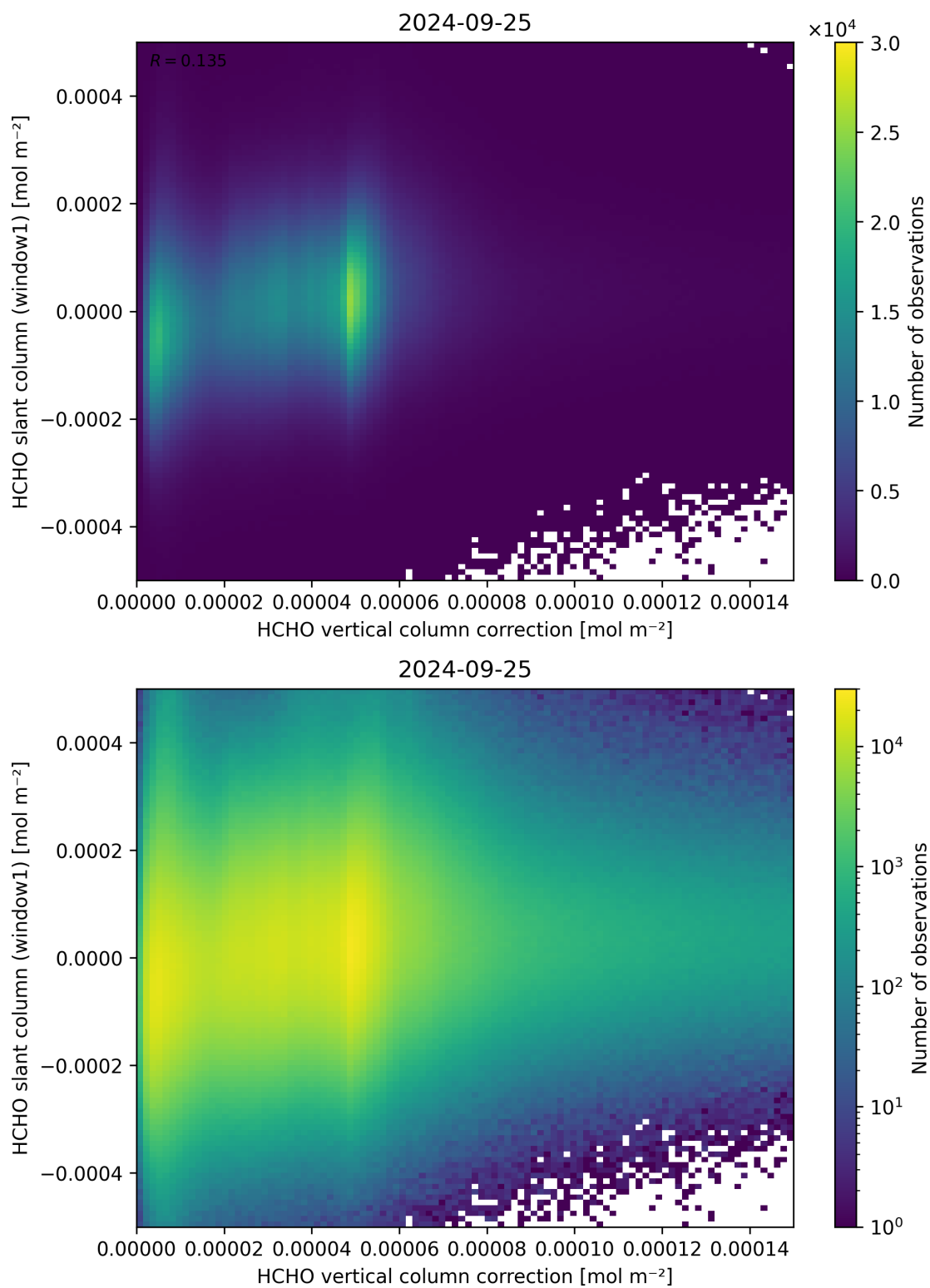
Figure 118: Scatter density plot of “HCHO vertical column correction” against “HCHO slant column (window1)” for 2024-09-24 to 2024-09-26.
