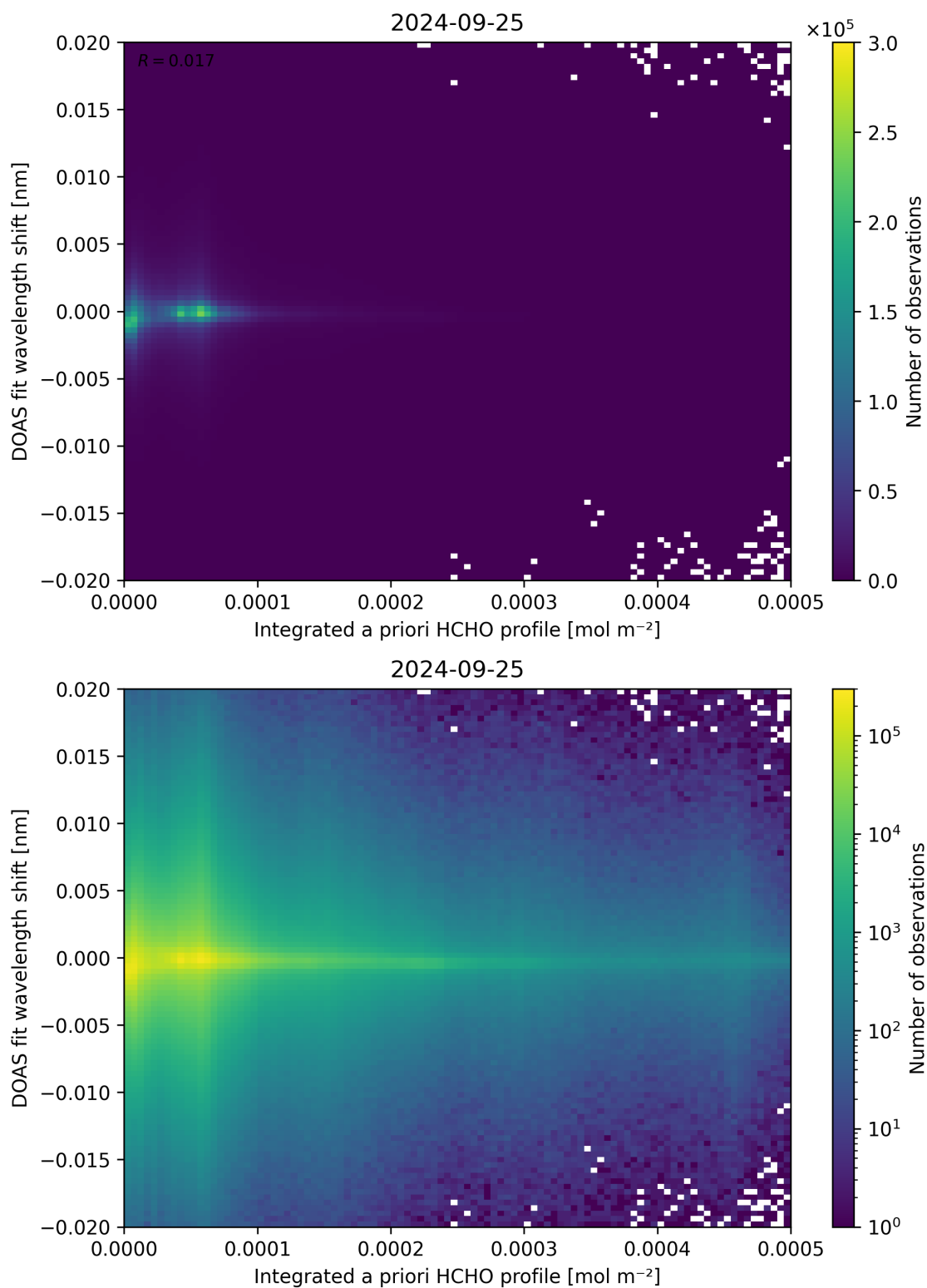
Figure 149: Scatter density plot of “Integrated a priori HCHO profile” against “DOAS fit wavelength shift” for 2024-09-24 to 2024-09-26.
