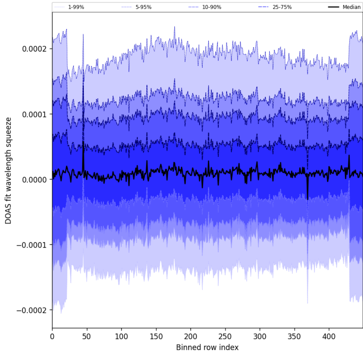
Figure 59: Along track statistics of “DOAS fit wavelength squeeze” for 2024-09-24 to 2024-09-26
