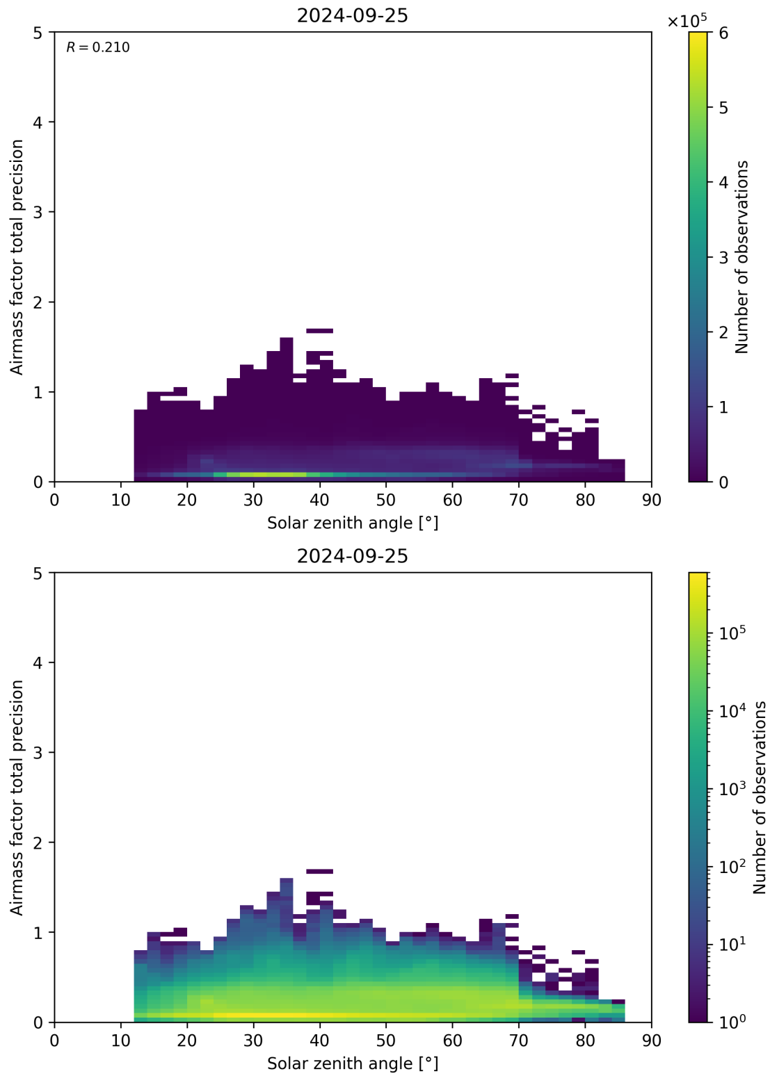
Figure 176: Scatter density plot of “Solar zenith angle” against “Airmass factor total precision” for 2024-09-24 to 2024-09-26.
