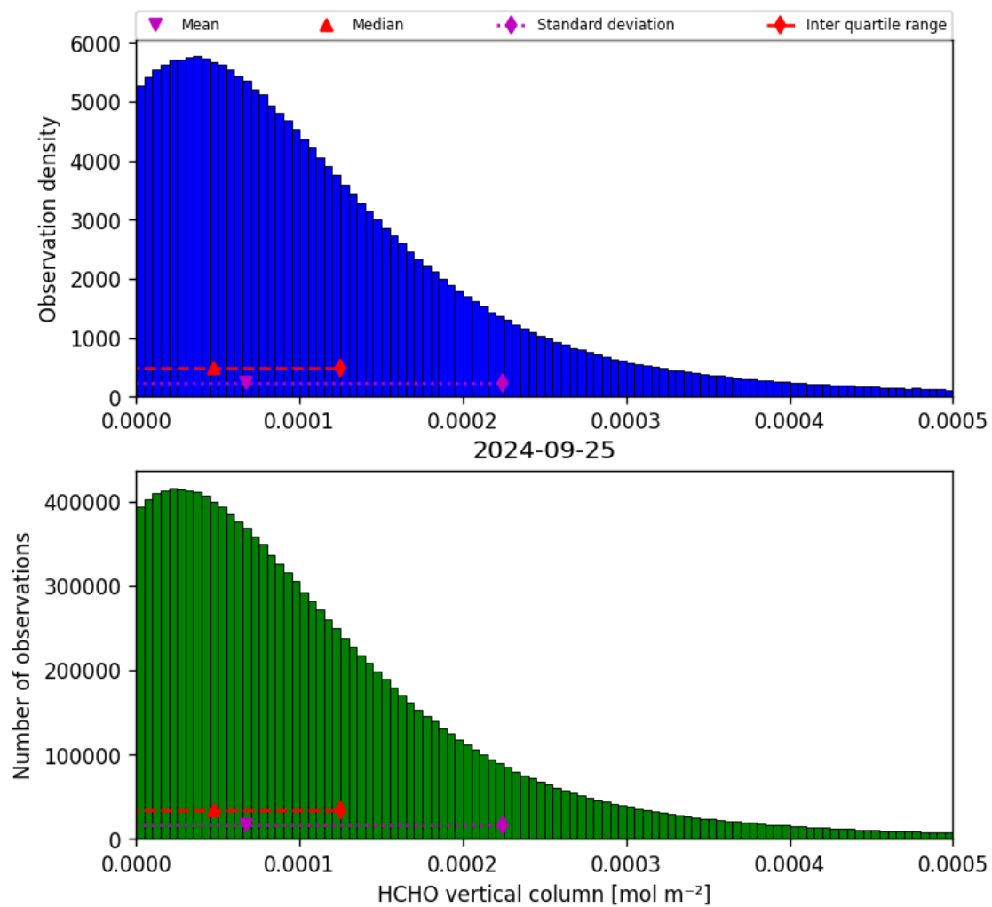
Figure 35: Histogram of “HCHO vertical column” for 2024-09-24 to 2024-09-26
