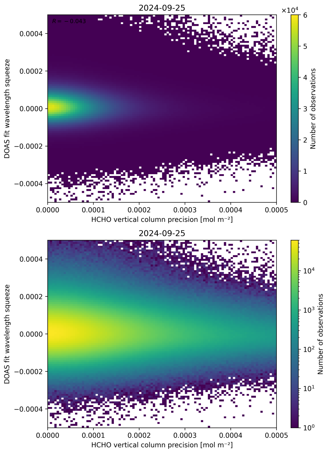
Figure 138: Scatter density plot of “HCHO vertical column precision” against “DOAS fit wavelength squeeze” for 2024-09-24 to 2024-09-26.
