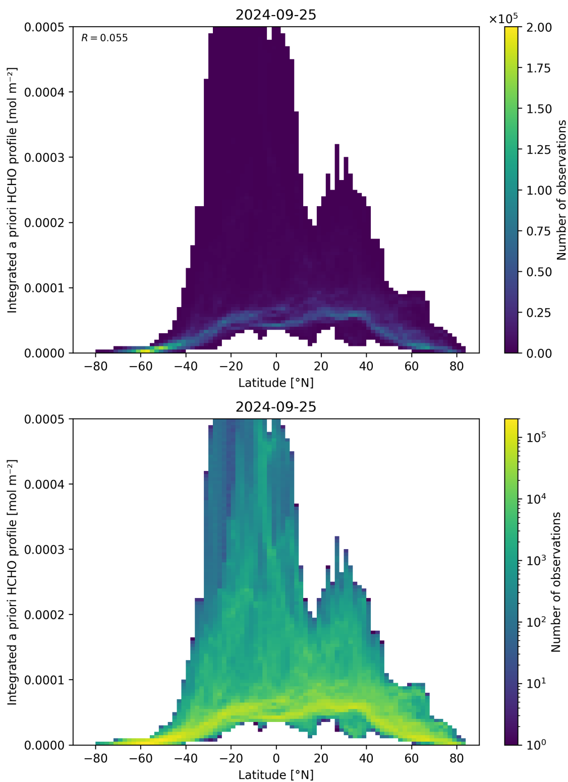
Figure 166: Scatter density plot of “Latitude” against “Integrated a priori HCHO profile” for 2024-09-24 to 2024-09-26.
