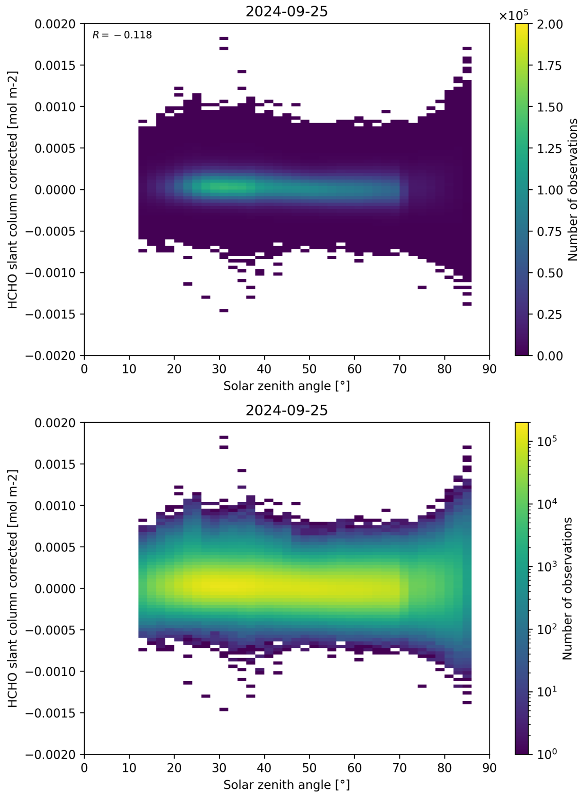
Figure 171: Scatter density plot of “Solar zenith angle” against “HCHO slant column corrected” for 2024-09-24 to 2024-09-26.
