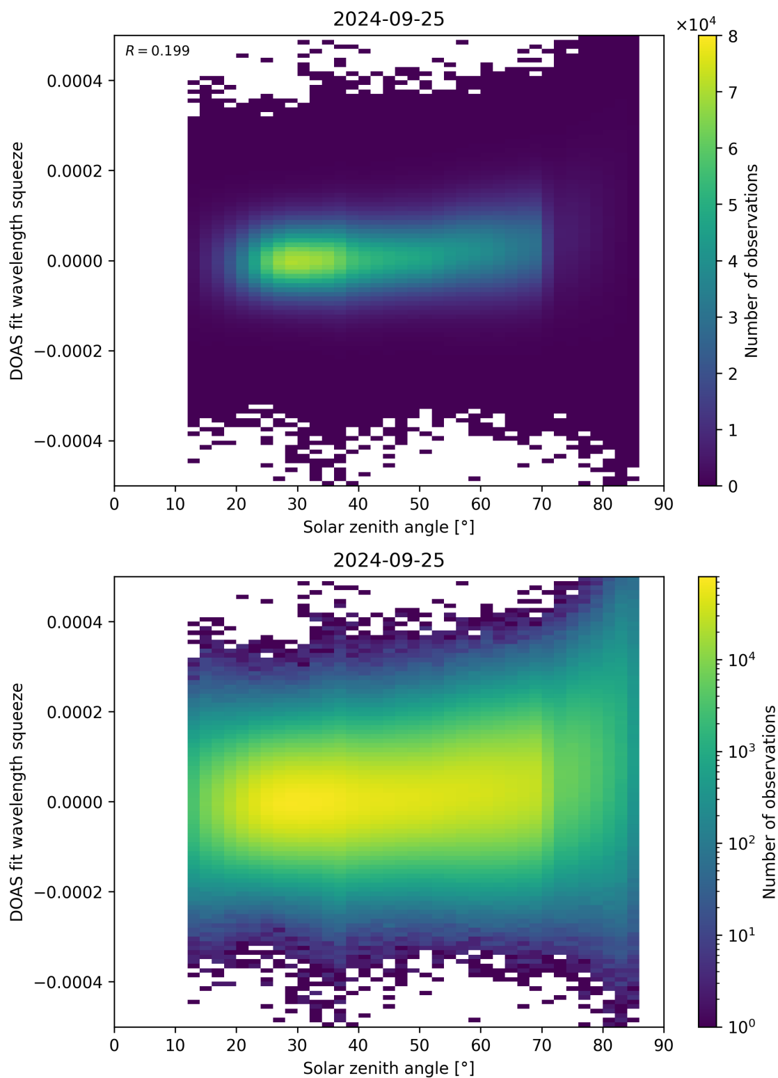
Figure 169: Scatter density plot of “Solar zenith angle” against “DOAS fit wavelength squeeze” for 2024-09-24 to 2024-09-26.
