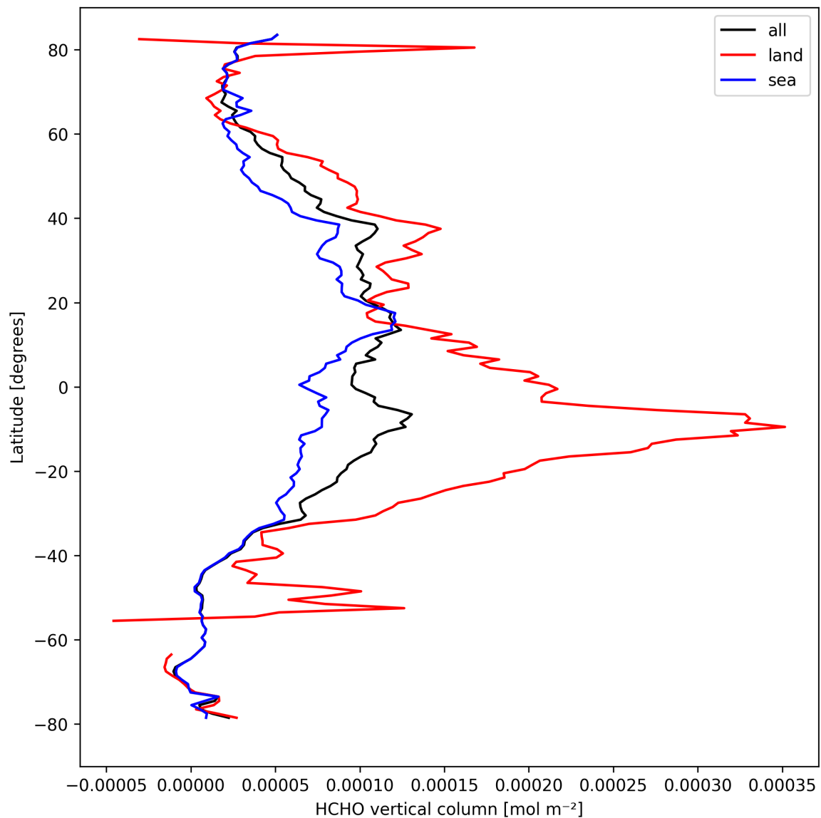
Figure 21: Zonal average of “HCHO vertical column” for 2024-09-24 to 2024-09-26.
