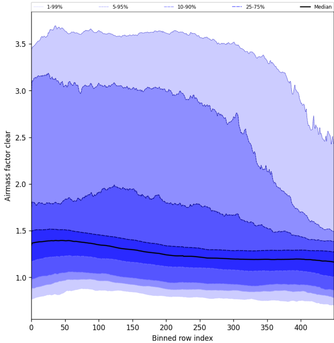
Figure 56: Along track statistics of “Airmass factor clear” for 2024-09-24 to 2024-09-26
