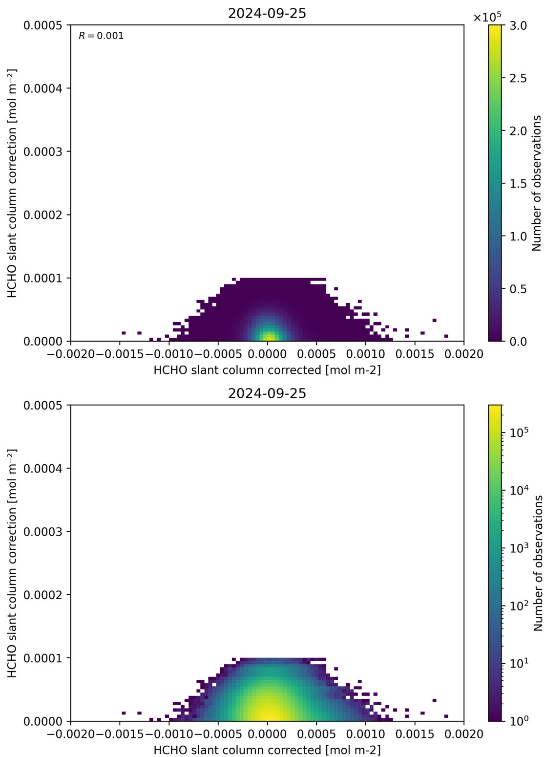
Figure 77: Scatter density plot of “HCHO slant column corrected” against “HCHO slant column correction” for 2024-09-24 to 2024-09-26.
