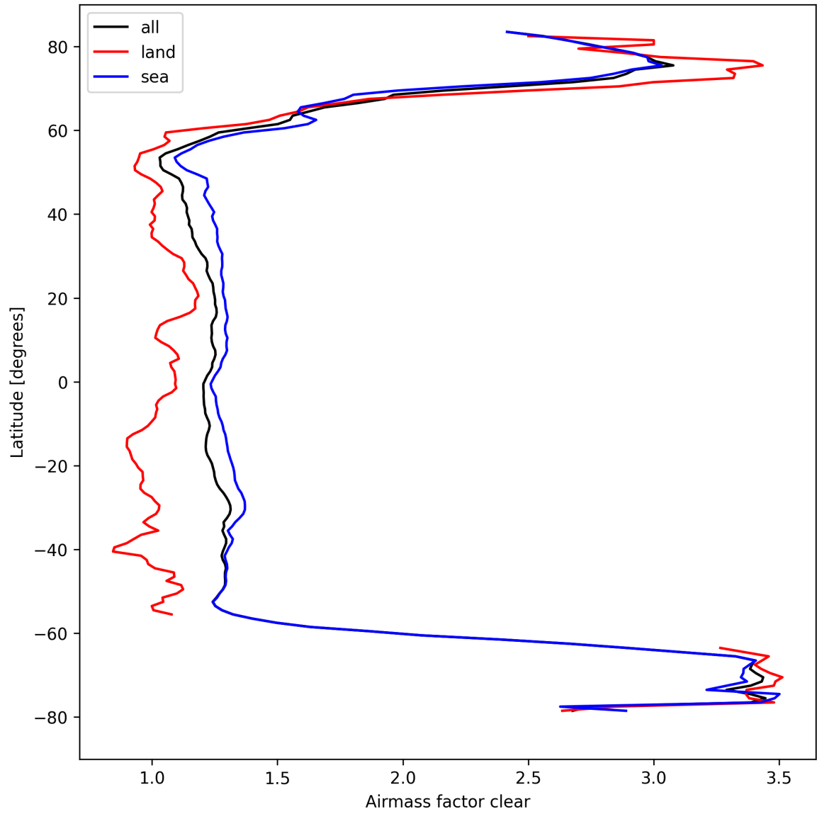
Figure 28: Zonal average of “Airmass factor clear” for 2024-09-24 to 2024-09-26.
