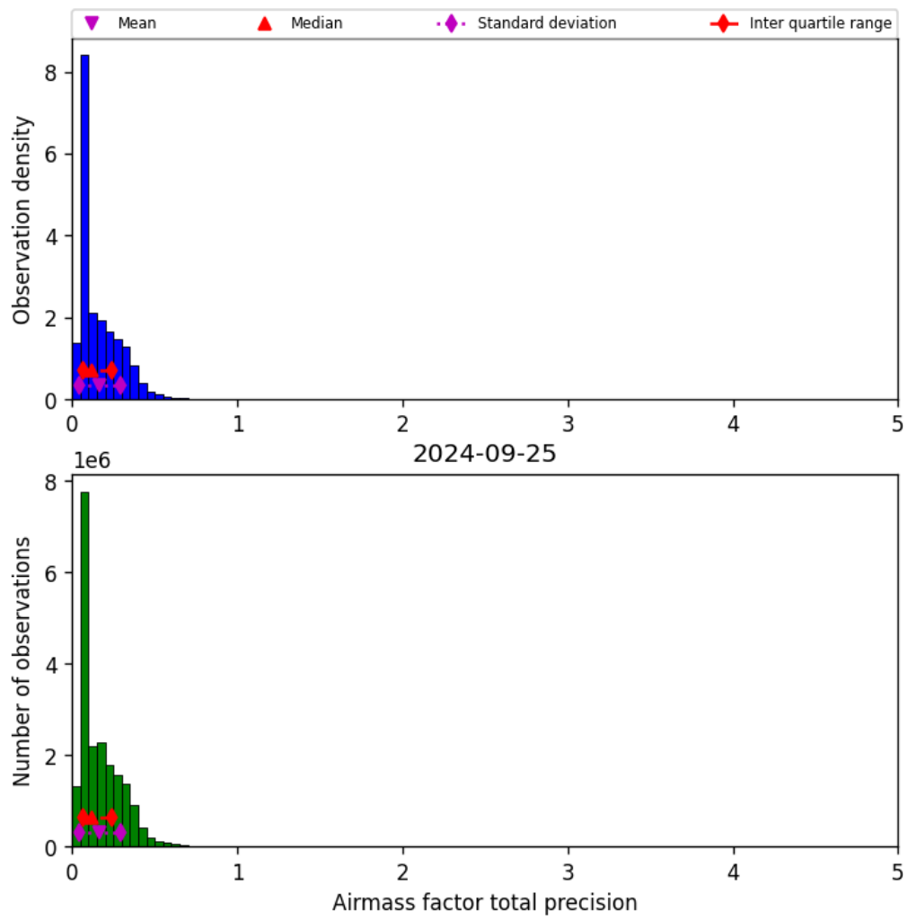
Figure 41: Histogram of “Airmass factor total precision” for 2024-09-24 to 2024-09-26
