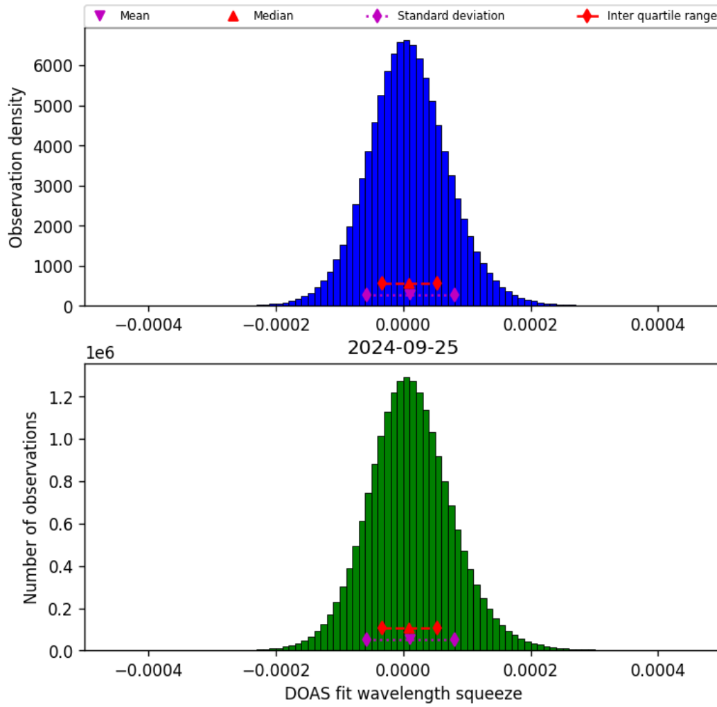
Figure 45: Histogram of “DOAS fit wavelength squeeze” for 2024-09-24 to 2024-09-26
