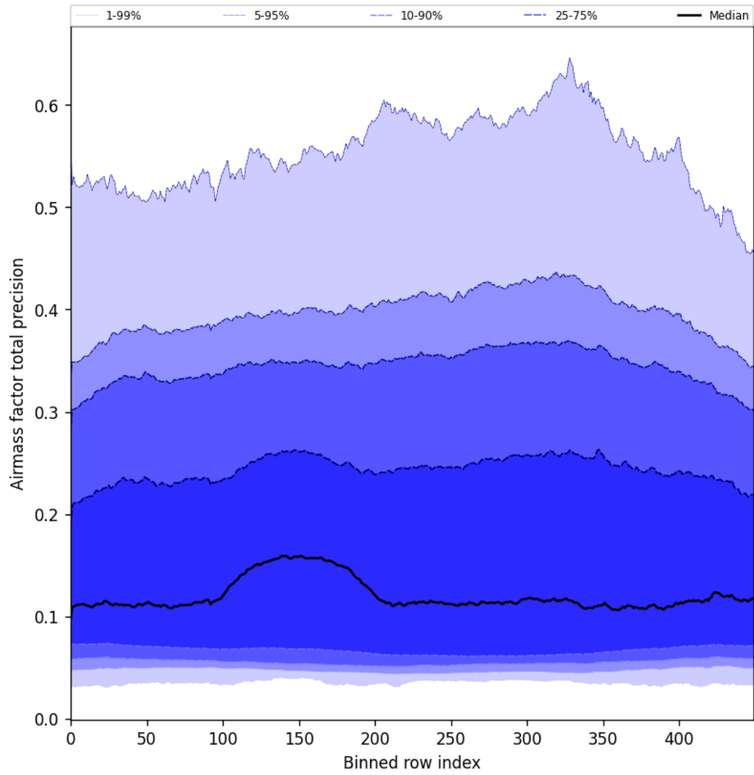
Figure 55: Along track statistics of “Airmass factor total precision” for 2024-09-24 to 2024-09-26
