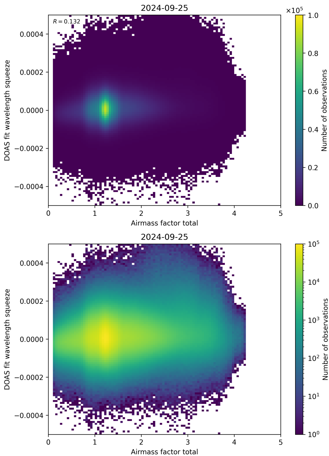
Figure 99: Scatter density plot of “Airmass factor total” against “DOAS fit wavelength squeeze” for 2024-09-24 to 2024-09-26.
