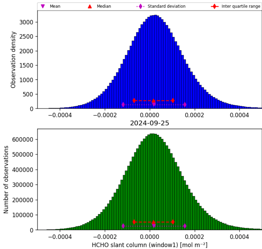
Figure 38: Histogram of “HCHO slant column (window1)” for 2024-09-24 to 2024-09-26
