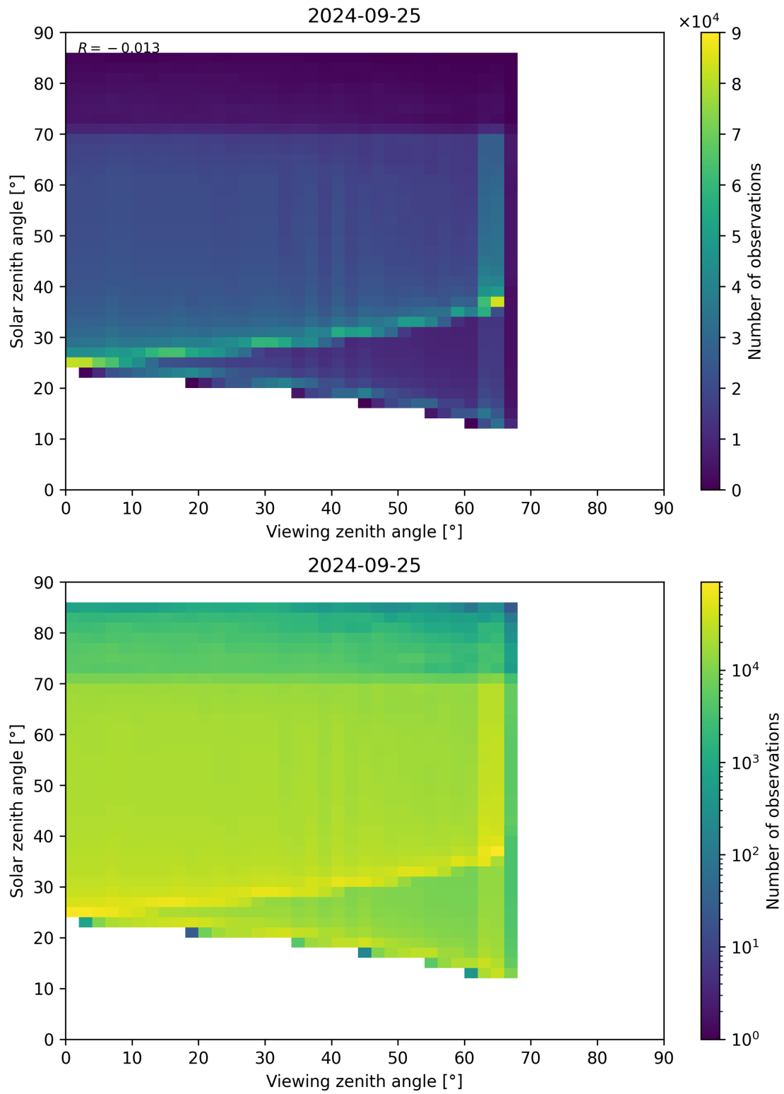
Figure 197: Scatter density plot of “Viewing zenith angle” against “Solar zenith angle” for 2024-09-24 to 2024-09-26.
