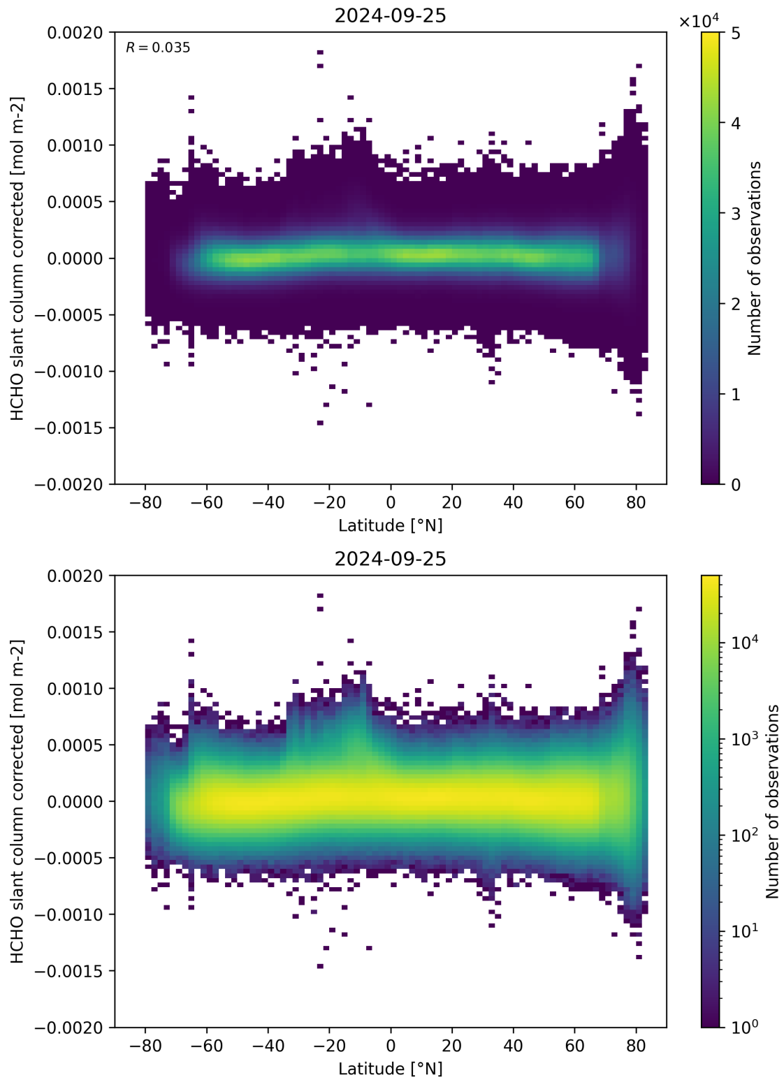
Figure 157: Scatter density plot of “Latitude” against “HCHO slant column corrected” for 2024-09-24 to 2024-09-26.
