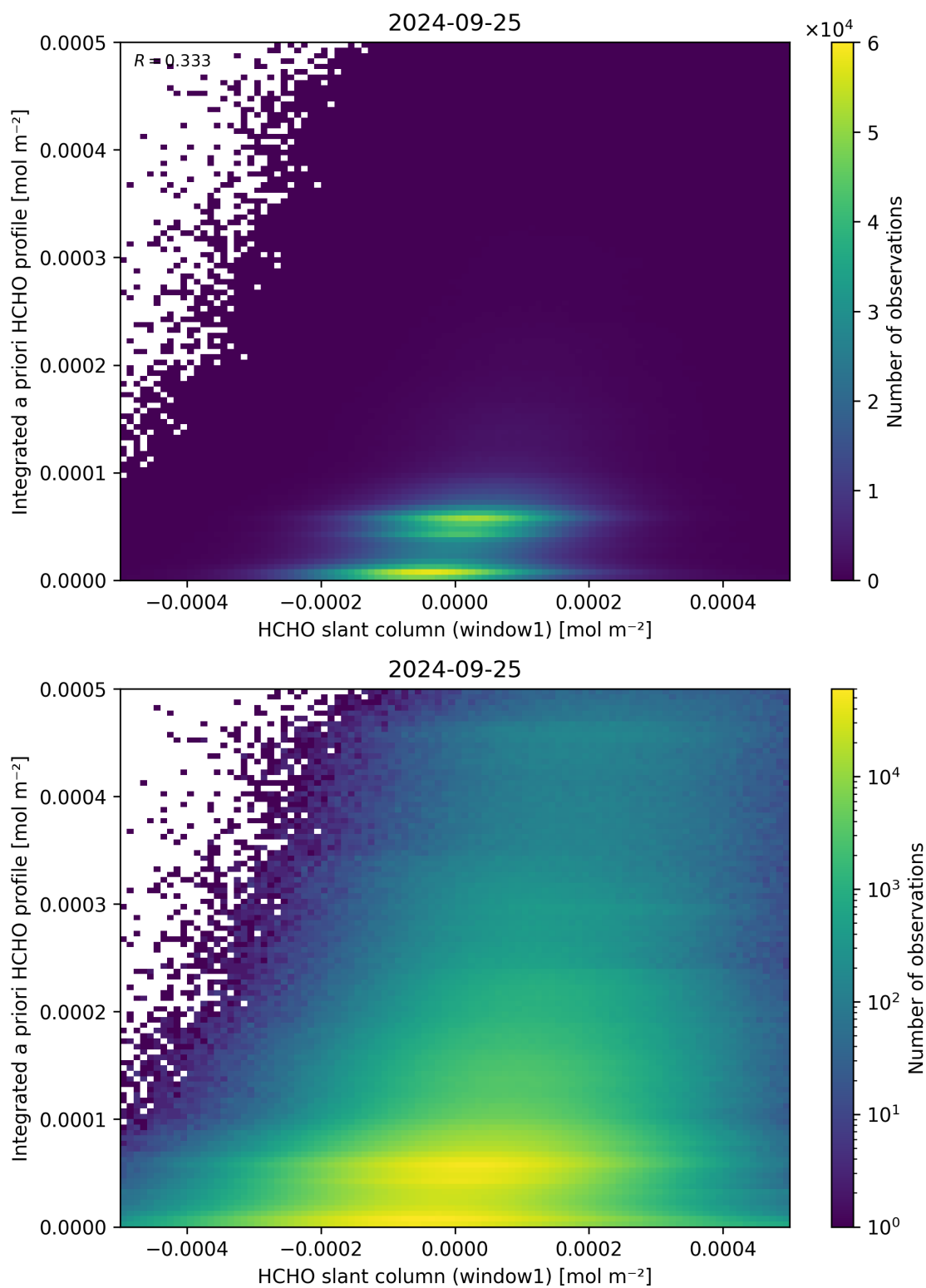
Figure 87: Scatter density plot of “HCHO slant column (window1)” against “Integrated a priori HCHO profile” for 2024-09-24 to 2024-09-26.
