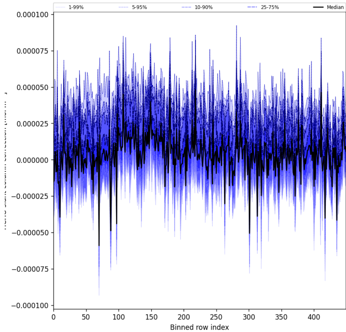
Figure 61: Along track statistics of “HCHO slant column correction” for 2024-09-24 to 2024-09-26
