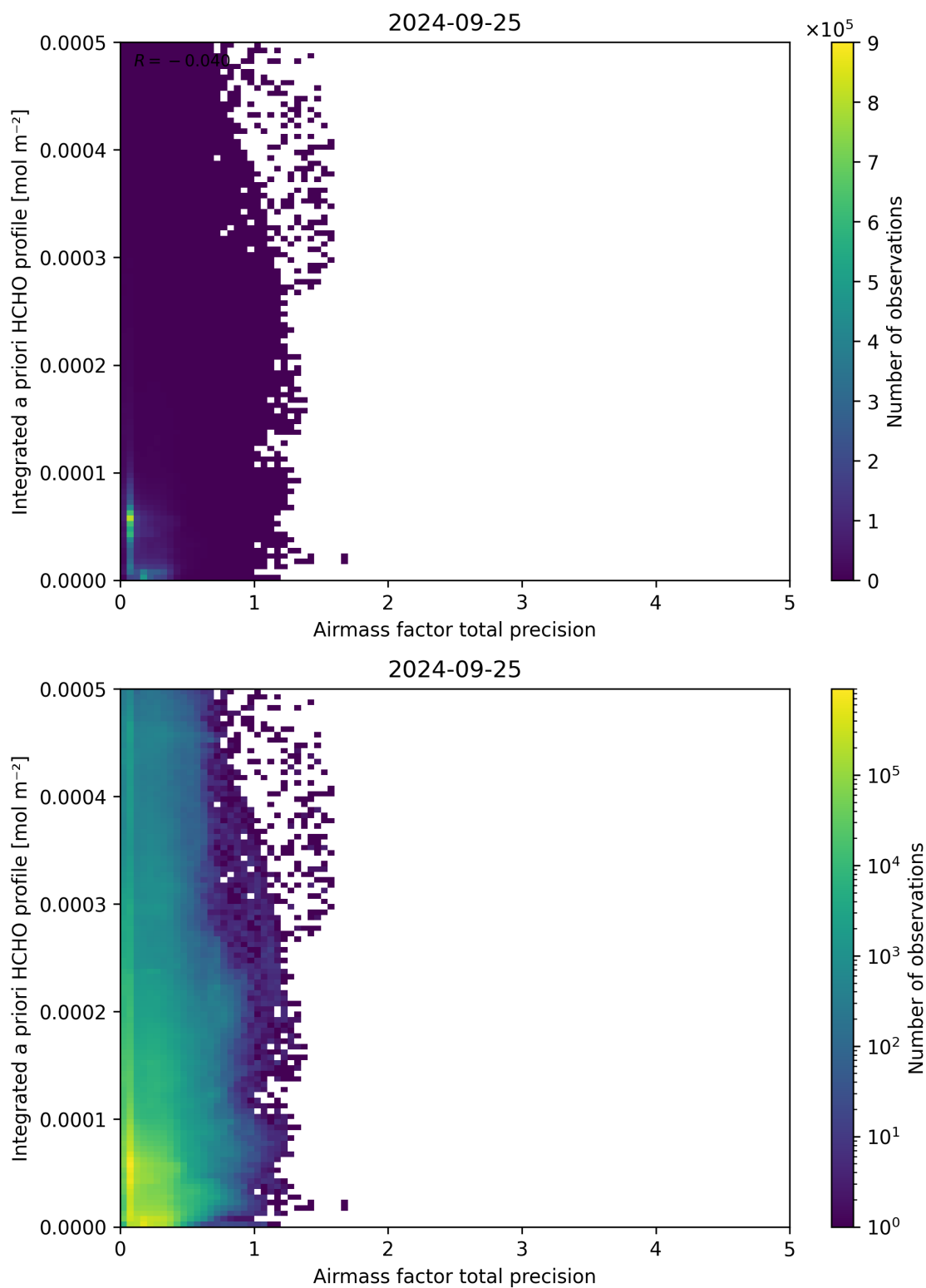
Figure 111: Scatter density plot of “Airmass factor total precision” against “Integrated a priori HCHO profile” for 2024-09-24 to 2024-09-26.
