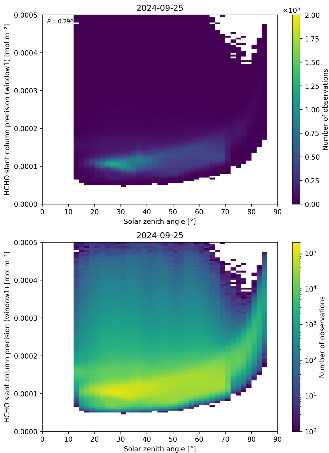
Figure 174: Scatter density plot of “Solar zenith angle” against “HCHO slant column precision (window1)” for 2024-09-24 to 2024-09-26.
