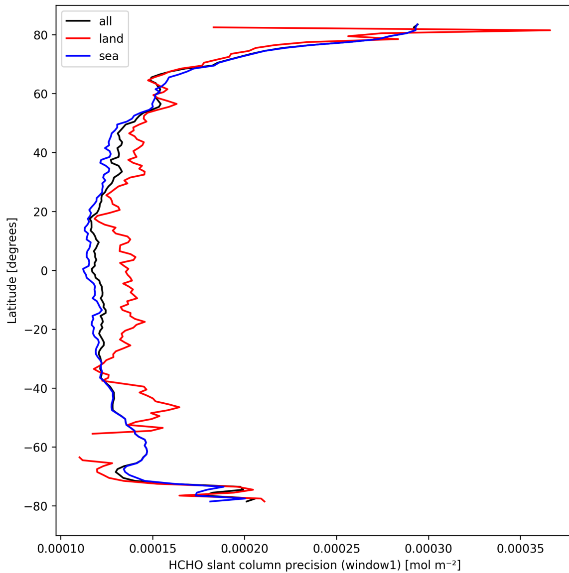
Figure 25: Zonal average of “HCHO slant column precision (window1)” for 2024-09-24 to 2024-09-26.
