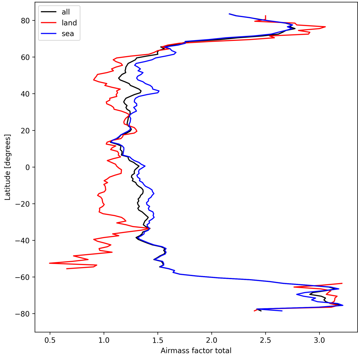
Figure 26: Zonal average of “Airmass factor total” for 2024-09-24 to 2024-09-26.
