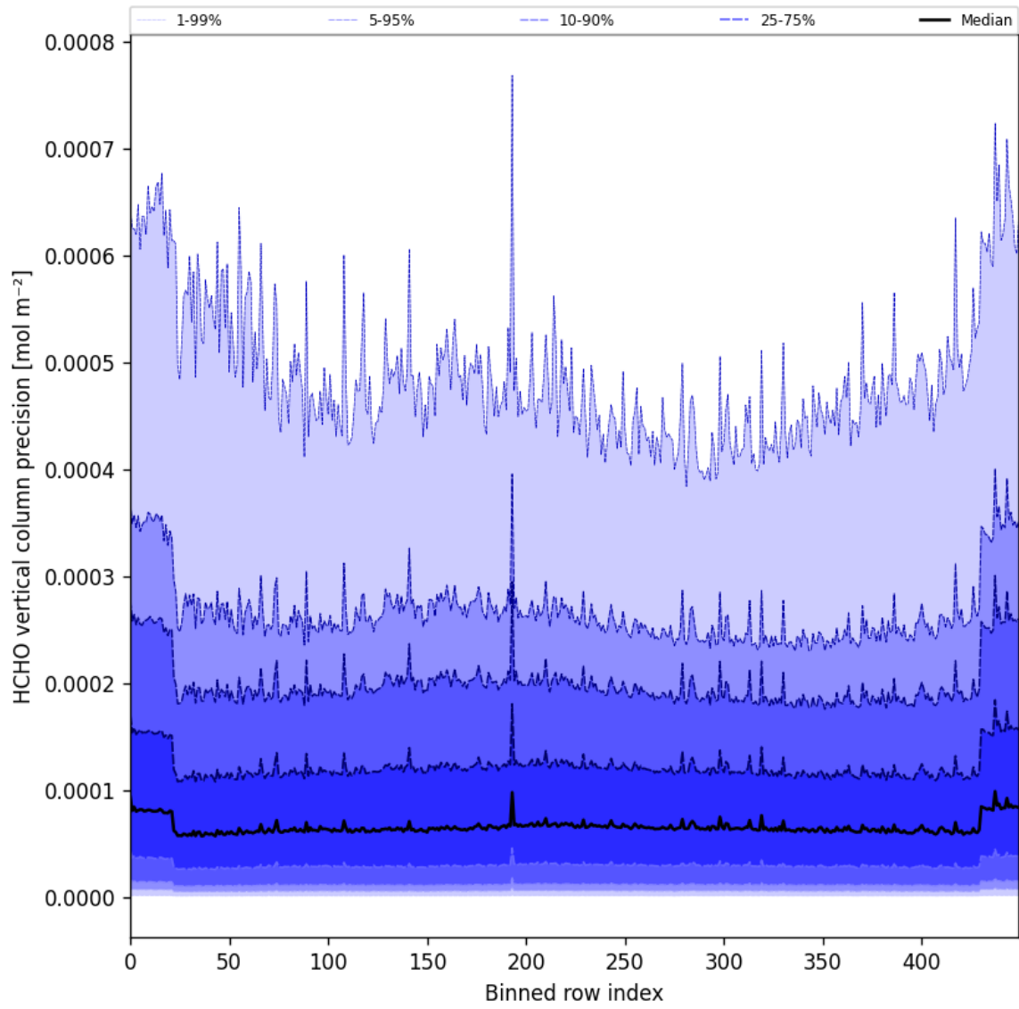
Figure 50: Along track statistics of “HCHO vertical column precision” for 2024-09-24 to 2024-09-26
