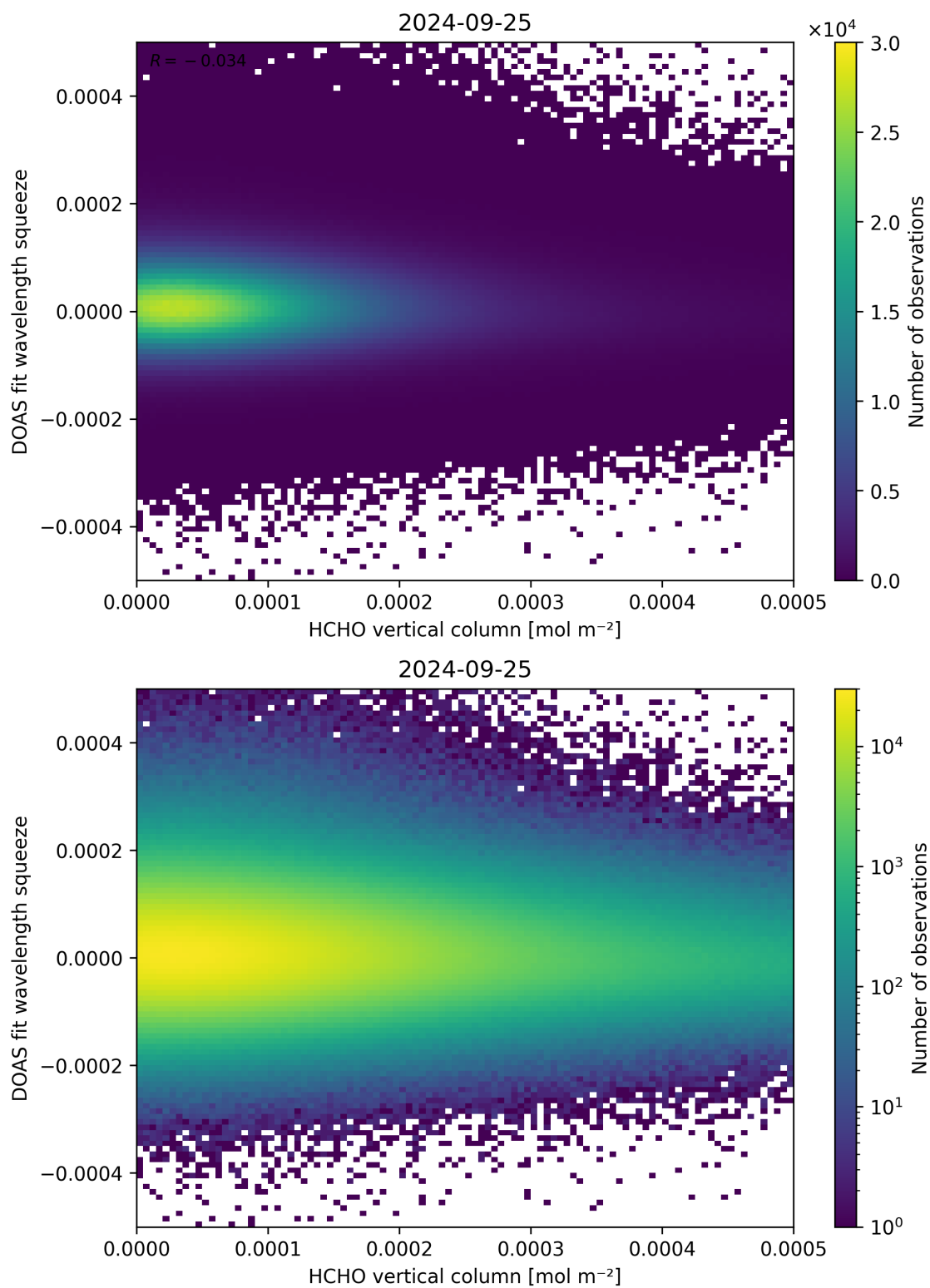
Figure 125: Scatter density plot of “HCHO vertical column” against “DOAS fit wavelength squeeze” for 2024-09-24 to 2024-09-26.
