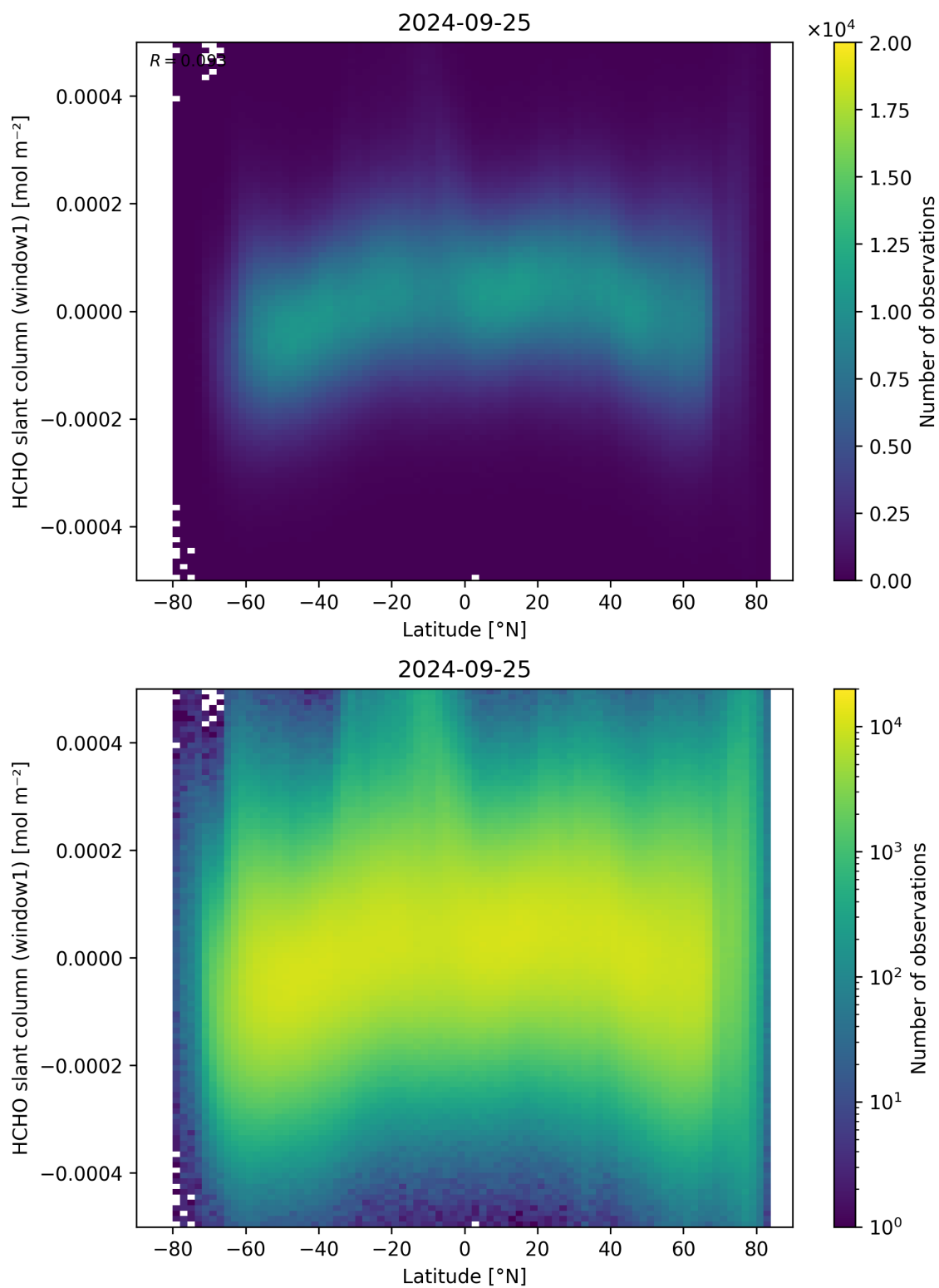
Figure 159: Scatter density plot of “Latitude” against “HCHO slant column (window1)” for 2024-09-24 to 2024-09-26.
