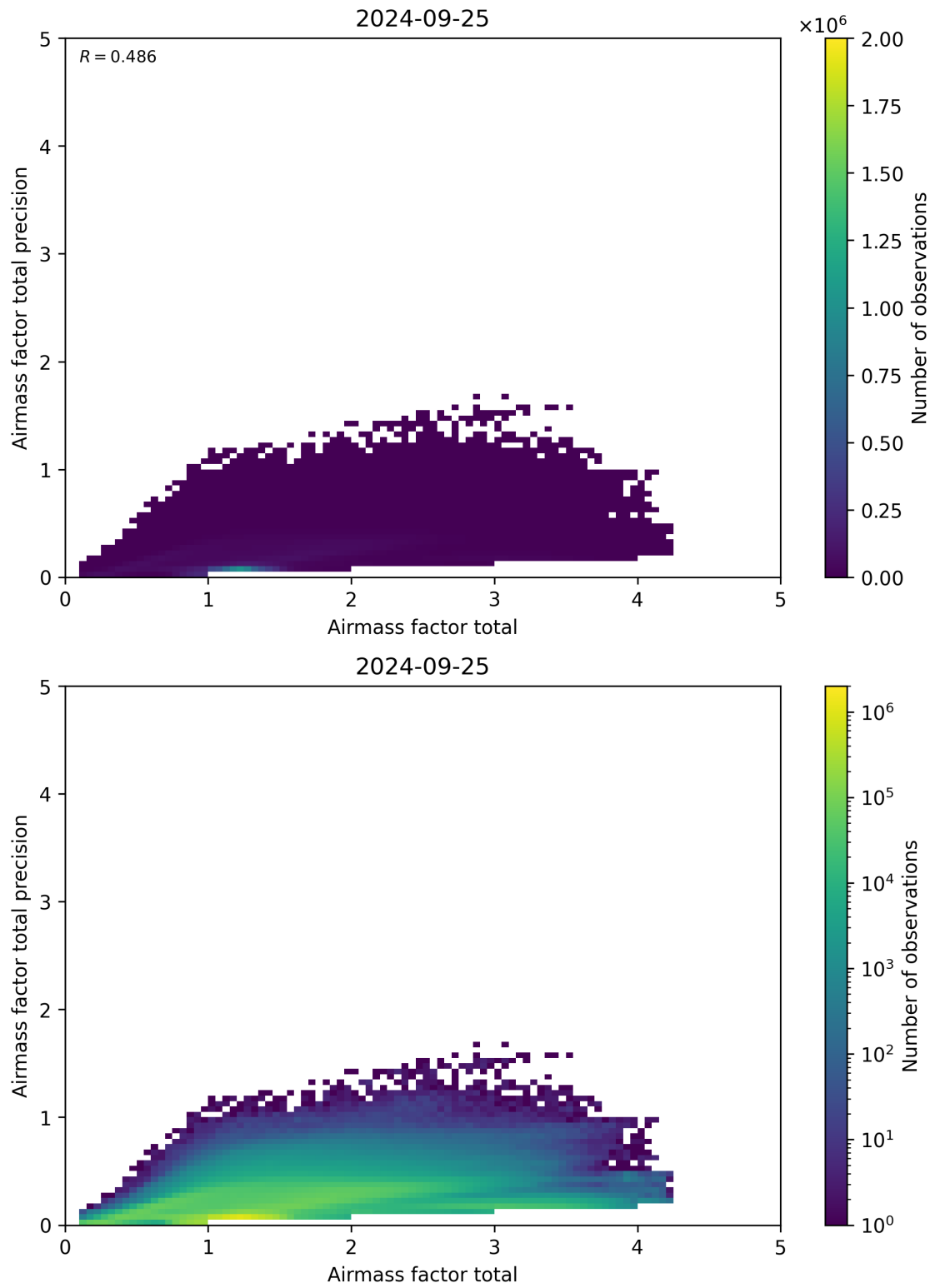
Figure 103: Scatter density plot of “Airmass factor total” against “Airmass factor total precision” for 2024-09-24 to 2024-09-26.
