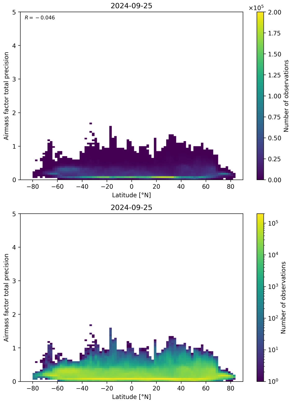
Figure 162: Scatter density plot of “Latitude” against “Airmass factor total precision” for 2024-09-24 to 2024-09-26.
