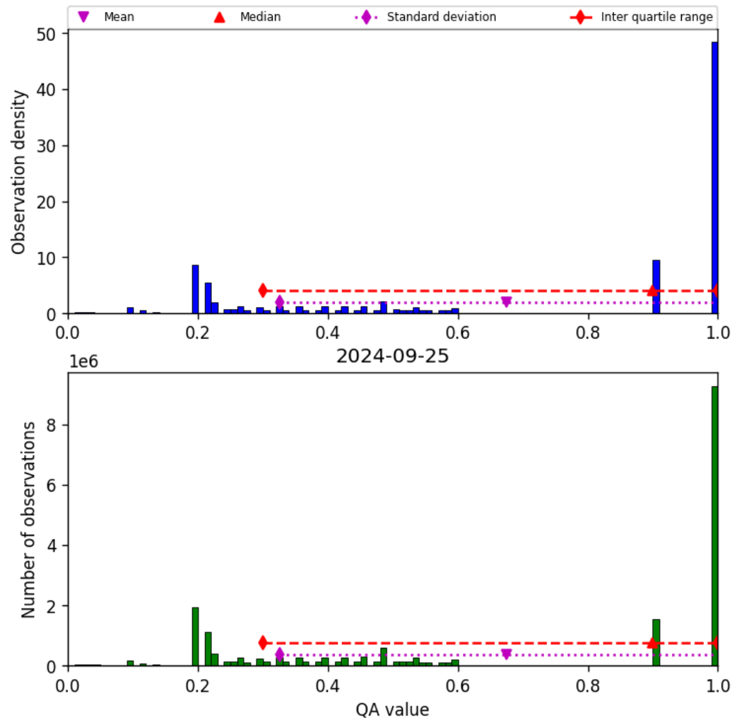
Figure 34: Histogram of “QA value” for 2024-09-24 to 2024-09-26
