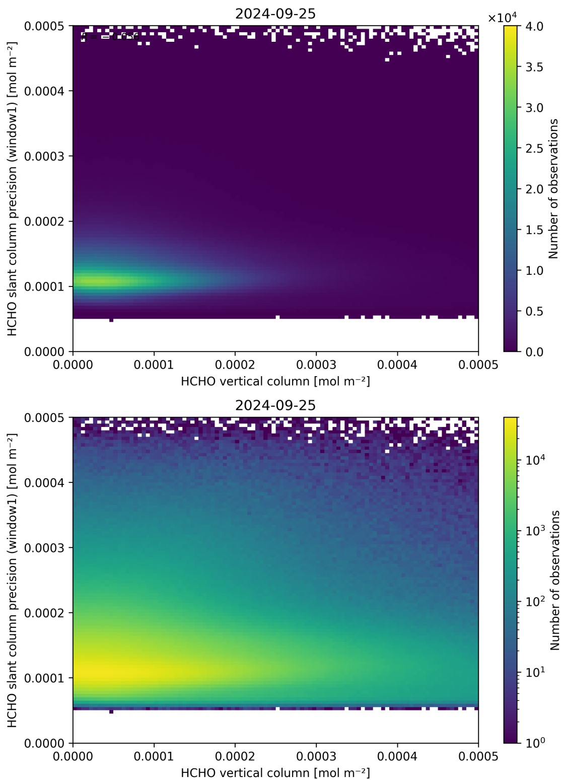
Figure 130: Scatter density plot of “HCHO vertical column” against “HCHO slant column precision (window1)” for 2024-09-24 to 2024-09-26.
