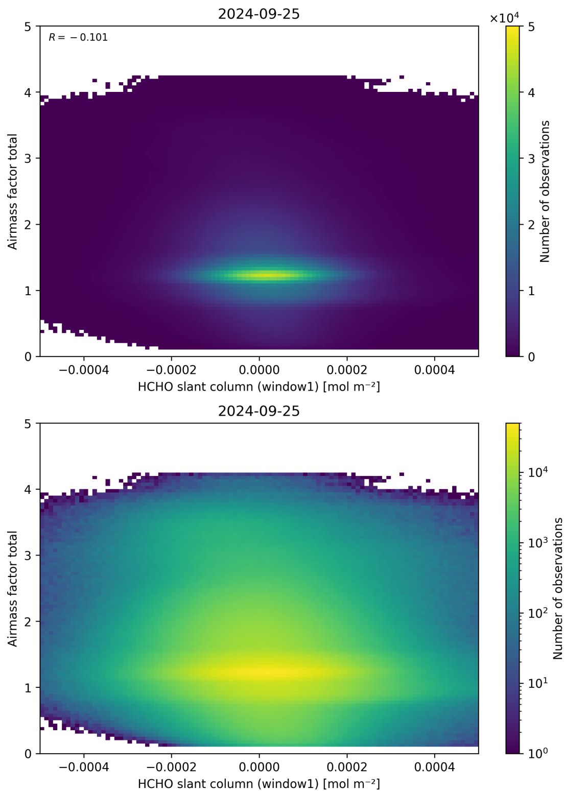
Figure 85: Scatter density plot of “HCHO slant column (window1)” against “Airmass factor total” for 2024-09-24 to 2024-09-26.
