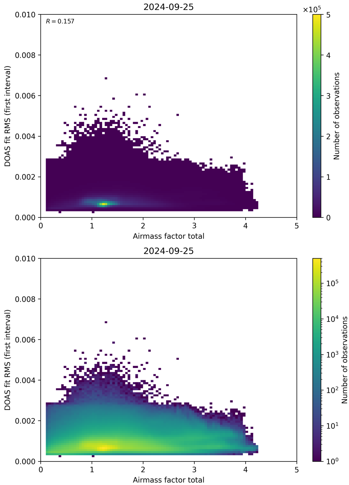
Figure 97: Scatter density plot of “Airmass factor total” against “DOAS fit RMS (first interval)” for 2024-09-24 to 2024-09-26.
