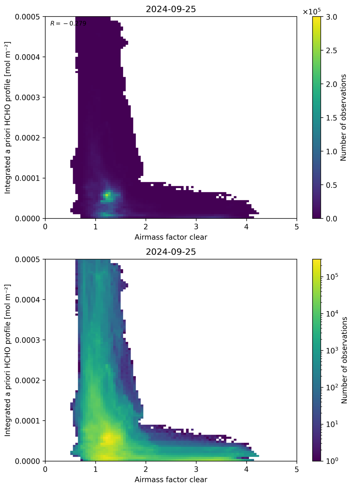
Figure 76: Scatter density plot of “Airmass factor clear” against “Integrated a priori HCHO profile” for 2024-09-24 to 2024-09-26.
