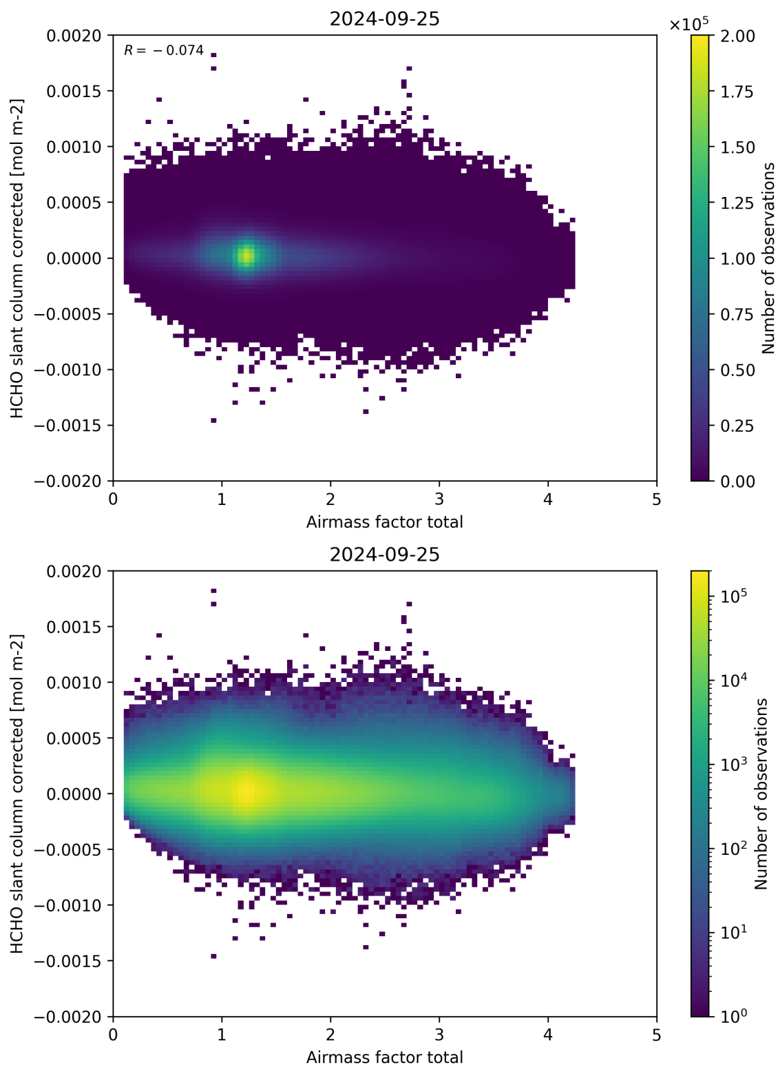
Figure 101: Scatter density plot of “Airmass factor total” against “HCHO slant column corrected” for 2024-09-24 to 2024-09-26.
