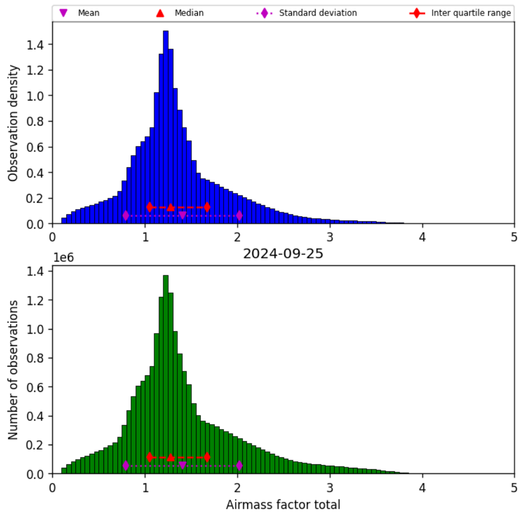
Figure 40: Histogram of “Airmass factor total” for 2024-09-24 to 2024-09-26
