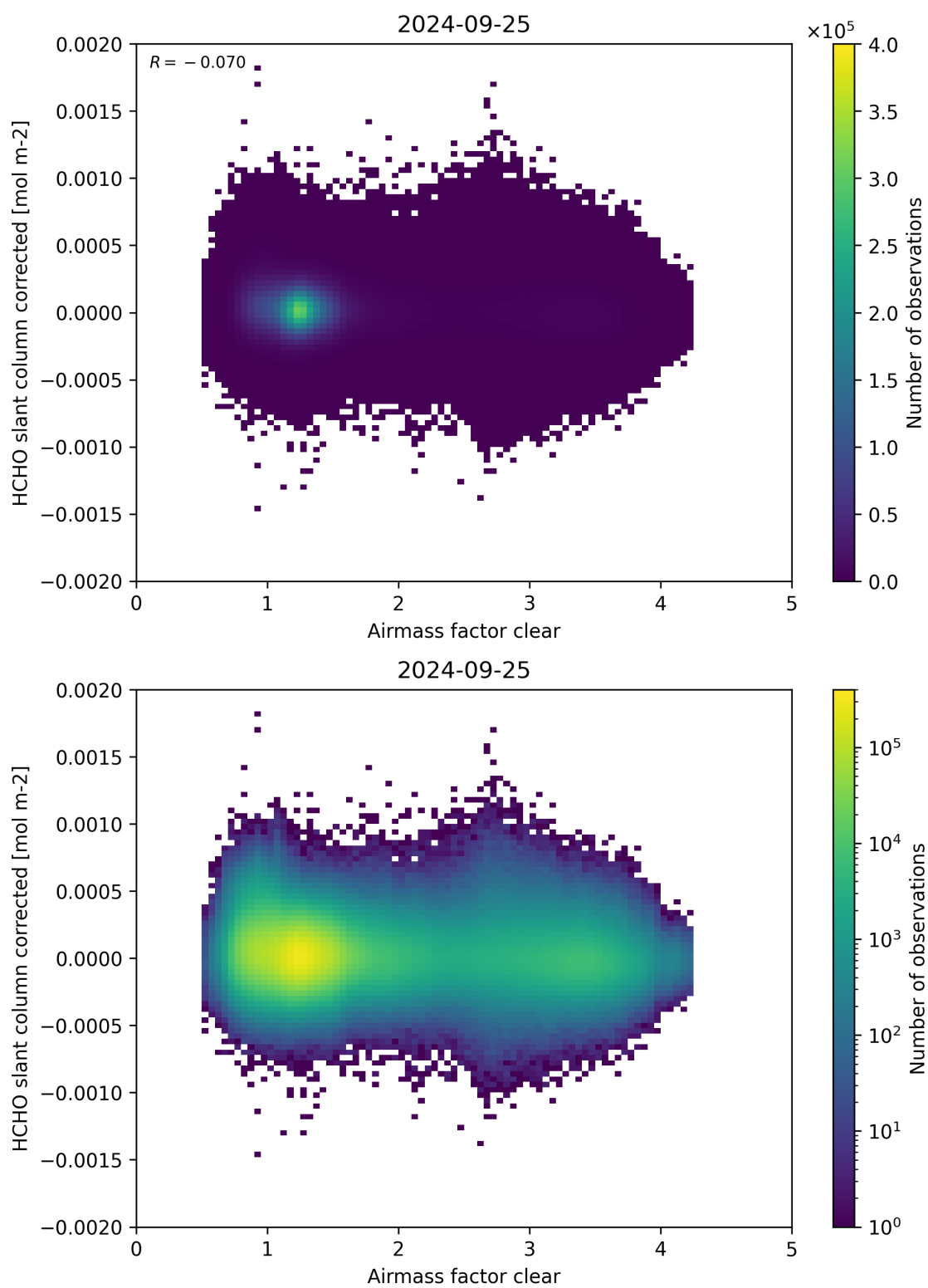
Figure 74: Scatter density plot of “Airmass factor clear” against “HCHO slant column corrected” for 2024-09-24 to 2024-09-26.
