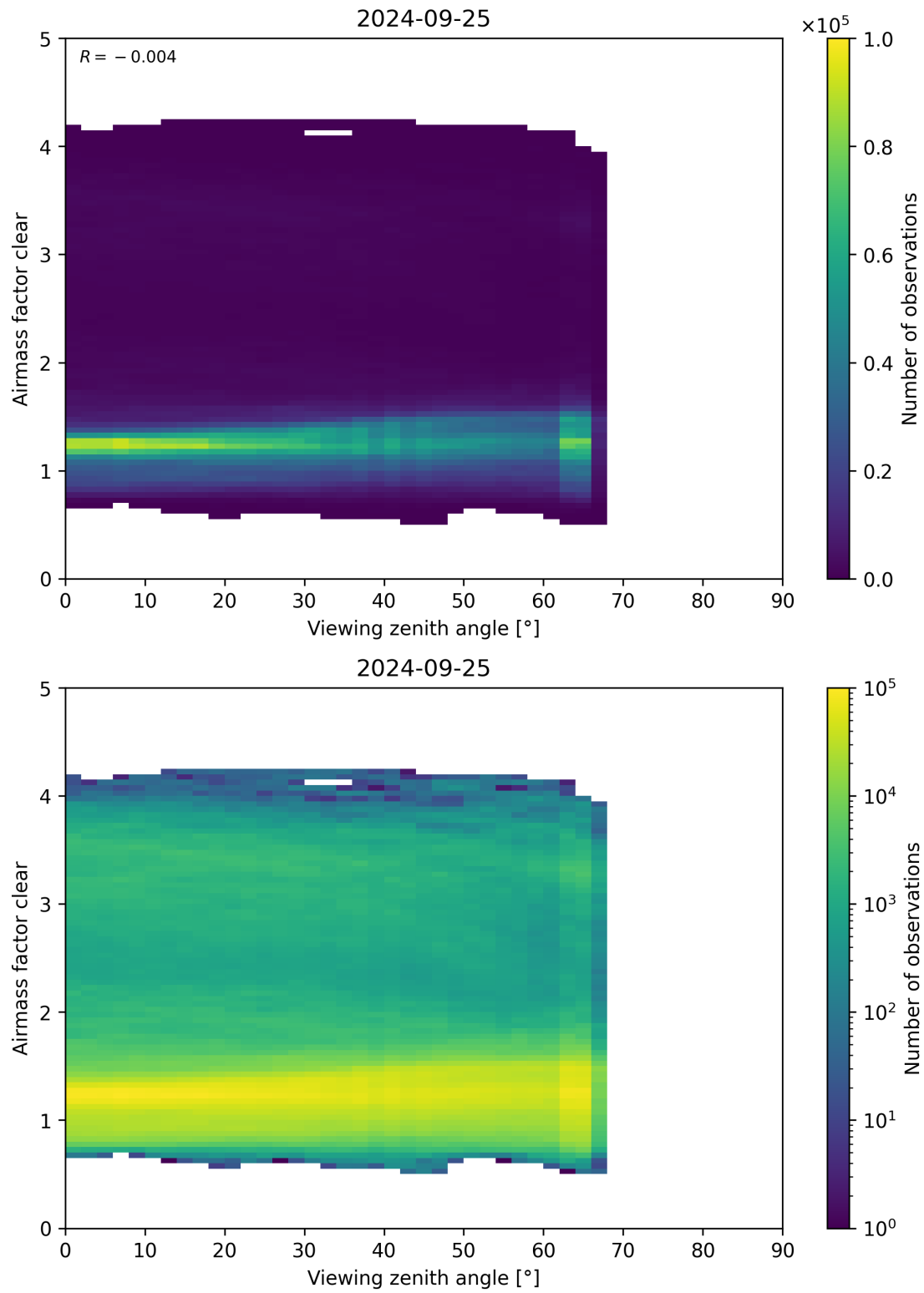
Figure 185: Scatter density plot of “Viewing zenith angle” against “Airmass factor clear” for 2024-09-24 to 2024-09-26.
