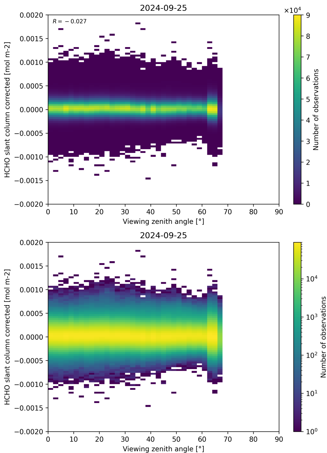
Figure 186: Scatter density plot of “Viewing zenith angle” against “HCHO slant column corrected” for 2024-09-24 to 2024-09-26.
