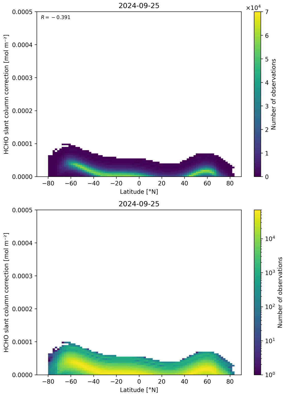
Figure 158: Scatter density plot of “Latitude” against “HCHO slant column correction” for 2024-09-24 to 2024-09-26.
