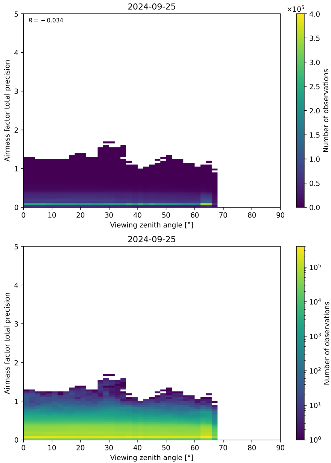
Figure 191: Scatter density plot of “Viewing zenith angle” against “Airmass factor total precision” for 2024-09-24 to 2024-09-26.
