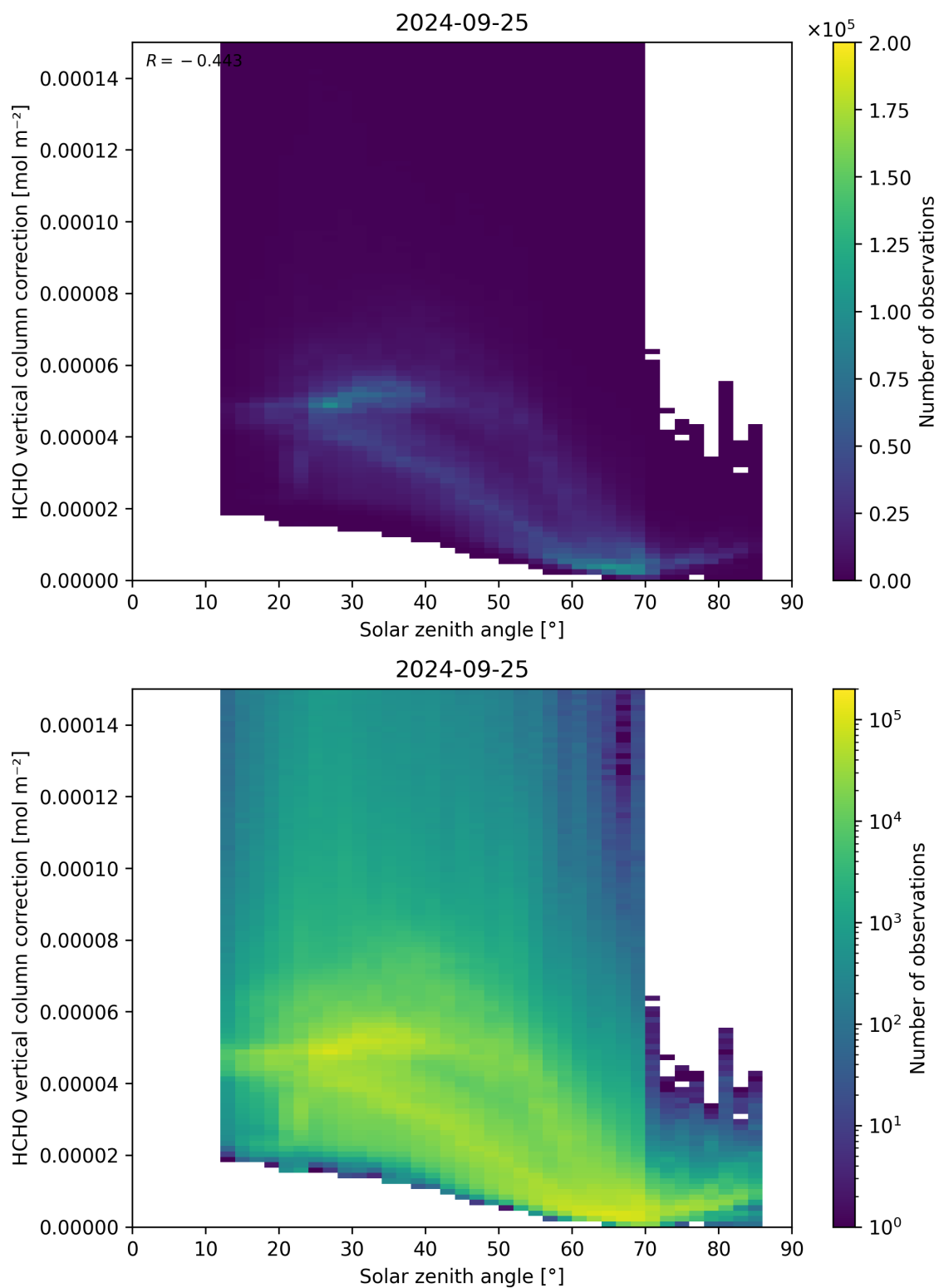
Figure 178: Scatter density plot of “Solar zenith angle” against “HCHO vertical column correction” for 2024-09-24 to 2024-09-26.
