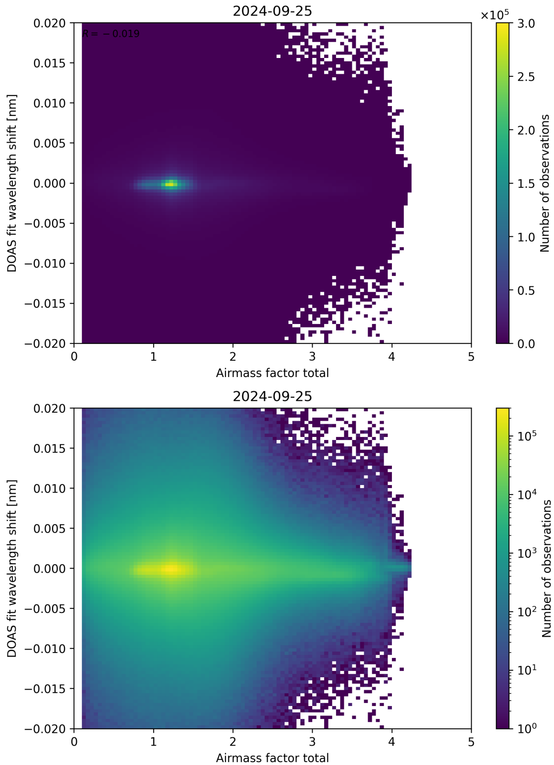
Figure 98: Scatter density plot of “Airmass factor total” against “DOAS fit wavelength shift” for 2024-09-24 to 2024-09-26.
