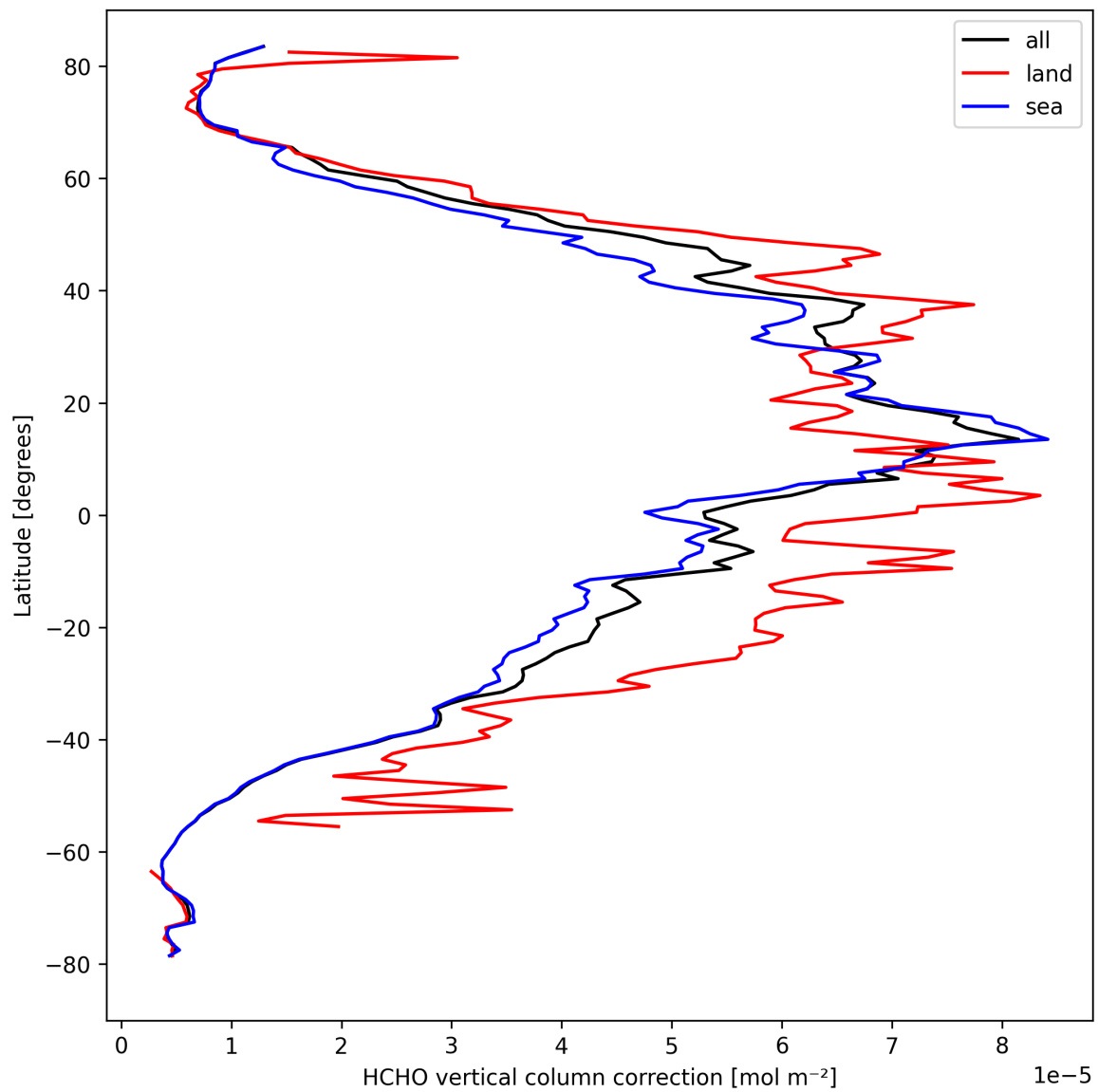
Figure 23: Zonal average of “HCHO vertical column correction” for 2024-09-24 to 2024-09-26.
