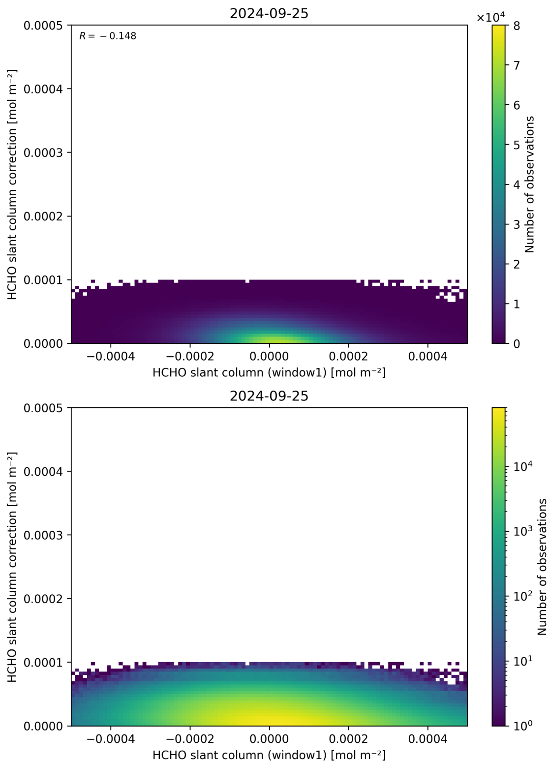
Figure 83: Scatter density plot of “HCHO slant column (window1)” against “HCHO slant column correction” for 2024-09-24 to 2024-09-26.
