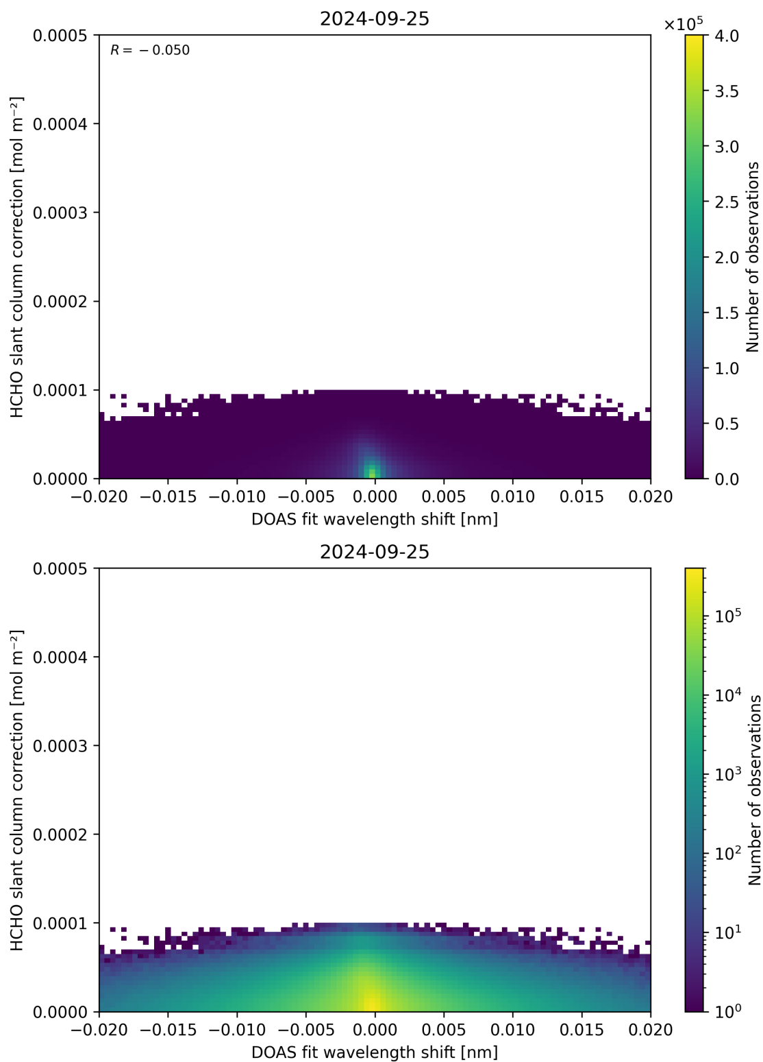
Figure 67: Scatter density plot of “DOAS fit wavelength shift” against “HCHO slant column correction” for 2024-09-24 to 2024-09-26.
