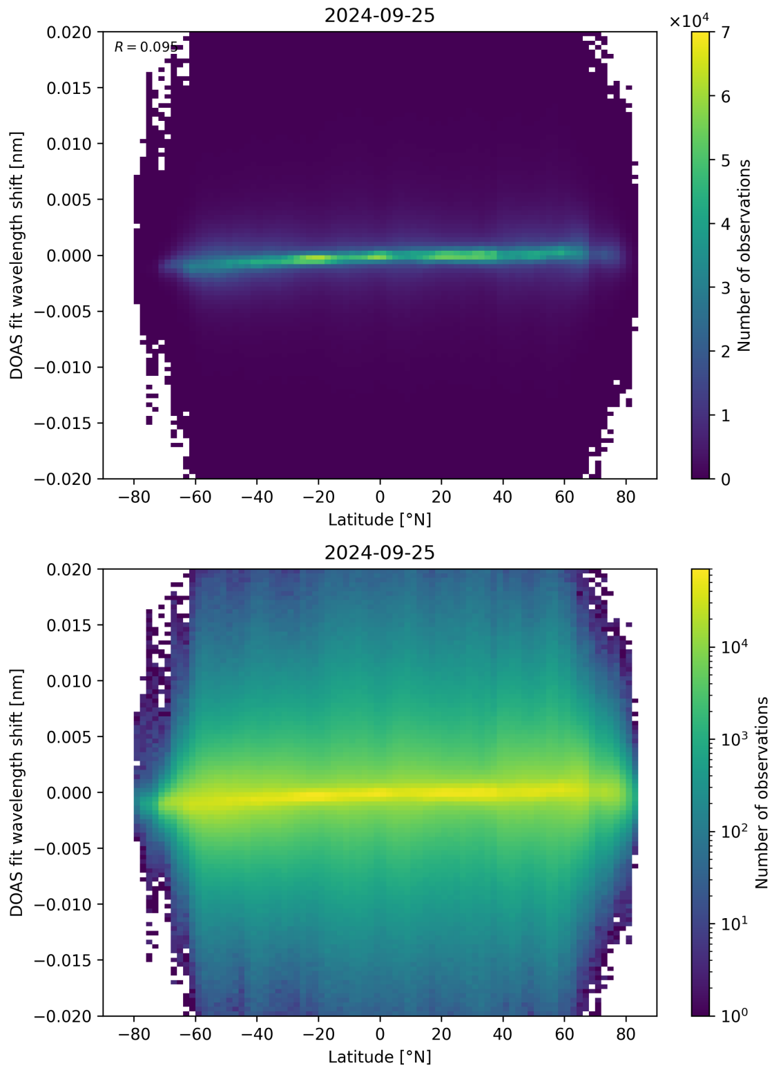
Figure 154: Scatter density plot of “Latitude” against “DOAS fit wavelength shift” for 2024-09-24 to 2024-09-26.
