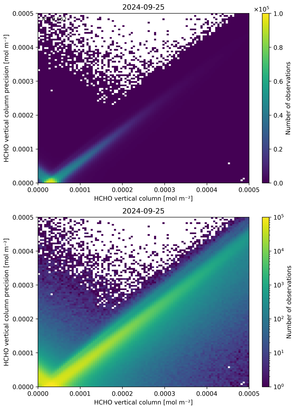
Figure 134: Scatter density plot of “HCHO vertical column” against “HCHO vertical column precision” for 2024-09-24 to 2024-09-26.
