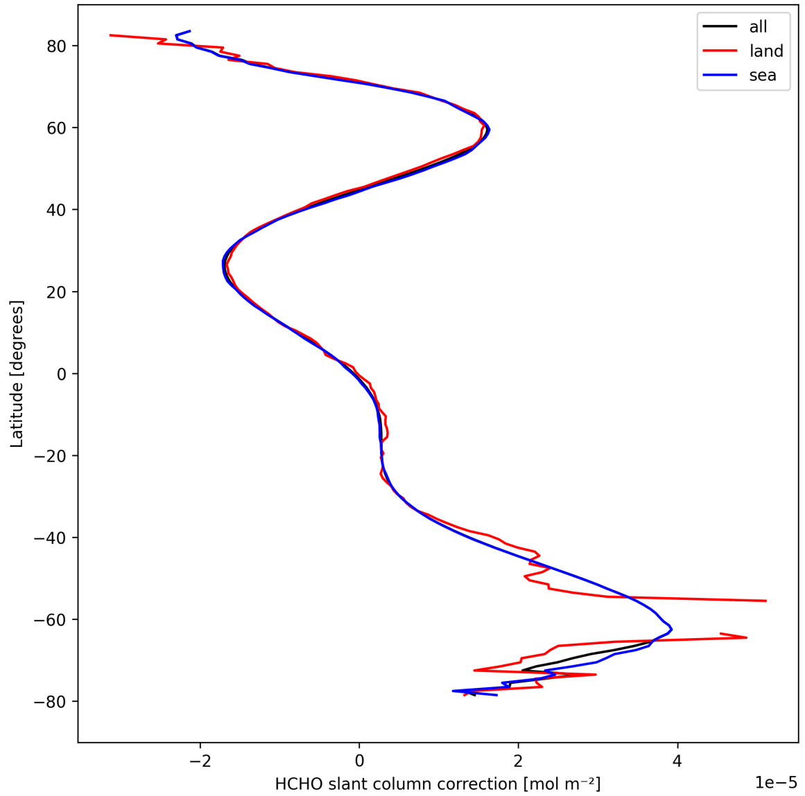
Figure 33: Zonal average of “HCHO slant column correction” for 2024-09-24 to 2024-09-26.
