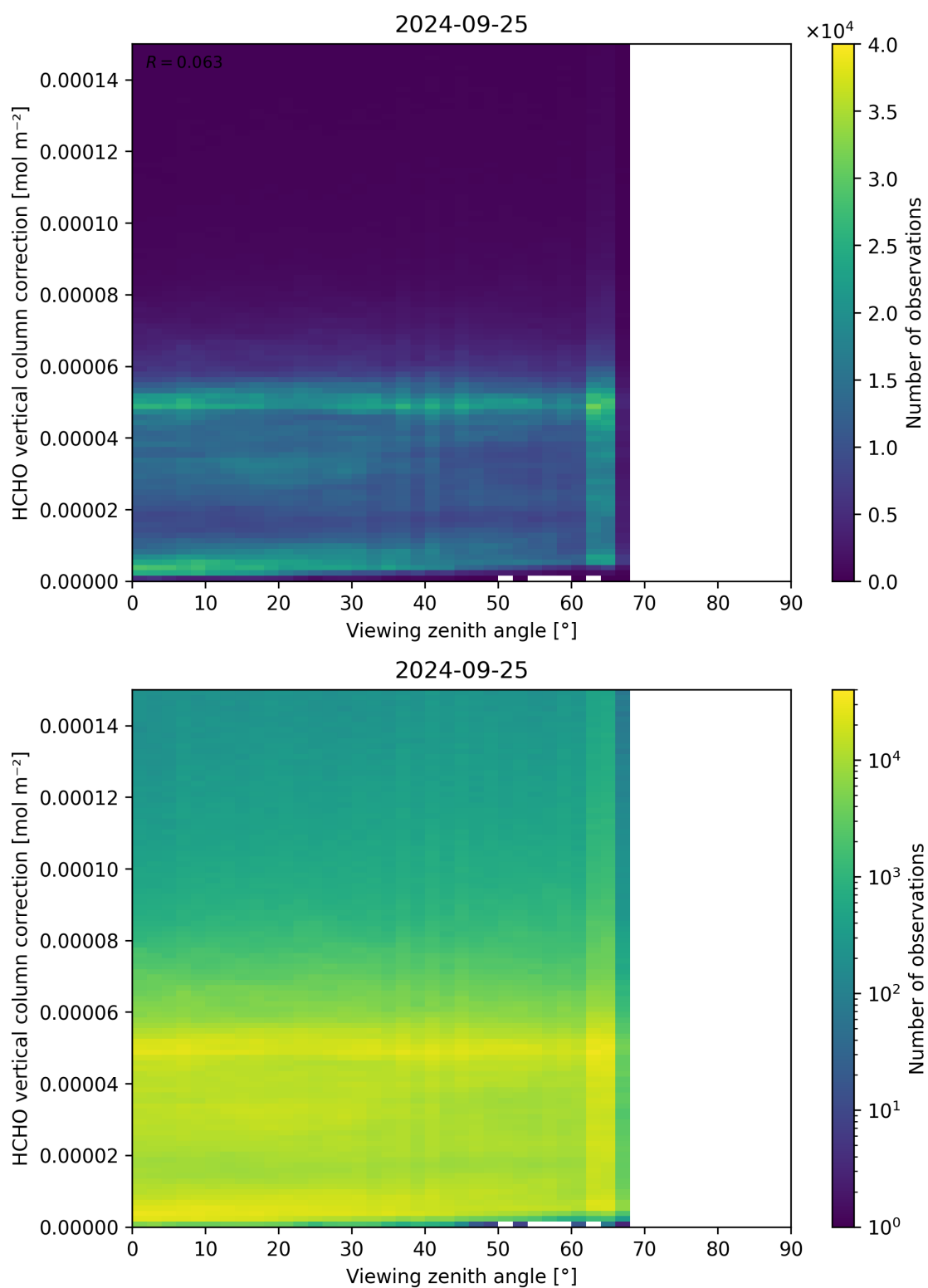
Figure 193: Scatter density plot of “Viewing zenith angle” against “HCHO vertical column correction” for 2024-09-24 to 2024-09-26.
