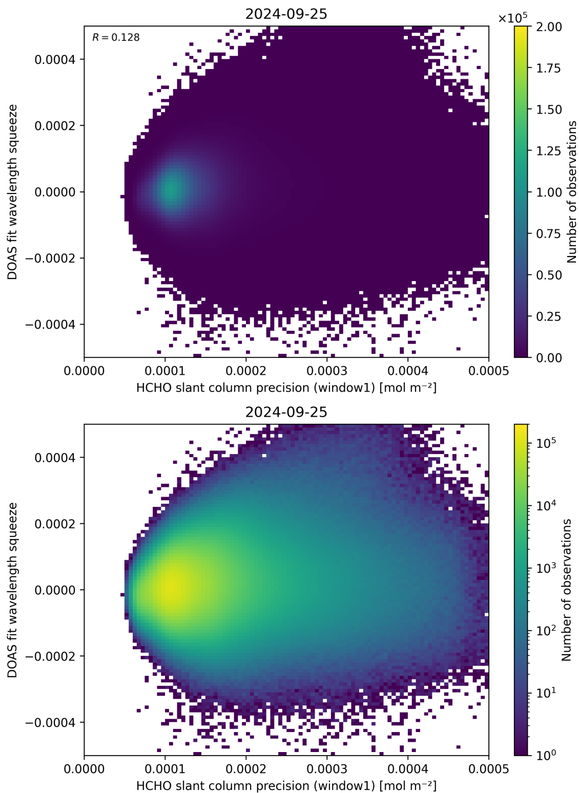
Figure 90: Scatter density plot of “HCHO slant column precision (window1)” against “DOAS fit wavelength squeeze” for 2024-09-24 to 2024-09-26.
