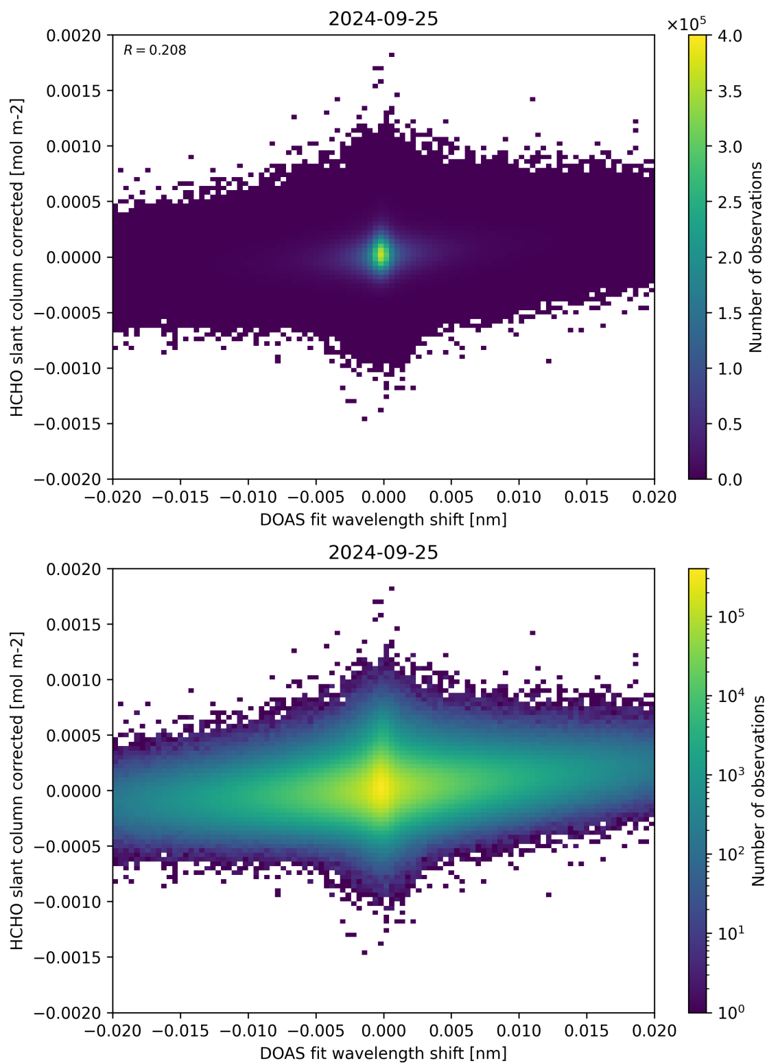
Figure 66: Scatter density plot of “DOAS fit wavelength shift” against “HCHO slant column corrected” for 2024-09-24 to 2024-09-26.
