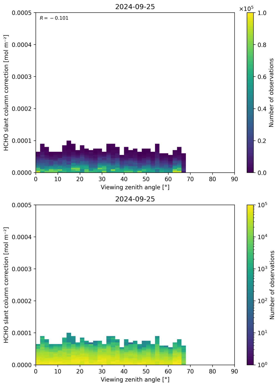
Figure 187: Scatter density plot of “Viewing zenith angle” against “HCHO slant column correction” for 2024-09-24 to 2024-09-26.
