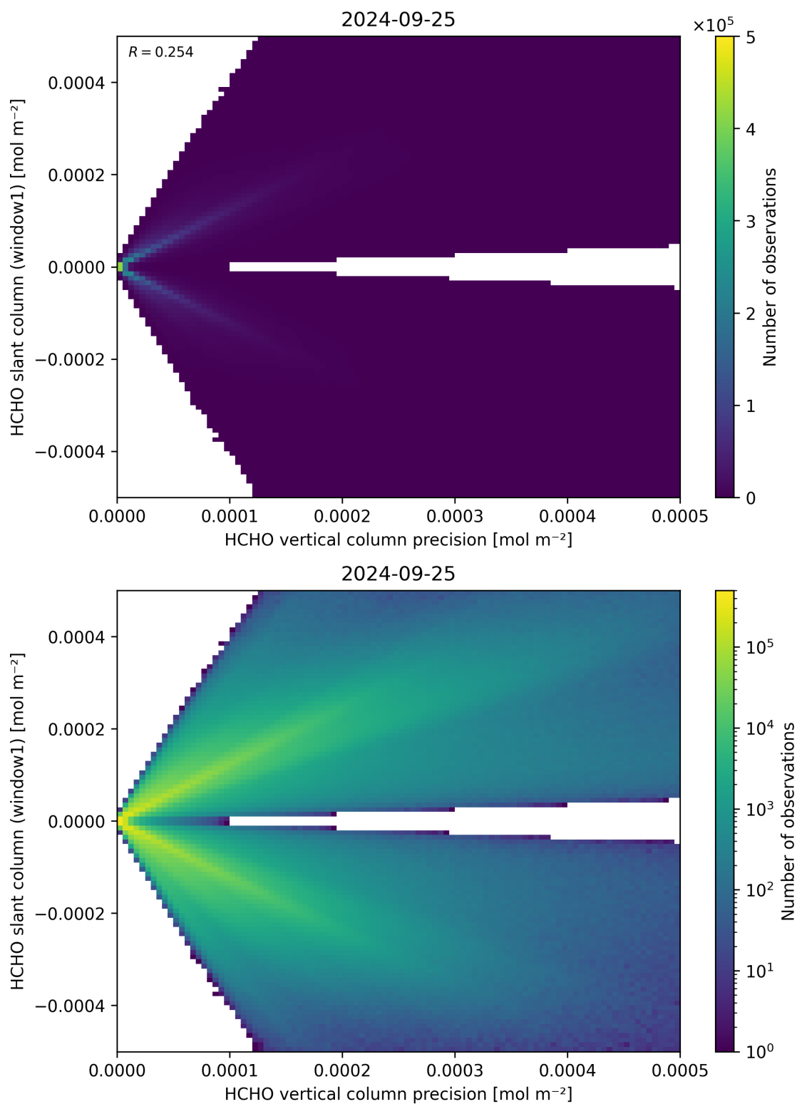
Figure 142: Scatter density plot of “HCHO vertical column precision” against “HCHO slant column (window1)” for 2024-09-24 to 2024-09-26.
