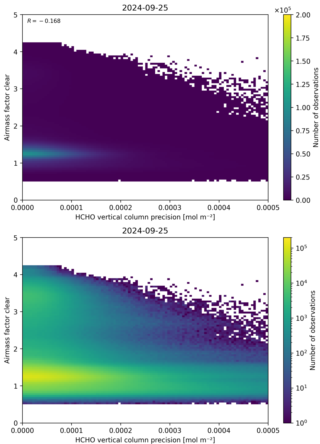
Figure 139: Scatter density plot of “HCHO vertical column precision” against “Airmass factor clear” for 2024-09-24 to 2024-09-26.
