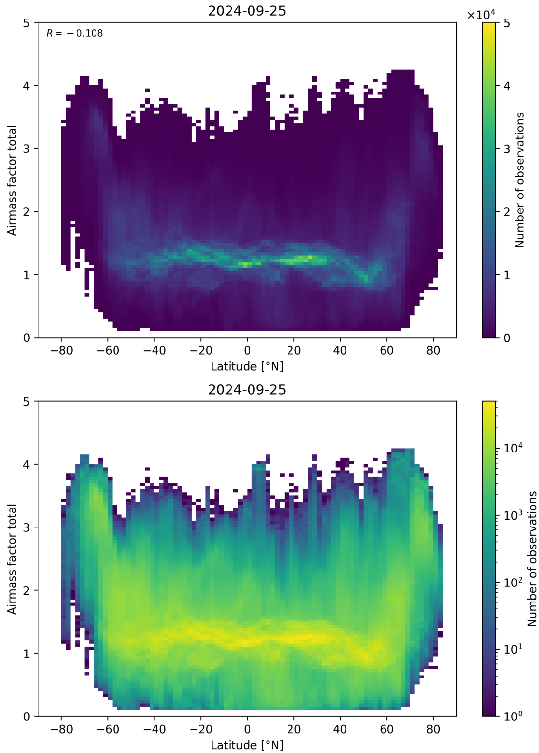
Figure 161: Scatter density plot of “Latitude” against “Airmass factor total” for 2024-09-24 to 2024-09-26.
