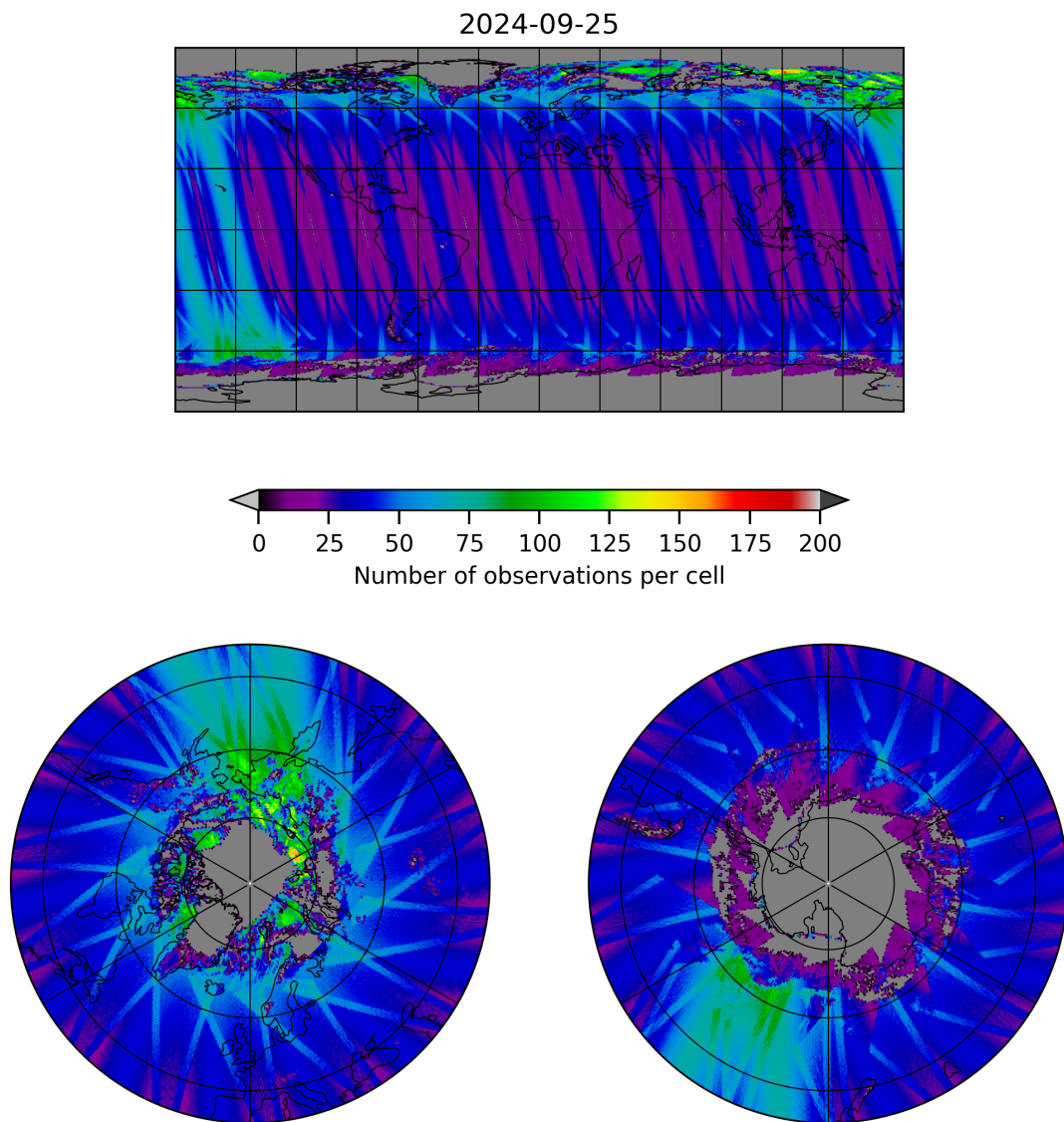
Figure 19: Map of the number of observations for 2024-09-24 to 2024-09-26
