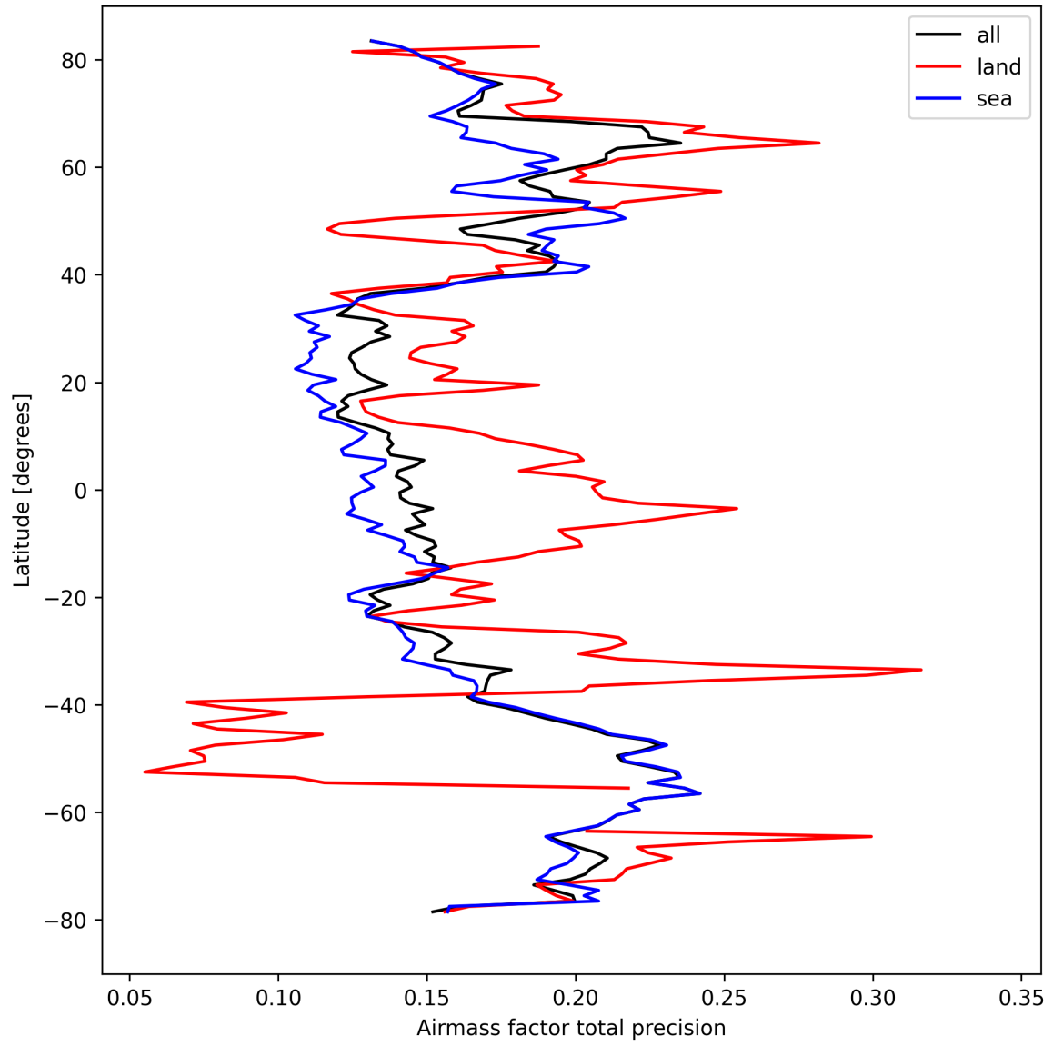
Figure 27: Zonal average of “Airmass factor total precision” for 2024-09-24 to 2024-09-26.
