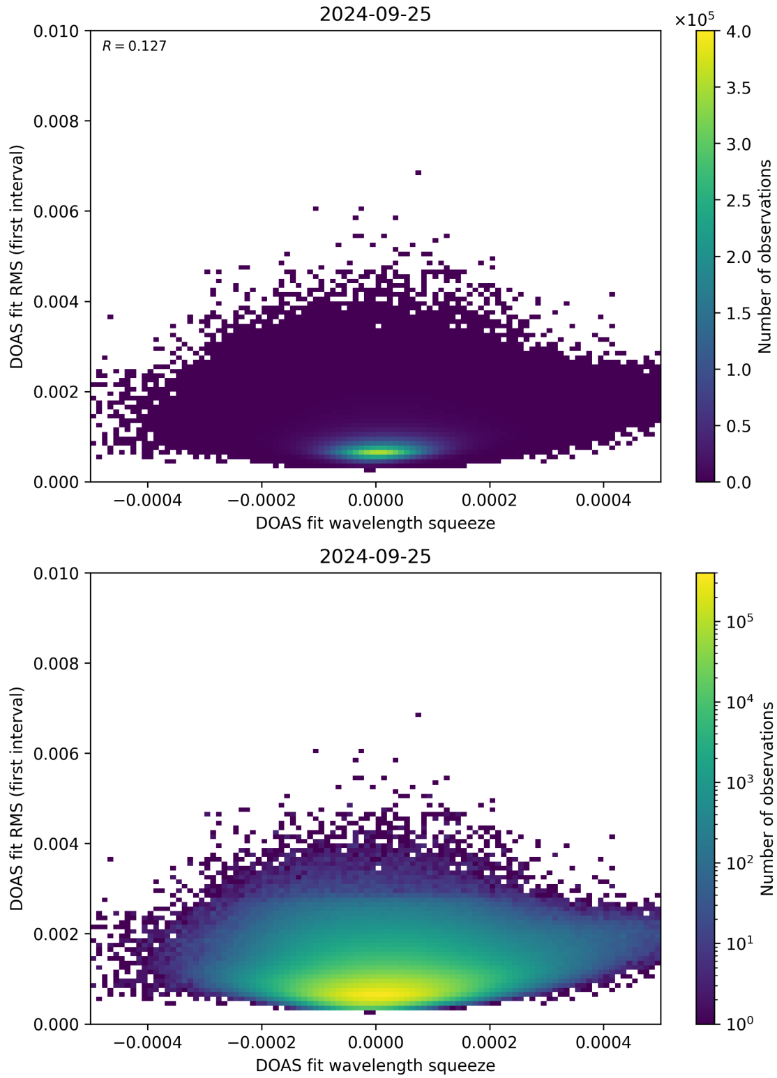
Figure 68: Scatter density plot of “DOAS fit wavelength squeeze” against “DOAS fit RMS (first interval)” for 2024-09-24 to 2024-09-26.
