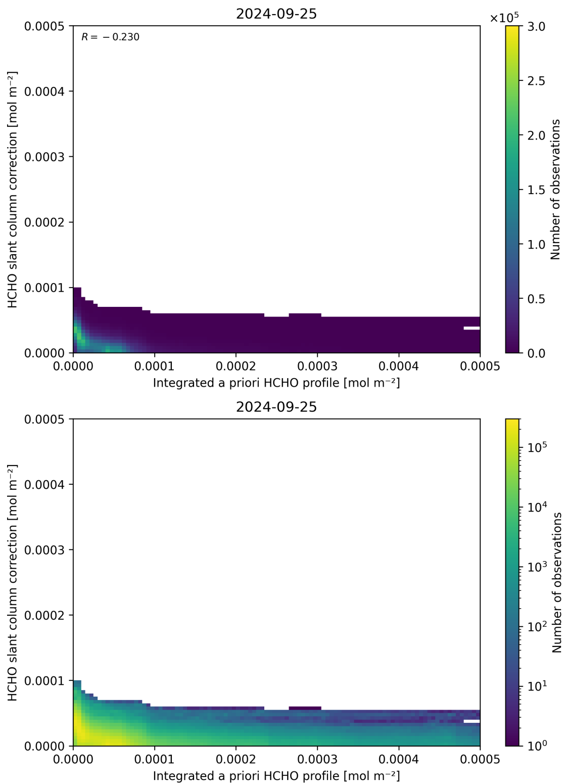
Figure 152: Scatter density plot of “Integrated a priori HCHO profile” against “HCHO slant column correction” for 2024-09-24 to 2024-09-26.
