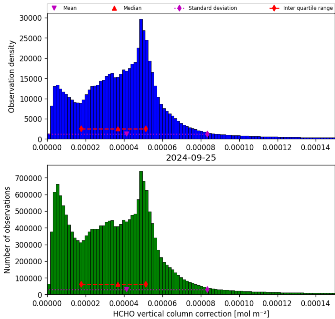
Figure 37: Histogram of “HCHO vertical column correction” for 2024-09-24 to 2024-09-26
