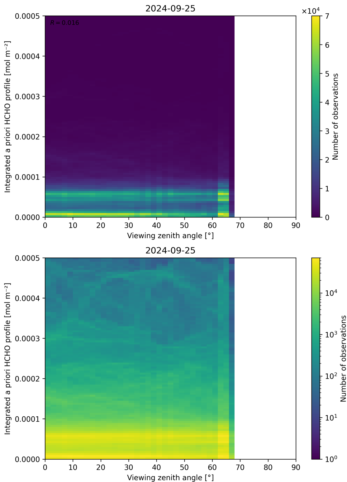
Figure 195: Scatter density plot of “Viewing zenith angle” against “Integrated a priori HCHO profile” for 2024-09-24 to 2024-09-26.
