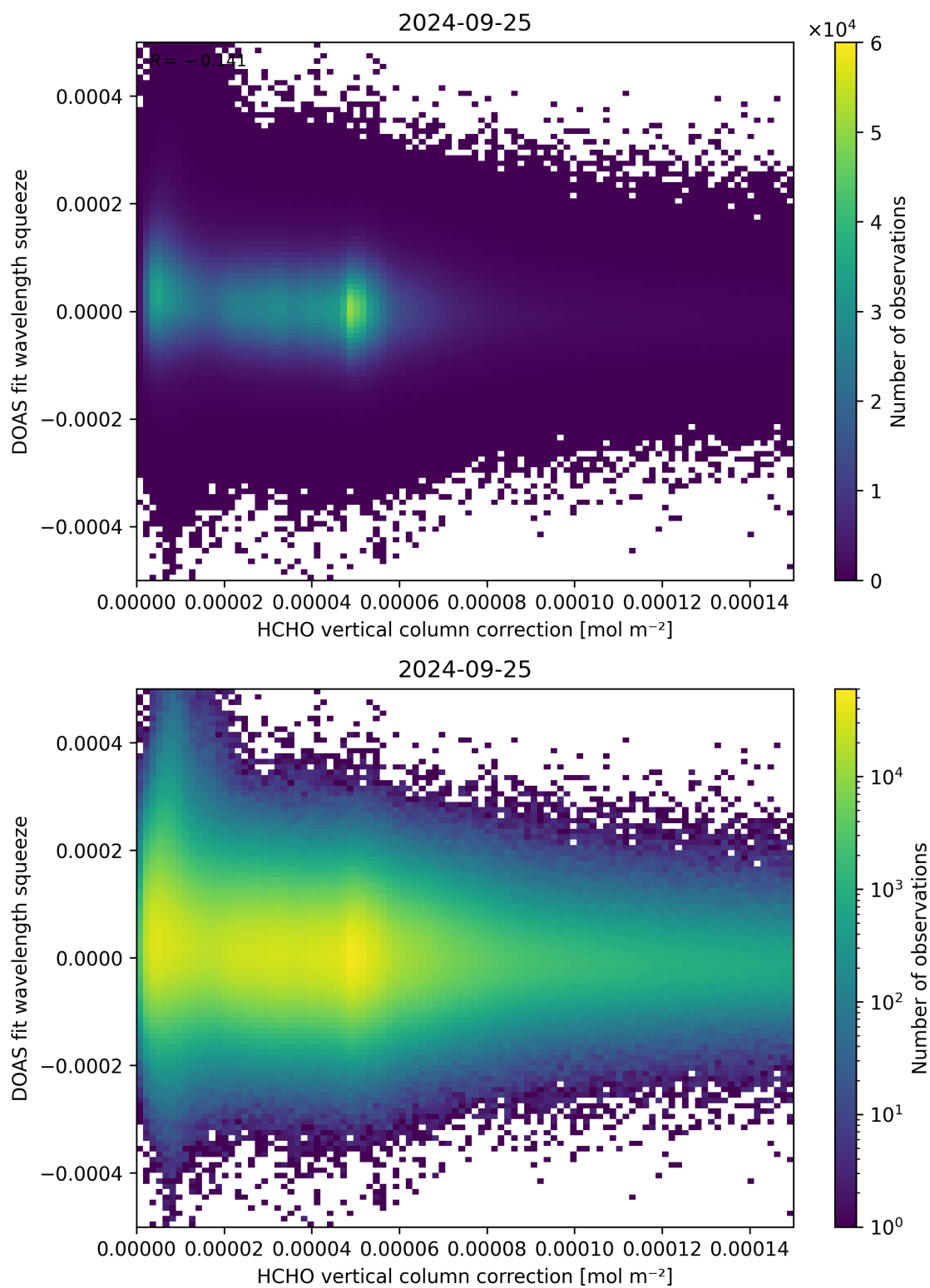
Figure 114: Scatter density plot of “HCHO vertical column correction” against “DOAS fit wavelength squeeze” for 2024-09-24 to 2024-09-26.
