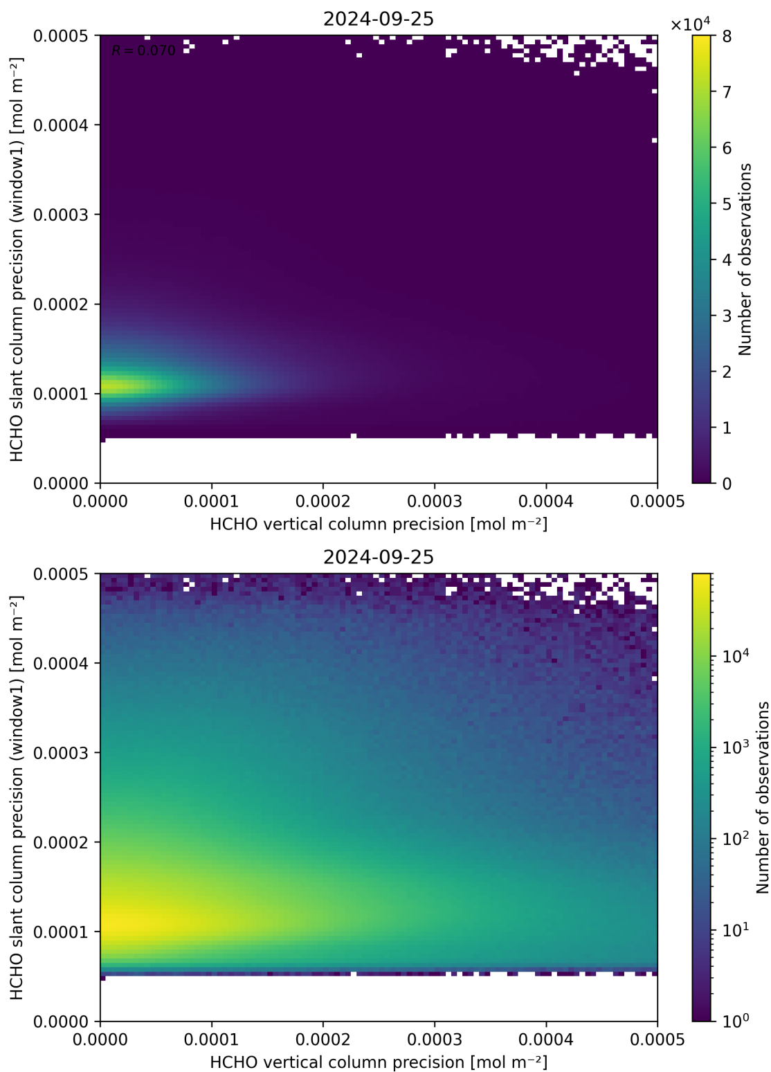
Figure 143: Scatter density plot of “HCHO vertical column precision” against “HCHO slant column precision (window1)” for 2024-09-24 to 2024-09-26.
