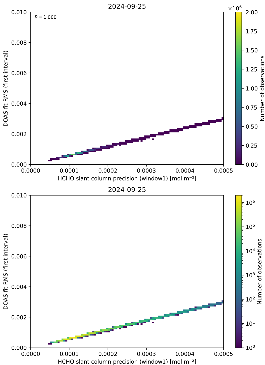
Figure 88: Scatter density plot of “HCHO slant column precision (window1)” against “DOAS fit RMS (first interval)” for 2024-09-24 to 2024-09-26.
