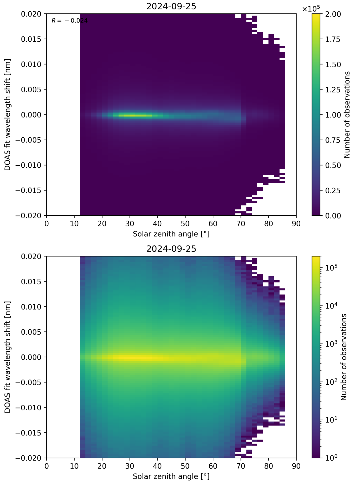
Figure 168: Scatter density plot of “Solar zenith angle” against “DOAS fit wavelength shift” for 2024-09-24 to 2024-09-26.
