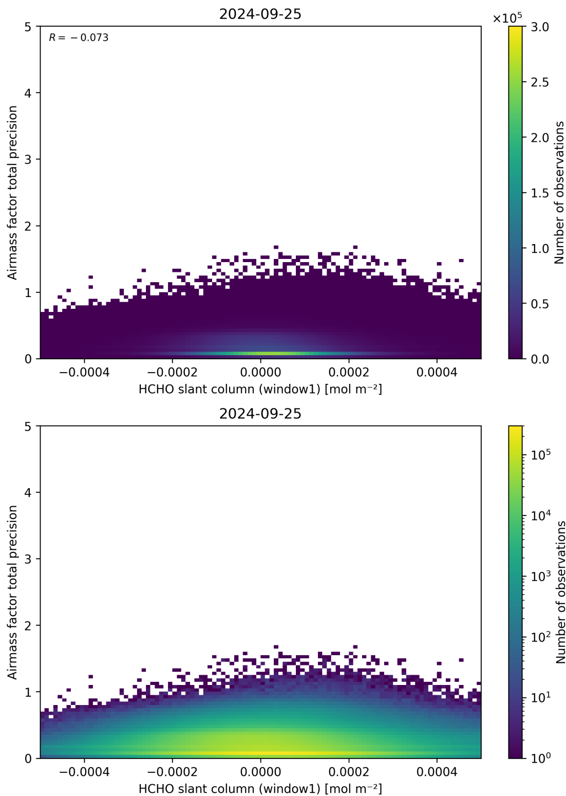
Figure 86: Scatter density plot of “HCHO slant column (window1)” against “Airmass factor total precision” for 2024-09-24 to 2024-09-26.
