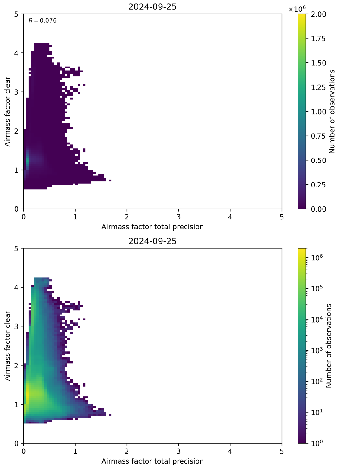
Figure 108: Scatter density plot of “Airmass factor total precision” against “Airmass factor clear” for 2024-09-24 to 2024-09-26.
