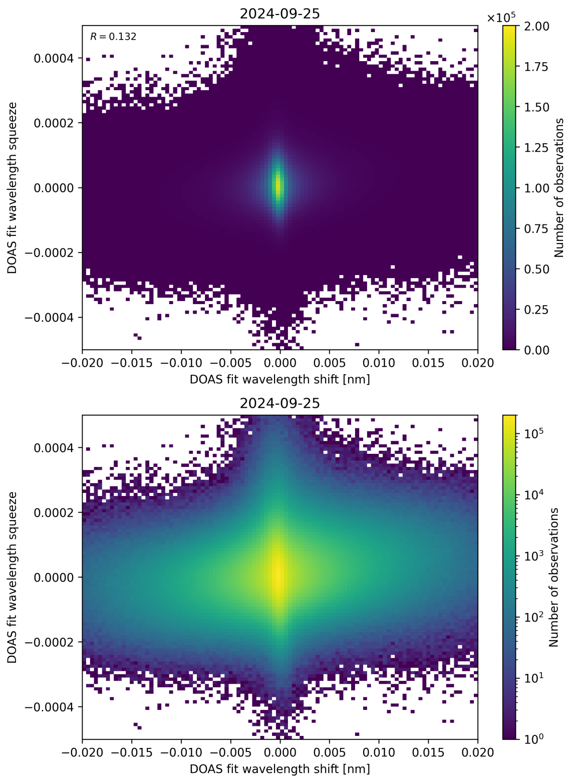
Figure 65: Scatter density plot of “DOAS fit wavelength shift” against “DOAS fit wavelength squeeze” for 2024-09-24 to 2024-09-26.
