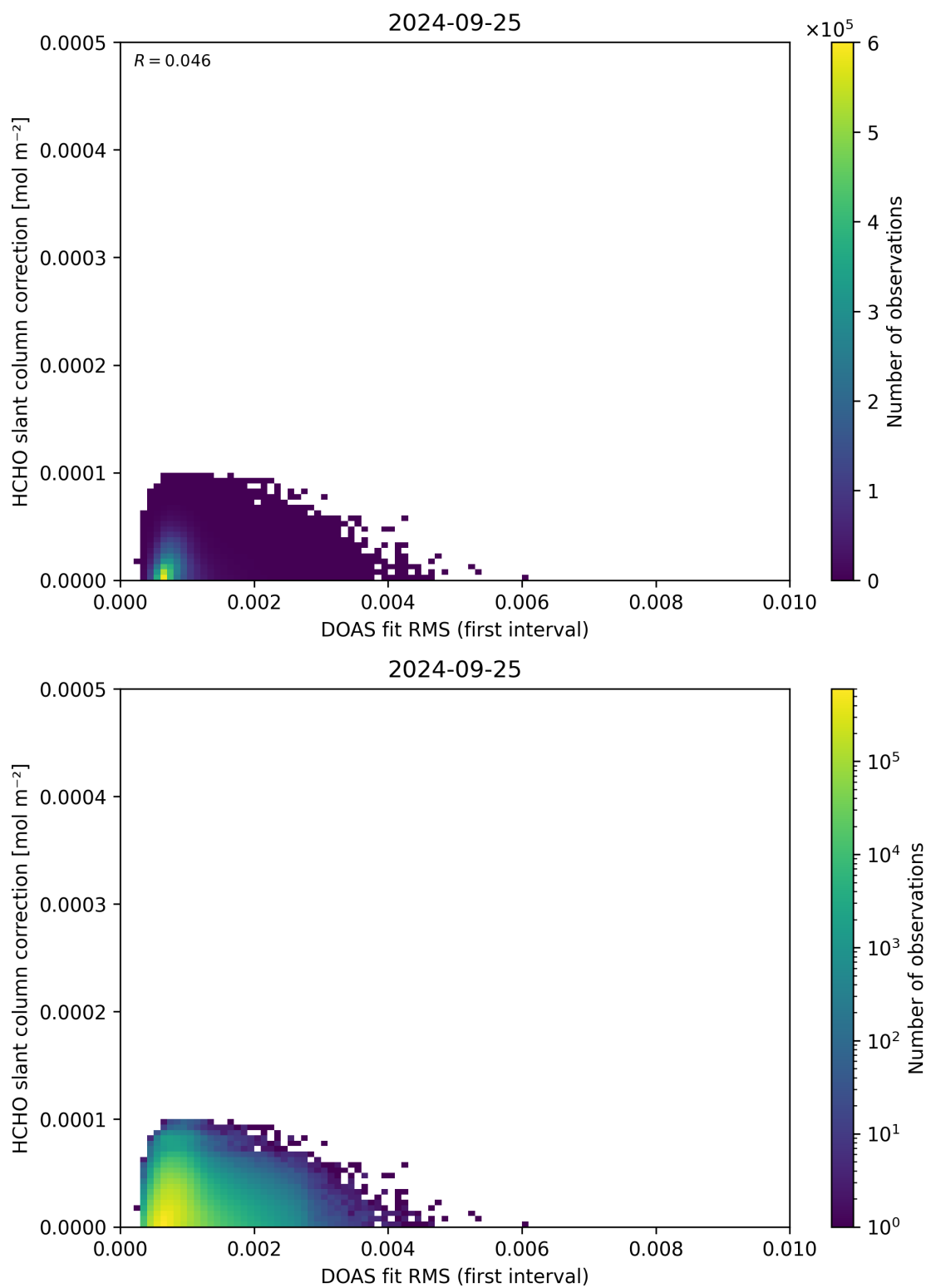
Figure 63: Scatter density plot of “DOAS fit RMS (first interval)” against “HCHO slant column correction” for 2024-09-24 to 2024-09-26.
