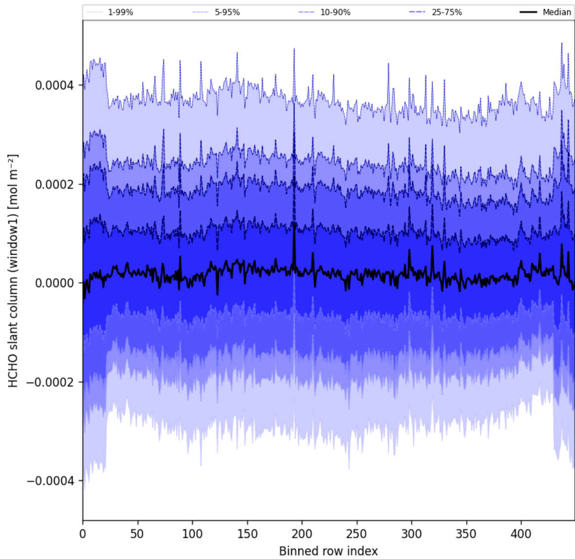
Figure 52: Along track statistics of “HCHO slant column (window1)” for 2024-09-24 to 2024-09-26
