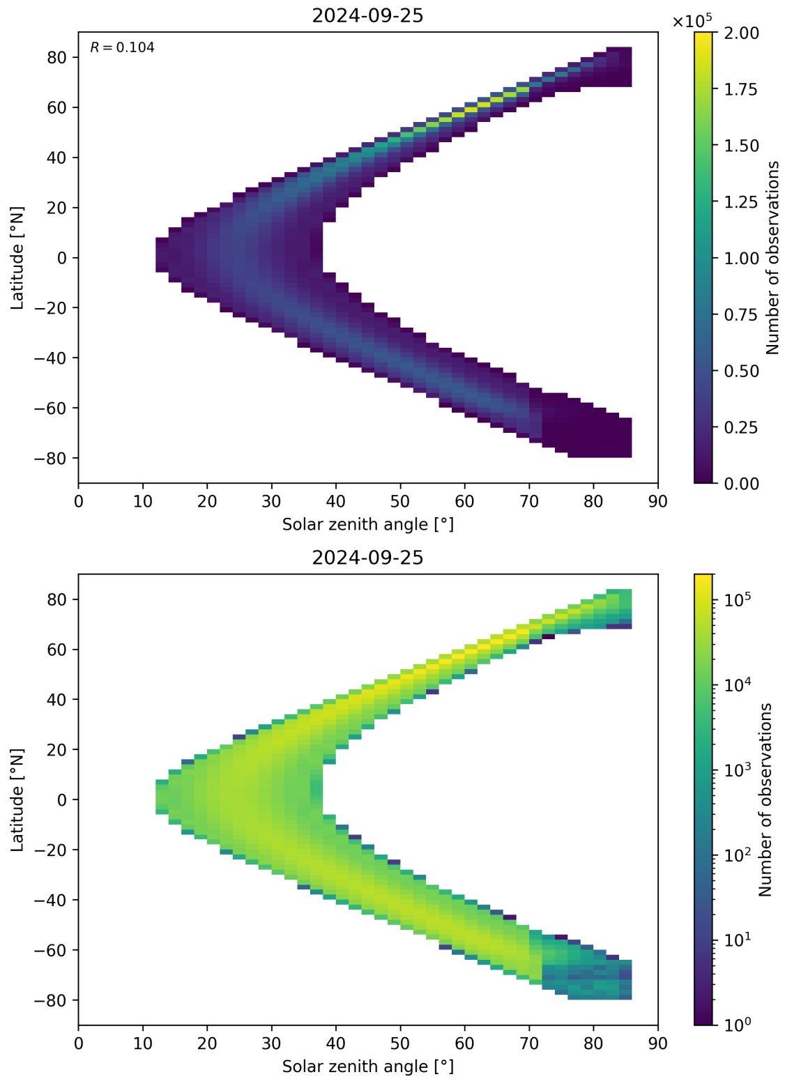
Figure 181: Scatter density plot of “Solar zenith angle” against “Latitude” for 2024-09-24 to 2024-09-26.
