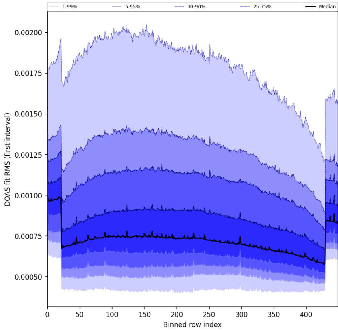
Figure 60: Along track statistics of “DOAS fit RMS (first interval)” for 2024-09-24 to 2024-09-26
