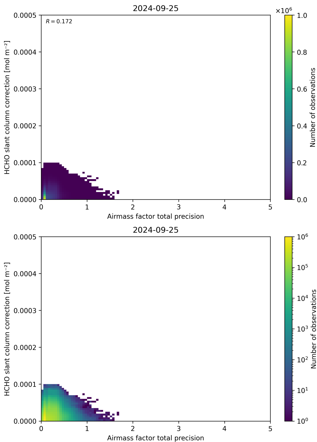
Figure 110: Scatter density plot of “Airmass factor total precision” against “HCHO slant column correction” for 2024-09-24 to 2024-09-26.
