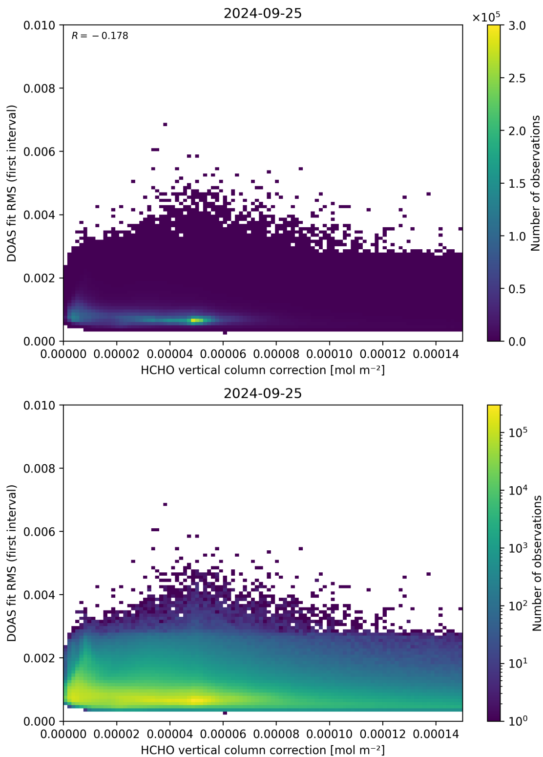
Figure 112: Scatter density plot of “HCHO vertical column correction” against “DOAS fit RMS (first interval)” for 2024-09-24 to 2024-09-26.
