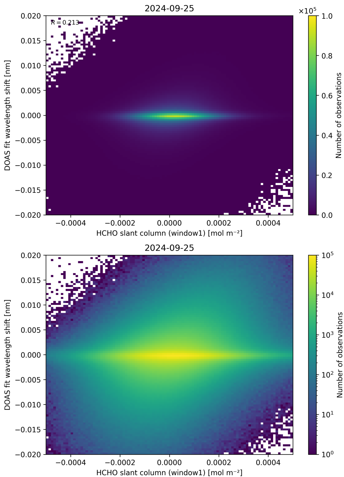
Figure 79: Scatter density plot of “HCHO slant column (window1)” against “DOAS fit wavelength shift” for 2024-09-24 to 2024-09-26.
