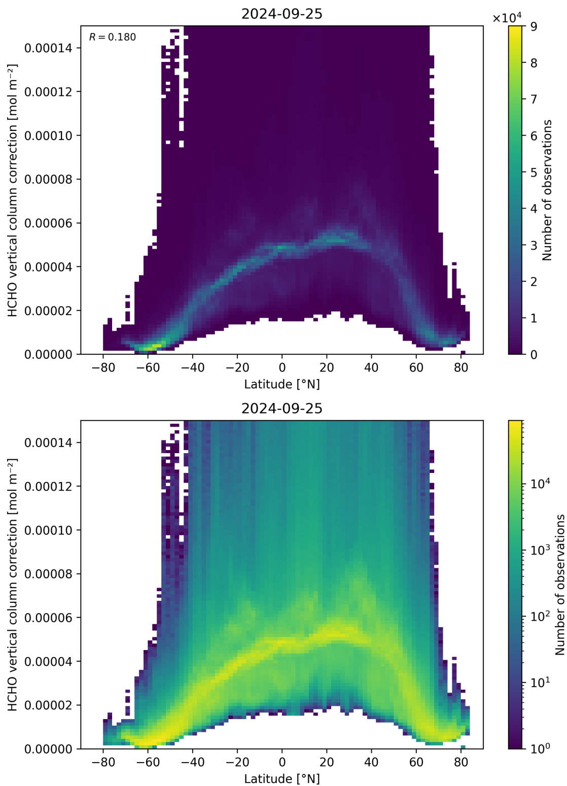
Figure 164: Scatter density plot of “Latitude” against “HCHO vertical column correction” for 2024-09-24 to 2024-09-26.
