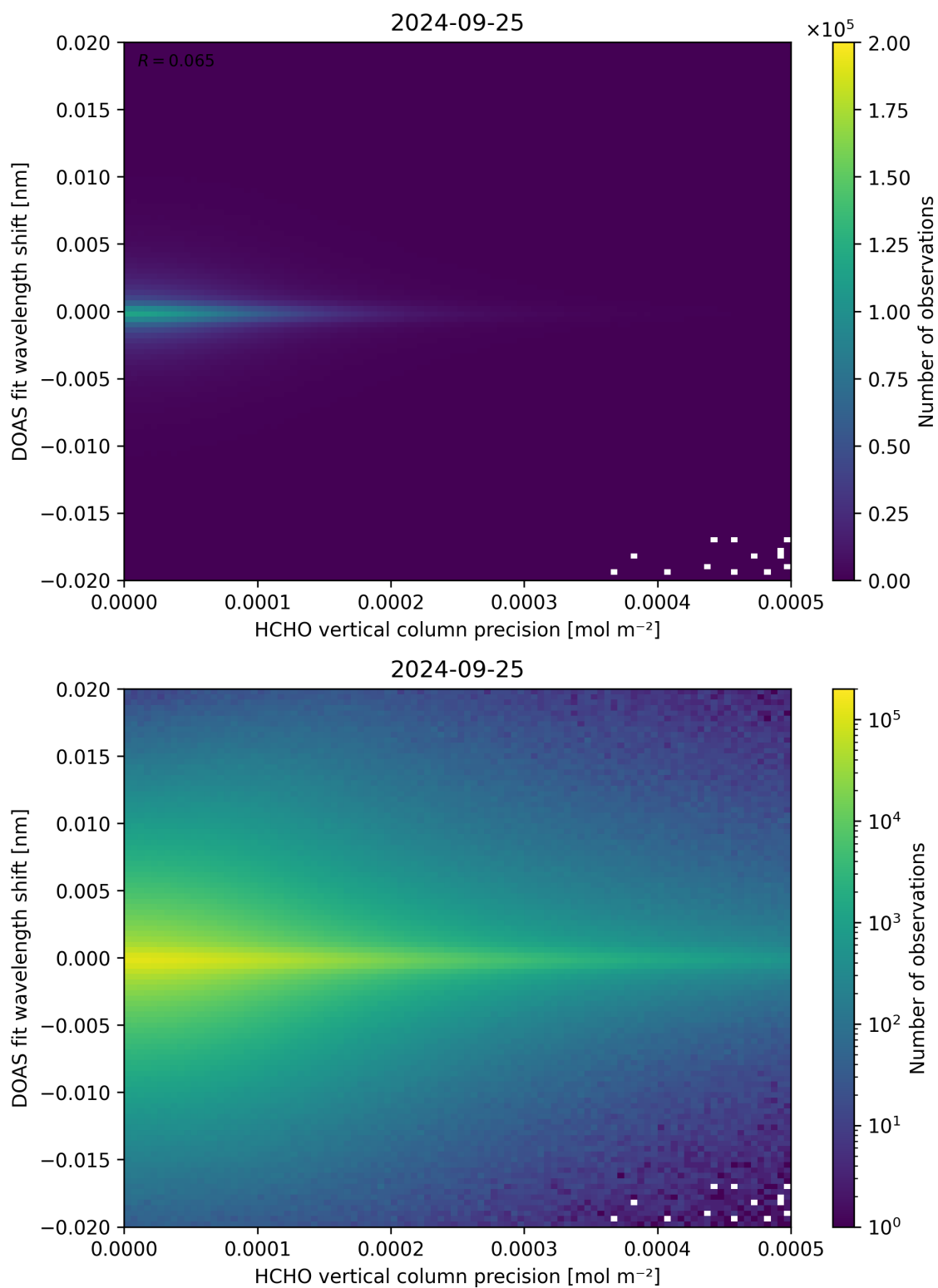
Figure 137: Scatter density plot of “HCHO vertical column precision” against “DOAS fit wavelength shift” for 2024-09-24 to 2024-09-26.
