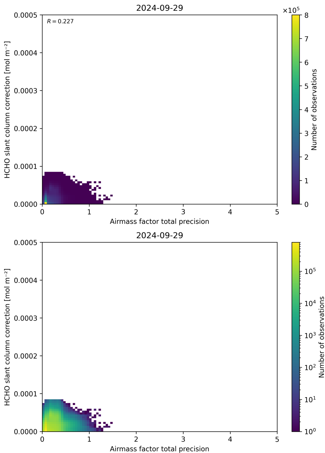
Figure 110: Scatter density plot of “Airmass factor total precision” against “HCHO slant column correction” for 2024-09-28 to 2024-09-30.
