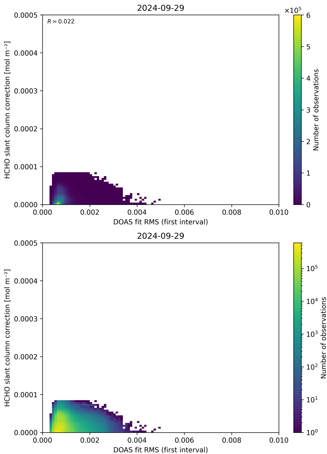
Figure 63: Scatter density plot of “DOAS fit RMS (first interval)” against “HCHO slant column correction” for 2024-09-28 to 2024-09-30.
