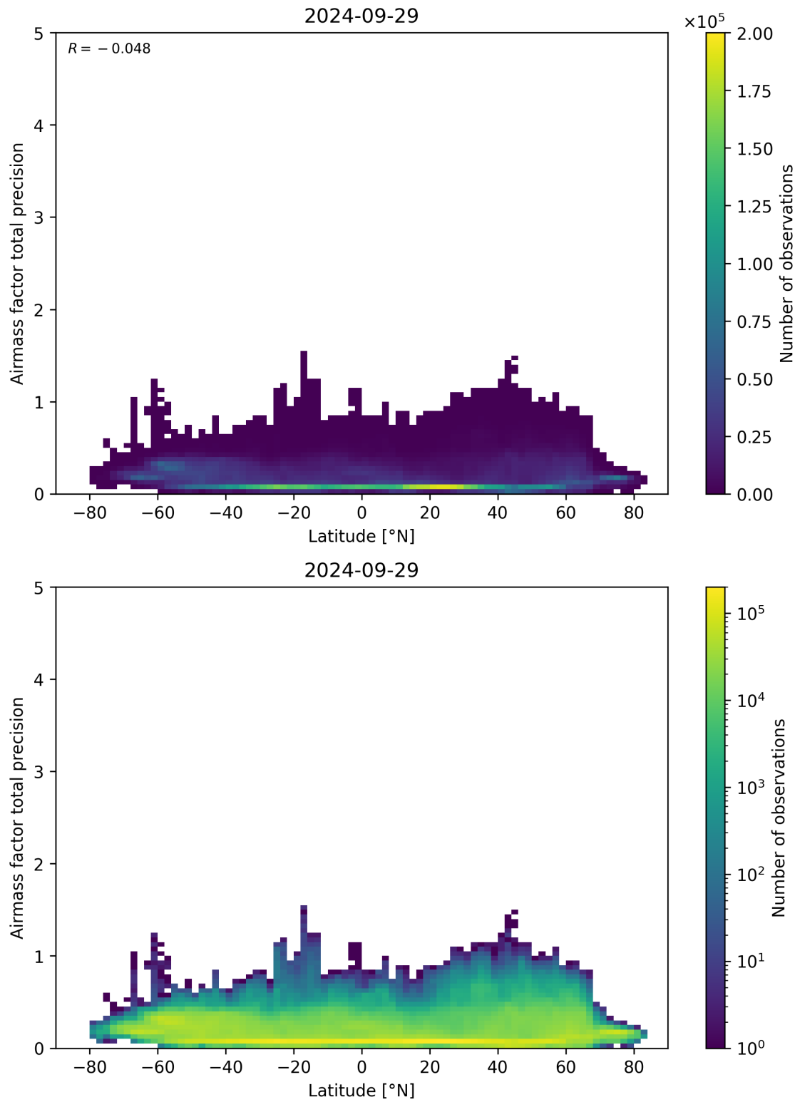
Figure 162: Scatter density plot of “Latitude” against “Airmass factor total precision” for 2024-09-28 to 2024-09-30.
