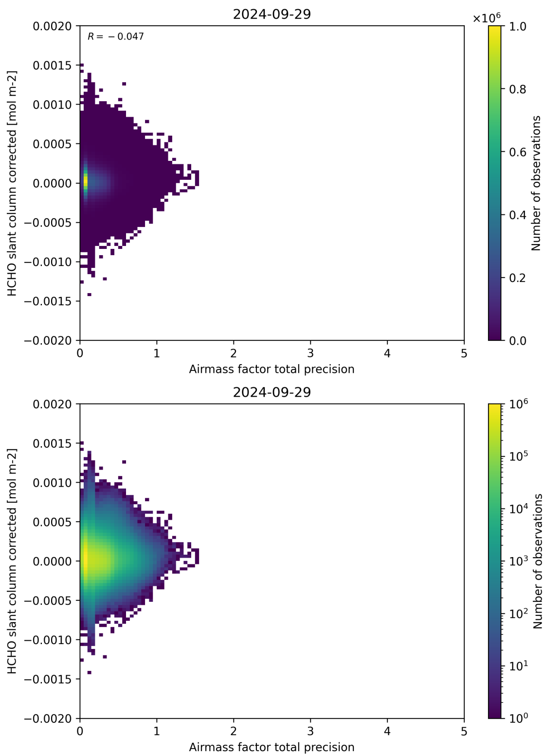
Figure 109: Scatter density plot of “Airmass factor total precision” against “HCHO slant column corrected” for 2024-09-28 to 2024-09-30.
