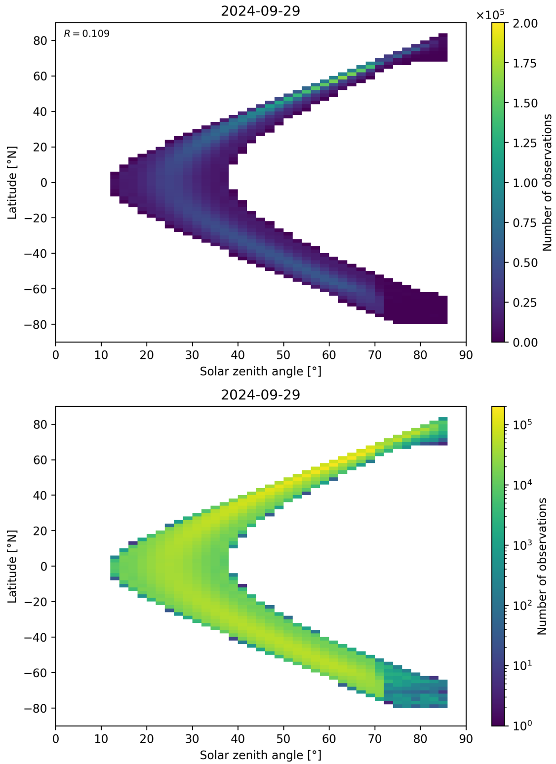
Figure 181: Scatter density plot of “Solar zenith angle” against “Latitude” for 2024-09-28 to 2024-09-30.
