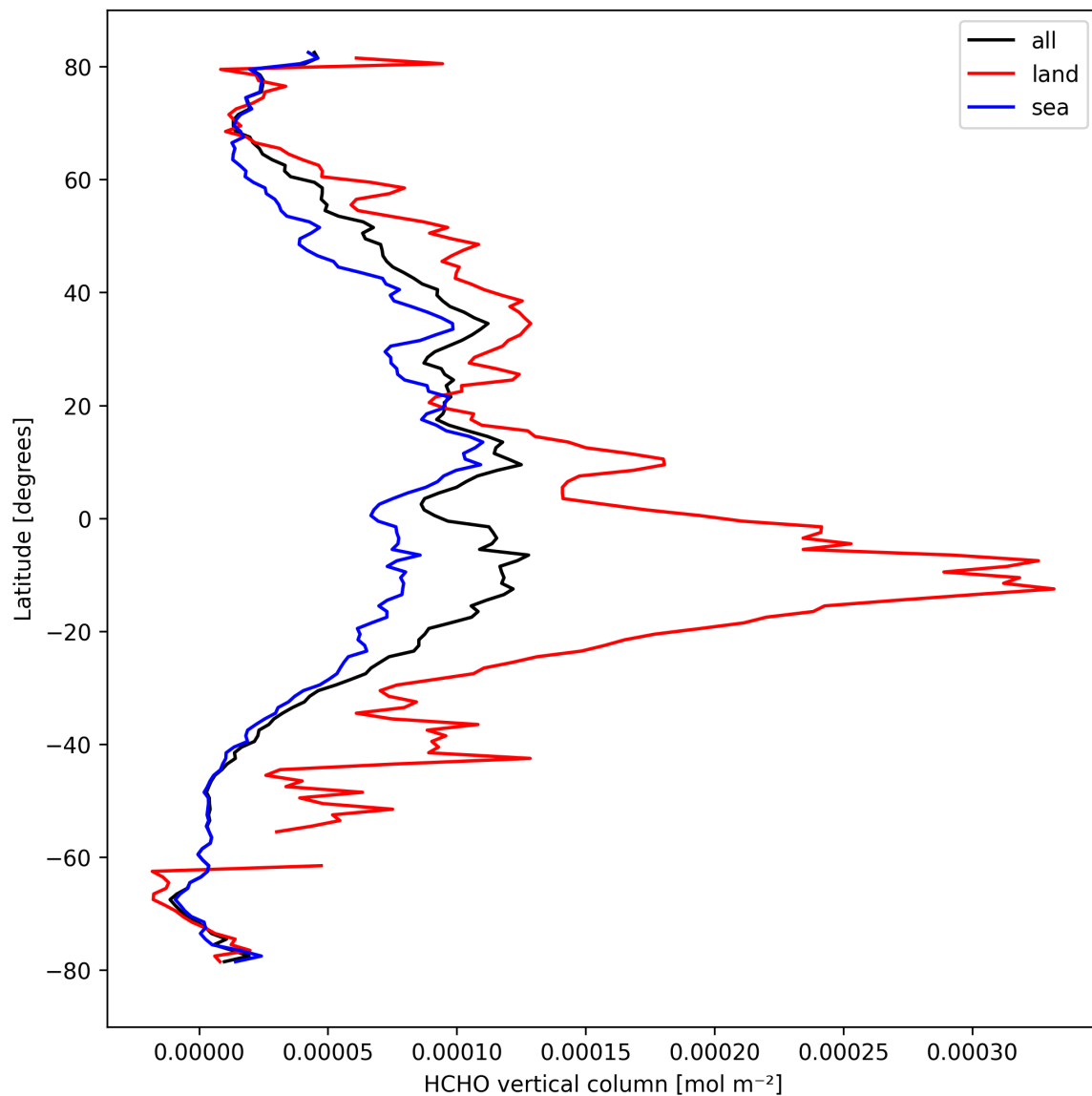
Figure 21: Zonal average of “HCHO vertical column” for 2024-09-28 to 2024-09-30.
