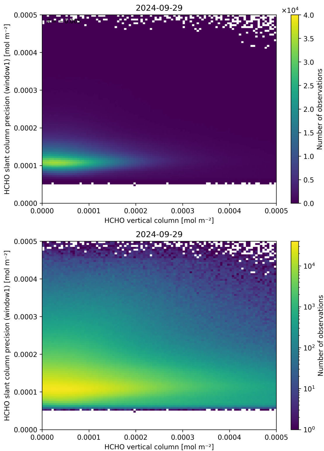
Figure 130: Scatter density plot of “HCHO vertical column” against “HCHO slant column precision (window1)” for 2024-09-28 to 2024-09-30.
