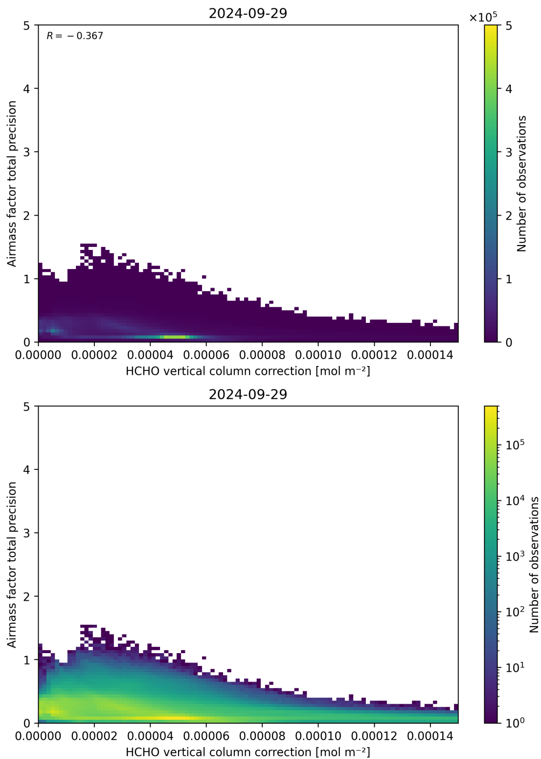
Figure 121: Scatter density plot of “HCHO vertical column correction” against “Airmass factor total precision” for 2024-09-28 to 2024-09-30.
