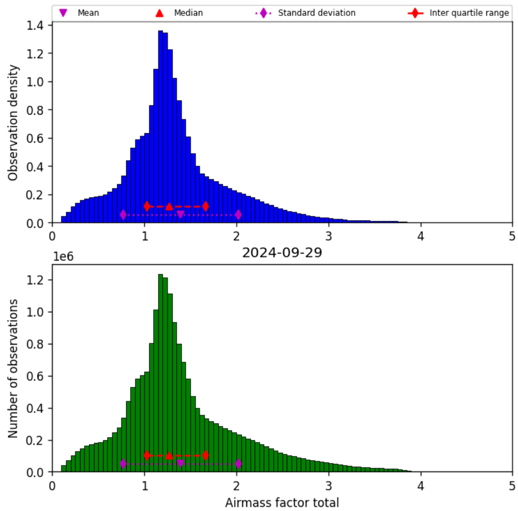
Figure 40: Histogram of “Airmass factor total” for 2024-09-28 to 2024-09-30
