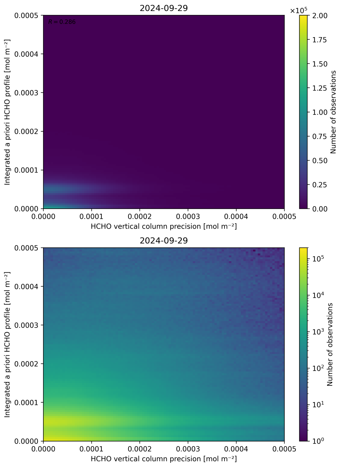
Figure 147: Scatter density plot of “HCHO vertical column precision” against “Integrated a priori HCHO profile” for 2024-09-28 to 2024-09-30.
