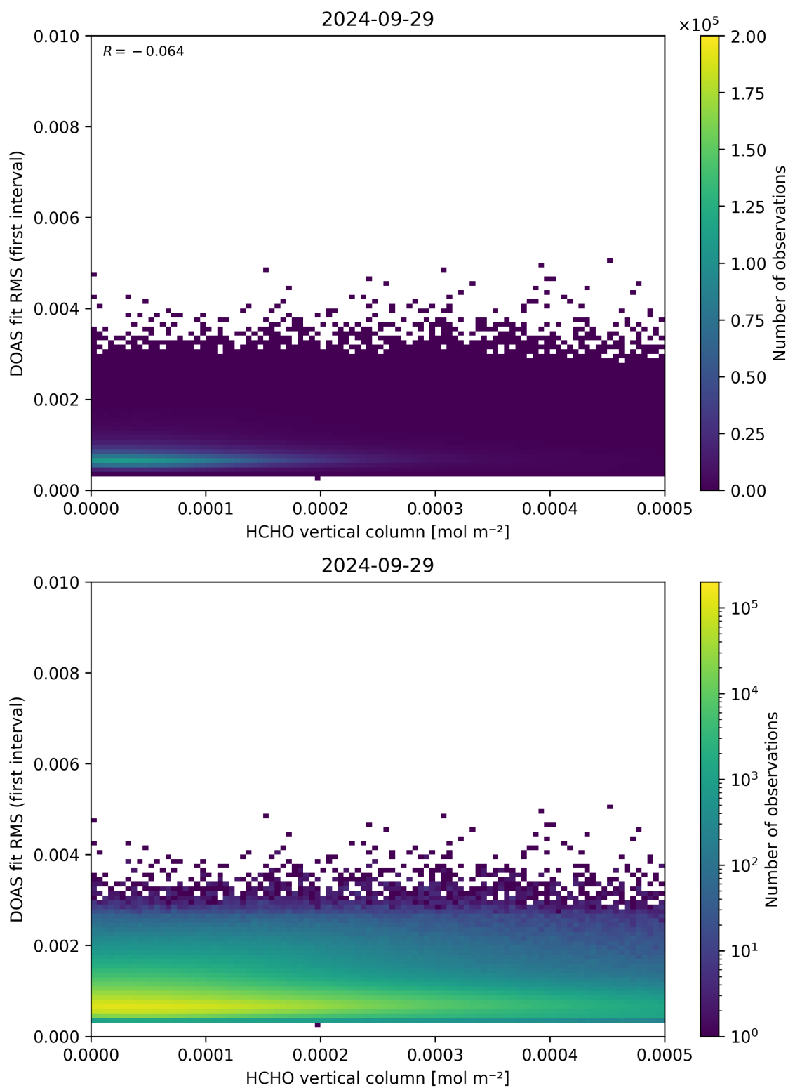
Figure 123: Scatter density plot of “HCHO vertical column” against “DOAS fit RMS (first interval)” for 2024-09-28 to 2024-09-30.
