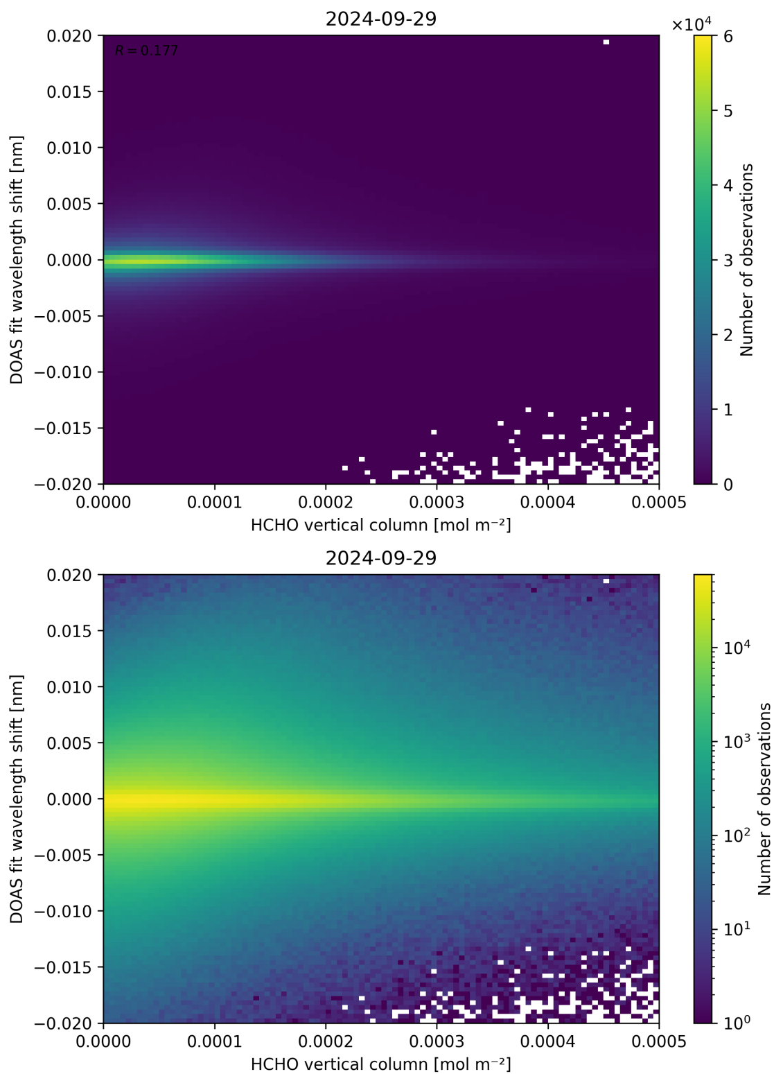
Figure 124: Scatter density plot of “HCHO vertical column” against “DOAS fit wavelength shift” for 2024-09-28 to 2024-09-30.
