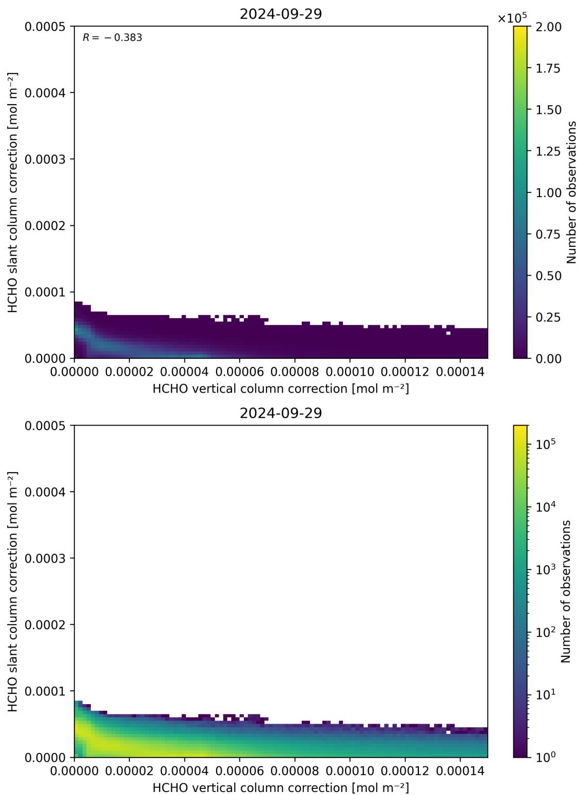
Figure 117: Scatter density plot of “HCHO vertical column correction” against “HCHO slant column correction” for 2024-09-28 to 2024-09-30.
