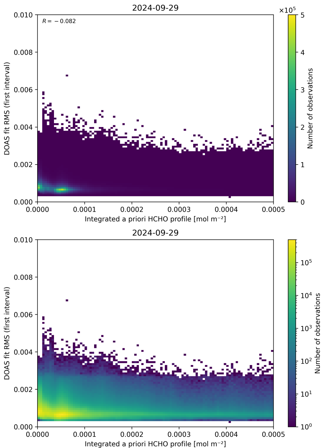
Figure 148: Scatter density plot of “Integrated a priori HCHO profile” against “DOAS fit RMS (first interval)” for 2024-09-28 to 2024-09-30.
