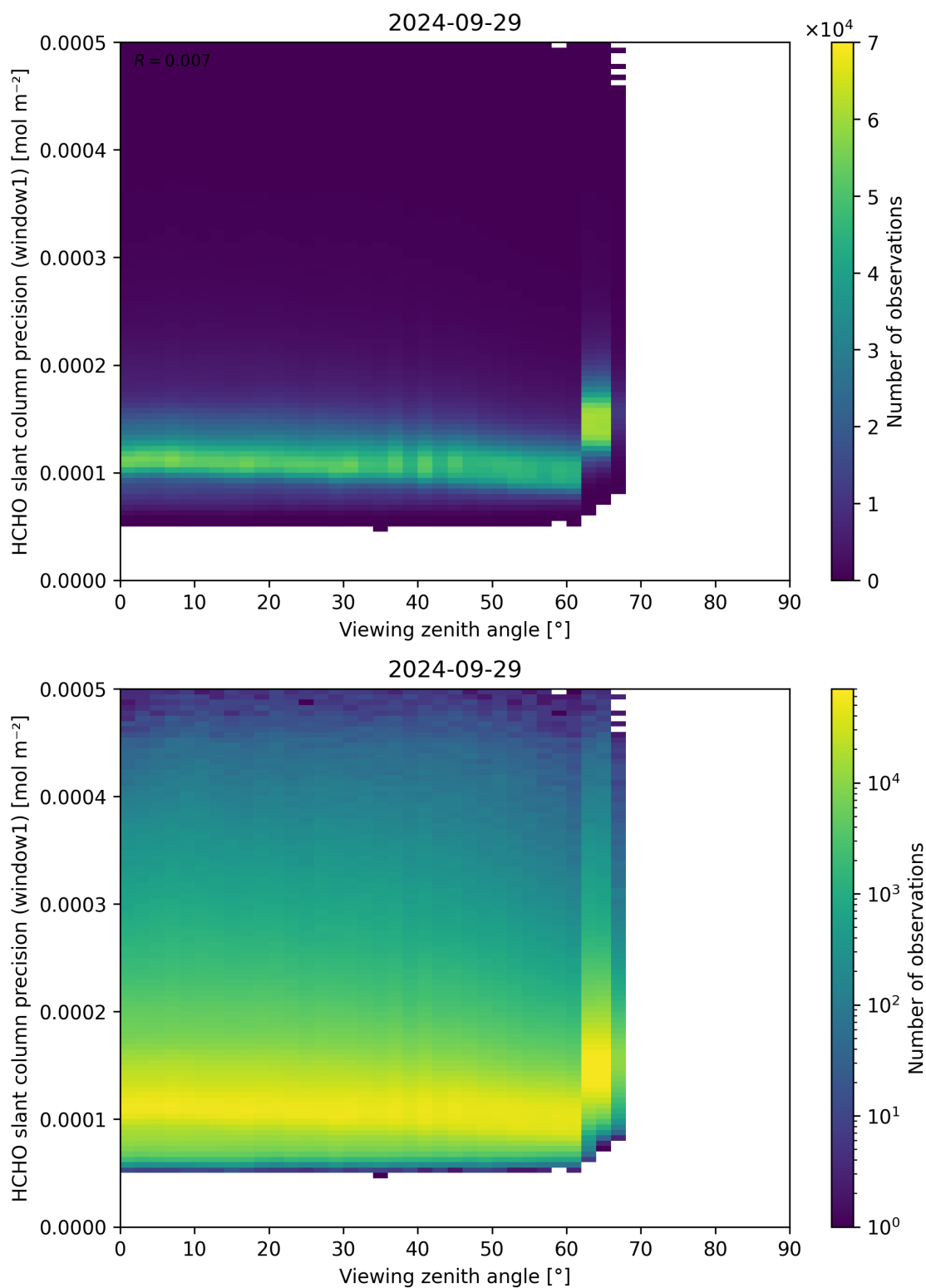
Figure 189: Scatter density plot of “Viewing zenith angle” against “HCHO slant column precision (window1)” for 2024-09-28 to 2024-09-30.
