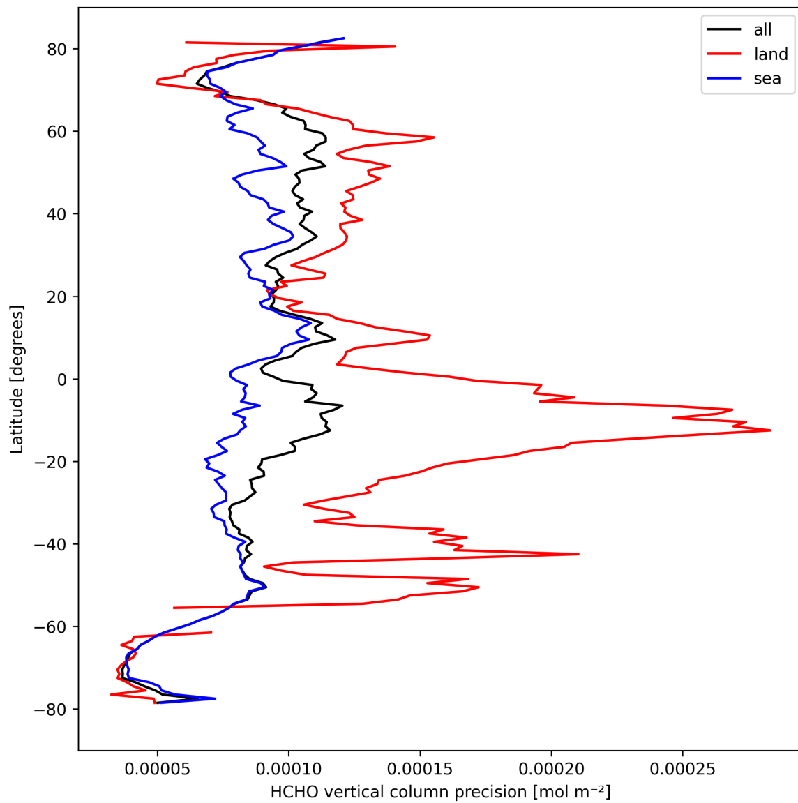
Figure 22: Zonal average of “HCHO vertical column precision” for 2024-09-28 to 2024-09-30.
