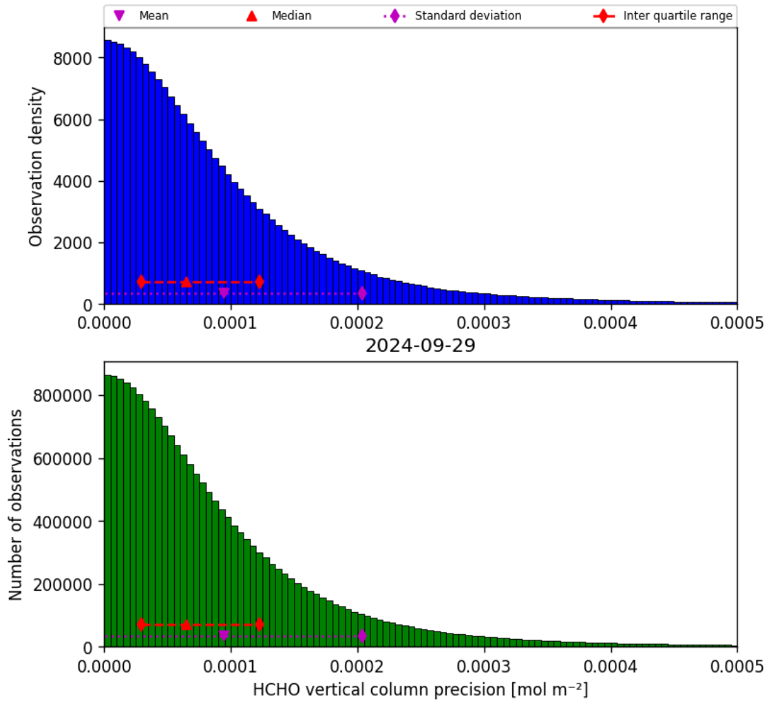
Figure 36: Histogram of “HCHO vertical column precision” for 2024-09-28 to 2024-09-30
