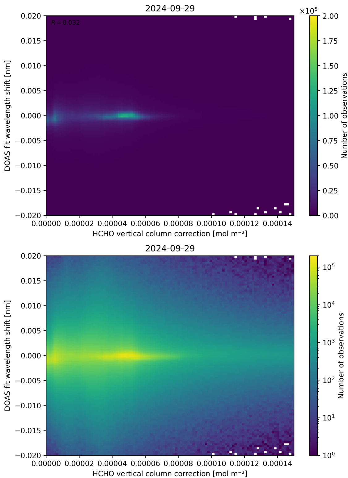
Figure 113: Scatter density plot of “HCHO vertical column correction” against “DOAS fit wavelength shift” for 2024-09-28 to 2024-09-30.
