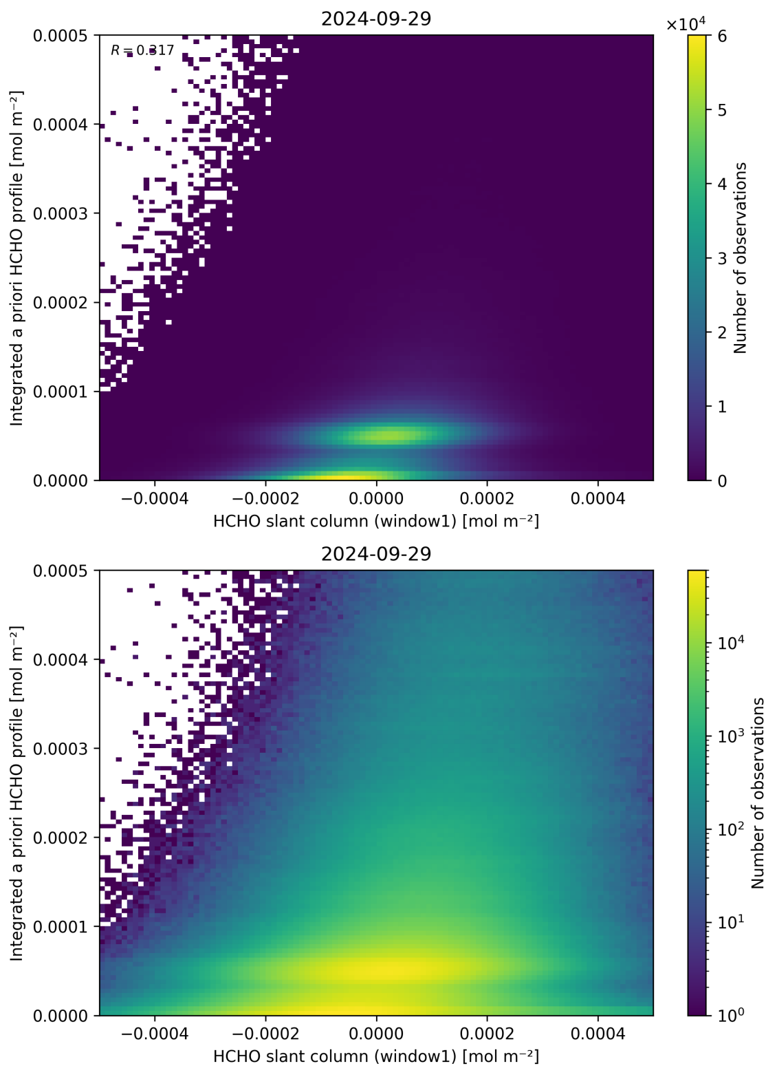
Figure 87: Scatter density plot of “HCHO slant column (window1)” against “Integrated a priori HCHO profile” for 2024-09-28 to 2024-09-30.
