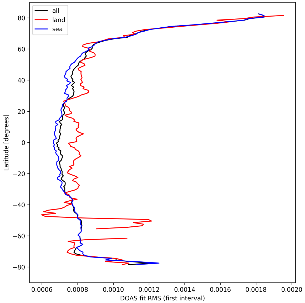
Figure 32: Zonal average of “DOAS fit RMS (first interval)” for 2024-09-28 to 2024-09-30.
