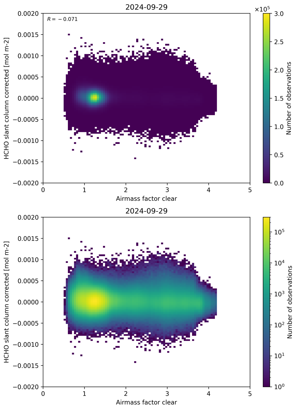
Figure 74: Scatter density plot of “Airmass factor clear” against “HCHO slant column corrected” for 2024-09-28 to 2024-09-30.
