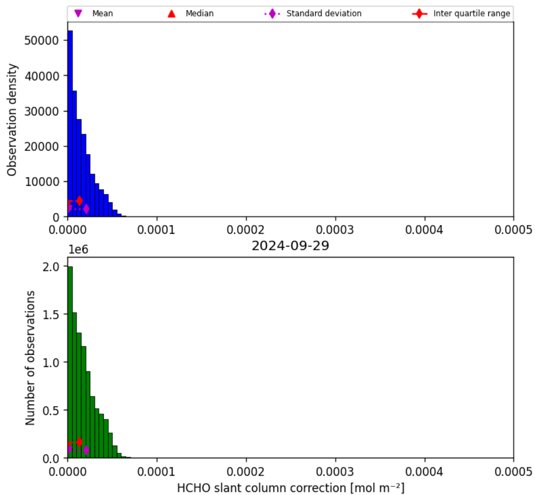
Figure 47: Histogram of “HCHO slant column correction” for 2024-09-28 to 2024-09-30
