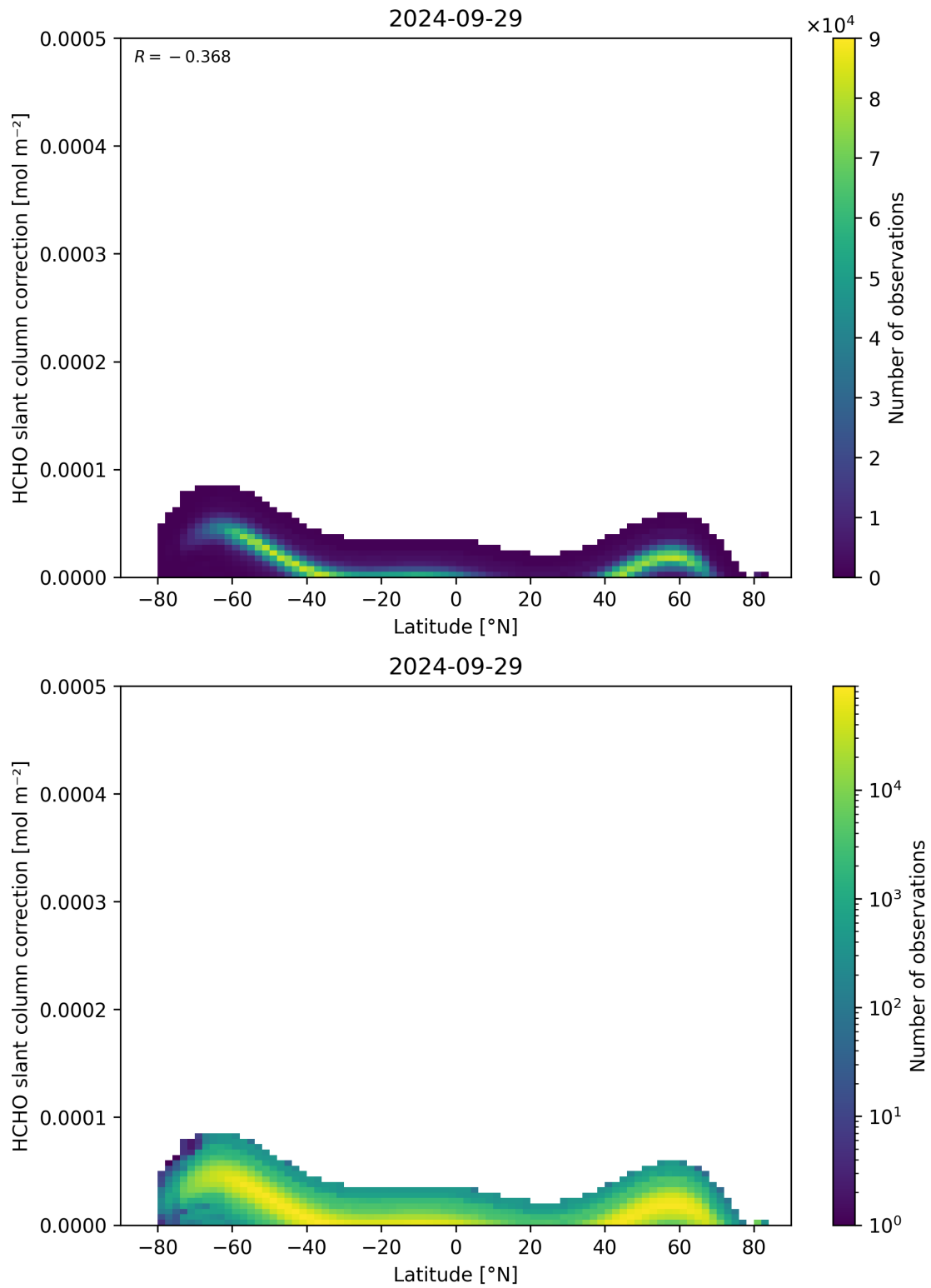
Figure 158: Scatter density plot of “Latitude” against “HCHO slant column correction” for 2024-09-28 to 2024-09-30.
