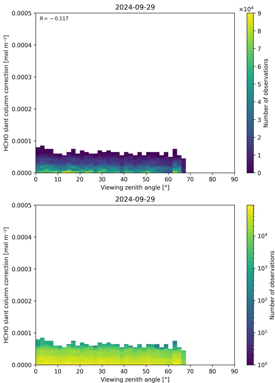
Figure 187: Scatter density plot of “Viewing zenith angle” against “HCHO slant column correction” for 2024-09-28 to 2024-09-30.
