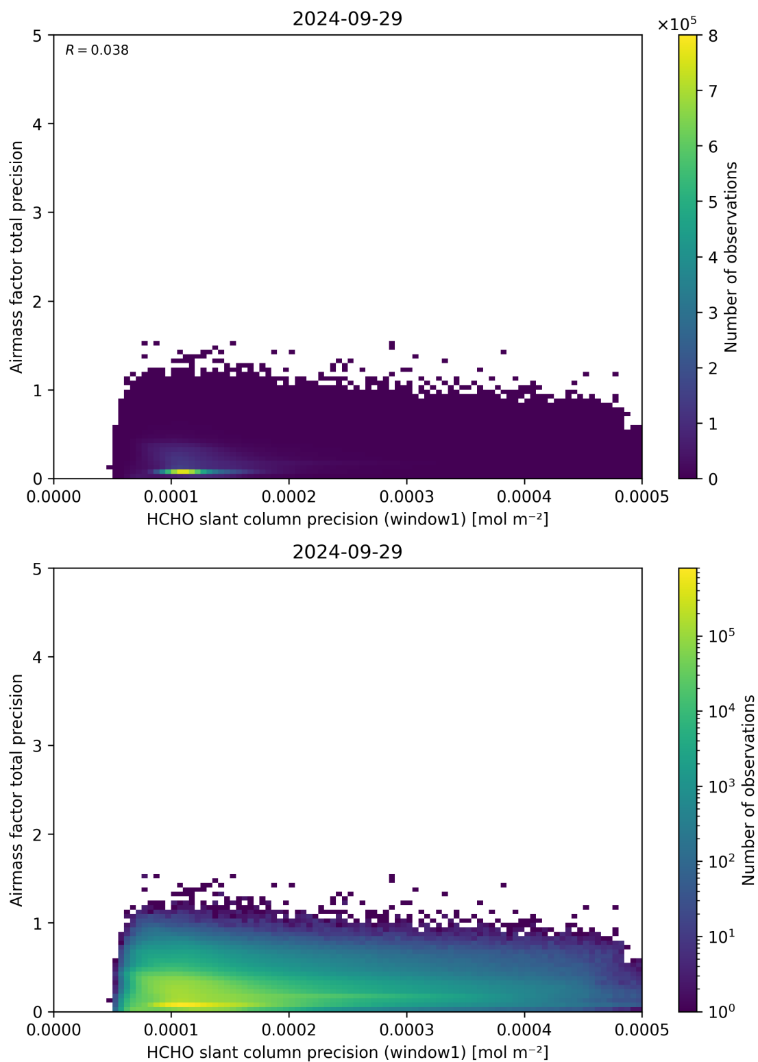
Figure 95: Scatter density plot of “HCHO slant column precision (window1)” against “Airmass factor total precision” for 2024-09-28 to 2024-09-30.
