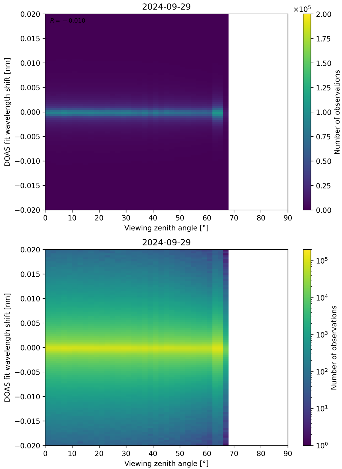
Figure 183: Scatter density plot of “Viewing zenith angle” against “DOAS fit wavelength shift” for 2024-09-28 to 2024-09-30.
