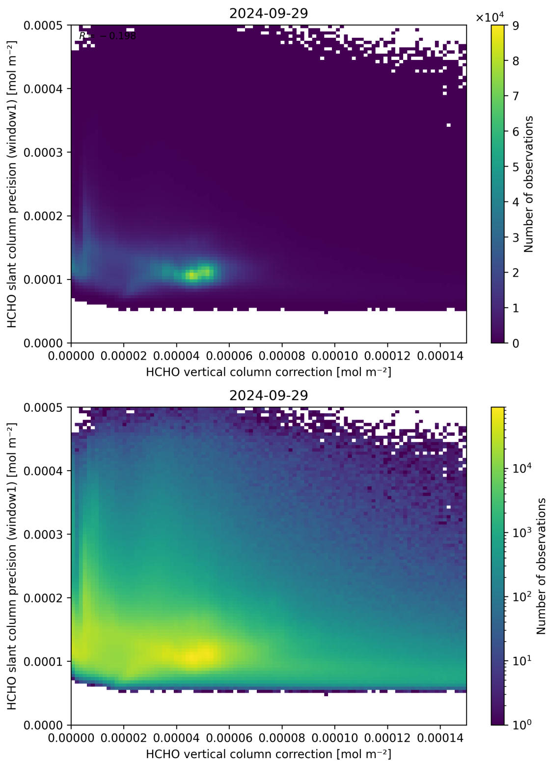
Figure 119: Scatter density plot of “HCHO vertical column correction” against “HCHO slant column precision (window1)” for 2024-09-28 to 2024-09-30.
