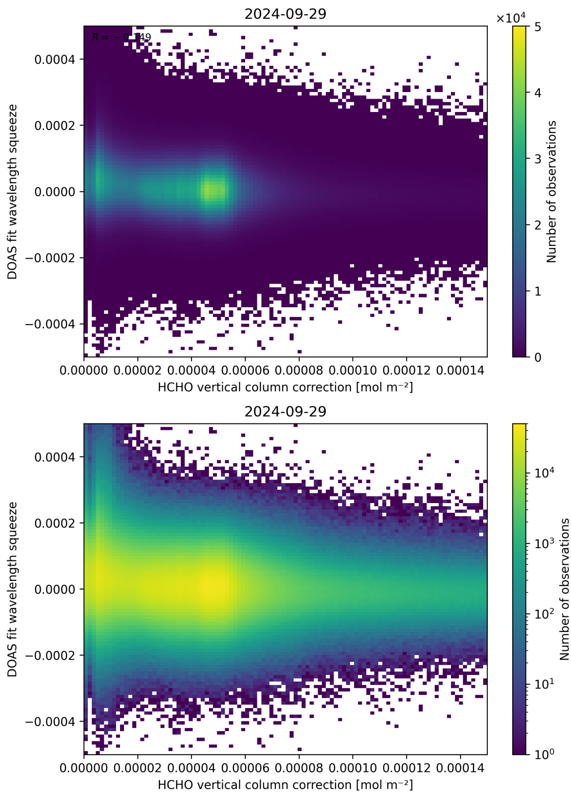
Figure 114: Scatter density plot of “HCHO vertical column correction” against “DOAS fit wavelength squeeze” for 2024-09-28 to 2024-09-30.
