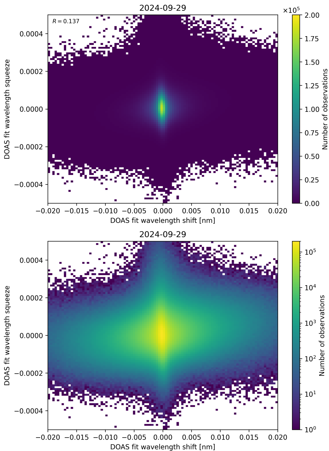
Figure 65: Scatter density plot of “DOAS fit wavelength shift” against “DOAS fit wavelength squeeze” for 2024-09-28 to 2024-09-30.
