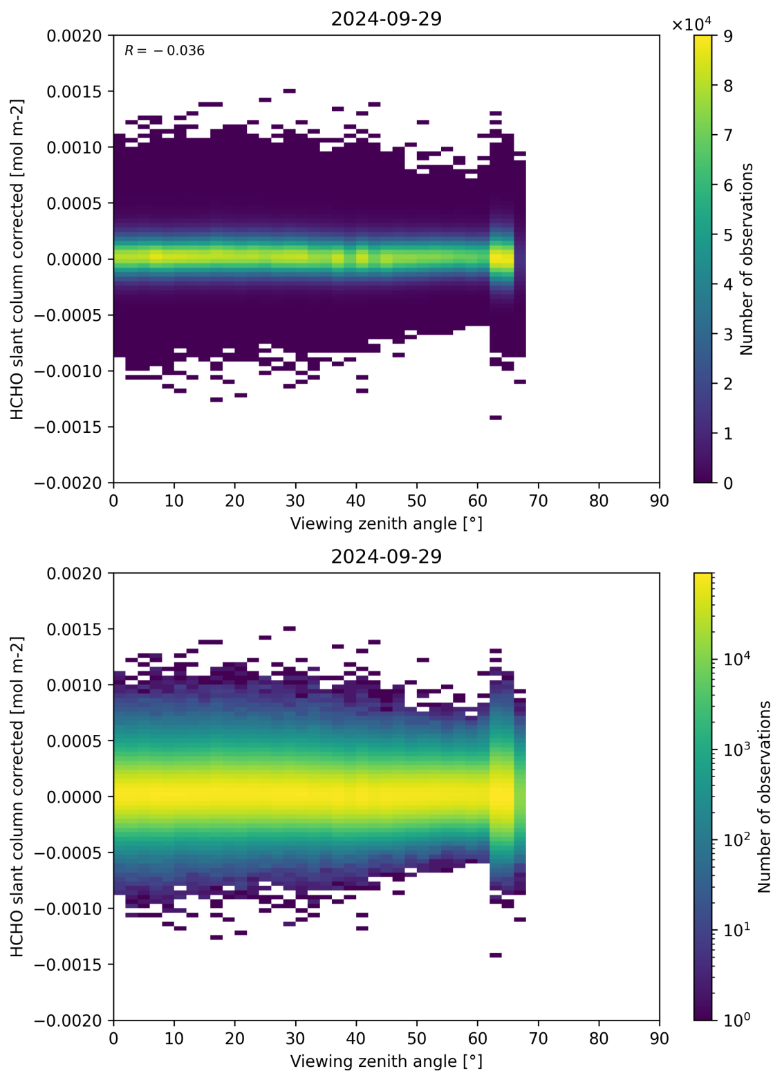
Figure 186: Scatter density plot of “Viewing zenith angle” against “HCHO slant column corrected” for 2024-09-28 to 2024-09-30.
