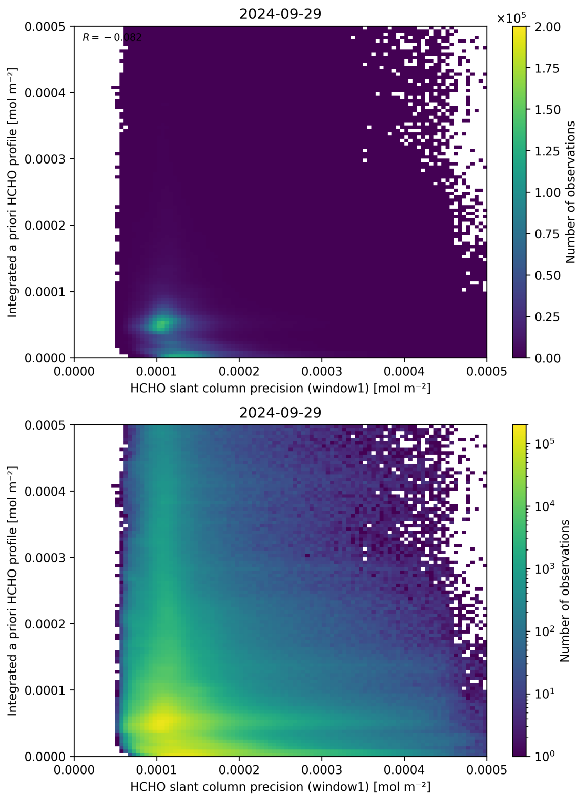
Figure 96: Scatter density plot of “HCHO slant column precision (window1)” against “Integrated a priori HCHO profile” for 2024-09-28 to 2024-09-30.
