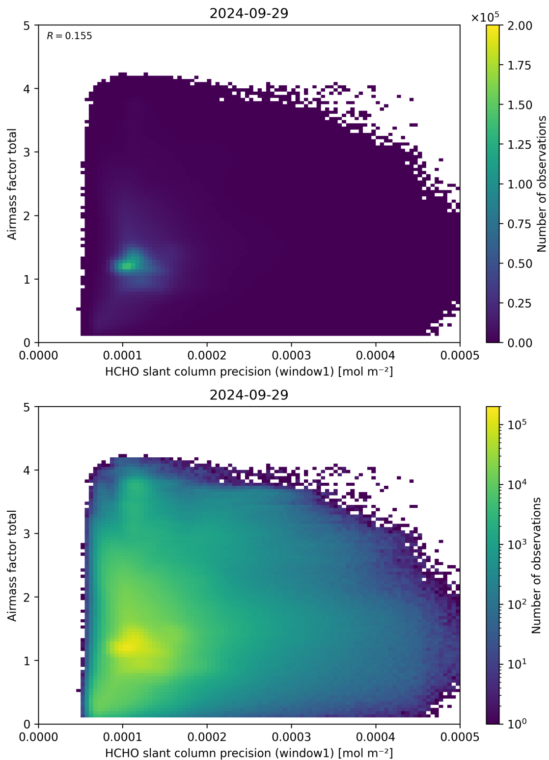
Figure 94: Scatter density plot of “HCHO slant column precision (window1)” against “Airmass factor total” for 2024-09-28 to 2024-09-30.
