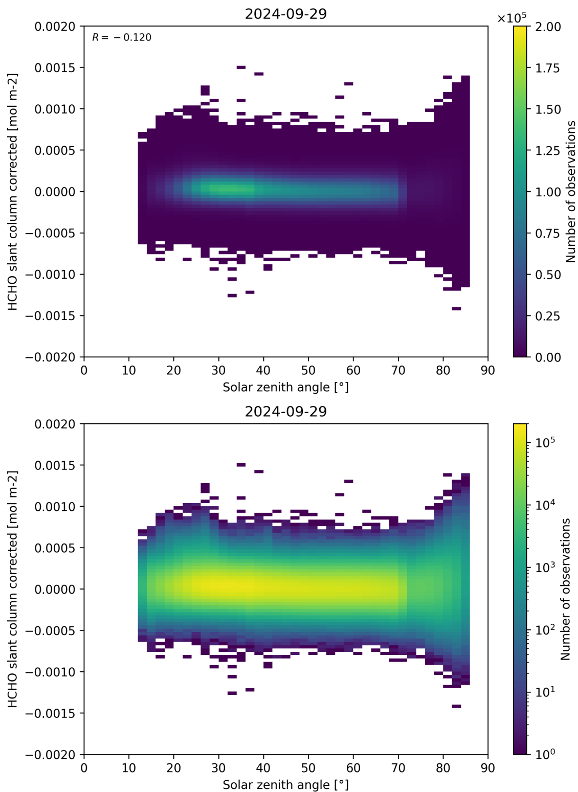
Figure 171: Scatter density plot of “Solar zenith angle” against “HCHO slant column corrected” for 2024-09-28 to 2024-09-30.
