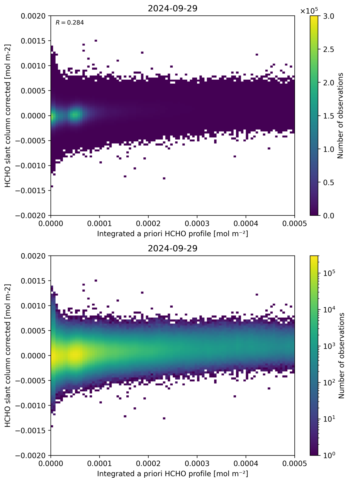
Figure 151: Scatter density plot of “Integrated a priori HCHO profile” against “HCHO slant column corrected” for 2024-09-28 to 2024-09-30.
