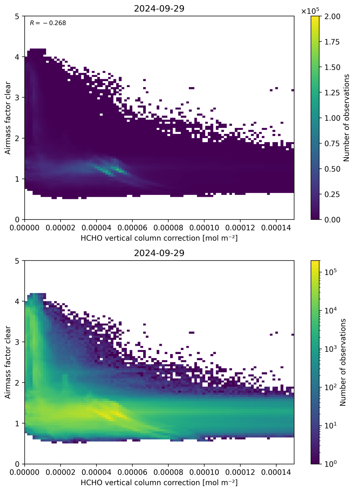
Figure 115: Scatter density plot of “HCHO vertical column correction” against “Airmass factor clear” for 2024-09-28 to 2024-09-30.
