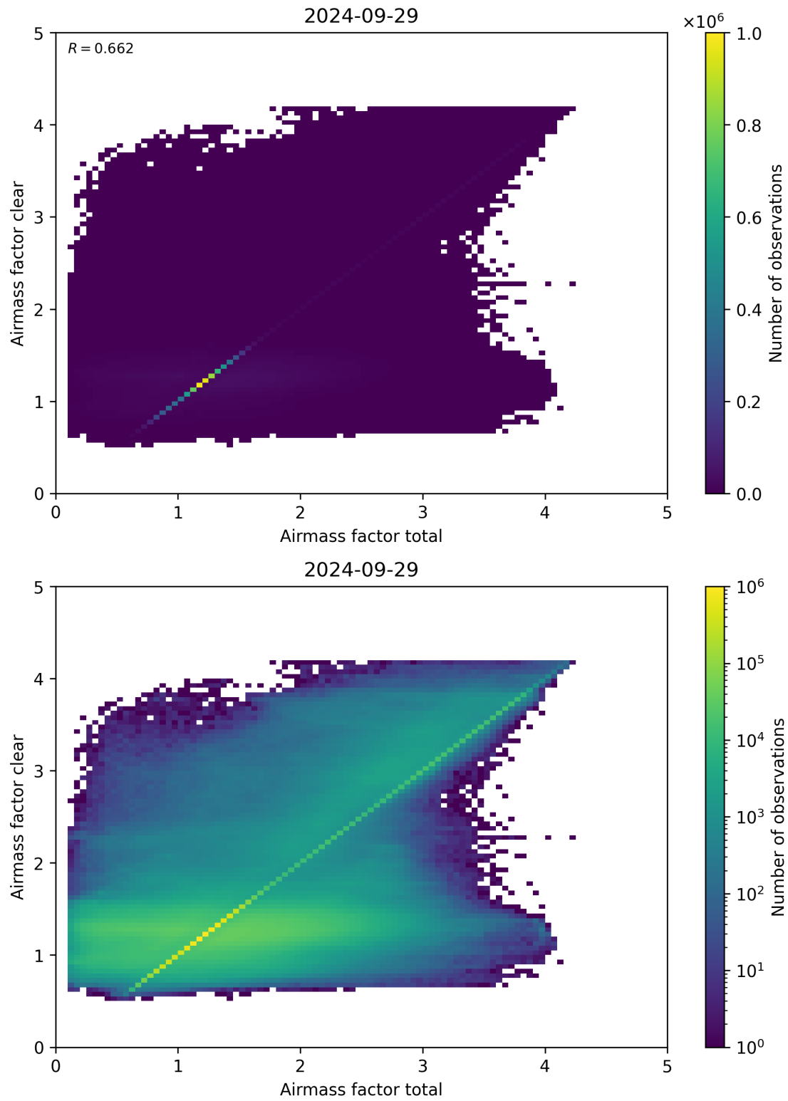
Figure 100: Scatter density plot of “Airmass factor total” against “Airmass factor clear” for 2024-09-28 to 2024-09-30.
