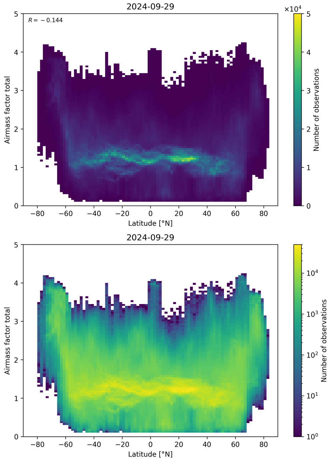
Figure 161: Scatter density plot of “Latitude” against “Airmass factor total” for 2024-09-28 to 2024-09-30.
