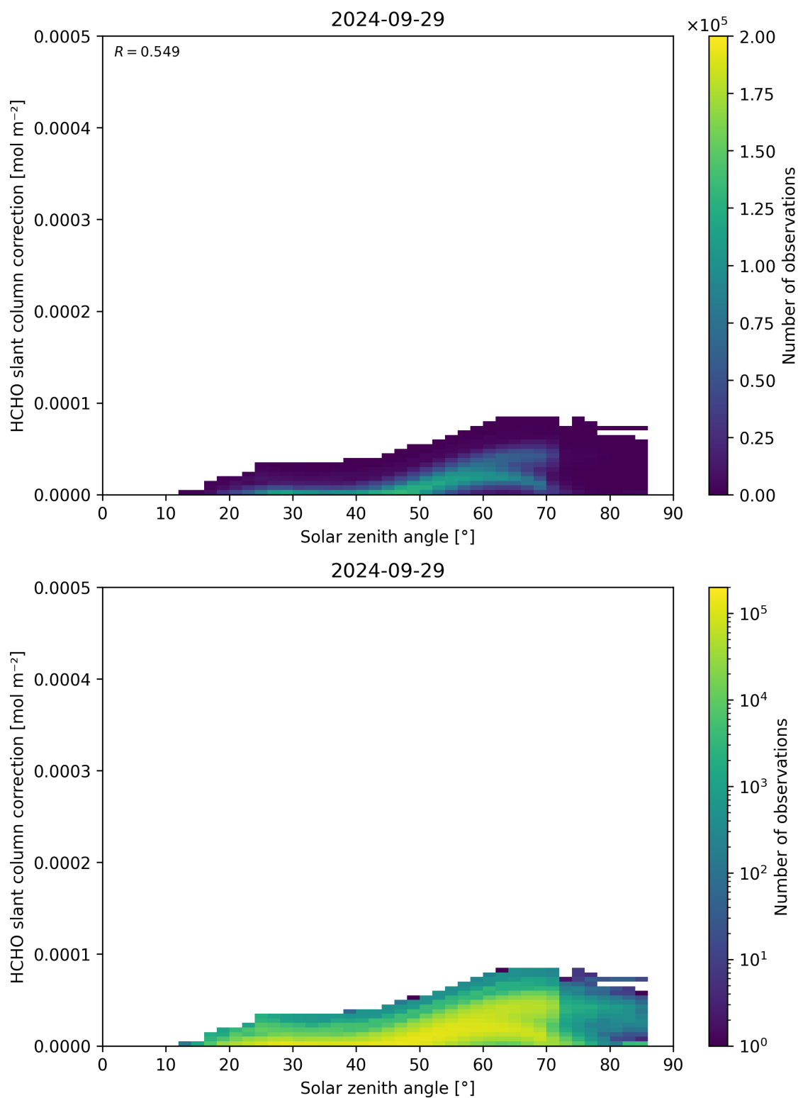
Figure 172: Scatter density plot of “Solar zenith angle” against “HCHO slant column correction” for 2024-09-28 to 2024-09-30.
