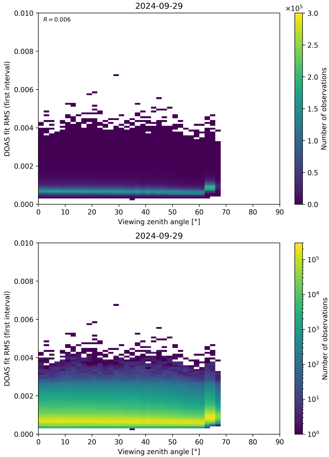
Figure 182: Scatter density plot of “Viewing zenith angle” against “DOAS fit RMS (first interval)” for 2024-09-28 to 2024-09-30.
