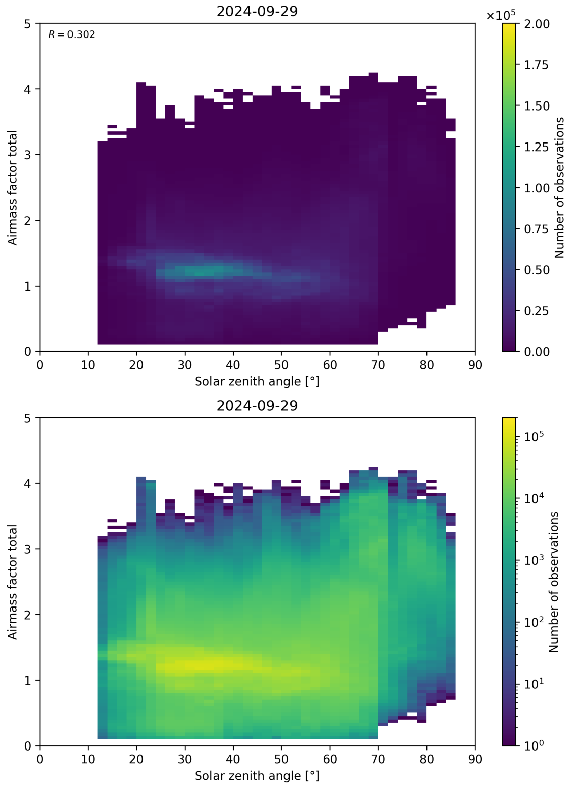
Figure 175: Scatter density plot of “Solar zenith angle” against “Airmass factor total” for 2024-09-28 to 2024-09-30.
