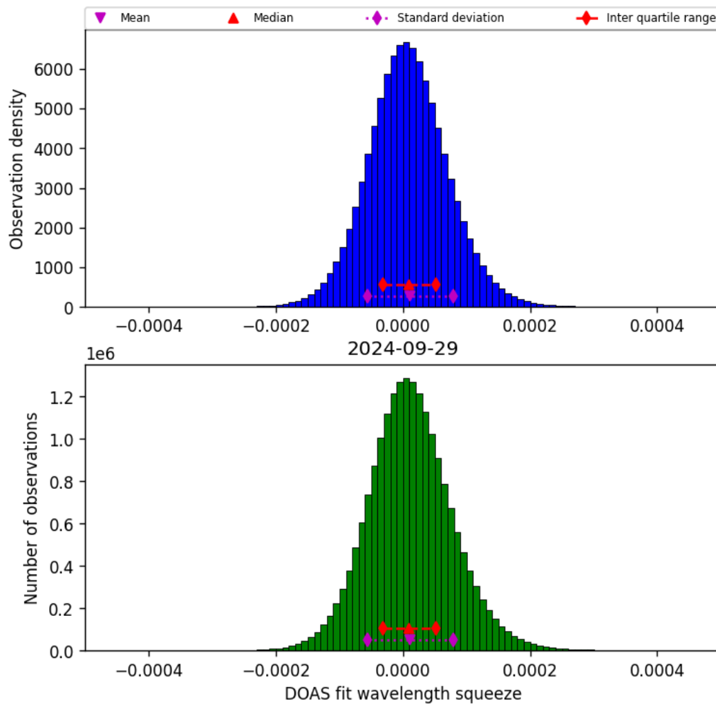
Figure 45: Histogram of “DOAS fit wavelength squeeze” for 2024-09-28 to 2024-09-30
