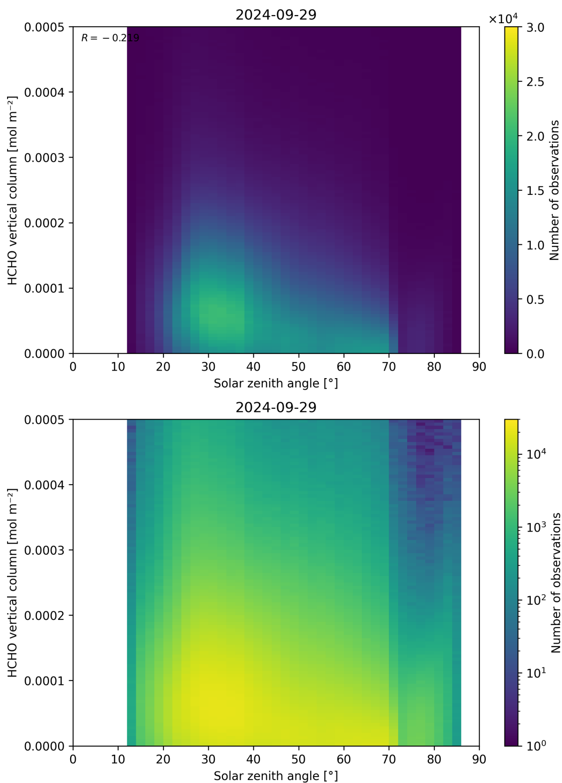
Figure 177: Scatter density plot of “Solar zenith angle” against “HCHO vertical column” for 2024-09-28 to 2024-09-30.
