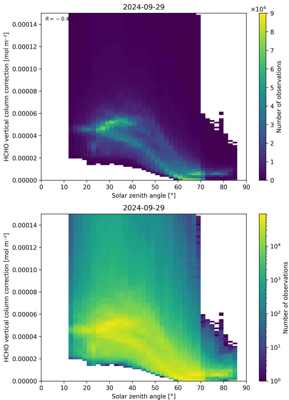
Figure 178: Scatter density plot of “Solar zenith angle” against “HCHO vertical column correction” for 2024-09-28 to 2024-09-30.
