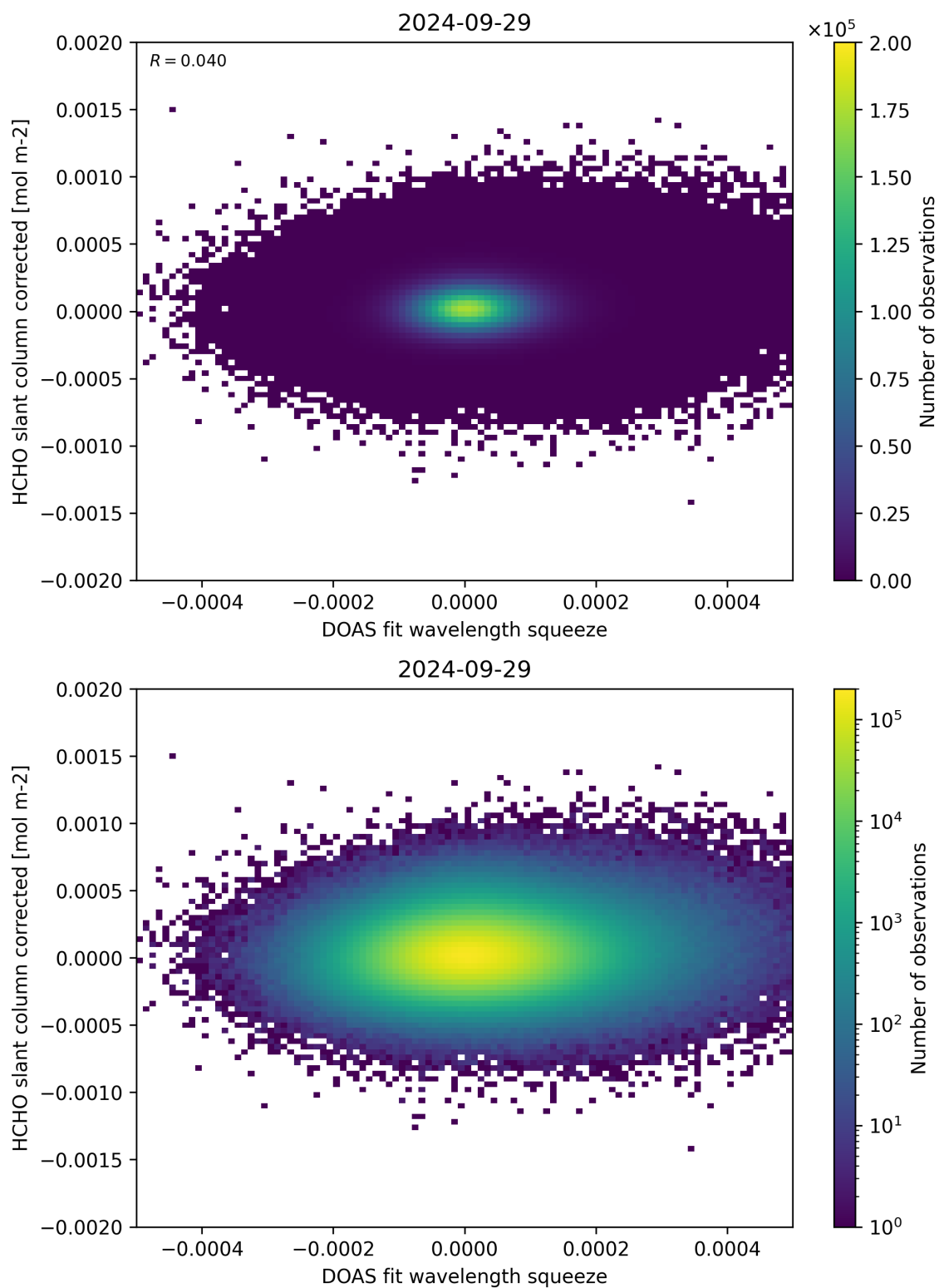
Figure 69: Scatter density plot of “DOAS fit wavelength squeeze” against “HCHO slant column corrected” for 2024-09-28 to 2024-09-30.
