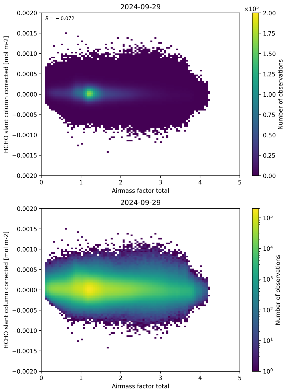
Figure 101: Scatter density plot of “Airmass factor total” against “HCHO slant column corrected” for 2024-09-28 to 2024-09-30.
