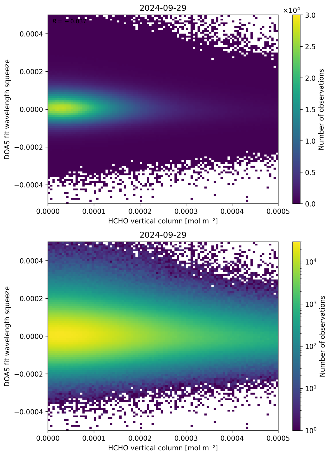
Figure 125: Scatter density plot of “HCHO vertical column” against “DOAS fit wavelength squeeze” for 2024-09-28 to 2024-09-30.
