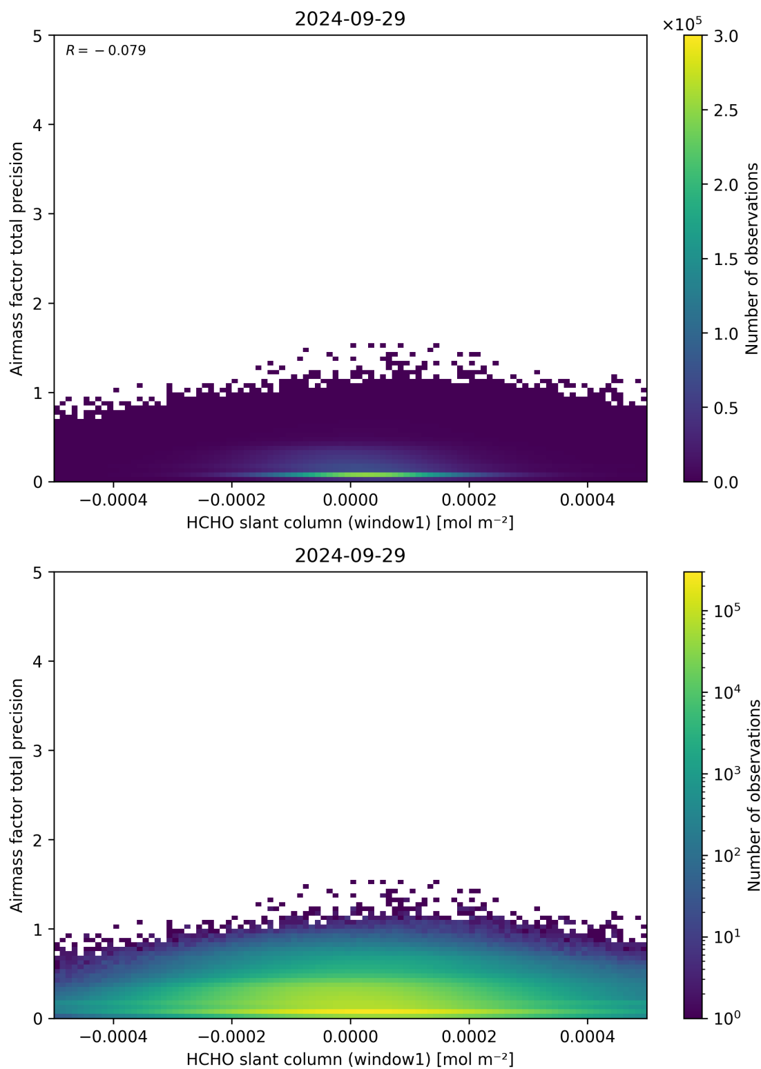
Figure 86: Scatter density plot of “HCHO slant column (window1)” against “Airmass factor total precision” for 2024-09-28 to 2024-09-30.
