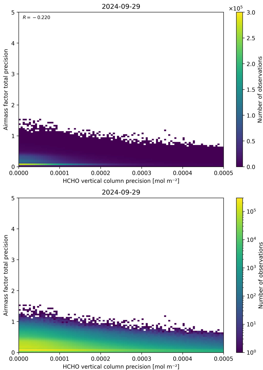
Figure 145: Scatter density plot of “HCHO vertical column precision” against “Airmass factor total precision” for 2024-09-28 to 2024-09-30.
