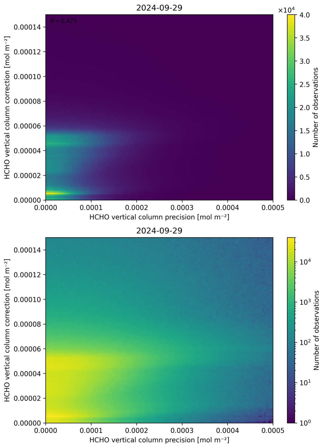
Figure 146: Scatter density plot of “HCHO vertical column precision” against “HCHO vertical column correction” for 2024-09-28 to 2024-09-30.
