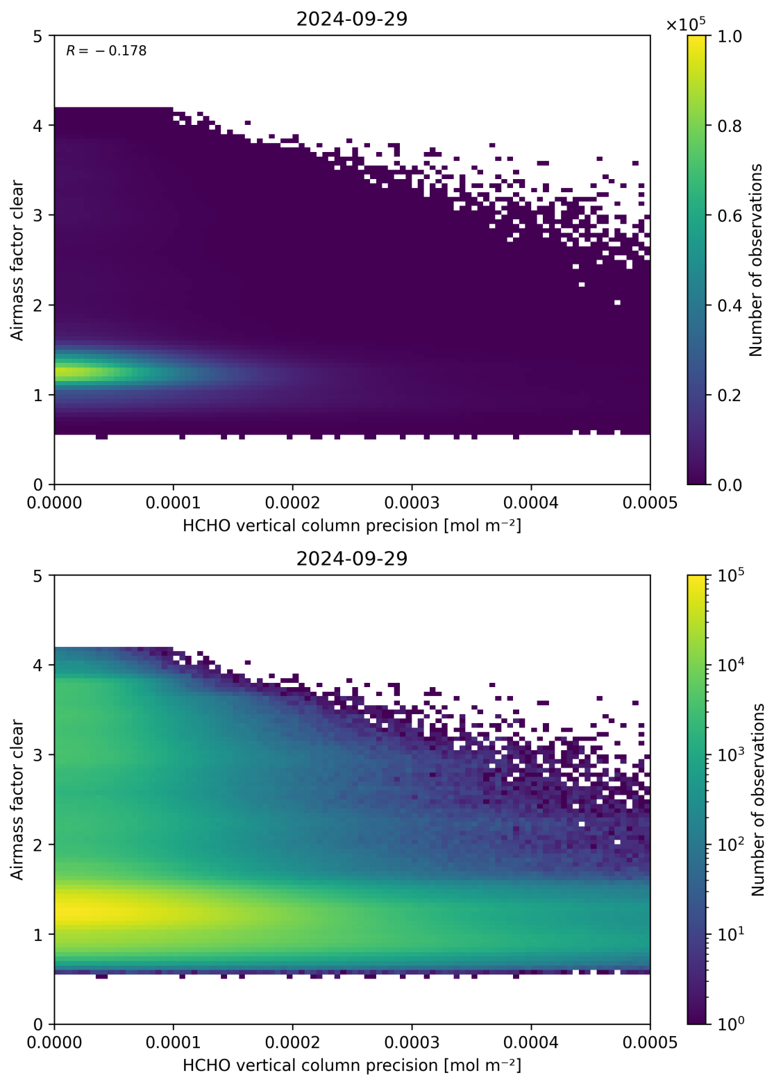
Figure 139: Scatter density plot of “HCHO vertical column precision” against “Airmass factor clear” for 2024-09-28 to 2024-09-30.
