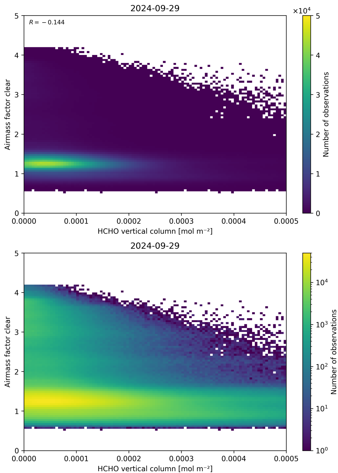
Figure 126: Scatter density plot of “HCHO vertical column” against “Airmass factor clear” for 2024-09-28 to 2024-09-30.
