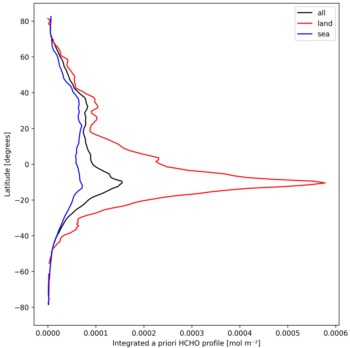
Figure 29: Zonal average of “Integrated a priori HCHO profile” for 2024-09-28 to 2024-09-30.
