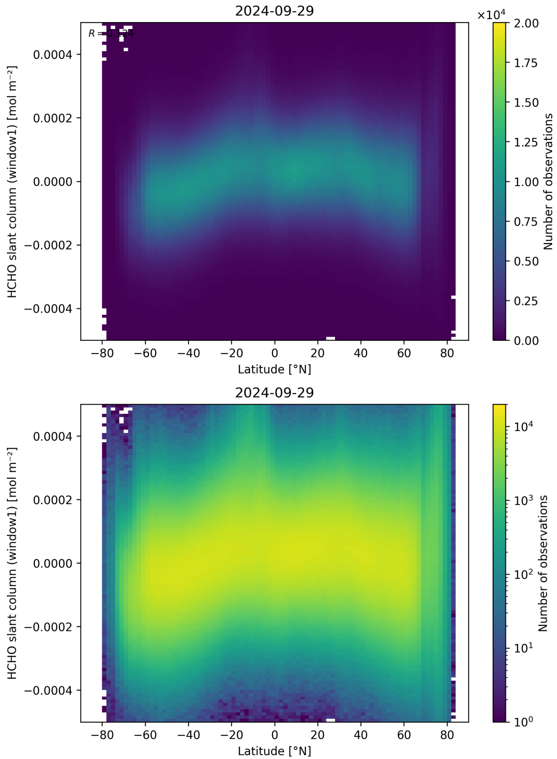
Figure 159: Scatter density plot of “Latitude” against “HCHO slant column (window1)” for 2024-09-28 to 2024-09-30.
