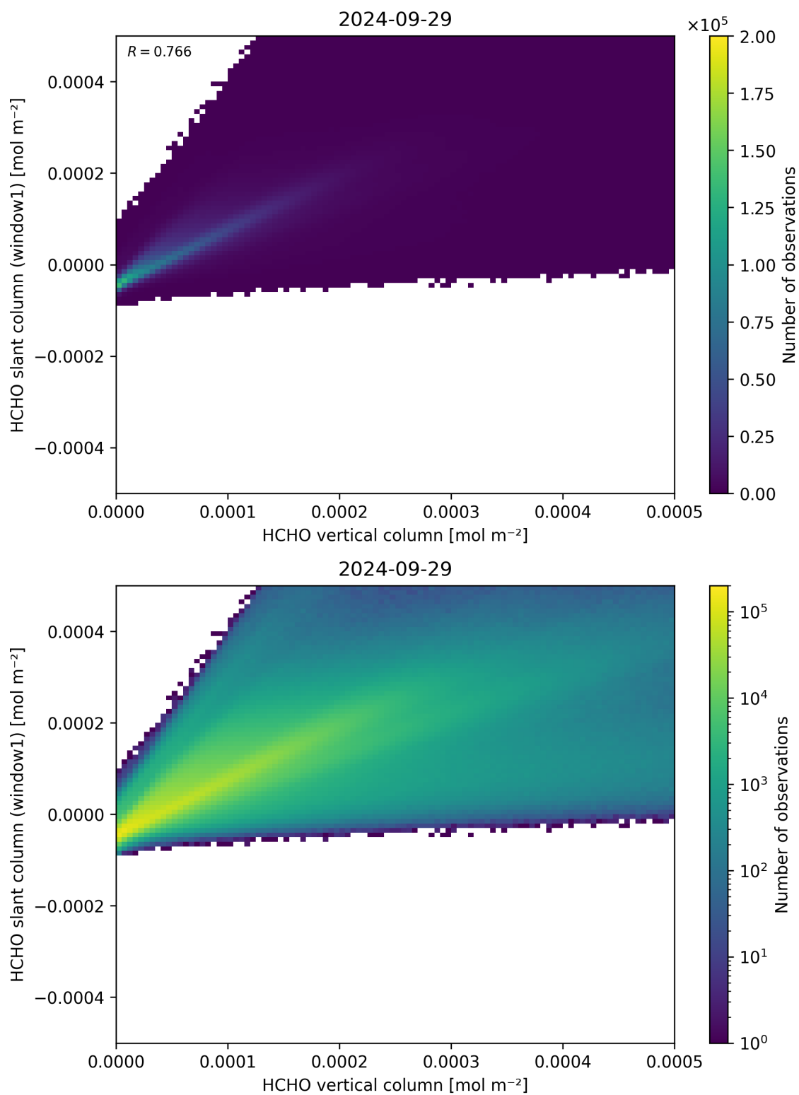
Figure 129: Scatter density plot of “HCHO vertical column” against “HCHO slant column (window1)” for 2024-09-28 to 2024-09-30.
