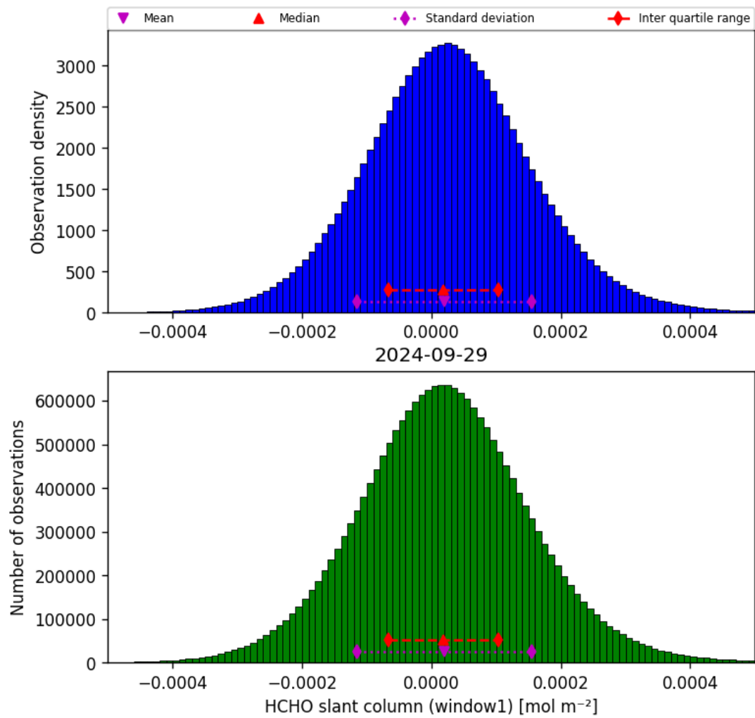
Figure 38: Histogram of “HCHO slant column (window1)” for 2024-09-28 to 2024-09-30
