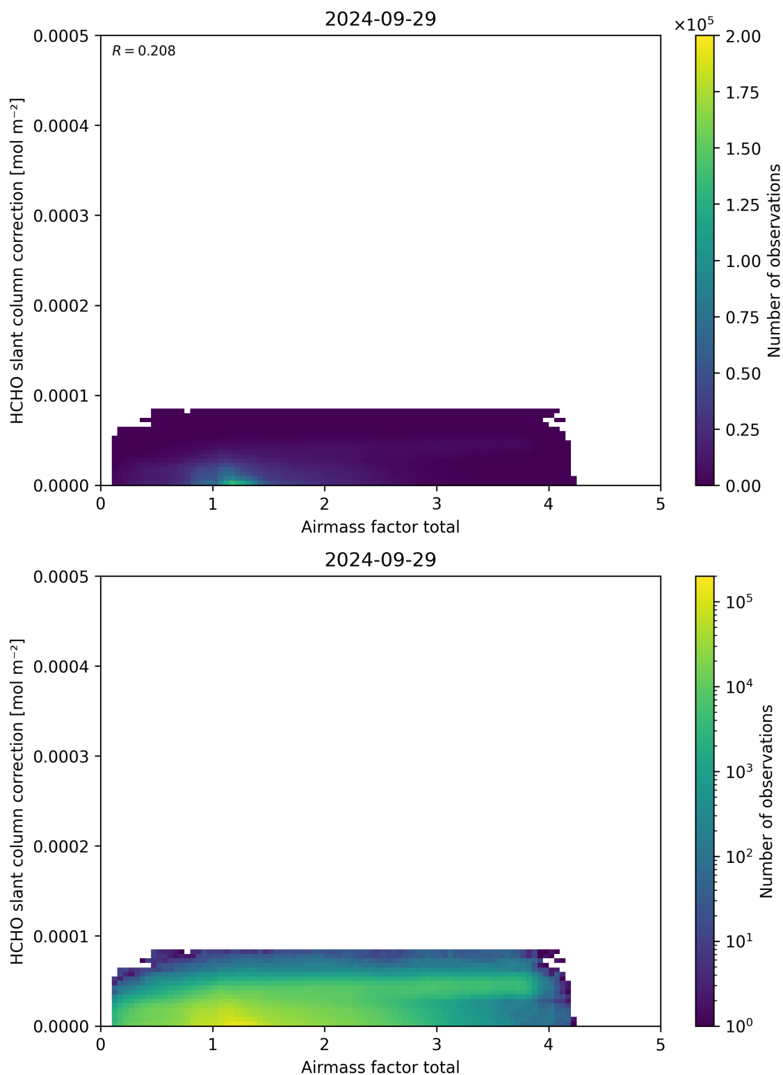
Figure 102: Scatter density plot of “Airmass factor total” against “HCHO slant column correction” for 2024-09-28 to 2024-09-30.
