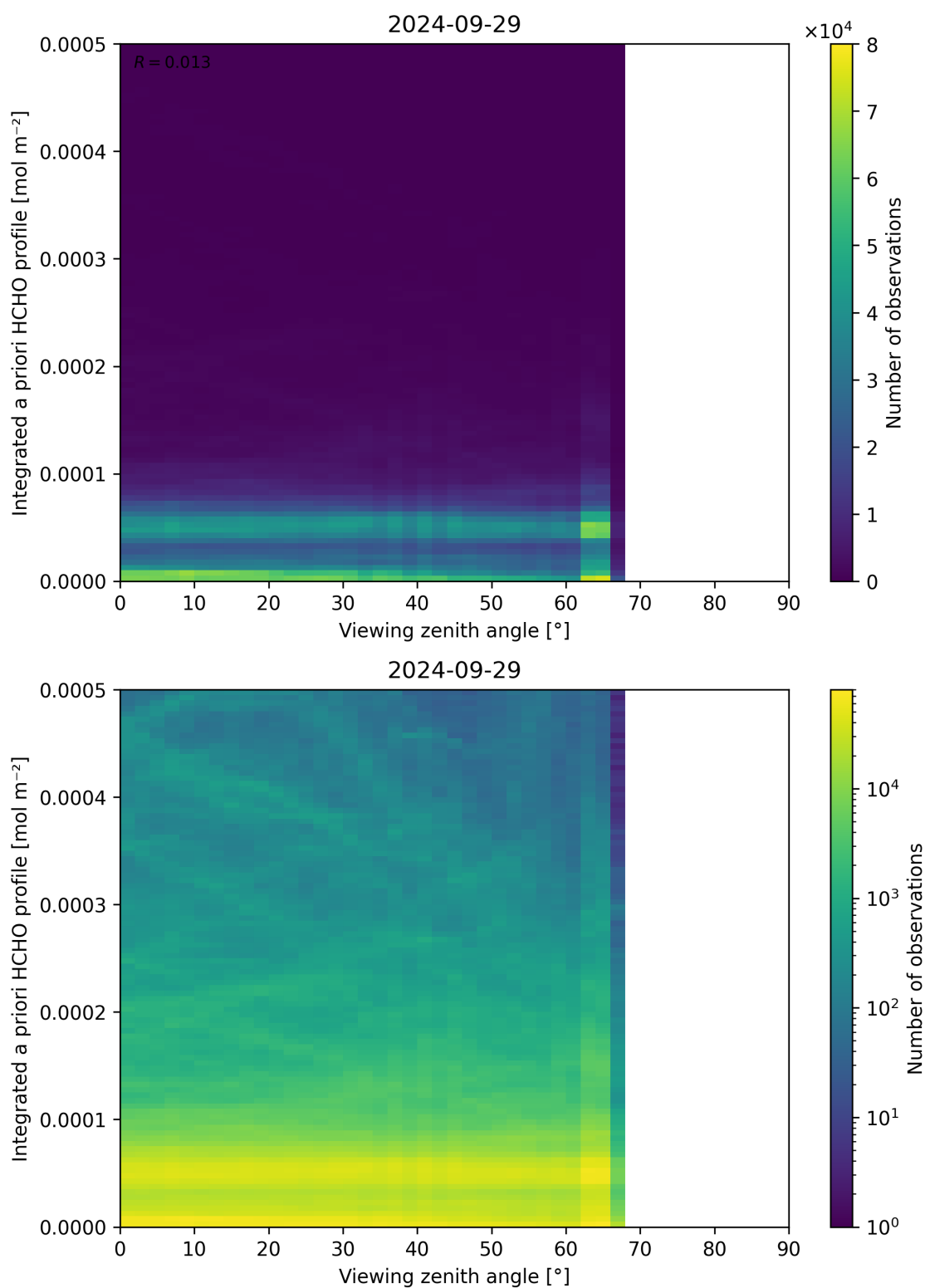
Figure 195: Scatter density plot of “Viewing zenith angle” against “Integrated a priori HCHO profile” for 2024-09-28 to 2024-09-30.
