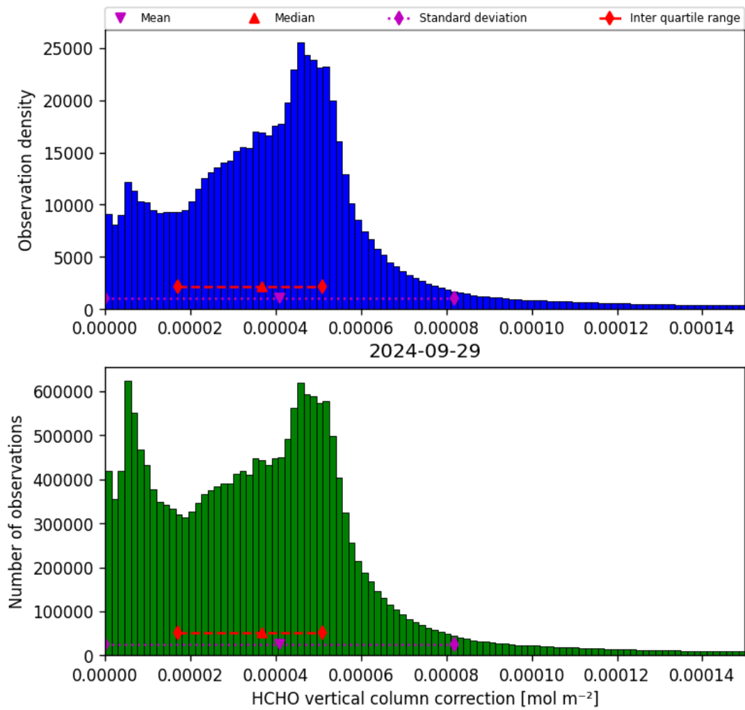
Figure 37: Histogram of “HCHO vertical column correction” for 2024-09-28 to 2024-09-30
