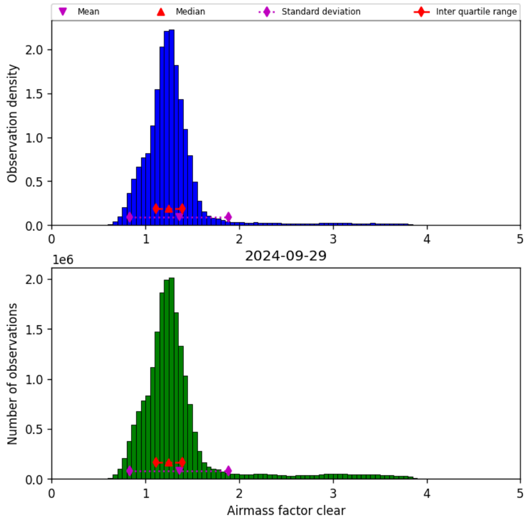
Figure 42: Histogram of “Airmass factor clear” for 2024-09-28 to 2024-09-30
