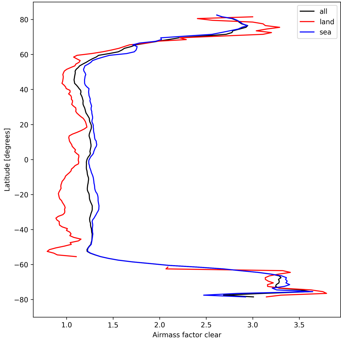
Figure 28: Zonal average of “Airmass factor clear” for 2024-09-28 to 2024-09-30.
