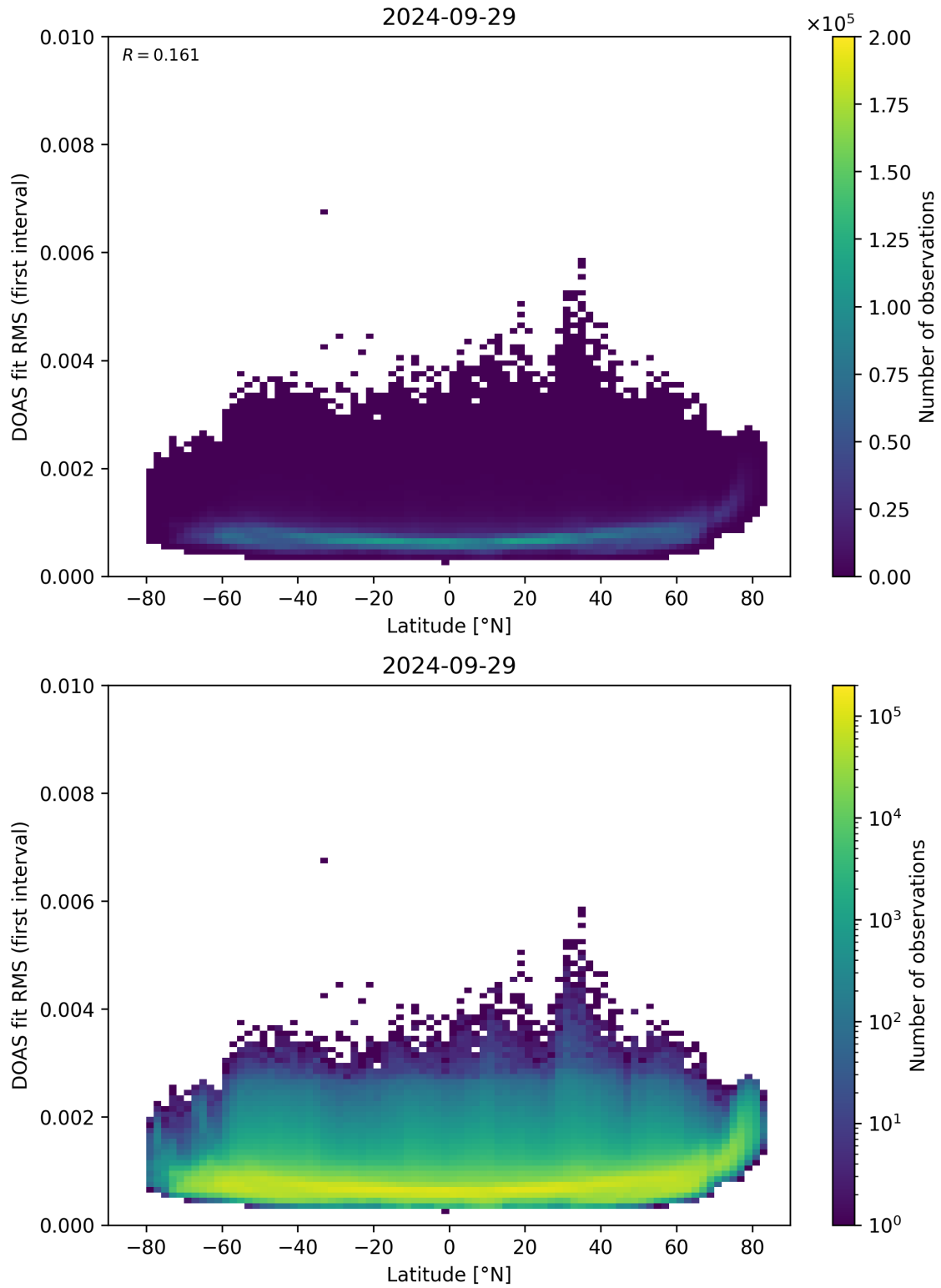
Figure 153: Scatter density plot of “Latitude” against “DOAS fit RMS (first interval)” for 2024-09-28 to 2024-09-30.
