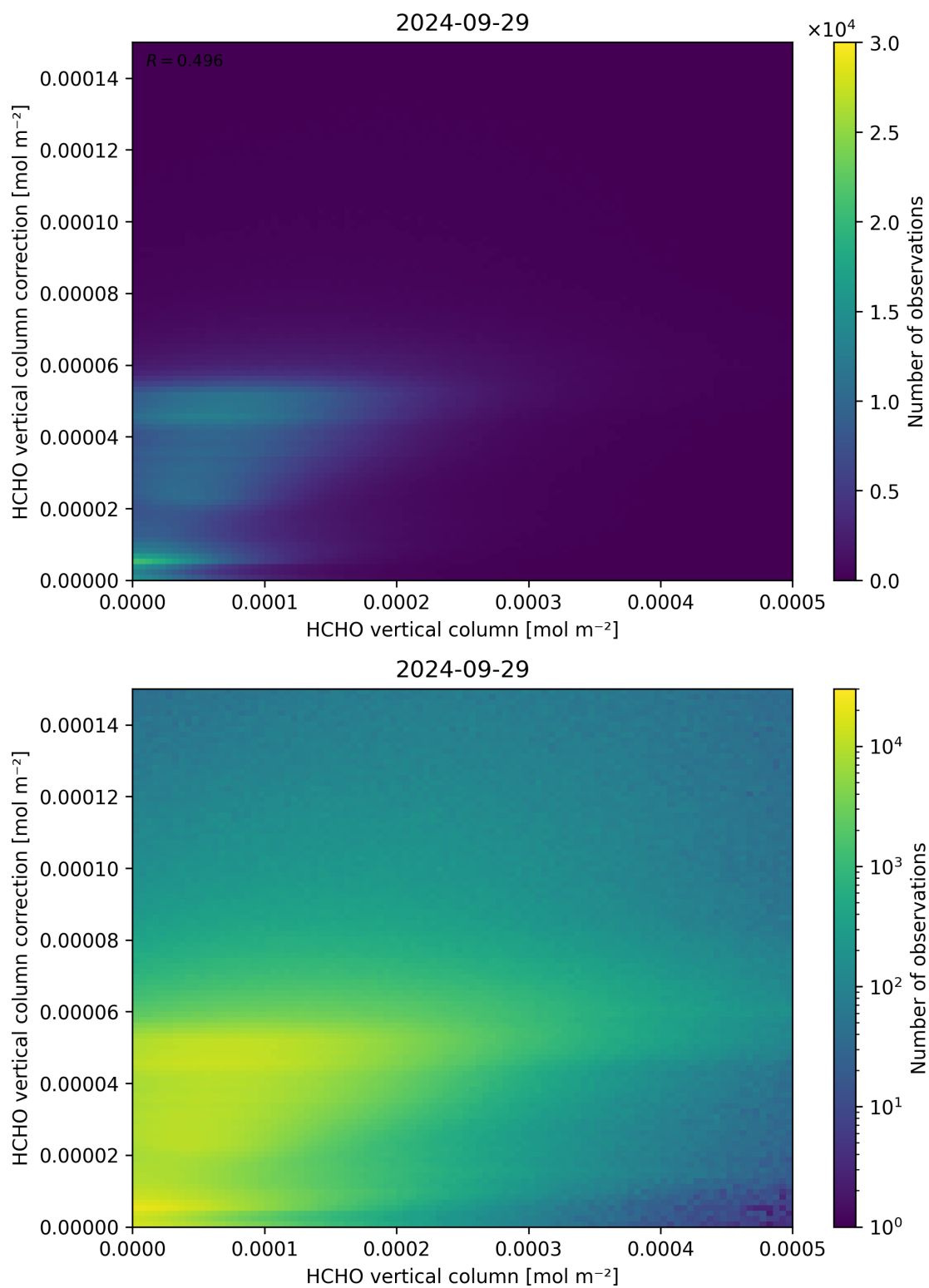
Figure 133: Scatter density plot of “HCHO vertical column” against “HCHO vertical column correction” for 2024-09-28 to 2024-09-30.
