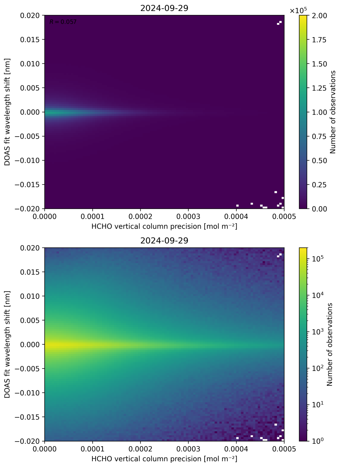
Figure 137: Scatter density plot of “HCHO vertical column precision” against “DOAS fit wavelength shift” for 2024-09-28 to 2024-09-30.
