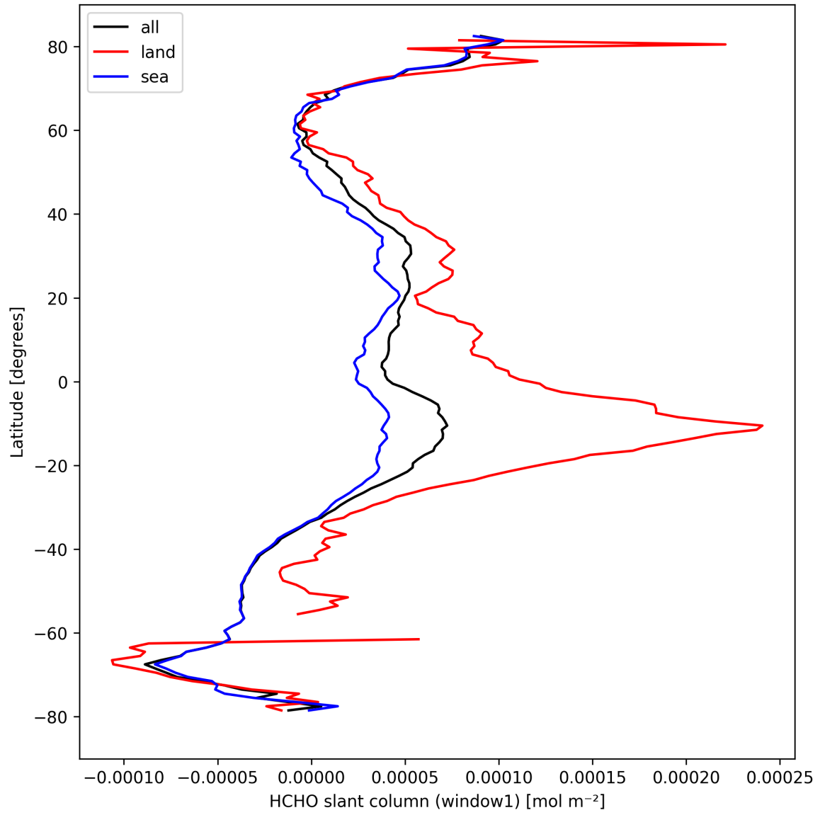
Figure 24: Zonal average of “HCHO slant column (window1)” for 2024-09-28 to 2024-09-30.
