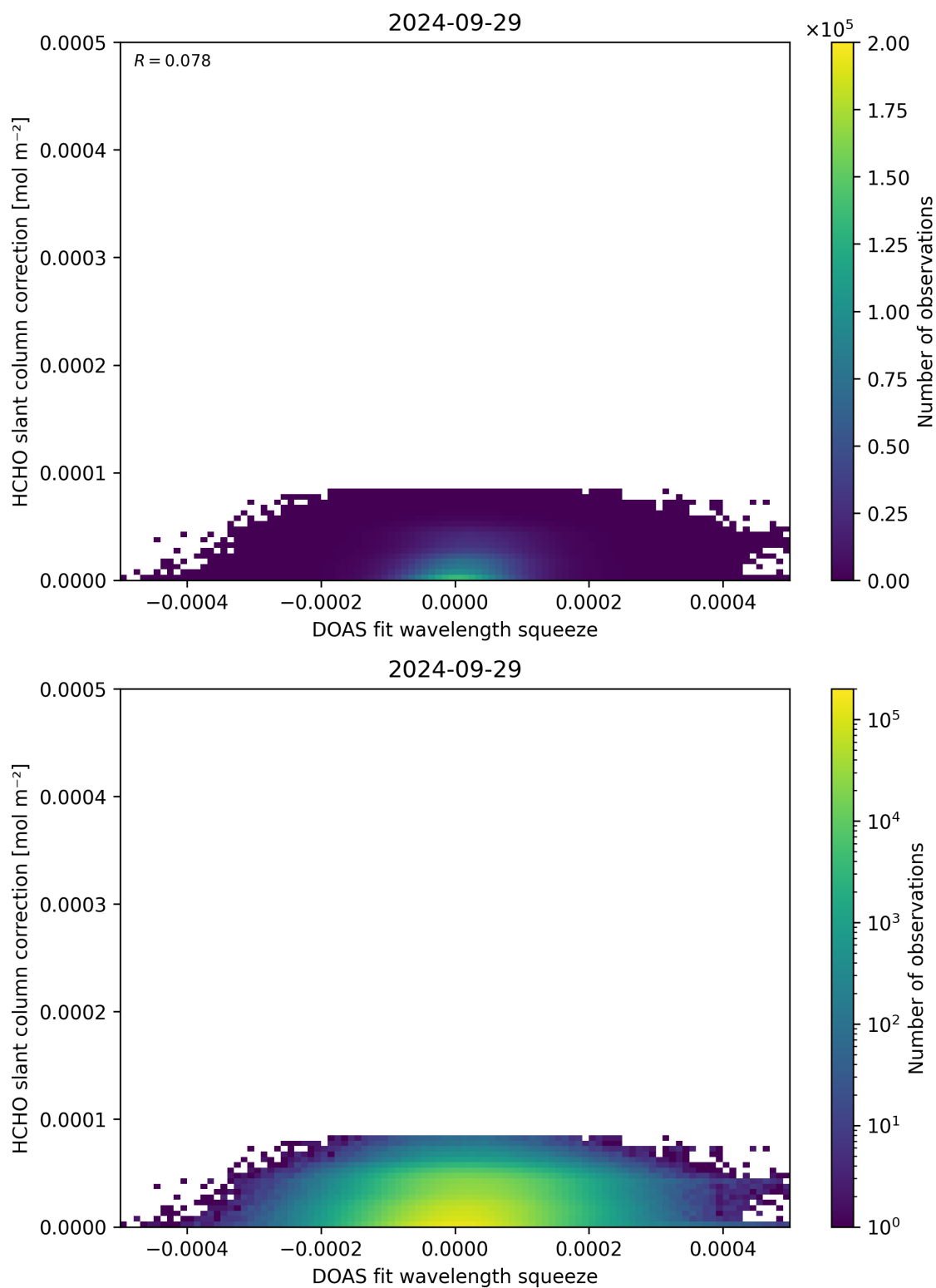
Figure 70: Scatter density plot of “DOAS fit wavelength squeeze” against “HCHO slant column correction” for 2024-09-28 to 2024-09-30.
