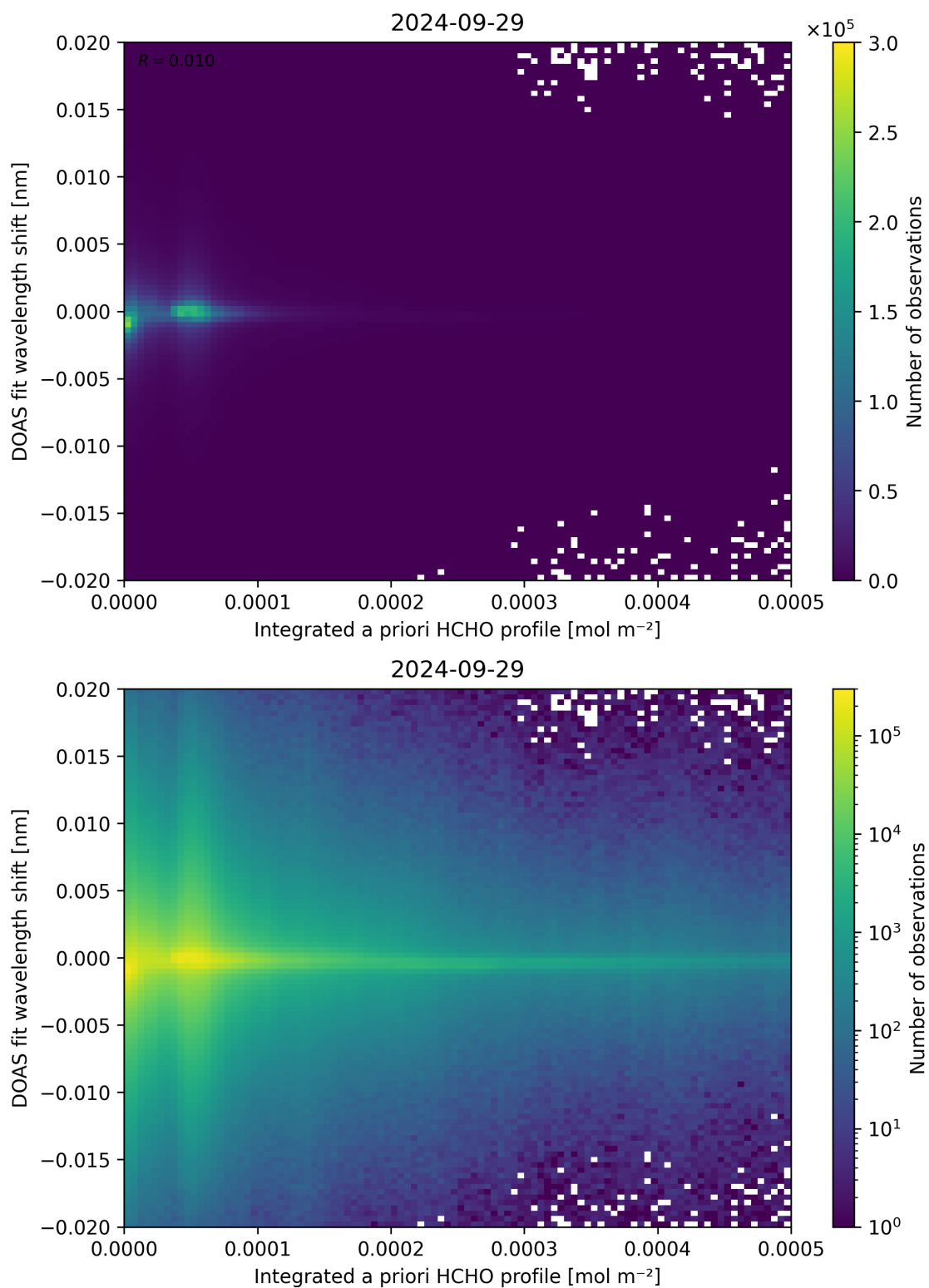
Figure 149: Scatter density plot of “Integrated a priori HCHO profile” against “DOAS fit wavelength shift” for 2024-09-28 to 2024-09-30.
