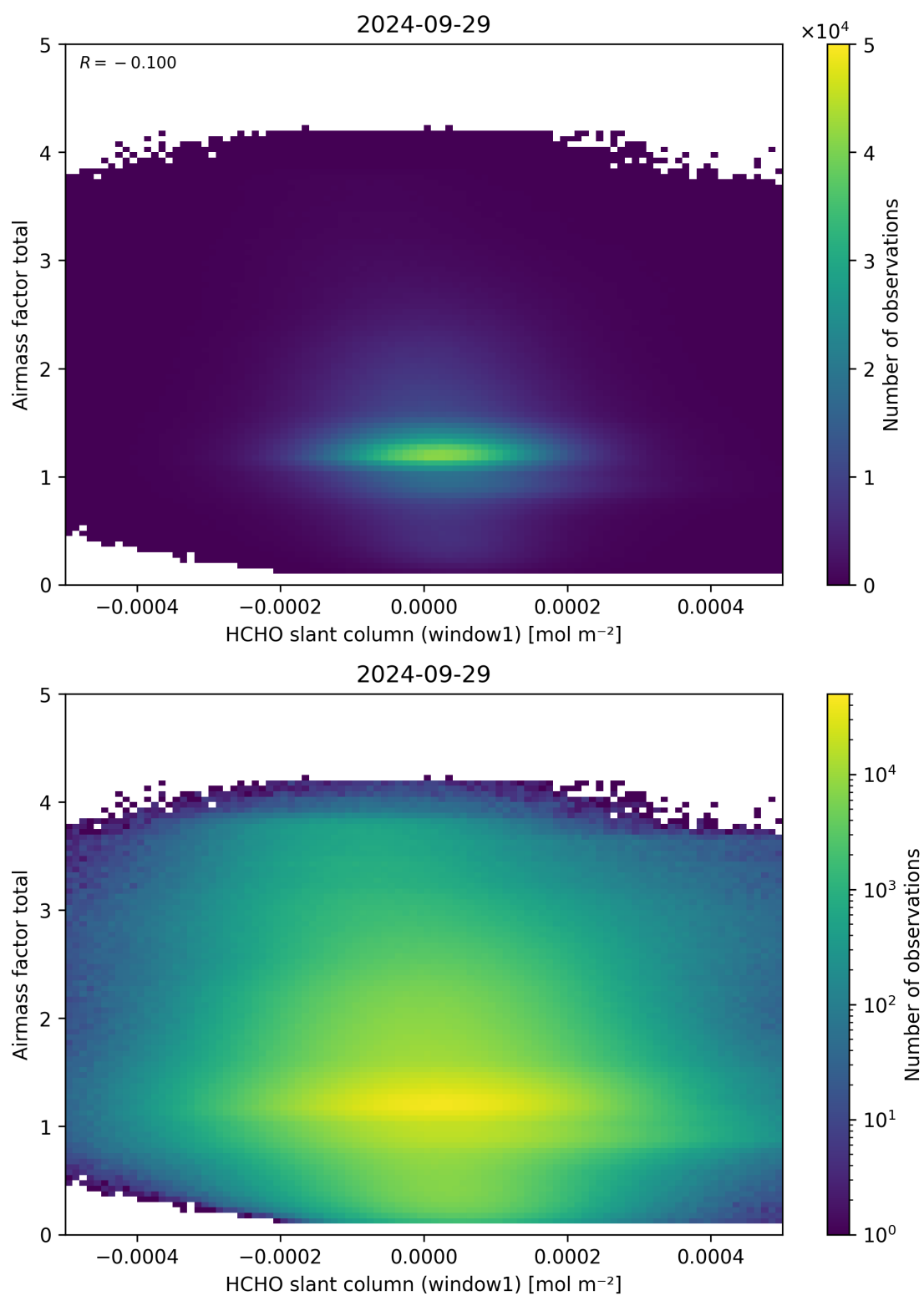
Figure 85: Scatter density plot of “HCHO slant column (window1)” against “Airmass factor total” for 2024-09-28 to 2024-09-30.
