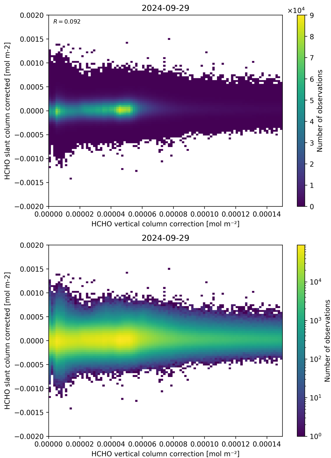
Figure 116: Scatter density plot of “HCHO vertical column correction” against “HCHO slant column corrected” for 2024-09-28 to 2024-09-30.
