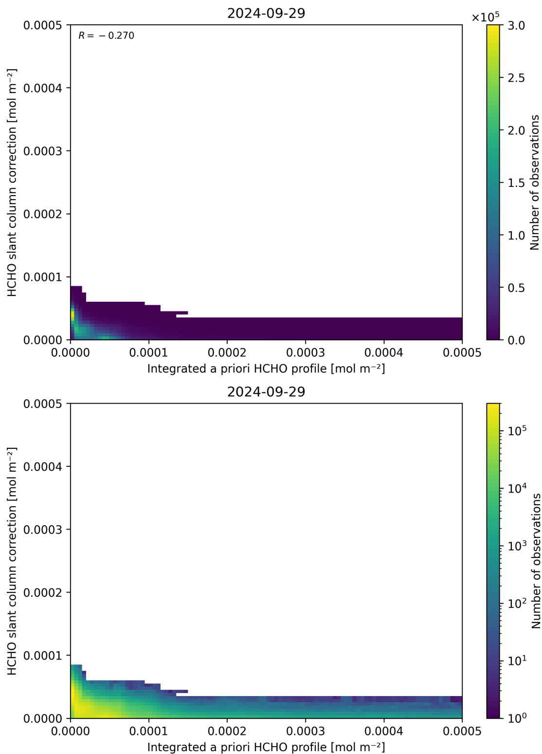
Figure 152: Scatter density plot of “Integrated a priori HCHO profile” against “HCHO slant column correction” for 2024-09-28 to 2024-09-30.
