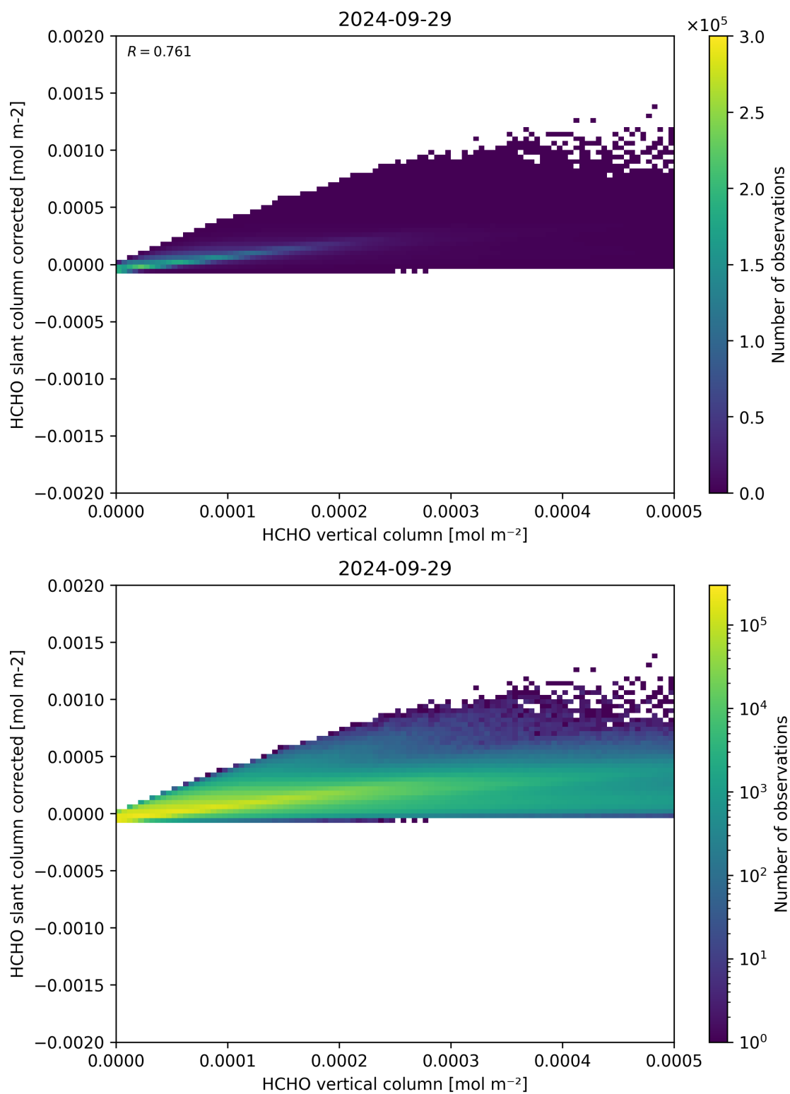
Figure 127: Scatter density plot of “HCHO vertical column” against “HCHO slant column corrected” for 2024-09-28 to 2024-09-30.
