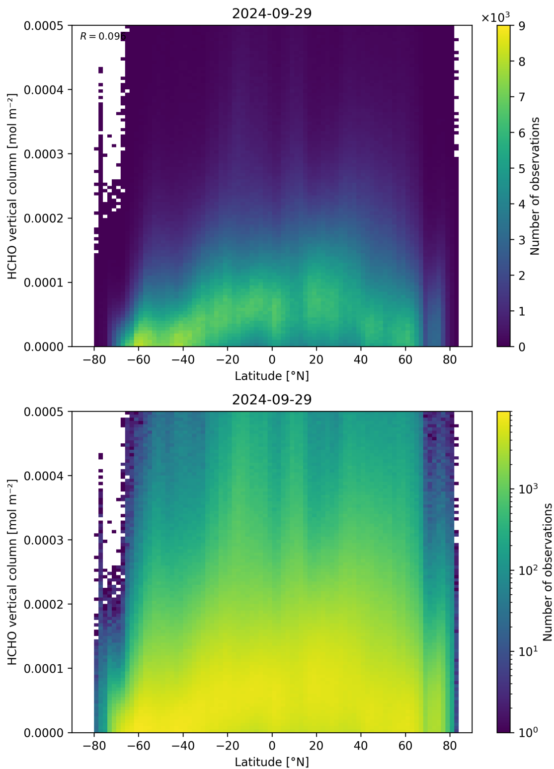
Figure 163: Scatter density plot of “Latitude” against “HCHO vertical column” for 2024-09-28 to 2024-09-30.
