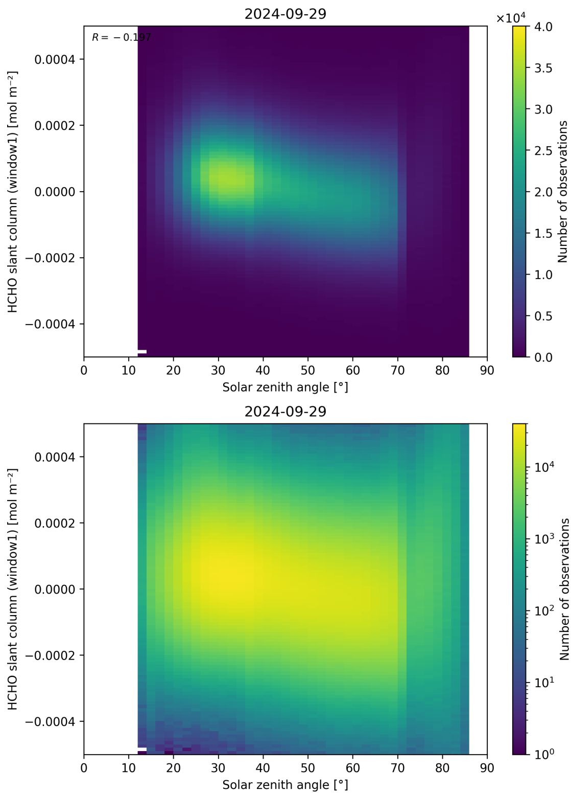
Figure 173: Scatter density plot of “Solar zenith angle” against “HCHO slant column (window1)” for 2024-09-28 to 2024-09-30.
