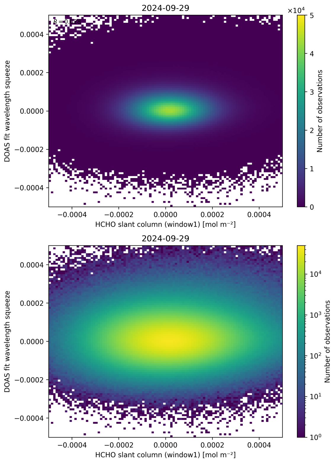
Figure 80: Scatter density plot of “HCHO slant column (window1)” against “DOAS fit wavelength squeeze” for 2024-09-28 to 2024-09-30.
