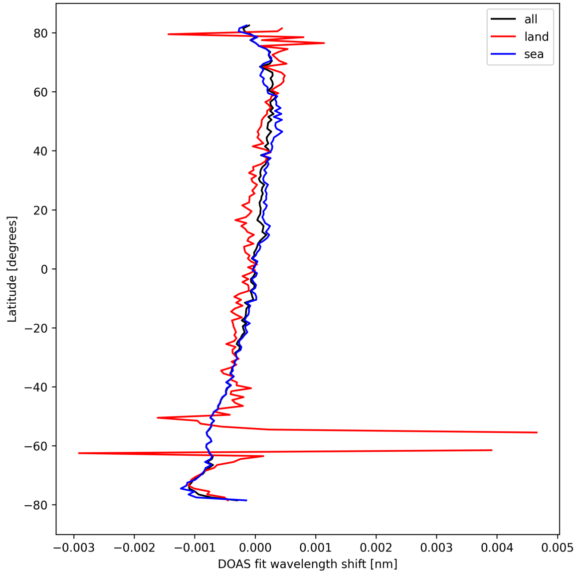
Figure 30: Zonal average of "DOAS fit wavelength shift" for 2024-09-28 to 2024-09-30.
