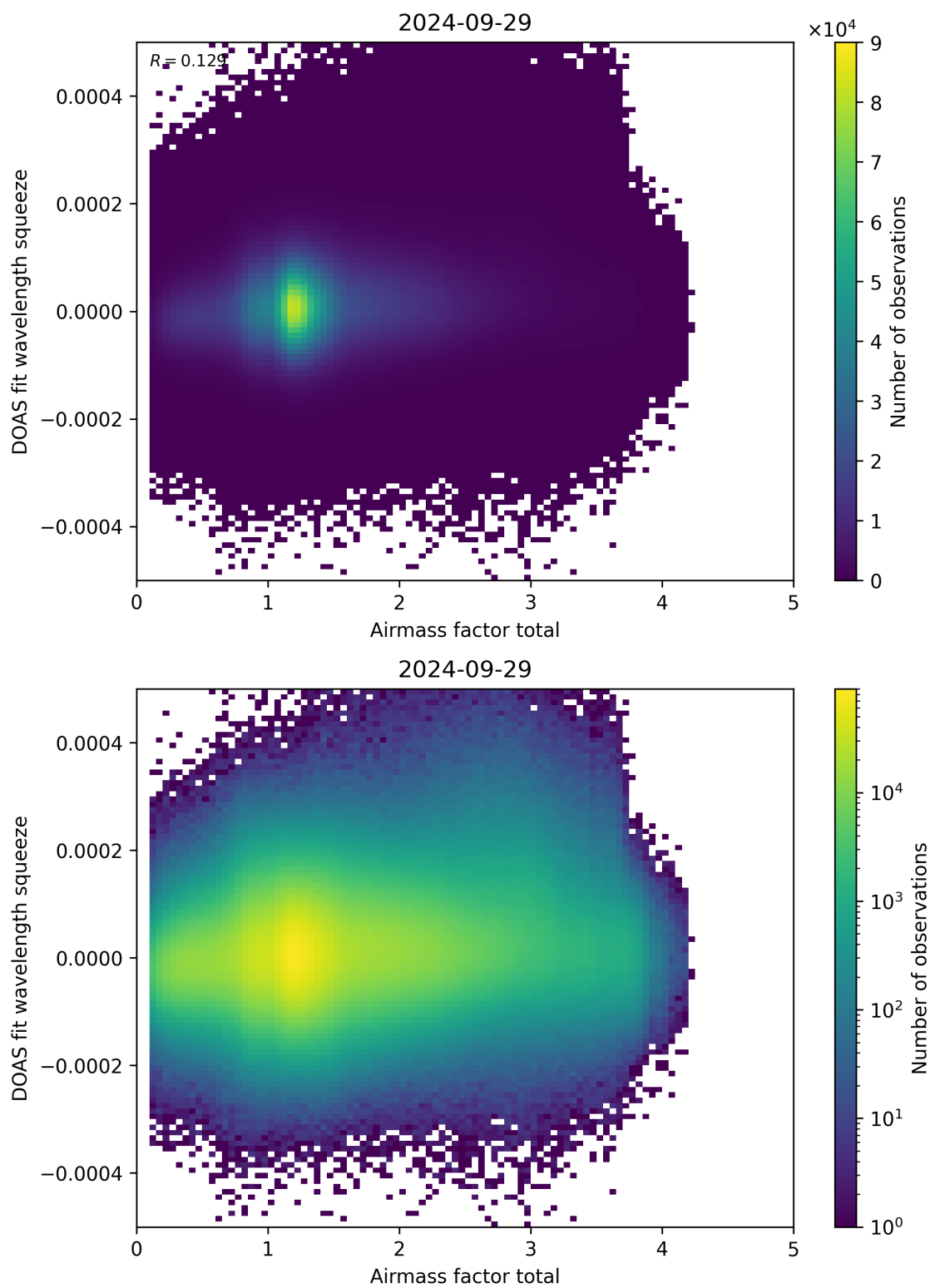
Figure 99: Scatter density plot of “Airmass factor total” against “DOAS fit wavelength squeeze” for 2024-09-28 to 2024-09-30.
