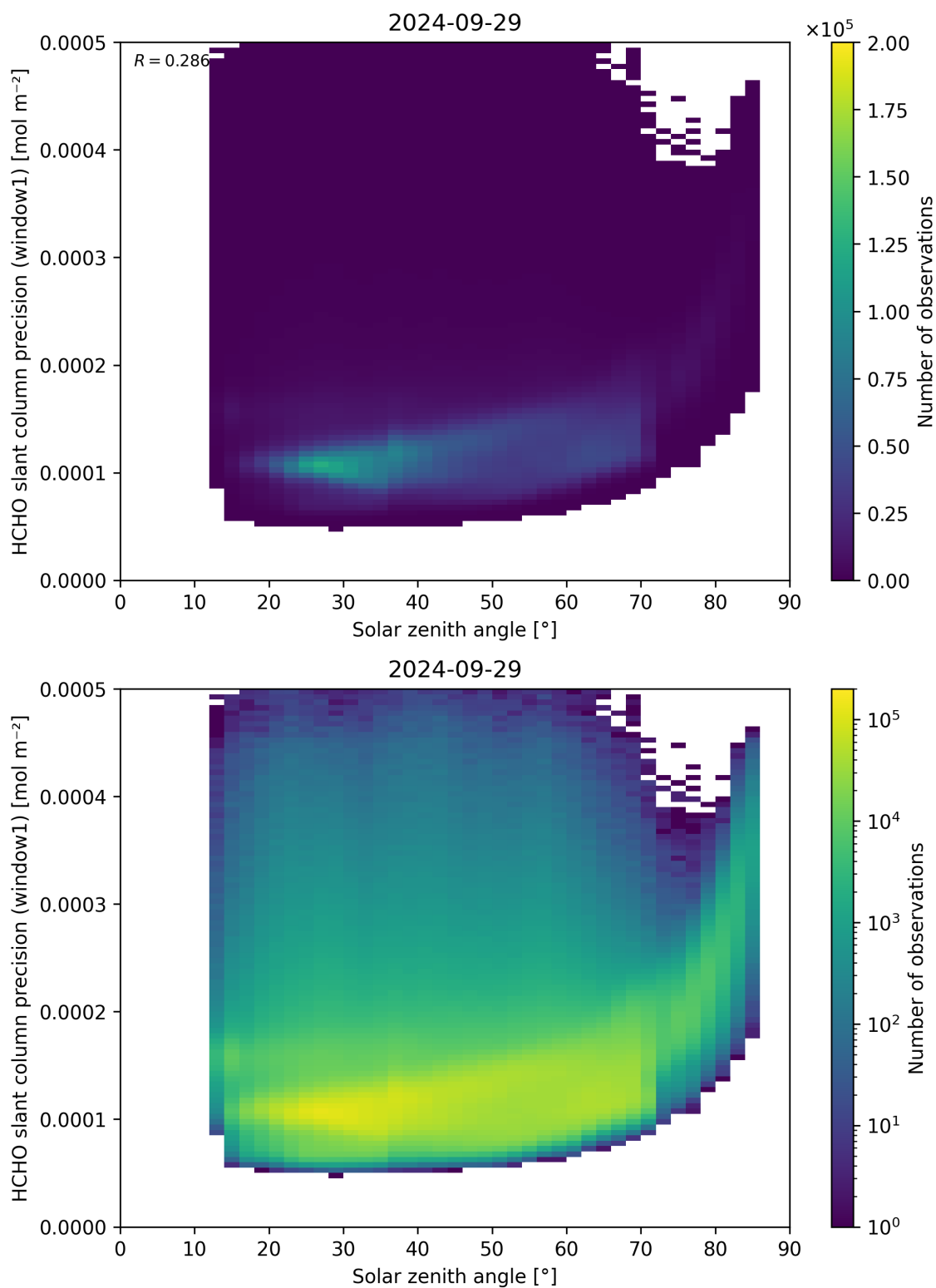
Figure 174: Scatter density plot of “Solar zenith angle” against “HCHO slant column precision (window1)” for 2024-09-28 to 2024-09-30.
