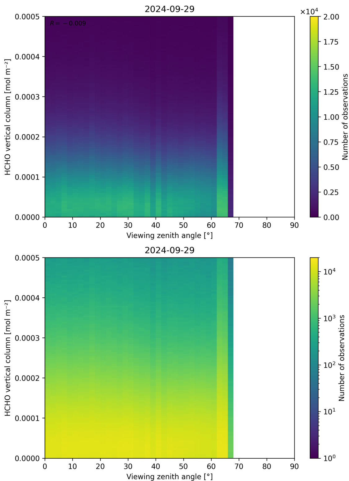
Figure 192: Scatter density plot of “Viewing zenith angle” against “HCHO vertical column” for 2024-09-28 to 2024-09-30.
