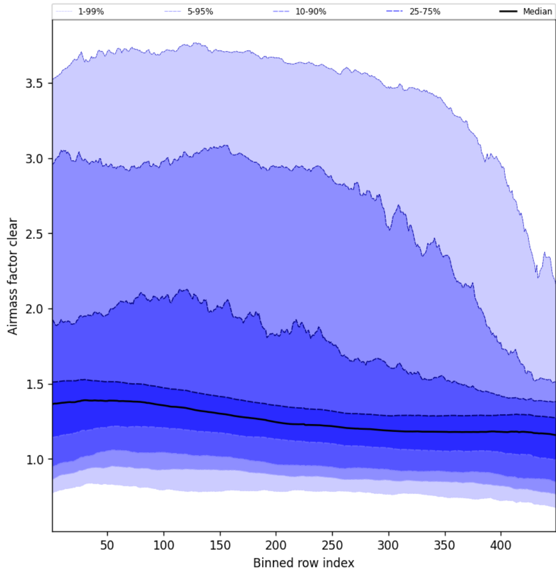
Figure 56: Along track statistics of “Airmass factor clear” for 2024-09-28 to 2024-09-30
