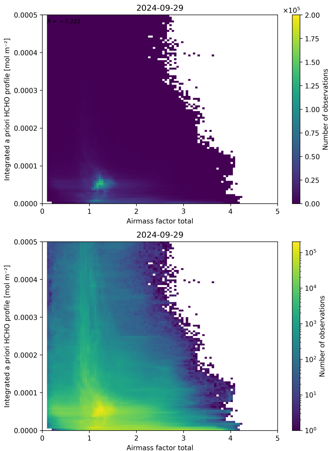
Figure 104: Scatter density plot of “Airmass factor total” against “Integrated a priori HCHO profile” for 2024-09-28 to 2024-09-30.
