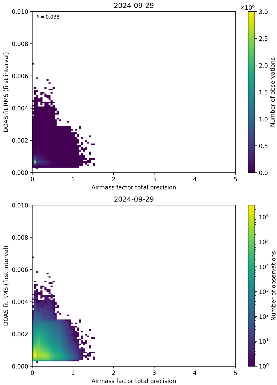
Figure 105: Scatter density plot of “Airmass factor total precision” against “DOAS fit RMS (first interval)” for 2024-09-28 to 2024-09-30.
