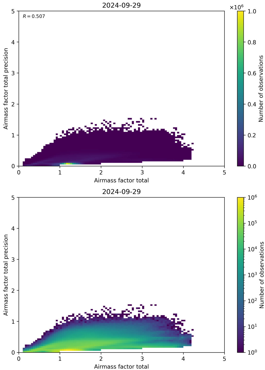
Figure 103: Scatter density plot of “Airmass factor total” against “Airmass factor total precision” for 2024-09-28 to 2024-09-30.
