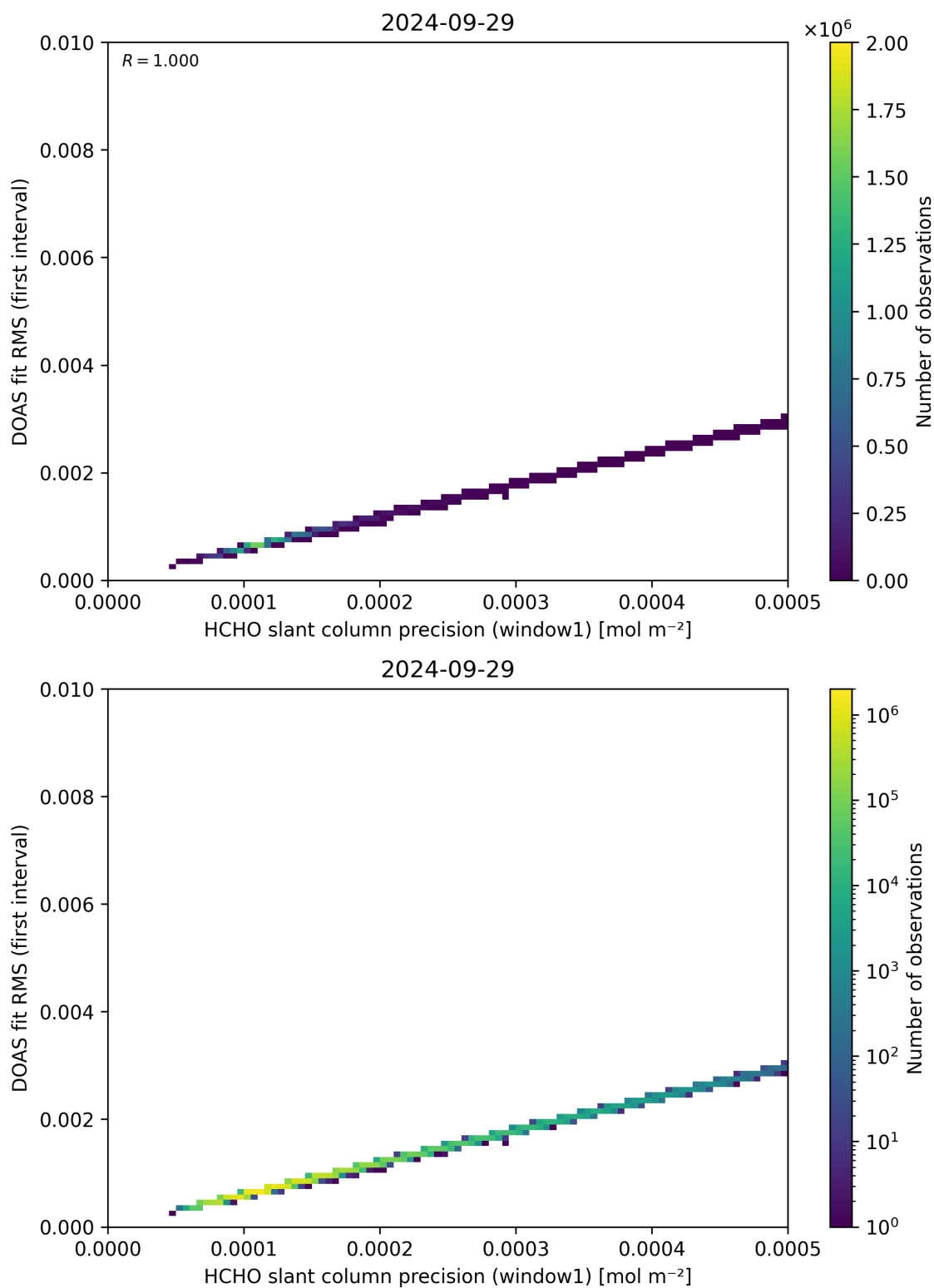
Figure 88: Scatter density plot of “HCHO slant column precision (window1)” against “DOAS fit RMS (first interval)” for 2024-09-28 to 2024-09-30.
