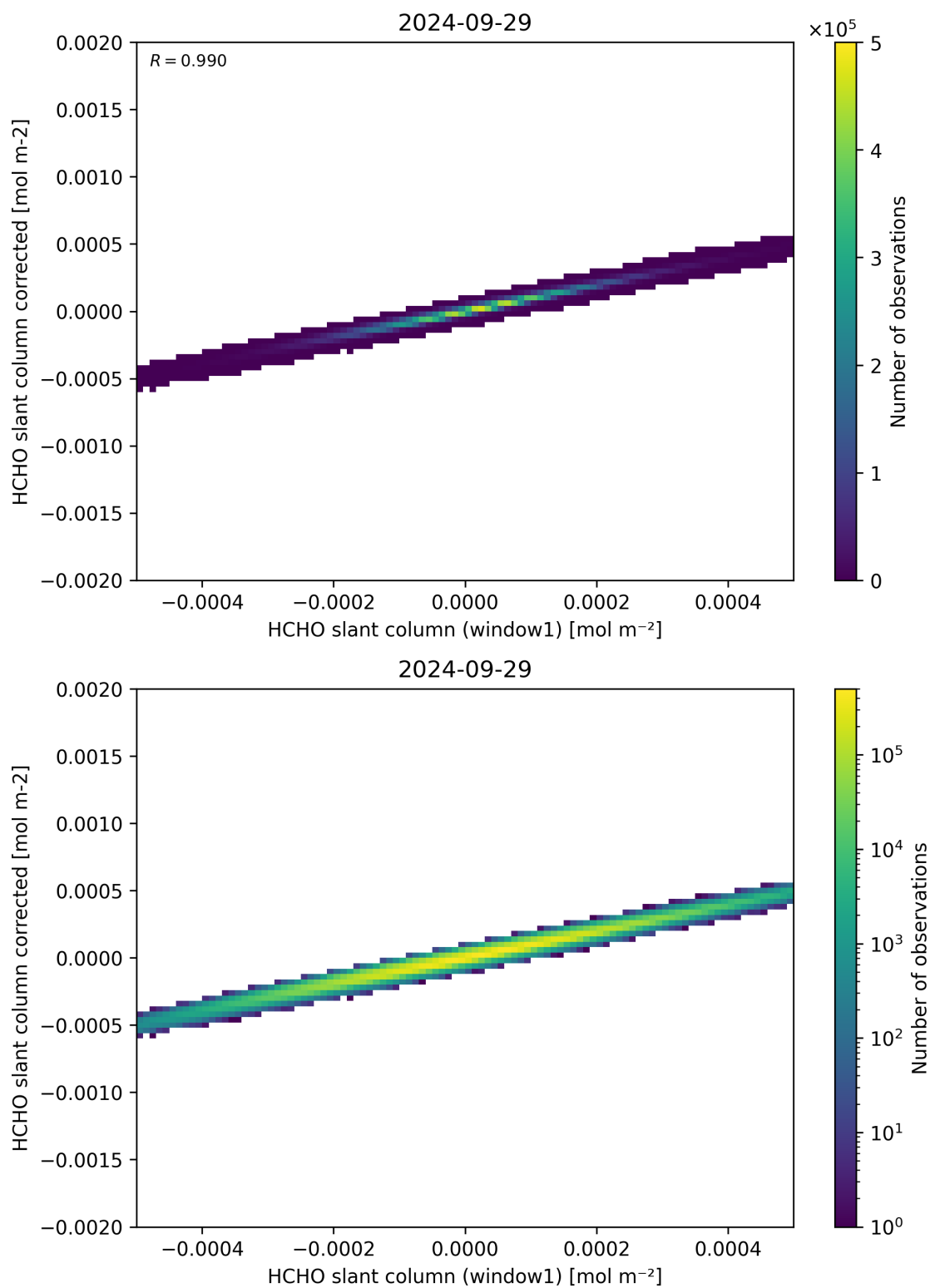
Figure 82: Scatter density plot of “HCHO slant column (window1)” against “HCHO slant column corrected” for 2024-09-28 to 2024-09-30.
