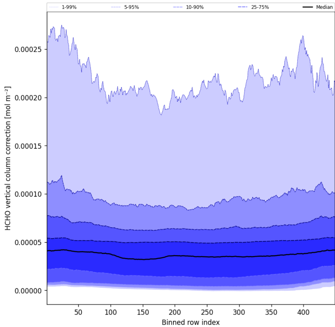
Figure 51: Along track statistics of “HCHO vertical column correction” for 2024-09-28 to 2024-09-30
