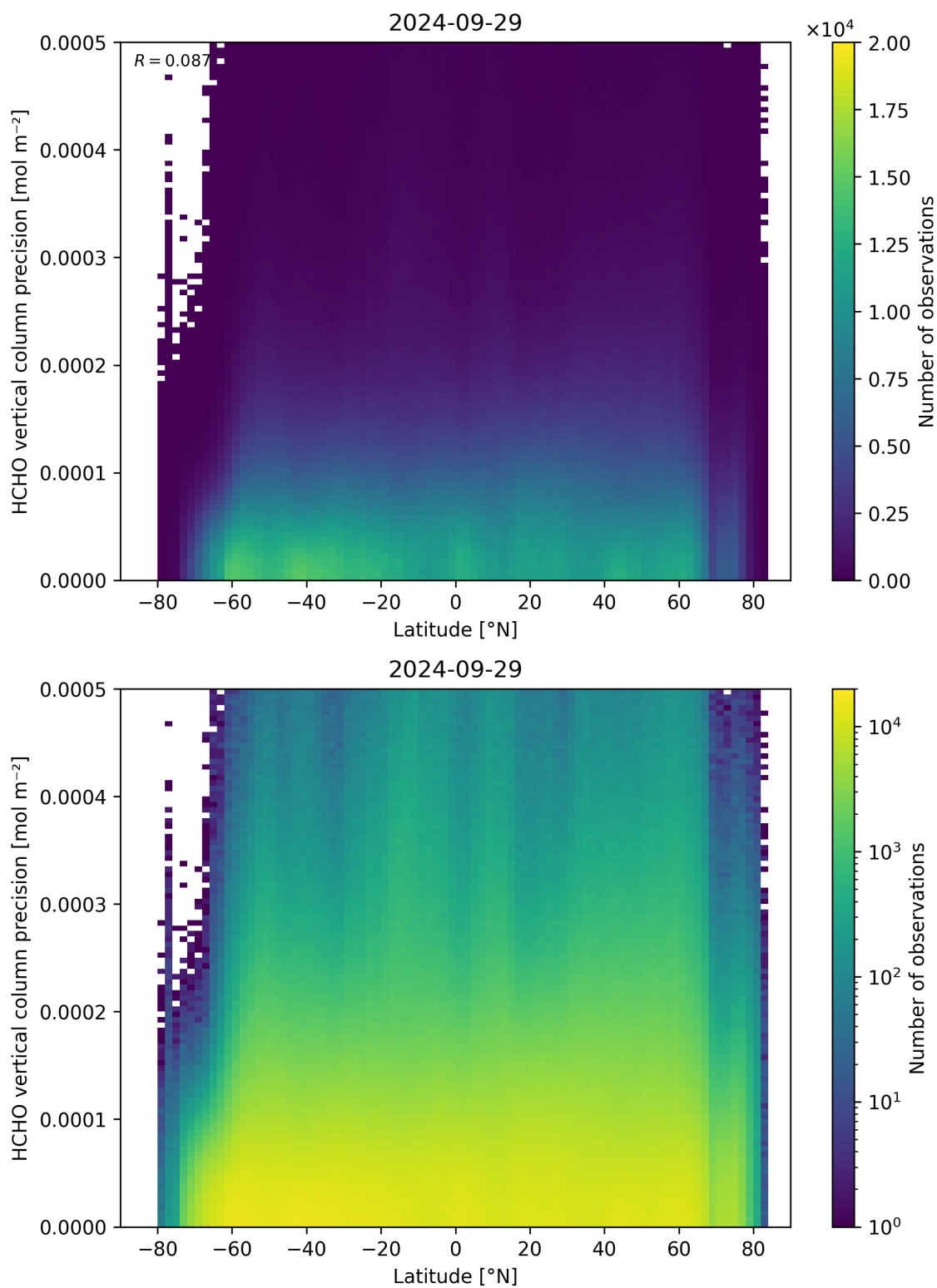
Figure 165: Scatter density plot of “Latitude” against “HCHO vertical column precision” for 2024-09-28 to 2024-09-30.
