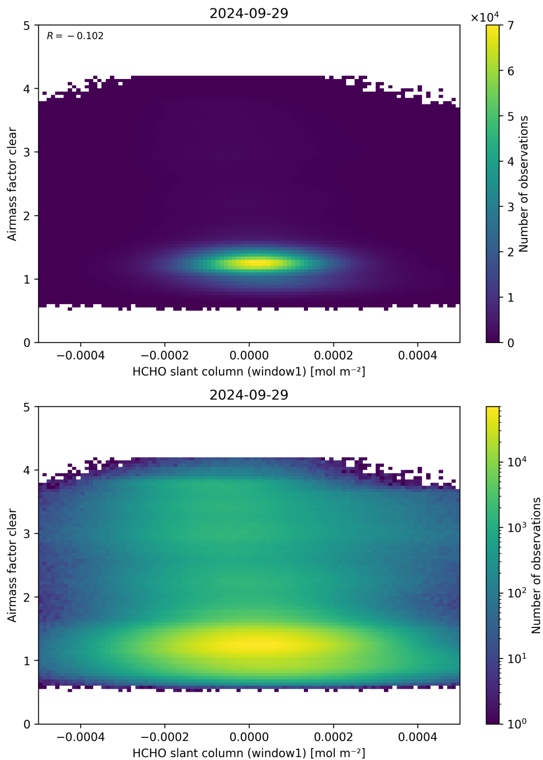
Figure 81: Scatter density plot of “HCHO slant column (window1)” against “Airmass factor clear” for 2024-09-28 to 2024-09-30.
