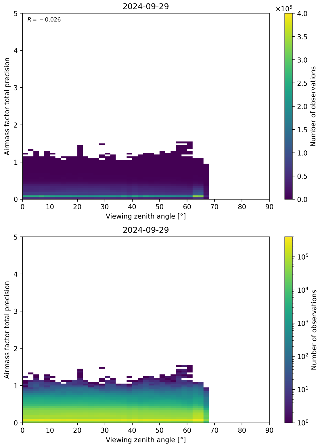
Figure 191: Scatter density plot of “Viewing zenith angle” against “Airmass factor total precision” for 2024-09-28 to 2024-09-30.
