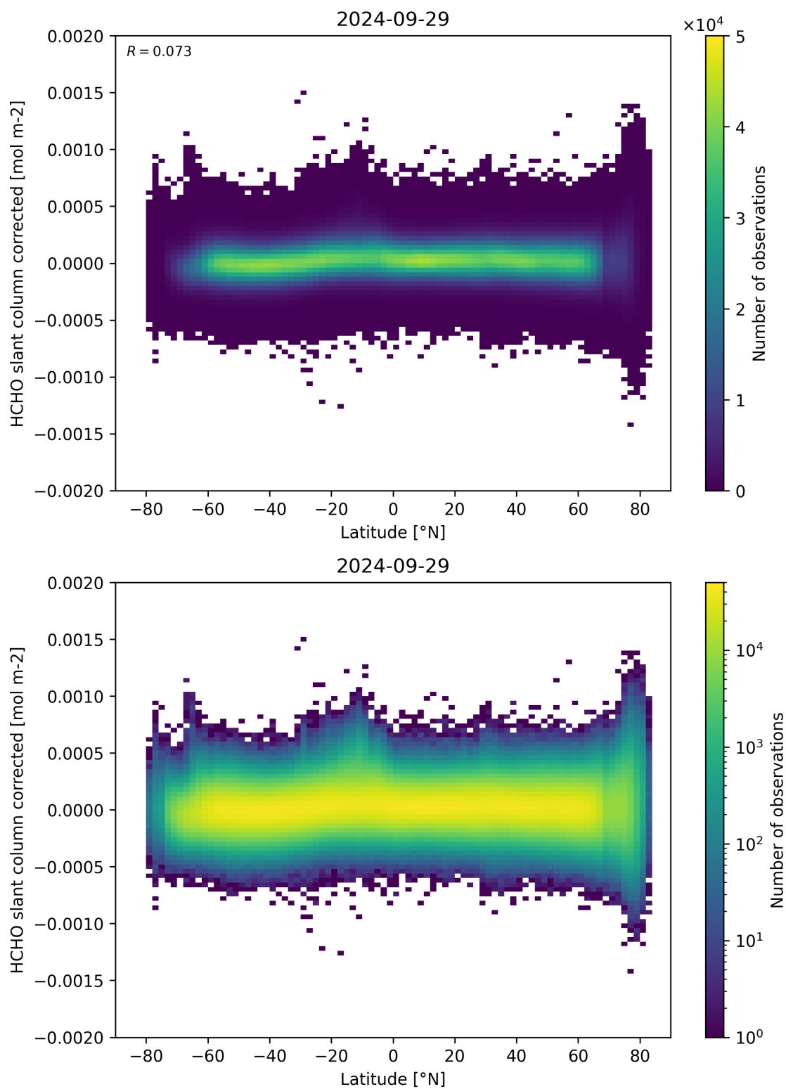
Figure 157: Scatter density plot of “Latitude” against “HCHO slant column corrected” for 2024-09-28 to 2024-09-30.
