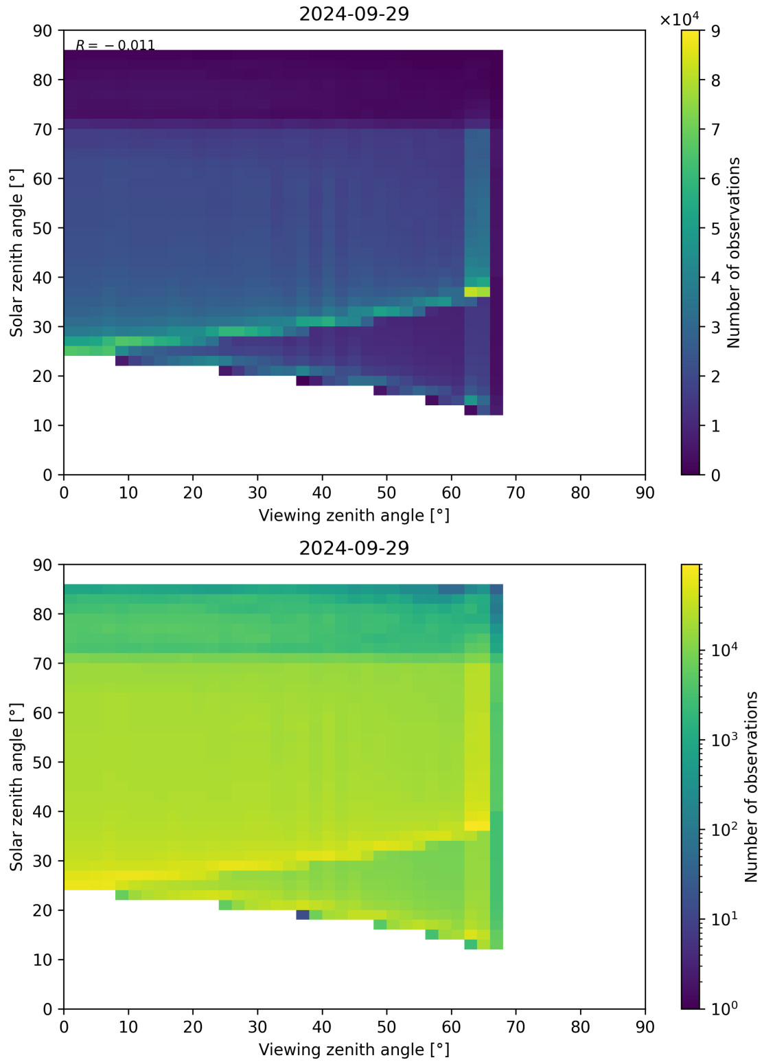
Figure 197: Scatter density plot of “Viewing zenith angle” against “Solar zenith angle” for 2024-09-28 to 2024-09-30.
