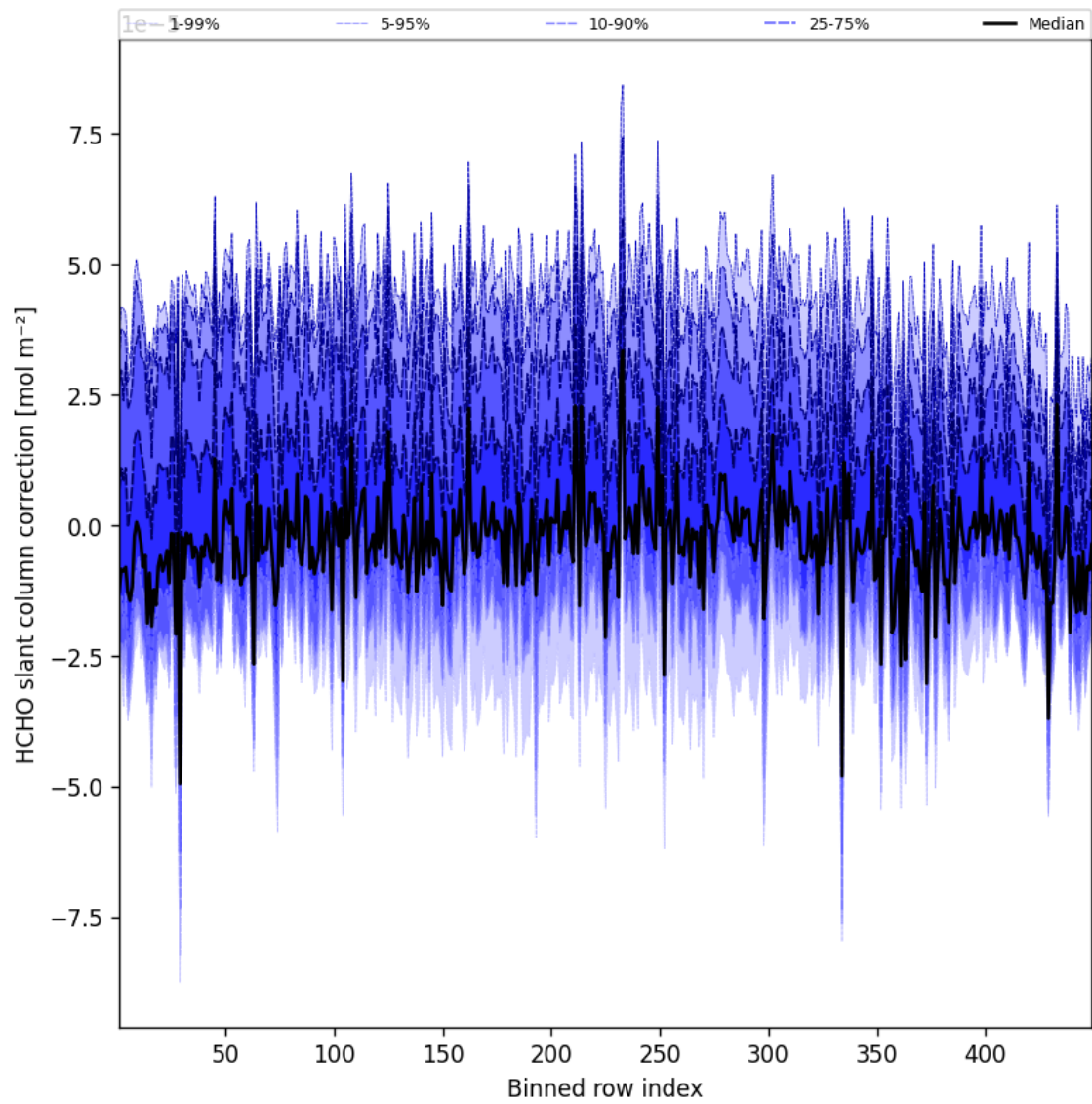
Figure 61: Along track statistics of "HCHO slant column correction" for 2024-09-28 to 2024-09-30
