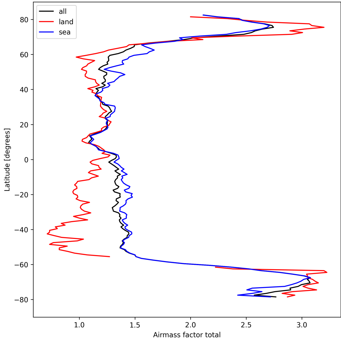
Figure 26: Zonal average of “Airmass factor total” for 2024-09-28 to 2024-09-30.
