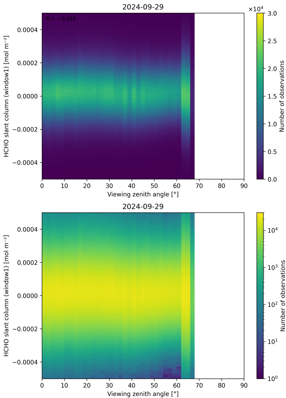
Figure 188: Scatter density plot of “Viewing zenith angle” against “HCHO slant column (window1)” for 2024-09-28 to 2024-09-30.
