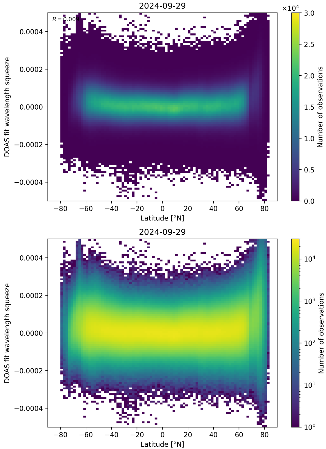
Figure 155: Scatter density plot of “Latitude” against “DOAS fit wavelength squeeze” for 2024-09-28 to 2024-09-30.
