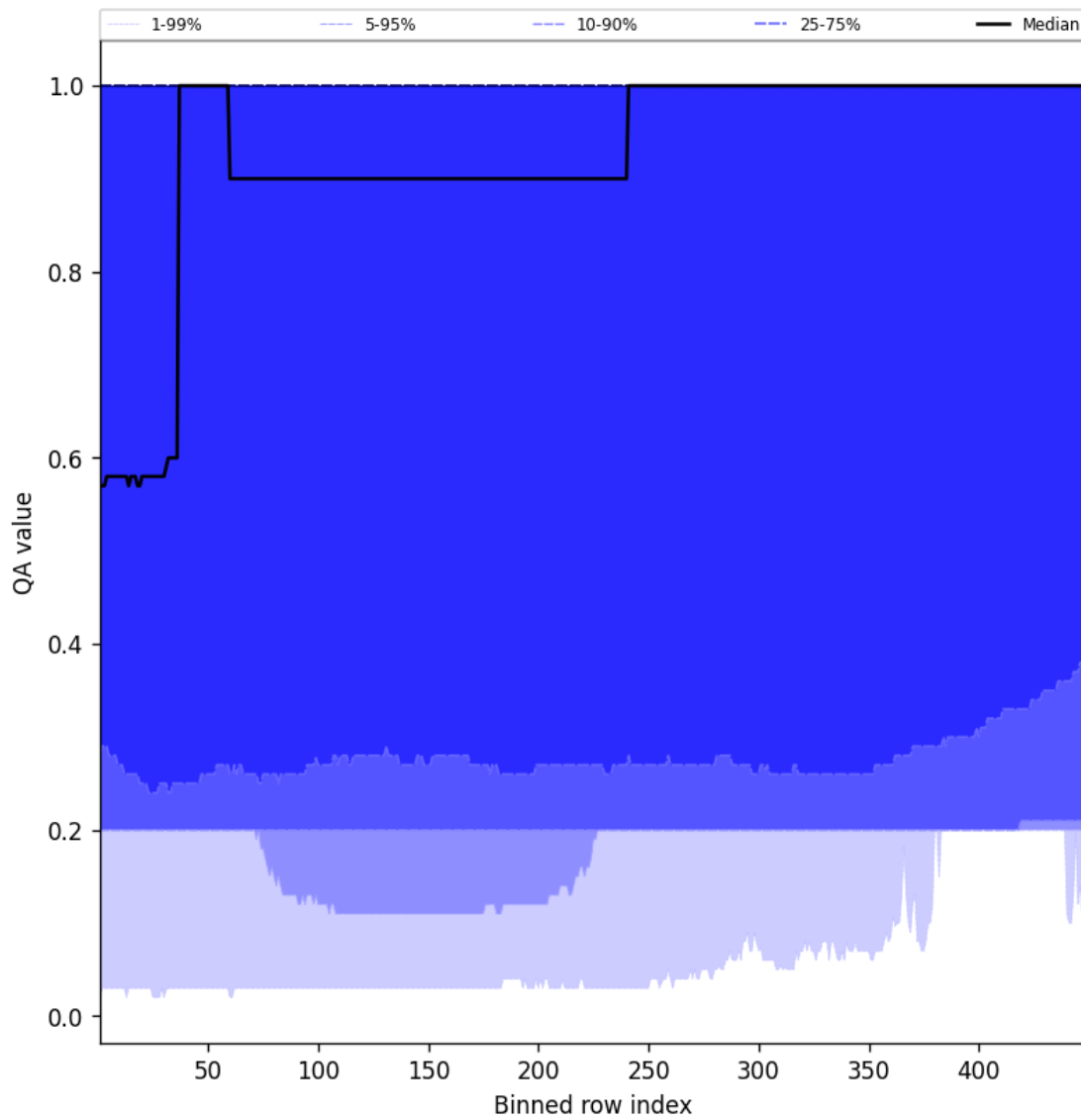
Figure 48: Along track statistics of “QA value” for 2024-09-28 to 2024-09-30
