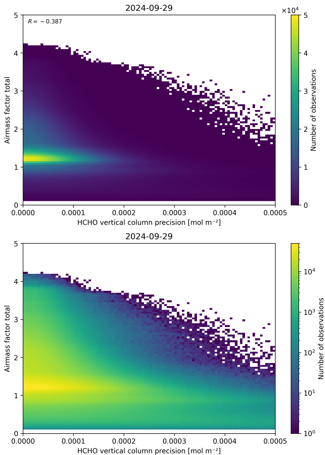
Figure 144: Scatter density plot of “HCHO vertical column precision” against “Airmass factor total” for 2024-09-28 to 2024-09-30.
