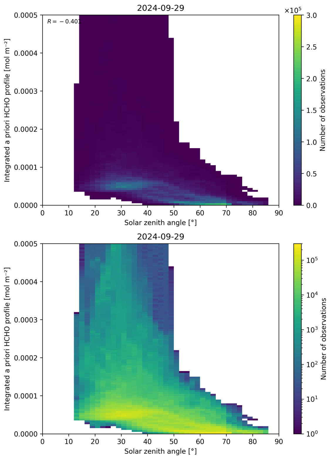
Figure 180: Scatter density plot of “Solar zenith angle” against “Integrated a priori HCHO profile” for 2024-09-28 to 2024-09-30.
