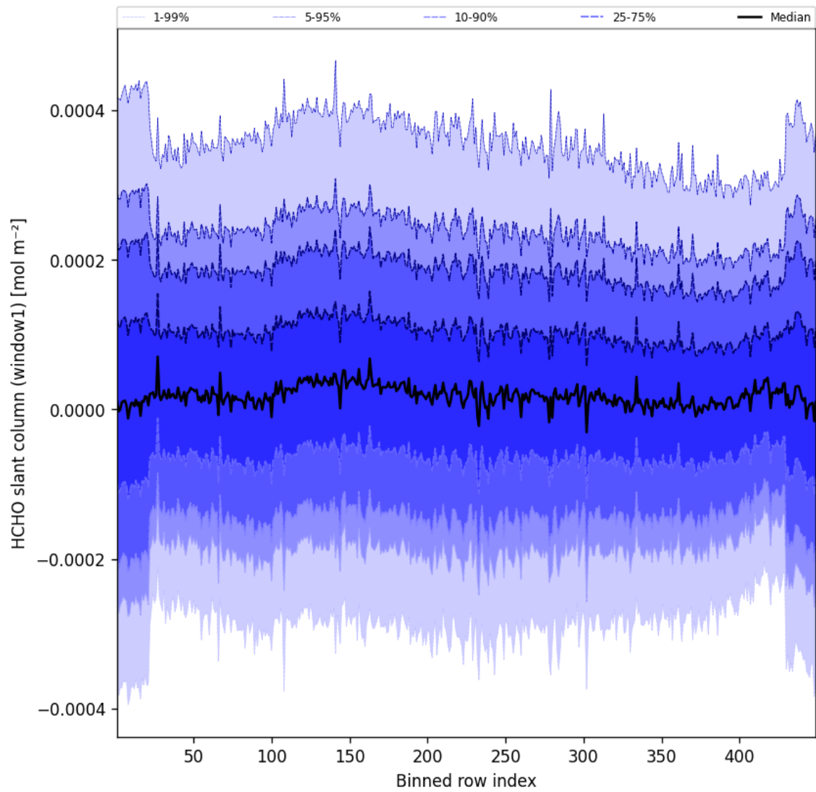
Figure 52: Along track statistics of “HCHO slant column (window1)” for 2024-09-28 to 2024-09-30
