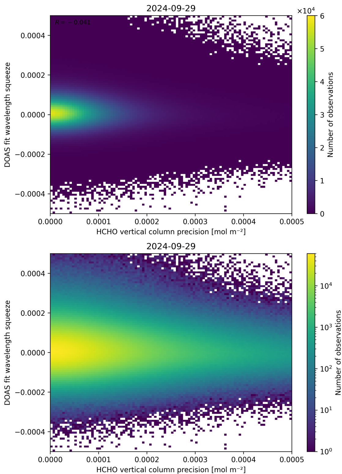
Figure 138: Scatter density plot of “HCHO vertical column precision” against “DOAS fit wavelength squeeze” for 2024-09-28 to 2024-09-30.
