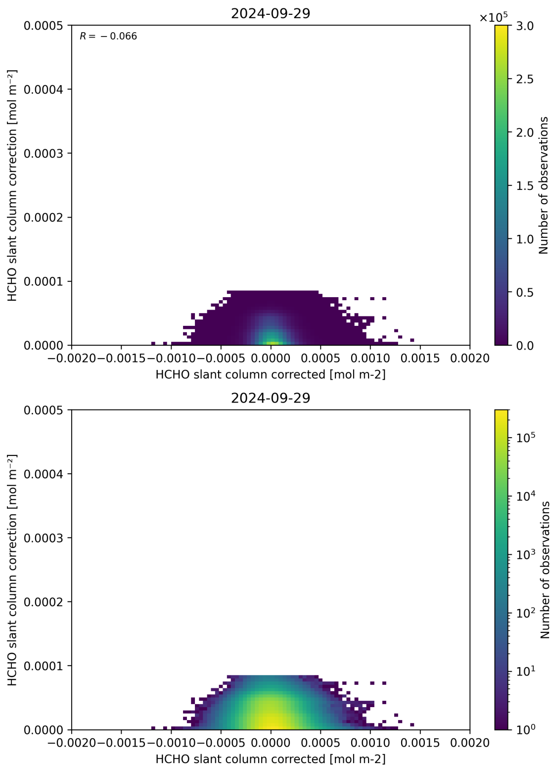
Figure 77: Scatter density plot of “HCHO slant column corrected” against “HCHO slant column correction” for 2024-09-28 to 2024-09-30.
