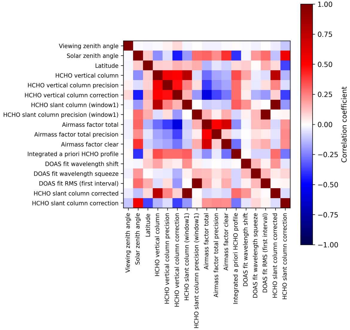
Figure 2: Map of correlation matrix for 2024-09-28 to 2024-09-30.
