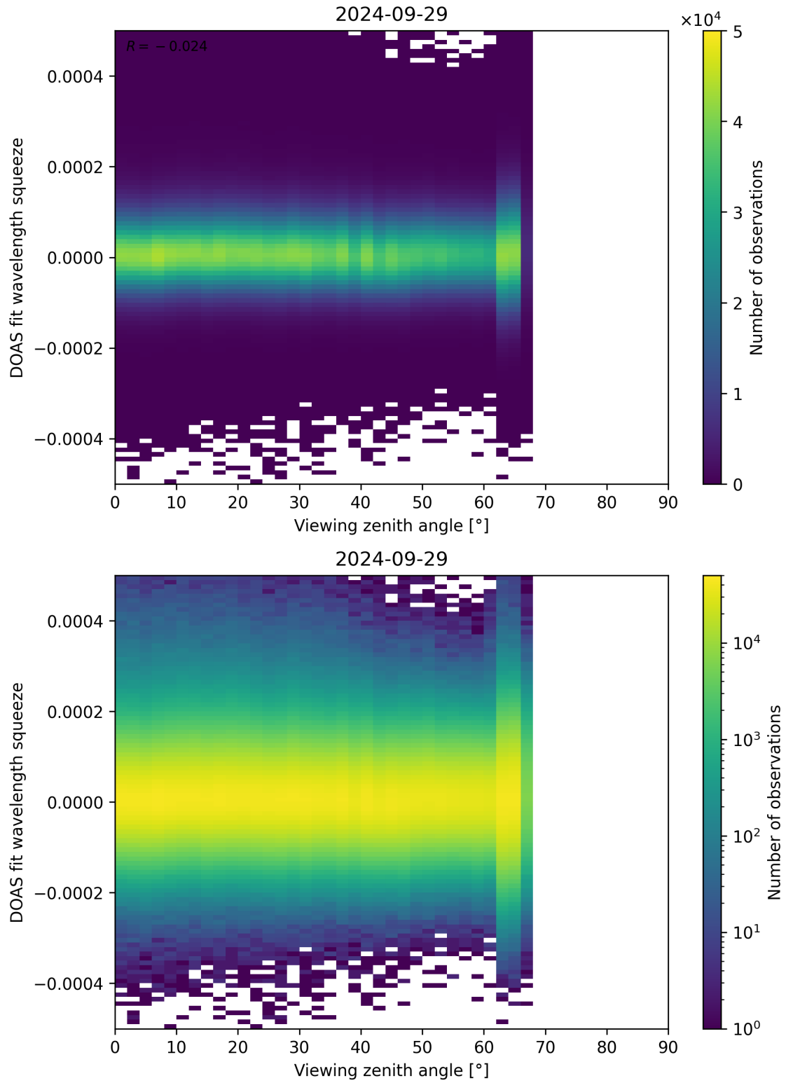
Figure 184: Scatter density plot of “Viewing zenith angle” against “DOAS fit wavelength squeeze” for 2024-09-28 to 2024-09-30.
