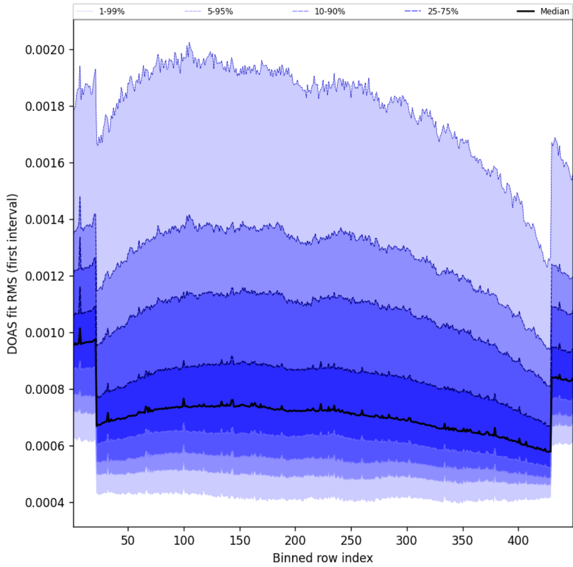
Figure 60: Along track statistics of “DOAS fit RMS (first interval)” for 2024-09-28 to 2024-09-30
