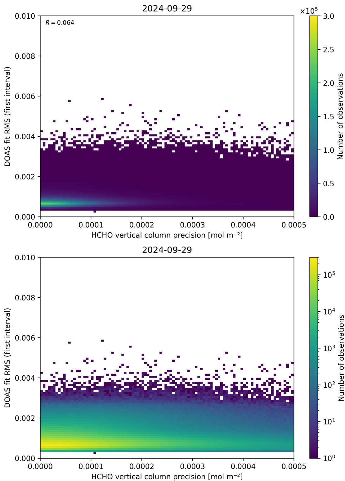
Figure 136: Scatter density plot of “HCHO vertical column precision” against “DOAS fit RMS (first interval)” for 2024-09-28 to 2024-09-30.
