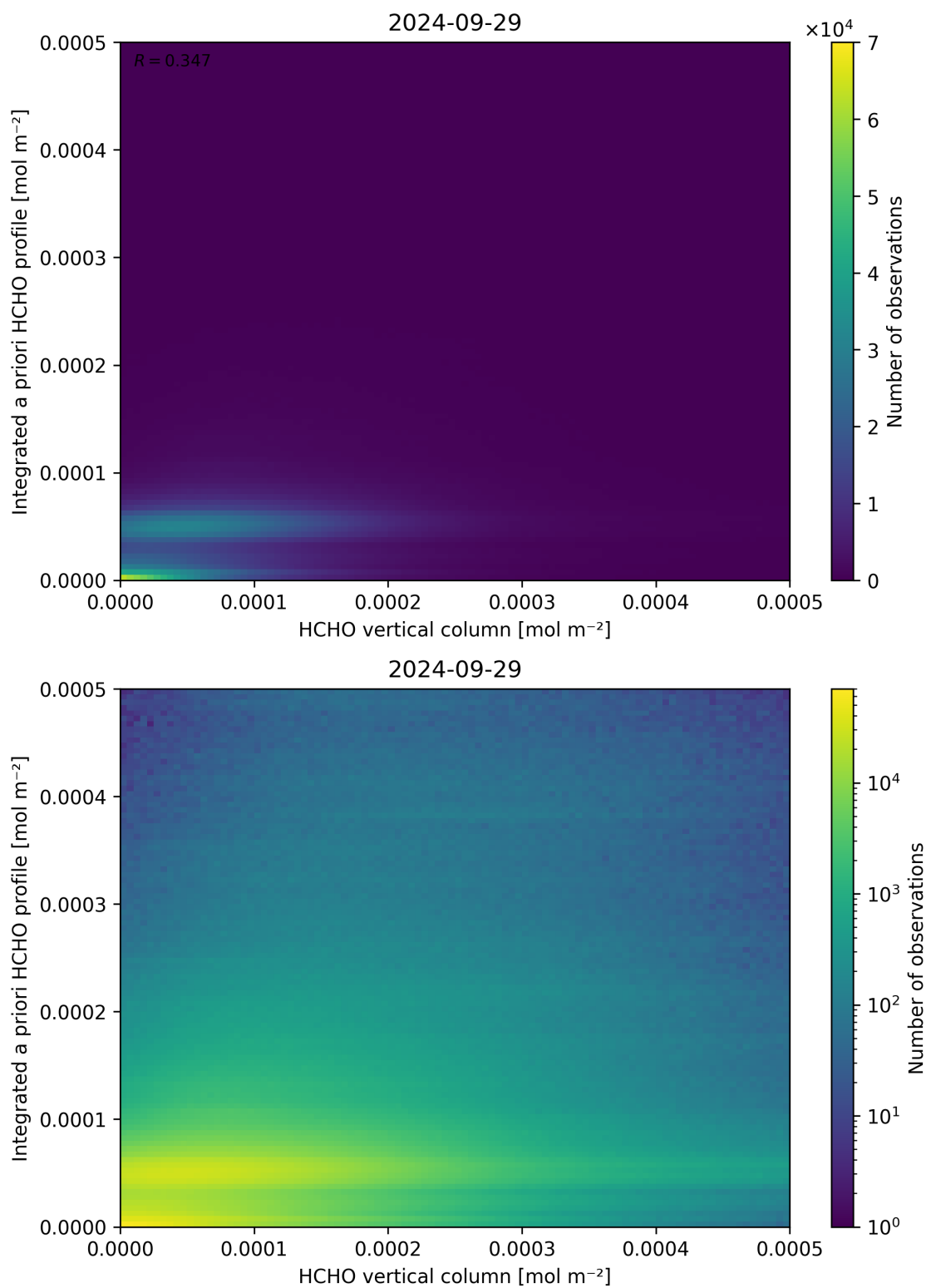
Figure 135: Scatter density plot of “HCHO vertical column” against “Integrated a priori HCHO profile” for 2024-09-28 to 2024-09-30.
