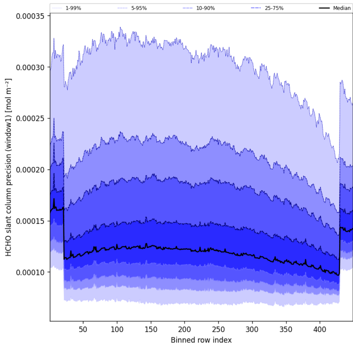
Figure 53: Along track statistics of “HCHO slant column precision (window1)” for 2024-09-28 to 2024-09-30
