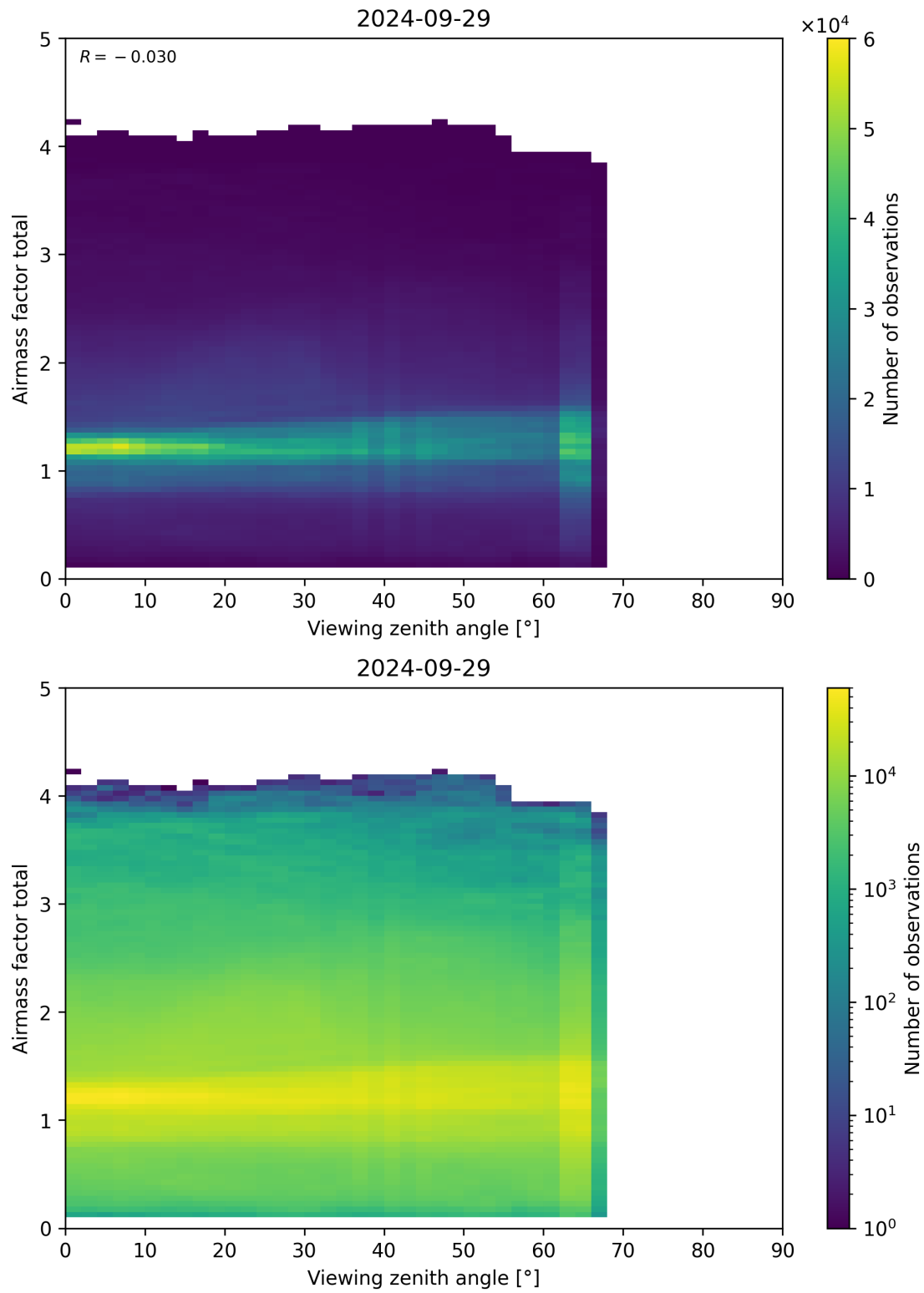
Figure 190: Scatter density plot of “Viewing zenith angle” against “Airmass factor total” for 2024-09-28 to 2024-09-30.
