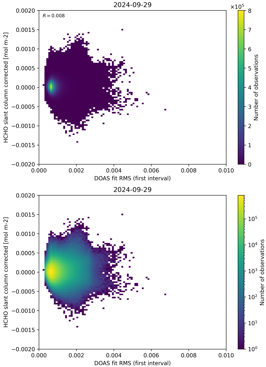
Figure 62: Scatter density plot of “DOAS fit RMS (first interval)” against “HCHO slant column corrected” for 2024-09-28 to 2024-09-30.
