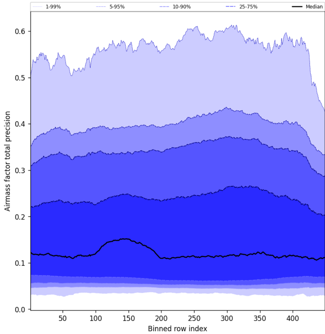
Figure 55: Along track statistics of “Airmass factor total precision” for 2024-09-28 to 2024-09-30
