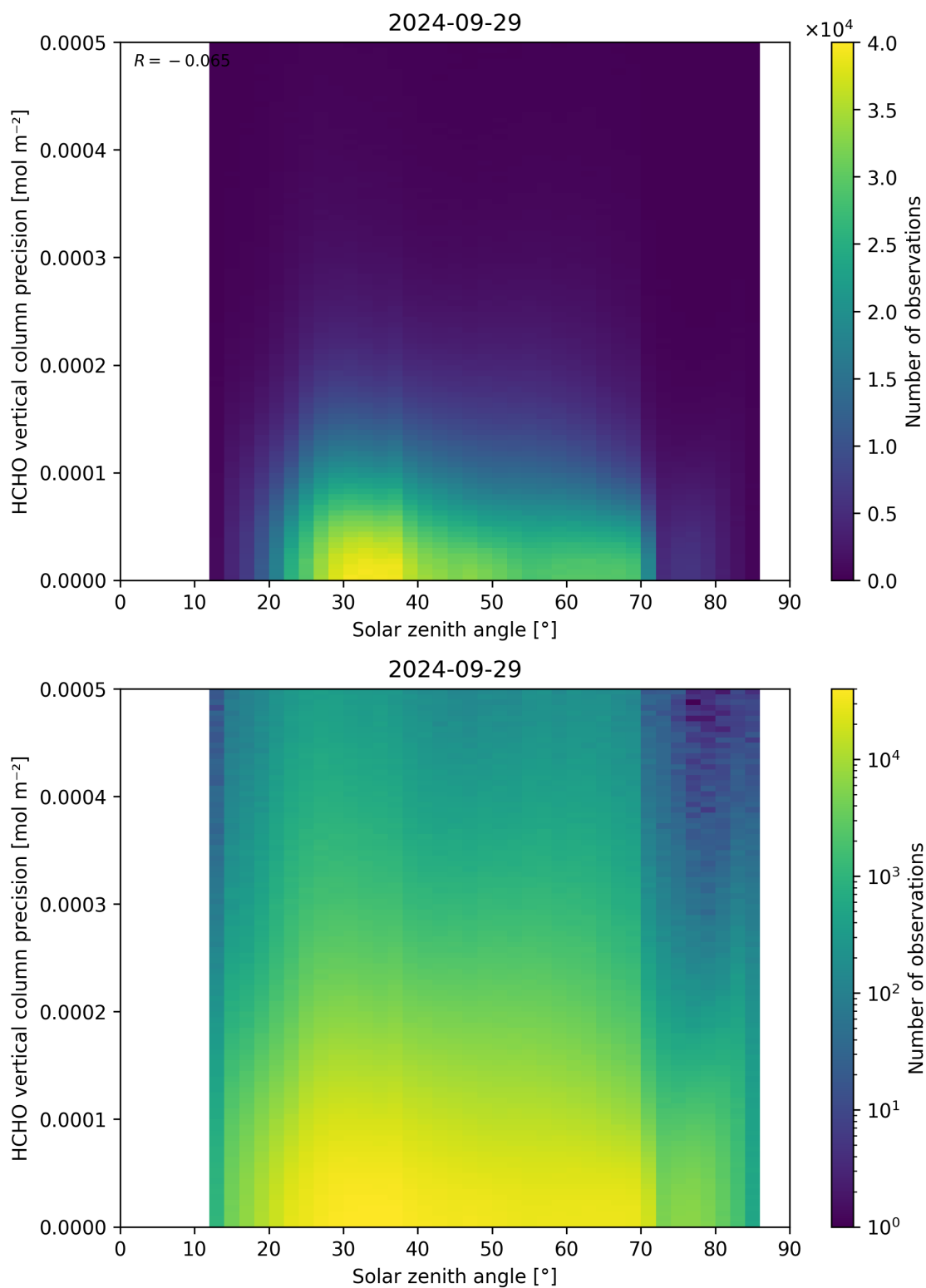
Figure 179: Scatter density plot of “Solar zenith angle” against “HCHO vertical column precision” for 2024-09-28 to 2024-09-30.
