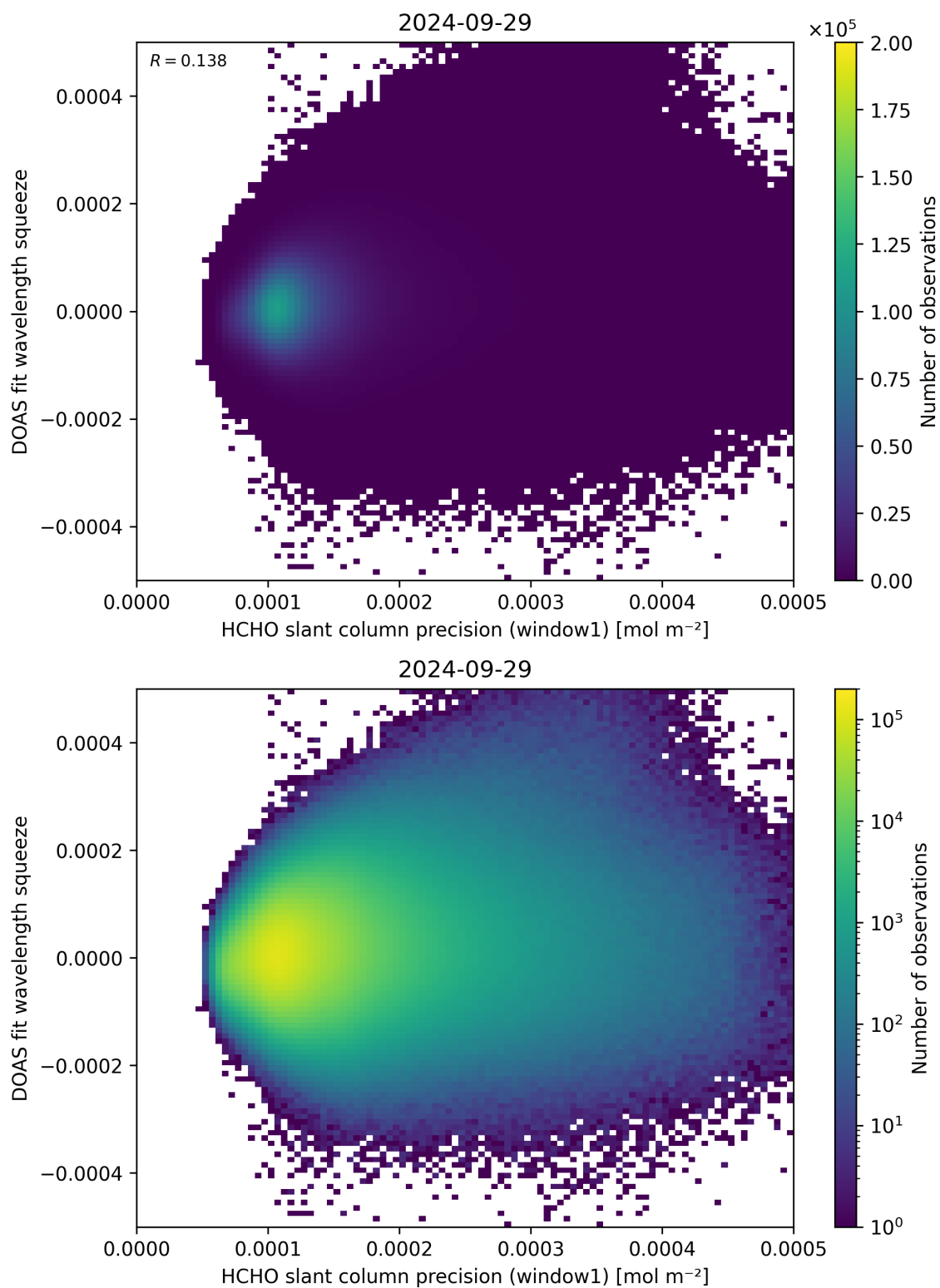
Figure 90: Scatter density plot of “HCHO slant column precision (window1)” against “DOAS fit wavelength squeeze” for 2024-09-28 to 2024-09-30.
