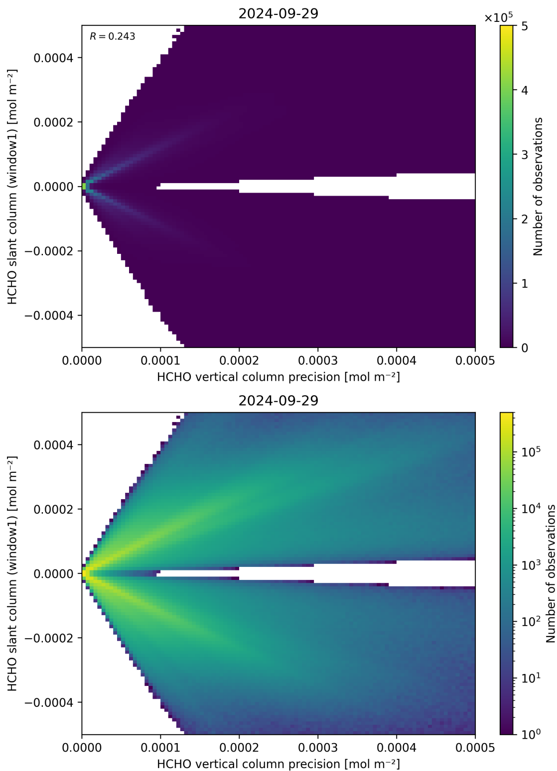
Figure 142: Scatter density plot of “HCHO vertical column precision” against “HCHO slant column (window1)” for 2024-09-28 to 2024-09-30.
