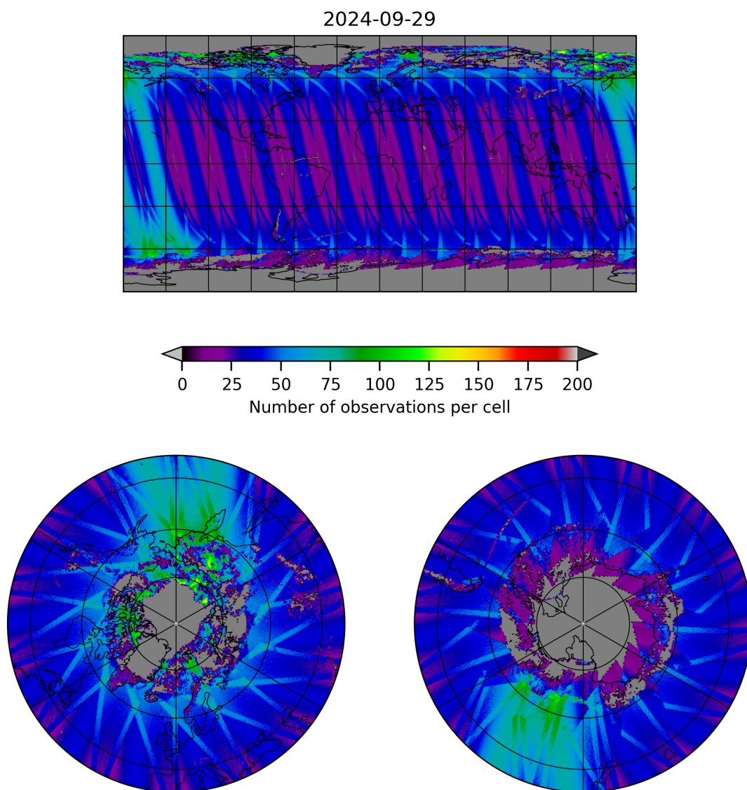
Figure 19: Map of the number of observations for 2024-09-28 to 2024-09-30
