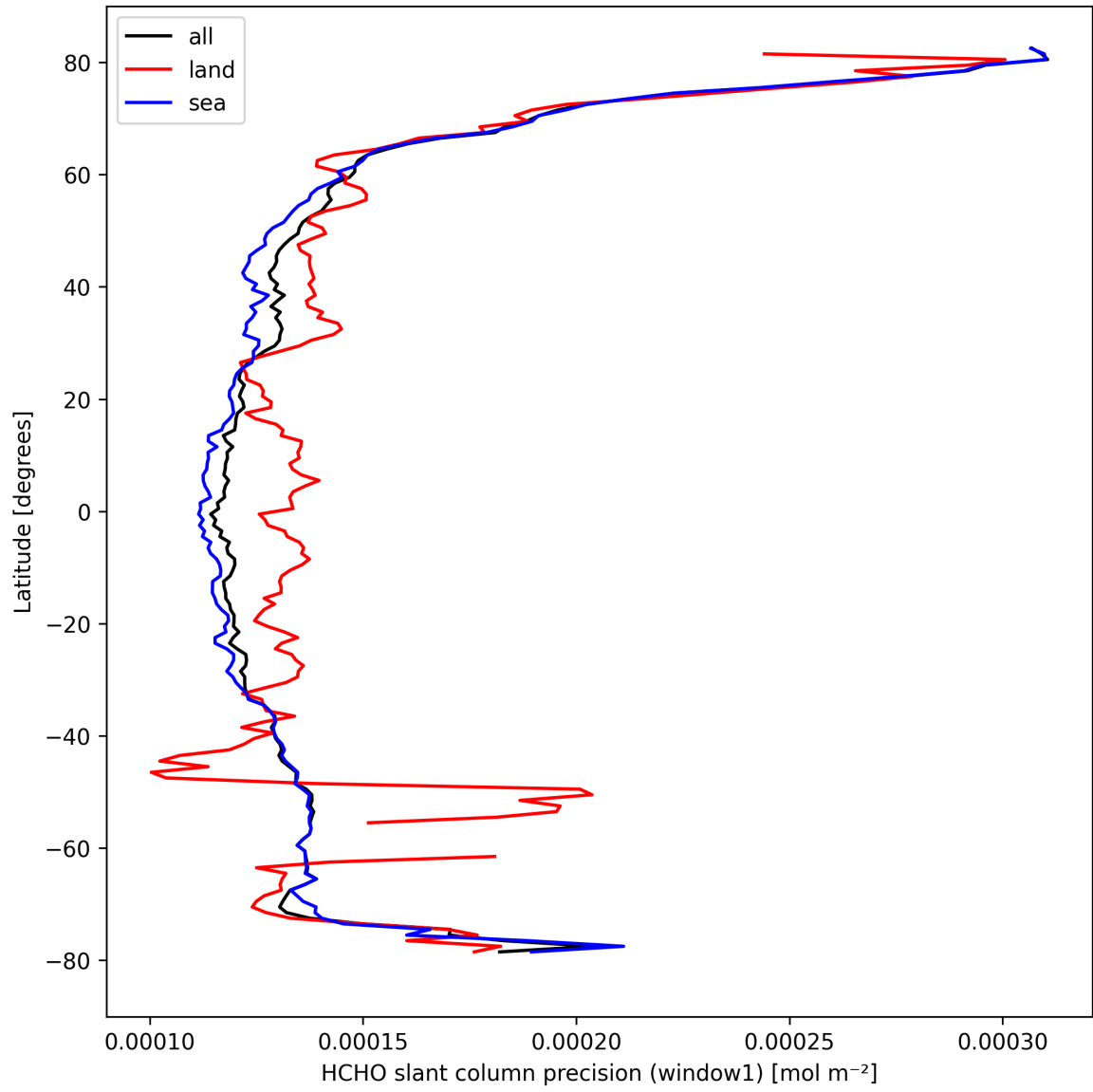
Figure 25: Zonal average of “HCHO slant column precision (window1)” for 2024-09-28 to 2024-09-30.
