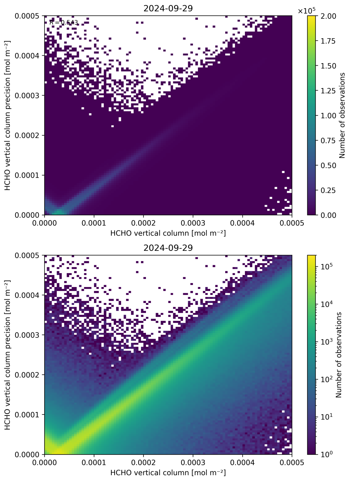
Figure 134: Scatter density plot of “HCHO vertical column” against “HCHO vertical column precision” for 2024-09-28 to 2024-09-30.
