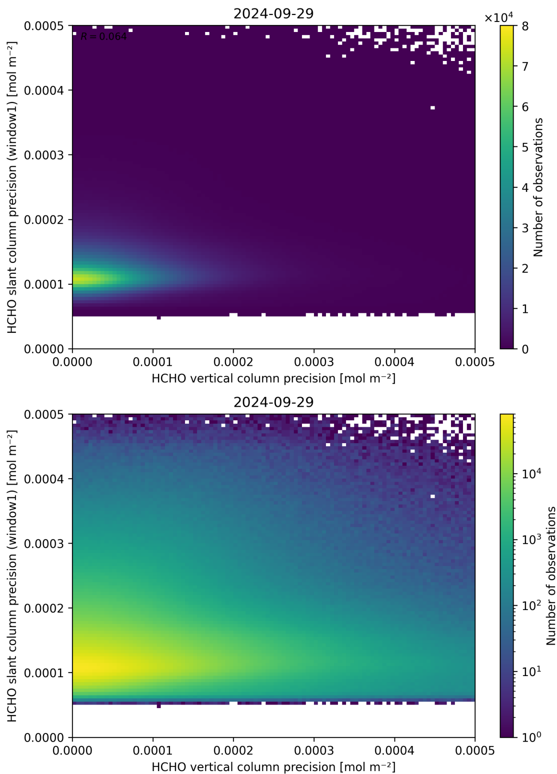
Figure 143: Scatter density plot of “HCHO vertical column precision” against “HCHO slant column precision (window1)” for 2024-09-28 to 2024-09-30.
