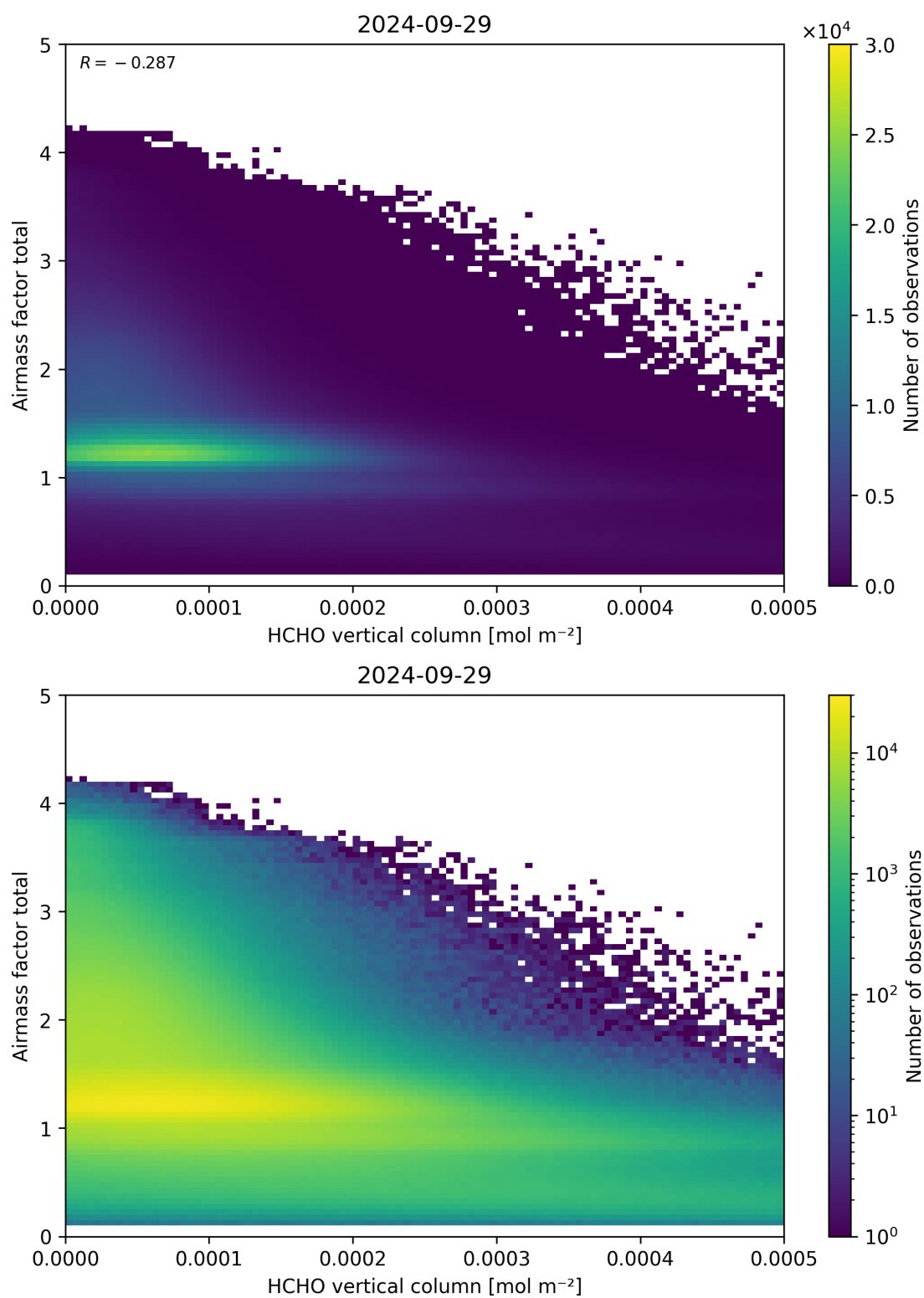
Figure 131: Scatter density plot of “HCHO vertical column” against “Airmass factor total” for 2024-09-28 to 2024-09-30.
