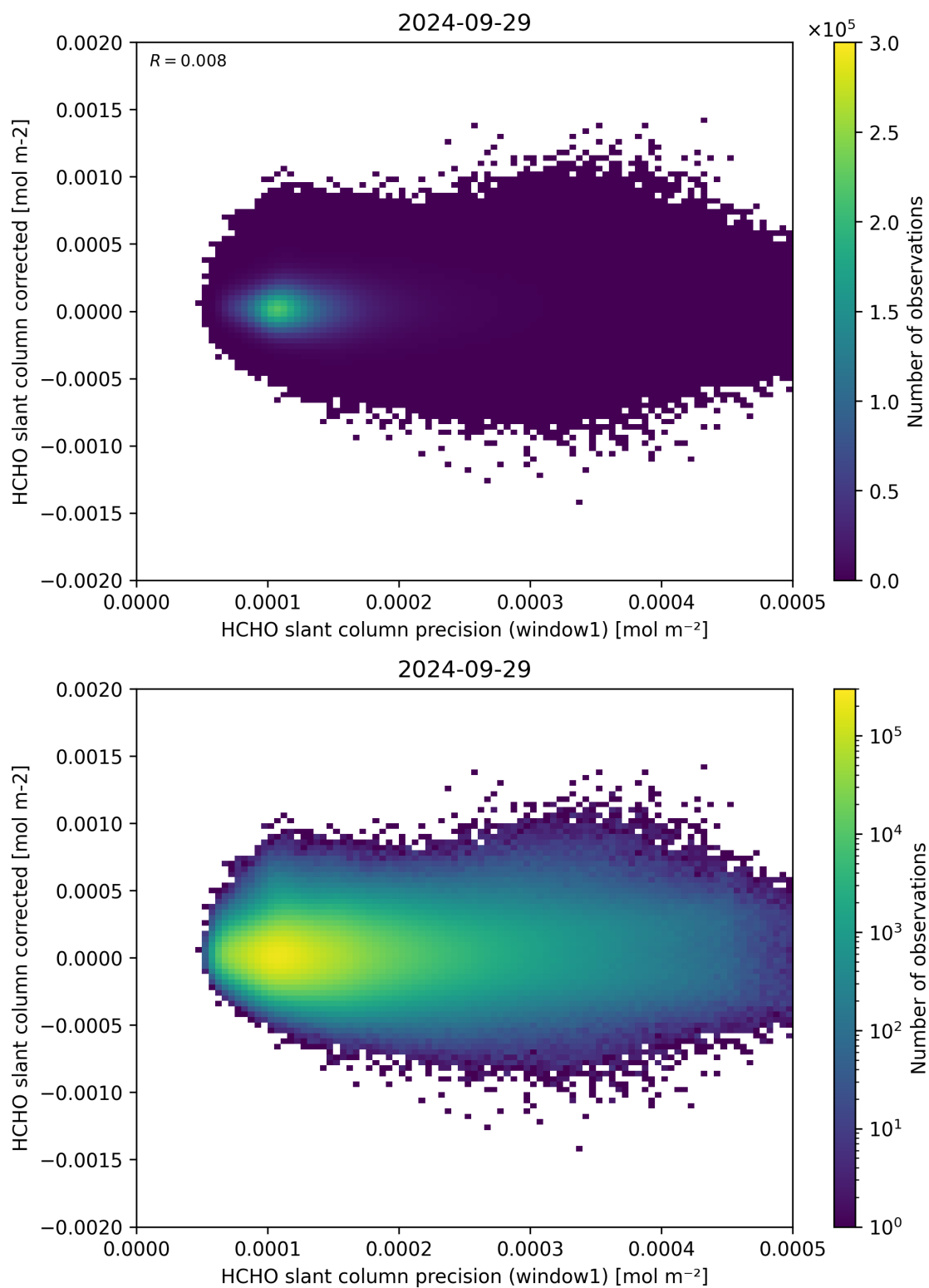
Figure 92: Scatter density plot of “HCHO slant column precision (window1)” against “HCHO slant column corrected” for 2024-09-28 to 2024-09-30.
