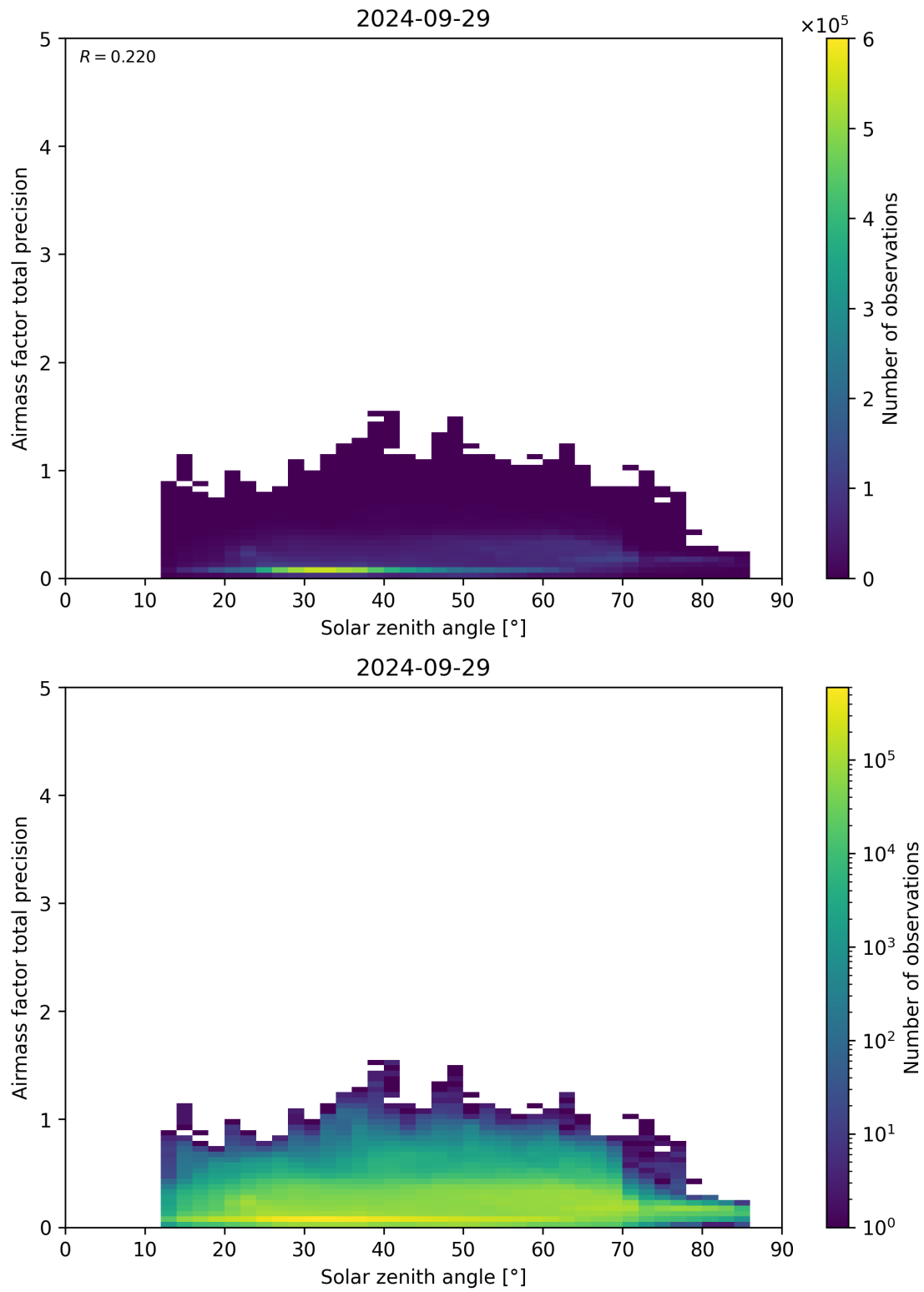
Figure 176: Scatter density plot of “Solar zenith angle” against “Airmass factor total precision” for 2024-09-28 to 2024-09-30.
