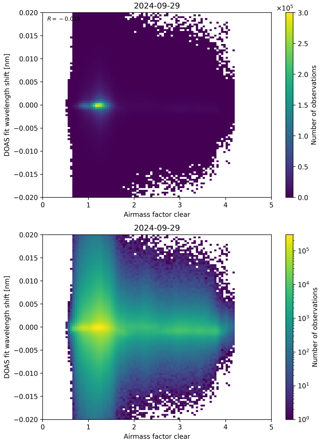
Figure 72: Scatter density plot of “Airmass factor clear” against “DOAS fit wavelength shift” for 2024-09-28 to 2024-09-30.
