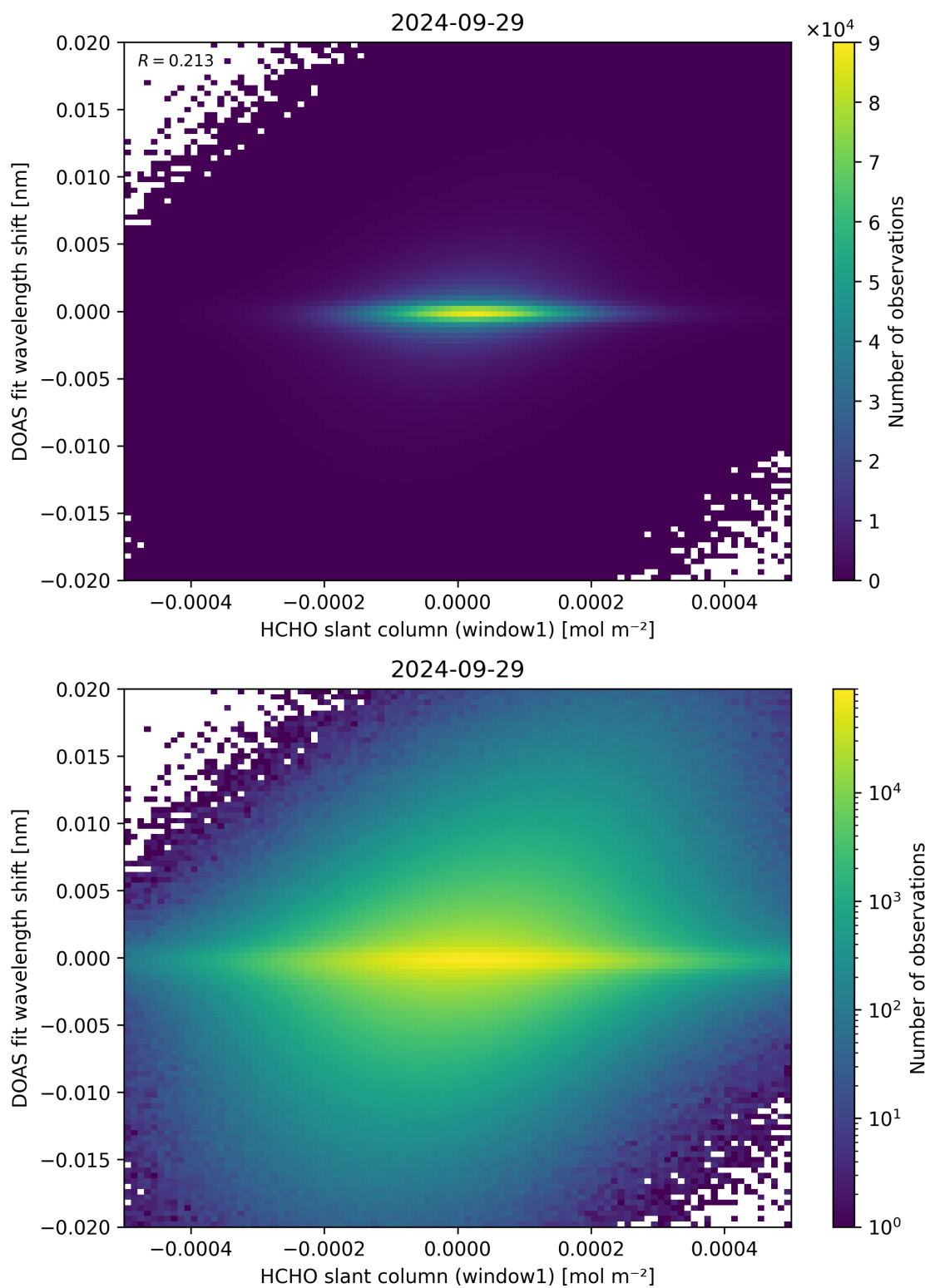
Figure 79: Scatter density plot of “HCHO slant column (window1)” against “DOAS fit wavelength shift” for 2024-09-28 to 2024-09-30.
