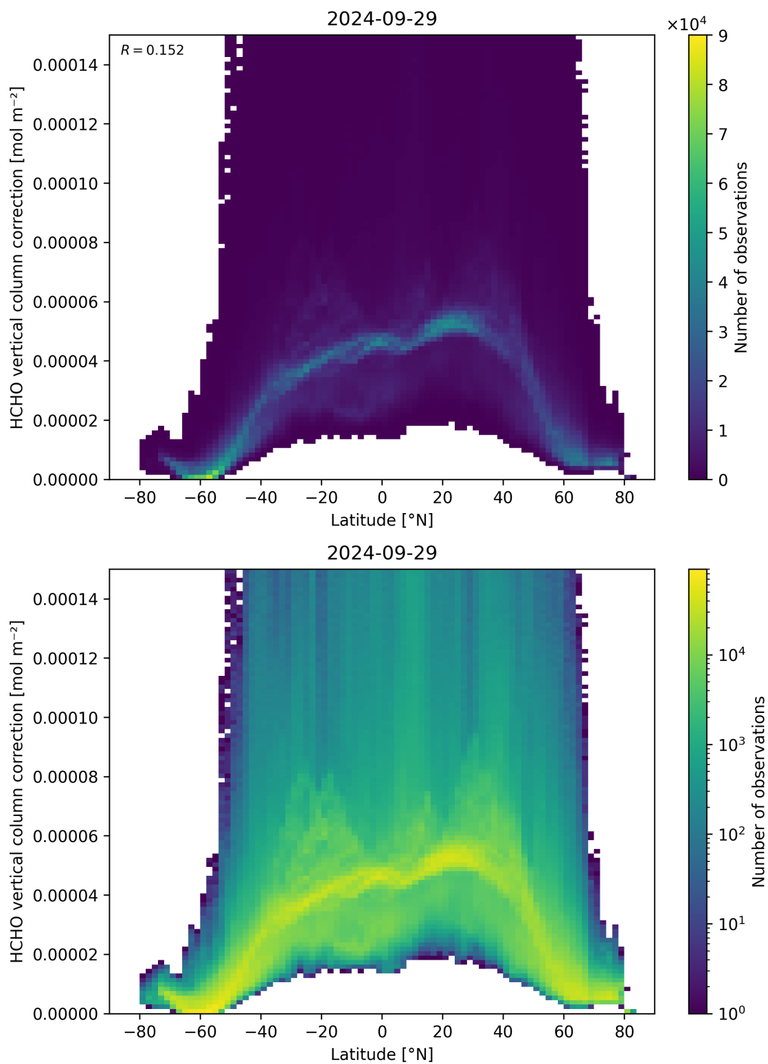
Figure 164: Scatter density plot of “Latitude” against “HCHO vertical column correction” for 2024-09-28 to 2024-09-30.
