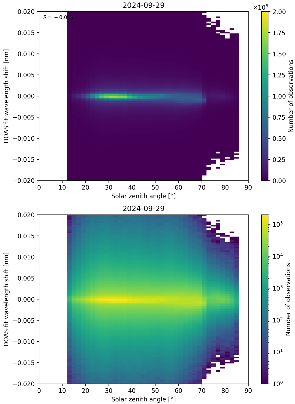
Figure 168: Scatter density plot of “Solar zenith angle” against “DOAS fit wavelength shift” for 2024-09-28 to 2024-09-30.
