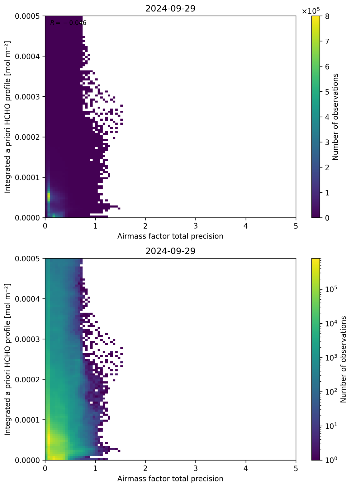
Figure 111: Scatter density plot of “Airmass factor total precision” against “Integrated a priori HCHO profile” for 2024-09-28 to 2024-09-30.
