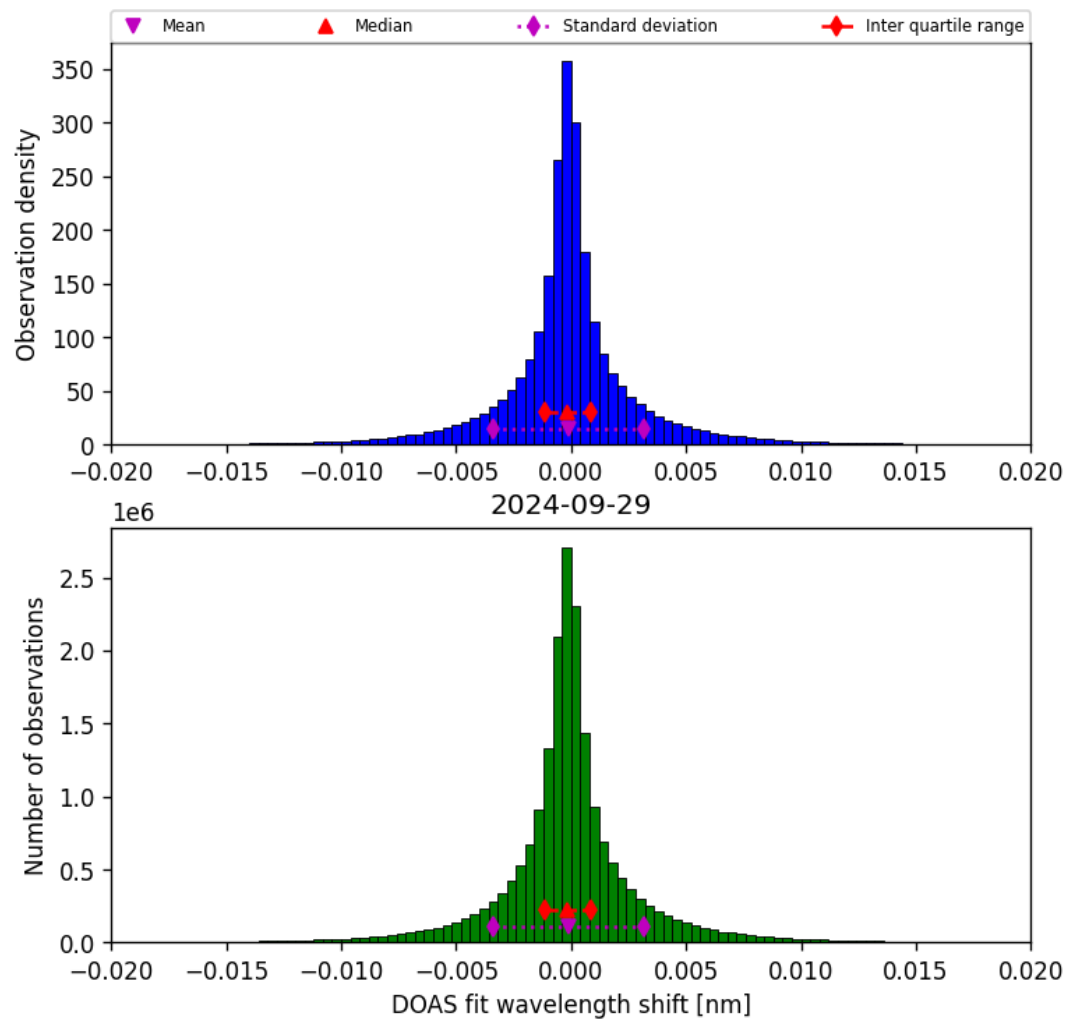
Figure 44: Histogram of “DOAS fit wavelength shift” for 2024-09-28 to 2024-09-30
