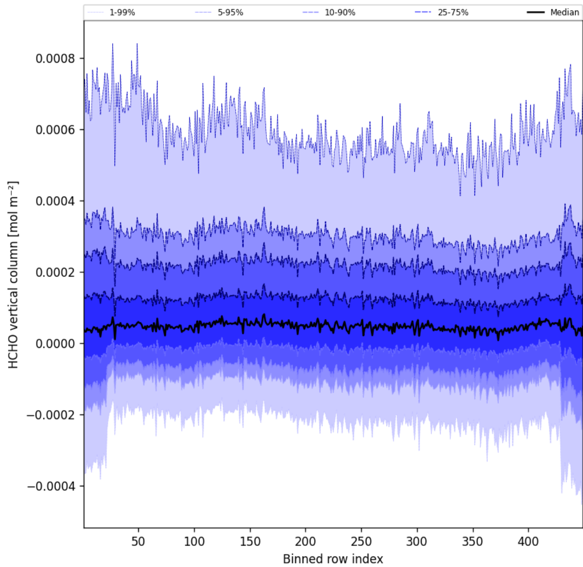
Figure 49: Along track statistics of “HCHO vertical column” for 2024-09-28 to 2024-09-30
