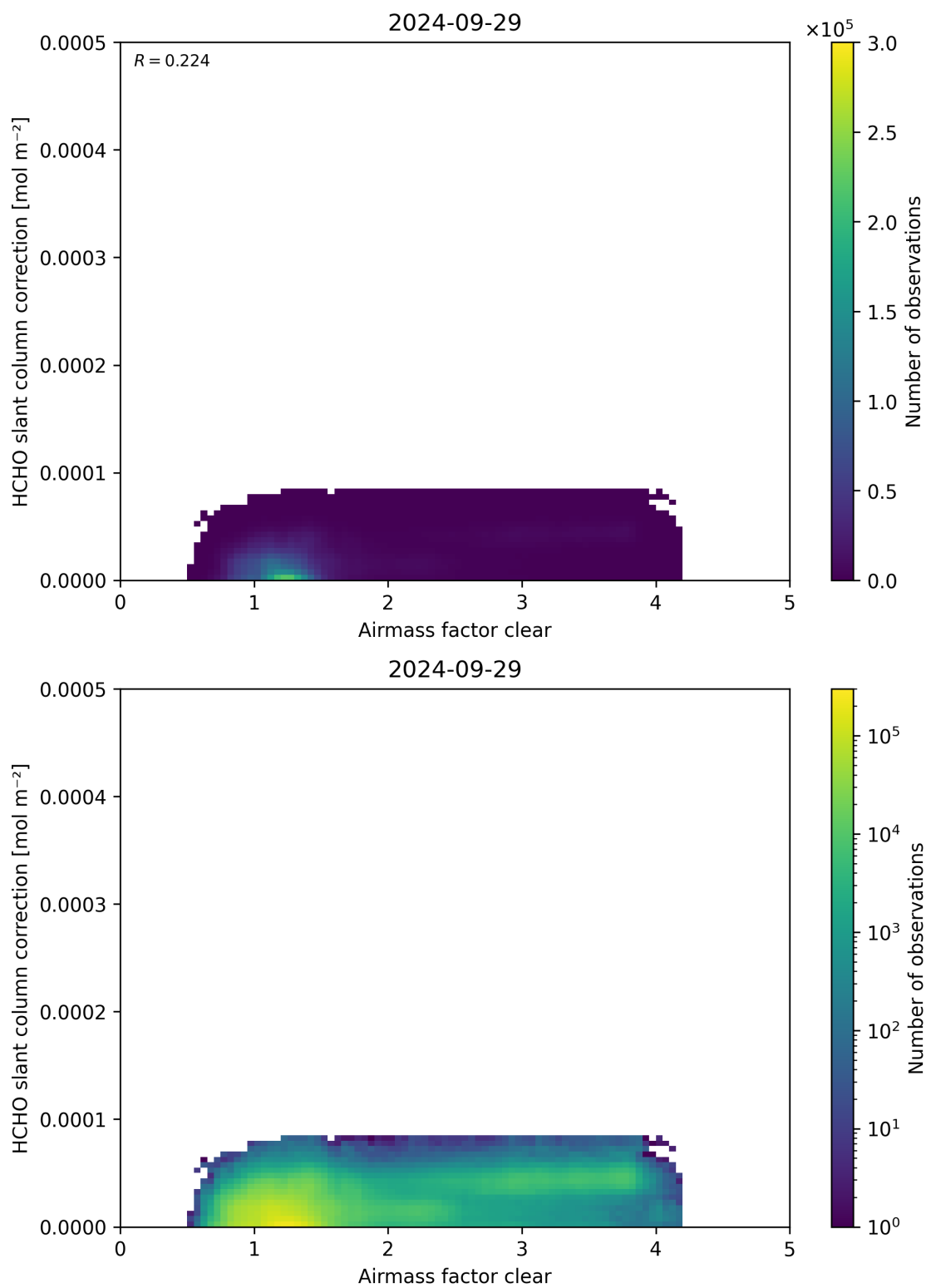
Figure 75: Scatter density plot of “Airmass factor clear” against “HCHO slant column correction” for 2024-09-28 to 2024-09-30.
