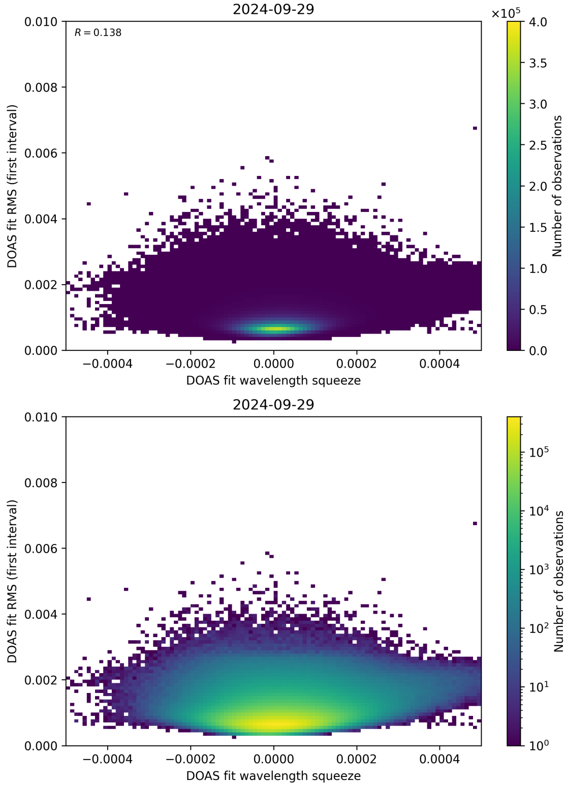
Figure 68: Scatter density plot of “DOAS fit wavelength squeeze” against “DOAS fit RMS (first interval)” for 2024-09-28 to 2024-09-30.
