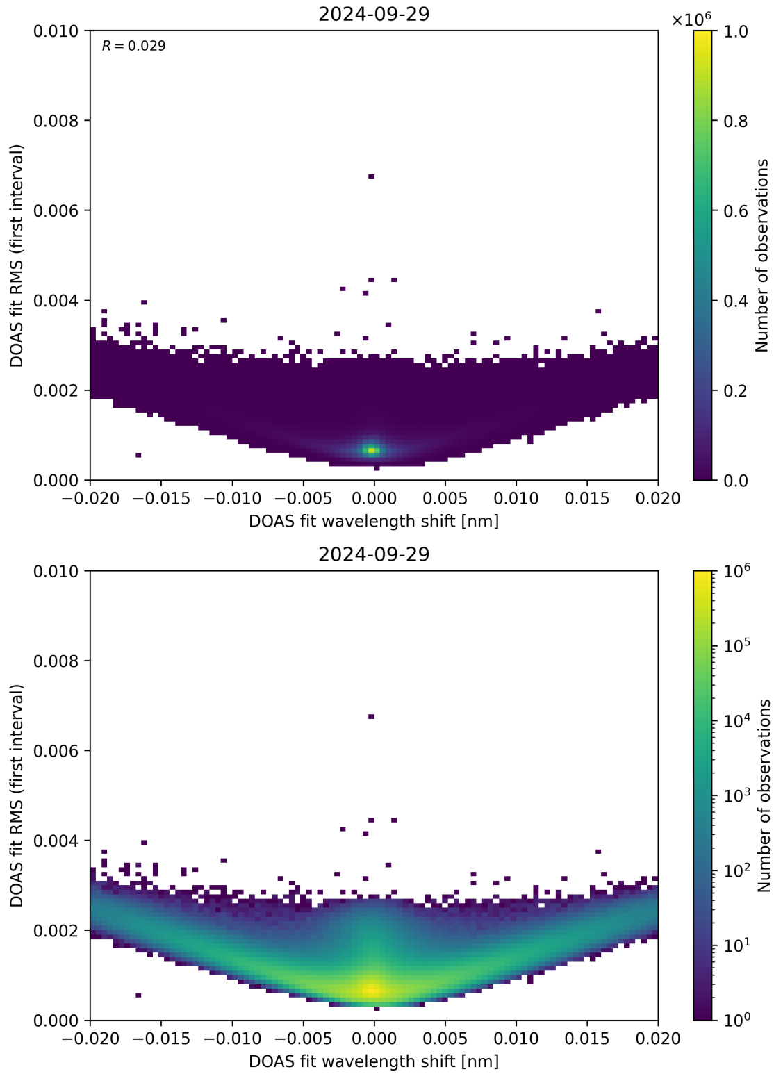
Figure 64: Scatter density plot of “DOAS fit wavelength shift” against “DOAS fit RMS (first interval)” for 2024-09-28 to 2024-09-30.
