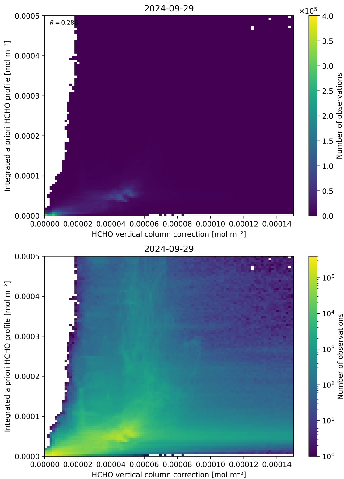
Figure 122: Scatter density plot of “HCHO vertical column correction” against “Integrated a priori HCHO profile” for 2024-09-28 to 2024-09-30.
