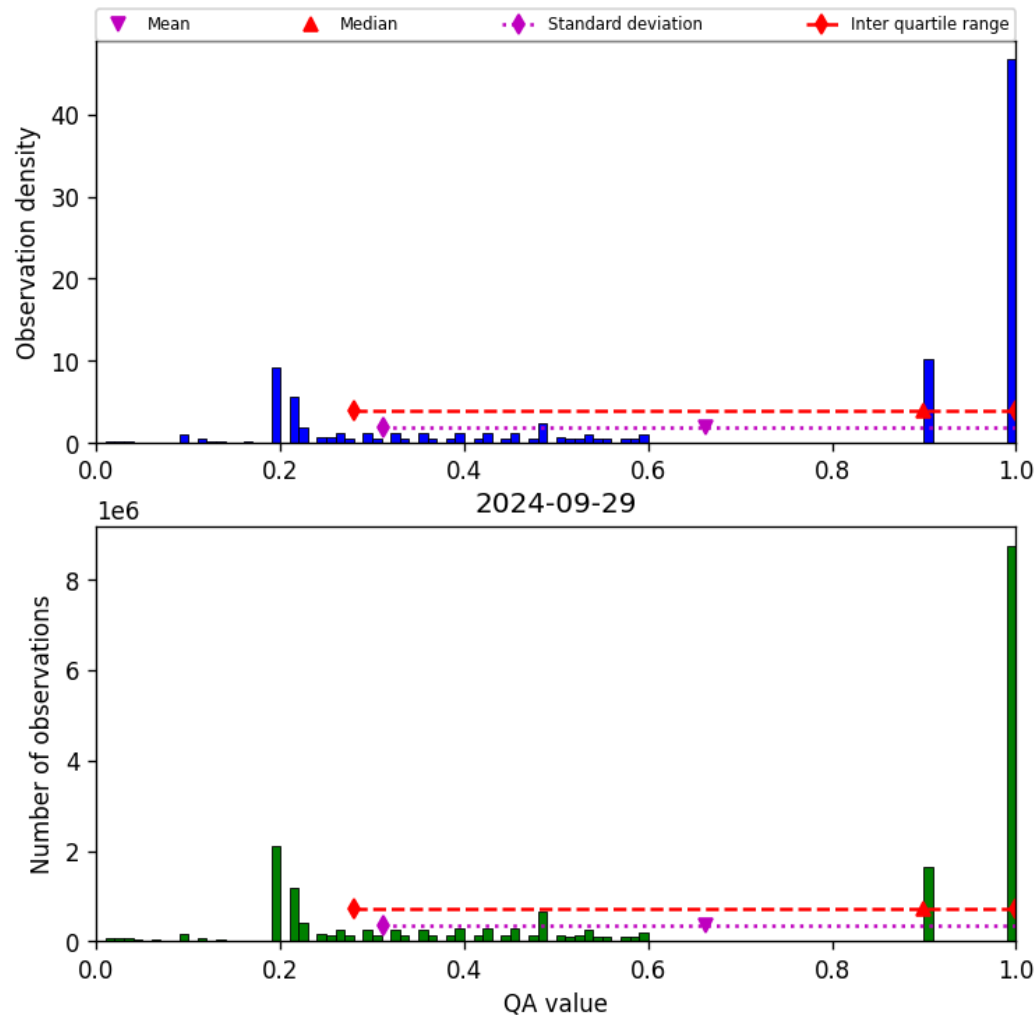
Figure 34: Histogram of “QA value” for 2024-09-28 to 2024-09-30
