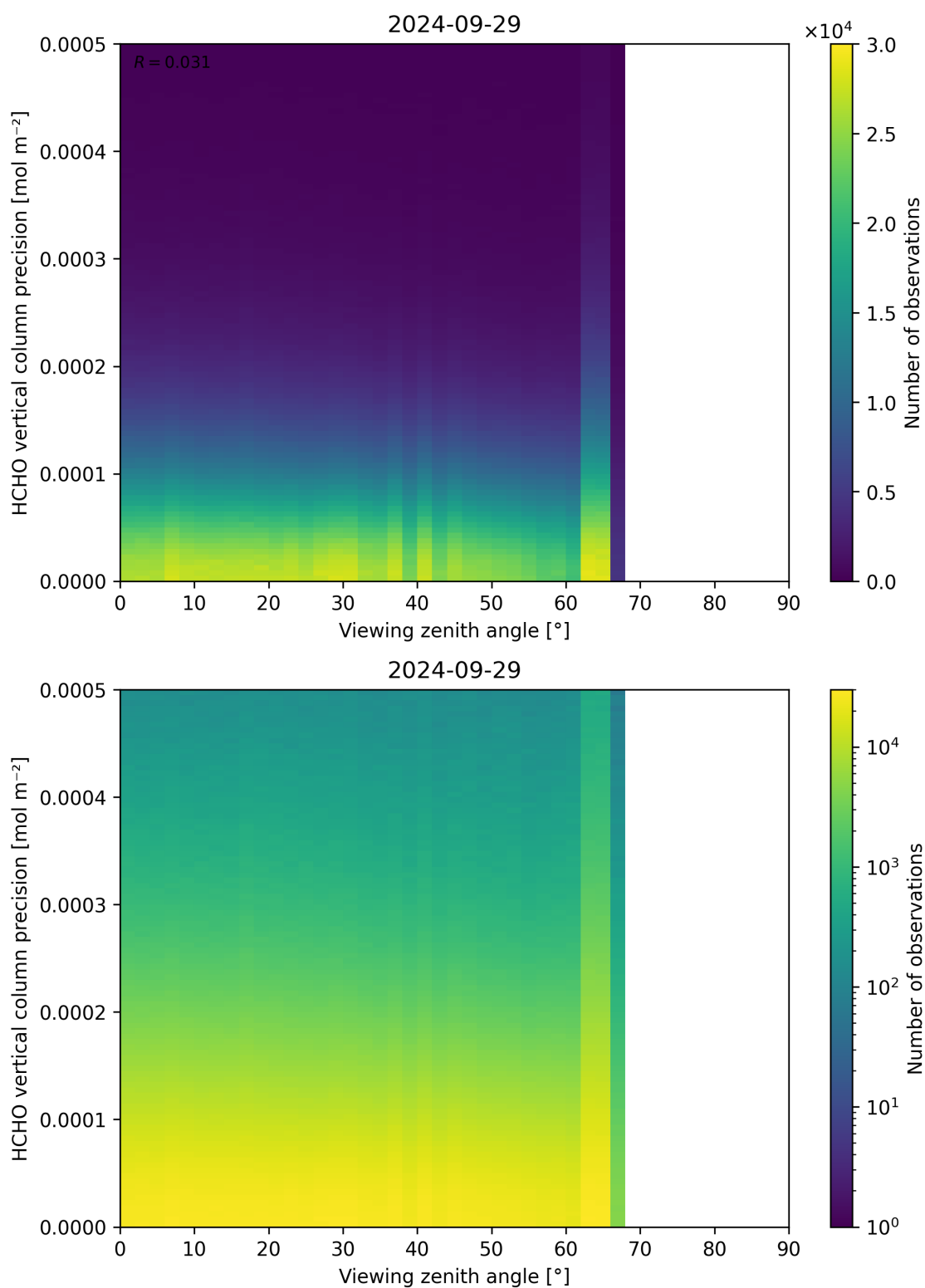
Figure 194: Scatter density plot of “Viewing zenith angle” against “HCHO vertical column precision” for 2024-09-28 to 2024-09-30.
