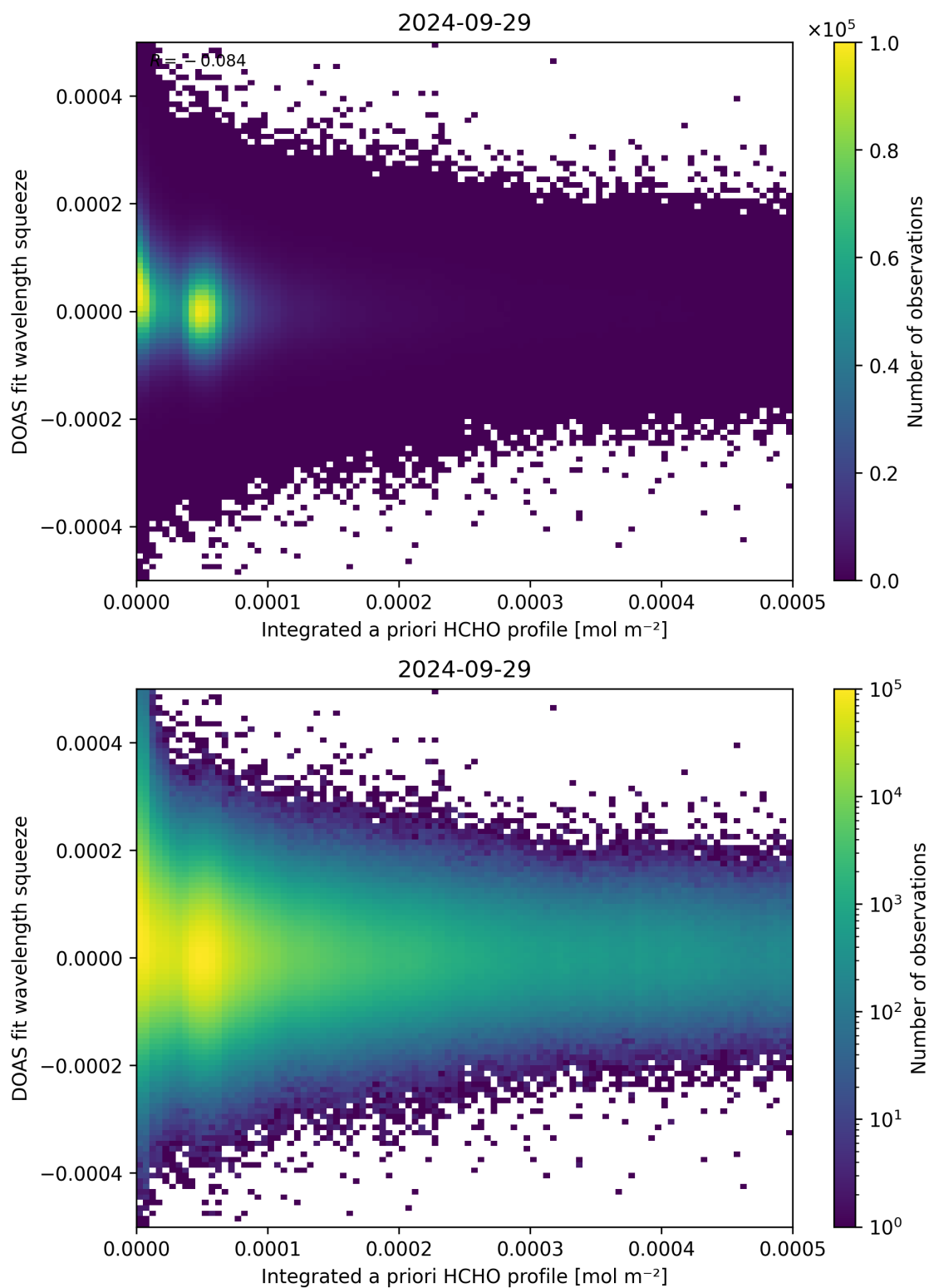
Figure 150: Scatter density plot of “Integrated a priori HCHO profile” against “DOAS fit wavelength squeeze” for 2024-09-28 to 2024-09-30.
