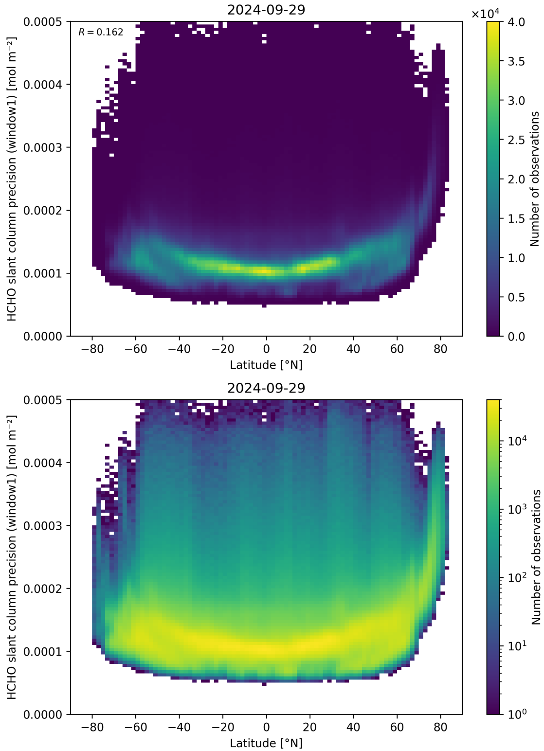
Figure 160: Scatter density plot of “Latitude” against “HCHO slant column precision (window1)” for 2024-09-28 to 2024-09-30.
