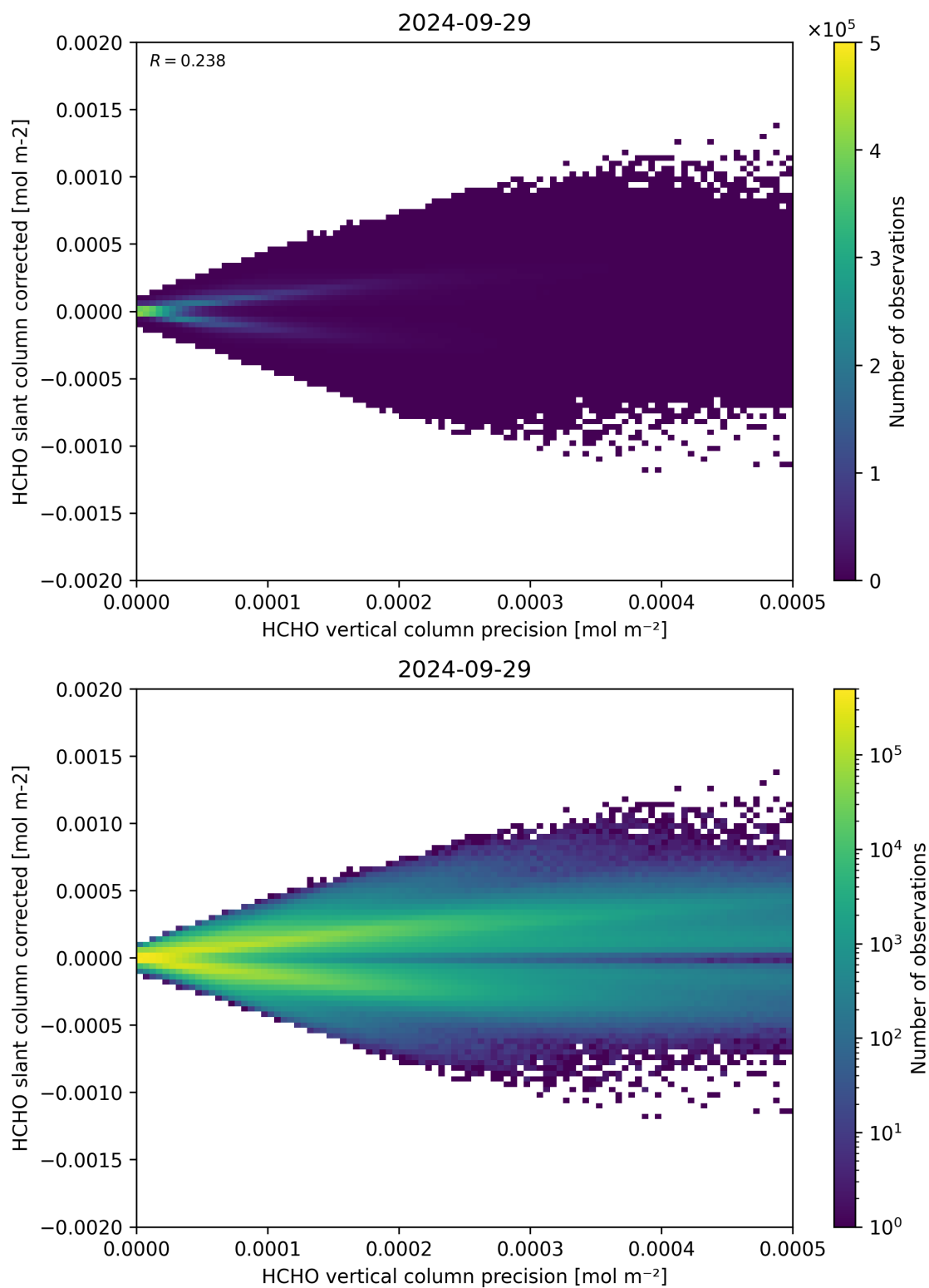
Figure 140: Scatter density plot of “HCHO vertical column precision” against “HCHO slant column corrected” for 2024-09-28 to 2024-09-30.
