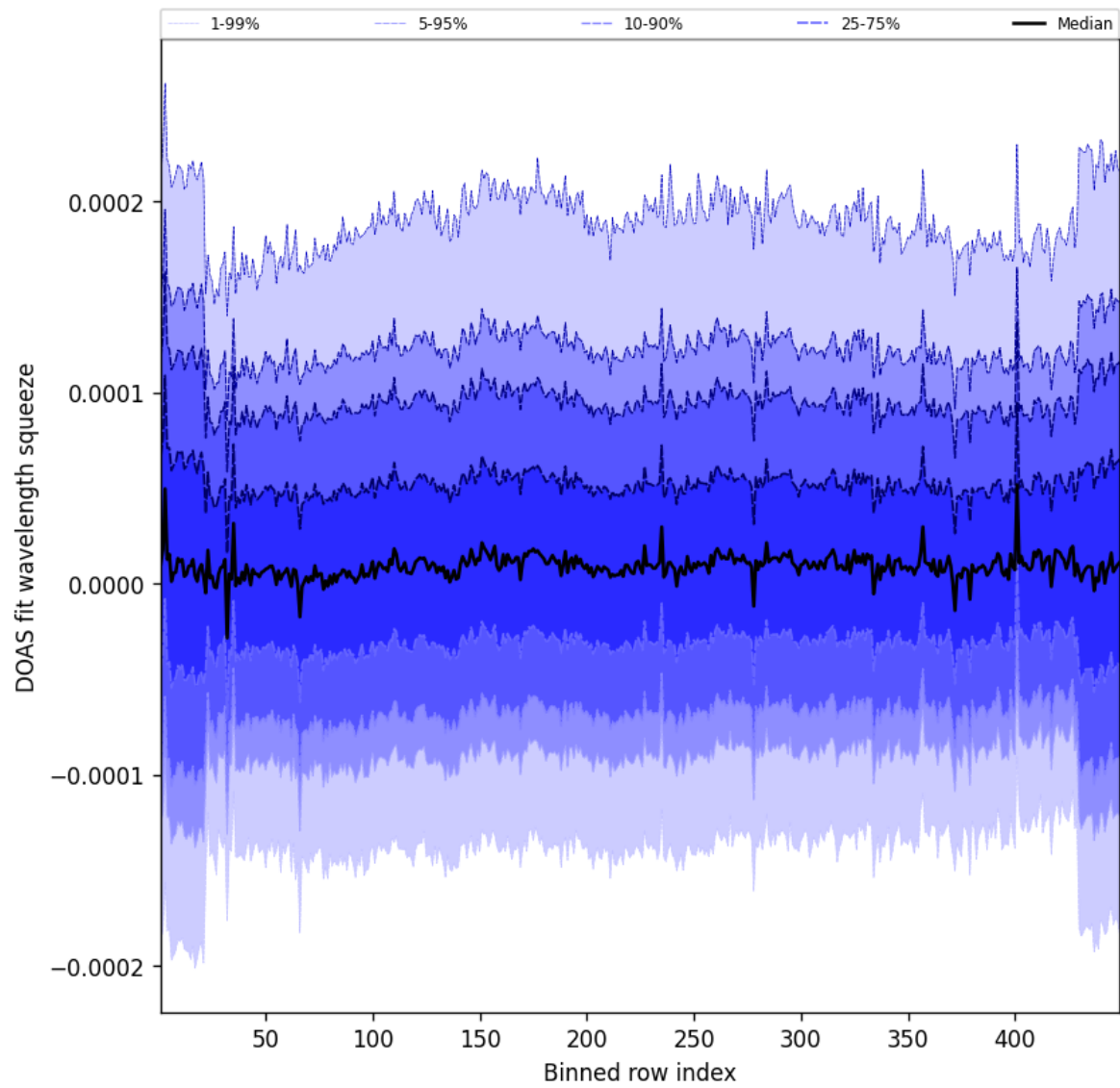
Figure 59: Along track statistics of “DOAS fit wavelength squeeze” for 2024-09-28 to 2024-09-30
