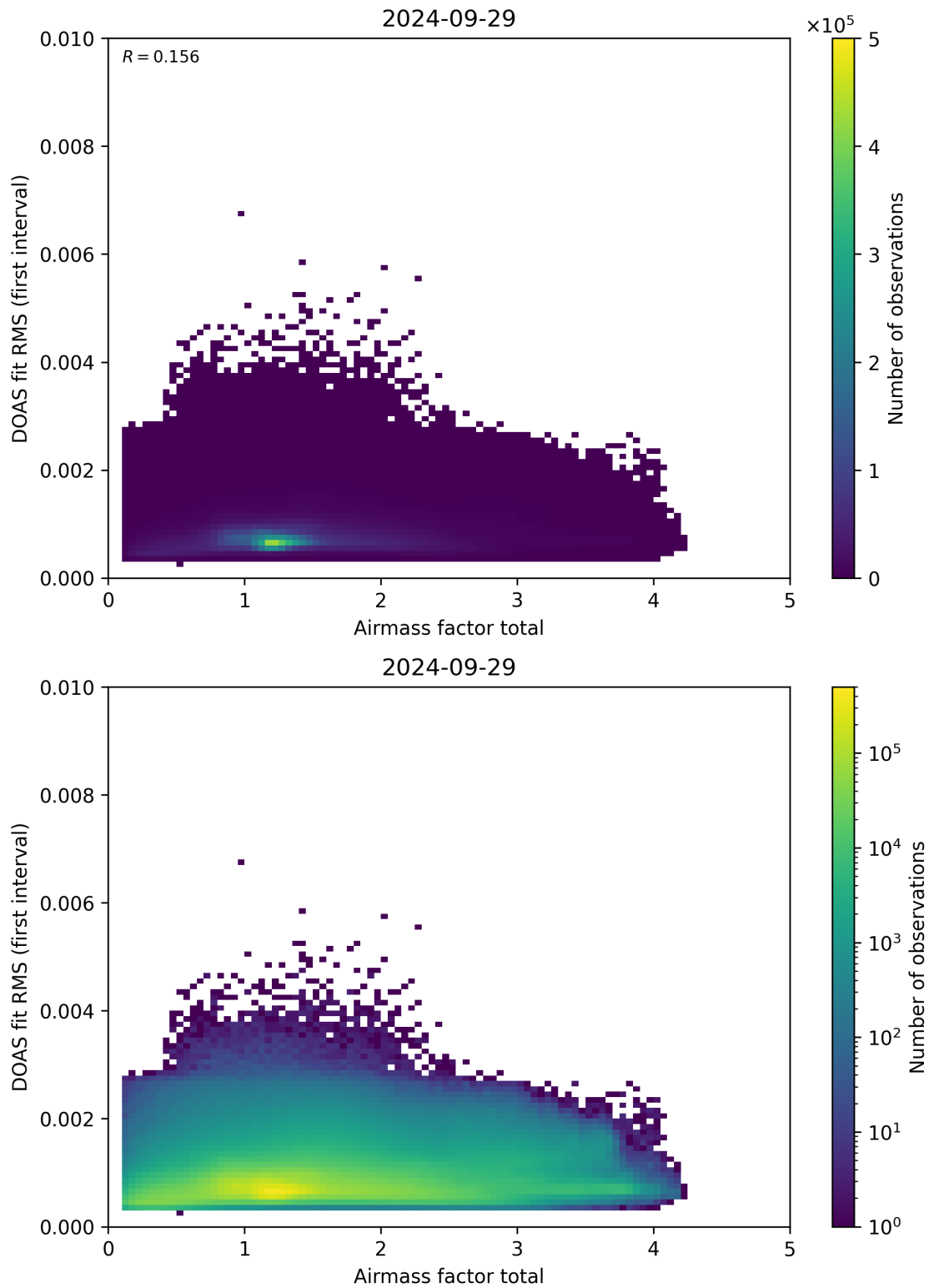
Figure 97: Scatter density plot of “Airmass factor total” against “DOAS fit RMS (first interval)” for 2024-09-28 to 2024-09-30.
