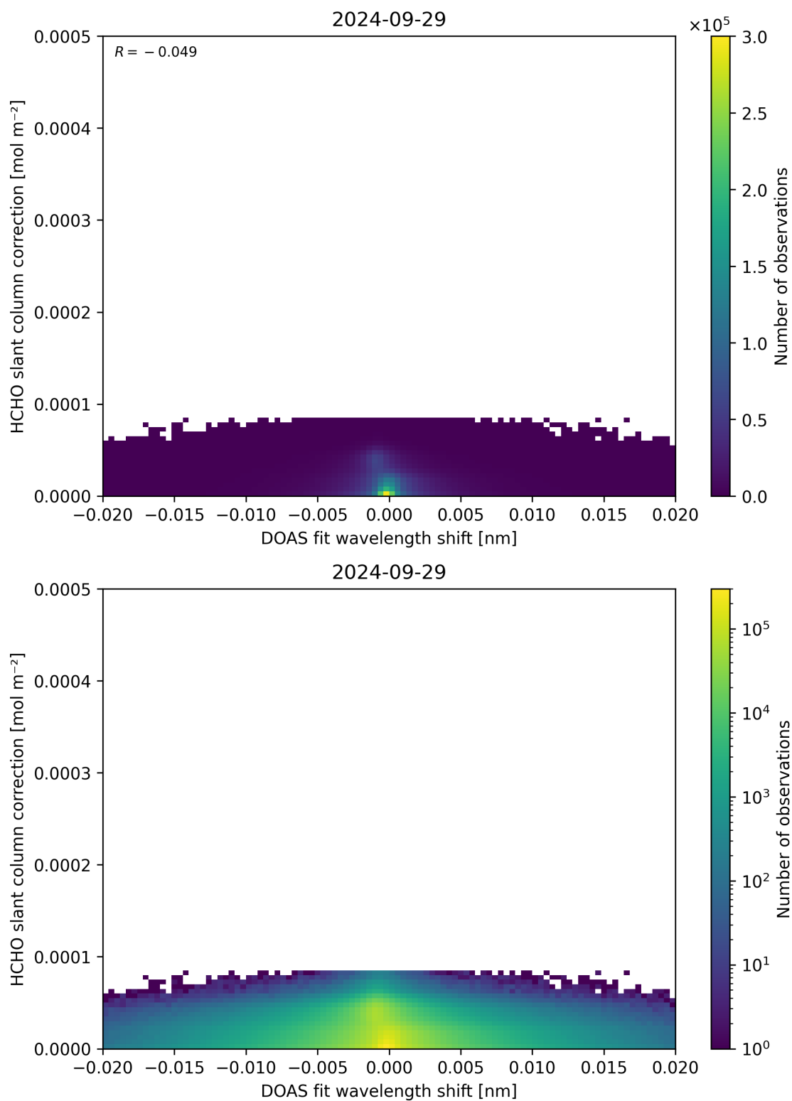
Figure 67: Scatter density plot of “DOAS fit wavelength shift” against “HCHO slant column correction” for 2024-09-28 to 2024-09-30.
