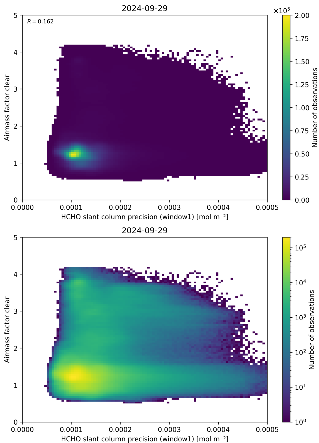
Figure 91: Scatter density plot of “HCHO slant column precision (window1)” against “Airmass factor clear” for 2024-09-28 to 2024-09-30.
