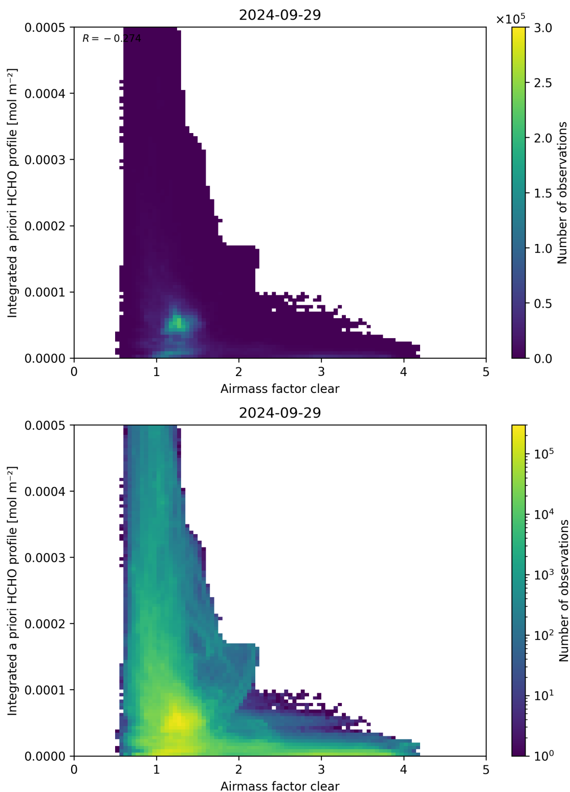
Figure 76: Scatter density plot of “Airmass factor clear” against “Integrated a priori HCHO profile” for 2024-09-28 to 2024-09-30.
