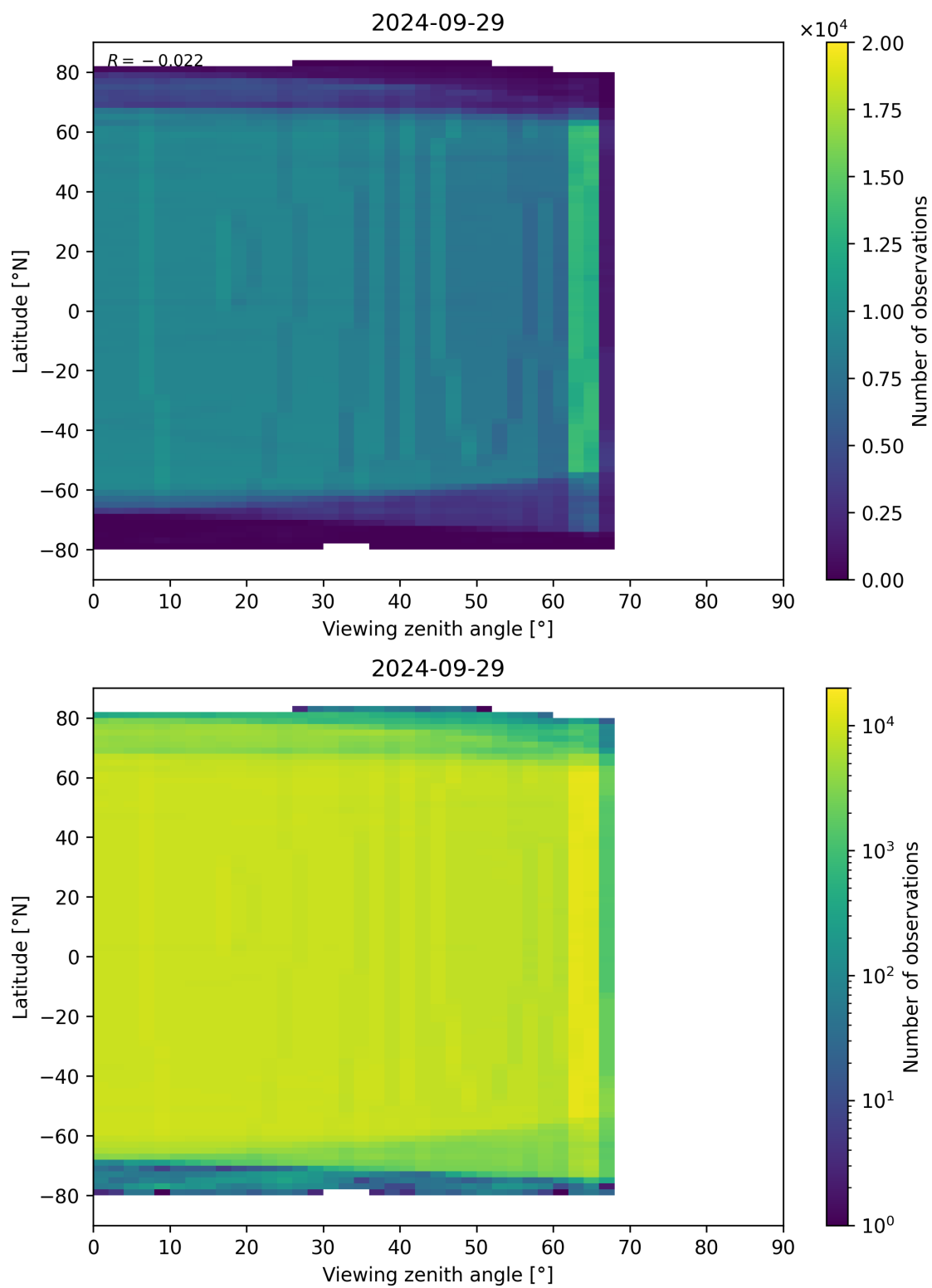
Figure 196: Scatter density plot of “Viewing zenith angle” against “Latitude” for 2024-09-28 to 2024-09-30.
