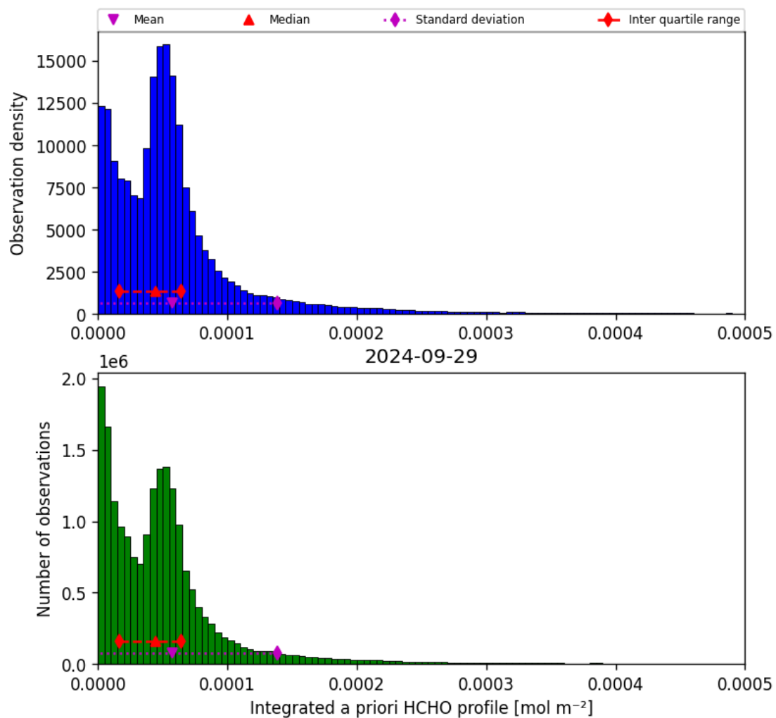
Figure 43: Histogram of “Integrated a priori HCHO profile” for 2024-09-28 to 2024-09-30
