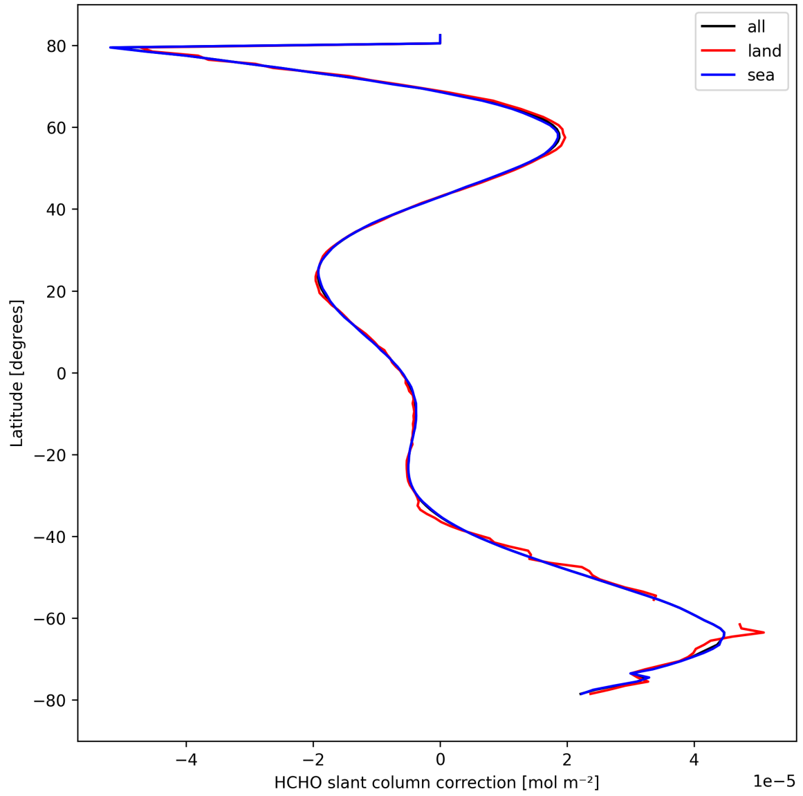
Figure 33: Zonal average of “HCHO slant column correction” for 2024-09-28 to 2024-09-30.
