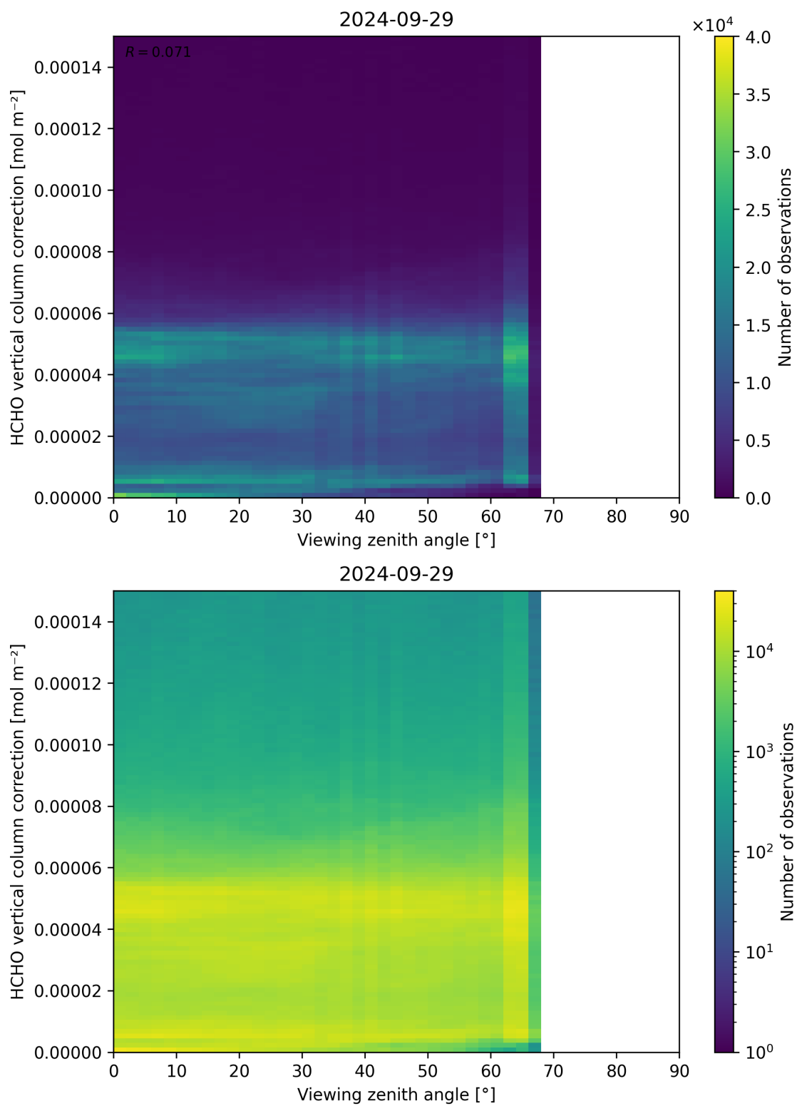
Figure 193: Scatter density plot of “Viewing zenith angle” against “HCHO vertical column correction” for 2024-09-28 to 2024-09-30.
