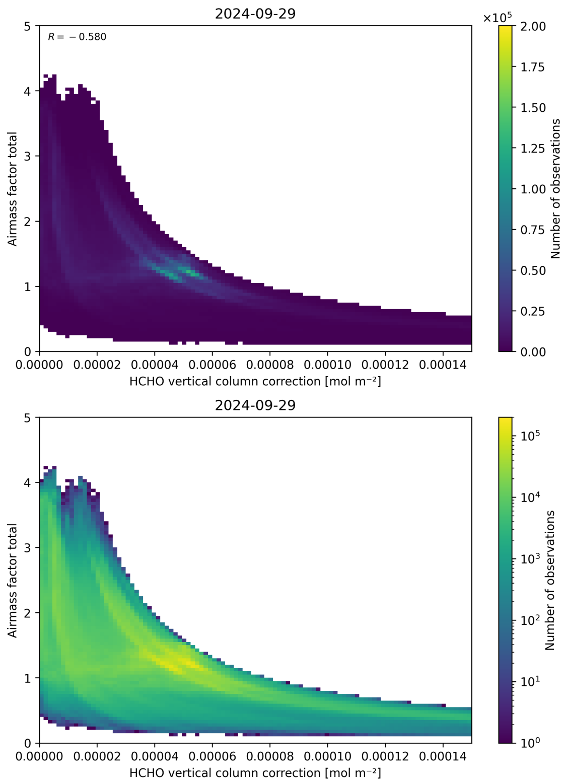
Figure 120: Scatter density plot of “HCHO vertical column correction” against “Airmass factor total” for 2024-09-28 to 2024-09-30.
