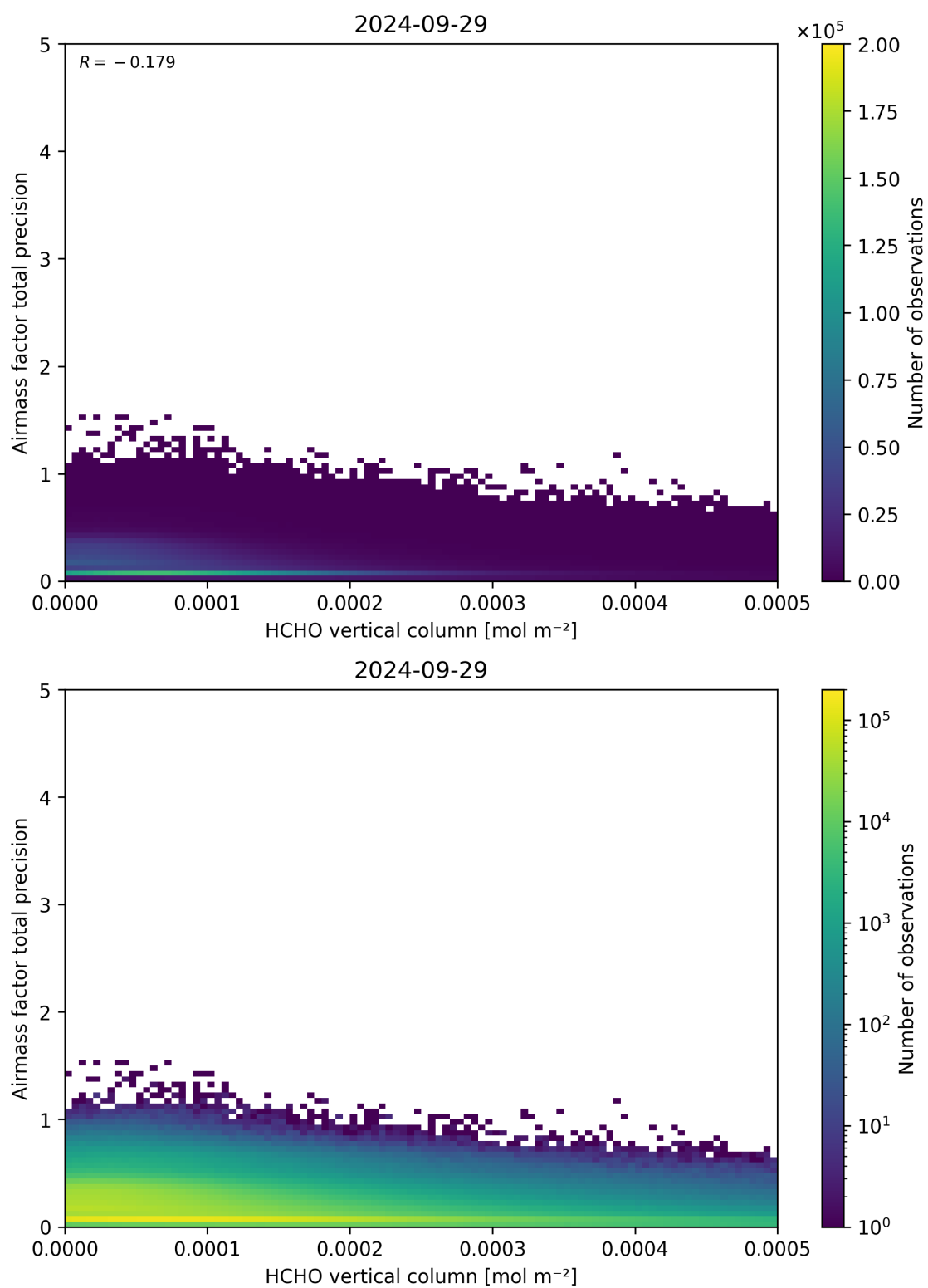
Figure 132: Scatter density plot of “HCHO vertical column” against “Airmass factor total precision” for 2024-09-28 to 2024-09-30.
