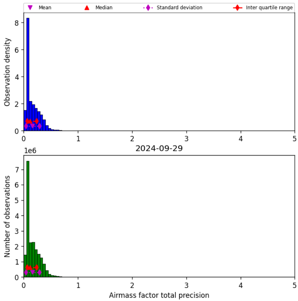
Figure 41: Histogram of “Airmass factor total precision” for 2024-09-28 to 2024-09-30
