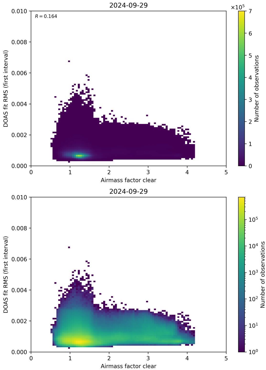
Figure 71: Scatter density plot of “Airmass factor clear” against “DOAS fit RMS (first interval)” for 2024-09-28 to 2024-09-30.
