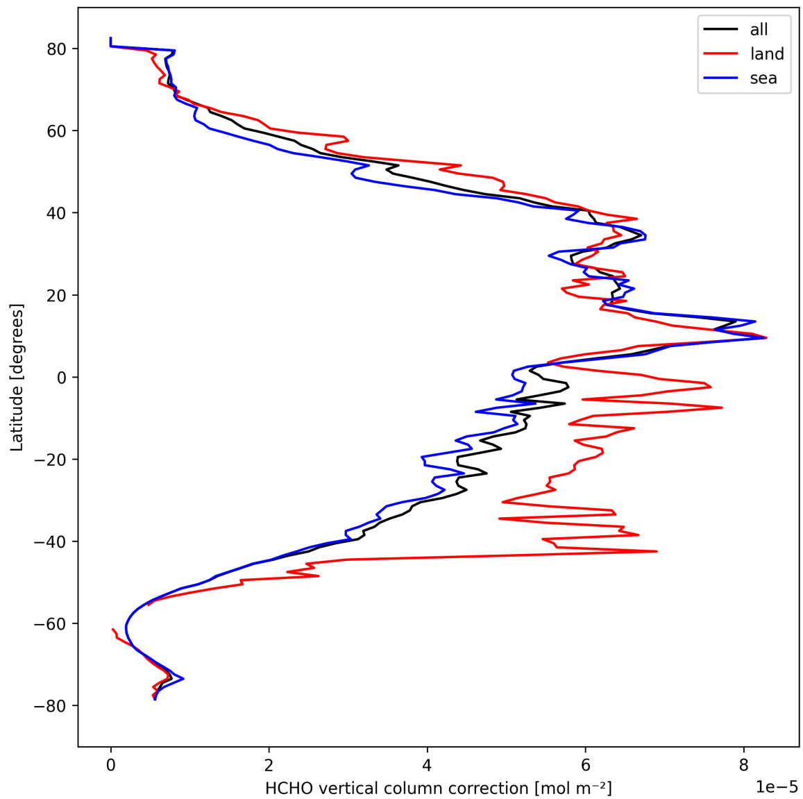
Figure 23: Zonal average of “HCHO vertical column correction” for 2024-09-28 to 2024-09-30.
