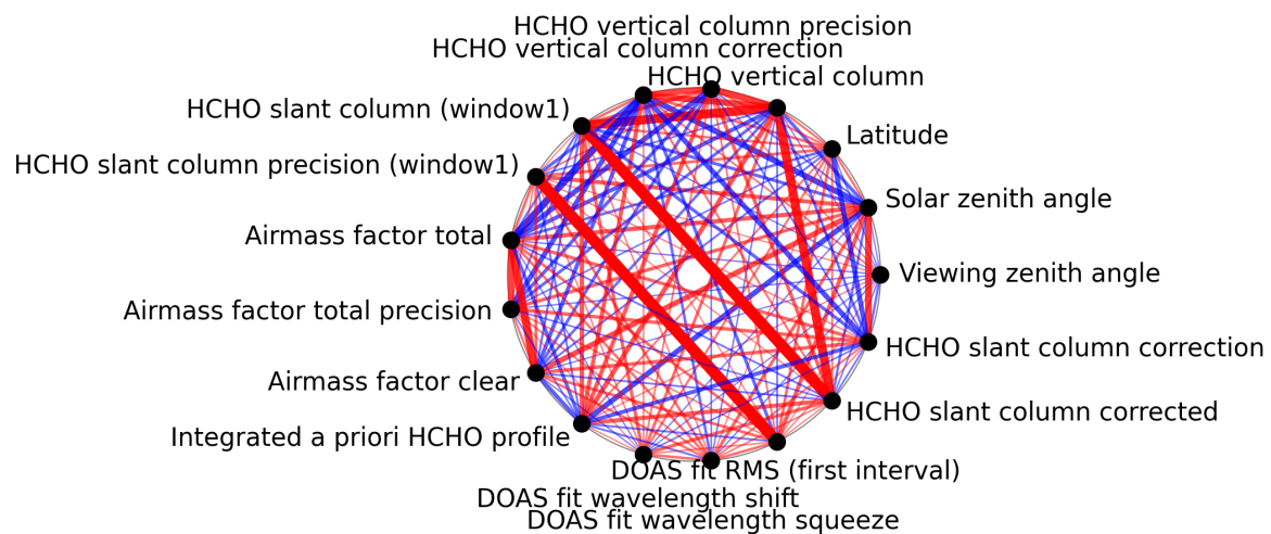
Figure 1: Map of correlation graph for 2024-09-28 to 2024-09-30.
