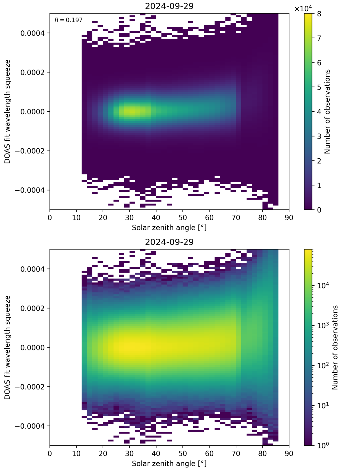
Figure 169: Scatter density plot of “Solar zenith angle” against “DOAS fit wavelength squeeze” for 2024-09-28 to 2024-09-30.
