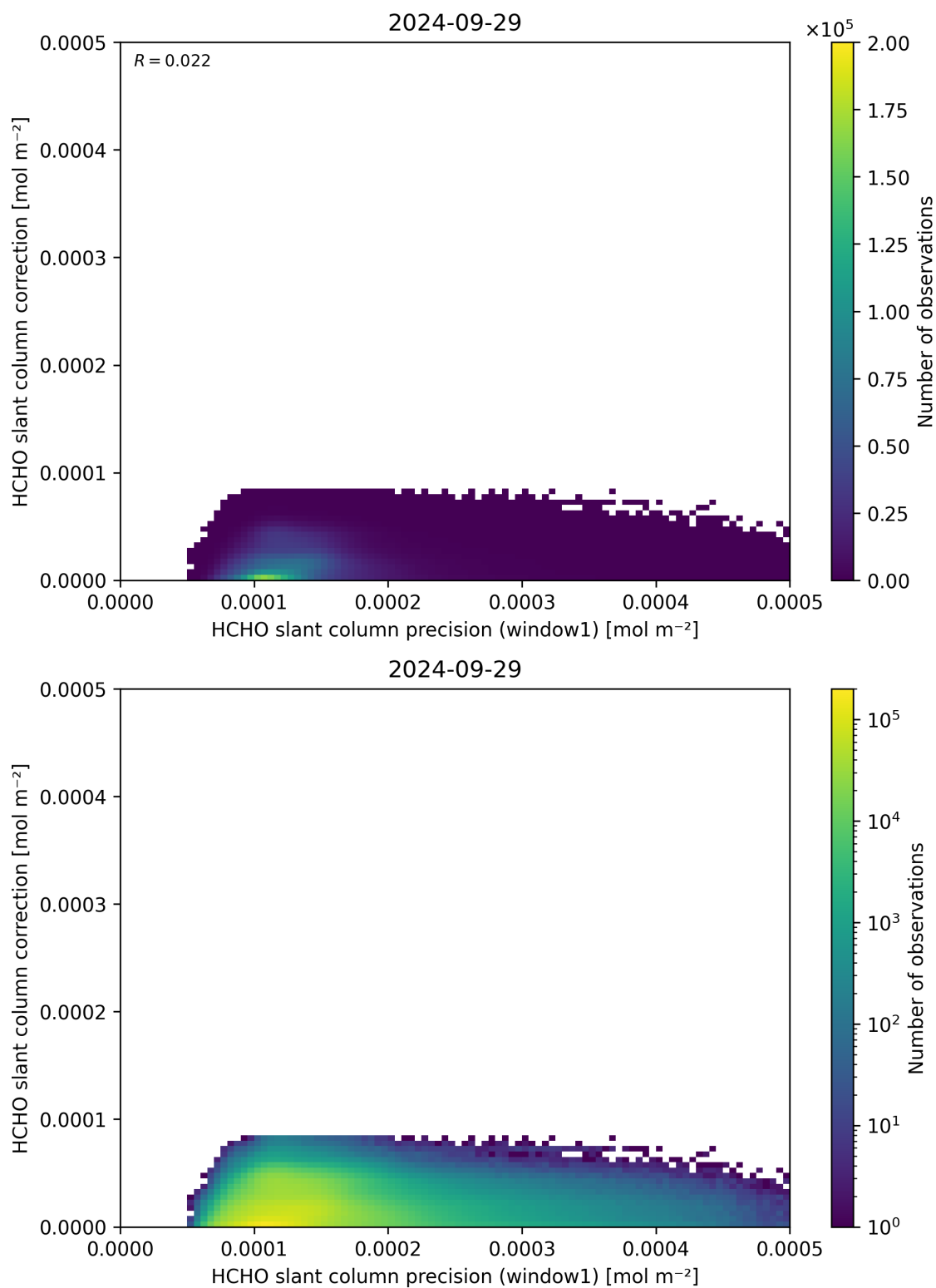
Figure 93: Scatter density plot of “HCHO slant column precision (window1)” against “HCHO slant column correction” for 2024-09-28 to 2024-09-30.
