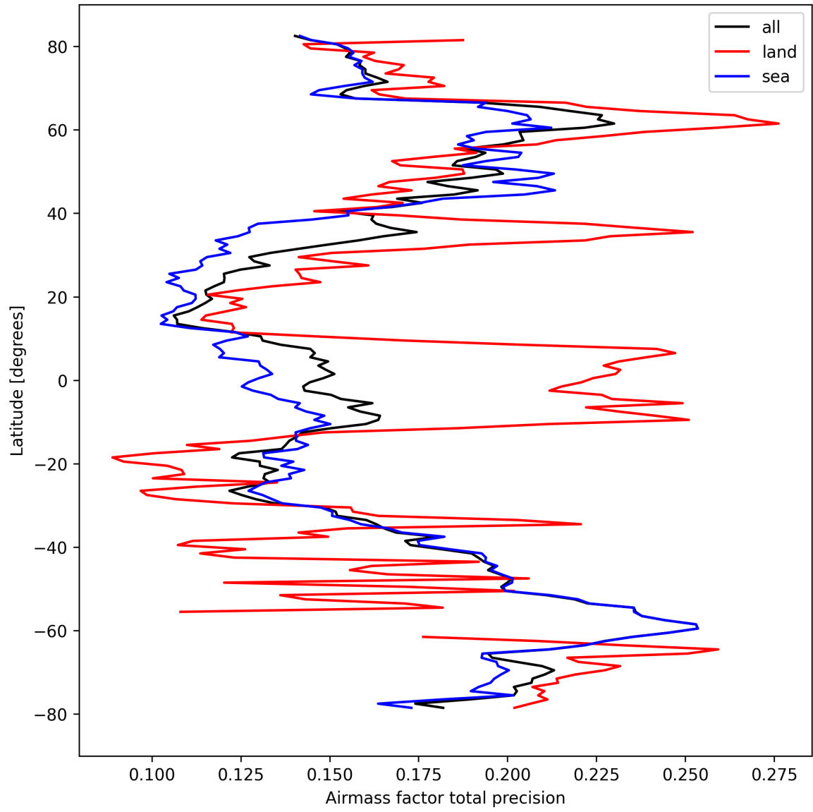
Figure 27: Zonal average of “Airmass factor total precision” for 2024-09-28 to 2024-09-30.
