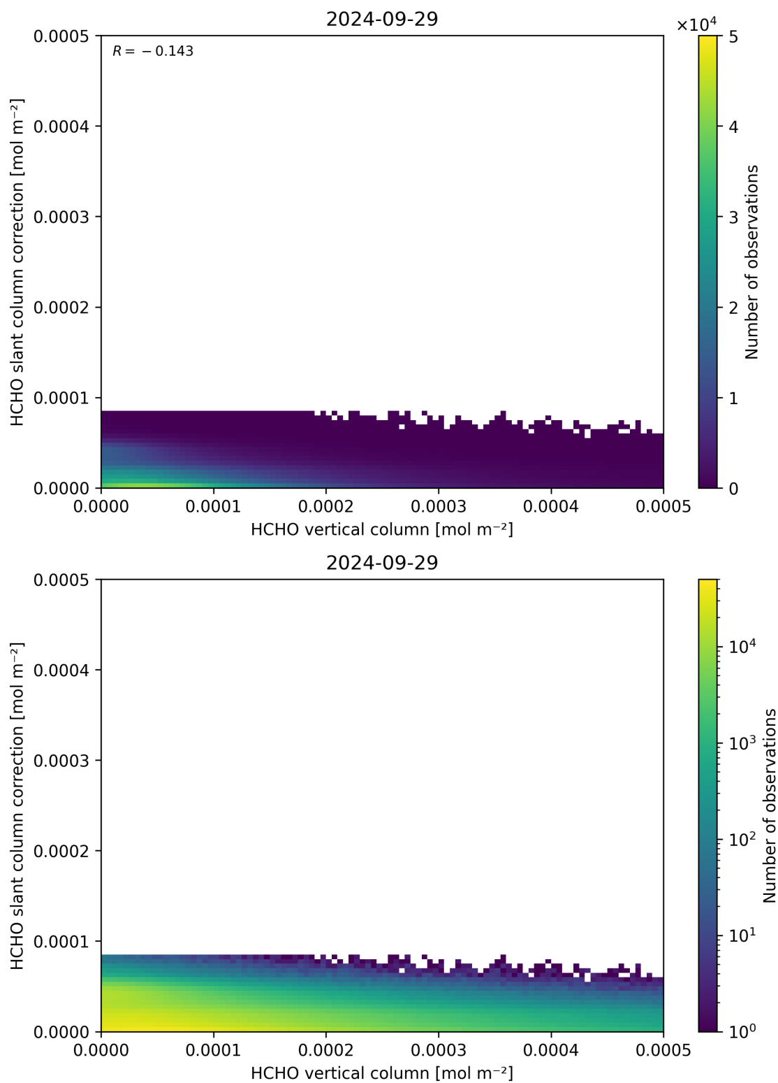
Figure 128: Scatter density plot of “HCHO vertical column” against “HCHO slant column correction” for 2024-09-28 to 2024-09-30.
