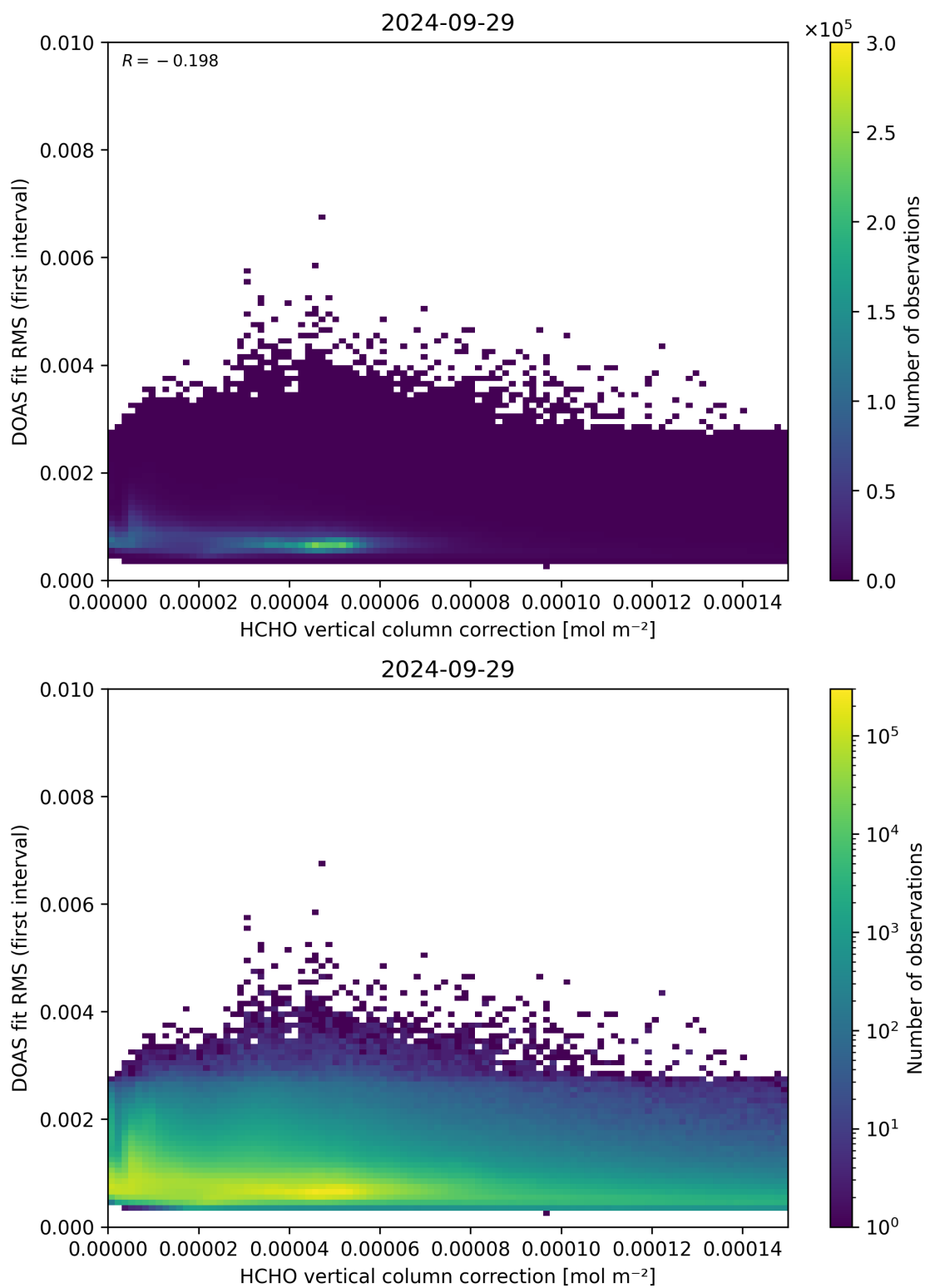
Figure 112: Scatter density plot of “HCHO vertical column correction” against “DOAS fit RMS (first interval)” for 2024-09-28 to 2024-09-30.
