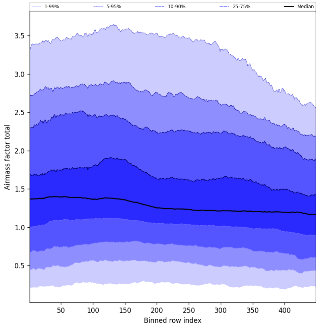
Figure 54: Along track statistics of “Airmass factor total” for 2024-09-28 to 2024-09-30
