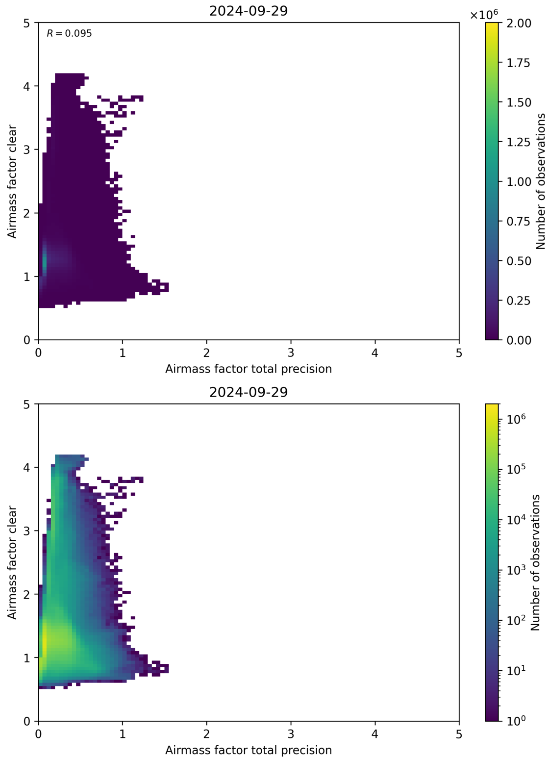
Figure 108: Scatter density plot of “Airmass factor total precision” against “Airmass factor clear” for 2024-09-28 to 2024-09-30.
