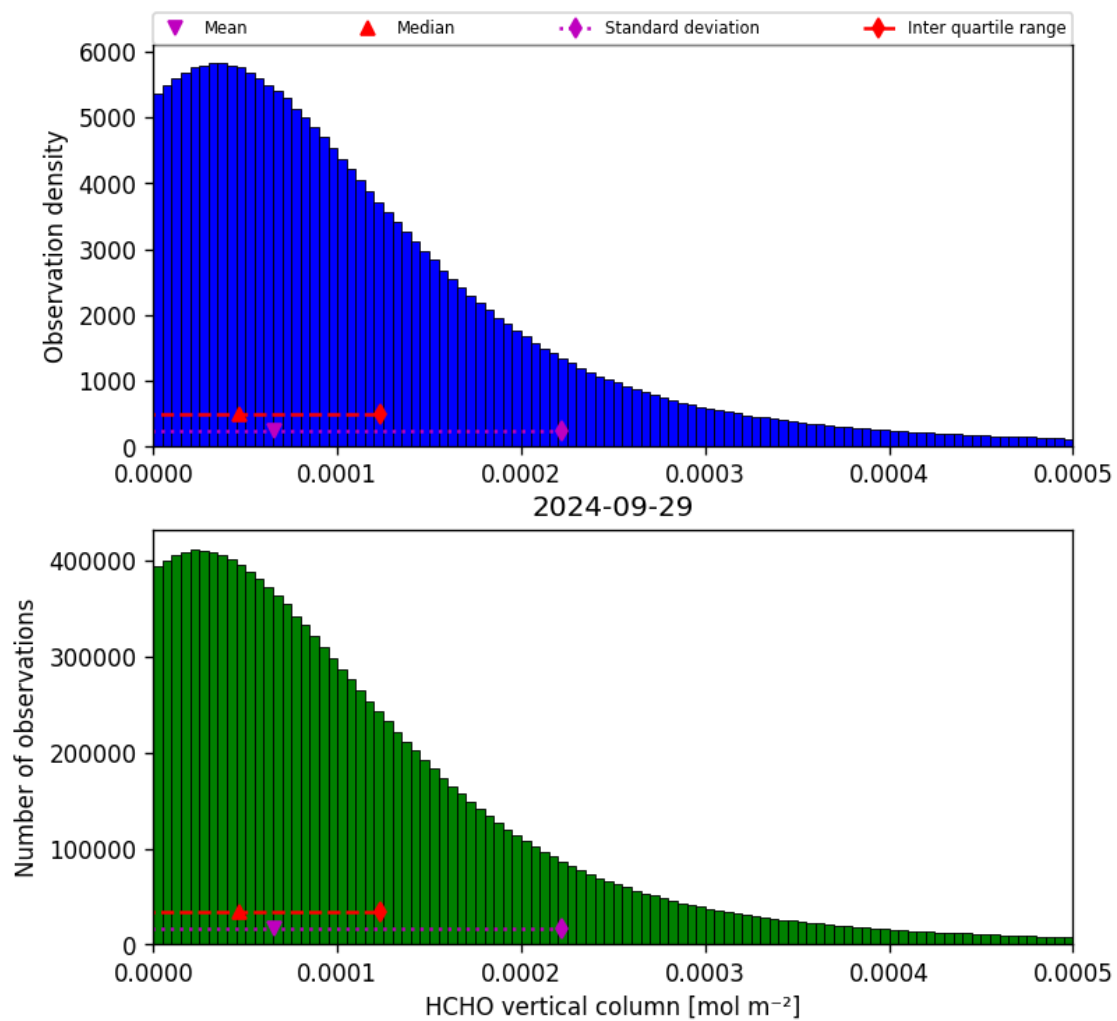
Figure 35: Histogram of “HCHO vertical column” for 2024-09-28 to 2024-09-30
