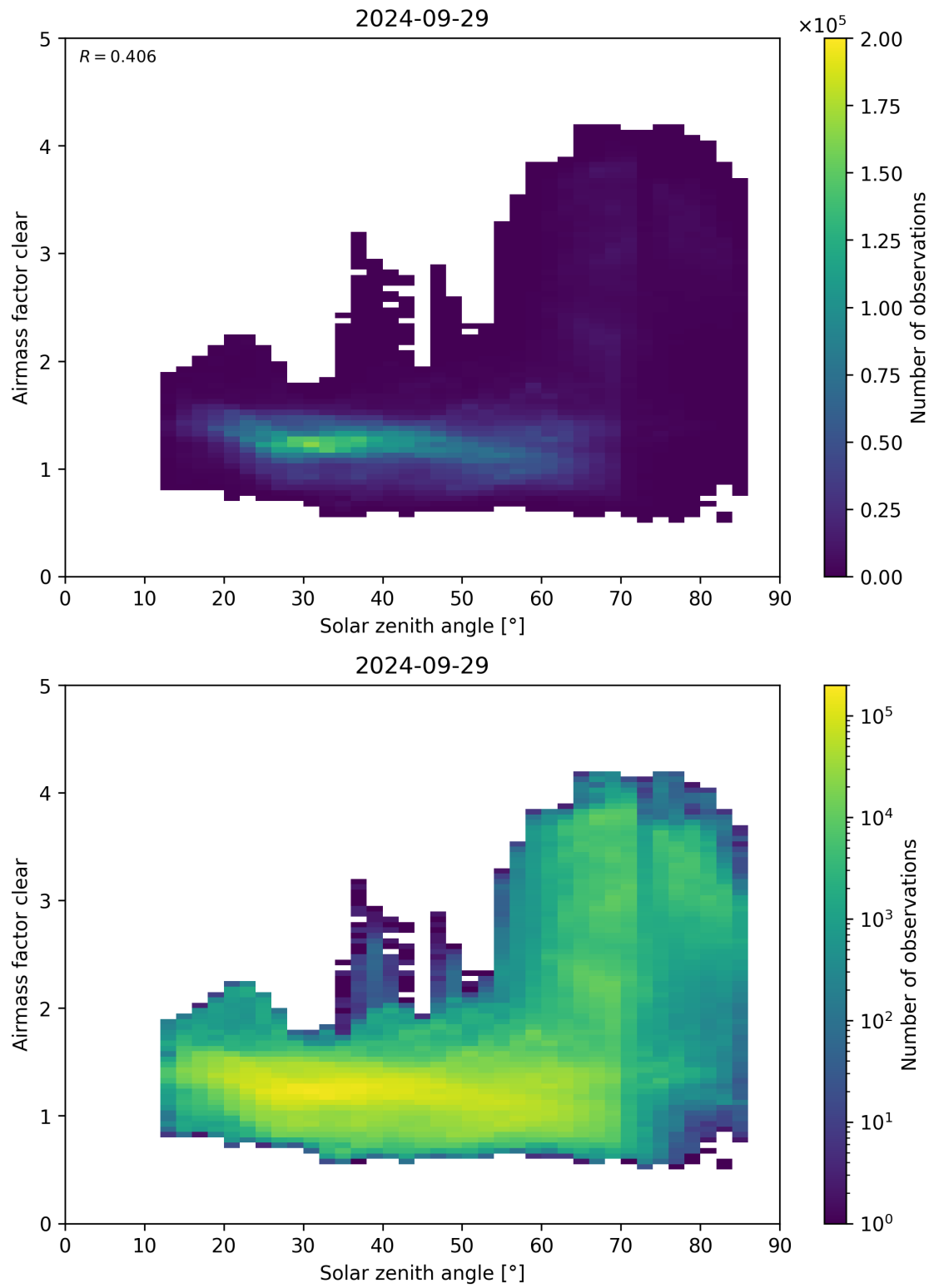
Figure 170: Scatter density plot of “Solar zenith angle” against “Airmass factor clear” for 2024-09-28 to 2024-09-30.
