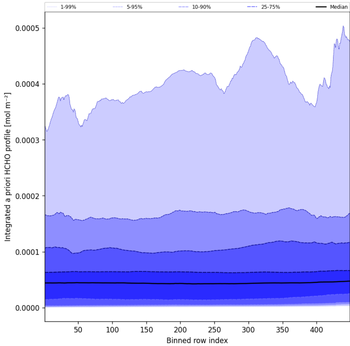
Figure 57: Along track statistics of “Integrated a priori HCHO profile” for 2024-09-28 to 2024-09-30
