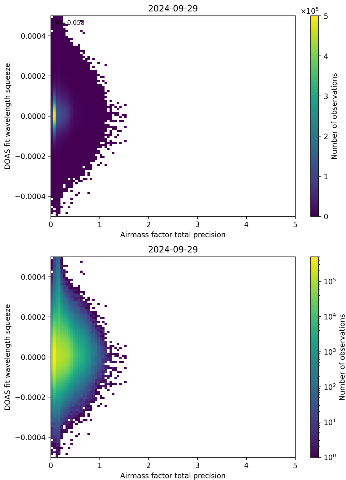
Figure 107: Scatter density plot of “Airmass factor total precision” against “DOAS fit wavelength squeeze” for 2024-09-28 to 2024-09-30.
