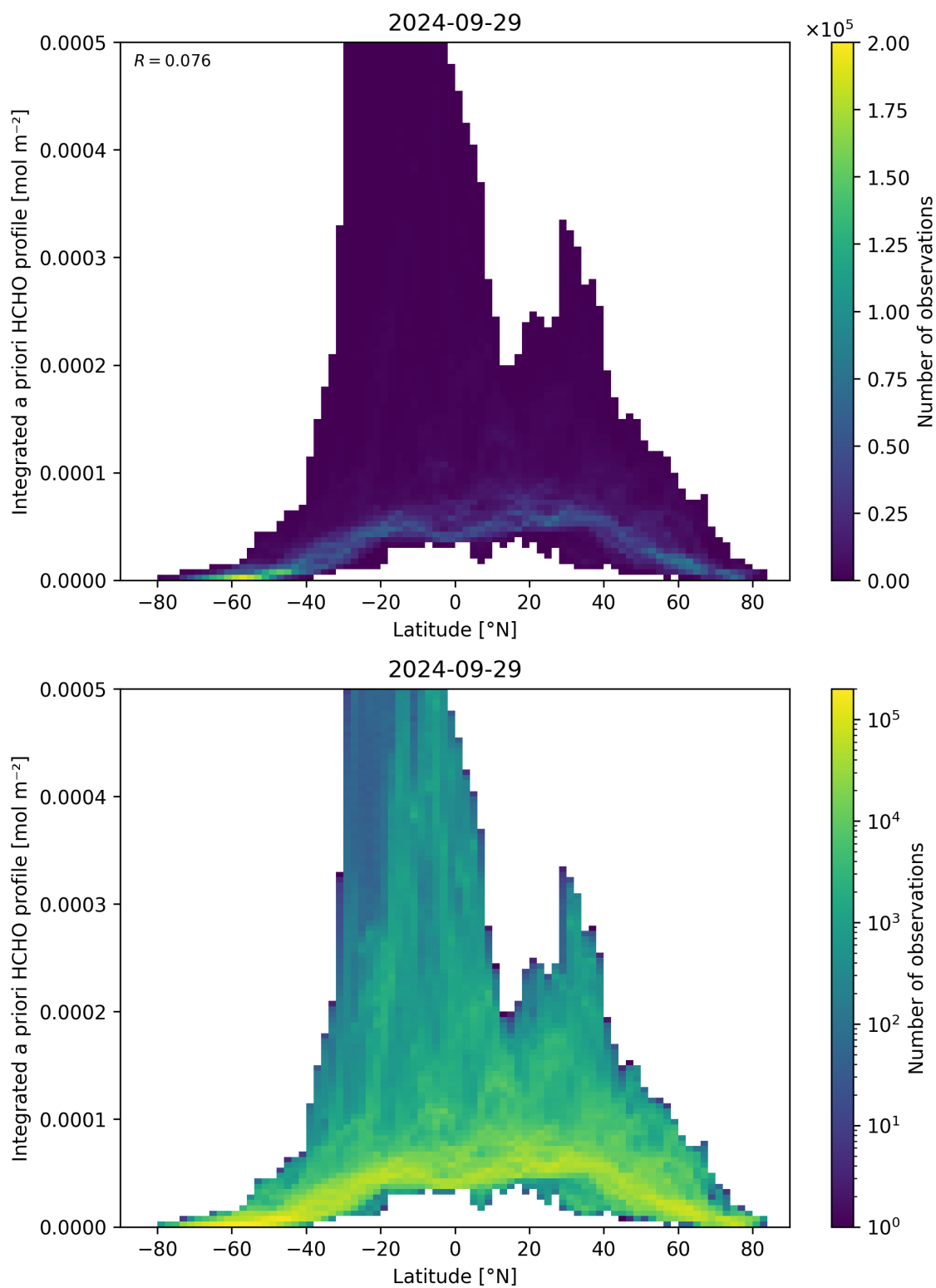
Figure 166: Scatter density plot of “Latitude” against “Integrated a priori HCHO profile” for 2024-09-28 to 2024-09-30.
