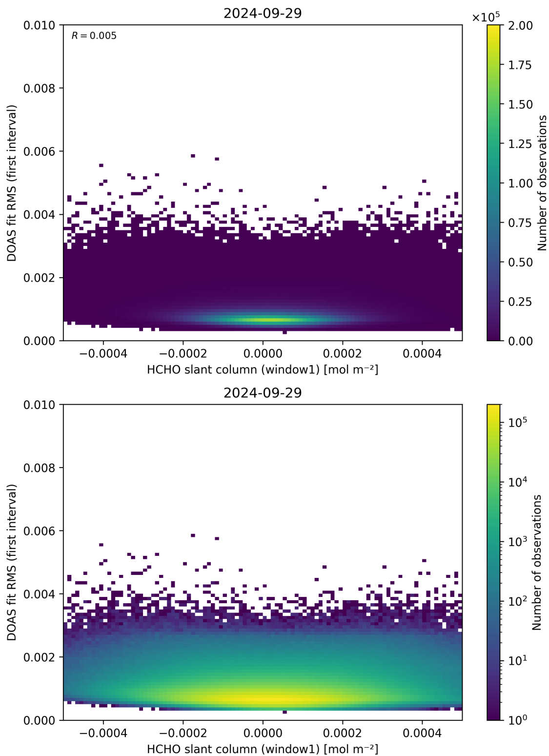
Figure 78: Scatter density plot of “HCHO slant column (window1)” against “DOAS fit RMS (first interval)” for 2024-09-28 to 2024-09-30.
