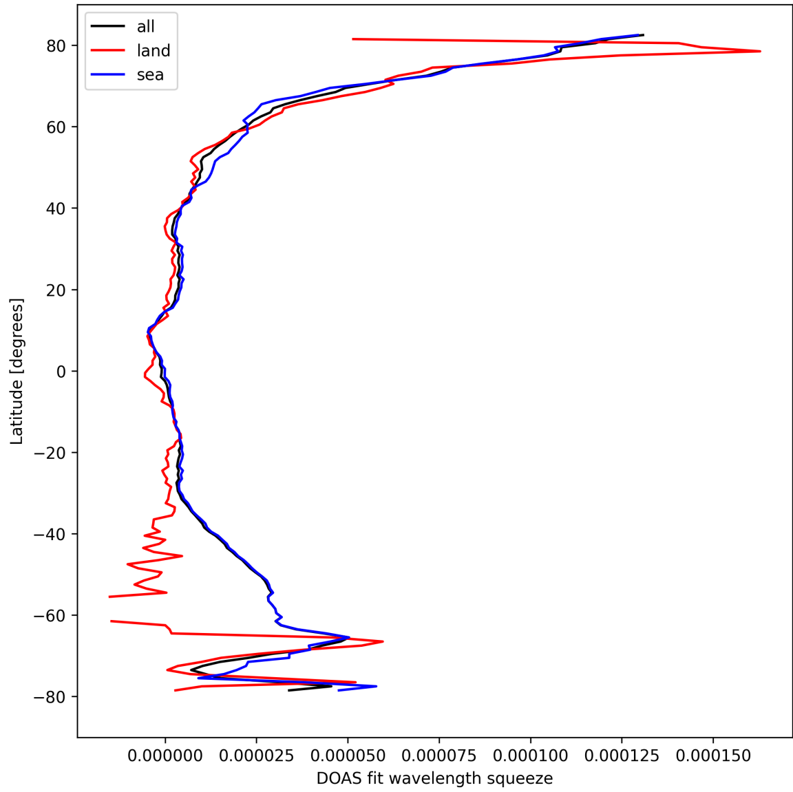
Figure 31: Zonal average of “DOAS fit wavelength squeeze” for 2024-09-28 to 2024-09-30.
