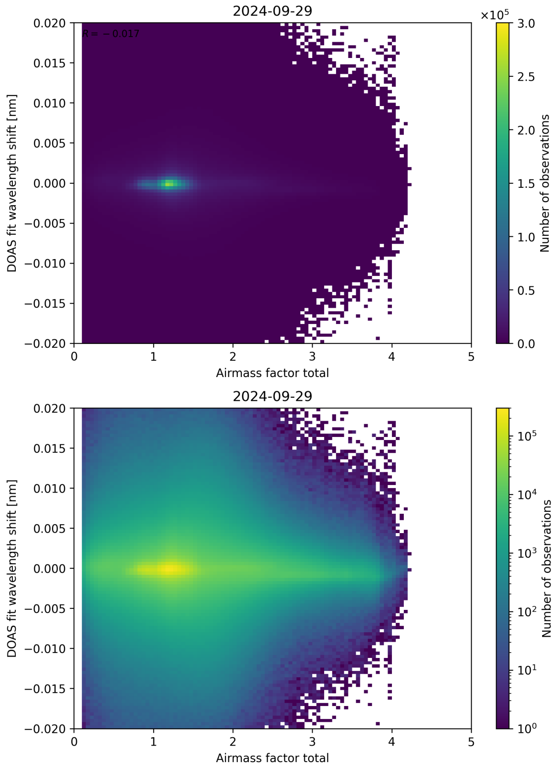
Figure 98: Scatter density plot of “Airmass factor total” against “DOAS fit wavelength shift” for 2024-09-28 to 2024-09-30.
