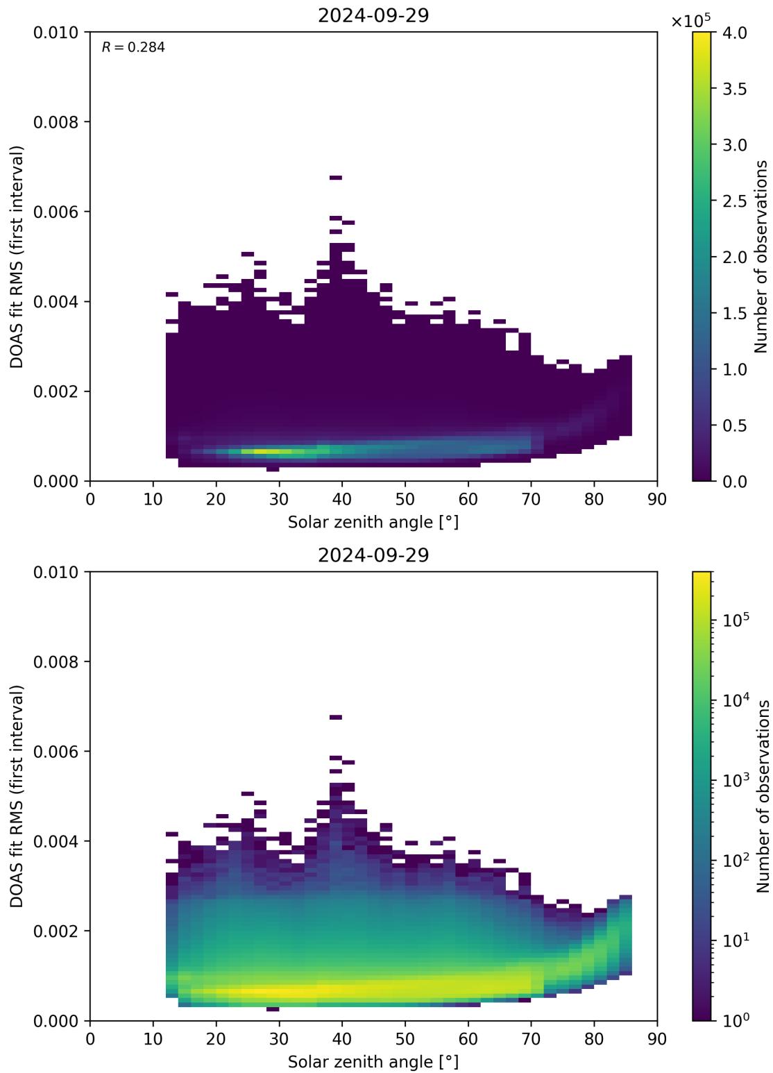
Figure 167: Scatter density plot of “Solar zenith angle” against “DOAS fit RMS (first interval)” for 2024-09-28 to 2024-09-30.
