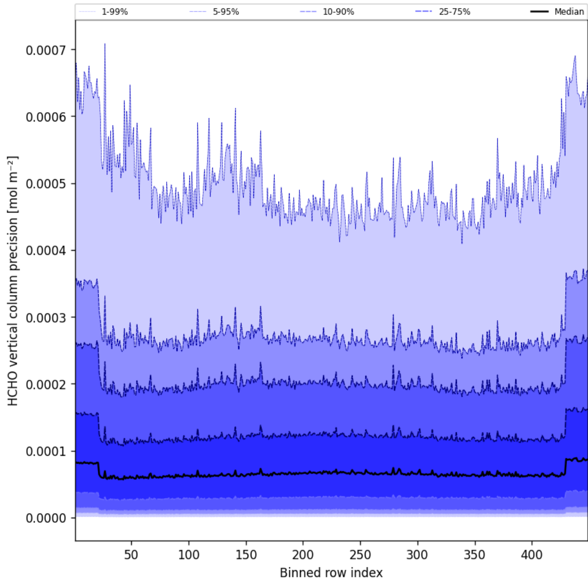
Figure 50: Along track statistics of “HCHO vertical column precision” for 2024-09-28 to 2024-09-30
