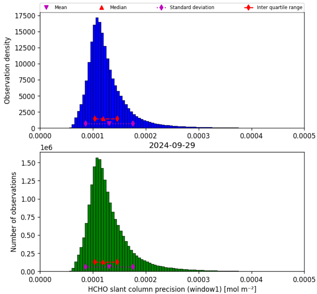
Figure 39: Histogram of “HCHO slant column precision (window1)” for 2024-09-28 to 2024-09-30
