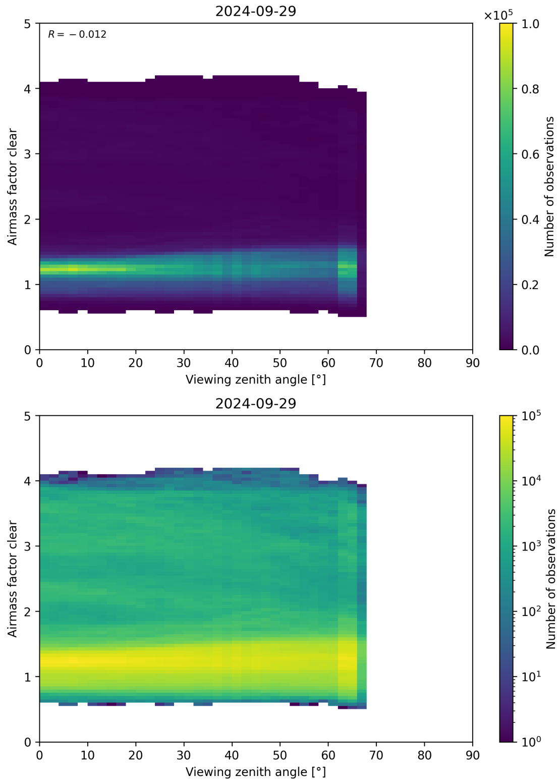
Figure 185: Scatter density plot of “Viewing zenith angle” against “Airmass factor clear” for 2024-09-28 to 2024-09-30.
