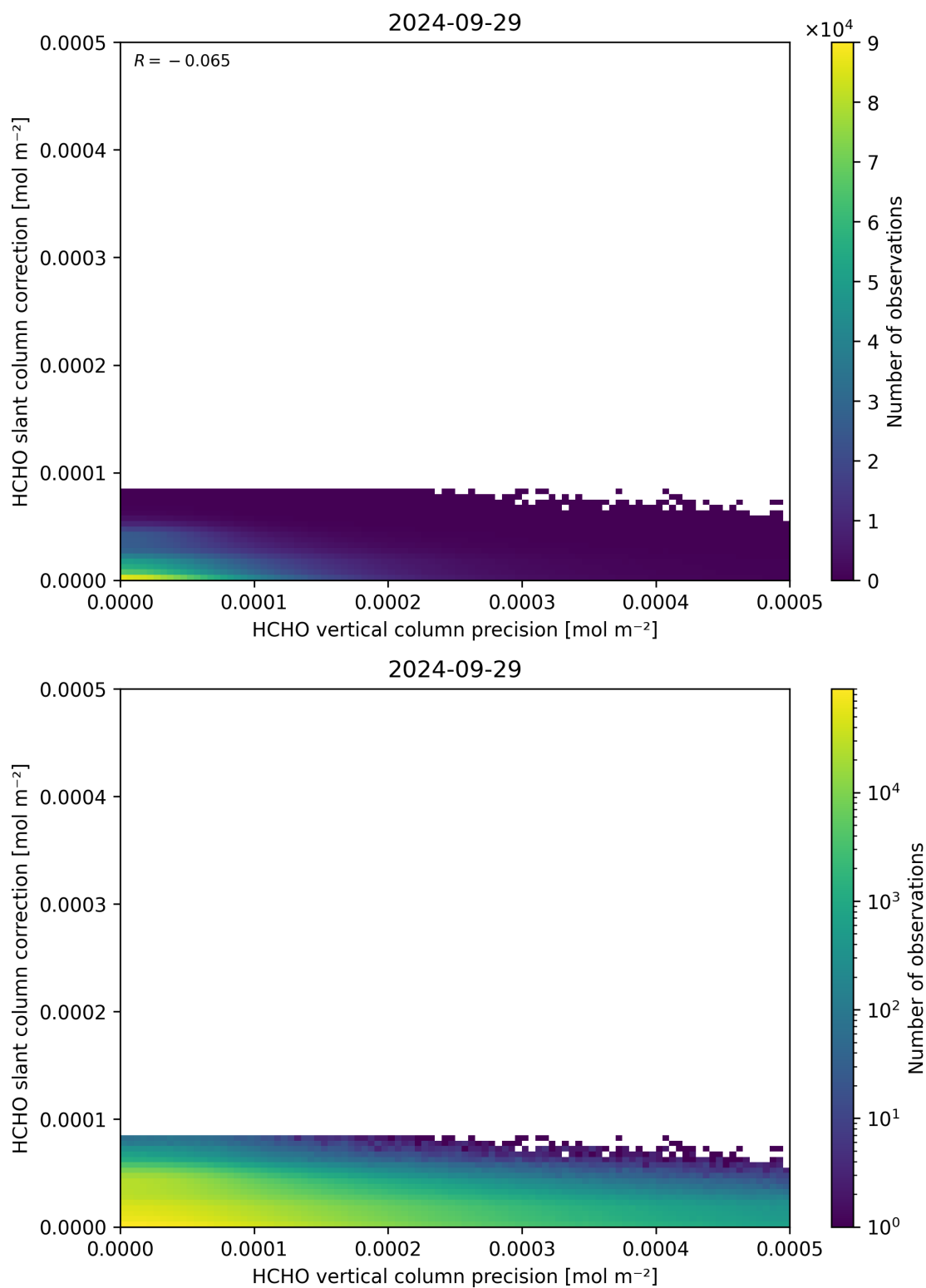
Figure 141: Scatter density plot of “HCHO vertical column precision” against “HCHO slant column correction” for 2024-09-28 to 2024-09-30.
