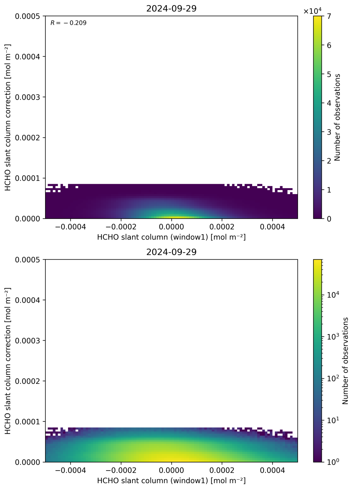
Figure 83: Scatter density plot of “HCHO slant column (window1)” against “HCHO slant column correction” for 2024-09-28 to 2024-09-30.
