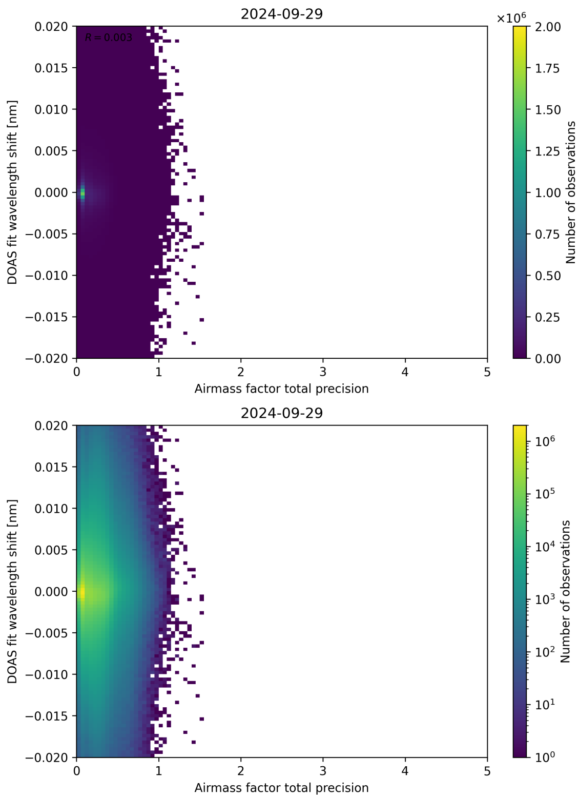
Figure 106: Scatter density plot of “Airmass factor total precision” against “DOAS fit wavelength shift” for 2024-09-28 to 2024-09-30.
