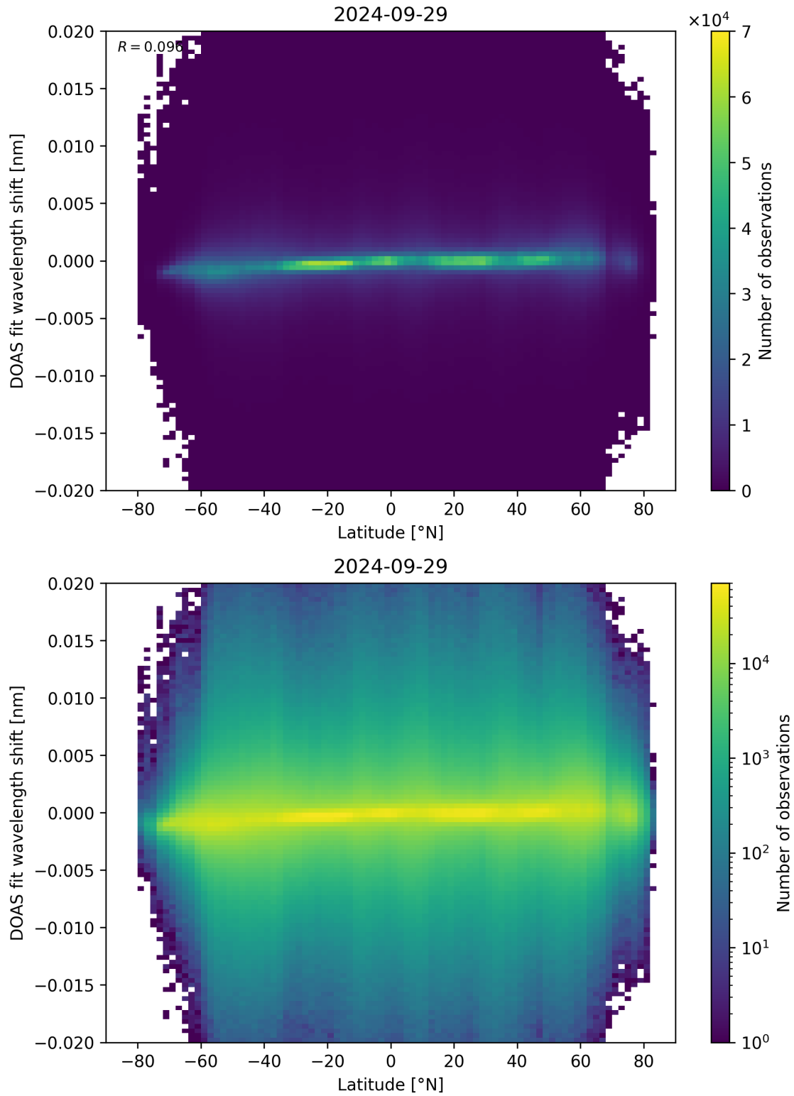
Figure 154: Scatter density plot of “Latitude” against “DOAS fit wavelength shift” for 2024-09-28 to 2024-09-30.
