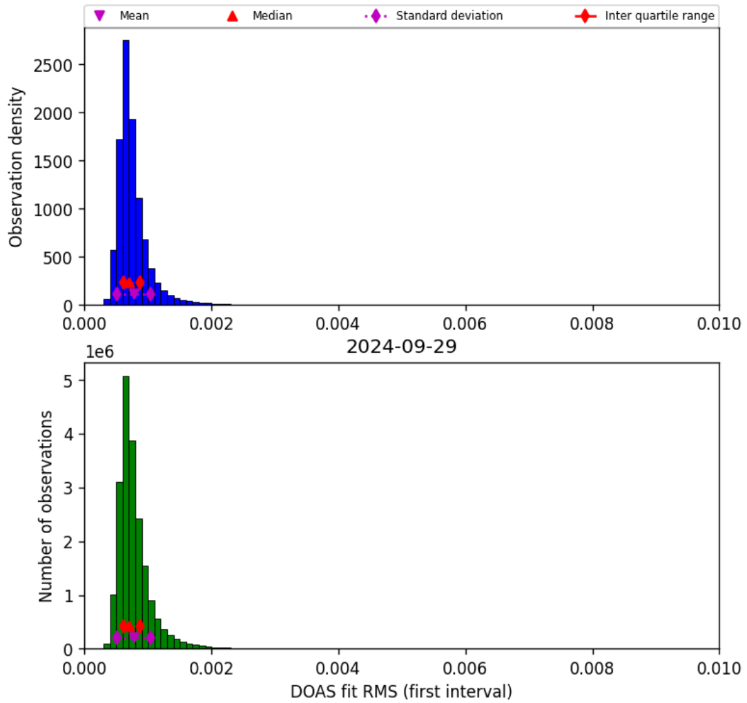
Figure 46: Histogram of “DOAS fit RMS (first interval)” for 2024-09-28 to 2024-09-30
