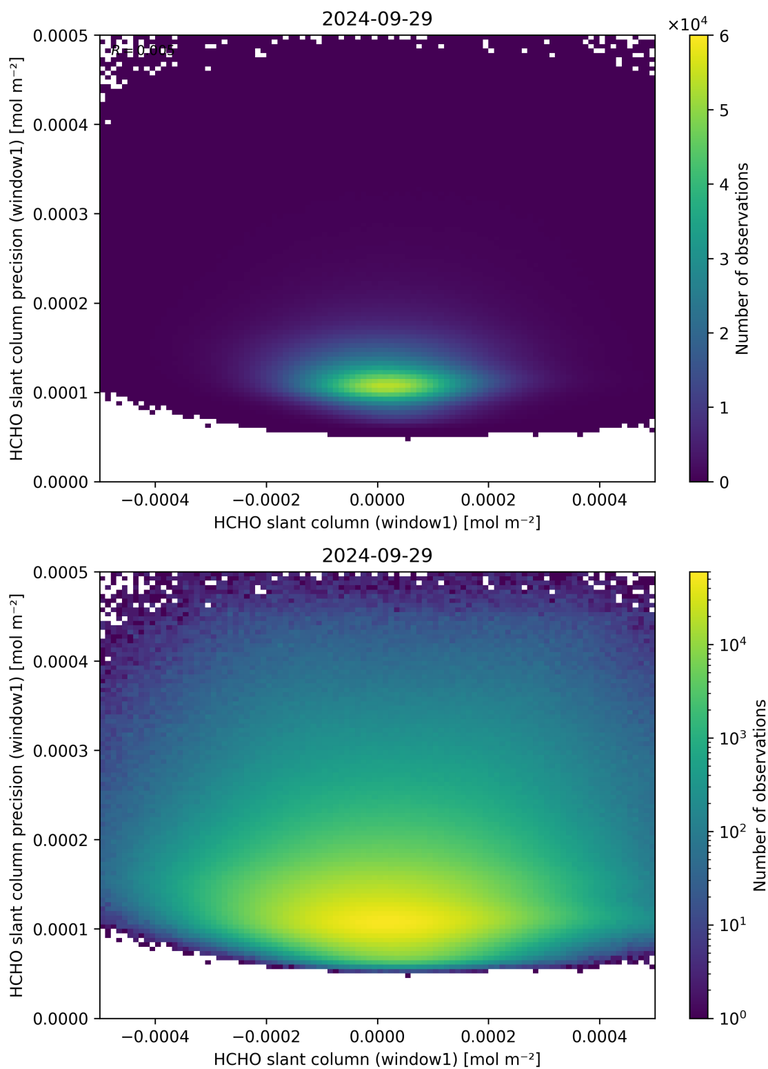
Figure 84: Scatter density plot of “HCHO slant column (window1)” against “HCHO slant column precision (window1)” for 2024-09-28 to 2024-09-30.
