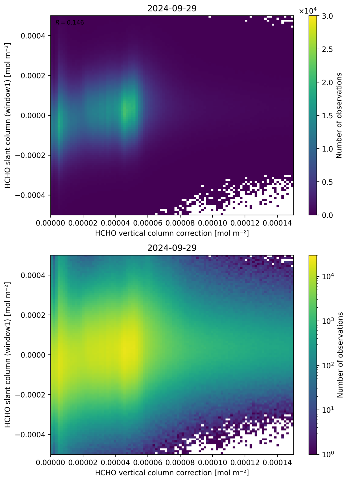
Figure 118: Scatter density plot of “HCHO vertical column correction” against “HCHO slant column (window1)” for 2024-09-28 to 2024-09-30.
