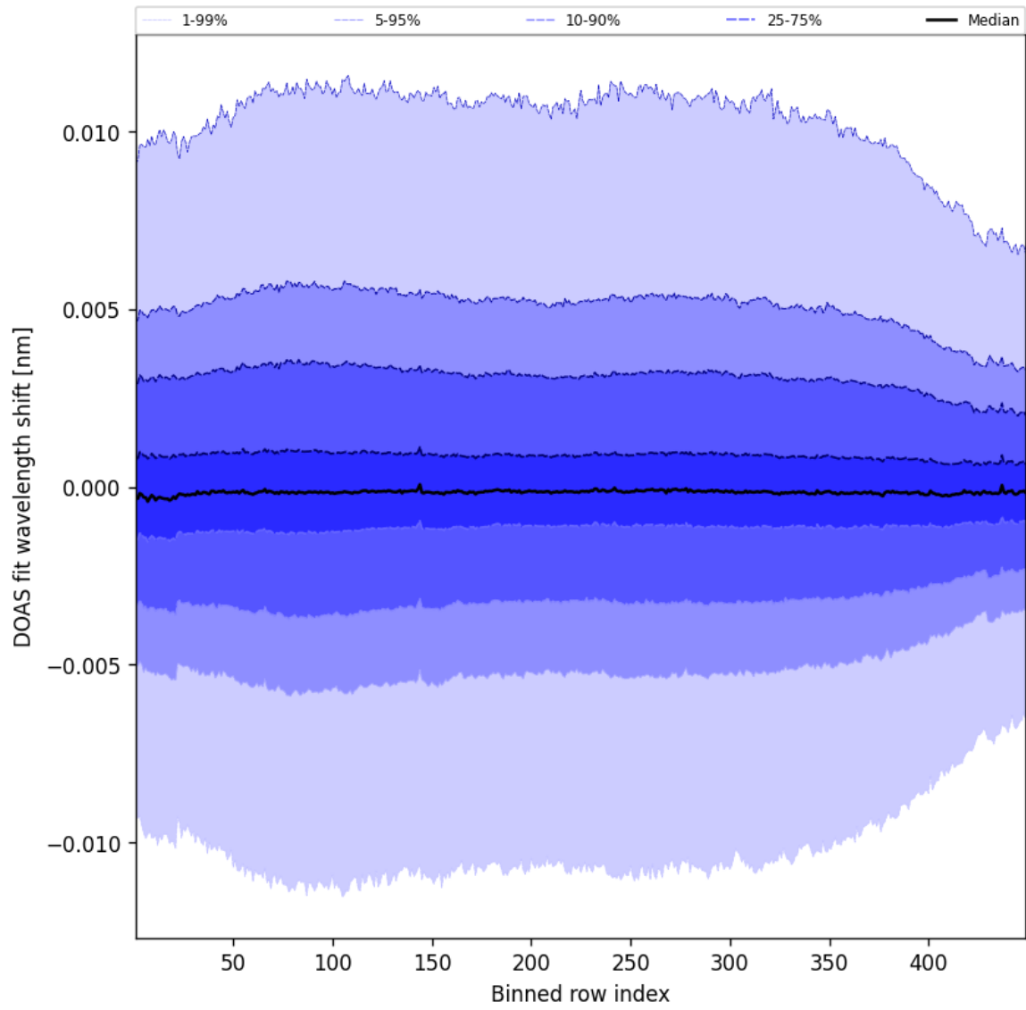
Figure 58: Along track statistics of “DOAS fit wavelength shift” for 2024-09-28 to 2024-09-30
