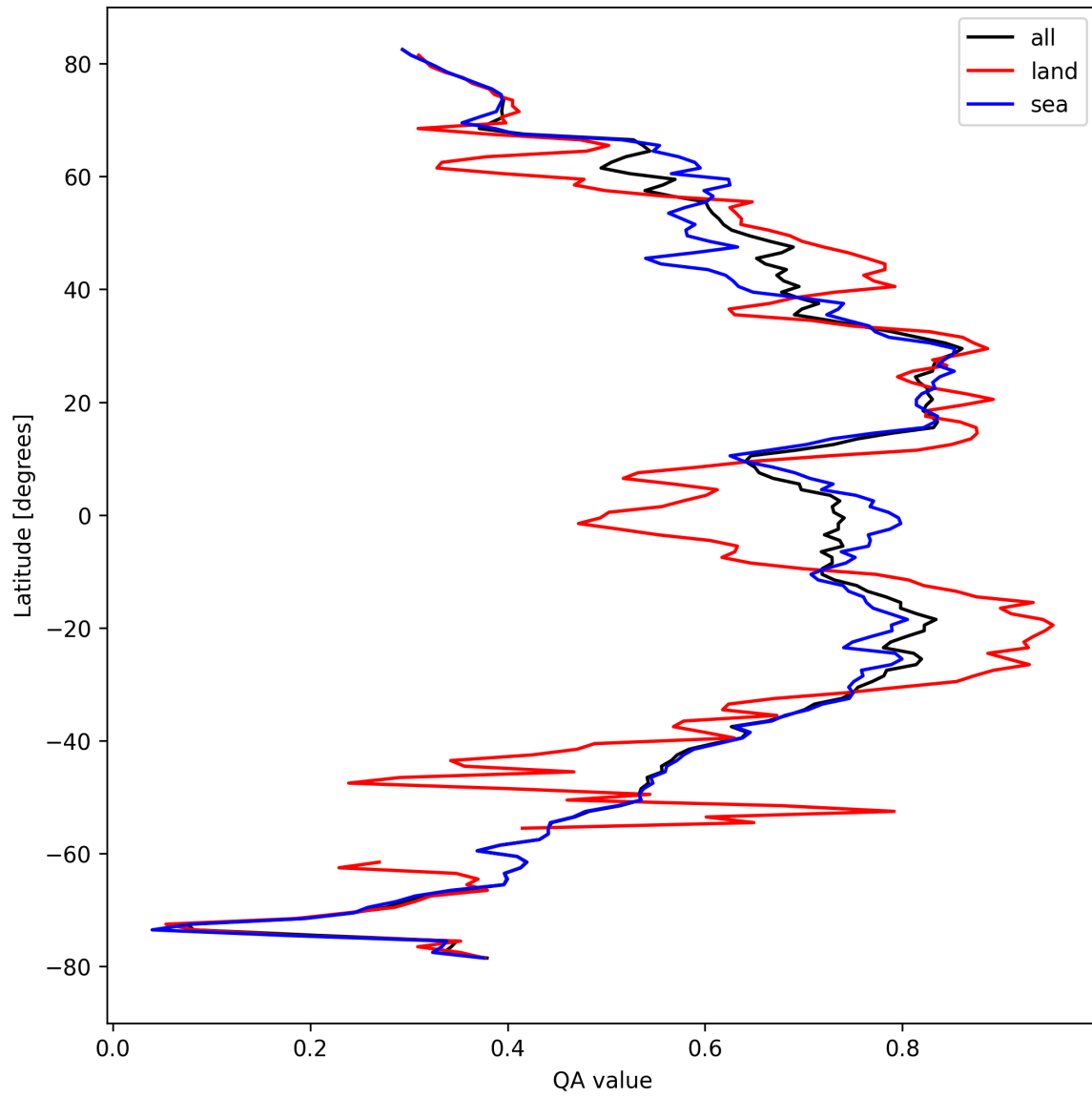
Figure 20: Zonal average of “QA value” for 2024-09-28 to 2024-09-30.
