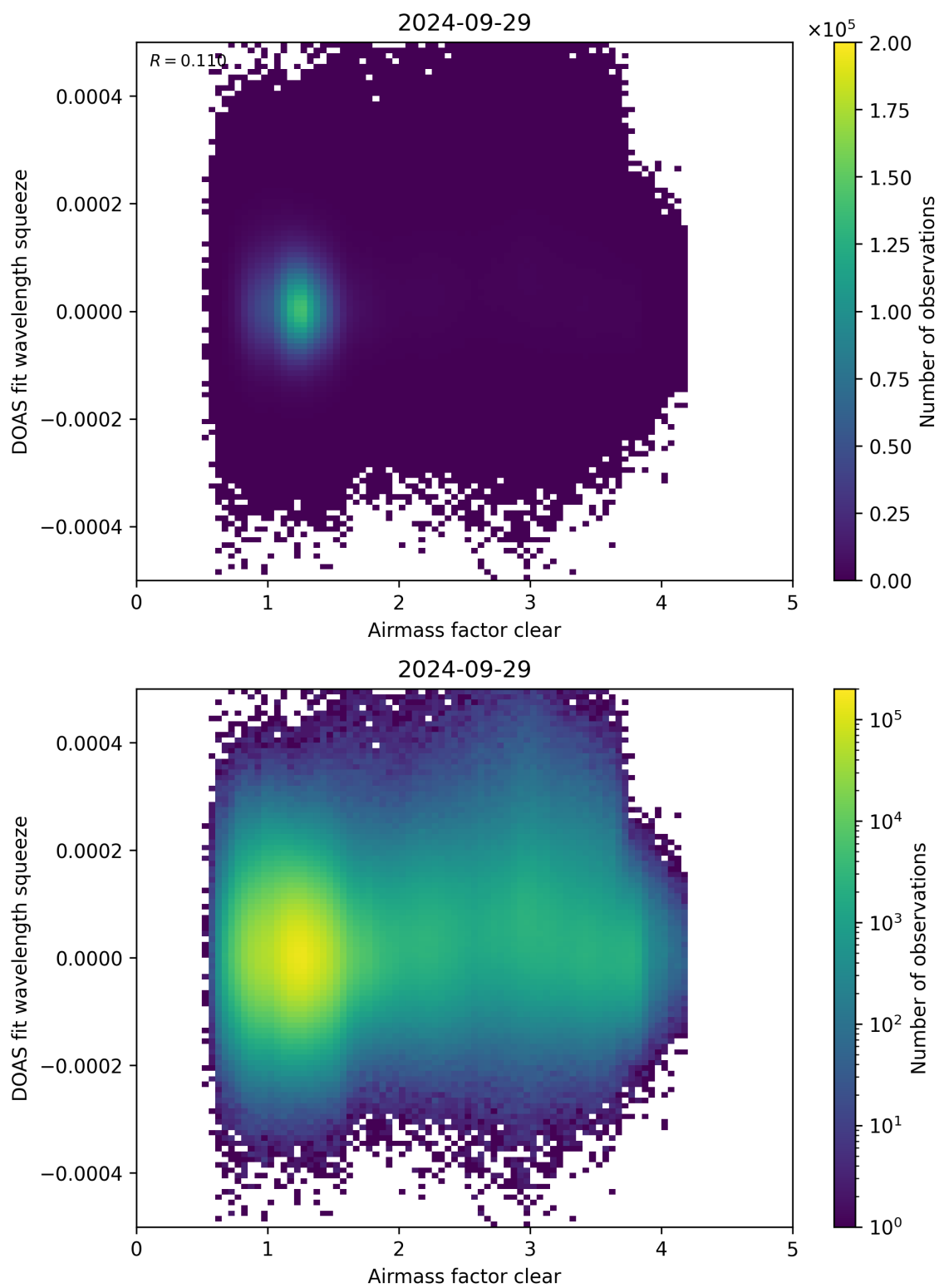
Figure 73: Scatter density plot of “Airmass factor clear” against “DOAS fit wavelength squeeze” for 2024-09-28 to 2024-09-30.
