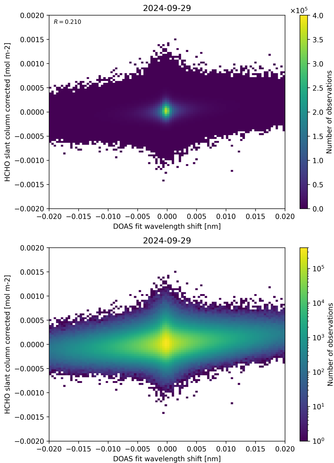
Figure 66: Scatter density plot of “DOAS fit wavelength shift” against “HCHO slant column corrected” for 2024-09-28 to 2024-09-30.
