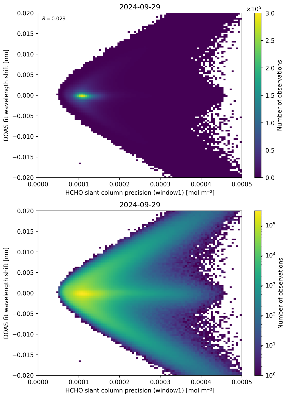
Figure 89: Scatter density plot of “HCHO slant column precision (window1)” against “DOAS fit wavelength shift” for 2024-09-28 to 2024-09-30.
