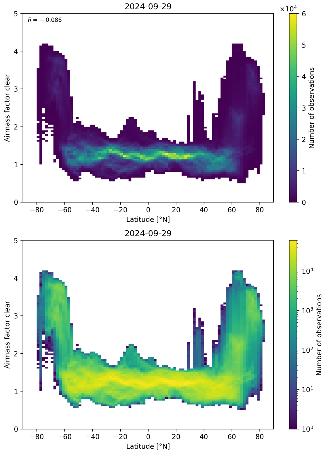
Figure 156: Scatter density plot of “Latitude” against “Airmass factor clear” for 2024-09-28 to 2024-09-30.
