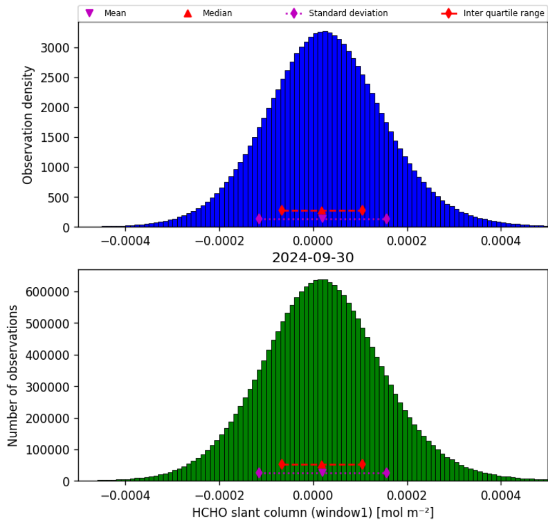
Figure 38: Histogram of “HCHO slant column (window1)” for 2024-09-29 to 2024-10-01
