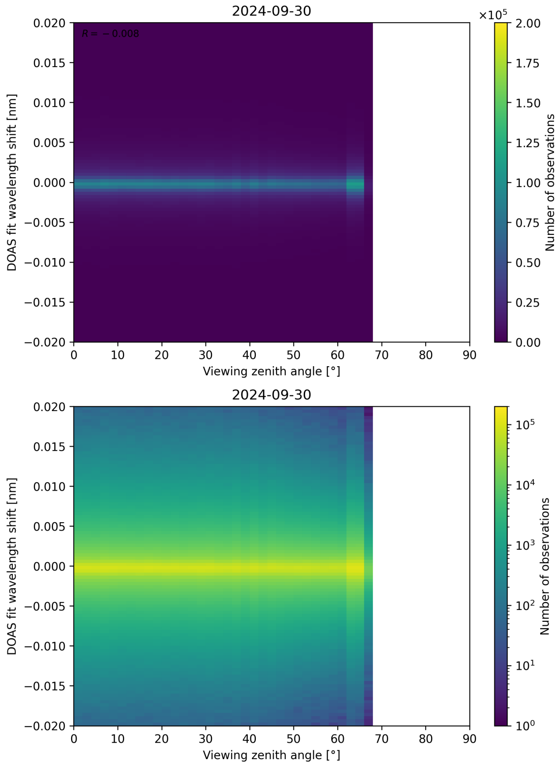
Figure 183: Scatter density plot of “Viewing zenith angle” against “DOAS fit wavelength shift” for 2024-09-29 to 2024-10-01.
