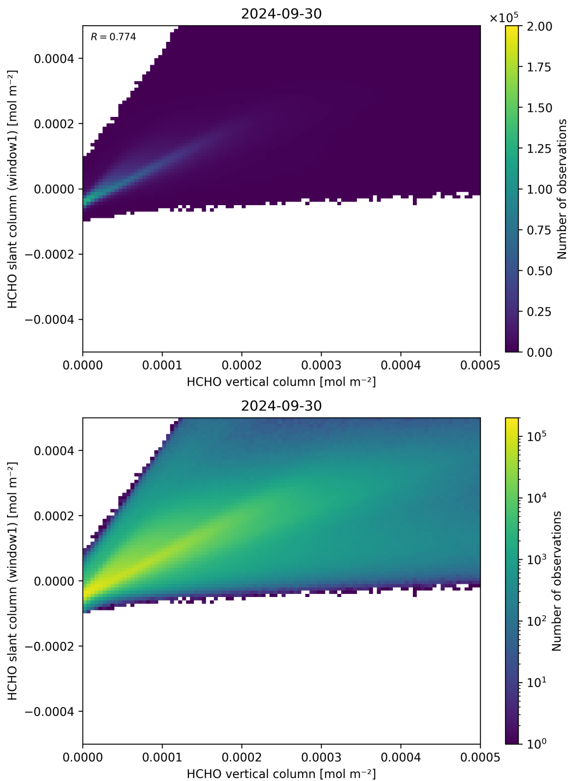
Figure 129: Scatter density plot of “HCHO vertical column” against “HCHO slant column (window1)” for 2024-09-29 to 2024-10-01.
