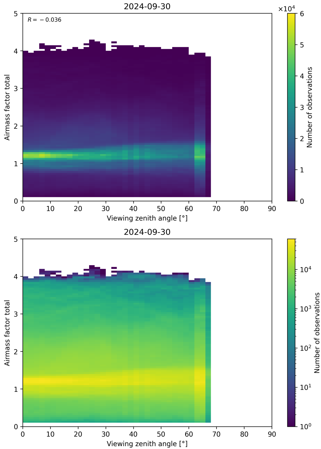
Figure 190: Scatter density plot of “Viewing zenith angle” against “Airmass factor total” for 2024-09-29 to 2024-10-01.
