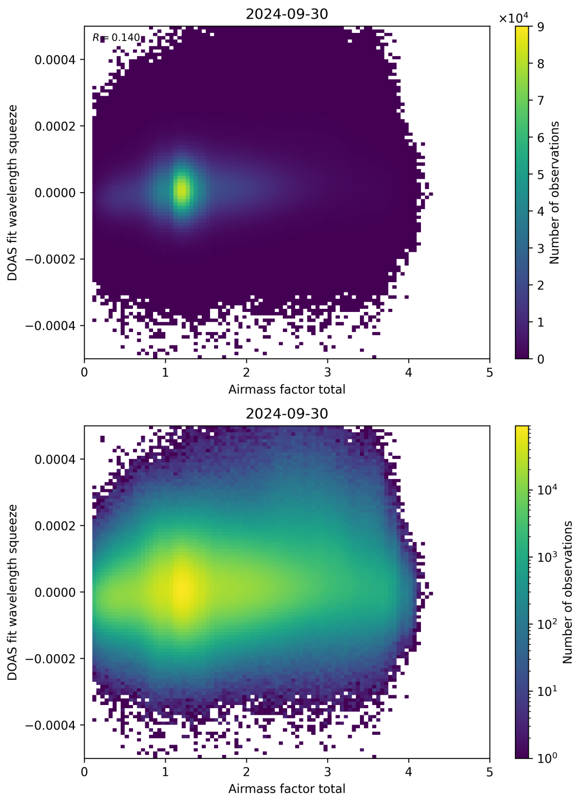
Figure 99: Scatter density plot of “Airmass factor total” against “DOAS fit wavelength squeeze” for 2024-09-29 to 2024-10-01.
