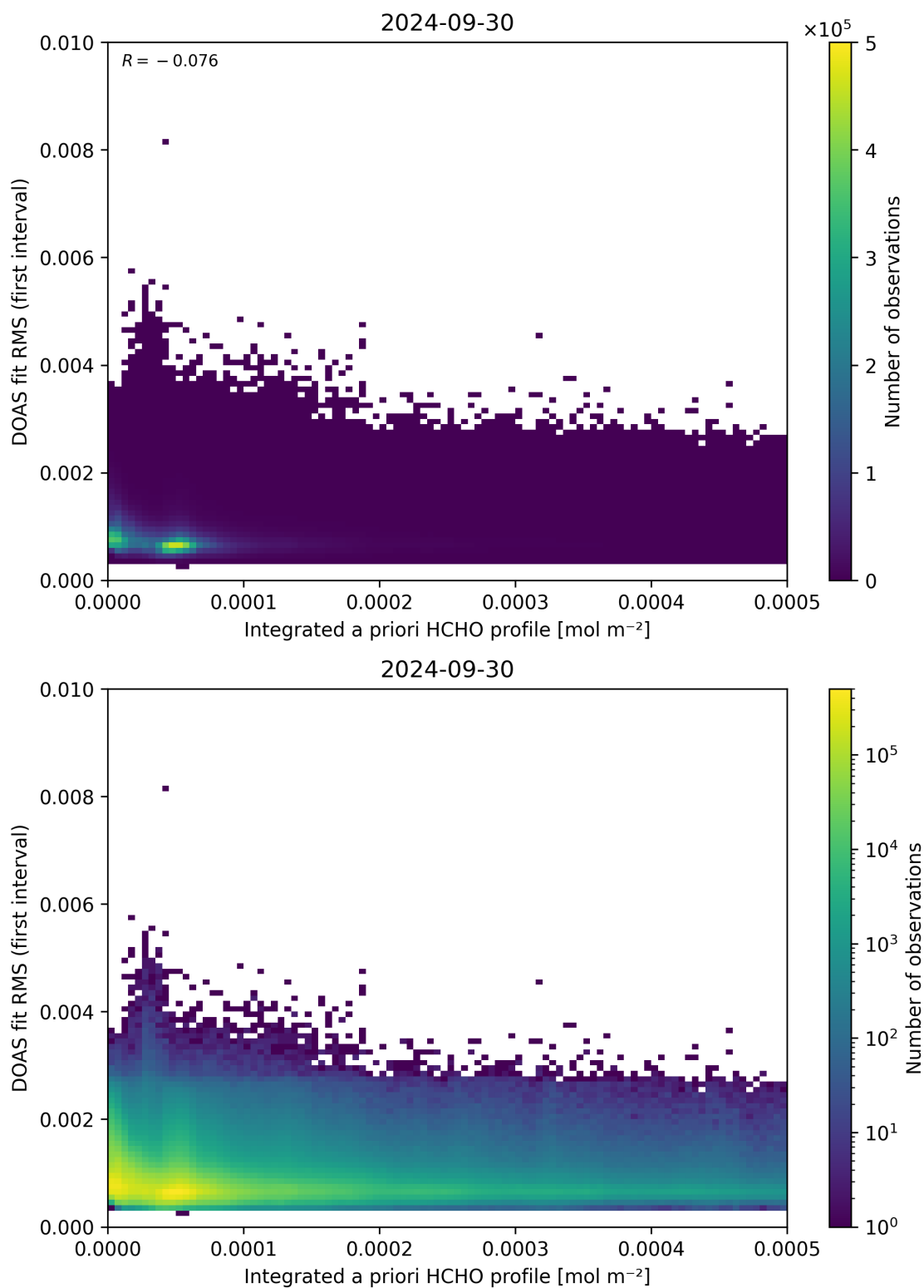
Figure 148: Scatter density plot of “Integrated a priori HCHO profile” against “DOAS fit RMS (first interval)” for 2024-09-29 to 2024-10-01.
