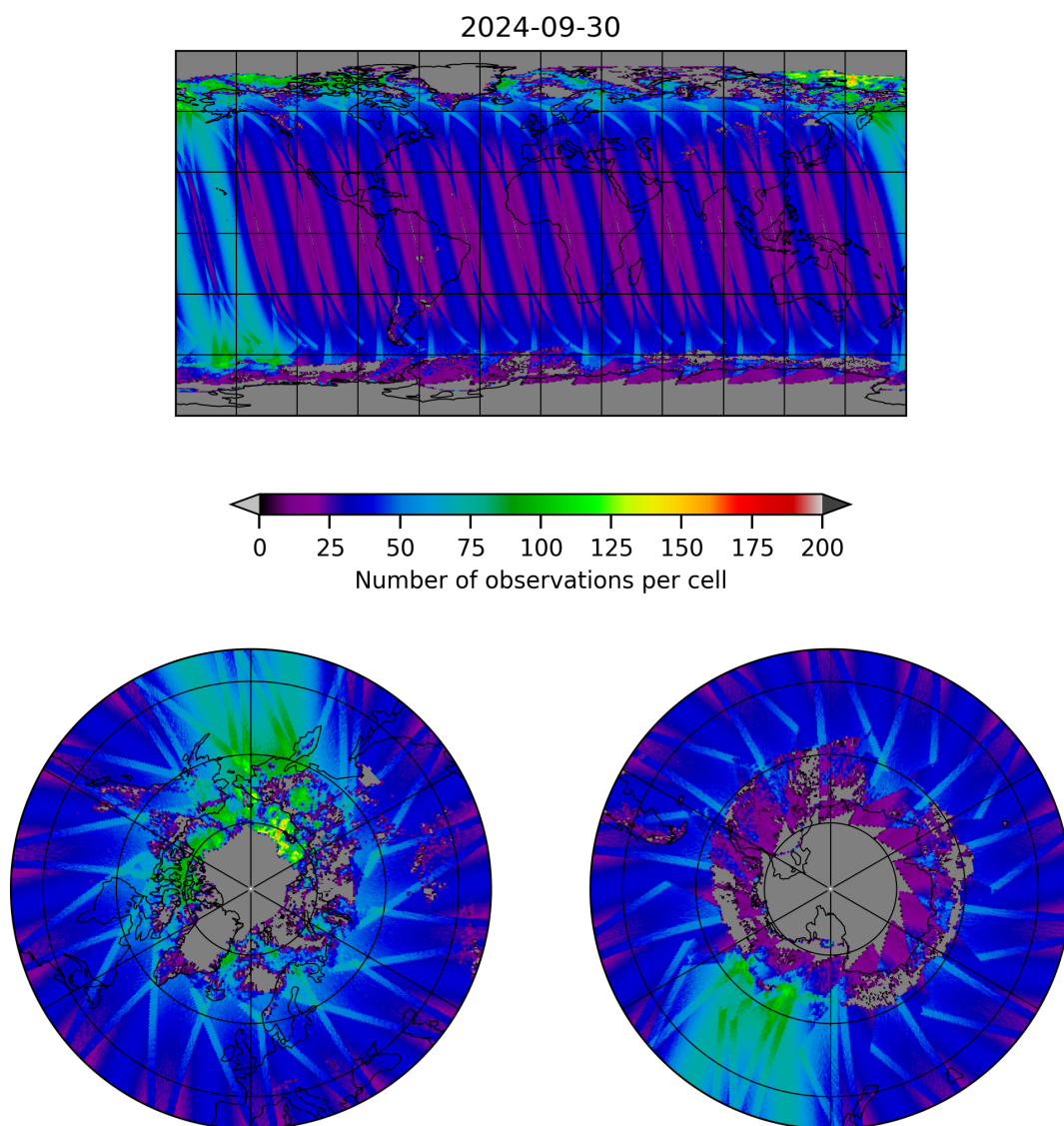
Figure 19: Map of the number of observations for 2024-09-29 to 2024-10-01
