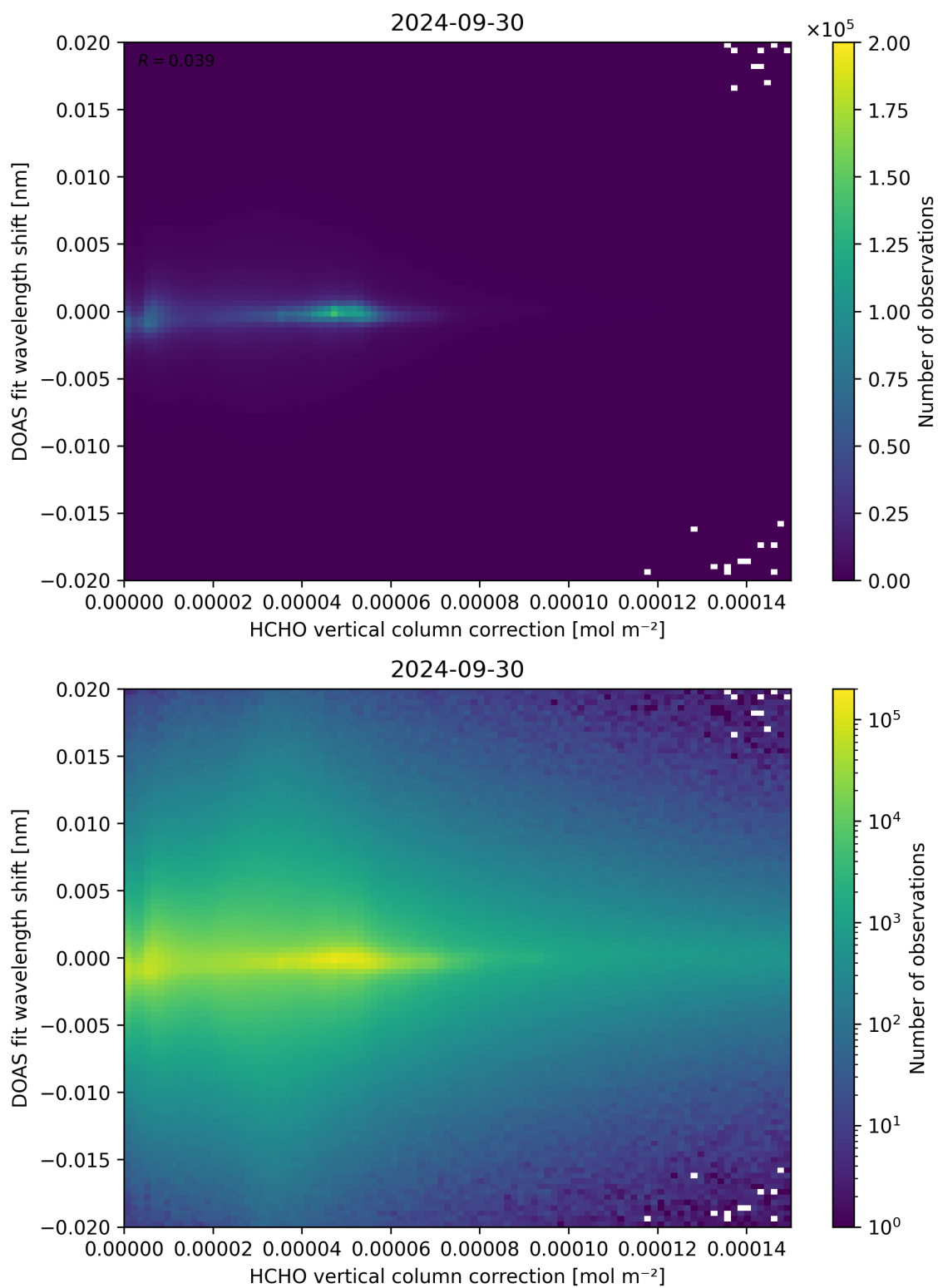
Figure 113: Scatter density plot of “HCHO vertical column correction” against “DOAS fit wavelength shift” for 2024-09-29 to 2024-10-01.
