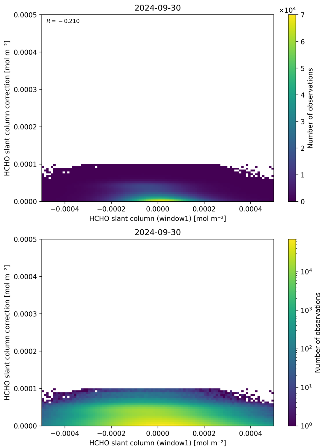
Figure 83: Scatter density plot of “HCHO slant column (window1)” against “HCHO slant column correction” for 2024-09-29 to 2024-10-01.
