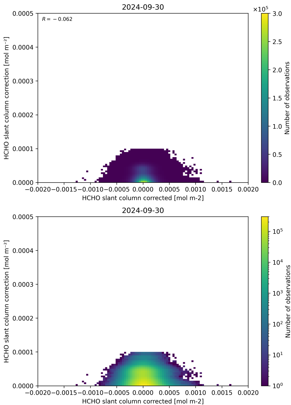
Figure 77: Scatter density plot of “HCHO slant column corrected” against “HCHO slant column correction” for 2024-09-29 to 2024-10-01.
