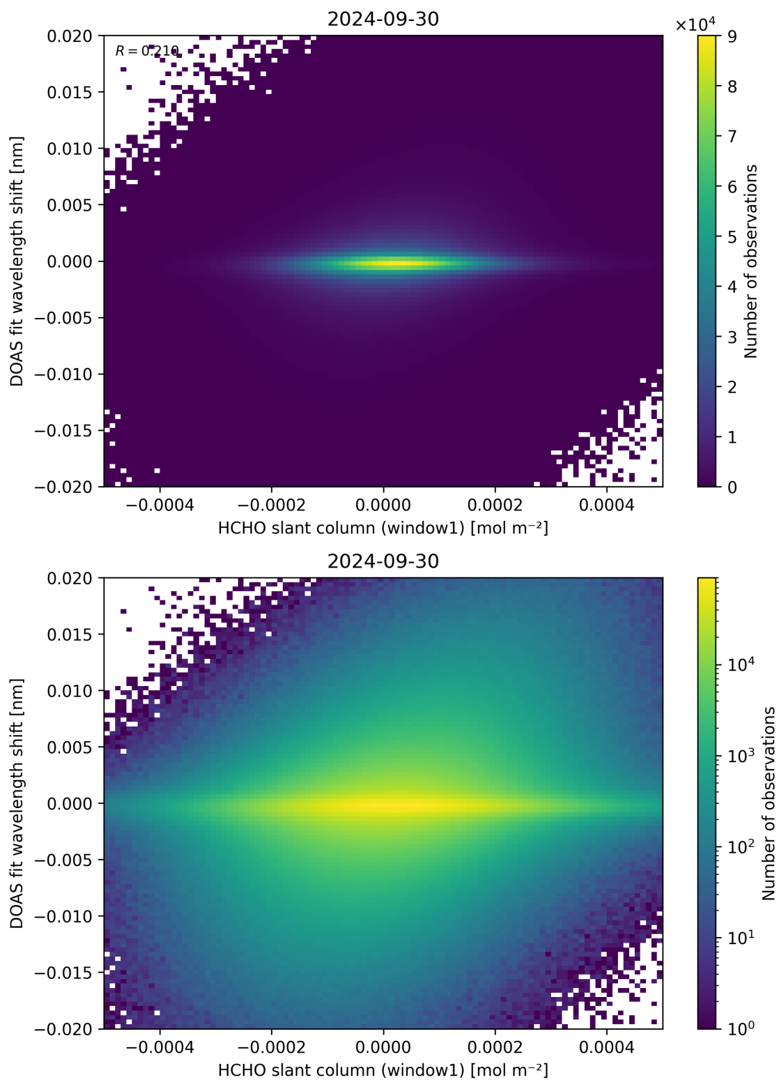
Figure 79: Scatter density plot of “HCHO slant column (window1)” against “DOAS fit wavelength shift” for 2024-09-29 to 2024-10-01.
