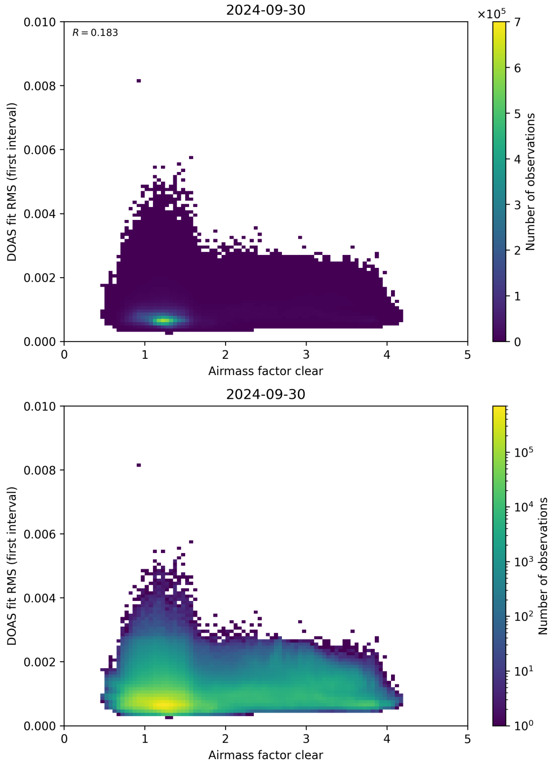
Figure 71: Scatter density plot of “Airmass factor clear” against “DOAS fit RMS (first interval)” for 2024-09-29 to 2024-10-01.
