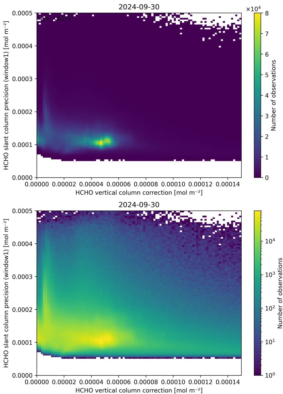
Figure 119: Scatter density plot of “HCHO vertical column correction” against “HCHO slant column precision (window1)” for 2024-09-29 to 2024-10-01.
