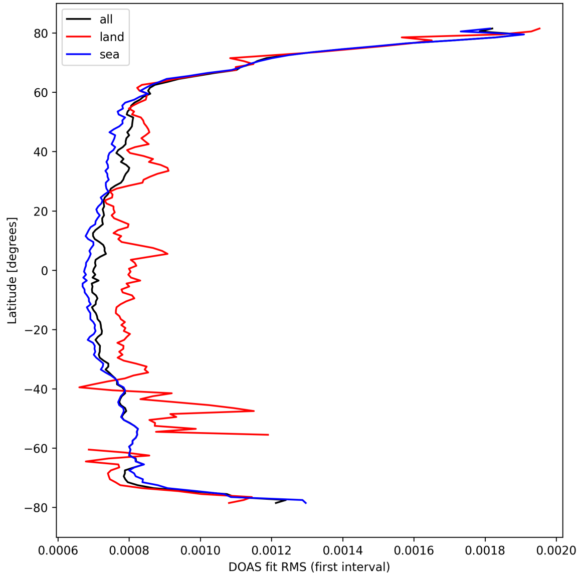
Figure 32: Zonal average of "DOAS fit RMS (first interval)" for 2024-09-29 to 2024-10-01.
