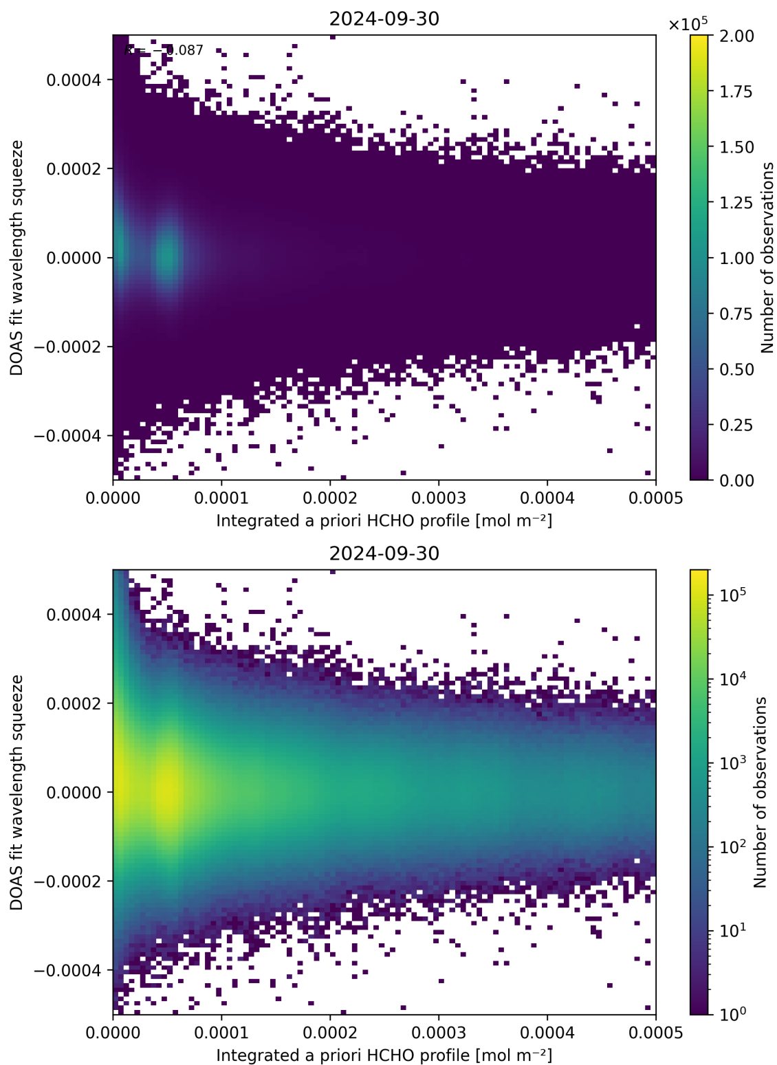
Figure 150: Scatter density plot of “Integrated a priori HCHO profile” against “DOAS fit wavelength squeeze” for 2024-09-29 to 2024-10-01.
