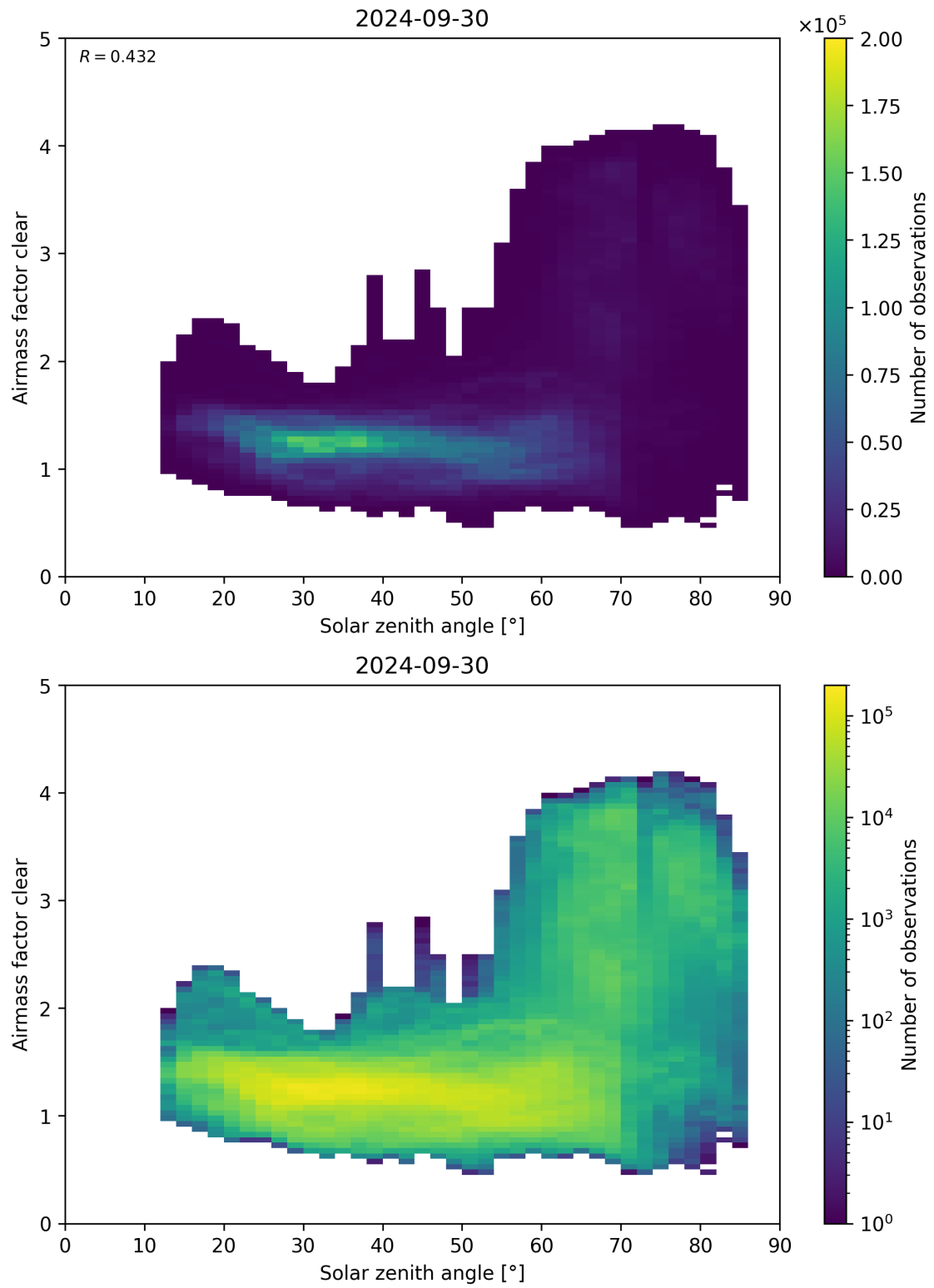
Figure 170: Scatter density plot of “Solar zenith angle” against “Airmass factor clear” for 2024-09-29 to 2024-10-01.
