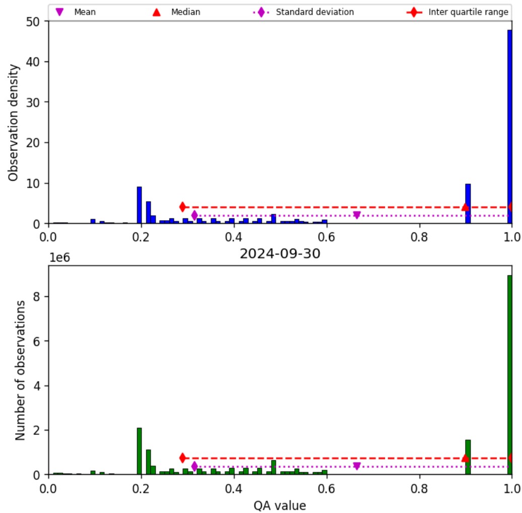
Figure 34: Histogram of “QA value” for 2024-09-29 to 2024-10-01
