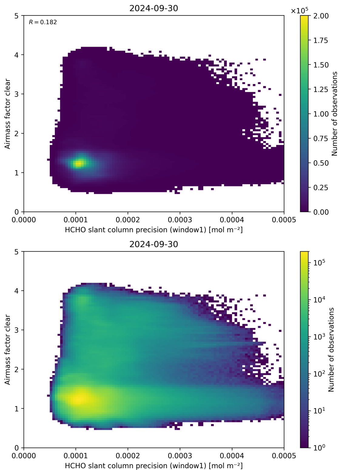
Figure 91: Scatter density plot of “HCHO slant column precision (window1)” against “Airmass factor clear” for 2024-09-29 to 2024-10-01.
