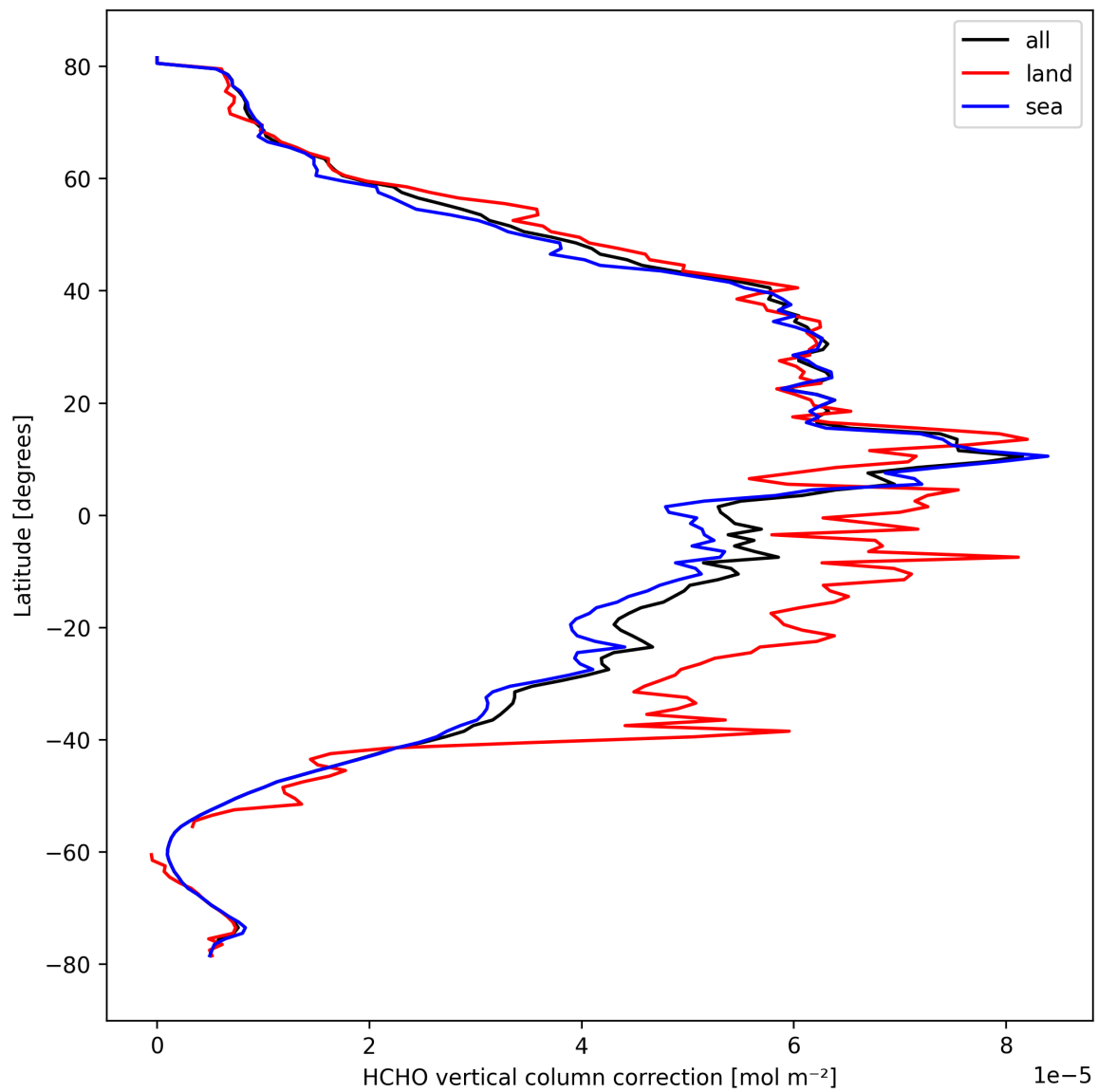
Figure 23: Zonal average of “HCHO vertical column correction” for 2024-09-29 to 2024-10-01.
