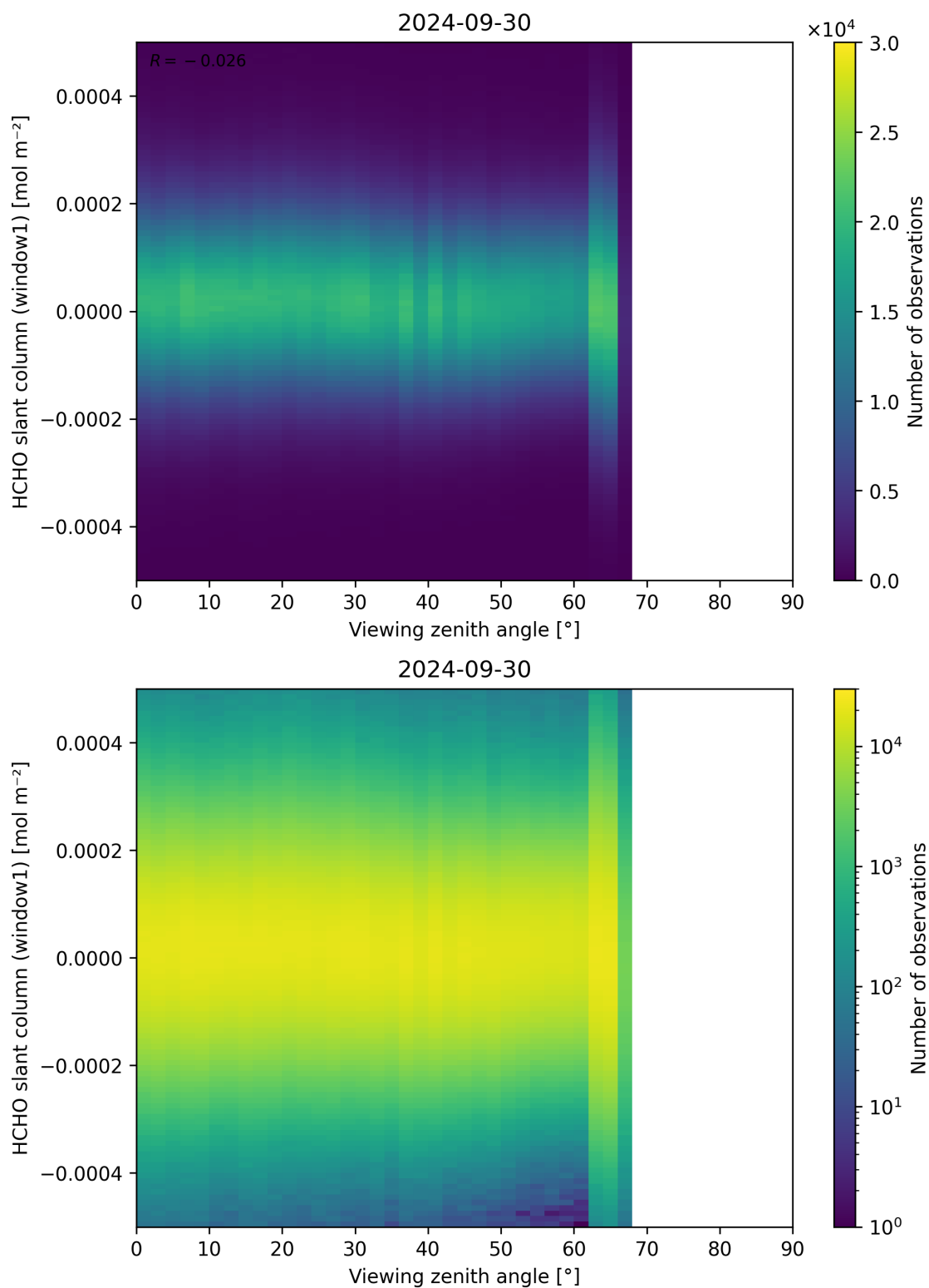
Figure 188: Scatter density plot of “Viewing zenith angle” against “HCHO slant column (window1)” for 2024-09-29 to 2024-10-01.
