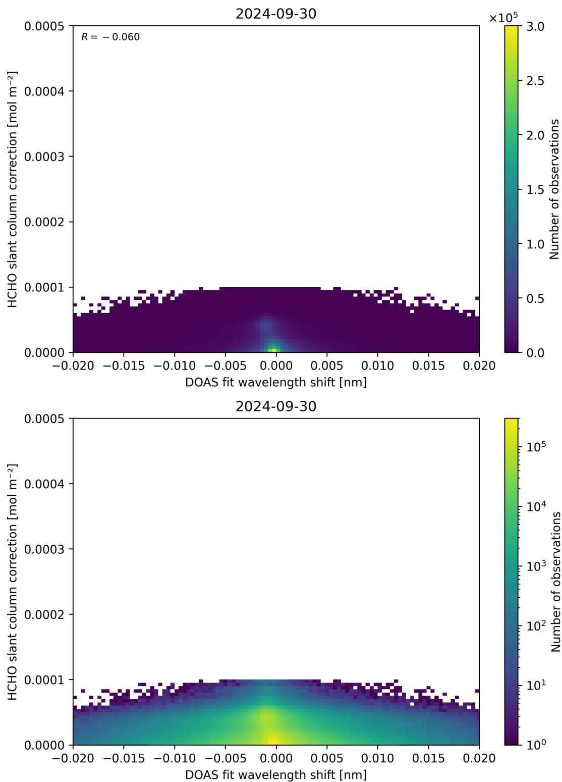
Figure 67: Scatter density plot of “DOAS fit wavelength shift” against “HCHO slant column correction” for 2024-09-29 to 2024-10-01.
