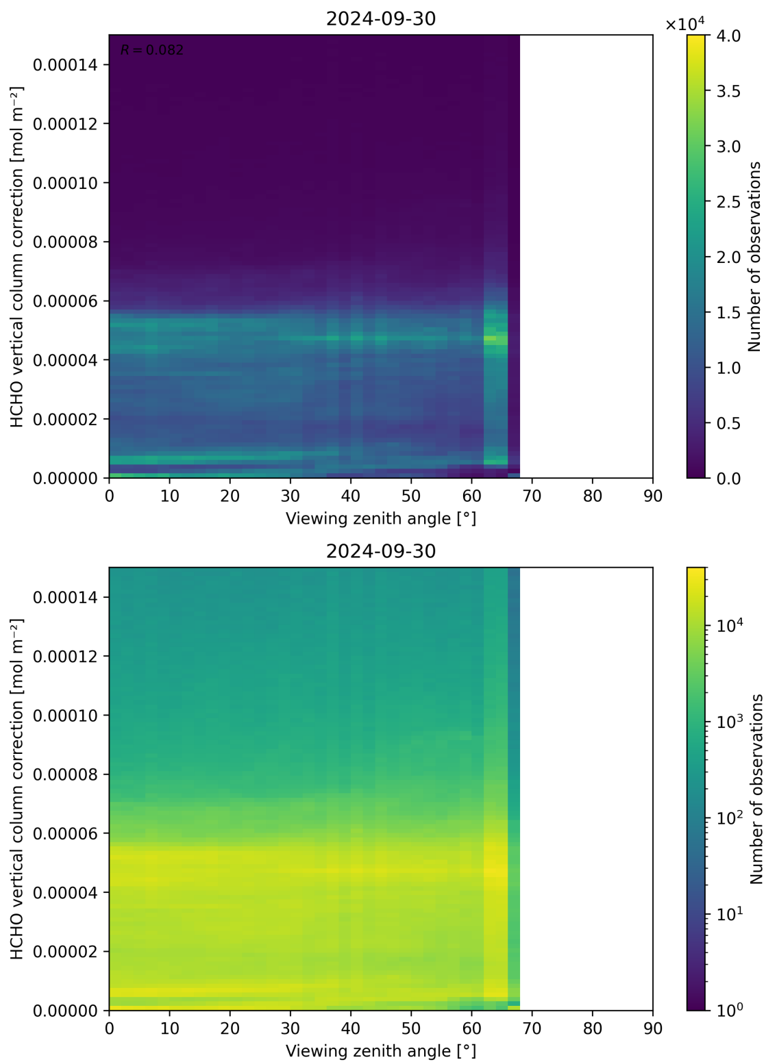
Figure 193: Scatter density plot of “Viewing zenith angle” against “HCHO vertical column correction” for 2024-09-29 to 2024-10-01.
