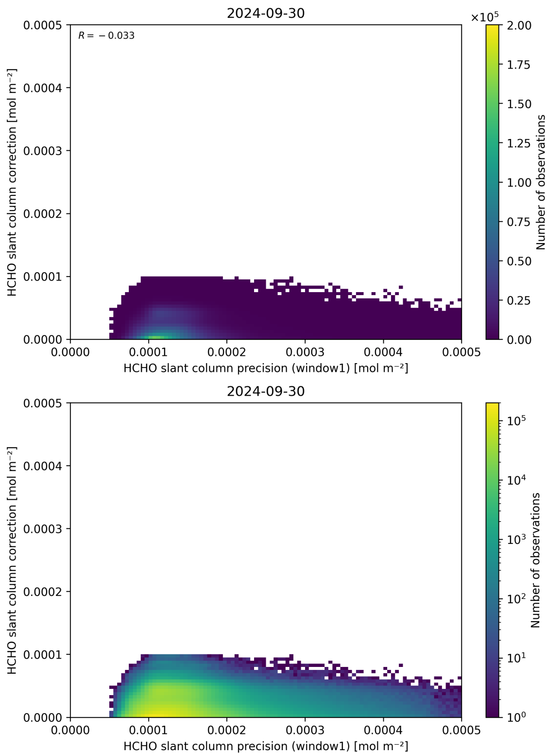
Figure 93: Scatter density plot of “HCHO slant column precision (window1)” against “HCHO slant column correction” for 2024-09-29 to 2024-10-01.
