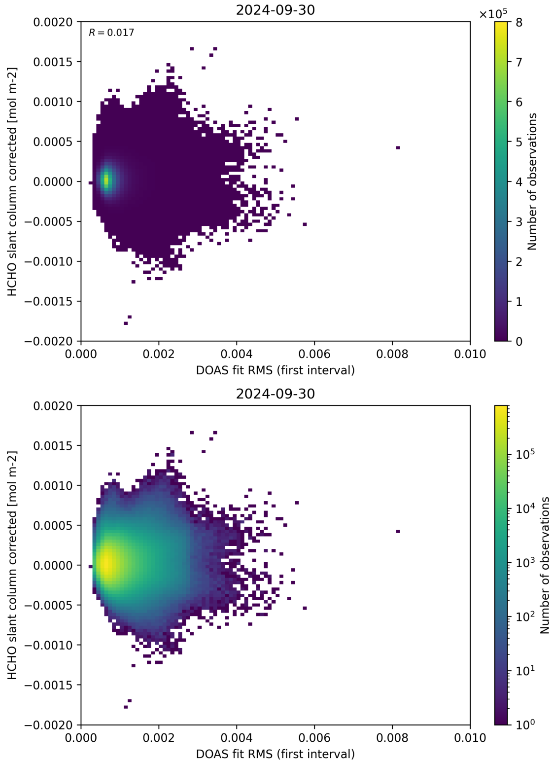
Figure 62: Scatter density plot of “DOAS fit RMS (first interval)” against “HCHO slant column corrected” for 2024-09-29 to 2024-10-01.
