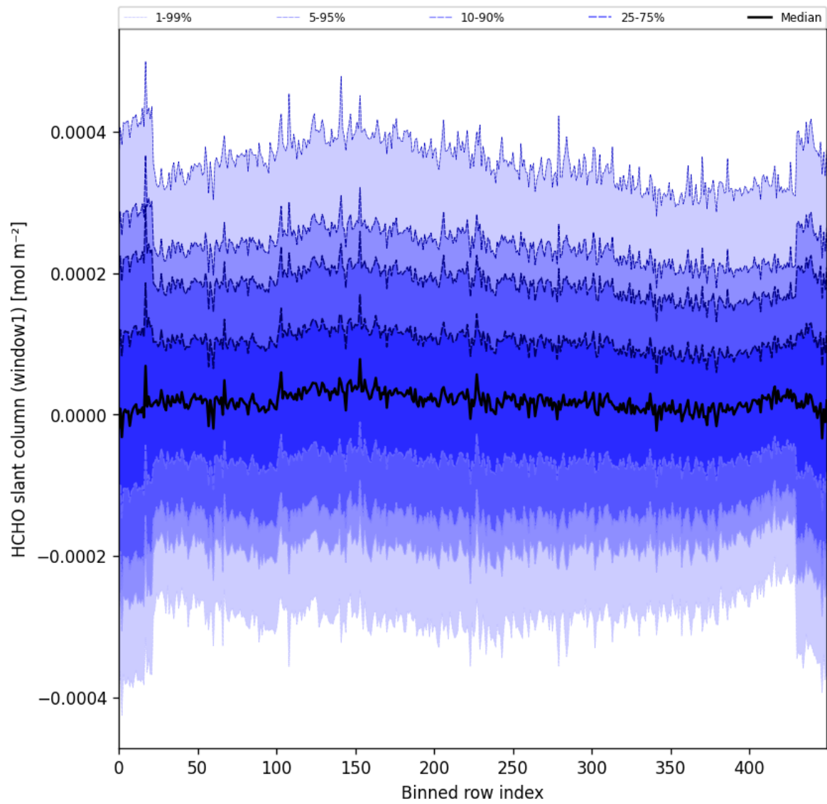
Figure 52: Along track statistics of “HCHO slant column (window1)” for 2024-09-29 to 2024-10-01
