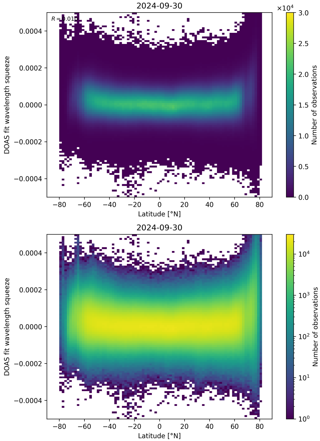
Figure 155: Scatter density plot of “Latitude” against “DOAS fit wavelength squeeze” for 2024-09-29 to 2024-10-01.
