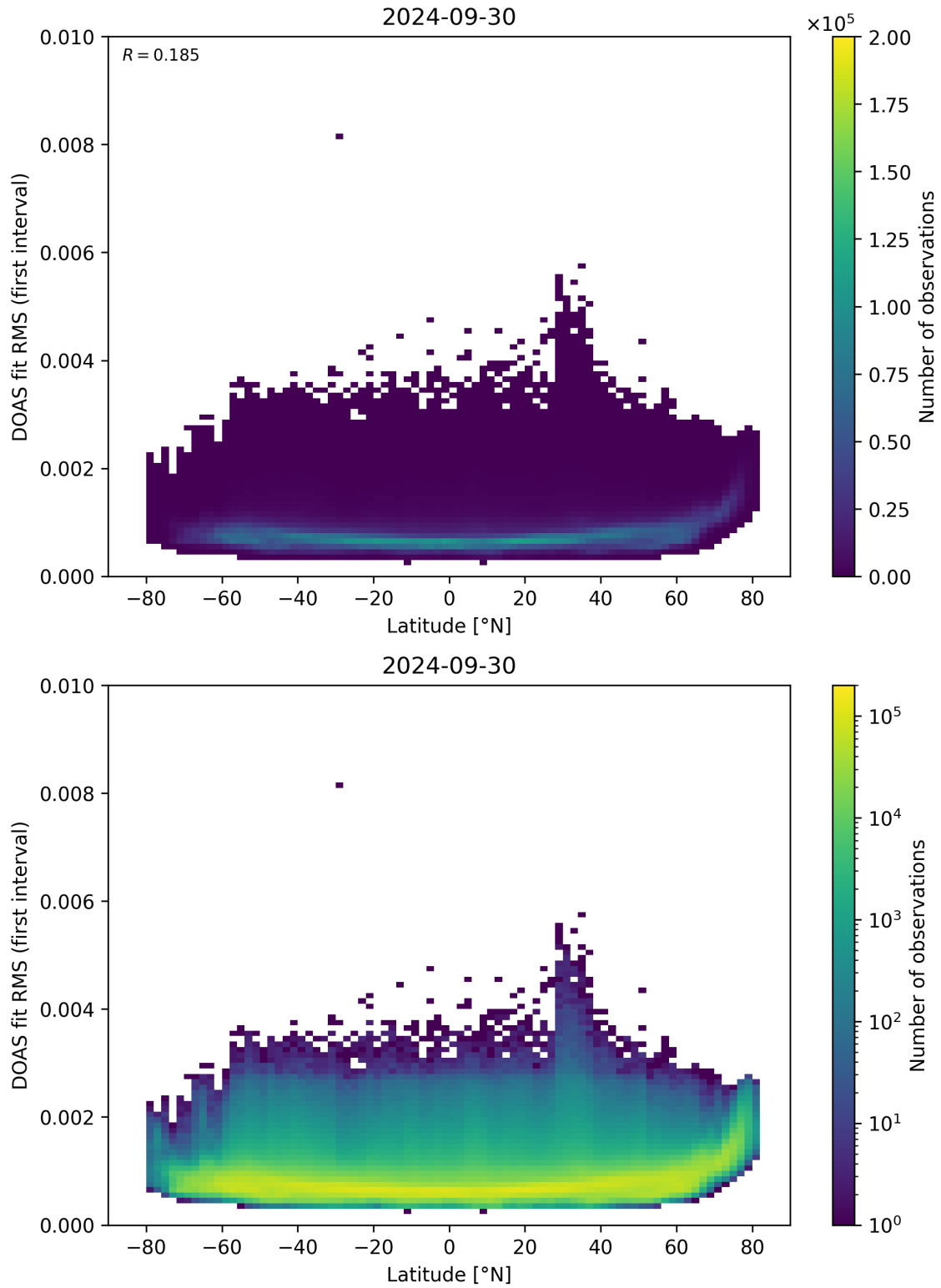
Figure 153: Scatter density plot of “Latitude” against “DOAS fit RMS (first interval)” for 2024-09-29 to 2024-10-01.
