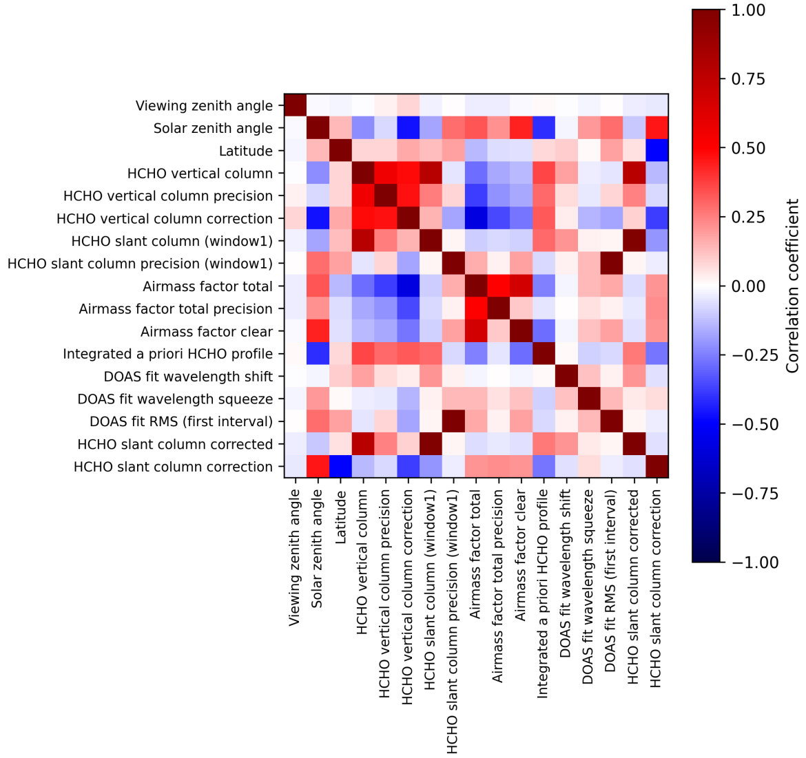
Figure 2: Map of correlation matrix for 2024-09-29 to 2024-10-01.
