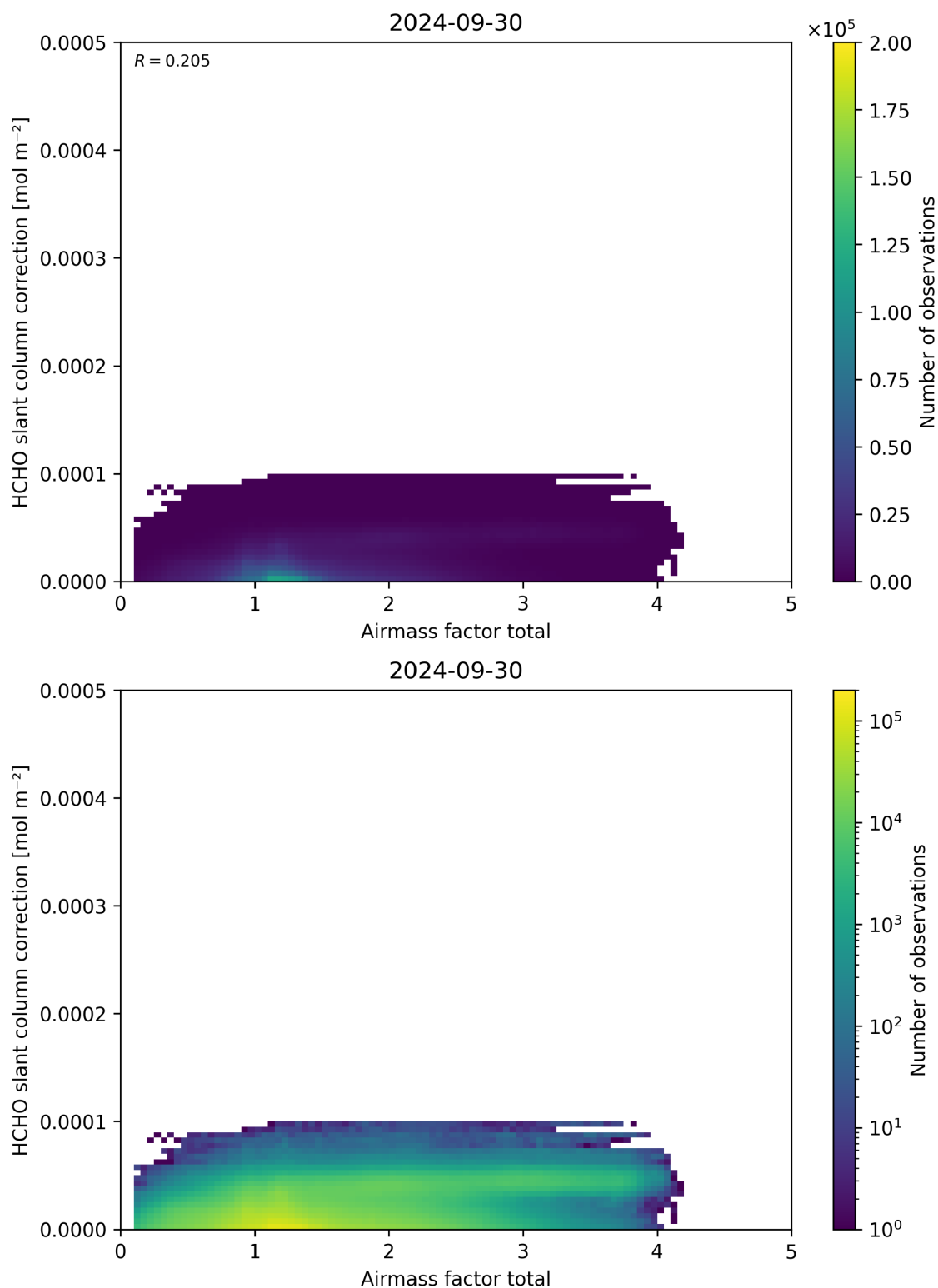
Figure 102: Scatter density plot of “Airmass factor total” against “HCHO slant column correction” for 2024-09-29 to 2024-10-01.
