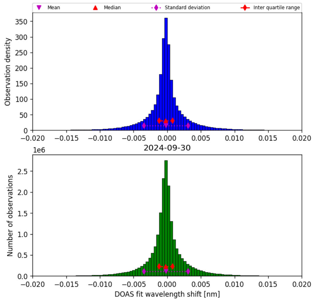
Figure 44: Histogram of “DOAS fit wavelength shift” for 2024-09-29 to 2024-10-01
