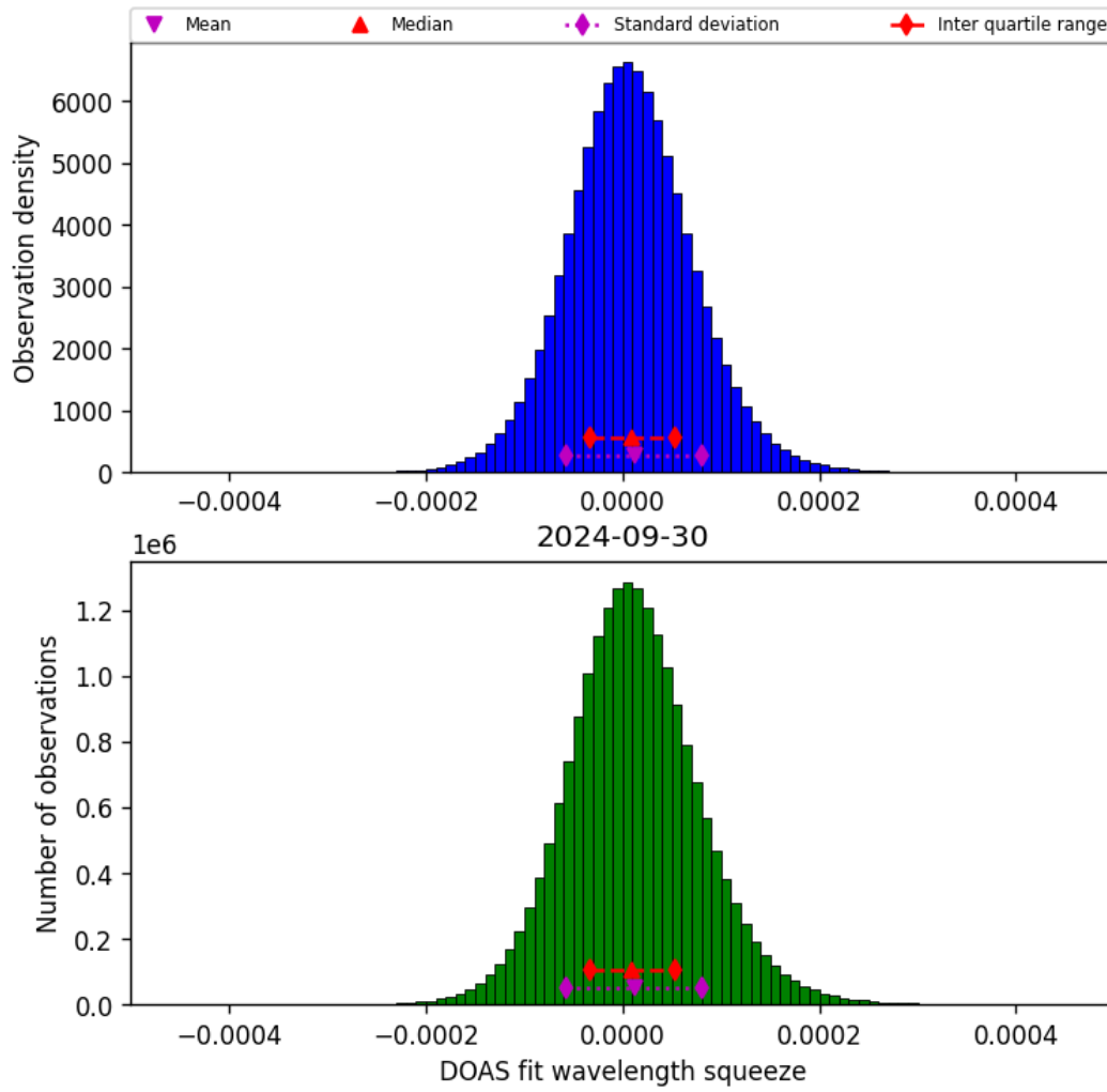
Figure 45: Histogram of “DOAS fit wavelength squeeze” for 2024-09-29 to 2024-10-01
