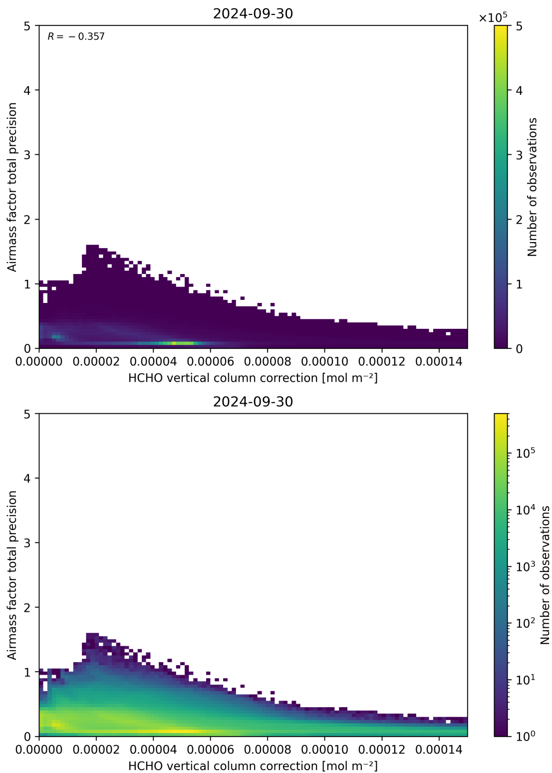
Figure 121: Scatter density plot of “HCHO vertical column correction” against “Airmass factor total precision” for 2024-09-29 to 2024-10-01.
