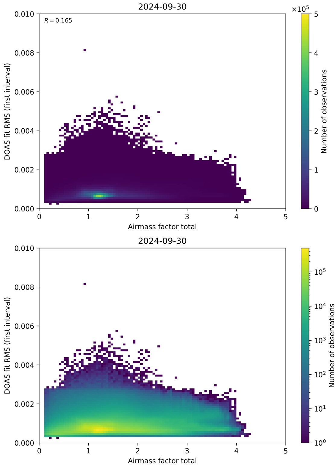
Figure 97: Scatter density plot of “Airmass factor total” against “DOAS fit RMS (first interval)” for 2024-09-29 to 2024-10-01.
