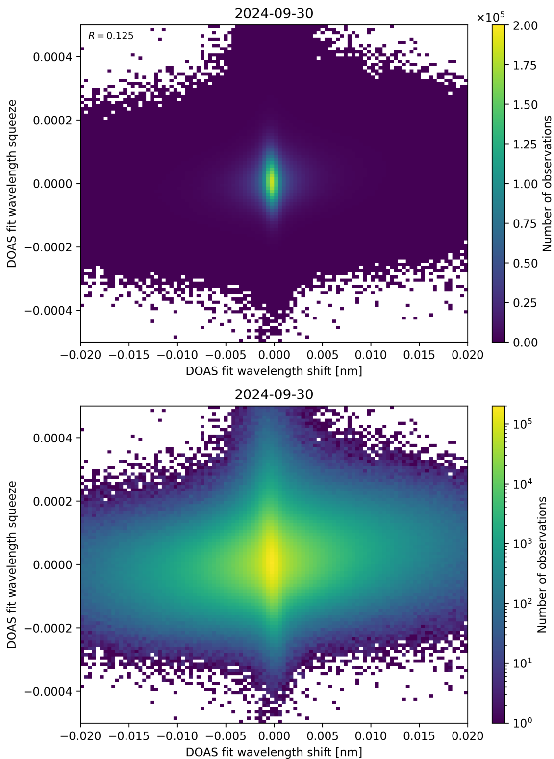
Figure 65: Scatter density plot of “DOAS fit wavelength shift” against “DOAS fit wavelength squeeze” for 2024-09-29 to 2024-10-01.
