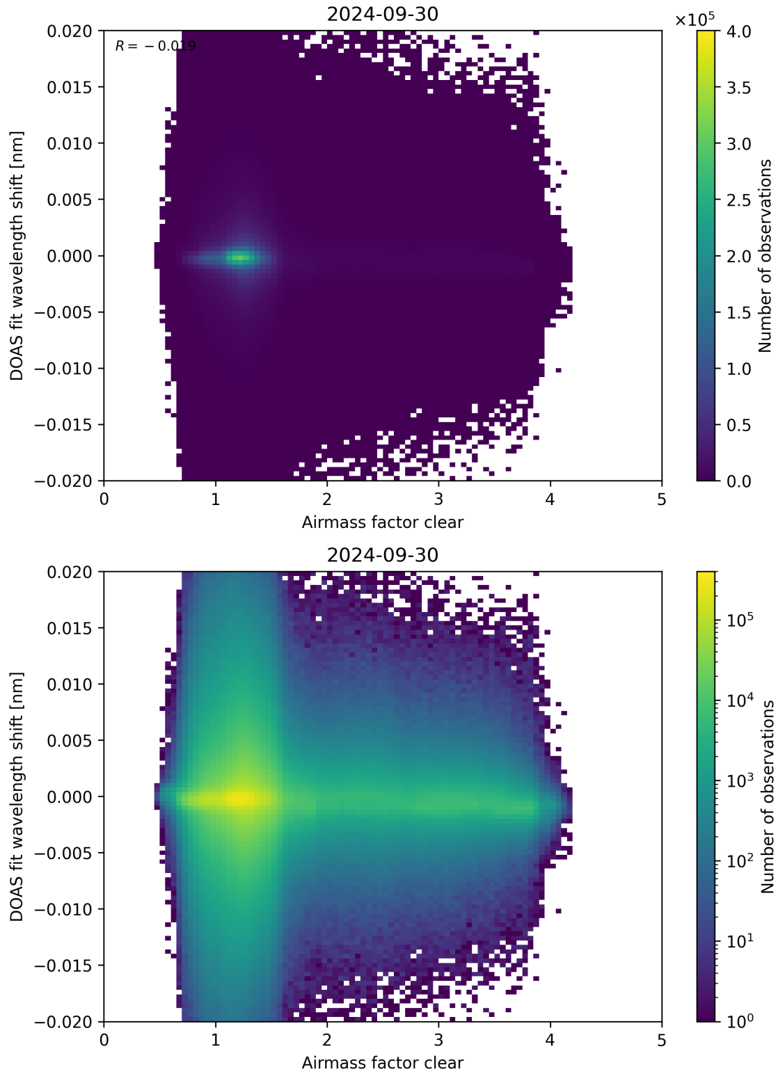
Figure 72: Scatter density plot of “Airmass factor clear” against “DOAS fit wavelength shift” for 2024-09-29 to 2024-10-01.
