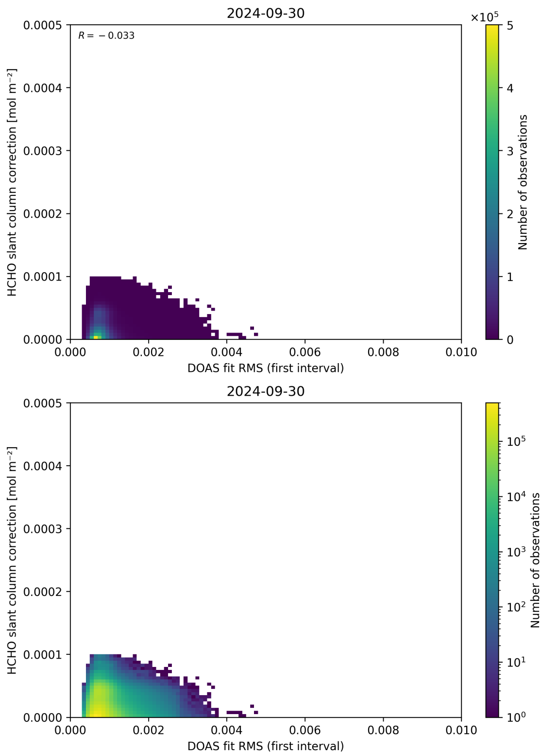
Figure 63: Scatter density plot of “DOAS fit RMS (first interval)” against “HCHO slant column correction” for 2024-09-29 to 2024-10-01.
