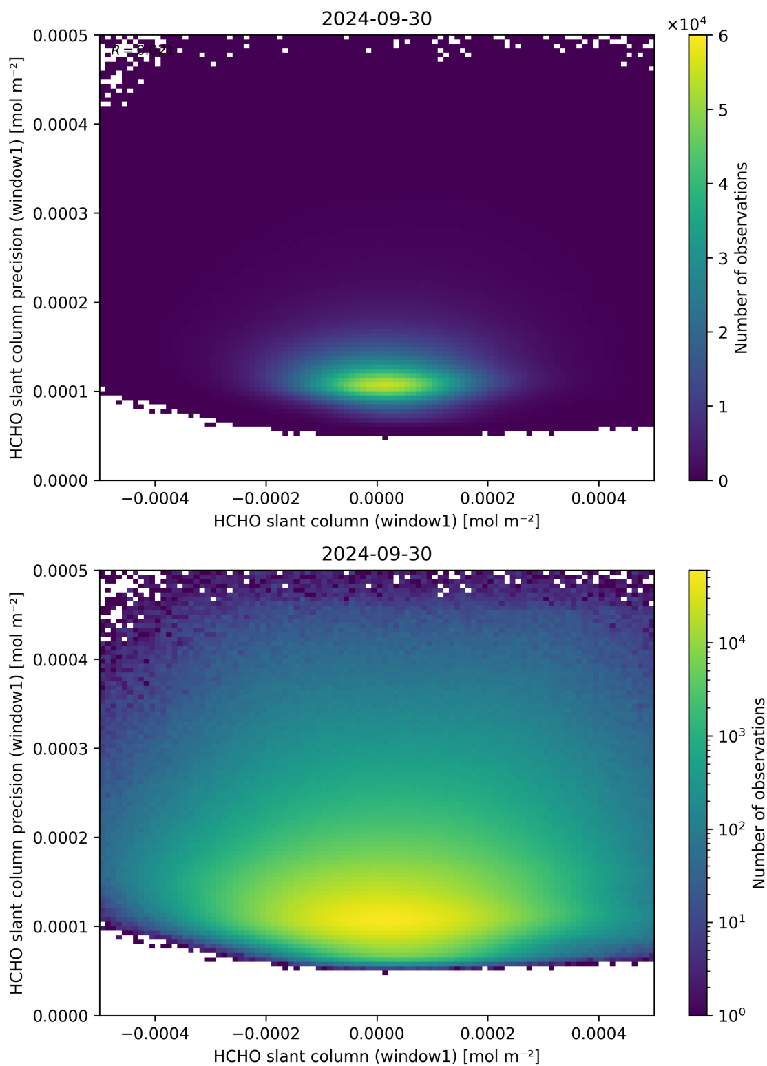
Figure 84: Scatter density plot of “HCHO slant column (window1)” against “HCHO slant column precision (window1)” for 2024-09-29 to 2024-10-01.
