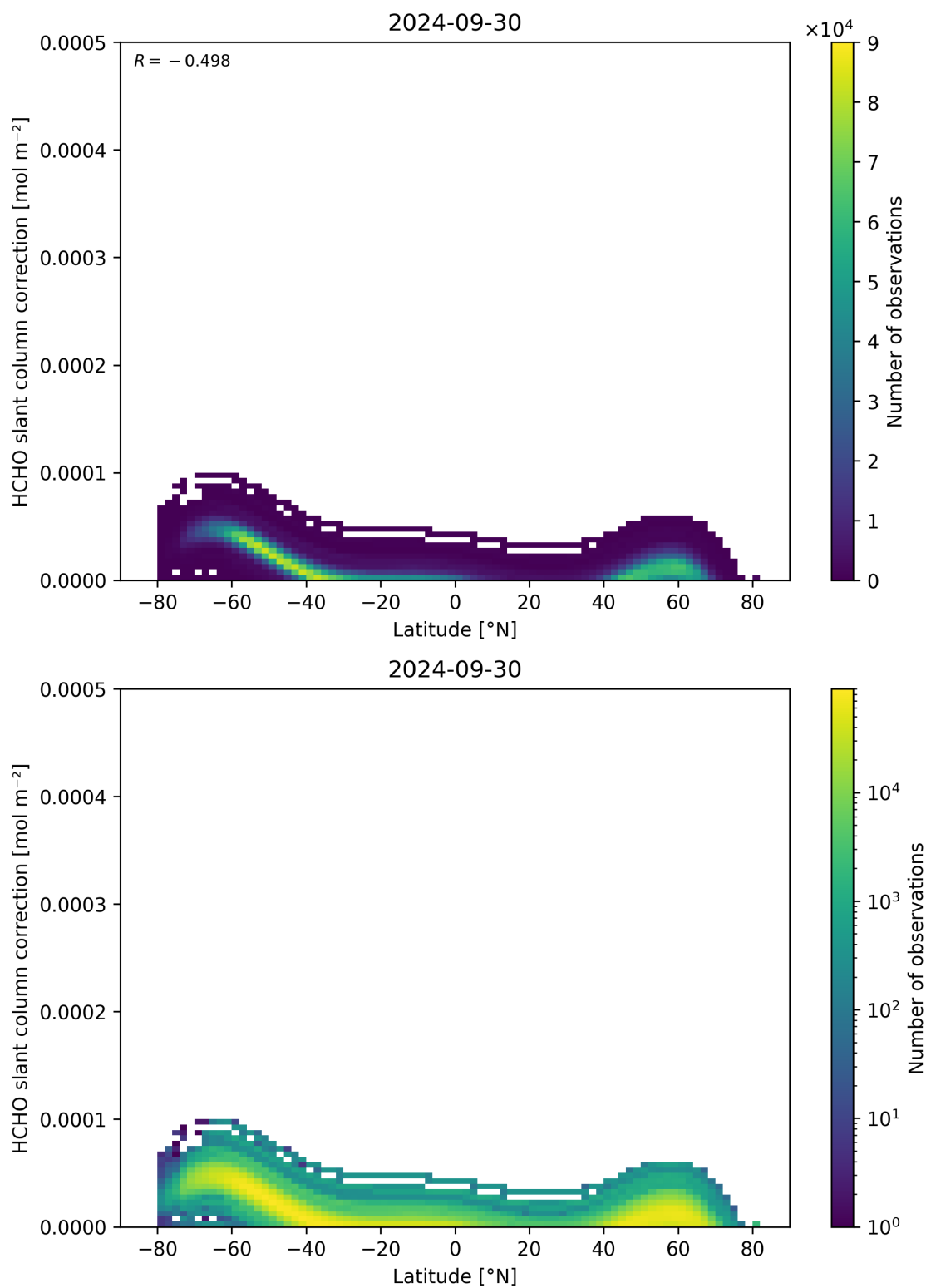
Figure 158: Scatter density plot of “Latitude” against “HCHO slant column correction” for 2024-09-29 to 2024-10-01.
