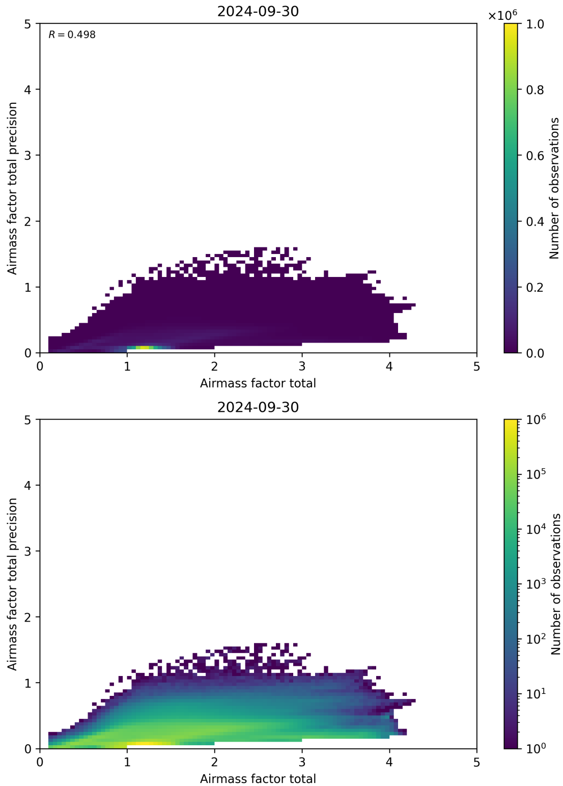
Figure 103: Scatter density plot of “Airmass factor total” against “Airmass factor total precision” for 2024-09-29 to 2024-10-01.
