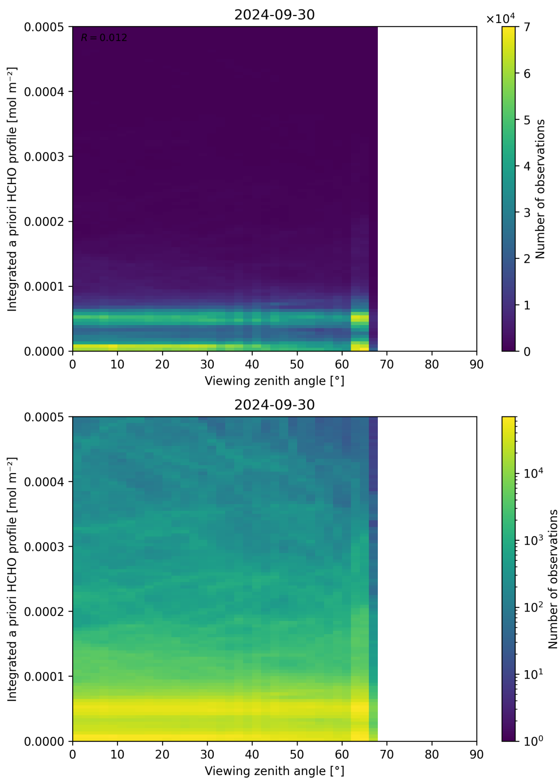
Figure 195: Scatter density plot of “Viewing zenith angle” against “Integrated a priori HCHO profile” for 2024-09-29 to 2024-10-01.
