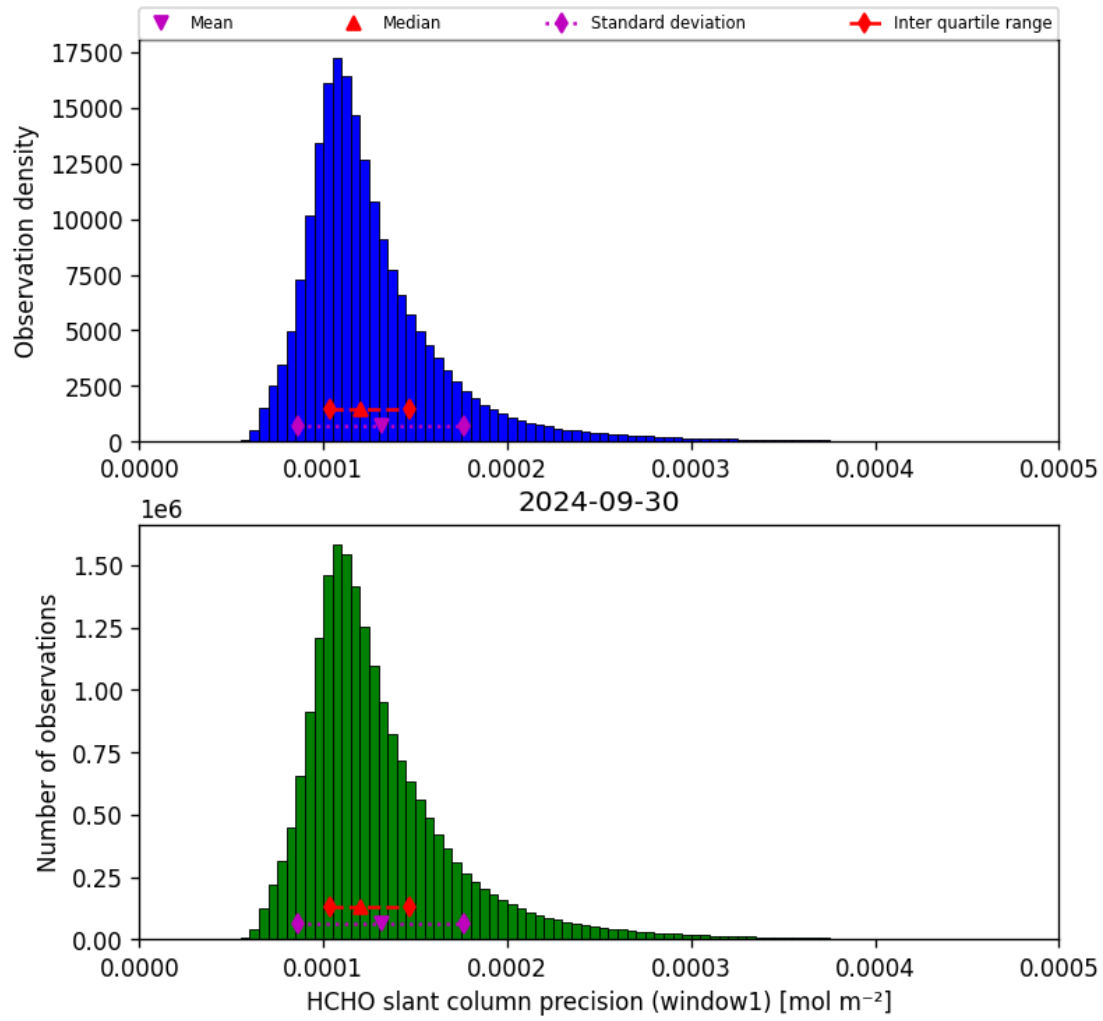
Figure 39: Histogram of “HCHO slant column precision (window1)” for 2024-09-29 to 2024-10-01
