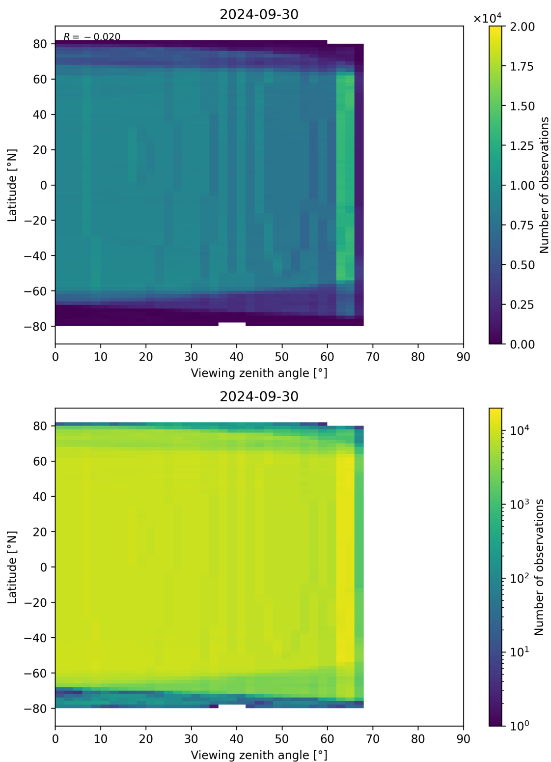
Figure 196: Scatter density plot of “Viewing zenith angle” against “Latitude” for 2024-09-29 to 2024-10-01.
