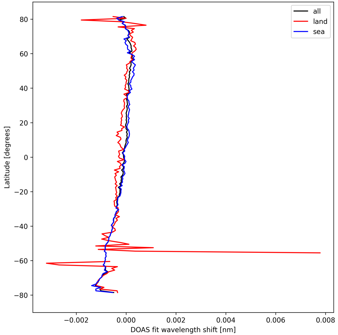
Figure 30: Zonal average of "DOAS fit wavelength shift" for 2024-09-29 to 2024-10-01.
