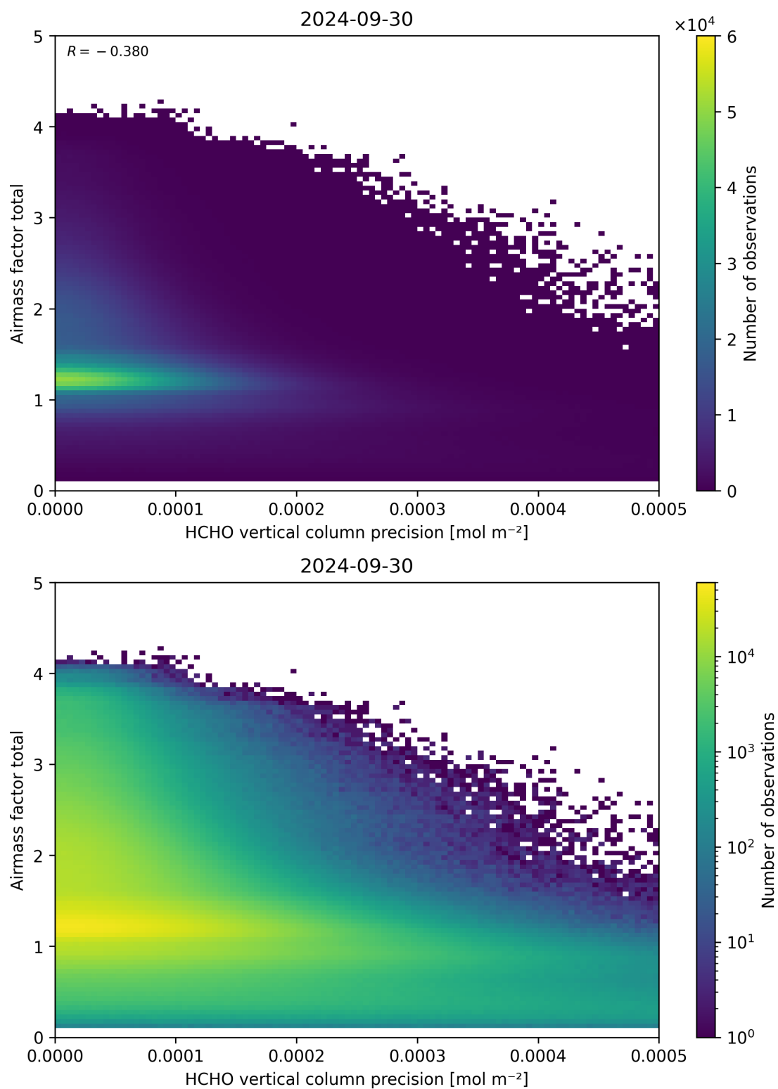
Figure 144: Scatter density plot of “HCHO vertical column precision” against “Airmass factor total” for 2024-09-29 to 2024-10-01.
