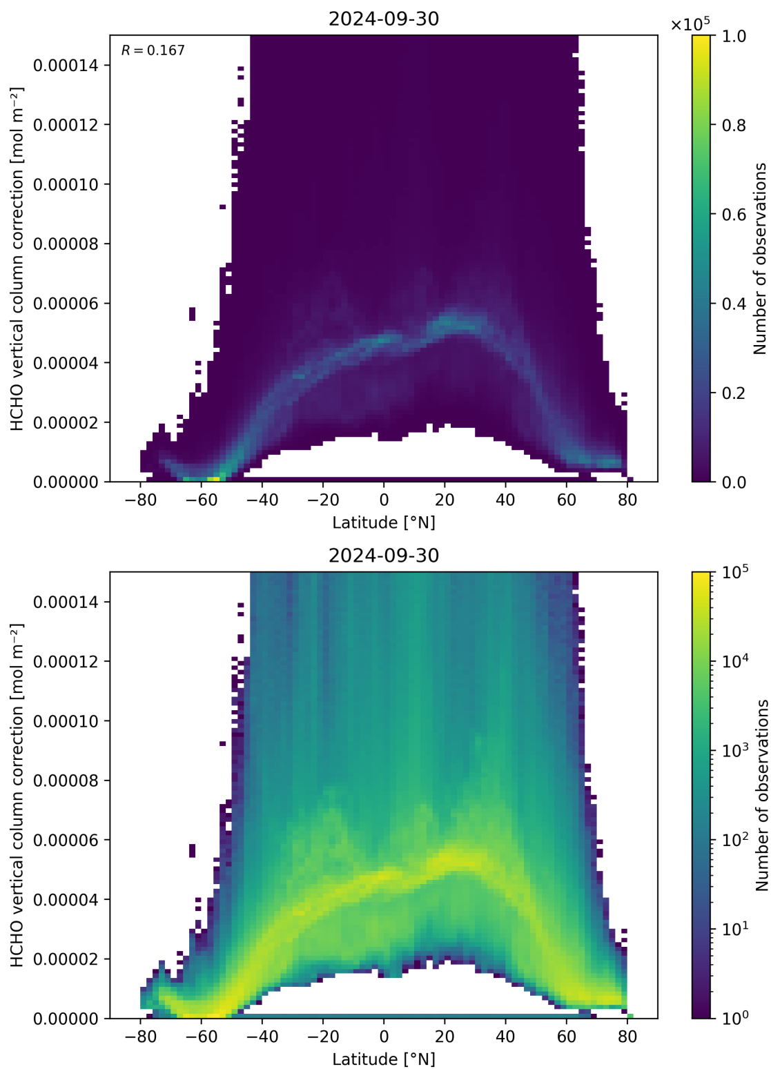
Figure 164: Scatter density plot of “Latitude” against “HCHO vertical column correction” for 2024-09-29 to 2024-10-01.
