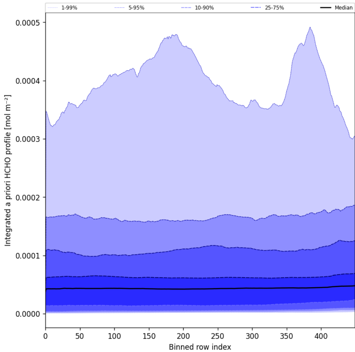
Figure 57: Along track statistics of “Integrated a priori HCHO profile” for 2024-09-29 to 2024-10-01
