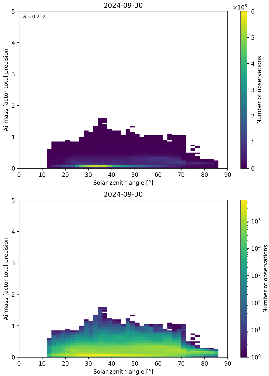
Figure 176: Scatter density plot of “Solar zenith angle” against “Airmass factor total precision” for 2024-09-29 to 2024-10-01.
