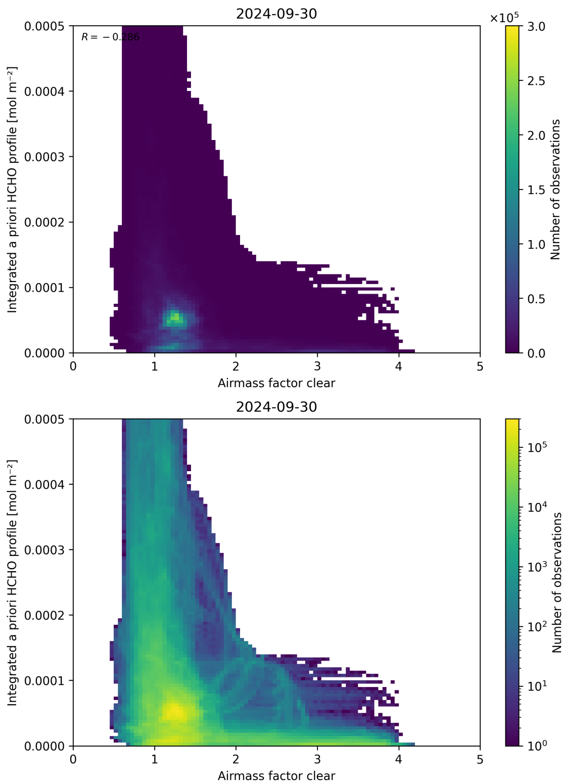
Figure 76: Scatter density plot of “Airmass factor clear” against “Integrated a priori HCHO profile” for 2024-09-29 to 2024-10-01.
