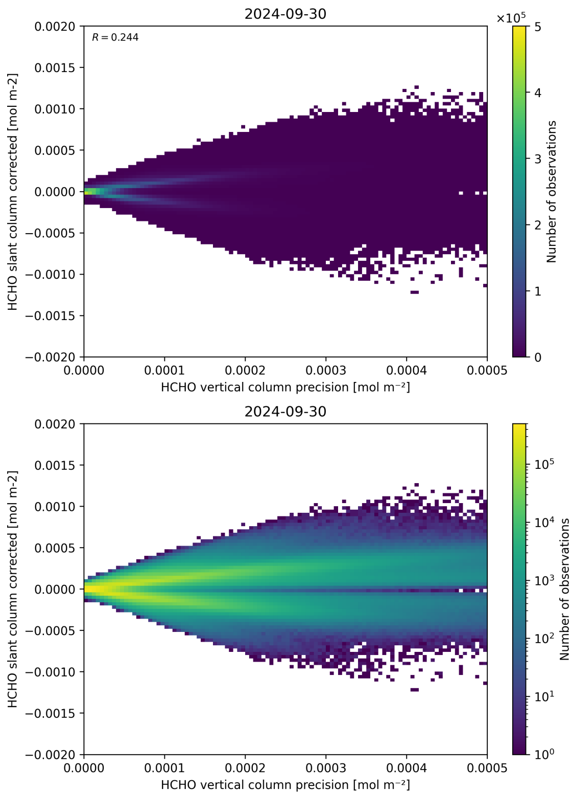
Figure 140: Scatter density plot of “HCHO vertical column precision” against “HCHO slant column corrected” for 2024-09-29 to 2024-10-01.
