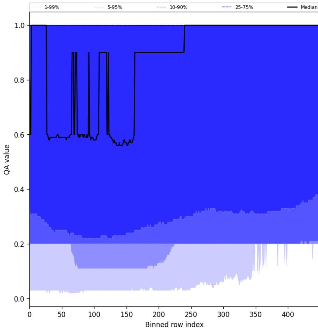
Figure 48: Along track statistics of “QA value” for 2024-09-29 to 2024-10-01
