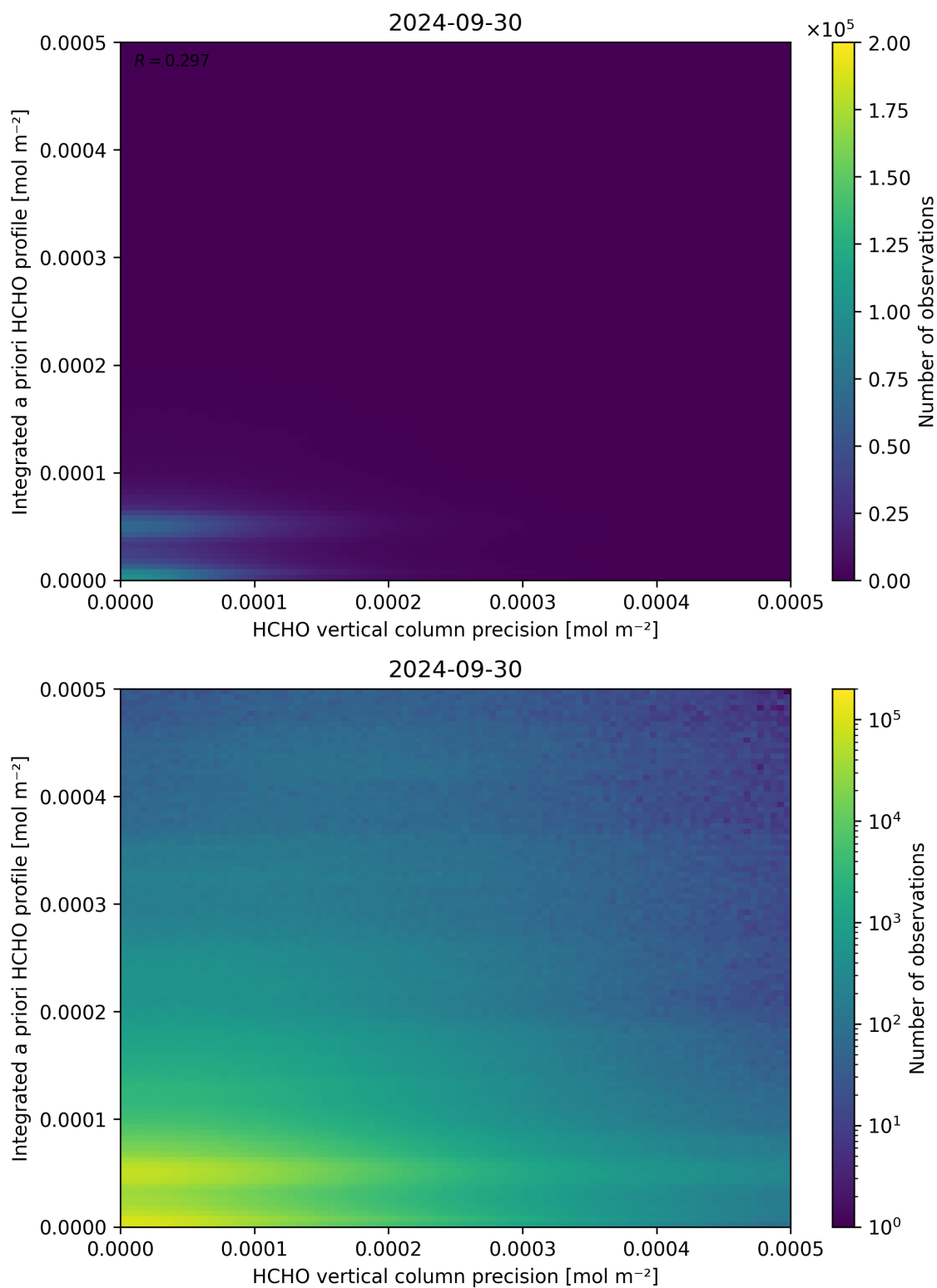
Figure 147: Scatter density plot of “HCHO vertical column precision” against “Integrated a priori HCHO profile” for 2024-09-29 to 2024-10-01.
