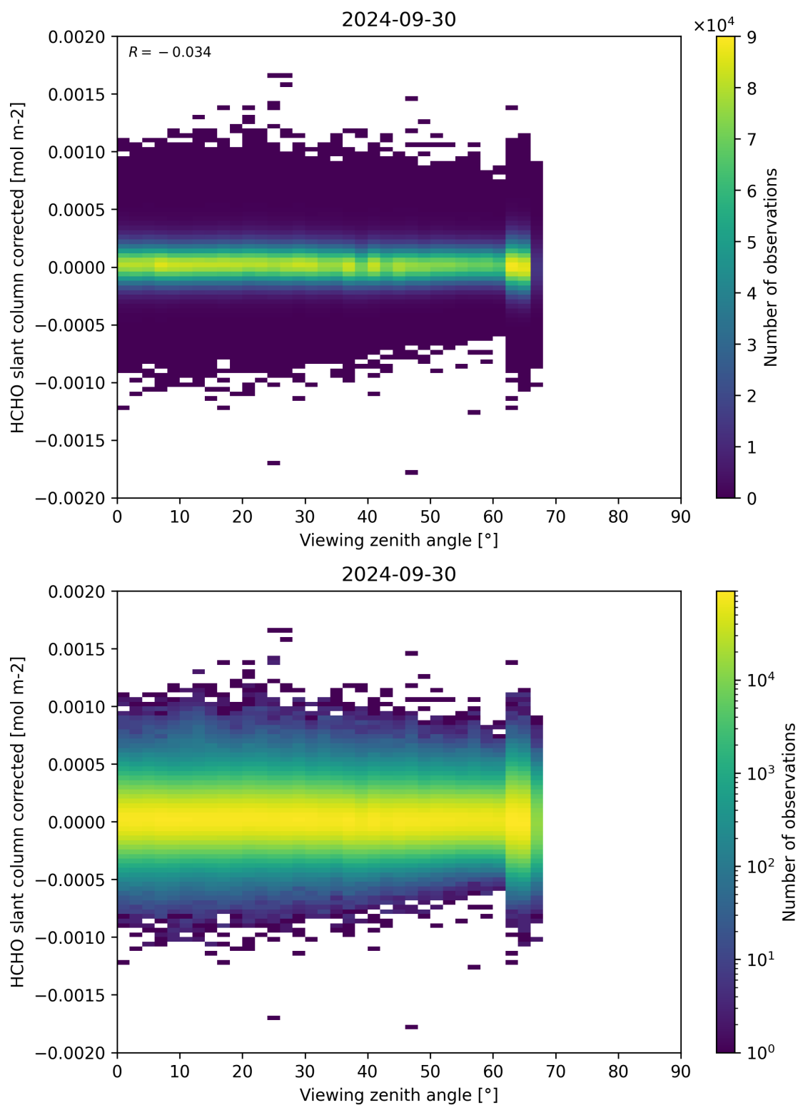
Figure 186: Scatter density plot of “Viewing zenith angle” against “HCHO slant column corrected” for 2024-09-29 to 2024-10-01.
