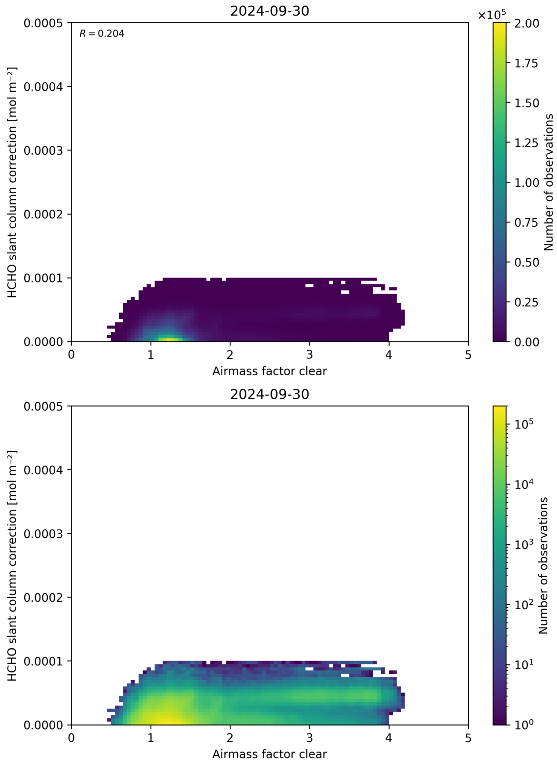
Figure 75: Scatter density plot of “Airmass factor clear” against “HCHO slant column correction” for 2024-09-29 to 2024-10-01.
