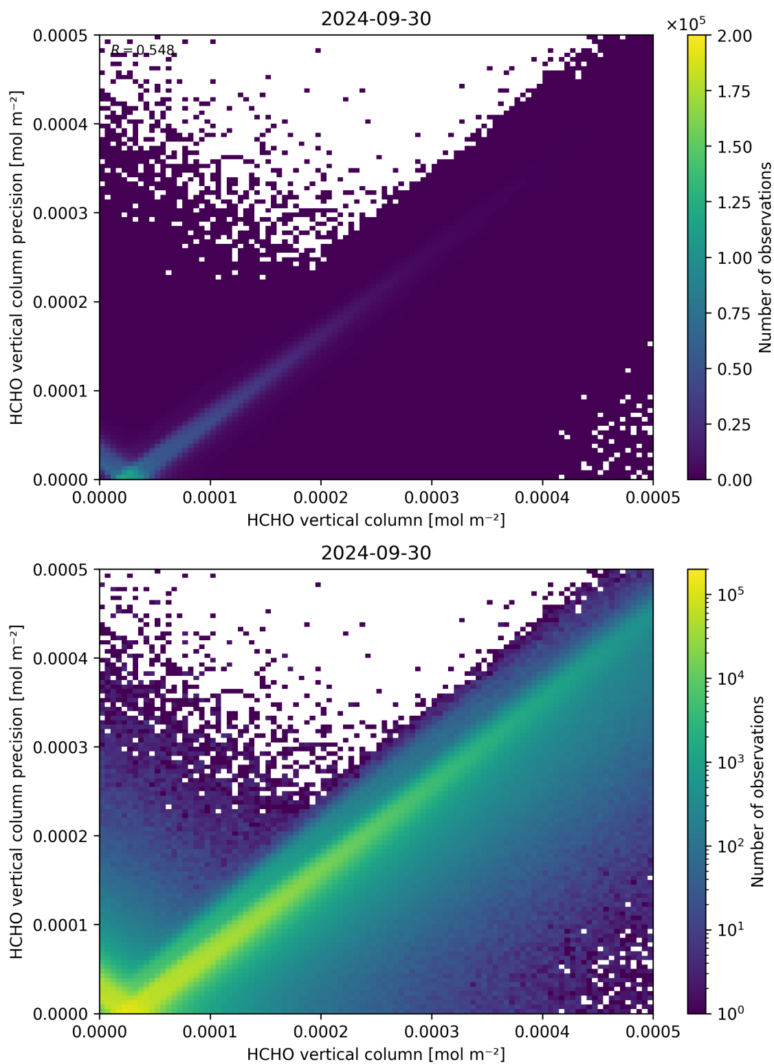
Figure 134: Scatter density plot of “HCHO vertical column” against “HCHO vertical column precision” for 2024-09-29 to 2024-10-01.
