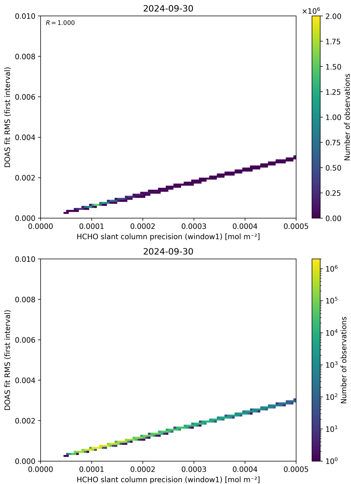
Figure 88: Scatter density plot of “HCHO slant column precision (window1)” against “DOAS fit RMS (first interval)” for 2024-09-29 to 2024-10-01.
