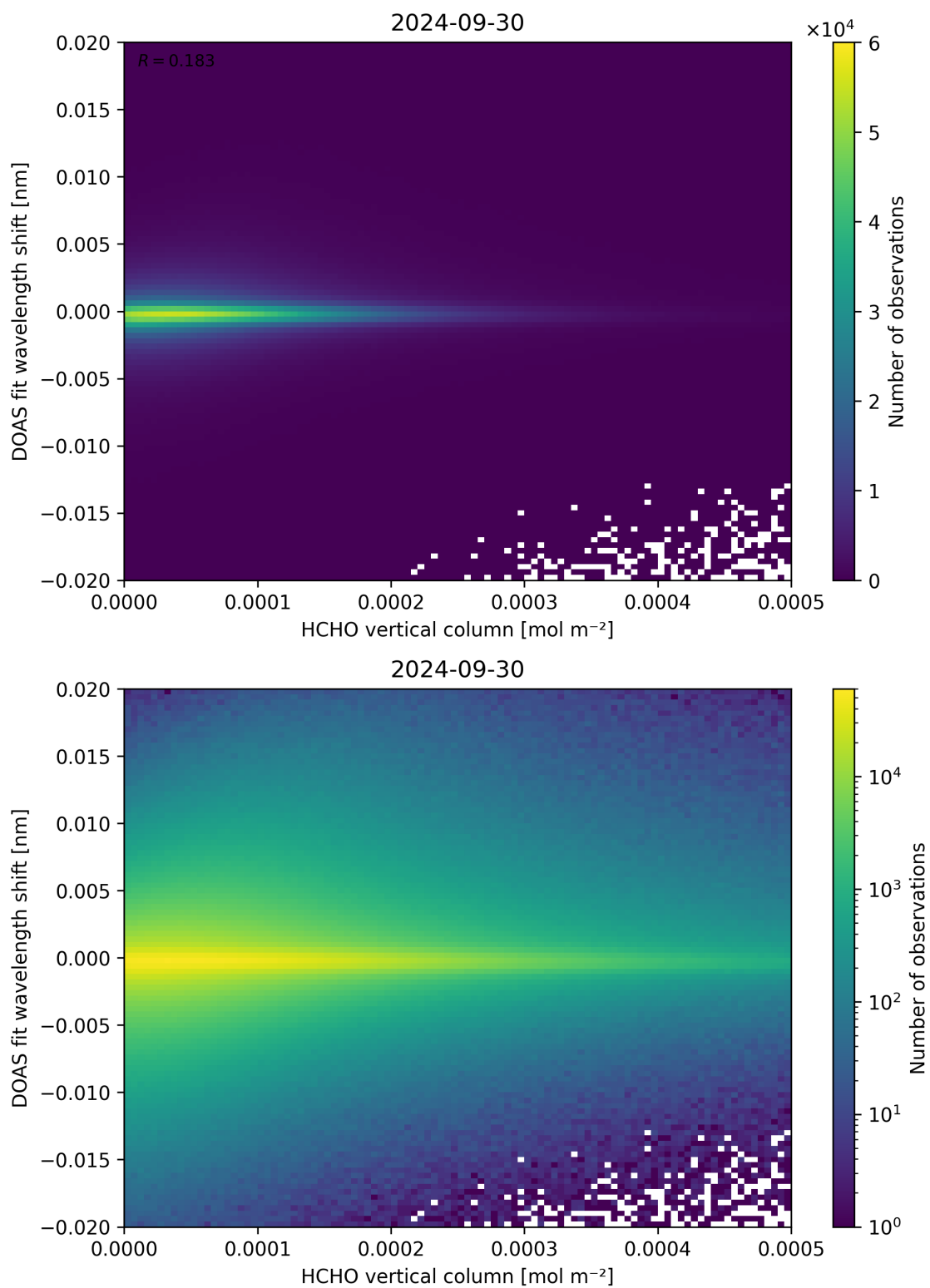
Figure 124: Scatter density plot of “HCHO vertical column” against “DOAS fit wavelength shift” for 2024-09-29 to 2024-10-01.
