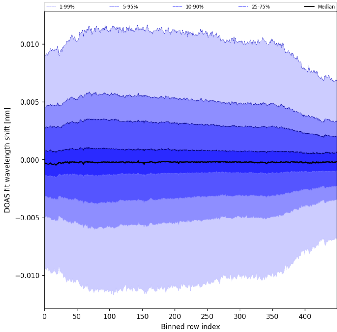
Figure 58: Along track statistics of “DOAS fit wavelength shift” for 2024-09-29 to 2024-10-01
