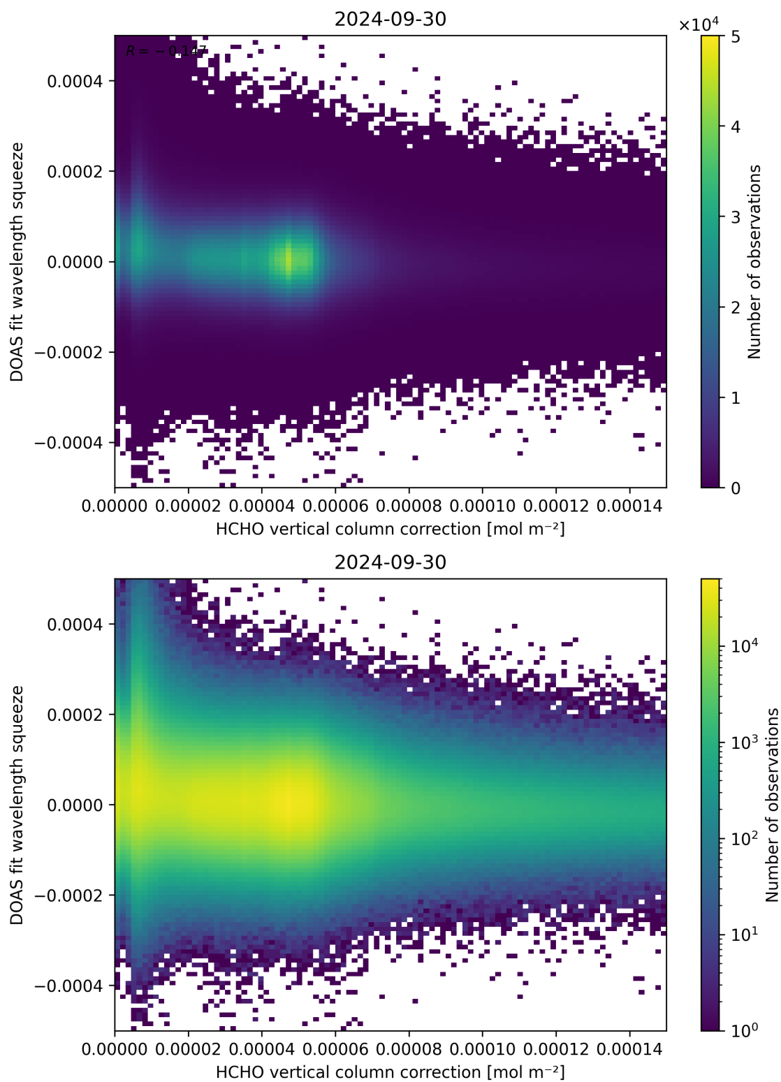
Figure 114: Scatter density plot of “HCHO vertical column correction” against “DOAS fit wavelength squeeze” for 2024-09-29 to 2024-10-01.
