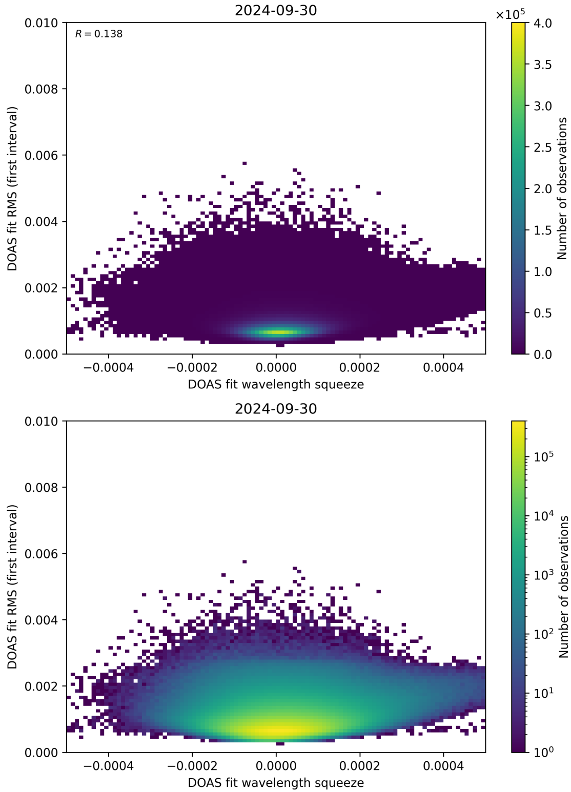
Figure 68: Scatter density plot of “DOAS fit wavelength squeeze” against “DOAS fit RMS (first interval)” for 2024-09-29 to 2024-10-01.
