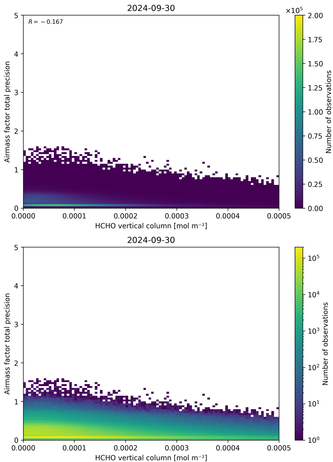
Figure 132: Scatter density plot of “HCHO vertical column” against “Airmass factor total precision” for 2024-09-29 to 2024-10-01.
