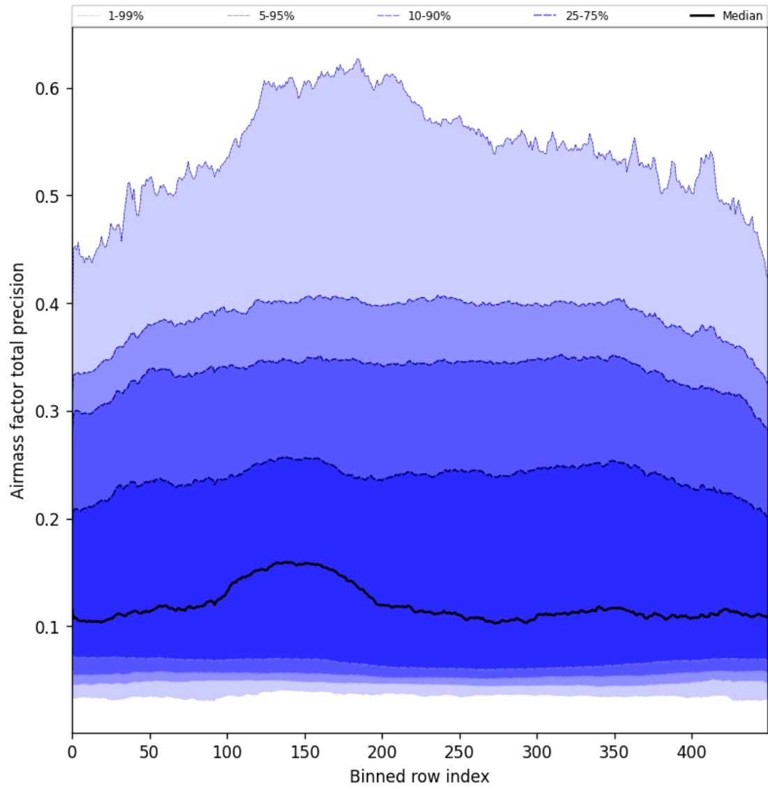
Figure 55: Along track statistics of “Airmass factor total precision” for 2024-09-29 to 2024-10-01
