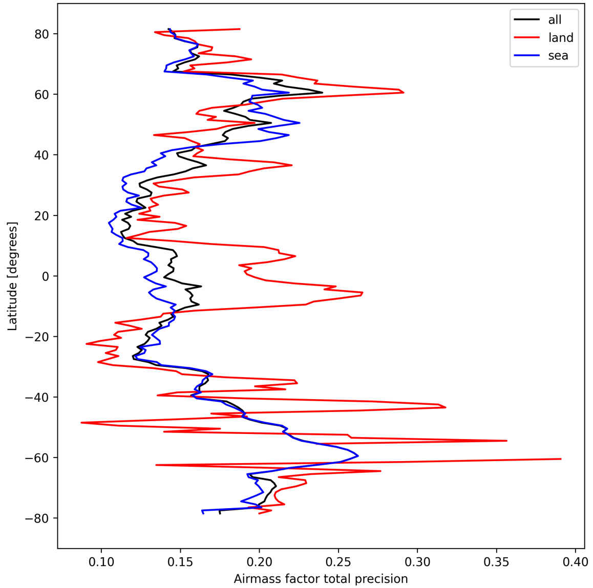
Figure 27: Zonal average of “Airmass factor total precision” for 2024-09-29 to 2024-10-01.
