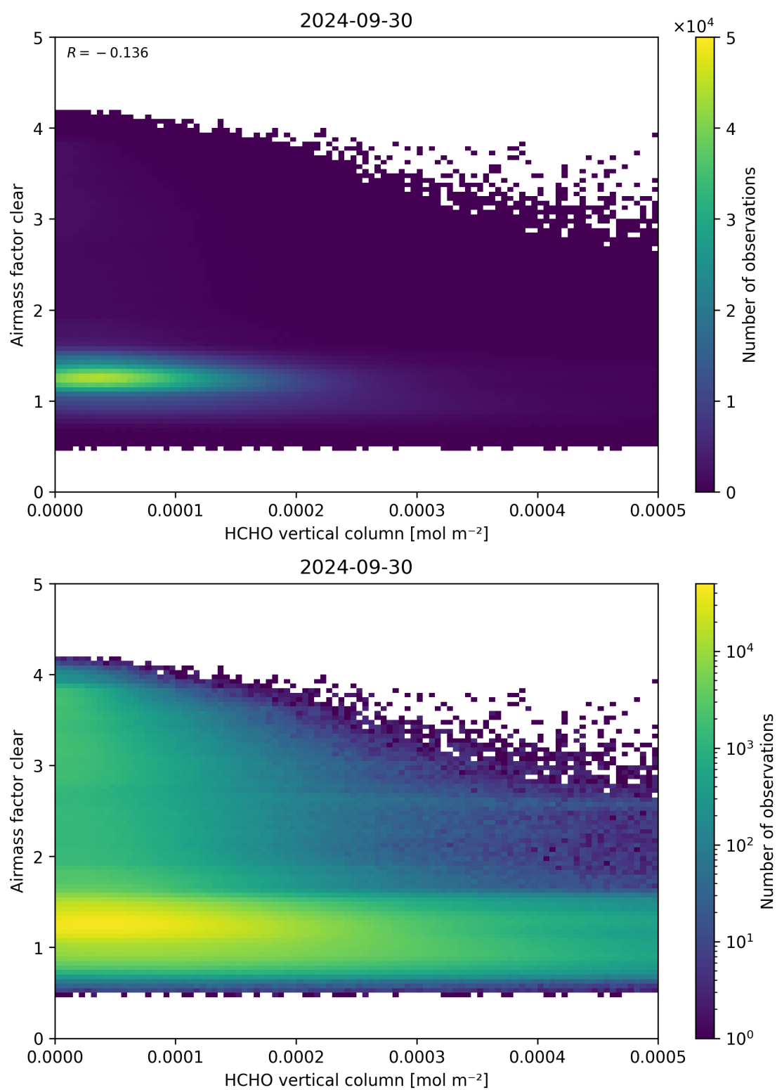
Figure 126: Scatter density plot of “HCHO vertical column” against “Airmass factor clear” for 2024-09-29 to 2024-10-01.
