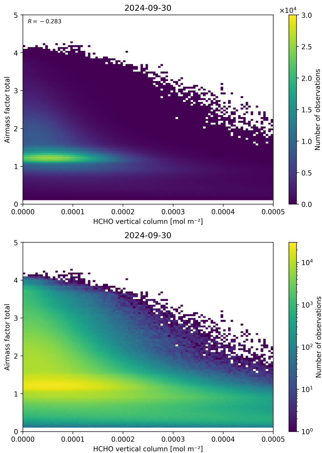
Figure 131: Scatter density plot of “HCHO vertical column” against “Airmass factor total” for 2024-09-29 to 2024-10-01.
