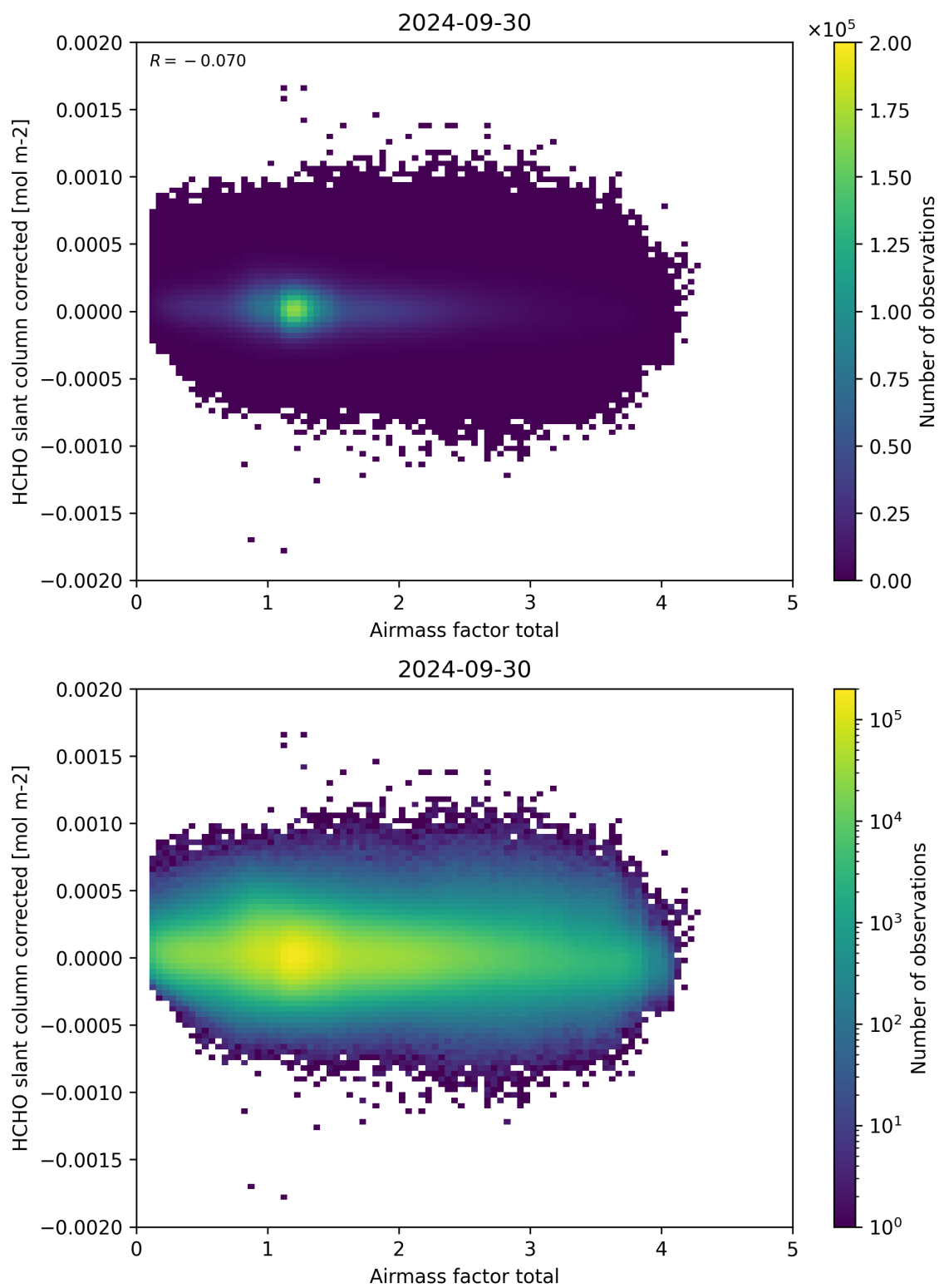
Figure 101: Scatter density plot of “Airmass factor total” against “HCHO slant column corrected” for 2024-09-29 to 2024-10-01.
