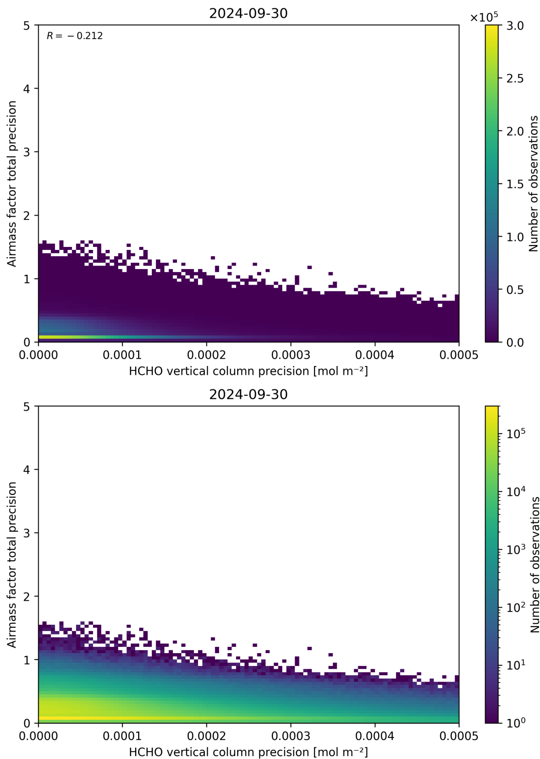
Figure 145: Scatter density plot of “HCHO vertical column precision” against “Airmass factor total precision” for 2024-09-29 to 2024-10-01.
