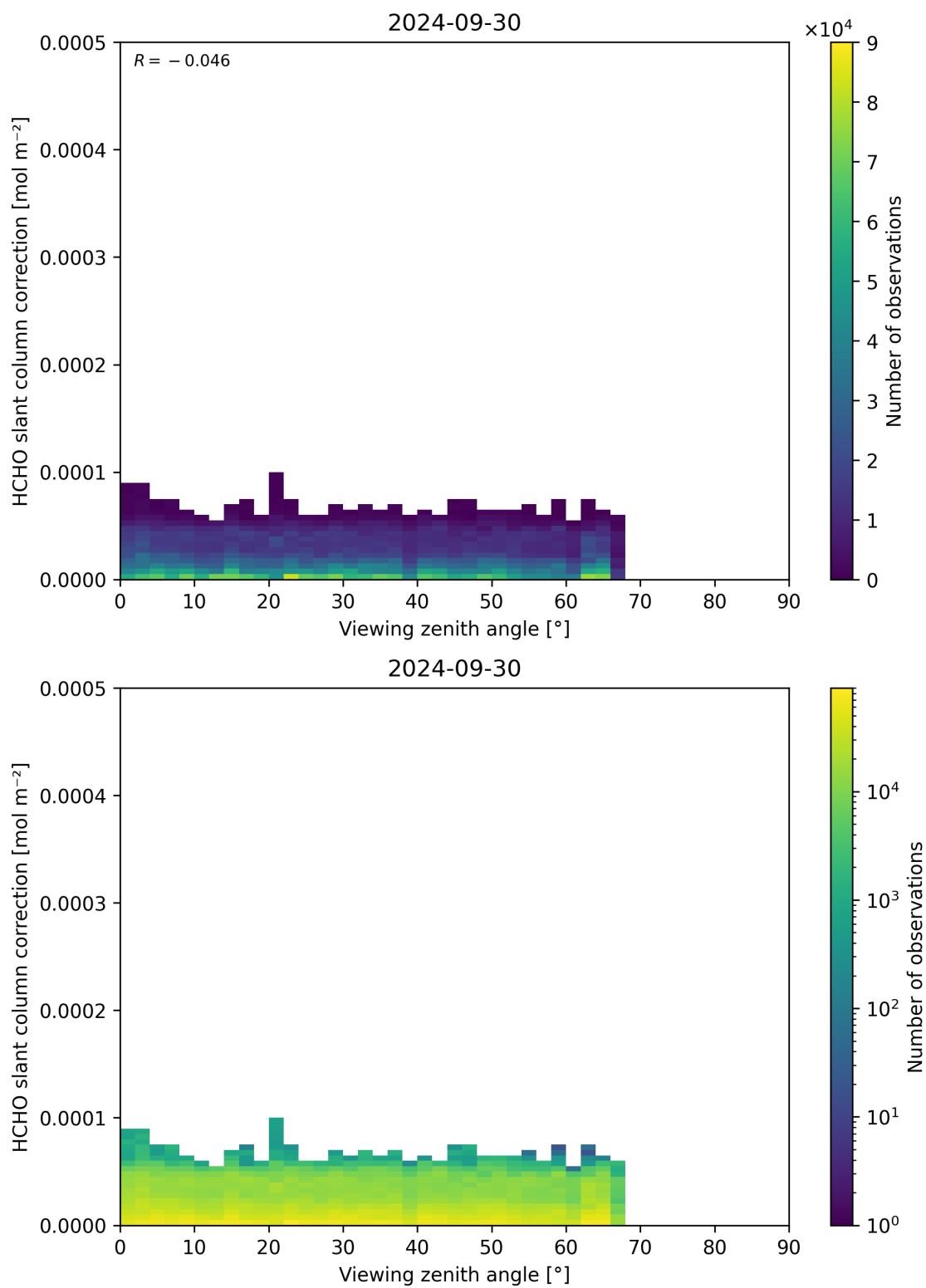
Figure 187: Scatter density plot of “Viewing zenith angle” against “HCHO slant column correction” for 2024-09-29 to 2024-10-01.
