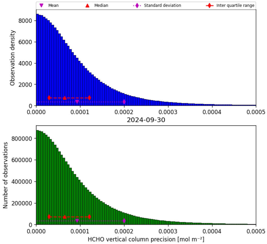
Figure 36: Histogram of “HCHO vertical column precision” for 2024-09-29 to 2024-10-01
