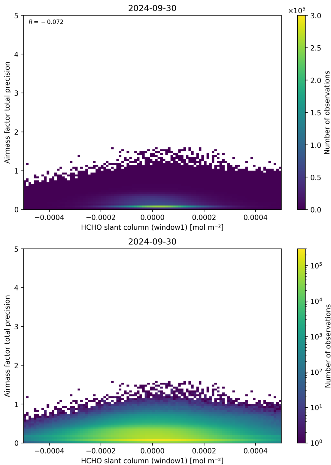
Figure 86: Scatter density plot of “HCHO slant column (window1)” against “Airmass factor total precision” for 2024-09-29 to 2024-10-01.
