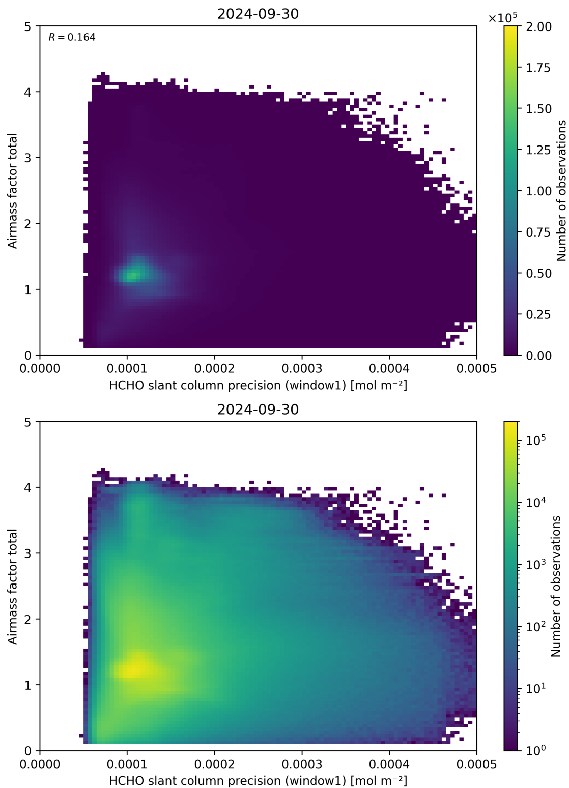
Figure 94: Scatter density plot of “HCHO slant column precision (window1)” against “Airmass factor total” for 2024-09-29 to 2024-10-01.
