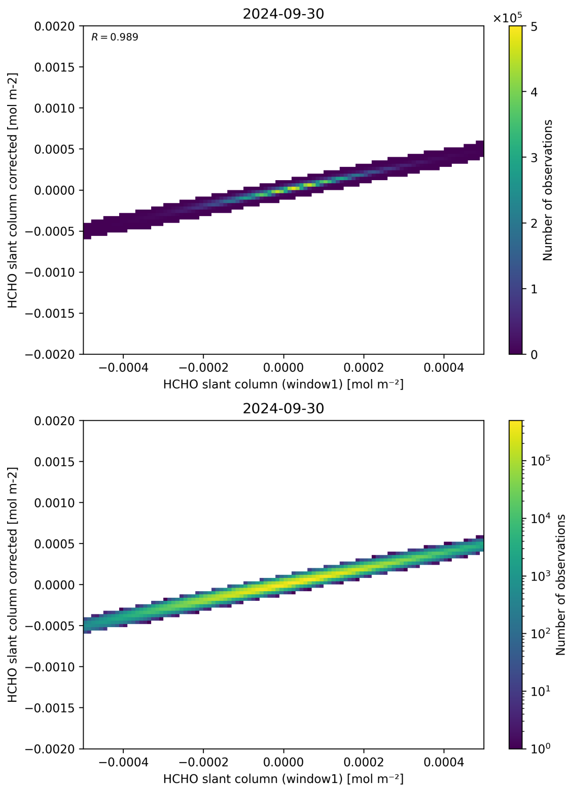
Figure 82: Scatter density plot of “HCHO slant column (window1)” against “HCHO slant column corrected” for 2024-09-29 to 2024-10-01.
