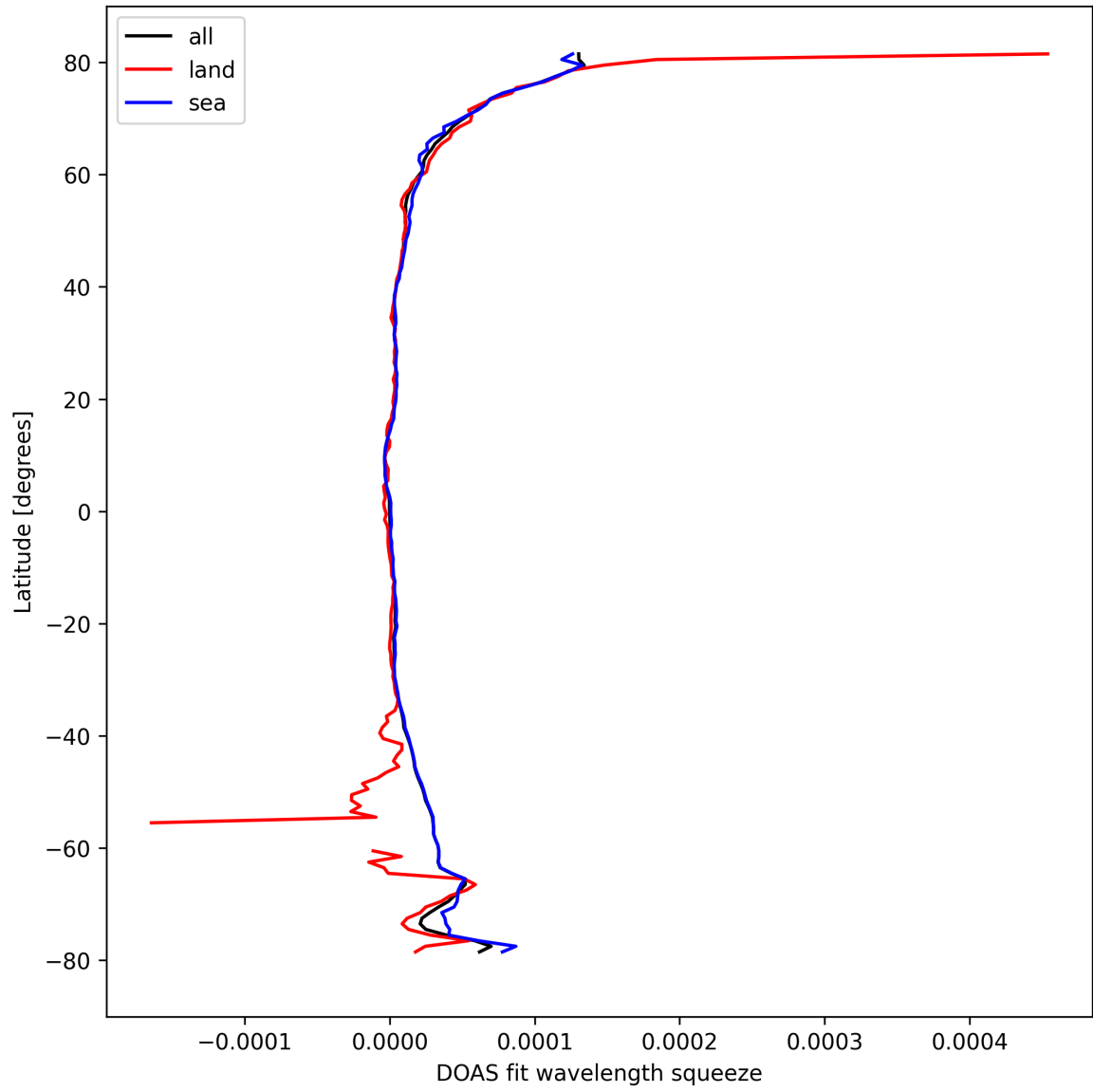
Figure 31: Zonal average of “DOAS fit wavelength squeeze” for 2024-09-29 to 2024-10-01.
