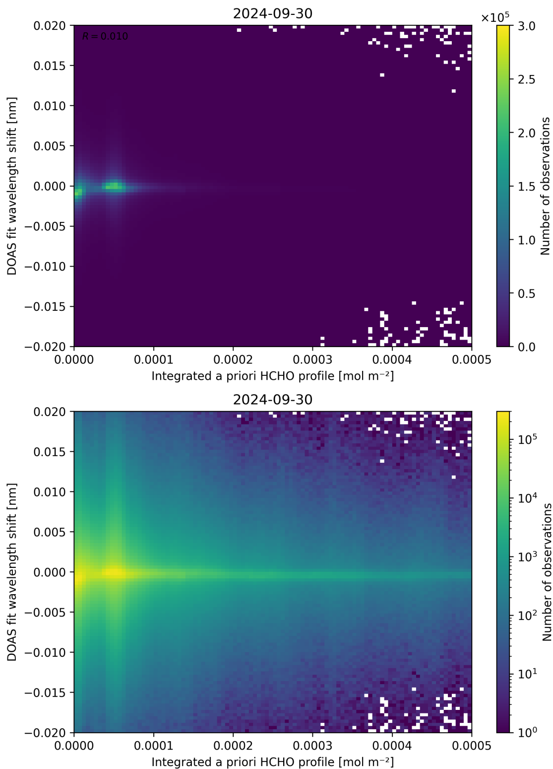
Figure 149: Scatter density plot of “Integrated a priori HCHO profile” against “DOAS fit wavelength shift” for 2024-09-29 to 2024-10-01.
