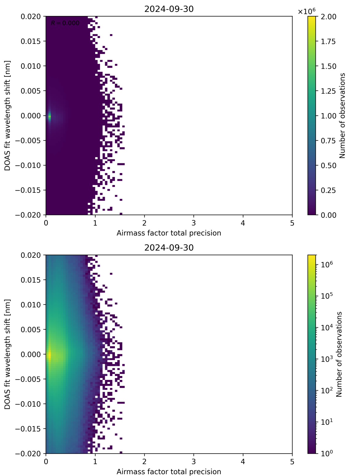
Figure 106: Scatter density plot of “Airmass factor total precision” against “DOAS fit wavelength shift” for 2024-09-29 to 2024-10-01.
