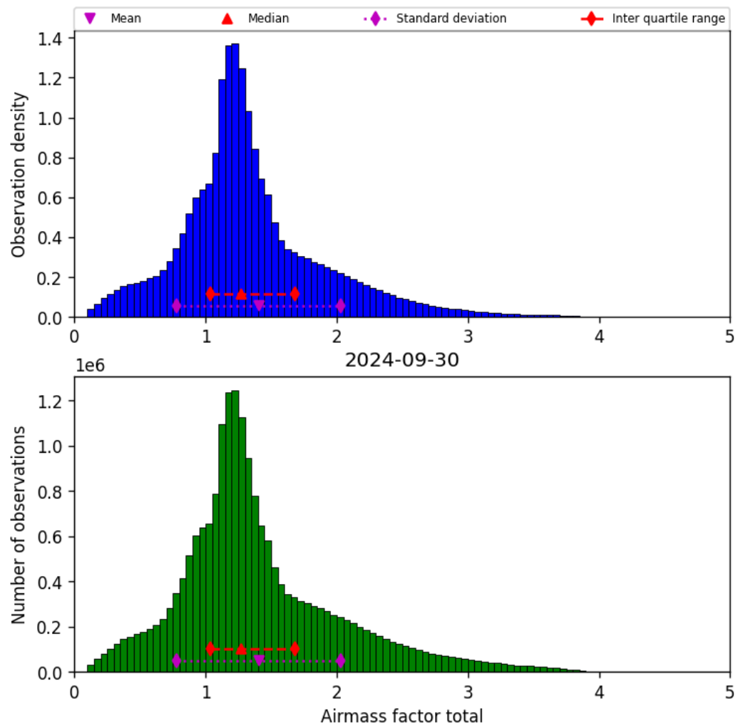
Figure 40: Histogram of “Airmass factor total” for 2024-09-29 to 2024-10-01
