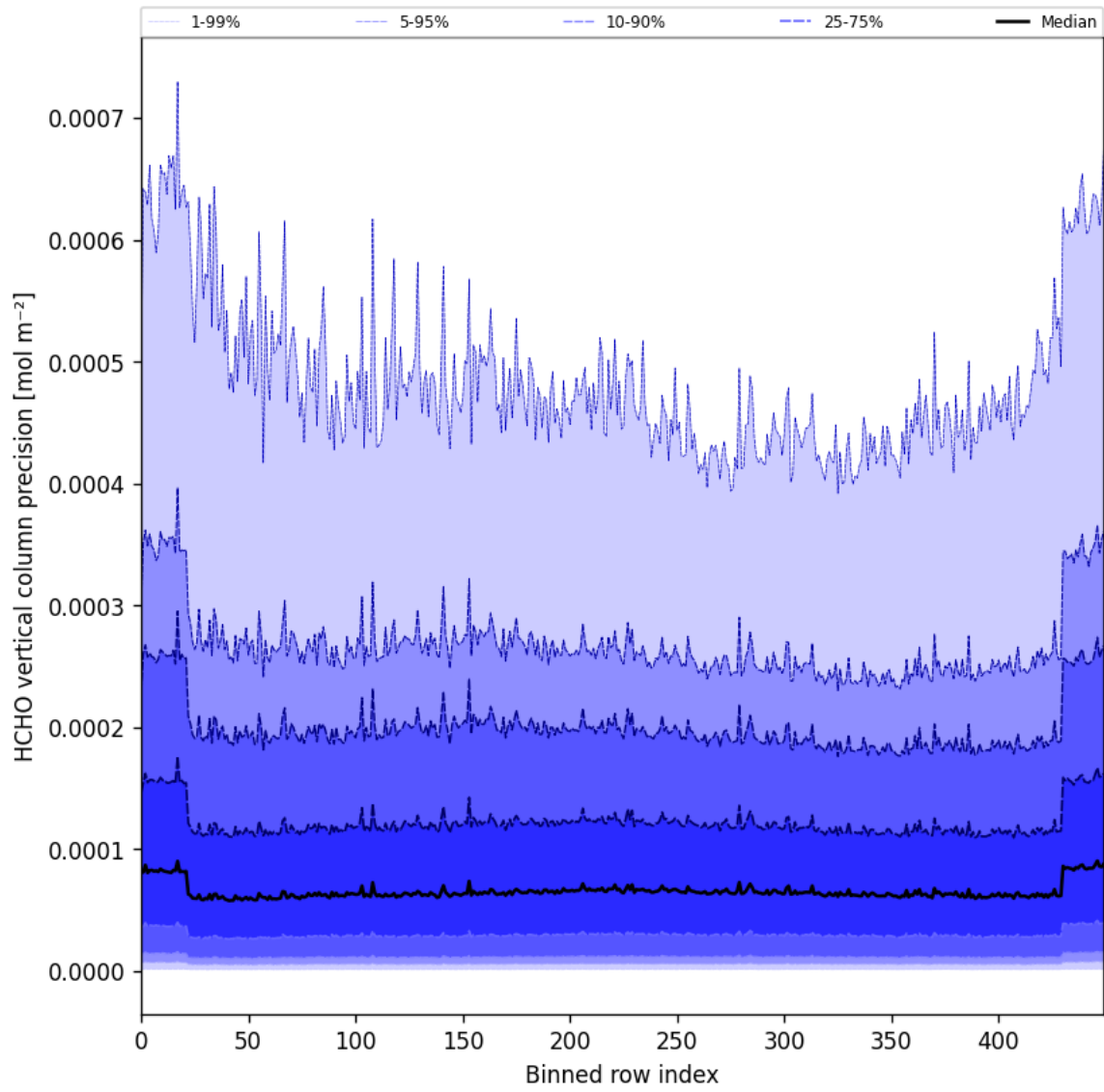
Figure 50: Along track statistics of “HCHO vertical column precision” for 2024-09-29 to 2024-10-01
