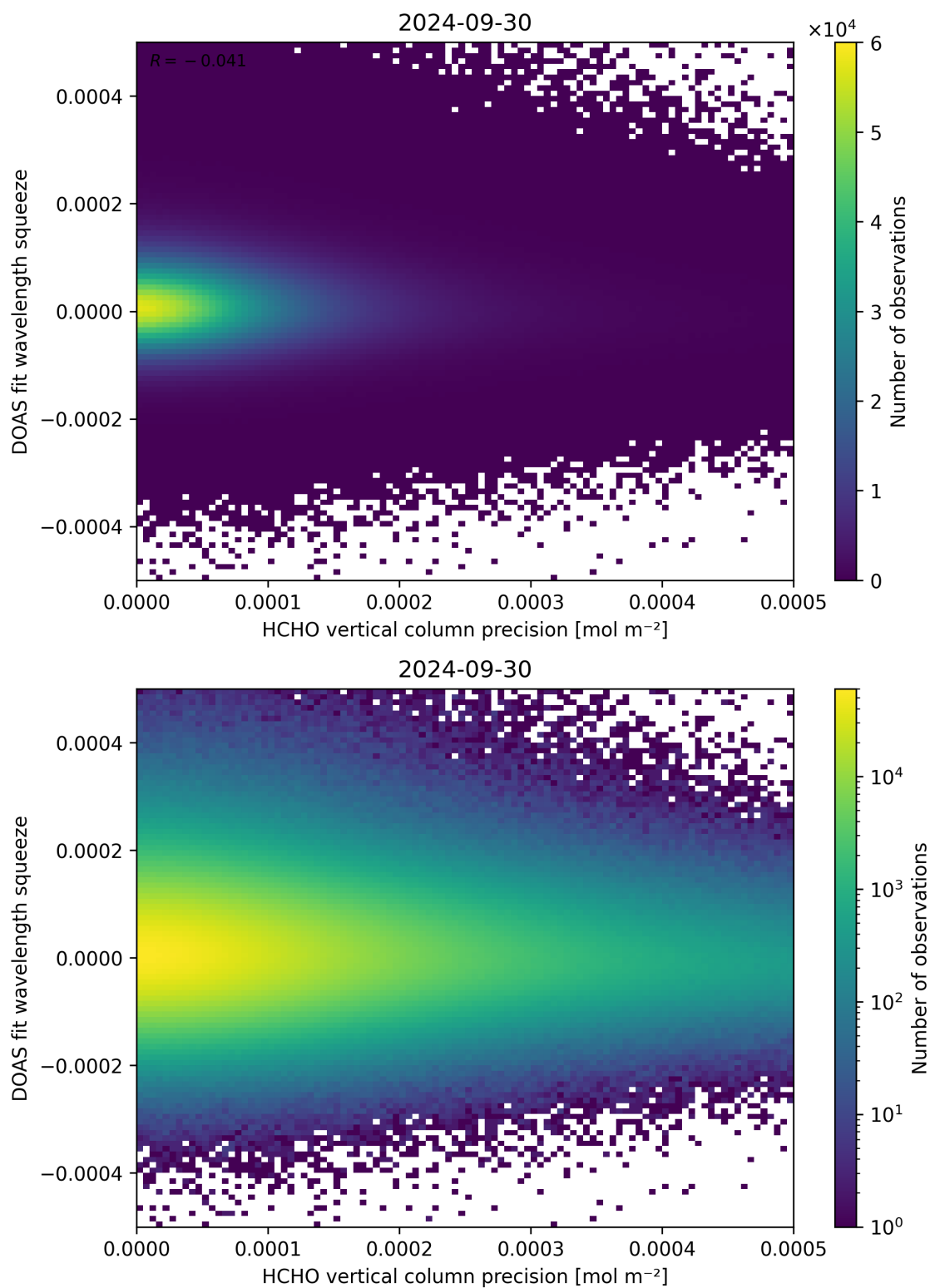
Figure 138: Scatter density plot of “HCHO vertical column precision” against “DOAS fit wavelength squeeze” for 2024-09-29 to 2024-10-01.
