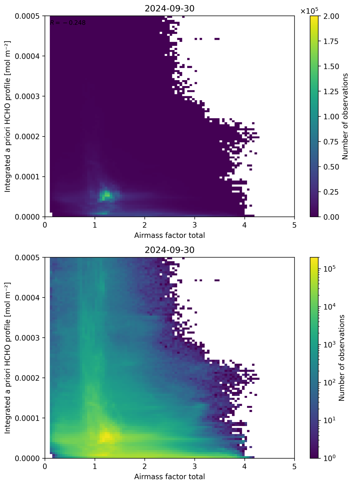
Figure 104: Scatter density plot of “Airmass factor total” against “Integrated a priori HCHO profile” for 2024-09-29 to 2024-10-01.
