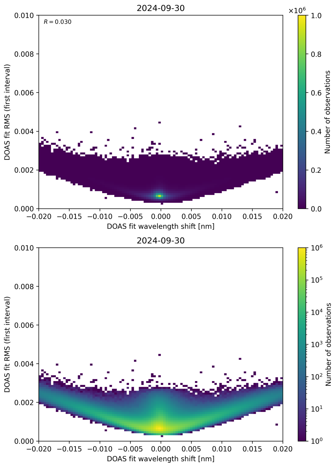
Figure 64: Scatter density plot of “DOAS fit wavelength shift” against “DOAS fit RMS (first interval)” for 2024-09-29 to 2024-10-01.
