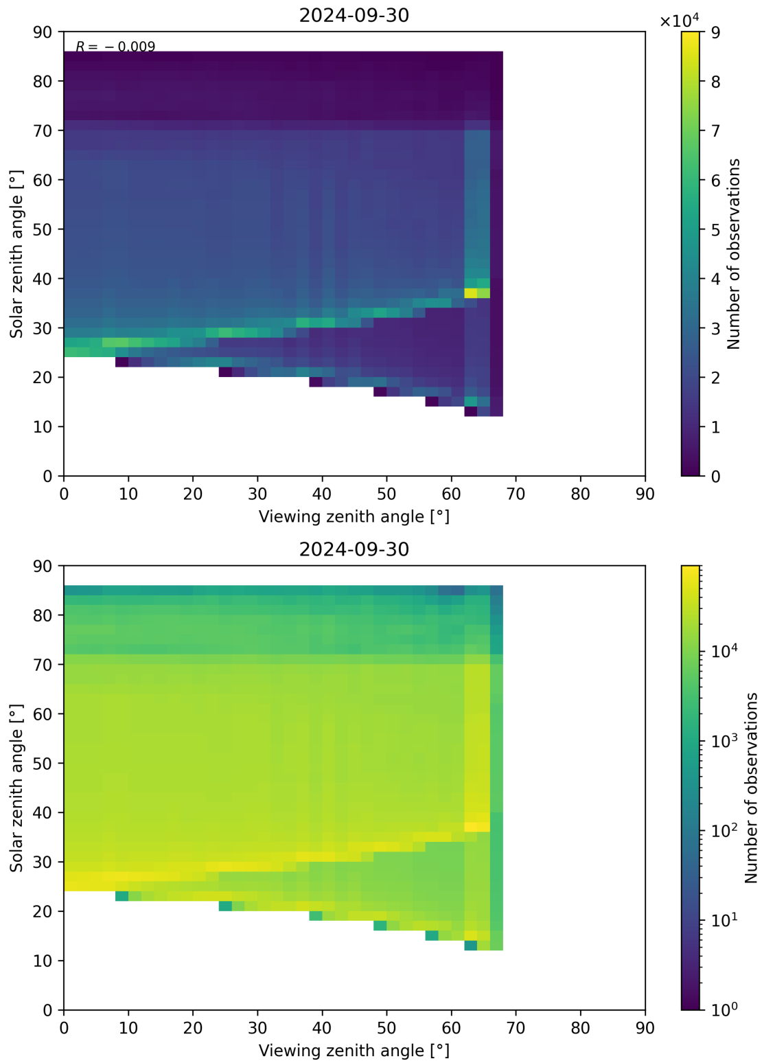
Figure 197: Scatter density plot of “Viewing zenith angle” against “Solar zenith angle” for 2024-09-29 to 2024-10-01.
