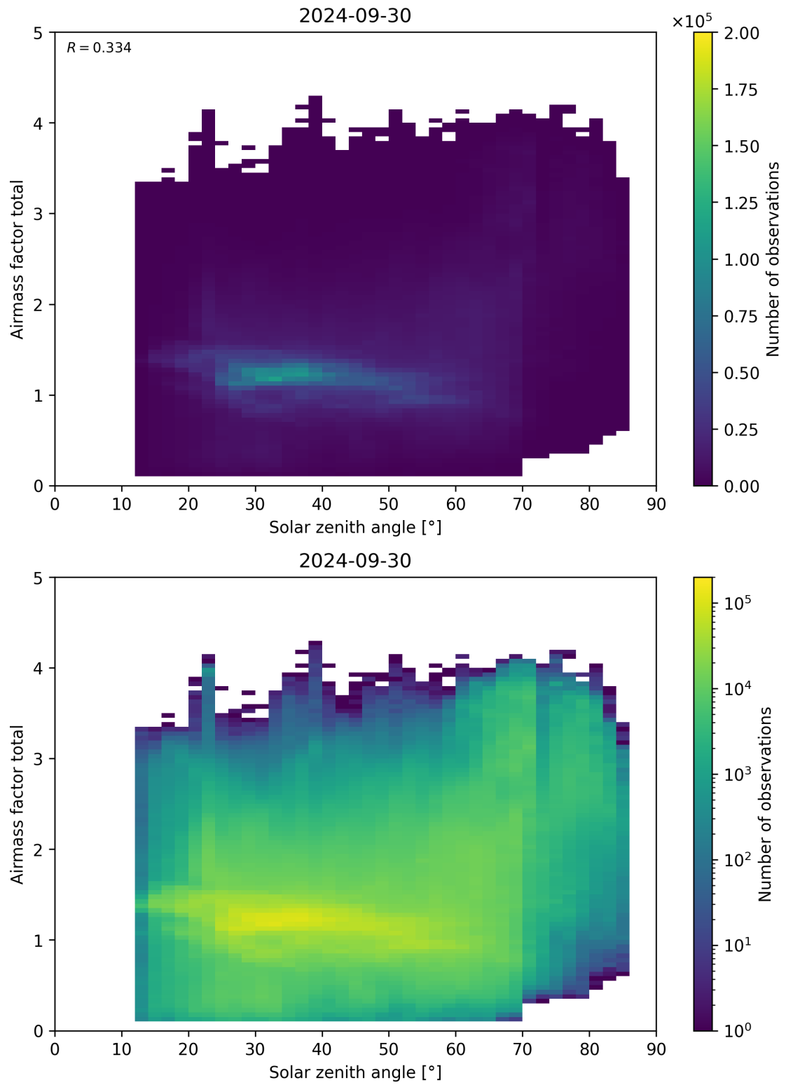
Figure 175: Scatter density plot of “Solar zenith angle” against “Airmass factor total” for 2024-09-29 to 2024-10-01.
