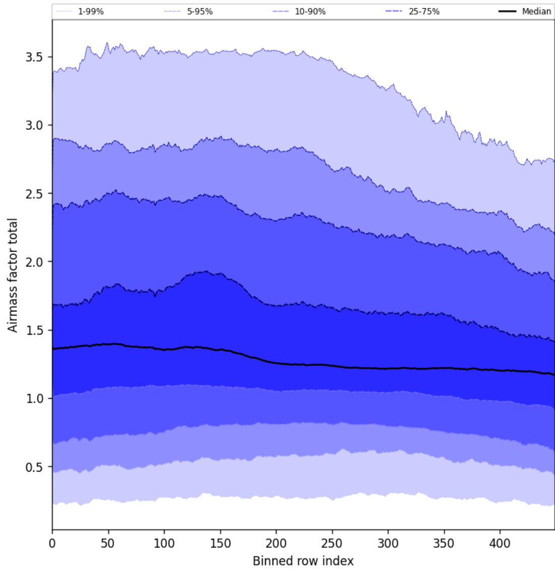
Figure 54: Along track statistics of “Airmass factor total” for 2024-09-29 to 2024-10-01
