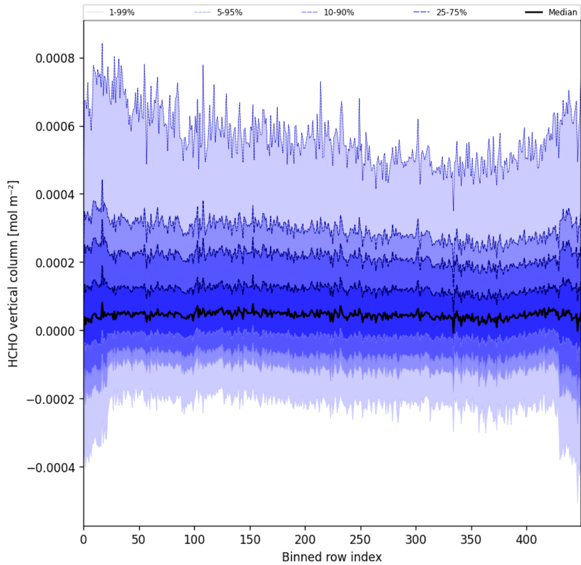
Figure 49: Along track statistics of “HCHO vertical column” for 2024-09-29 to 2024-10-01
