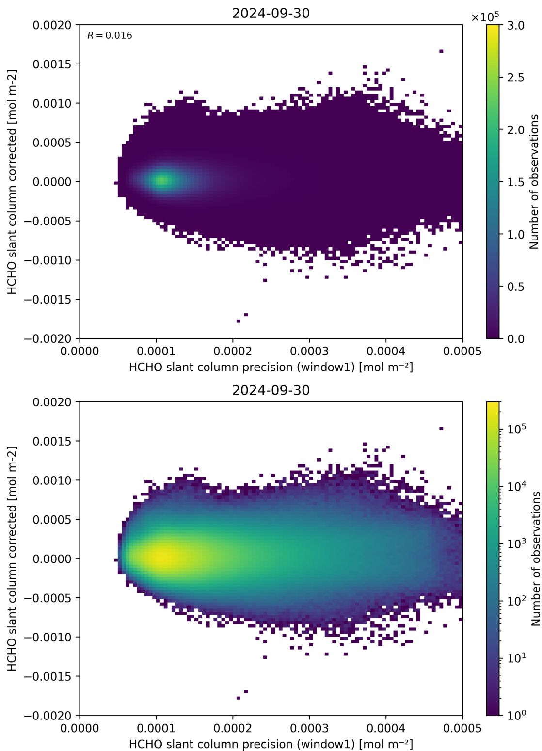
Figure 92: Scatter density plot of “HCHO slant column precision (window1)” against “HCHO slant column corrected” for 2024-09-29 to 2024-10-01.
