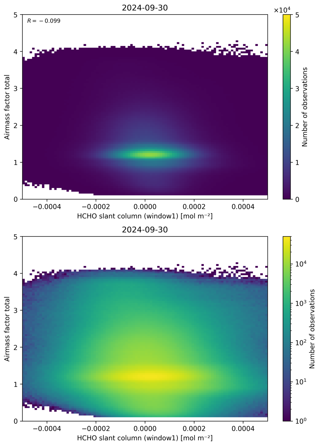
Figure 85: Scatter density plot of “HCHO slant column (window1)” against “Airmass factor total” for 2024-09-29 to 2024-10-01.
