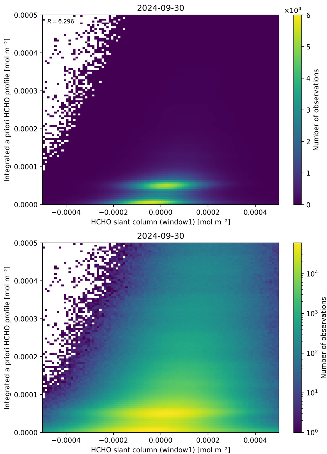
Figure 87: Scatter density plot of “HCHO slant column (window1)” against “Integrated a priori HCHO profile” for 2024-09-29 to 2024-10-01.
