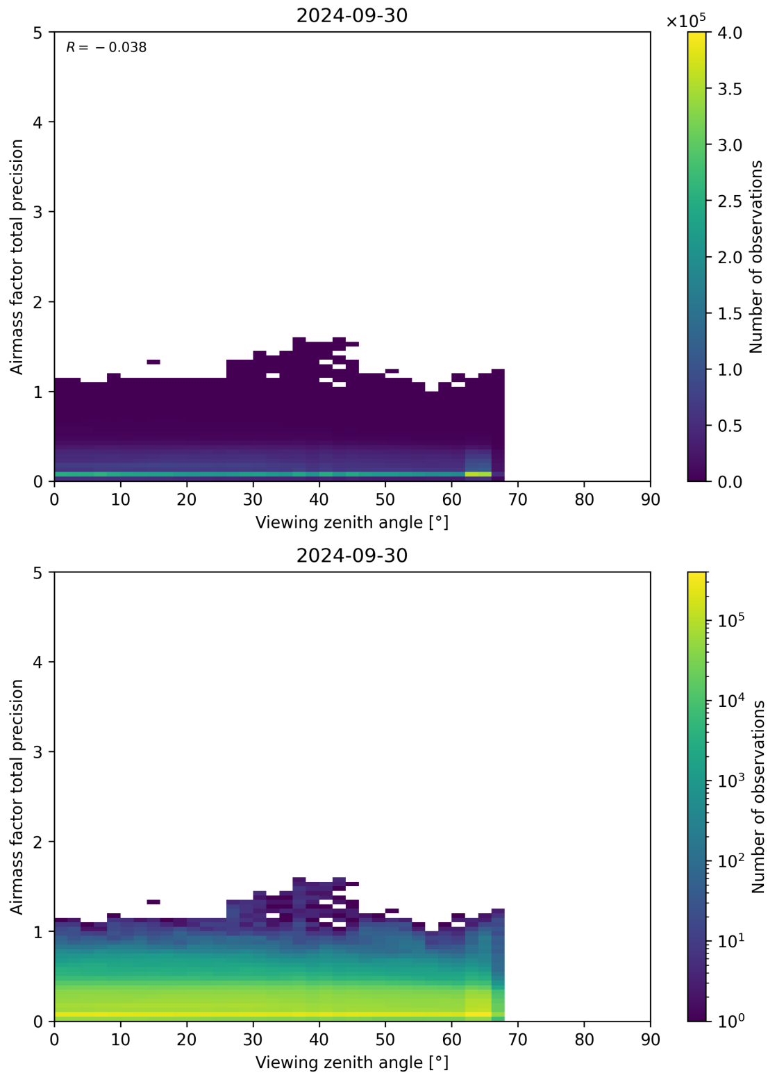
Figure 191: Scatter density plot of “Viewing zenith angle” against “Airmass factor total precision” for 2024-09-29 to 2024-10-01.
