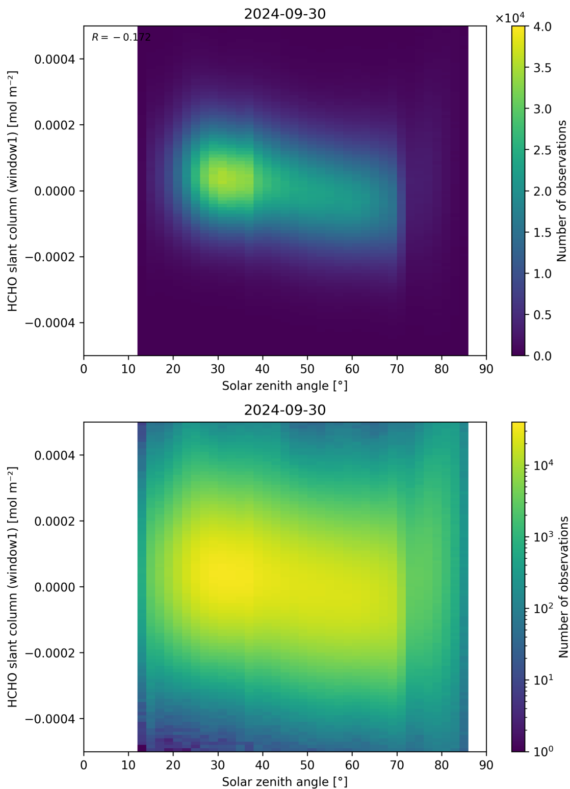
Figure 173: Scatter density plot of “Solar zenith angle” against “HCHO slant column (window1)” for 2024-09-29 to 2024-10-01.
