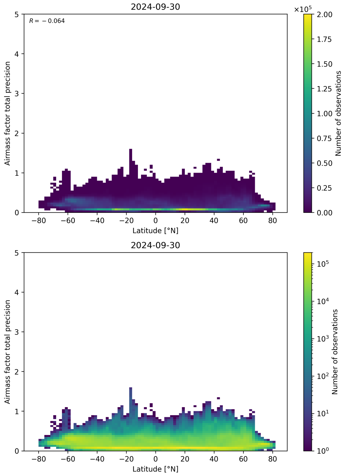
Figure 162: Scatter density plot of “Latitude” against “Airmass factor total precision” for 2024-09-29 to 2024-10-01.
