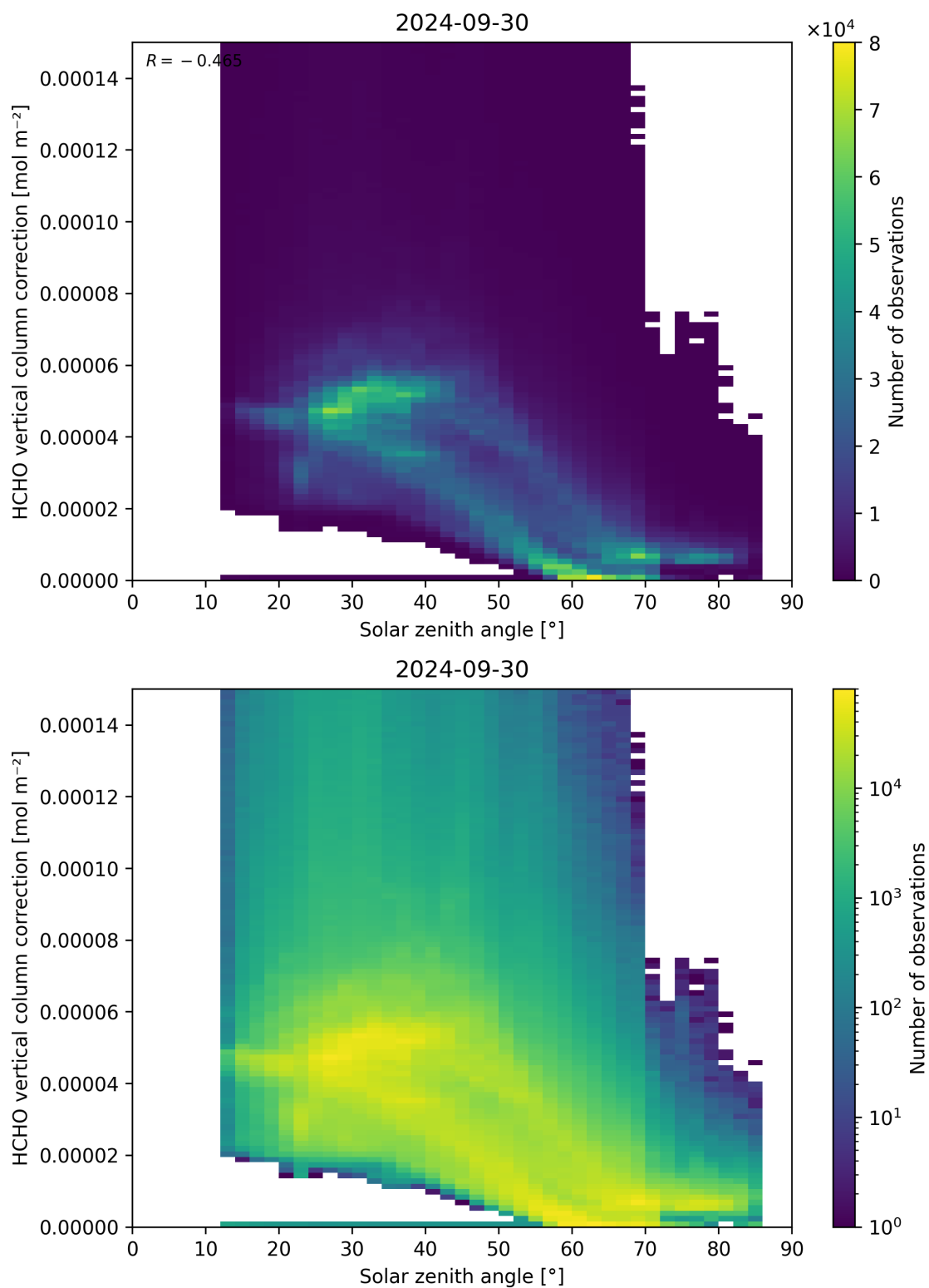
Figure 178: Scatter density plot of “Solar zenith angle” against “HCHO vertical column correction” for 2024-09-29 to 2024-10-01.
