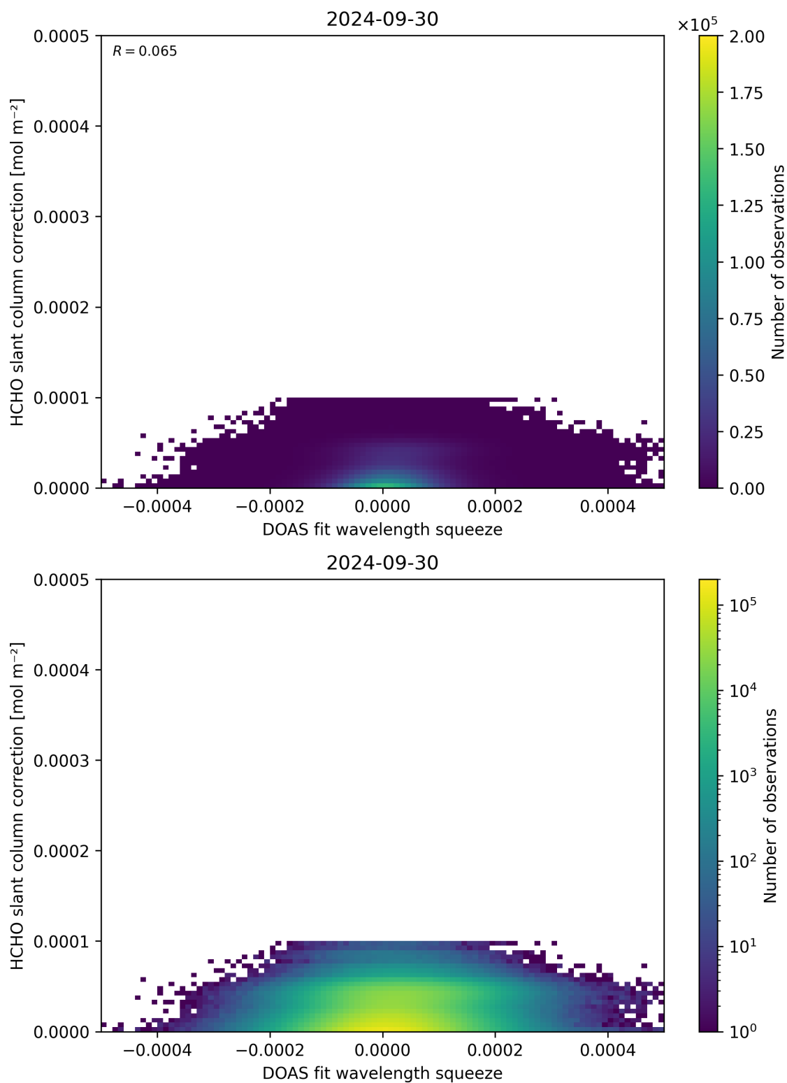
Figure 70: Scatter density plot of “DOAS fit wavelength squeeze” against “HCHO slant column correction” for 2024-09-29 to 2024-10-01.
