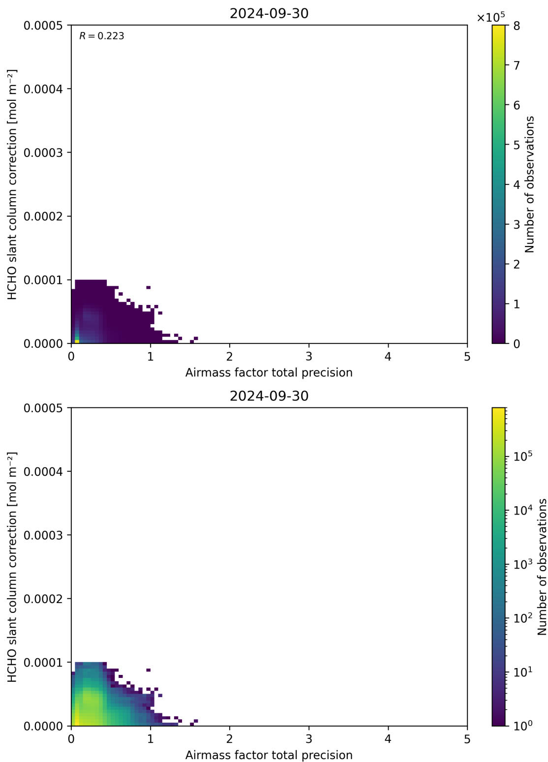
Figure 110: Scatter density plot of “Airmass factor total precision” against “HCHO slant column correction” for 2024-09-29 to 2024-10-01.
