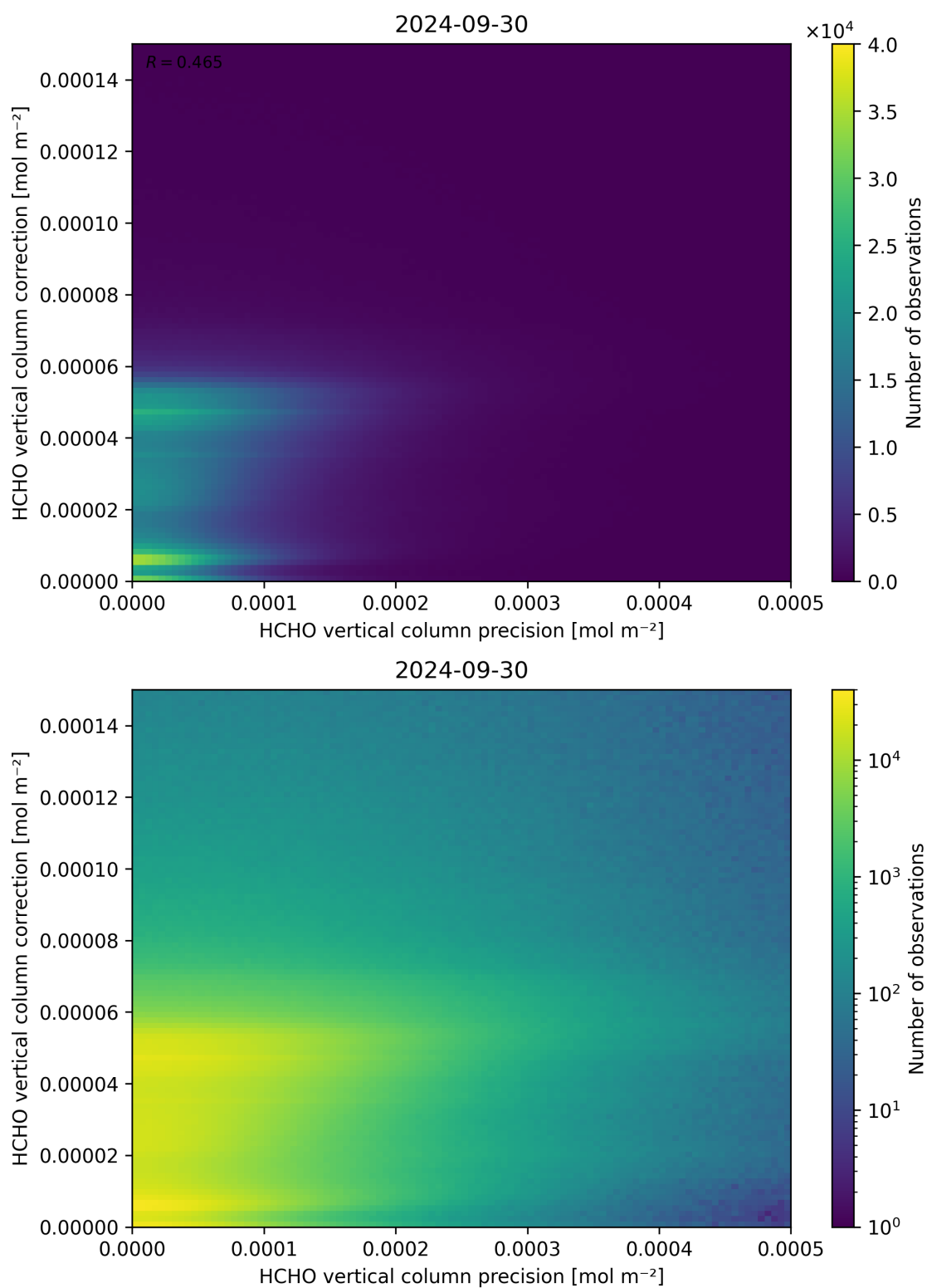
Figure 146: Scatter density plot of “HCHO vertical column precision” against “HCHO vertical column correction” for 2024-09-29 to 2024-10-01.
