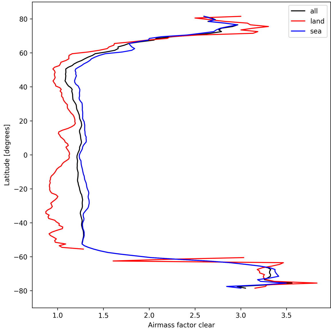
Figure 28: Zonal average of “Airmass factor clear” for 2024-09-29 to 2024-10-01.
