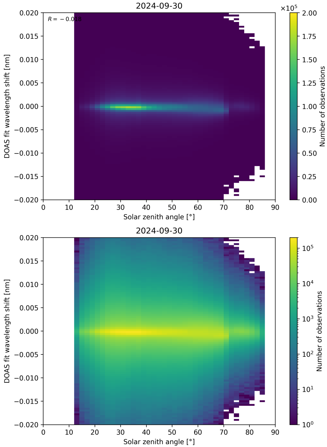
Figure 168: Scatter density plot of “Solar zenith angle” against “DOAS fit wavelength shift” for 2024-09-29 to 2024-10-01.
