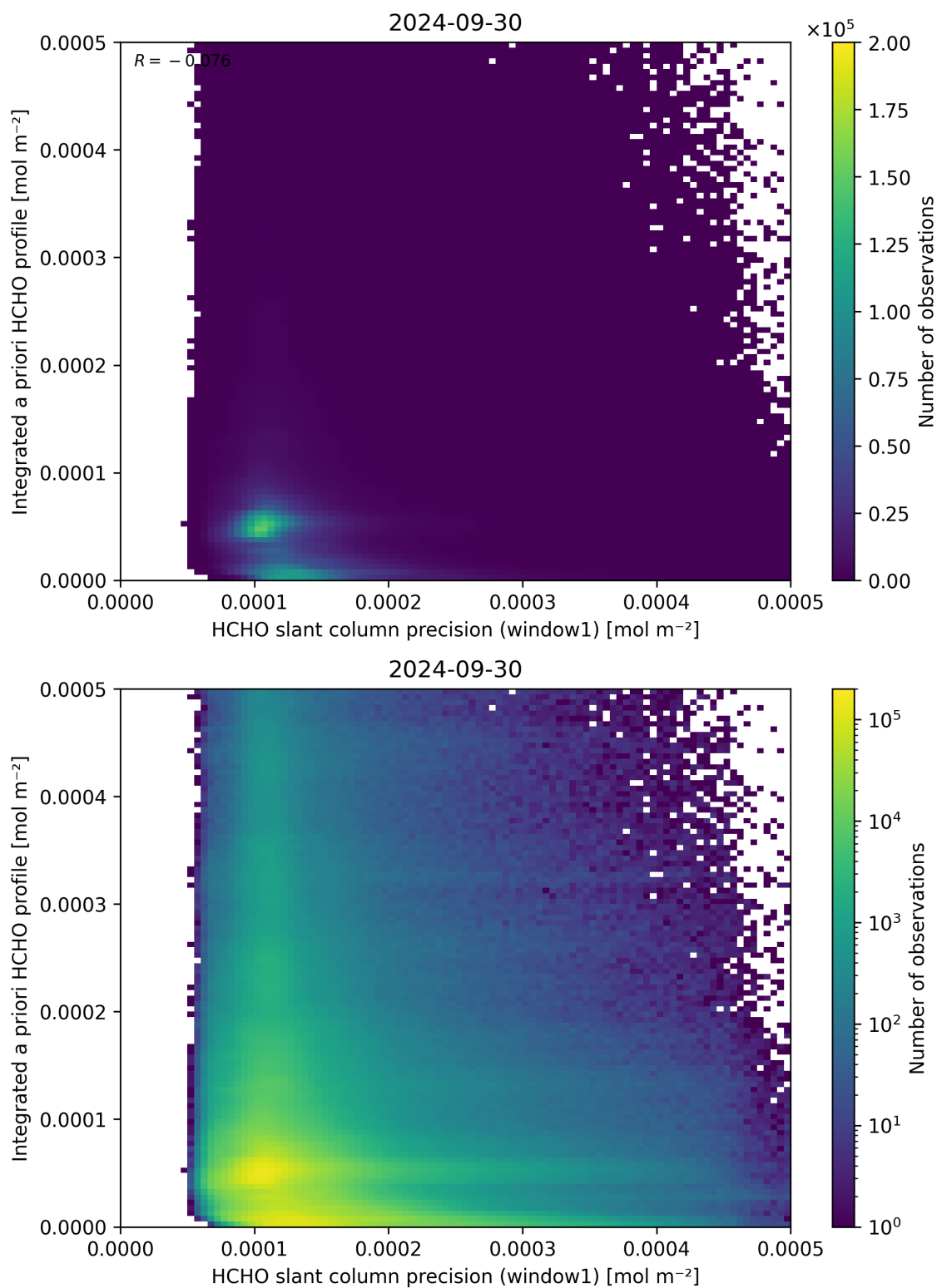
Figure 96: Scatter density plot of “HCHO slant column precision (window1)” against “Integrated a priori HCHO profile” for 2024-09-29 to 2024-10-01.
