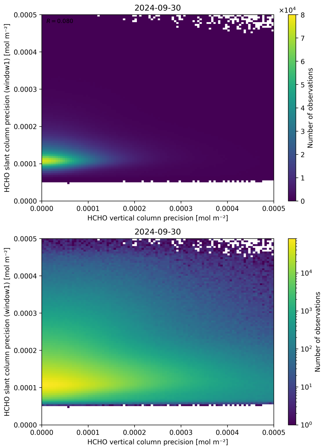
Figure 143: Scatter density plot of “HCHO vertical column precision” against “HCHO slant column precision (window1)” for 2024-09-29 to 2024-10-01.
