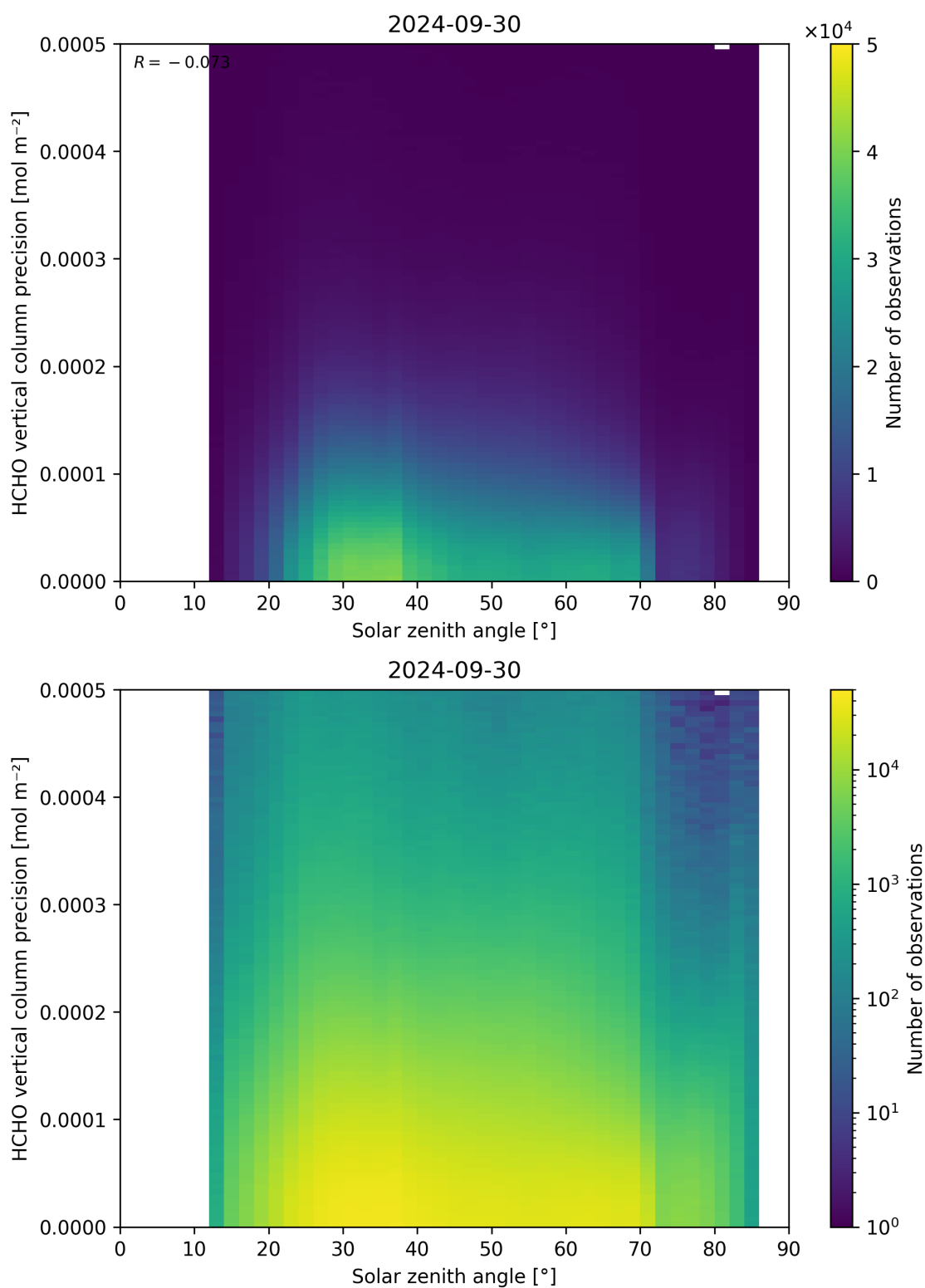
Figure 179: Scatter density plot of “Solar zenith angle” against “HCHO vertical column precision” for 2024-09-29 to 2024-10-01.
