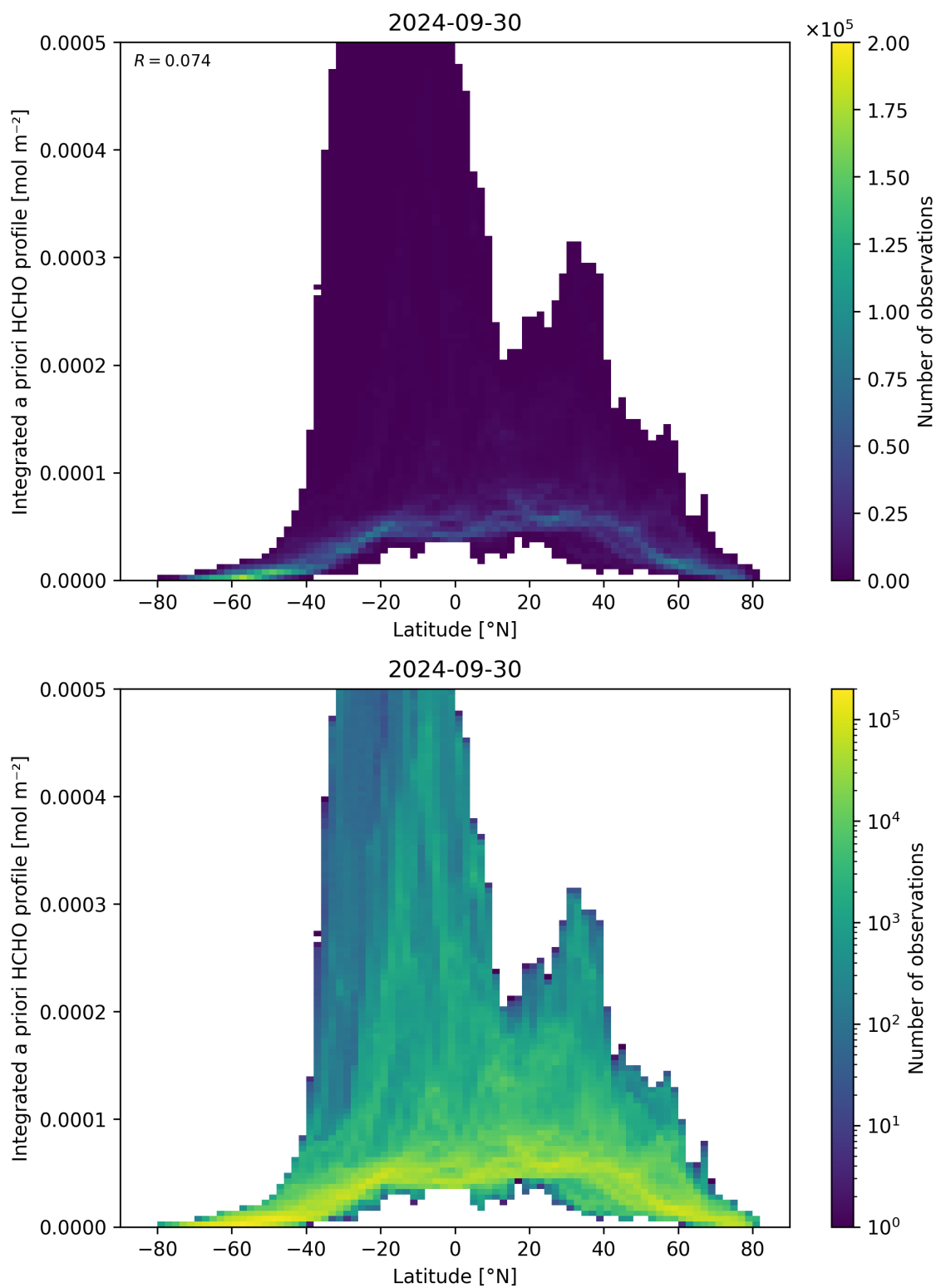
Figure 166: Scatter density plot of “Latitude” against “Integrated a priori HCHO profile” for 2024-09-29 to 2024-10-01.
