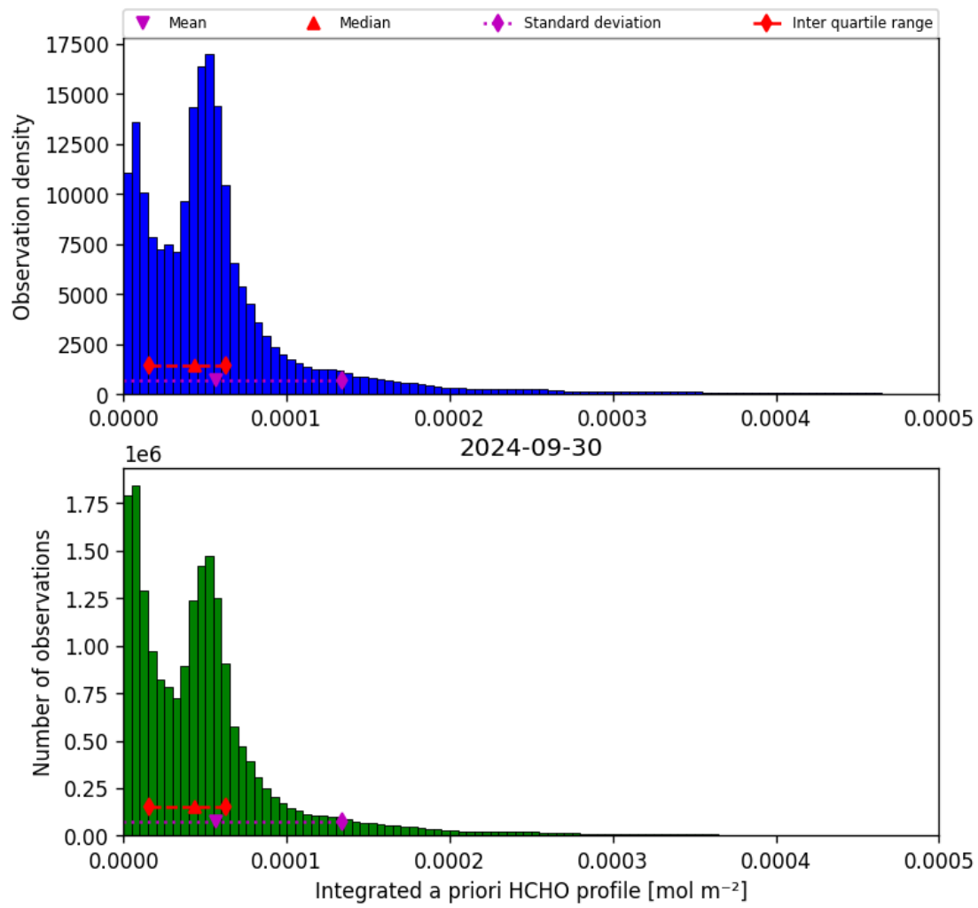
Figure 43: Histogram of “Integrated a priori HCHO profile” for 2024-09-29 to 2024-10-01
