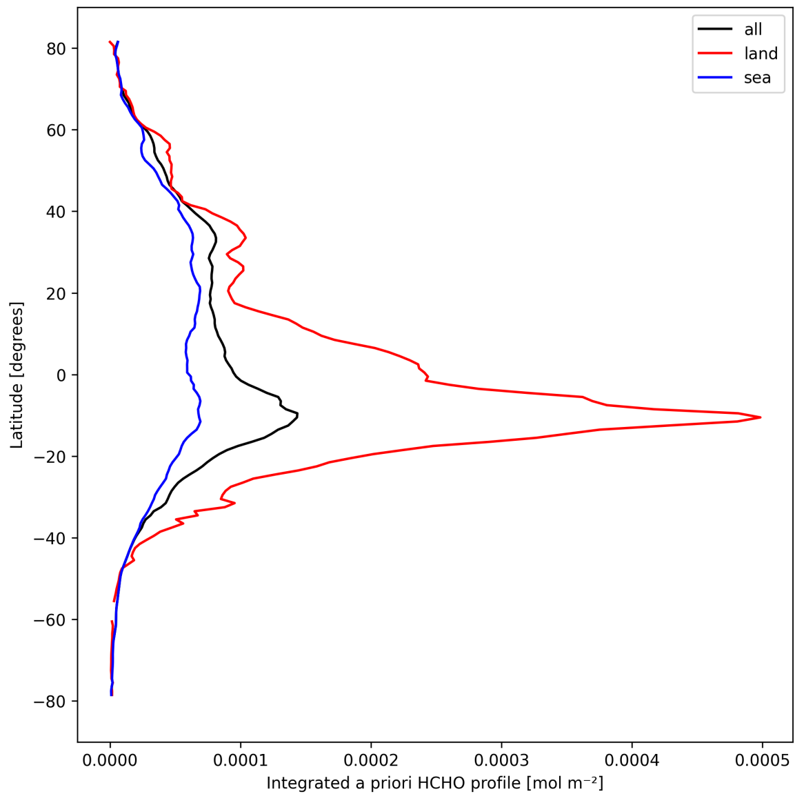
Figure 29: Zonal average of “Integrated a priori HCHO profile” for 2024-09-29 to 2024-10-01.
