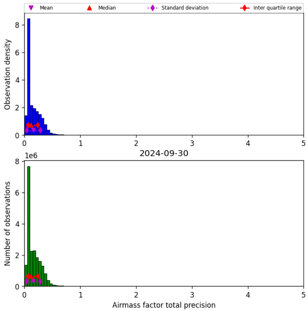
Figure 41: Histogram of “Airmass factor total precision” for 2024-09-29 to 2024-10-01
