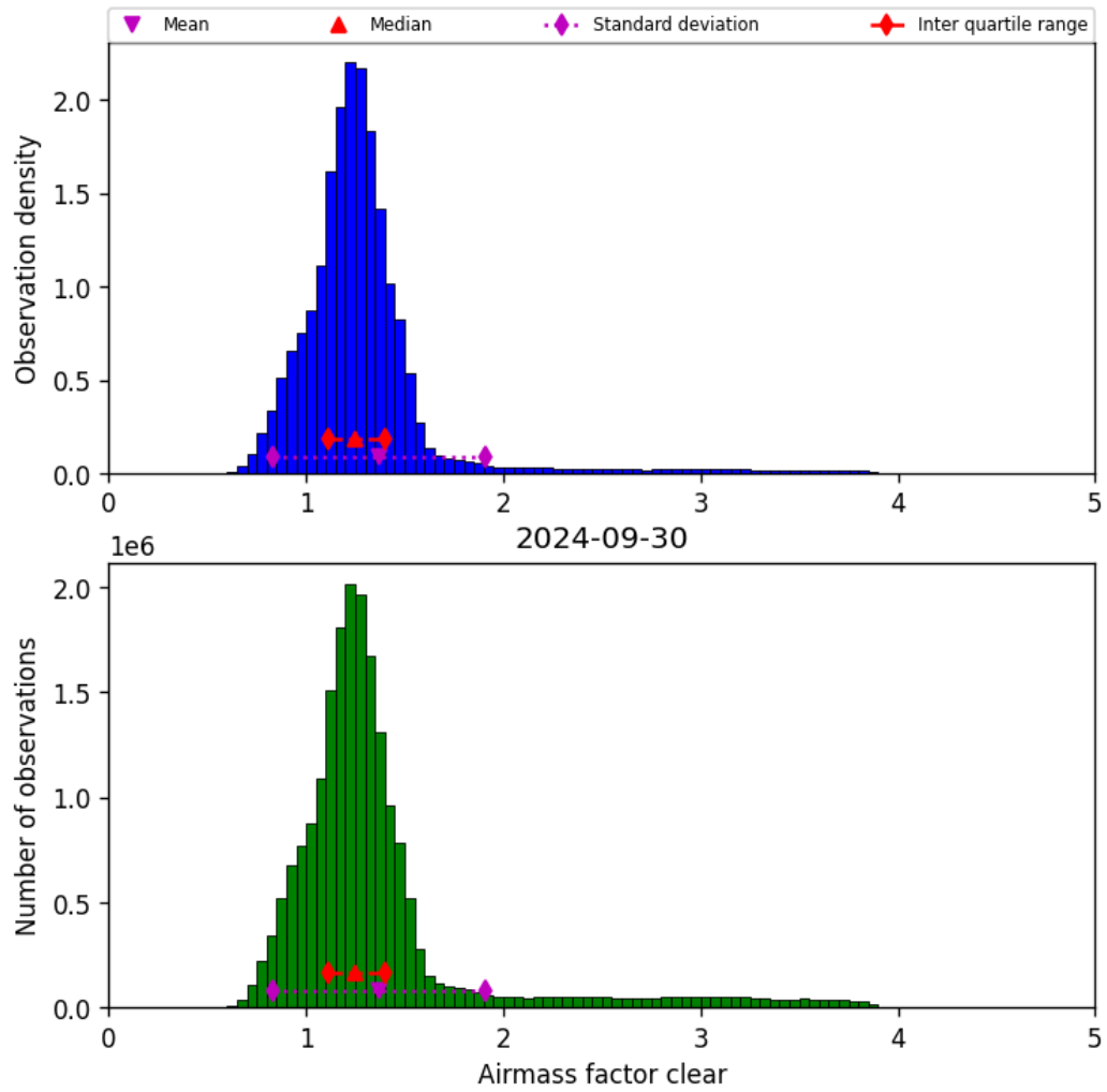
Figure 42: Histogram of “Airmass factor clear” for 2024-09-29 to 2024-10-01
