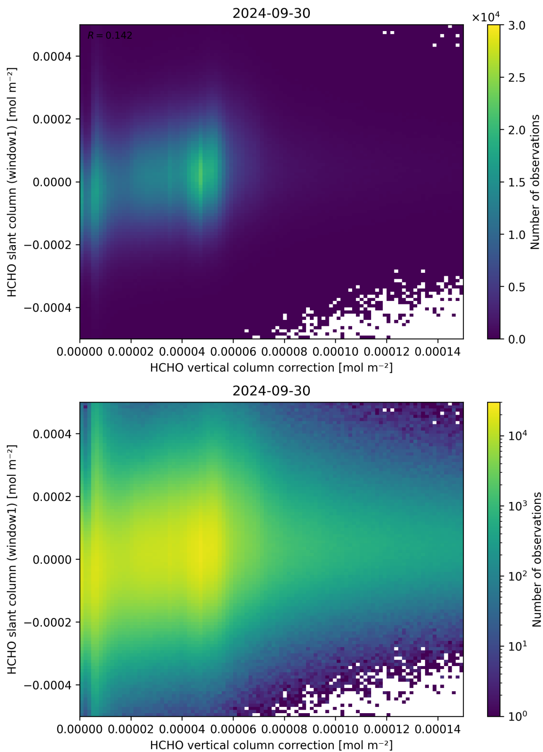
Figure 118: Scatter density plot of “HCHO vertical column correction” against “HCHO slant column (window1)” for 2024-09-29 to 2024-10-01.
