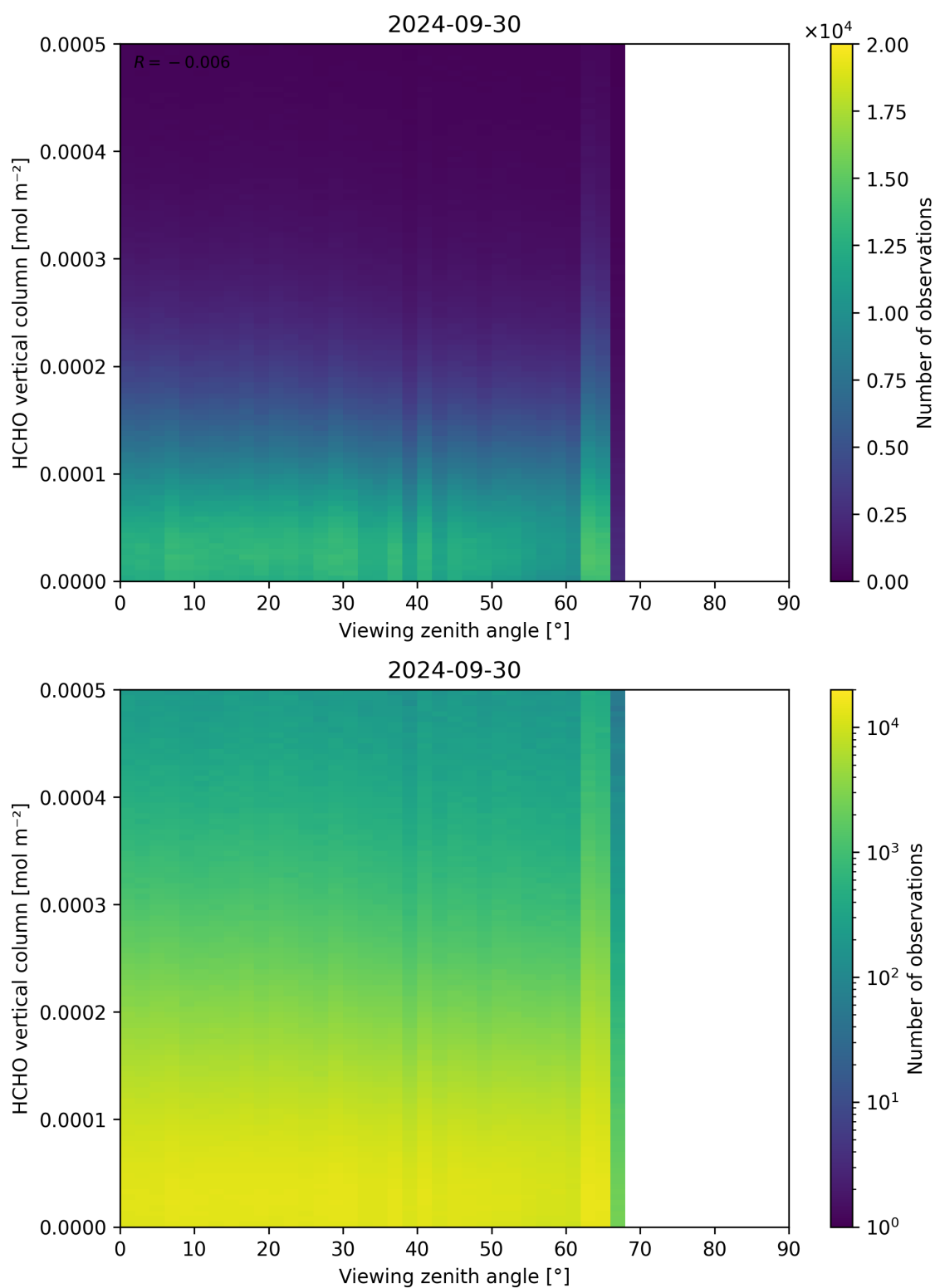
Figure 192: Scatter density plot of “Viewing zenith angle” against “HCHO vertical column” for 2024-09-29 to 2024-10-01.
