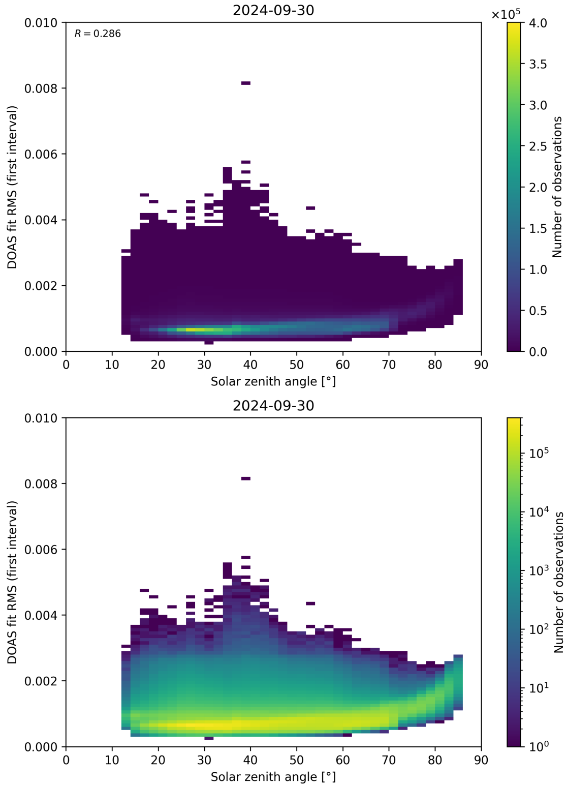
Figure 167: Scatter density plot of “Solar zenith angle” against “DOAS fit RMS (first interval)” for 2024-09-29 to 2024-10-01.
