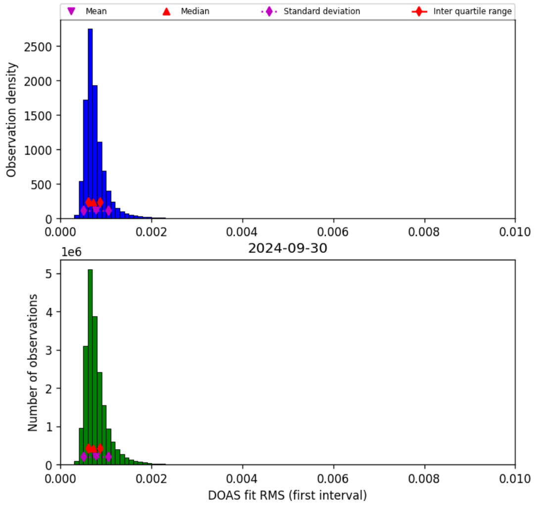
Figure 46: Histogram of “DOAS fit RMS (first interval)” for 2024-09-29 to 2024-10-01
