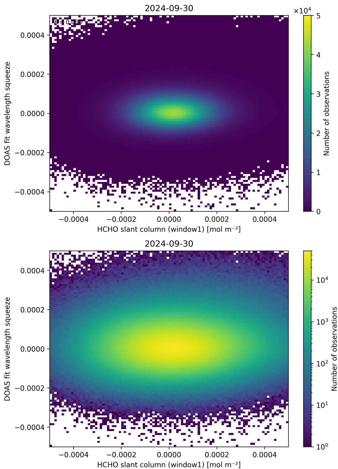
Figure 80: Scatter density plot of “HCHO slant column (window1)” against “DOAS fit wavelength squeeze” for 2024-09-29 to 2024-10-01.
