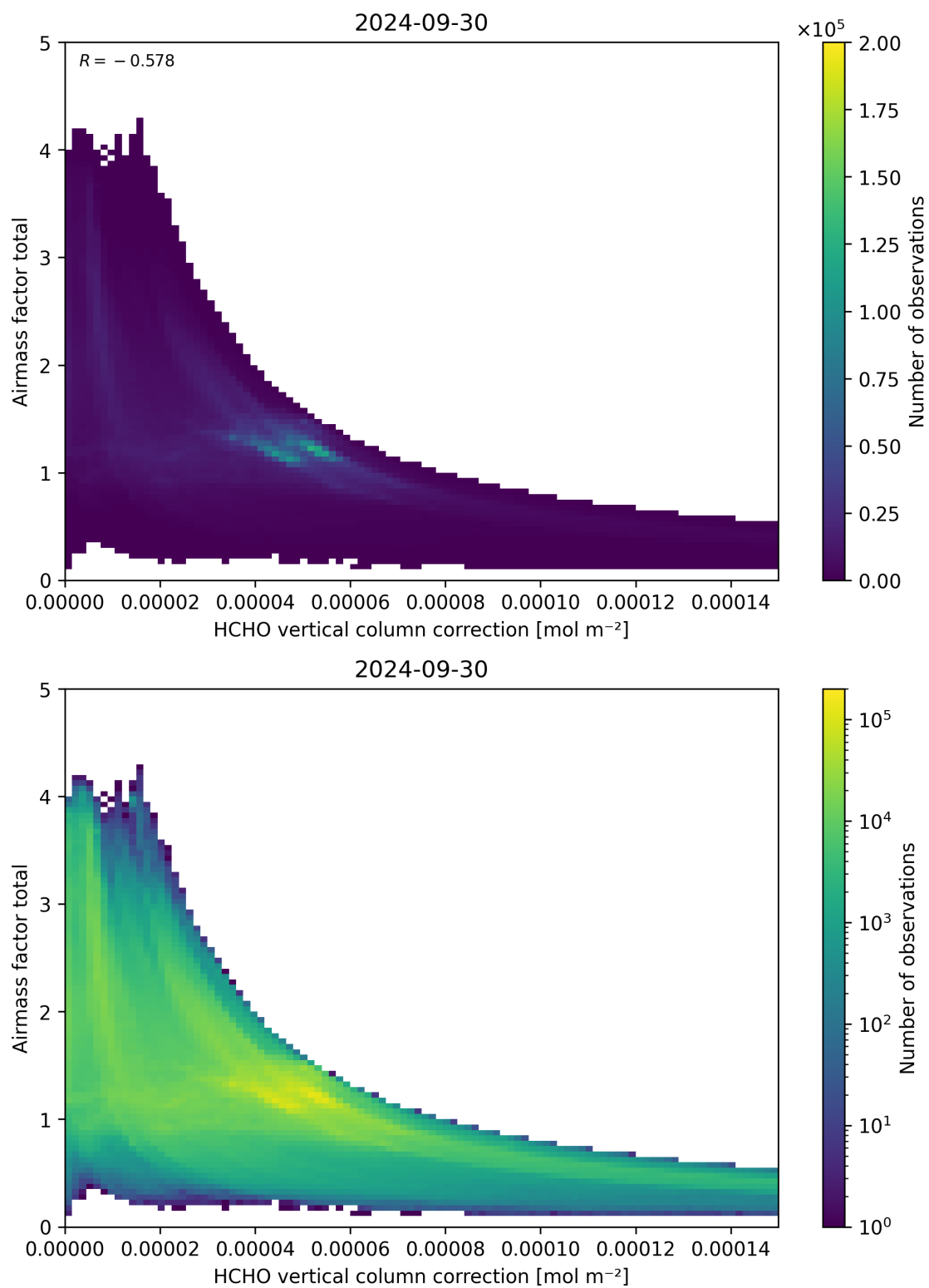
Figure 120: Scatter density plot of “HCHO vertical column correction” against “Airmass factor total” for 2024-09-29 to 2024-10-01.
