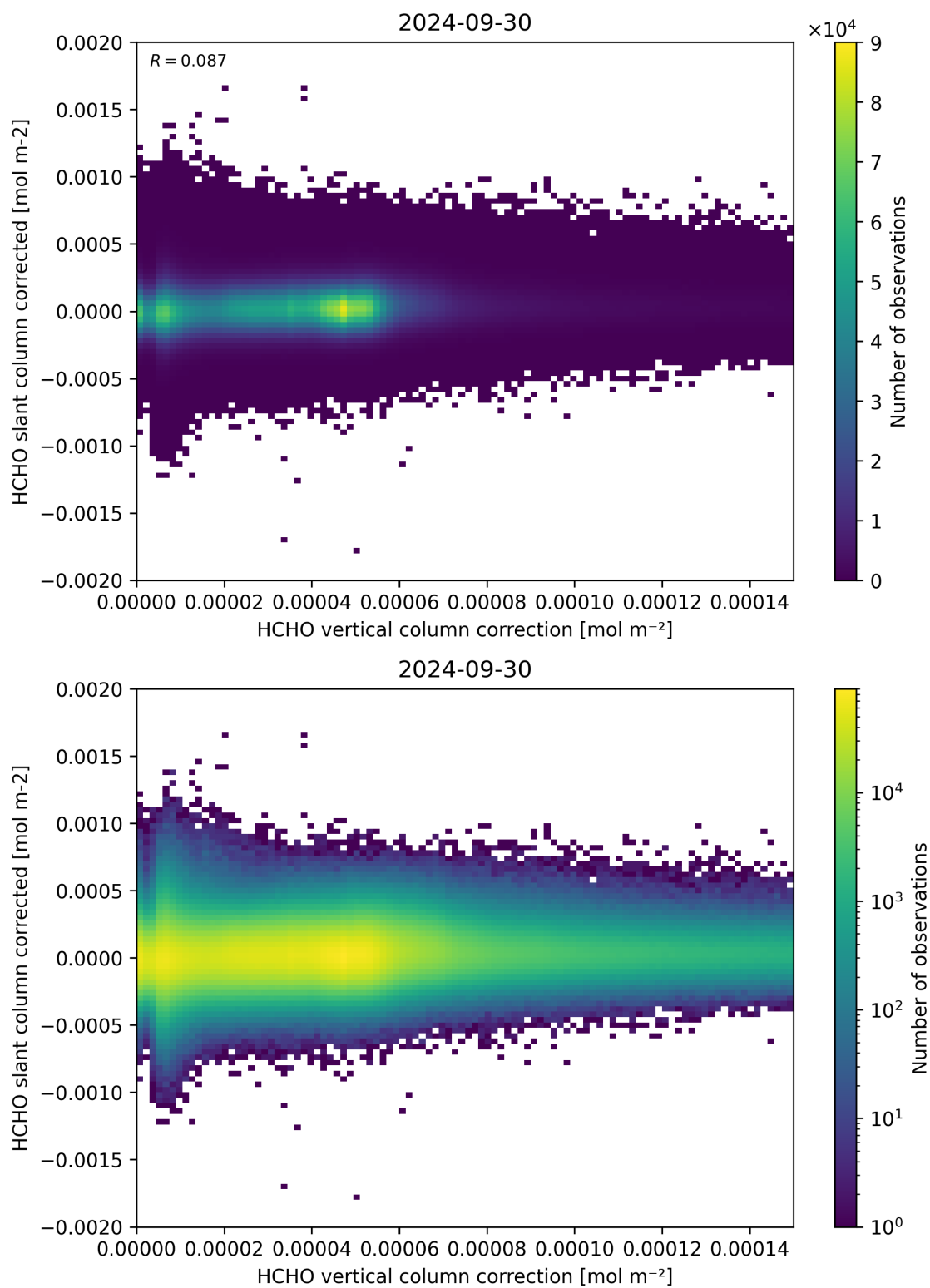
Figure 116: Scatter density plot of “HCHO vertical column correction” against “HCHO slant column corrected” for 2024-09-29 to 2024-10-01.
