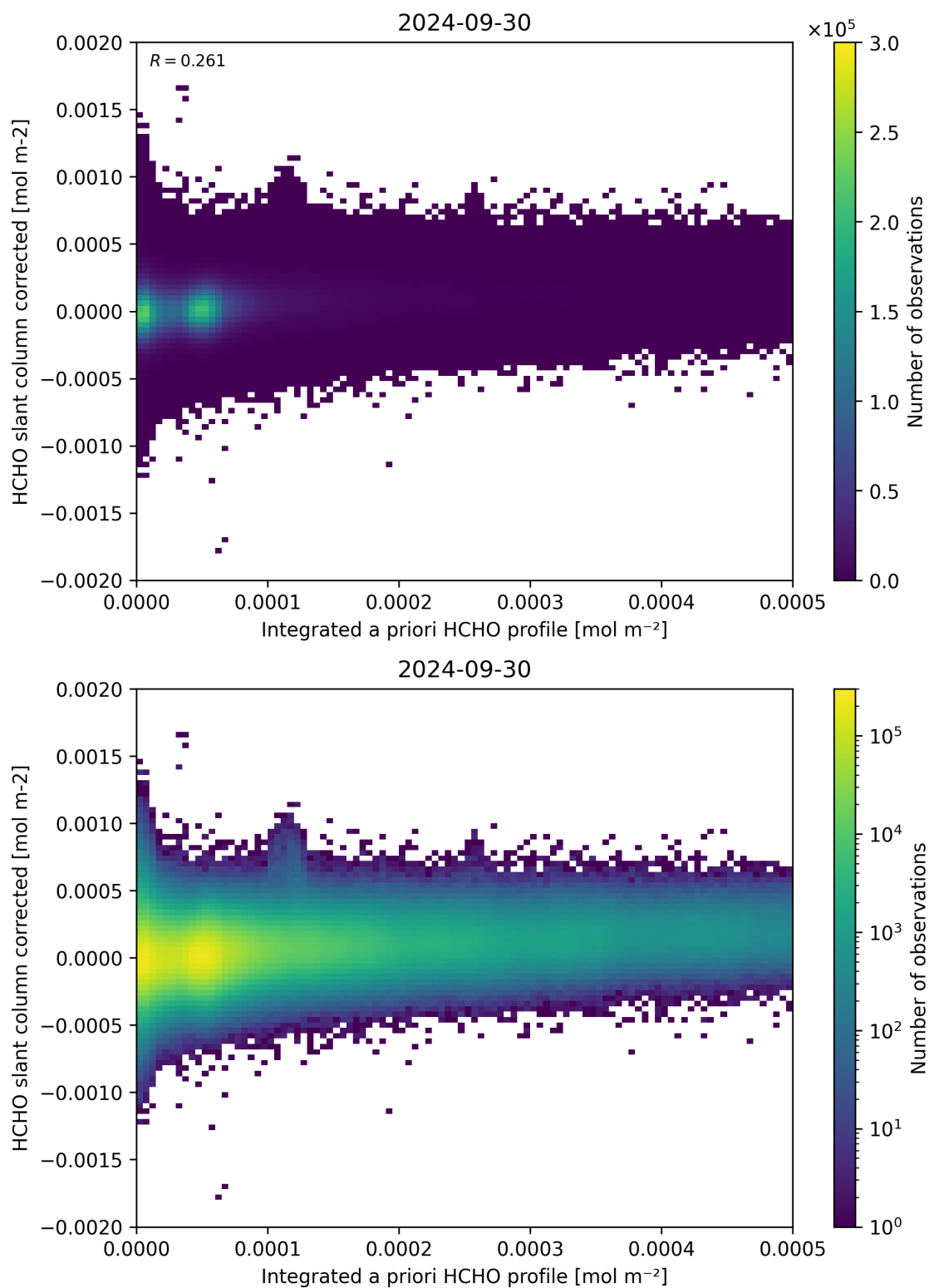
Figure 151: Scatter density plot of “Integrated a priori HCHO profile” against “HCHO slant column corrected” for 2024-09-29 to 2024-10-01.
