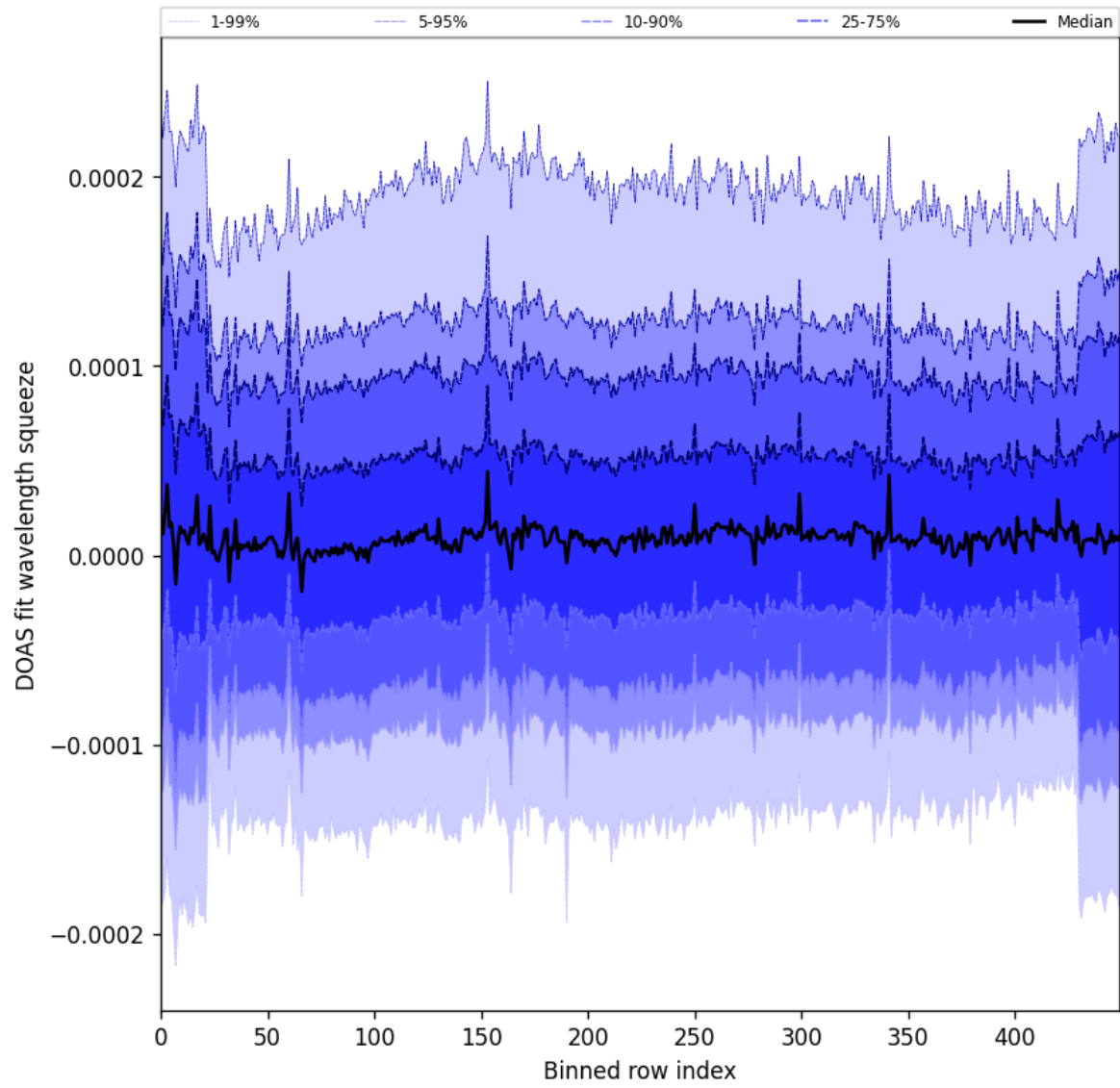
Figure 59: Along track statistics of “DOAS fit wavelength squeeze” for 2024-09-29 to 2024-10-01
