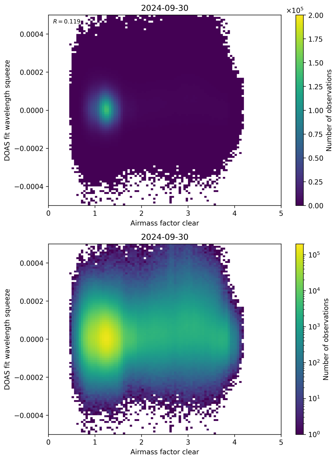
Figure 73: Scatter density plot of “Airmass factor clear” against “DOAS fit wavelength squeeze” for 2024-09-29 to 2024-10-01.
