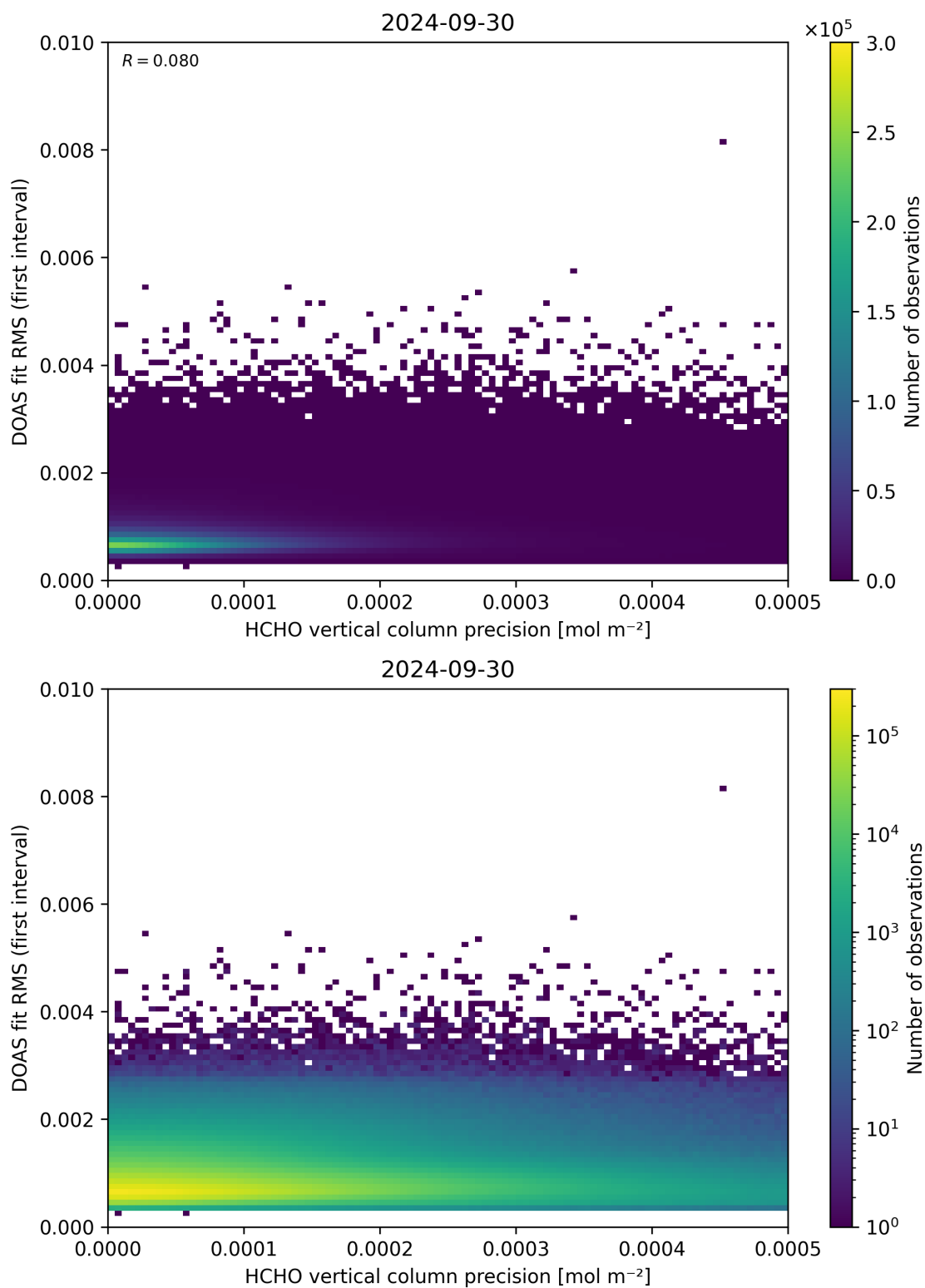
Figure 136: Scatter density plot of “HCHO vertical column precision” against “DOAS fit RMS (first interval)” for 2024-09-29 to 2024-10-01.
