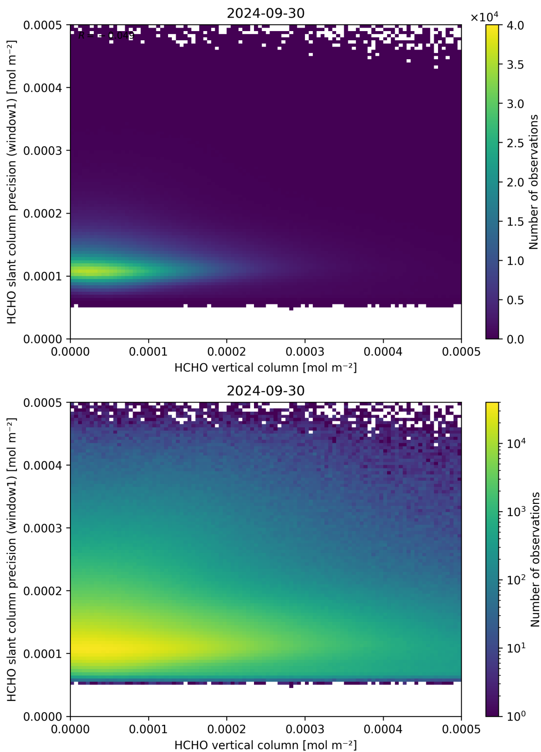
Figure 130: Scatter density plot of “HCHO vertical column” against “HCHO slant column precision (window1)” for 2024-09-29 to 2024-10-01.
