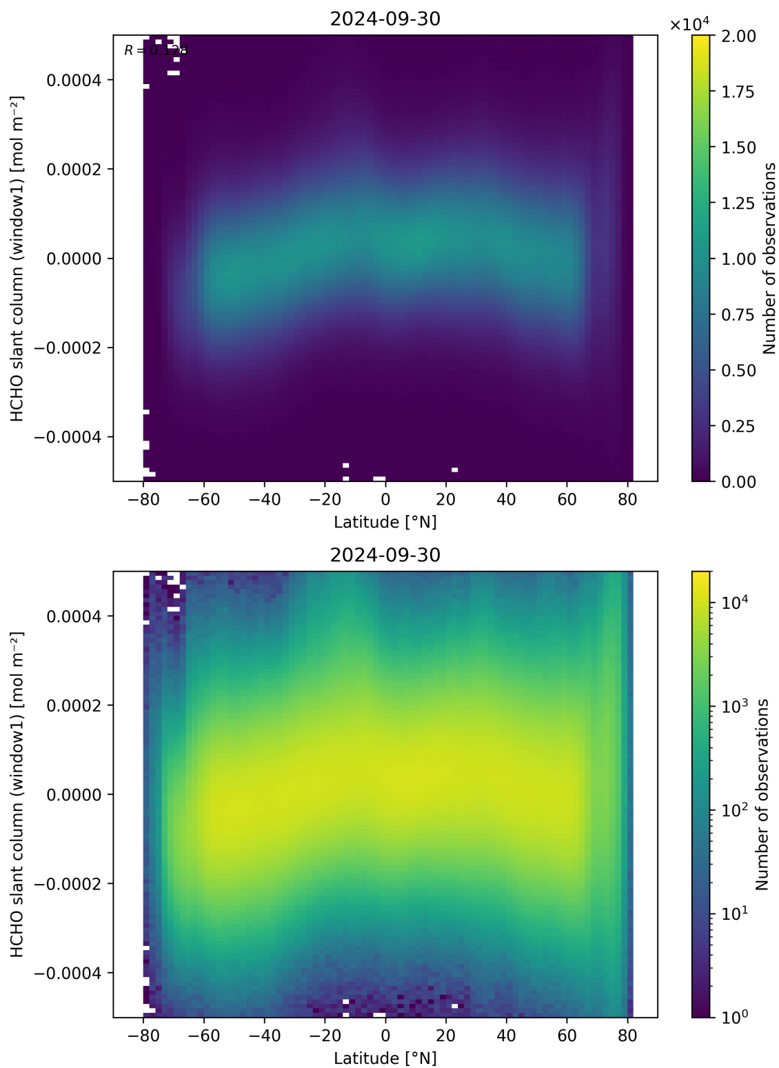
Figure 159: Scatter density plot of “Latitude” against “HCHO slant column (window1)” for 2024-09-29 to 2024-10-01.
