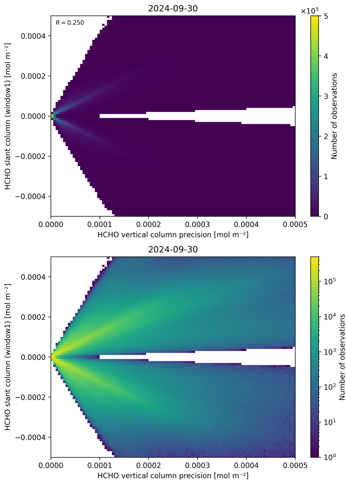
Figure 142: Scatter density plot of “HCHO vertical column precision” against “HCHO slant column (window1)” for 2024-09-29 to 2024-10-01.
