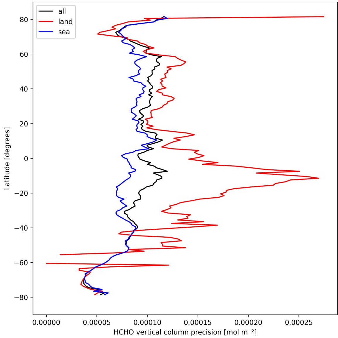
Figure 22: Zonal average of "HCHO vertical column precision" for 2024-09-29 to 2024-10-01.
