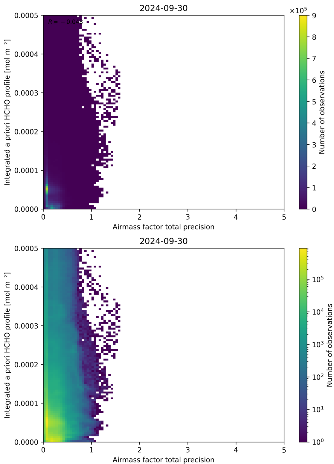
Figure 111: Scatter density plot of “Airmass factor total precision” against “Integrated a priori HCHO profile” for 2024-09-29 to 2024-10-01.
