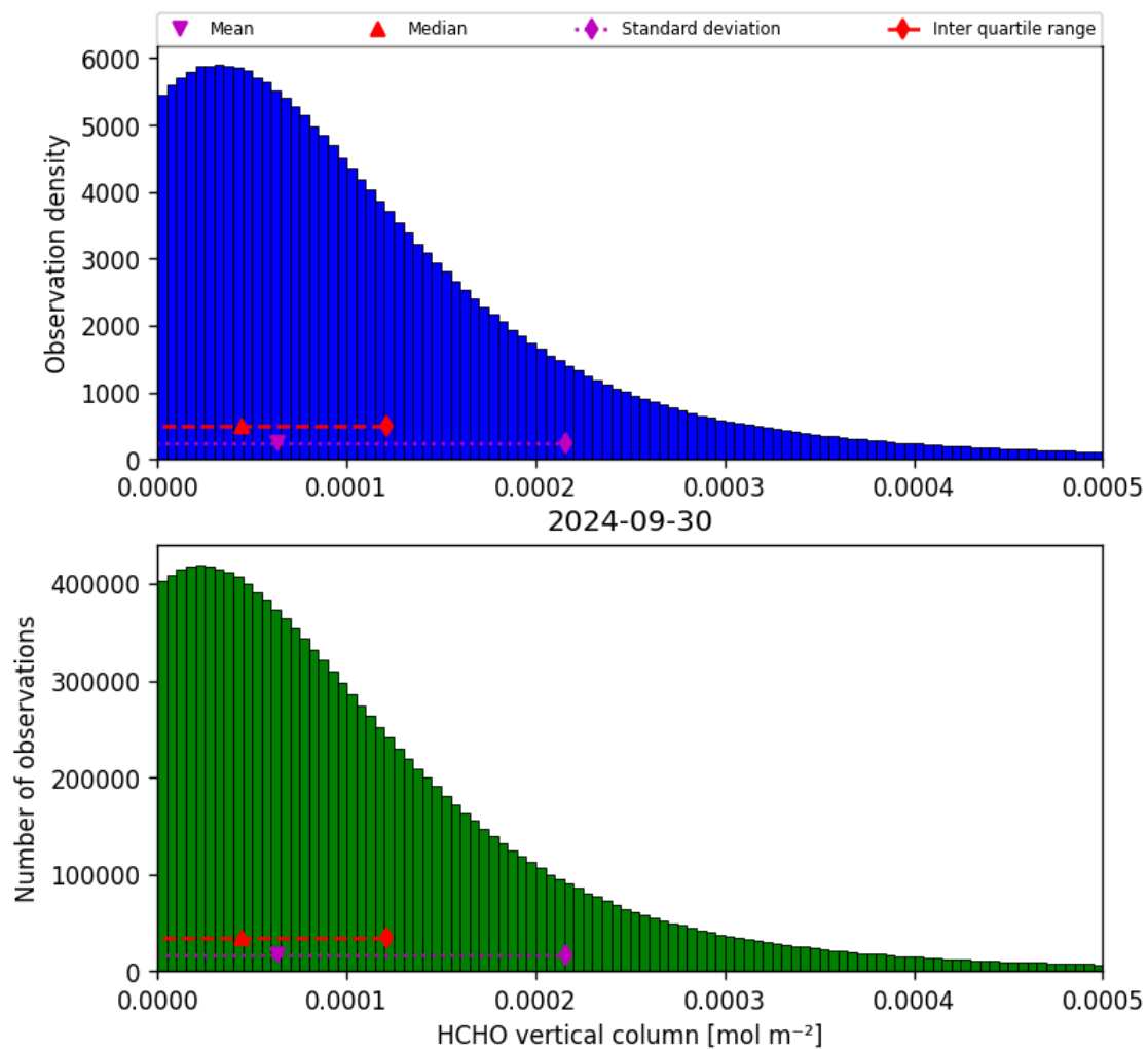
Figure 35: Histogram of “HCHO vertical column” for 2024-09-29 to 2024-10-01
