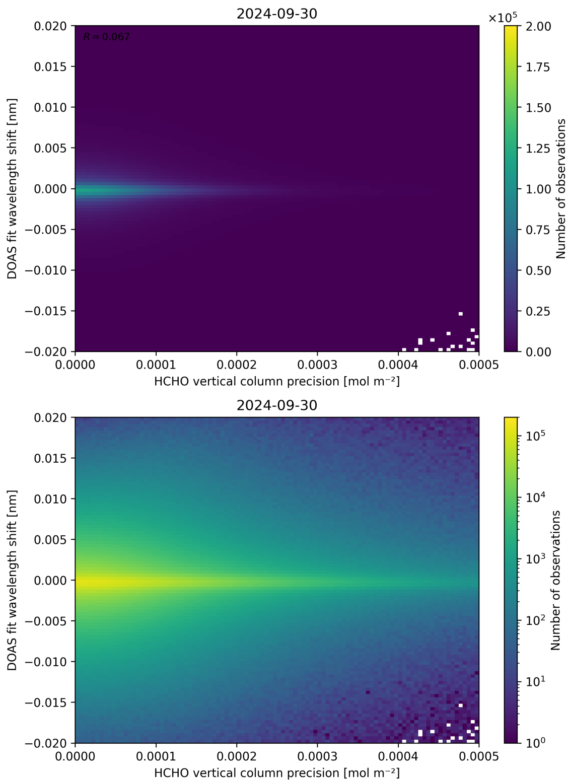
Figure 137: Scatter density plot of “HCHO vertical column precision” against “DOAS fit wavelength shift” for 2024-09-29 to 2024-10-01.
