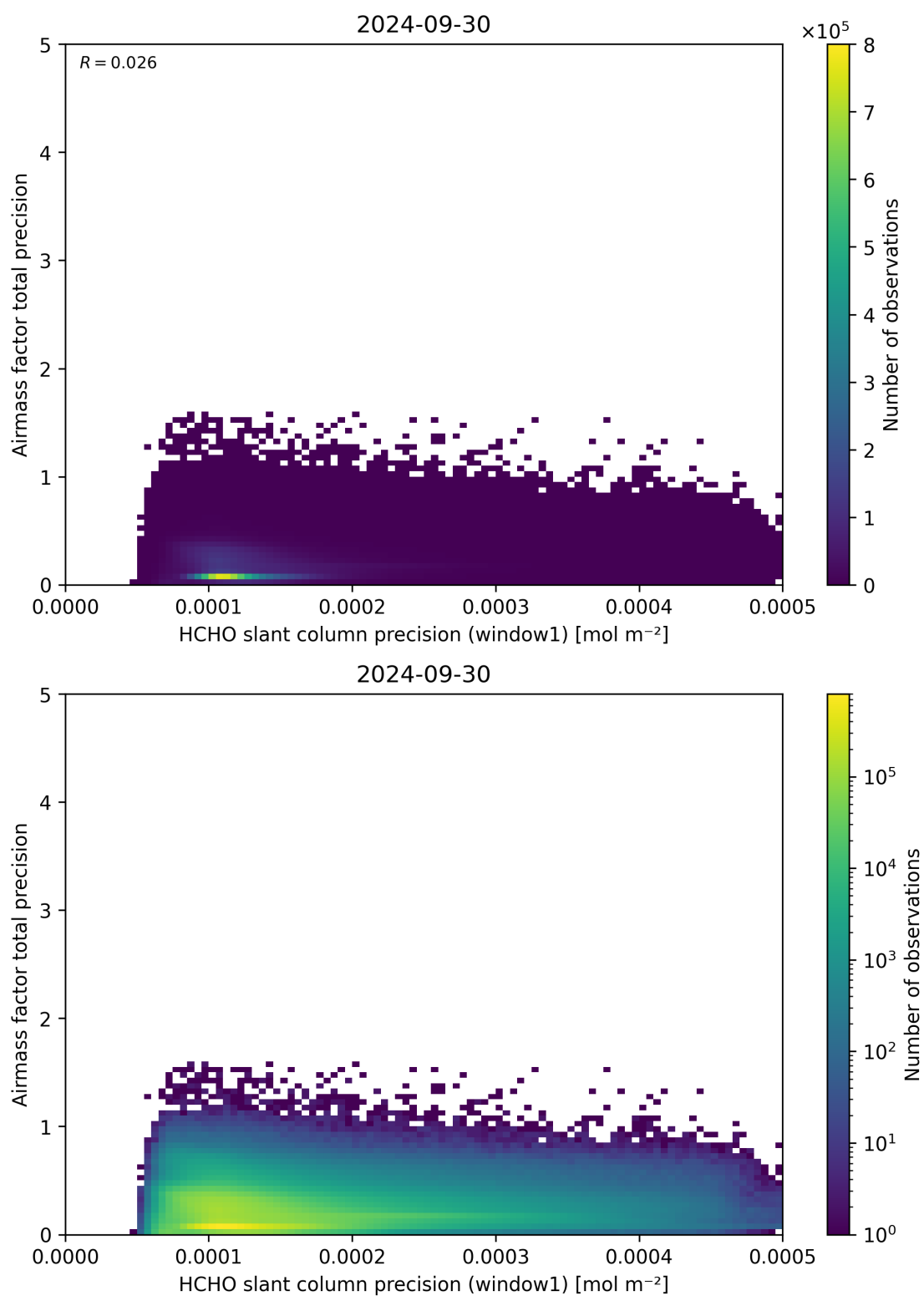
Figure 95: Scatter density plot of “HCHO slant column precision (window1)” against “Airmass factor total precision” for 2024-09-29 to 2024-10-01.
