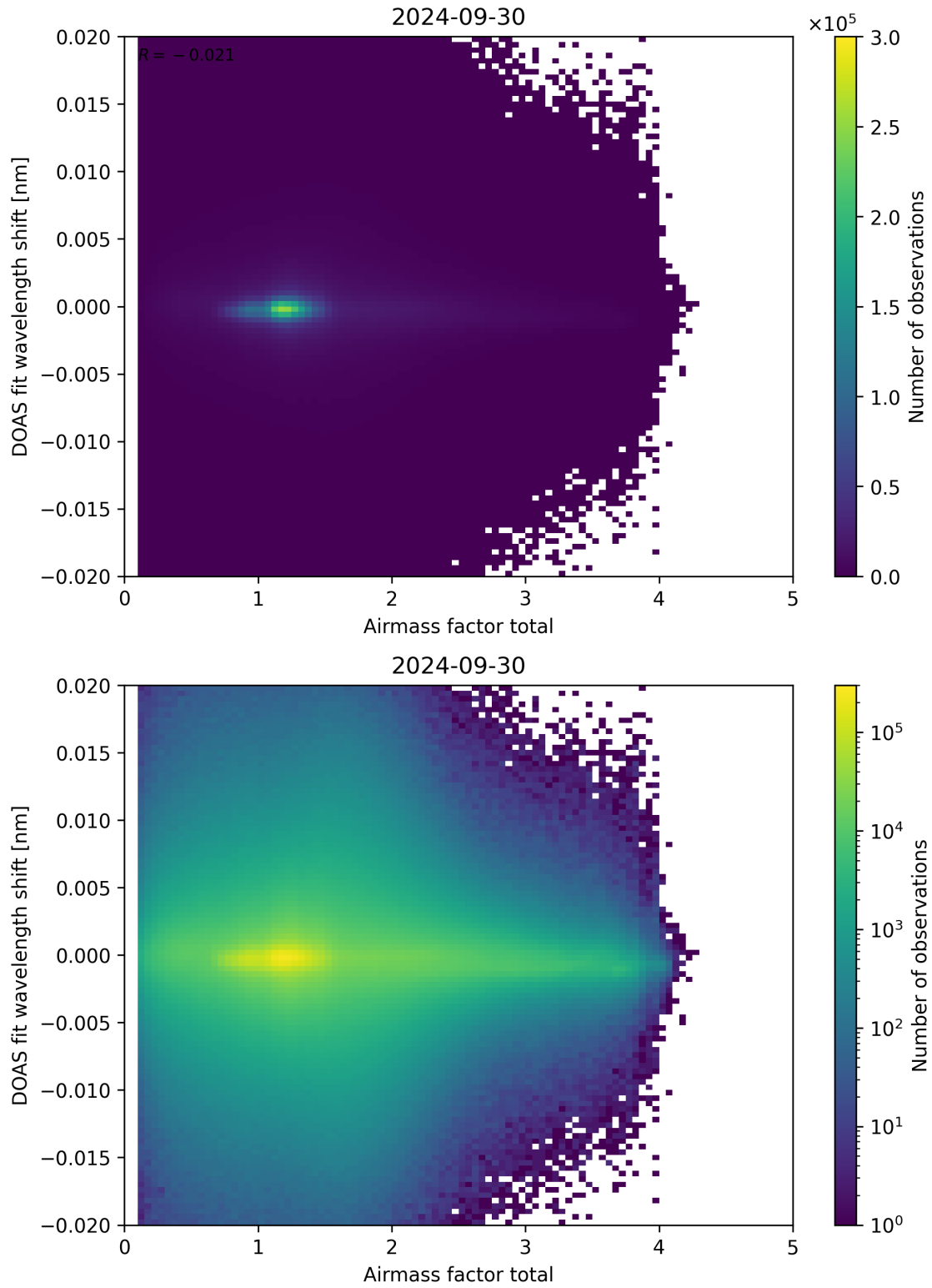
Figure 98: Scatter density plot of “Airmass factor total” against “DOAS fit wavelength shift” for 2024-09-29 to 2024-10-01.
