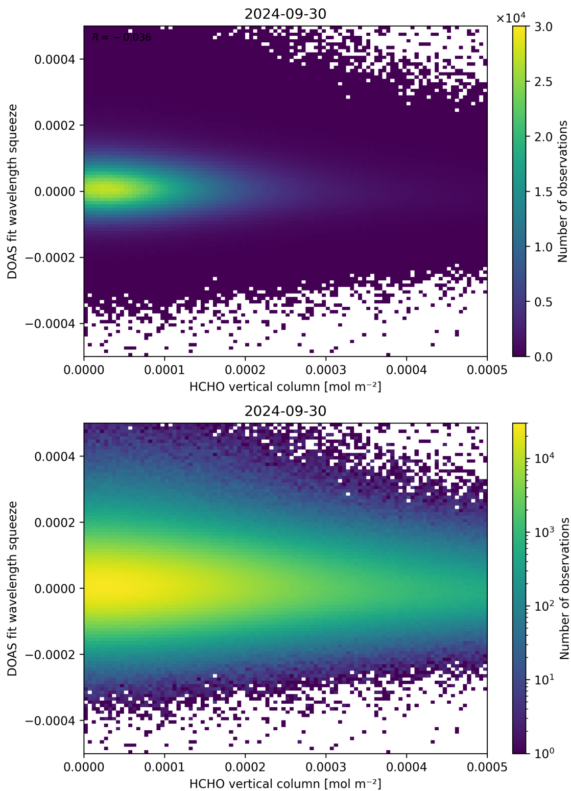
Figure 125: Scatter density plot of “HCHO vertical column” against “DOAS fit wavelength squeeze” for 2024-09-29 to 2024-10-01.
