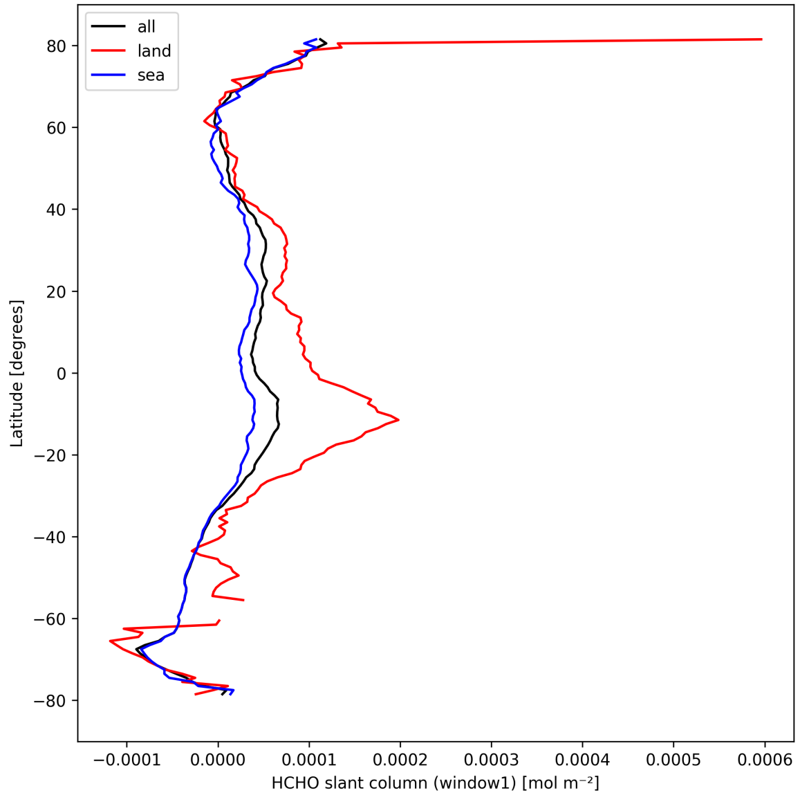
Figure 24: Zonal average of “HCHO slant column (window1)” for 2024-09-29 to 2024-10-01.
