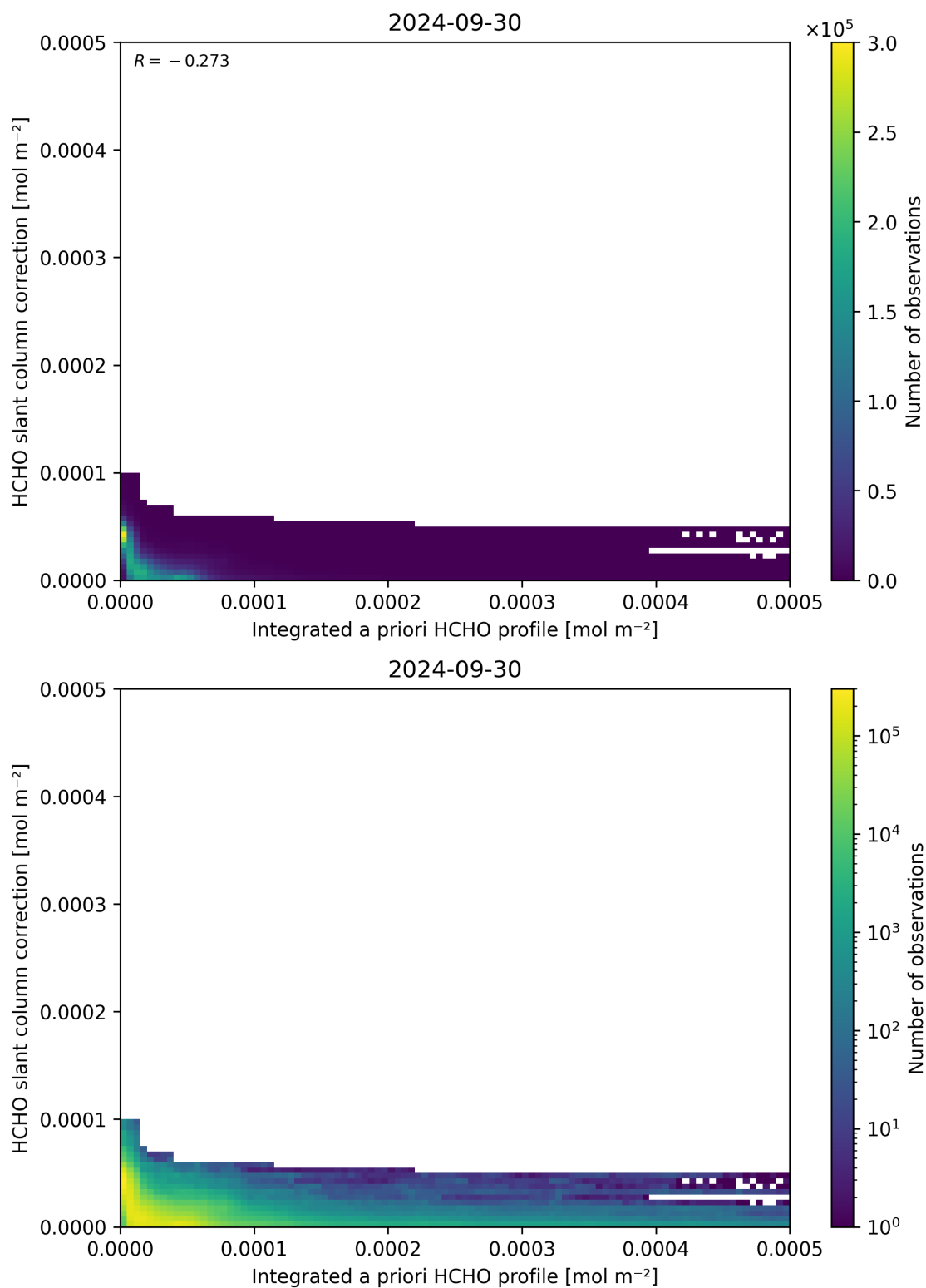
Figure 152: Scatter density plot of “Integrated a priori HCHO profile” against “HCHO slant column correction” for 2024-09-29 to 2024-10-01.
