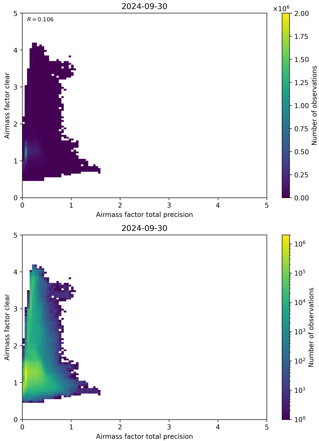
Figure 108: Scatter density plot of “Airmass factor total precision” against “Airmass factor clear” for 2024-09-29 to 2024-10-01.
