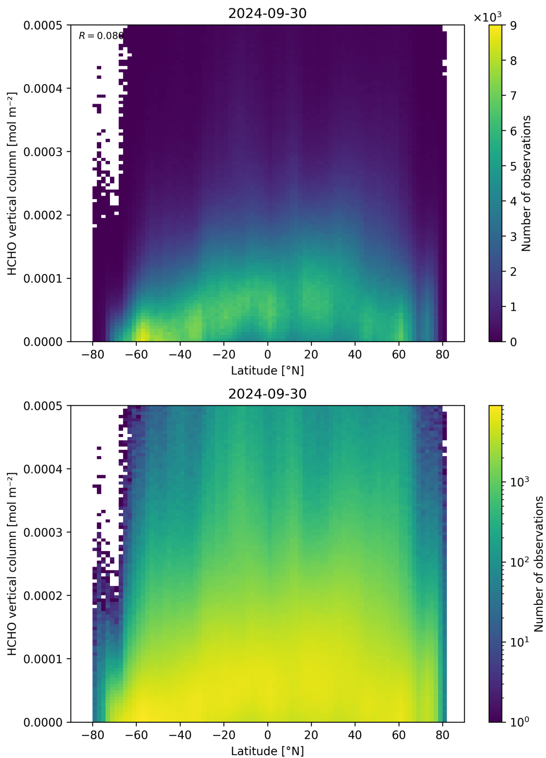
Figure 163: Scatter density plot of “Latitude” against “HCHO vertical column” for 2024-09-29 to 2024-10-01.
