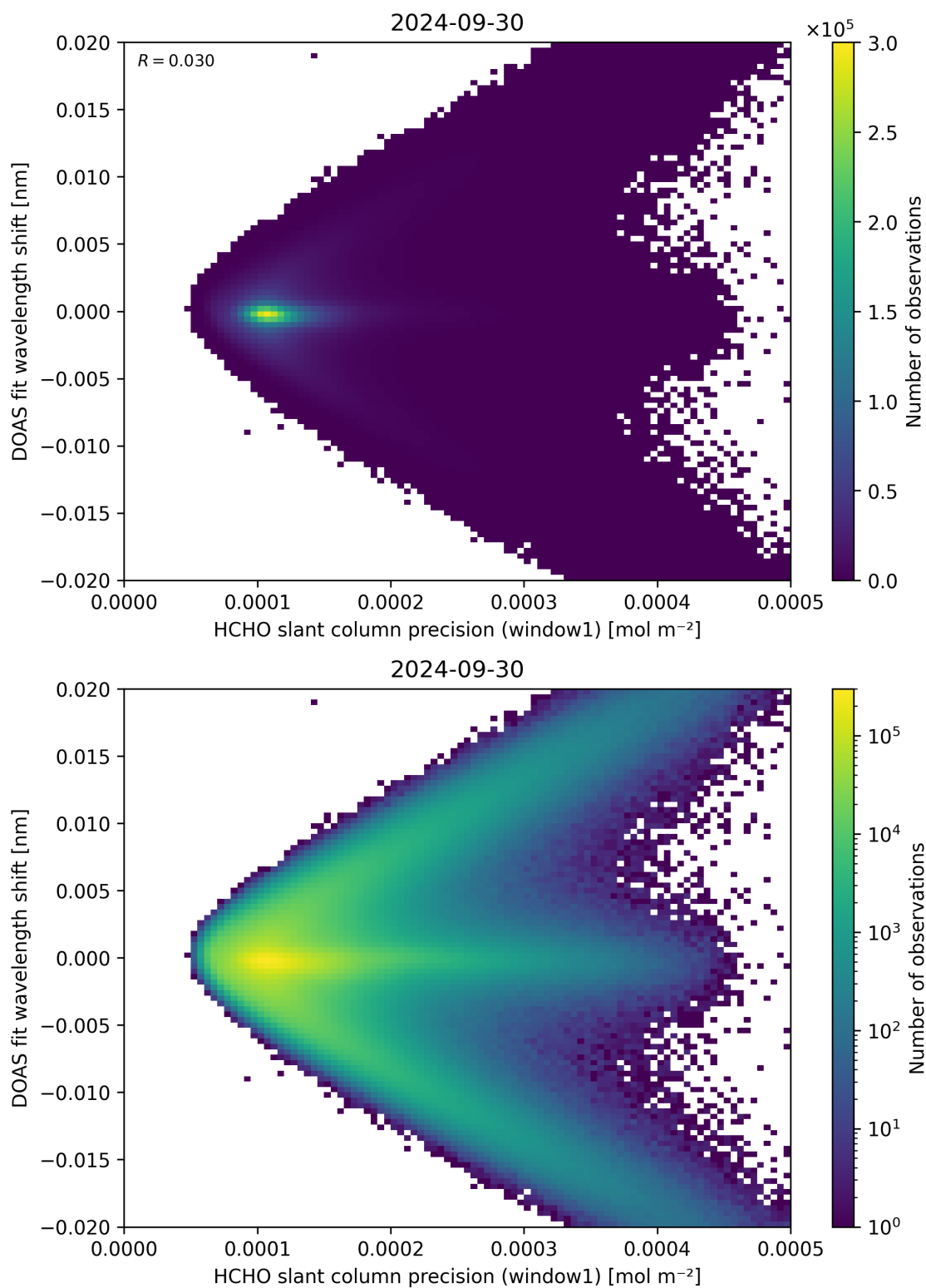
Figure 89: Scatter density plot of “HCHO slant column precision (window1)” against “DOAS fit wavelength shift” for 2024-09-29 to 2024-10-01.
