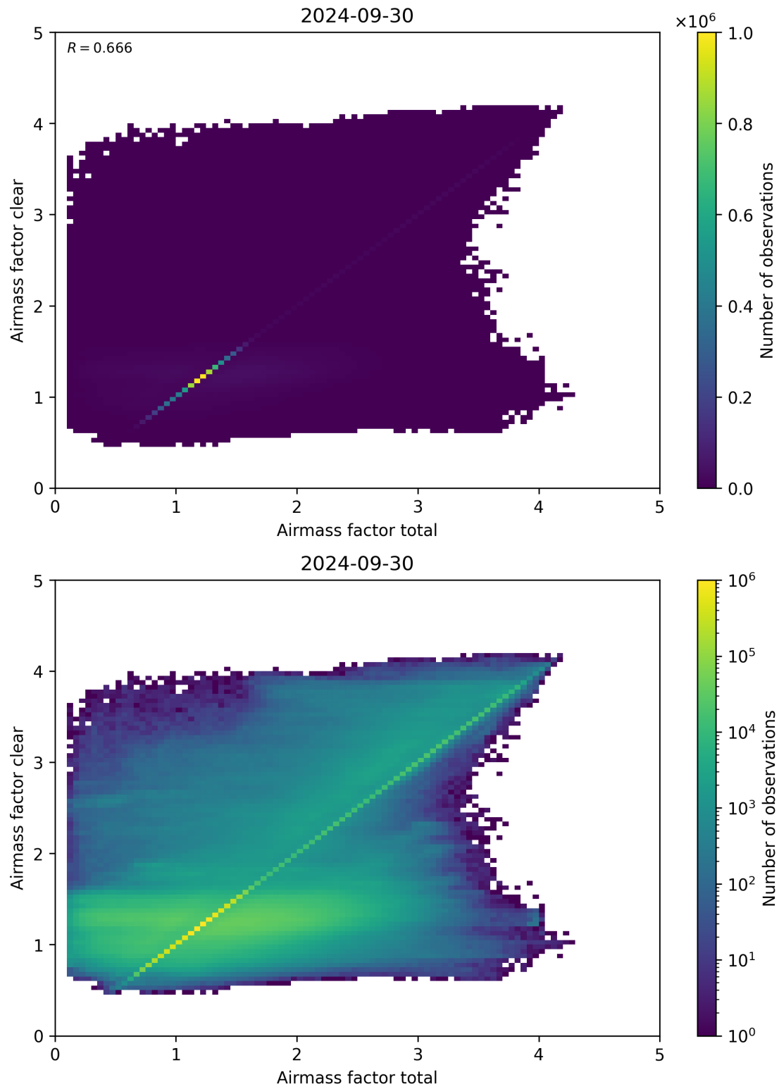
Figure 100: Scatter density plot of “Airmass factor total” against “Airmass factor clear” for 2024-09-29 to 2024-10-01.
