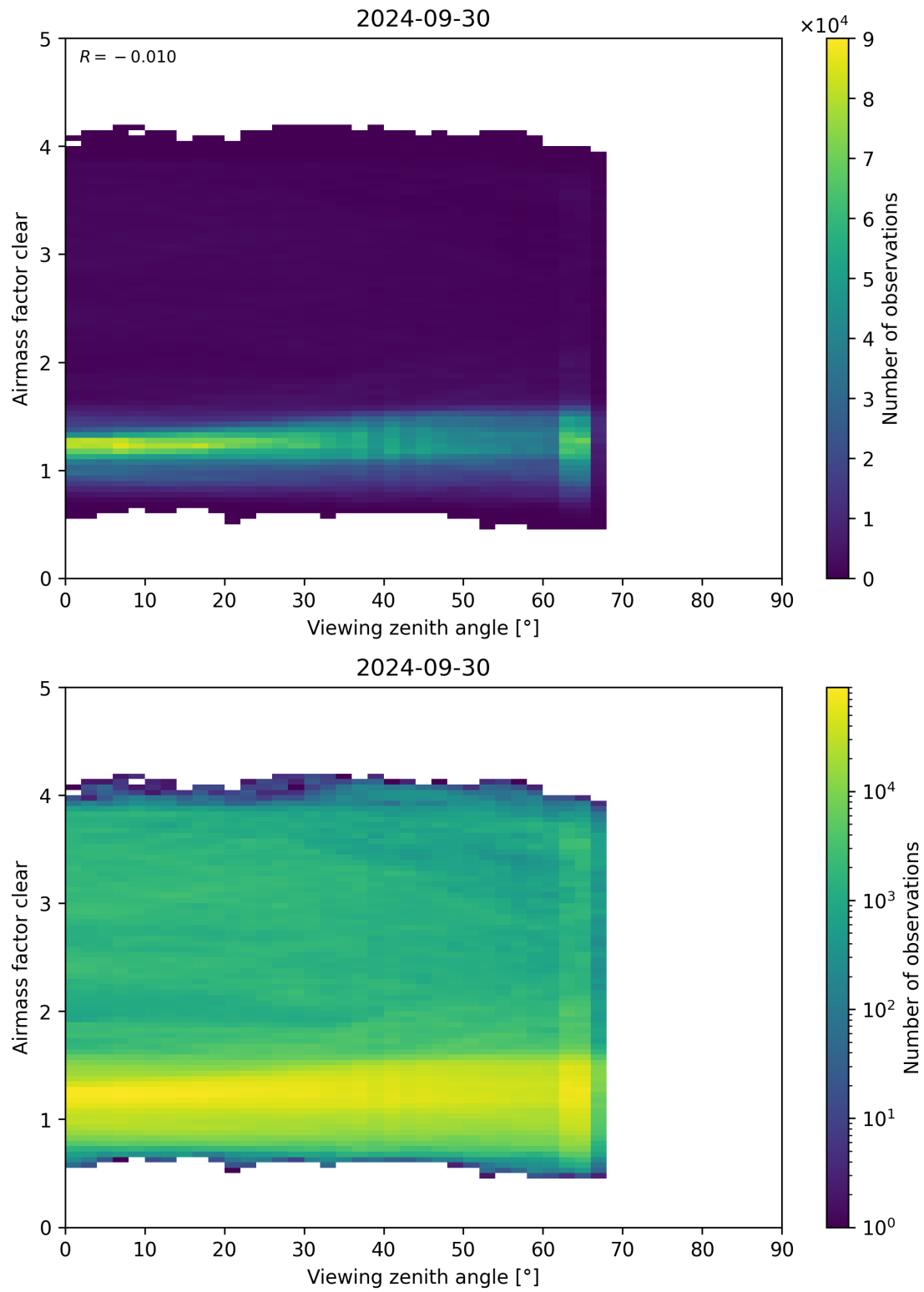
Figure 185: Scatter density plot of “Viewing zenith angle” against “Airmass factor clear” for 2024-09-29 to 2024-10-01.
