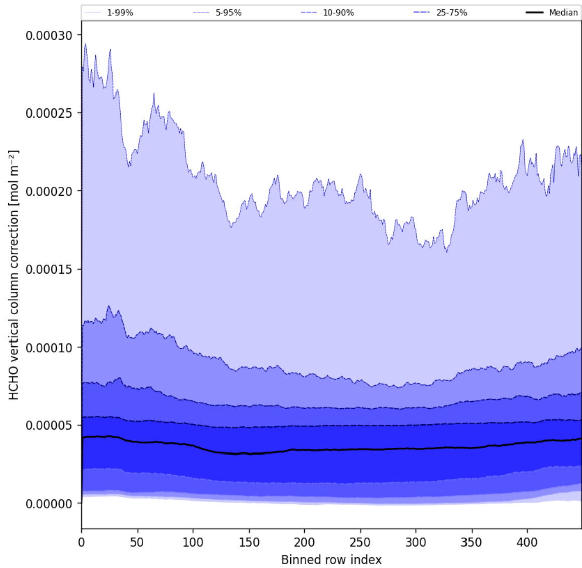
Figure 51: Along track statistics of “HCHO vertical column correction” for 2024-09-29 to 2024-10-01
