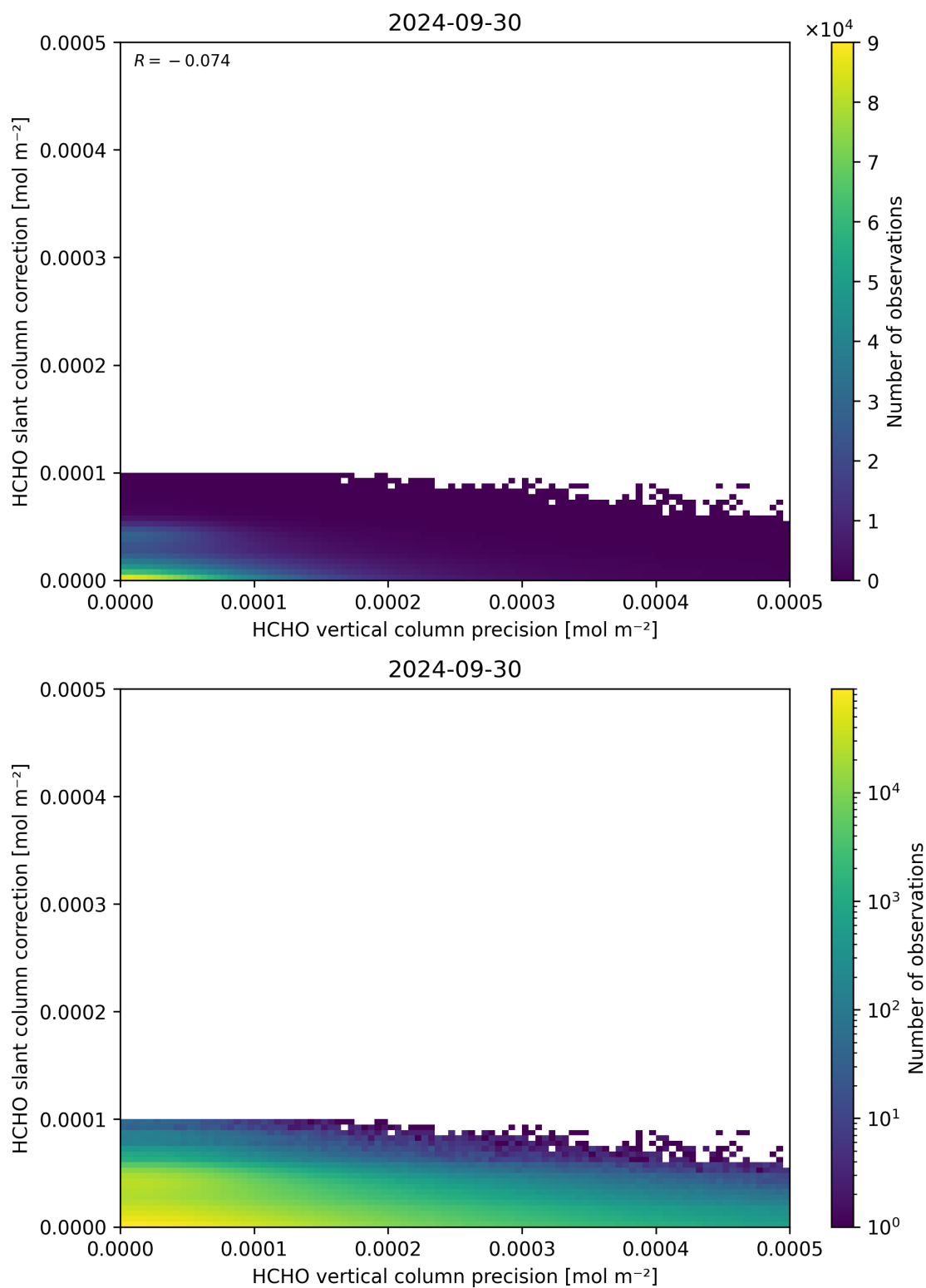
Figure 141: Scatter density plot of “HCHO vertical column precision” against “HCHO slant column correction” for 2024-09-29 to 2024-10-01.
