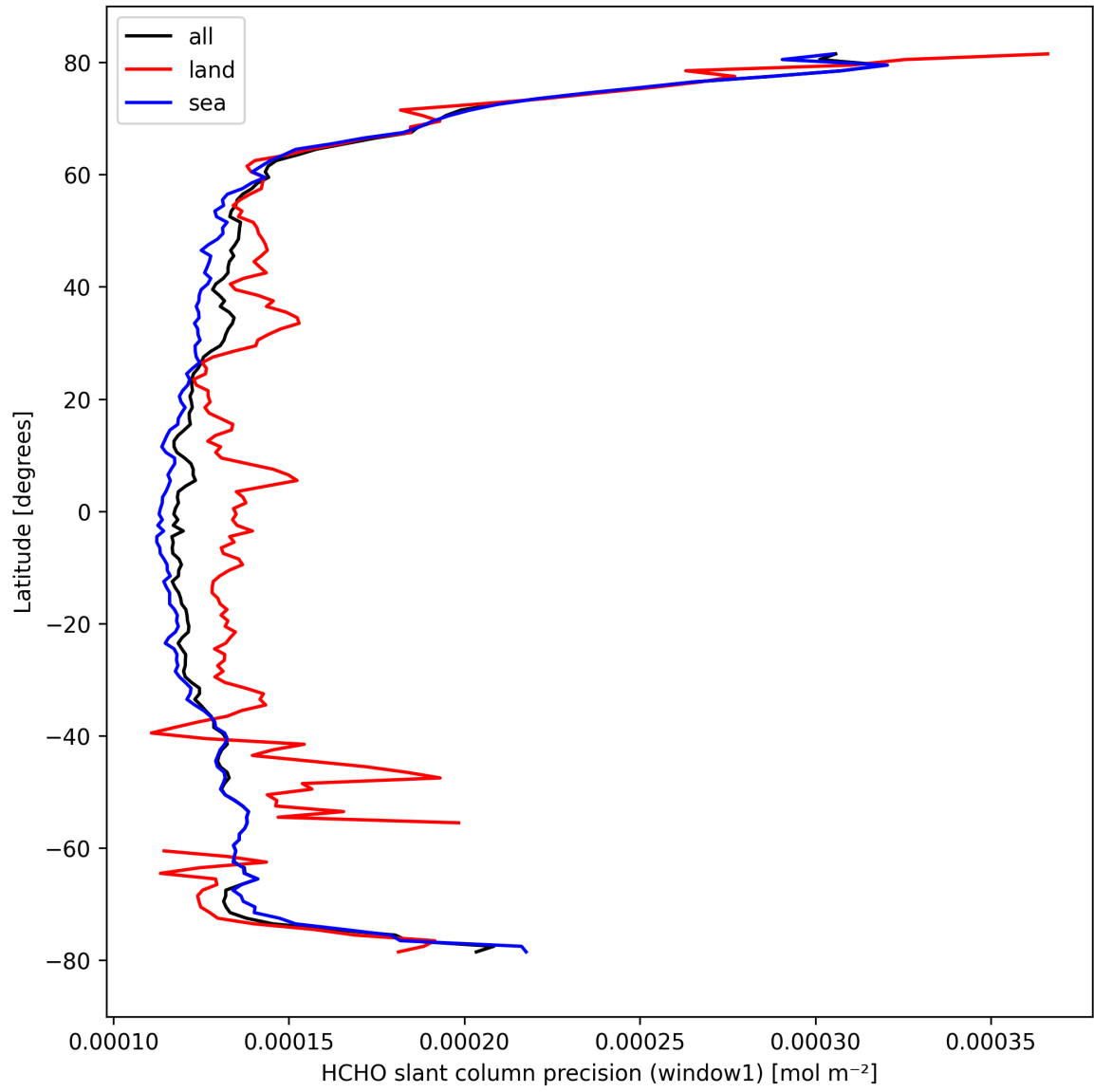
Figure 25: Zonal average of "HCHO slant column precision (window1)" for 2024-09-29 to 2024-10-01.
