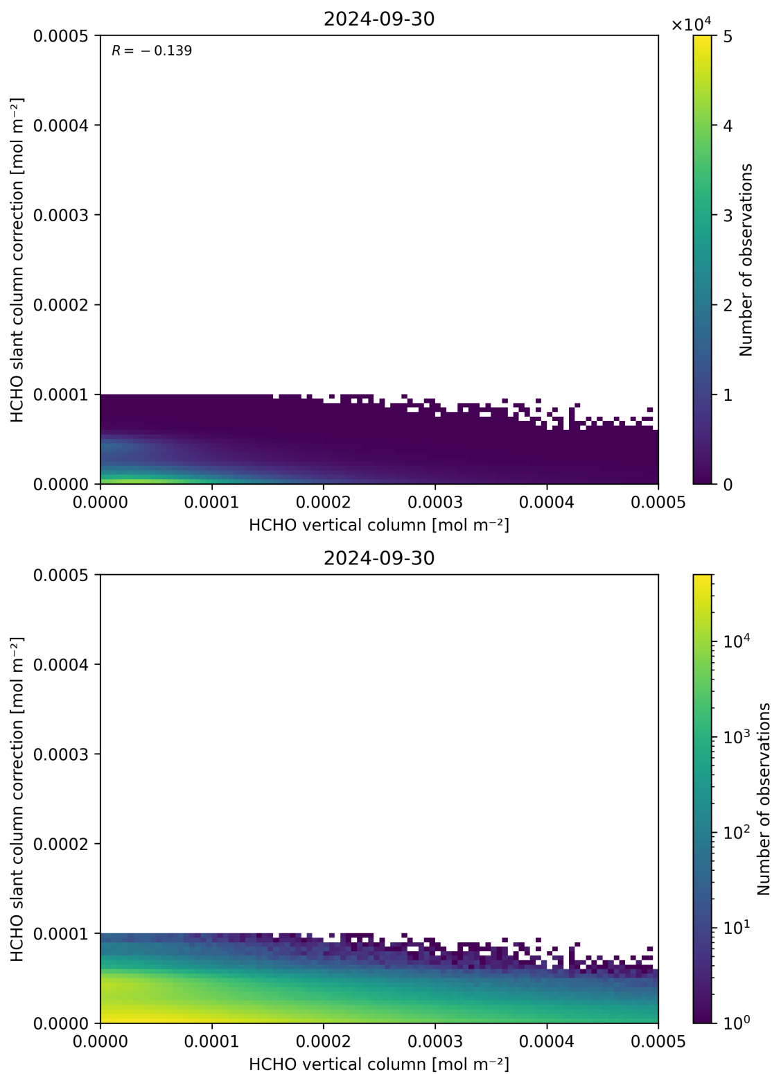
Figure 128: Scatter density plot of “HCHO vertical column” against “HCHO slant column correction” for 2024-09-29 to 2024-10-01.
