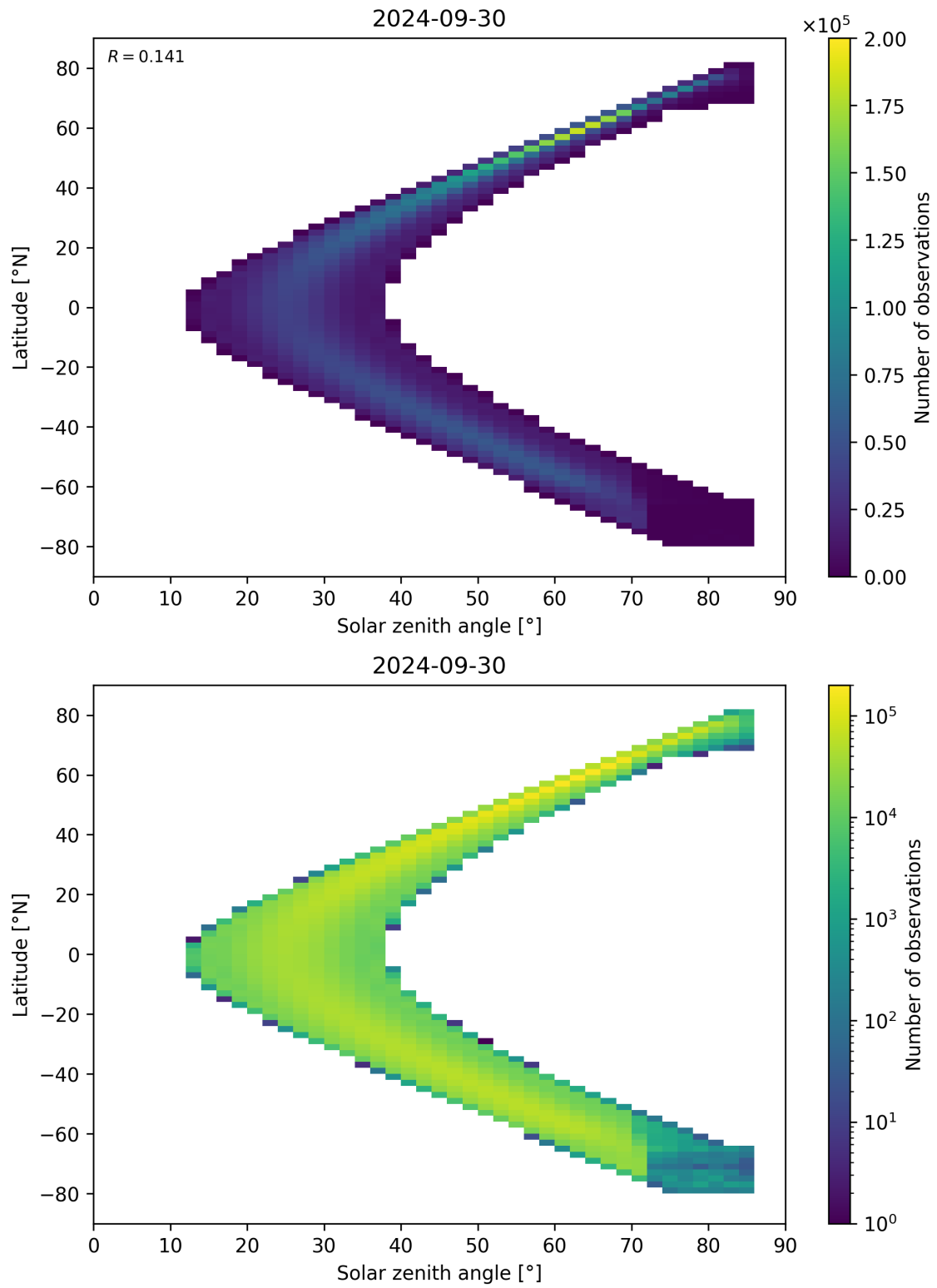
Figure 181: Scatter density plot of “Solar zenith angle” against “Latitude” for 2024-09-29 to 2024-10-01.
