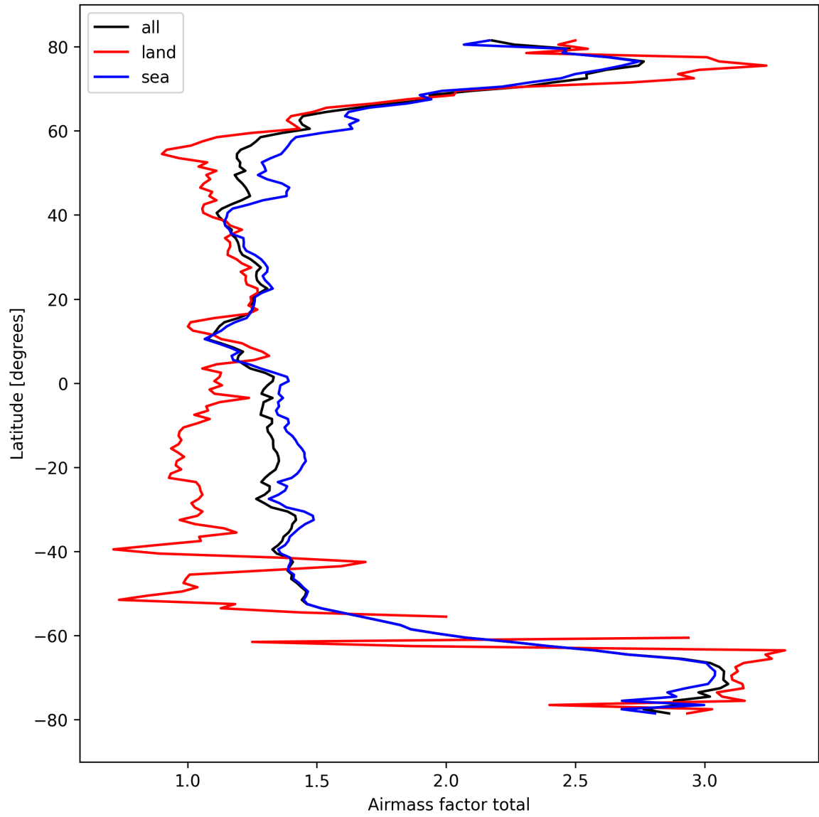
Figure 26: Zonal average of “Airmass factor total” for 2024-09-29 to 2024-10-01.
