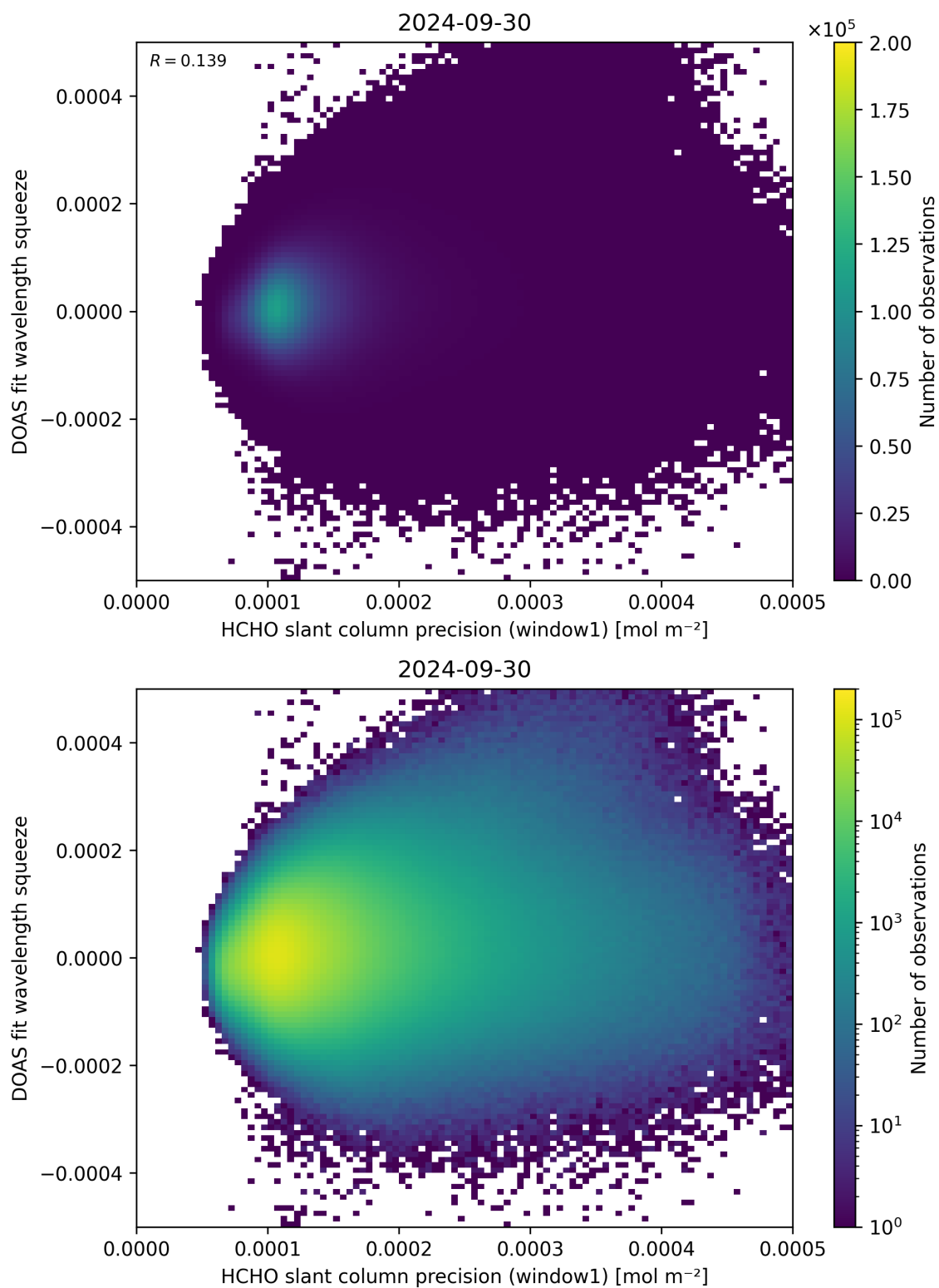
Figure 90: Scatter density plot of “HCHO slant column precision (window1)” against “DOAS fit wavelength squeeze” for 2024-09-29 to 2024-10-01.
