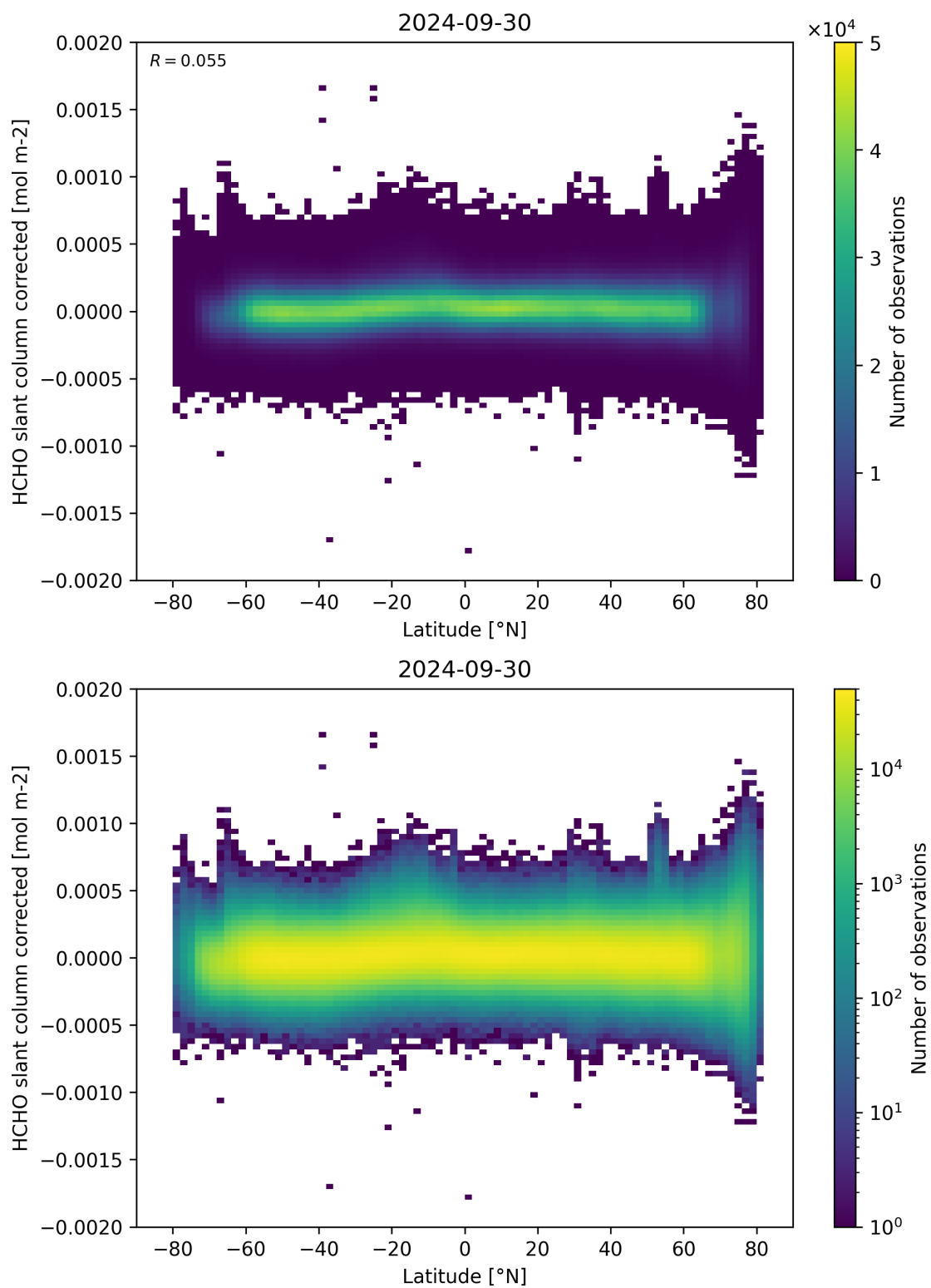
Figure 157: Scatter density plot of “Latitude” against “HCHO slant column corrected” for 2024-09-29 to 2024-10-01.
