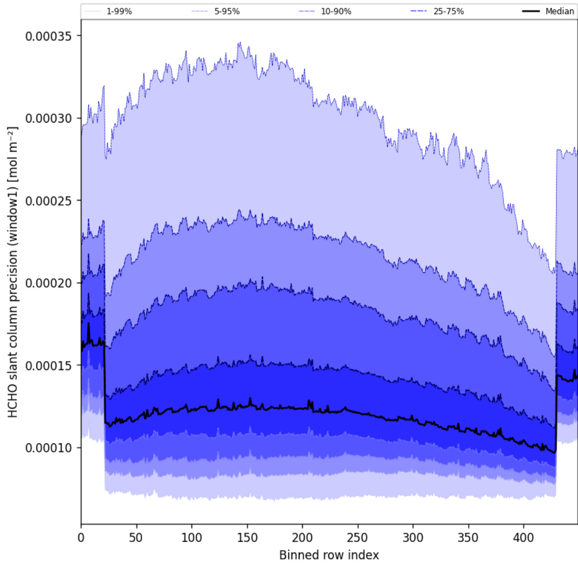
Figure 53: Along track statistics of “HCHO slant column precision (window1)” for 2024-09-29 to 2024-10-01
