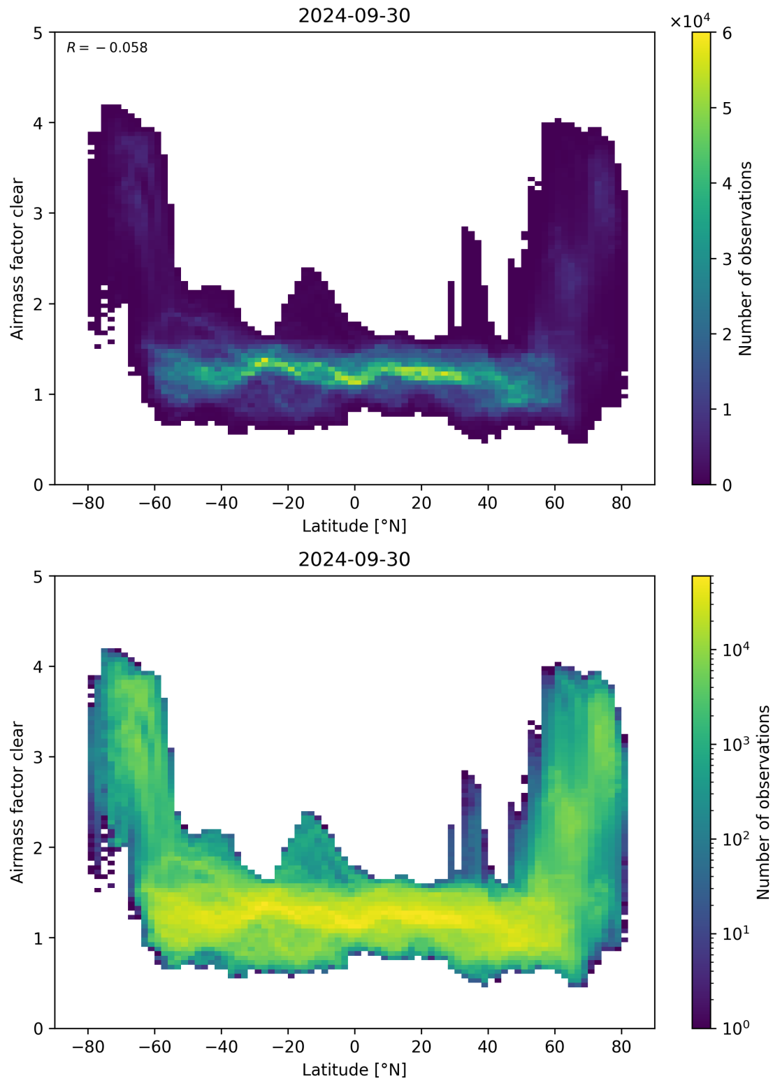
Figure 156: Scatter density plot of “Latitude” against “Airmass factor clear” for 2024-09-29 to 2024-10-01.
