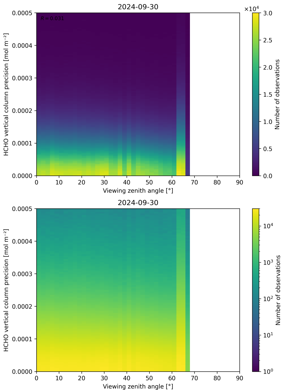
Figure 194: Scatter density plot of “Viewing zenith angle” against “HCHO vertical column precision” for 2024-09-29 to 2024-10-01.
