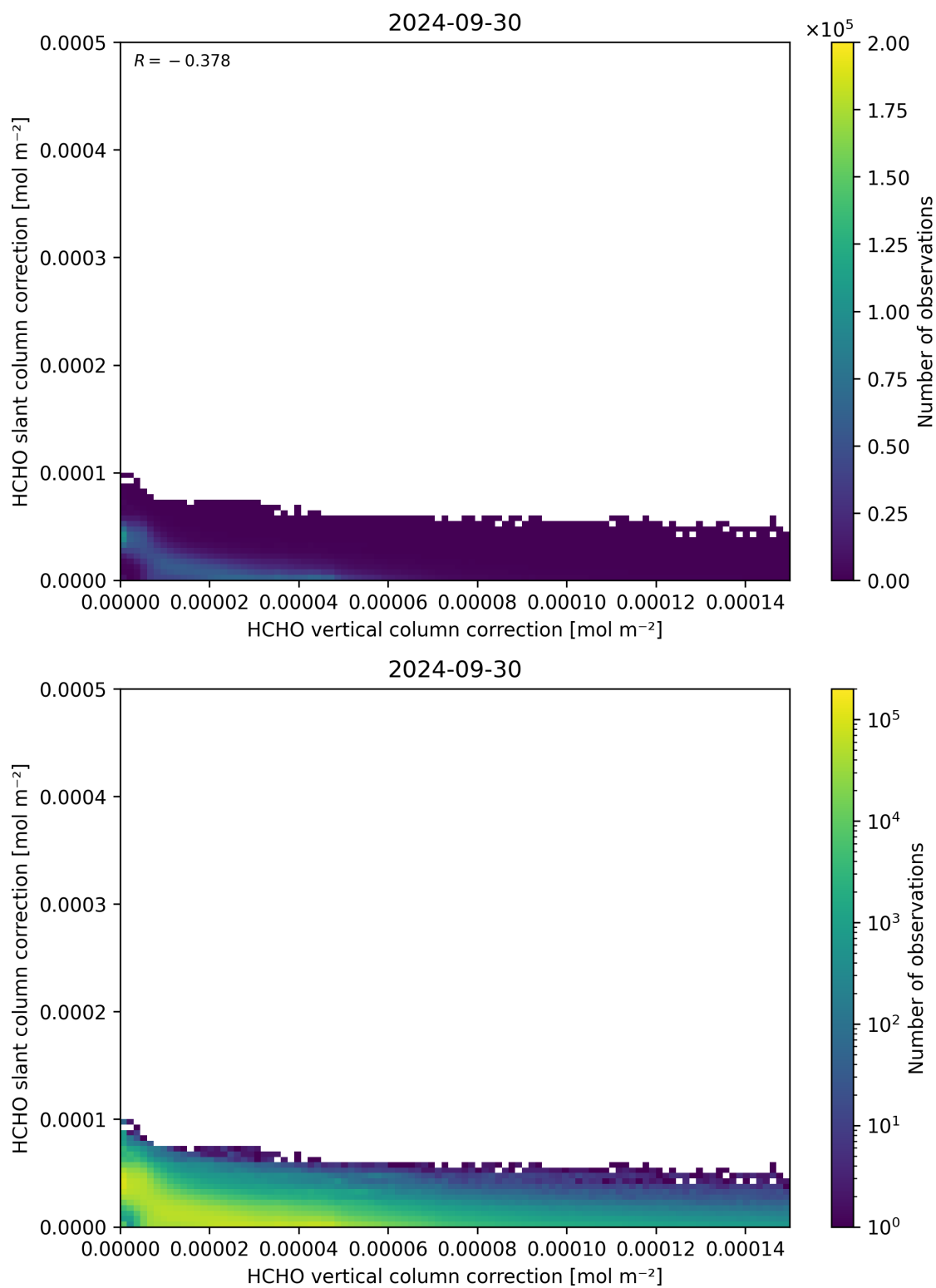
Figure 117: Scatter density plot of “HCHO vertical column correction” against “HCHO slant column correction” for 2024-09-29 to 2024-10-01.
