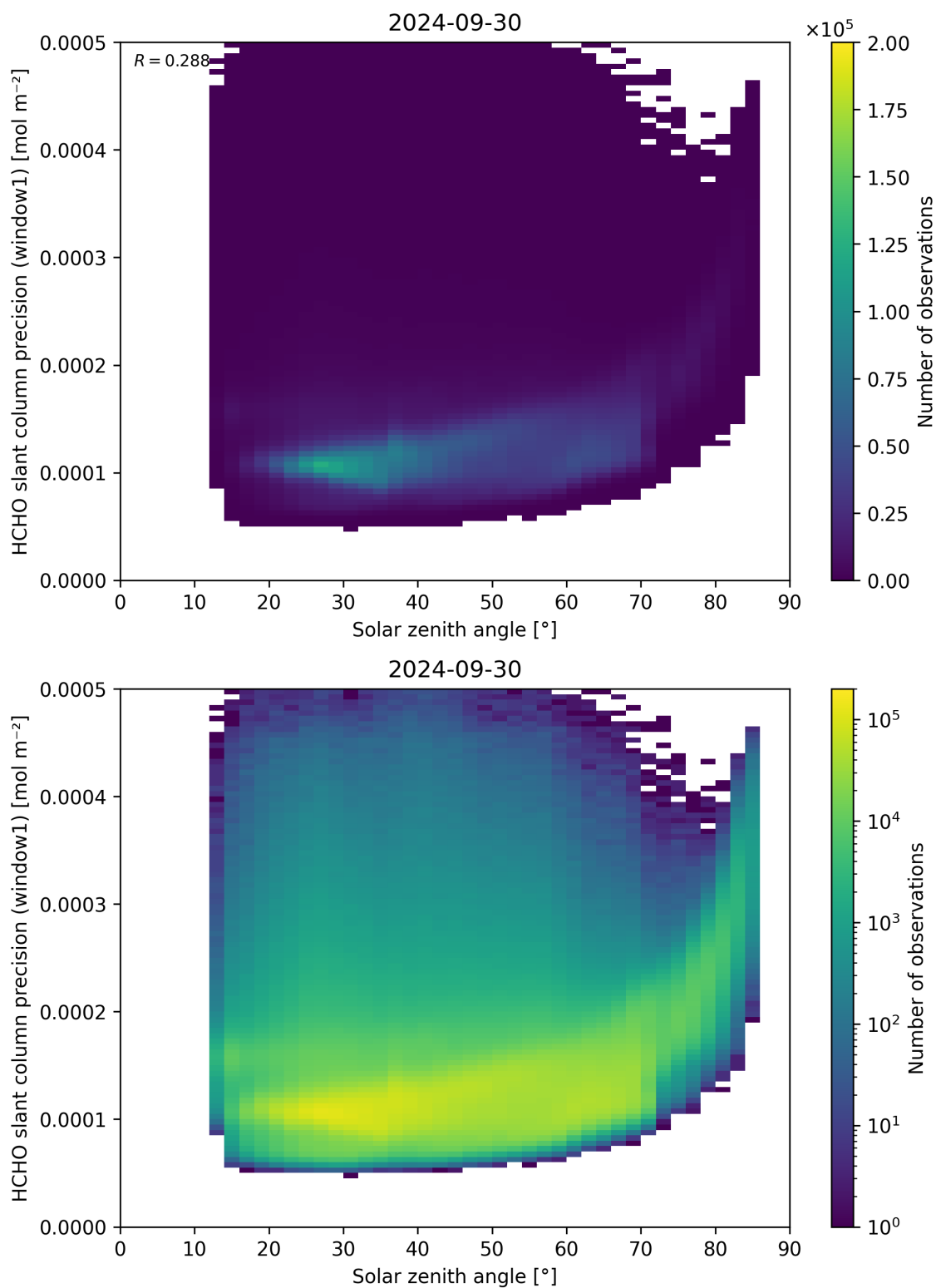
Figure 174: Scatter density plot of “Solar zenith angle” against “HCHO slant column precision (window1)” for 2024-09-29 to 2024-10-01.
