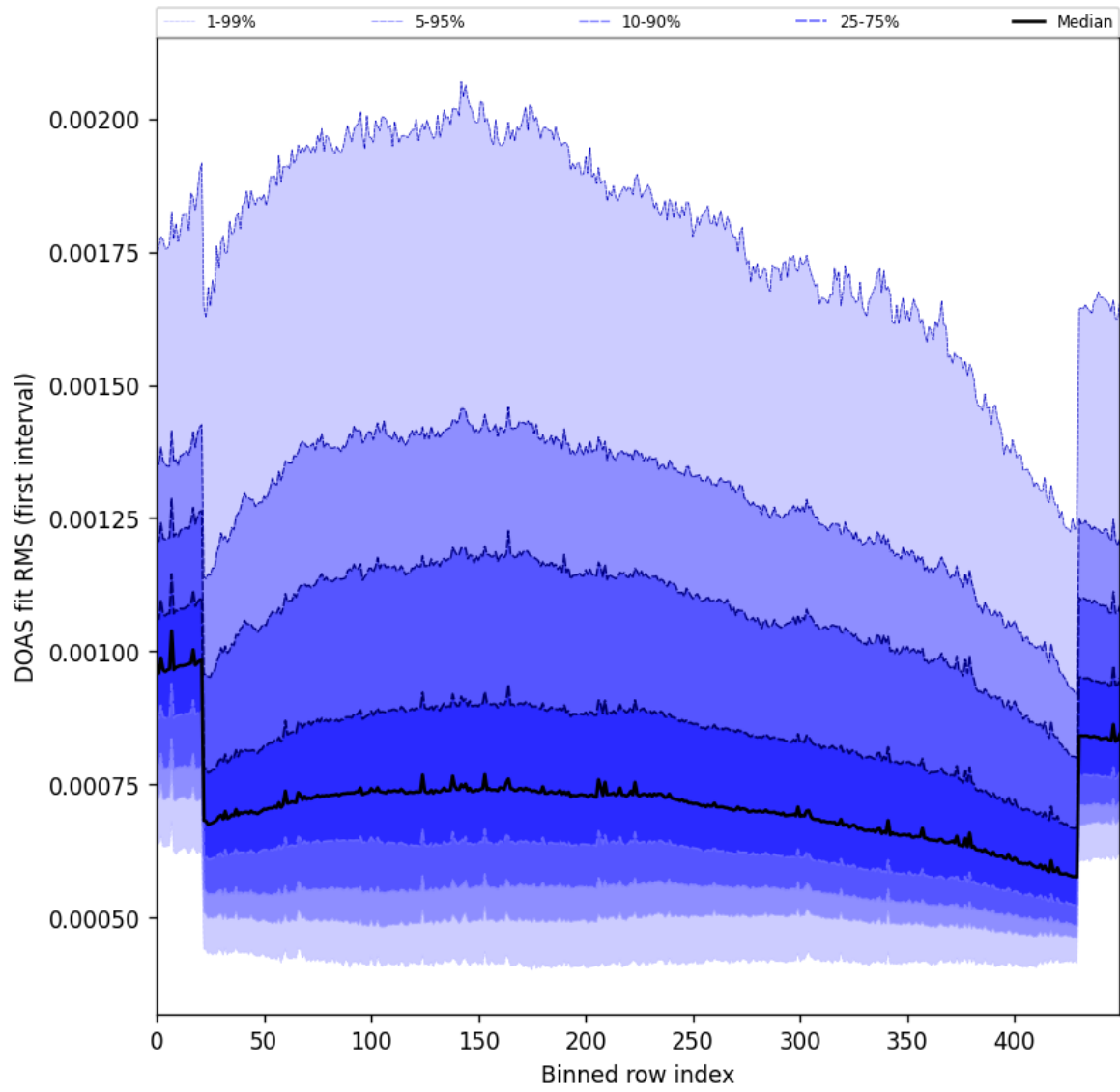
Figure 60: Along track statistics of “DOAS fit RMS (first interval)” for 2024-09-29 to 2024-10-01
