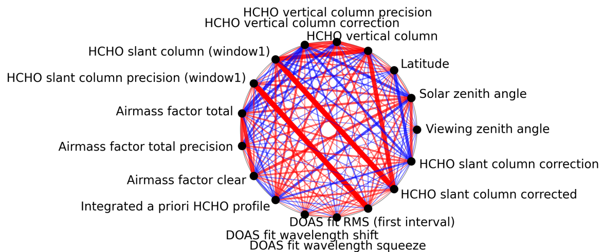
Figure 1: Map of correlation graph for 2024-09-29 to 2024-10-01.
