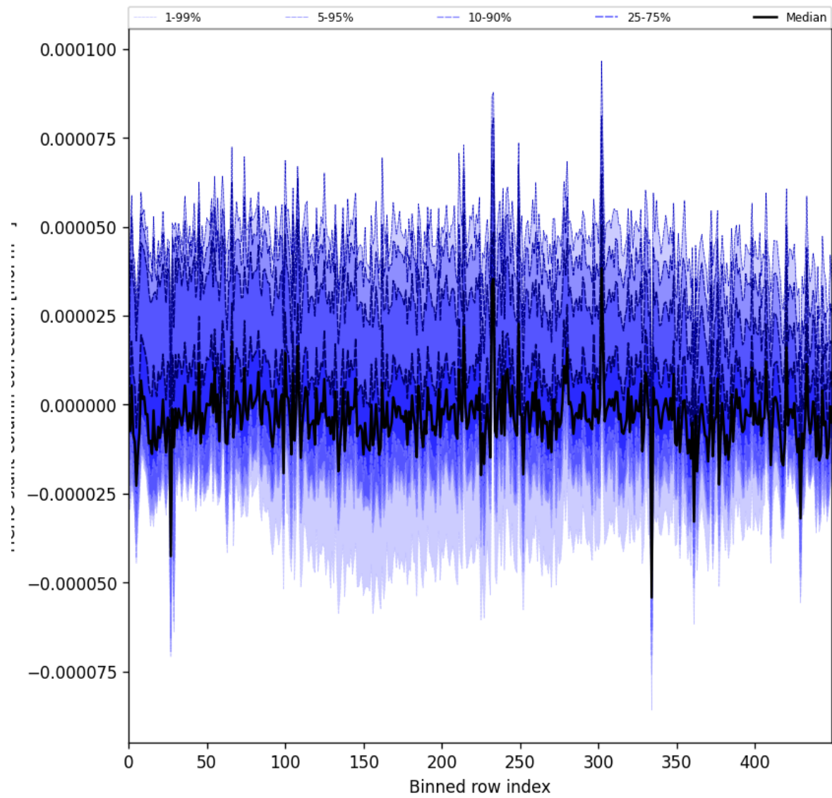
Figure 61: Along track statistics of “HCHO slant column correction” for 2024-09-29 to 2024-10-01
