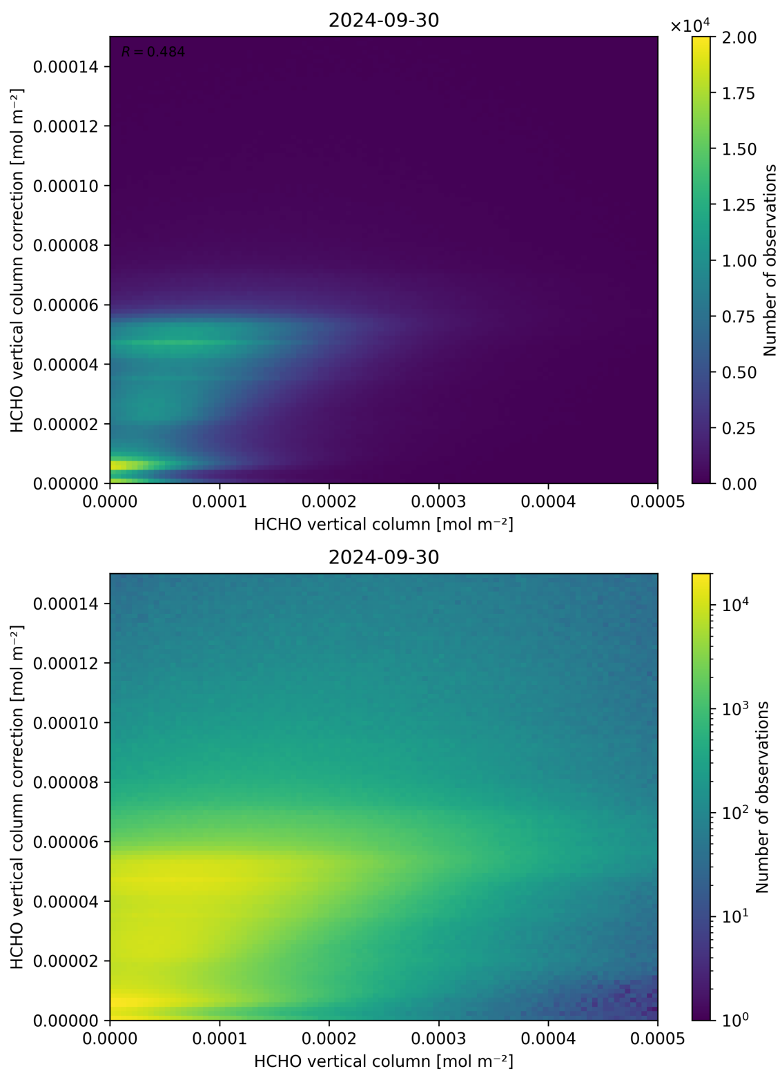
Figure 133: Scatter density plot of “HCHO vertical column” against “HCHO vertical column correction” for 2024-09-29 to 2024-10-01.
