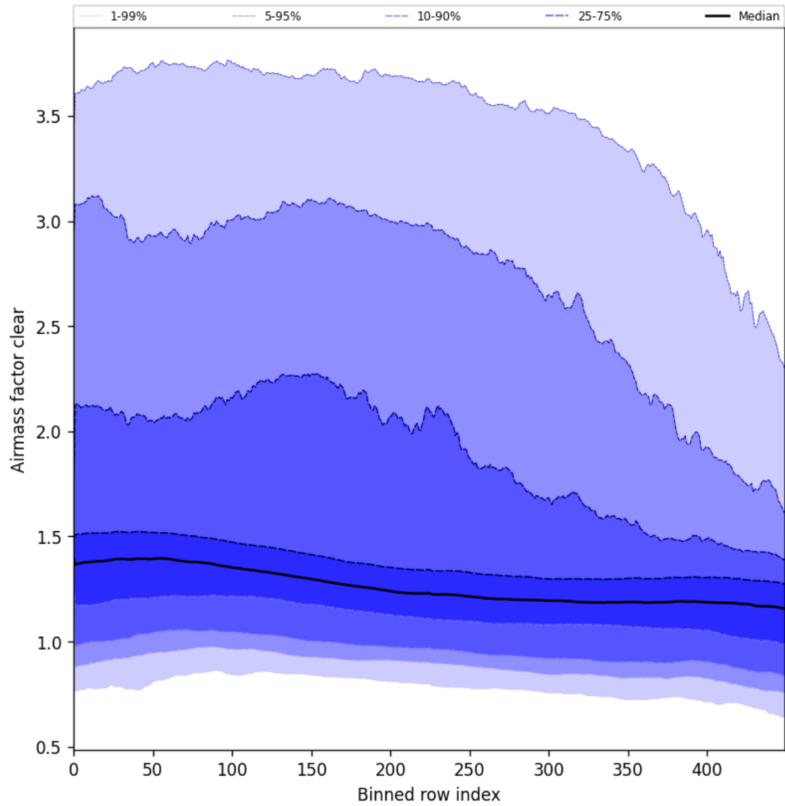
Figure 56: Along track statistics of “Airmass factor clear” for 2024-09-29 to 2024-10-01
