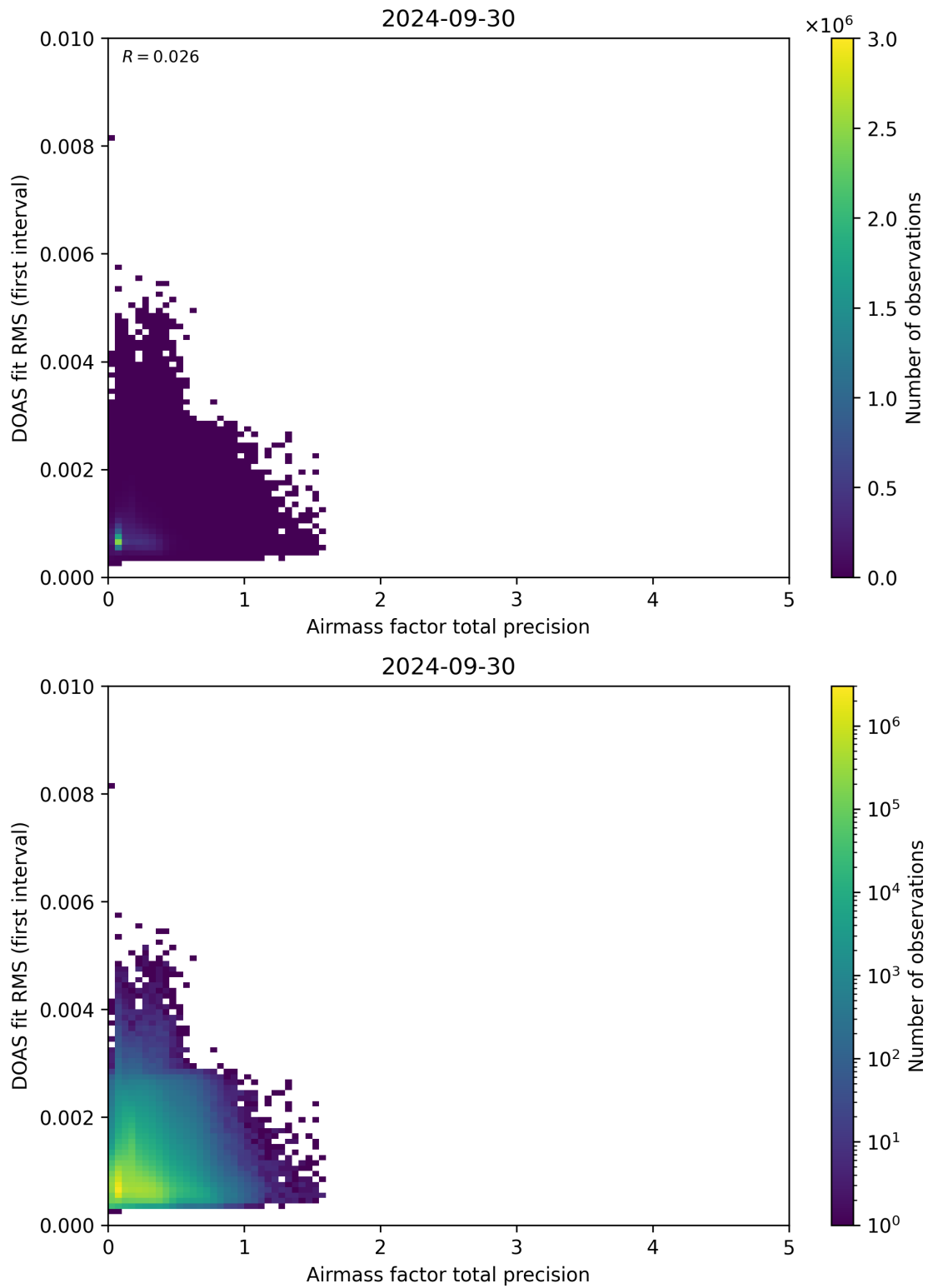
Figure 105: Scatter density plot of “Airmass factor total precision” against “DOAS fit RMS (first interval)” for 2024-09-29 to 2024-10-01.
