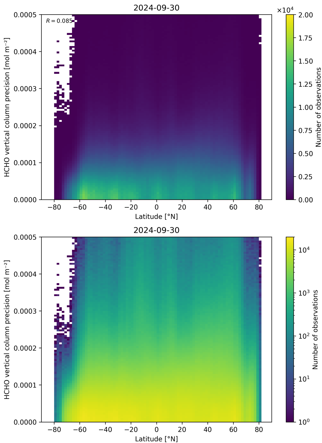
Figure 165: Scatter density plot of “Latitude” against “HCHO vertical column precision” for 2024-09-29 to 2024-10-01.
