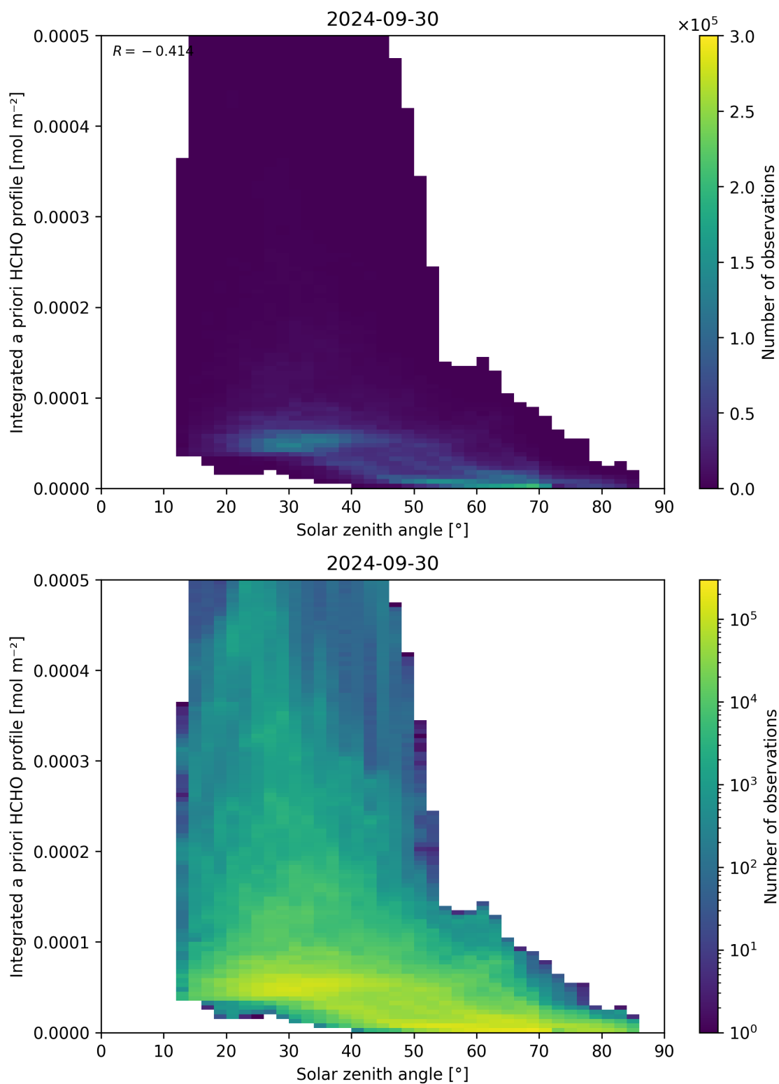
Figure 180: Scatter density plot of “Solar zenith angle” against “Integrated a priori HCHO profile” for 2024-09-29 to 2024-10-01.
