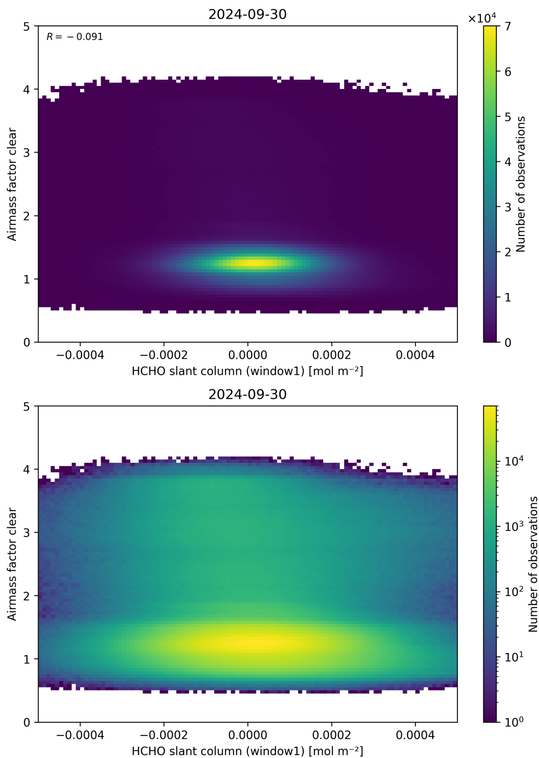
Figure 81: Scatter density plot of “HCHO slant column (window1)” against “Airmass factor clear” for 2024-09-29 to 2024-10-01.
