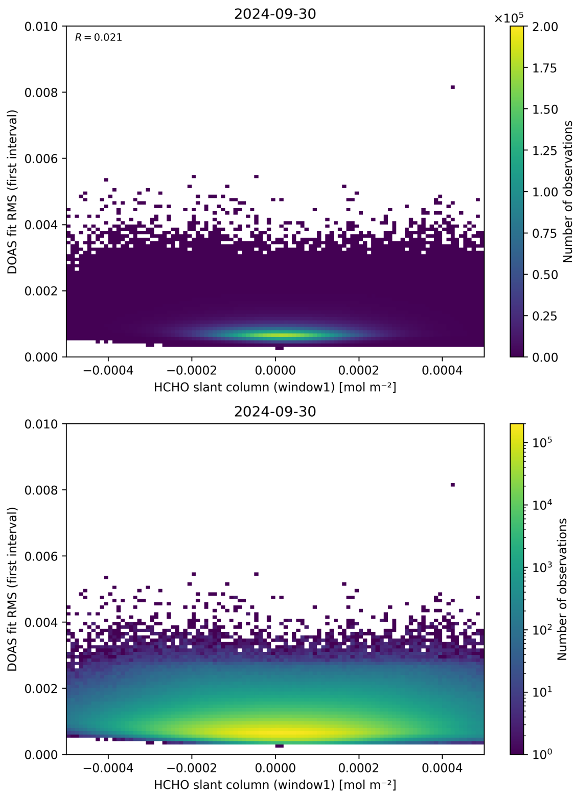
Figure 78: Scatter density plot of “HCHO slant column (window1)” against “DOAS fit RMS (first interval)” for 2024-09-29 to 2024-10-01.
