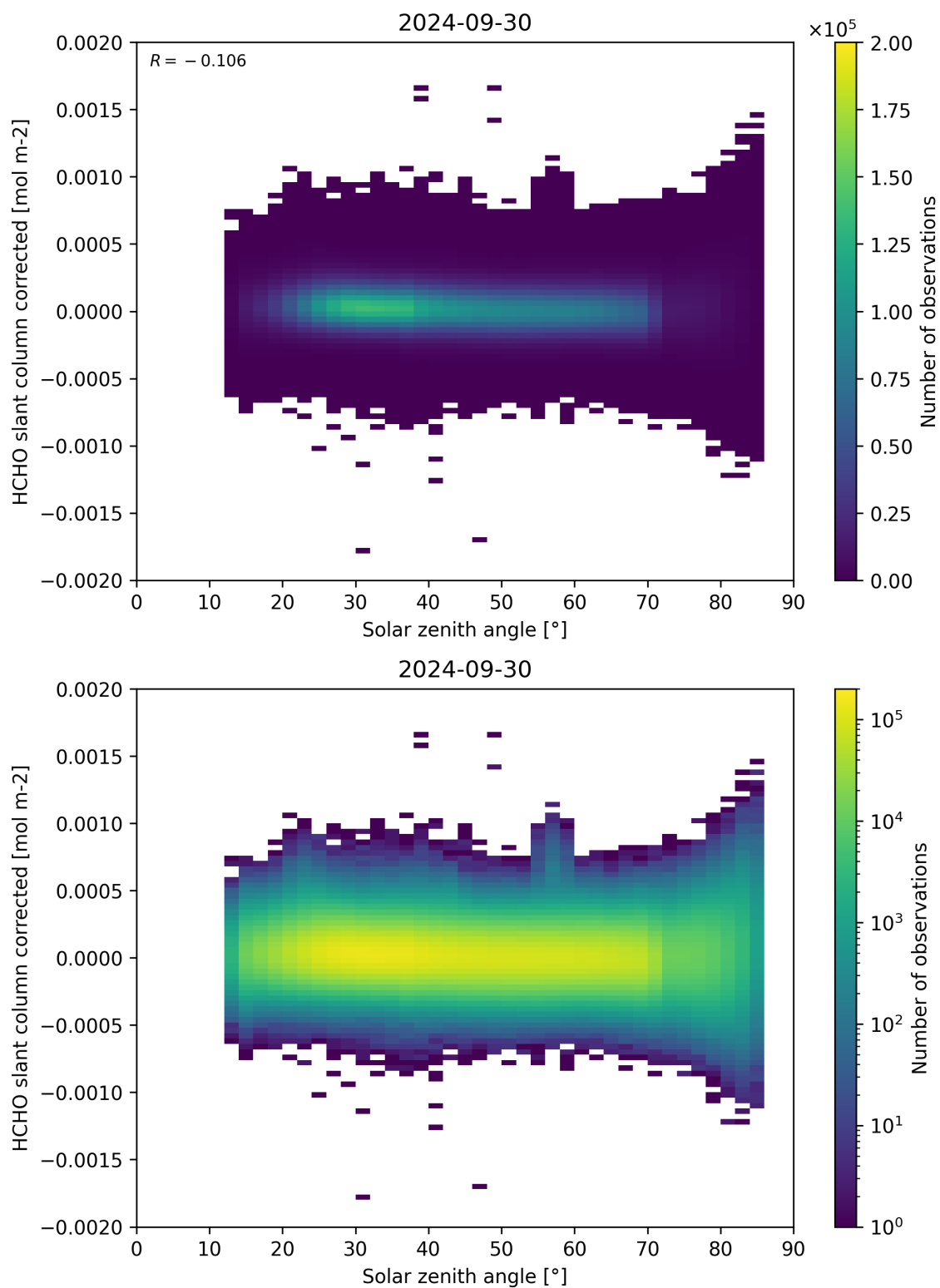
Figure 171: Scatter density plot of “Solar zenith angle” against “HCHO slant column corrected” for 2024-09-29 to 2024-10-01.
