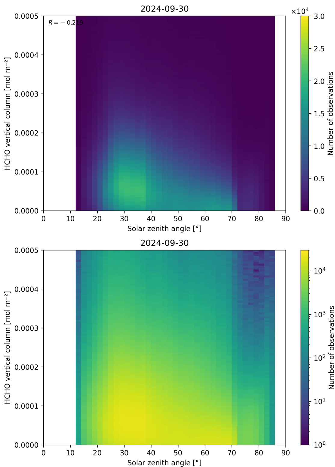
Figure 177: Scatter density plot of “Solar zenith angle” against “HCHO vertical column” for 2024-09-29 to 2024-10-01.
