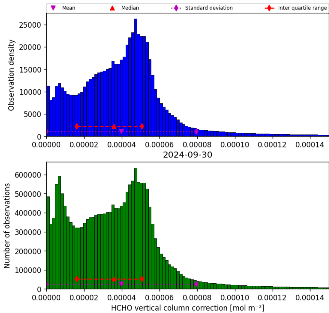
Figure 37: Histogram of “HCHO vertical column correction” for 2024-09-29 to 2024-10-01
