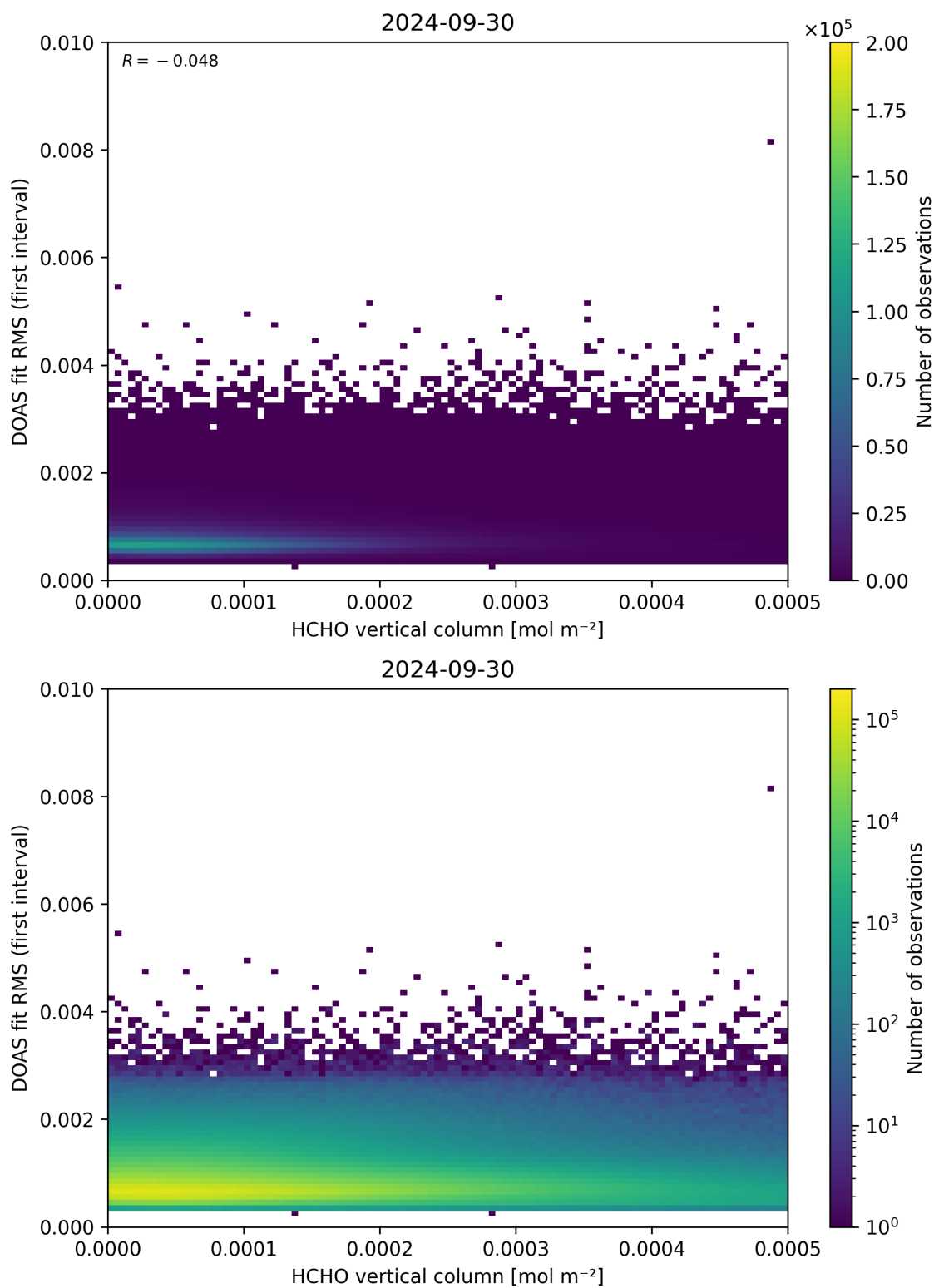
Figure 123: Scatter density plot of “HCHO vertical column” against “DOAS fit RMS (first interval)” for 2024-09-29 to 2024-10-01.
