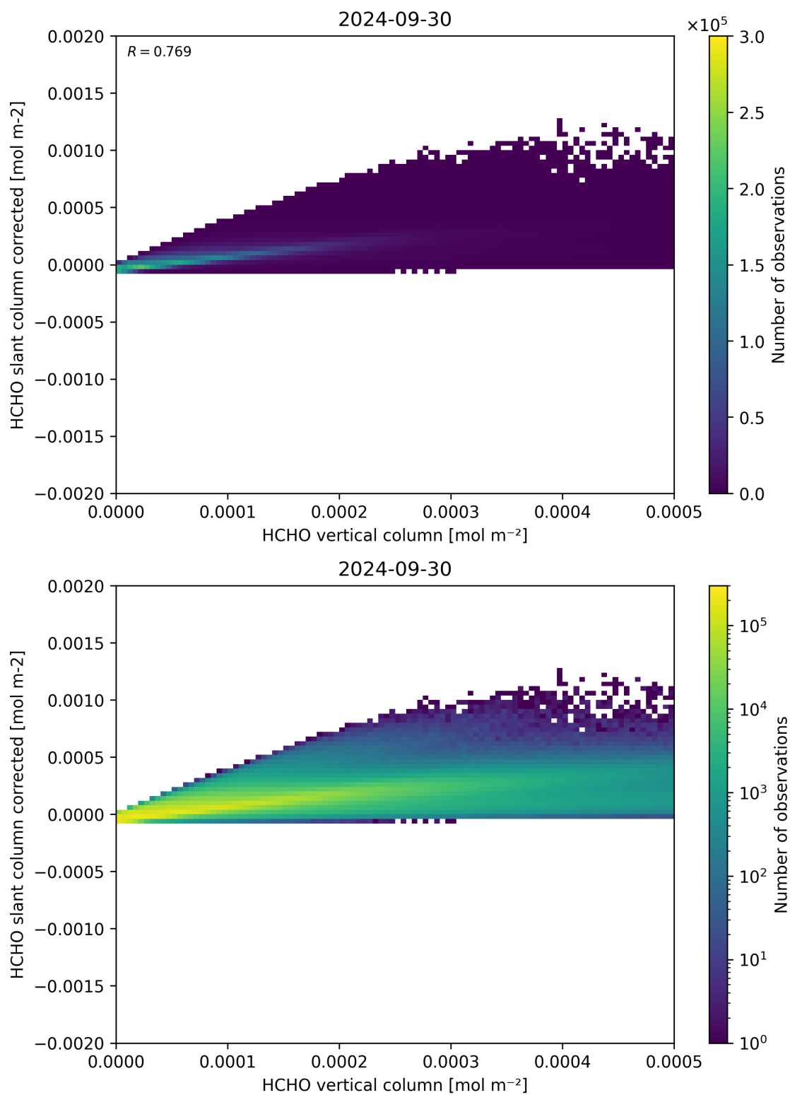
Figure 127: Scatter density plot of “HCHO vertical column” against “HCHO slant column corrected” for 2024-09-29 to 2024-10-01.
