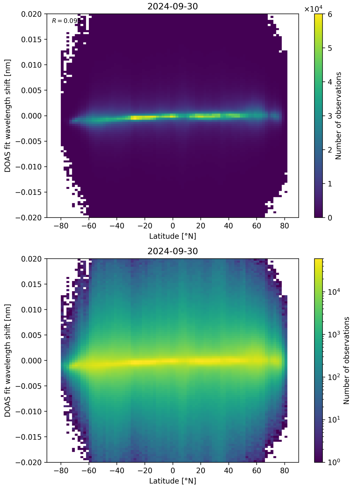
Figure 154: Scatter density plot of “Latitude” against “DOAS fit wavelength shift” for 2024-09-29 to 2024-10-01.
