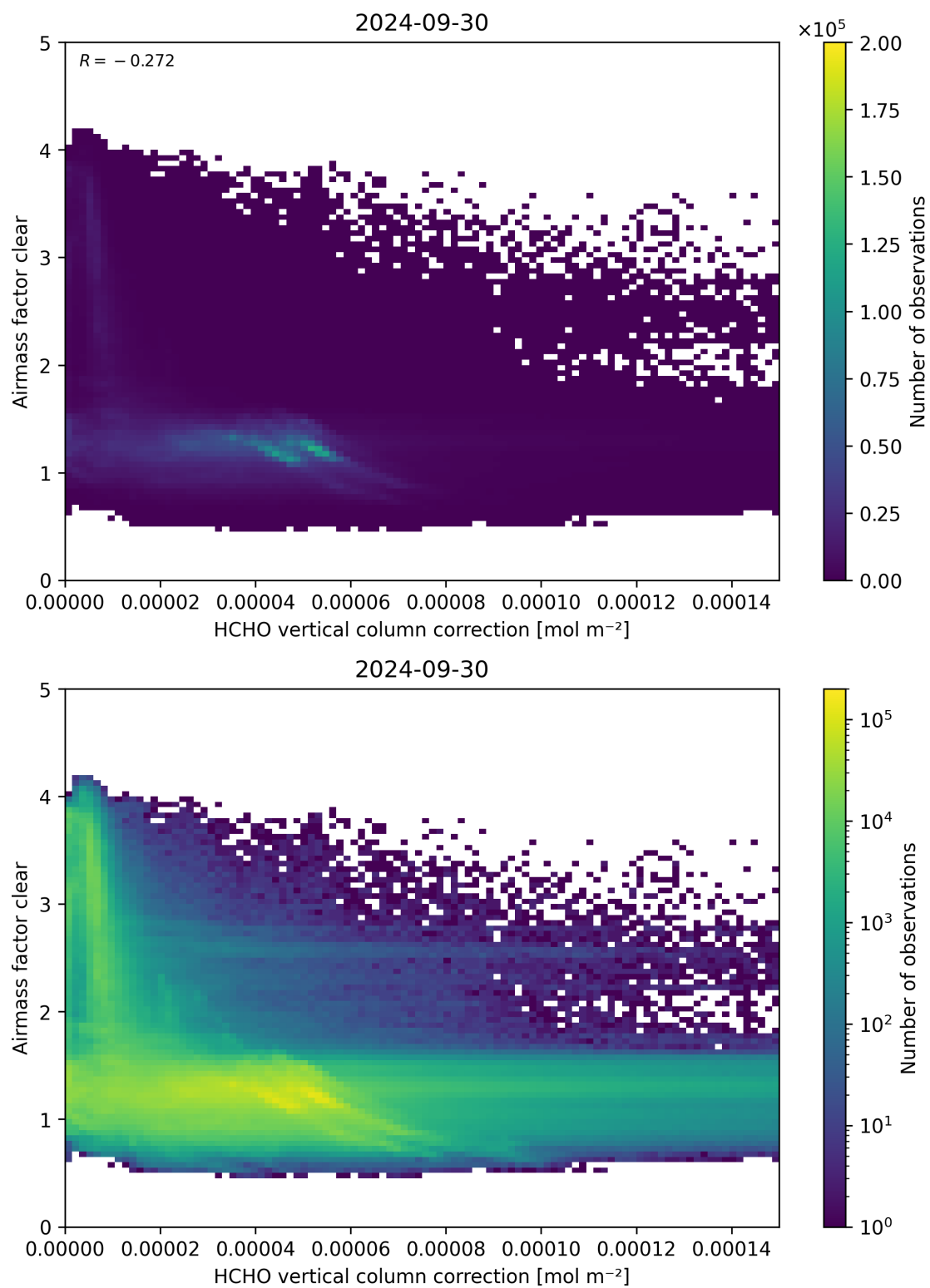
Figure 115: Scatter density plot of “HCHO vertical column correction” against “Airmass factor clear” for 2024-09-29 to 2024-10-01.
