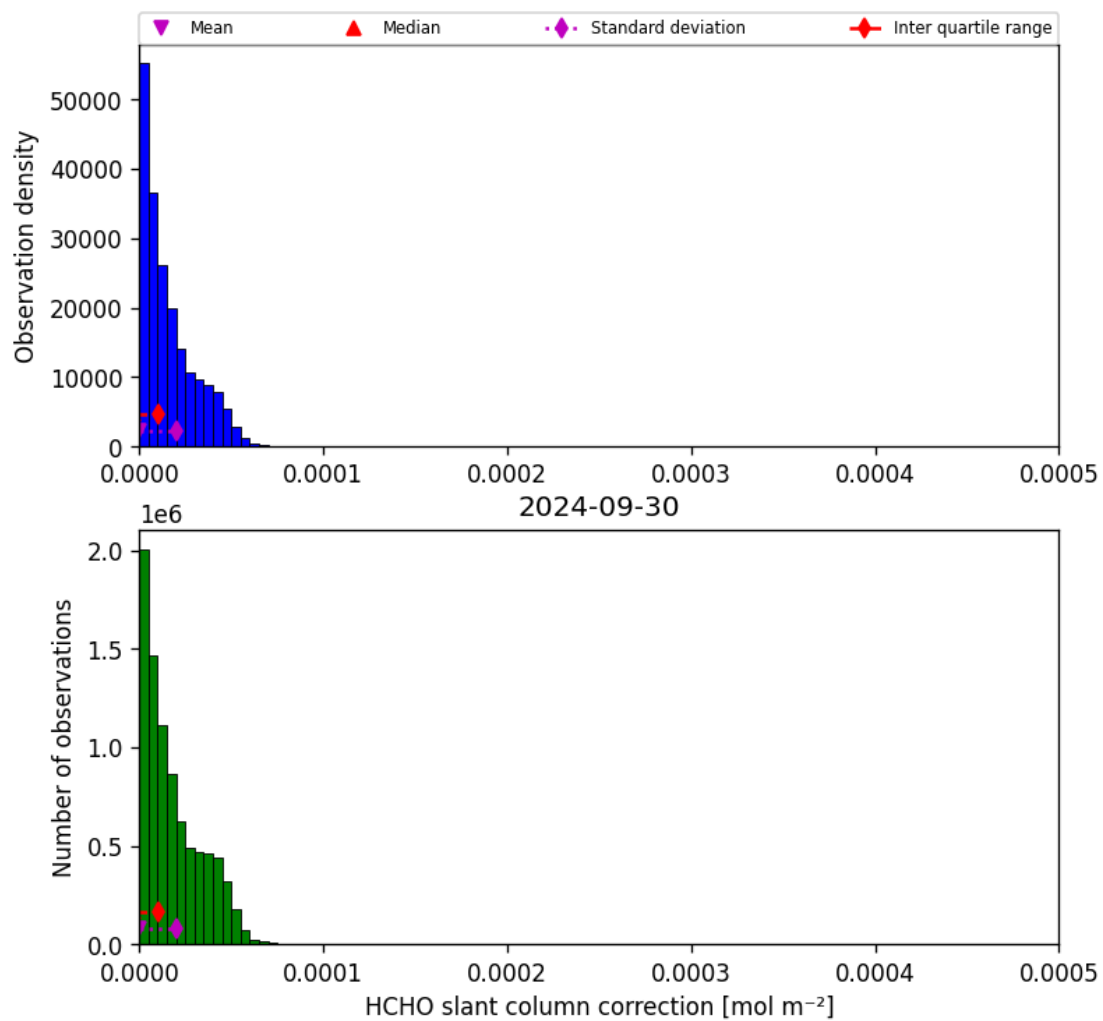
Figure 47: Histogram of “HCHO slant column correction” for 2024-09-29 to 2024-10-01
