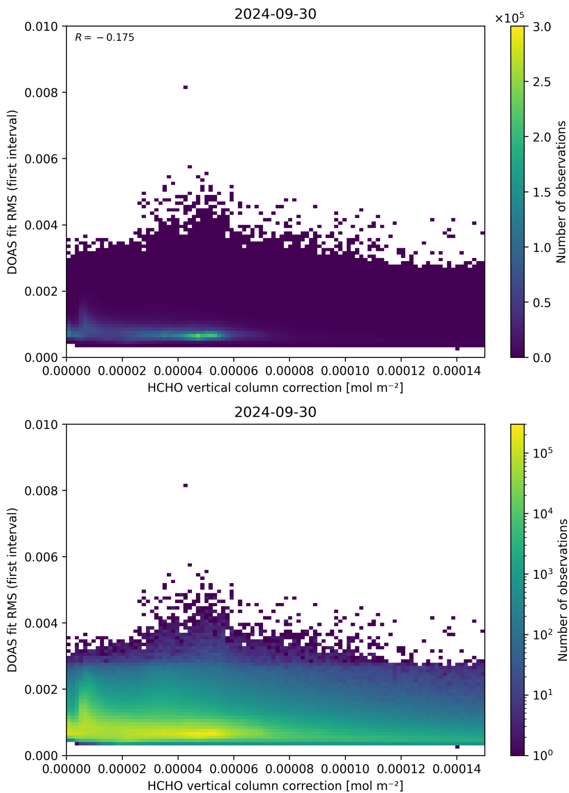
Figure 112: Scatter density plot of “HCHO vertical column correction” against “DOAS fit RMS (first interval)” for 2024-09-29 to 2024-10-01.
