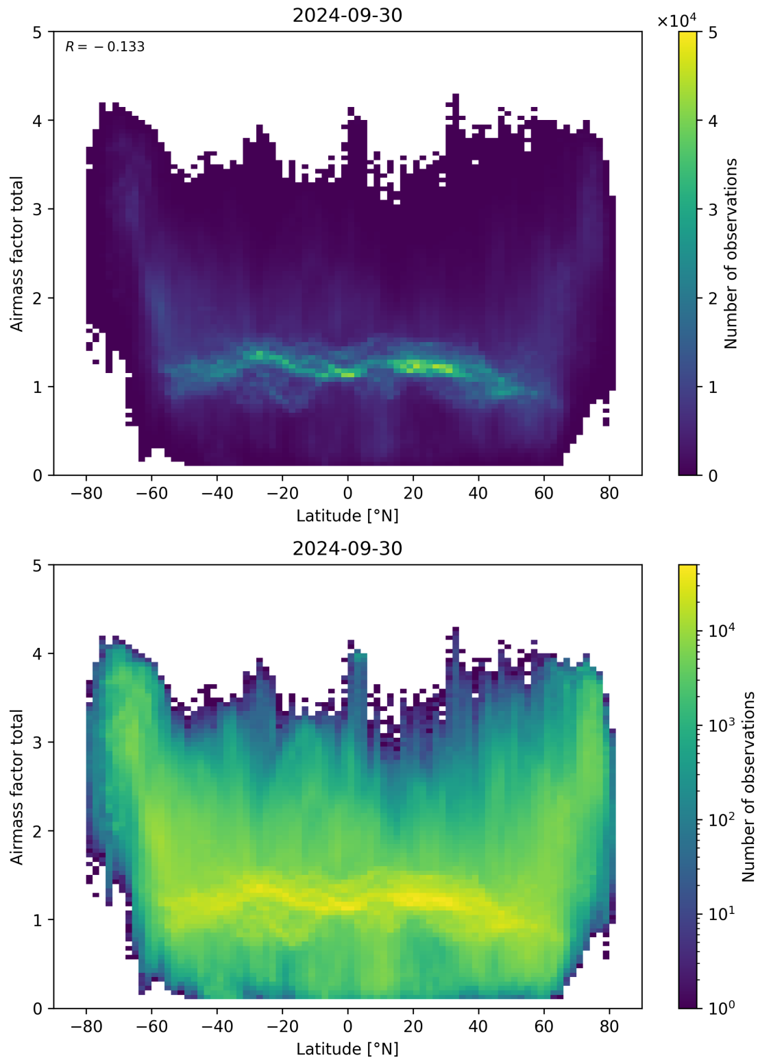
Figure 161: Scatter density plot of “Latitude” against “Airmass factor total” for 2024-09-29 to 2024-10-01.
