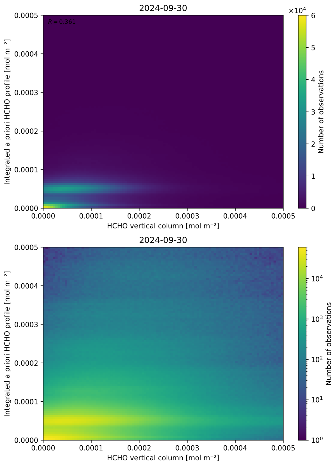
Figure 135: Scatter density plot of “HCHO vertical column” against “Integrated a priori HCHO profile” for 2024-09-29 to 2024-10-01.
