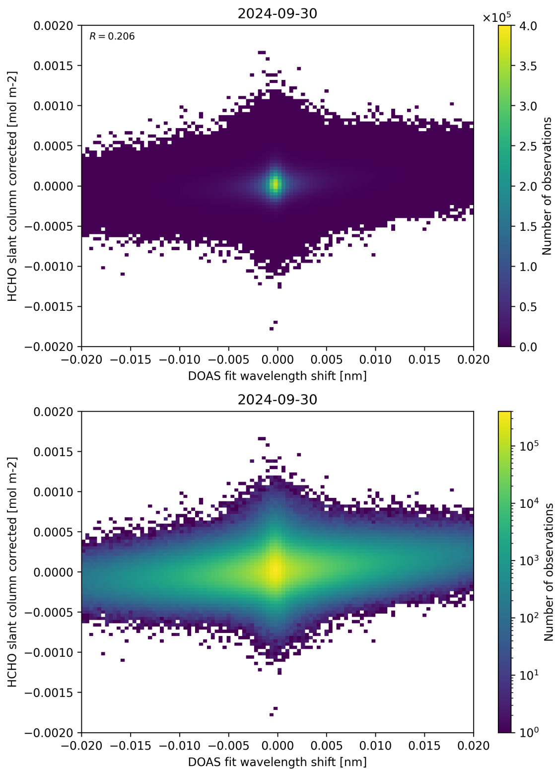
Figure 66: Scatter density plot of “DOAS fit wavelength shift” against “HCHO slant column corrected” for 2024-09-29 to 2024-10-01.
