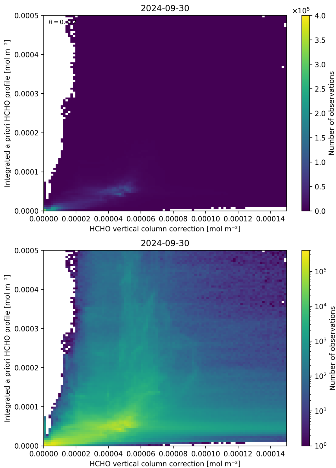
Figure 122: Scatter density plot of “HCHO vertical column correction” against “Integrated a priori HCHO profile” for 2024-09-29 to 2024-10-01.
