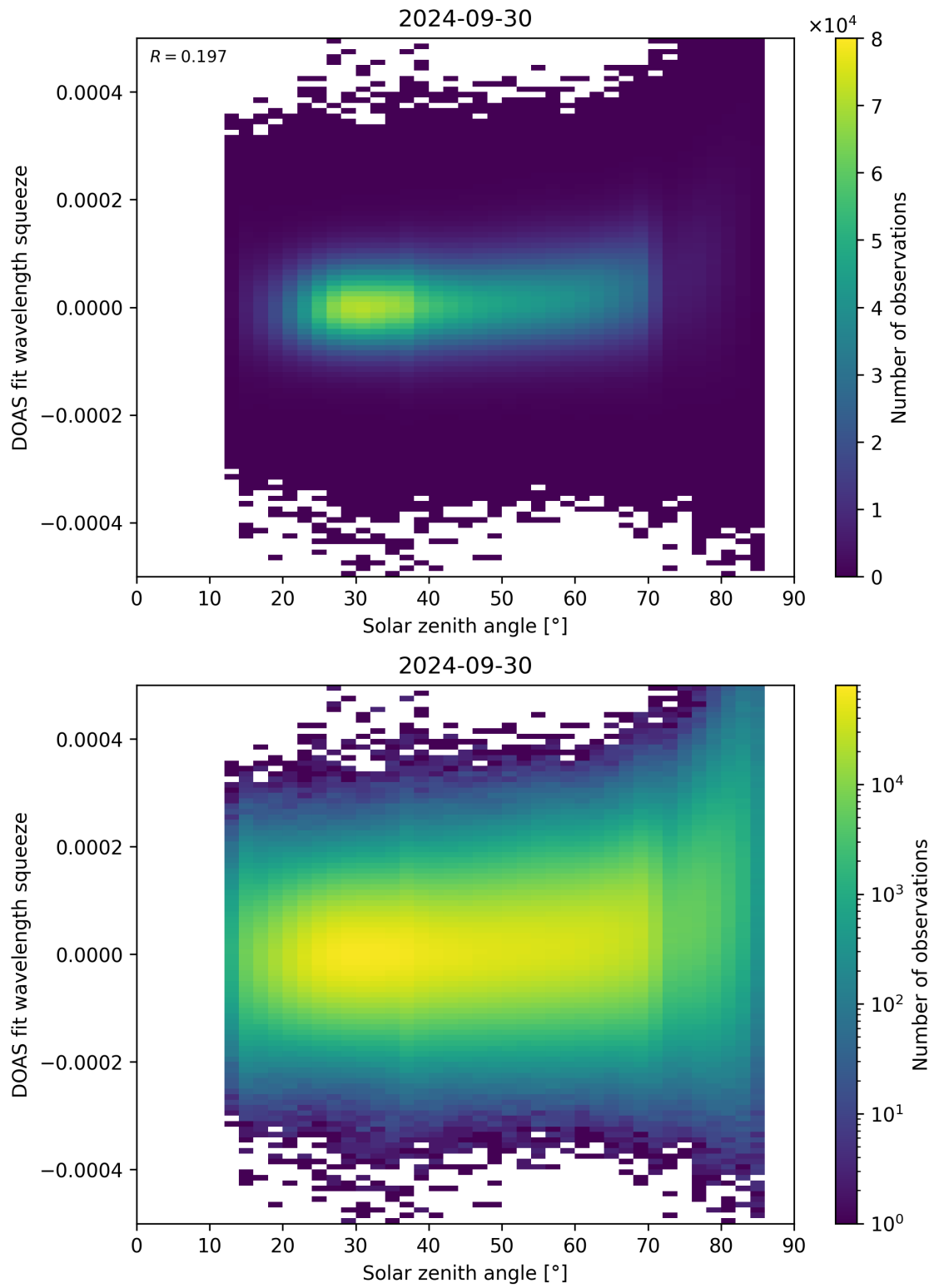
Figure 169: Scatter density plot of “Solar zenith angle” against “DOAS fit wavelength squeeze” for 2024-09-29 to 2024-10-01.
