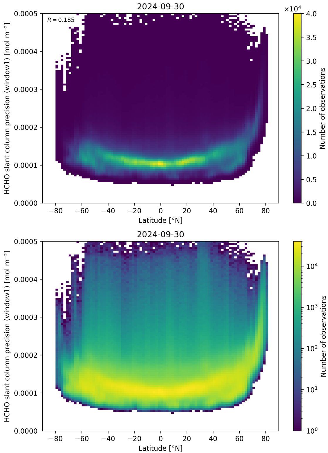
Figure 160: Scatter density plot of “Latitude” against “HCHO slant column precision (window1)” for 2024-09-29 to 2024-10-01.
