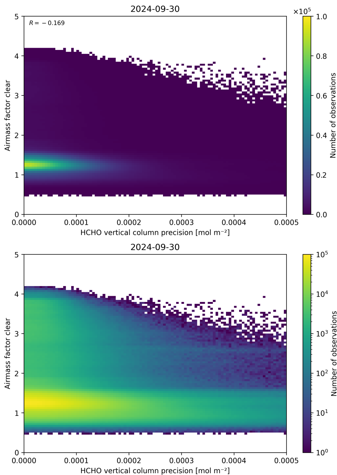
Figure 139: Scatter density plot of “HCHO vertical column precision” against “Airmass factor clear” for 2024-09-29 to 2024-10-01.
