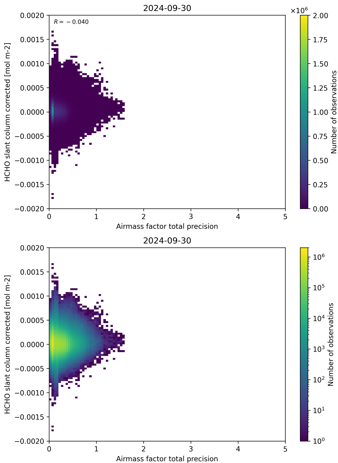
Figure 109: Scatter density plot of “Airmass factor total precision” against “HCHO slant column corrected” for 2024-09-29 to 2024-10-01.
