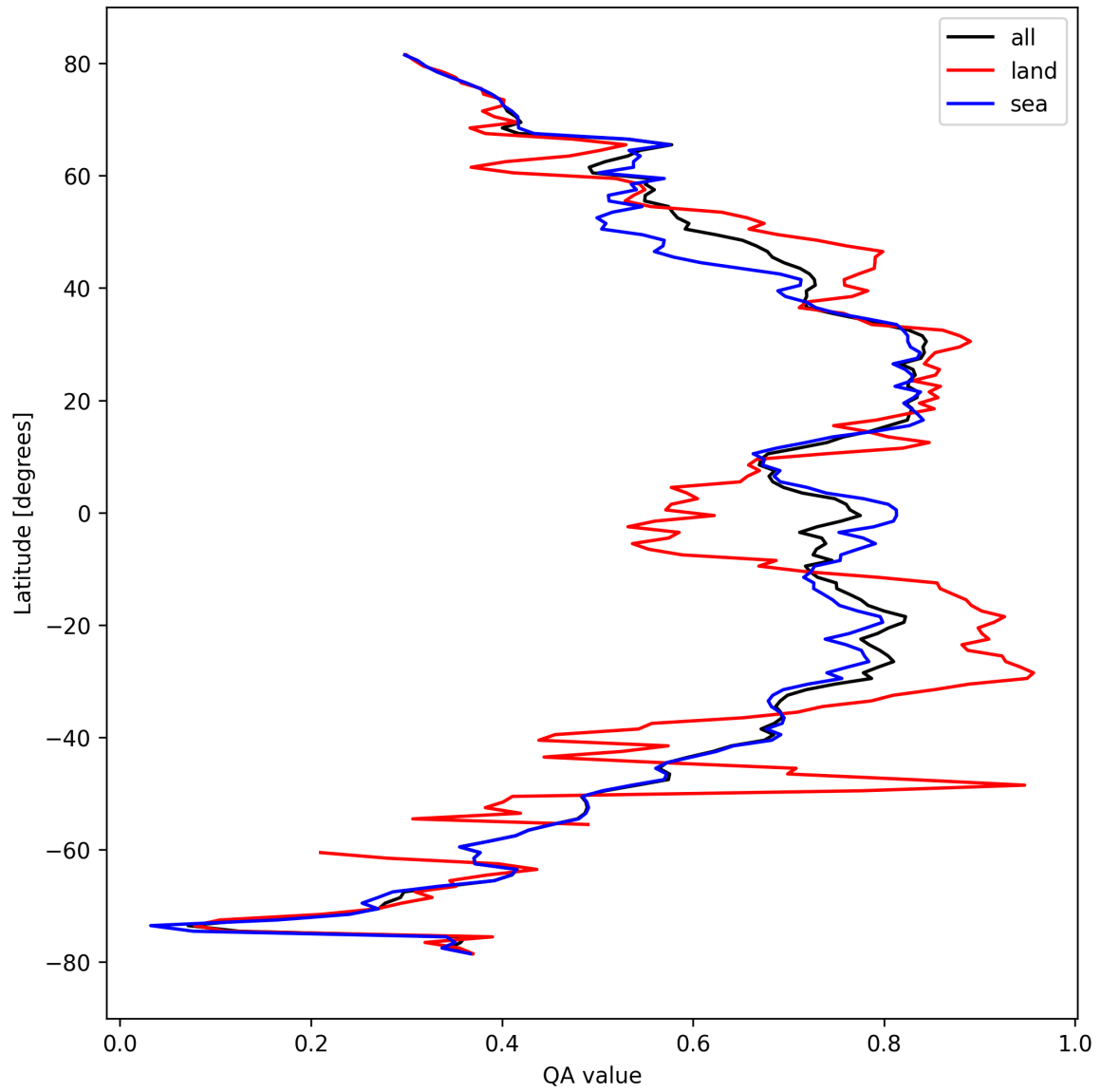
Figure 20: Zonal average of “QA value” for 2024-09-29 to 2024-10-01.
