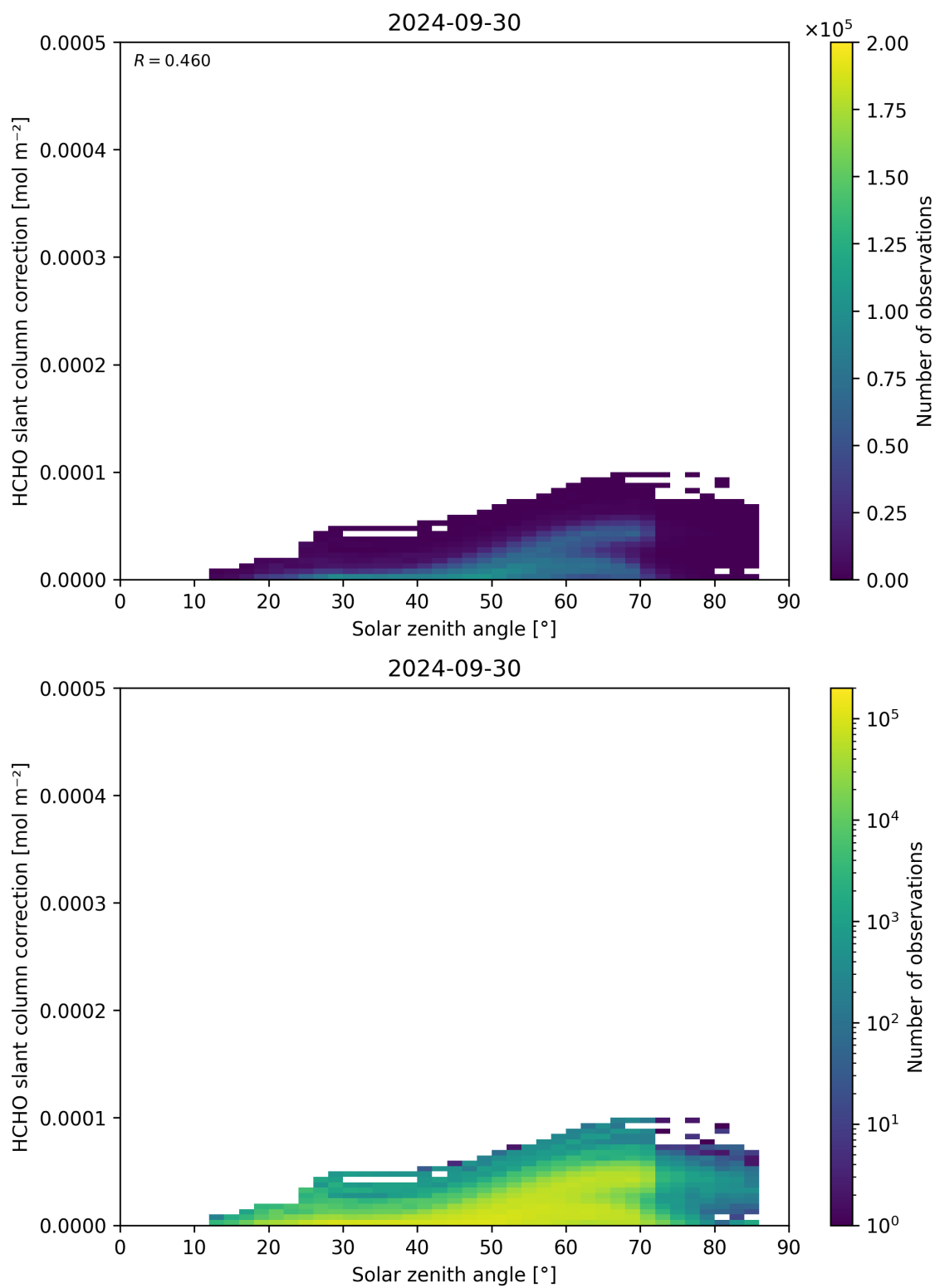
Figure 172: Scatter density plot of “Solar zenith angle” against “HCHO slant column correction” for 2024-09-29 to 2024-10-01.
