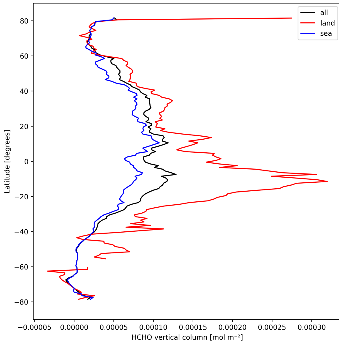
Figure 21: Zonal average of “HCHO vertical column” for 2024-09-29 to 2024-10-01.
