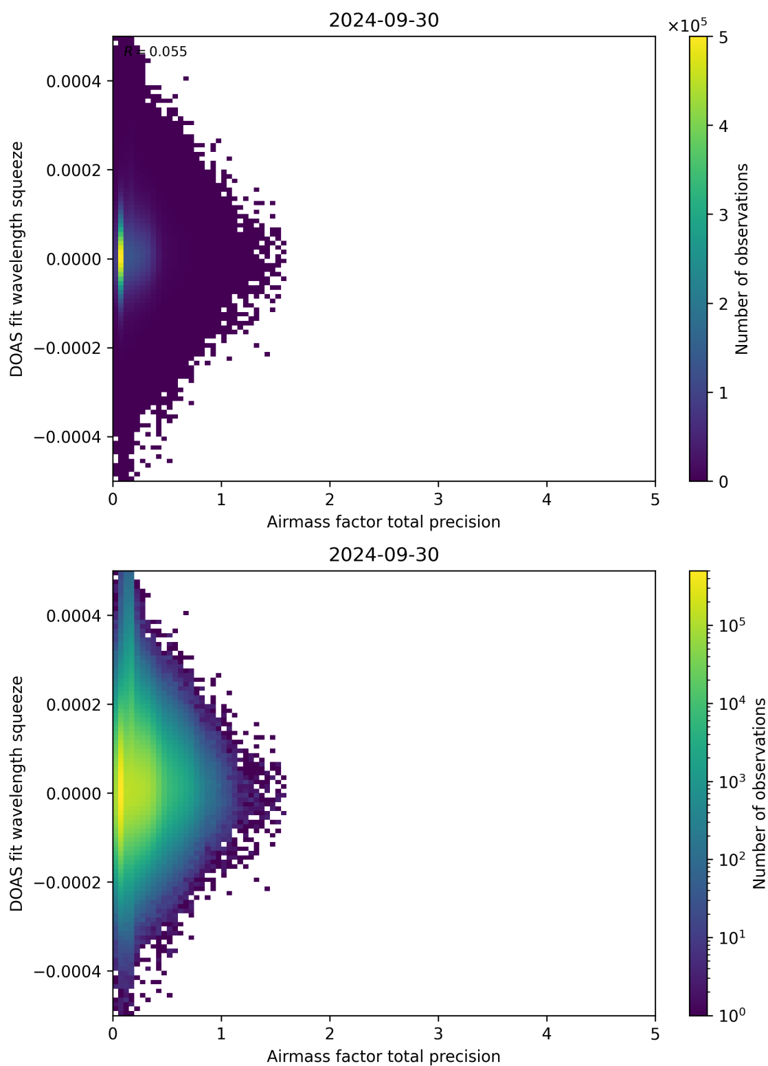
Figure 107: Scatter density plot of “Airmass factor total precision” against “DOAS fit wavelength squeeze” for 2024-09-29 to 2024-10-01.
