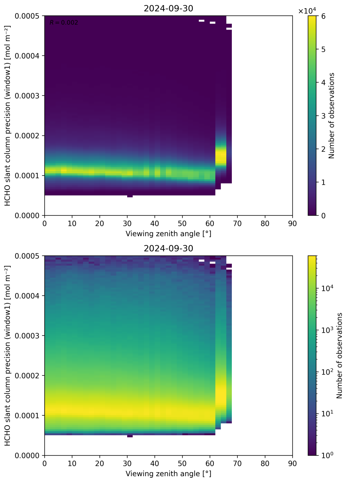
Figure 189: Scatter density plot of “Viewing zenith angle” against “HCHO slant column precision (window1)” for 2024-09-29 to 2024-10-01.
