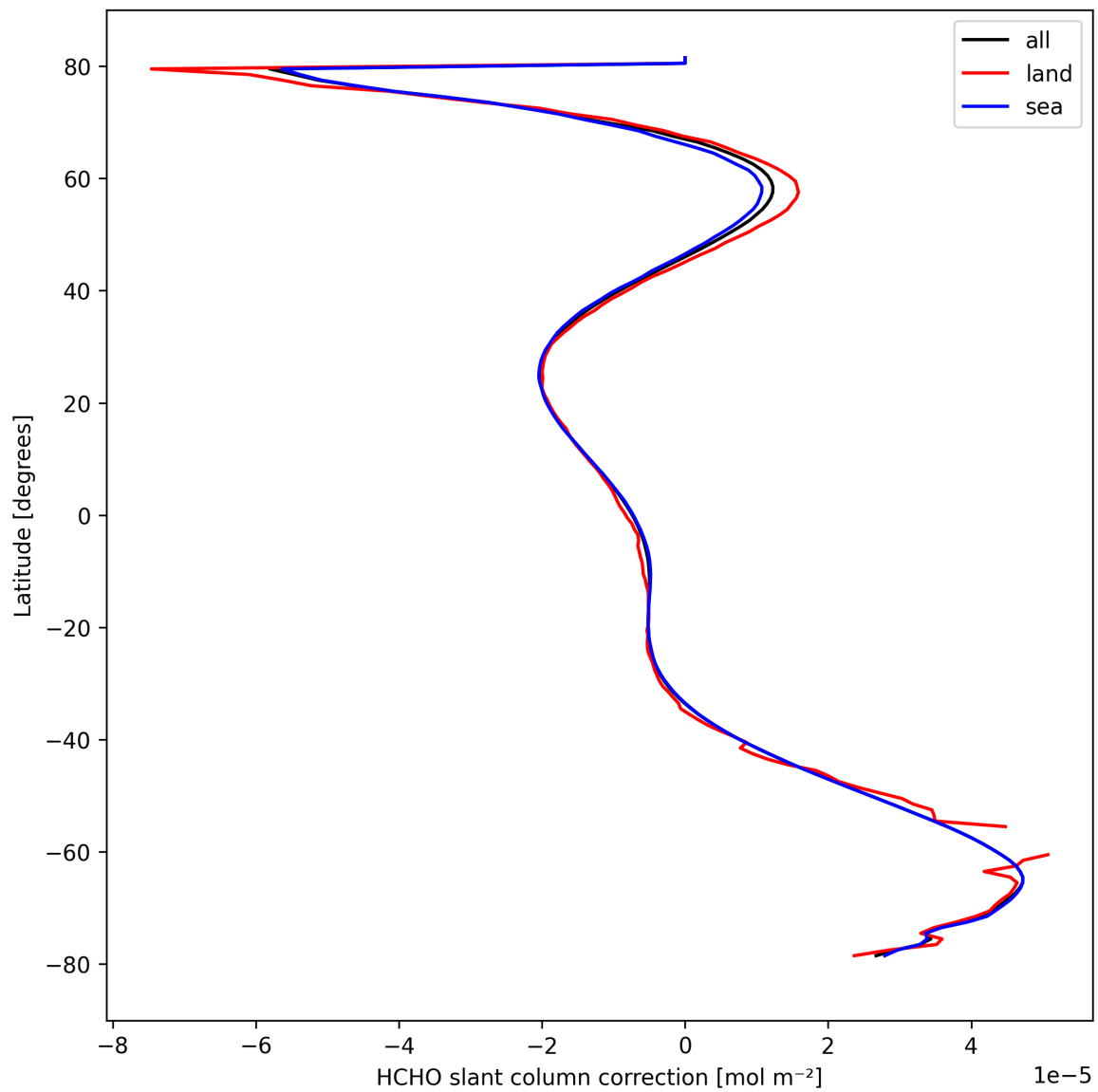
Figure 33: Zonal average of "HCHO slant column correction" for 2024-09-29 to 2024-10-01.
