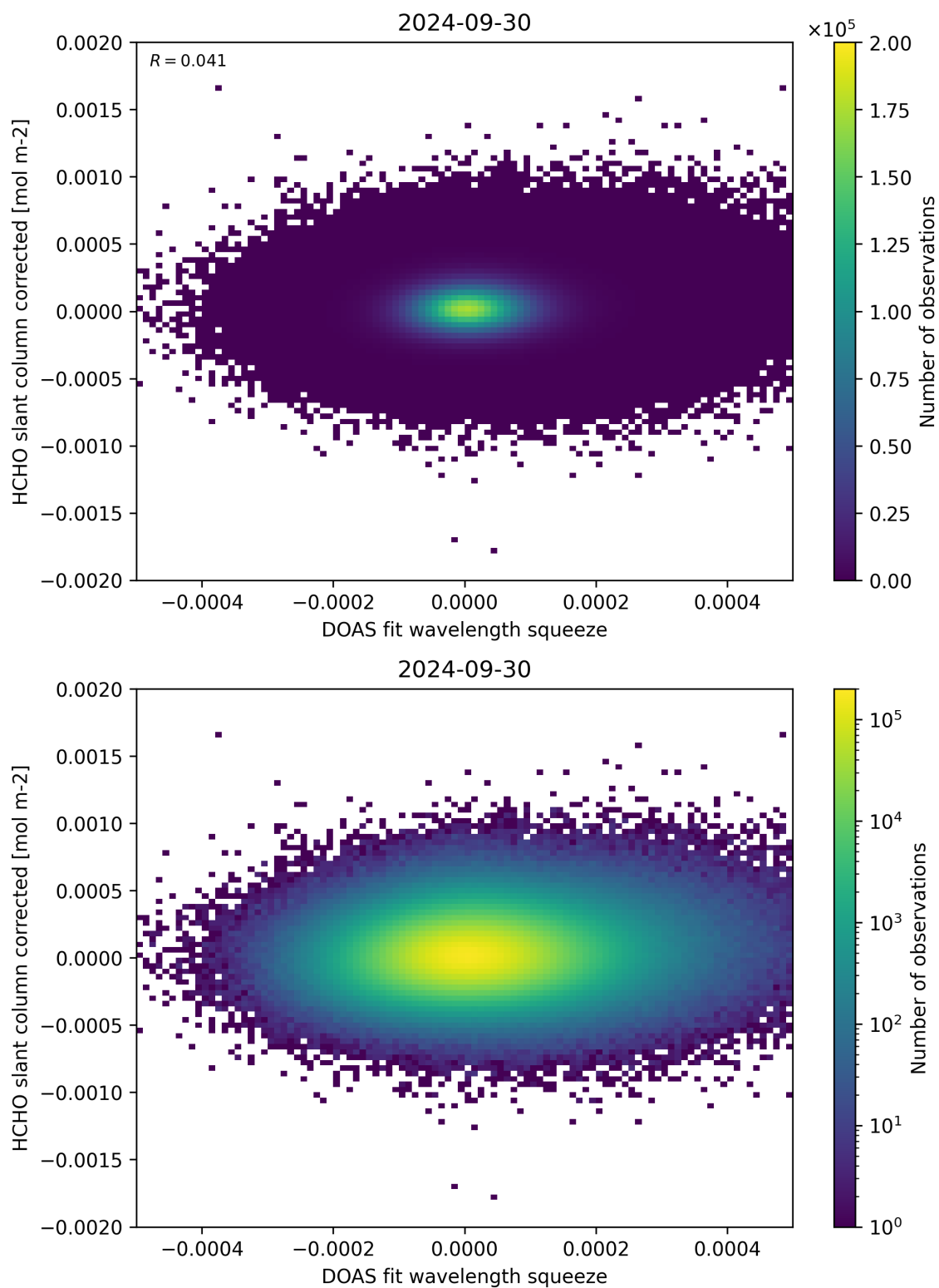
Figure 69: Scatter density plot of “DOAS fit wavelength squeeze” against “HCHO slant column corrected” for 2024-09-29 to 2024-10-01.
