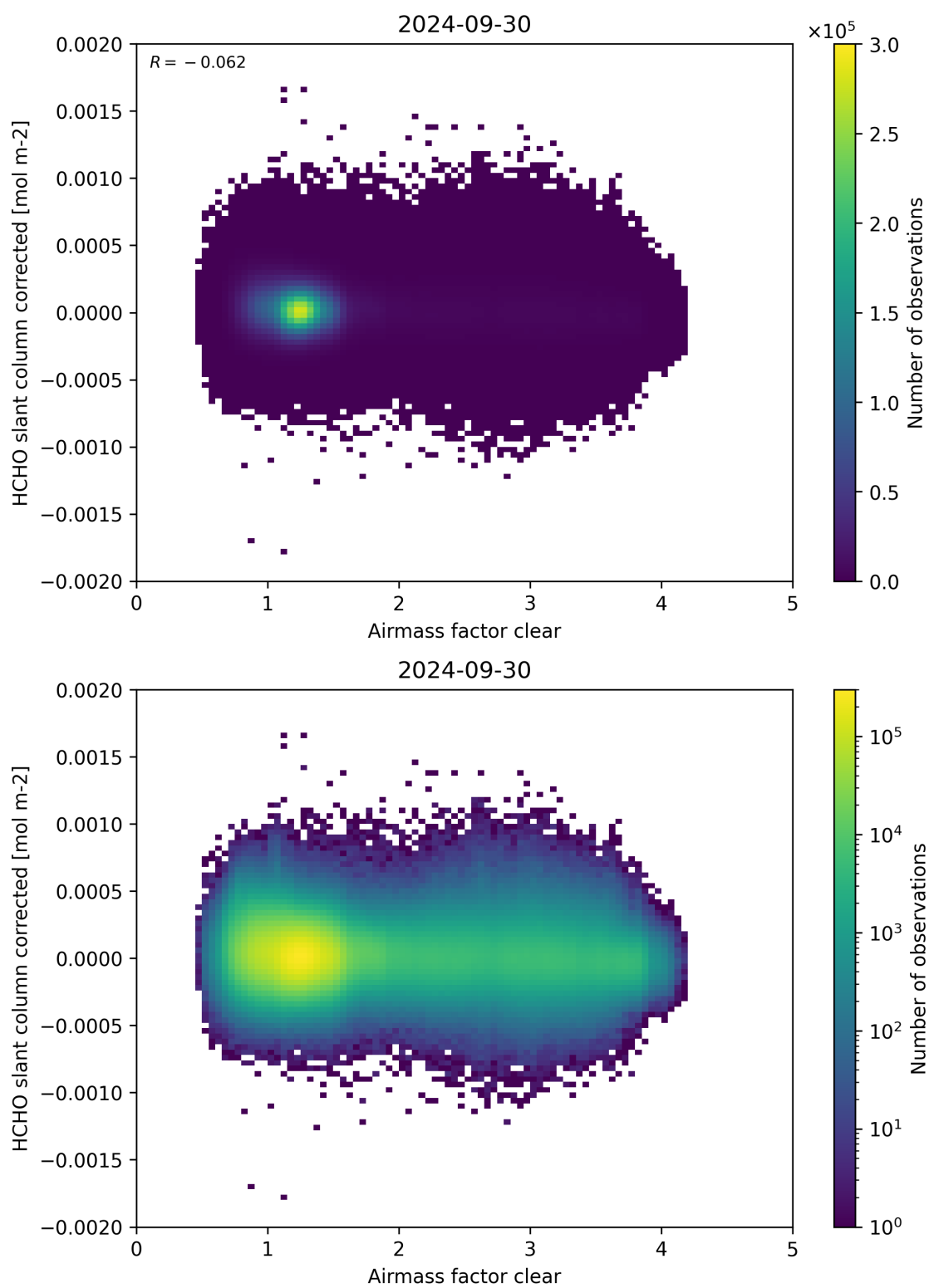
Figure 74: Scatter density plot of “Airmass factor clear” against “HCHO slant column corrected” for 2024-09-29 to 2024-10-01.
