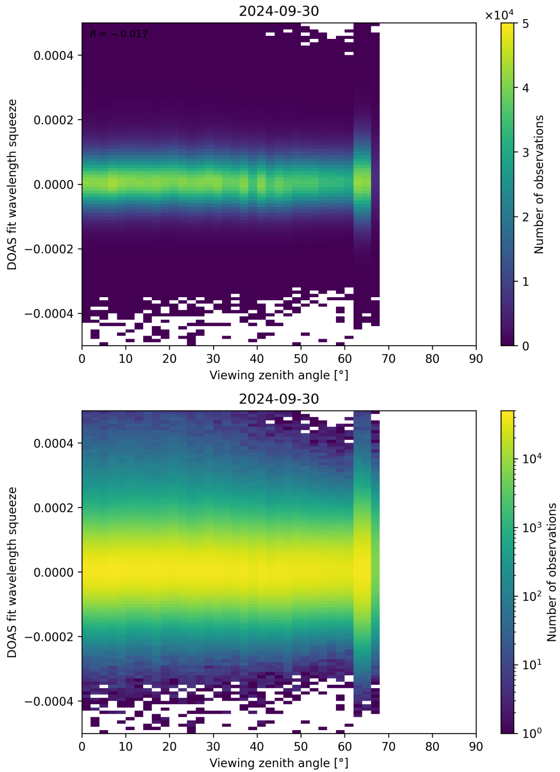
Figure 184: Scatter density plot of “Viewing zenith angle” against “DOAS fit wavelength squeeze” for 2024-09-29 to 2024-10-01.
