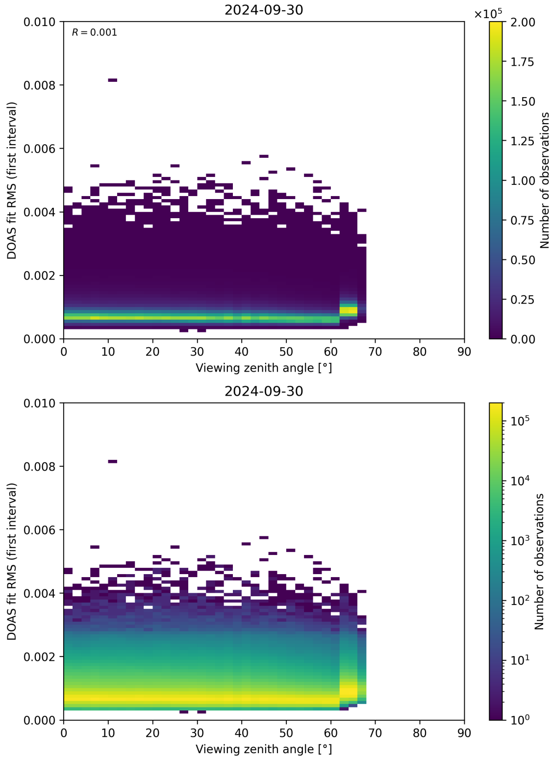
Figure 182: Scatter density plot of “Viewing zenith angle” against “DOAS fit RMS (first interval)” for 2024-09-29 to 2024-10-01.
