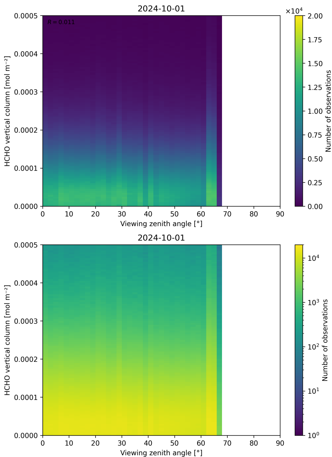
Figure 192: Scatter density plot of “Viewing zenith angle” against “HCHO vertical column” for 2024-09-30 to 2024-10-02.
