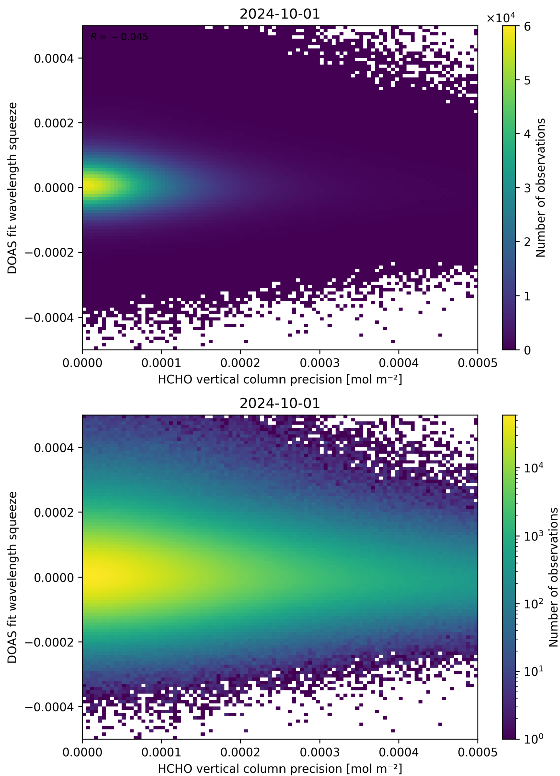
Figure 138: Scatter density plot of “HCHO vertical column precision” against “DOAS fit wavelength squeeze” for 2024-09-30 to 2024-10-02.
