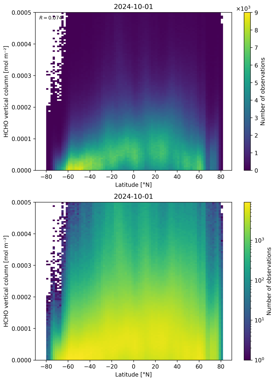
Figure 163: Scatter density plot of “Latitude” against “HCHO vertical column” for 2024-09-30 to 2024-10-02.
