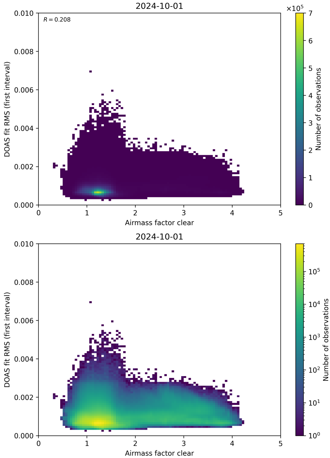
Figure 71: Scatter density plot of “Airmass factor clear” against “DOAS fit RMS (first interval)” for 2024-09-30 to 2024-10-02.
