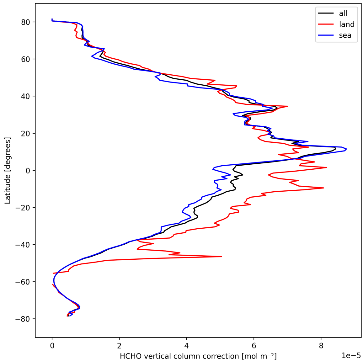
Figure 23: Zonal average of “HCHO vertical column correction” for 2024-09-30 to 2024-10-02.
