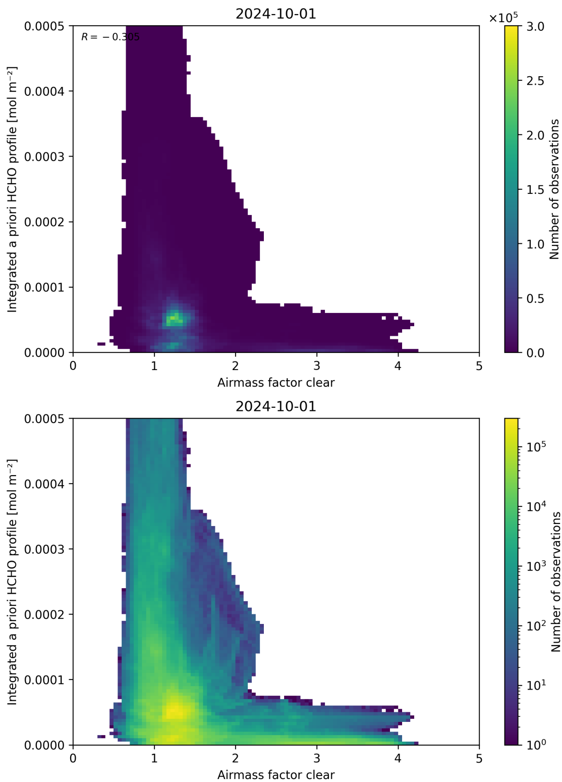
Figure 76: Scatter density plot of “Airmass factor clear” against “Integrated a priori HCHO profile” for 2024-09-30 to 2024-10-02.
