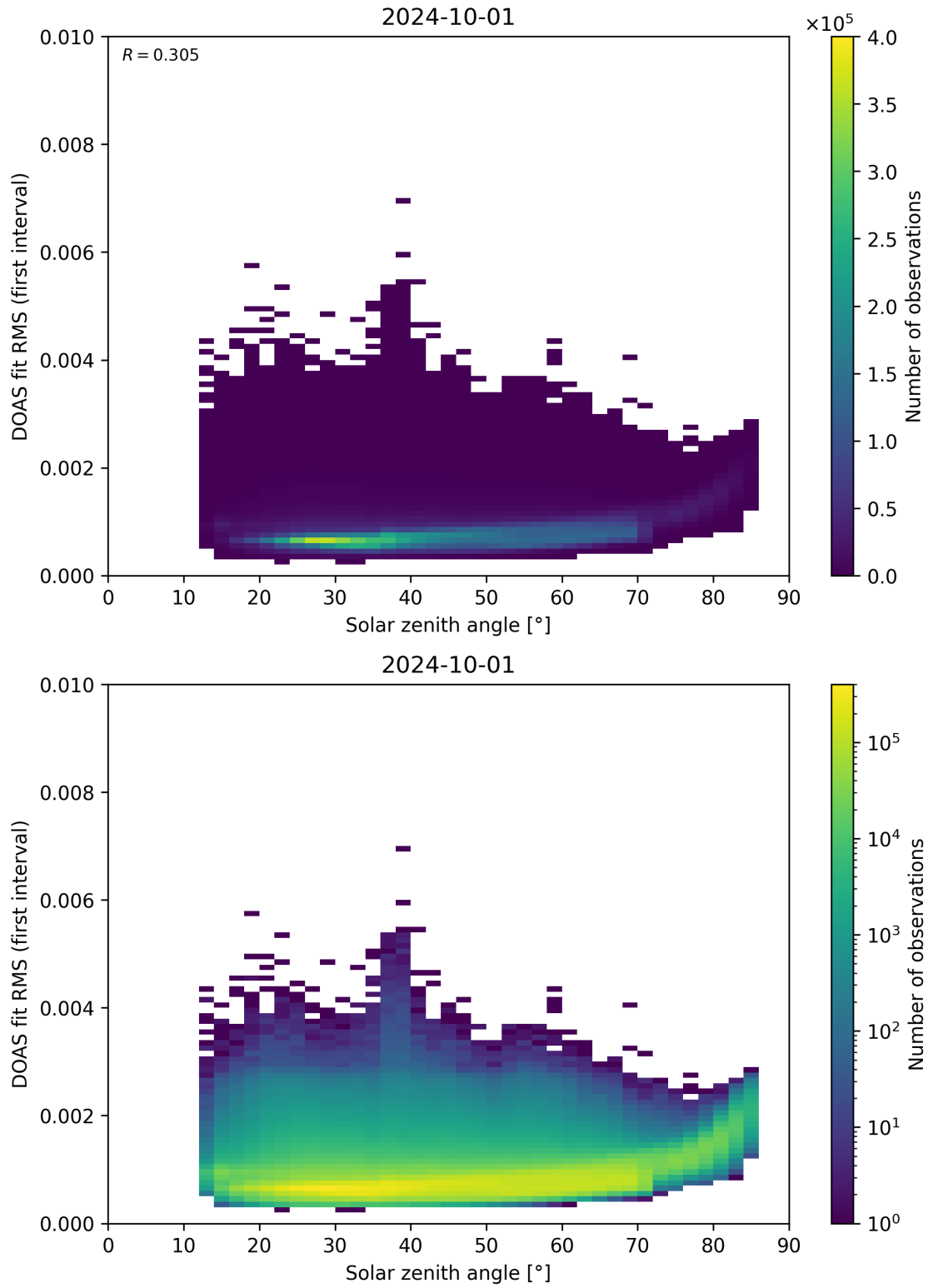
Figure 167: Scatter density plot of “Solar zenith angle” against “DOAS fit RMS (first interval)” for 2024-09-30 to 2024-10-02.
