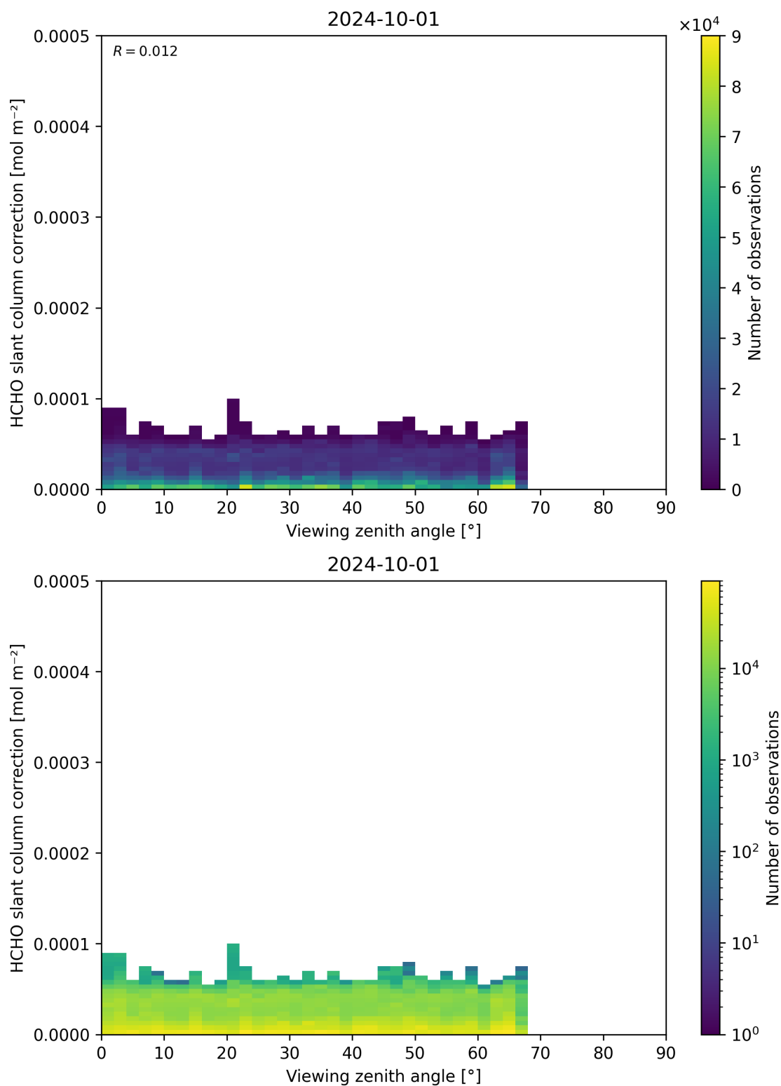
Figure 187: Scatter density plot of “Viewing zenith angle” against “HCHO slant column correction” for 2024-09-30 to 2024-10-02.
