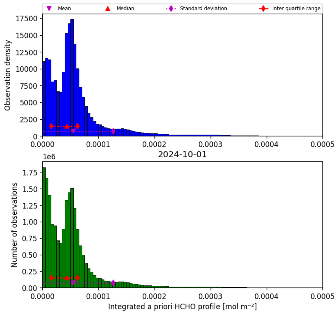
Figure 43: Histogram of “Integrated a priori HCHO profile” for 2024-09-30 to 2024-10-02
