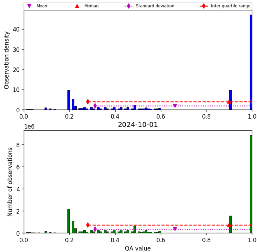
Figure 34: Histogram of “QA value” for 2024-09-30 to 2024-10-02
