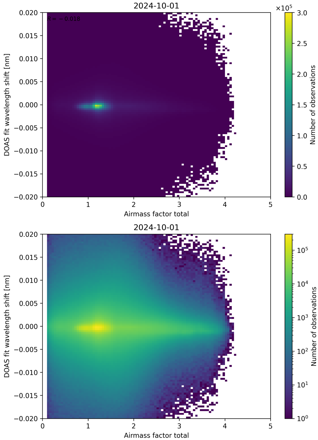
Figure 98: Scatter density plot of “Airmass factor total” against “DOAS fit wavelength shift” for 2024-09-30 to 2024-10-02.
