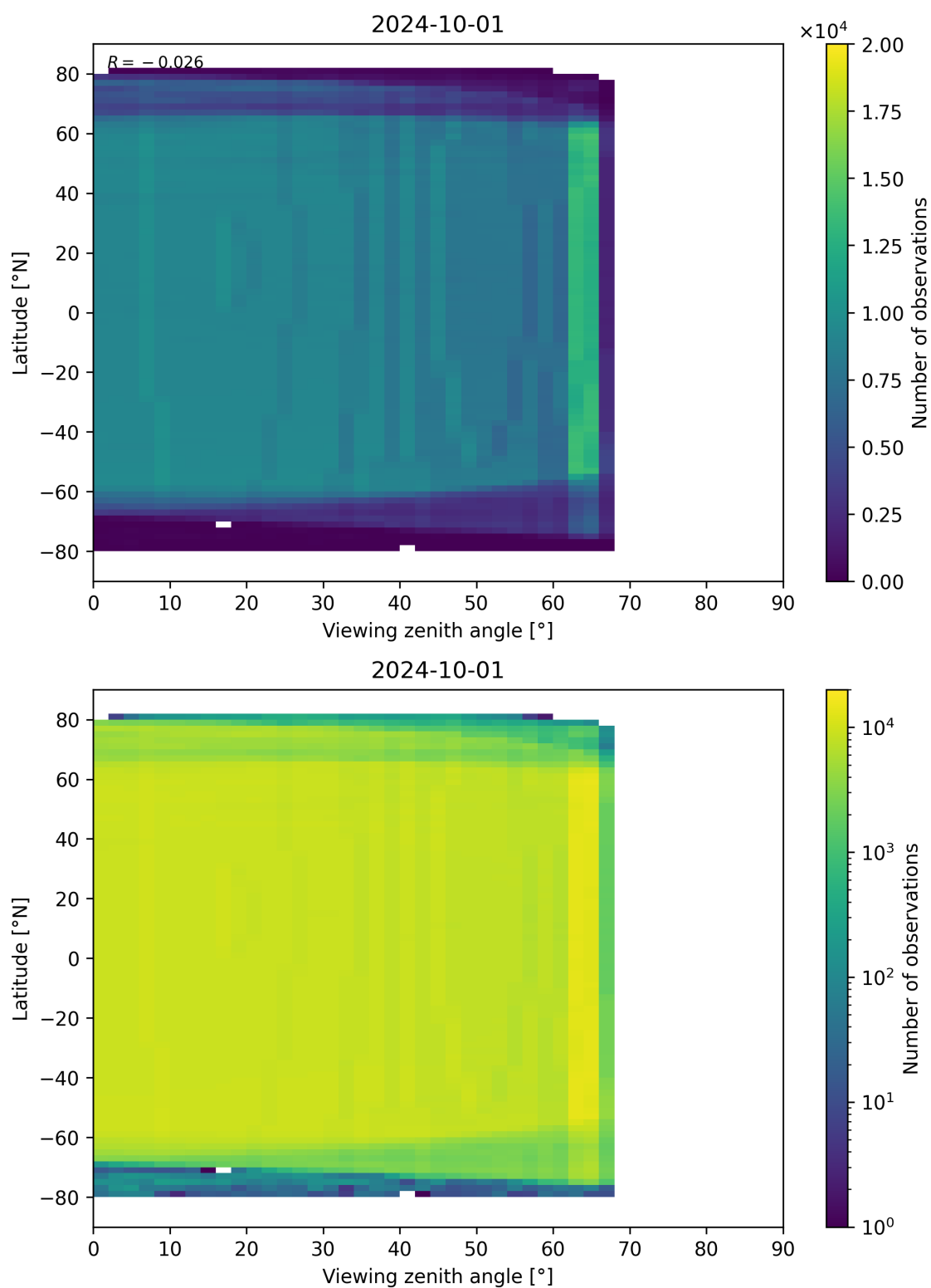
Figure 196: Scatter density plot of “Viewing zenith angle” against “Latitude” for 2024-09-30 to 2024-10-02.
