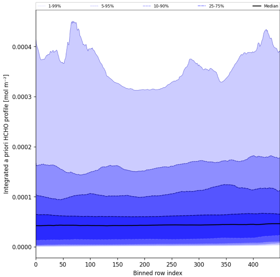
Figure 57: Along track statistics of “Integrated a priori HCHO profile” for 2024-09-30 to 2024-10-02
