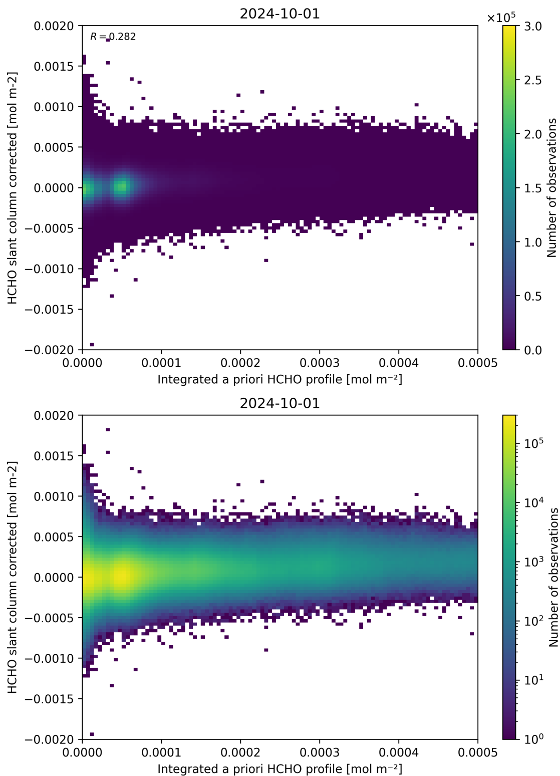
Figure 151: Scatter density plot of “Integrated a priori HCHO profile” against “HCHO slant column corrected” for 2024-09-30 to 2024-10-02.
