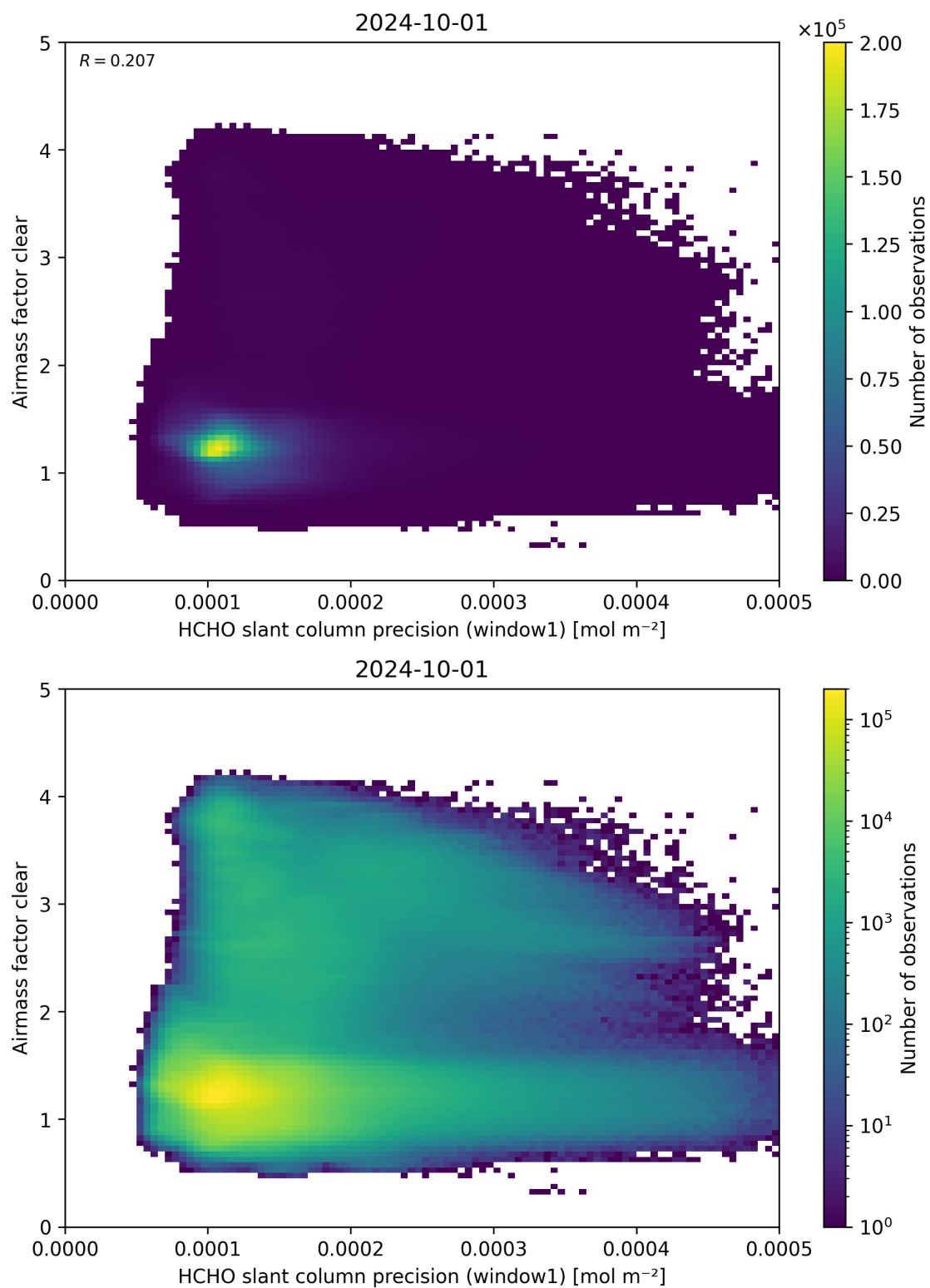
Figure 91: Scatter density plot of “HCHO slant column precision (window1)” against “Airmass factor clear” for 2024-09-30 to 2024-10-02.
