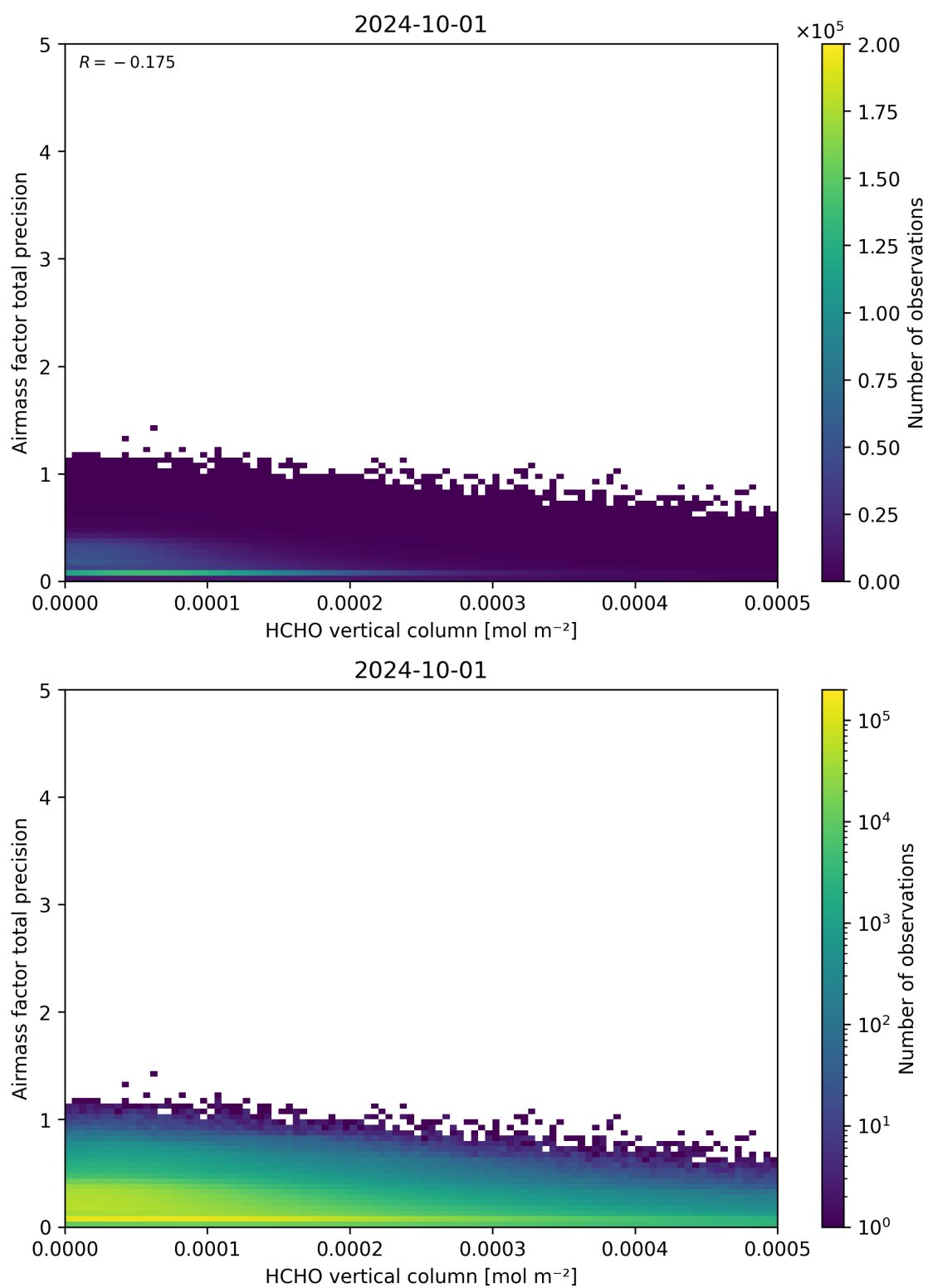
Figure 132: Scatter density plot of “HCHO vertical column” against “Airmass factor total precision” for 2024-09-30 to 2024-10-02.
