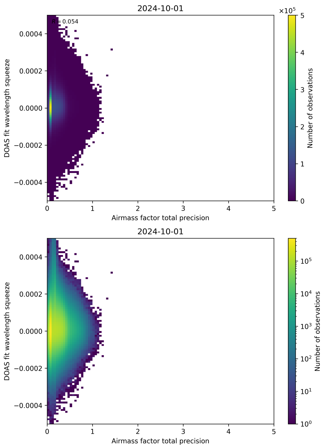
Figure 107: Scatter density plot of “Airmass factor total precision” against “DOAS fit wavelength squeeze” for 2024-09-30 to 2024-10-02.
