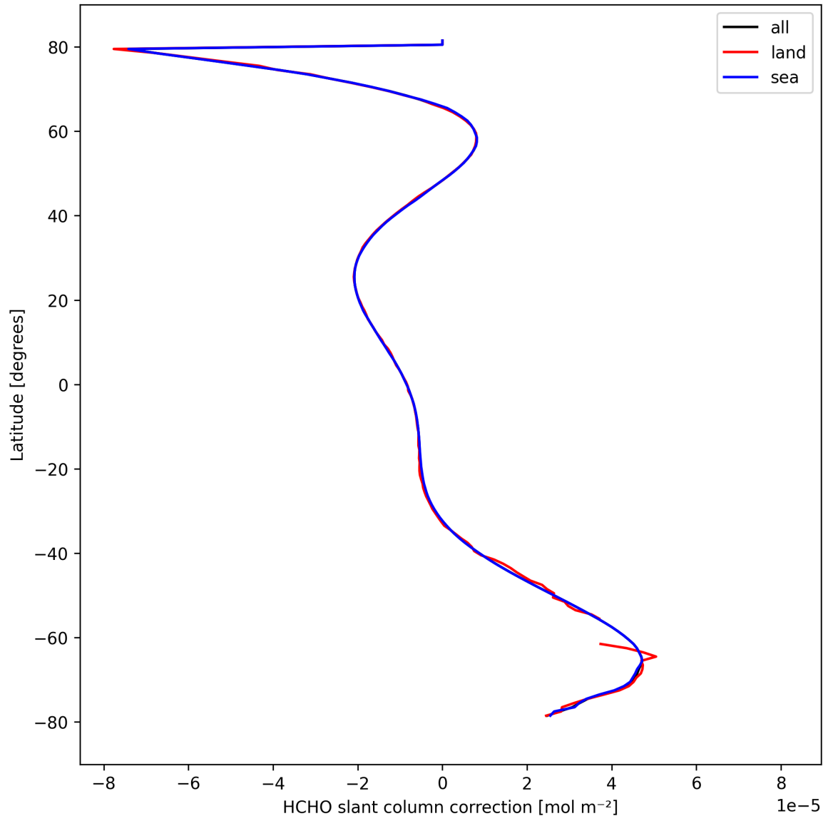
Figure 33: Zonal average of “HCHO slant column correction” for 2024-09-30 to 2024-10-02.
