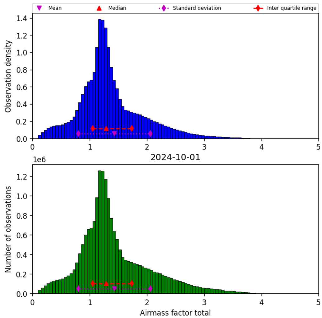
Figure 40: Histogram of “Airmass factor total” for 2024-09-30 to 2024-10-02
