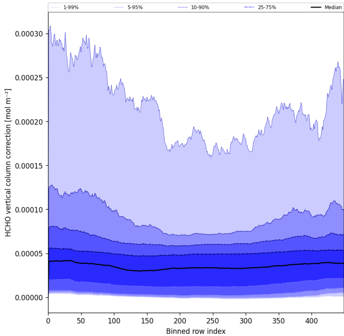
Figure 51: Along track statistics of “HCHO vertical column correction” for 2024-09-30 to 2024-10-02
