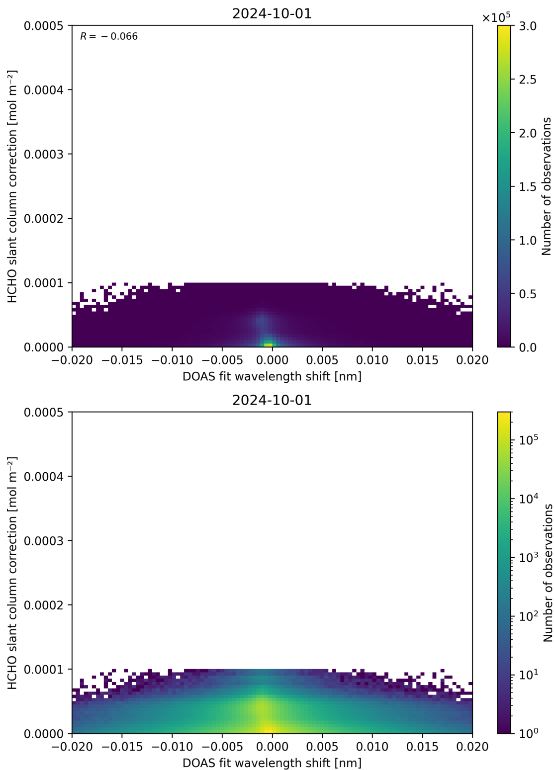
Figure 67: Scatter density plot of “DOAS fit wavelength shift” against “HCHO slant column correction” for 2024-09-30 to 2024-10-02.
