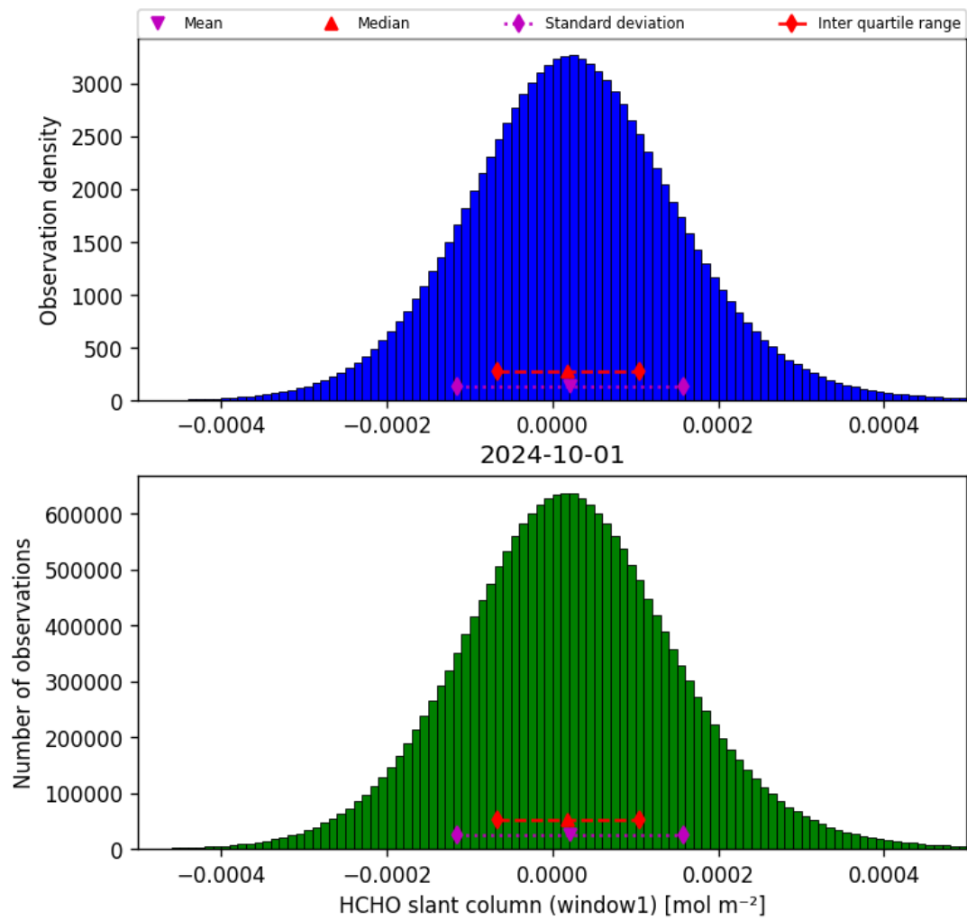
Figure 38: Histogram of “HCHO slant column (window1)” for 2024-09-30 to 2024-10-02
