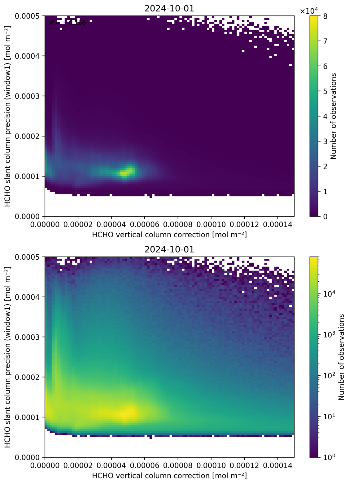
Figure 119: Scatter density plot of “HCHO vertical column correction” against “HCHO slant column precision (window1)” for 2024-09-30 to 2024-10-02.
