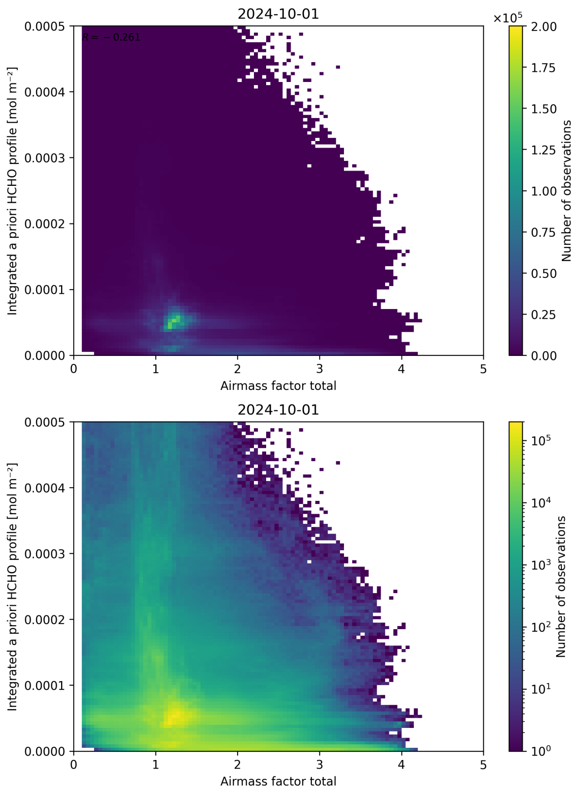
Figure 104: Scatter density plot of “Airmass factor total” against “Integrated a priori HCHO profile” for 2024-09-30 to 2024-10-02.
