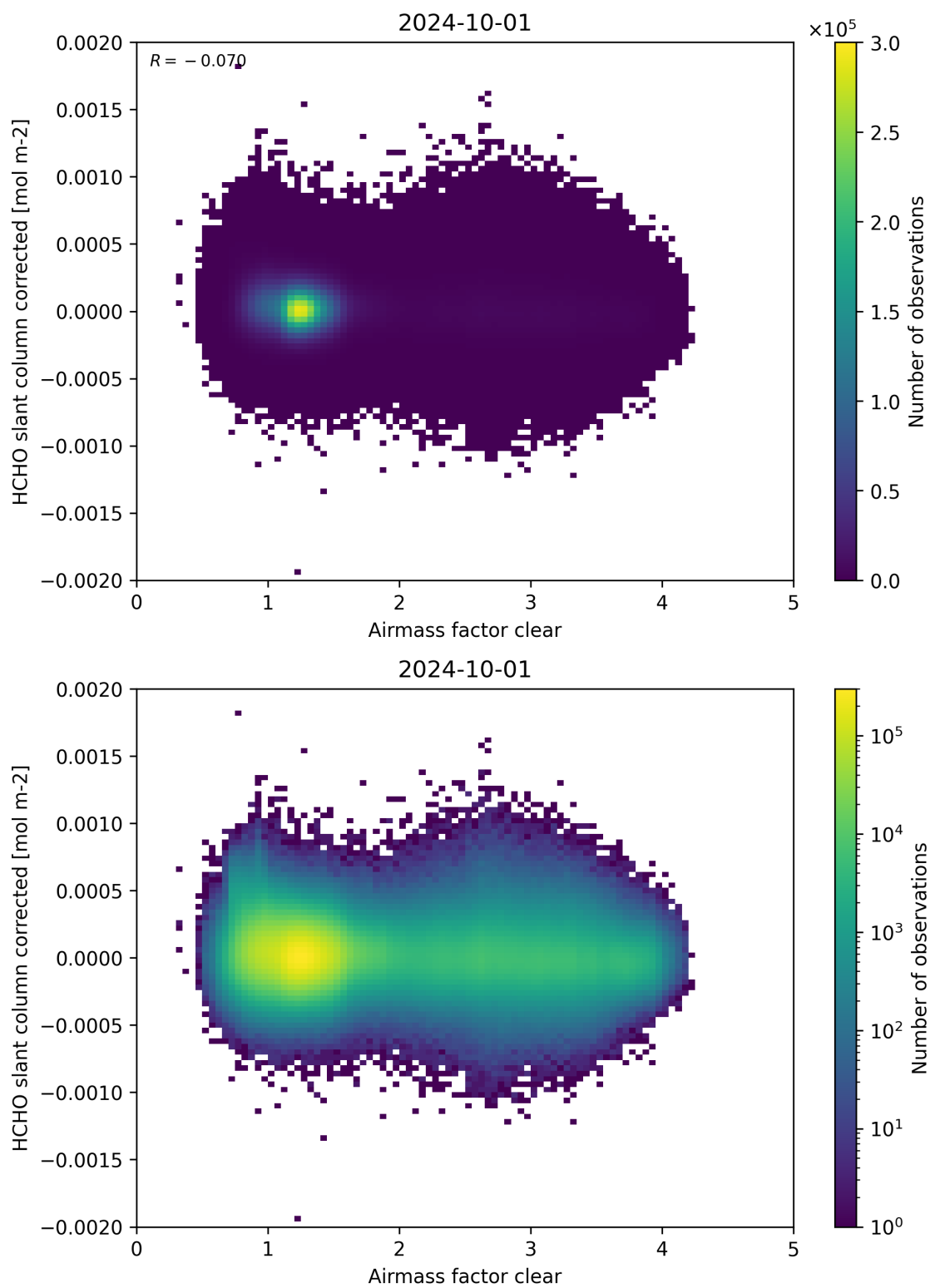
Figure 74: Scatter density plot of “Airmass factor clear” against “HCHO slant column corrected” for 2024-09-30 to 2024-10-02.
