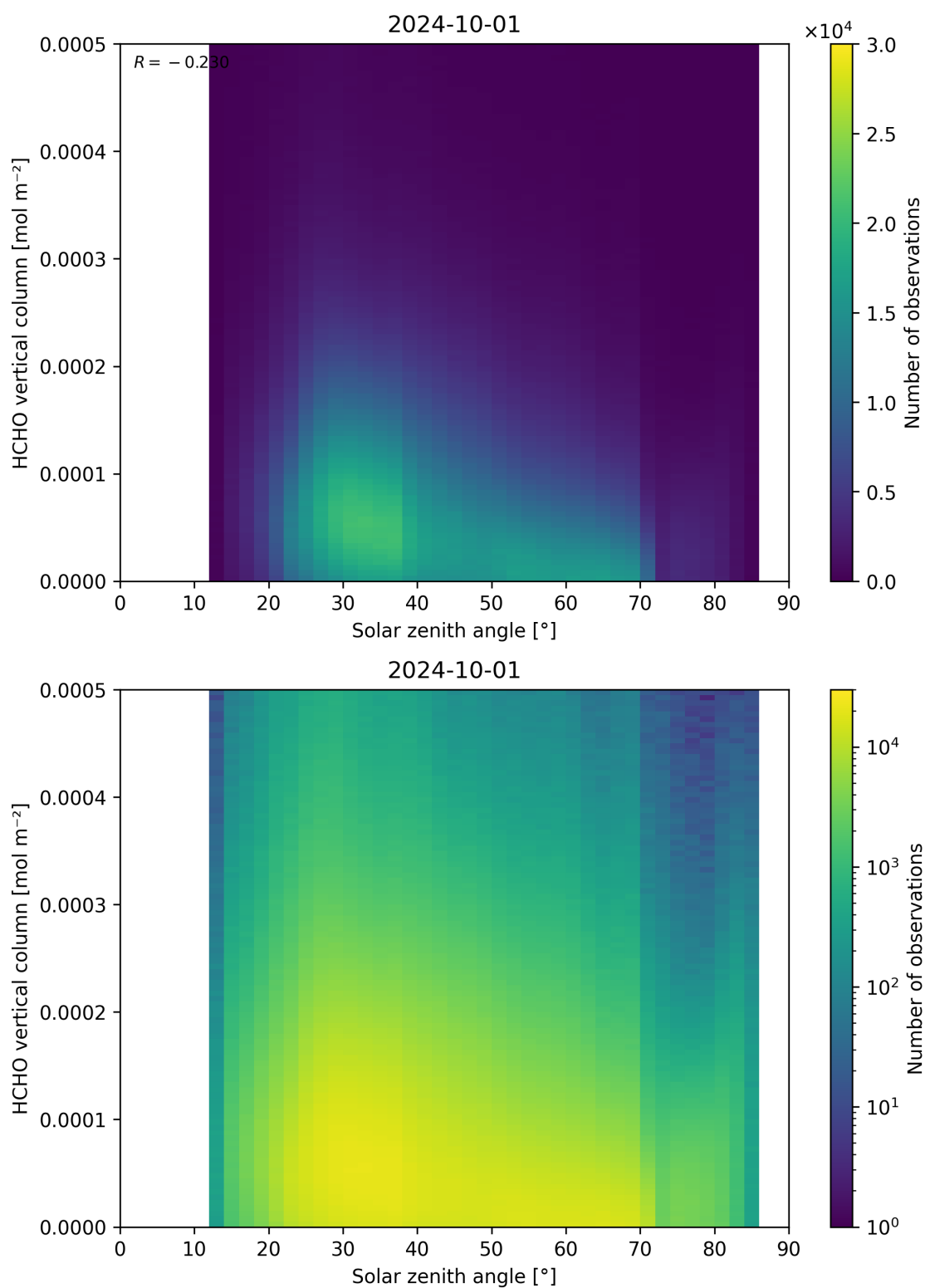
Figure 177: Scatter density plot of “Solar zenith angle” against “HCHO vertical column” for 2024-09-30 to 2024-10-02.
