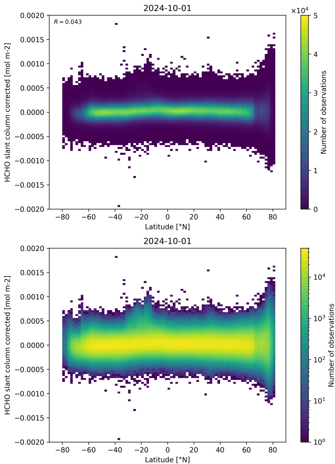
Figure 157: Scatter density plot of “Latitude” against “HCHO slant column corrected” for 2024-09-30 to 2024-10-02.
