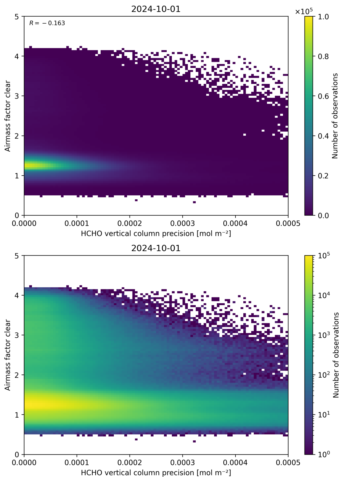
Figure 139: Scatter density plot of “HCHO vertical column precision” against “Airmass factor clear” for 2024-09-30 to 2024-10-02.
