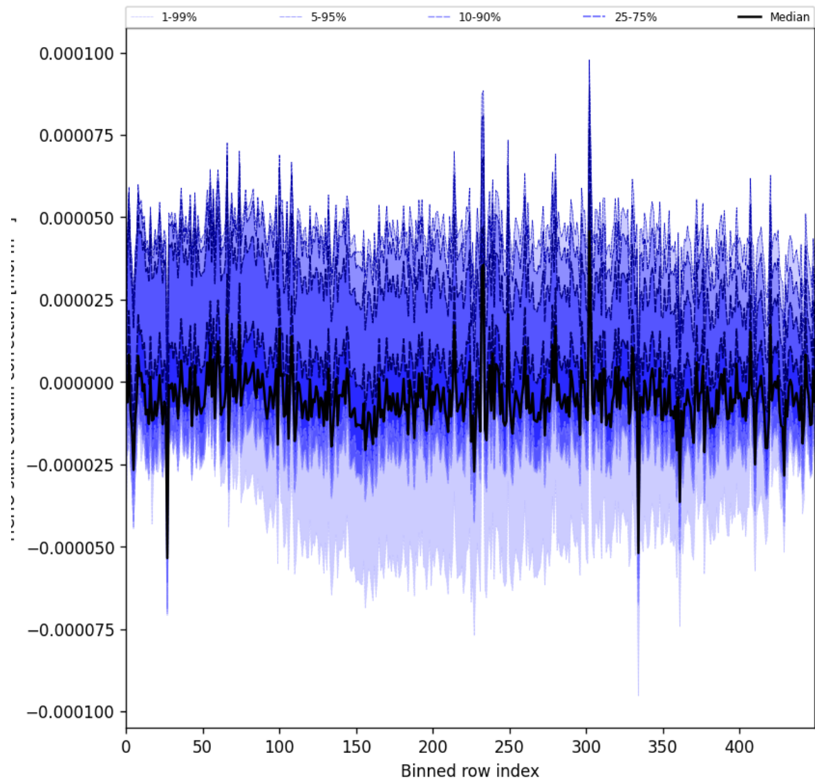
Figure 61: Along track statistics of “HCHO slant column correction” for 2024-09-30 to 2024-10-02
