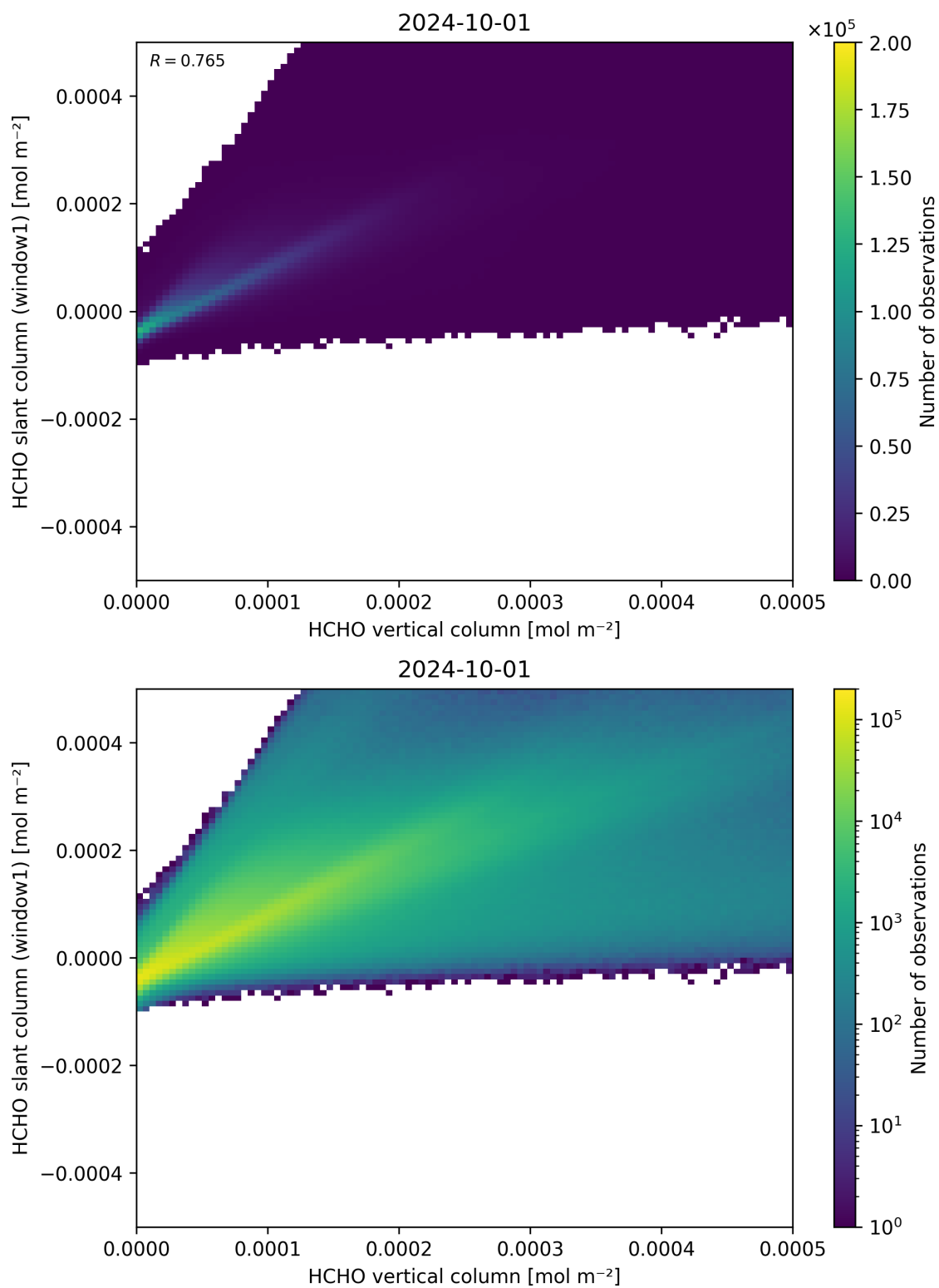
Figure 129: Scatter density plot of “HCHO vertical column” against “HCHO slant column (window1)” for 2024-09-30 to 2024-10-02.
