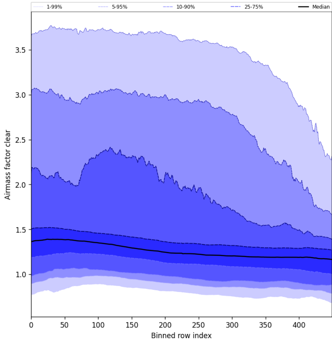
Figure 56: Along track statistics of “Airmass factor clear” for 2024-09-30 to 2024-10-02
