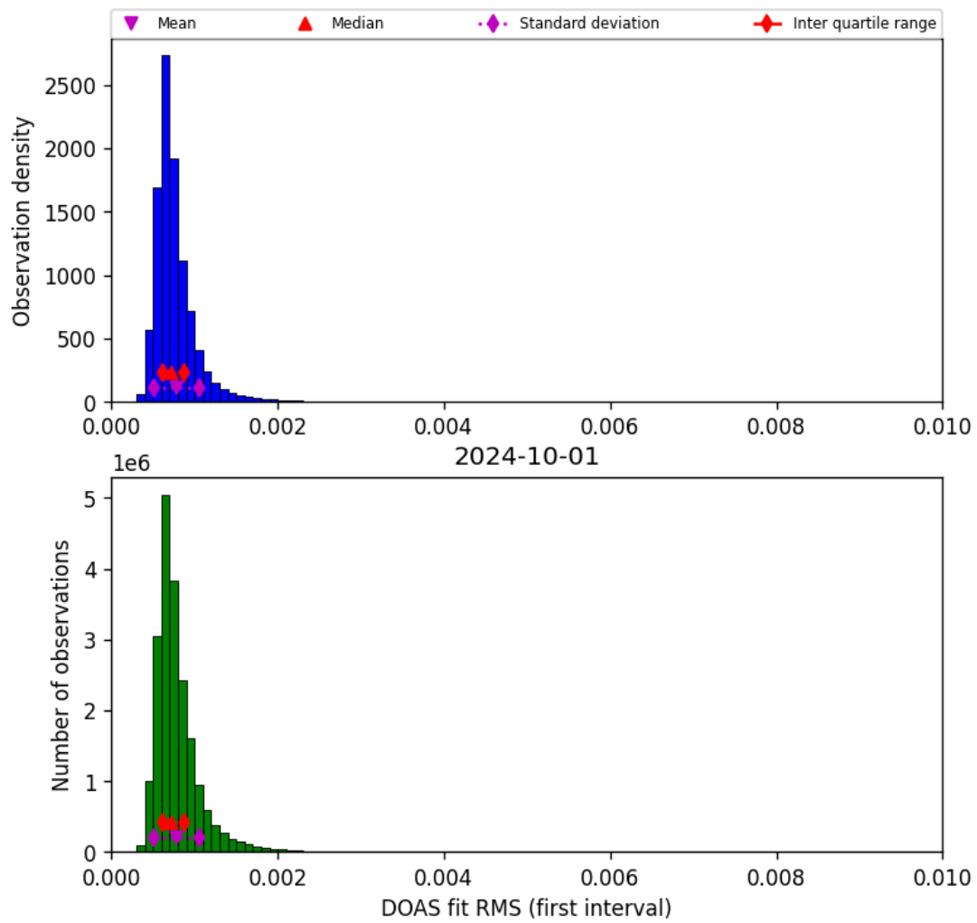
Figure 46: Histogram of “DOAS fit RMS (first interval)” for 2024-09-30 to 2024-10-02
