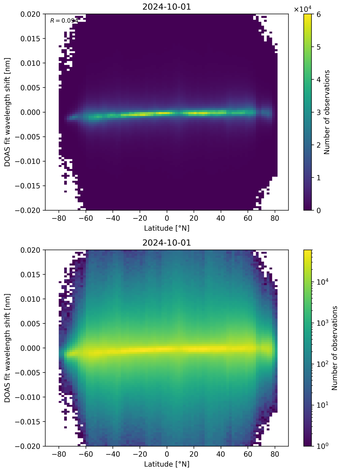
Figure 154: Scatter density plot of “Latitude” against “DOAS fit wavelength shift” for 2024-09-30 to 2024-10-02.
