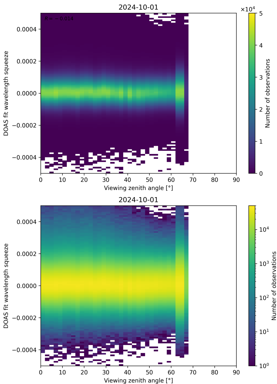
Figure 184: Scatter density plot of “Viewing zenith angle” against “DOAS fit wavelength squeeze” for 2024-09-30 to 2024-10-02.
