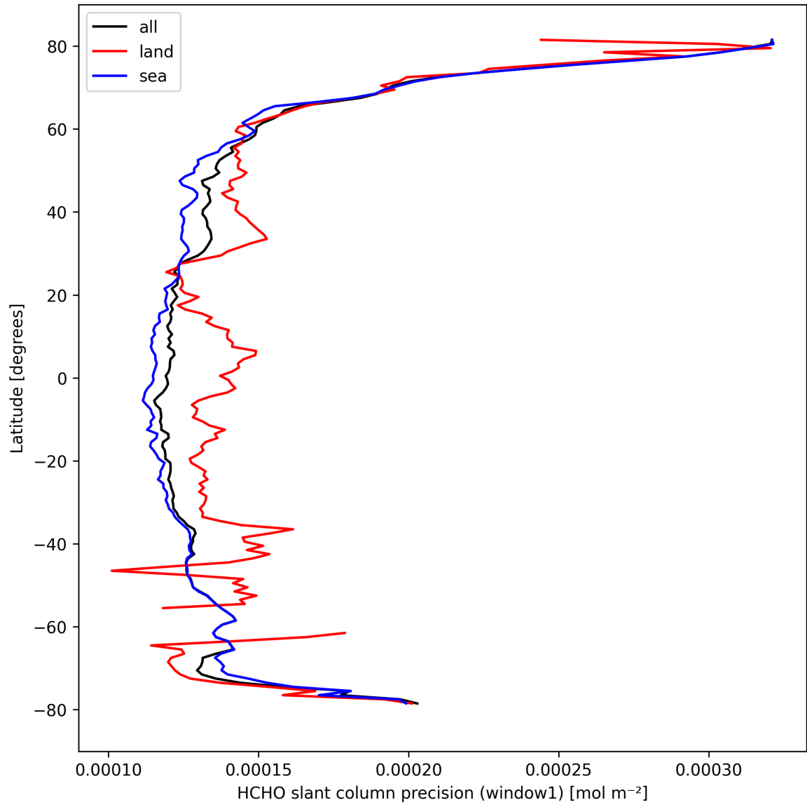
Figure 25: Zonal average of "HCHO slant column precision (window1)" for 2024-09-30 to 2024-10-02.
