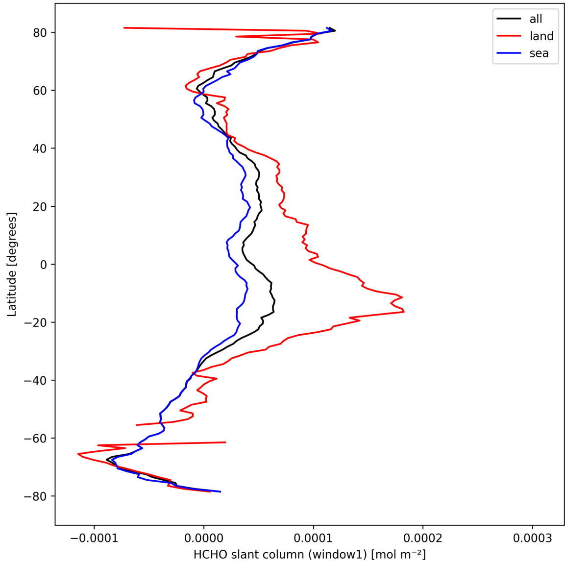
Figure 24: Zonal average of “HCHO slant column (window1)” for 2024-09-30 to 2024-10-02.
