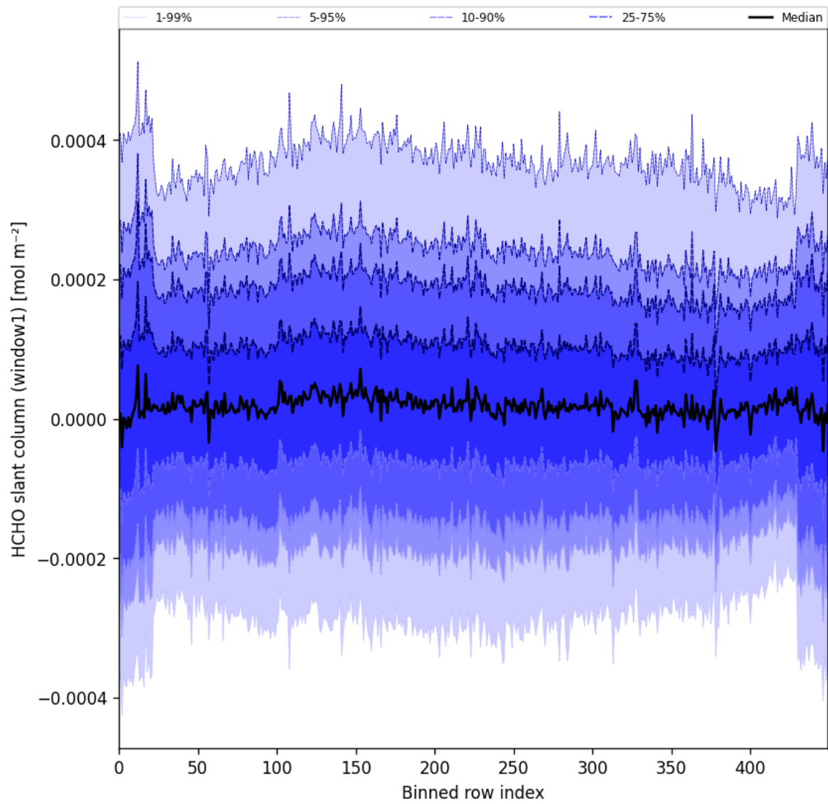
Figure 52: Along track statistics of “HCHO slant column (window1)” for 2024-09-30 to 2024-10-02
