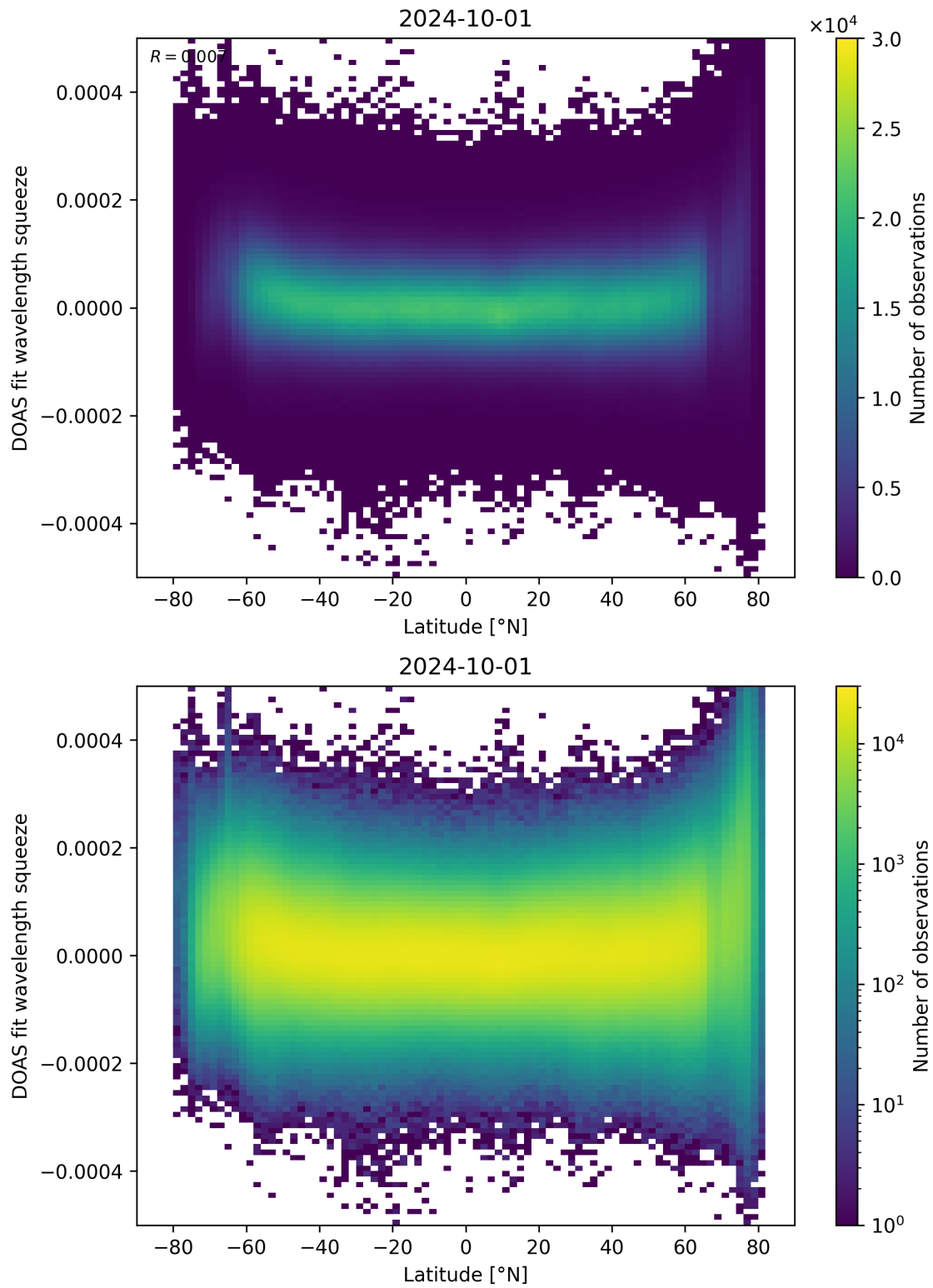
Figure 155: Scatter density plot of “Latitude” against “DOAS fit wavelength squeeze” for 2024-09-30 to 2024-10-02.
