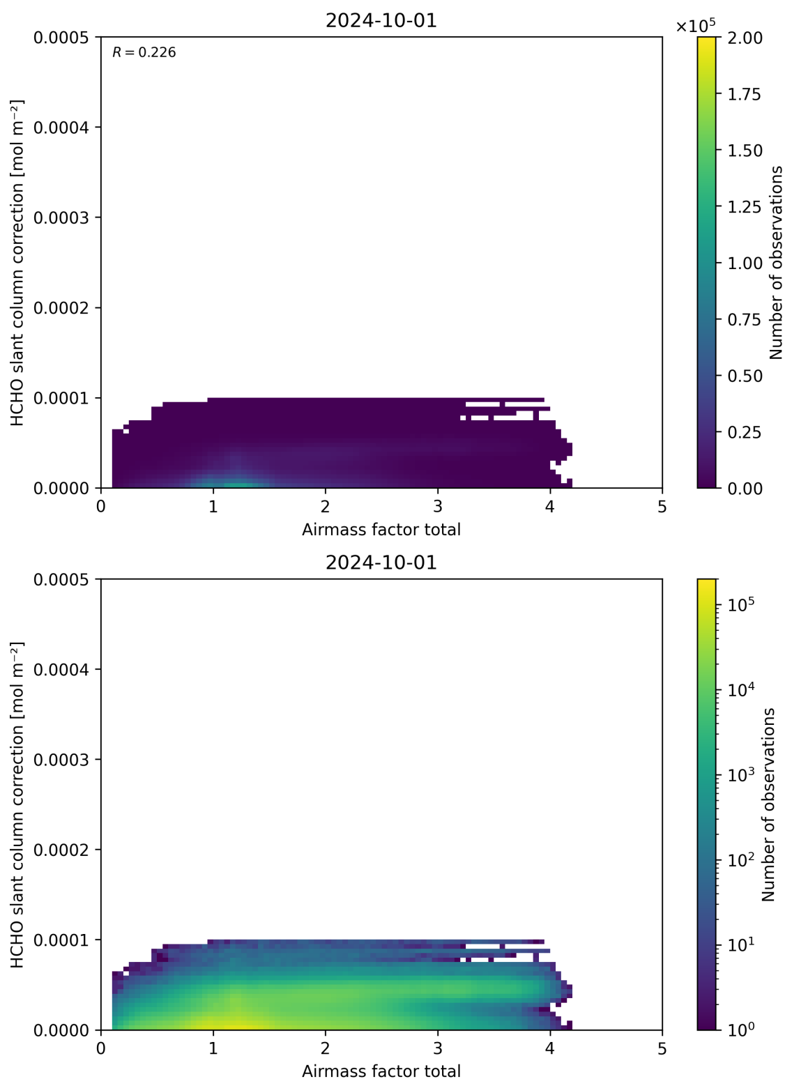
Figure 102: Scatter density plot of “Airmass factor total” against “HCHO slant column correction” for 2024-09-30 to 2024-10-02.
