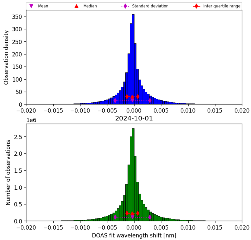
Figure 44: Histogram of “DOAS fit wavelength shift” for 2024-09-30 to 2024-10-02
