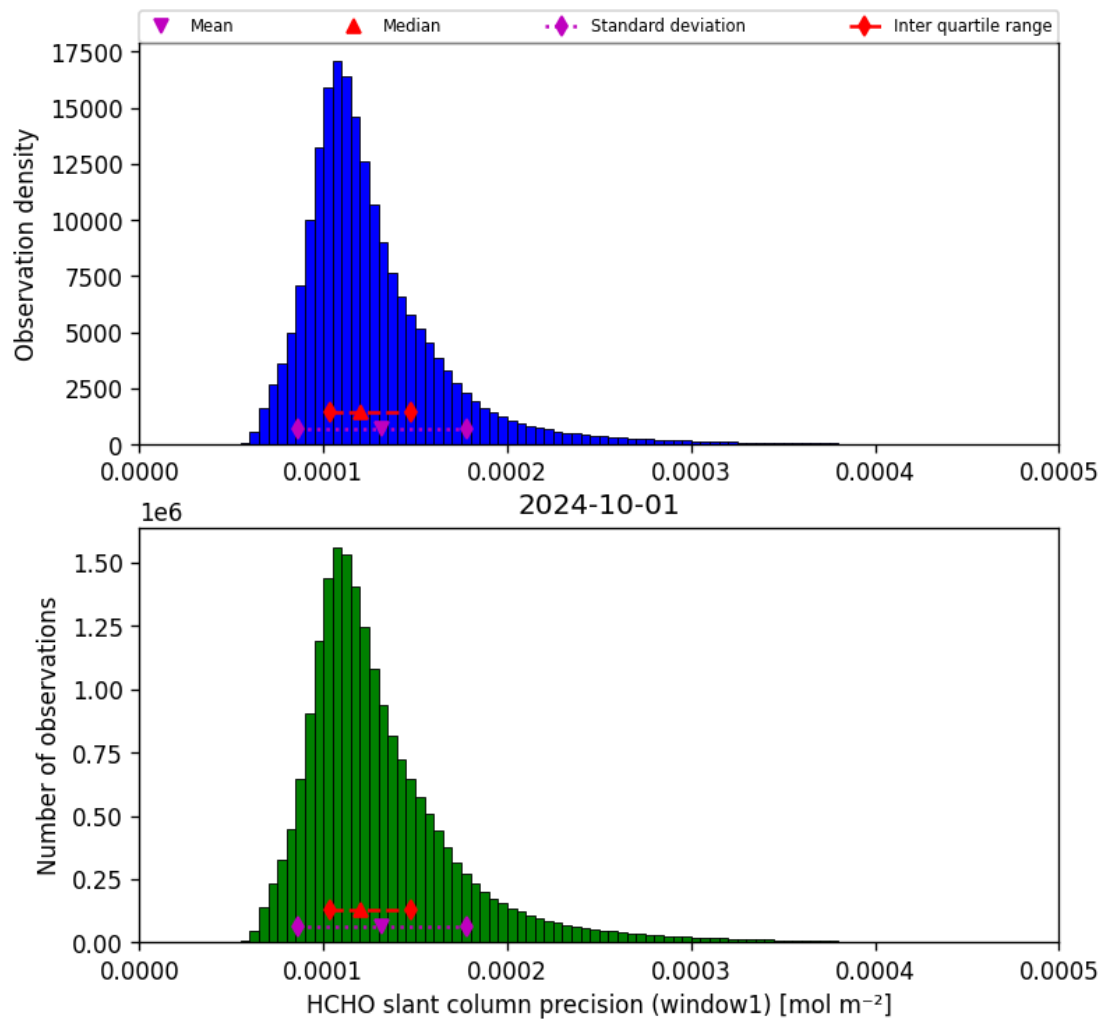
Figure 39: Histogram of “HCHO slant column precision (window1)” for 2024-09-30 to 2024-10-02
