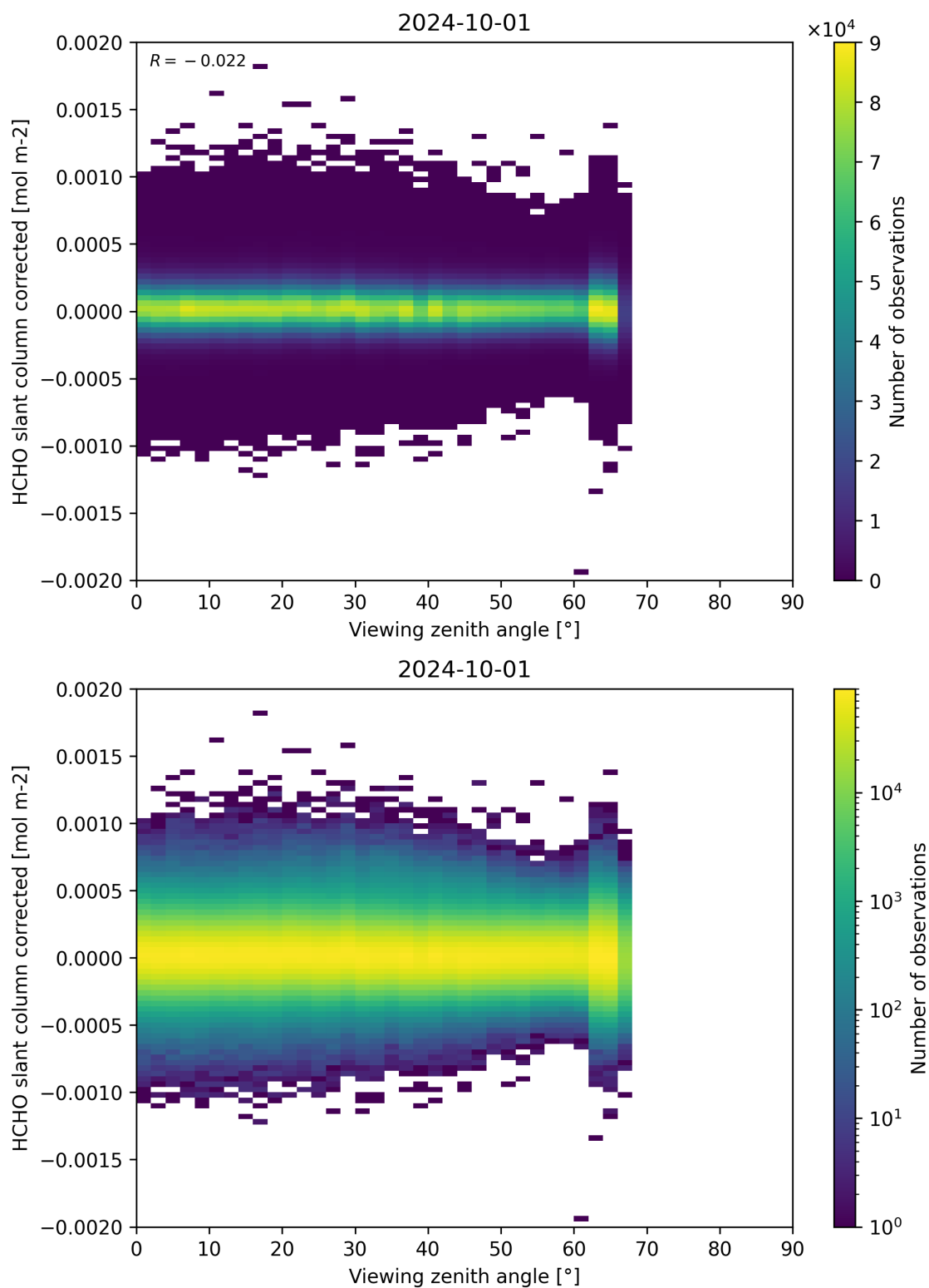
Figure 186: Scatter density plot of “Viewing zenith angle” against “HCHO slant column corrected” for 2024-09-30 to 2024-10-02.
