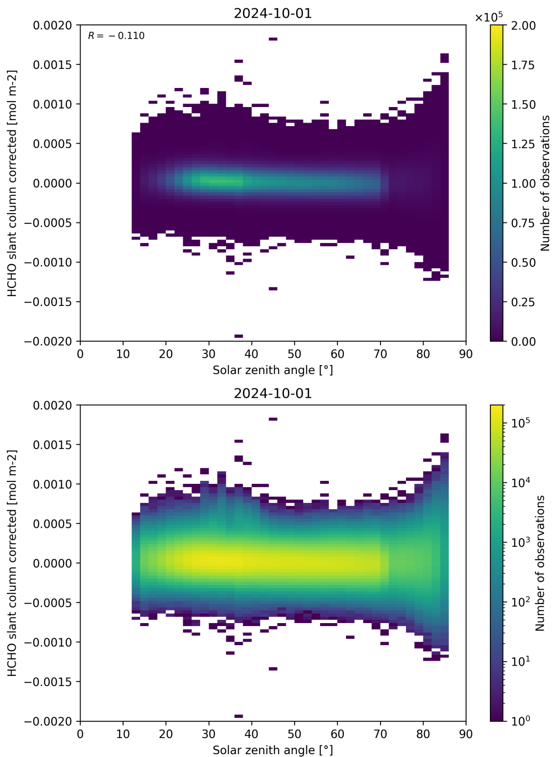
Figure 171: Scatter density plot of “Solar zenith angle” against “HCHO slant column corrected” for 2024-09-30 to 2024-10-02.
