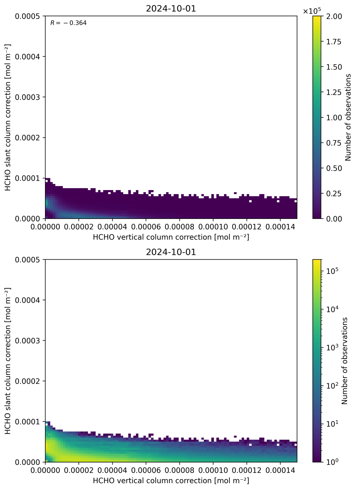
Figure 117: Scatter density plot of “HCHO vertical column correction” against “HCHO slant column correction” for 2024-09-30 to 2024-10-02.
