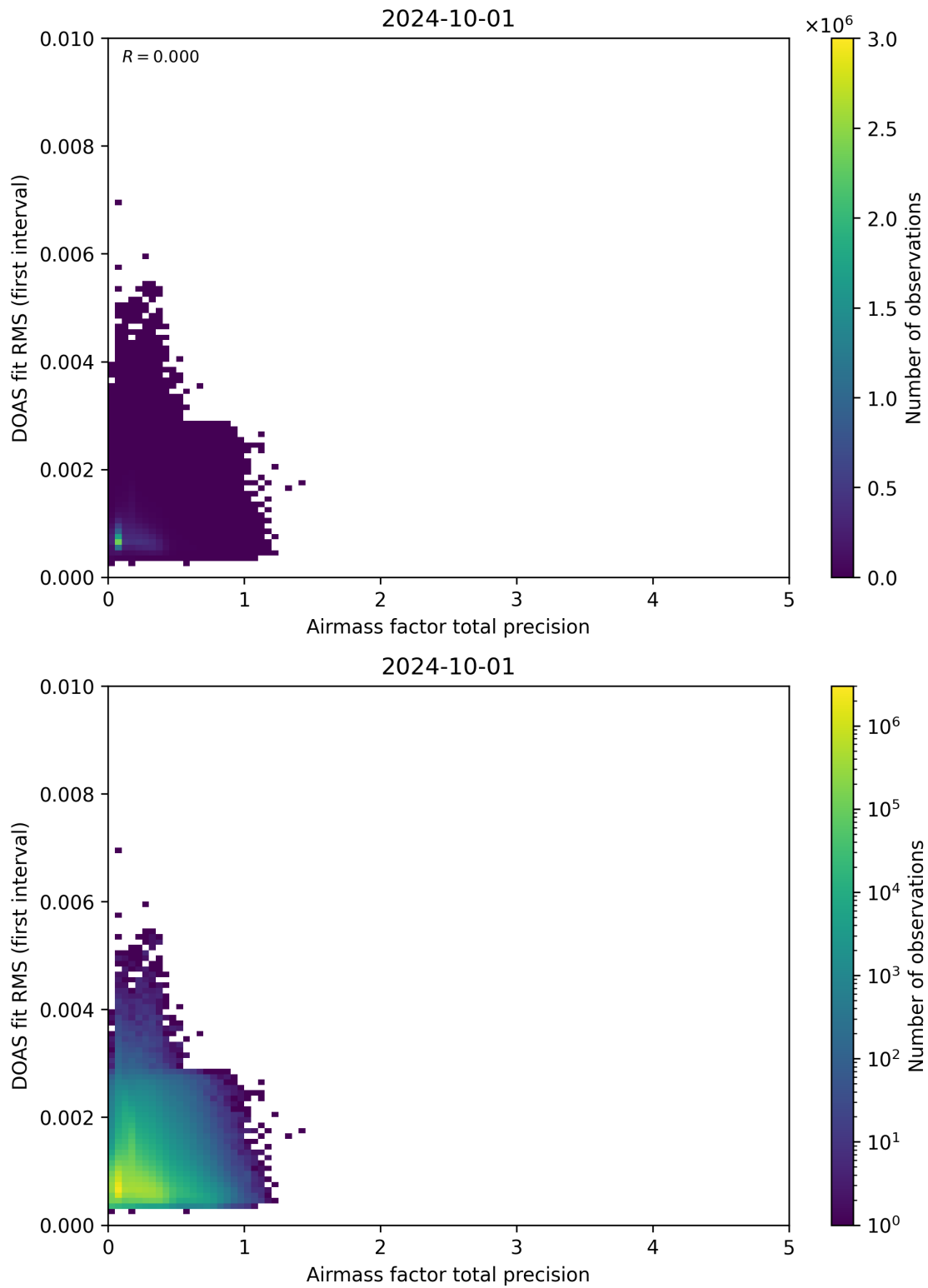
Figure 105: Scatter density plot of “Airmass factor total precision” against “DOAS fit RMS (first interval)” for 2024-09-30 to 2024-10-02.
