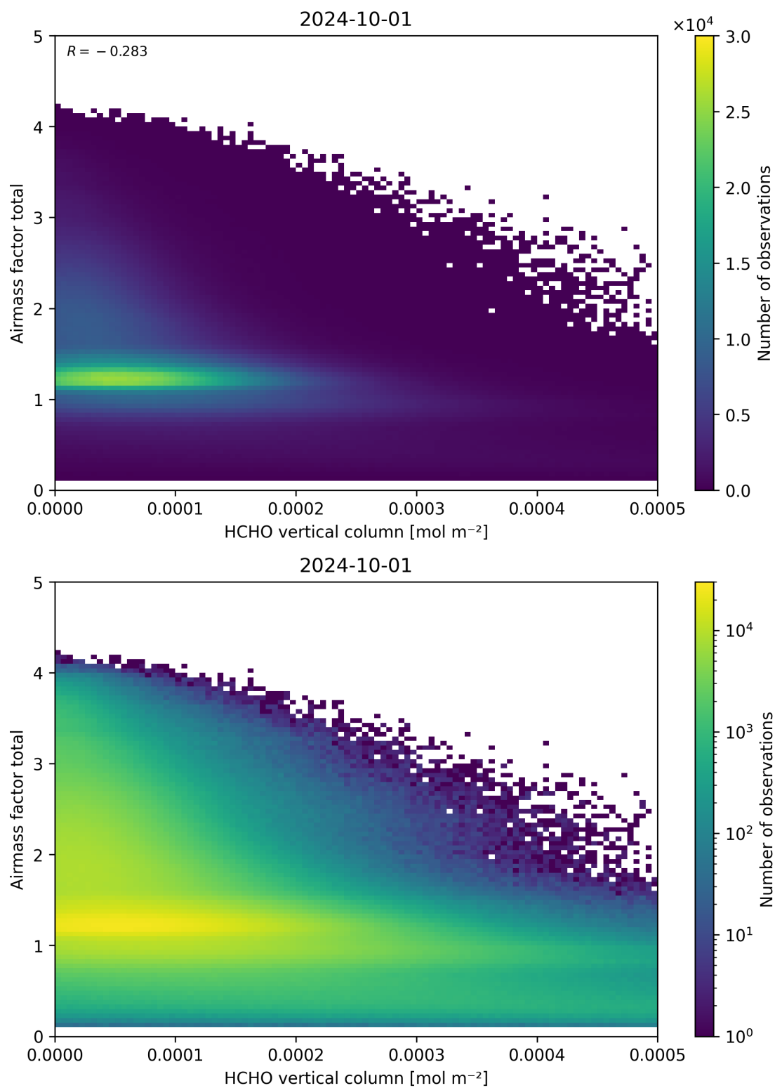
Figure 131: Scatter density plot of “HCHO vertical column” against “Airmass factor total” for 2024-09-30 to 2024-10-02.
