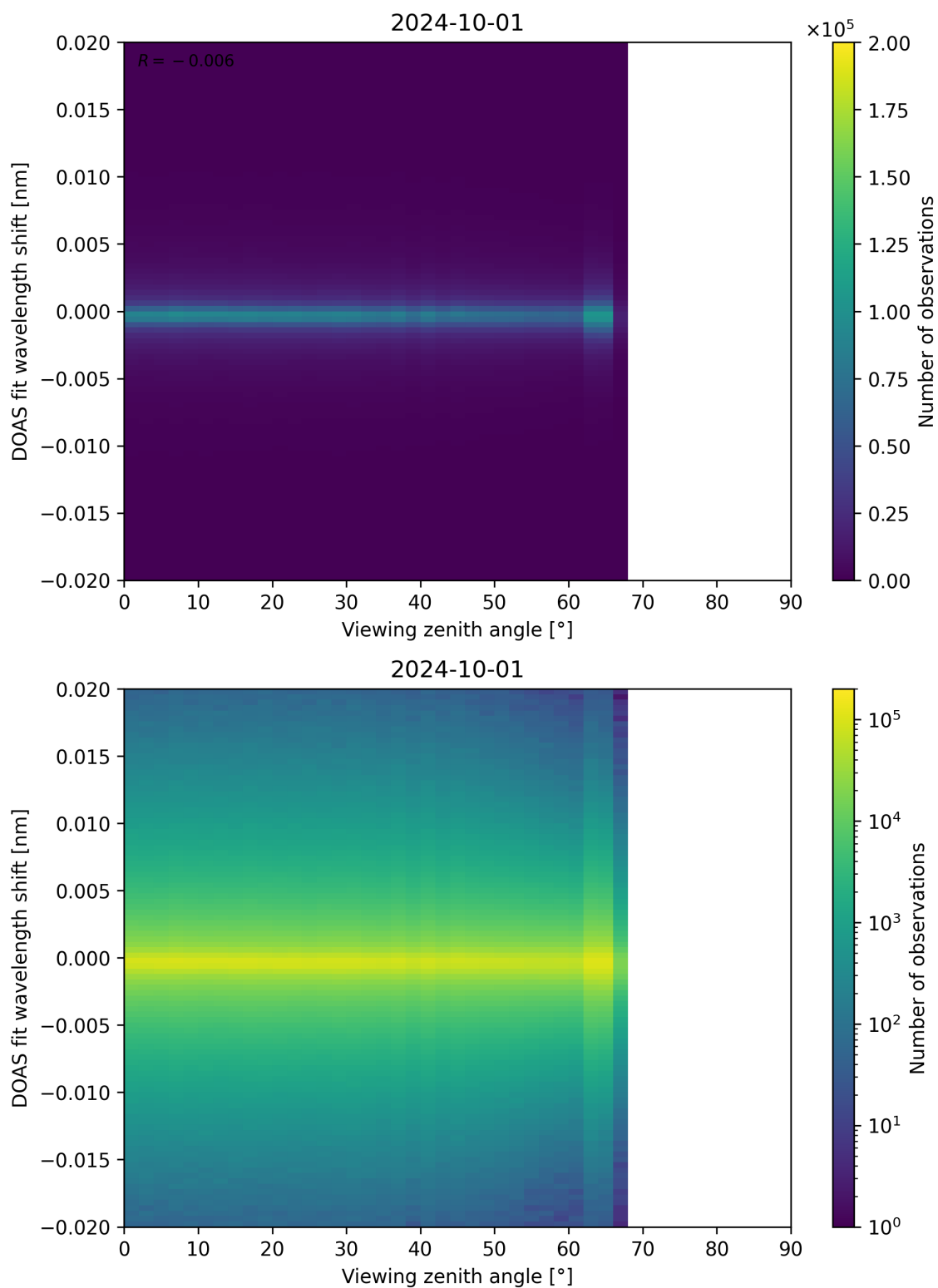
Figure 183: Scatter density plot of “Viewing zenith angle” against “DOAS fit wavelength shift” for 2024-09-30 to 2024-10-02.
