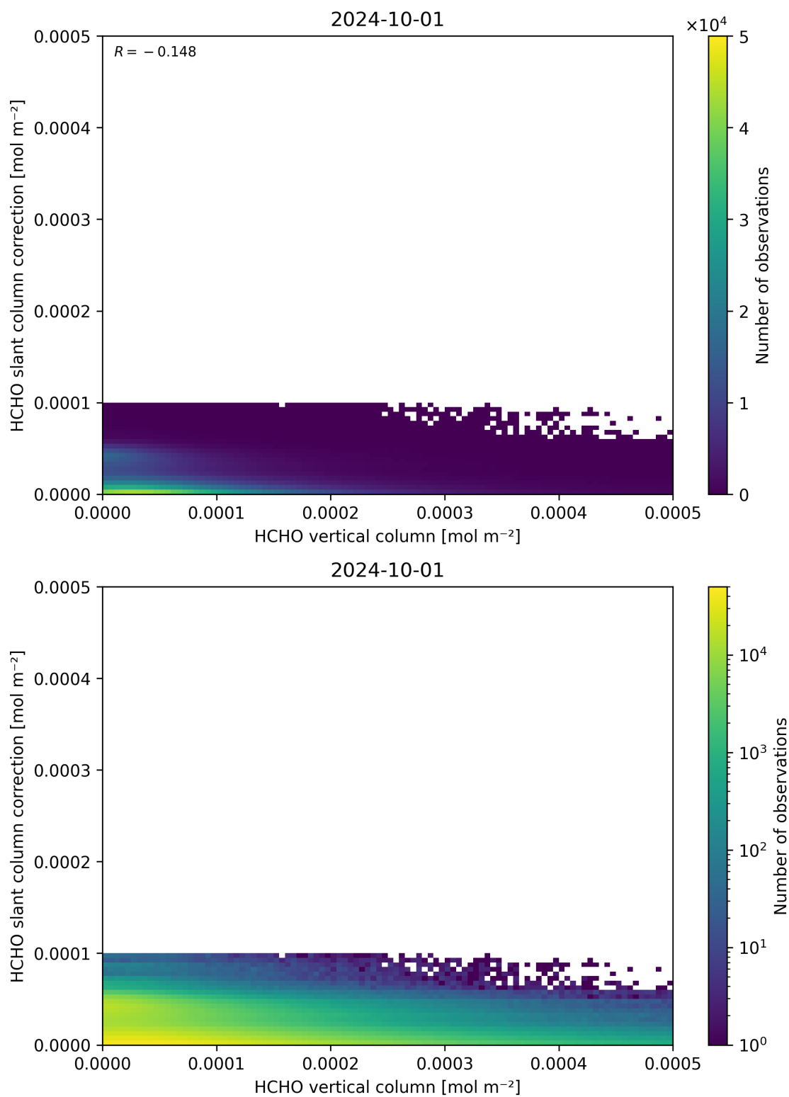
Figure 128: Scatter density plot of “HCHO vertical column” against “HCHO slant column correction” for 2024-09-30 to 2024-10-02.
