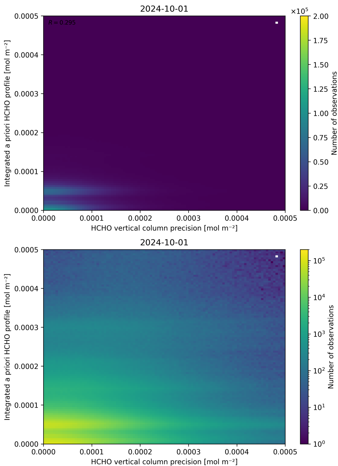
Figure 147: Scatter density plot of “HCHO vertical column precision” against “Integrated a priori HCHO profile” for 2024-09-30 to 2024-10-02.
