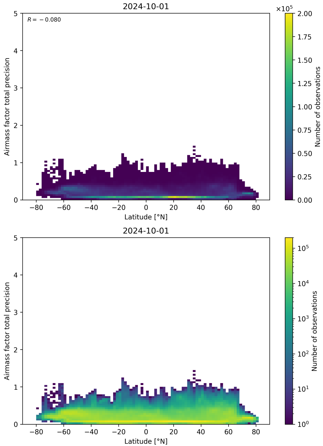
Figure 162: Scatter density plot of “Latitude” against “Airmass factor total precision” for 2024-09-30 to 2024-10-02.
