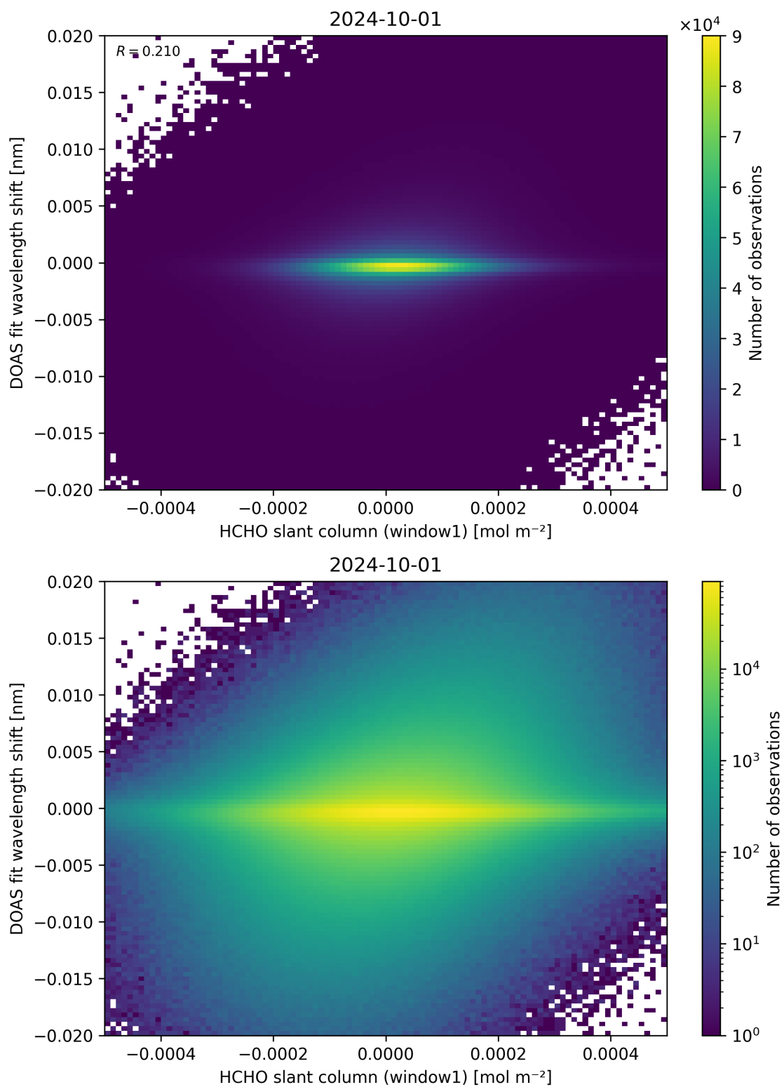
Figure 79: Scatter density plot of “HCHO slant column (window1)” against “DOAS fit wavelength shift” for 2024-09-30 to 2024-10-02.
