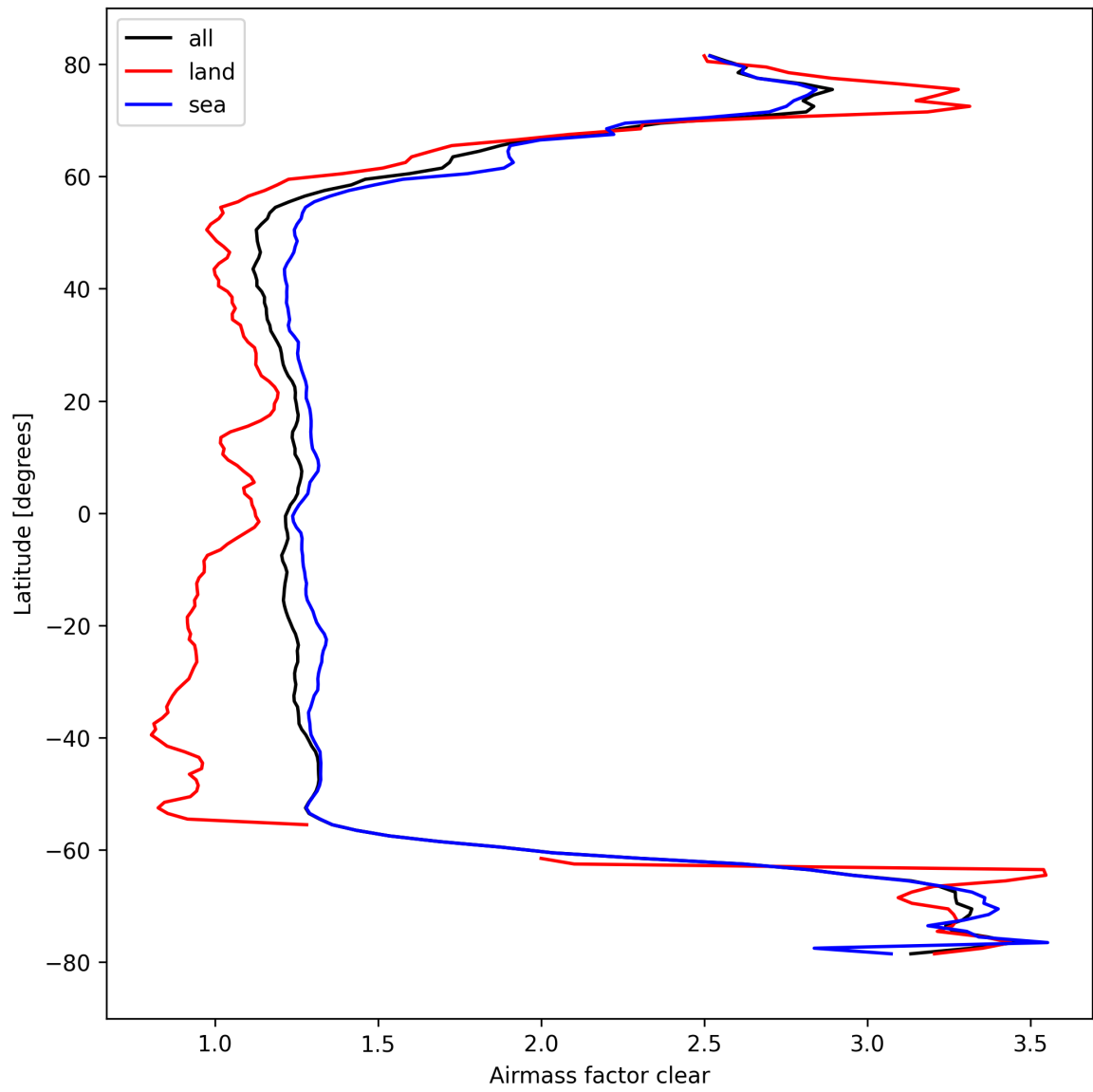
Figure 28: Zonal average of “Airmass factor clear” for 2024-09-30 to 2024-10-02.
