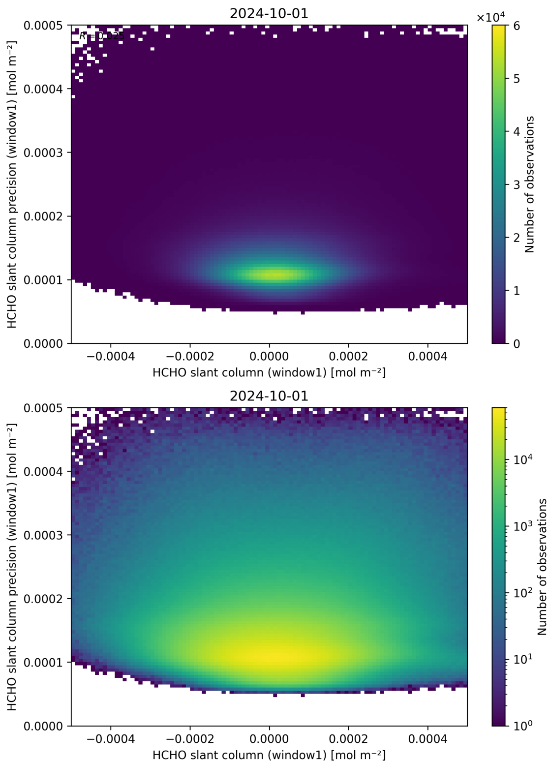
Figure 84: Scatter density plot of “HCHO slant column (window1)” against “HCHO slant column precision (window1)” for 2024-09-30 to 2024-10-02.
