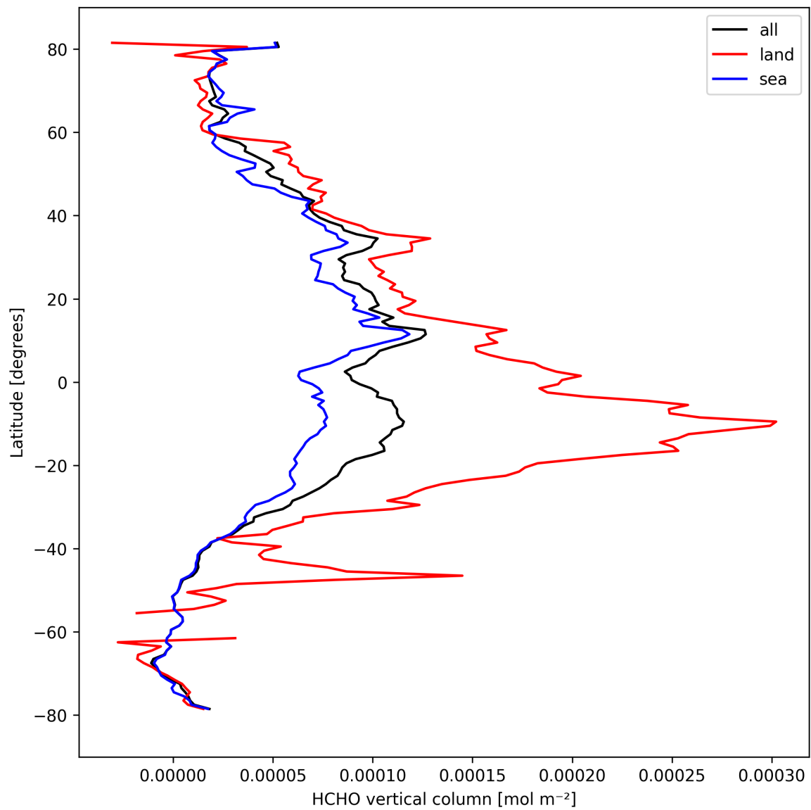
Figure 21: Zonal average of “HCHO vertical column” for 2024-09-30 to 2024-10-02.
