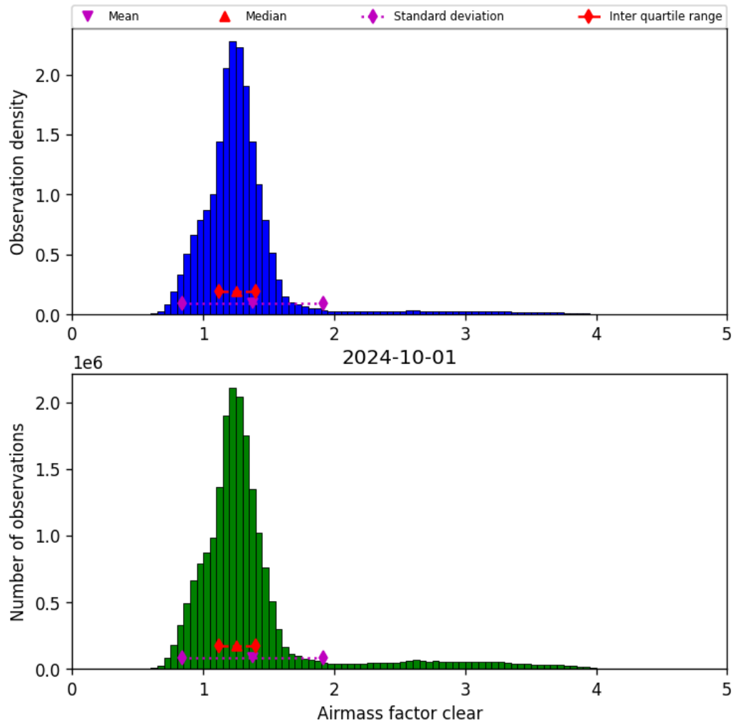
Figure 42: Histogram of “Airmass factor clear” for 2024-09-30 to 2024-10-02
