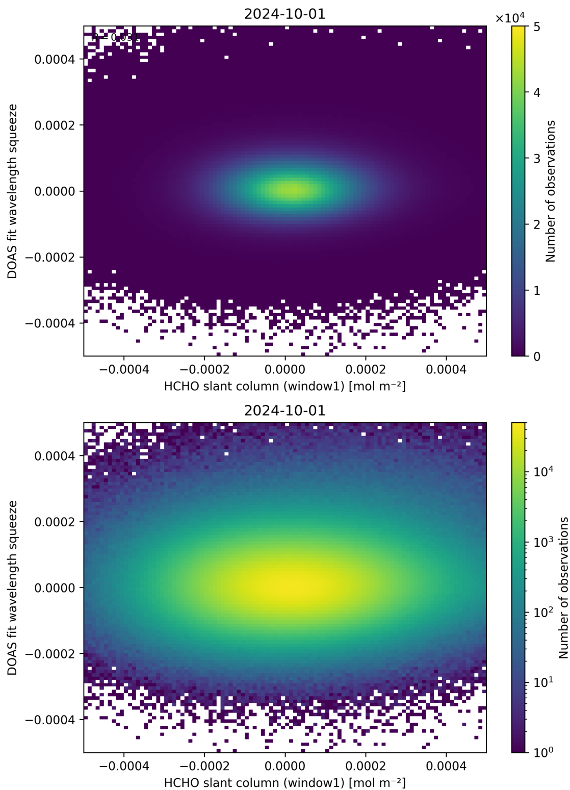
Figure 80: Scatter density plot of “HCHO slant column (window1)” against “DOAS fit wavelength squeeze” for 2024-09-30 to 2024-10-02.
