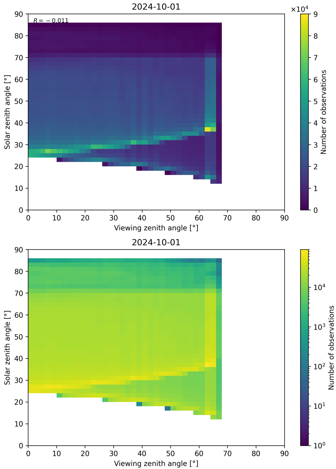
Figure 197: Scatter density plot of “Viewing zenith angle” against “Solar zenith angle” for 2024-09-30 to 2024-10-02.
