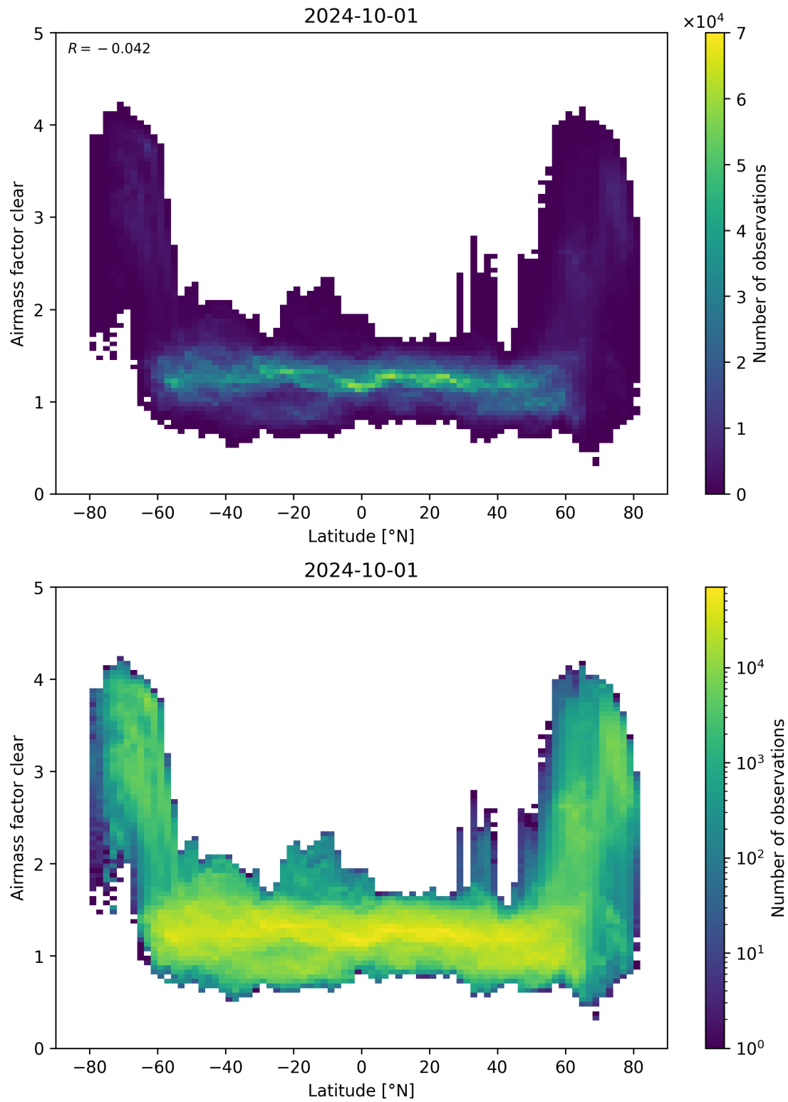
Figure 156: Scatter density plot of “Latitude” against “Airmass factor clear” for 2024-09-30 to 2024-10-02.
