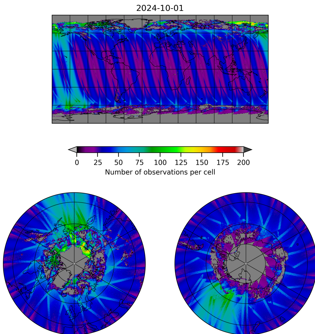
Figure 19: Map of the number of observations for 2024-09-30 to 2024-10-02
