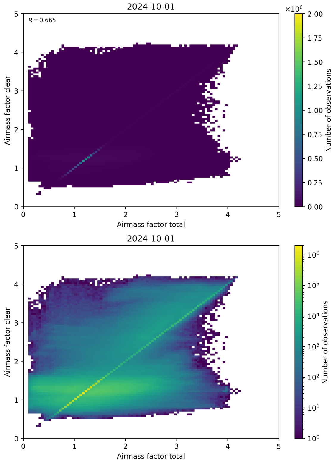
Figure 100: Scatter density plot of “Airmass factor total” against “Airmass factor clear” for 2024-09-30 to 2024-10-02.
