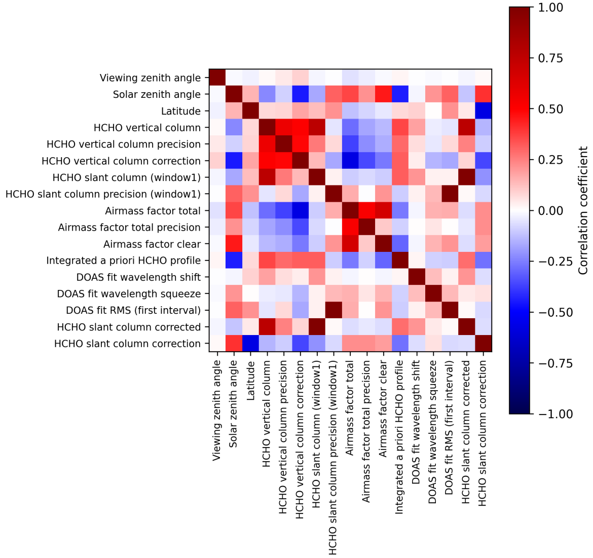
Figure 2: Map of correlation matrix for 2024-09-30 to 2024-10-02.
