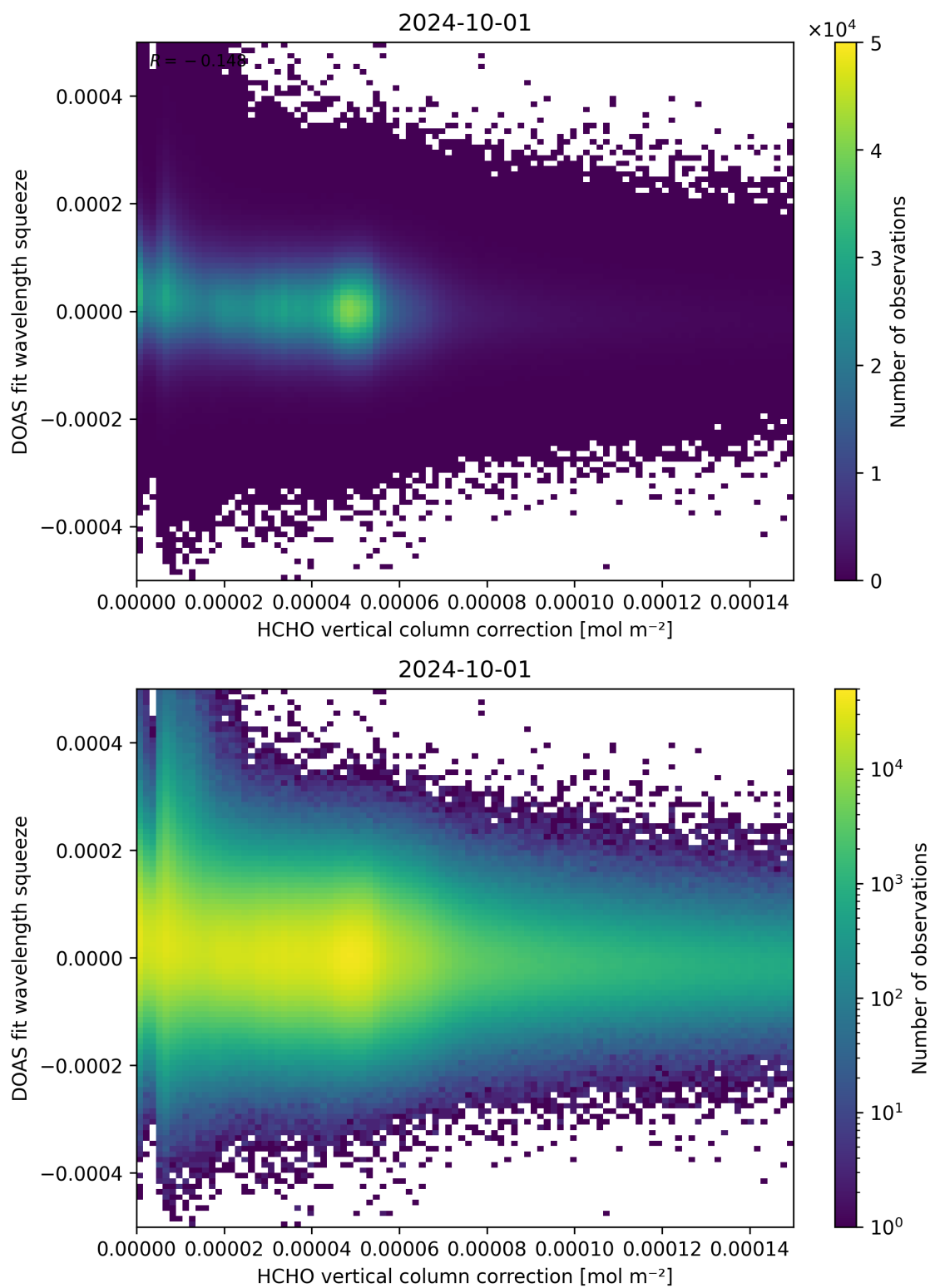
Figure 114: Scatter density plot of “HCHO vertical column correction” against “DOAS fit wavelength squeeze” for 2024-09-30 to 2024-10-02.
