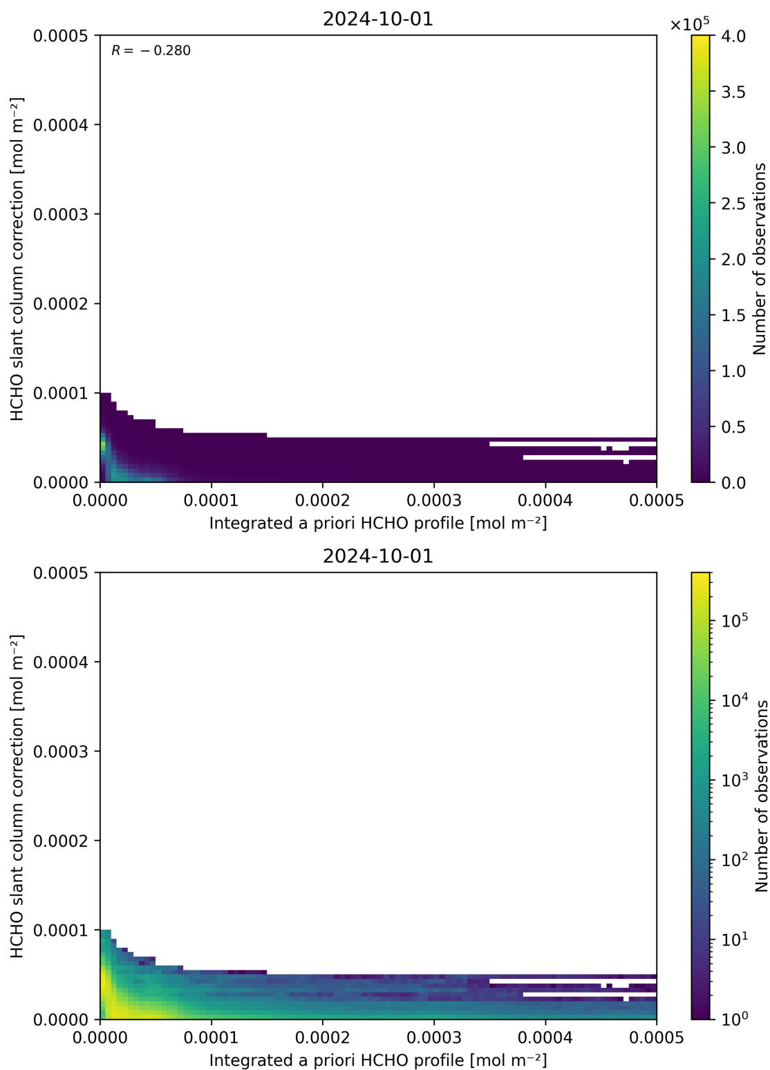
Figure 152: Scatter density plot of “Integrated a priori HCHO profile” against “HCHO slant column correction” for 2024-09-30 to 2024-10-02.
