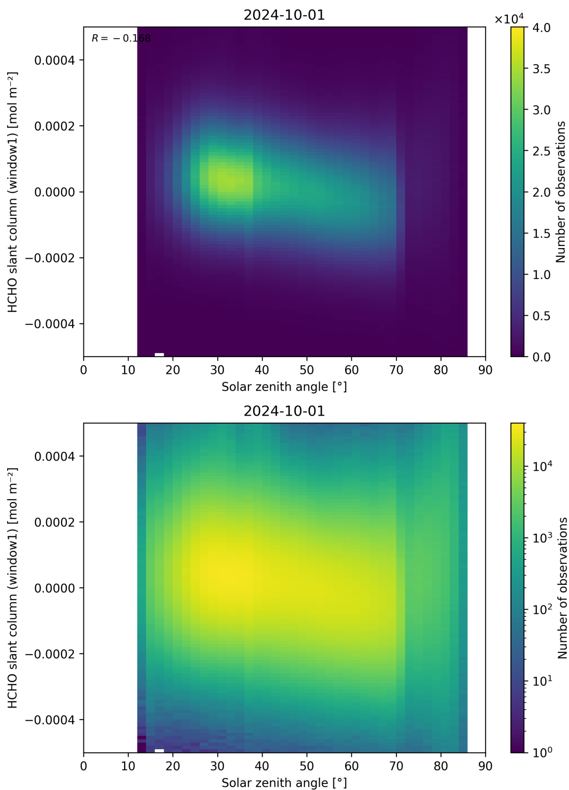
Figure 173: Scatter density plot of “Solar zenith angle” against “HCHO slant column (window1)” for 2024-09-30 to 2024-10-02.
