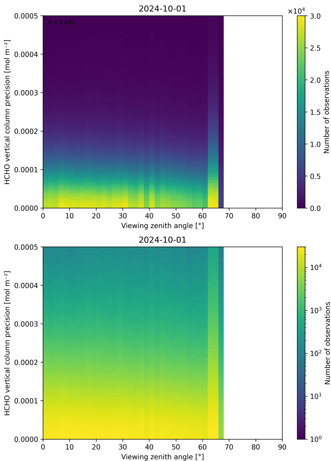
Figure 194: Scatter density plot of “Viewing zenith angle” against “HCHO vertical column precision” for 2024-09-30 to 2024-10-02.
