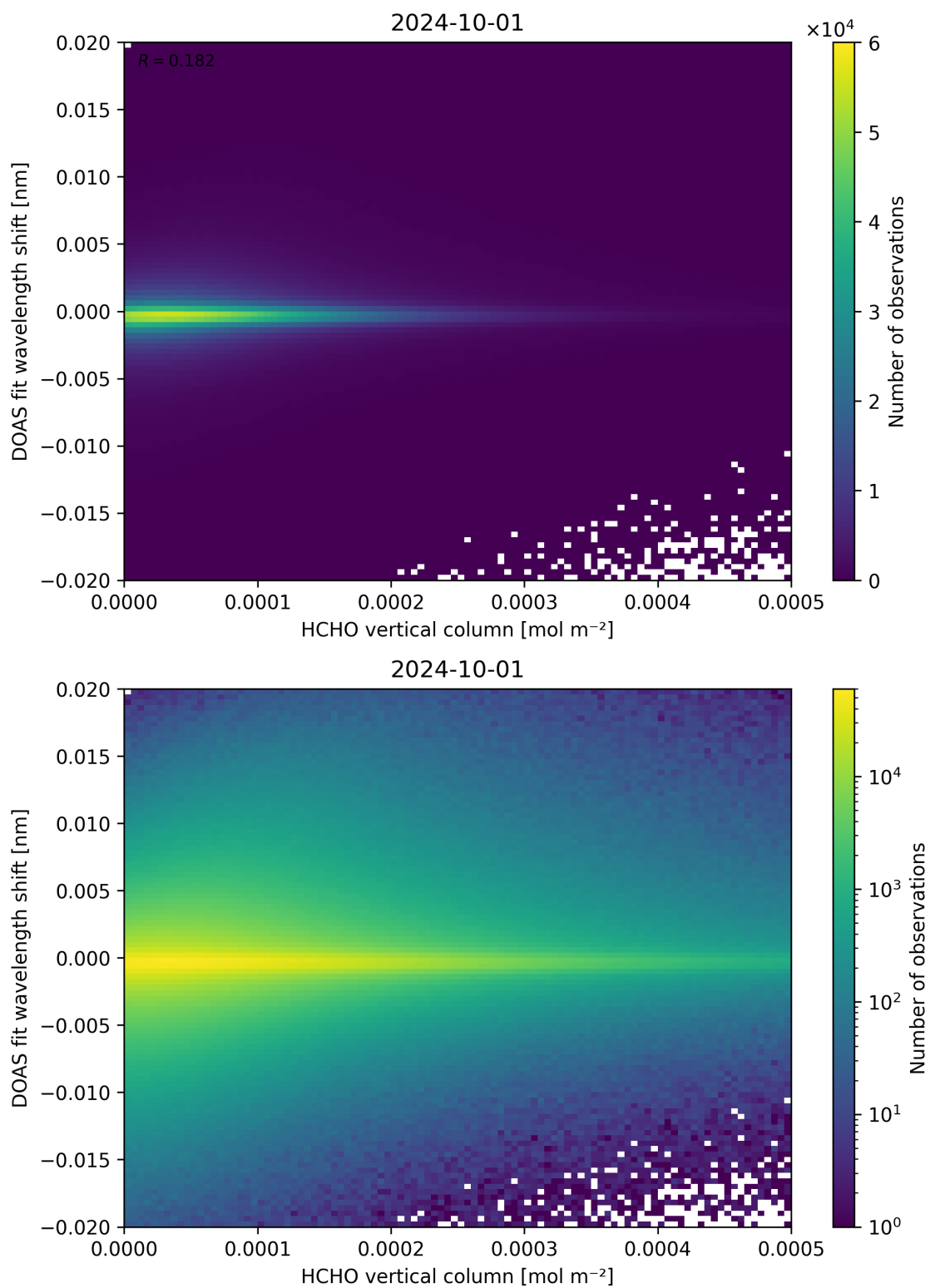
Figure 124: Scatter density plot of “HCHO vertical column” against “DOAS fit wavelength shift” for 2024-09-30 to 2024-10-02.
