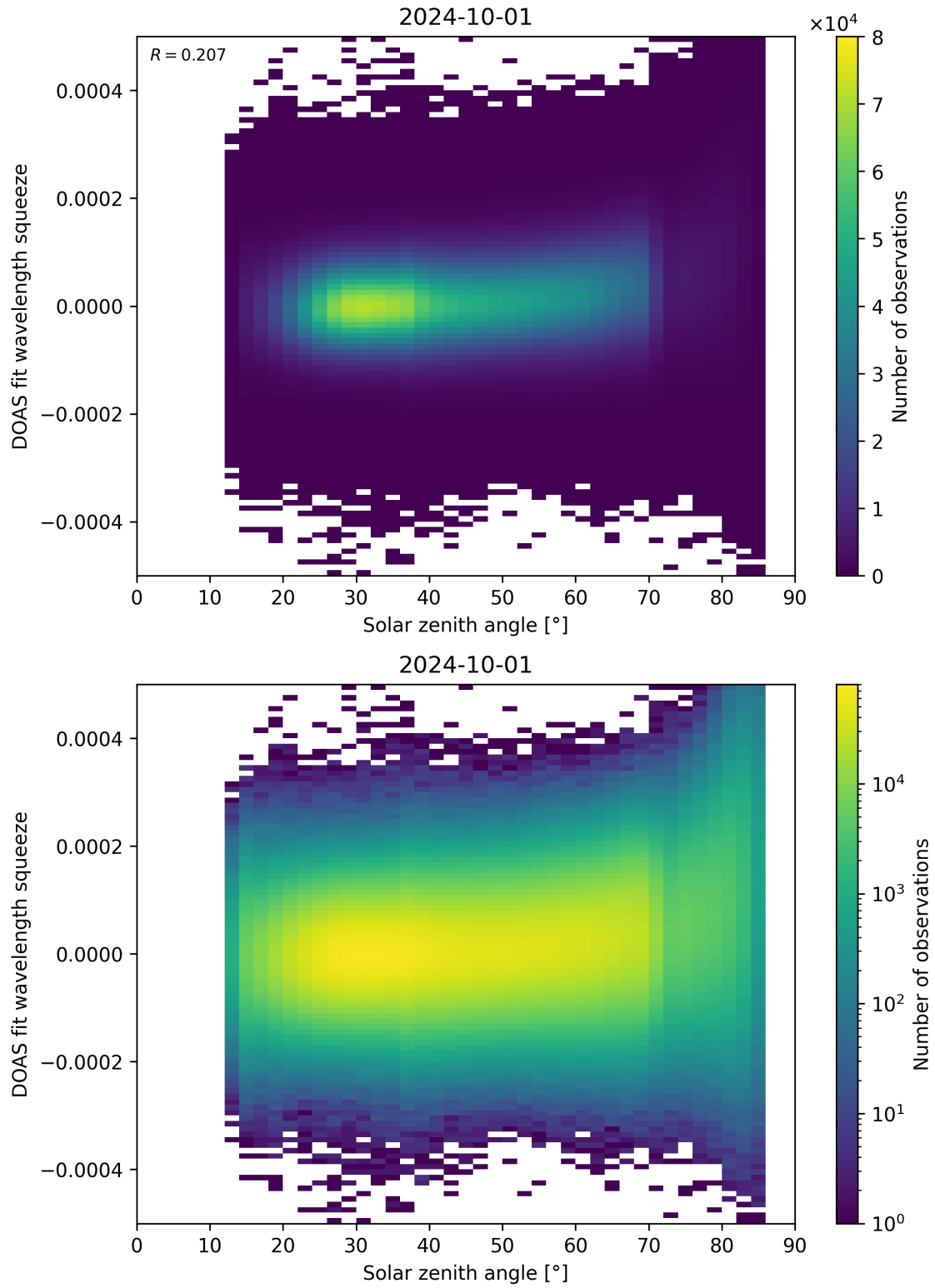
Figure 169: Scatter density plot of “Solar zenith angle” against “DOAS fit wavelength squeeze” for 2024-09-30 to 2024-10-02.
