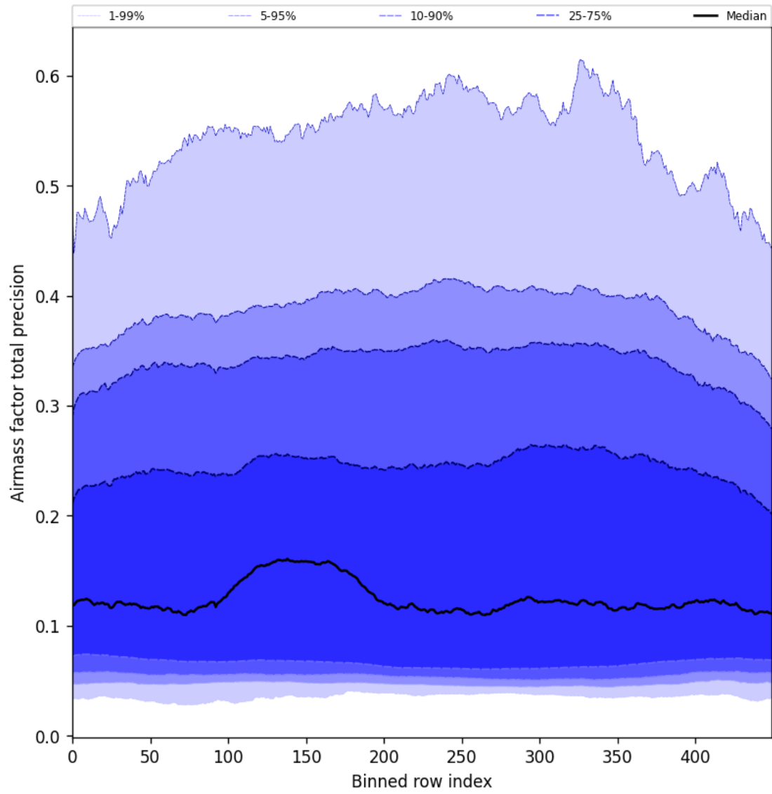
Figure 55: Along track statistics of “Airmass factor total precision” for 2024-09-30 to 2024-10-02
