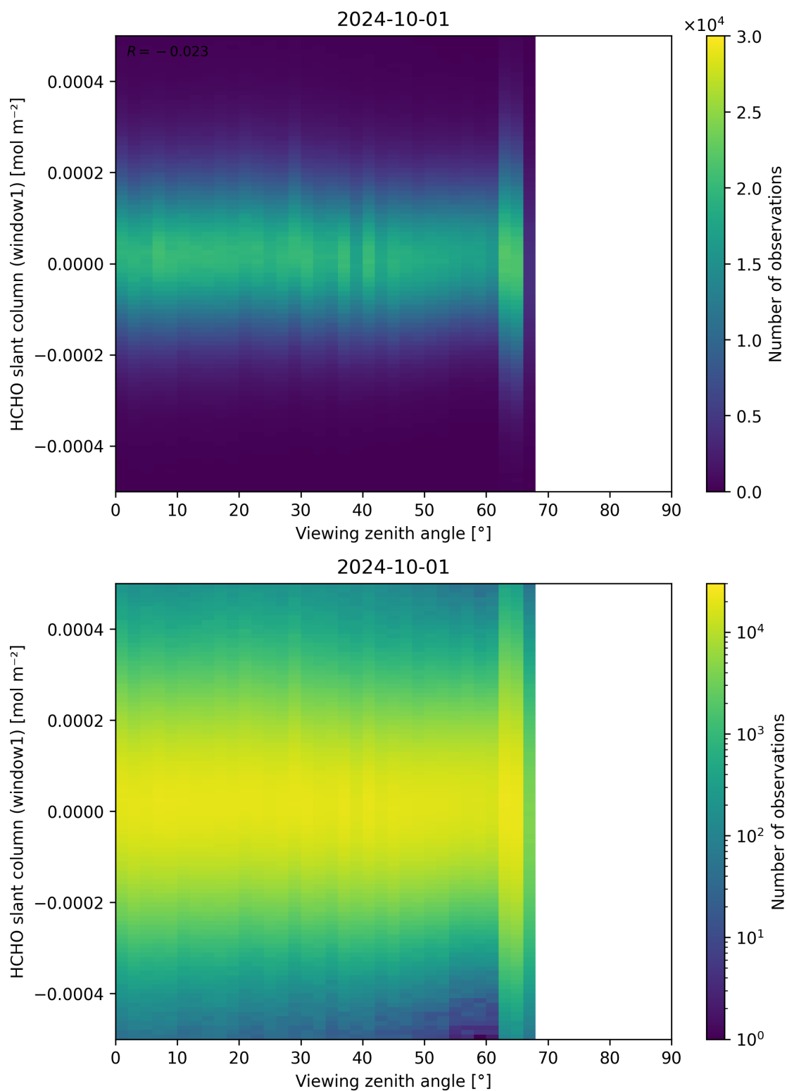
Figure 188: Scatter density plot of “Viewing zenith angle” against “HCHO slant column (window1)” for 2024-09-30 to 2024-10-02.
