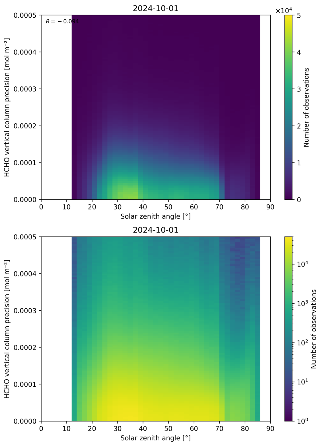
Figure 179: Scatter density plot of “Solar zenith angle” against “HCHO vertical column precision” for 2024-09-30 to 2024-10-02.
