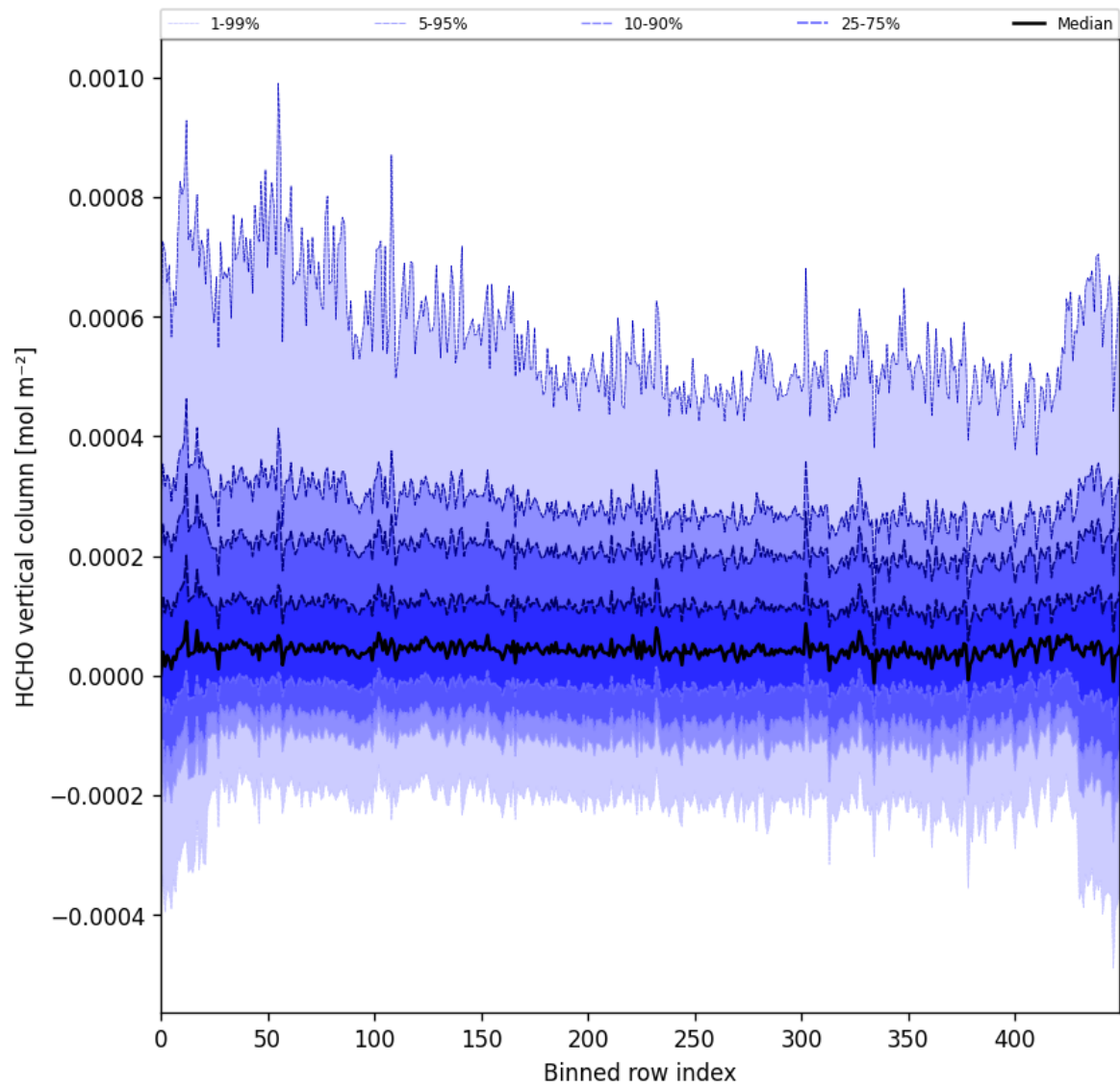
Figure 49: Along track statistics of “HCHO vertical column” for 2024-09-30 to 2024-10-02
