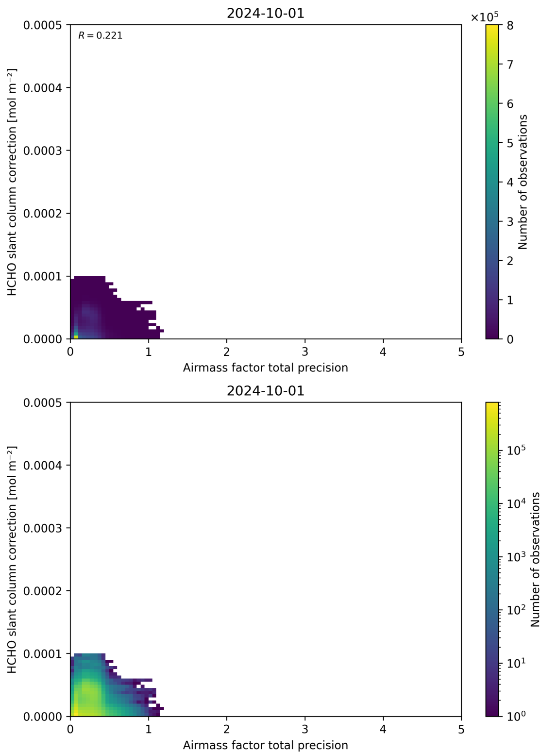
Figure 110: Scatter density plot of “Airmass factor total precision” against “HCHO slant column correction” for 2024-09-30 to 2024-10-02.
