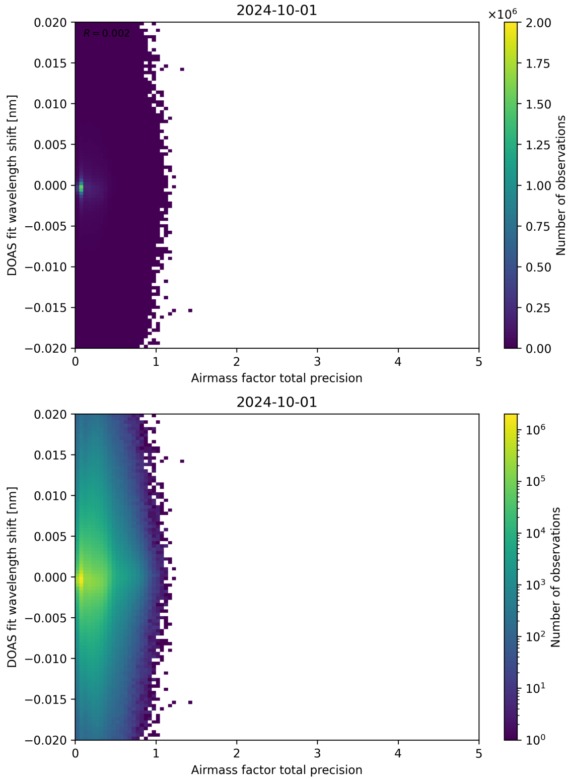
Figure 106: Scatter density plot of “Airmass factor total precision” against “DOAS fit wavelength shift” for 2024-09-30 to 2024-10-02.
