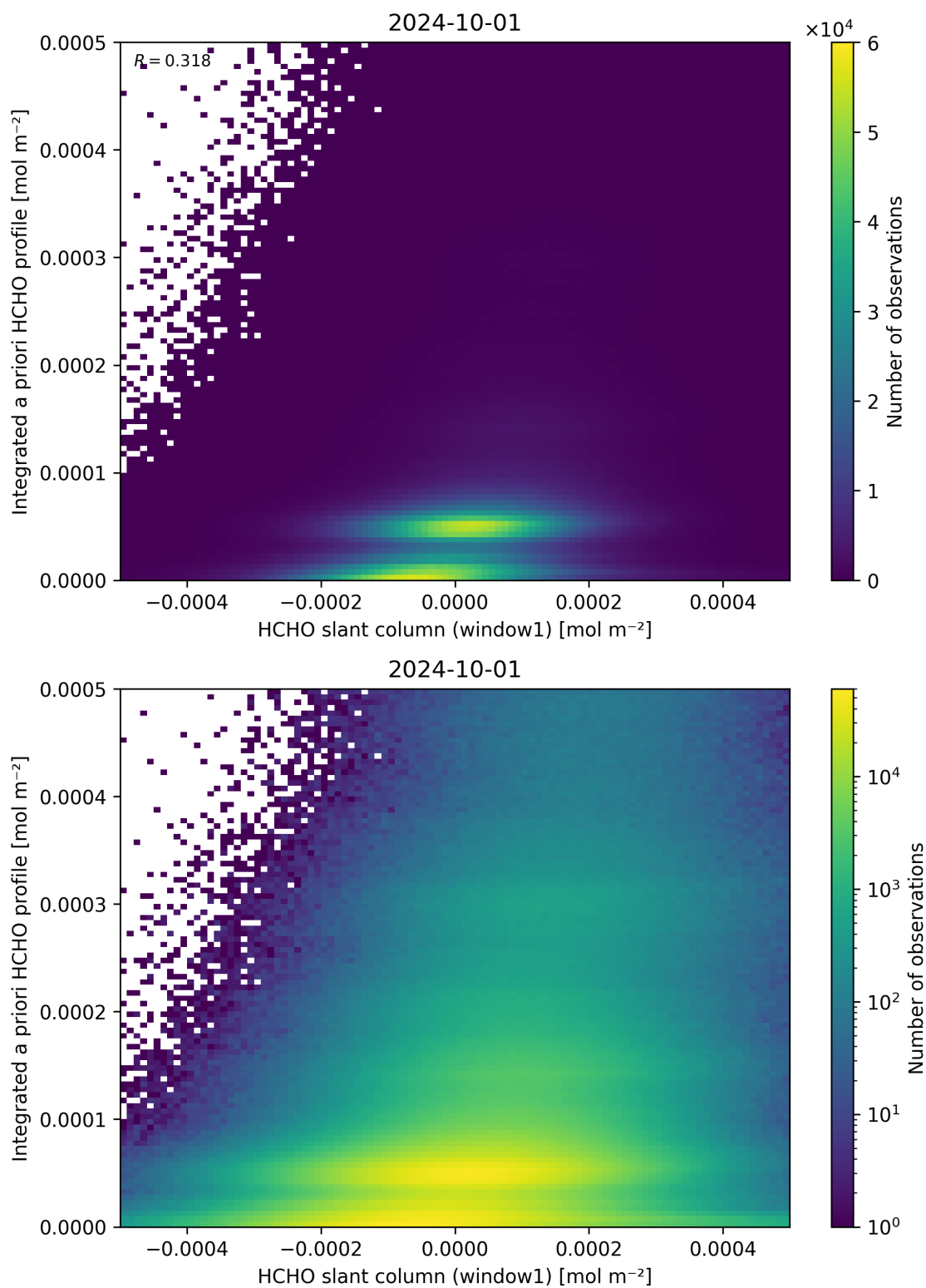
Figure 87: Scatter density plot of “HCHO slant column (window1)” against “Integrated a priori HCHO profile” for 2024-09-30 to 2024-10-02.
