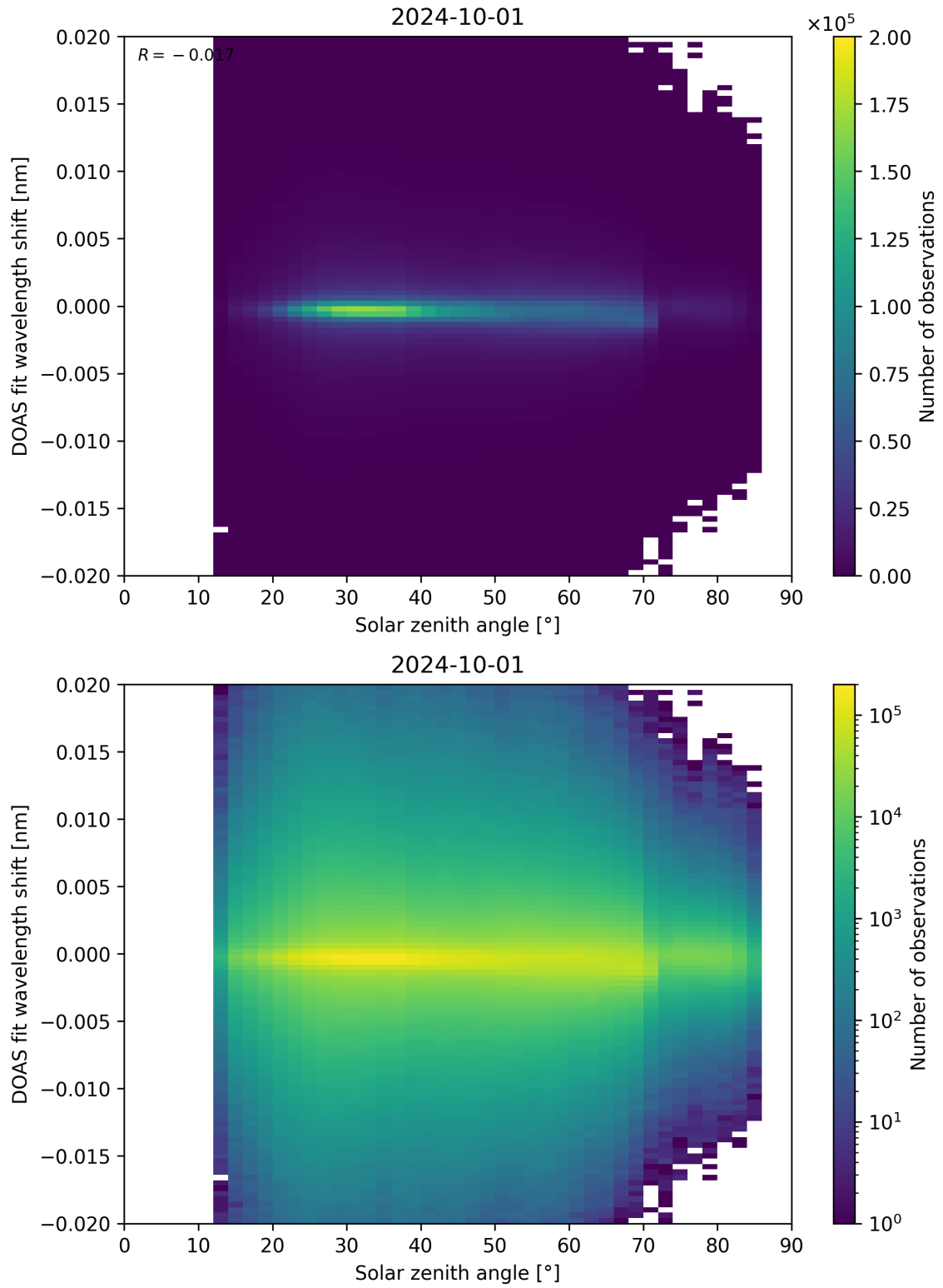
Figure 168: Scatter density plot of “Solar zenith angle” against “DOAS fit wavelength shift” for 2024-09-30 to 2024-10-02.
