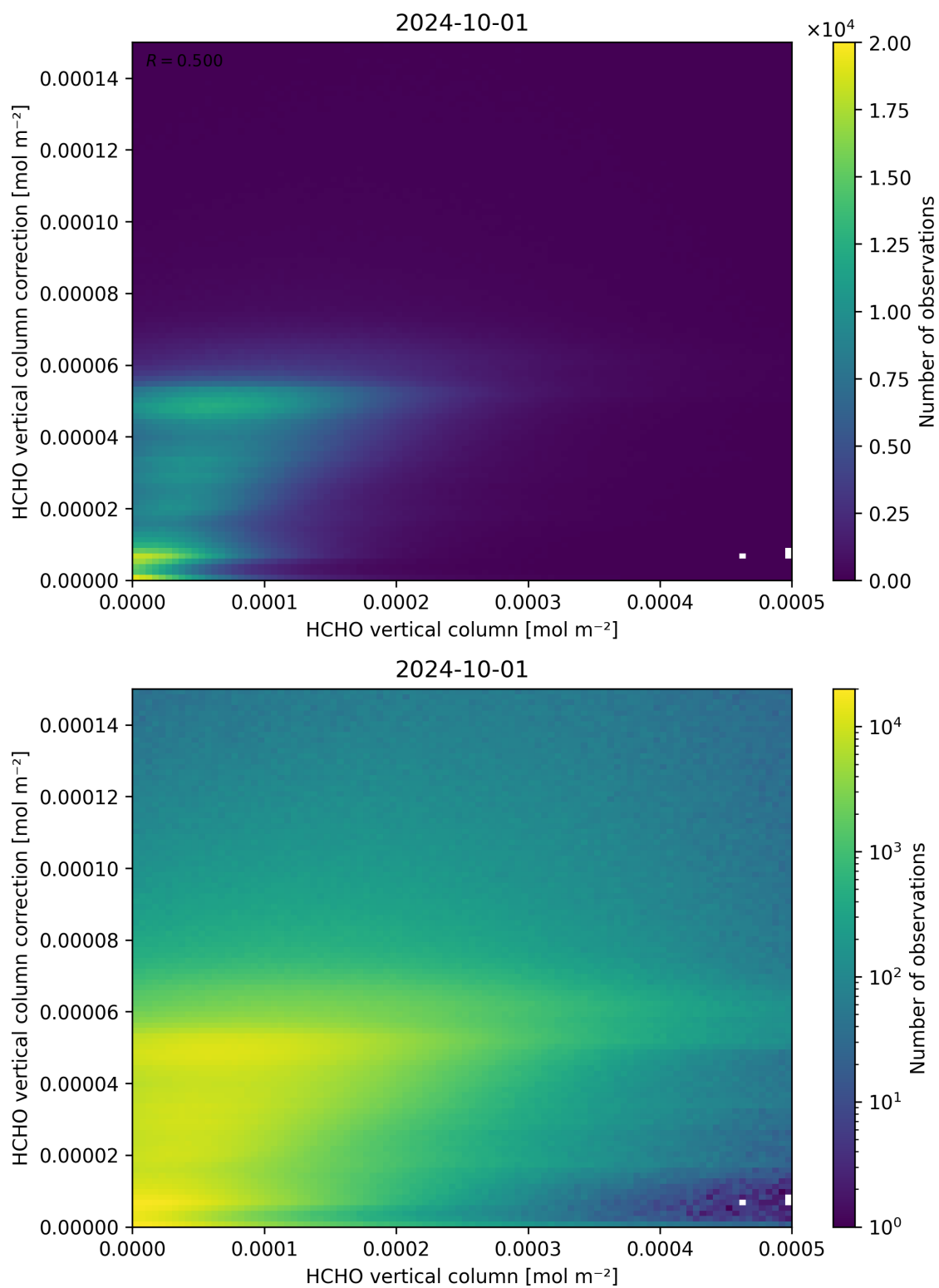
Figure 133: Scatter density plot of “HCHO vertical column” against “HCHO vertical column correction” for 2024-09-30 to 2024-10-02.
