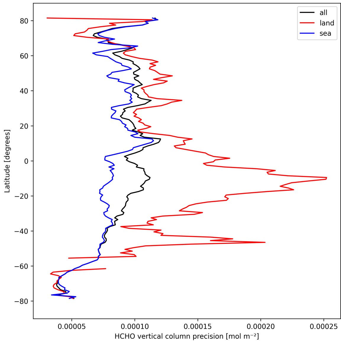
Figure 22: Zonal average of “HCHO vertical column precision” for 2024-09-30 to 2024-10-02.
