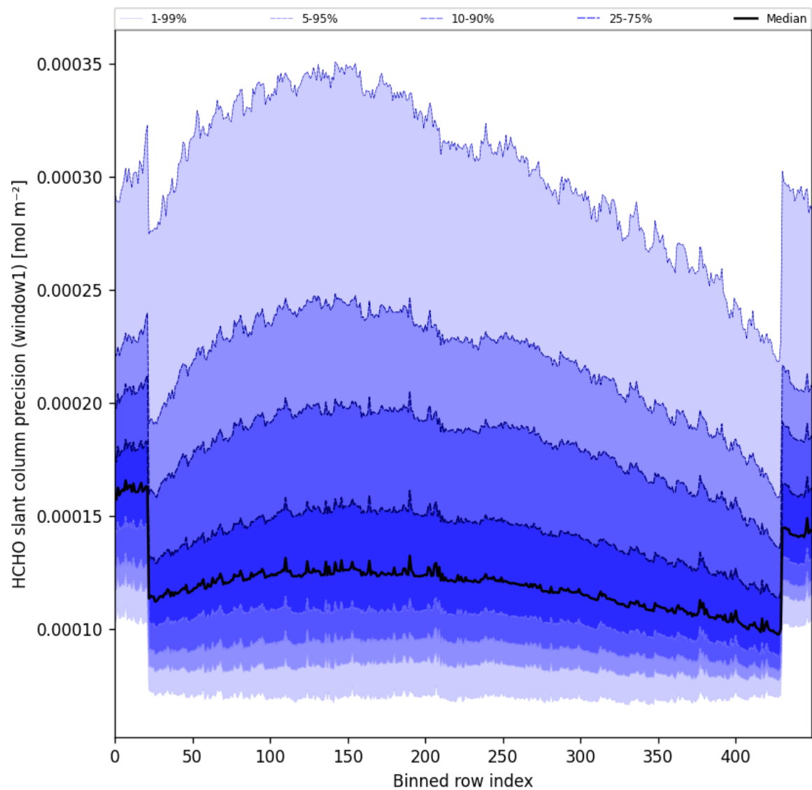
Figure 53: Along track statistics of “HCHO slant column precision (window1)” for 2024-09-30 to 2024-10-02
