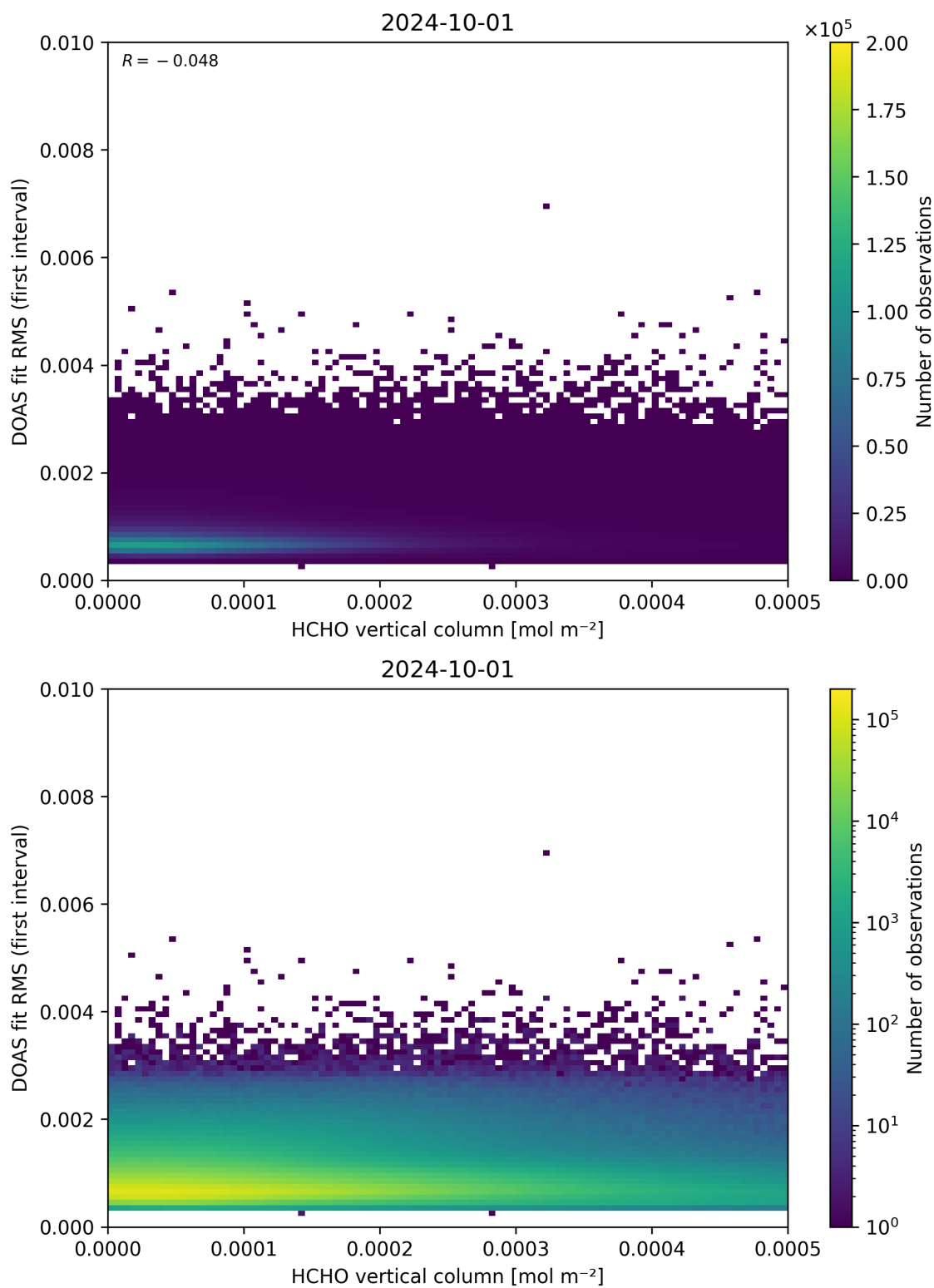
Figure 123: Scatter density plot of “HCHO vertical column” against “DOAS fit RMS (first interval)” for 2024-09-30 to 2024-10-02.
