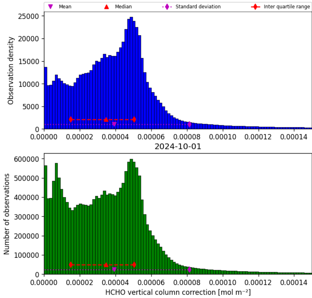
Figure 37: Histogram of “HCHO vertical column correction” for 2024-09-30 to 2024-10-02
