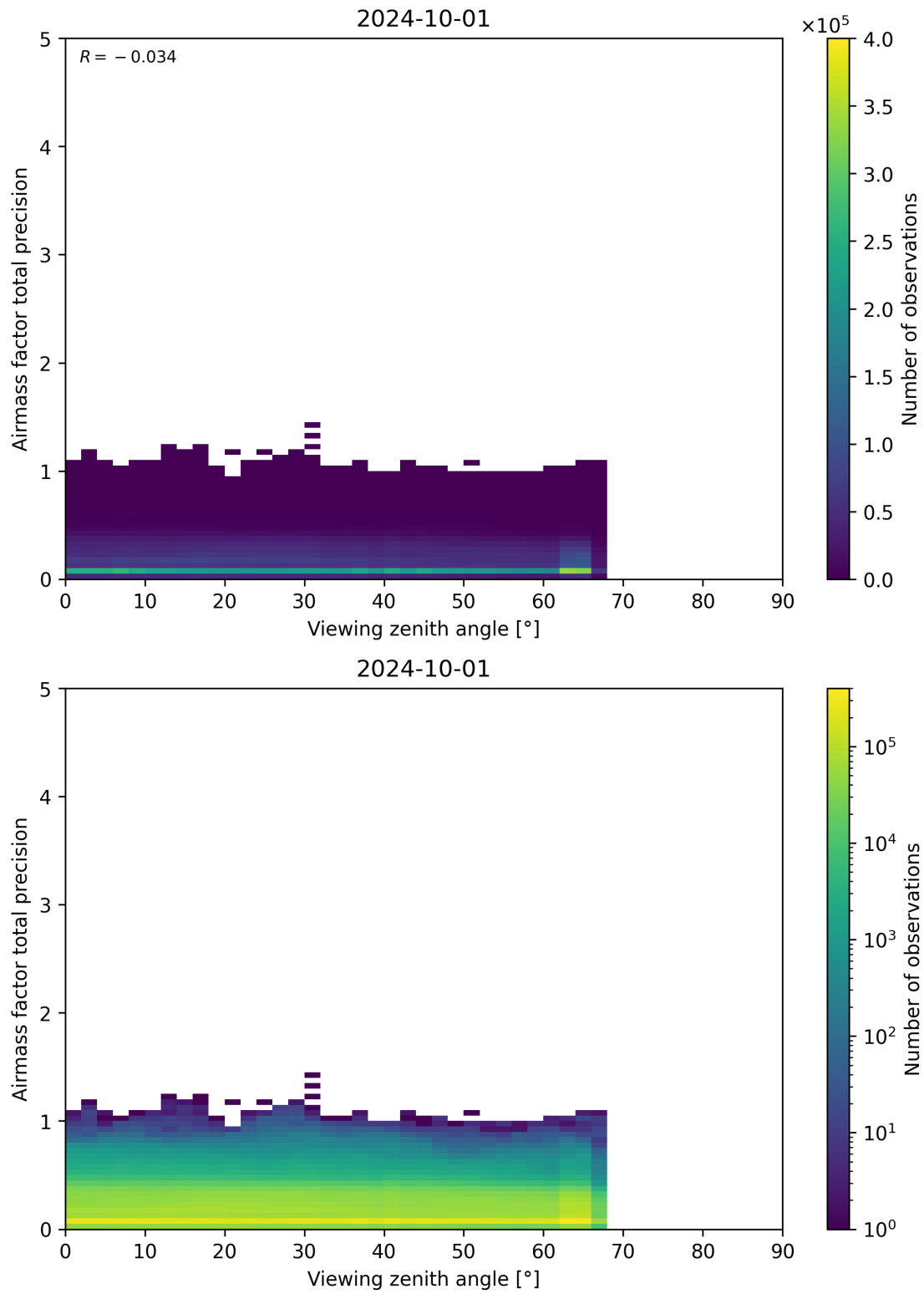
Figure 191: Scatter density plot of “Viewing zenith angle” against “Airmass factor total precision” for 2024-09-30 to 2024-10-02.
