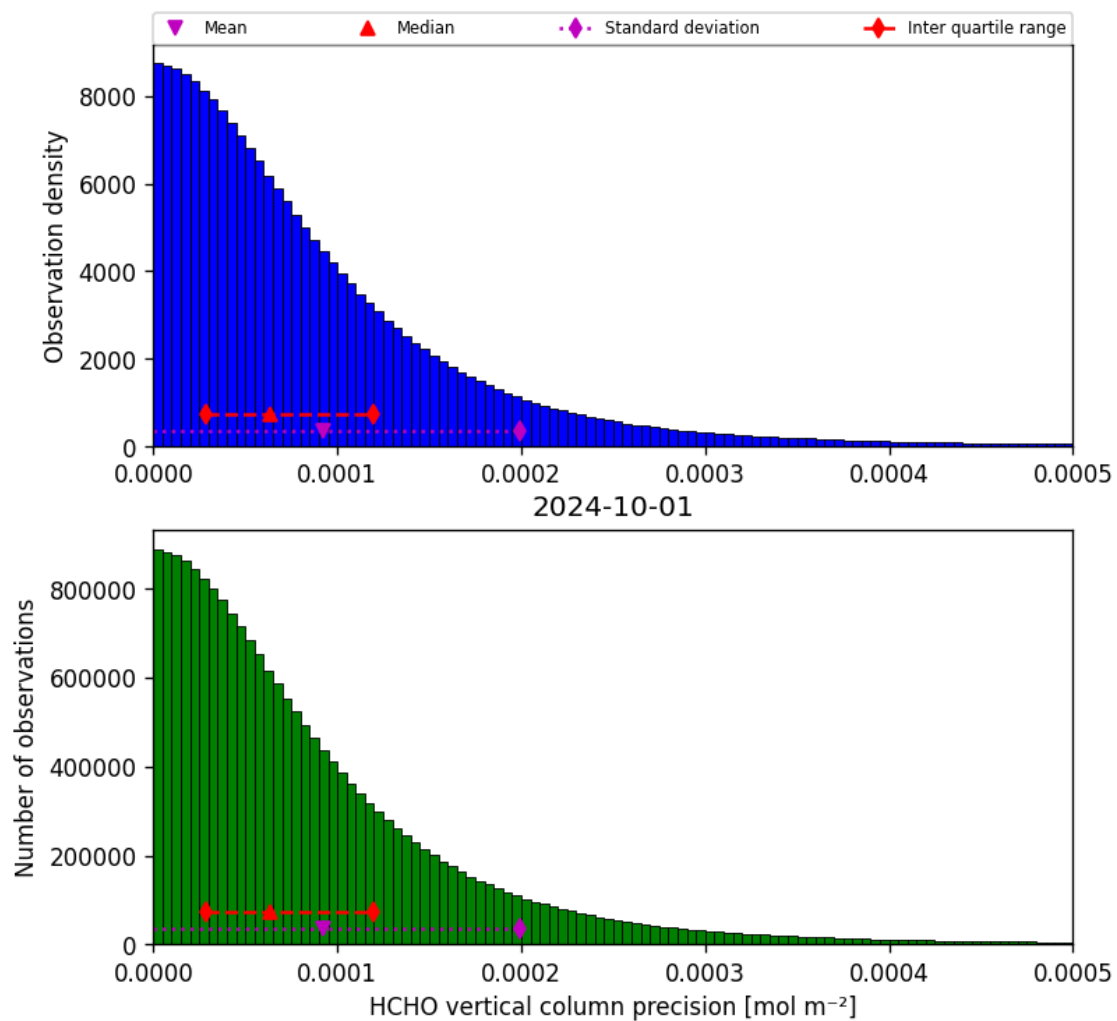
Figure 36: Histogram of “HCHO vertical column precision” for 2024-09-30 to 2024-10-02
