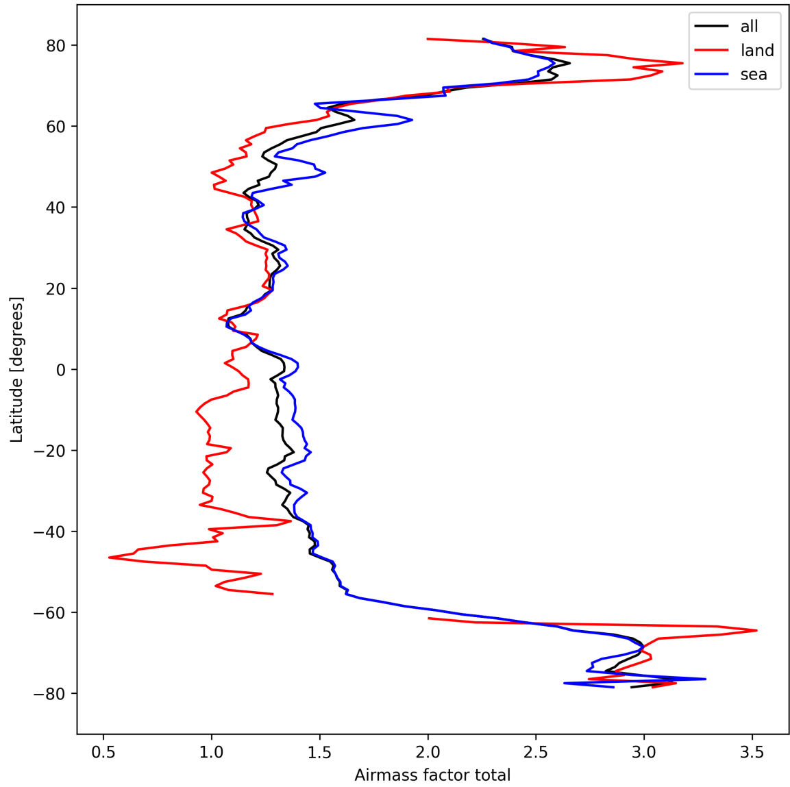
Figure 26: Zonal average of “Airmass factor total” for 2024-09-30 to 2024-10-02.
