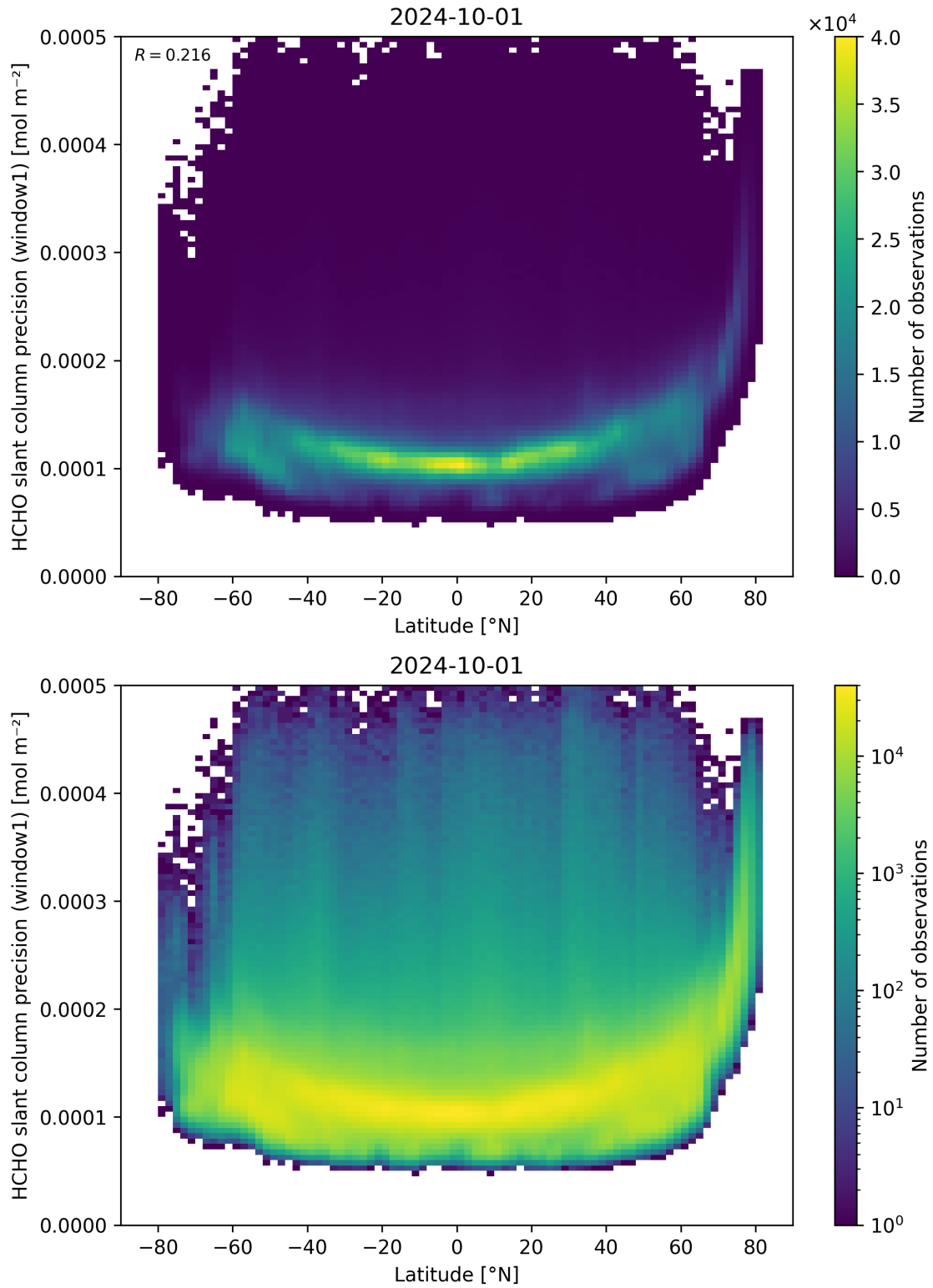
Figure 160: Scatter density plot of “Latitude” against “HCHO slant column precision (window1)” for 2024-09-30 to 2024-10-02.
