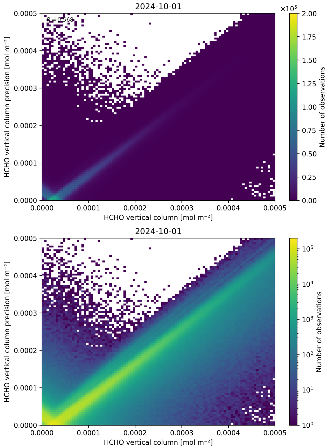
Figure 134: Scatter density plot of “HCHO vertical column” against “HCHO vertical column precision” for 2024-09-30 to 2024-10-02.
