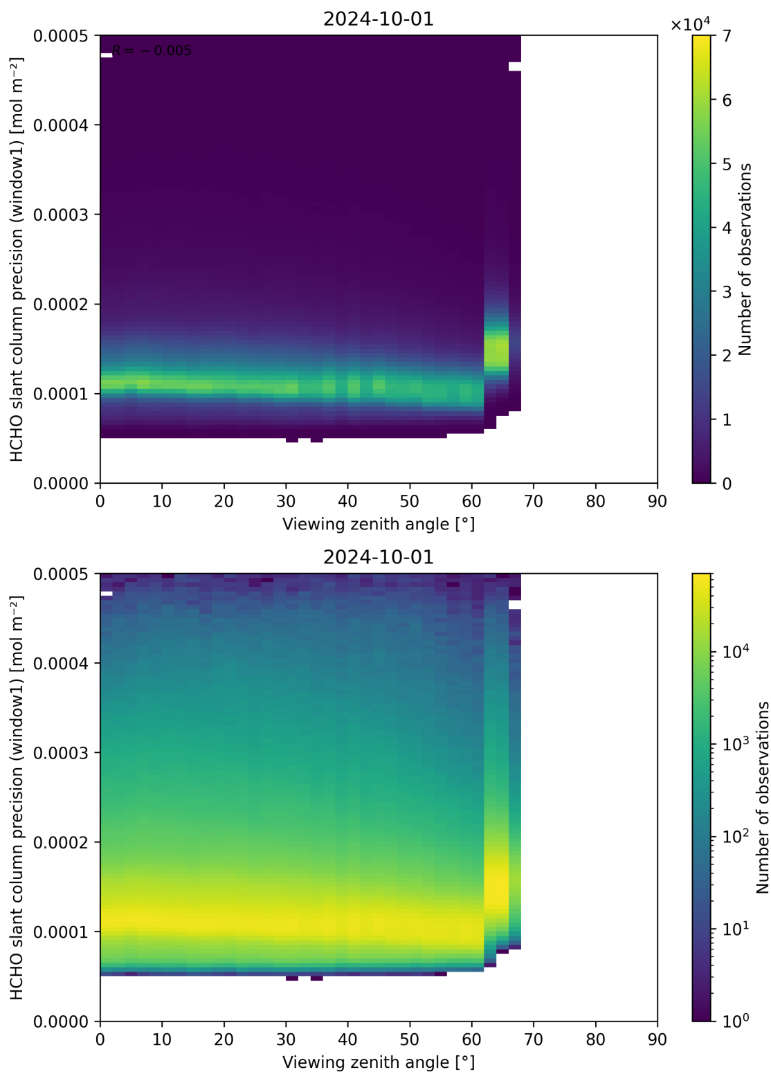
Figure 189: Scatter density plot of “Viewing zenith angle” against “HCHO slant column precision (window1)” for 2024-09-30 to 2024-10-02.
