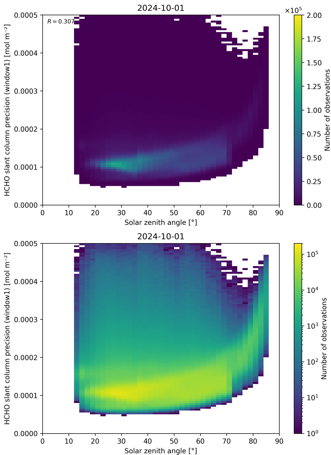
Figure 174: Scatter density plot of “Solar zenith angle” against “HCHO slant column precision (window1)” for 2024-09-30 to 2024-10-02.
