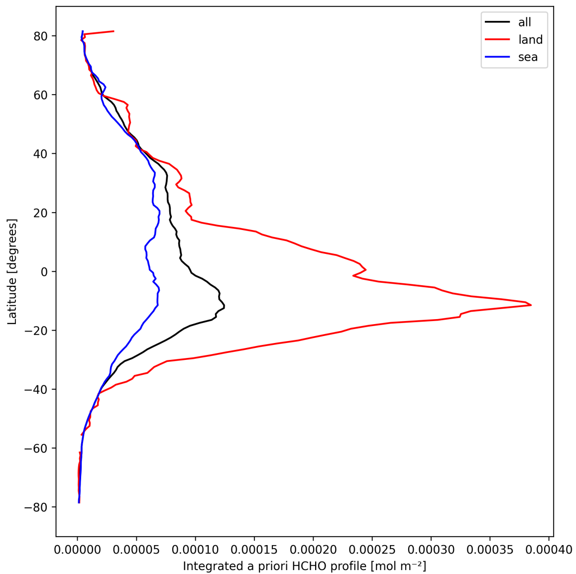
Figure 29: Zonal average of “Integrated a priori HCHO profile” for 2024-09-30 to 2024-10-02.
