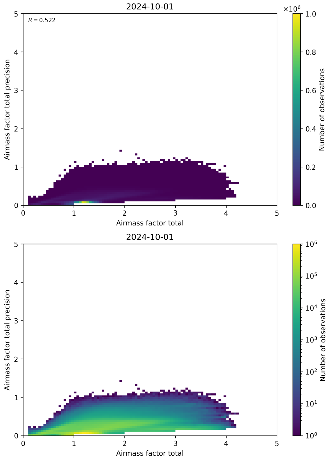
Figure 103: Scatter density plot of “Airmass factor total” against “Airmass factor total precision” for 2024-09-30 to 2024-10-02.
