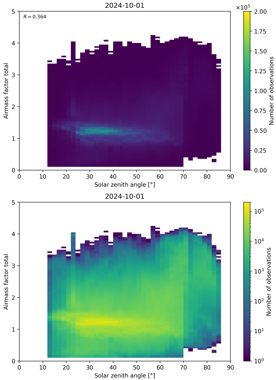
Figure 175: Scatter density plot of “Solar zenith angle” against “Airmass factor total” for 2024-09-30 to 2024-10-02.
