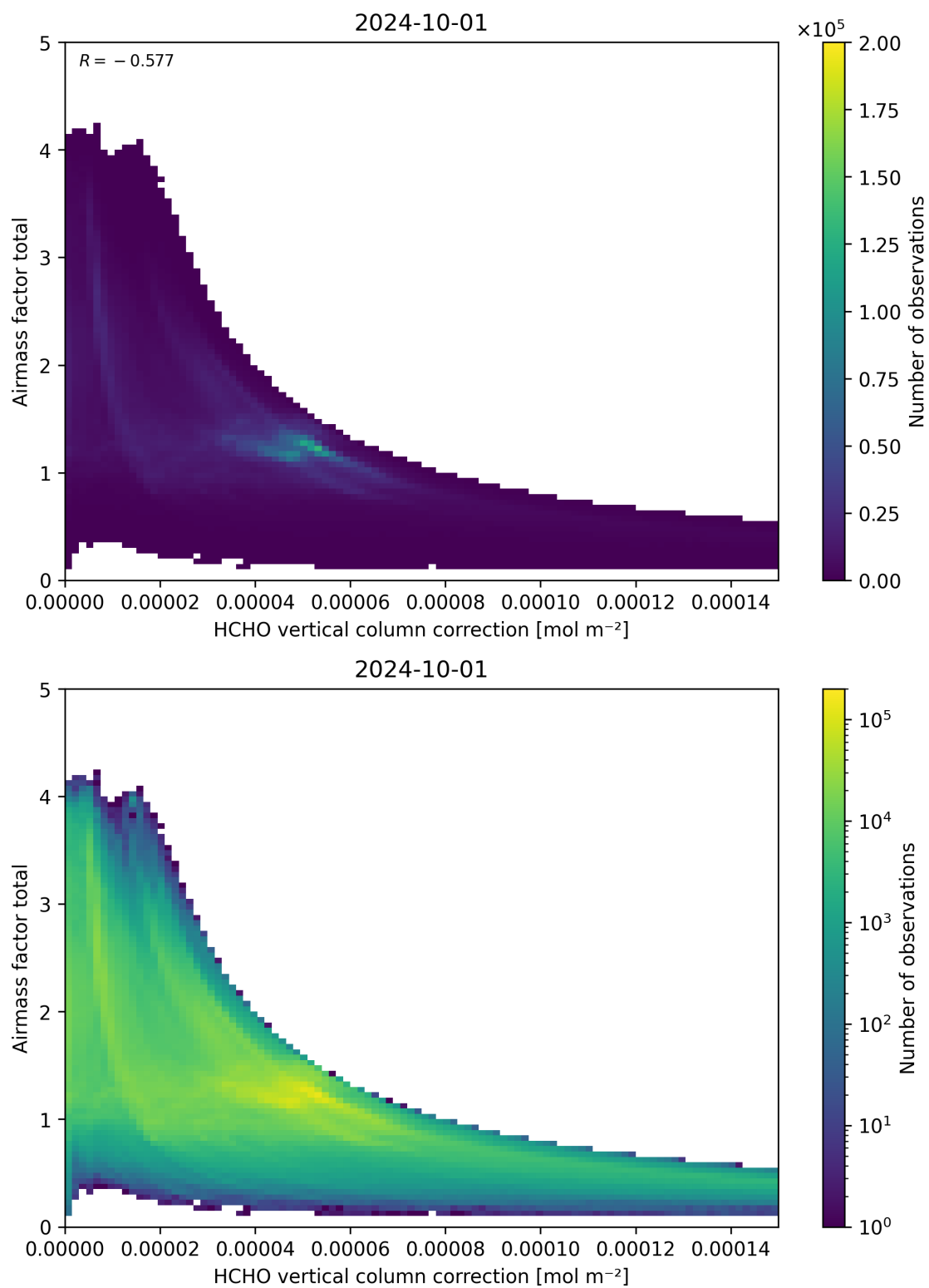
Figure 120: Scatter density plot of “HCHO vertical column correction” against “Airmass factor total” for 2024-09-30 to 2024-10-02.
