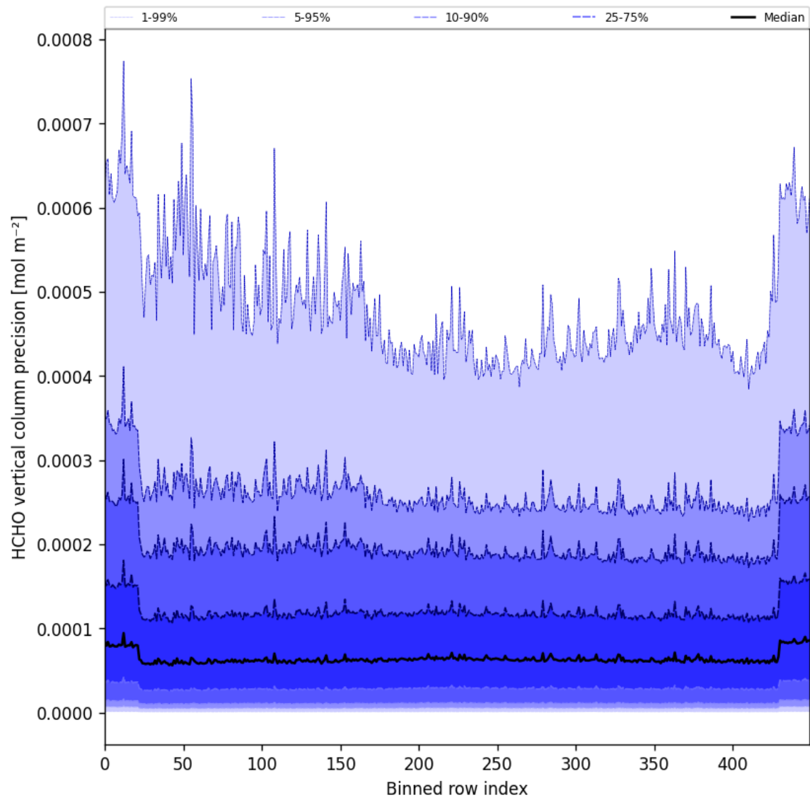
Figure 50: Along track statistics of “HCHO vertical column precision” for 2024-09-30 to 2024-10-02
