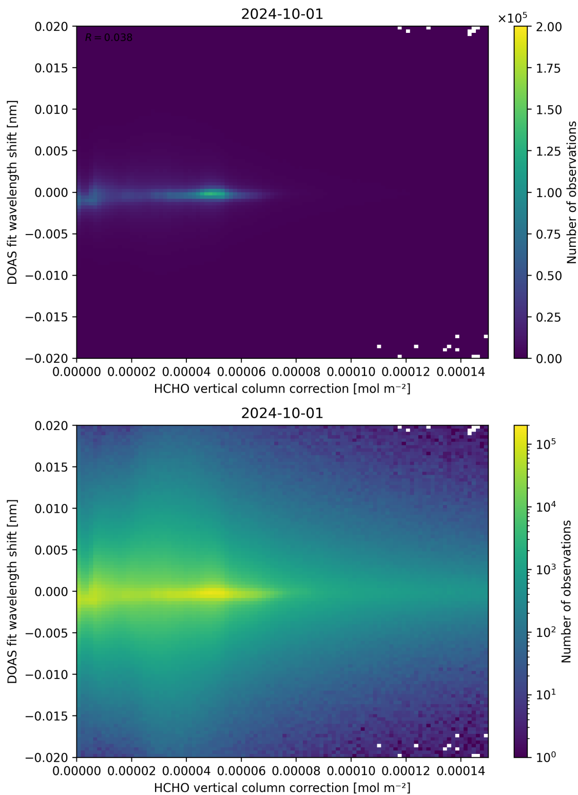
Figure 113: Scatter density plot of “HCHO vertical column correction” against “DOAS fit wavelength shift” for 2024-09-30 to 2024-10-02.
