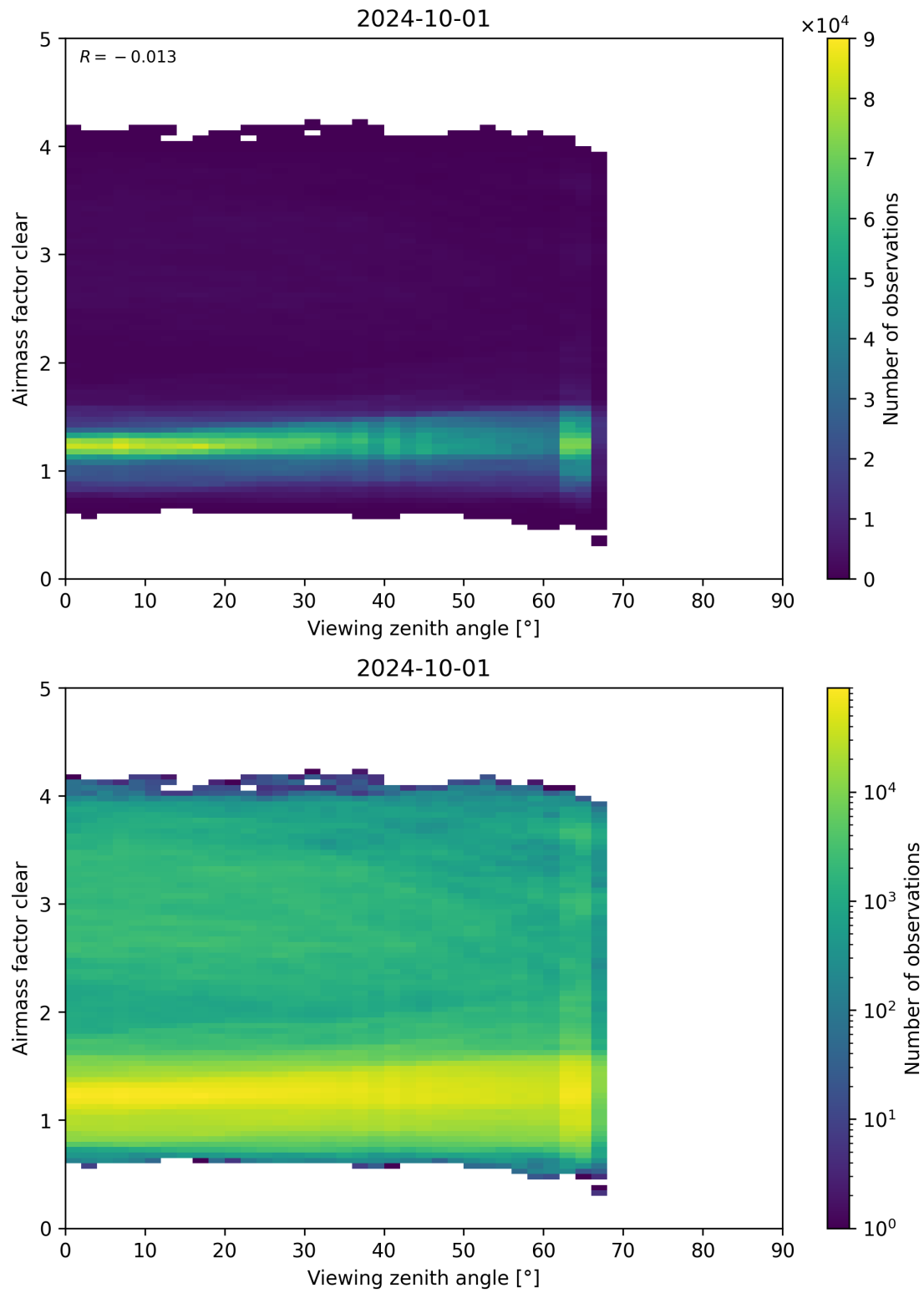
Figure 185: Scatter density plot of “Viewing zenith angle” against “Airmass factor clear” for 2024-09-30 to 2024-10-02.
