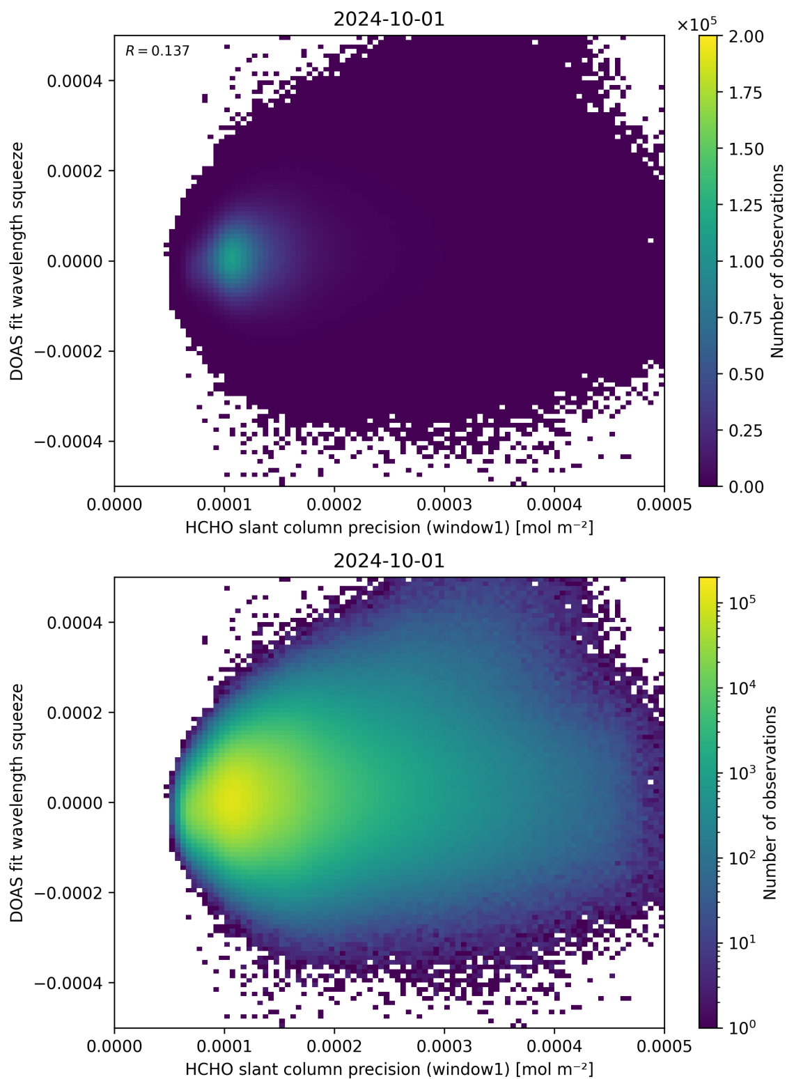
Figure 90: Scatter density plot of “HCHO slant column precision (window1)” against “DOAS fit wavelength squeeze” for 2024-09-30 to 2024-10-02.
