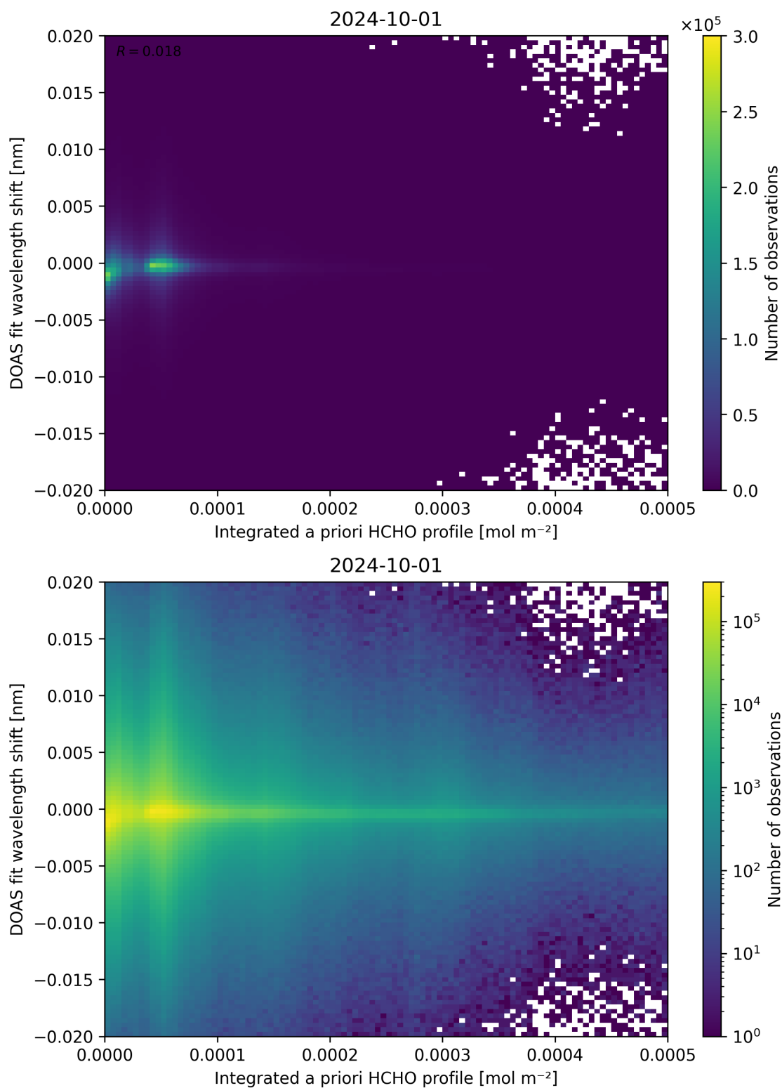
Figure 149: Scatter density plot of “Integrated a priori HCHO profile” against “DOAS fit wavelength shift” for 2024-09-30 to 2024-10-02.
