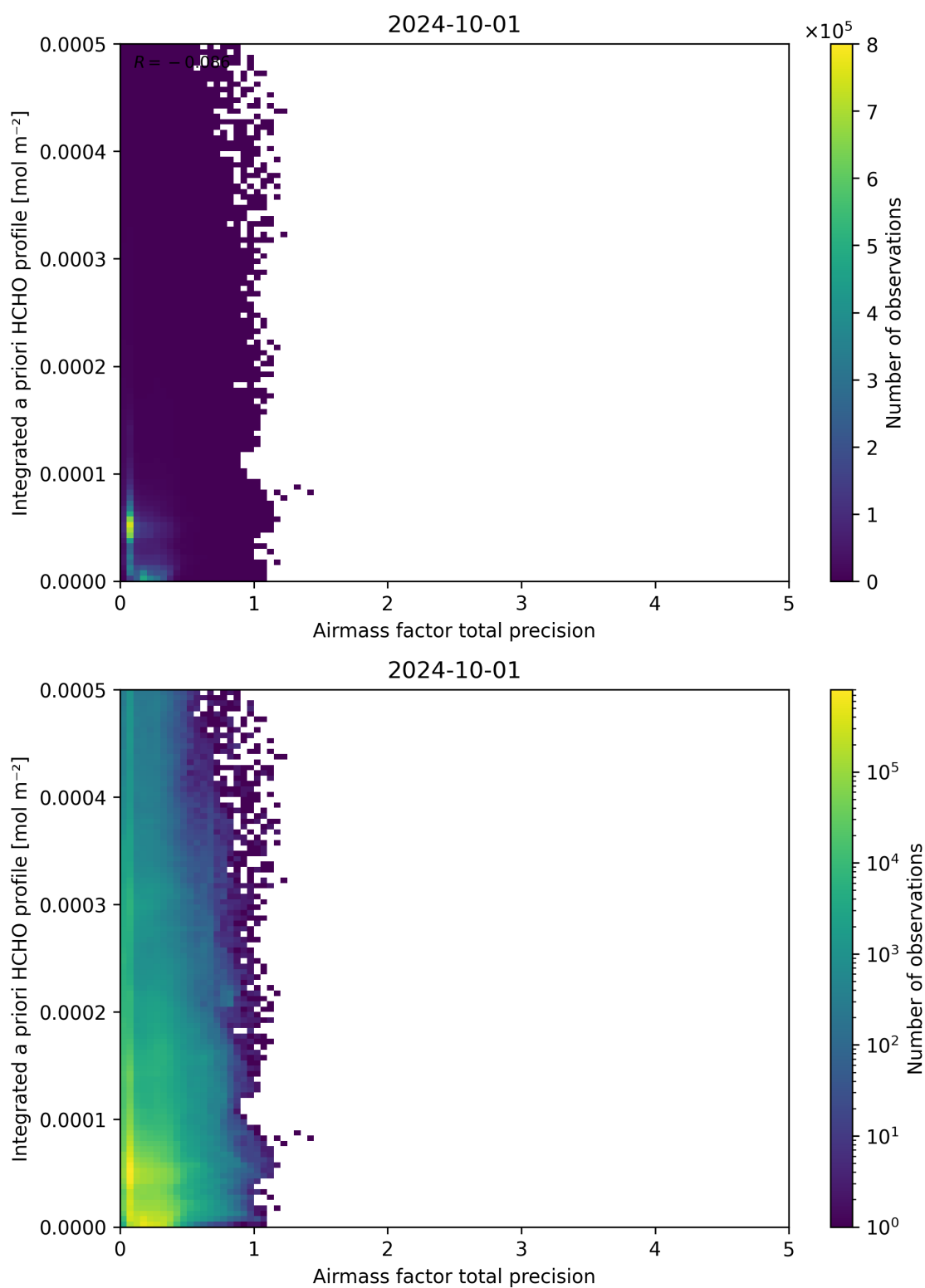
Figure 111: Scatter density plot of “Airmass factor total precision” against “Integrated a priori HCHO profile” for 2024-09-30 to 2024-10-02.
