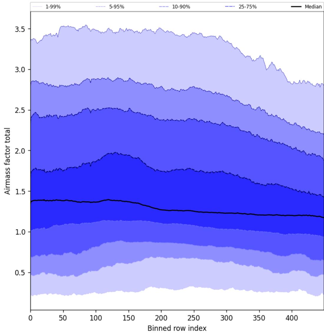
Figure 54: Along track statistics of “Airmass factor total” for 2024-09-30 to 2024-10-02
