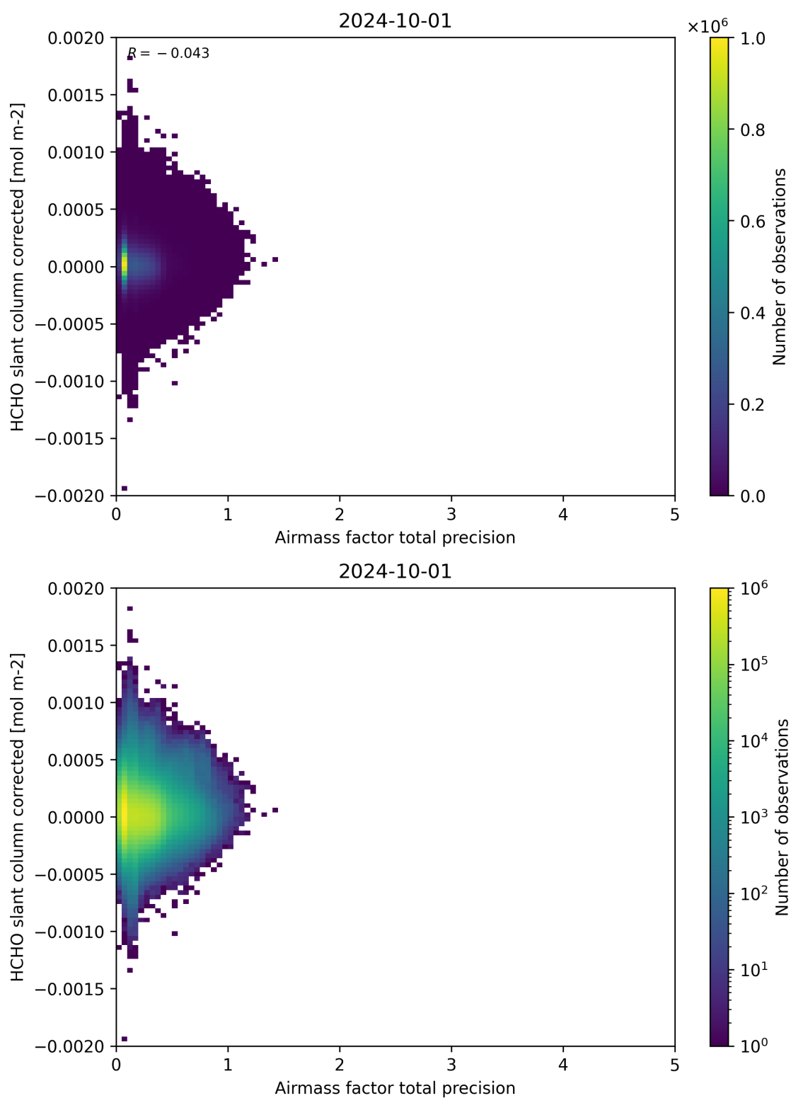
Figure 109: Scatter density plot of “Airmass factor total precision” against “HCHO slant column corrected” for 2024-09-30 to 2024-10-02.
