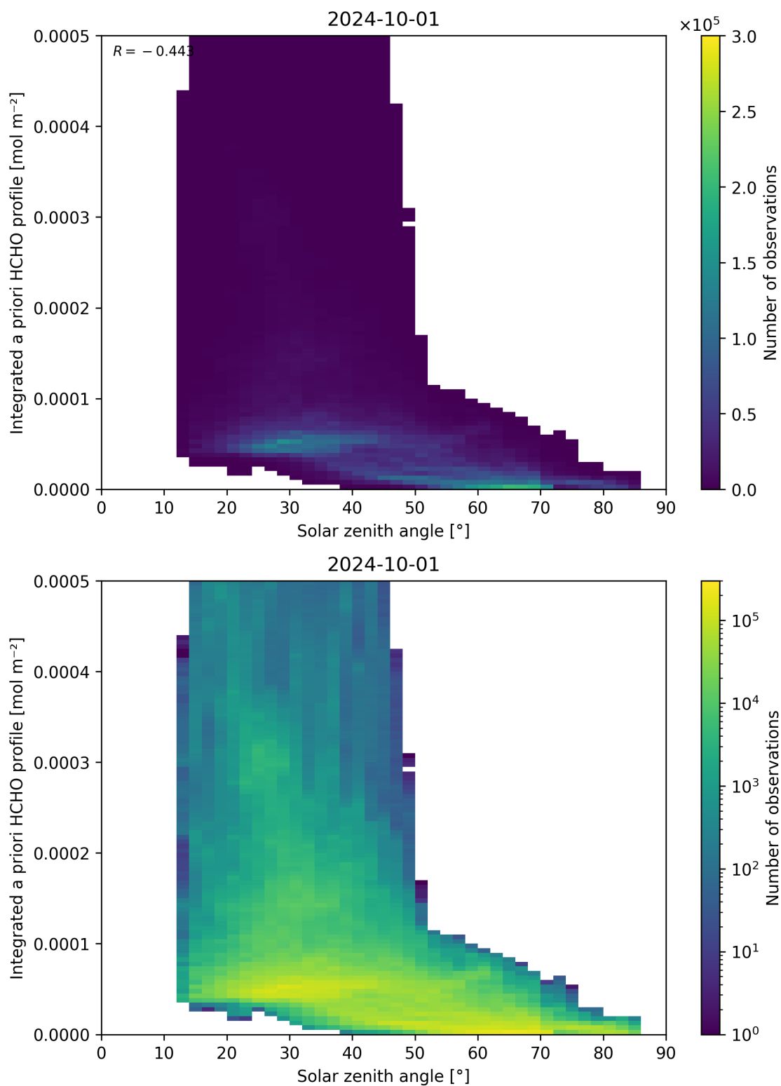
Figure 180: Scatter density plot of “Solar zenith angle” against “Integrated a priori HCHO profile” for 2024-09-30 to 2024-10-02.
