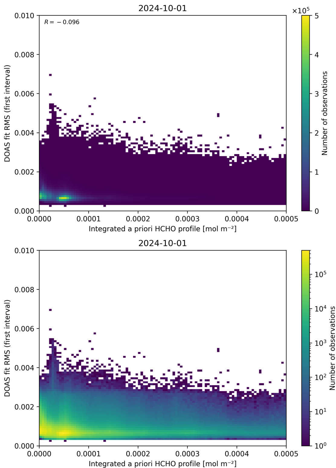
Figure 148: Scatter density plot of “Integrated a priori HCHO profile” against “DOAS fit RMS (first interval)” for 2024-09-30 to 2024-10-02.
