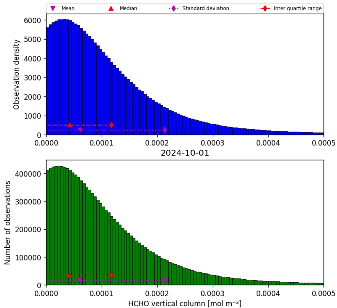
Figure 35: Histogram of “HCHO vertical column” for 2024-09-30 to 2024-10-02
