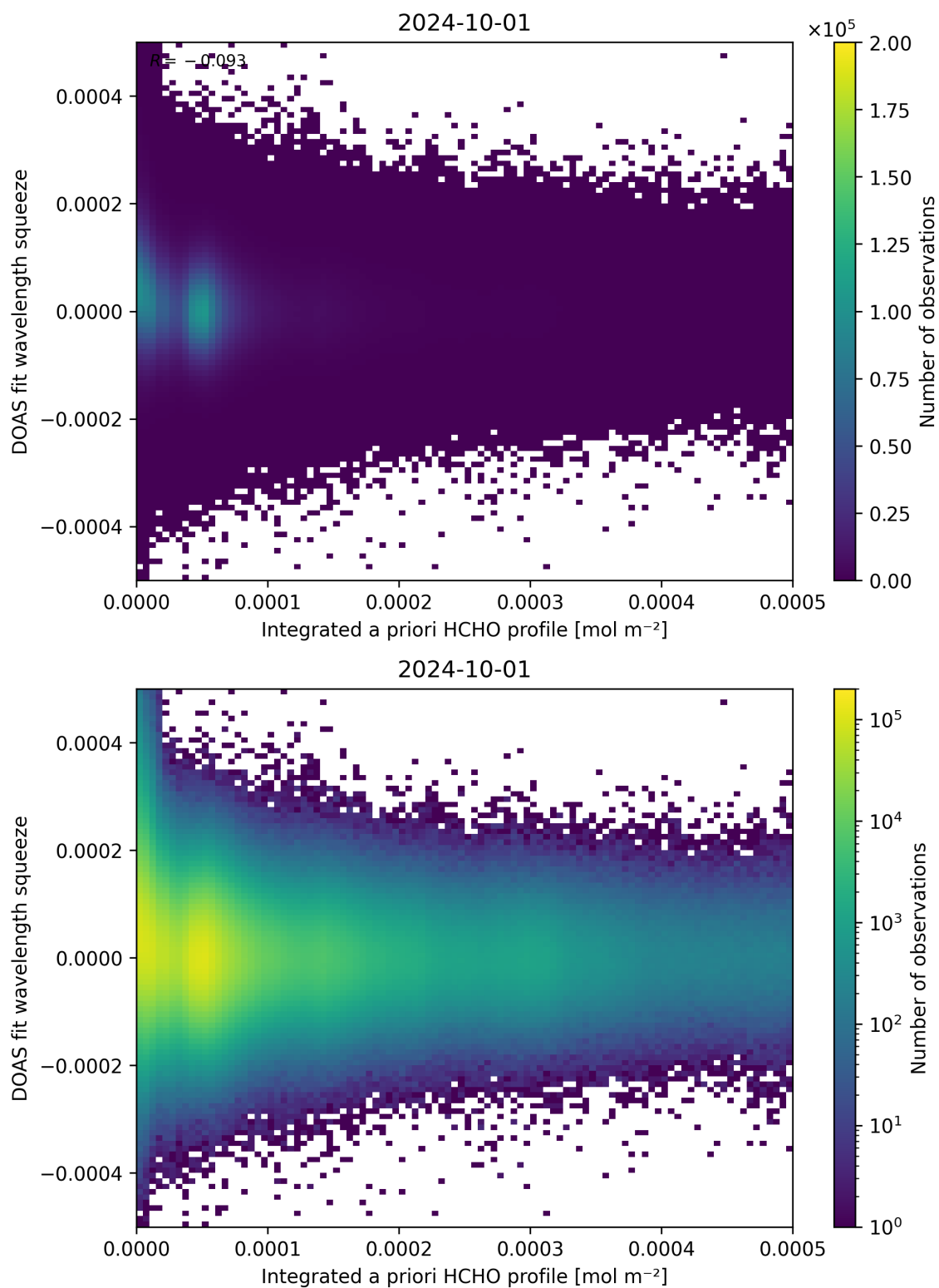
Figure 150: Scatter density plot of “Integrated a priori HCHO profile” against “DOAS fit wavelength squeeze” for 2024-09-30 to 2024-10-02.
