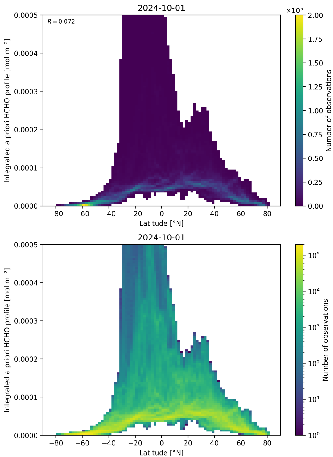
Figure 166: Scatter density plot of “Latitude” against “Integrated a priori HCHO profile” for 2024-09-30 to 2024-10-02.
