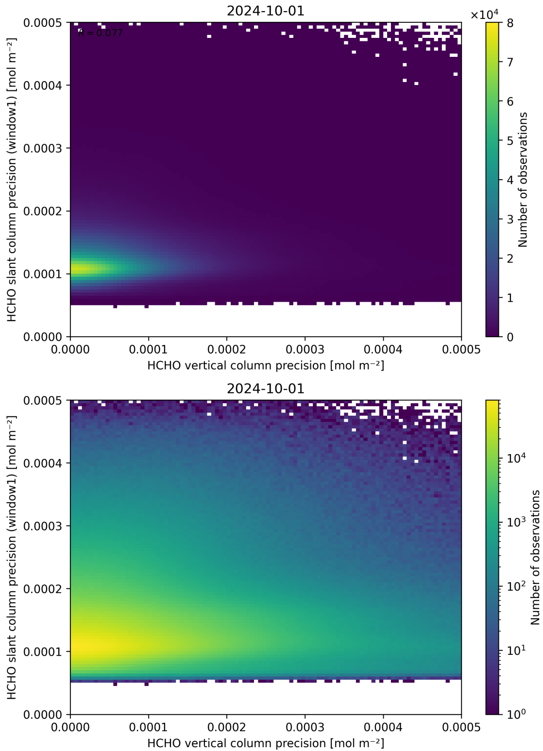
Figure 143: Scatter density plot of “HCHO vertical column precision” against “HCHO slant column precision (window1)” for 2024-09-30 to 2024-10-02.
