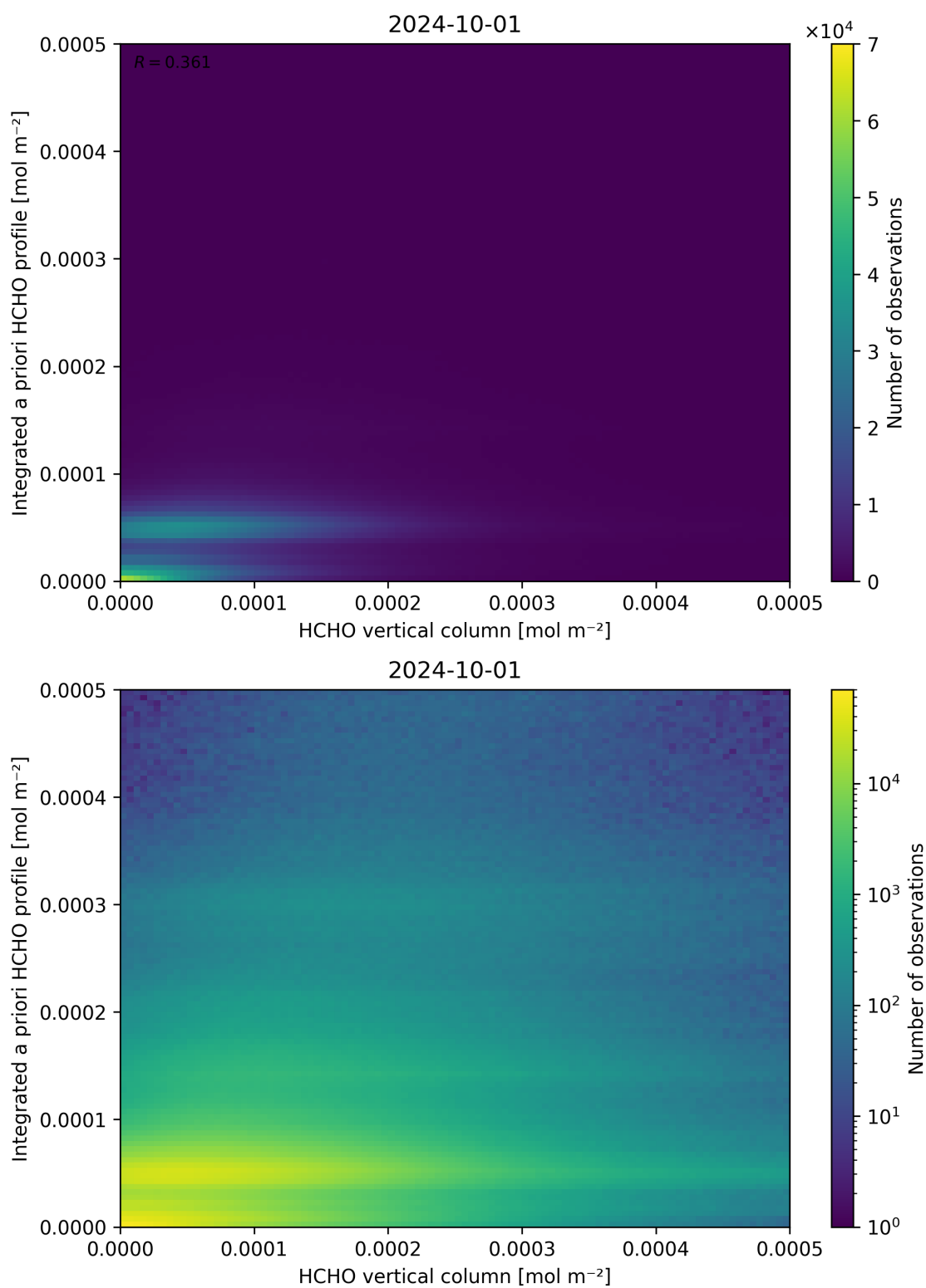
Figure 135: Scatter density plot of “HCHO vertical column” against “Integrated a priori HCHO profile” for 2024-09-30 to 2024-10-02.
