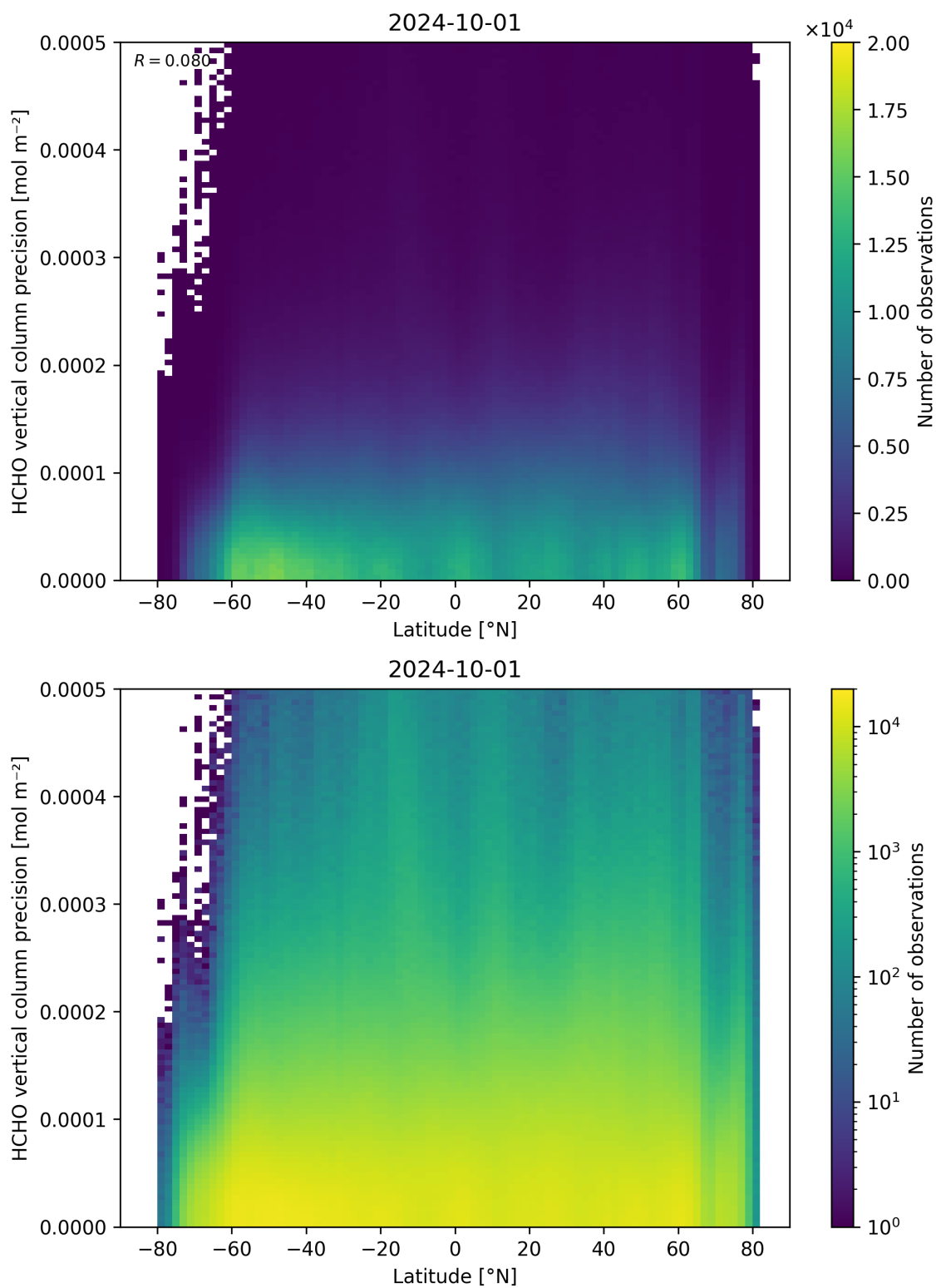
Figure 165: Scatter density plot of “Latitude” against “HCHO vertical column precision” for 2024-09-30 to 2024-10-02.
