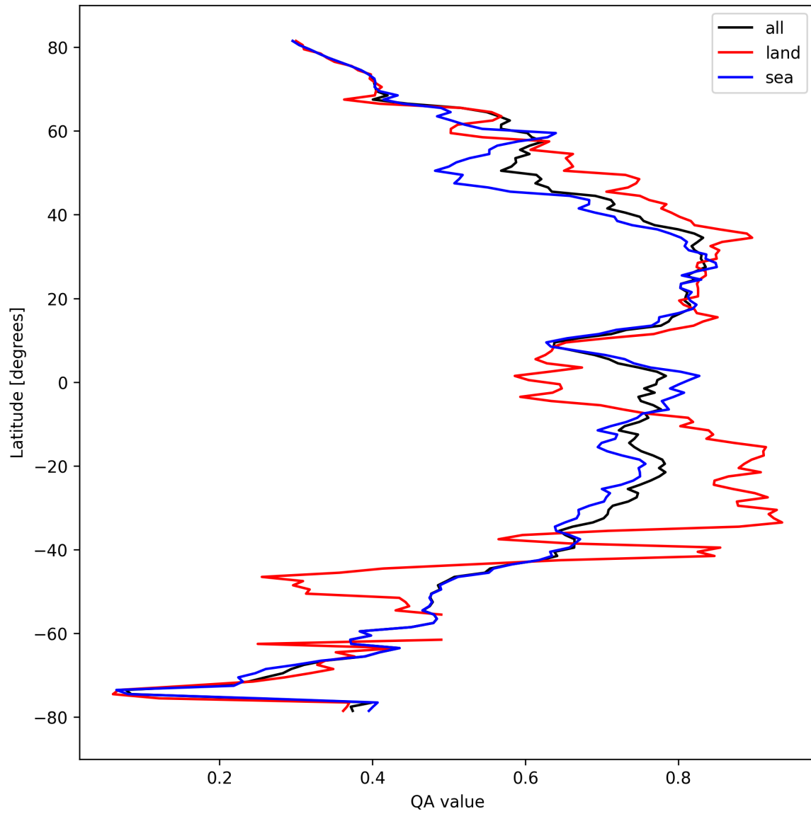
Figure 20: Zonal average of “QA value” for 2024-09-30 to 2024-10-02.
