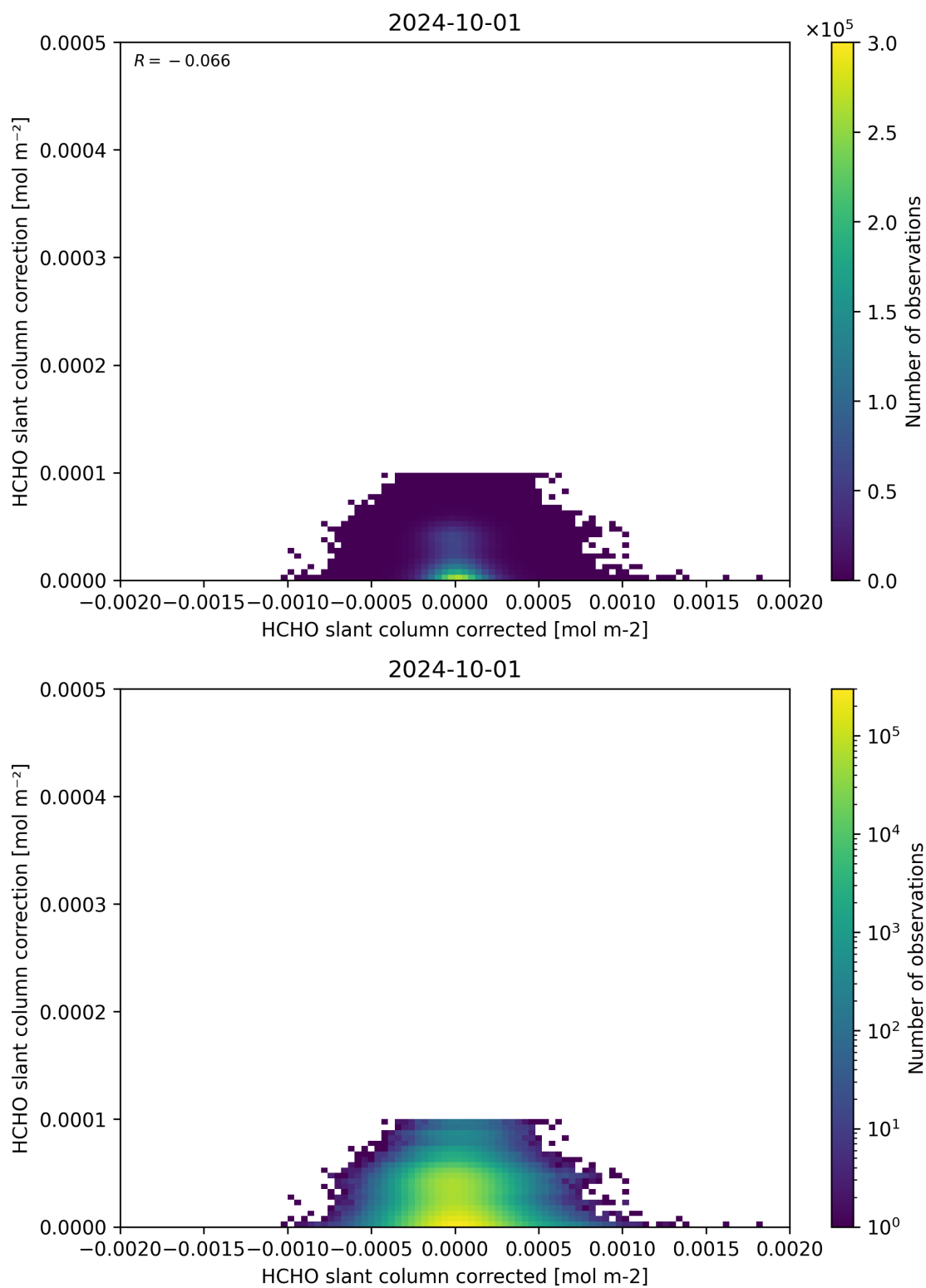
Figure 77: Scatter density plot of “HCHO slant column corrected” against “HCHO slant column correction” for 2024-09-30 to 2024-10-02.
