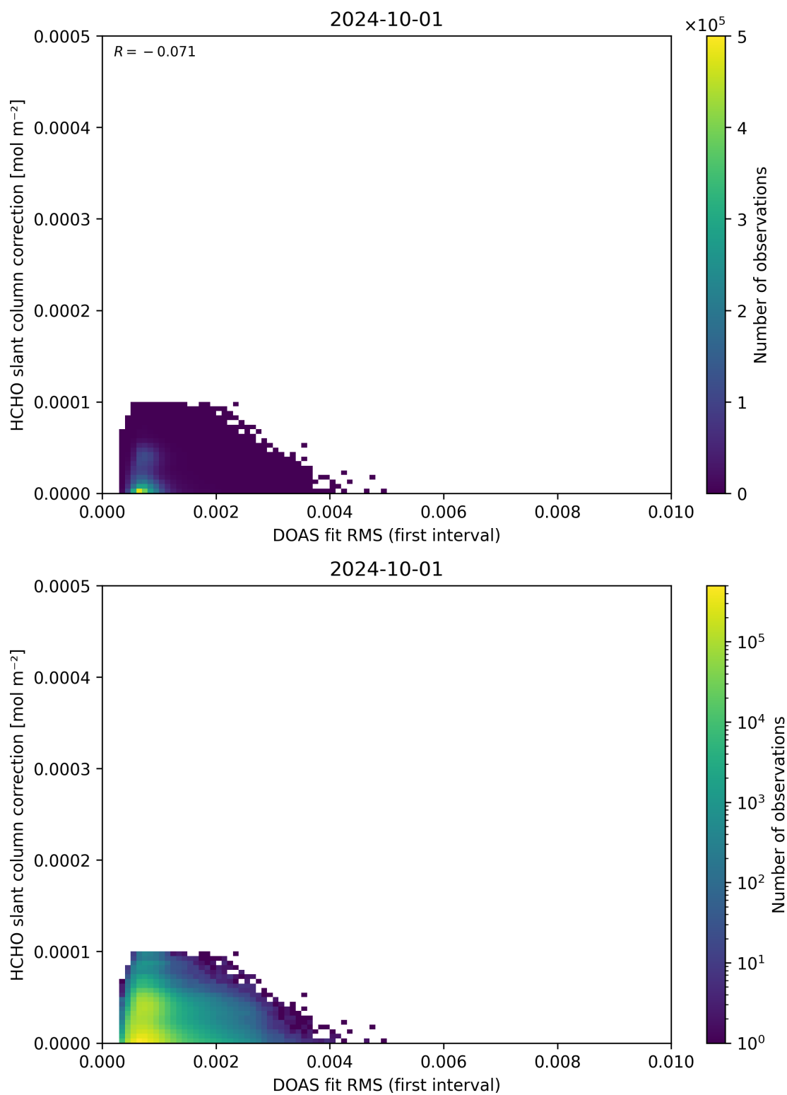
Figure 63: Scatter density plot of “DOAS fit RMS (first interval)” against “HCHO slant column correction” for 2024-09-30 to 2024-10-02.
