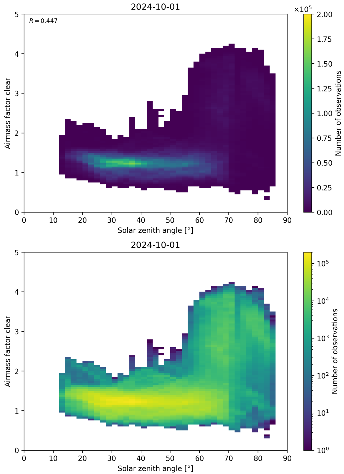
Figure 170: Scatter density plot of “Solar zenith angle” against “Airmass factor clear” for 2024-09-30 to 2024-10-02.
