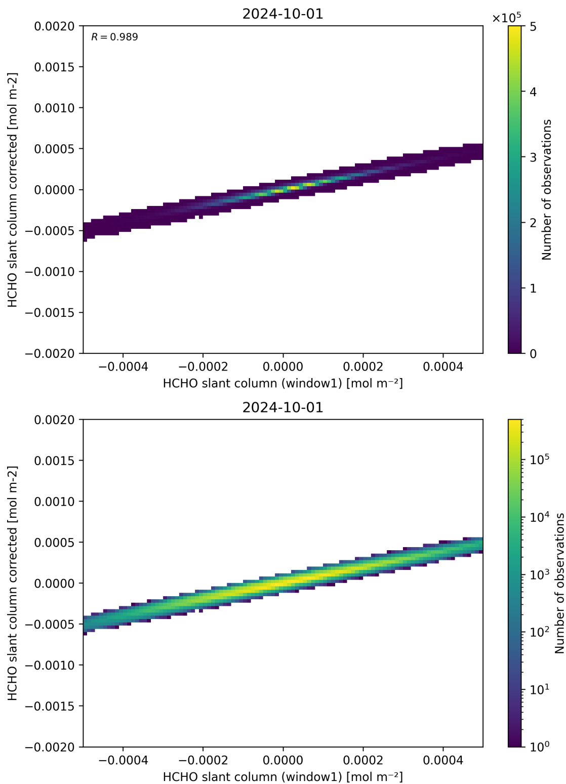
Figure 82: Scatter density plot of “HCHO slant column (window1)” against “HCHO slant column corrected” for 2024-09-30 to 2024-10-02.
