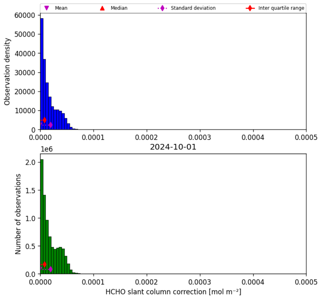
Figure 47: Histogram of “HCHO slant column correction” for 2024-09-30 to 2024-10-02
