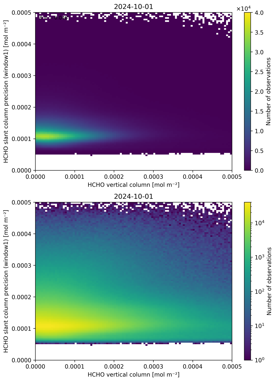
Figure 130: Scatter density plot of “HCHO vertical column” against “HCHO slant column precision (window1)” for 2024-09-30 to 2024-10-02.
