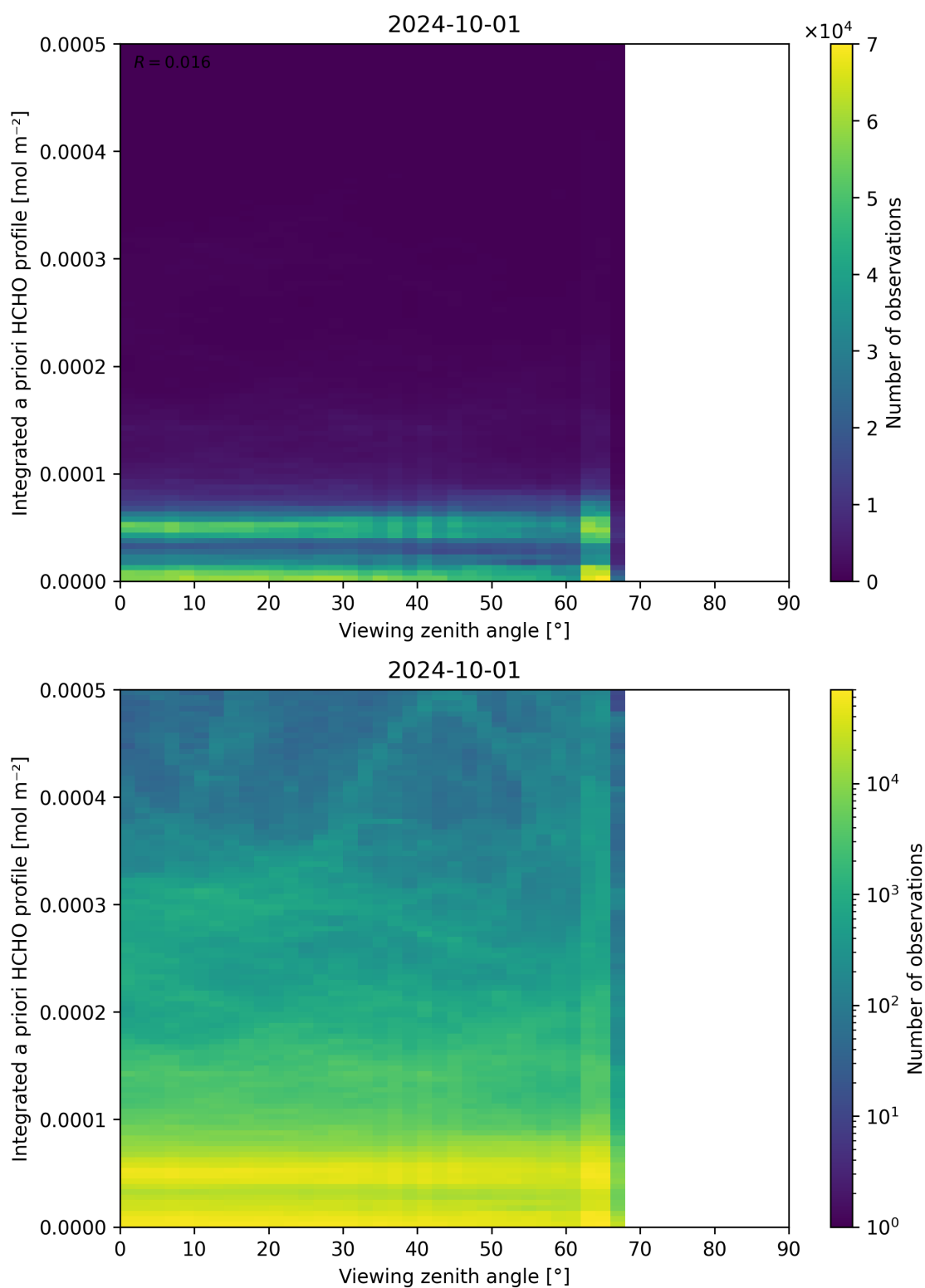
Figure 195: Scatter density plot of “Viewing zenith angle” against “Integrated a priori HCHO profile” for 2024-09-30 to 2024-10-02.
