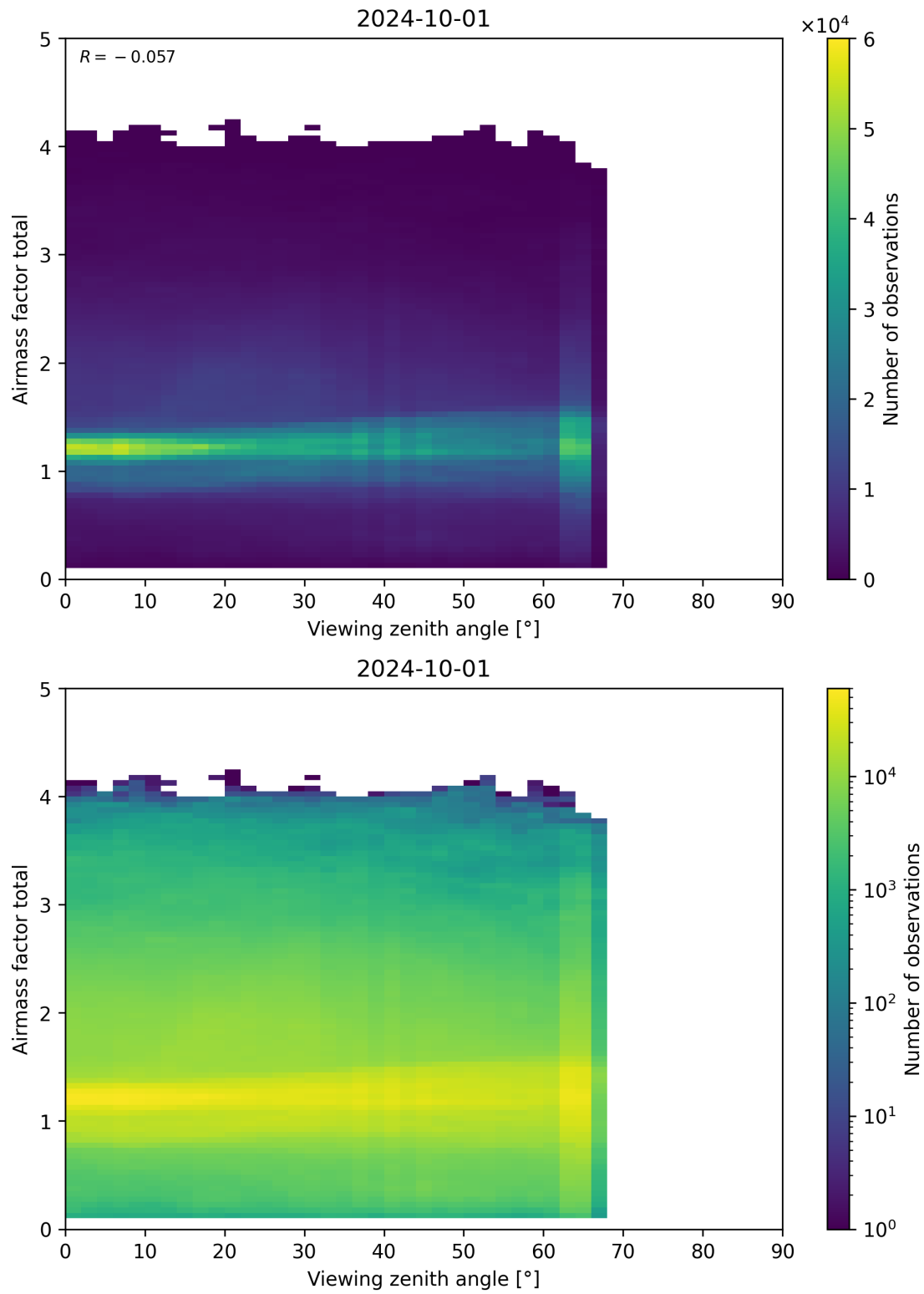
Figure 190: Scatter density plot of “Viewing zenith angle” against “Airmass factor total” for 2024-09-30 to 2024-10-02.
