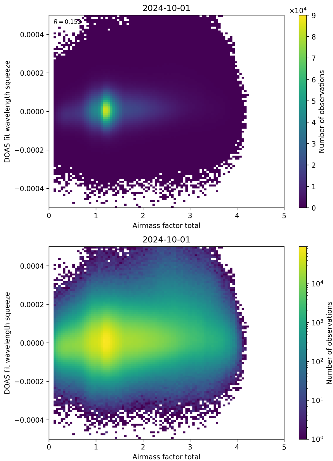
Figure 99: Scatter density plot of “Airmass factor total” against “DOAS fit wavelength squeeze” for 2024-09-30 to 2024-10-02.
