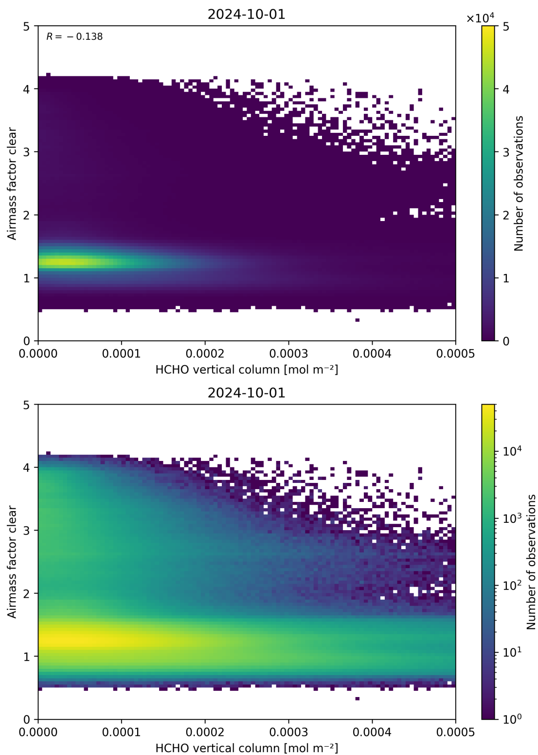
Figure 126: Scatter density plot of “HCHO vertical column” against “Airmass factor clear” for 2024-09-30 to 2024-10-02.
