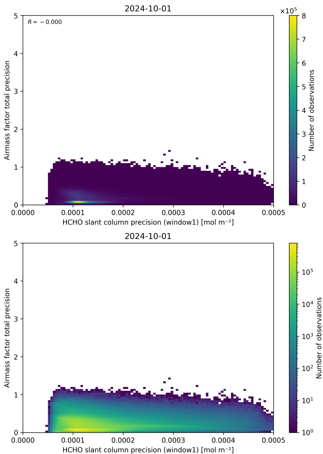
Figure 95: Scatter density plot of “HCHO slant column precision (window1)” against “Airmass factor total precision” for 2024-09-30 to 2024-10-02.
