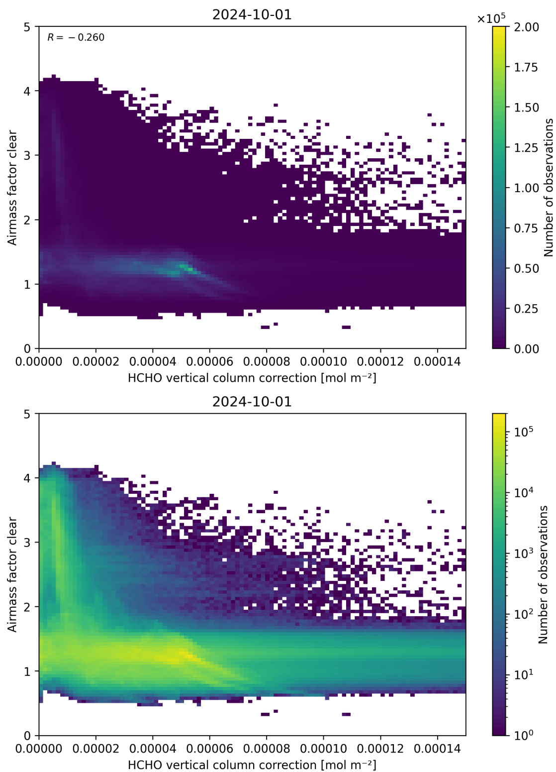
Figure 115: Scatter density plot of “HCHO vertical column correction” against “Airmass factor clear” for 2024-09-30 to 2024-10-02.
