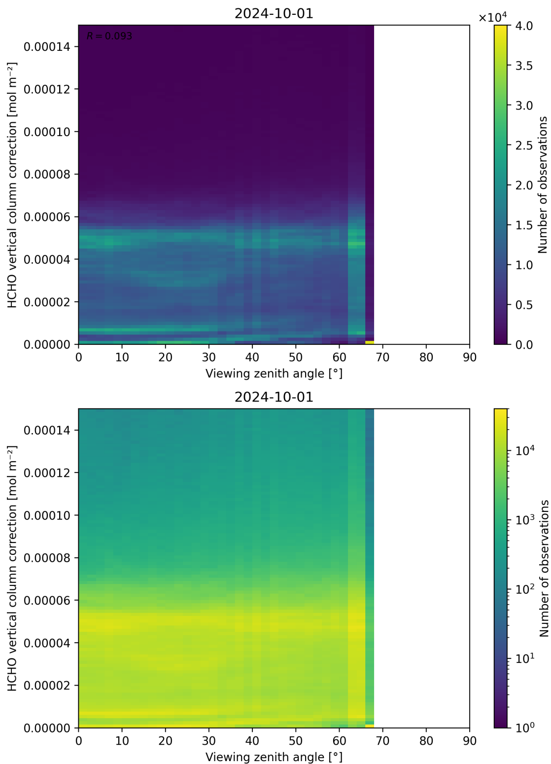
Figure 193: Scatter density plot of “Viewing zenith angle” against “HCHO vertical column correction” for 2024-09-30 to 2024-10-02.
