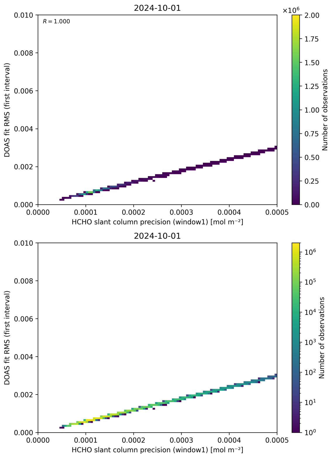
Figure 88: Scatter density plot of “HCHO slant column precision (window1)” against “DOAS fit RMS (first interval)” for 2024-09-30 to 2024-10-02.
