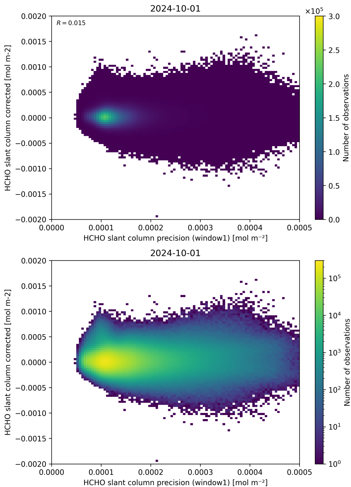
Figure 92: Scatter density plot of “HCHO slant column precision (window1)” against “HCHO slant column corrected” for 2024-09-30 to 2024-10-02.
