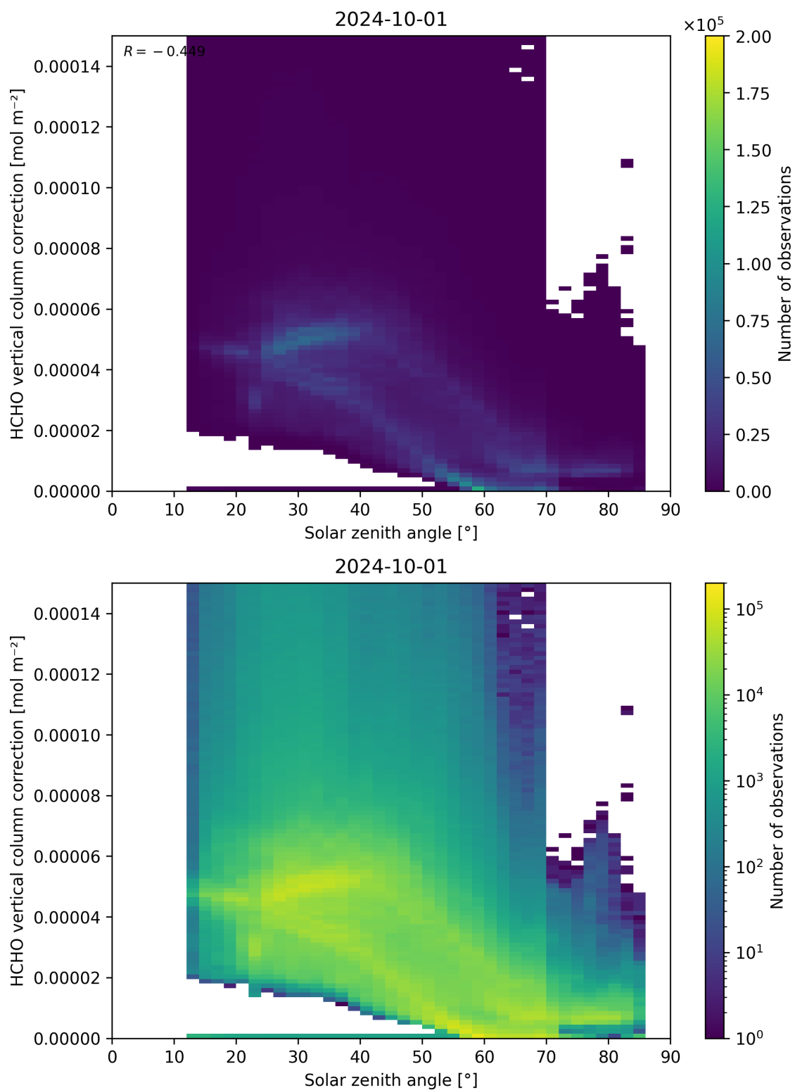
Figure 178: Scatter density plot of “Solar zenith angle” against “HCHO vertical column correction” for 2024-09-30 to 2024-10-02.
