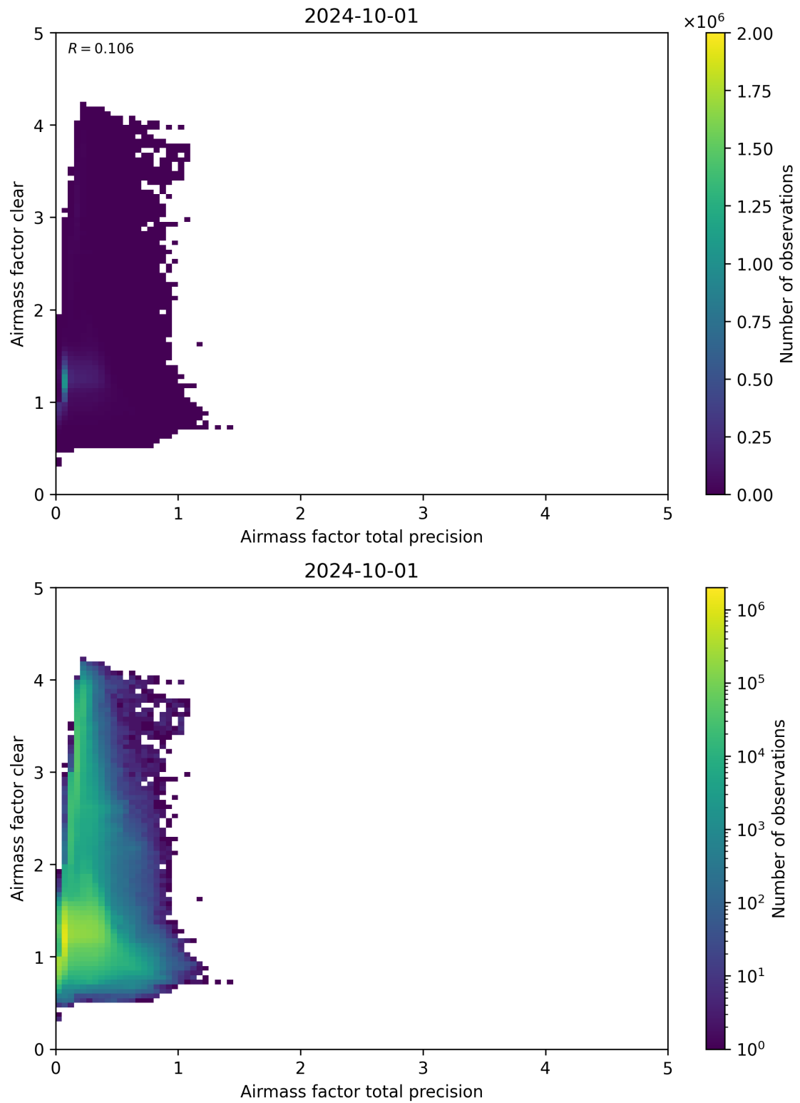
Figure 108: Scatter density plot of “Airmass factor total precision” against “Airmass factor clear” for 2024-09-30 to 2024-10-02.
