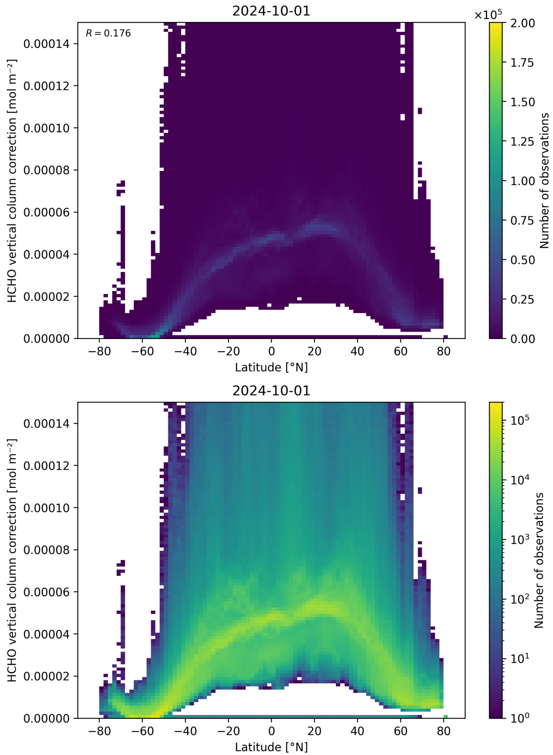
Figure 164: Scatter density plot of “Latitude” against “HCHO vertical column correction” for 2024-09-30 to 2024-10-02.
