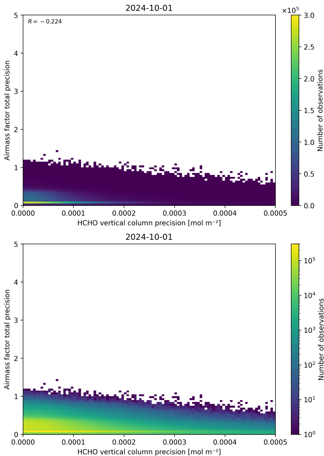
Figure 145: Scatter density plot of “HCHO vertical column precision” against “Airmass factor total precision” for 2024-09-30 to 2024-10-02.
