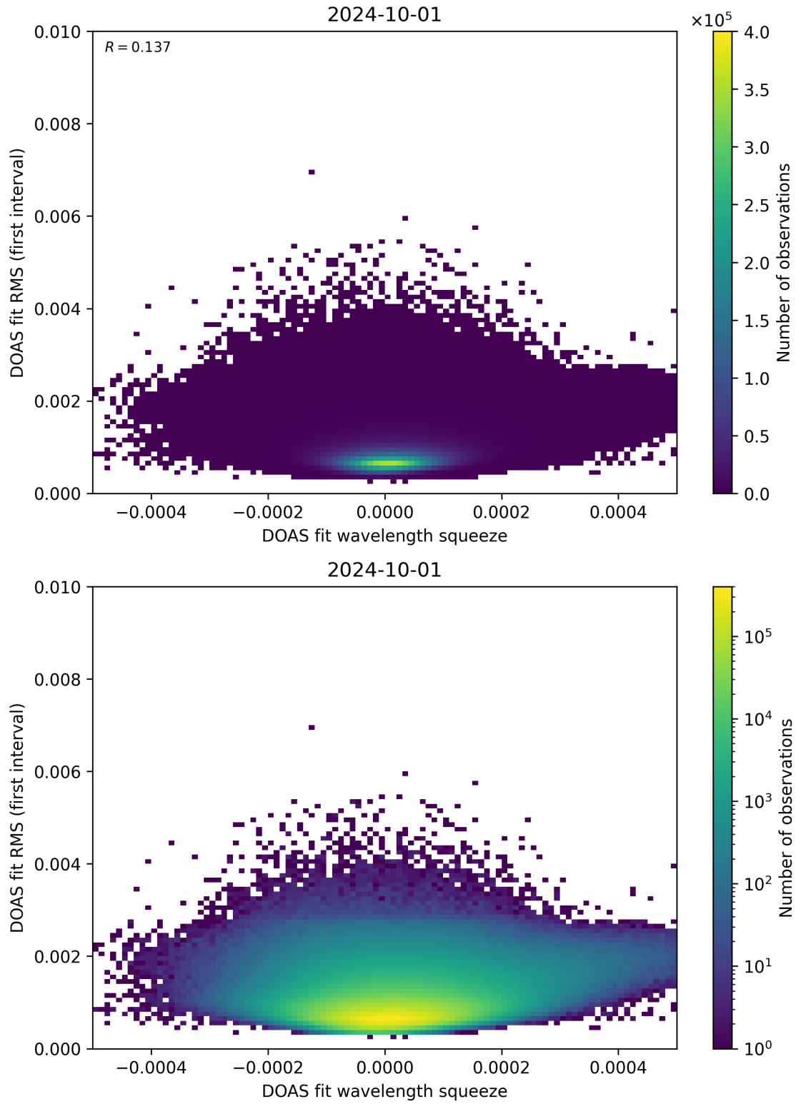
Figure 68: Scatter density plot of “DOAS fit wavelength squeeze” against “DOAS fit RMS (first interval)” for 2024-09-30 to 2024-10-02.
