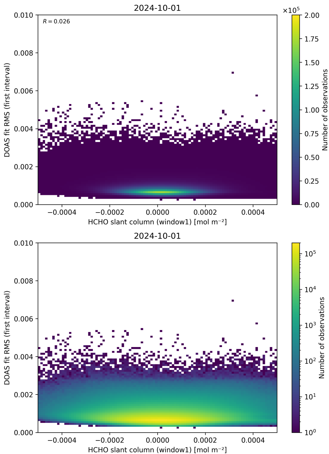
Figure 78: Scatter density plot of “HCHO slant column (window1)” against “DOAS fit RMS (first interval)” for 2024-09-30 to 2024-10-02.
