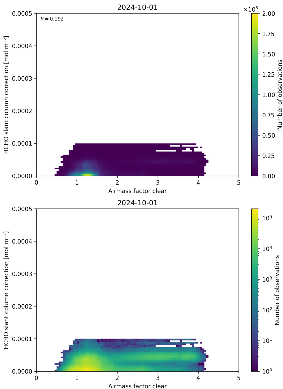
Figure 75: Scatter density plot of “Airmass factor clear” against “HCHO slant column correction” for 2024-09-30 to 2024-10-02.
