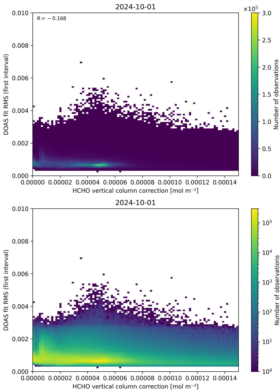
Figure 112: Scatter density plot of “HCHO vertical column correction” against “DOAS fit RMS (first interval)” for 2024-09-30 to 2024-10-02.
