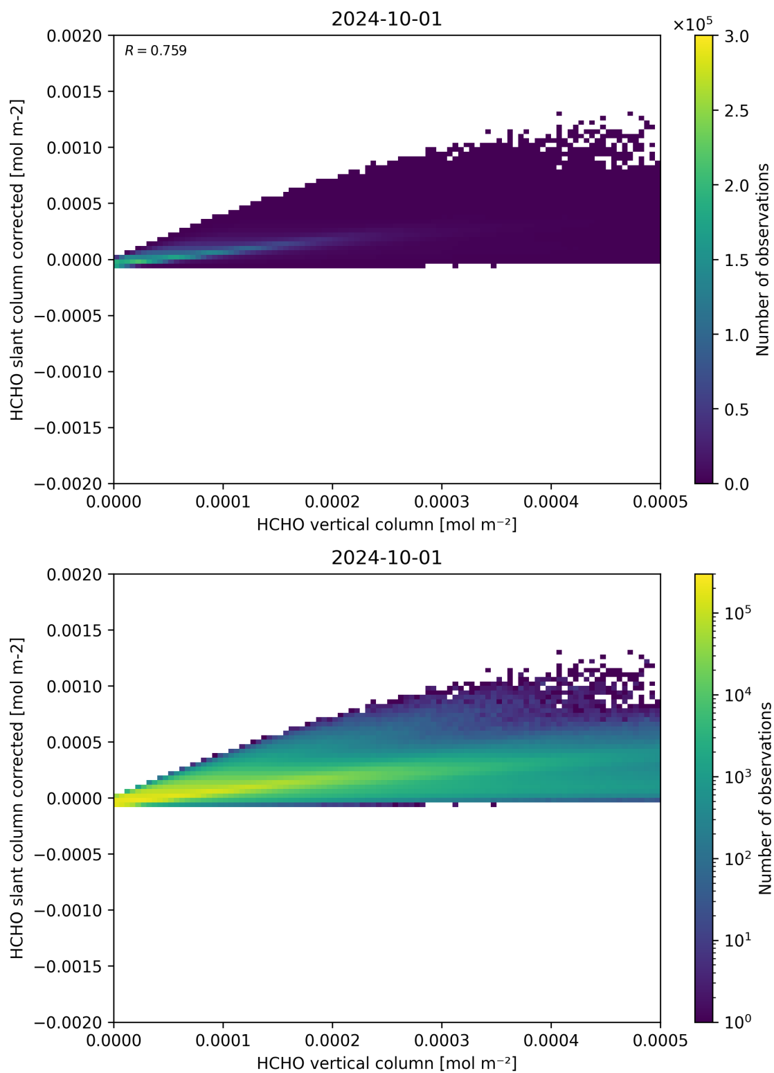
Figure 127: Scatter density plot of “HCHO vertical column” against “HCHO slant column corrected” for 2024-09-30 to 2024-10-02.
