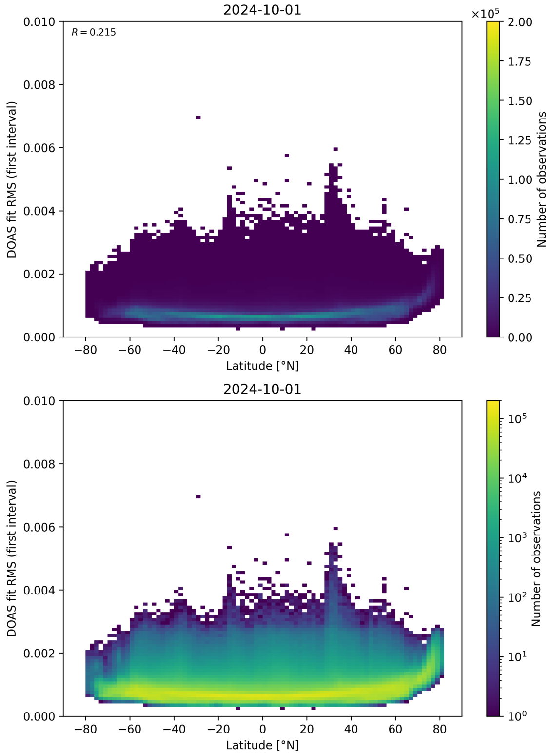
Figure 153: Scatter density plot of “Latitude” against “DOAS fit RMS (first interval)” for 2024-09-30 to 2024-10-02.
