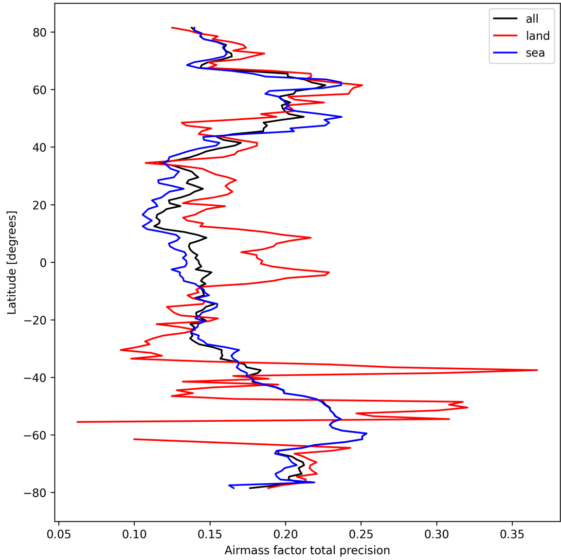
Figure 27: Zonal average of “Airmass factor total precision” for 2024-09-30 to 2024-10-02.
