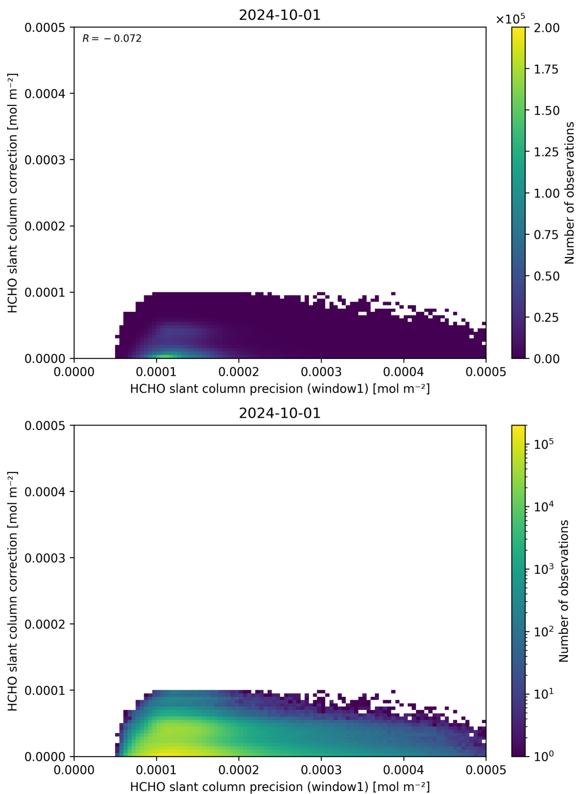
Figure 93: Scatter density plot of “HCHO slant column precision (window1)” against “HCHO slant column correction” for 2024-09-30 to 2024-10-02.
