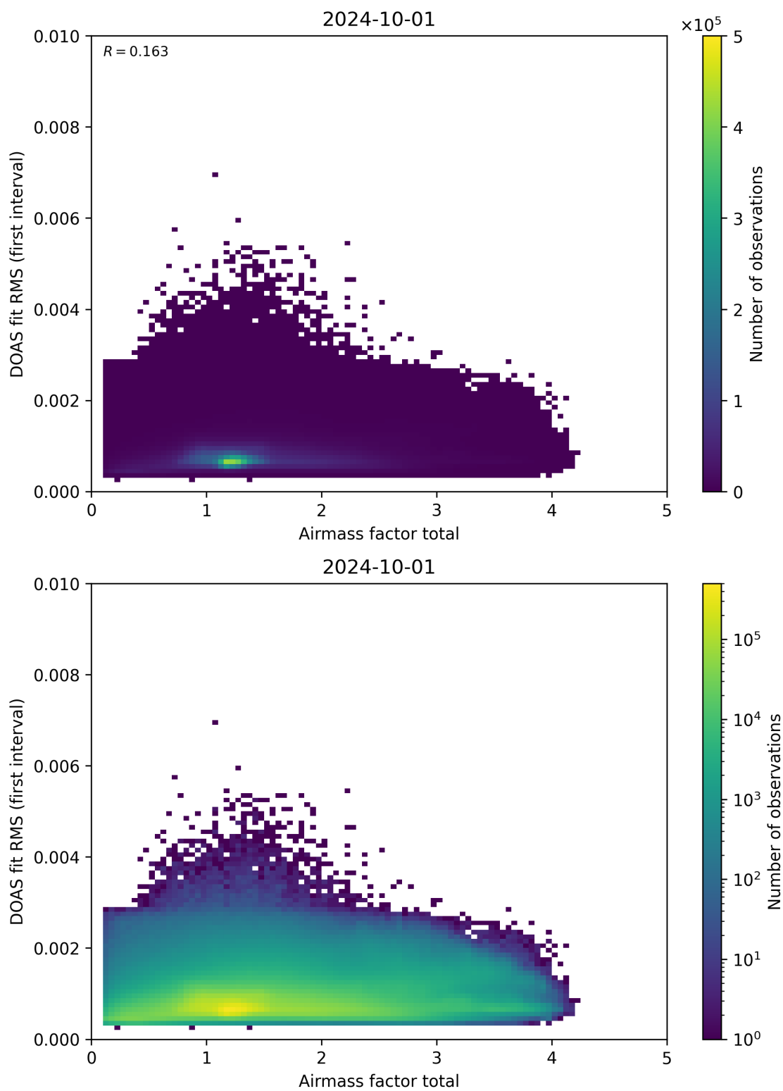
Figure 97: Scatter density plot of “Airmass factor total” against “DOAS fit RMS (first interval)” for 2024-09-30 to 2024-10-02.
