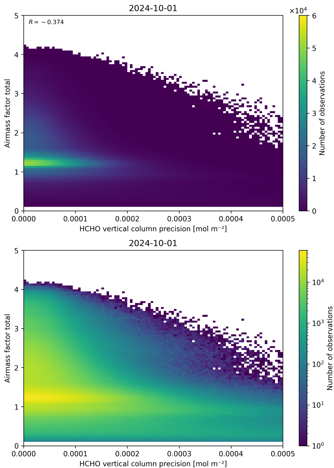
Figure 144: Scatter density plot of “HCHO vertical column precision” against “Airmass factor total” for 2024-09-30 to 2024-10-02.
