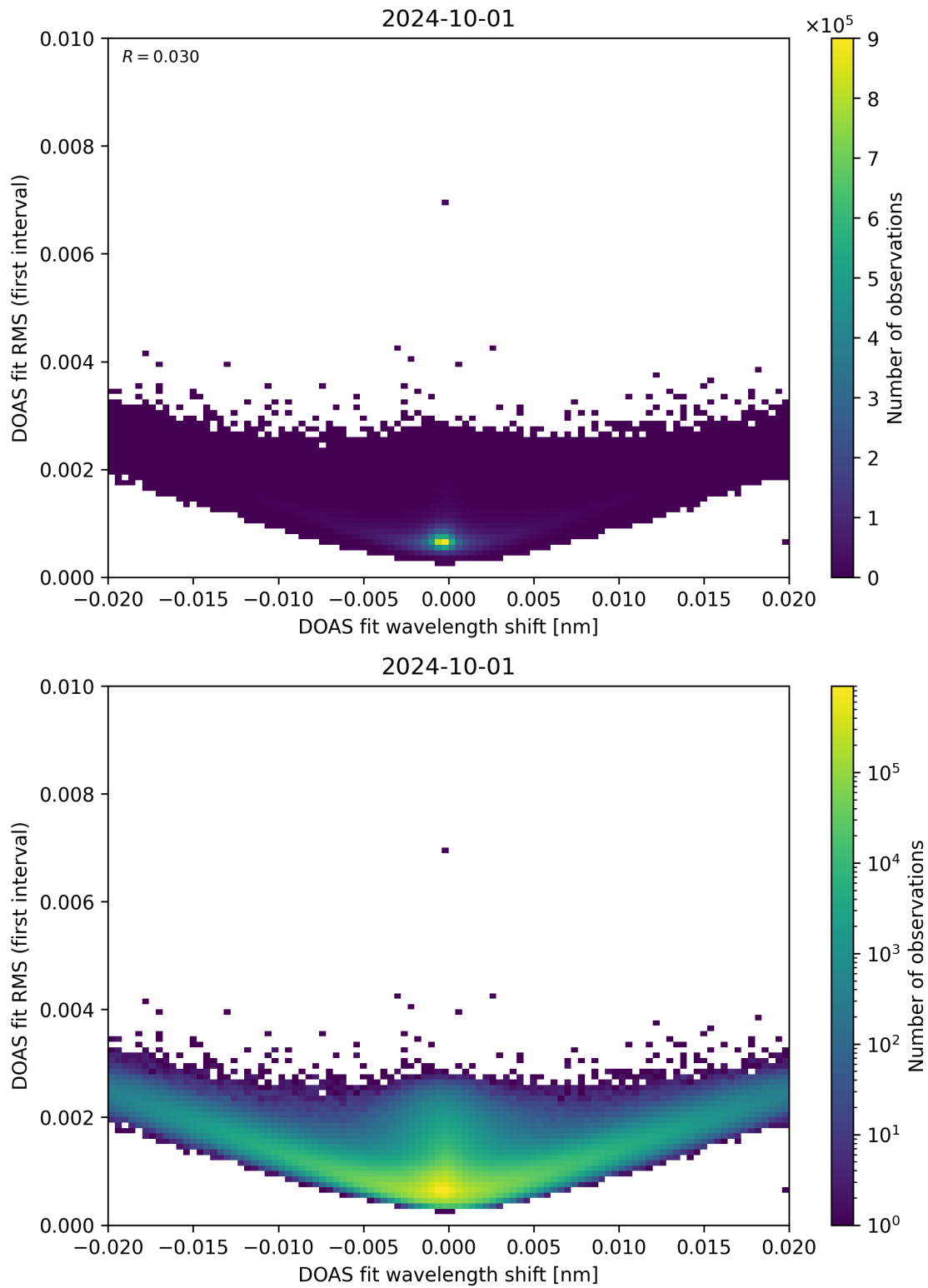
Figure 64: Scatter density plot of “DOAS fit wavelength shift” against “DOAS fit RMS (first interval)” for 2024-09-30 to 2024-10-02.
