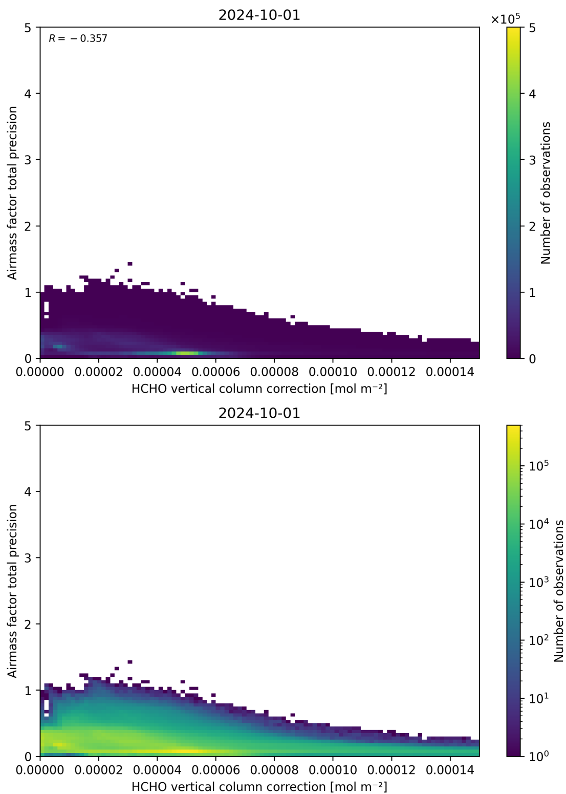
Figure 121: Scatter density plot of “HCHO vertical column correction” against “Airmass factor total precision” for 2024-09-30 to 2024-10-02.
