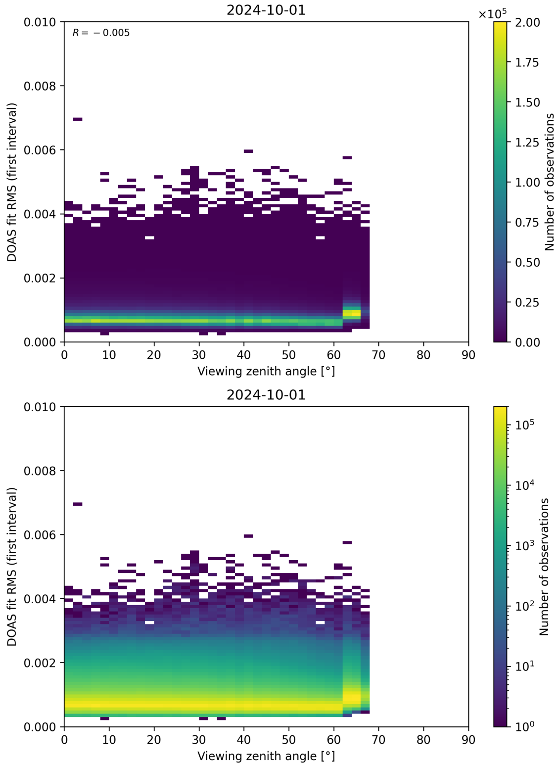
Figure 182: Scatter density plot of “Viewing zenith angle” against “DOAS fit RMS (first interval)” for 2024-09-30 to 2024-10-02.
