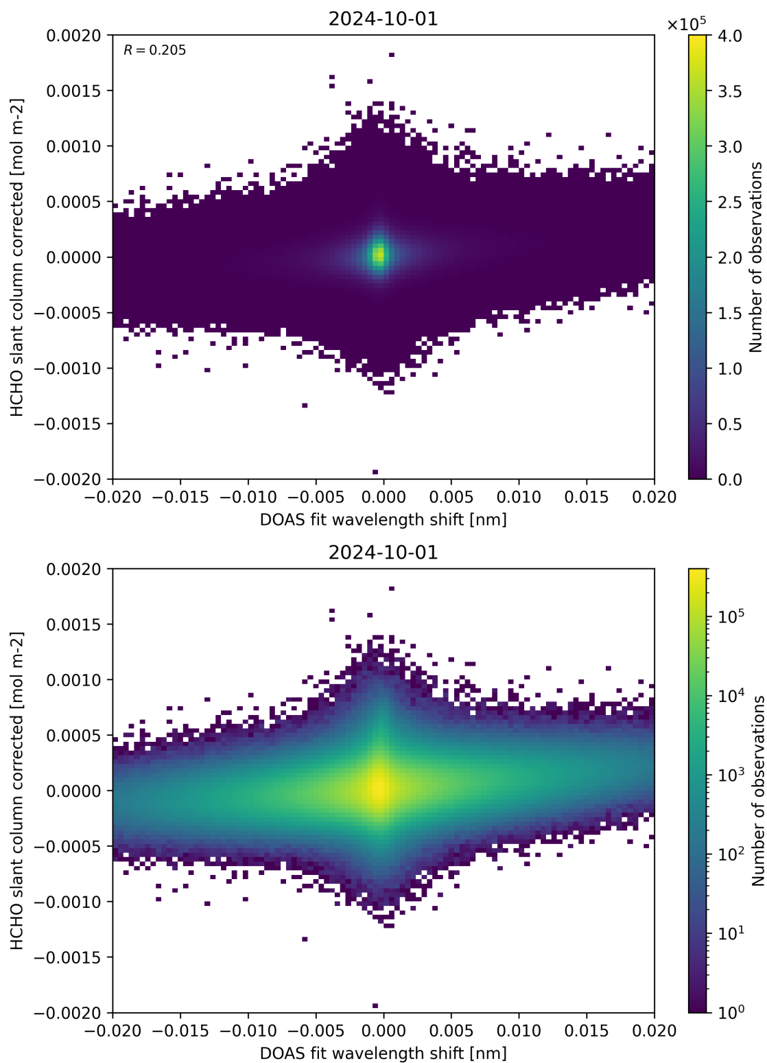
Figure 66: Scatter density plot of “DOAS fit wavelength shift” against “HCHO slant column corrected” for 2024-09-30 to 2024-10-02.
