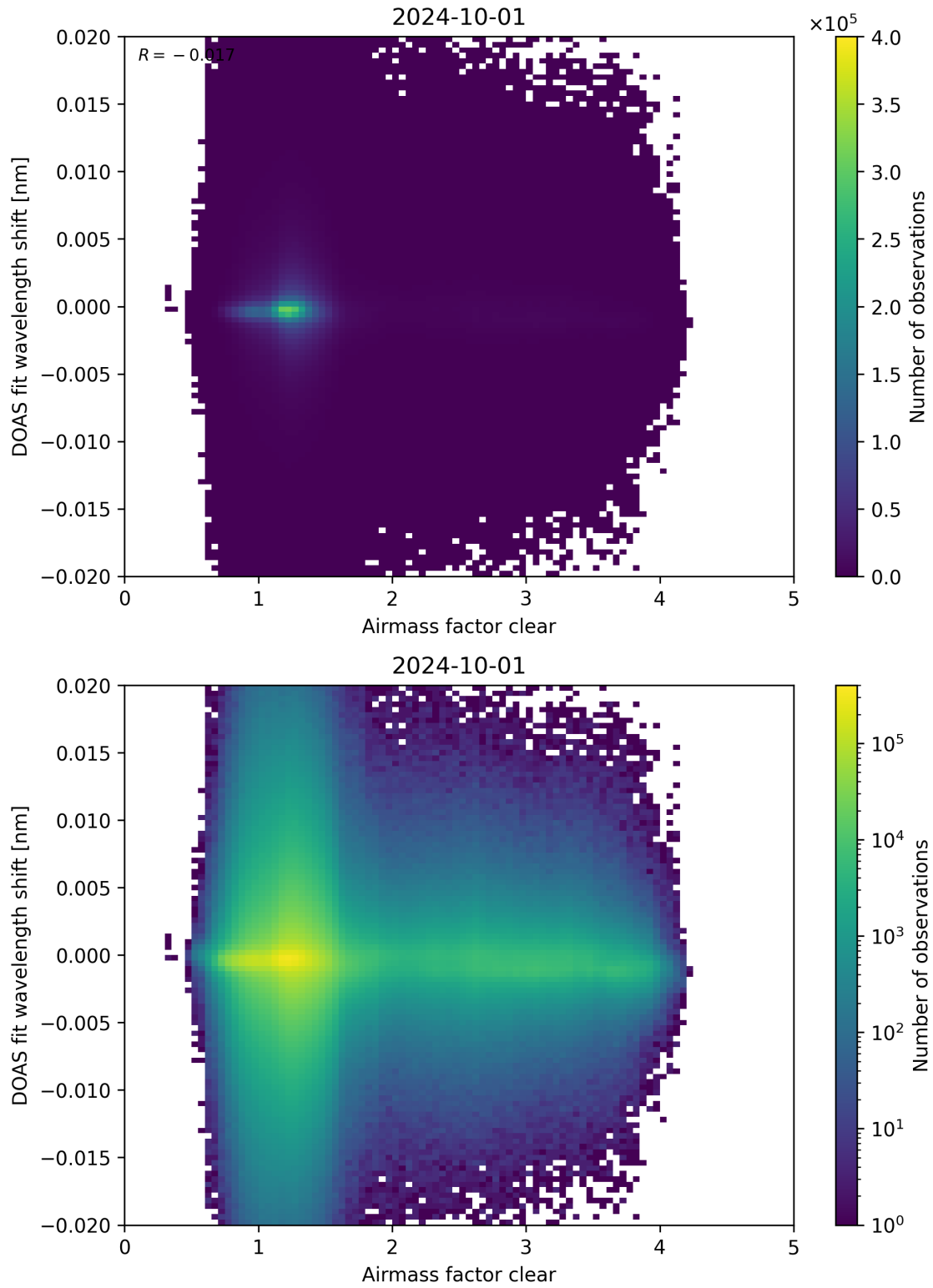
Figure 72: Scatter density plot of “Airmass factor clear” against “DOAS fit wavelength shift” for 2024-09-30 to 2024-10-02.
