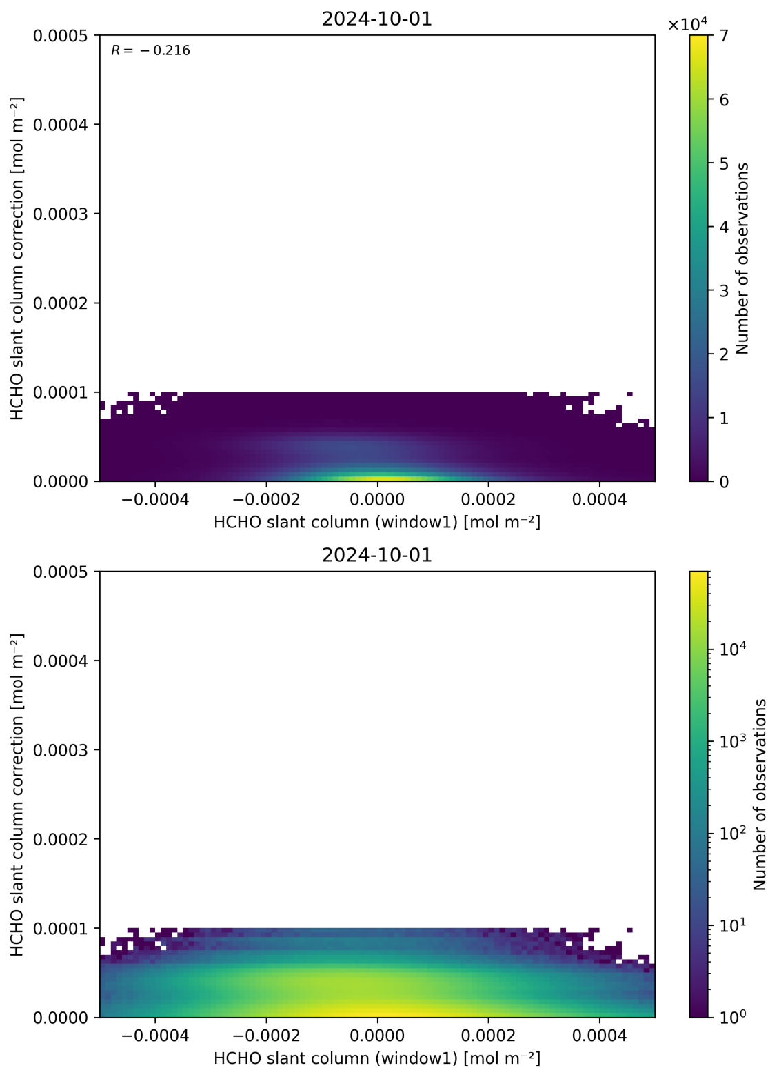
Figure 83: Scatter density plot of “HCHO slant column (window1)” against “HCHO slant column correction” for 2024-09-30 to 2024-10-02.
