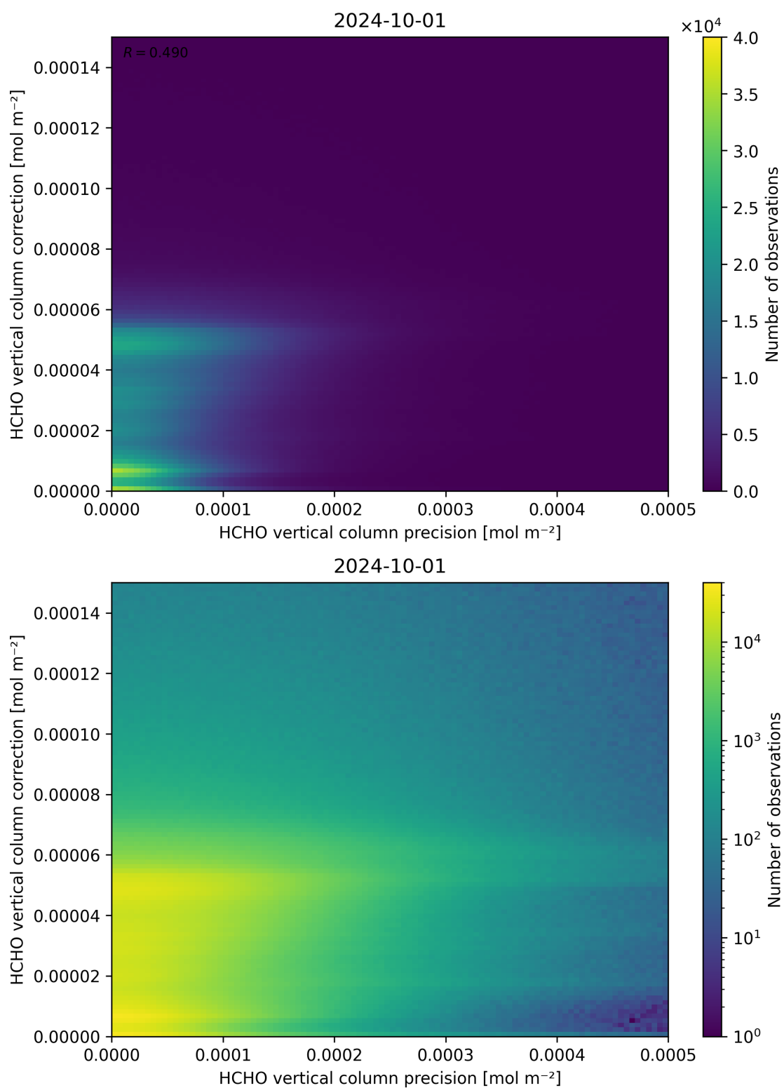
Figure 146: Scatter density plot of “HCHO vertical column precision” against “HCHO vertical column correction” for 2024-09-30 to 2024-10-02.
