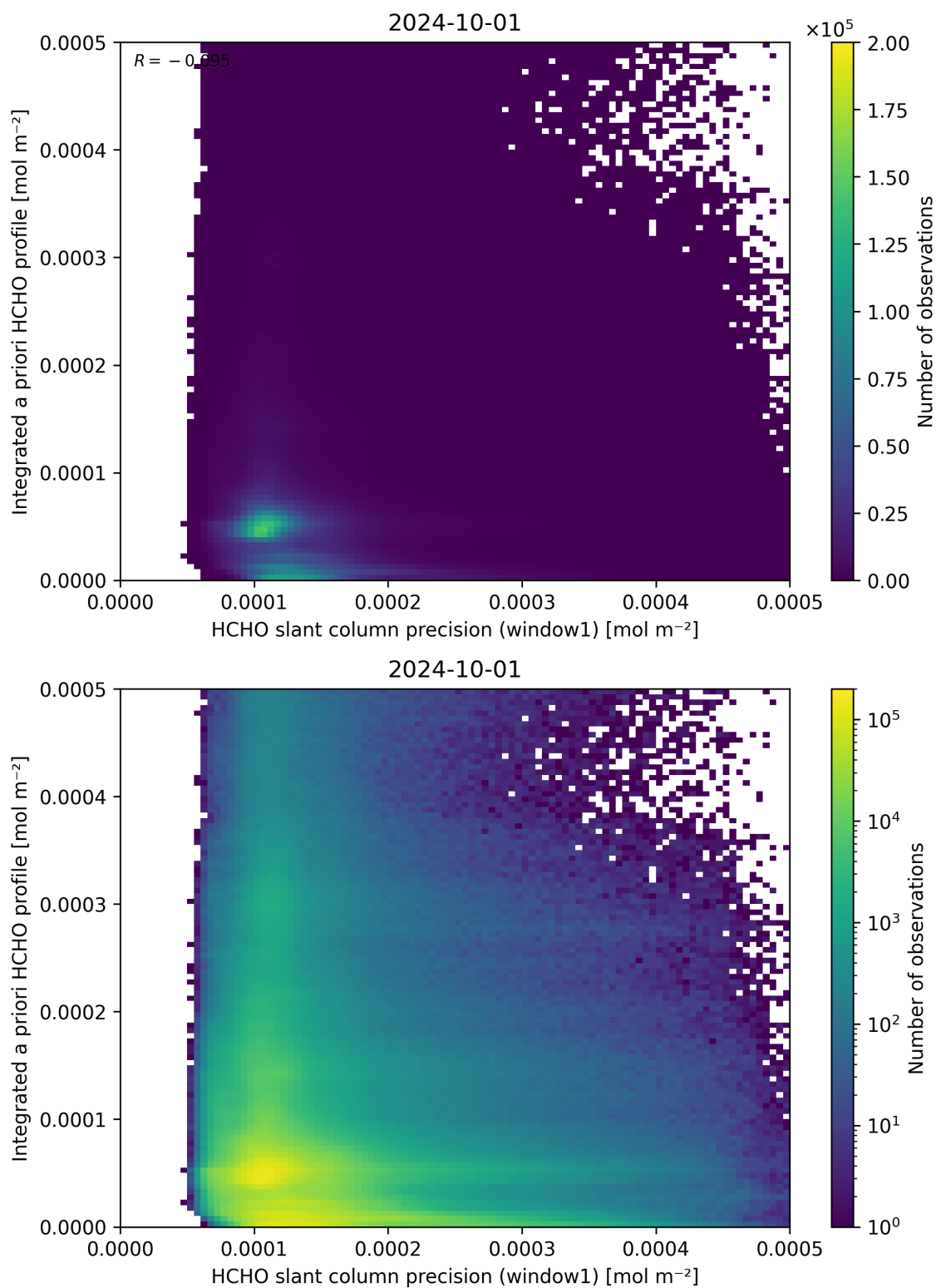
Figure 96: Scatter density plot of “HCHO slant column precision (window1)” against “Integrated a priori HCHO profile” for 2024-09-30 to 2024-10-02.
