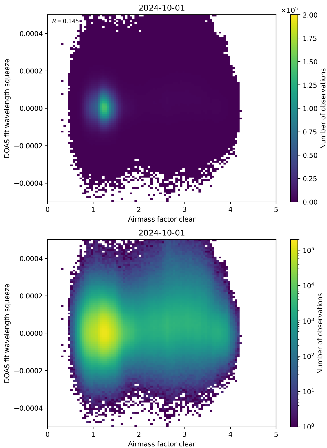
Figure 73: Scatter density plot of “Airmass factor clear” against “DOAS fit wavelength squeeze” for 2024-09-30 to 2024-10-02.
