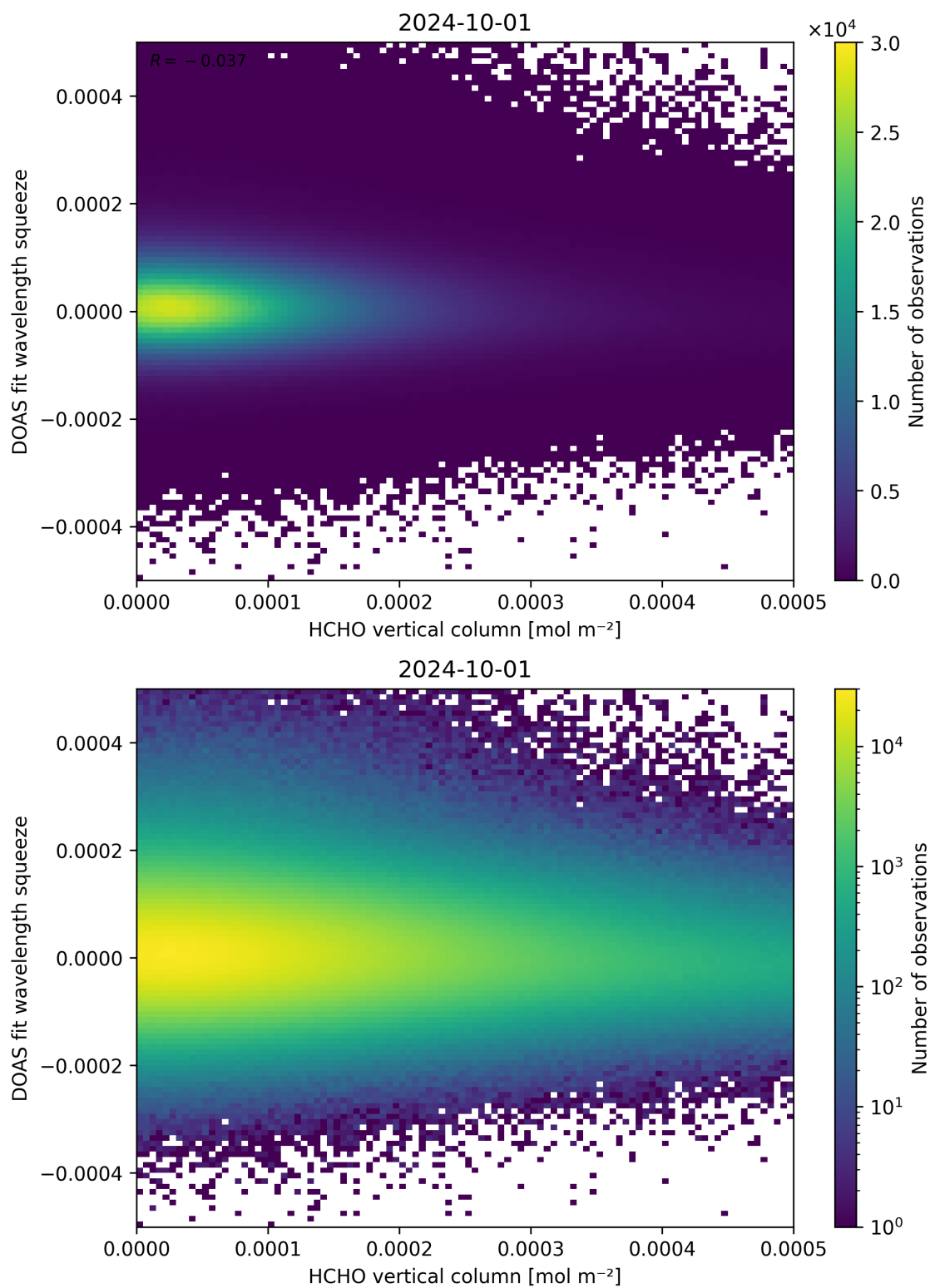
Figure 125: Scatter density plot of “HCHO vertical column” against “DOAS fit wavelength squeeze” for 2024-09-30 to 2024-10-02.
