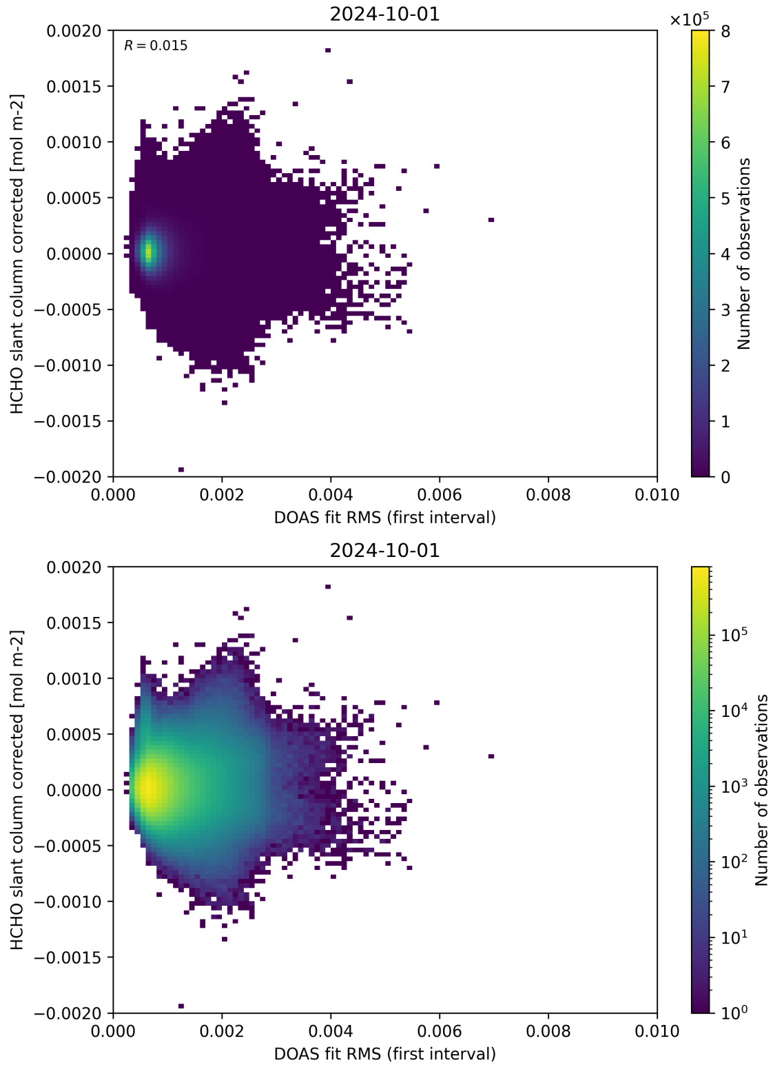
Figure 62: Scatter density plot of “DOAS fit RMS (first interval)” against “HCHO slant column corrected” for 2024-09-30 to 2024-10-02.
