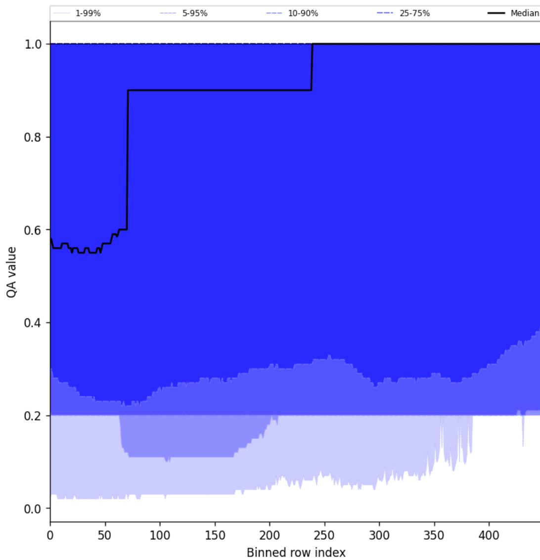
Figure 48: Along track statistics of “QA value” for 2024-09-30 to 2024-10-02
