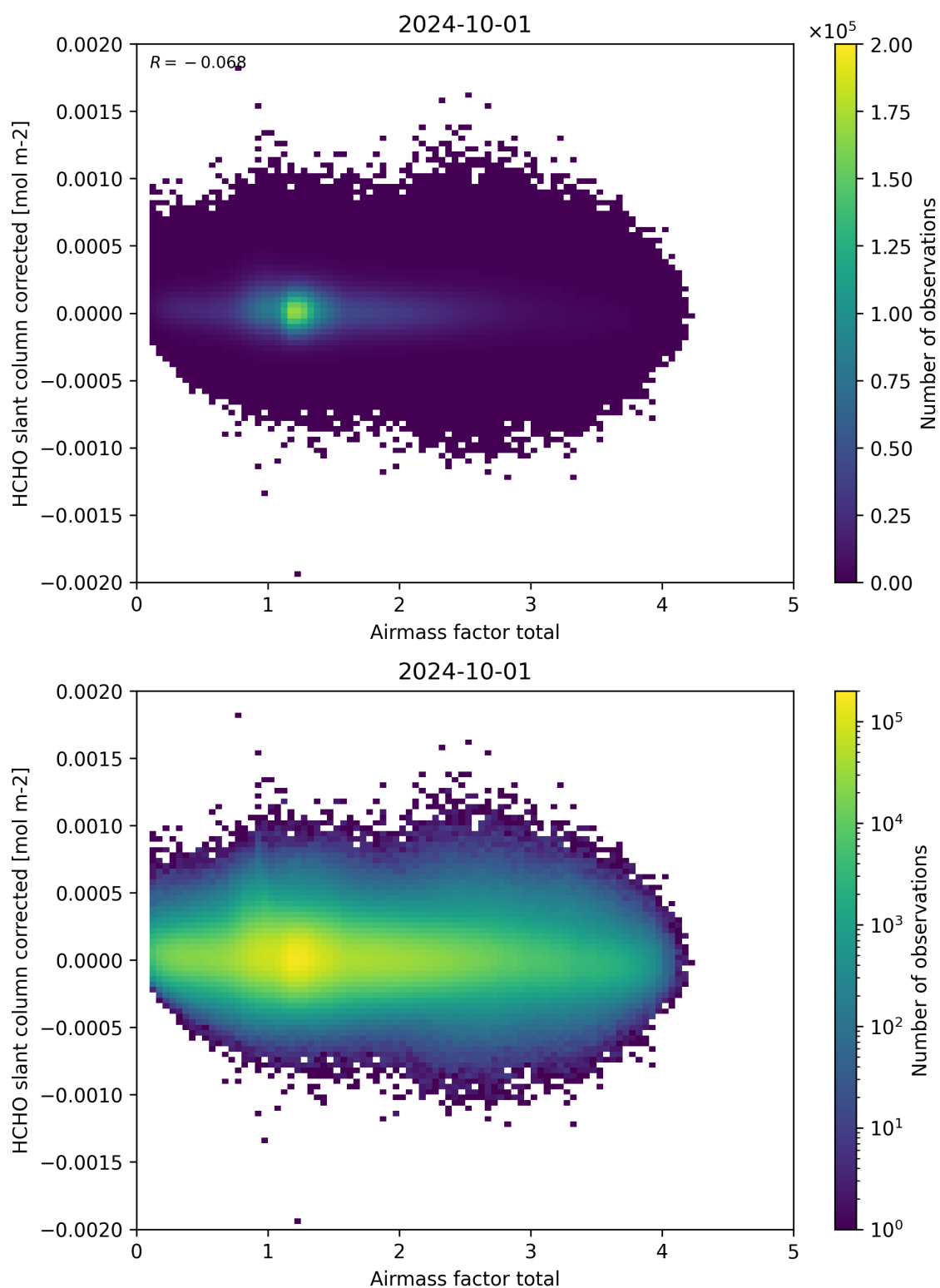
Figure 101: Scatter density plot of “Airmass factor total” against “HCHO slant column corrected” for 2024-09-30 to 2024-10-02.
