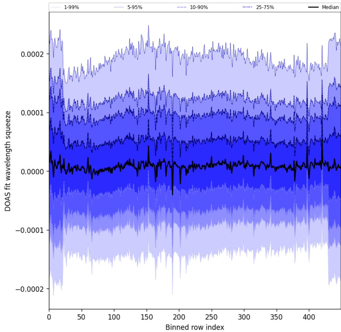
Figure 59: Along track statistics of “DOAS fit wavelength squeeze” for 2024-09-30 to 2024-10-02
