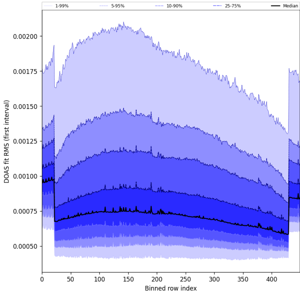
Figure 60: Along track statistics of “DOAS fit RMS (first interval)” for 2024-09-30 to 2024-10-02
