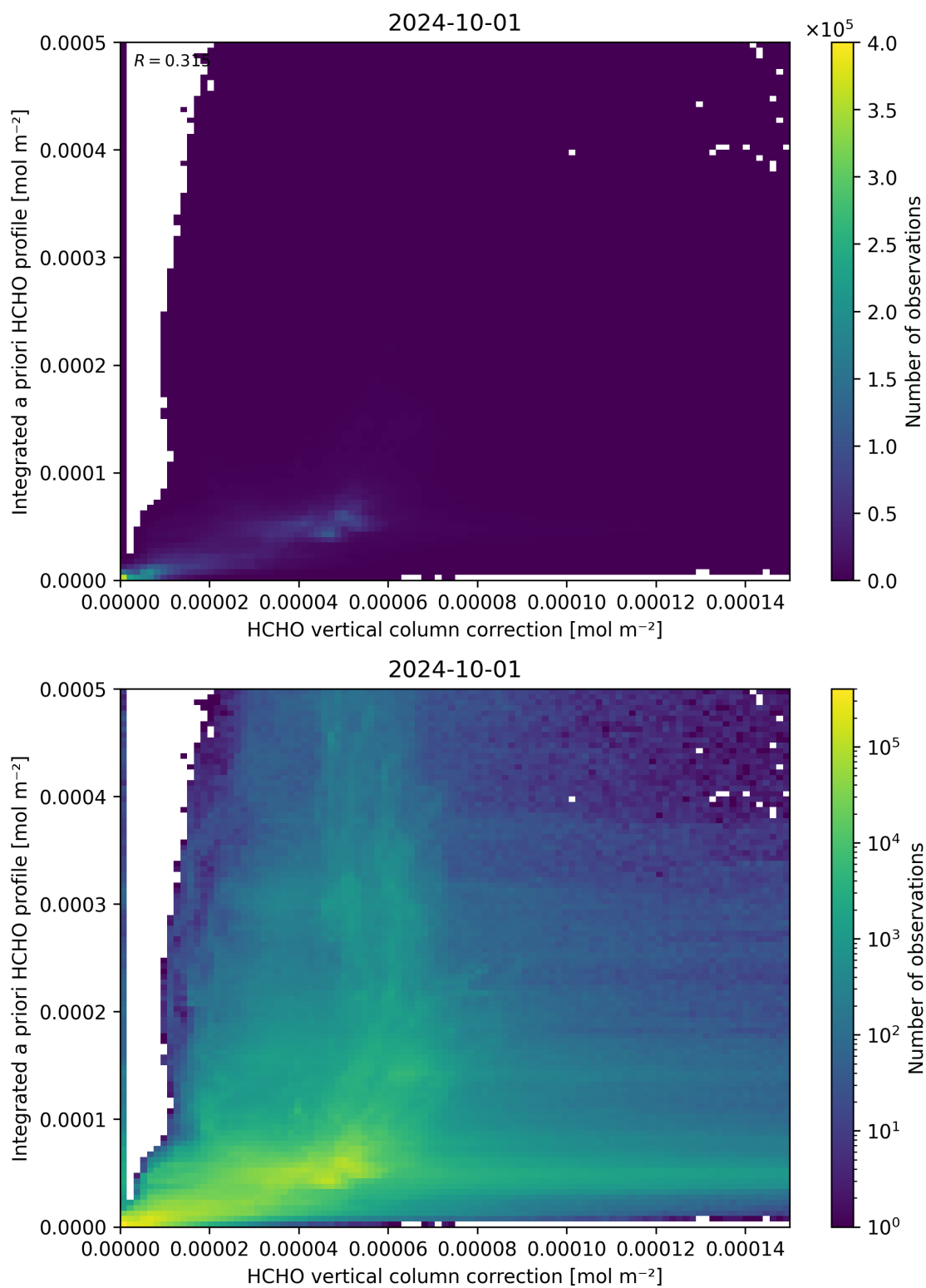
Figure 122: Scatter density plot of “HCHO vertical column correction” against “Integrated a priori HCHO profile” for 2024-09-30 to 2024-10-02.
