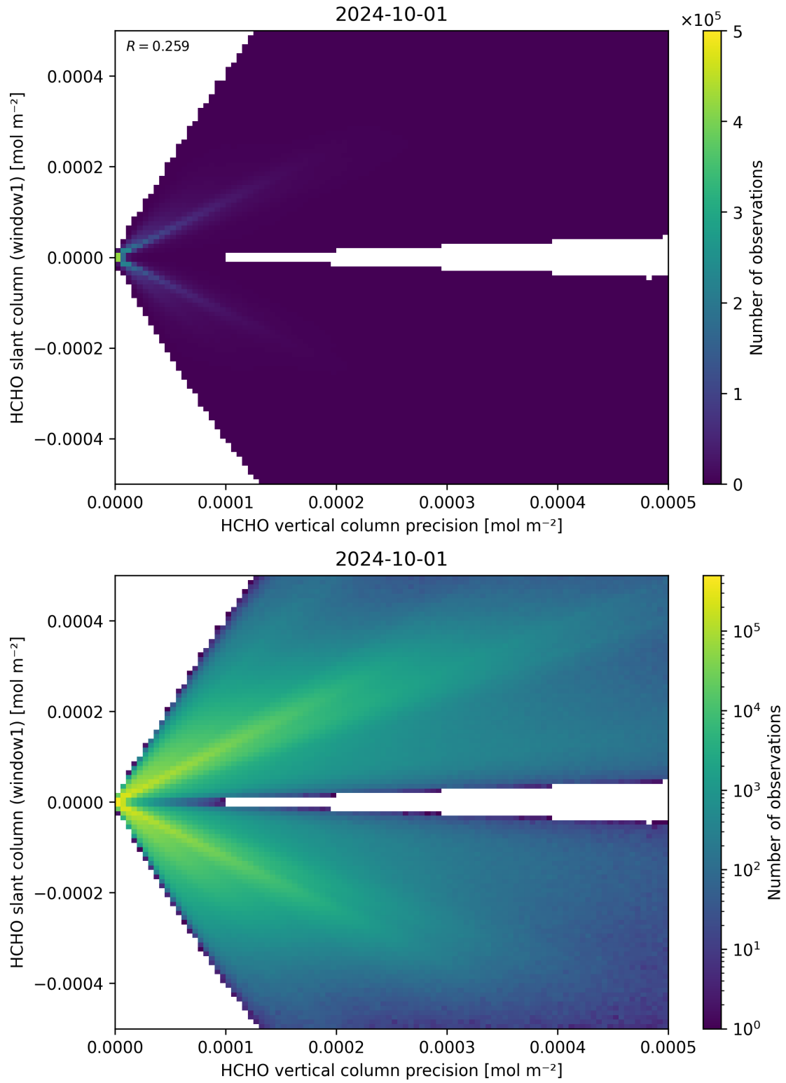
Figure 142: Scatter density plot of “HCHO vertical column precision” against “HCHO slant column (window1)” for 2024-09-30 to 2024-10-02.
