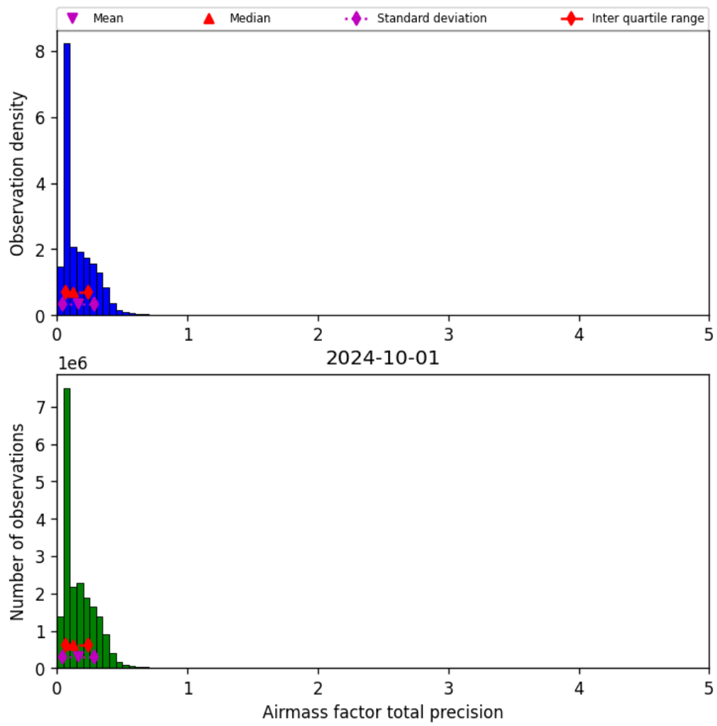
Figure 41: Histogram of “Airmass factor total precision” for 2024-09-30 to 2024-10-02
