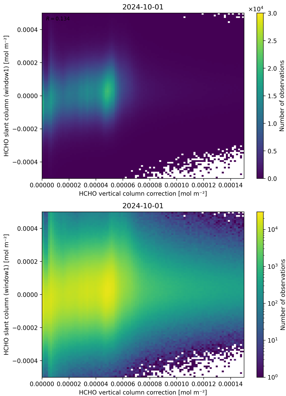
Figure 118: Scatter density plot of “HCHO vertical column correction” against “HCHO slant column (window1)” for 2024-09-30 to 2024-10-02.
