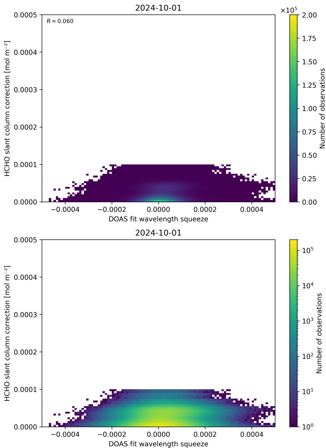
Figure 70: Scatter density plot of “DOAS fit wavelength squeeze” against “HCHO slant column correction” for 2024-09-30 to 2024-10-02.
