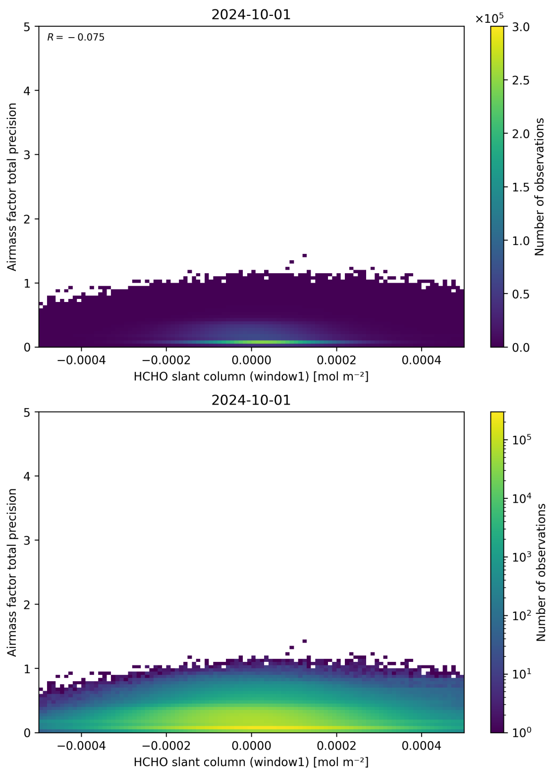
Figure 86: Scatter density plot of “HCHO slant column (window1)” against “Airmass factor total precision” for 2024-09-30 to 2024-10-02.
