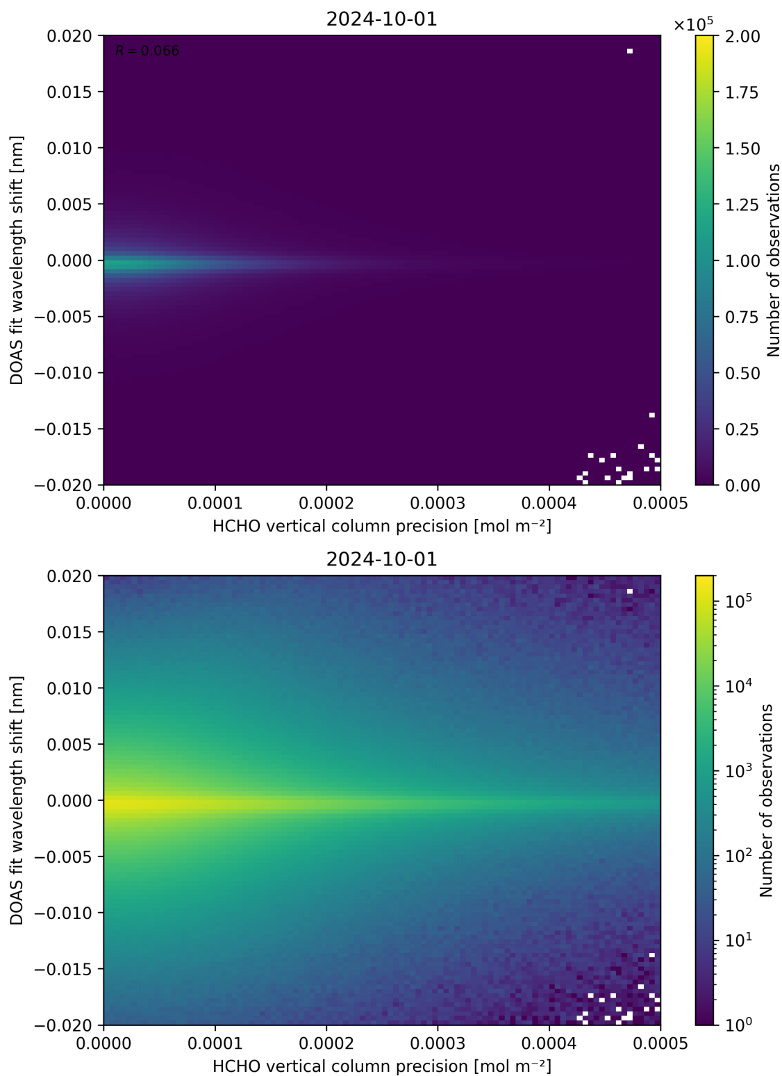
Figure 137: Scatter density plot of “HCHO vertical column precision” against “DOAS fit wavelength shift” for 2024-09-30 to 2024-10-02.
