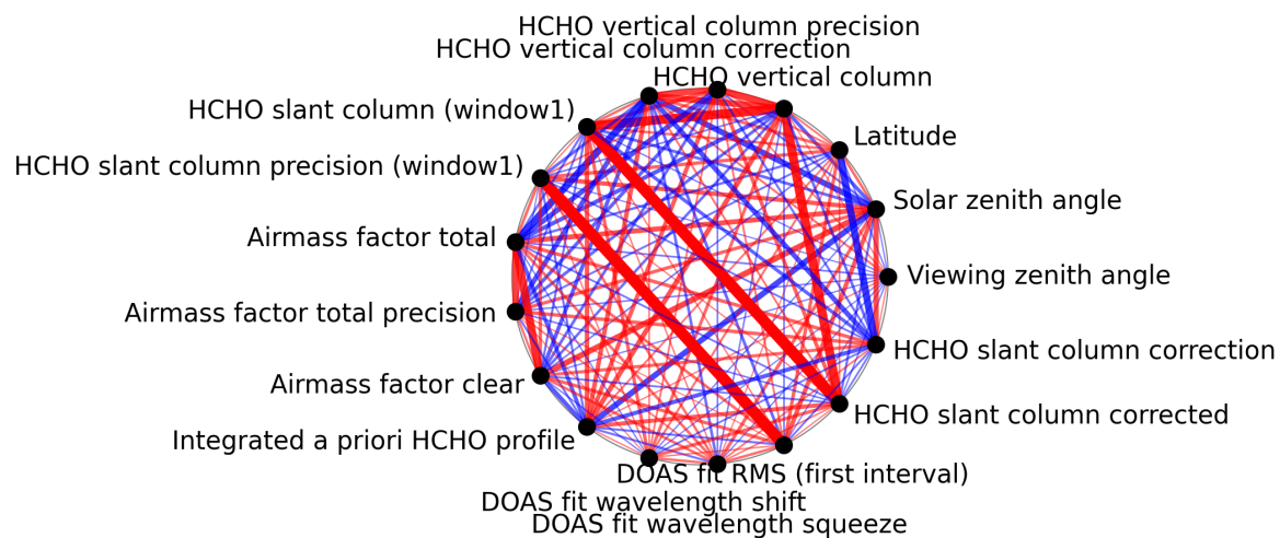
Figure 1: Map of correlation graph for 2024-09-30 to 2024-10-02.
