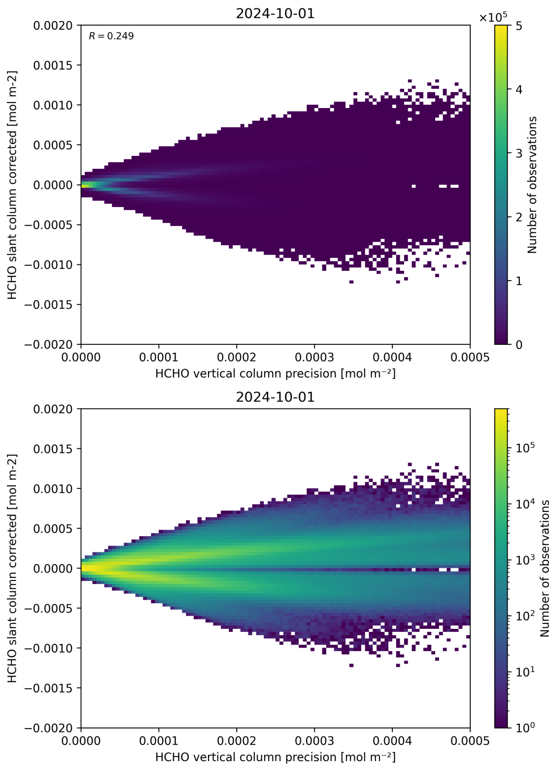
Figure 140: Scatter density plot of “HCHO vertical column precision” against “HCHO slant column corrected” for 2024-09-30 to 2024-10-02.
