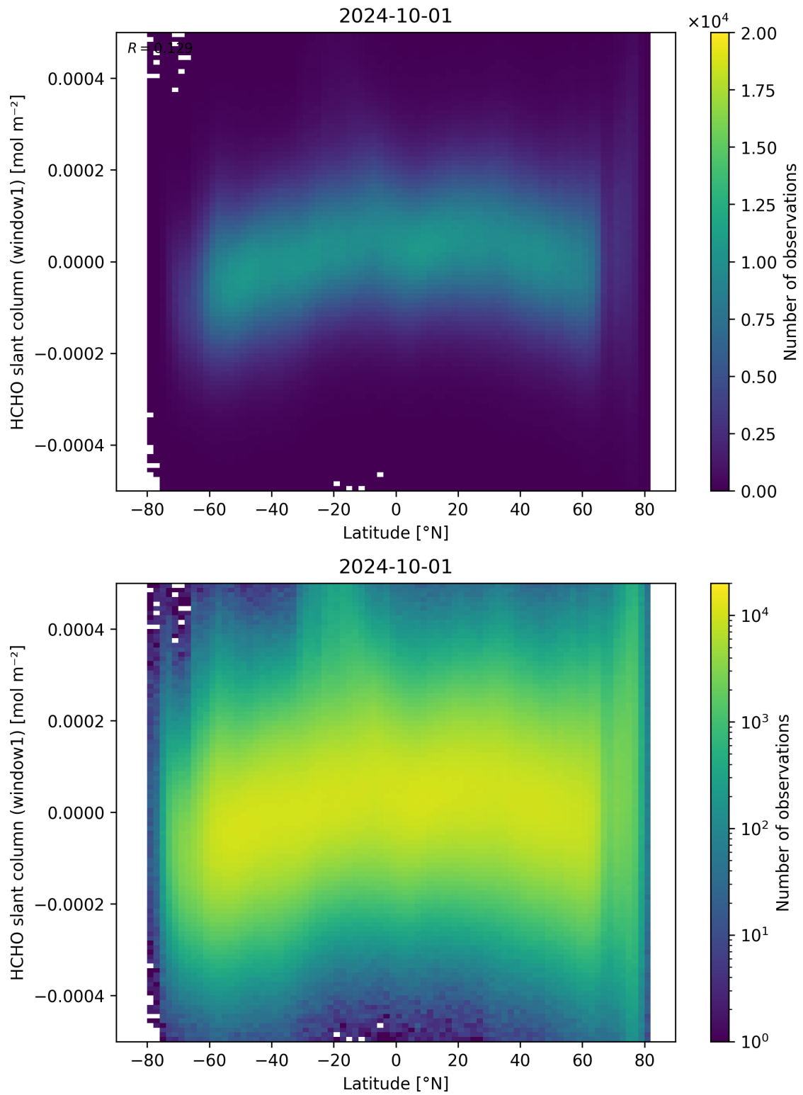
Figure 159: Scatter density plot of “Latitude” against “HCHO slant column (window1)” for 2024-09-30 to 2024-10-02.
