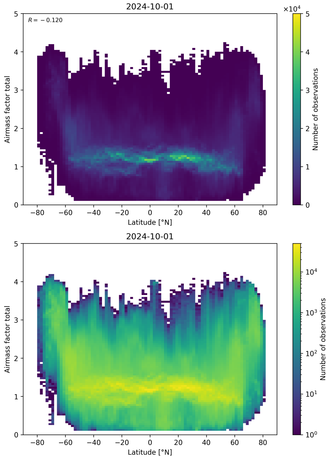
Figure 161: Scatter density plot of “Latitude” against “Airmass factor total” for 2024-09-30 to 2024-10-02.
