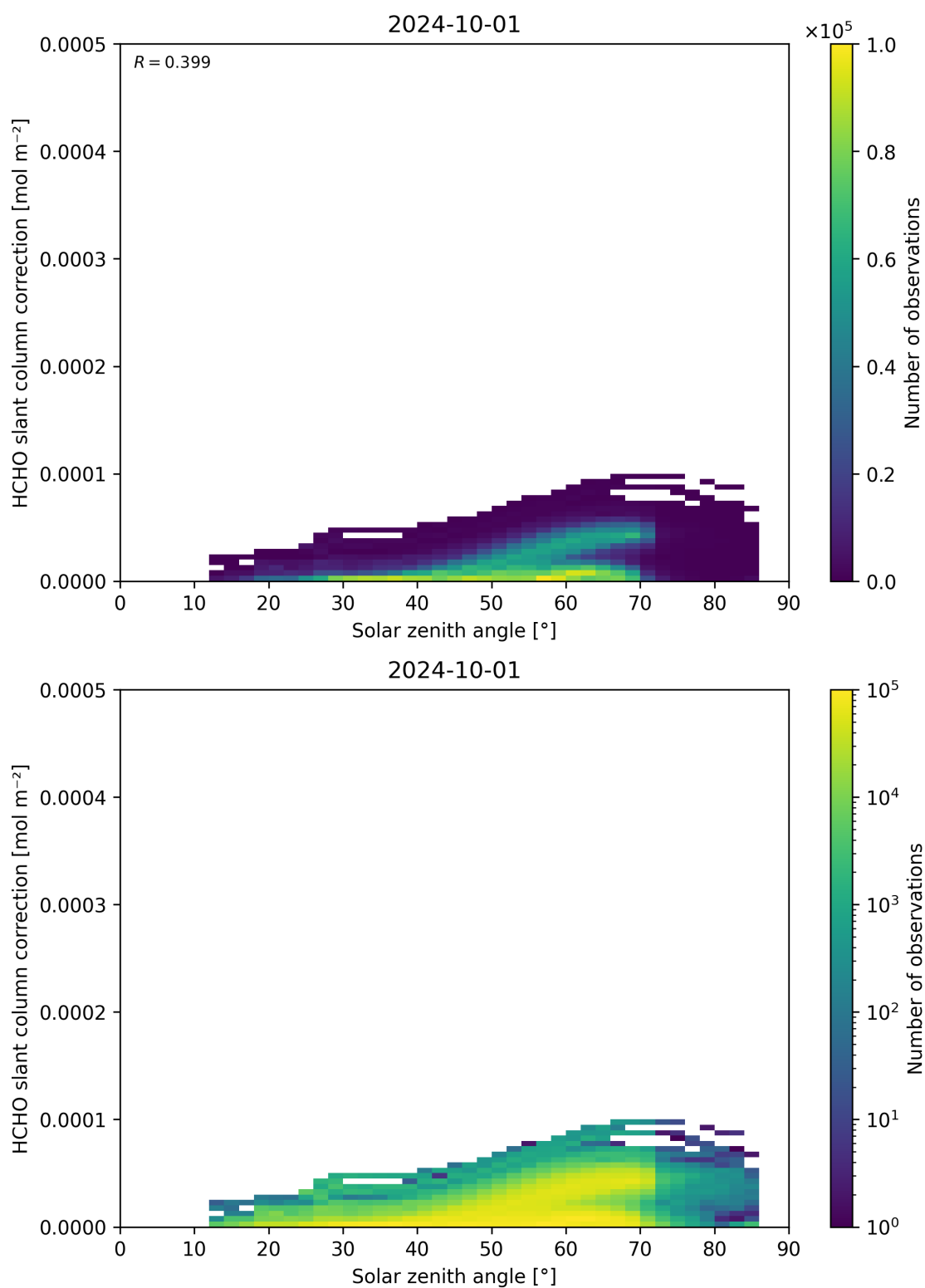
Figure 172: Scatter density plot of “Solar zenith angle” against “HCHO slant column correction” for 2024-09-30 to 2024-10-02.
