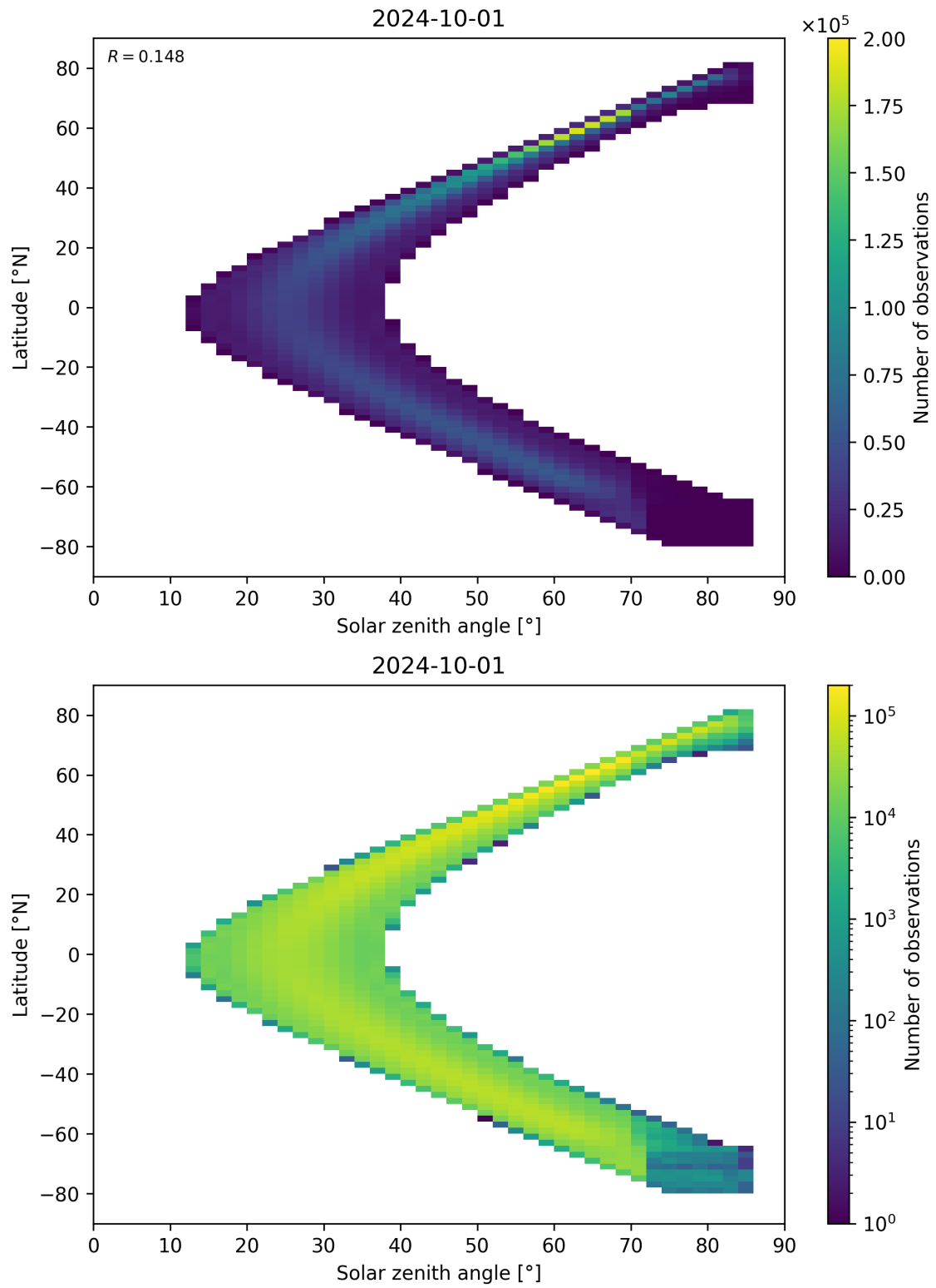
Figure 181: Scatter density plot of “Solar zenith angle” against “Latitude” for 2024-09-30 to 2024-10-02.
