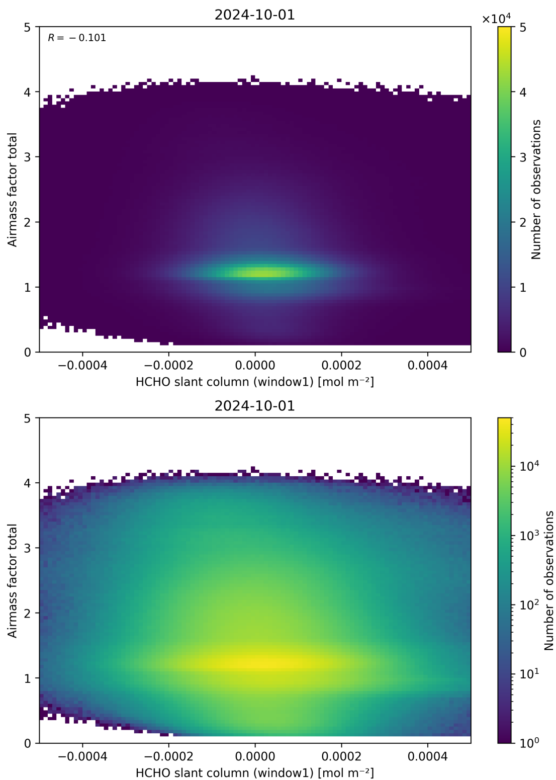
Figure 85: Scatter density plot of “HCHO slant column (window1)” against “Airmass factor total” for 2024-09-30 to 2024-10-02.
