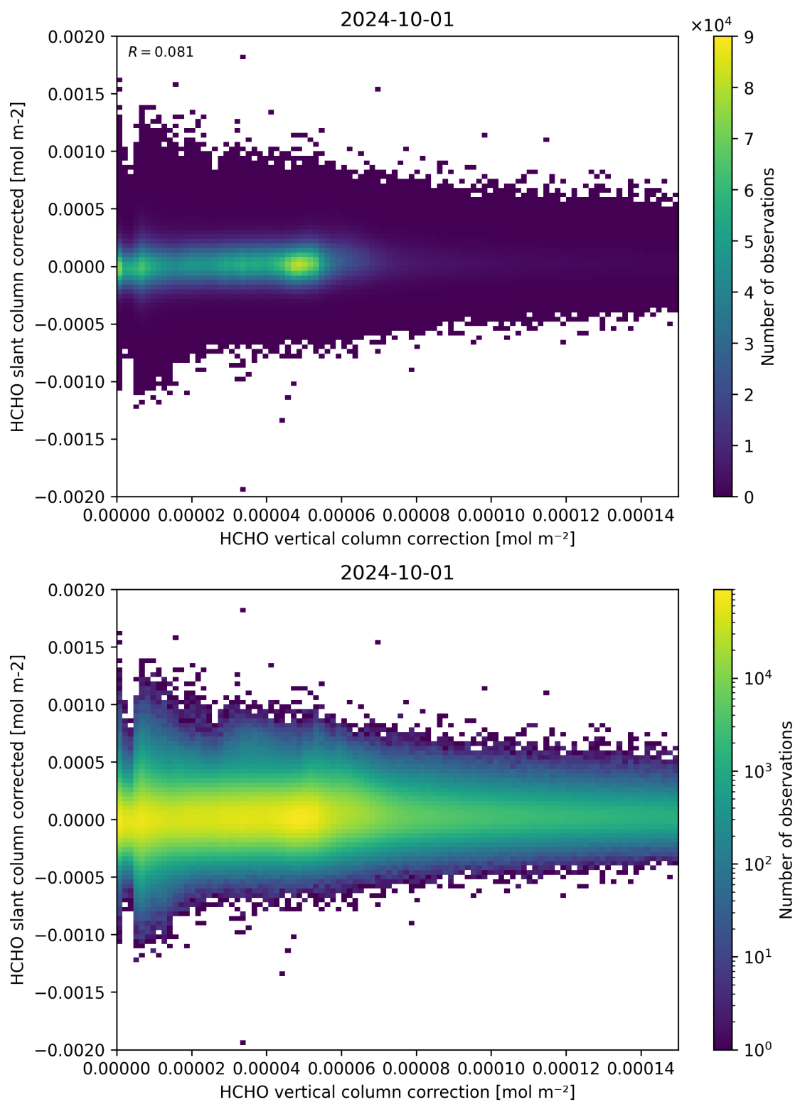
Figure 116: Scatter density plot of “HCHO vertical column correction” against “HCHO slant column corrected” for 2024-09-30 to 2024-10-02.
