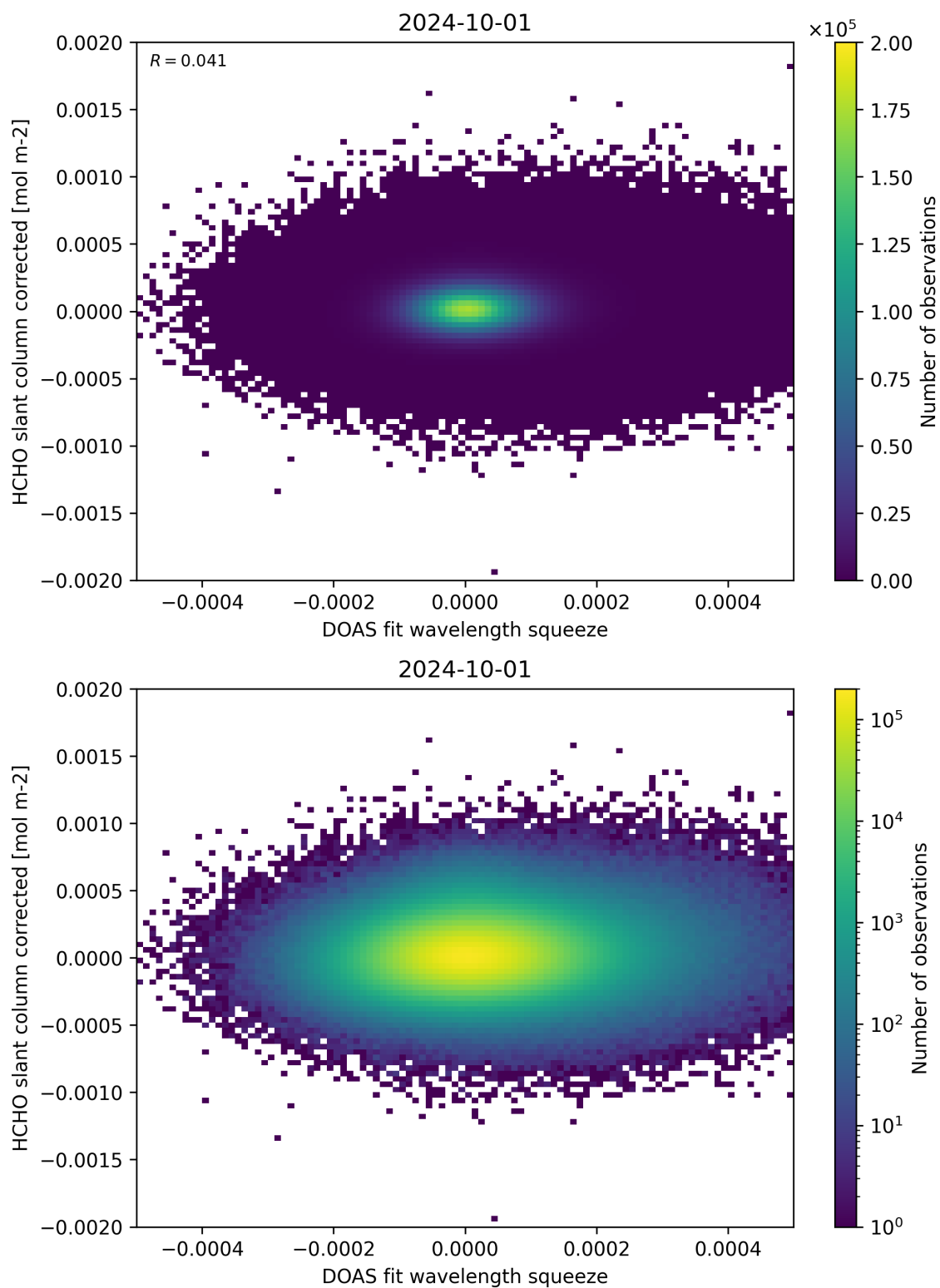
Figure 69: Scatter density plot of “DOAS fit wavelength squeeze” against “HCHO slant column corrected” for 2024-09-30 to 2024-10-02.
