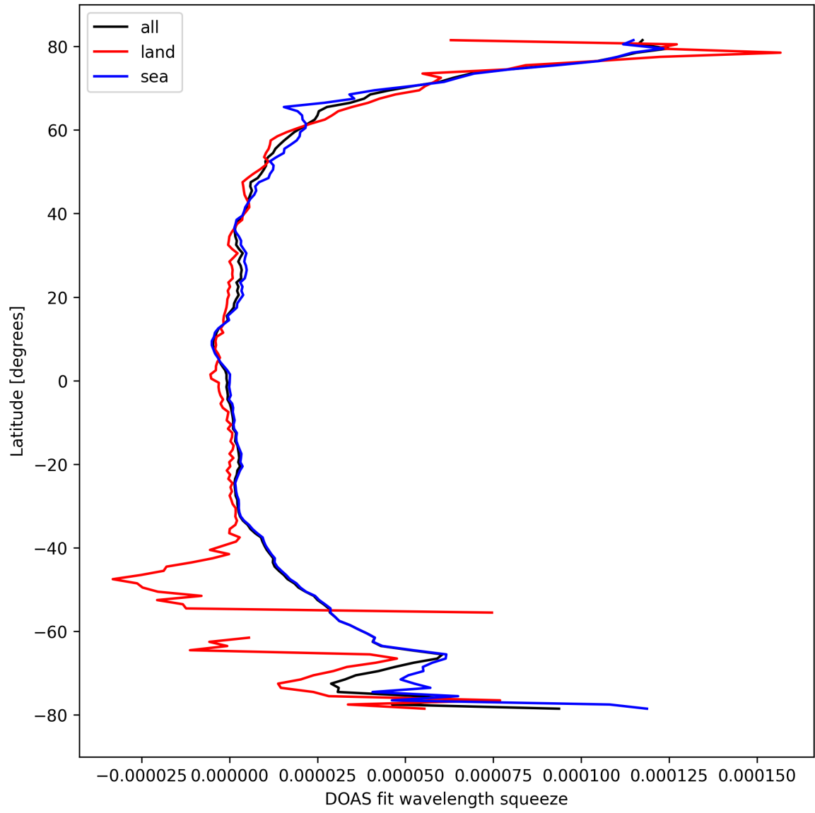
Figure 31: Zonal average of “DOAS fit wavelength squeeze” for 2024-09-30 to 2024-10-02.
