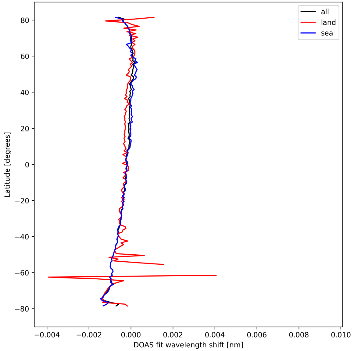
Figure 30: Zonal average of “DOAS fit wavelength shift” for 2024-09-30 to 2024-10-02.
