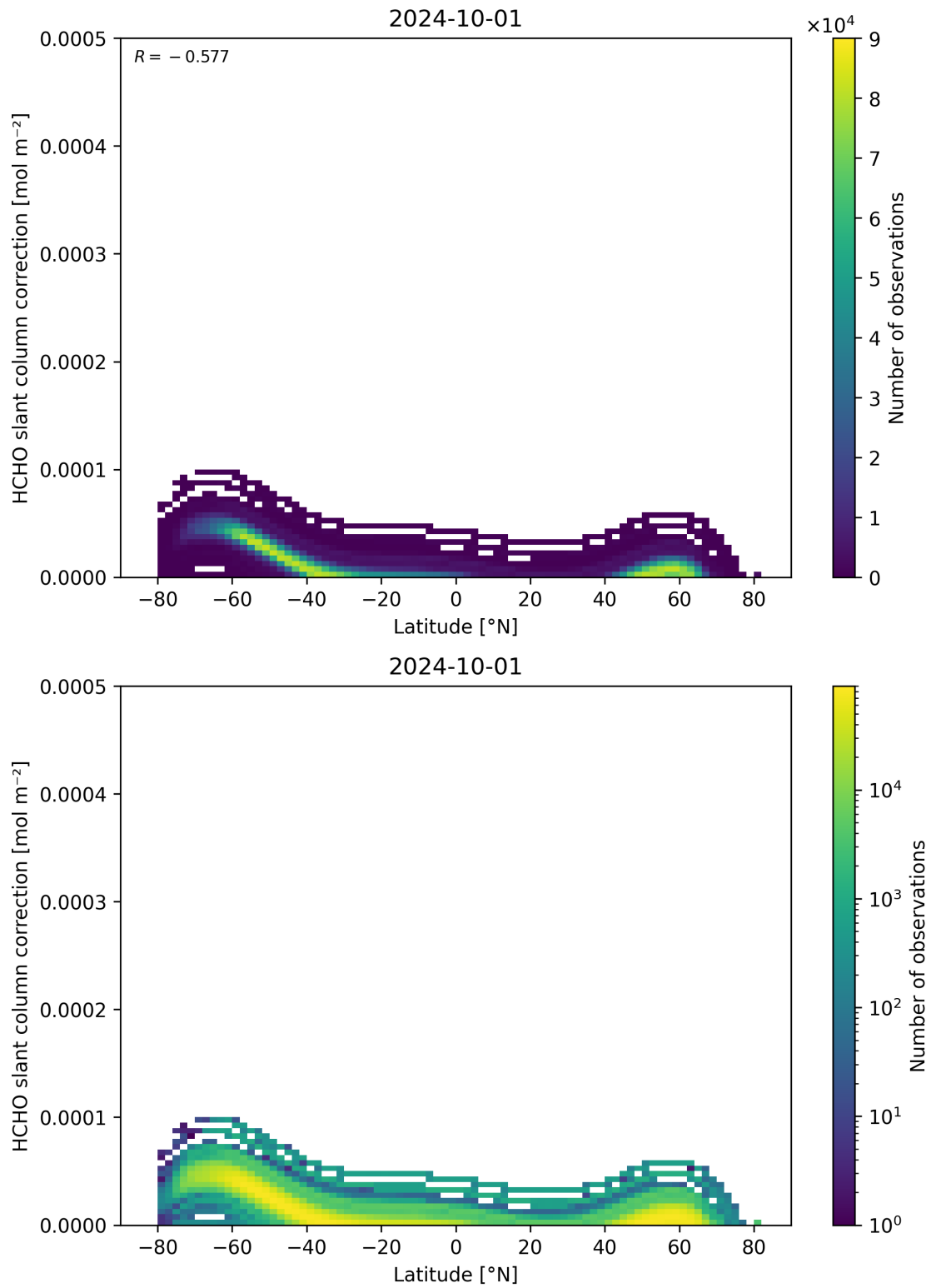
Figure 158: Scatter density plot of “Latitude” against “HCHO slant column correction” for 2024-09-30 to 2024-10-02.
