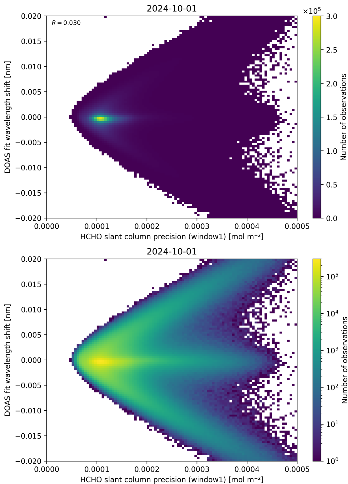
Figure 89: Scatter density plot of “HCHO slant column precision (window1)” against “DOAS fit wavelength shift” for 2024-09-30 to 2024-10-02.
