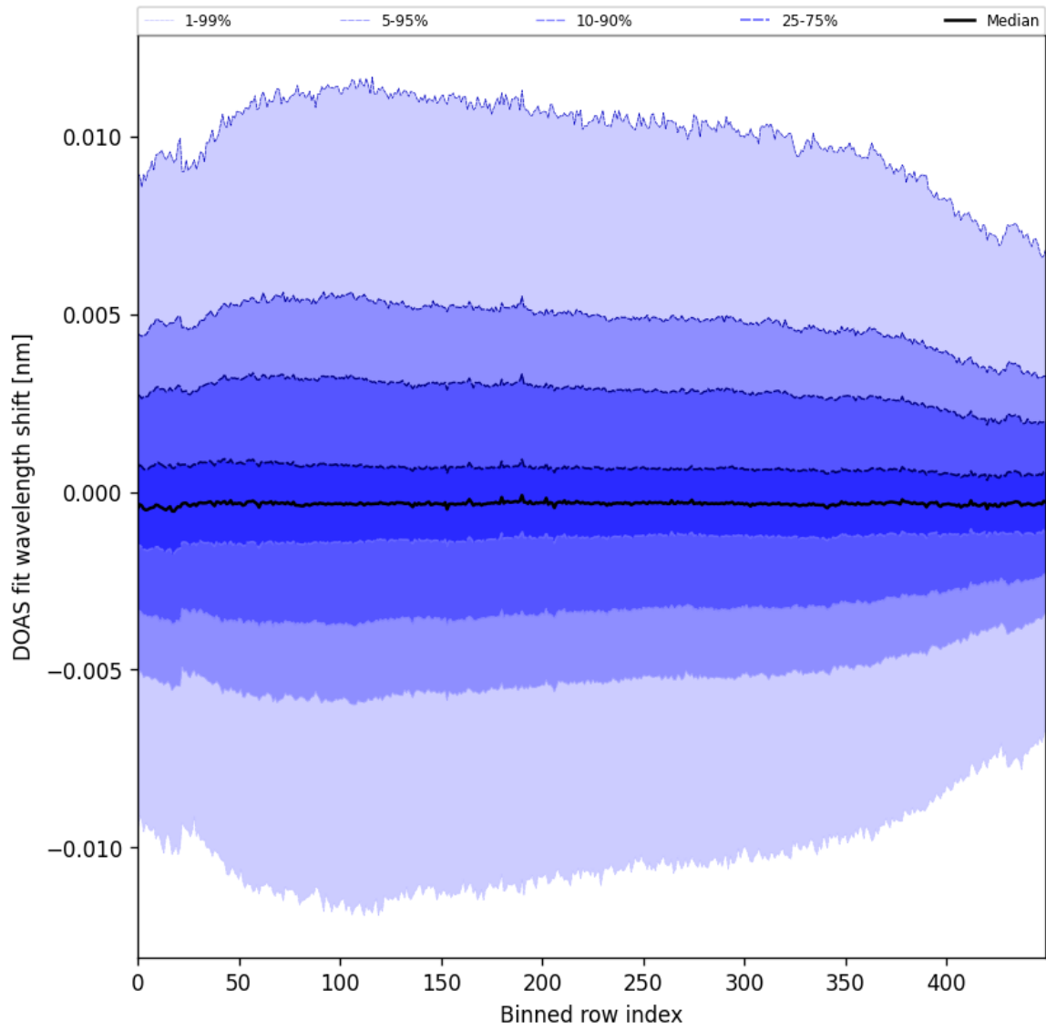
Figure 58: Along track statistics of “DOAS fit wavelength shift” for 2024-09-30 to 2024-10-02
