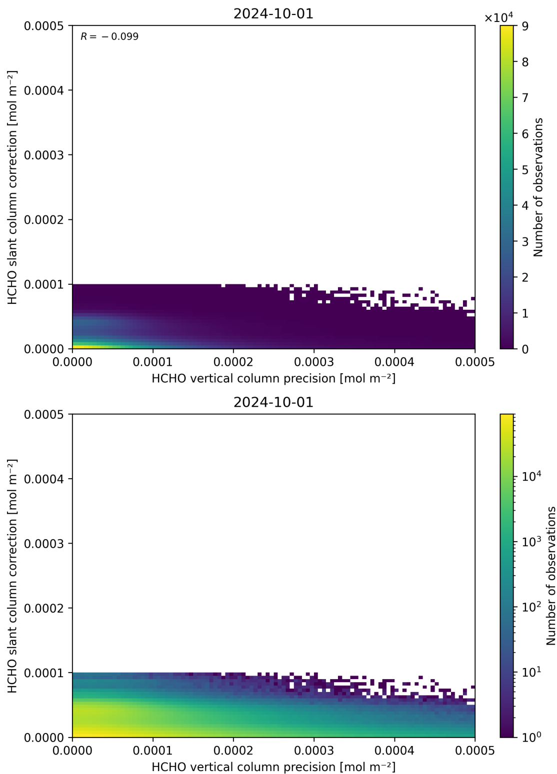
Figure 141: Scatter density plot of “HCHO vertical column precision” against “HCHO slant column correction” for 2024-09-30 to 2024-10-02.
