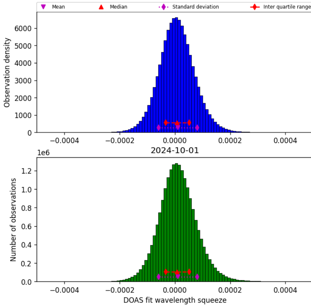
Figure 45: Histogram of “DOAS fit wavelength squeeze” for 2024-09-30 to 2024-10-02
