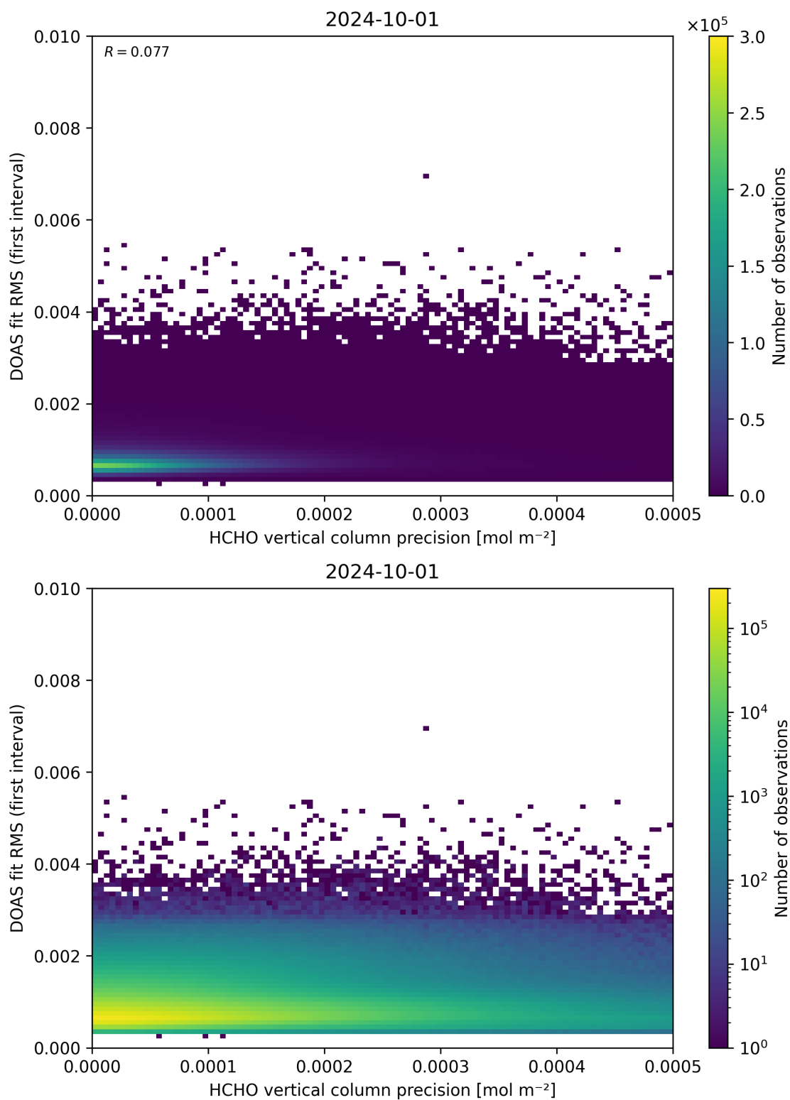
Figure 136: Scatter density plot of “HCHO vertical column precision” against “DOAS fit RMS (first interval)” for 2024-09-30 to 2024-10-02.
