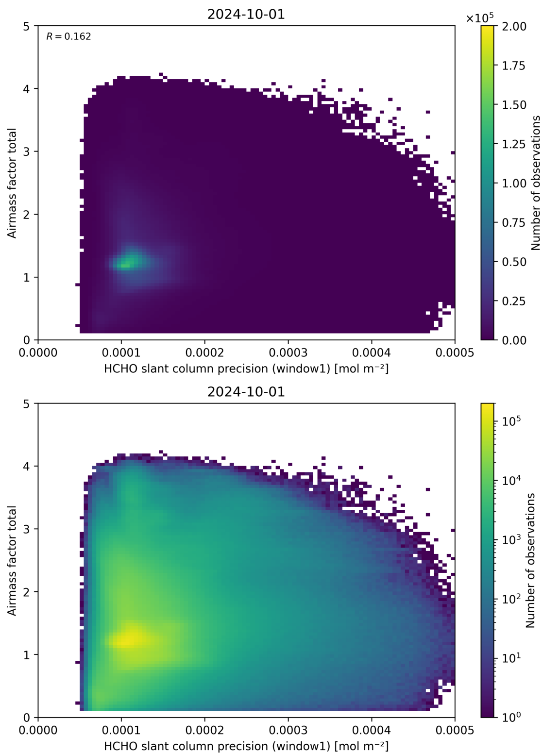
Figure 94: Scatter density plot of “HCHO slant column precision (window1)” against “Airmass factor total” for 2024-09-30 to 2024-10-02.
