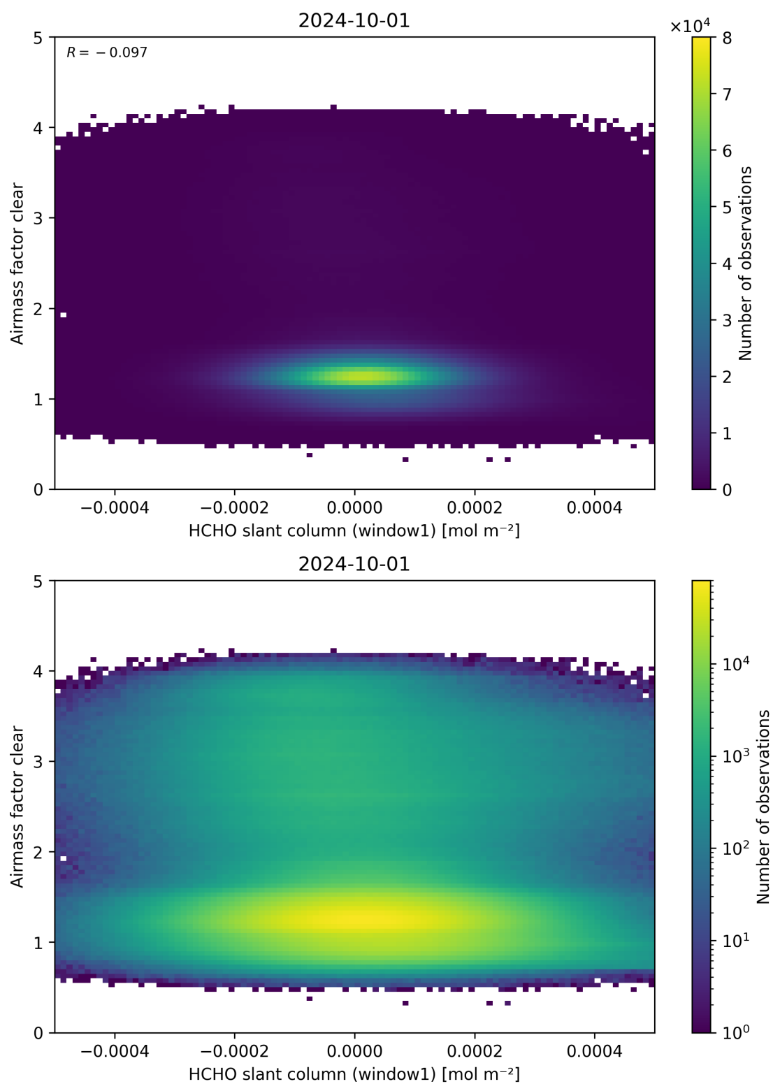
Figure 81: Scatter density plot of “HCHO slant column (window1)” against “Airmass factor clear” for 2024-09-30 to 2024-10-02.
