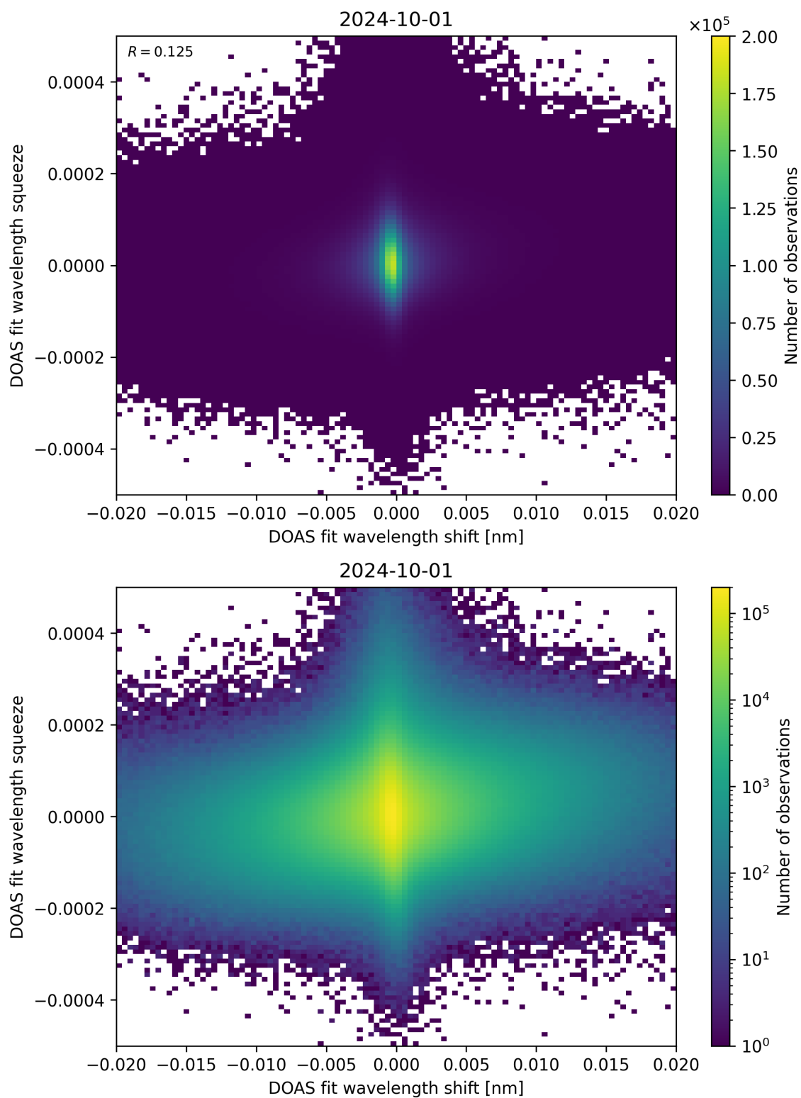
Figure 65: Scatter density plot of “DOAS fit wavelength shift” against “DOAS fit wavelength squeeze” for 2024-09-30 to 2024-10-02.
