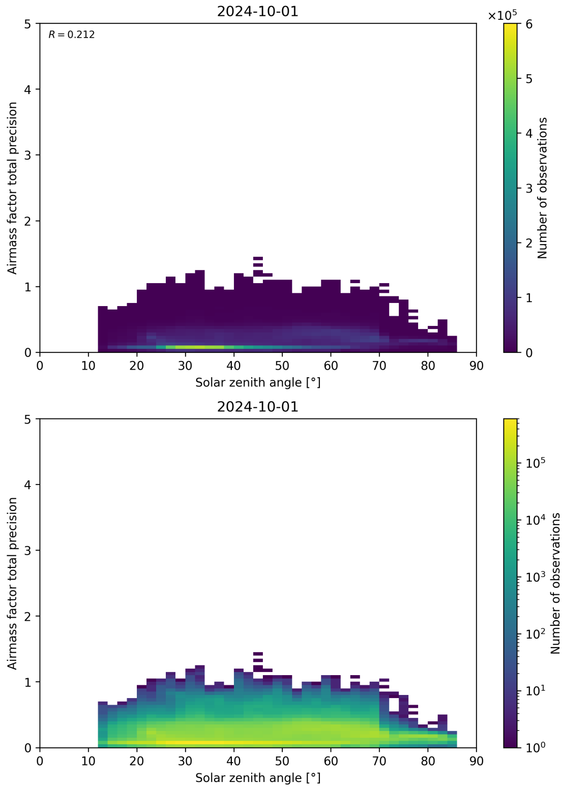
Figure 176: Scatter density plot of “Solar zenith angle” against “Airmass factor total precision” for 2024-09-30 to 2024-10-02.
