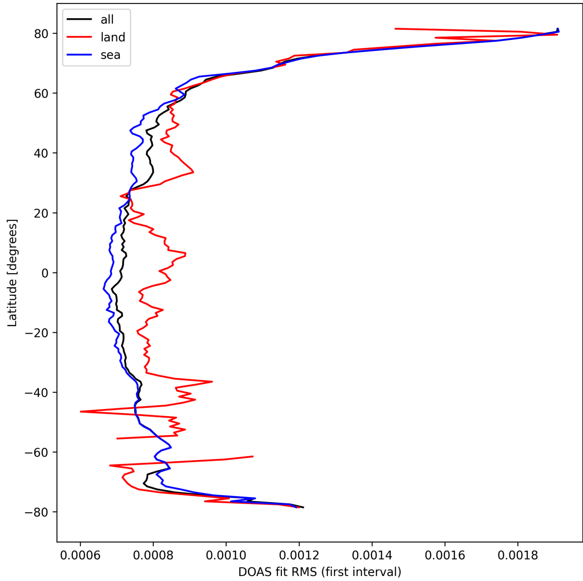
Figure 32: Zonal average of “DOAS fit RMS (first interval)” for 2024-09-30 to 2024-10-02.
