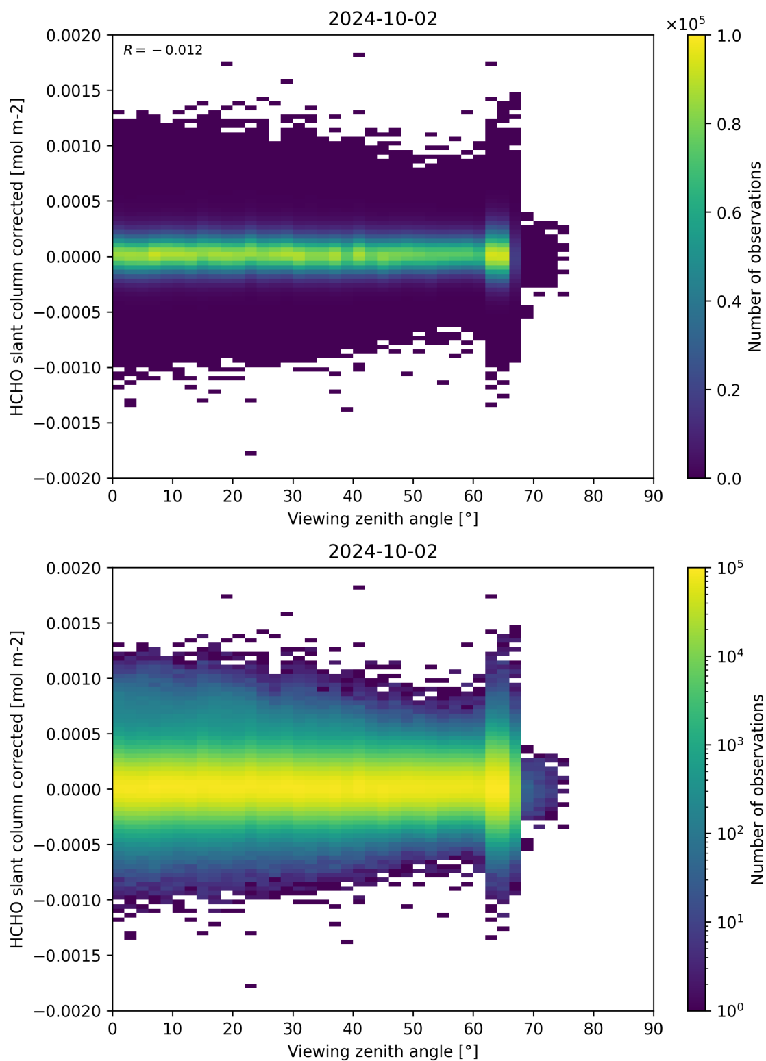
Figure 186: Scatter density plot of “Viewing zenith angle” against “HCHO slant column corrected” for 2024-10-01 to 2024-10-03.
