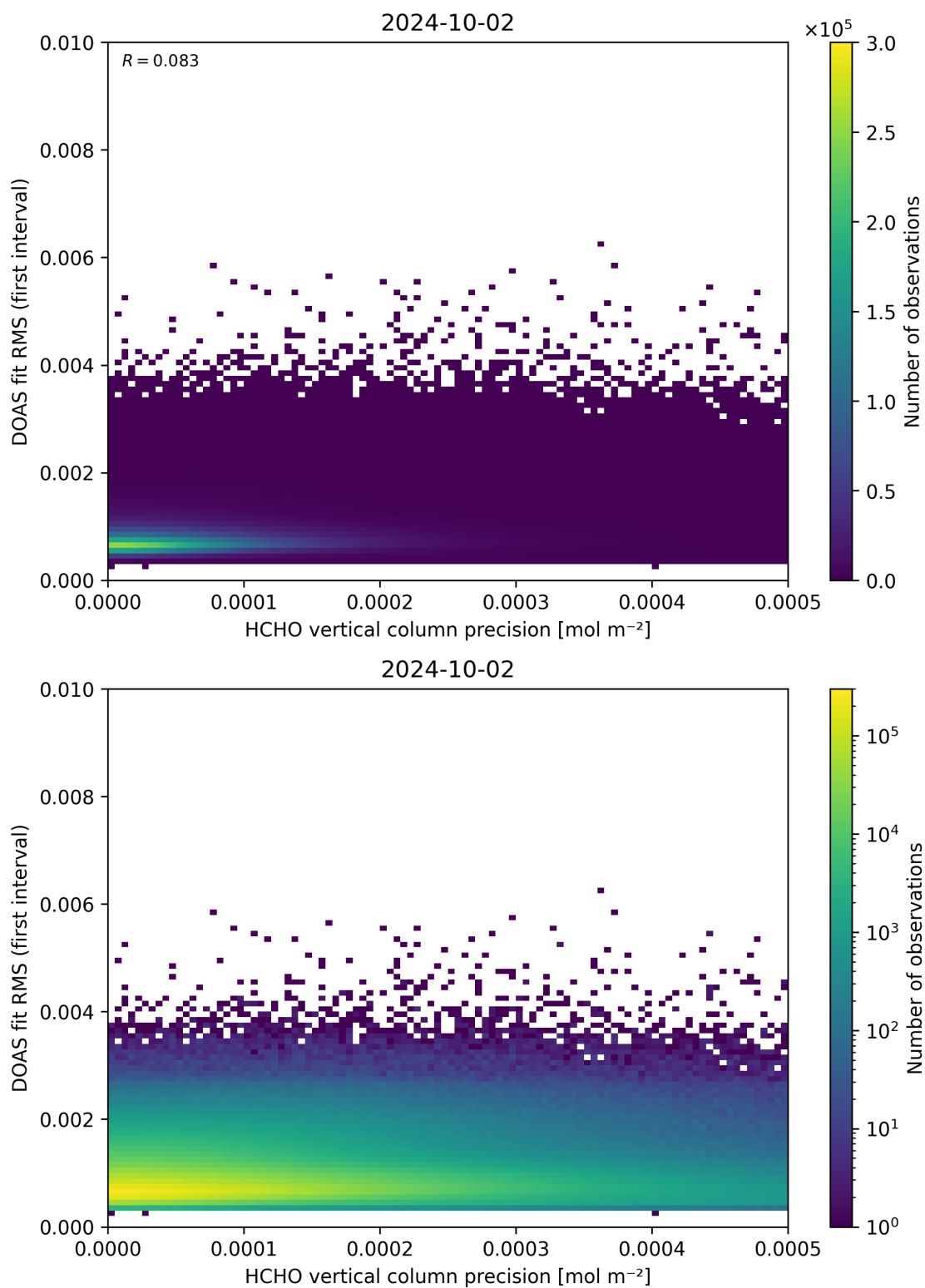
Figure 136: Scatter density plot of “HCHO vertical column precision” against “DOAS fit RMS (first interval)” for 2024-10-01 to 2024-10-03.
