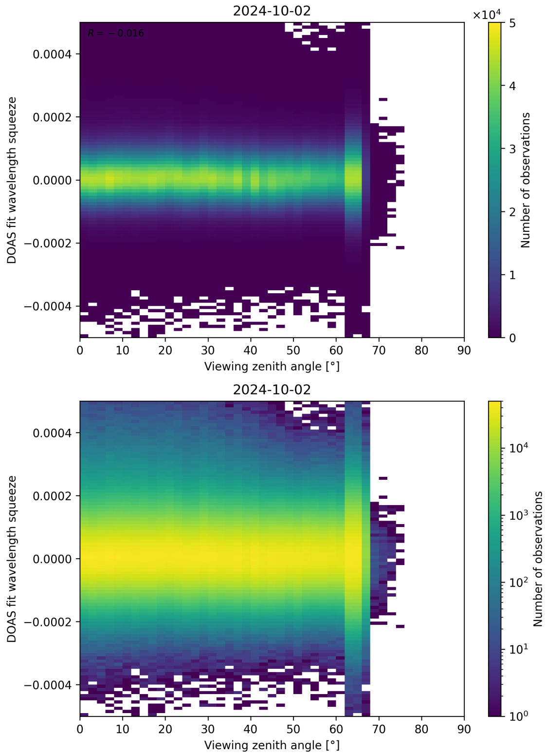
Figure 184: Scatter density plot of “Viewing zenith angle” against “DOAS fit wavelength squeeze” for 2024-10-01 to 2024-10-03.
