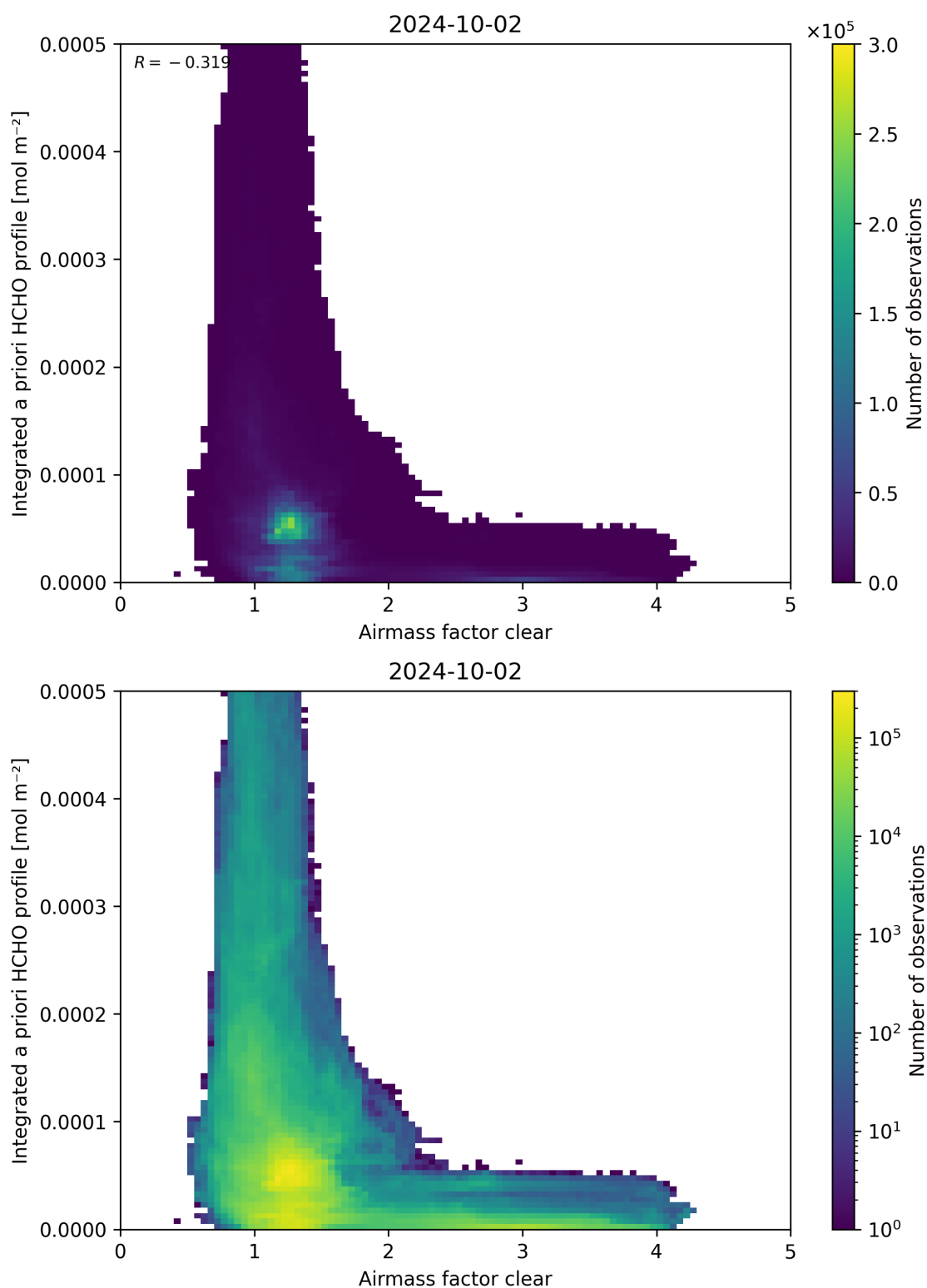
Figure 76: Scatter density plot of “Airmass factor clear” against “Integrated a priori HCHO profile” for 2024-10-01 to 2024-10-03.
