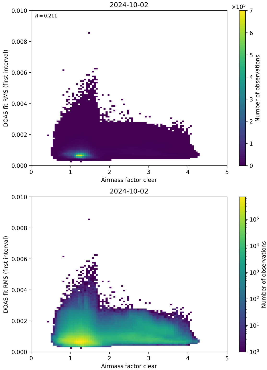
Figure 71: Scatter density plot of “Airmass factor clear” against “DOAS fit RMS (first interval)” for 2024-10-01 to 2024-10-03.
