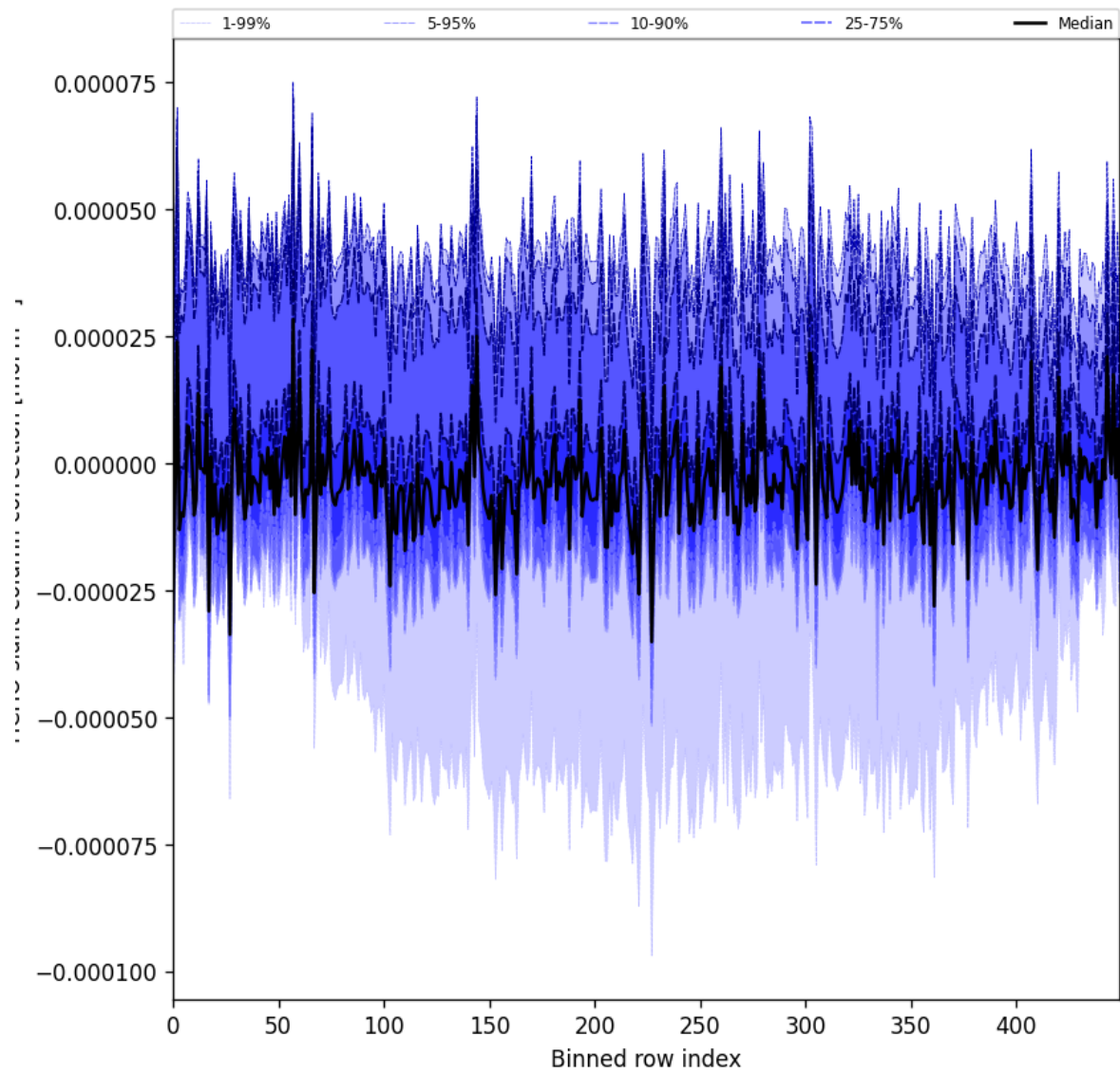
Figure 61: Along track statistics of “HCHO slant column correction” for 2024-10-01 to 2024-10-03
