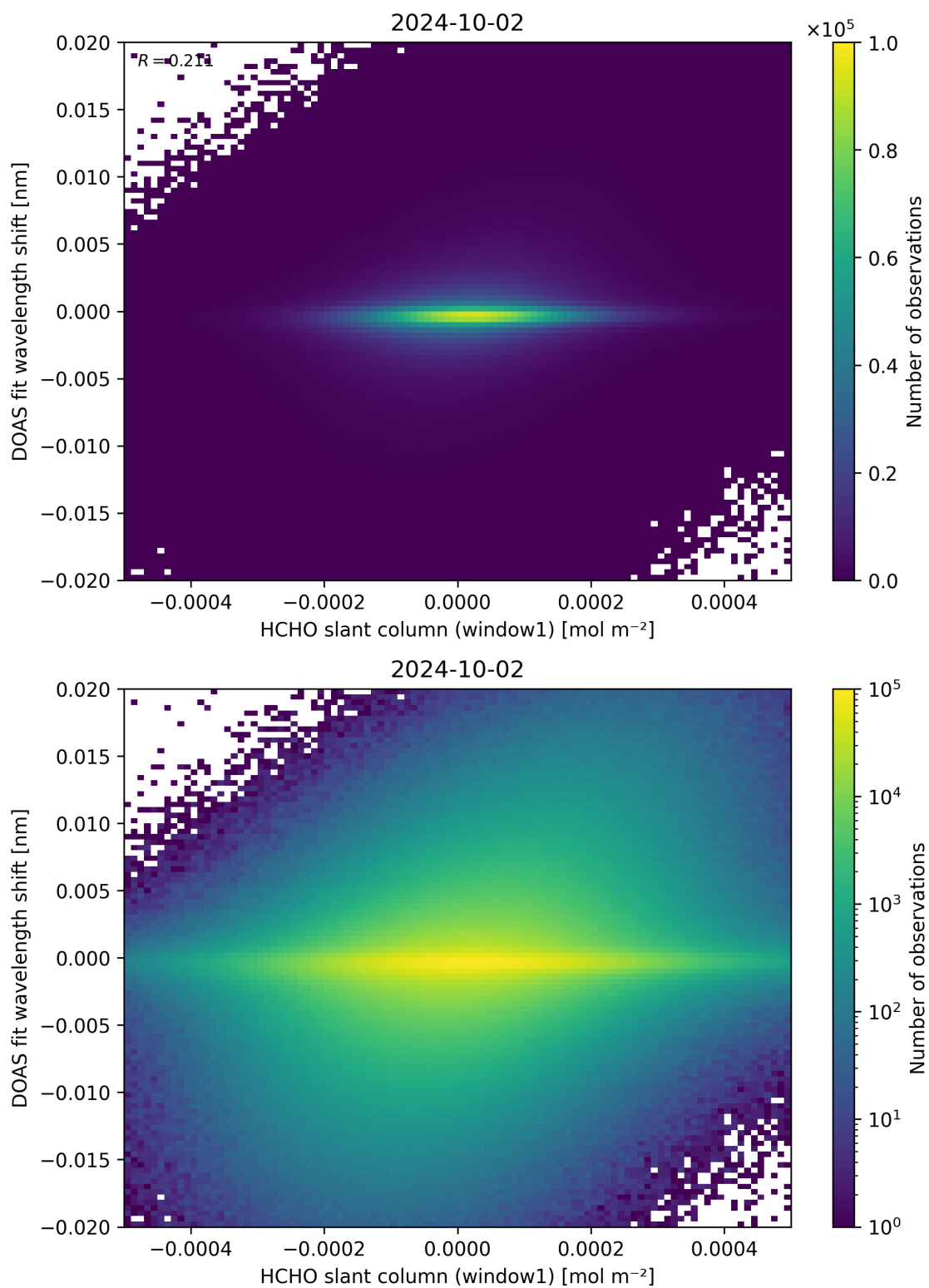
Figure 79: Scatter density plot of “HCHO slant column (window1)” against “DOAS fit wavelength shift” for 2024-10-01 to 2024-10-03.
