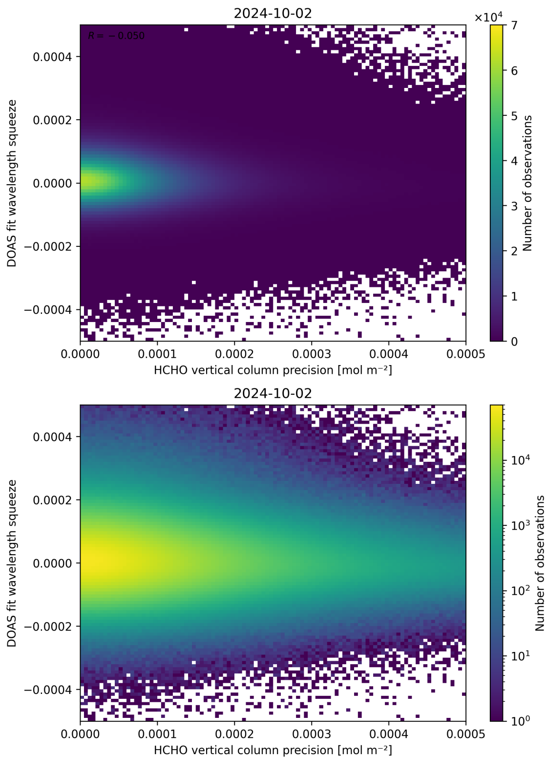
Figure 138: Scatter density plot of “HCHO vertical column precision” against “DOAS fit wavelength squeeze” for 2024-10-01 to 2024-10-03.
