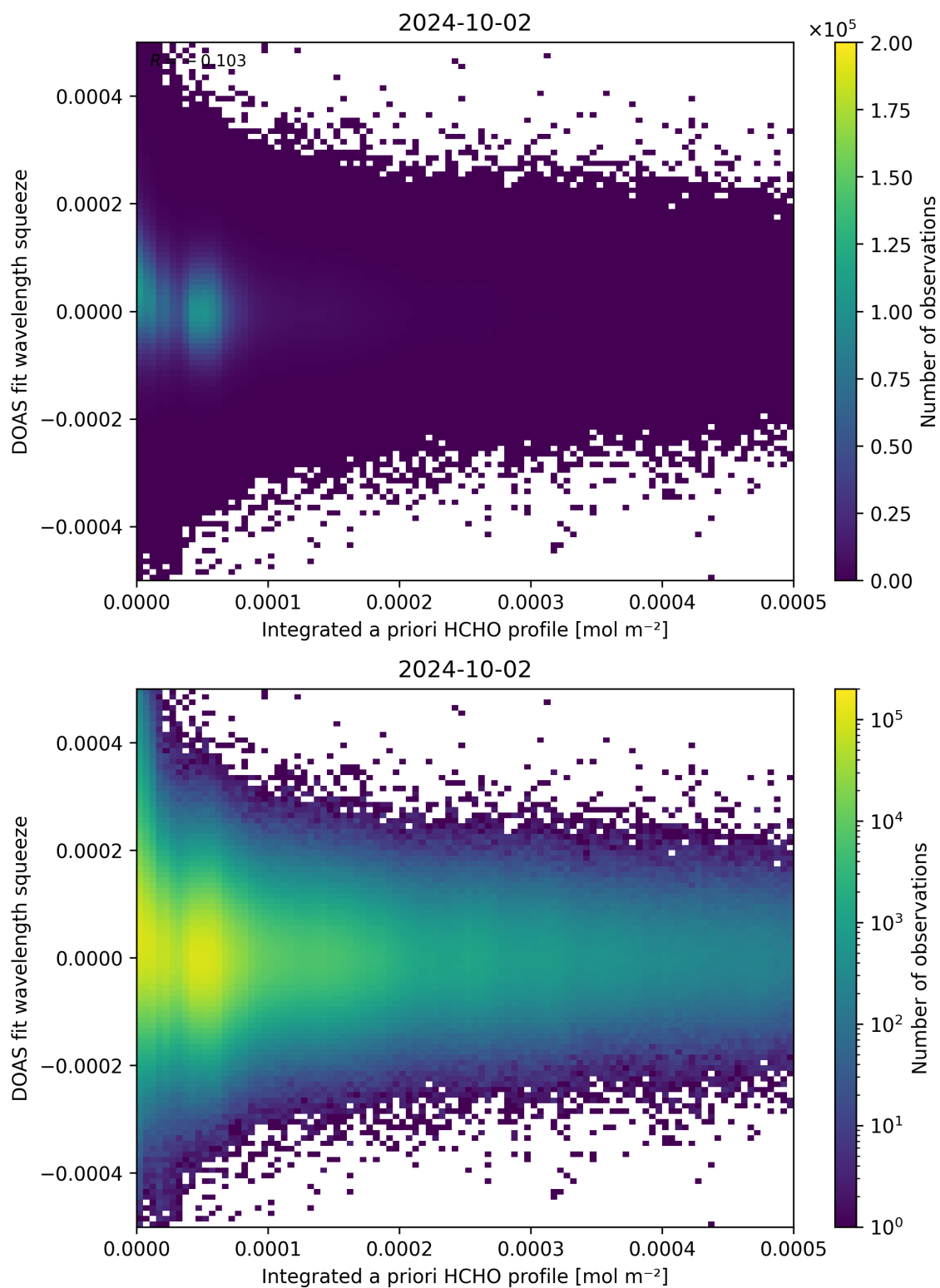
Figure 150: Scatter density plot of “Integrated a priori HCHO profile” against “DOAS fit wavelength squeeze” for 2024-10-01 to 2024-10-03.
