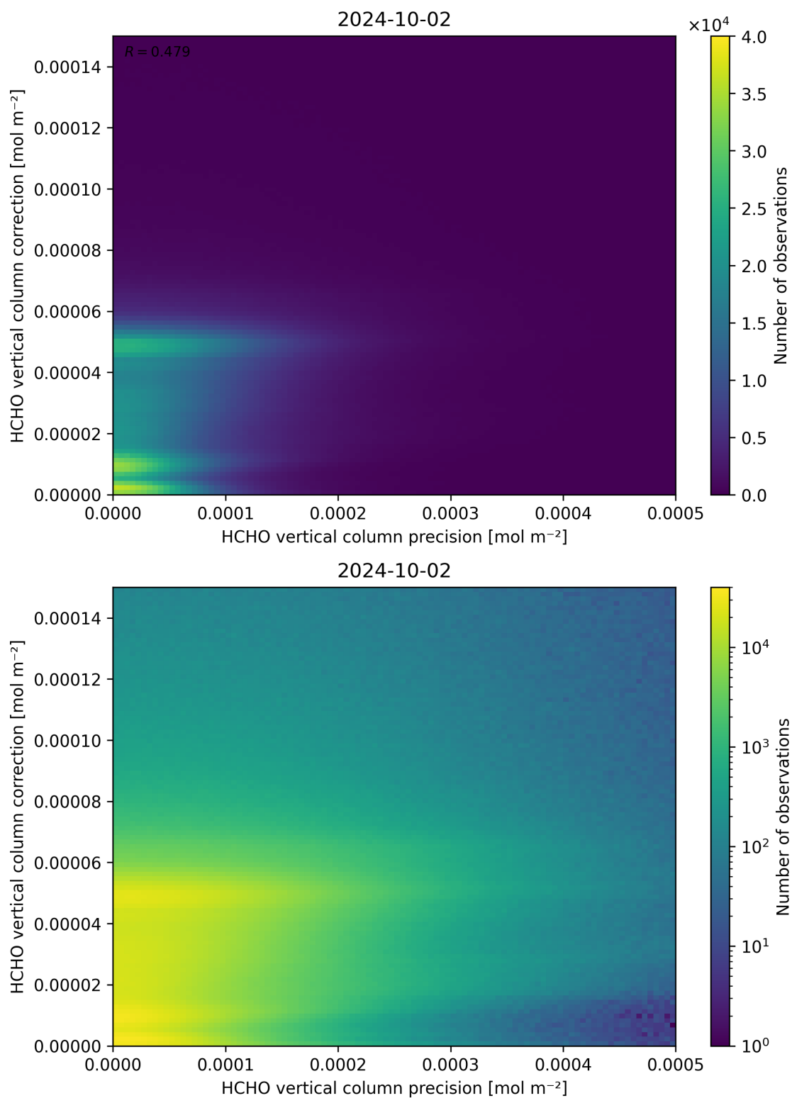
Figure 146: Scatter density plot of “HCHO vertical column precision” against “HCHO vertical column correction” for 2024-10-01 to 2024-10-03.
