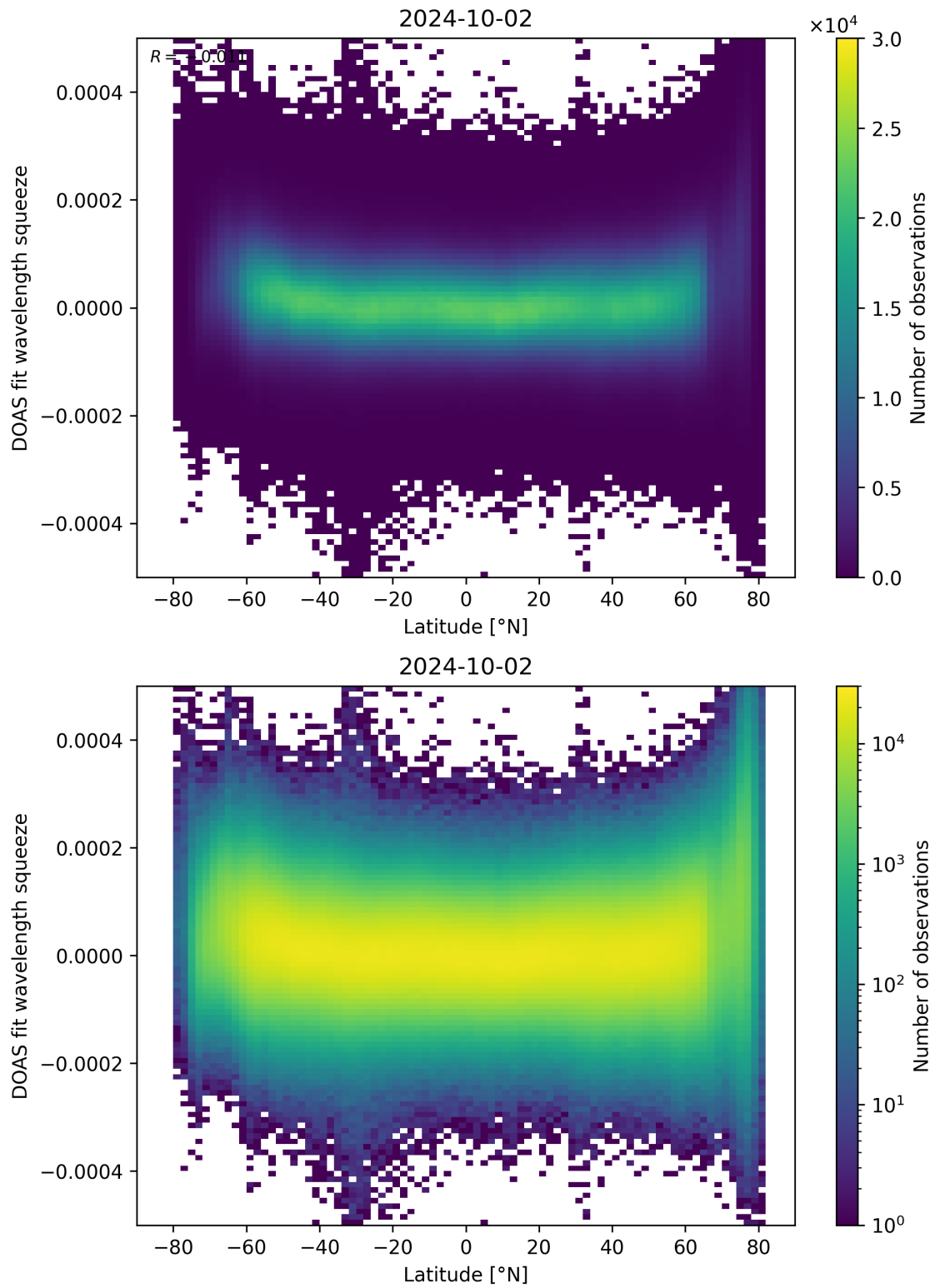
Figure 155: Scatter density plot of “Latitude” against “DOAS fit wavelength squeeze” for 2024-10-01 to 2024-10-03.
