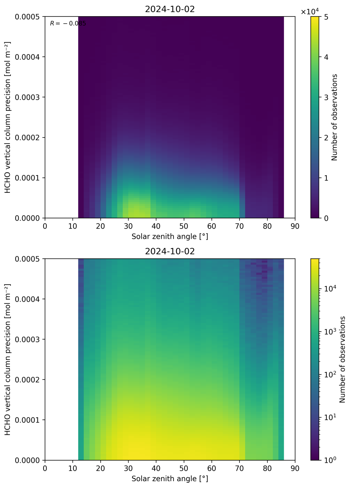
Figure 179: Scatter density plot of “Solar zenith angle” against “HCHO vertical column precision” for 2024-10-01 to 2024-10-03.
