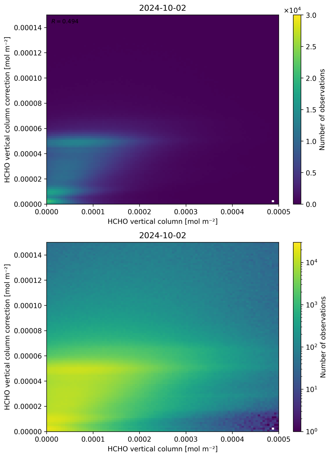
Figure 133: Scatter density plot of “HCHO vertical column” against “HCHO vertical column correction” for 2024-10-01 to 2024-10-03.
