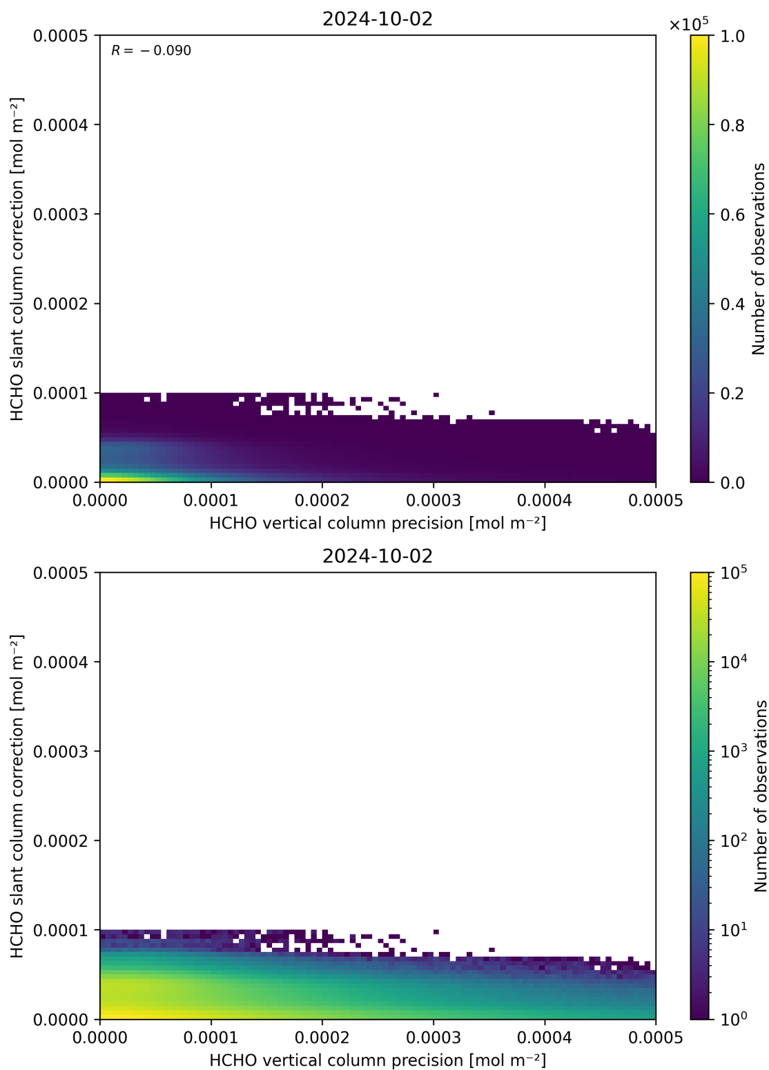
Figure 141: Scatter density plot of “HCHO vertical column precision” against “HCHO slant column correction” for 2024-10-01 to 2024-10-03.
