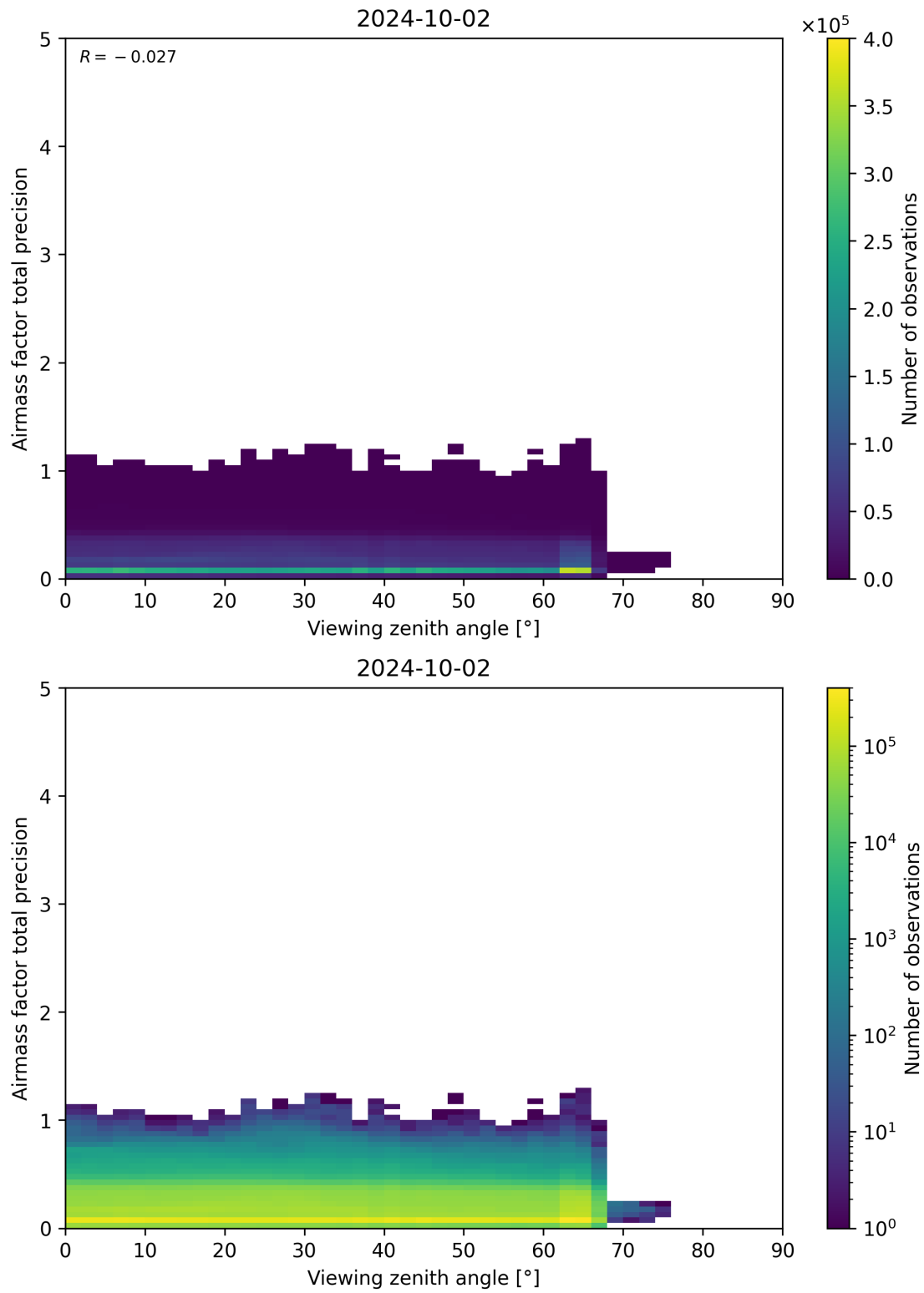
Figure 191: Scatter density plot of “Viewing zenith angle” against “Airmass factor total precision” for 2024-10-01 to 2024-10-03.
