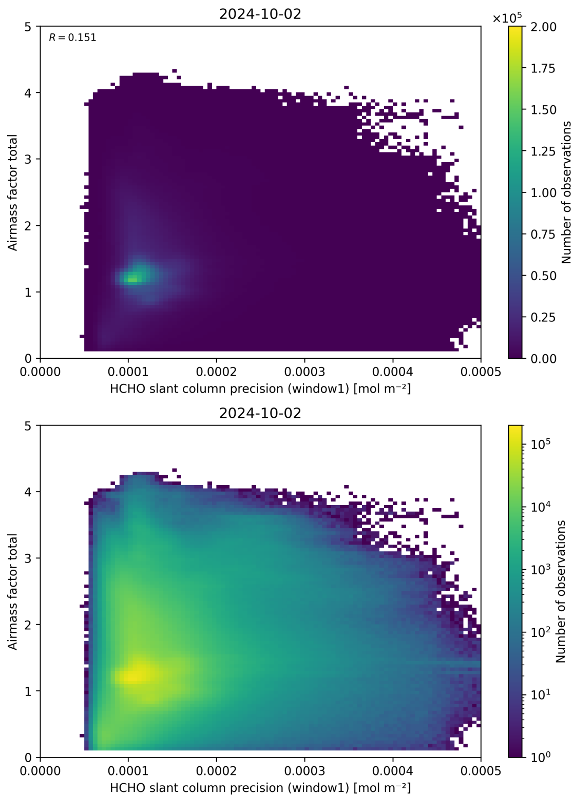
Figure 94: Scatter density plot of “HCHO slant column precision (window1)” against “Airmass factor total” for 2024-10-01 to 2024-10-03.
