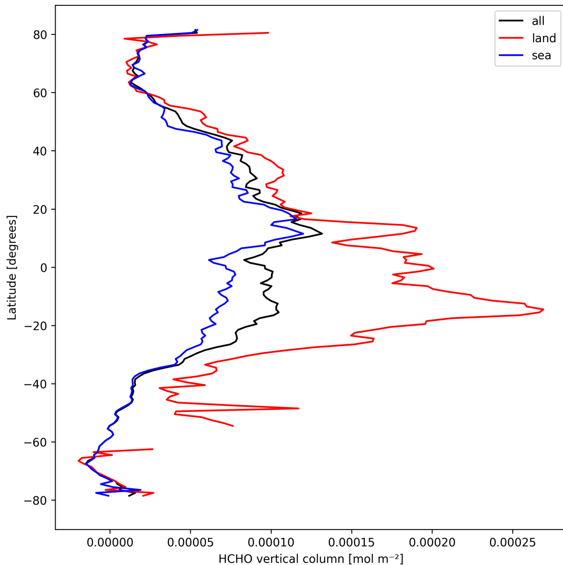
Figure 21: Zonal average of “HCHO vertical column” for 2024-10-01 to 2024-10-03.
