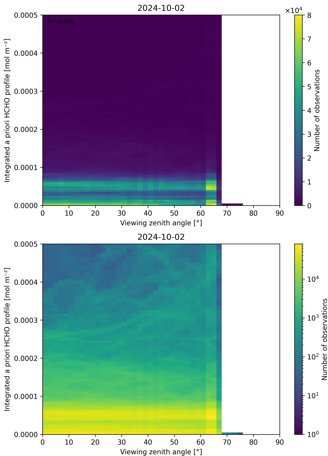
Figure 195: Scatter density plot of “Viewing zenith angle” against “Integrated a priori HCHO profile” for 2024-10-01 to 2024-10-03.
