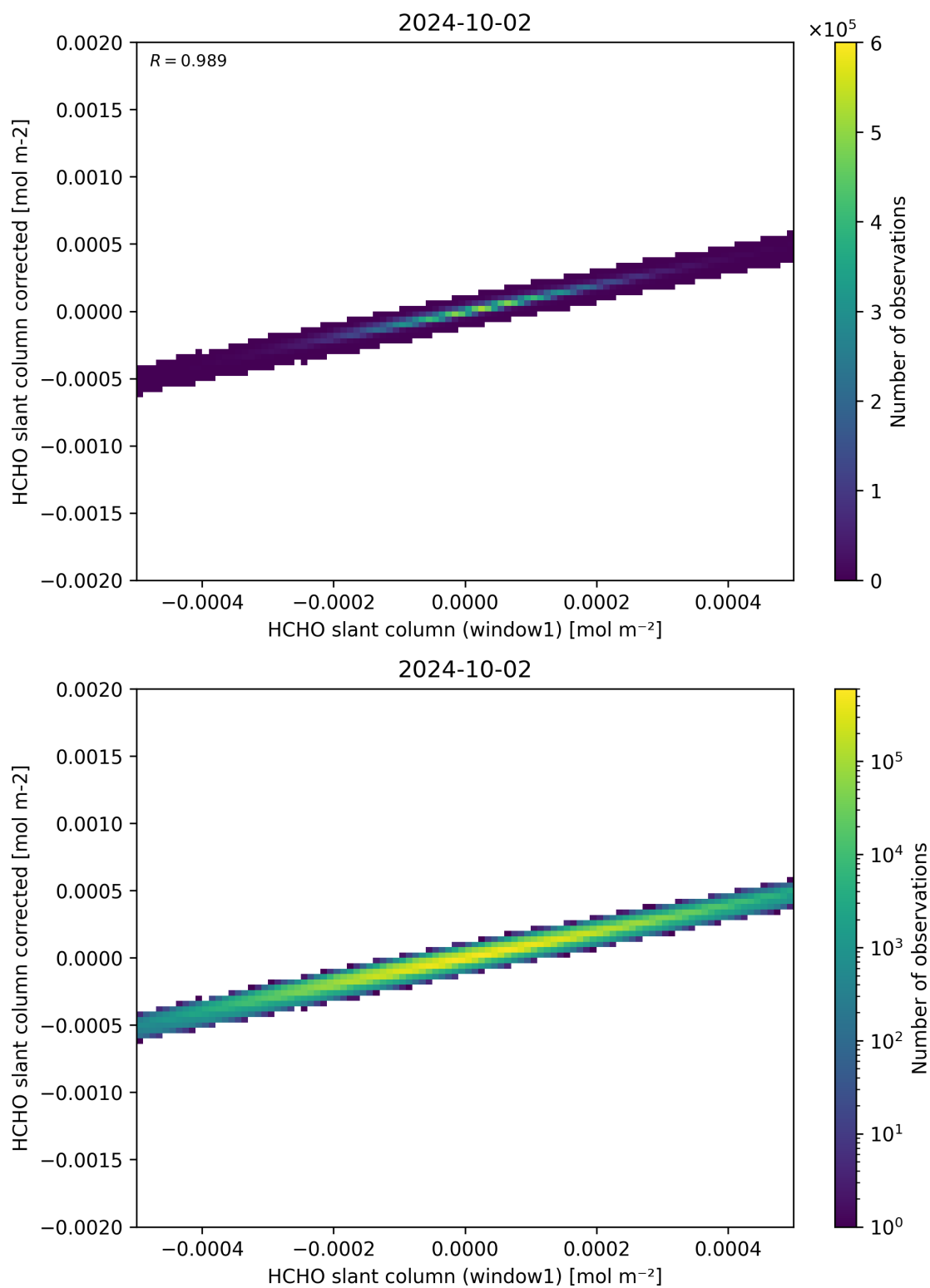
Figure 82: Scatter density plot of “HCHO slant column (window1)” against “HCHO slant column corrected” for 2024-10-01 to 2024-10-03.
