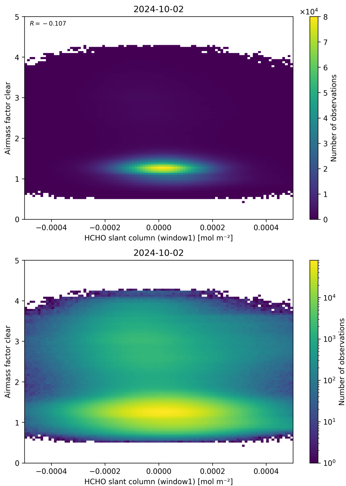
Figure 81: Scatter density plot of “HCHO slant column (window1)” against “Airmass factor clear” for 2024-10-01 to 2024-10-03.
