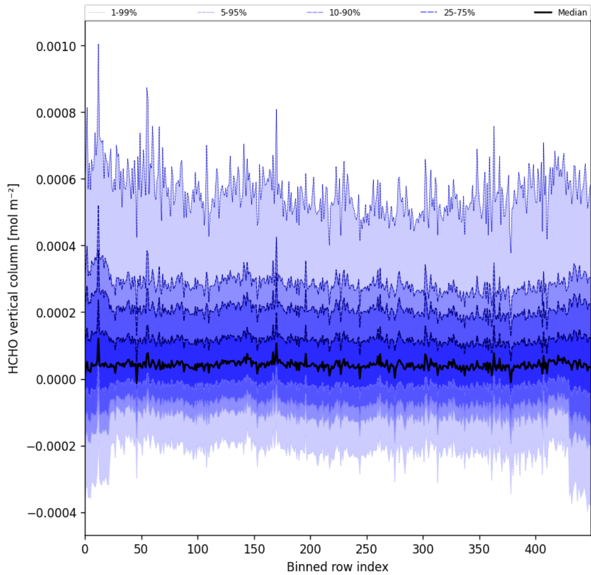
Figure 49: Along track statistics of “HCHO vertical column” for 2024-10-01 to 2024-10-03
