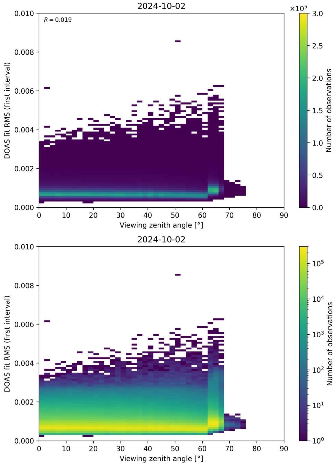
Figure 182: Scatter density plot of “Viewing zenith angle” against “DOAS fit RMS (first interval)” for 2024-10-01 to 2024-10-03.
