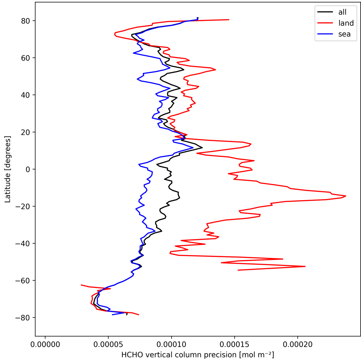
Figure 22: Zonal average of “HCHO vertical column precision” for 2024-10-01 to 2024-10-03.
