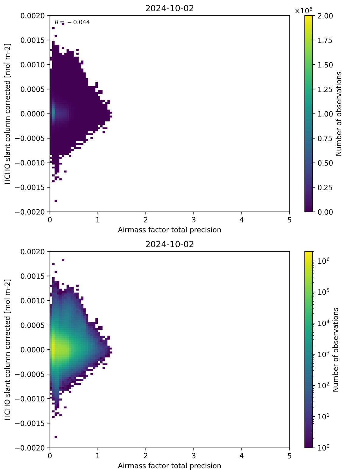
Figure 109: Scatter density plot of “Airmass factor total precision” against “HCHO slant column corrected” for 2024-10-01 to 2024-10-03.
