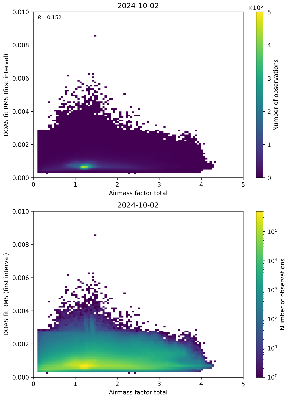
Figure 97: Scatter density plot of “Airmass factor total” against “DOAS fit RMS (first interval)” for 2024-10-01 to 2024-10-03.
