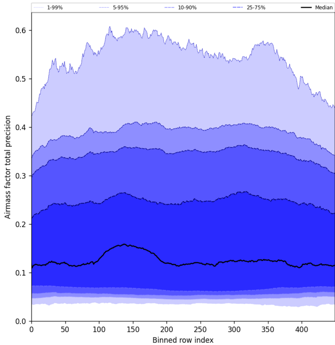
Figure 55: Along track statistics of “Airmass factor total precision” for 2024-10-01 to 2024-10-03
