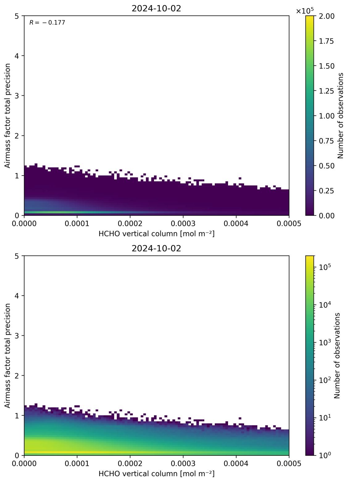
Figure 132: Scatter density plot of “HCHO vertical column” against “Airmass factor total precision” for 2024-10-01 to 2024-10-03.
