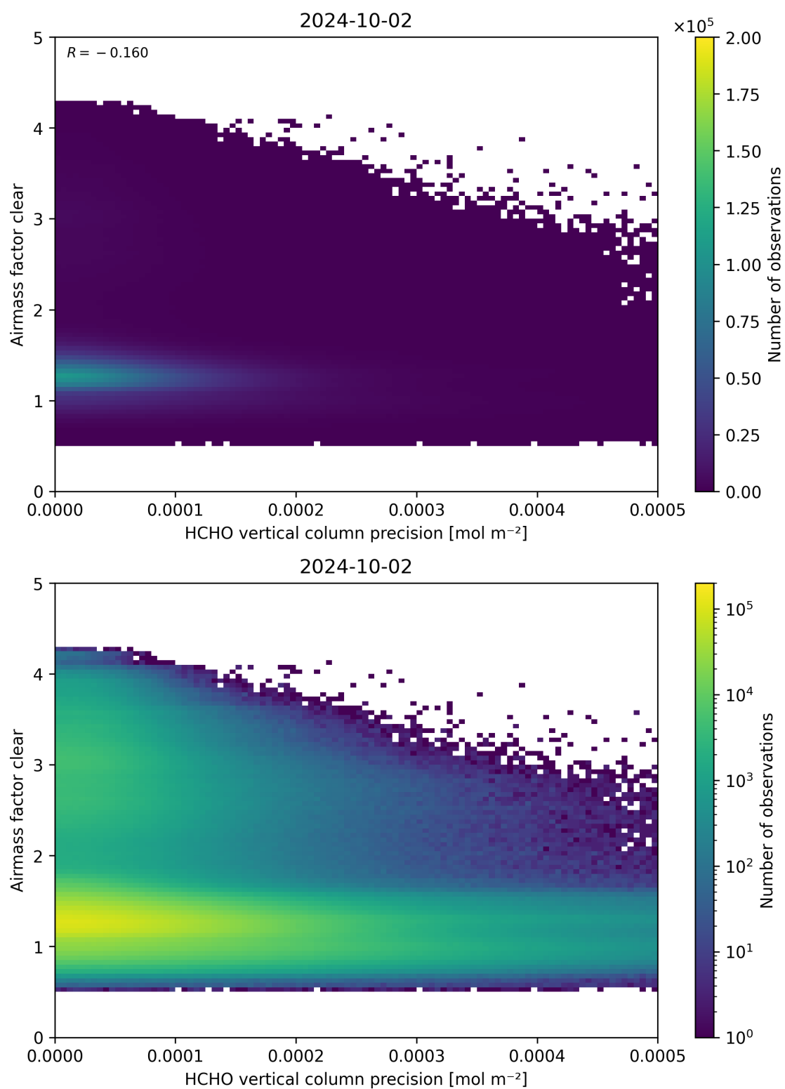
Figure 139: Scatter density plot of “HCHO vertical column precision” against “Airmass factor clear” for 2024-10-01 to 2024-10-03.
