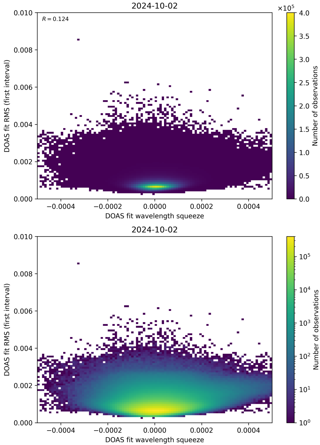
Figure 68: Scatter density plot of “DOAS fit wavelength squeeze” against “DOAS fit RMS (first interval)” for 2024-10-01 to 2024-10-03.
