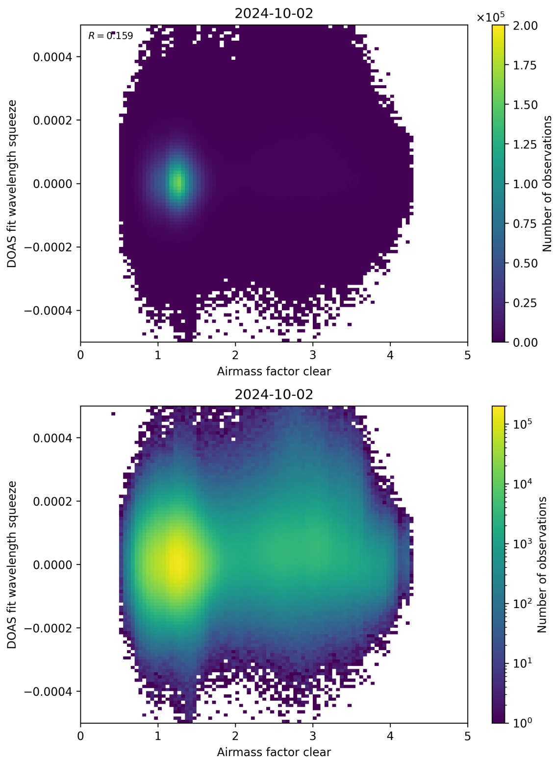
Figure 73: Scatter density plot of “Airmass factor clear” against “DOAS fit wavelength squeeze” for 2024-10-01 to 2024-10-03.
