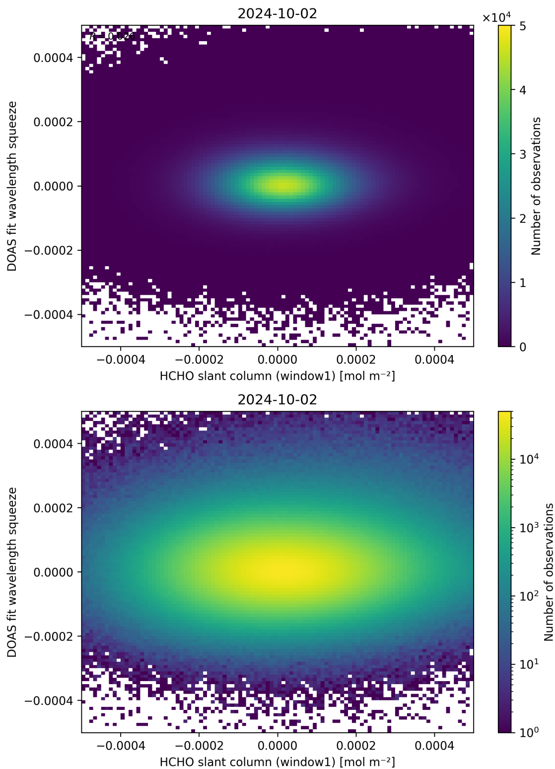
Figure 80: Scatter density plot of “HCHO slant column (window1)” against “DOAS fit wavelength squeeze” for 2024-10-01 to 2024-10-03.
