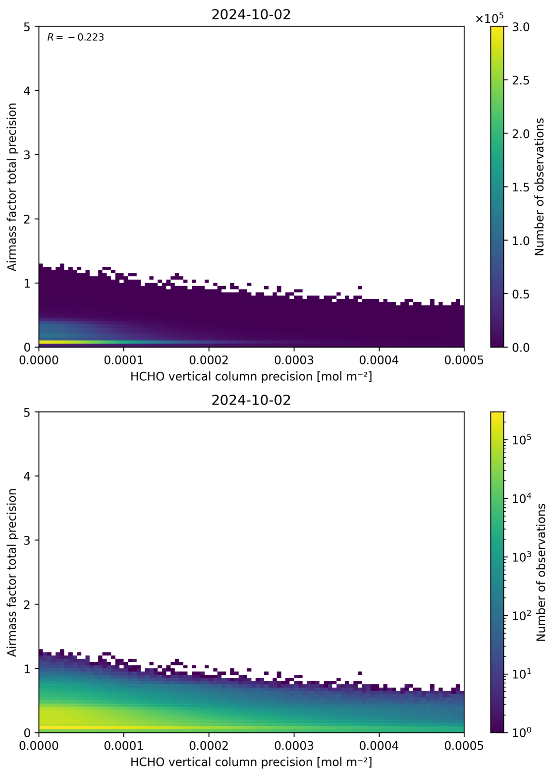
Figure 145: Scatter density plot of “HCHO vertical column precision” against “Airmass factor total precision” for 2024-10-01 to 2024-10-03.
