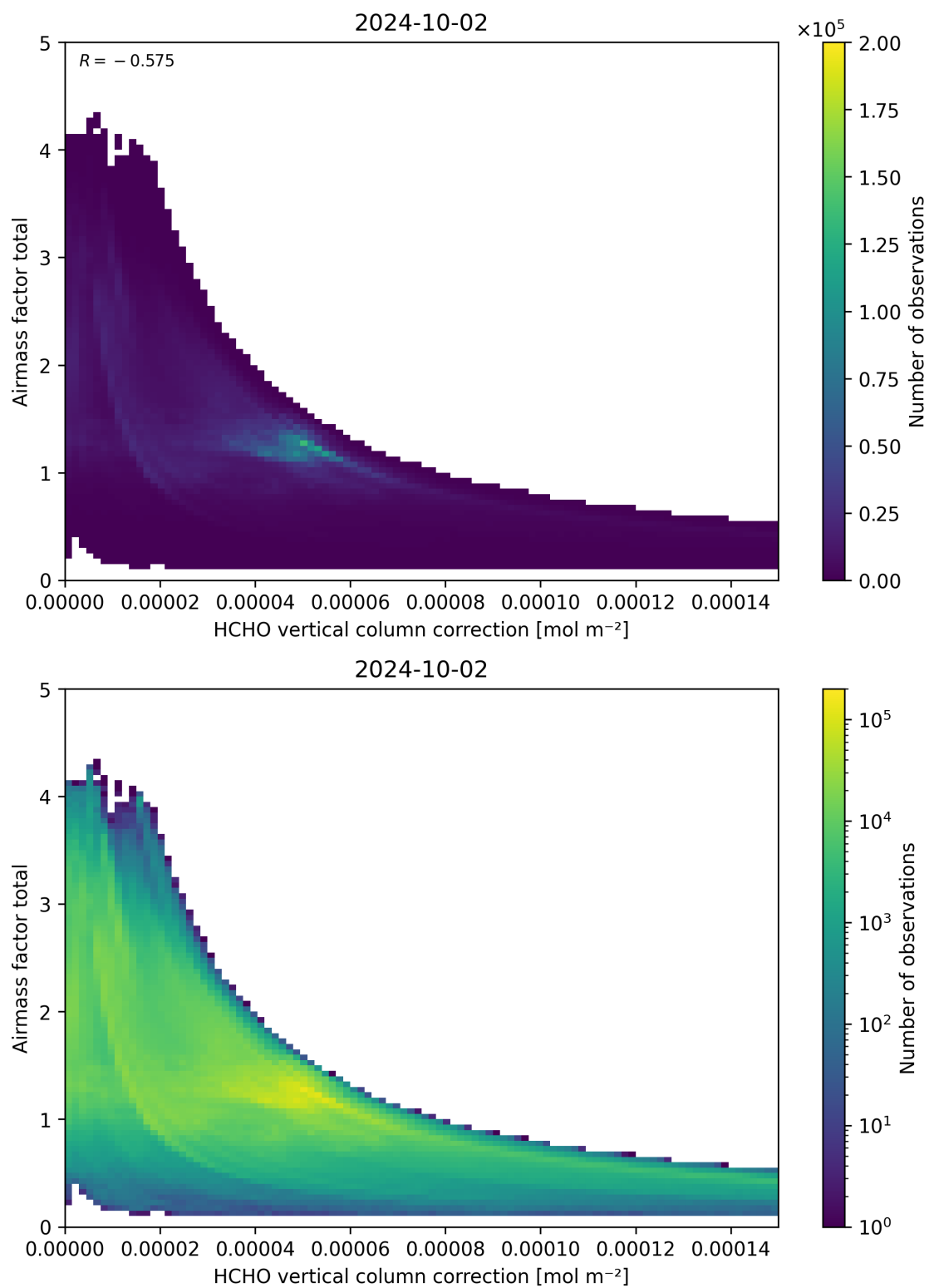
Figure 120: Scatter density plot of “HCHO vertical column correction” against “Airmass factor total” for 2024-10-01 to 2024-10-03.
