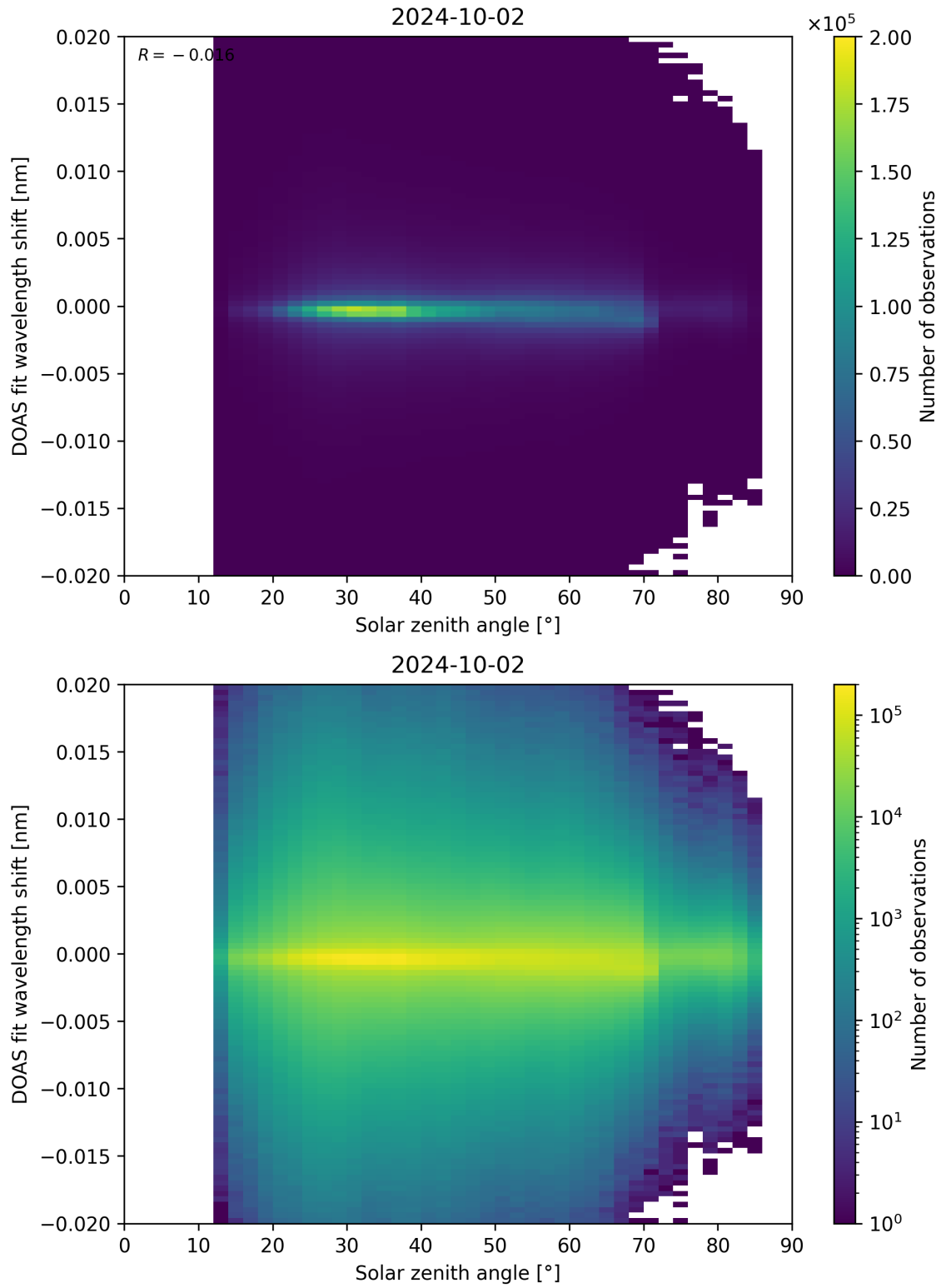
Figure 168: Scatter density plot of “Solar zenith angle” against “DOAS fit wavelength shift” for 2024-10-01 to 2024-10-03.
