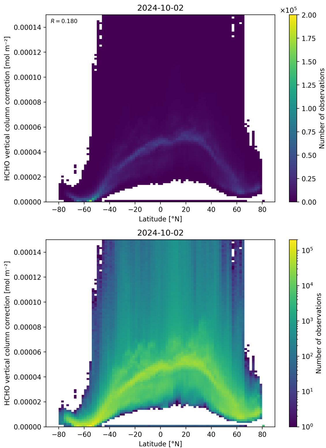
Figure 164: Scatter density plot of “Latitude” against “HCHO vertical column correction” for 2024-10-01 to 2024-10-03.
