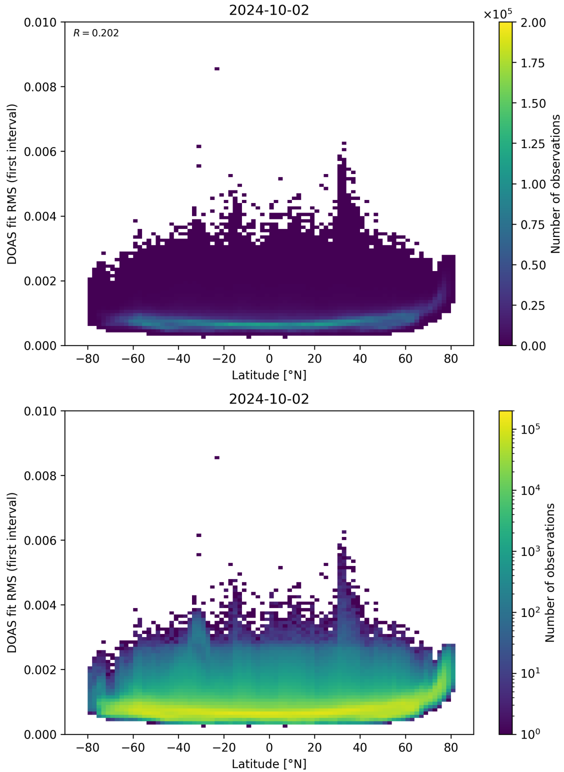
Figure 153: Scatter density plot of “Latitude” against “DOAS fit RMS (first interval)” for 2024-10-01 to 2024-10-03.
