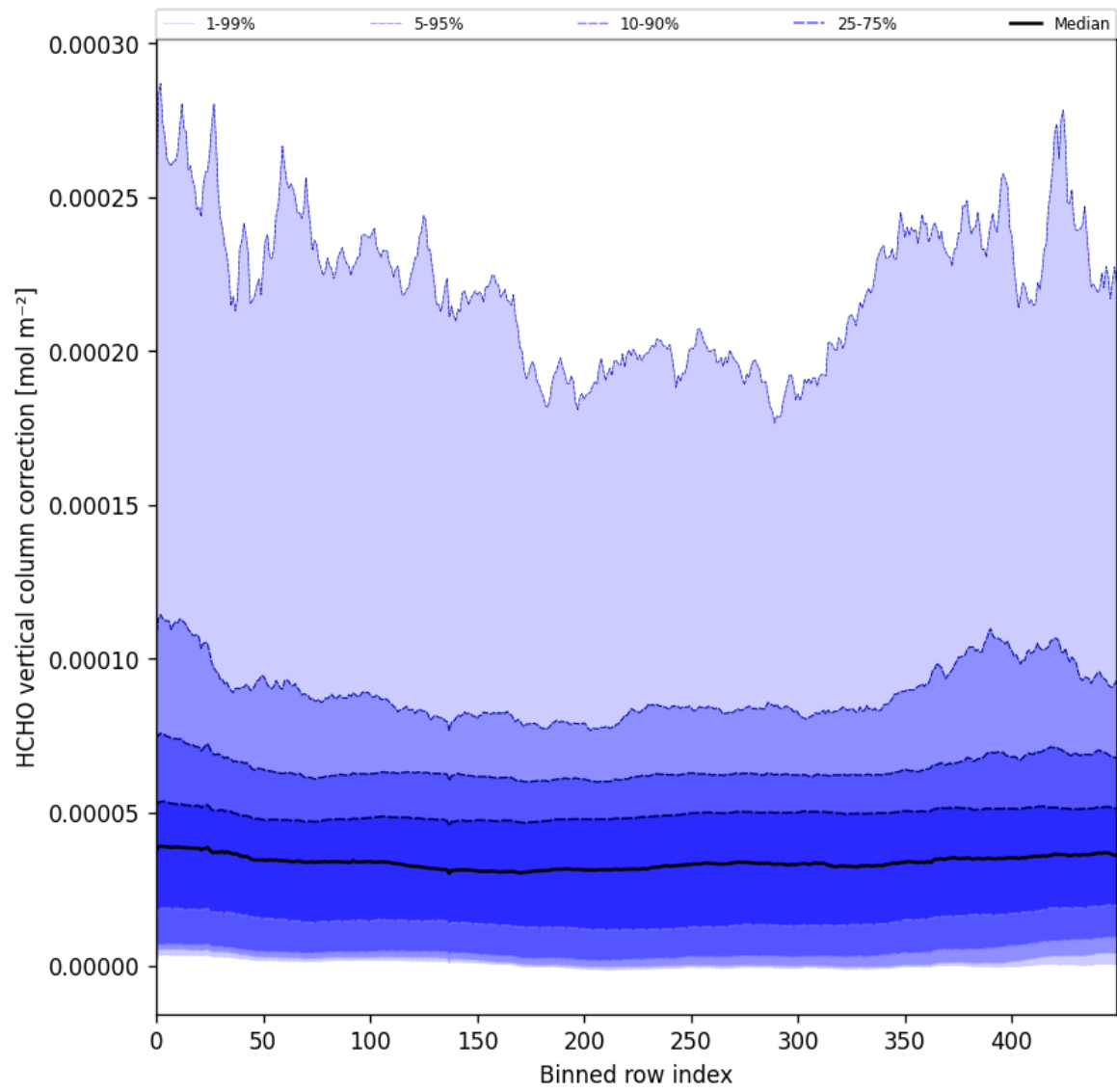
Figure 51: Along track statistics of “HCHO vertical column correction” for 2024-10-01 to 2024-10-03
