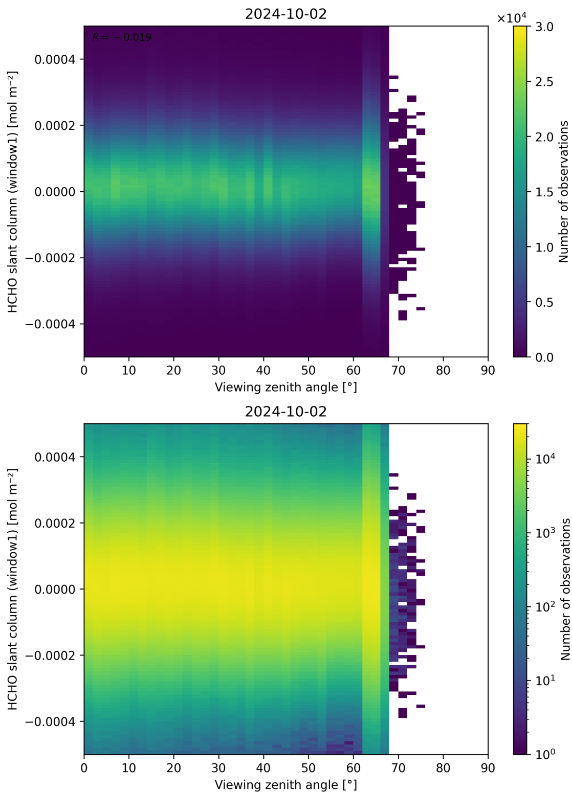
Figure 188: Scatter density plot of “Viewing zenith angle” against “HCHO slant column (window1)” for 2024-10-01 to 2024-10-03.
