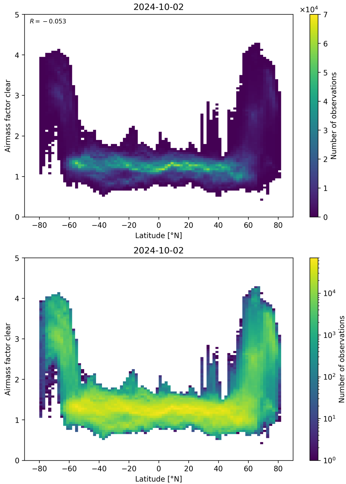
Figure 156: Scatter density plot of “Latitude” against “Airmass factor clear” for 2024-10-01 to 2024-10-03.
