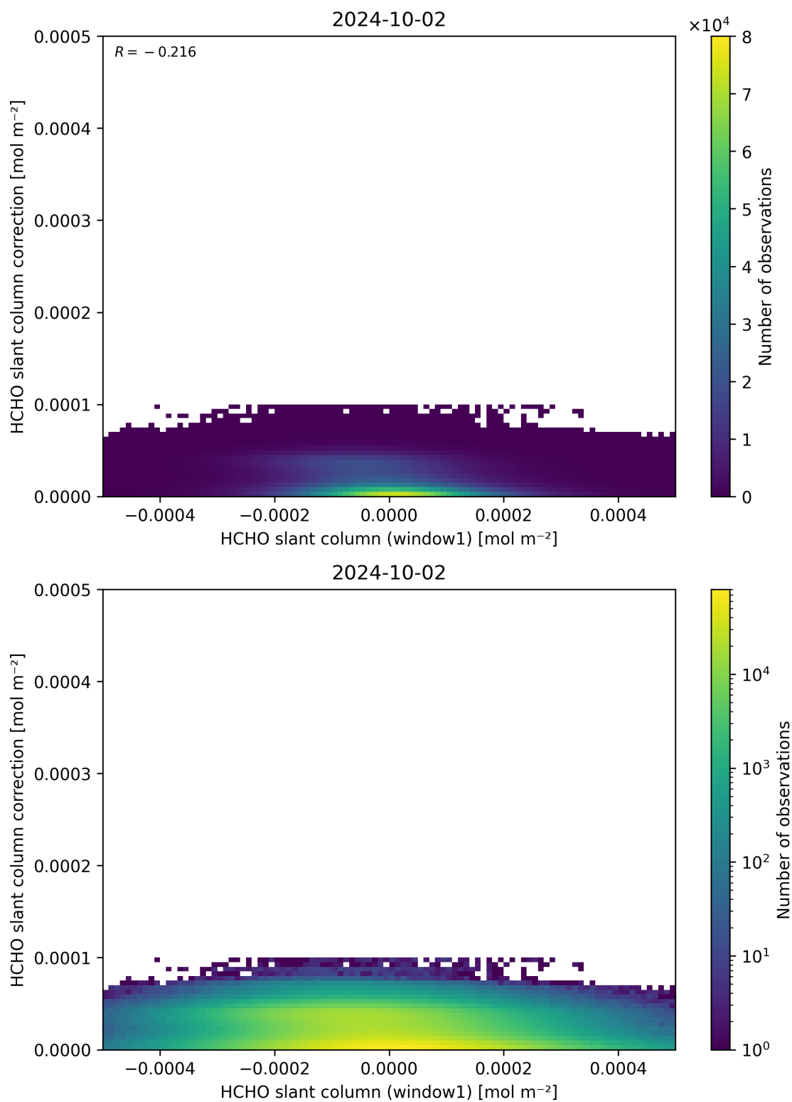
Figure 83: Scatter density plot of “HCHO slant column (window1)” against “HCHO slant column correction” for 2024-10-01 to 2024-10-03.
