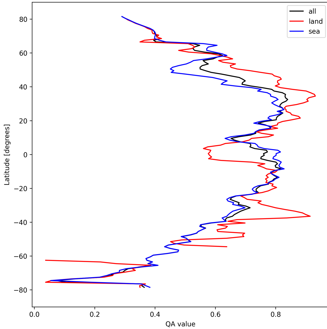
Figure 20: Zonal average of “QA value” for 2024-10-01 to 2024-10-03.
