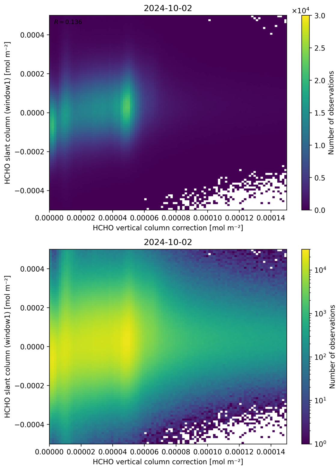
Figure 118: Scatter density plot of “HCHO vertical column correction” against “HCHO slant column (window1)” for 2024-10-01 to 2024-10-03.
