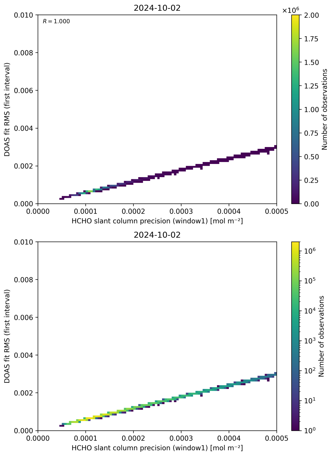
Figure 88: Scatter density plot of “HCHO slant column precision (window1)” against “DOAS fit RMS (first interval)” for 2024-10-01 to 2024-10-03.
