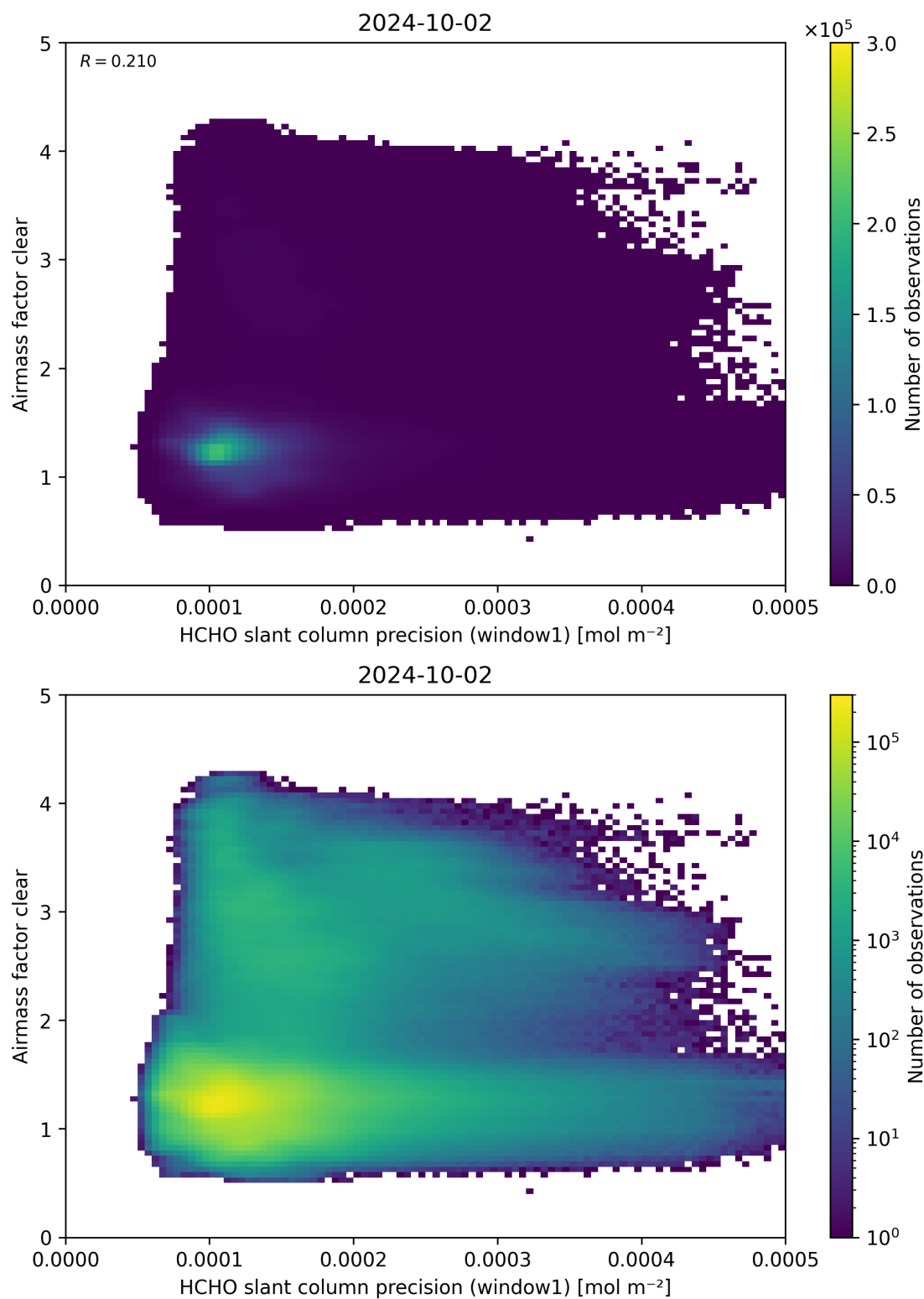
Figure 91: Scatter density plot of “HCHO slant column precision (window1)” against “Airmass factor clear” for 2024-10-01 to 2024-10-03.
