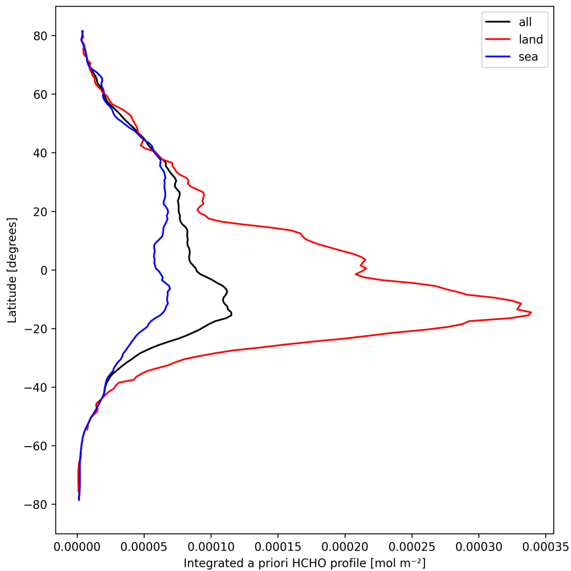
Figure 29: Zonal average of “Integrated a priori HCHO profile” for 2024-10-01 to 2024-10-03.
