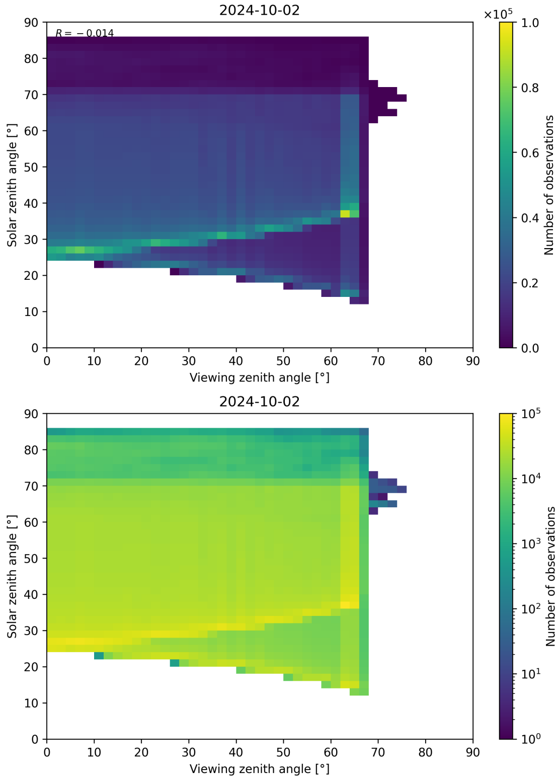
Figure 197: Scatter density plot of “Viewing zenith angle” against “Solar zenith angle” for 2024-10-01 to 2024-10-03.
