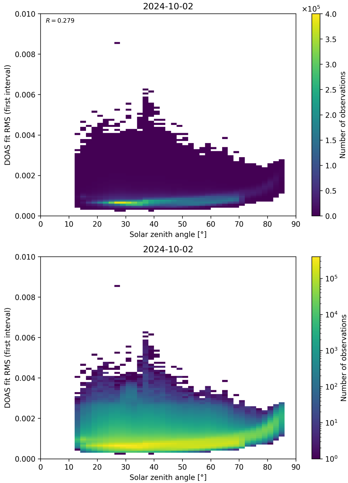
Figure 167: Scatter density plot of “Solar zenith angle” against “DOAS fit RMS (first interval)” for 2024-10-01 to 2024-10-03.
