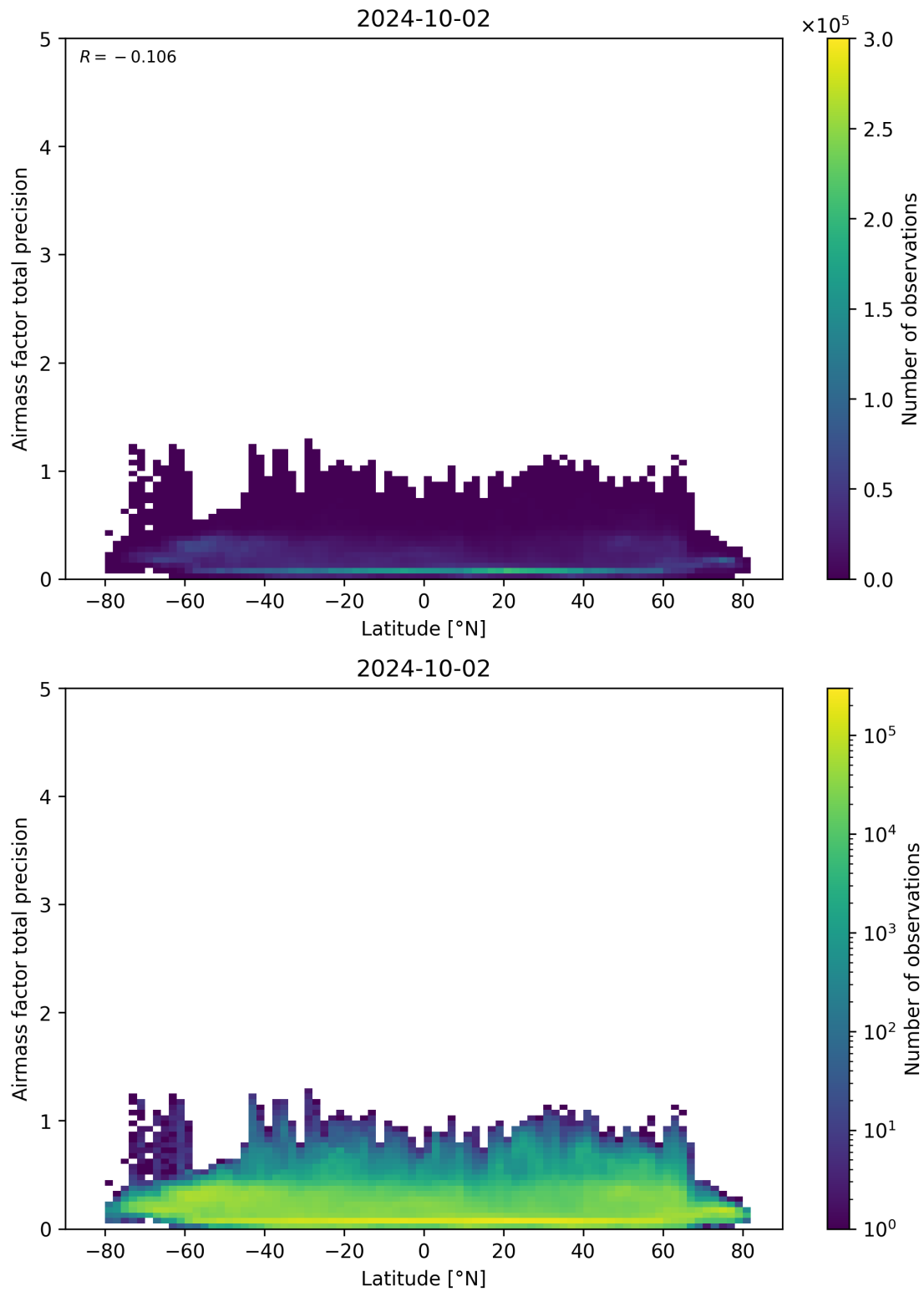
Figure 162: Scatter density plot of “Latitude” against “Airmass factor total precision” for 2024-10-01 to 2024-10-03.
