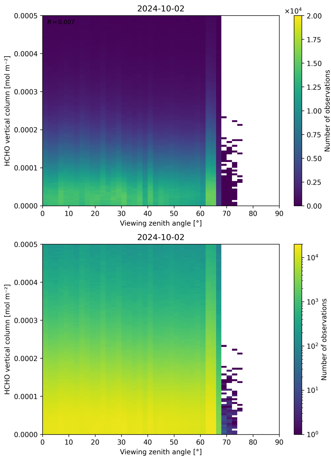
Figure 192: Scatter density plot of “Viewing zenith angle” against “HCHO vertical column” for 2024-10-01 to 2024-10-03.
