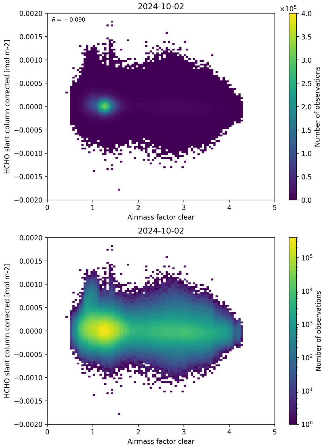
Figure 74: Scatter density plot of “Airmass factor clear” against “HCHO slant column corrected” for 2024-10-01 to 2024-10-03.
