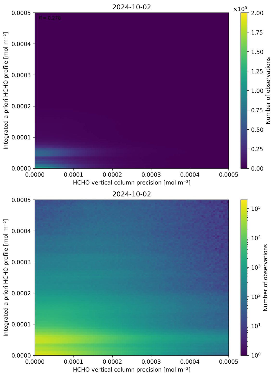
Figure 147: Scatter density plot of “HCHO vertical column precision” against “Integrated a priori HCHO profile” for 2024-10-01 to 2024-10-03.
