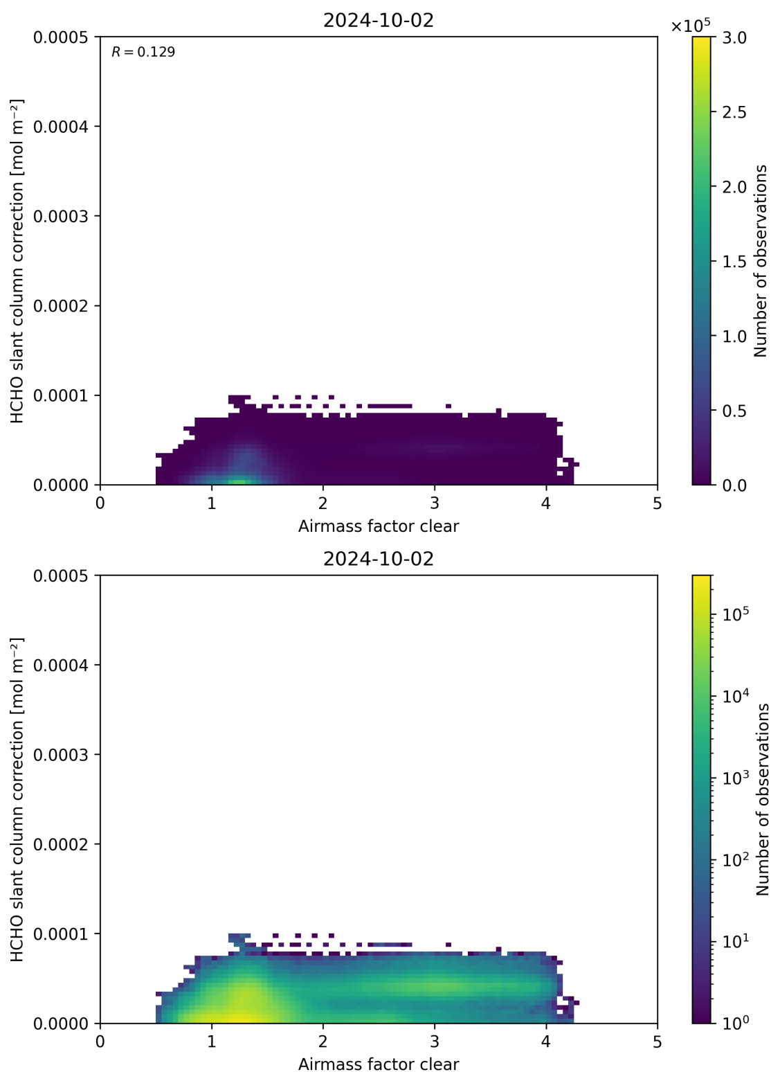
Figure 75: Scatter density plot of “Airmass factor clear” against “HCHO slant column correction” for 2024-10-01 to 2024-10-03.
