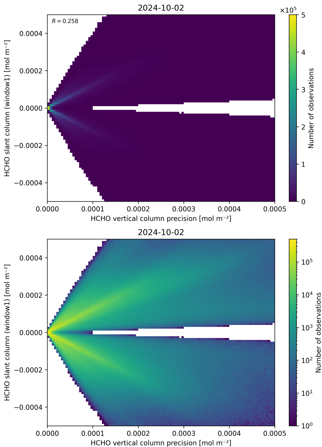
Figure 142: Scatter density plot of “HCHO vertical column precision” against “HCHO slant column (window1)” for 2024-10-01 to 2024-10-03.
