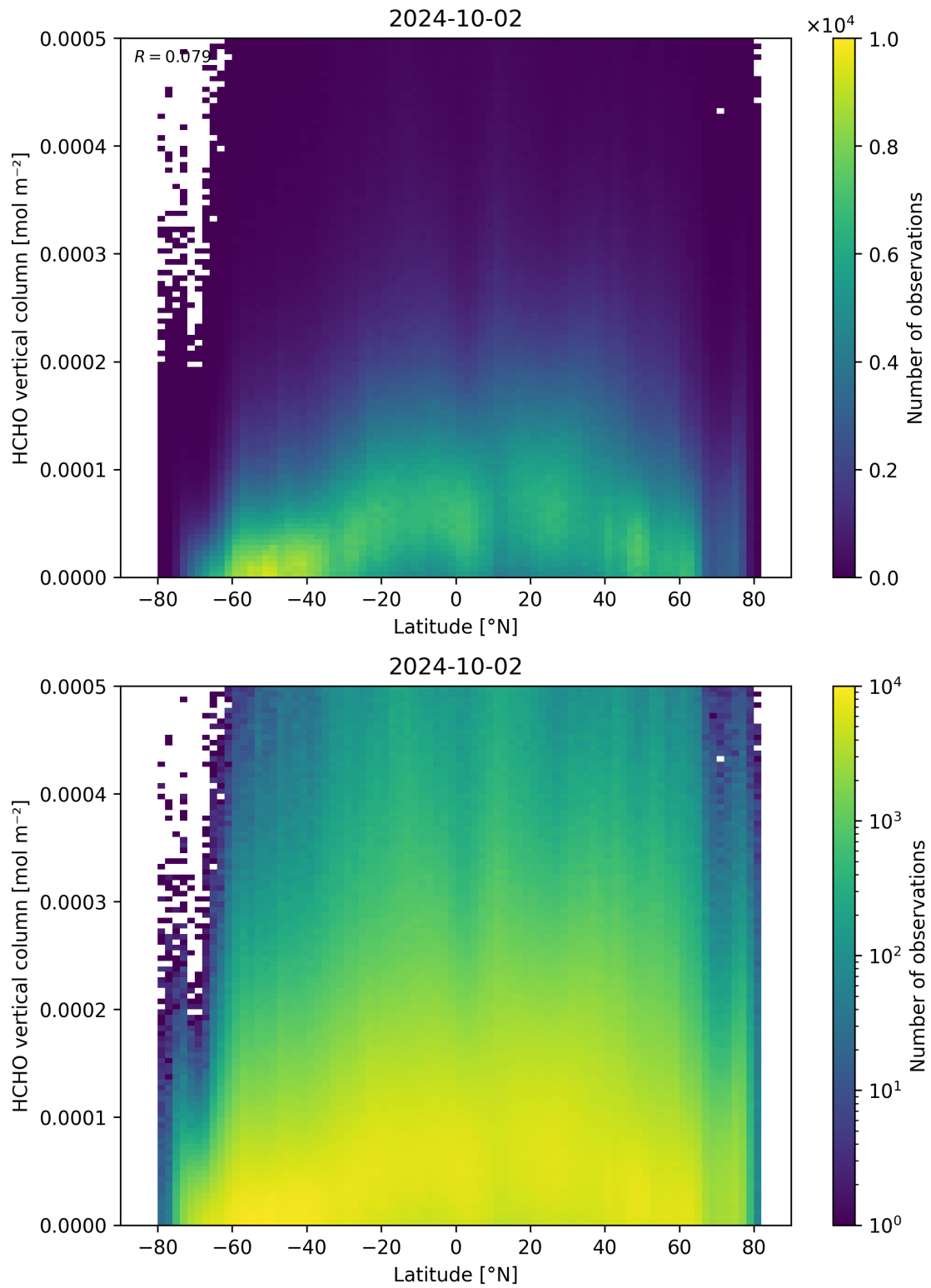
Figure 163: Scatter density plot of “Latitude” against “HCHO vertical column” for 2024-10-01 to 2024-10-03.
