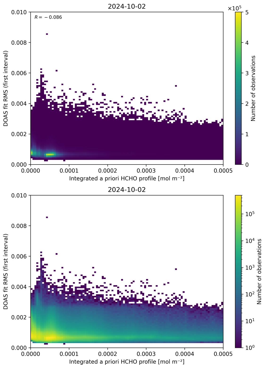
Figure 148: Scatter density plot of “Integrated a priori HCHO profile” against “DOAS fit RMS (first interval)” for 2024-10-01 to 2024-10-03.
