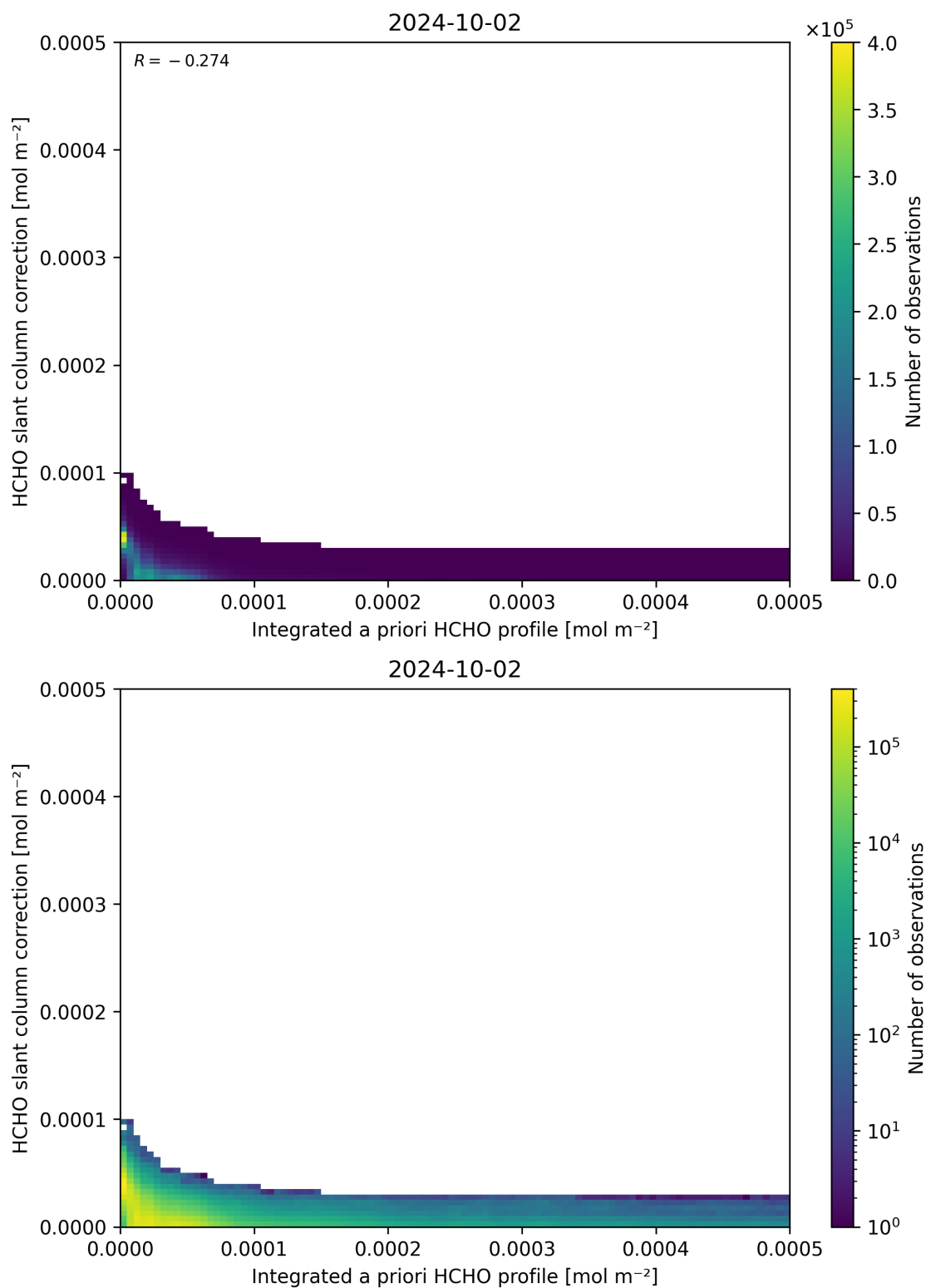
Figure 152: Scatter density plot of “Integrated a priori HCHO profile” against “HCHO slant column correction” for 2024-10-01 to 2024-10-03.
