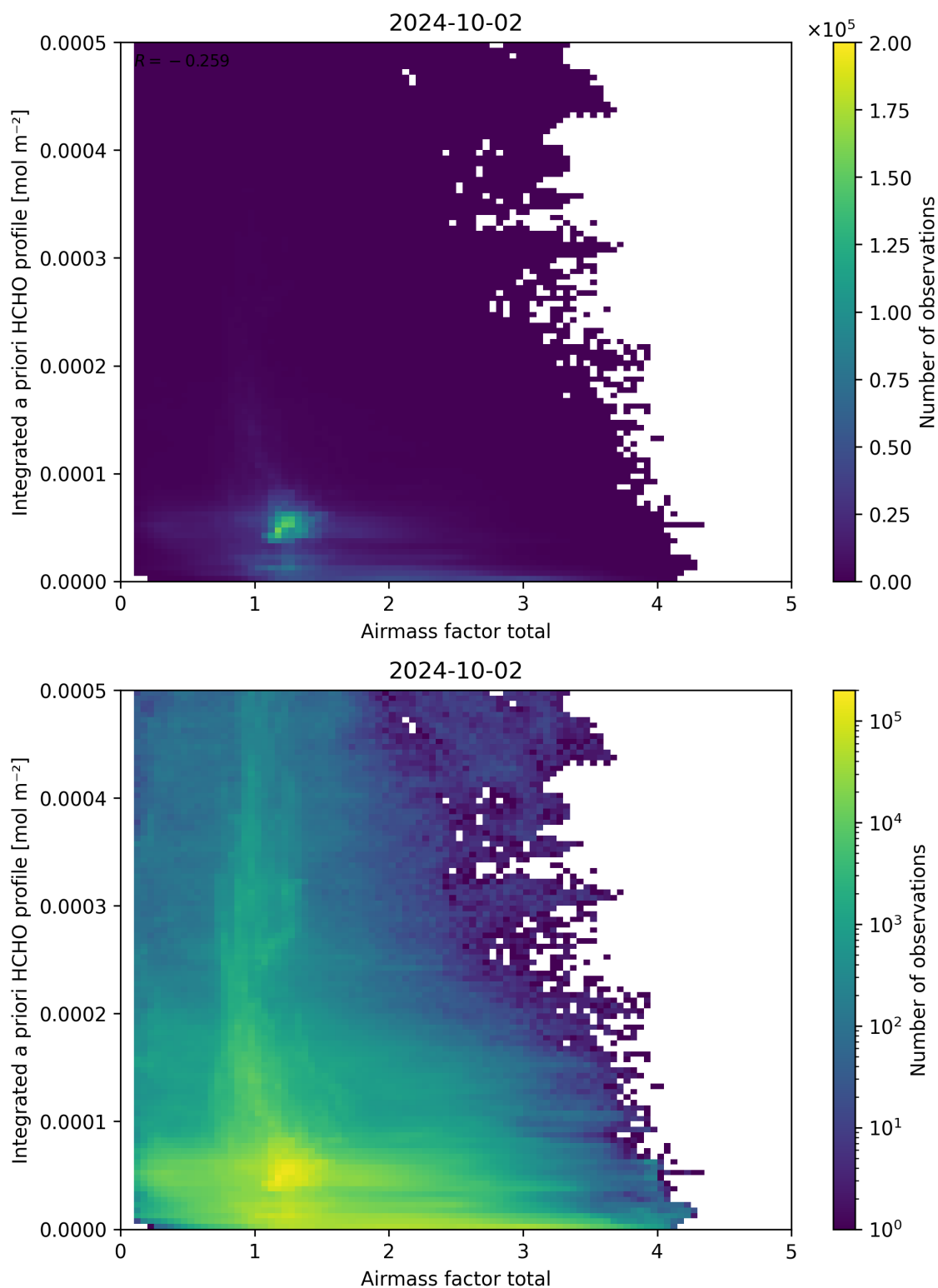
Figure 104: Scatter density plot of “Airmass factor total” against “Integrated a priori HCHO profile” for 2024-10-01 to 2024-10-03.
