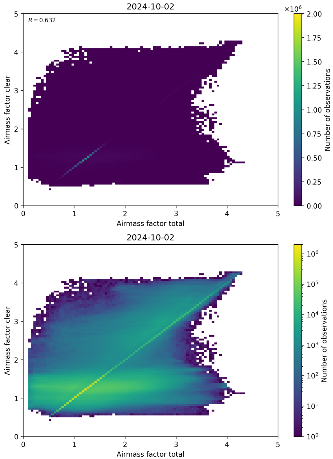
Figure 100: Scatter density plot of “Airmass factor total” against “Airmass factor clear” for 2024-10-01 to 2024-10-03.
