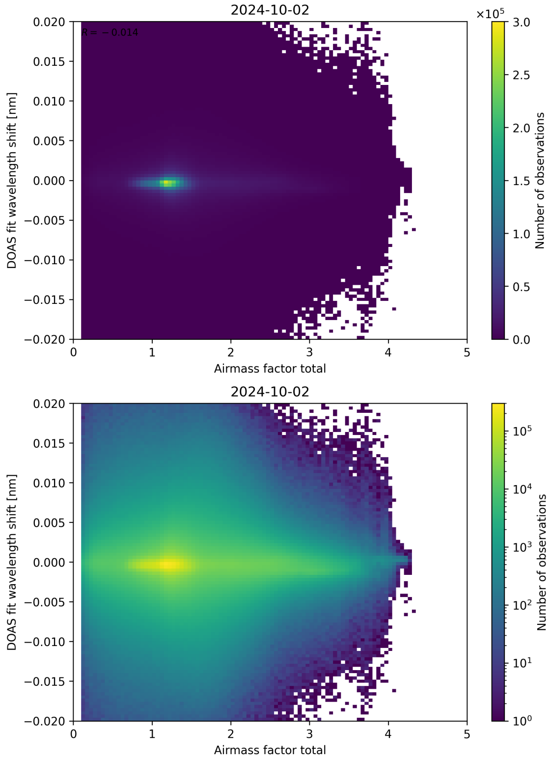
Figure 98: Scatter density plot of “Airmass factor total” against “DOAS fit wavelength shift” for 2024-10-01 to 2024-10-03.
