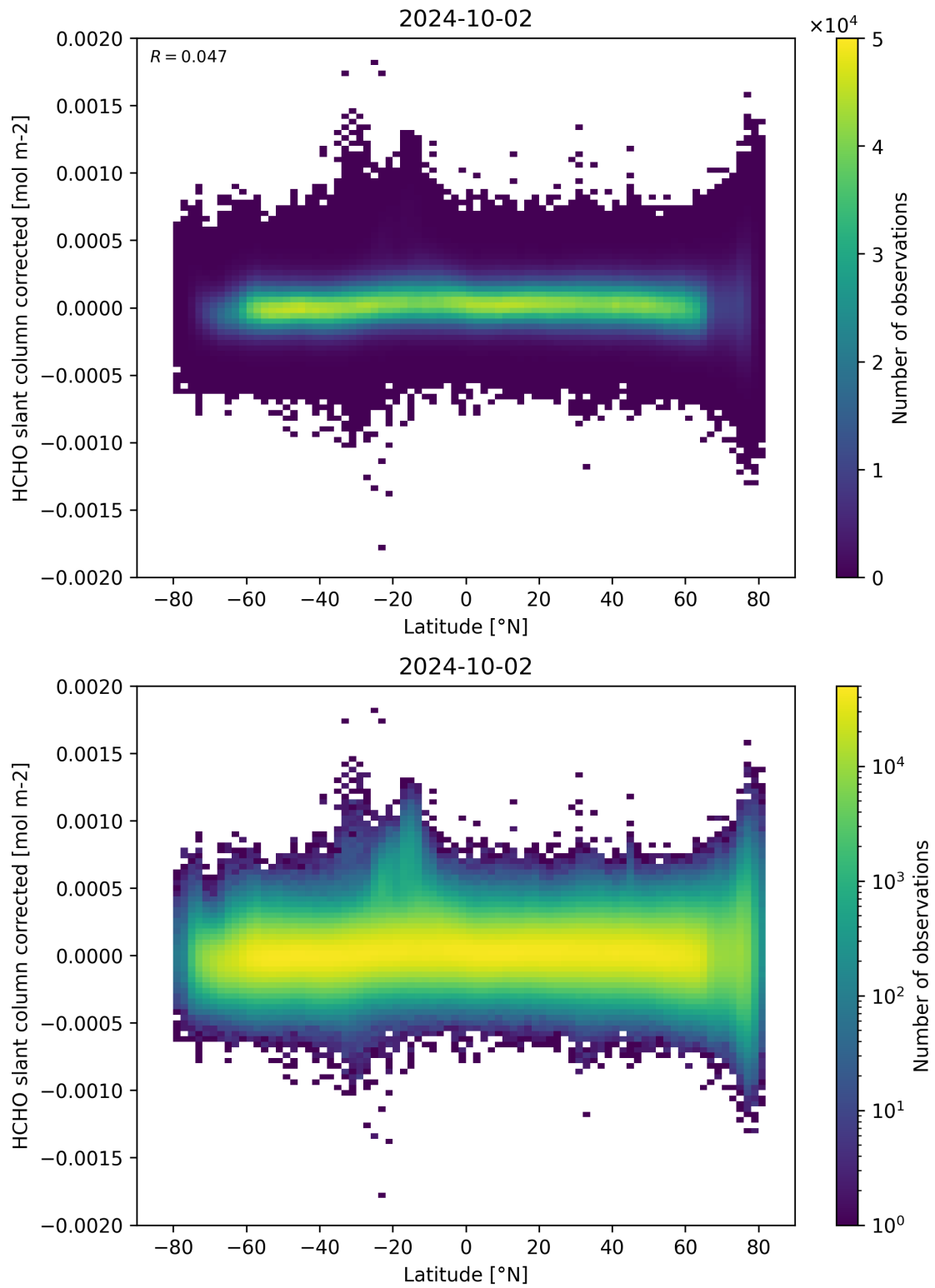
Figure 157: Scatter density plot of “Latitude” against “HCHO slant column corrected” for 2024-10-01 to 2024-10-03.
