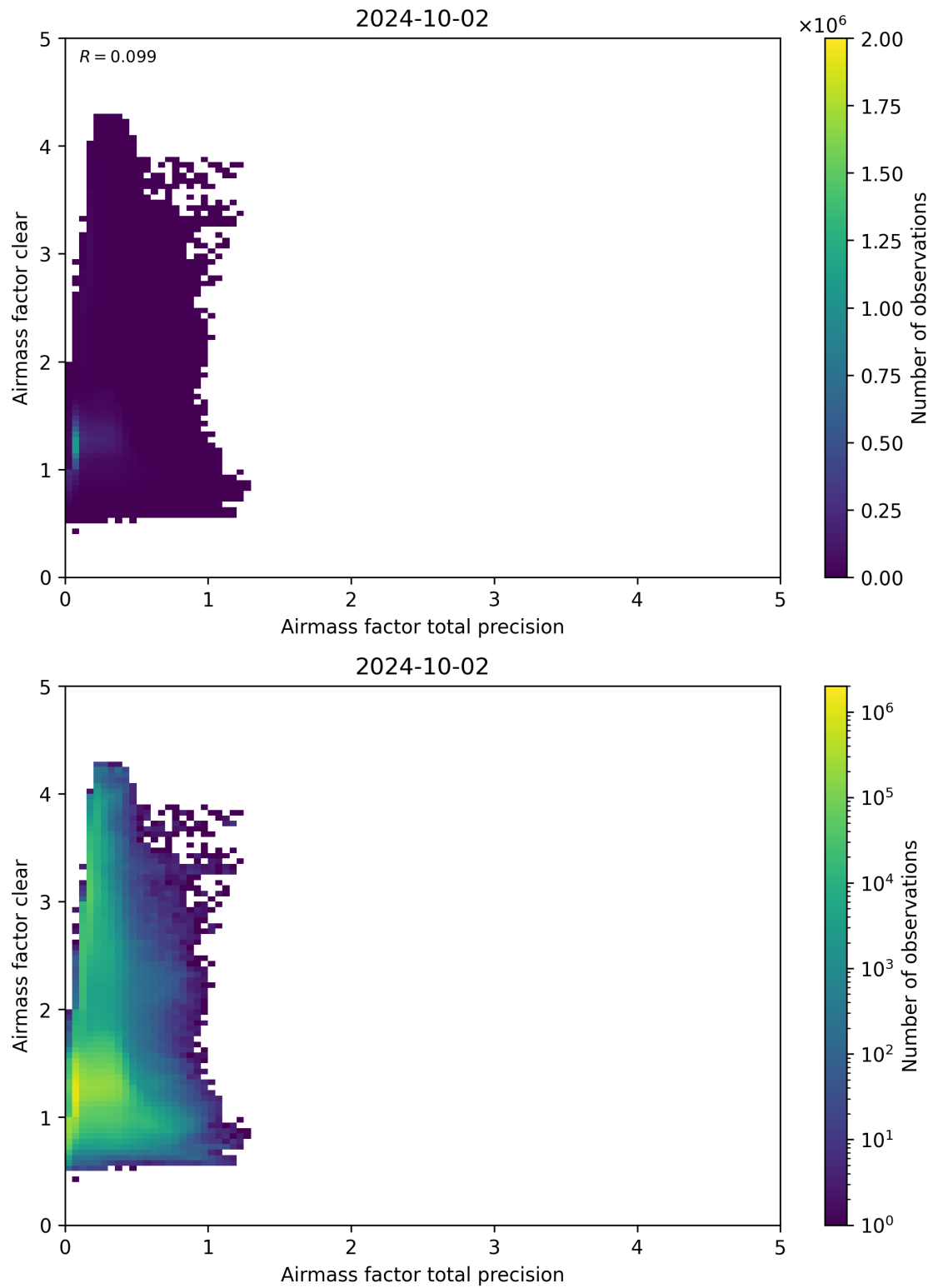
Figure 108: Scatter density plot of “Airmass factor total precision” against “Airmass factor clear” for 2024-10-01 to 2024-10-03.
