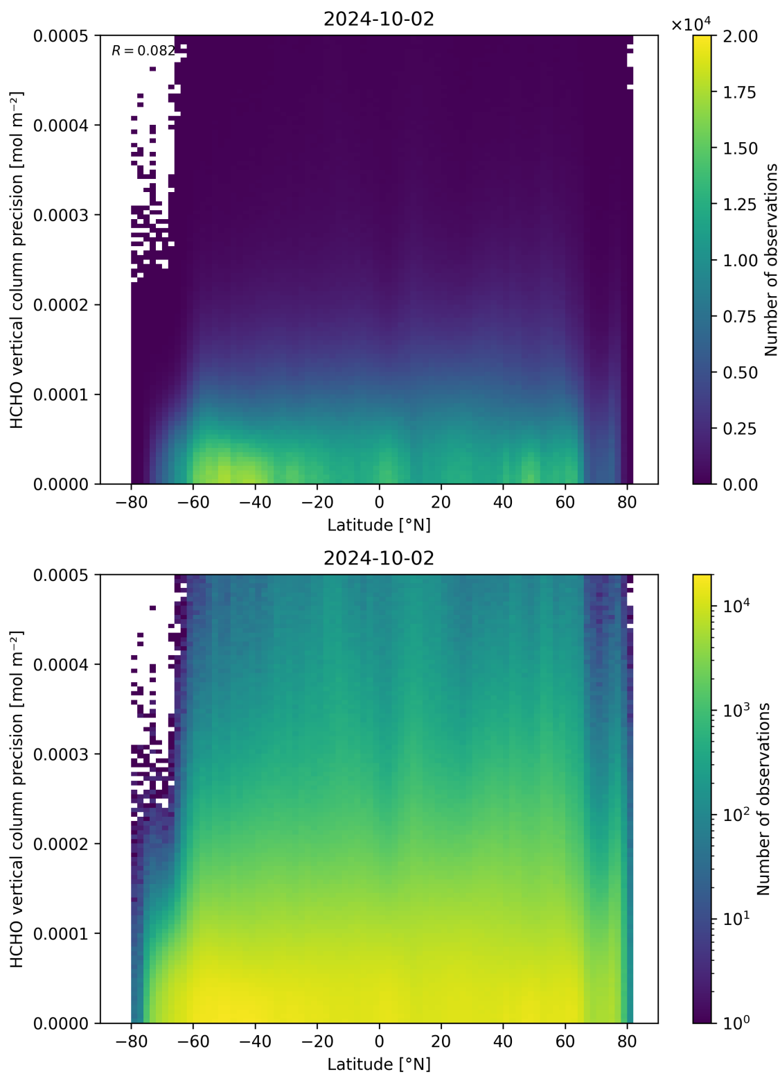
Figure 165: Scatter density plot of “Latitude” against “HCHO vertical column precision” for 2024-10-01 to 2024-10-03.
