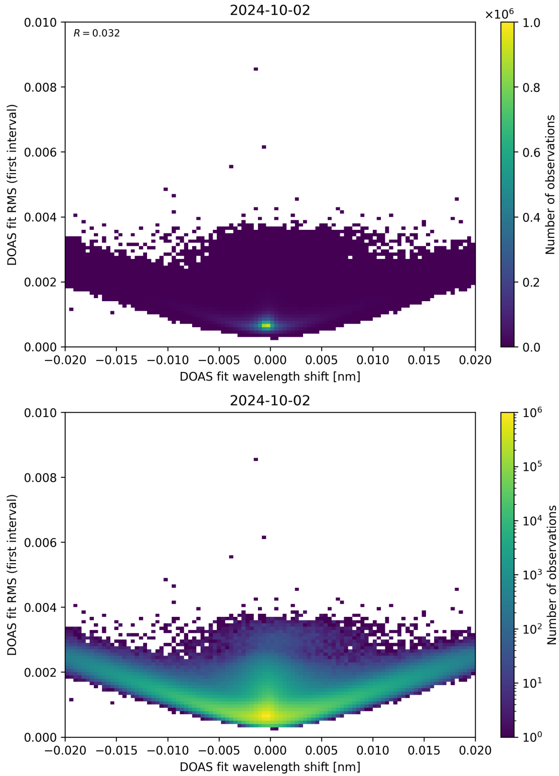
Figure 64: Scatter density plot of “DOAS fit wavelength shift” against “DOAS fit RMS (first interval)” for 2024-10-01 to 2024-10-03.
