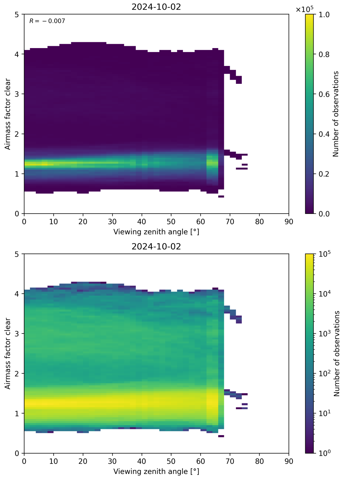
Figure 185: Scatter density plot of “Viewing zenith angle” against “Airmass factor clear” for 2024-10-01 to 2024-10-03.
