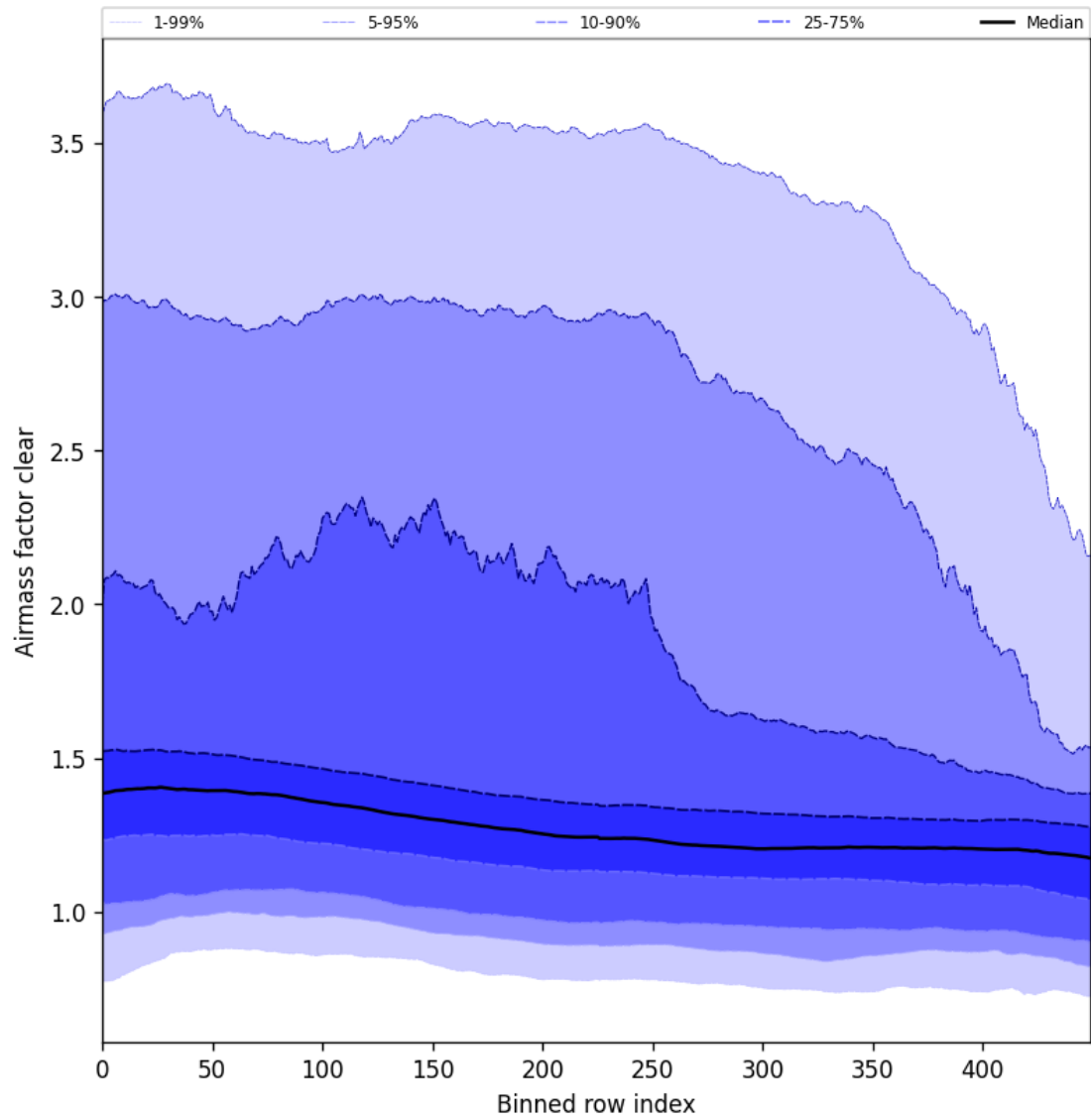
Figure 56: Along track statistics of “Airmass factor clear” for 2024-10-01 to 2024-10-03
