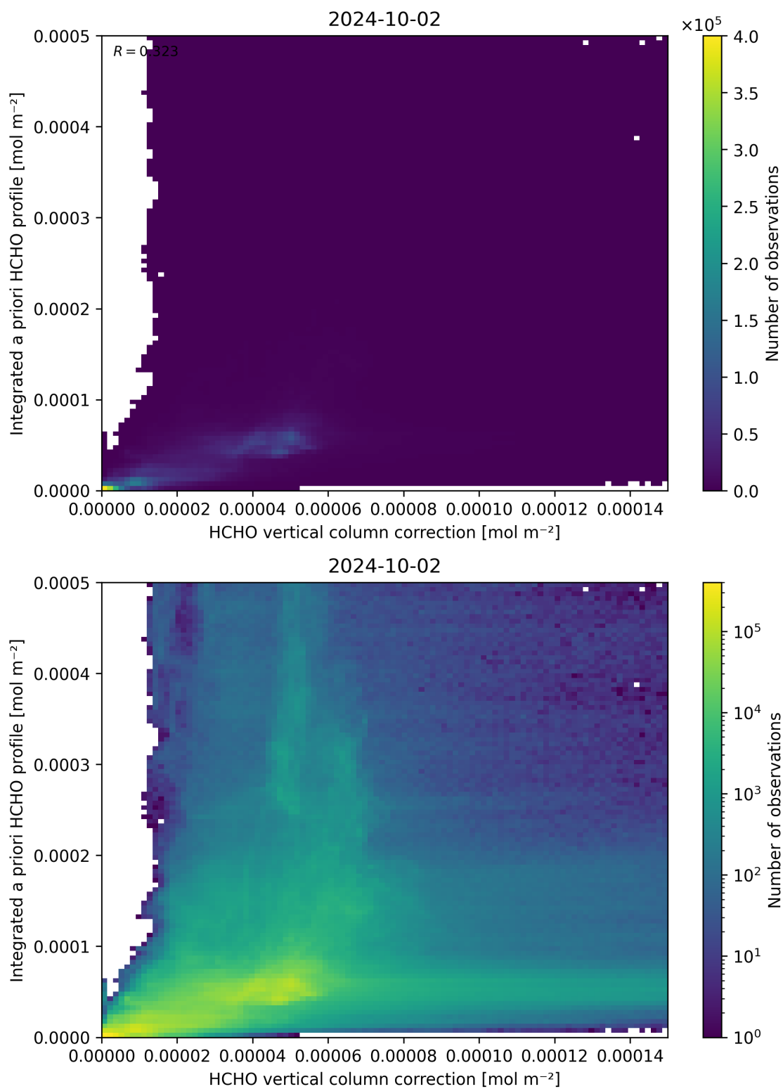
Figure 122: Scatter density plot of “HCHO vertical column correction” against “Integrated a priori HCHO profile” for 2024-10-01 to 2024-10-03.
