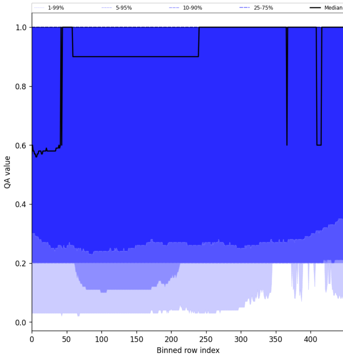
Figure 48: Along track statistics of “QA value” for 2024-10-01 to 2024-10-03
