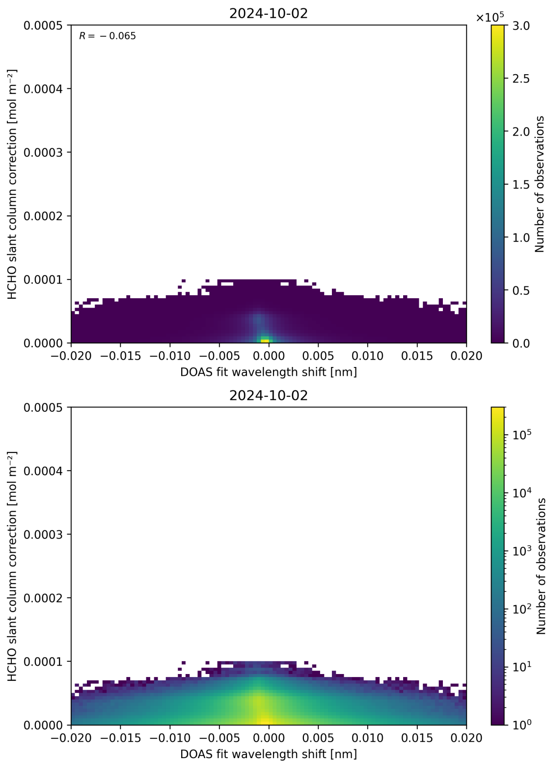
Figure 67: Scatter density plot of “DOAS fit wavelength shift” against “HCHO slant column correction” for 2024-10-01 to 2024-10-03.
