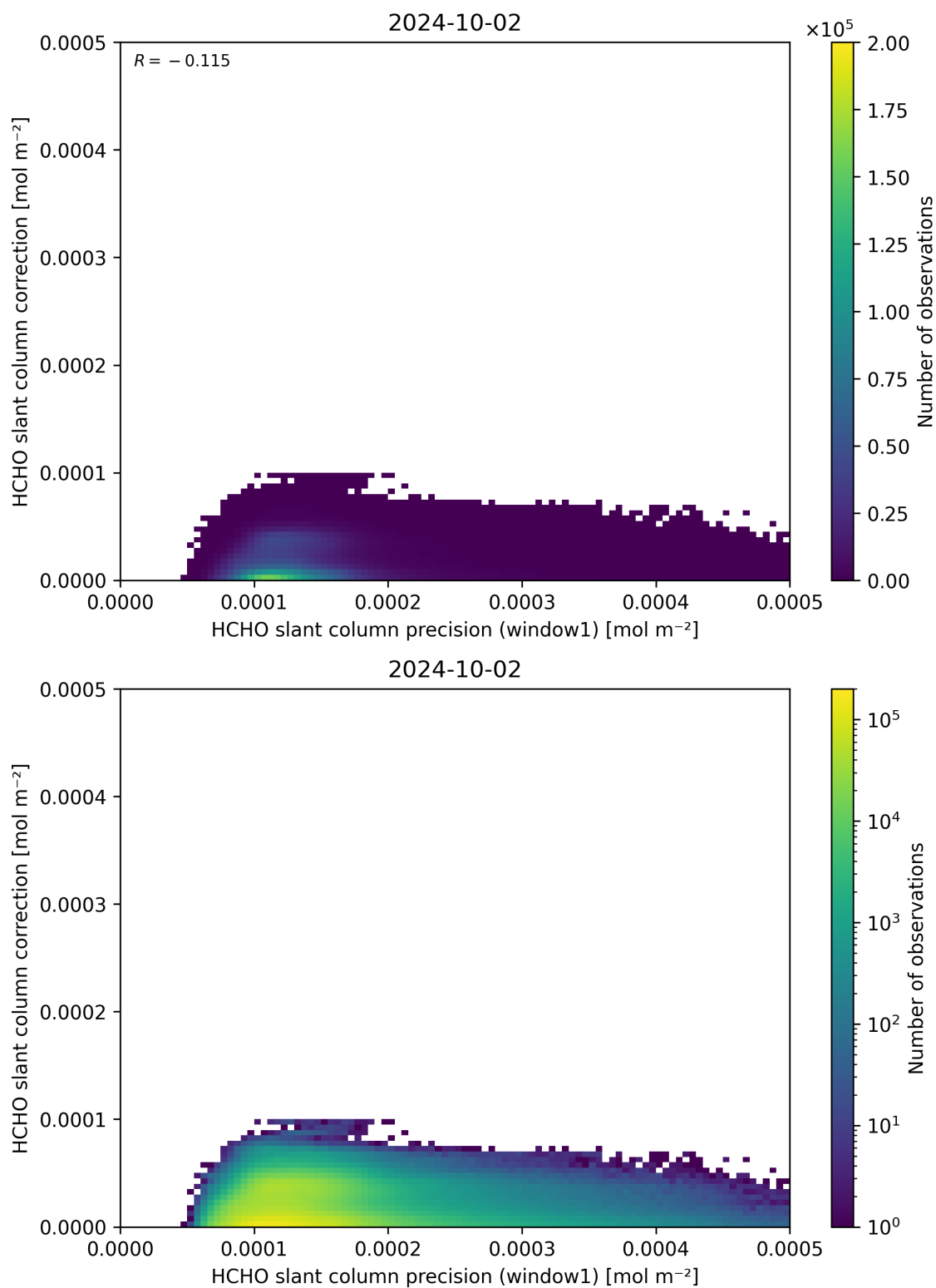
Figure 93: Scatter density plot of “HCHO slant column precision (window1)” against “HCHO slant column correction” for 2024-10-01 to 2024-10-03.
