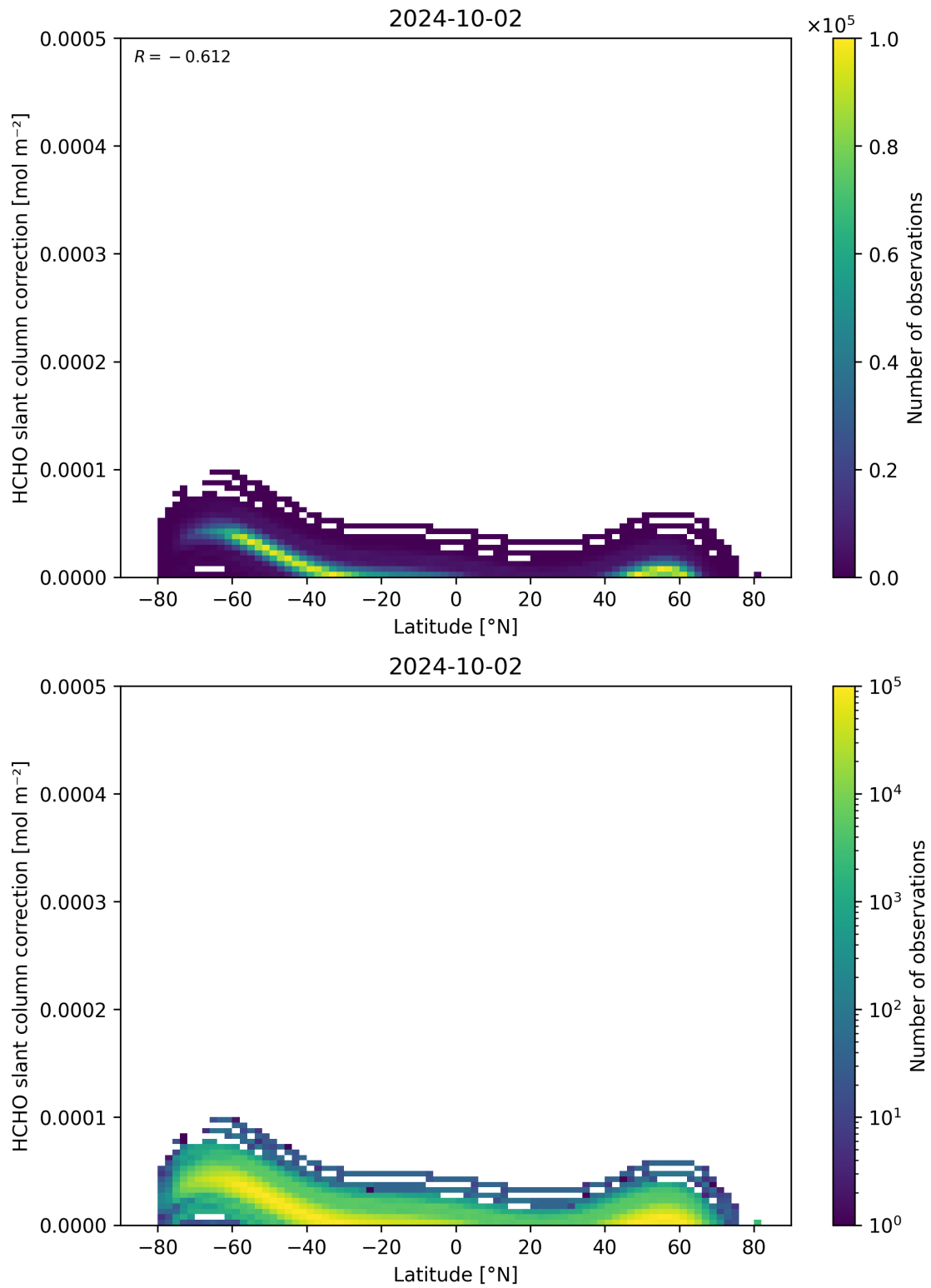
Figure 158: Scatter density plot of “Latitude” against “HCHO slant column correction” for 2024-10-01 to 2024-10-03.
