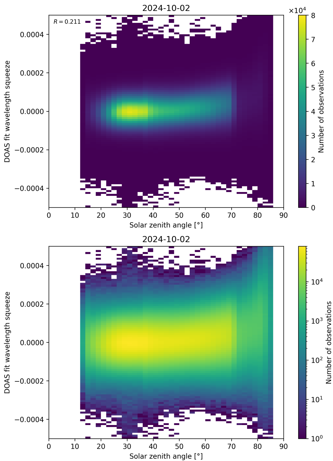
Figure 169: Scatter density plot of “Solar zenith angle” against “DOAS fit wavelength squeeze” for 2024-10-01 to 2024-10-03.
