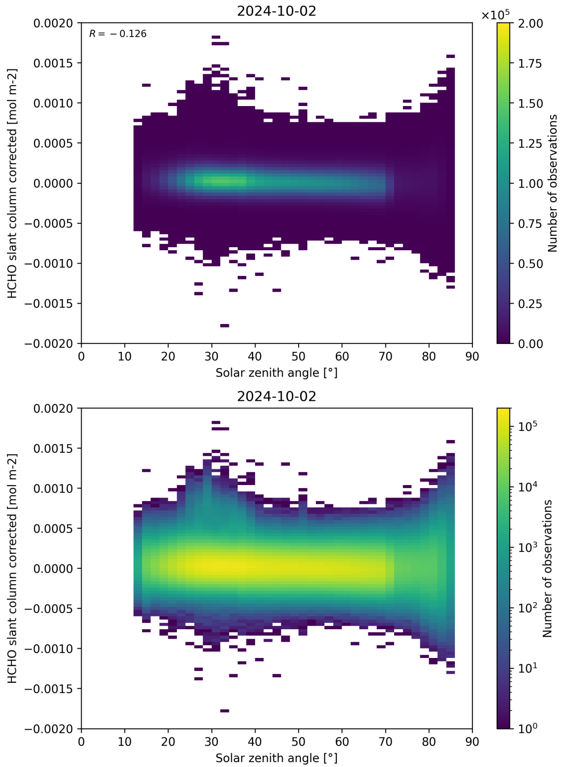
Figure 171: Scatter density plot of “Solar zenith angle” against “HCHO slant column corrected” for 2024-10-01 to 2024-10-03.
