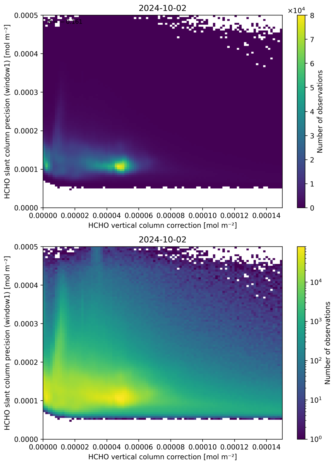
Figure 119: Scatter density plot of “HCHO vertical column correction” against “HCHO slant column precision (window1)” for 2024-10-01 to 2024-10-03.
