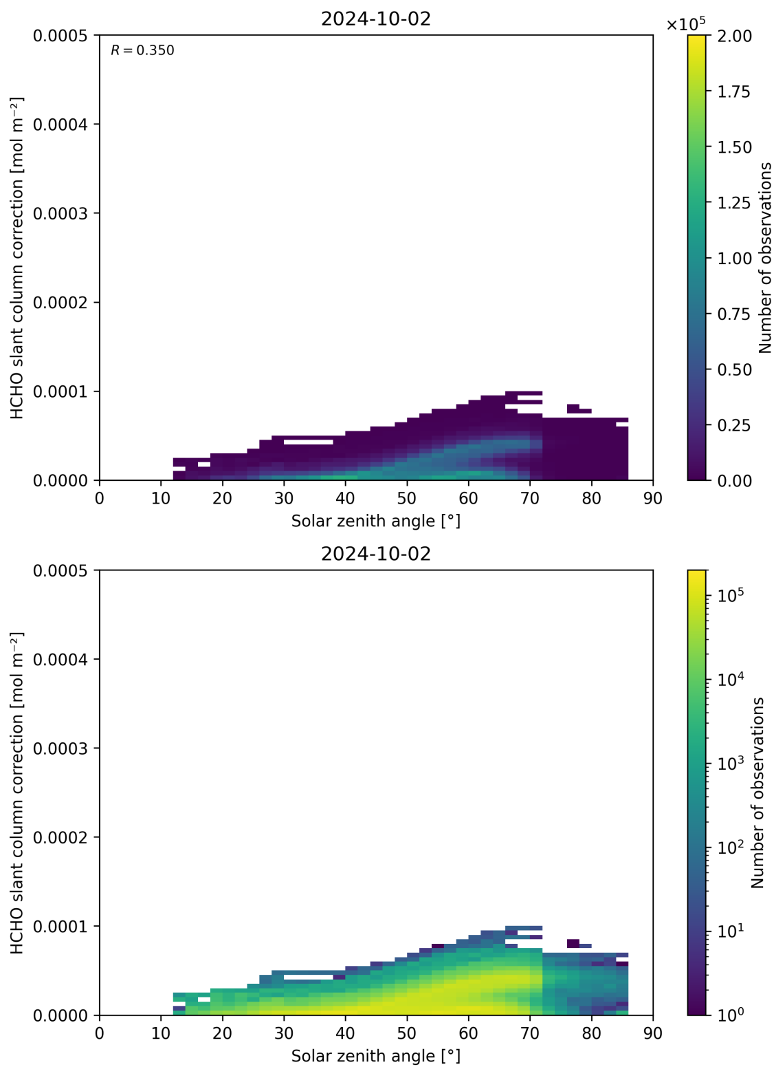
Figure 172: Scatter density plot of “Solar zenith angle” against “HCHO slant column correction” for 2024-10-01 to 2024-10-03.
