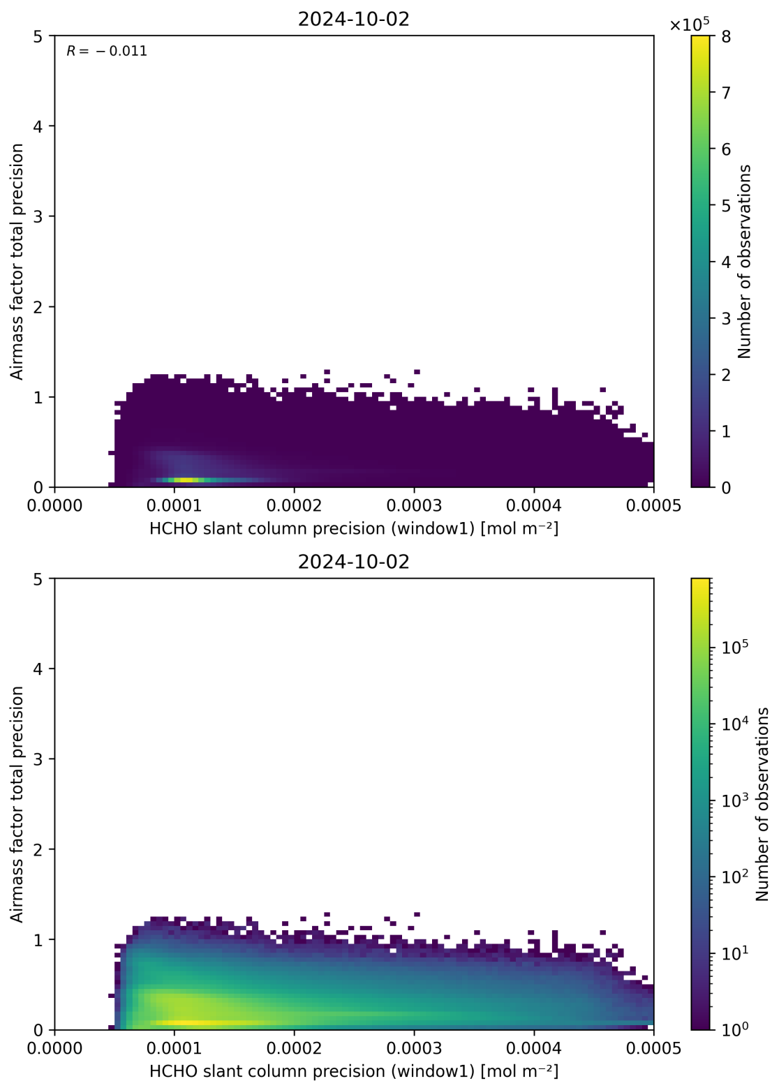
Figure 95: Scatter density plot of “HCHO slant column precision (window1)” against “Airmass factor total precision” for 2024-10-01 to 2024-10-03.
