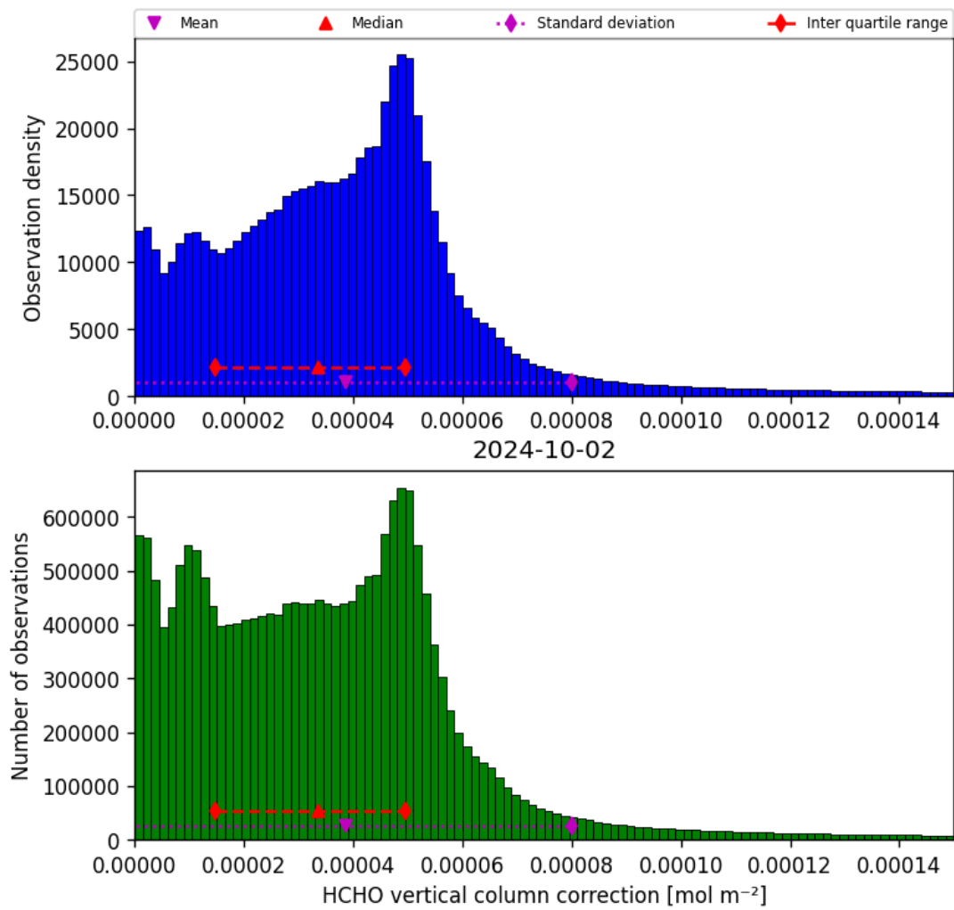
Figure 37: Histogram of “HCHO vertical column correction” for 2024-10-01 to 2024-10-03
