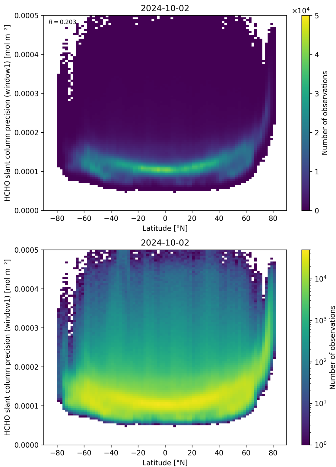
Figure 160: Scatter density plot of “Latitude” against “HCHO slant column precision (window1)” for 2024-10-01 to 2024-10-03.
