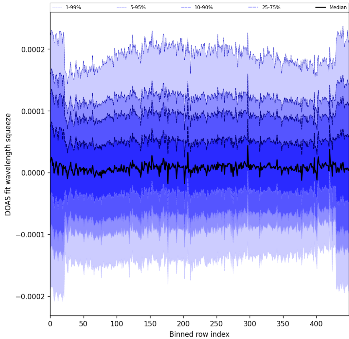
Figure 59: Along track statistics of “DOAS fit wavelength squeeze” for 2024-10-01 to 2024-10-03
