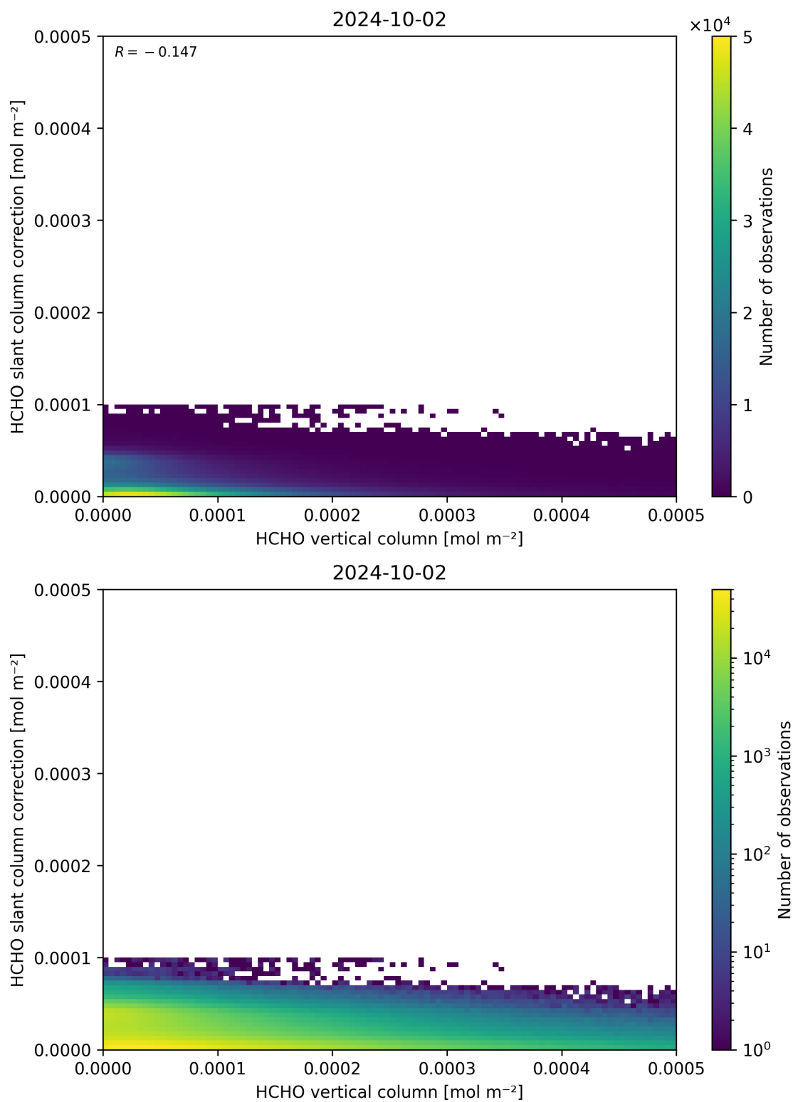
Figure 128: Scatter density plot of “HCHO vertical column” against “HCHO slant column correction” for 2024-10-01 to 2024-10-03.
