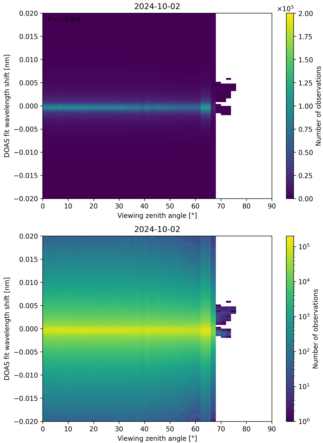
Figure 183: Scatter density plot of “Viewing zenith angle” against “DOAS fit wavelength shift” for 2024-10-01 to 2024-10-03.
