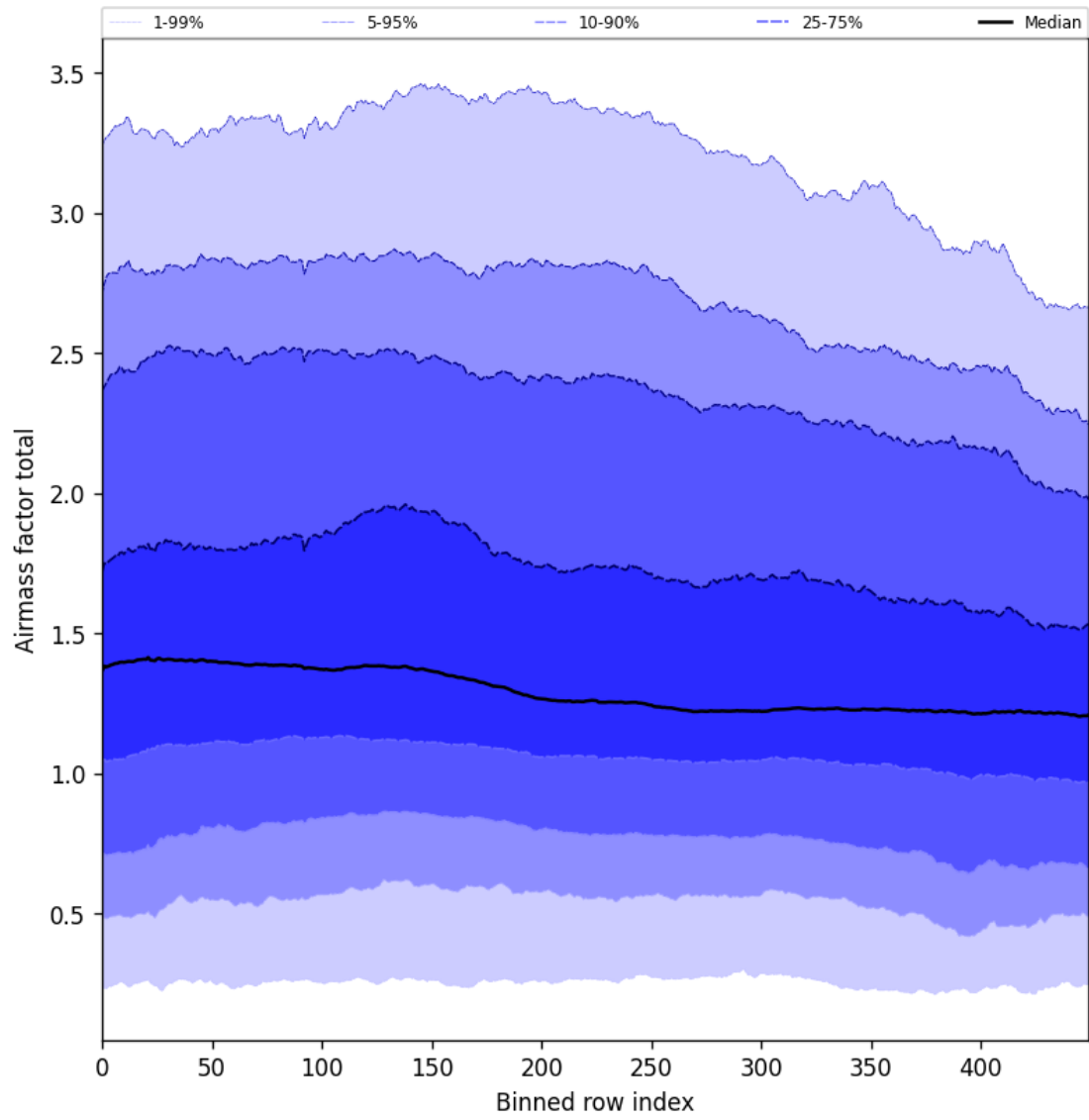
Figure 54: Along track statistics of “Airmass factor total” for 2024-10-01 to 2024-10-03
