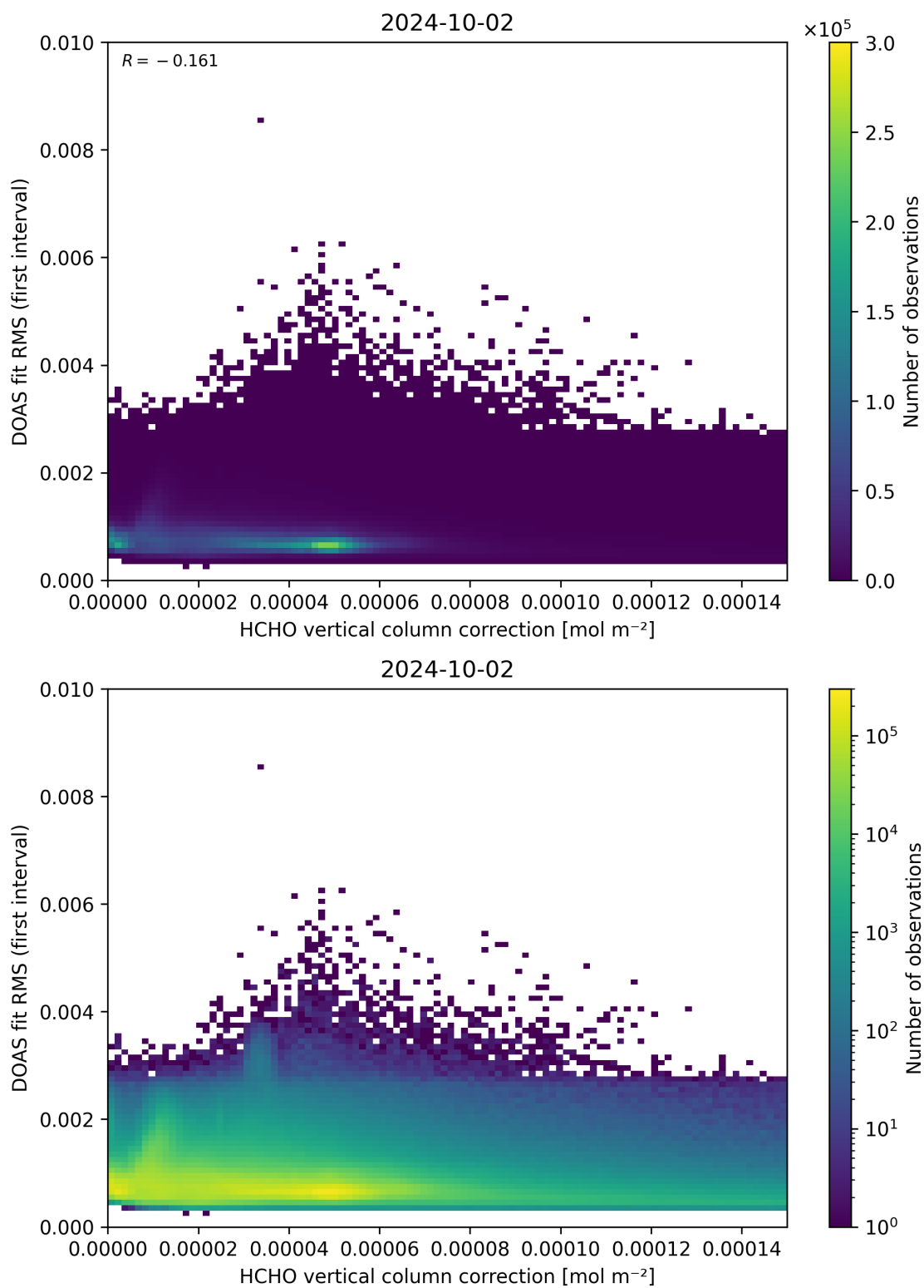
Figure 112: Scatter density plot of “HCHO vertical column correction” against “DOAS fit RMS (first interval)” for 2024-10-01 to 2024-10-03.
