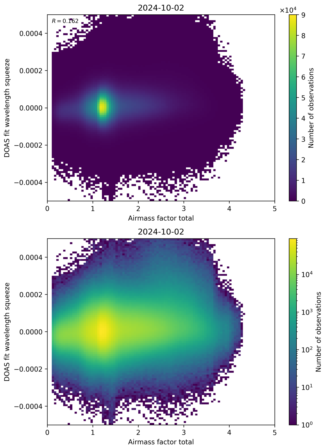
Figure 99: Scatter density plot of “Airmass factor total” against “DOAS fit wavelength squeeze” for 2024-10-01 to 2024-10-03.
