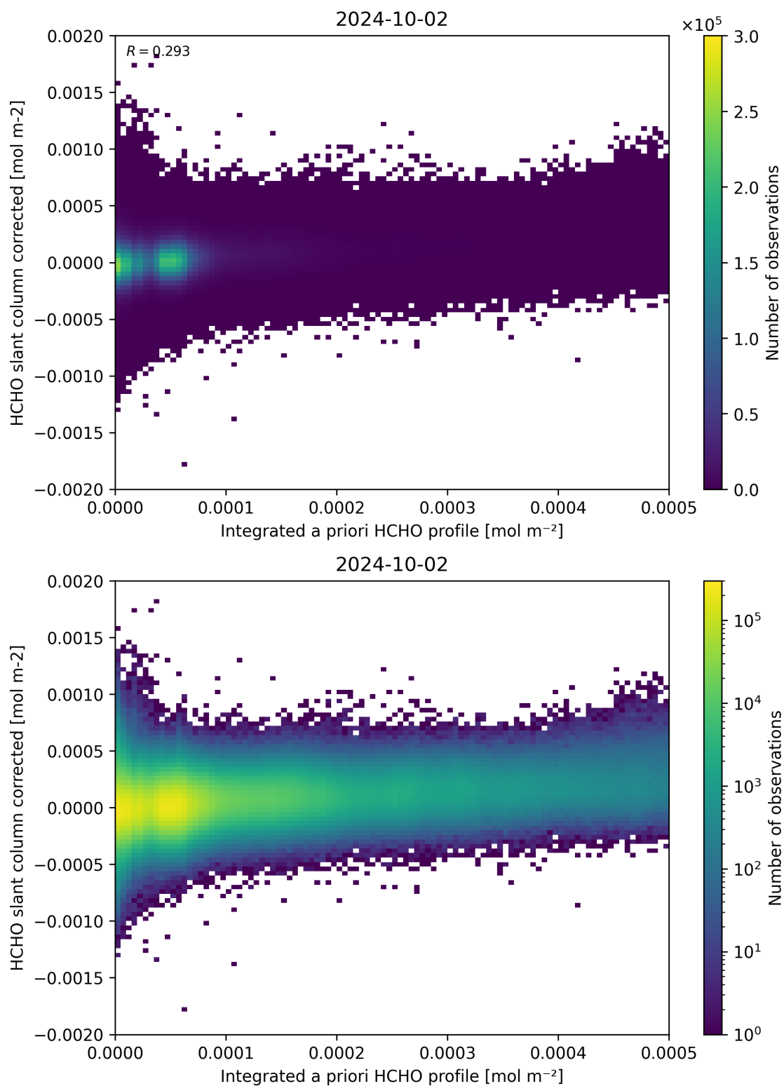
Figure 151: Scatter density plot of “Integrated a priori HCHO profile” against “HCHO slant column corrected” for 2024-10-01 to 2024-10-03.
