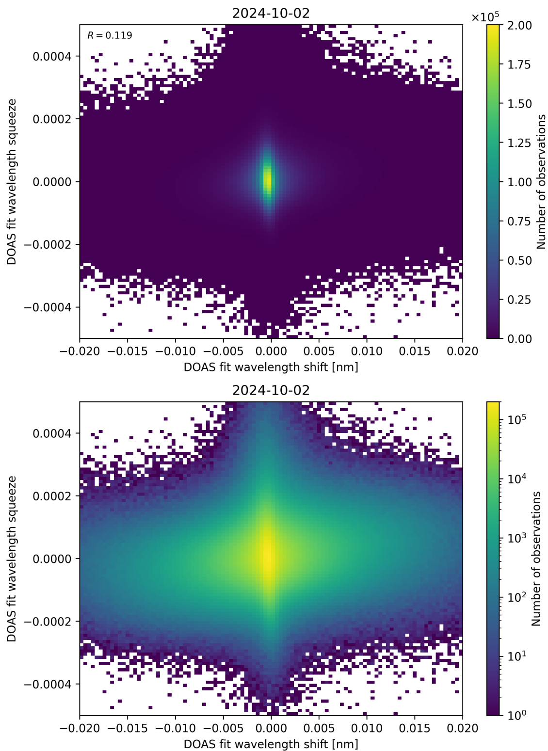
Figure 65: Scatter density plot of “DOAS fit wavelength shift” against “DOAS fit wavelength squeeze” for 2024-10-01 to 2024-10-03.
