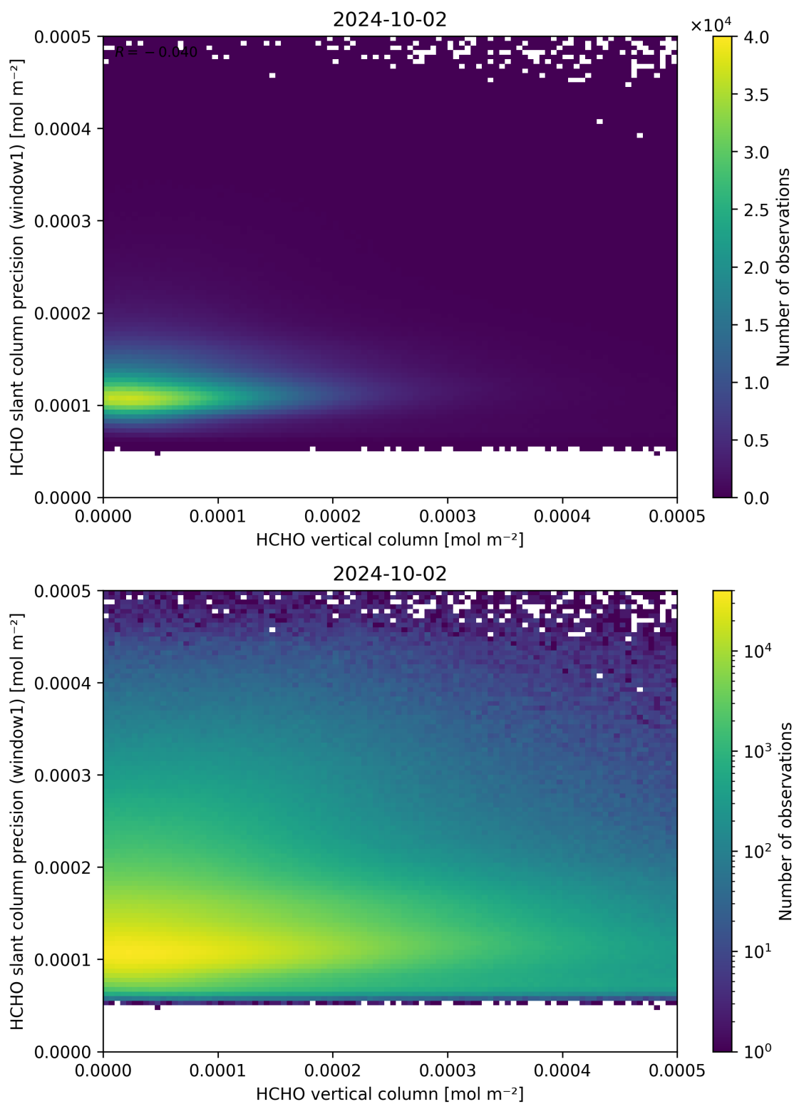
Figure 130: Scatter density plot of “HCHO vertical column” against “HCHO slant column precision (window1)” for 2024-10-01 to 2024-10-03.
