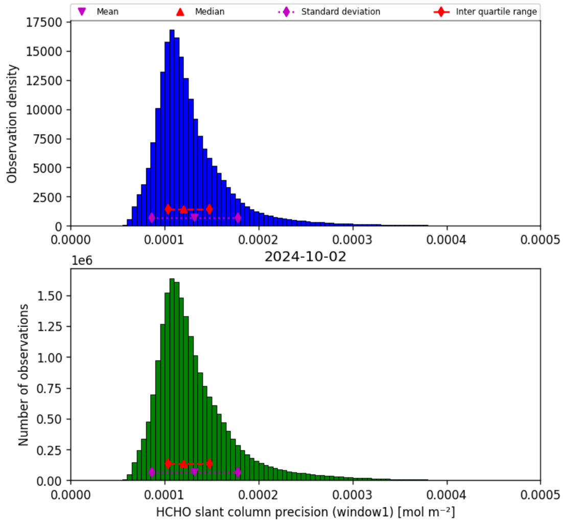
Figure 39: Histogram of “HCHO slant column precision (window1)” for 2024-10-01 to 2024-10-03
