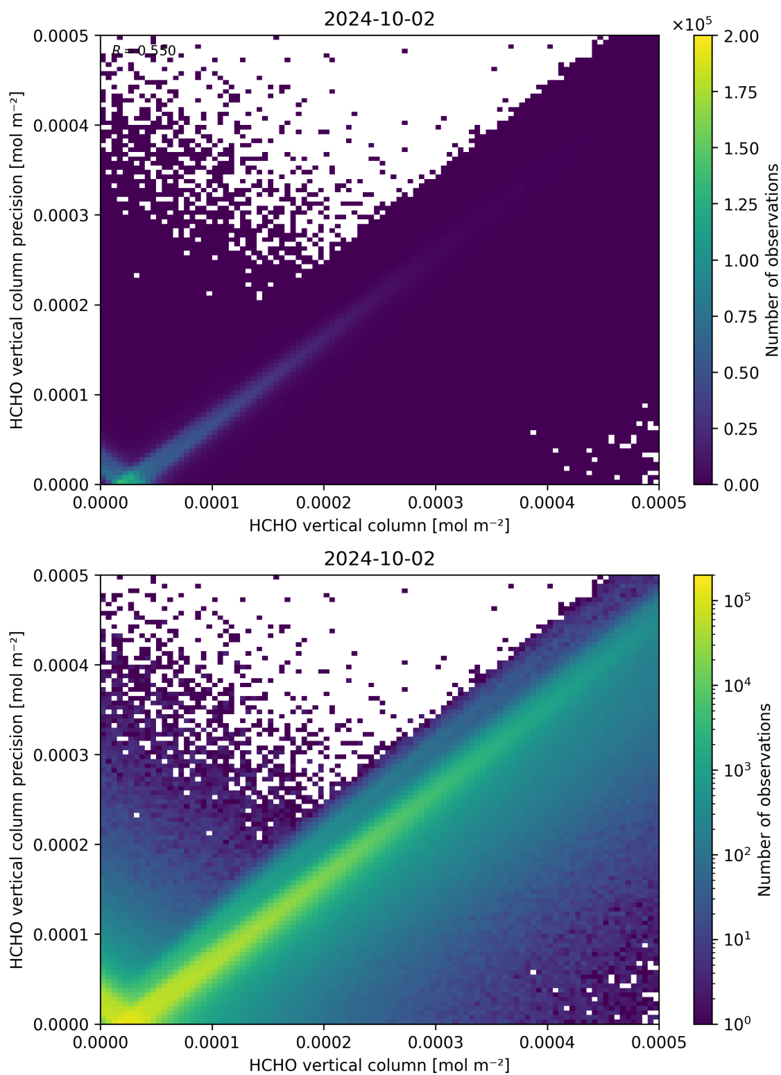
Figure 134: Scatter density plot of “HCHO vertical column” against “HCHO vertical column precision” for 2024-10-01 to 2024-10-03.
