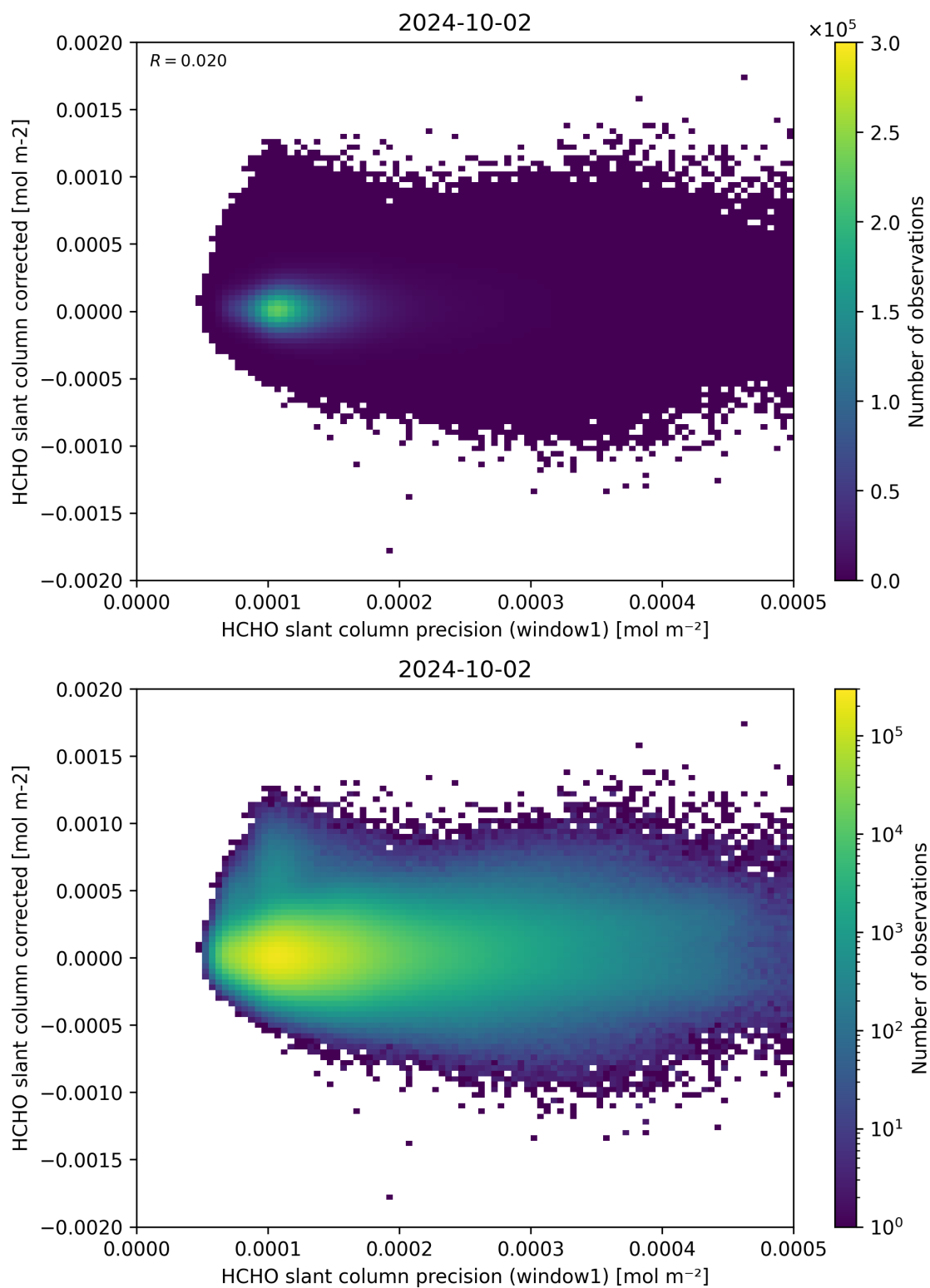
Figure 92: Scatter density plot of “HCHO slant column precision (window1)” against “HCHO slant column corrected” for 2024-10-01 to 2024-10-03.
