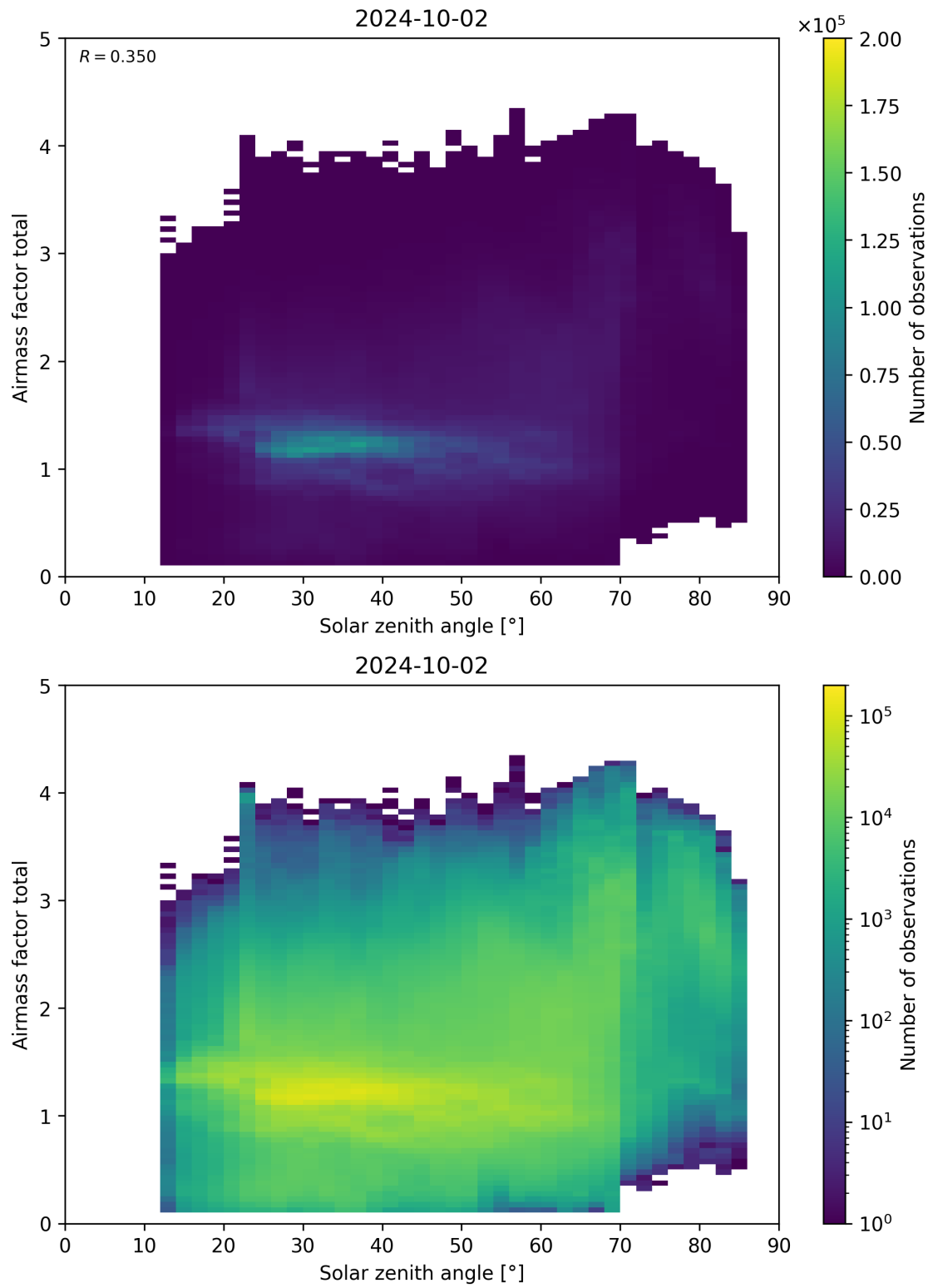
Figure 175: Scatter density plot of “Solar zenith angle” against “Airmass factor total” for 2024-10-01 to 2024-10-03.
