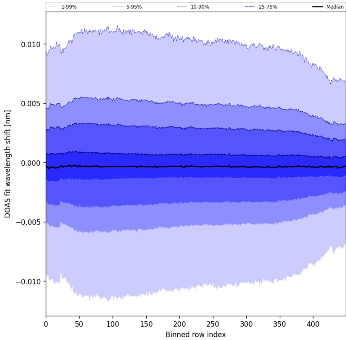
Figure 58: Along track statistics of “DOAS fit wavelength shift” for 2024-10-01 to 2024-10-03
