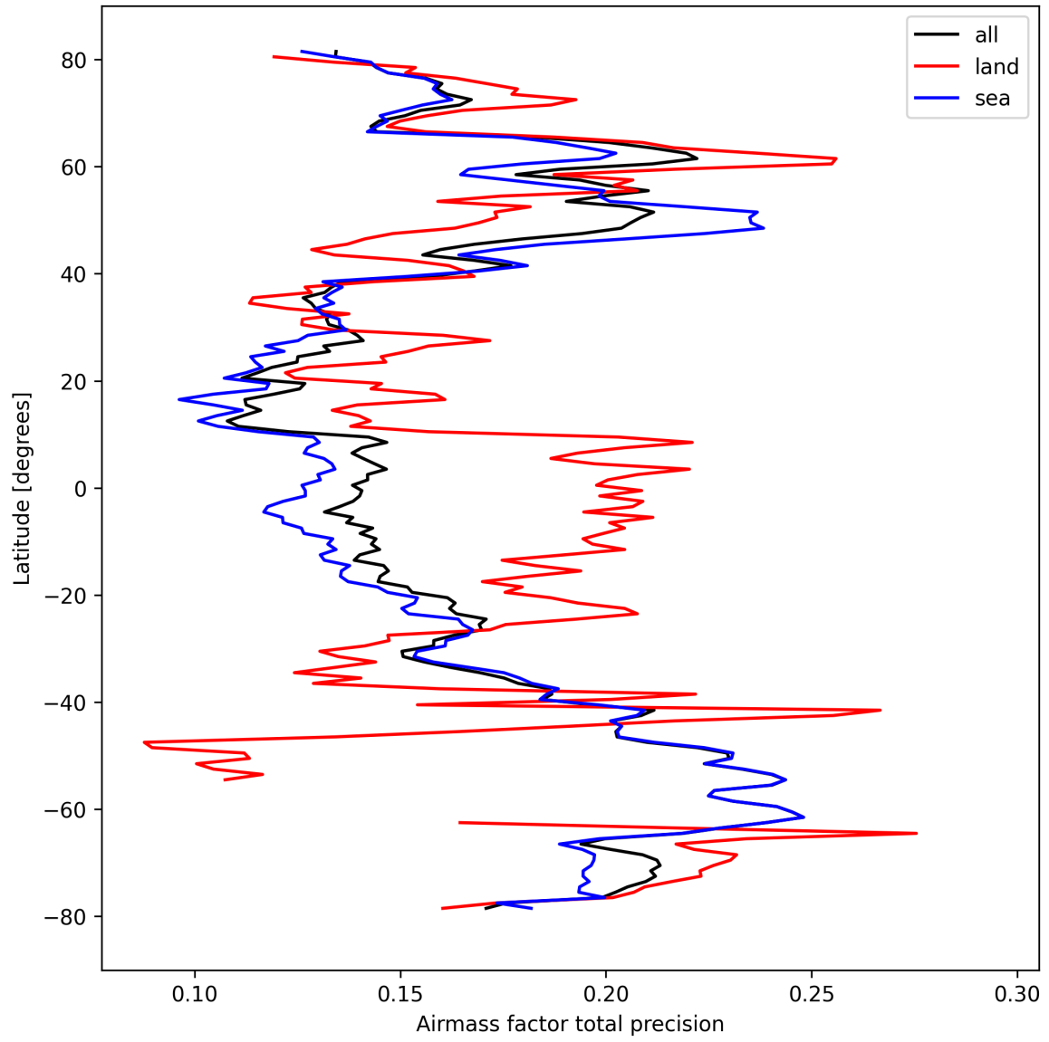
Figure 27: Zonal average of “Airmass factor total precision” for 2024-10-01 to 2024-10-03.
