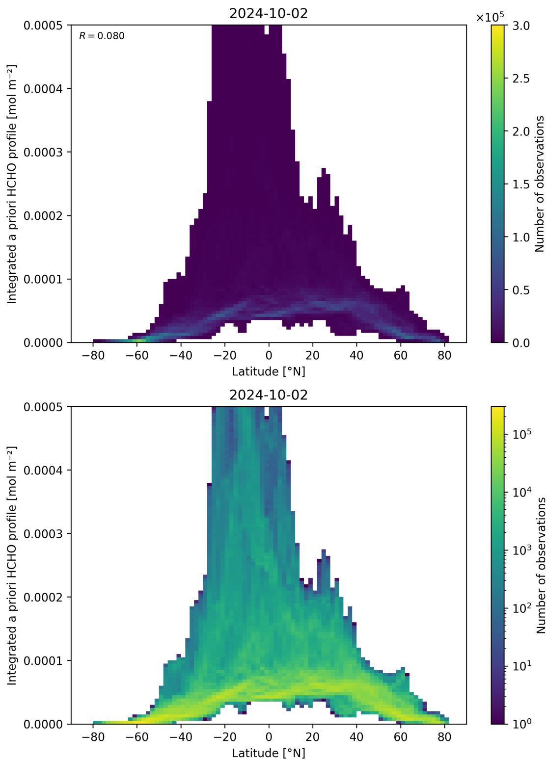
Figure 166: Scatter density plot of “Latitude” against “Integrated a priori HCHO profile” for 2024-10-01 to 2024-10-03.
