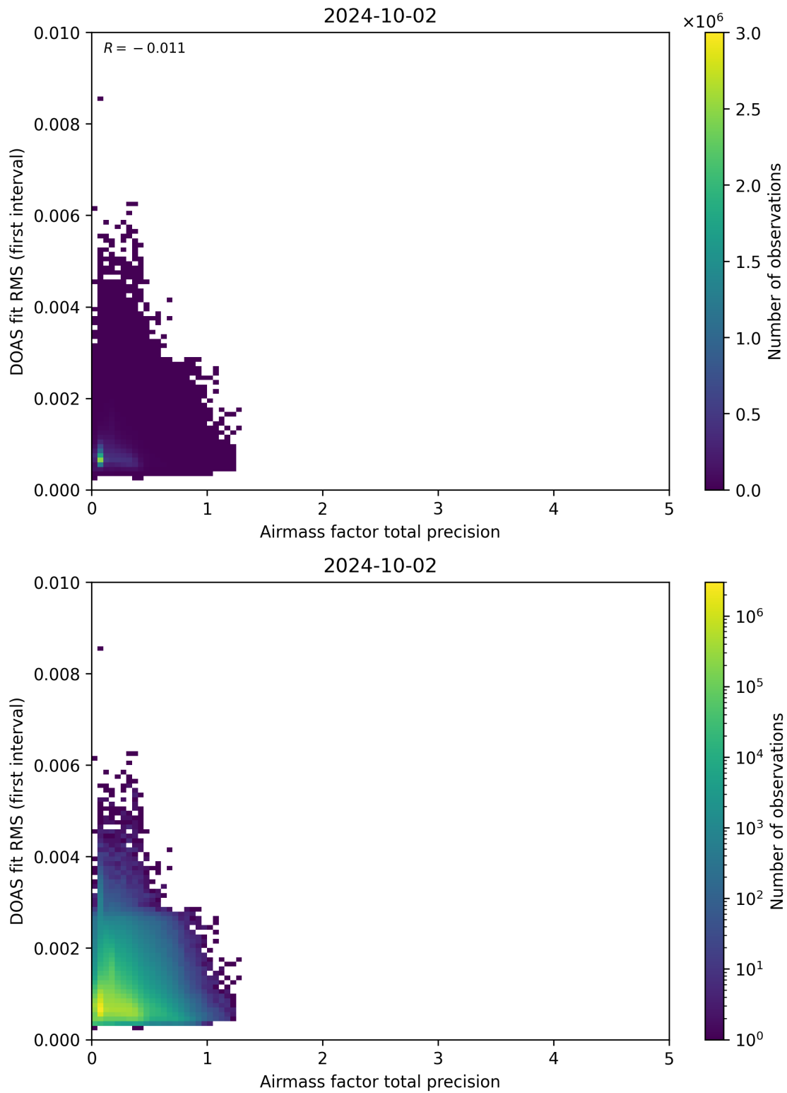
Figure 105: Scatter density plot of “Airmass factor total precision” against “DOAS fit RMS (first interval)” for 2024-10-01 to 2024-10-03.
