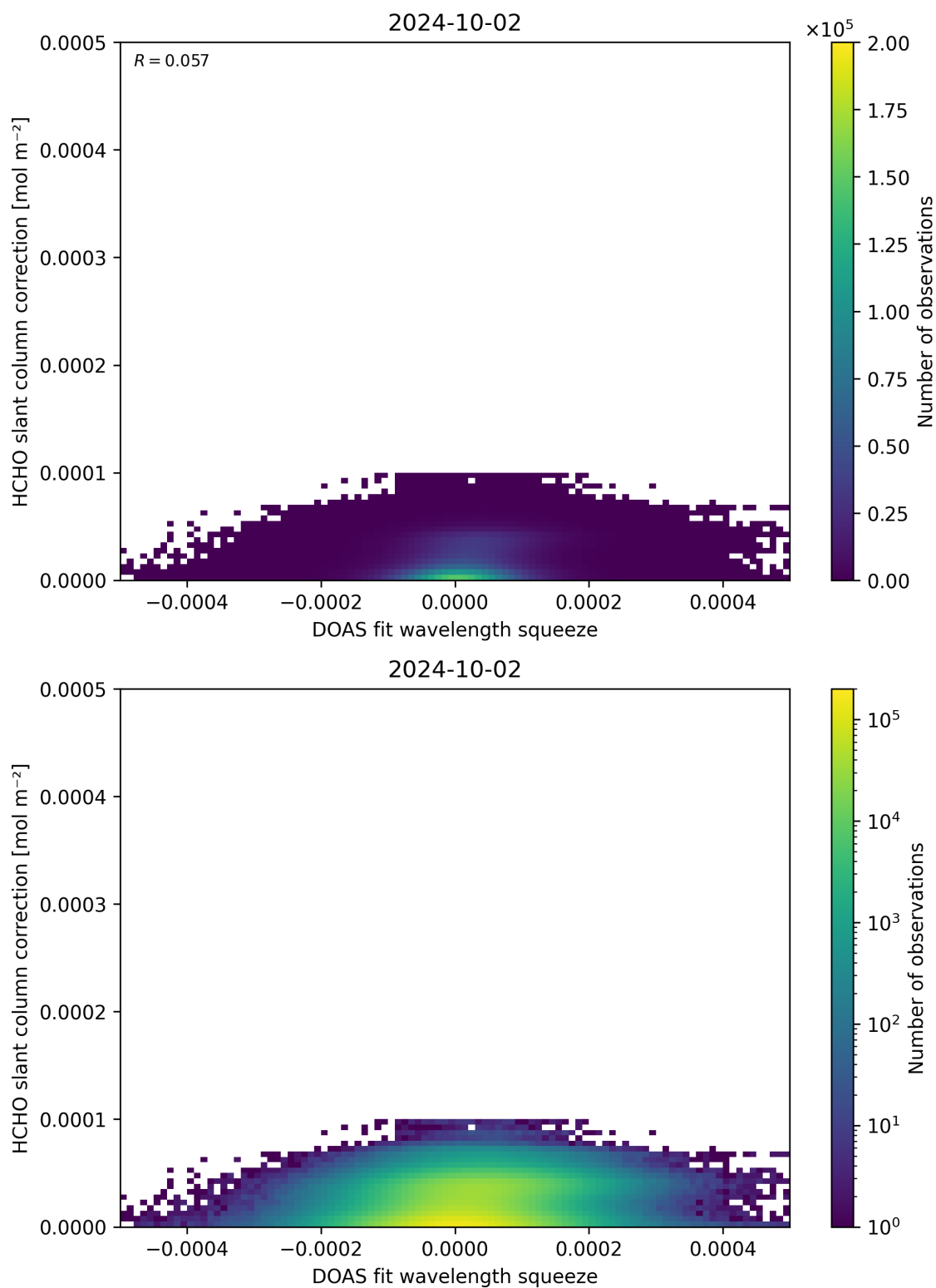
Figure 70: Scatter density plot of “DOAS fit wavelength squeeze” against “HCHO slant column correction” for 2024-10-01 to 2024-10-03.
