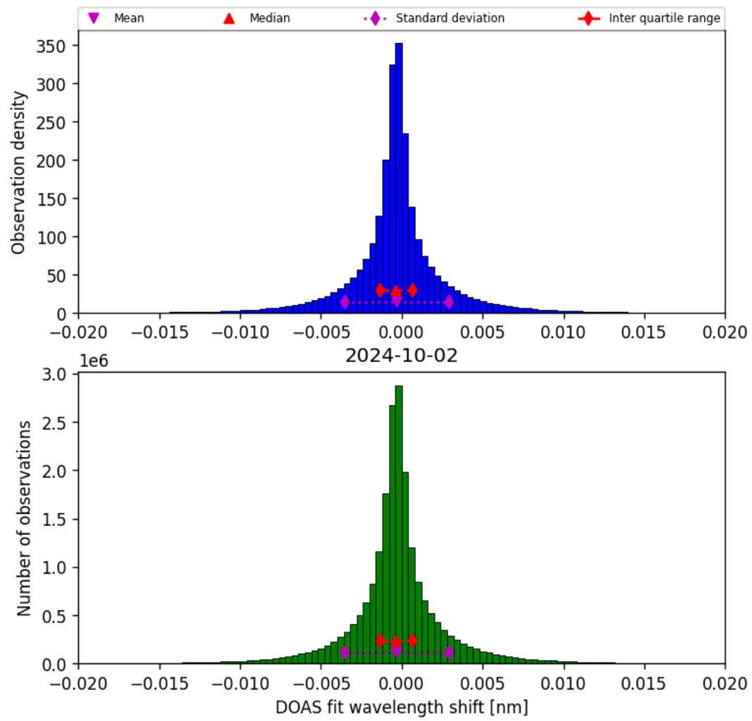
Figure 44: Histogram of “DOAS fit wavelength shift” for 2024-10-01 to 2024-10-03
