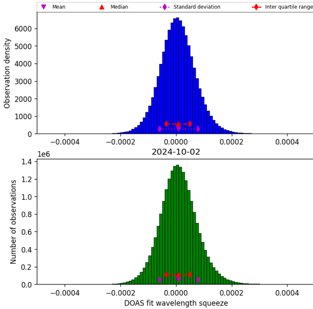
Figure 45: Histogram of “DOAS fit wavelength squeeze” for 2024-10-01 to 2024-10-03
