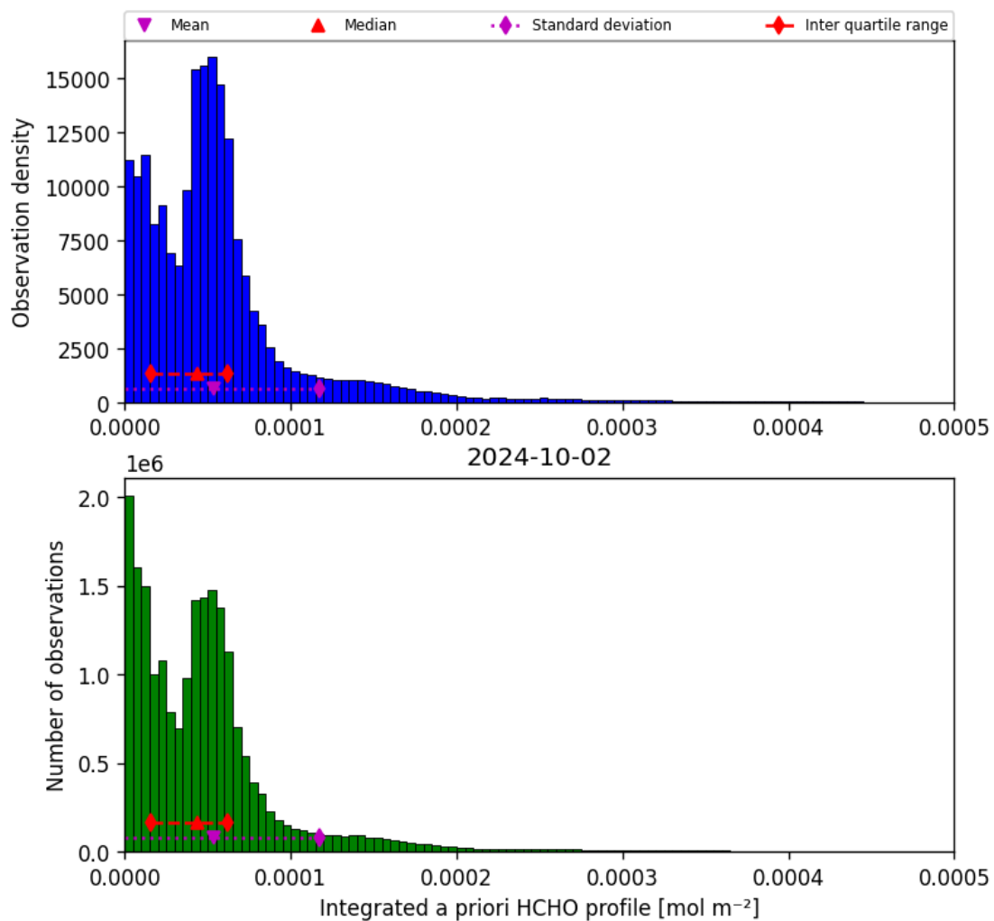
Figure 43: Histogram of “Integrated a priori HCHO profile” for 2024-10-01 to 2024-10-03
