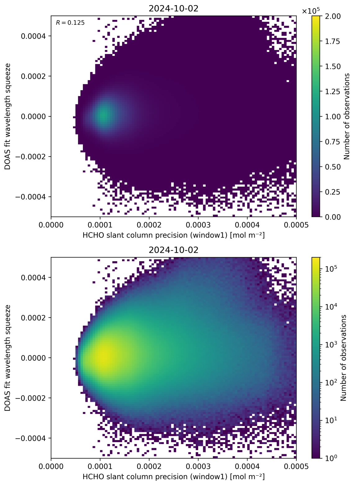
Figure 90: Scatter density plot of “HCHO slant column precision (window1)” against “DOAS fit wavelength squeeze” for 2024-10-01 to 2024-10-03.
