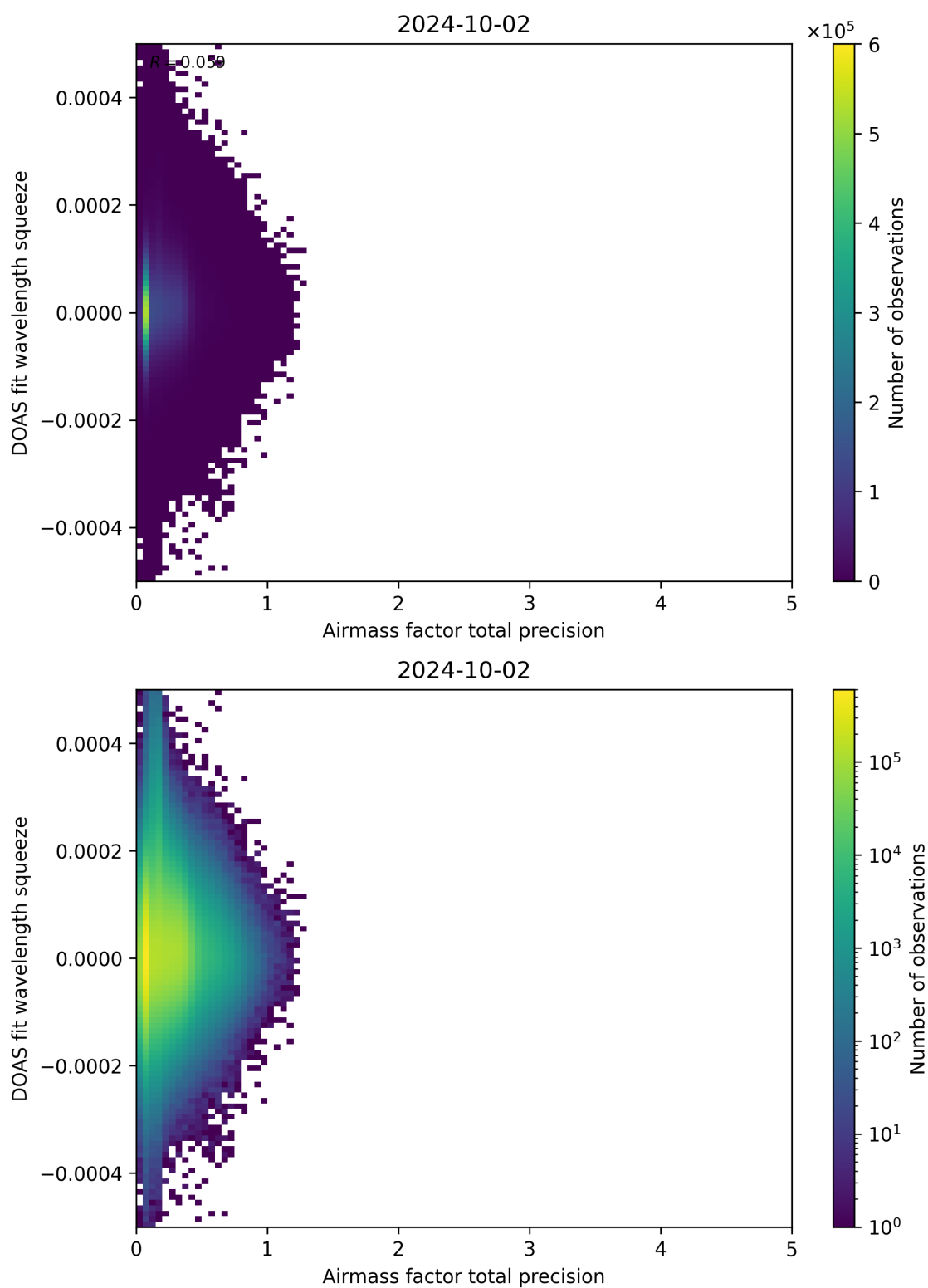
Figure 107: Scatter density plot of “Airmass factor total precision” against “DOAS fit wavelength squeeze” for 2024-10-01 to 2024-10-03.
