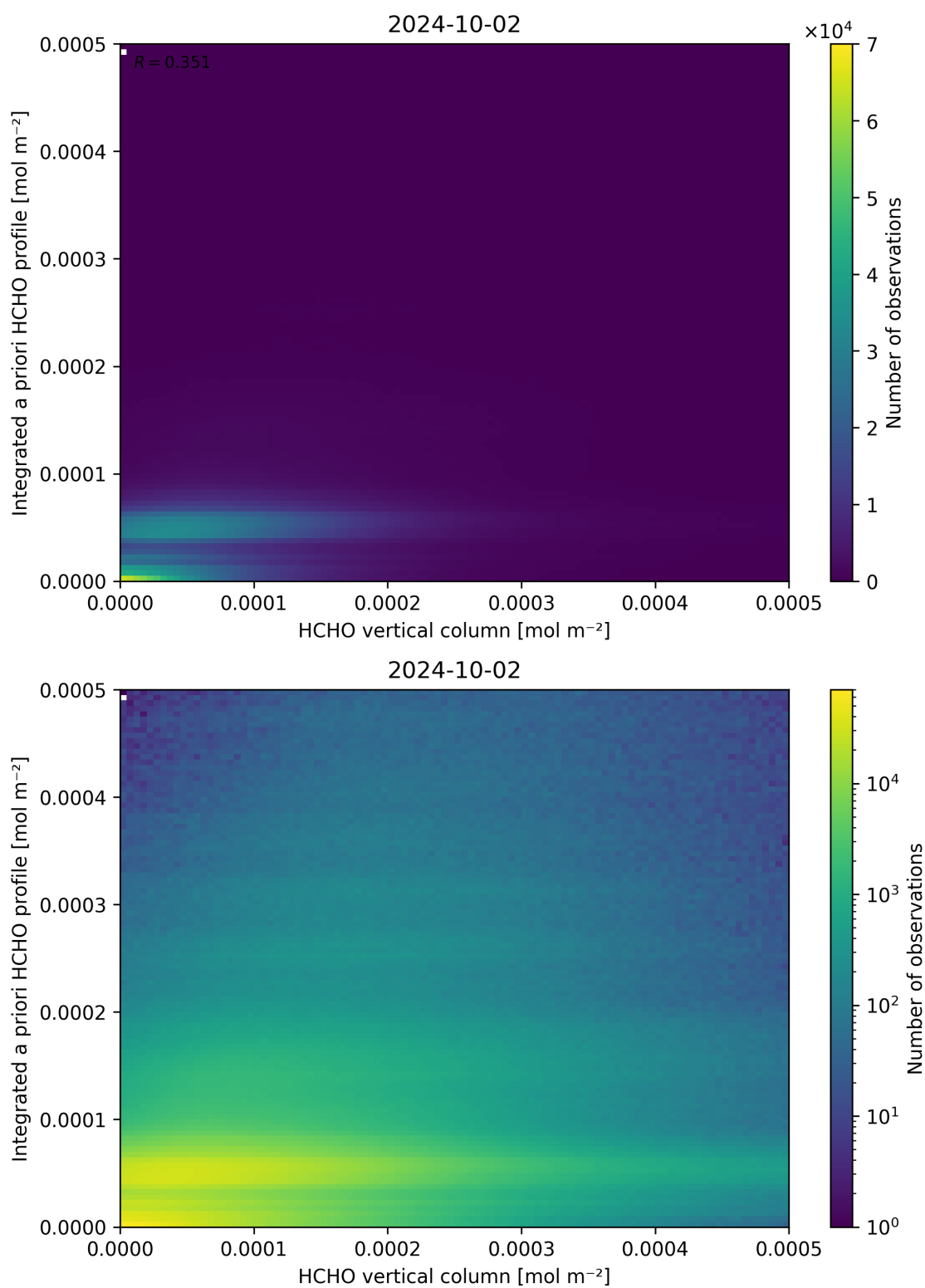
Figure 135: Scatter density plot of “HCHO vertical column” against “Integrated a priori HCHO profile” for 2024-10-01 to 2024-10-03.
