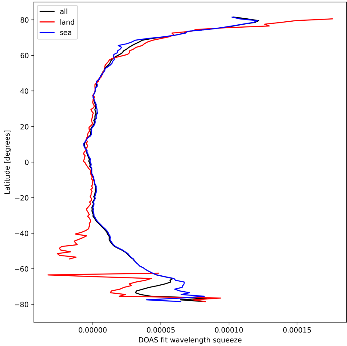
Figure 31: Zonal average of “DOAS fit wavelength squeeze” for 2024-10-01 to 2024-10-03.
