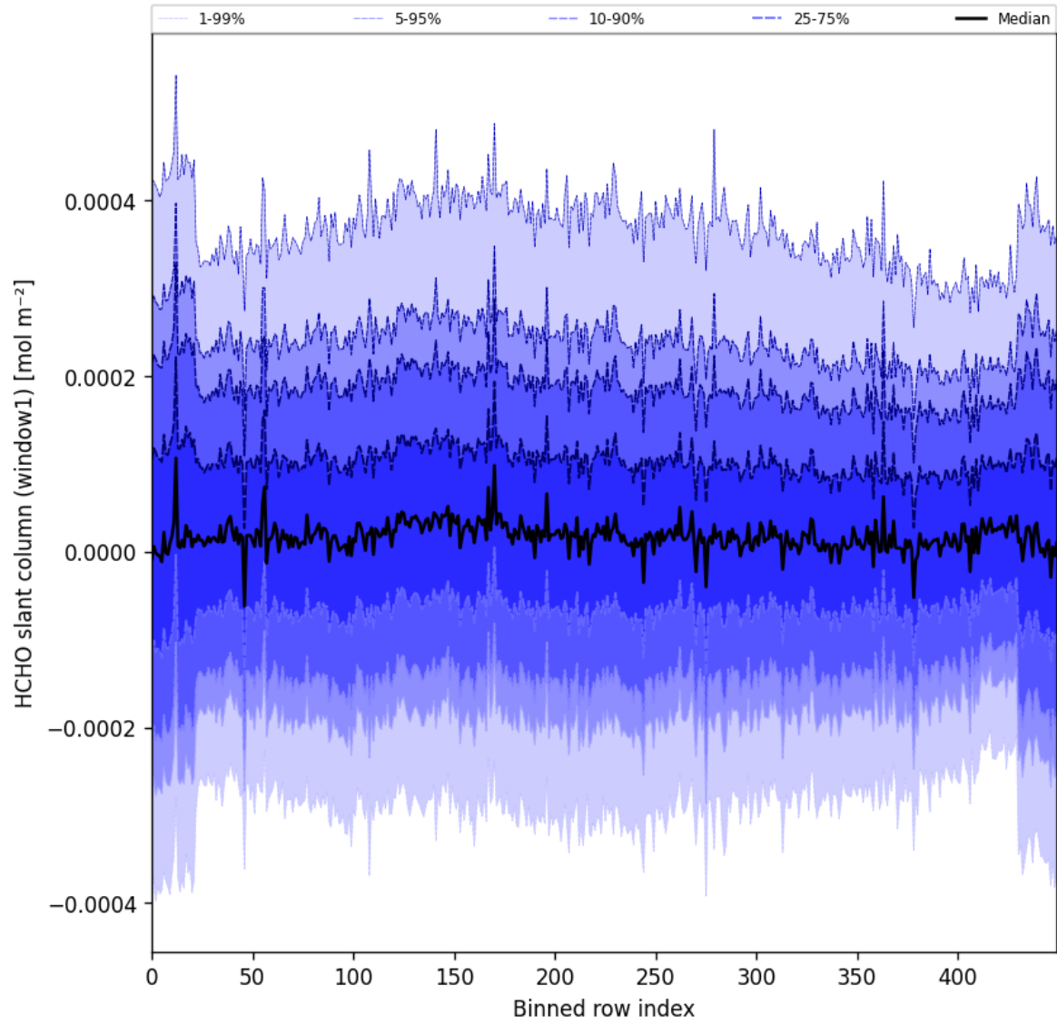
Figure 52: Along track statistics of “HCHO slant column (window1)” for 2024-10-01 to 2024-10-03
