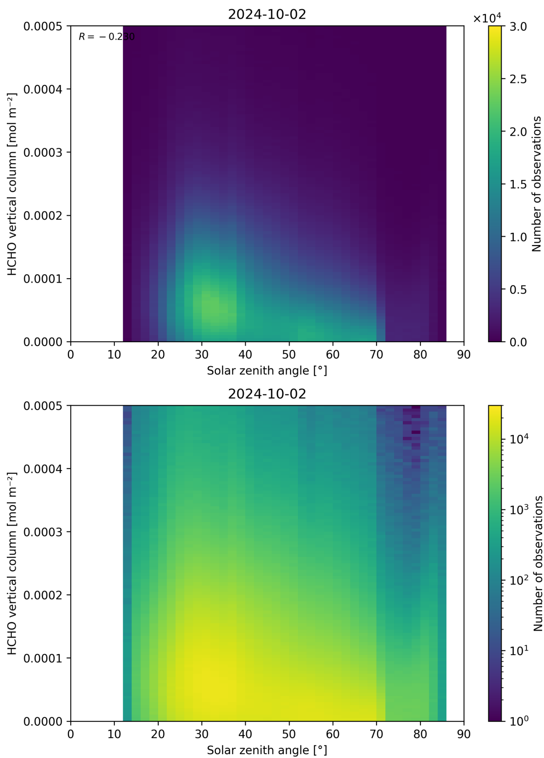
Figure 177: Scatter density plot of “Solar zenith angle” against “HCHO vertical column” for 2024-10-01 to 2024-10-03.
