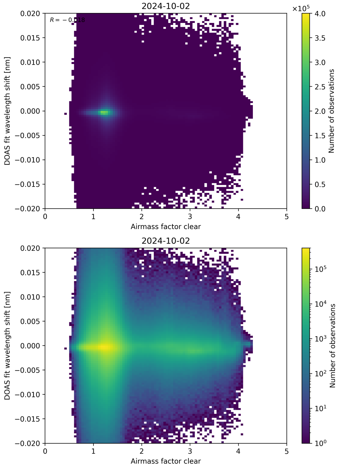
Figure 72: Scatter density plot of “Airmass factor clear” against “DOAS fit wavelength shift” for 2024-10-01 to 2024-10-03.
