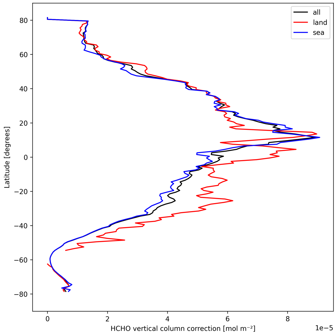
Figure 23: Zonal average of “HCHO vertical column correction” for 2024-10-01 to 2024-10-03.
