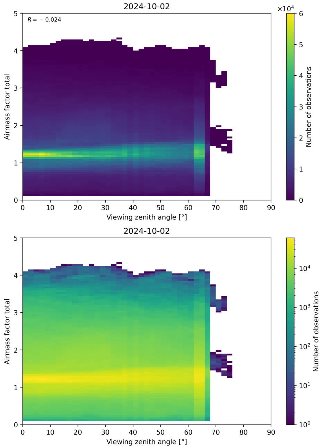
Figure 190: Scatter density plot of “Viewing zenith angle” against “Airmass factor total” for 2024-10-01 to 2024-10-03.
