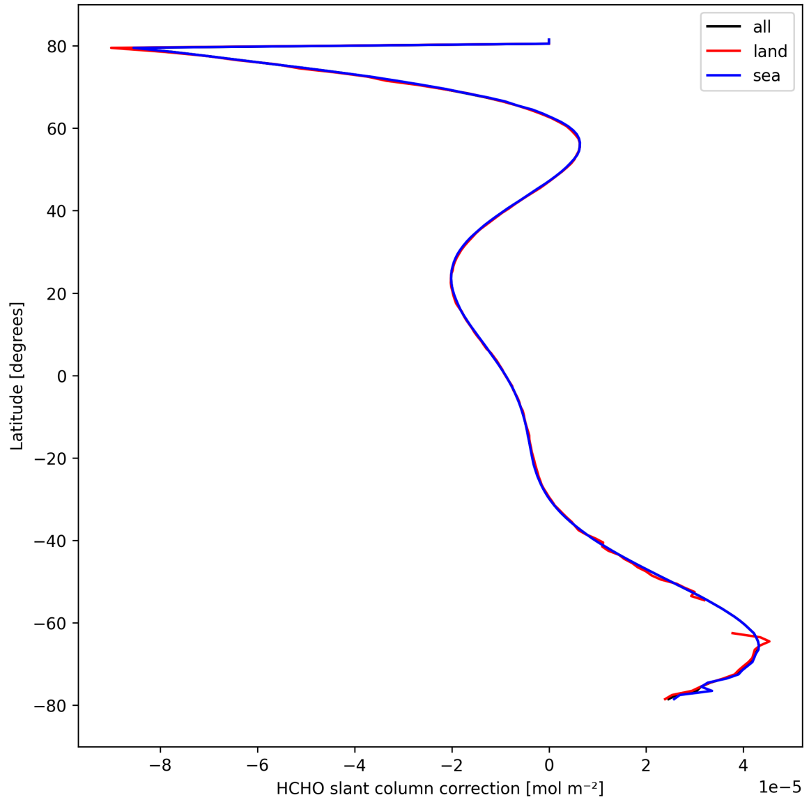
Figure 33: Zonal average of “HCHO slant column correction” for 2024-10-01 to 2024-10-03.
