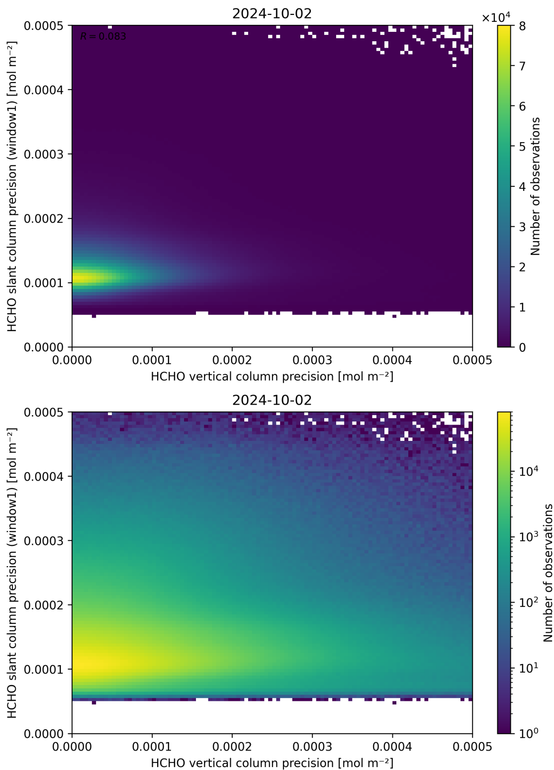
Figure 143: Scatter density plot of “HCHO vertical column precision” against “HCHO slant column precision (window1)” for 2024-10-01 to 2024-10-03.
