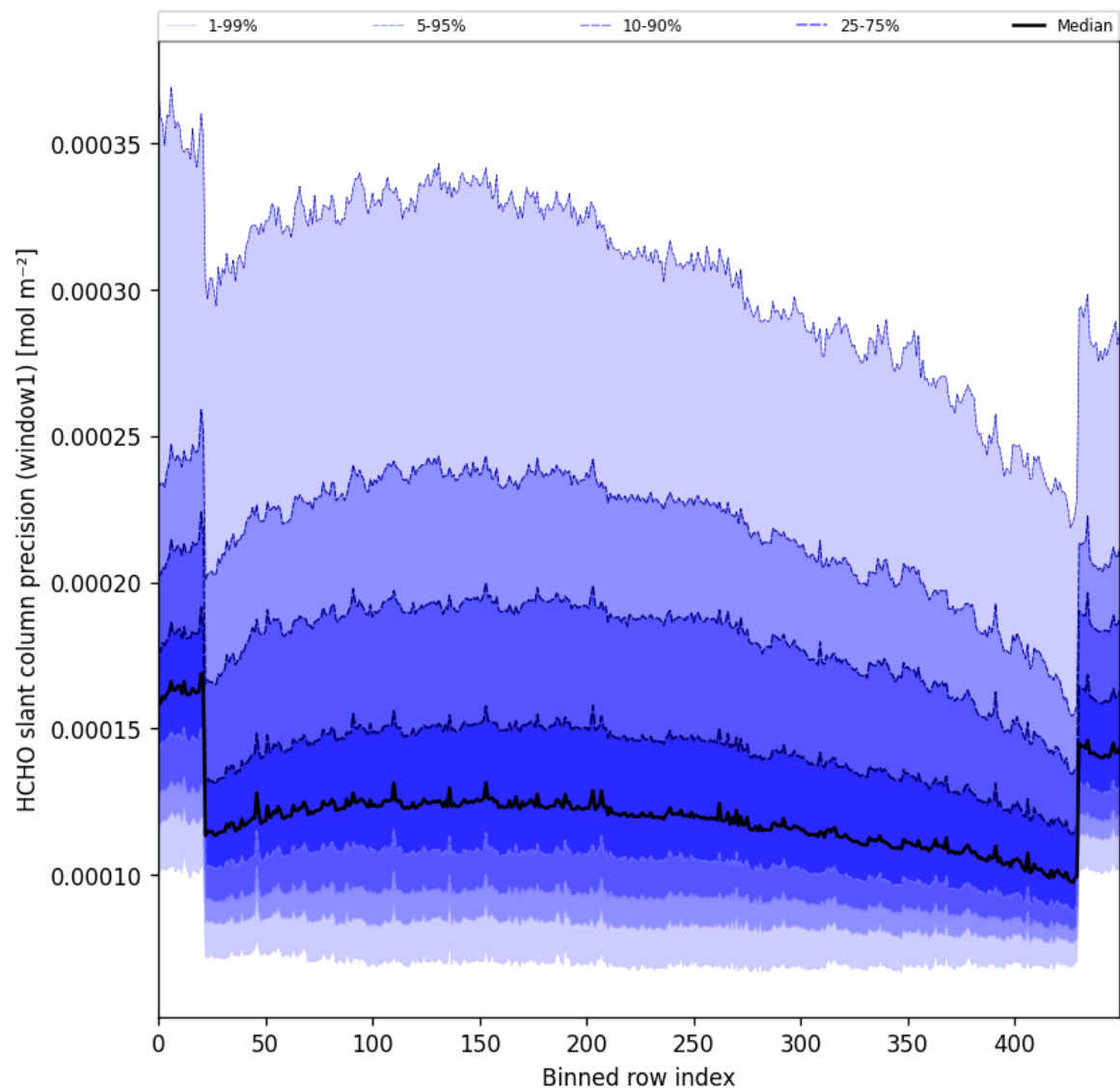
Figure 53: Along track statistics of “HCHO slant column precision (window1)” for 2024-10-01 to 2024-10-03
