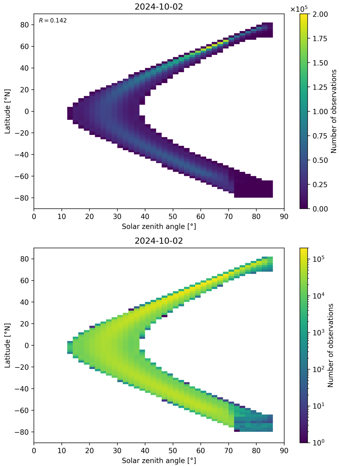
Figure 181: Scatter density plot of “Solar zenith angle” against “Latitude” for 2024-10-01 to 2024-10-03.
