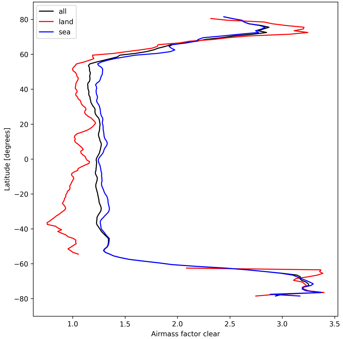
Figure 28: Zonal average of “Airmass factor clear” for 2024-10-01 to 2024-10-03.
