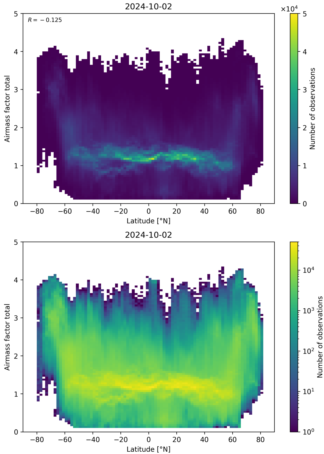
Figure 161: Scatter density plot of “Latitude” against “Airmass factor total” for 2024-10-01 to 2024-10-03.
