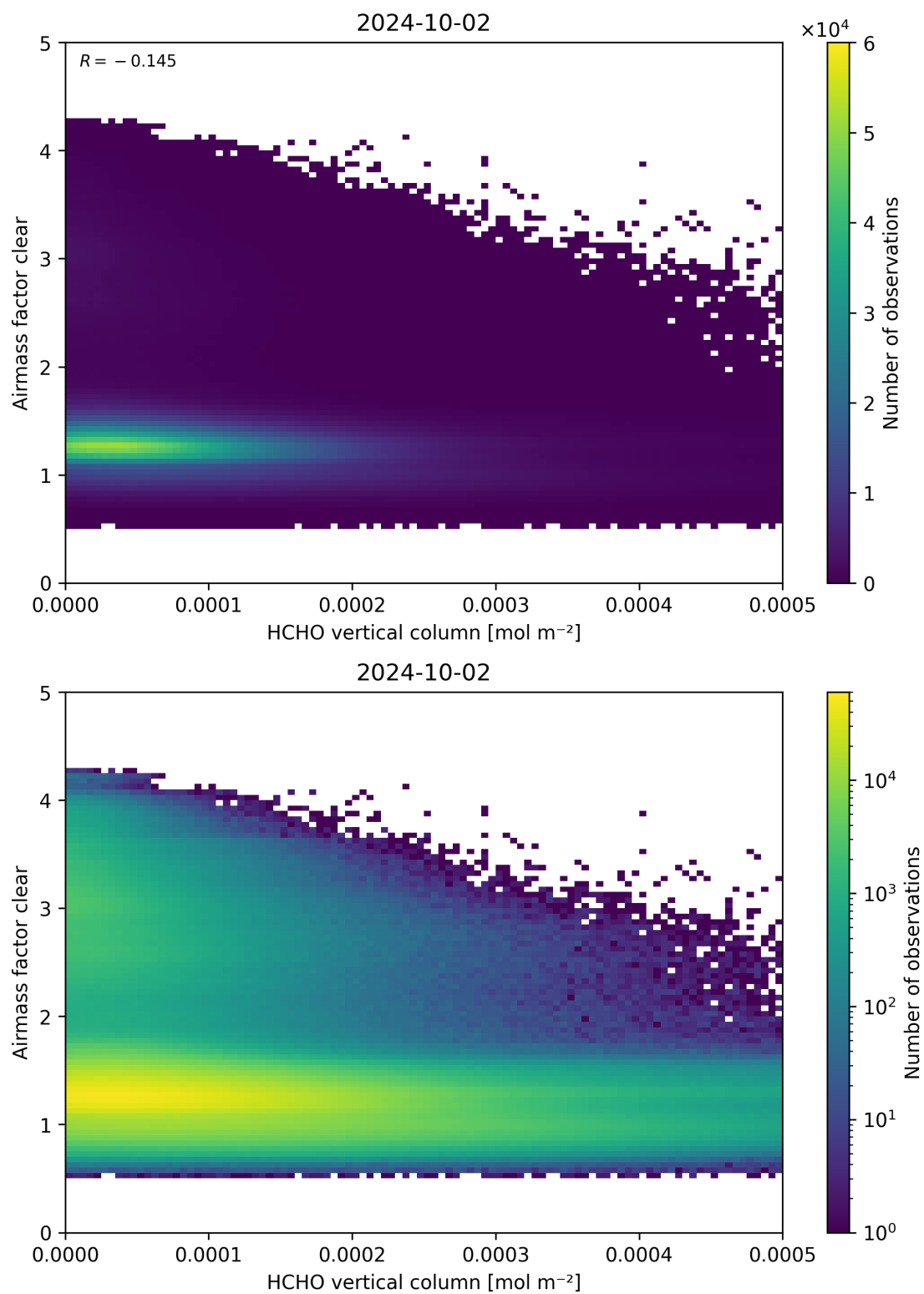
Figure 126: Scatter density plot of “HCHO vertical column” against “Airmass factor clear” for 2024-10-01 to 2024-10-03.
