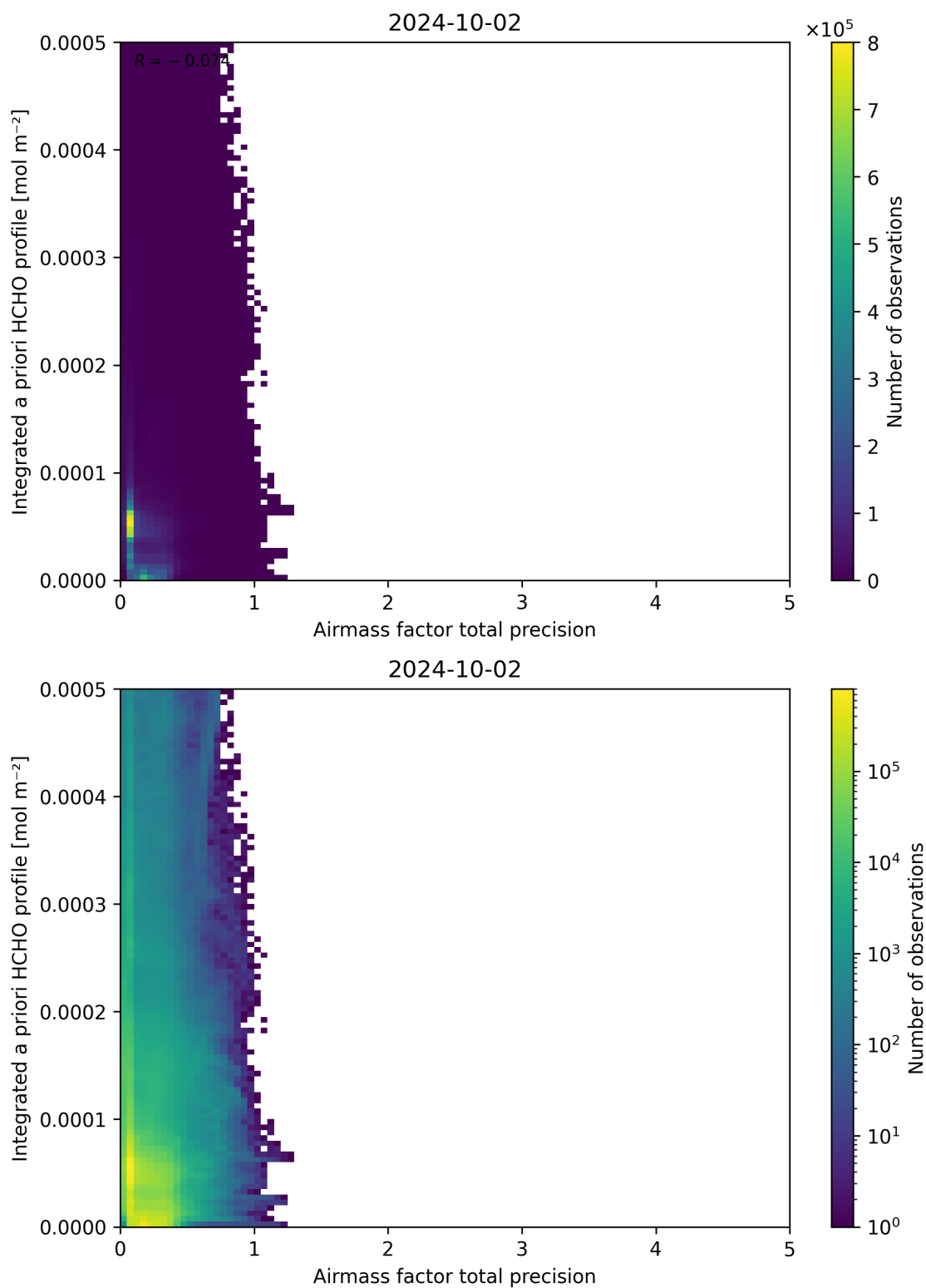
Figure 111: Scatter density plot of “Airmass factor total precision” against “Integrated a priori HCHO profile” for 2024-10-01 to 2024-10-03.
