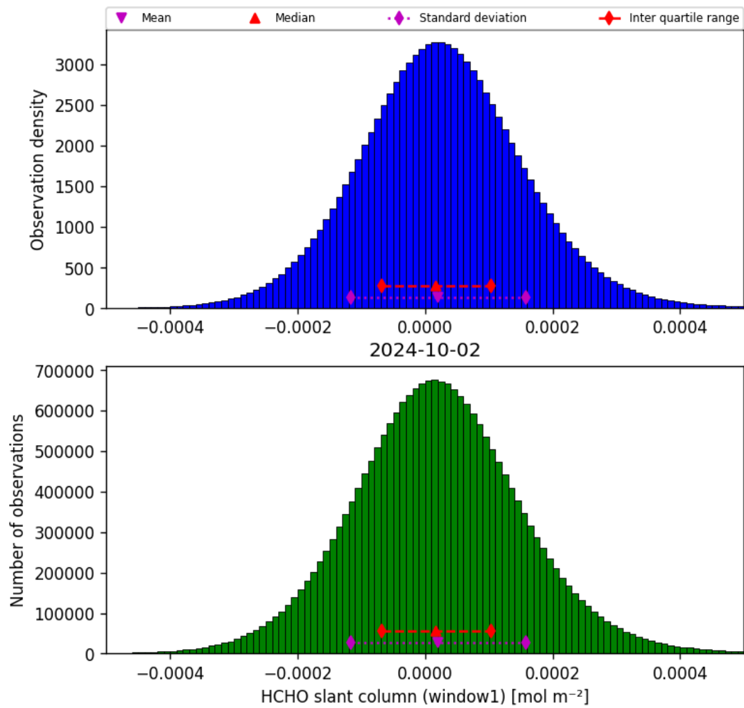
Figure 38: Histogram of “HCHO slant column (window1)” for 2024-10-01 to 2024-10-03
