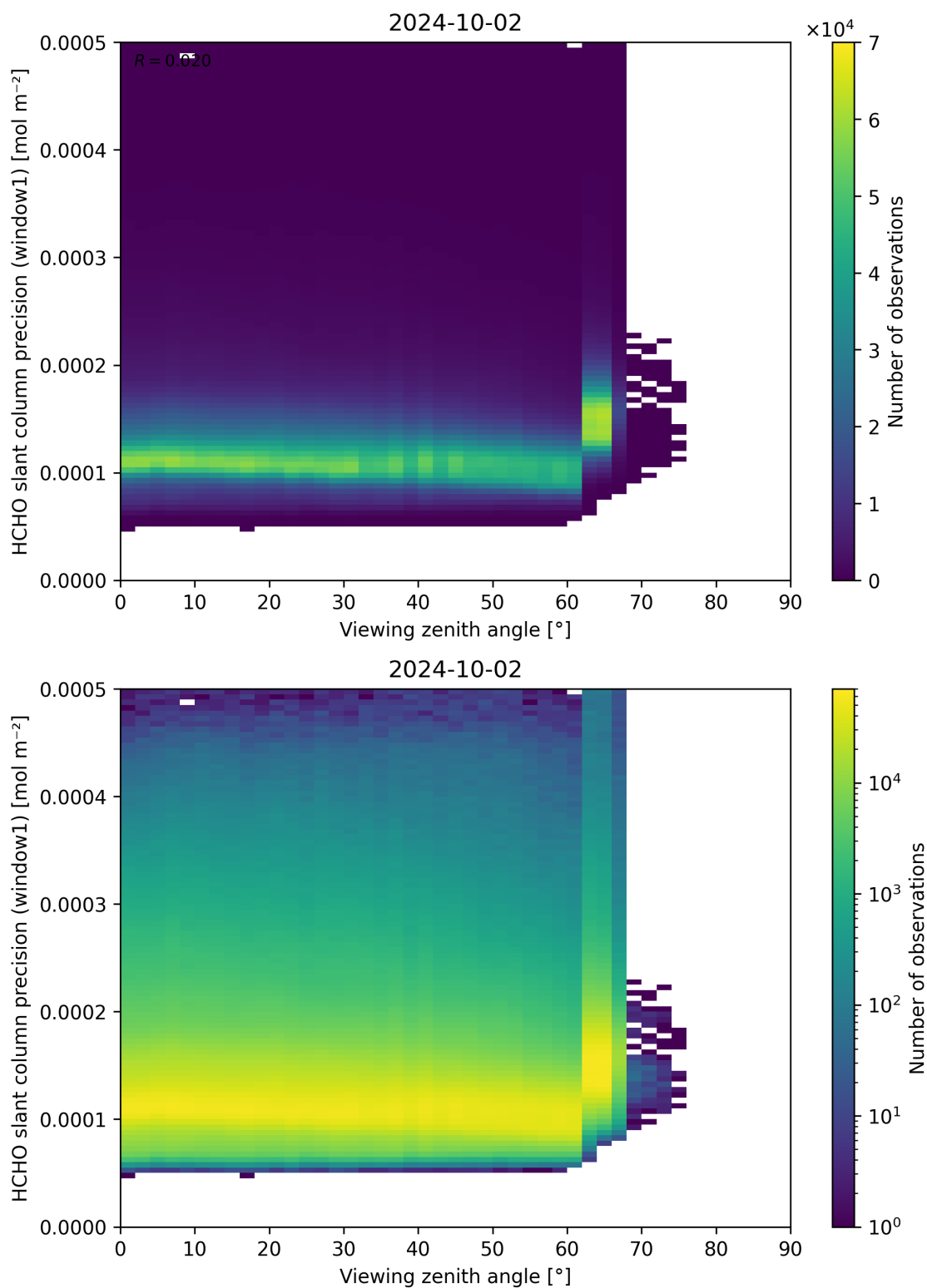
Figure 189: Scatter density plot of “Viewing zenith angle” against “HCHO slant column precision (window1)” for 2024-10-01 to 2024-10-03.
