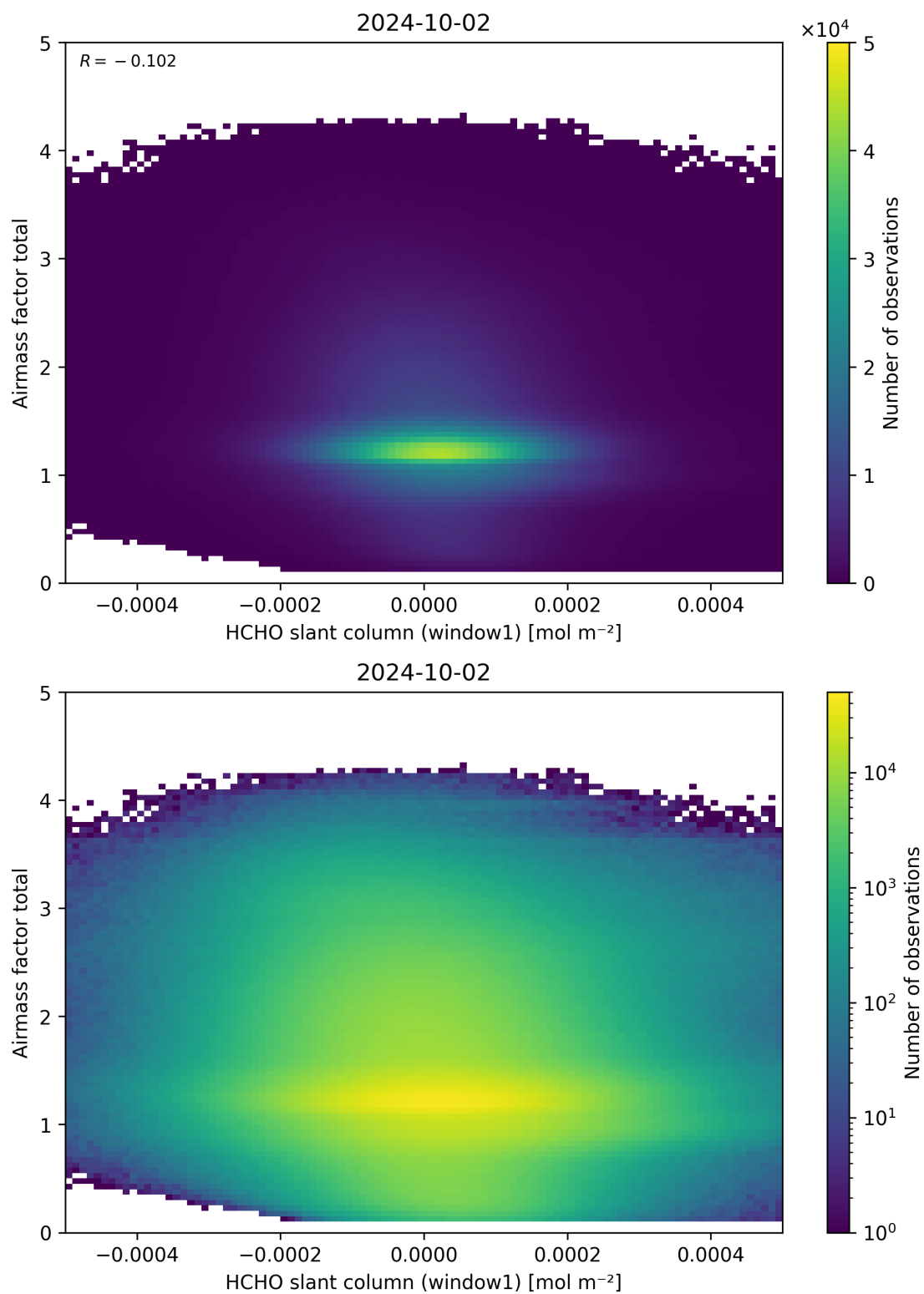
Figure 85: Scatter density plot of “HCHO slant column (window1)” against “Airmass factor total” for 2024-10-01 to 2024-10-03.
