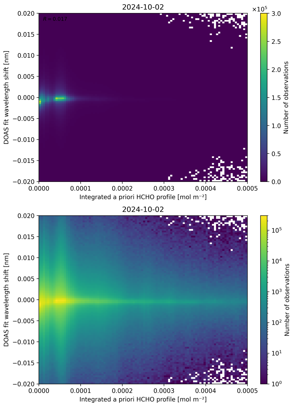
Figure 149: Scatter density plot of “Integrated a priori HCHO profile” against “DOAS fit wavelength shift” for 2024-10-01 to 2024-10-03.
