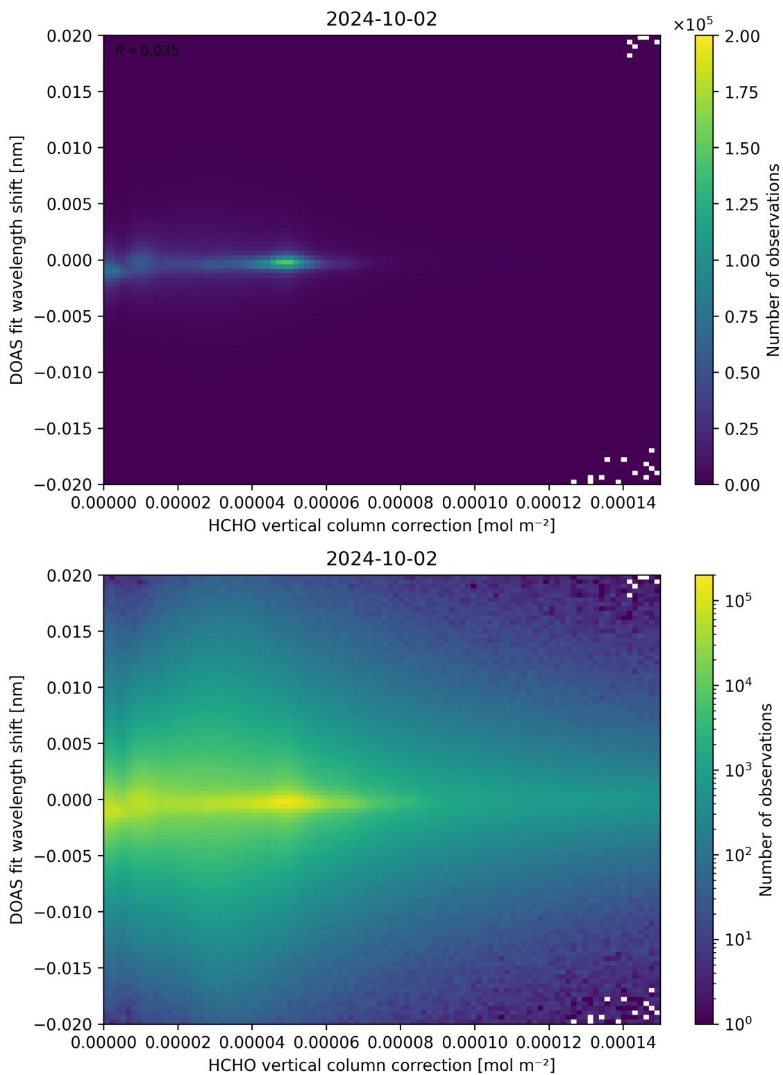
Figure 113: Scatter density plot of “HCHO vertical column correction” against “DOAS fit wavelength shift” for 2024-10-01 to 2024-10-03.
