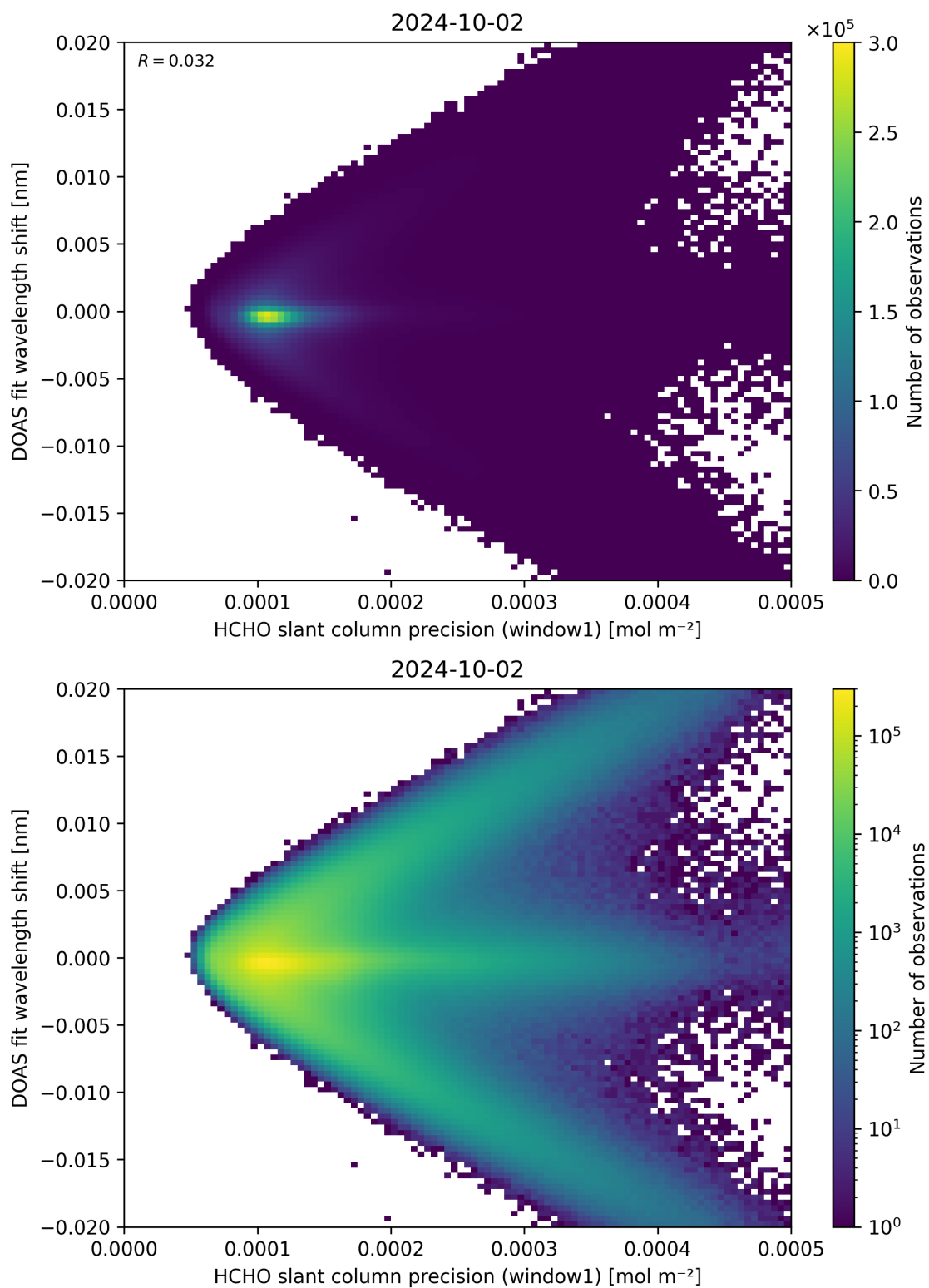
Figure 89: Scatter density plot of “HCHO slant column precision (window1)” against “DOAS fit wavelength shift” for 2024-10-01 to 2024-10-03.
