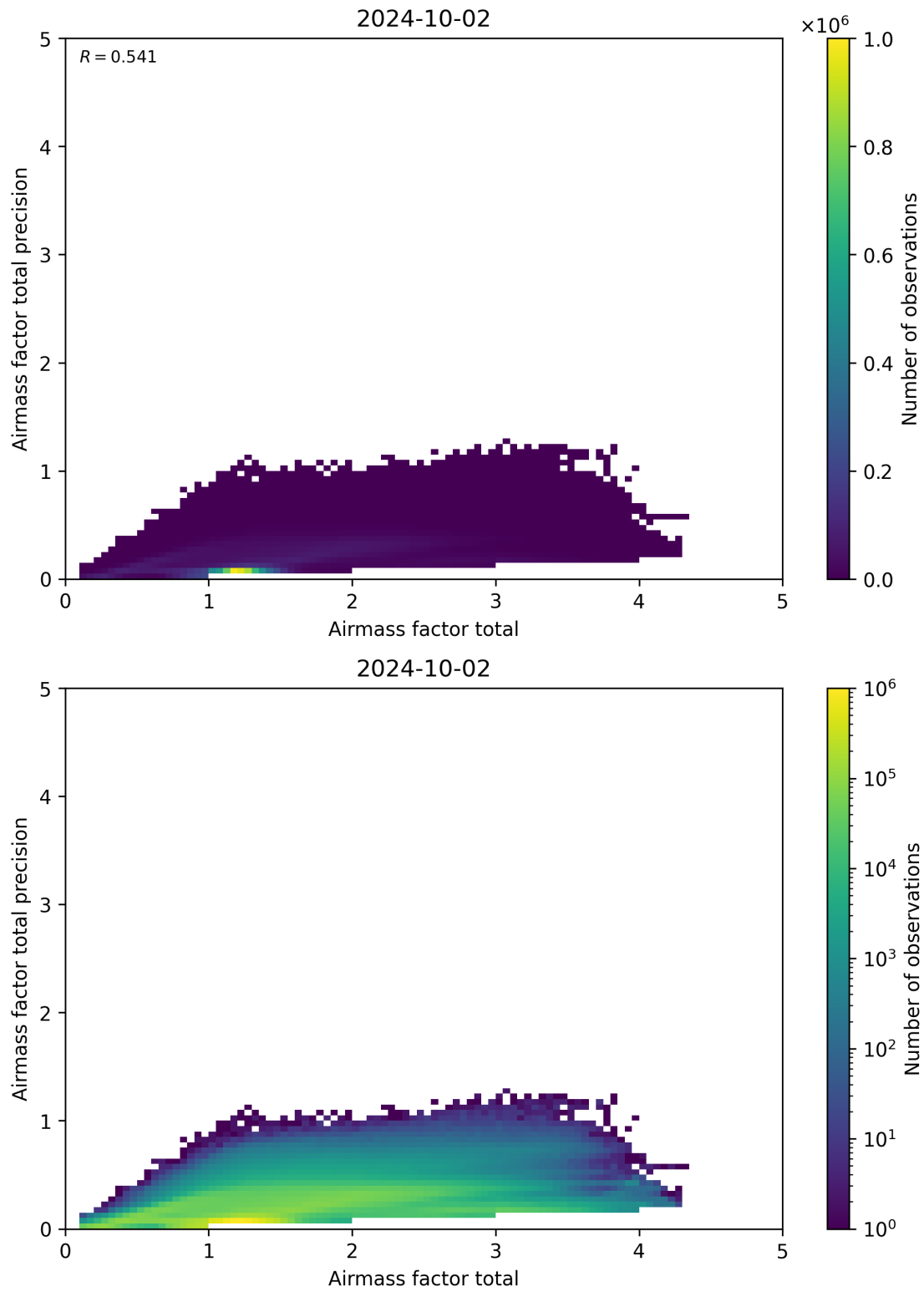
Figure 103: Scatter density plot of “Airmass factor total” against “Airmass factor total precision” for 2024-10-01 to 2024-10-03.
