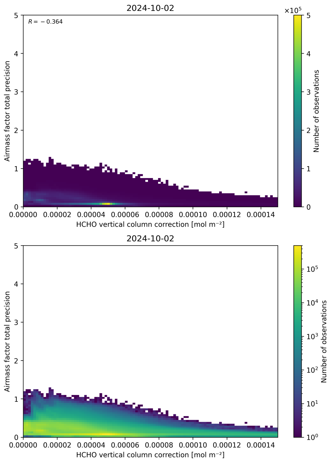
Figure 121: Scatter density plot of “HCHO vertical column correction” against “Airmass factor total precision” for 2024-10-01 to 2024-10-03.
