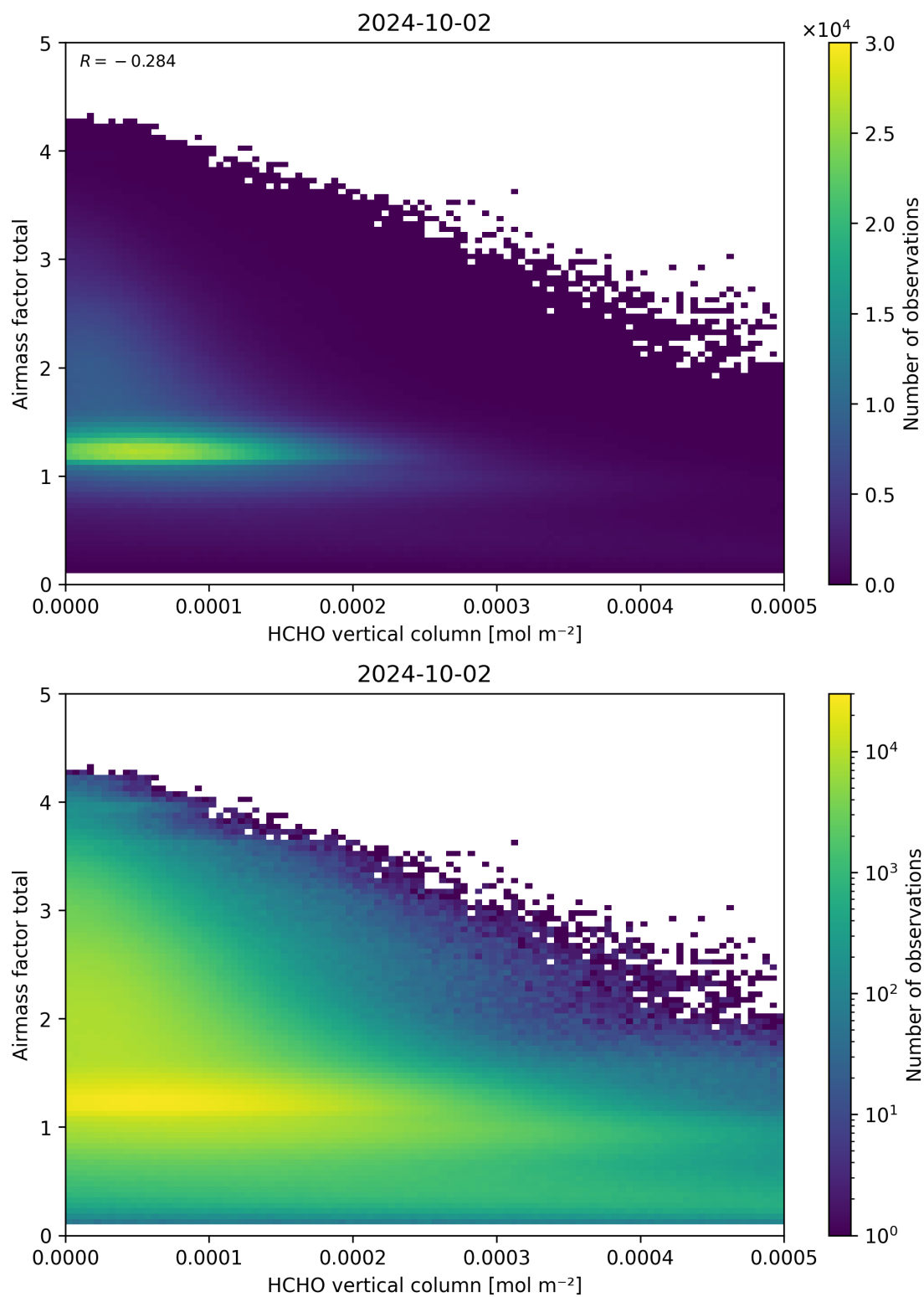
Figure 131: Scatter density plot of “HCHO vertical column” against “Airmass factor total” for 2024-10-01 to 2024-10-03.
