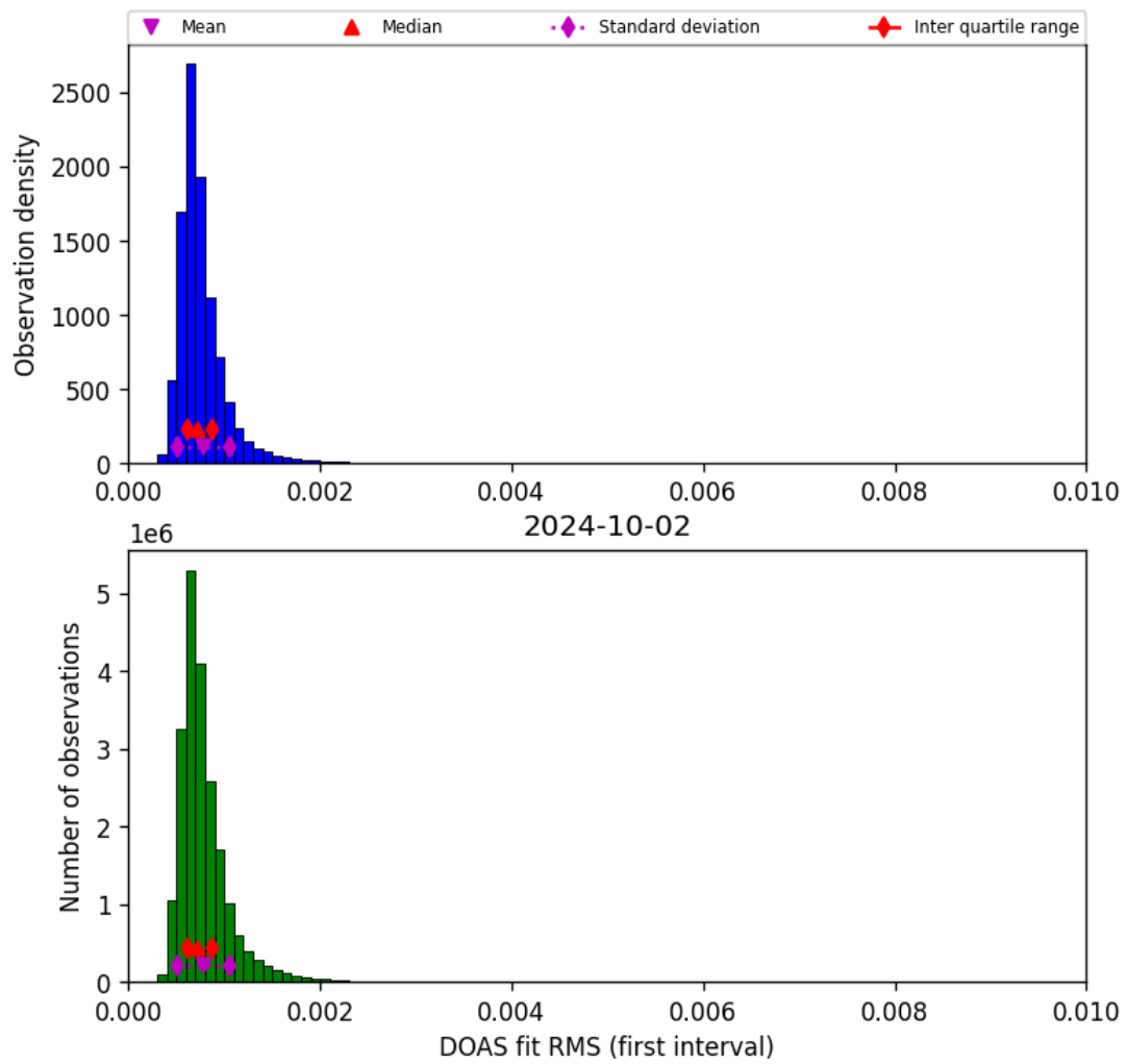
Figure 46: Histogram of “DOAS fit RMS (first interval)” for 2024-10-01 to 2024-10-03
