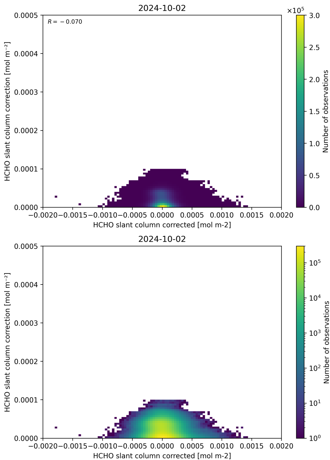
Figure 77: Scatter density plot of “HCHO slant column corrected” against “HCHO slant column correction” for 2024-10-01 to 2024-10-03.
