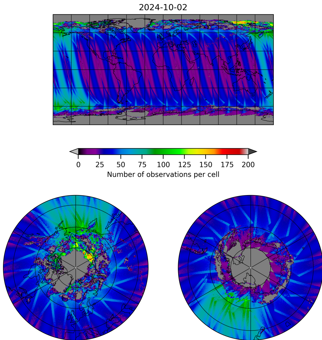
Figure 19: Map of the number of observations for 2024-10-01 to 2024-10-03
