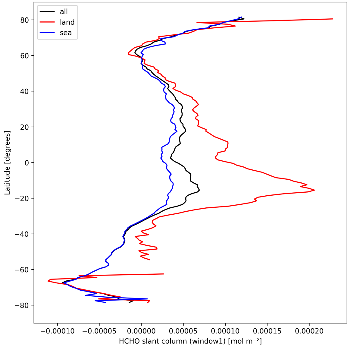
Figure 24: Zonal average of “HCHO slant column (window1)” for 2024-10-01 to 2024-10-03.
