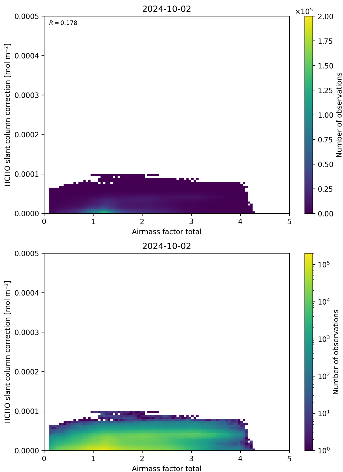
Figure 102: Scatter density plot of “Airmass factor total” against “HCHO slant column correction” for 2024-10-01 to 2024-10-03.
