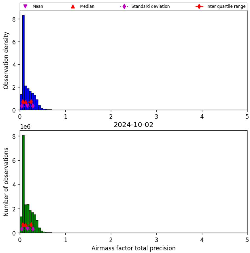
Figure 41: Histogram of “Airmass factor total precision” for 2024-10-01 to 2024-10-03
