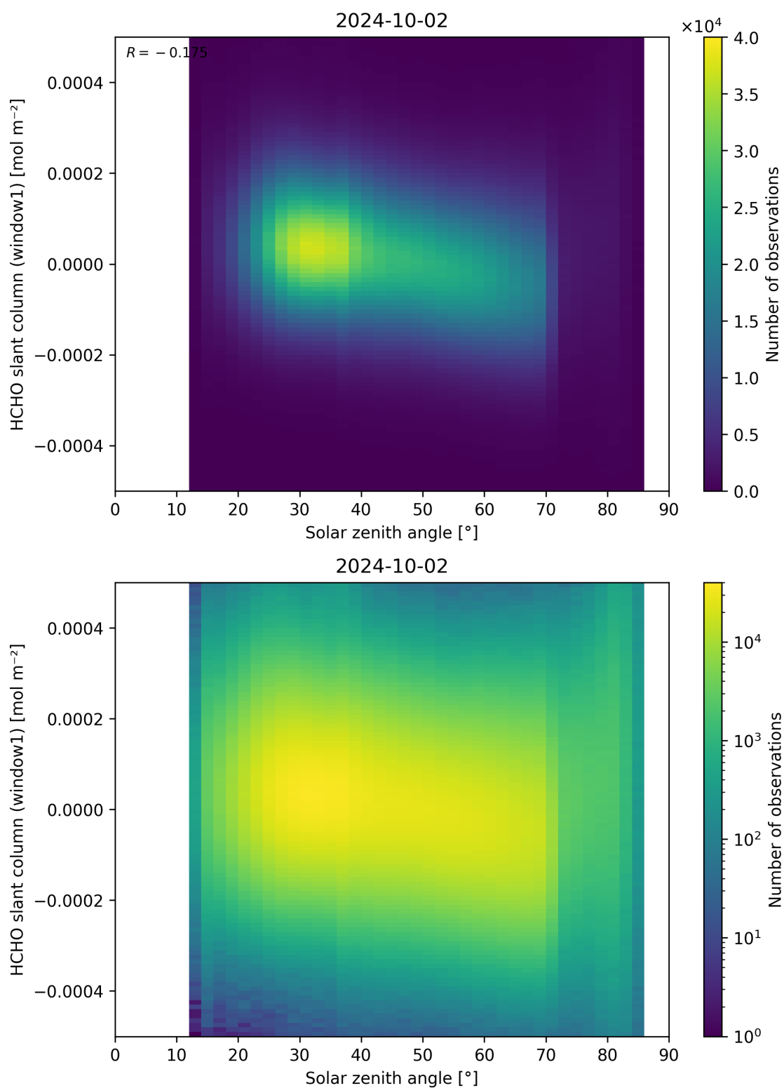
Figure 173: Scatter density plot of “Solar zenith angle” against “HCHO slant column (window1)” for 2024-10-01 to 2024-10-03.
