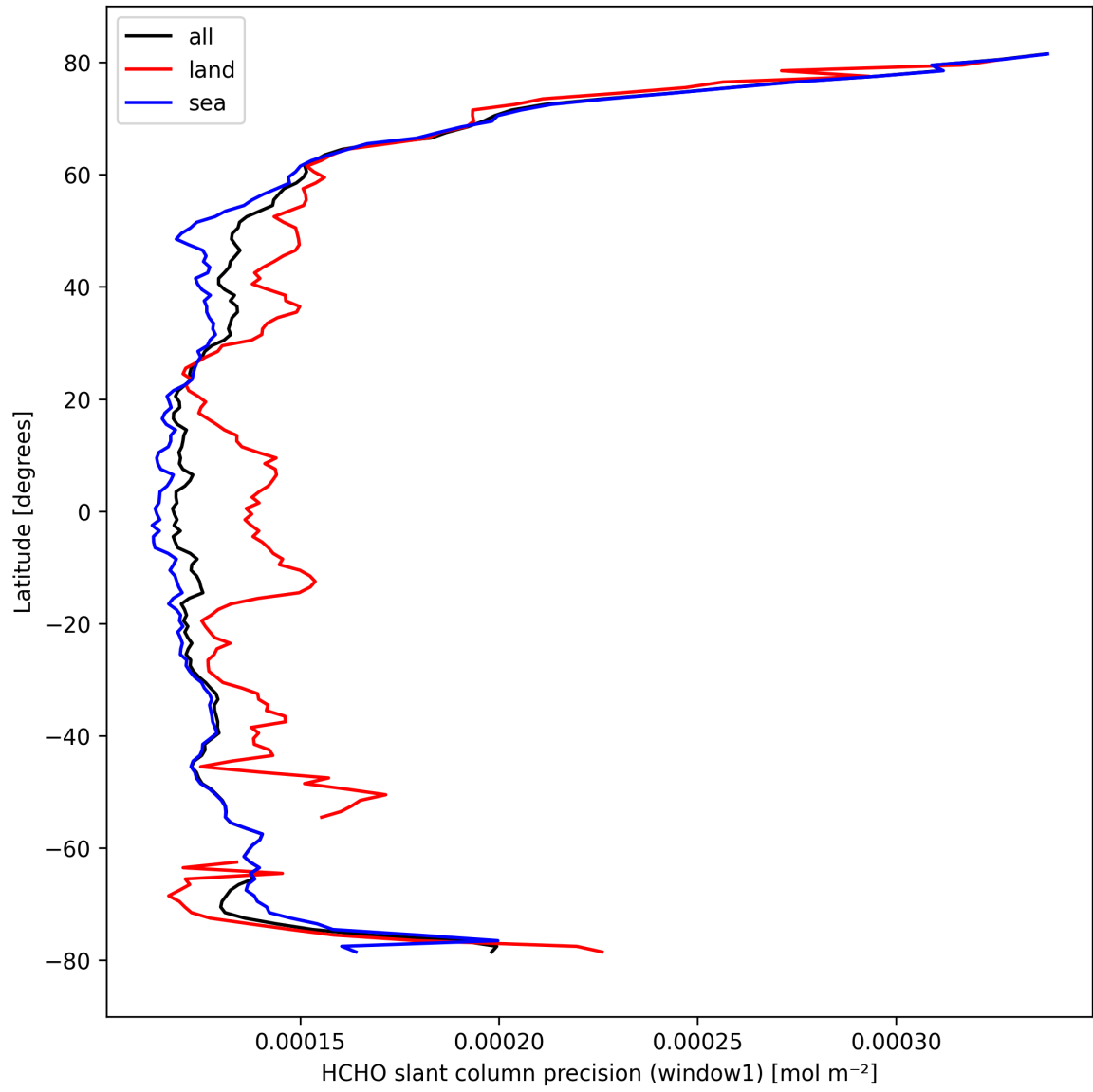
Figure 25: Zonal average of "HCHO slant column precision (window1)" for 2024-10-01 to 2024-10-03.
