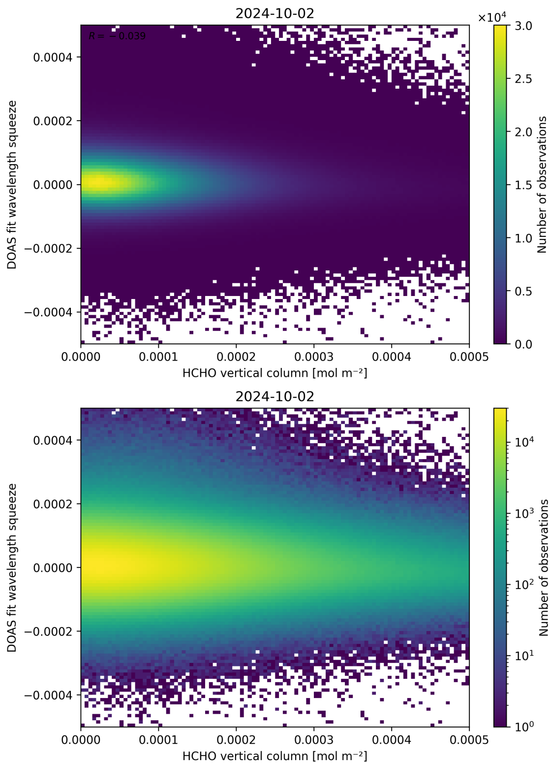
Figure 125: Scatter density plot of “HCHO vertical column” against “DOAS fit wavelength squeeze” for 2024-10-01 to 2024-10-03.
