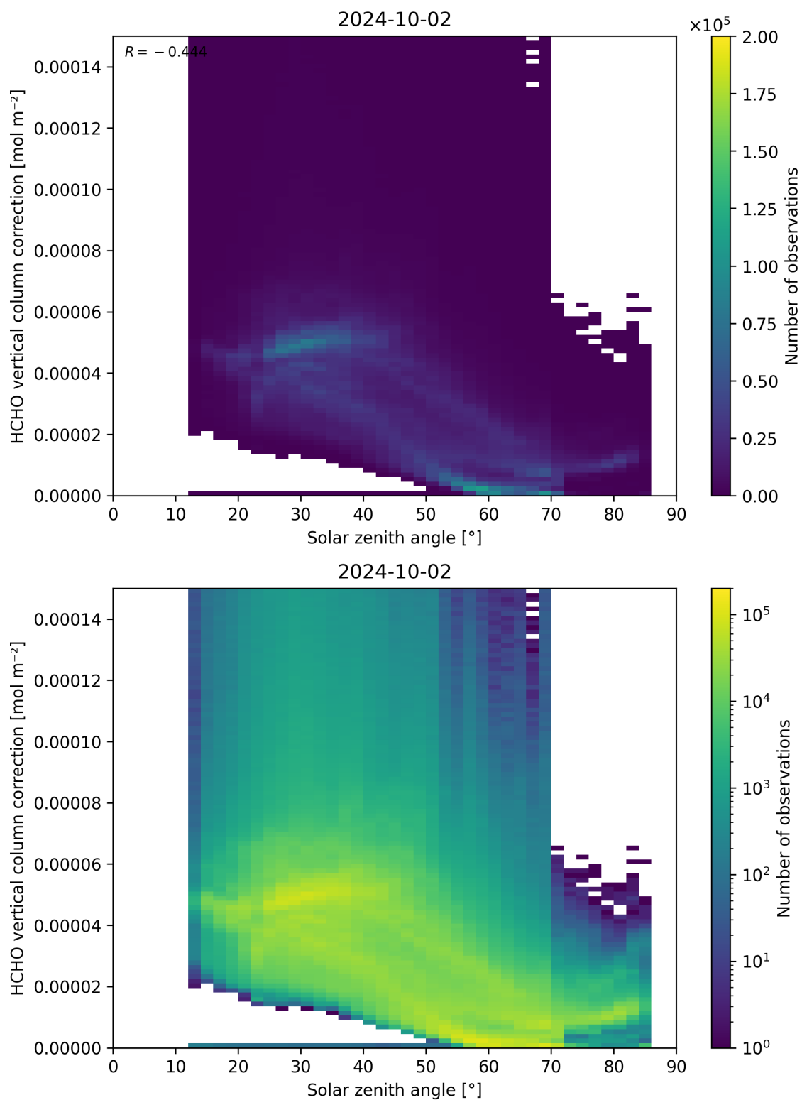
Figure 178: Scatter density plot of “Solar zenith angle” against “HCHO vertical column correction” for 2024-10-01 to 2024-10-03.
