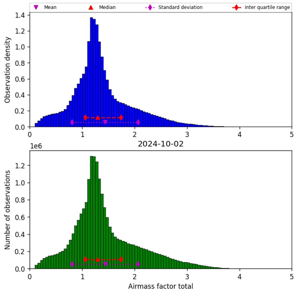
Figure 40: Histogram of “Airmass factor total” for 2024-10-01 to 2024-10-03
