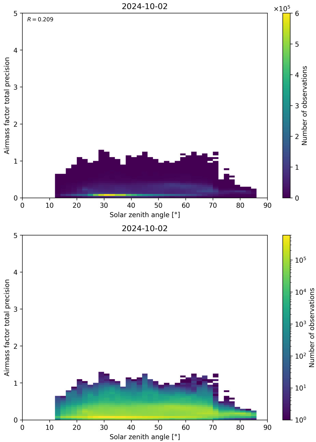
Figure 176: Scatter density plot of “Solar zenith angle” against “Airmass factor total precision” for 2024-10-01 to 2024-10-03.
