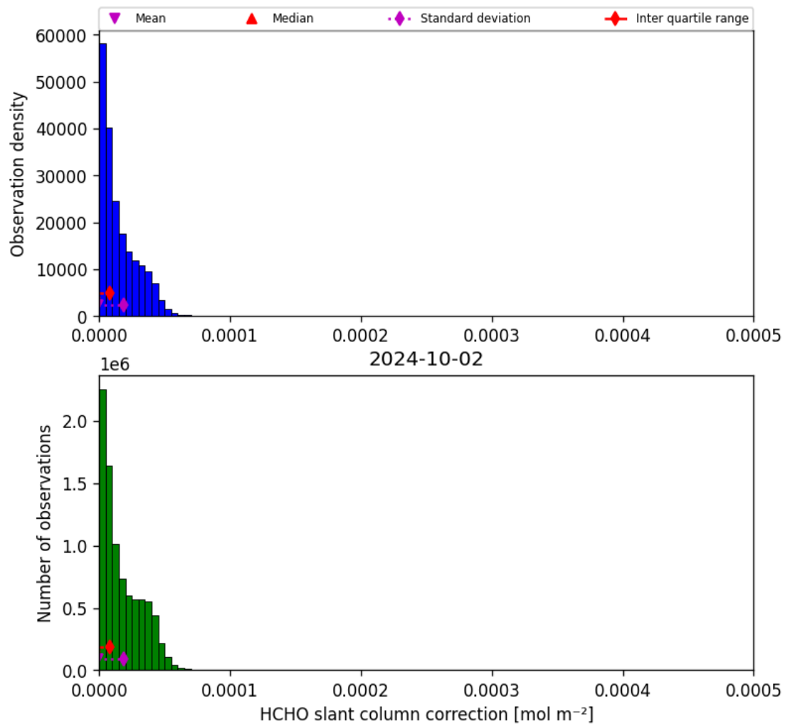
Figure 47: Histogram of “HCHO slant column correction” for 2024-10-01 to 2024-10-03
