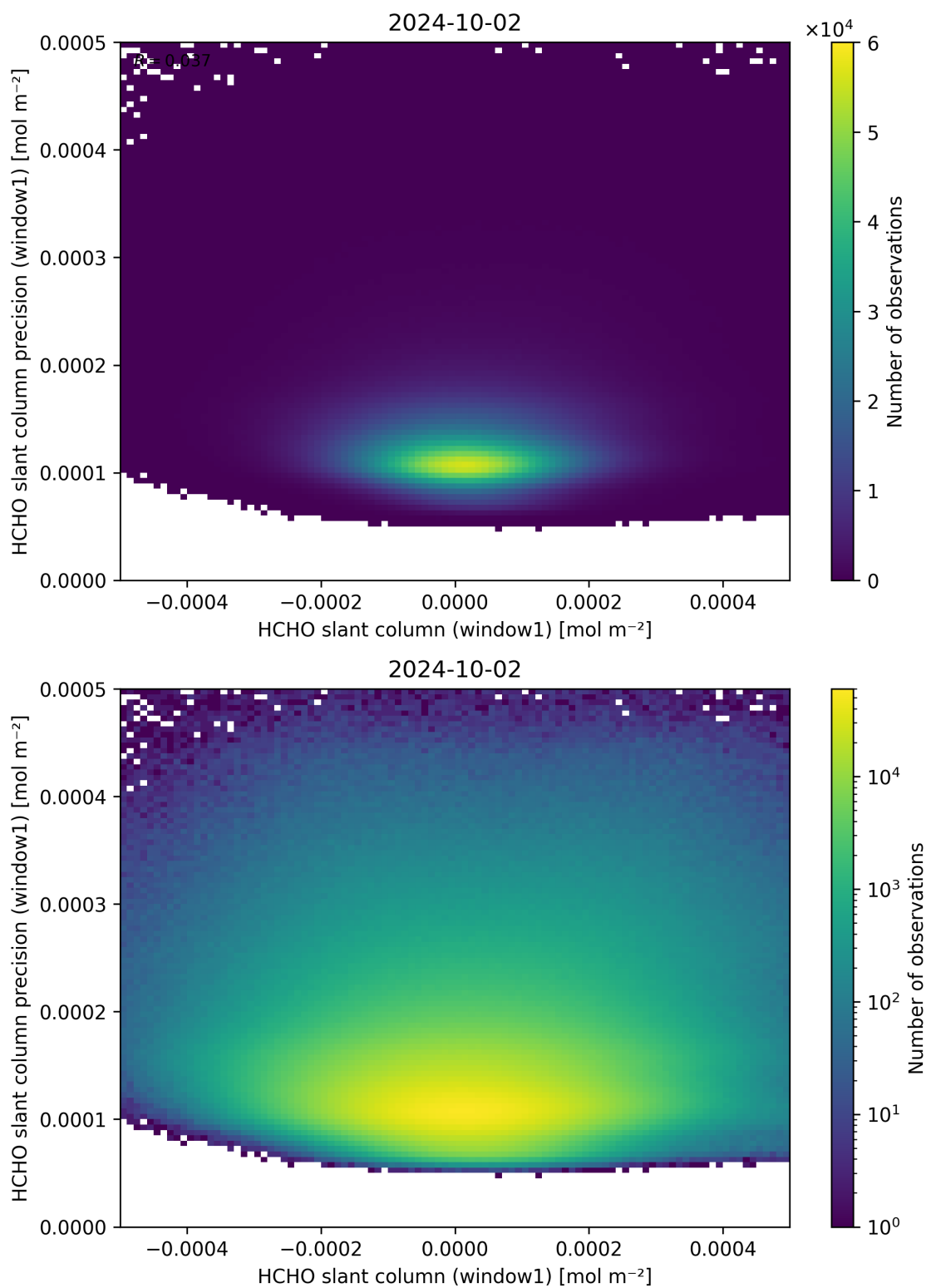
Figure 84: Scatter density plot of “HCHO slant column (window1)” against “HCHO slant column precision (window1)” for 2024-10-01 to 2024-10-03.
