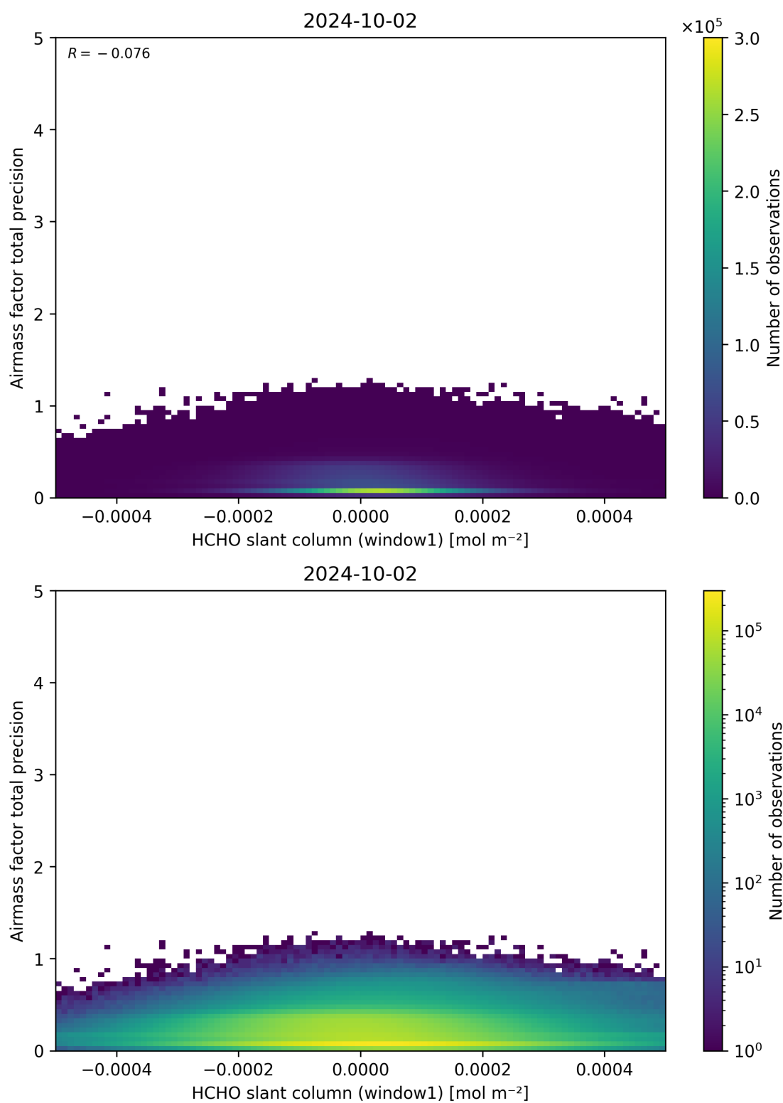
Figure 86: Scatter density plot of “HCHO slant column (window1)” against “Airmass factor total precision” for 2024-10-01 to 2024-10-03.
