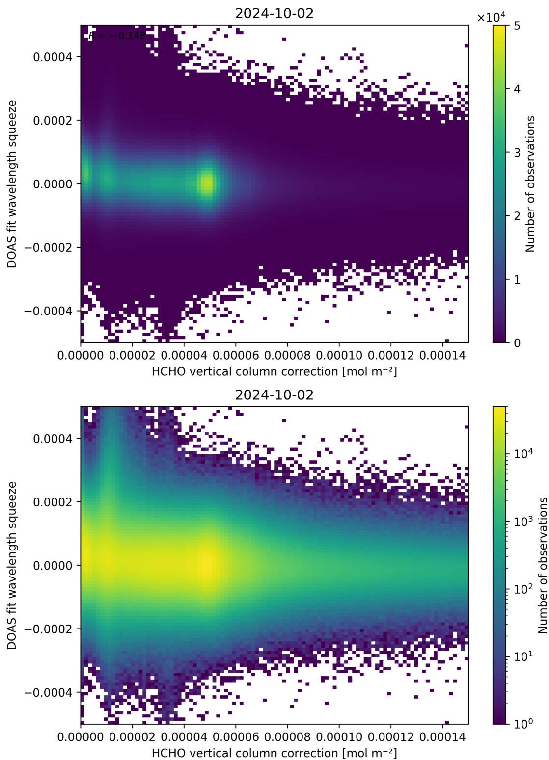
Figure 114: Scatter density plot of “HCHO vertical column correction” against “DOAS fit wavelength squeeze” for 2024-10-01 to 2024-10-03.
