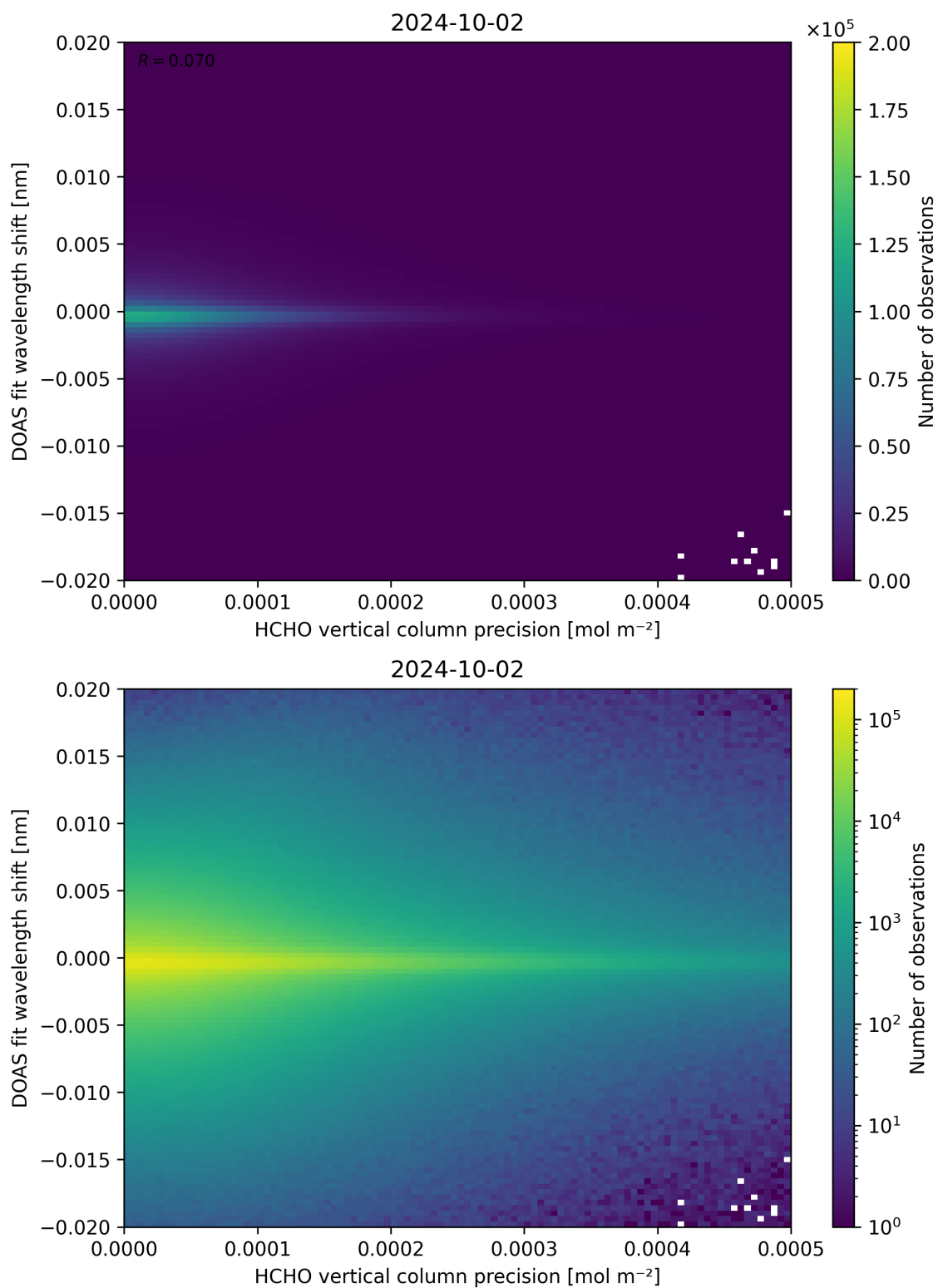
Figure 137: Scatter density plot of “HCHO vertical column precision” against “DOAS fit wavelength shift” for 2024-10-01 to 2024-10-03.
