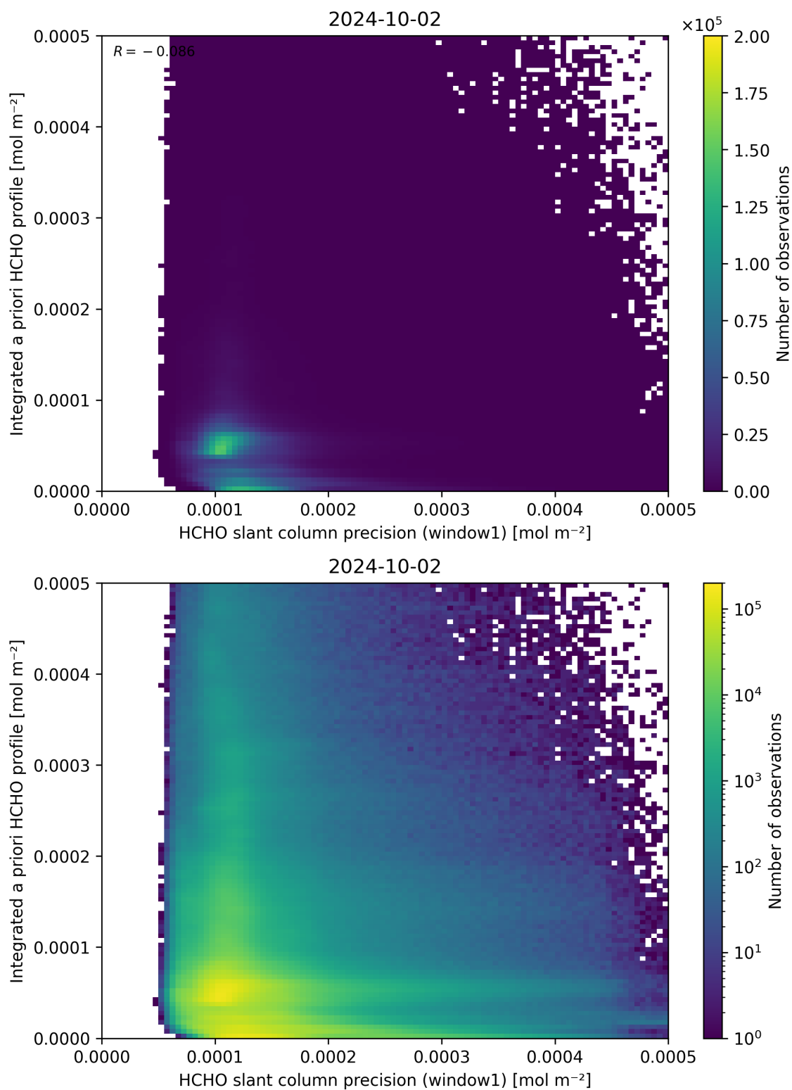
Figure 96: Scatter density plot of “HCHO slant column precision (window1)” against “Integrated a priori HCHO profile” for 2024-10-01 to 2024-10-03.
