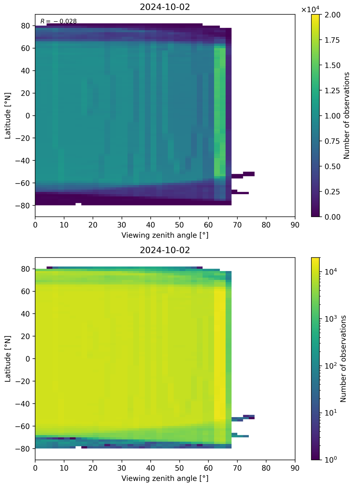
Figure 196: Scatter density plot of “Viewing zenith angle” against “Latitude” for 2024-10-01 to 2024-10-03.
