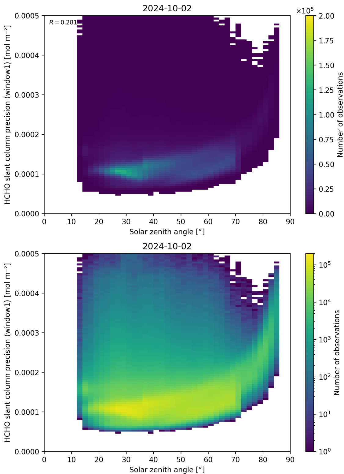
Figure 174: Scatter density plot of “Solar zenith angle” against “HCHO slant column precision (window1)” for 2024-10-01 to 2024-10-03.
