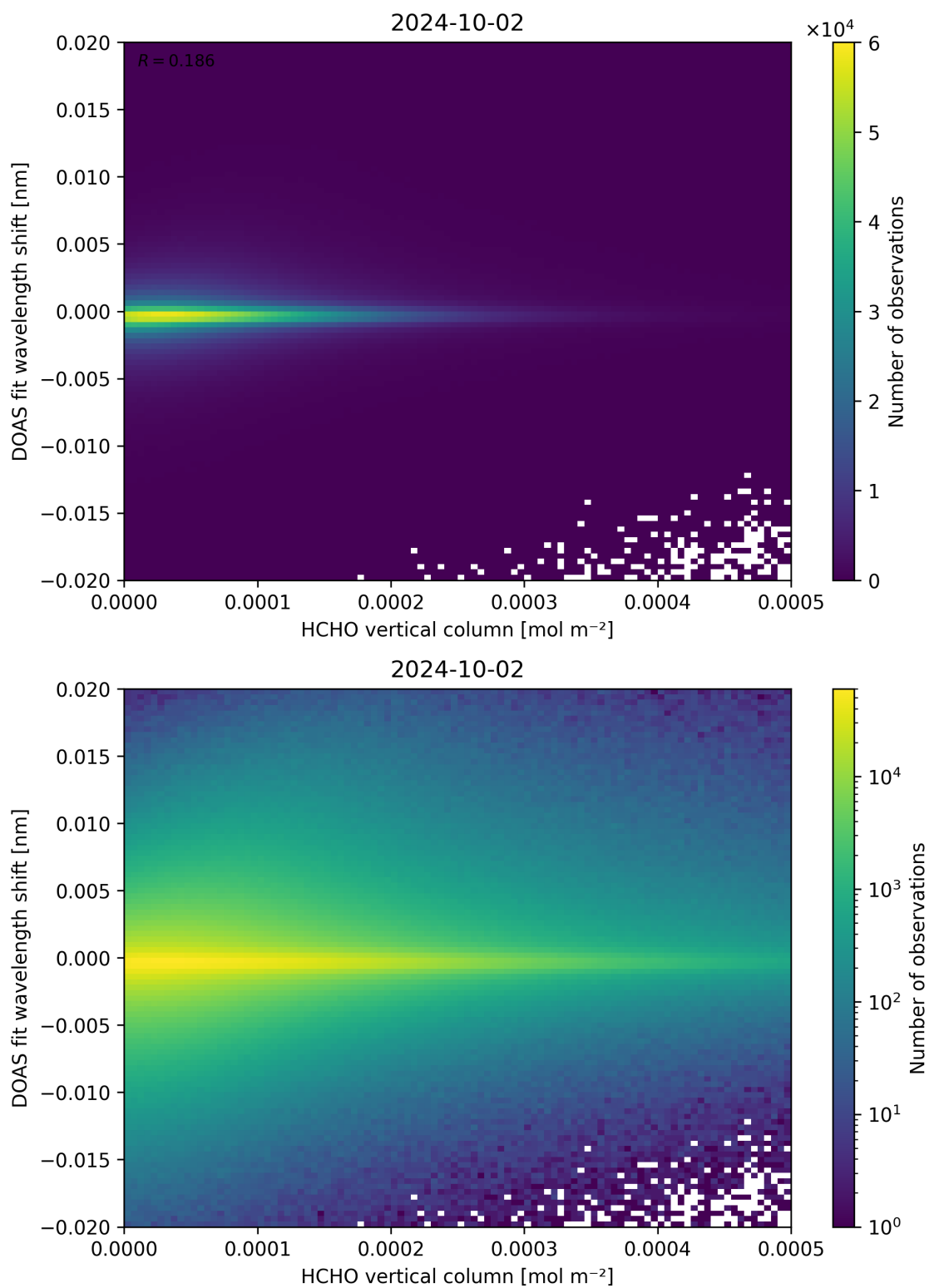
Figure 124: Scatter density plot of “HCHO vertical column” against “DOAS fit wavelength shift” for 2024-10-01 to 2024-10-03.
