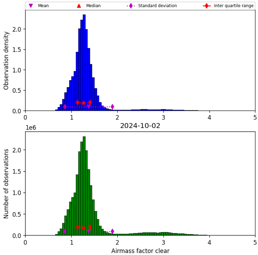
Figure 42: Histogram of “Airmass factor clear” for 2024-10-01 to 2024-10-03
