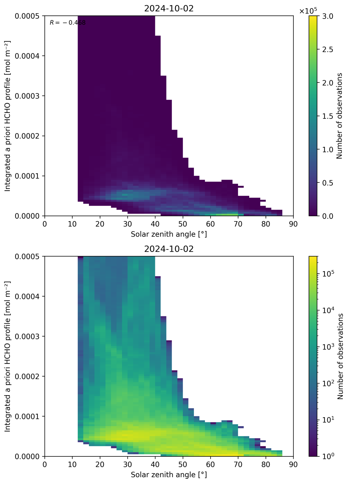
Figure 180: Scatter density plot of “Solar zenith angle” against “Integrated a priori HCHO profile” for 2024-10-01 to 2024-10-03.
