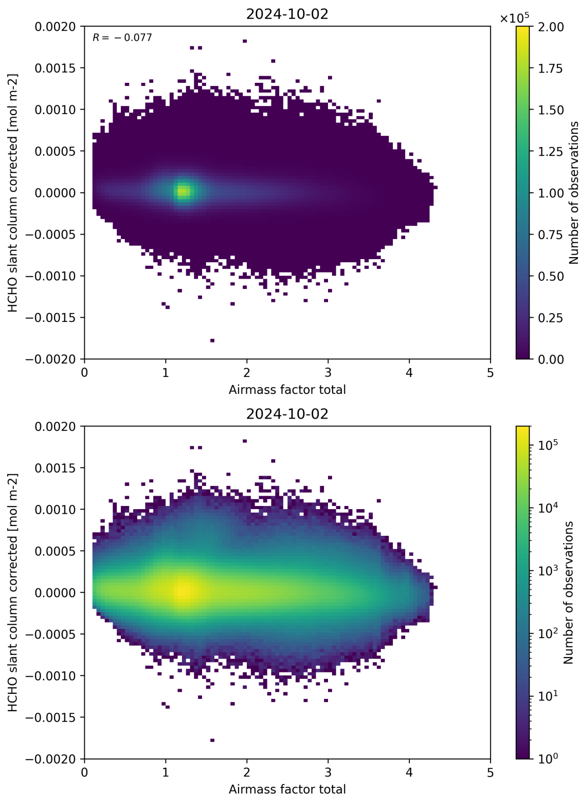
Figure 101: Scatter density plot of “Airmass factor total” against “HCHO slant column corrected” for 2024-10-01 to 2024-10-03.
