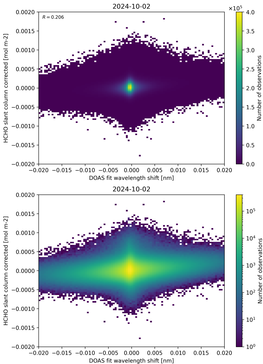
Figure 66: Scatter density plot of “DOAS fit wavelength shift” against “HCHO slant column corrected” for 2024-10-01 to 2024-10-03.
