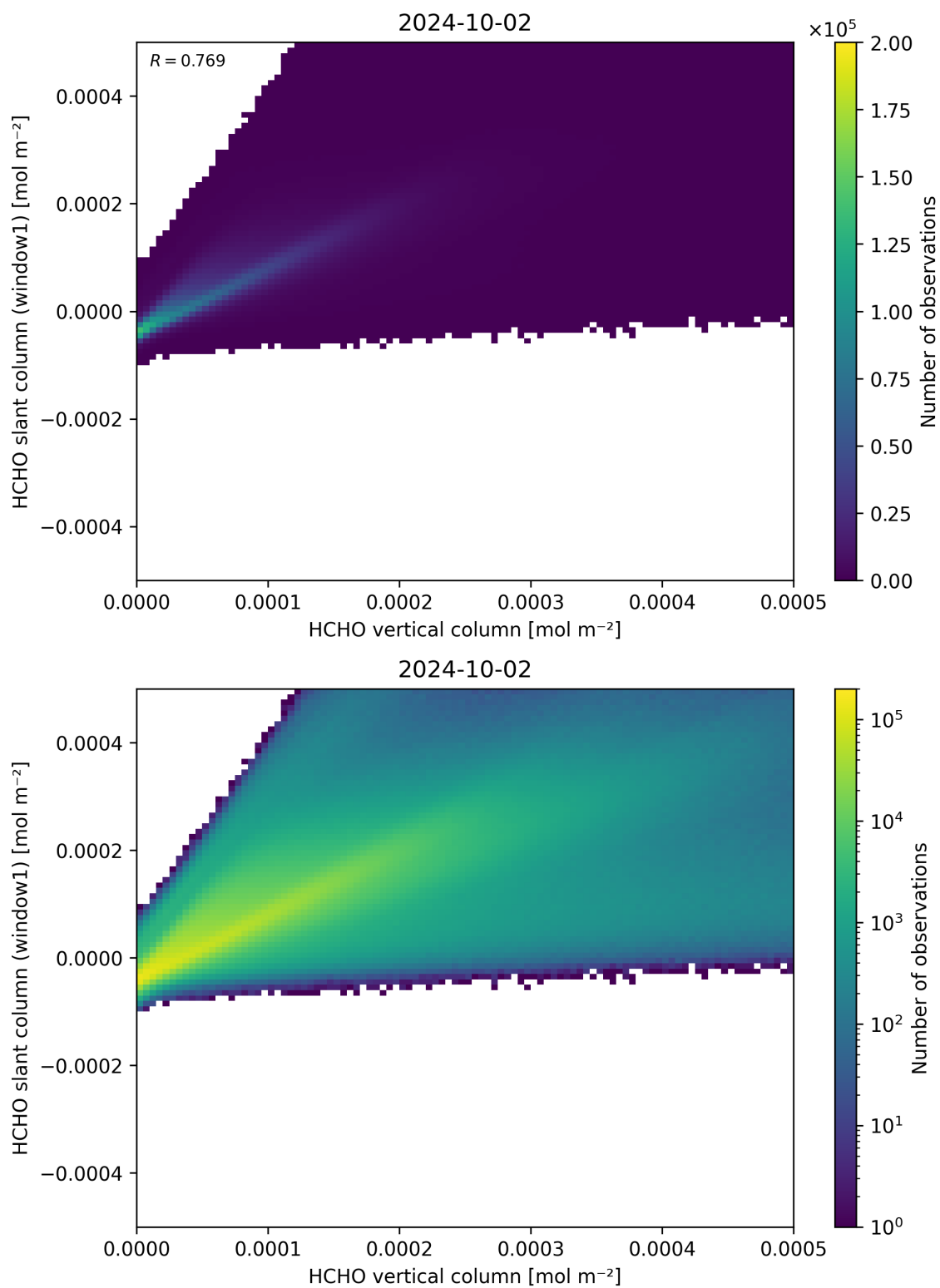
Figure 129: Scatter density plot of “HCHO vertical column” against “HCHO slant column (window1)” for 2024-10-01 to 2024-10-03.
