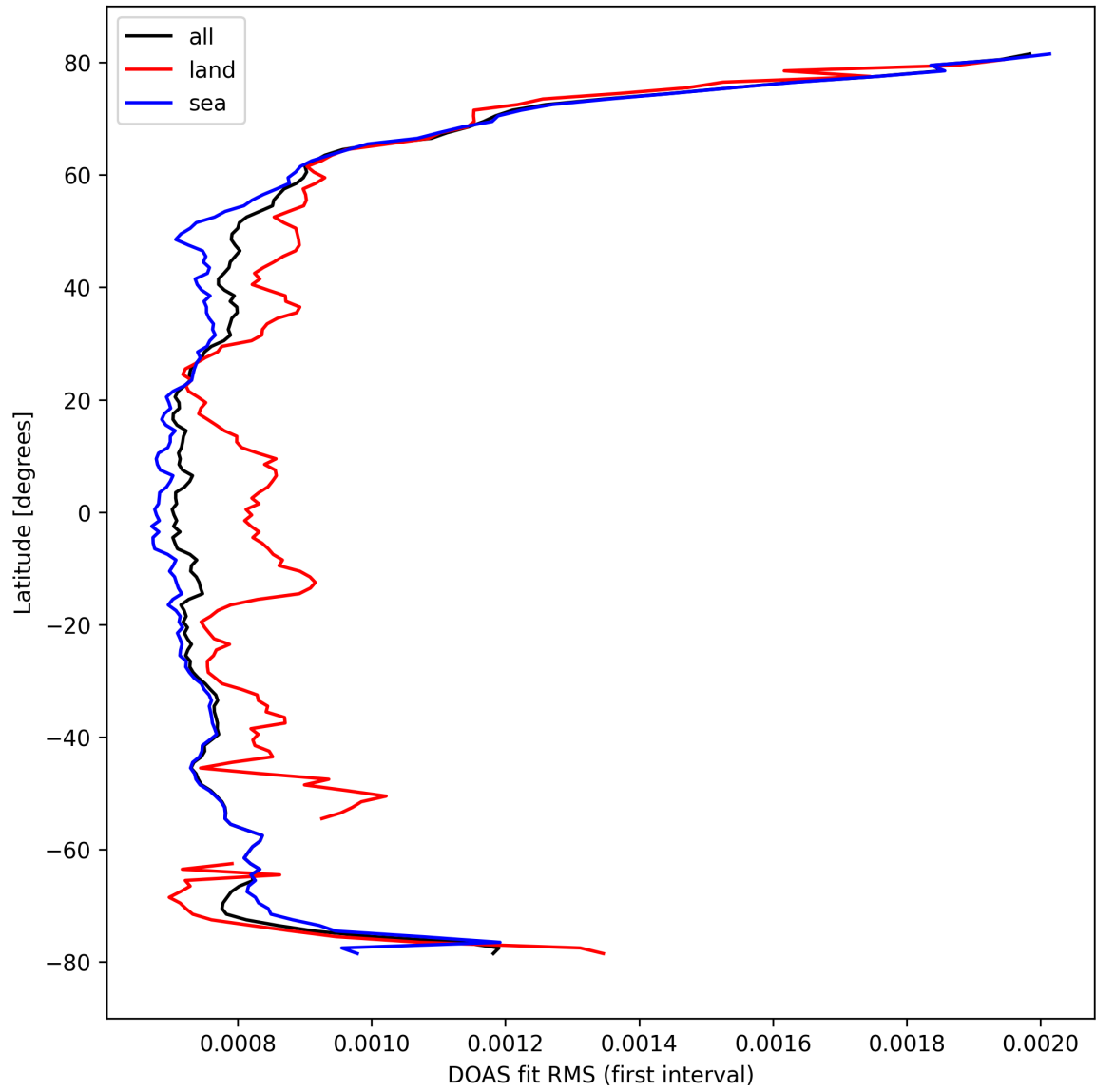
Figure 32: Zonal average of "DOAS fit RMS (first interval)" for 2024-10-01 to 2024-10-03.
