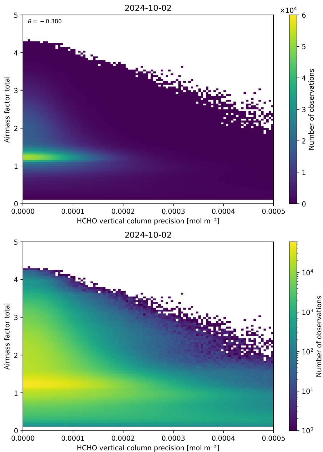
Figure 144: Scatter density plot of “HCHO vertical column precision” against “Airmass factor total” for 2024-10-01 to 2024-10-03.
