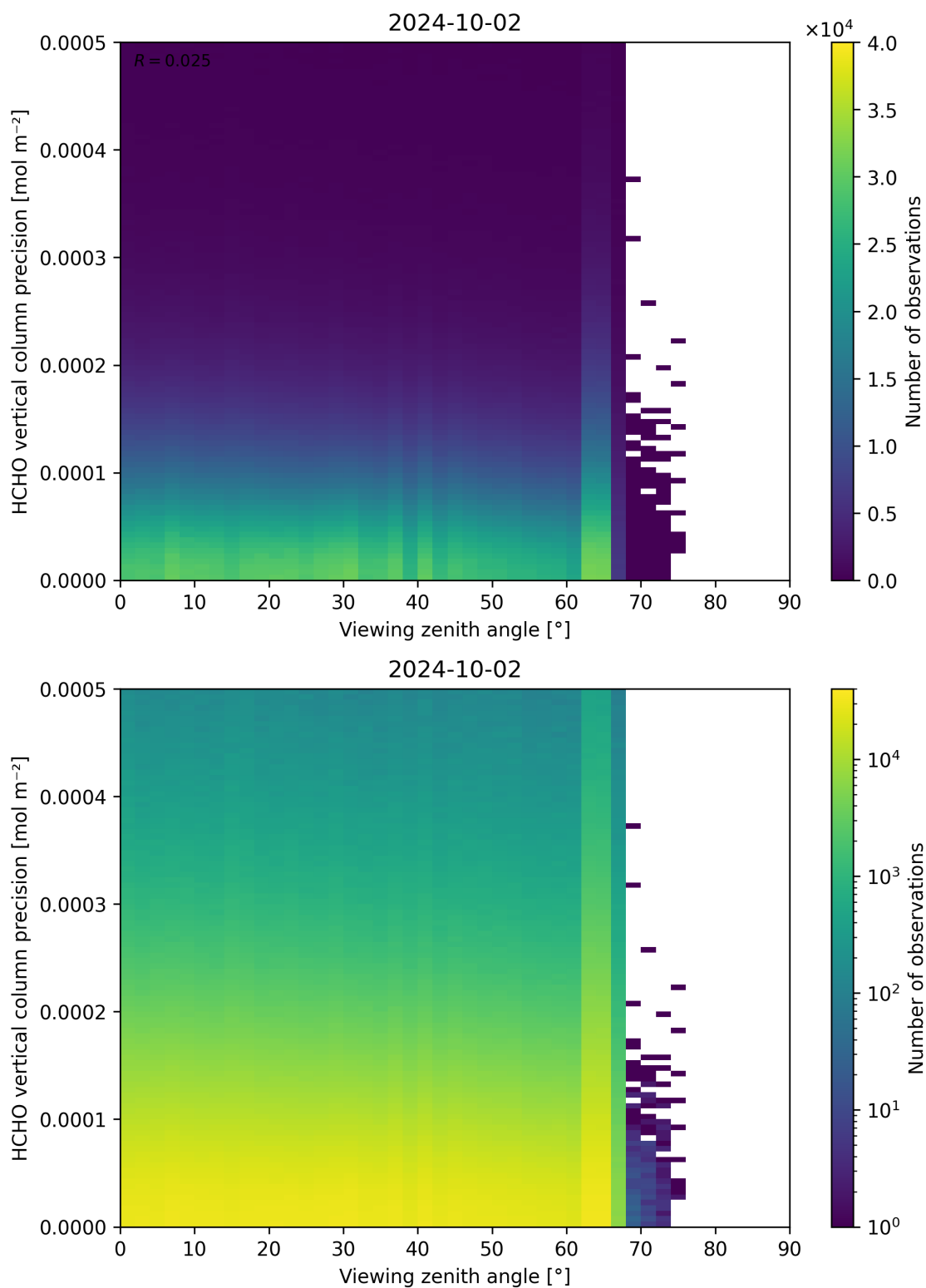
Figure 194: Scatter density plot of “Viewing zenith angle” against “HCHO vertical column precision” for 2024-10-01 to 2024-10-03.
