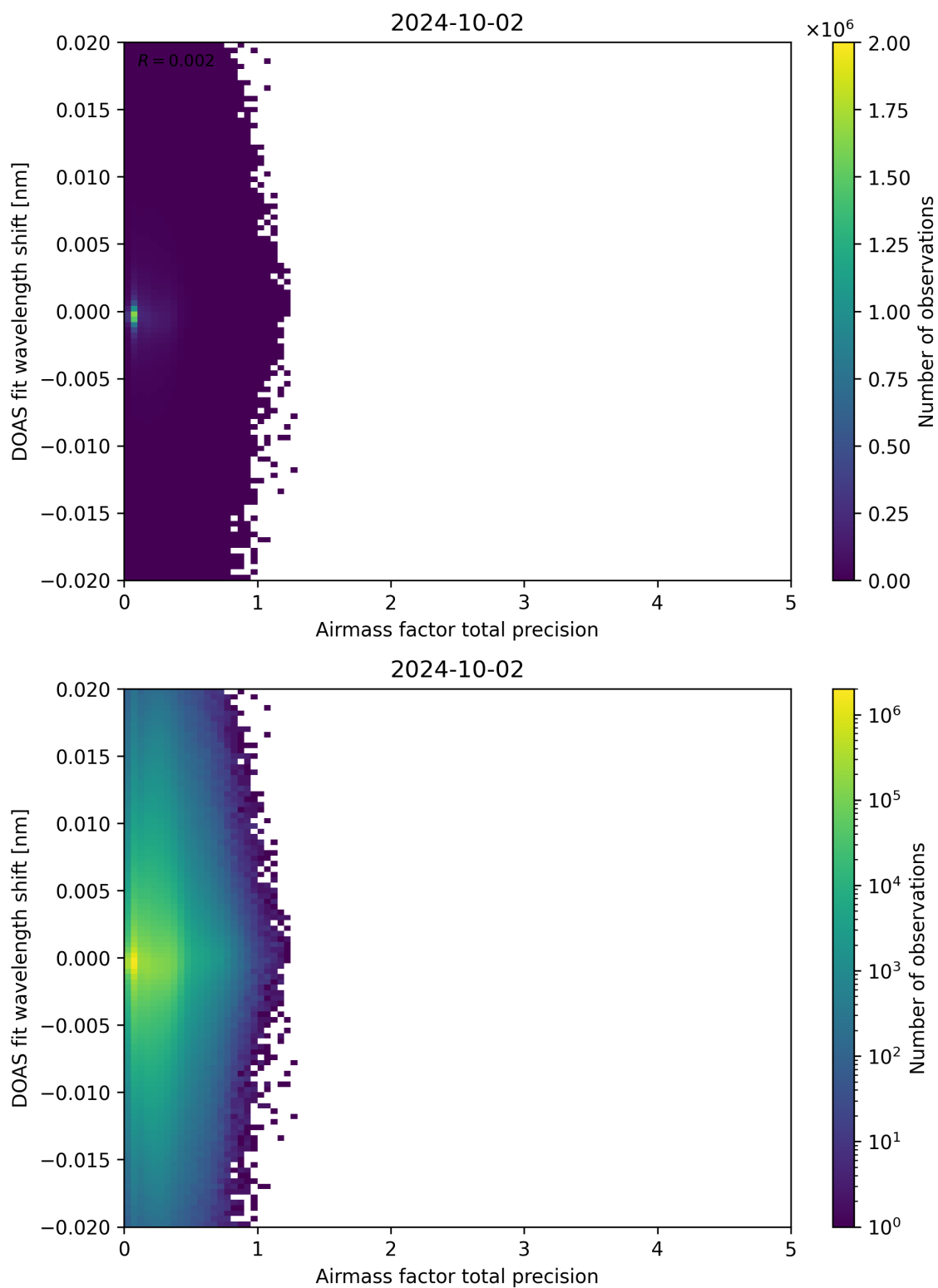
Figure 106: Scatter density plot of “Airmass factor total precision” against “DOAS fit wavelength shift” for 2024-10-01 to 2024-10-03.
