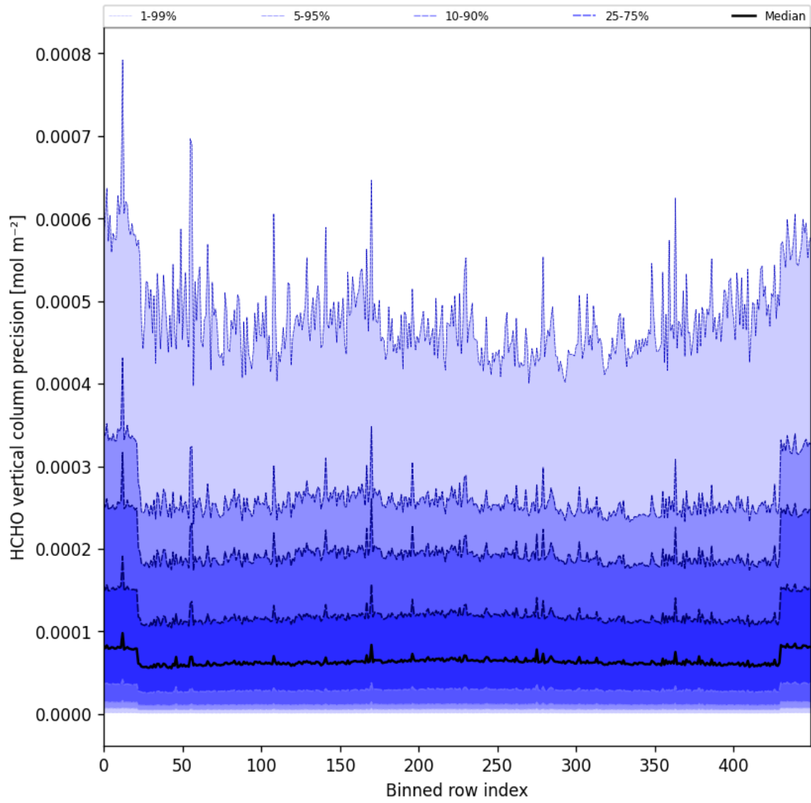
Figure 50: Along track statistics of “HCHO vertical column precision” for 2024-10-01 to 2024-10-03
