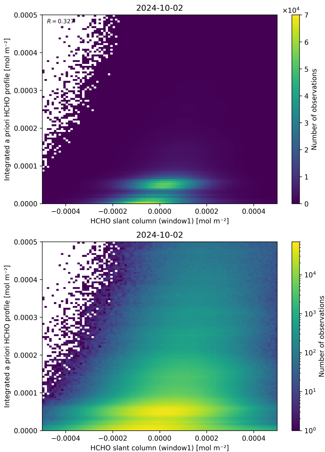
Figure 87: Scatter density plot of “HCHO slant column (window1)” against “Integrated a priori HCHO profile” for 2024-10-01 to 2024-10-03.
