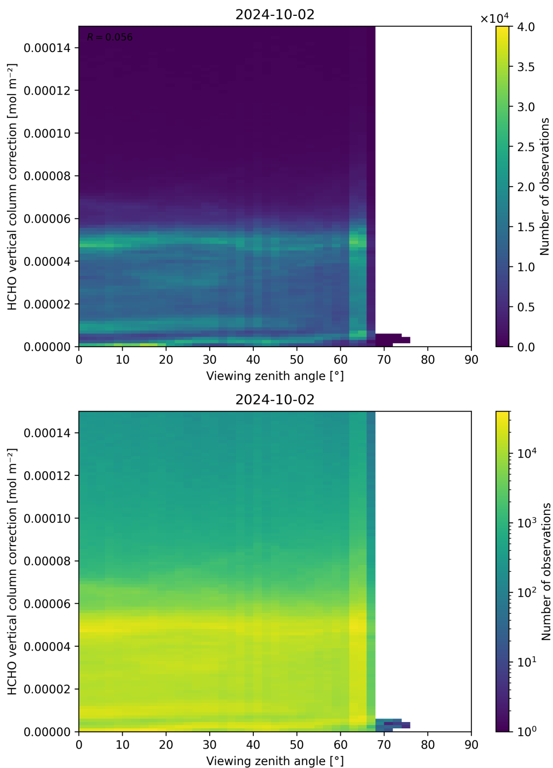
Figure 193: Scatter density plot of “Viewing zenith angle” against “HCHO vertical column correction” for 2024-10-01 to 2024-10-03.
