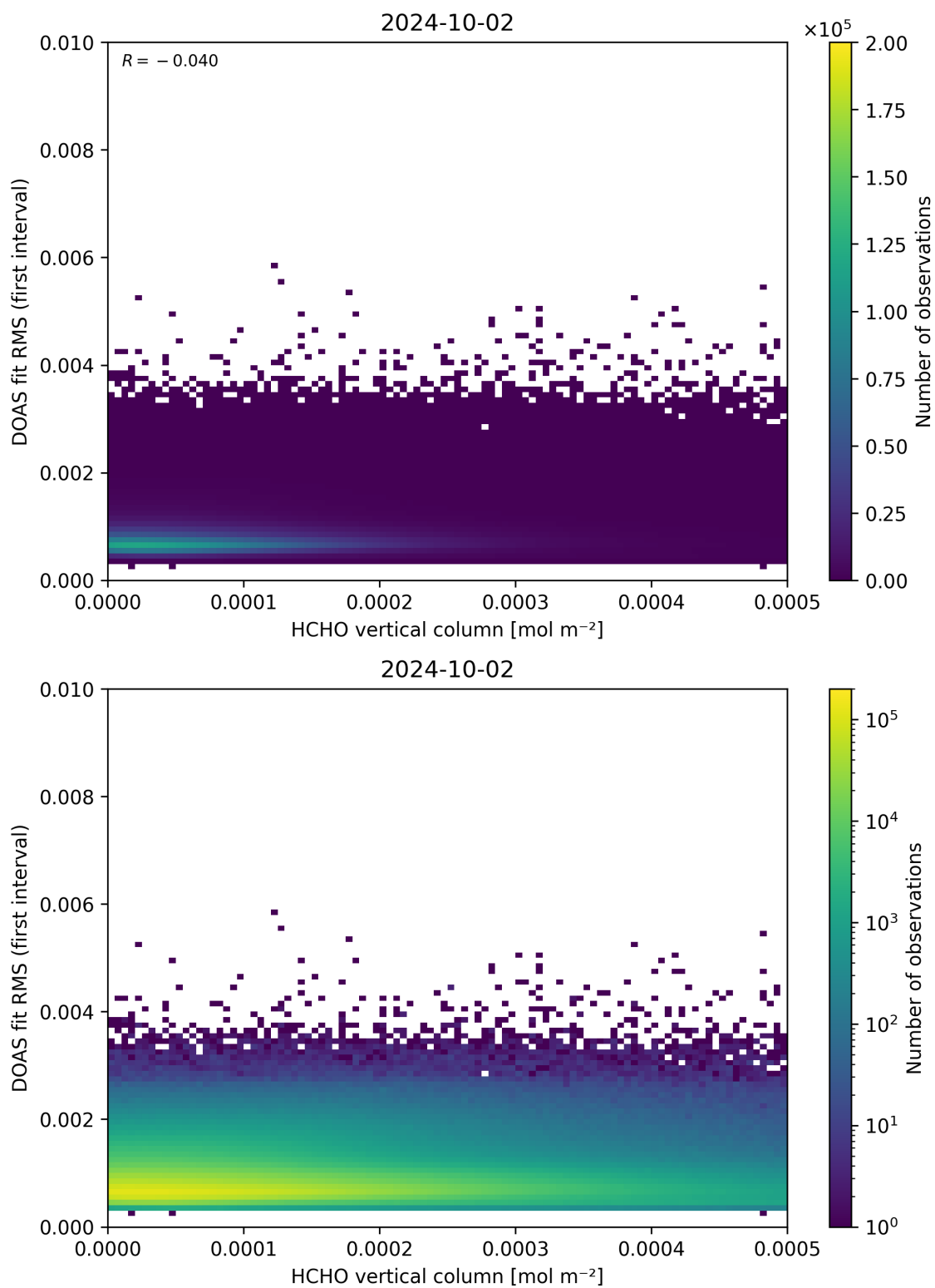
Figure 123: Scatter density plot of “HCHO vertical column” against “DOAS fit RMS (first interval)” for 2024-10-01 to 2024-10-03.
