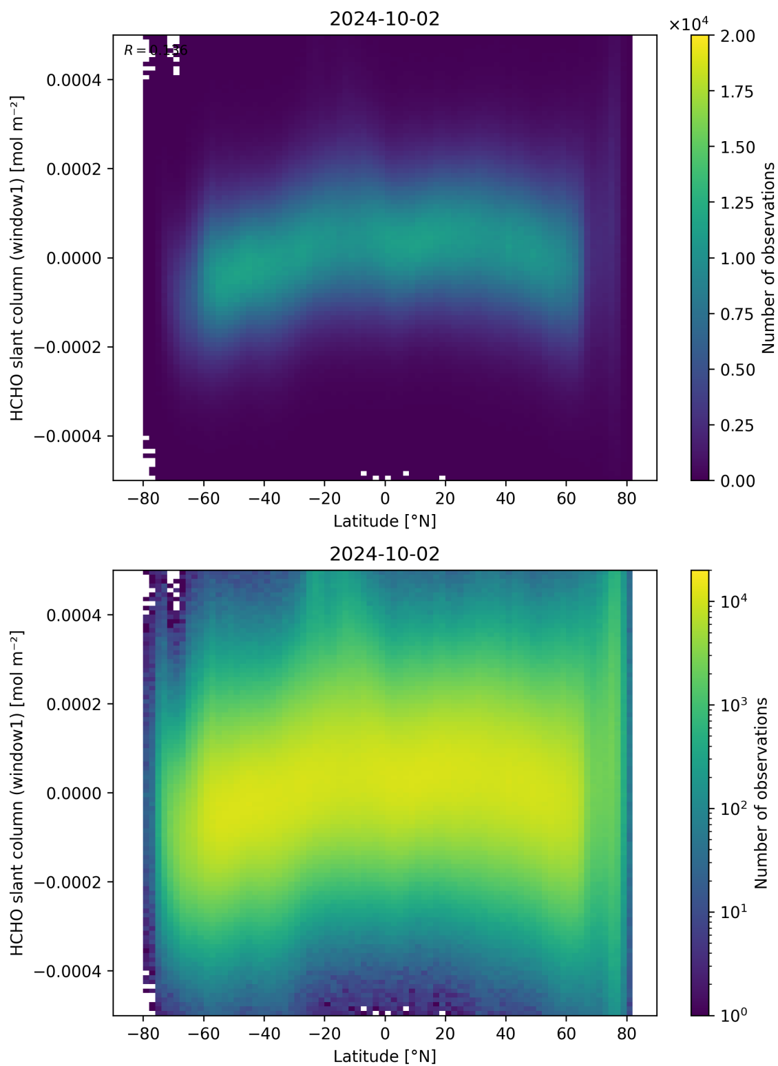
Figure 159: Scatter density plot of “Latitude” against “HCHO slant column (window1)” for 2024-10-01 to 2024-10-03.
