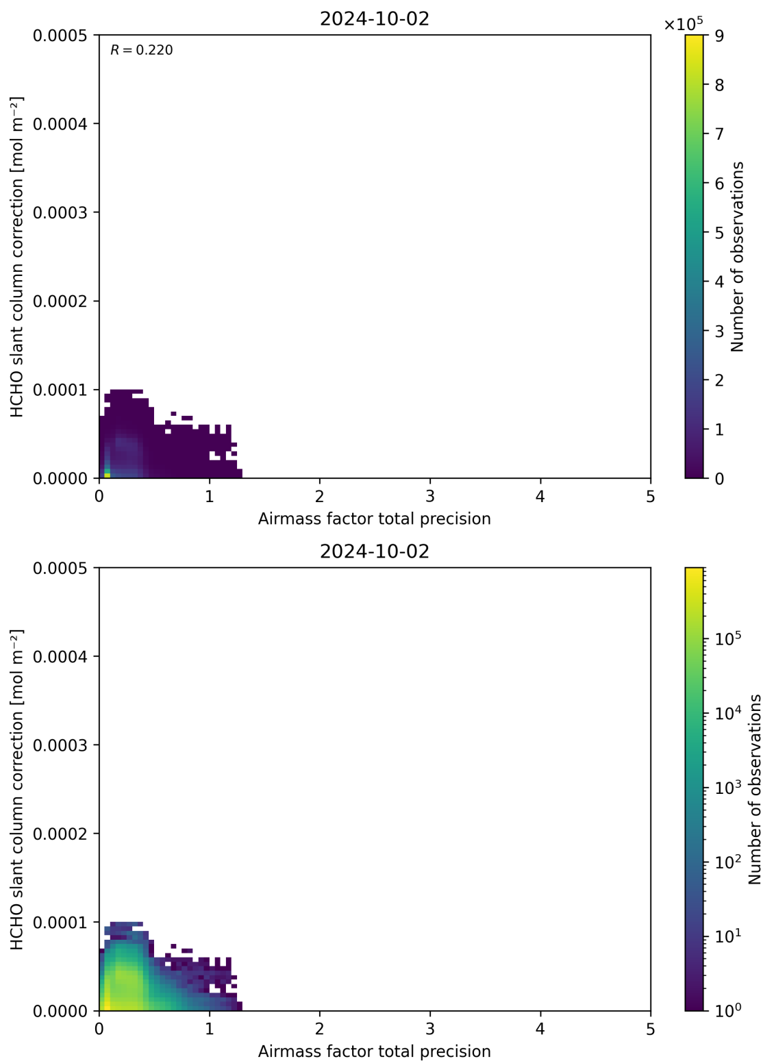
Figure 110: Scatter density plot of “Airmass factor total precision” against “HCHO slant column correction” for 2024-10-01 to 2024-10-03.
