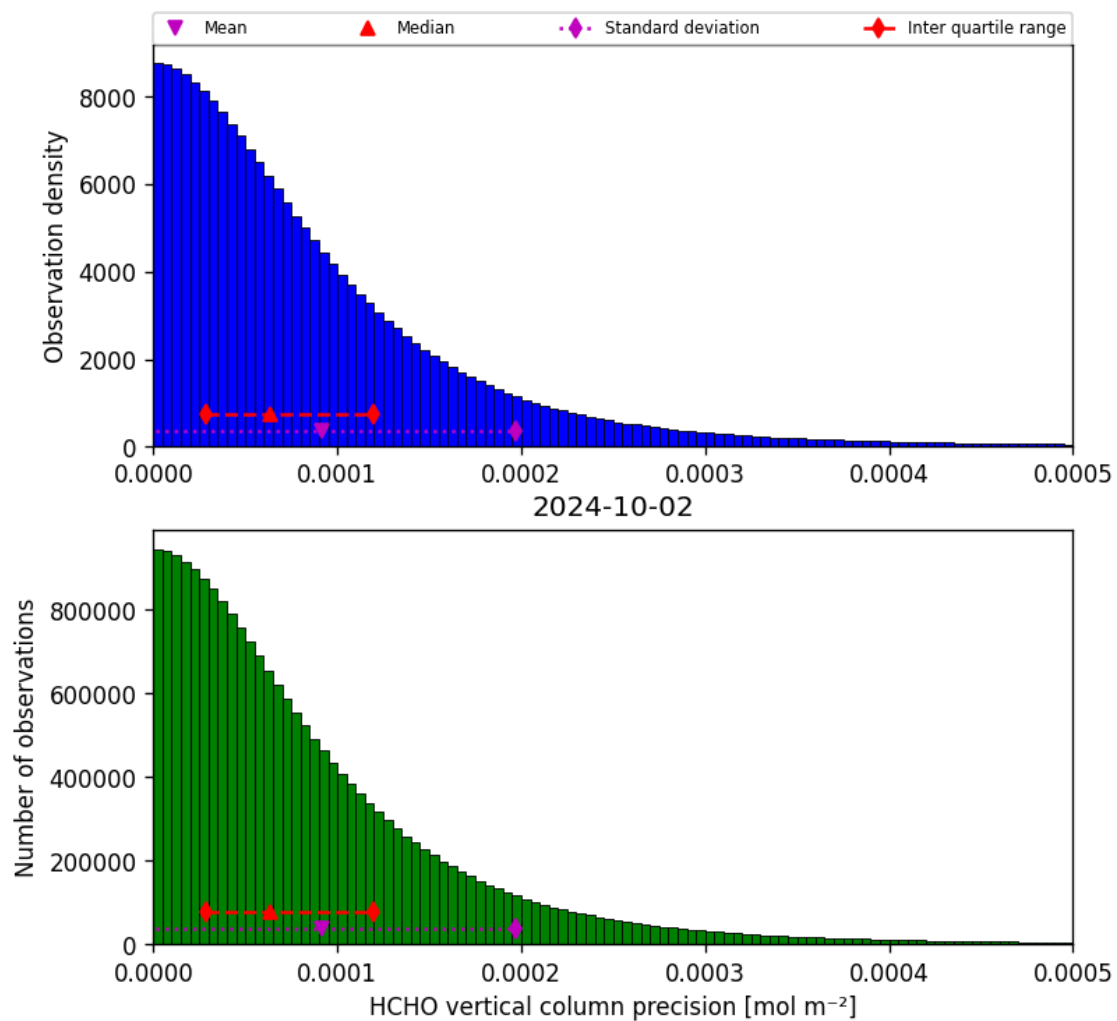
Figure 36: Histogram of “HCHO vertical column precision” for 2024-10-01 to 2024-10-03
