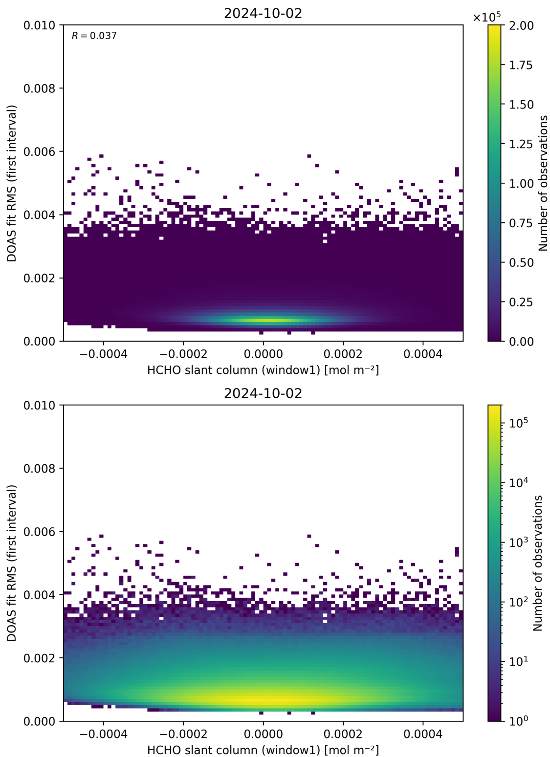
Figure 78: Scatter density plot of “HCHO slant column (window1)” against “DOAS fit RMS (first interval)” for 2024-10-01 to 2024-10-03.
