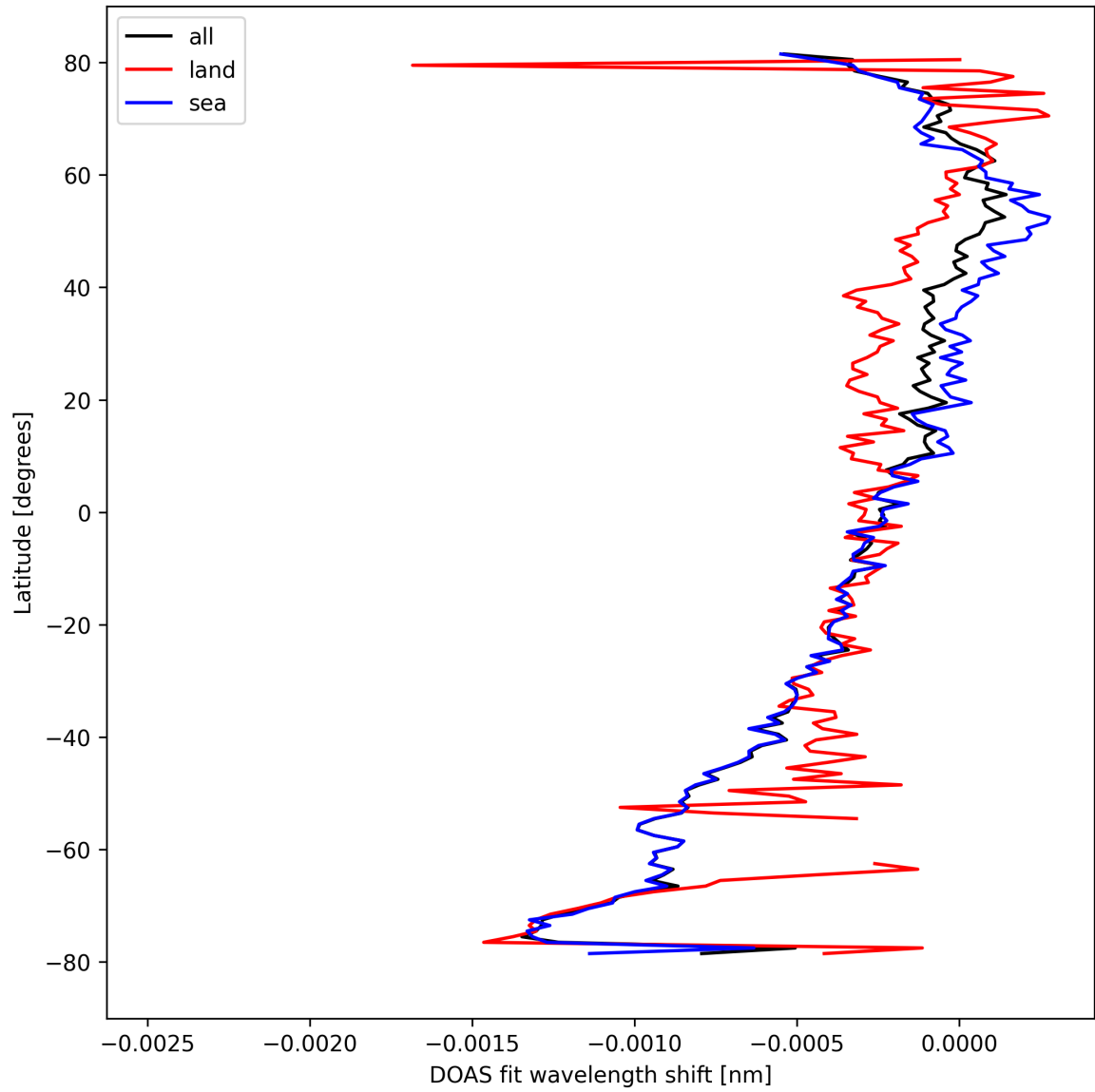
Figure 30: Zonal average of “DOAS fit wavelength shift” for 2024-10-01 to 2024-10-03.
