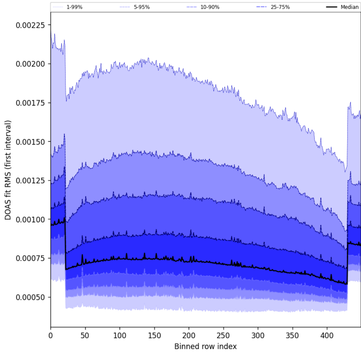
Figure 60: Along track statistics of “DOAS fit RMS (first interval)” for 2024-10-01 to 2024-10-03
