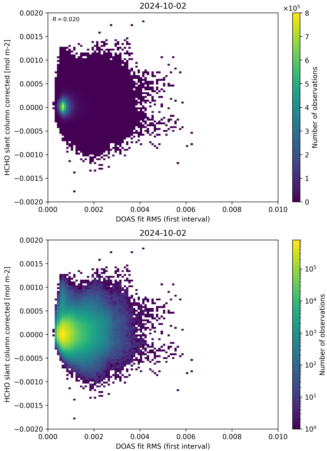
Figure 62: Scatter density plot of “DOAS fit RMS (first interval)” against “HCHO slant column corrected” for 2024-10-01 to 2024-10-03.
