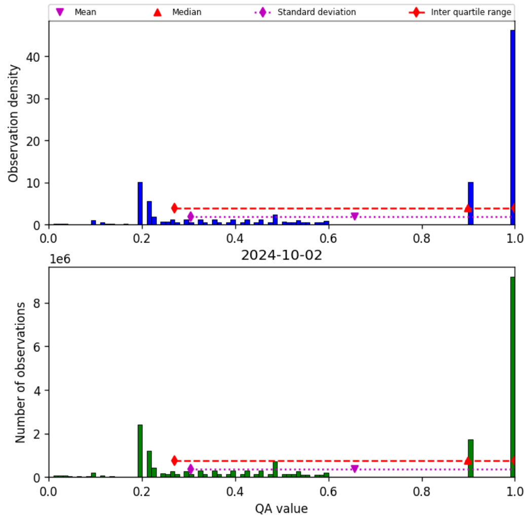
Figure 34: Histogram of “QA value” for 2024-10-01 to 2024-10-03
