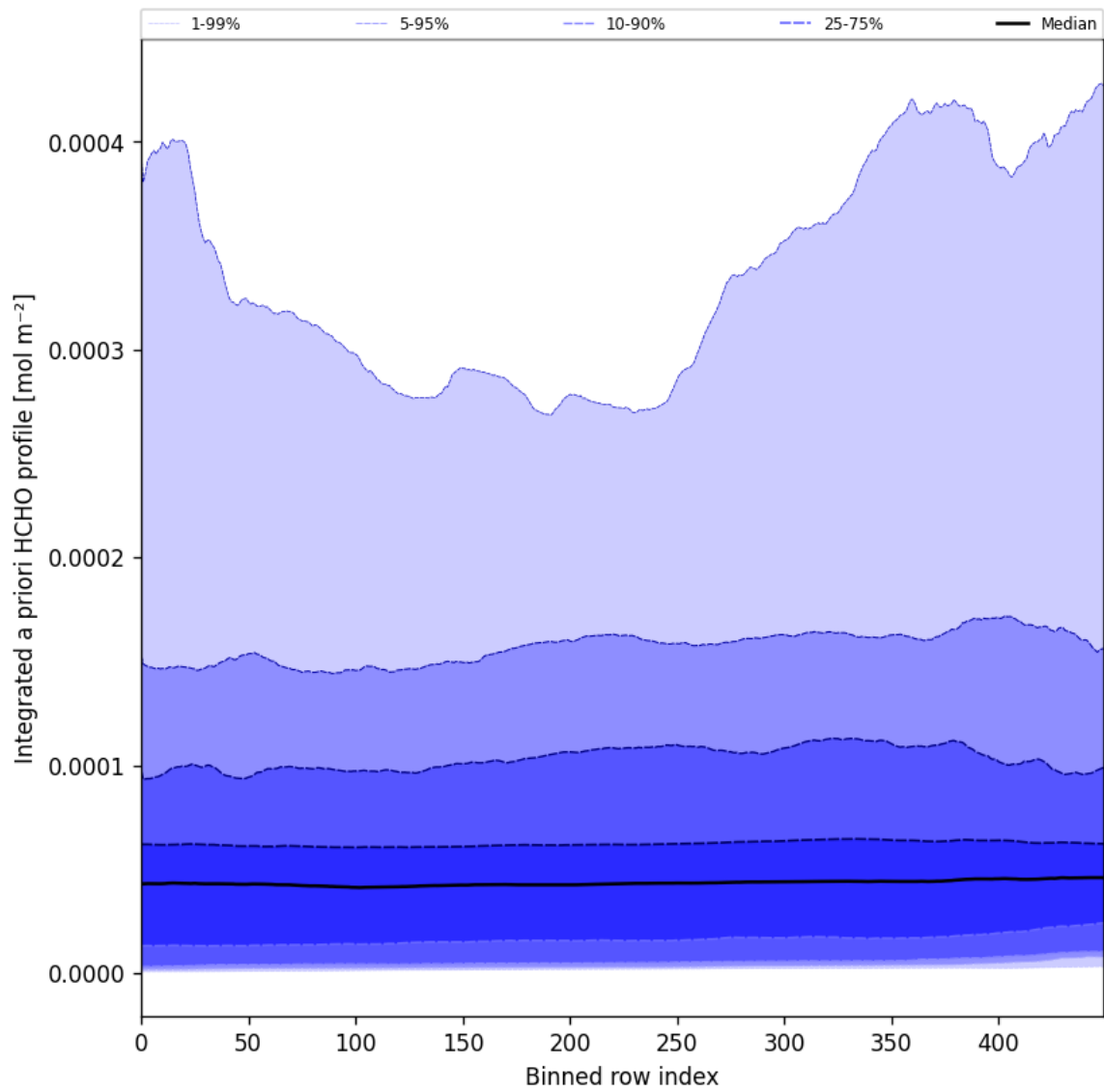
Figure 57: Along track statistics of "Integrated a priori HCHO profile" for 2024-10-01 to 2024-10-03
