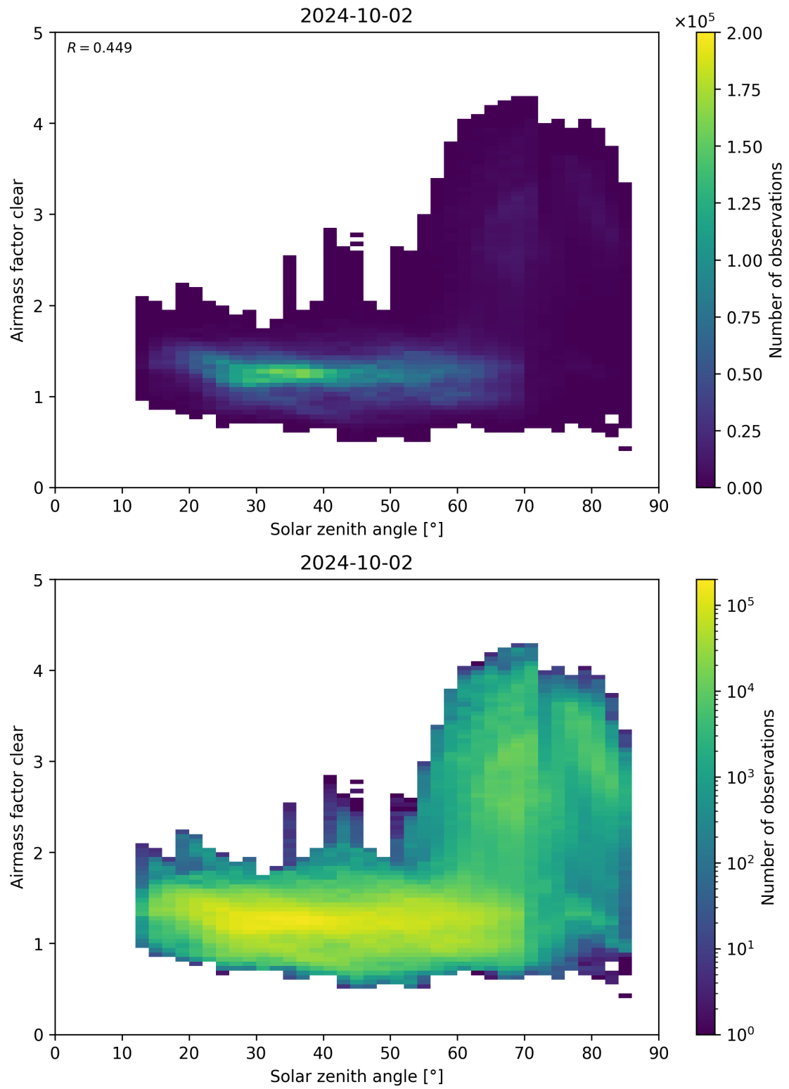
Figure 170: Scatter density plot of “Solar zenith angle” against “Airmass factor clear” for 2024-10-01 to 2024-10-03.
