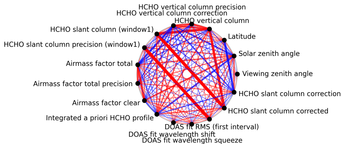
Figure 1: Map of correlation graph for 2024-10-01 to 2024-10-03.
