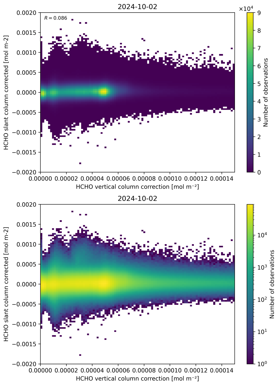
Figure 116: Scatter density plot of “HCHO vertical column correction” against “HCHO slant column corrected” for 2024-10-01 to 2024-10-03.
