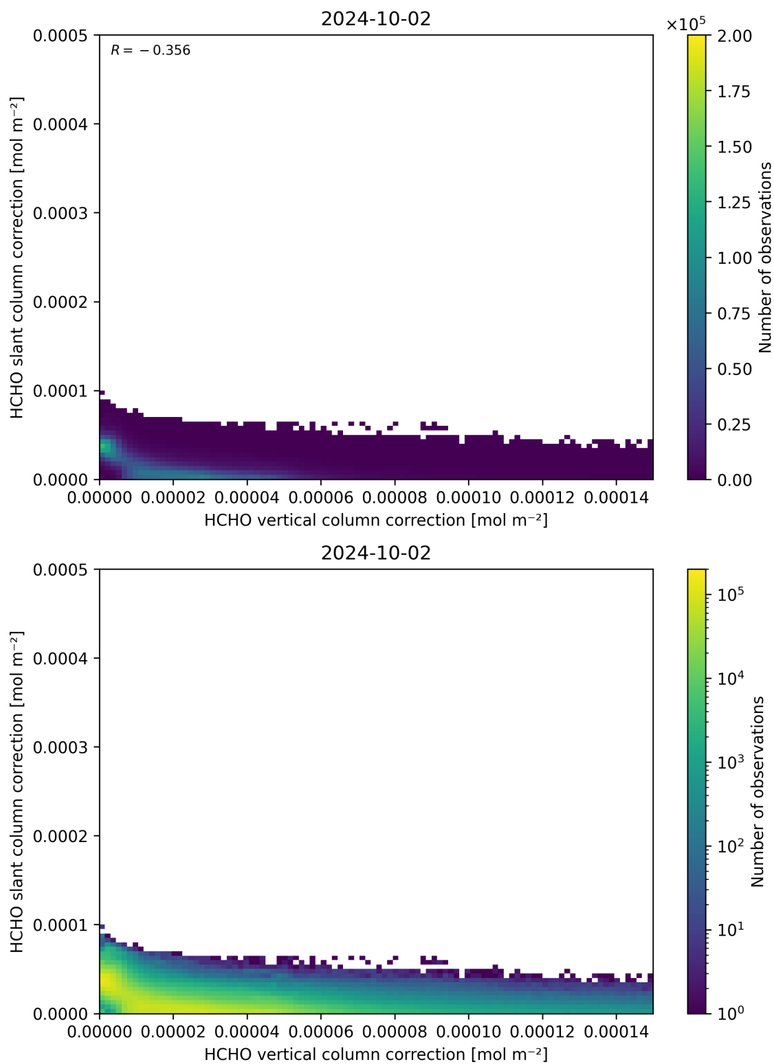
Figure 117: Scatter density plot of “HCHO vertical column correction” against “HCHO slant column correction” for 2024-10-01 to 2024-10-03.
