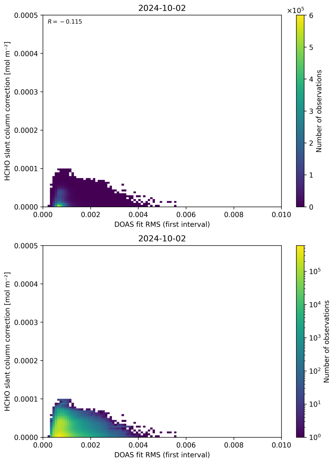
Figure 63: Scatter density plot of “DOAS fit RMS (first interval)” against “HCHO slant column correction” for 2024-10-01 to 2024-10-03.
