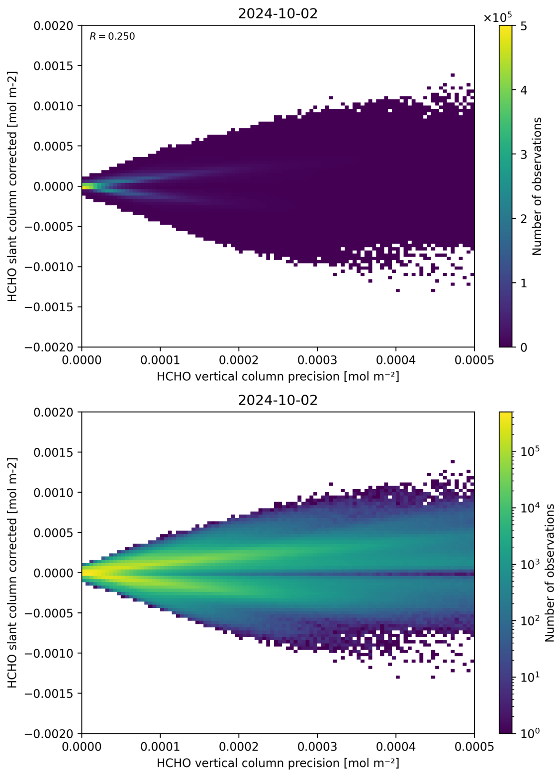
Figure 140: Scatter density plot of “HCHO vertical column precision” against “HCHO slant column corrected” for 2024-10-01 to 2024-10-03.
