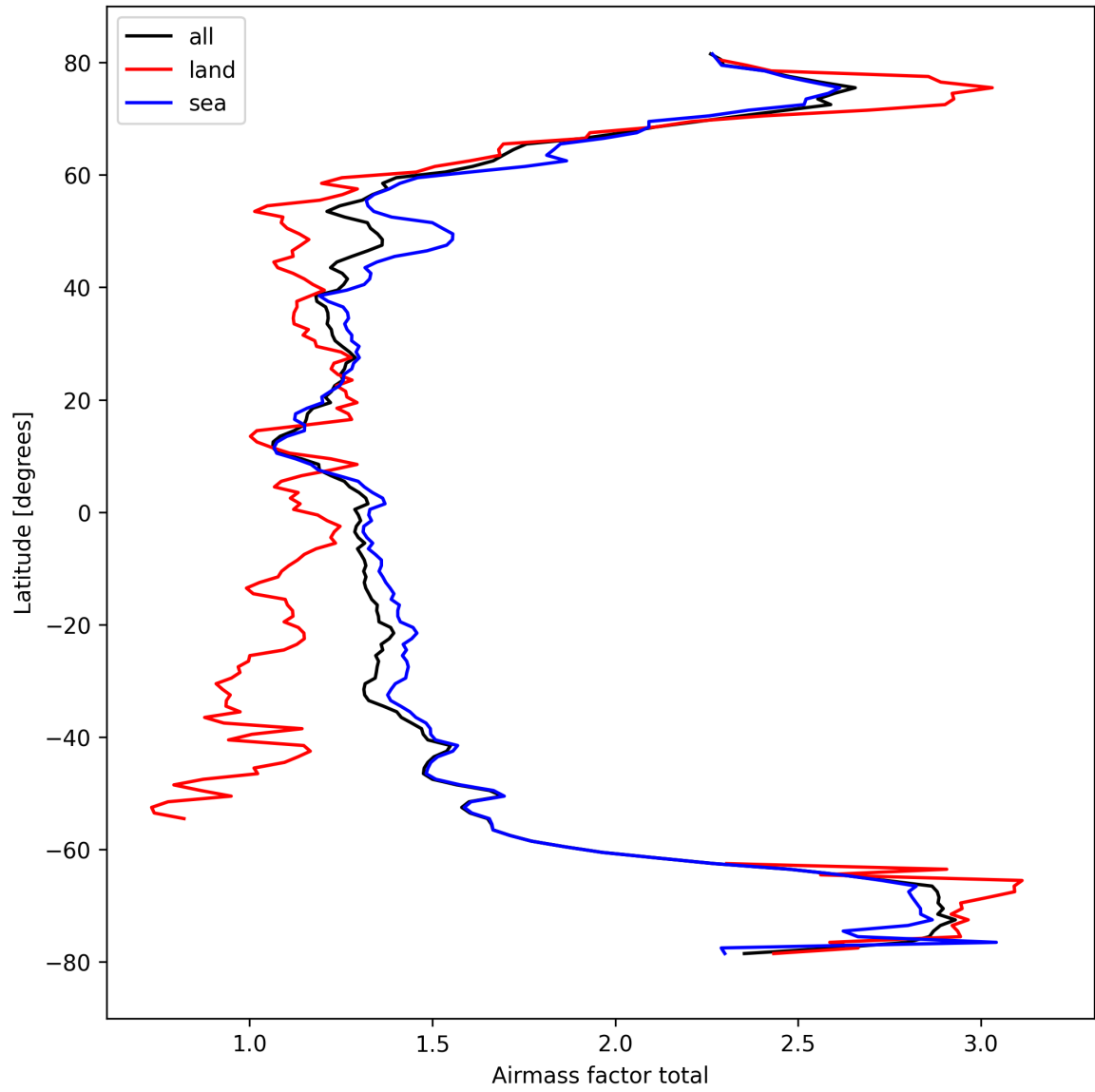
Figure 26: Zonal average of “Airmass factor total” for 2024-10-01 to 2024-10-03.
