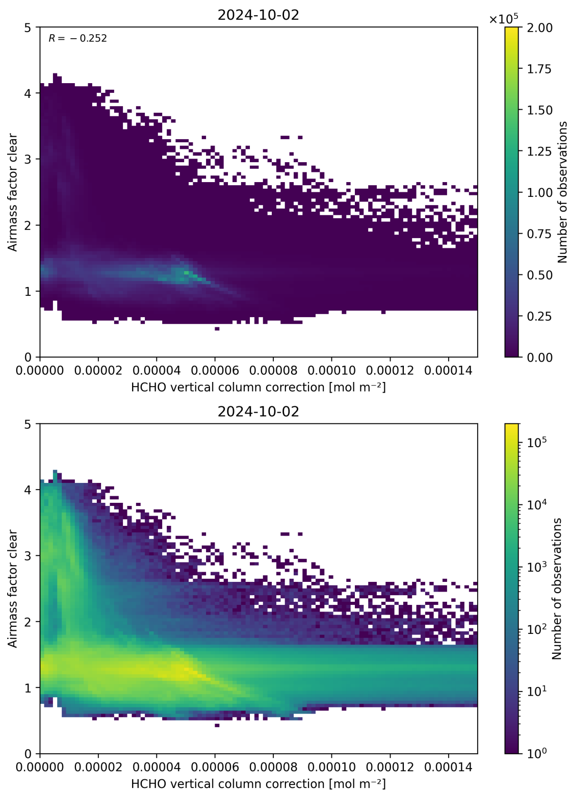
Figure 115: Scatter density plot of “HCHO vertical column correction” against “Airmass factor clear” for 2024-10-01 to 2024-10-03.
