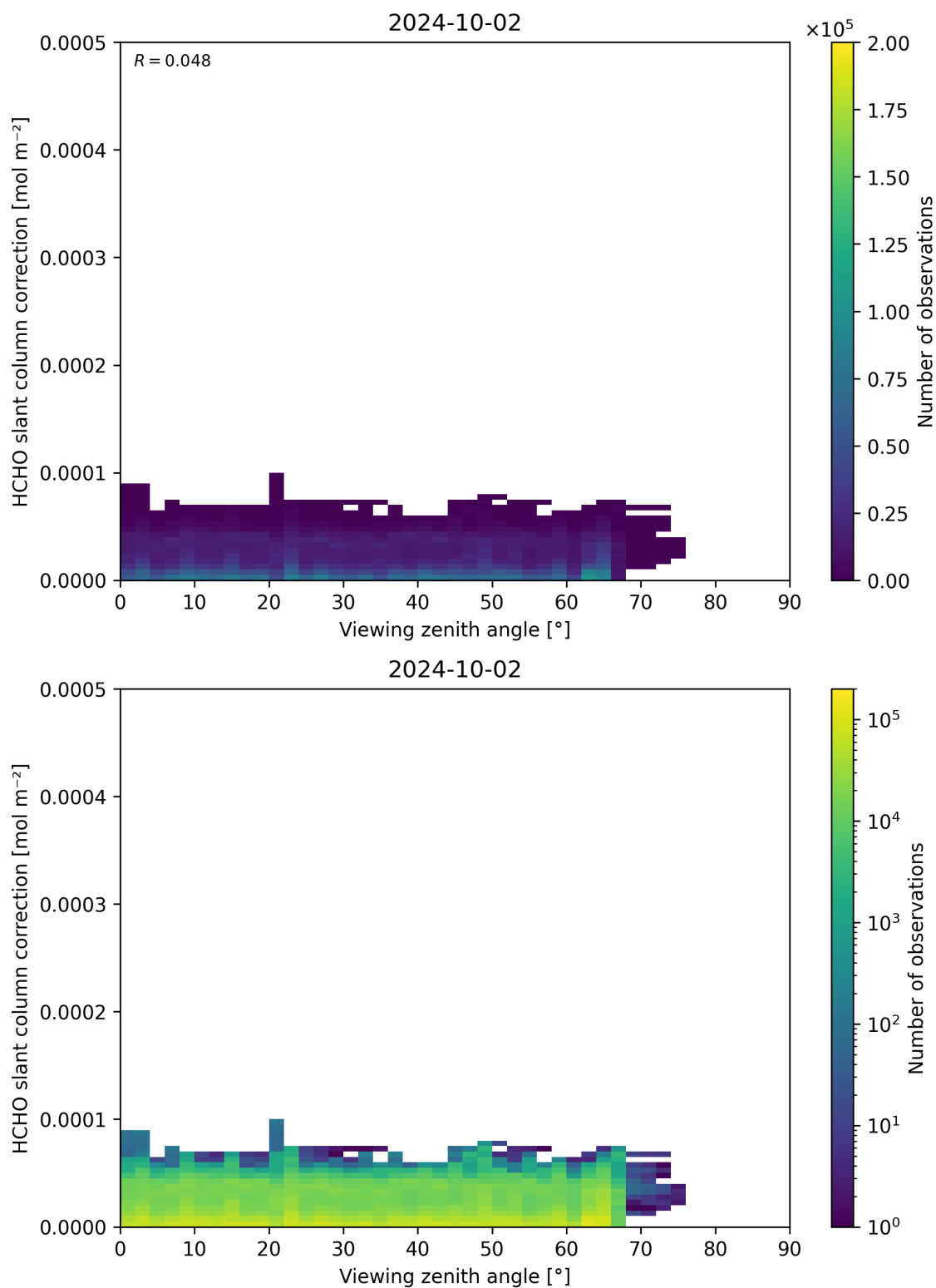
Figure 187: Scatter density plot of “Viewing zenith angle” against “HCHO slant column correction” for 2024-10-01 to 2024-10-03.
