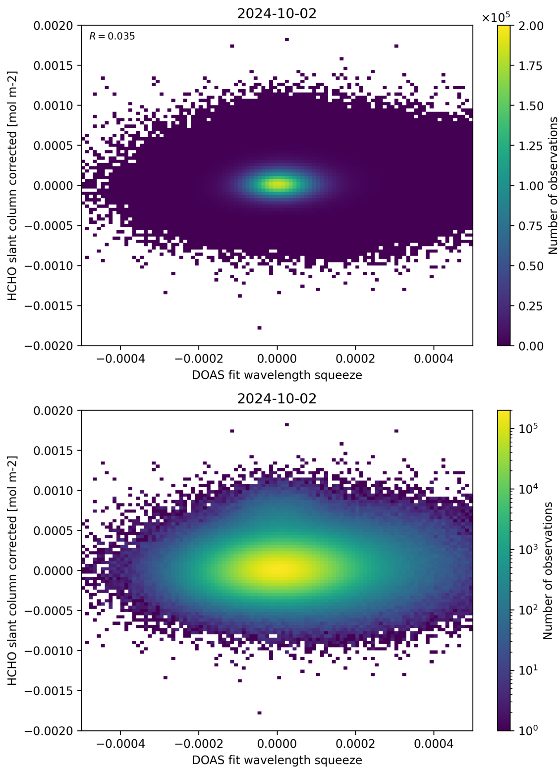
Figure 69: Scatter density plot of “DOAS fit wavelength squeeze” against “HCHO slant column corrected” for 2024-10-01 to 2024-10-03.
