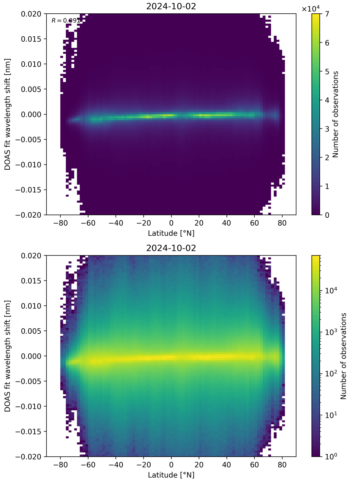
Figure 154: Scatter density plot of “Latitude” against “DOAS fit wavelength shift” for 2024-10-01 to 2024-10-03.
