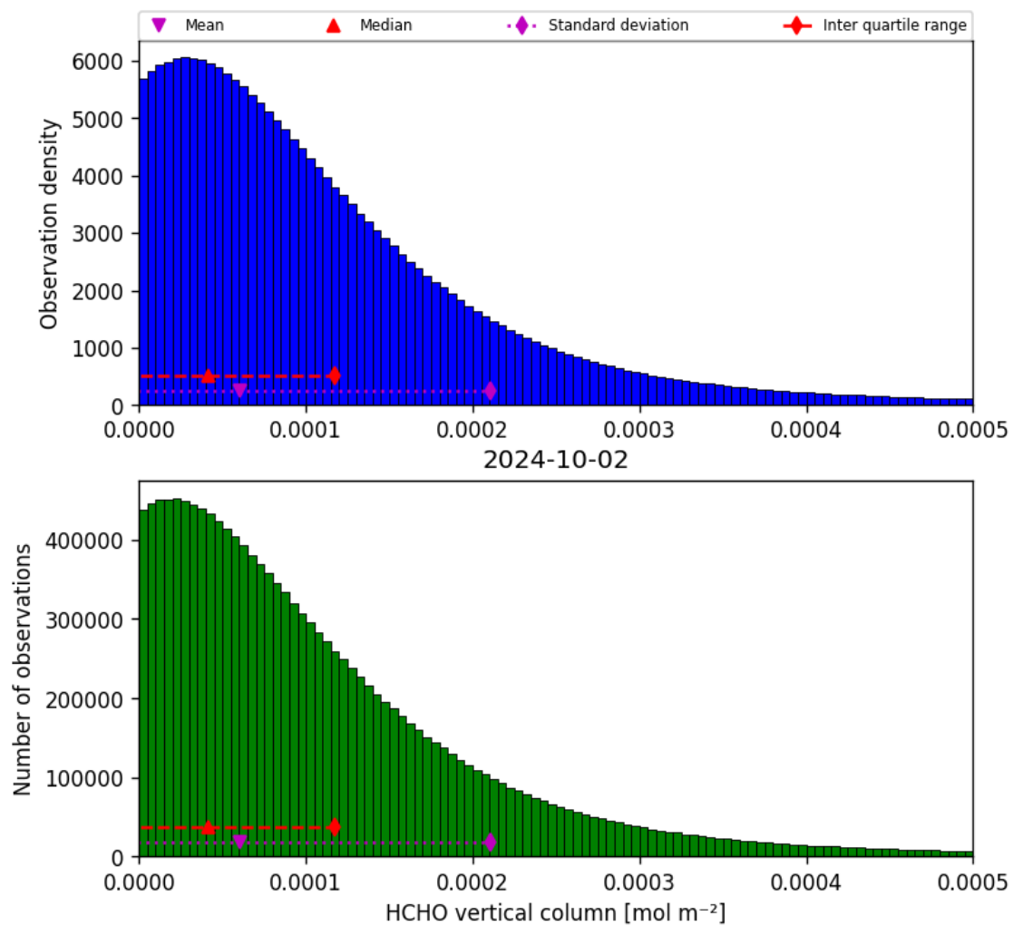
Figure 35: Histogram of “HCHO vertical column” for 2024-10-01 to 2024-10-03
