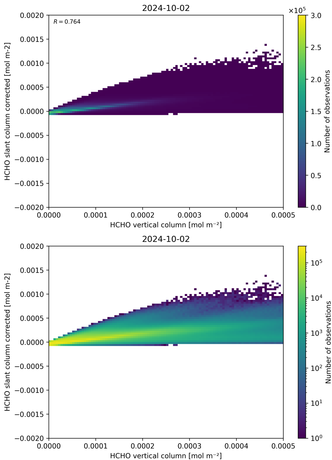
Figure 127: Scatter density plot of “HCHO vertical column” against “HCHO slant column corrected” for 2024-10-01 to 2024-10-03.
