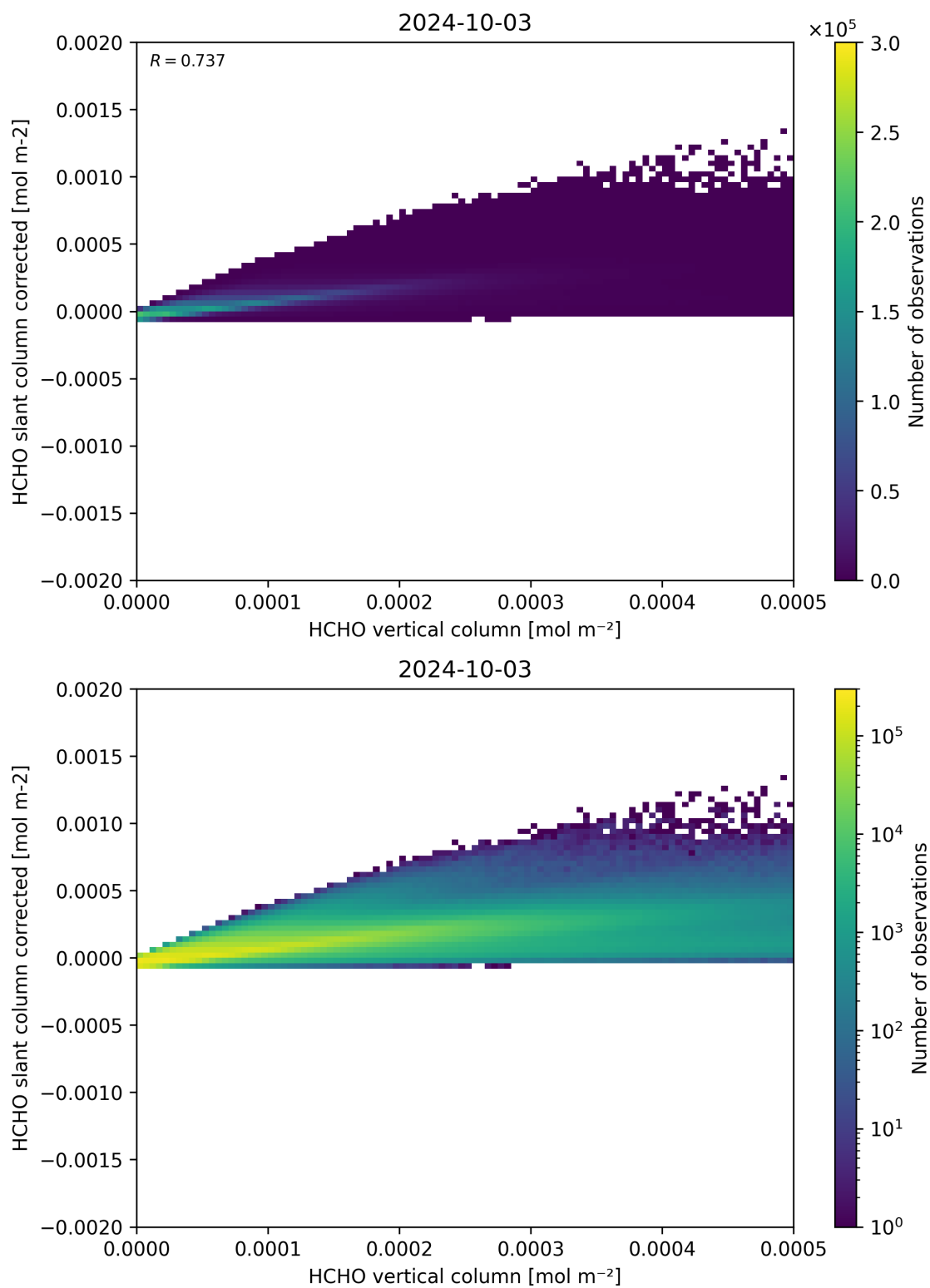
Figure 127: Scatter density plot of “HCHO vertical column” against “HCHO slant column corrected” for 2024-10-03 to 2024-10-04.
