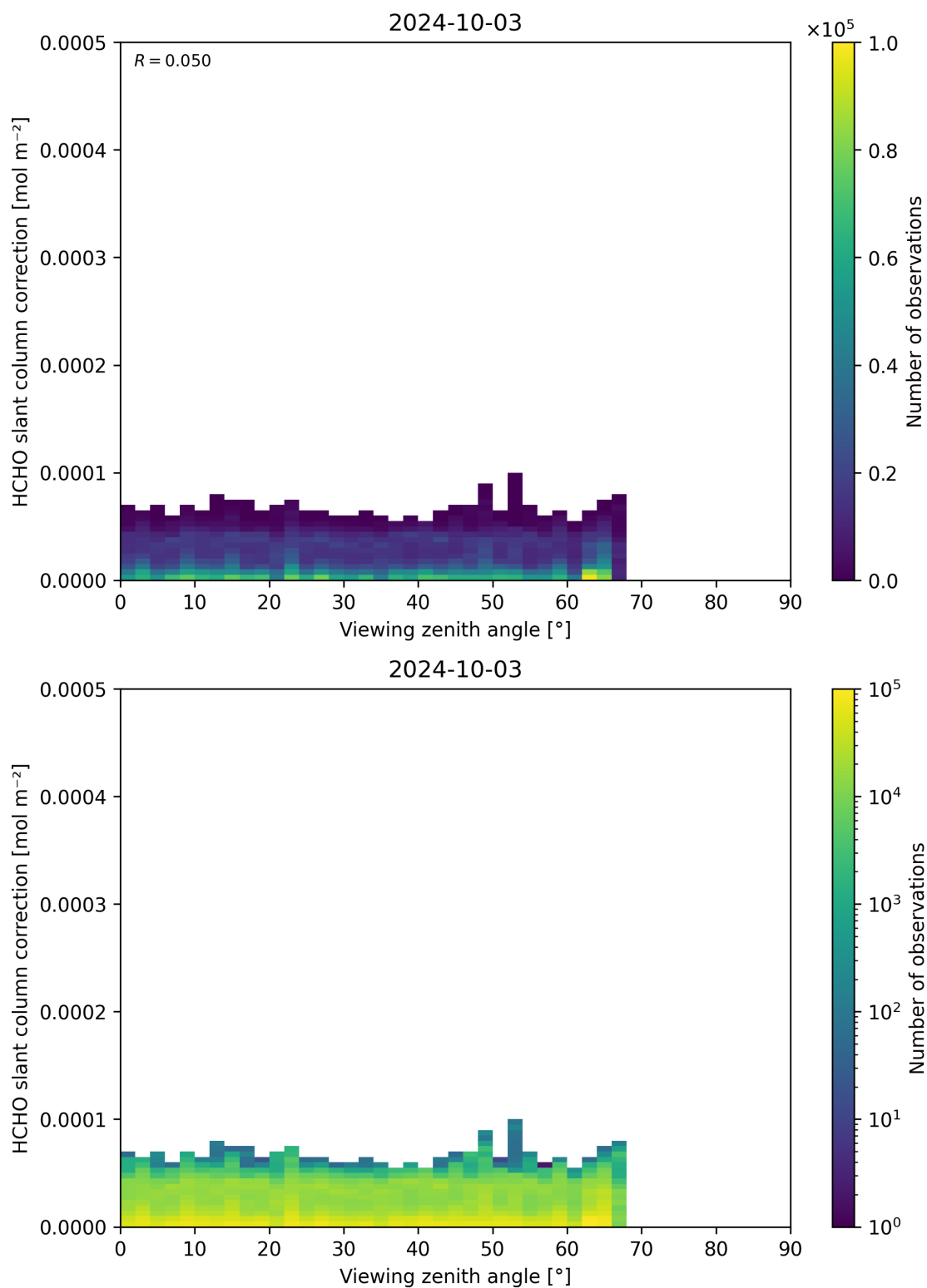
Figure 187: Scatter density plot of “Viewing zenith angle” against “HCHO slant column correction” for 2024-10-03 to 2024-10-04.
