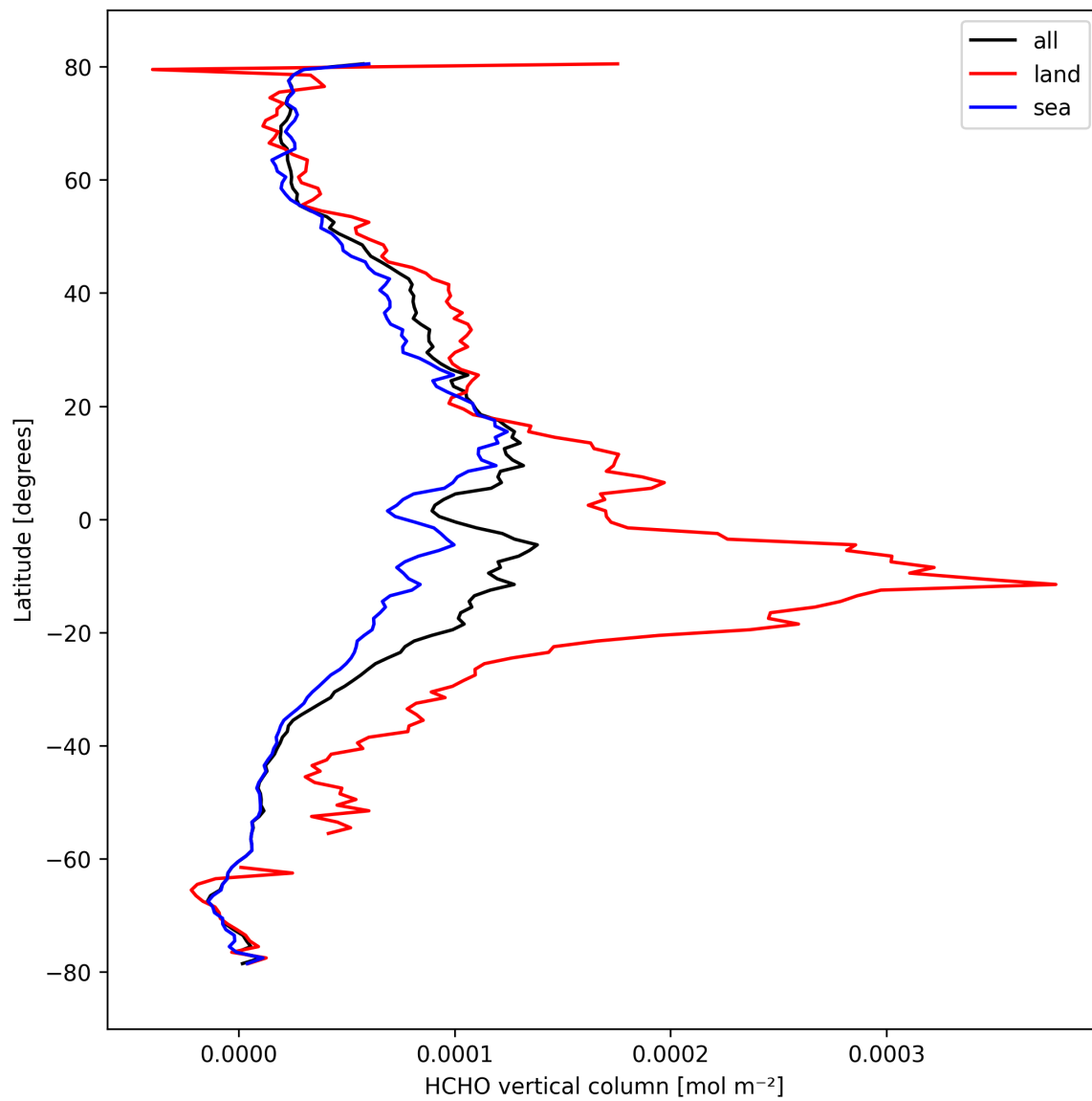
Figure 21: Zonal average of “HCHO vertical column” for 2024-10-03 to 2024-10-04.
