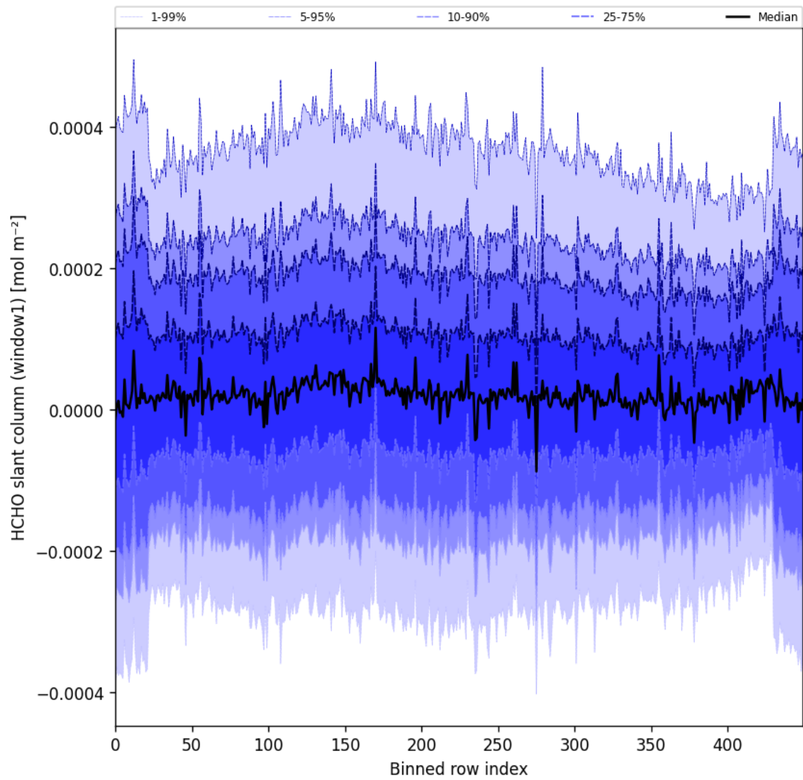
Figure 52: Along track statistics of “HCHO slant column (window1)” for 2024-10-03 to 2024-10-04
