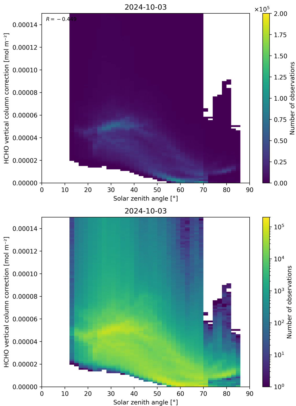
Figure 178: Scatter density plot of “Solar zenith angle” against “HCHO vertical column correction” for 2024-10-03 to 2024-10-04.
