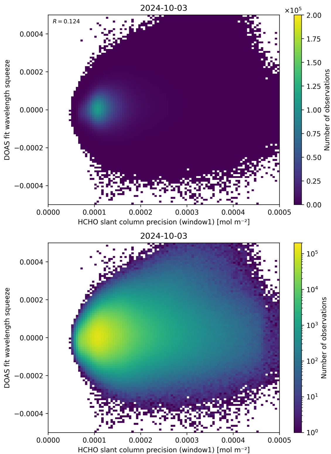
Figure 90: Scatter density plot of “HCHO slant column precision (window1)” against “DOAS fit wavelength squeeze” for 2024-10-03 to 2024-10-04.
