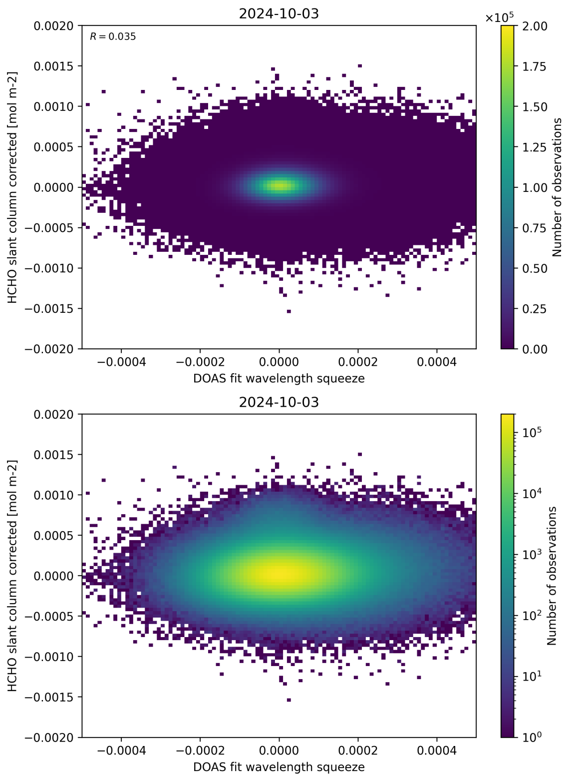
Figure 69: Scatter density plot of “DOAS fit wavelength squeeze” against “HCHO slant column corrected” for 2024-10-03 to 2024-10-04.
