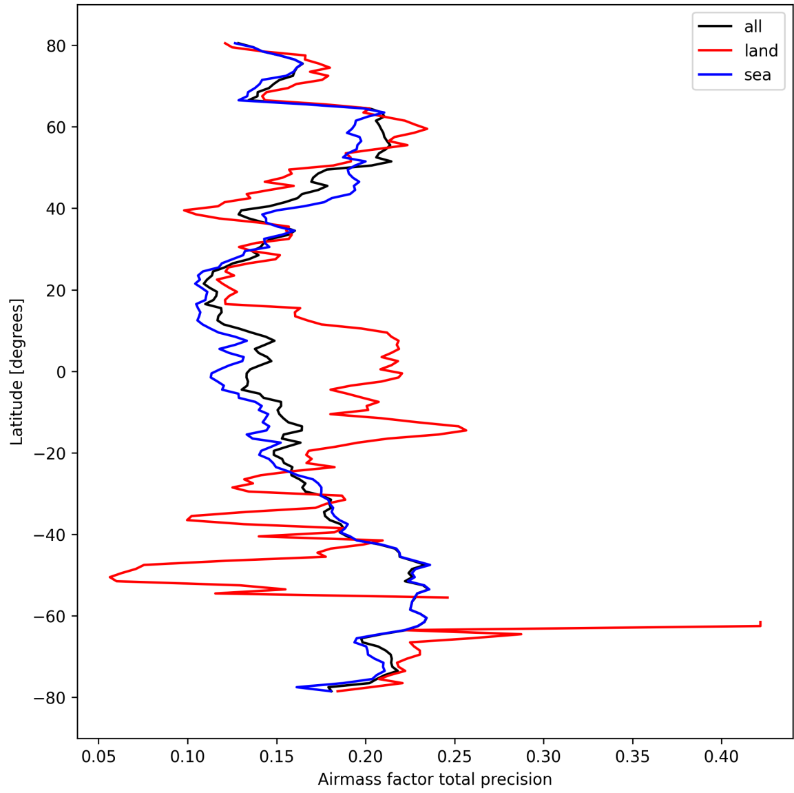
Figure 27: Zonal average of “Airmass factor total precision” for 2024-10-03 to 2024-10-04.
