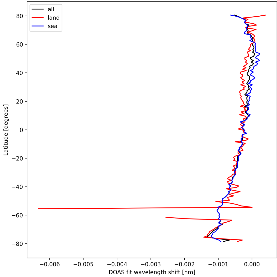
Figure 30: Zonal average of “DOAS fit wavelength shift” for 2024-10-03 to 2024-10-04.
