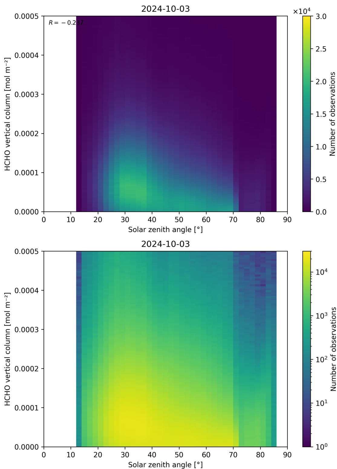
Figure 177: Scatter density plot of “Solar zenith angle” against “HCHO vertical column” for 2024-10-03 to 2024-10-04.
