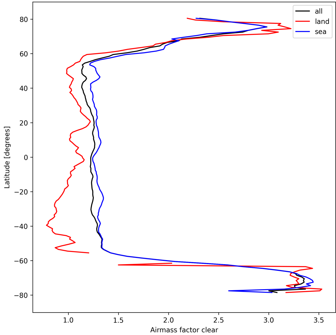
Figure 28: Zonal average of “Airmass factor clear” for 2024-10-03 to 2024-10-04.
