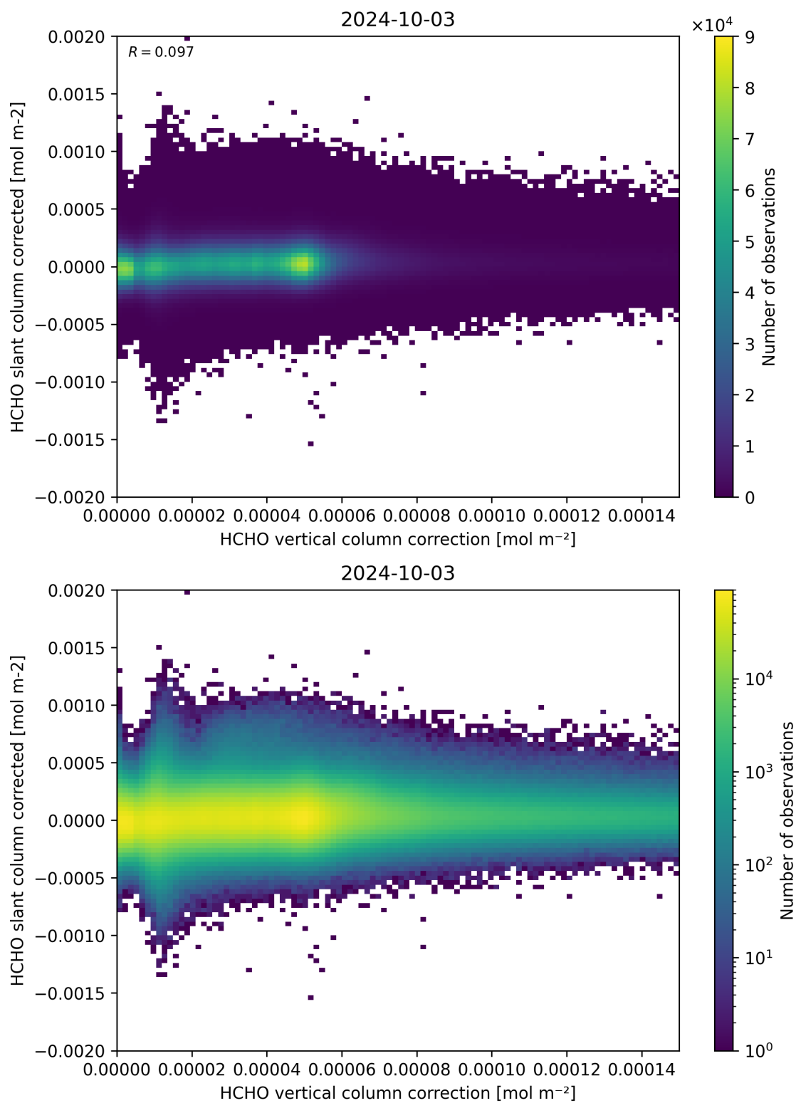
Figure 116: Scatter density plot of “HCHO vertical column correction” against “HCHO slant column corrected” for 2024-10-03 to 2024-10-04.
