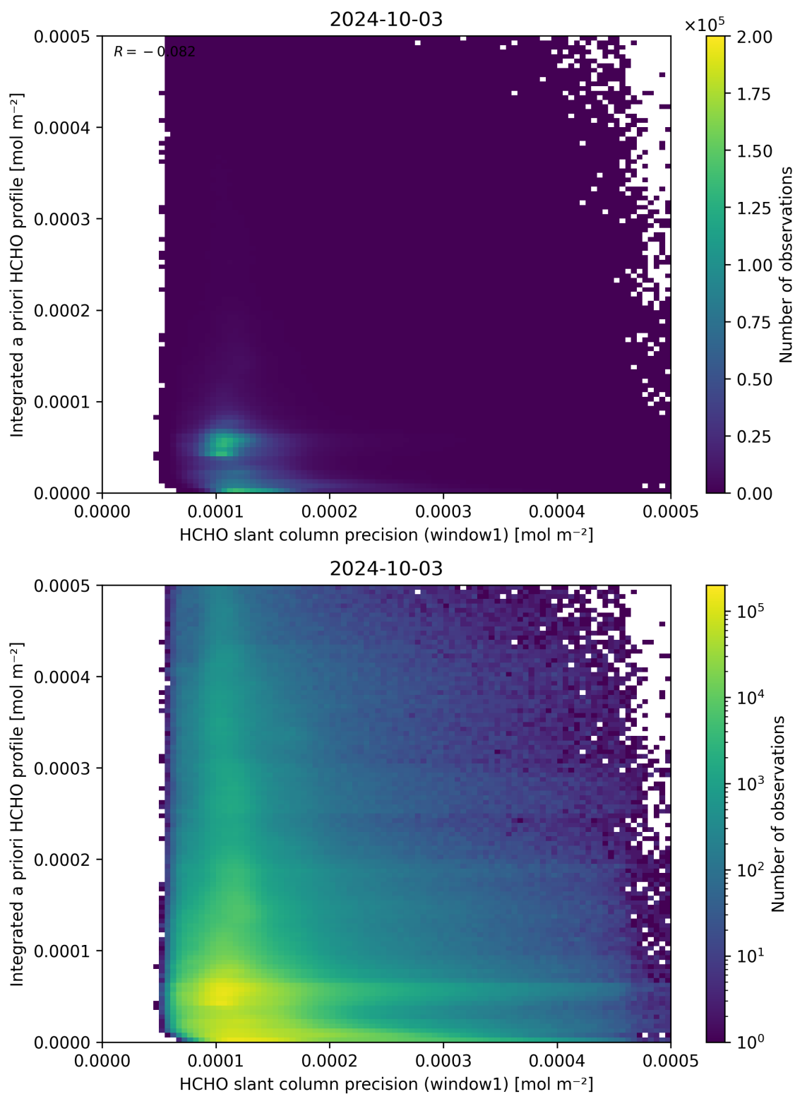
Figure 96: Scatter density plot of “HCHO slant column precision (window1)” against “Integrated a priori HCHO profile” for 2024-10-03 to 2024-10-04.
