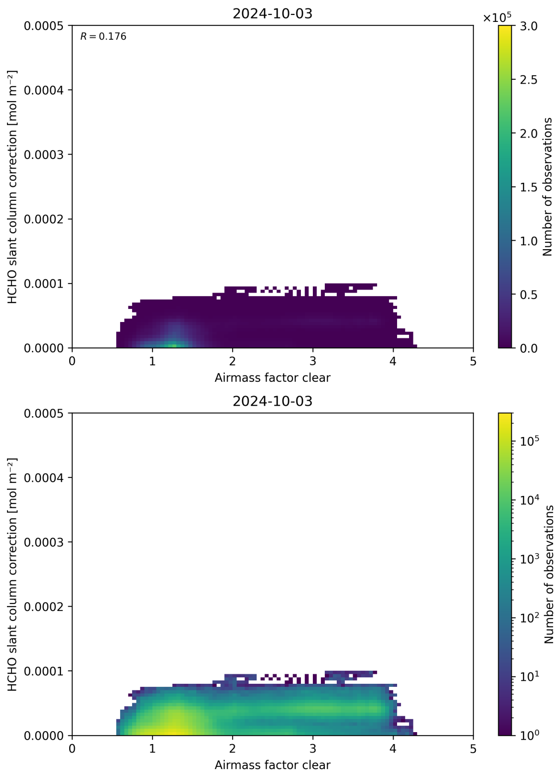
Figure 75: Scatter density plot of “Airmass factor clear” against “HCHO slant column correction” for 2024-10-03 to 2024-10-04.
