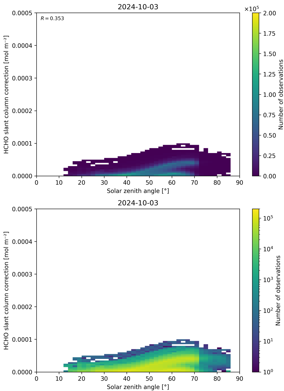
Figure 172: Scatter density plot of “Solar zenith angle” against “HCHO slant column correction” for 2024-10-03 to 2024-10-04.
