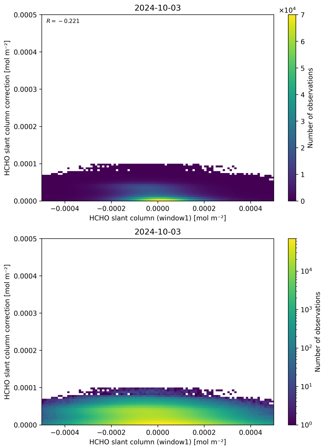
Figure 83: Scatter density plot of “HCHO slant column (window1)” against “HCHO slant column correction” for 2024-10-03 to 2024-10-04.
