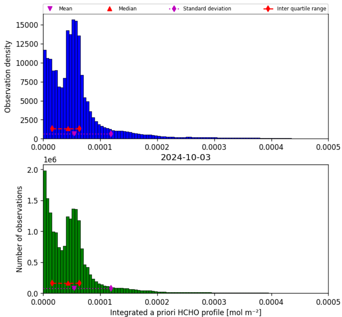
Figure 43: Histogram of “Integrated a priori HCHO profile” for 2024-10-03 to 2024-10-04
