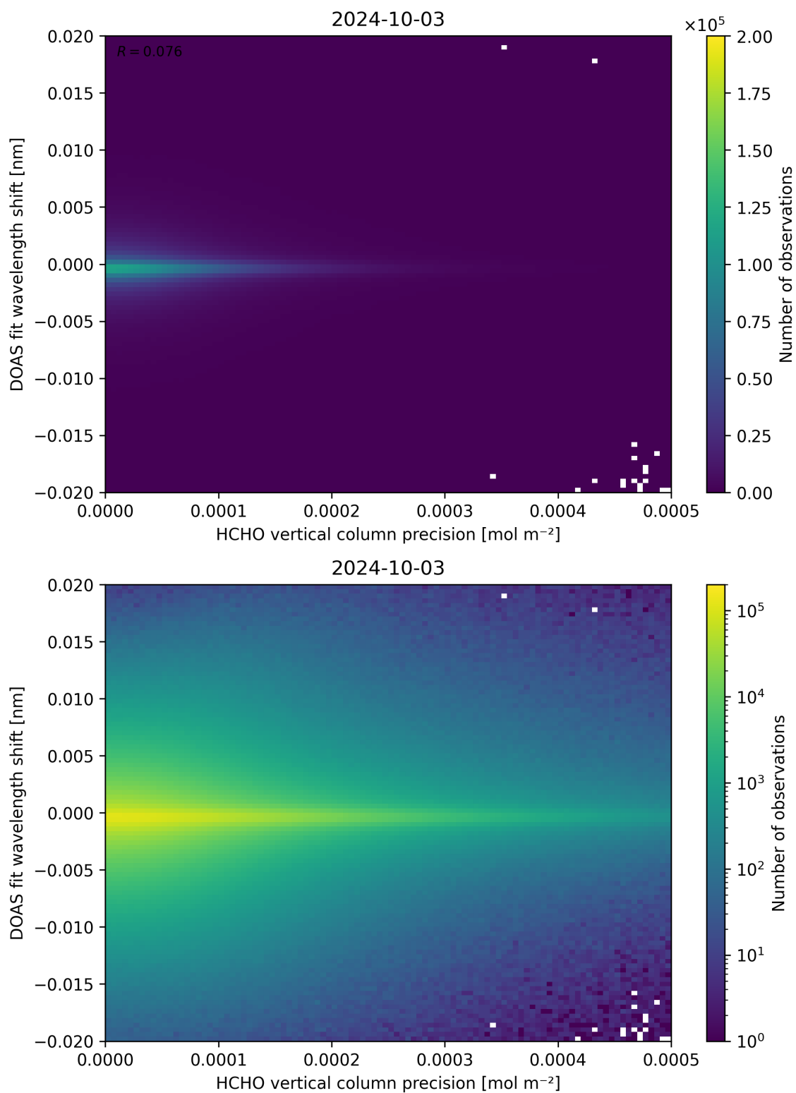
Figure 137: Scatter density plot of “HCHO vertical column precision” against “DOAS fit wavelength shift” for 2024-10-03 to 2024-10-04.
