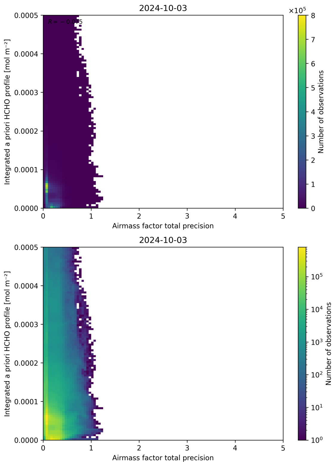
Figure 111: Scatter density plot of “Airmass factor total precision” against “Integrated a priori HCHO profile” for 2024-10-03 to 2024-10-04.
