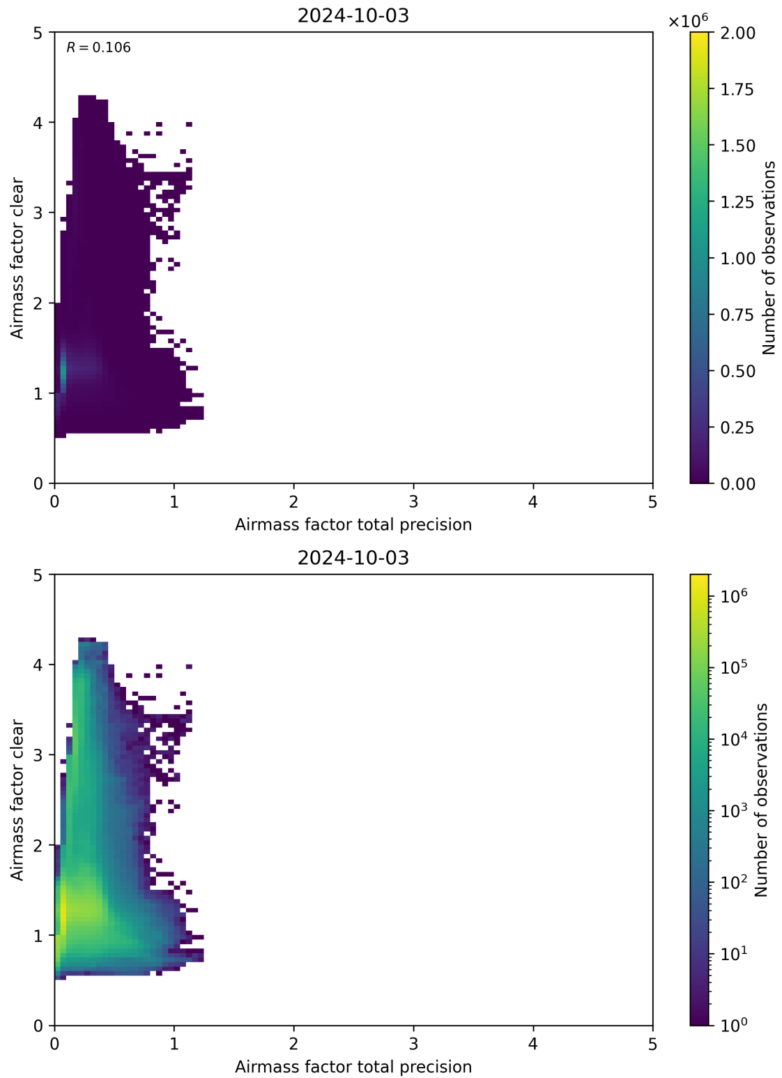
Figure 108: Scatter density plot of “Airmass factor total precision” against “Airmass factor clear” for 2024-10-03 to 2024-10-04.
