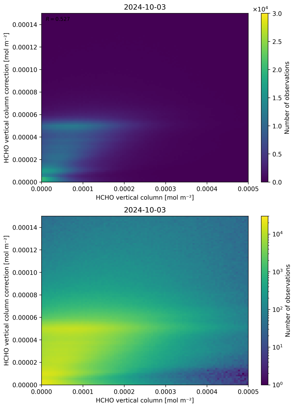
Figure 133: Scatter density plot of “HCHO vertical column” against “HCHO vertical column correction” for 2024-10-03 to 2024-10-04.
