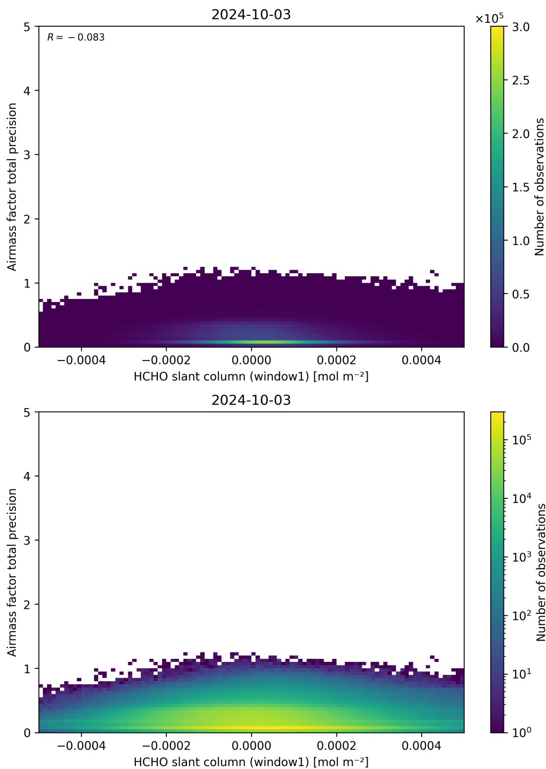
Figure 86: Scatter density plot of “HCHO slant column (window1)” against “Airmass factor total precision” for 2024-10-03 to 2024-10-04.
