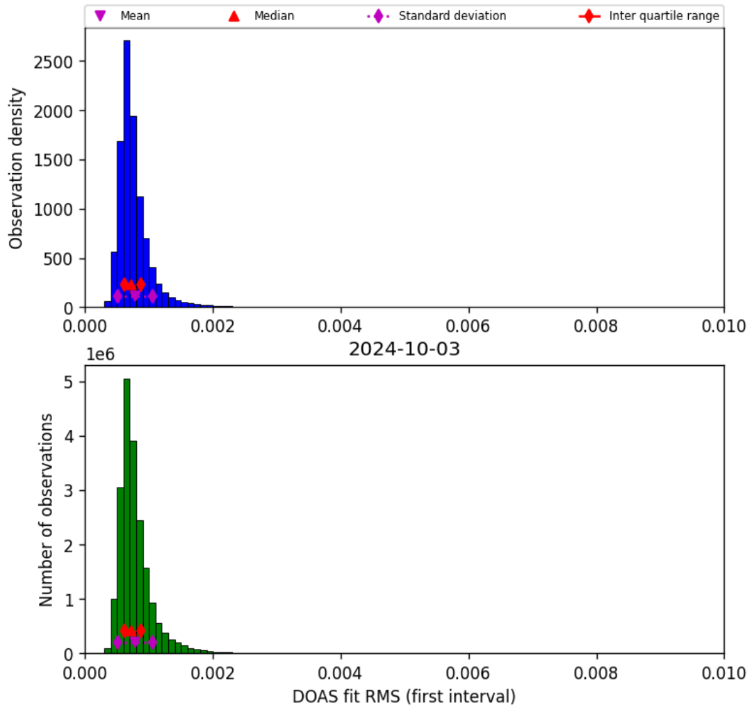
Figure 46: Histogram of “DOAS fit RMS (first interval)” for 2024-10-03 to 2024-10-04
