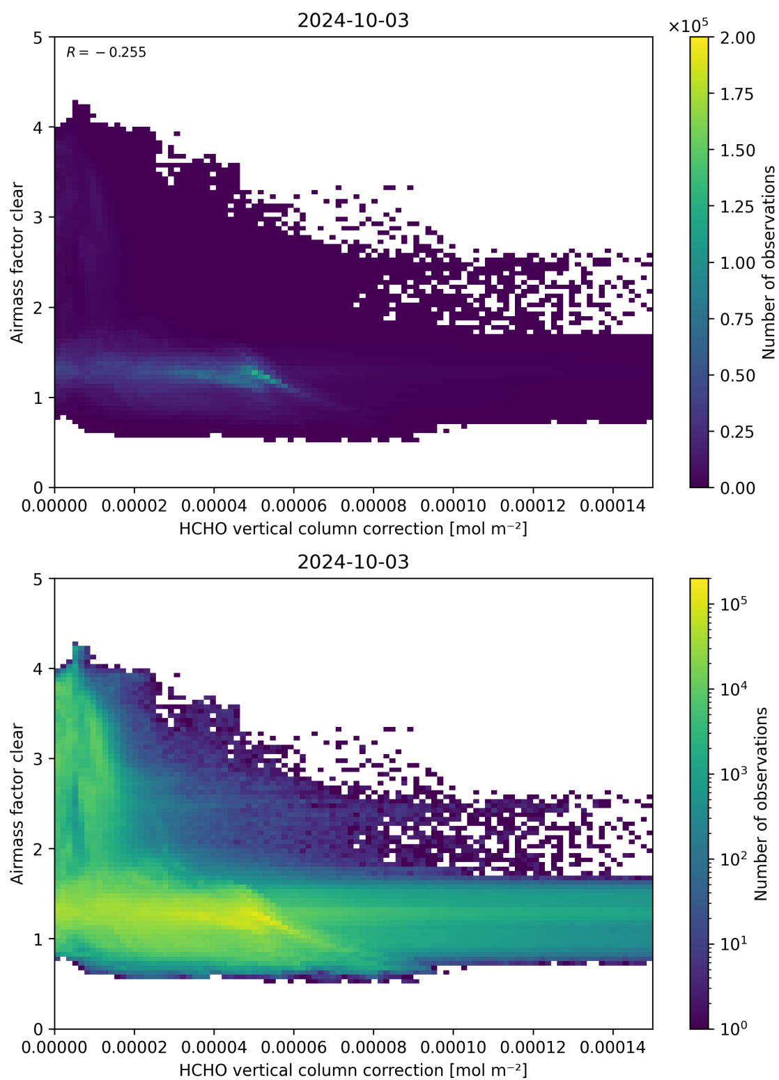
Figure 115: Scatter density plot of “HCHO vertical column correction” against “Airmass factor clear” for 2024-10-03 to 2024-10-04.
