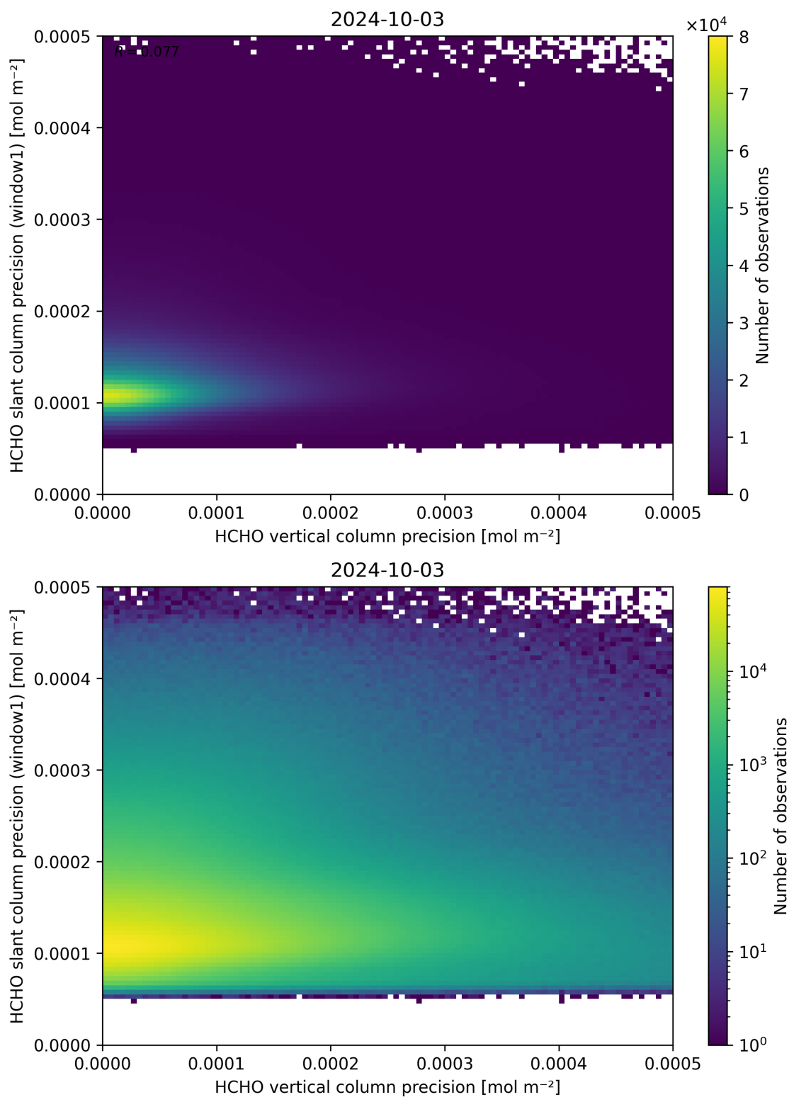
Figure 143: Scatter density plot of “HCHO vertical column precision” against “HCHO slant column precision (window1)” for 2024-10-03 to 2024-10-04.
