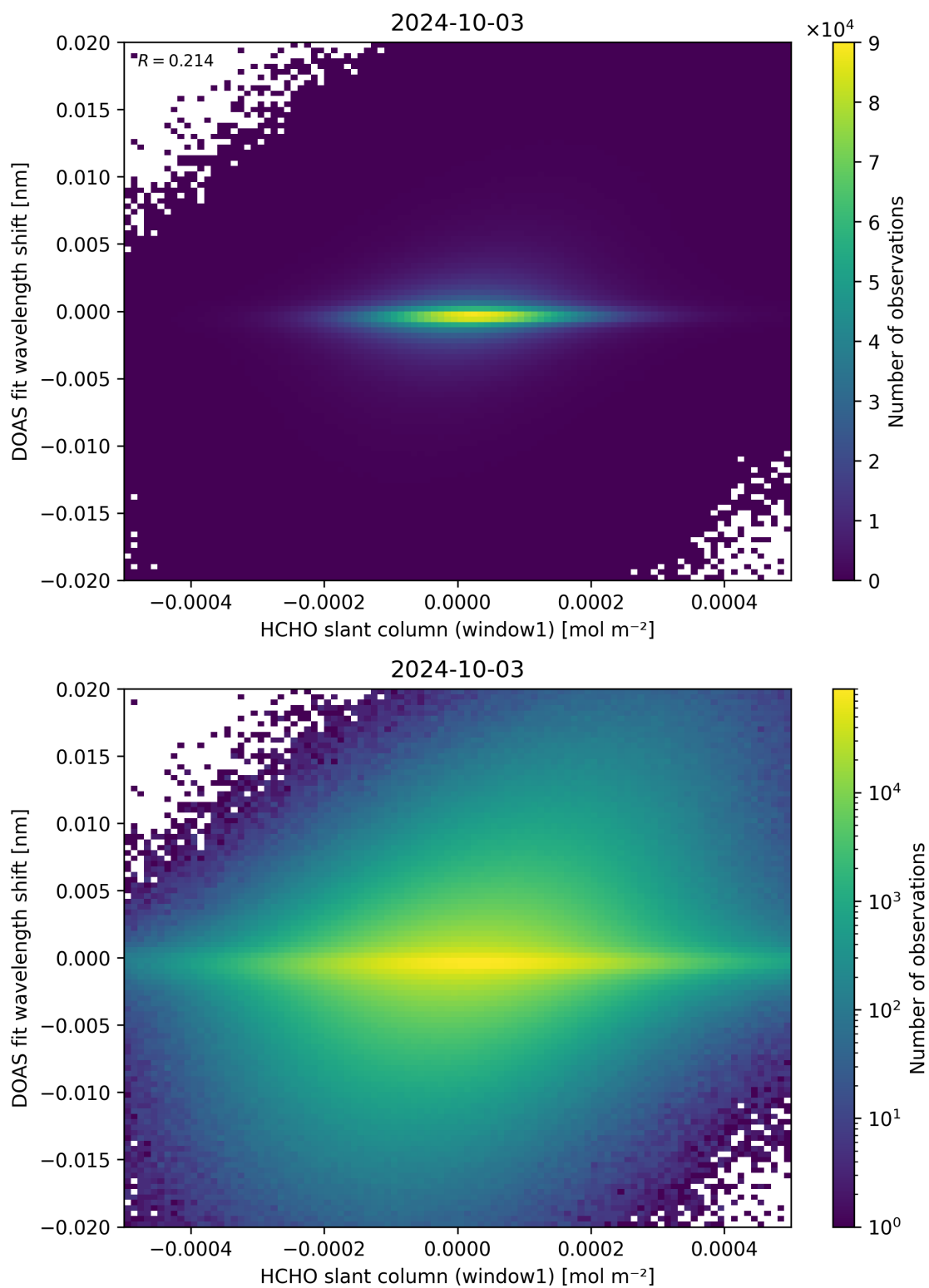
Figure 79: Scatter density plot of “HCHO slant column (window1)” against “DOAS fit wavelength shift” for 2024-10-03 to 2024-10-04.
