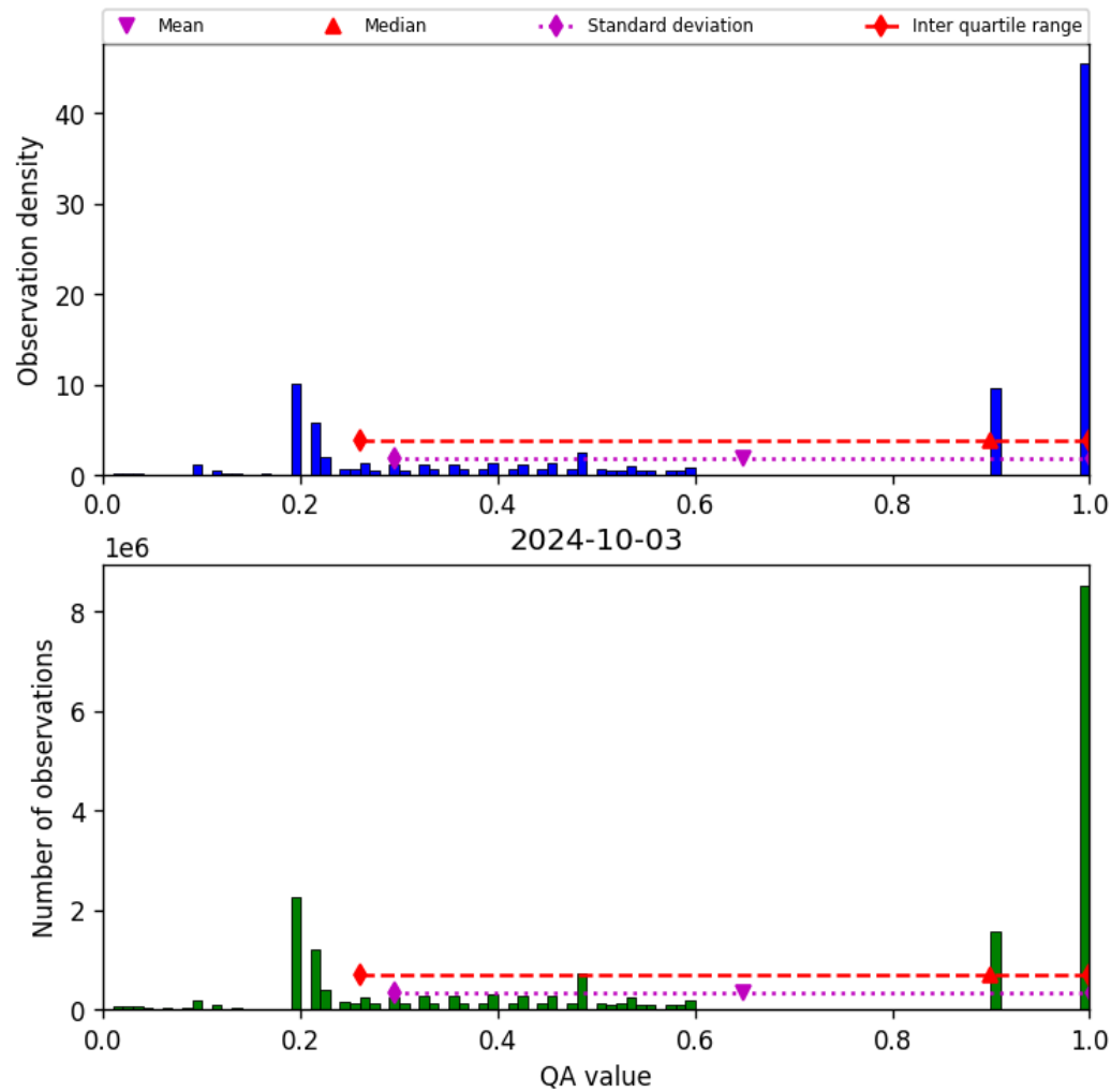
Figure 34: Histogram of “QA value” for 2024-10-03 to 2024-10-04
