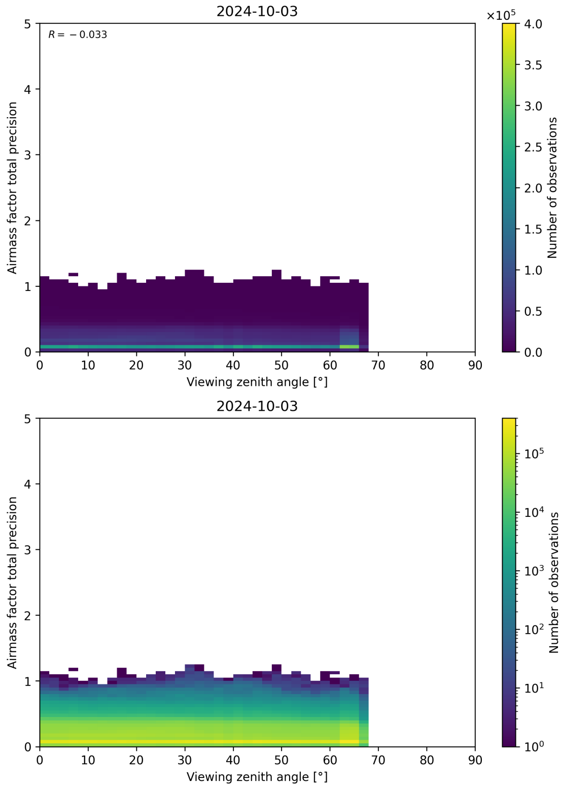
Figure 191: Scatter density plot of “Viewing zenith angle” against “Airmass factor total precision” for 2024-10-03 to 2024-10-04.
