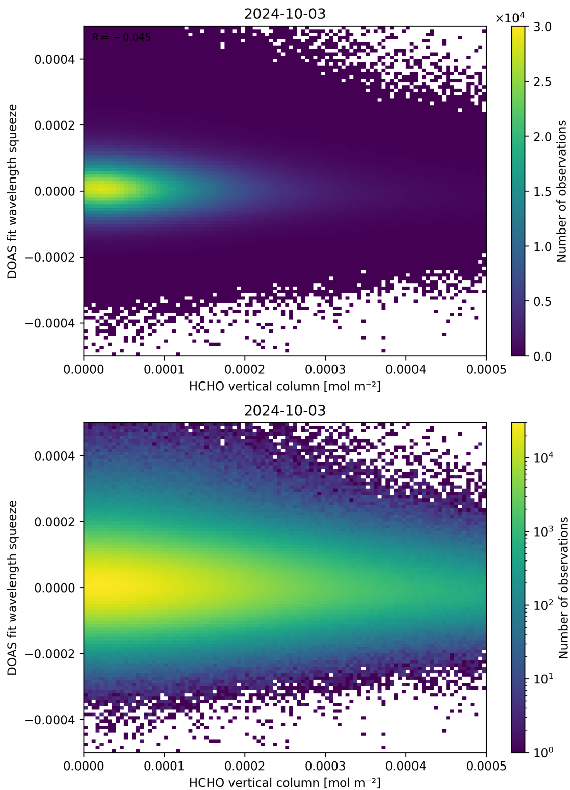
Figure 125: Scatter density plot of “HCHO vertical column” against “DOAS fit wavelength squeeze” for 2024-10-03 to 2024-10-04.
