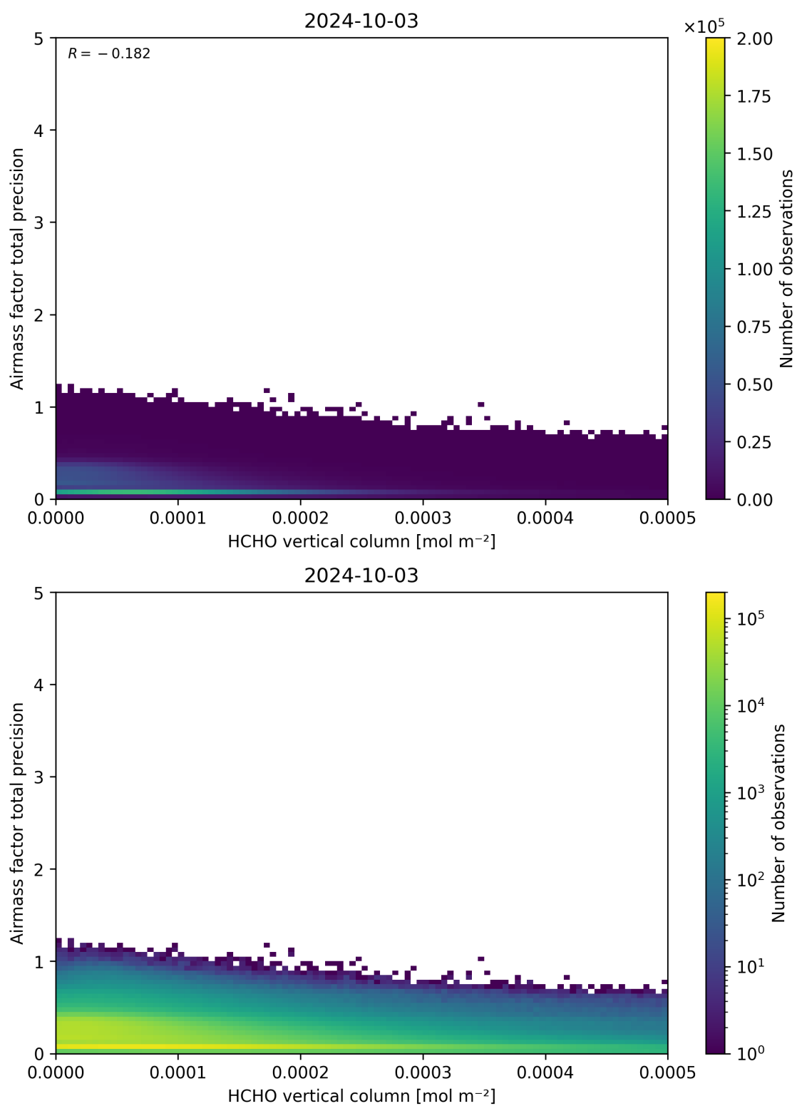
Figure 132: Scatter density plot of “HCHO vertical column” against “Airmass factor total precision” for 2024-10-03 to 2024-10-04.
