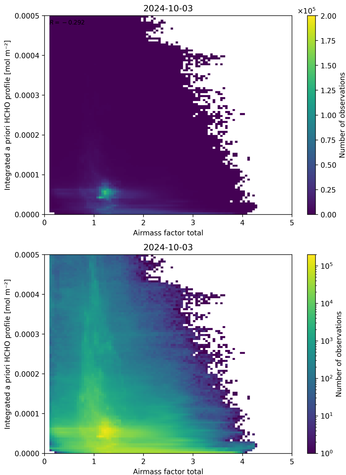
Figure 104: Scatter density plot of “Airmass factor total” against “Integrated a priori HCHO profile” for 2024-10-03 to 2024-10-04.
