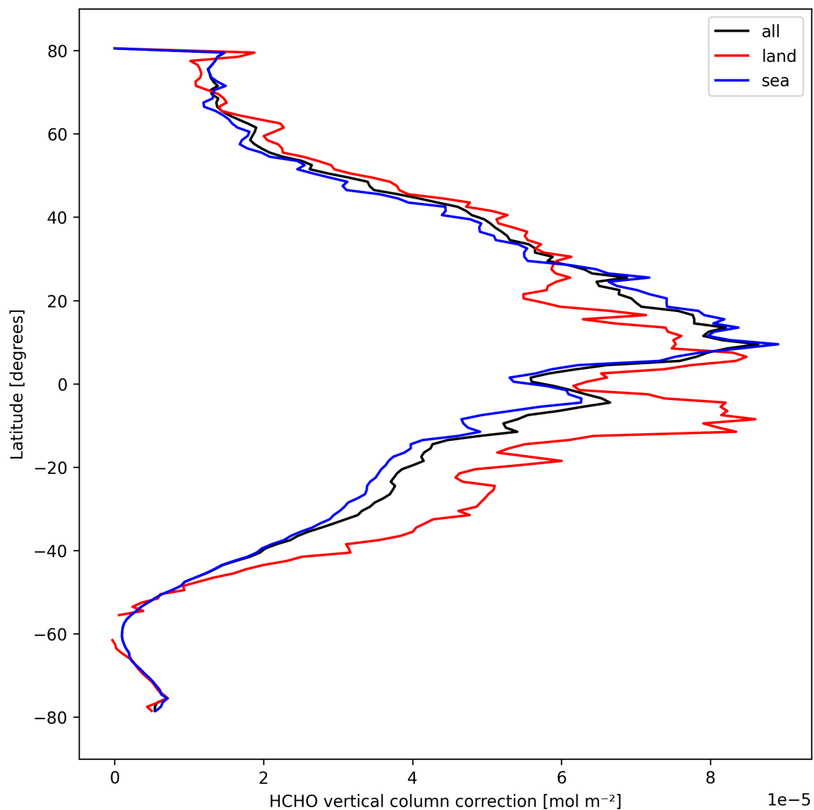
Figure 23: Zonal average of “HCHO vertical column correction” for 2024-10-03 to 2024-10-04.
