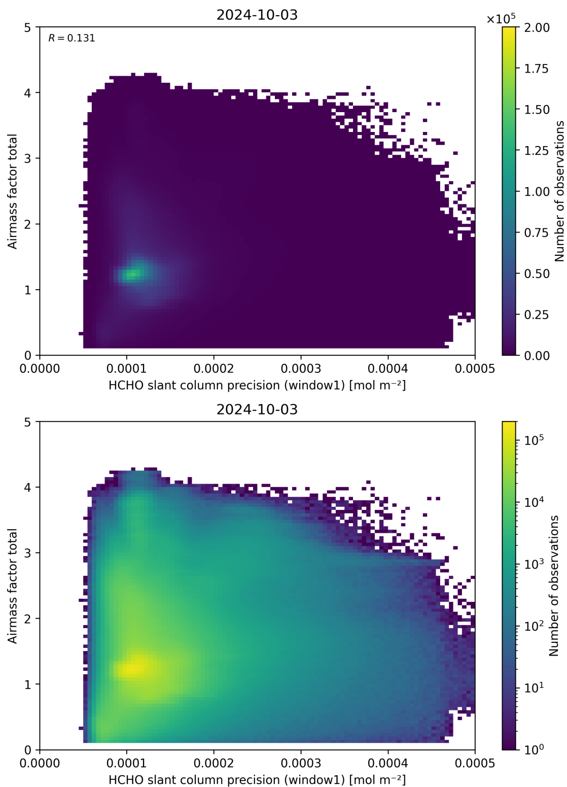
Figure 94: Scatter density plot of “HCHO slant column precision (window1)” against “Airmass factor total” for 2024-10-03 to 2024-10-04.
