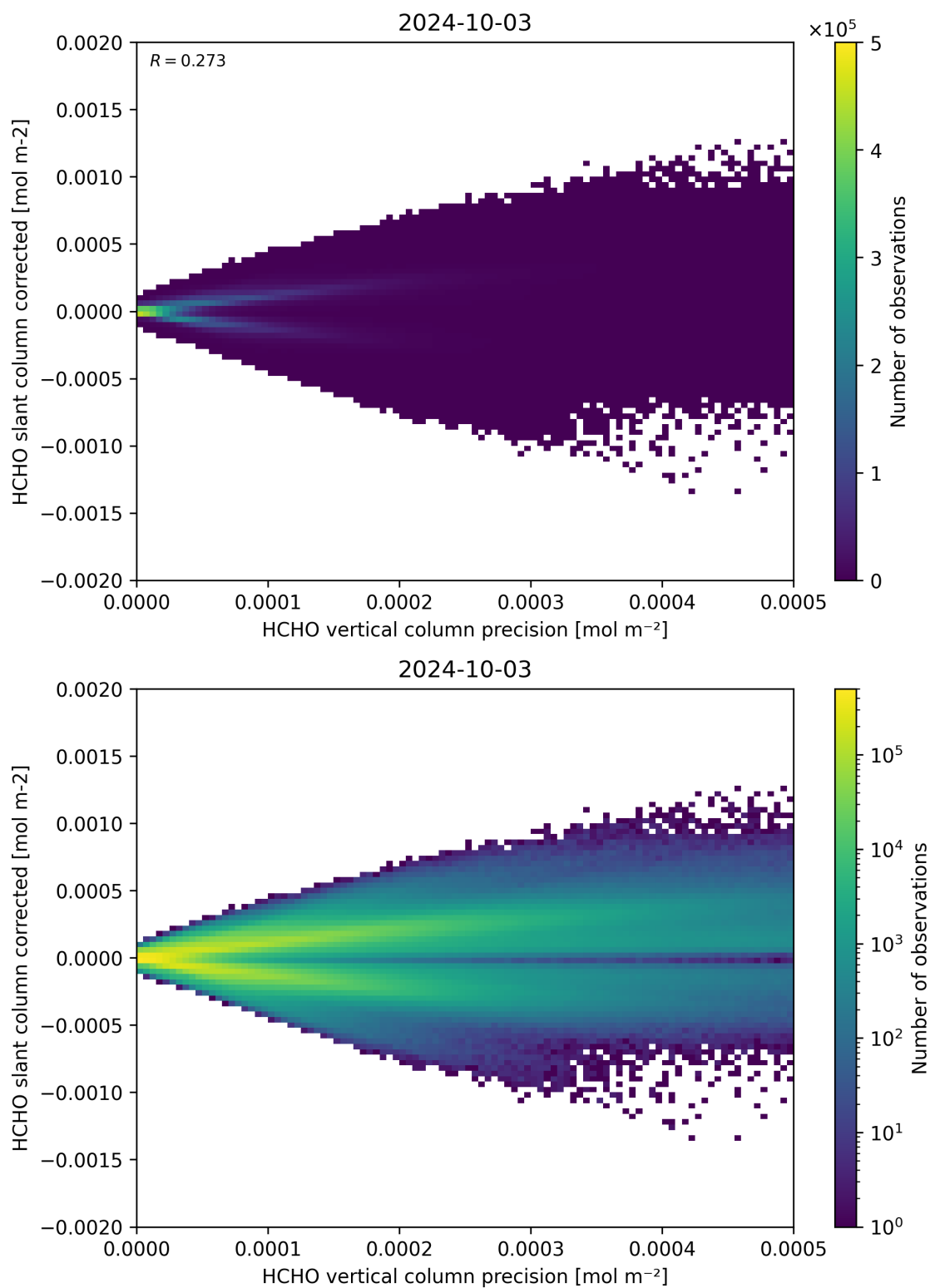
Figure 140: Scatter density plot of “HCHO vertical column precision” against “HCHO slant column corrected” for 2024-10-03 to 2024-10-04.
