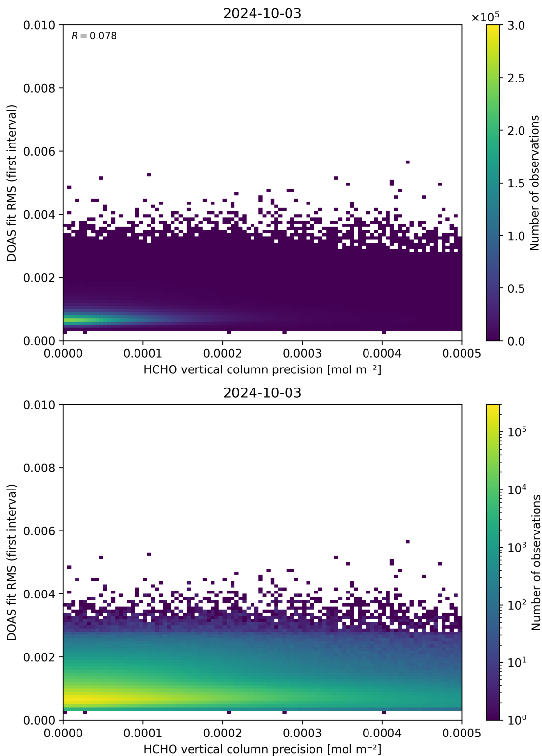
Figure 136: Scatter density plot of “HCHO vertical column precision” against “DOAS fit RMS (first interval)” for 2024-10-03 to 2024-10-04.
