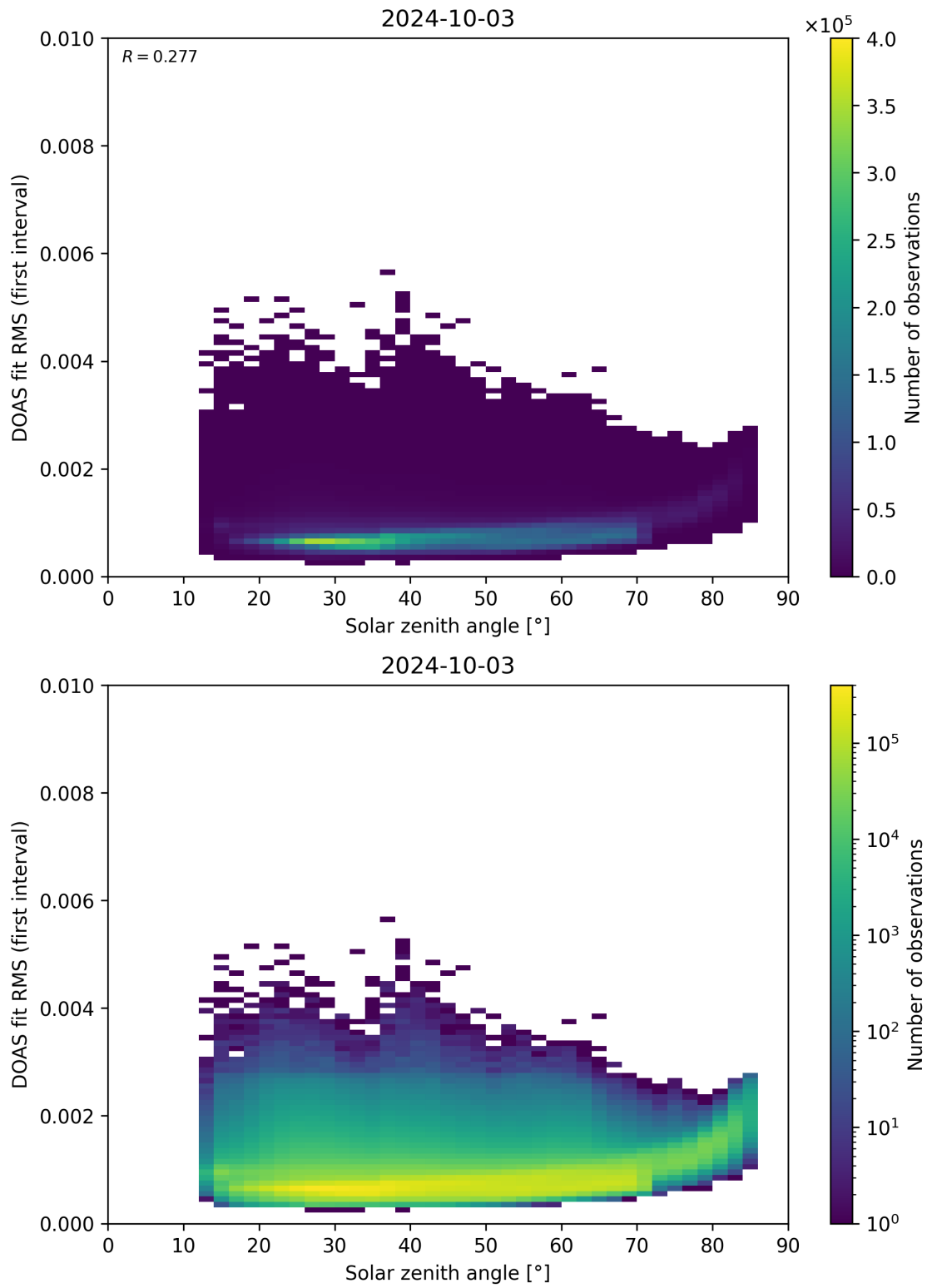
Figure 167: Scatter density plot of “Solar zenith angle” against “DOAS fit RMS (first interval)” for 2024-10-03 to 2024-10-04.
