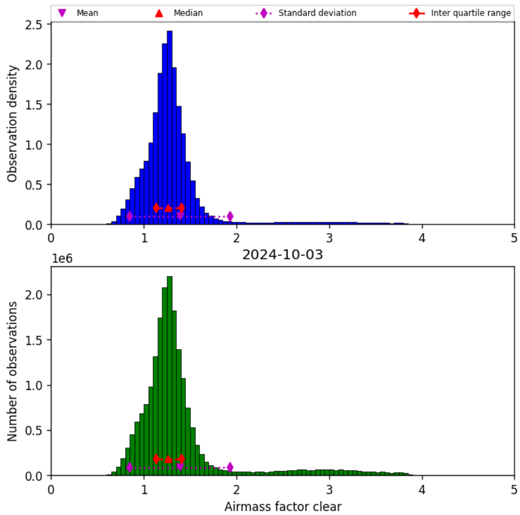
Figure 42: Histogram of “Airmass factor clear” for 2024-10-03 to 2024-10-04
