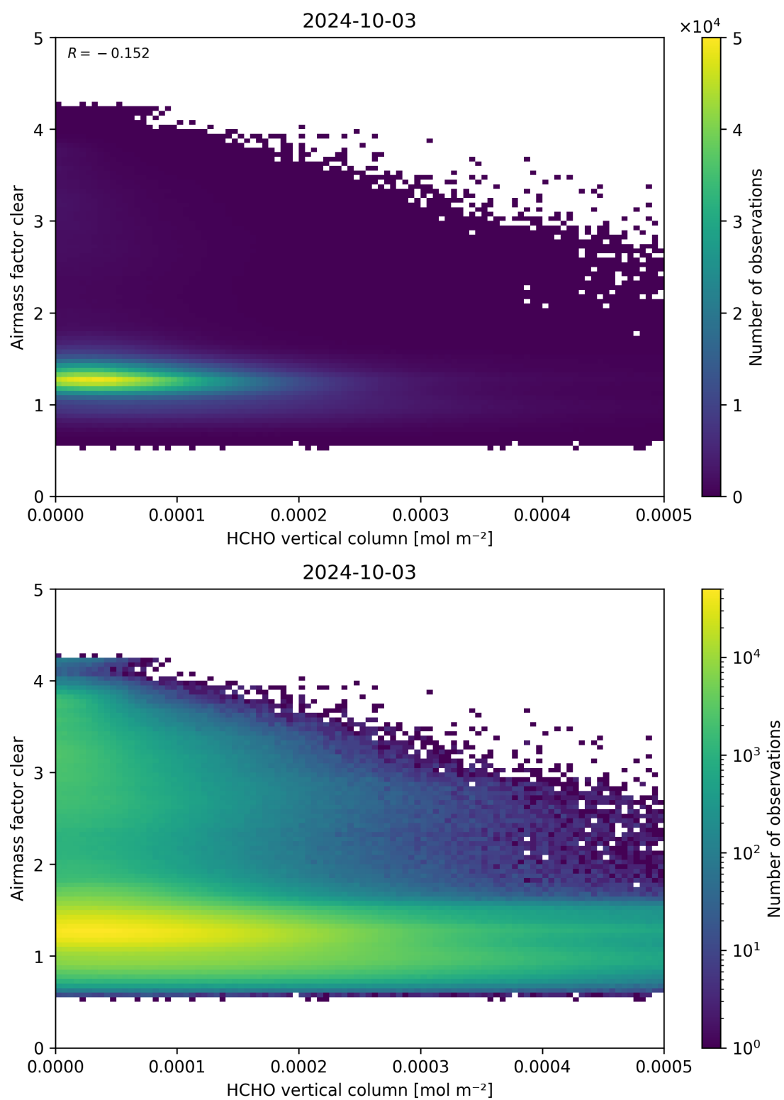
Figure 126: Scatter density plot of “HCHO vertical column” against “Airmass factor clear” for 2024-10-03 to 2024-10-04.
