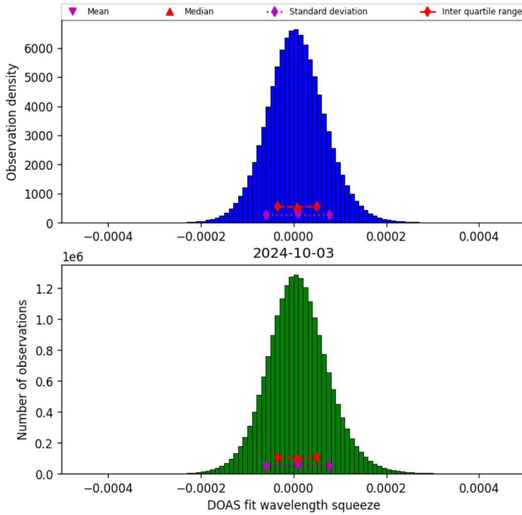
Figure 45: Histogram of “DOAS fit wavelength squeeze” for 2024-10-03 to 2024-10-04
