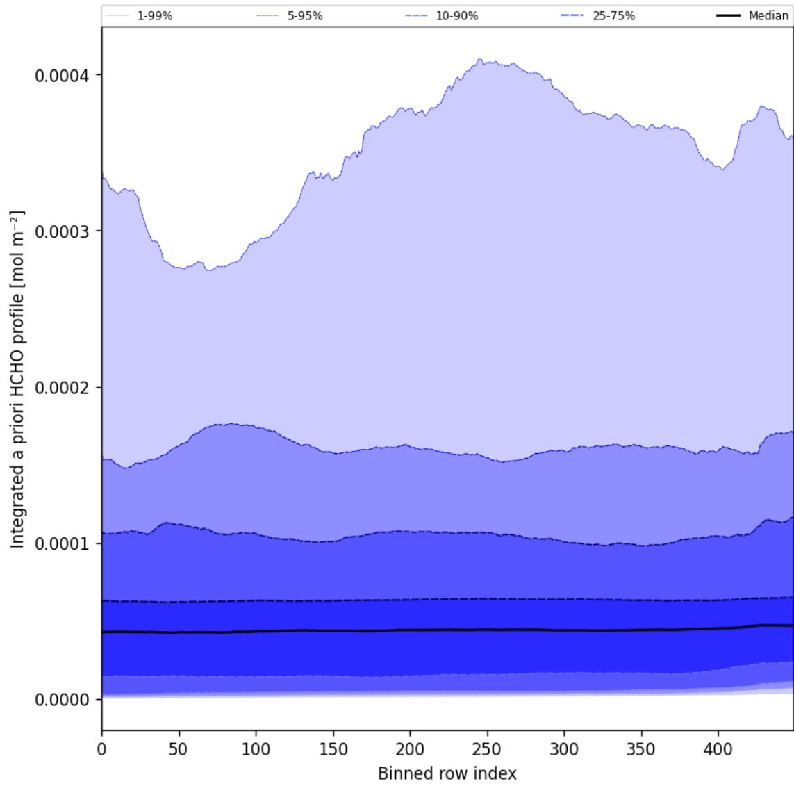
Figure 57: Along track statistics of “Integrated a priori HCHO profile” for 2024-10-03 to 2024-10-04
