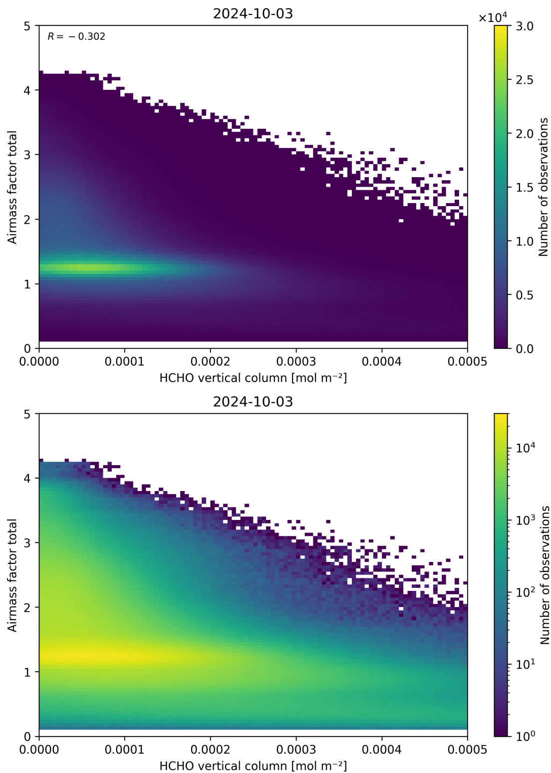
Figure 131: Scatter density plot of “HCHO vertical column” against “Airmass factor total” for 2024-10-03 to 2024-10-04.
