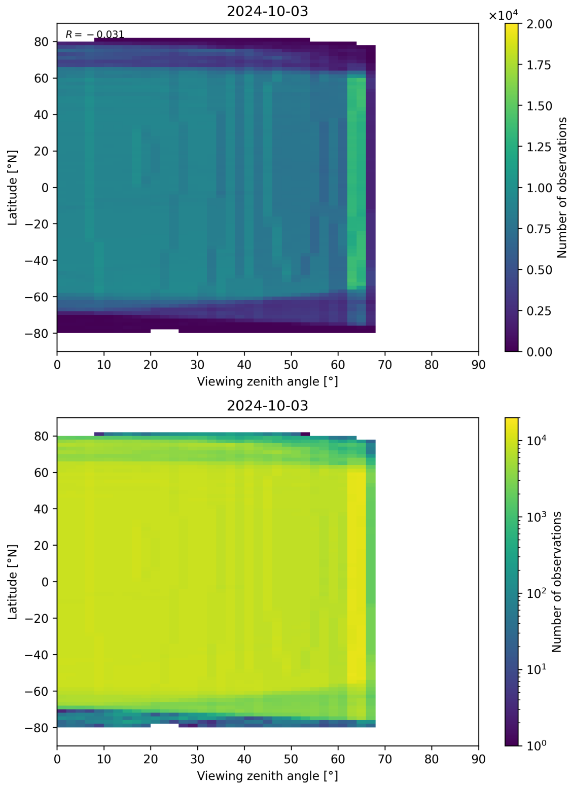
Figure 196: Scatter density plot of “Viewing zenith angle” against “Latitude” for 2024-10-03 to 2024-10-04.
