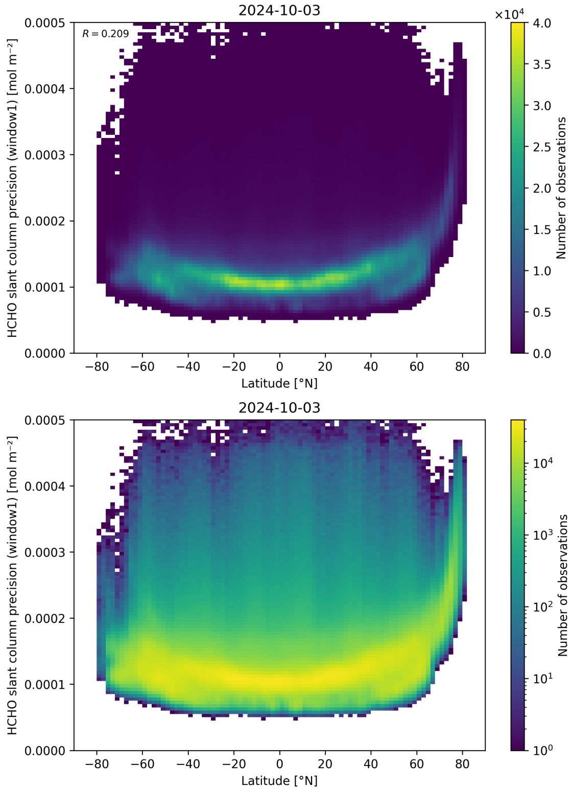
Figure 160: Scatter density plot of “Latitude” against “HCHO slant column precision (window1)” for 2024-10-03 to 2024-10-04.
