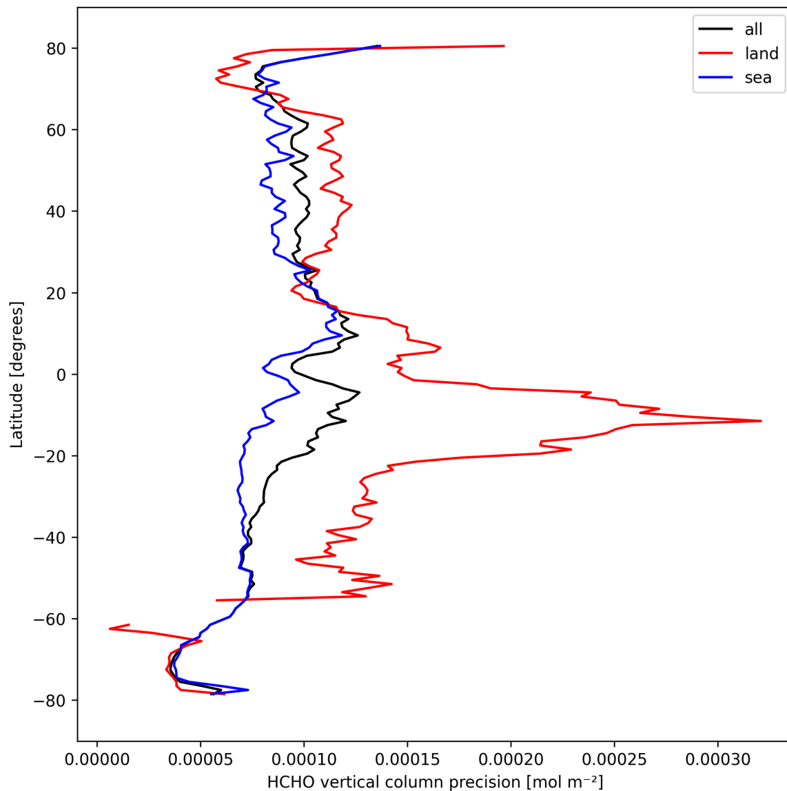
Figure 22: Zonal average of “HCHO vertical column precision” for 2024-10-03 to 2024-10-04.
