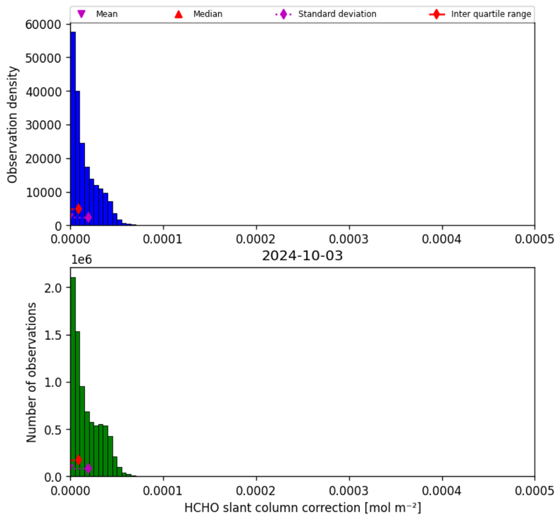
Figure 47: Histogram of “HCHO slant column correction” for 2024-10-03 to 2024-10-04
