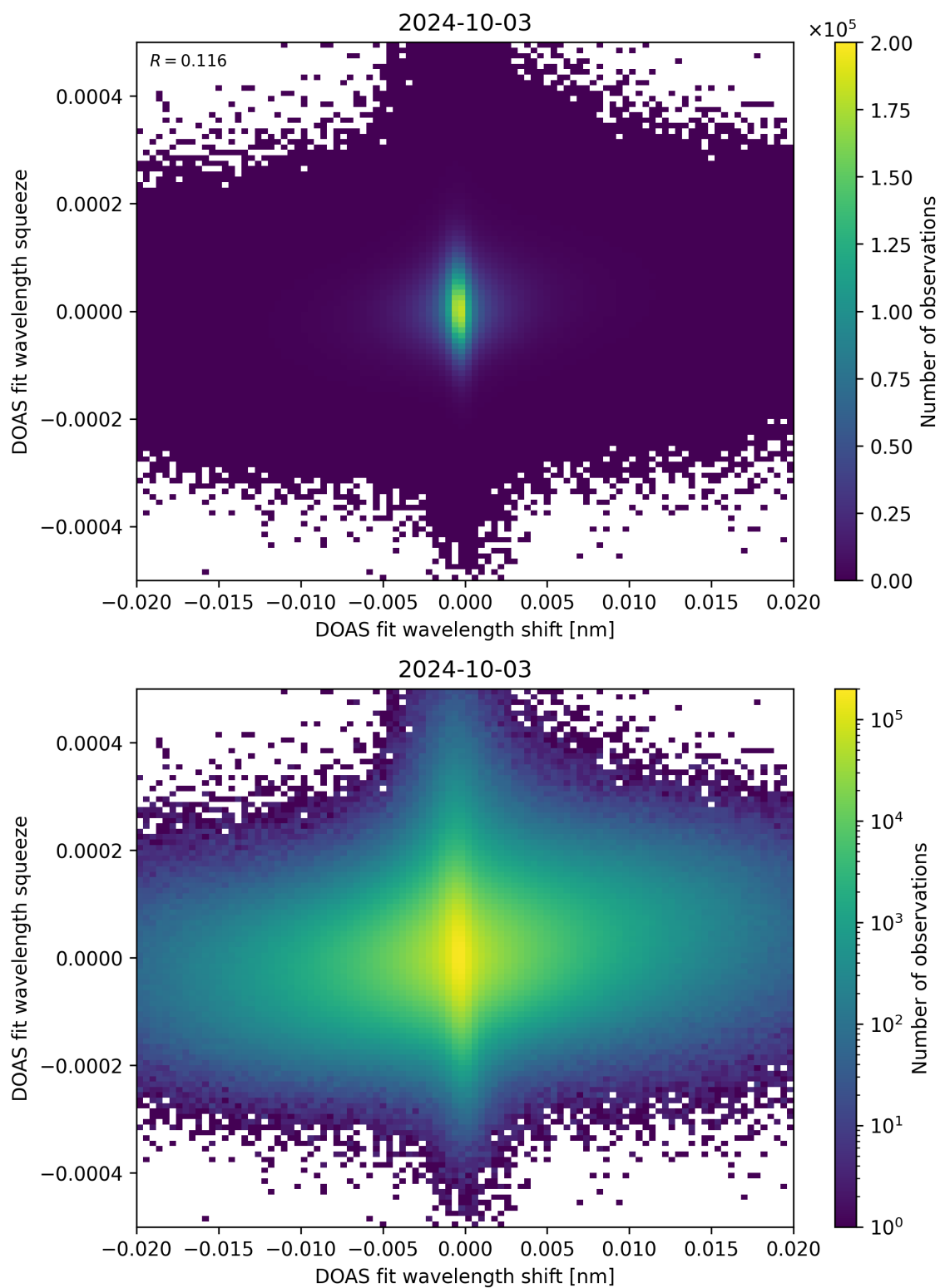
Figure 65: Scatter density plot of “DOAS fit wavelength shift” against “DOAS fit wavelength squeeze” for 2024-10-03 to 2024-10-04.
