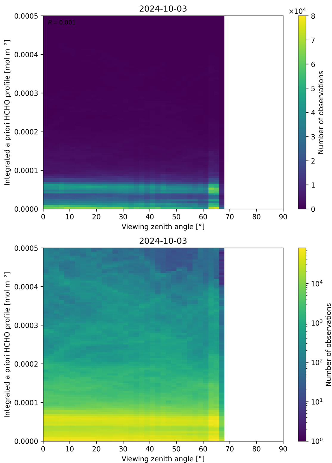
Figure 195: Scatter density plot of “Viewing zenith angle” against “Integrated a priori HCHO profile” for 2024-10-03 to 2024-10-04.
