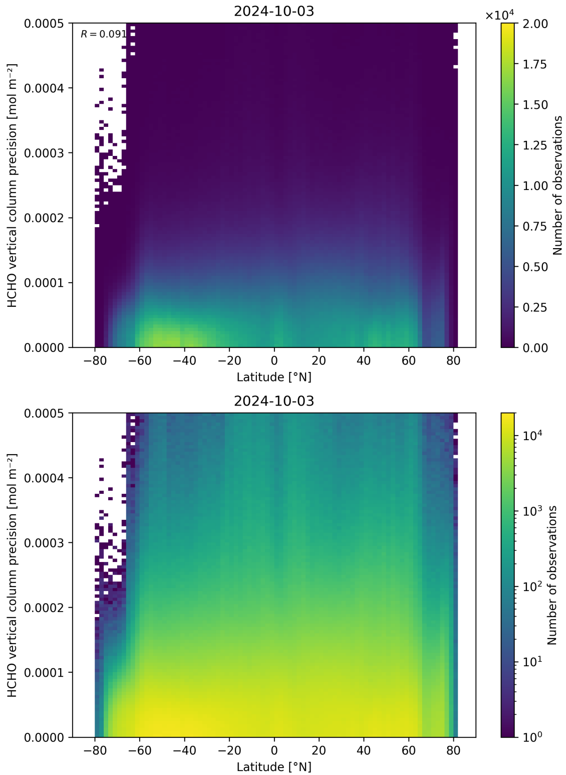
Figure 165: Scatter density plot of “Latitude” against “HCHO vertical column precision” for 2024-10-03 to 2024-10-04.
