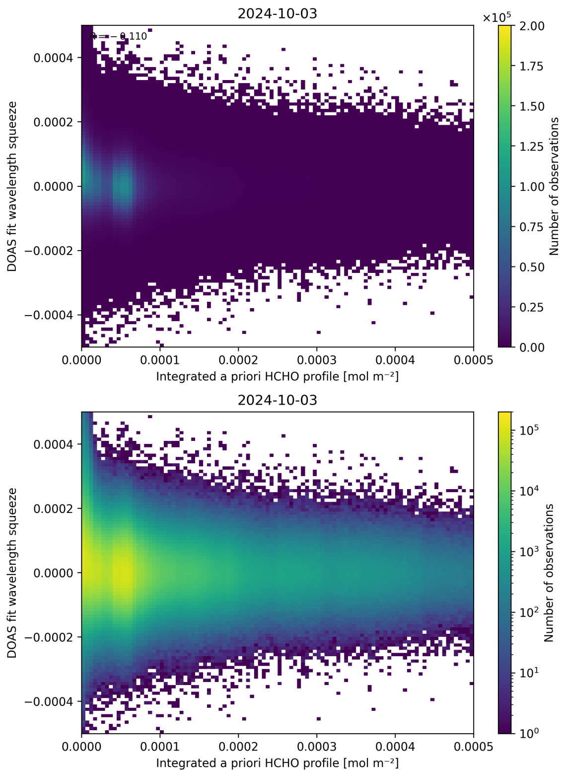
Figure 150: Scatter density plot of “Integrated a priori HCHO profile” against “DOAS fit wavelength squeeze” for 2024-10-03 to 2024-10-04.
