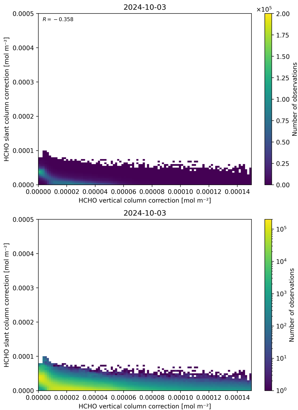
Figure 117: Scatter density plot of “HCHO vertical column correction” against “HCHO slant column correction” for 2024-10-03 to 2024-10-04.
