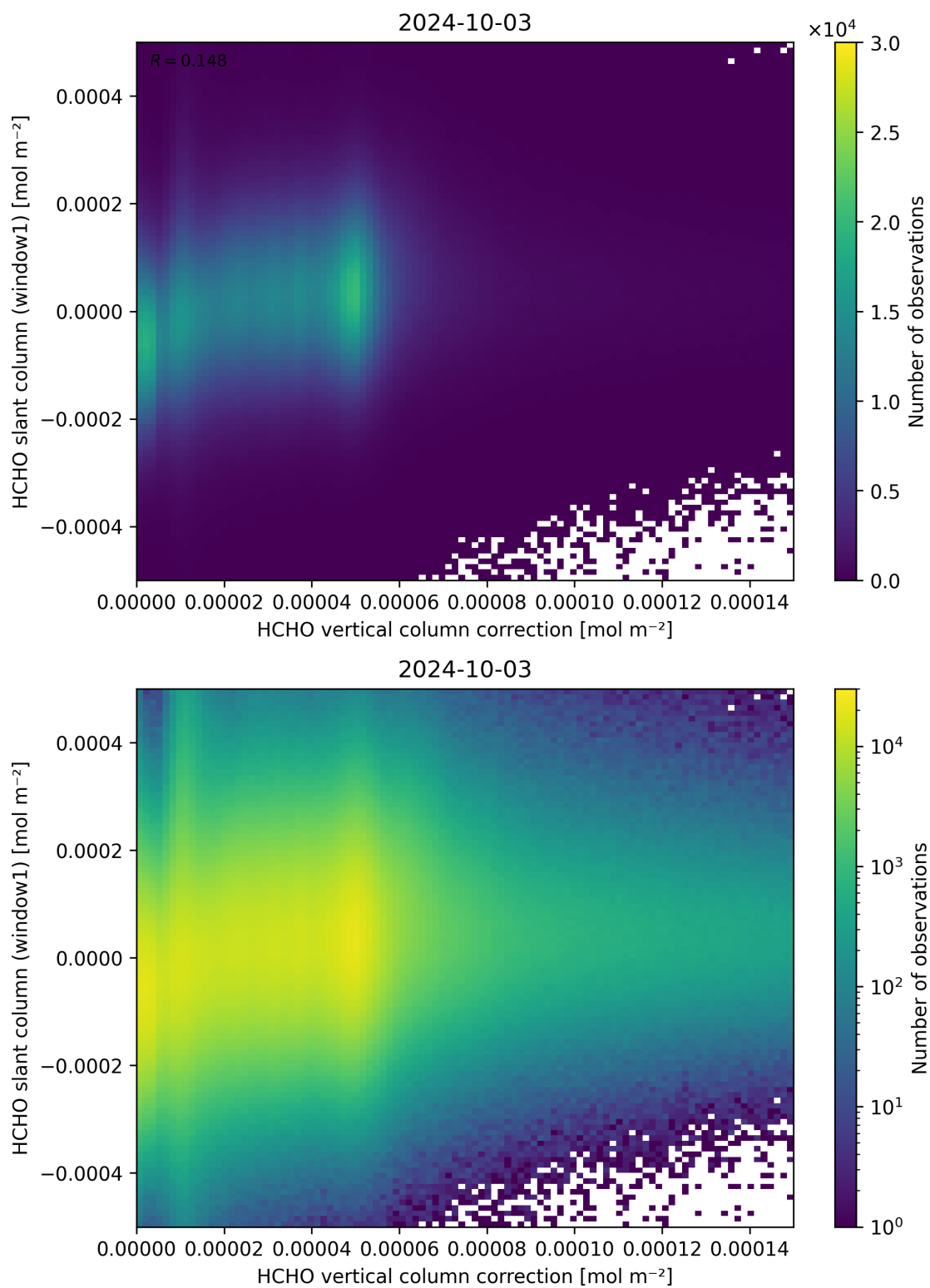
Figure 118: Scatter density plot of “HCHO vertical column correction” against “HCHO slant column (window1)” for 2024-10-03 to 2024-10-04.
