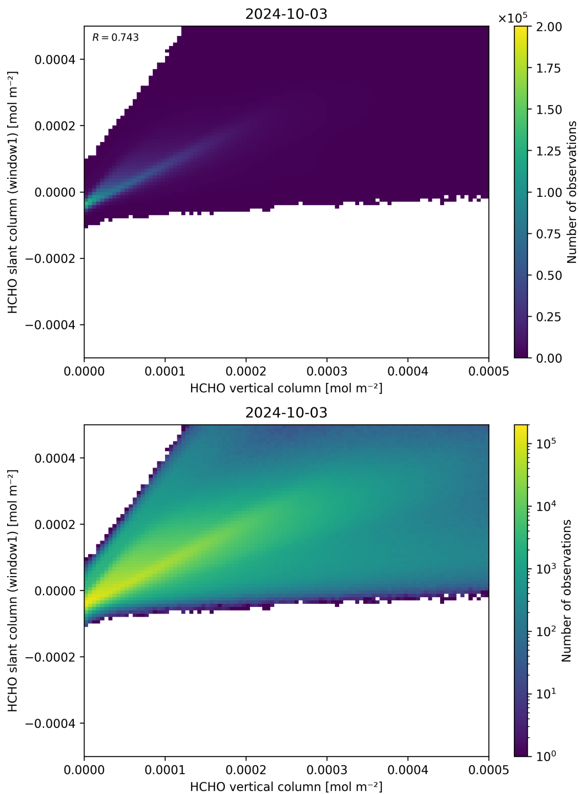
Figure 129: Scatter density plot of “HCHO vertical column” against “HCHO slant column (window1)” for 2024-10-03 to 2024-10-04.
