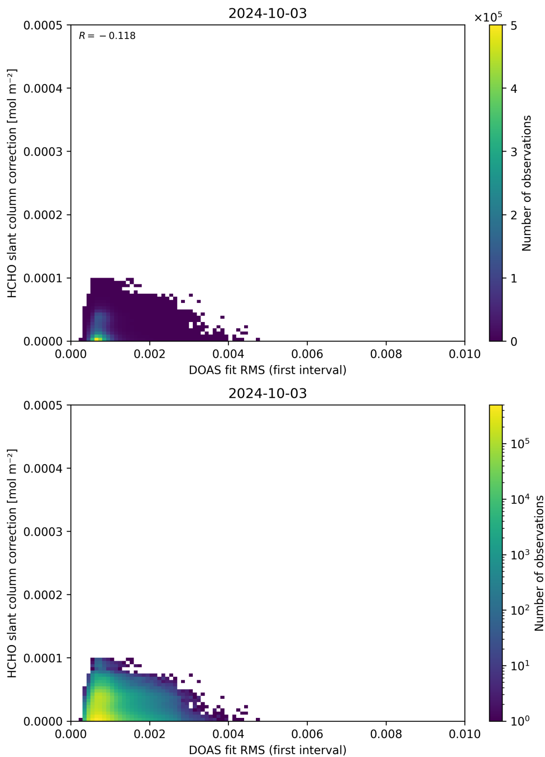
Figure 63: Scatter density plot of “DOAS fit RMS (first interval)” against “HCHO slant column correction” for 2024-10-03 to 2024-10-04.
