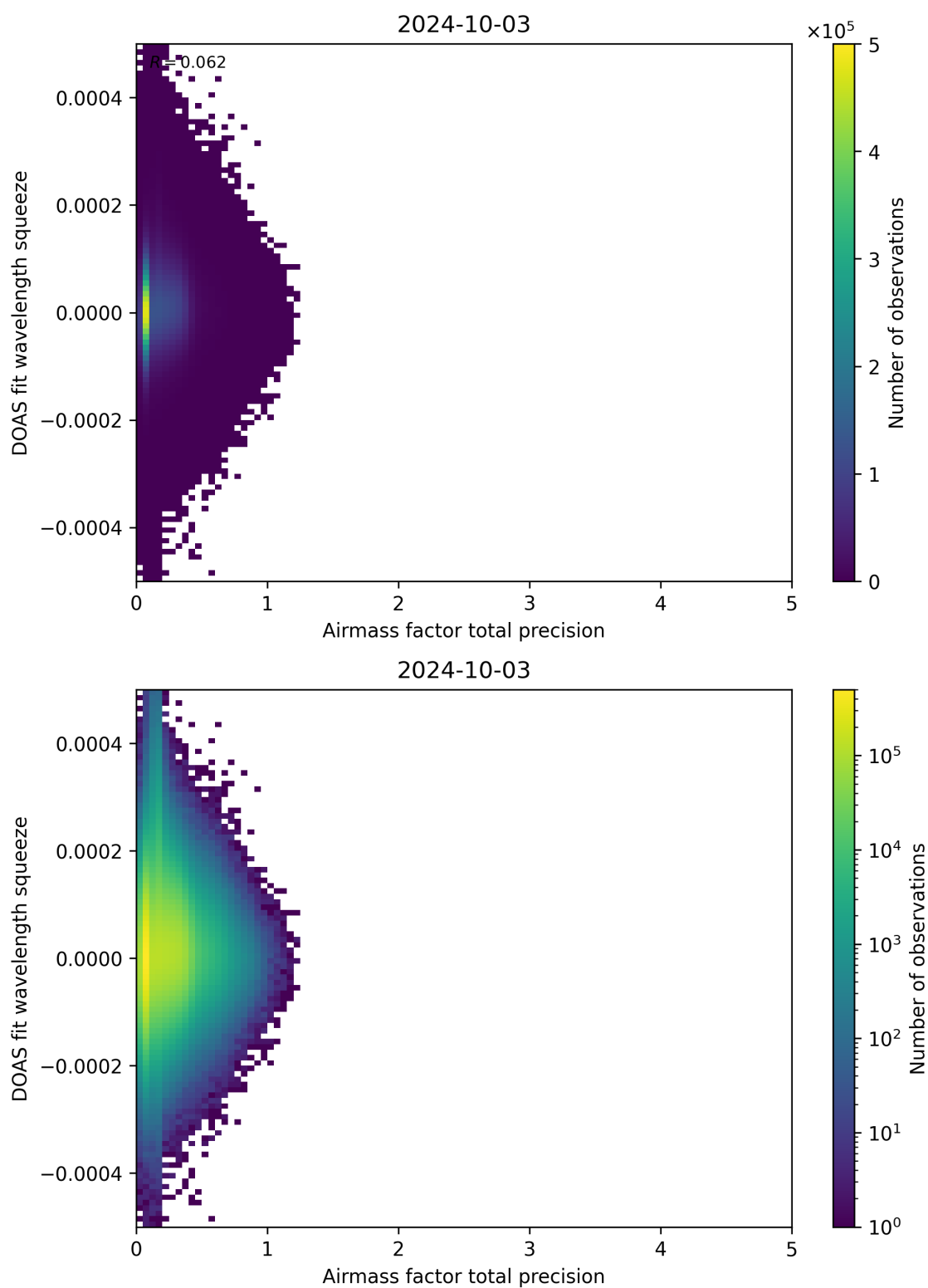
Figure 107: Scatter density plot of “Airmass factor total precision” against “DOAS fit wavelength squeeze” for 2024-10-03 to 2024-10-04.
