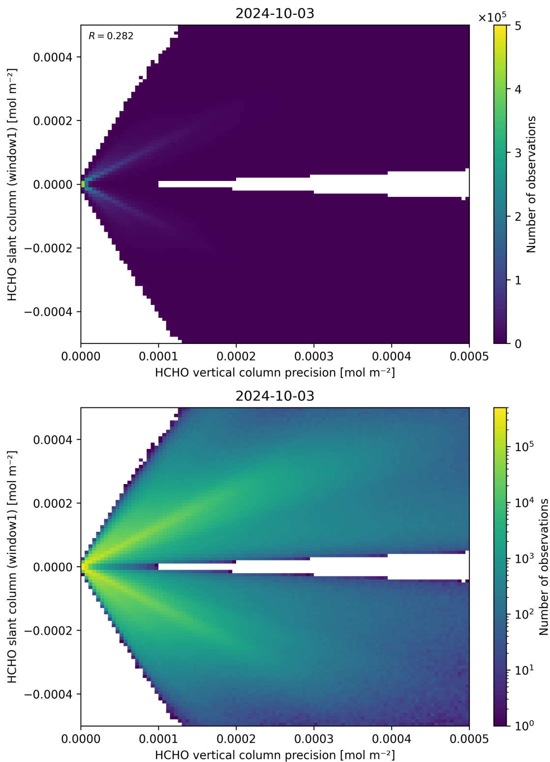
Figure 142: Scatter density plot of “HCHO vertical column precision” against “HCHO slant column (window1)” for 2024-10-03 to 2024-10-04.
