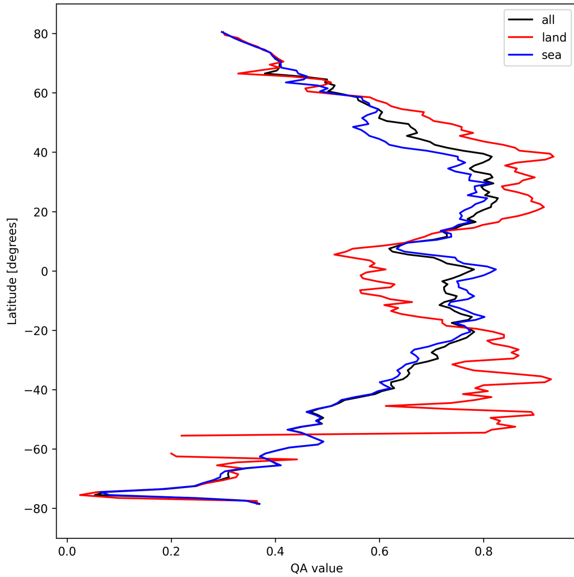
Figure 20: Zonal average of “QA value” for 2024-10-03 to 2024-10-04.
