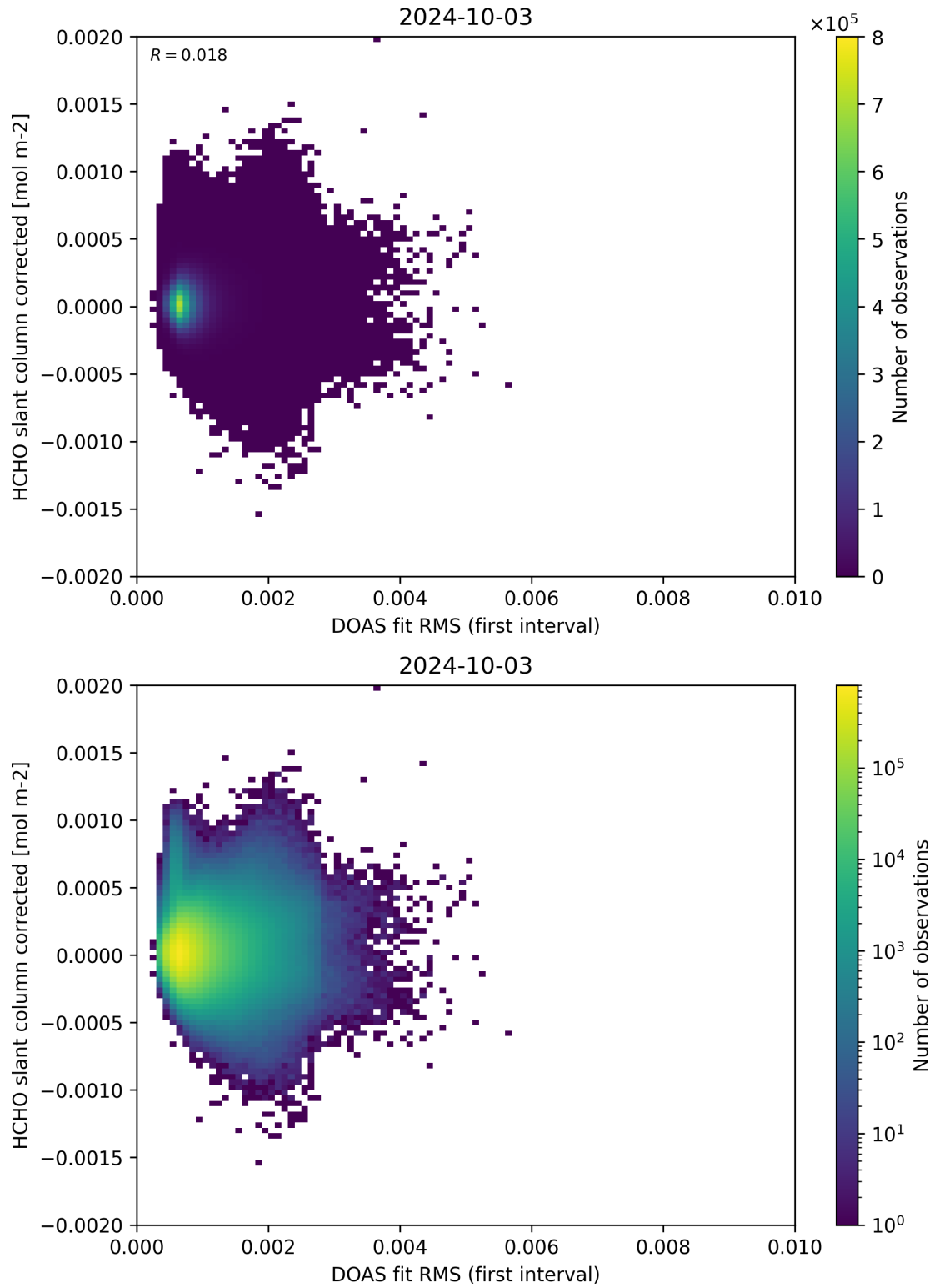
Figure 62: Scatter density plot of “DOAS fit RMS (first interval)” against “HCHO slant column corrected” for 2024-10-03 to 2024-10-04.
