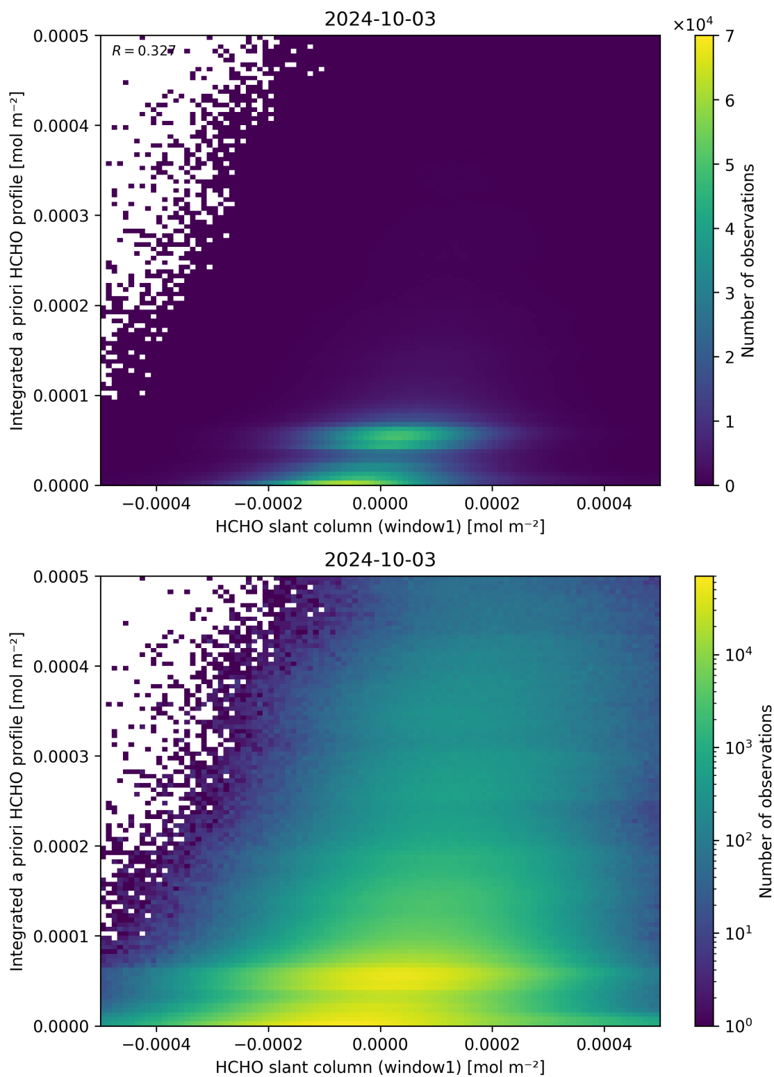
Figure 87: Scatter density plot of “HCHO slant column (window1)” against “Integrated a priori HCHO profile” for 2024-10-03 to 2024-10-04.
