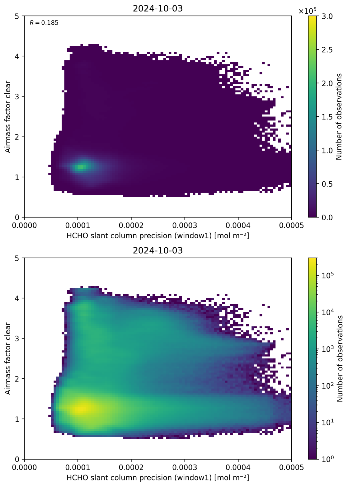
Figure 91: Scatter density plot of “HCHO slant column precision (window1)” against “Airmass factor clear” for 2024-10-03 to 2024-10-04.
