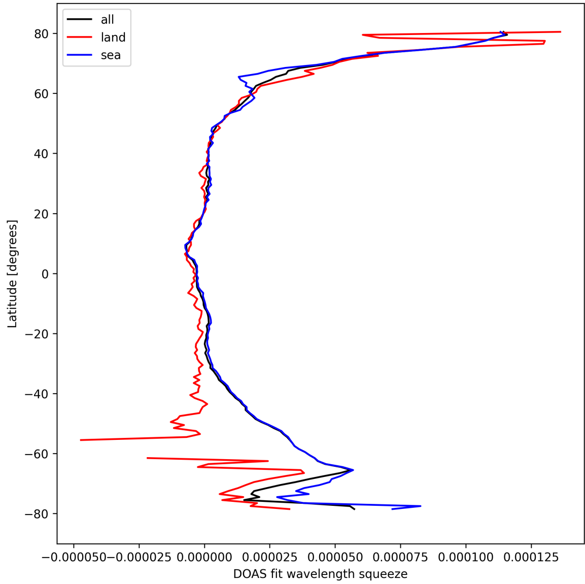
Figure 31: Zonal average of “DOAS fit wavelength squeeze” for 2024-10-03 to 2024-10-04.
