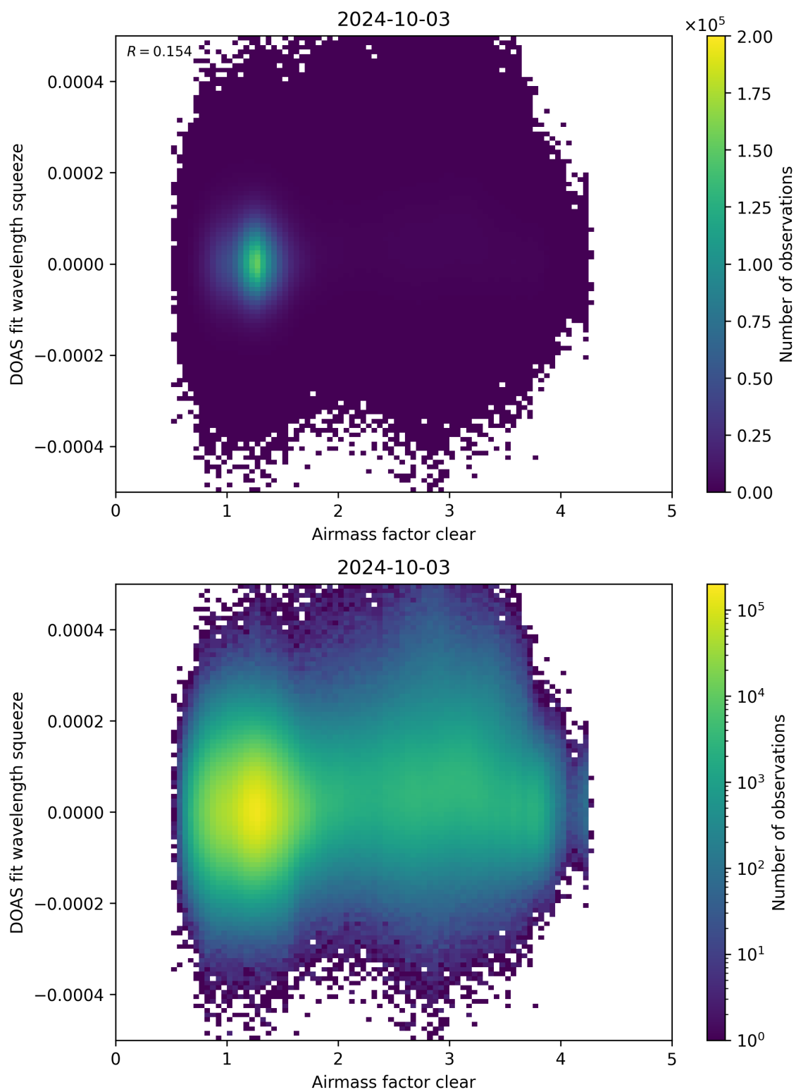
Figure 73: Scatter density plot of “Airmass factor clear” against “DOAS fit wavelength squeeze” for 2024-10-03 to 2024-10-04.
