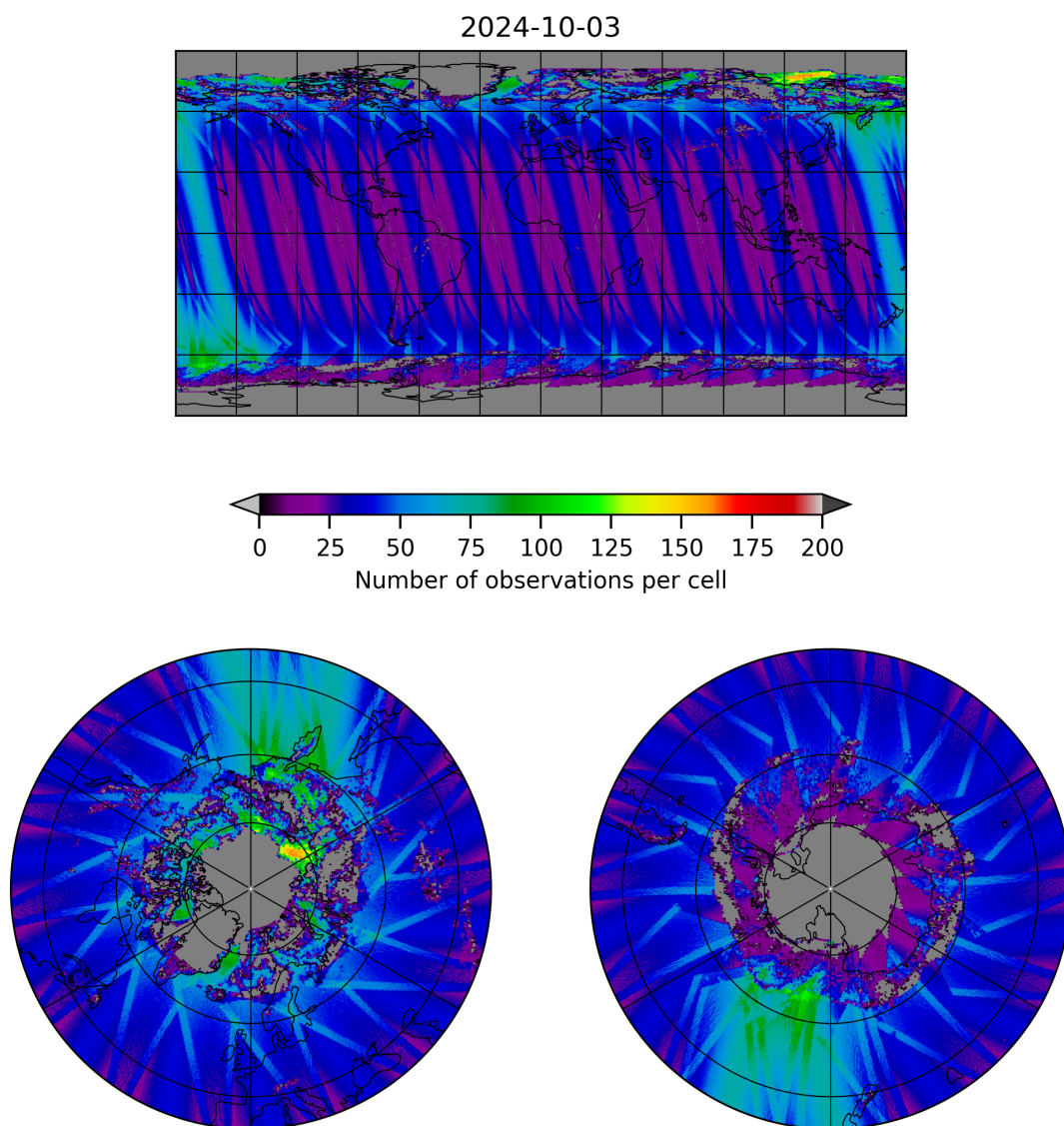
Figure 19: Map of the number of observations for 2024-10-03 to 2024-10-04
