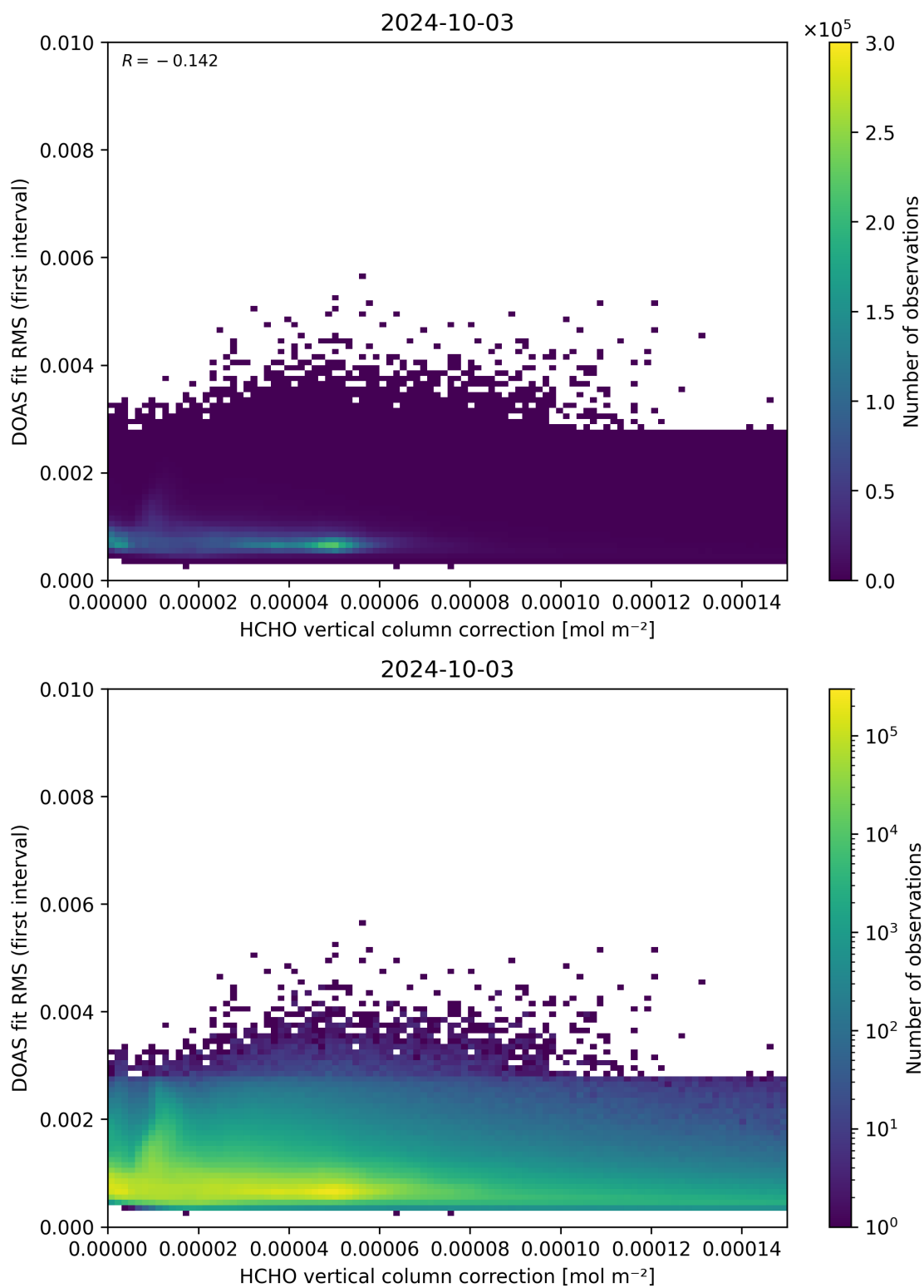
Figure 112: Scatter density plot of “HCHO vertical column correction” against “DOAS fit RMS (first interval)” for 2024-10-03 to 2024-10-04.
