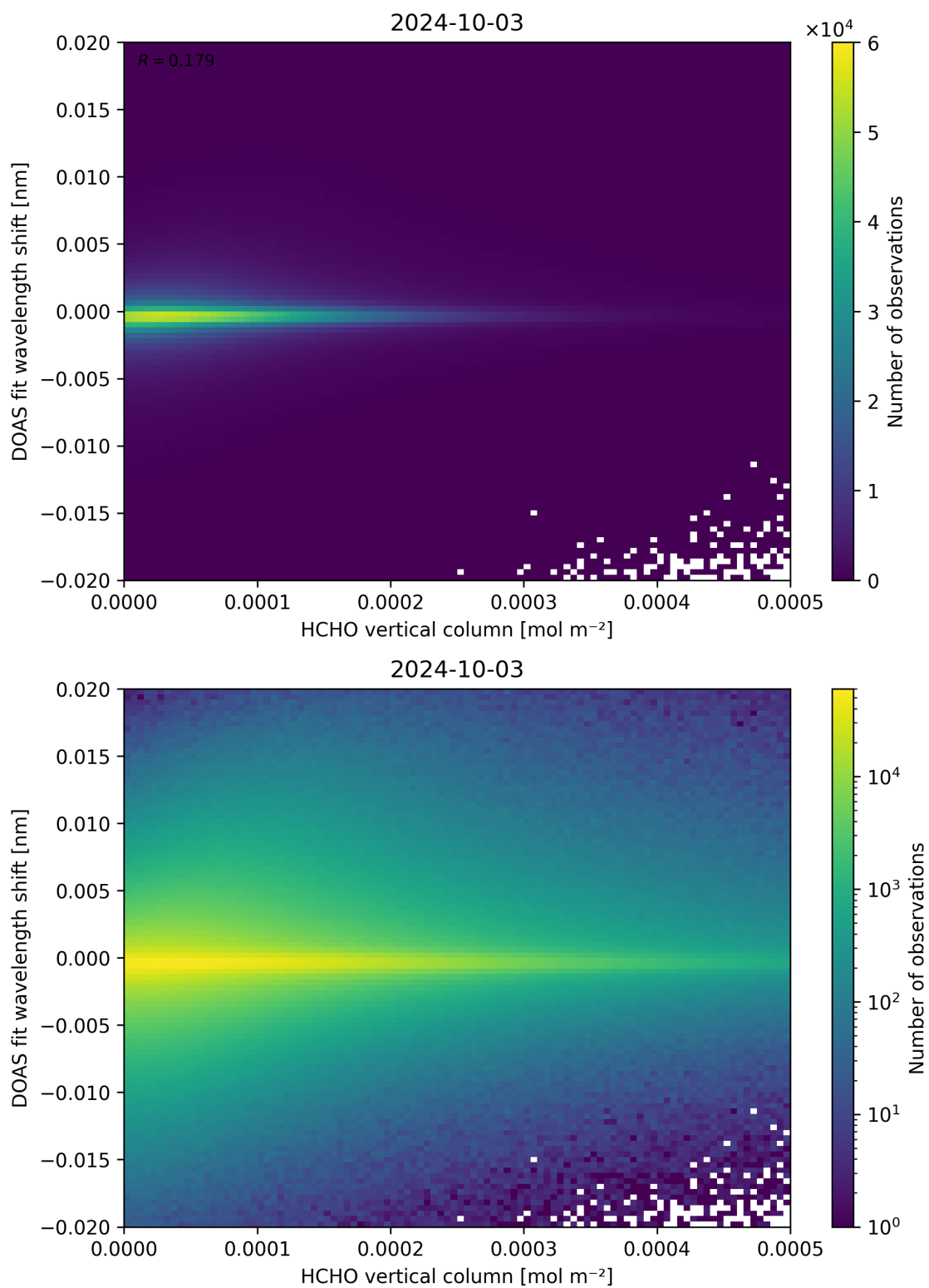
Figure 124: Scatter density plot of “HCHO vertical column” against “DOAS fit wavelength shift” for 2024-10-03 to 2024-10-04.
