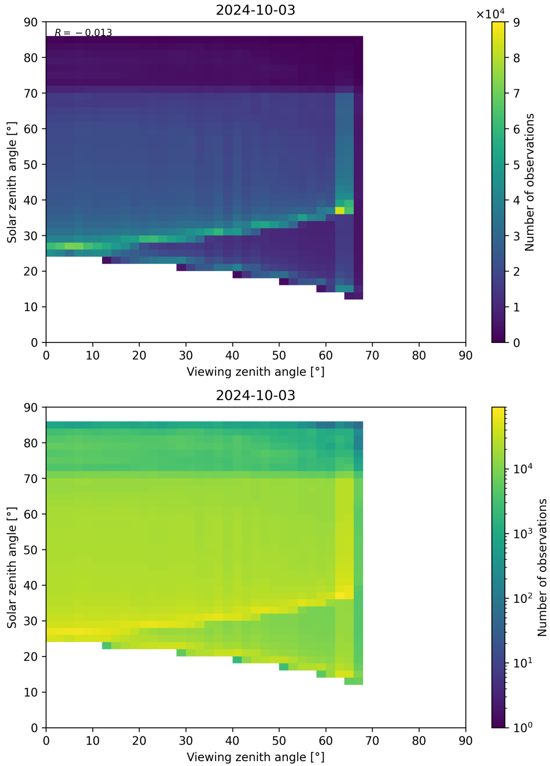
Figure 197: Scatter density plot of “Viewing zenith angle” against “Solar zenith angle” for 2024-10-03 to 2024-10-04.
