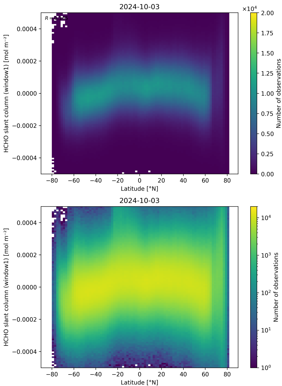
Figure 159: Scatter density plot of “Latitude” against “HCHO slant column (window1)” for 2024-10-03 to 2024-10-04.
