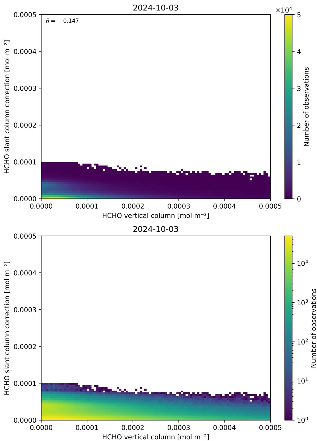
Figure 128: Scatter density plot of “HCHO vertical column” against “HCHO slant column correction” for 2024-10-03 to 2024-10-04.
