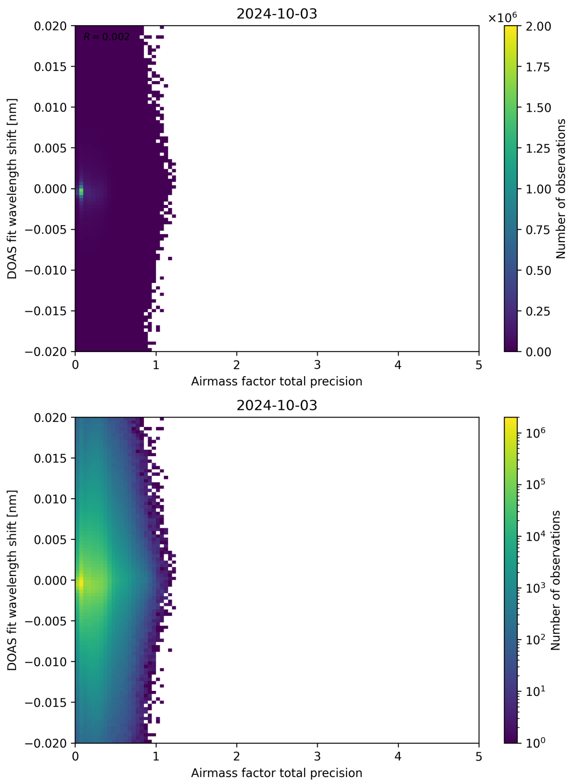
Figure 106: Scatter density plot of “Airmass factor total precision” against “DOAS fit wavelength shift” for 2024-10-03 to 2024-10-04.
