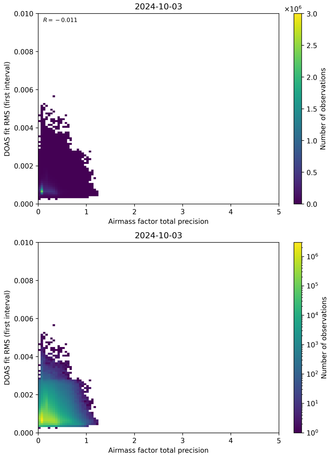
Figure 105: Scatter density plot of “Airmass factor total precision” against “DOAS fit RMS (first interval)” for 2024-10-03 to 2024-10-04.
