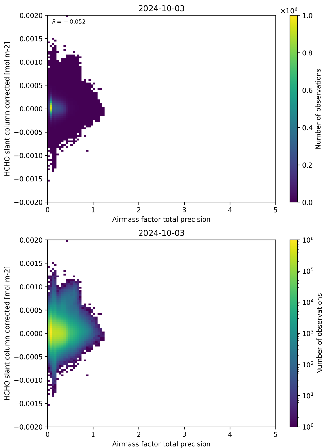
Figure 109: Scatter density plot of “Airmass factor total precision” against “HCHO slant column corrected” for 2024-10-03 to 2024-10-04.
