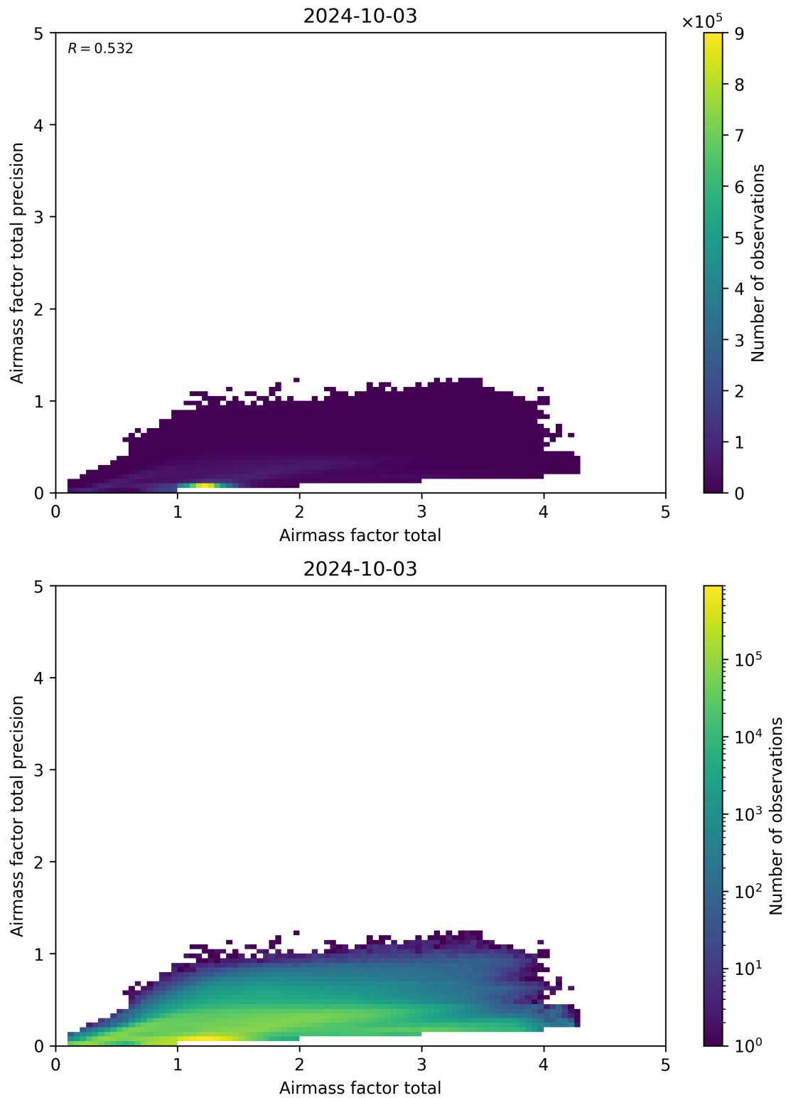
Figure 103: Scatter density plot of “Airmass factor total” against “Airmass factor total precision” for 2024-10-03 to 2024-10-04.
