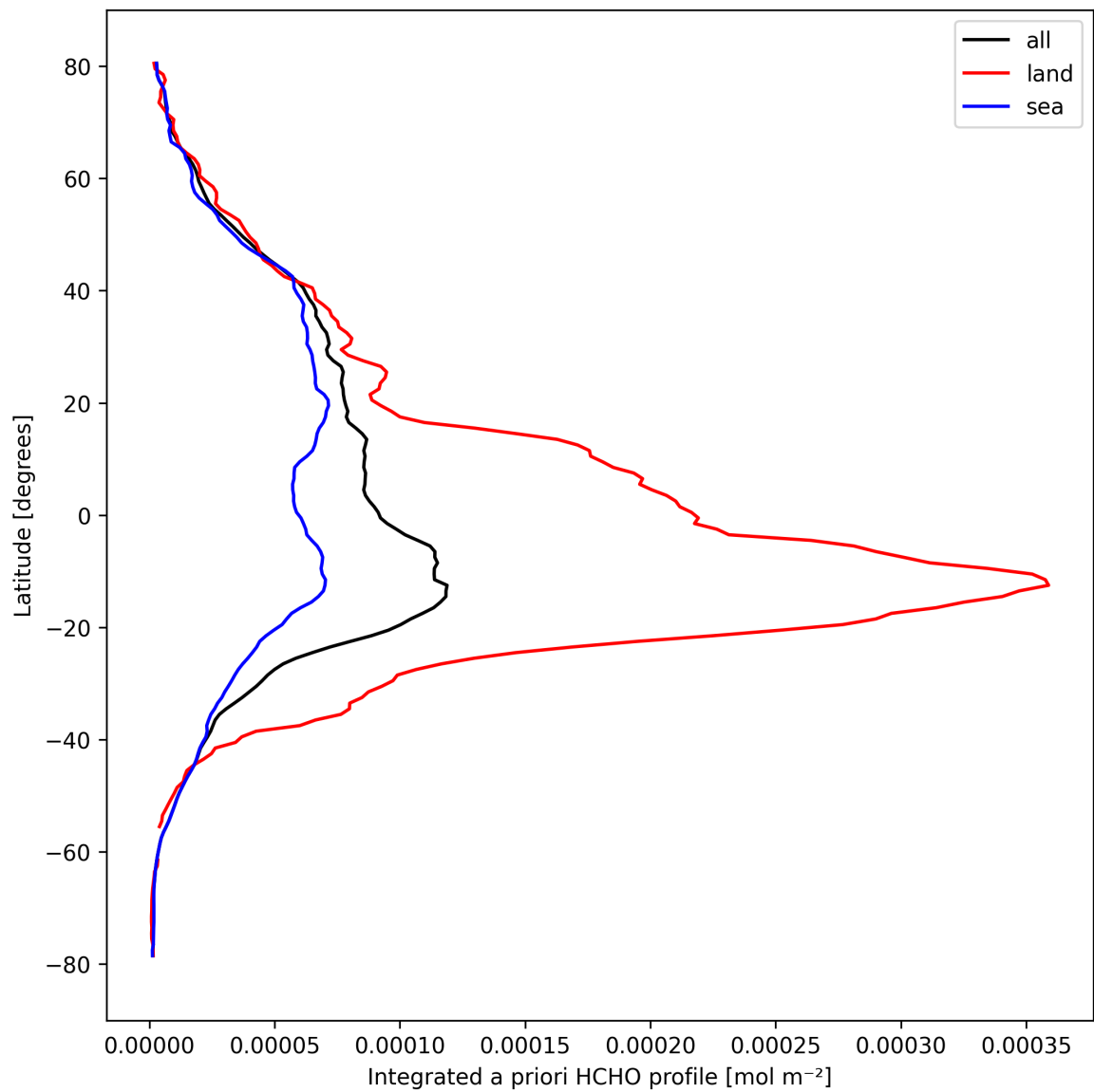
Figure 29: Zonal average of “Integrated a priori HCHO profile” for 2024-10-03 to 2024-10-04.
