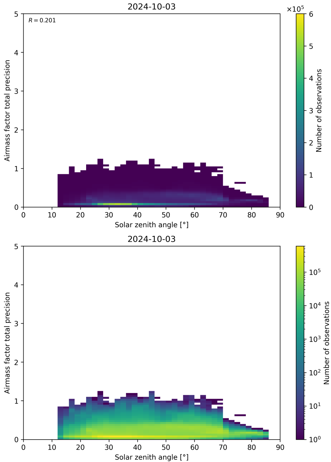
Figure 176: Scatter density plot of “Solar zenith angle” against “Airmass factor total precision” for 2024-10-03 to 2024-10-04.
