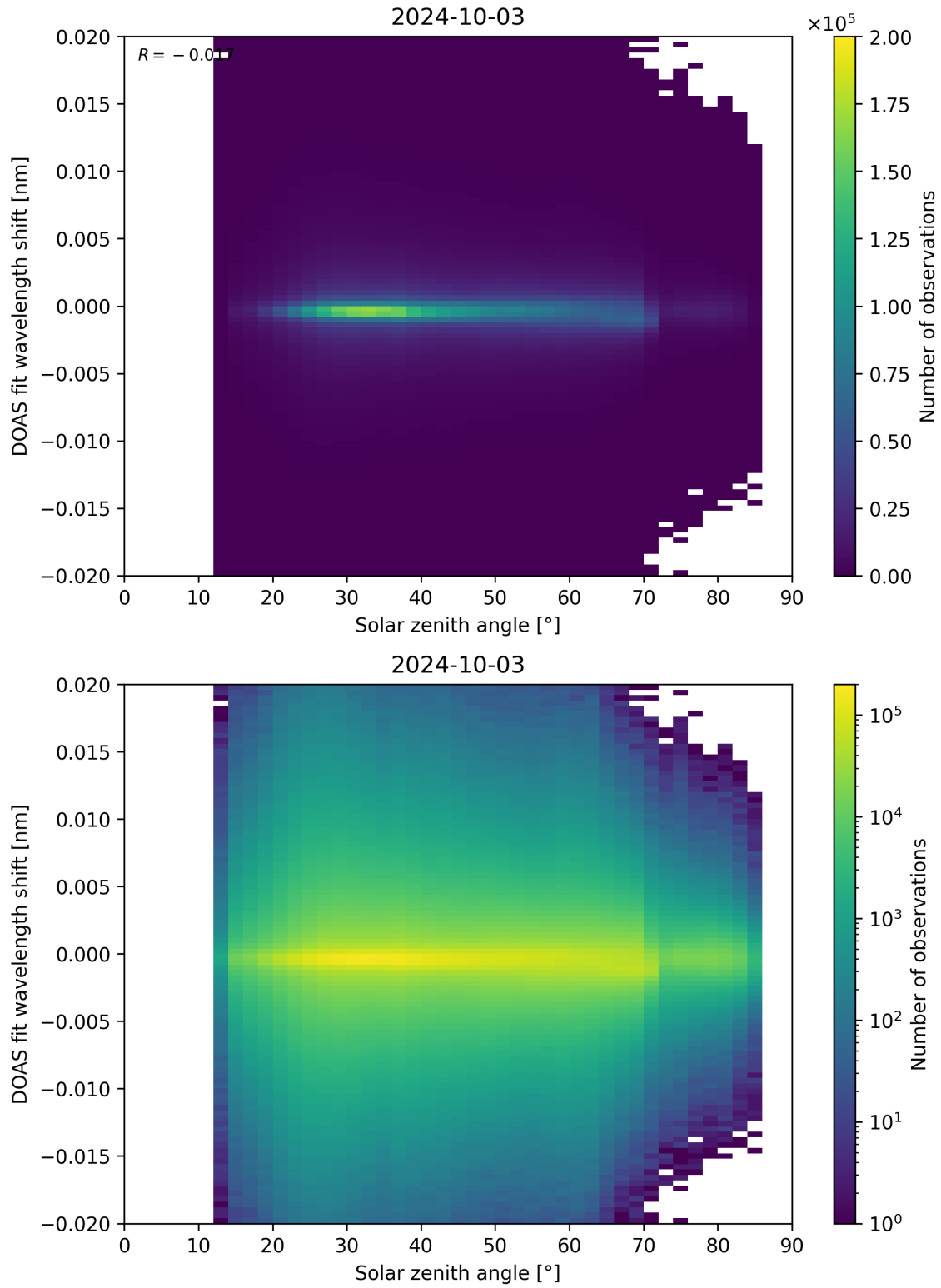
Figure 168: Scatter density plot of “Solar zenith angle” against “DOAS fit wavelength shift” for 2024-10-03 to 2024-10-04.
