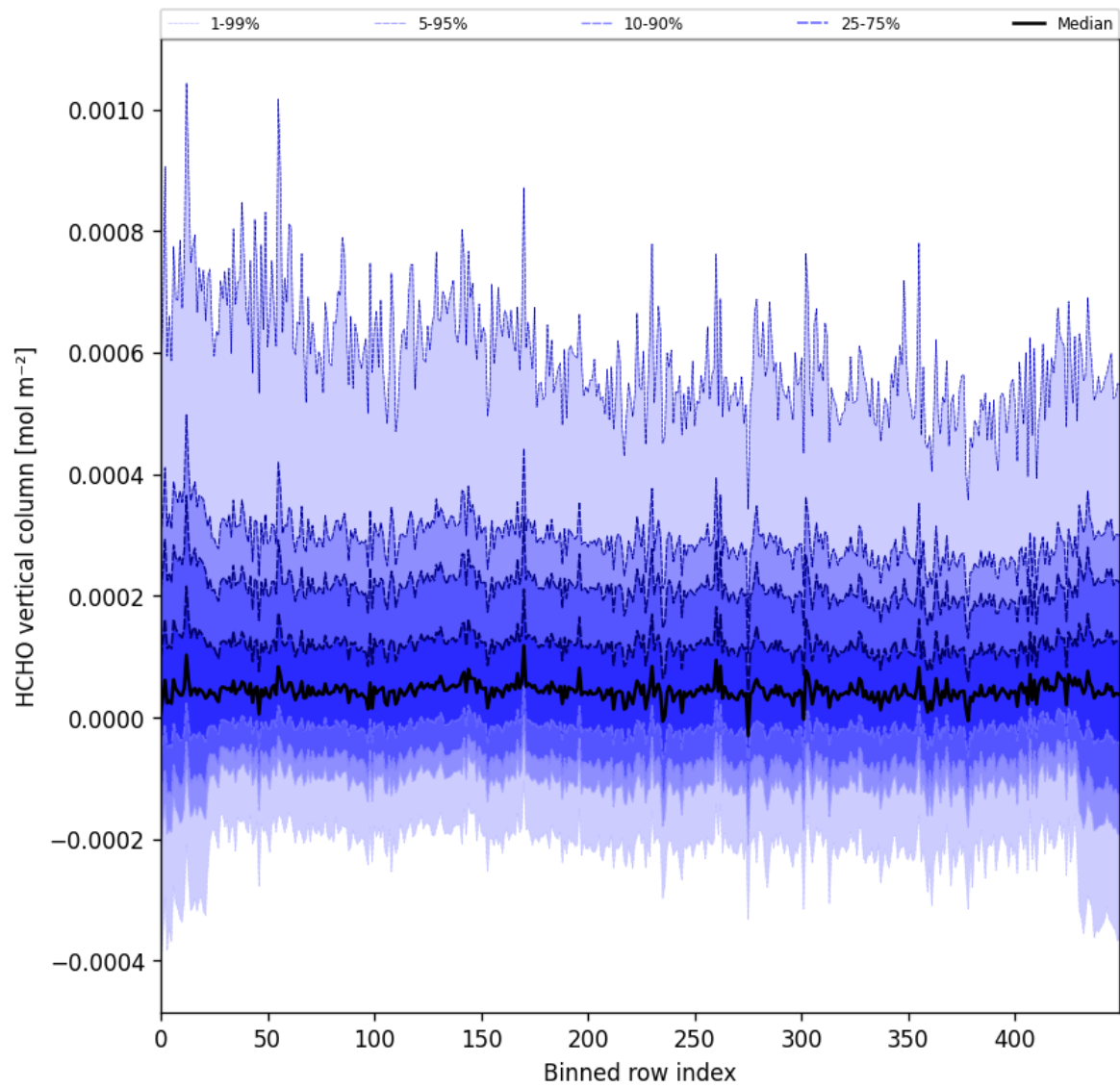
Figure 49: Along track statistics of “HCHO vertical column” for 2024-10-03 to 2024-10-04
