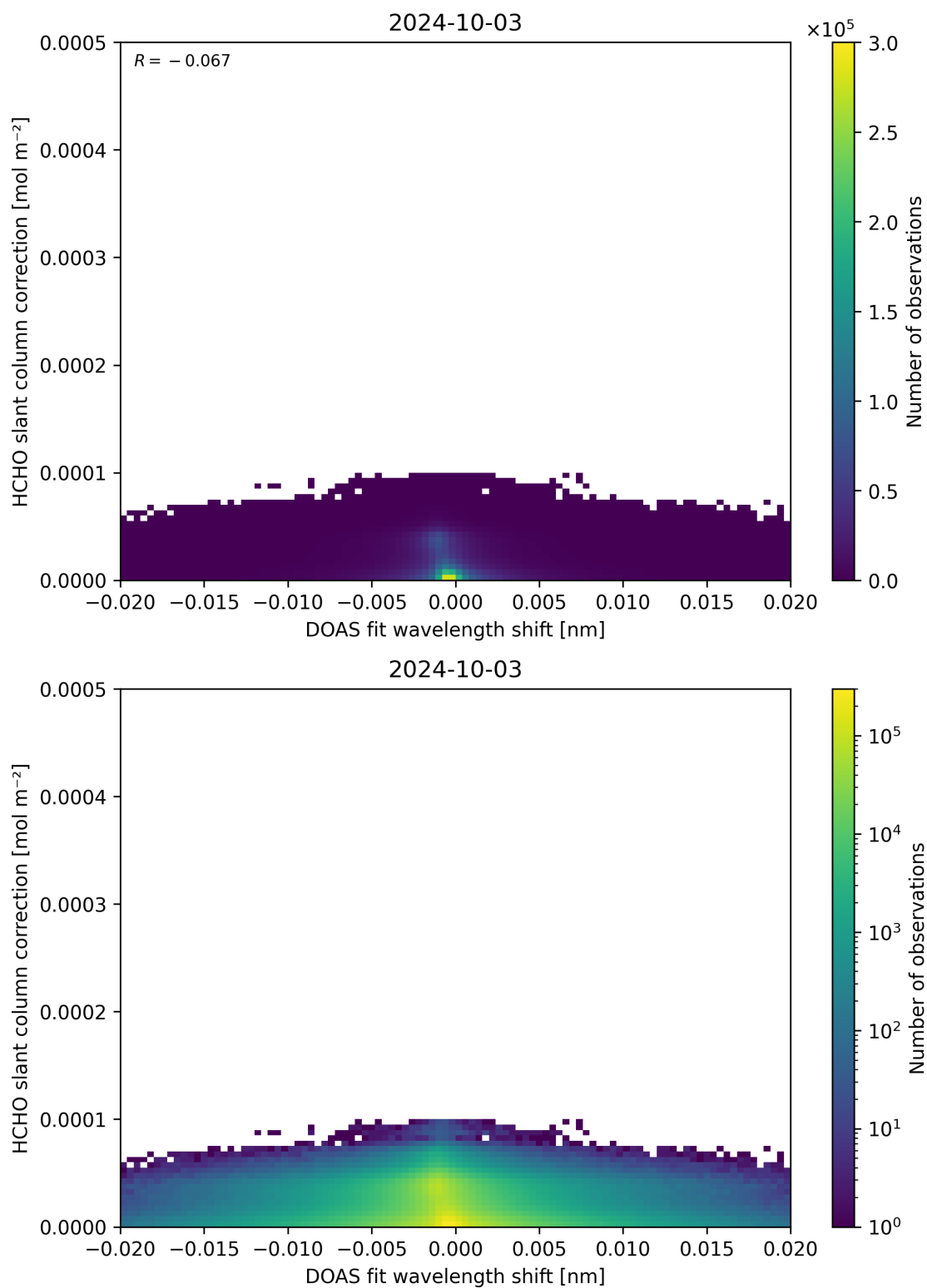
Figure 67: Scatter density plot of “DOAS fit wavelength shift” against “HCHO slant column correction” for 2024-10-03 to 2024-10-04.
