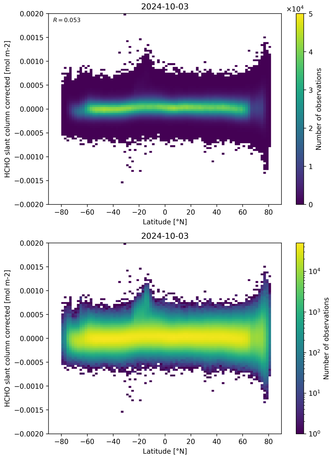
Figure 157: Scatter density plot of “Latitude” against “HCHO slant column corrected” for 2024-10-03 to 2024-10-04.
