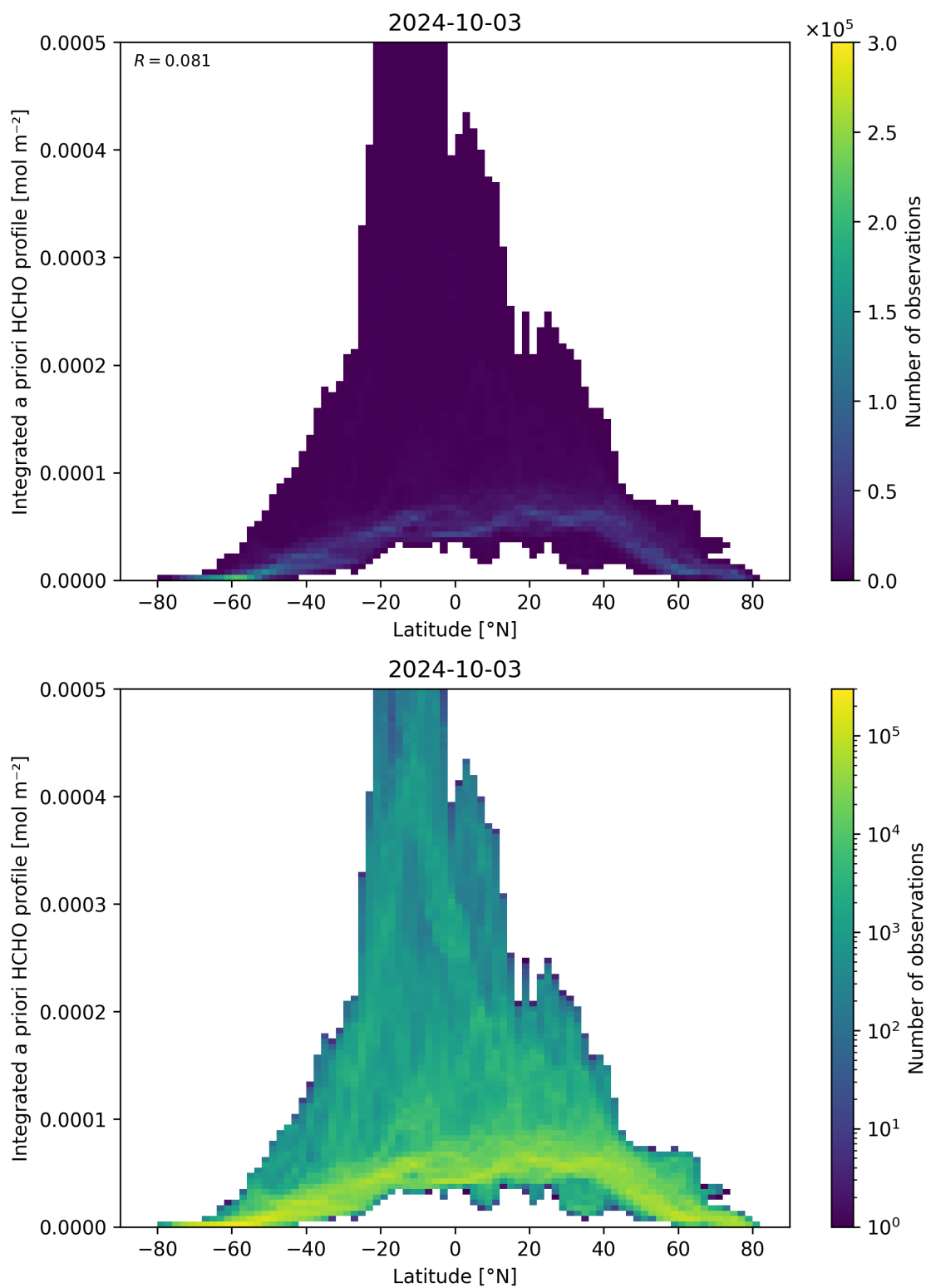
Figure 166: Scatter density plot of “Latitude” against “Integrated a priori HCHO profile” for 2024-10-03 to 2024-10-04.
