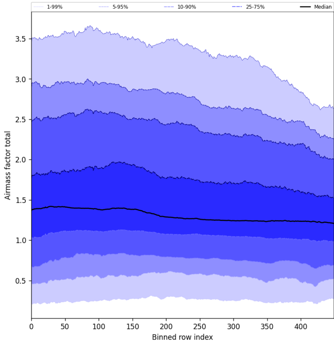
Figure 54: Along track statistics of “Airmass factor total” for 2024-10-03 to 2024-10-04
