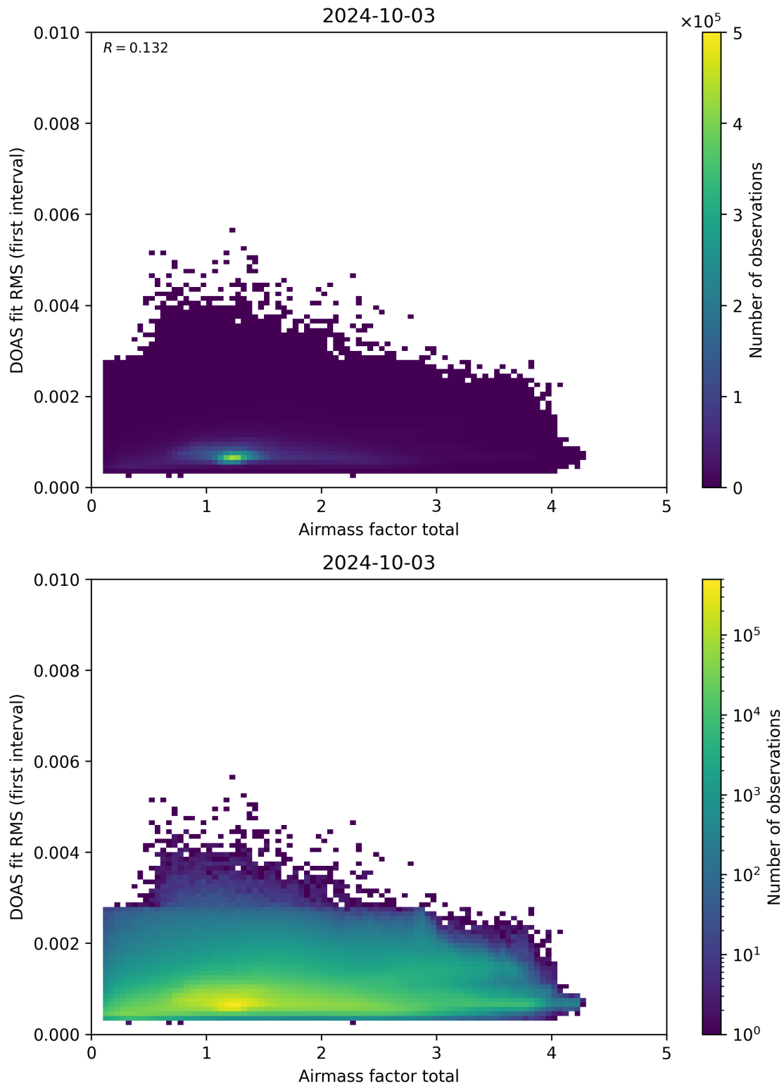
Figure 97: Scatter density plot of “Airmass factor total” against “DOAS fit RMS (first interval)” for 2024-10-03 to 2024-10-04.
