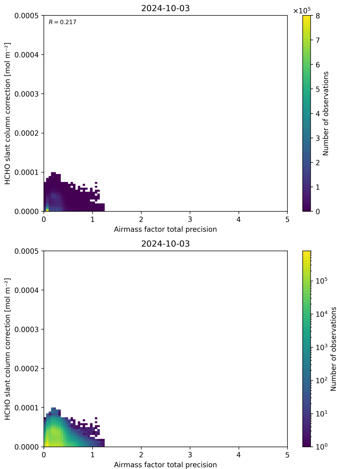
Figure 110: Scatter density plot of “Airmass factor total precision” against “HCHO slant column correction” for 2024-10-03 to 2024-10-04.
