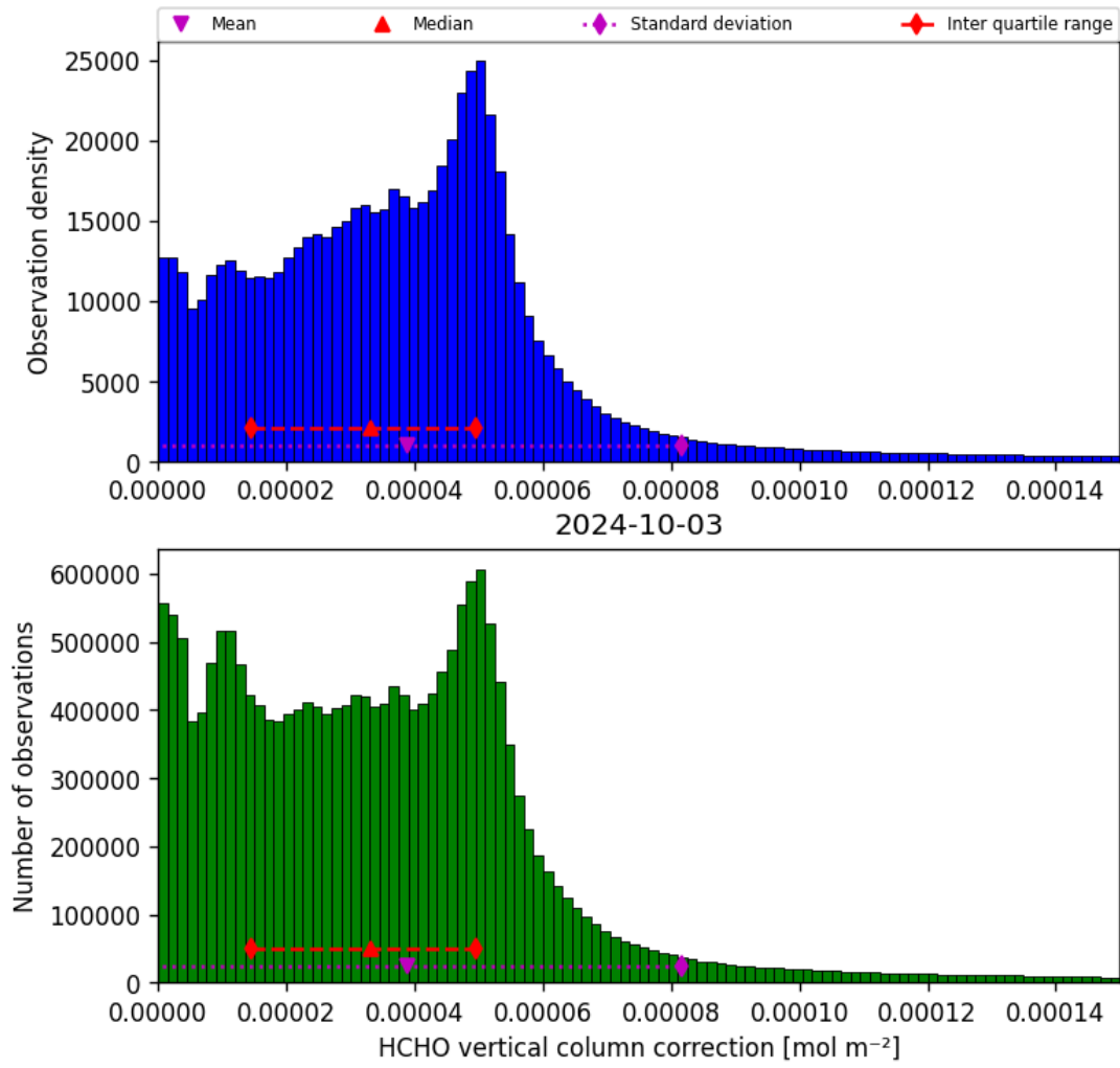
Figure 37: Histogram of “HCHO vertical column correction” for 2024-10-03 to 2024-10-04
