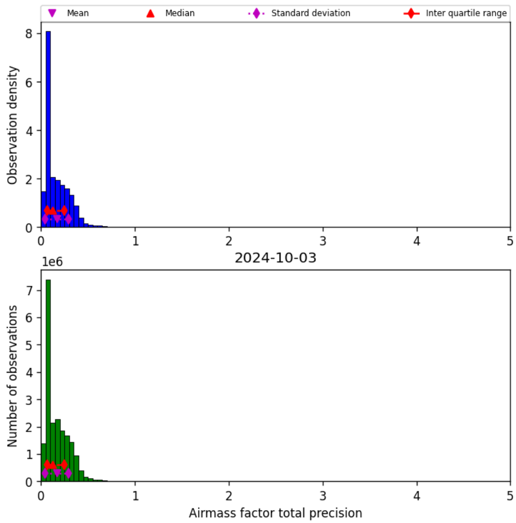
Figure 41: Histogram of “Airmass factor total precision” for 2024-10-03 to 2024-10-04
