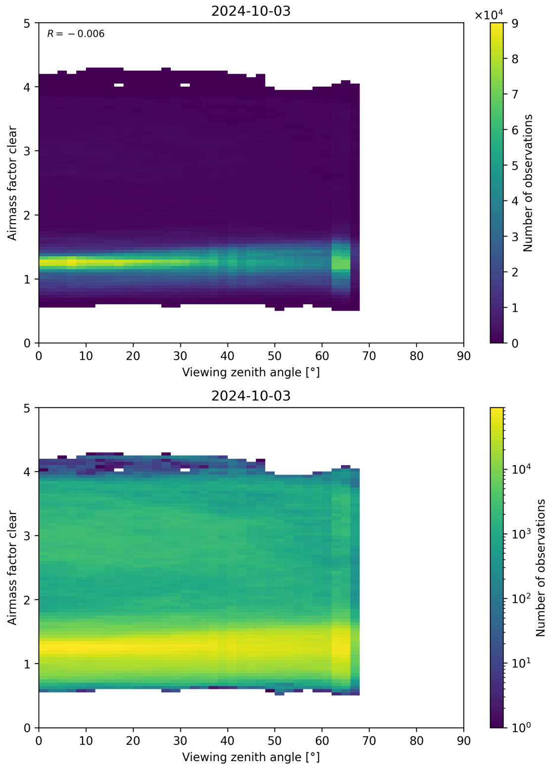
Figure 185: Scatter density plot of “Viewing zenith angle” against “Airmass factor clear” for 2024-10-03 to 2024-10-04.
