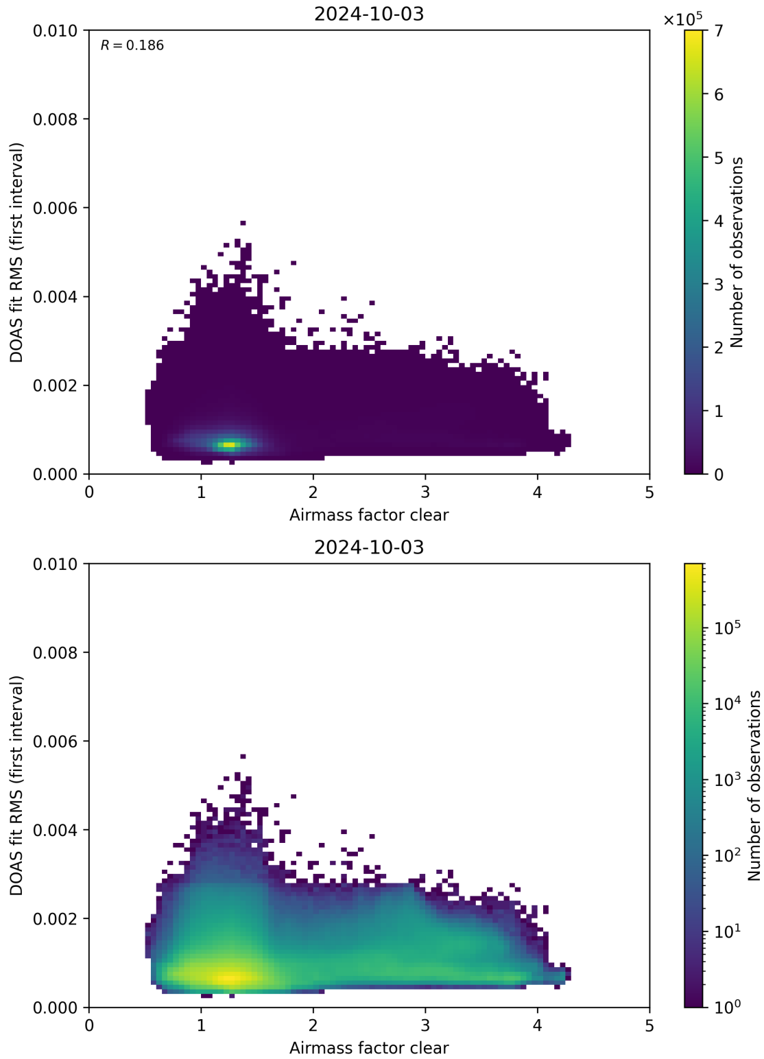
Figure 71: Scatter density plot of “Airmass factor clear” against “DOAS fit RMS (first interval)” for 2024-10-03 to 2024-10-04.
