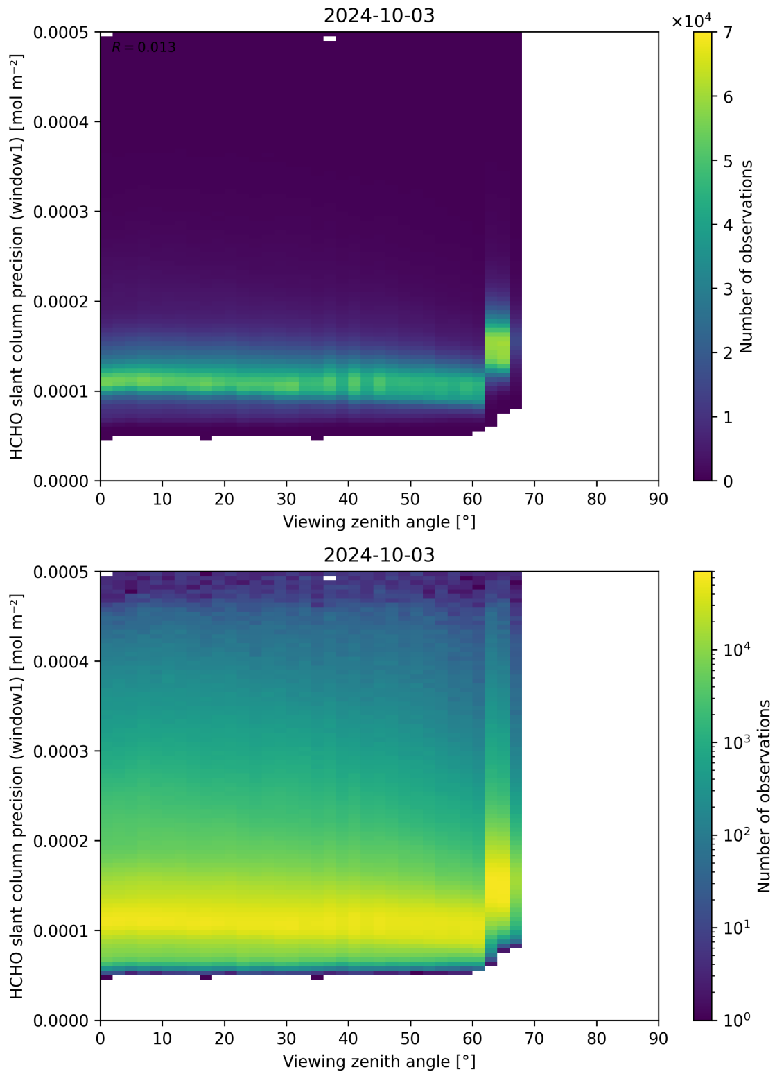
Figure 189: Scatter density plot of “Viewing zenith angle” against “HCHO slant column precision (window1)” for 2024-10-03 to 2024-10-04.
