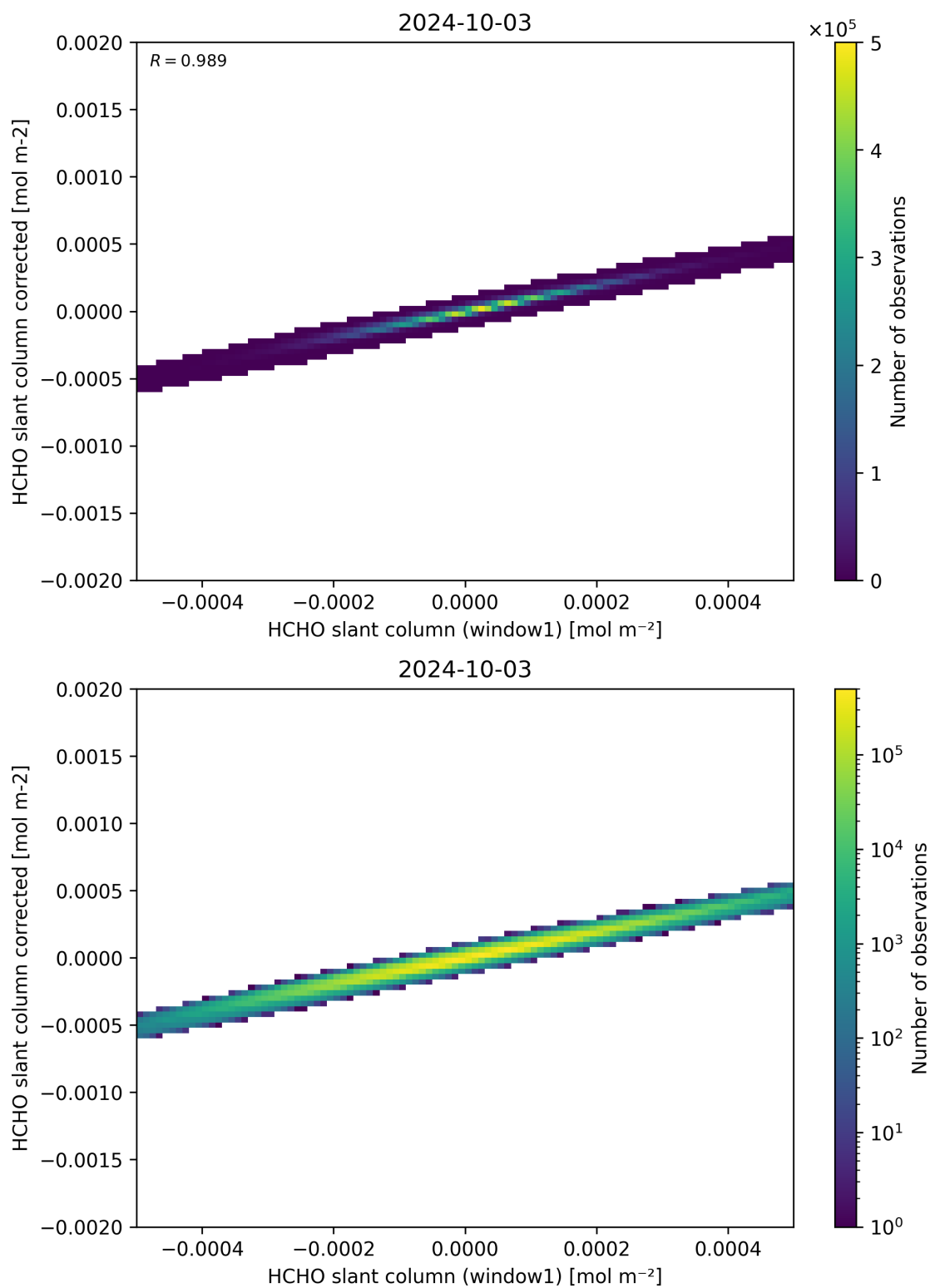
Figure 82: Scatter density plot of “HCHO slant column (window1)” against “HCHO slant column corrected” for 2024-10-03 to 2024-10-04.
