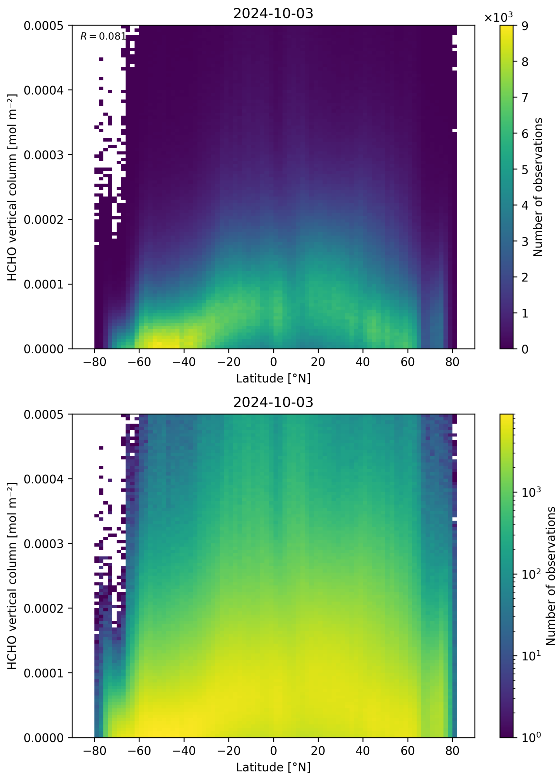
Figure 163: Scatter density plot of “Latitude” against “HCHO vertical column” for 2024-10-03 to 2024-10-04.
