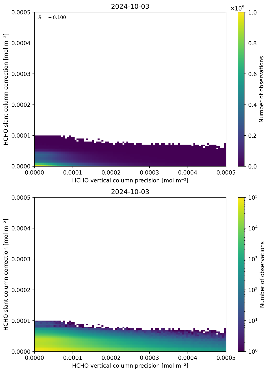
Figure 141: Scatter density plot of “HCHO vertical column precision” against “HCHO slant column correction” for 2024-10-03 to 2024-10-04.
