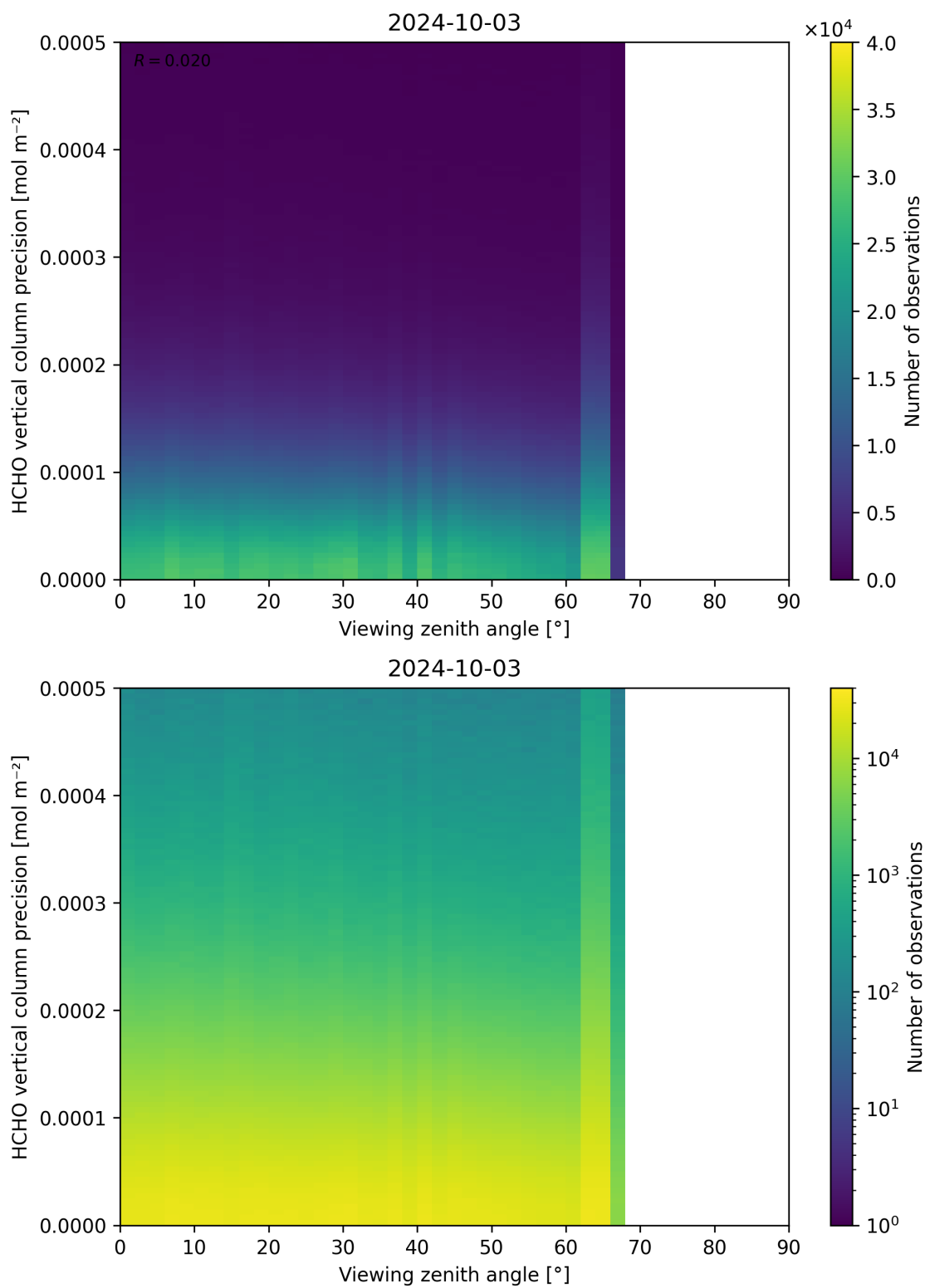
Figure 194: Scatter density plot of “Viewing zenith angle” against “HCHO vertical column precision” for 2024-10-03 to 2024-10-04.
