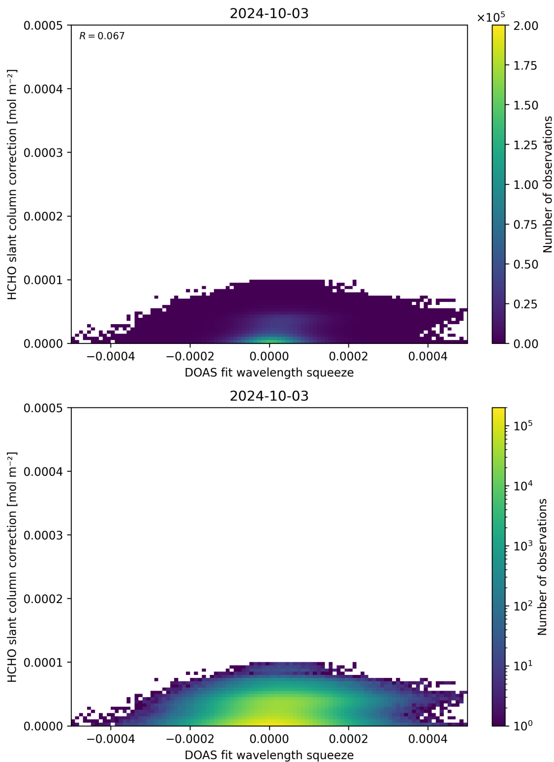
Figure 70: Scatter density plot of “DOAS fit wavelength squeeze” against “HCHO slant column correction” for 2024-10-03 to 2024-10-04.
