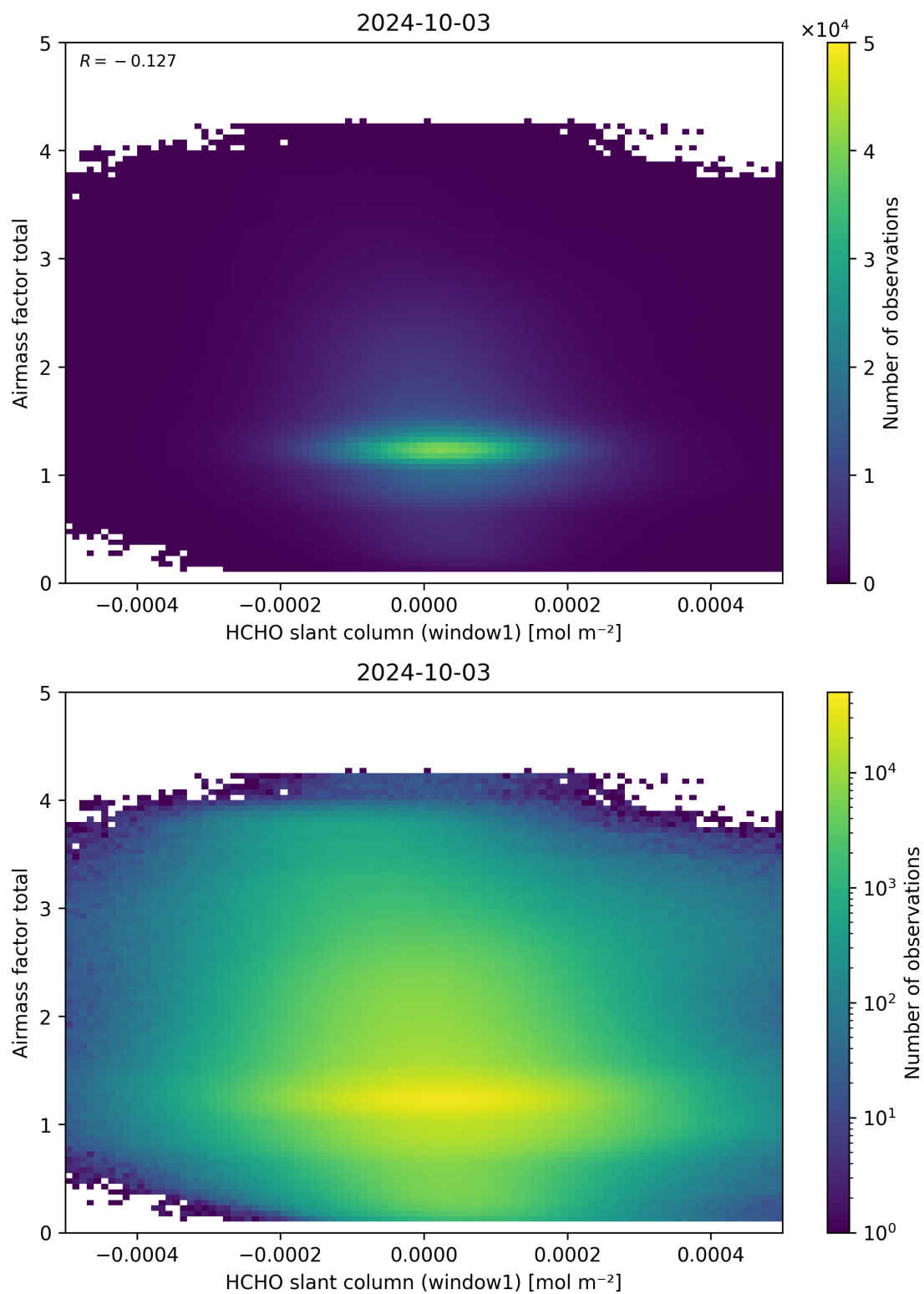
Figure 85: Scatter density plot of “HCHO slant column (window1)” against “Airmass factor total” for 2024-10-03 to 2024-10-04.
