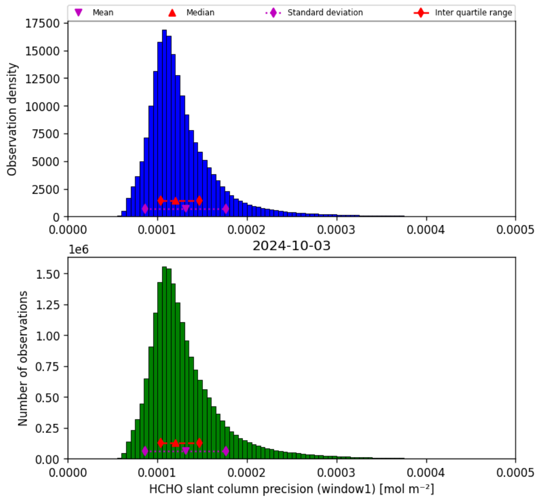
Figure 39: Histogram of “HCHO slant column precision (window1)” for 2024-10-03 to 2024-10-04
