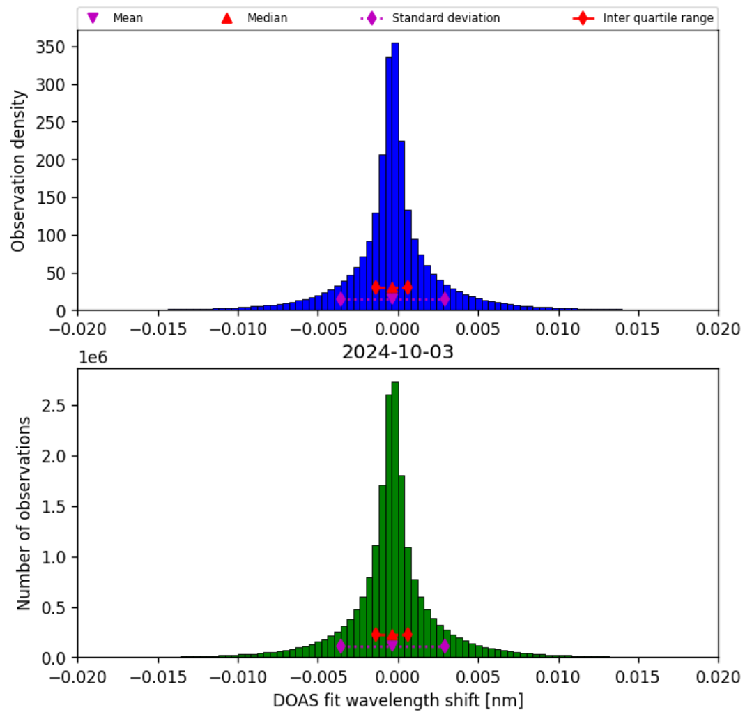
Figure 44: Histogram of “DOAS fit wavelength shift” for 2024-10-03 to 2024-10-04
