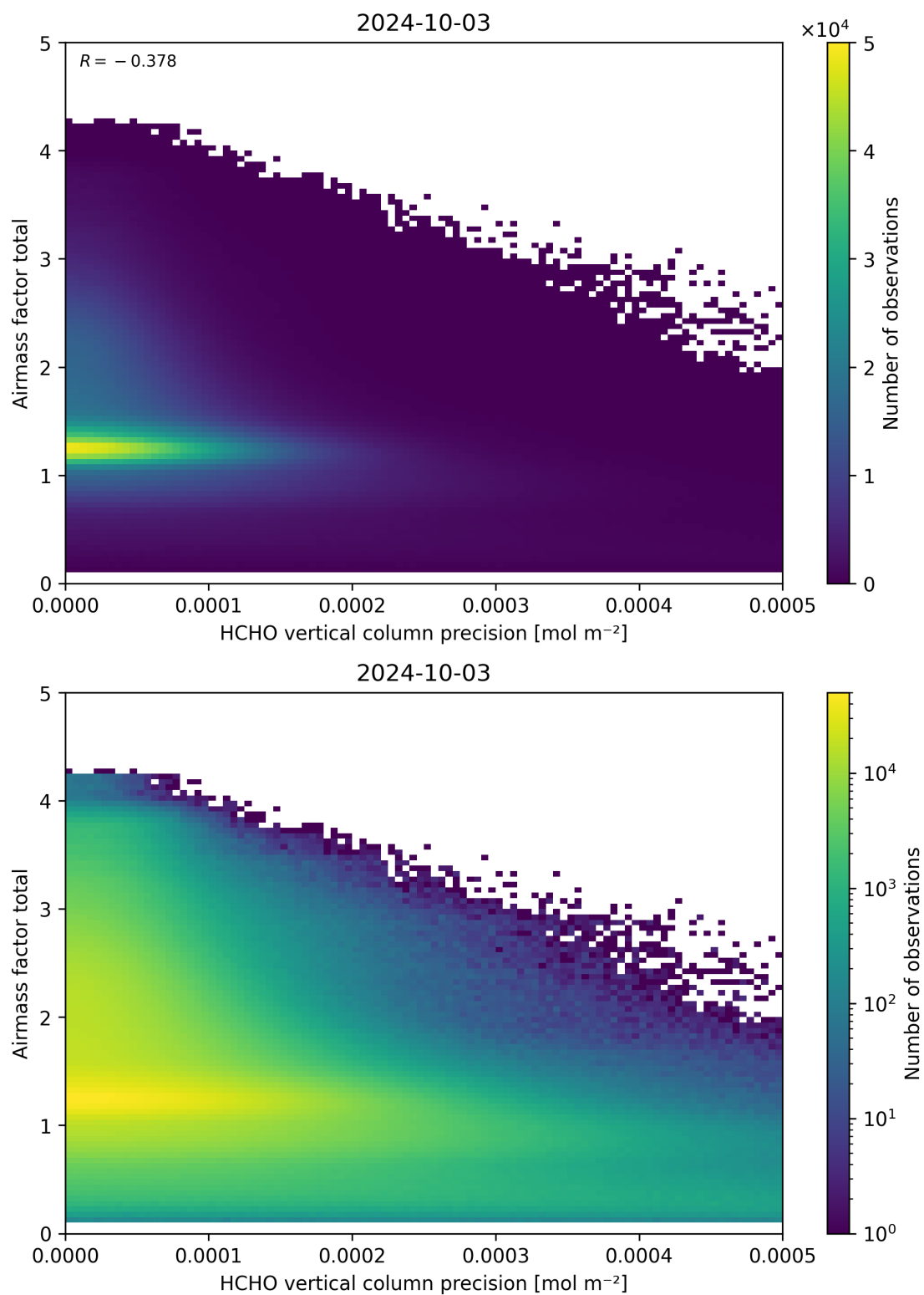
Figure 144: Scatter density plot of “HCHO vertical column precision” against “Airmass factor total” for 2024-10-03 to 2024-10-04.
