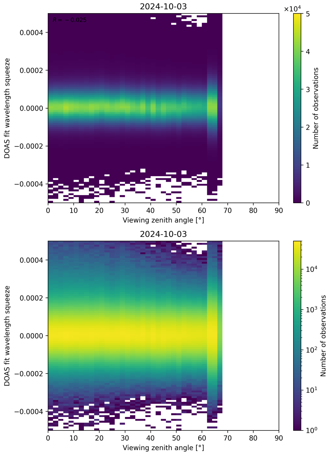
Figure 184: Scatter density plot of “Viewing zenith angle” against “DOAS fit wavelength squeeze” for 2024-10-03 to 2024-10-04.
