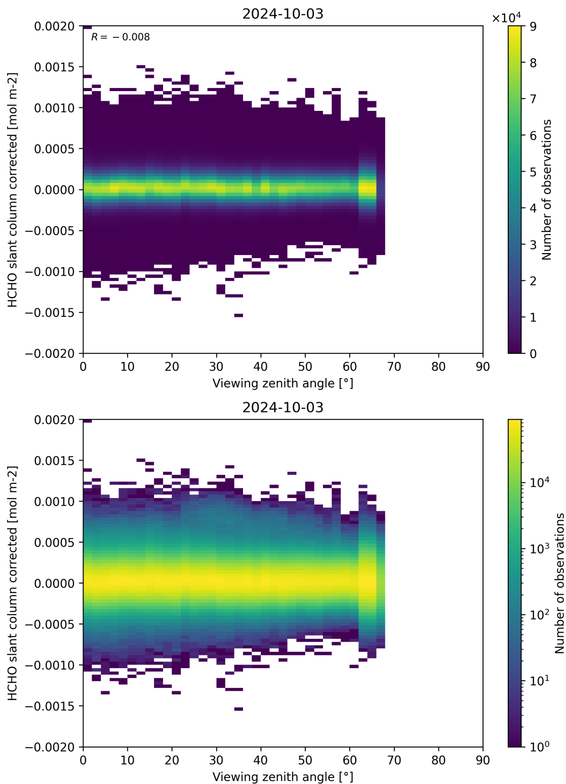
Figure 186: Scatter density plot of “Viewing zenith angle” against “HCHO slant column corrected” for 2024-10-03 to 2024-10-04.
