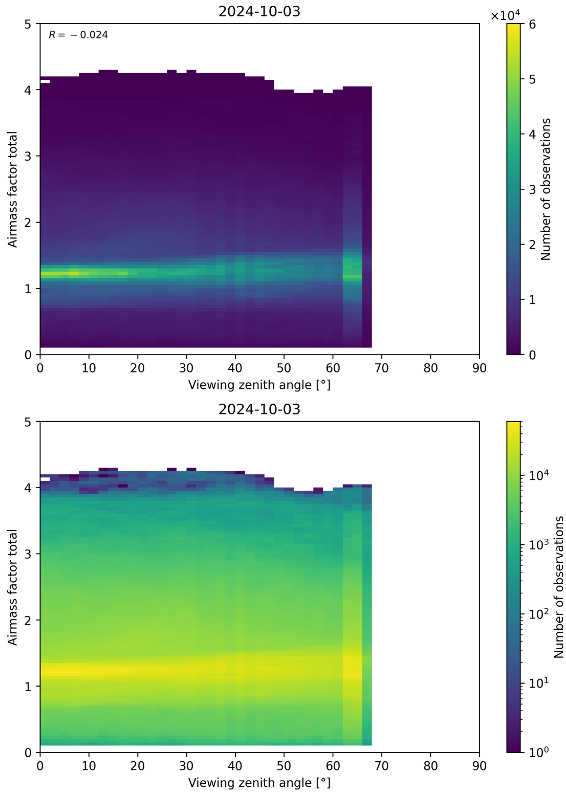
Figure 190: Scatter density plot of “Viewing zenith angle” against “Airmass factor total” for 2024-10-03 to 2024-10-04.
