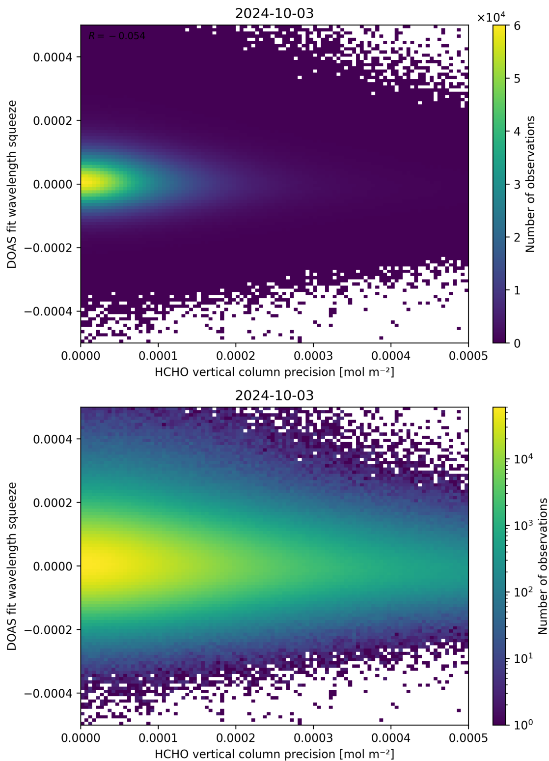
Figure 138: Scatter density plot of “HCHO vertical column precision” against “DOAS fit wavelength squeeze” for 2024-10-03 to 2024-10-04.
