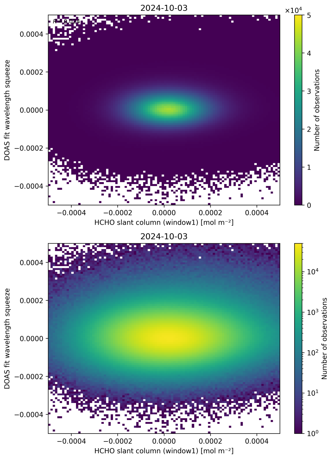
Figure 80: Scatter density plot of “HCHO slant column (window1)” against “DOAS fit wavelength squeeze” for 2024-10-03 to 2024-10-04.
