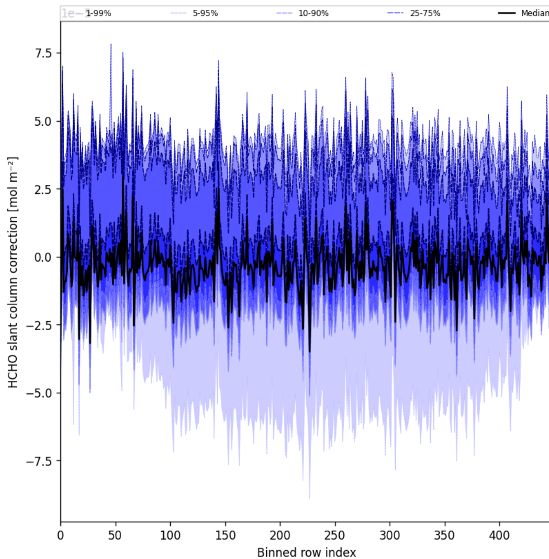
Figure 61: Along track statistics of “HCHO slant column correction” for 2024-10-03 to 2024-10-04
