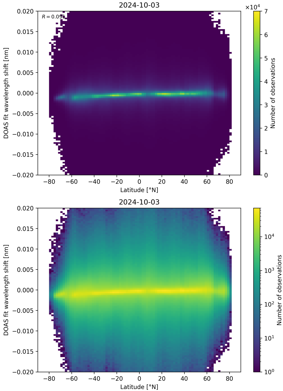
Figure 154: Scatter density plot of “Latitude” against “DOAS fit wavelength shift” for 2024-10-03 to 2024-10-04.
