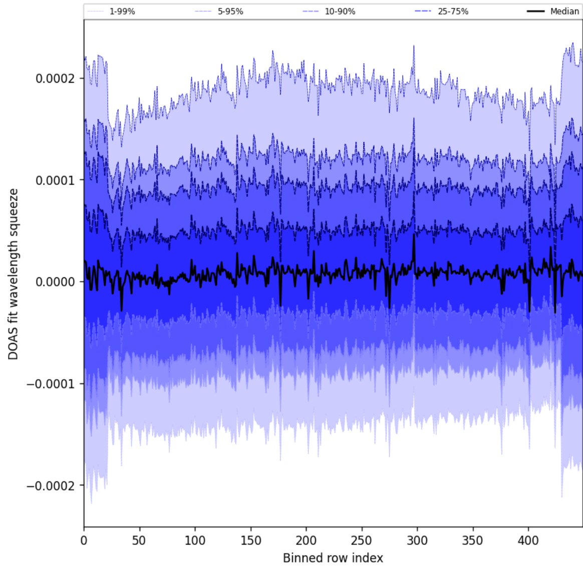
Figure 59: Along track statistics of “DOAS fit wavelength squeeze” for 2024-10-03 to 2024-10-04
