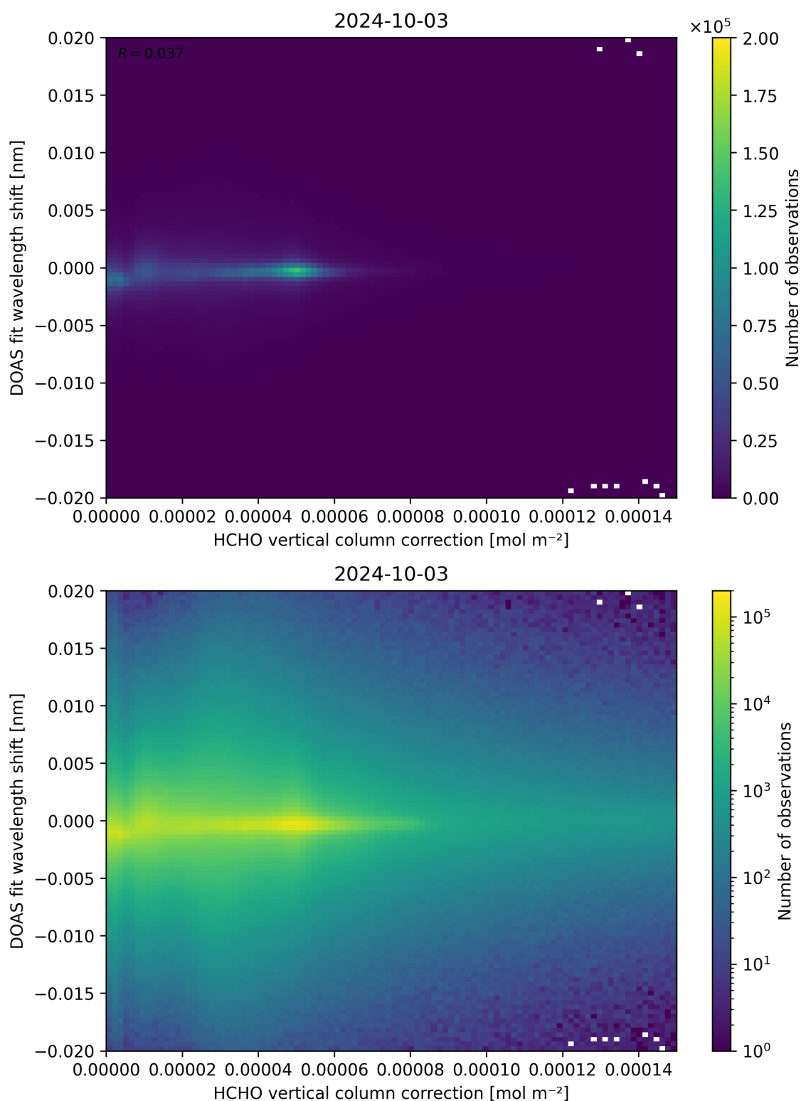
Figure 113: Scatter density plot of “HCHO vertical column correction” against “DOAS fit wavelength shift” for 2024-10-03 to 2024-10-04.
