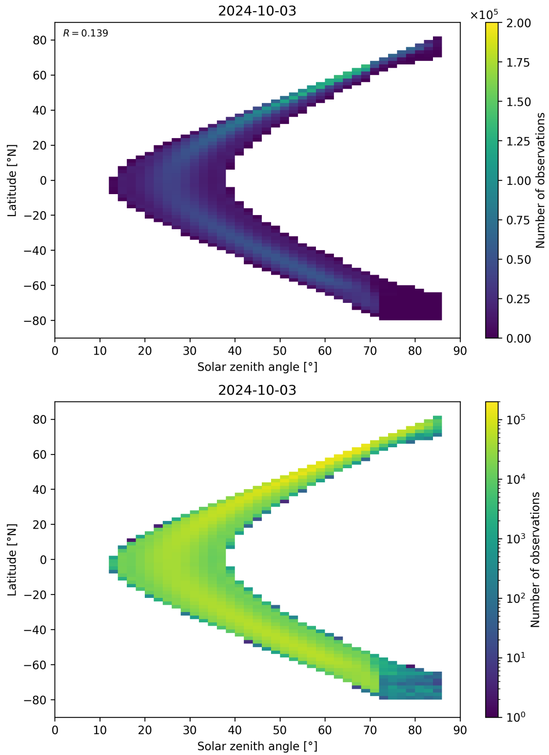
Figure 181: Scatter density plot of “Solar zenith angle” against “Latitude” for 2024-10-03 to 2024-10-04.
