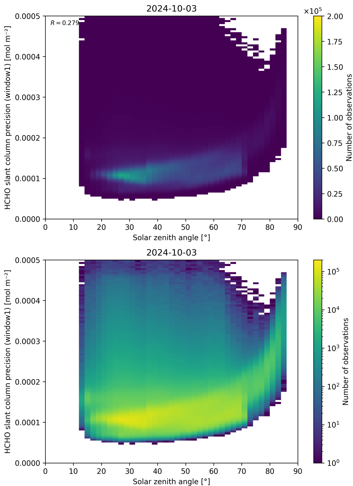
Figure 174: Scatter density plot of “Solar zenith angle” against “HCHO slant column precision (window1)” for 2024-10-03 to 2024-10-04.
