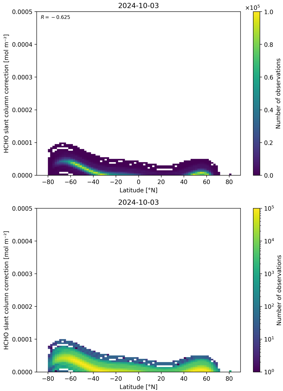
Figure 158: Scatter density plot of “Latitude” against “HCHO slant column correction” for 2024-10-03 to 2024-10-04.
