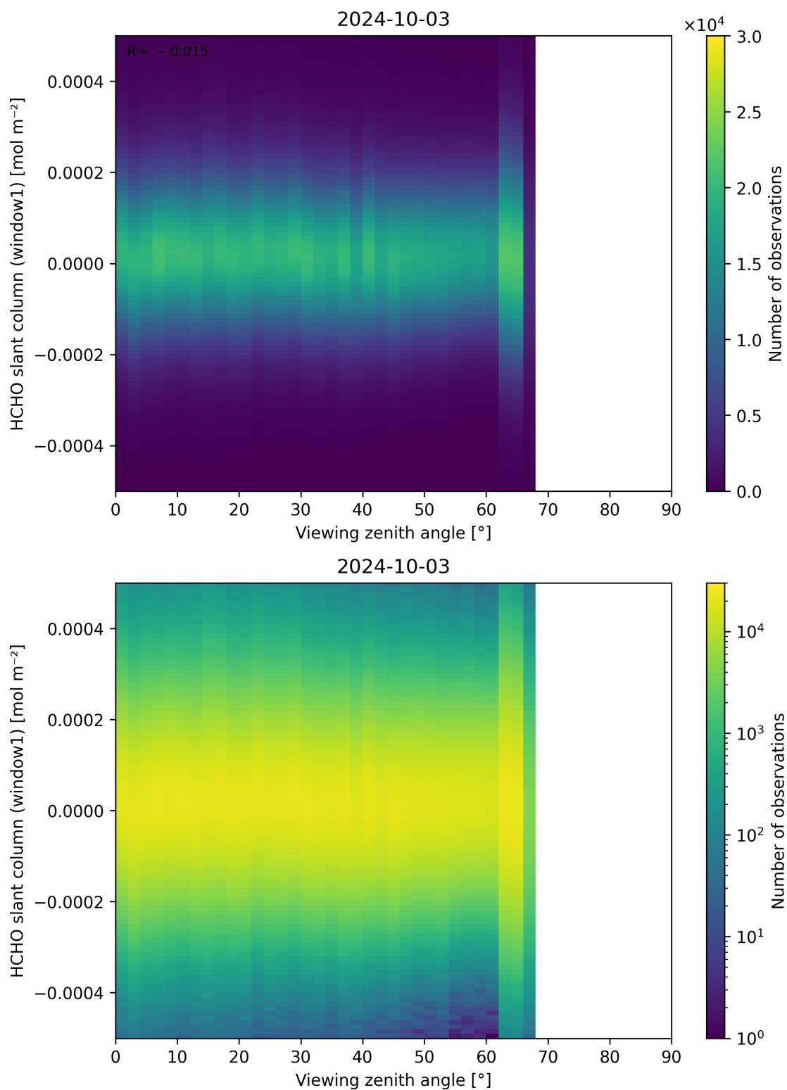
Figure 188: Scatter density plot of “Viewing zenith angle” against “HCHO slant column (window1)” for 2024-10-03 to 2024-10-04.
