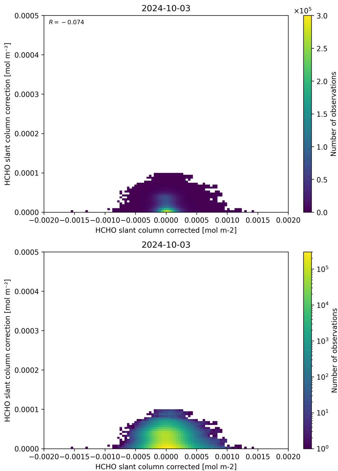
Figure 77: Scatter density plot of “HCHO slant column corrected” against “HCHO slant column correction” for 2024-10-03 to 2024-10-04.
