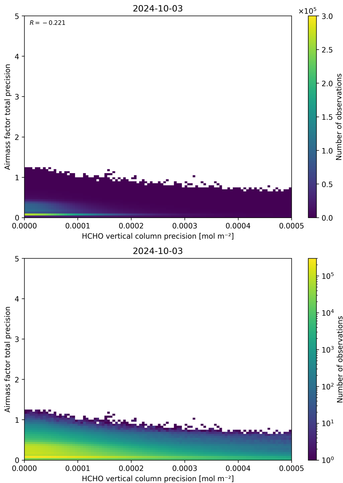
Figure 145: Scatter density plot of “HCHO vertical column precision” against “Airmass factor total precision” for 2024-10-03 to 2024-10-04.
