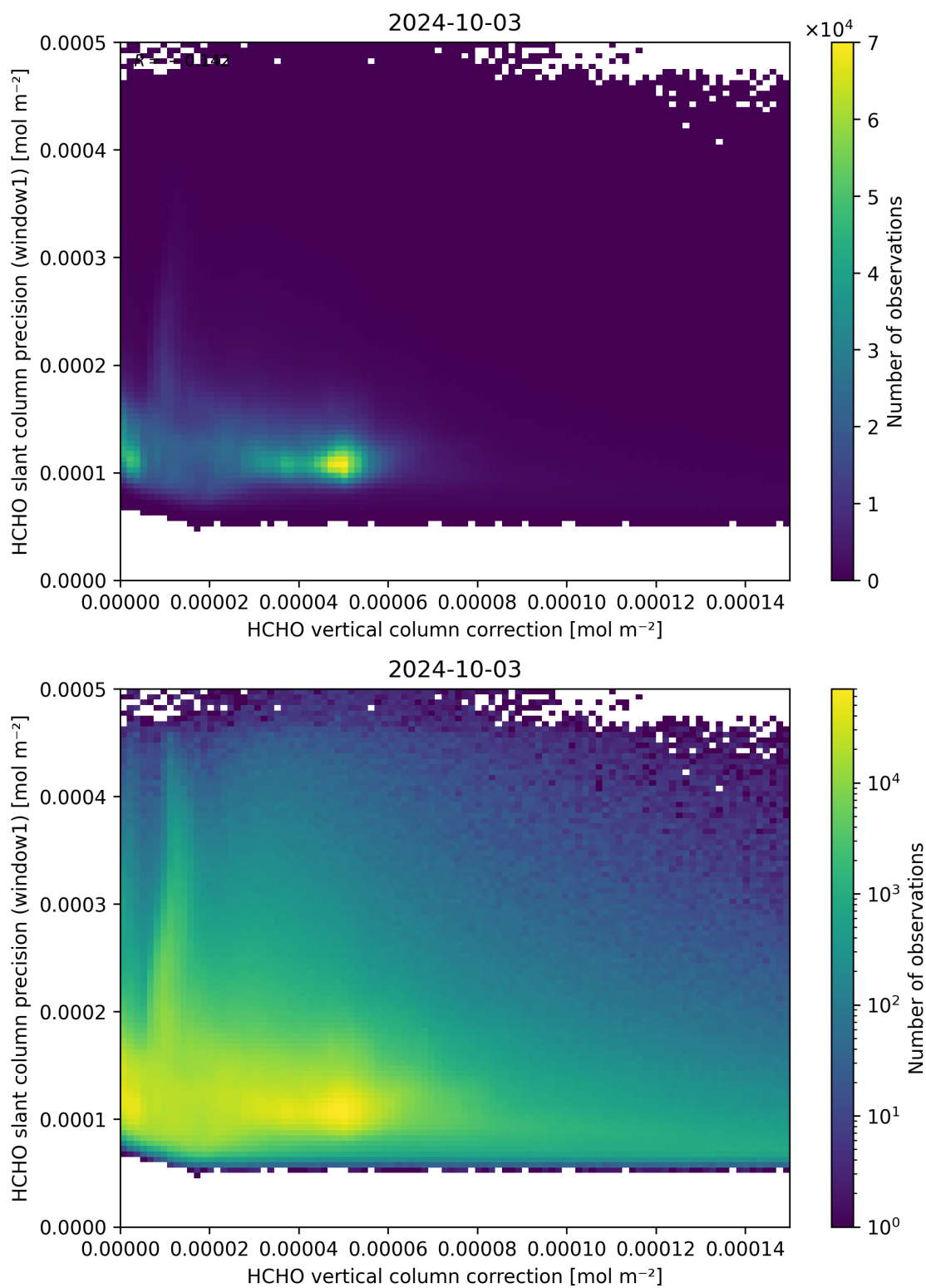
Figure 119: Scatter density plot of “HCHO vertical column correction” against “HCHO slant column precision (window1)” for 2024-10-03 to 2024-10-04.
