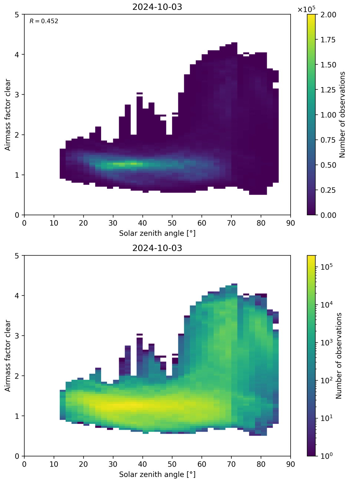
Figure 170: Scatter density plot of “Solar zenith angle” against “Airmass factor clear” for 2024-10-03 to 2024-10-04.
