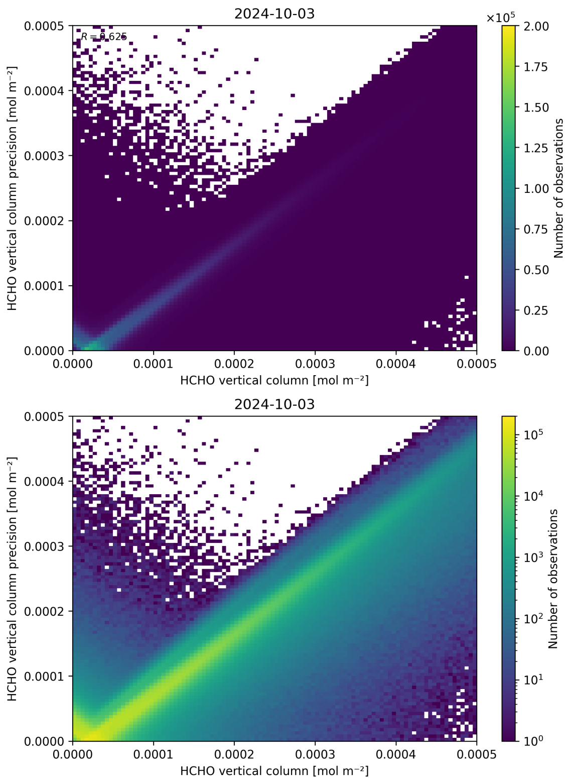
Figure 134: Scatter density plot of “HCHO vertical column” against “HCHO vertical column precision” for 2024-10-03 to 2024-10-04.
