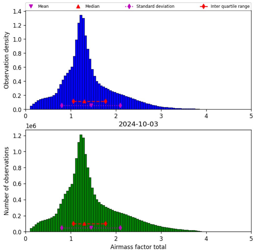
Figure 40: Histogram of “Airmass factor total” for 2024-10-03 to 2024-10-04
