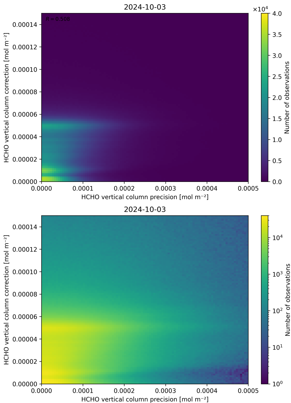
Figure 146: Scatter density plot of “HCHO vertical column precision” against “HCHO vertical column correction” for 2024-10-03 to 2024-10-04.
