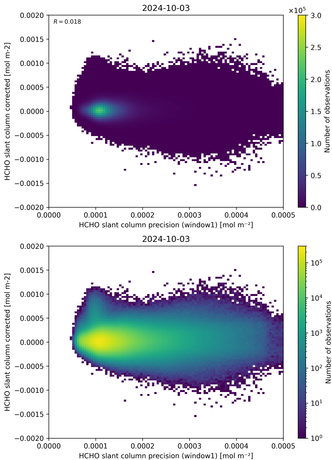
Figure 92: Scatter density plot of “HCHO slant column precision (window1)” against “HCHO slant column corrected” for 2024-10-03 to 2024-10-04.
