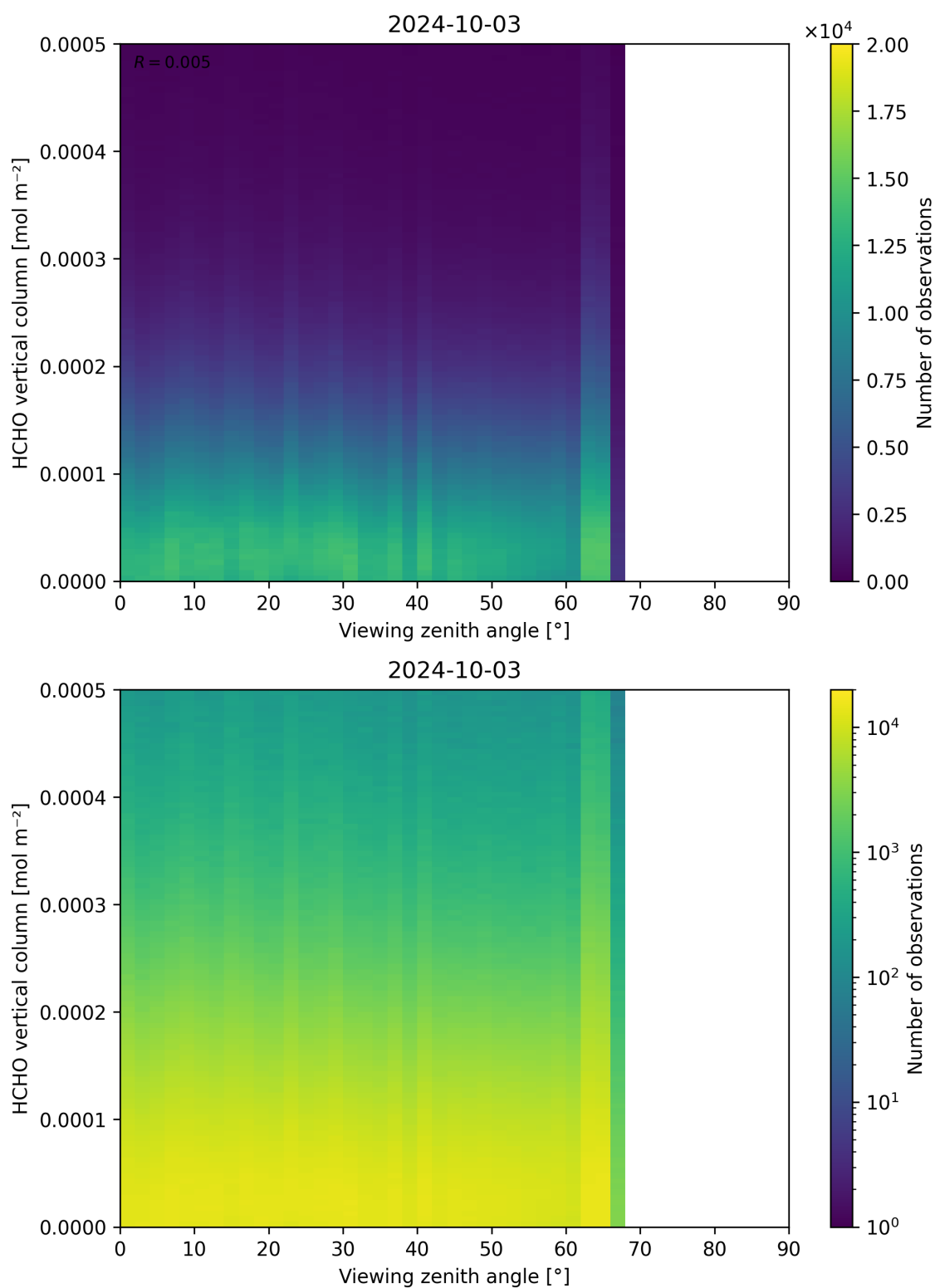
Figure 192: Scatter density plot of “Viewing zenith angle” against “HCHO vertical column” for 2024-10-03 to 2024-10-04.
