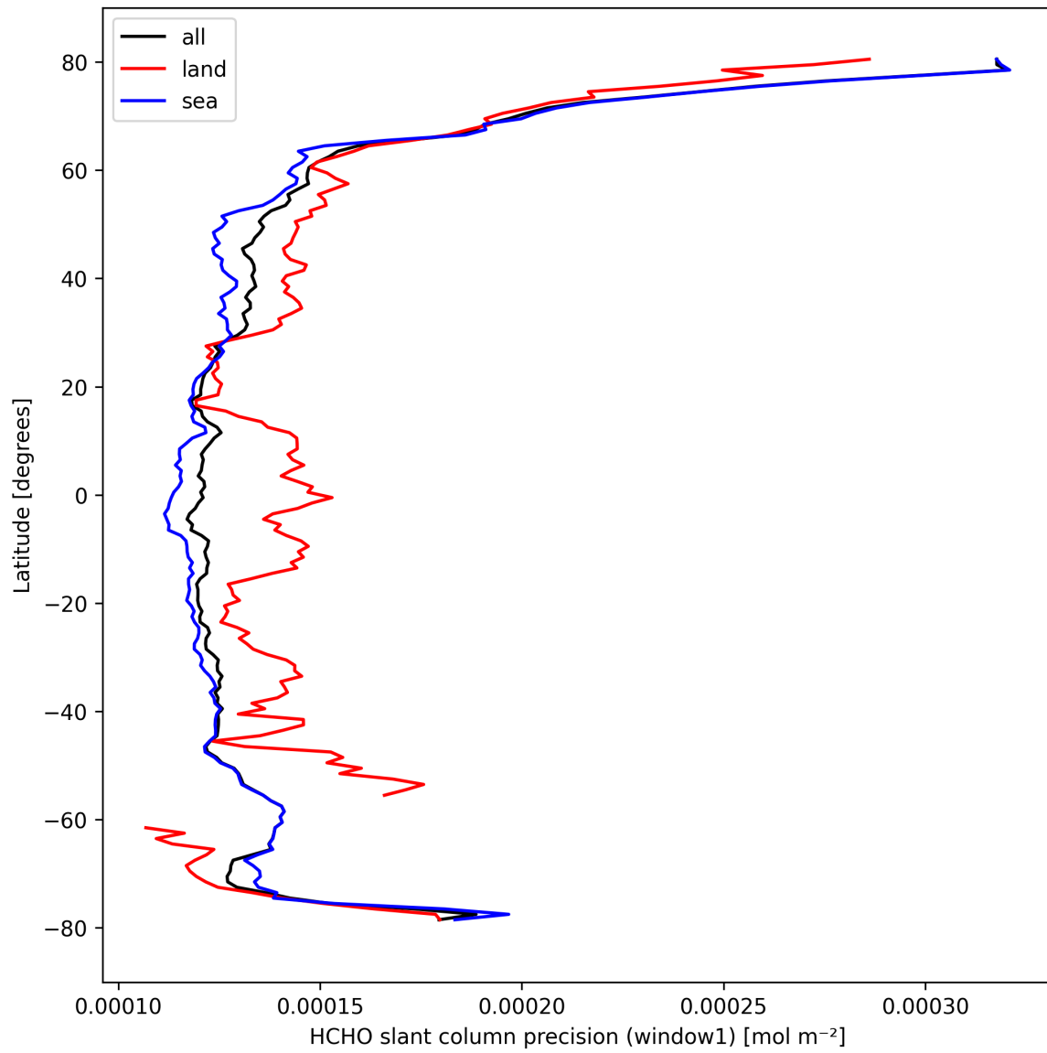
Figure 25: Zonal average of “HCHO slant column precision (window1)” for 2024-10-03 to 2024-10-04.
