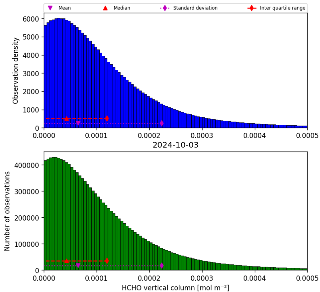
Figure 35: Histogram of “HCHO vertical column” for 2024-10-03 to 2024-10-04
