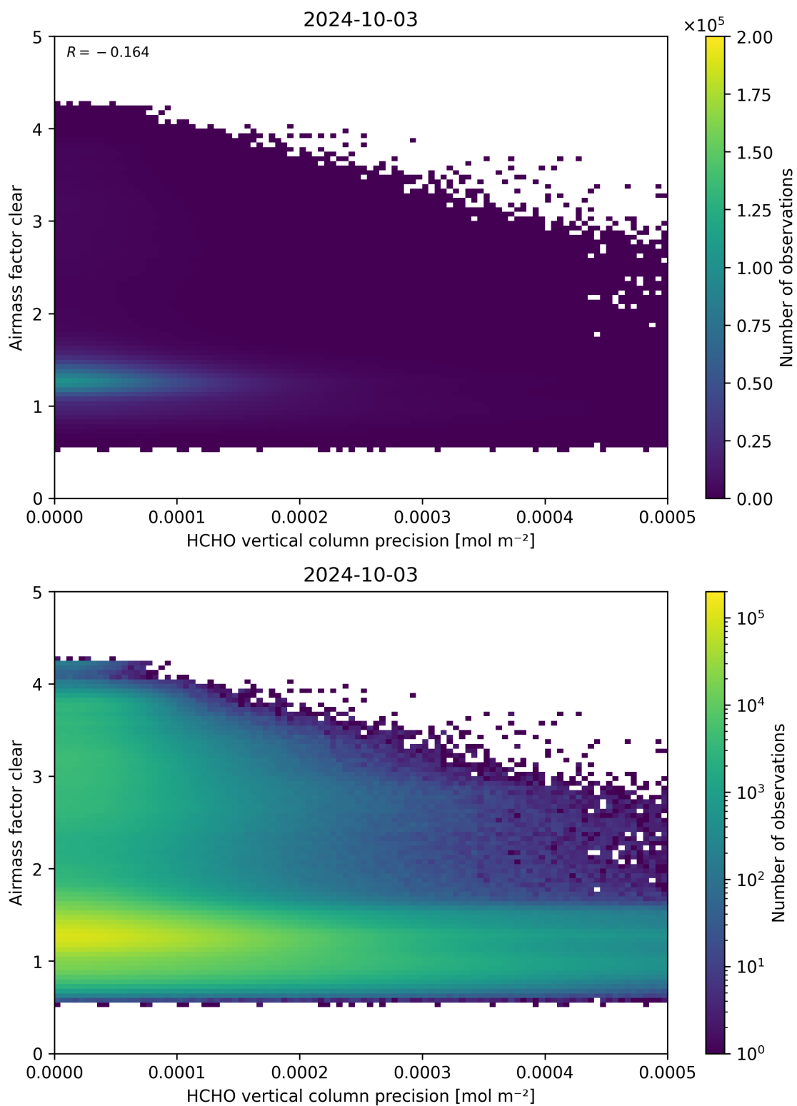
Figure 139: Scatter density plot of “HCHO vertical column precision” against “Airmass factor clear” for 2024-10-03 to 2024-10-04.
