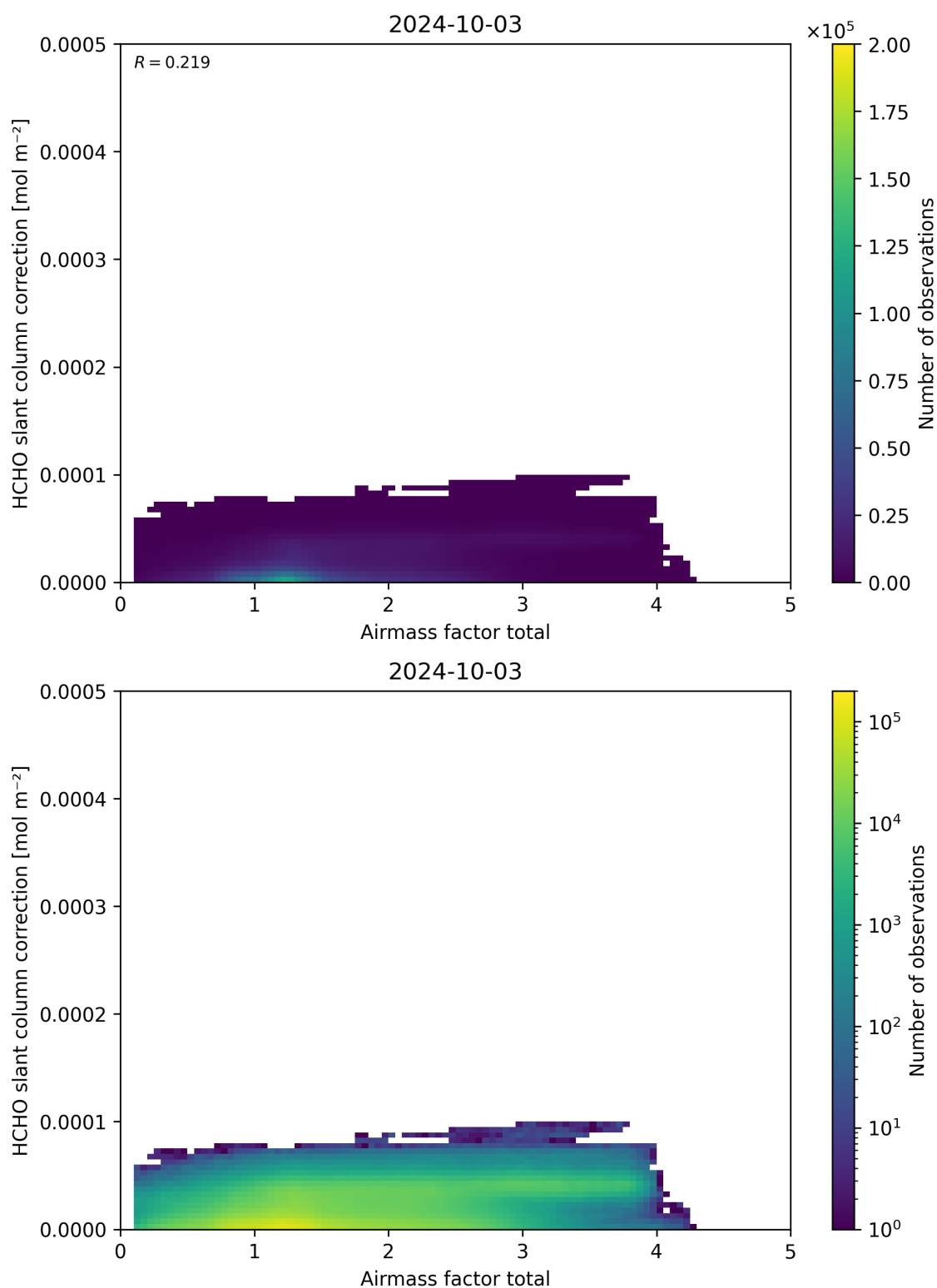
Figure 102: Scatter density plot of “Airmass factor total” against “HCHO slant column correction” for 2024-10-03 to 2024-10-04.
