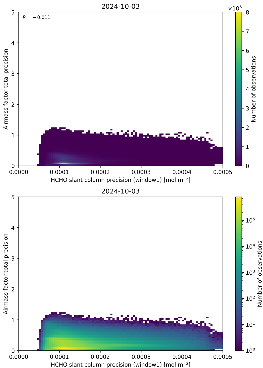
Figure 95: Scatter density plot of “HCHO slant column precision (window1)” against “Airmass factor total precision” for 2024-10-03 to 2024-10-04.
