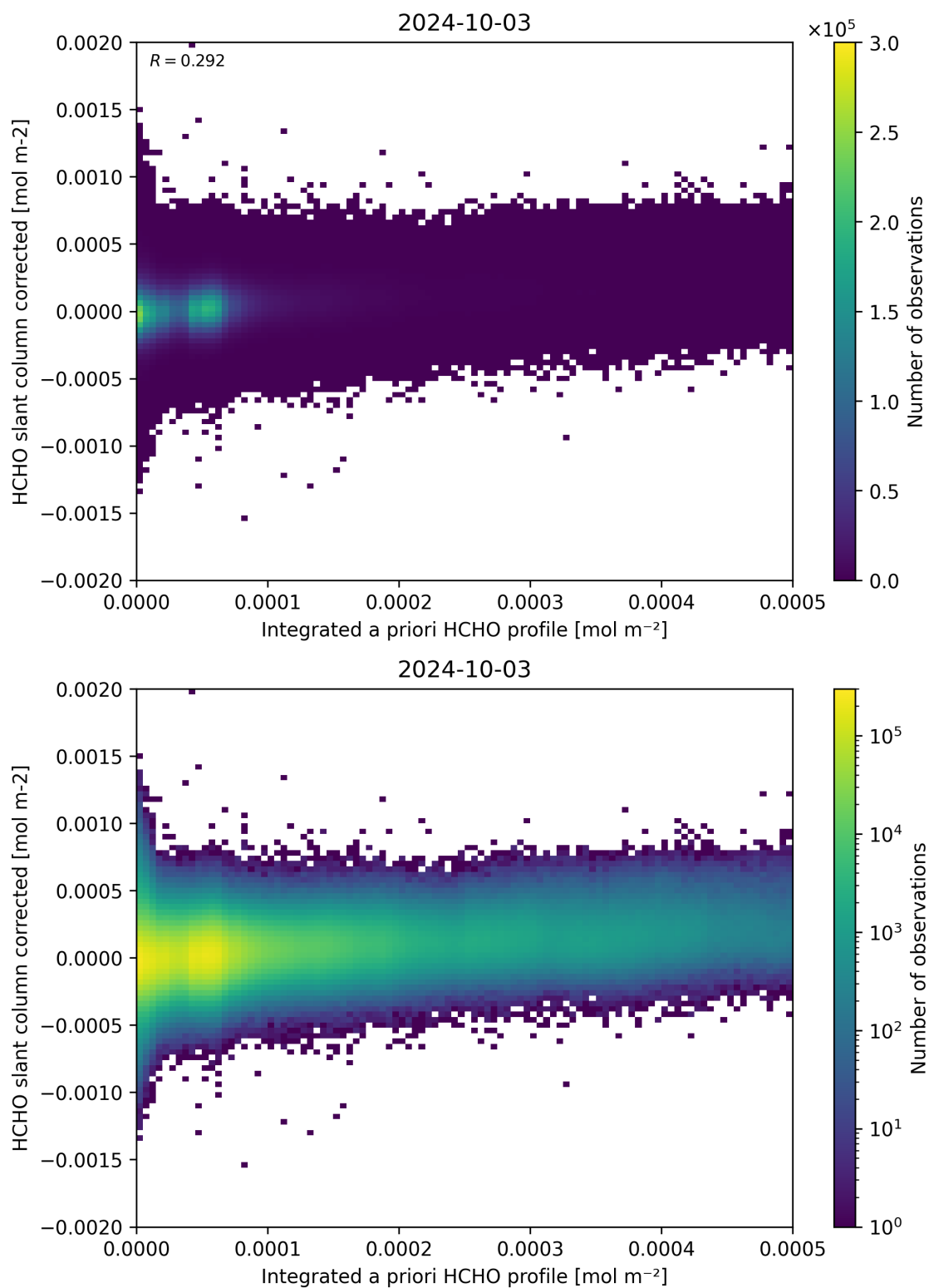
Figure 151: Scatter density plot of “Integrated a priori HCHO profile” against “HCHO slant column corrected” for 2024-10-03 to 2024-10-04.
