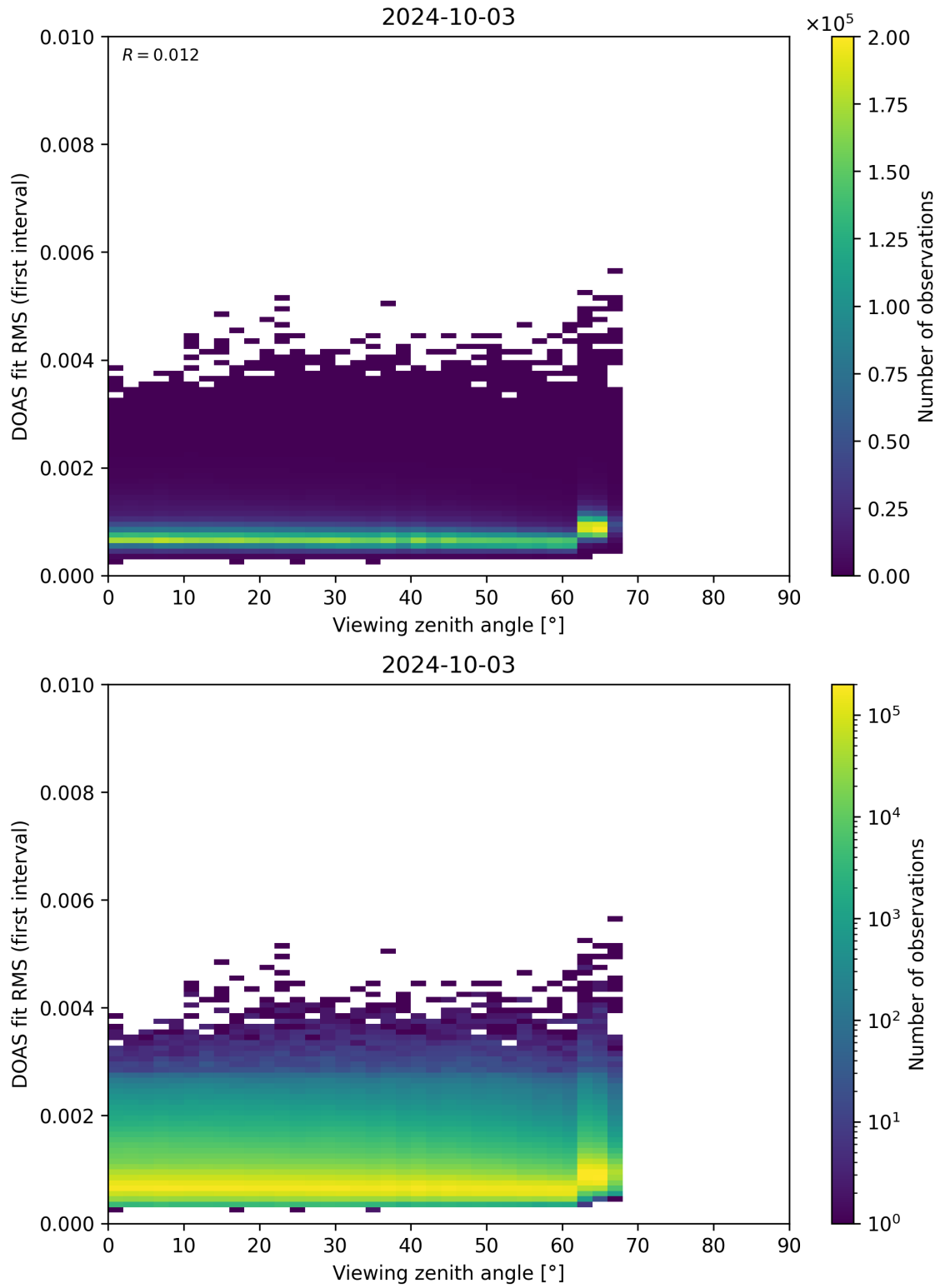
Figure 182: Scatter density plot of “Viewing zenith angle” against “DOAS fit RMS (first interval)” for 2024-10-03 to 2024-10-04.
