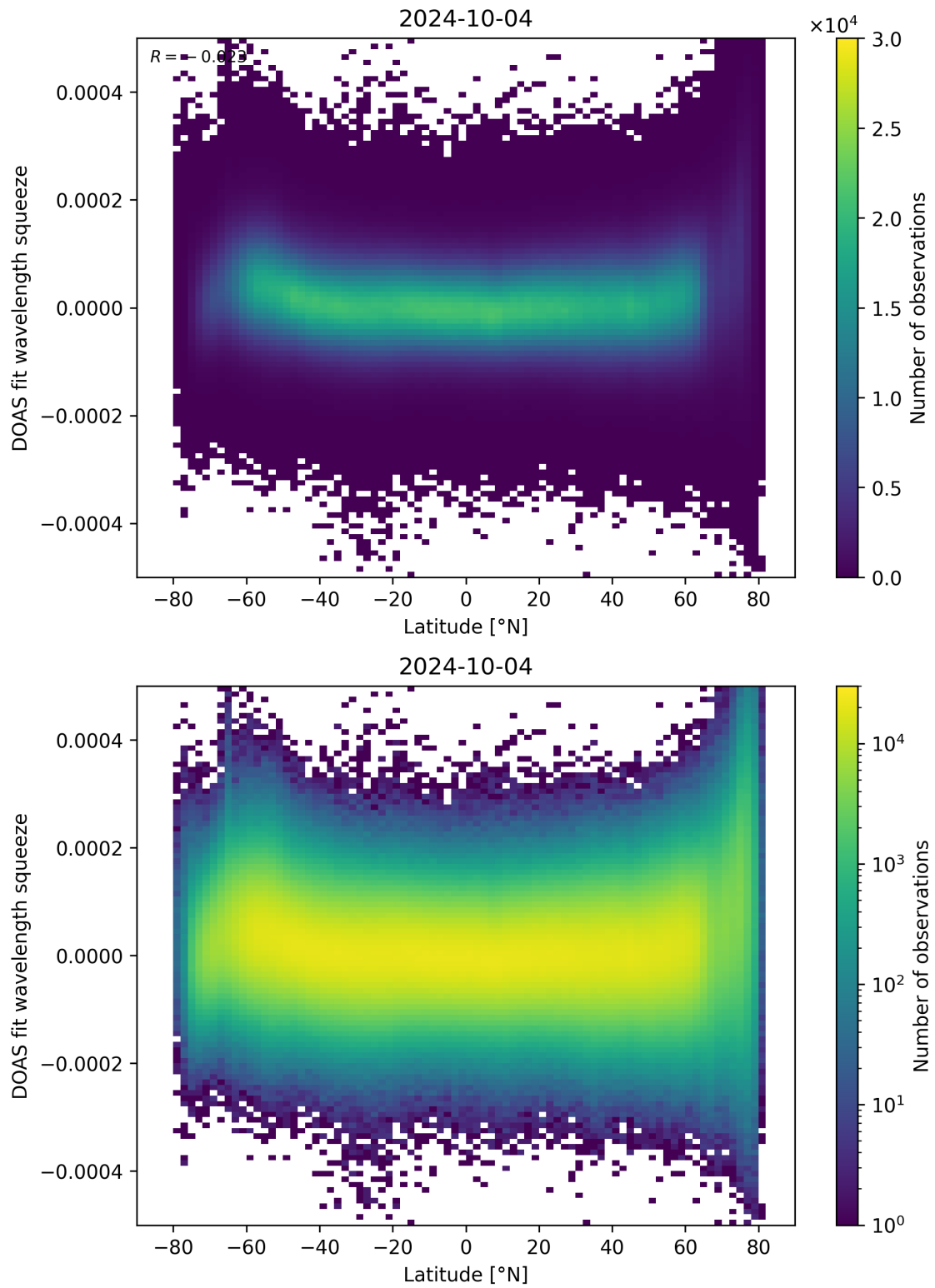
Figure 155: Scatter density plot of “Latitude” against “DOAS fit wavelength squeeze” for 2024-10-03 to 2024-10-05.
