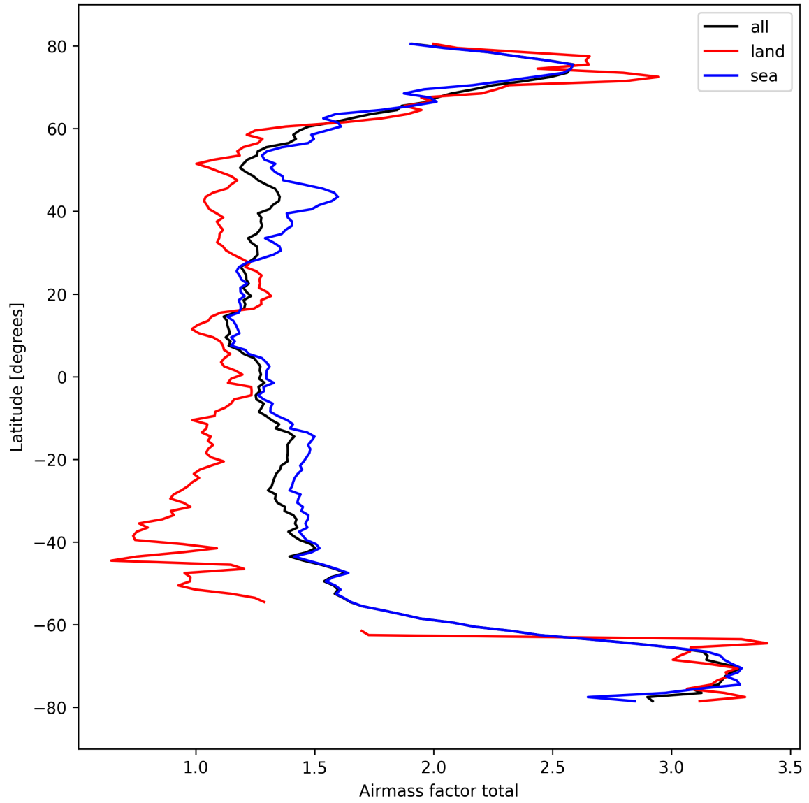
Figure 26: Zonal average of “Airmass factor total” for 2024-10-03 to 2024-10-05.
