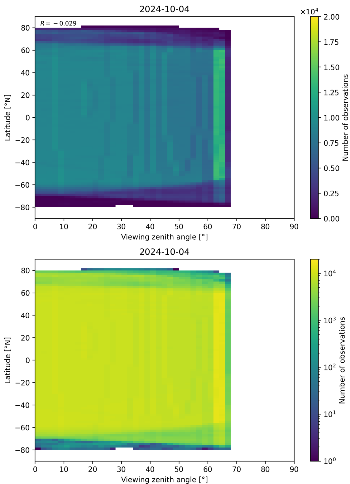
Figure 196: Scatter density plot of “Viewing zenith angle” against “Latitude” for 2024-10-03 to 2024-10-05.
