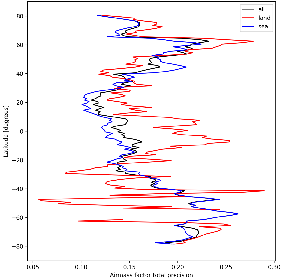
Figure 27: Zonal average of “Airmass factor total precision” for 2024-10-03 to 2024-10-05.
