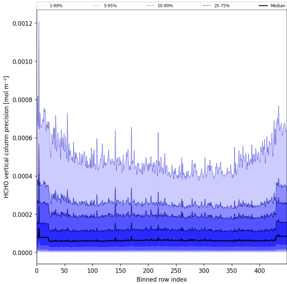
Figure 50: Along track statistics of “HCHO vertical column precision” for 2024-10-03 to 2024-10-05
