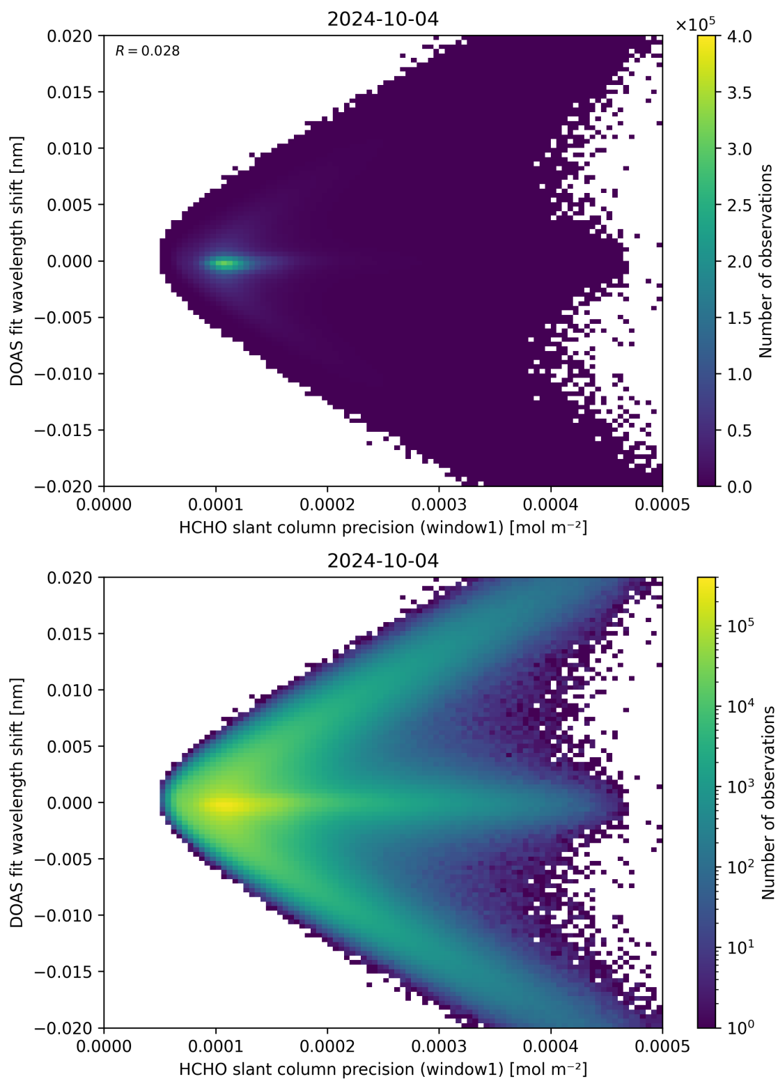
Figure 89: Scatter density plot of “HCHO slant column precision (window1)” against “DOAS fit wavelength shift” for 2024-10-03 to 2024-10-05.
