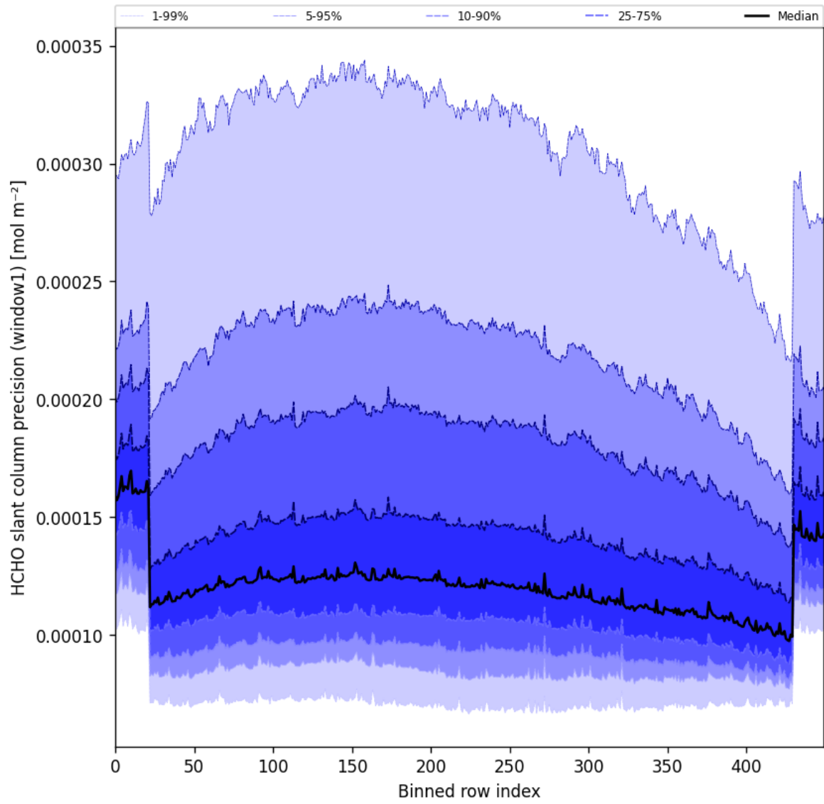
Figure 53: Along track statistics of “HCHO slant column precision (window1)” for 2024-10-03 to 2024-10-05
