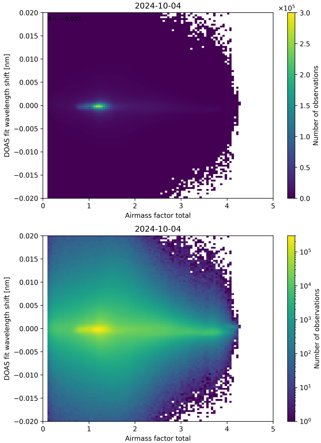
Figure 98: Scatter density plot of “Airmass factor total” against “DOAS fit wavelength shift” for 2024-10-03 to 2024-10-05.
