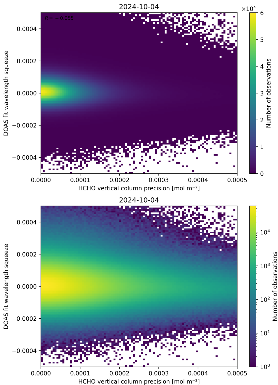
Figure 138: Scatter density plot of “HCHO vertical column precision” against “DOAS fit wavelength squeeze” for 2024-10-03 to 2024-10-05.
