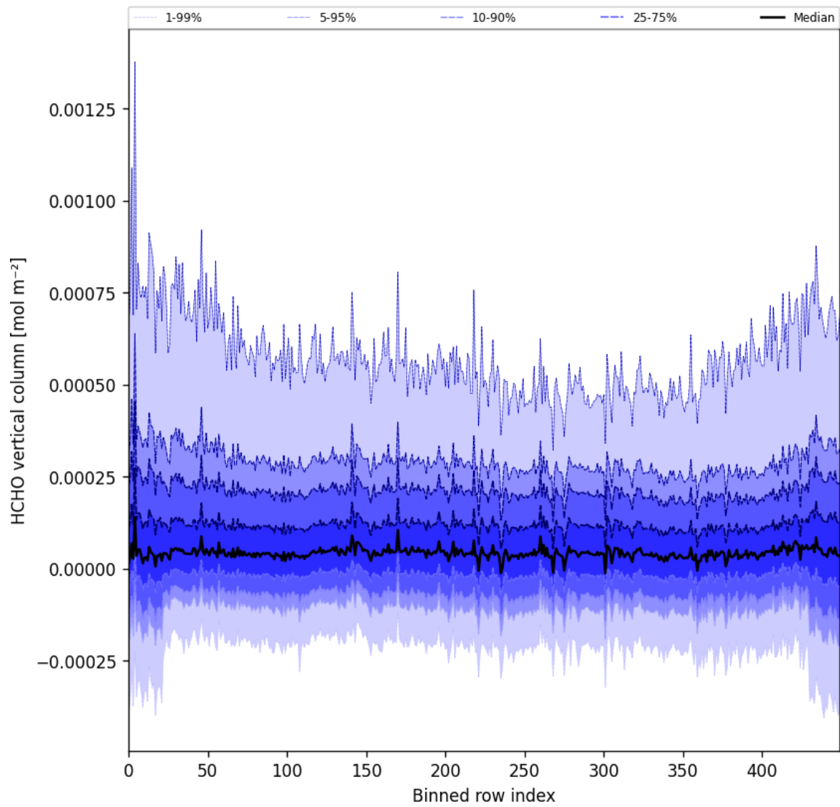
Figure 49: Along track statistics of “HCHO vertical column” for 2024-10-03 to 2024-10-05
