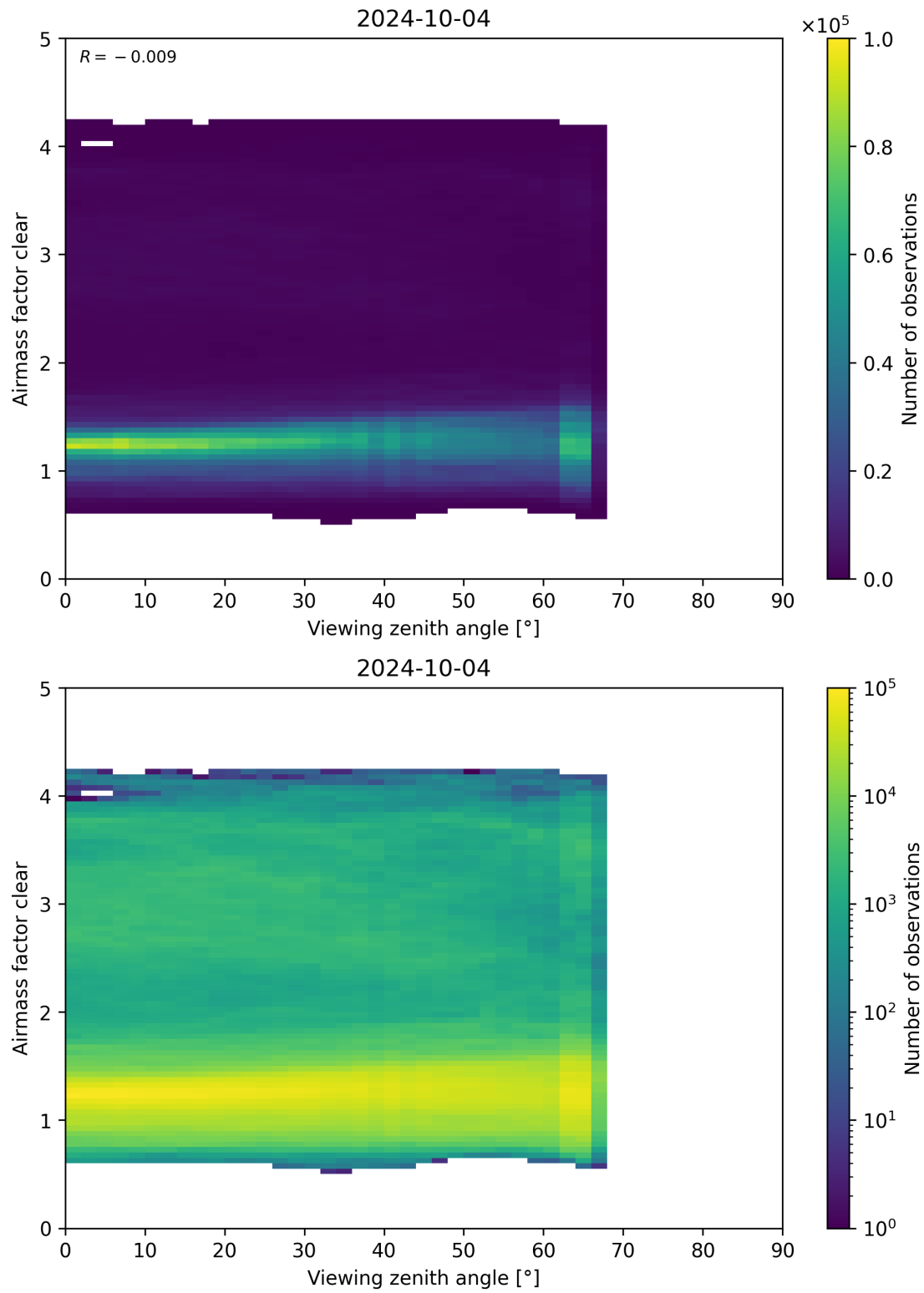
Figure 185: Scatter density plot of “Viewing zenith angle” against “Airmass factor clear” for 2024-10-03 to 2024-10-05.
