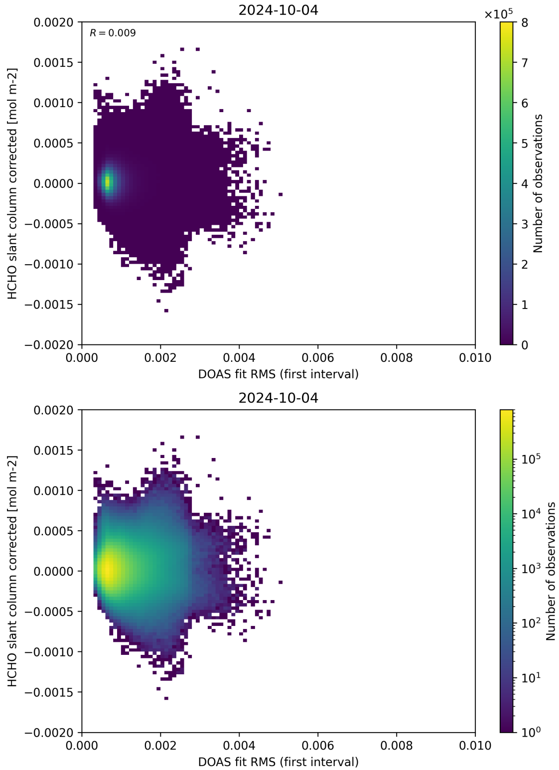
Figure 62: Scatter density plot of “DOAS fit RMS (first interval)” against “HCHO slant column corrected” for 2024-10-03 to 2024-10-05.
