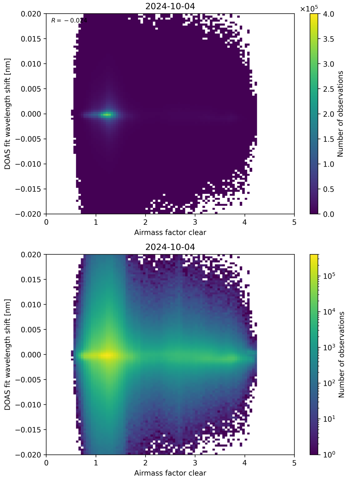
Figure 72: Scatter density plot of “Airmass factor clear” against “DOAS fit wavelength shift” for 2024-10-03 to 2024-10-05.
