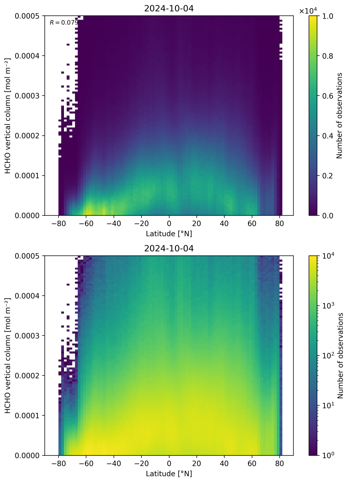
Figure 163: Scatter density plot of “Latitude” against “HCHO vertical column” for 2024-10-03 to 2024-10-05.
