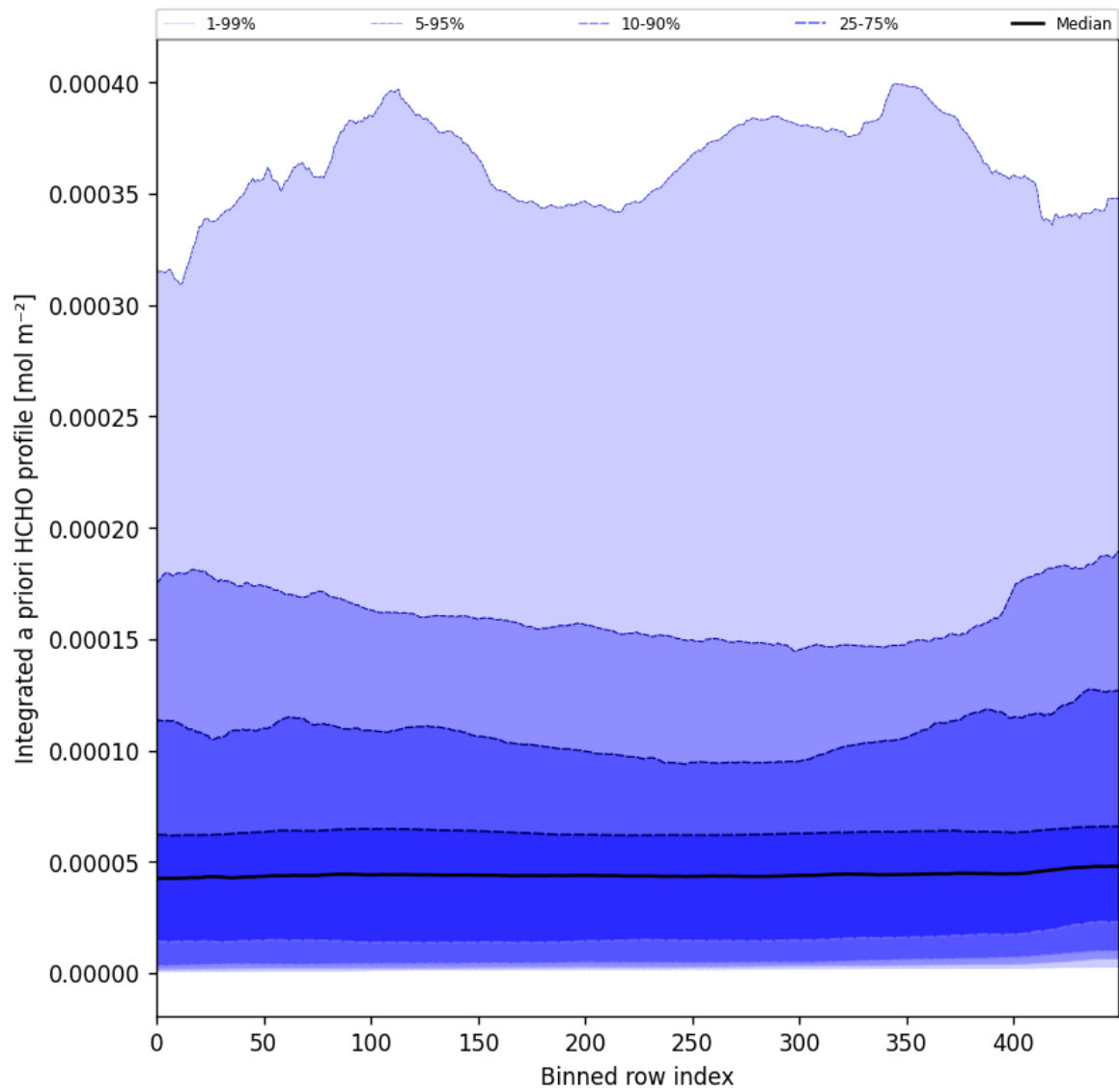
Figure 57: Along track statistics of "Integrated a priori HCHO profile" for 2024-10-03 to 2024-10-05
