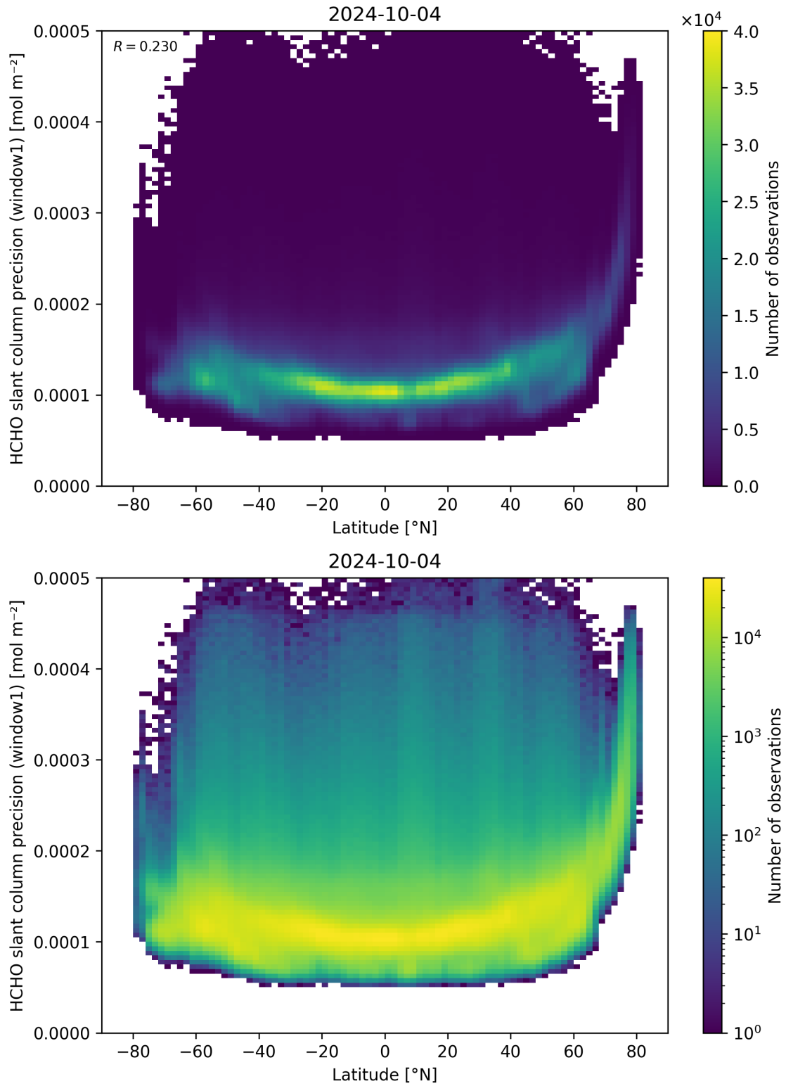
Figure 160: Scatter density plot of “Latitude” against “HCHO slant column precision (window1)” for 2024-10-03 to 2024-10-05.
