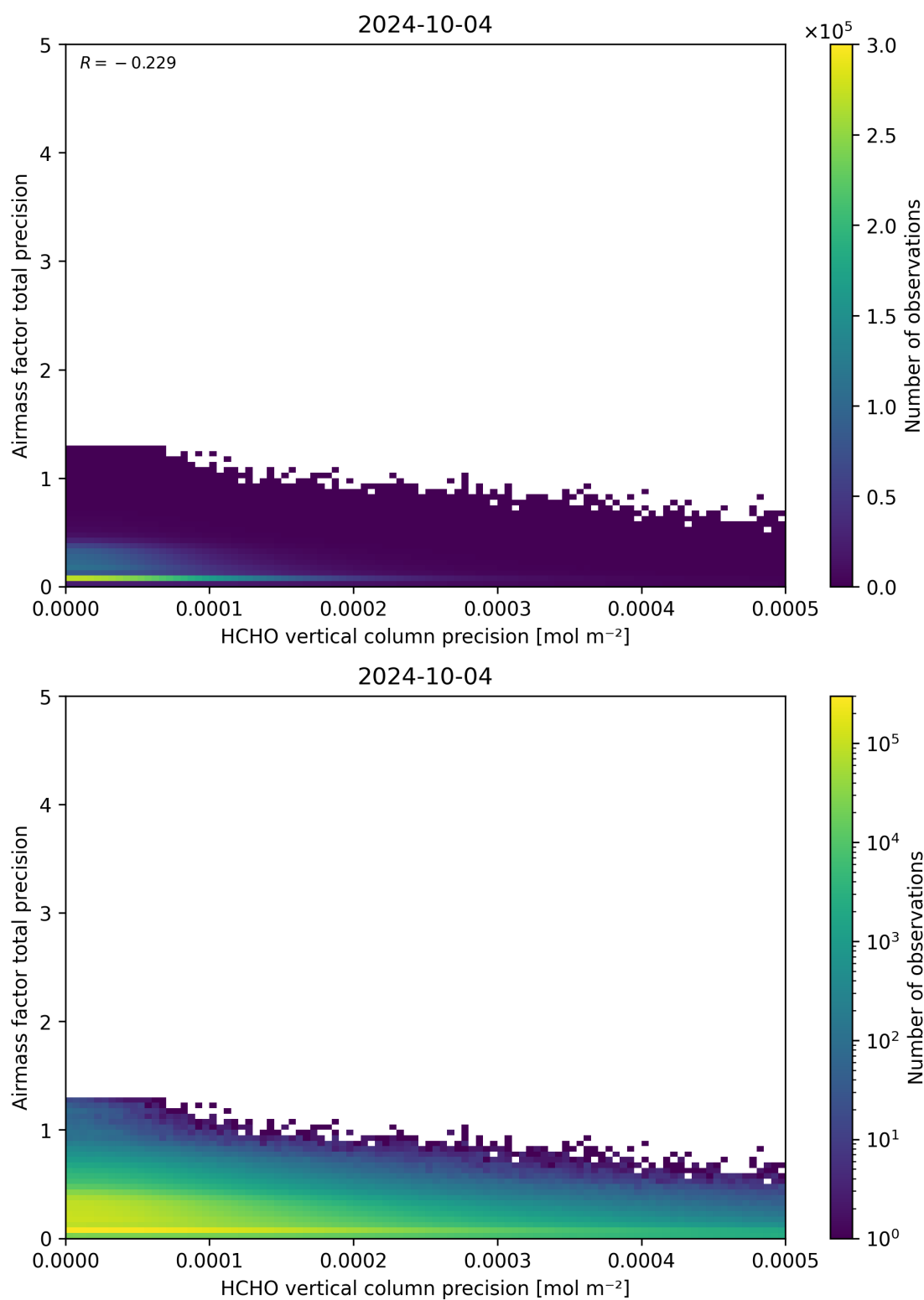
Figure 145: Scatter density plot of “HCHO vertical column precision” against “Airmass factor total precision” for 2024-10-03 to 2024-10-05.
