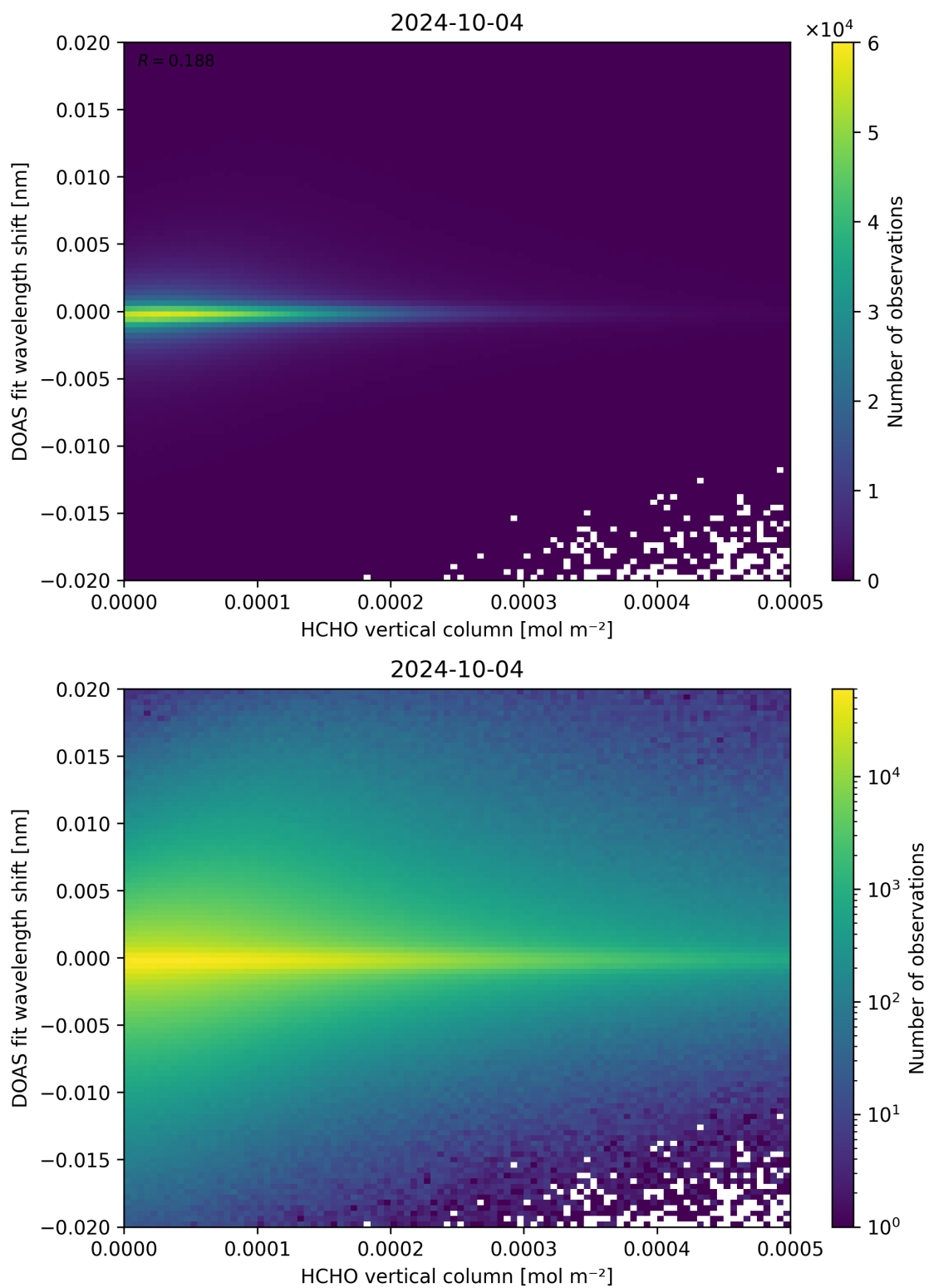
Figure 124: Scatter density plot of “HCHO vertical column” against “DOAS fit wavelength shift” for 2024-10-03 to 2024-10-05.
