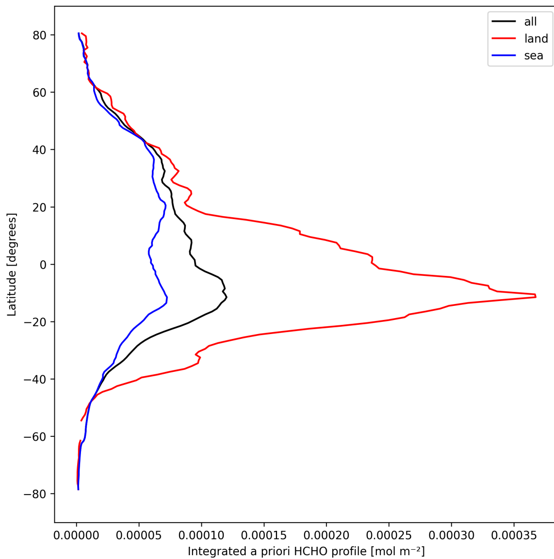
Figure 29: Zonal average of “Integrated a priori HCHO profile” for 2024-10-03 to 2024-10-05.
