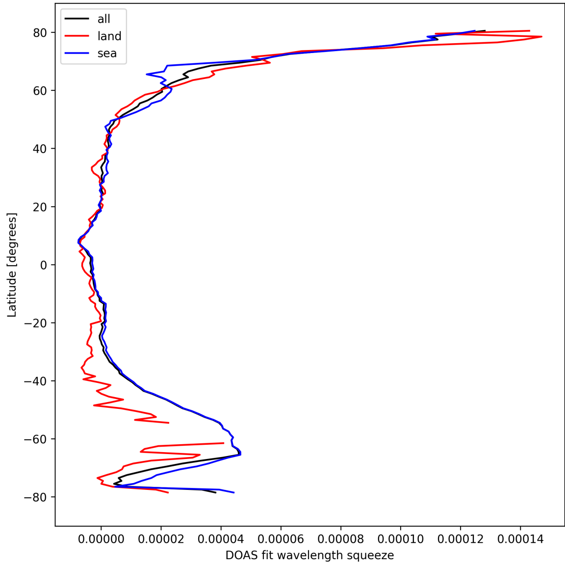
Figure 31: Zonal average of “DOAS fit wavelength squeeze” for 2024-10-03 to 2024-10-05.
