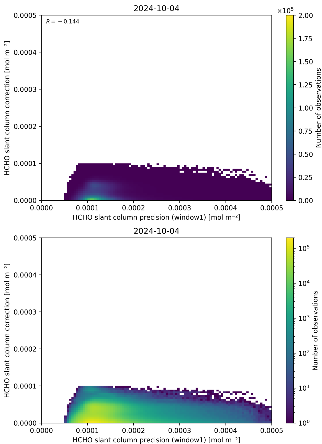
Figure 93: Scatter density plot of “HCHO slant column precision (window1)” against “HCHO slant column correction” for 2024-10-03 to 2024-10-05.
