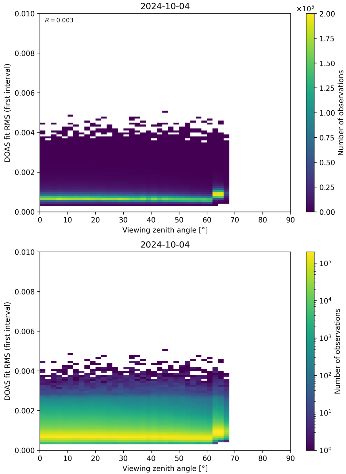
Figure 182: Scatter density plot of “Viewing zenith angle” against “DOAS fit RMS (first interval)” for 2024-10-03 to 2024-10-05.
