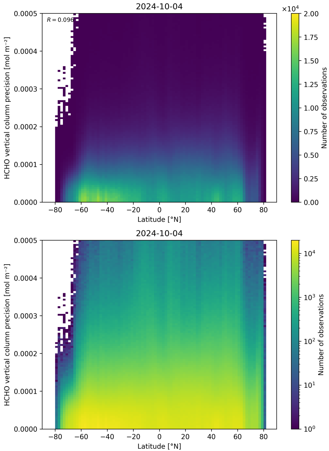
Figure 165: Scatter density plot of “Latitude” against “HCHO vertical column precision” for 2024-10-03 to 2024-10-05.
