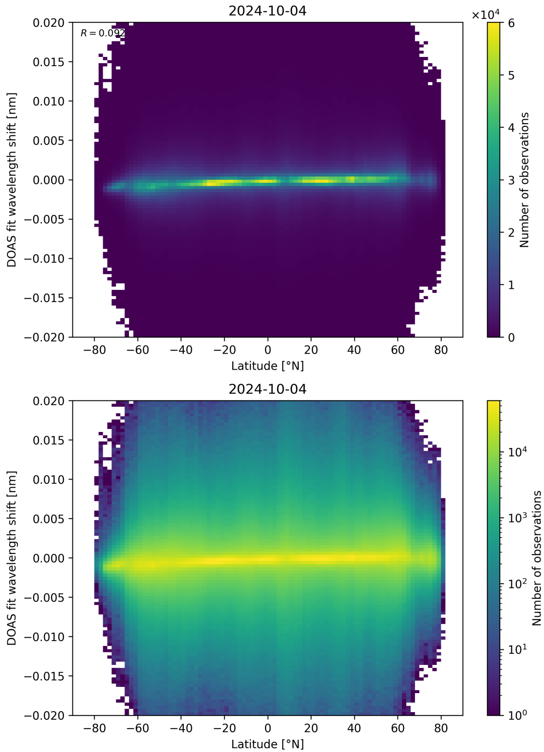
Figure 154: Scatter density plot of “Latitude” against “DOAS fit wavelength shift” for 2024-10-03 to 2024-10-05.
