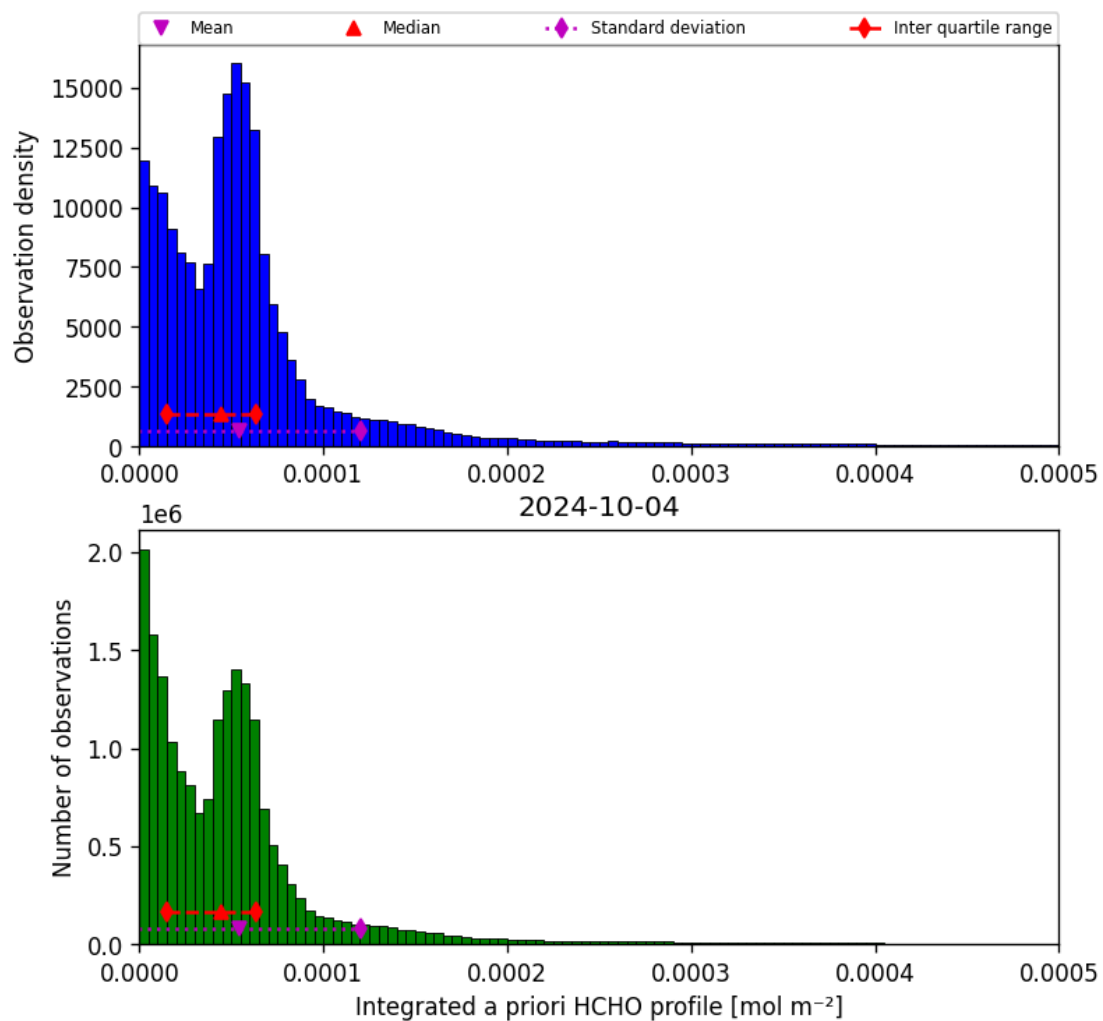
Figure 43: Histogram of “Integrated a priori HCHO profile” for 2024-10-03 to 2024-10-05
