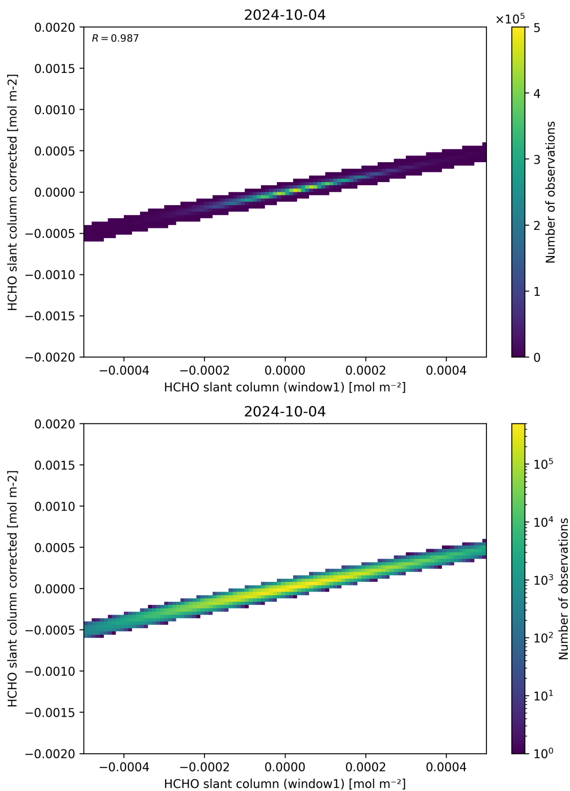
Figure 82: Scatter density plot of “HCHO slant column (window1)” against “HCHO slant column corrected” for 2024-10-03 to 2024-10-05.
