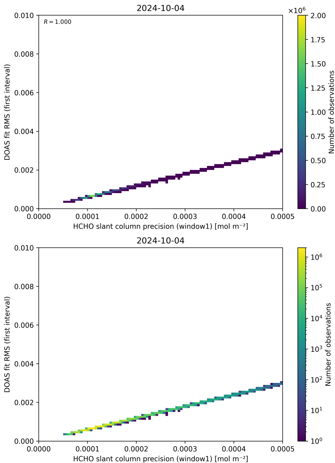
Figure 88: Scatter density plot of “HCHO slant column precision (window1)” against “DOAS fit RMS (first interval)” for 2024-10-03 to 2024-10-05.
