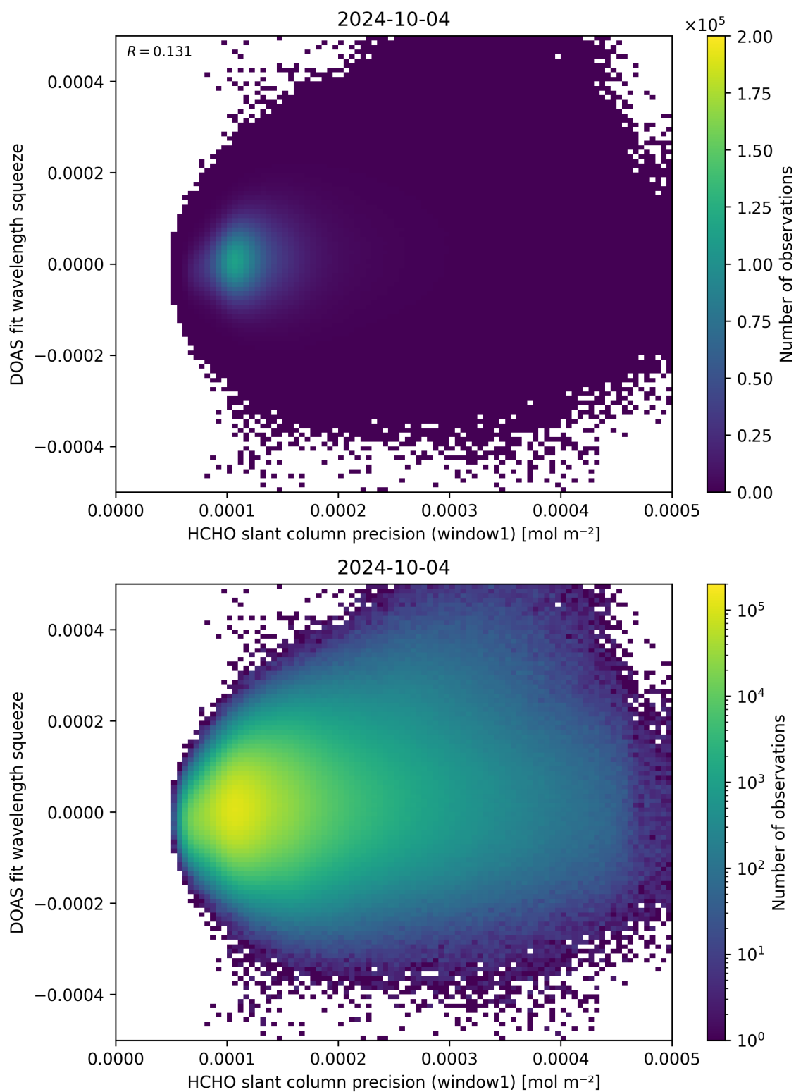
Figure 90: Scatter density plot of “HCHO slant column precision (window1)” against “DOAS fit wavelength squeeze” for 2024-10-03 to 2024-10-05.
