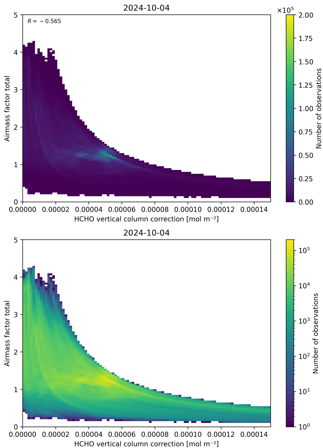
Figure 120: Scatter density plot of “HCHO vertical column correction” against “Airmass factor total” for 2024-10-03 to 2024-10-05.
