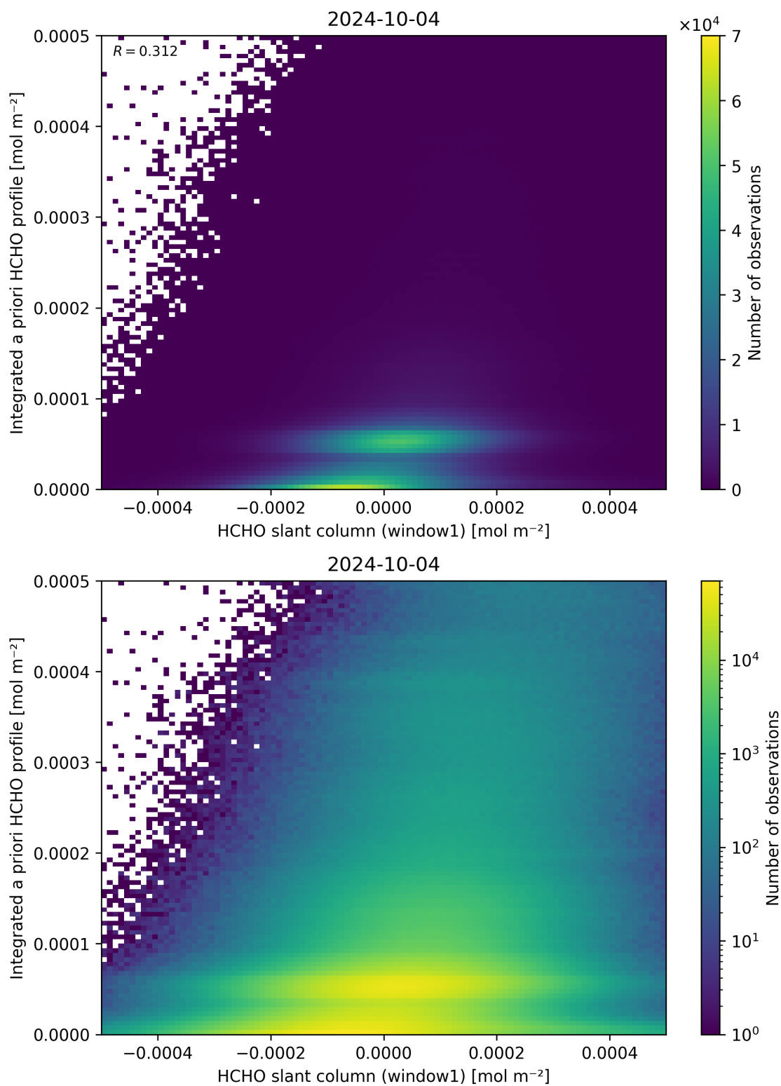
Figure 87: Scatter density plot of “HCHO slant column (window1)” against “Integrated a priori HCHO profile” for 2024-10-03 to 2024-10-05.
