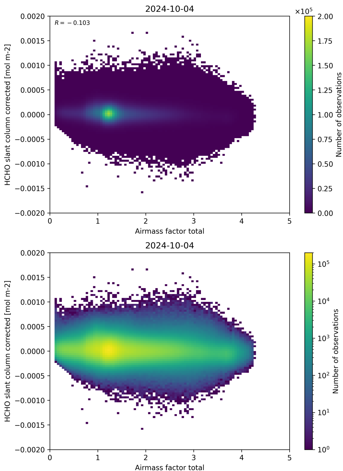
Figure 101: Scatter density plot of “Airmass factor total” against “HCHO slant column corrected” for 2024-10-03 to 2024-10-05.
