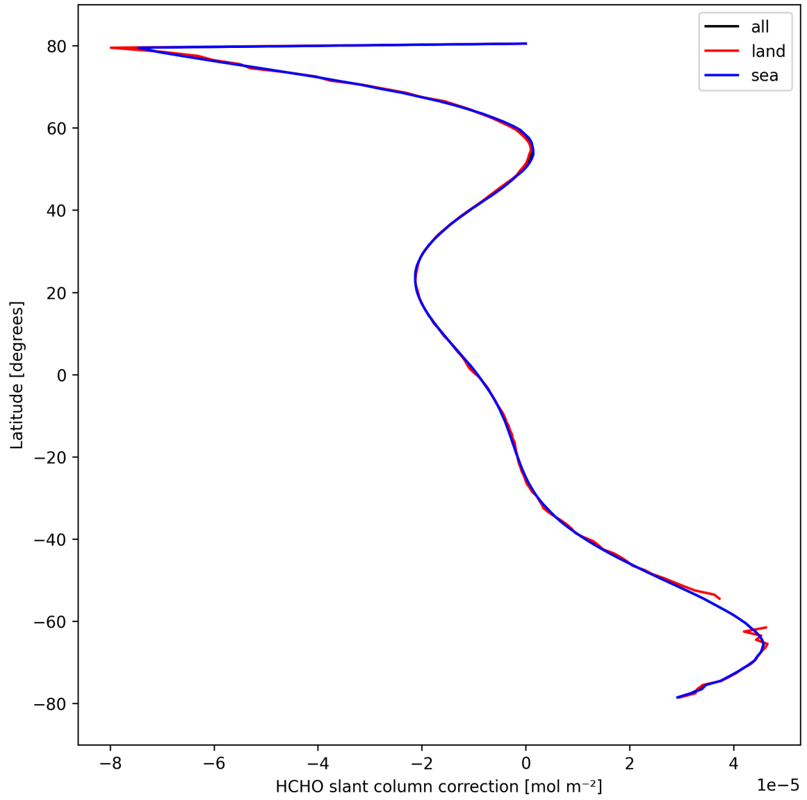
Figure 33: Zonal average of "HCHO slant column correction" for 2024-10-03 to 2024-10-05.
