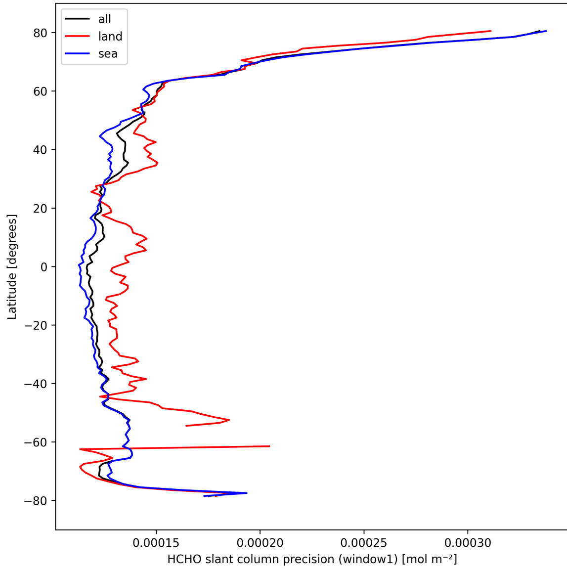
Figure 25: Zonal average of “HCHO slant column precision (window1)” for 2024-10-03 to 2024-10-05.
