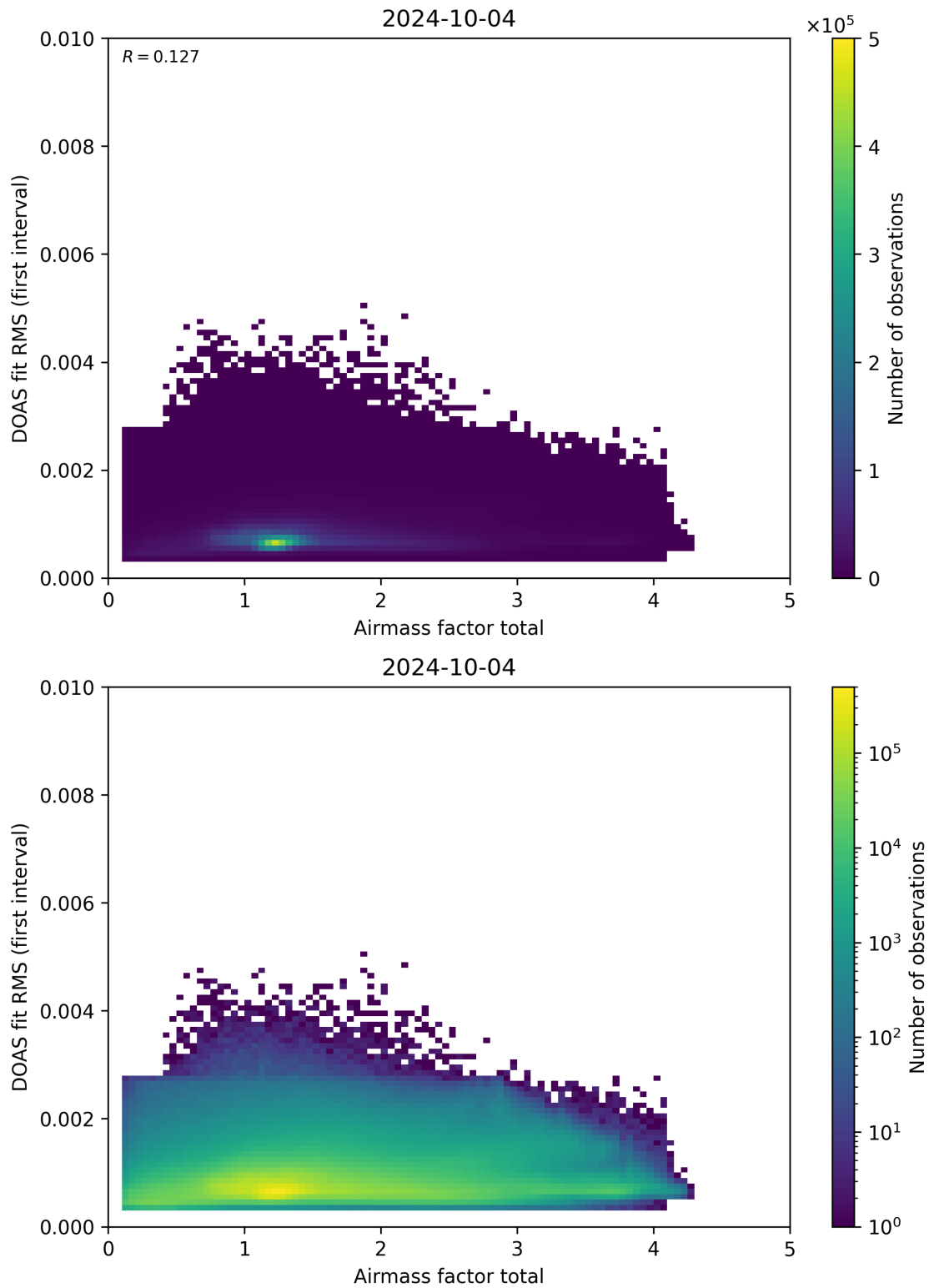
Figure 97: Scatter density plot of “Airmass factor total” against “DOAS fit RMS (first interval)” for 2024-10-03 to 2024-10-05.
