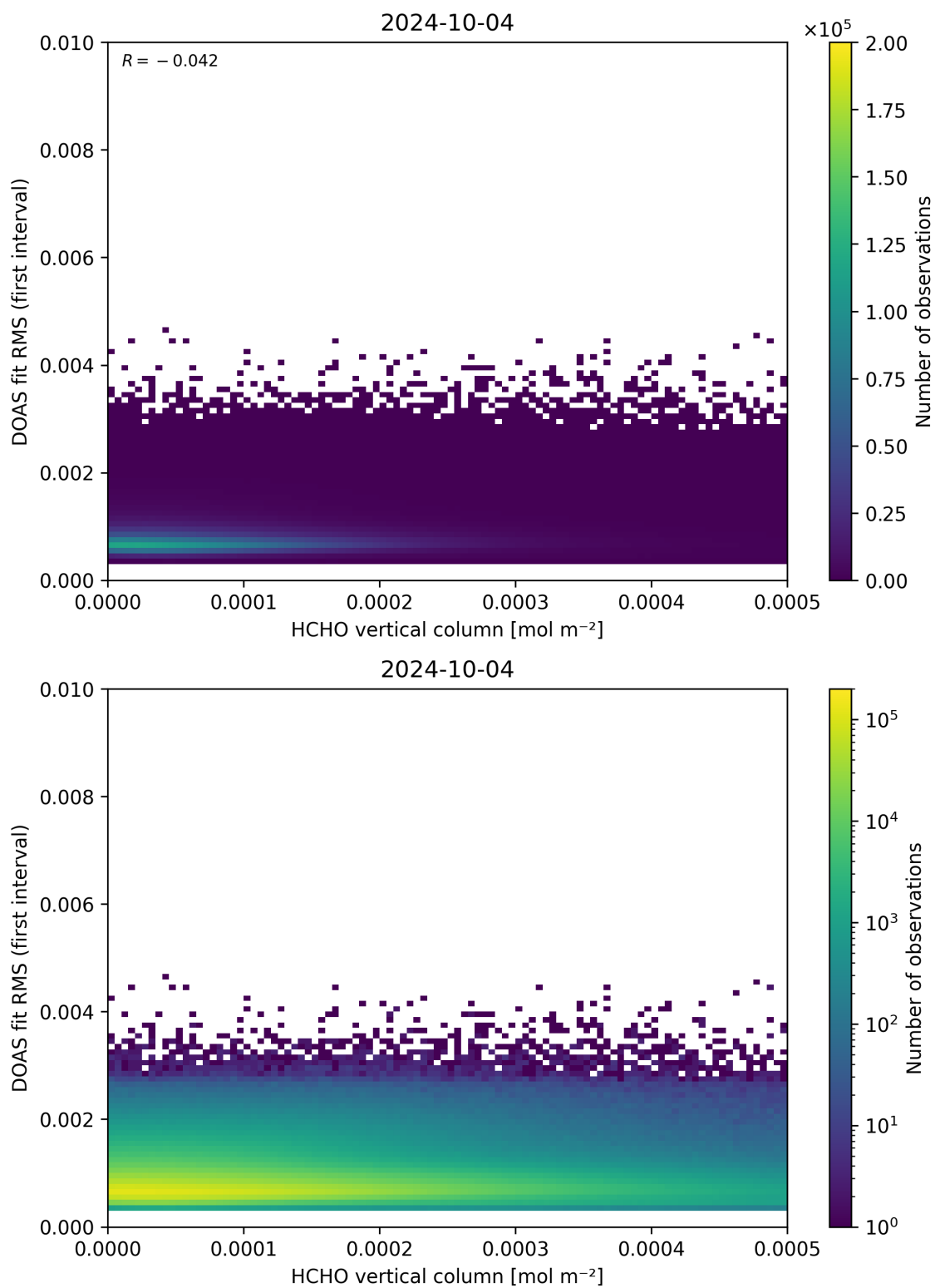
Figure 123: Scatter density plot of “HCHO vertical column” against “DOAS fit RMS (first interval)” for 2024-10-03 to 2024-10-05.
