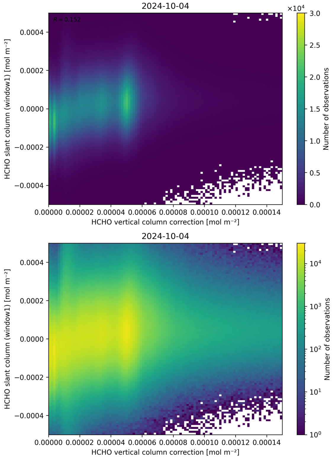
Figure 118: Scatter density plot of “HCHO vertical column correction” against “HCHO slant column (window1)” for 2024-10-03 to 2024-10-05.
