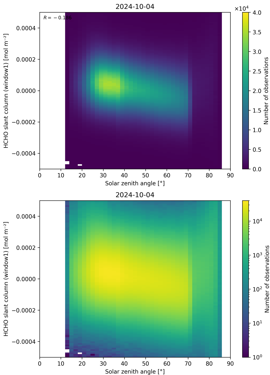
Figure 173: Scatter density plot of “Solar zenith angle” against “HCHO slant column (window1)” for 2024-10-03 to 2024-10-05.
