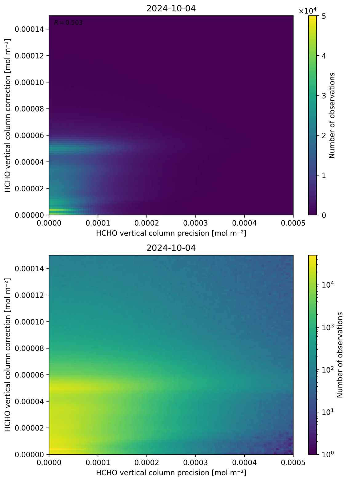
Figure 146: Scatter density plot of “HCHO vertical column precision” against “HCHO vertical column correction” for 2024-10-03 to 2024-10-05.
