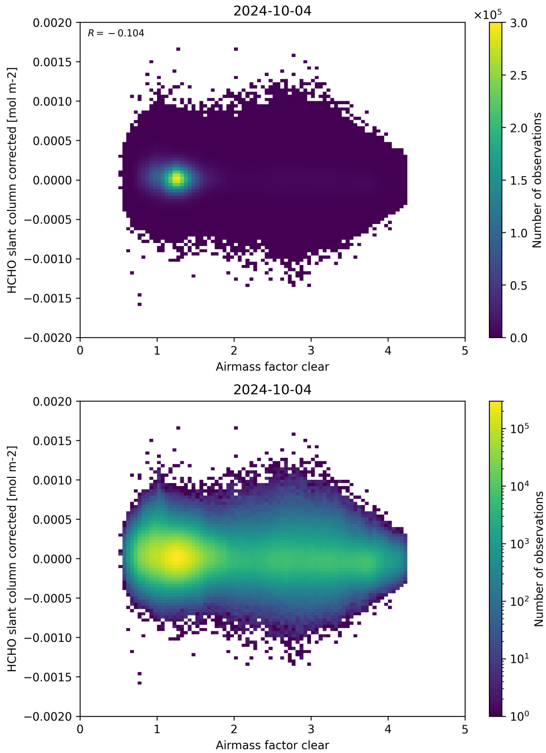
Figure 74: Scatter density plot of “Airmass factor clear” against “HCHO slant column corrected” for 2024-10-03 to 2024-10-05.
