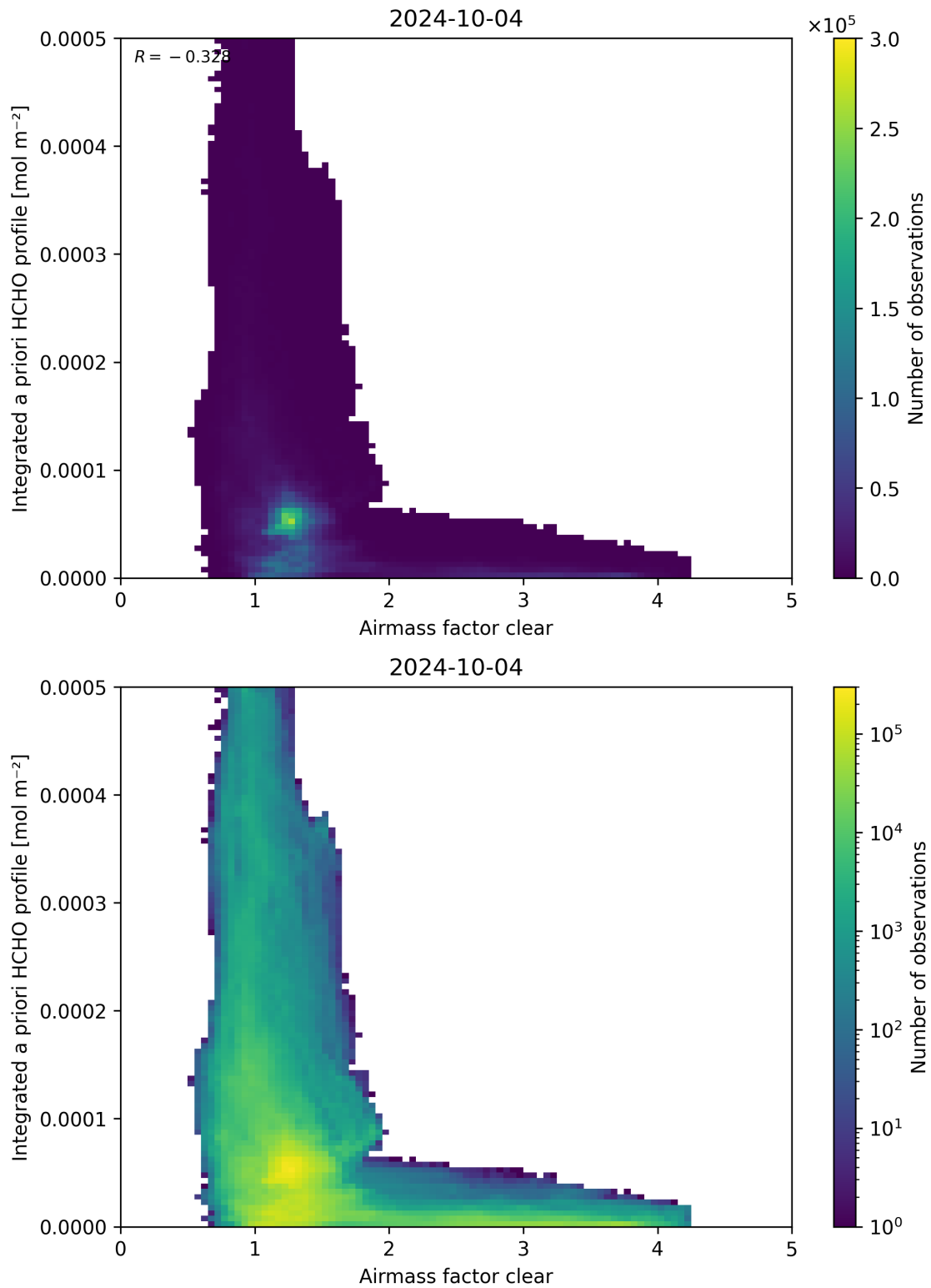
Figure 76: Scatter density plot of “Airmass factor clear” against “Integrated a priori HCHO profile” for 2024-10-03 to 2024-10-05.
