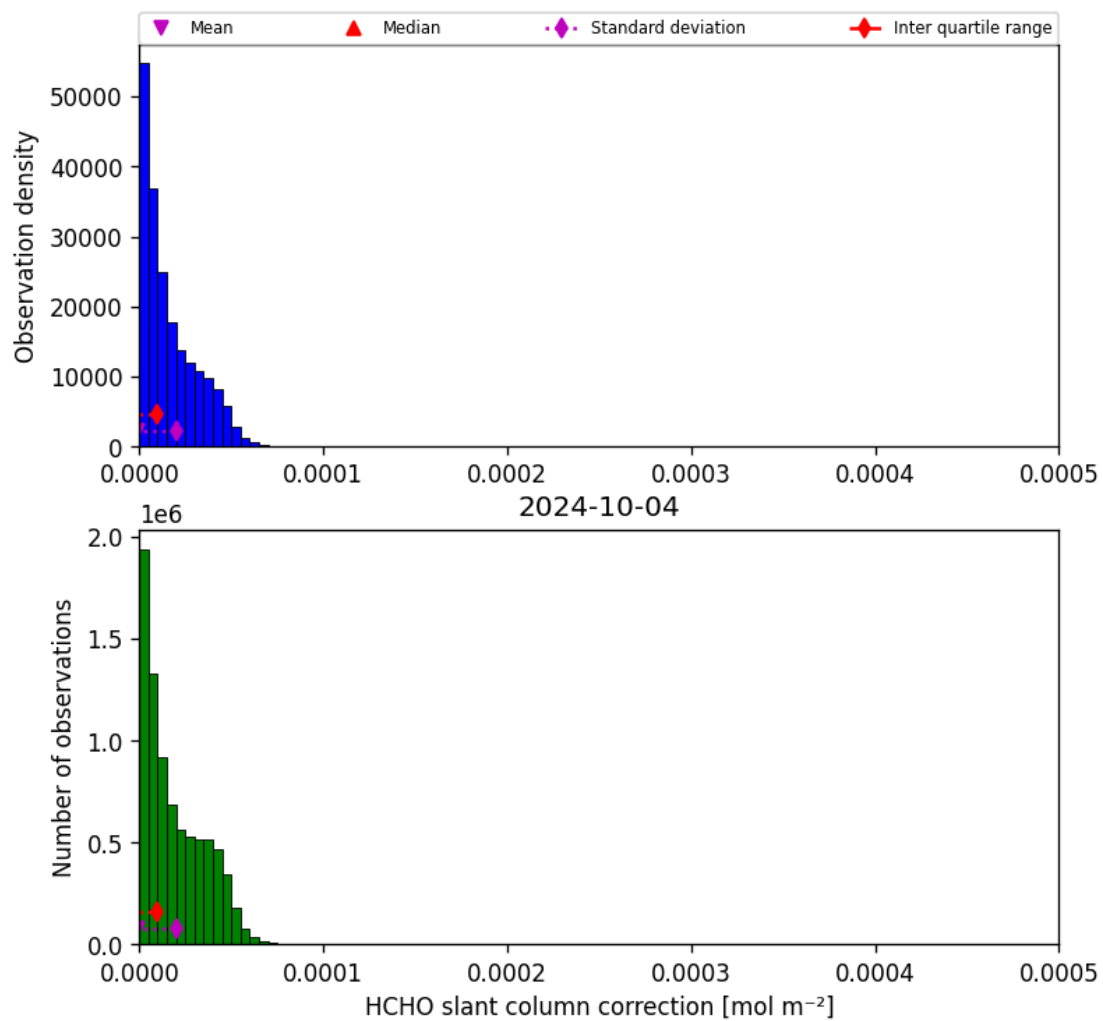
Figure 47: Histogram of “HCHO slant column correction” for 2024-10-03 to 2024-10-05
