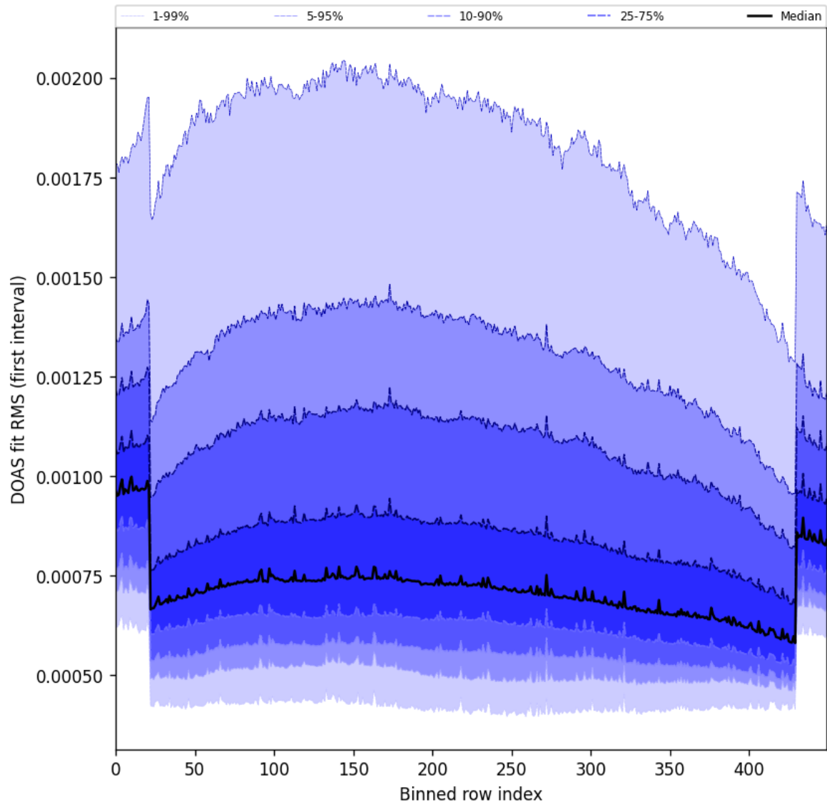
Figure 60: Along track statistics of “DOAS fit RMS (first interval)” for 2024-10-03 to 2024-10-05
