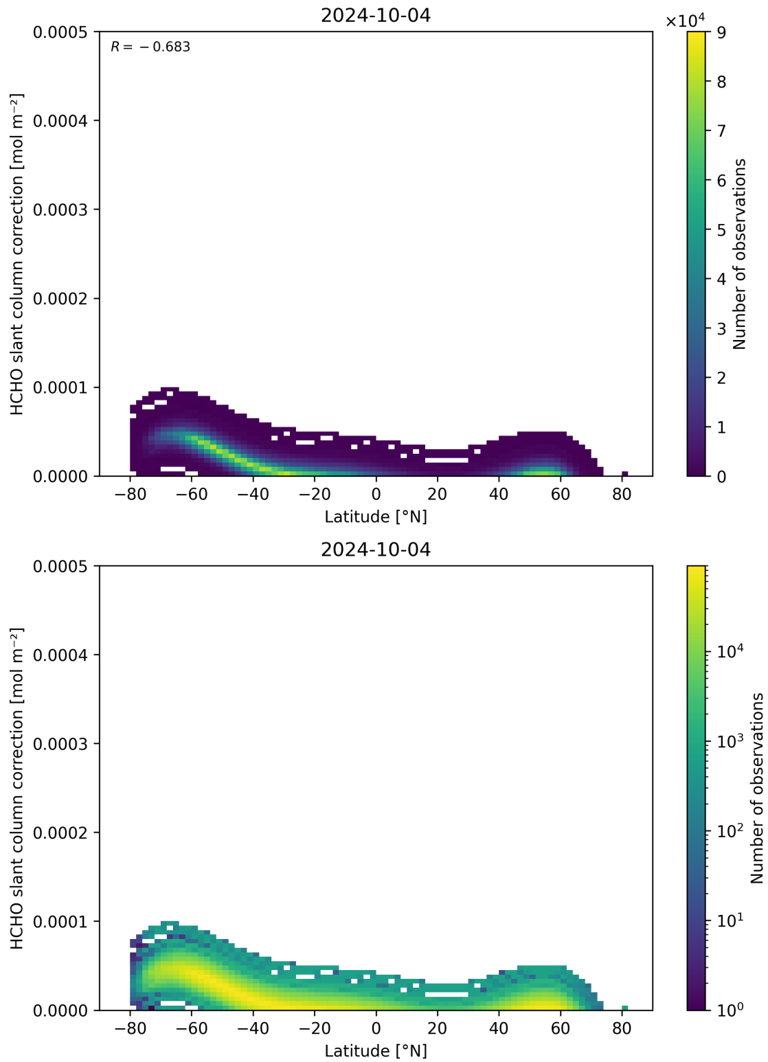
Figure 158: Scatter density plot of “Latitude” against “HCHO slant column correction” for 2024-10-03 to 2024-10-05.
