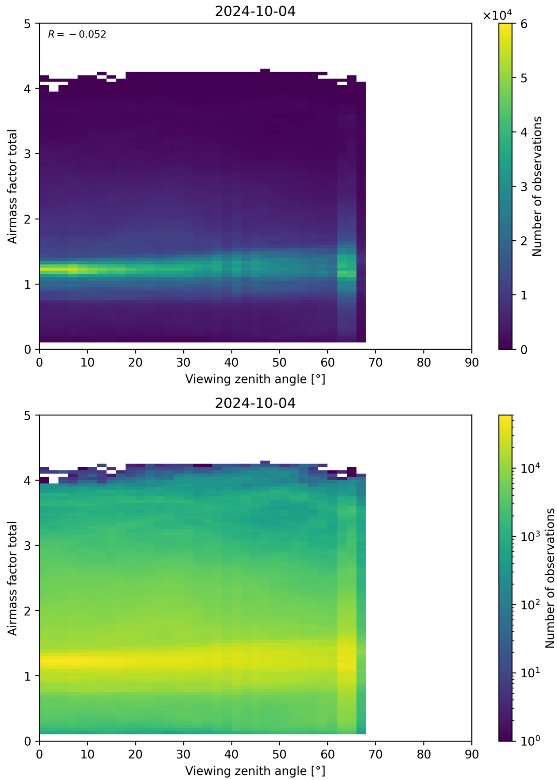
Figure 190: Scatter density plot of “Viewing zenith angle” against “Airmass factor total” for 2024-10-03 to 2024-10-05.
