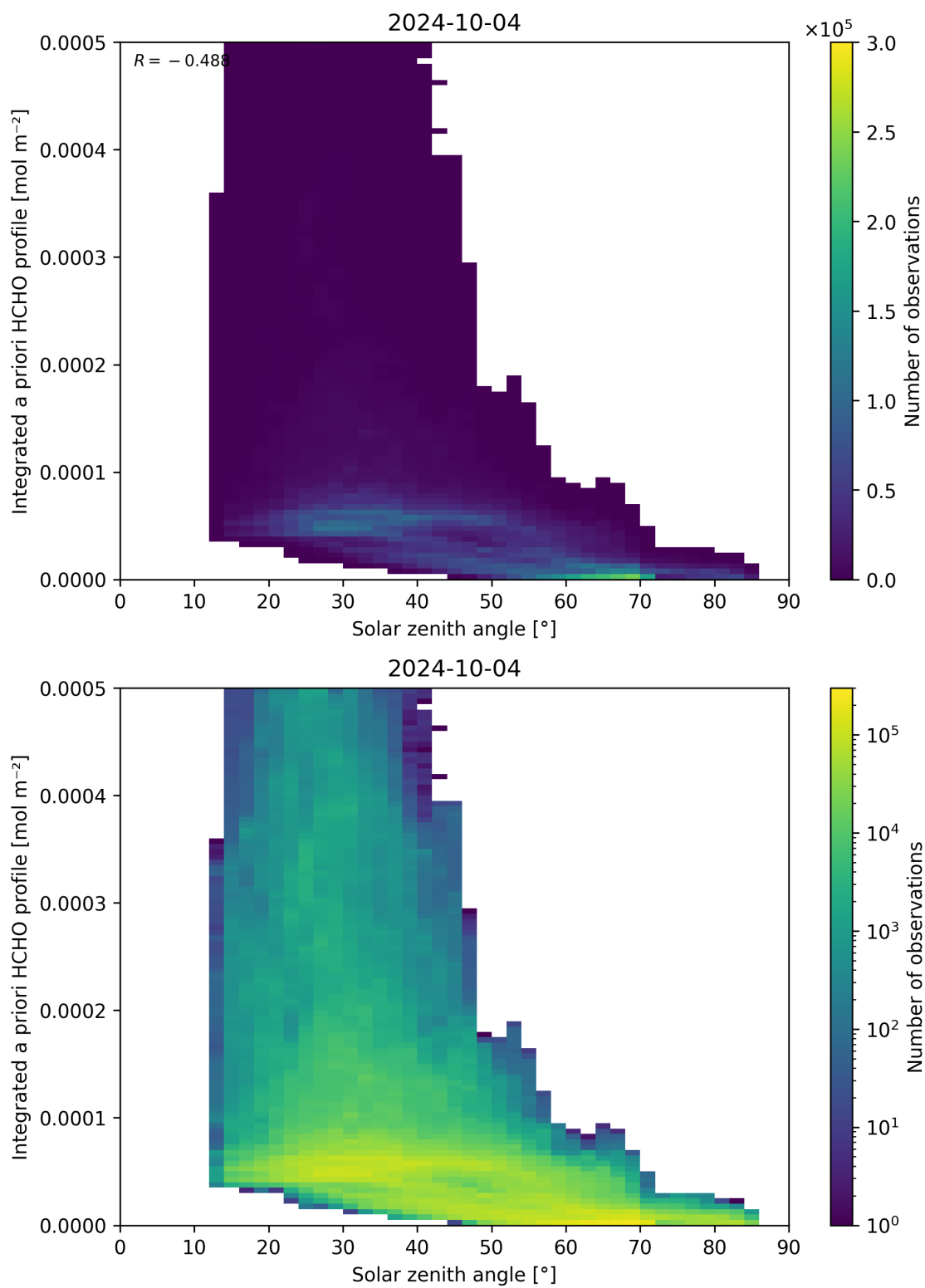
Figure 180: Scatter density plot of “Solar zenith angle” against “Integrated a priori HCHO profile” for 2024-10-03 to 2024-10-05.
