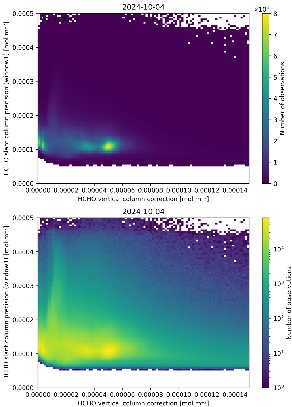
Figure 119: Scatter density plot of “HCHO vertical column correction” against “HCHO slant column precision (window1)” for 2024-10-03 to 2024-10-05.
