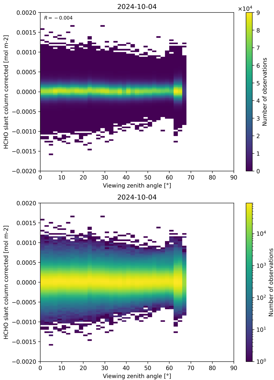
Figure 186: Scatter density plot of “Viewing zenith angle” against “HCHO slant column corrected” for 2024-10-03 to 2024-10-05.
