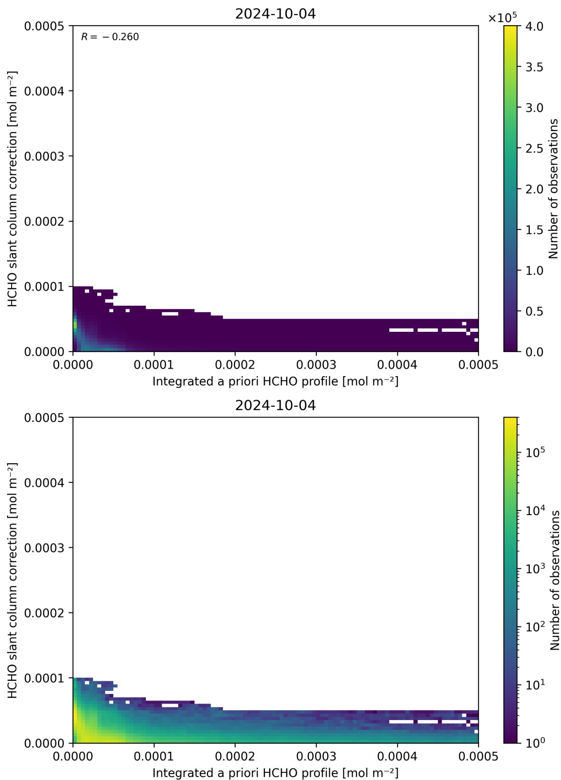
Figure 152: Scatter density plot of “Integrated a priori HCHO profile” against “HCHO slant column correction” for 2024-10-03 to 2024-10-05.
