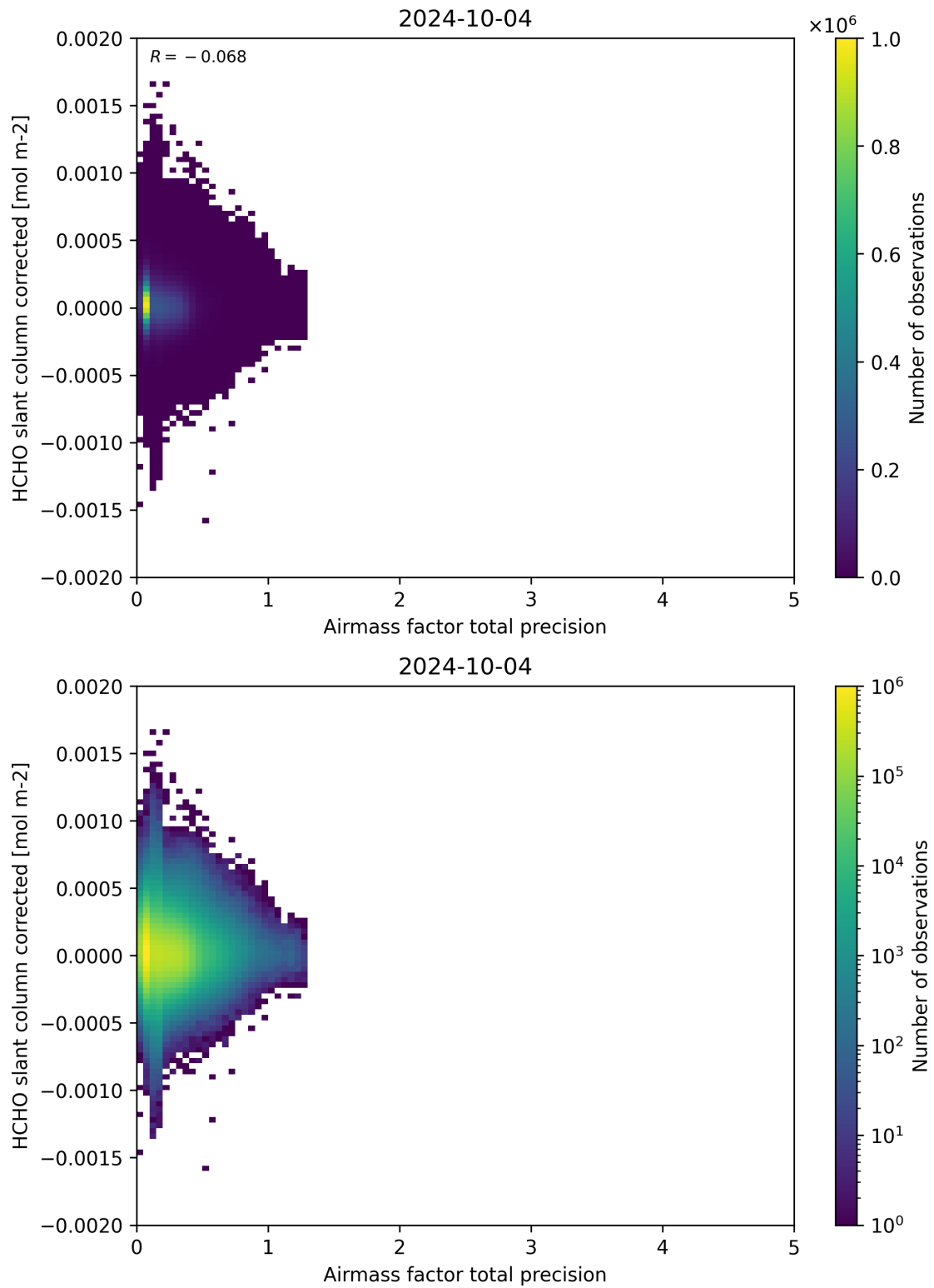
Figure 109: Scatter density plot of “Airmass factor total precision” against “HCHO slant column corrected” for 2024-10-03 to 2024-10-05.
