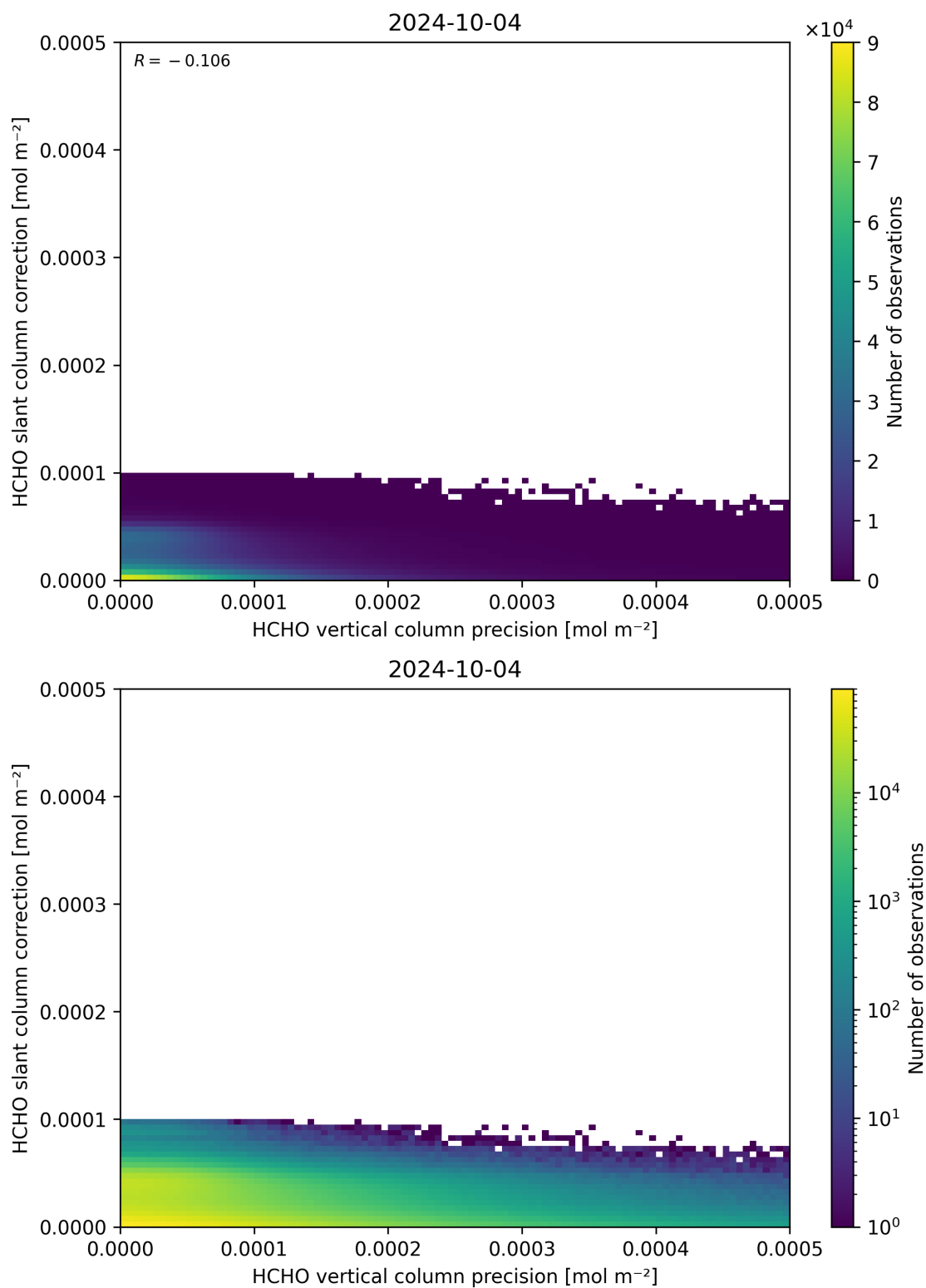
Figure 141: Scatter density plot of “HCHO vertical column precision” against “HCHO slant column correction” for 2024-10-03 to 2024-10-05.
