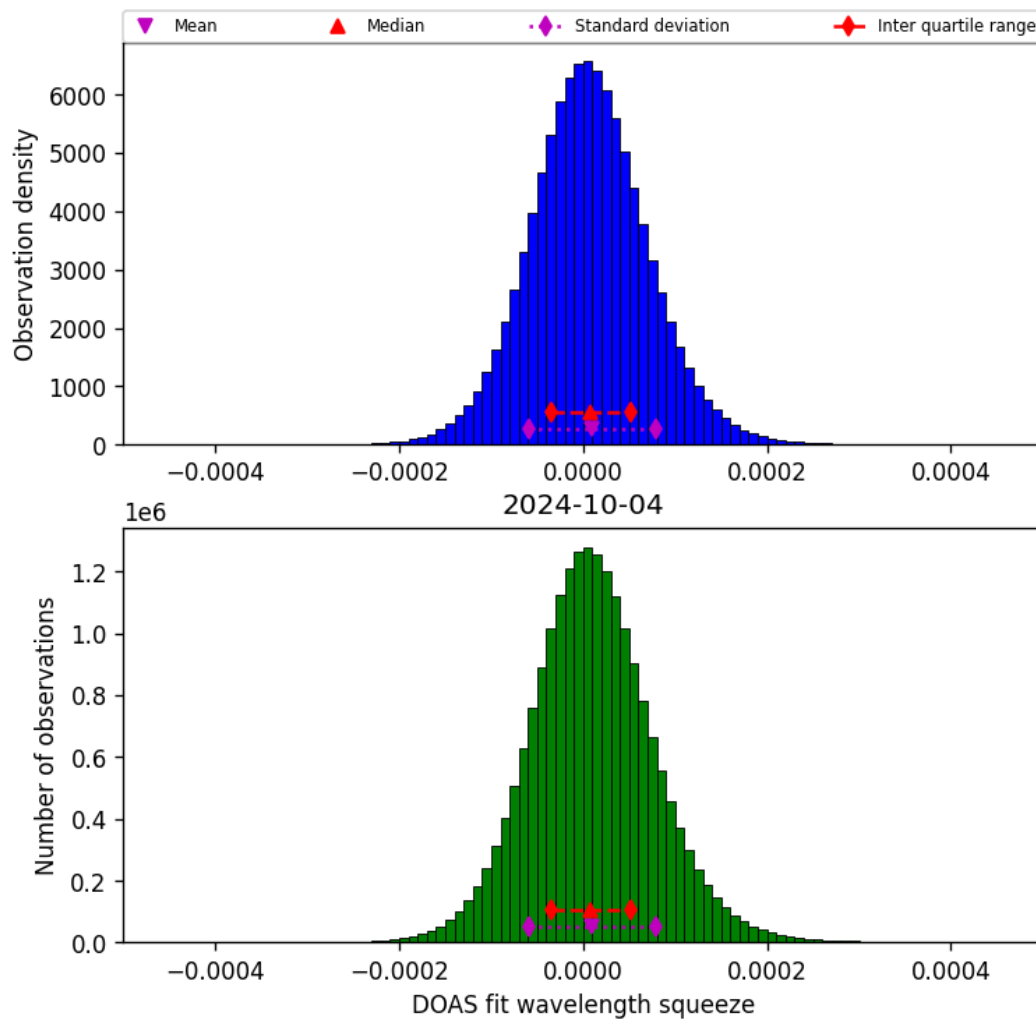
Figure 45: Histogram of “DOAS fit wavelength squeeze” for 2024-10-03 to 2024-10-05
