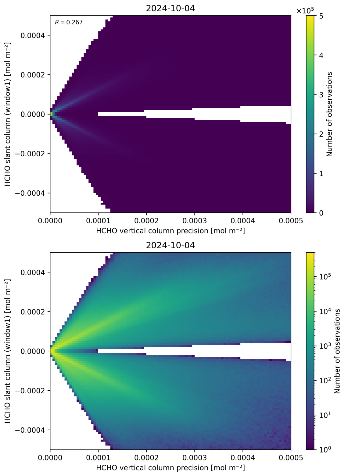
Figure 142: Scatter density plot of “HCHO vertical column precision” against “HCHO slant column (window1)” for 2024-10-03 to 2024-10-05.
