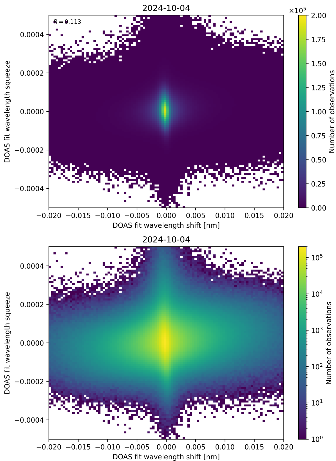
Figure 65: Scatter density plot of “DOAS fit wavelength shift” against “DOAS fit wavelength squeeze” for 2024-10-03 to 2024-10-05.
