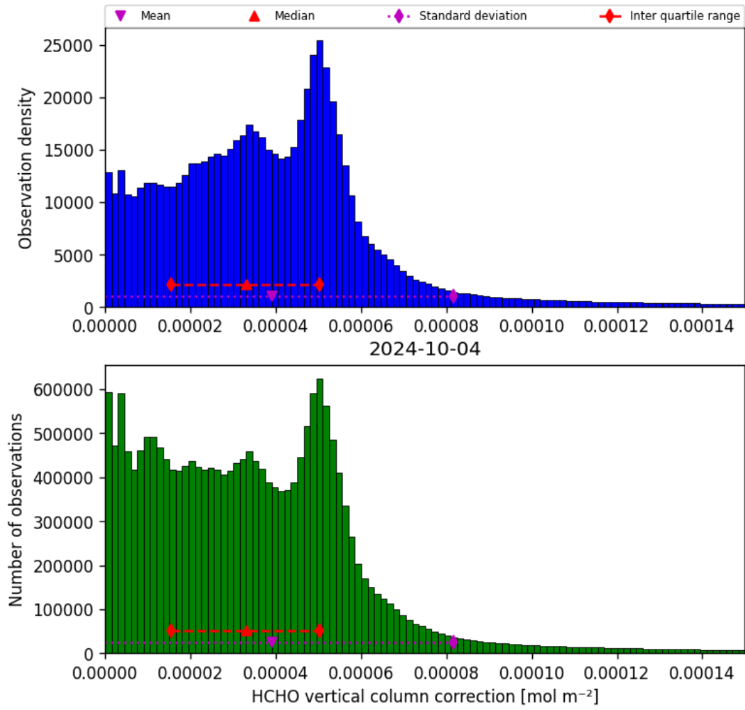
Figure 37: Histogram of “HCHO vertical column correction” for 2024-10-03 to 2024-10-05
