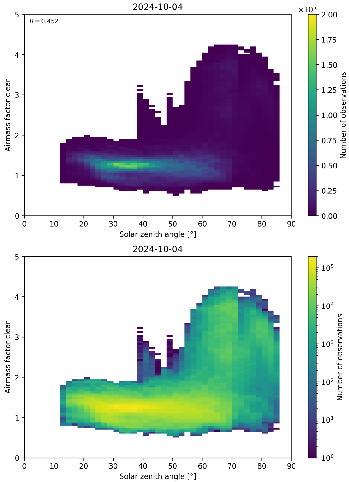
Figure 170: Scatter density plot of “Solar zenith angle” against “Airmass factor clear” for 2024-10-03 to 2024-10-05.
