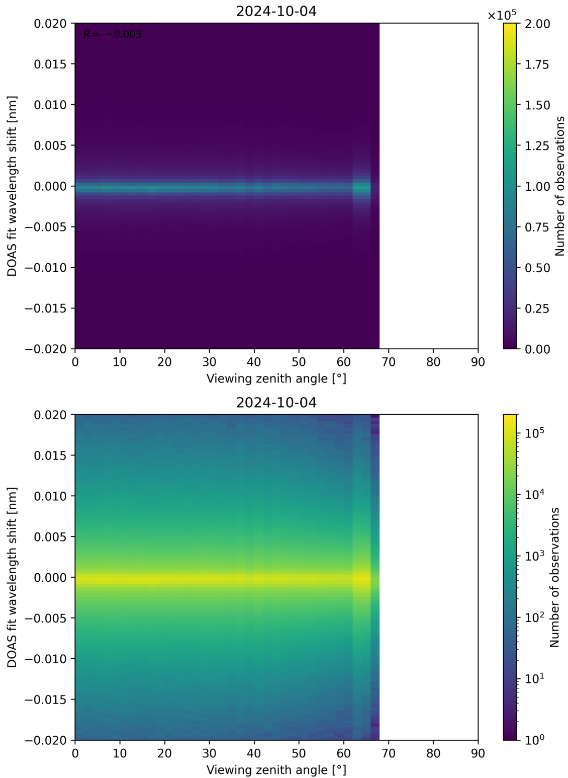
Figure 183: Scatter density plot of “Viewing zenith angle” against “DOAS fit wavelength shift” for 2024-10-03 to 2024-10-05.
