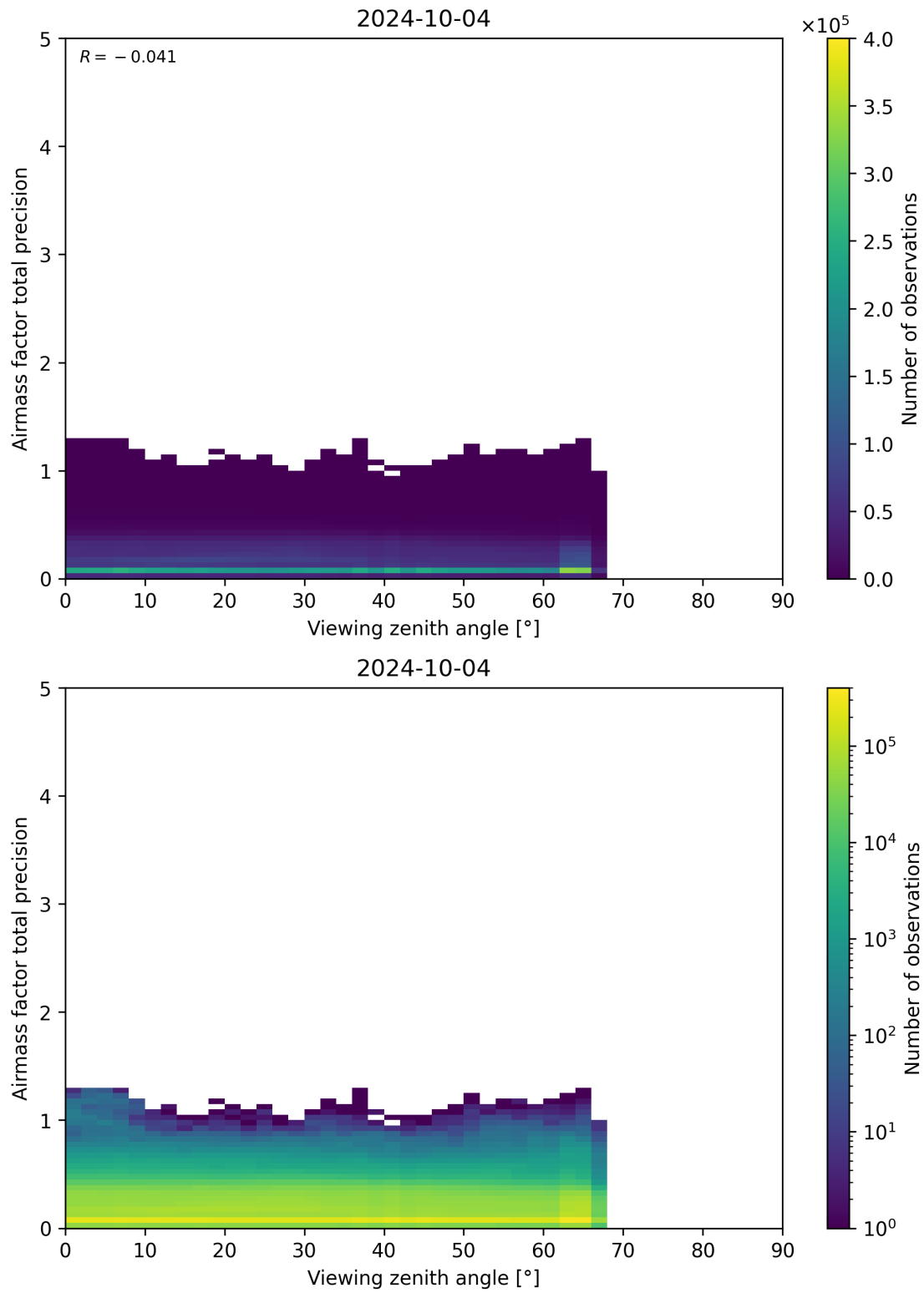
Figure 191: Scatter density plot of “Viewing zenith angle” against “Airmass factor total precision” for 2024-10-03 to 2024-10-05.
