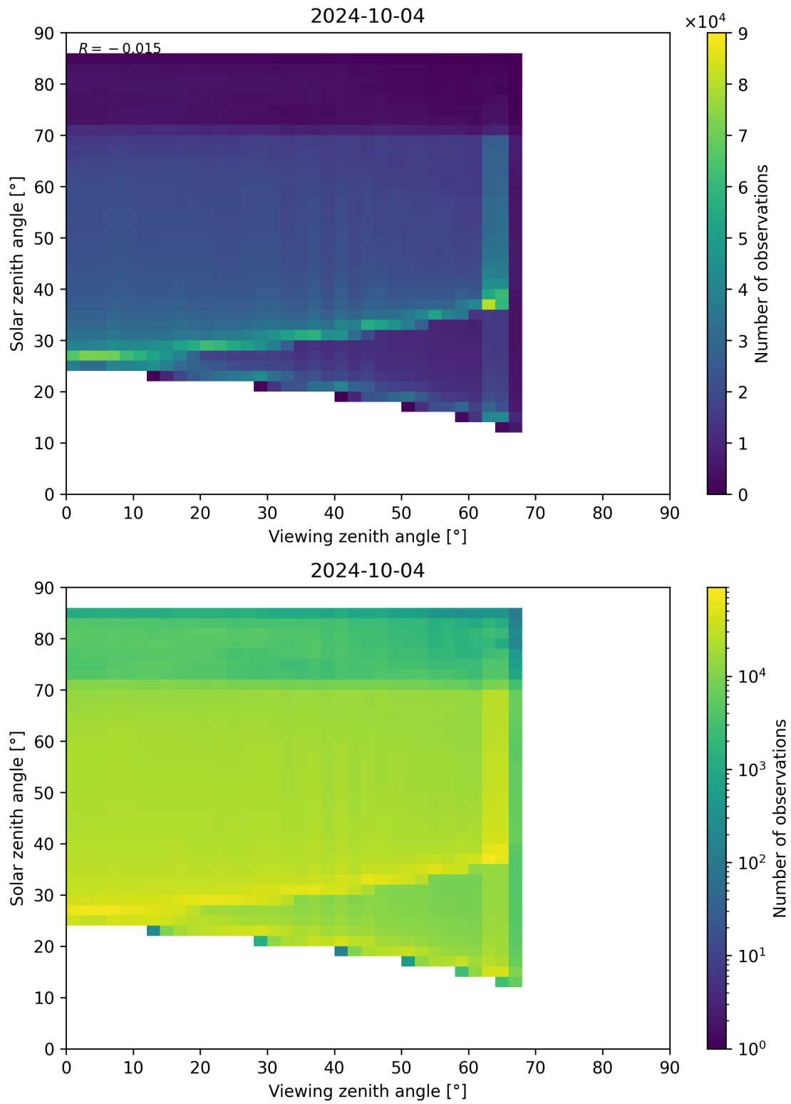
Figure 197: Scatter density plot of “Viewing zenith angle” against “Solar zenith angle” for 2024-10-03 to 2024-10-05.
