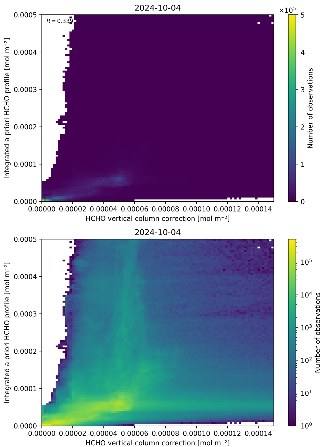
Figure 122: Scatter density plot of “HCHO vertical column correction” against “Integrated a priori HCHO profile” for 2024-10-03 to 2024-10-05.
