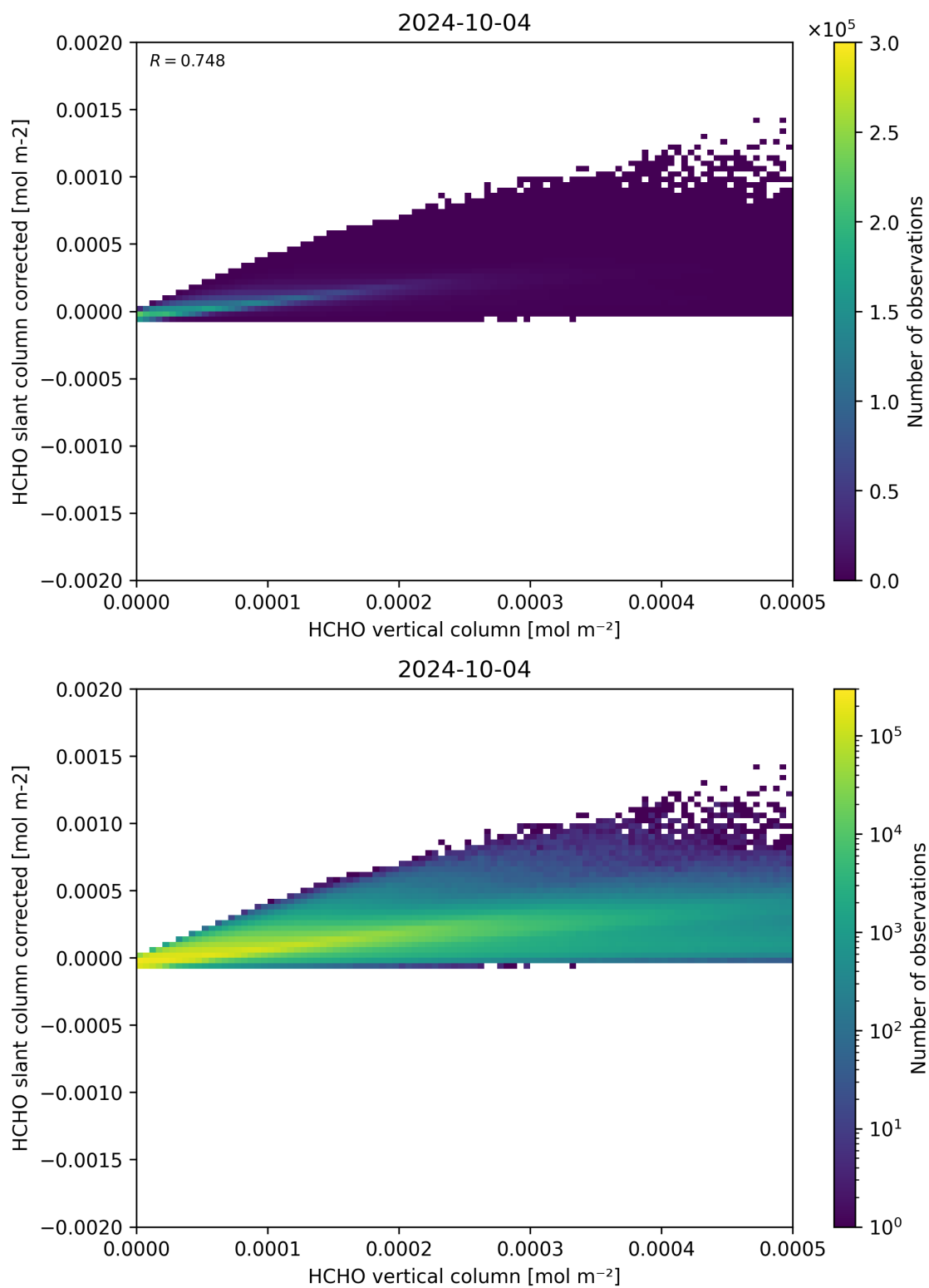
Figure 127: Scatter density plot of “HCHO vertical column” against “HCHO slant column corrected” for 2024-10-03 to 2024-10-05.
