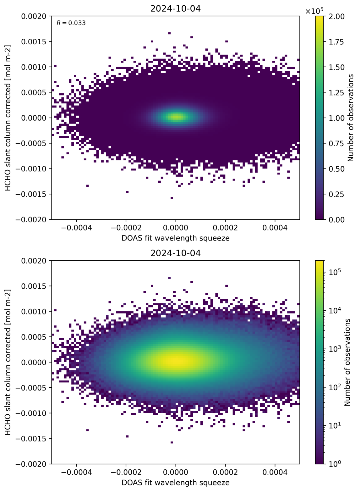
Figure 69: Scatter density plot of “DOAS fit wavelength squeeze” against “HCHO slant column corrected” for 2024-10-03 to 2024-10-05.
