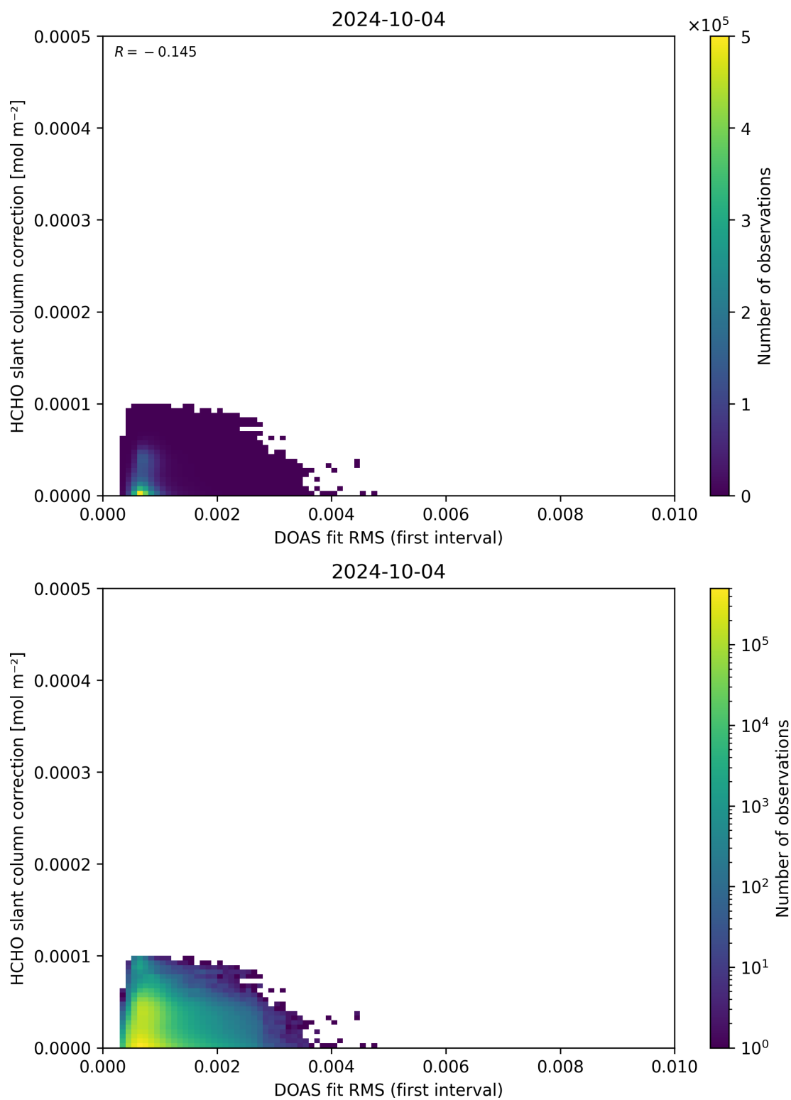
Figure 63: Scatter density plot of “DOAS fit RMS (first interval)” against “HCHO slant column correction” for 2024-10-03 to 2024-10-05.
