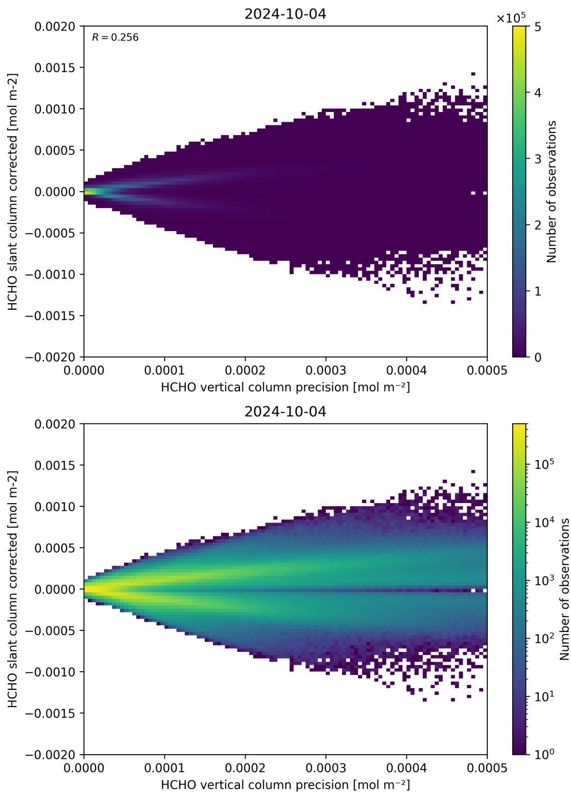
Figure 140: Scatter density plot of “HCHO vertical column precision” against “HCHO slant column corrected” for 2024-10-03 to 2024-10-05.
