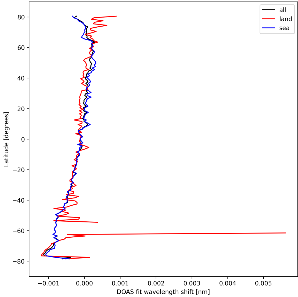
Figure 30: Zonal average of “DOAS fit wavelength shift” for 2024-10-03 to 2024-10-05.
