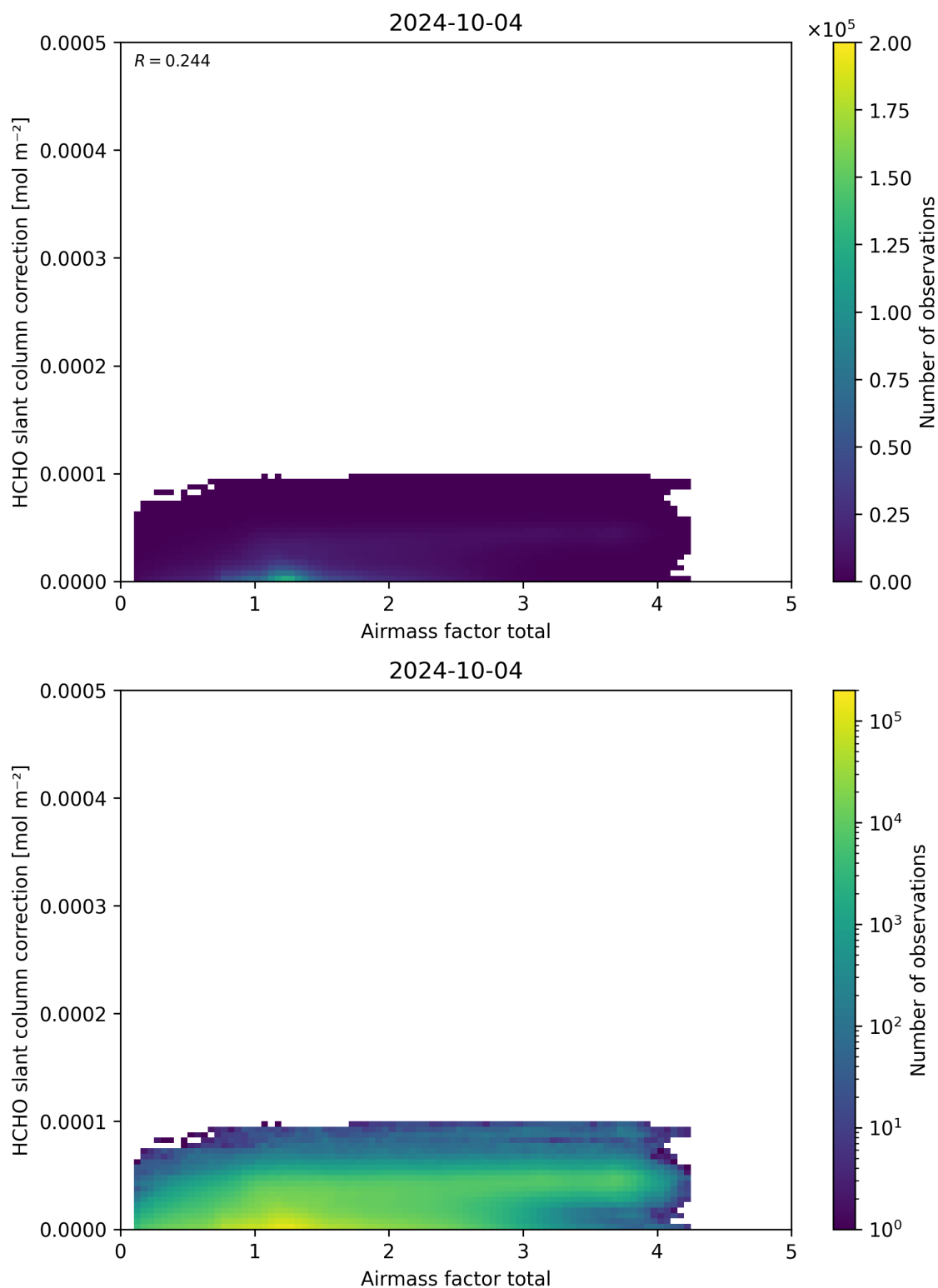
Figure 102: Scatter density plot of “Airmass factor total” against “HCHO slant column correction” for 2024-10-03 to 2024-10-05.
