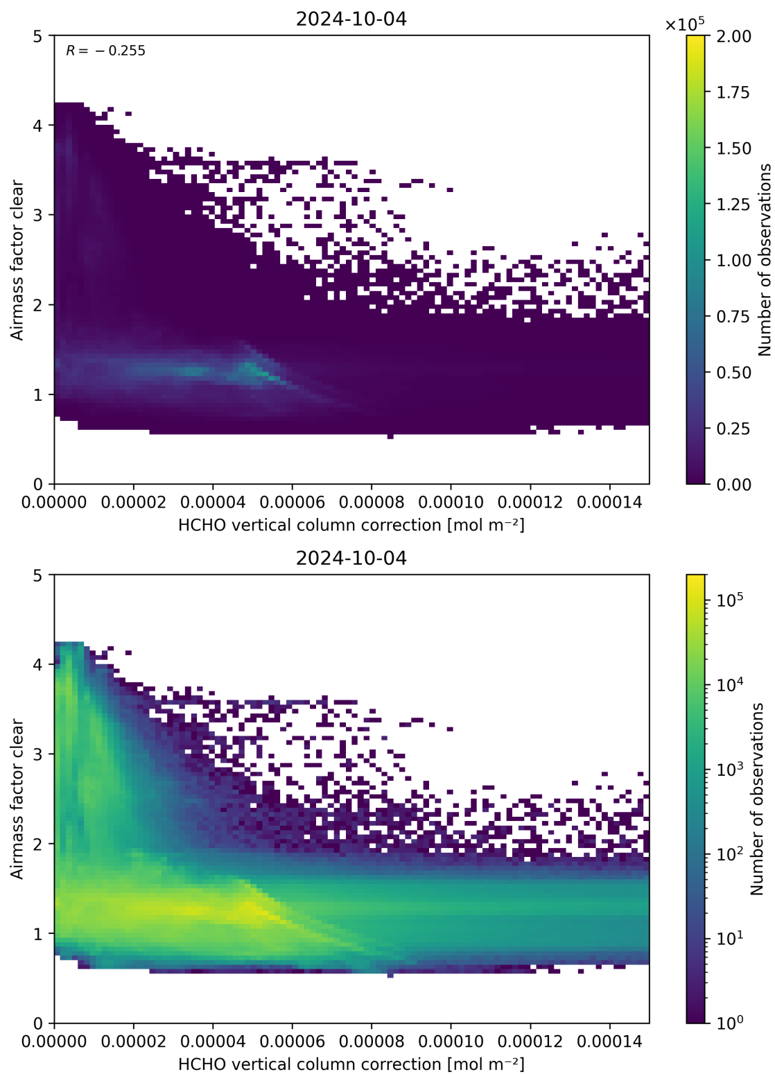
Figure 115: Scatter density plot of “HCHO vertical column correction” against “Airmass factor clear” for 2024-10-03 to 2024-10-05.
