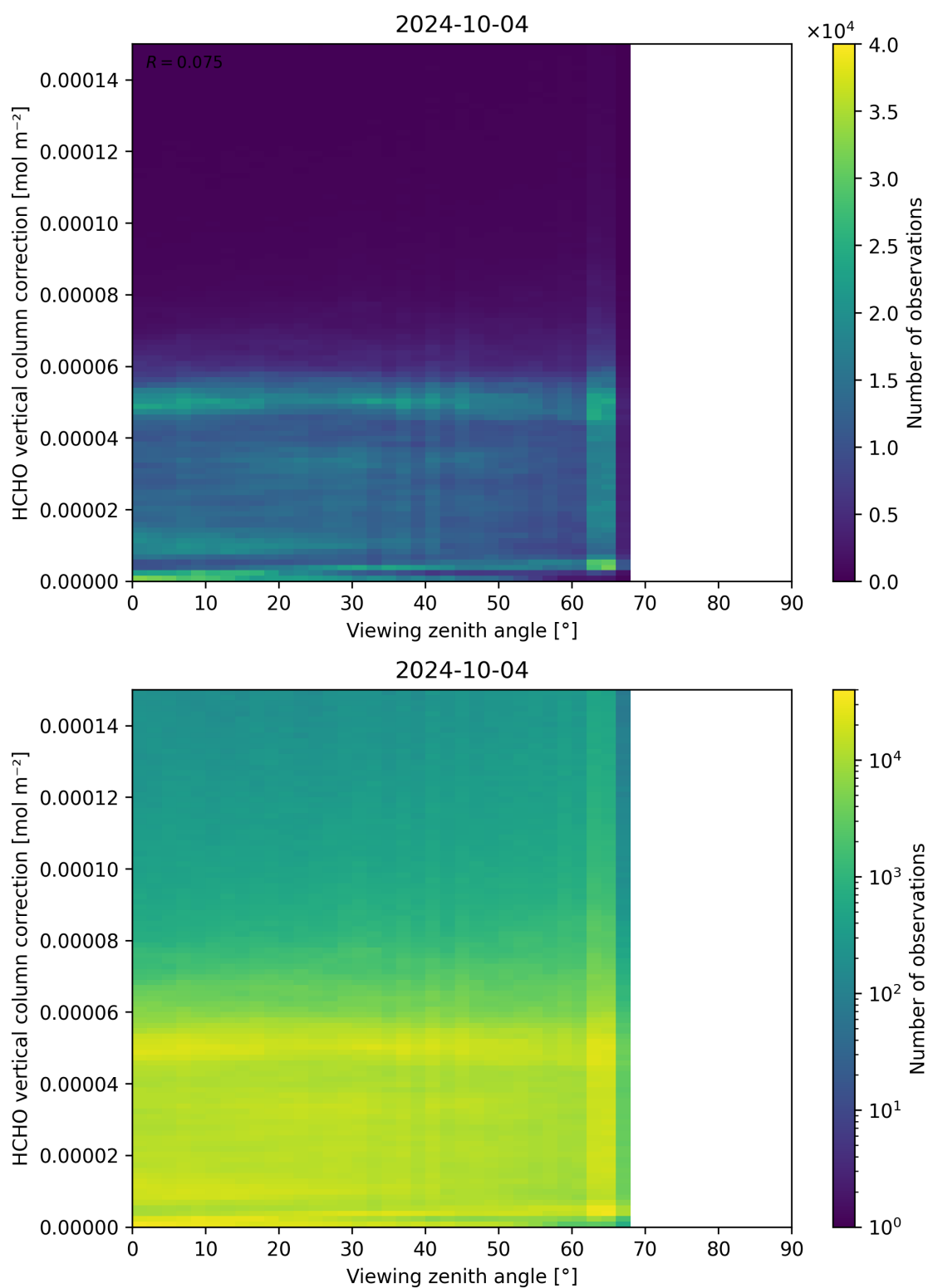
Figure 193: Scatter density plot of “Viewing zenith angle” against “HCHO vertical column correction” for 2024-10-03 to 2024-10-05.
