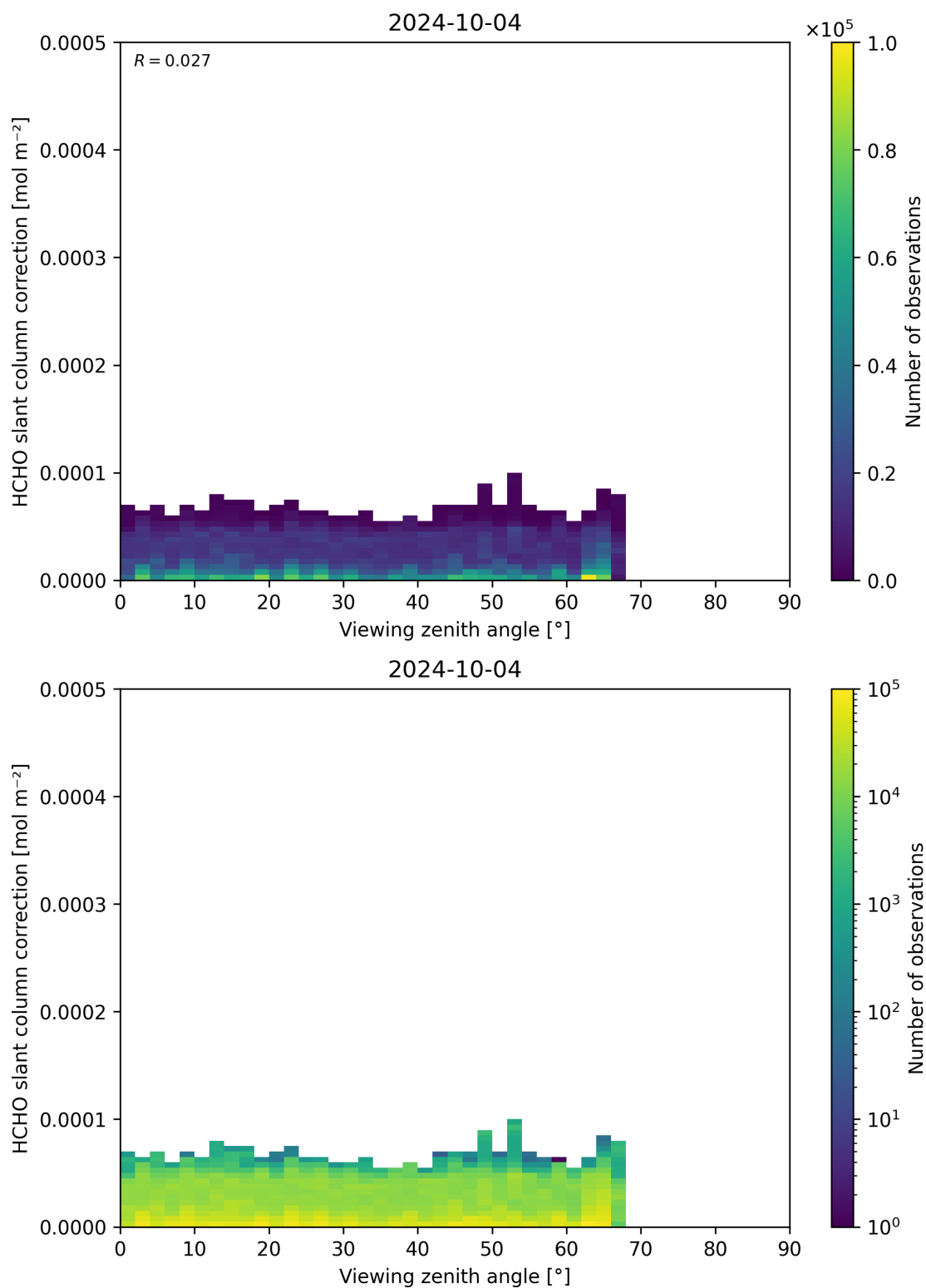
Figure 187: Scatter density plot of “Viewing zenith angle” against “HCHO slant column correction” for 2024-10-03 to 2024-10-05.
