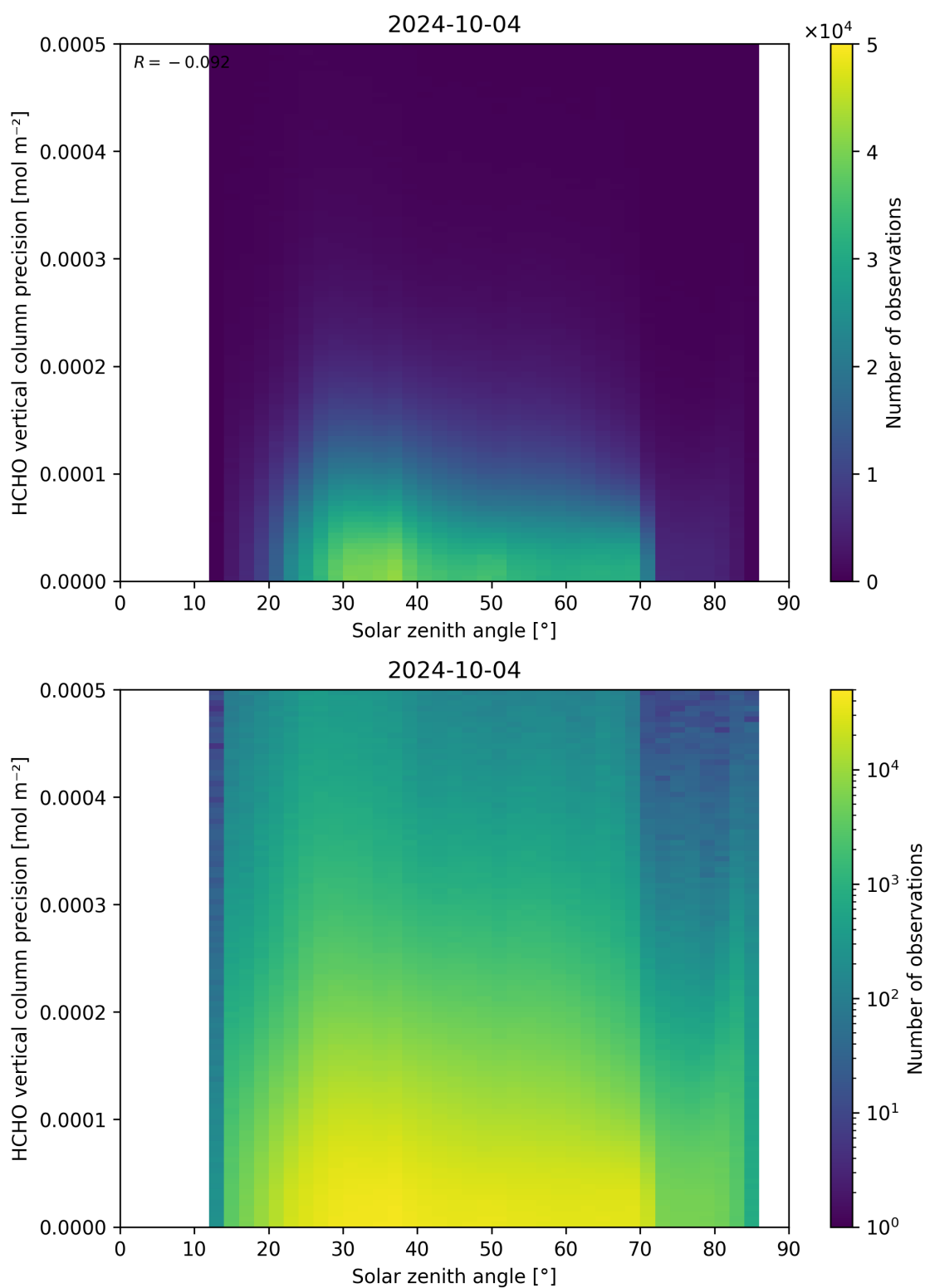
Figure 179: Scatter density plot of “Solar zenith angle” against “HCHO vertical column precision” for 2024-10-03 to 2024-10-05.
