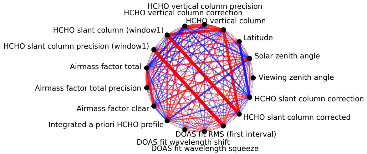
Figure 1: Map of correlation graph for 2024-10-03 to 2024-10-05.
