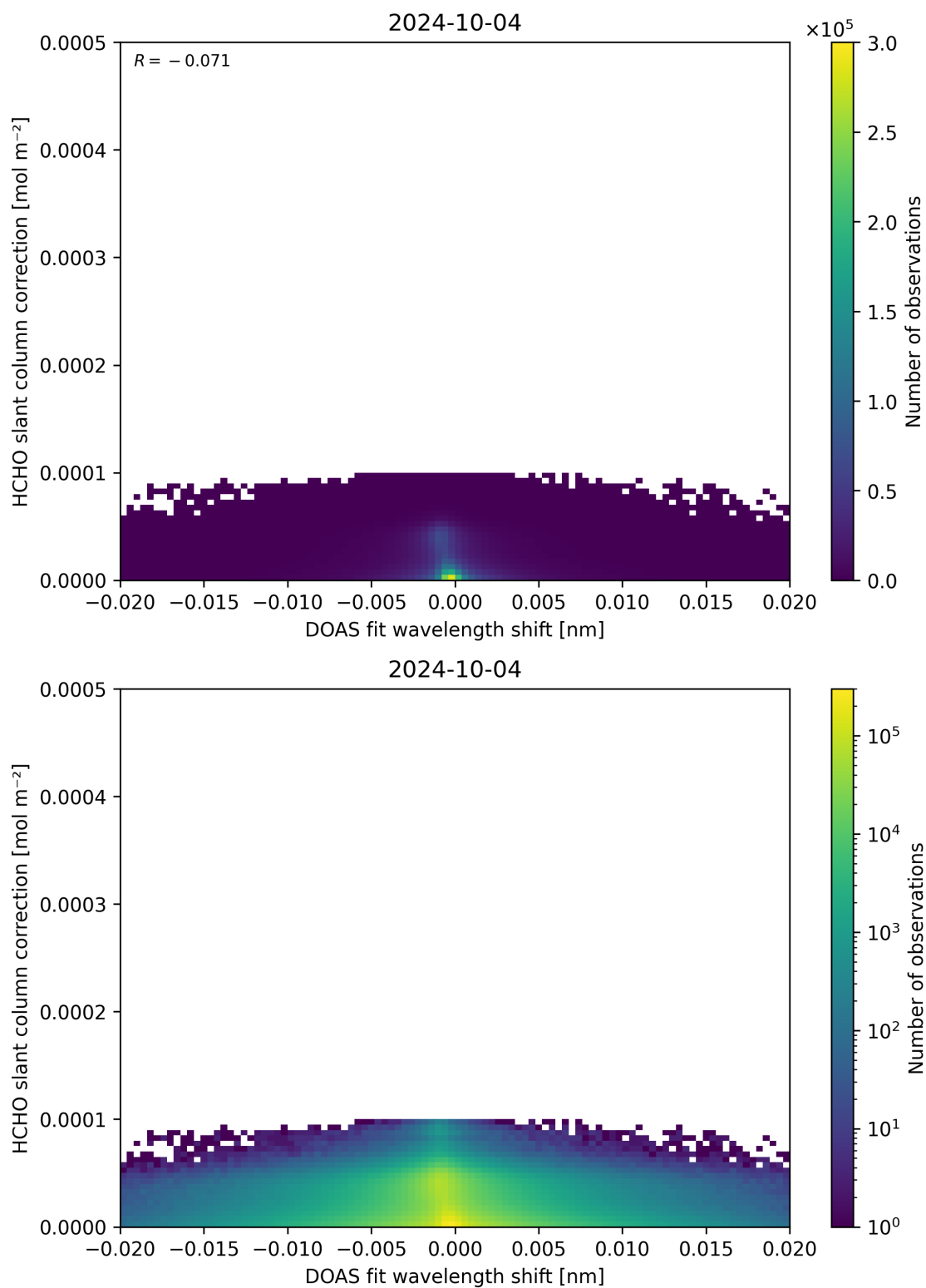
Figure 67: Scatter density plot of “DOAS fit wavelength shift” against “HCHO slant column correction” for 2024-10-03 to 2024-10-05.
