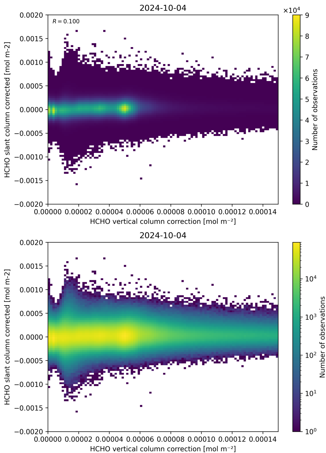
Figure 116: Scatter density plot of “HCHO vertical column correction” against “HCHO slant column corrected” for 2024-10-03 to 2024-10-05.
