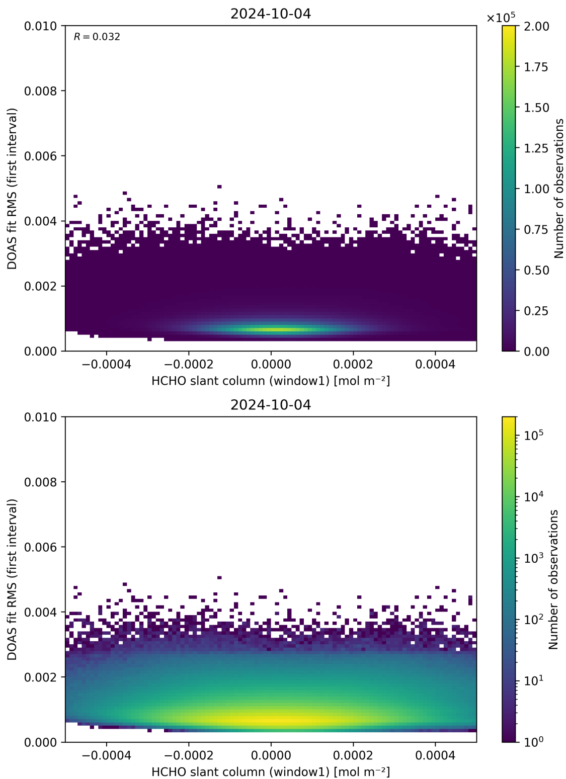
Figure 78: Scatter density plot of “HCHO slant column (window1)” against “DOAS fit RMS (first interval)” for 2024-10-03 to 2024-10-05.
