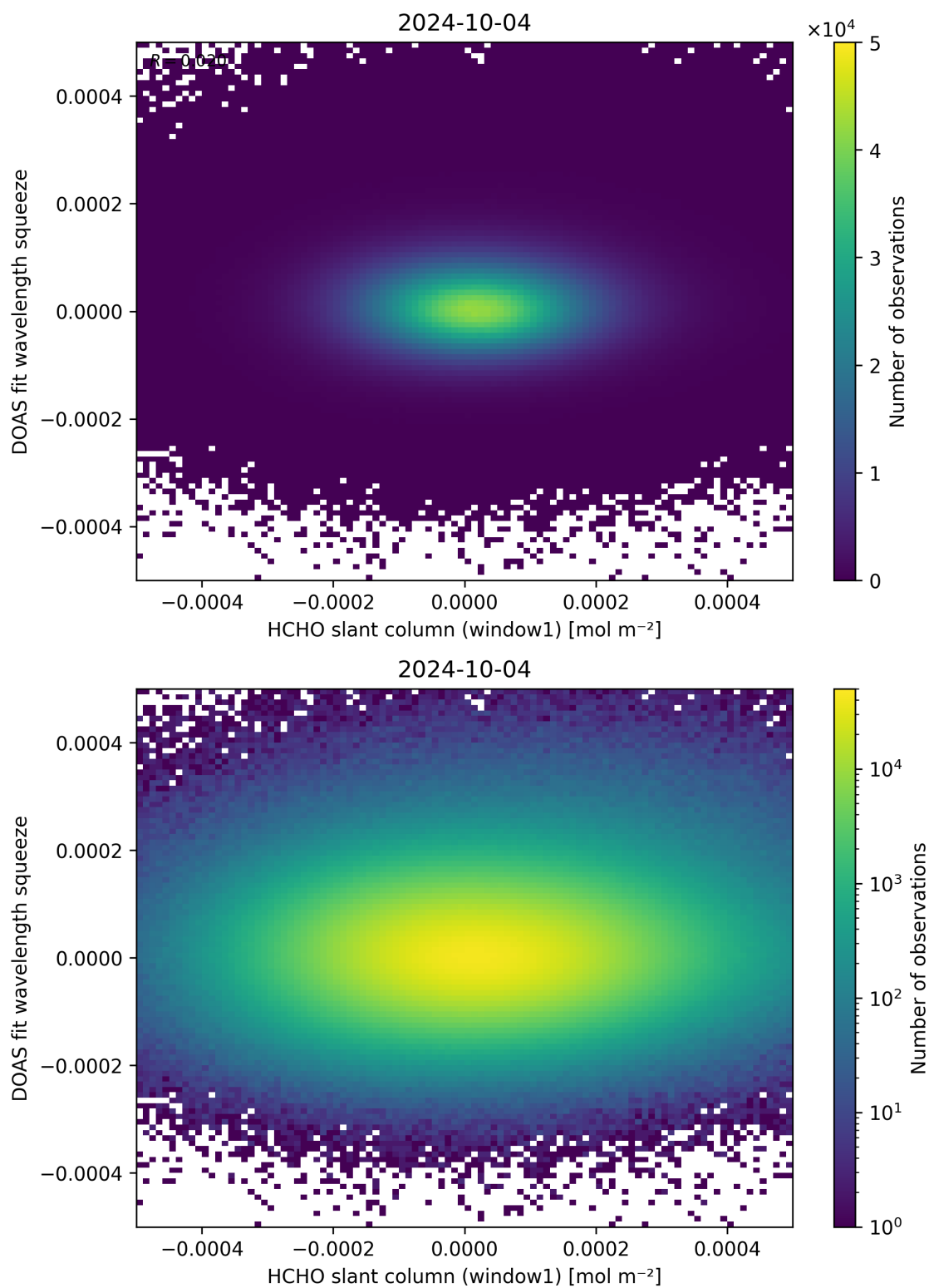
Figure 80: Scatter density plot of “HCHO slant column (window1)” against “DOAS fit wavelength squeeze” for 2024-10-03 to 2024-10-05.
