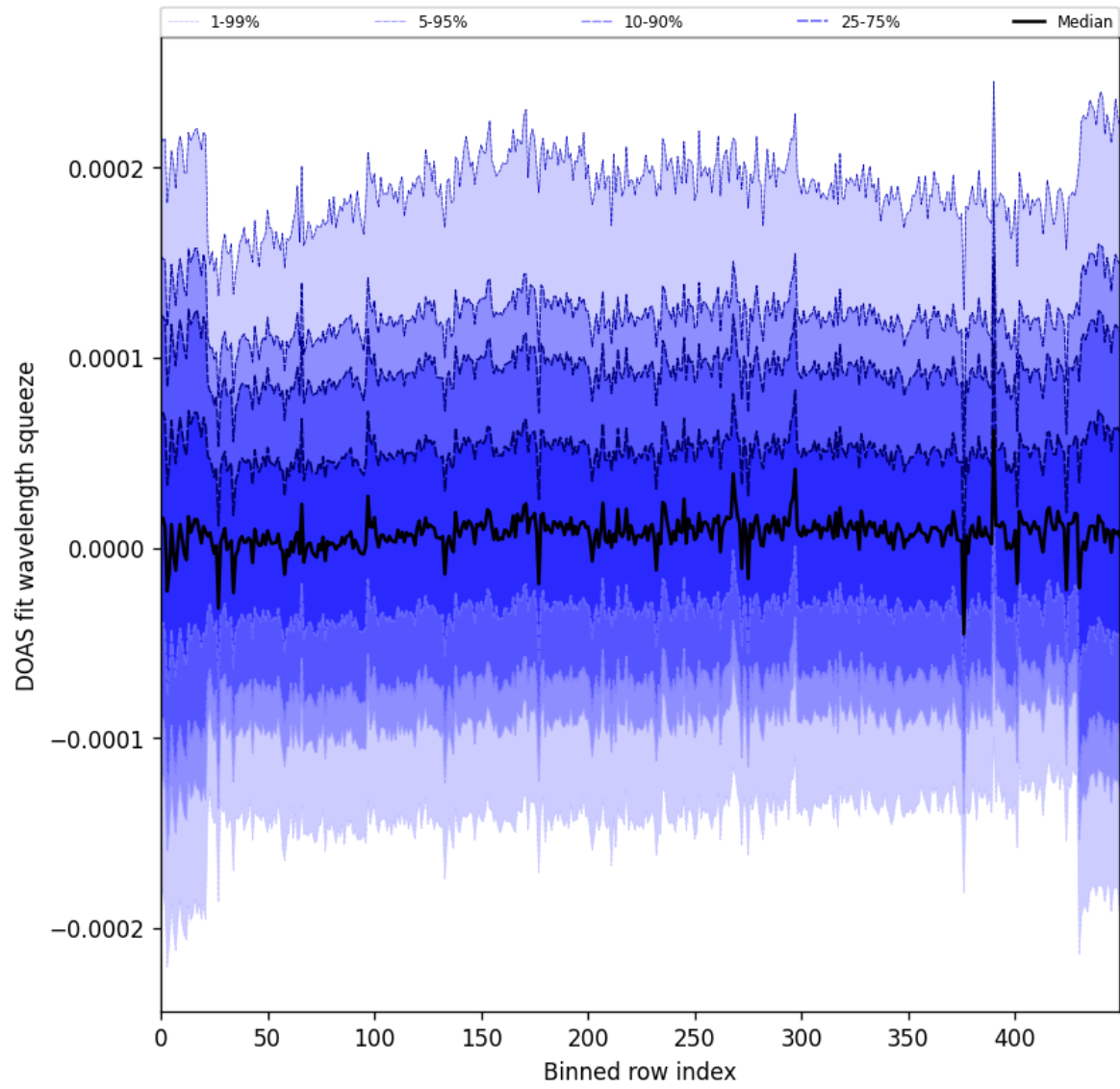
Figure 59: Along track statistics of “DOAS fit wavelength squeeze” for 2024-10-03 to 2024-10-05
