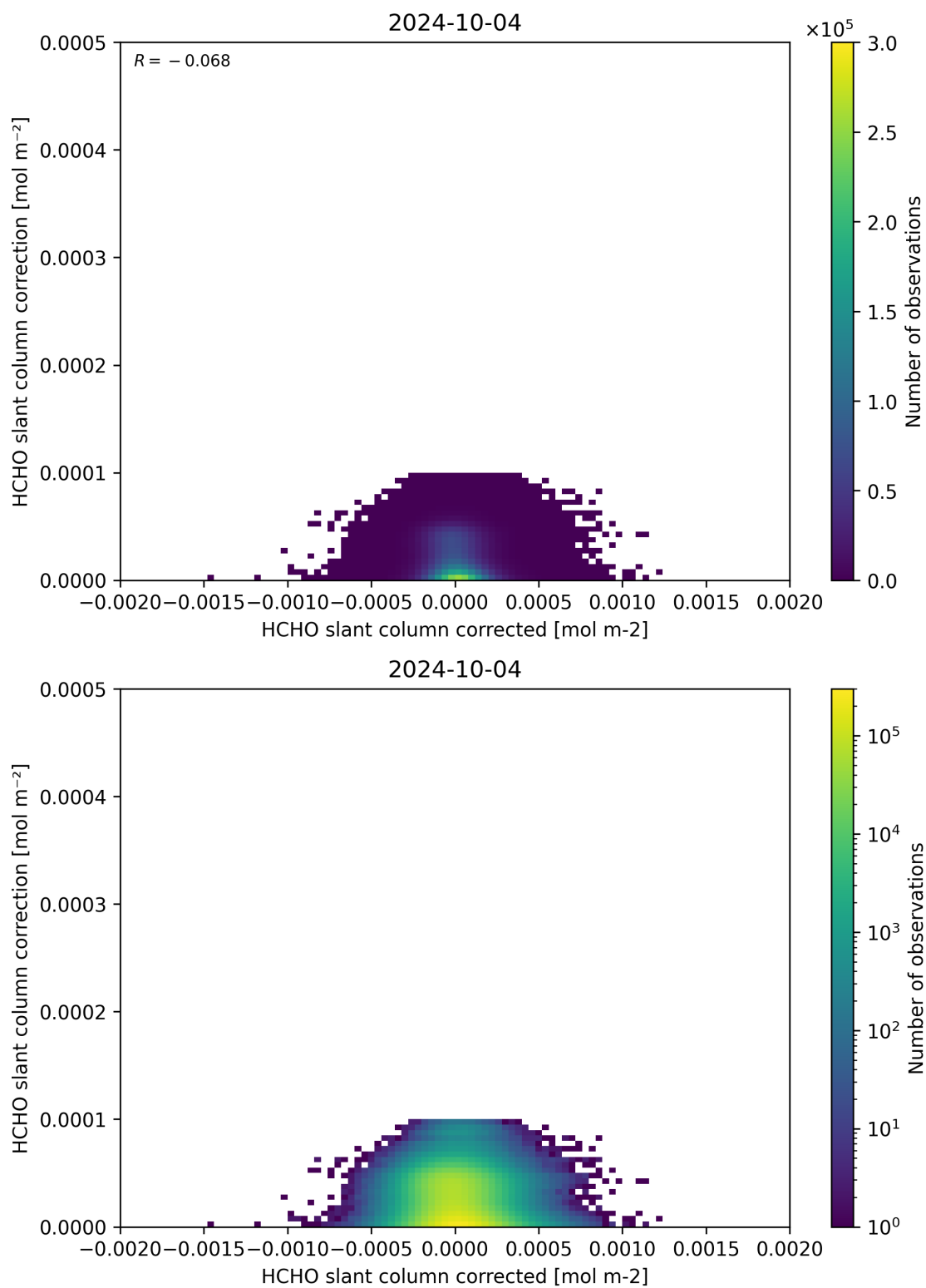
Figure 77: Scatter density plot of “HCHO slant column corrected” against “HCHO slant column correction” for 2024-10-03 to 2024-10-05.
