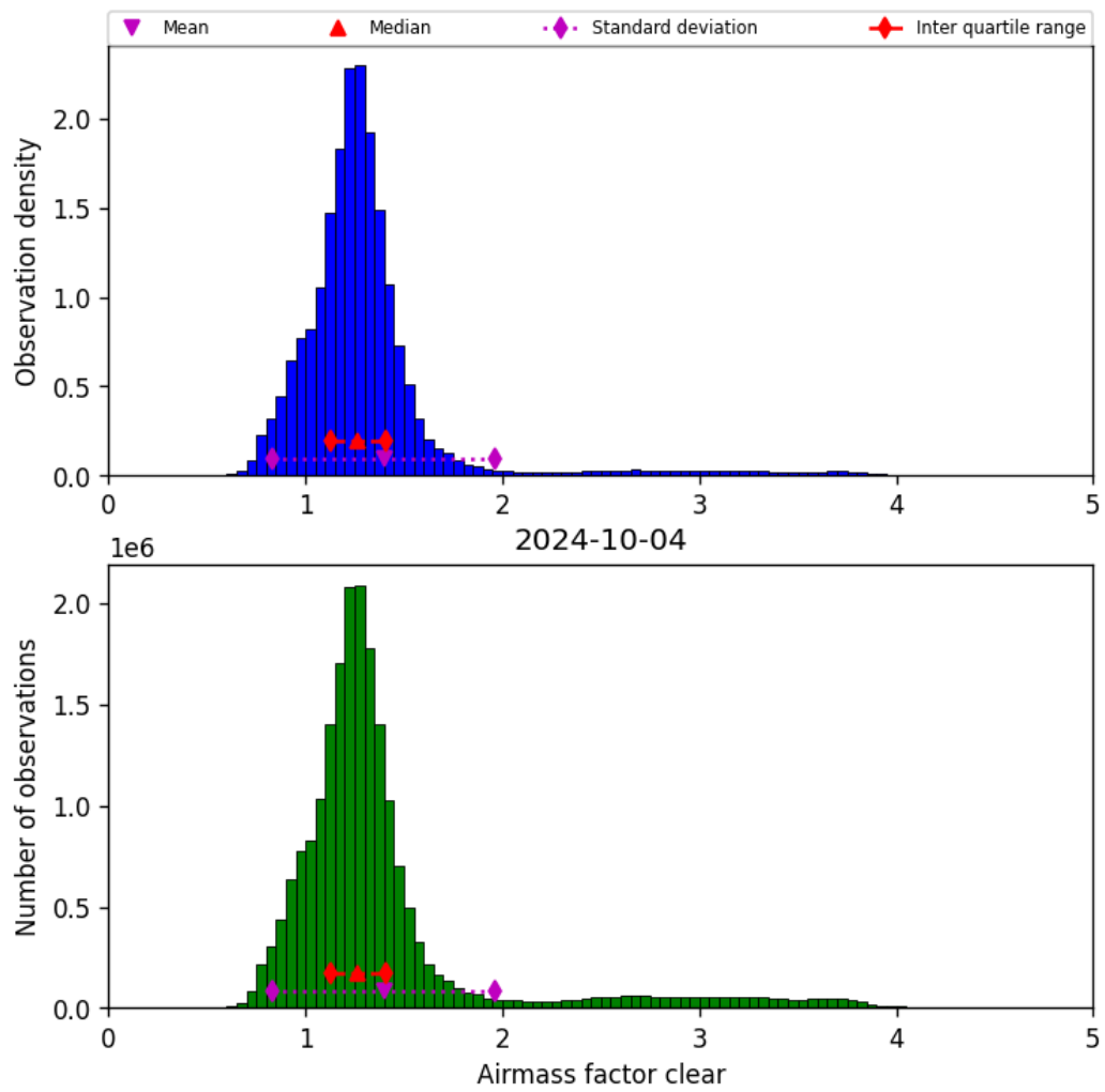
Figure 42: Histogram of “Airmass factor clear” for 2024-10-03 to 2024-10-05
