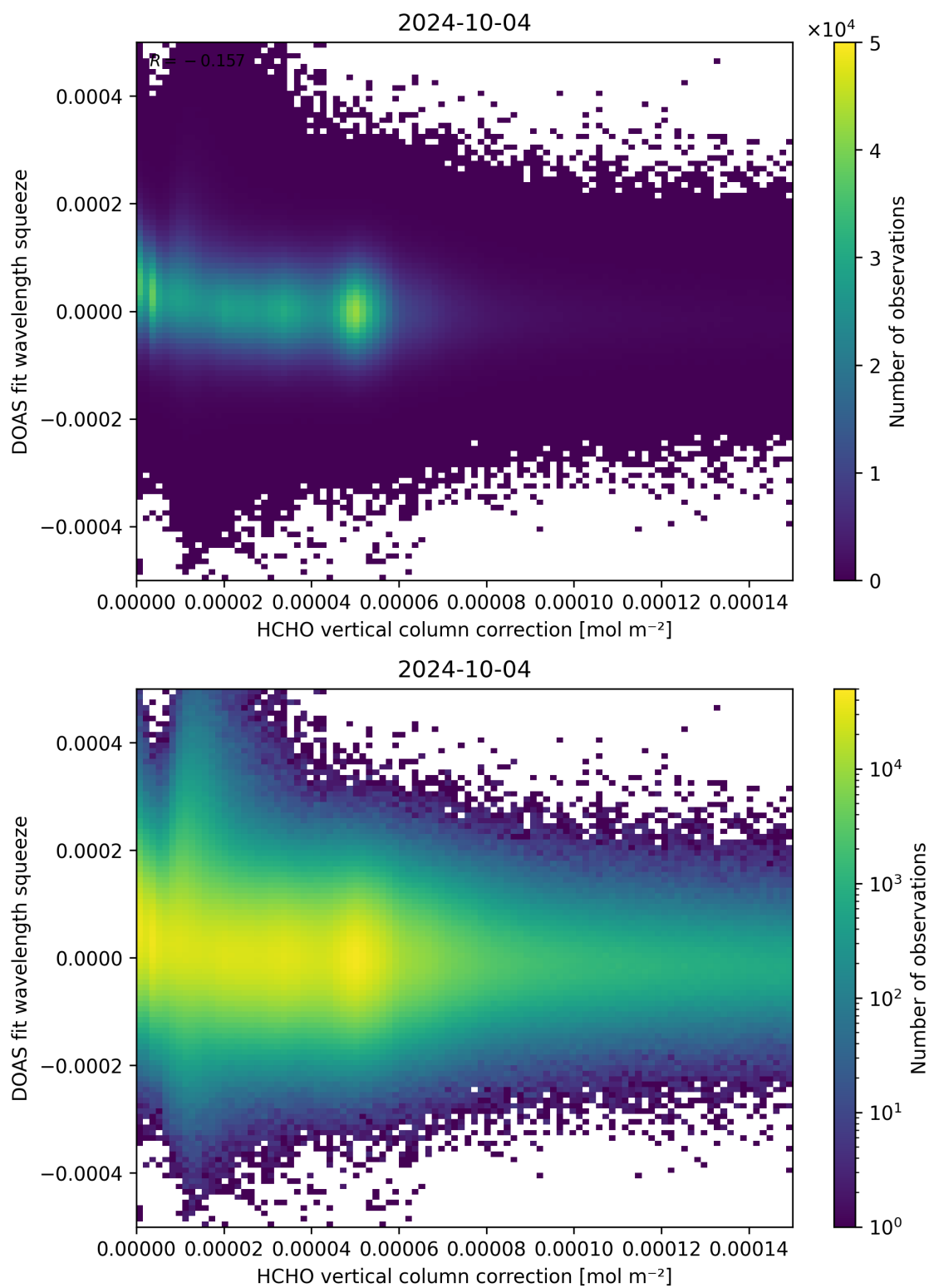
Figure 114: Scatter density plot of “HCHO vertical column correction” against “DOAS fit wavelength squeeze” for 2024-10-03 to 2024-10-05.
