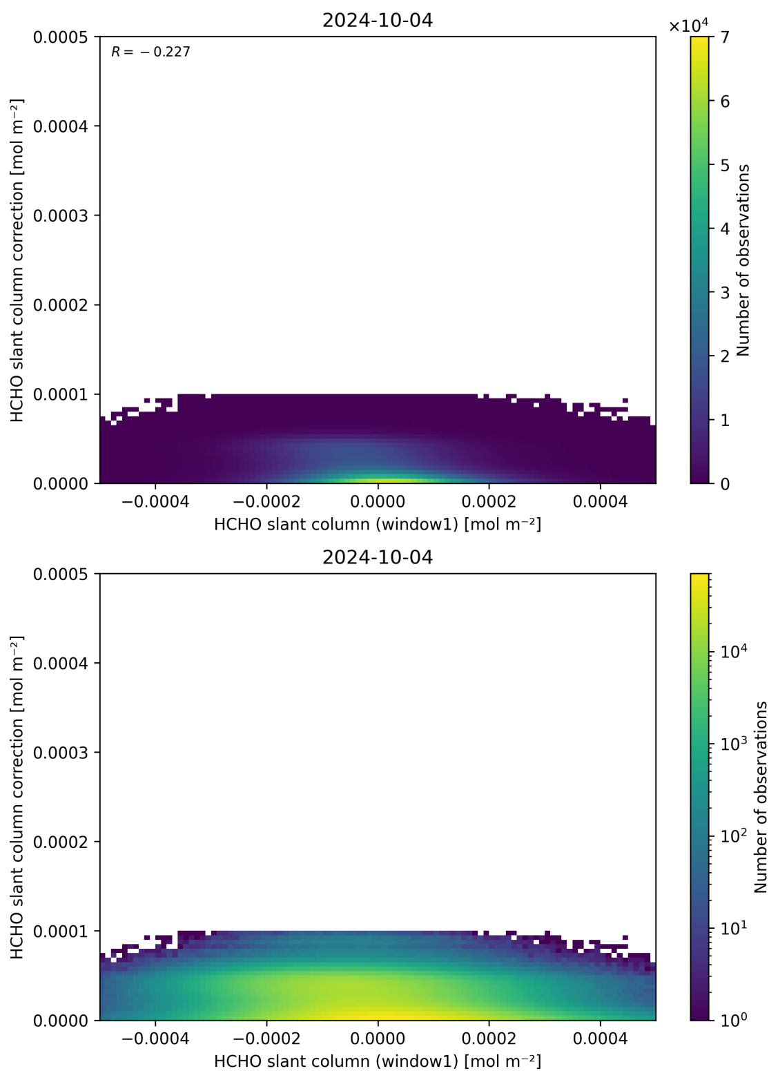
Figure 83: Scatter density plot of “HCHO slant column (window1)” against “HCHO slant column correction” for 2024-10-03 to 2024-10-05.
