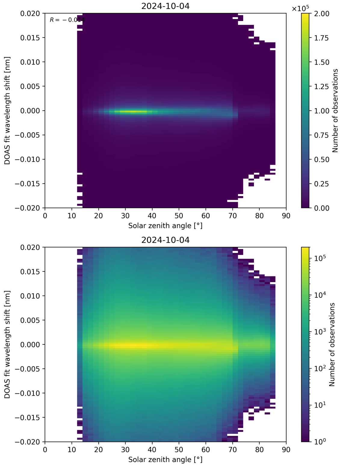
Figure 168: Scatter density plot of “Solar zenith angle” against “DOAS fit wavelength shift” for 2024-10-03 to 2024-10-05.
