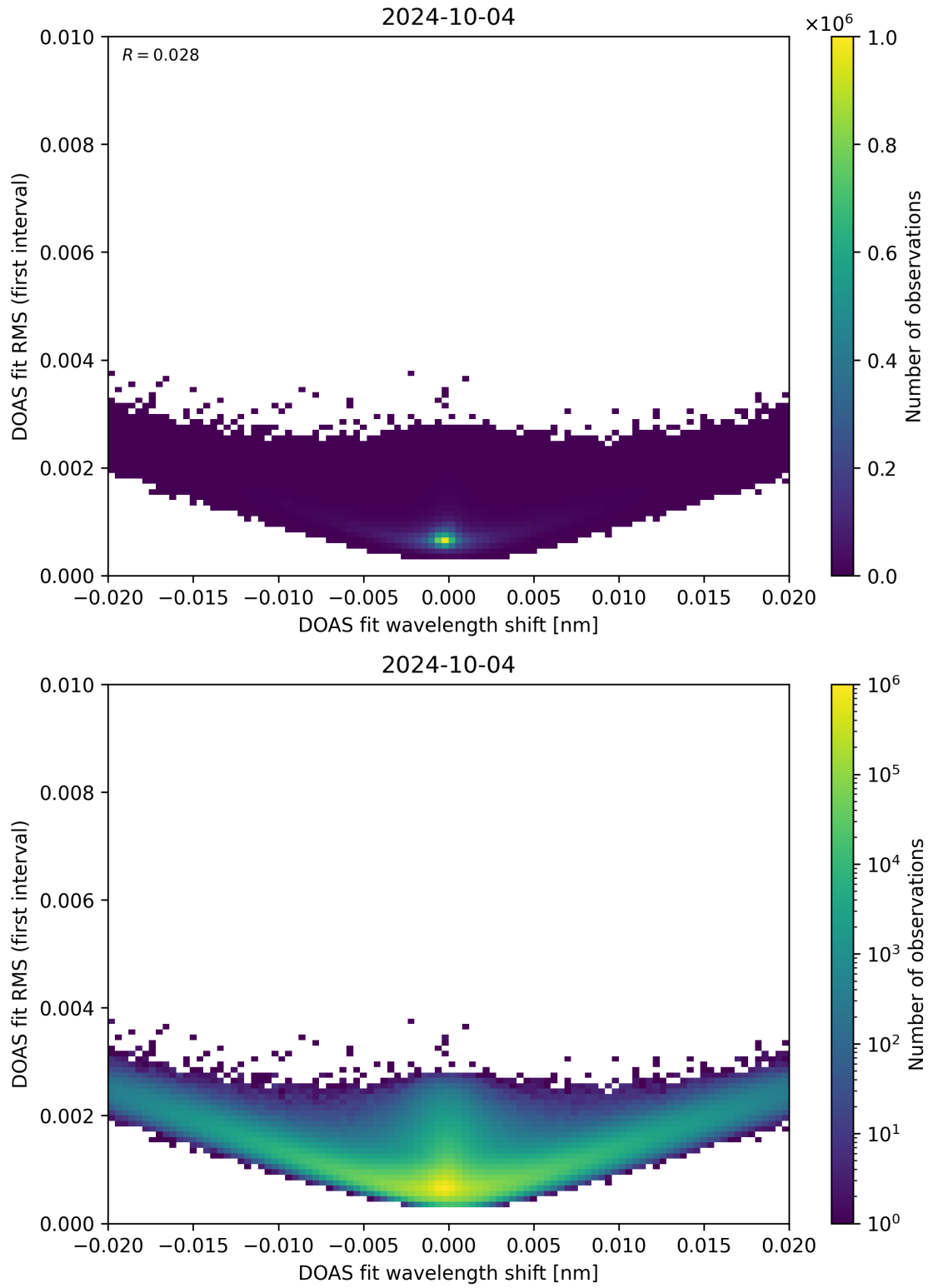
Figure 64: Scatter density plot of “DOAS fit wavelength shift” against “DOAS fit RMS (first interval)” for 2024-10-03 to 2024-10-05.
