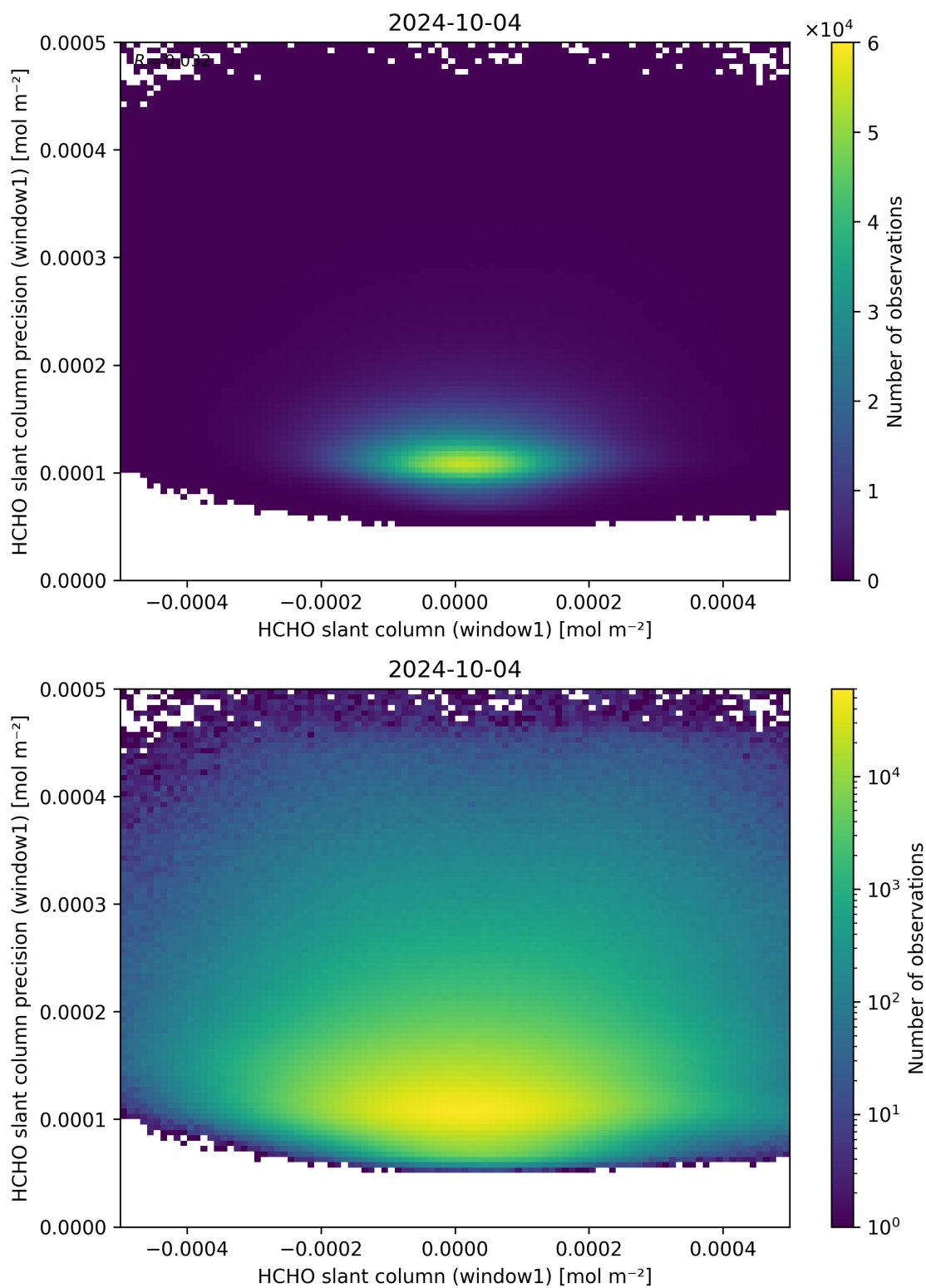
Figure 84: Scatter density plot of “HCHO slant column (window1)” against “HCHO slant column precision (window1)” for 2024-10-03 to 2024-10-05.
