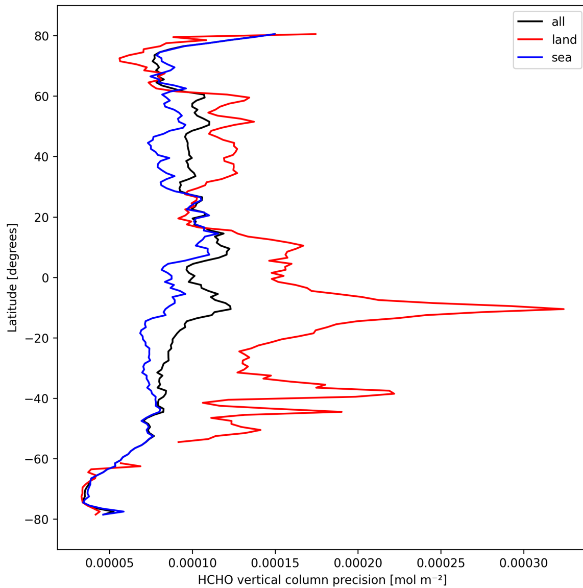
Figure 22: Zonal average of “HCHO vertical column precision” for 2024-10-03 to 2024-10-05.
