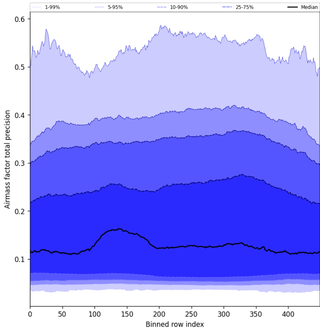
Figure 55: Along track statistics of “Airmass factor total precision” for 2024-10-03 to 2024-10-05
