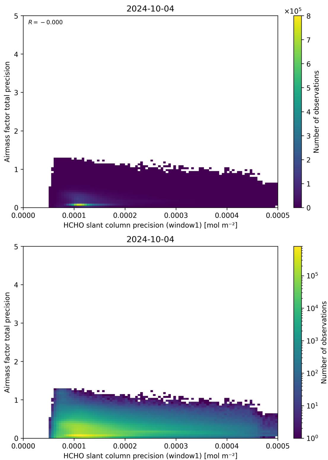
Figure 95: Scatter density plot of “HCHO slant column precision (window1)” against “Airmass factor total precision” for 2024-10-03 to 2024-10-05.
