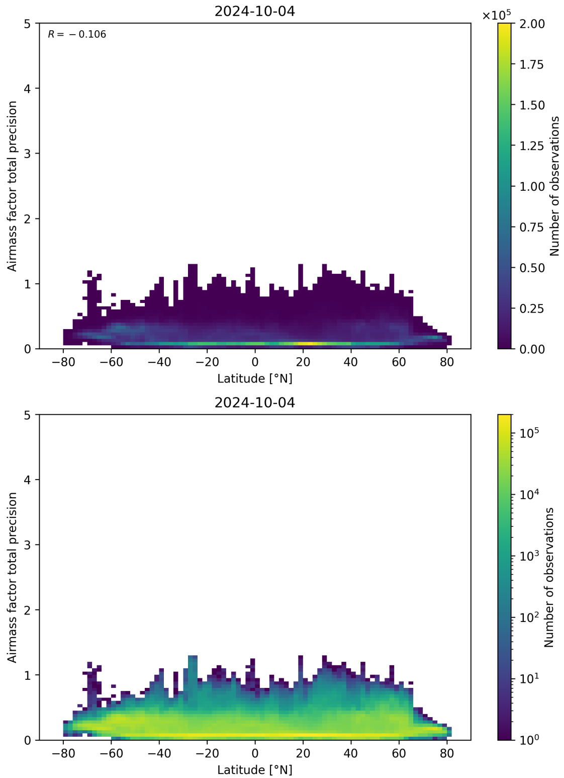
Figure 162: Scatter density plot of “Latitude” against “Airmass factor total precision” for 2024-10-03 to 2024-10-05.
