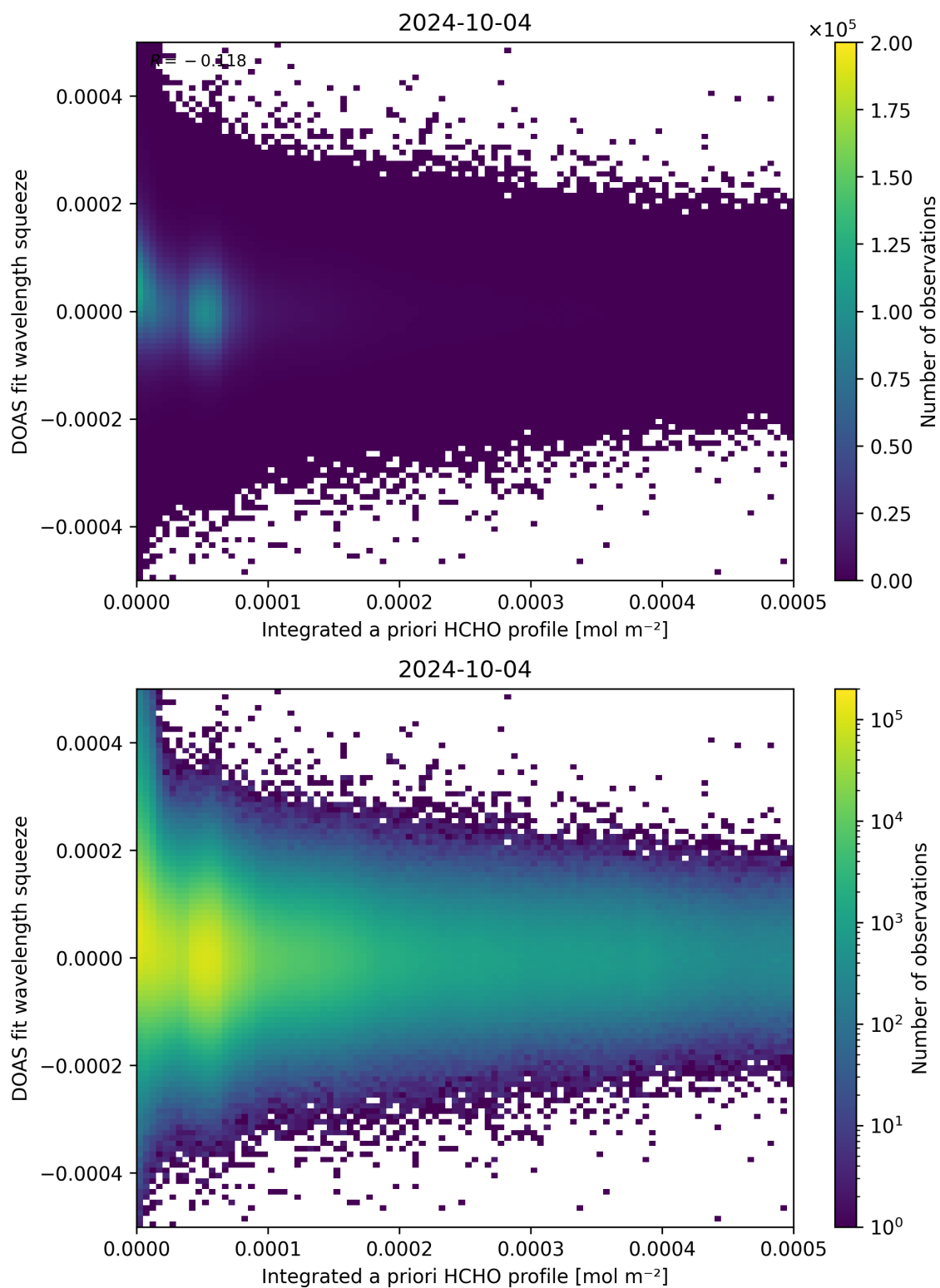
Figure 150: Scatter density plot of “Integrated a priori HCHO profile” against “DOAS fit wavelength squeeze” for 2024-10-03 to 2024-10-05.
