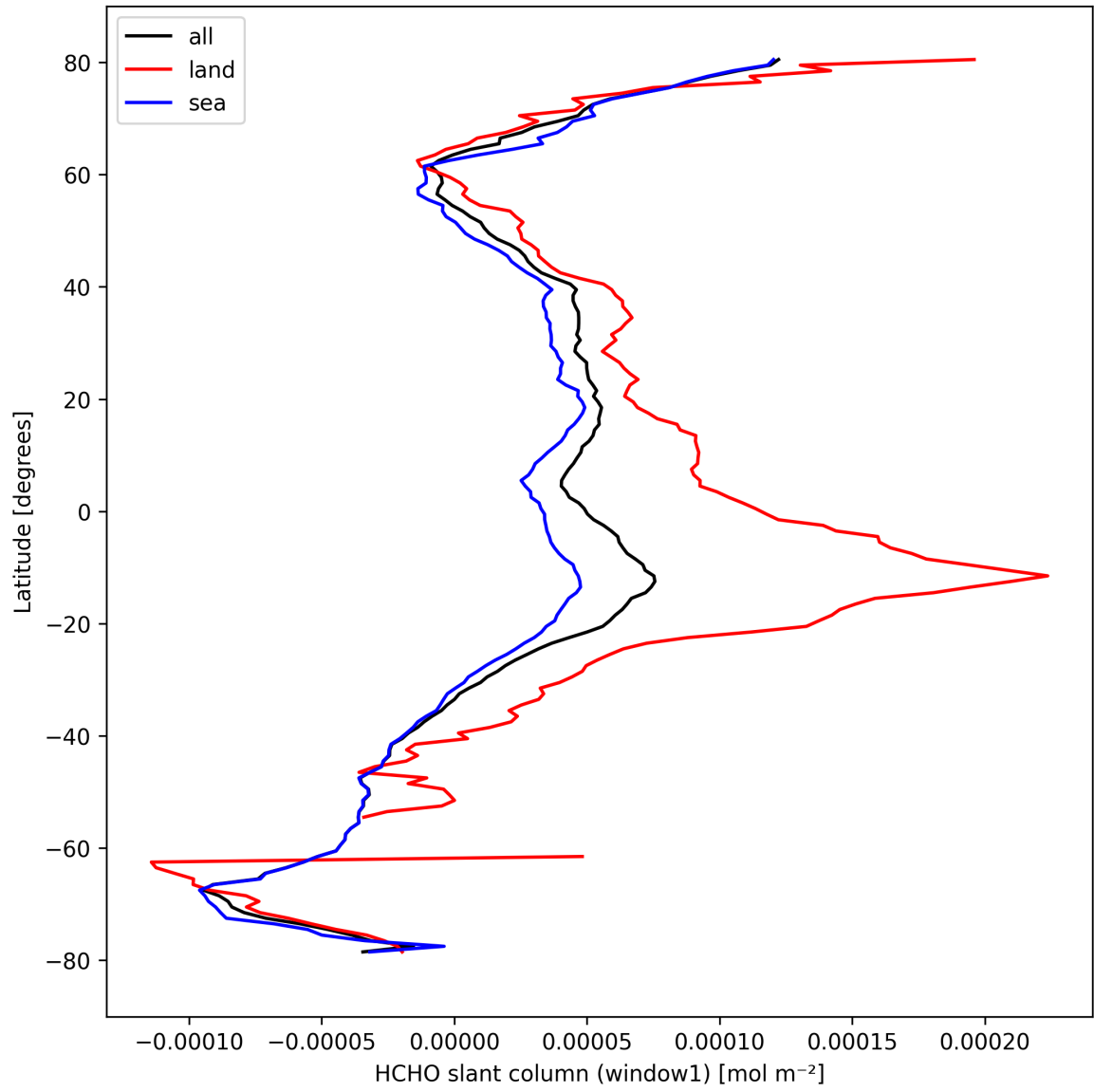
Figure 24: Zonal average of “HCHO slant column (window1)” for 2024-10-03 to 2024-10-05.
