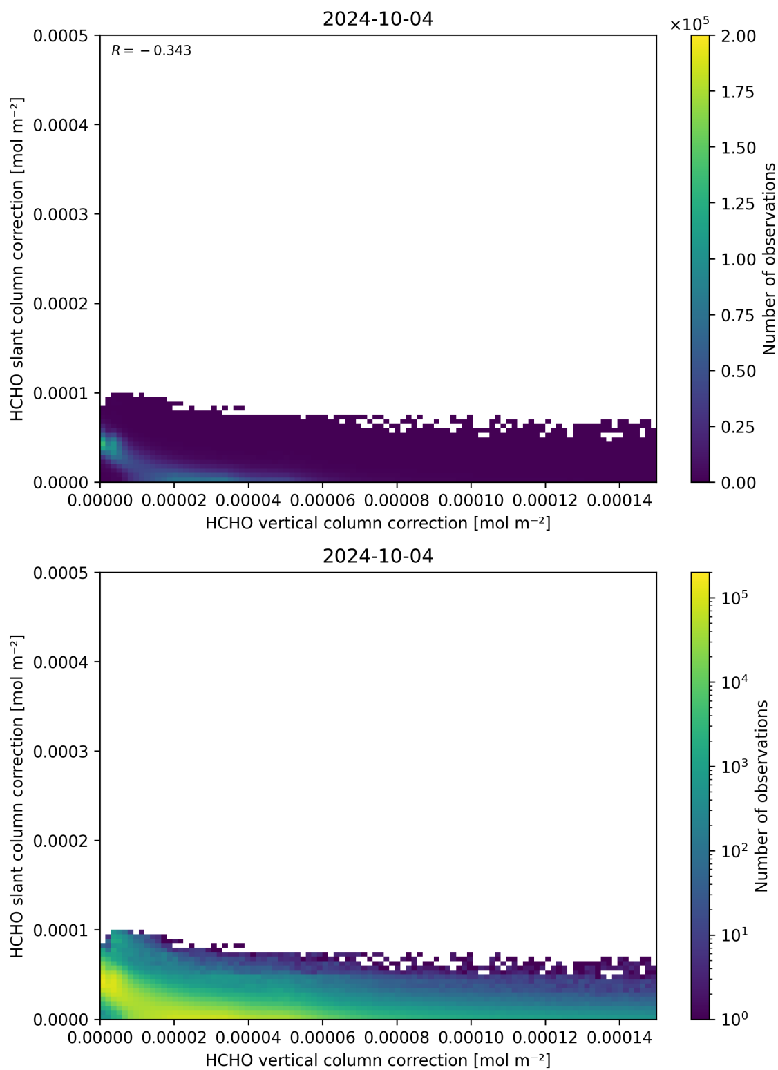
Figure 117: Scatter density plot of “HCHO vertical column correction” against “HCHO slant column correction” for 2024-10-03 to 2024-10-05.
