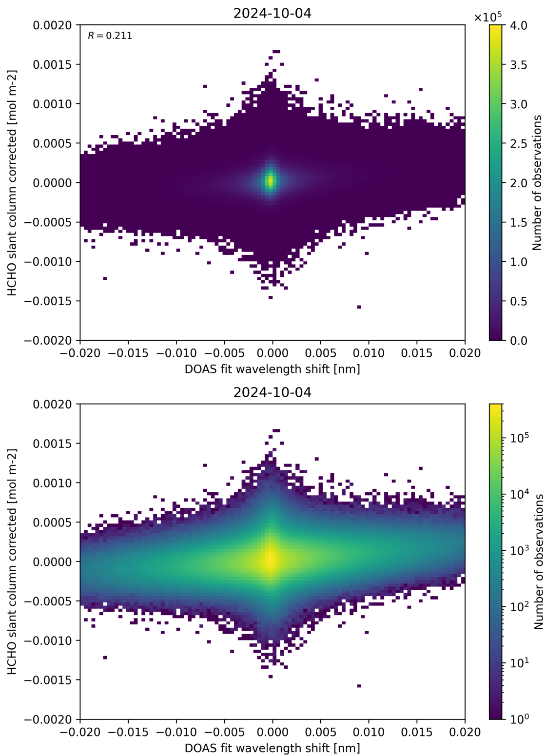
Figure 66: Scatter density plot of “DOAS fit wavelength shift” against “HCHO slant column corrected” for 2024-10-03 to 2024-10-05.
