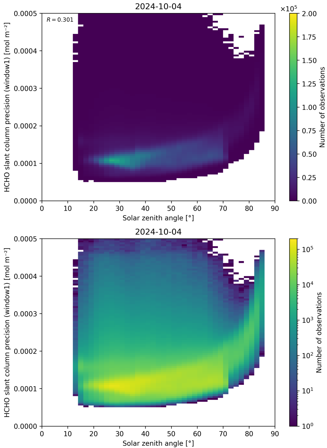
Figure 174: Scatter density plot of “Solar zenith angle” against “HCHO slant column precision (window1)” for 2024-10-03 to 2024-10-05.
