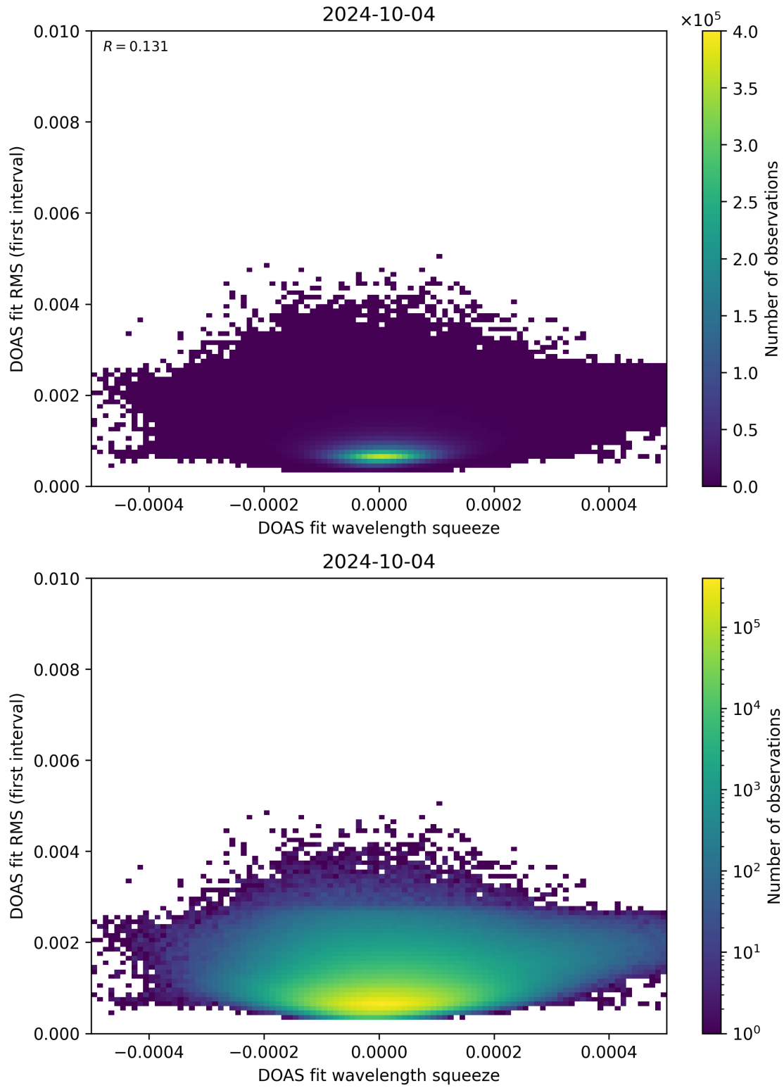
Figure 68: Scatter density plot of “DOAS fit wavelength squeeze” against “DOAS fit RMS (first interval)” for 2024-10-03 to 2024-10-05.
