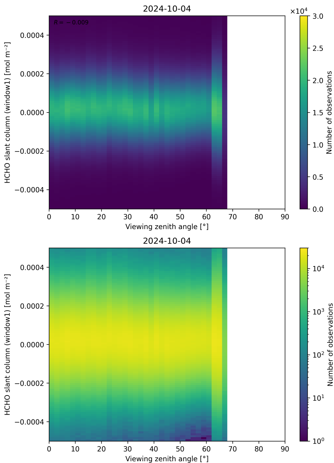
Figure 188: Scatter density plot of “Viewing zenith angle” against “HCHO slant column (window1)” for 2024-10-03 to 2024-10-05.
