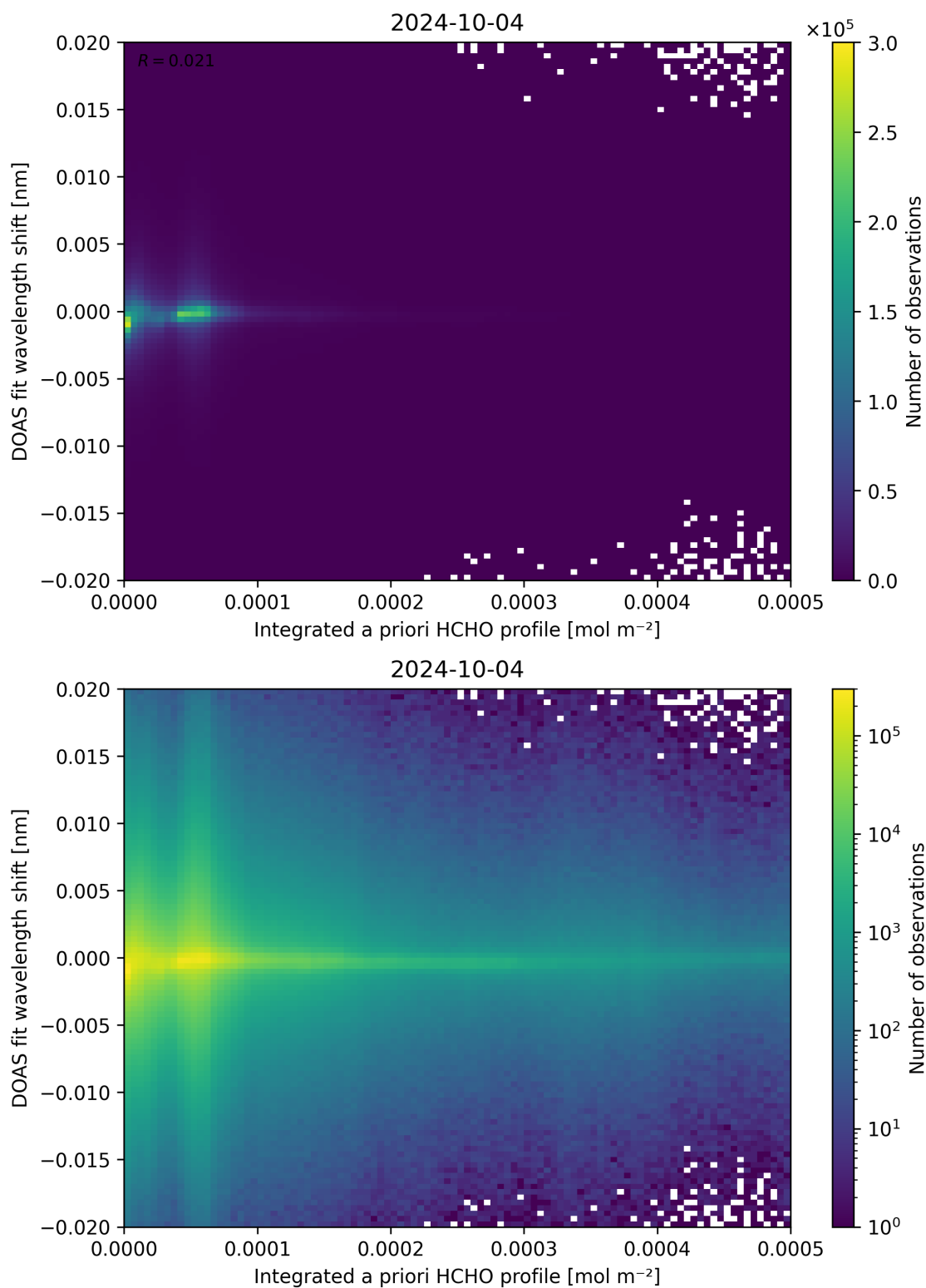
Figure 149: Scatter density plot of “Integrated a priori HCHO profile” against “DOAS fit wavelength shift” for 2024-10-03 to 2024-10-05.
