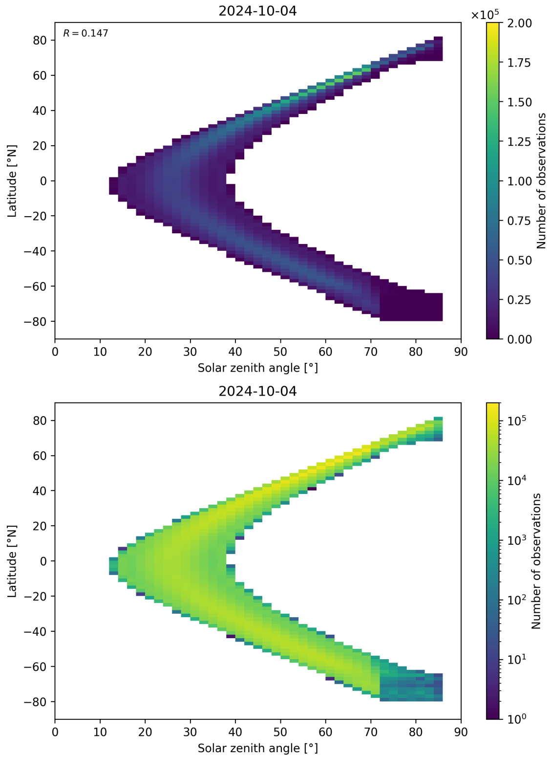
Figure 181: Scatter density plot of “Solar zenith angle” against “Latitude” for 2024-10-03 to 2024-10-05.
