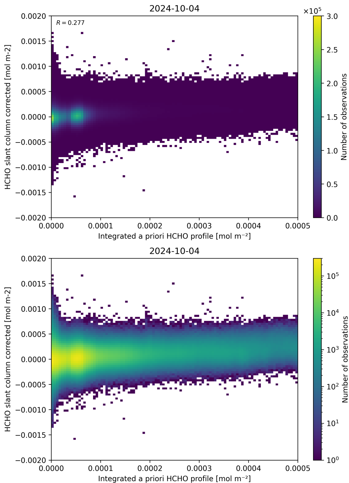
Figure 151: Scatter density plot of “Integrated a priori HCHO profile” against “HCHO slant column corrected” for 2024-10-03 to 2024-10-05.
