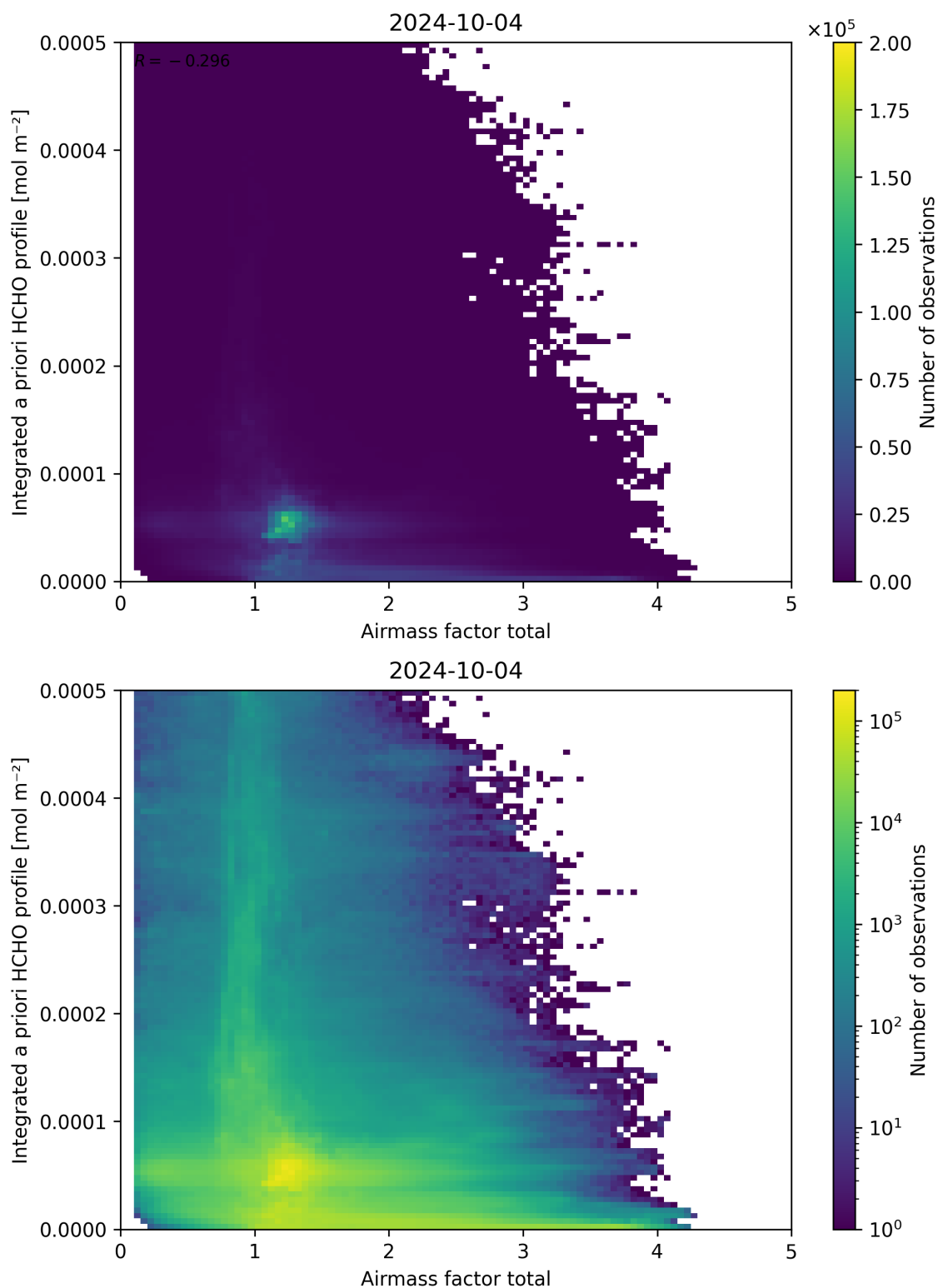
Figure 104: Scatter density plot of “Airmass factor total” against “Integrated a priori HCHO profile” for 2024-10-03 to 2024-10-05.
