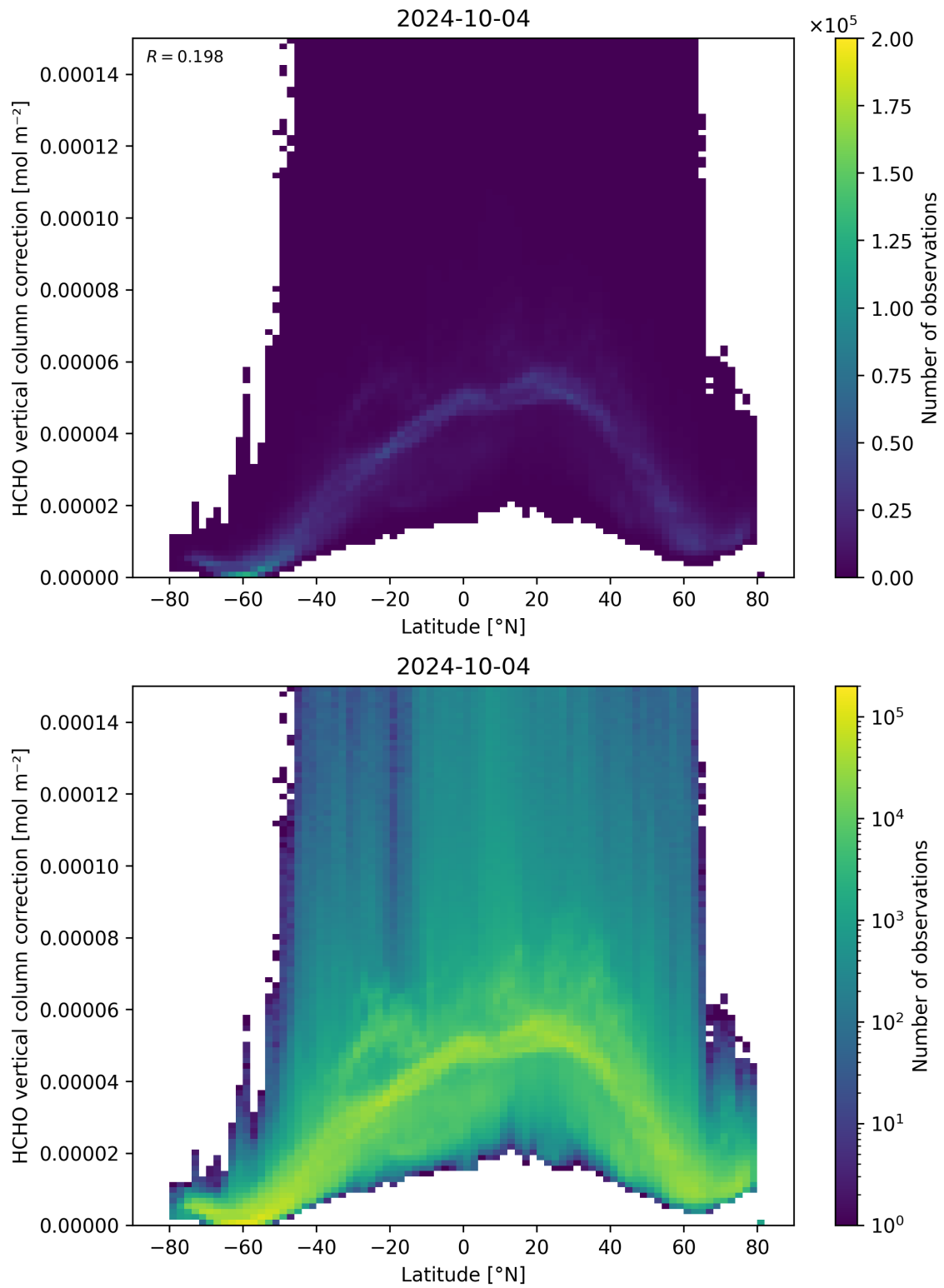
Figure 164: Scatter density plot of “Latitude” against “HCHO vertical column correction” for 2024-10-03 to 2024-10-05.
