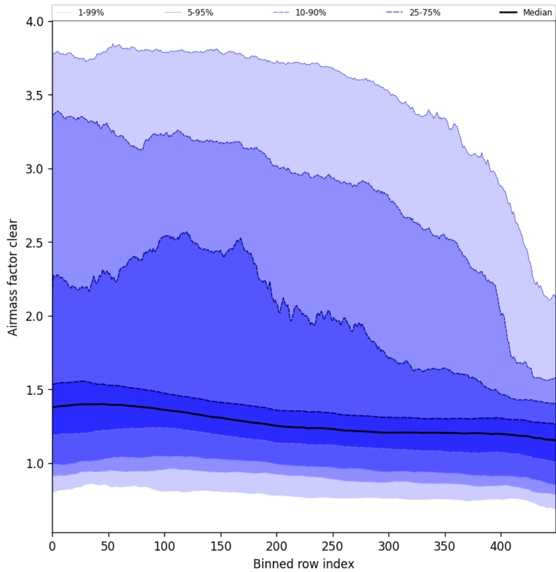
Figure 56: Along track statistics of “Airmass factor clear” for 2024-10-03 to 2024-10-05
