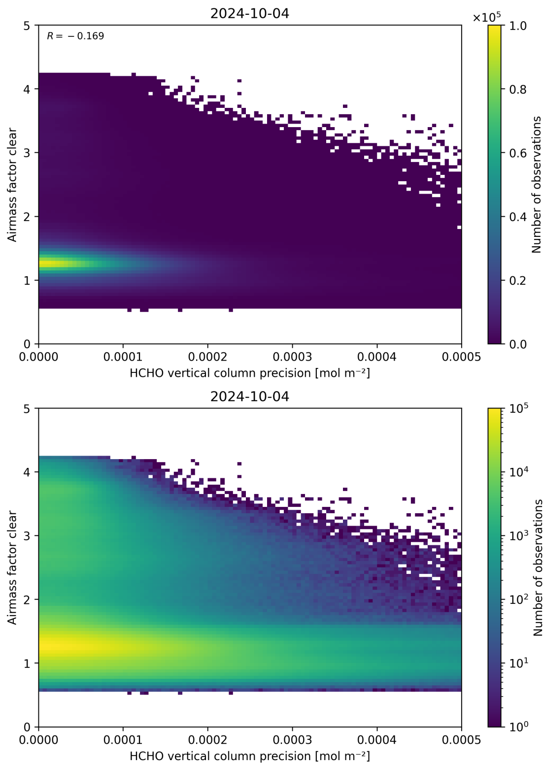
Figure 139: Scatter density plot of “HCHO vertical column precision” against “Airmass factor clear” for 2024-10-03 to 2024-10-05.
