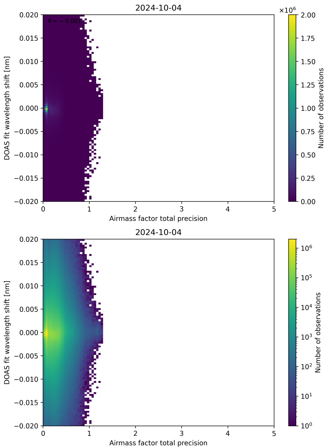
Figure 106: Scatter density plot of “Airmass factor total precision” against “DOAS fit wavelength shift” for 2024-10-03 to 2024-10-05.
