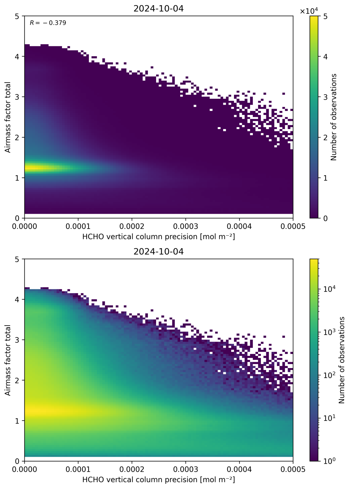
Figure 144: Scatter density plot of “HCHO vertical column precision” against “Airmass factor total” for 2024-10-03 to 2024-10-05.
