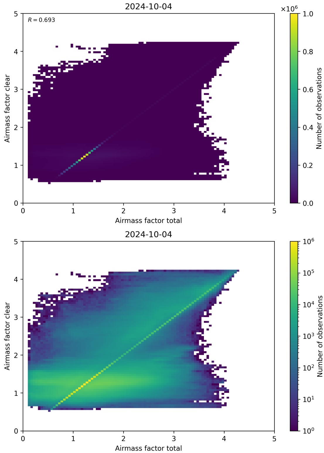
Figure 100: Scatter density plot of “Airmass factor total” against “Airmass factor clear” for 2024-10-03 to 2024-10-05.
