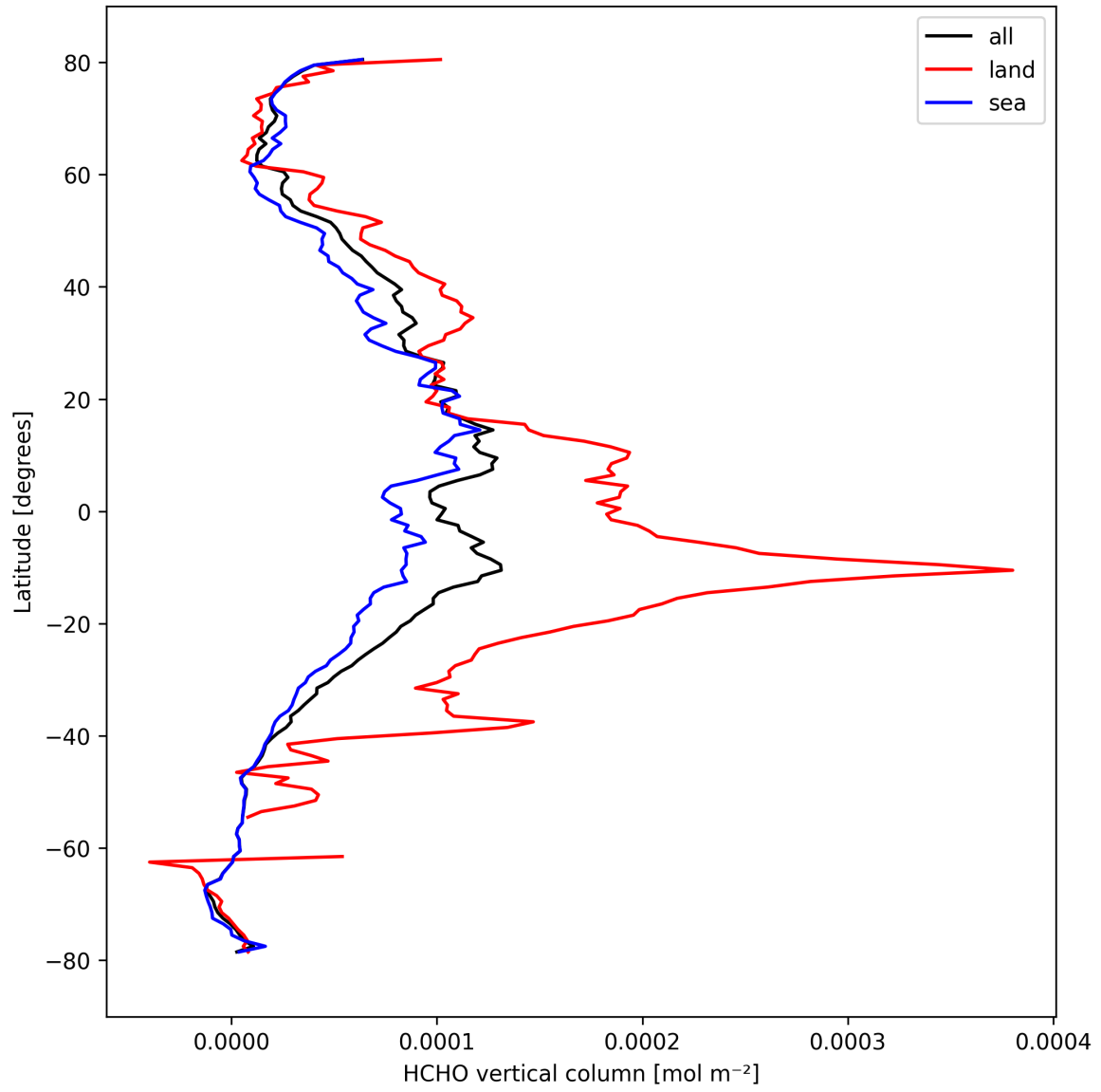
Figure 21: Zonal average of “HCHO vertical column” for 2024-10-03 to 2024-10-05.
