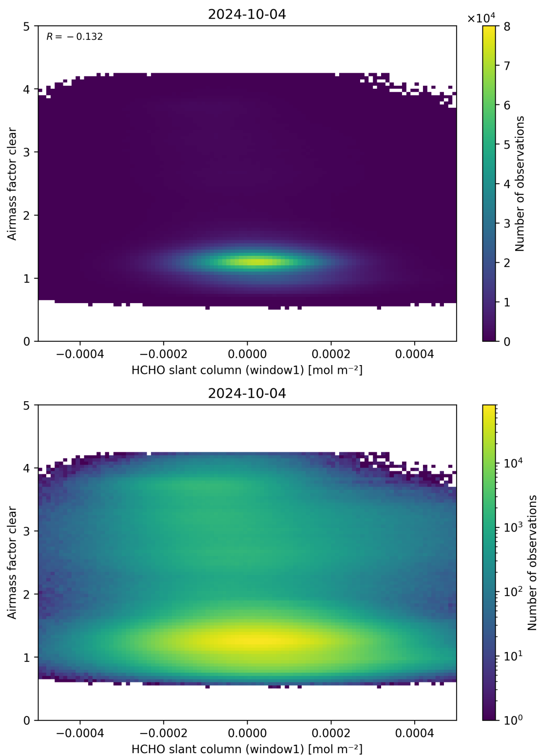
Figure 81: Scatter density plot of “HCHO slant column (window1)” against “Airmass factor clear” for 2024-10-03 to 2024-10-05.
