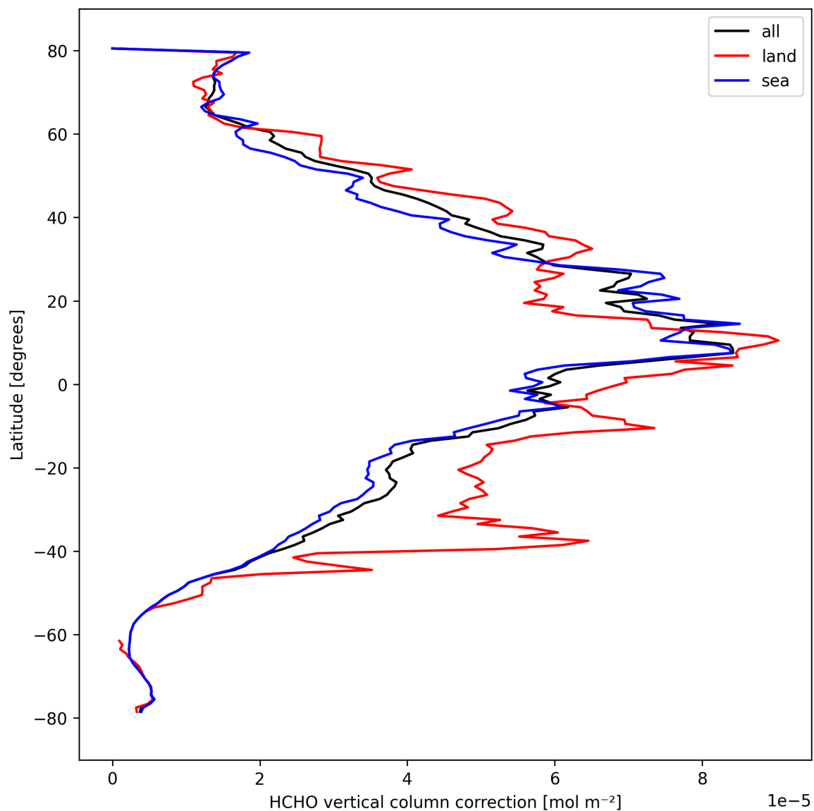
Figure 23: Zonal average of “HCHO vertical column correction” for 2024-10-03 to 2024-10-05.
