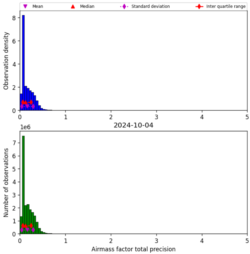
Figure 41: Histogram of “Airmass factor total precision” for 2024-10-03 to 2024-10-05
