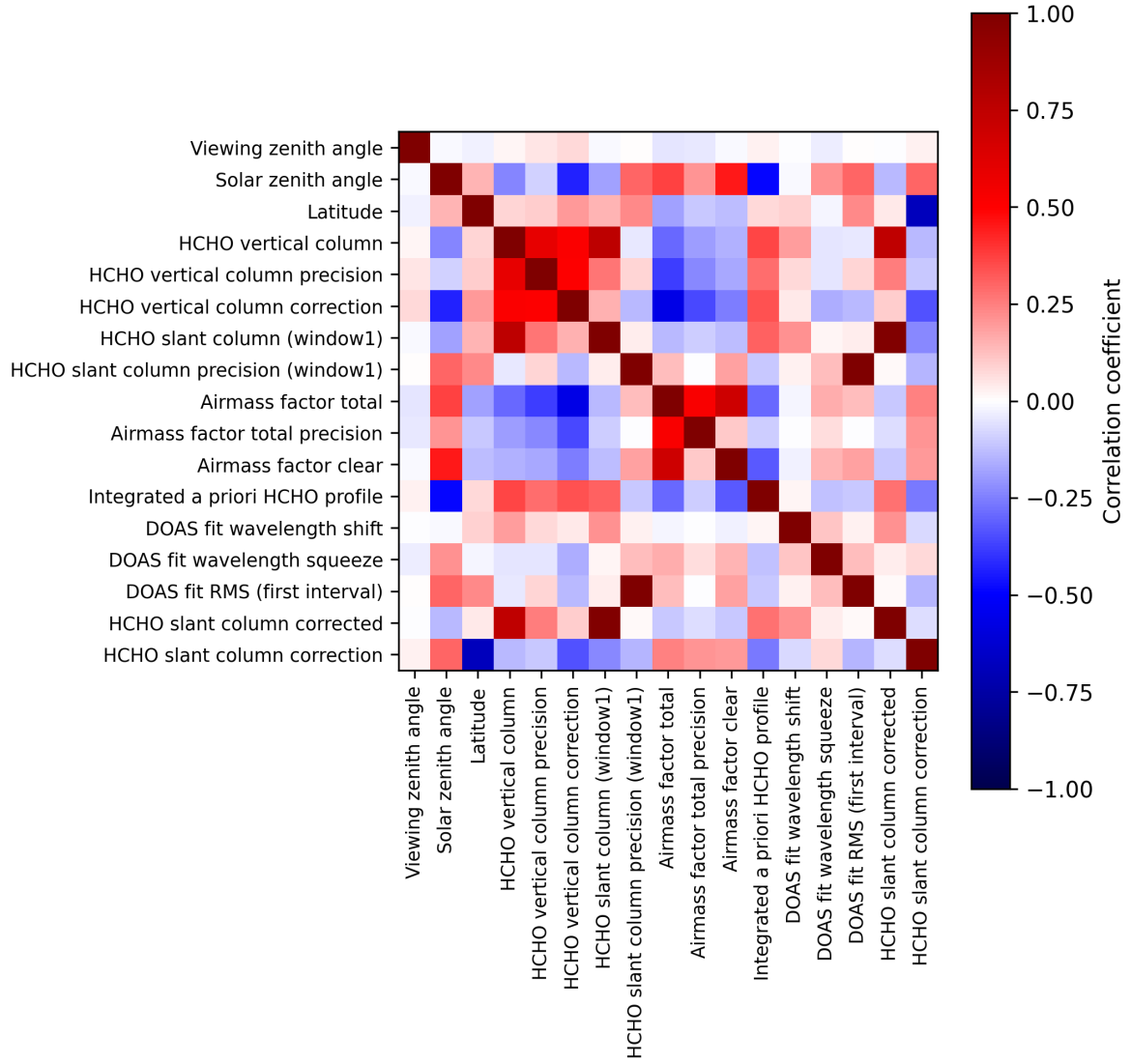
Figure 2: Map of correlation matrix for 2024-10-03 to 2024-10-05.
