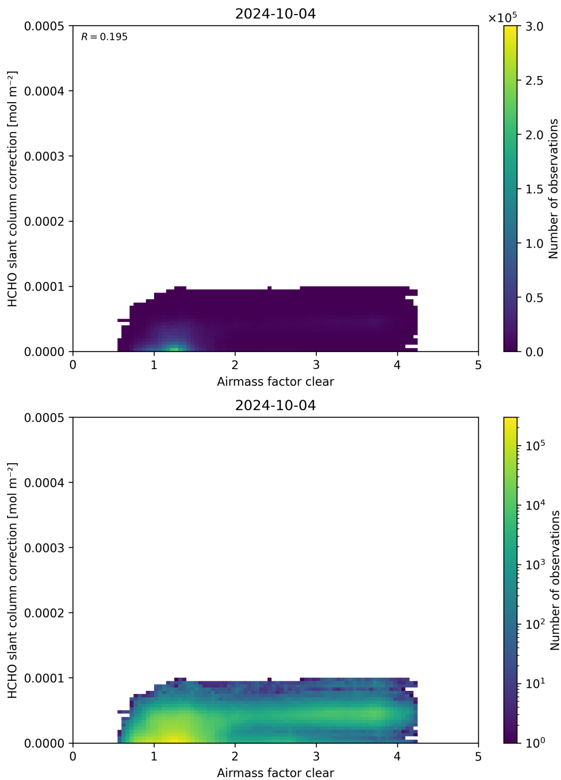
Figure 75: Scatter density plot of “Airmass factor clear” against “HCHO slant column correction” for 2024-10-03 to 2024-10-05.
