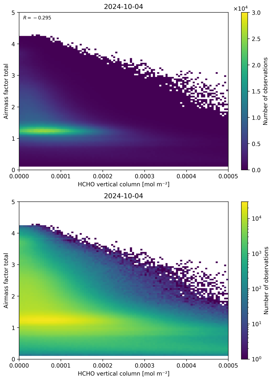
Figure 131: Scatter density plot of “HCHO vertical column” against “Airmass factor total” for 2024-10-03 to 2024-10-05.
