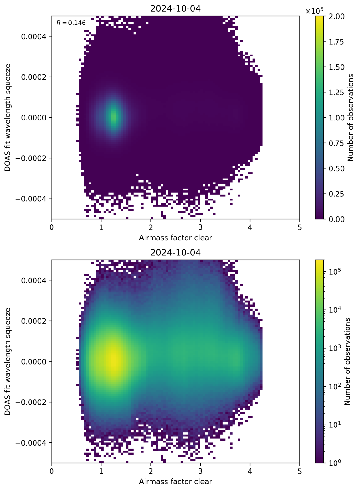
Figure 73: Scatter density plot of “Airmass factor clear” against “DOAS fit wavelength squeeze” for 2024-10-03 to 2024-10-05.
