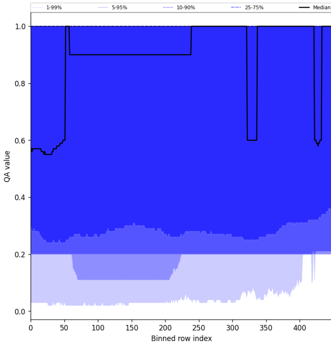
Figure 48: Along track statistics of “QA value” for 2024-10-03 to 2024-10-05
