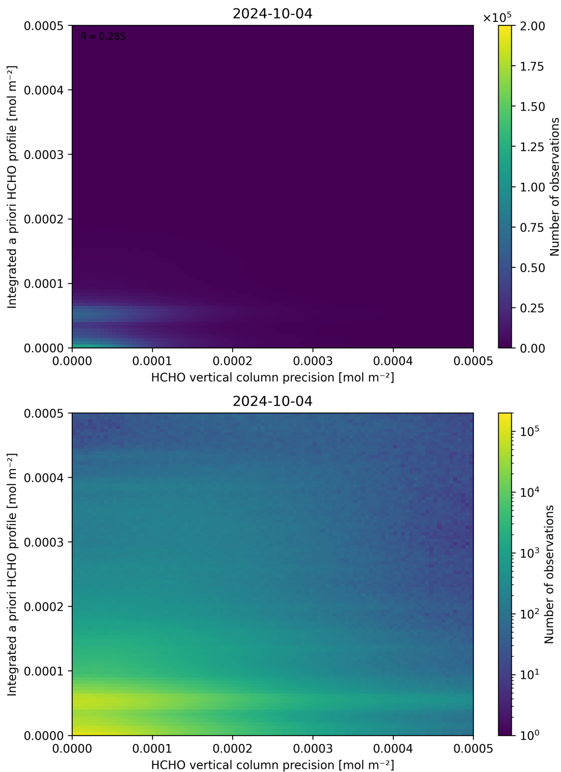
Figure 147: Scatter density plot of “HCHO vertical column precision” against “Integrated a priori HCHO profile” for 2024-10-03 to 2024-10-05.
