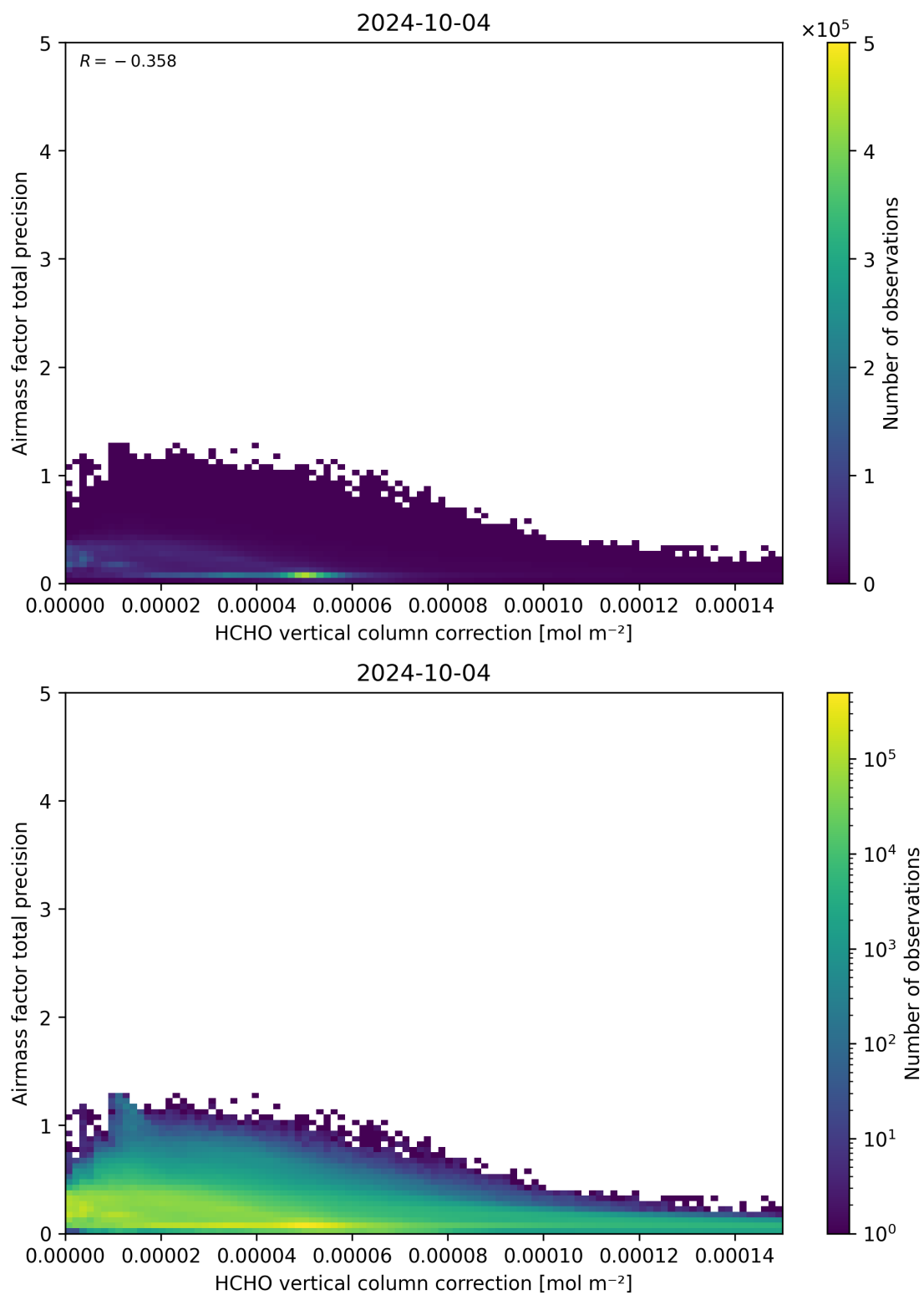
Figure 121: Scatter density plot of “HCHO vertical column correction” against “Airmass factor total precision” for 2024-10-03 to 2024-10-05.
