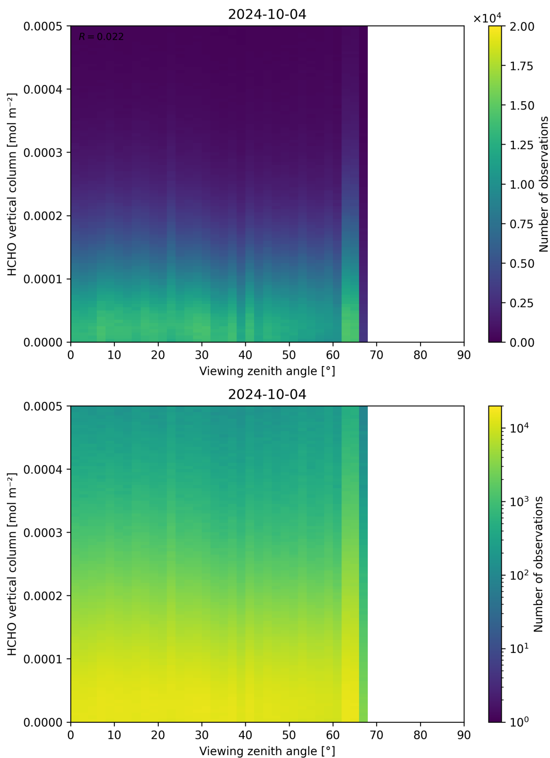
Figure 192: Scatter density plot of “Viewing zenith angle” against “HCHO vertical column” for 2024-10-03 to 2024-10-05.
