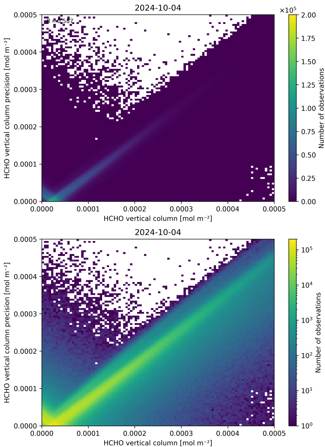
Figure 134: Scatter density plot of “HCHO vertical column” against “HCHO vertical column precision” for 2024-10-03 to 2024-10-05.
