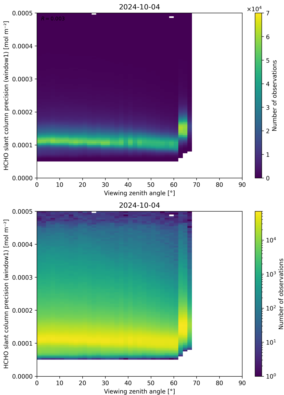
Figure 189: Scatter density plot of “Viewing zenith angle” against “HCHO slant column precision (window1)” for 2024-10-03 to 2024-10-05.
