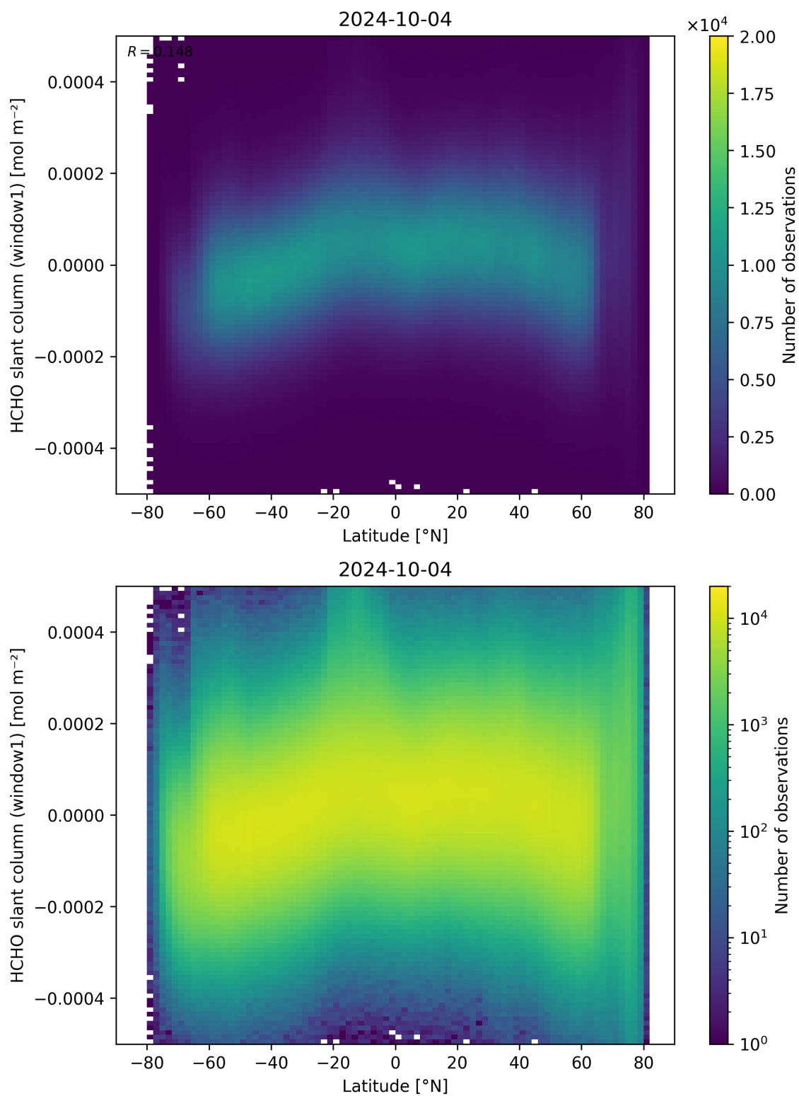
Figure 159: Scatter density plot of “Latitude” against “HCHO slant column (window1)” for 2024-10-03 to 2024-10-05.
