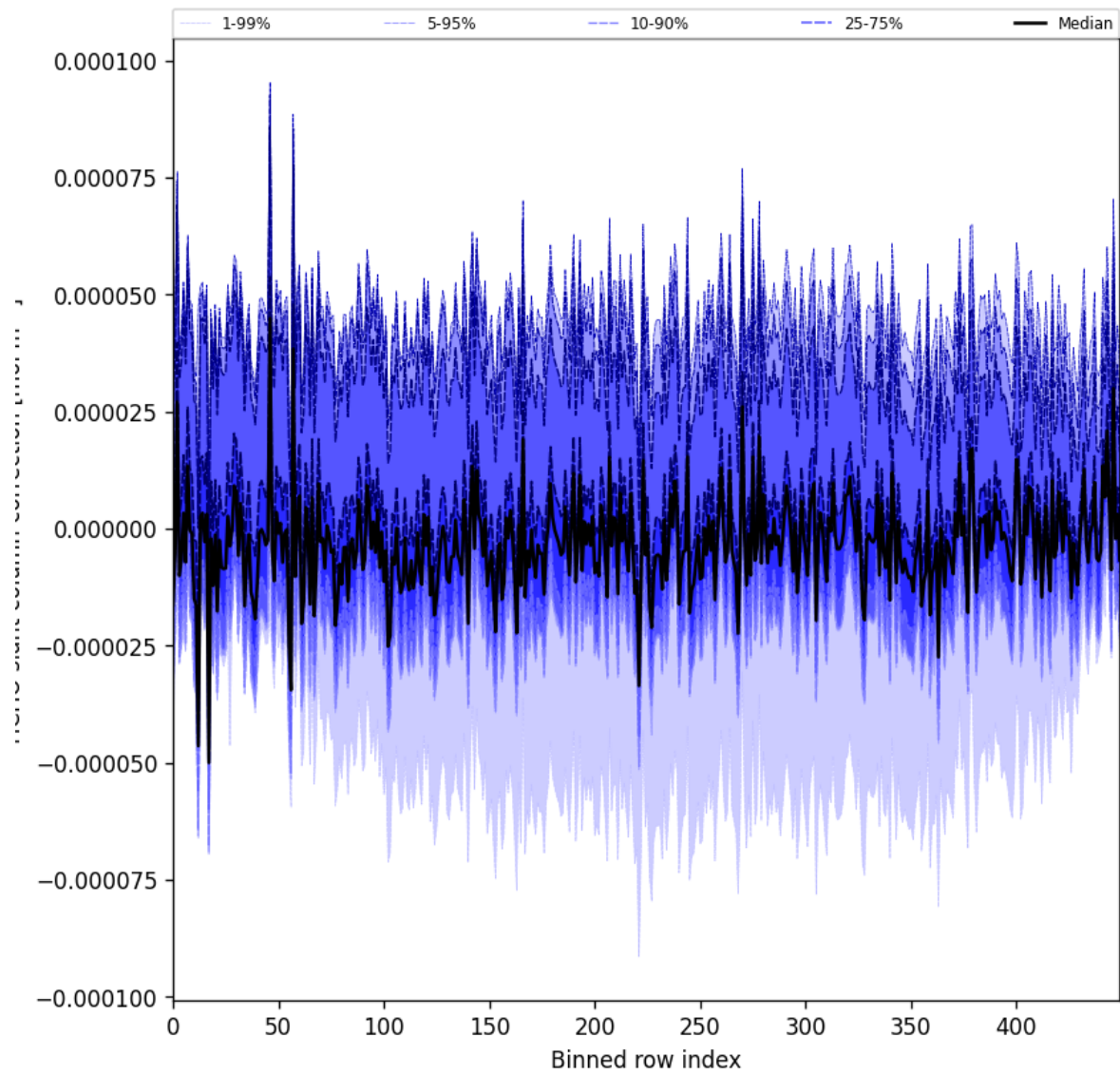
Figure 61: Along track statistics of “HCHO slant column correction” for 2024-10-03 to 2024-10-05
