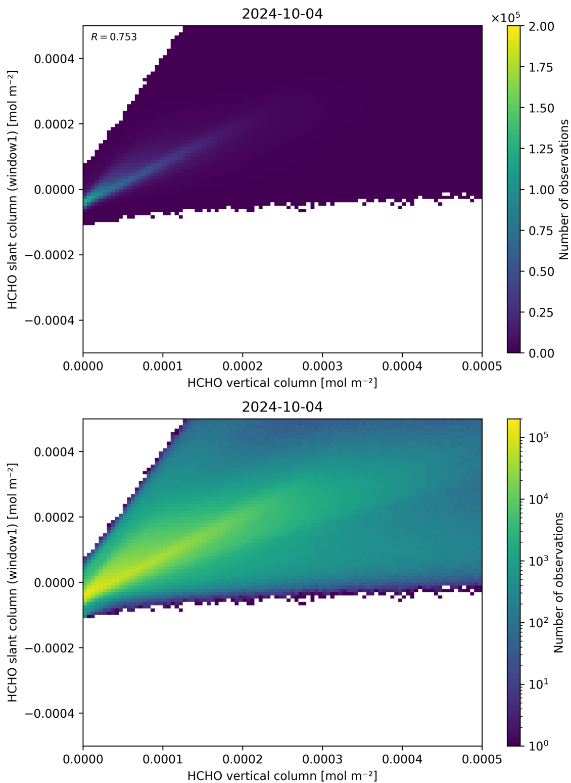
Figure 129: Scatter density plot of “HCHO vertical column” against “HCHO slant column (window1)” for 2024-10-03 to 2024-10-05.
