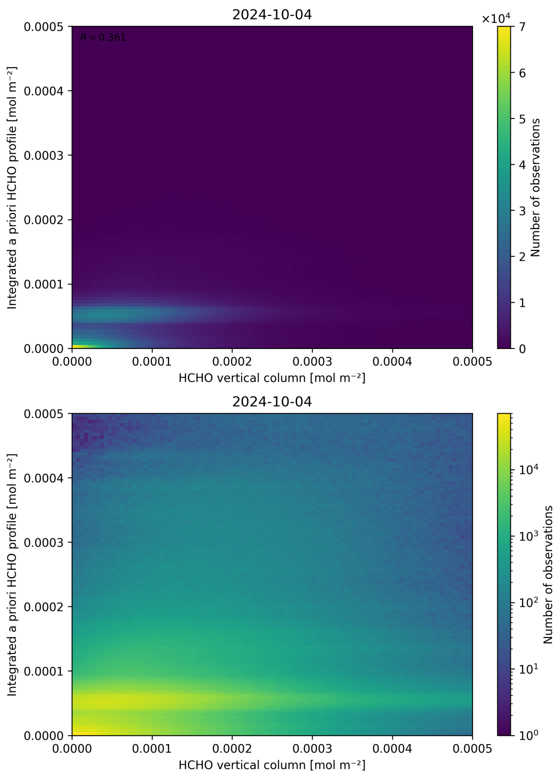
Figure 135: Scatter density plot of “HCHO vertical column” against “Integrated a priori HCHO profile” for 2024-10-03 to 2024-10-05.
