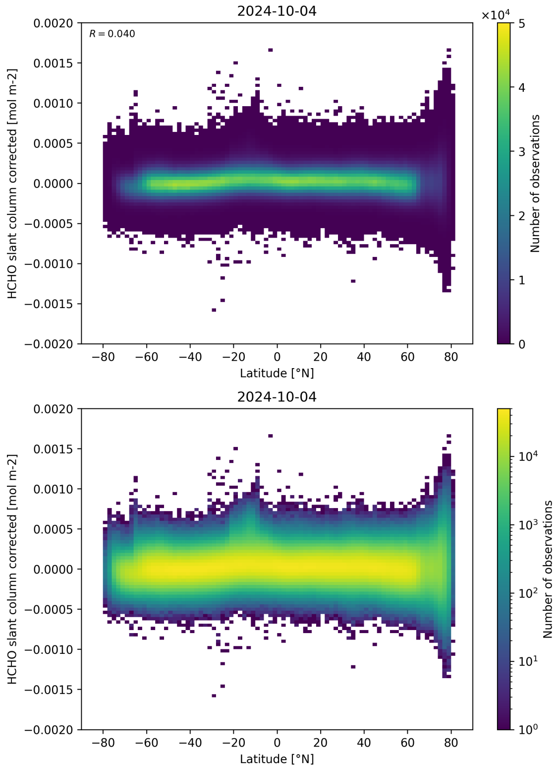
Figure 157: Scatter density plot of “Latitude” against “HCHO slant column corrected” for 2024-10-03 to 2024-10-05.
