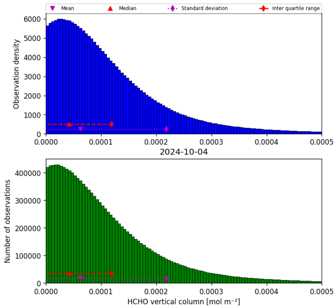
Figure 35: Histogram of “HCHO vertical column” for 2024-10-03 to 2024-10-05
