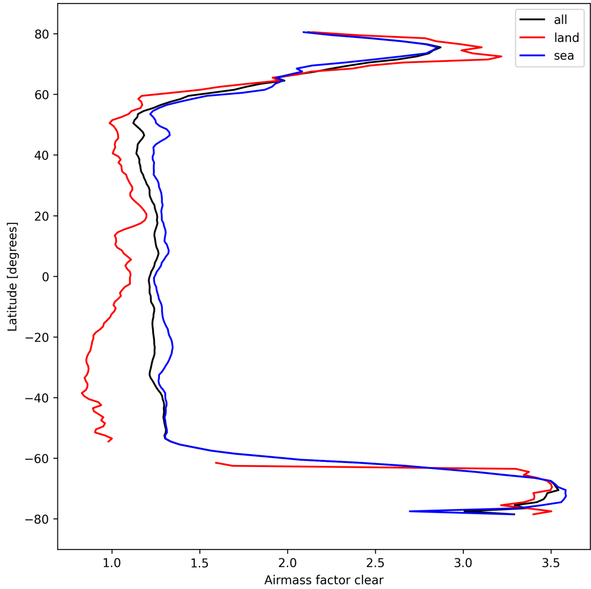
Figure 28: Zonal average of “Airmass factor clear” for 2024-10-03 to 2024-10-05.
