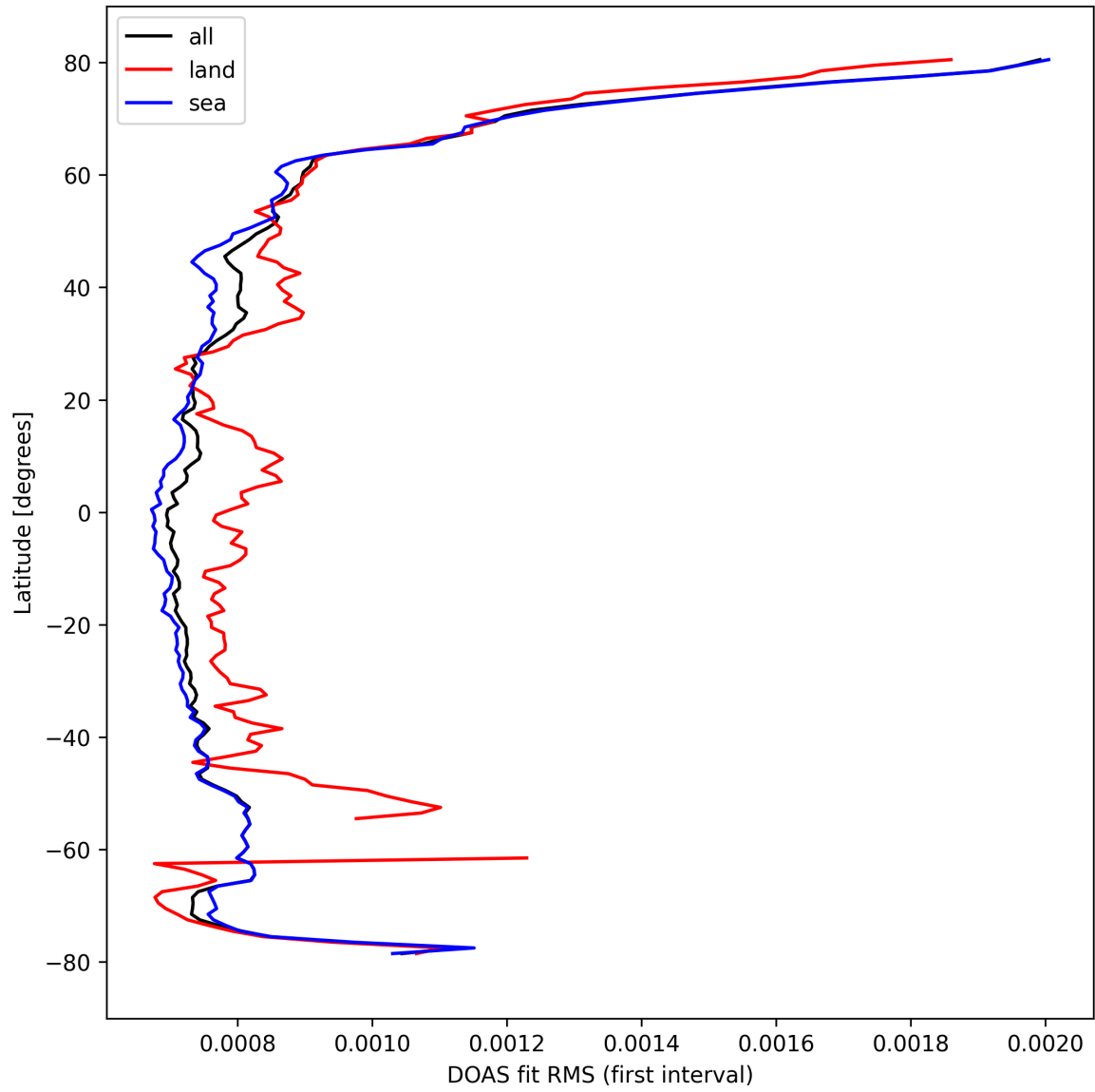
Figure 32: Zonal average of "DOAS fit RMS (first interval)" for 2024-10-03 to 2024-10-05.
