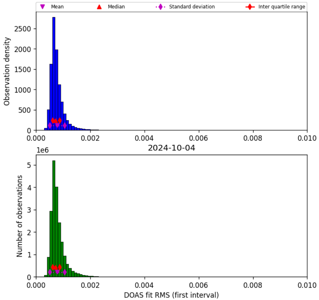
Figure 46: Histogram of “DOAS fit RMS (first interval)” for 2024-10-03 to 2024-10-05
