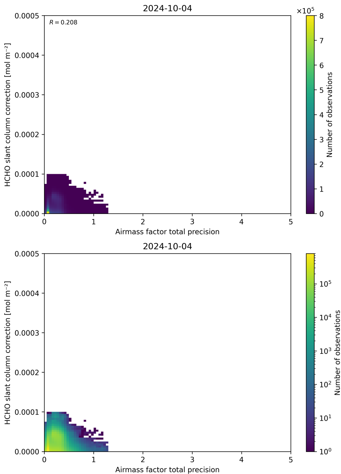
Figure 110: Scatter density plot of “Airmass factor total precision” against “HCHO slant column correction” for 2024-10-03 to 2024-10-05.
