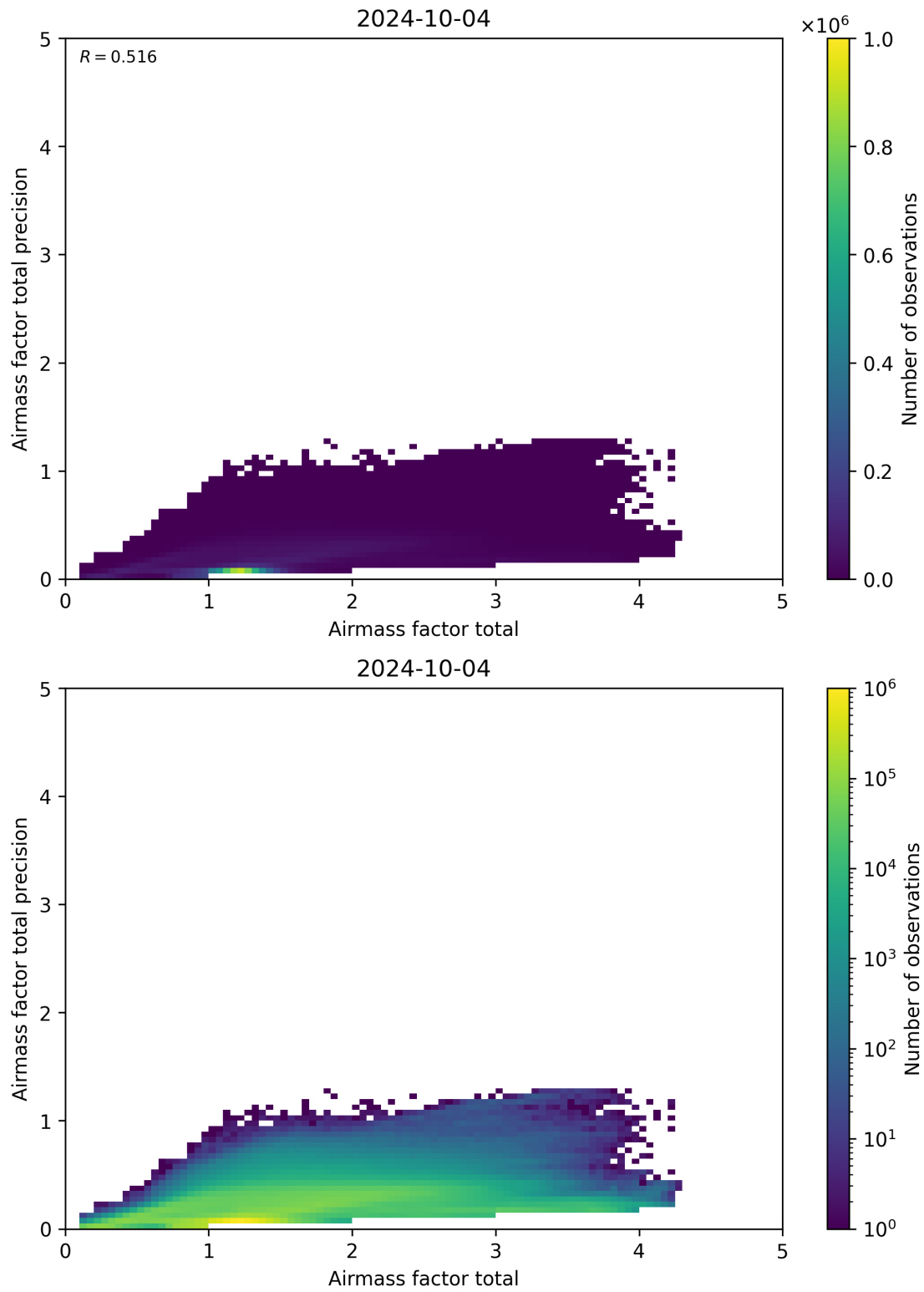
Figure 103: Scatter density plot of “Airmass factor total” against “Airmass factor total precision” for 2024-10-03 to 2024-10-05.
