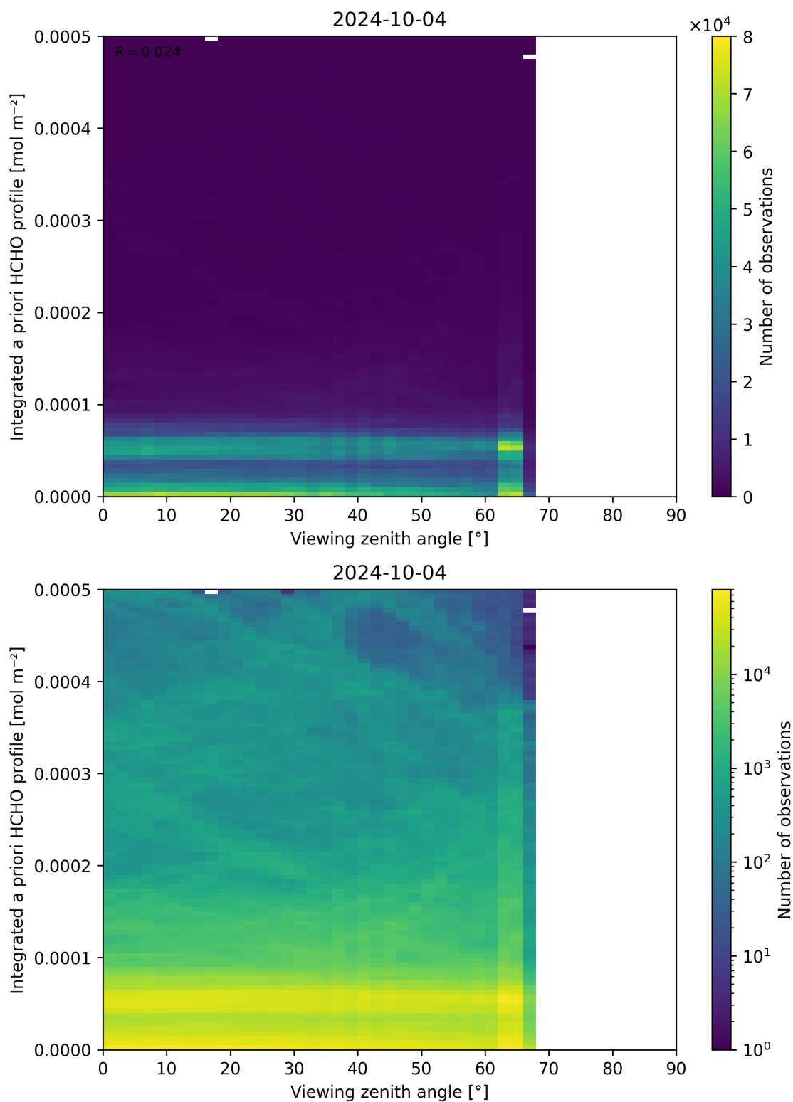
Figure 195: Scatter density plot of “Viewing zenith angle” against “Integrated a priori HCHO profile” for 2024-10-03 to 2024-10-05.
