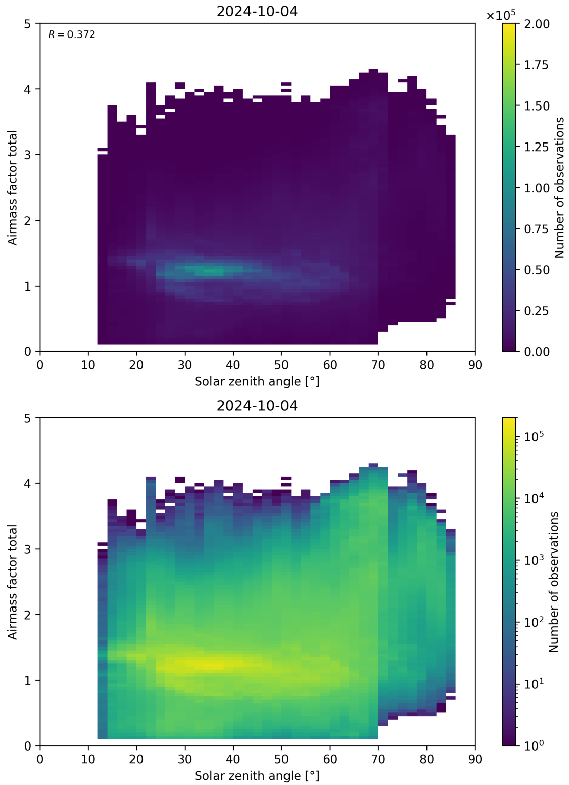
Figure 175: Scatter density plot of “Solar zenith angle” against “Airmass factor total” for 2024-10-03 to 2024-10-05.
