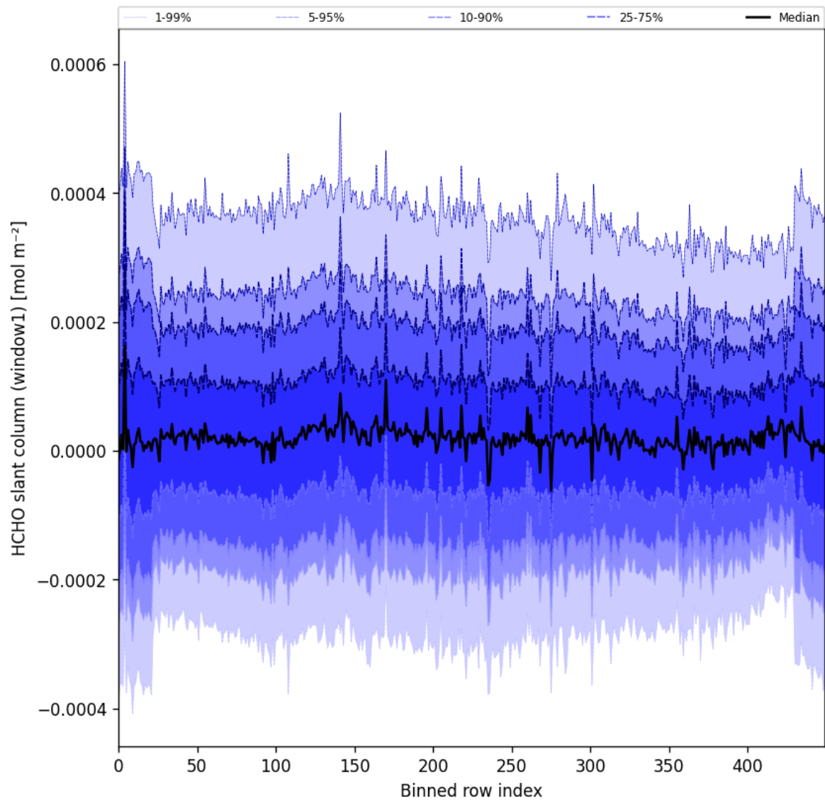
Figure 52: Along track statistics of “HCHO slant column (window1)” for 2024-10-03 to 2024-10-05
