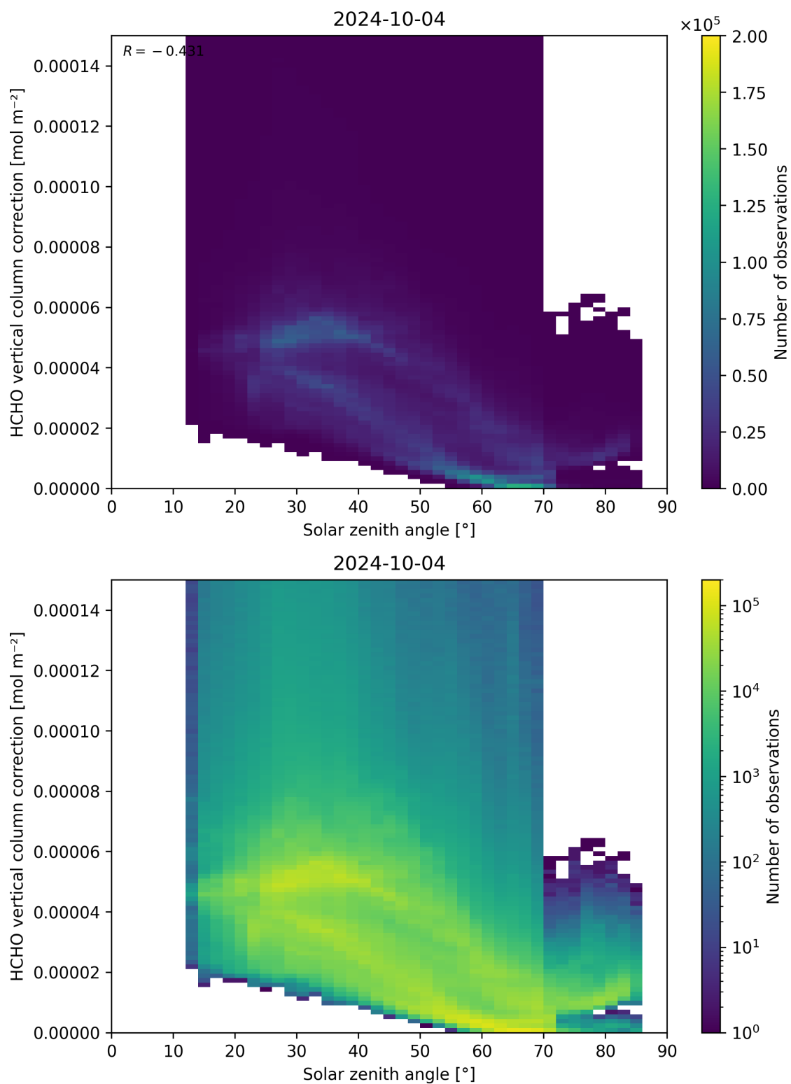
Figure 178: Scatter density plot of “Solar zenith angle” against “HCHO vertical column correction” for 2024-10-03 to 2024-10-05.
