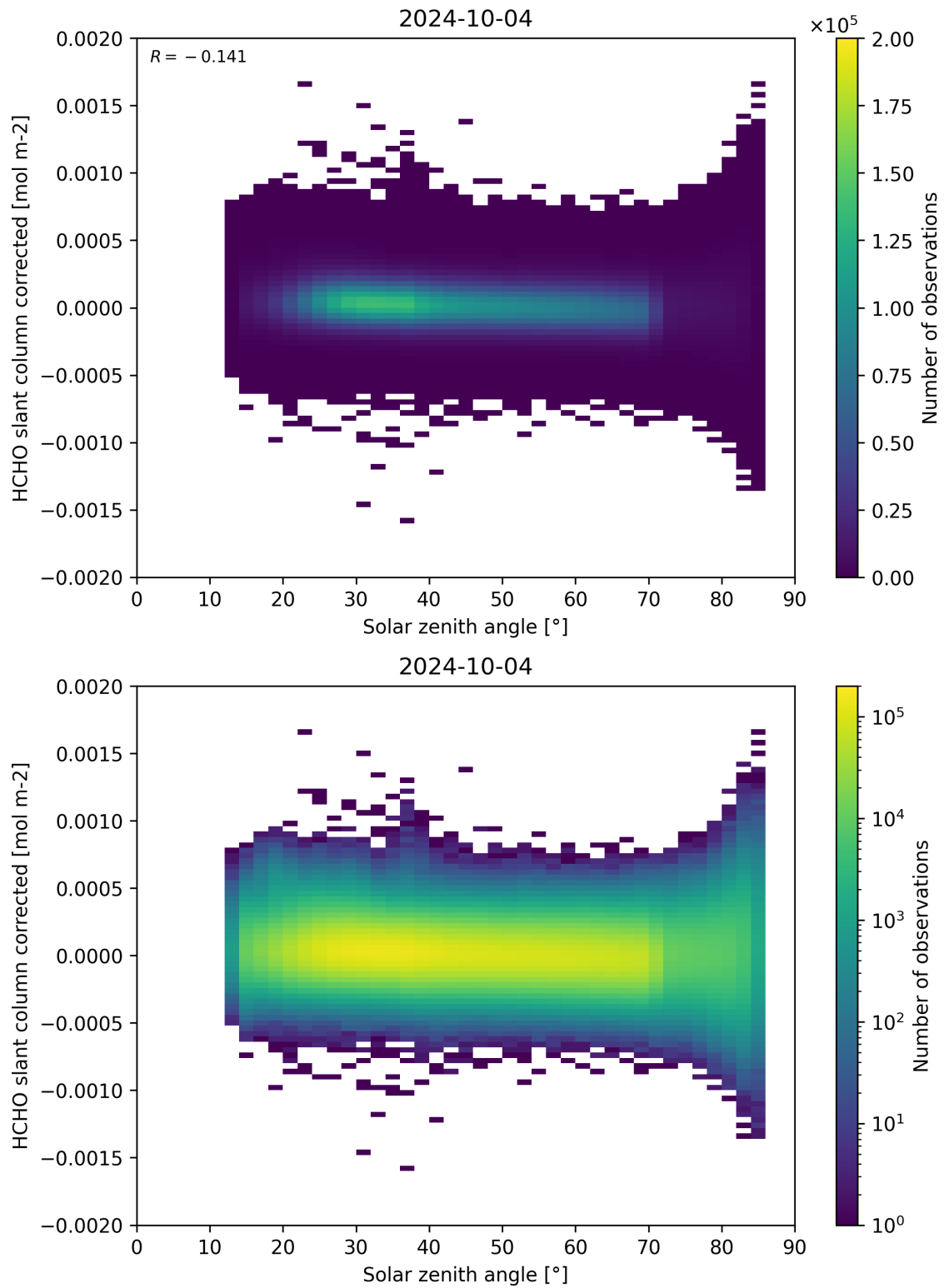
Figure 171: Scatter density plot of “Solar zenith angle” against “HCHO slant column corrected” for 2024-10-03 to 2024-10-05.
