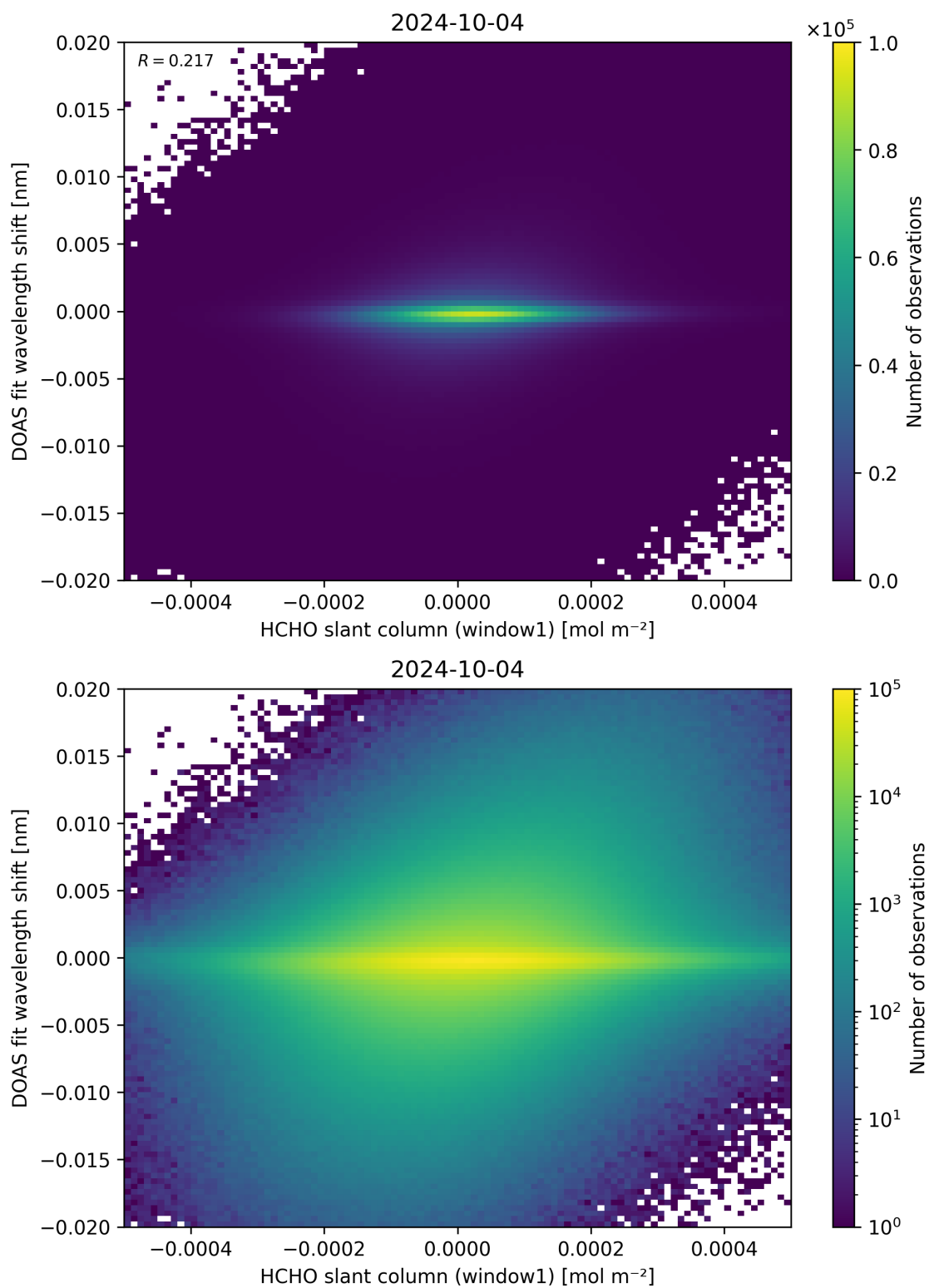
Figure 79: Scatter density plot of “HCHO slant column (window1)” against “DOAS fit wavelength shift” for 2024-10-03 to 2024-10-05.
