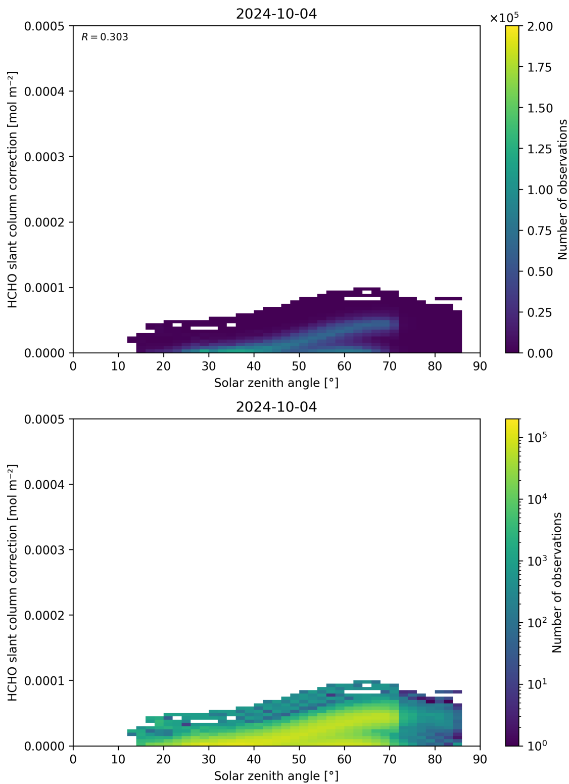
Figure 172: Scatter density plot of “Solar zenith angle” against “HCHO slant column correction” for 2024-10-03 to 2024-10-05.
