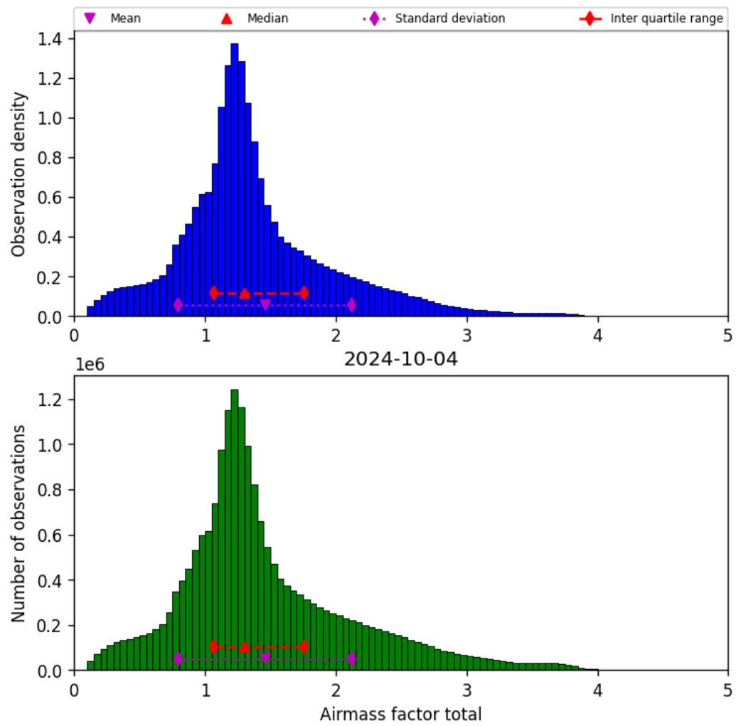
Figure 40: Histogram of “Airmass factor total” for 2024-10-03 to 2024-10-05
