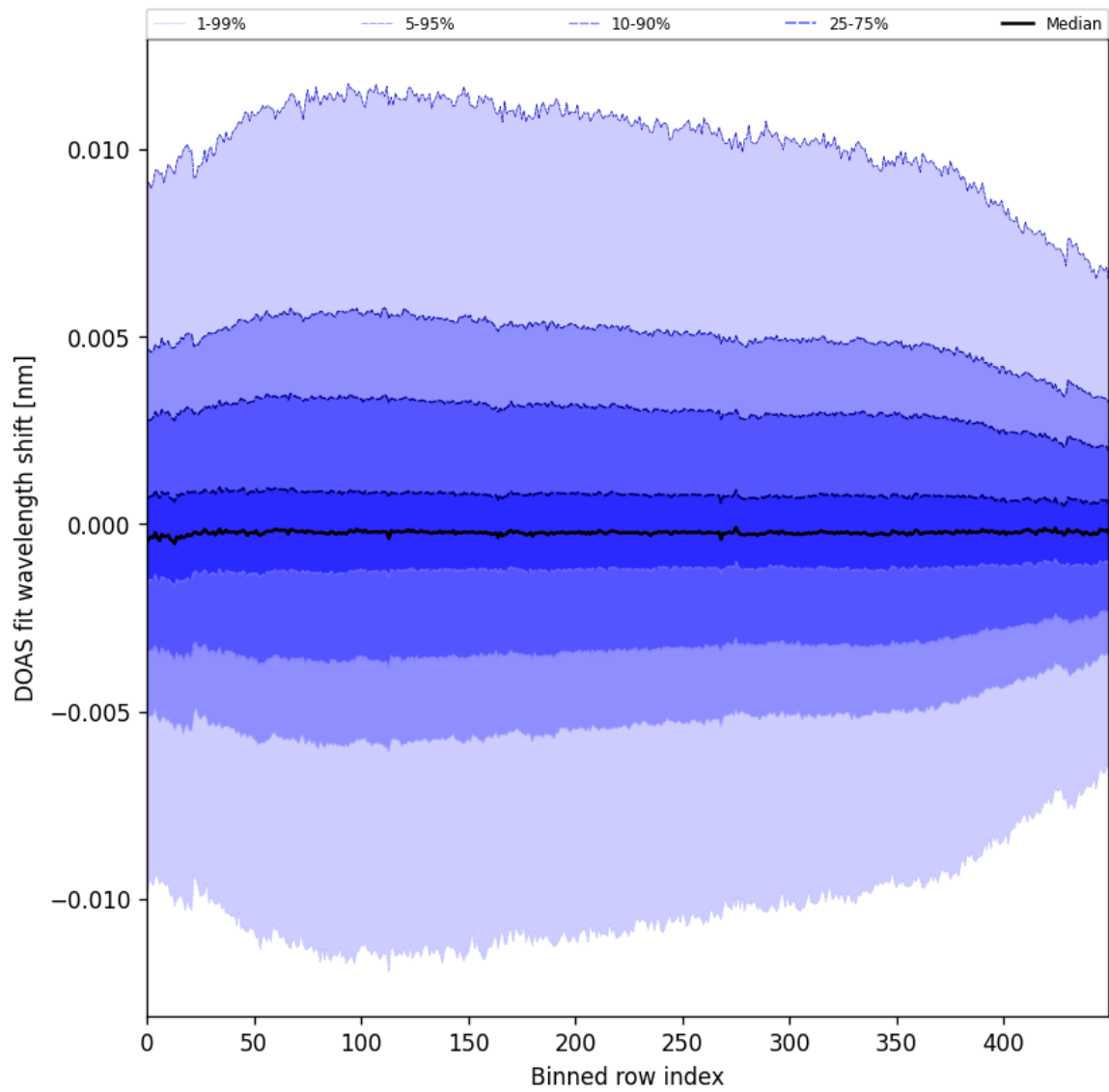
Figure 58: Along track statistics of “DOAS fit wavelength shift” for 2024-10-03 to 2024-10-05
