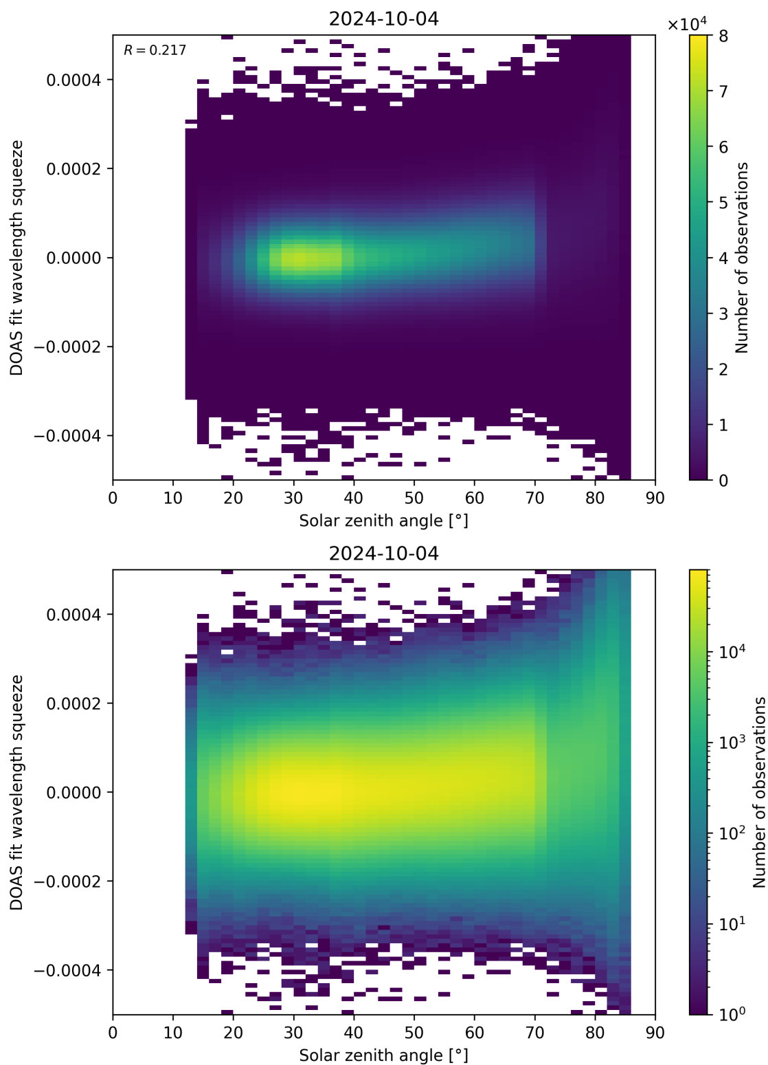
Figure 169: Scatter density plot of “Solar zenith angle” against “DOAS fit wavelength squeeze” for 2024-10-03 to 2024-10-05.
