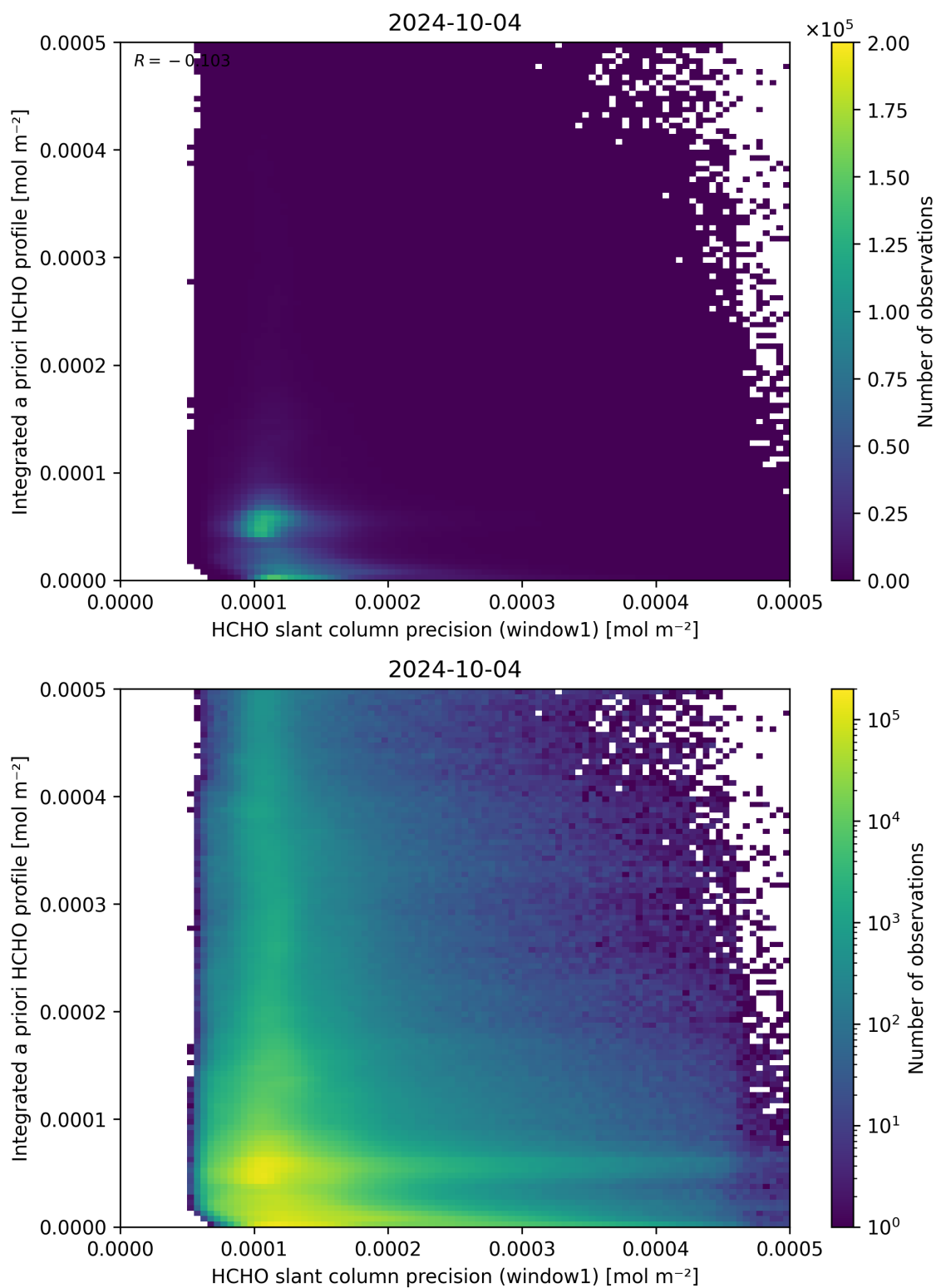
Figure 96: Scatter density plot of “HCHO slant column precision (window1)” against “Integrated a priori HCHO profile” for 2024-10-03 to 2024-10-05.
