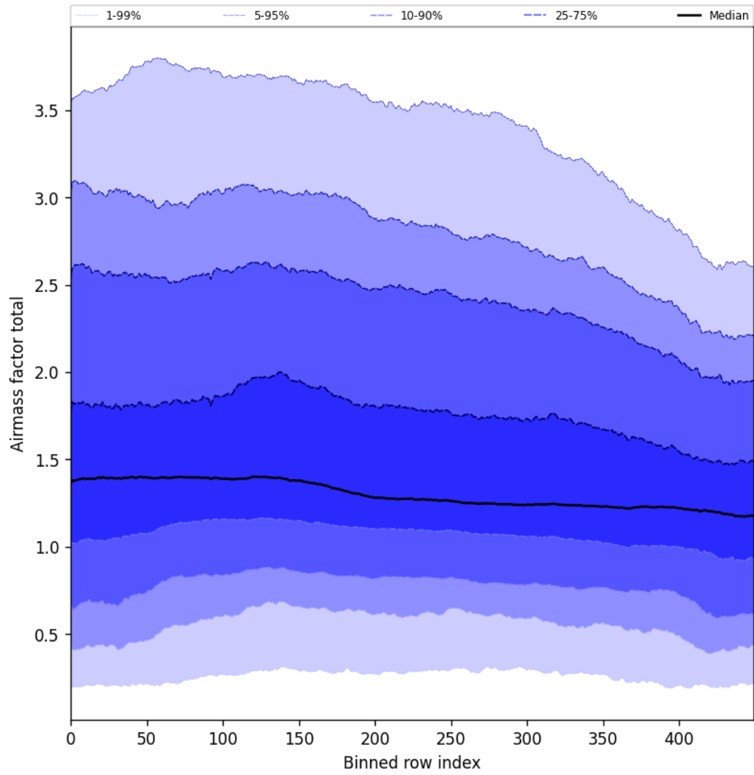
Figure 54: Along track statistics of “Airmass factor total” for 2024-10-03 to 2024-10-05
