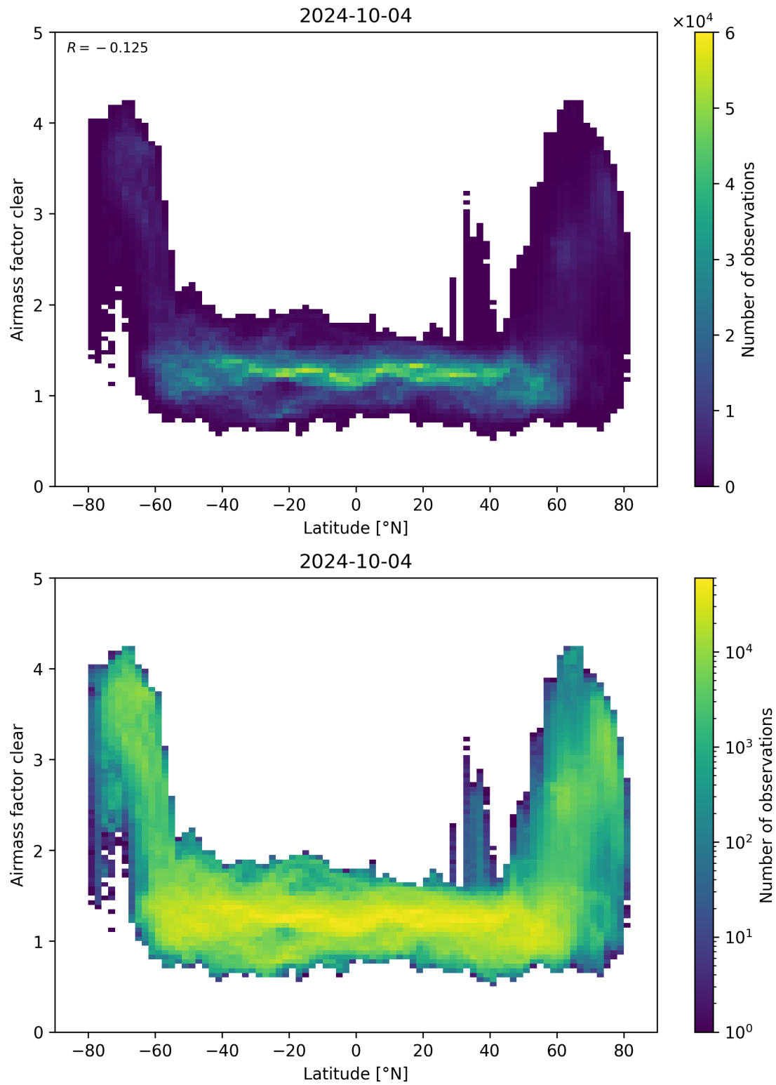
Figure 156: Scatter density plot of “Latitude” against “Airmass factor clear” for 2024-10-03 to 2024-10-05.
