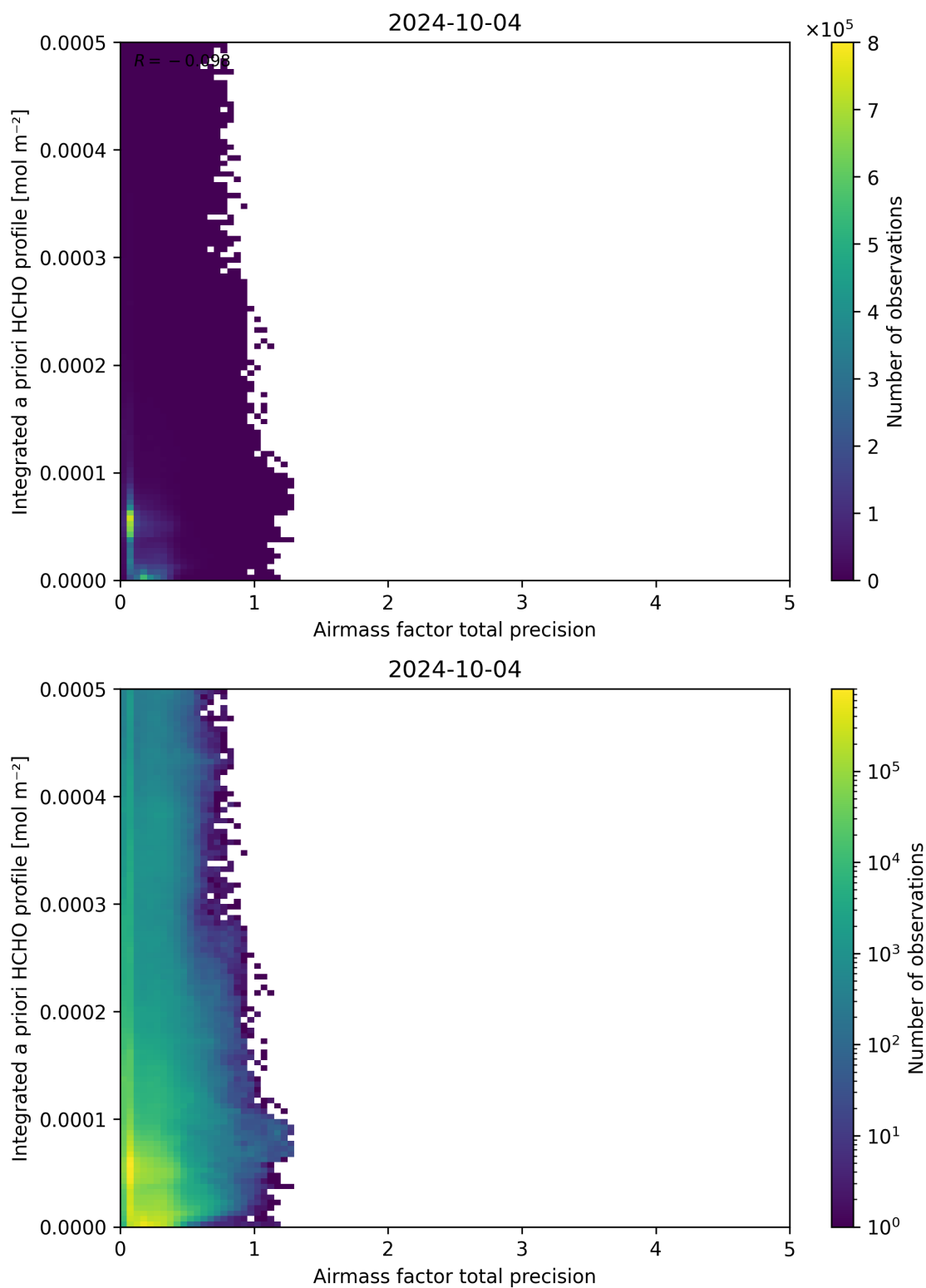
Figure 111: Scatter density plot of “Airmass factor total precision” against “Integrated a priori HCHO profile” for 2024-10-03 to 2024-10-05.
