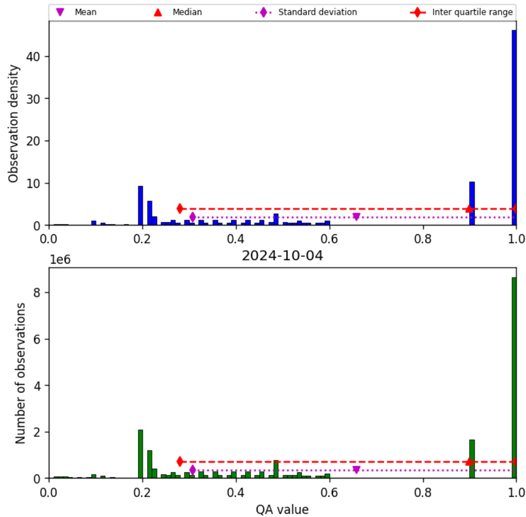
Figure 34: Histogram of “QA value” for 2024-10-03 to 2024-10-05
