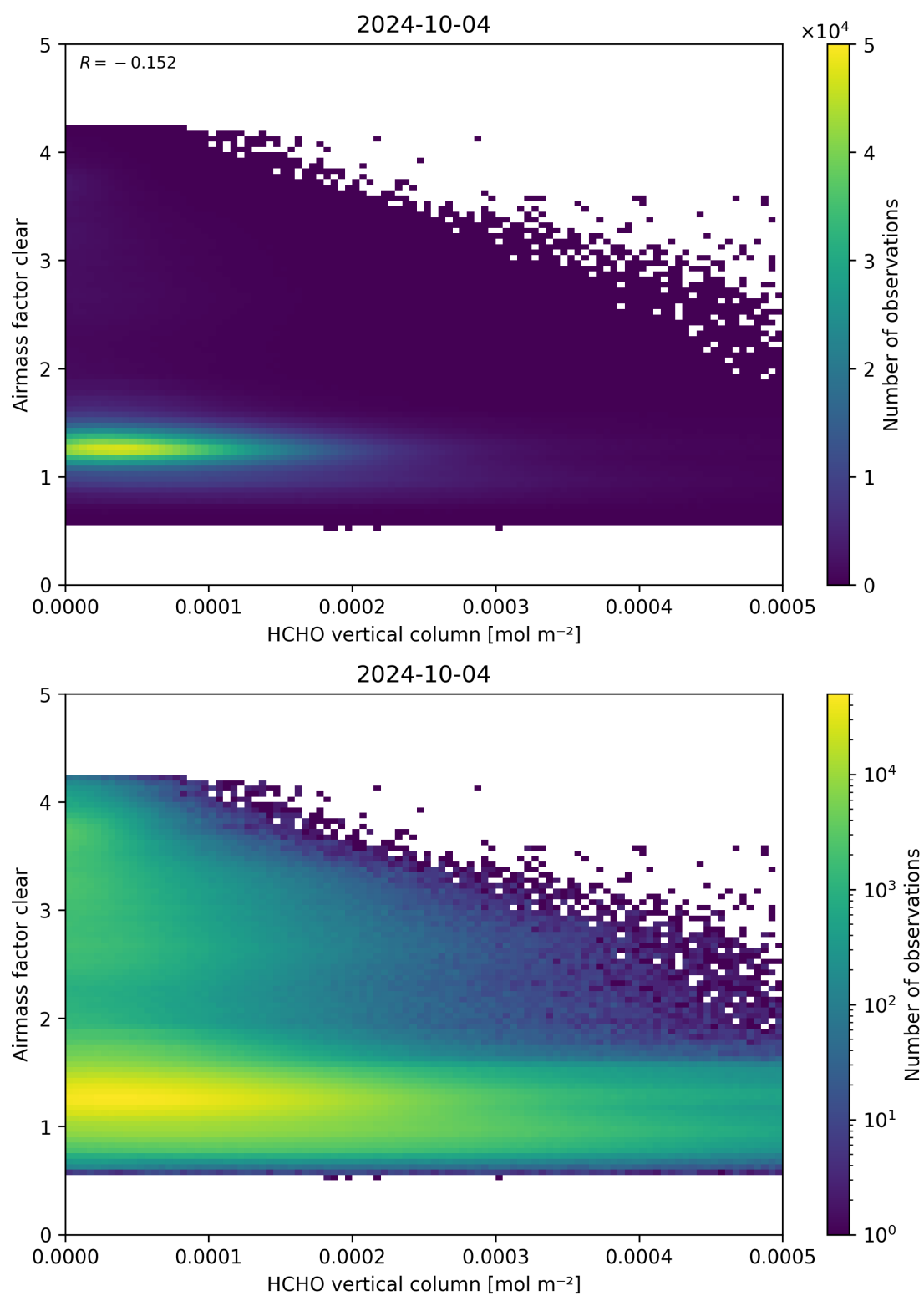
Figure 126: Scatter density plot of “HCHO vertical column” against “Airmass factor clear” for 2024-10-03 to 2024-10-05.
