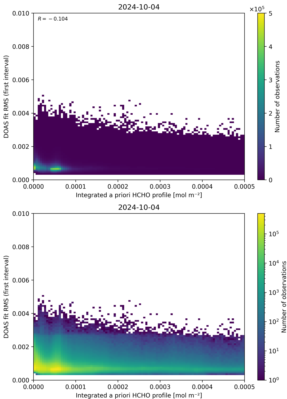
Figure 148: Scatter density plot of “Integrated a priori HCHO profile” against “DOAS fit RMS (first interval)” for 2024-10-03 to 2024-10-05.
