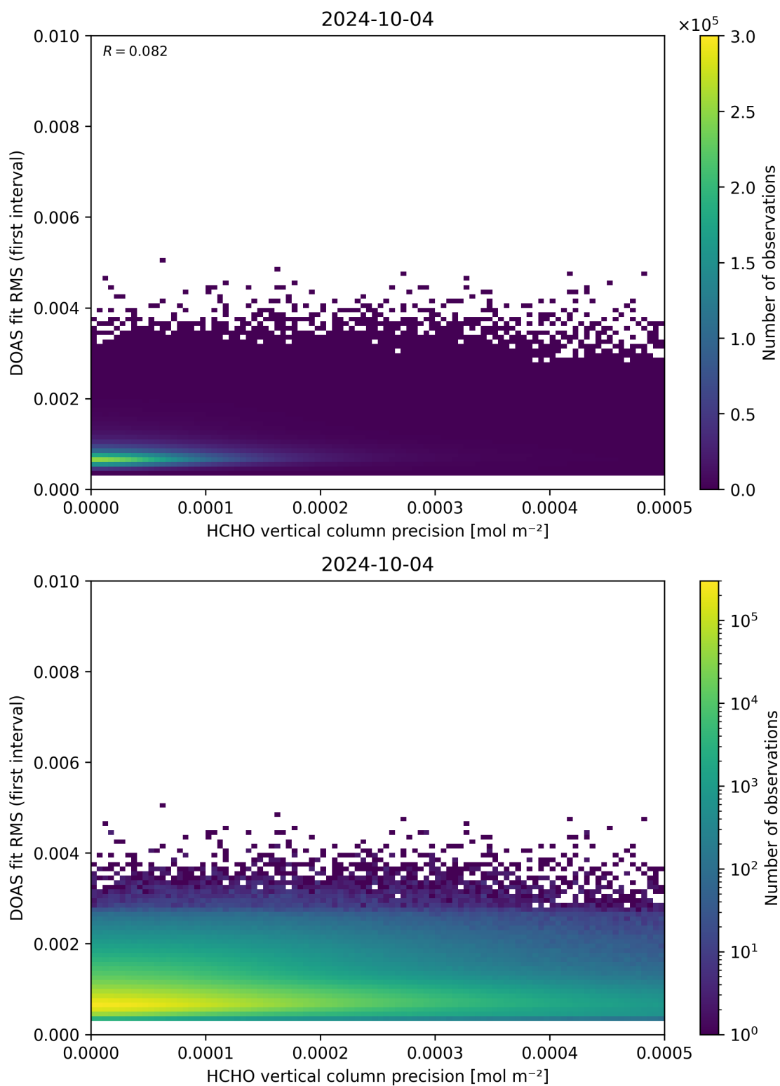
Figure 136: Scatter density plot of “HCHO vertical column precision” against “DOAS fit RMS (first interval)” for 2024-10-03 to 2024-10-05.
