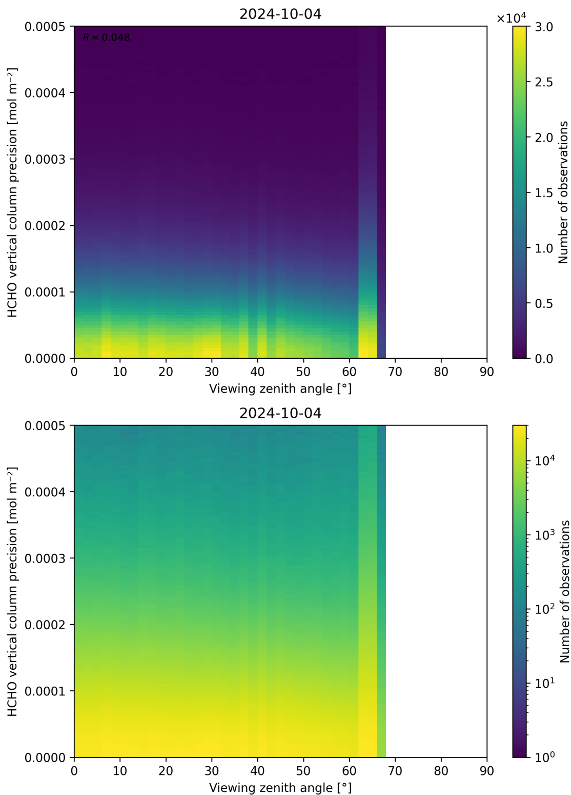
Figure 194: Scatter density plot of “Viewing zenith angle” against “HCHO vertical column precision” for 2024-10-03 to 2024-10-05.
