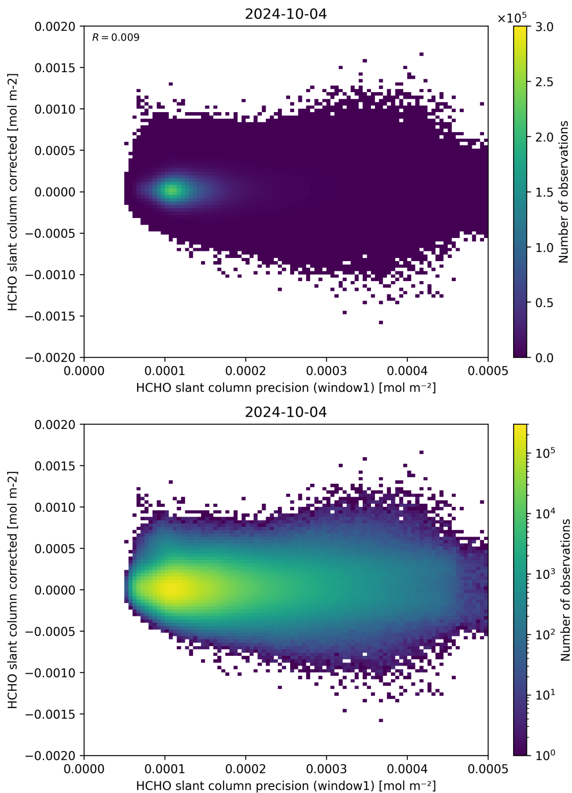
Figure 92: Scatter density plot of “HCHO slant column precision (window1)” against “HCHO slant column corrected” for 2024-10-03 to 2024-10-05.
