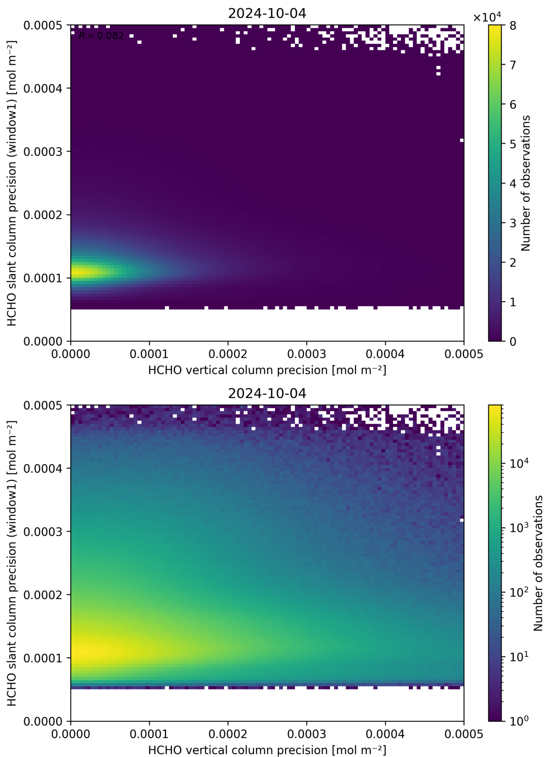
Figure 143: Scatter density plot of “HCHO vertical column precision” against “HCHO slant column precision (window1)” for 2024-10-03 to 2024-10-05.
