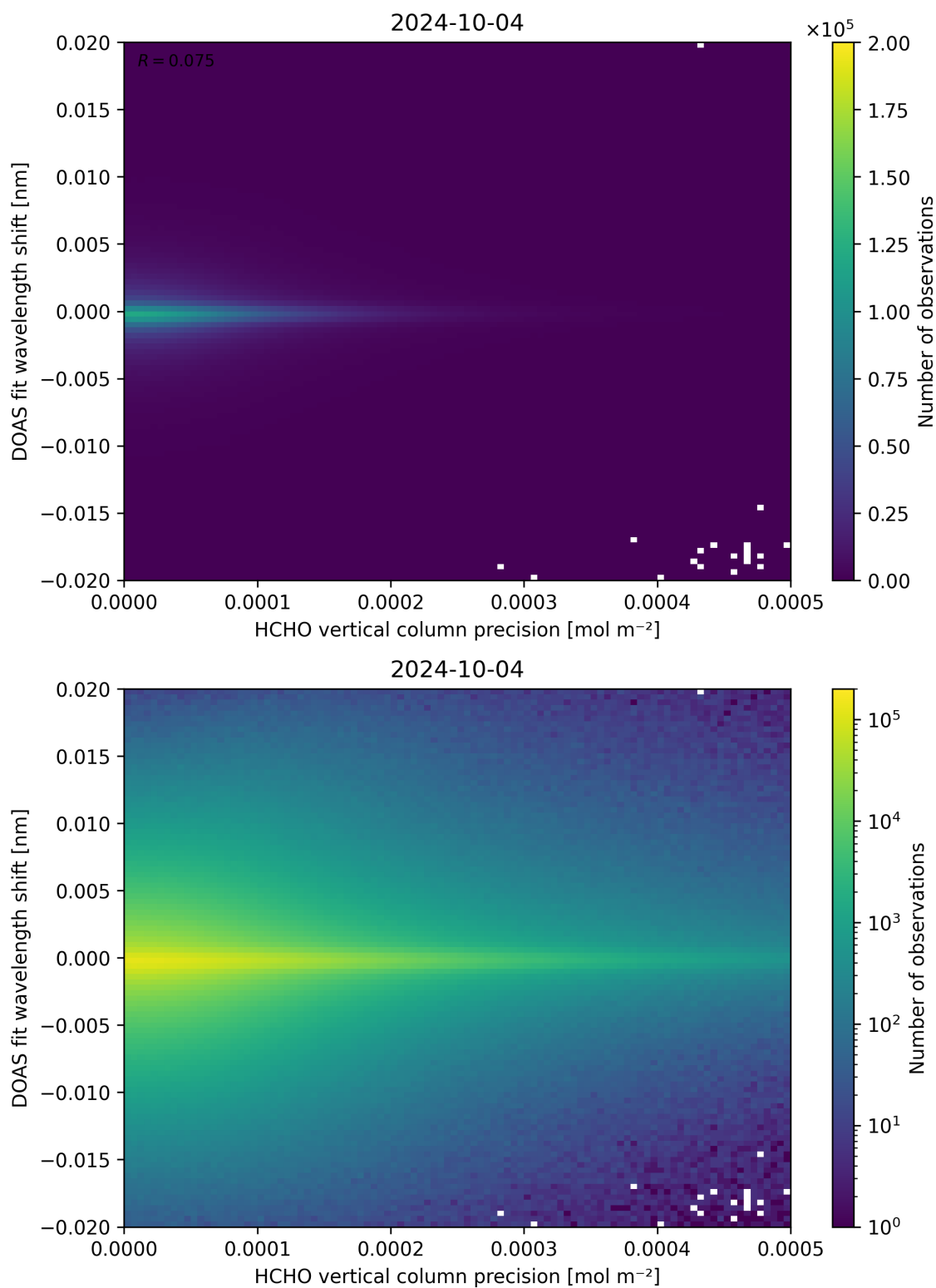
Figure 137: Scatter density plot of “HCHO vertical column precision” against “DOAS fit wavelength shift” for 2024-10-03 to 2024-10-05.
