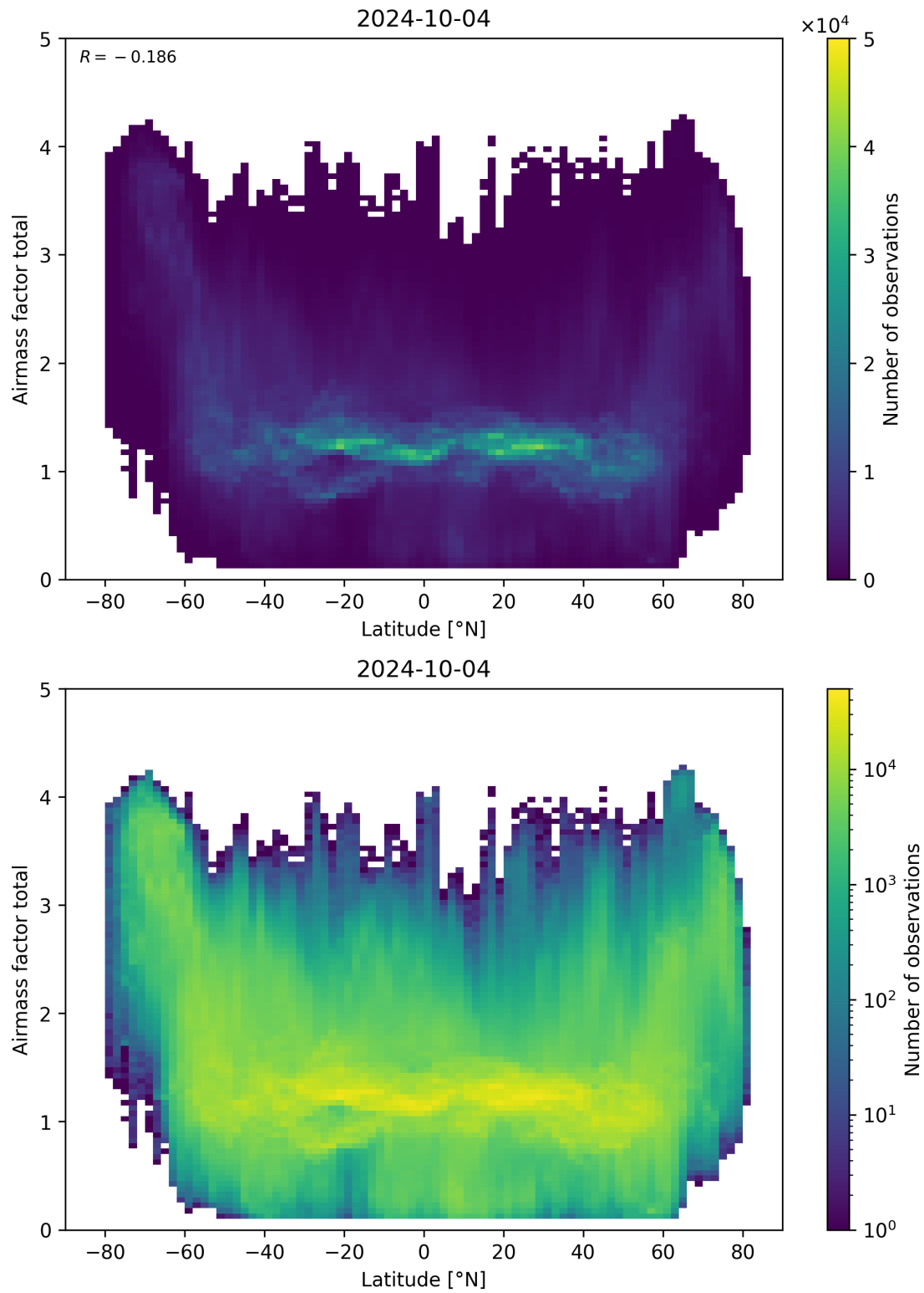
Figure 161: Scatter density plot of “Latitude” against “Airmass factor total” for 2024-10-03 to 2024-10-05.
