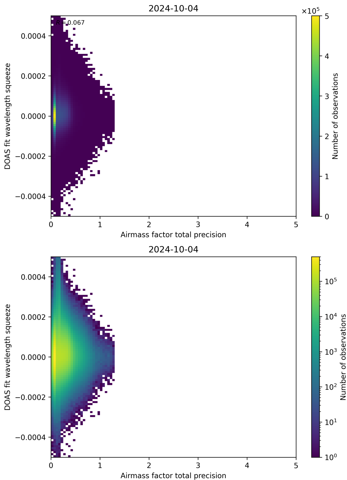
Figure 107: Scatter density plot of “Airmass factor total precision” against “DOAS fit wavelength squeeze” for 2024-10-03 to 2024-10-05.
