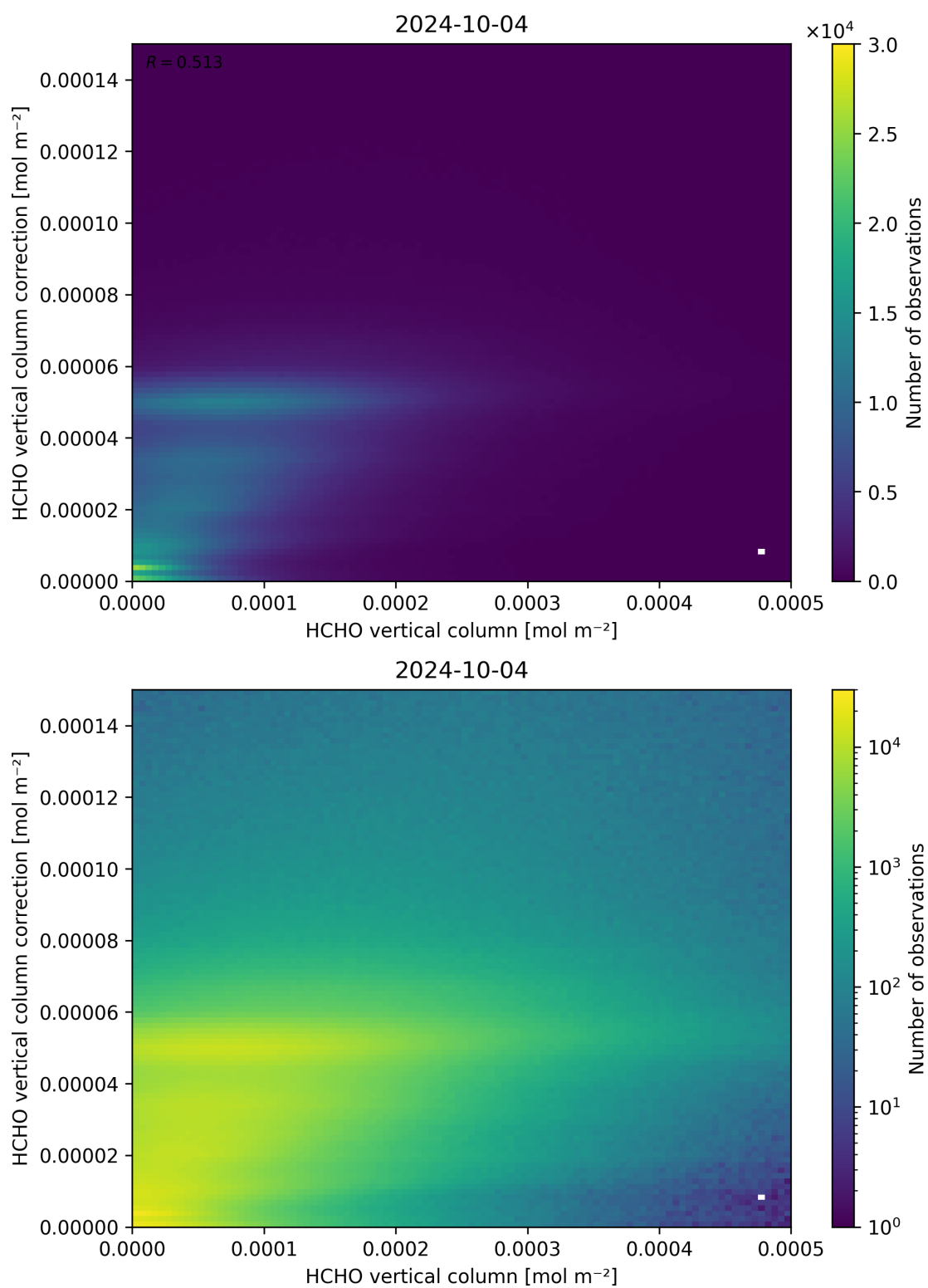
Figure 133: Scatter density plot of “HCHO vertical column” against “HCHO vertical column correction” for 2024-10-03 to 2024-10-05.
