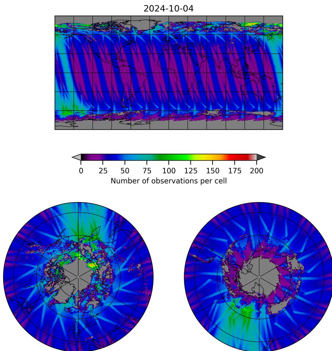
Figure 19: Map of the number of observations for 2024-10-03 to 2024-10-05
