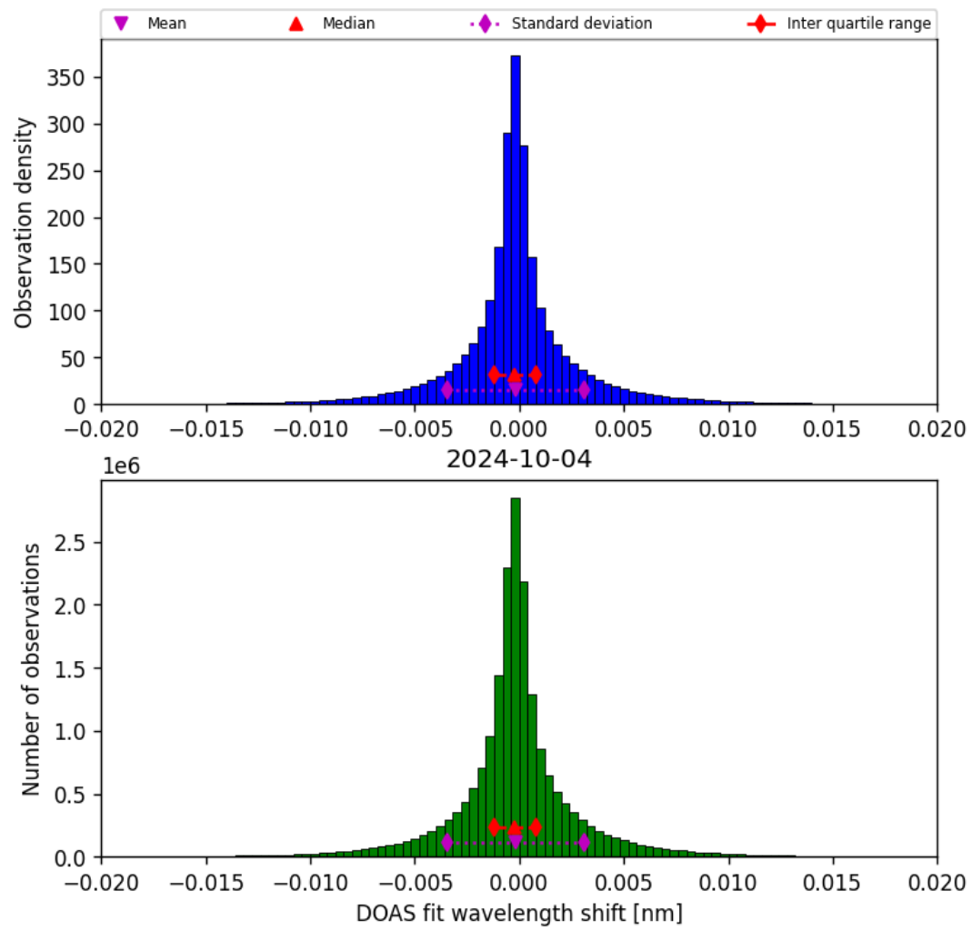
Figure 44: Histogram of “DOAS fit wavelength shift” for 2024-10-03 to 2024-10-05
