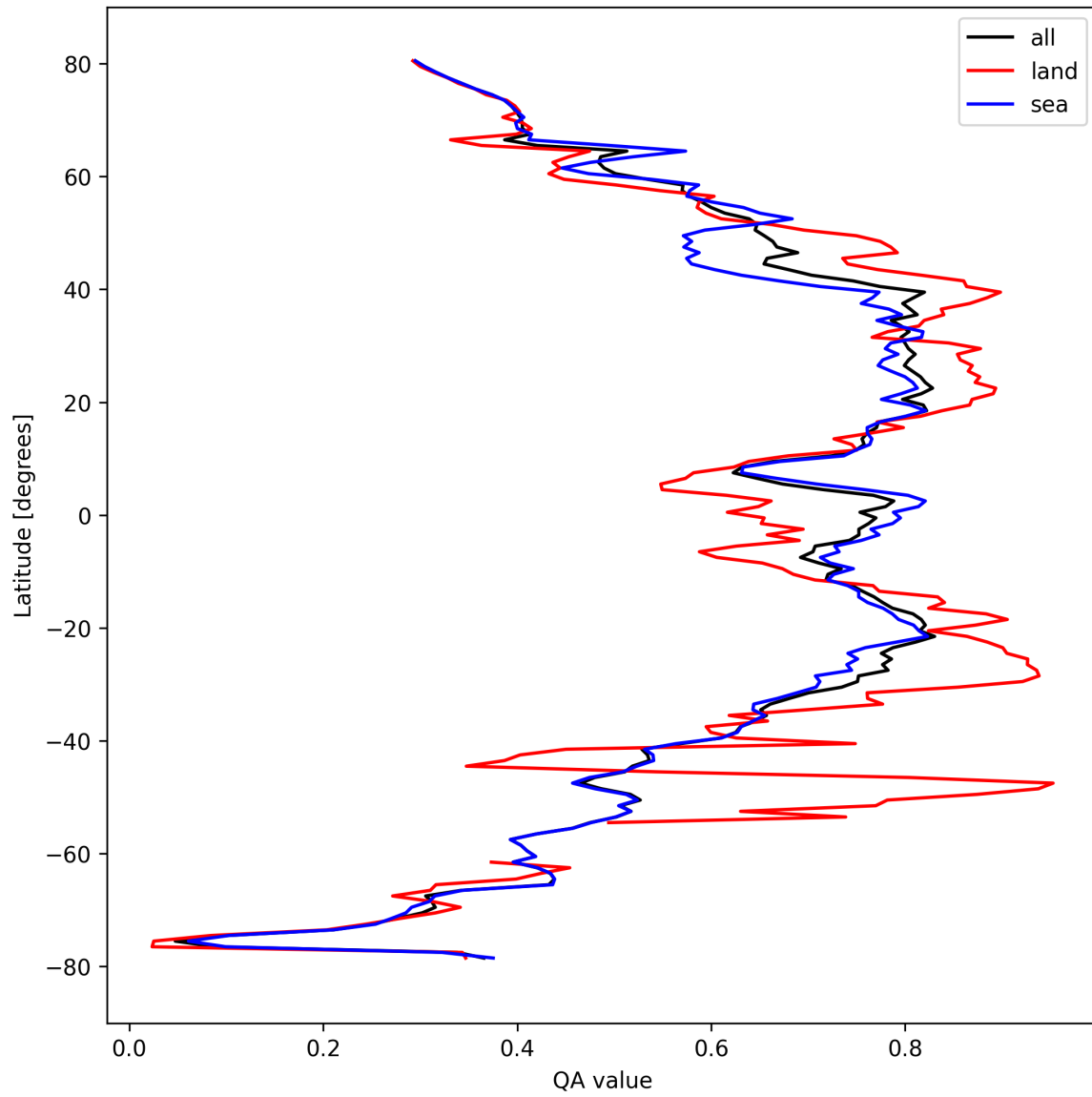
Figure 20: Zonal average of “QA value” for 2024-10-03 to 2024-10-05.
