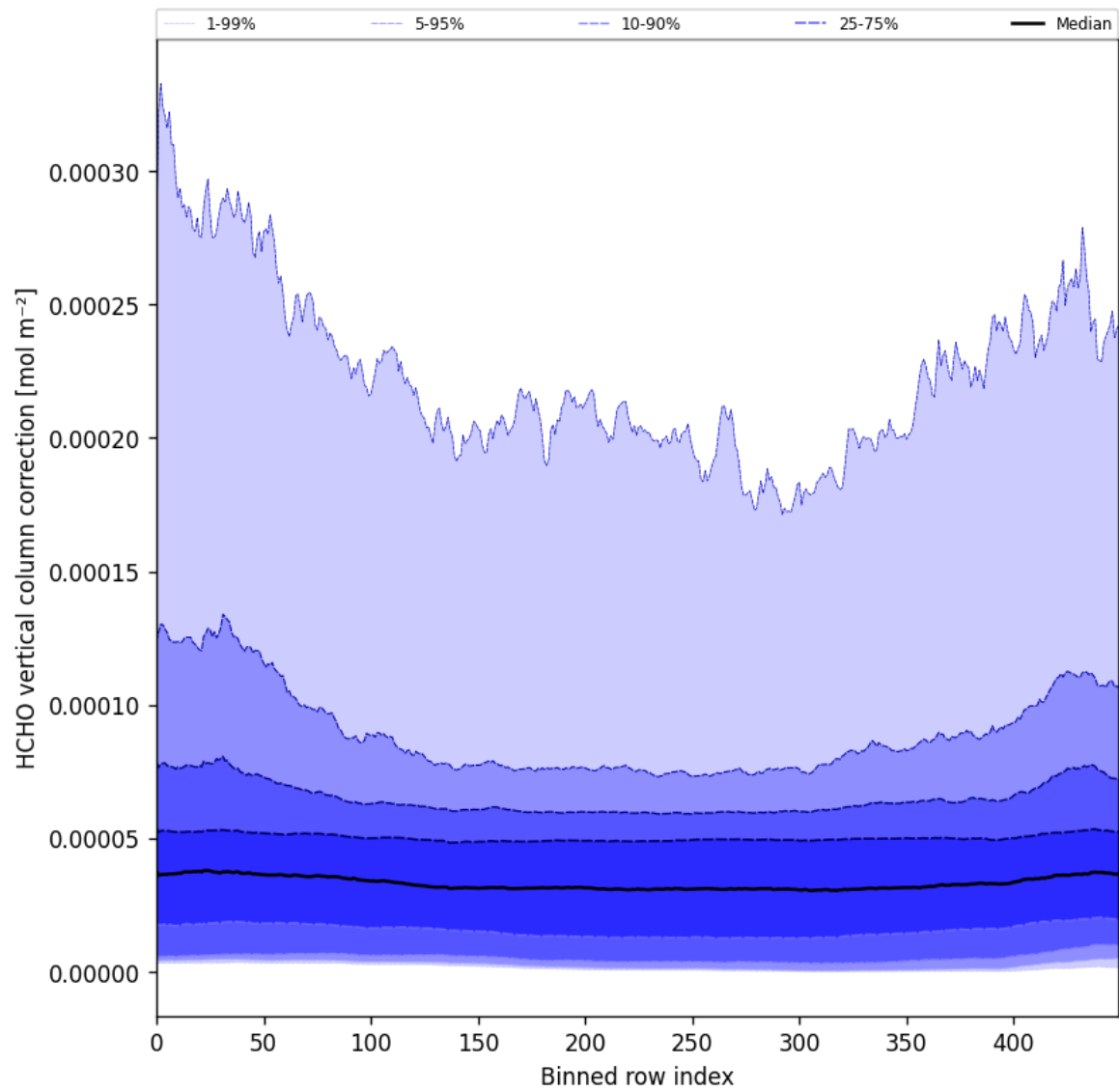
Figure 51: Along track statistics of “HCHO vertical column correction” for 2024-10-03 to 2024-10-05
