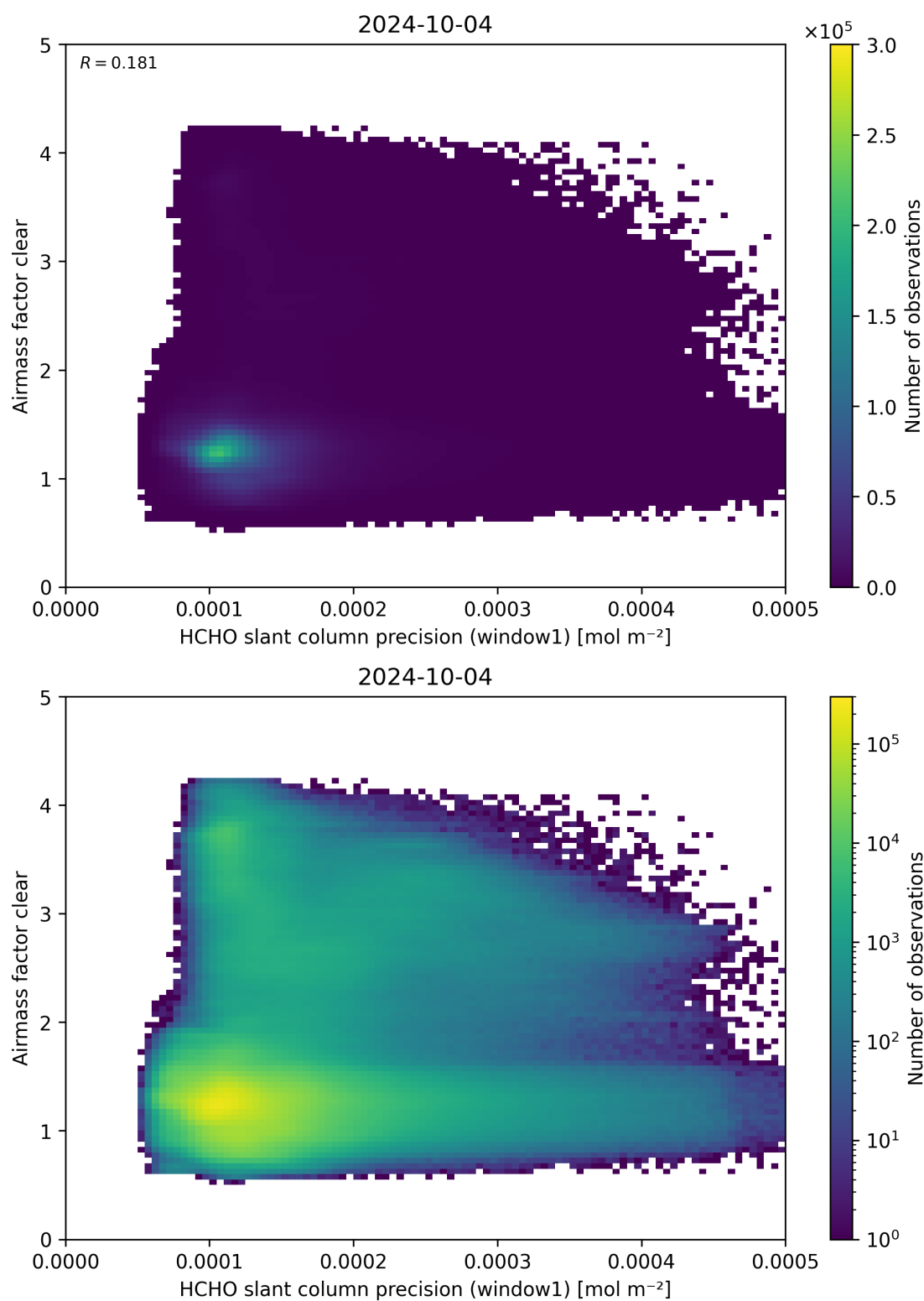
Figure 91: Scatter density plot of “HCHO slant column precision (window1)” against “Airmass factor clear” for 2024-10-03 to 2024-10-05.
