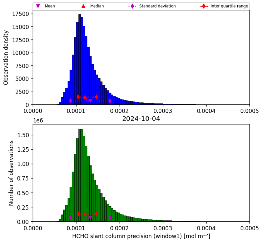
Figure 39: Histogram of “HCHO slant column precision (window1)” for 2024-10-03 to 2024-10-05
