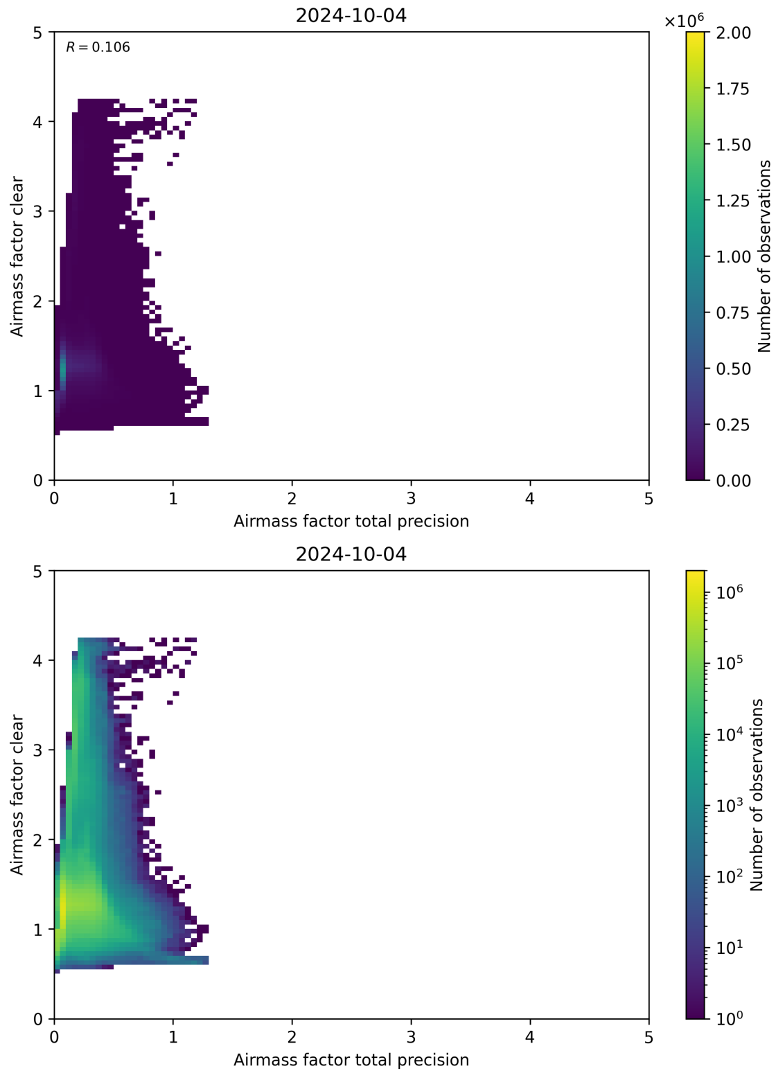
Figure 108: Scatter density plot of “Airmass factor total precision” against “Airmass factor clear” for 2024-10-03 to 2024-10-05.
