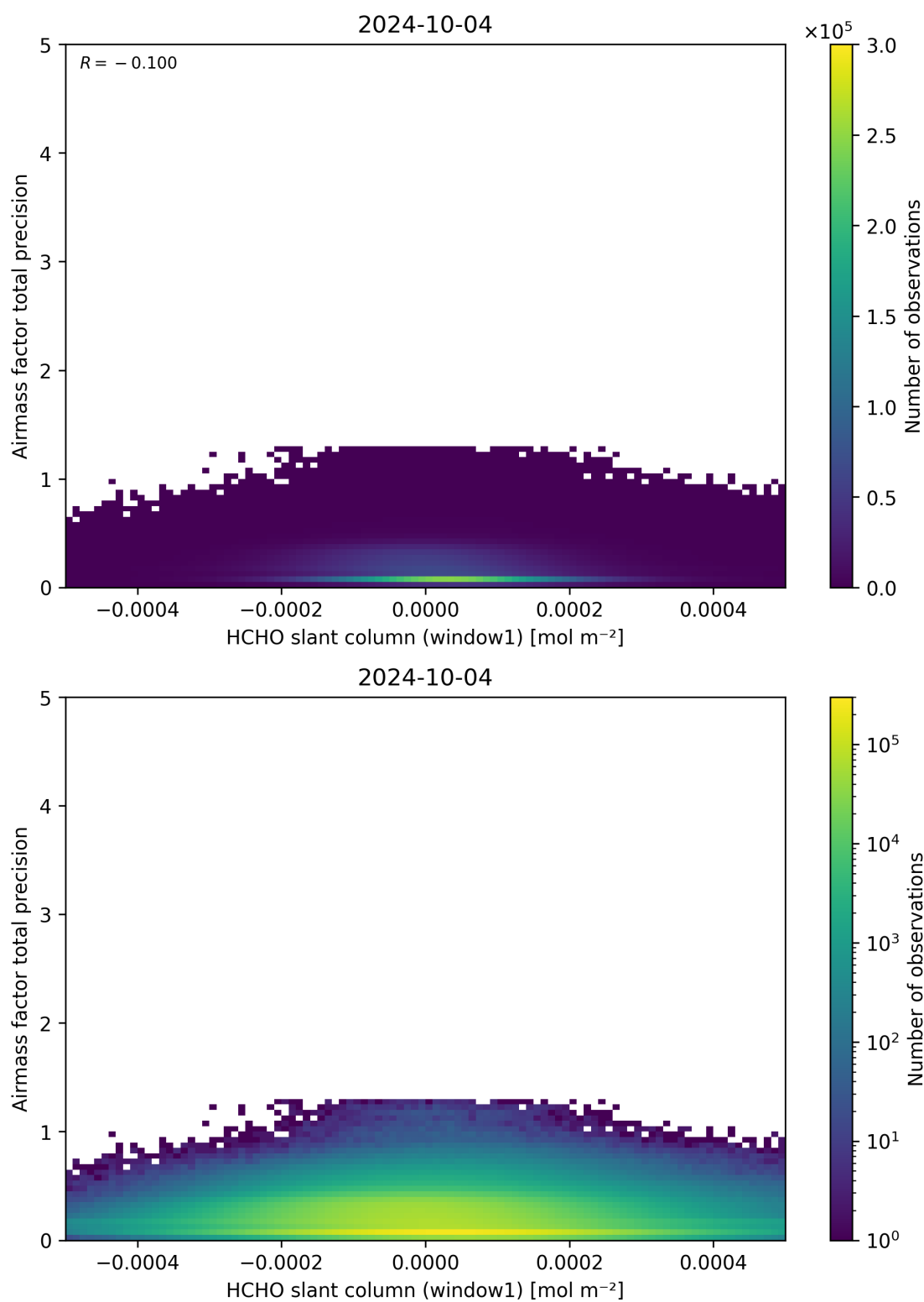
Figure 86: Scatter density plot of “HCHO slant column (window1)” against “Airmass factor total precision” for 2024-10-03 to 2024-10-05.
