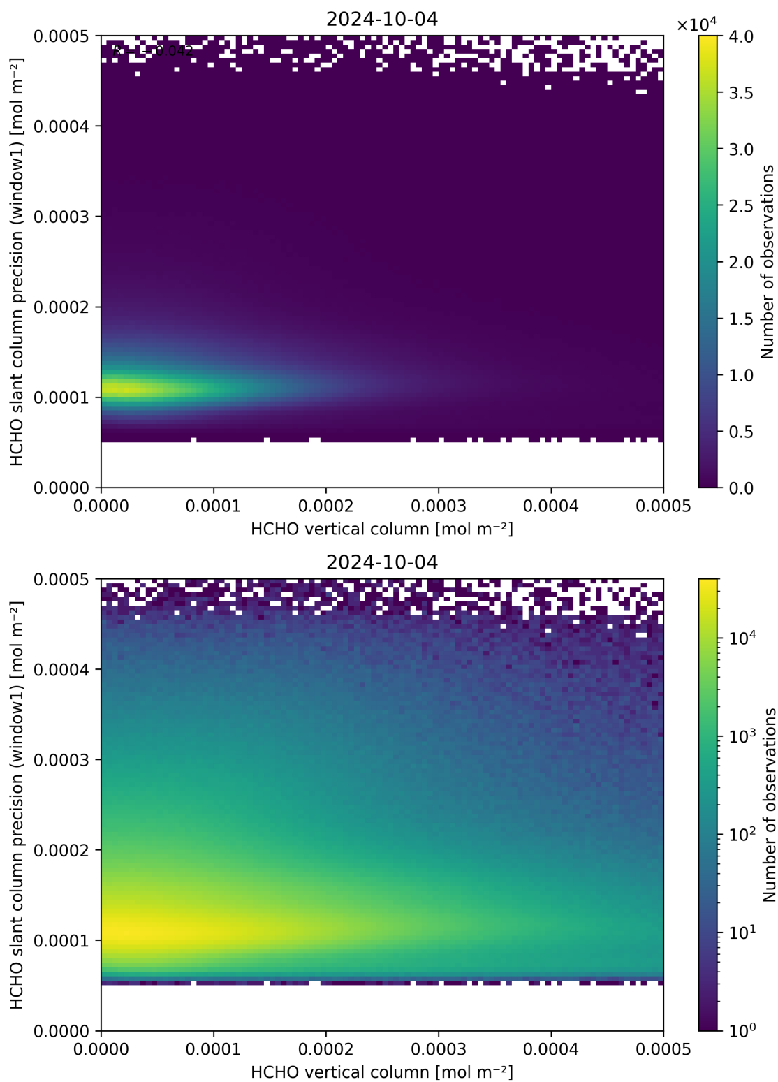
Figure 130: Scatter density plot of “HCHO vertical column” against “HCHO slant column precision (window1)” for 2024-10-03 to 2024-10-05.
