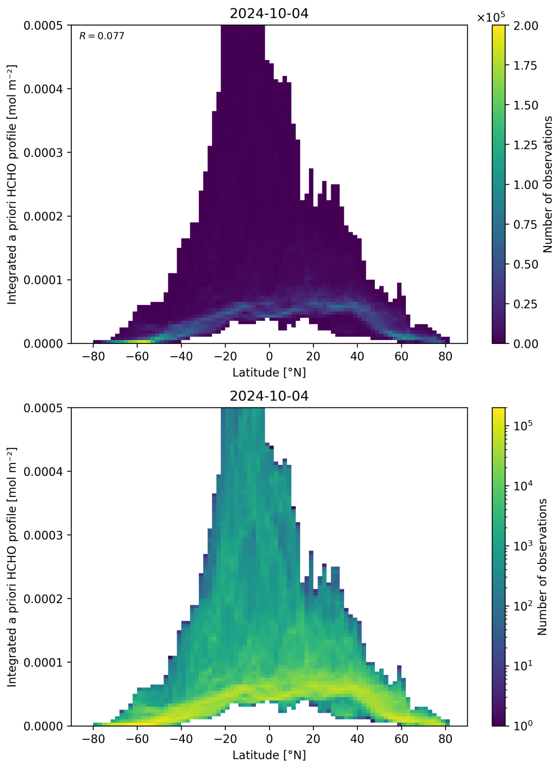
Figure 166: Scatter density plot of “Latitude” against “Integrated a priori HCHO profile” for 2024-10-03 to 2024-10-05.
