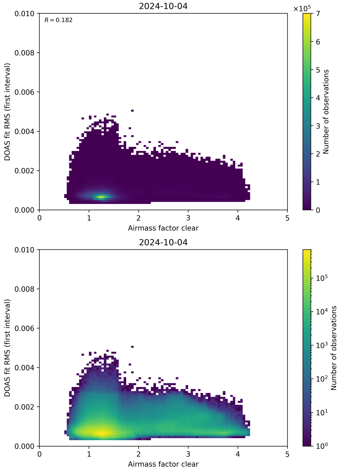
Figure 71: Scatter density plot of “Airmass factor clear” against “DOAS fit RMS (first interval)” for 2024-10-03 to 2024-10-05.
