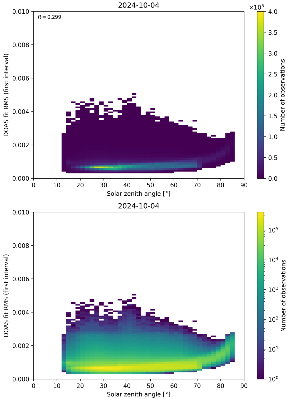
Figure 167: Scatter density plot of “Solar zenith angle” against “DOAS fit RMS (first interval)” for 2024-10-03 to 2024-10-05.
