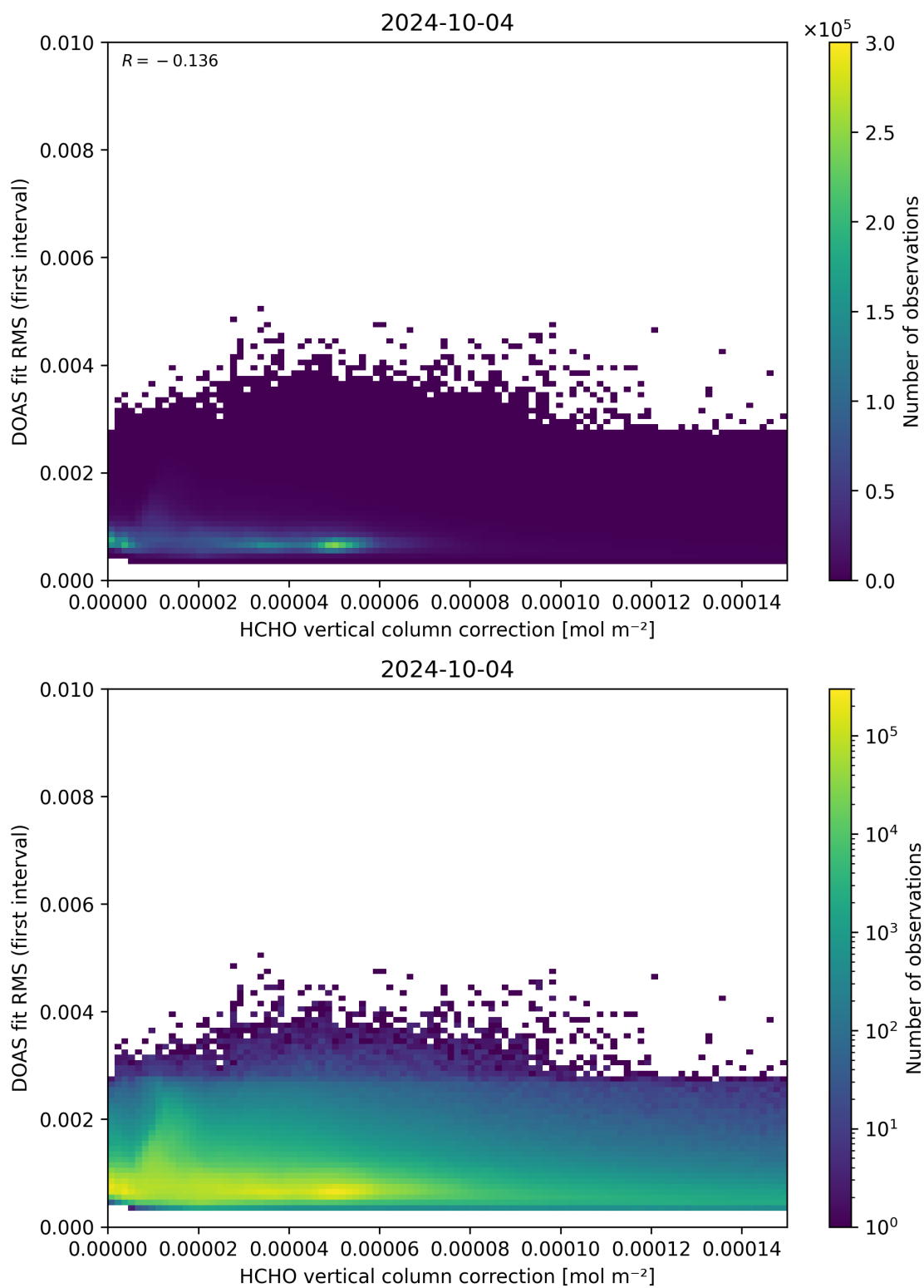
Figure 112: Scatter density plot of “HCHO vertical column correction” against “DOAS fit RMS (first interval)” for 2024-10-03 to 2024-10-05.
