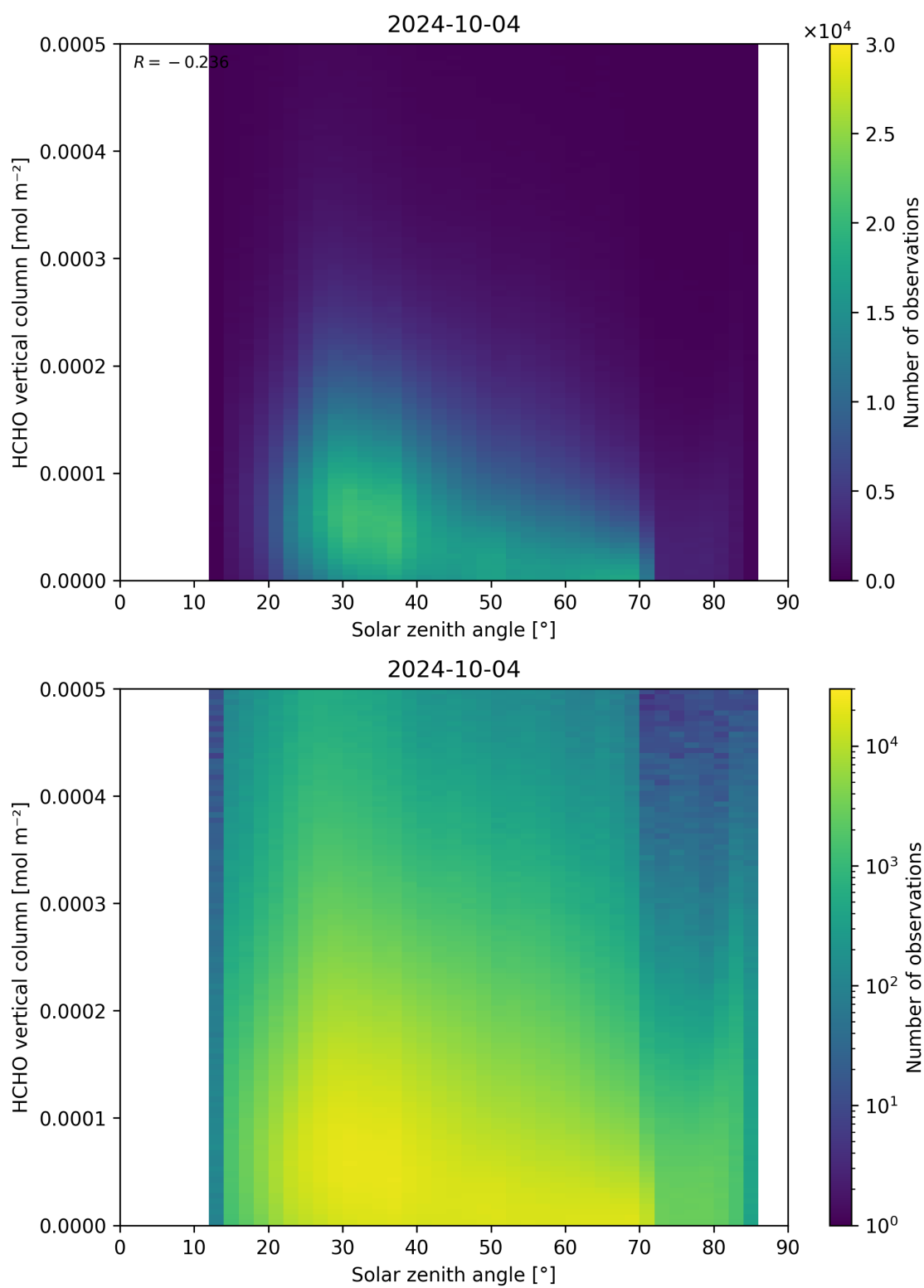
Figure 177: Scatter density plot of “Solar zenith angle” against “HCHO vertical column” for 2024-10-03 to 2024-10-05.
