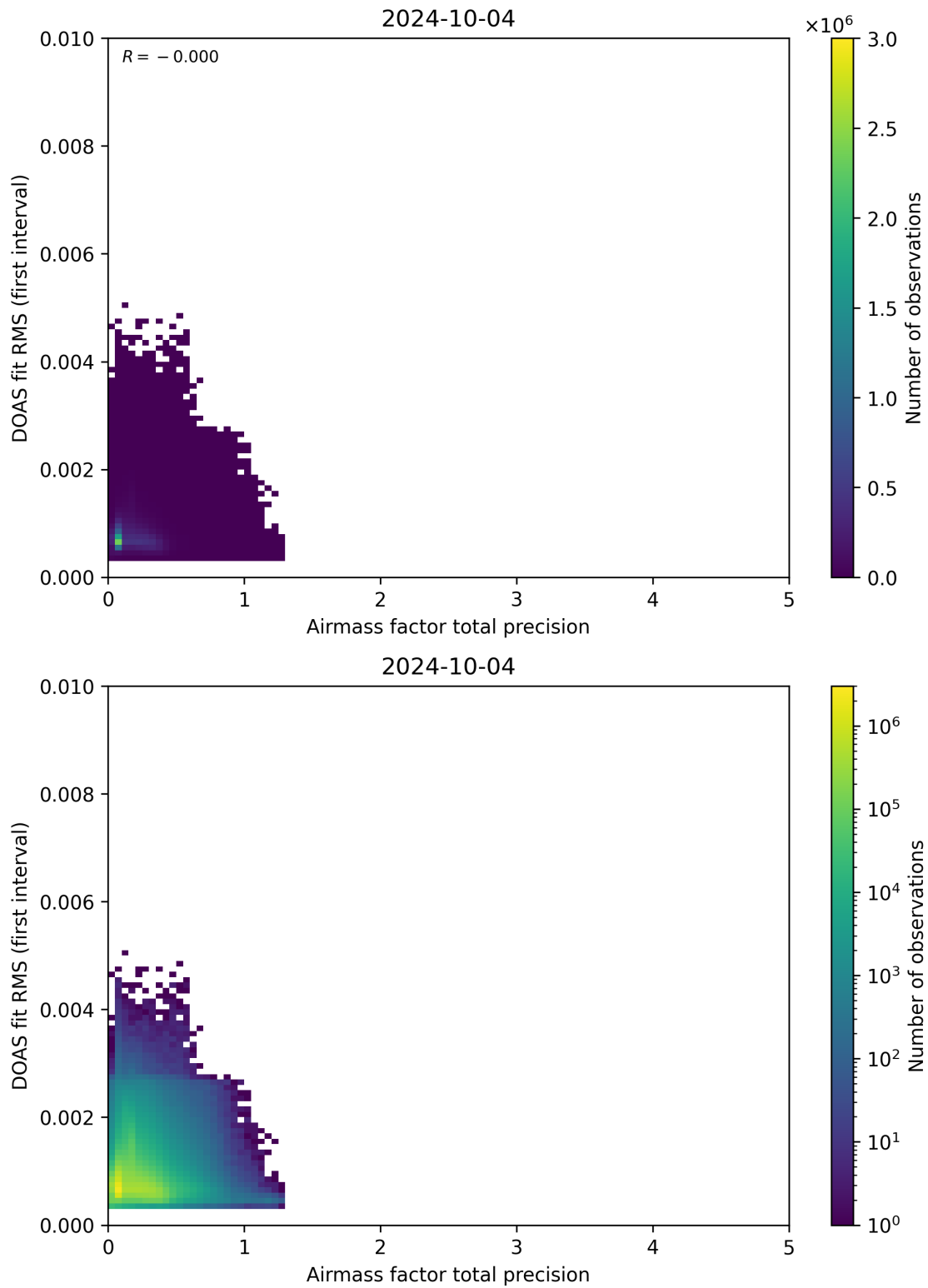
Figure 105: Scatter density plot of “Airmass factor total precision” against “DOAS fit RMS (first interval)” for 2024-10-03 to 2024-10-05.
