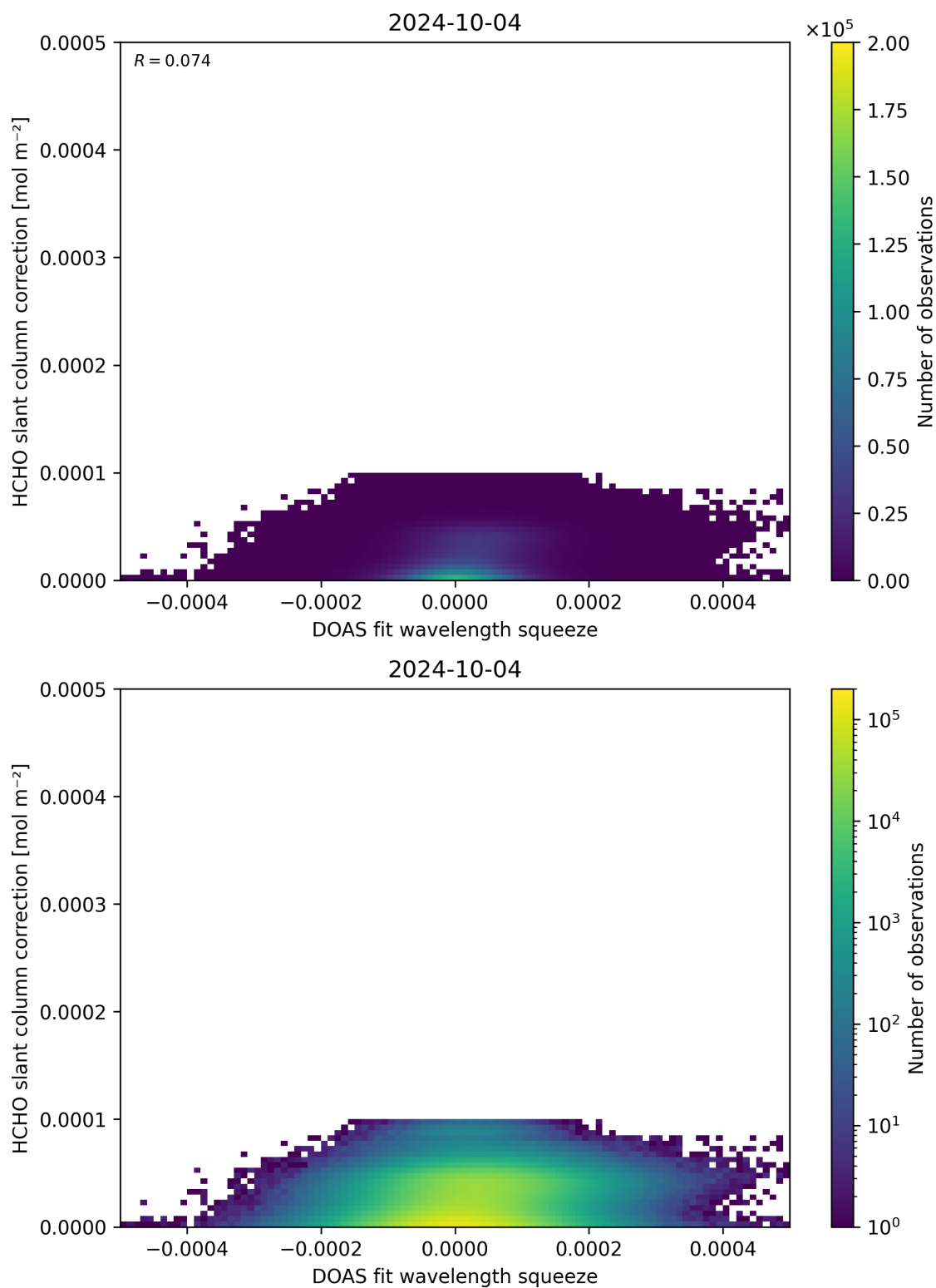
Figure 70: Scatter density plot of “DOAS fit wavelength squeeze” against “HCHO slant column correction” for 2024-10-03 to 2024-10-05.
