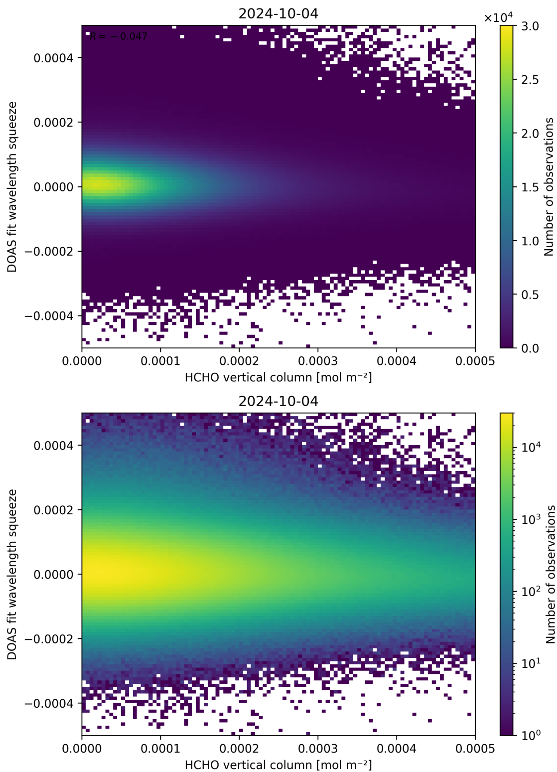
Figure 125: Scatter density plot of “HCHO vertical column” against “DOAS fit wavelength squeeze” for 2024-10-03 to 2024-10-05.
