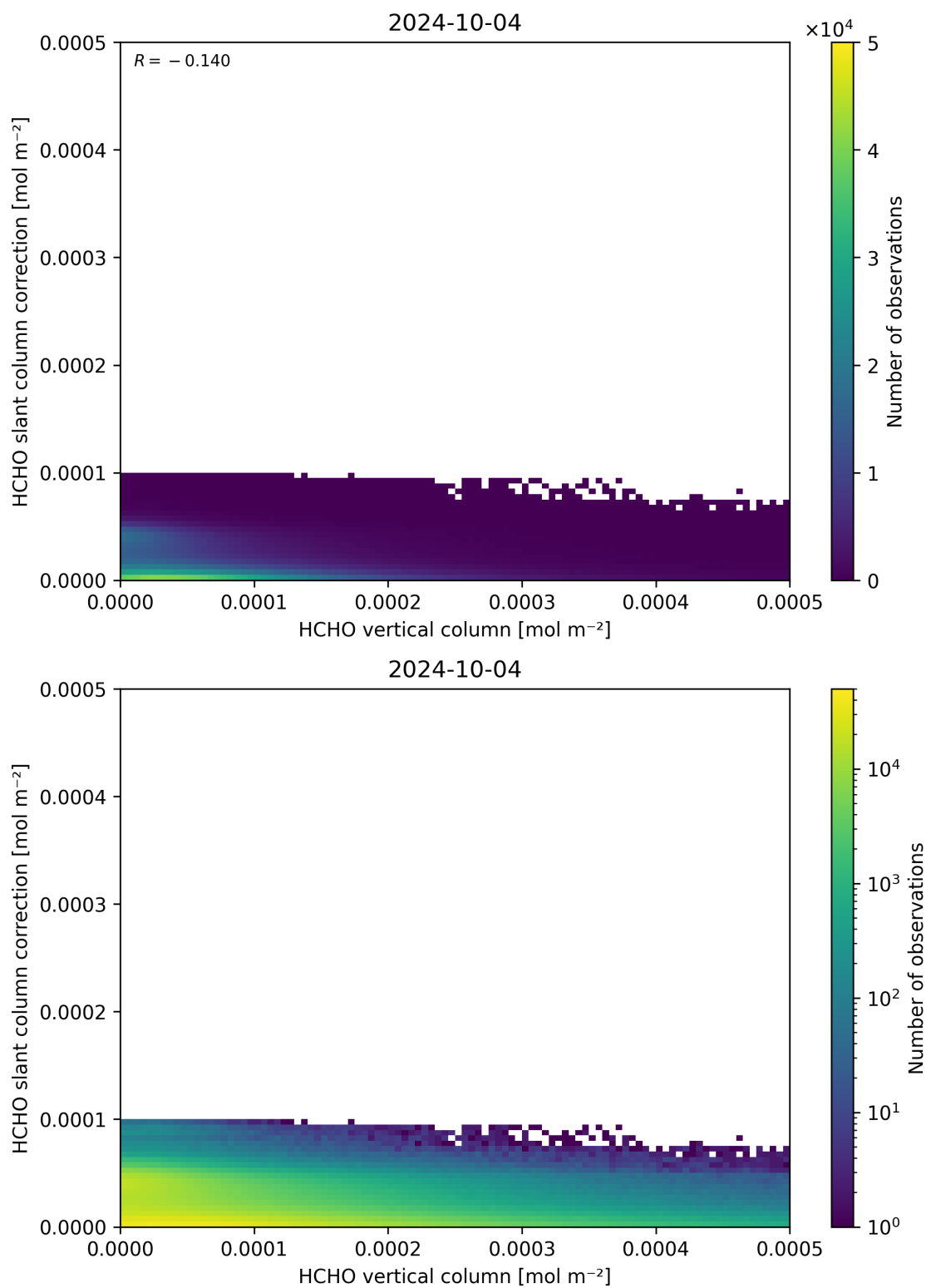
Figure 128: Scatter density plot of “HCHO vertical column” against “HCHO slant column correction” for 2024-10-03 to 2024-10-05.
