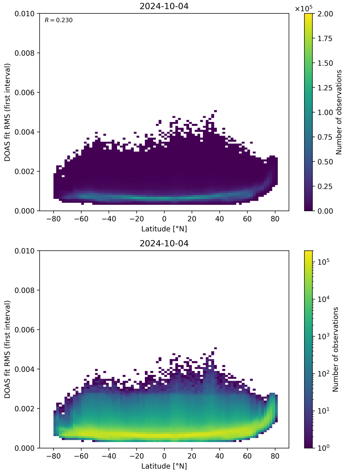
Figure 153: Scatter density plot of “Latitude” against “DOAS fit RMS (first interval)” for 2024-10-03 to 2024-10-05.
