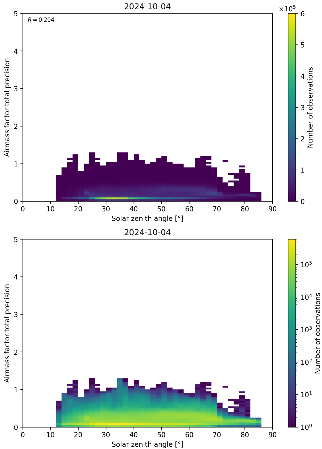
Figure 176: Scatter density plot of “Solar zenith angle” against “Airmass factor total precision” for 2024-10-03 to 2024-10-05.
