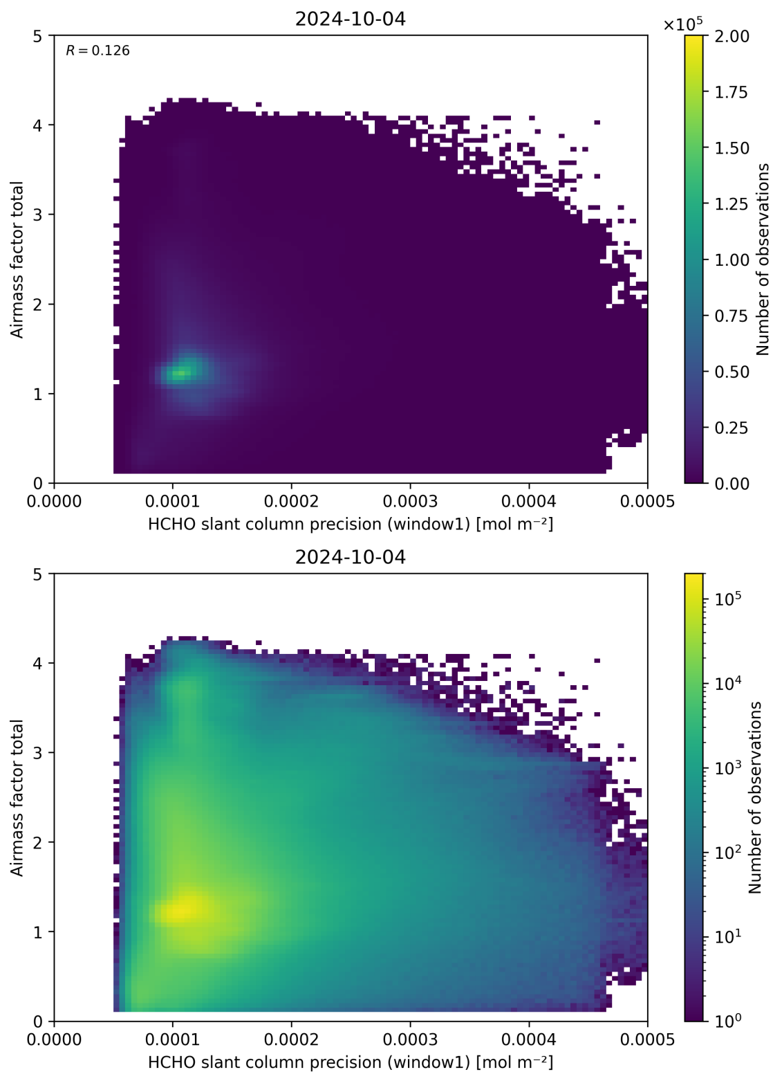
Figure 94: Scatter density plot of “HCHO slant column precision (window1)” against “Airmass factor total” for 2024-10-03 to 2024-10-05.
