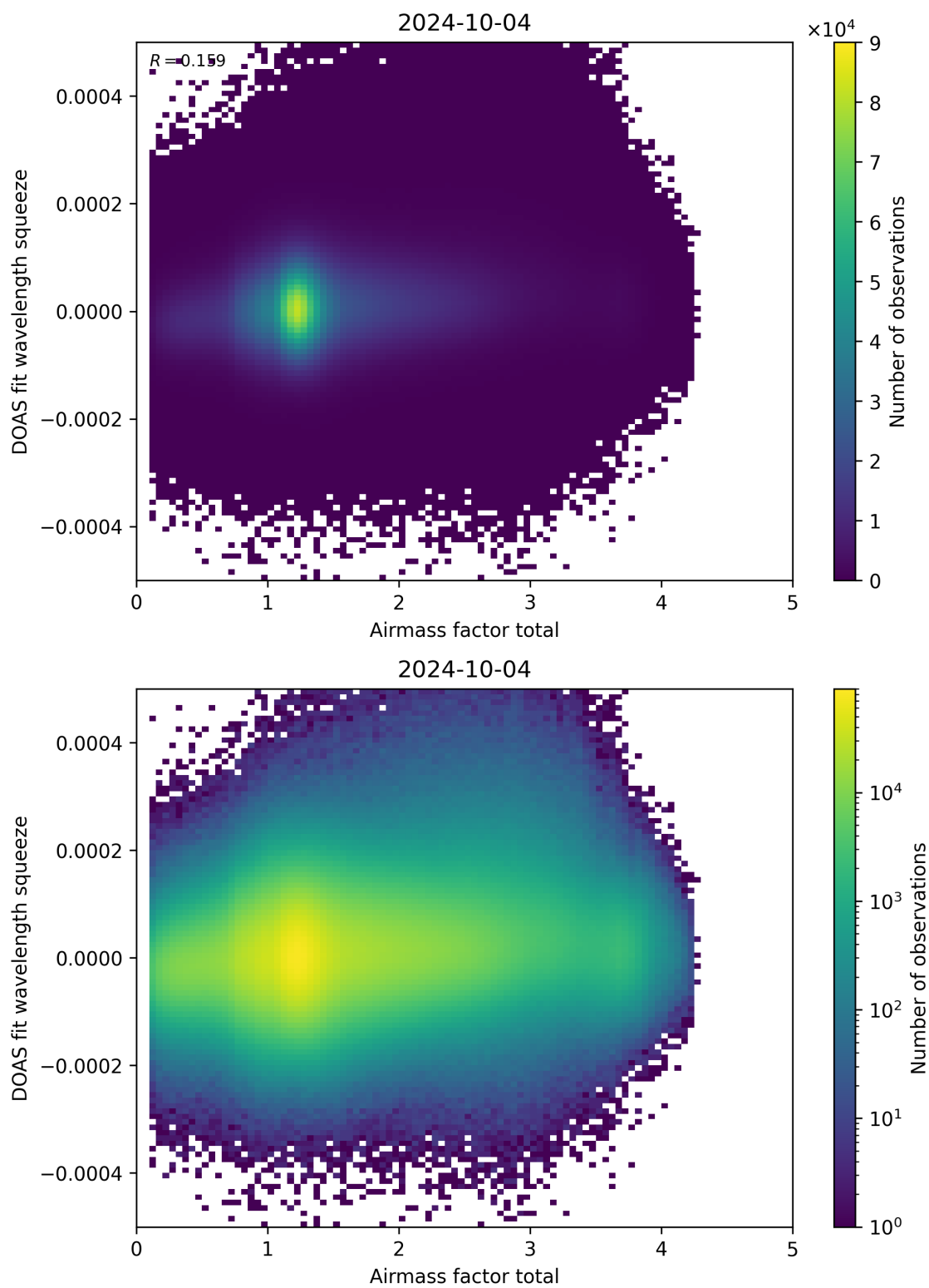
Figure 99: Scatter density plot of “Airmass factor total” against “DOAS fit wavelength squeeze” for 2024-10-03 to 2024-10-05.
