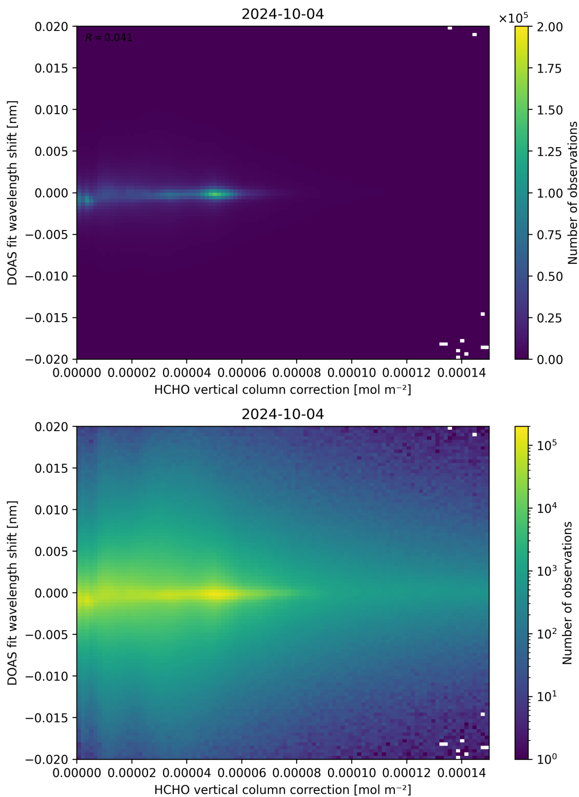
Figure 113: Scatter density plot of “HCHO vertical column correction” against “DOAS fit wavelength shift” for 2024-10-03 to 2024-10-05.
