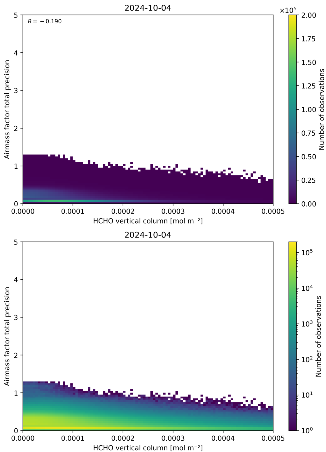
Figure 132: Scatter density plot of “HCHO vertical column” against “Airmass factor total precision” for 2024-10-03 to 2024-10-05.
