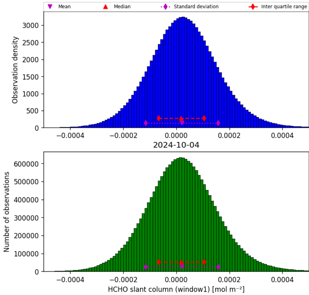
Figure 38: Histogram of “HCHO slant column (window1)” for 2024-10-03 to 2024-10-05
