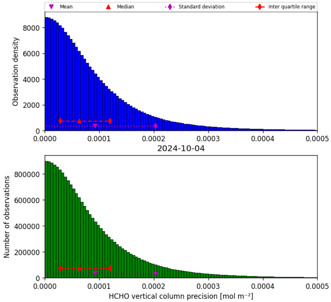
Figure 36: Histogram of “HCHO vertical column precision” for 2024-10-03 to 2024-10-05
