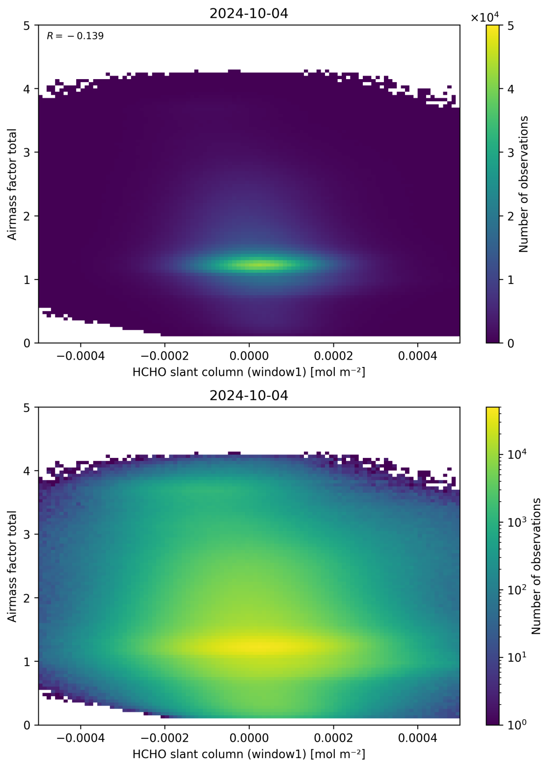
Figure 85: Scatter density plot of “HCHO slant column (window1)” against “Airmass factor total” for 2024-10-03 to 2024-10-05.
