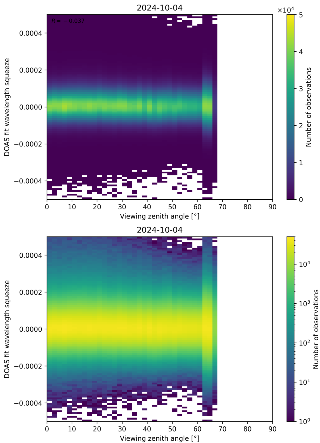
Figure 184: Scatter density plot of “Viewing zenith angle” against “DOAS fit wavelength squeeze” for 2024-10-03 to 2024-10-05.
