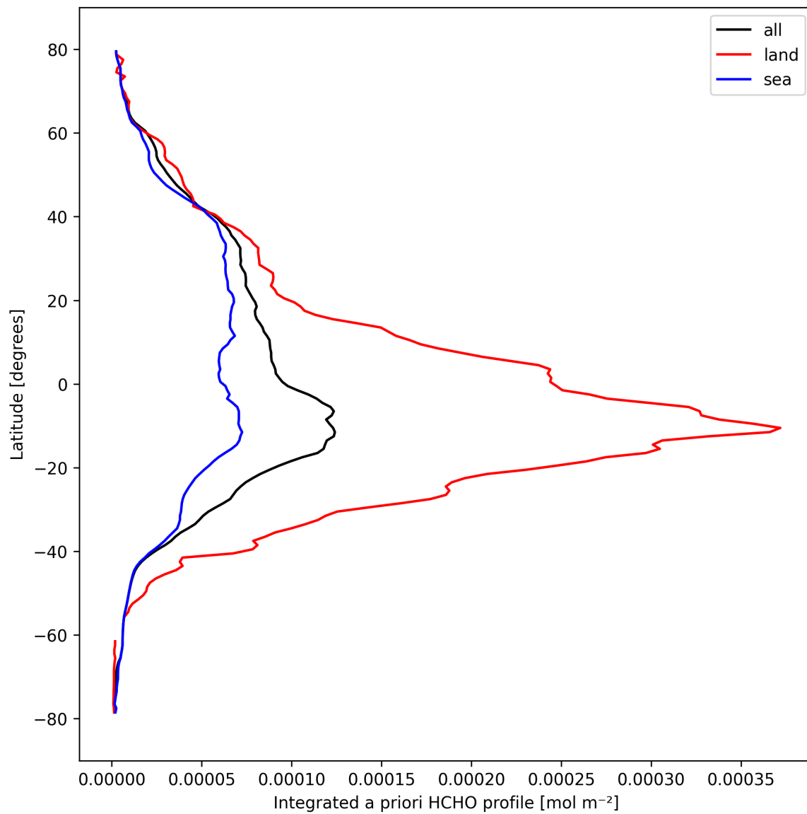
Figure 29: Zonal average of “Integrated a priori HCHO profile” for 2024-10-05 to 2024-10-07.
