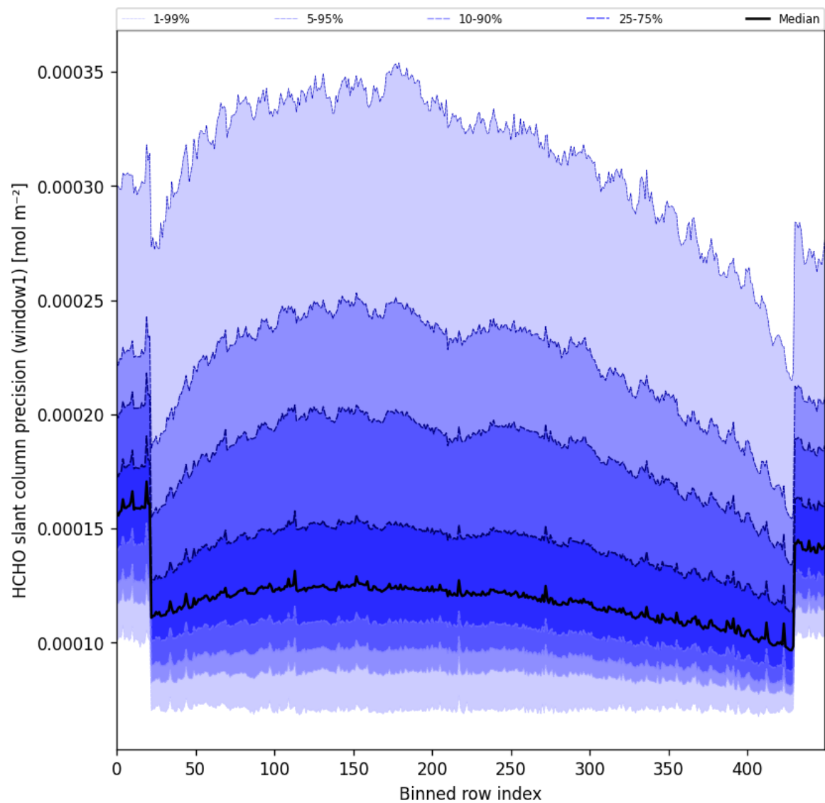
Figure 53: Along track statistics of “HCHO slant column precision (window1)” for 2024-10-05 to 2024-10-07
