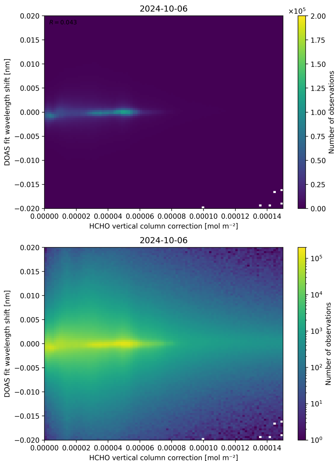
Figure 113: Scatter density plot of “HCHO vertical column correction” against “DOAS fit wavelength shift” for 2024-10-05 to 2024-10-07.
