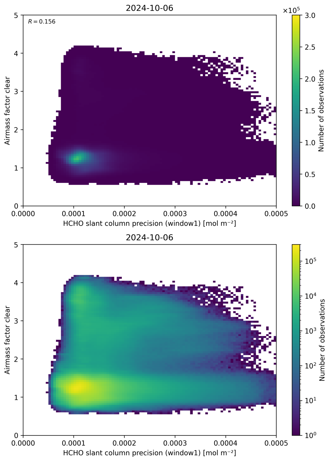
Figure 91: Scatter density plot of “HCHO slant column precision (window1)” against “Airmass factor clear” for 2024-10-05 to 2024-10-07.
