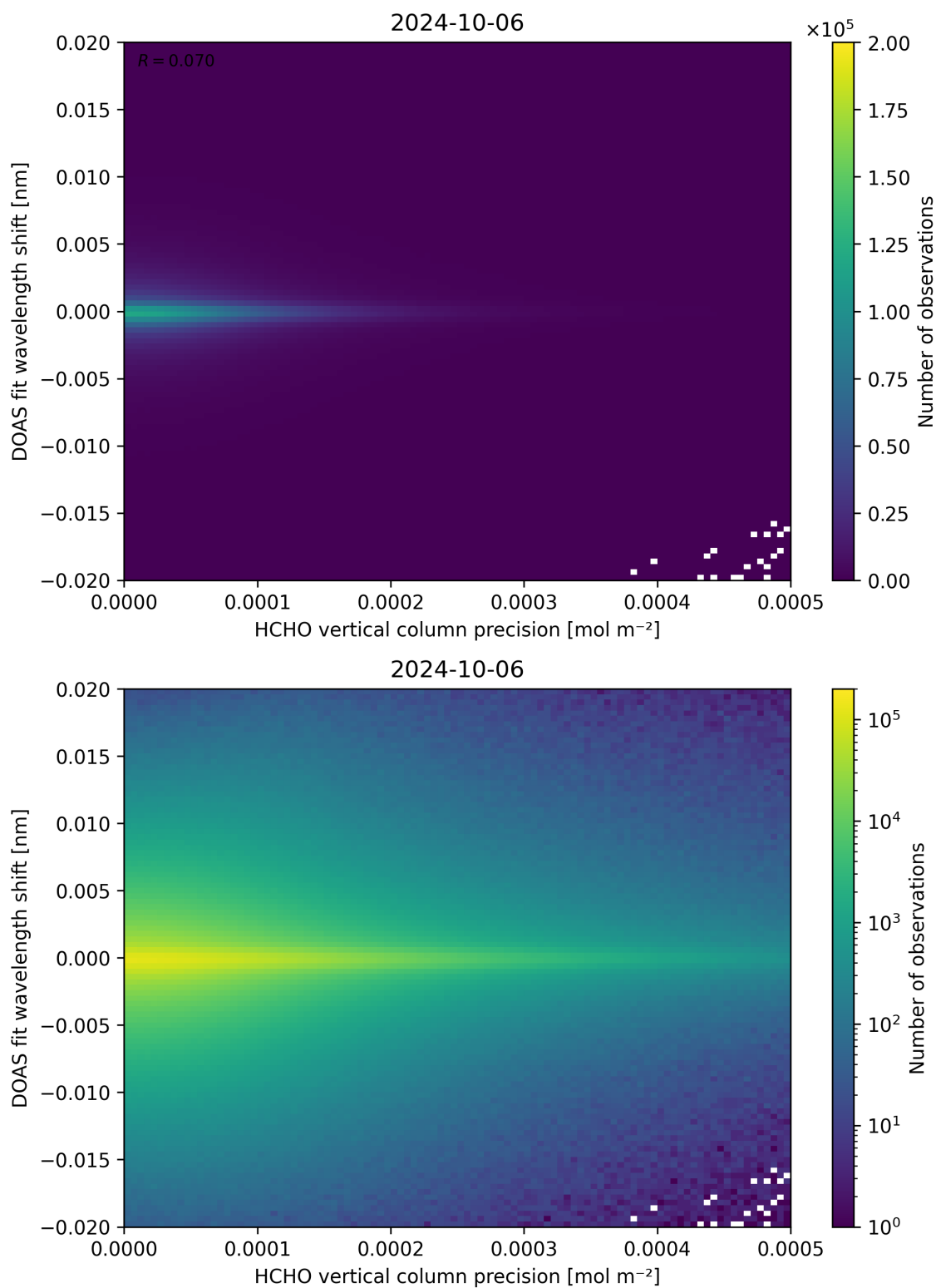
Figure 137: Scatter density plot of “HCHO vertical column precision” against “DOAS fit wavelength shift” for 2024-10-05 to 2024-10-07.
