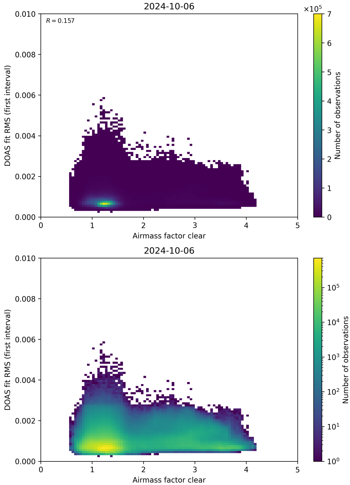
Figure 71: Scatter density plot of “Airmass factor clear” against “DOAS fit RMS (first interval)” for 2024-10-05 to 2024-10-07.
