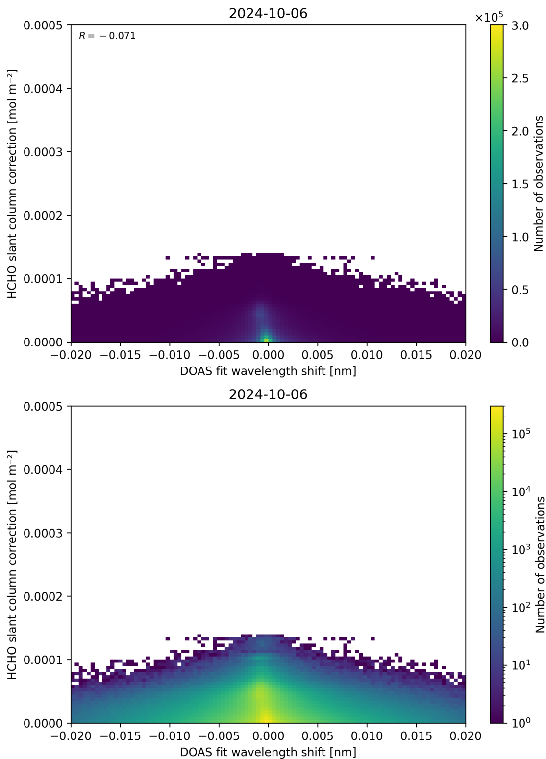
Figure 67: Scatter density plot of “DOAS fit wavelength shift” against “HCHO slant column correction” for 2024-10-05 to 2024-10-07.
