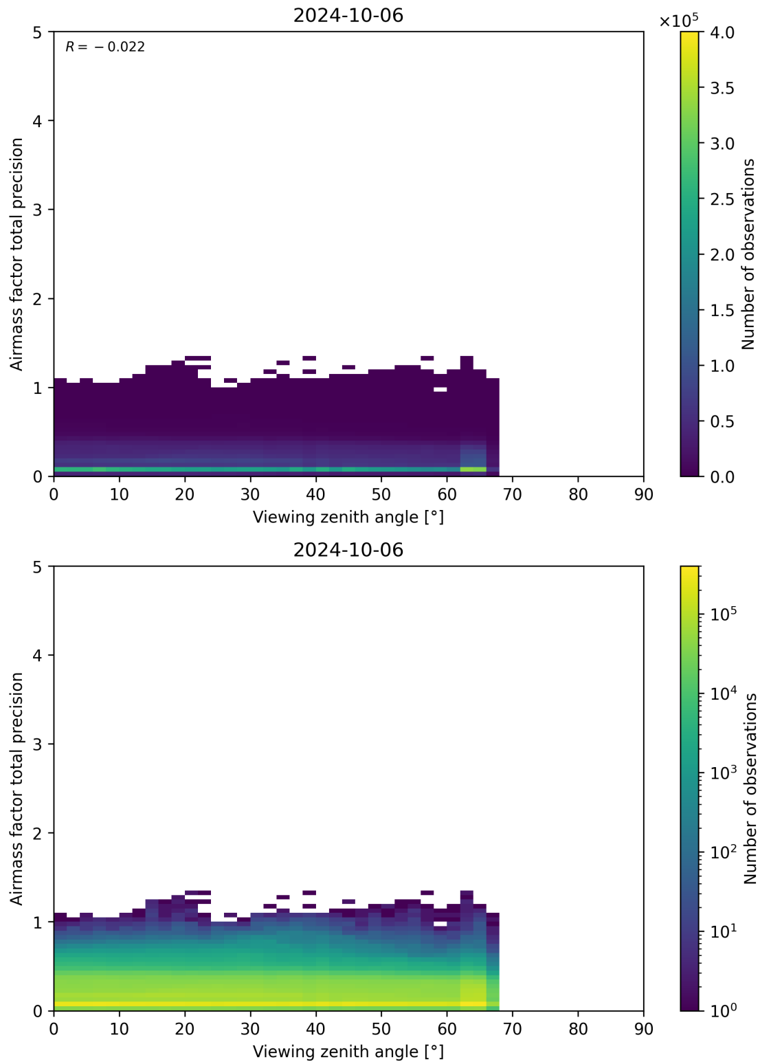
Figure 191: Scatter density plot of “Viewing zenith angle” against “Airmass factor total precision” for 2024-10-05 to 2024-10-07.
