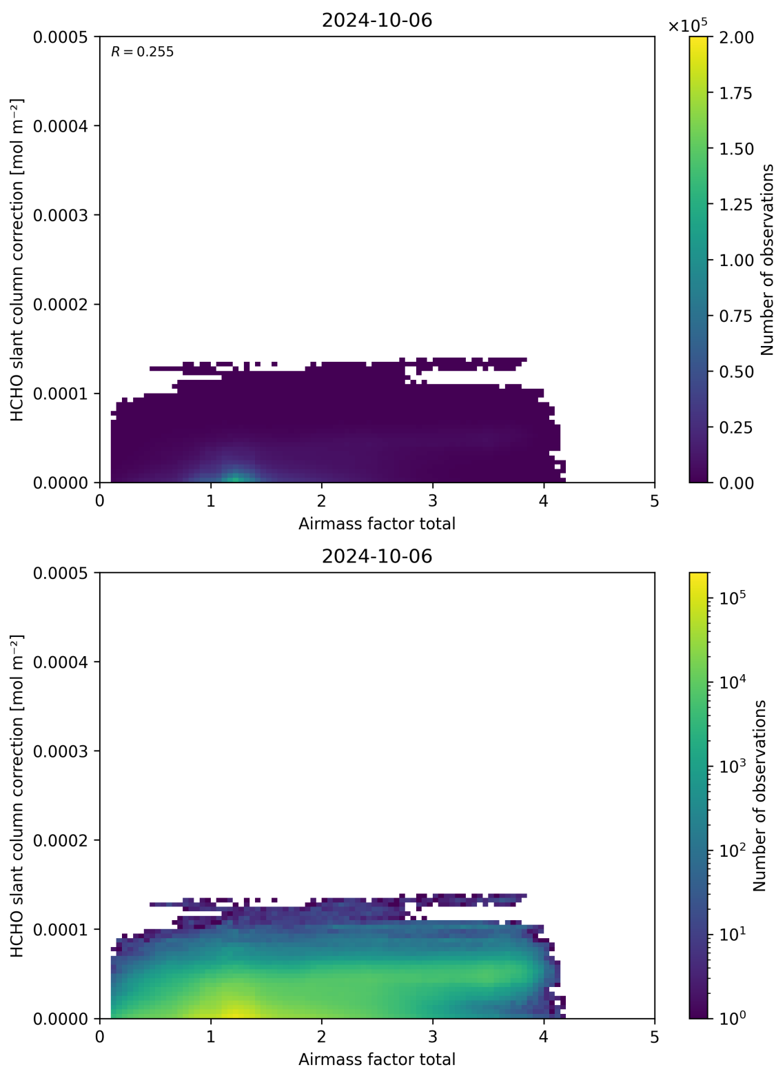
Figure 102: Scatter density plot of “Airmass factor total” against “HCHO slant column correction” for 2024-10-05 to 2024-10-07.
