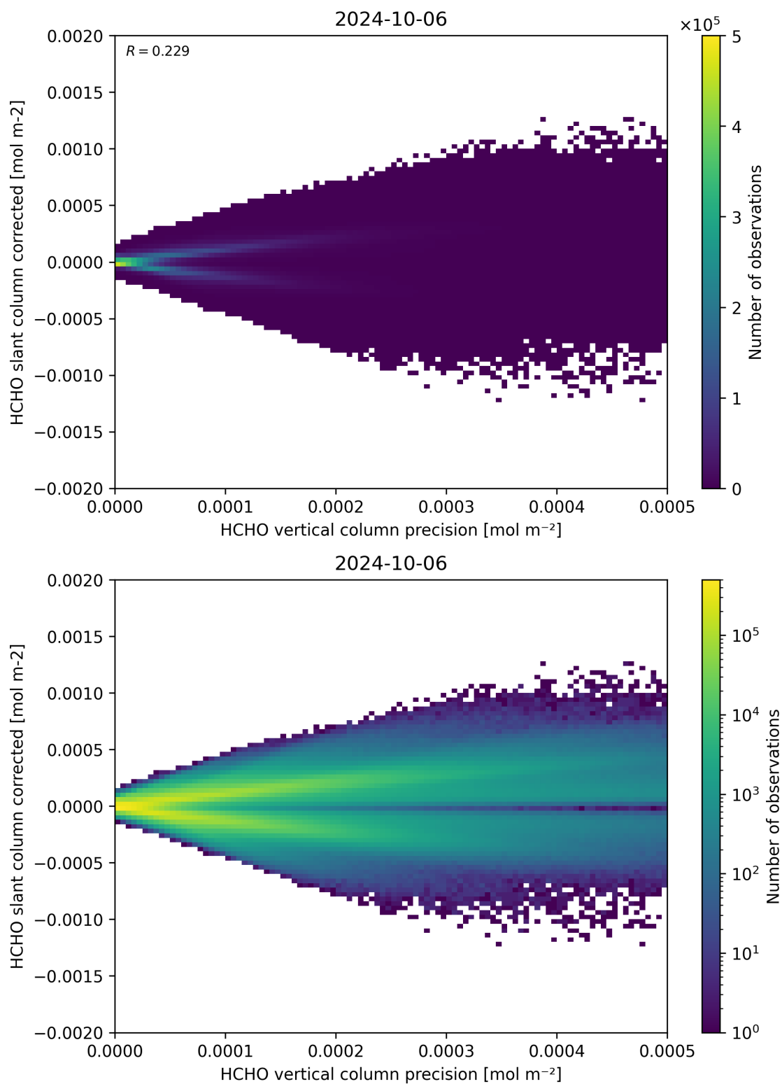
Figure 140: Scatter density plot of “HCHO vertical column precision” against “HCHO slant column corrected” for 2024-10-05 to 2024-10-07.
