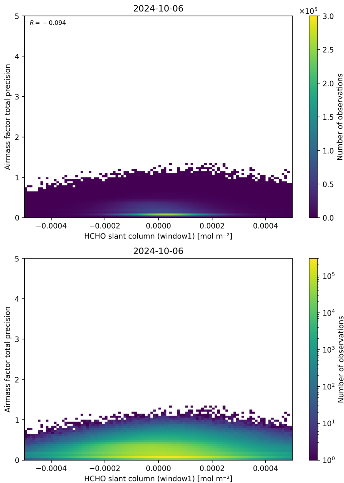
Figure 86: Scatter density plot of “HCHO slant column (window1)” against “Airmass factor total precision” for 2024-10-05 to 2024-10-07.
