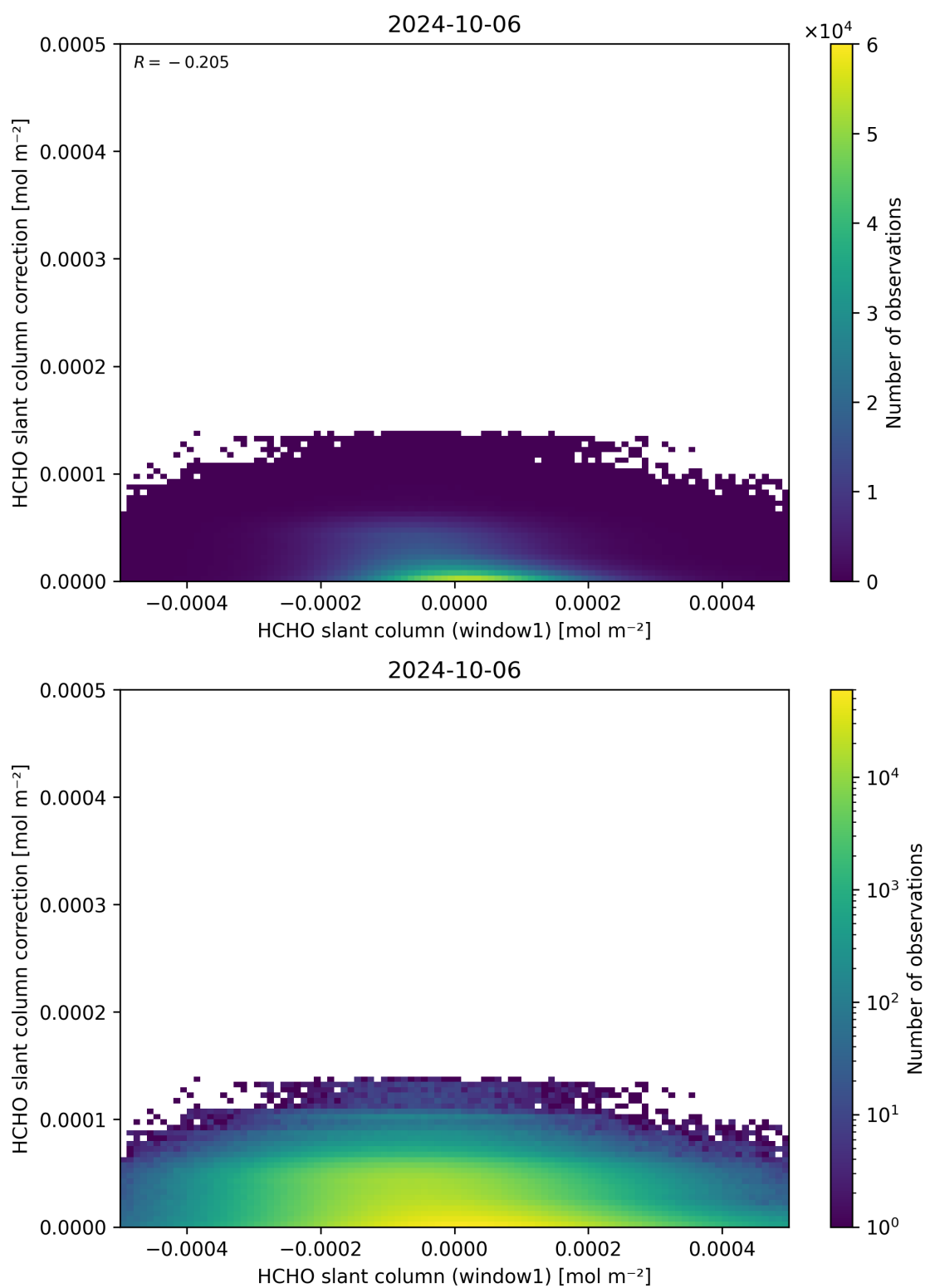
Figure 83: Scatter density plot of “HCHO slant column (window1)” against “HCHO slant column correction” for 2024-10-05 to 2024-10-07.
