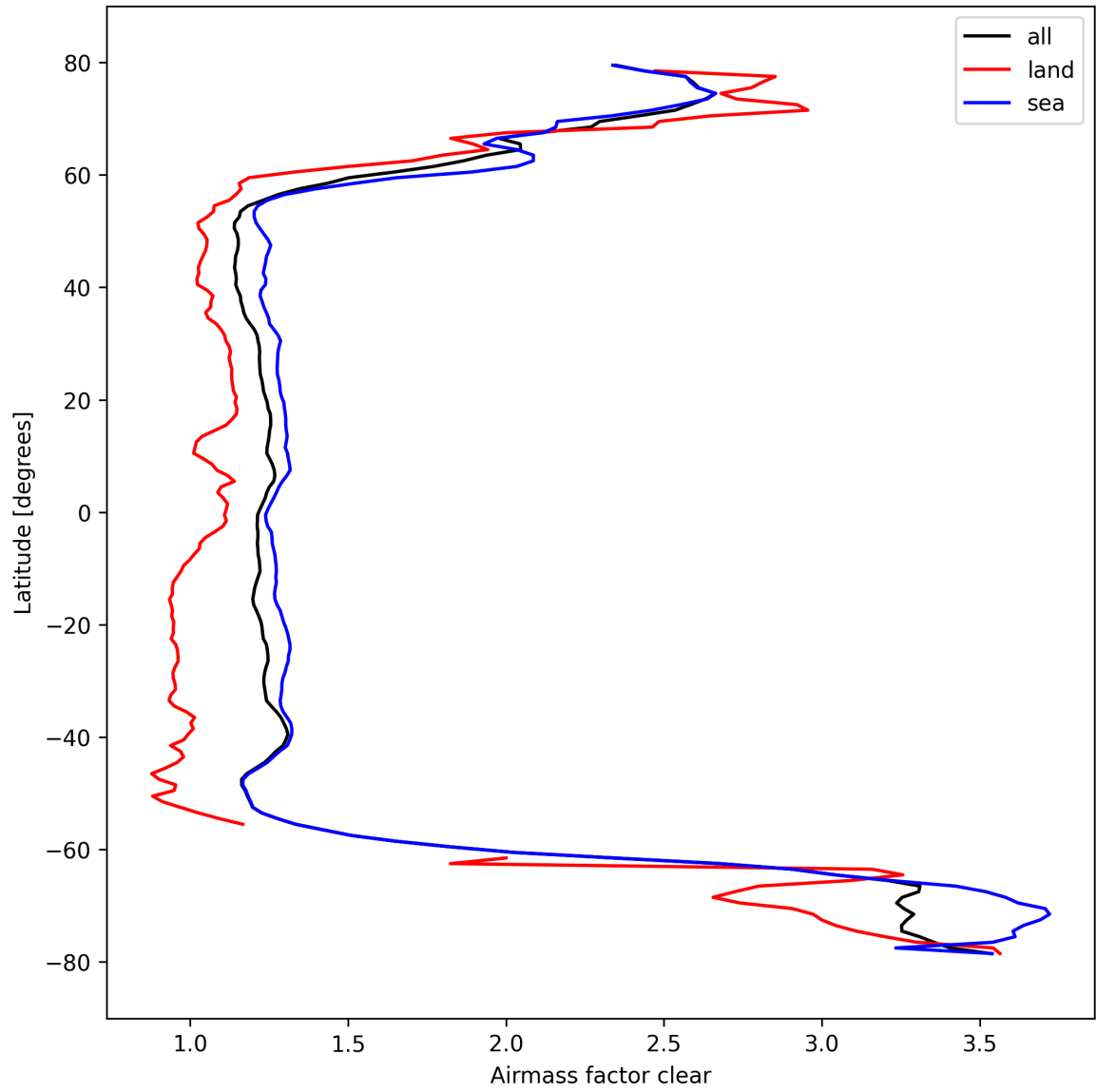
Figure 28: Zonal average of “Airmass factor clear” for 2024-10-05 to 2024-10-07.
