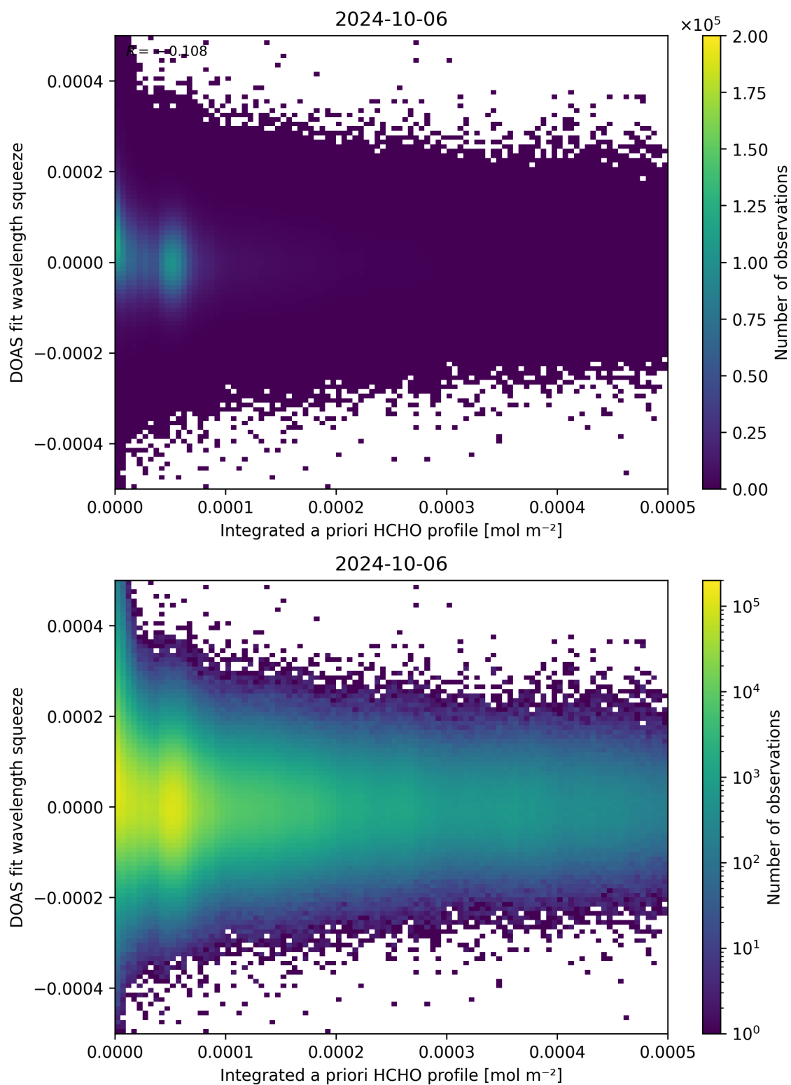
Figure 150: Scatter density plot of “Integrated a priori HCHO profile” against “DOAS fit wavelength squeeze” for 2024-10-05 to 2024-10-07.
