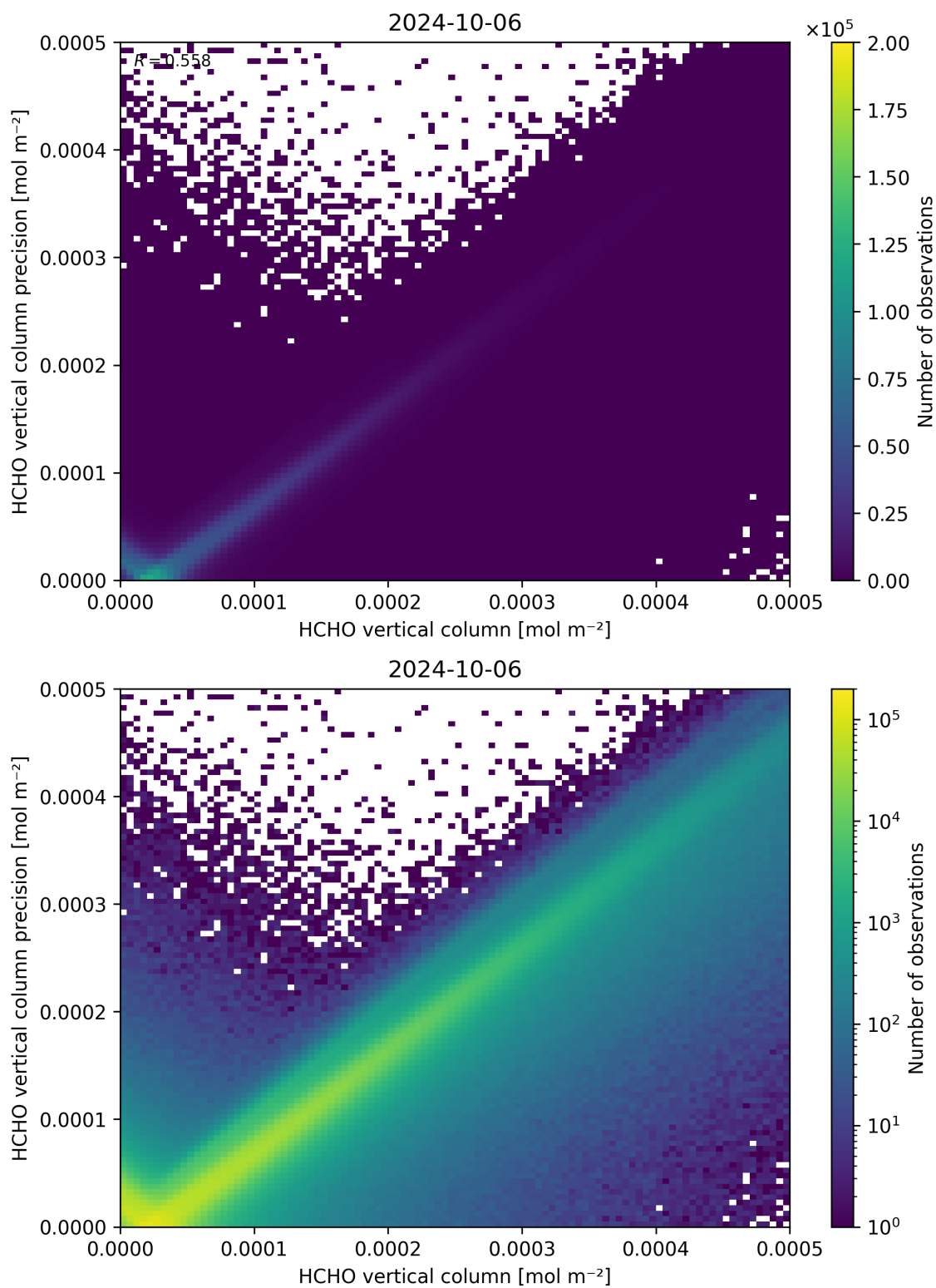
Figure 134: Scatter density plot of “HCHO vertical column” against “HCHO vertical column precision” for 2024-10-05 to 2024-10-07.
