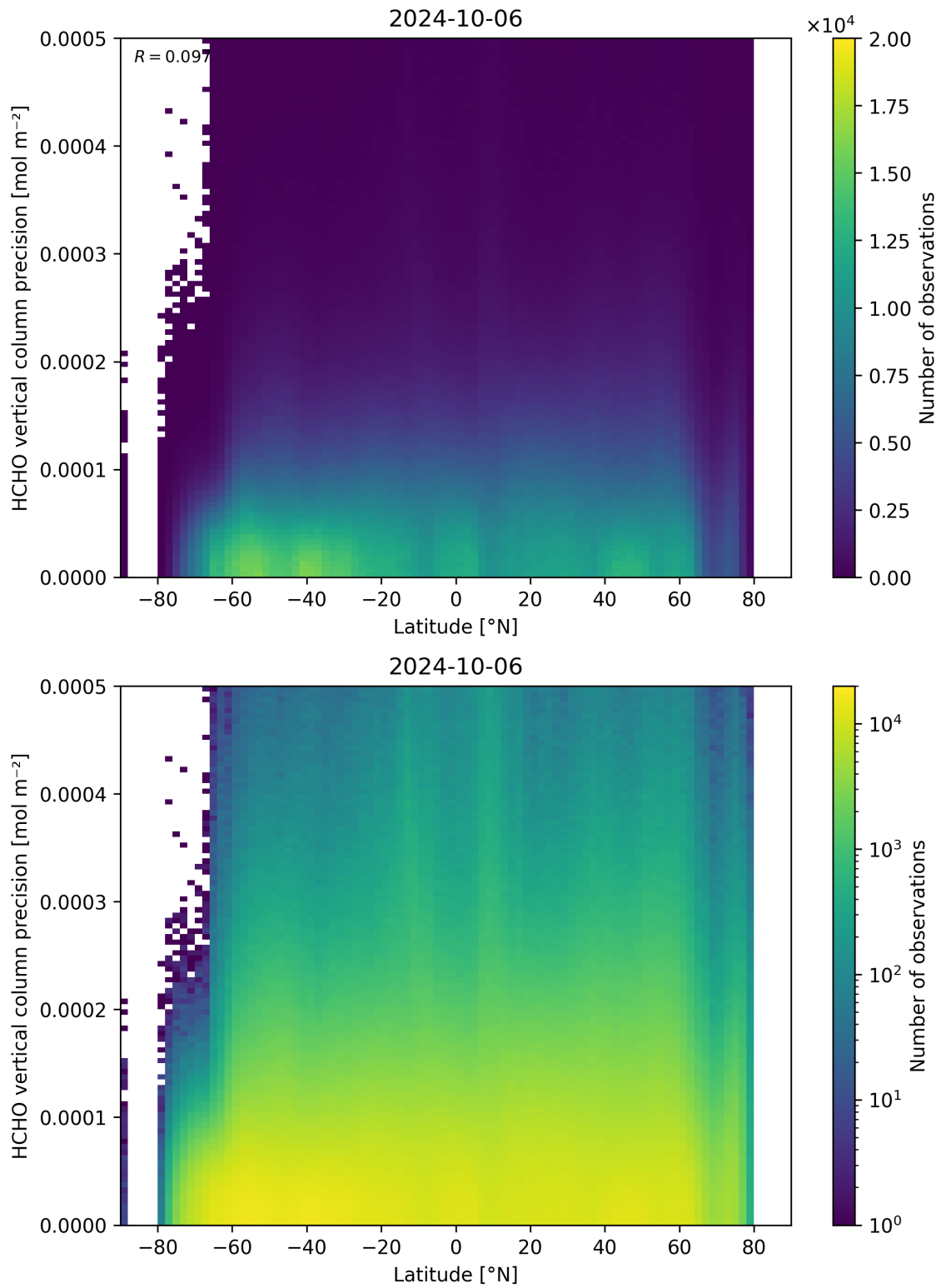
Figure 165: Scatter density plot of “Latitude” against “HCHO vertical column precision” for 2024-10-05 to 2024-10-07.
