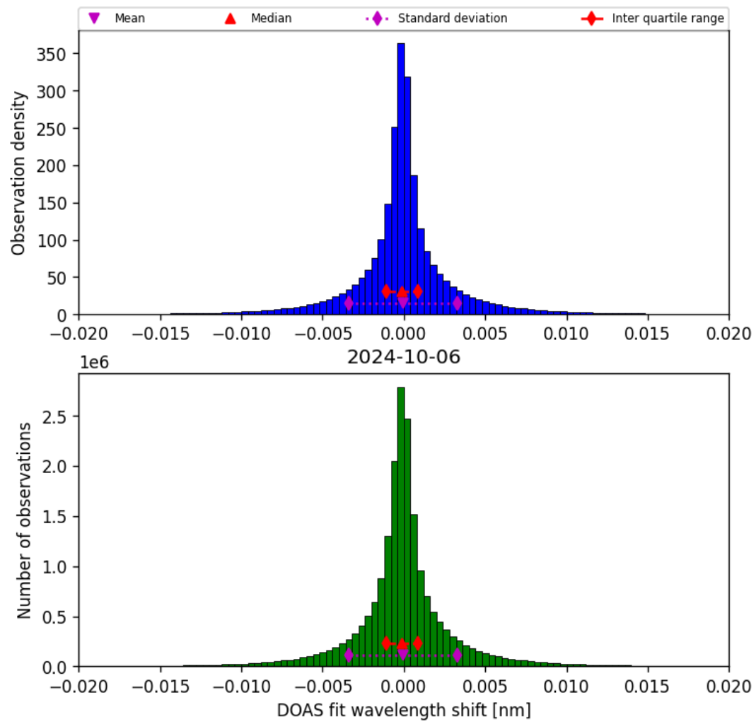
Figure 44: Histogram of “DOAS fit wavelength shift” for 2024-10-05 to 2024-10-07
