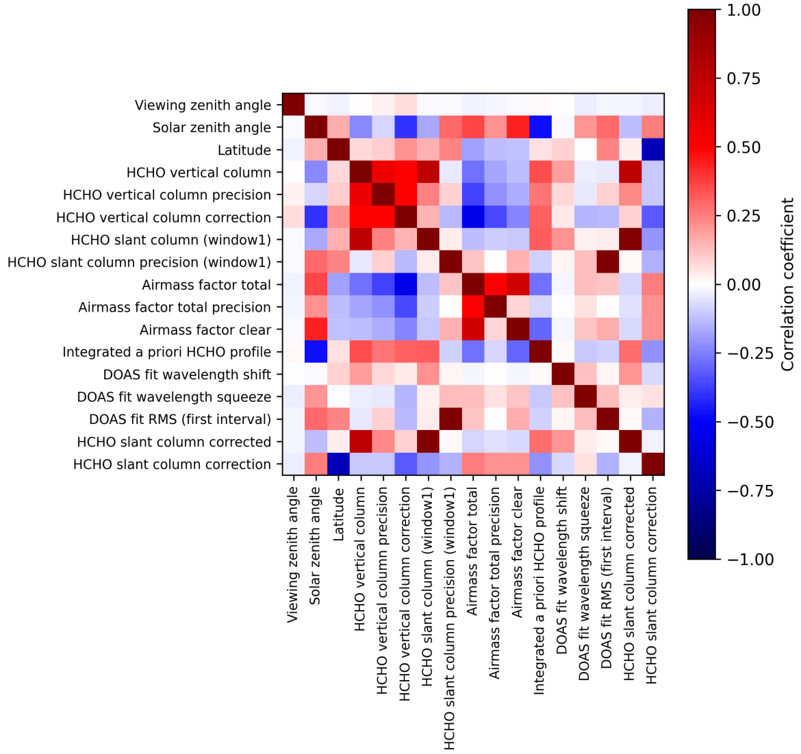
Figure 2: Map of correlation matrix for 2024-10-05 to 2024-10-07.
