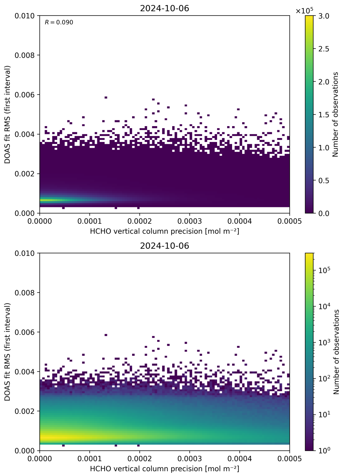
Figure 136: Scatter density plot of “HCHO vertical column precision” against “DOAS fit RMS (first interval)” for 2024-10-05 to 2024-10-07.
