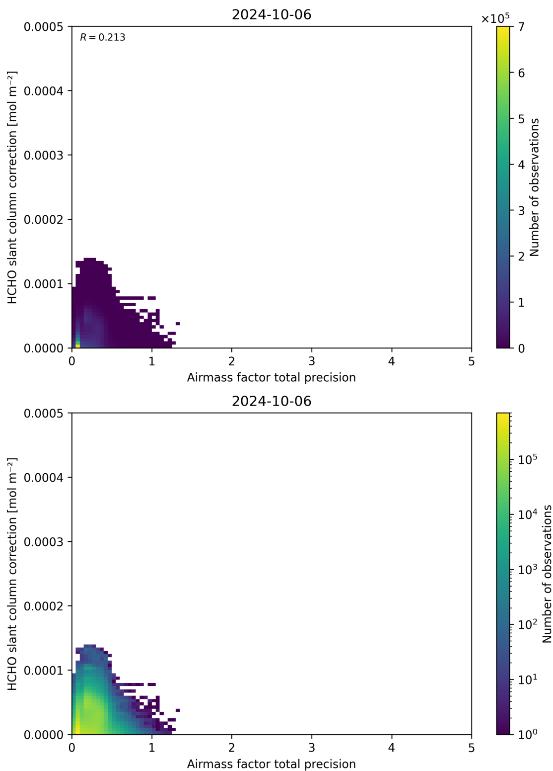
Figure 110: Scatter density plot of “Airmass factor total precision” against “HCHO slant column correction” for 2024-10-05 to 2024-10-07.
