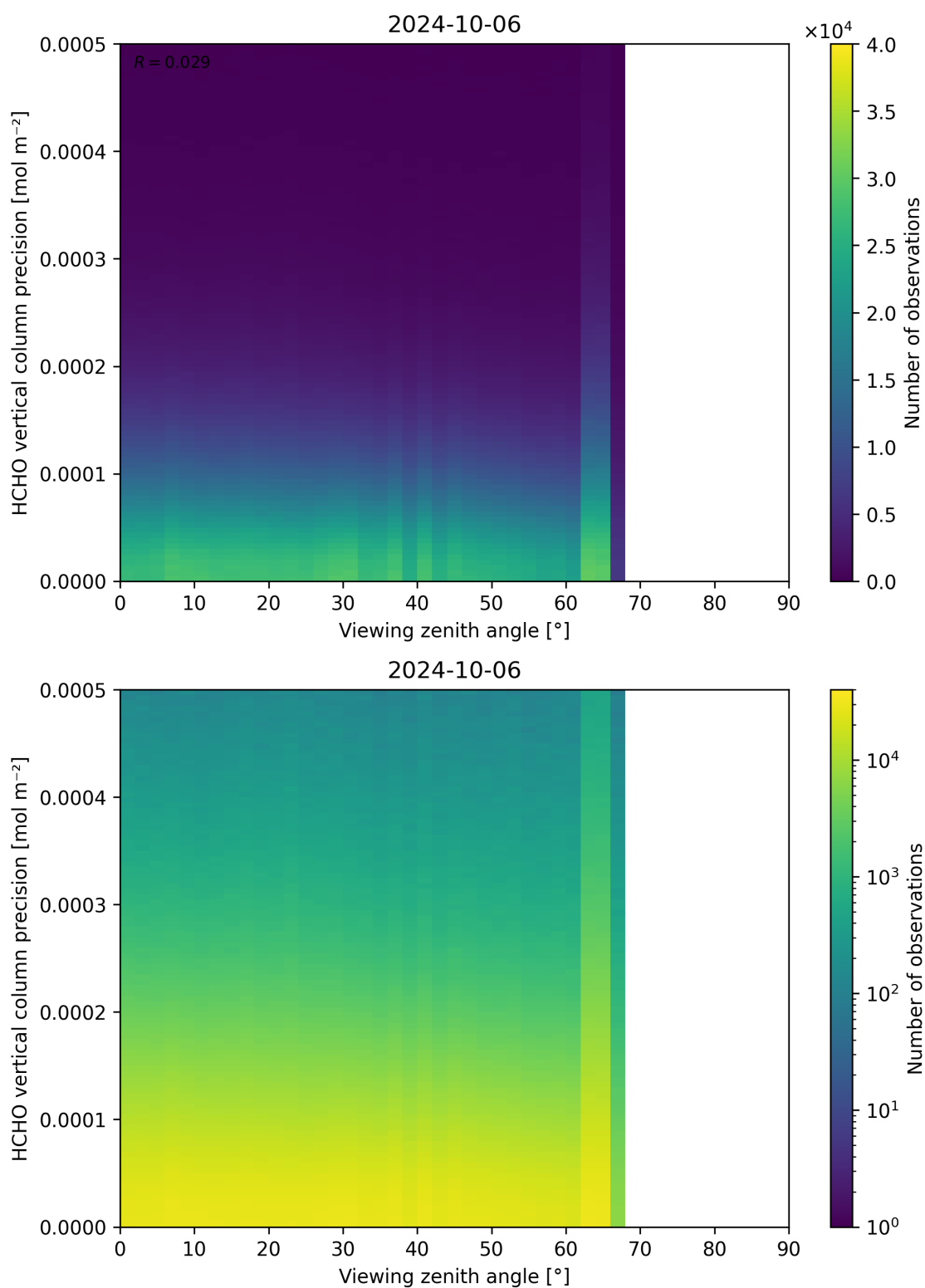
Figure 194: Scatter density plot of “Viewing zenith angle” against “HCHO vertical column precision” for 2024-10-05 to 2024-10-07.
