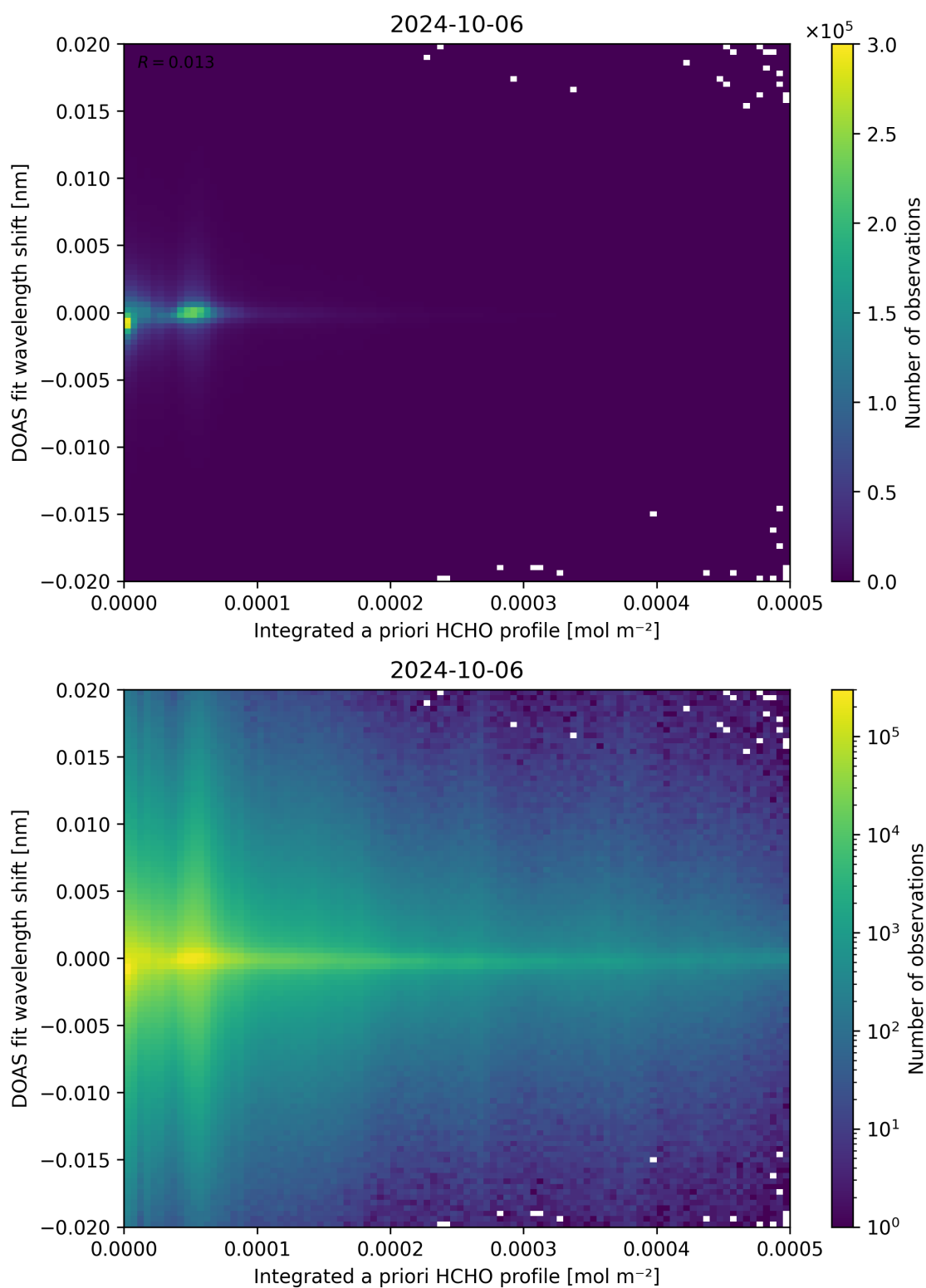
Figure 149: Scatter density plot of “Integrated a priori HCHO profile” against “DOAS fit wavelength shift” for 2024-10-05 to 2024-10-07.
