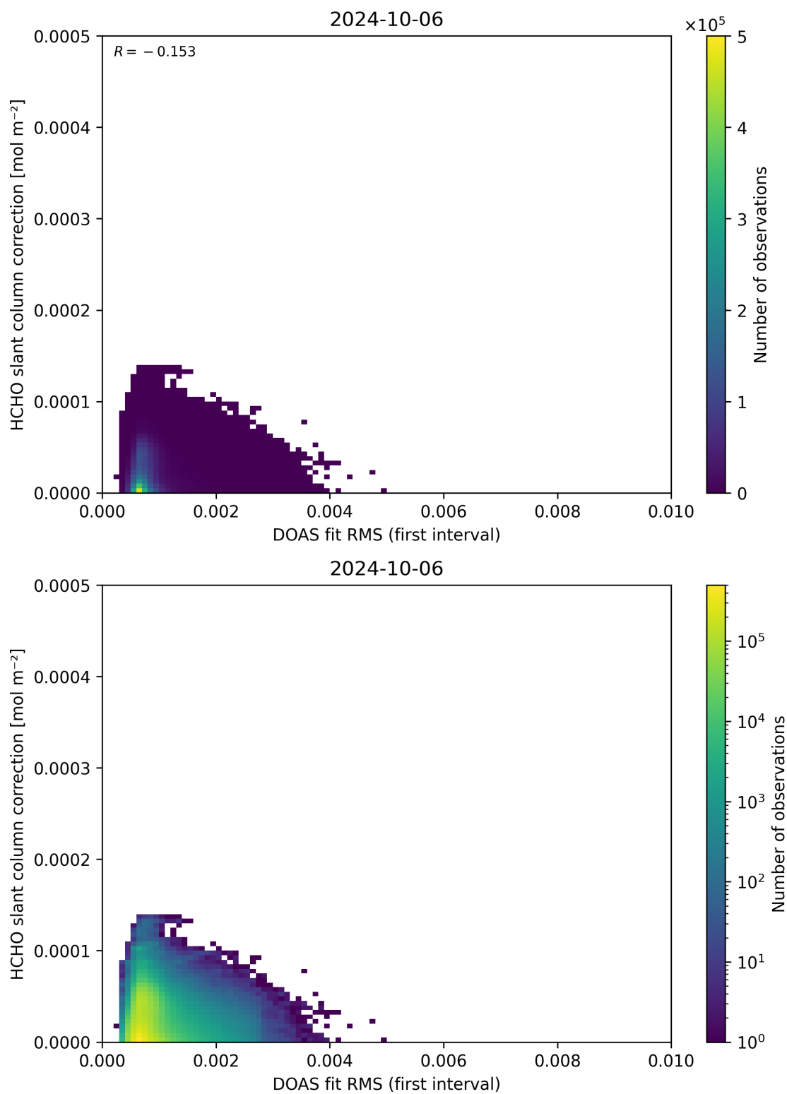
Figure 63: Scatter density plot of “DOAS fit RMS (first interval)” against “HCHO slant column correction” for 2024-10-05 to 2024-10-07.
