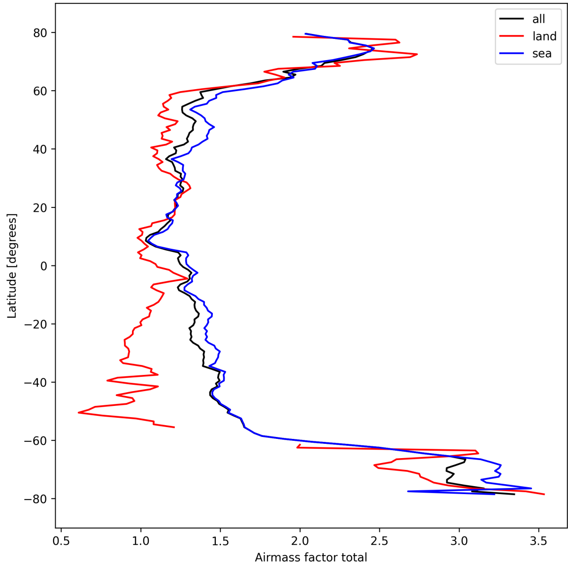
Figure 26: Zonal average of “Airmass factor total” for 2024-10-05 to 2024-10-07.
