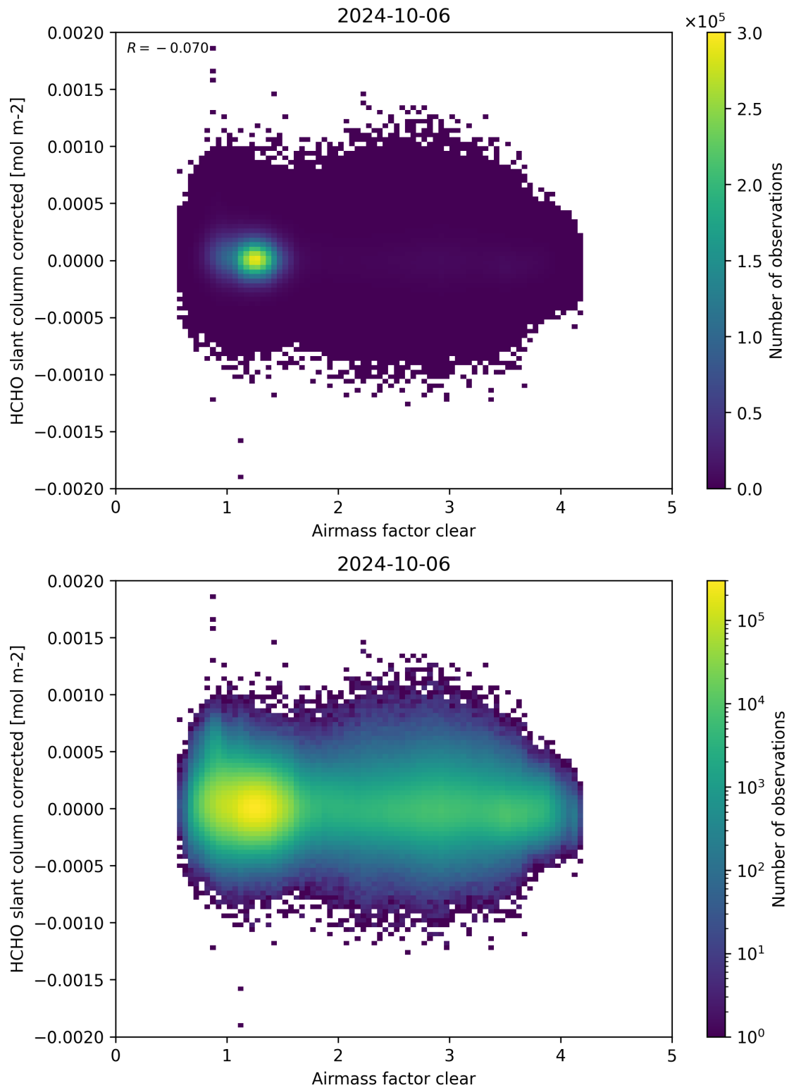
Figure 74: Scatter density plot of “Airmass factor clear” against “HCHO slant column corrected” for 2024-10-05 to 2024-10-07.
