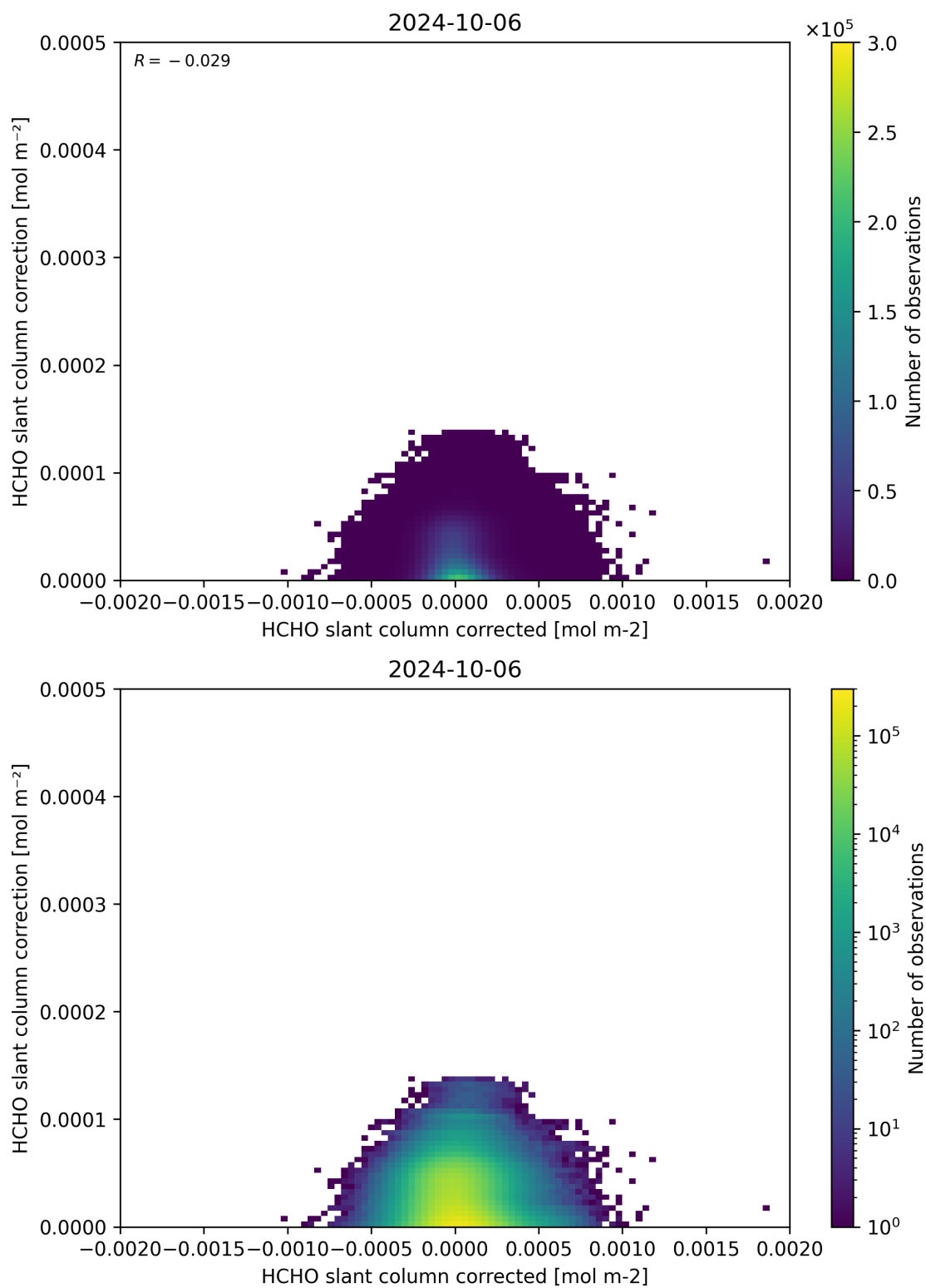
Figure 77: Scatter density plot of “HCHO slant column corrected” against “HCHO slant column correction” for 2024-10-05 to 2024-10-07.
