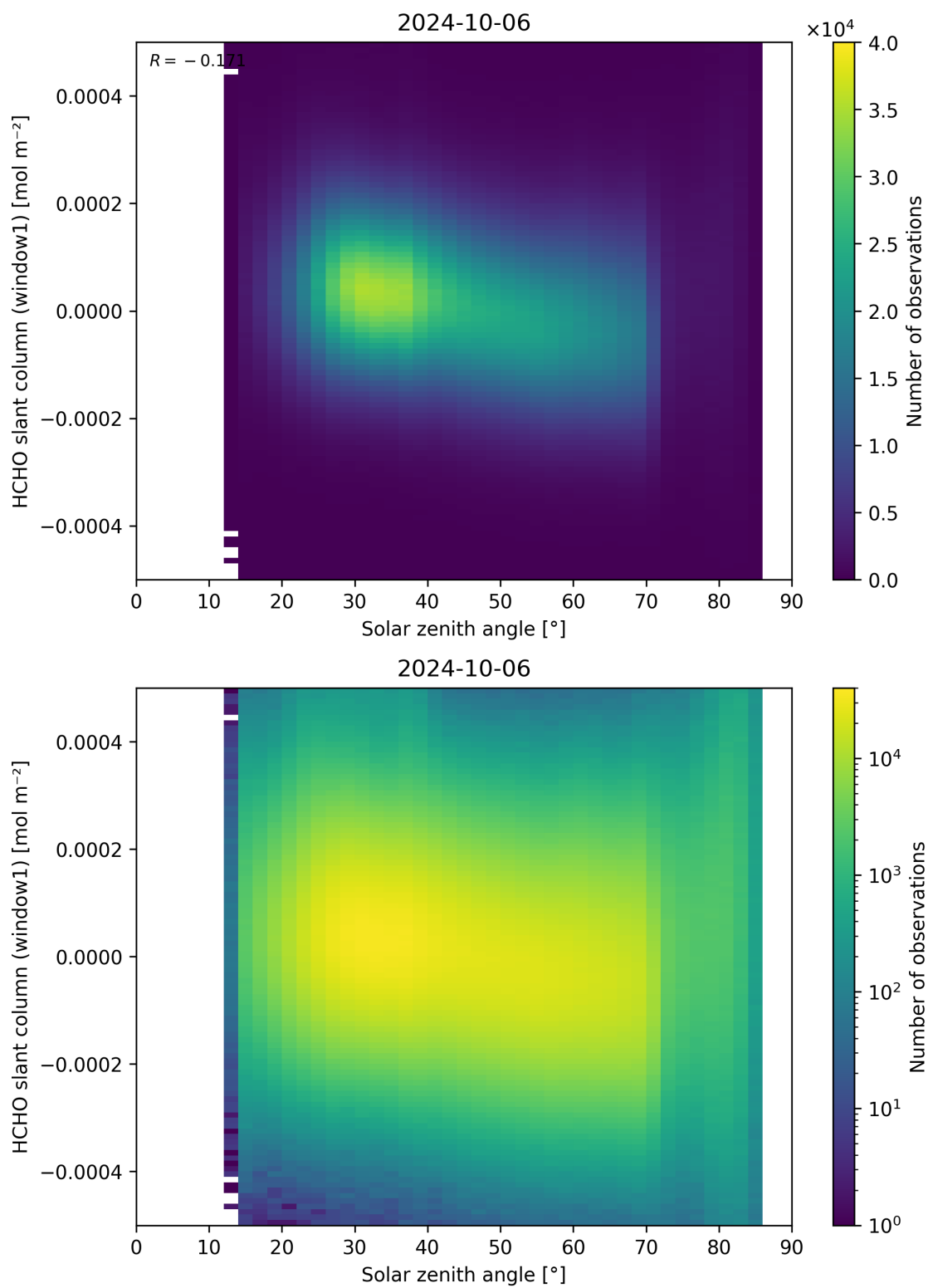
Figure 173: Scatter density plot of “Solar zenith angle” against “HCHO slant column (window1)” for 2024-10-05 to 2024-10-07.
