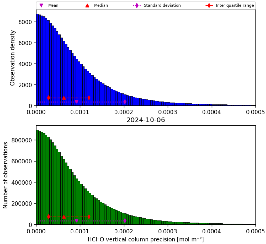
Figure 36: Histogram of “HCHO vertical column precision” for 2024-10-05 to 2024-10-07
