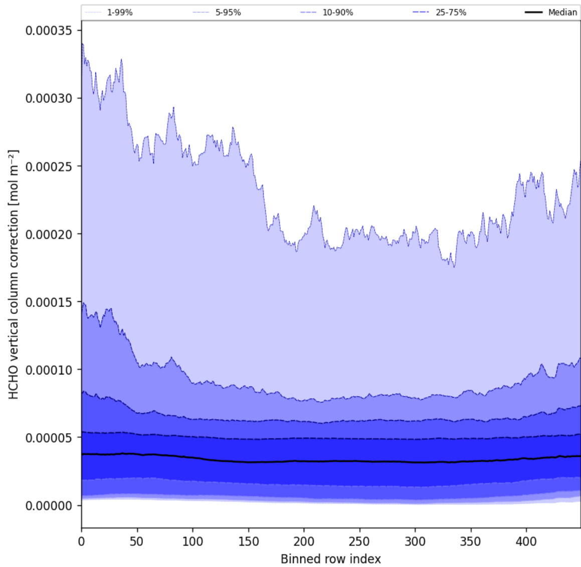
Figure 51: Along track statistics of “HCHO vertical column correction” for 2024-10-05 to 2024-10-07
