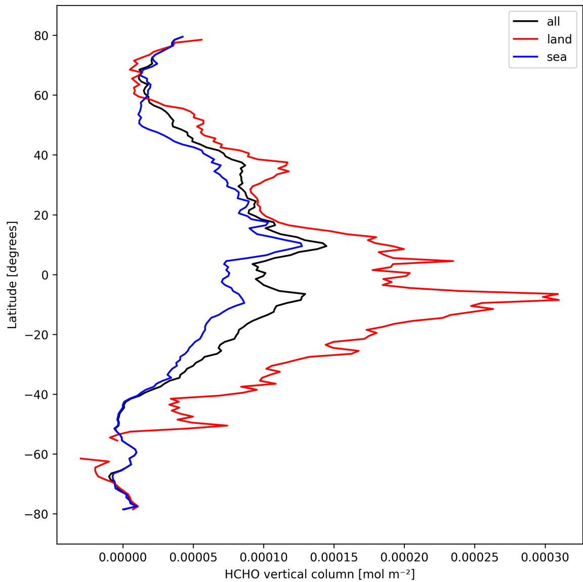
Figure 21: Zonal average of “HCHO vertical column” for 2024-10-05 to 2024-10-07.
