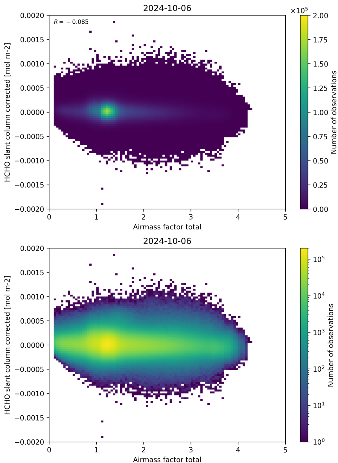
Figure 101: Scatter density plot of “Airmass factor total” against “HCHO slant column corrected” for 2024-10-05 to 2024-10-07.
