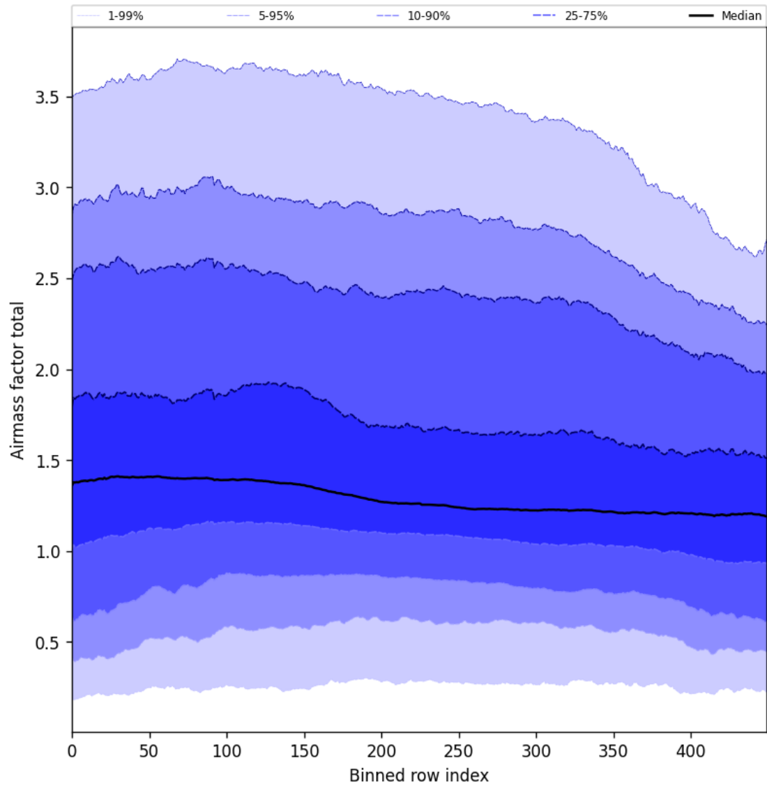
Figure 54: Along track statistics of “Airmass factor total” for 2024-10-05 to 2024-10-07
