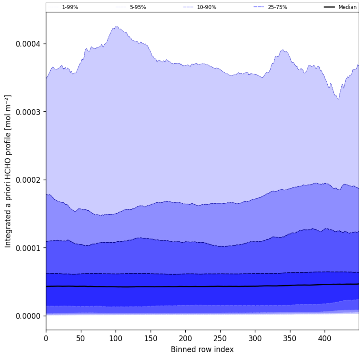
Figure 57: Along track statistics of “Integrated a priori HCHO profile” for 2024-10-05 to 2024-10-07
