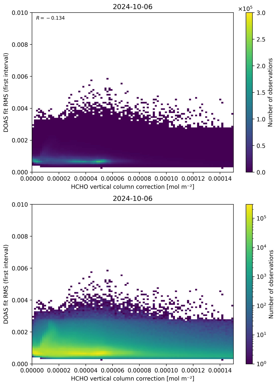
Figure 112: Scatter density plot of “HCHO vertical column correction” against “DOAS fit RMS (first interval)” for 2024-10-05 to 2024-10-07.
