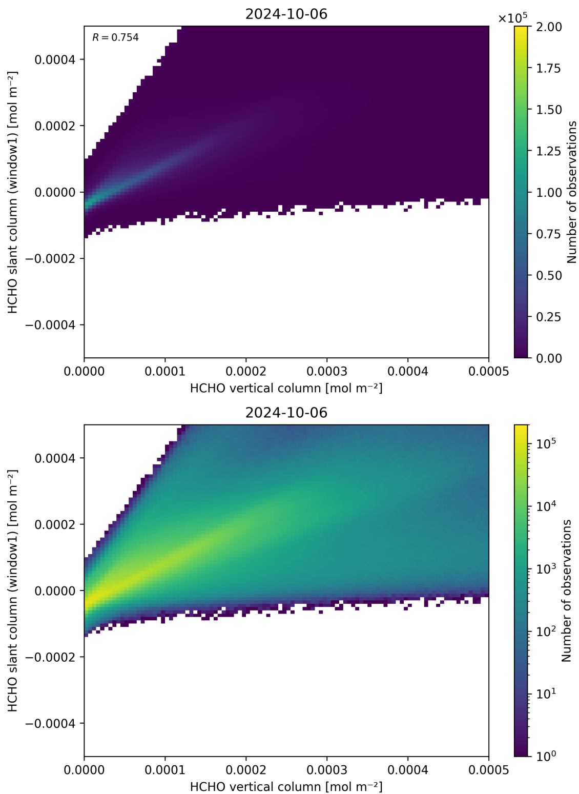
Figure 129: Scatter density plot of “HCHO vertical column” against “HCHO slant column (window1)” for 2024-10-05 to 2024-10-07.
