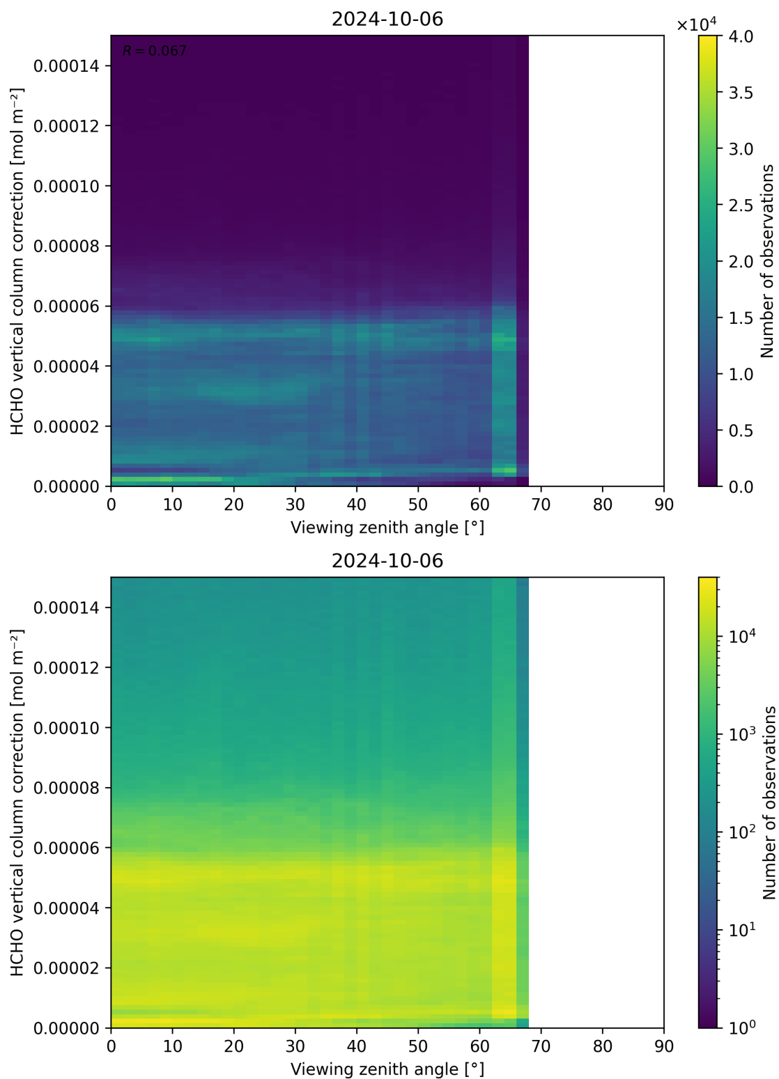
Figure 193: Scatter density plot of “Viewing zenith angle” against “HCHO vertical column correction” for 2024-10-05 to 2024-10-07.
