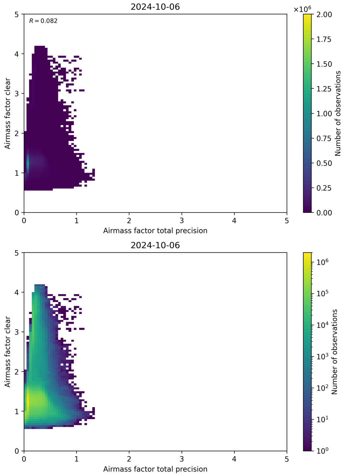
Figure 108: Scatter density plot of “Airmass factor total precision” against “Airmass factor clear” for 2024-10-05 to 2024-10-07.
