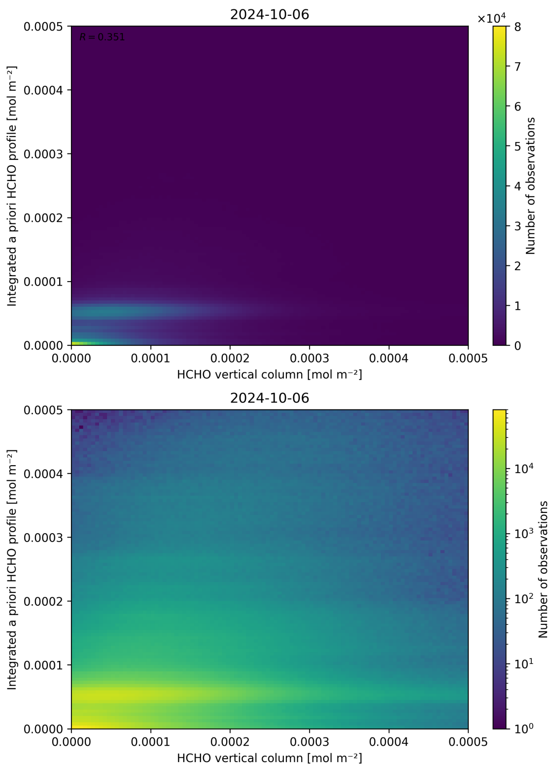
Figure 135: Scatter density plot of “HCHO vertical column” against “Integrated a priori HCHO profile” for 2024-10-05 to 2024-10-07.
