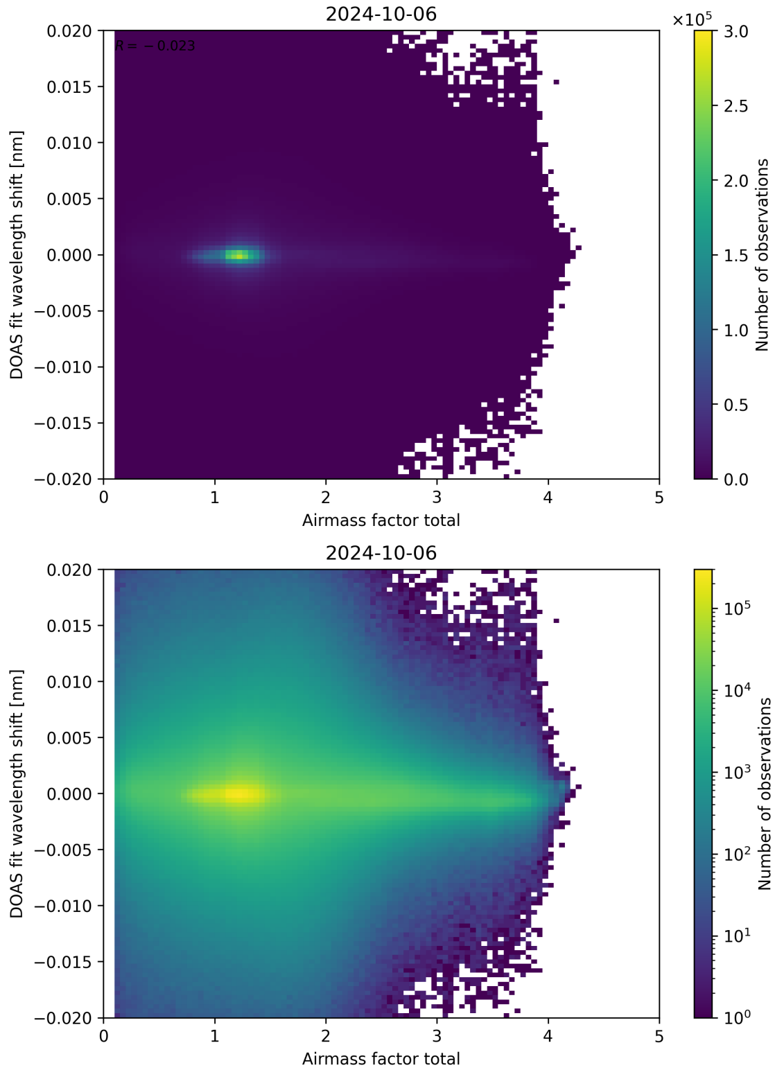
Figure 98: Scatter density plot of “Airmass factor total” against “DOAS fit wavelength shift” for 2024-10-05 to 2024-10-07.
