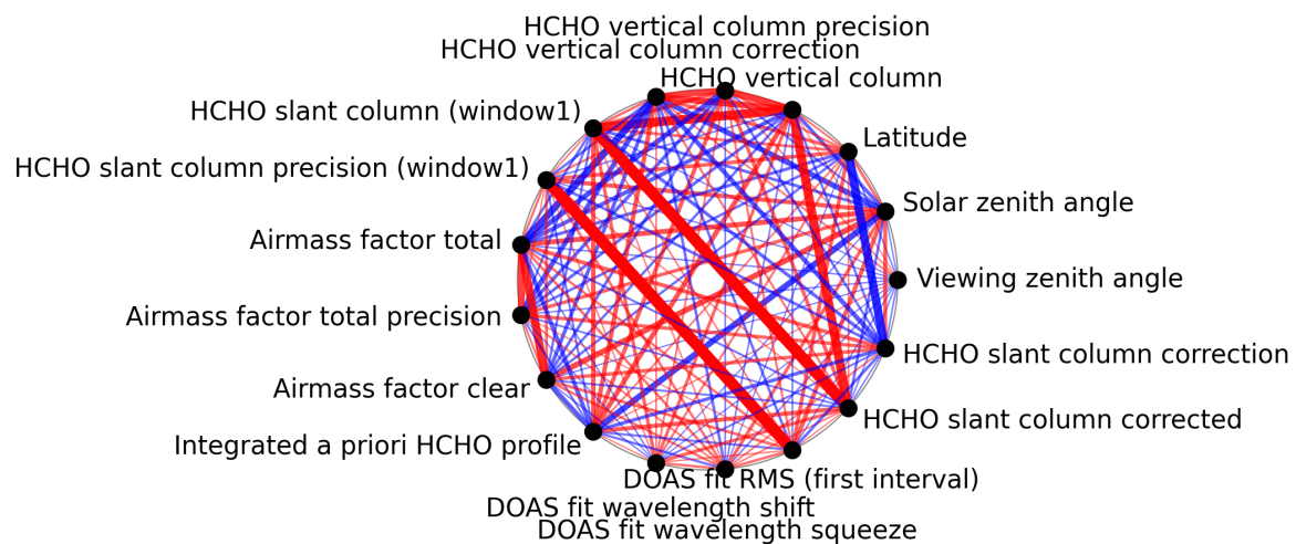
Figure 1: Map of correlation graph for 2024-10-05 to 2024-10-07.
