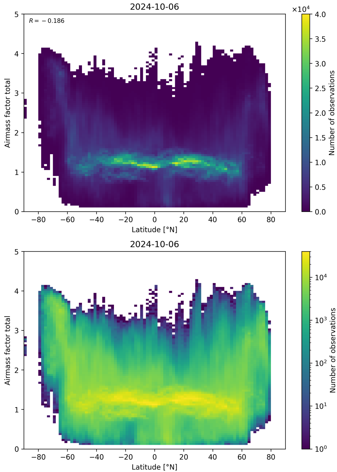
Figure 161: Scatter density plot of “Latitude” against “Airmass factor total” for 2024-10-05 to 2024-10-07.
