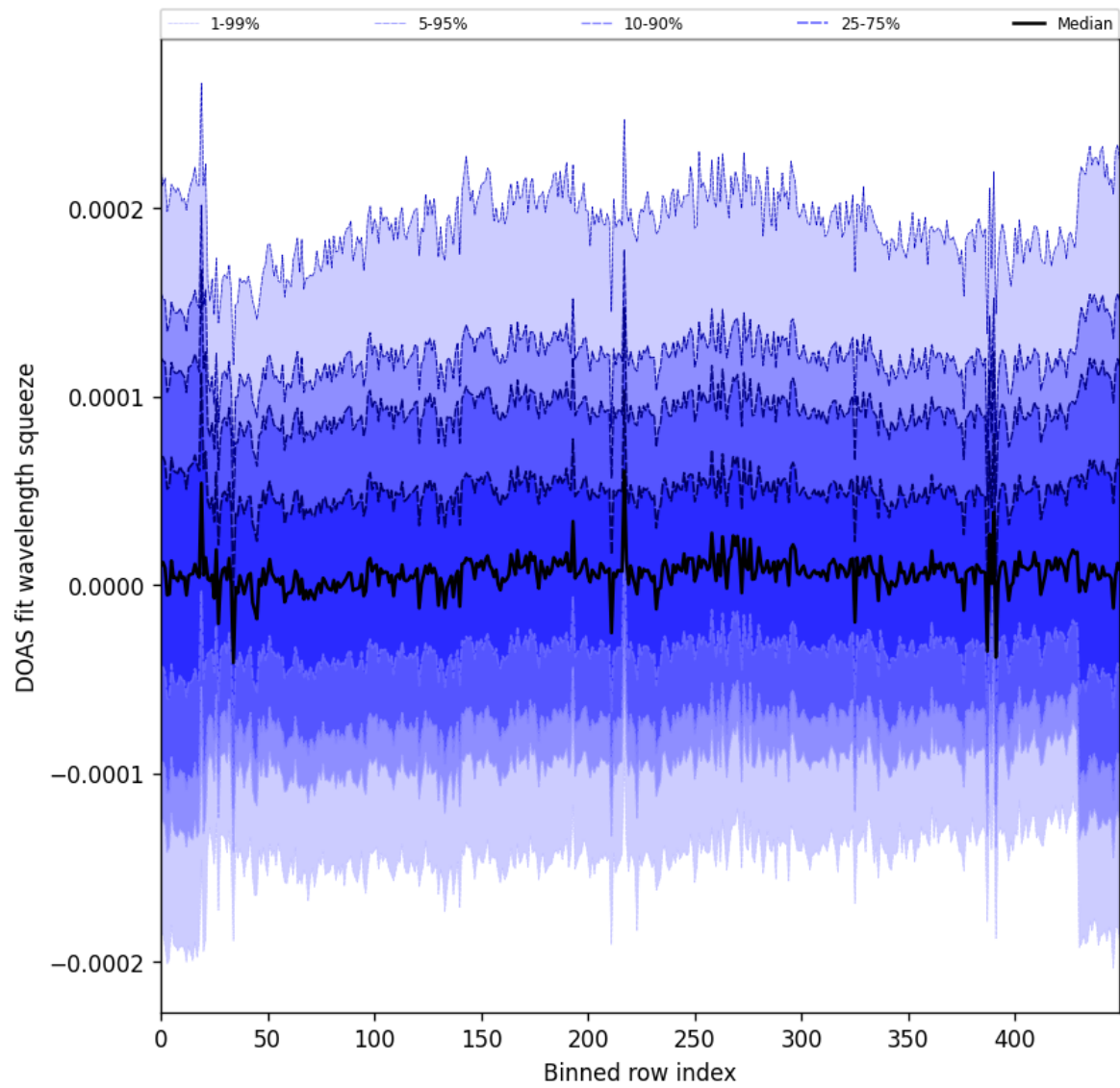
Figure 59: Along track statistics of “DOAS fit wavelength squeeze” for 2024-10-05 to 2024-10-07
