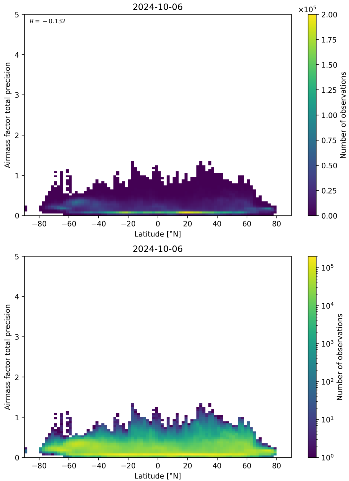
Figure 162: Scatter density plot of “Latitude” against “Airmass factor total precision” for 2024-10-05 to 2024-10-07.
