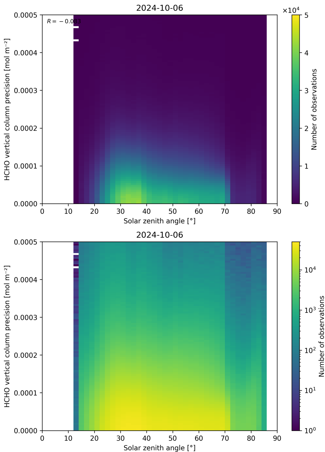
Figure 179: Scatter density plot of “Solar zenith angle” against “HCHO vertical column precision” for 2024-10-05 to 2024-10-07.
