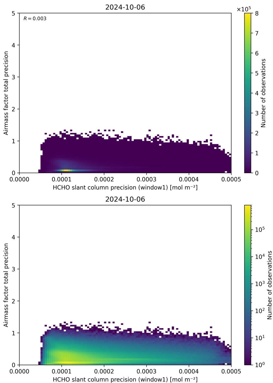
Figure 95: Scatter density plot of “HCHO slant column precision (window1)” against “Airmass factor total precision” for 2024-10-05 to 2024-10-07.
