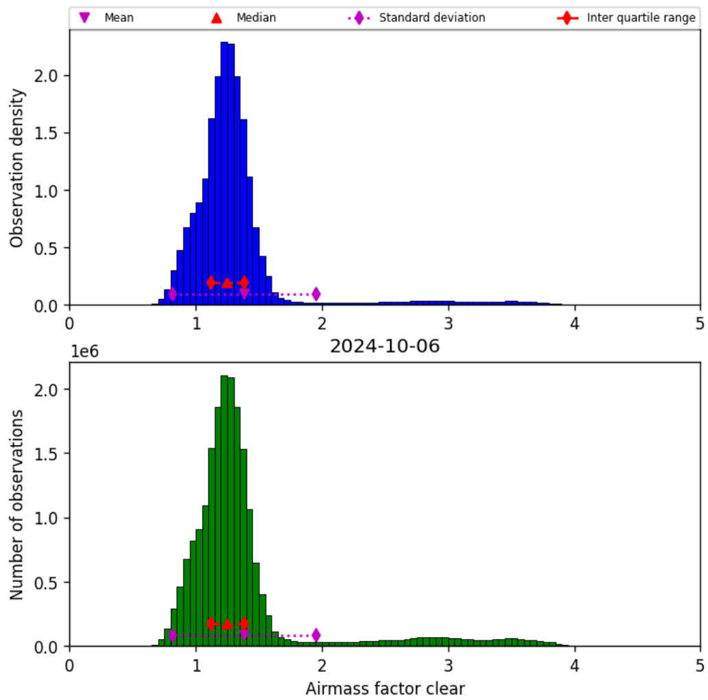
Figure 42: Histogram of “Airmass factor clear” for 2024-10-05 to 2024-10-07
