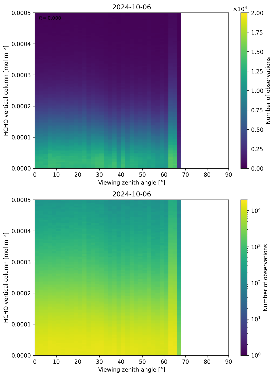
Figure 192: Scatter density plot of “Viewing zenith angle” against “HCHO vertical column” for 2024-10-05 to 2024-10-07.
