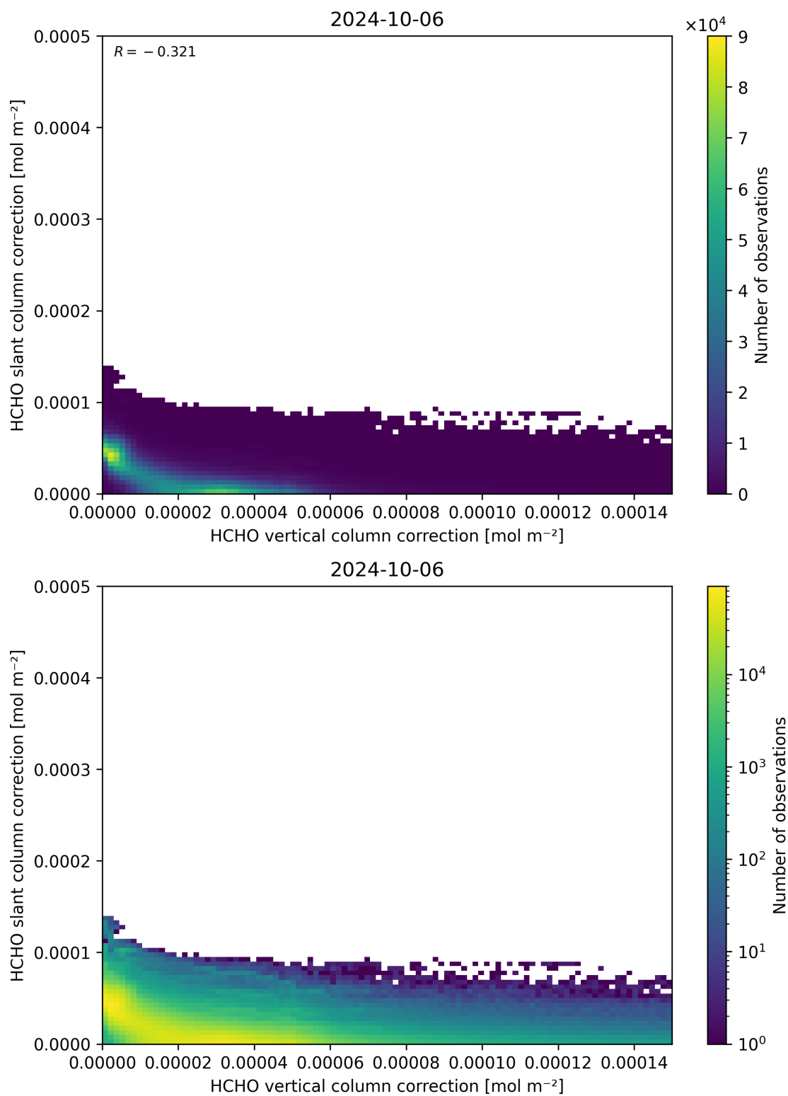
Figure 117: Scatter density plot of “HCHO vertical column correction” against “HCHO slant column correction” for 2024-10-05 to 2024-10-07.
