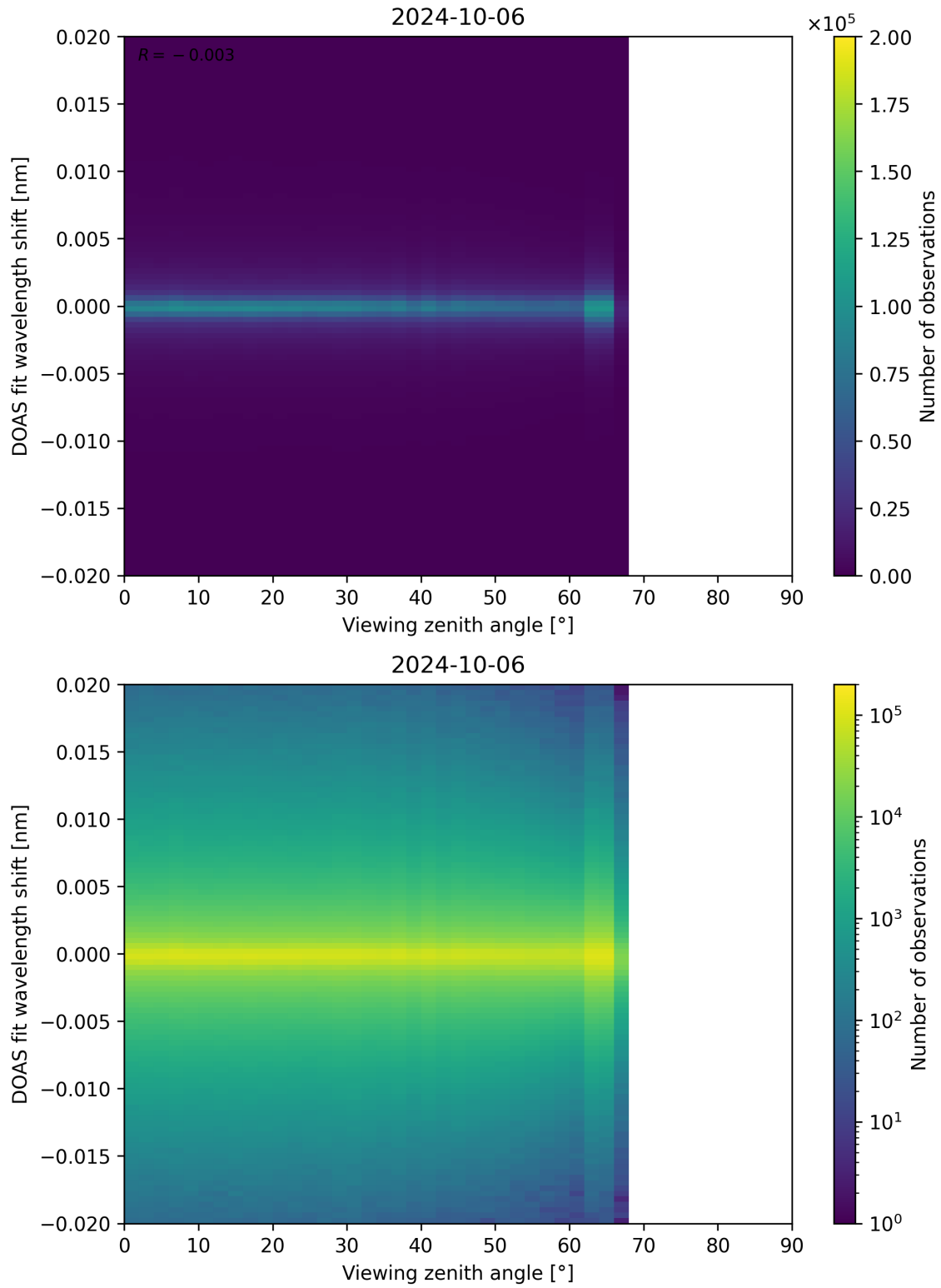
Figure 183: Scatter density plot of “Viewing zenith angle” against “DOAS fit wavelength shift” for 2024-10-05 to 2024-10-07.
