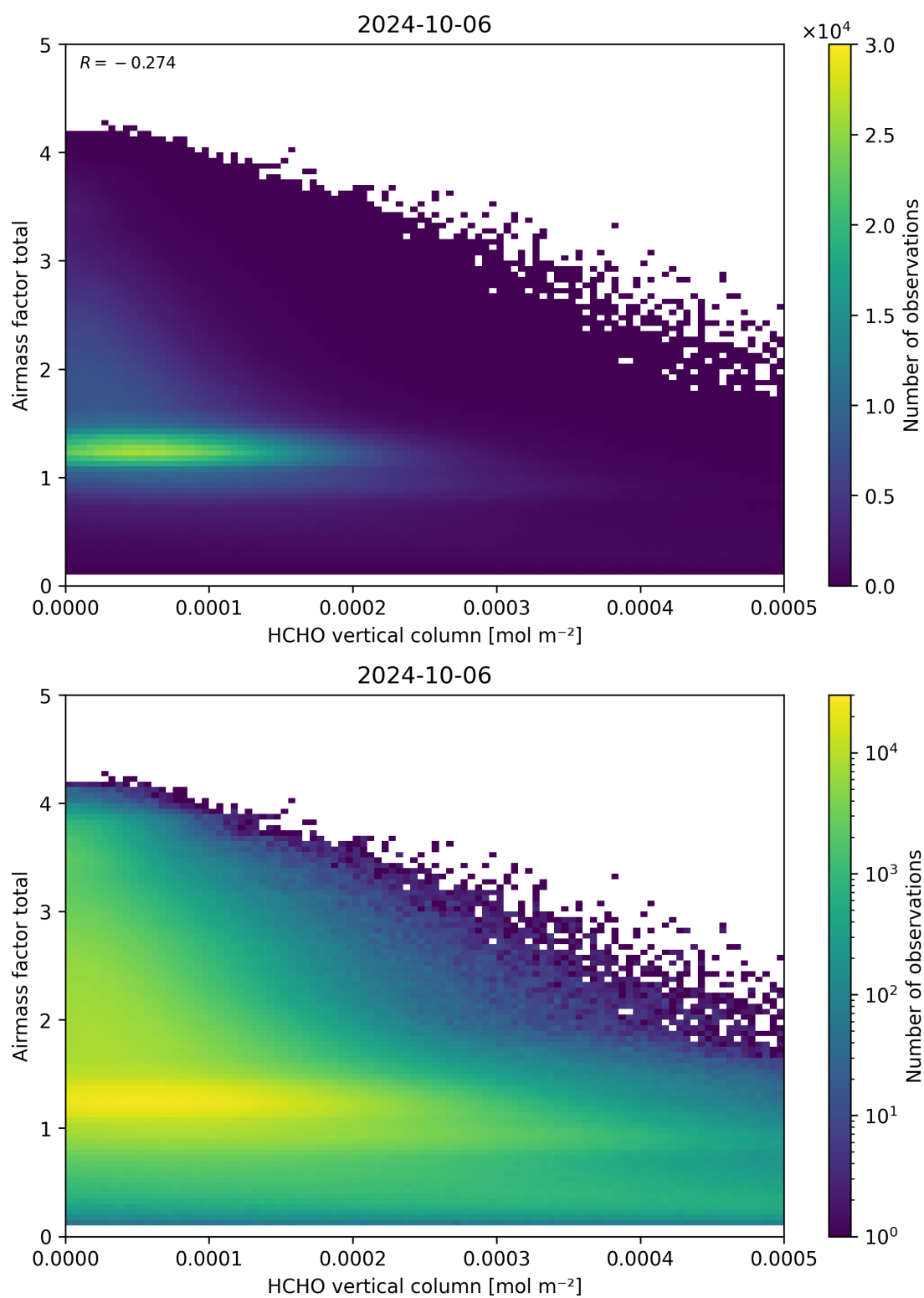
Figure 131: Scatter density plot of “HCHO vertical column” against “Airmass factor total” for 2024-10-05 to 2024-10-07.
