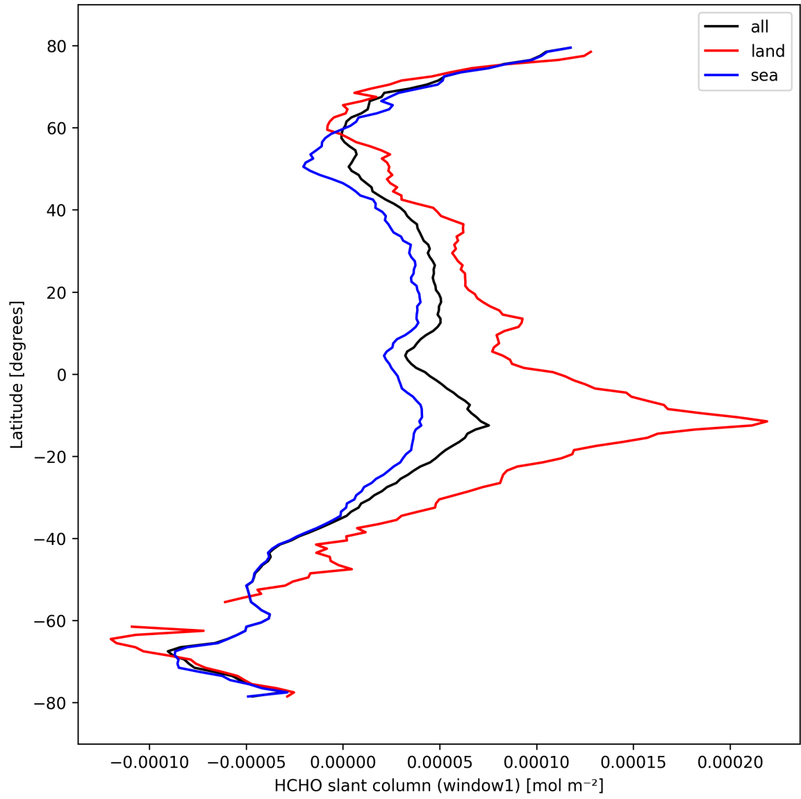
Figure 24: Zonal average of “HCHO slant column (window1)” for 2024-10-05 to 2024-10-07.
