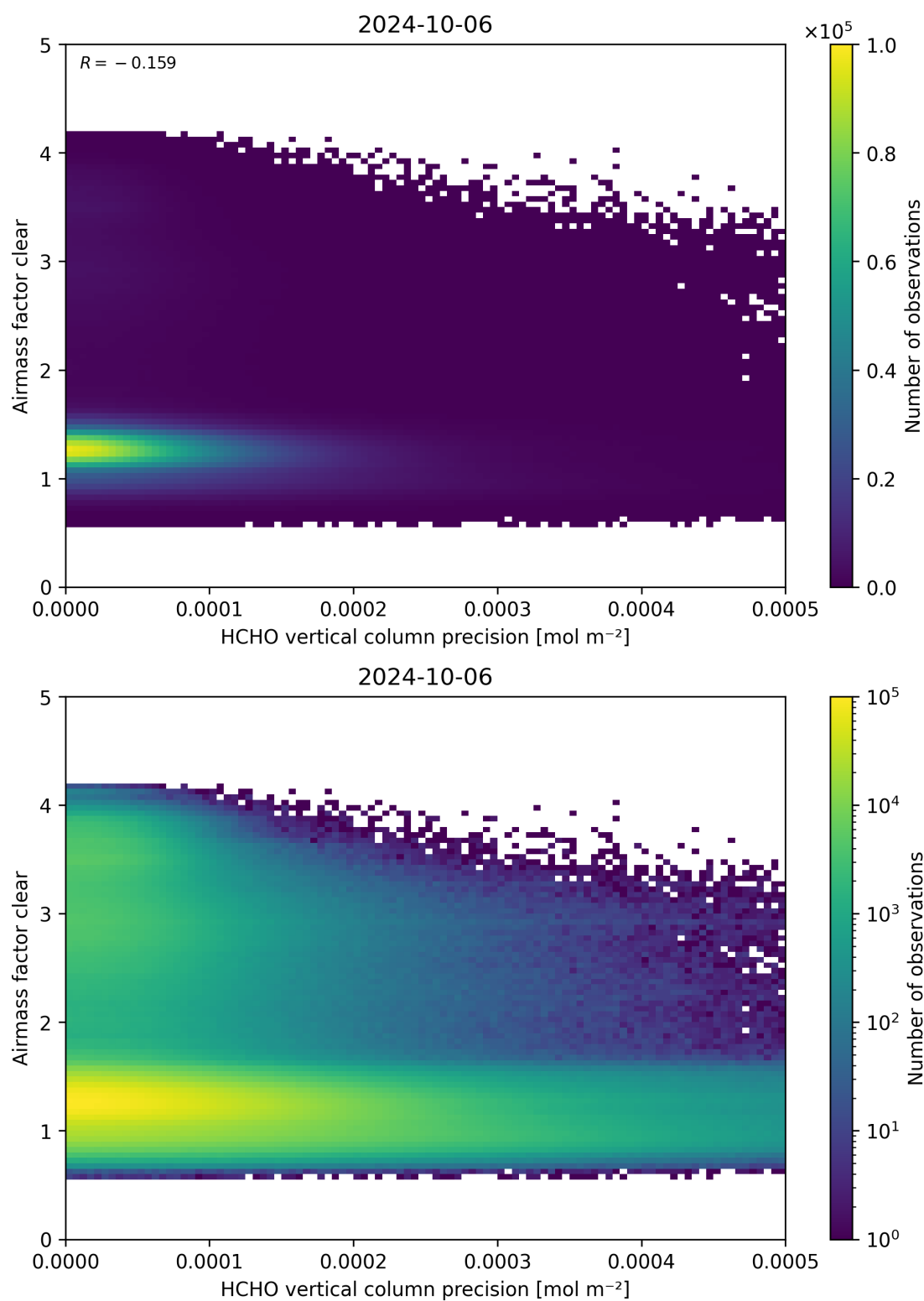
Figure 139: Scatter density plot of “HCHO vertical column precision” against “Airmass factor clear” for 2024-10-05 to 2024-10-07.
