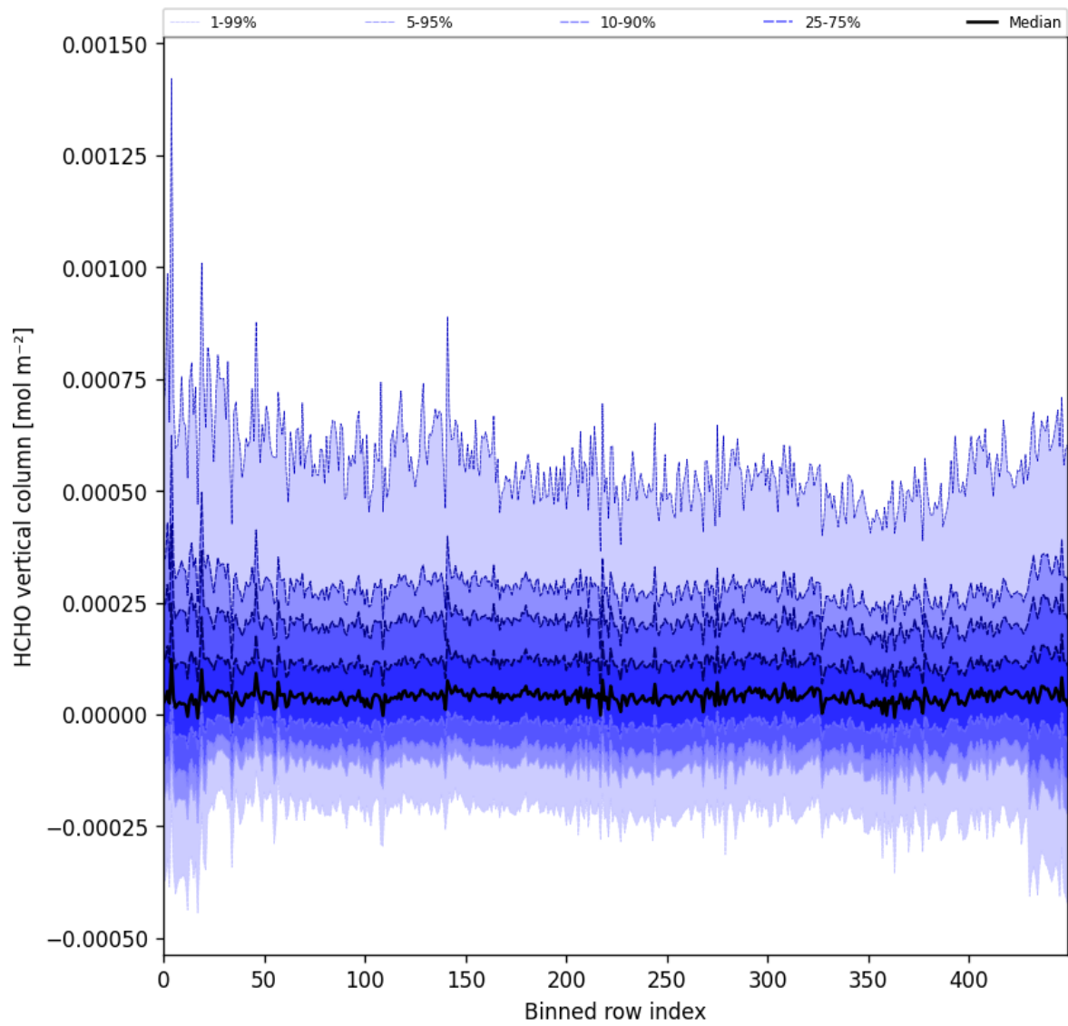
Figure 49: Along track statistics of “HCHO vertical column” for 2024-10-05 to 2024-10-07
