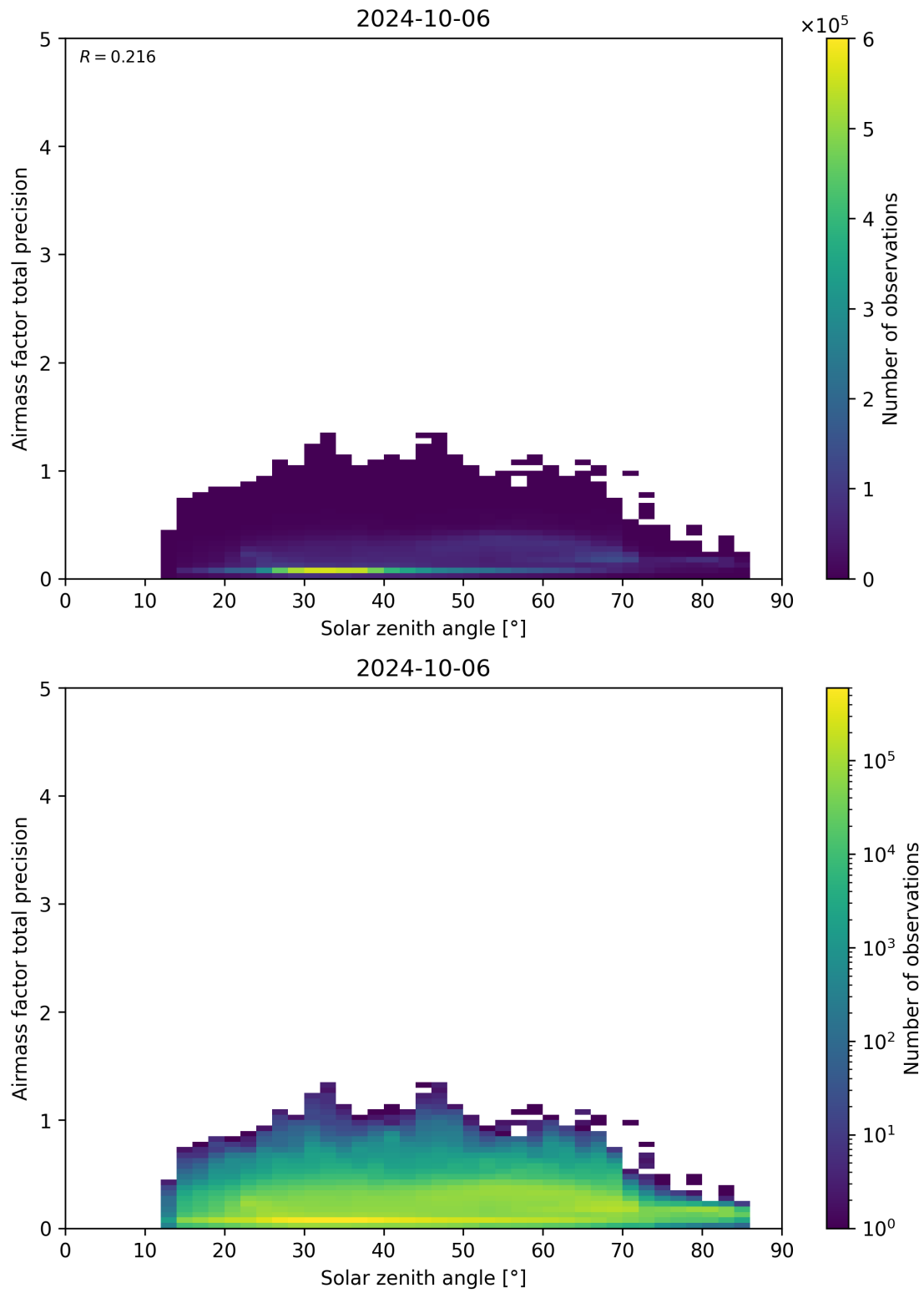
Figure 176: Scatter density plot of “Solar zenith angle” against “Airmass factor total precision” for 2024-10-05 to 2024-10-07.
