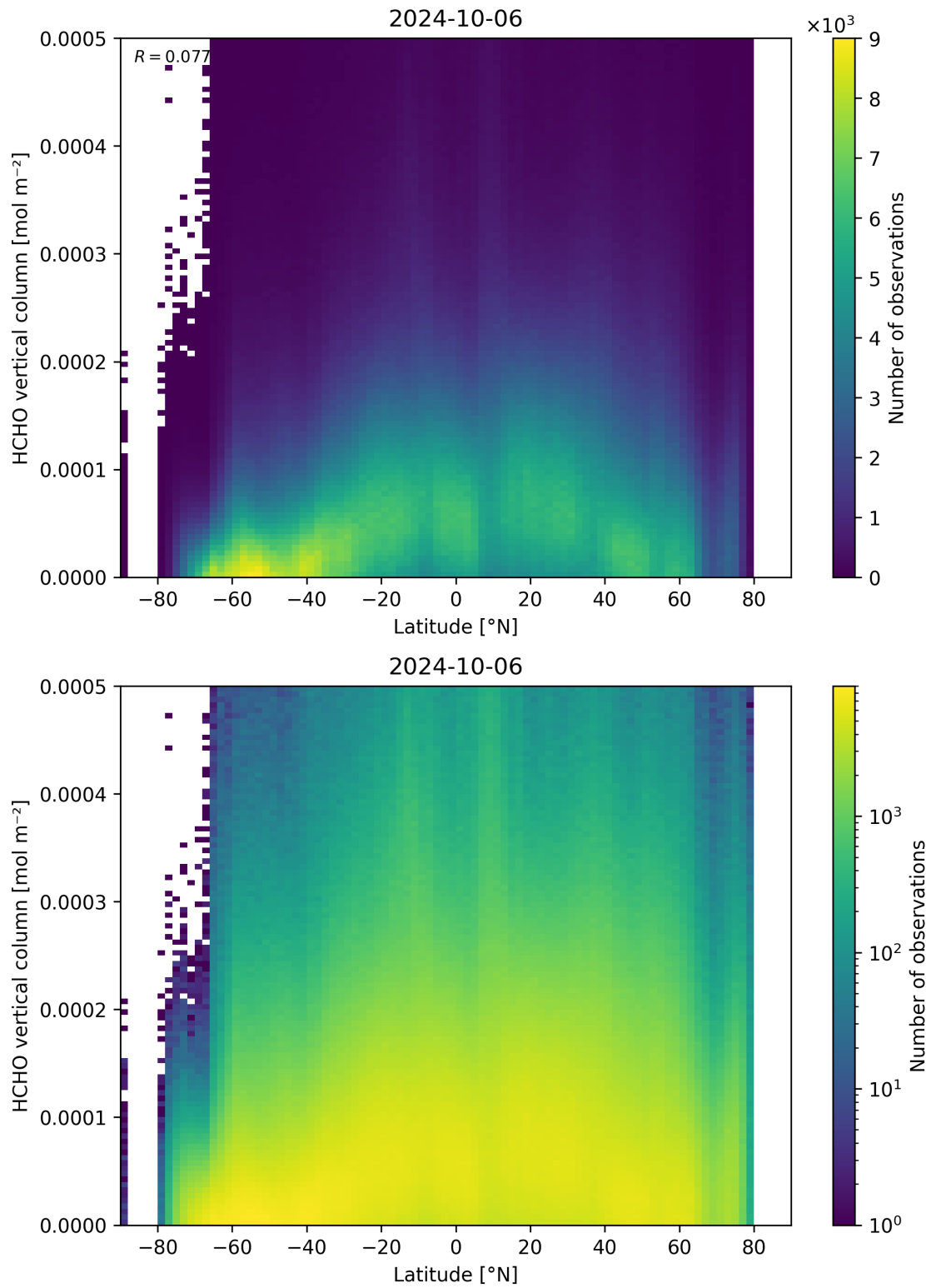
Figure 163: Scatter density plot of “Latitude” against “HCHO vertical column” for 2024-10-05 to 2024-10-07.
