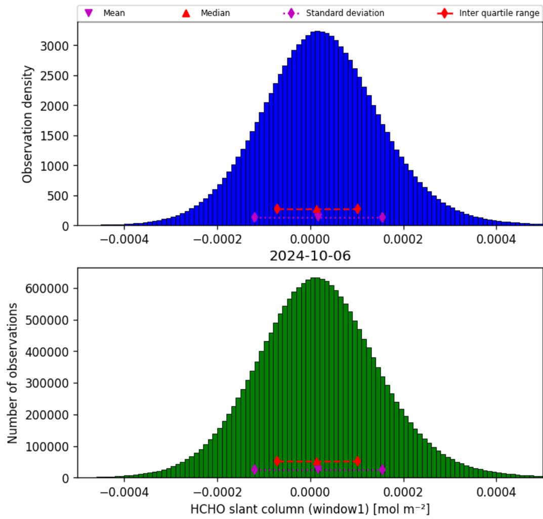
Figure 38: Histogram of “HCHO slant column (window1)” for 2024-10-05 to 2024-10-07
