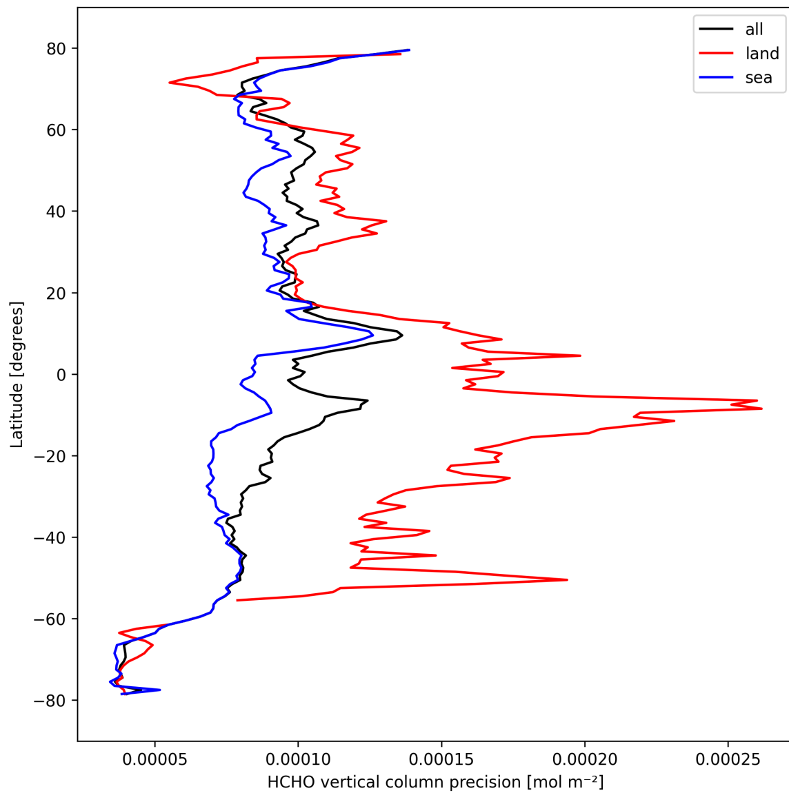
Figure 22: Zonal average of “HCHO vertical column precision” for 2024-10-05 to 2024-10-07.
