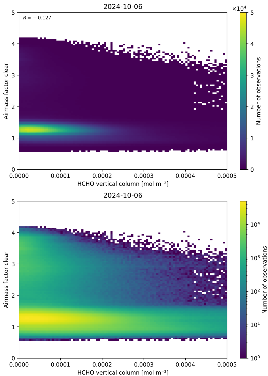
Figure 126: Scatter density plot of “HCHO vertical column” against “Airmass factor clear” for 2024-10-05 to 2024-10-07.
