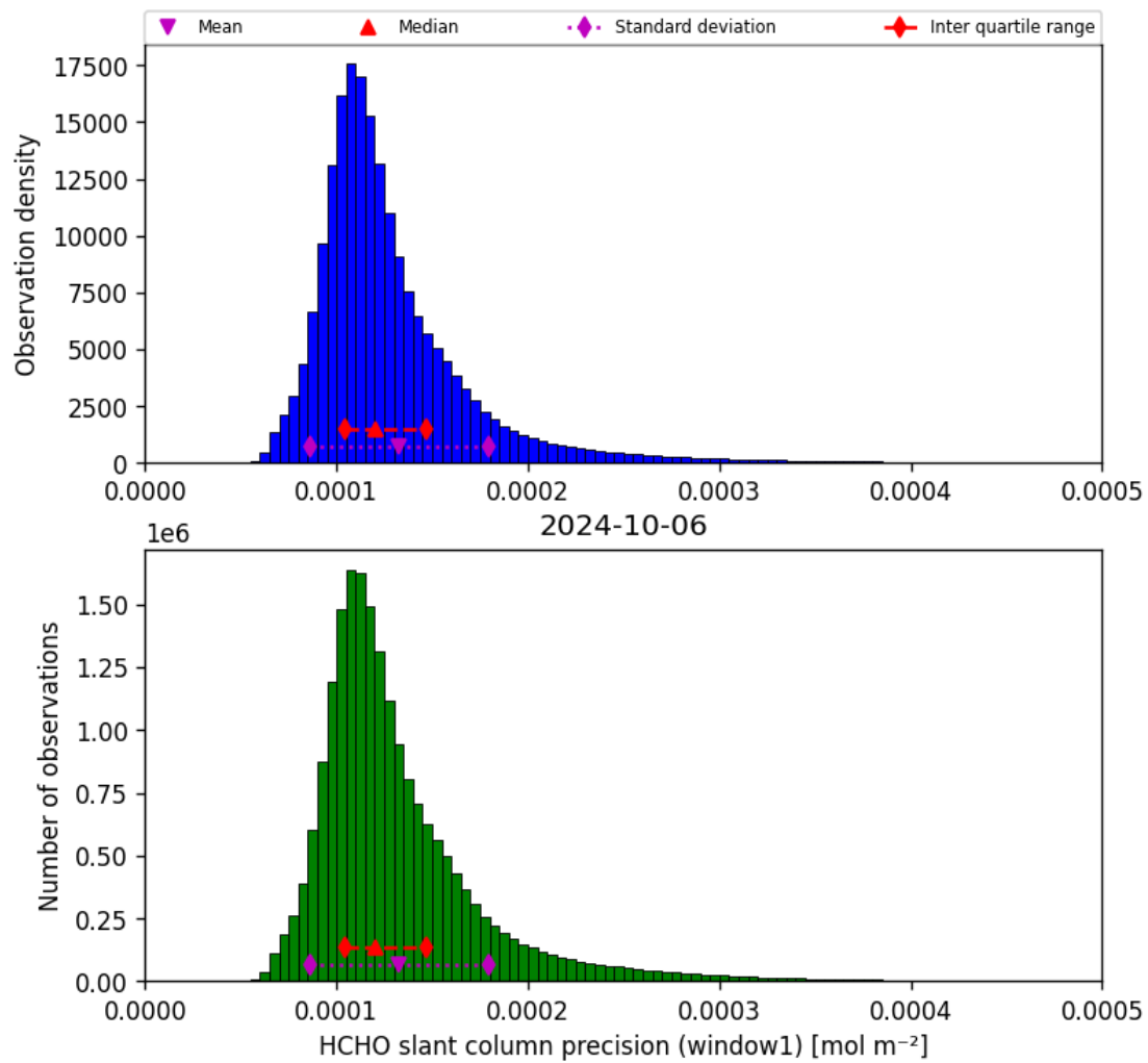
Figure 39: Histogram of “HCHO slant column precision (window1)” for 2024-10-05 to 2024-10-07
