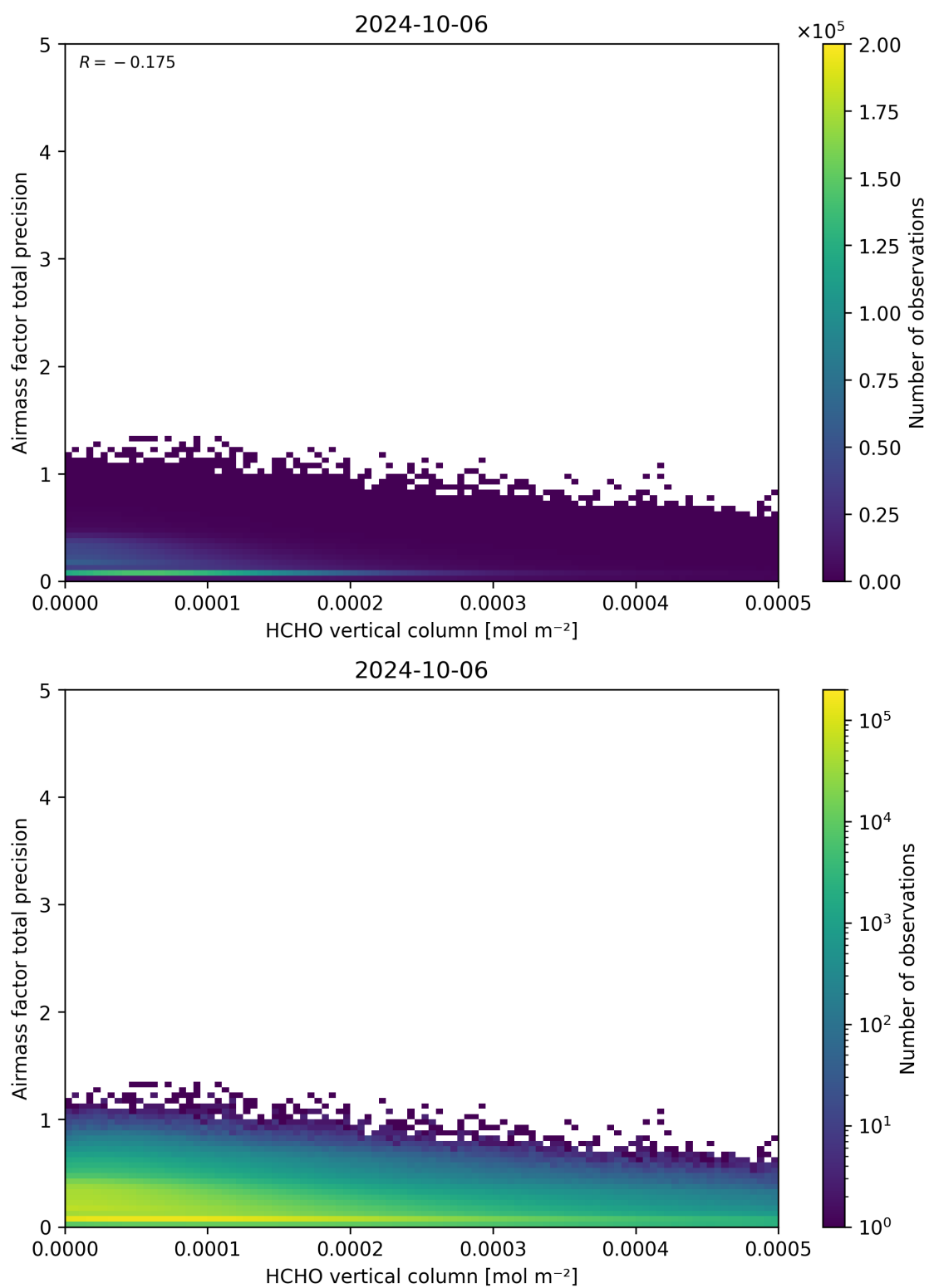
Figure 132: Scatter density plot of “HCHO vertical column” against “Airmass factor total precision” for 2024-10-05 to 2024-10-07.
