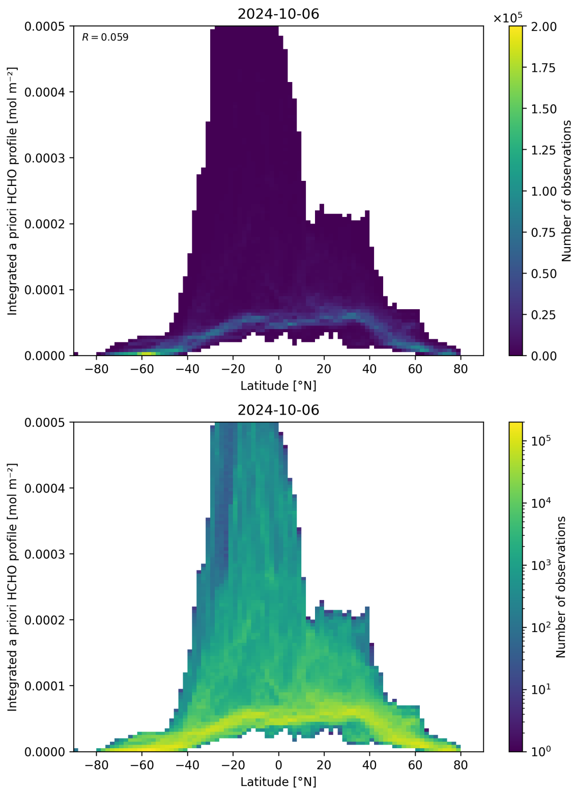
Figure 166: Scatter density plot of “Latitude” against “Integrated a priori HCHO profile” for 2024-10-05 to 2024-10-07.
