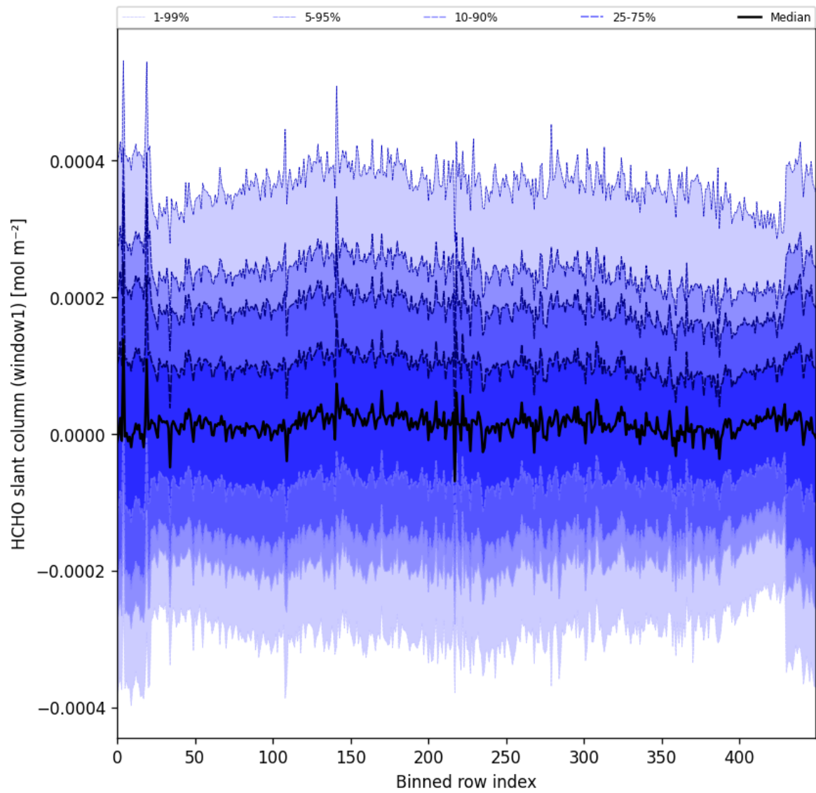
Figure 52: Along track statistics of “HCHO slant column (window1)” for 2024-10-05 to 2024-10-07
