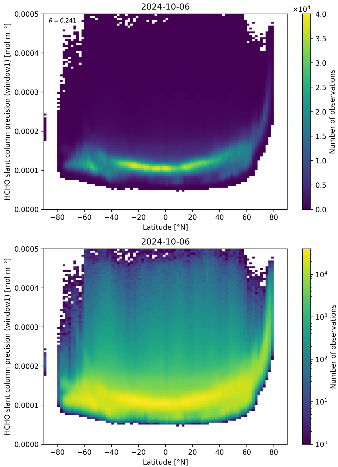
Figure 160: Scatter density plot of “Latitude” against “HCHO slant column precision (window1)” for 2024-10-05 to 2024-10-07.
