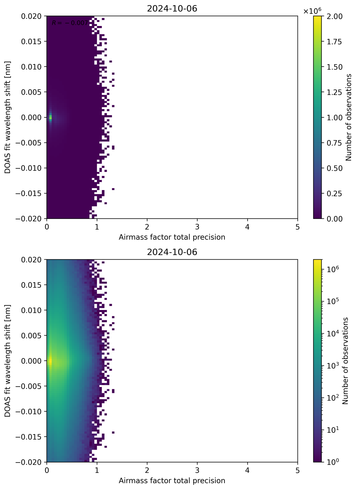
Figure 106: Scatter density plot of “Airmass factor total precision” against “DOAS fit wavelength shift” for 2024-10-05 to 2024-10-07.
