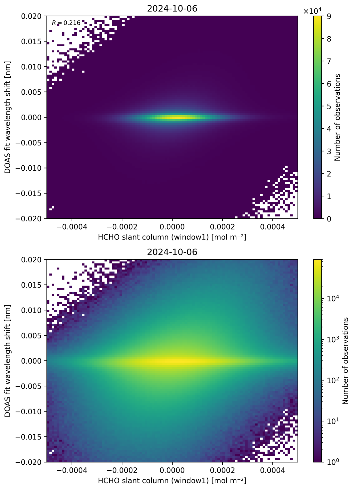
Figure 79: Scatter density plot of “HCHO slant column (window1)” against “DOAS fit wavelength shift” for 2024-10-05 to 2024-10-07.
