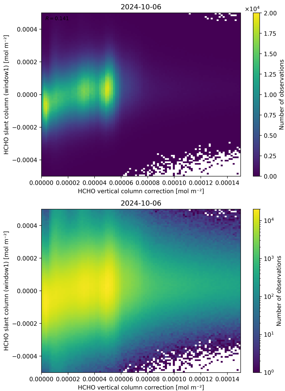
Figure 118: Scatter density plot of “HCHO vertical column correction” against “HCHO slant column (window1)” for 2024-10-05 to 2024-10-07.
