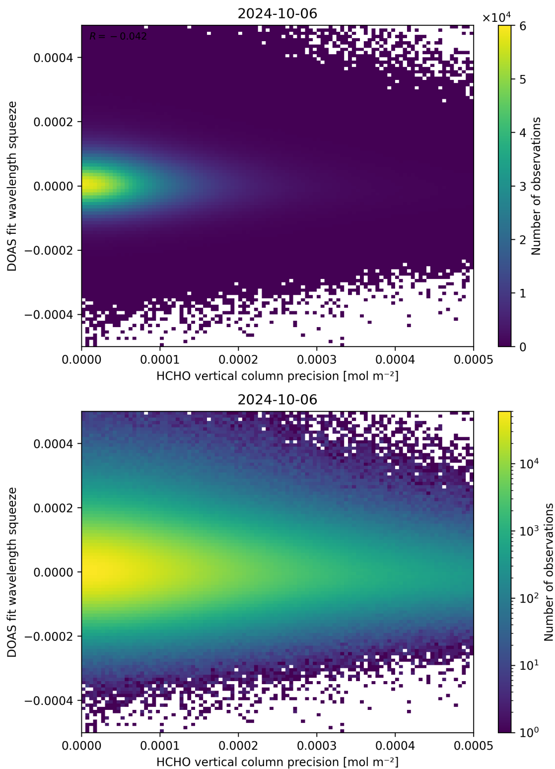
Figure 138: Scatter density plot of “HCHO vertical column precision” against “DOAS fit wavelength squeeze” for 2024-10-05 to 2024-10-07.
