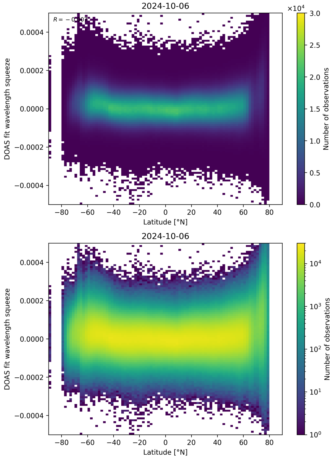
Figure 155: Scatter density plot of “Latitude” against “DOAS fit wavelength squeeze” for 2024-10-05 to 2024-10-07.
