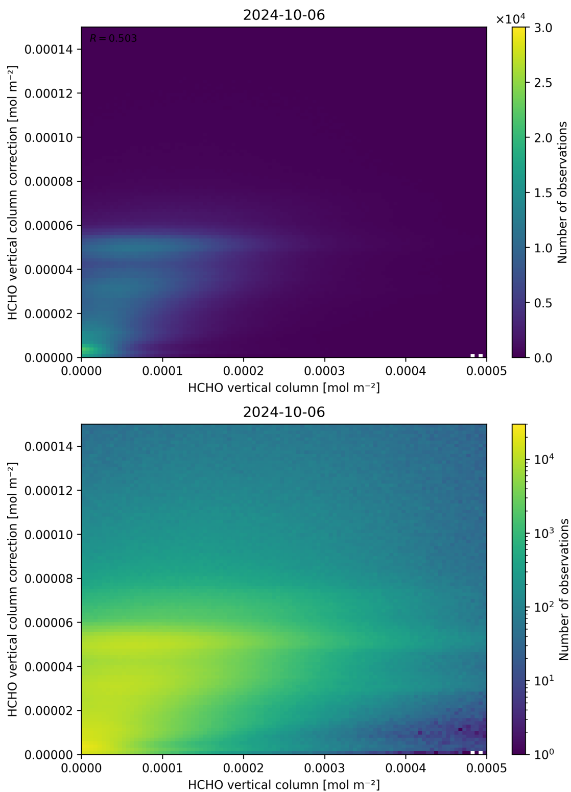
Figure 133: Scatter density plot of “HCHO vertical column” against “HCHO vertical column correction” for 2024-10-05 to 2024-10-07.
