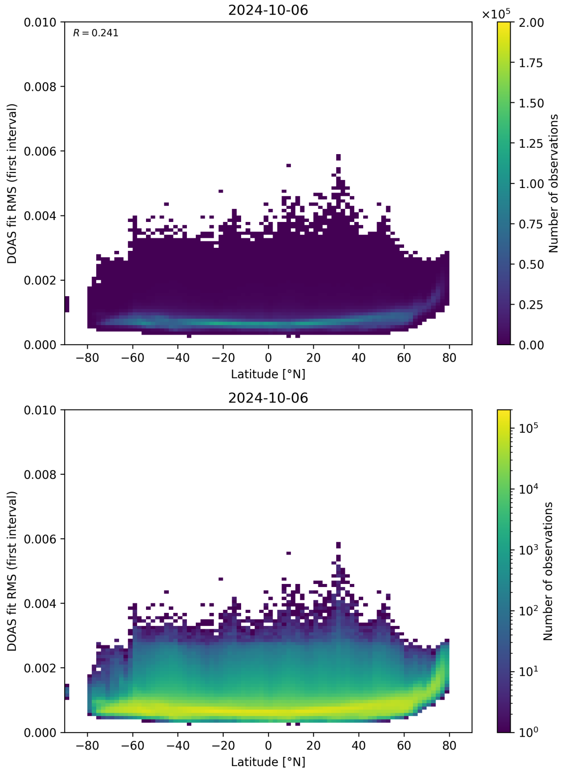
Figure 153: Scatter density plot of “Latitude” against “DOAS fit RMS (first interval)” for 2024-10-05 to 2024-10-07.
