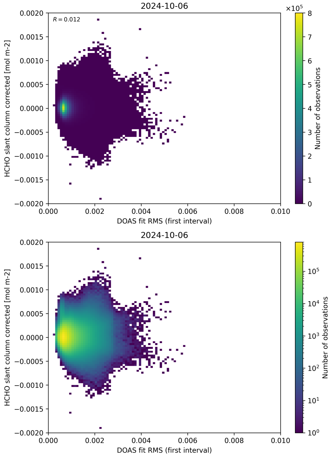
Figure 62: Scatter density plot of “DOAS fit RMS (first interval)” against “HCHO slant column corrected” for 2024-10-05 to 2024-10-07.
