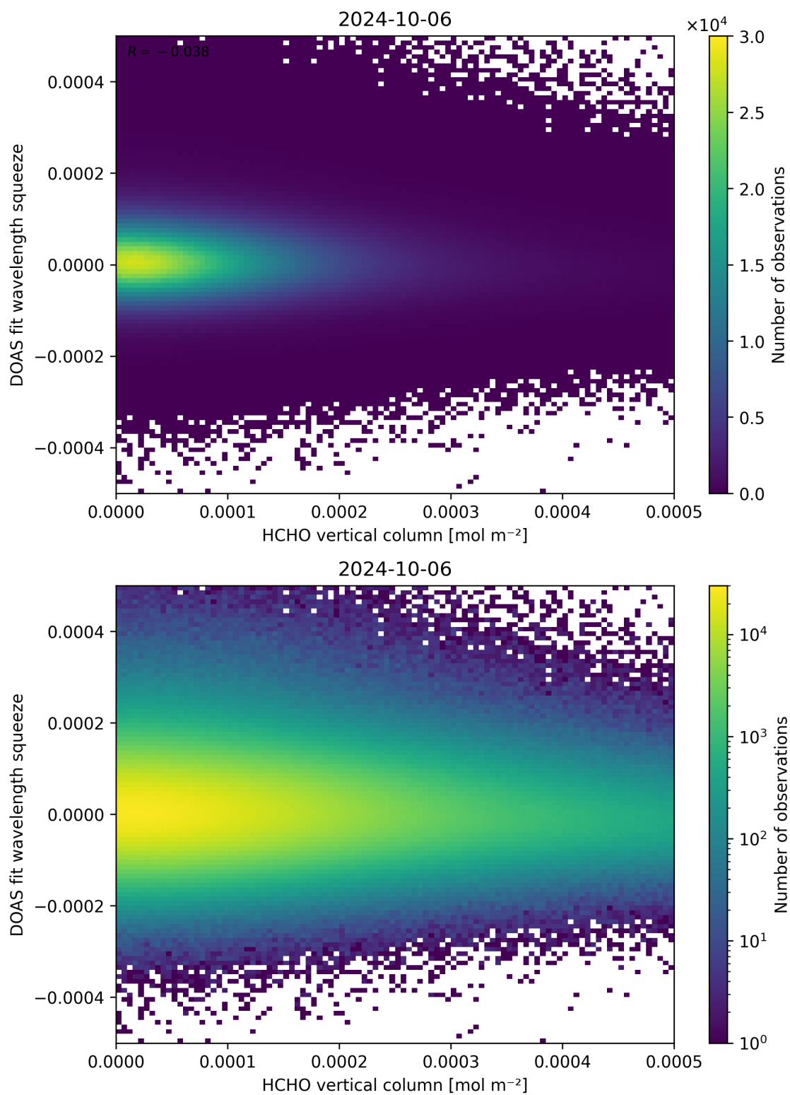
Figure 125: Scatter density plot of “HCHO vertical column” against “DOAS fit wavelength squeeze” for 2024-10-05 to 2024-10-07.
