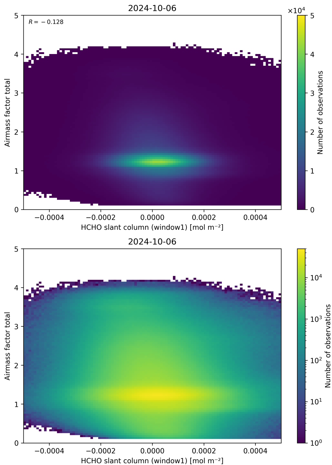
Figure 85: Scatter density plot of “HCHO slant column (window1)” against “Airmass factor total” for 2024-10-05 to 2024-10-07.
