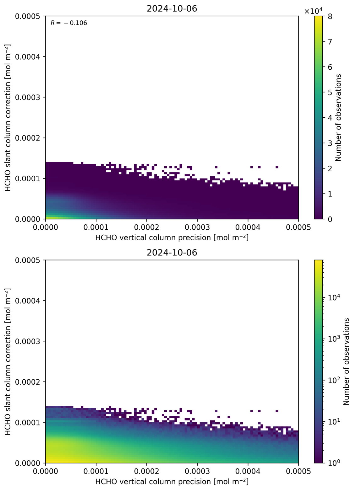
Figure 141: Scatter density plot of “HCHO vertical column precision” against “HCHO slant column correction” for 2024-10-05 to 2024-10-07.
