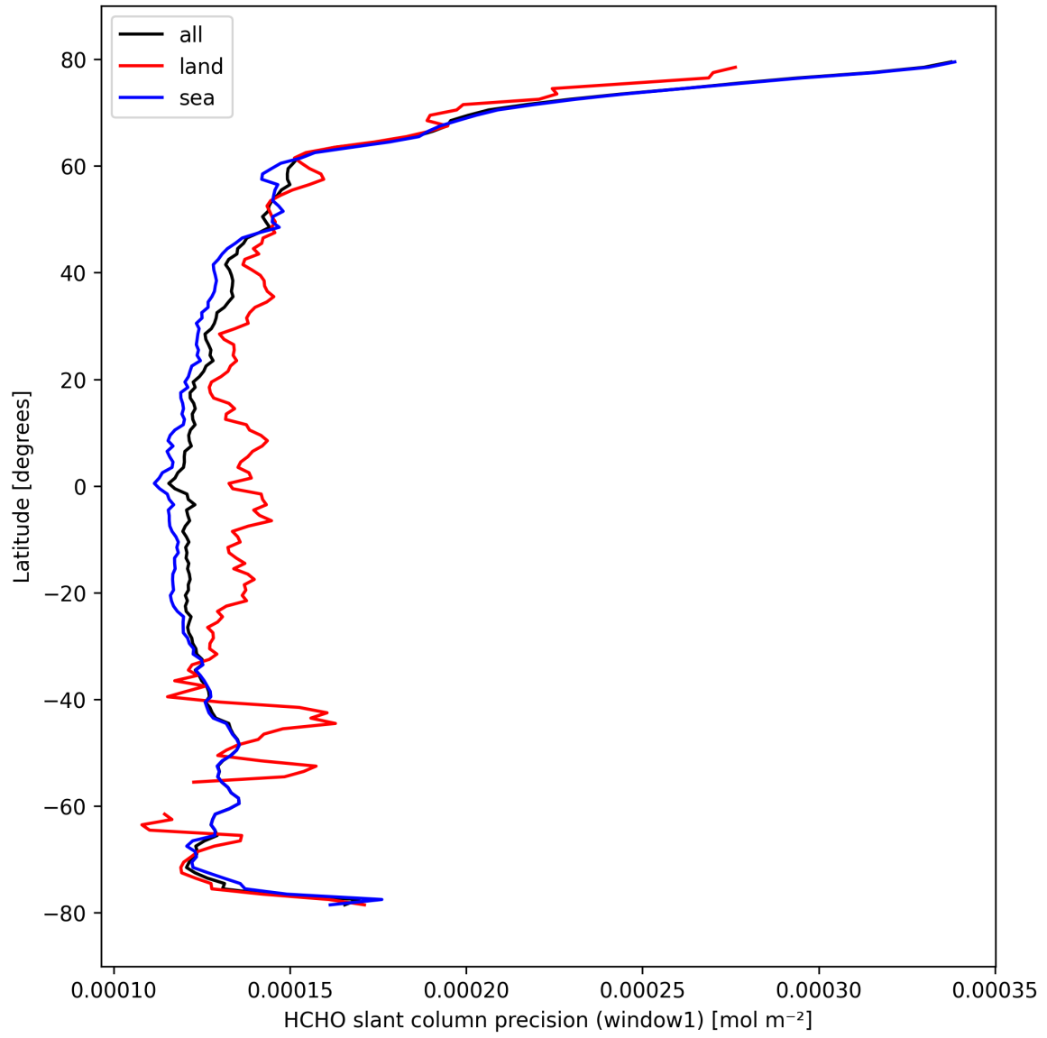
Figure 25: Zonal average of “HCHO slant column precision (window1)” for 2024-10-05 to 2024-10-07.
