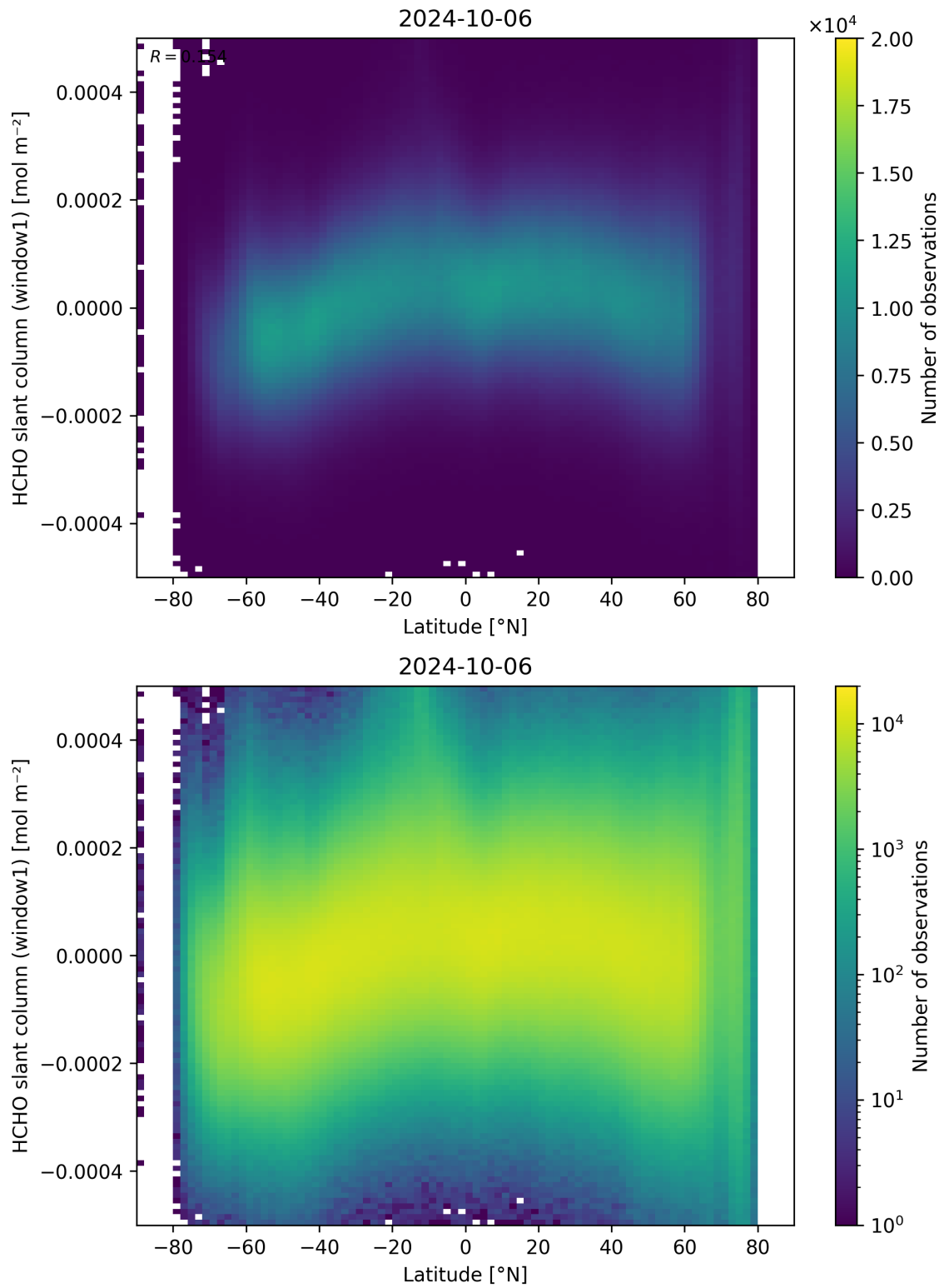
Figure 159: Scatter density plot of “Latitude” against “HCHO slant column (window1)” for 2024-10-05 to 2024-10-07.
