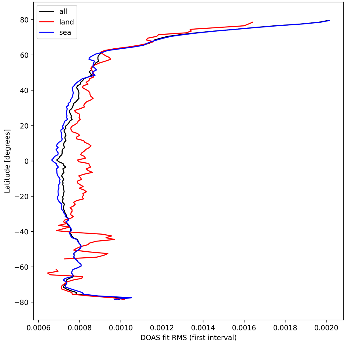
Figure 32: Zonal average of “DOAS fit RMS (first interval)” for 2024-10-05 to 2024-10-07.
