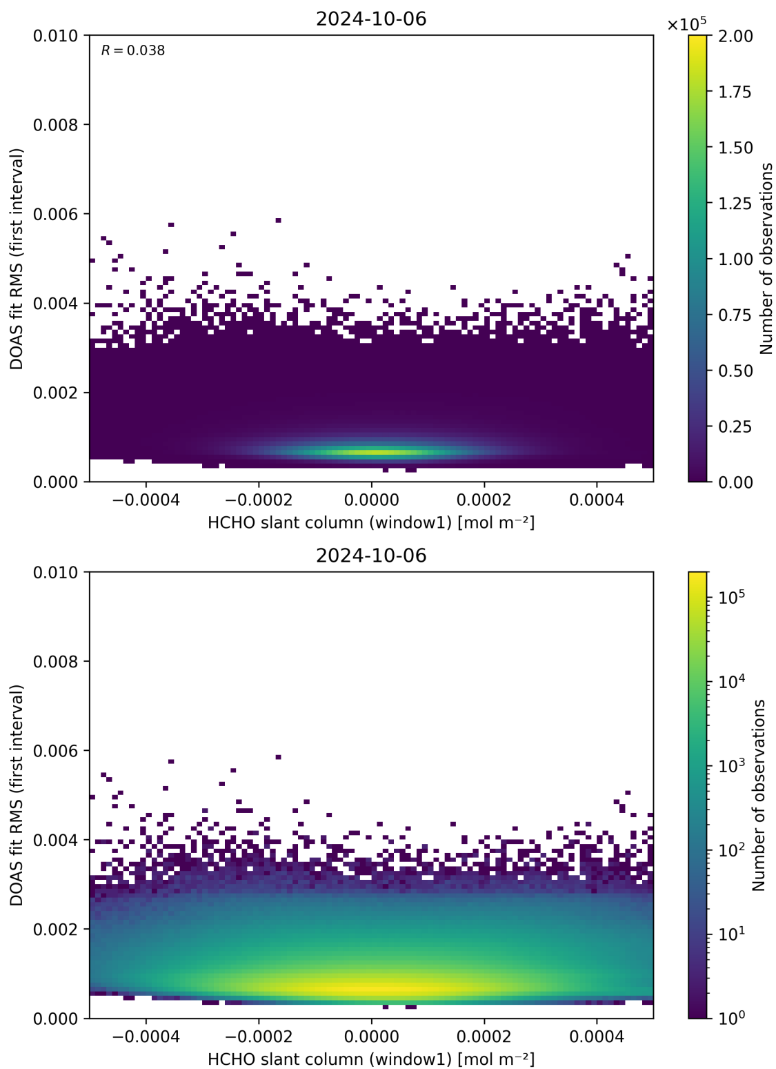
Figure 78: Scatter density plot of “HCHO slant column (window1)” against “DOAS fit RMS (first interval)” for 2024-10-05 to 2024-10-07.
