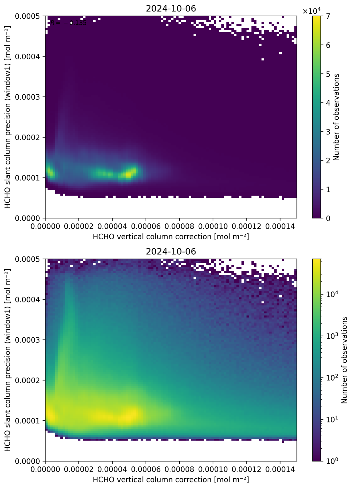
Figure 119: Scatter density plot of “HCHO vertical column correction” against “HCHO slant column precision (window1)” for 2024-10-05 to 2024-10-07.
