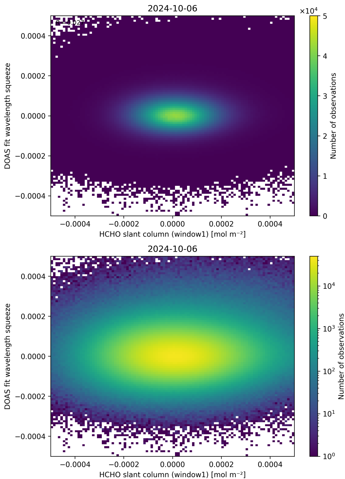
Figure 80: Scatter density plot of “HCHO slant column (window1)” against “DOAS fit wavelength squeeze” for 2024-10-05 to 2024-10-07.
