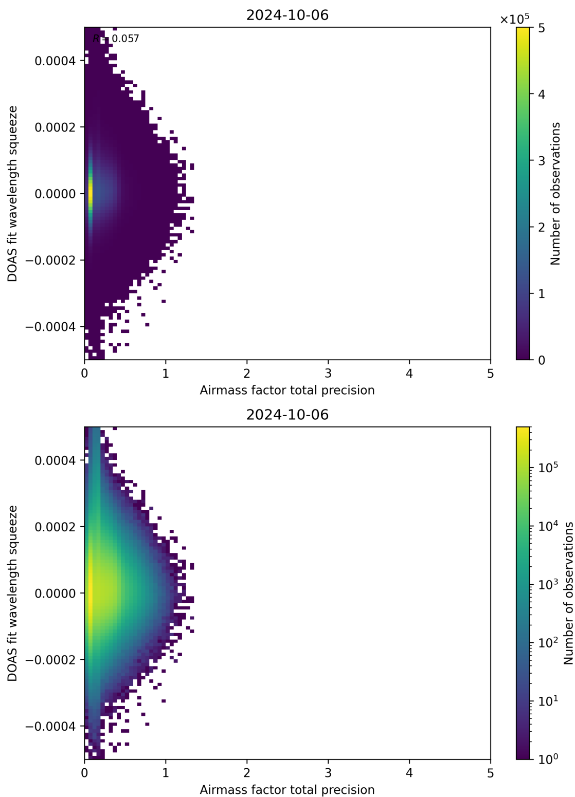
Figure 107: Scatter density plot of “Airmass factor total precision” against “DOAS fit wavelength squeeze” for 2024-10-05 to 2024-10-07.
