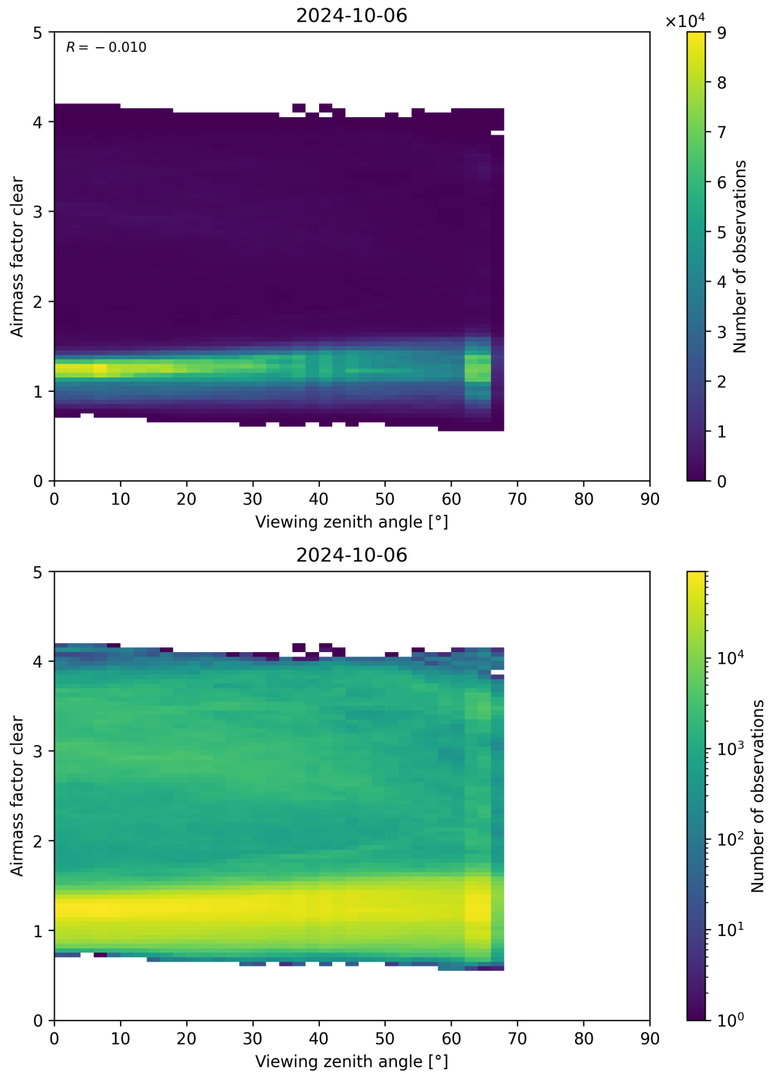
Figure 185: Scatter density plot of “Viewing zenith angle” against “Airmass factor clear” for 2024-10-05 to 2024-10-07.
