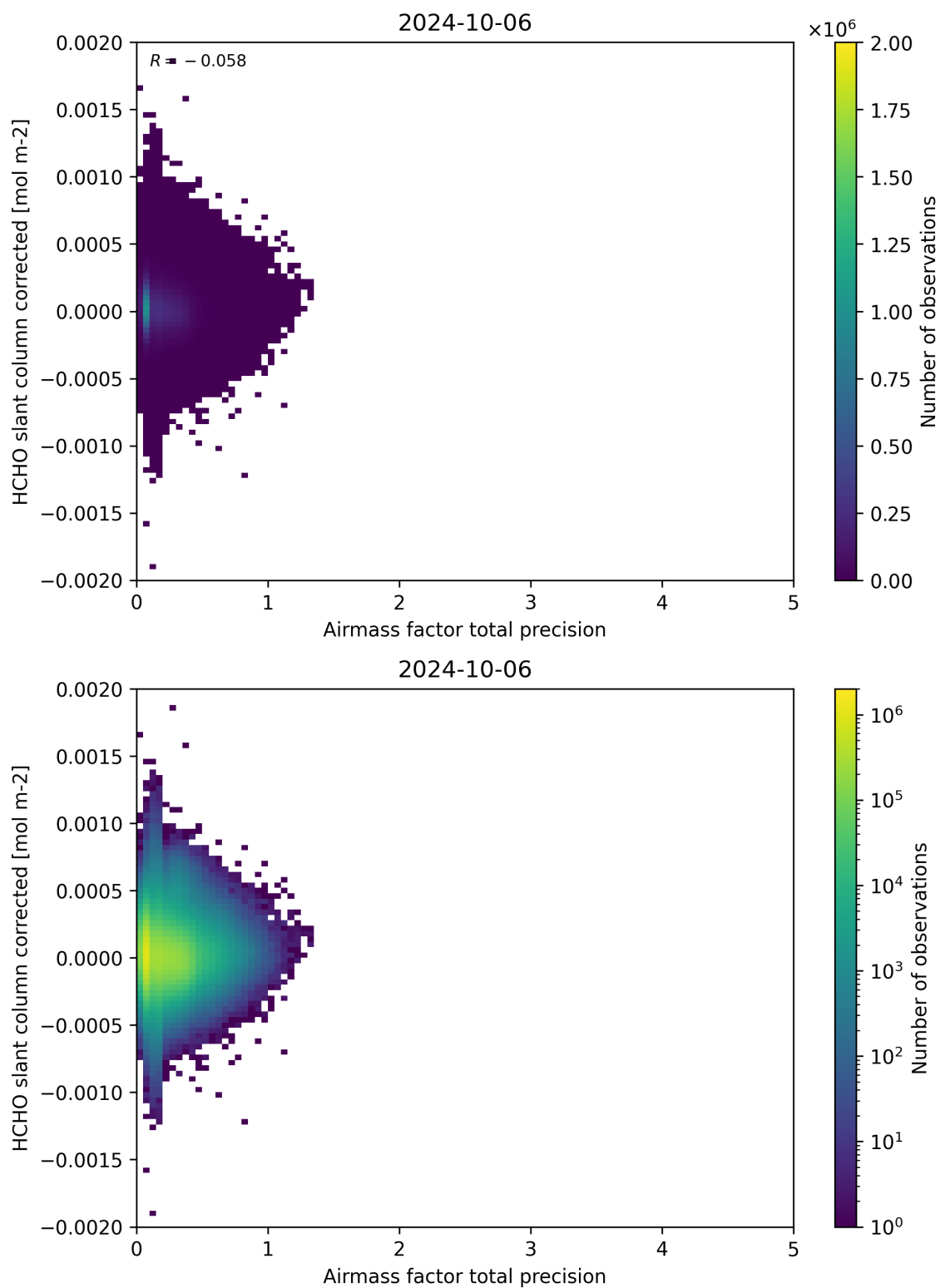
Figure 109: Scatter density plot of “Airmass factor total precision” against “HCHO slant column corrected” for 2024-10-05 to 2024-10-07.
