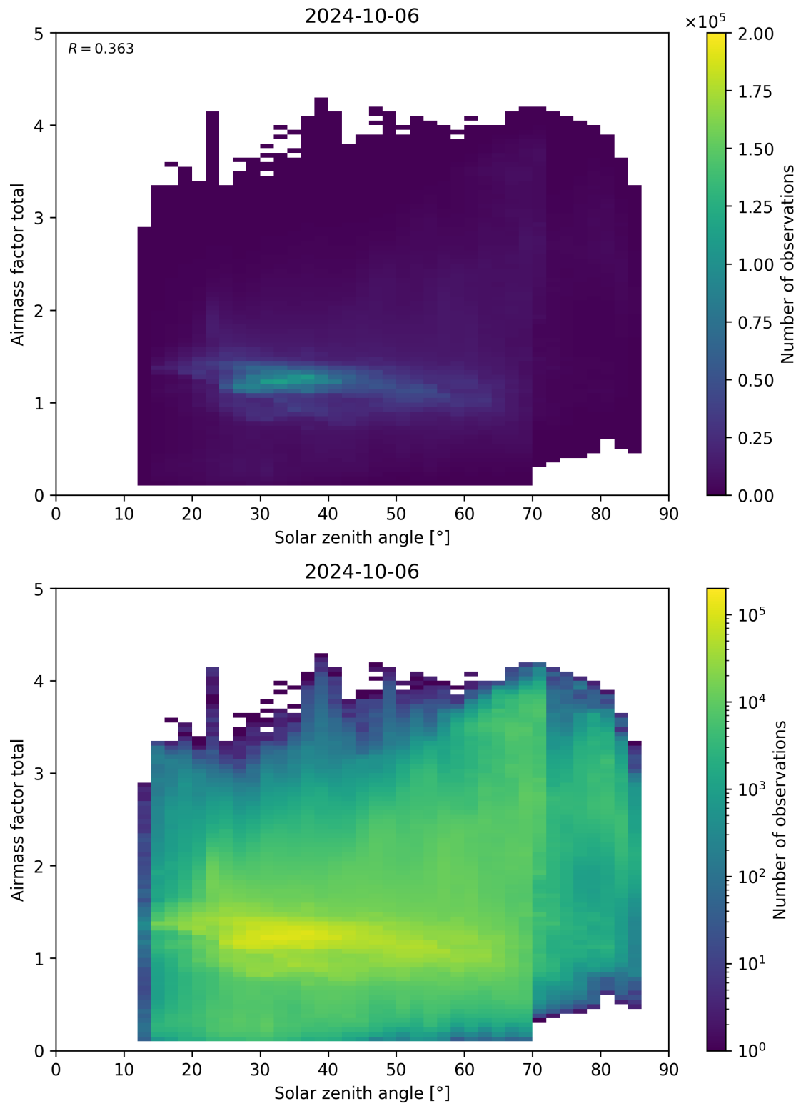
Figure 175: Scatter density plot of “Solar zenith angle” against “Airmass factor total” for 2024-10-05 to 2024-10-07.
