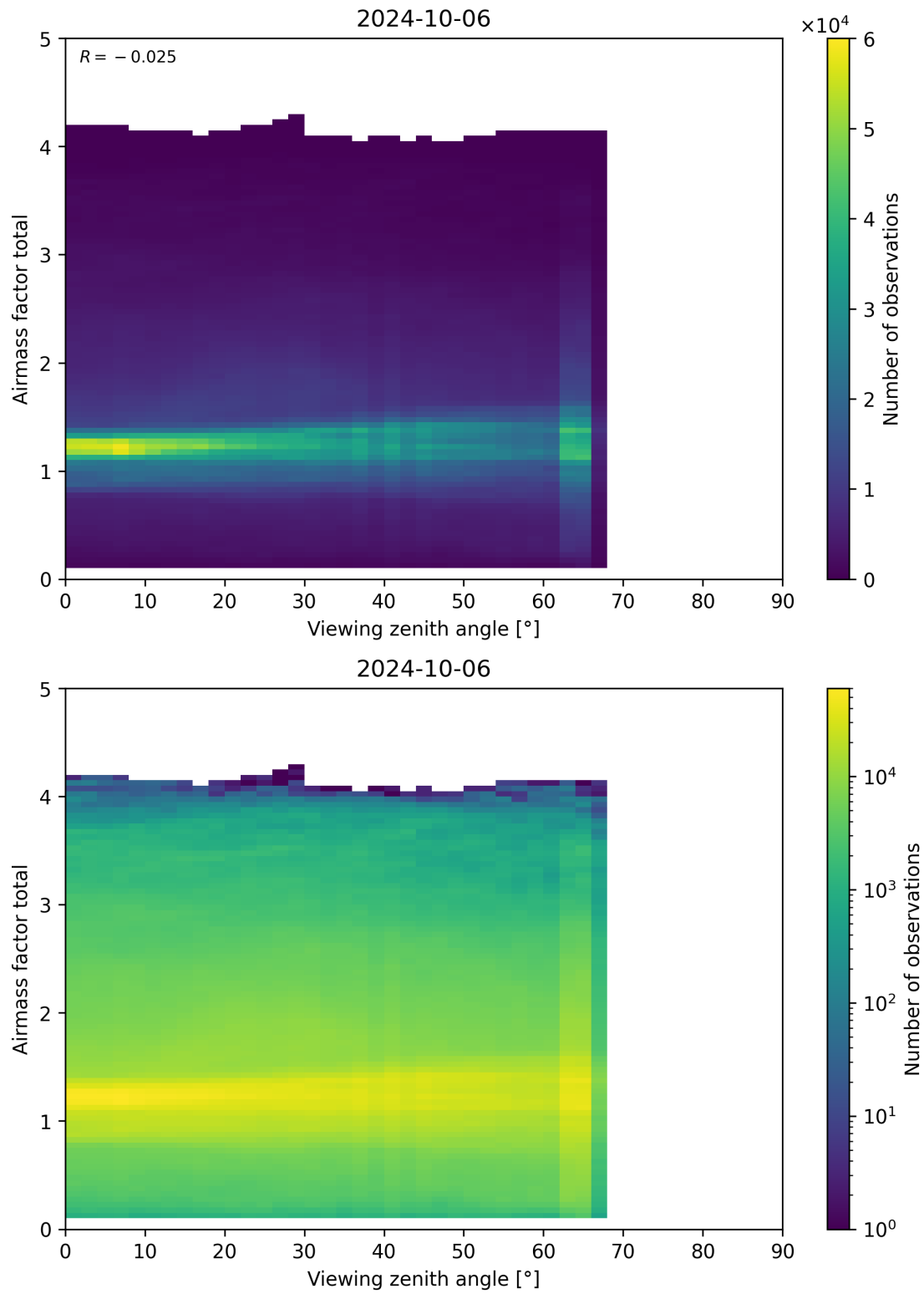
Figure 190: Scatter density plot of “Viewing zenith angle” against “Airmass factor total” for 2024-10-05 to 2024-10-07.
