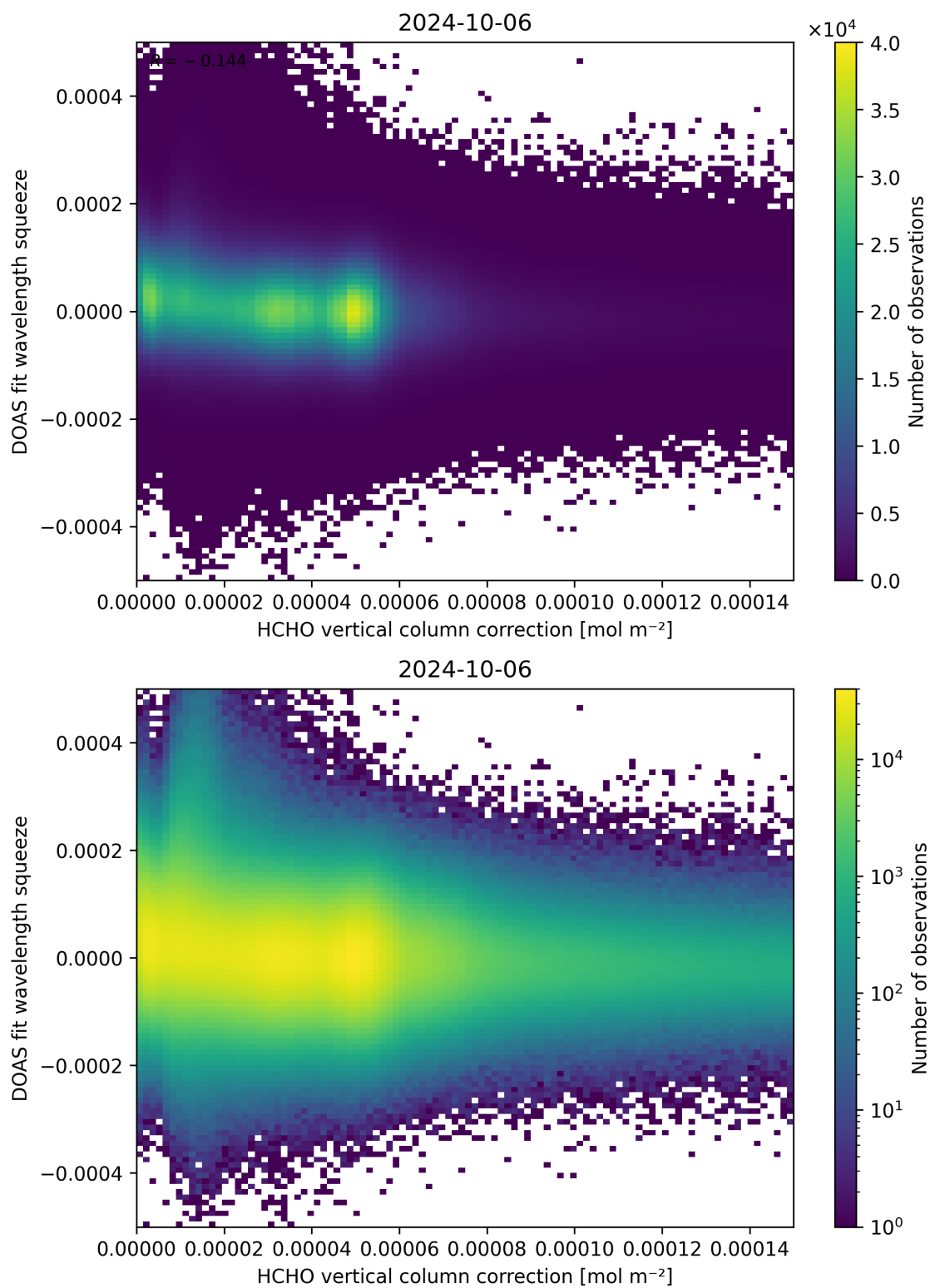
Figure 114: Scatter density plot of “HCHO vertical column correction” against “DOAS fit wavelength squeeze” for 2024-10-05 to 2024-10-07.
