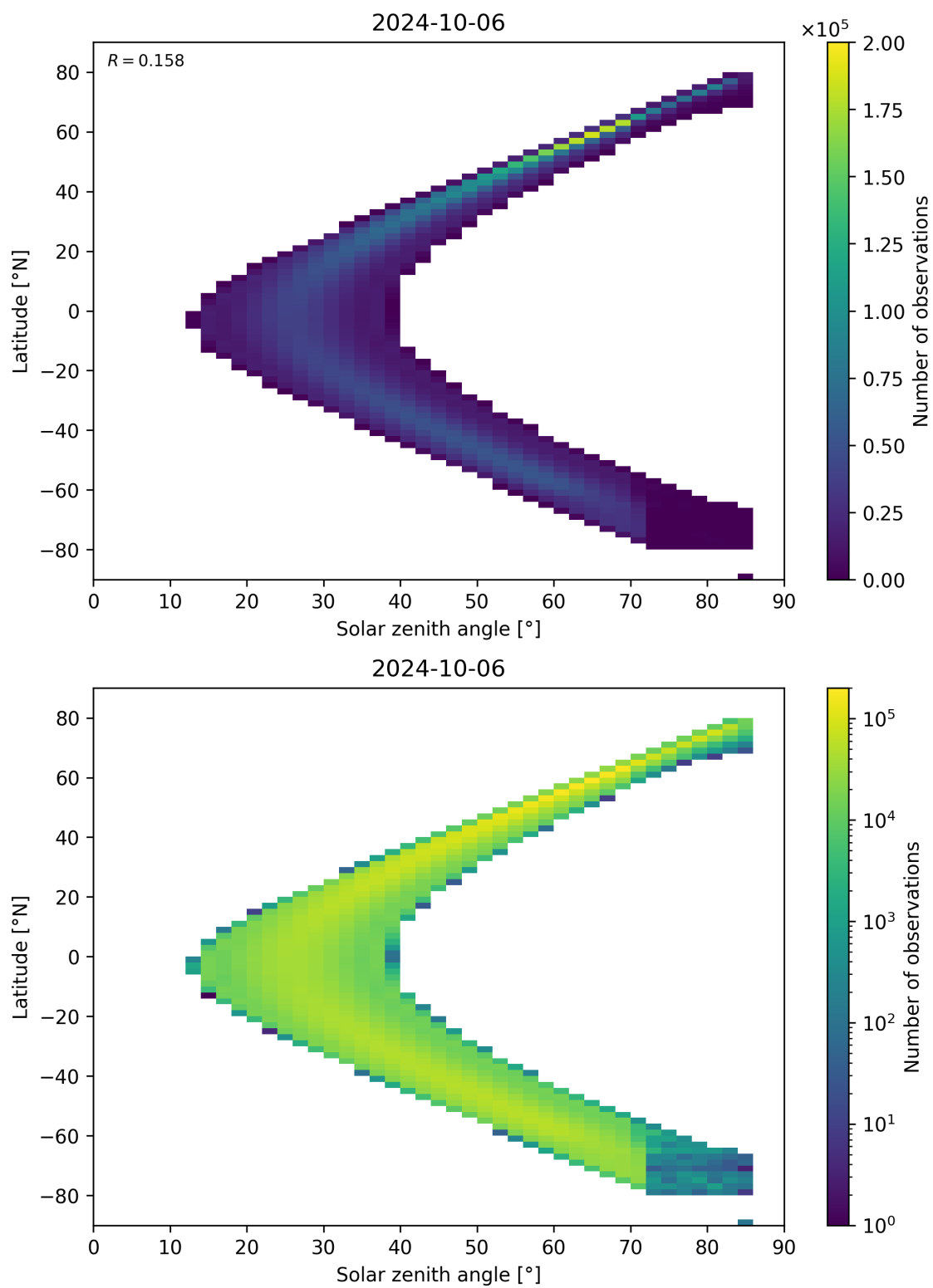
Figure 181: Scatter density plot of “Solar zenith angle” against “Latitude” for 2024-10-05 to 2024-10-07.
