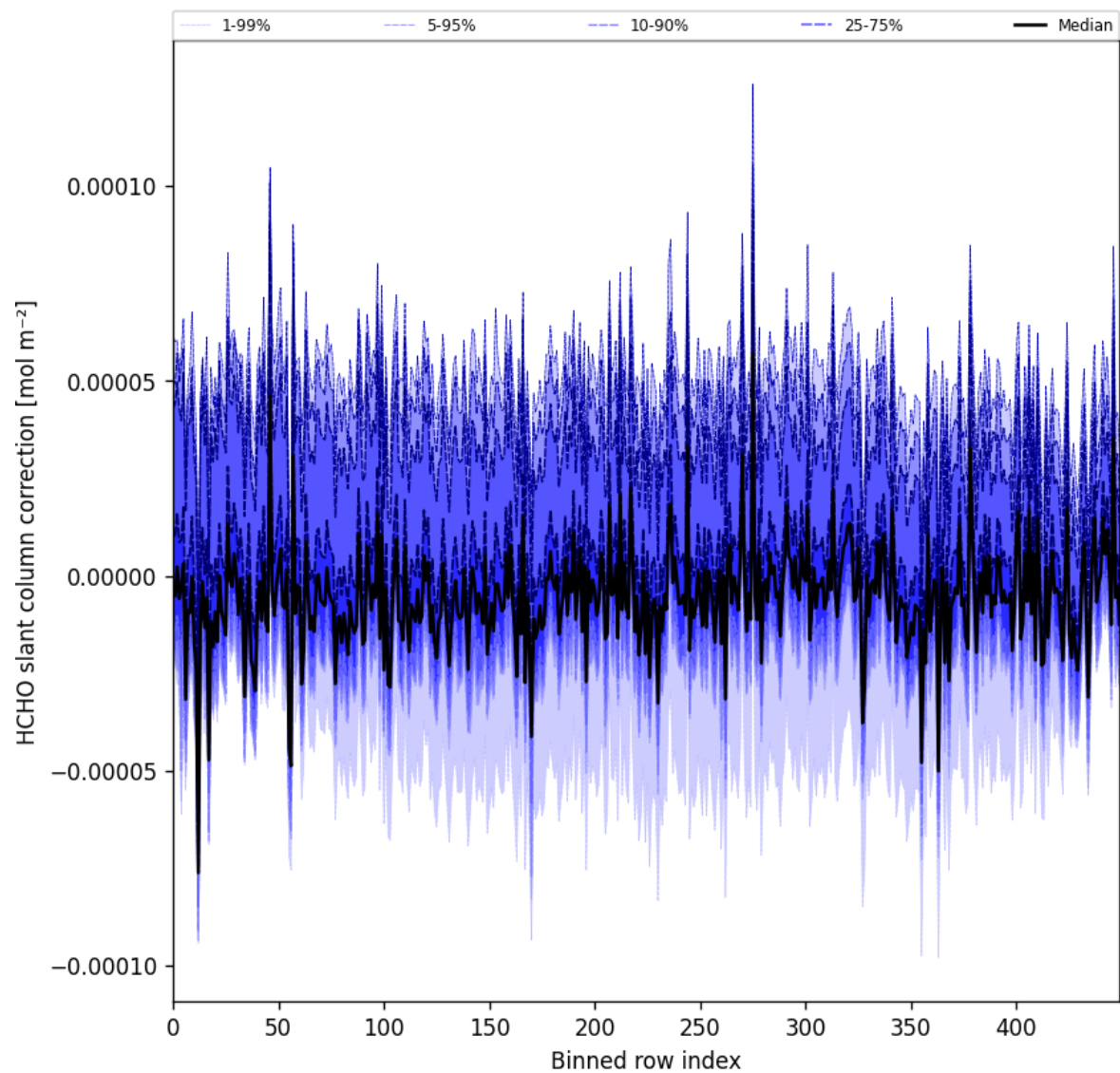
Figure 61: Along track statistics of “HCHO slant column correction” for 2024-10-05 to 2024-10-07
