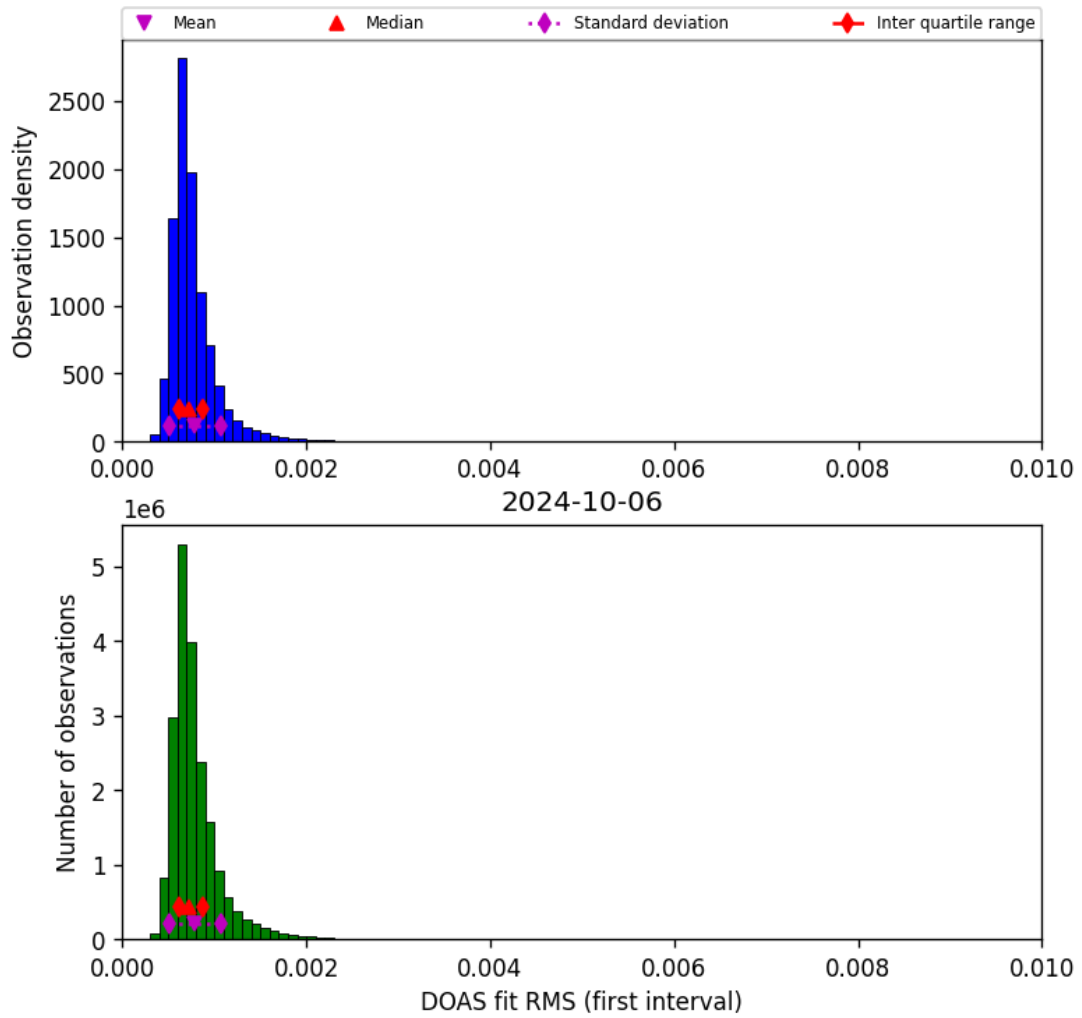
Figure 46: Histogram of “DOAS fit RMS (first interval)” for 2024-10-05 to 2024-10-07
