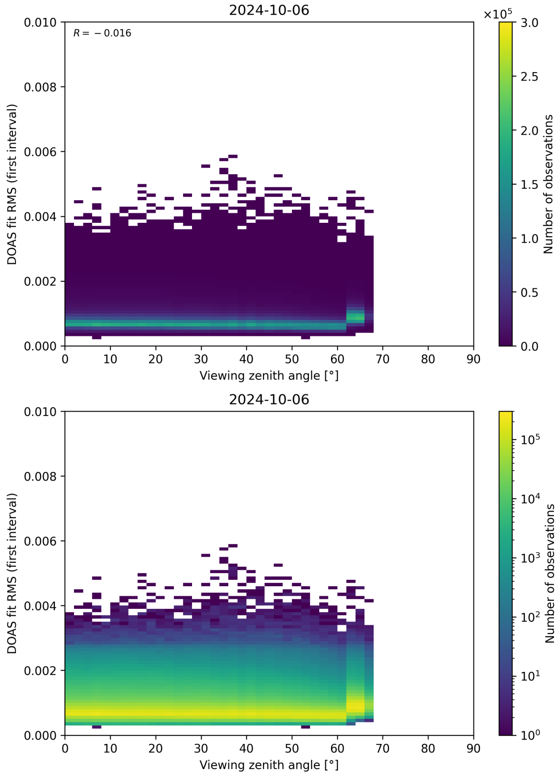
Figure 182: Scatter density plot of “Viewing zenith angle” against “DOAS fit RMS (first interval)” for 2024-10-05 to 2024-10-07.
