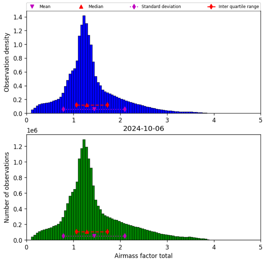
Figure 40: Histogram of “Airmass factor total” for 2024-10-05 to 2024-10-07
