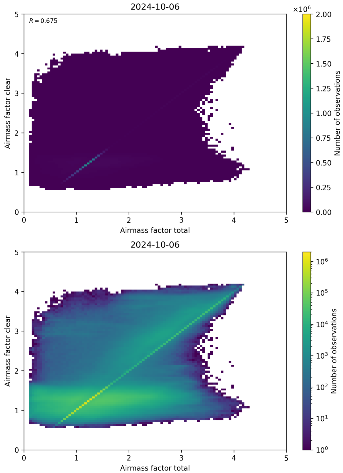
Figure 100: Scatter density plot of “Airmass factor total” against “Airmass factor clear” for 2024-10-05 to 2024-10-07.
