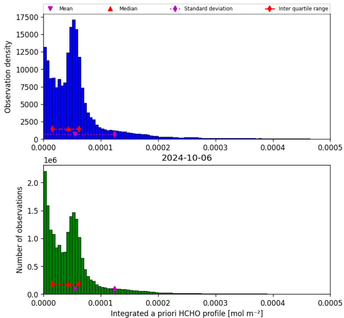
Figure 43: Histogram of “Integrated a priori HCHO profile” for 2024-10-05 to 2024-10-07
