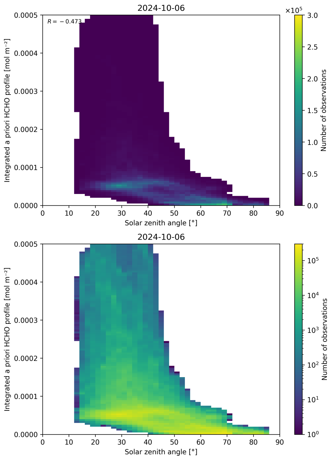
Figure 180: Scatter density plot of “Solar zenith angle” against “Integrated a priori HCHO profile” for 2024-10-05 to 2024-10-07.
