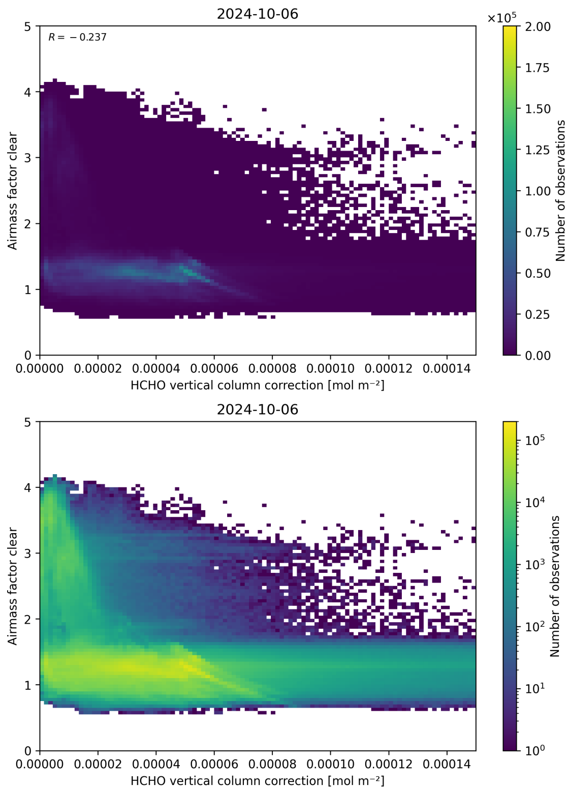
Figure 115: Scatter density plot of “HCHO vertical column correction” against “Airmass factor clear” for 2024-10-05 to 2024-10-07.
