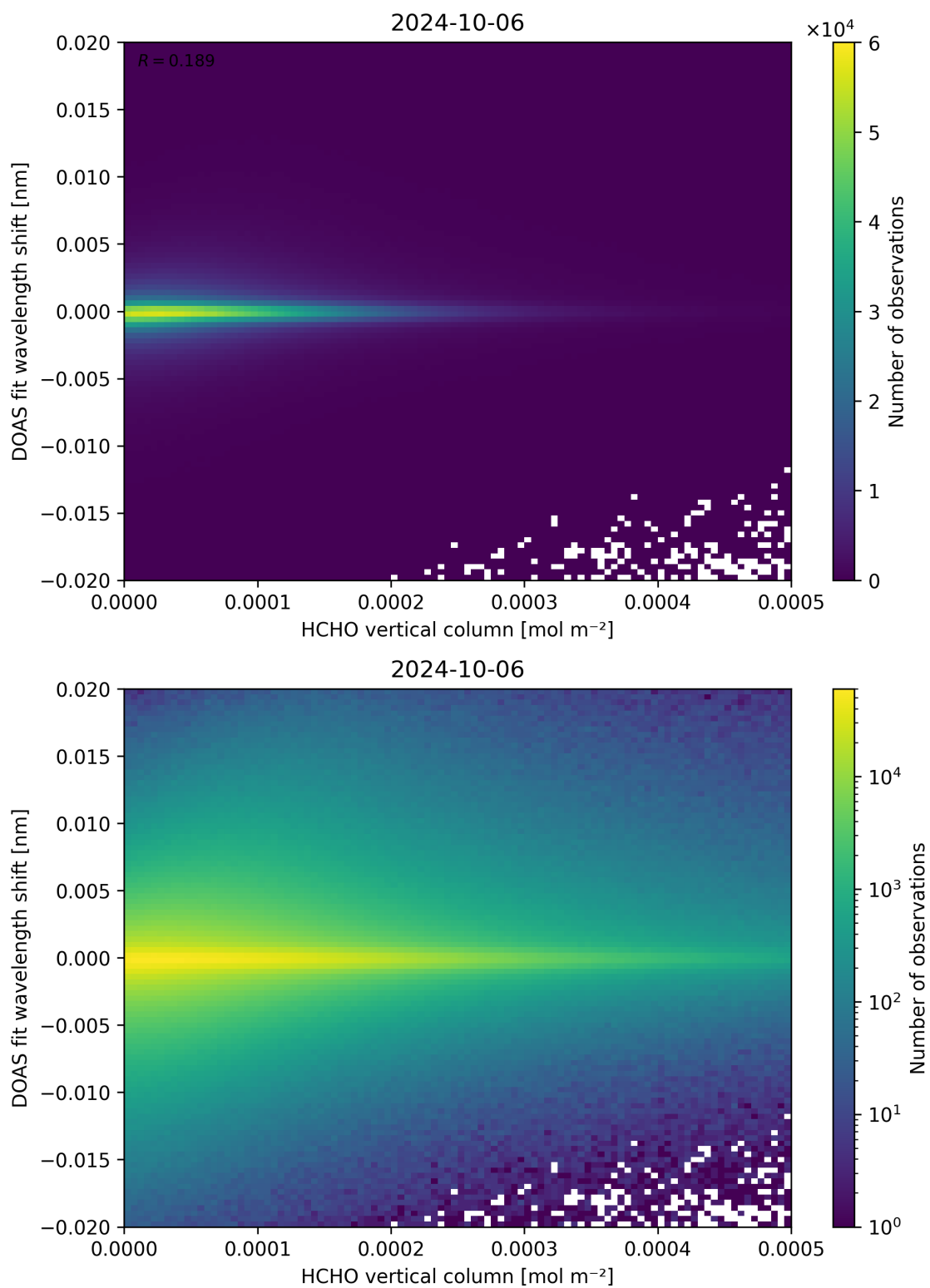
Figure 124: Scatter density plot of “HCHO vertical column” against “DOAS fit wavelength shift” for 2024-10-05 to 2024-10-07.
