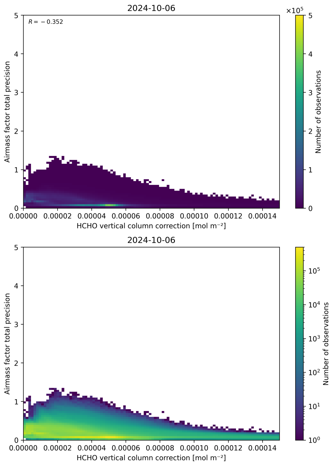
Figure 121: Scatter density plot of “HCHO vertical column correction” against “Airmass factor total precision” for 2024-10-05 to 2024-10-07.
