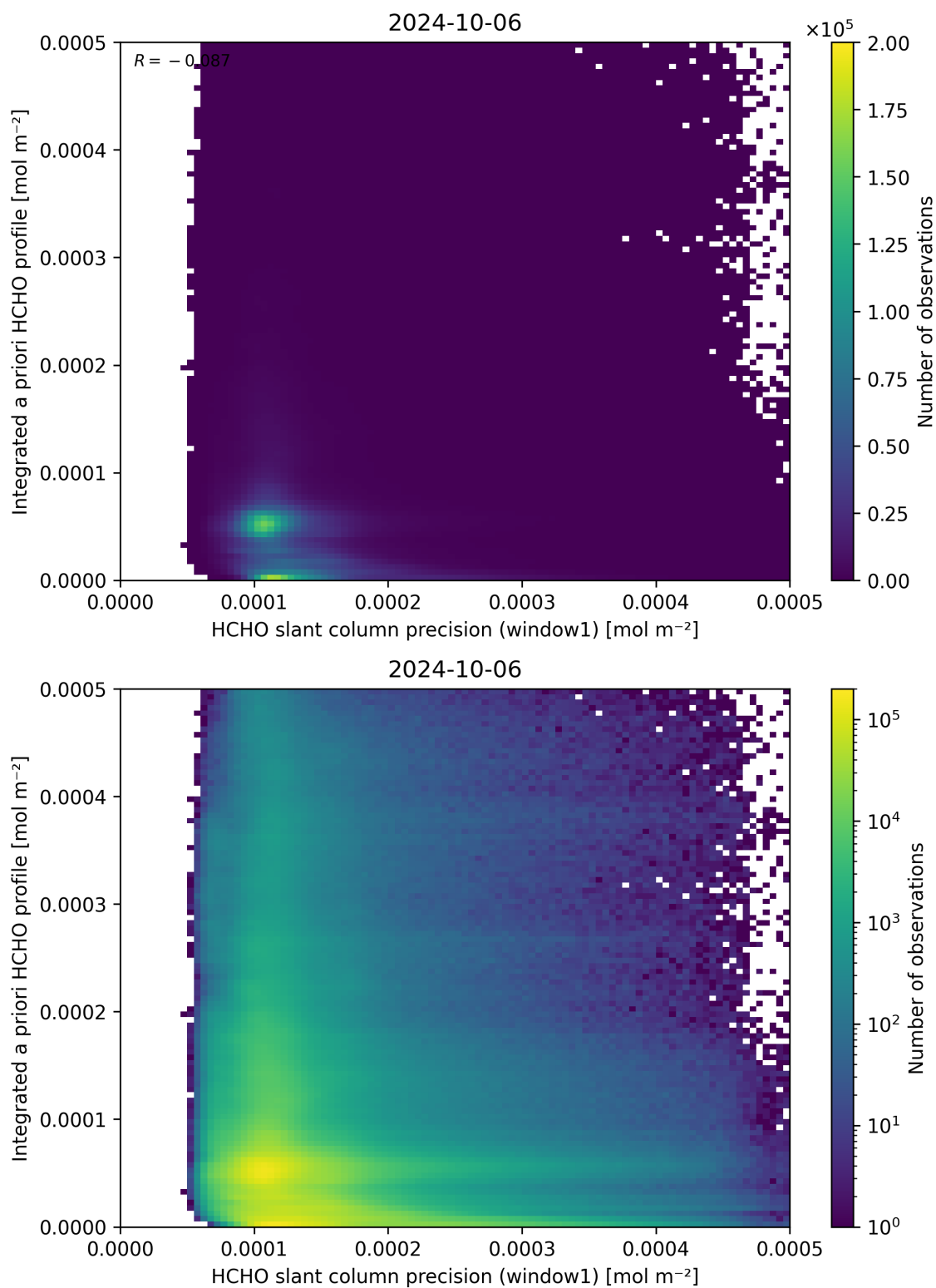
Figure 96: Scatter density plot of “HCHO slant column precision (window1)” against “Integrated a priori HCHO profile” for 2024-10-05 to 2024-10-07.
