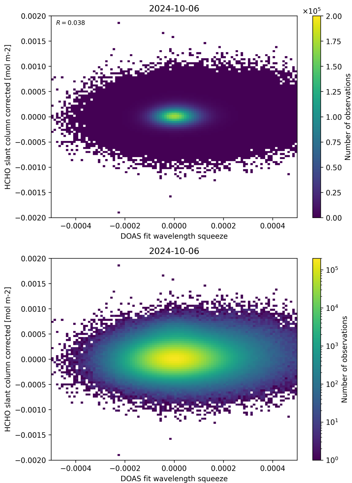
Figure 69: Scatter density plot of “DOAS fit wavelength squeeze” against “HCHO slant column corrected” for 2024-10-05 to 2024-10-07.
