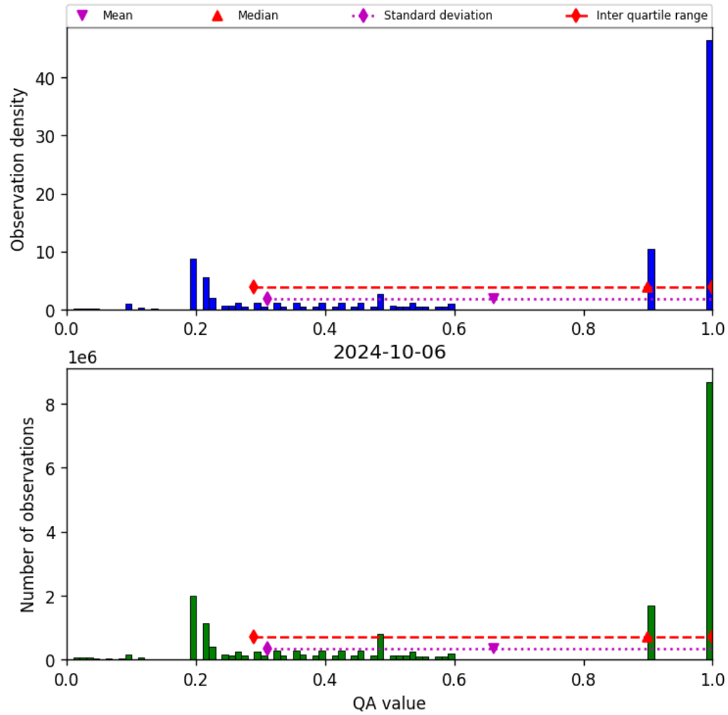
Figure 34: Histogram of “QA value” for 2024-10-05 to 2024-10-07
