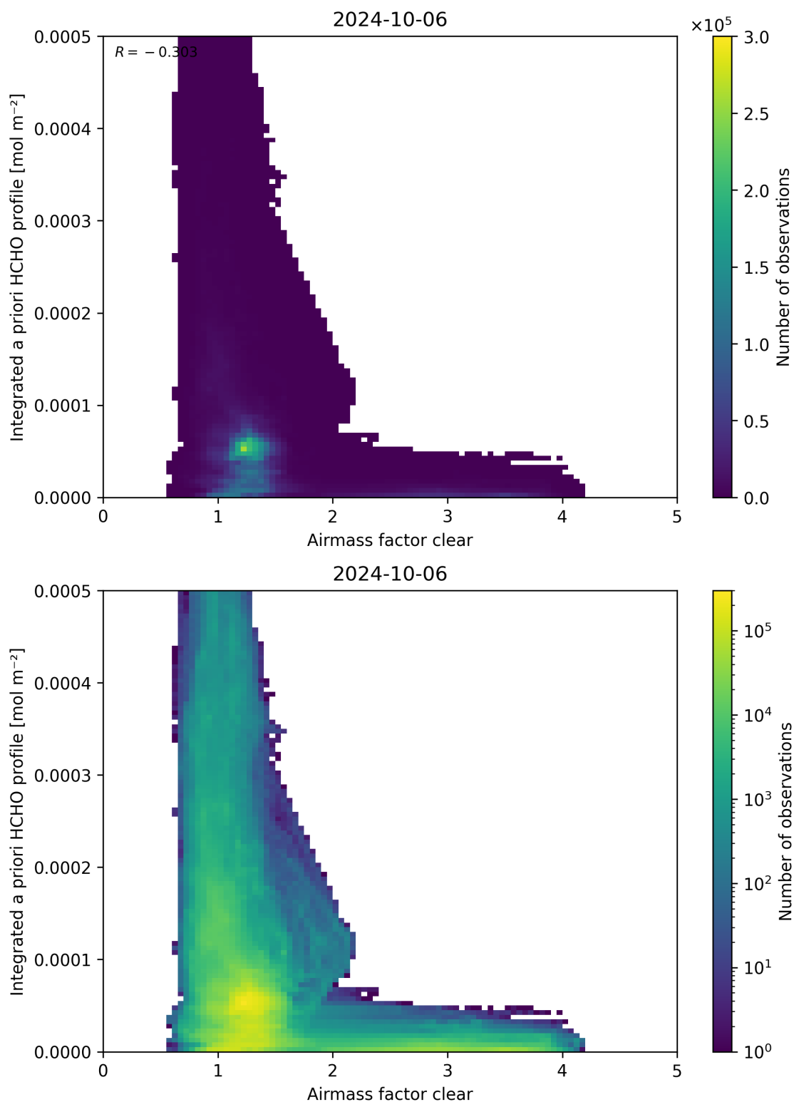
Figure 76: Scatter density plot of “Airmass factor clear” against “Integrated a priori HCHO profile” for 2024-10-05 to 2024-10-07.
