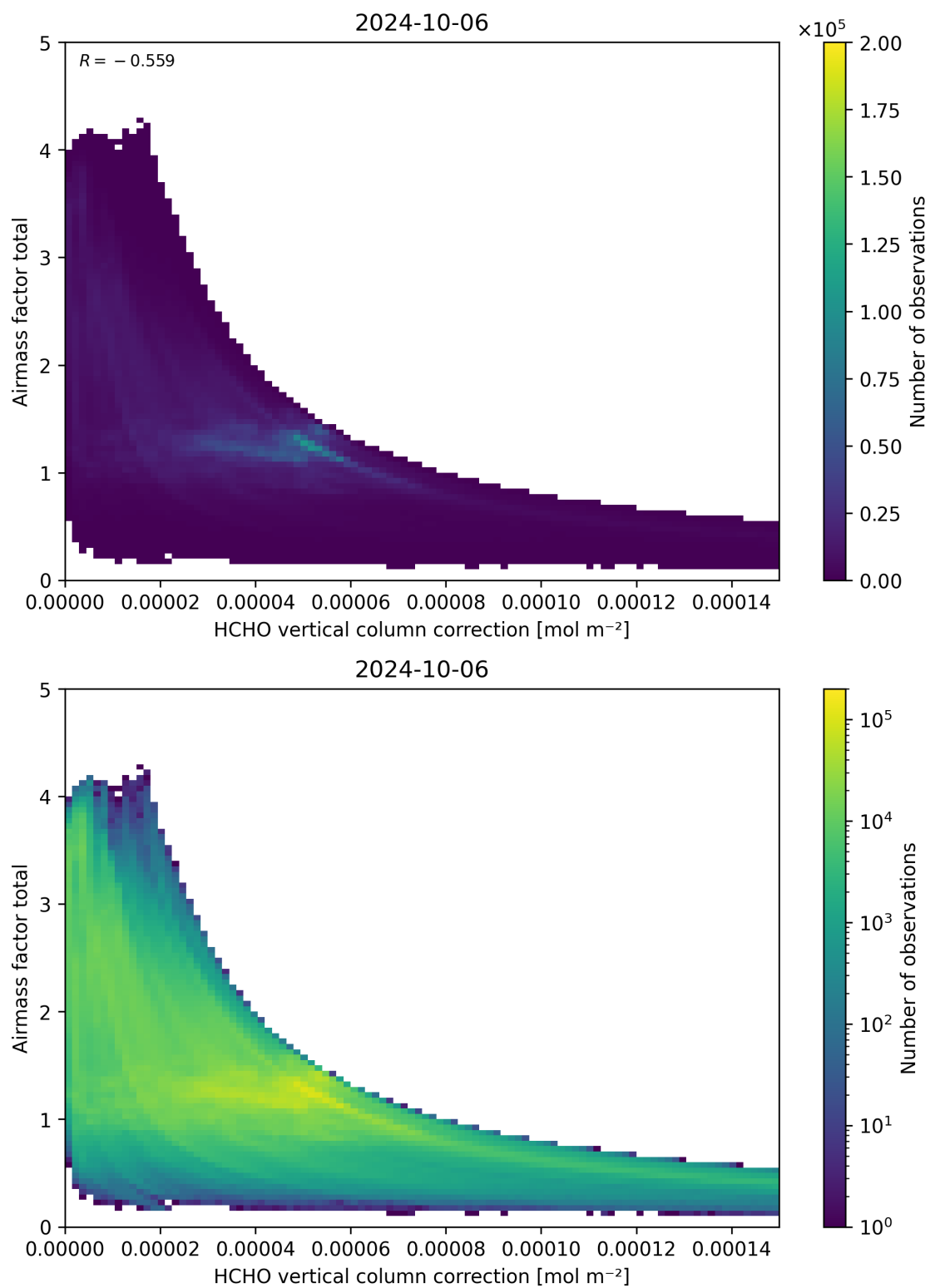
Figure 120: Scatter density plot of “HCHO vertical column correction” against “Airmass factor total” for 2024-10-05 to 2024-10-07.
