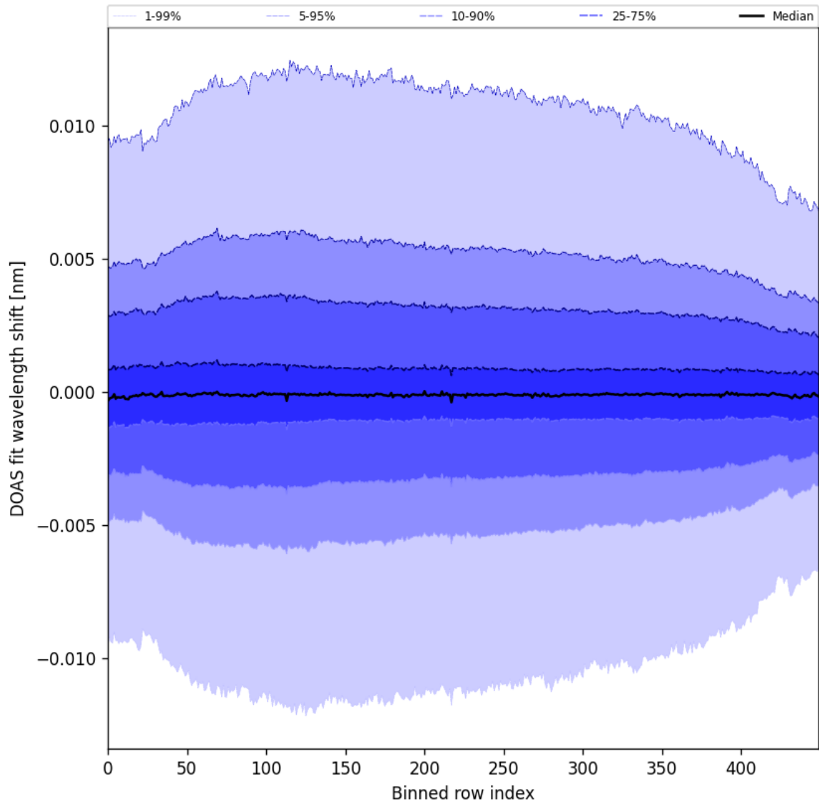
Figure 58: Along track statistics of “DOAS fit wavelength shift” for 2024-10-05 to 2024-10-07
