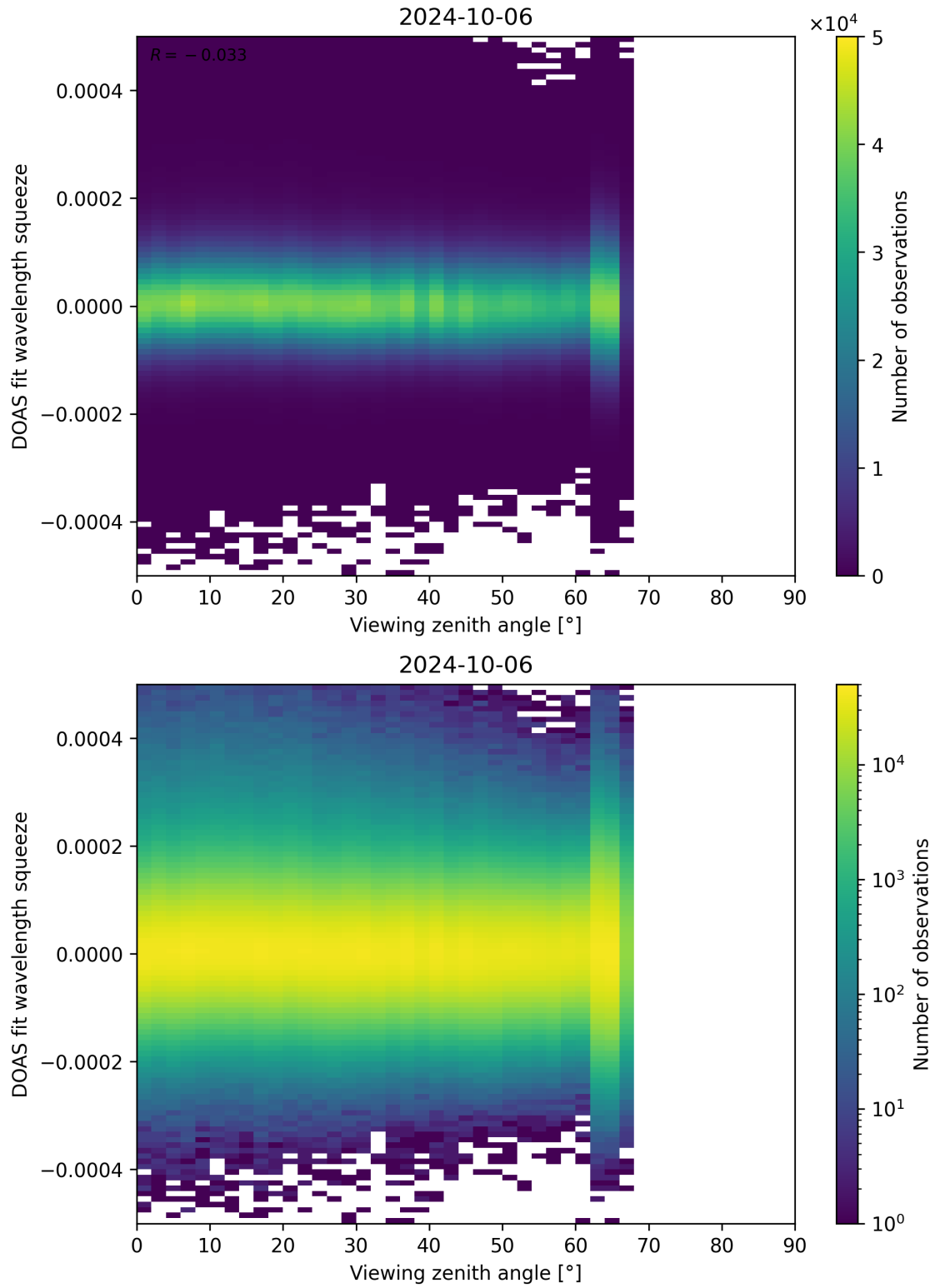
Figure 184: Scatter density plot of “Viewing zenith angle” against “DOAS fit wavelength squeeze” for 2024-10-05 to 2024-10-07.
