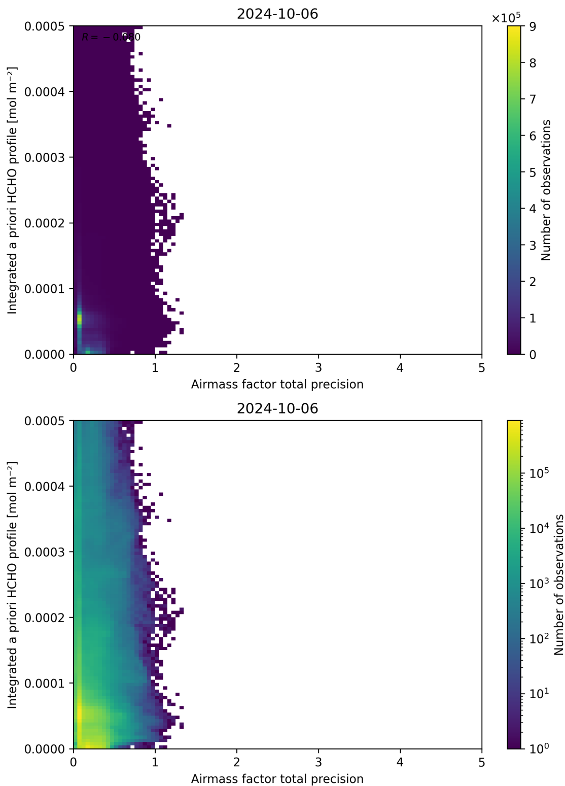
Figure 111: Scatter density plot of “Airmass factor total precision” against “Integrated a priori HCHO profile” for 2024-10-05 to 2024-10-07.
