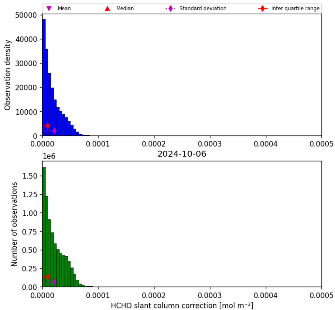
Figure 47: Histogram of “HCHO slant column correction” for 2024-10-05 to 2024-10-07
