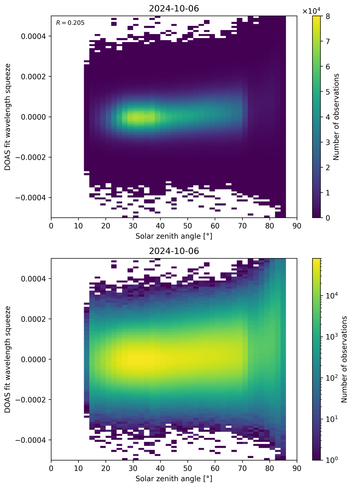
Figure 169: Scatter density plot of “Solar zenith angle” against “DOAS fit wavelength squeeze” for 2024-10-05 to 2024-10-07.
