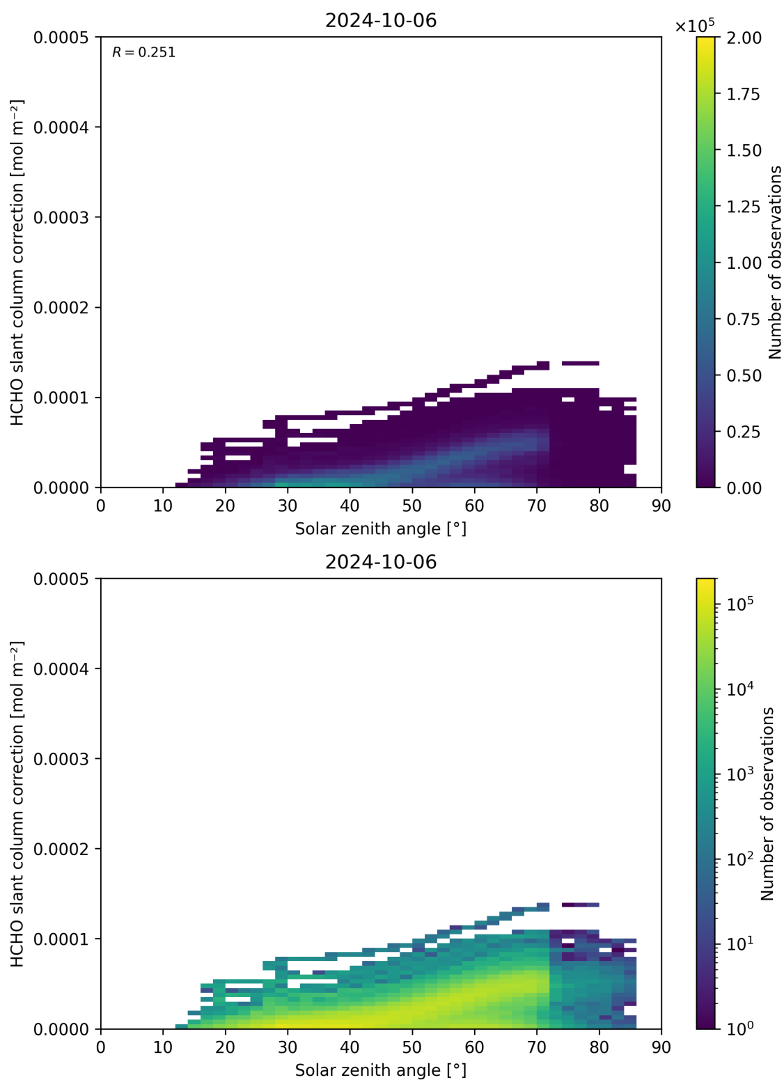
Figure 172: Scatter density plot of “Solar zenith angle” against “HCHO slant column correction” for 2024-10-05 to 2024-10-07.
