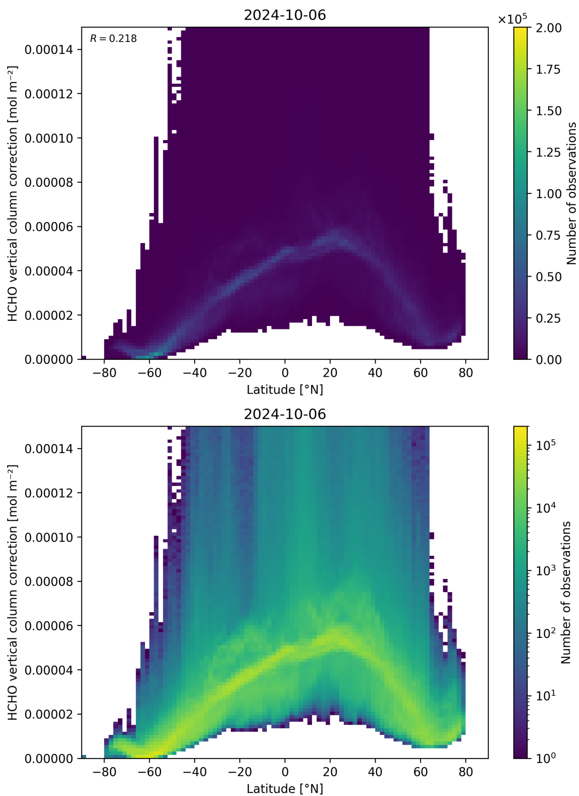
Figure 164: Scatter density plot of “Latitude” against “HCHO vertical column correction” for 2024-10-05 to 2024-10-07.
