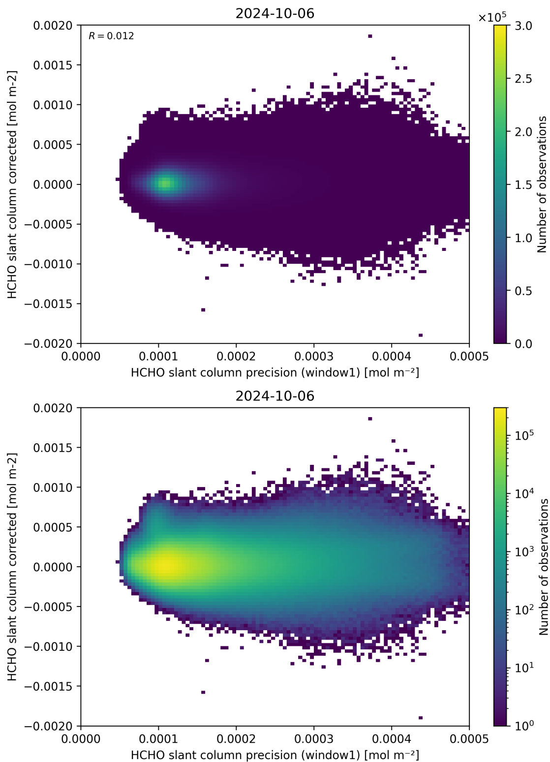
Figure 92: Scatter density plot of “HCHO slant column precision (window1)” against “HCHO slant column corrected” for 2024-10-05 to 2024-10-07.
