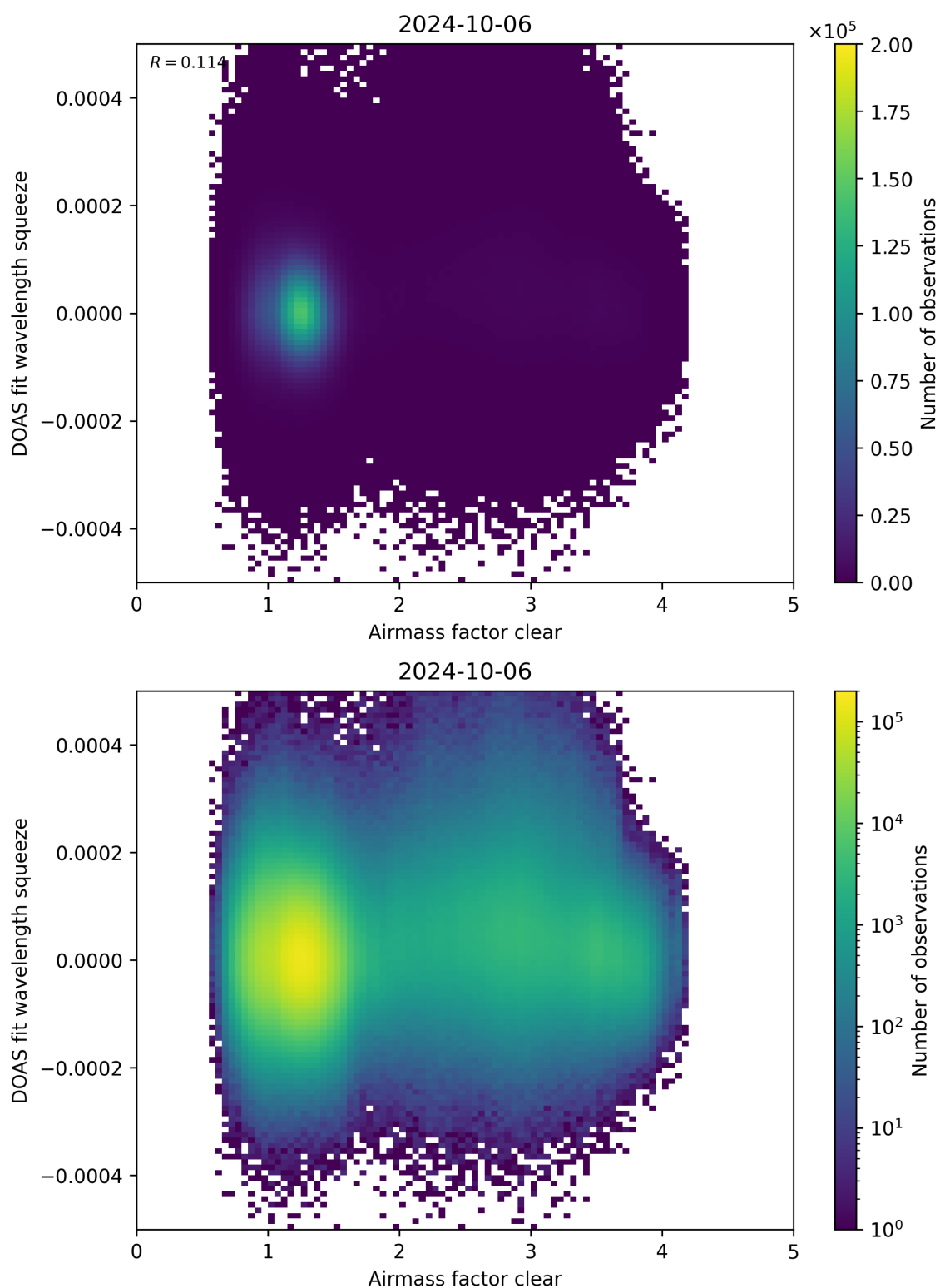
Figure 73: Scatter density plot of “Airmass factor clear” against “DOAS fit wavelength squeeze” for 2024-10-05 to 2024-10-07.
