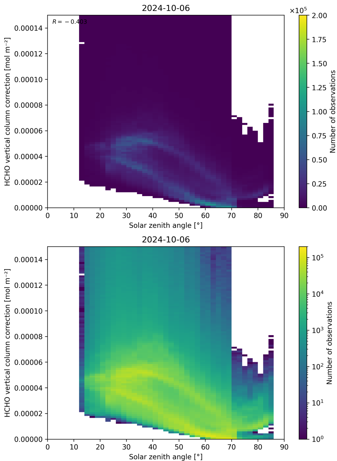
Figure 178: Scatter density plot of “Solar zenith angle” against “HCHO vertical column correction” for 2024-10-05 to 2024-10-07.
