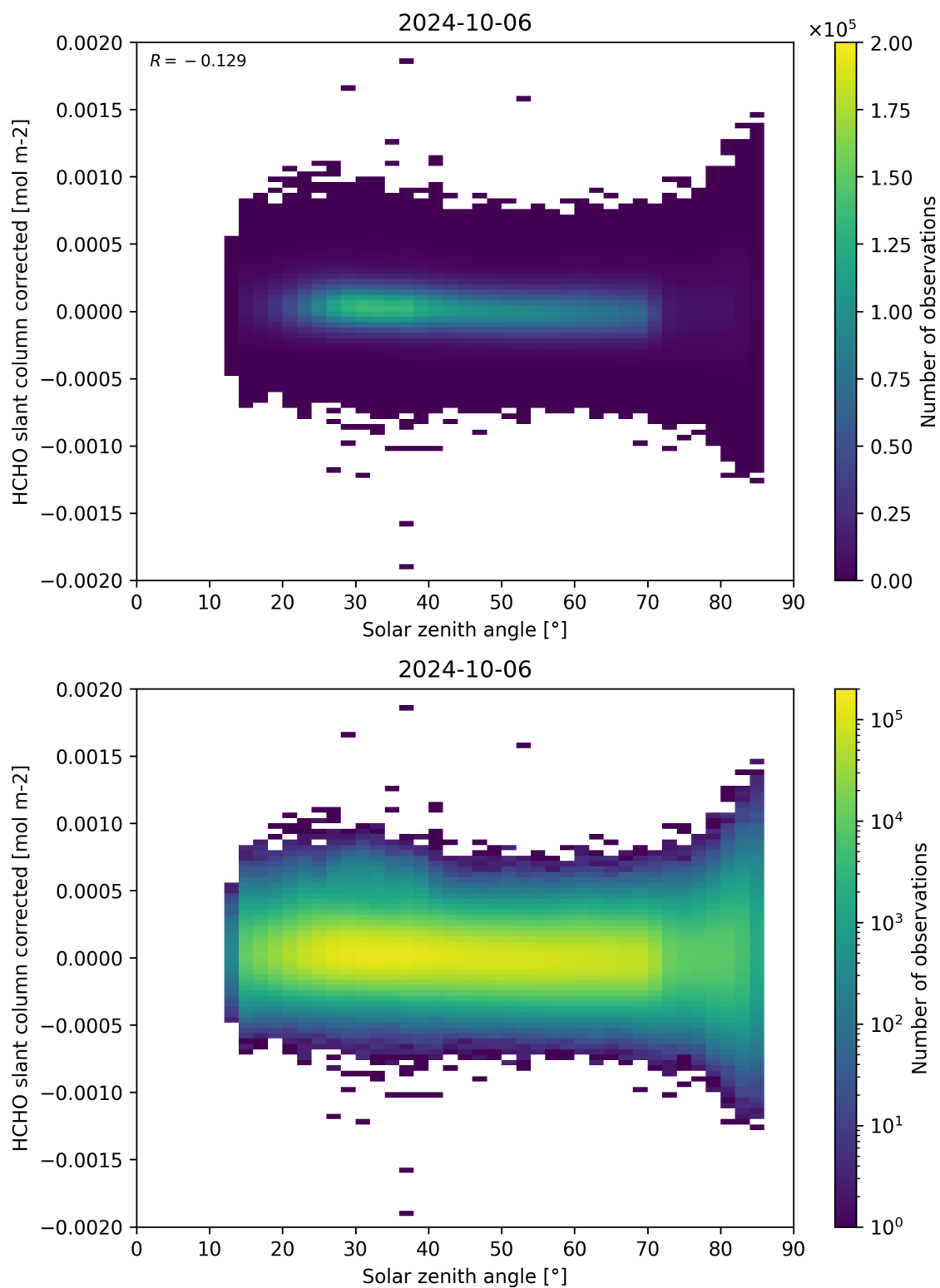
Figure 171: Scatter density plot of “Solar zenith angle” against “HCHO slant column corrected” for 2024-10-05 to 2024-10-07.
