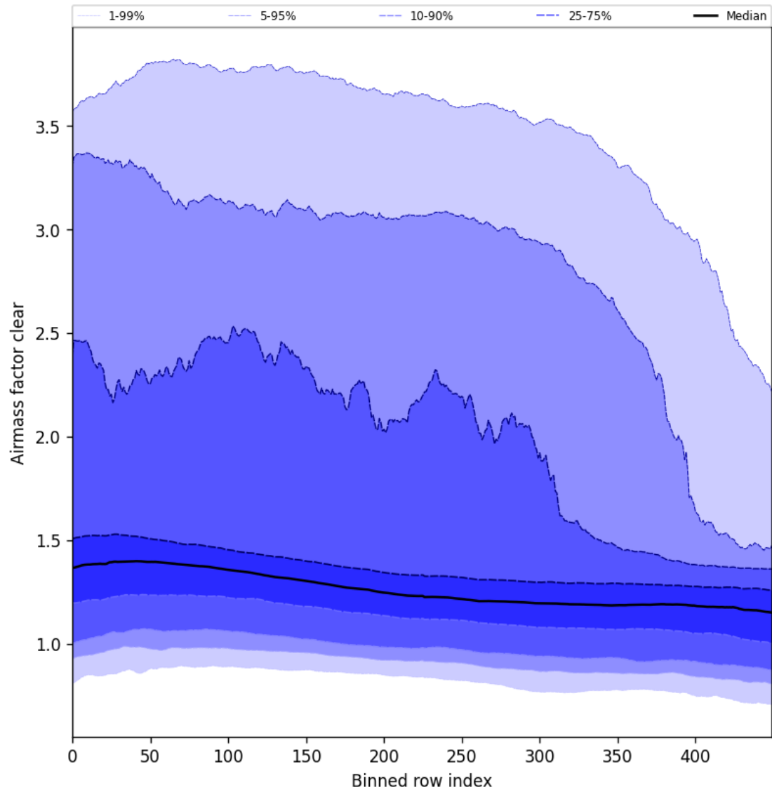
Figure 56: Along track statistics of “Airmass factor clear” for 2024-10-05 to 2024-10-07
