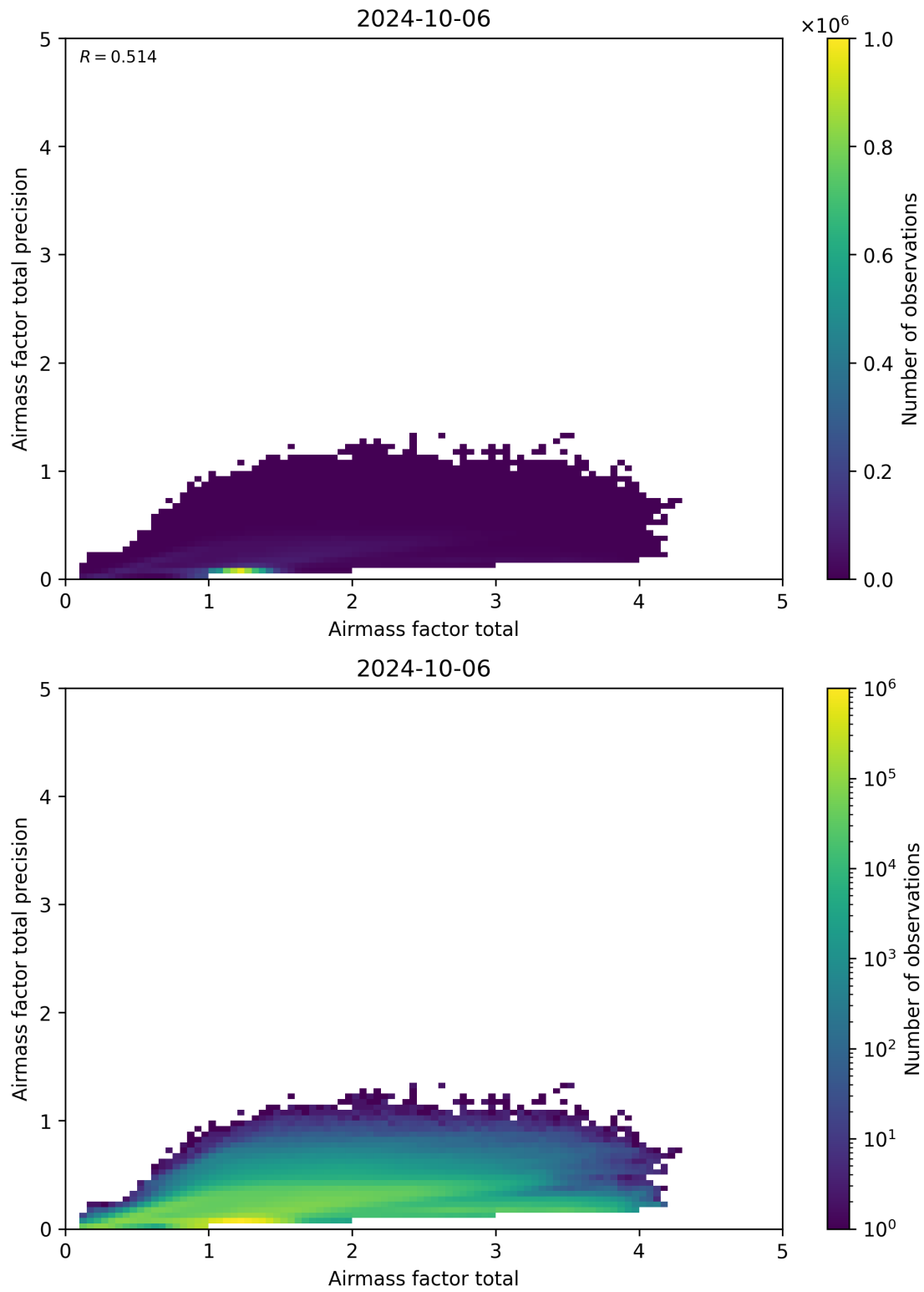
Figure 103: Scatter density plot of “Airmass factor total” against “Airmass factor total precision” for 2024-10-05 to 2024-10-07.
