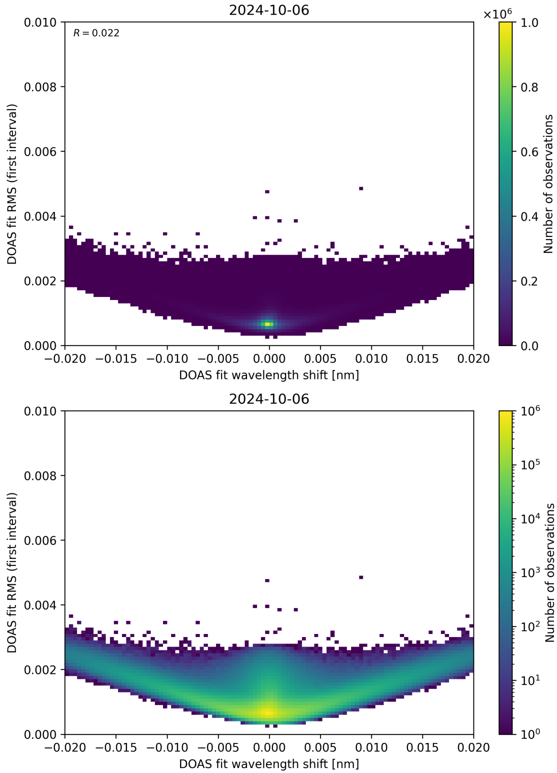
Figure 64: Scatter density plot of “DOAS fit wavelength shift” against “DOAS fit RMS (first interval)” for 2024-10-05 to 2024-10-07.
