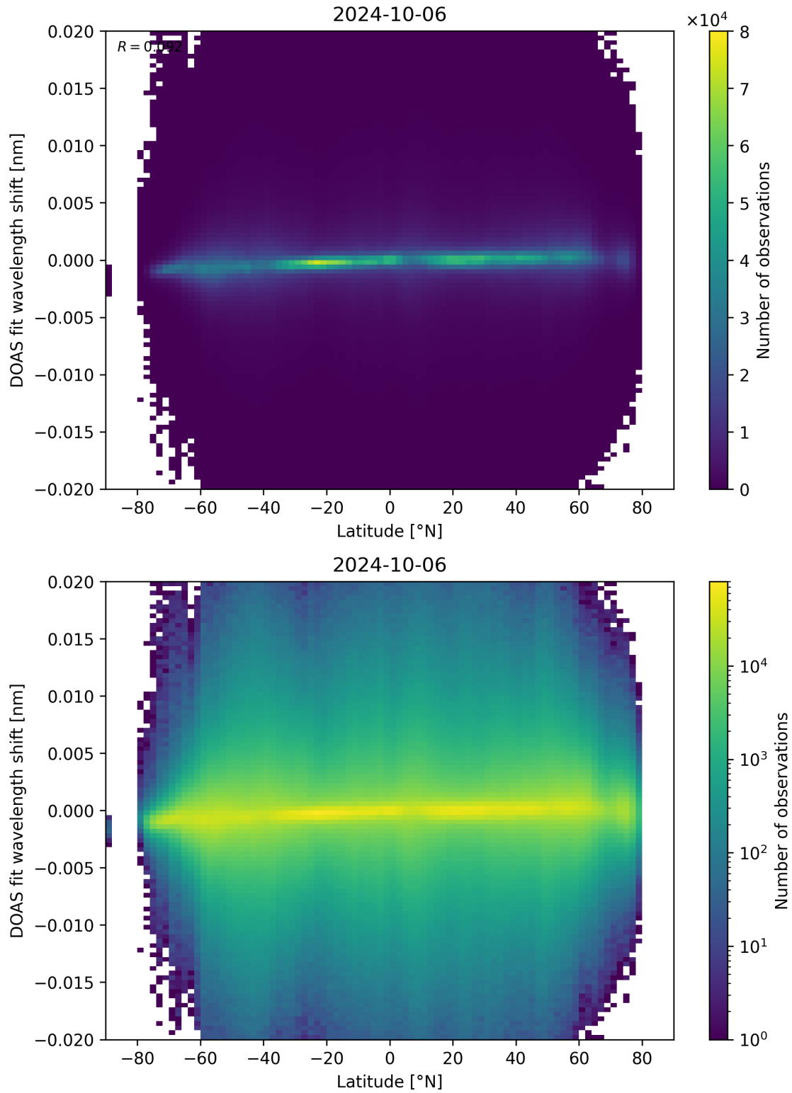
Figure 154: Scatter density plot of “Latitude” against “DOAS fit wavelength shift” for 2024-10-05 to 2024-10-07.
