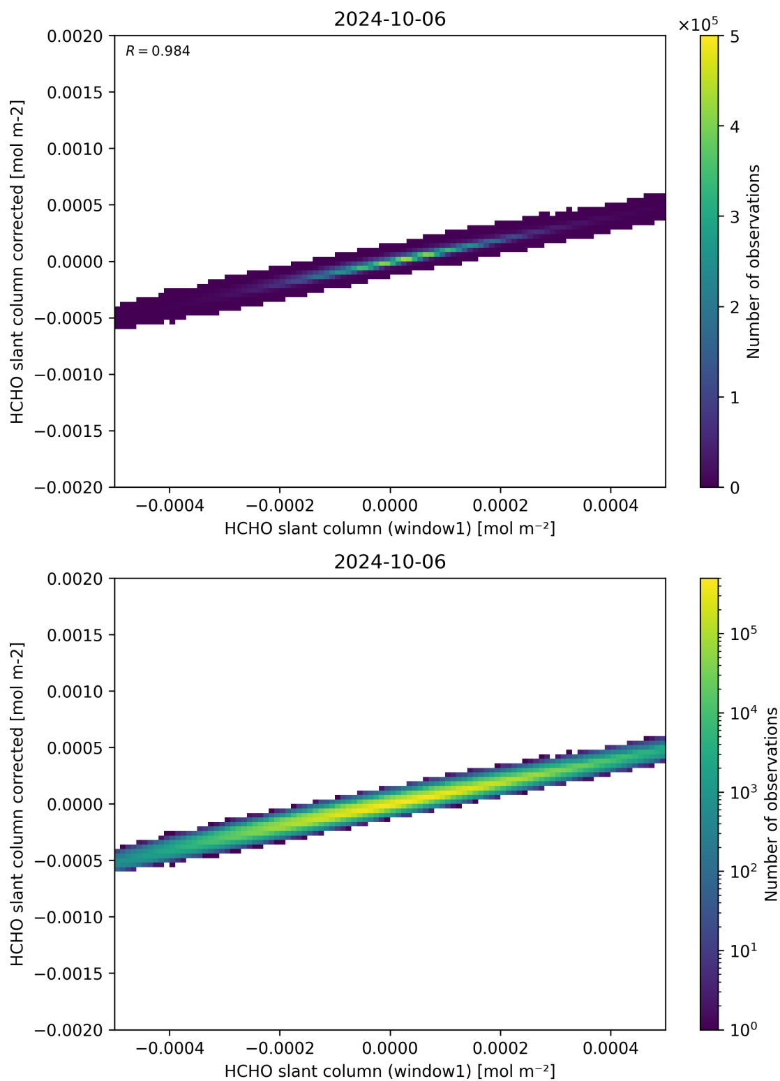
Figure 82: Scatter density plot of “HCHO slant column (window1)” against “HCHO slant column corrected” for 2024-10-05 to 2024-10-07.
