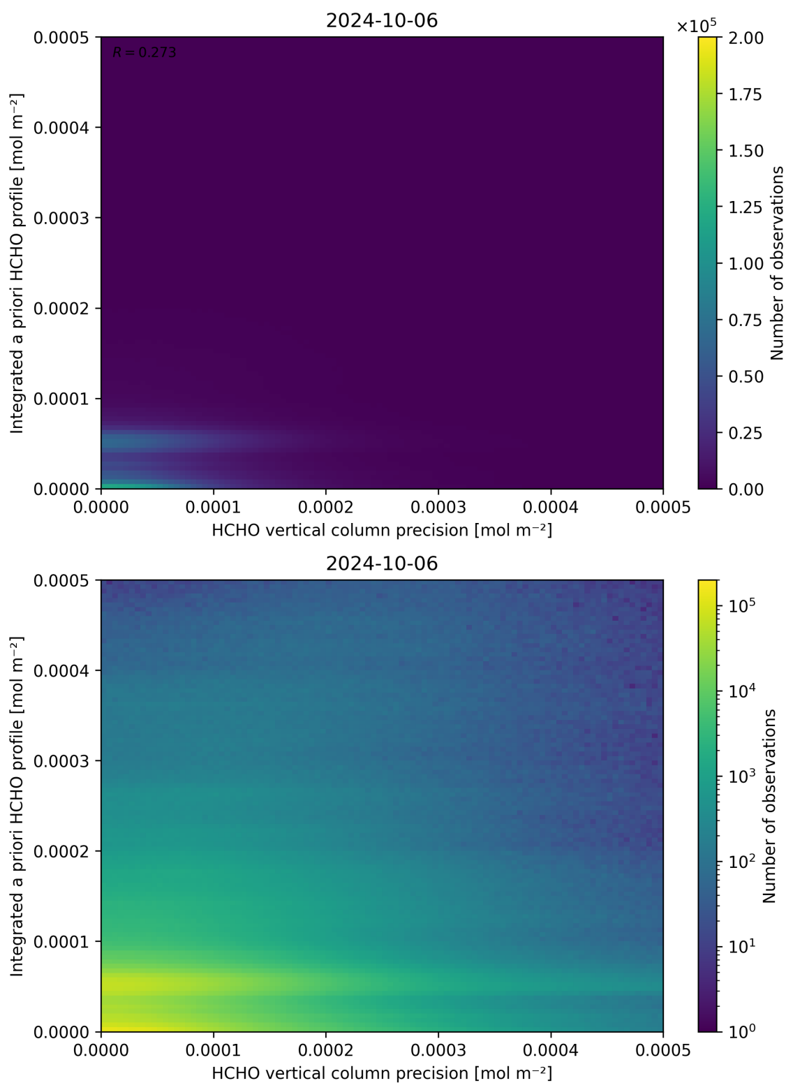
Figure 147: Scatter density plot of “HCHO vertical column precision” against “Integrated a priori HCHO profile” for 2024-10-05 to 2024-10-07.
