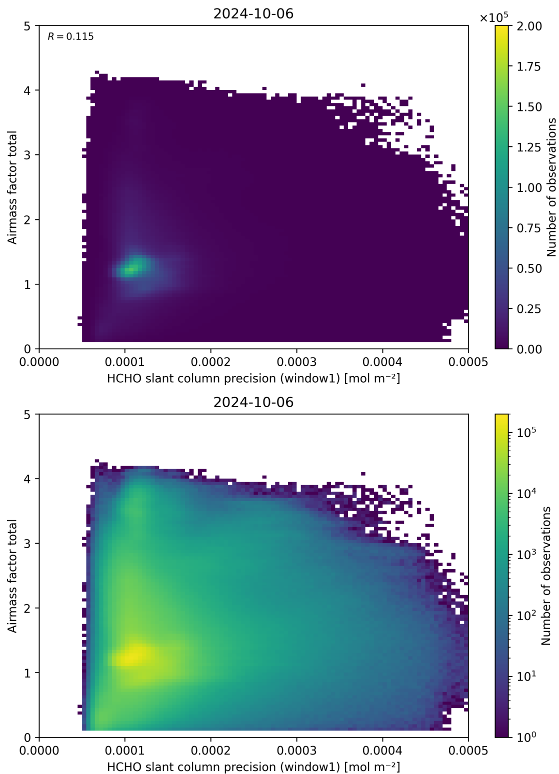
Figure 94: Scatter density plot of “HCHO slant column precision (window1)” against “Airmass factor total” for 2024-10-05 to 2024-10-07.
