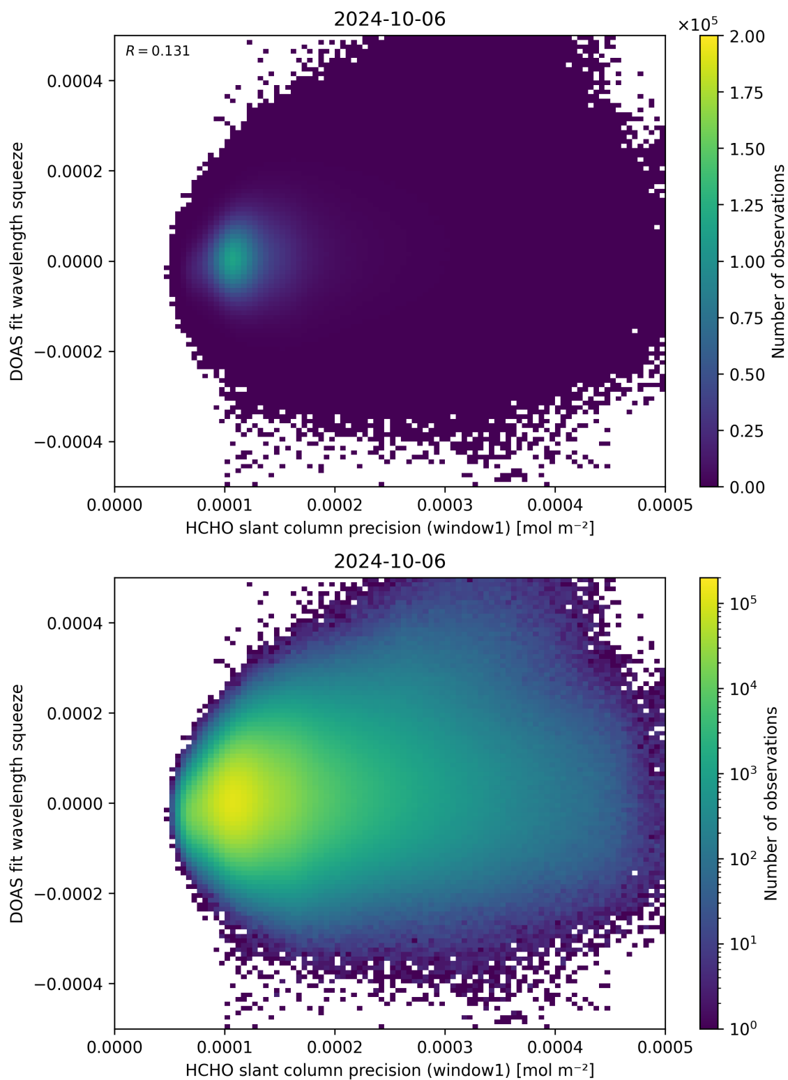
Figure 90: Scatter density plot of “HCHO slant column precision (window1)” against “DOAS fit wavelength squeeze” for 2024-10-05 to 2024-10-07.
