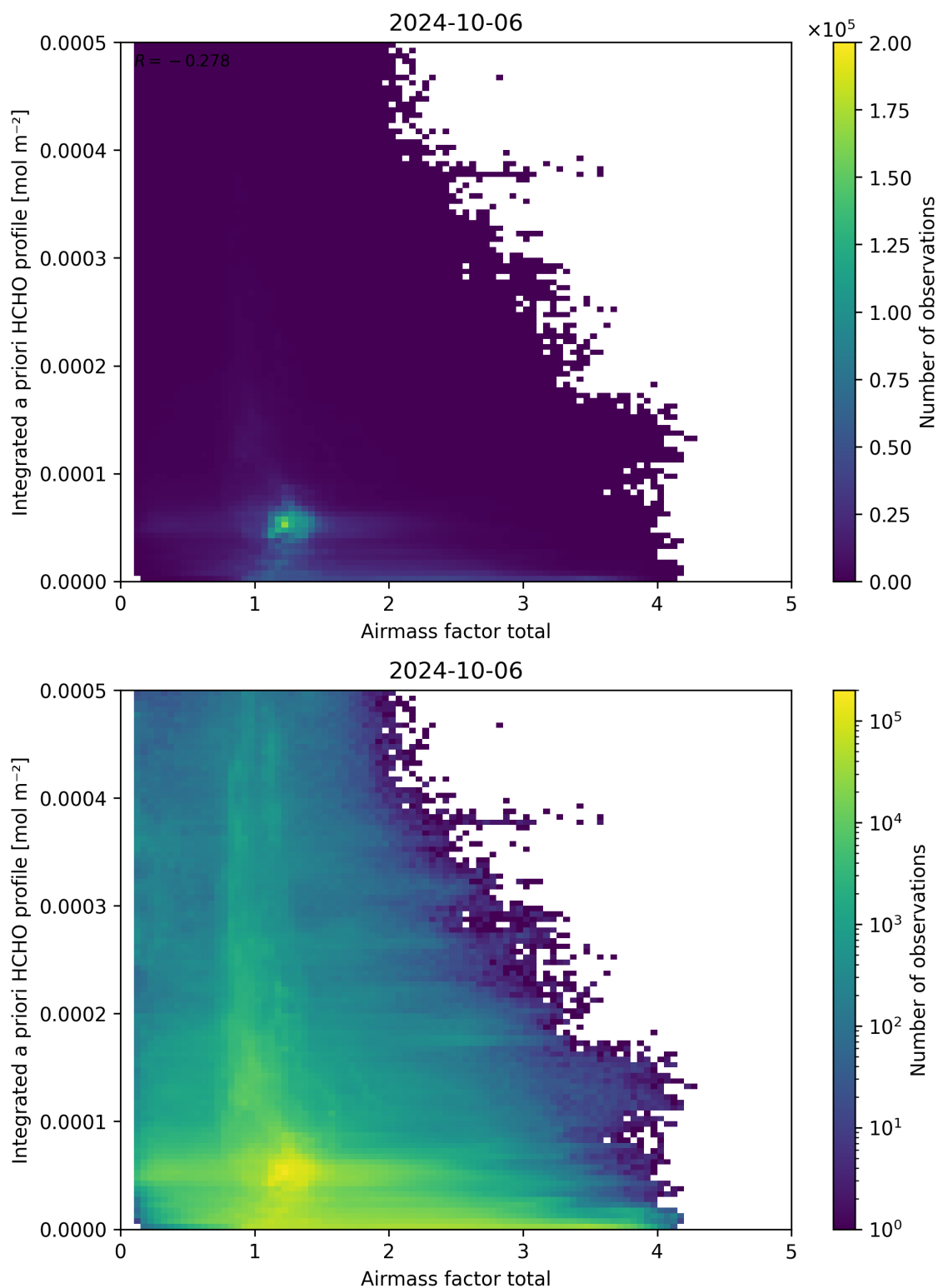
Figure 104: Scatter density plot of “Airmass factor total” against “Integrated a priori HCHO profile” for 2024-10-05 to 2024-10-07.
