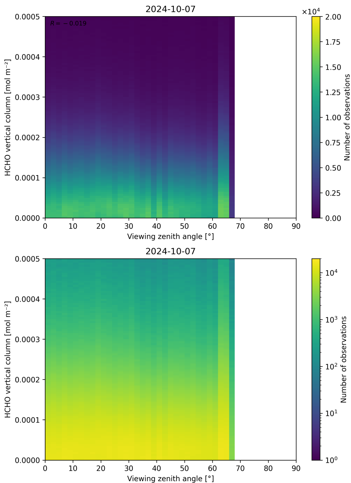
Figure 192: Scatter density plot of “Viewing zenith angle” against “HCHO vertical column” for 2024-10-06 to 2024-10-08.
