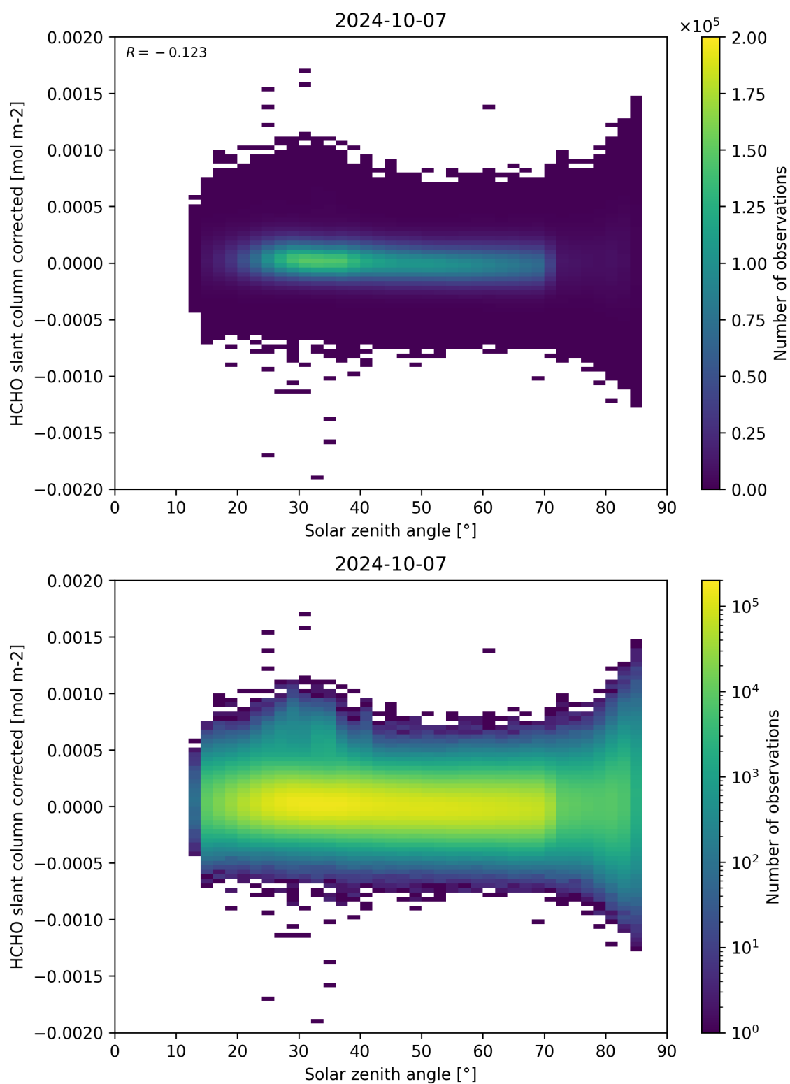
Figure 171: Scatter density plot of “Solar zenith angle” against “HCHO slant column corrected” for 2024-10-06 to 2024-10-08.
