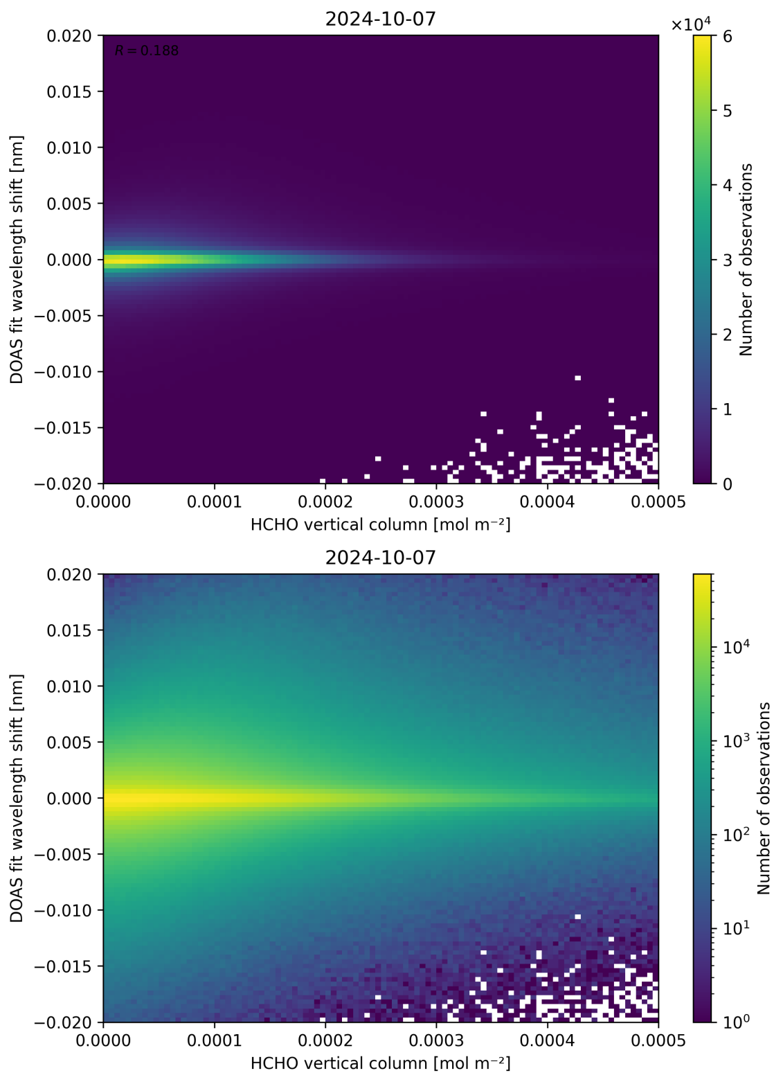
Figure 124: Scatter density plot of “HCHO vertical column” against “DOAS fit wavelength shift” for 2024-10-06 to 2024-10-08.
