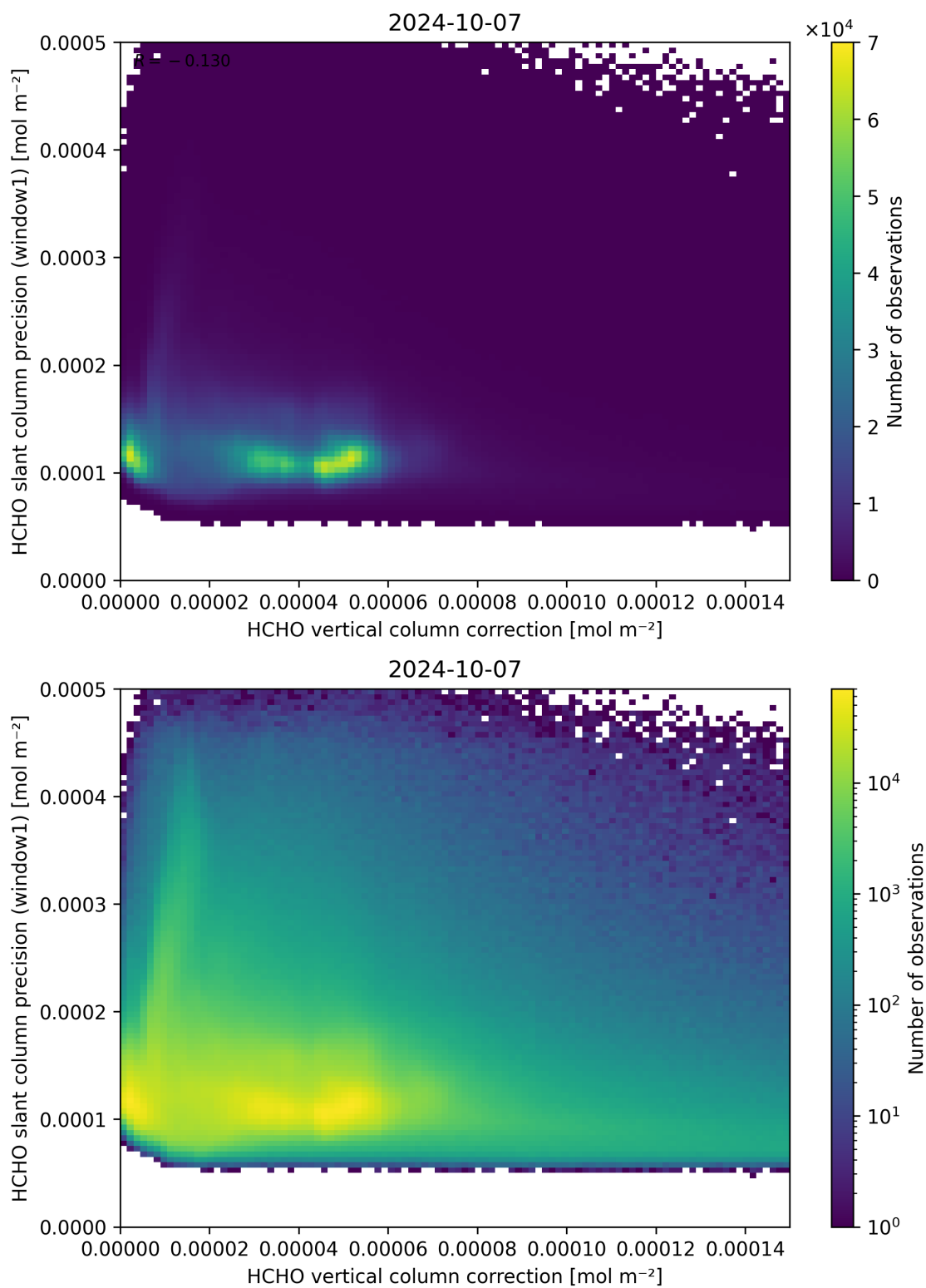
Figure 119: Scatter density plot of “HCHO vertical column correction” against “HCHO slant column precision (window1)” for 2024-10-06 to 2024-10-08.
