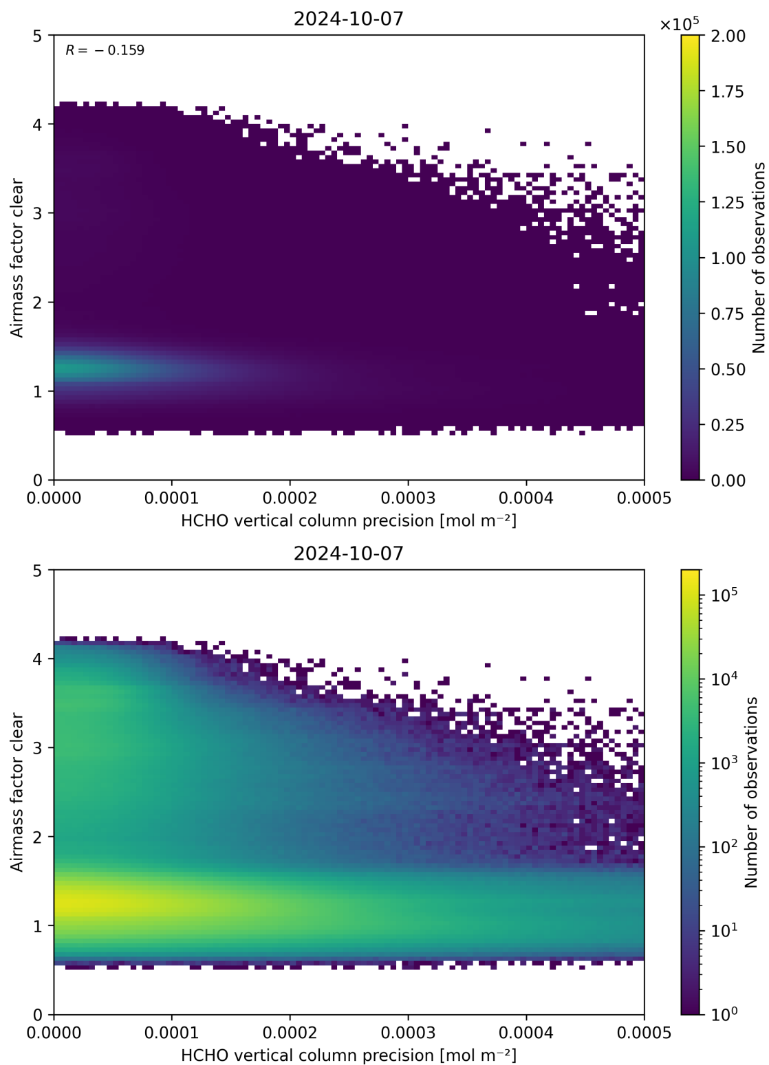
Figure 139: Scatter density plot of “HCHO vertical column precision” against “Airmass factor clear” for 2024-10-06 to 2024-10-08.
