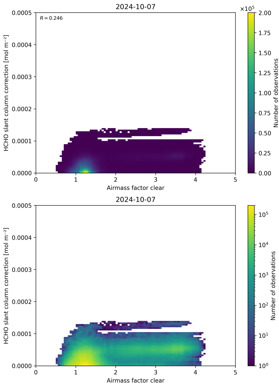
Figure 75: Scatter density plot of “Airmass factor clear” against “HCHO slant column correction” for 2024-10-06 to 2024-10-08.
