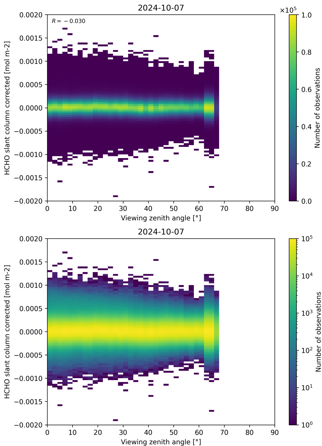
Figure 186: Scatter density plot of “Viewing zenith angle” against “HCHO slant column corrected” for 2024-10-06 to 2024-10-08.
