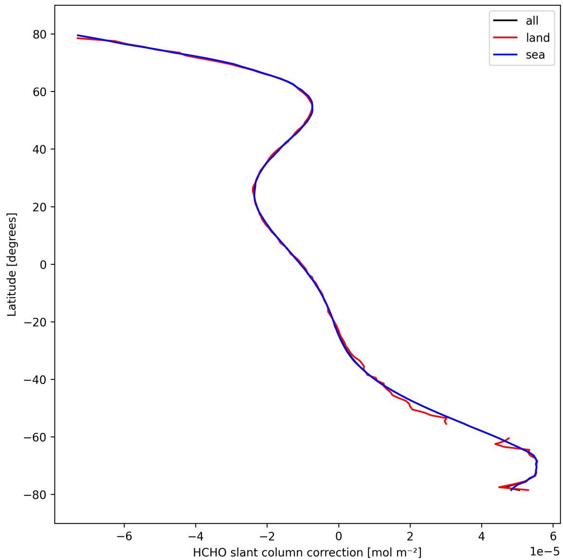
Figure 33: Zonal average of “HCHO slant column correction” for 2024-10-06 to 2024-10-08.
