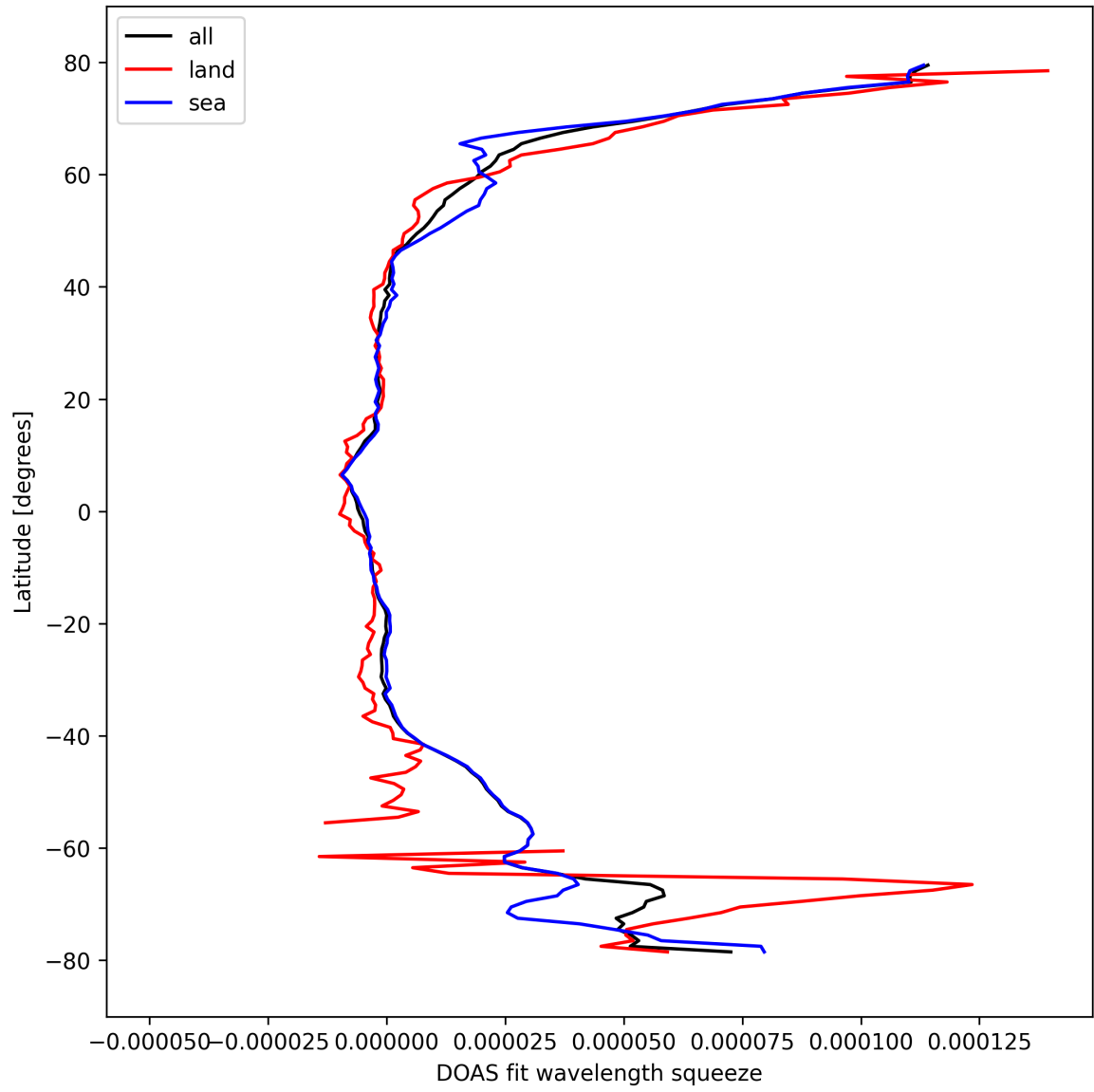
Figure 31: Zonal average of “DOAS fit wavelength squeeze” for 2024-10-06 to 2024-10-08.
