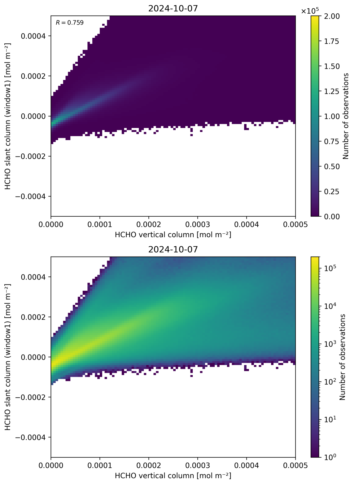
Figure 129: Scatter density plot of “HCHO vertical column” against “HCHO slant column (window1)” for 2024-10-06 to 2024-10-08.
