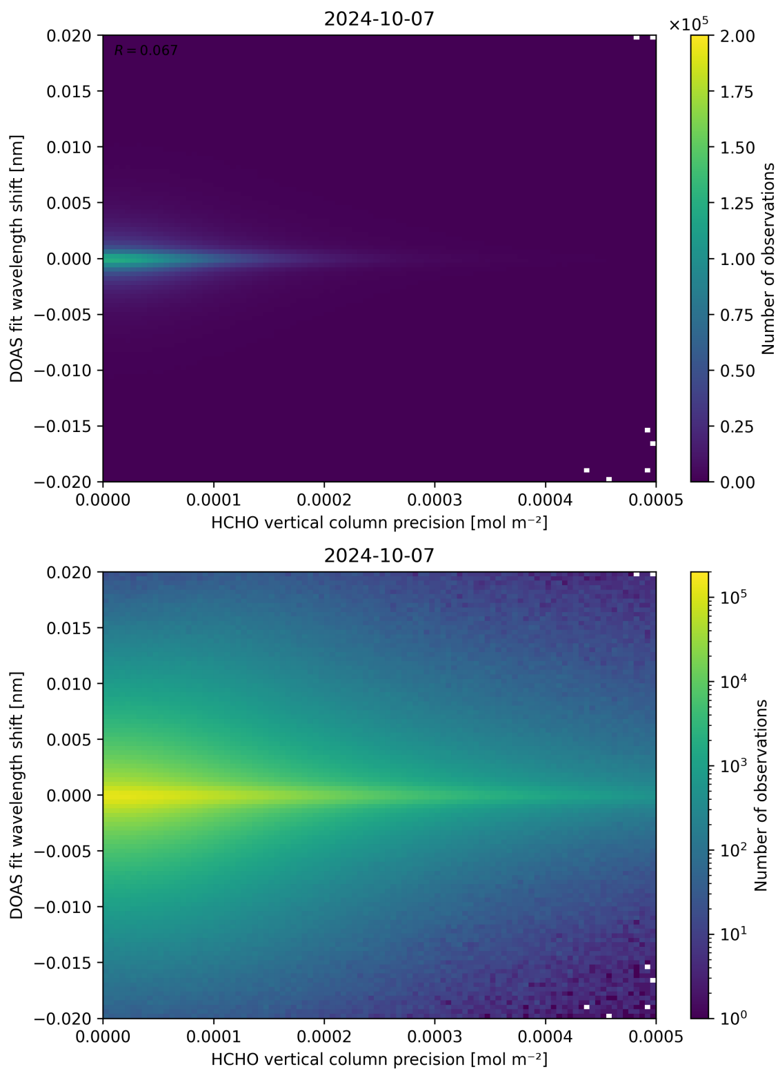
Figure 137: Scatter density plot of “HCHO vertical column precision” against “DOAS fit wavelength shift” for 2024-10-06 to 2024-10-08.
