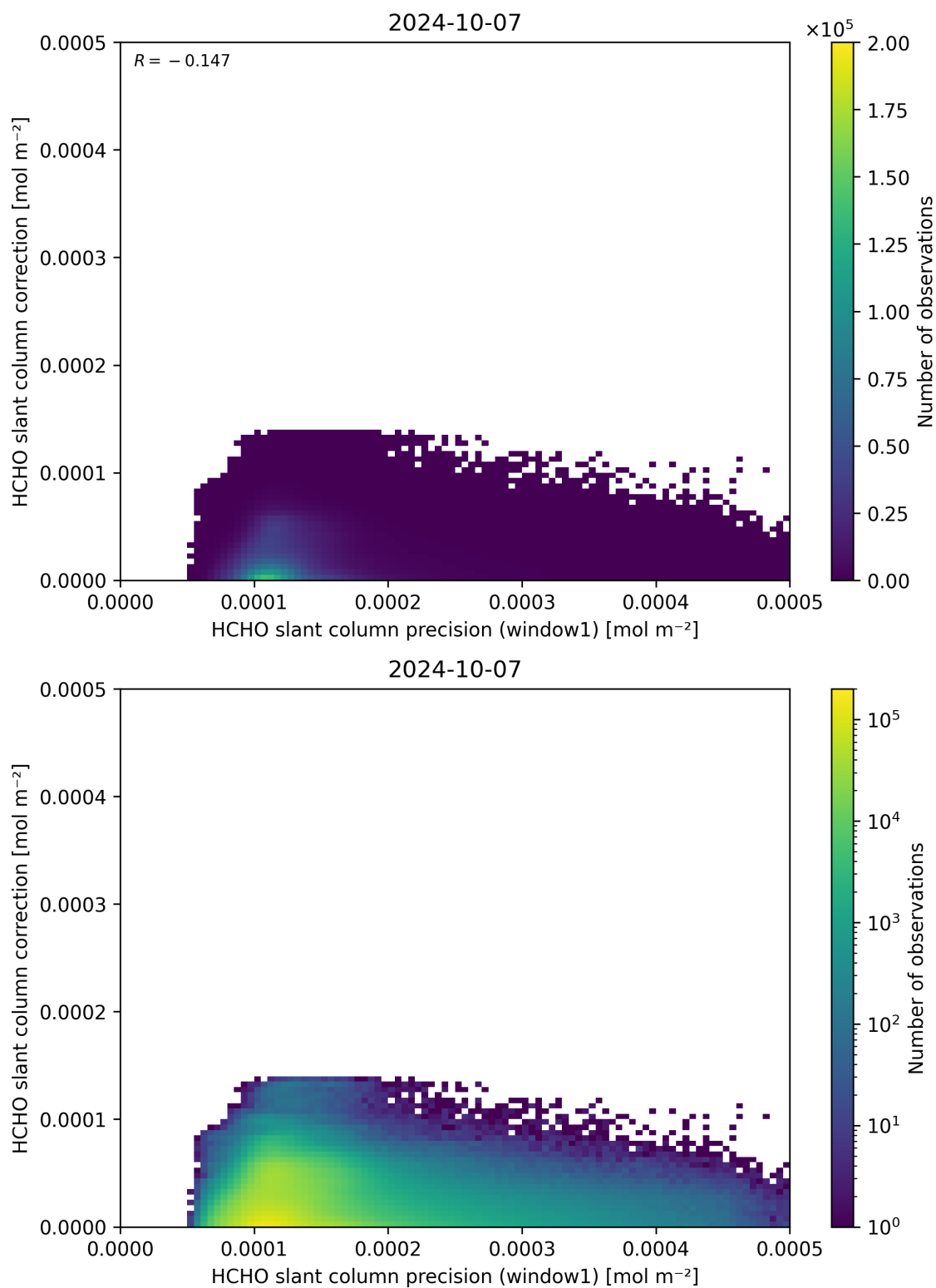
Figure 93: Scatter density plot of “HCHO slant column precision (window1)” against “HCHO slant column correction” for 2024-10-06 to 2024-10-08.
