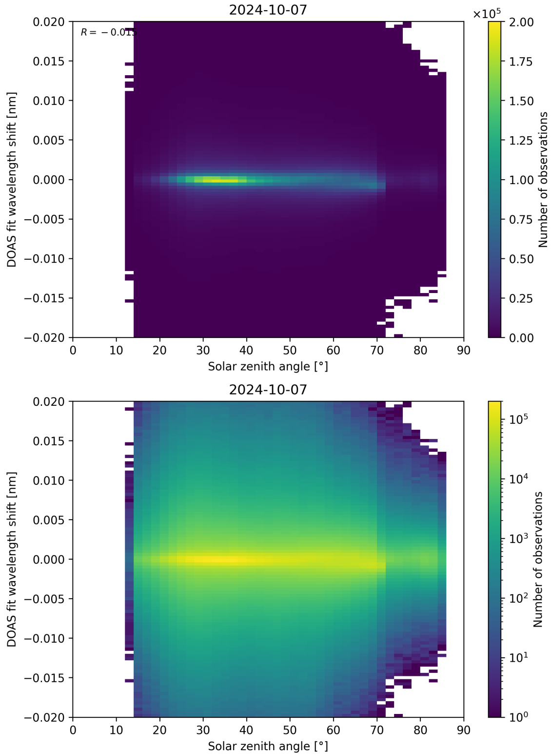
Figure 168: Scatter density plot of “Solar zenith angle” against “DOAS fit wavelength shift” for 2024-10-06 to 2024-10-08.
