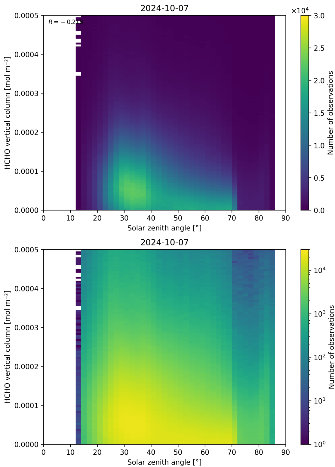
Figure 177: Scatter density plot of “Solar zenith angle” against “HCHO vertical column” for 2024-10-06 to 2024-10-08.
