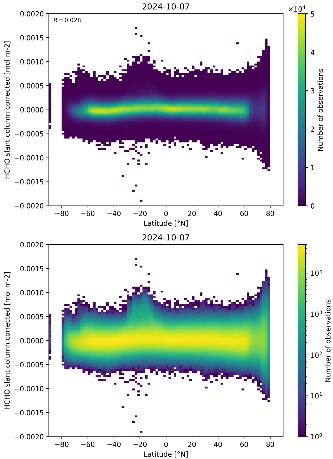
Figure 157: Scatter density plot of “Latitude” against “HCHO slant column corrected” for 2024-10-06 to 2024-10-08.
