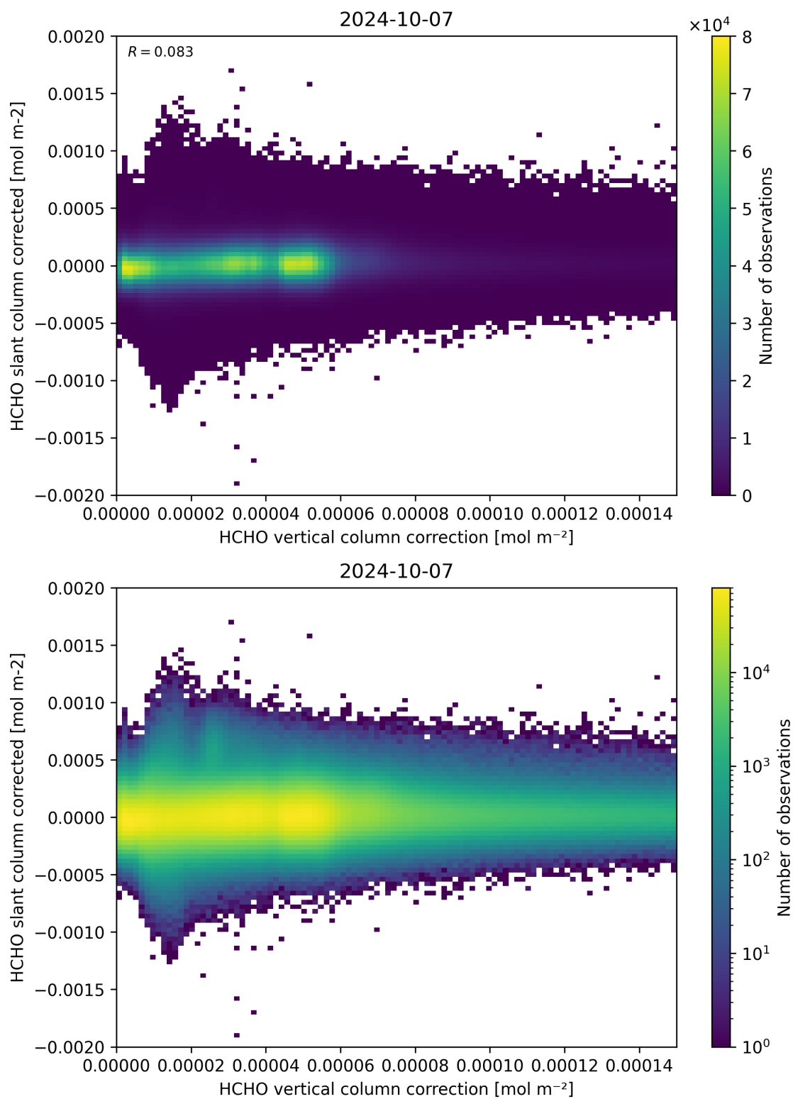
Figure 116: Scatter density plot of “HCHO vertical column correction” against “HCHO slant column corrected” for 2024-10-06 to 2024-10-08.
