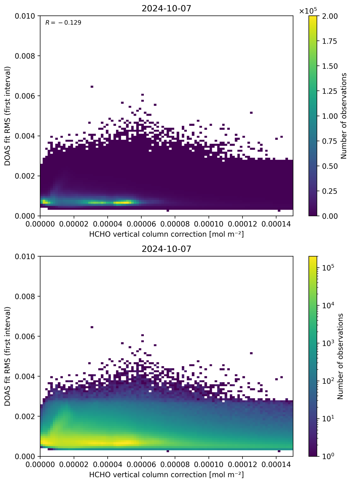
Figure 112: Scatter density plot of “HCHO vertical column correction” against “DOAS fit RMS (first interval)” for 2024-10-06 to 2024-10-08.
