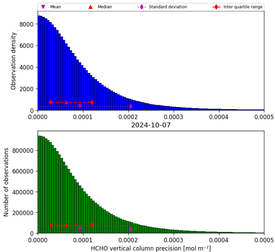
Figure 36: Histogram of “HCHO vertical column precision” for 2024-10-06 to 2024-10-08
