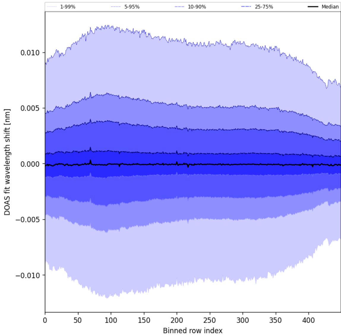
Figure 58: Along track statistics of “DOAS fit wavelength shift” for 2024-10-06 to 2024-10-08
