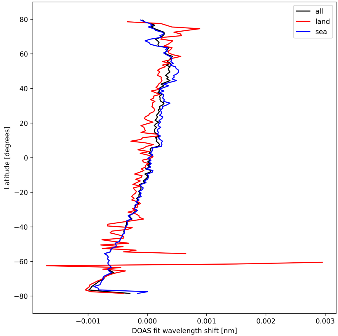
Figure 30: Zonal average of “DOAS fit wavelength shift” for 2024-10-06 to 2024-10-08.
