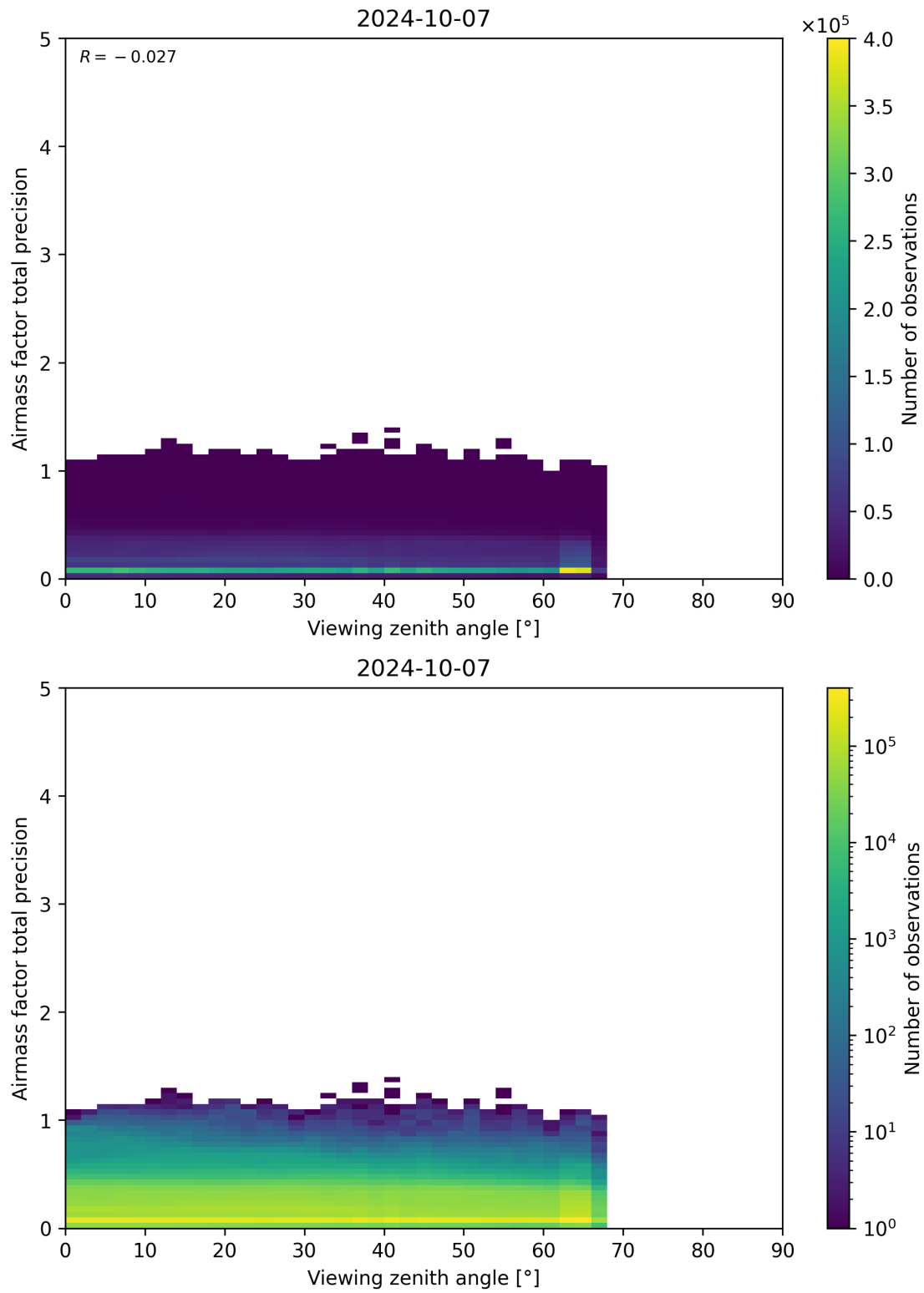
Figure 191: Scatter density plot of “Viewing zenith angle” against “Airmass factor total precision” for 2024-10-06 to 2024-10-08.
