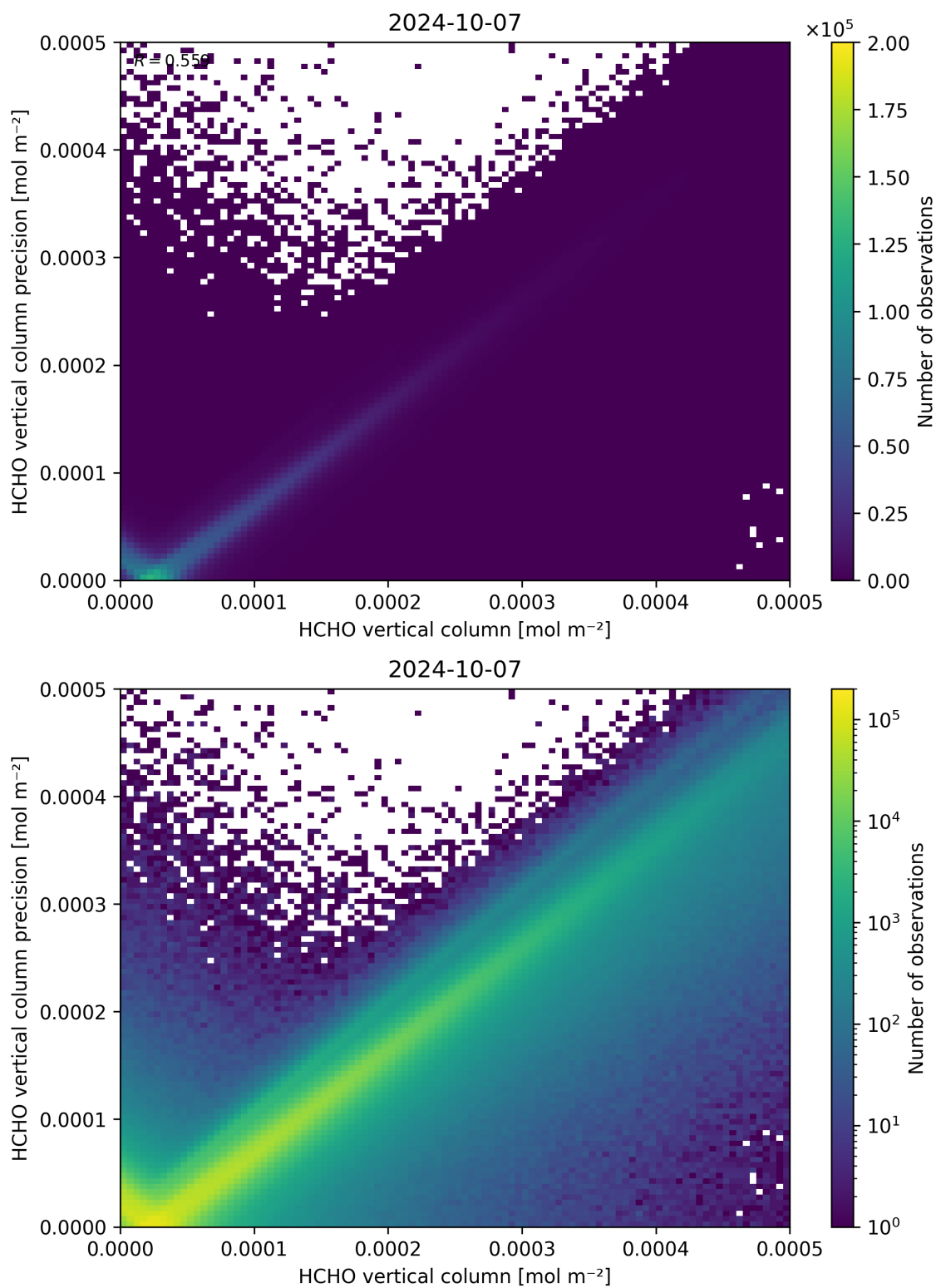
Figure 134: Scatter density plot of “HCHO vertical column” against “HCHO vertical column precision” for 2024-10-06 to 2024-10-08.
