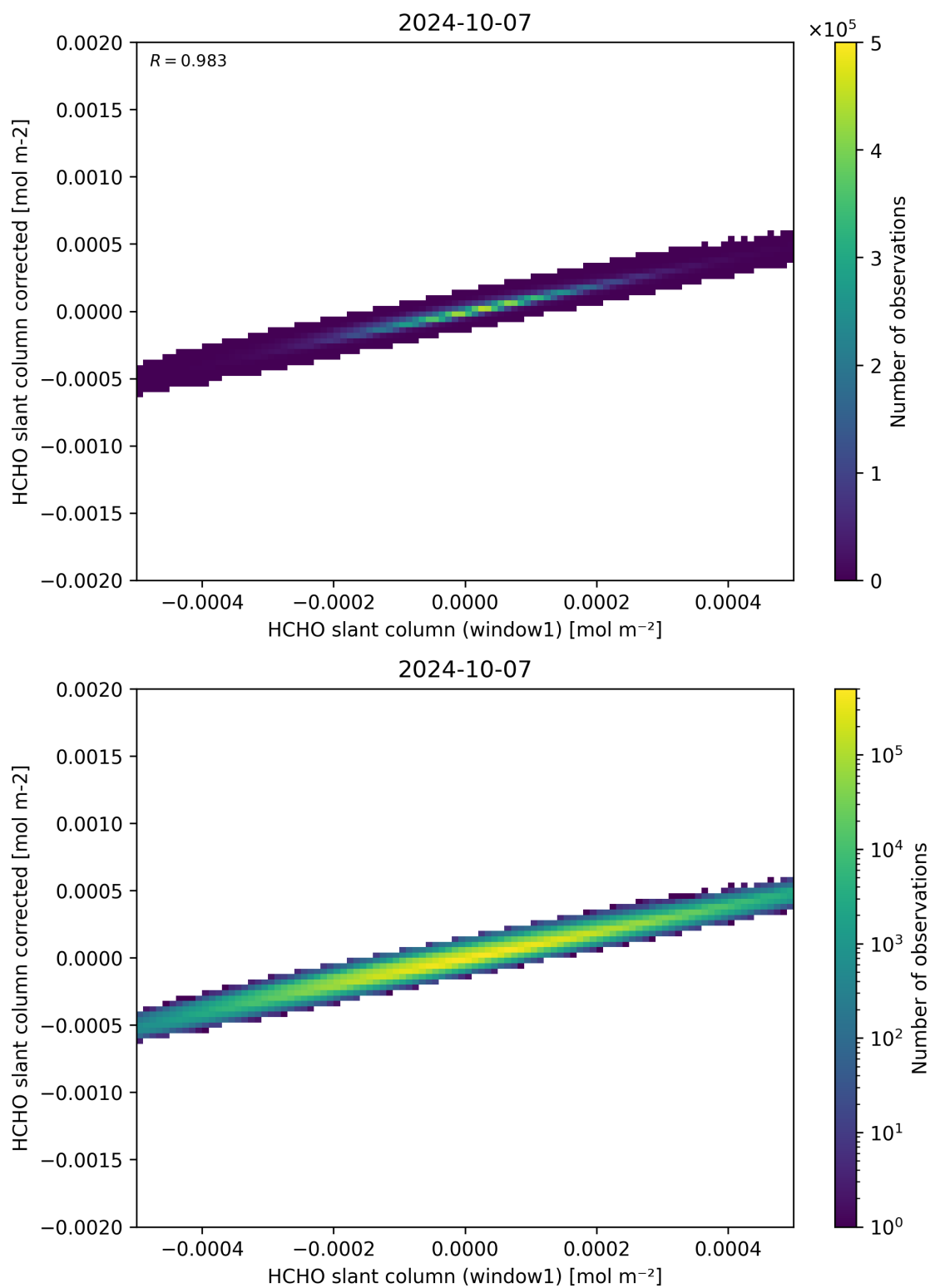
Figure 82: Scatter density plot of “HCHO slant column (window1)” against “HCHO slant column corrected” for 2024-10-06 to 2024-10-08.
