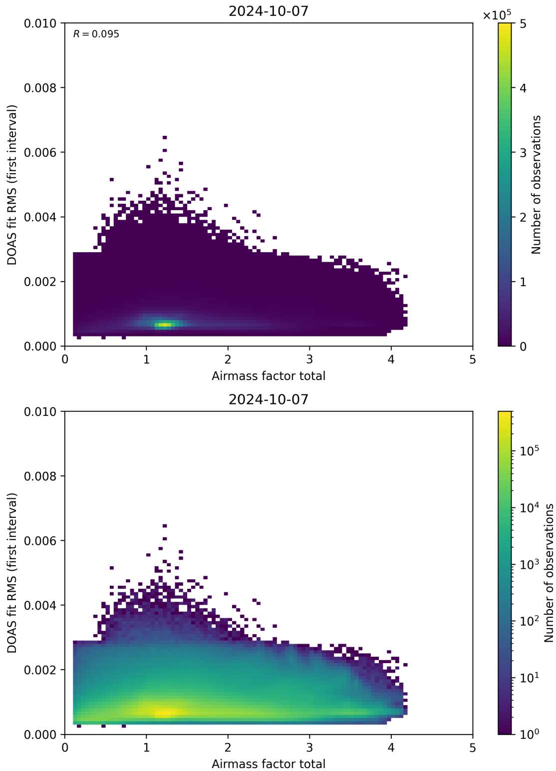
Figure 97: Scatter density plot of “Airmass factor total” against “DOAS fit RMS (first interval)” for 2024-10-06 to 2024-10-08.
