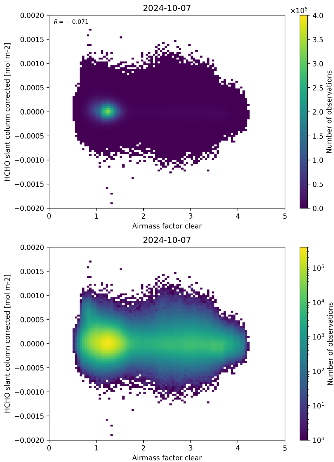
Figure 74: Scatter density plot of “Airmass factor clear” against “HCHO slant column corrected” for 2024-10-06 to 2024-10-08.
