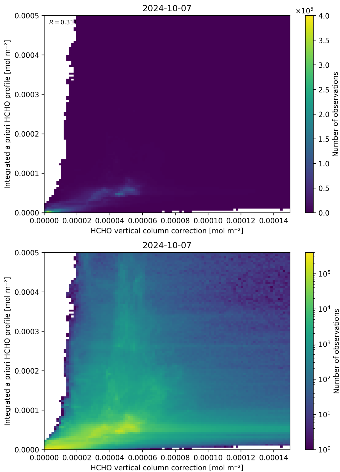
Figure 122: Scatter density plot of “HCHO vertical column correction” against “Integrated a priori HCHO profile” for 2024-10-06 to 2024-10-08.
