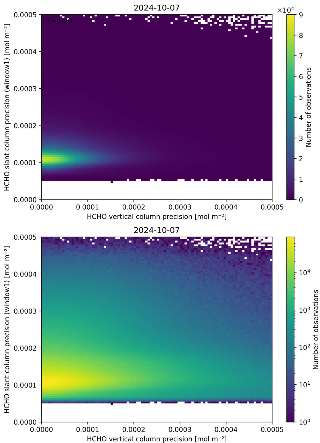
Figure 143: Scatter density plot of “HCHO vertical column precision” against “HCHO slant column precision (window1)” for 2024-10-06 to 2024-10-08.
