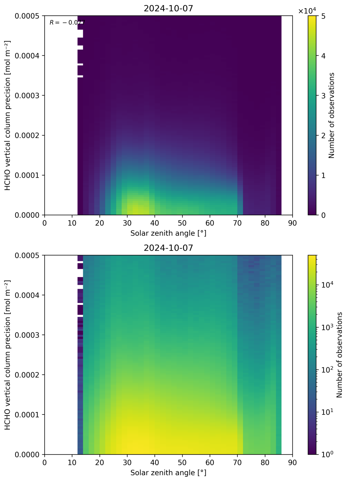
Figure 179: Scatter density plot of “Solar zenith angle” against “HCHO vertical column precision” for 2024-10-06 to 2024-10-08.
