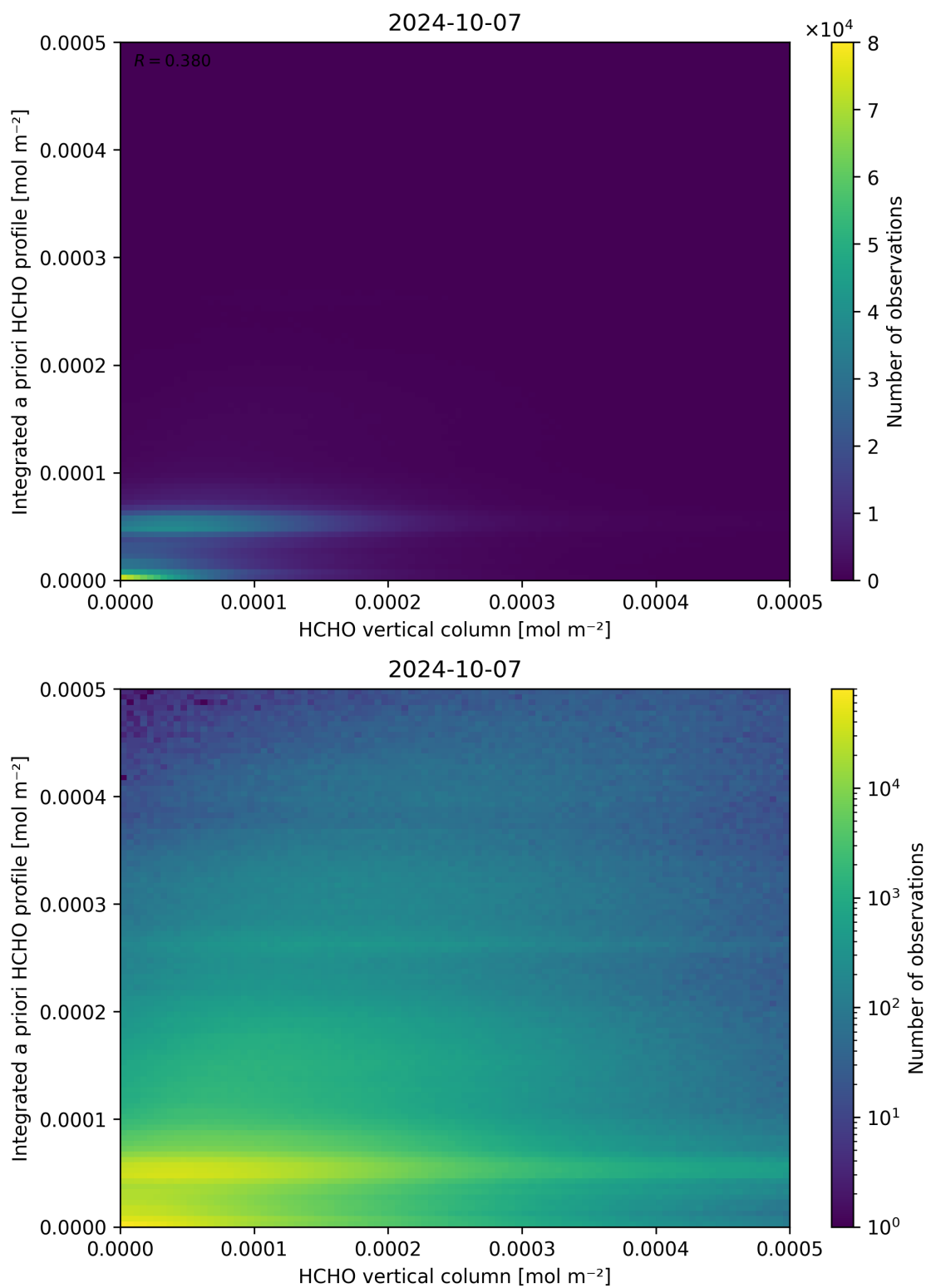
Figure 135: Scatter density plot of “HCHO vertical column” against “Integrated a priori HCHO profile” for 2024-10-06 to 2024-10-08.
