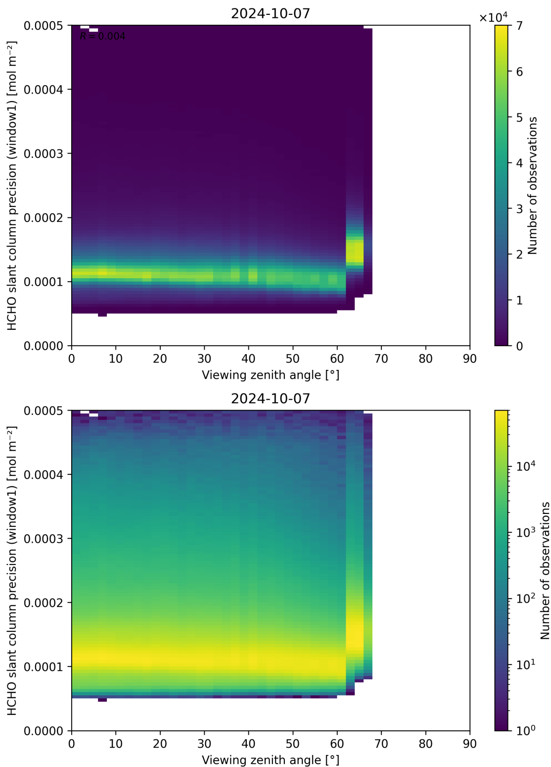
Figure 189: Scatter density plot of “Viewing zenith angle” against “HCHO slant column precision (window1)” for 2024-10-06 to 2024-10-08.
