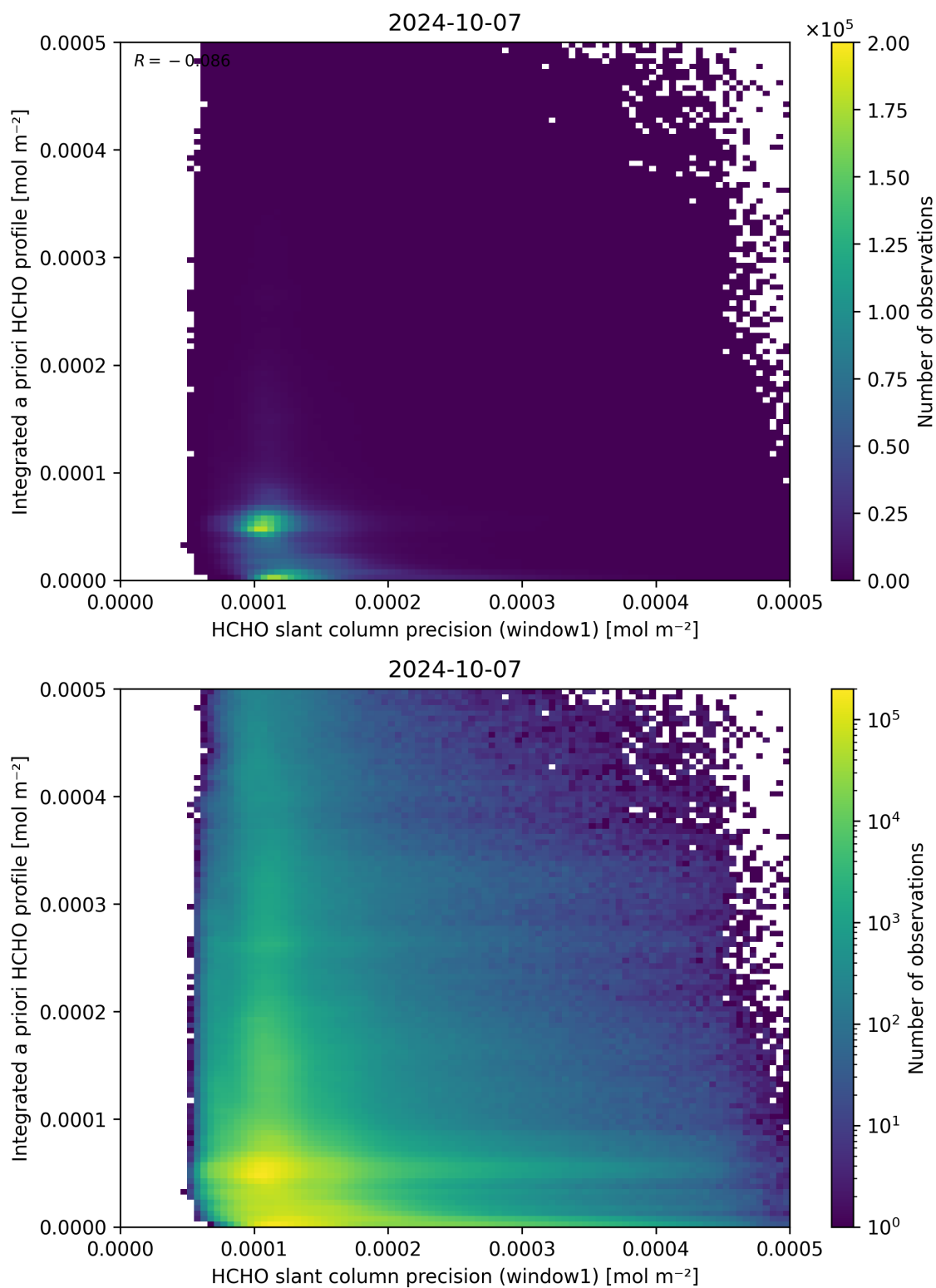
Figure 96: Scatter density plot of “HCHO slant column precision (window1)” against “Integrated a priori HCHO profile” for 2024-10-06 to 2024-10-08.
