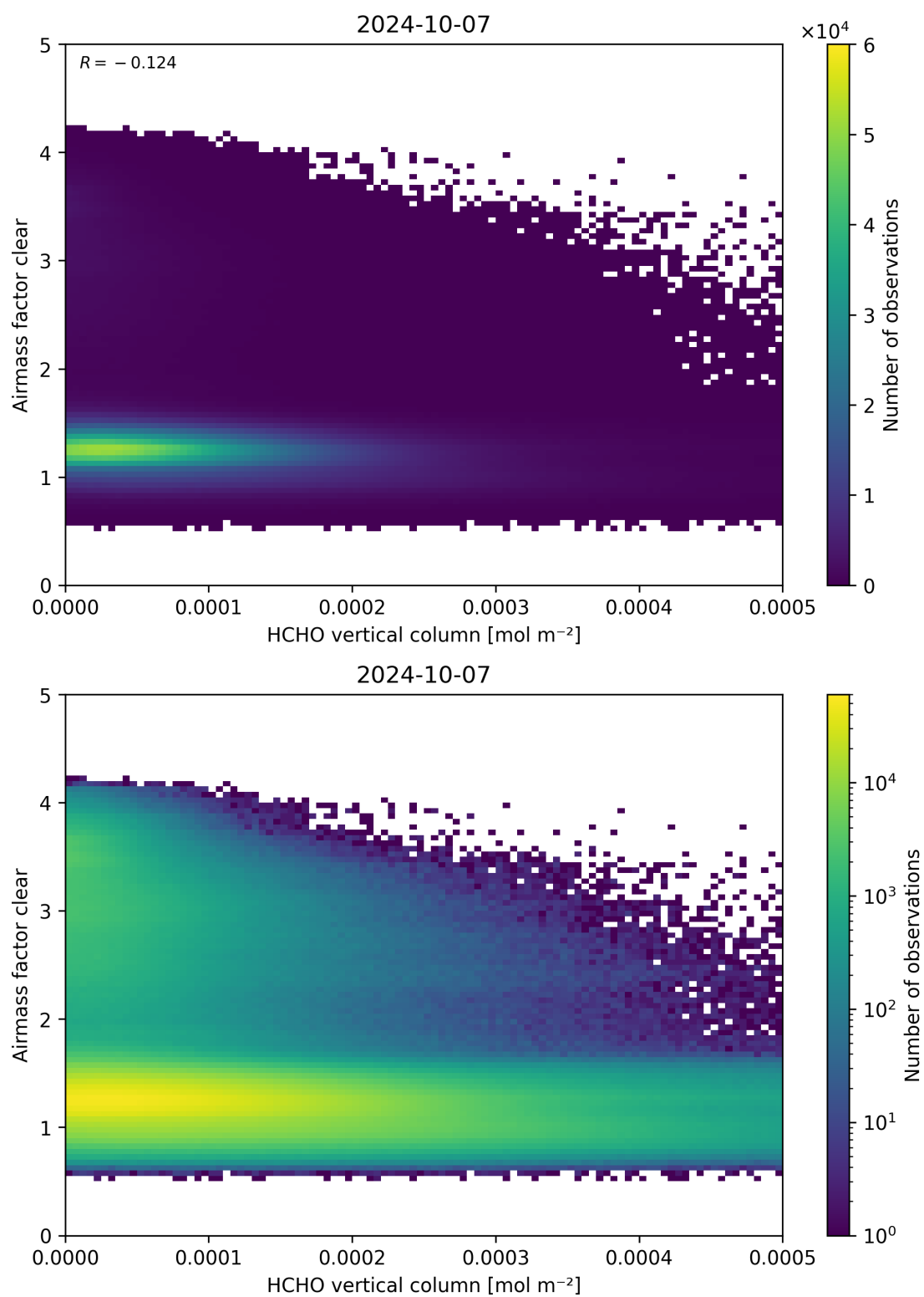
Figure 126: Scatter density plot of “HCHO vertical column” against “Airmass factor clear” for 2024-10-06 to 2024-10-08.
