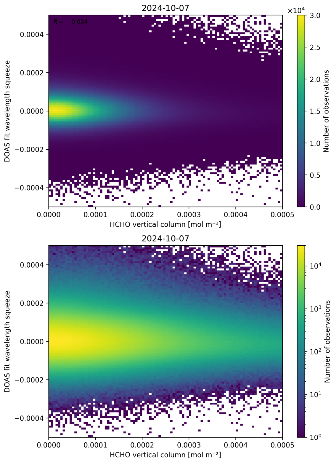
Figure 125: Scatter density plot of “HCHO vertical column” against “DOAS fit wavelength squeeze” for 2024-10-06 to 2024-10-08.
