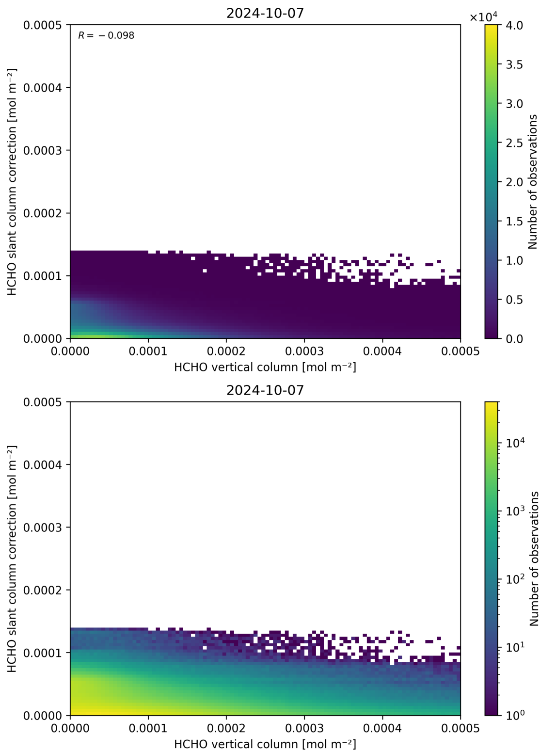
Figure 128: Scatter density plot of “HCHO vertical column” against “HCHO slant column correction” for 2024-10-06 to 2024-10-08.
