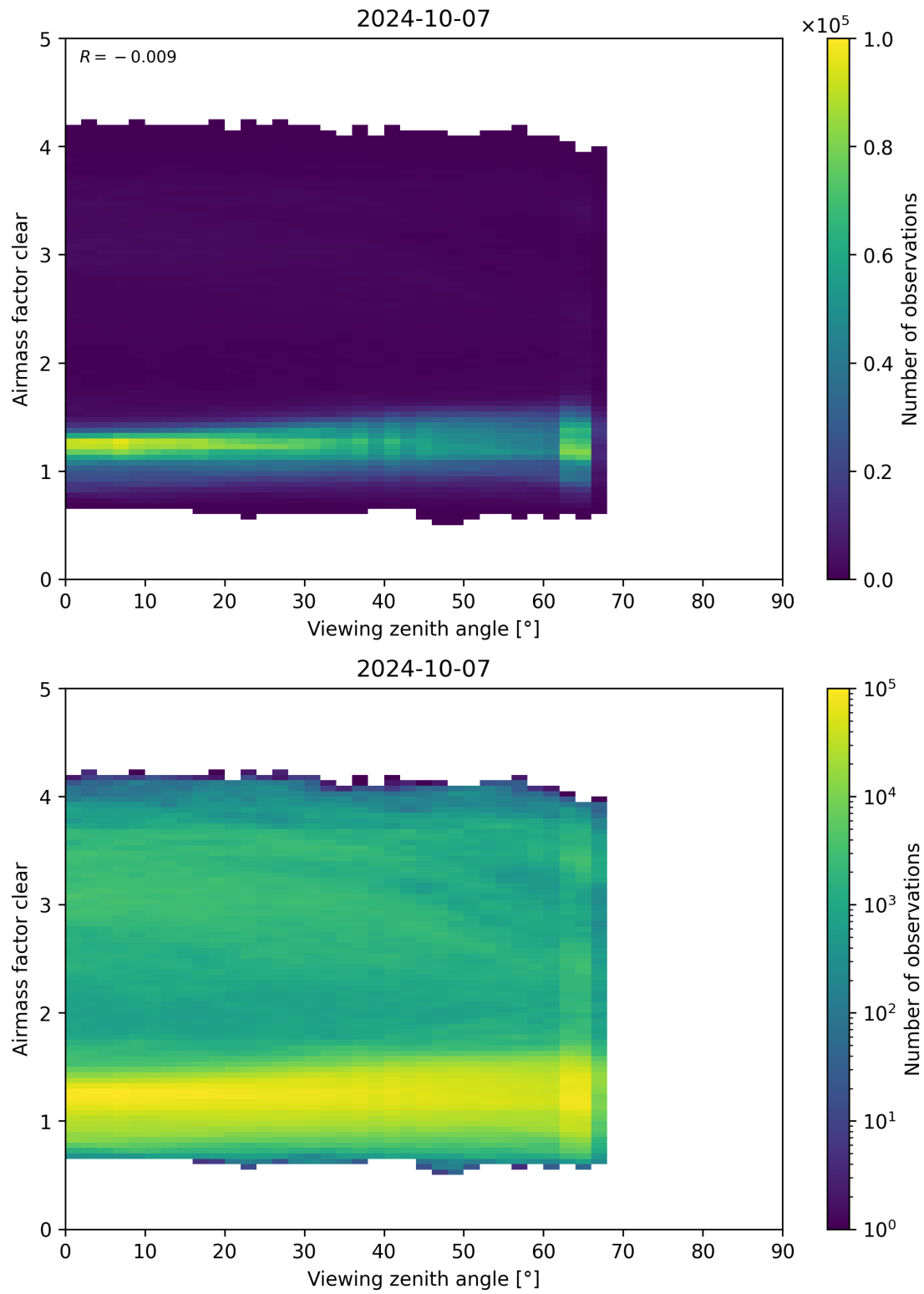
Figure 185: Scatter density plot of “Viewing zenith angle” against “Airmass factor clear” for 2024-10-06 to 2024-10-08.
