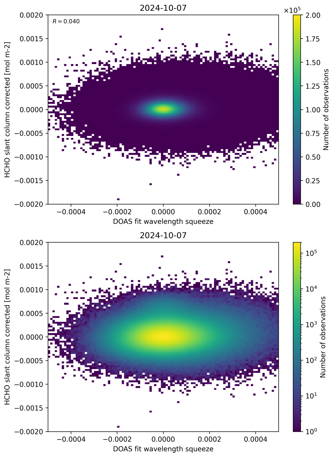
Figure 69: Scatter density plot of “DOAS fit wavelength squeeze” against “HCHO slant column corrected” for 2024-10-06 to 2024-10-08.
