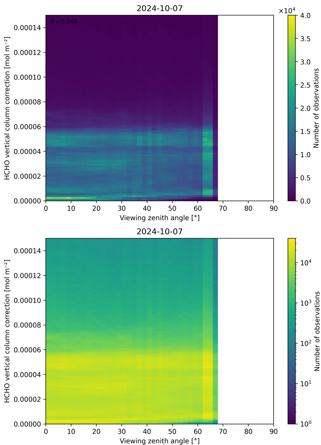
Figure 193: Scatter density plot of “Viewing zenith angle” against “HCHO vertical column correction” for 2024-10-06 to 2024-10-08.
