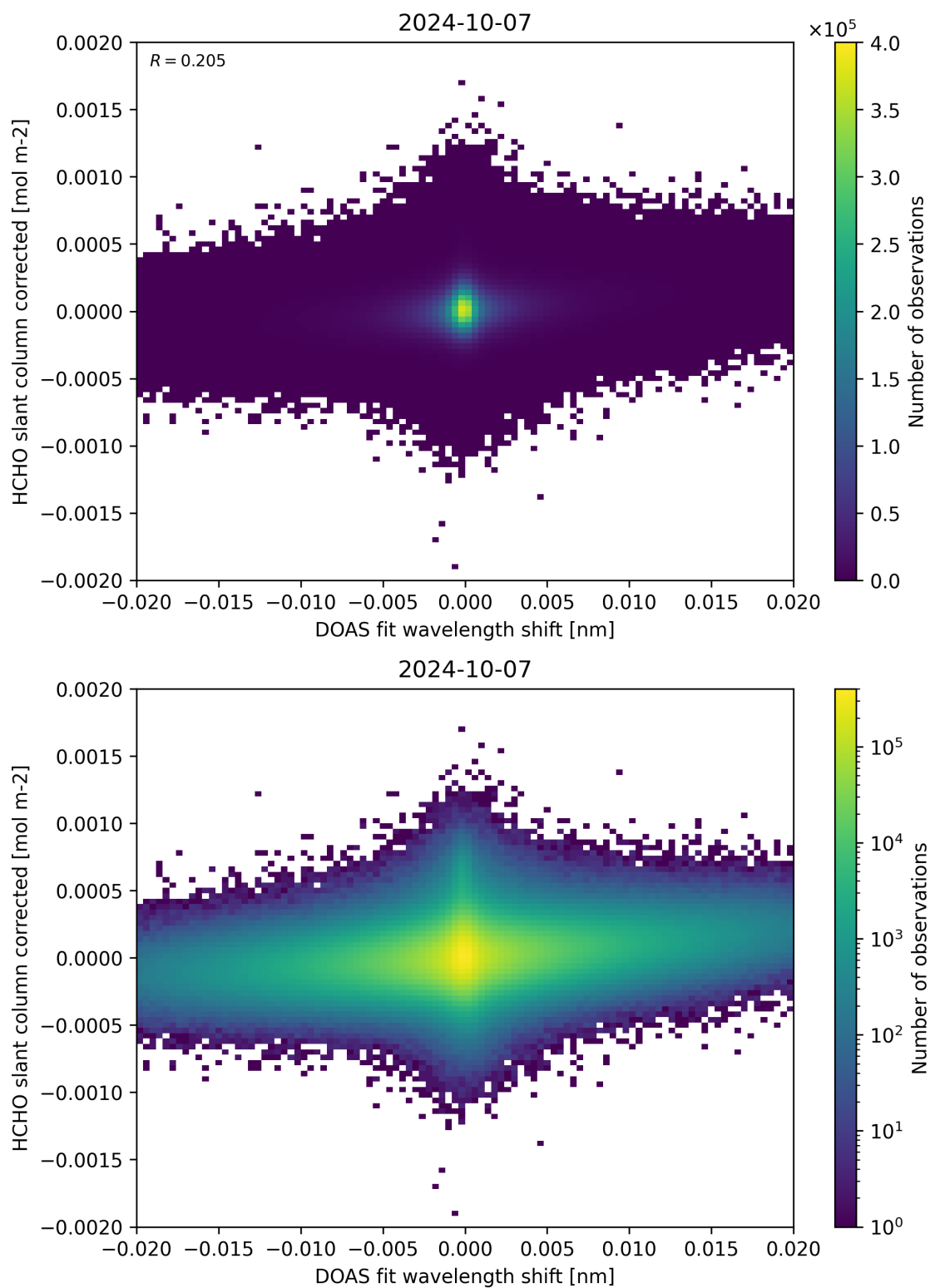
Figure 66: Scatter density plot of “DOAS fit wavelength shift” against “HCHO slant column corrected” for 2024-10-06 to 2024-10-08.
