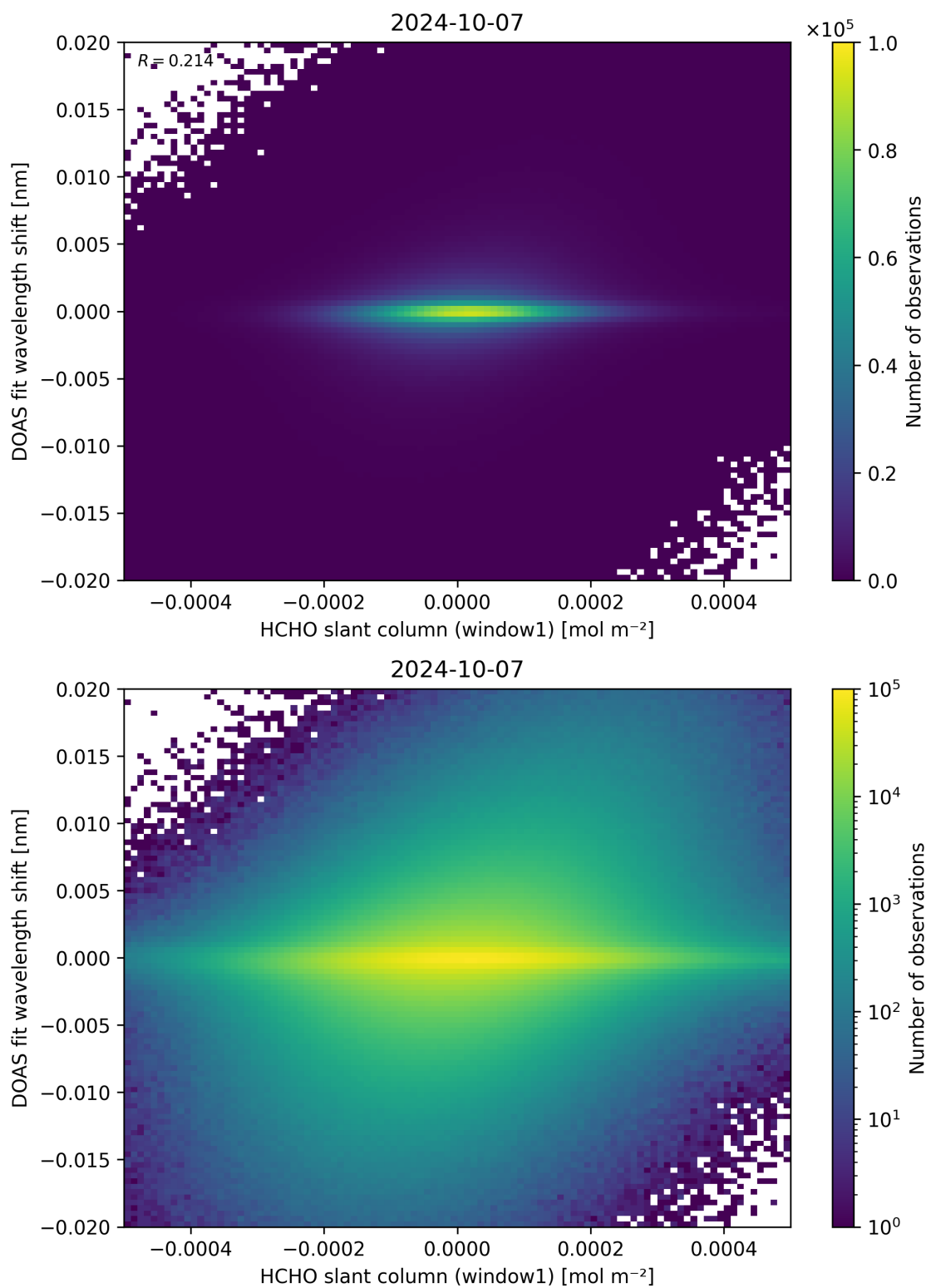
Figure 79: Scatter density plot of “HCHO slant column (window1)” against “DOAS fit wavelength shift” for 2024-10-06 to 2024-10-08.
