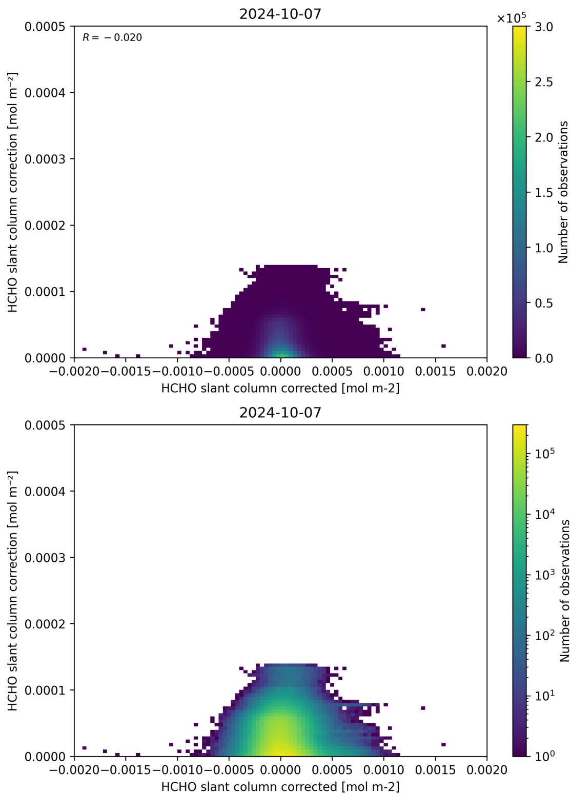
Figure 77: Scatter density plot of “HCHO slant column corrected” against “HCHO slant column correction” for 2024-10-06 to 2024-10-08.
