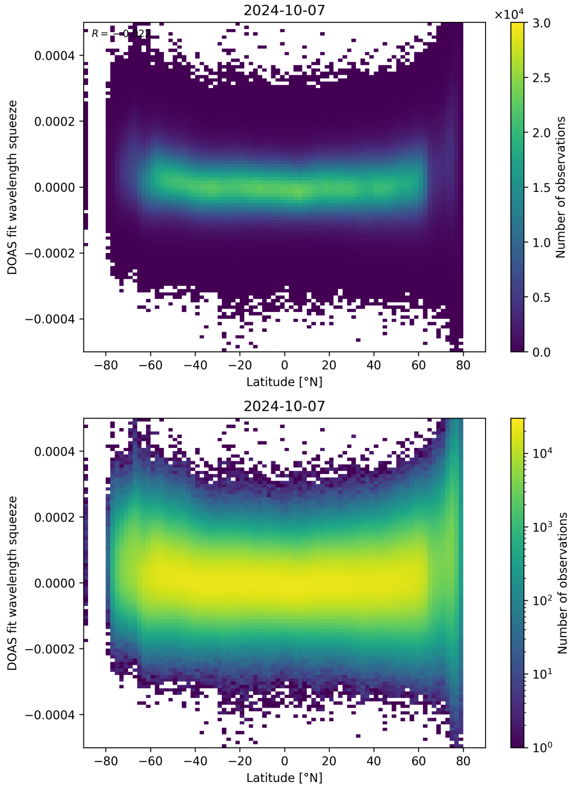
Figure 155: Scatter density plot of “Latitude” against “DOAS fit wavelength squeeze” for 2024-10-06 to 2024-10-08.
