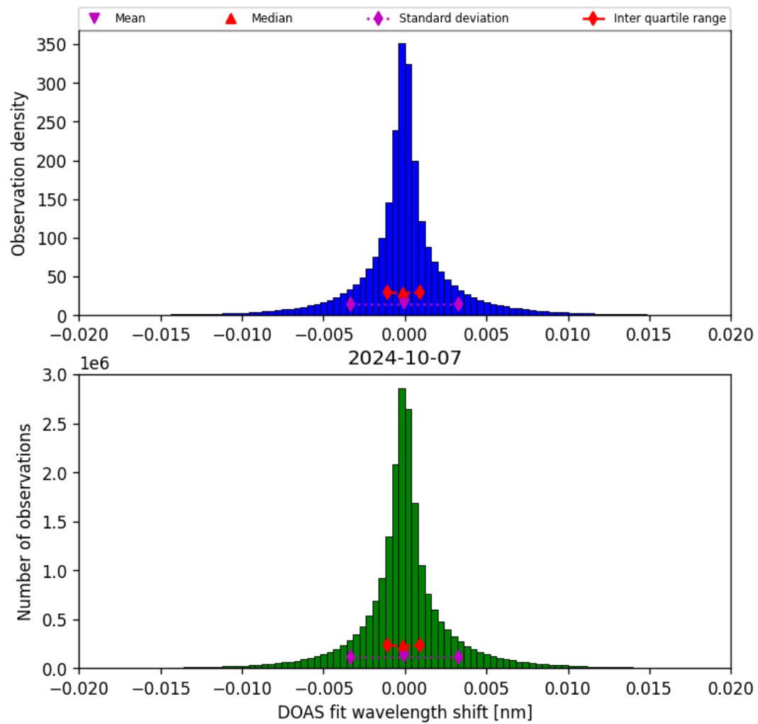
Figure 44: Histogram of “DOAS fit wavelength shift” for 2024-10-06 to 2024-10-08
