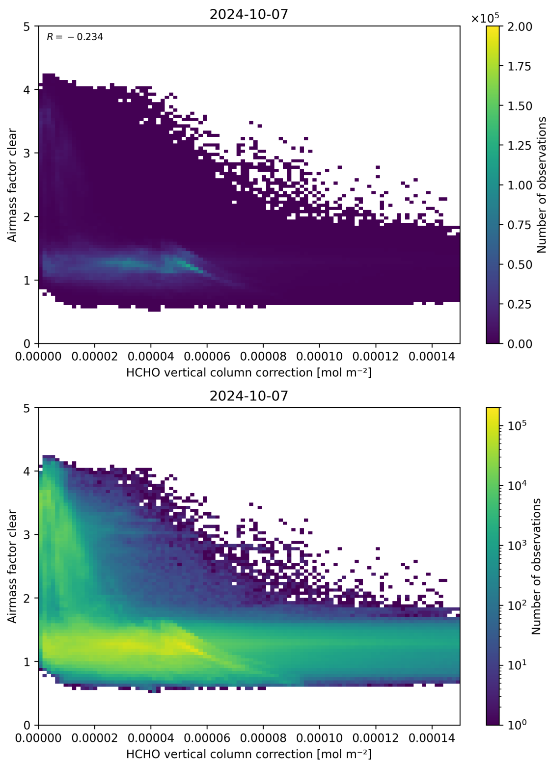
Figure 115: Scatter density plot of “HCHO vertical column correction” against “Airmass factor clear” for 2024-10-06 to 2024-10-08.
