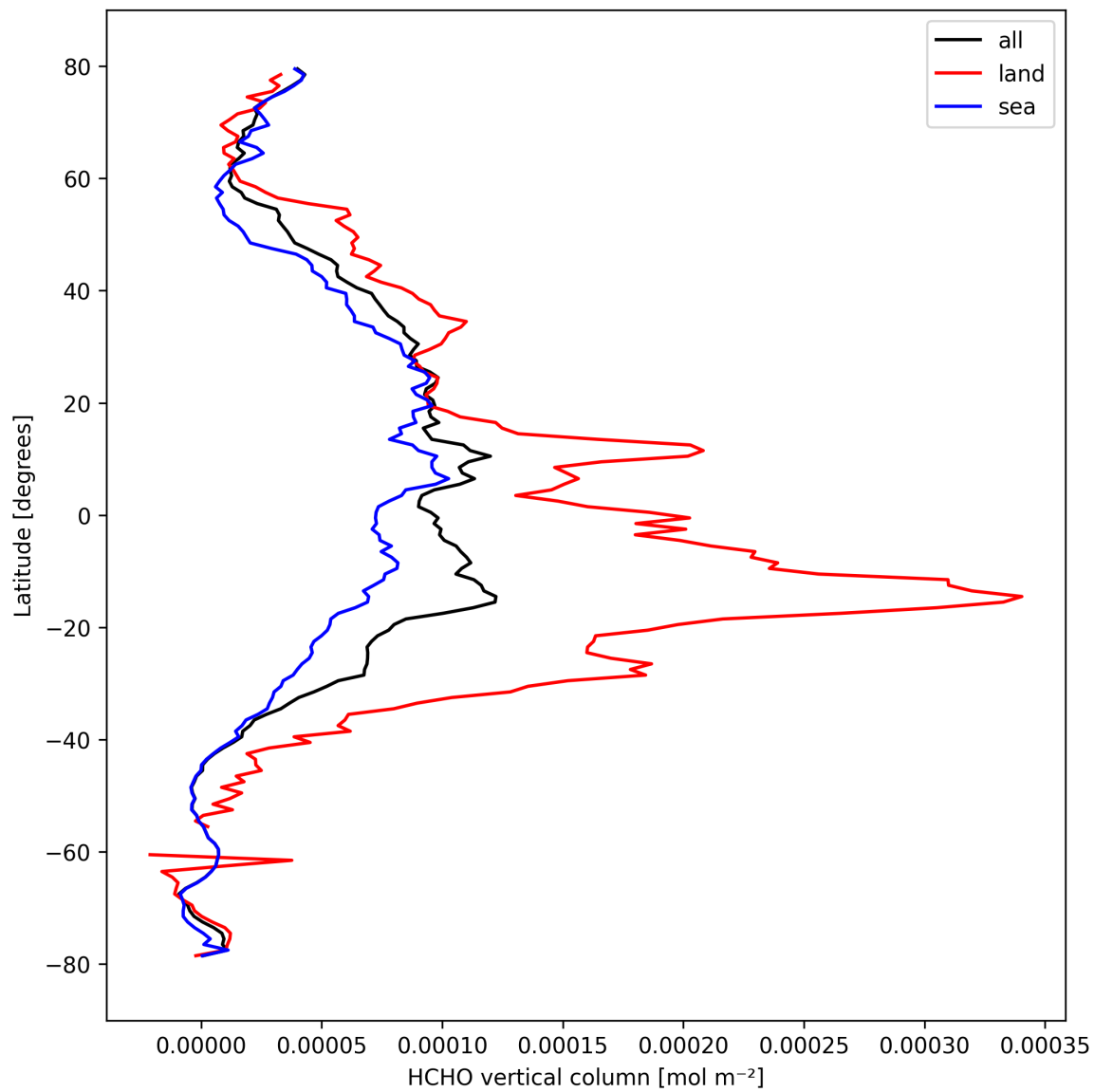
Figure 21: Zonal average of “HCHO vertical column” for 2024-10-06 to 2024-10-08.
