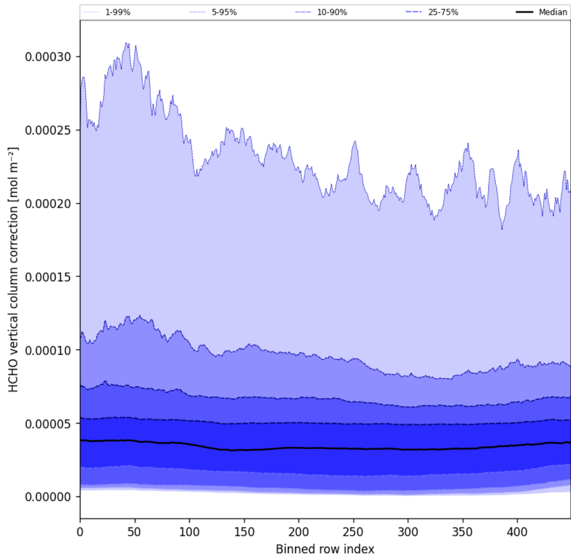
Figure 51: Along track statistics of “HCHO vertical column correction” for 2024-10-06 to 2024-10-08
