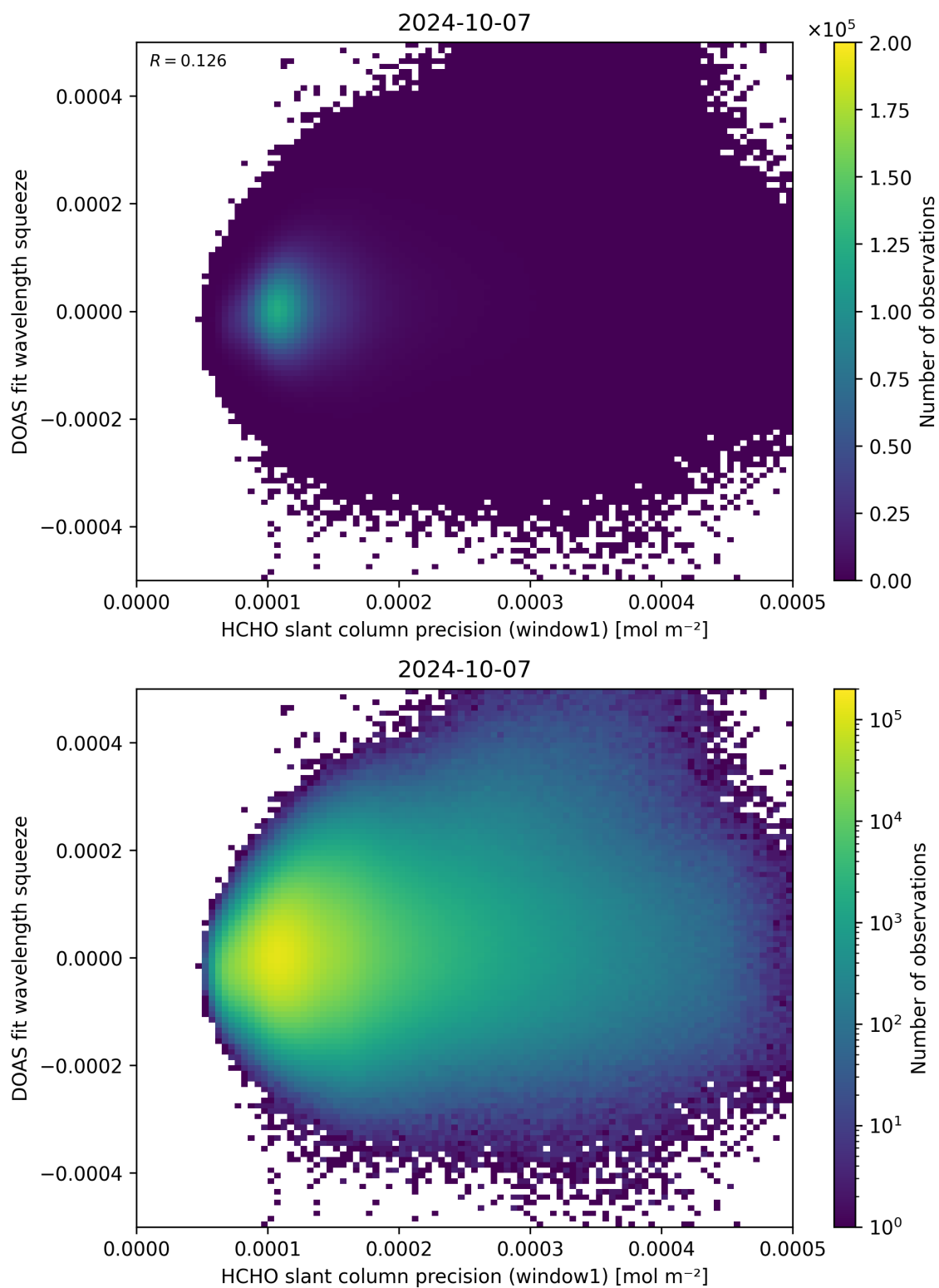
Figure 90: Scatter density plot of “HCHO slant column precision (window1)” against “DOAS fit wavelength squeeze” for 2024-10-06 to 2024-10-08.
