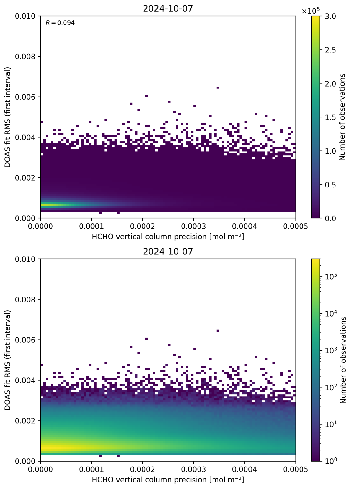
Figure 136: Scatter density plot of “HCHO vertical column precision” against “DOAS fit RMS (first interval)” for 2024-10-06 to 2024-10-08.
