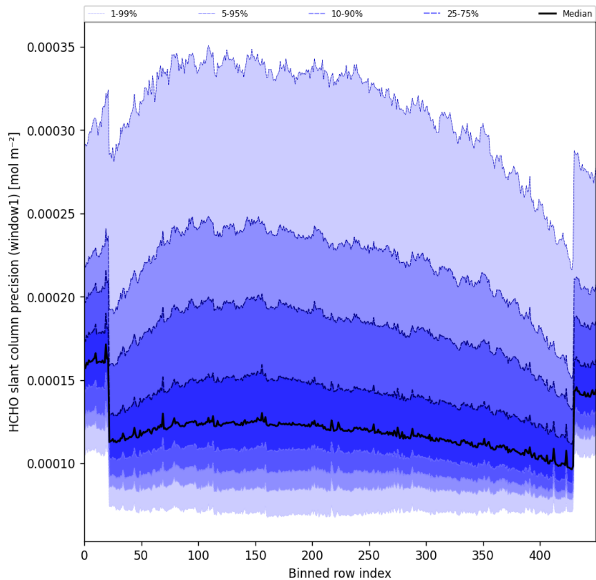
Figure 53: Along track statistics of “HCHO slant column precision (window1)” for 2024-10-06 to 2024-10-08
