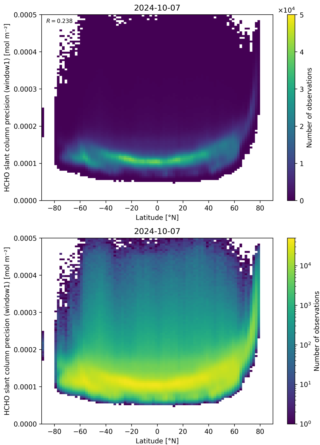
Figure 160: Scatter density plot of “Latitude” against “HCHO slant column precision (window1)” for 2024-10-06 to 2024-10-08.
