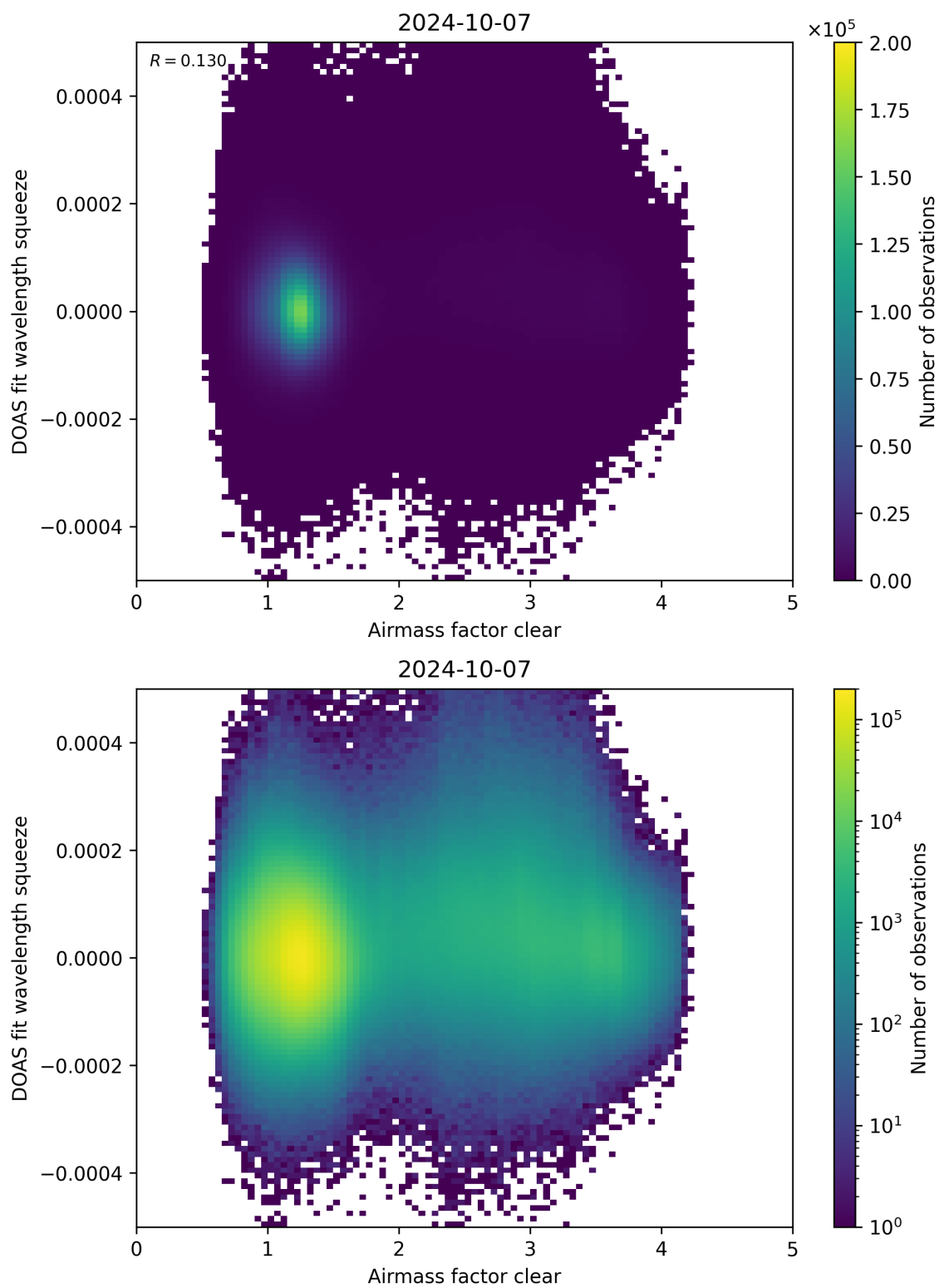
Figure 73: Scatter density plot of “Airmass factor clear” against “DOAS fit wavelength squeeze” for 2024-10-06 to 2024-10-08.
