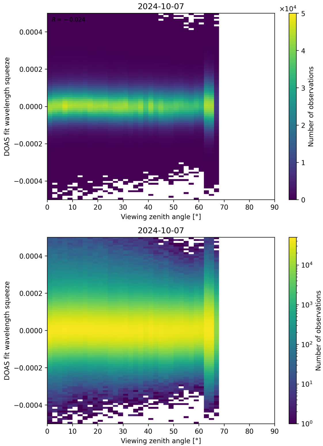
Figure 184: Scatter density plot of “Viewing zenith angle” against “DOAS fit wavelength squeeze” for 2024-10-06 to 2024-10-08.
