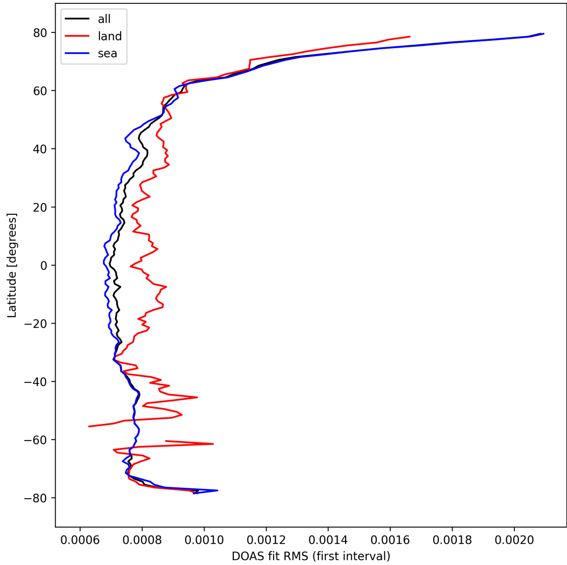
Figure 32: Zonal average of “DOAS fit RMS (first interval)” for 2024-10-06 to 2024-10-08.
