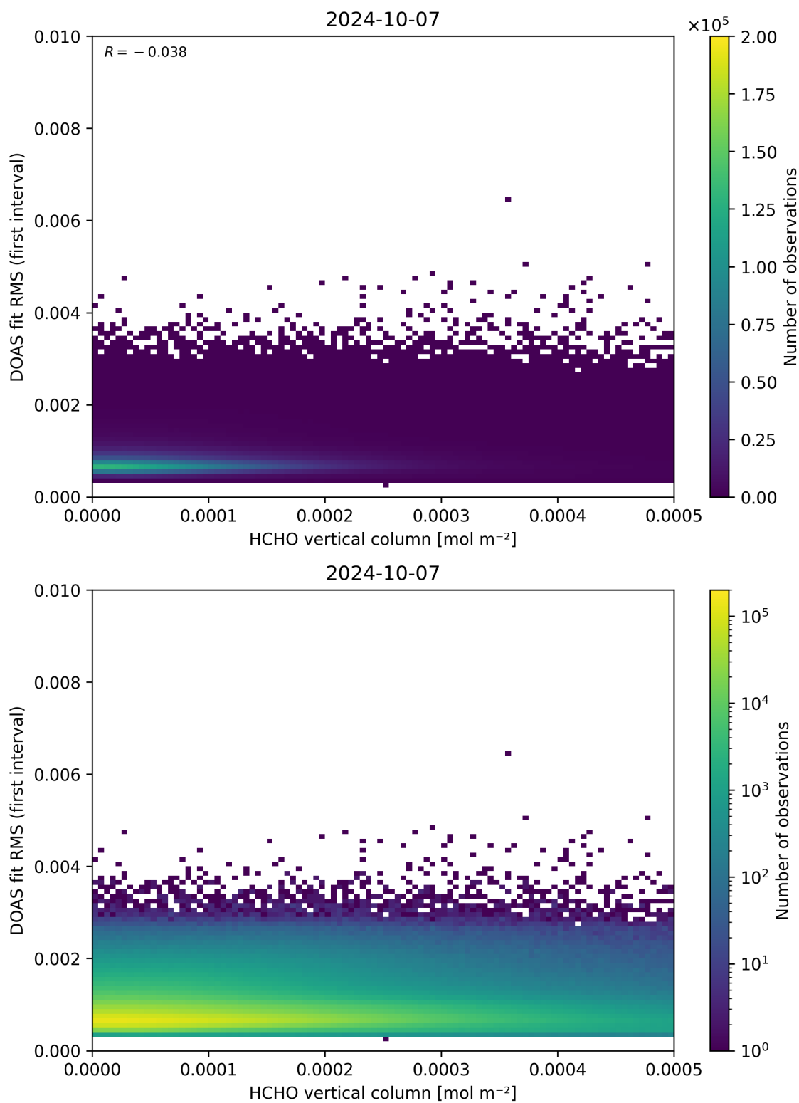
Figure 123: Scatter density plot of “HCHO vertical column” against “DOAS fit RMS (first interval)” for 2024-10-06 to 2024-10-08.
