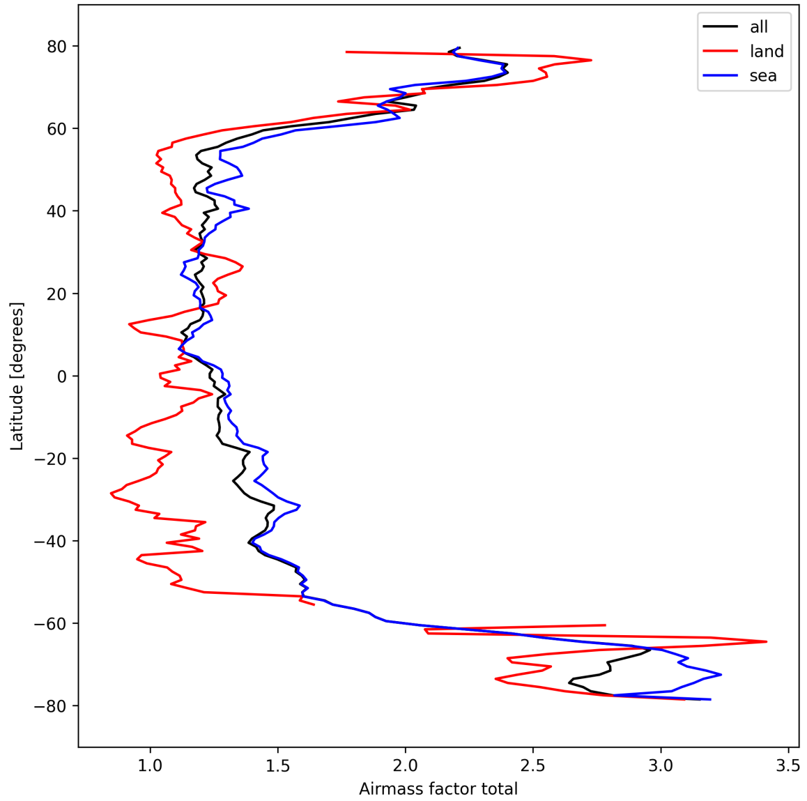
Figure 26: Zonal average of “Airmass factor total” for 2024-10-06 to 2024-10-08.
