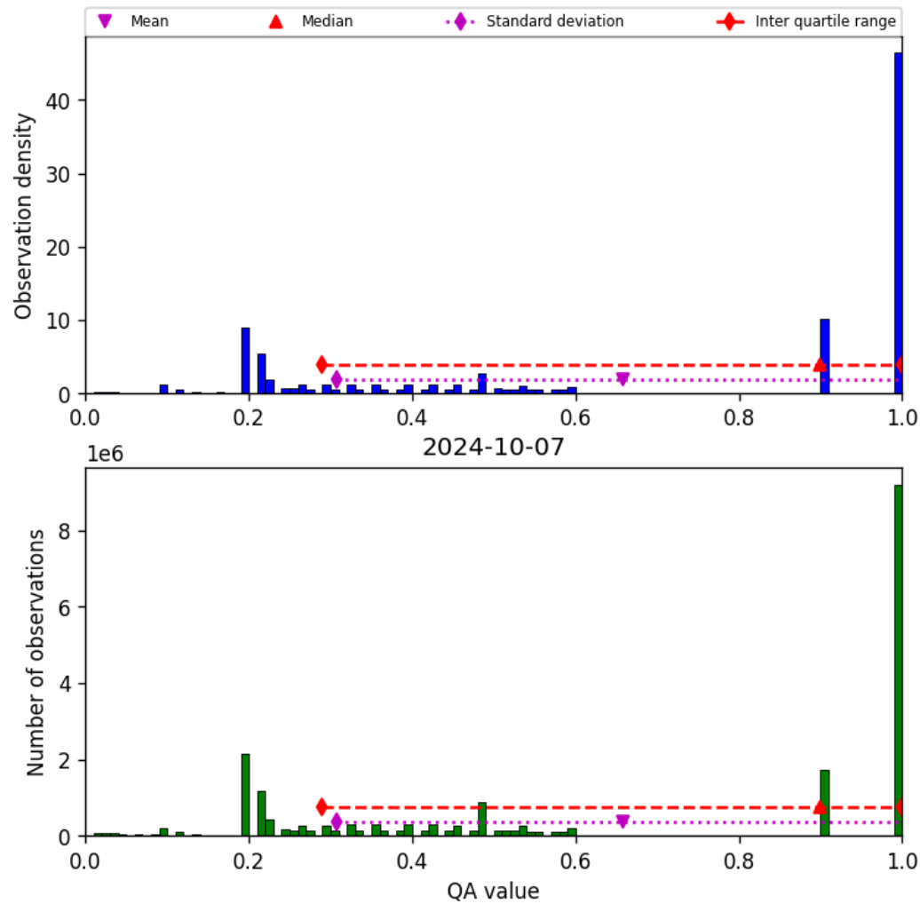
Figure 34: Histogram of “QA value” for 2024-10-06 to 2024-10-08
