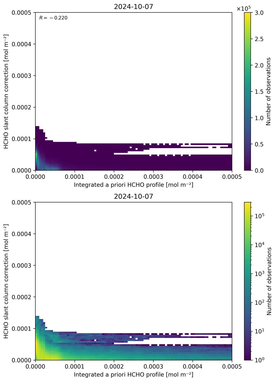
Figure 152: Scatter density plot of “Integrated a priori HCHO profile” against “HCHO slant column correction” for 2024-10-06 to 2024-10-08.
