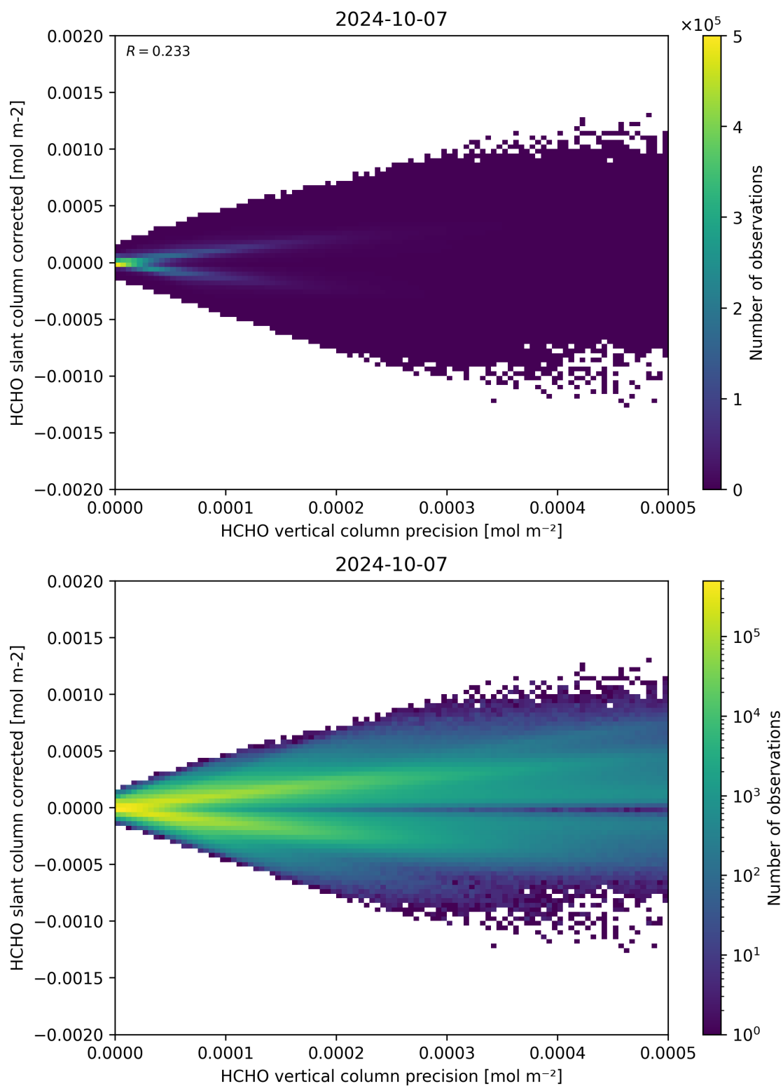
Figure 140: Scatter density plot of “HCHO vertical column precision” against “HCHO slant column corrected” for 2024-10-06 to 2024-10-08.
