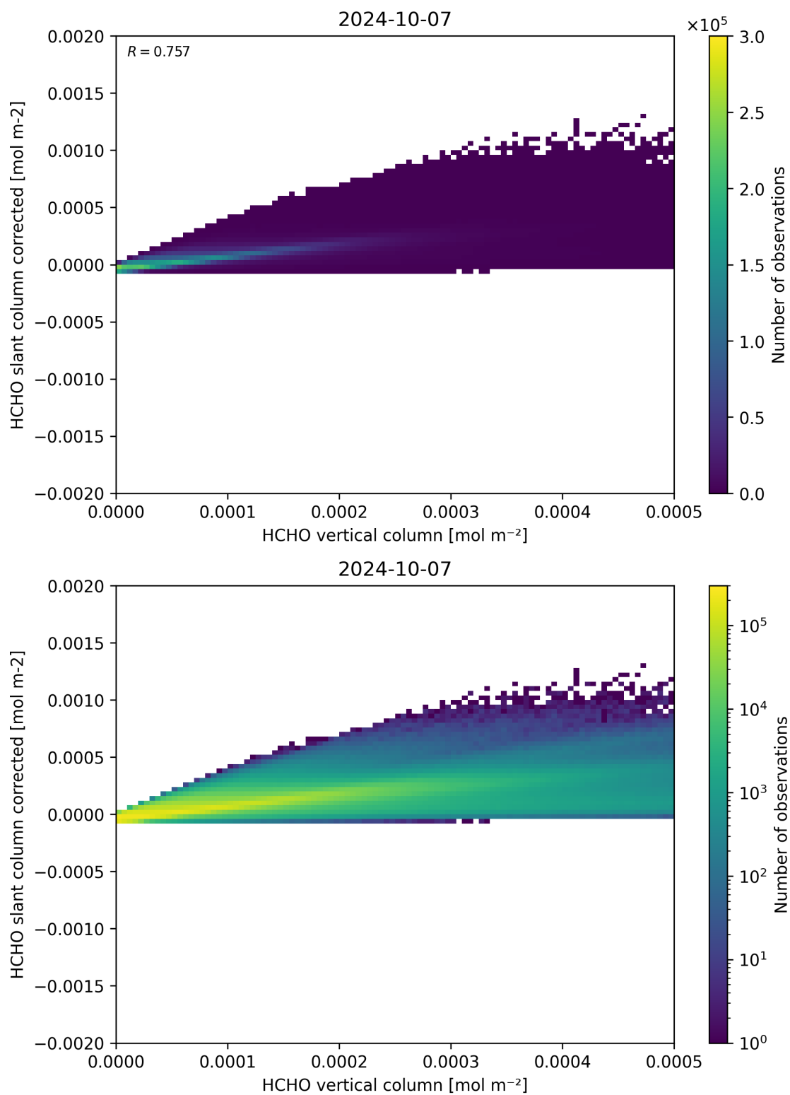
Figure 127: Scatter density plot of “HCHO vertical column” against “HCHO slant column corrected” for 2024-10-06 to 2024-10-08.
