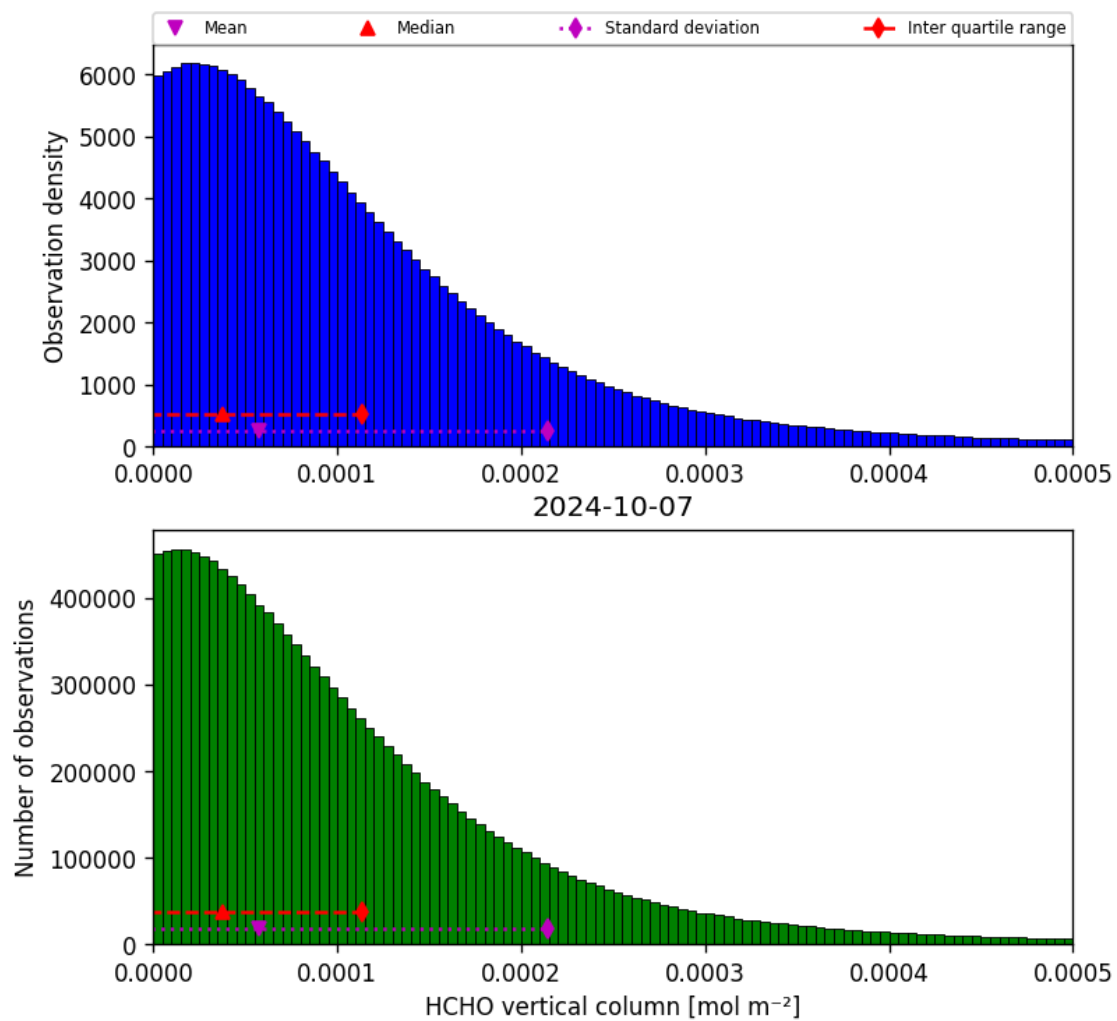
Figure 35: Histogram of “HCHO vertical column” for 2024-10-06 to 2024-10-08
