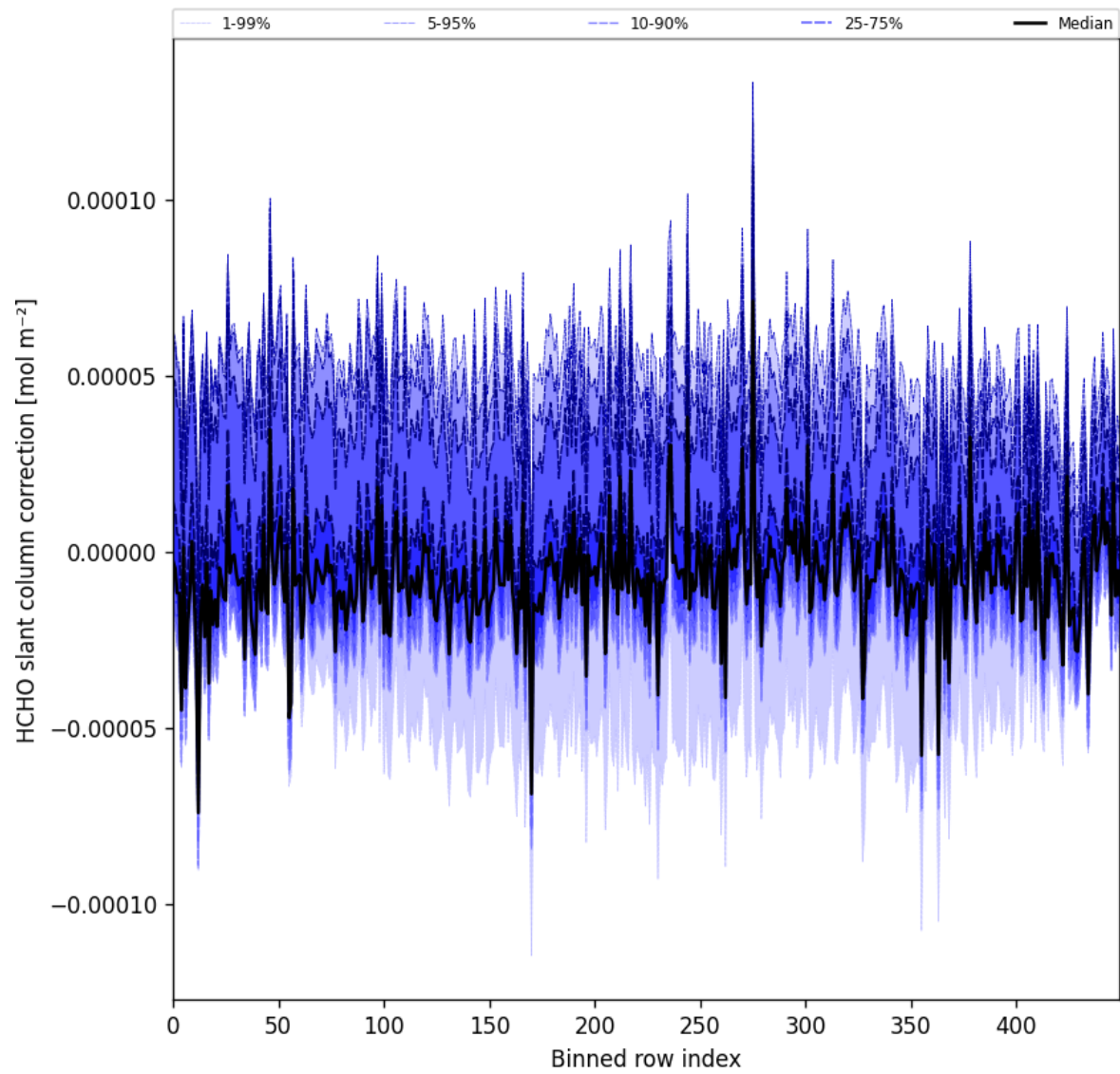
Figure 61: Along track statistics of “HCHO slant column correction” for 2024-10-06 to 2024-10-08
