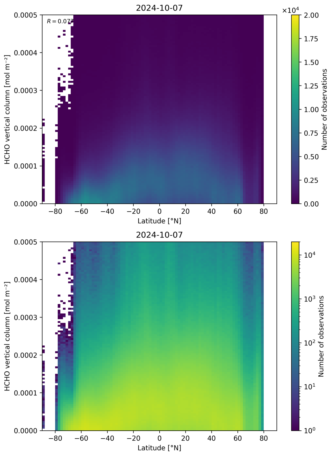
Figure 163: Scatter density plot of “Latitude” against “HCHO vertical column” for 2024-10-06 to 2024-10-08.
