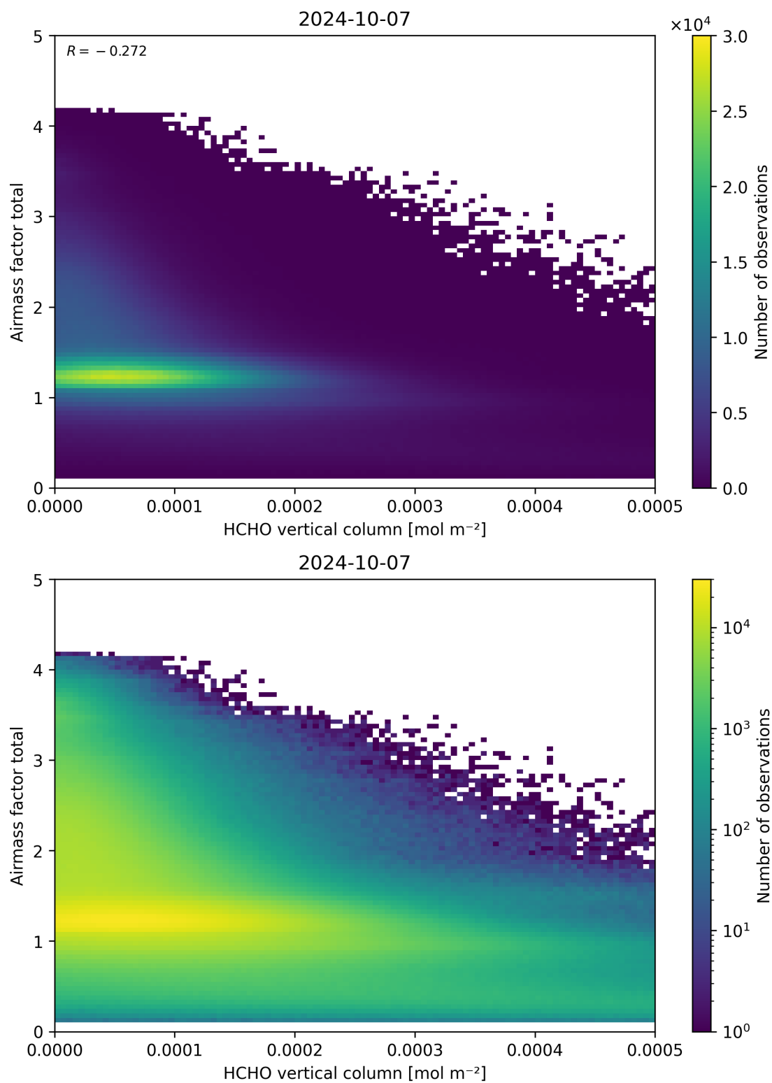
Figure 131: Scatter density plot of “HCHO vertical column” against “Airmass factor total” for 2024-10-06 to 2024-10-08.
