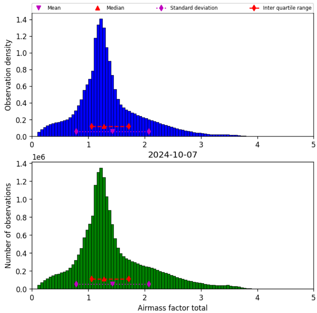
Figure 40: Histogram of “Airmass factor total” for 2024-10-06 to 2024-10-08
