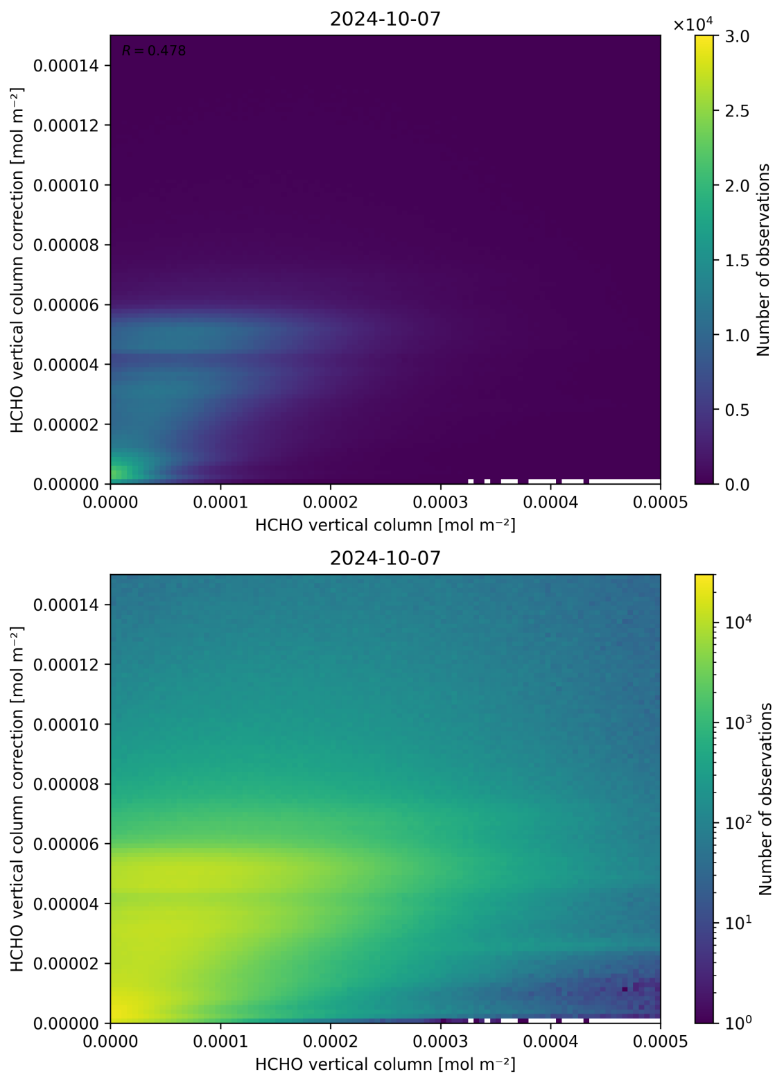
Figure 133: Scatter density plot of “HCHO vertical column” against “HCHO vertical column correction” for 2024-10-06 to 2024-10-08.
