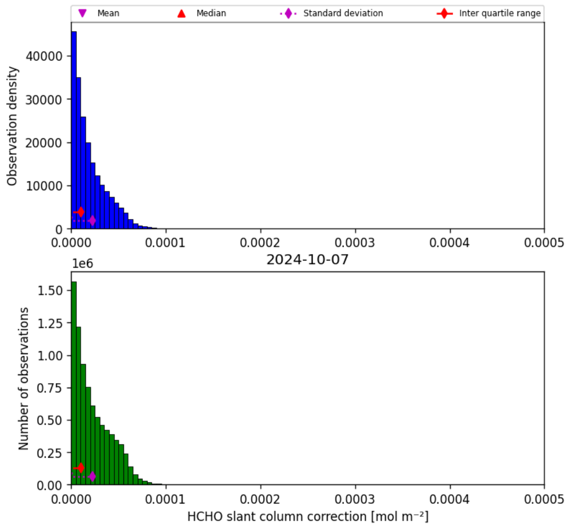
Figure 47: Histogram of “HCHO slant column correction” for 2024-10-06 to 2024-10-08
