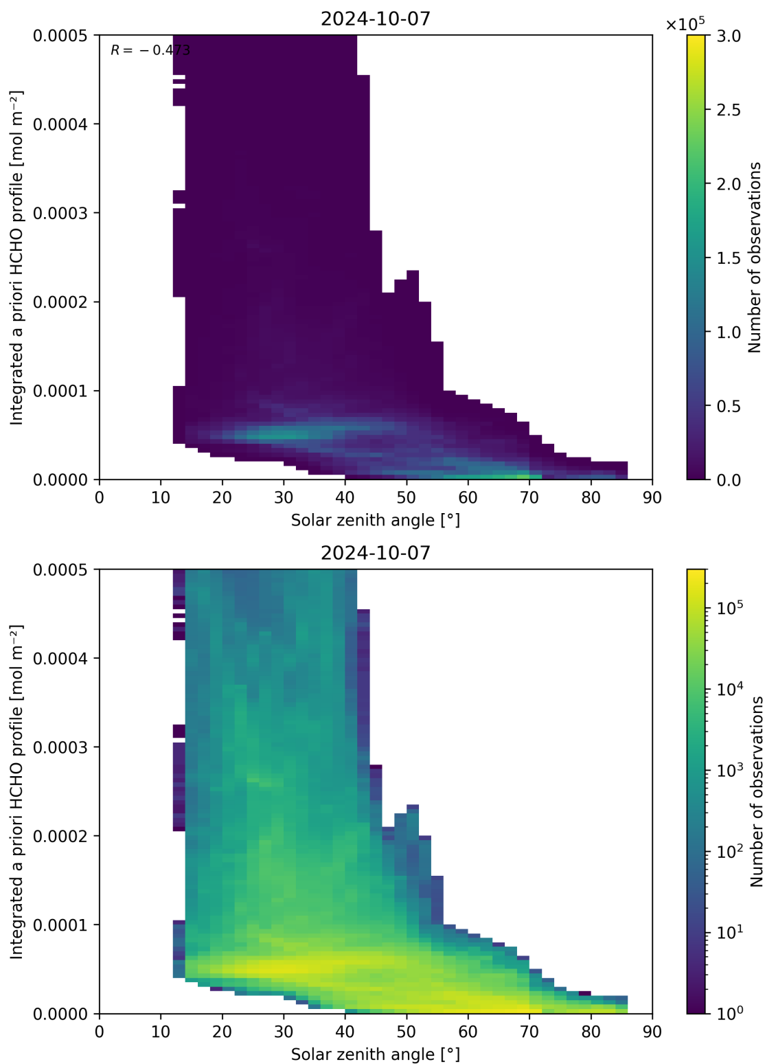
Figure 180: Scatter density plot of “Solar zenith angle” against “Integrated a priori HCHO profile” for 2024-10-06 to 2024-10-08.
