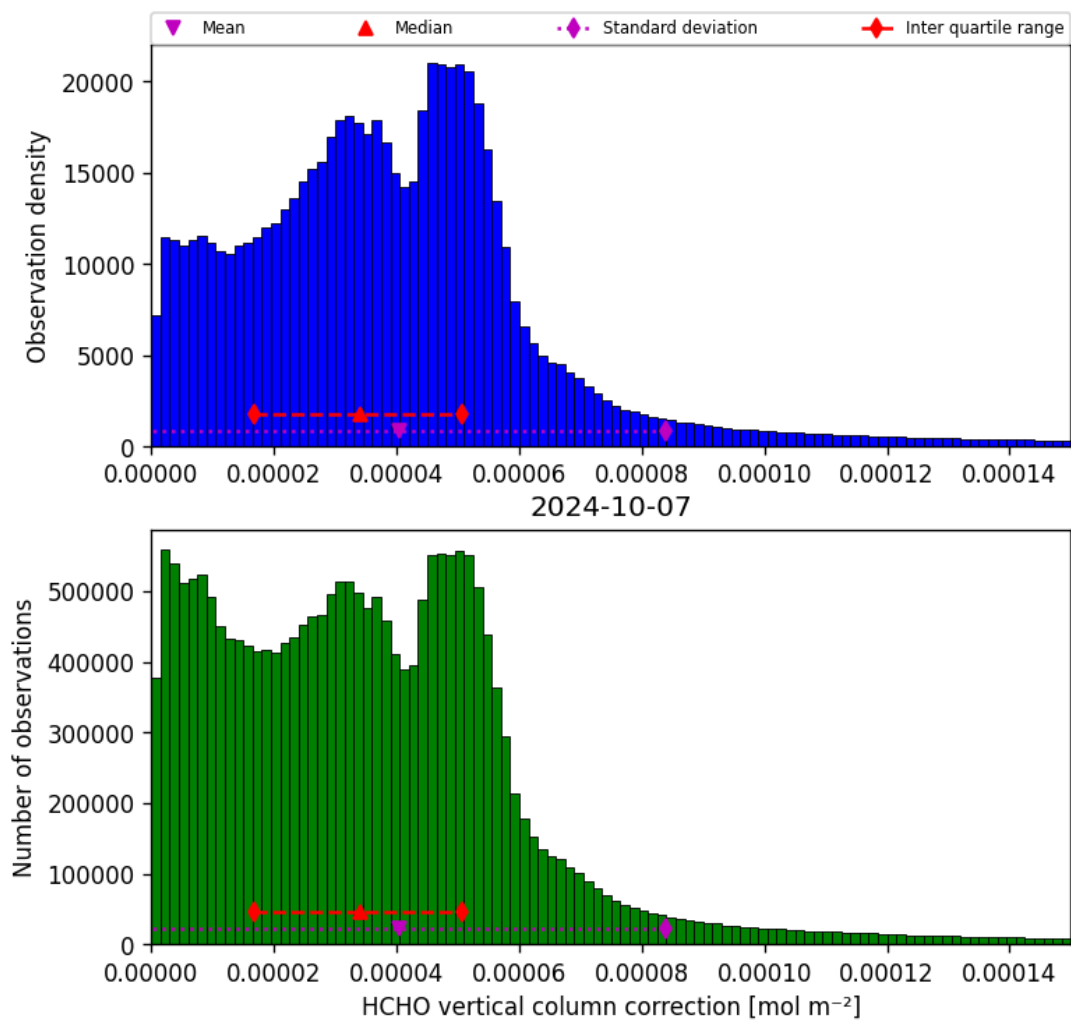
Figure 37: Histogram of “HCHO vertical column correction” for 2024-10-06 to 2024-10-08
