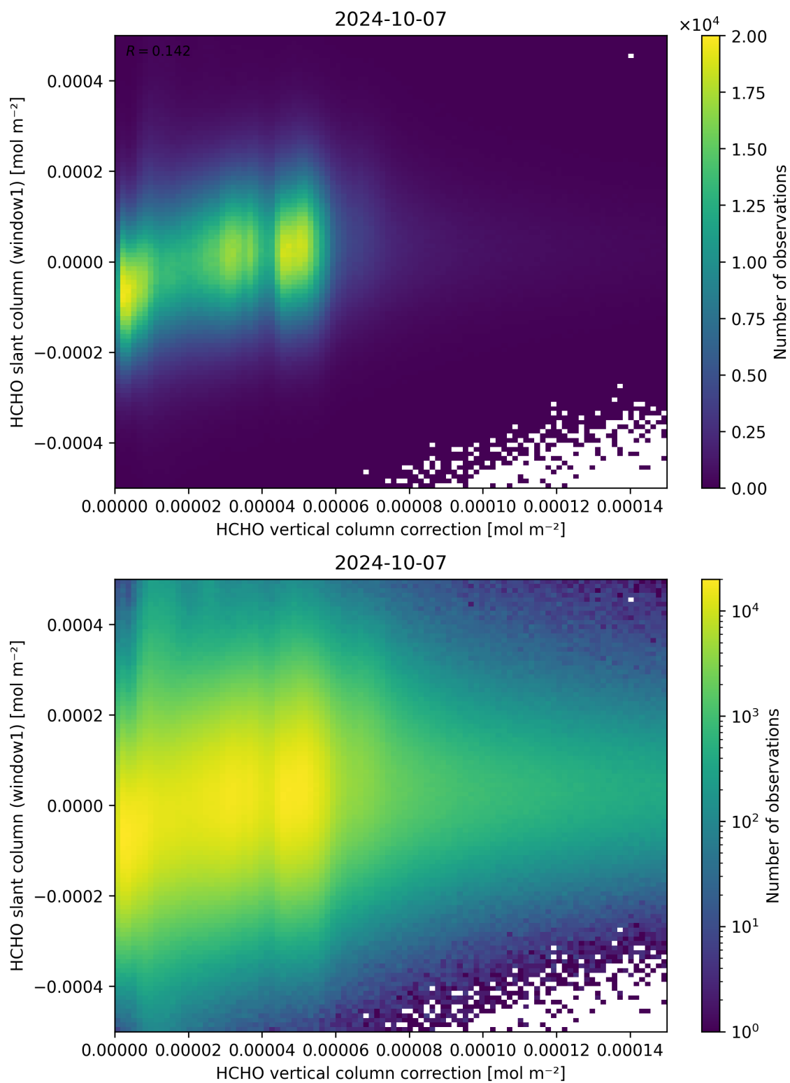
Figure 118: Scatter density plot of “HCHO vertical column correction” against “HCHO slant column (window1)” for 2024-10-06 to 2024-10-08.
