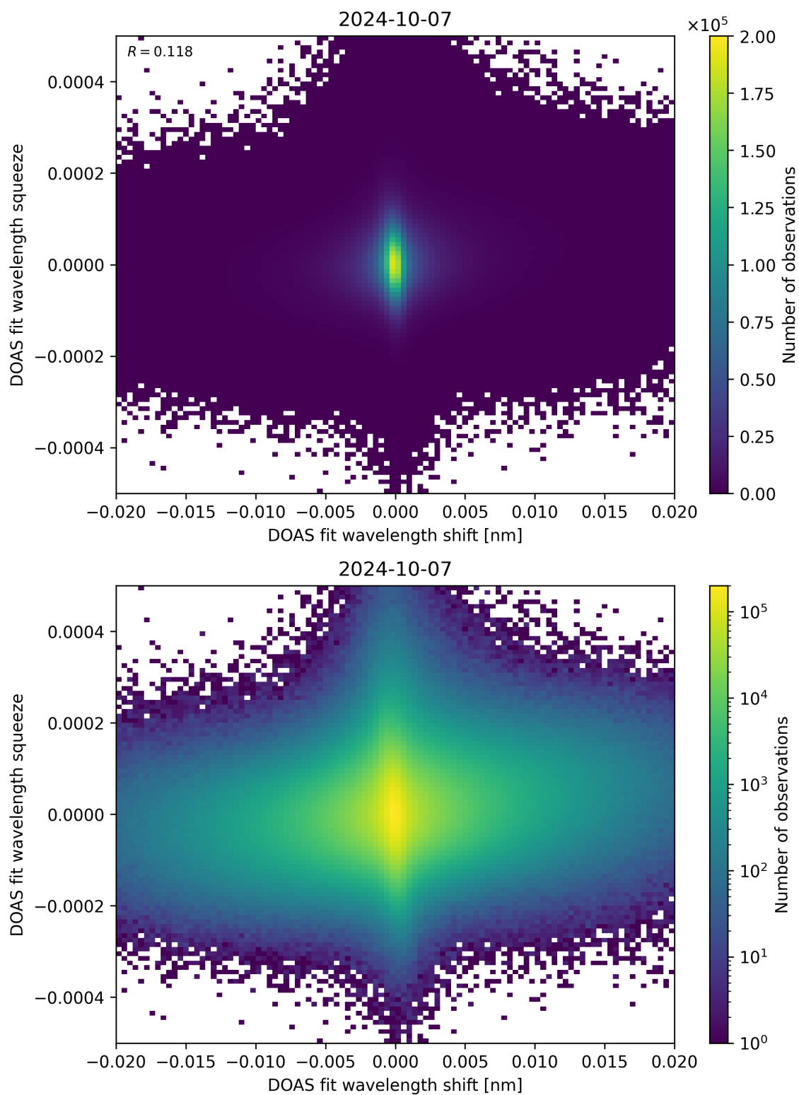
Figure 65: Scatter density plot of “DOAS fit wavelength shift” against “DOAS fit wavelength squeeze” for 2024-10-06 to 2024-10-08.
