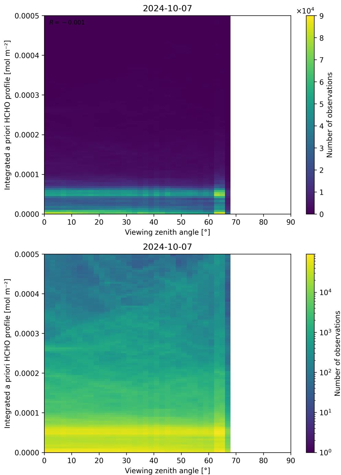
Figure 195: Scatter density plot of “Viewing zenith angle” against “Integrated a priori HCHO profile” for 2024-10-06 to 2024-10-08.
