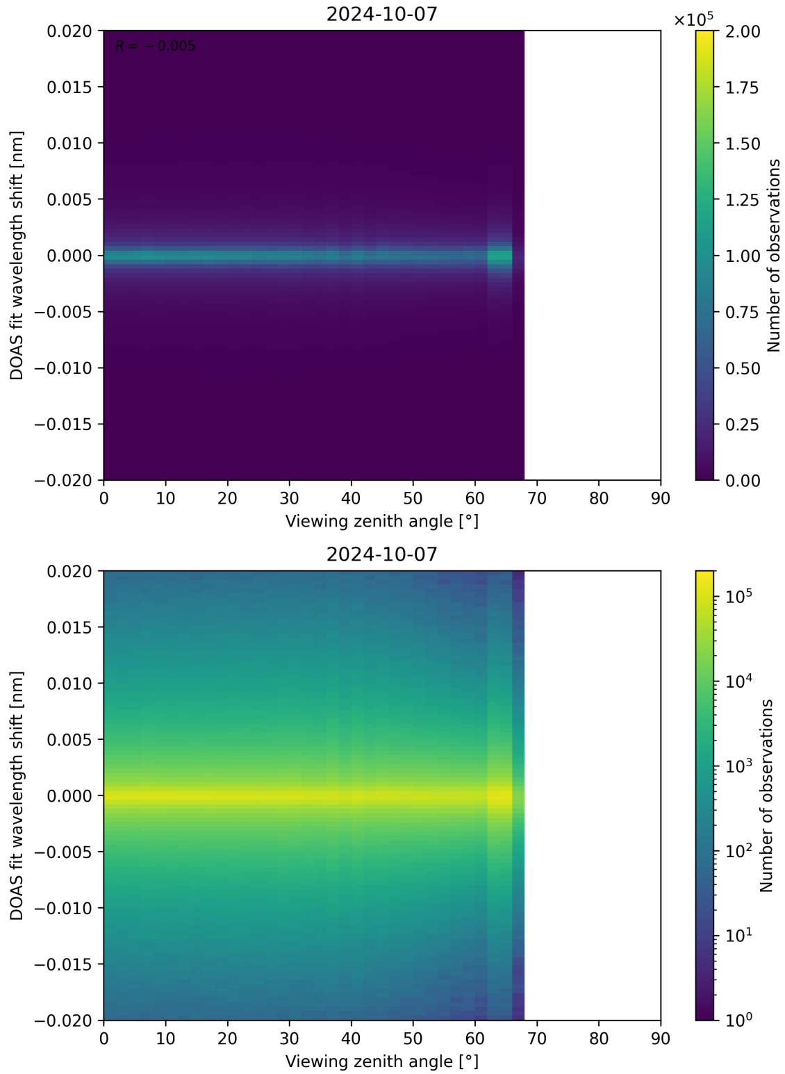
Figure 183: Scatter density plot of “Viewing zenith angle” against “DOAS fit wavelength shift” for 2024-10-06 to 2024-10-08.
