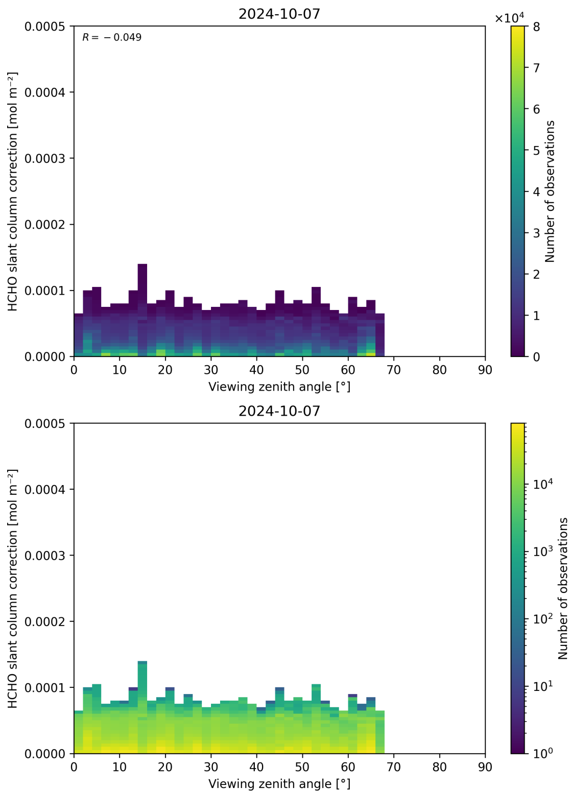
Figure 187: Scatter density plot of “Viewing zenith angle” against “HCHO slant column correction” for 2024-10-06 to 2024-10-08.
