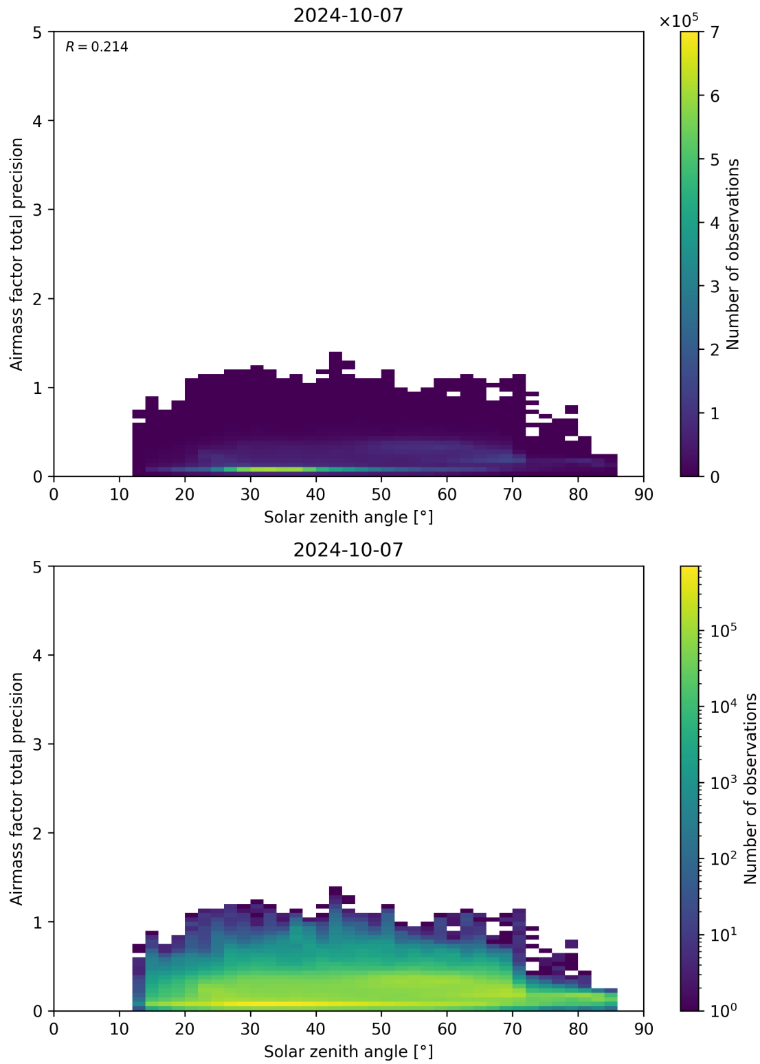
Figure 176: Scatter density plot of “Solar zenith angle” against “Airmass factor total precision” for 2024-10-06 to 2024-10-08.
