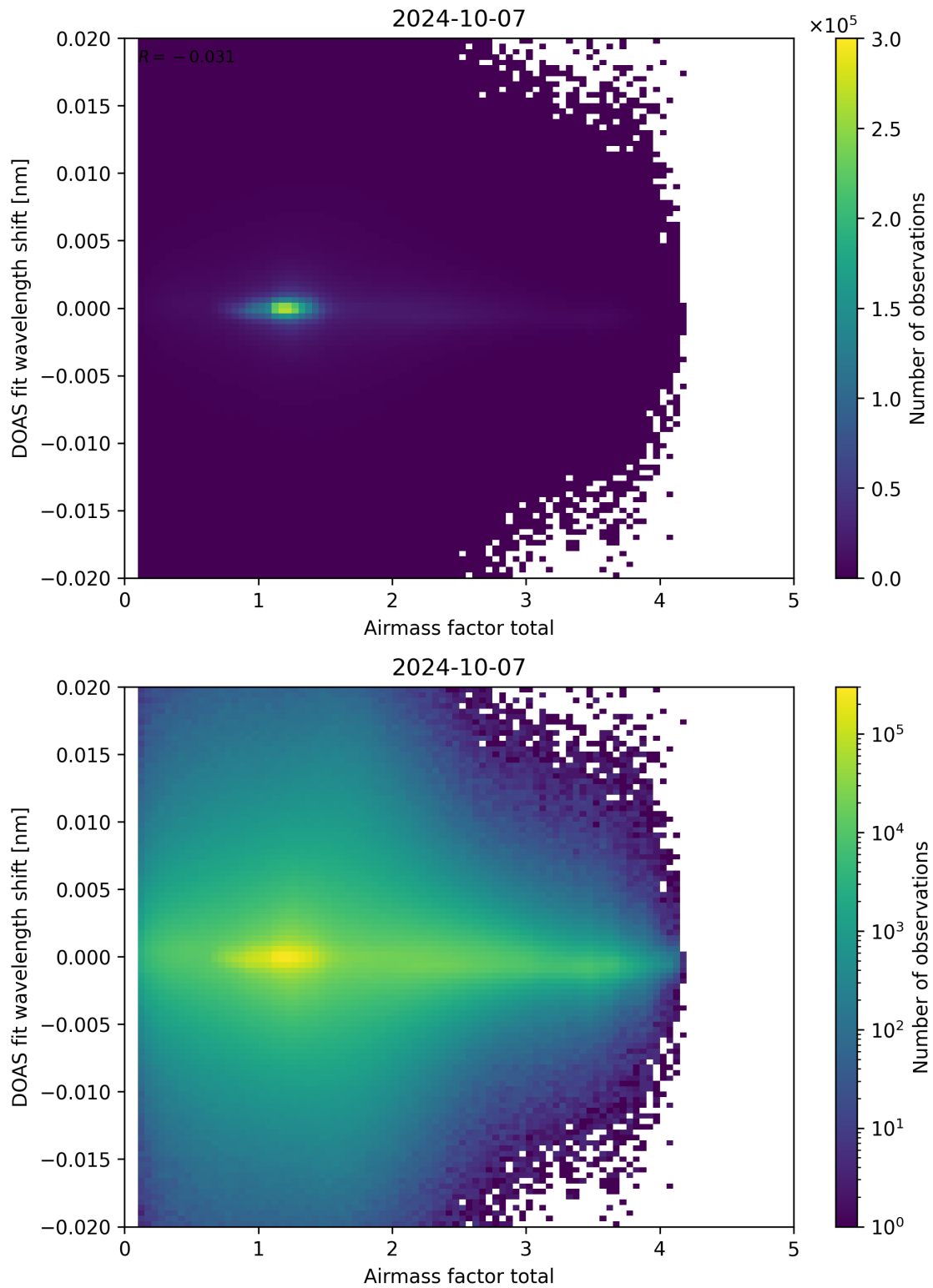
Figure 98: Scatter density plot of “Airmass factor total” against “DOAS fit wavelength shift” for 2024-10-06 to 2024-10-08.
