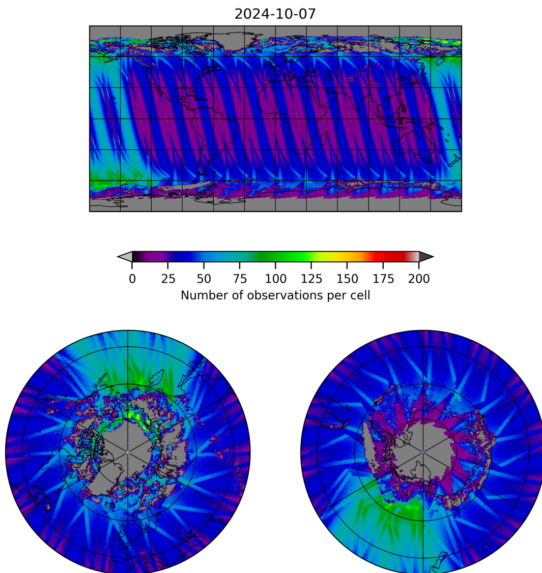
Figure 19: Map of the number of observations for 2024-10-06 to 2024-10-08
