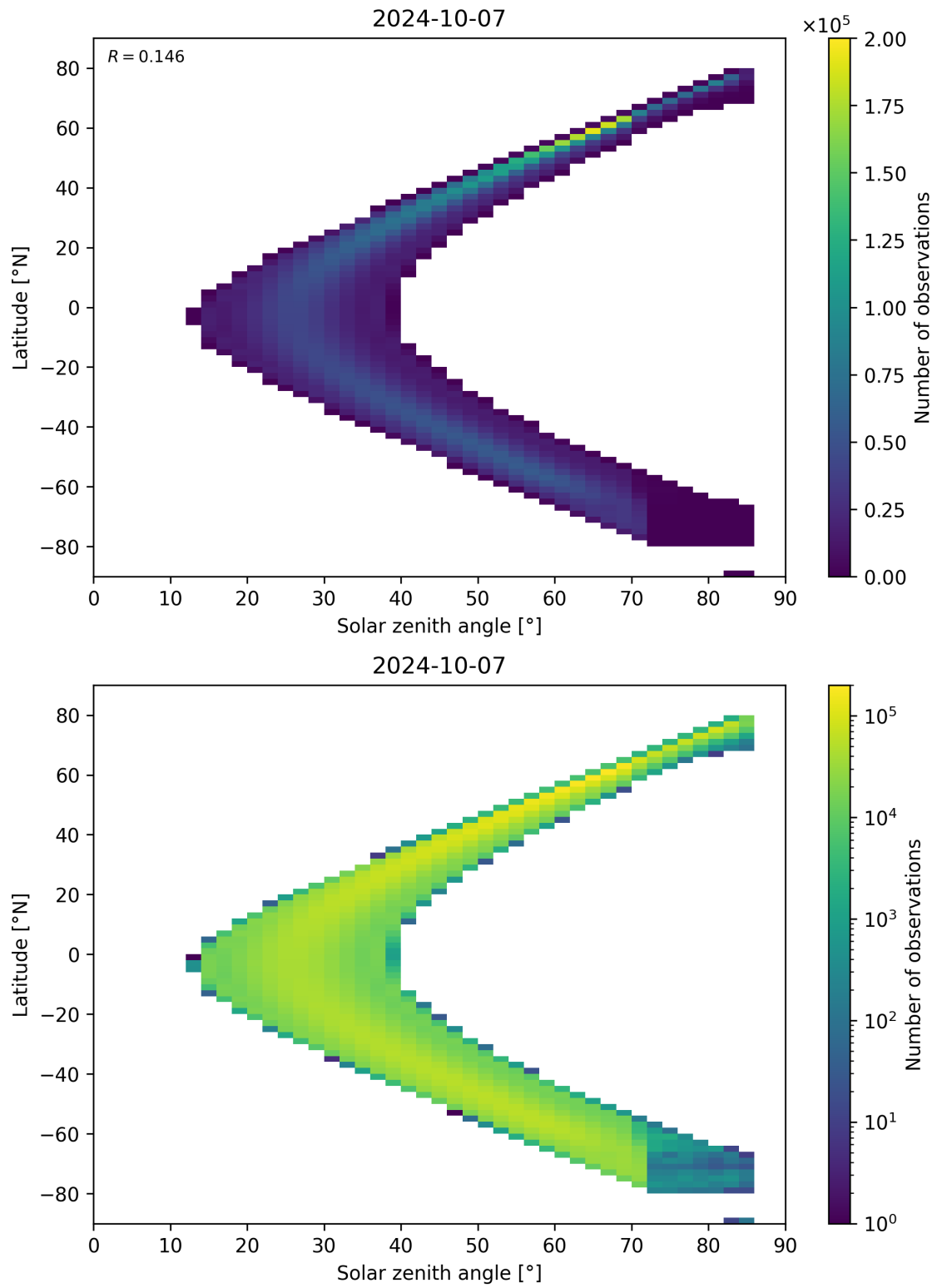
Figure 181: Scatter density plot of “Solar zenith angle” against “Latitude” for 2024-10-06 to 2024-10-08.
