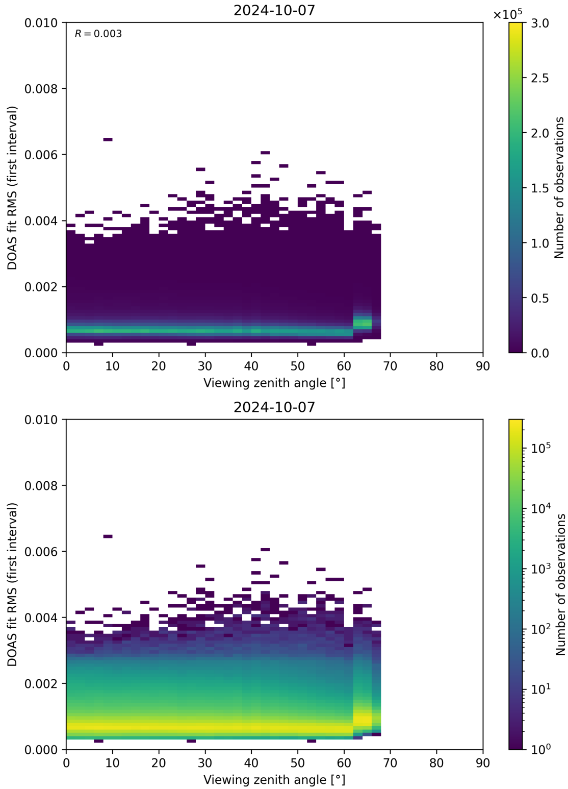
Figure 182: Scatter density plot of “Viewing zenith angle” against “DOAS fit RMS (first interval)” for 2024-10-06 to 2024-10-08.
