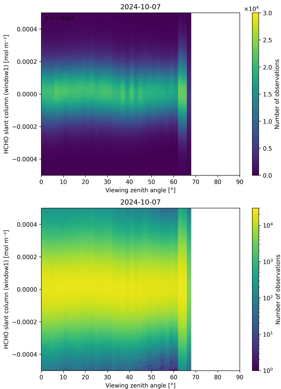
Figure 188: Scatter density plot of “Viewing zenith angle” against “HCHO slant column (window1)” for 2024-10-06 to 2024-10-08.
