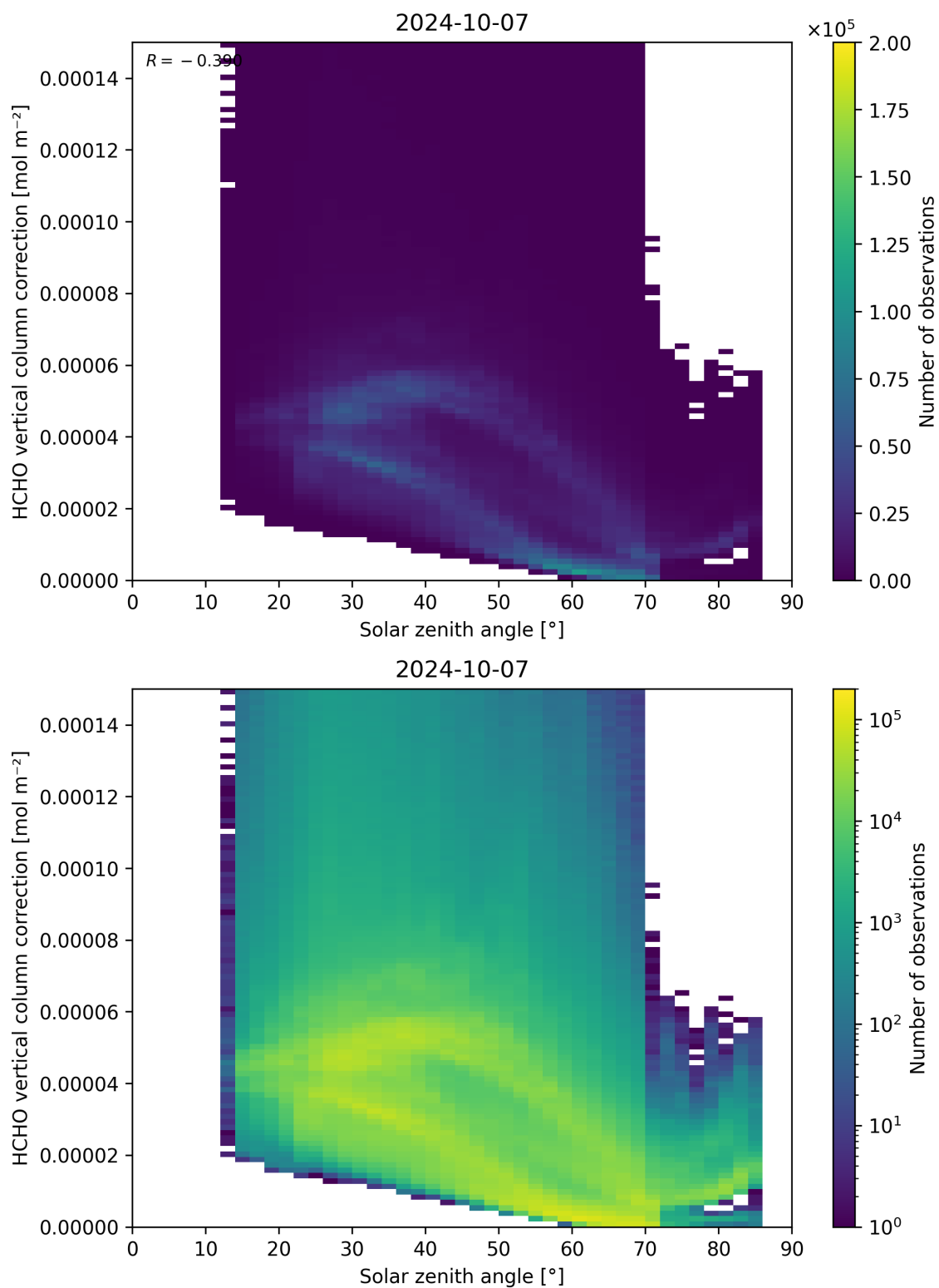
Figure 178: Scatter density plot of “Solar zenith angle” against “HCHO vertical column correction” for 2024-10-06 to 2024-10-08.
