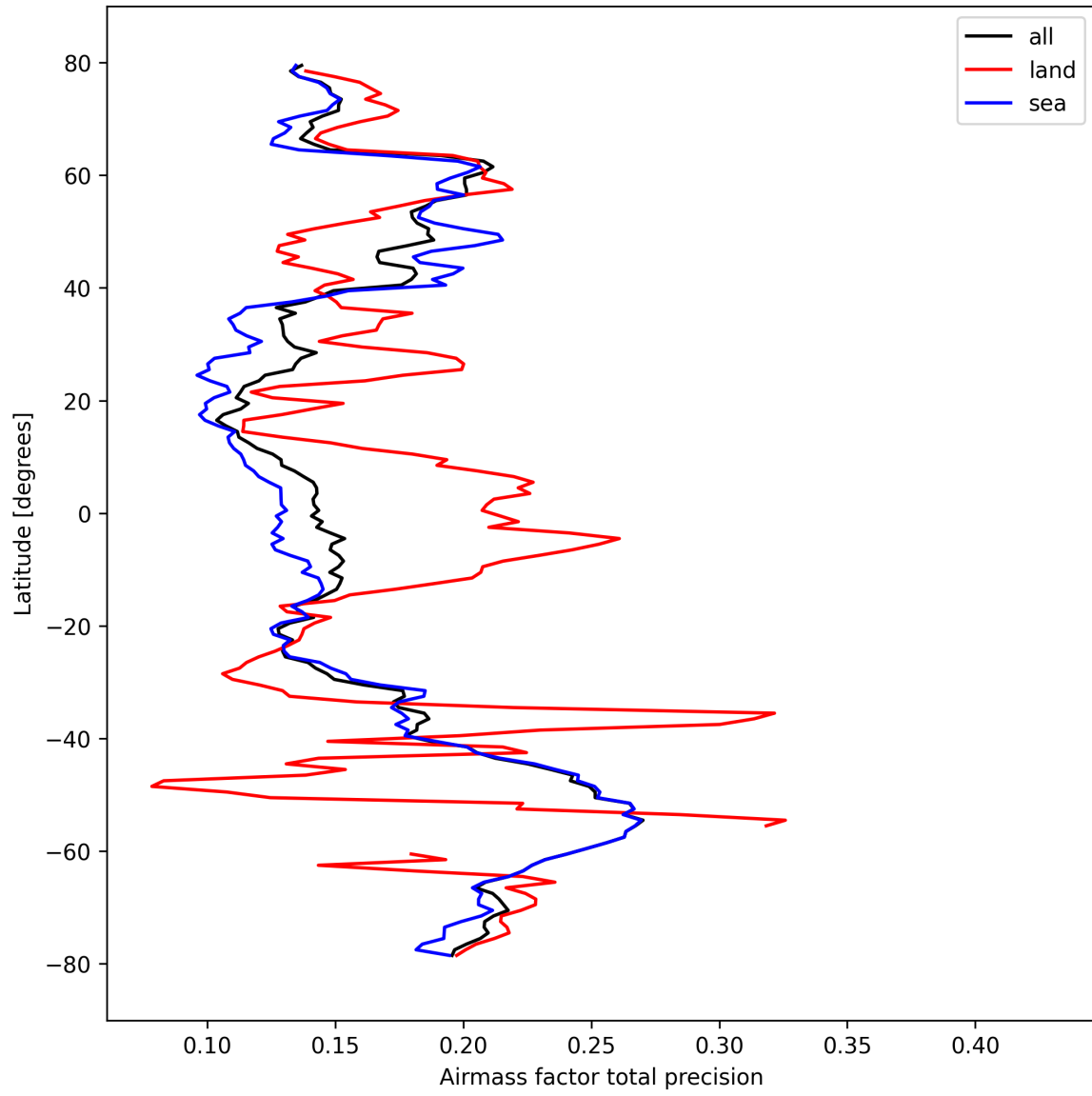
Figure 27: Zonal average of “Airmass factor total precision” for 2024-10-06 to 2024-10-08.
