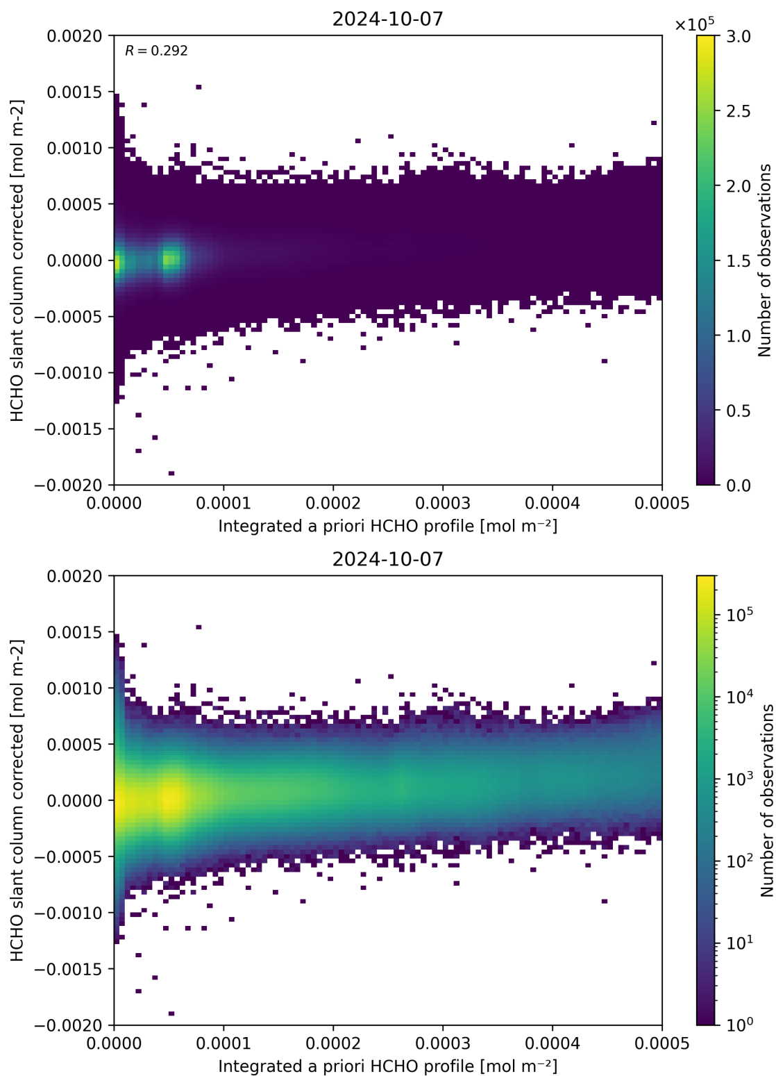
Figure 151: Scatter density plot of “Integrated a priori HCHO profile” against “HCHO slant column corrected” for 2024-10-06 to 2024-10-08.
