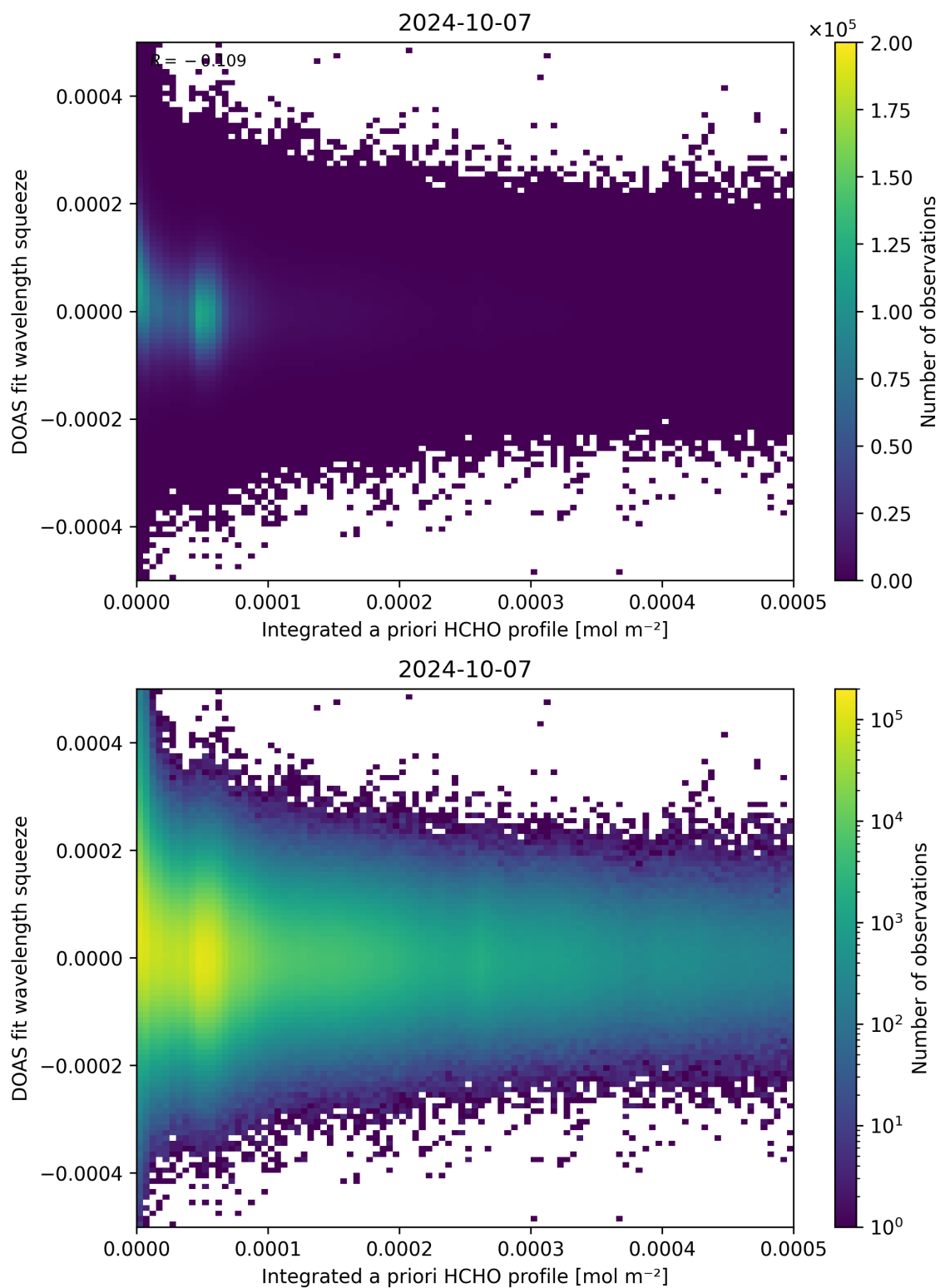
Figure 150: Scatter density plot of “Integrated a priori HCHO profile” against “DOAS fit wavelength squeeze” for 2024-10-06 to 2024-10-08.
