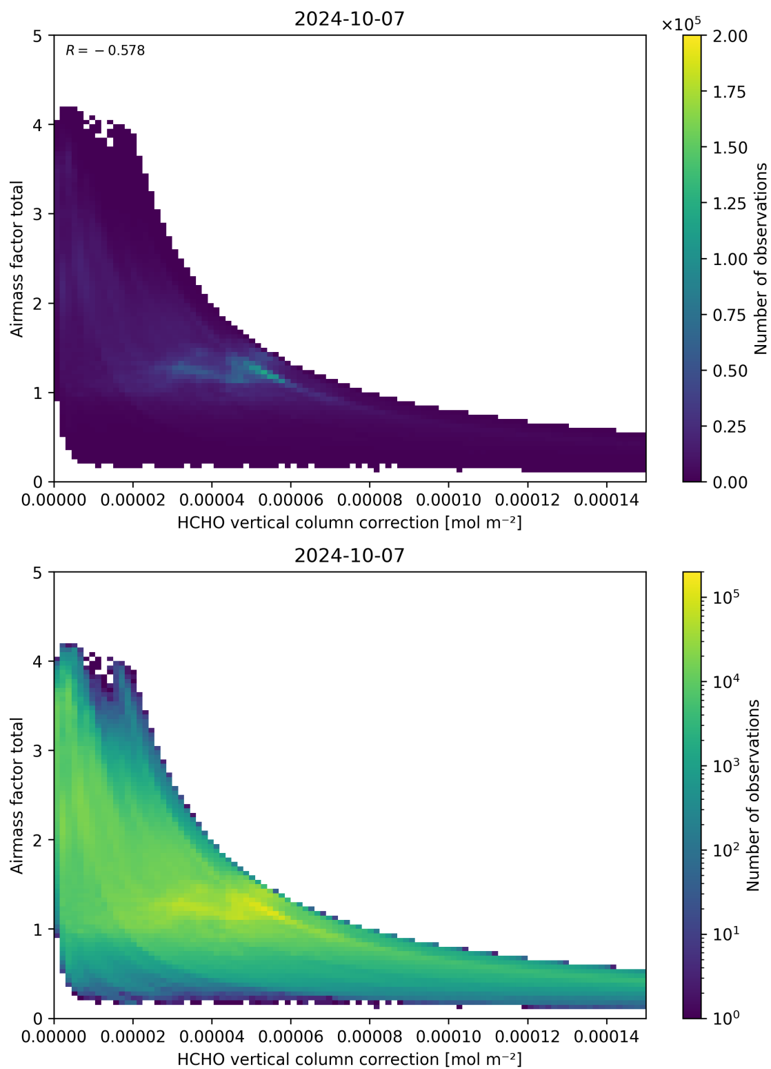
Figure 120: Scatter density plot of “HCHO vertical column correction” against “Airmass factor total” for 2024-10-06 to 2024-10-08.
