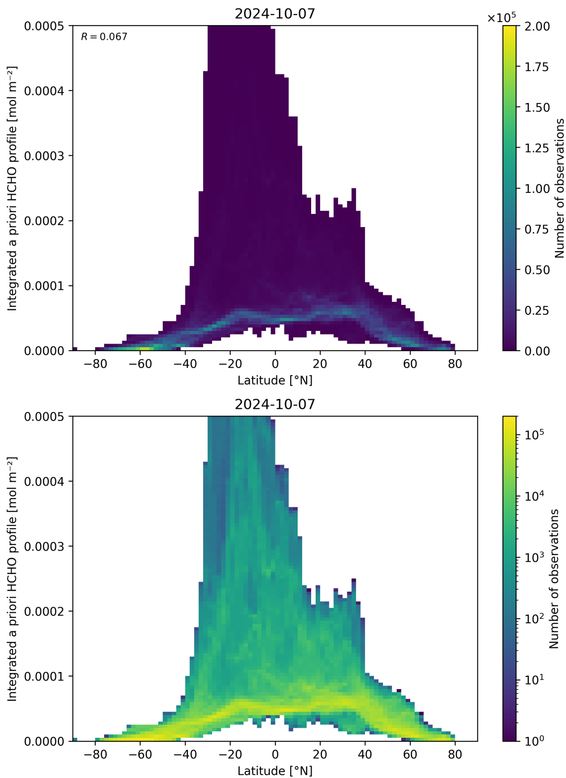
Figure 166: Scatter density plot of “Latitude” against “Integrated a priori HCHO profile” for 2024-10-06 to 2024-10-08.
