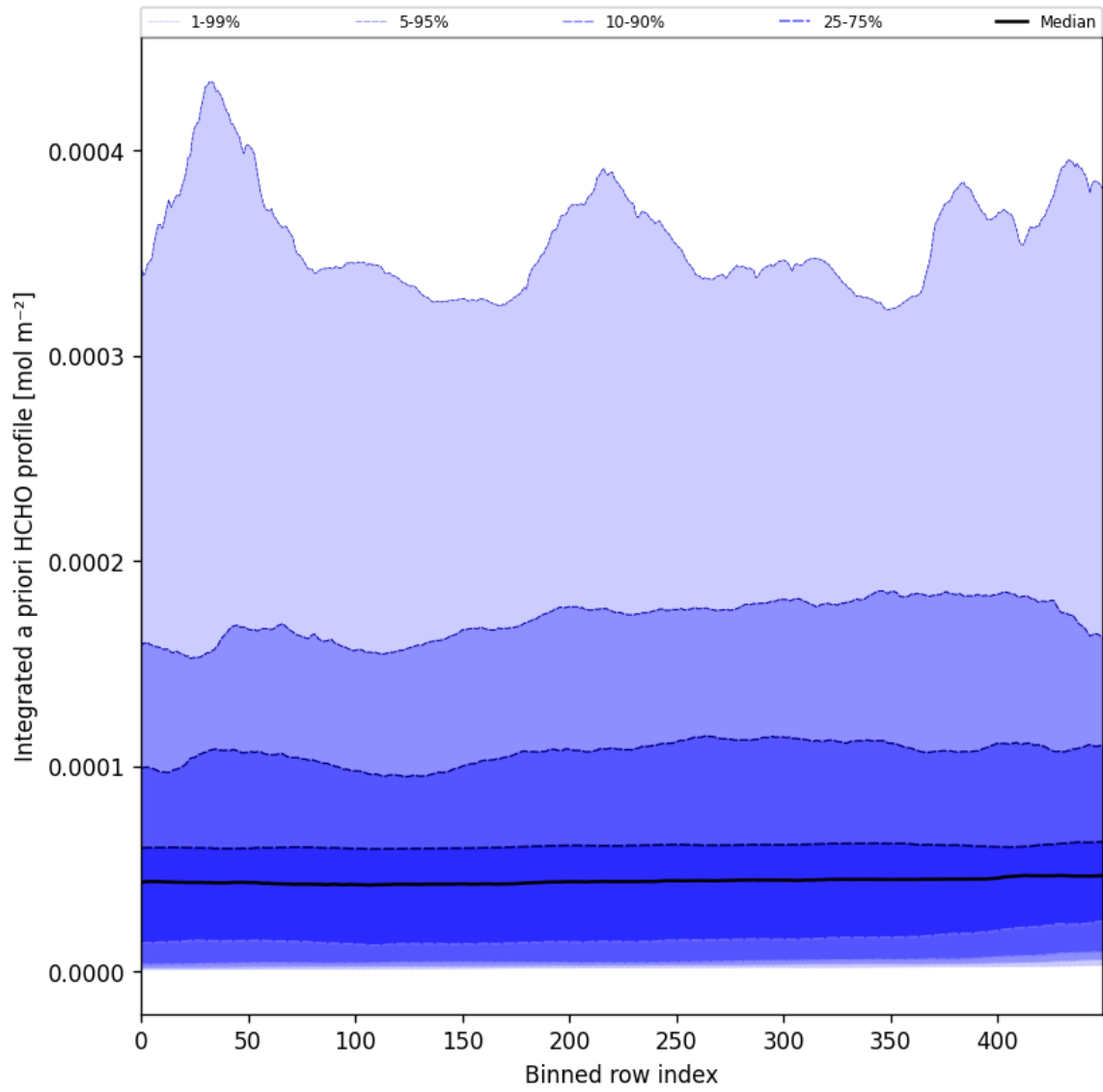
Figure 57: Along track statistics of “Integrated a priori HCHO profile” for 2024-10-06 to 2024-10-08
