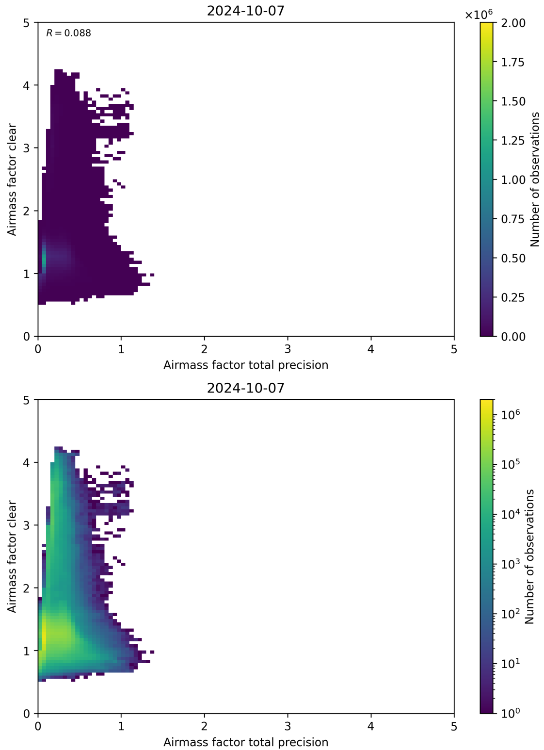
Figure 108: Scatter density plot of “Airmass factor total precision” against “Airmass factor clear” for 2024-10-06 to 2024-10-08.
