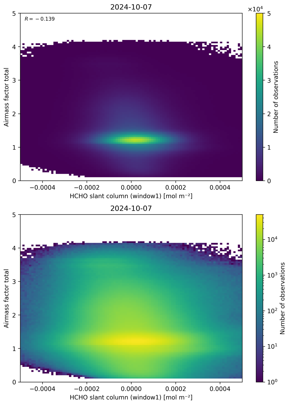
Figure 85: Scatter density plot of “HCHO slant column (window1)” against “Airmass factor total” for 2024-10-06 to 2024-10-08.
