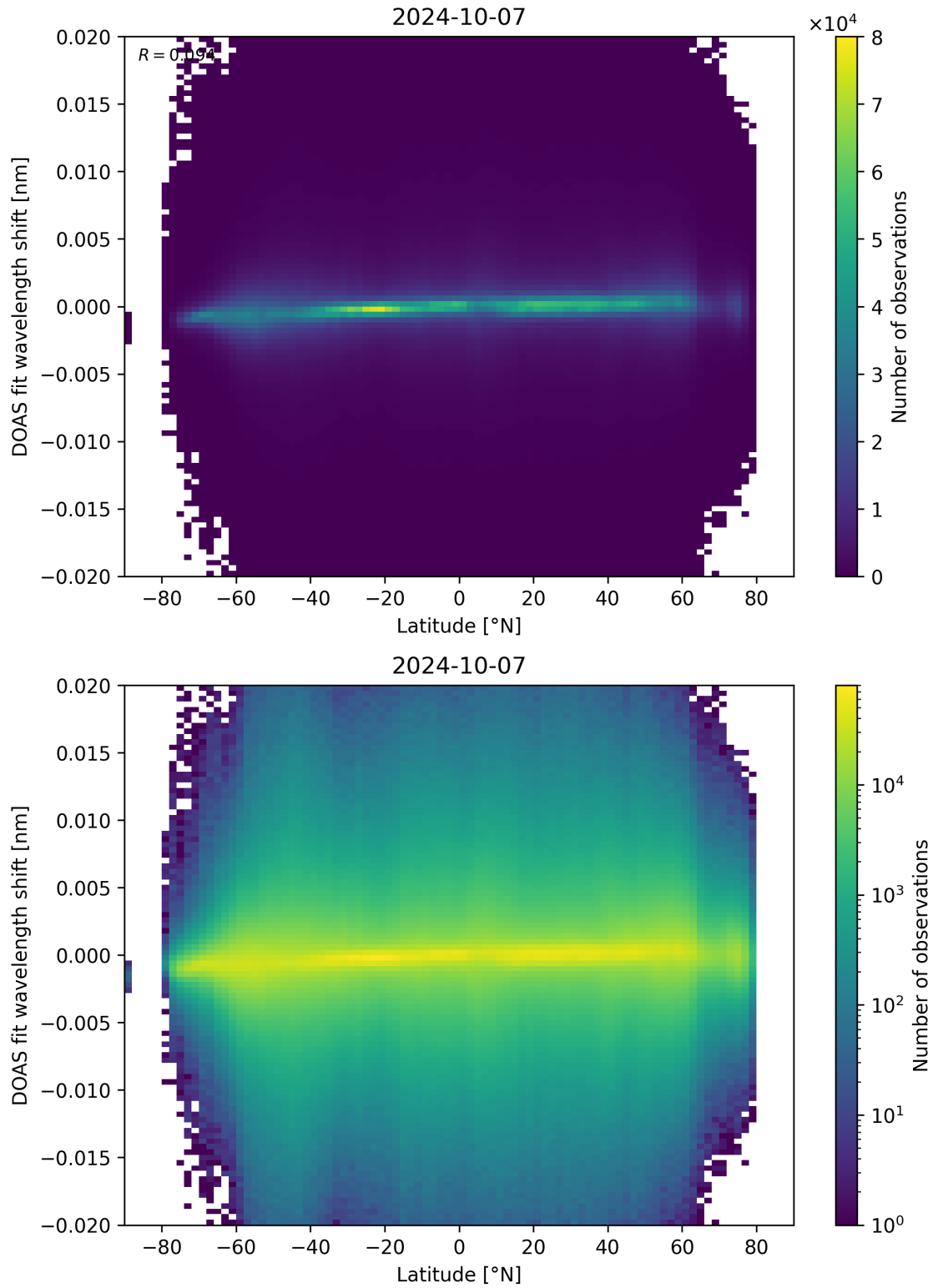
Figure 154: Scatter density plot of “Latitude” against “DOAS fit wavelength shift” for 2024-10-06 to 2024-10-08.
