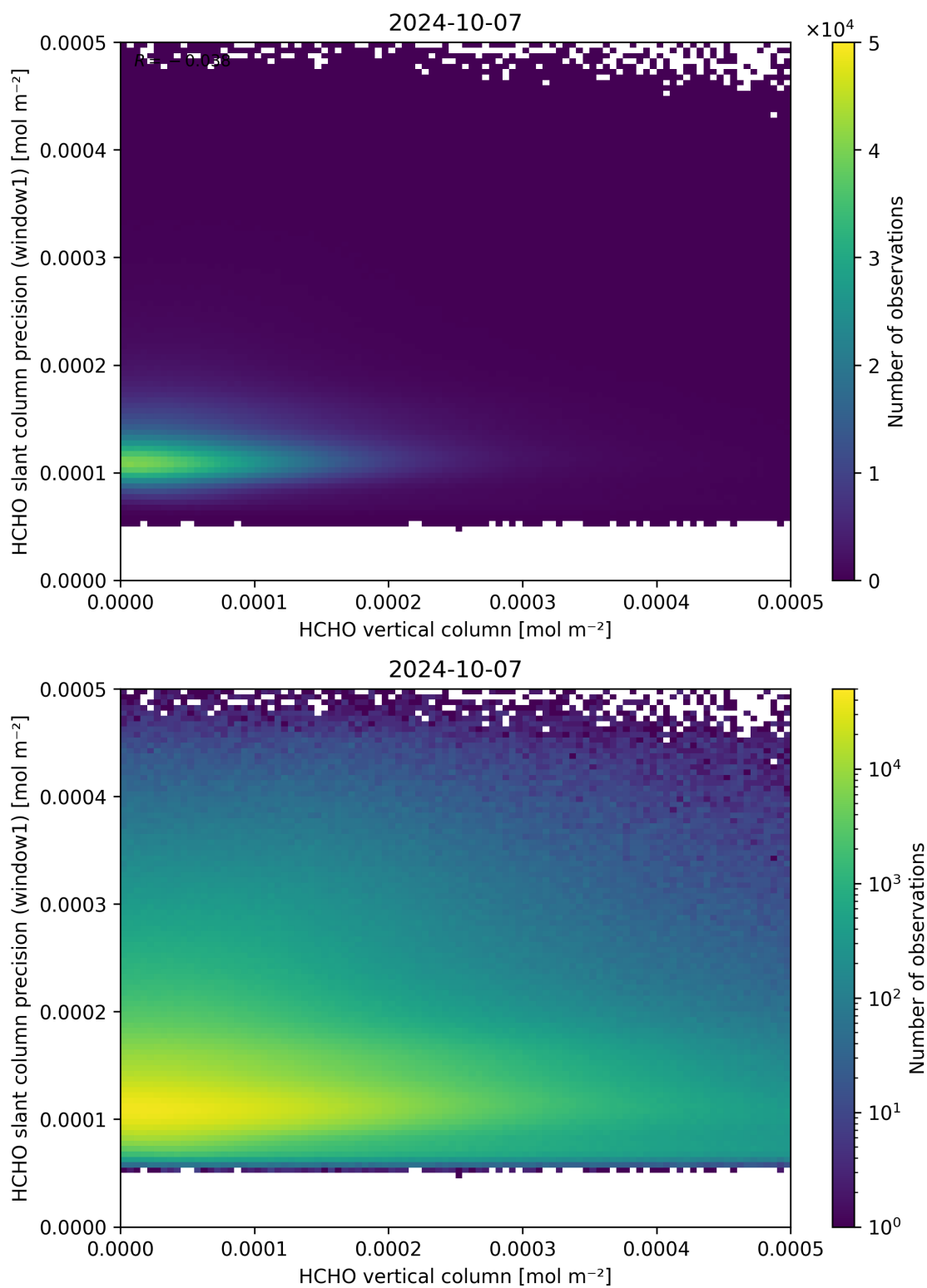
Figure 130: Scatter density plot of “HCHO vertical column” against “HCHO slant column precision (window1)” for 2024-10-06 to 2024-10-08.
