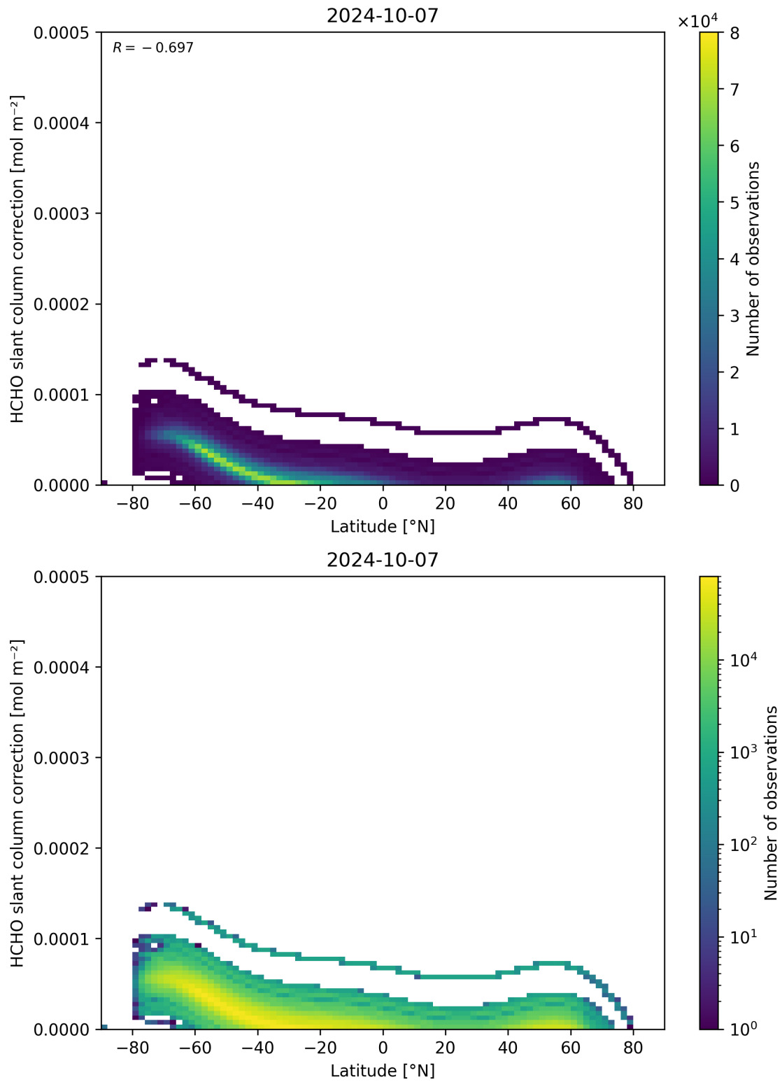
Figure 158: Scatter density plot of “Latitude” against “HCHO slant column correction” for 2024-10-06 to 2024-10-08.
