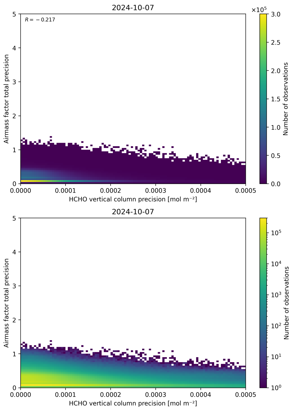
Figure 145: Scatter density plot of “HCHO vertical column precision” against “Airmass factor total precision” for 2024-10-06 to 2024-10-08.
