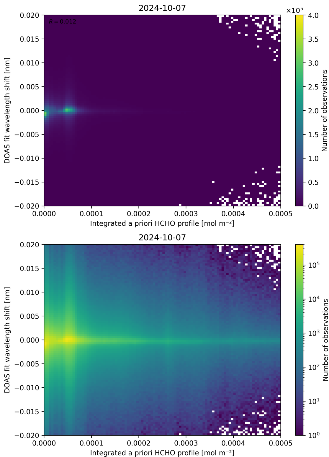
Figure 149: Scatter density plot of “Integrated a priori HCHO profile” against “DOAS fit wavelength shift” for 2024-10-06 to 2024-10-08.
