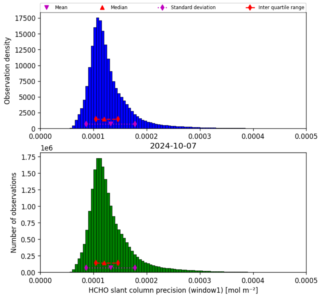
Figure 39: Histogram of “HCHO slant column precision (window1)” for 2024-10-06 to 2024-10-08
