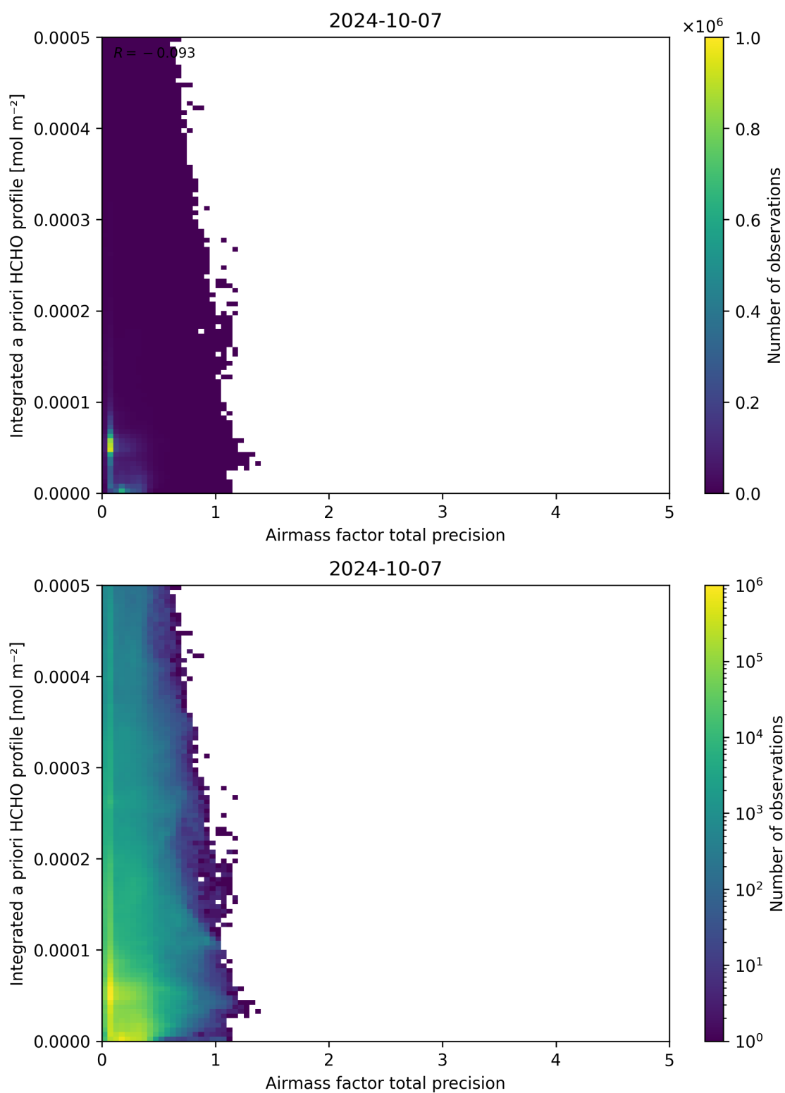
Figure 111: Scatter density plot of “Airmass factor total precision” against “Integrated a priori HCHO profile” for 2024-10-06 to 2024-10-08.
