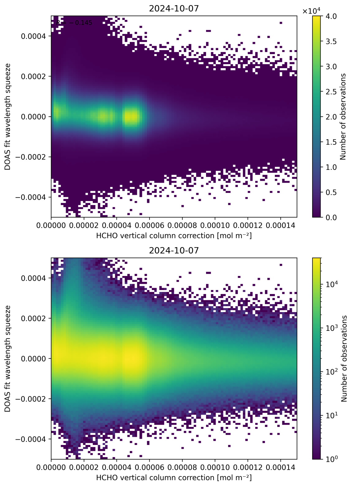
Figure 114: Scatter density plot of “HCHO vertical column correction” against “DOAS fit wavelength squeeze” for 2024-10-06 to 2024-10-08.
