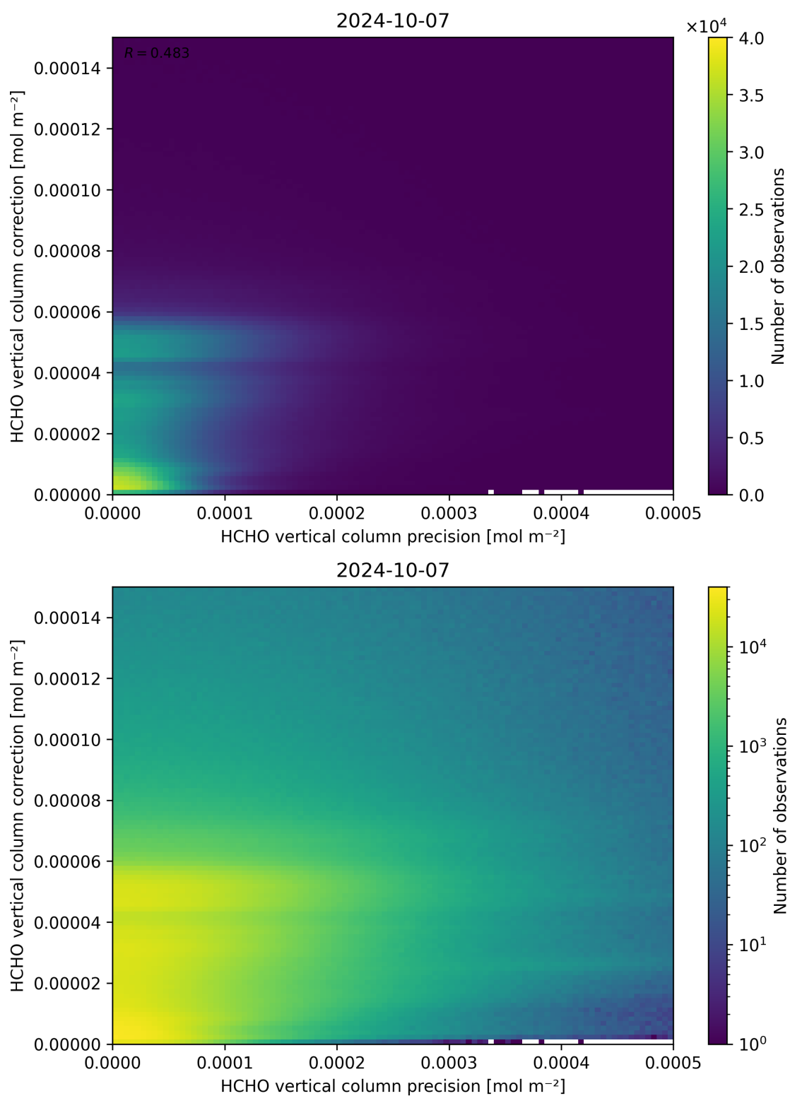
Figure 146: Scatter density plot of “HCHO vertical column precision” against “HCHO vertical column correction” for 2024-10-06 to 2024-10-08.
