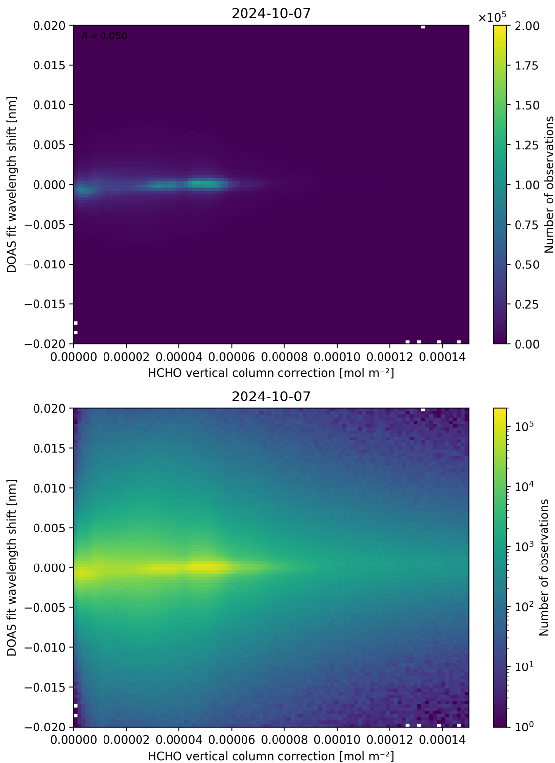
Figure 113: Scatter density plot of “HCHO vertical column correction” against “DOAS fit wavelength shift” for 2024-10-06 to 2024-10-08.
