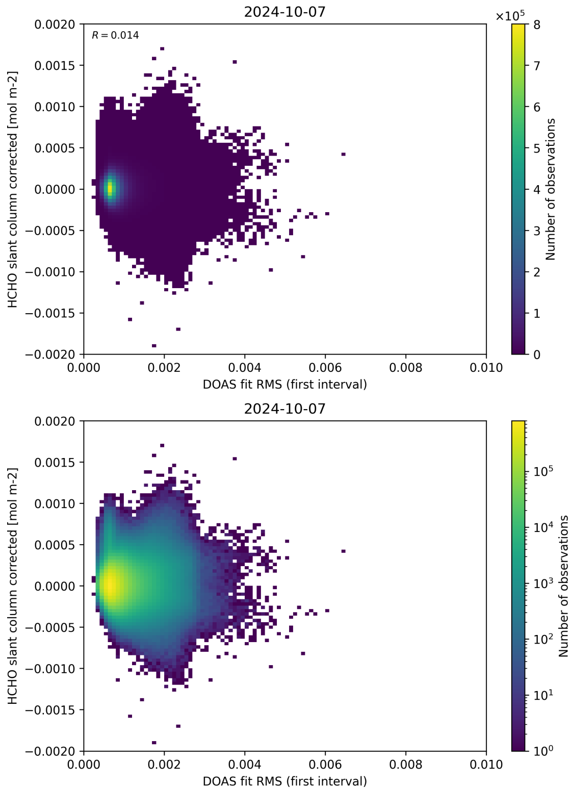
Figure 62: Scatter density plot of “DOAS fit RMS (first interval)” against “HCHO slant column corrected” for 2024-10-06 to 2024-10-08.
