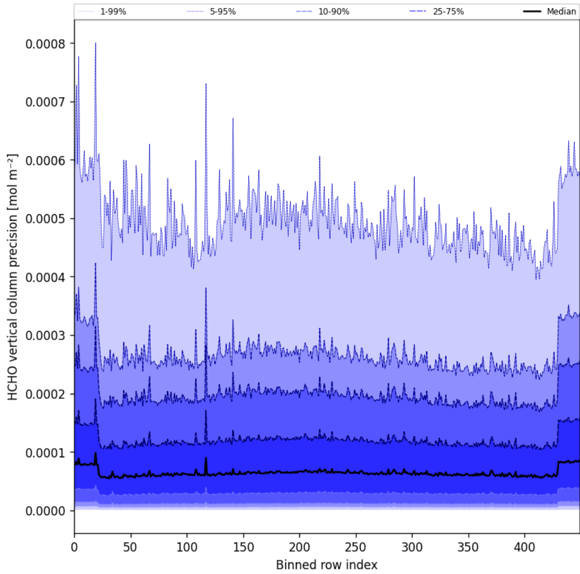
Figure 50: Along track statistics of “HCHO vertical column precision” for 2024-10-06 to 2024-10-08
