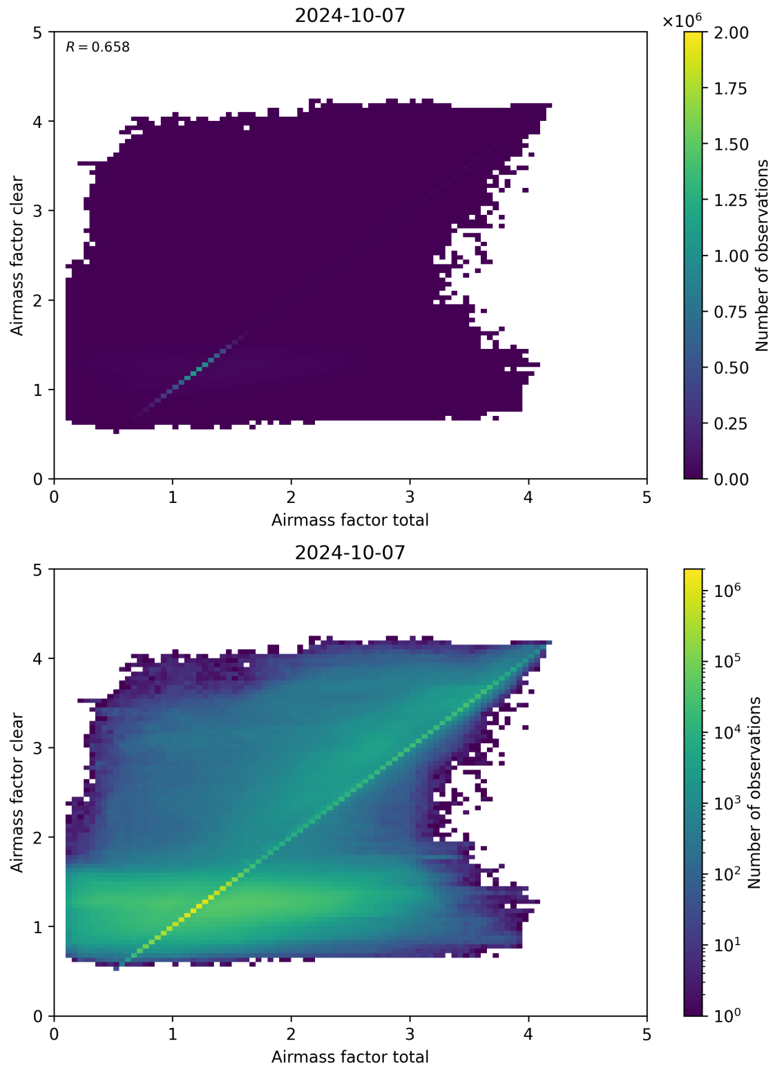
Figure 100: Scatter density plot of “Airmass factor total” against “Airmass factor clear” for 2024-10-06 to 2024-10-08.
