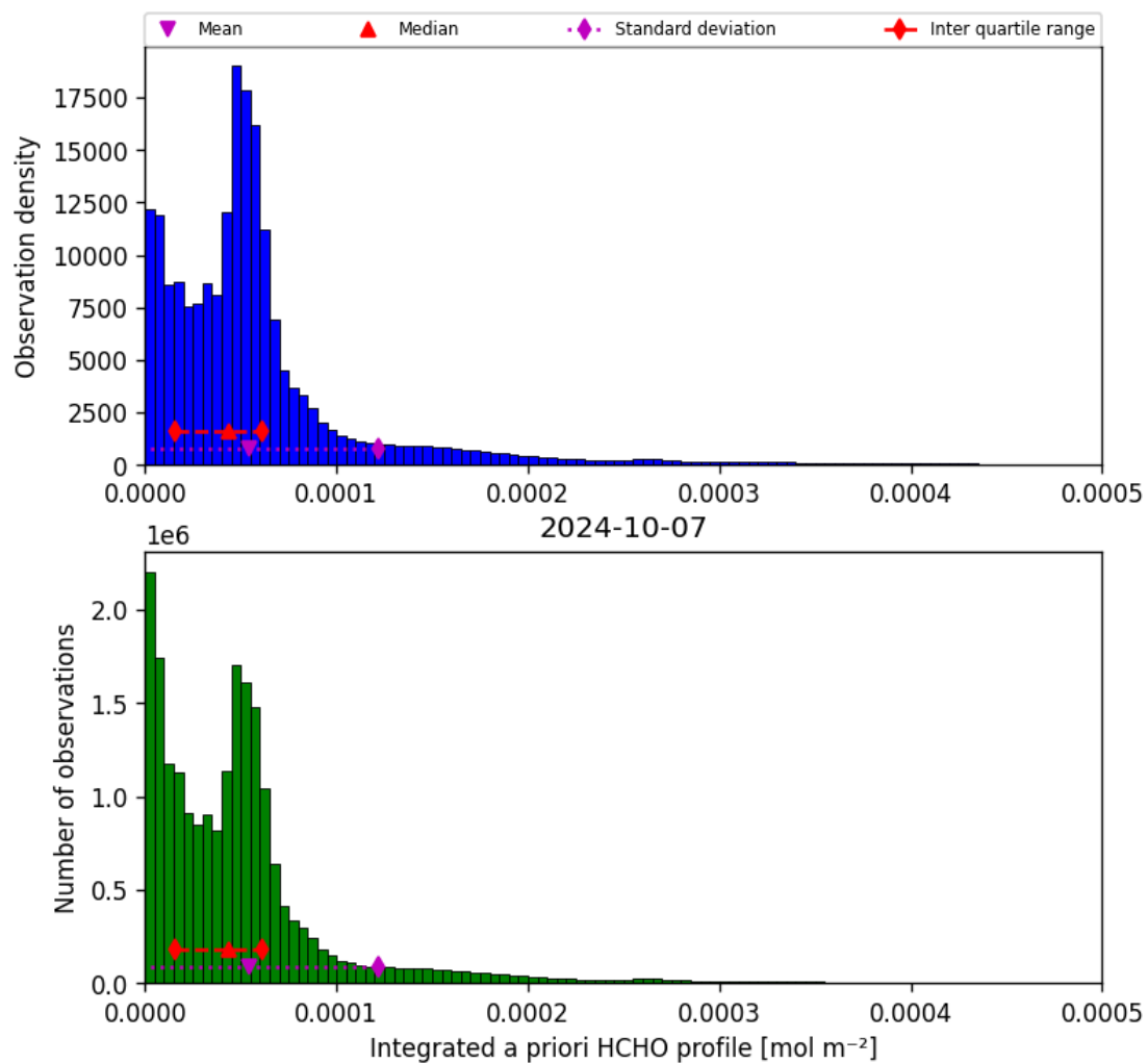
Figure 43: Histogram of “Integrated a priori HCHO profile” for 2024-10-06 to 2024-10-08
