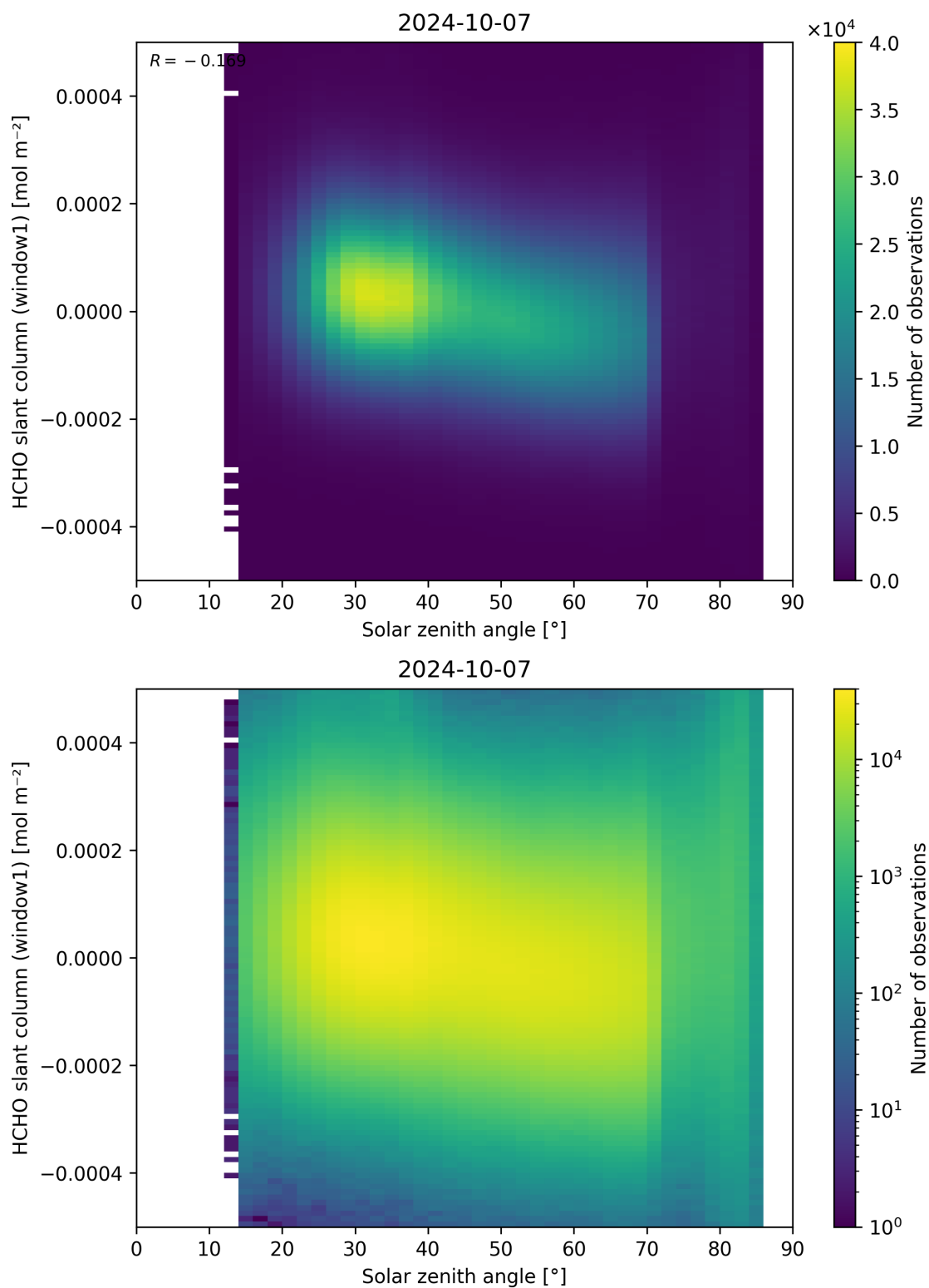
Figure 173: Scatter density plot of “Solar zenith angle” against “HCHO slant column (window1)” for 2024-10-06 to 2024-10-08.
