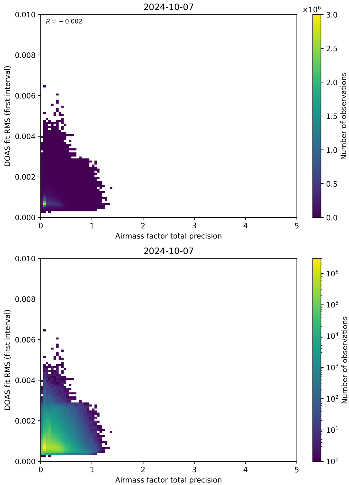
Figure 105: Scatter density plot of “Airmass factor total precision” against “DOAS fit RMS (first interval)” for 2024-10-06 to 2024-10-08.
