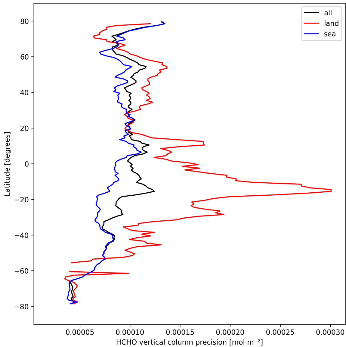
Figure 22: Zonal average of “HCHO vertical column precision” for 2024-10-06 to 2024-10-08.
