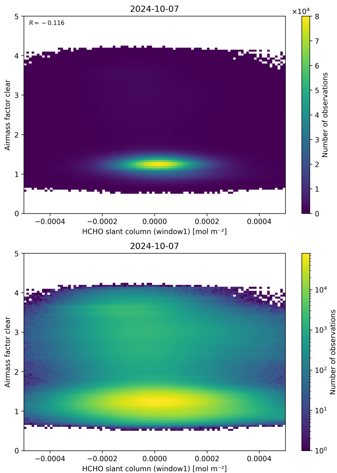
Figure 81: Scatter density plot of “HCHO slant column (window1)” against “Airmass factor clear” for 2024-10-06 to 2024-10-08.
