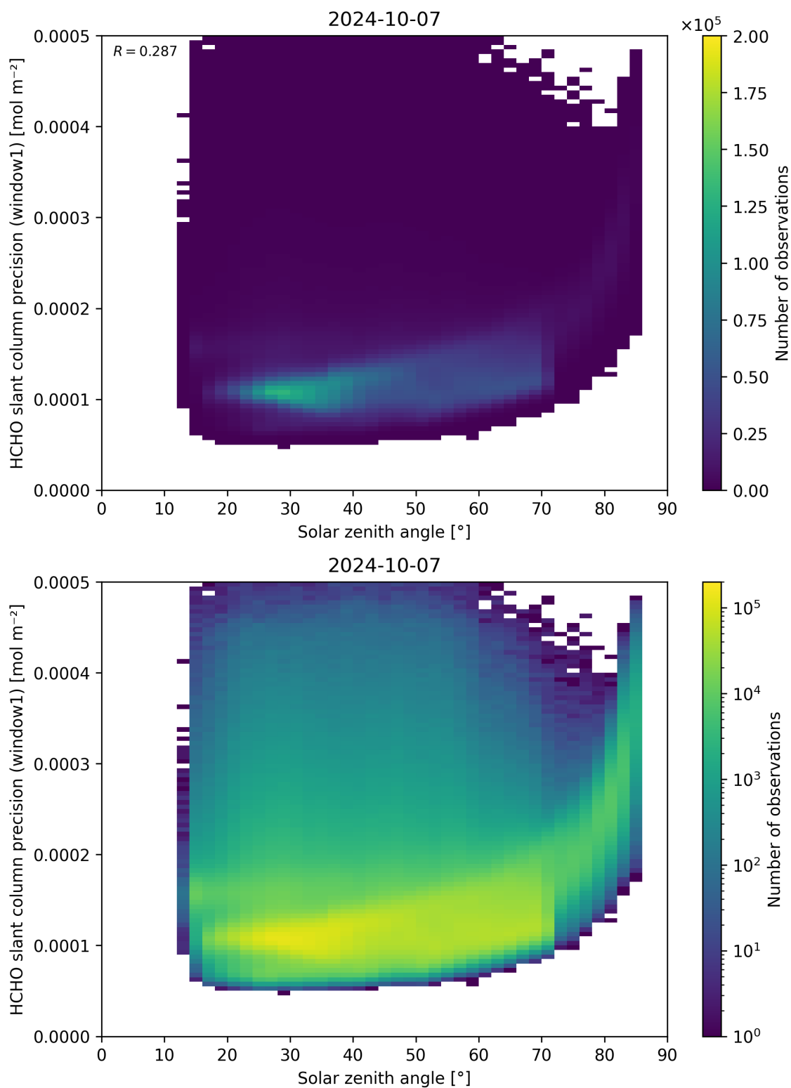
Figure 174: Scatter density plot of “Solar zenith angle” against “HCHO slant column precision (window1)” for 2024-10-06 to 2024-10-08.
