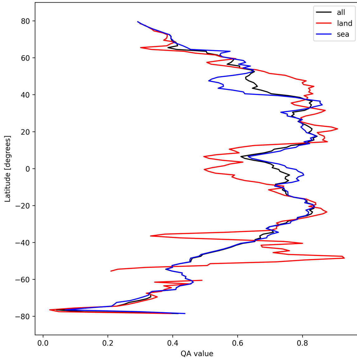
Figure 20: Zonal average of “QA value” for 2024-10-06 to 2024-10-08.
