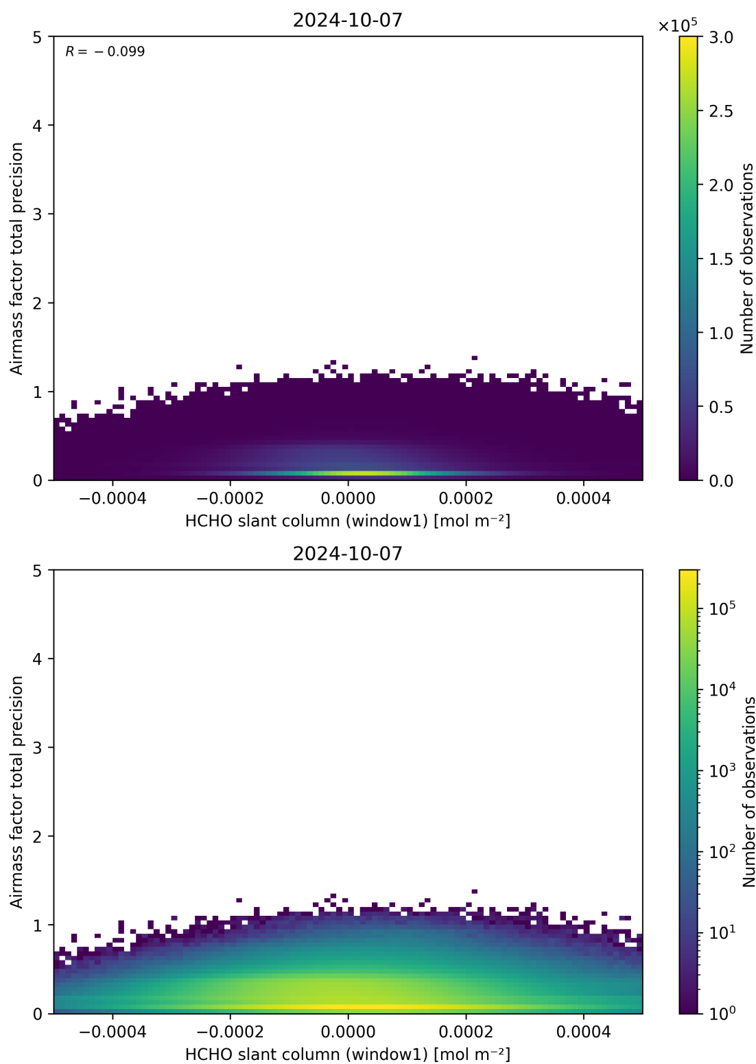
Figure 86: Scatter density plot of “HCHO slant column (window1)” against “Airmass factor total precision” for 2024-10-06 to 2024-10-08.
