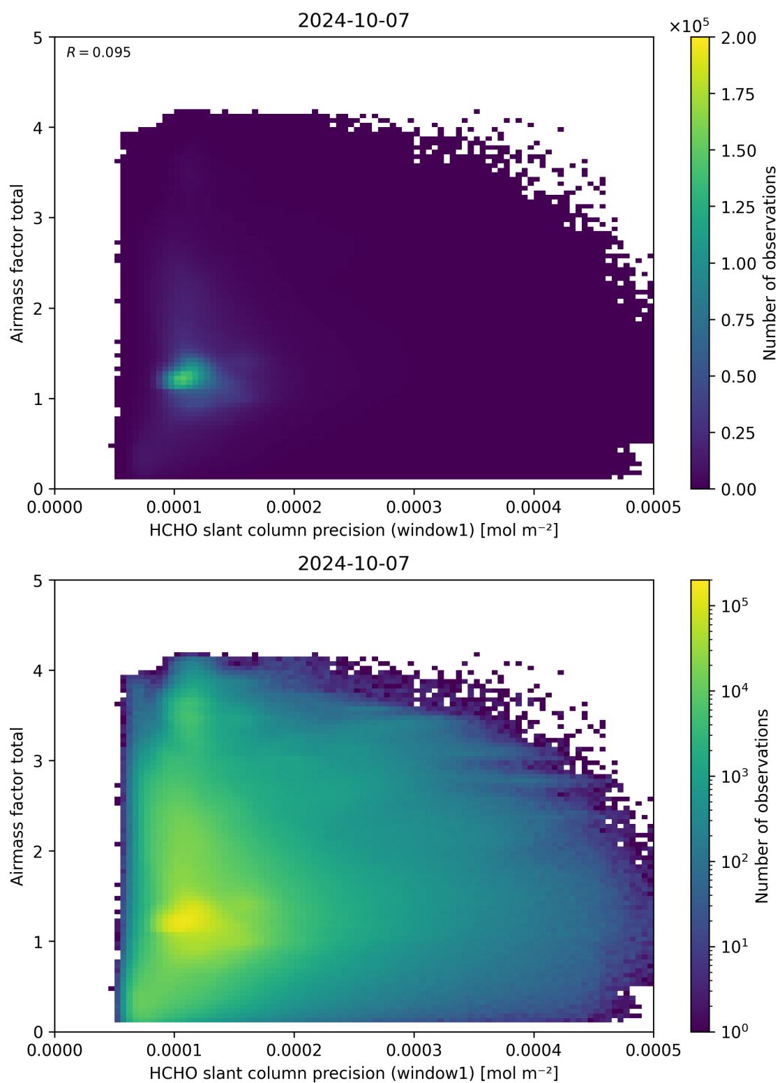
Figure 94: Scatter density plot of “HCHO slant column precision (window1)” against “Airmass factor total” for 2024-10-06 to 2024-10-08.
