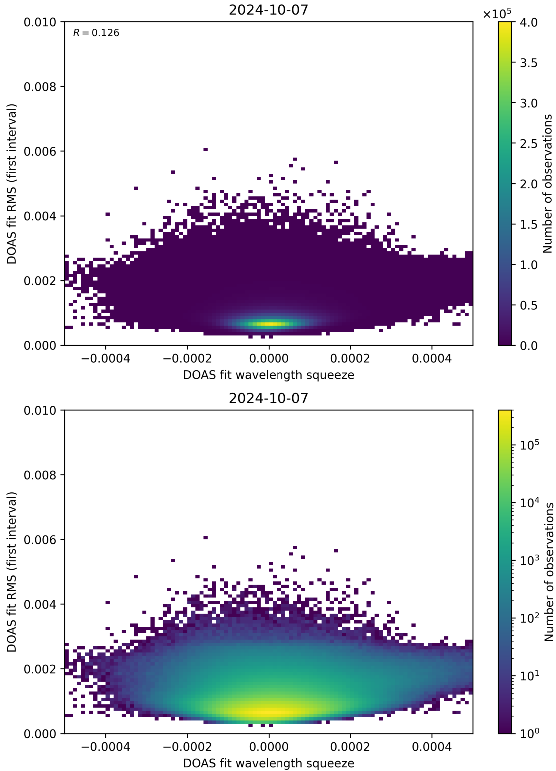
Figure 68: Scatter density plot of “DOAS fit wavelength squeeze” against “DOAS fit RMS (first interval)” for 2024-10-06 to 2024-10-08.
