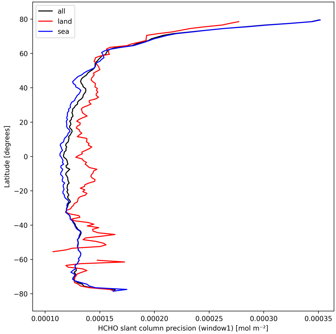
Figure 25: Zonal average of “HCHO slant column precision (window1)” for 2024-10-06 to 2024-10-08.
