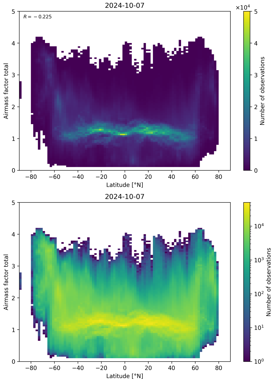
Figure 161: Scatter density plot of “Latitude” against “Airmass factor total” for 2024-10-06 to 2024-10-08.
