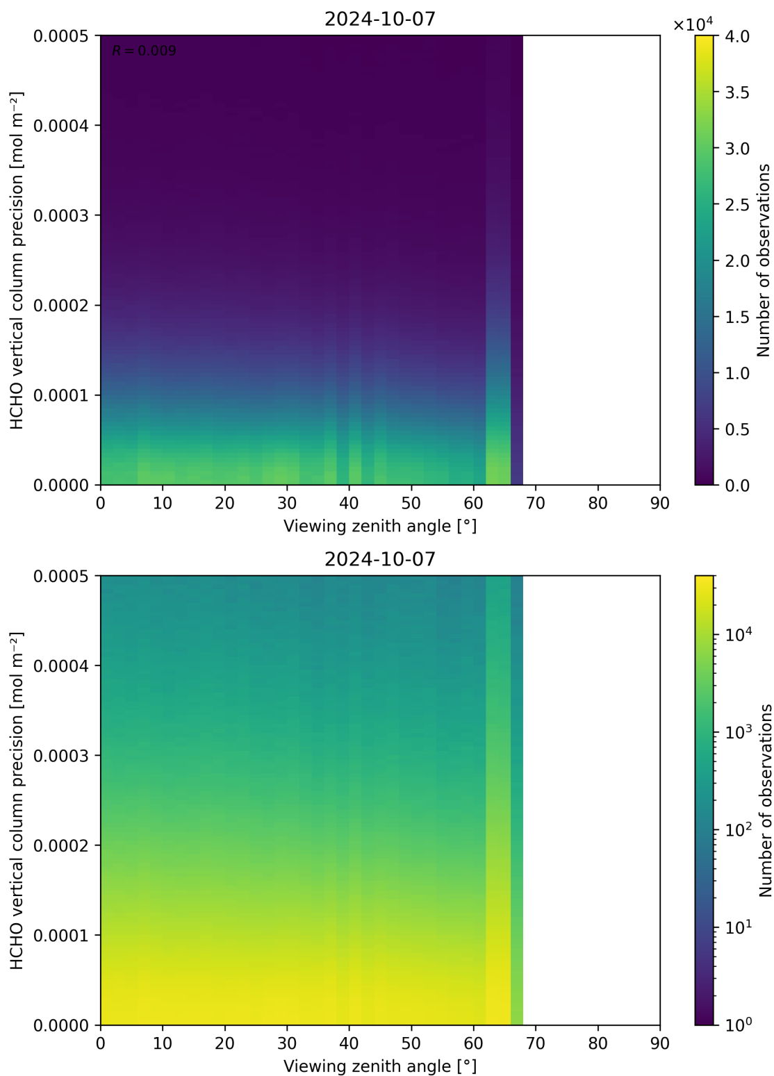
Figure 194: Scatter density plot of “Viewing zenith angle” against “HCHO vertical column precision” for 2024-10-06 to 2024-10-08.
