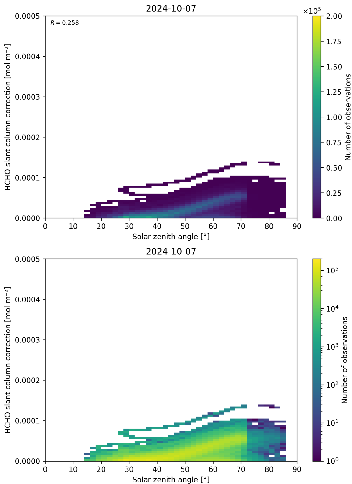
Figure 172: Scatter density plot of “Solar zenith angle” against “HCHO slant column correction” for 2024-10-06 to 2024-10-08.
