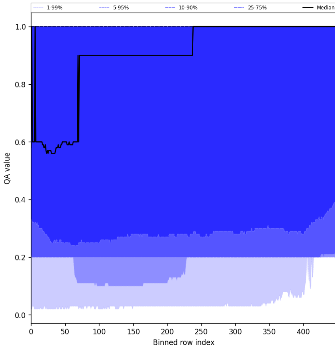
Figure 48: Along track statistics of “QA value” for 2024-10-06 to 2024-10-08
