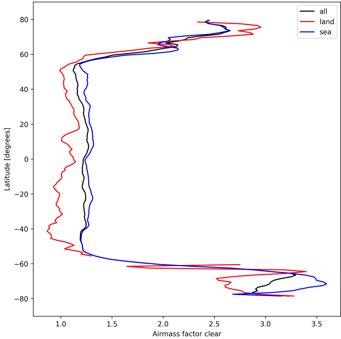
Figure 28: Zonal average of “Airmass factor clear” for 2024-10-06 to 2024-10-08.
