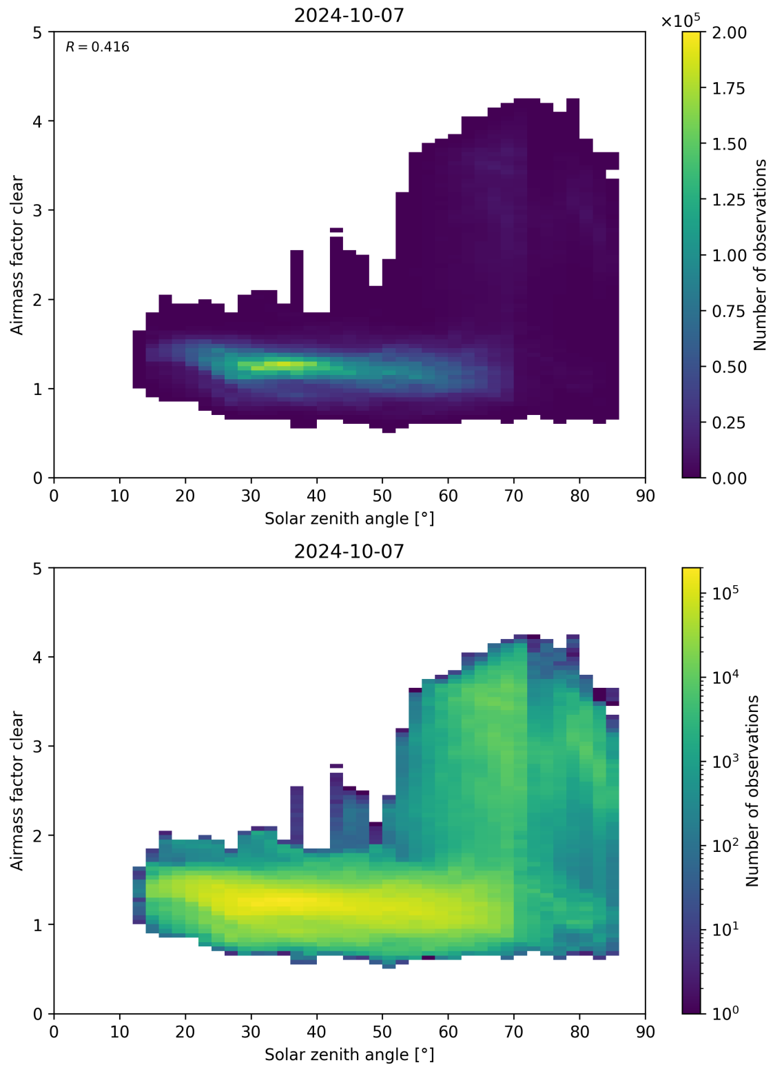
Figure 170: Scatter density plot of “Solar zenith angle” against “Airmass factor clear” for 2024-10-06 to 2024-10-08.
