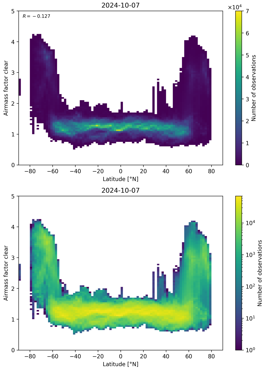
Figure 156: Scatter density plot of “Latitude” against “Airmass factor clear” for 2024-10-06 to 2024-10-08.
