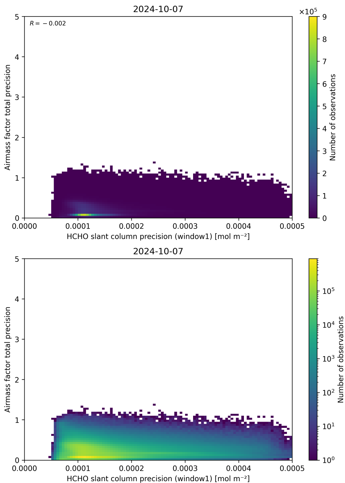
Figure 95: Scatter density plot of “HCHO slant column precision (window1)” against “Airmass factor total precision” for 2024-10-06 to 2024-10-08.
