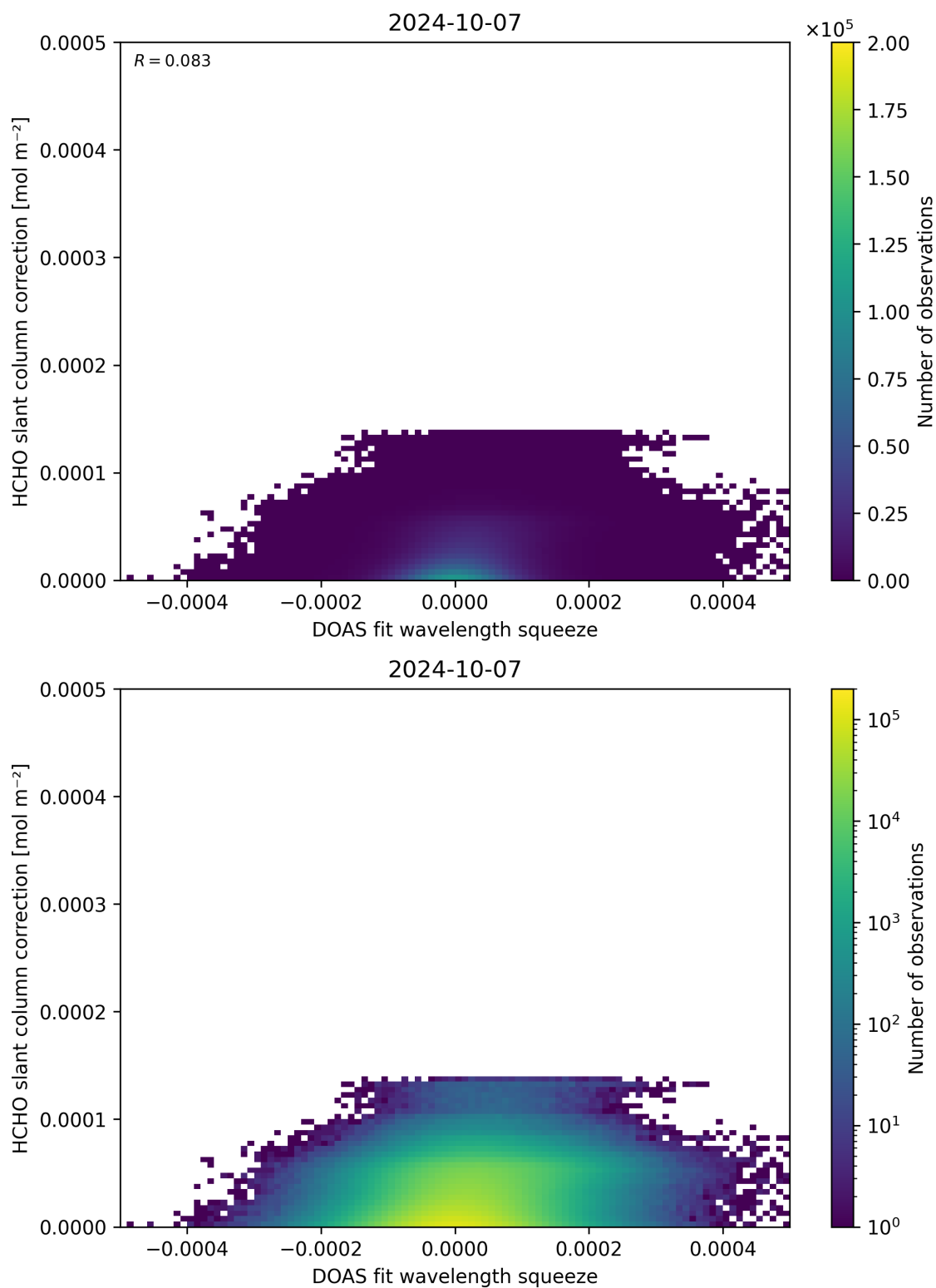
Figure 70: Scatter density plot of “DOAS fit wavelength squeeze” against “HCHO slant column correction” for 2024-10-06 to 2024-10-08.
