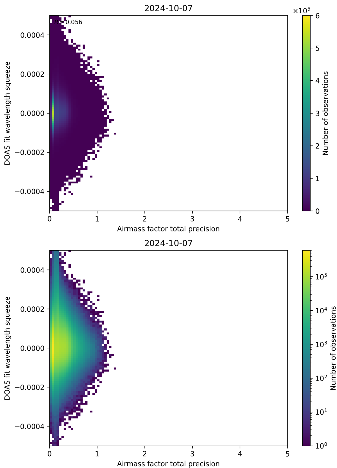
Figure 107: Scatter density plot of “Airmass factor total precision” against “DOAS fit wavelength squeeze” for 2024-10-06 to 2024-10-08.
