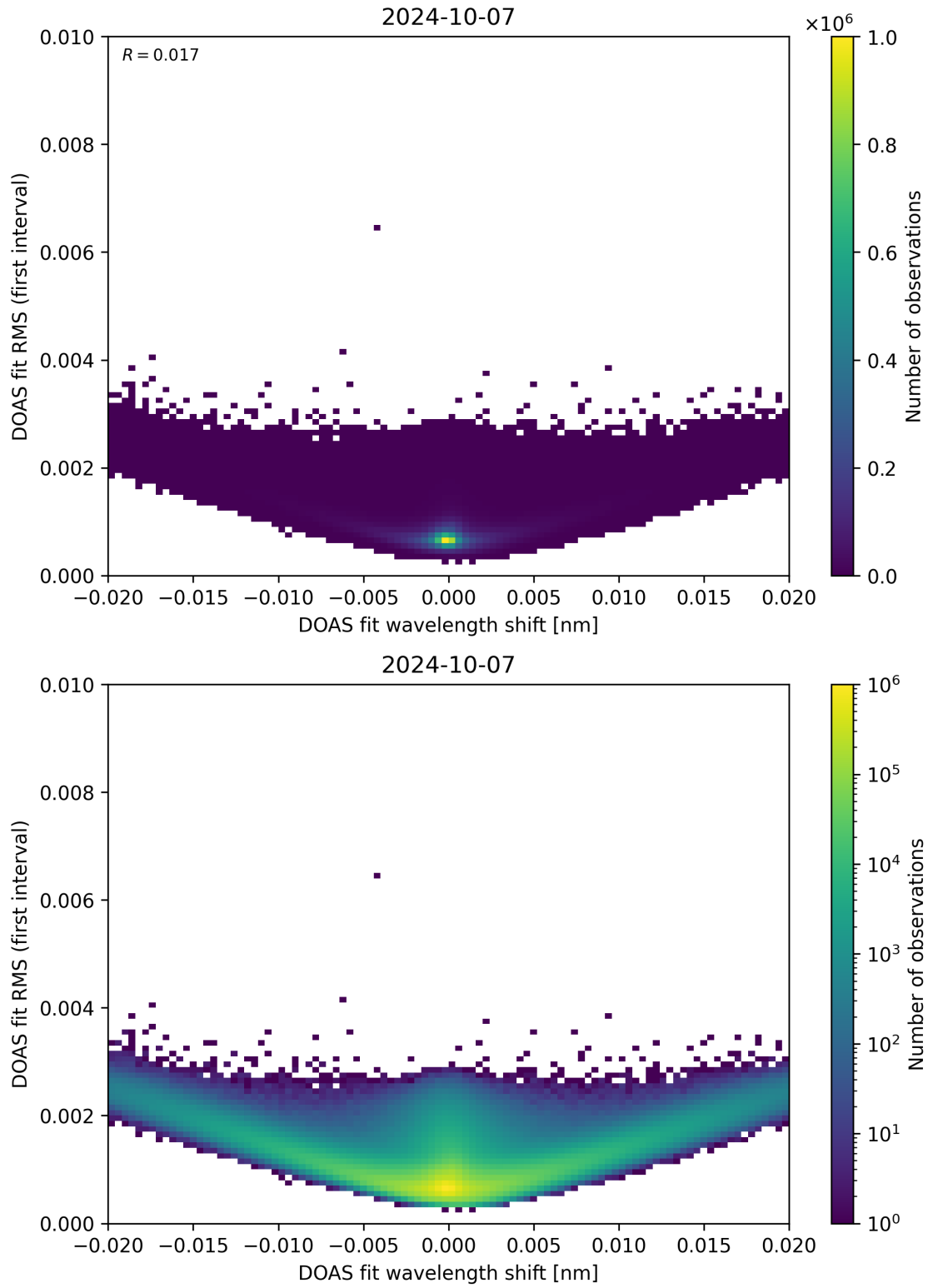
Figure 64: Scatter density plot of “DOAS fit wavelength shift” against “DOAS fit RMS (first interval)” for 2024-10-06 to 2024-10-08.
