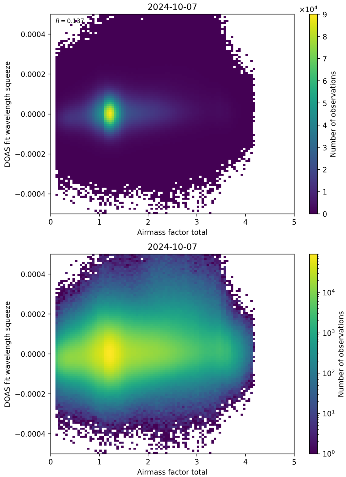
Figure 99: Scatter density plot of “Airmass factor total” against “DOAS fit wavelength squeeze” for 2024-10-06 to 2024-10-08.
