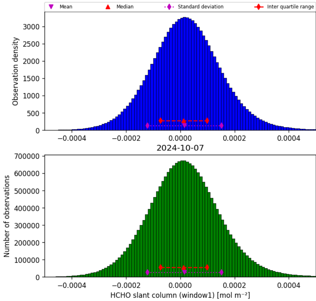
Figure 38: Histogram of “HCHO slant column (window1)” for 2024-10-06 to 2024-10-08
