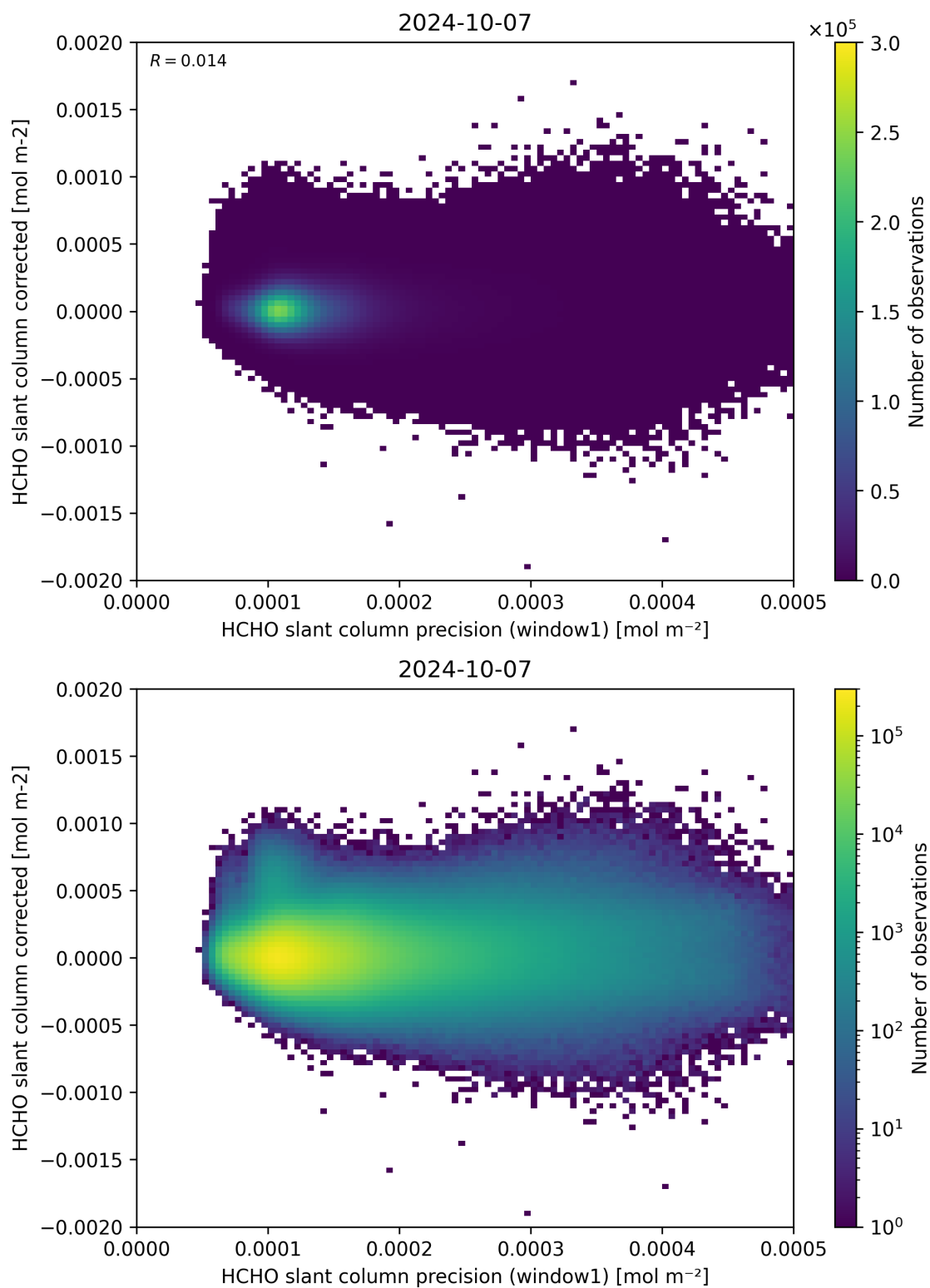
Figure 92: Scatter density plot of “HCHO slant column precision (window1)” against “HCHO slant column corrected” for 2024-10-06 to 2024-10-08.
