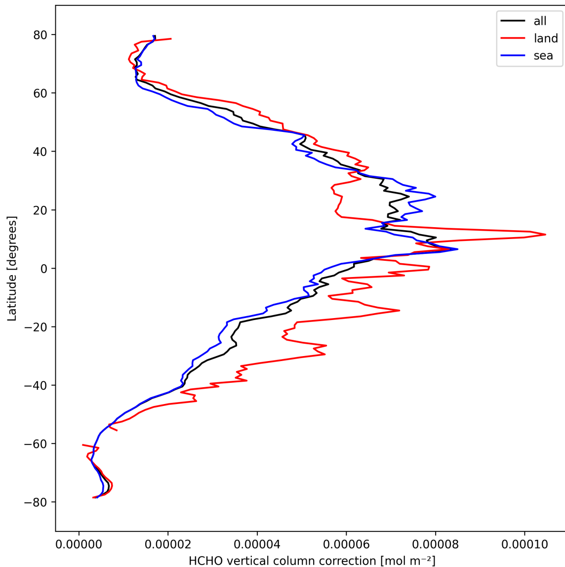
Figure 23: Zonal average of “HCHO vertical column correction” for 2024-10-06 to 2024-10-08.
