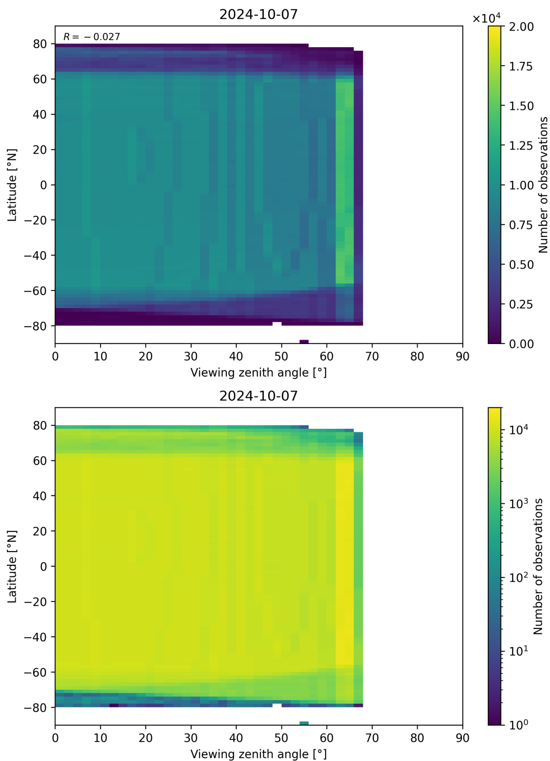
Figure 196: Scatter density plot of “Viewing zenith angle” against “Latitude” for 2024-10-06 to 2024-10-08.
