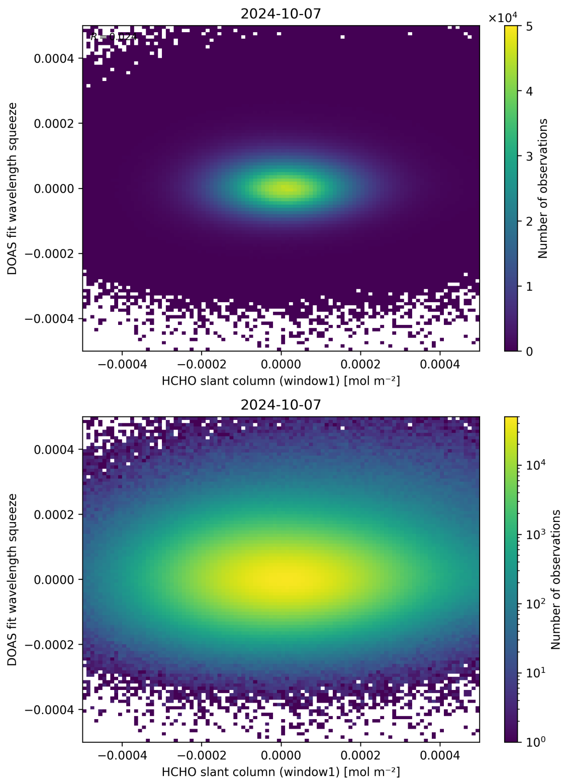
Figure 80: Scatter density plot of “HCHO slant column (window1)” against “DOAS fit wavelength squeeze” for 2024-10-06 to 2024-10-08.
