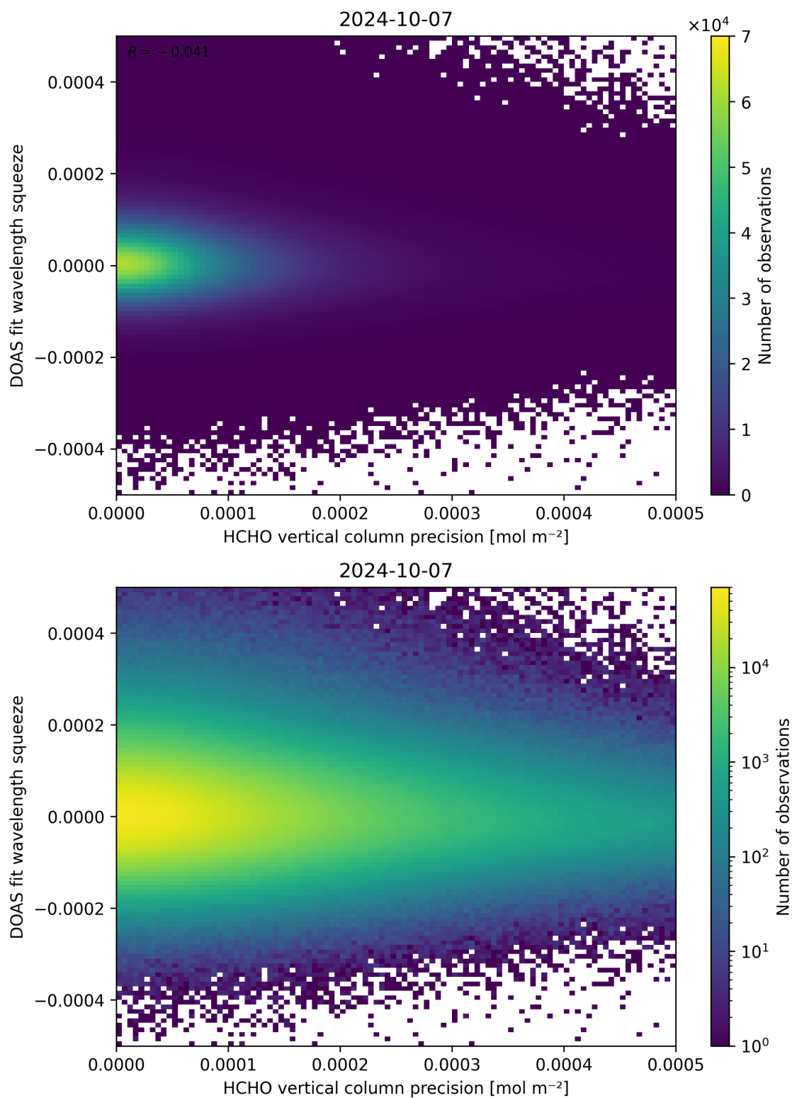
Figure 138: Scatter density plot of “HCHO vertical column precision” against “DOAS fit wavelength squeeze” for 2024-10-06 to 2024-10-08.
