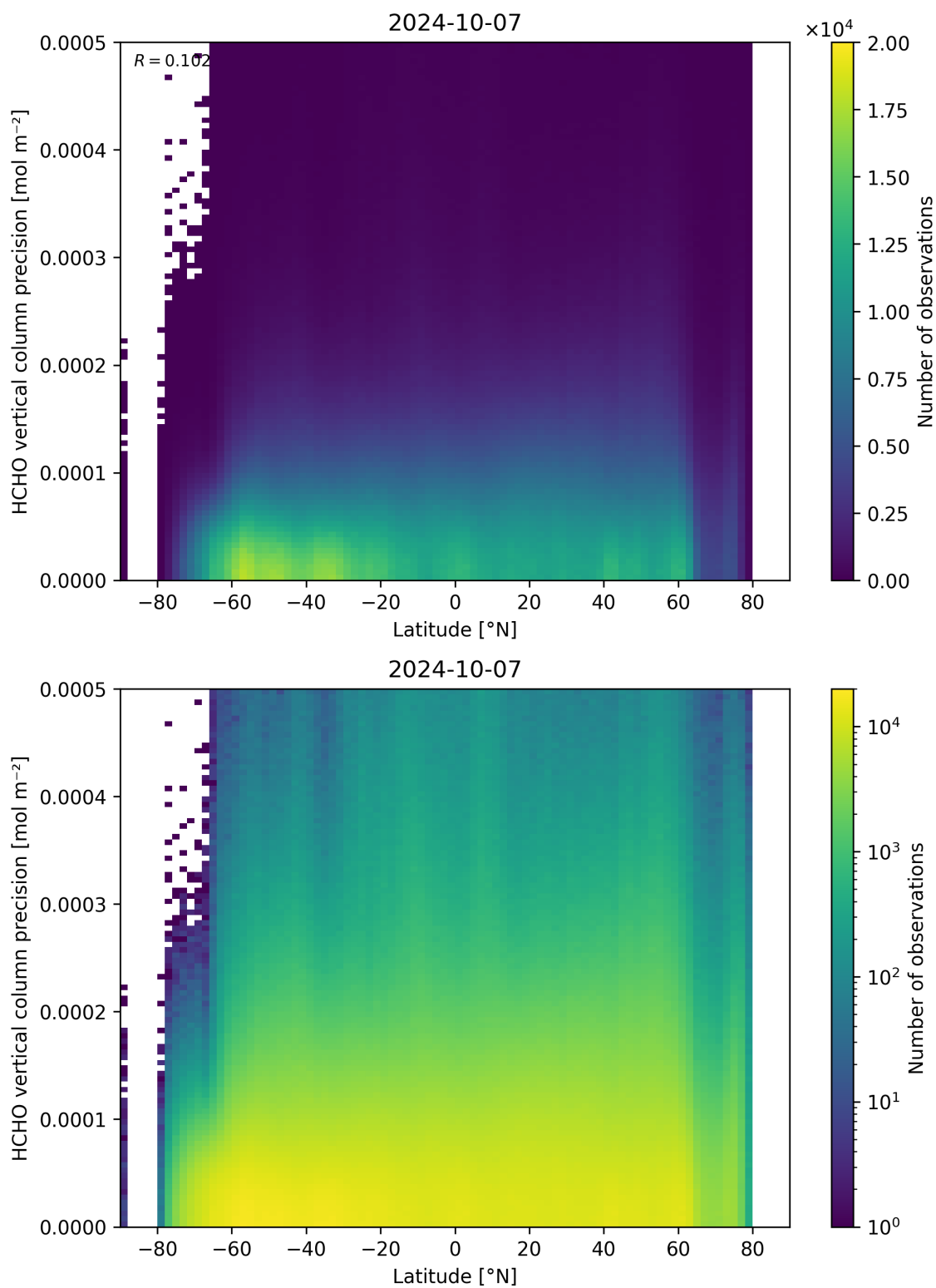
Figure 165: Scatter density plot of “Latitude” against “HCHO vertical column precision” for 2024-10-06 to 2024-10-08.
