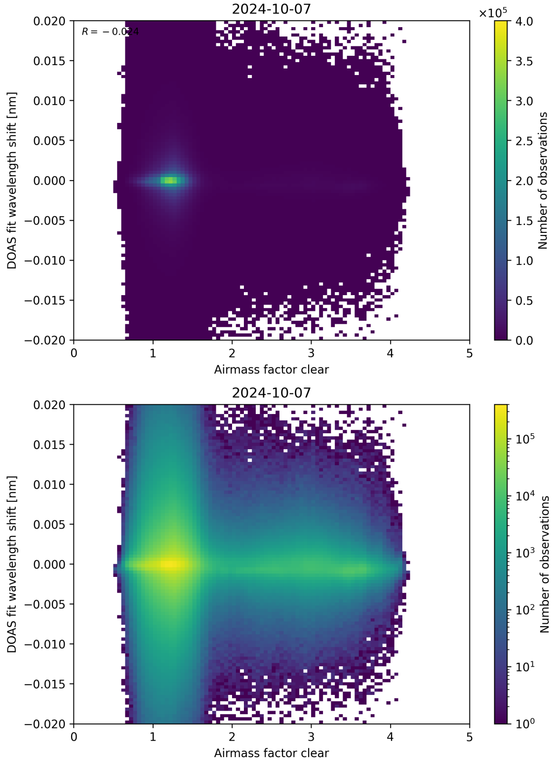
Figure 72: Scatter density plot of “Airmass factor clear” against “DOAS fit wavelength shift” for 2024-10-06 to 2024-10-08.
