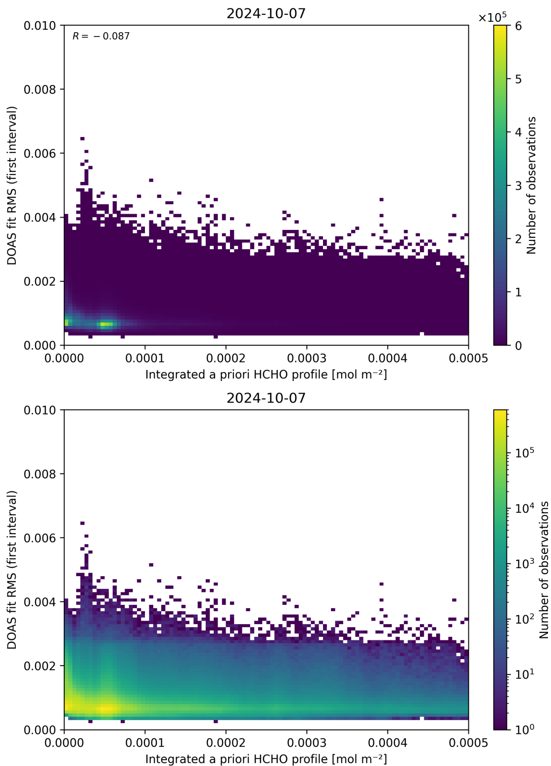
Figure 148: Scatter density plot of “Integrated a priori HCHO profile” against “DOAS fit RMS (first interval)” for 2024-10-06 to 2024-10-08.
