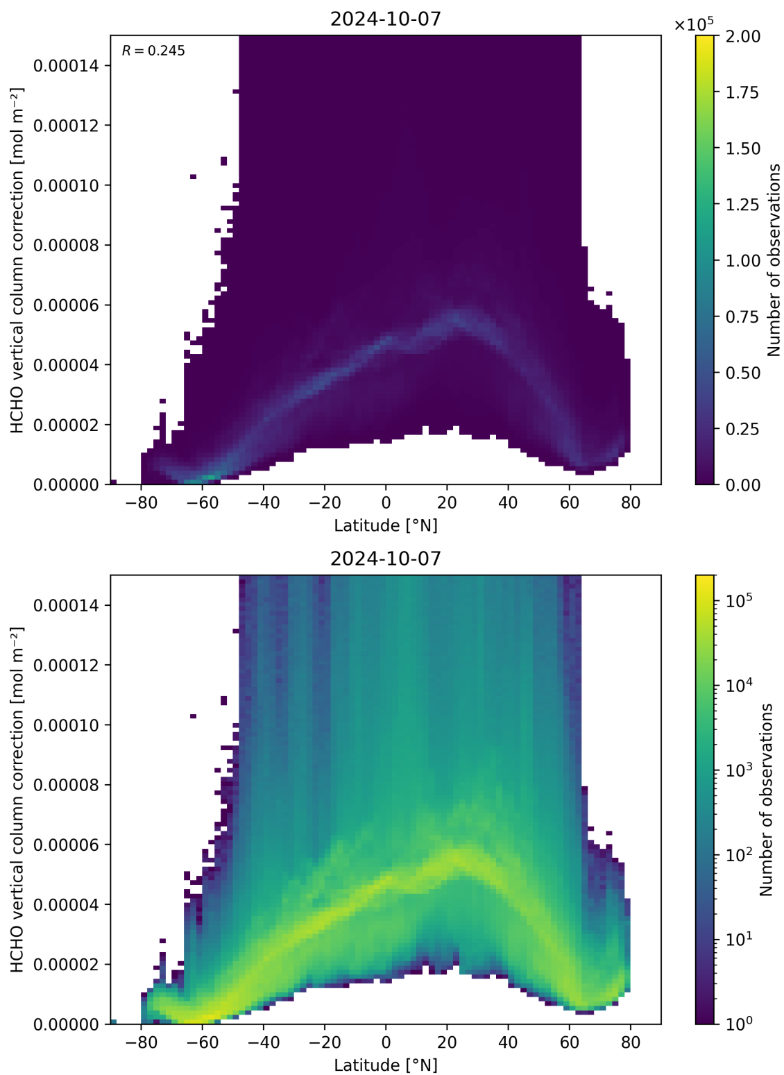
Figure 164: Scatter density plot of “Latitude” against “HCHO vertical column correction” for 2024-10-06 to 2024-10-08.
