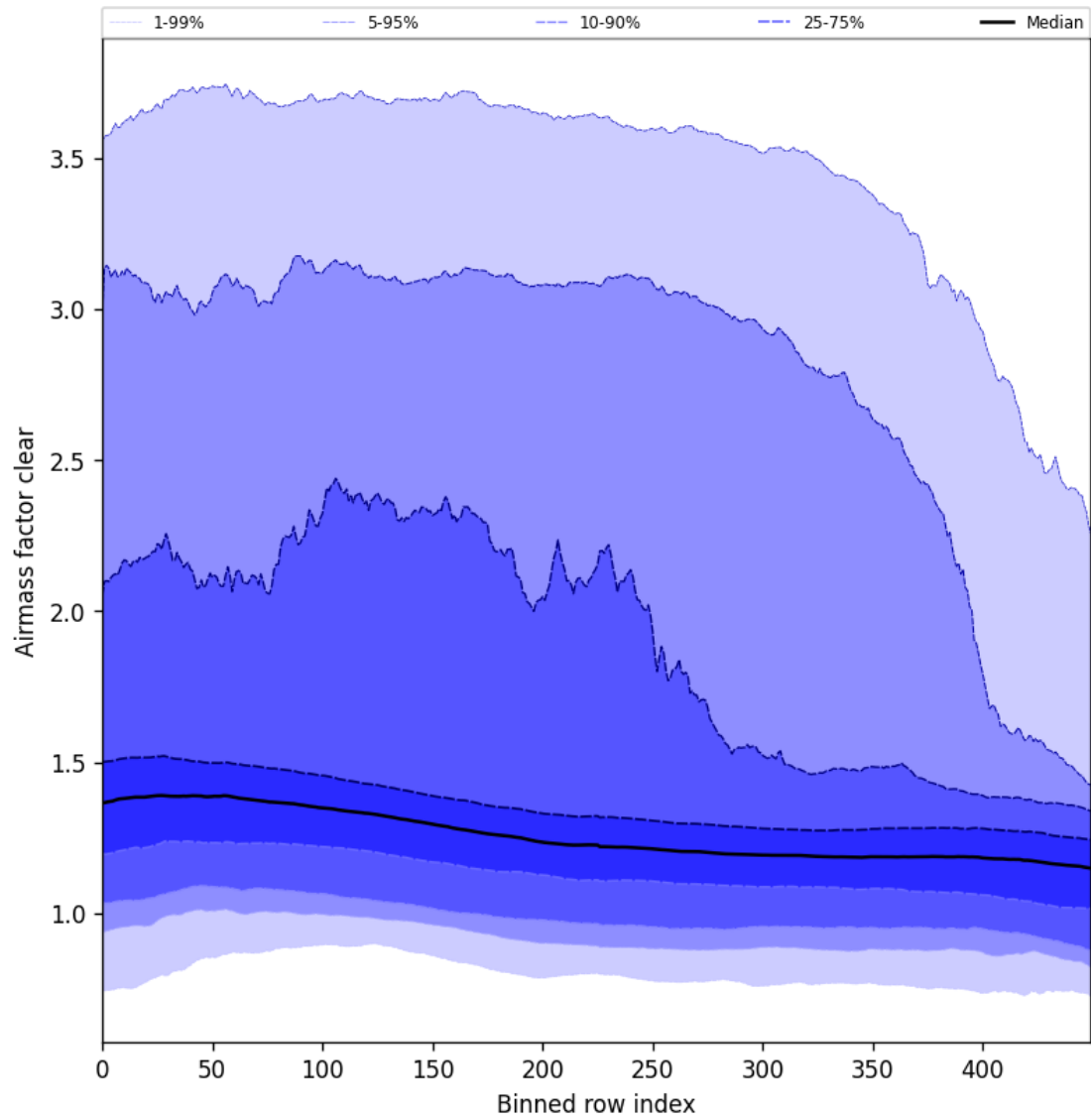
Figure 56: Along track statistics of “Airmass factor clear” for 2024-10-06 to 2024-10-08
