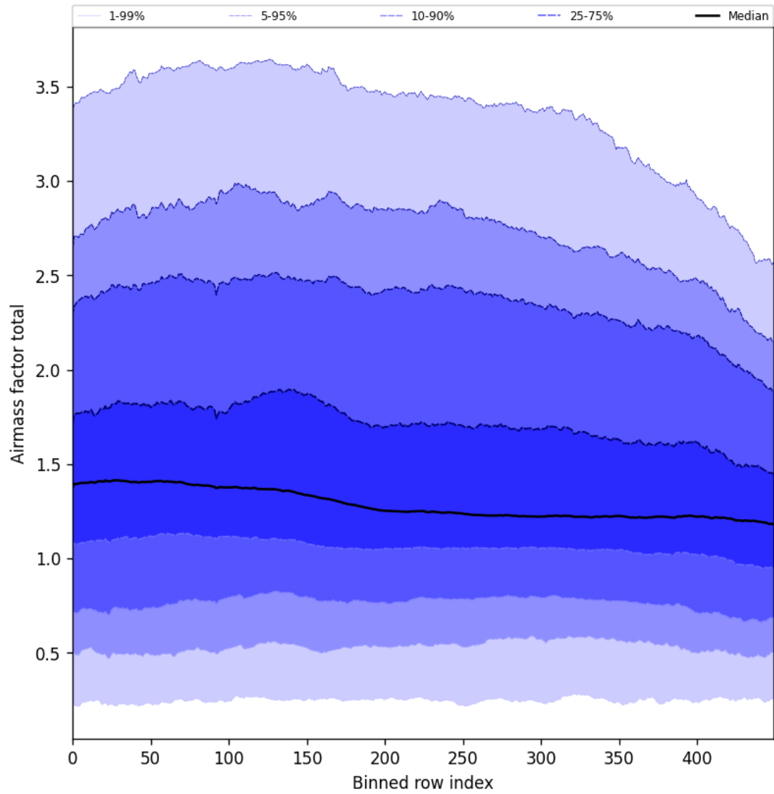
Figure 54: Along track statistics of “Airmass factor total” for 2024-10-06 to 2024-10-08
