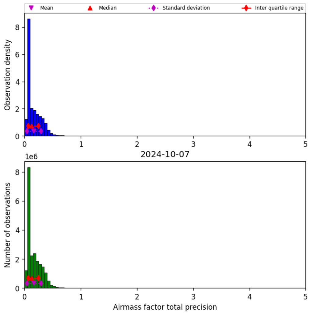
Figure 41: Histogram of “Airmass factor total precision” for 2024-10-06 to 2024-10-08
