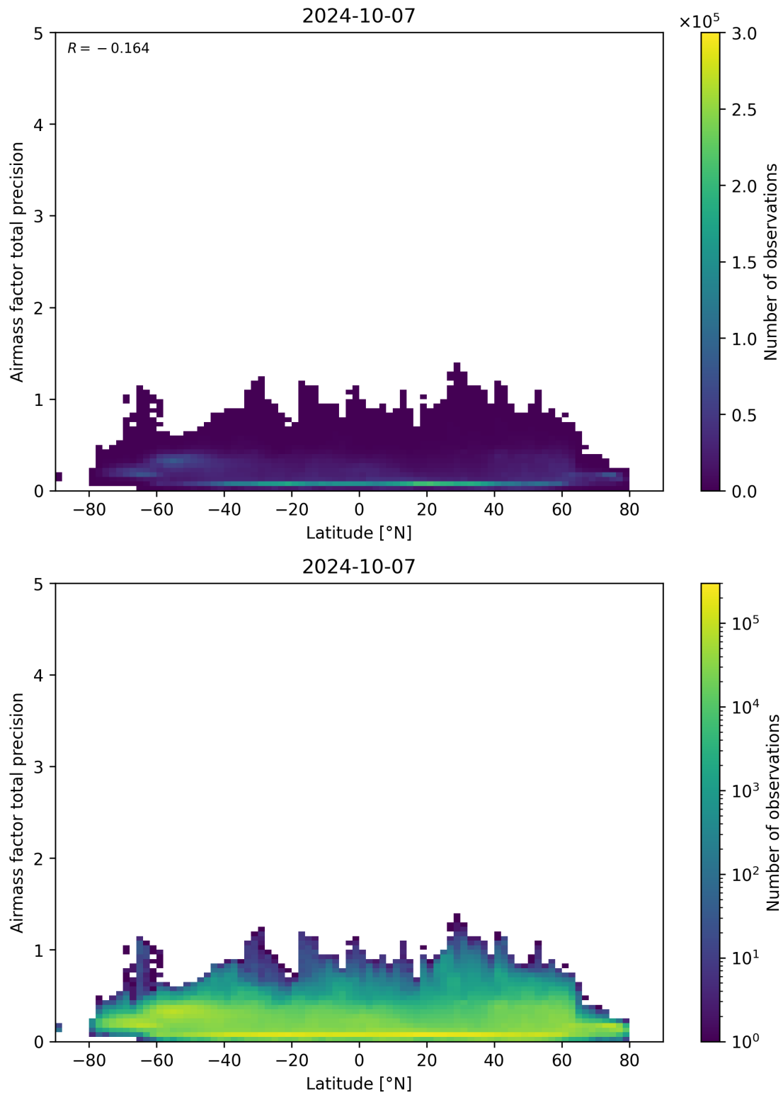
Figure 162: Scatter density plot of “Latitude” against “Airmass factor total precision” for 2024-10-06 to 2024-10-08.
