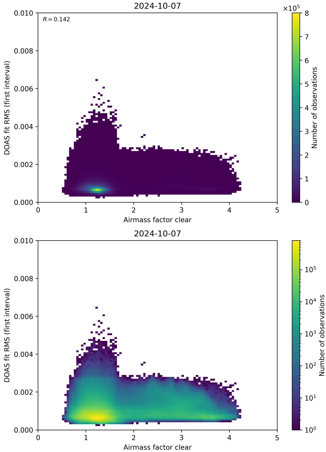
Figure 71: Scatter density plot of “Airmass factor clear” against “DOAS fit RMS (first interval)” for 2024-10-06 to 2024-10-08.
