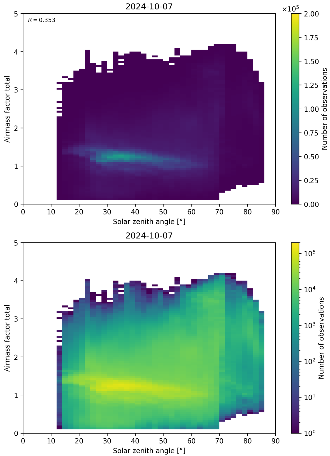
Figure 175: Scatter density plot of “Solar zenith angle” against “Airmass factor total” for 2024-10-06 to 2024-10-08.
