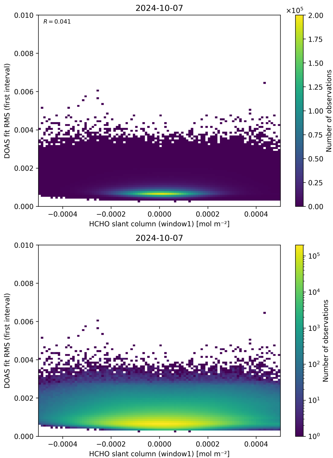
Figure 78: Scatter density plot of “HCHO slant column (window1)” against “DOAS fit RMS (first interval)” for 2024-10-06 to 2024-10-08.
