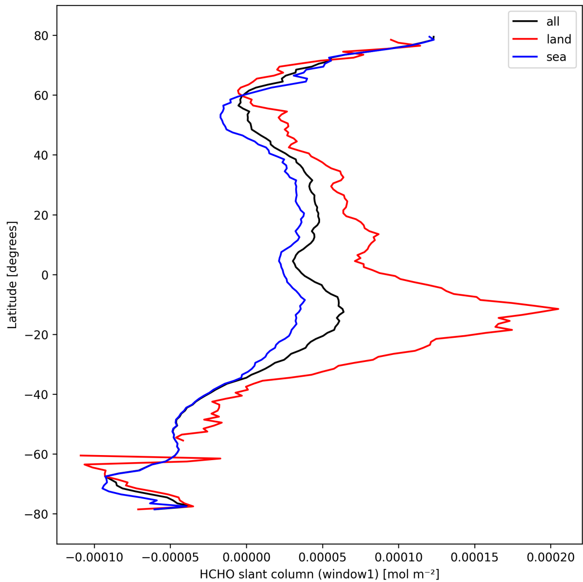
Figure 24: Zonal average of “HCHO slant column (window1)” for 2024-10-06 to 2024-10-08.
