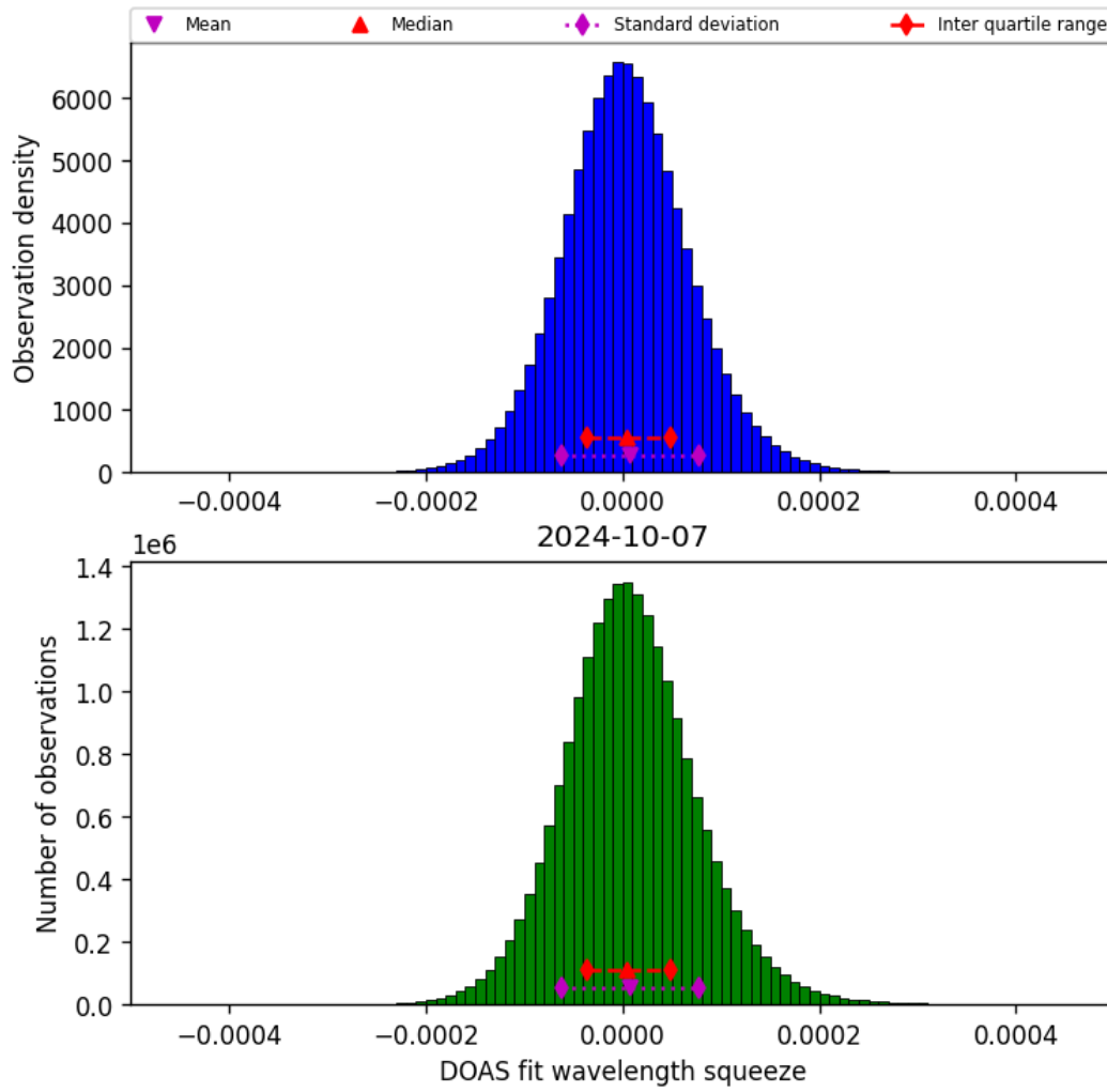
Figure 45: Histogram of “DOAS fit wavelength squeeze” for 2024-10-06 to 2024-10-08
