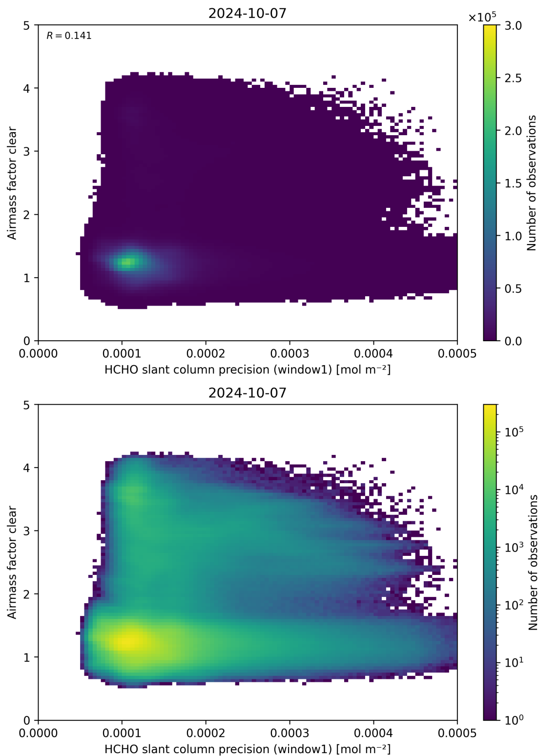
Figure 91: Scatter density plot of “HCHO slant column precision (window1)” against “Airmass factor clear” for 2024-10-06 to 2024-10-08.
