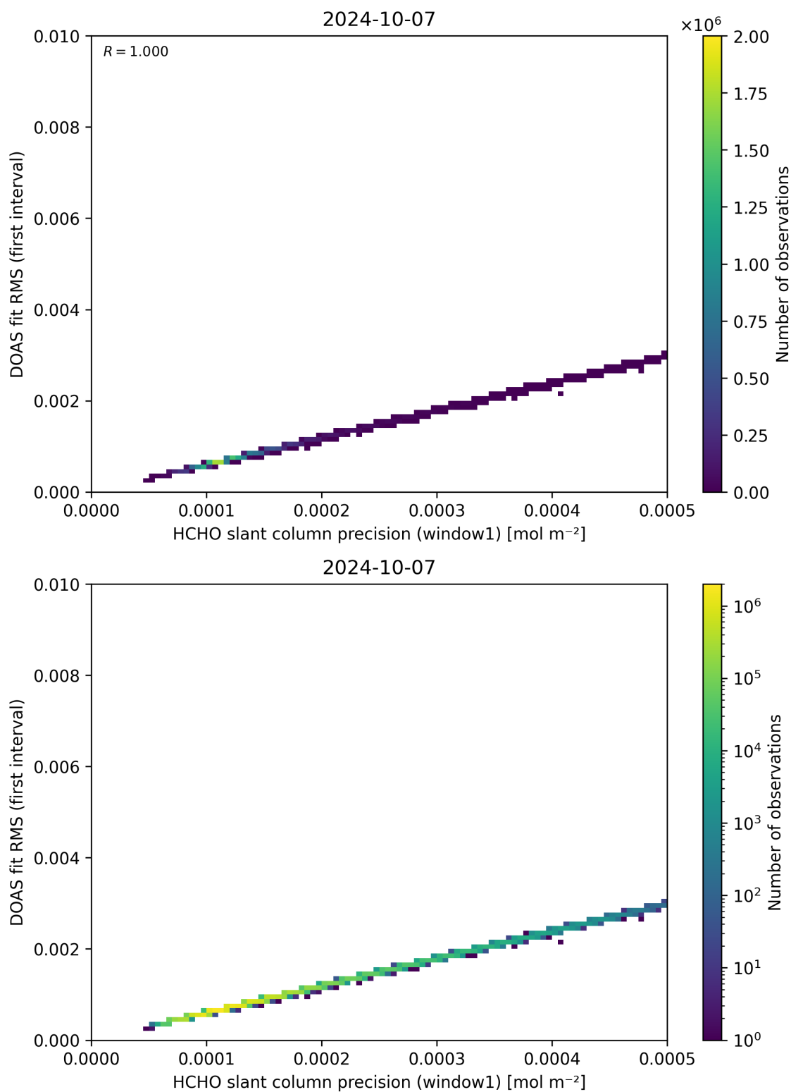
Figure 88: Scatter density plot of “HCHO slant column precision (window1)” against “DOAS fit RMS (first interval)” for 2024-10-06 to 2024-10-08.
