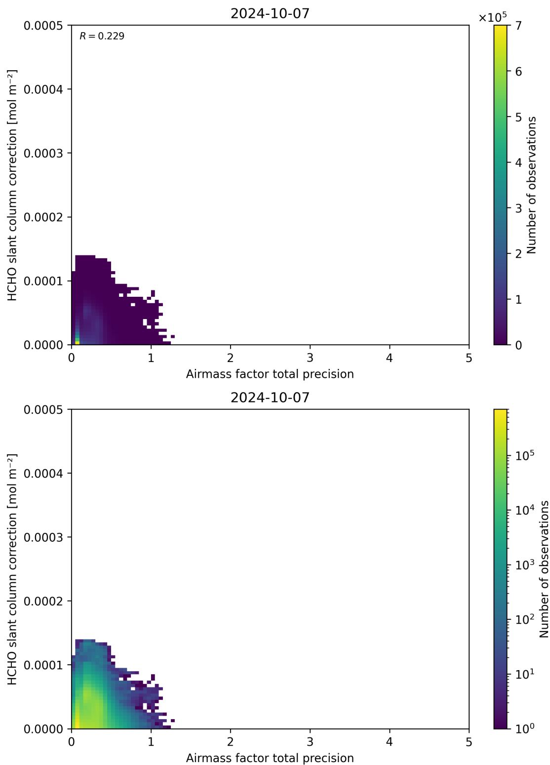
Figure 110: Scatter density plot of “Airmass factor total precision” against “HCHO slant column correction” for 2024-10-06 to 2024-10-08.
