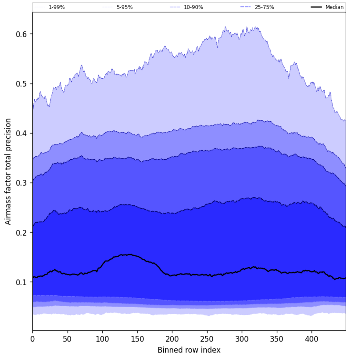
Figure 55: Along track statistics of “Airmass factor total precision” for 2024-10-06 to 2024-10-08
