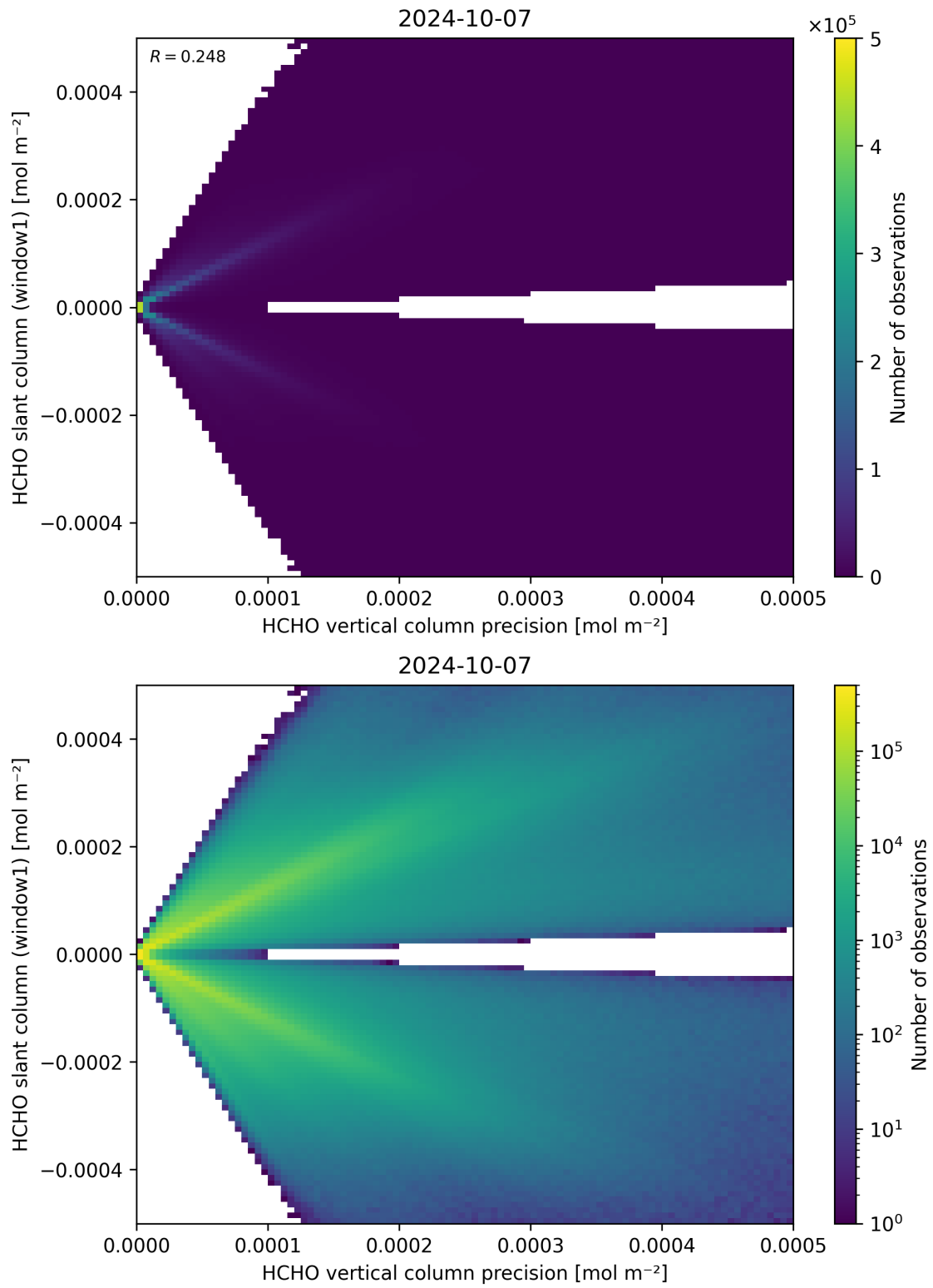
Figure 142: Scatter density plot of “HCHO vertical column precision” against “HCHO slant column (window1)” for 2024-10-06 to 2024-10-08.
