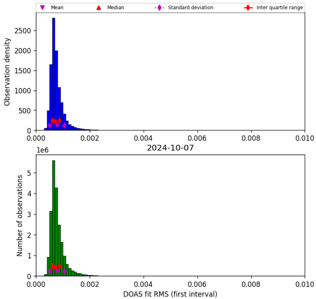
Figure 46: Histogram of “DOAS fit RMS (first interval)” for 2024-10-06 to 2024-10-08
