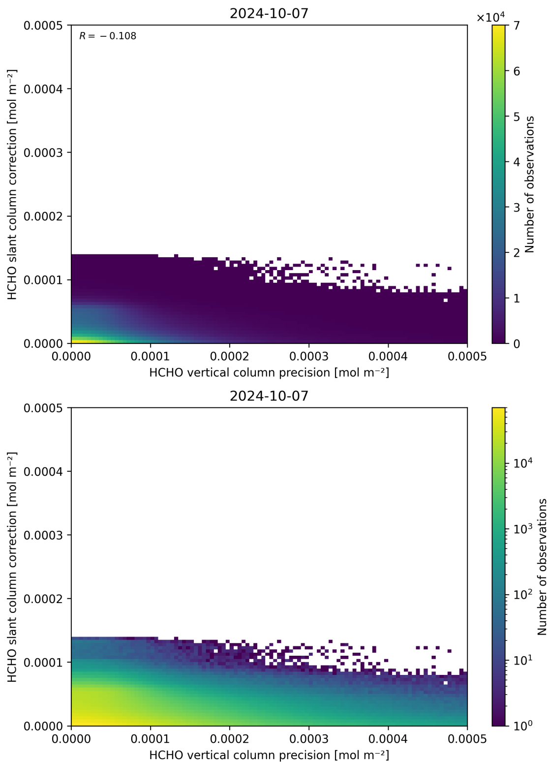
Figure 141: Scatter density plot of “HCHO vertical column precision” against “HCHO slant column correction” for 2024-10-06 to 2024-10-08.
