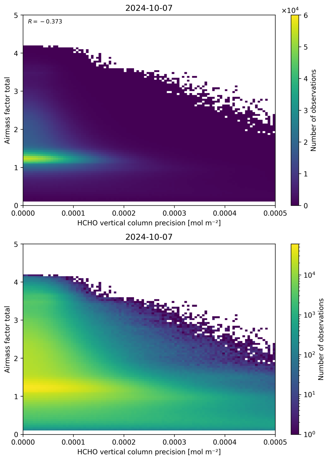
Figure 144: Scatter density plot of “HCHO vertical column precision” against “Airmass factor total” for 2024-10-06 to 2024-10-08.
