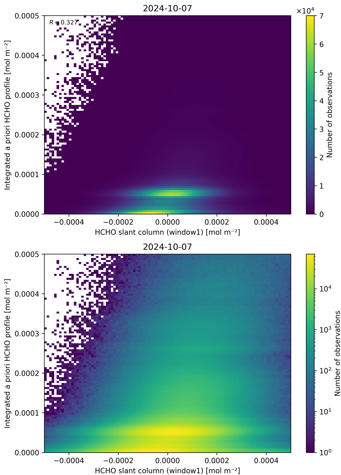
Figure 87: Scatter density plot of “HCHO slant column (window1)” against “Integrated a priori HCHO profile” for 2024-10-06 to 2024-10-08.
