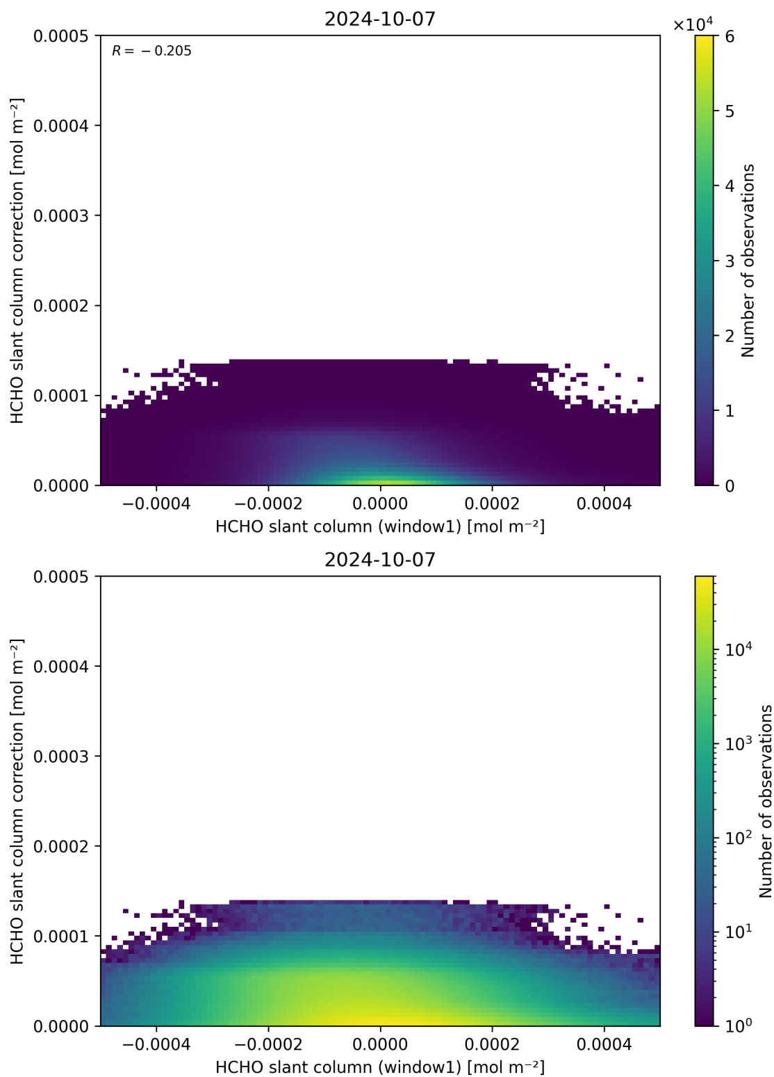
Figure 83: Scatter density plot of “HCHO slant column (window1)” against “HCHO slant column correction” for 2024-10-06 to 2024-10-08.
