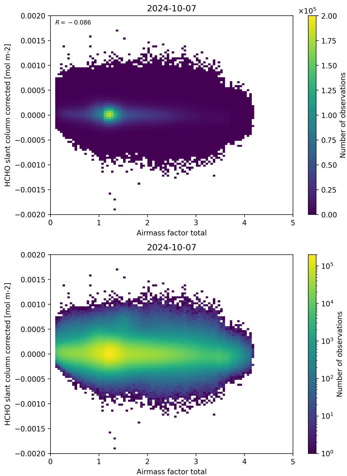
Figure 101: Scatter density plot of “Airmass factor total” against “HCHO slant column corrected” for 2024-10-06 to 2024-10-08.
