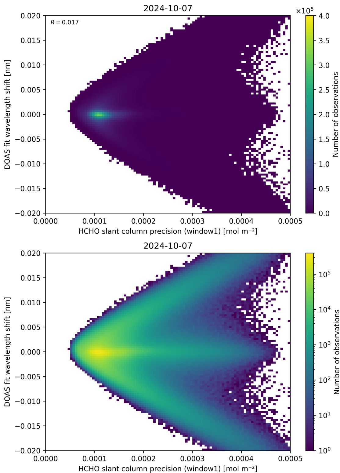
Figure 89: Scatter density plot of “HCHO slant column precision (window1)” against “DOAS fit wavelength shift” for 2024-10-06 to 2024-10-08.
