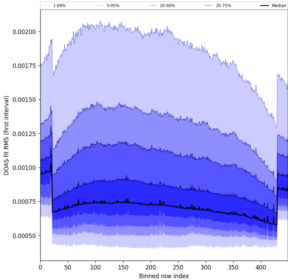
Figure 60: Along track statistics of “DOAS fit RMS (first interval)” for 2024-10-06 to 2024-10-08
