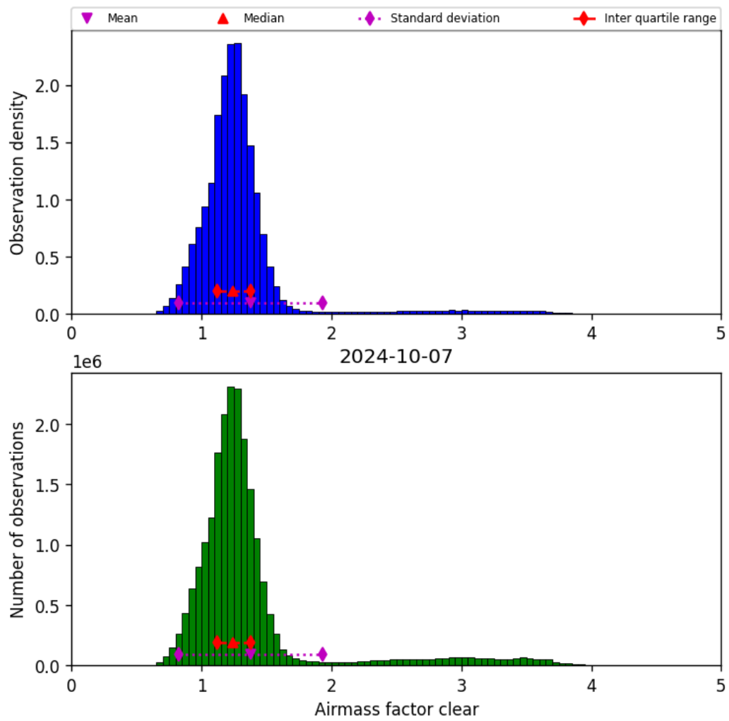
Figure 42: Histogram of “Airmass factor clear” for 2024-10-06 to 2024-10-08
