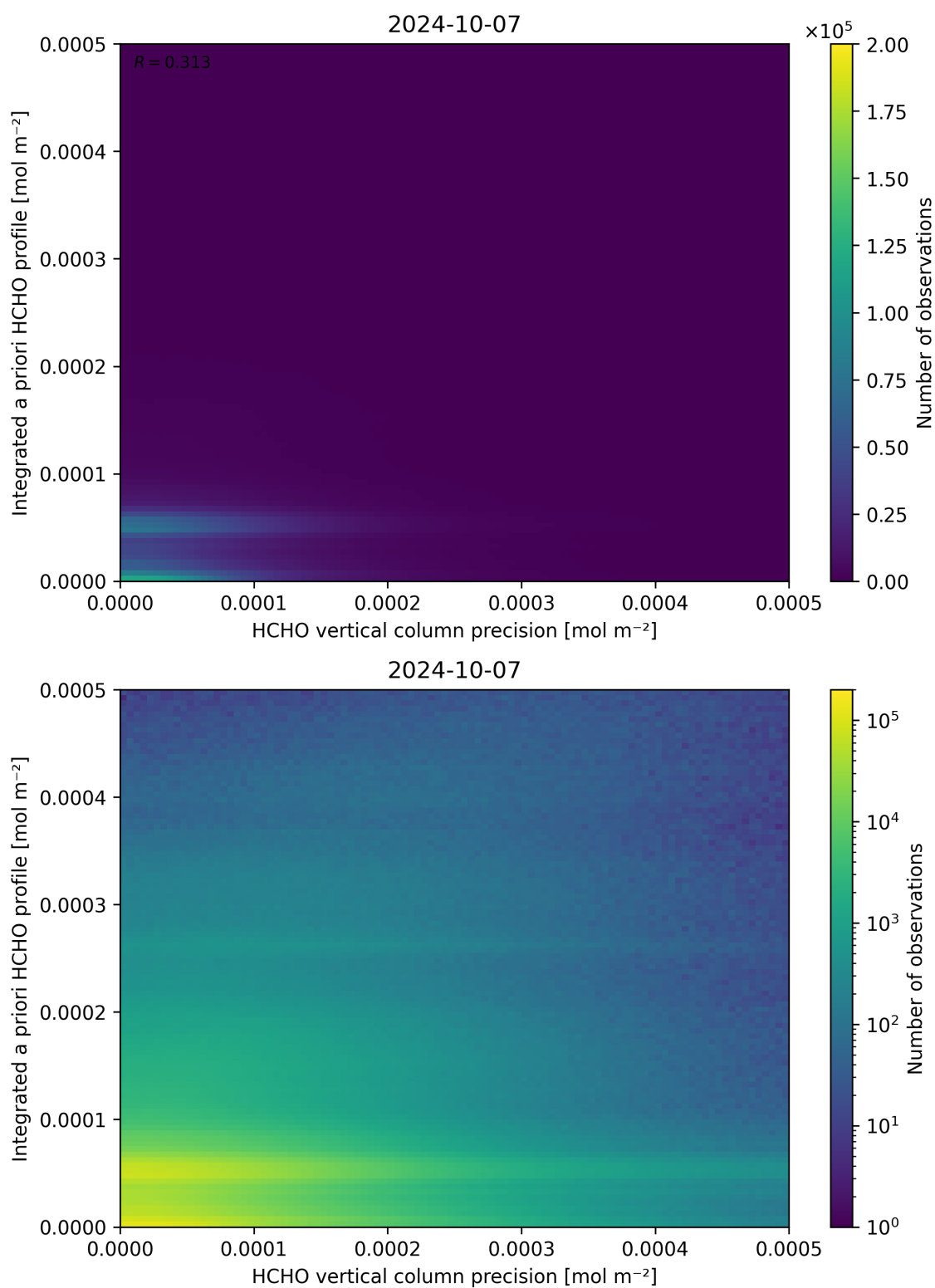
Figure 147: Scatter density plot of “HCHO vertical column precision” against “Integrated a priori HCHO profile” for 2024-10-06 to 2024-10-08.
