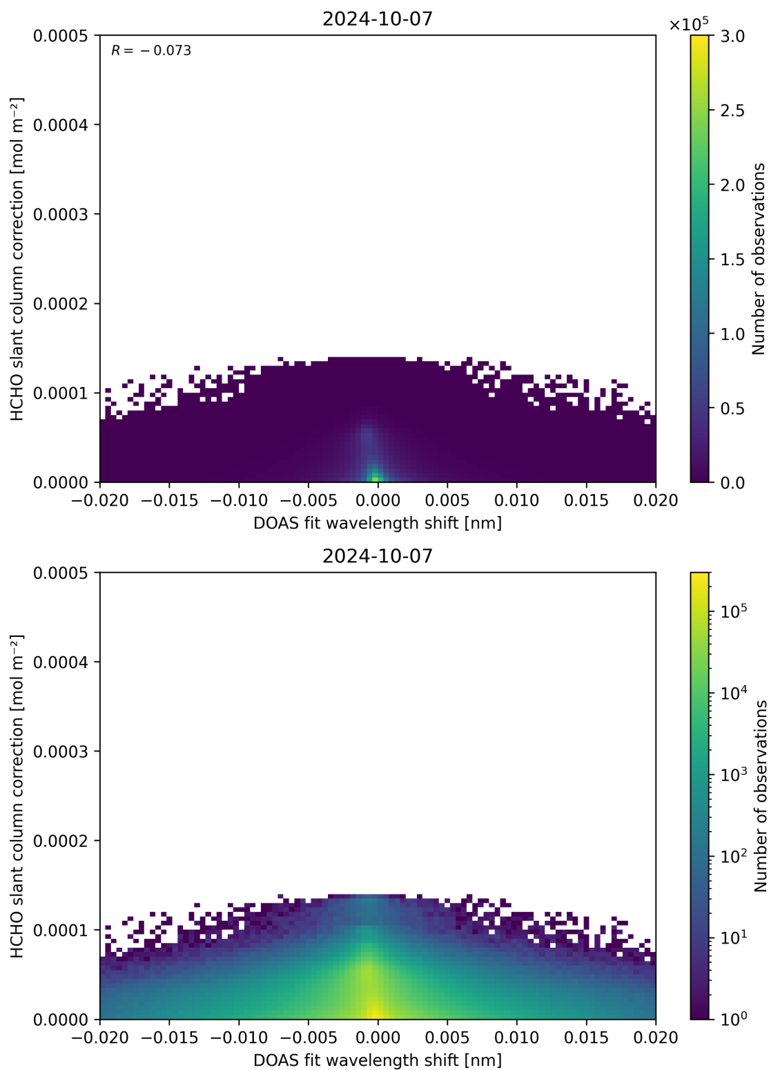
Figure 67: Scatter density plot of “DOAS fit wavelength shift” against “HCHO slant column correction” for 2024-10-06 to 2024-10-08.
