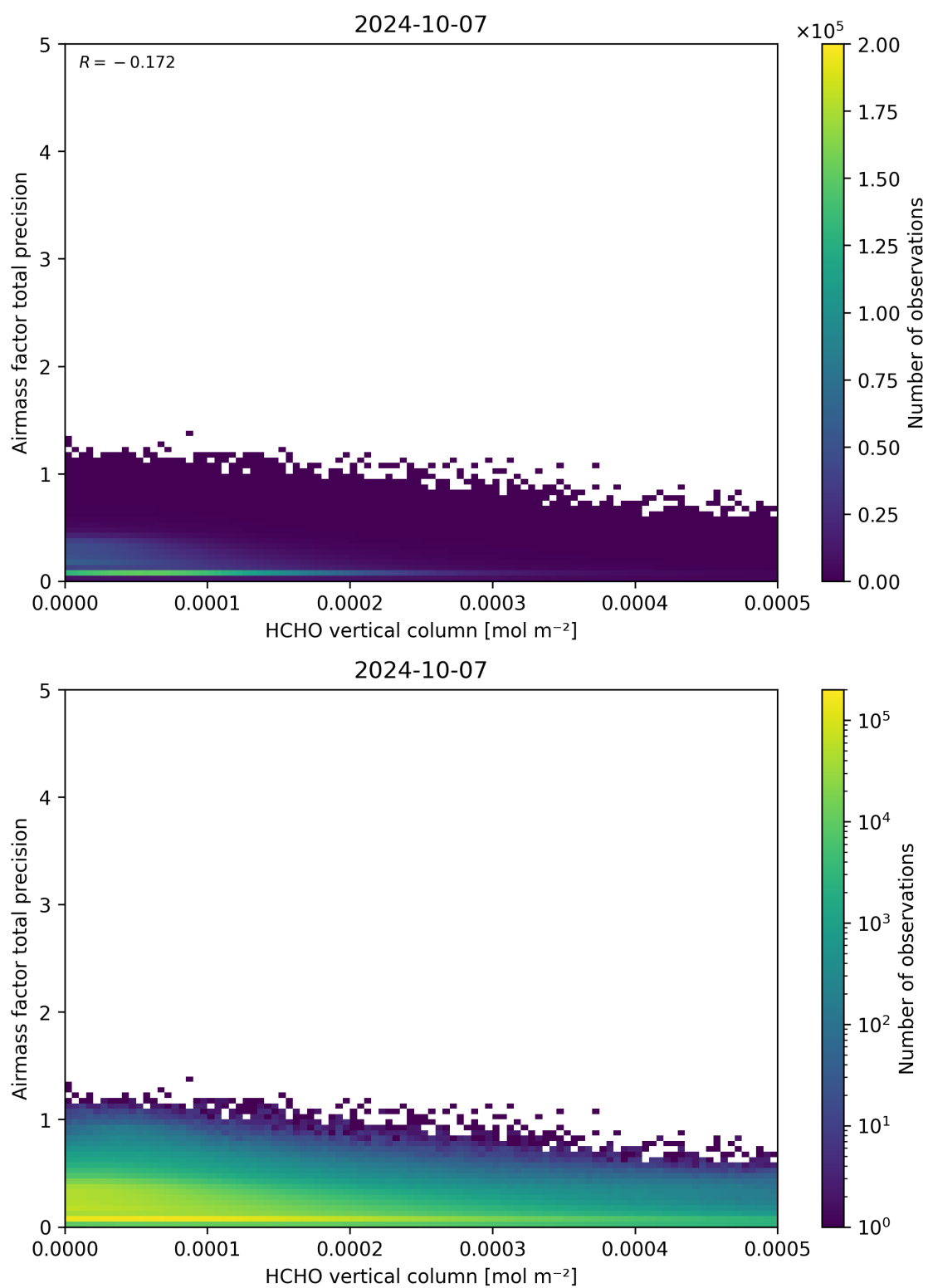
Figure 132: Scatter density plot of “HCHO vertical column” against “Airmass factor total precision” for 2024-10-06 to 2024-10-08.
