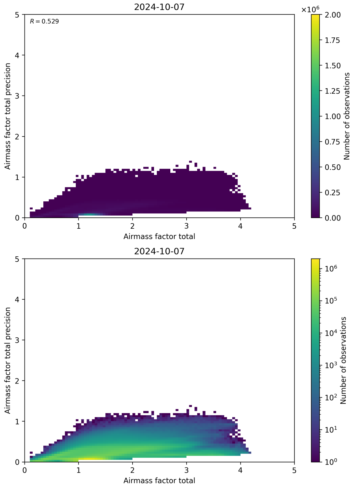
Figure 103: Scatter density plot of “Airmass factor total” against “Airmass factor total precision” for 2024-10-06 to 2024-10-08.
