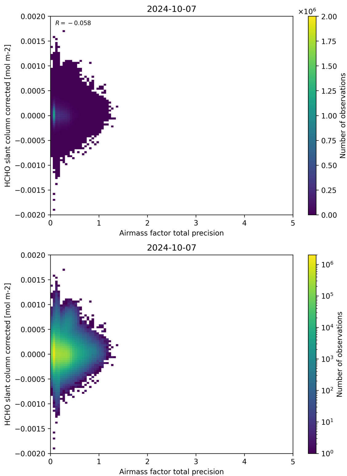
Figure 109: Scatter density plot of “Airmass factor total precision” against “HCHO slant column corrected” for 2024-10-06 to 2024-10-08.
