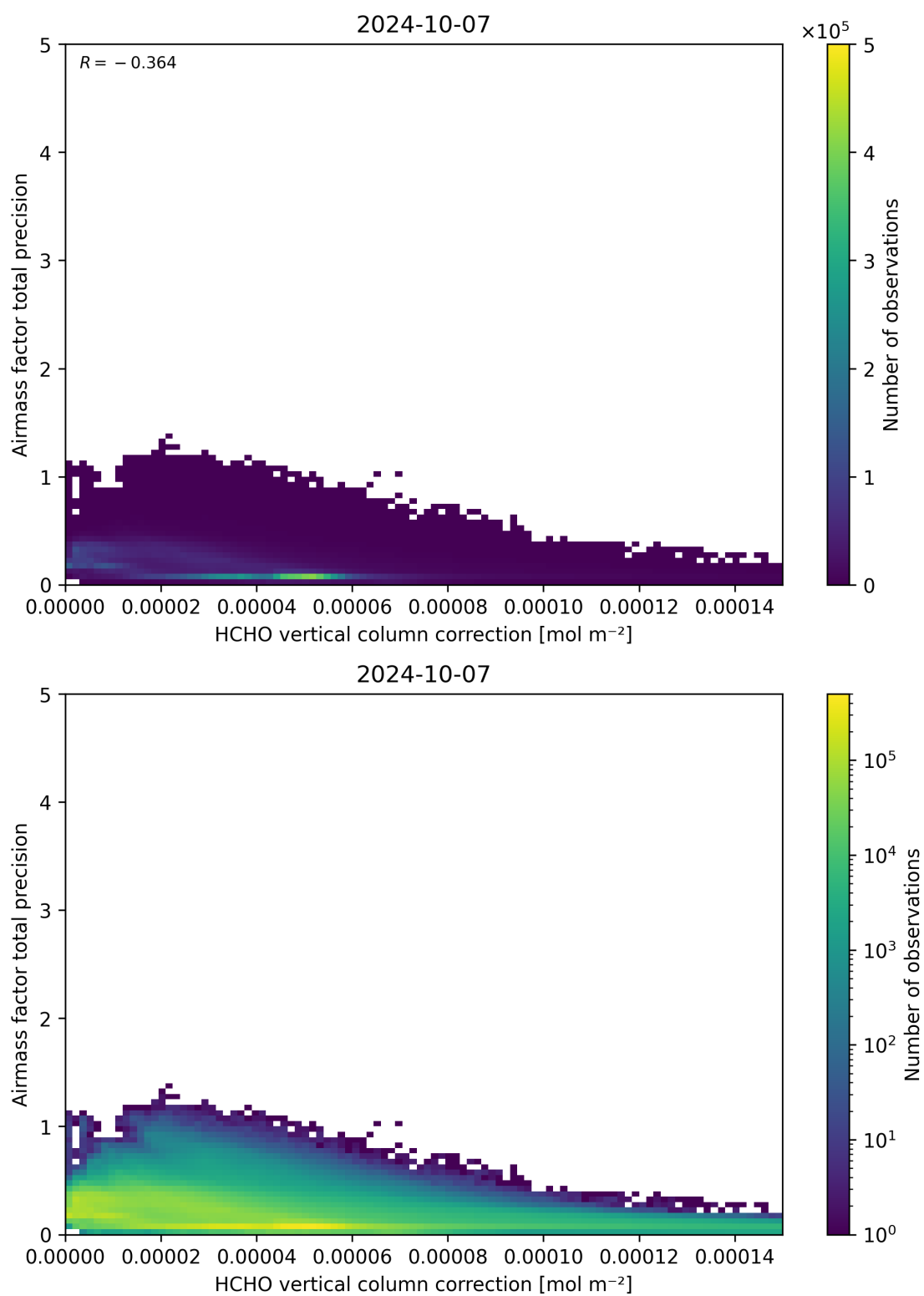
Figure 121: Scatter density plot of “HCHO vertical column correction” against “Airmass factor total precision” for 2024-10-06 to 2024-10-08.
