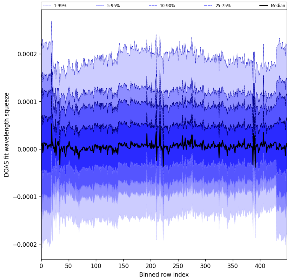
Figure 59: Along track statistics of “DOAS fit wavelength squeeze” for 2024-10-06 to 2024-10-08
