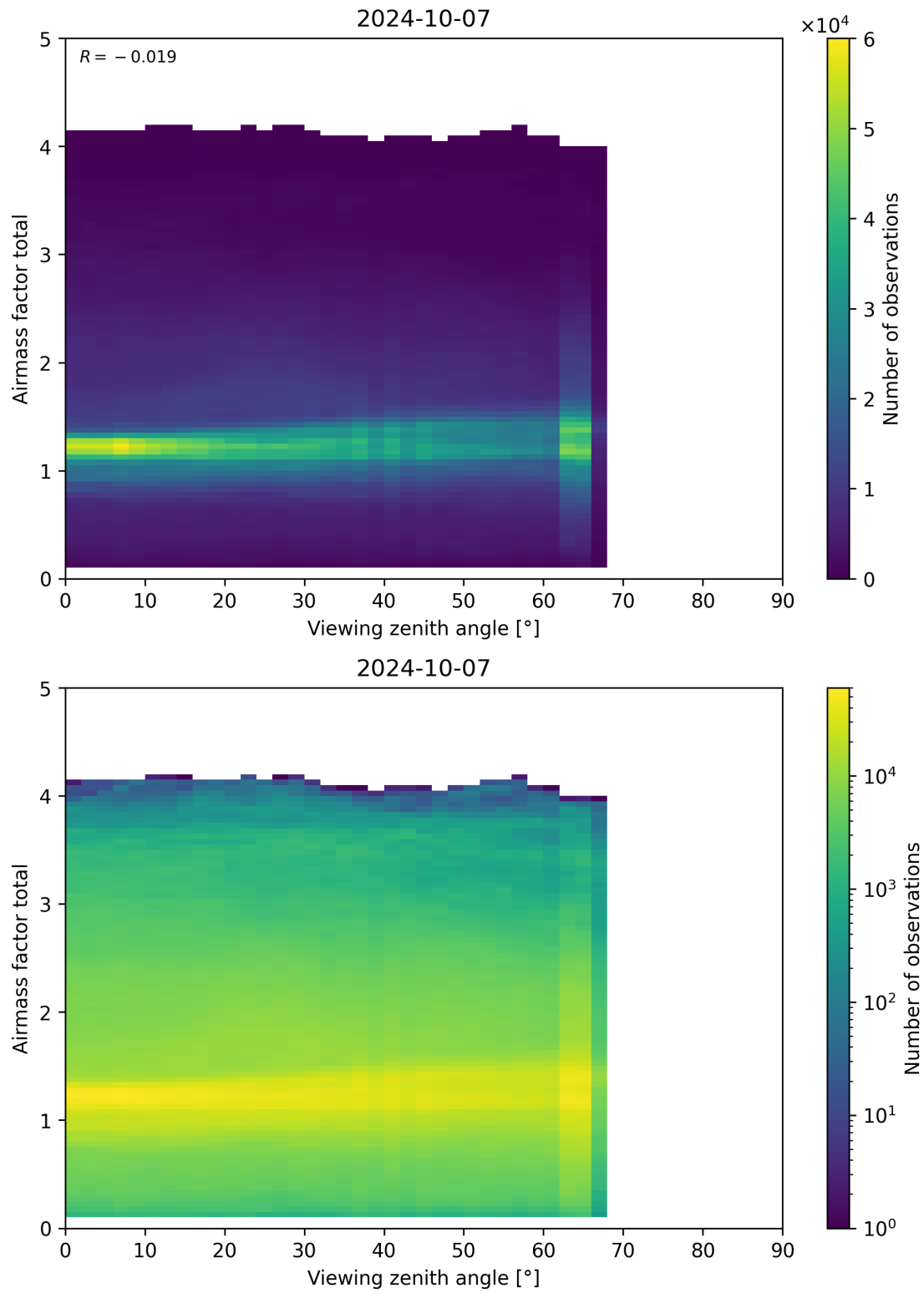
Figure 190: Scatter density plot of “Viewing zenith angle” against “Airmass factor total” for 2024-10-06 to 2024-10-08.
