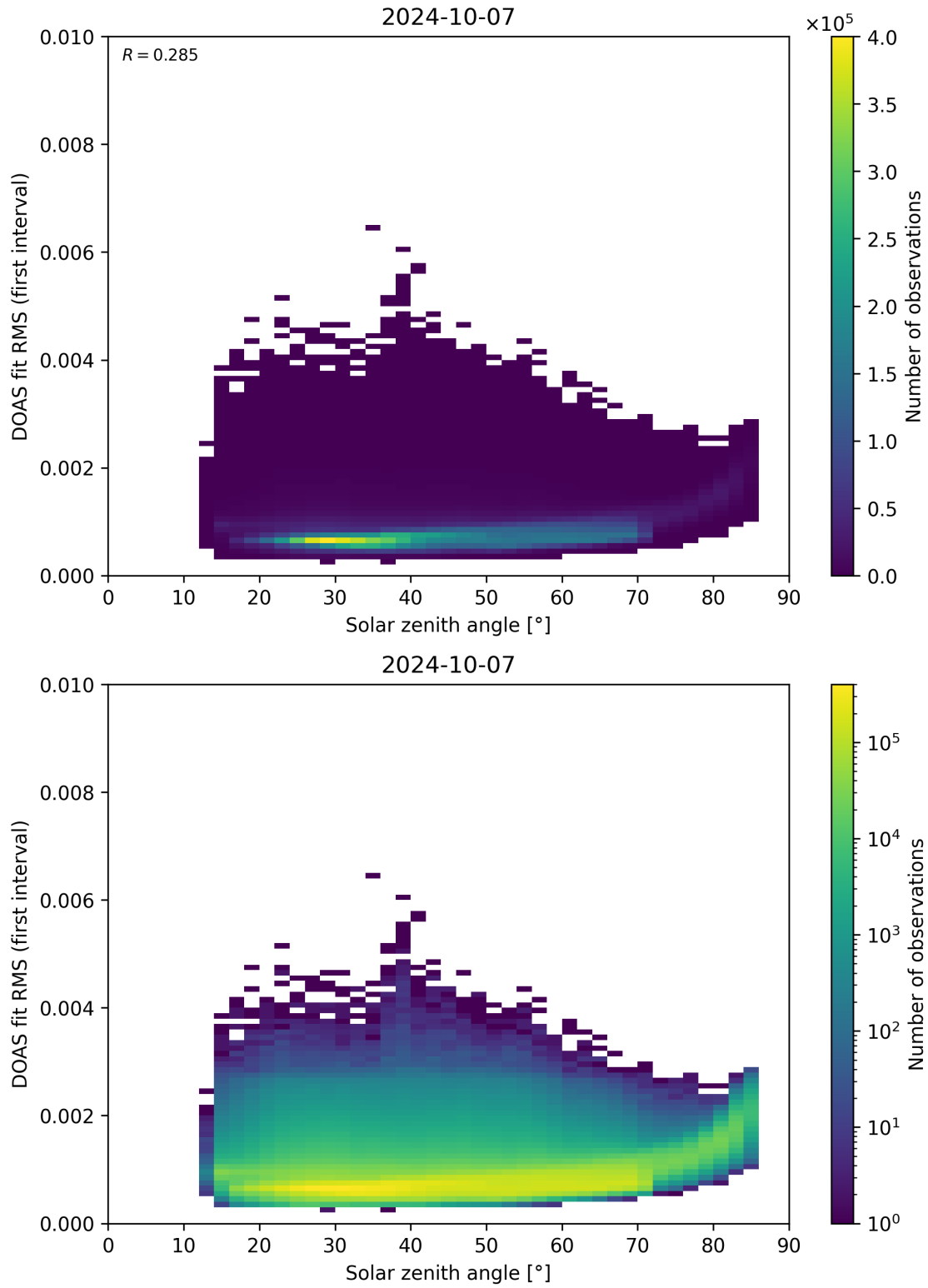
Figure 167: Scatter density plot of “Solar zenith angle” against “DOAS fit RMS (first interval)” for 2024-10-06 to 2024-10-08.
