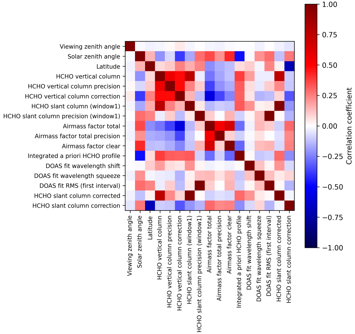
Figure 2: Map of correlation matrix for 2024-10-06 to 2024-10-08.
