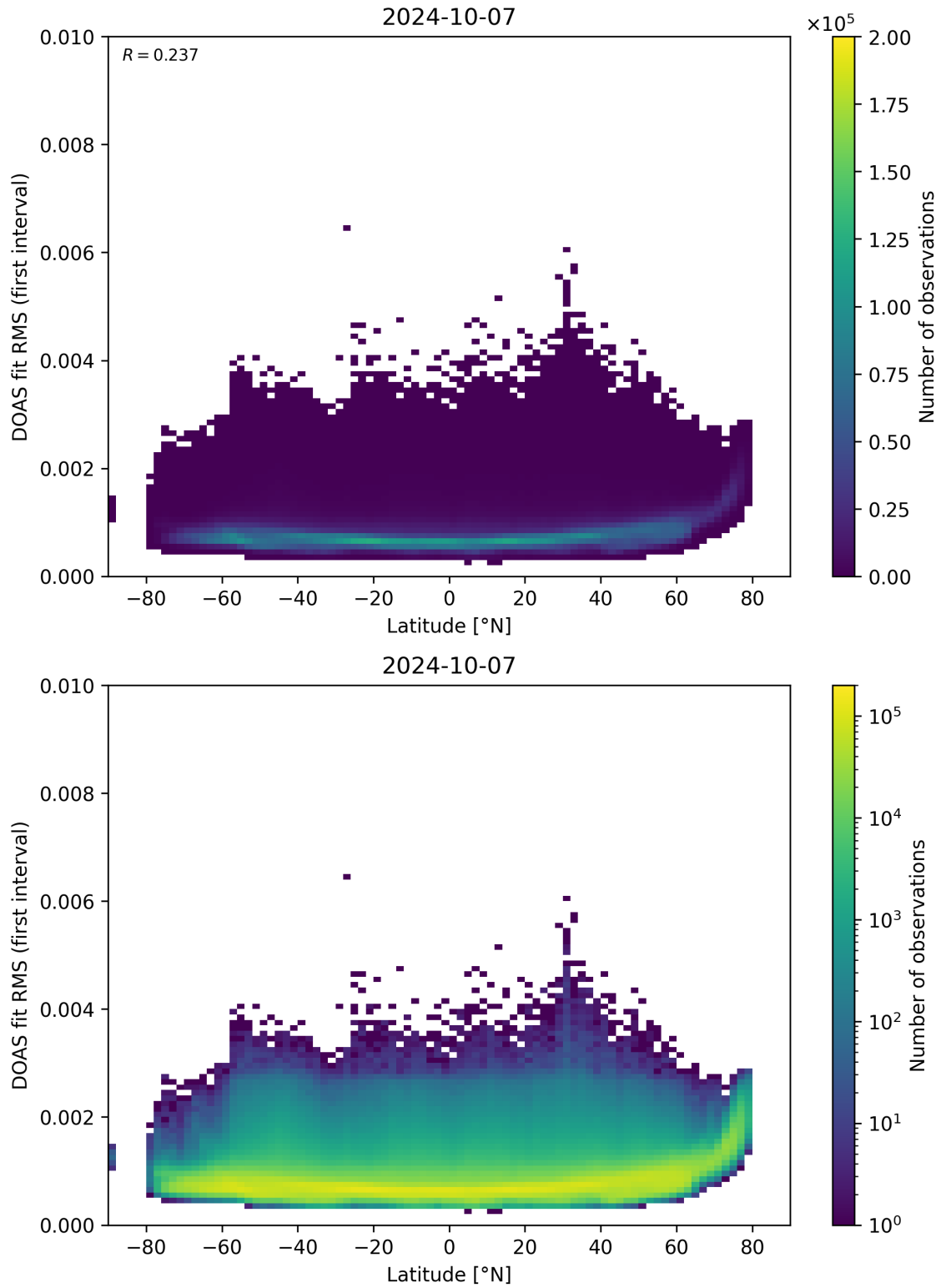
Figure 153: Scatter density plot of “Latitude” against “DOAS fit RMS (first interval)” for 2024-10-06 to 2024-10-08.
