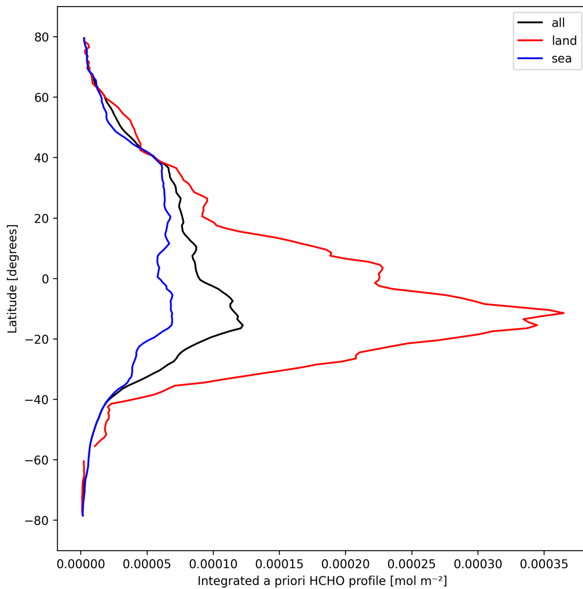
Figure 29: Zonal average of “Integrated a priori HCHO profile” for 2024-10-06 to 2024-10-08.
