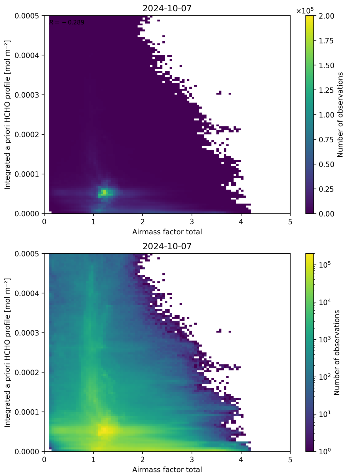
Figure 104: Scatter density plot of “Airmass factor total” against “Integrated a priori HCHO profile” for 2024-10-06 to 2024-10-08.
