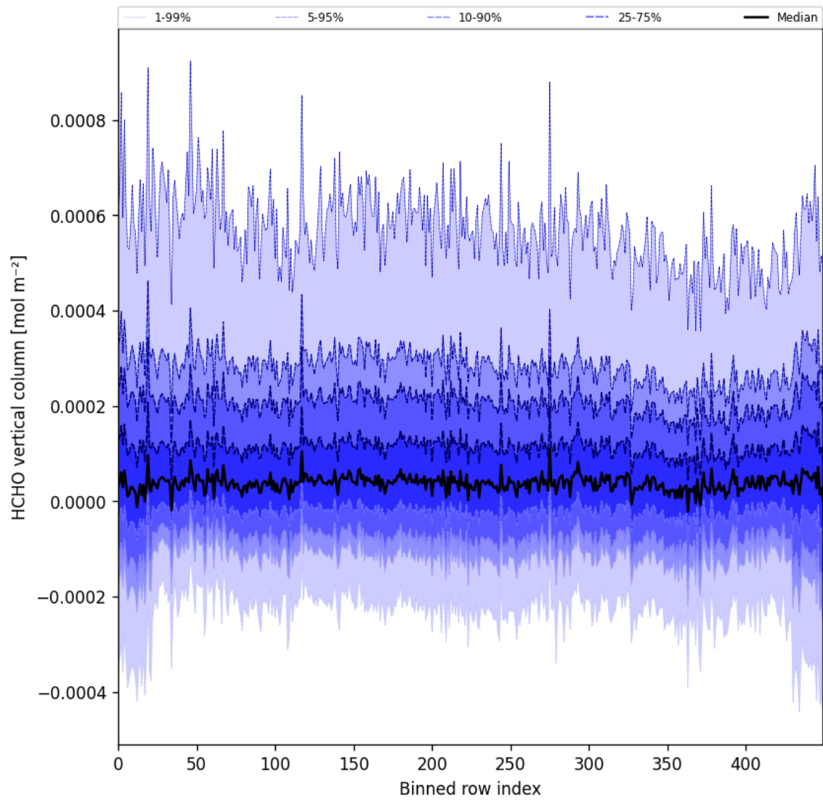
Figure 49: Along track statistics of “HCHO vertical column” for 2024-10-06 to 2024-10-08
