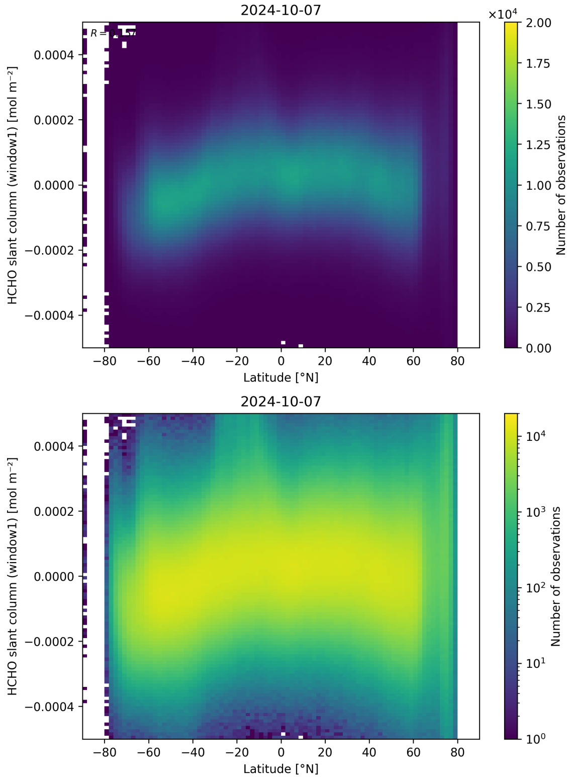
Figure 159: Scatter density plot of “Latitude” against “HCHO slant column (window1)” for 2024-10-06 to 2024-10-08.
