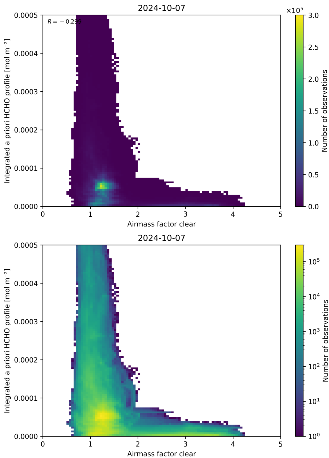
Figure 76: Scatter density plot of “Airmass factor clear” against “Integrated a priori HCHO profile” for 2024-10-06 to 2024-10-08.
