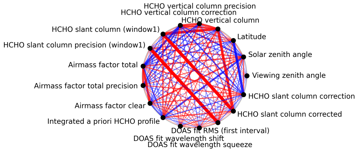
Figure 1: Map of correlation graph for 2024-10-06 to 2024-10-08.
