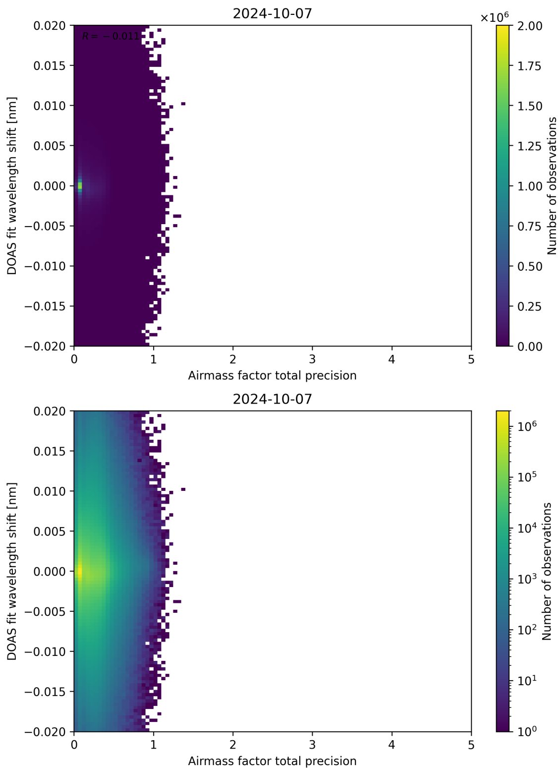
Figure 106: Scatter density plot of “Airmass factor total precision” against “DOAS fit wavelength shift” for 2024-10-06 to 2024-10-08.
