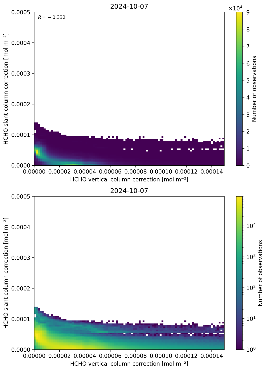
Figure 117: Scatter density plot of “HCHO vertical column correction” against “HCHO slant column correction” for 2024-10-06 to 2024-10-08.
