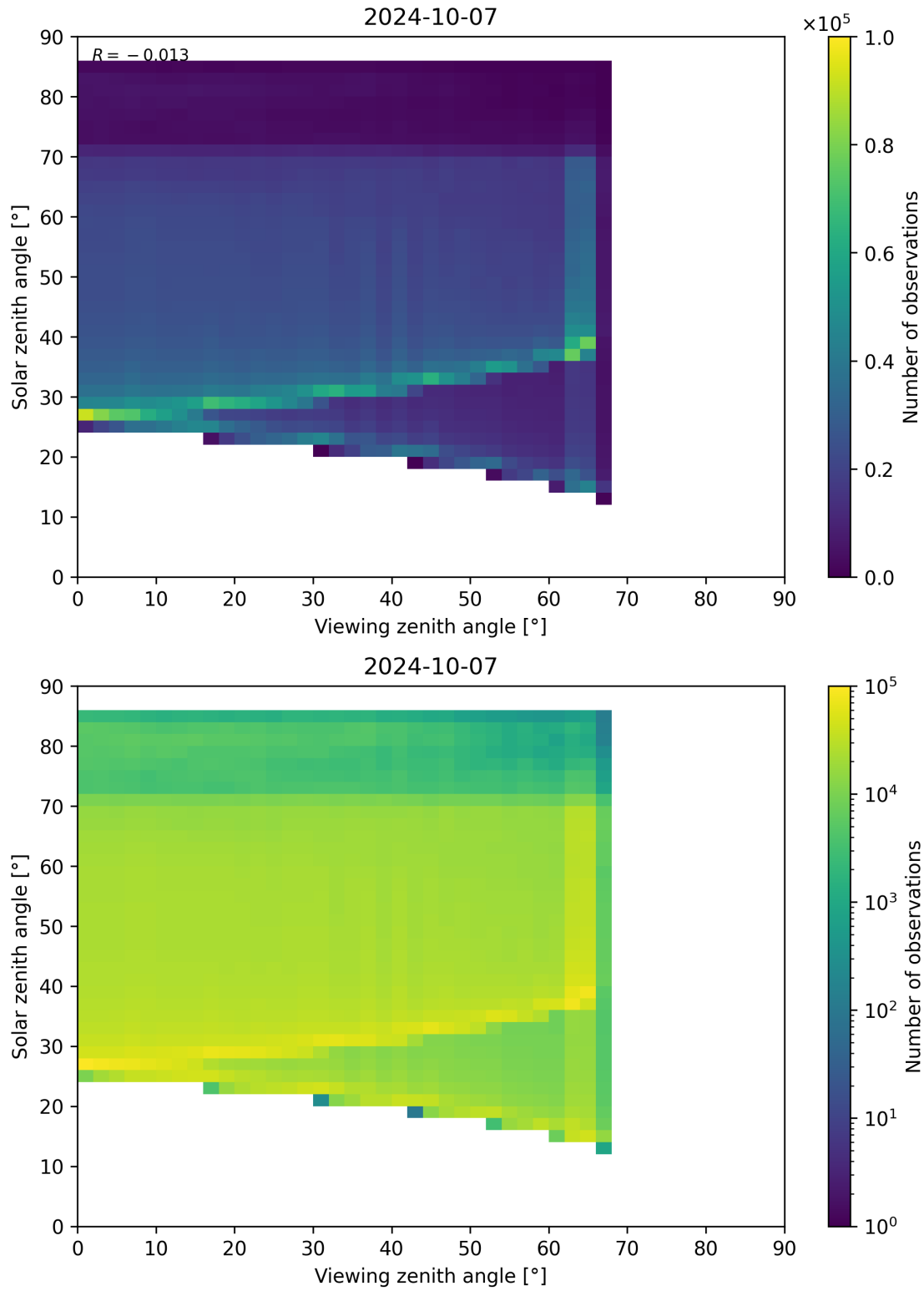
Figure 197: Scatter density plot of “Viewing zenith angle” against “Solar zenith angle” for 2024-10-06 to 2024-10-08.
