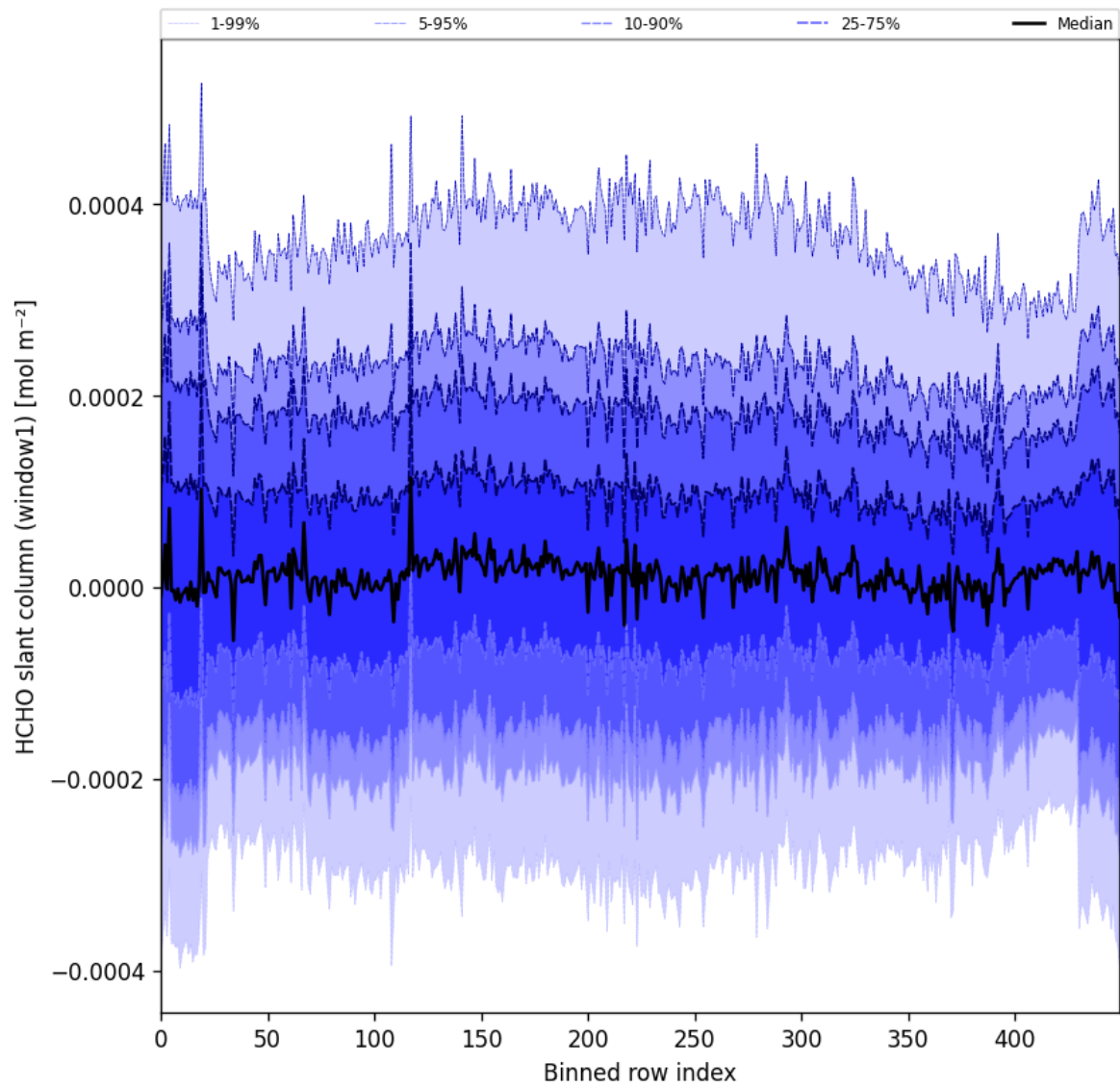
Figure 52: Along track statistics of “HCHO slant column (window1)” for 2024-10-06 to 2024-10-08
