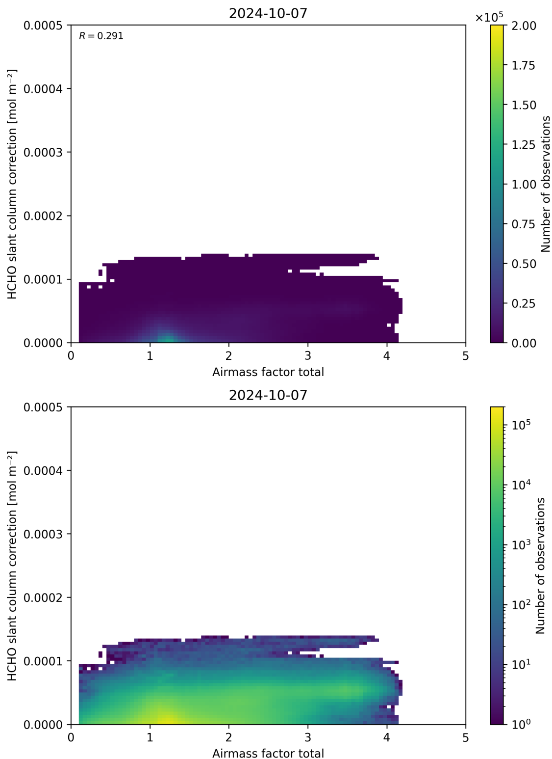
Figure 102: Scatter density plot of “Airmass factor total” against “HCHO slant column correction” for 2024-10-06 to 2024-10-08.
