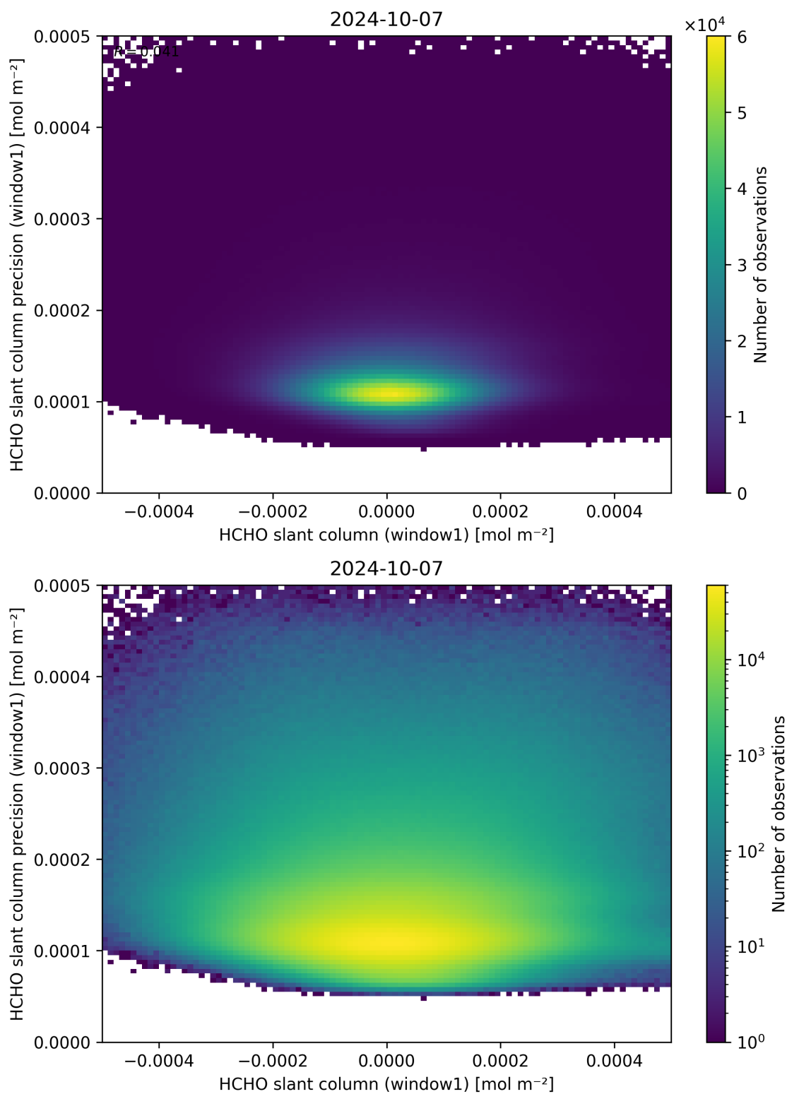
Figure 84: Scatter density plot of “HCHO slant column (window1)” against “HCHO slant column precision (window1)” for 2024-10-06 to 2024-10-08.
