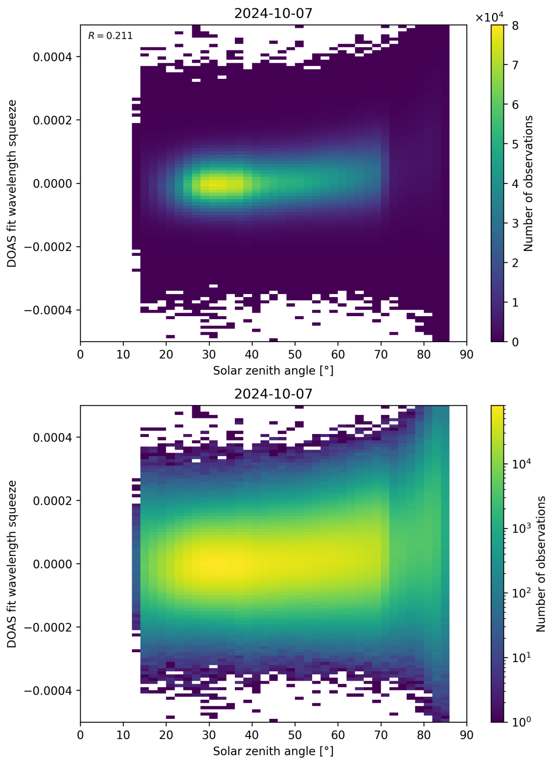
Figure 169: Scatter density plot of “Solar zenith angle” against “DOAS fit wavelength squeeze” for 2024-10-06 to 2024-10-08.
