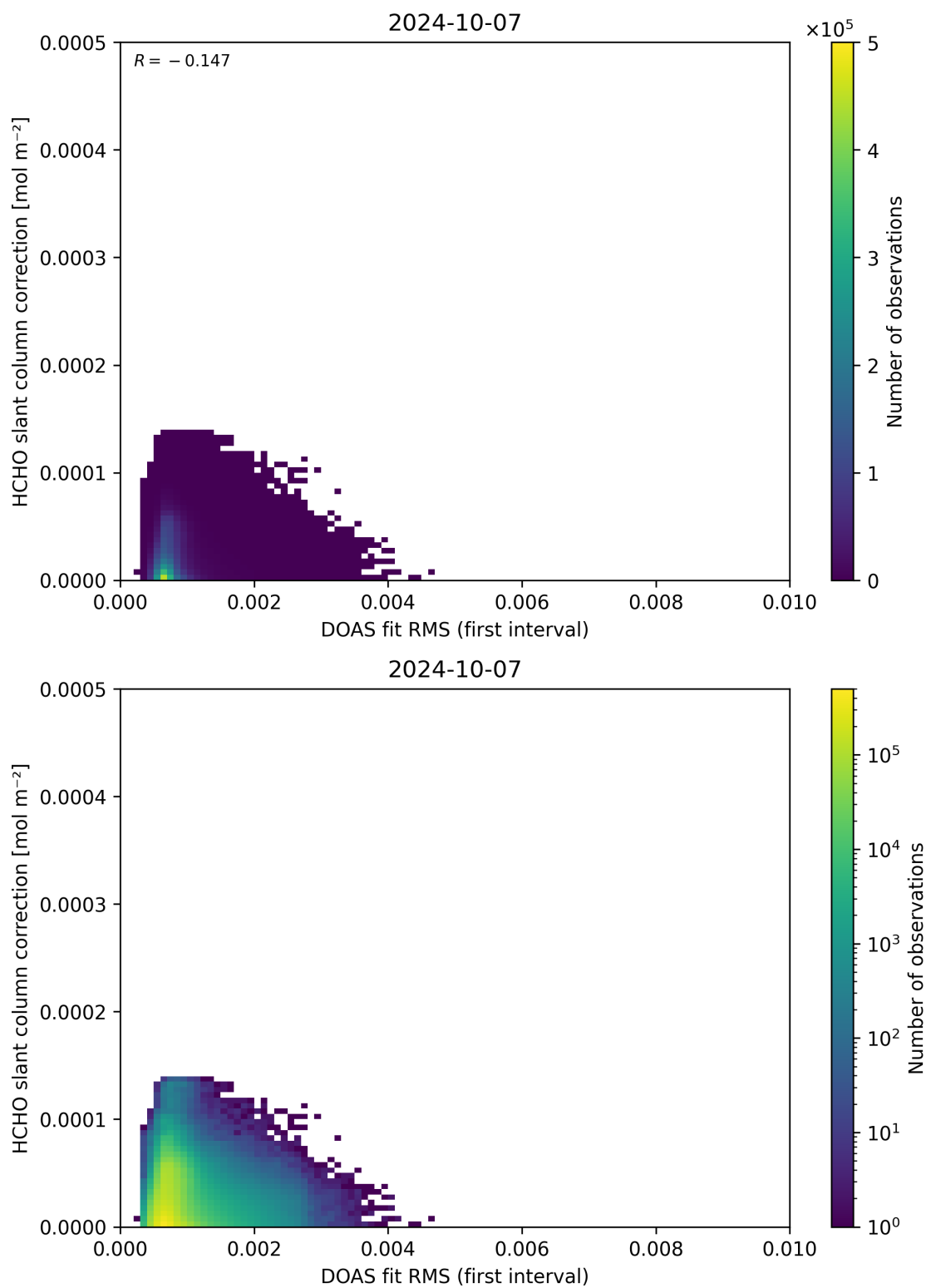
Figure 63: Scatter density plot of “DOAS fit RMS (first interval)” against “HCHO slant column correction” for 2024-10-06 to 2024-10-08.
