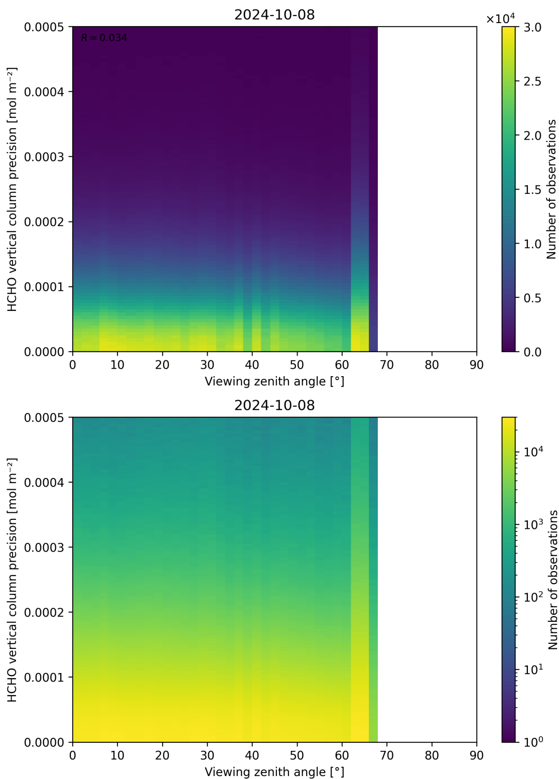
Figure 194: Scatter density plot of “Viewing zenith angle” against “HCHO vertical column precision” for 2024-10-08 to 2024-10-09.
