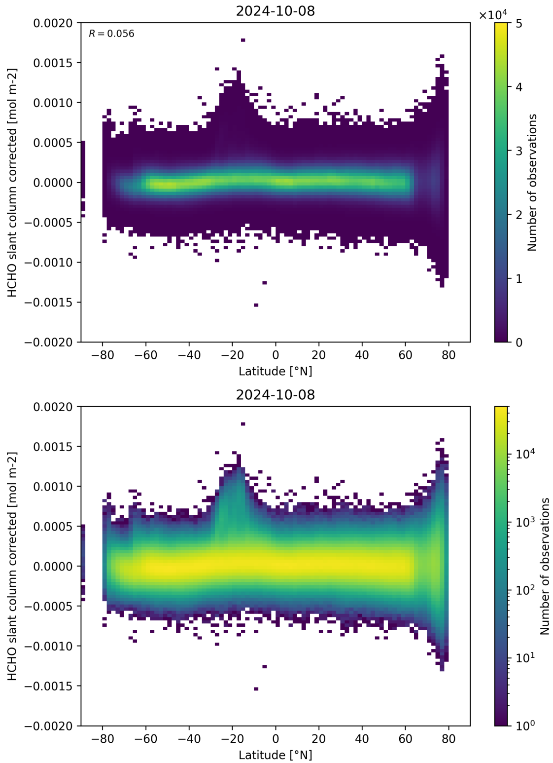
Figure 157: Scatter density plot of “Latitude” against “HCHO slant column corrected” for 2024-10-08 to 2024-10-09.
