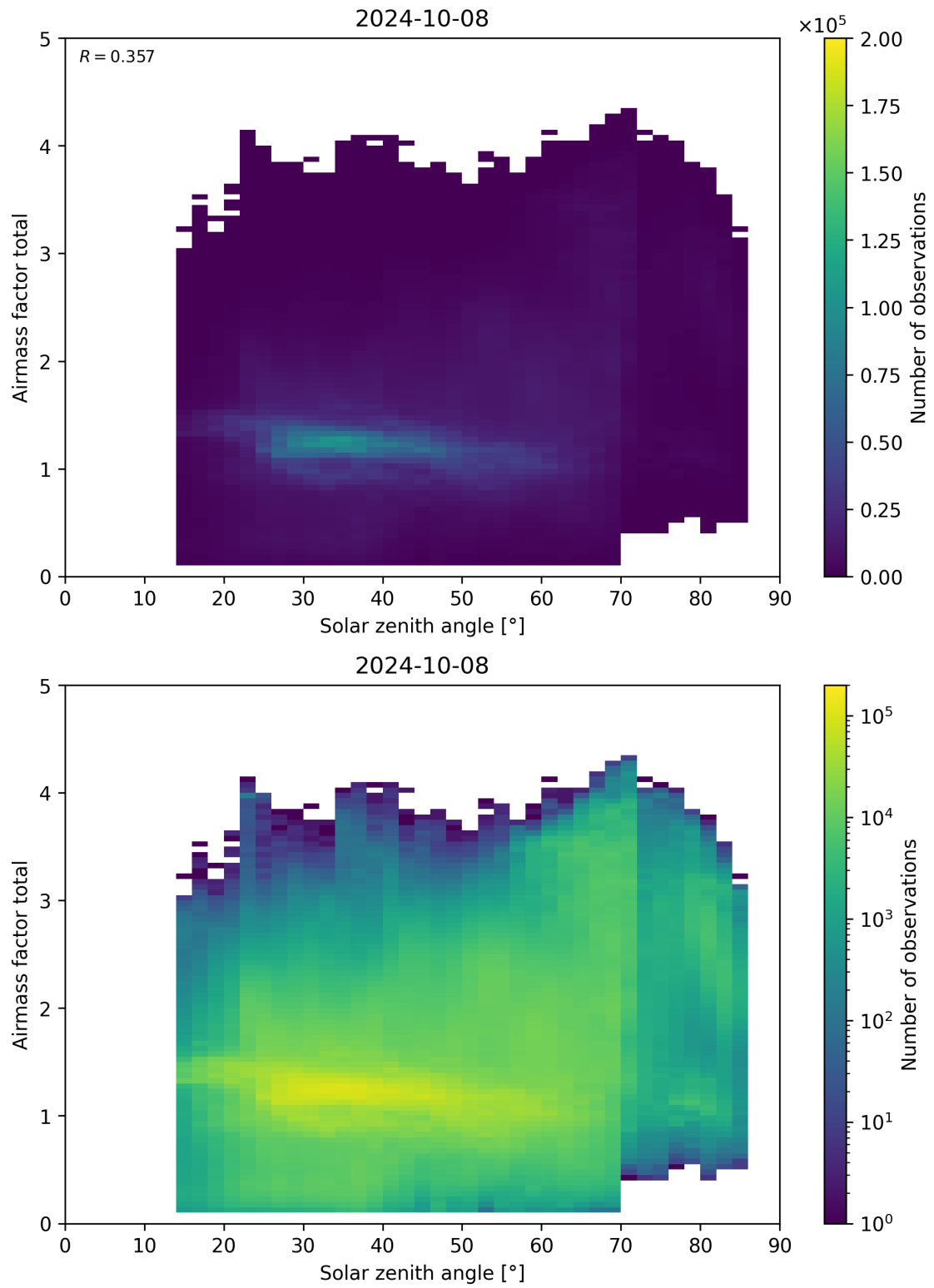
Figure 175: Scatter density plot of “Solar zenith angle” against “Airmass factor total” for 2024-10-08 to 2024-10-09.
