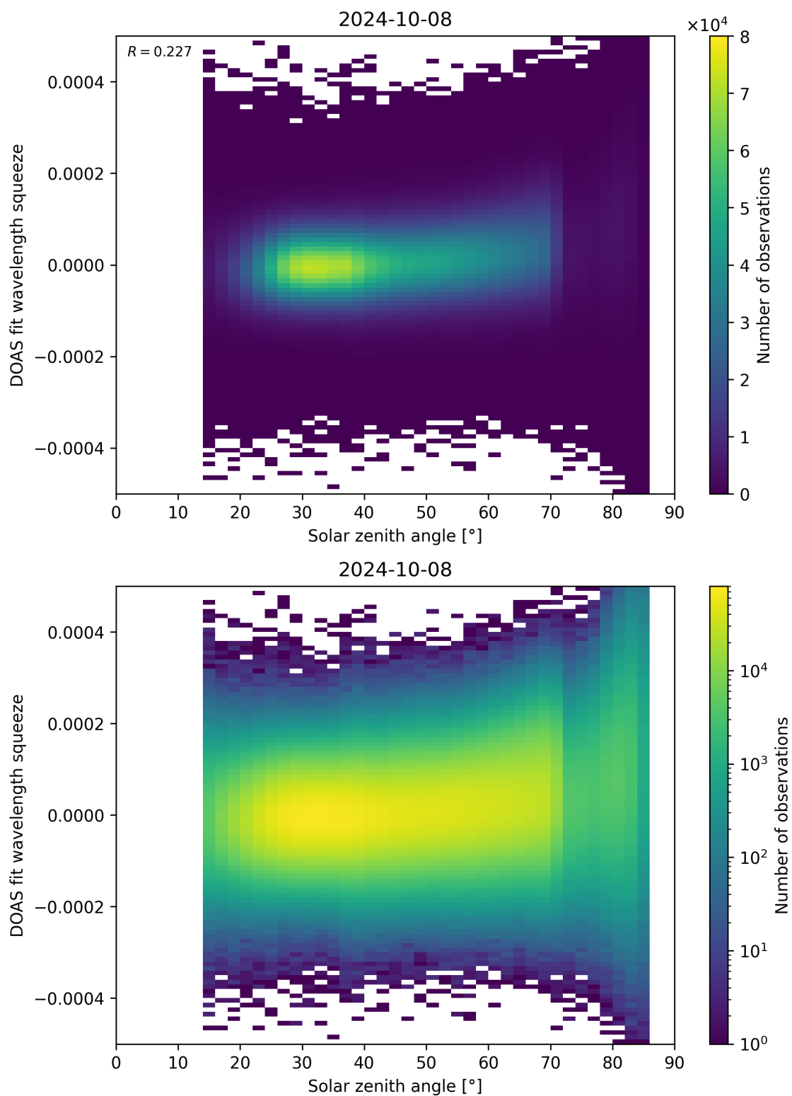
Figure 169: Scatter density plot of “Solar zenith angle” against “DOAS fit wavelength squeeze” for 2024-10-08 to 2024-10-09.
