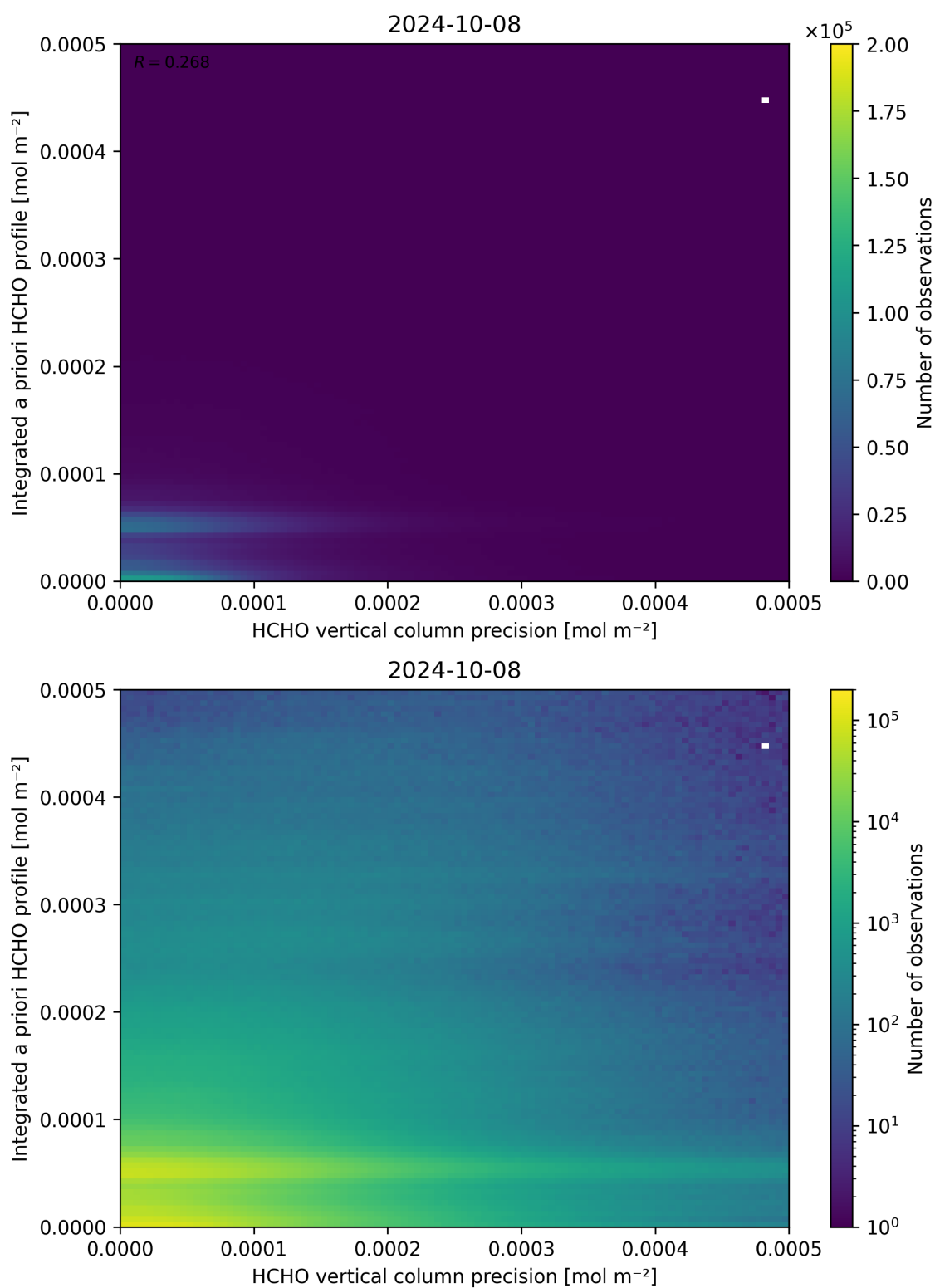
Figure 147: Scatter density plot of “HCHO vertical column precision” against “Integrated a priori HCHO profile” for 2024-10-08 to 2024-10-09.
