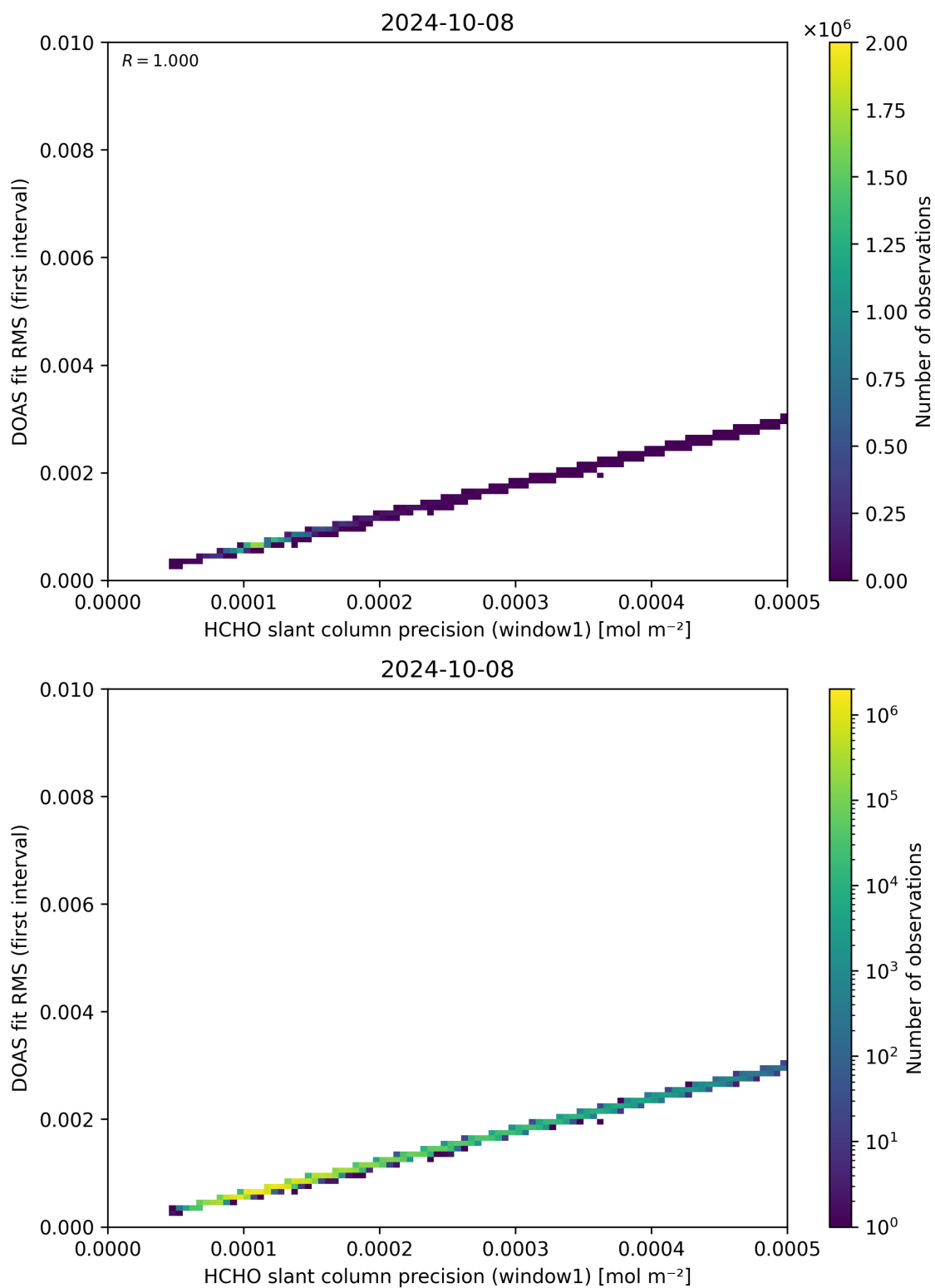
Figure 88: Scatter density plot of “HCHO slant column precision (window1)” against “DOAS fit RMS (first interval)” for 2024-10-08 to 2024-10-09.
