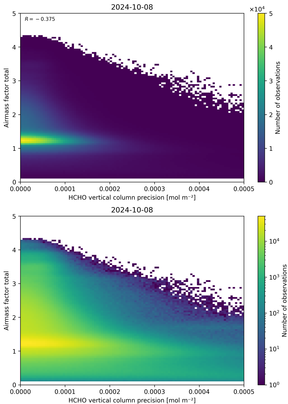
Figure 144: Scatter density plot of “HCHO vertical column precision” against “Airmass factor total” for 2024-10-08 to 2024-10-09.
