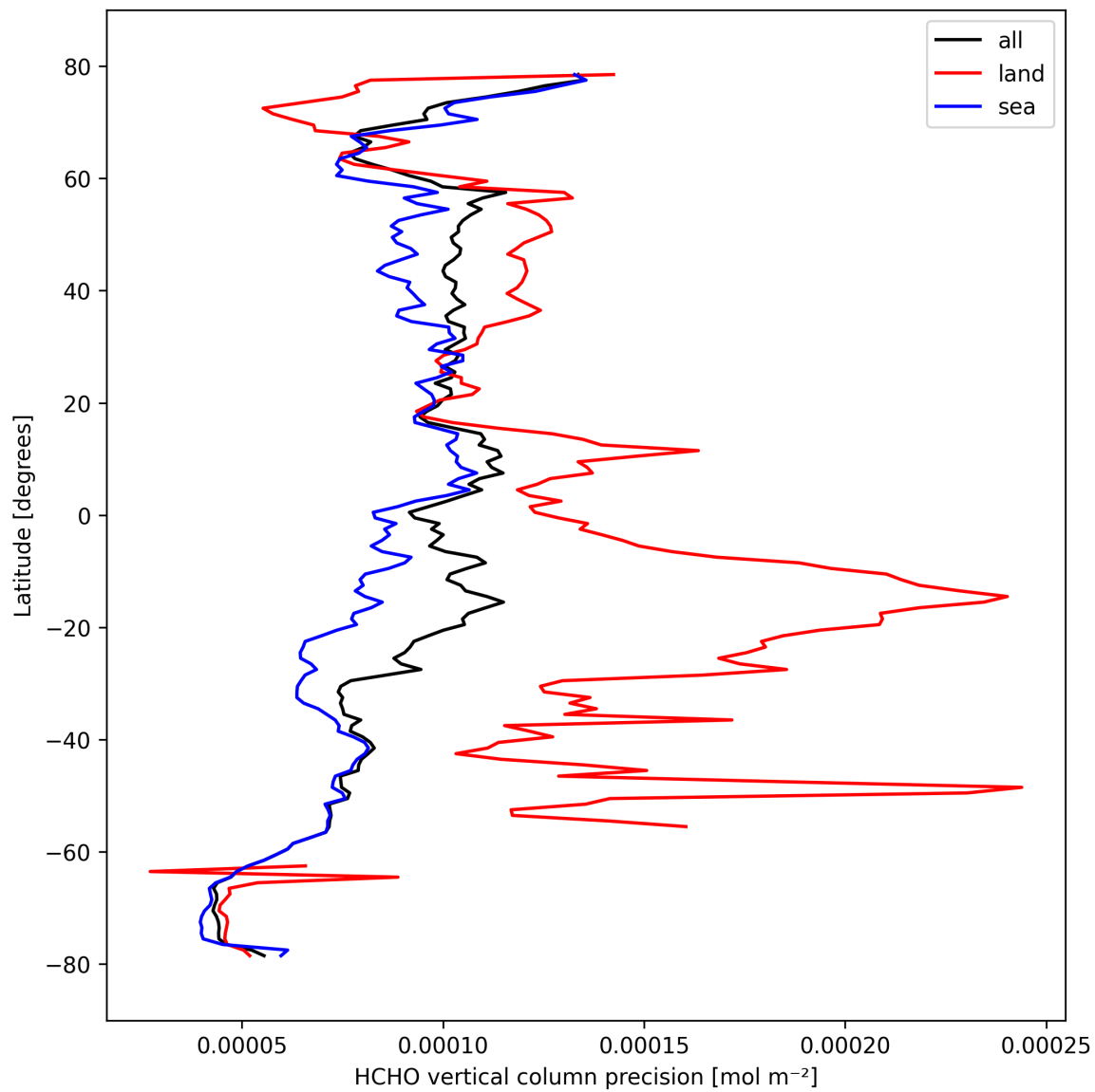
Figure 22: Zonal average of “HCHO vertical column precision” for 2024-10-08 to 2024-10-09.
