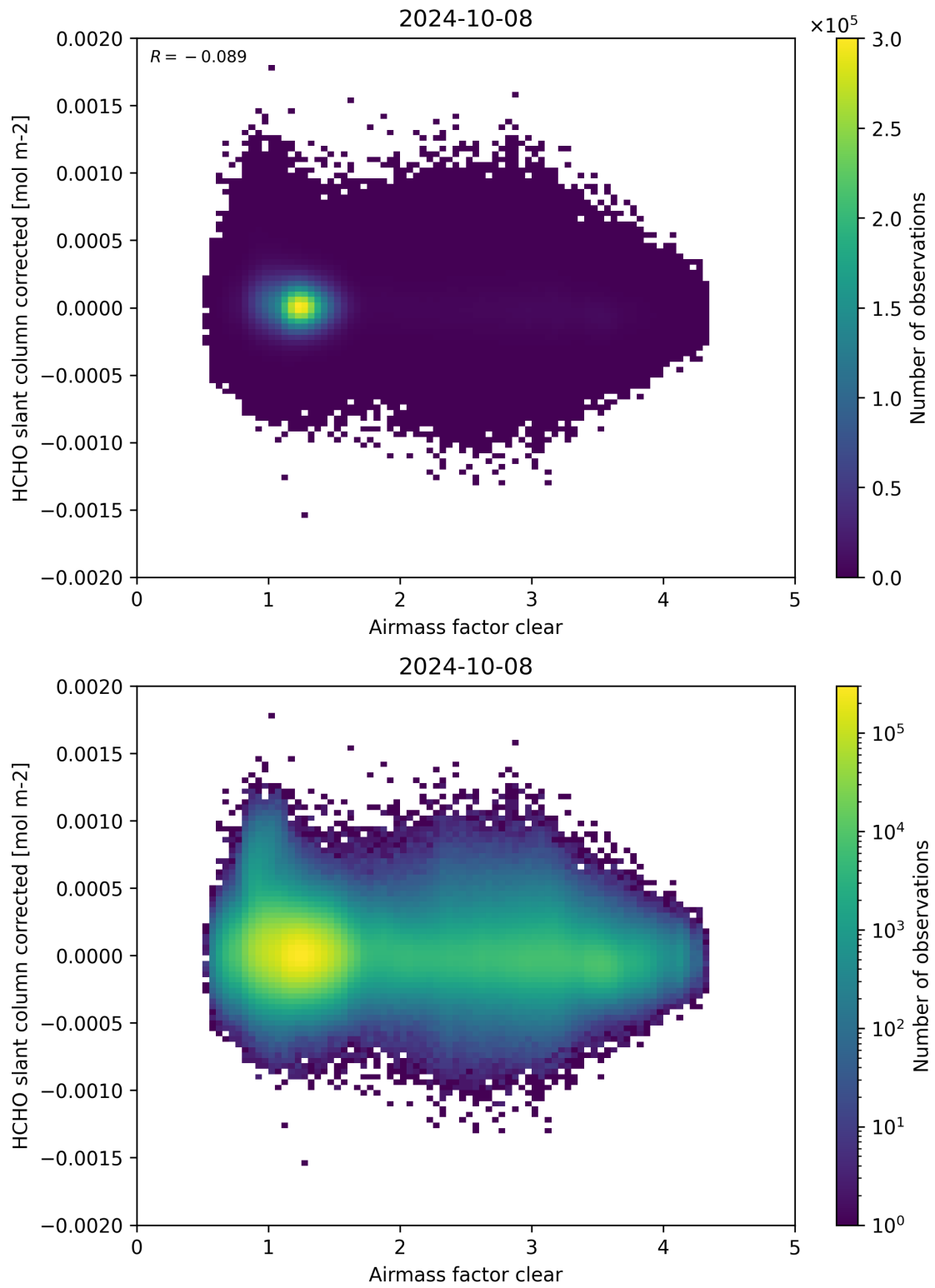
Figure 74: Scatter density plot of “Airmass factor clear” against “HCHO slant column corrected” for 2024-10-08 to 2024-10-09.
