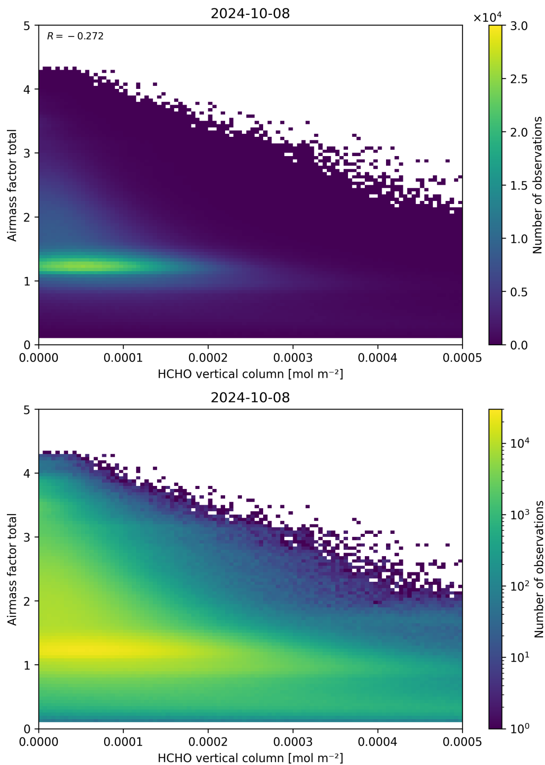
Figure 131: Scatter density plot of “HCHO vertical column” against “Airmass factor total” for 2024-10-08 to 2024-10-09.
