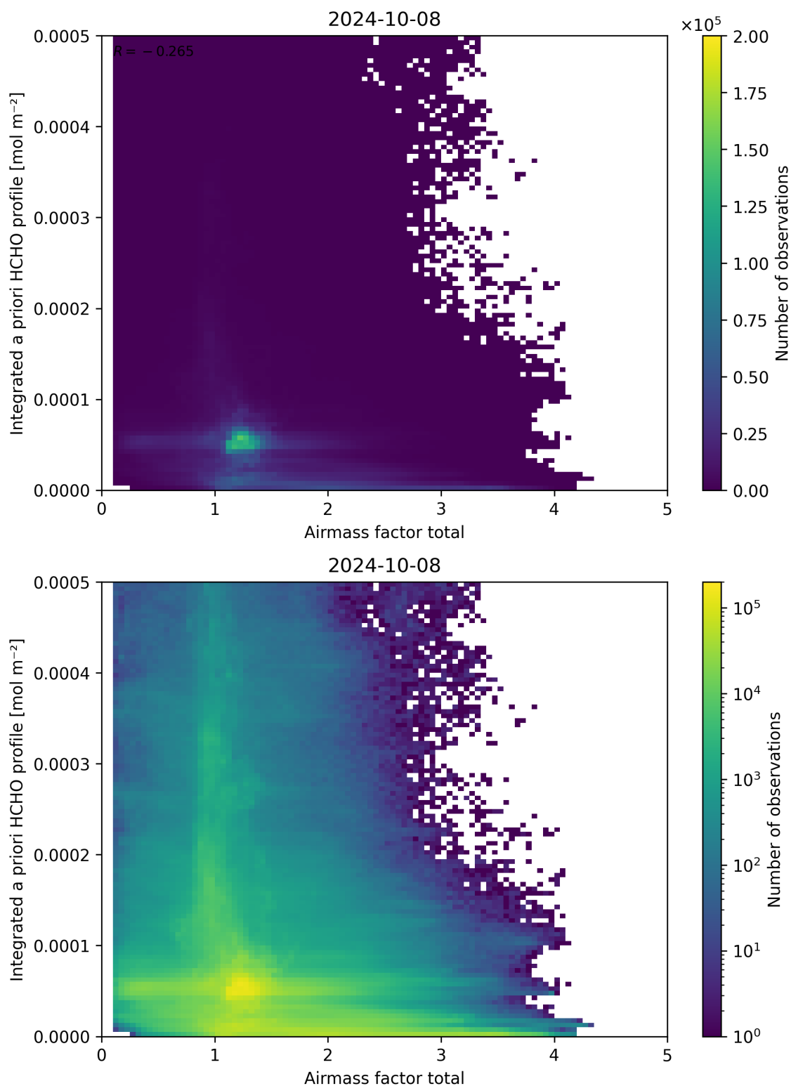
Figure 104: Scatter density plot of “Airmass factor total” against “Integrated a priori HCHO profile” for 2024-10-08 to 2024-10-09.
