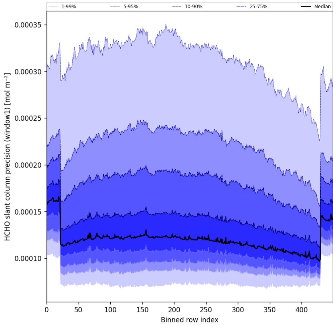
Figure 53: Along track statistics of “HCHO slant column precision (window1)” for 2024-10-08 to 2024-10-09
