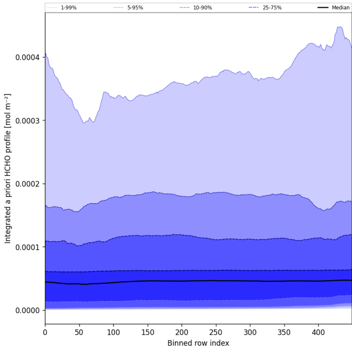
Figure 57: Along track statistics of “Integrated a priori HCHO profile” for 2024-10-08 to 2024-10-09
