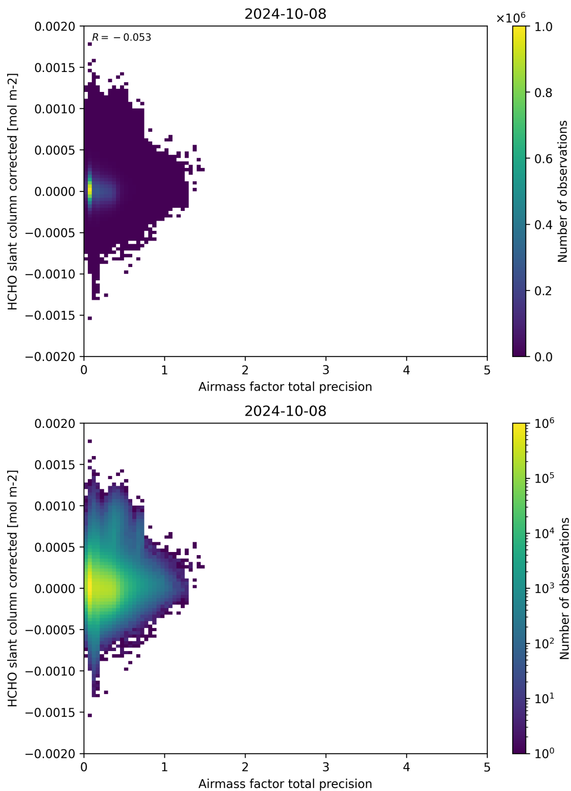
Figure 109: Scatter density plot of “Airmass factor total precision” against “HCHO slant column corrected” for 2024-10-08 to 2024-10-09.
