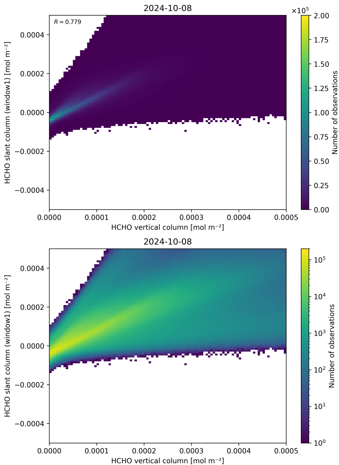
Figure 129: Scatter density plot of “HCHO vertical column” against “HCHO slant column (window1)” for 2024-10-08 to 2024-10-09.
