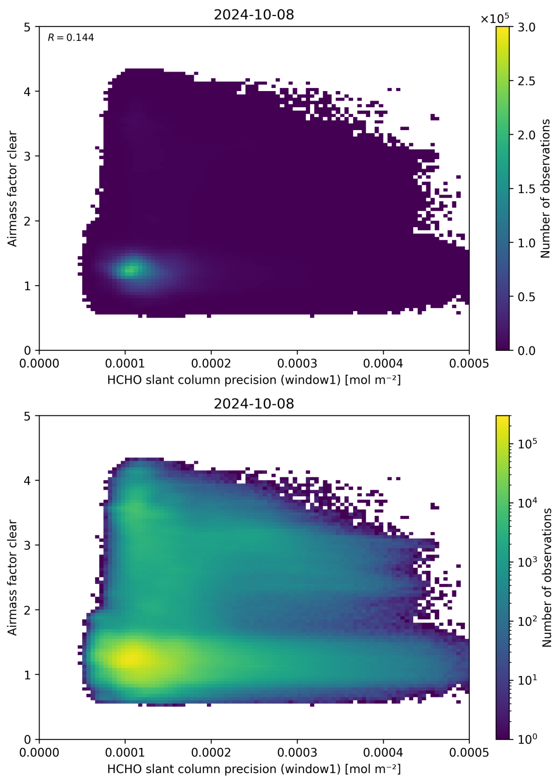
Figure 91: Scatter density plot of “HCHO slant column precision (window1)” against “Airmass factor clear” for 2024-10-08 to 2024-10-09.
