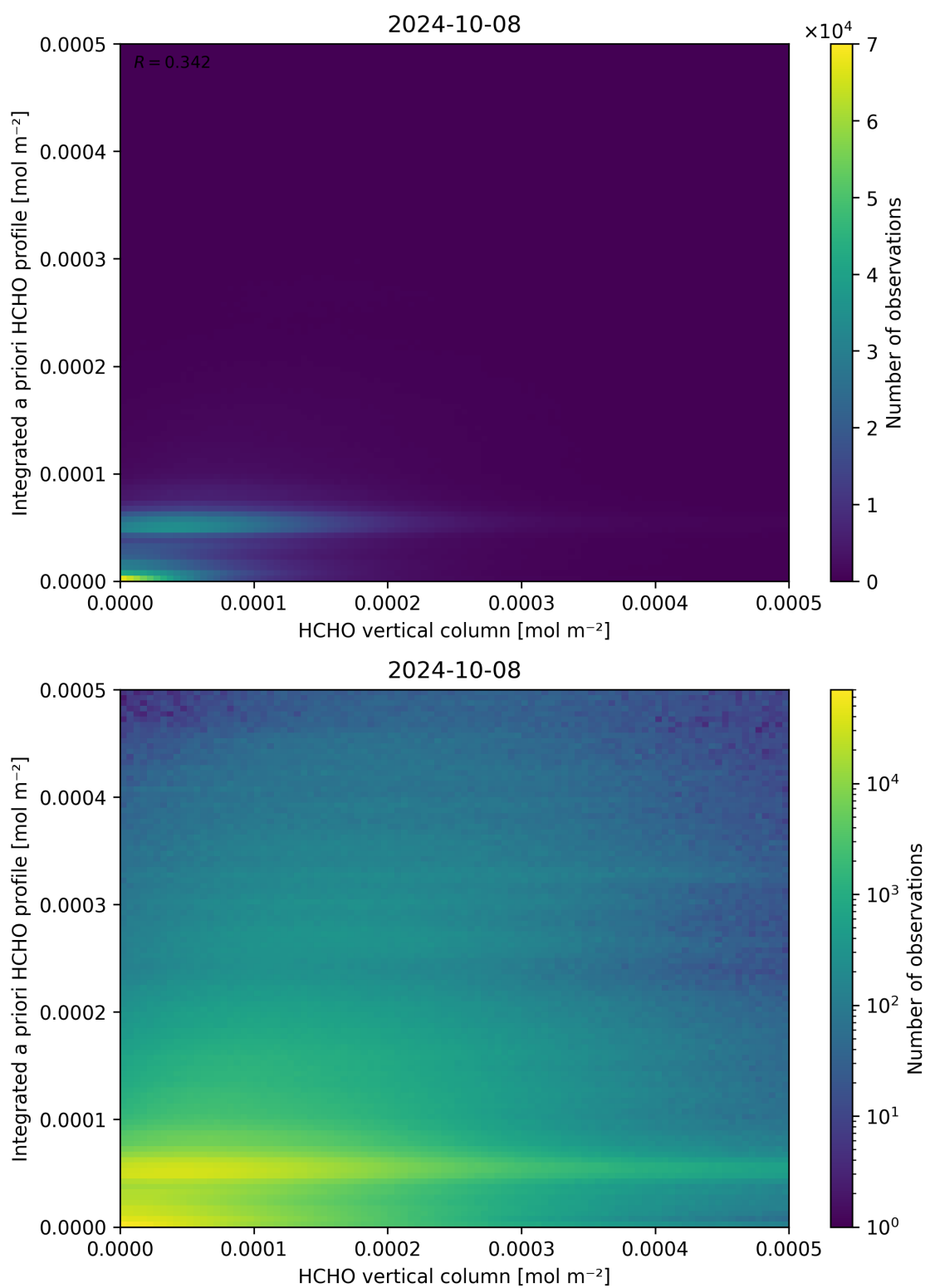
Figure 135: Scatter density plot of “HCHO vertical column” against “Integrated a priori HCHO profile” for 2024-10-08 to 2024-10-09.
