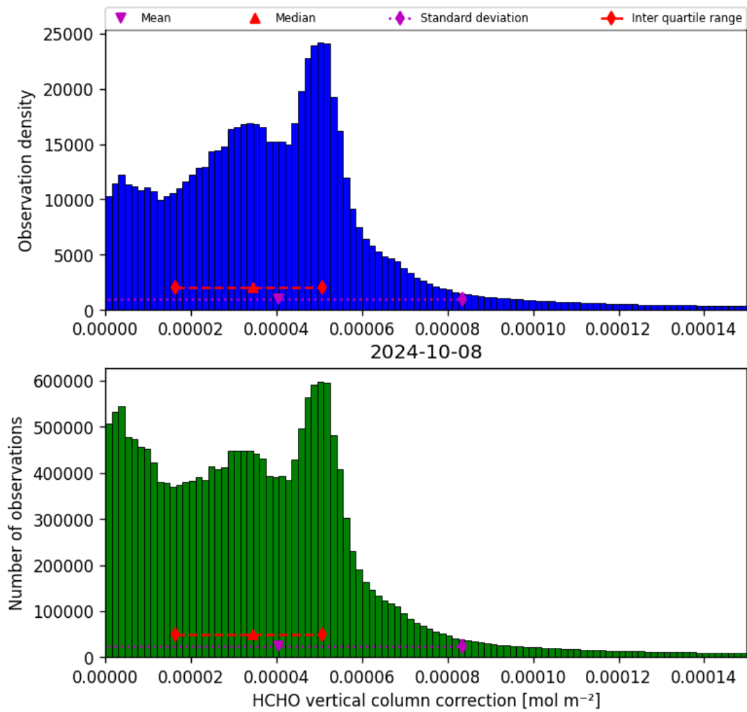
Figure 37: Histogram of “HCHO vertical column correction” for 2024-10-08 to 2024-10-09
