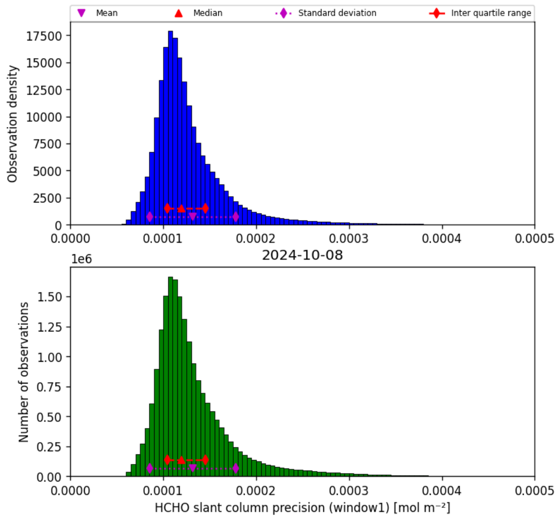
Figure 39: Histogram of “HCHO slant column precision (window1)” for 2024-10-08 to 2024-10-09
