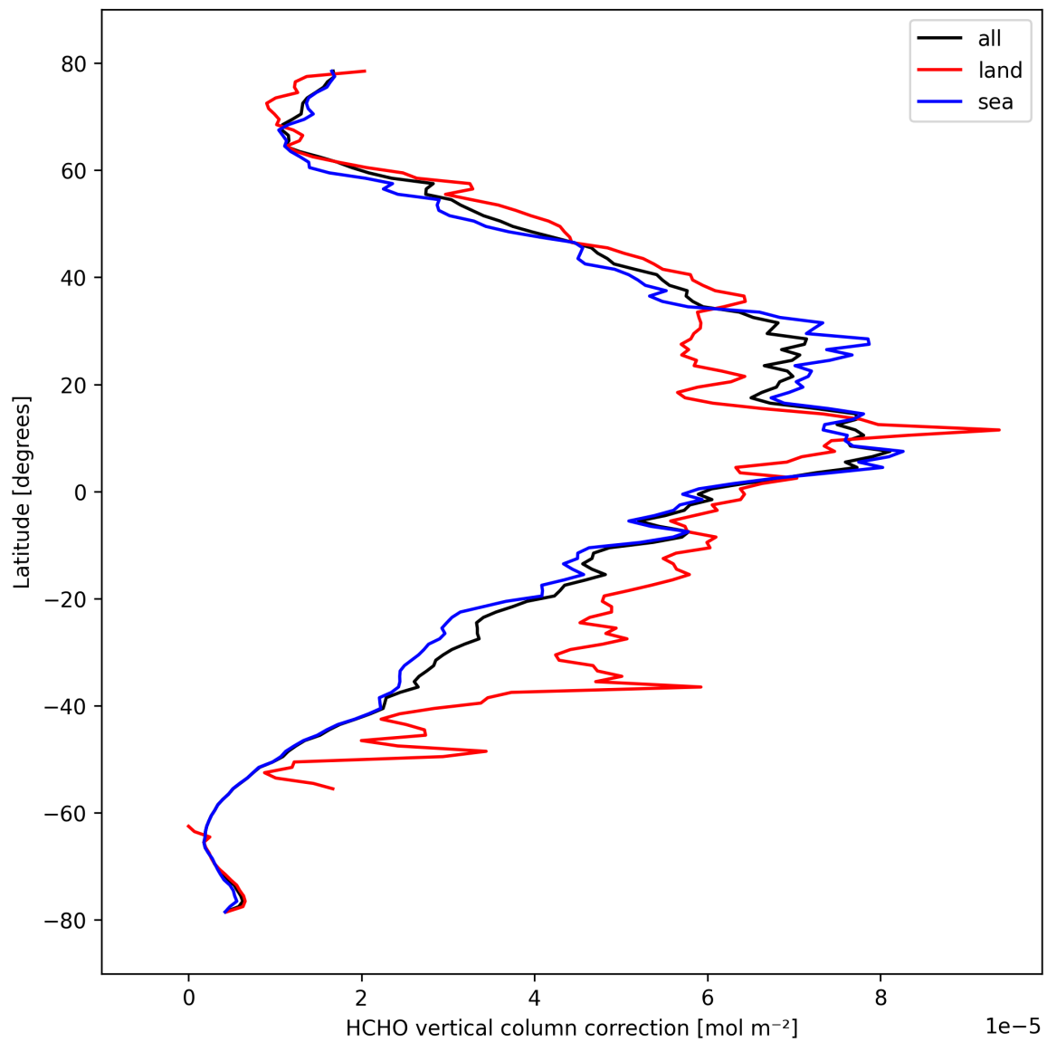
Figure 23: Zonal average of “HCHO vertical column correction” for 2024-10-08 to 2024-10-09.
