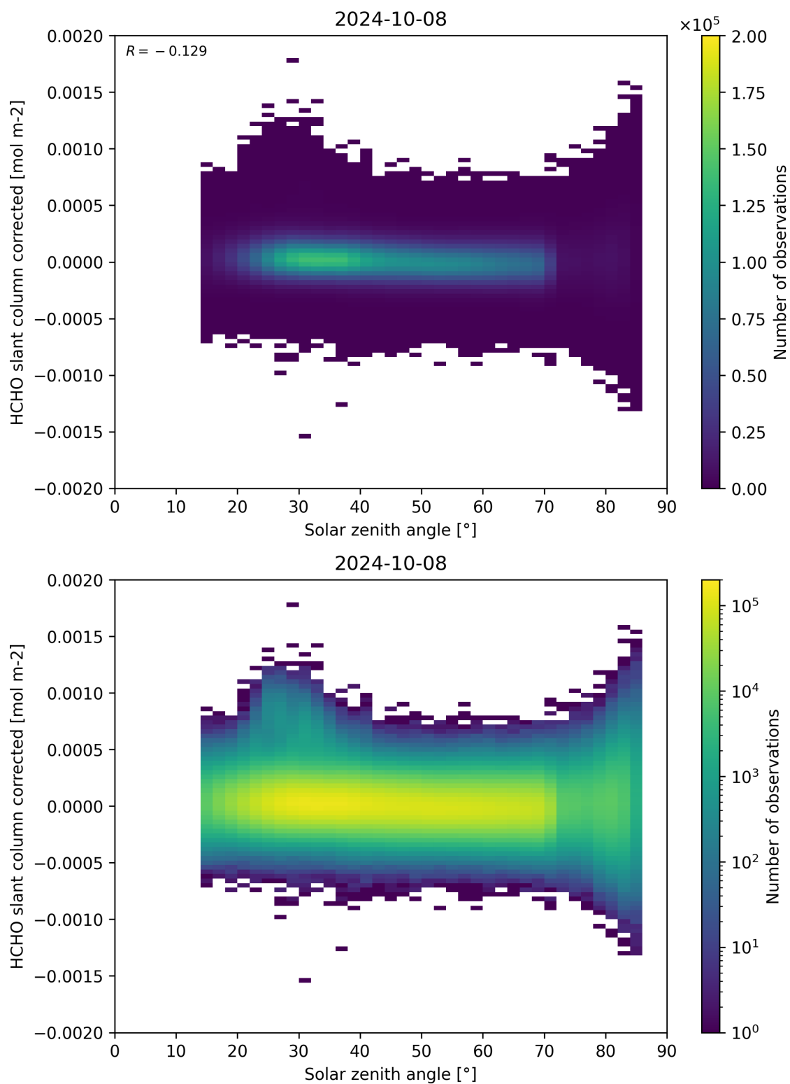
Figure 171: Scatter density plot of “Solar zenith angle” against “HCHO slant column corrected” for 2024-10-08 to 2024-10-09.
