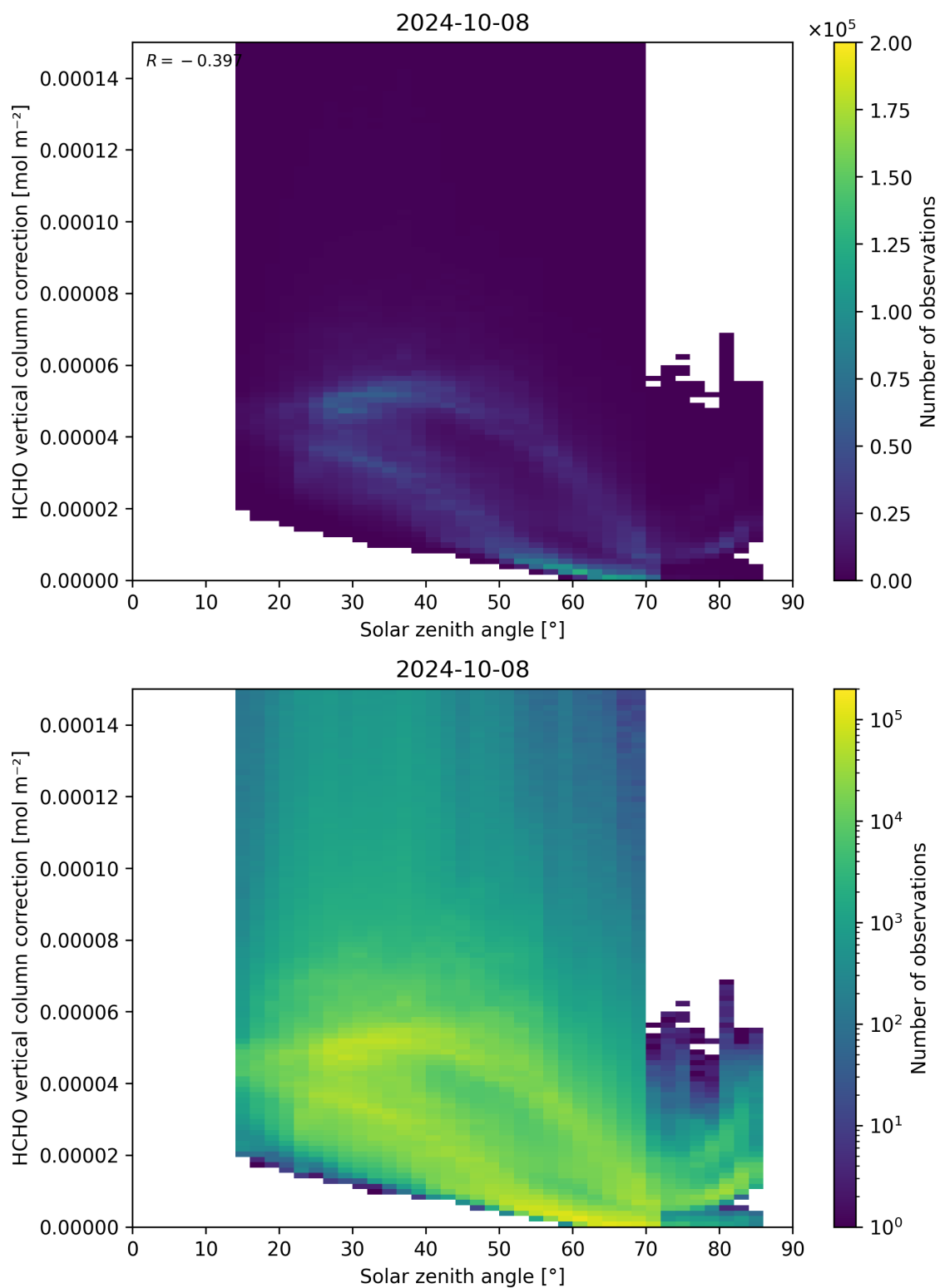
Figure 178: Scatter density plot of “Solar zenith angle” against “HCHO vertical column correction” for 2024-10-08 to 2024-10-09.
