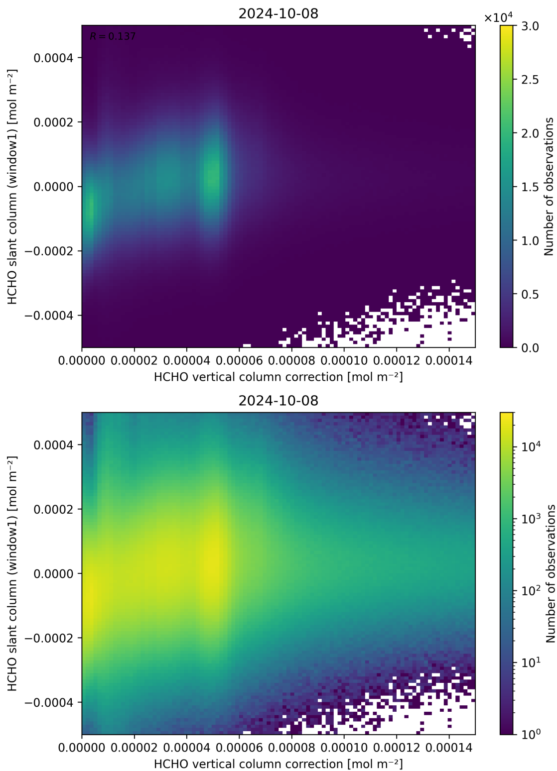
Figure 118: Scatter density plot of “HCHO vertical column correction” against “HCHO slant column (window1)” for 2024-10-08 to 2024-10-09.
