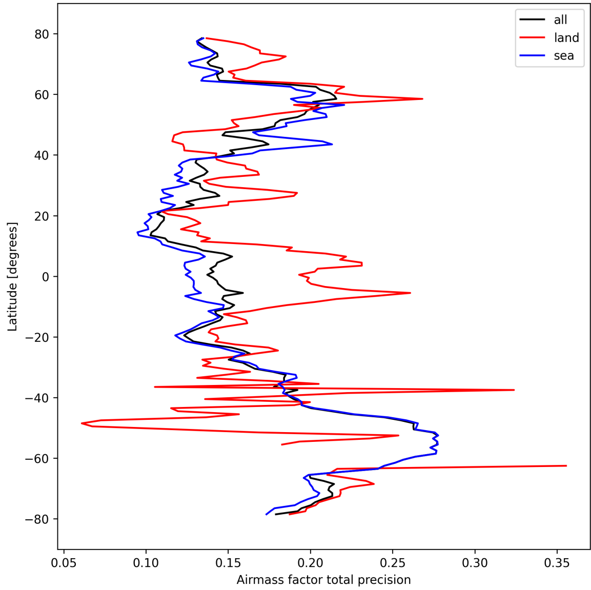
Figure 27: Zonal average of “Airmass factor total precision” for 2024-10-08 to 2024-10-09.
