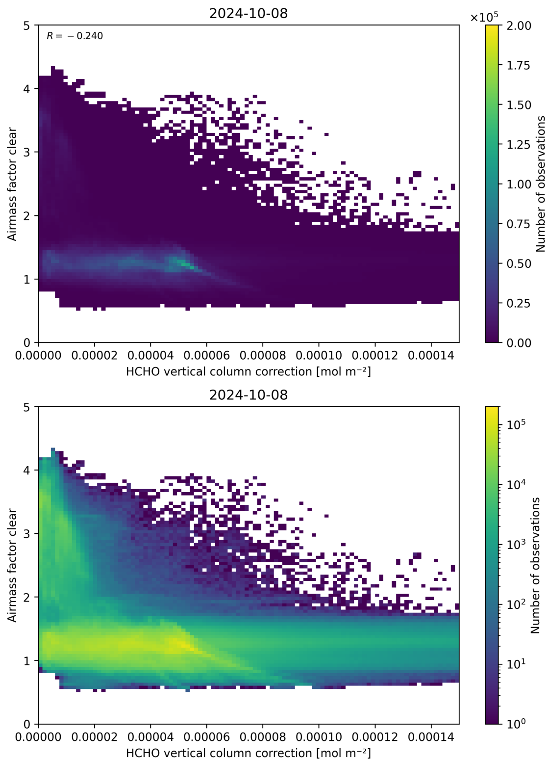
Figure 115: Scatter density plot of “HCHO vertical column correction” against “Airmass factor clear” for 2024-10-08 to 2024-10-09.
