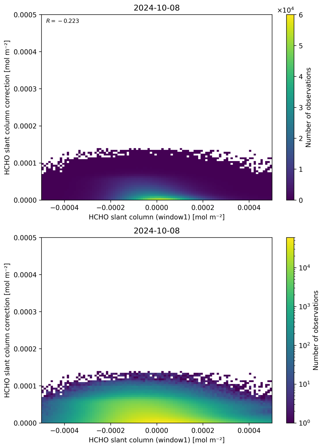
Figure 83: Scatter density plot of “HCHO slant column (window1)” against “HCHO slant column correction” for 2024-10-08 to 2024-10-09.
