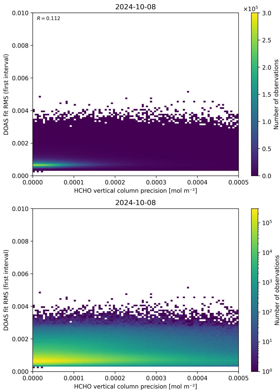
Figure 136: Scatter density plot of “HCHO vertical column precision” against “DOAS fit RMS (first interval)” for 2024-10-08 to 2024-10-09.
