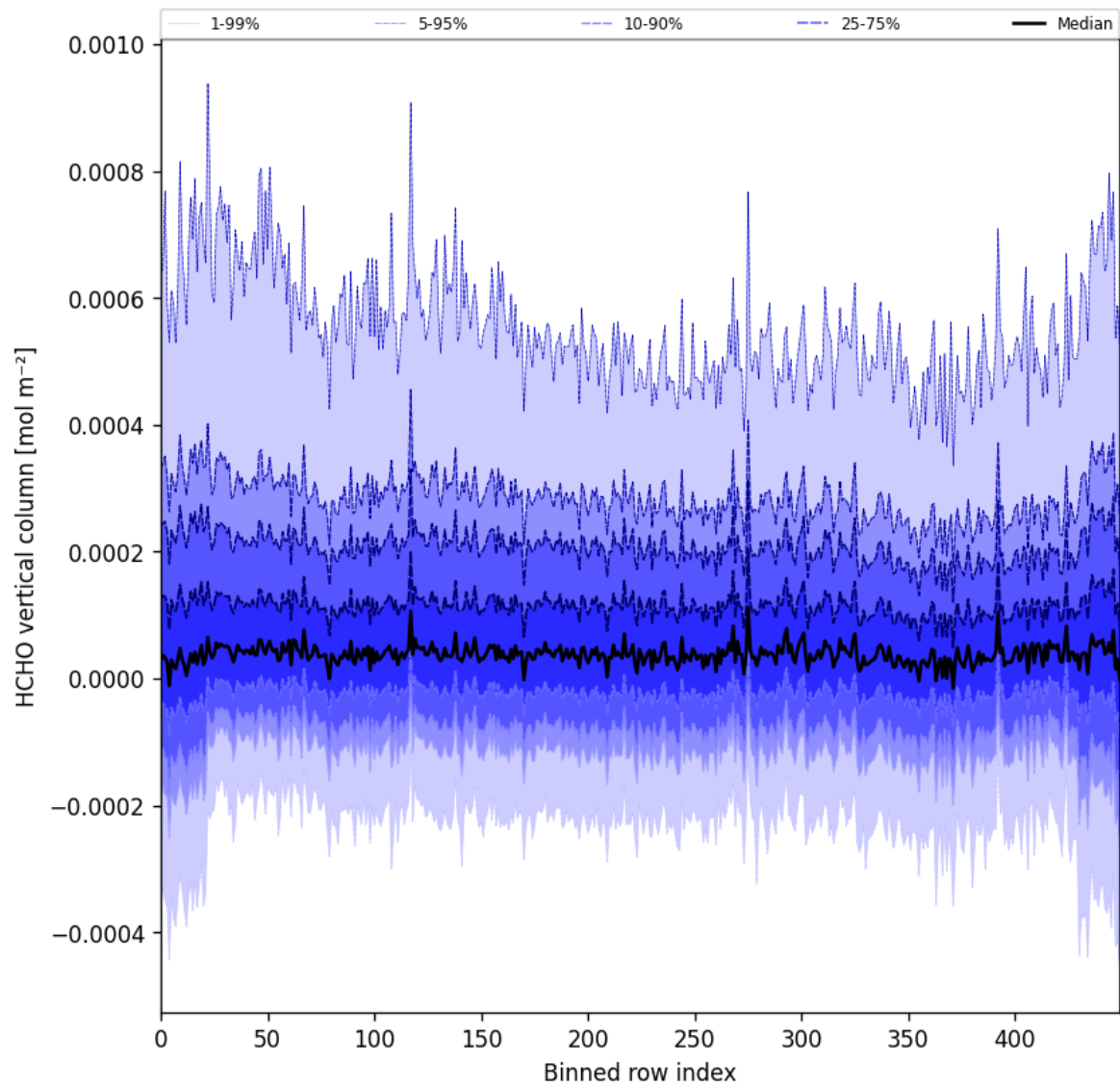
Figure 49: Along track statistics of “HCHO vertical column” for 2024-10-08 to 2024-10-09
