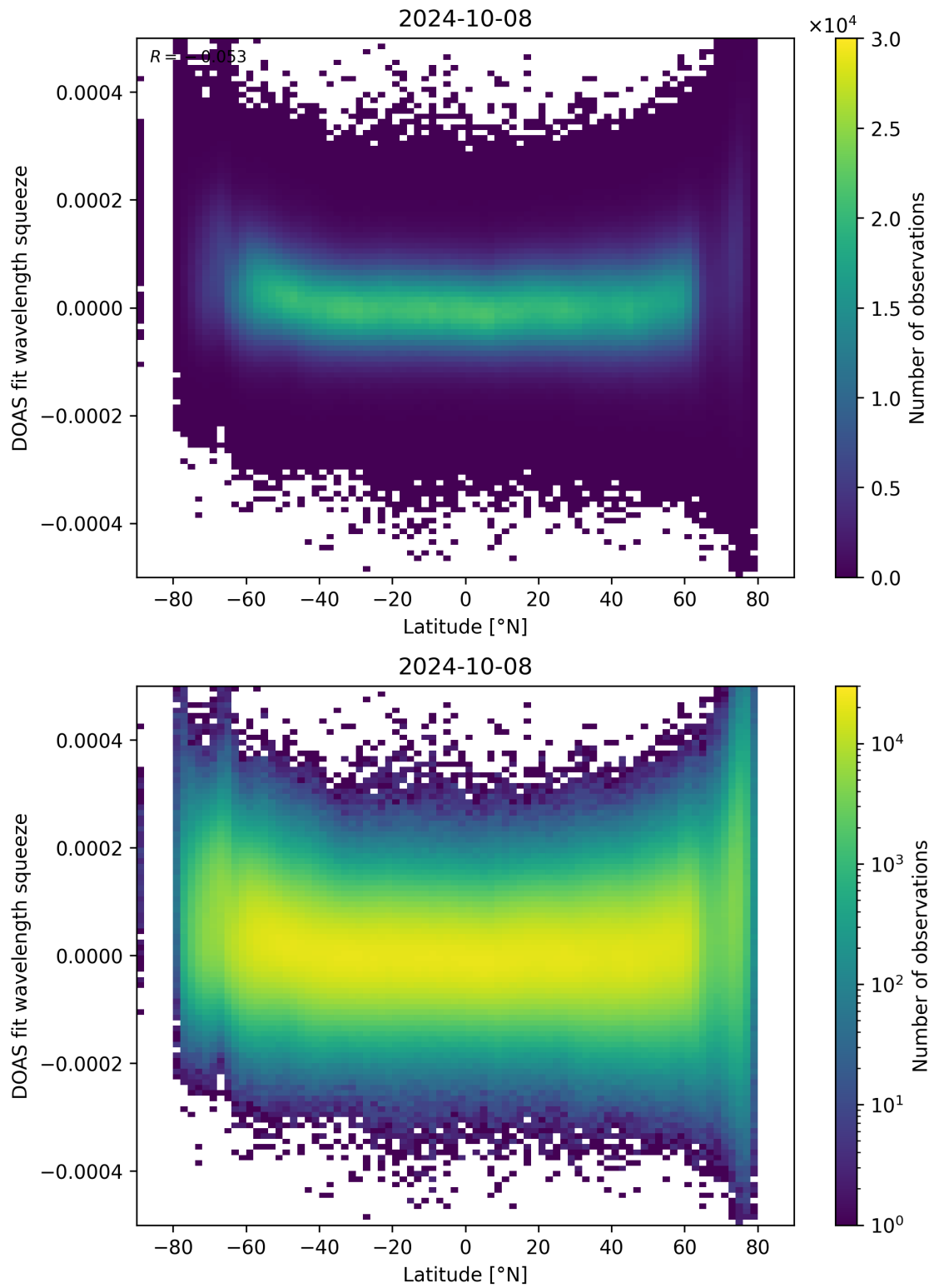
Figure 155: Scatter density plot of “Latitude” against “DOAS fit wavelength squeeze” for 2024-10-08 to 2024-10-09.
