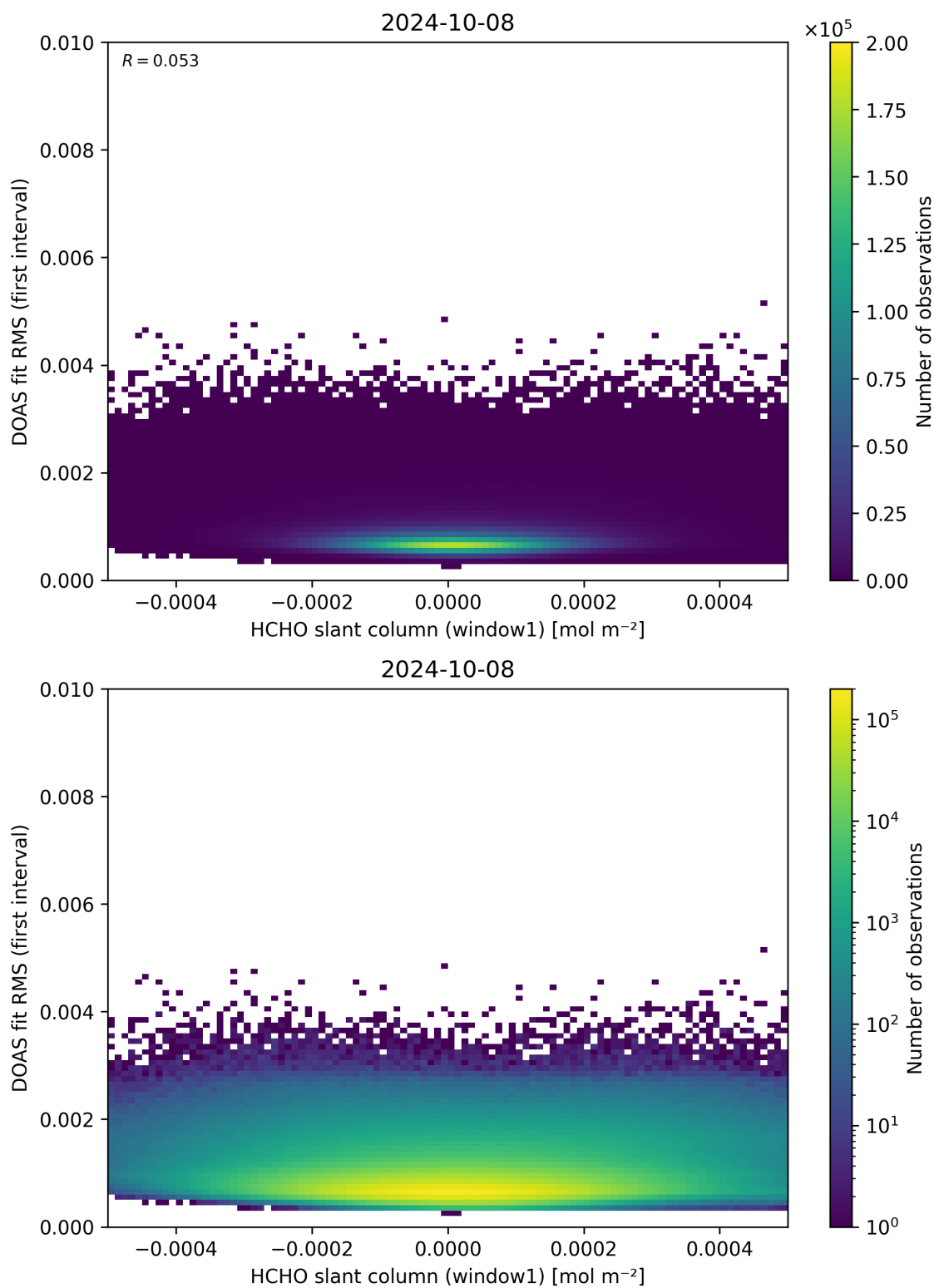
Figure 78: Scatter density plot of “HCHO slant column (window1)” against “DOAS fit RMS (first interval)” for 2024-10-08 to 2024-10-09.
