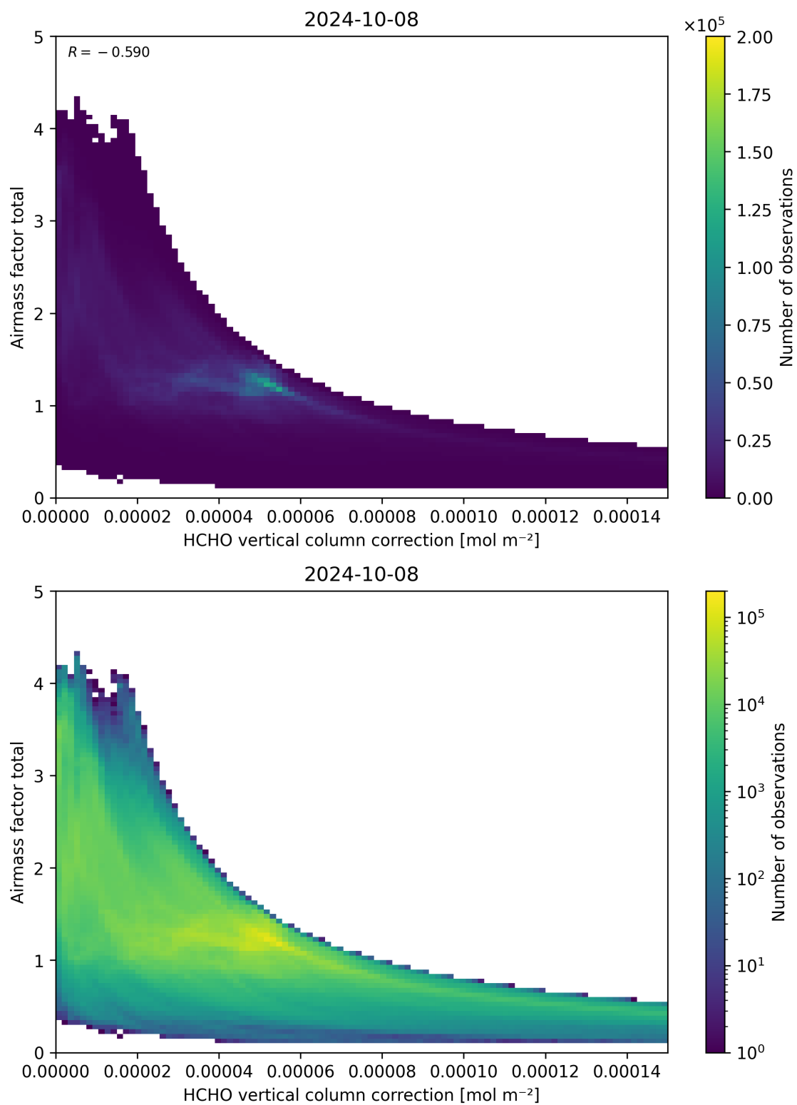
Figure 120: Scatter density plot of “HCHO vertical column correction” against “Airmass factor total” for 2024-10-08 to 2024-10-09.
