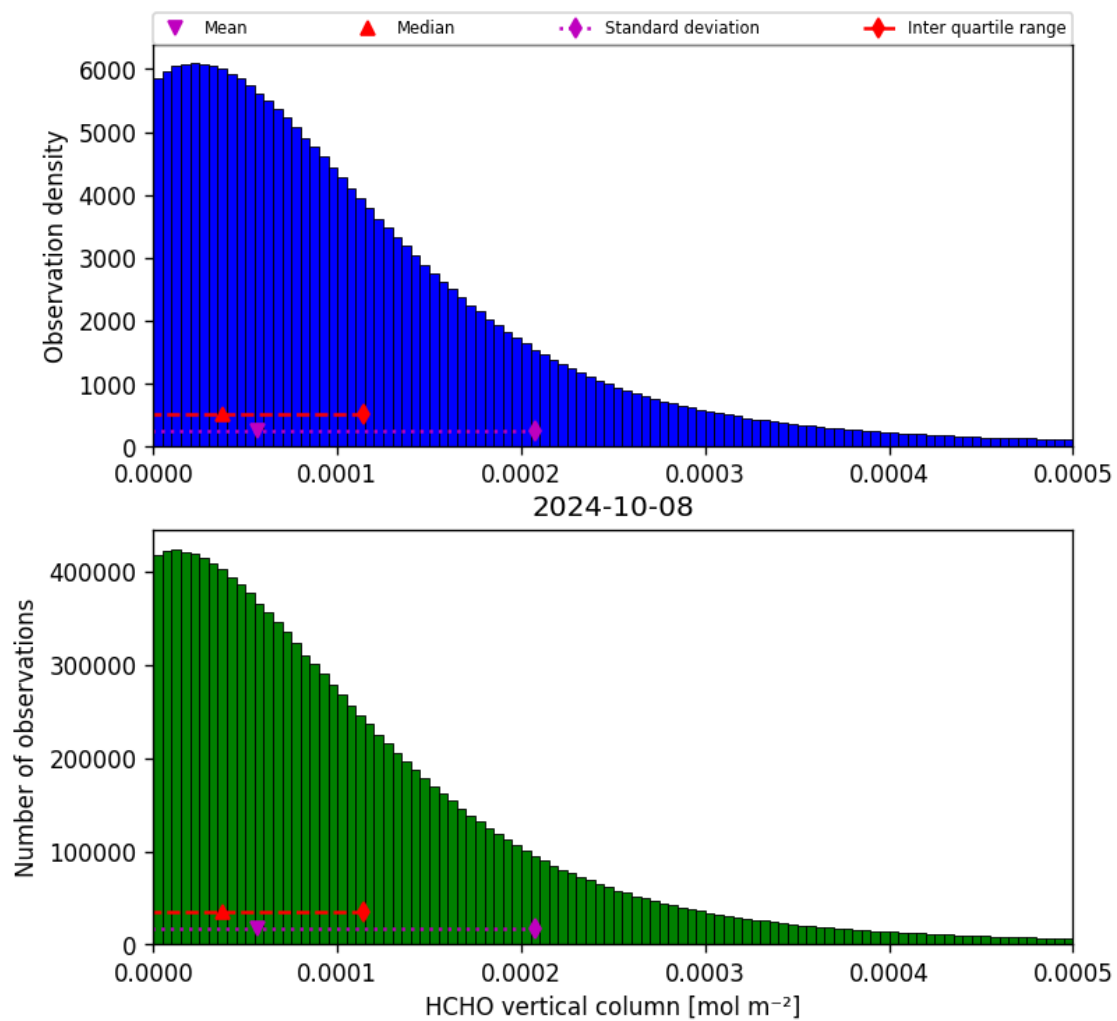
Figure 35: Histogram of “HCHO vertical column” for 2024-10-08 to 2024-10-09
