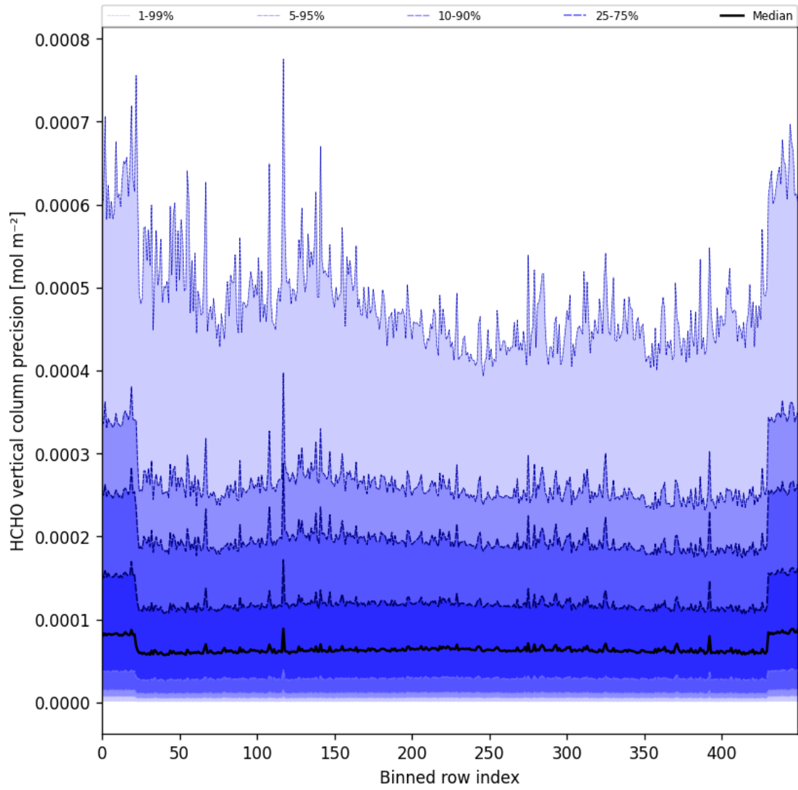
Figure 50: Along track statistics of “HCHO vertical column precision” for 2024-10-08 to 2024-10-09
