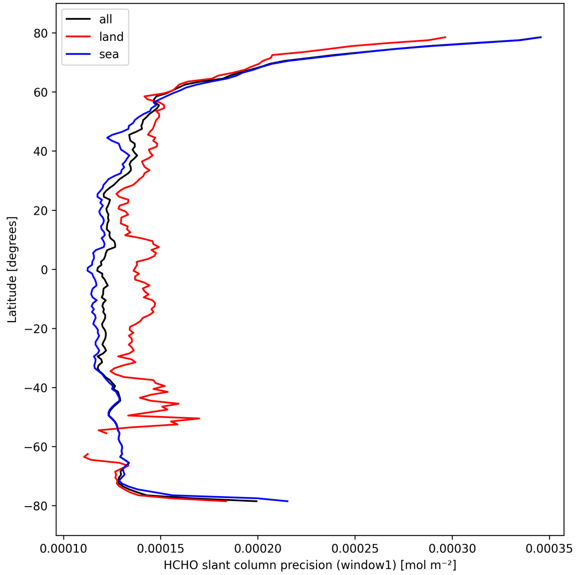
Figure 25: Zonal average of “HCHO slant column precision (window1)” for 2024-10-08 to 2024-10-09.
