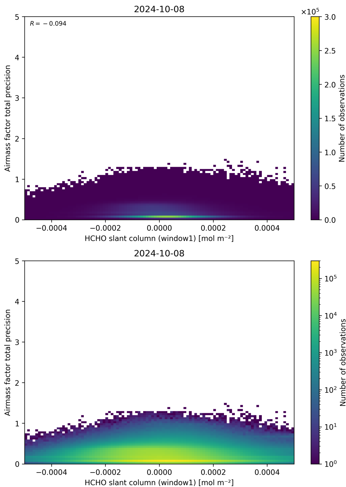
Figure 86: Scatter density plot of “HCHO slant column (window1)” against “Airmass factor total precision” for 2024-10-08 to 2024-10-09.
