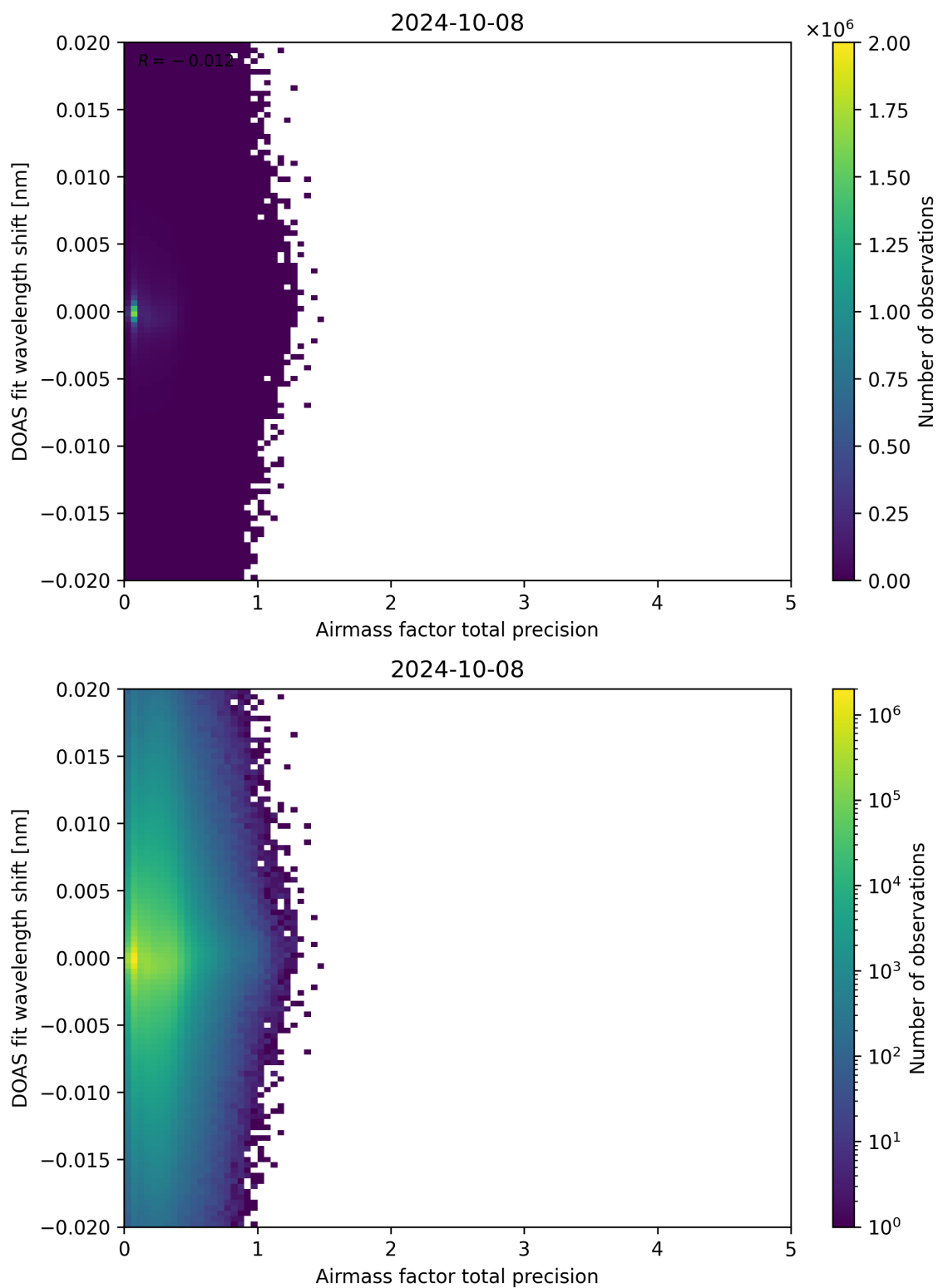
Figure 106: Scatter density plot of “Airmass factor total precision” against “DOAS fit wavelength shift” for 2024-10-08 to 2024-10-09.
