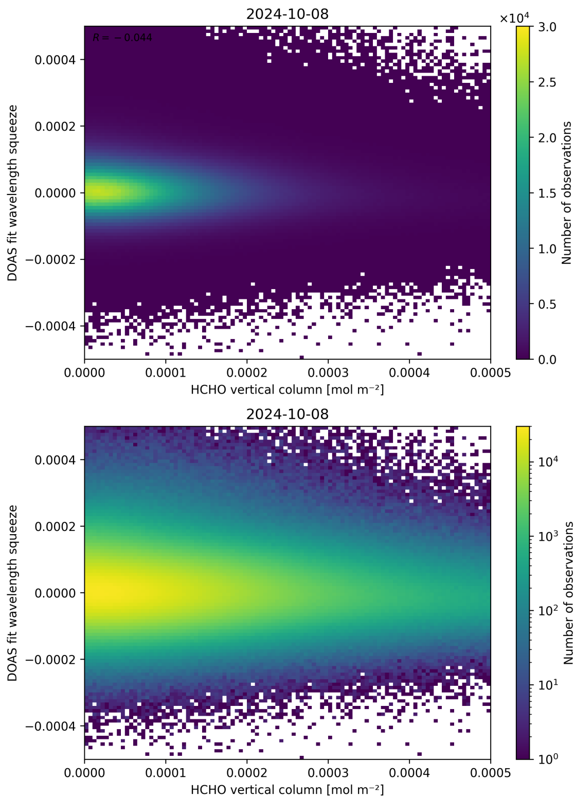
Figure 125: Scatter density plot of “HCHO vertical column” against “DOAS fit wavelength squeeze” for 2024-10-08 to 2024-10-09.
