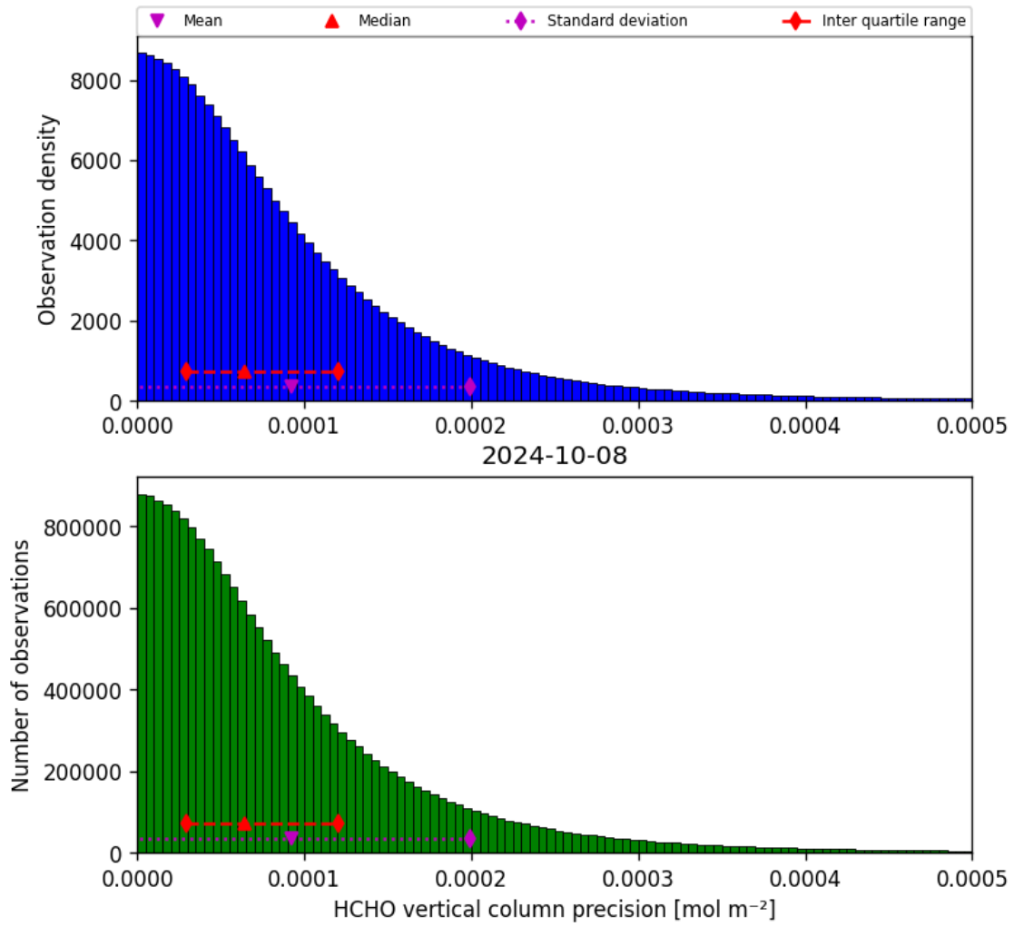
Figure 36: Histogram of “HCHO vertical column precision” for 2024-10-08 to 2024-10-09
