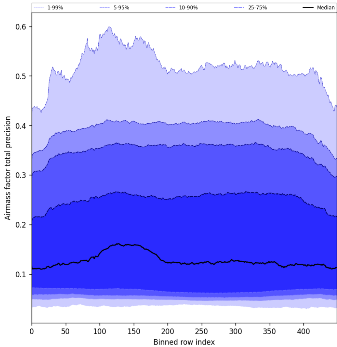
Figure 55: Along track statistics of “Airmass factor total precision” for 2024-10-08 to 2024-10-09
