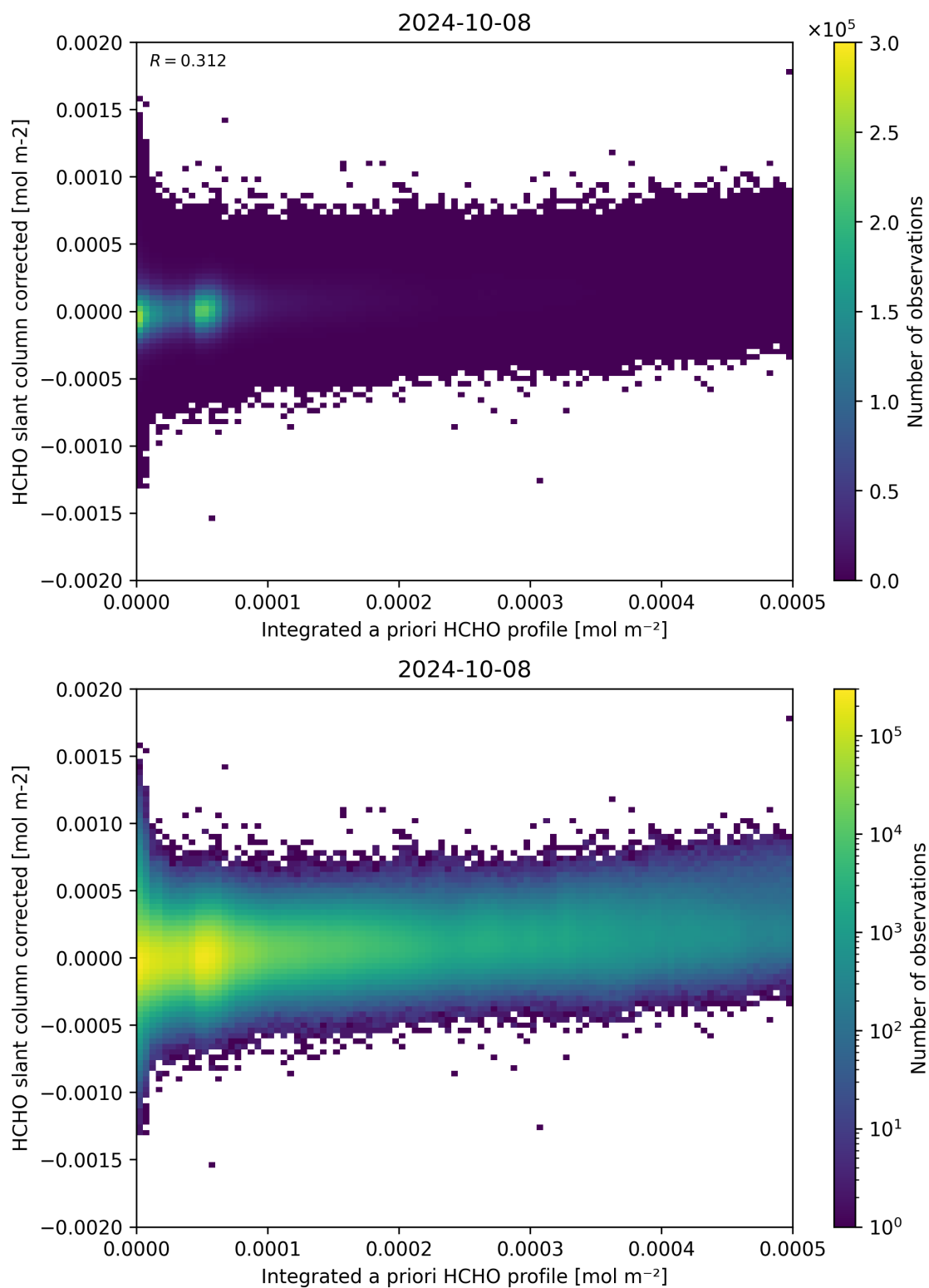
Figure 151: Scatter density plot of “Integrated a priori HCHO profile” against “HCHO slant column corrected” for 2024-10-08 to 2024-10-09.
