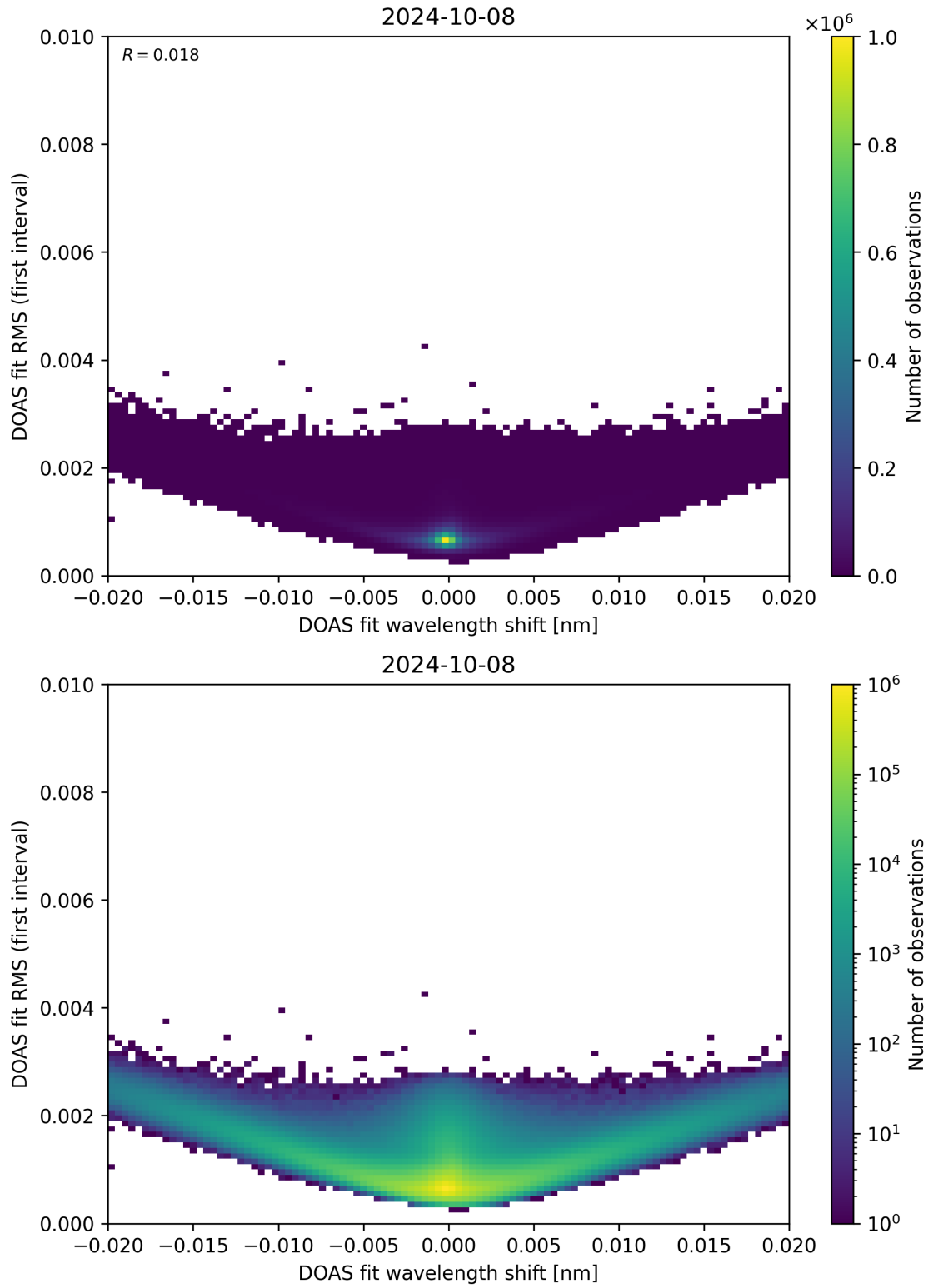
Figure 64: Scatter density plot of “DOAS fit wavelength shift” against “DOAS fit RMS (first interval)” for 2024-10-08 to 2024-10-09.
