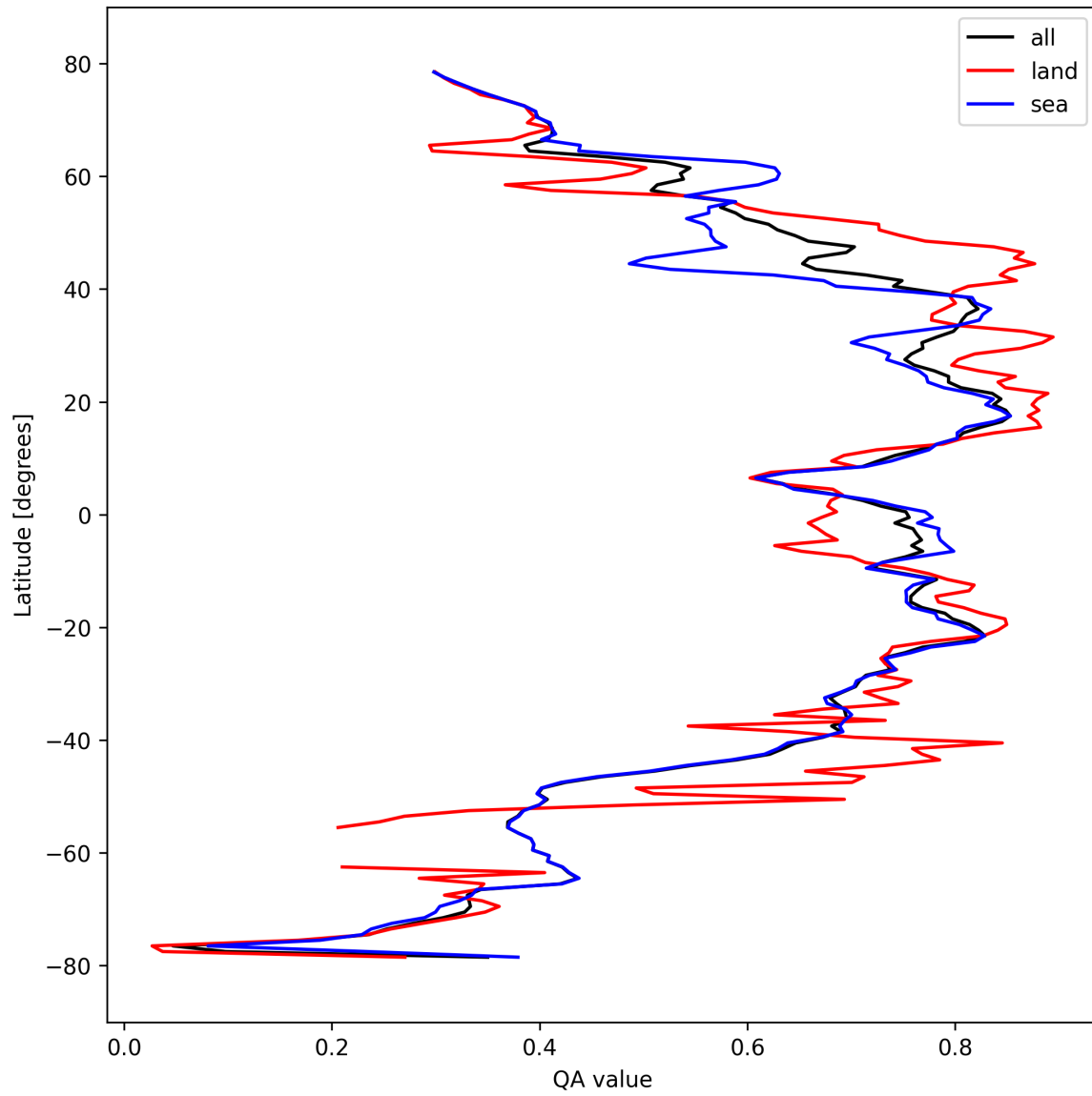
Figure 20: Zonal average of “QA value” for 2024-10-08 to 2024-10-09.
