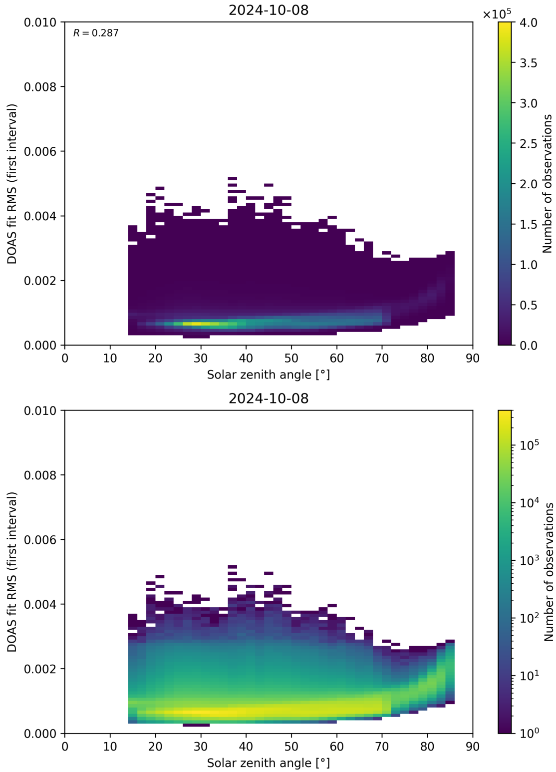
Figure 167: Scatter density plot of “Solar zenith angle” against “DOAS fit RMS (first interval)” for 2024-10-08 to 2024-10-09.
