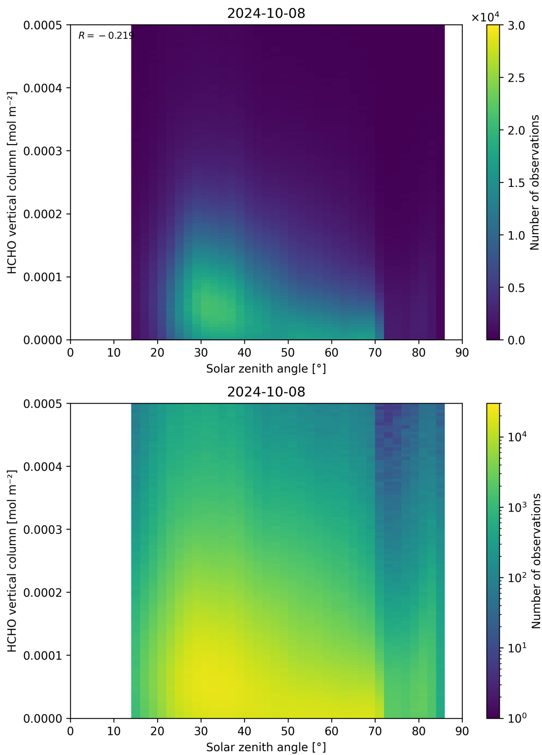
Figure 177: Scatter density plot of “Solar zenith angle” against “HCHO vertical column” for 2024-10-08 to 2024-10-09.
