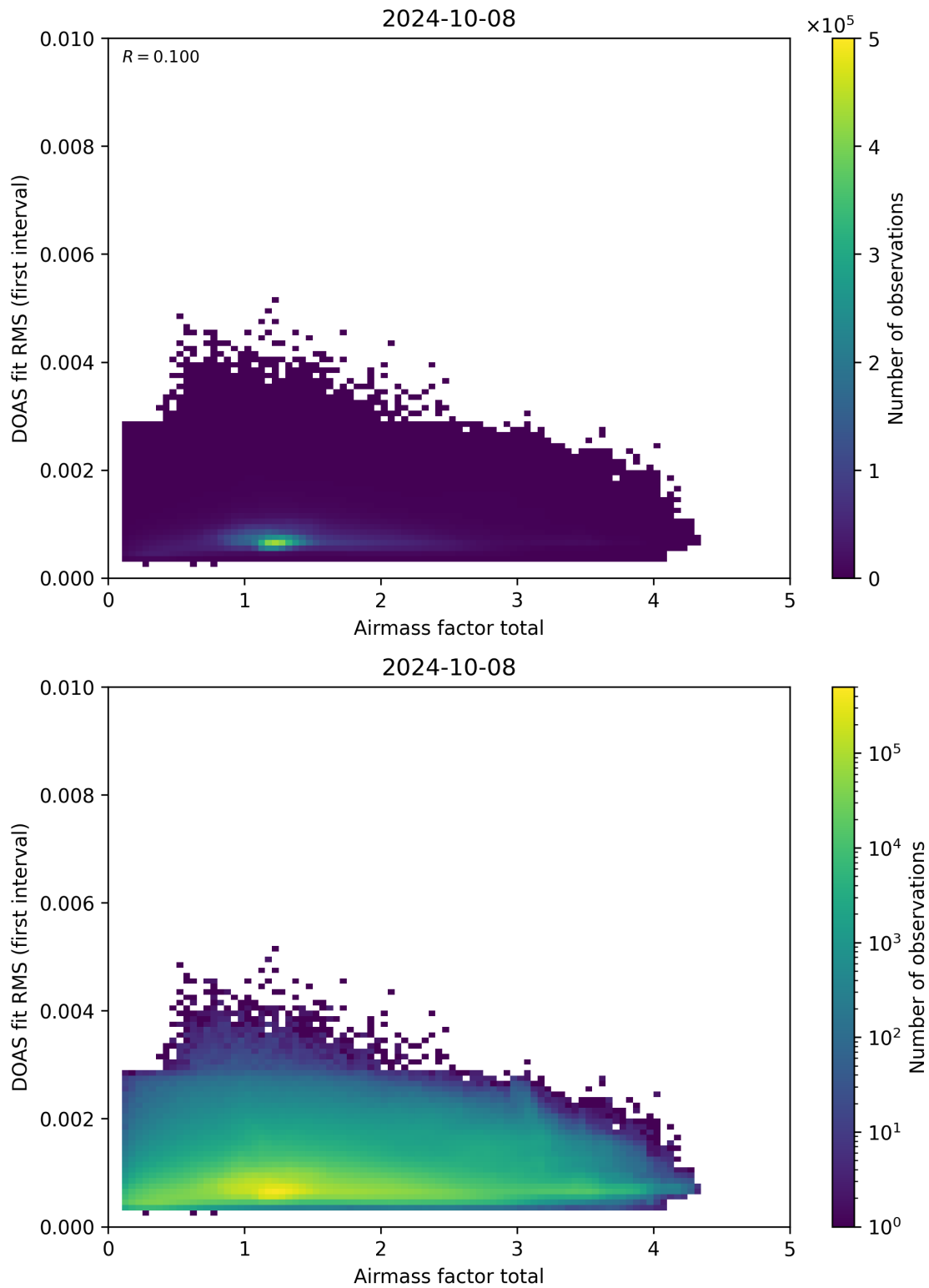
Figure 97: Scatter density plot of “Airmass factor total” against “DOAS fit RMS (first interval)” for 2024-10-08 to 2024-10-09.
