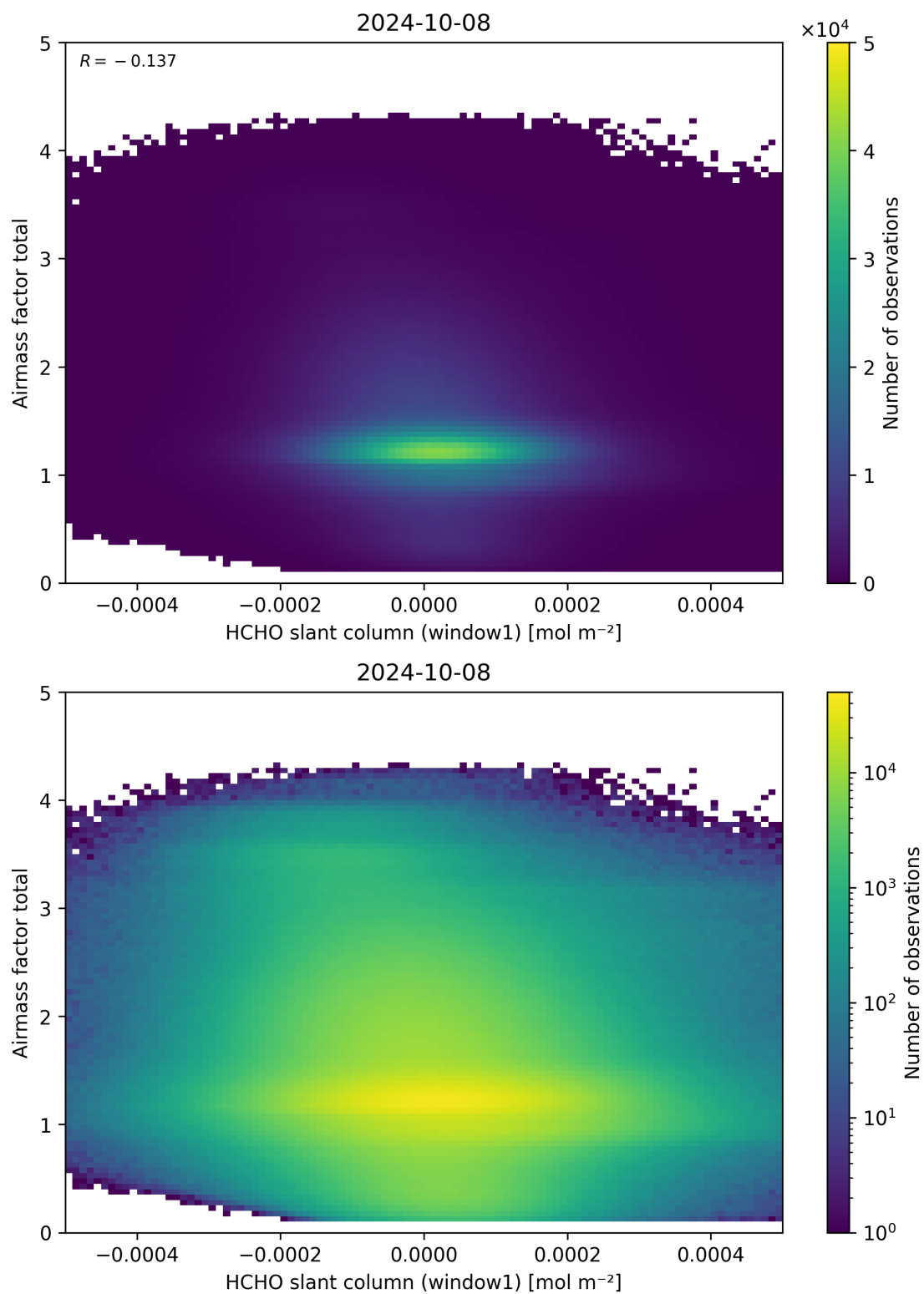
Figure 85: Scatter density plot of “HCHO slant column (window1)” against “Airmass factor total” for 2024-10-08 to 2024-10-09.
