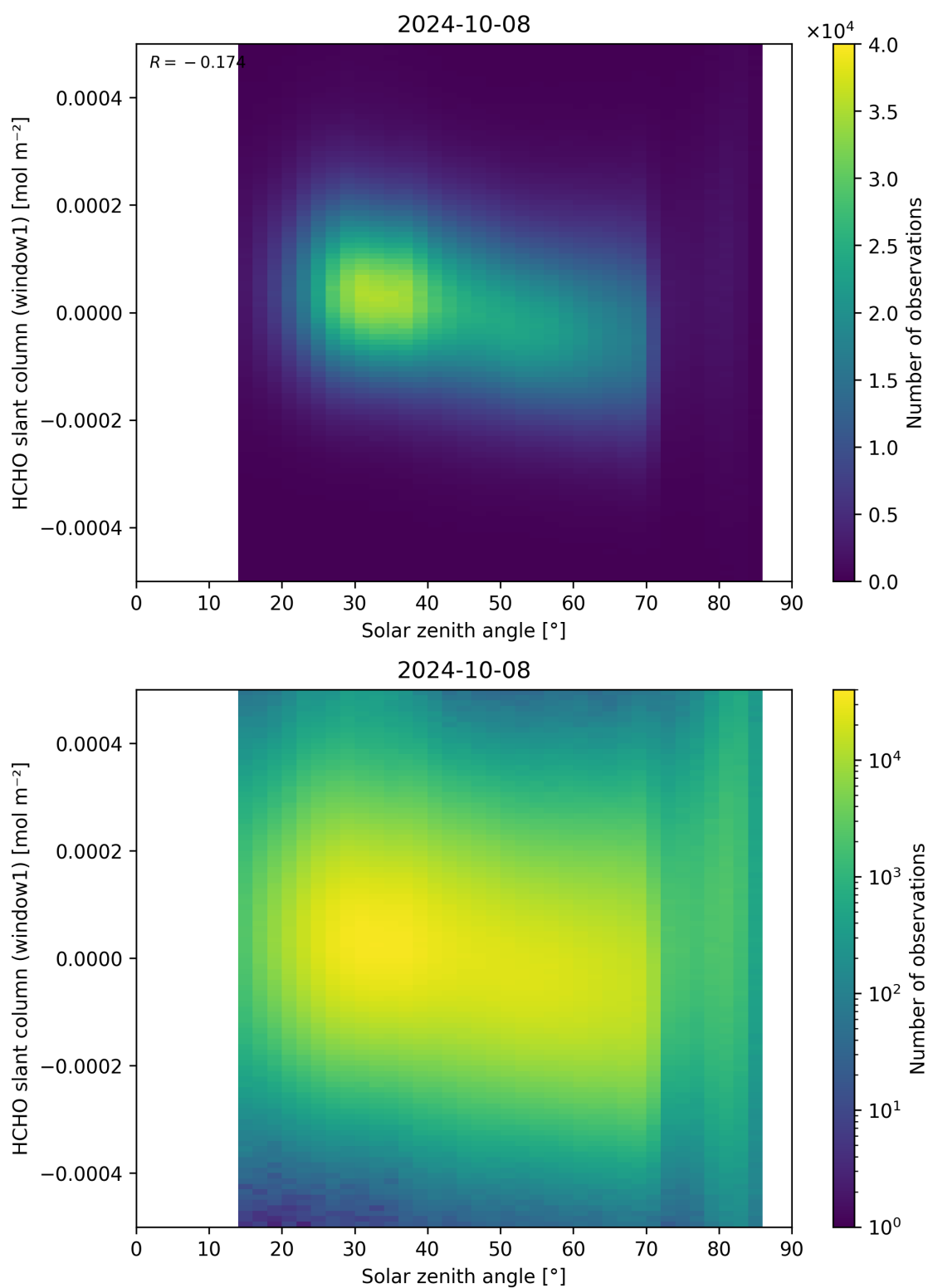
Figure 173: Scatter density plot of “Solar zenith angle” against “HCHO slant column (window1)” for 2024-10-08 to 2024-10-09.
