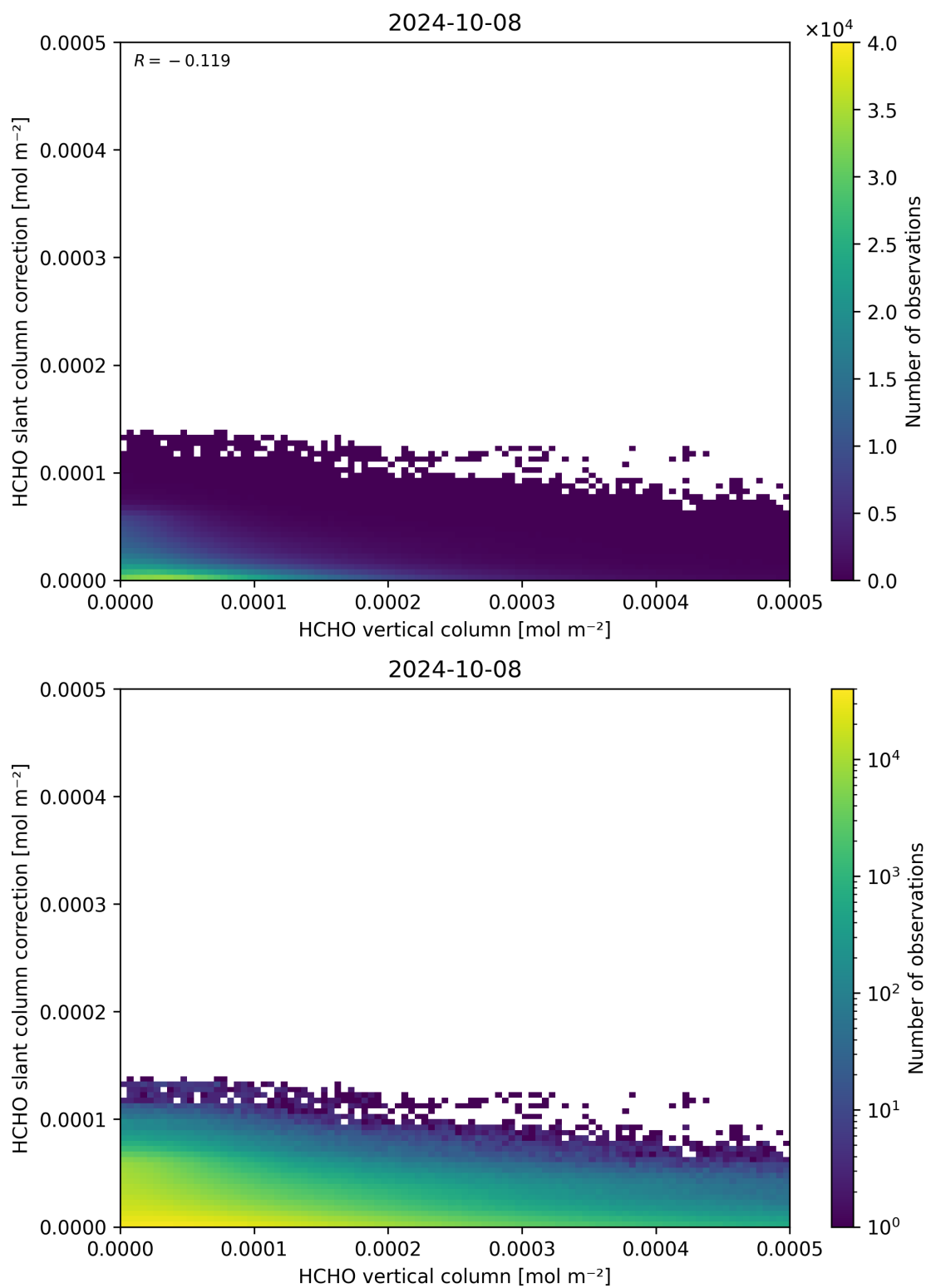
Figure 128: Scatter density plot of “HCHO vertical column” against “HCHO slant column correction” for 2024-10-08 to 2024-10-09.
