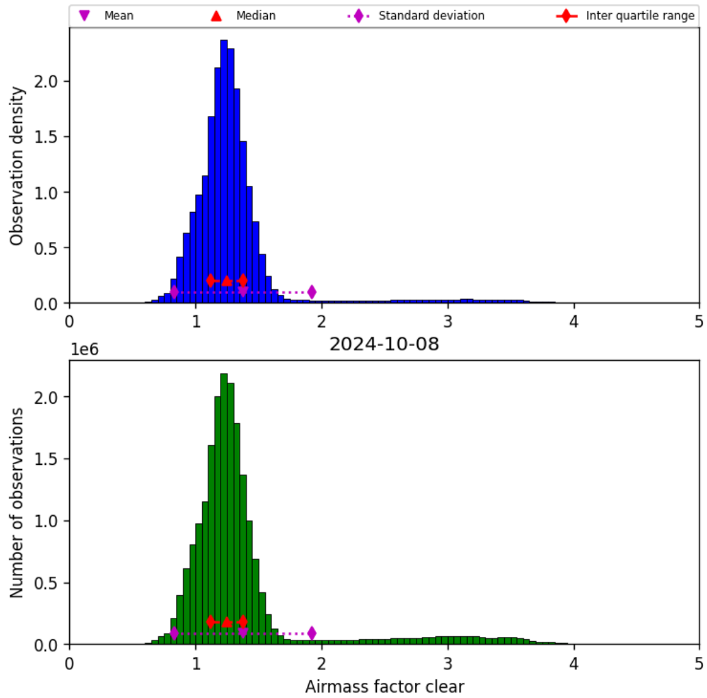
Figure 42: Histogram of “Airmass factor clear” for 2024-10-08 to 2024-10-09
