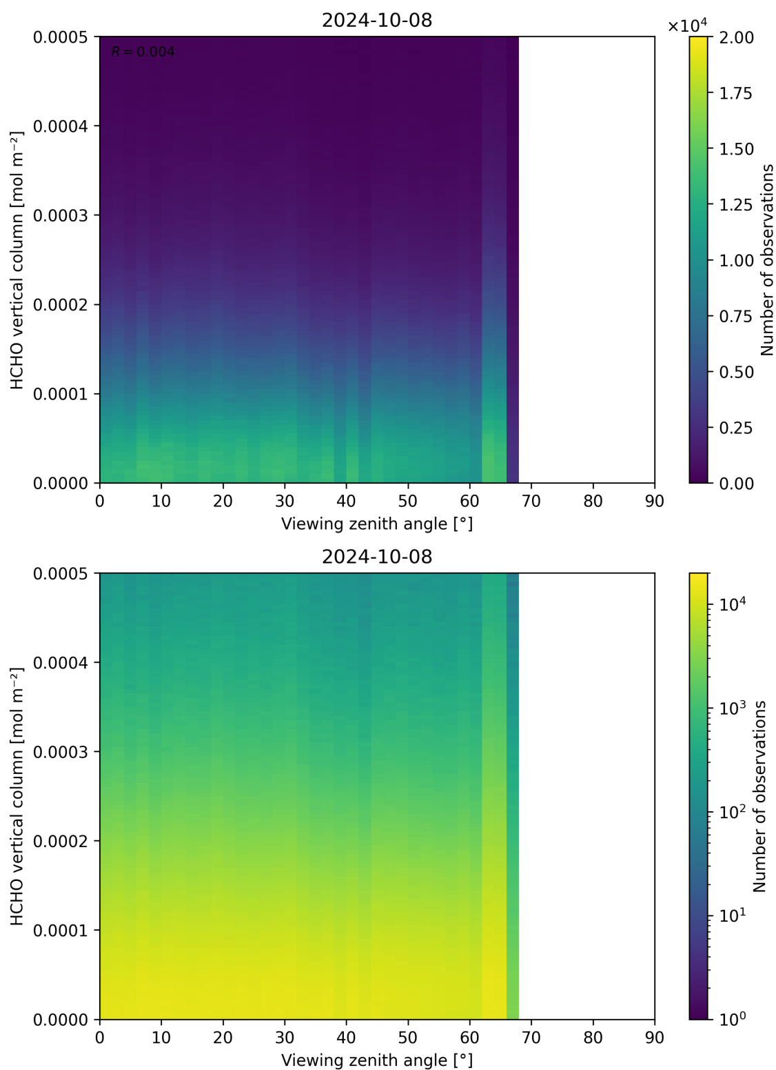
Figure 192: Scatter density plot of “Viewing zenith angle” against “HCHO vertical column” for 2024-10-08 to 2024-10-09.
