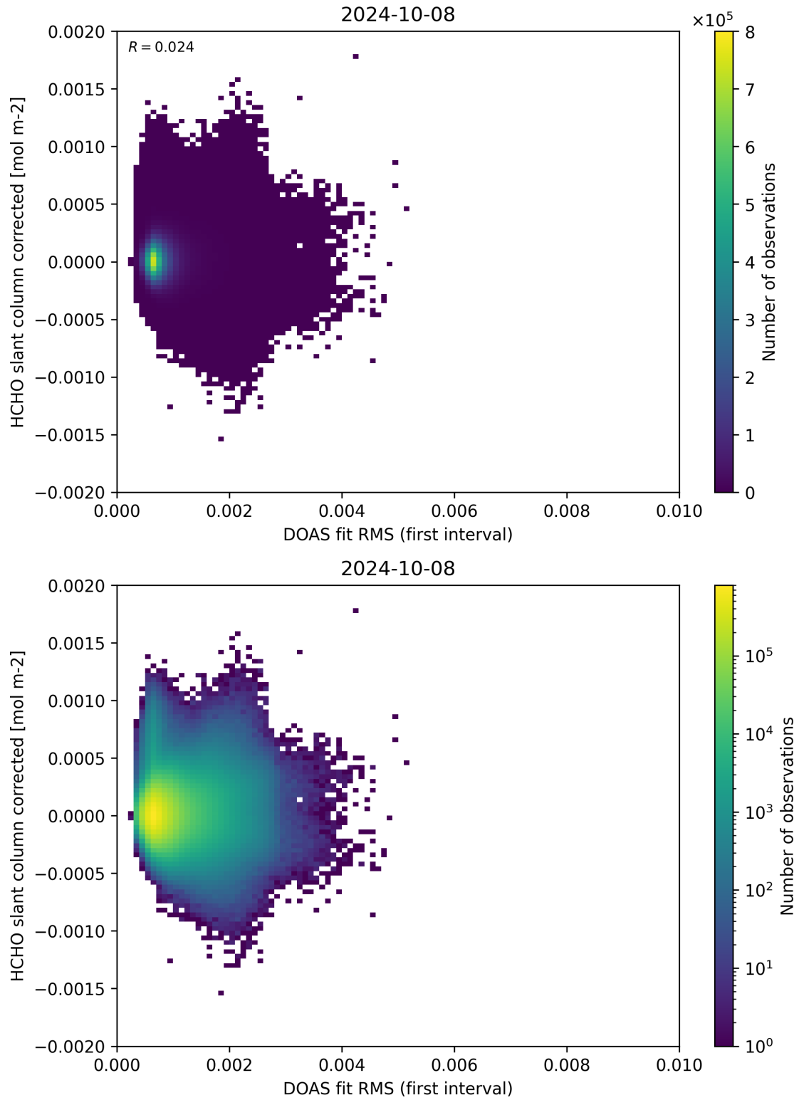
Figure 62: Scatter density plot of “DOAS fit RMS (first interval)” against “HCHO slant column corrected” for 2024-10-08 to 2024-10-09.
