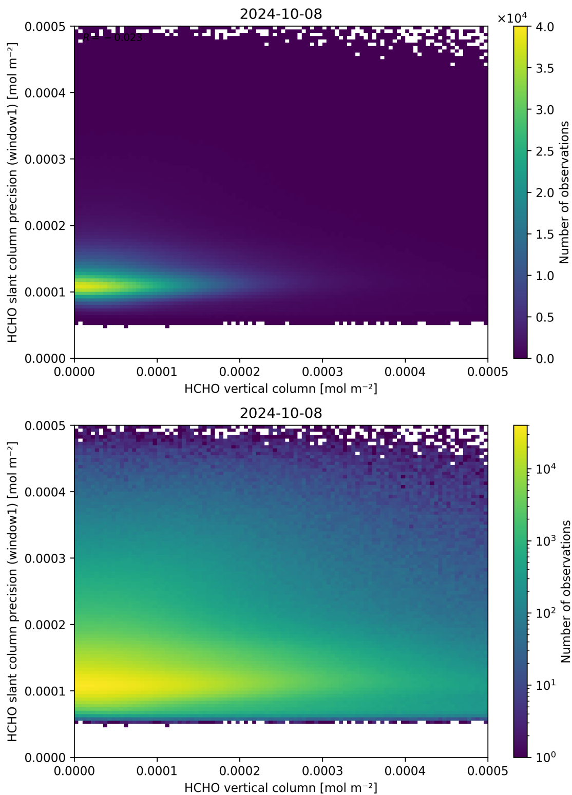
Figure 130: Scatter density plot of “HCHO vertical column” against “HCHO slant column precision (window1)” for 2024-10-08 to 2024-10-09.
