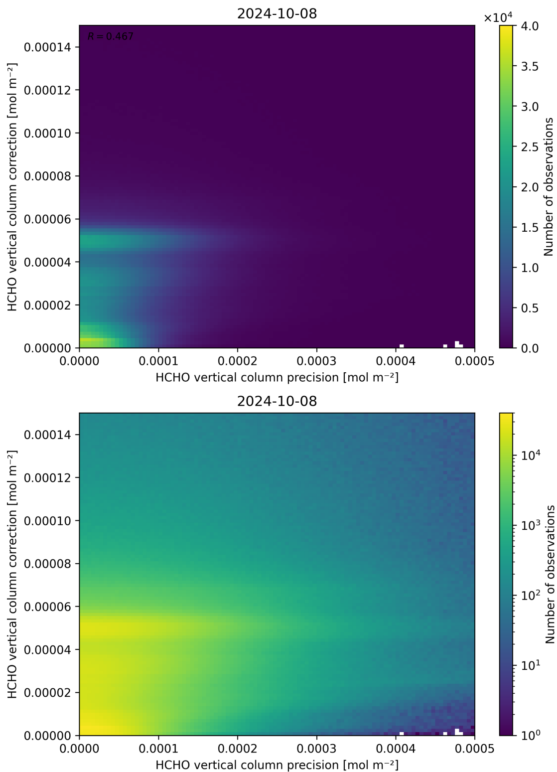
Figure 146: Scatter density plot of “HCHO vertical column precision” against “HCHO vertical column correction” for 2024-10-08 to 2024-10-09.
