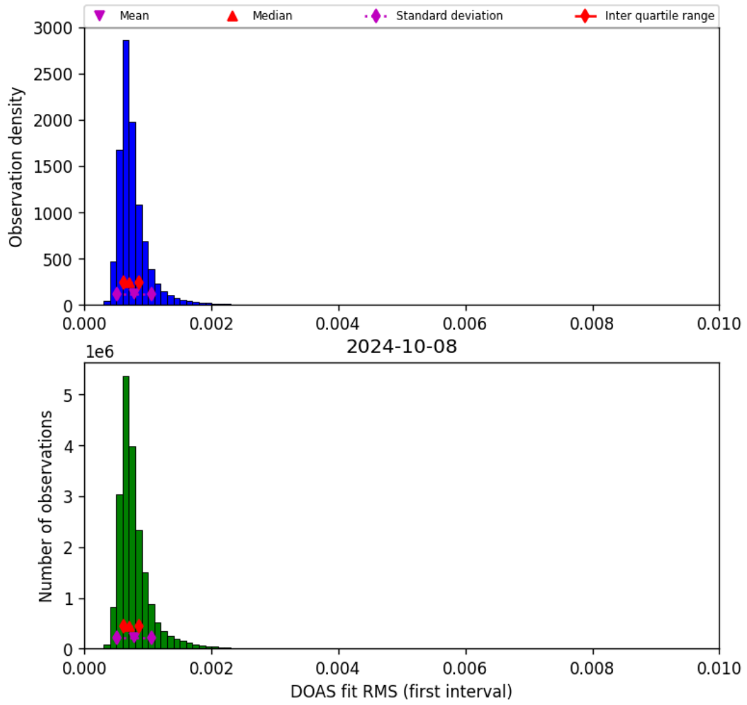
Figure 46: Histogram of “DOAS fit RMS (first interval)” for 2024-10-08 to 2024-10-09
