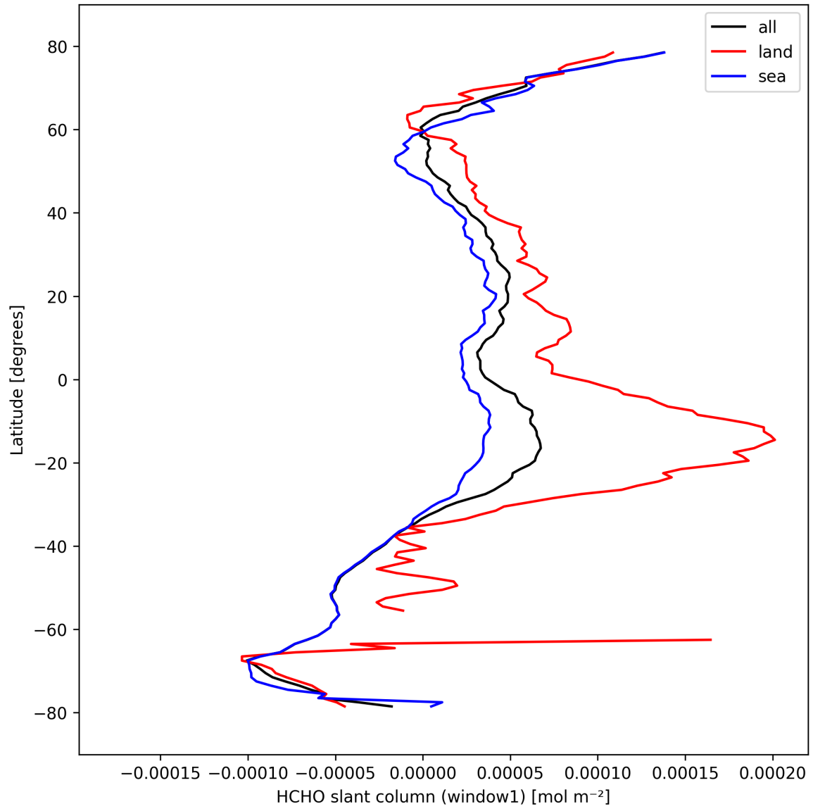
Figure 24: Zonal average of “HCHO slant column (window1)” for 2024-10-08 to 2024-10-09.
