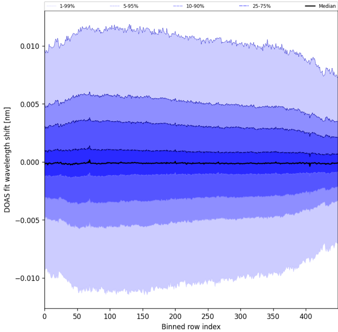
Figure 58: Along track statistics of “DOAS fit wavelength shift” for 2024-10-08 to 2024-10-09
