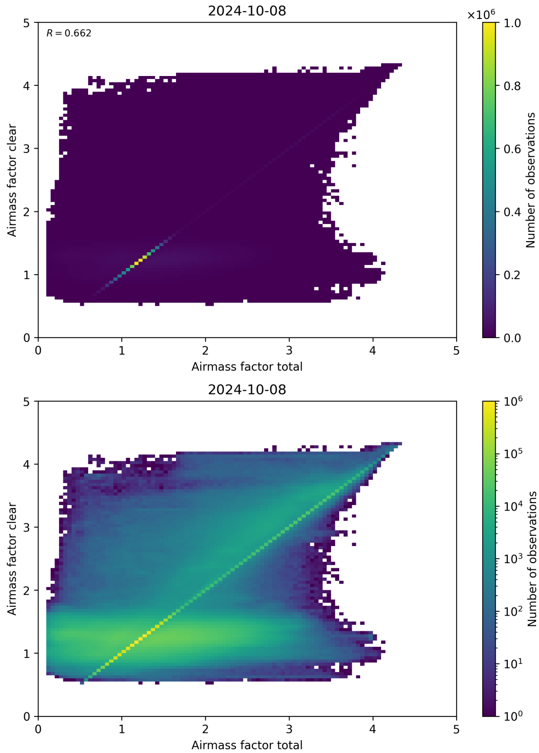
Figure 100: Scatter density plot of “Airmass factor total” against “Airmass factor clear” for 2024-10-08 to 2024-10-09.
