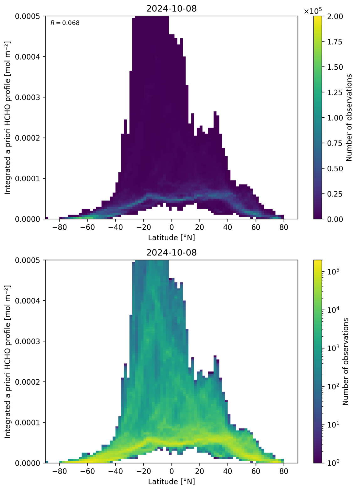
Figure 166: Scatter density plot of “Latitude” against “Integrated a priori HCHO profile” for 2024-10-08 to 2024-10-09.
