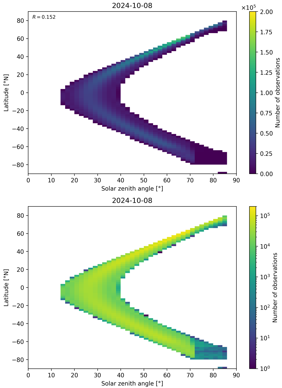
Figure 181: Scatter density plot of “Solar zenith angle” against “Latitude” for 2024-10-08 to 2024-10-09.
