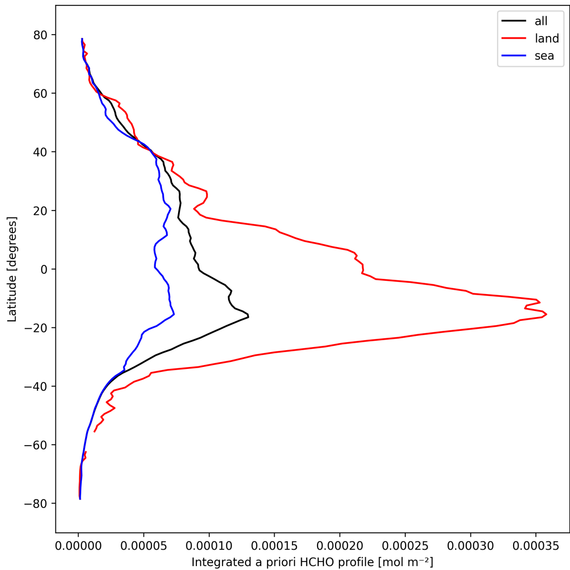
Figure 29: Zonal average of “Integrated a priori HCHO profile” for 2024-10-08 to 2024-10-09.
