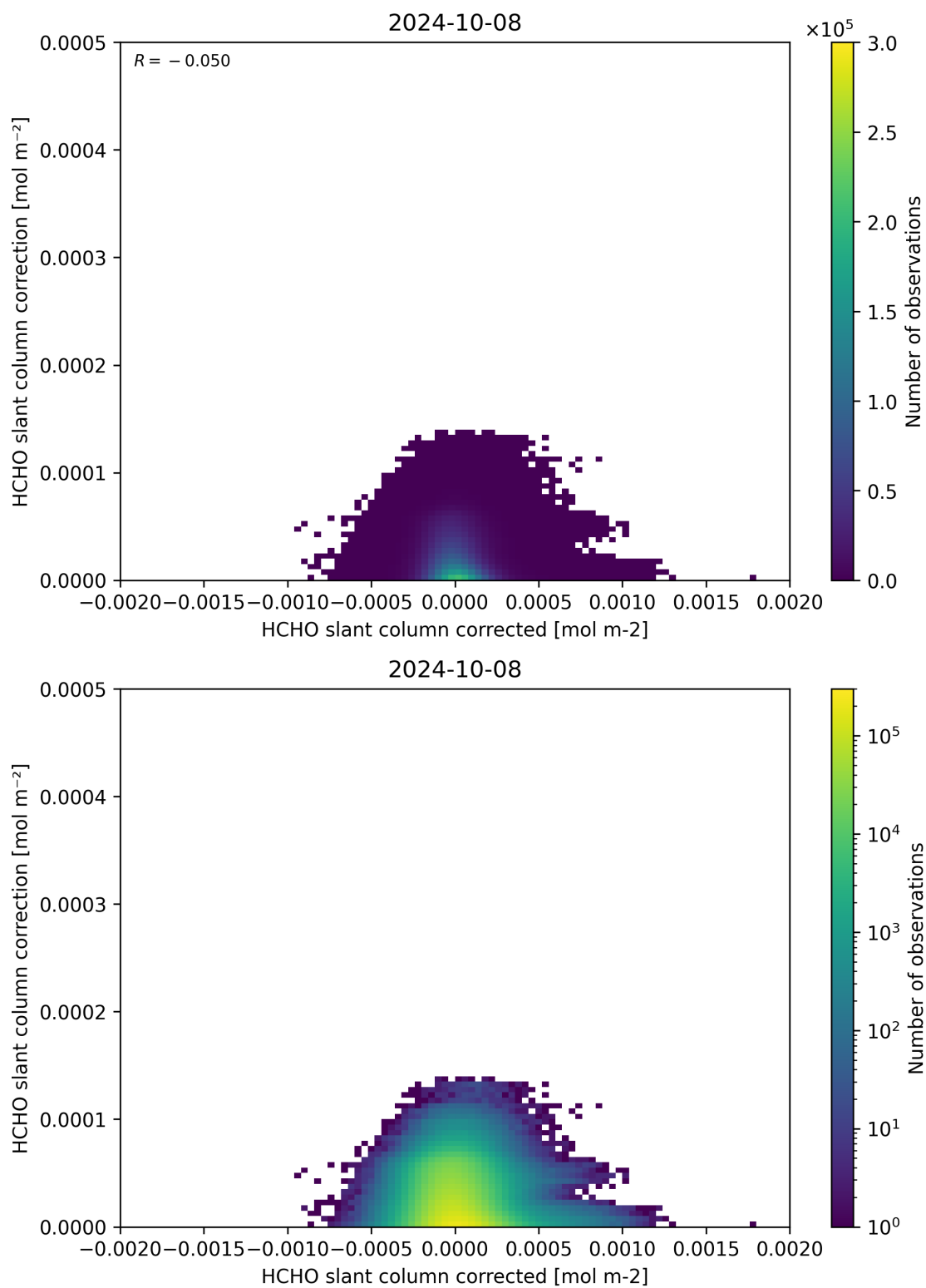
Figure 77: Scatter density plot of “HCHO slant column corrected” against “HCHO slant column correction” for 2024-10-08 to 2024-10-09.
