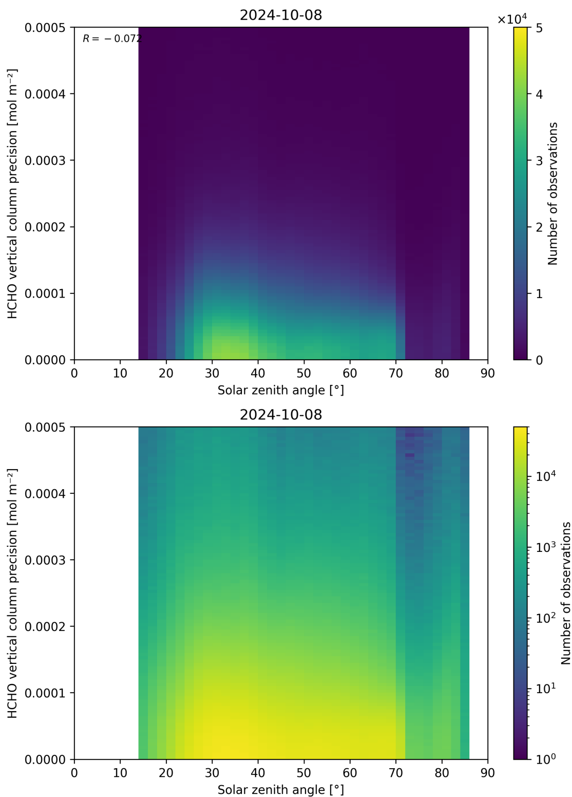
Figure 179: Scatter density plot of “Solar zenith angle” against “HCHO vertical column precision” for 2024-10-08 to 2024-10-09.
