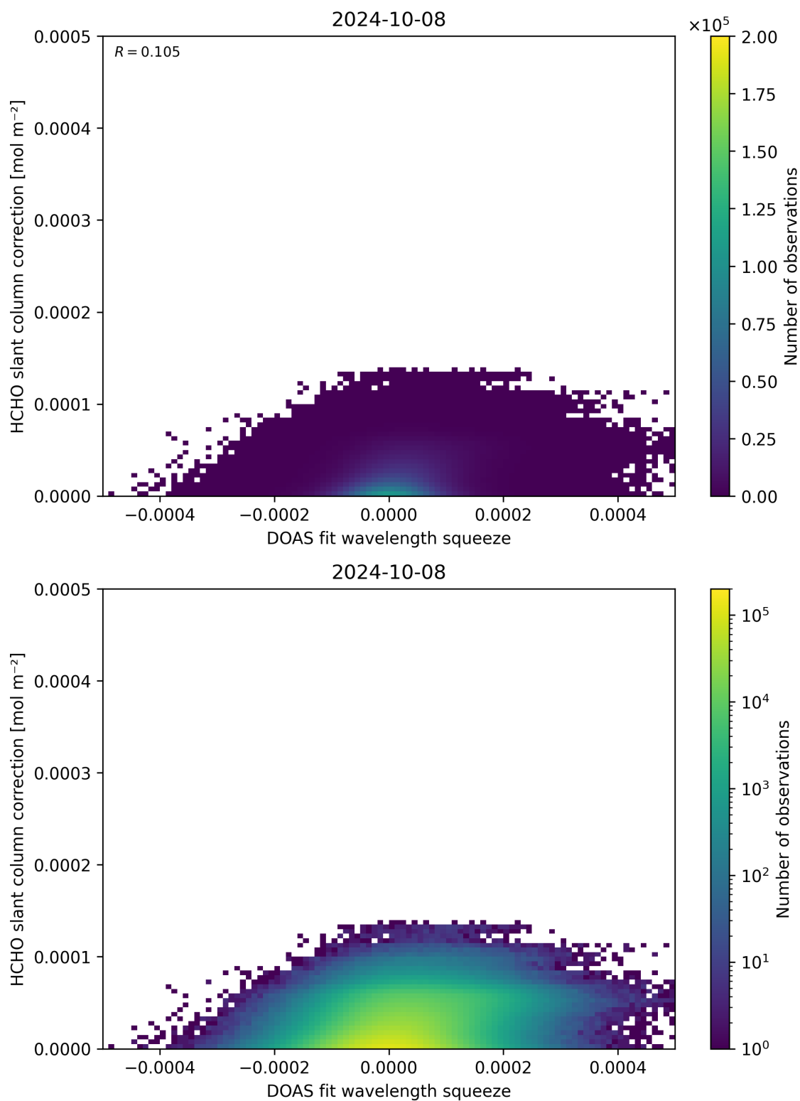
Figure 70: Scatter density plot of “DOAS fit wavelength squeeze” against “HCHO slant column correction” for 2024-10-08 to 2024-10-09.
