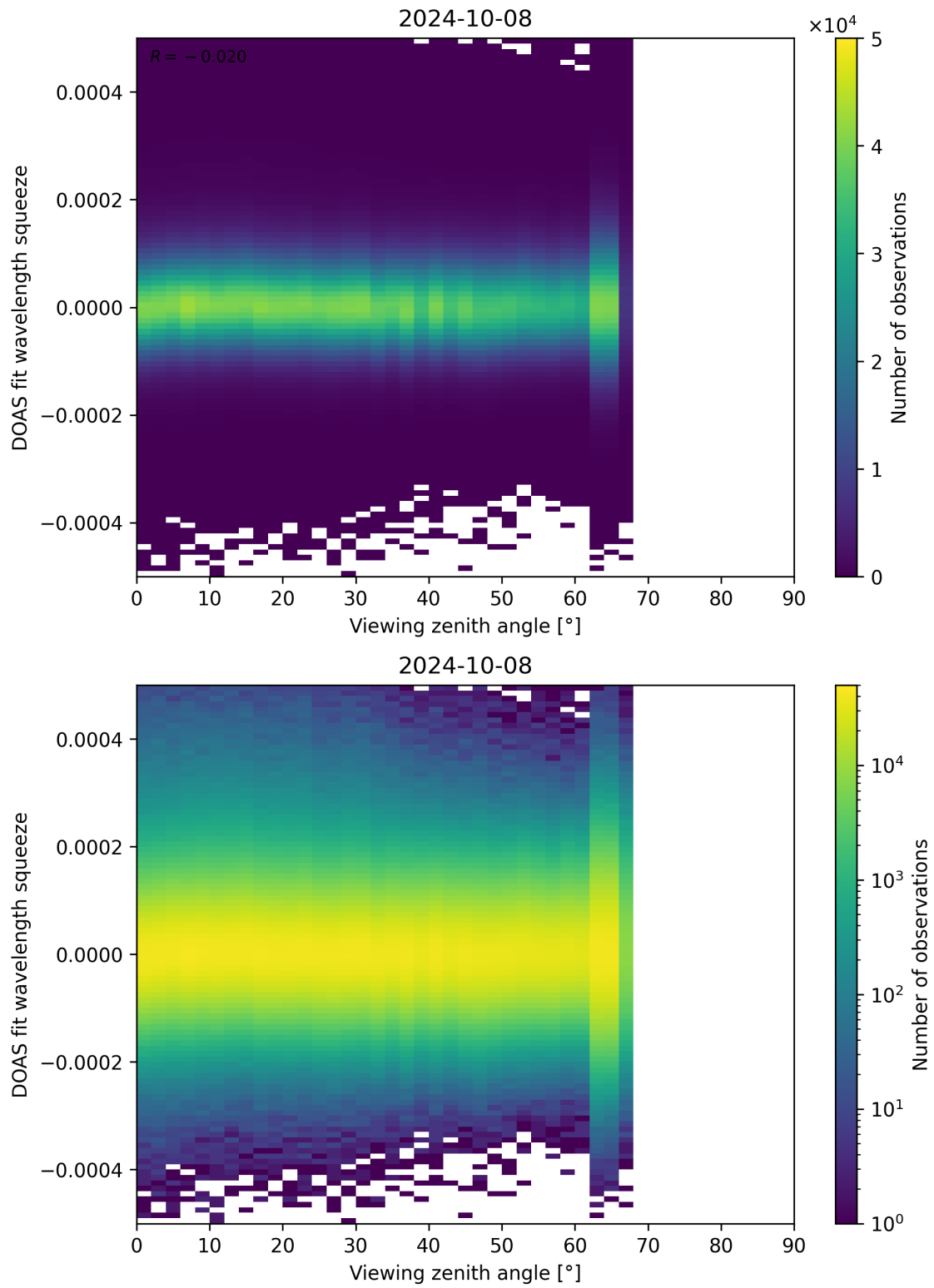
Figure 184: Scatter density plot of “Viewing zenith angle” against “DOAS fit wavelength squeeze” for 2024-10-08 to 2024-10-09.
