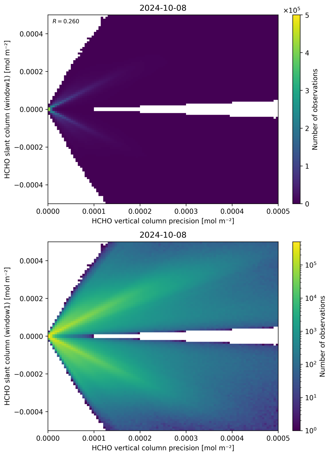
Figure 142: Scatter density plot of “HCHO vertical column precision” against “HCHO slant column (window1)” for 2024-10-08 to 2024-10-09.
