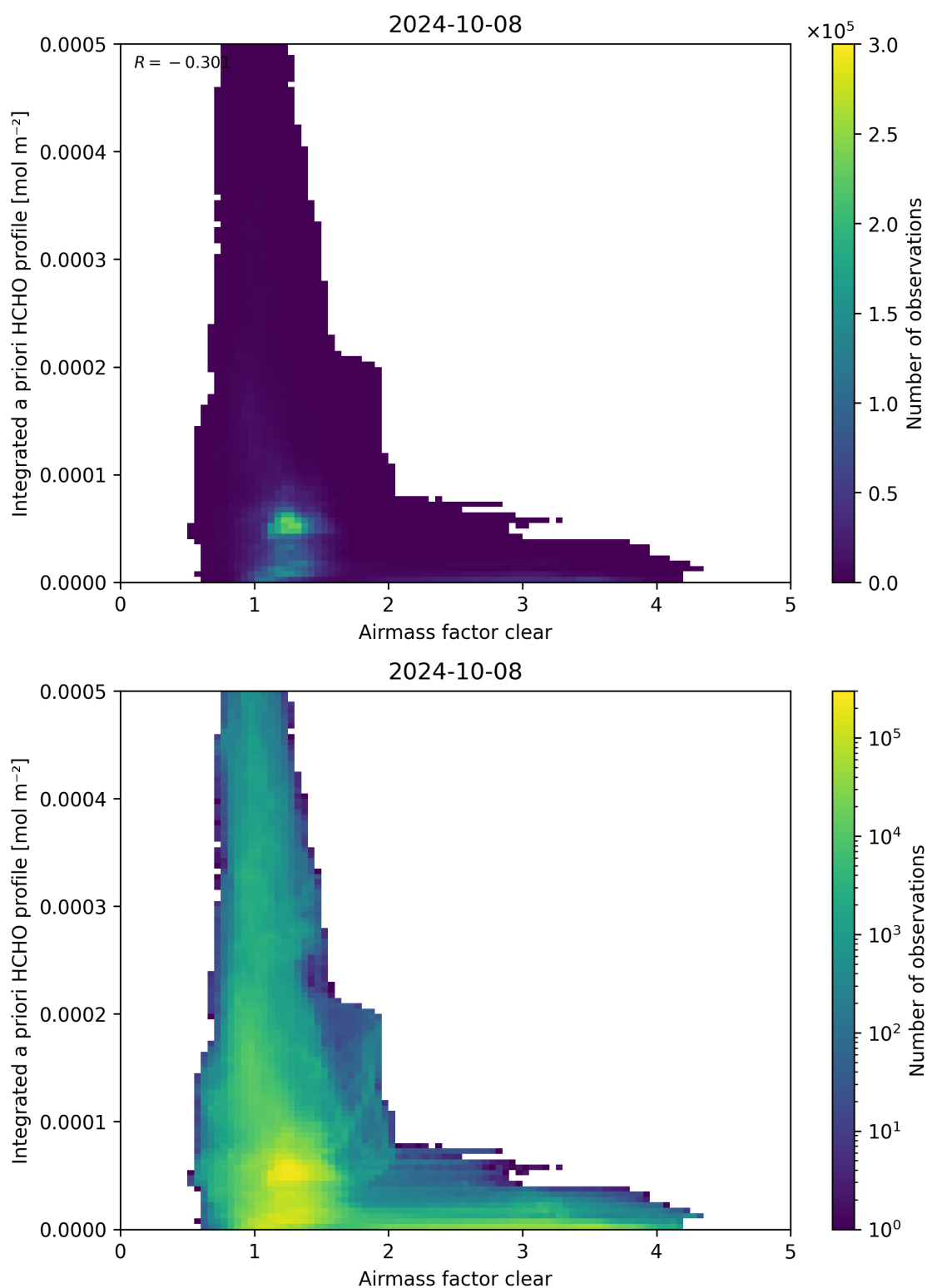
Figure 76: Scatter density plot of “Airmass factor clear” against “Integrated a priori HCHO profile” for 2024-10-08 to 2024-10-09.
