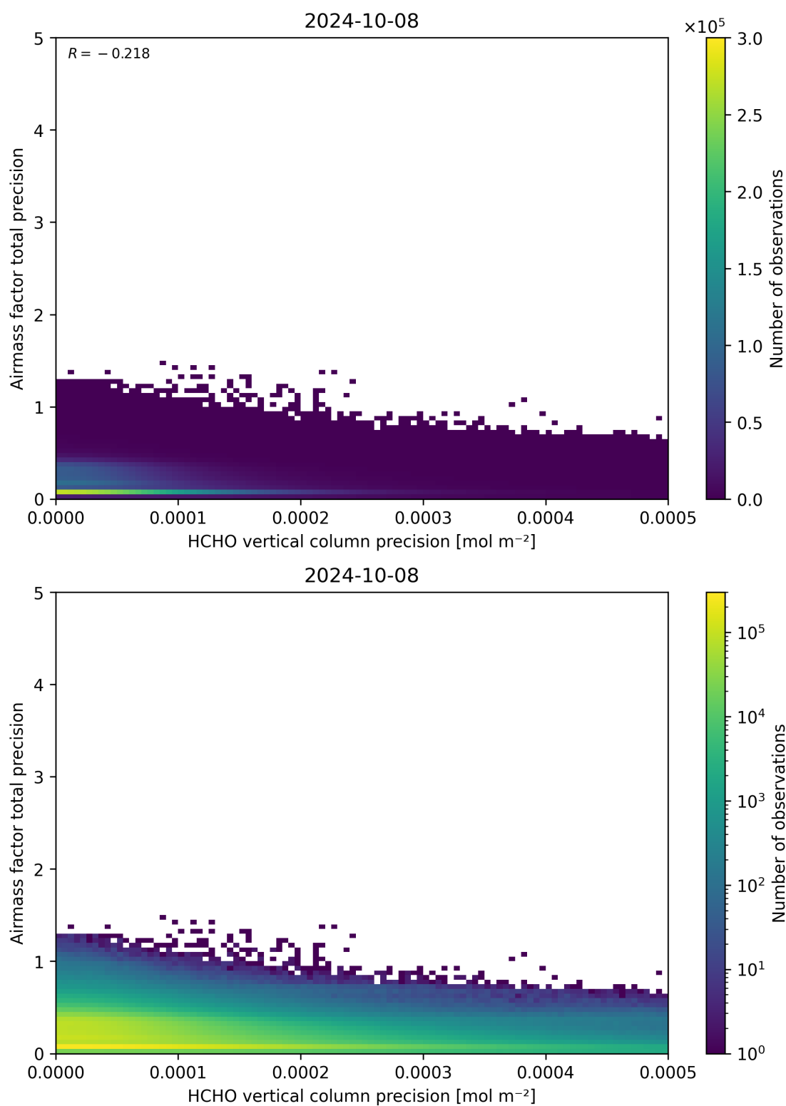
Figure 145: Scatter density plot of “HCHO vertical column precision” against “Airmass factor total precision” for 2024-10-08 to 2024-10-09.
