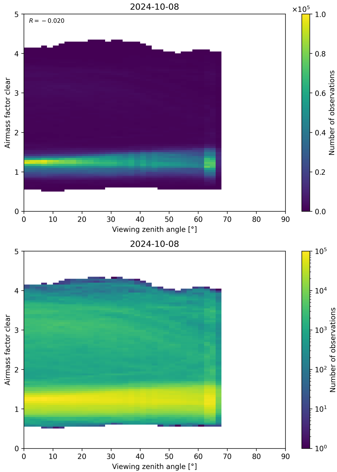
Figure 185: Scatter density plot of “Viewing zenith angle” against “Airmass factor clear” for 2024-10-08 to 2024-10-09.
