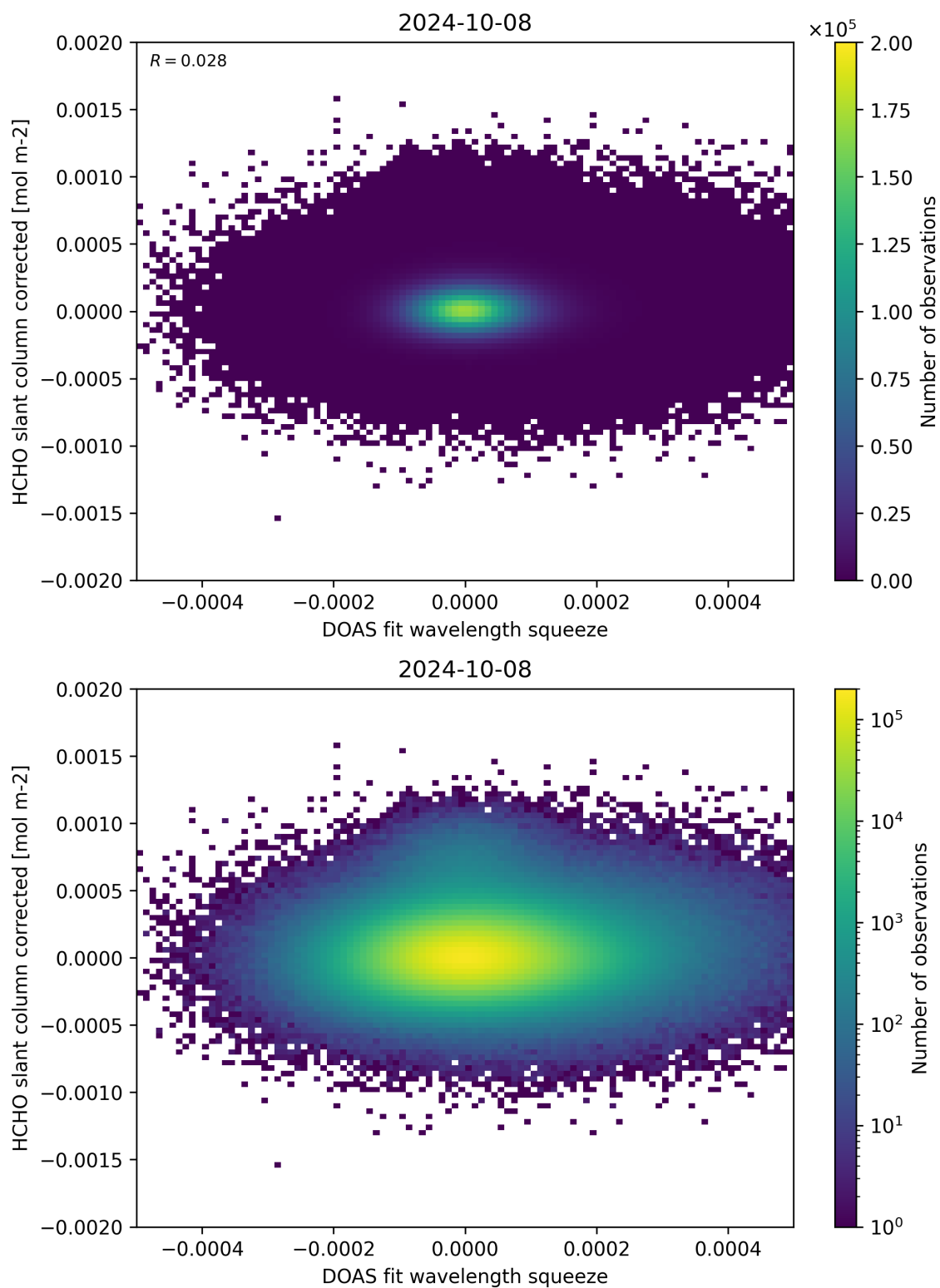
Figure 69: Scatter density plot of “DOAS fit wavelength squeeze” against “HCHO slant column corrected” for 2024-10-08 to 2024-10-09.
