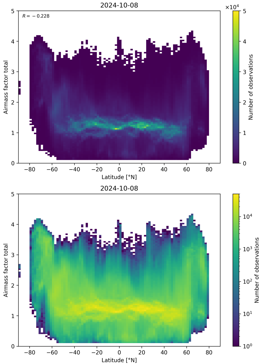
Figure 161: Scatter density plot of “Latitude” against “Airmass factor total” for 2024-10-08 to 2024-10-09.
