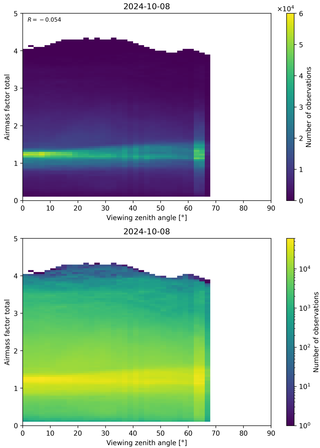
Figure 190: Scatter density plot of “Viewing zenith angle” against “Airmass factor total” for 2024-10-08 to 2024-10-09.
