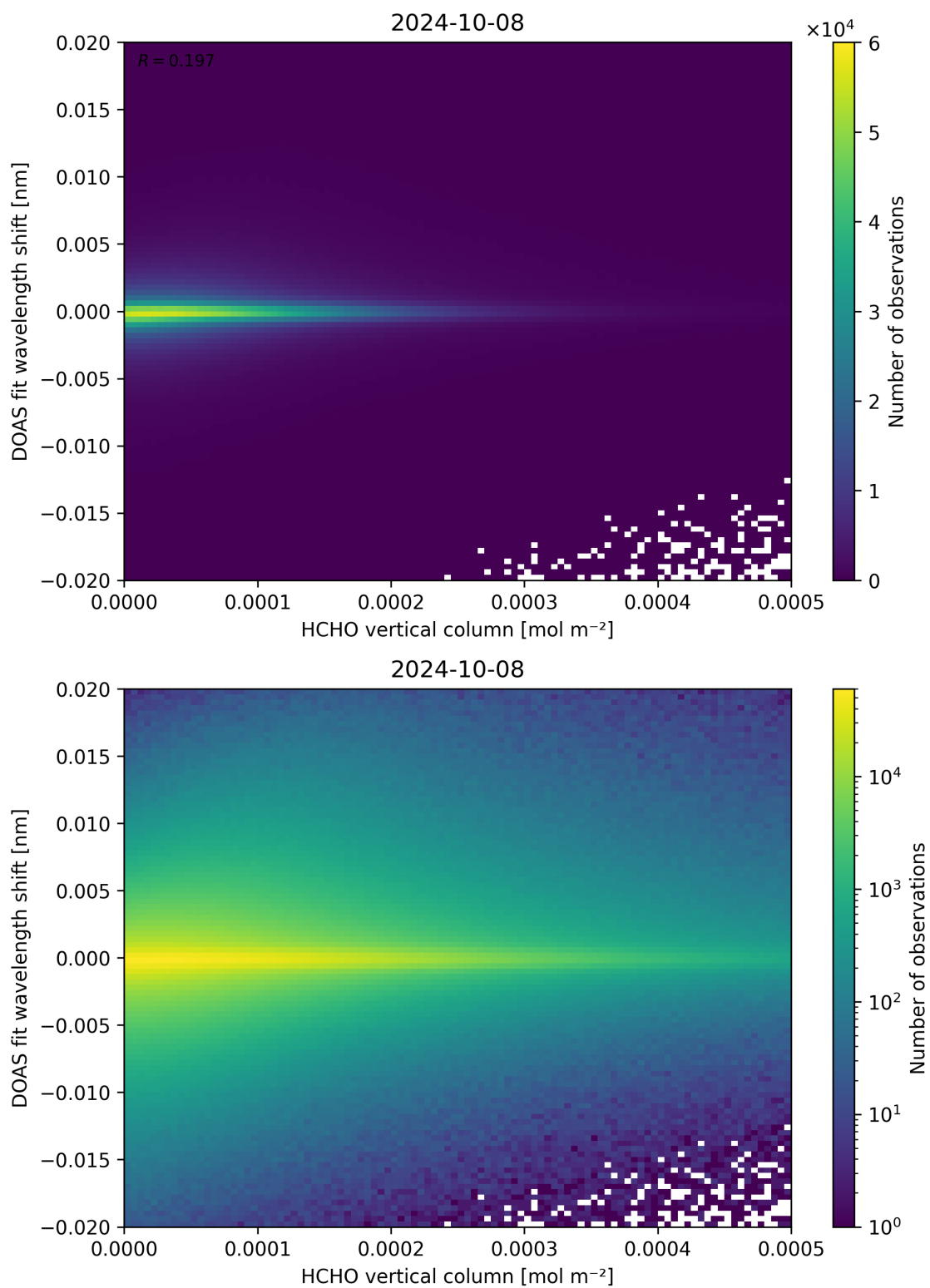
Figure 124: Scatter density plot of “HCHO vertical column” against “DOAS fit wavelength shift” for 2024-10-08 to 2024-10-09.
