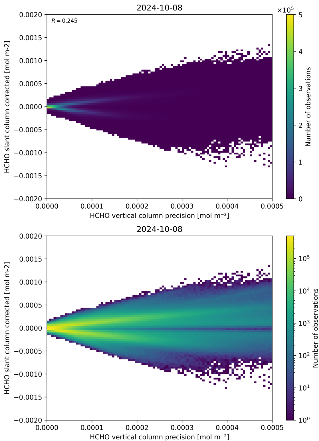
Figure 140: Scatter density plot of “HCHO vertical column precision” against “HCHO slant column corrected” for 2024-10-08 to 2024-10-09.
