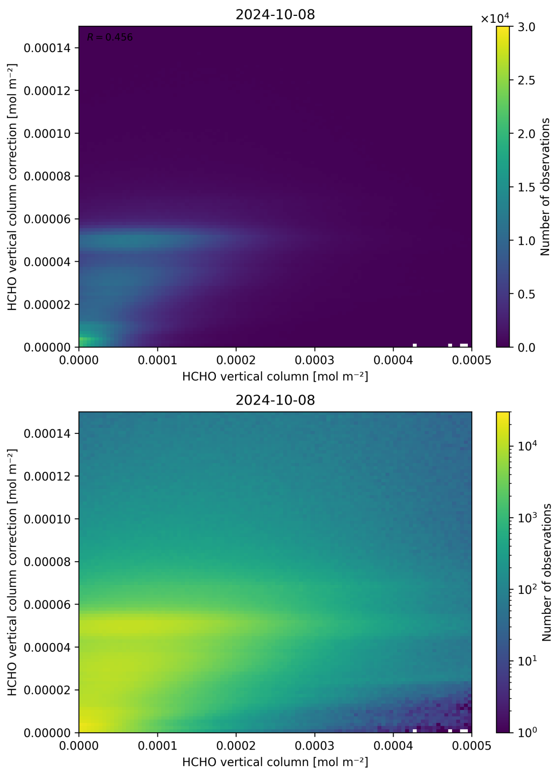
Figure 133: Scatter density plot of “HCHO vertical column” against “HCHO vertical column correction” for 2024-10-08 to 2024-10-09.
