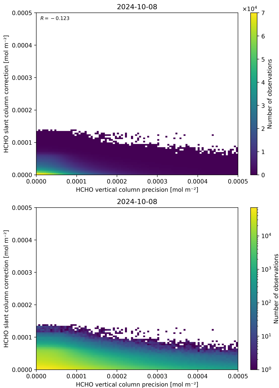
Figure 141: Scatter density plot of “HCHO vertical column precision” against “HCHO slant column correction” for 2024-10-08 to 2024-10-09.
