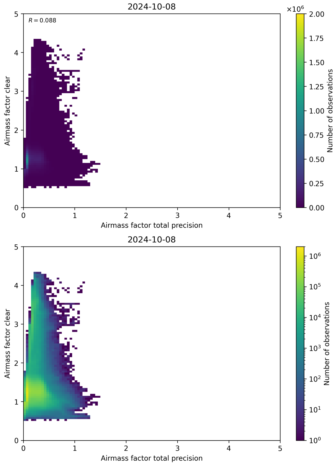
Figure 108: Scatter density plot of “Airmass factor total precision” against “Airmass factor clear” for 2024-10-08 to 2024-10-09.
