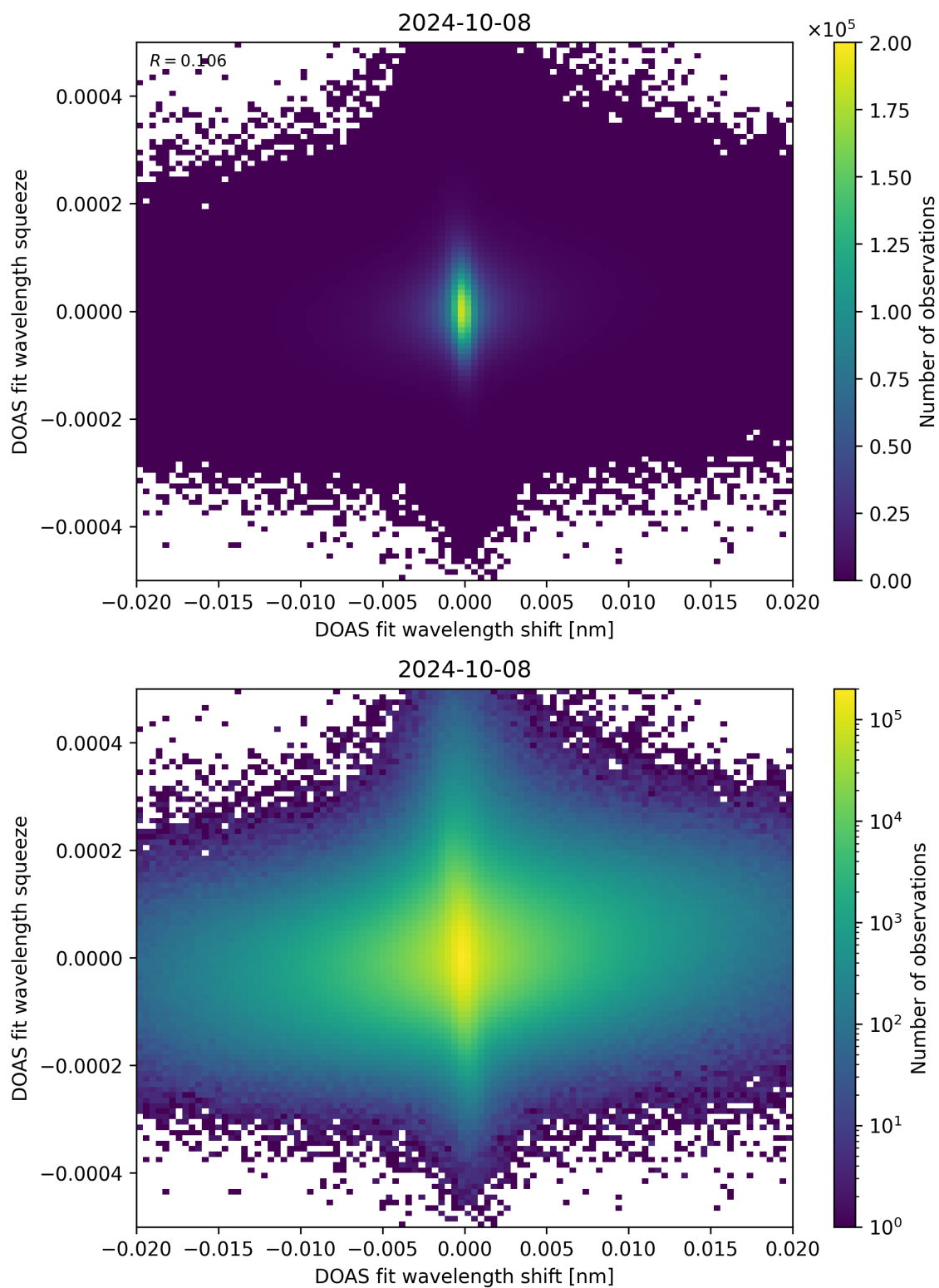
Figure 65: Scatter density plot of “DOAS fit wavelength shift” against “DOAS fit wavelength squeeze” for 2024-10-08 to 2024-10-09.
