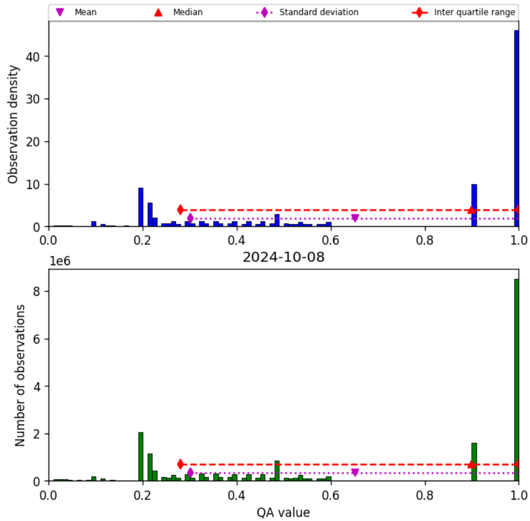
Figure 34: Histogram of “QA value” for 2024-10-08 to 2024-10-09
