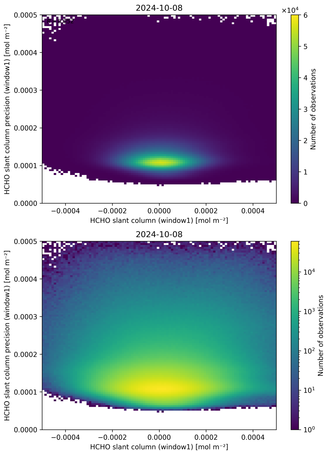
Figure 84: Scatter density plot of “HCHO slant column (window1)” against “HCHO slant column precision (window1)” for 2024-10-08 to 2024-10-09.
