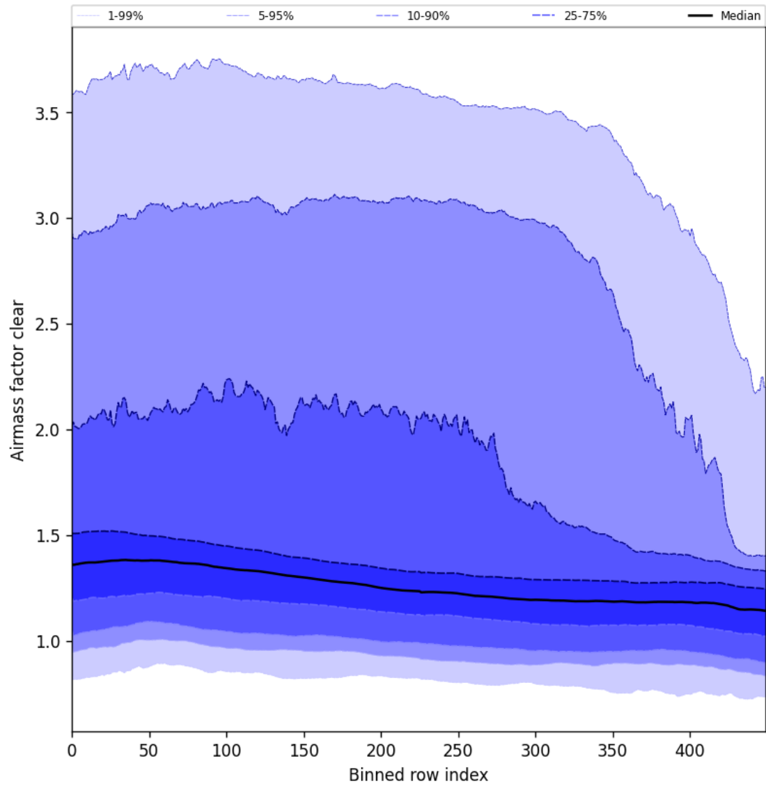
Figure 56: Along track statistics of “Airmass factor clear” for 2024-10-08 to 2024-10-09
