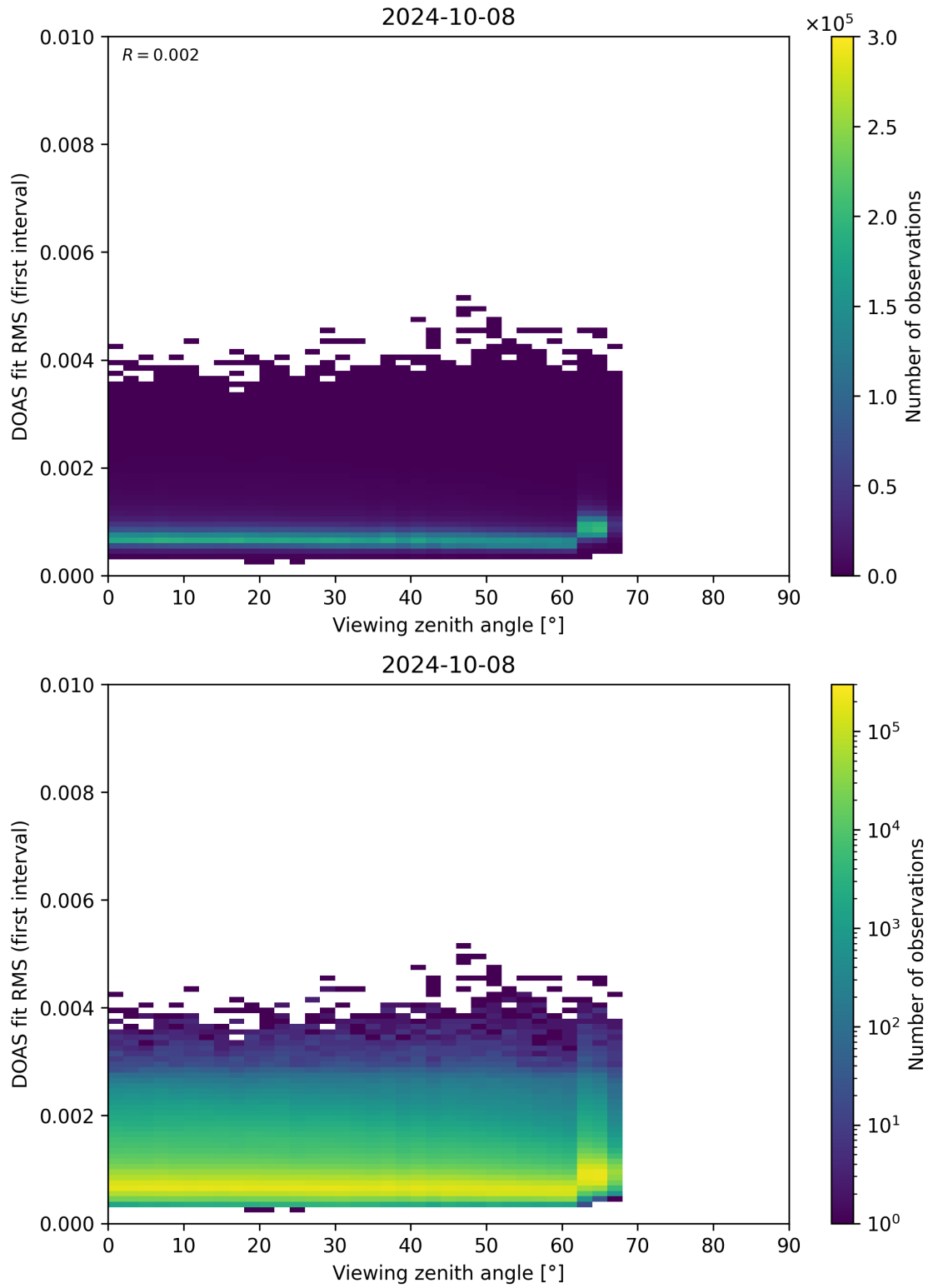
Figure 182: Scatter density plot of “Viewing zenith angle” against “DOAS fit RMS (first interval)” for 2024-10-08 to 2024-10-09.
