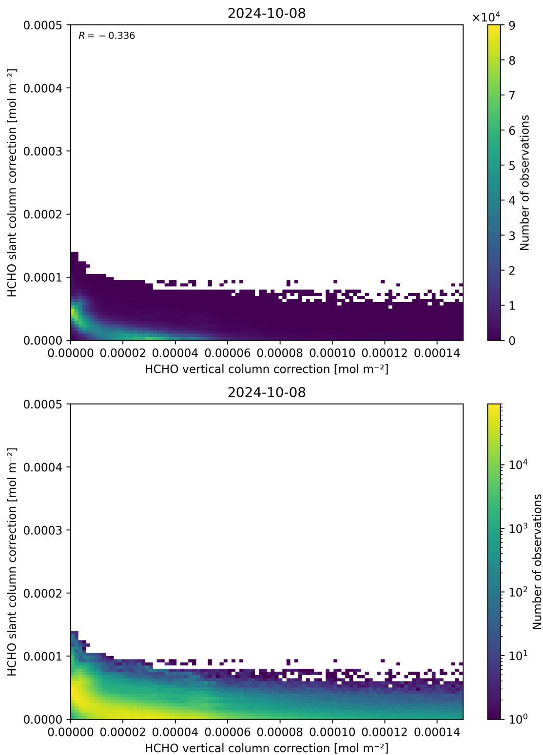
Figure 117: Scatter density plot of “HCHO vertical column correction” against “HCHO slant column correction” for 2024-10-08 to 2024-10-09.
