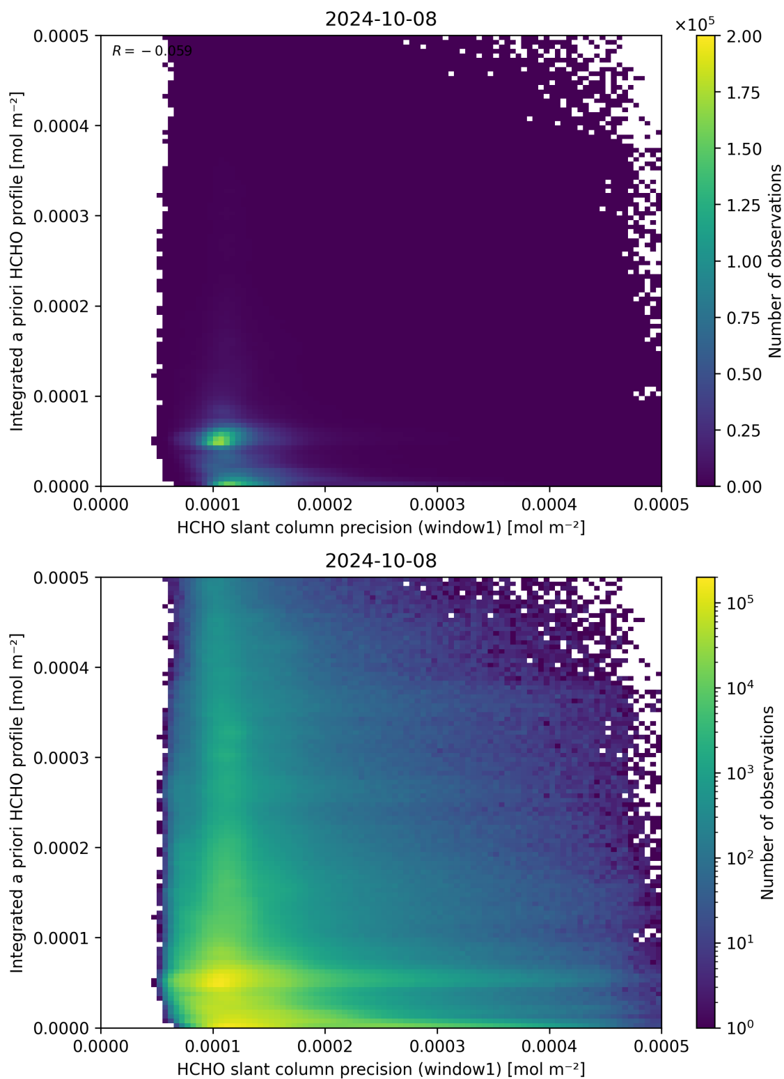
Figure 96: Scatter density plot of “HCHO slant column precision (window1)” against “Integrated a priori HCHO profile” for 2024-10-08 to 2024-10-09.
