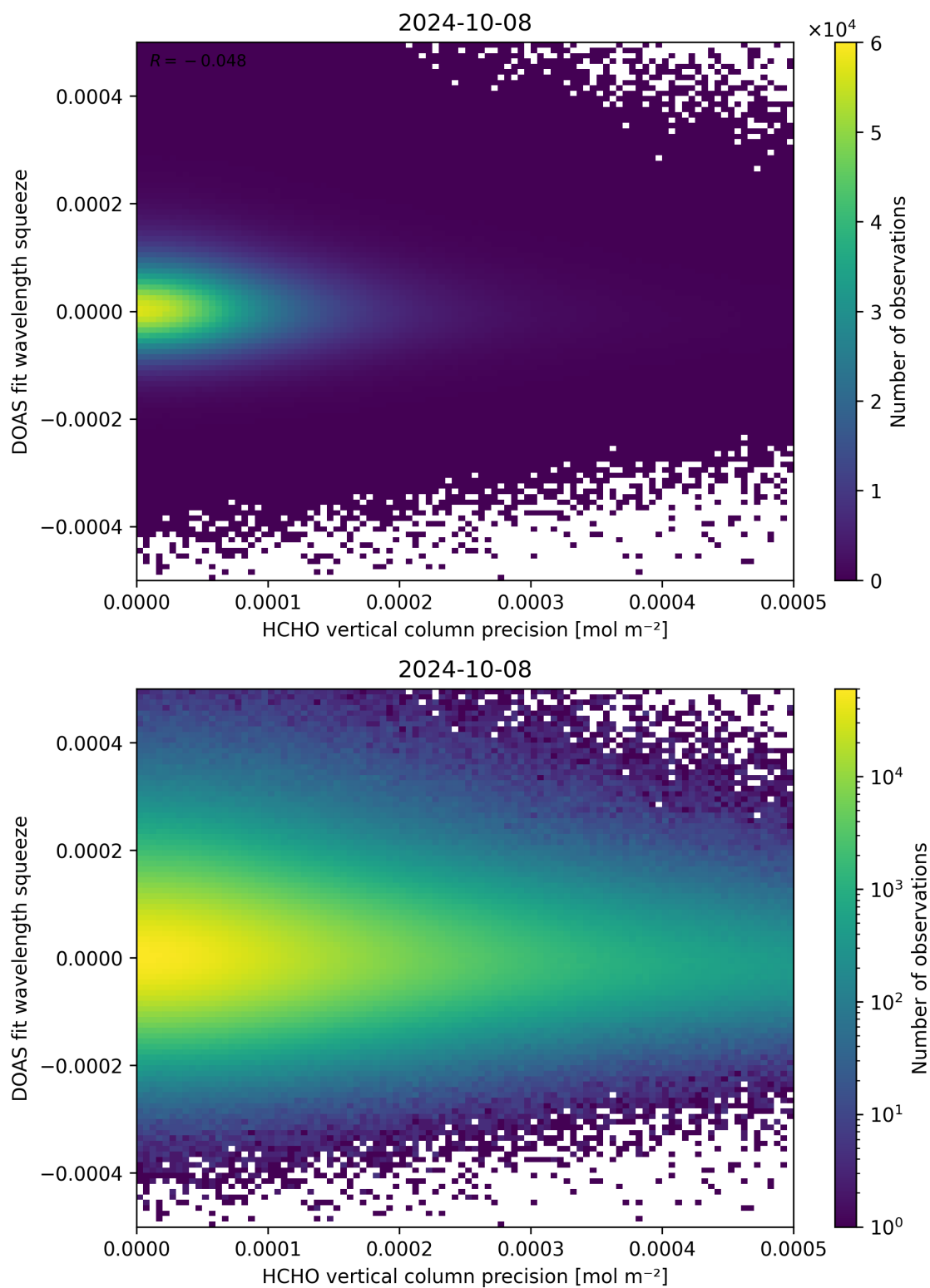
Figure 138: Scatter density plot of “HCHO vertical column precision” against “DOAS fit wavelength squeeze” for 2024-10-08 to 2024-10-09.
