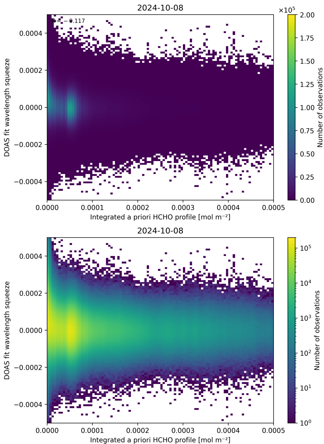
Figure 150: Scatter density plot of “Integrated a priori HCHO profile” against “DOAS fit wavelength squeeze” for 2024-10-08 to 2024-10-09.
