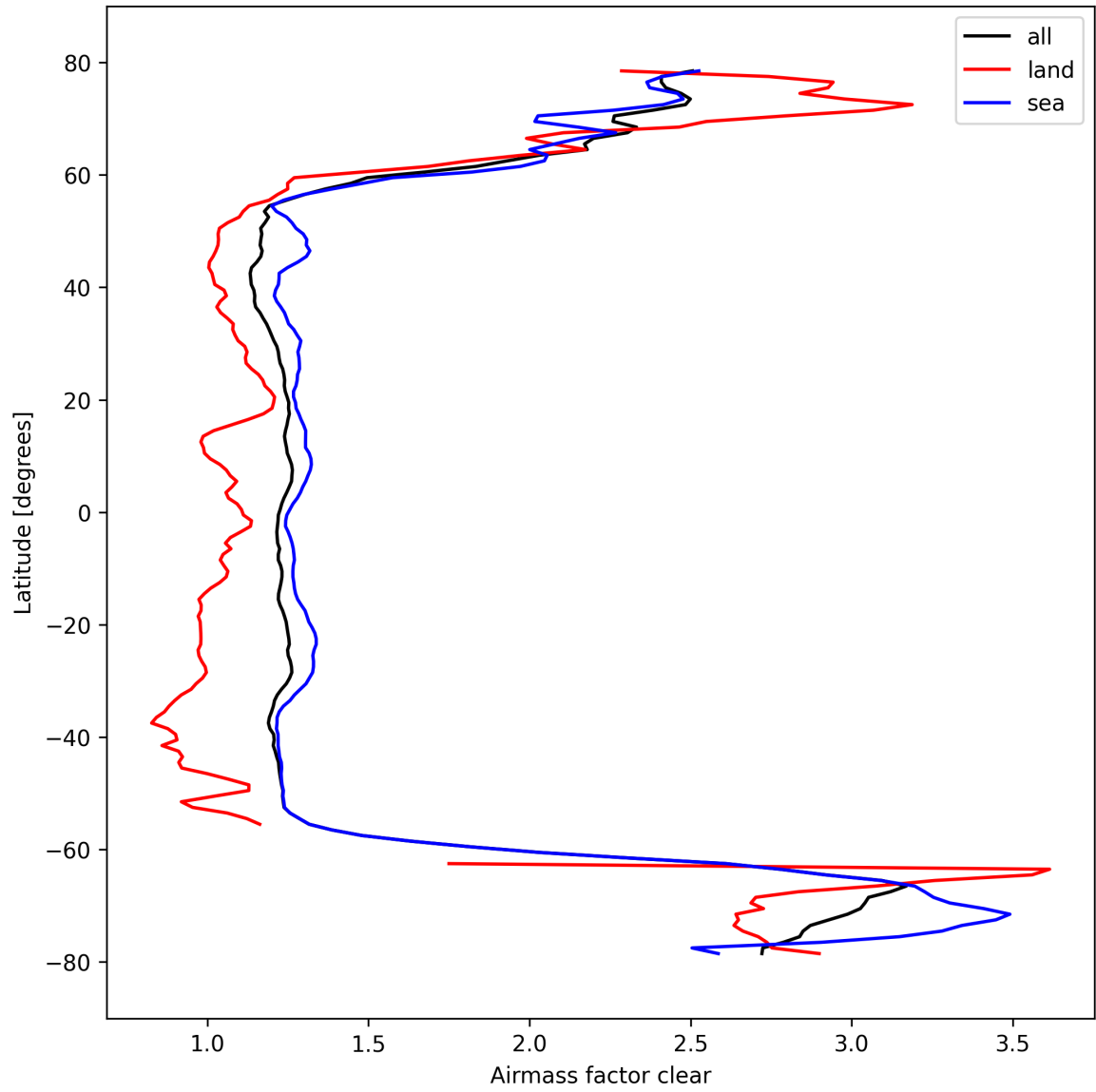
Figure 28: Zonal average of “Airmass factor clear” for 2024-10-08 to 2024-10-09.
