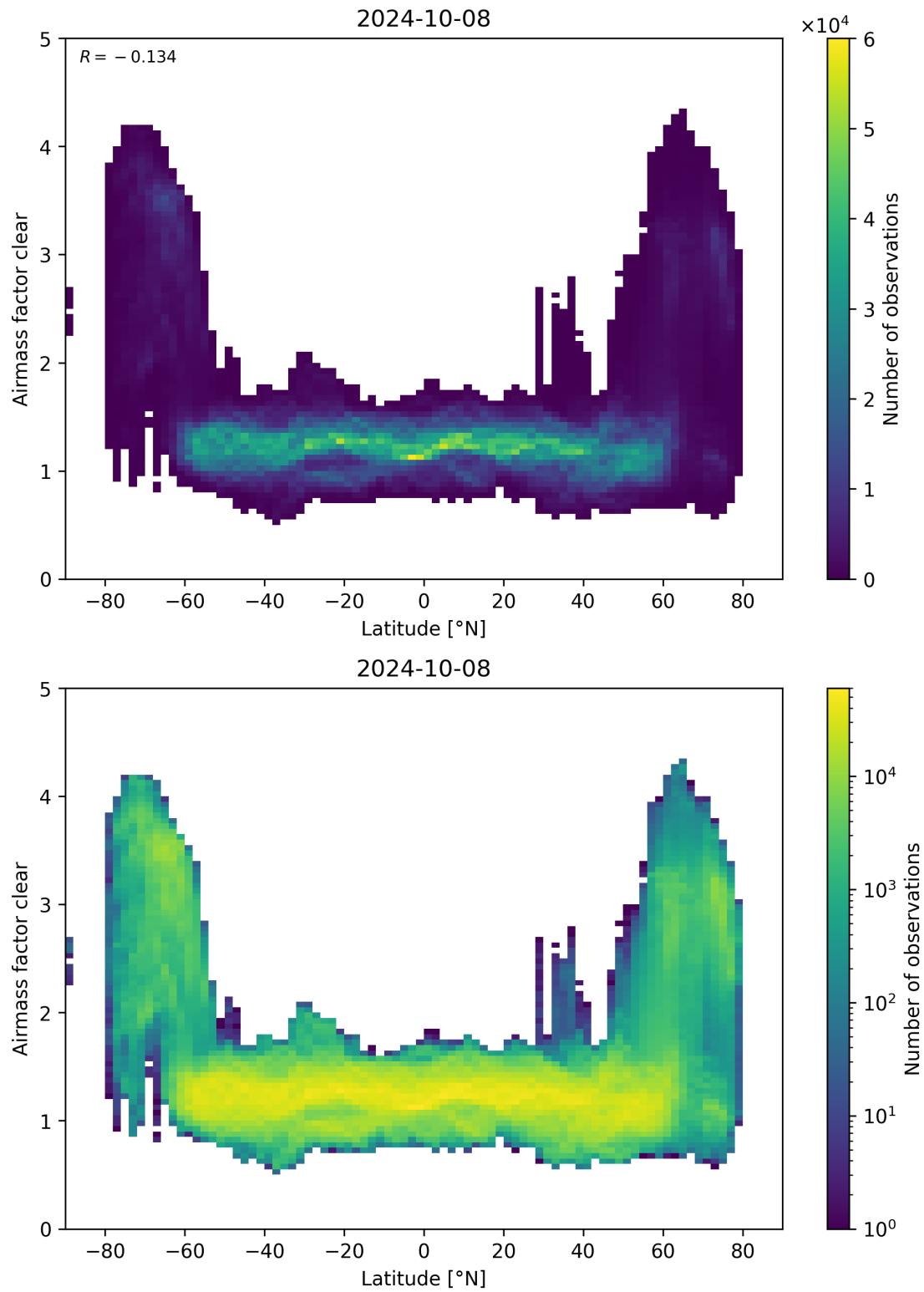
Figure 156: Scatter density plot of “Latitude” against “Airmass factor clear” for 2024-10-08 to 2024-10-09.
