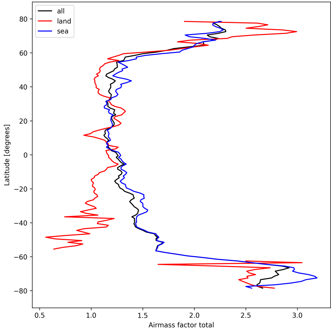
Figure 26: Zonal average of “Airmass factor total” for 2024-10-08 to 2024-10-09.
