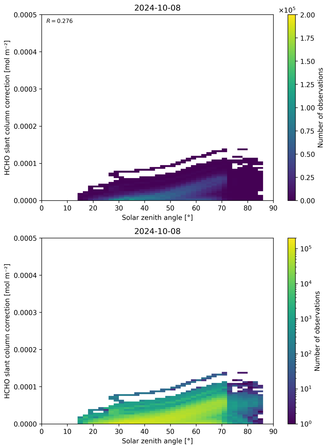
Figure 172: Scatter density plot of “Solar zenith angle” against “HCHO slant column correction” for 2024-10-08 to 2024-10-09.
