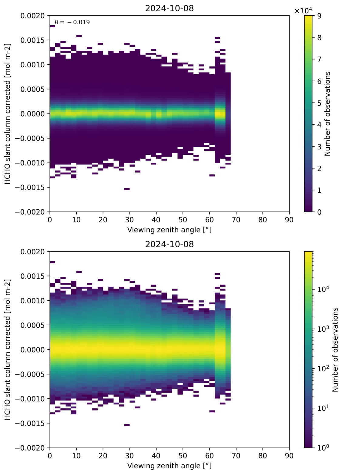
Figure 186: Scatter density plot of “Viewing zenith angle” against “HCHO slant column corrected” for 2024-10-08 to 2024-10-09.
