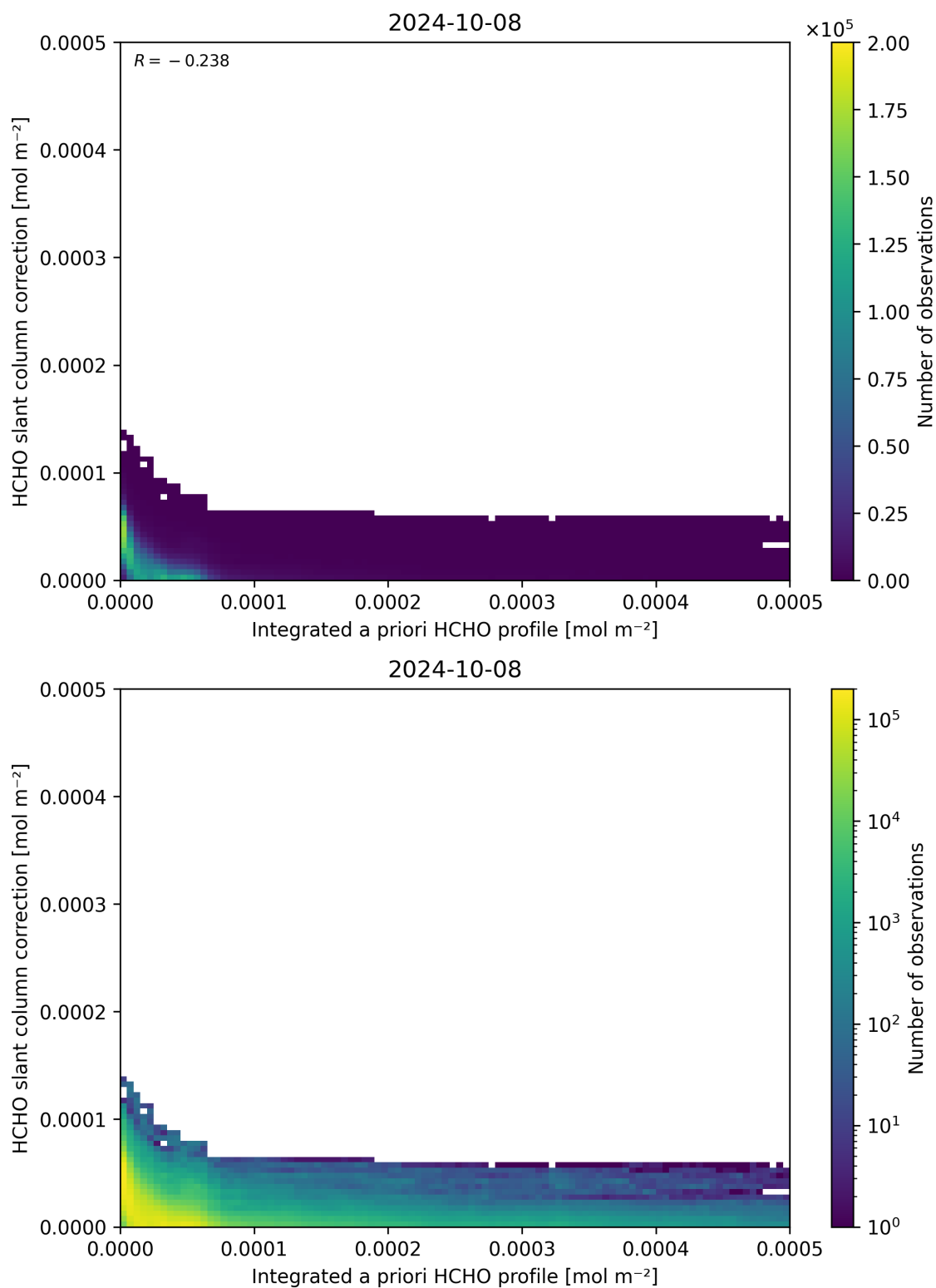
Figure 152: Scatter density plot of “Integrated a priori HCHO profile” against “HCHO slant column correction” for 2024-10-08 to 2024-10-09.
