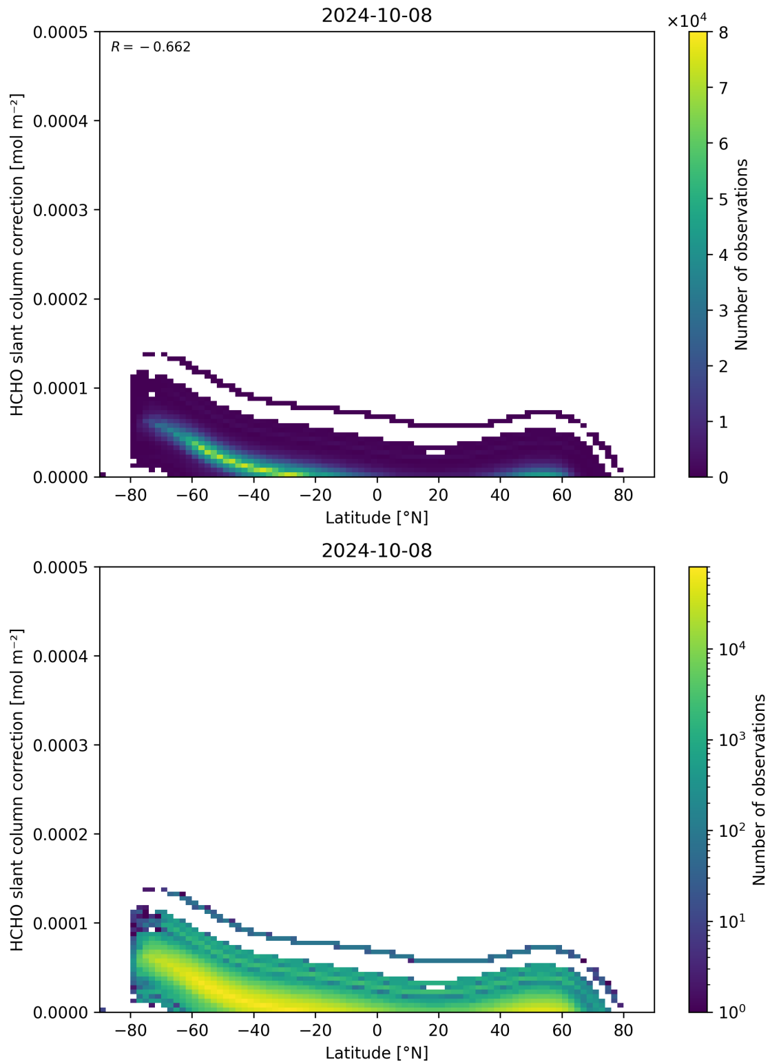
Figure 158: Scatter density plot of “Latitude” against “HCHO slant column correction” for 2024-10-08 to 2024-10-09.
