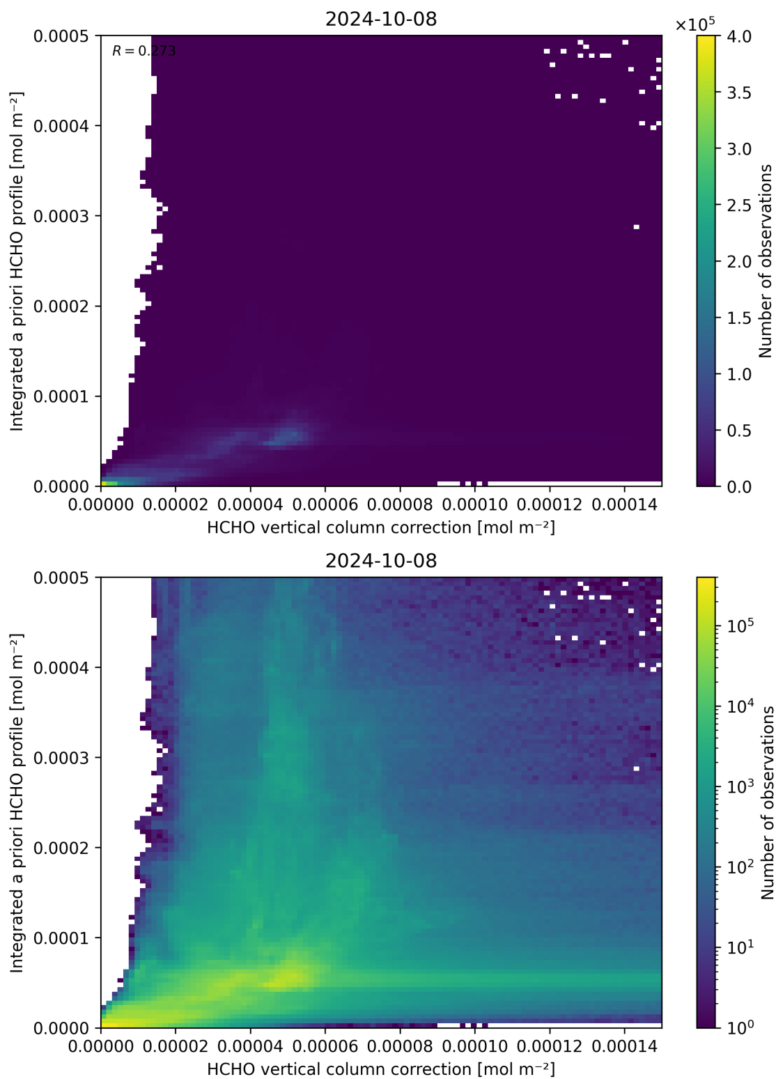
Figure 122: Scatter density plot of “HCHO vertical column correction” against “Integrated a priori HCHO profile” for 2024-10-08 to 2024-10-09.
