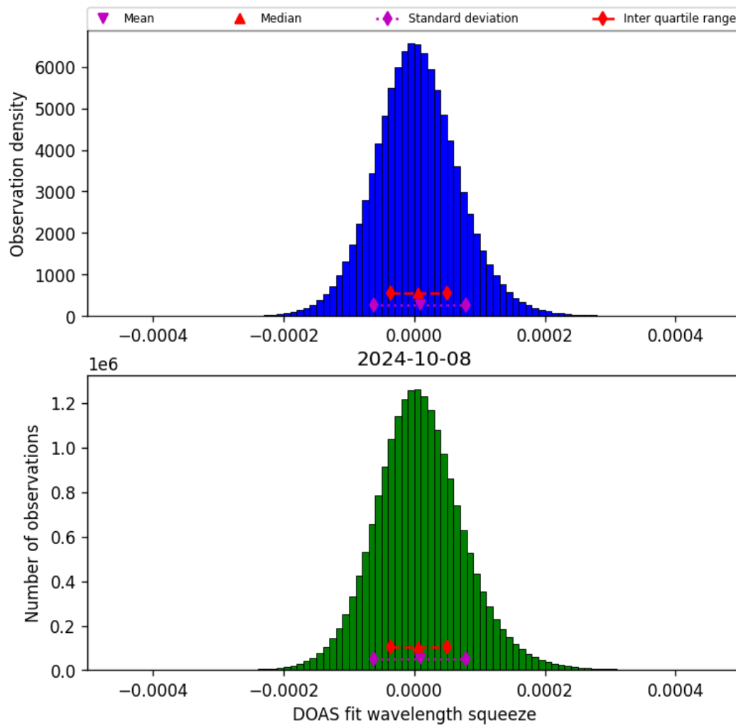
Figure 45: Histogram of “DOAS fit wavelength squeeze” for 2024-10-08 to 2024-10-09
