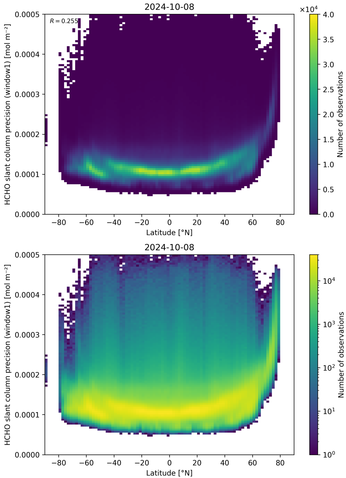
Figure 160: Scatter density plot of “Latitude” against “HCHO slant column precision (window1)” for 2024-10-08 to 2024-10-09.
