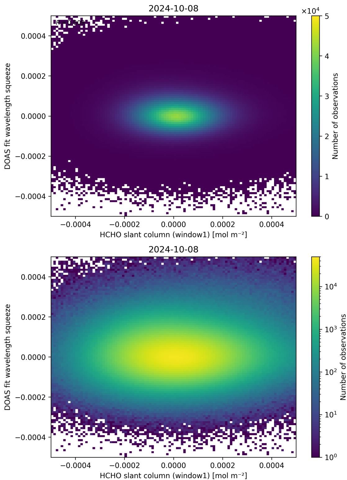
Figure 80: Scatter density plot of “HCHO slant column (window1)” against “DOAS fit wavelength squeeze” for 2024-10-08 to 2024-10-09.
