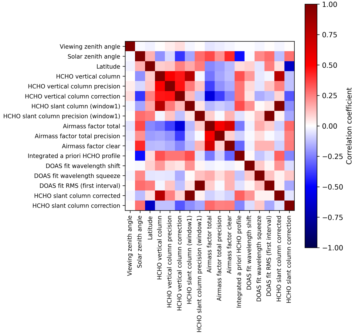
Figure 2: Map of correlation matrix for 2024-10-08 to 2024-10-09.
