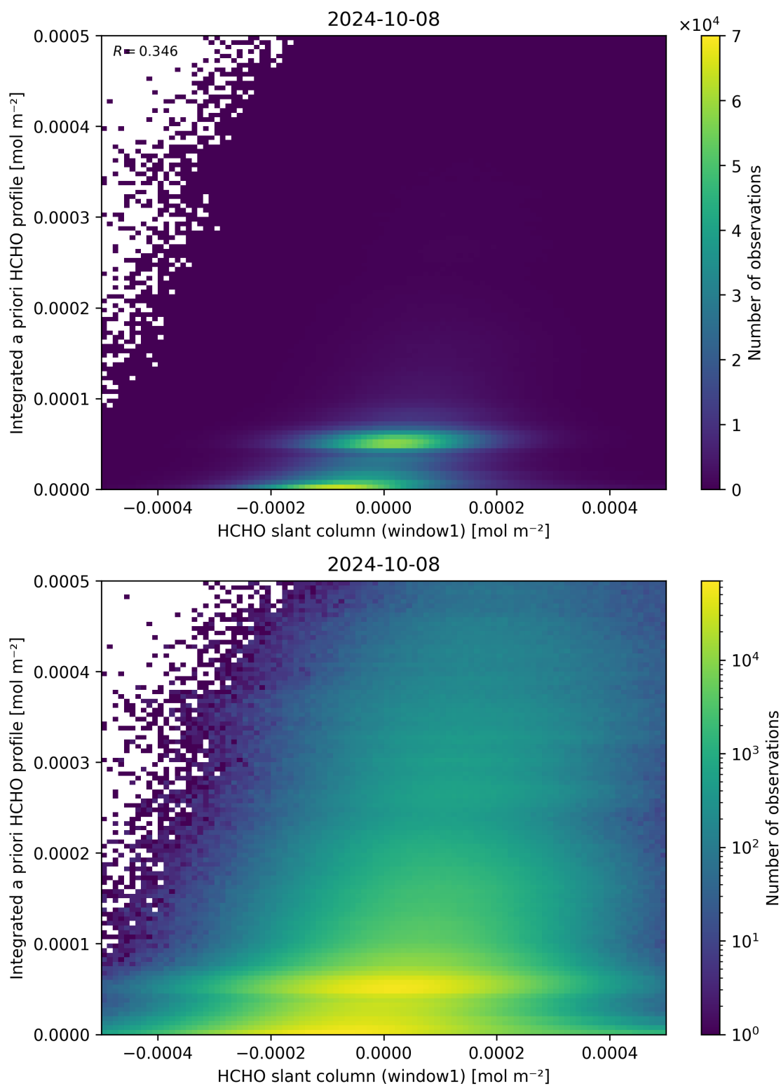
Figure 87: Scatter density plot of “HCHO slant column (window1)” against “Integrated a priori HCHO profile” for 2024-10-08 to 2024-10-09.
