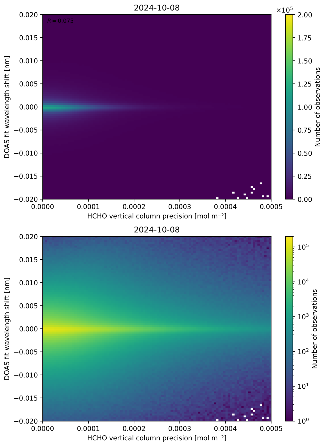
Figure 137: Scatter density plot of “HCHO vertical column precision” against “DOAS fit wavelength shift” for 2024-10-08 to 2024-10-09.
