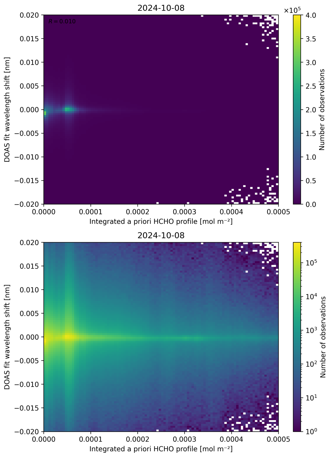
Figure 149: Scatter density plot of “Integrated a priori HCHO profile” against “DOAS fit wavelength shift” for 2024-10-08 to 2024-10-09.
