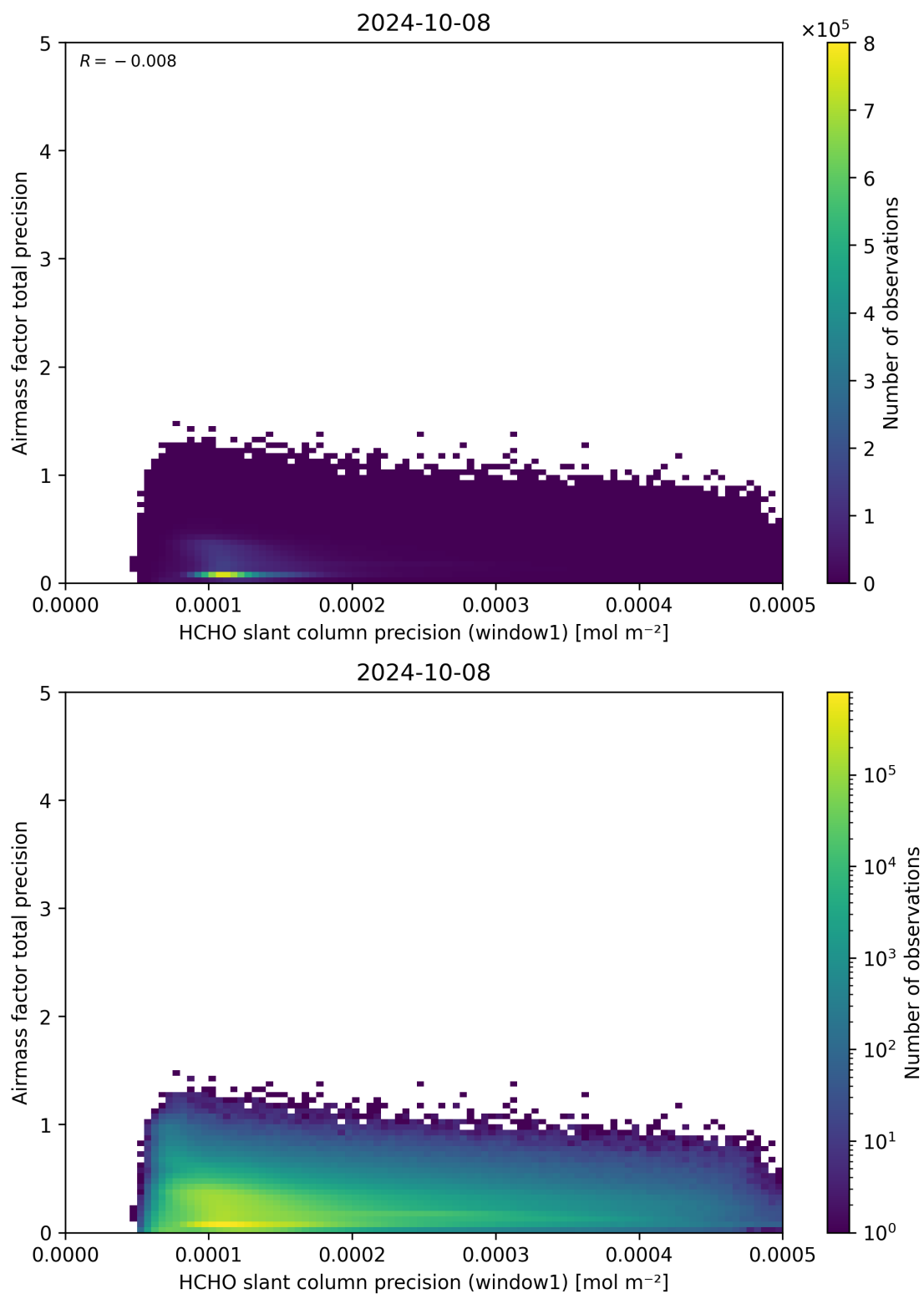
Figure 95: Scatter density plot of “HCHO slant column precision (window1)” against “Airmass factor total precision” for 2024-10-08 to 2024-10-09.
