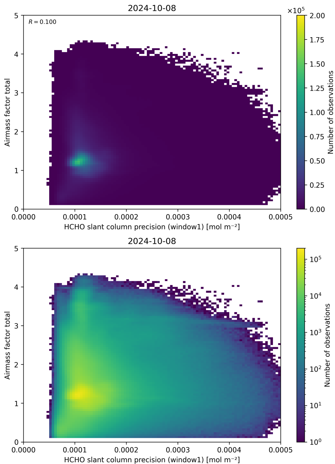
Figure 94: Scatter density plot of “HCHO slant column precision (window1)” against “Airmass factor total” for 2024-10-08 to 2024-10-09.
