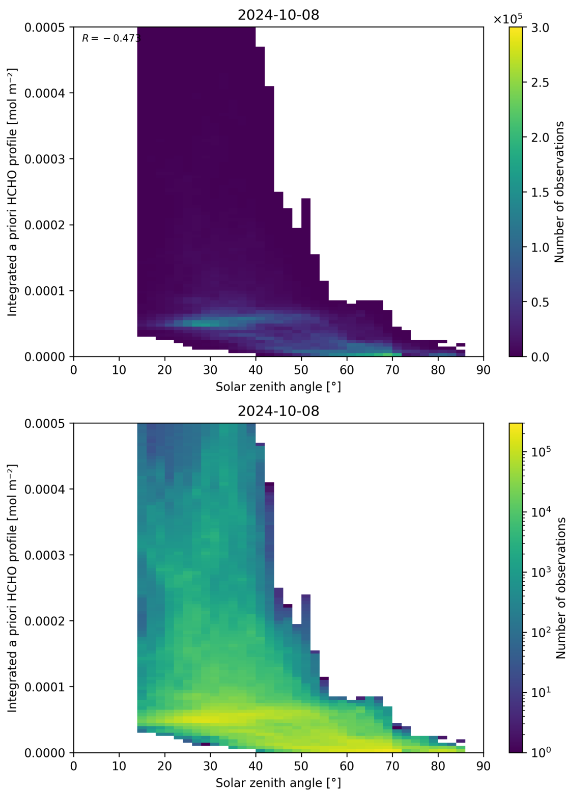
Figure 180: Scatter density plot of “Solar zenith angle” against “Integrated a priori HCHO profile” for 2024-10-08 to 2024-10-09.
