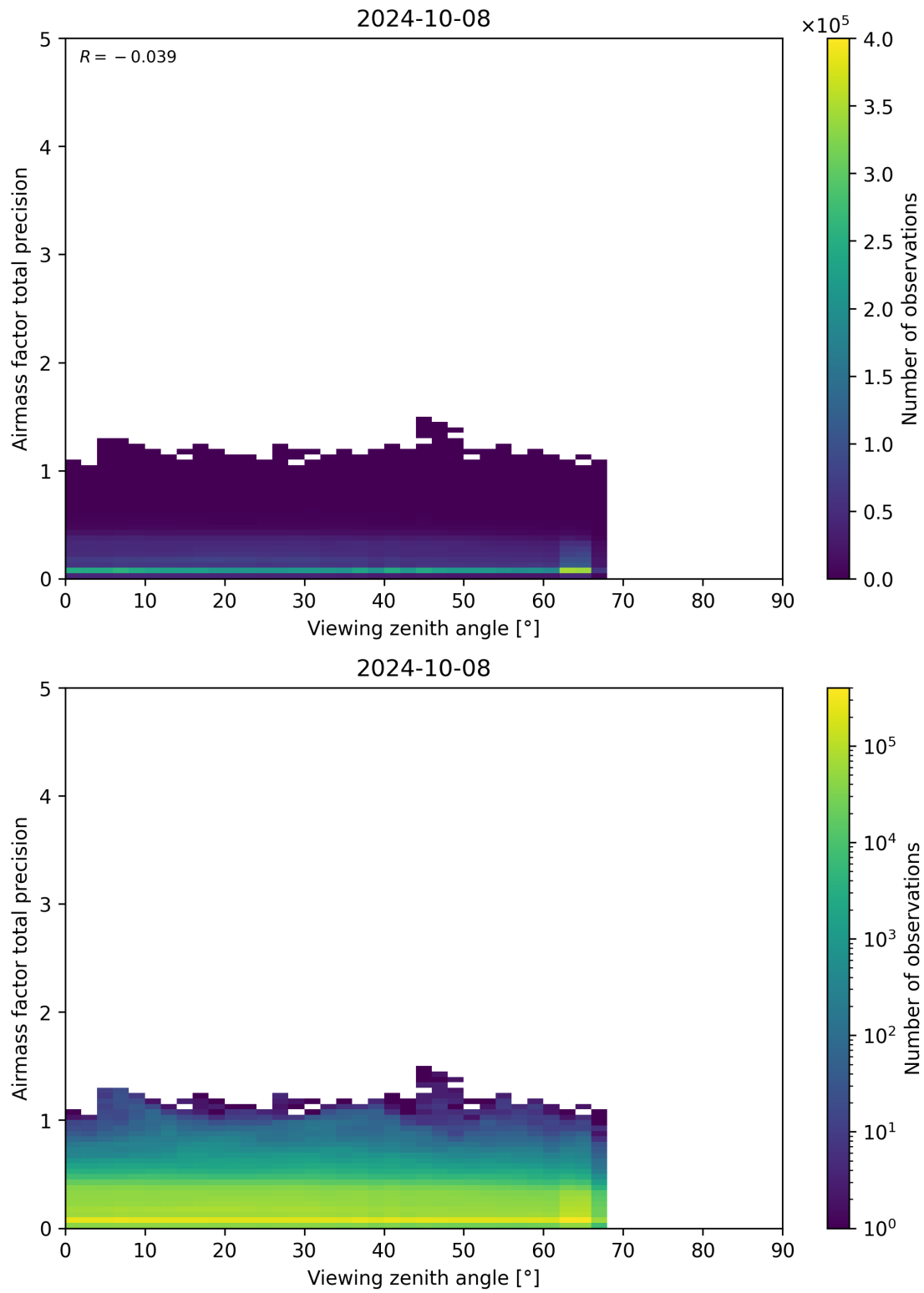
Figure 191: Scatter density plot of “Viewing zenith angle” against “Airmass factor total precision” for 2024-10-08 to 2024-10-09.
