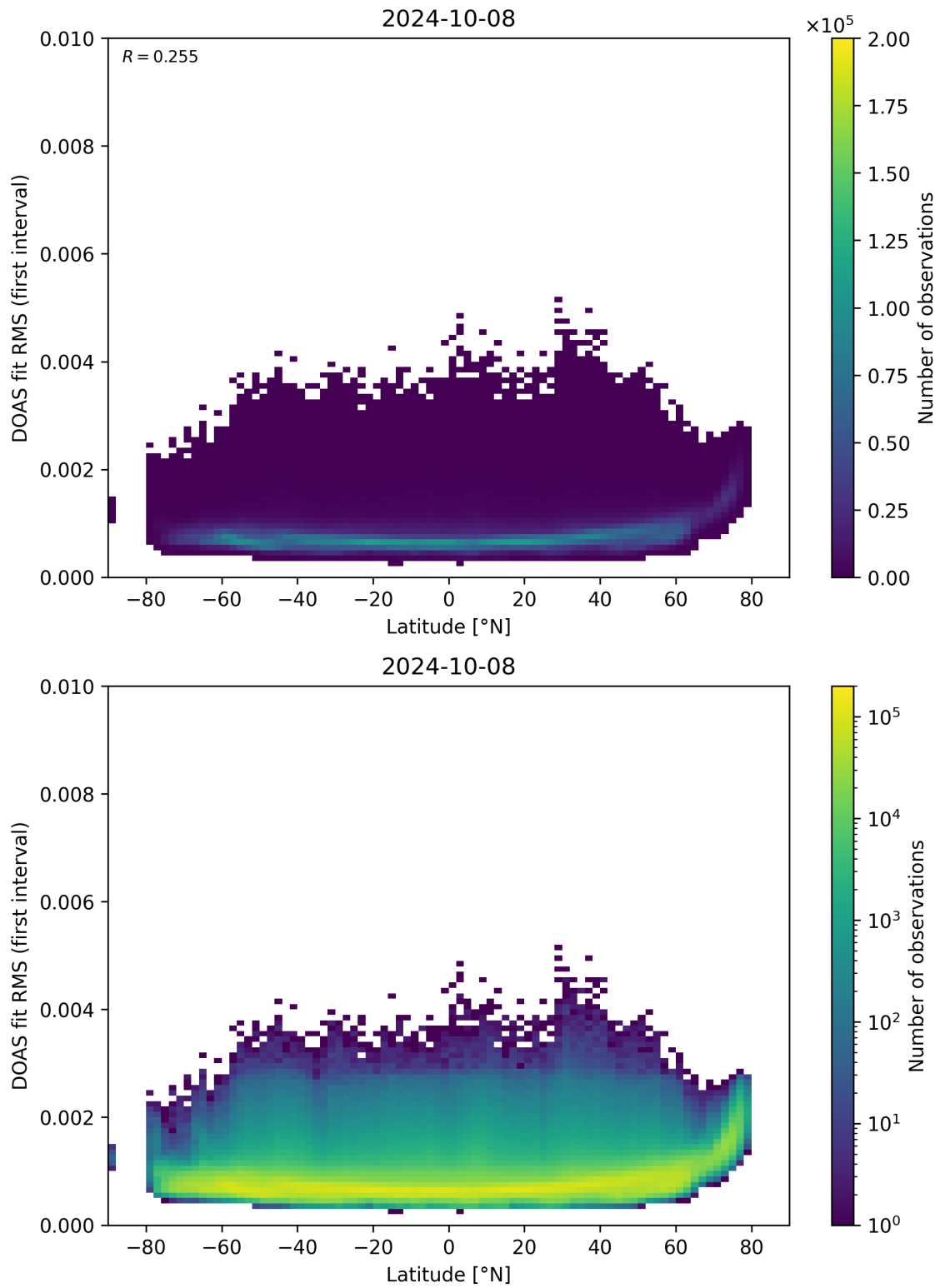
Figure 153: Scatter density plot of “Latitude” against “DOAS fit RMS (first interval)” for 2024-10-08 to 2024-10-09.
