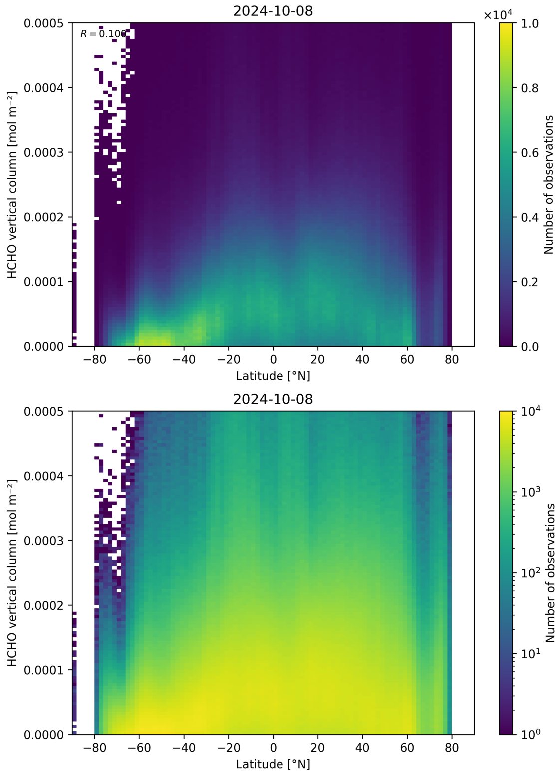
Figure 163: Scatter density plot of “Latitude” against “HCHO vertical column” for 2024-10-08 to 2024-10-09.
