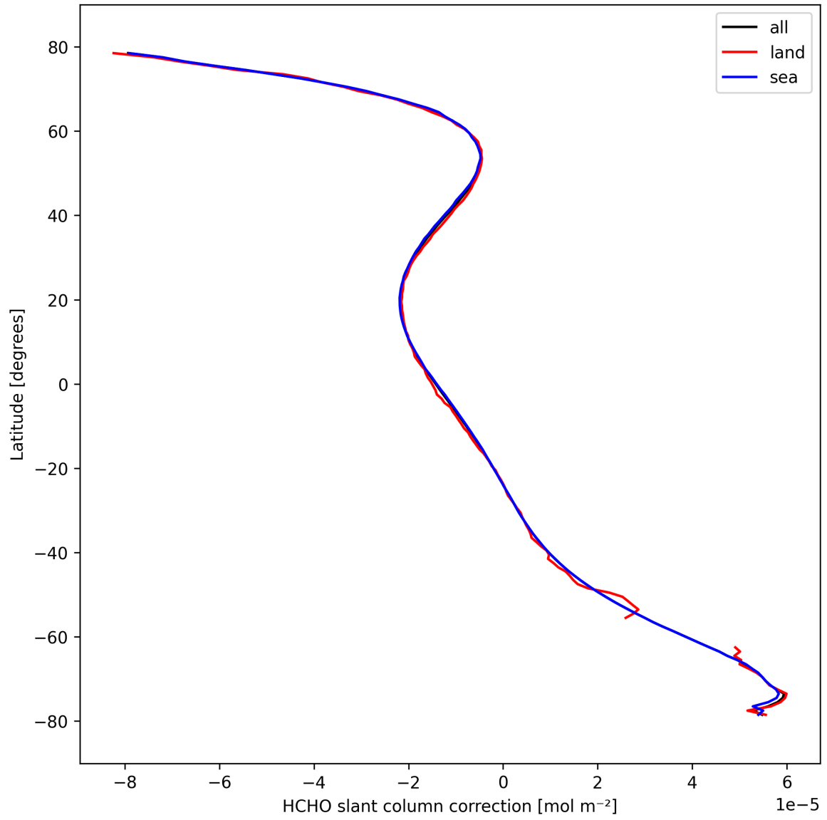
Figure 33: Zonal average of “HCHO slant column correction” for 2024-10-08 to 2024-10-09.
