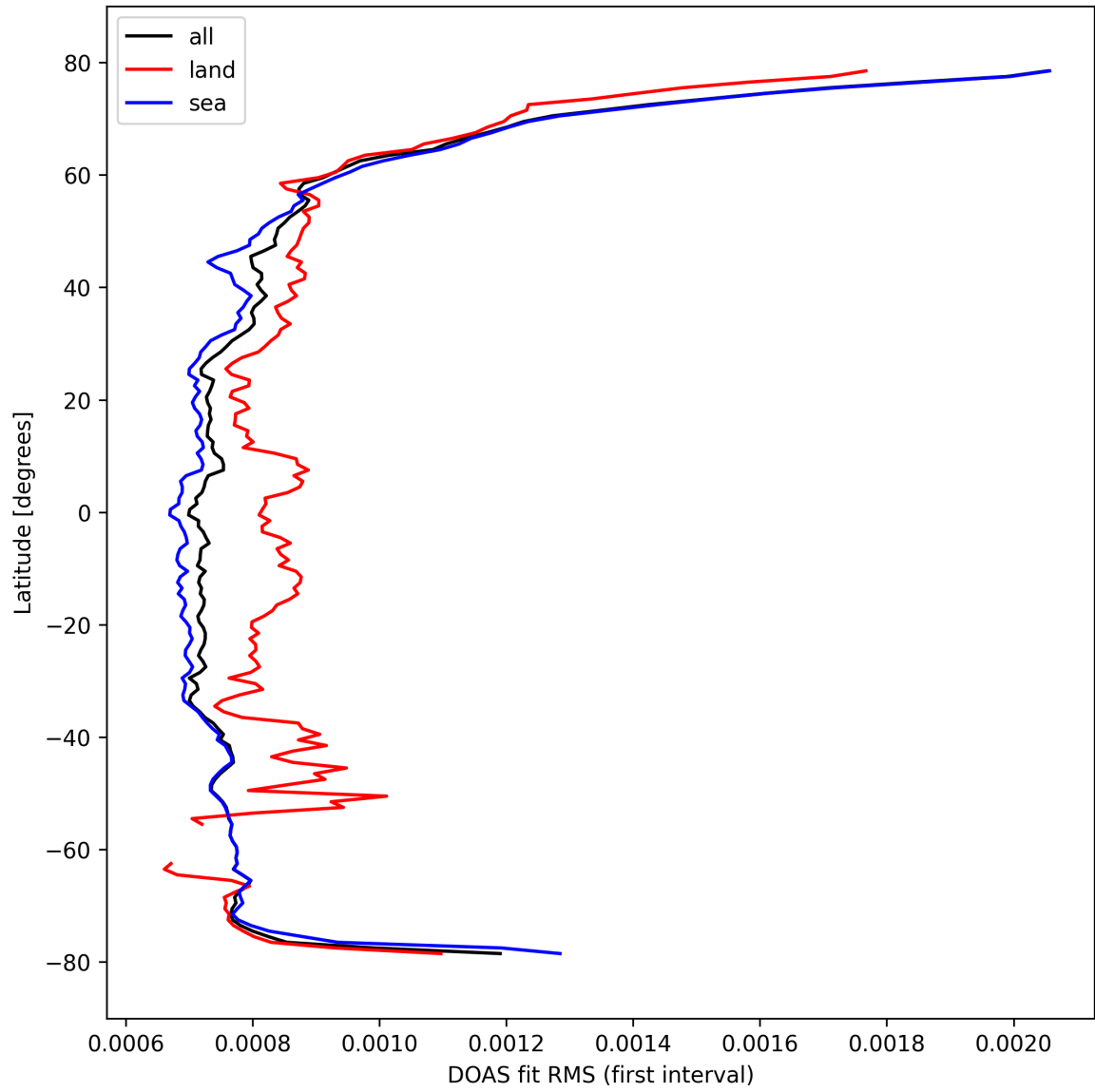
Figure 32: Zonal average of “DOAS fit RMS (first interval)” for 2024-10-08 to 2024-10-09.
