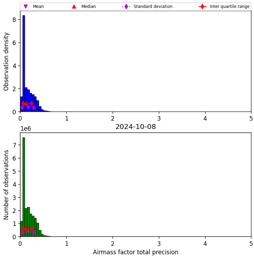
Figure 41: Histogram of “Airmass factor total precision” for 2024-10-08 to 2024-10-09
