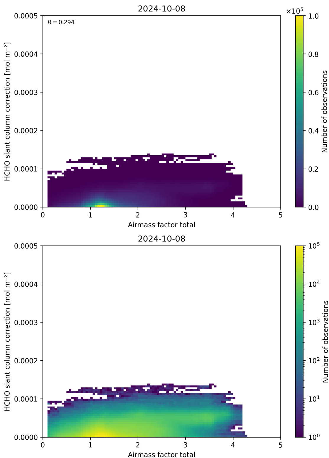
Figure 102: Scatter density plot of “Airmass factor total” against “HCHO slant column correction” for 2024-10-08 to 2024-10-09.
