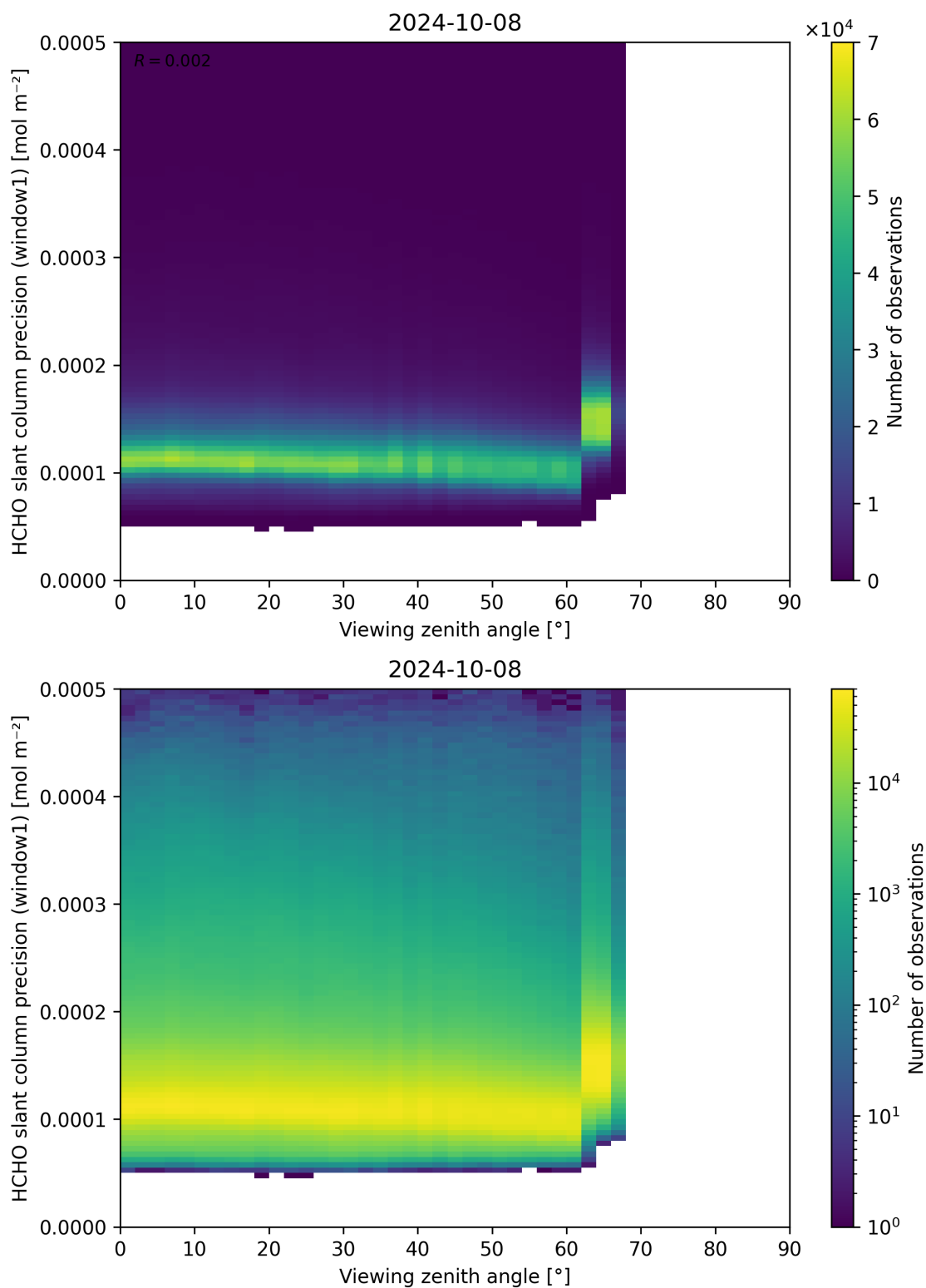
Figure 189: Scatter density plot of “Viewing zenith angle” against “HCHO slant column precision (window1)” for 2024-10-08 to 2024-10-09.
