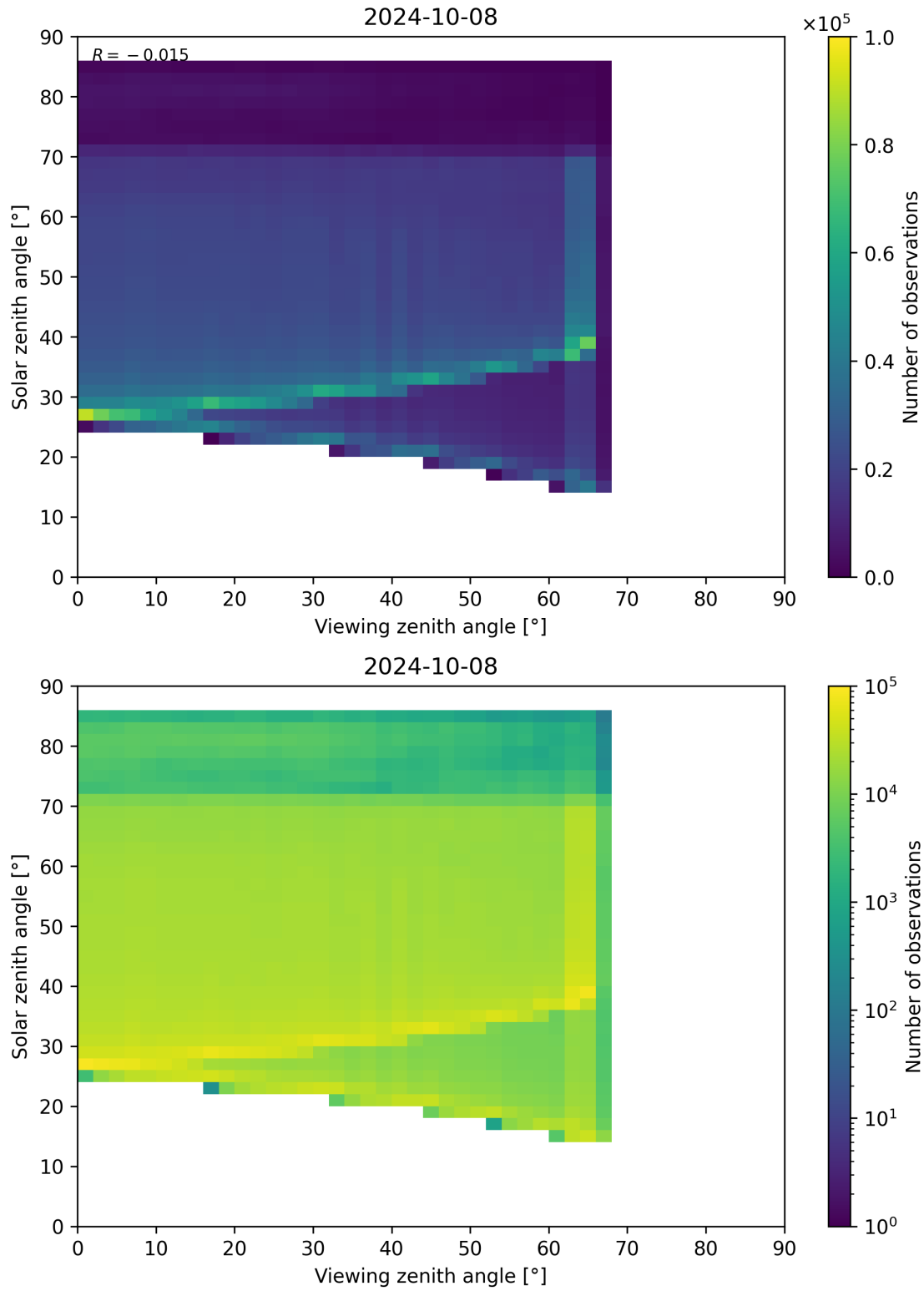
Figure 197: Scatter density plot of “Viewing zenith angle” against “Solar zenith angle” for 2024-10-08 to 2024-10-09.
