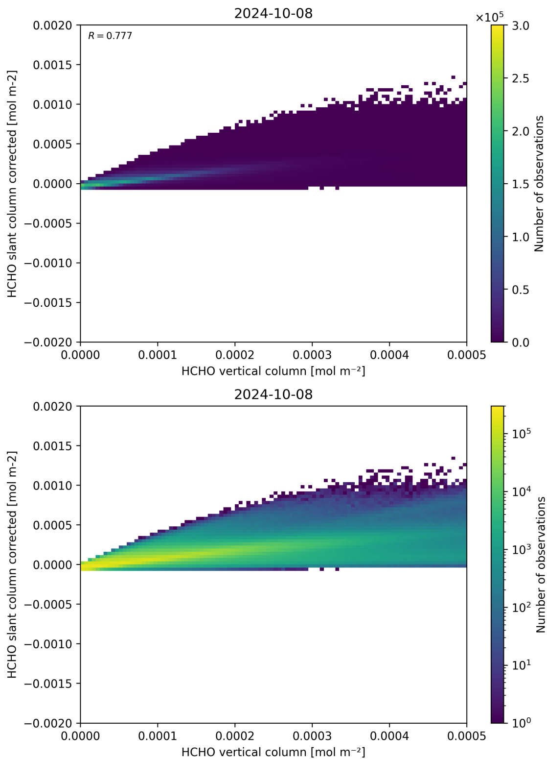
Figure 127: Scatter density plot of “HCHO vertical column” against “HCHO slant column corrected” for 2024-10-08 to 2024-10-09.
