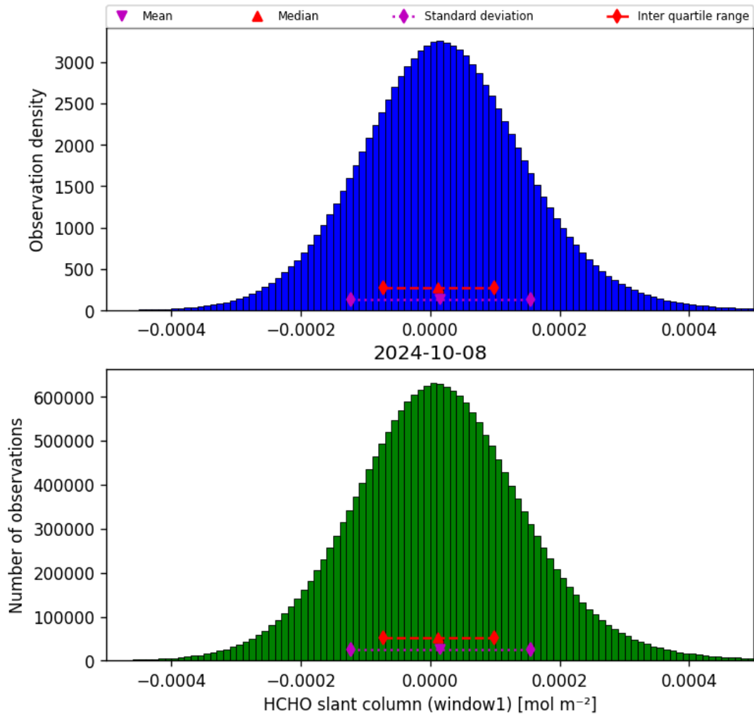
Figure 38: Histogram of “HCHO slant column (window1)” for 2024-10-08 to 2024-10-09
