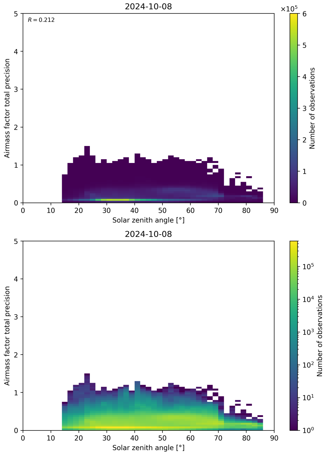
Figure 176: Scatter density plot of “Solar zenith angle” against “Airmass factor total precision” for 2024-10-08 to 2024-10-09.
