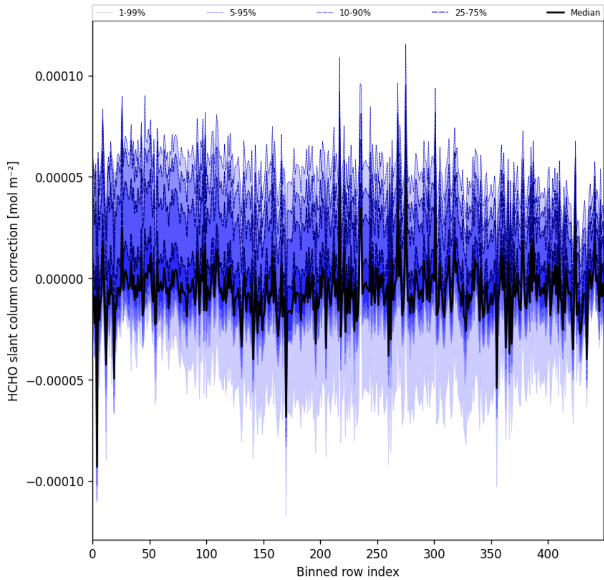
Figure 61: Along track statistics of “HCHO slant column correction” for 2024-10-08 to 2024-10-09
