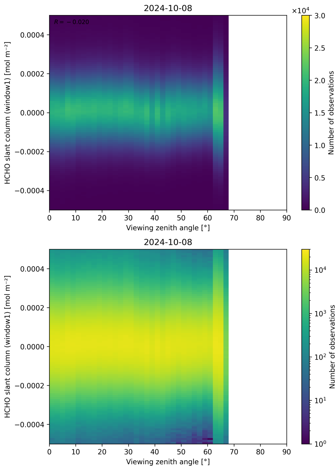
Figure 188: Scatter density plot of “Viewing zenith angle” against “HCHO slant column (window1)” for 2024-10-08 to 2024-10-09.
