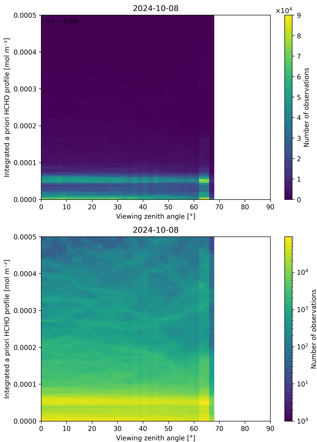
Figure 195: Scatter density plot of “Viewing zenith angle” against “Integrated a priori HCHO profile” for 2024-10-08 to 2024-10-09.
