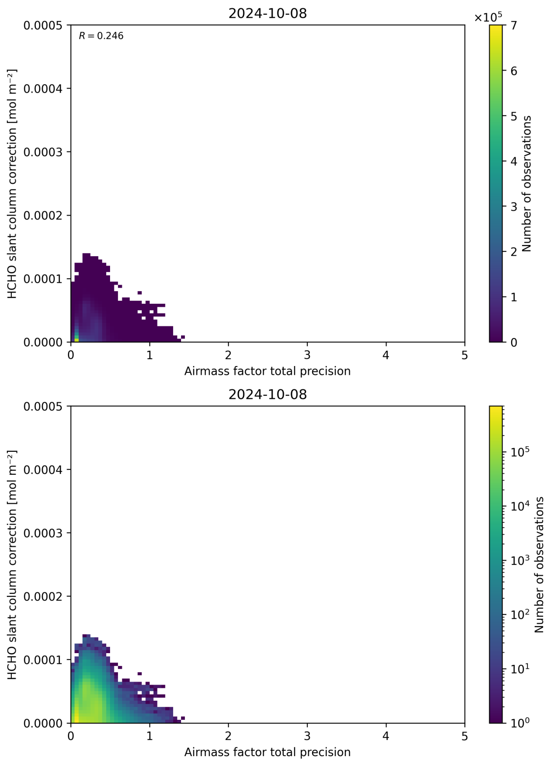
Figure 110: Scatter density plot of “Airmass factor total precision” against “HCHO slant column correction” for 2024-10-08 to 2024-10-09.
