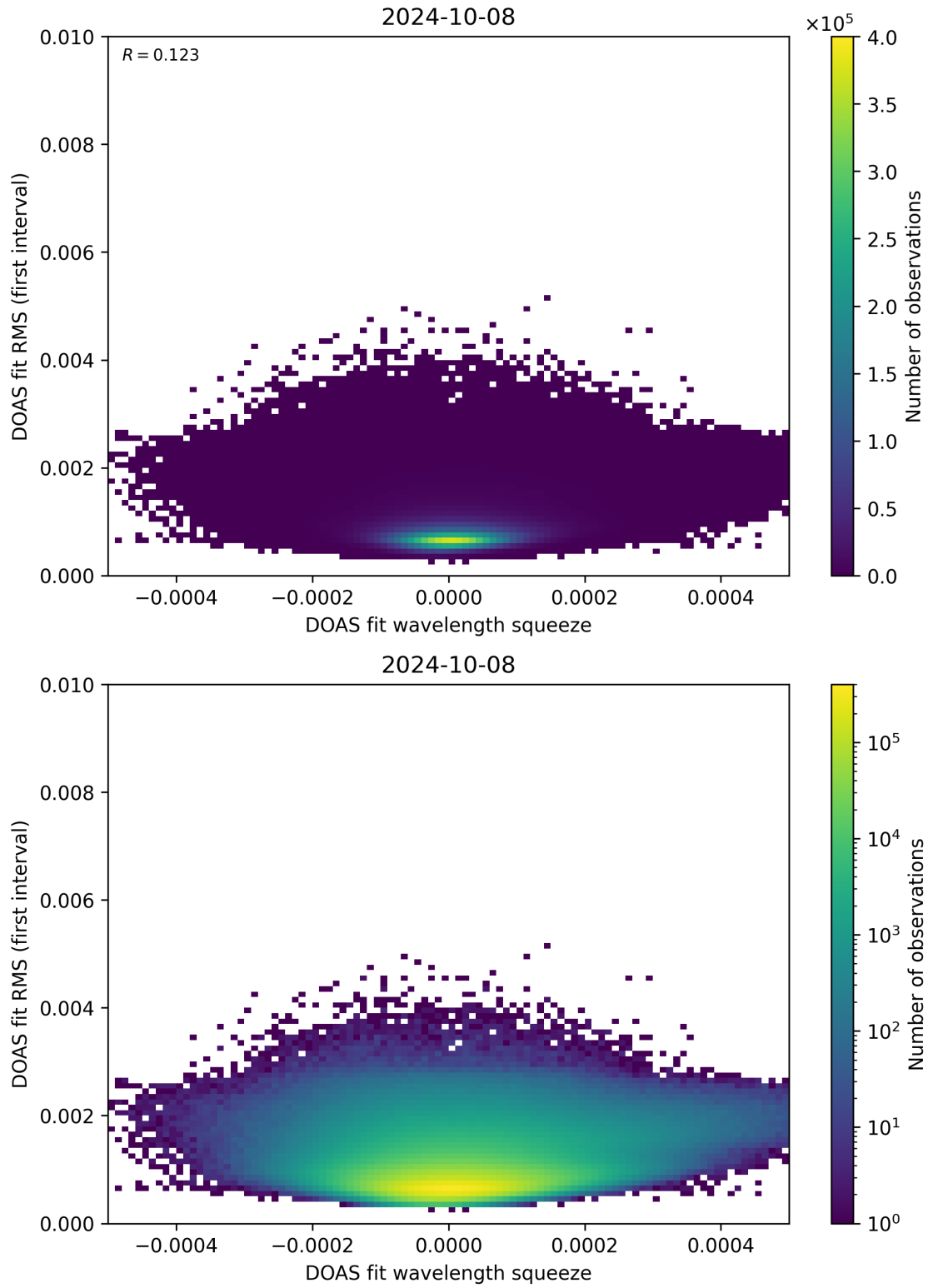
Figure 68: Scatter density plot of “DOAS fit wavelength squeeze” against “DOAS fit RMS (first interval)” for 2024-10-08 to 2024-10-09.
