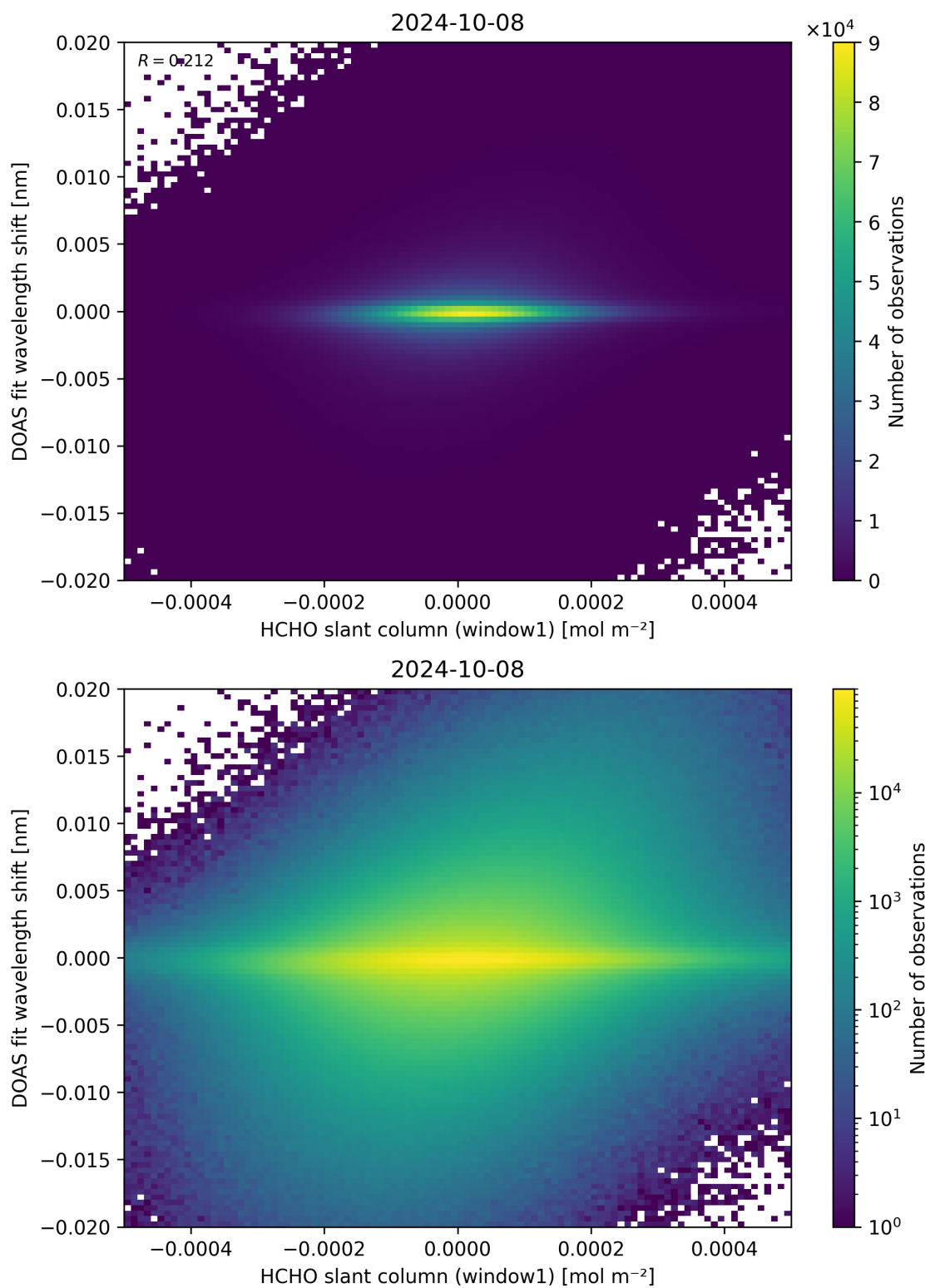
Figure 79: Scatter density plot of “HCHO slant column (window1)” against “DOAS fit wavelength shift” for 2024-10-08 to 2024-10-09.
