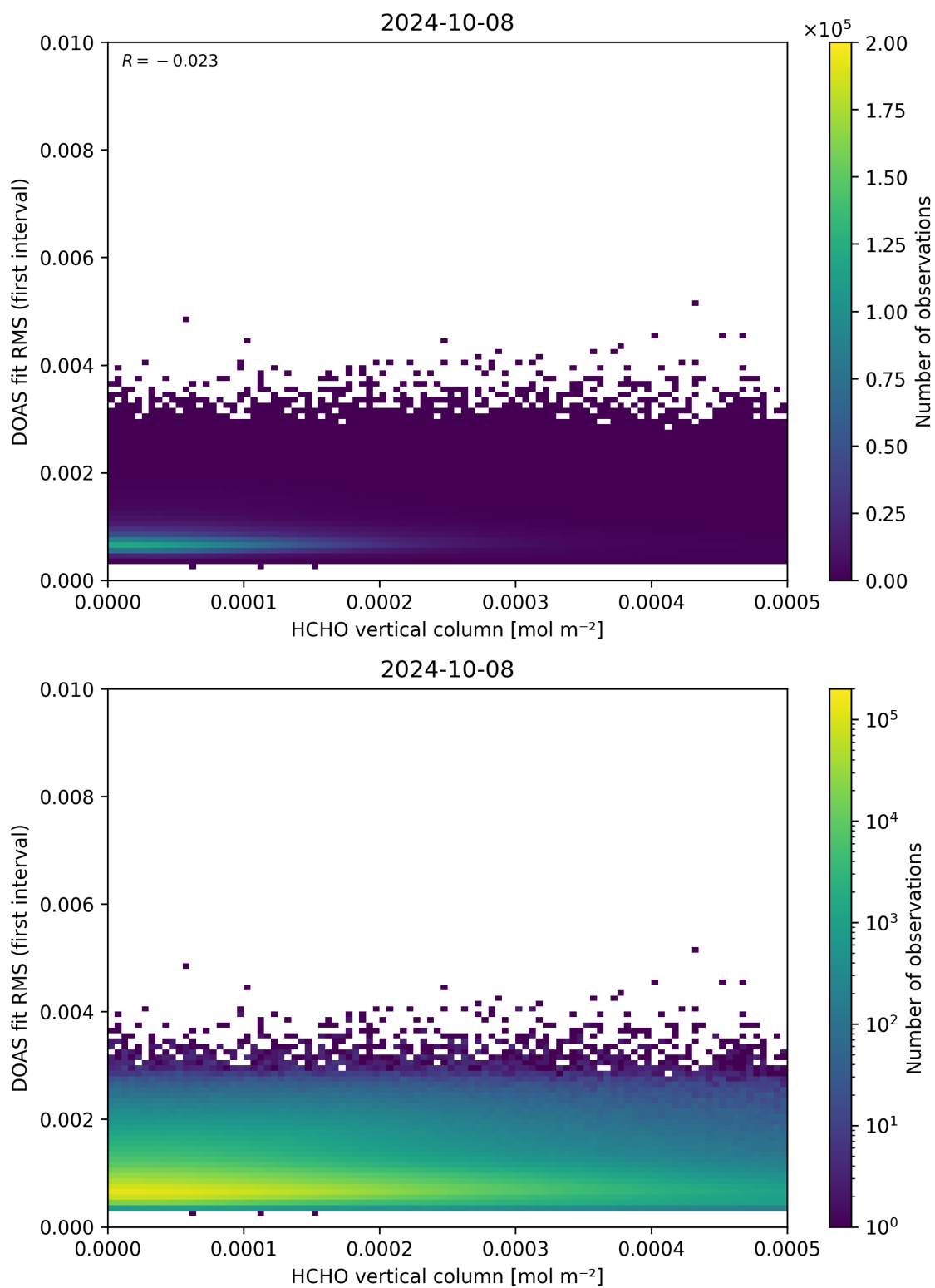
Figure 123: Scatter density plot of “HCHO vertical column” against “DOAS fit RMS (first interval)” for 2024-10-08 to 2024-10-09.
