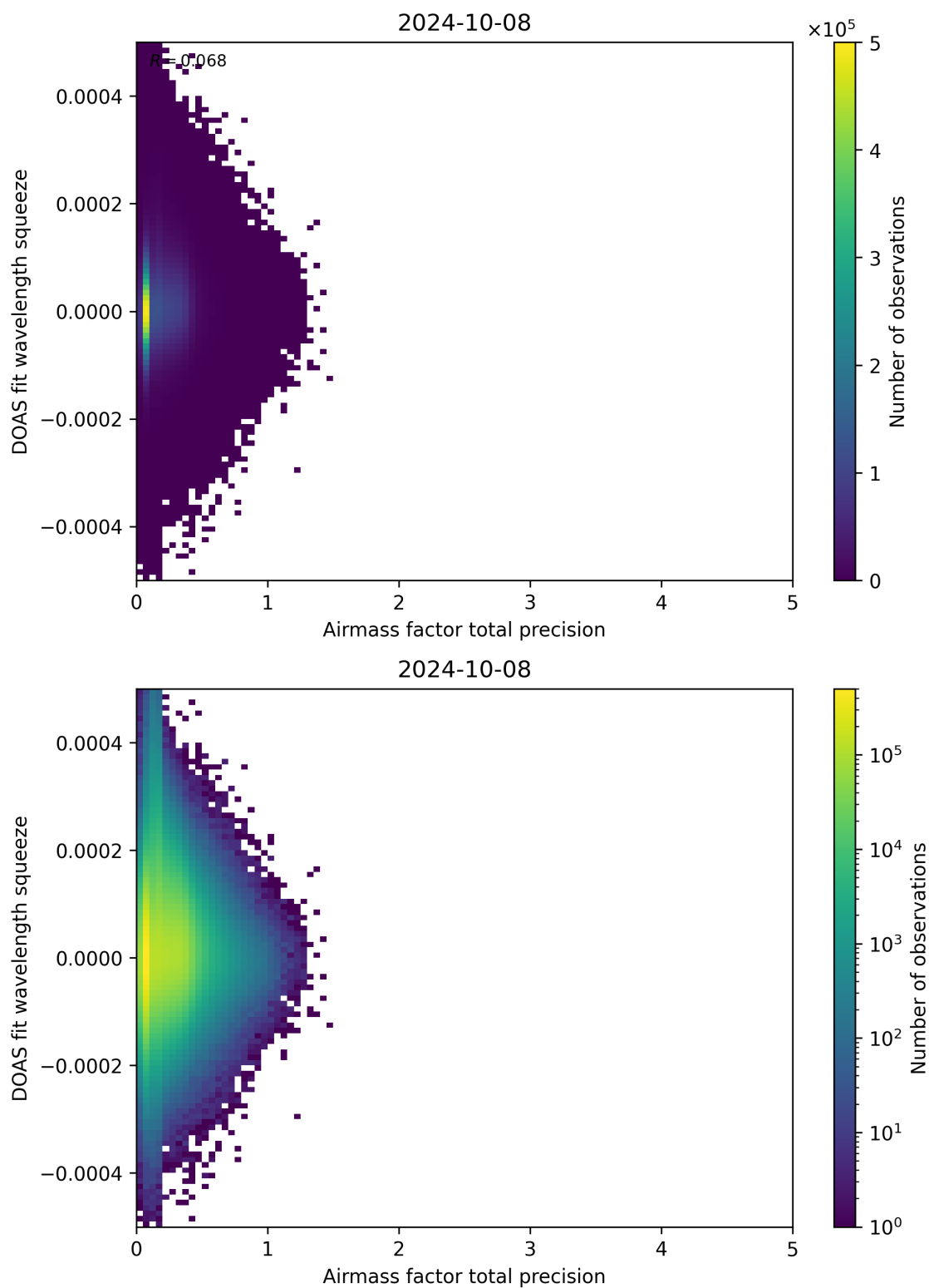
Figure 107: Scatter density plot of “Airmass factor total precision” against “DOAS fit wavelength squeeze” for 2024-10-08 to 2024-10-09.
