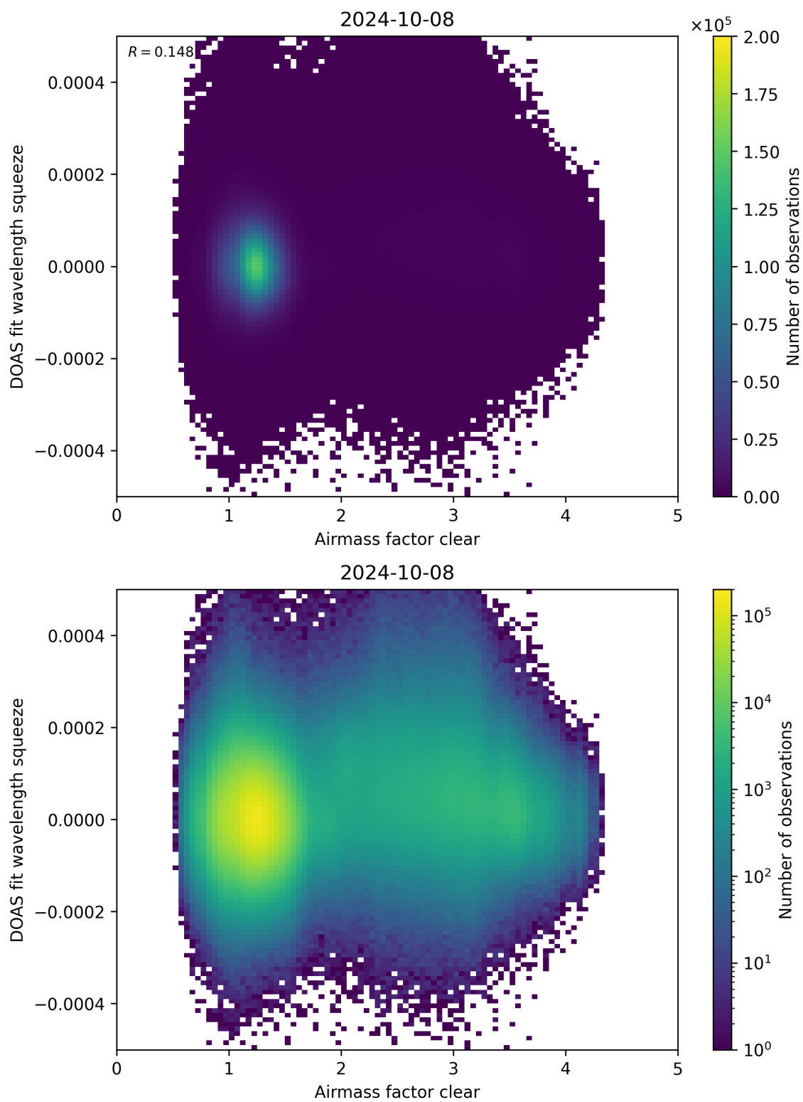
Figure 73: Scatter density plot of “Airmass factor clear” against “DOAS fit wavelength squeeze” for 2024-10-08 to 2024-10-09.
