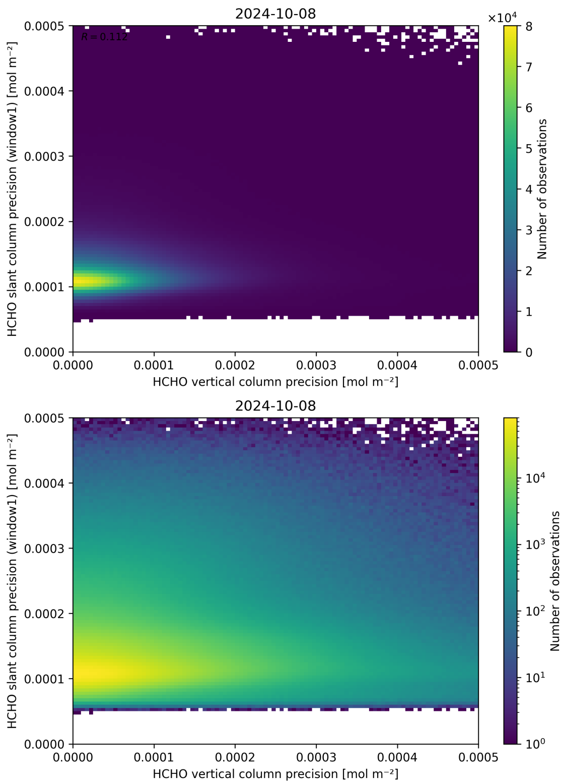
Figure 143: Scatter density plot of “HCHO vertical column precision” against “HCHO slant column precision (window1)” for 2024-10-08 to 2024-10-09.
