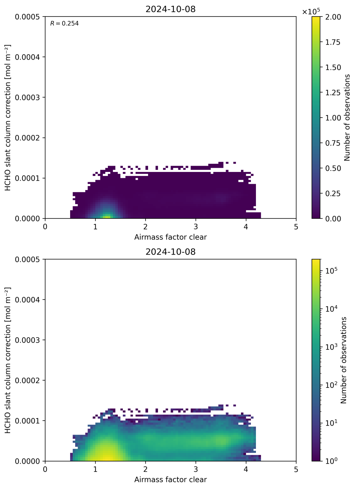
Figure 75: Scatter density plot of “Airmass factor clear” against “HCHO slant column correction” for 2024-10-08 to 2024-10-09.
