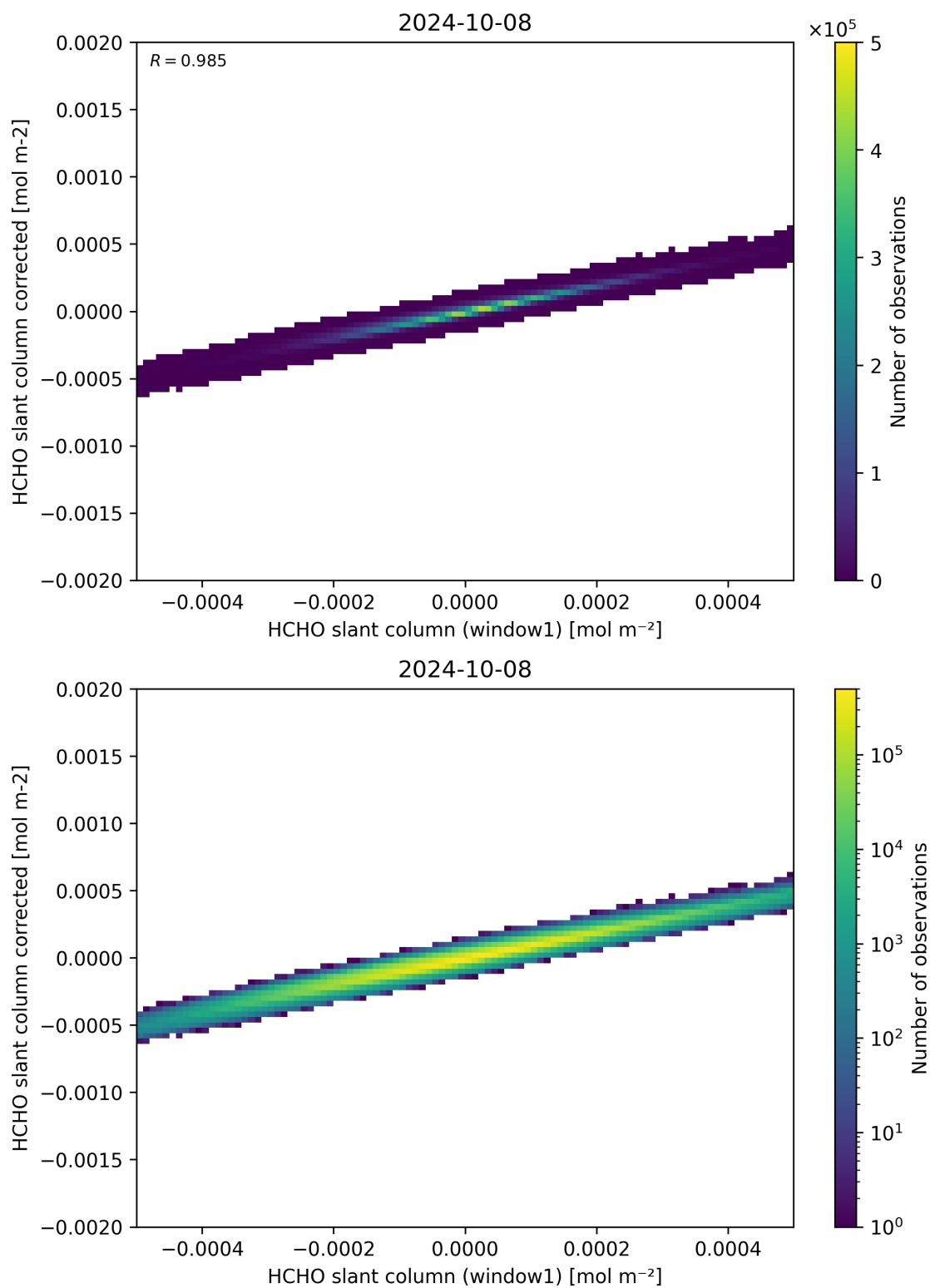
Figure 82: Scatter density plot of “HCHO slant column (window1)” against “HCHO slant column corrected” for 2024-10-08 to 2024-10-09.
