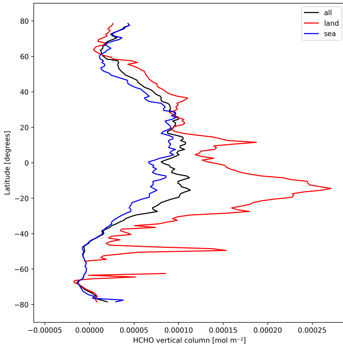
Figure 21: Zonal average of “HCHO vertical column” for 2024-10-08 to 2024-10-09.
