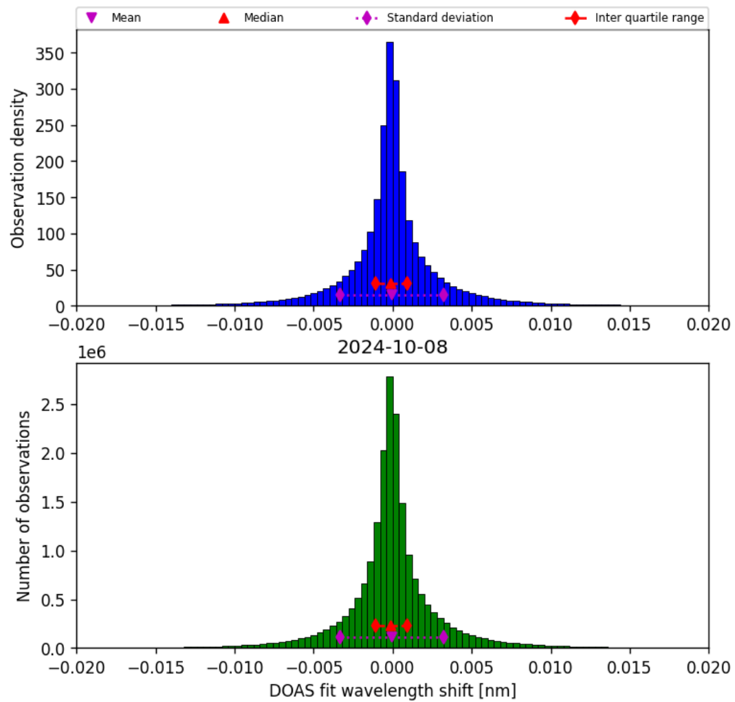
Figure 44: Histogram of “DOAS fit wavelength shift” for 2024-10-08 to 2024-10-09
