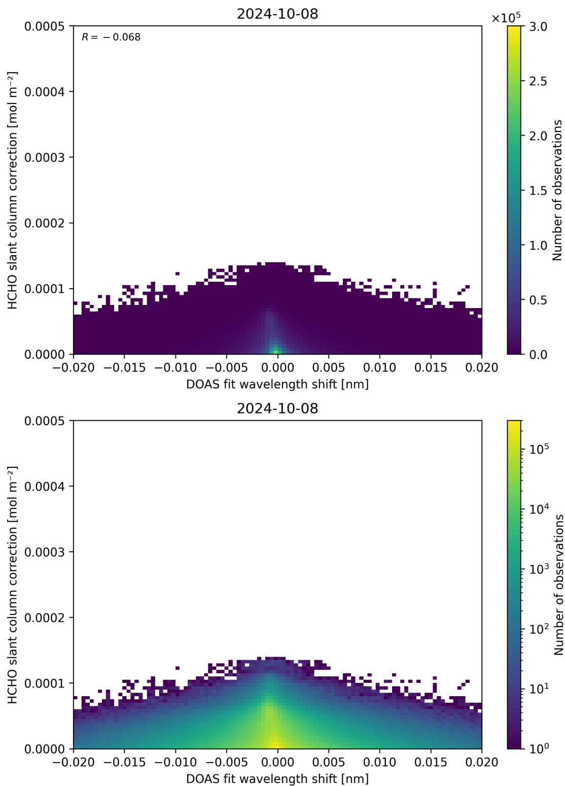
Figure 67: Scatter density plot of “DOAS fit wavelength shift” against “HCHO slant column correction” for 2024-10-08 to 2024-10-09.
