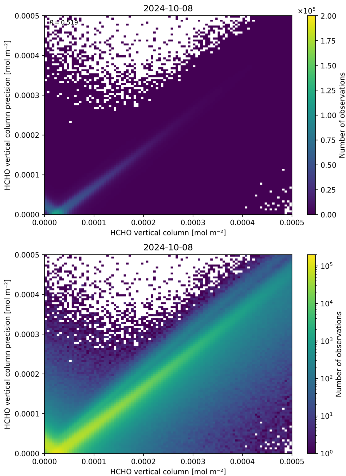
Figure 134: Scatter density plot of “HCHO vertical column” against “HCHO vertical column precision” for 2024-10-08 to 2024-10-09.
