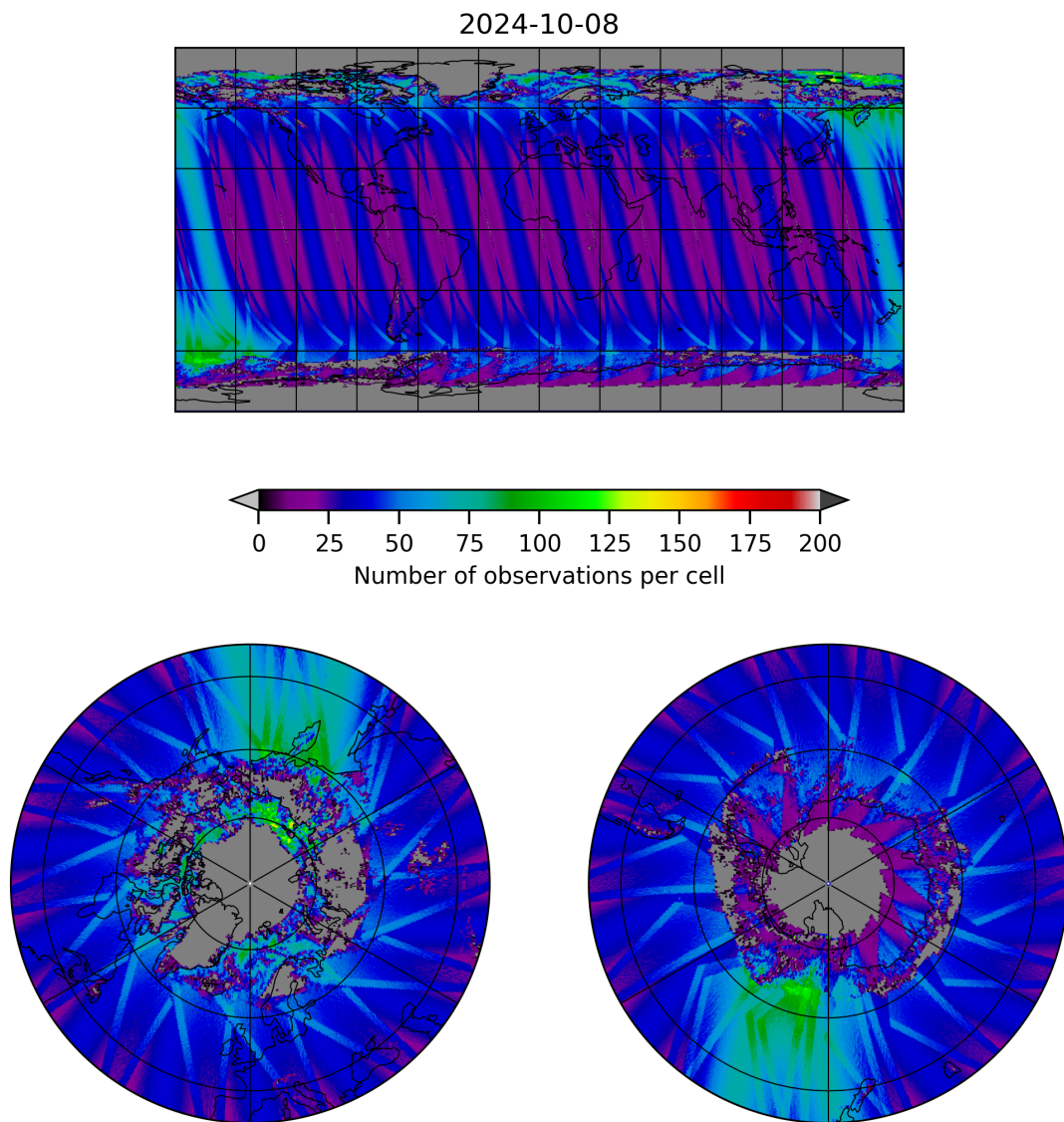
Figure 19: Map of the number of observations for 2024-10-08 to 2024-10-09
