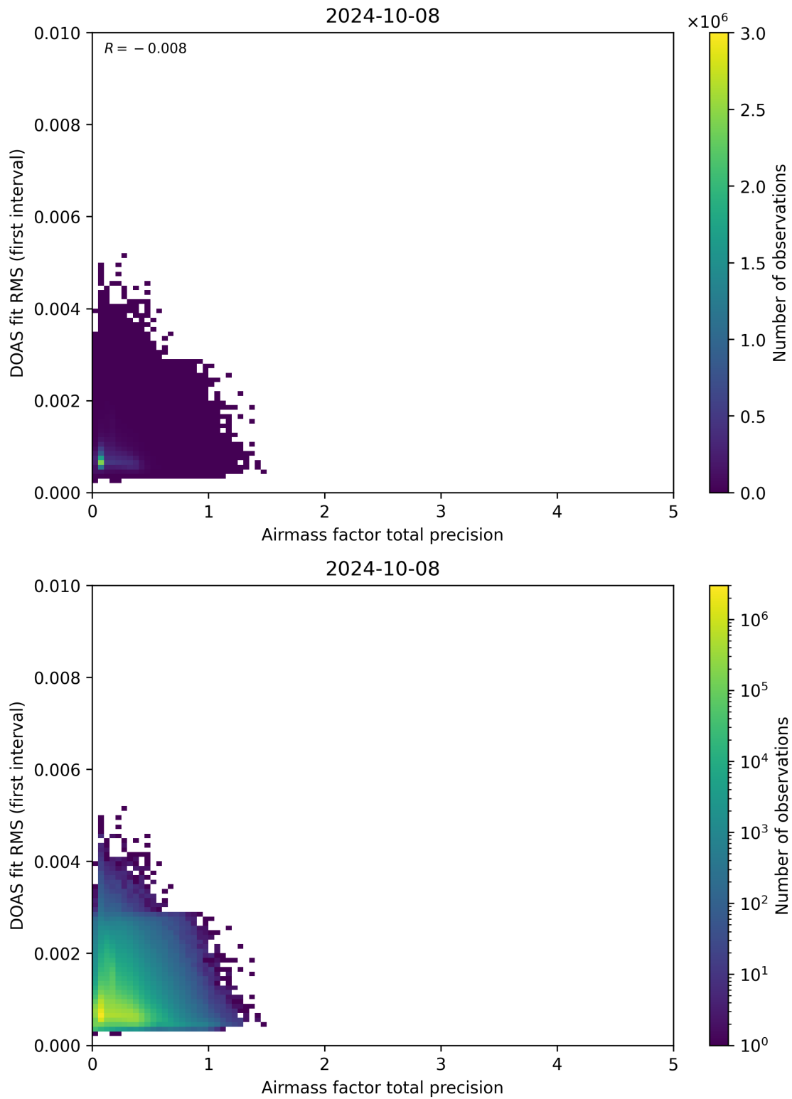
Figure 105: Scatter density plot of “Airmass factor total precision” against “DOAS fit RMS (first interval)” for 2024-10-08 to 2024-10-09.
