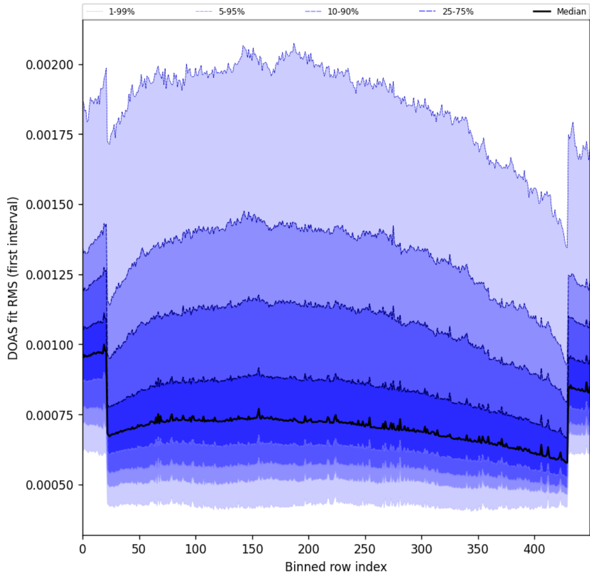
Figure 60: Along track statistics of “DOAS fit RMS (first interval)” for 2024-10-08 to 2024-10-09
