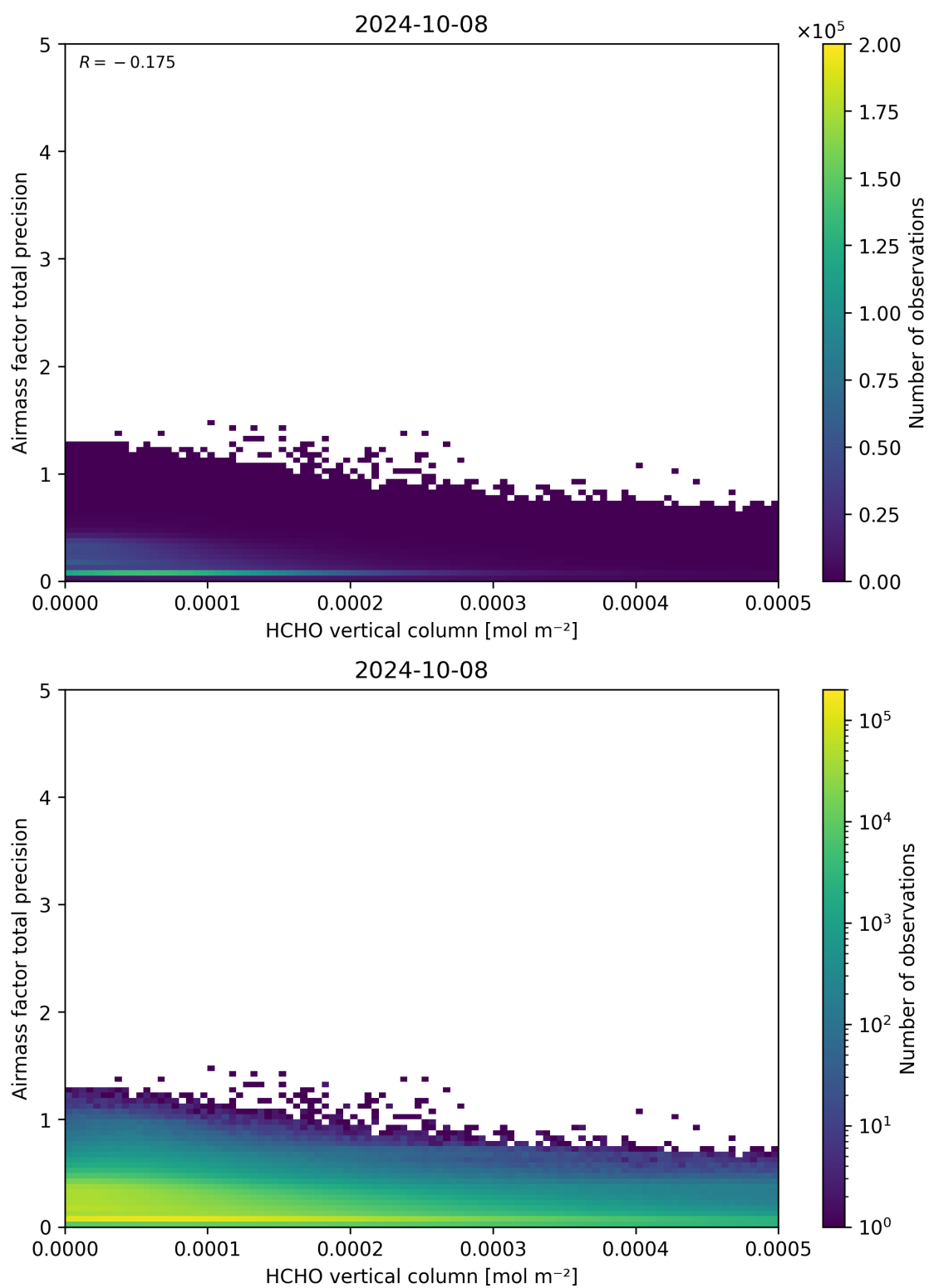
Figure 132: Scatter density plot of “HCHO vertical column” against “Airmass factor total precision” for 2024-10-08 to 2024-10-09.
