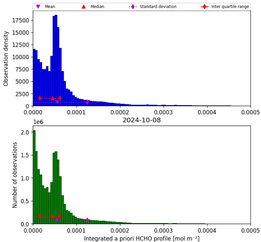
Figure 43: Histogram of “Integrated a priori HCHO profile” for 2024-10-08 to 2024-10-09
