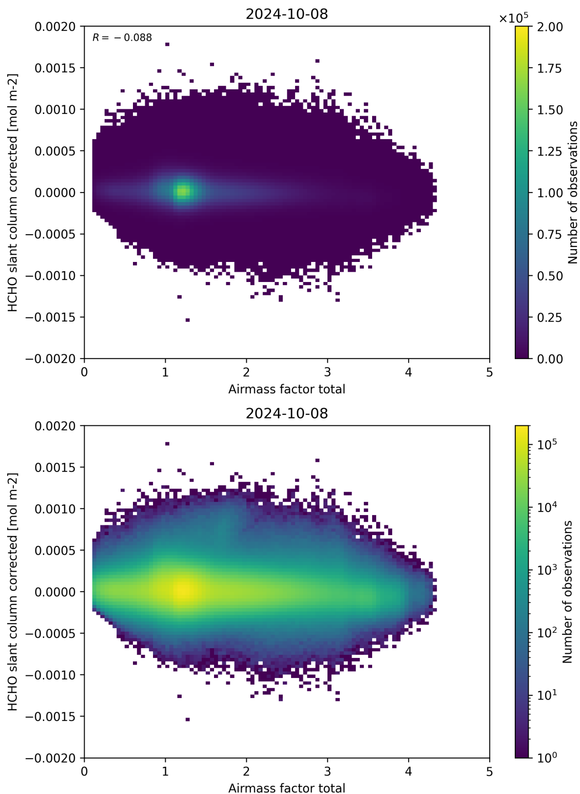
Figure 101: Scatter density plot of “Airmass factor total” against “HCHO slant column corrected” for 2024-10-08 to 2024-10-09.
