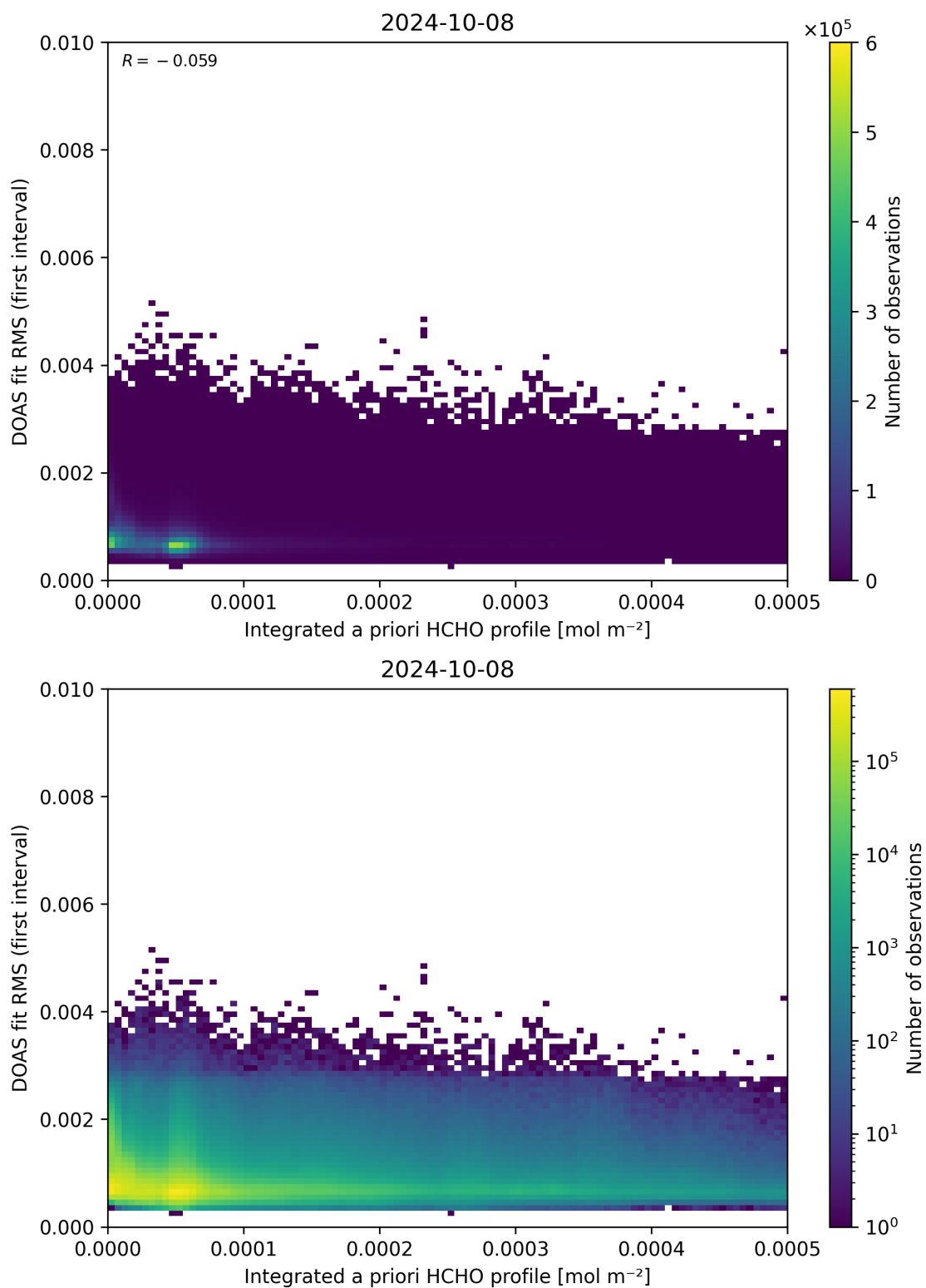
Figure 148: Scatter density plot of “Integrated a priori HCHO profile” against “DOAS fit RMS (first interval)” for 2024-10-08 to 2024-10-09.
