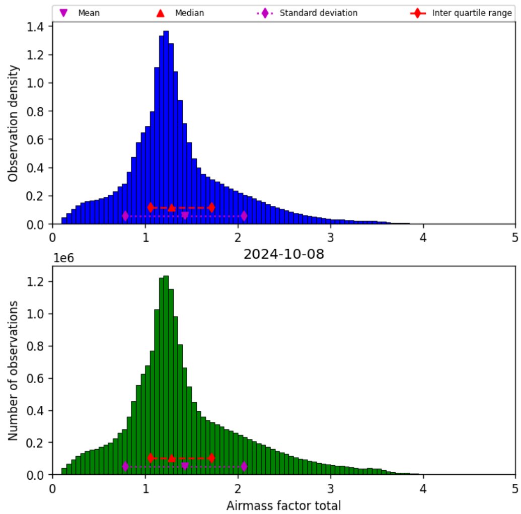
Figure 40: Histogram of “Airmass factor total” for 2024-10-08 to 2024-10-09
