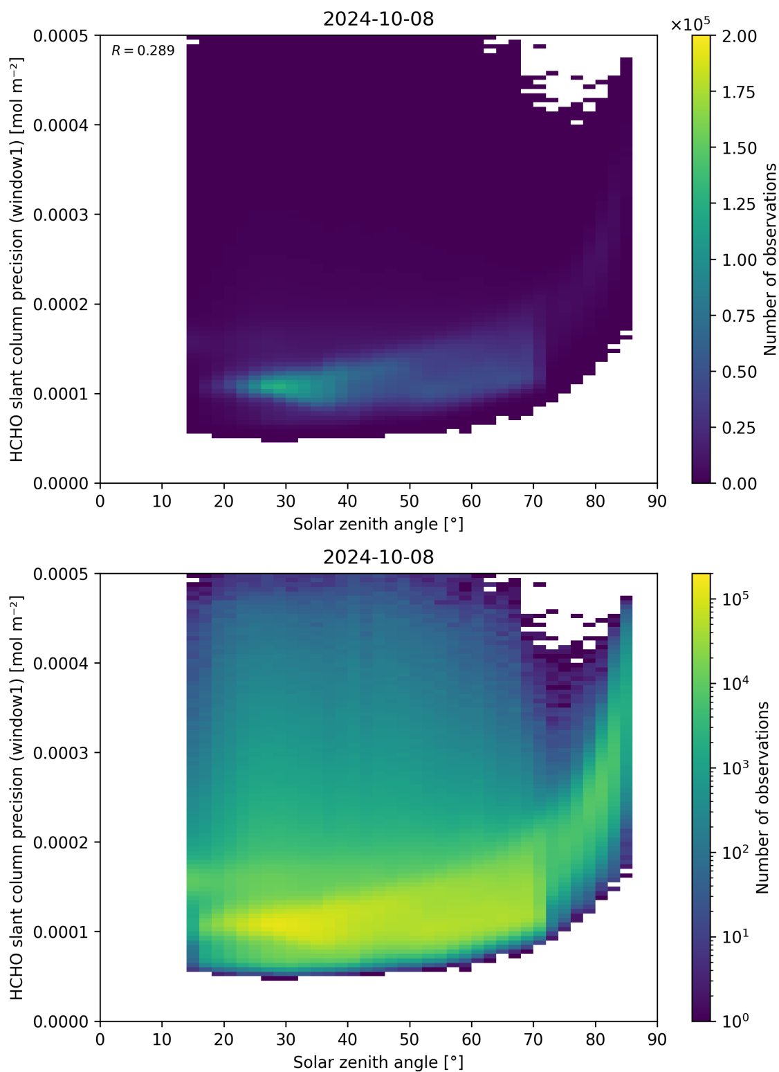
Figure 174: Scatter density plot of “Solar zenith angle” against “HCHO slant column precision (window1)” for 2024-10-08 to 2024-10-09.
