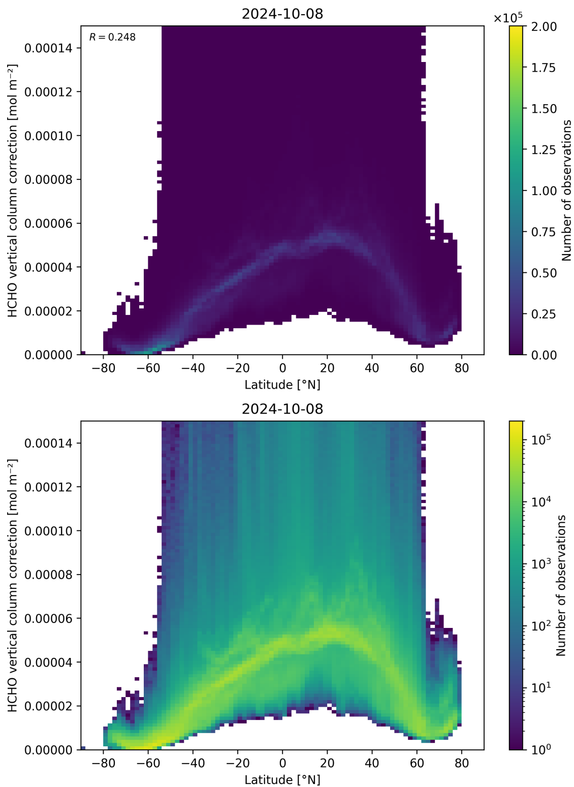
Figure 164: Scatter density plot of “Latitude” against “HCHO vertical column correction” for 2024-10-08 to 2024-10-09.
