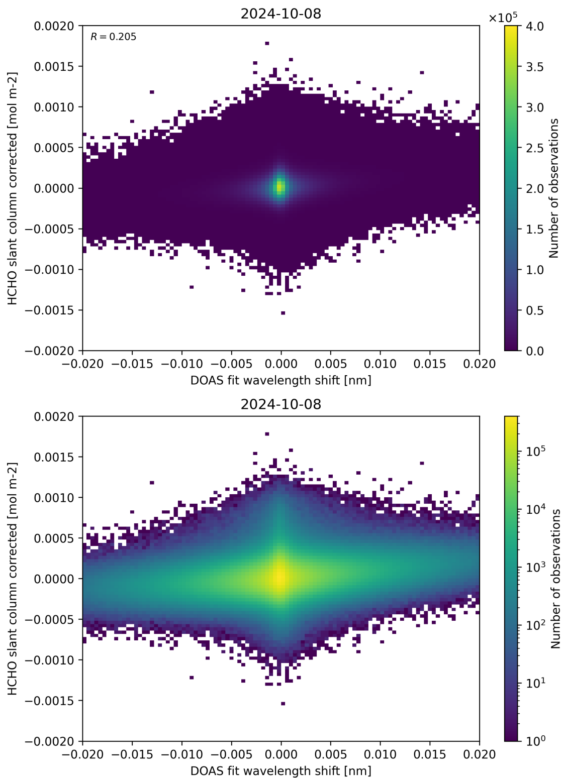
Figure 66: Scatter density plot of “DOAS fit wavelength shift” against “HCHO slant column corrected” for 2024-10-08 to 2024-10-09.
