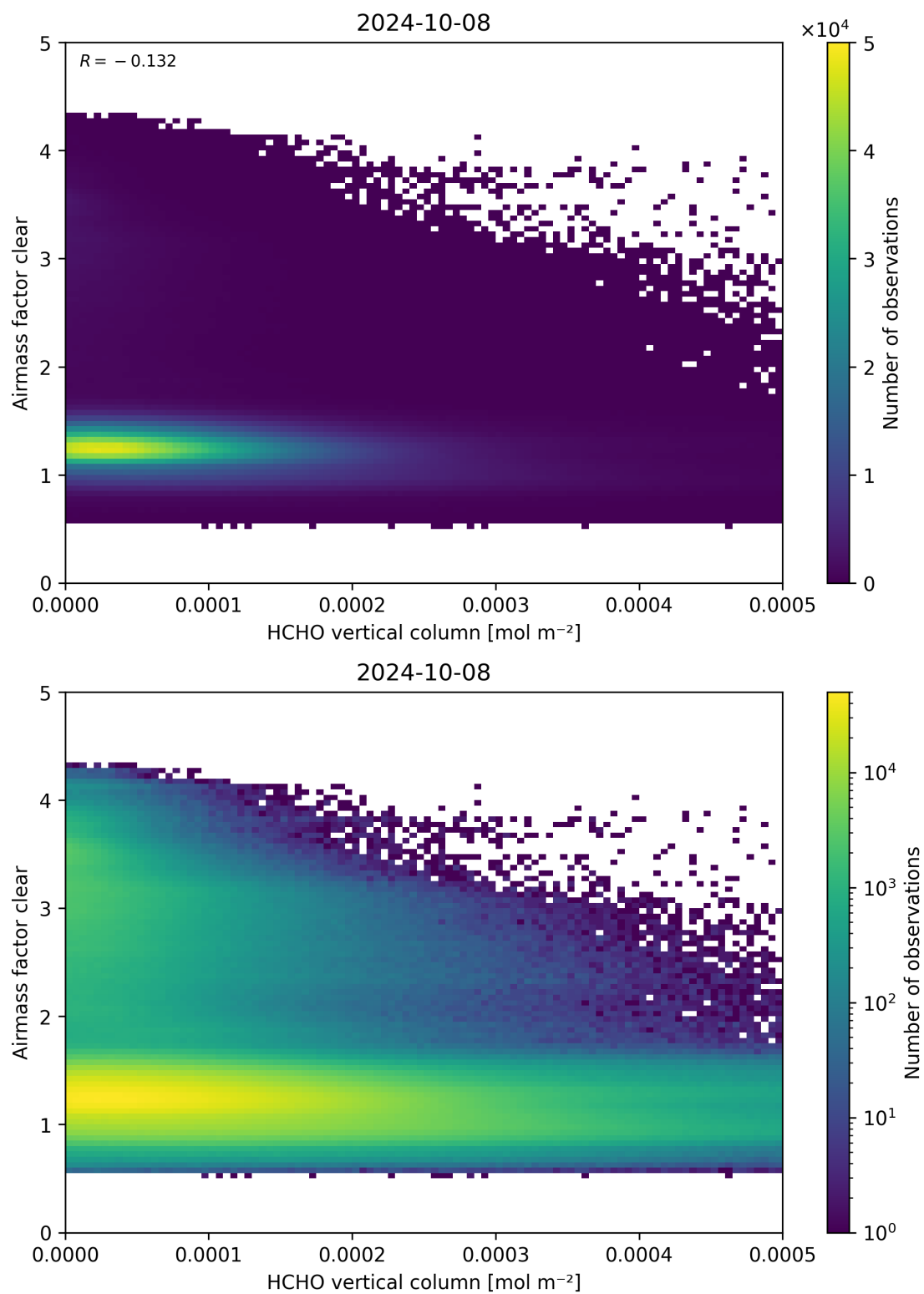
Figure 126: Scatter density plot of “HCHO vertical column” against “Airmass factor clear” for 2024-10-08 to 2024-10-09.
