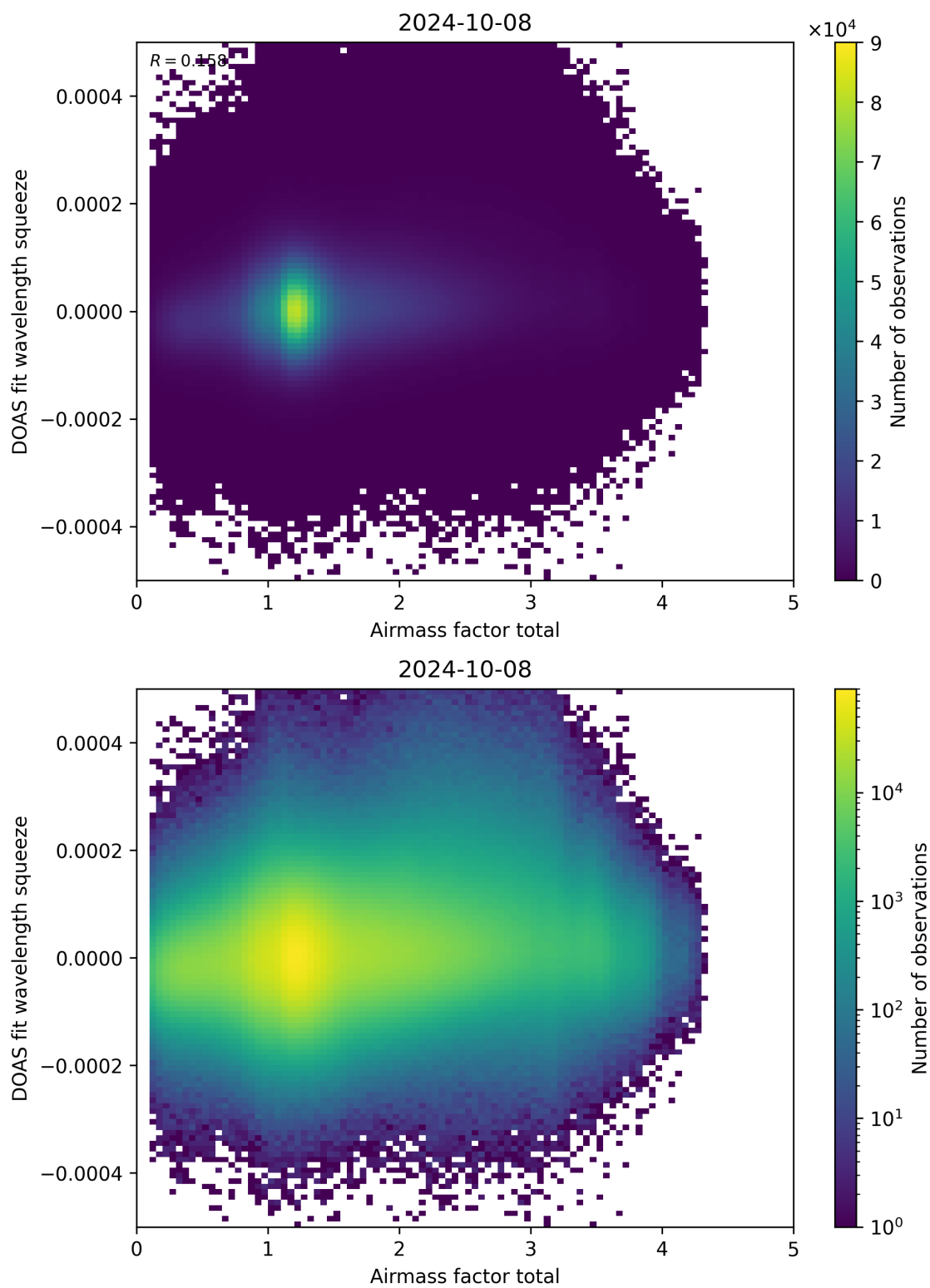
Figure 99: Scatter density plot of “Airmass factor total” against “DOAS fit wavelength squeeze” for 2024-10-08 to 2024-10-09.
