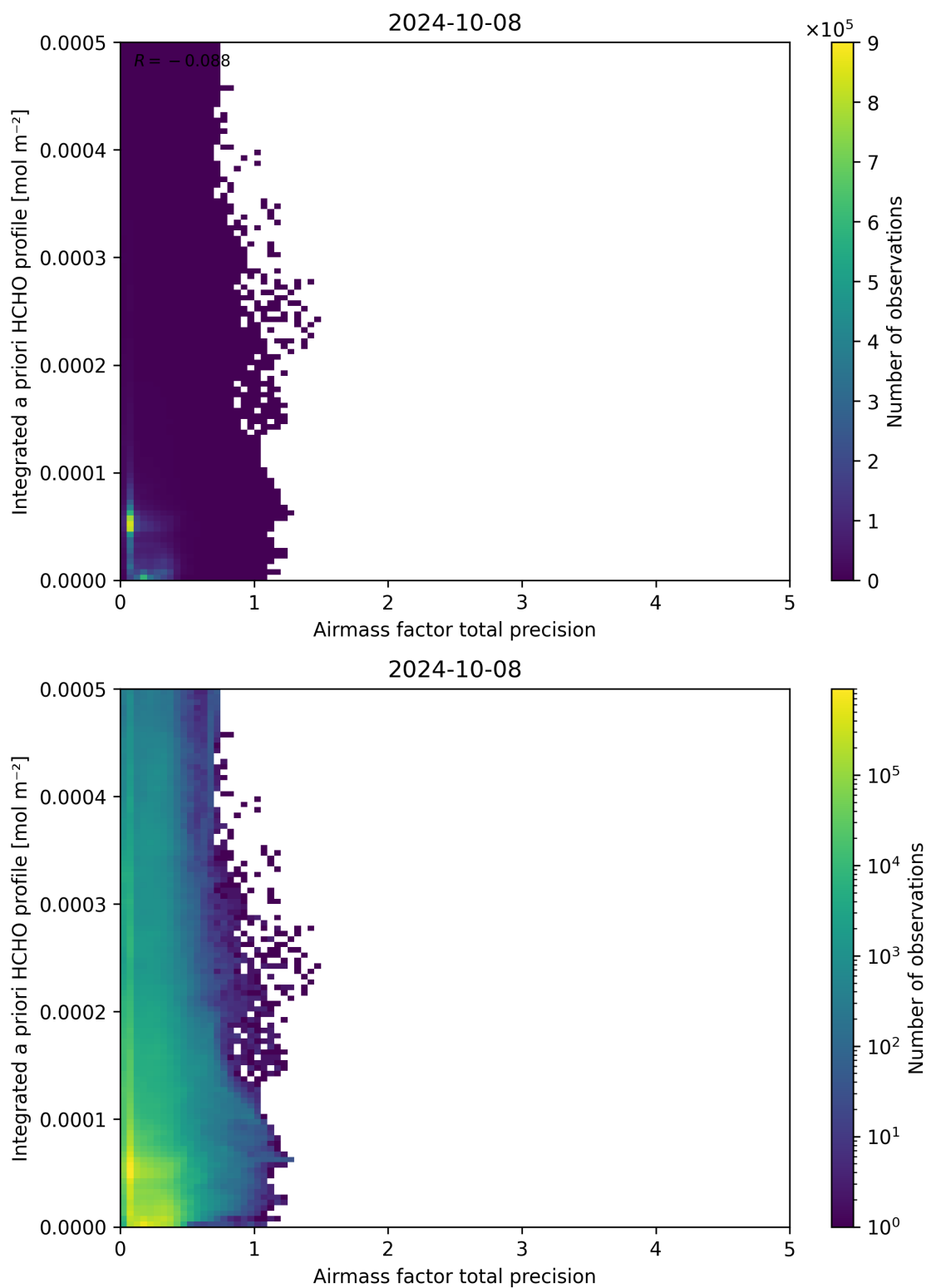
Figure 111: Scatter density plot of “Airmass factor total precision” against “Integrated a priori HCHO profile” for 2024-10-08 to 2024-10-09.
