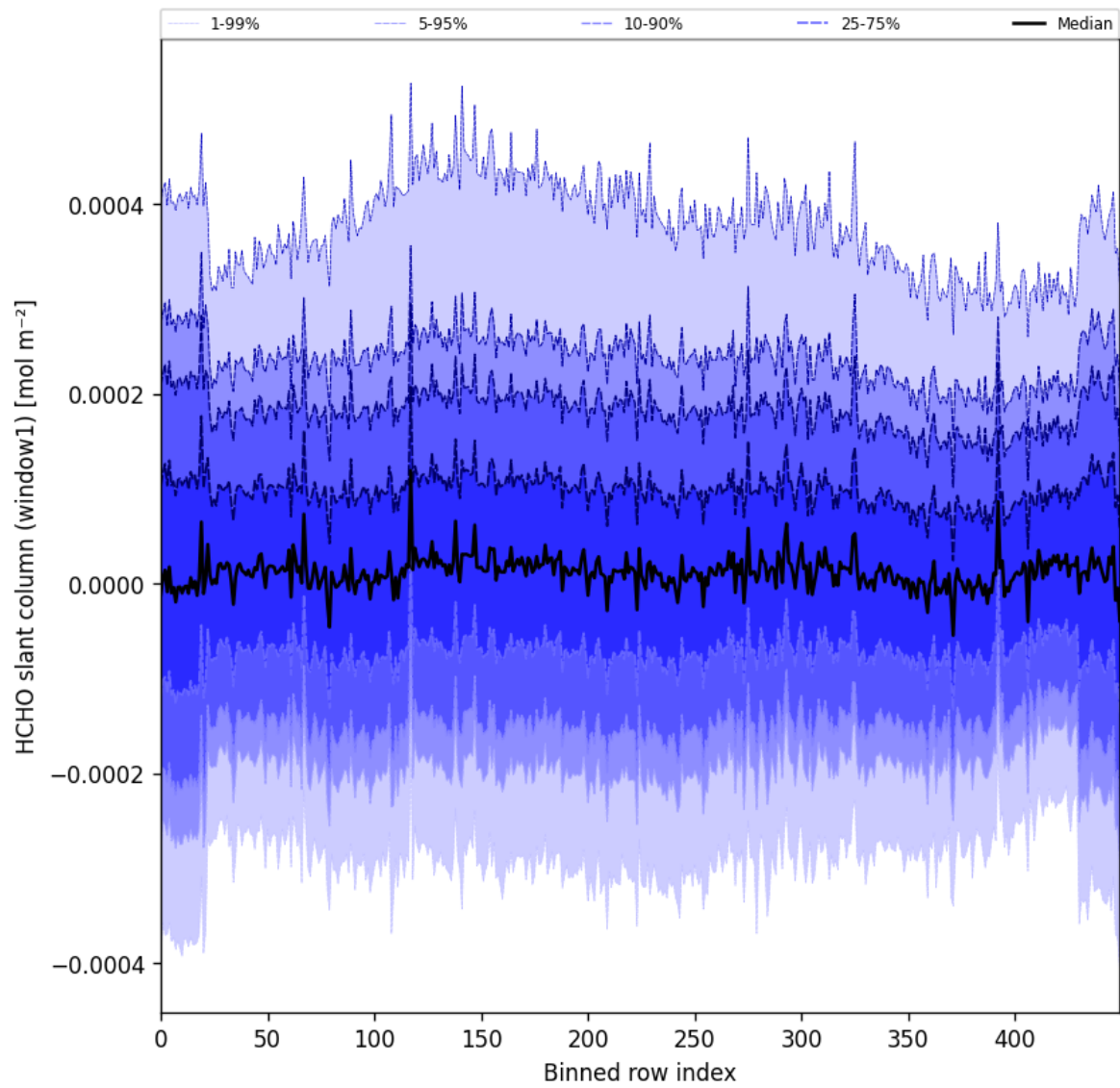
Figure 52: Along track statistics of “HCHO slant column (window1)” for 2024-10-08 to 2024-10-09
