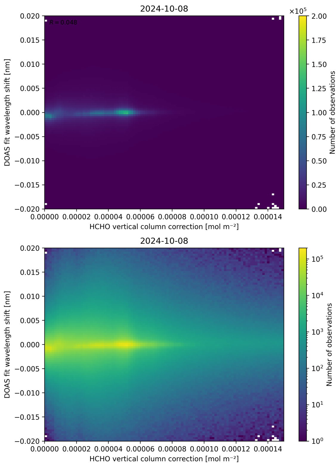
Figure 113: Scatter density plot of “HCHO vertical column correction” against “DOAS fit wavelength shift” for 2024-10-08 to 2024-10-09.
