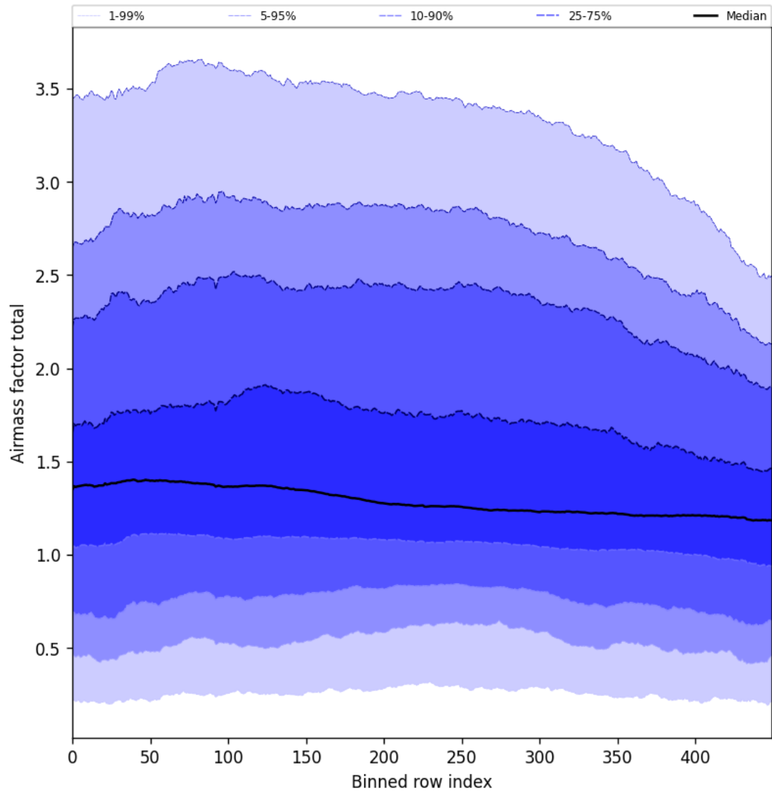
Figure 54: Along track statistics of “Airmass factor total” for 2024-10-08 to 2024-10-09
