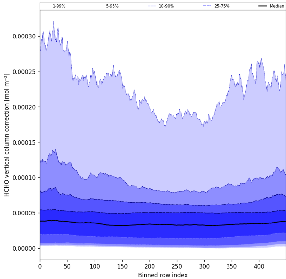
Figure 51: Along track statistics of “HCHO vertical column correction” for 2024-10-08 to 2024-10-09
