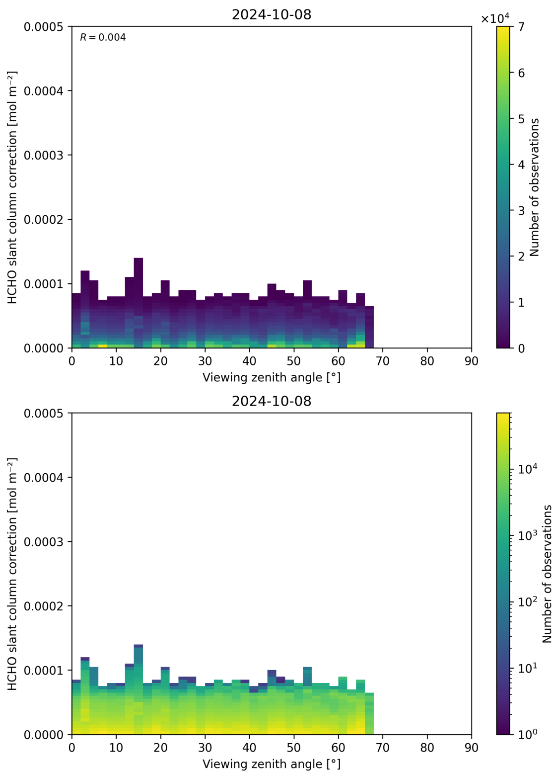
Figure 187: Scatter density plot of “Viewing zenith angle” against “HCHO slant column correction” for 2024-10-08 to 2024-10-09.
