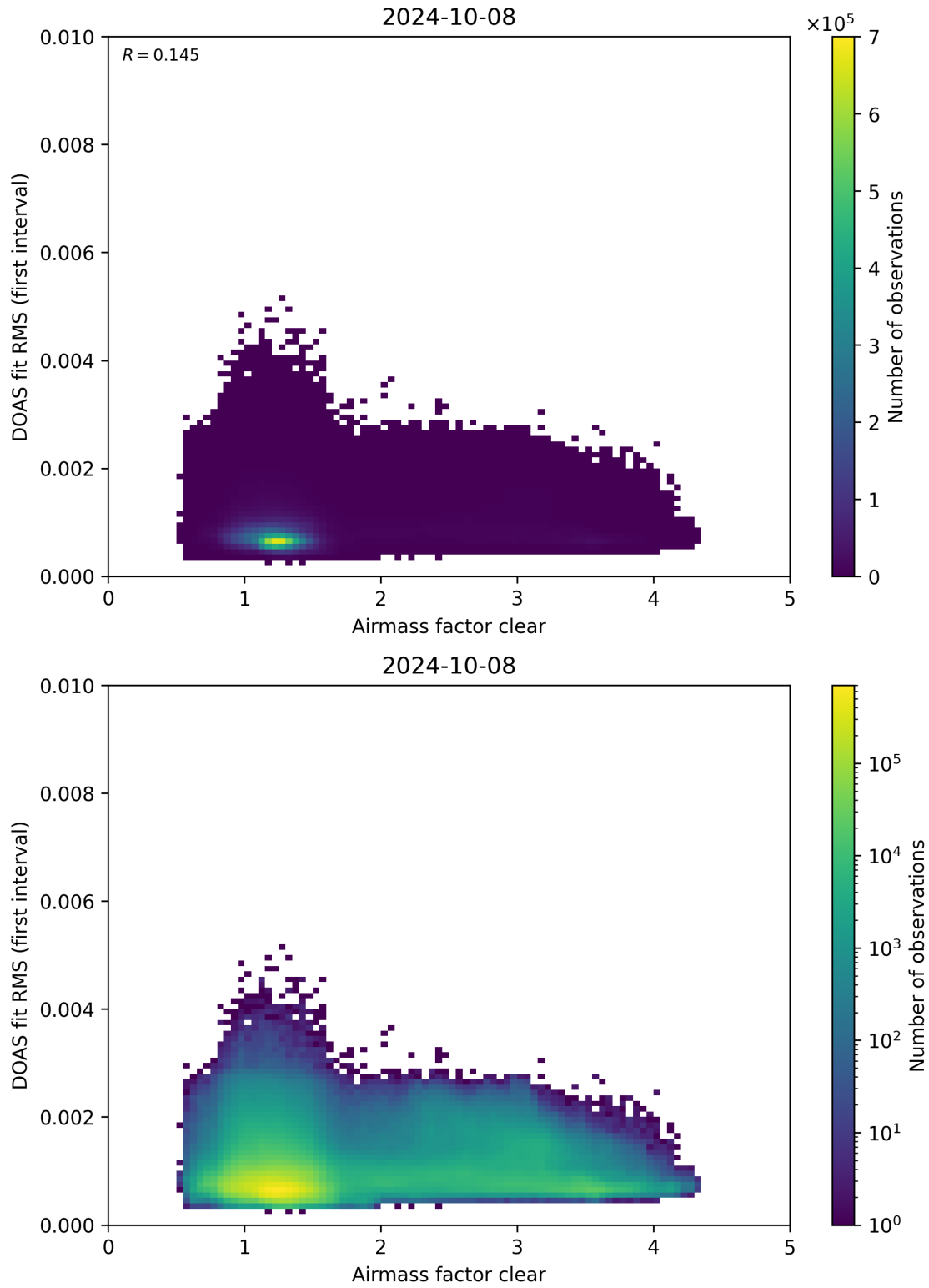
Figure 71: Scatter density plot of “Airmass factor clear” against “DOAS fit RMS (first interval)” for 2024-10-08 to 2024-10-09.
