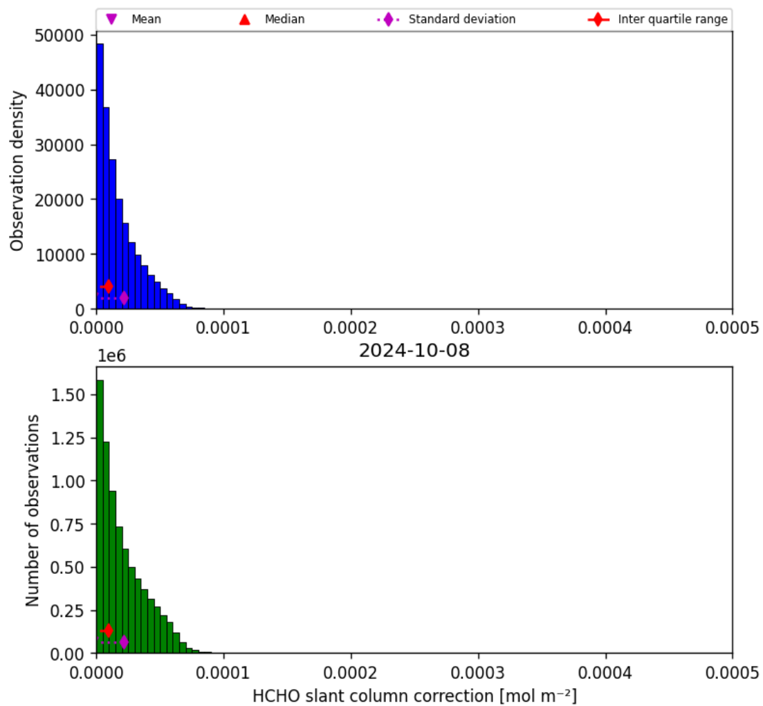
Figure 47: Histogram of “HCHO slant column correction” for 2024-10-08 to 2024-10-09
