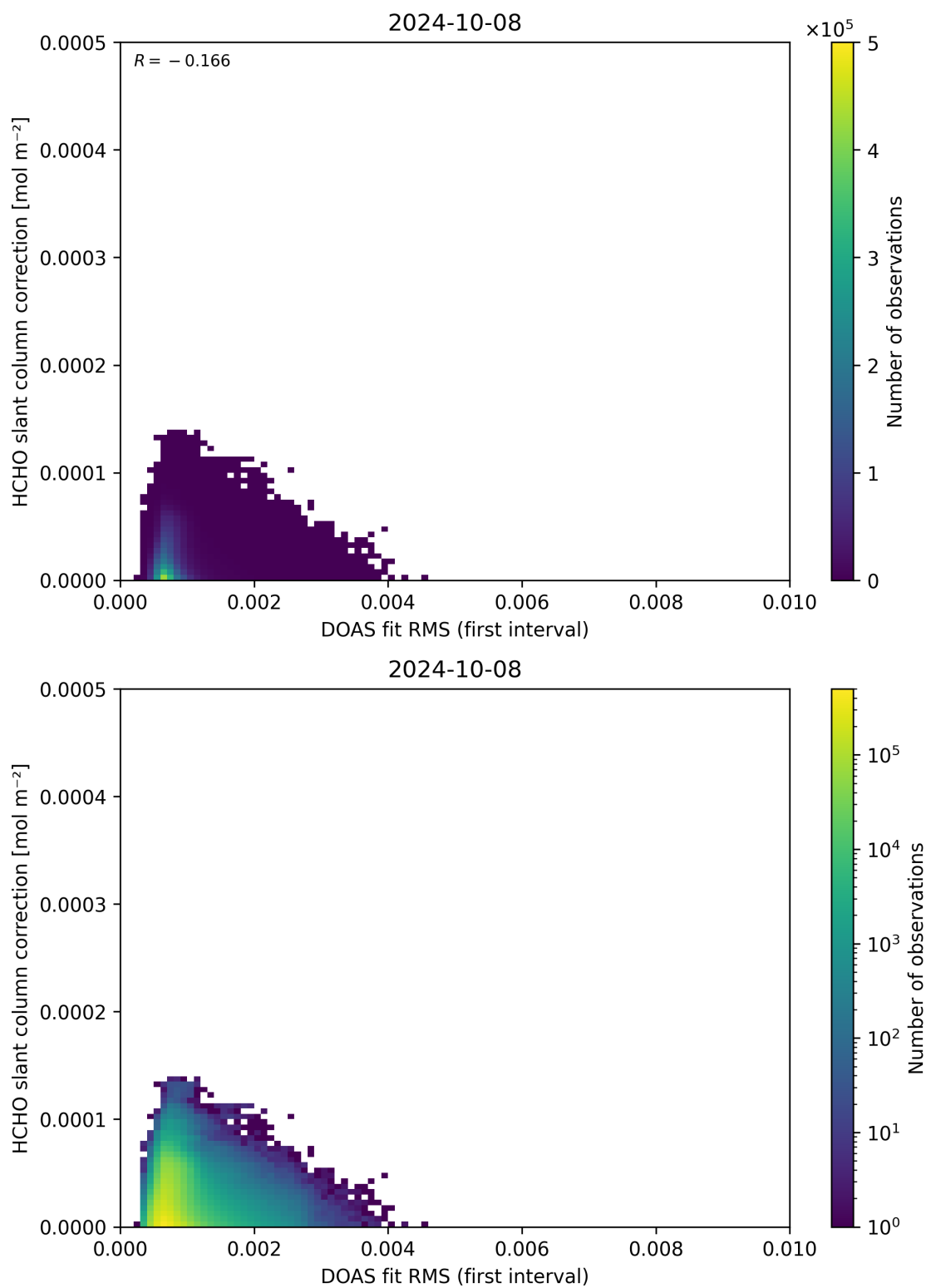
Figure 63: Scatter density plot of “DOAS fit RMS (first interval)” against “HCHO slant column correction” for 2024-10-08 to 2024-10-09.
