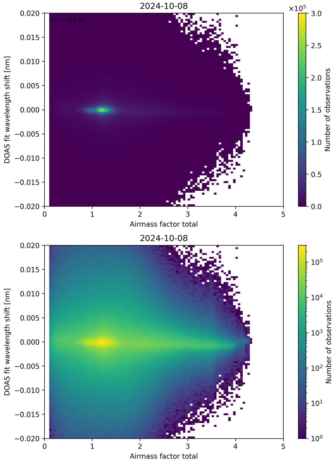
Figure 98: Scatter density plot of “Airmass factor total” against “DOAS fit wavelength shift” for 2024-10-08 to 2024-10-09.
