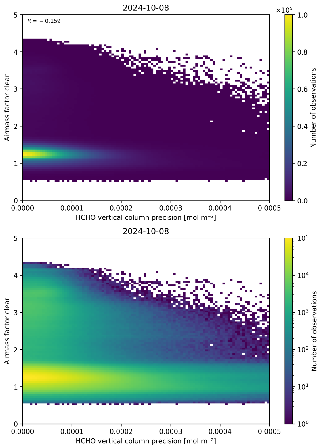
Figure 139: Scatter density plot of “HCHO vertical column precision” against “Airmass factor clear” for 2024-10-08 to 2024-10-09.
