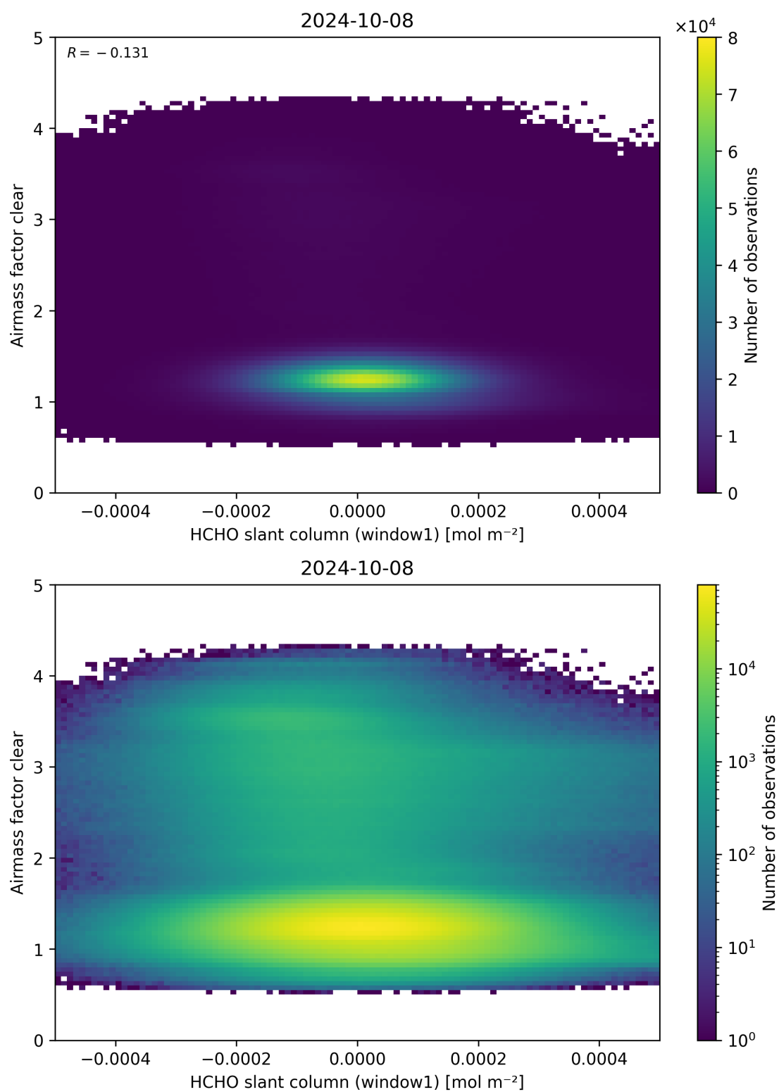
Figure 81: Scatter density plot of “HCHO slant column (window1)” against “Airmass factor clear” for 2024-10-08 to 2024-10-09.
