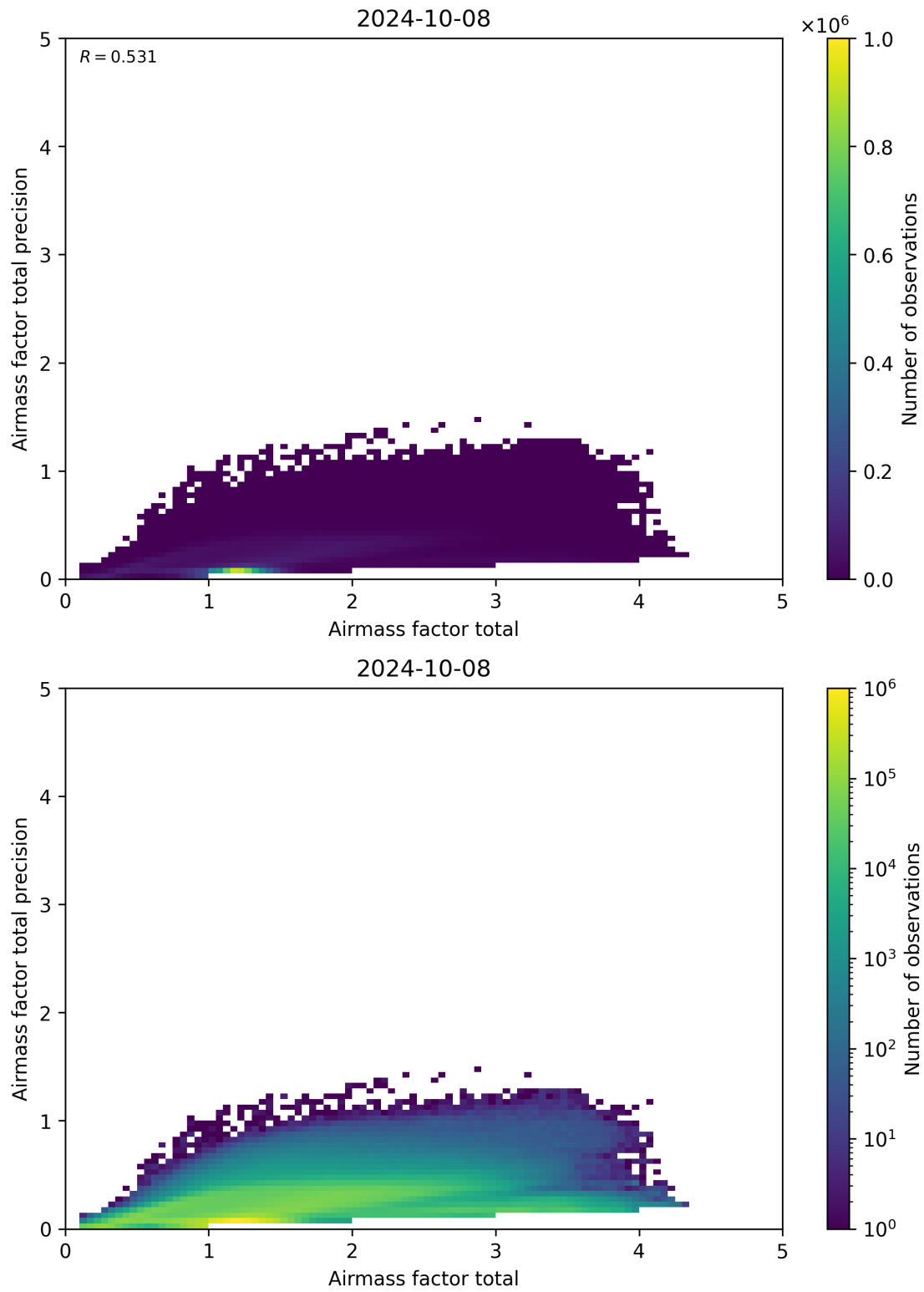
Figure 103: Scatter density plot of “Airmass factor total” against “Airmass factor total precision” for 2024-10-08 to 2024-10-09.
