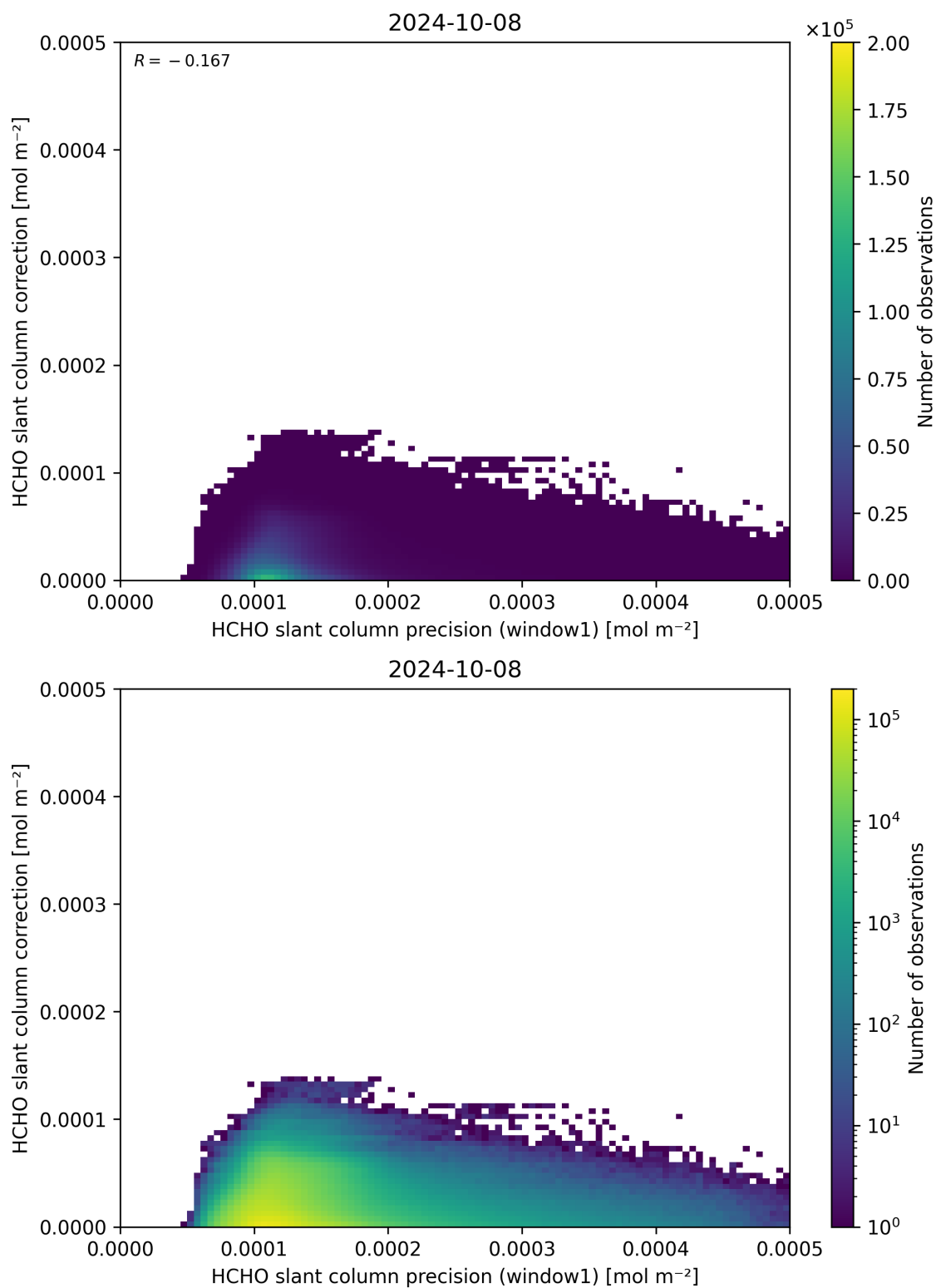
Figure 93: Scatter density plot of “HCHO slant column precision (window1)” against “HCHO slant column correction” for 2024-10-08 to 2024-10-09.
