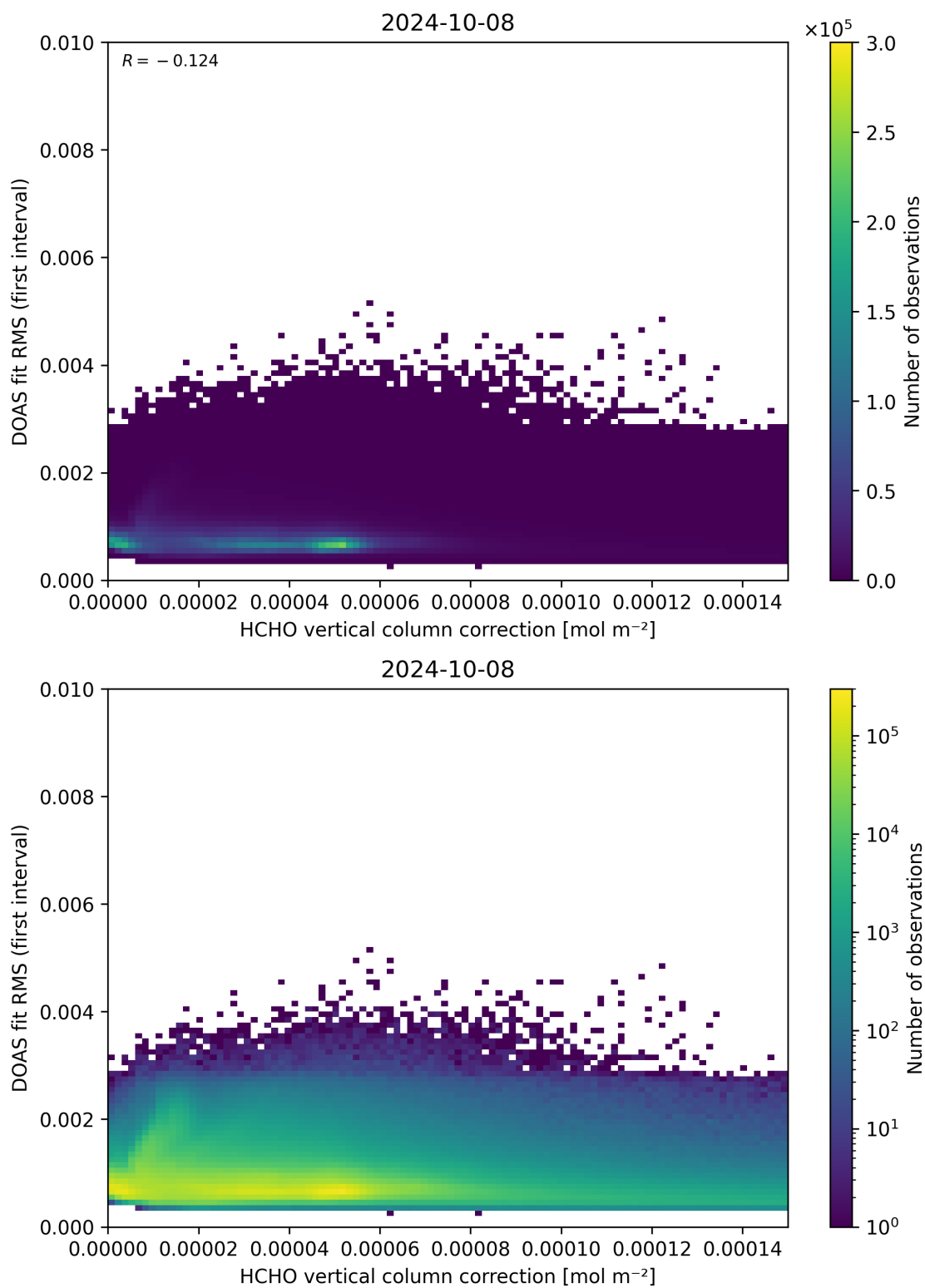
Figure 112: Scatter density plot of “HCHO vertical column correction” against “DOAS fit RMS (first interval)” for 2024-10-08 to 2024-10-09.
