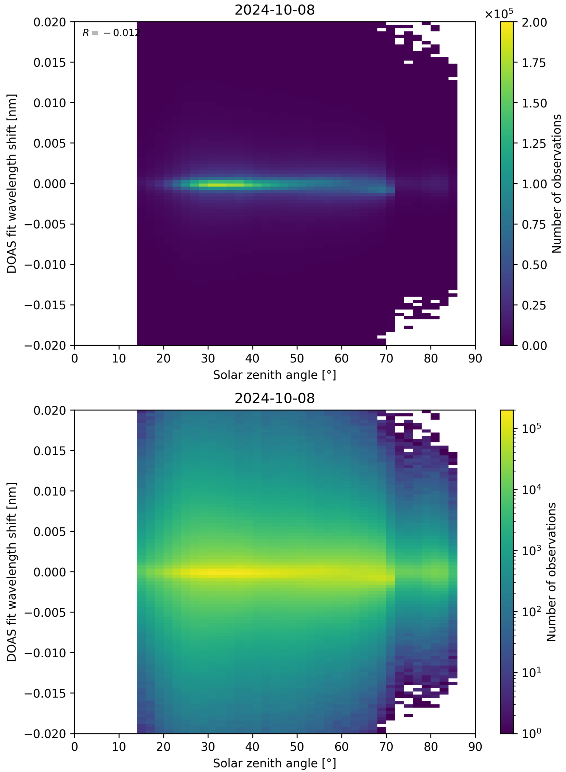
Figure 168: Scatter density plot of “Solar zenith angle” against “DOAS fit wavelength shift” for 2024-10-08 to 2024-10-09.
