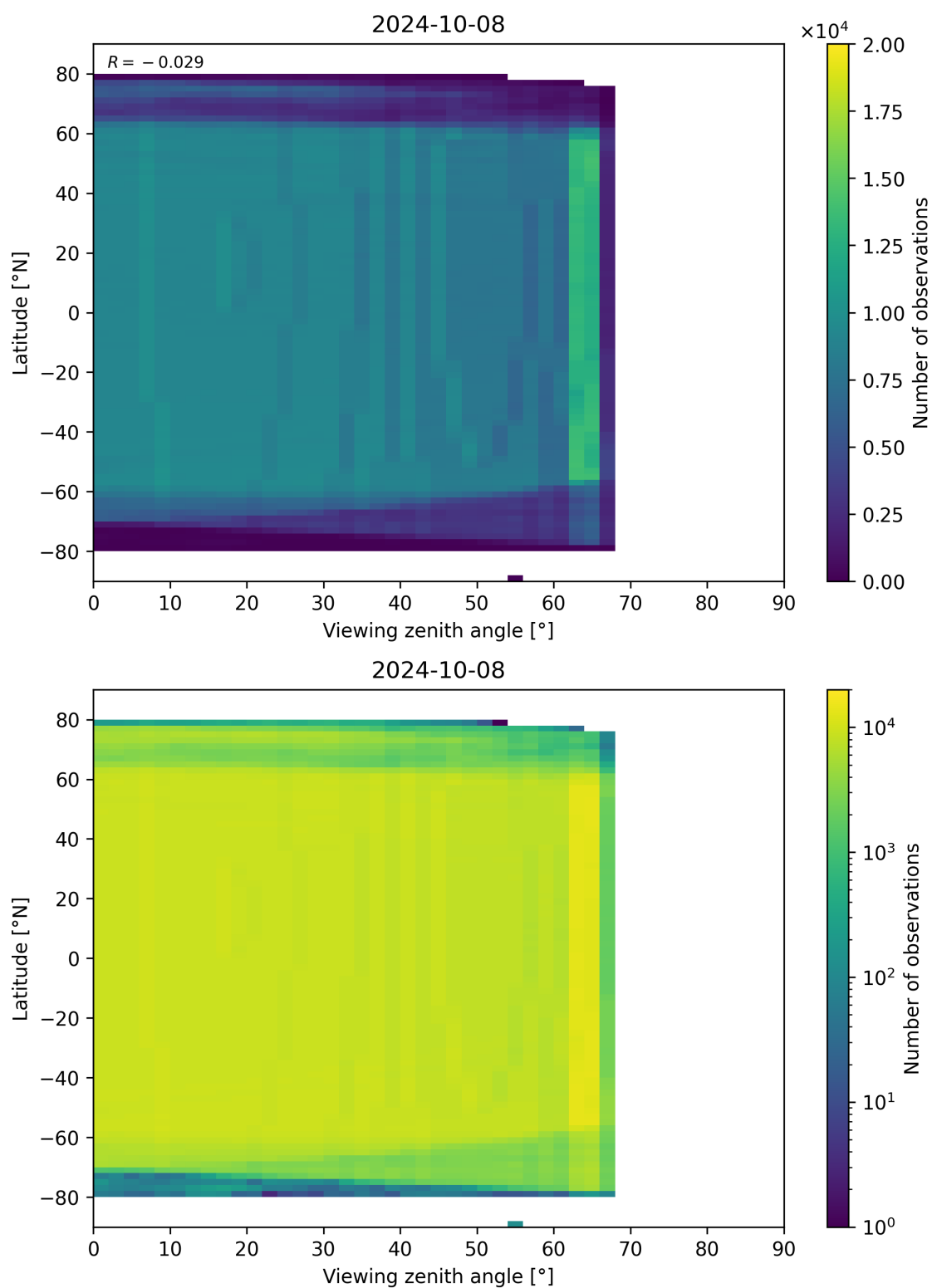
Figure 196: Scatter density plot of “Viewing zenith angle” against “Latitude” for 2024-10-08 to 2024-10-09.
