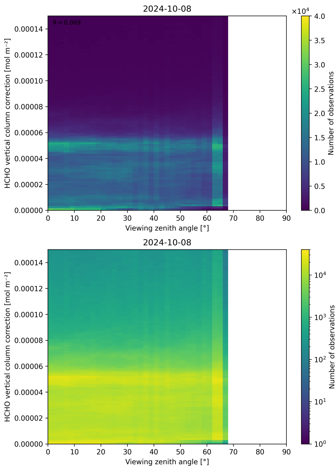
Figure 193: Scatter density plot of “Viewing zenith angle” against “HCHO vertical column correction” for 2024-10-08 to 2024-10-09.
