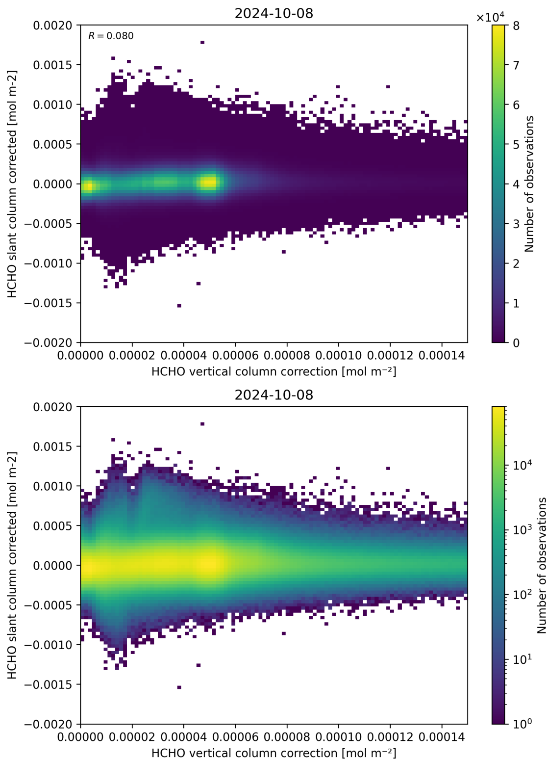
Figure 116: Scatter density plot of “HCHO vertical column correction” against “HCHO slant column corrected” for 2024-10-08 to 2024-10-09.
