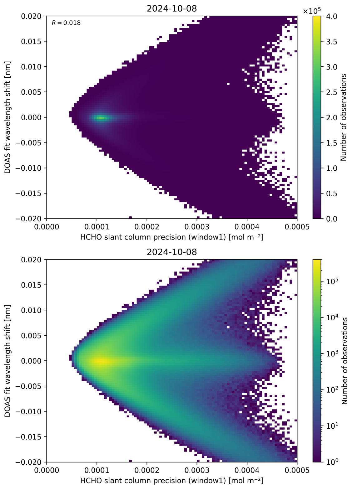
Figure 89: Scatter density plot of “HCHO slant column precision (window1)” against “DOAS fit wavelength shift” for 2024-10-08 to 2024-10-09.
