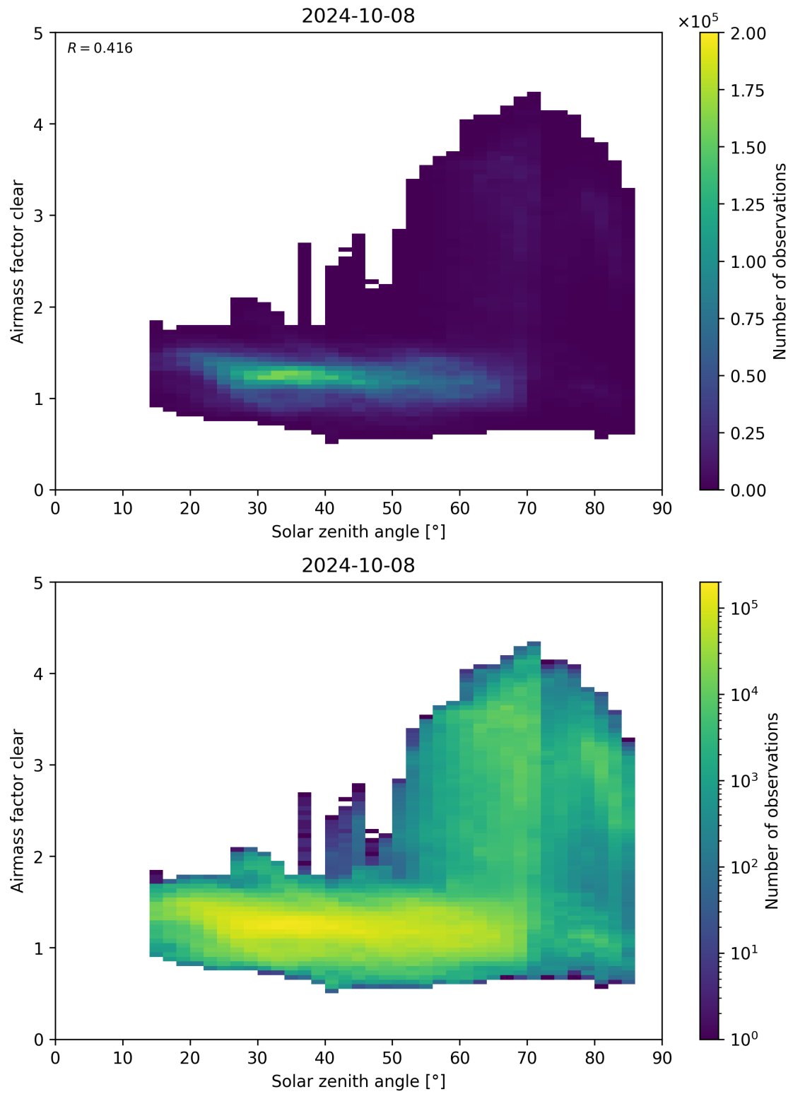
Figure 170: Scatter density plot of “Solar zenith angle” against “Airmass factor clear” for 2024-10-08 to 2024-10-09.
