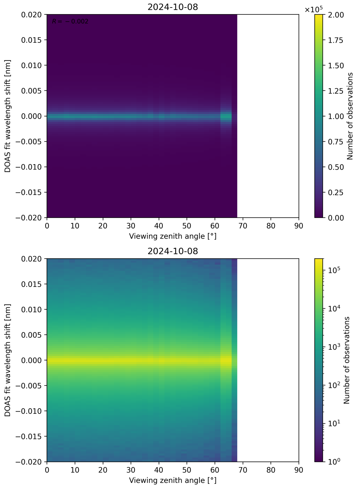
Figure 183: Scatter density plot of “Viewing zenith angle” against “DOAS fit wavelength shift” for 2024-10-08 to 2024-10-09.
