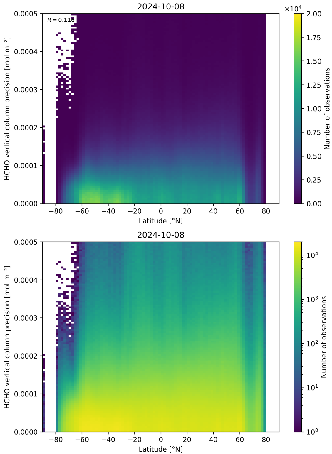
Figure 165: Scatter density plot of “Latitude” against “HCHO vertical column precision” for 2024-10-08 to 2024-10-09.
