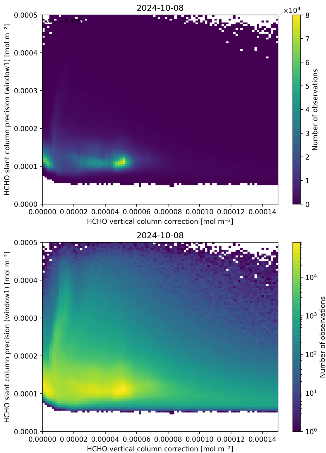
Figure 119: Scatter density plot of “HCHO vertical column correction” against “HCHO slant column precision (window1)” for 2024-10-08 to 2024-10-09.
