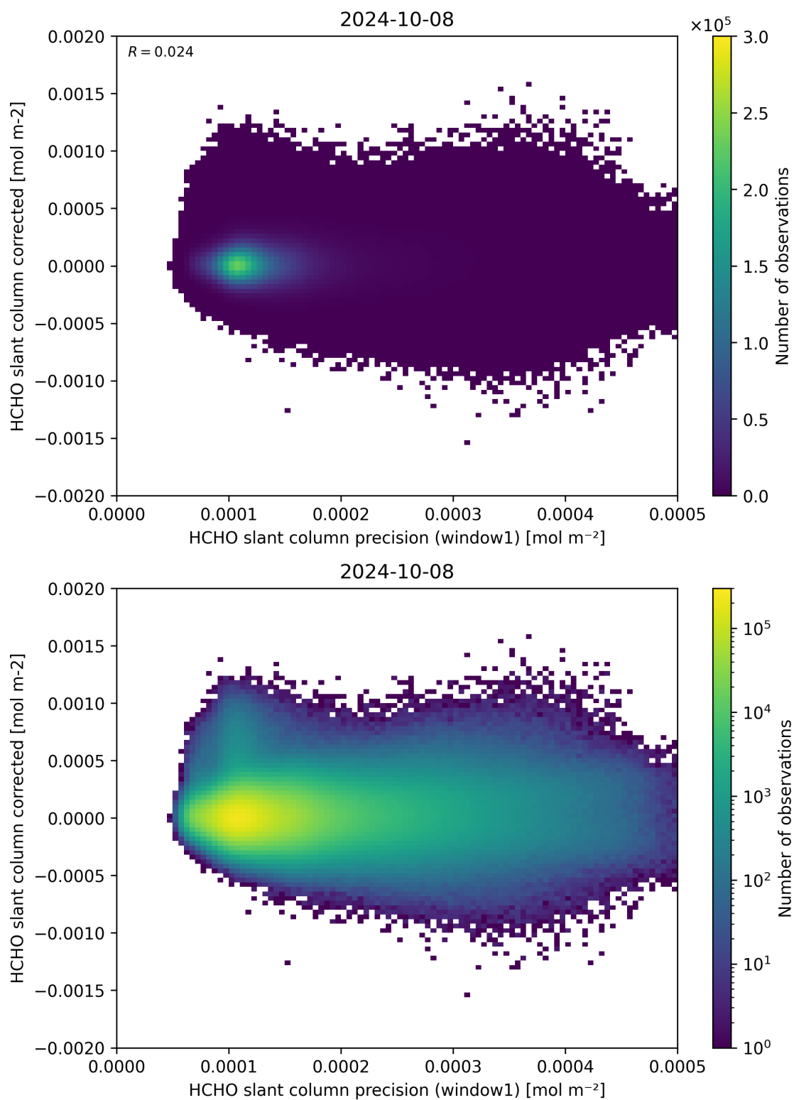
Figure 92: Scatter density plot of “HCHO slant column precision (window1)” against “HCHO slant column corrected” for 2024-10-08 to 2024-10-09.
