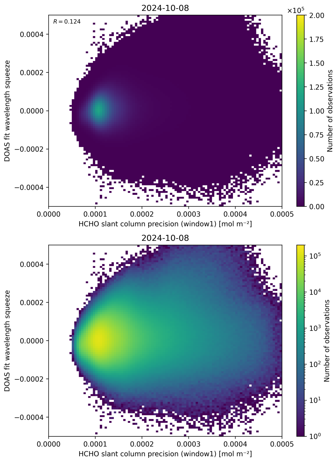
Figure 90: Scatter density plot of “HCHO slant column precision (window1)” against “DOAS fit wavelength squeeze” for 2024-10-08 to 2024-10-09.
