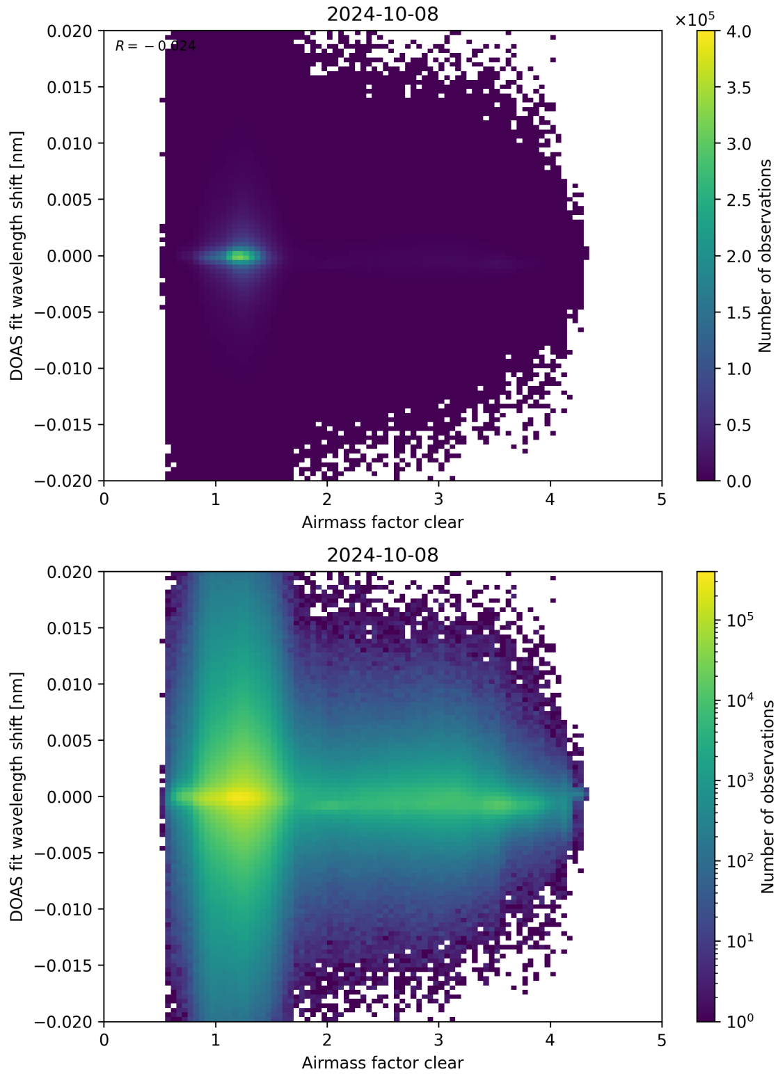
Figure 72: Scatter density plot of “Airmass factor clear” against “DOAS fit wavelength shift” for 2024-10-08 to 2024-10-09.
