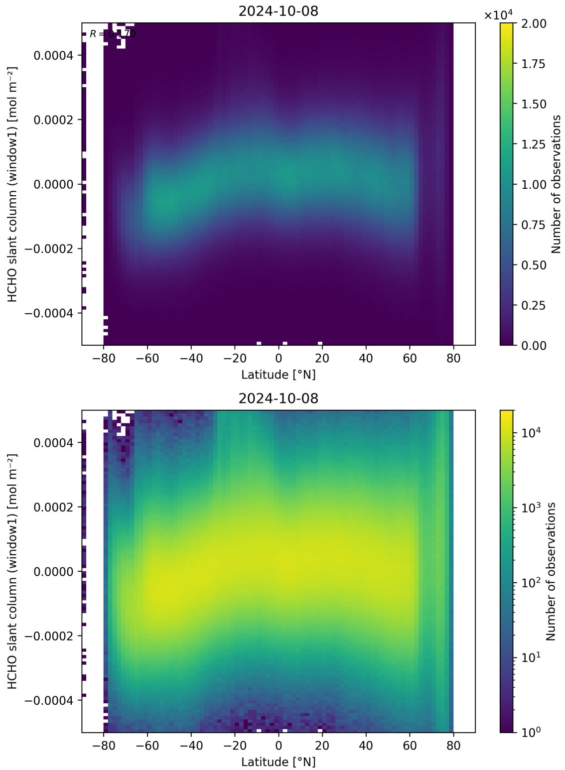
Figure 159: Scatter density plot of “Latitude” against “HCHO slant column (window1)” for 2024-10-08 to 2024-10-09.
