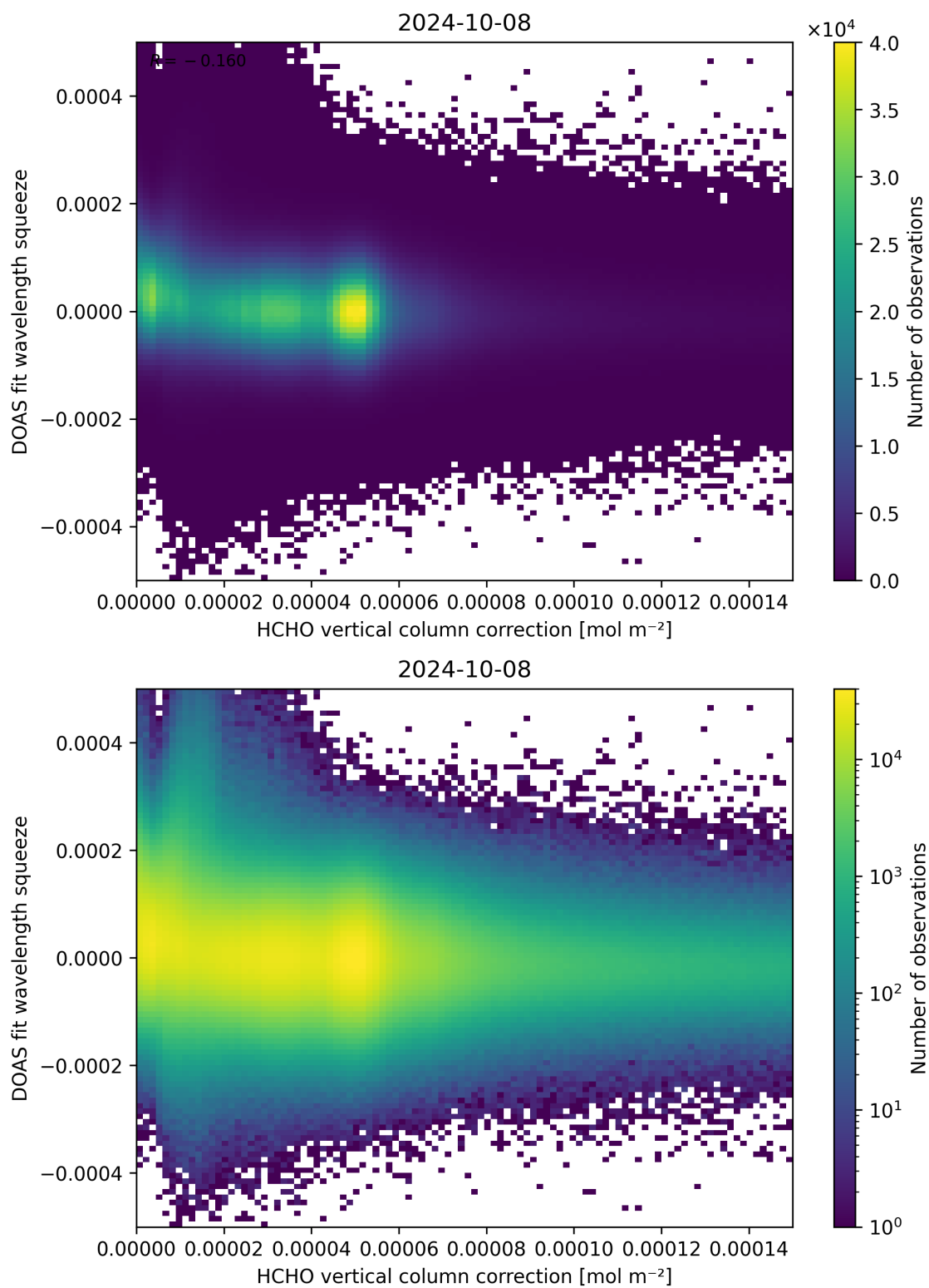
Figure 114: Scatter density plot of “HCHO vertical column correction” against “DOAS fit wavelength squeeze” for 2024-10-08 to 2024-10-09.
