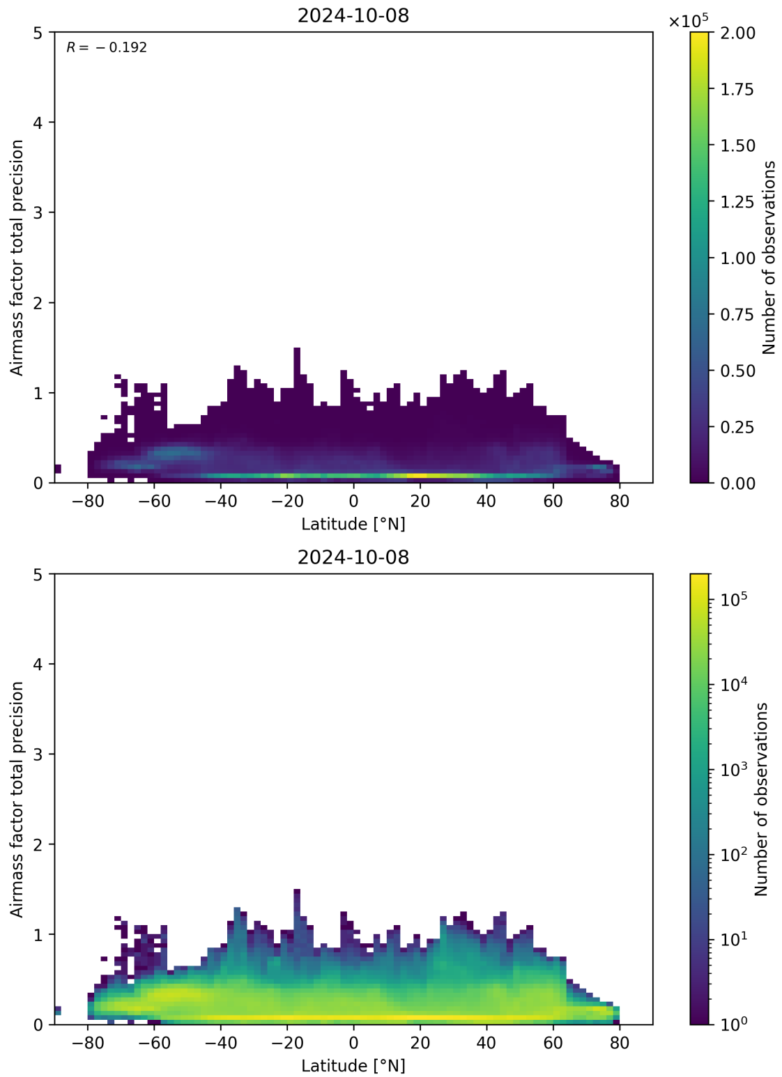
Figure 162: Scatter density plot of “Latitude” against “Airmass factor total precision” for 2024-10-08 to 2024-10-09.
