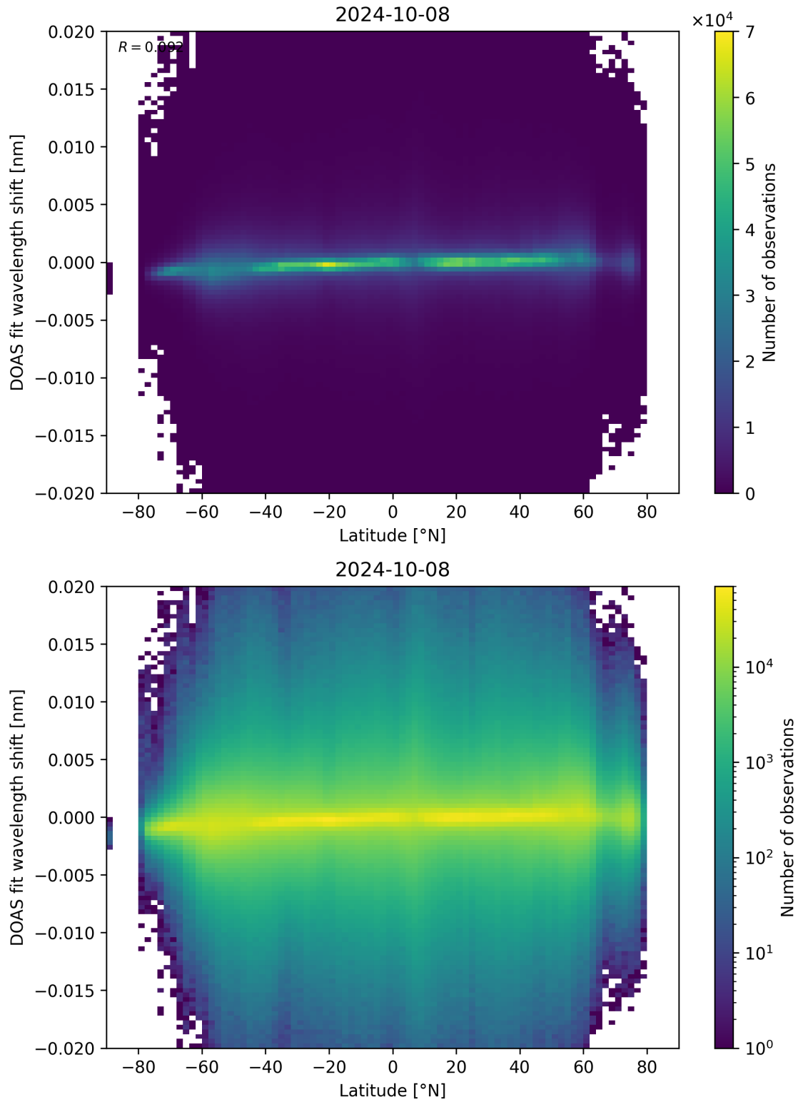
Figure 154: Scatter density plot of “Latitude” against “DOAS fit wavelength shift” for 2024-10-08 to 2024-10-09.
