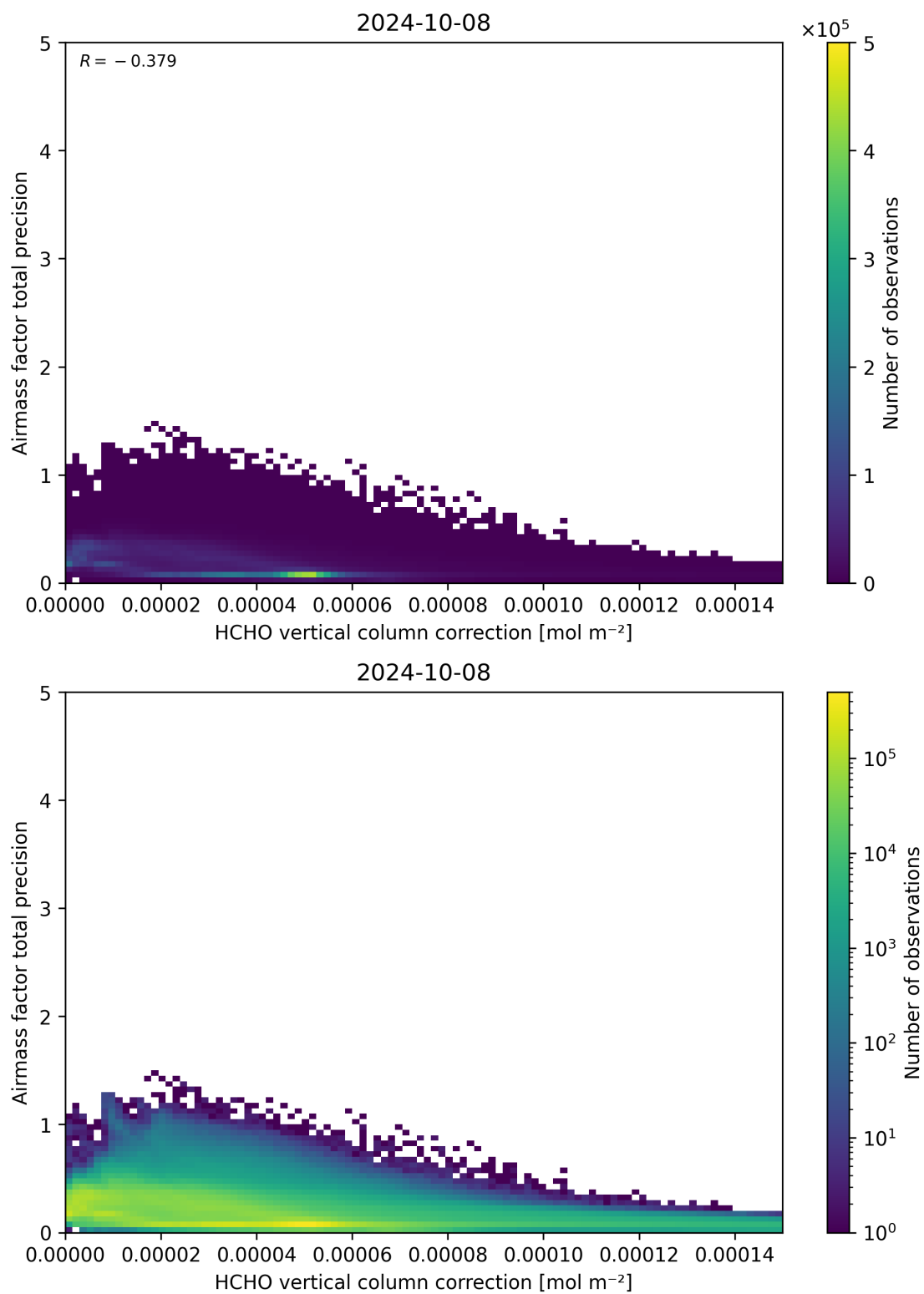
Figure 121: Scatter density plot of “HCHO vertical column correction” against “Airmass factor total precision” for 2024-10-08 to 2024-10-09.
