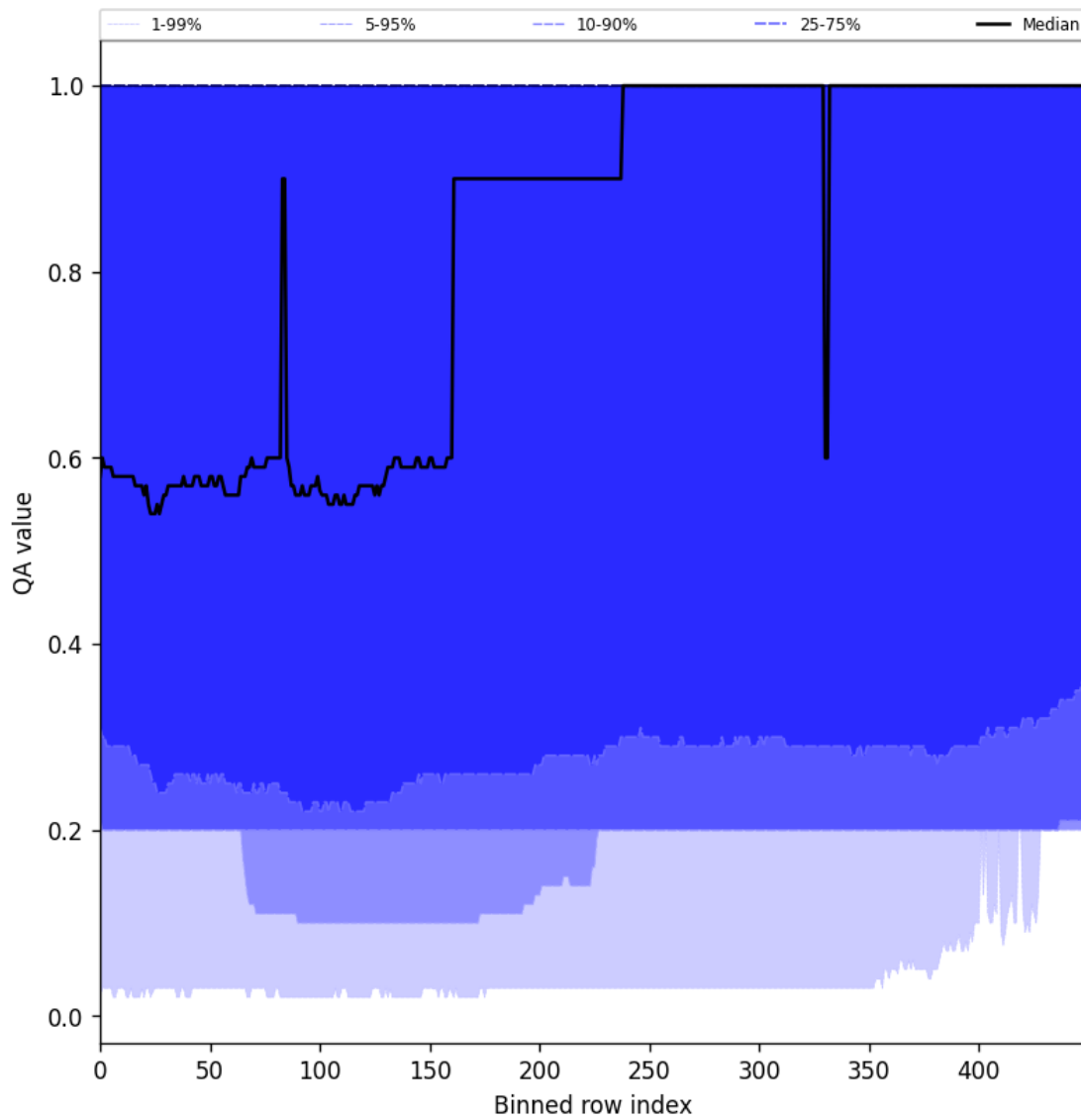
Figure 48: Along track statistics of “QA value” for 2024-10-08 to 2024-10-09
