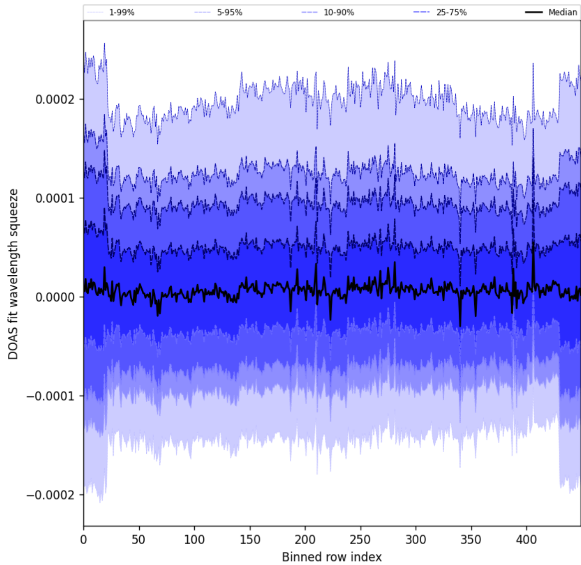
Figure 59: Along track statistics of “DOAS fit wavelength squeeze” for 2024-10-08 to 2024-10-09
