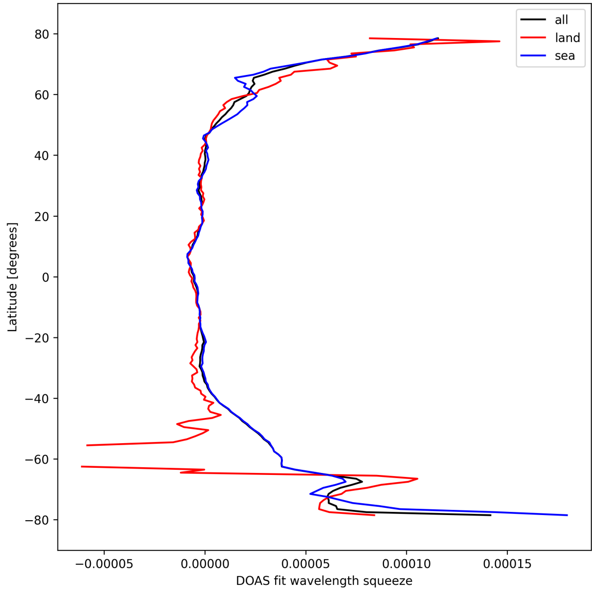
Figure 31: Zonal average of “DOAS fit wavelength squeeze” for 2024-10-08 to 2024-10-09.
