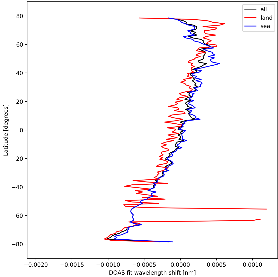
Figure 30: Zonal average of “DOAS fit wavelength shift” for 2024-10-08 to 2024-10-09.
