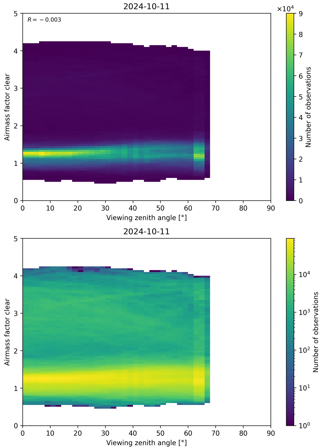
Figure 185: Scatter density plot of “Viewing zenith angle” against “Airmass factor clear” for 2024-10-10 to 2024-10-12.
