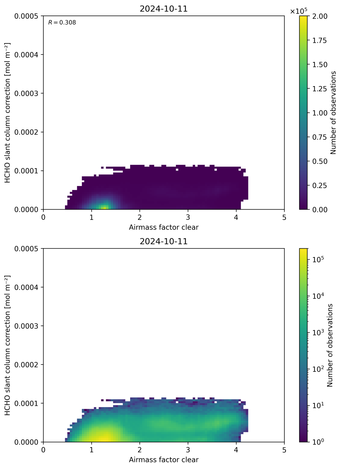
Figure 75: Scatter density plot of “Airmass factor clear” against “HCHO slant column correction” for 2024-10-10 to 2024-10-12.
