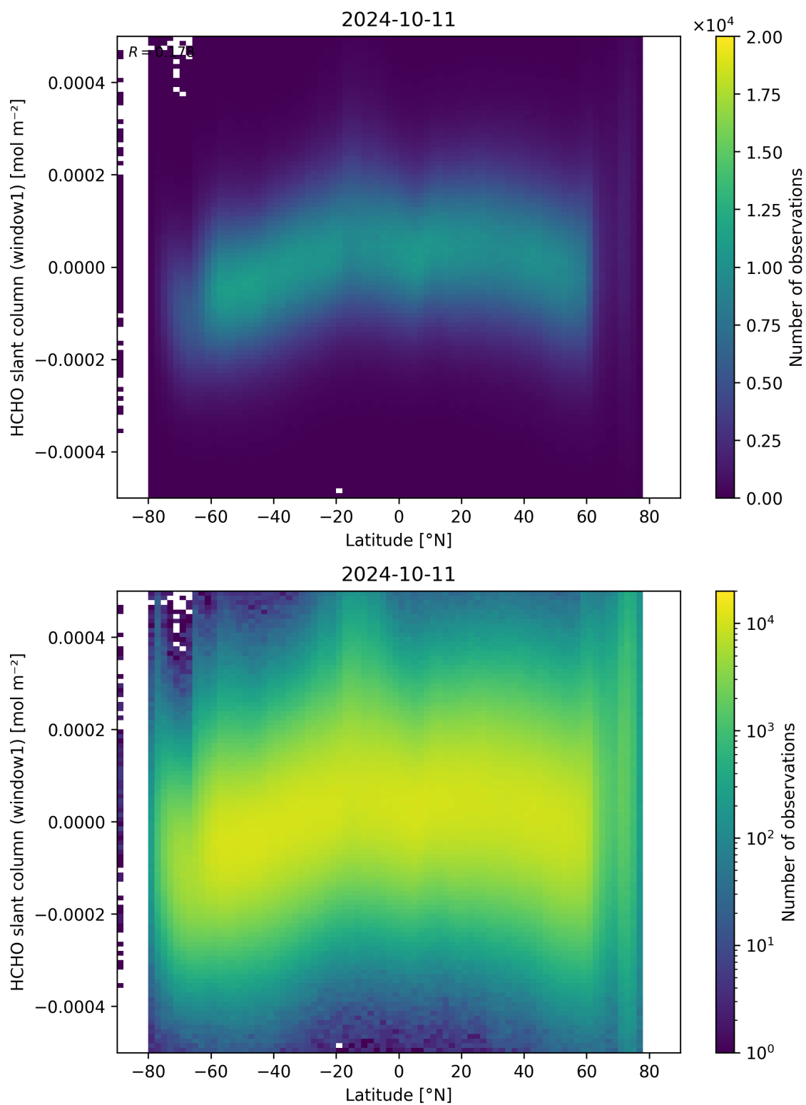
Figure 159: Scatter density plot of “Latitude” against “HCHO slant column (window1)” for 2024-10-10 to 2024-10-12.
