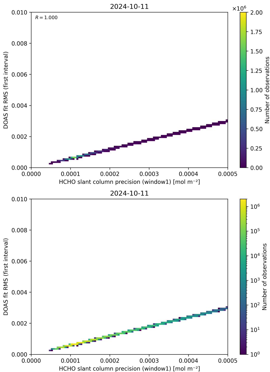
Figure 88: Scatter density plot of “HCHO slant column precision (window1)” against “DOAS fit RMS (first interval)” for 2024-10-10 to 2024-10-12.
