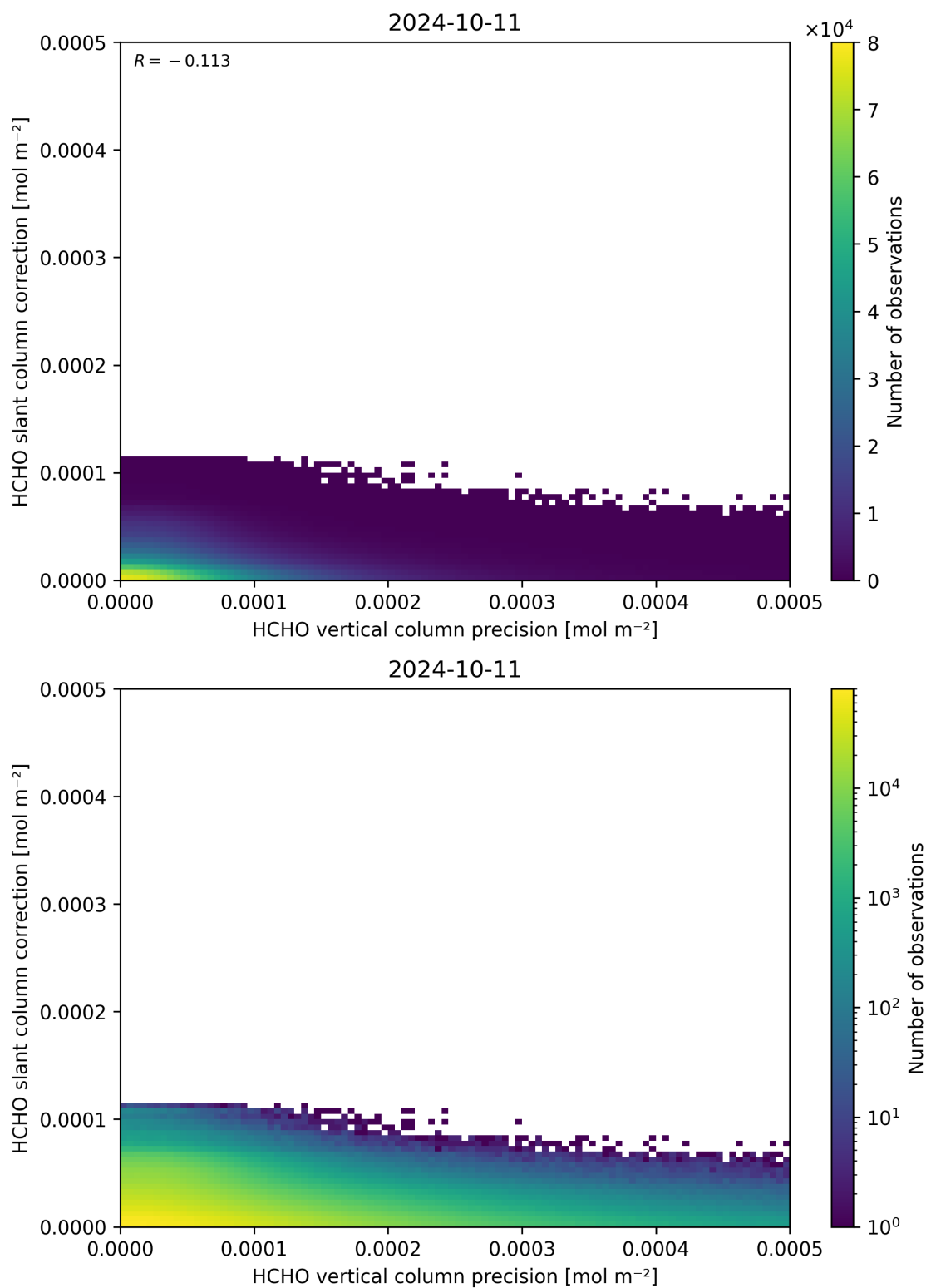
Figure 141: Scatter density plot of “HCHO vertical column precision” against “HCHO slant column correction” for 2024-10-10 to 2024-10-12.
