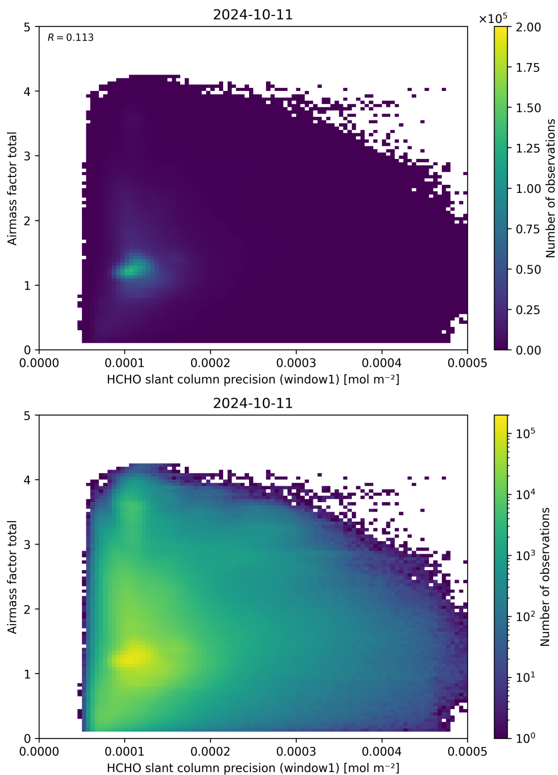
Figure 94: Scatter density plot of “HCHO slant column precision (window1)” against “Airmass factor total” for 2024-10-10 to 2024-10-12.
