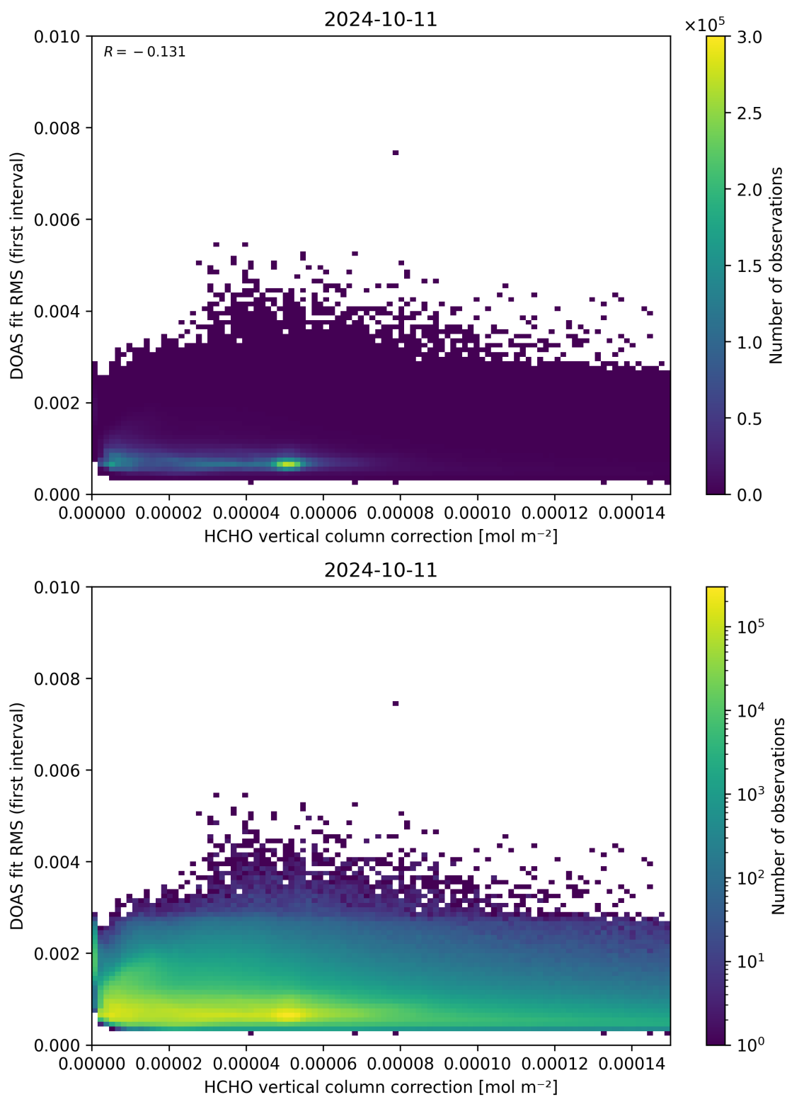
Figure 112: Scatter density plot of “HCHO vertical column correction” against “DOAS fit RMS (first interval)” for 2024-10-10 to 2024-10-12.
