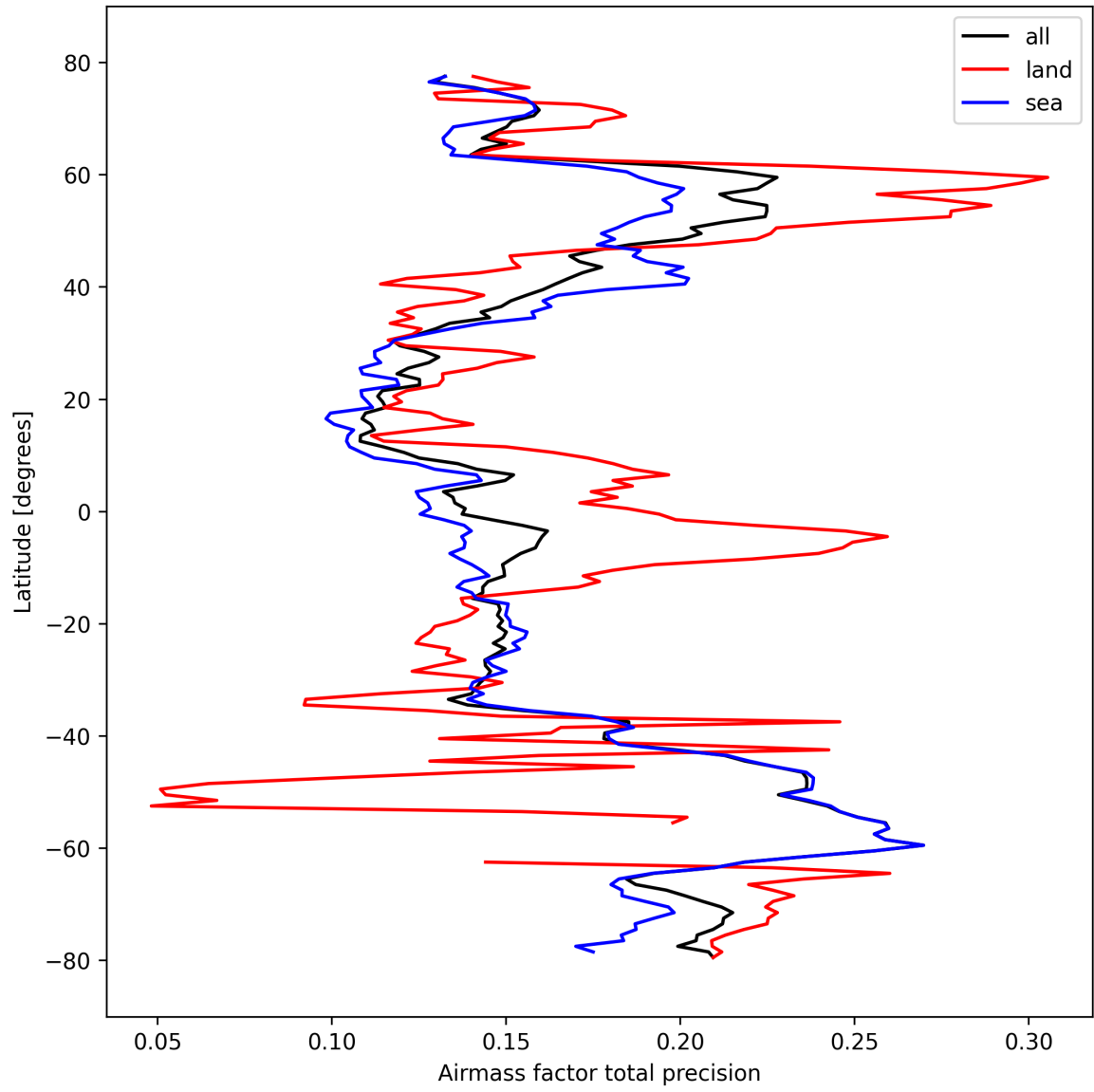
Figure 27: Zonal average of “Airmass factor total precision” for 2024-10-10 to 2024-10-12.
