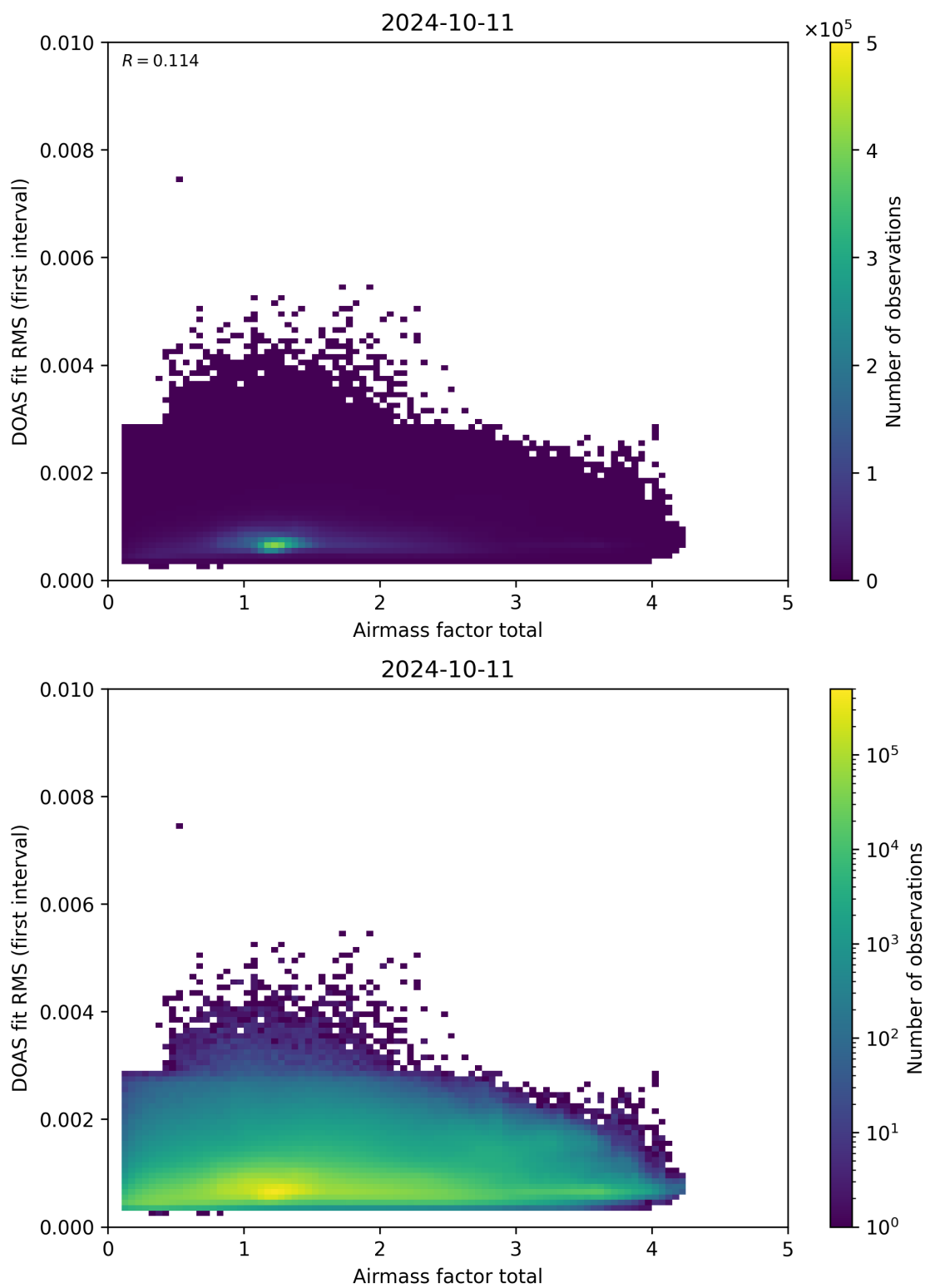
Figure 97: Scatter density plot of “Airmass factor total” against “DOAS fit RMS (first interval)” for 2024-10-10 to 2024-10-12.
