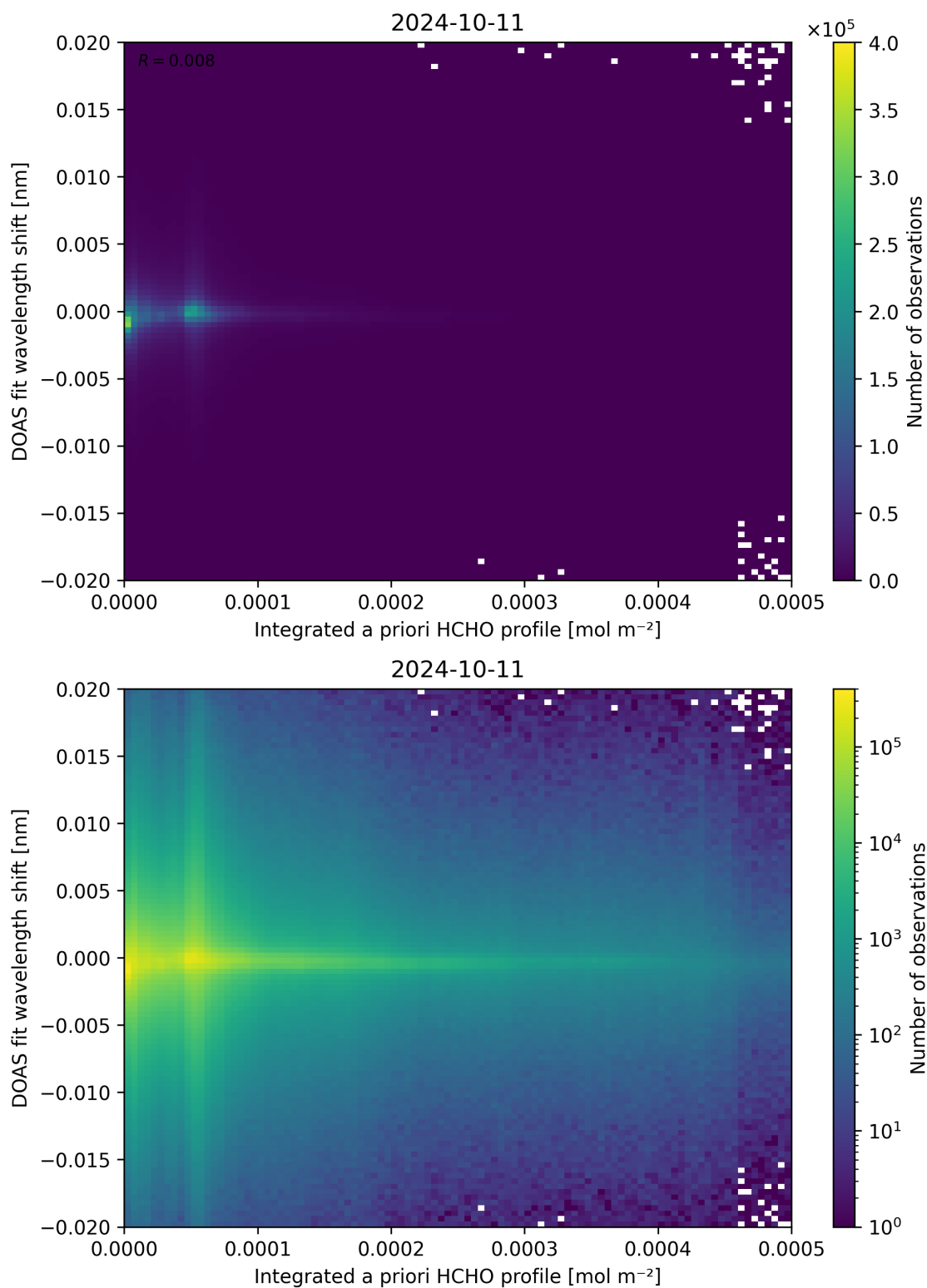
Figure 149: Scatter density plot of “Integrated a priori HCHO profile” against “DOAS fit wavelength shift” for 2024-10-10 to 2024-10-12.
