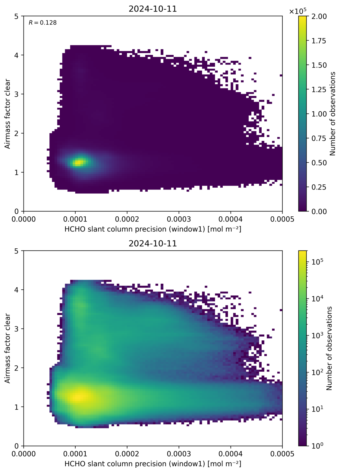
Figure 91: Scatter density plot of “HCHO slant column precision (window1)” against “Airmass factor clear” for 2024-10-10 to 2024-10-12.
