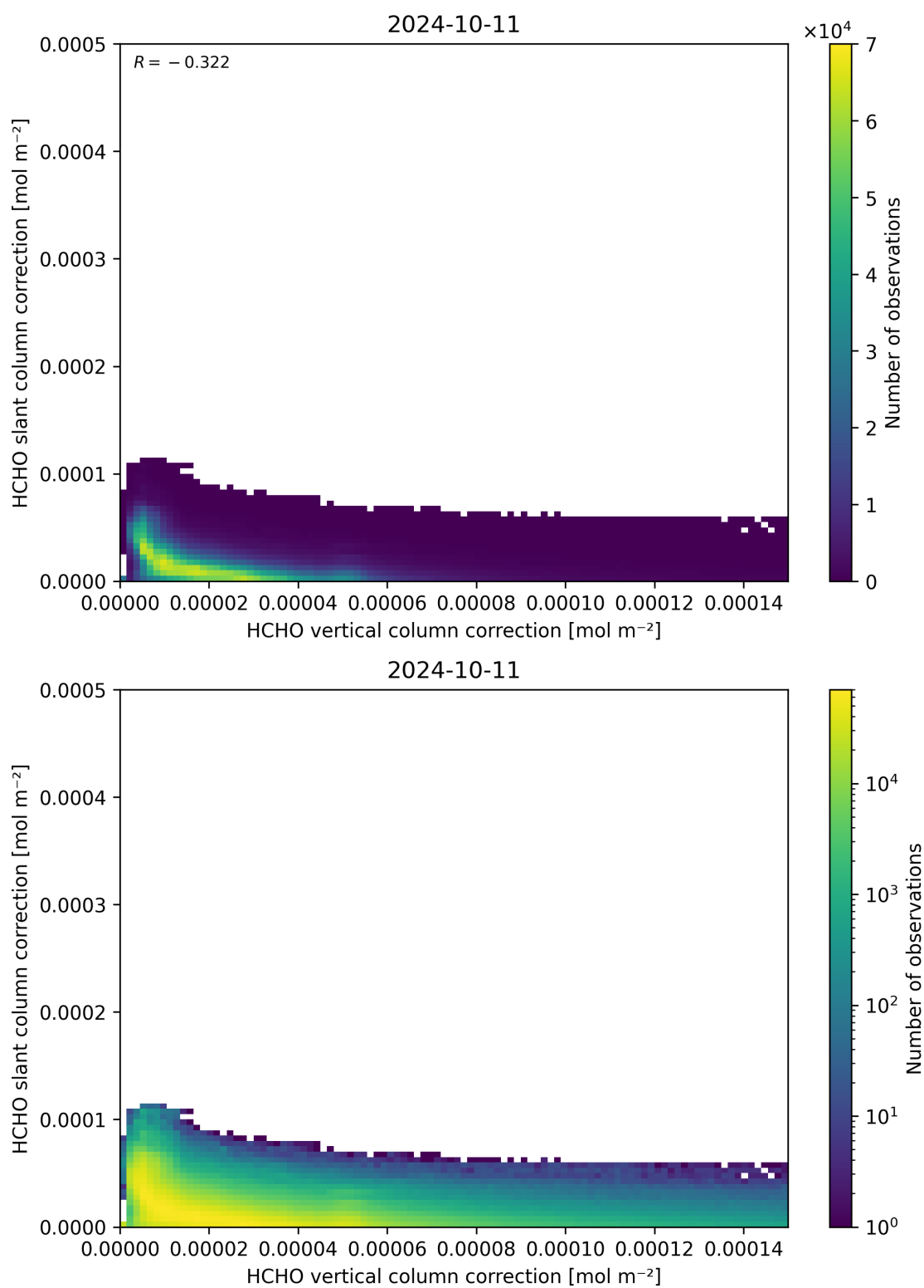
Figure 117: Scatter density plot of “HCHO vertical column correction” against “HCHO slant column correction” for 2024-10-10 to 2024-10-12.
