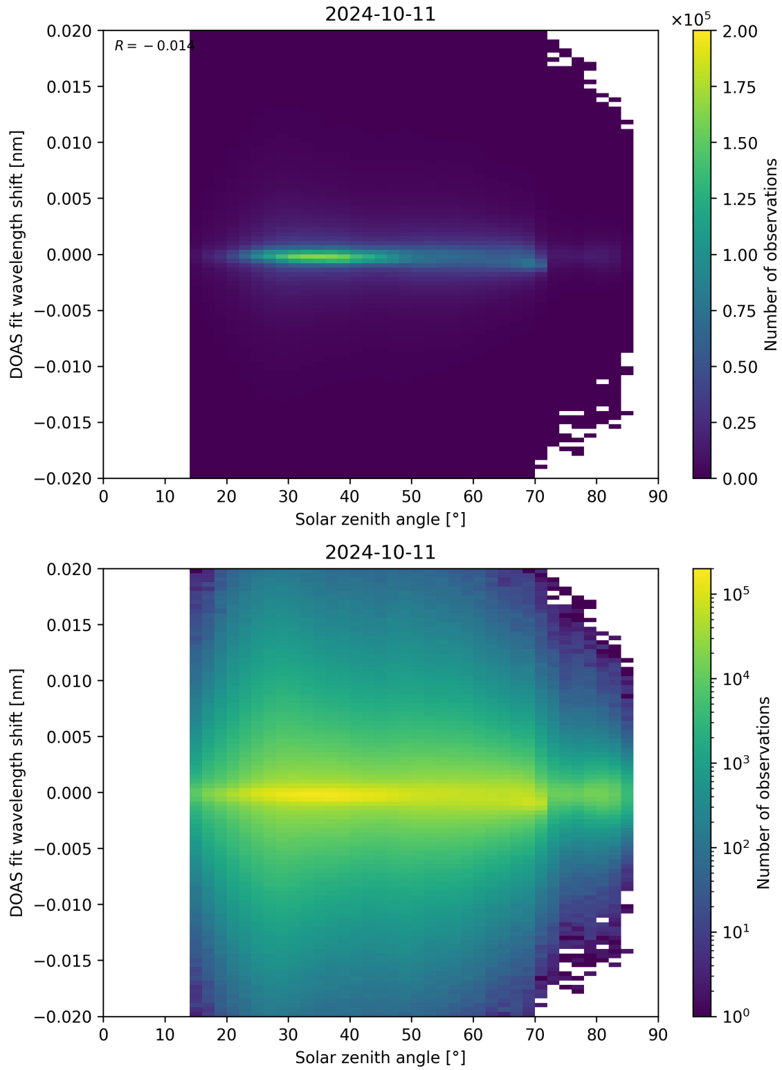
Figure 168: Scatter density plot of “Solar zenith angle” against “DOAS fit wavelength shift” for 2024-10-10 to 2024-10-12.
