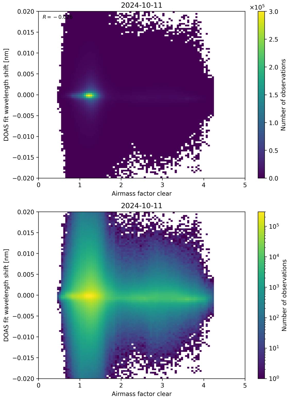
Figure 72: Scatter density plot of “Airmass factor clear” against “DOAS fit wavelength shift” for 2024-10-10 to 2024-10-12.
