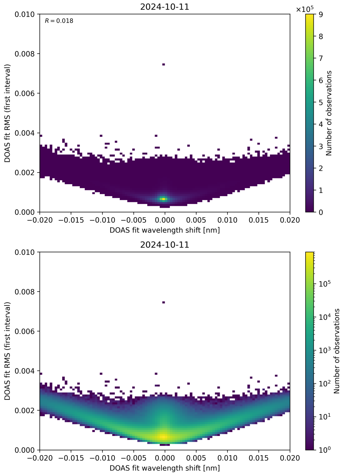
Figure 64: Scatter density plot of “DOAS fit wavelength shift” against “DOAS fit RMS (first interval)” for 2024-10-10 to 2024-10-12.
