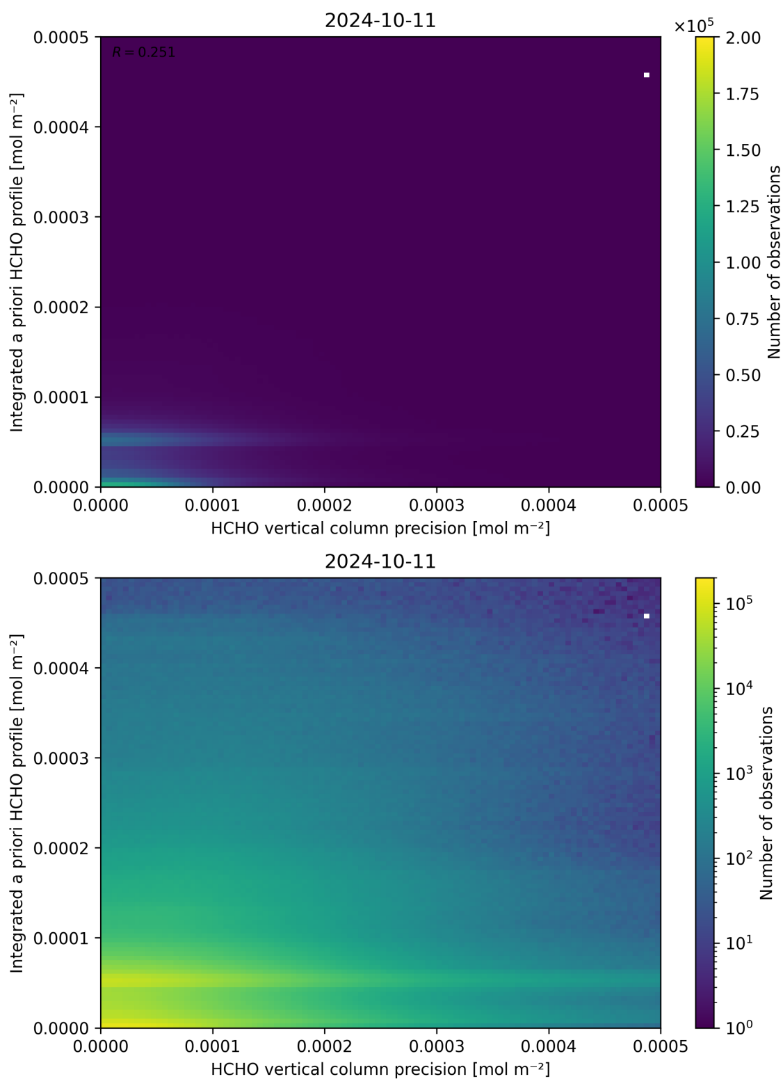
Figure 147: Scatter density plot of “HCHO vertical column precision” against “Integrated a priori HCHO profile” for 2024-10-10 to 2024-10-12.
