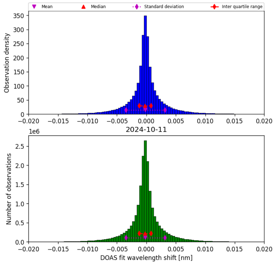
Figure 44: Histogram of “DOAS fit wavelength shift” for 2024-10-10 to 2024-10-12
