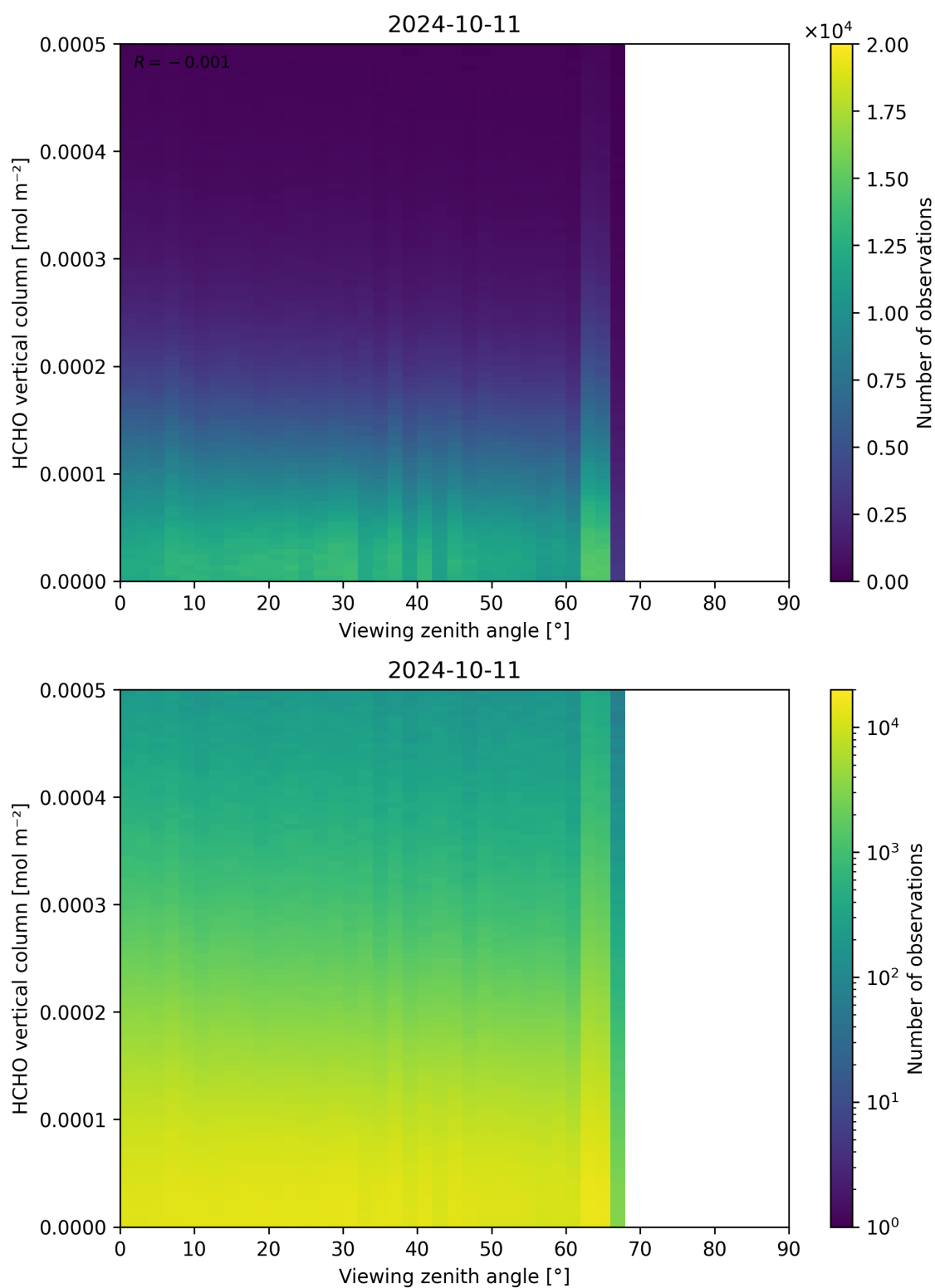
Figure 192: Scatter density plot of “Viewing zenith angle” against “HCHO vertical column” for 2024-10-10 to 2024-10-12.
