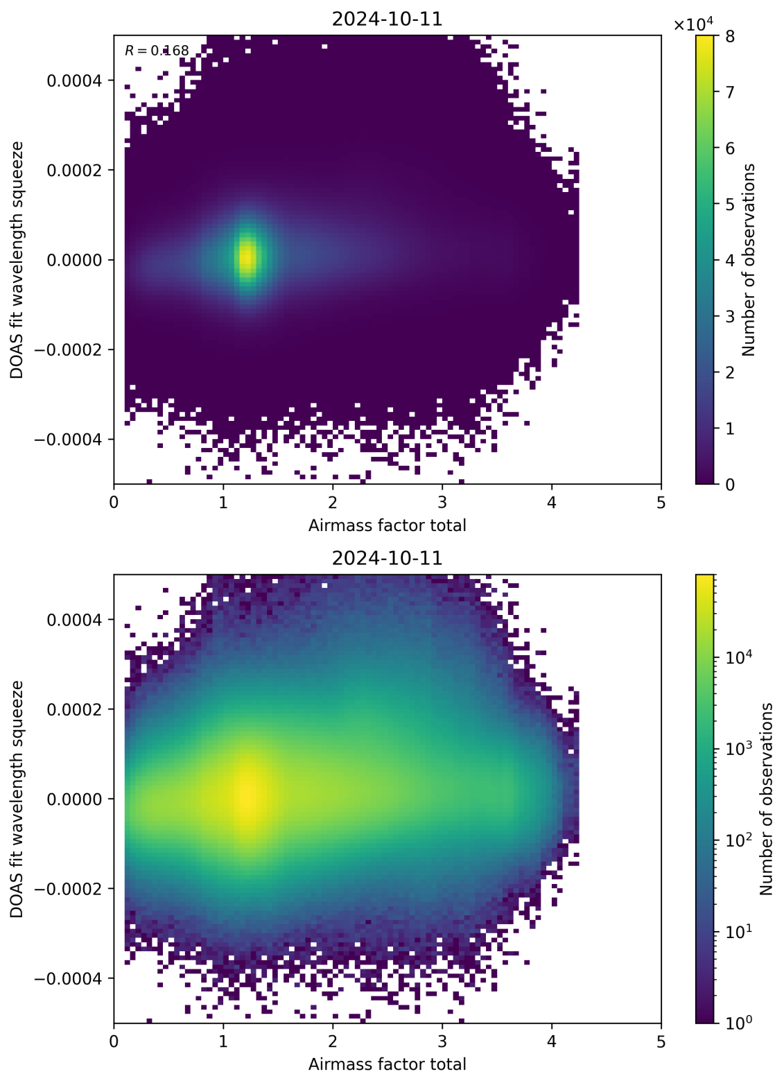
Figure 99: Scatter density plot of “Airmass factor total” against “DOAS fit wavelength squeeze” for 2024-10-10 to 2024-10-12.
