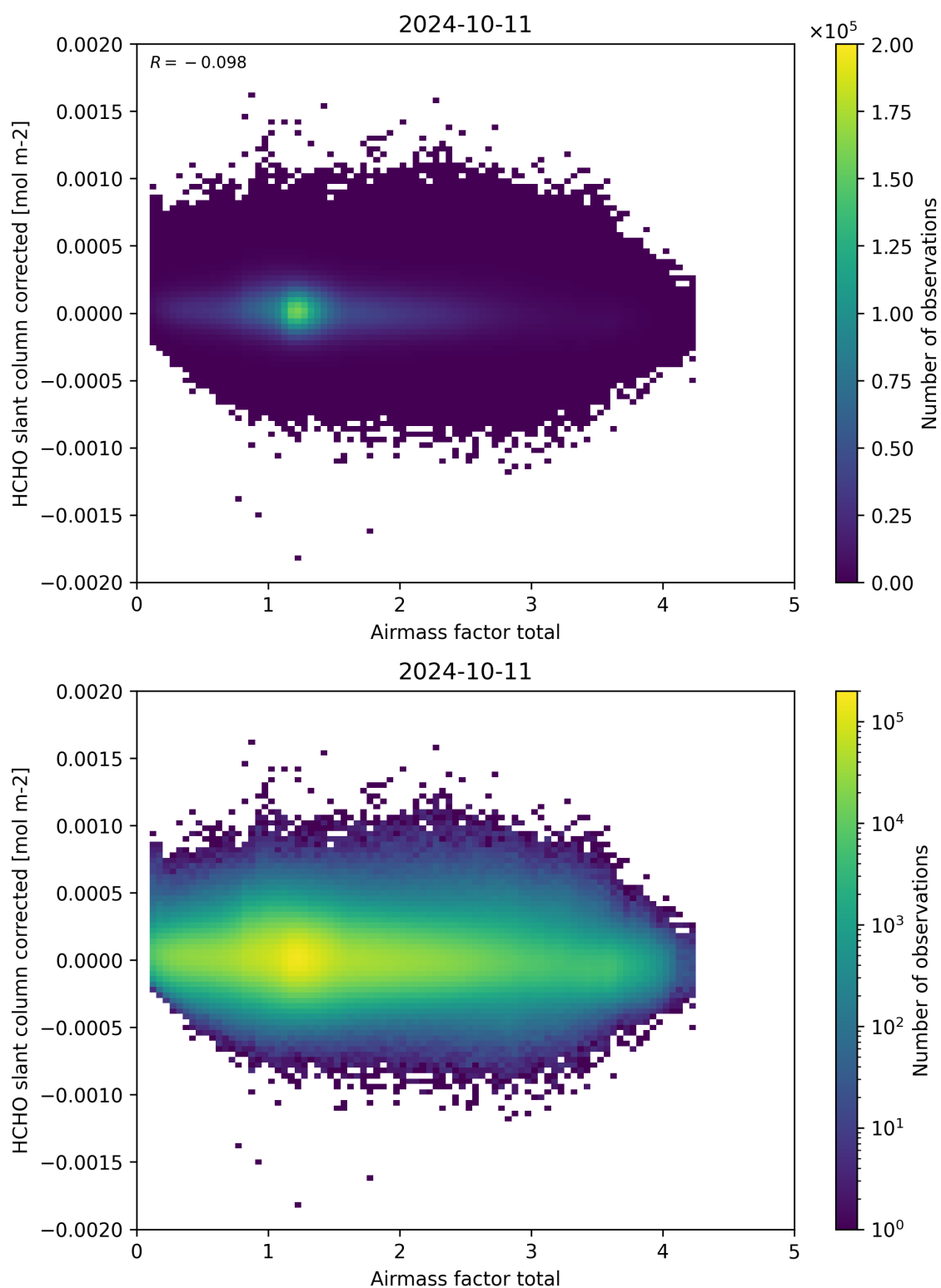
Figure 101: Scatter density plot of “Airmass factor total” against “HCHO slant column corrected” for 2024-10-10 to 2024-10-12.
