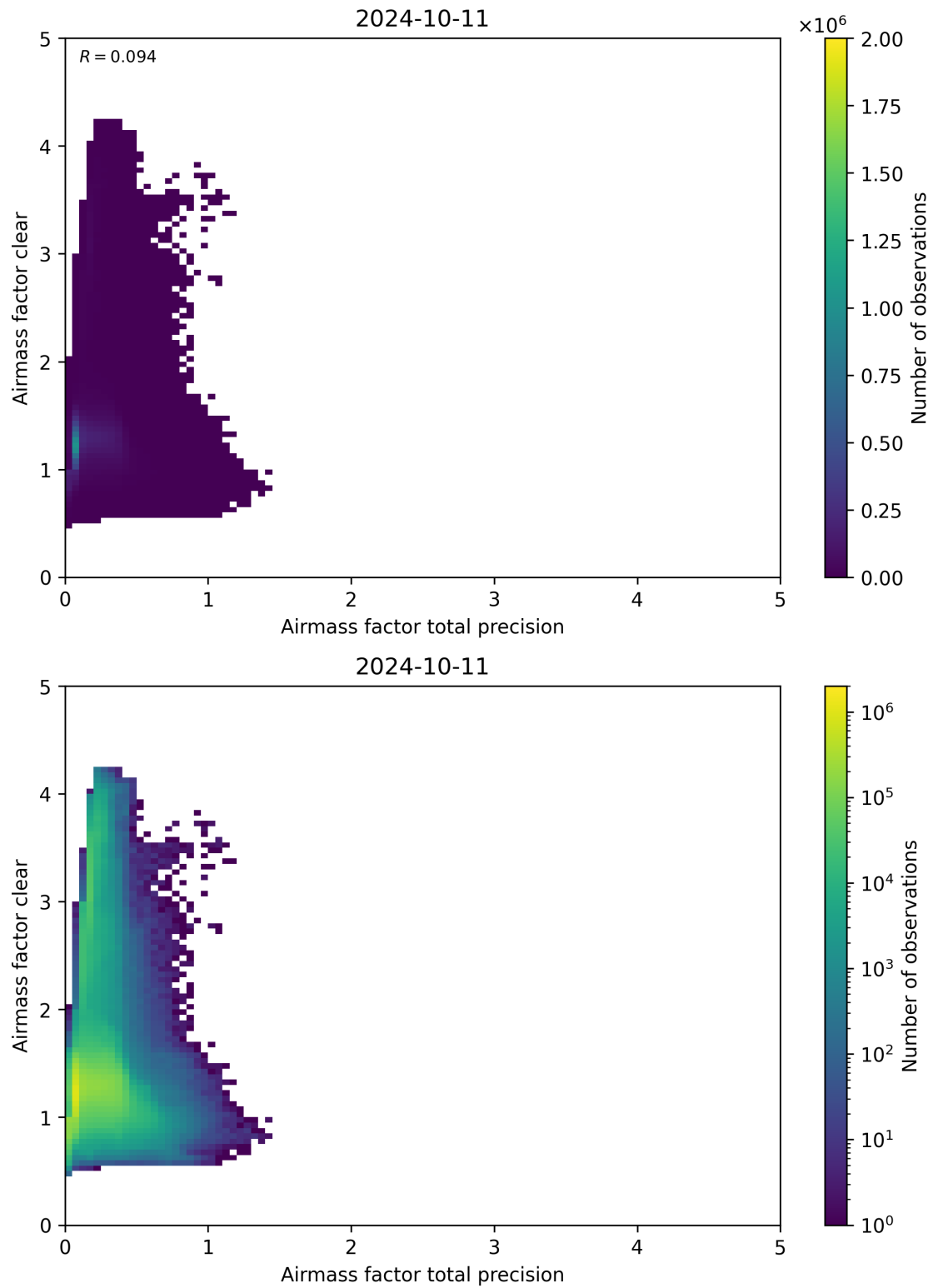
Figure 108: Scatter density plot of “Airmass factor total precision” against “Airmass factor clear” for 2024-10-10 to 2024-10-12.
