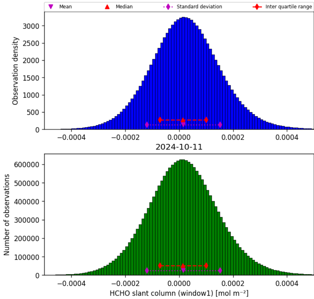
Figure 38: Histogram of “HCHO slant column (window1)” for 2024-10-10 to 2024-10-12
