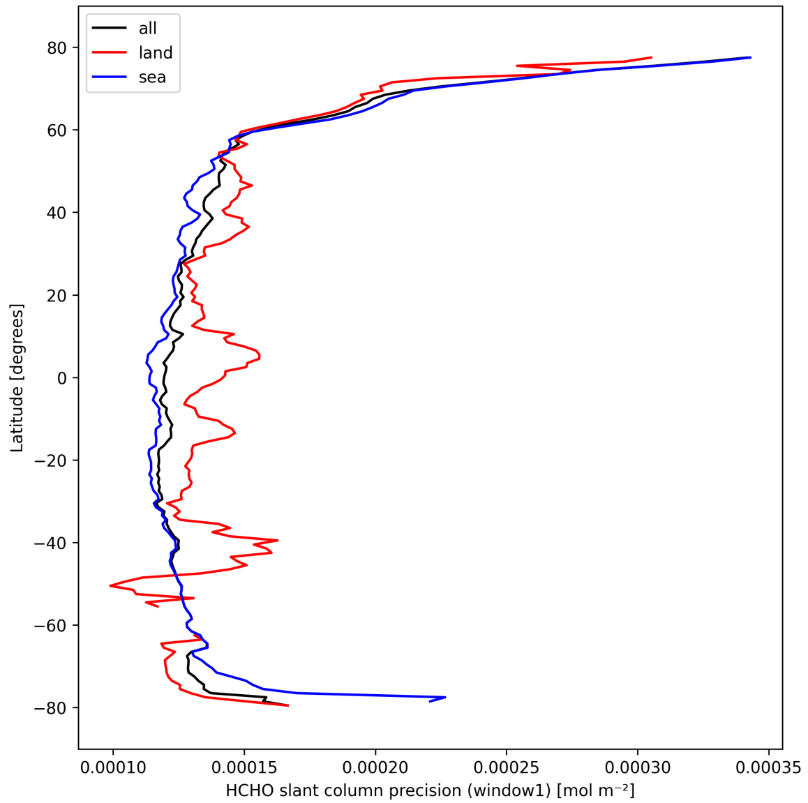
Figure 25: Zonal average of “HCHO slant column precision (window1)” for 2024-10-10 to 2024-10-12.
