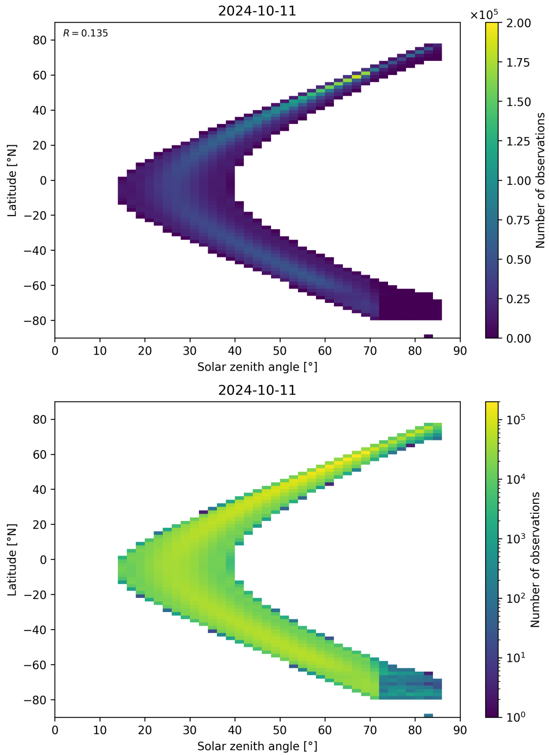
Figure 181: Scatter density plot of “Solar zenith angle” against “Latitude” for 2024-10-10 to 2024-10-12.
