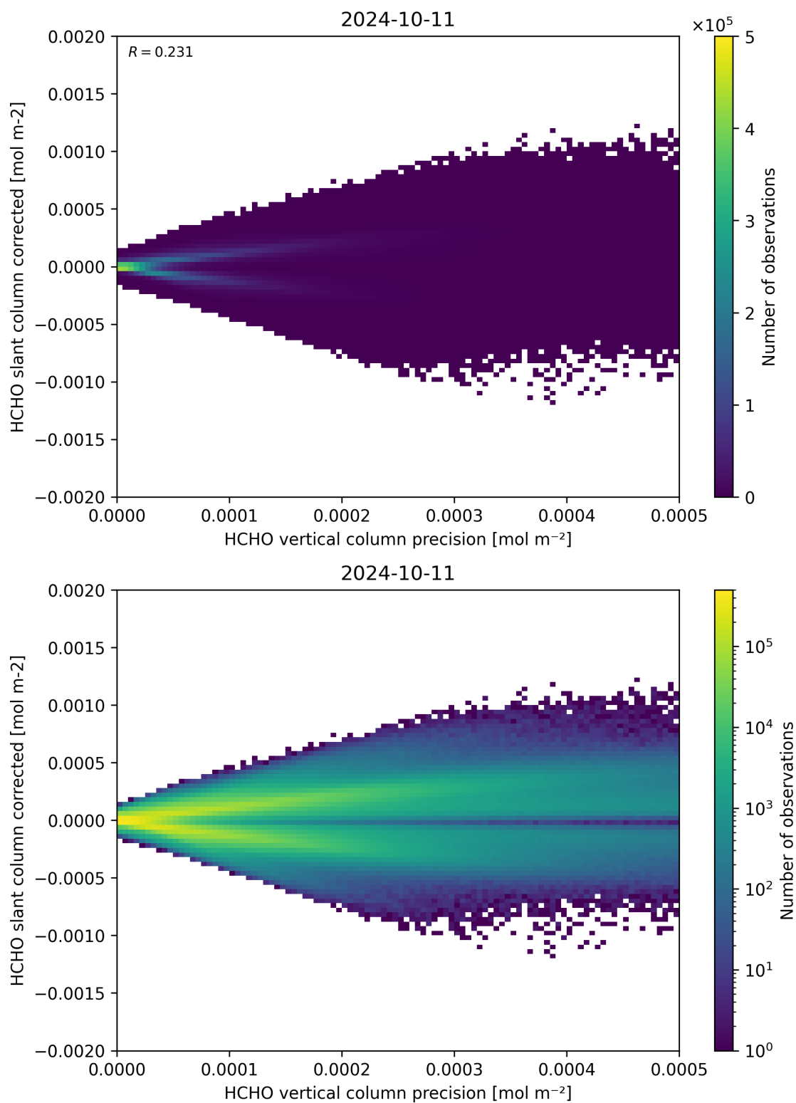
Figure 140: Scatter density plot of “HCHO vertical column precision” against “HCHO slant column corrected” for 2024-10-10 to 2024-10-12.
