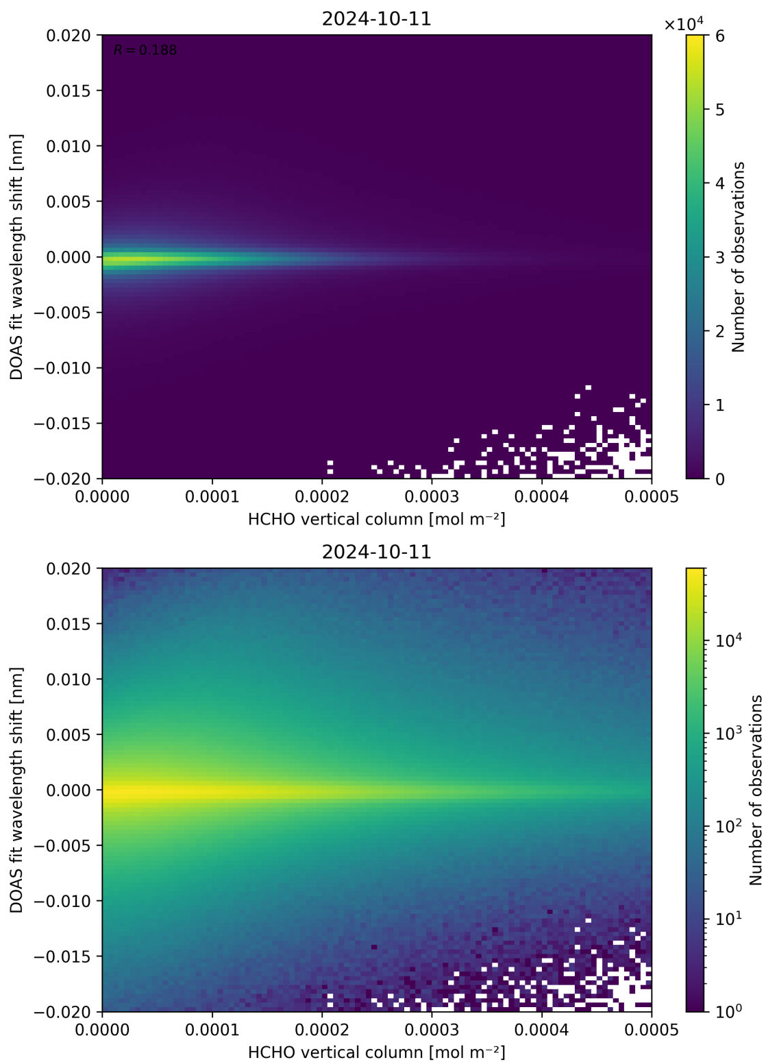
Figure 124: Scatter density plot of “HCHO vertical column” against “DOAS fit wavelength shift” for 2024-10-10 to 2024-10-12.
