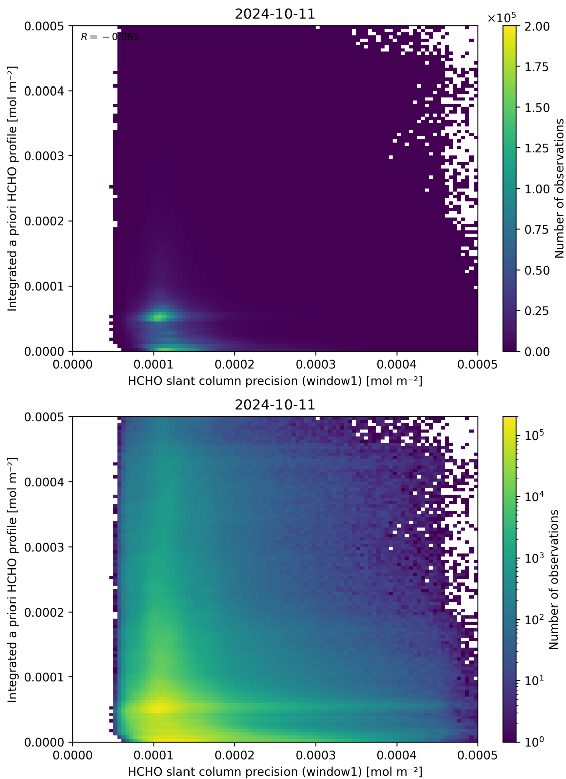
Figure 96: Scatter density plot of “HCHO slant column precision (window1)” against “Integrated a priori HCHO profile” for 2024-10-10 to 2024-10-12.
