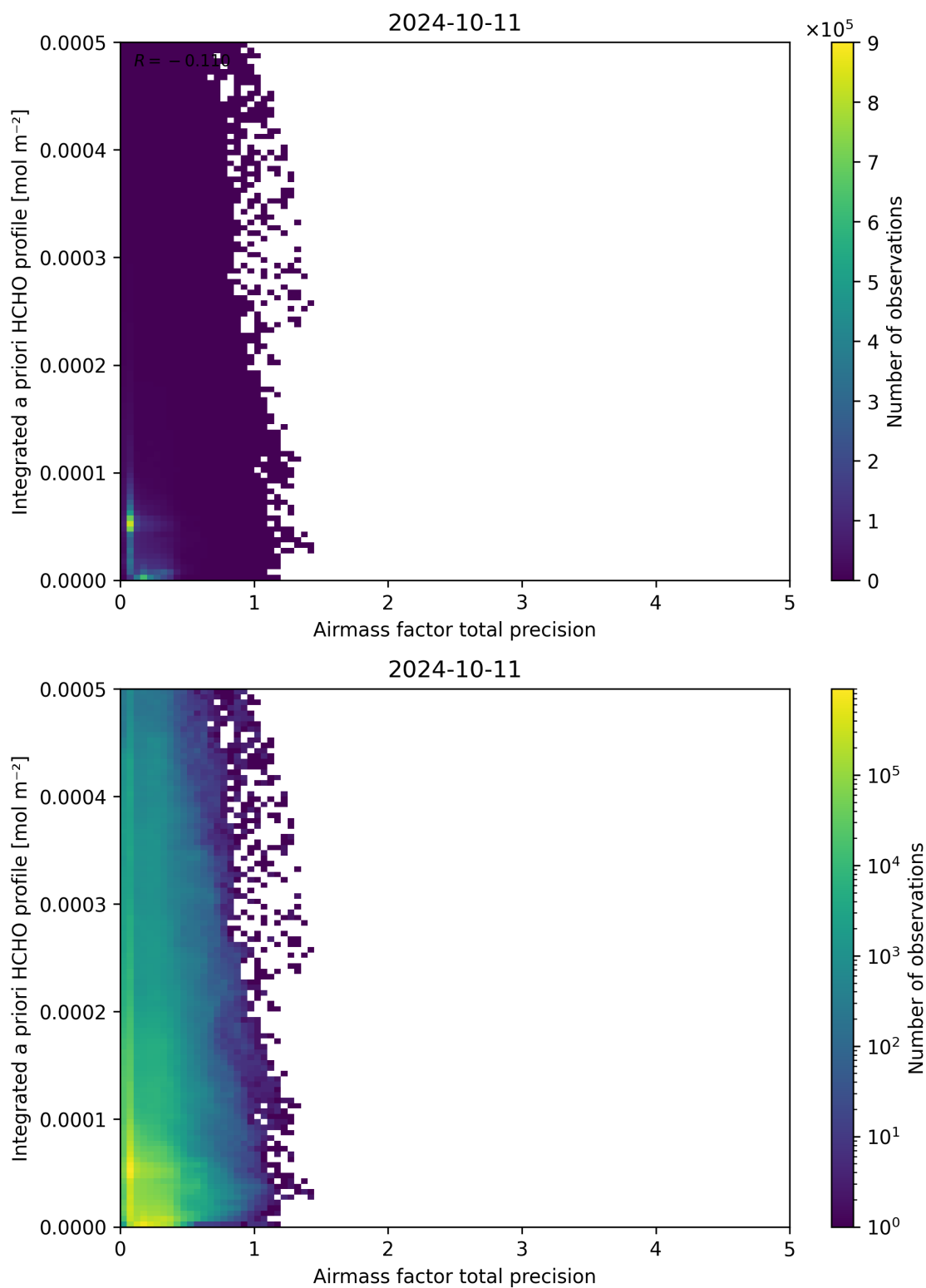
Figure 111: Scatter density plot of “Airmass factor total precision” against “Integrated a priori HCHO profile” for 2024-10-10 to 2024-10-12.
