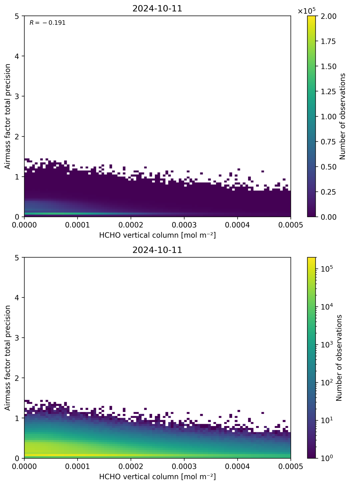
Figure 132: Scatter density plot of “HCHO vertical column” against “Airmass factor total precision” for 2024-10-10 to 2024-10-12.
