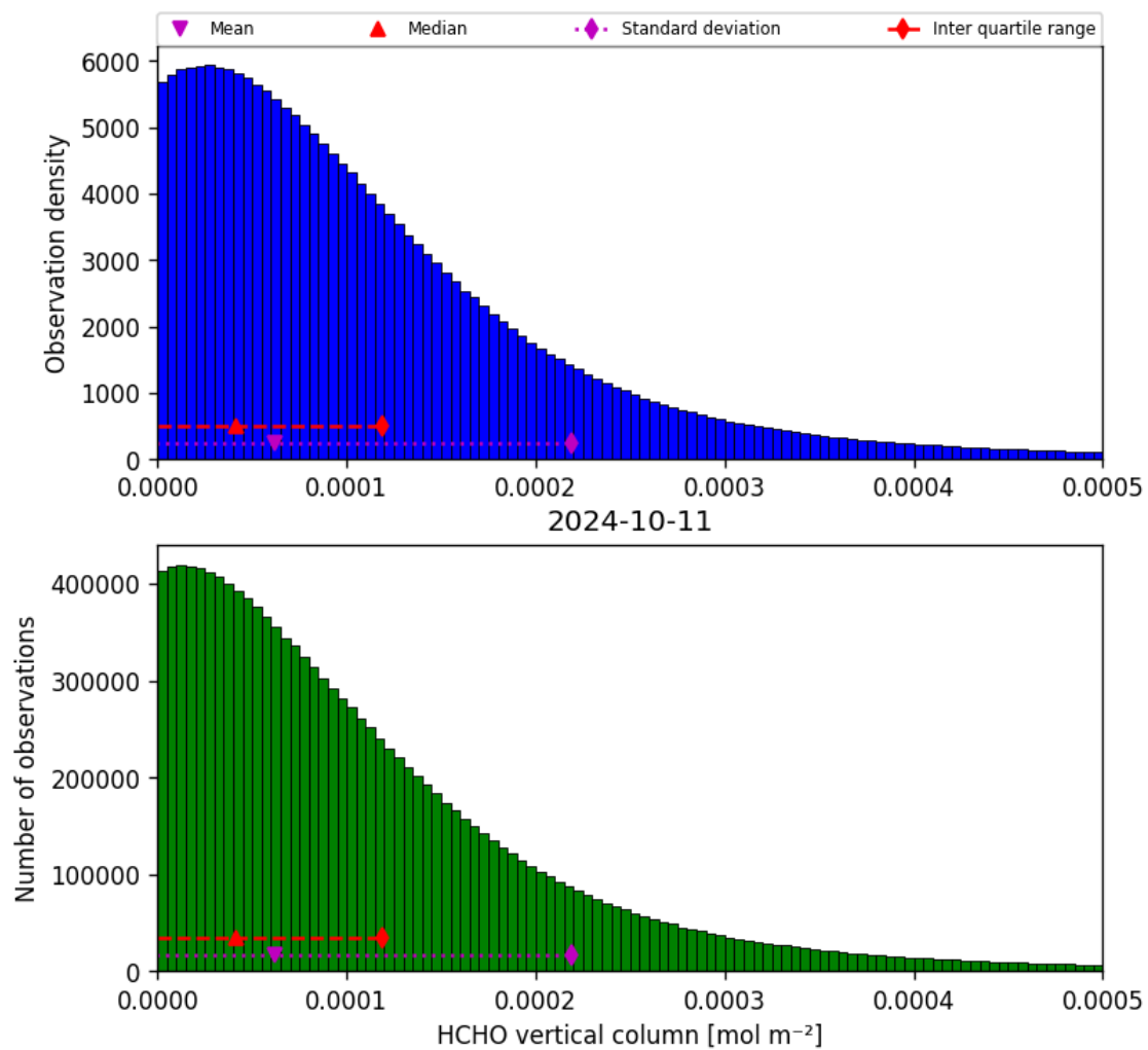
Figure 35: Histogram of “HCHO vertical column” for 2024-10-10 to 2024-10-12
