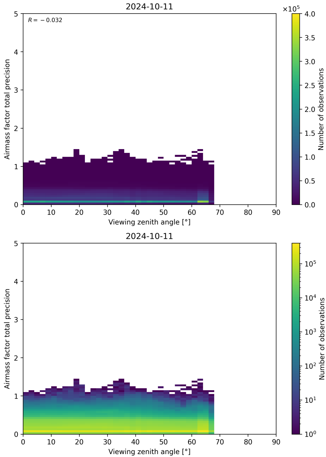
Figure 191: Scatter density plot of “Viewing zenith angle” against “Airmass factor total precision” for 2024-10-10 to 2024-10-12.
