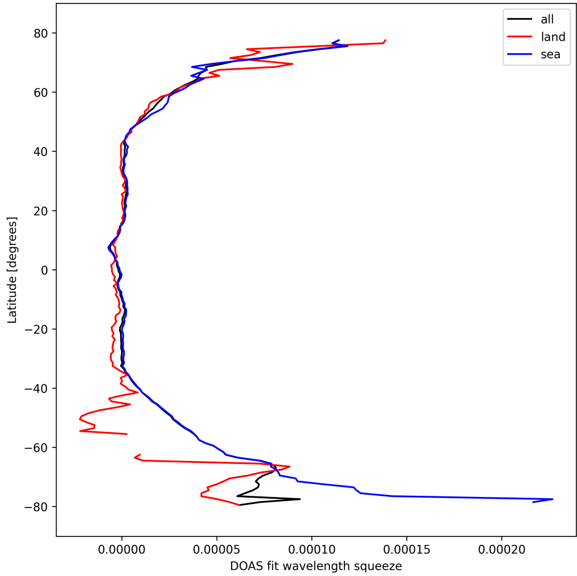
Figure 31: Zonal average of “DOAS fit wavelength squeeze” for 2024-10-10 to 2024-10-12.
