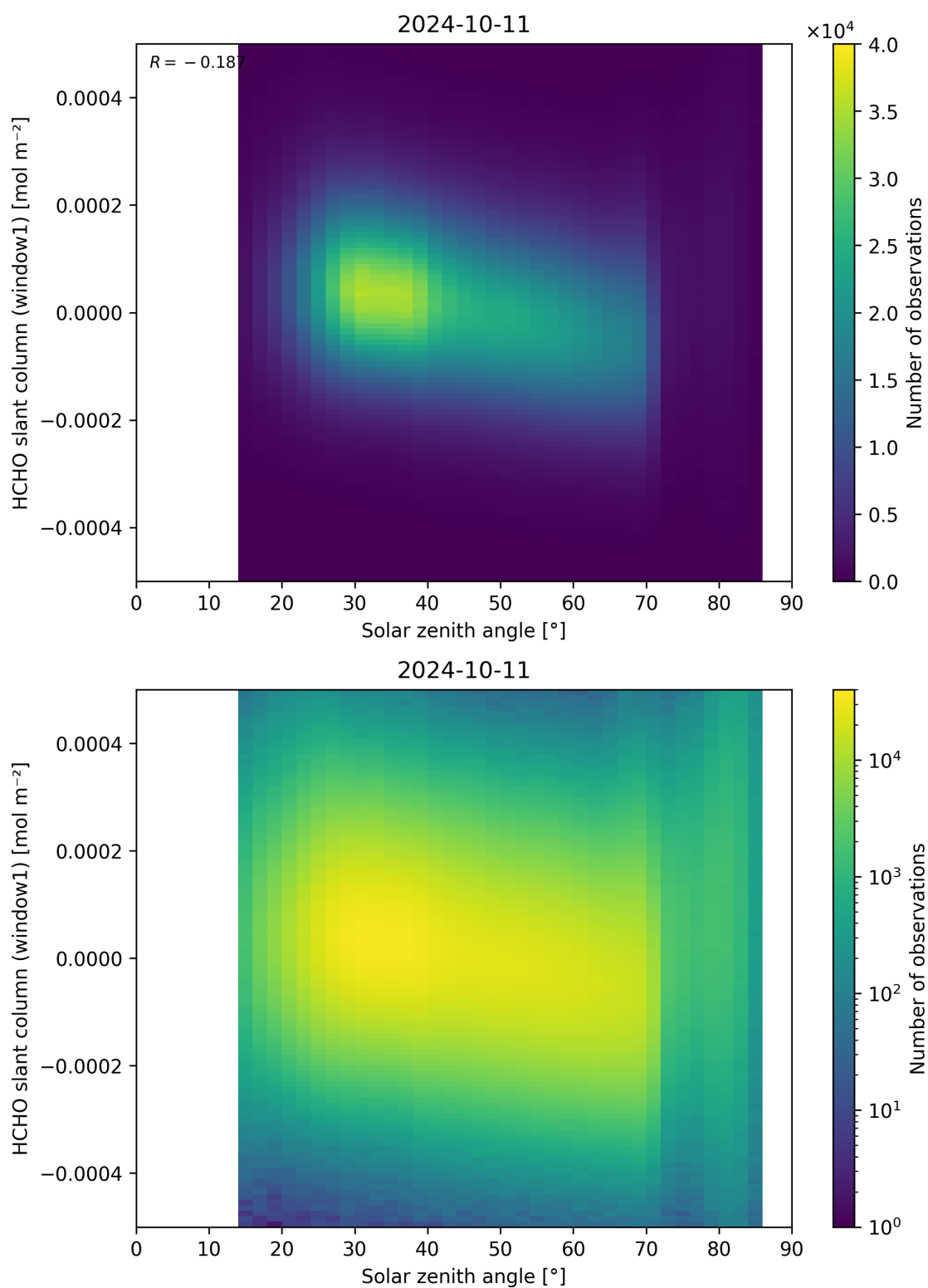
Figure 173: Scatter density plot of “Solar zenith angle” against “HCHO slant column (window1)” for 2024-10-10 to 2024-10-12.
