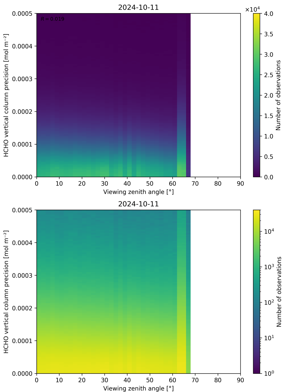
Figure 194: Scatter density plot of “Viewing zenith angle” against “HCHO vertical column precision” for 2024-10-10 to 2024-10-12.
