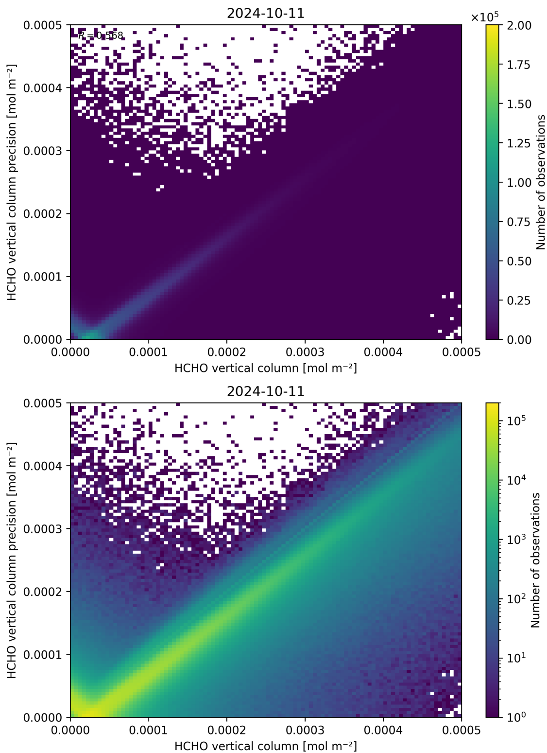
Figure 134: Scatter density plot of “HCHO vertical column” against “HCHO vertical column precision” for 2024-10-10 to 2024-10-12.
