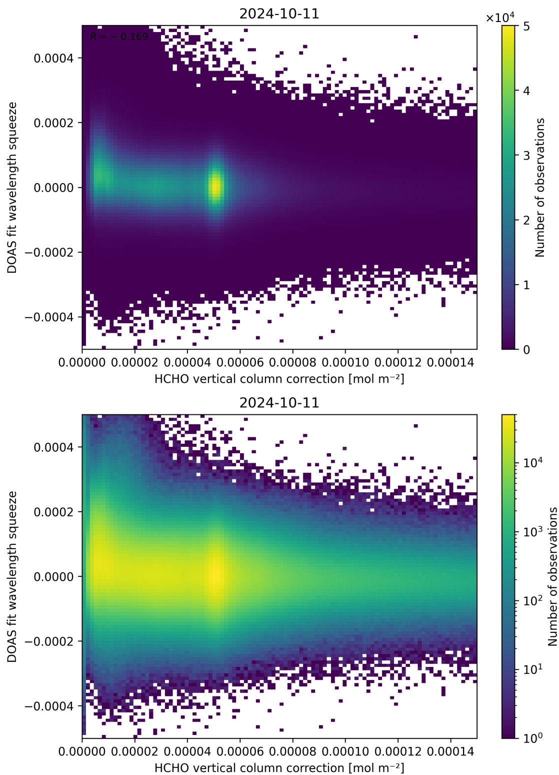
Figure 114: Scatter density plot of “HCHO vertical column correction” against “DOAS fit wavelength squeeze” for 2024-10-10 to 2024-10-12.
