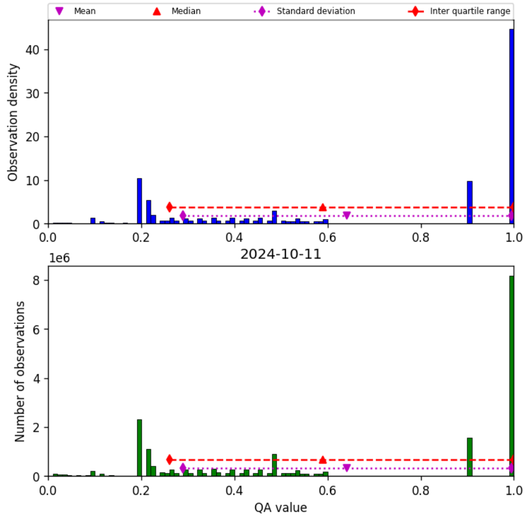
Figure 34: Histogram of “QA value” for 2024-10-10 to 2024-10-12
