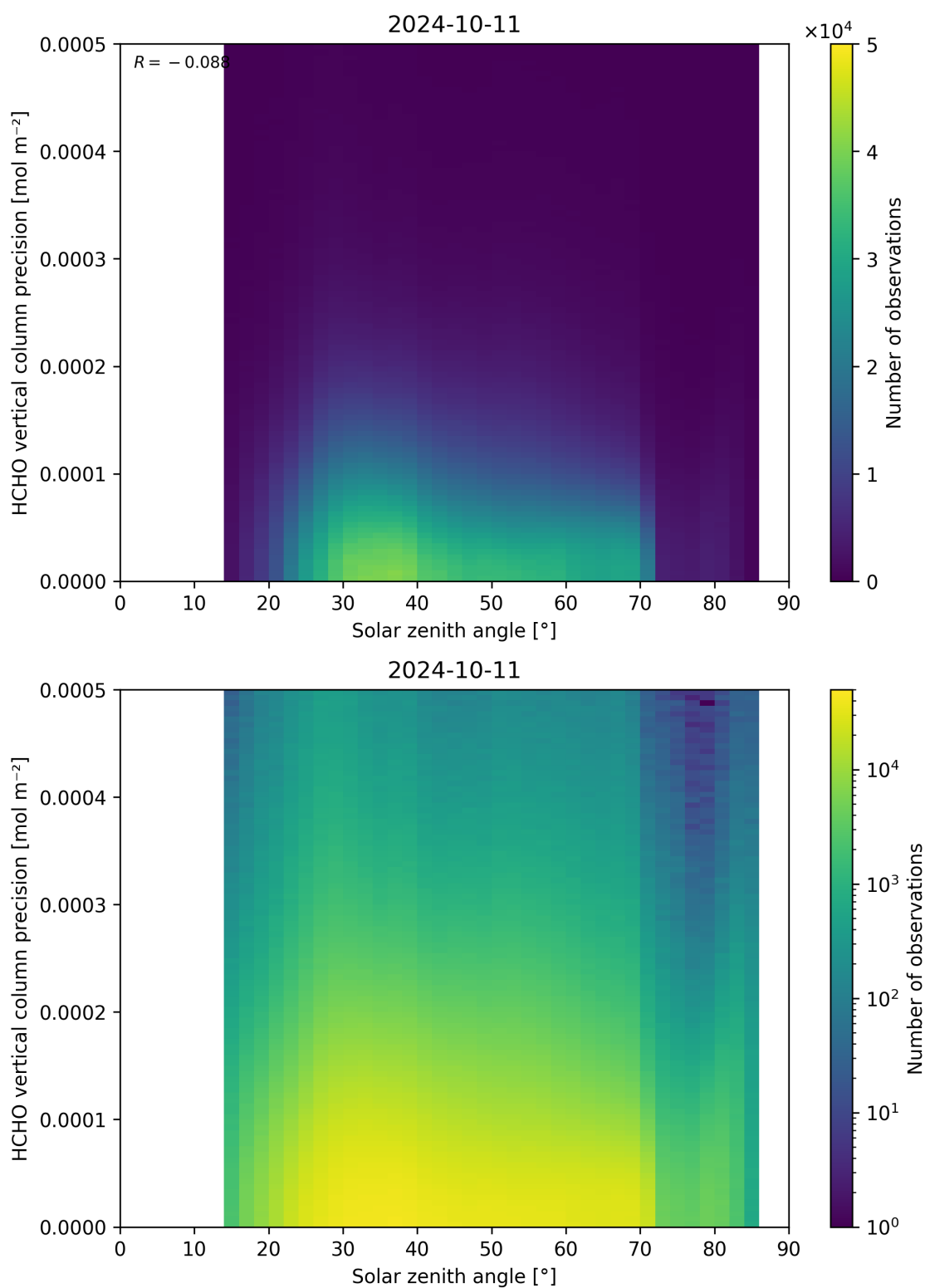
Figure 179: Scatter density plot of “Solar zenith angle” against “HCHO vertical column precision” for 2024-10-10 to 2024-10-12.
