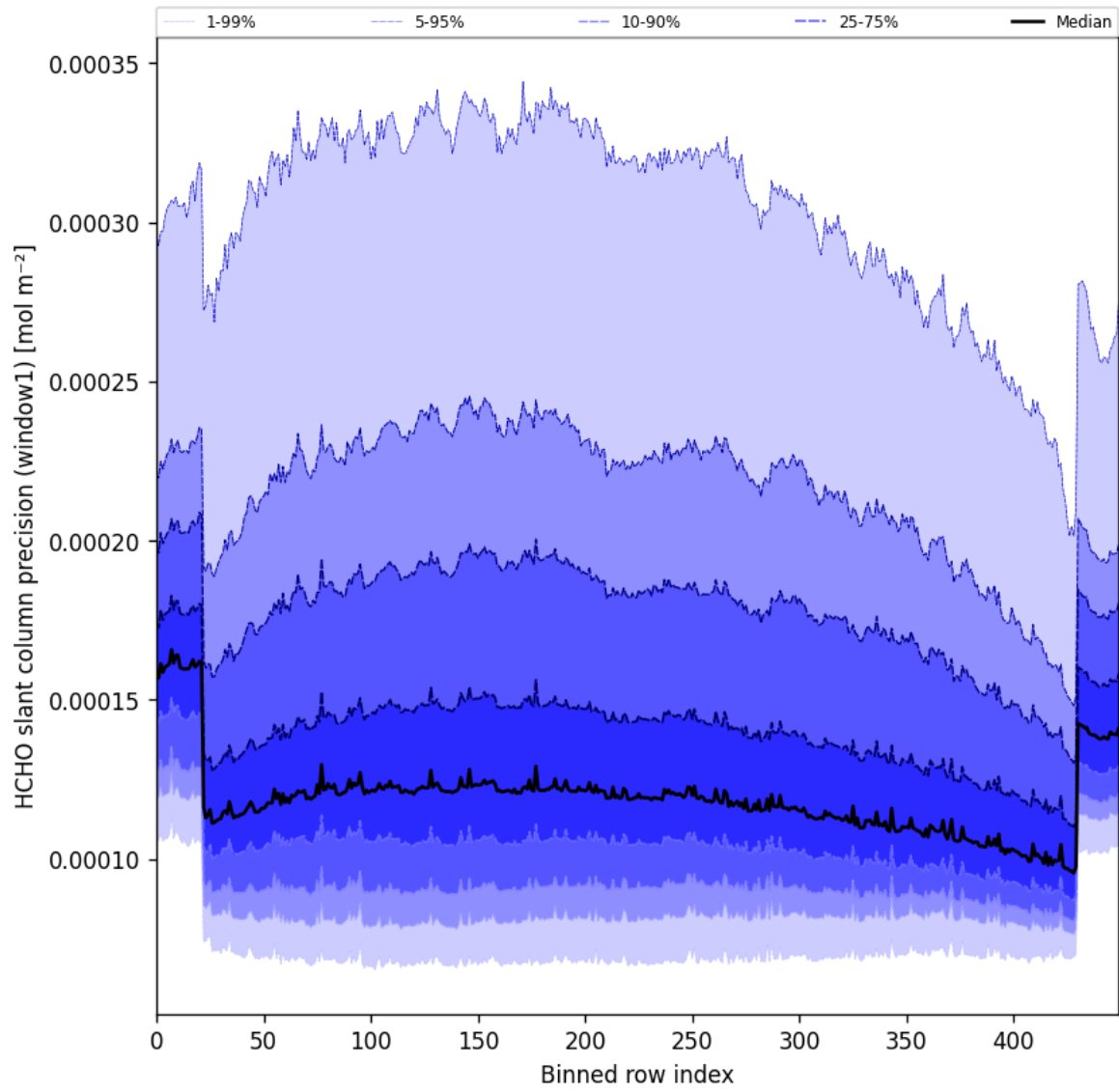
Figure 53: Along track statistics of "HCHO slant column precision (window1)" for 2024-10-10 to 2024-10-12
