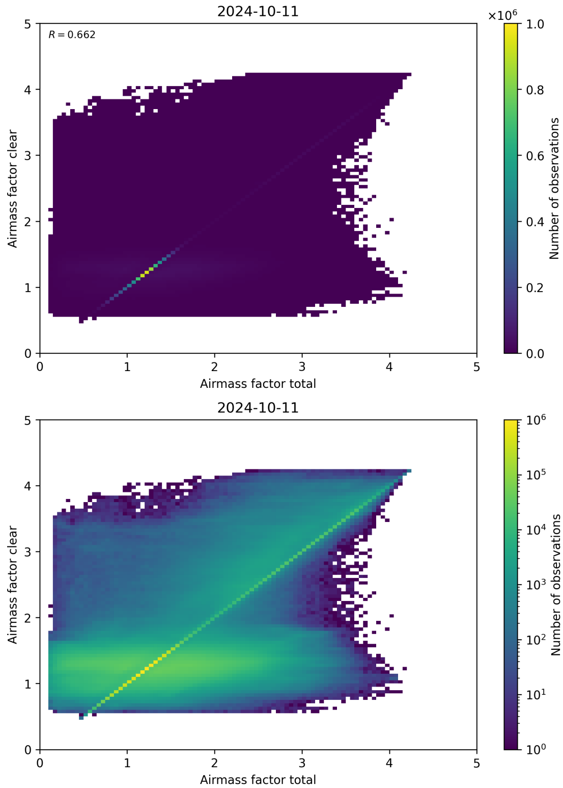
Figure 100: Scatter density plot of “Airmass factor total” against “Airmass factor clear” for 2024-10-10 to 2024-10-12.
