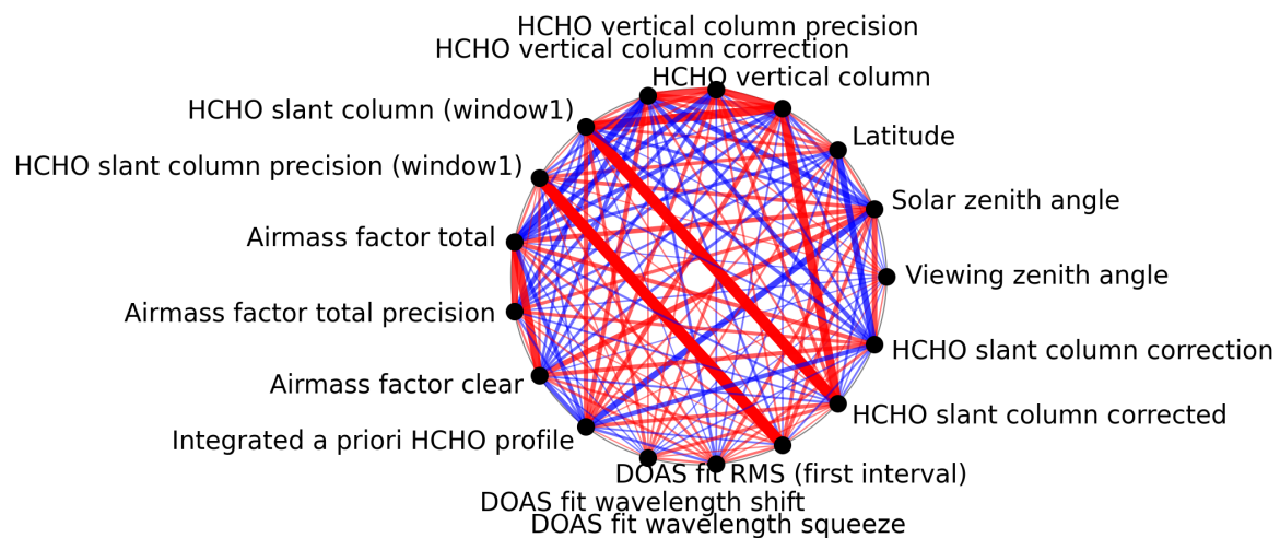
Figure 1: Map of correlation graph for 2024-10-10 to 2024-10-12.
