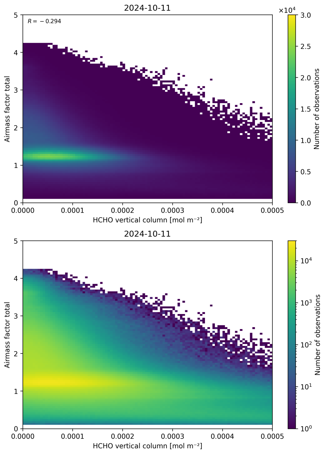
Figure 131: Scatter density plot of “HCHO vertical column” against “Airmass factor total” for 2024-10-10 to 2024-10-12.
