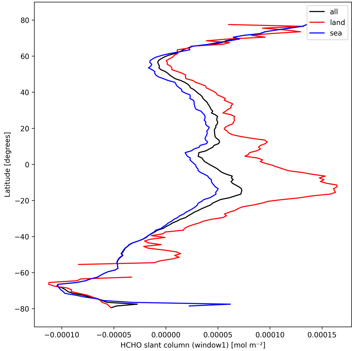
Figure 24: Zonal average of “HCHO slant column (window1)” for 2024-10-10 to 2024-10-12.
