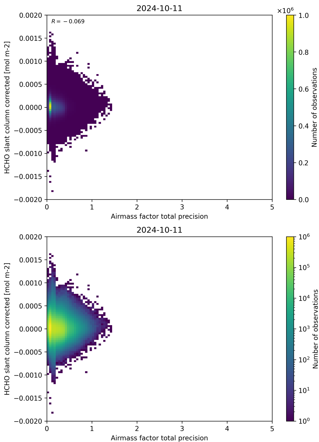
Figure 109: Scatter density plot of “Airmass factor total precision” against “HCHO slant column corrected” for 2024-10-10 to 2024-10-12.
