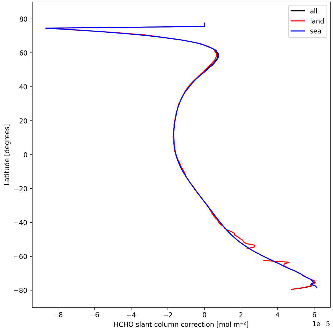
Figure 33: Zonal average of “HCHO slant column correction” for 2024-10-10 to 2024-10-12.
