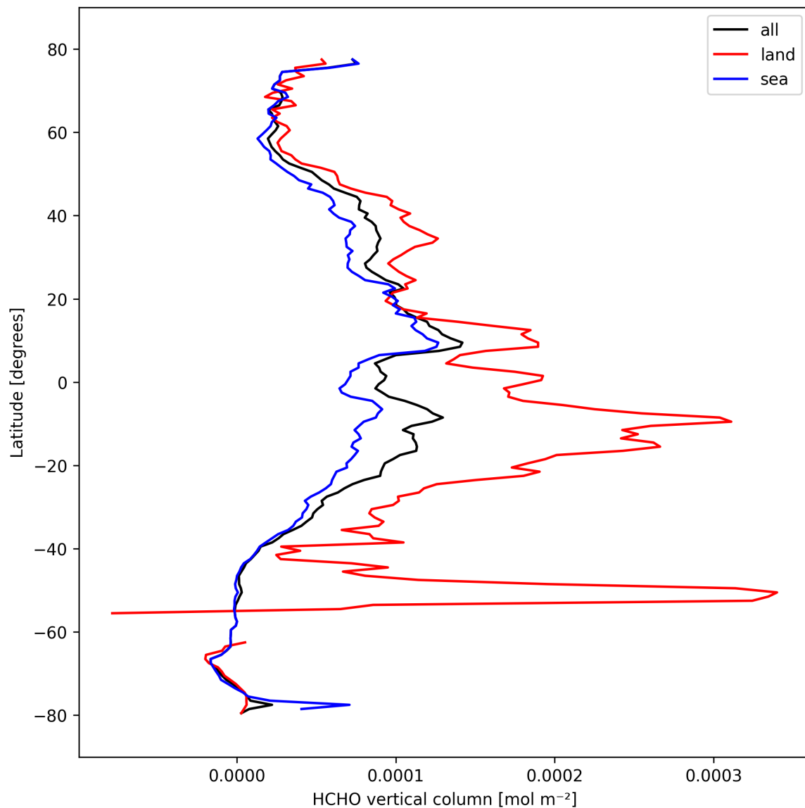
Figure 21: Zonal average of “HCHO vertical column” for 2024-10-10 to 2024-10-12.
