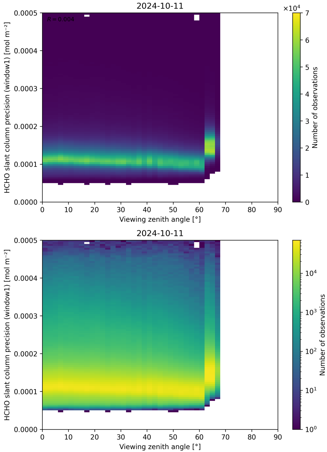
Figure 189: Scatter density plot of “Viewing zenith angle” against “HCHO slant column precision (window1)” for 2024-10-10 to 2024-10-12.
