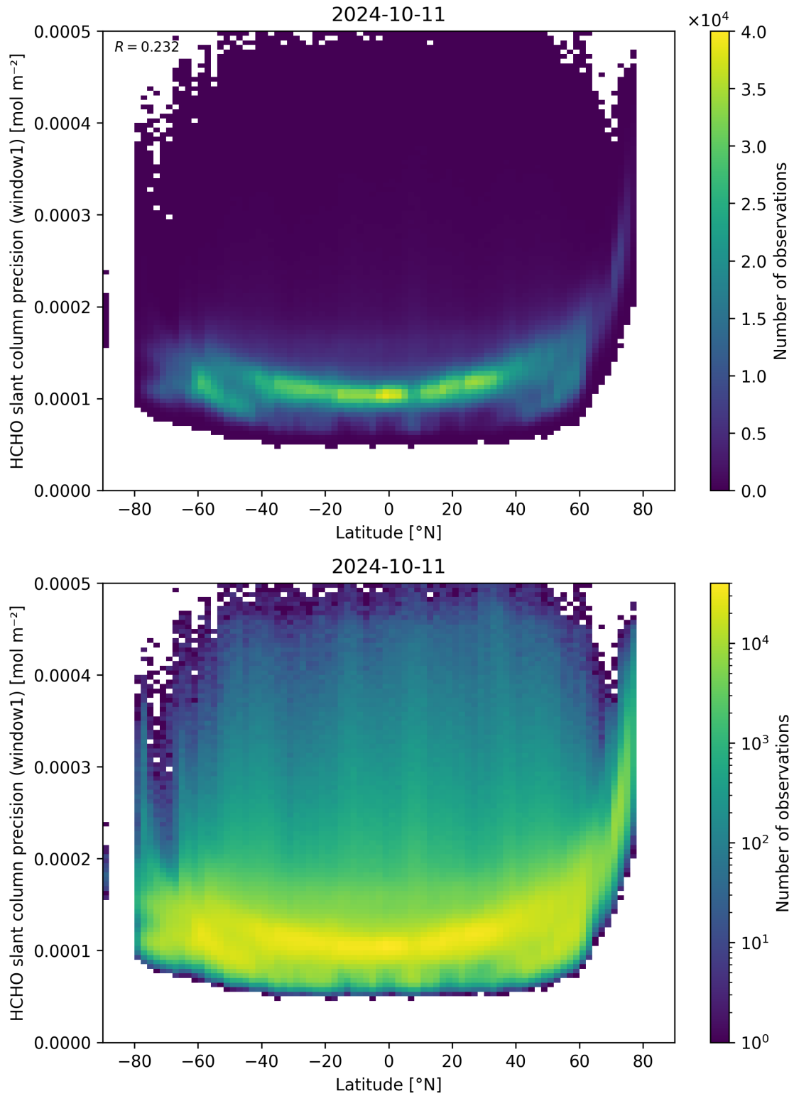
Figure 160: Scatter density plot of “Latitude” against “HCHO slant column precision (window1)” for 2024-10-10 to 2024-10-12.
