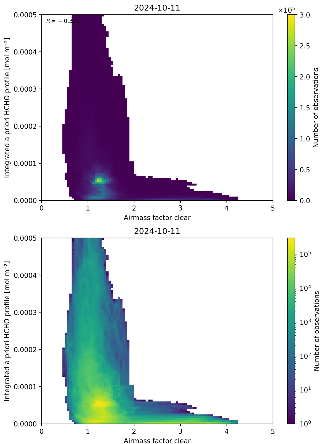
Figure 76: Scatter density plot of “Airmass factor clear” against “Integrated a priori HCHO profile” for 2024-10-10 to 2024-10-12.
