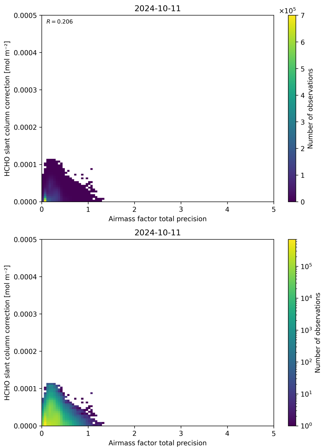
Figure 110: Scatter density plot of “Airmass factor total precision” against “HCHO slant column correction” for 2024-10-10 to 2024-10-12.
