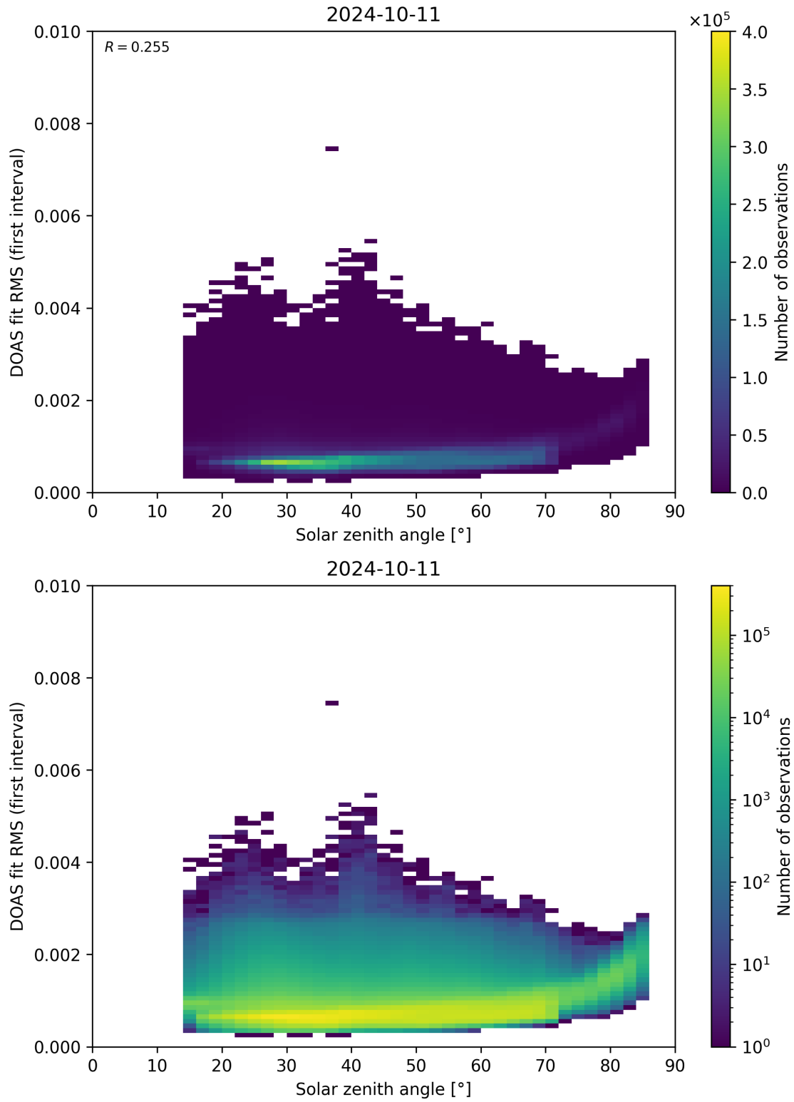
Figure 167: Scatter density plot of “Solar zenith angle” against “DOAS fit RMS (first interval)” for 2024-10-10 to 2024-10-12.
