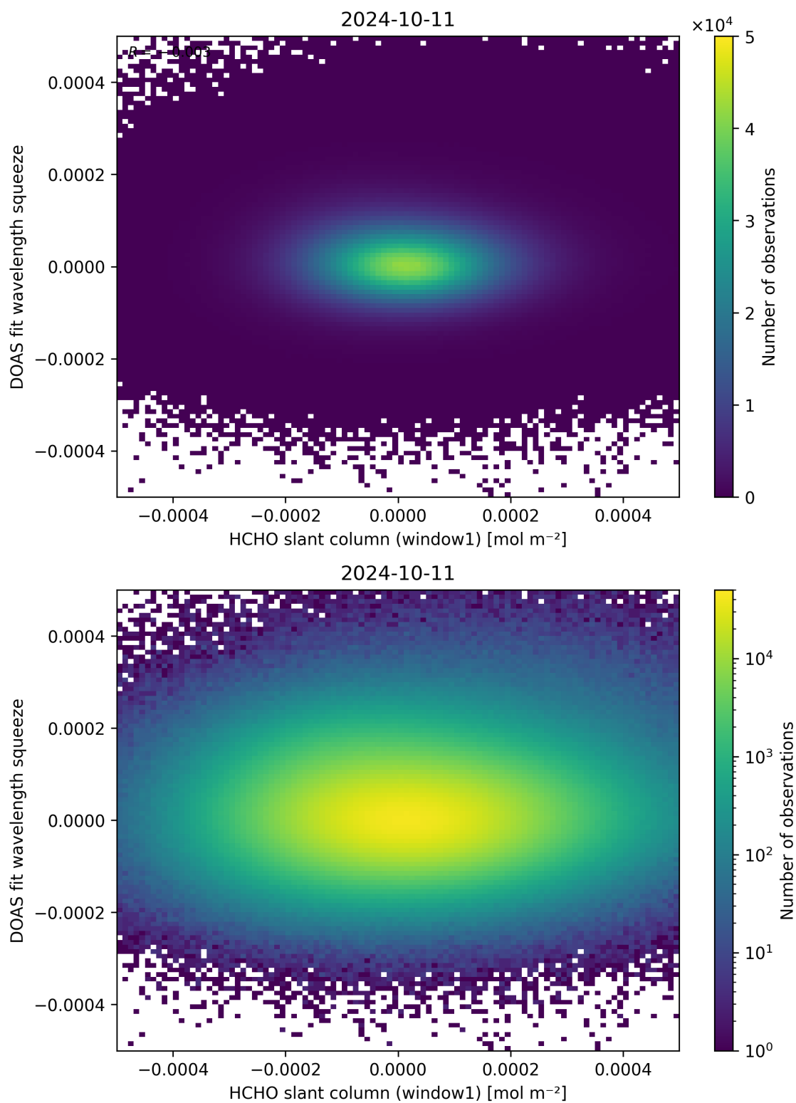
Figure 80: Scatter density plot of “HCHO slant column (window1)” against “DOAS fit wavelength squeeze” for 2024-10-10 to 2024-10-12.
