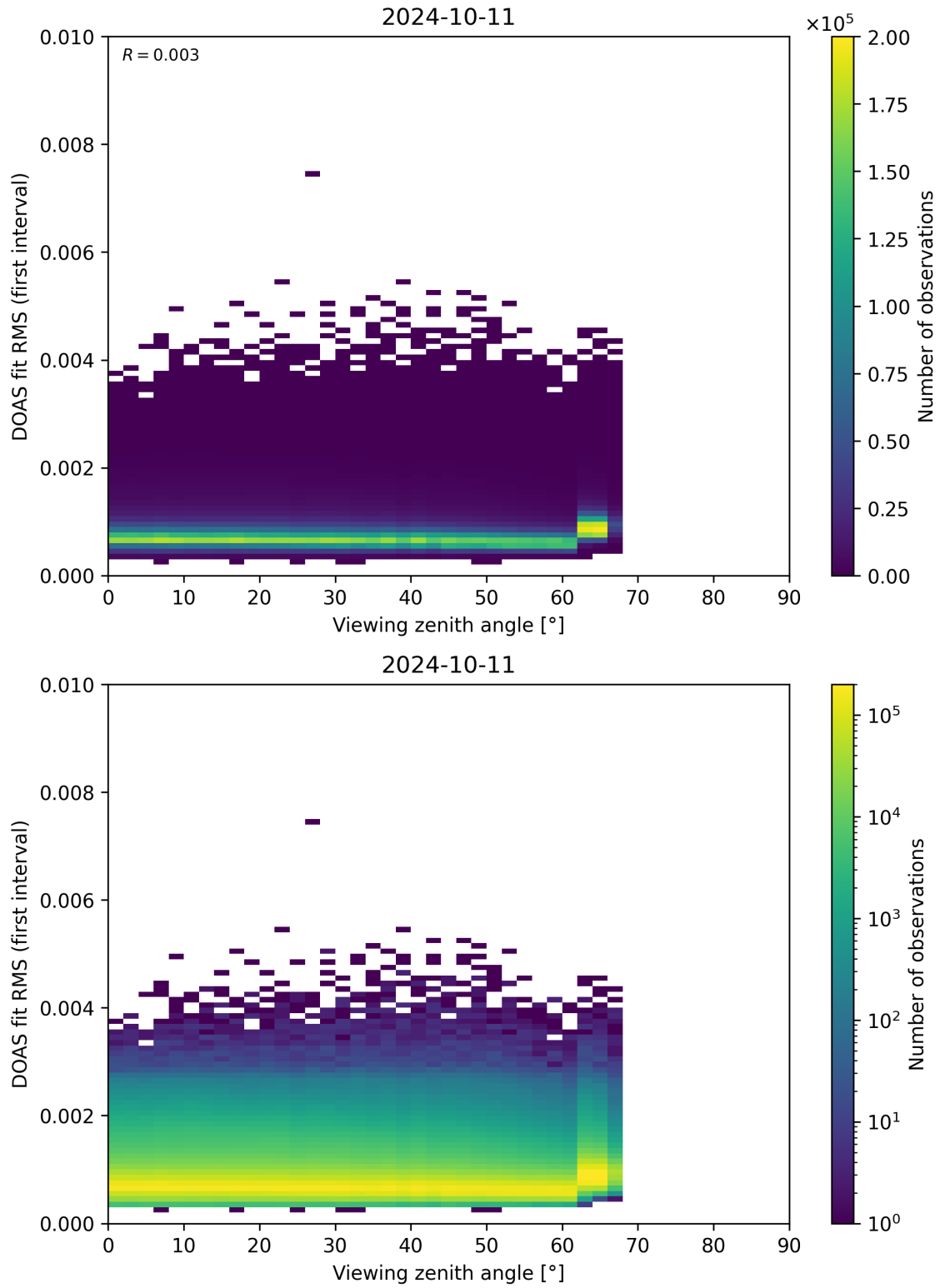
Figure 182: Scatter density plot of “Viewing zenith angle” against “DOAS fit RMS (first interval)” for 2024-10-10 to 2024-10-12.
