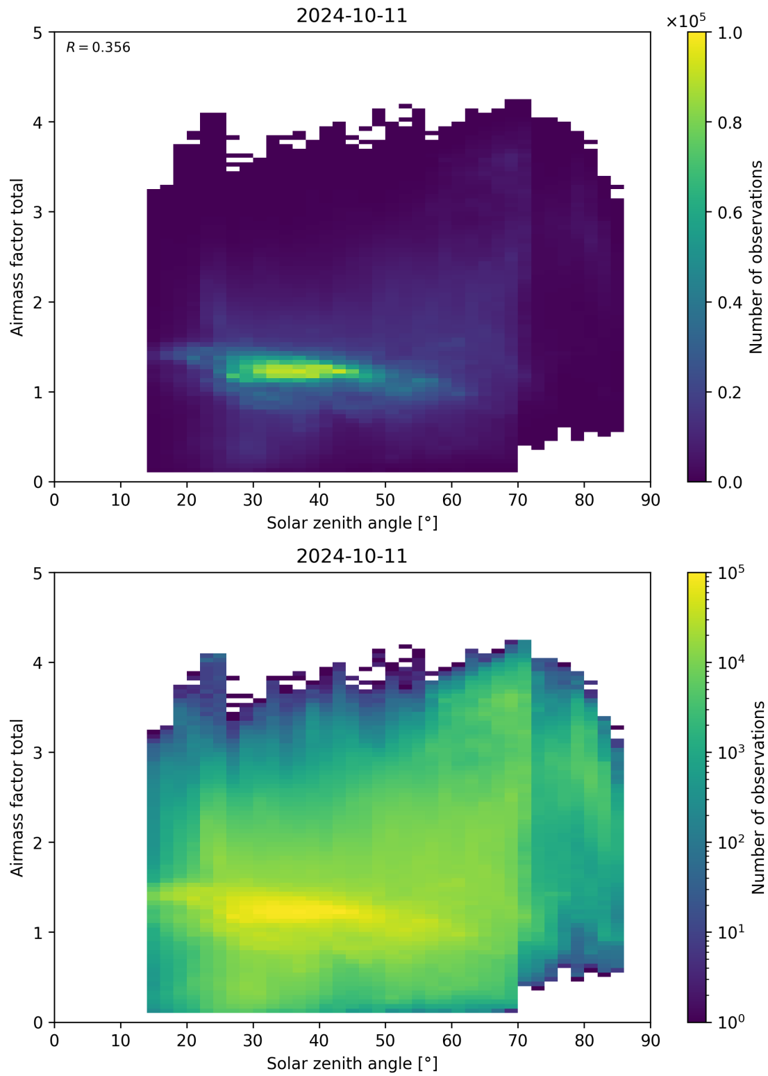
Figure 175: Scatter density plot of “Solar zenith angle” against “Airmass factor total” for 2024-10-10 to 2024-10-12.
