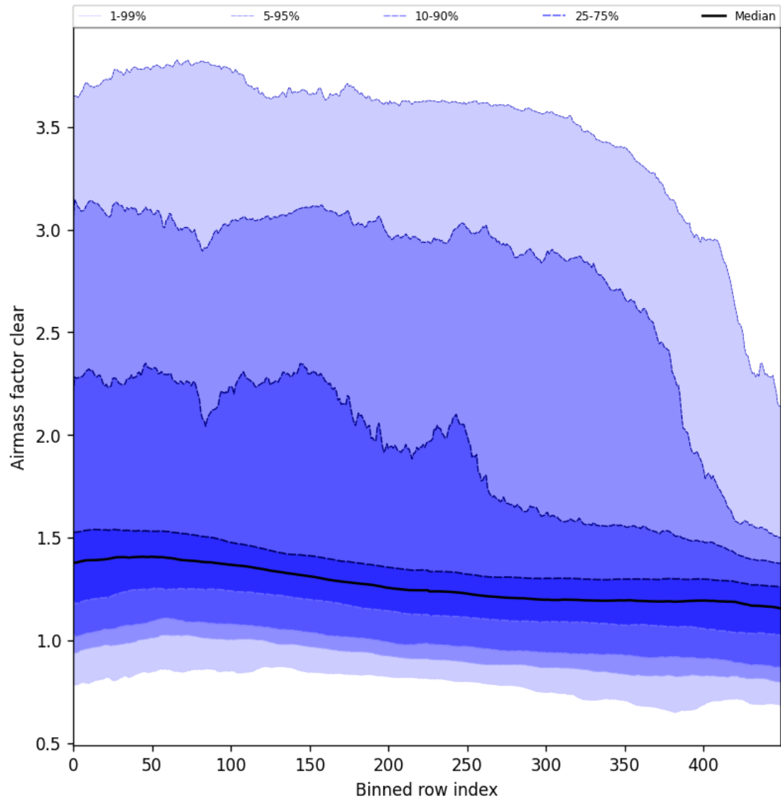
Figure 56: Along track statistics of “Airmass factor clear” for 2024-10-10 to 2024-10-12
