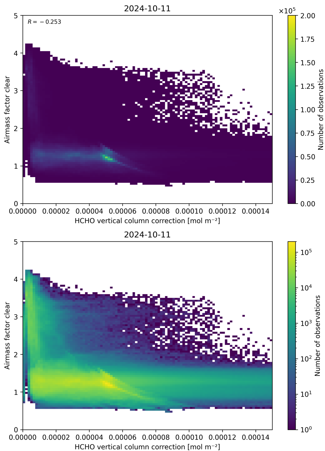
Figure 115: Scatter density plot of “HCHO vertical column correction” against “Airmass factor clear” for 2024-10-10 to 2024-10-12.
