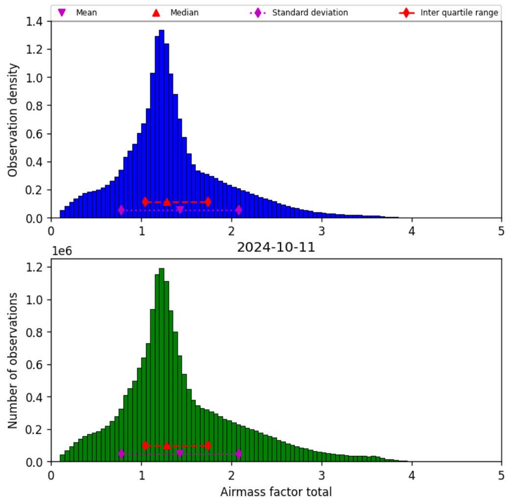
Figure 40: Histogram of “Airmass factor total” for 2024-10-10 to 2024-10-12
