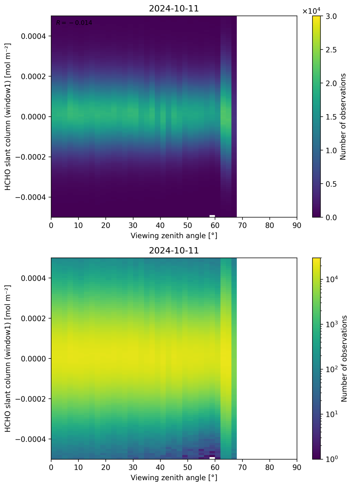
Figure 188: Scatter density plot of “Viewing zenith angle” against “HCHO slant column (window1)” for 2024-10-10 to 2024-10-12.
