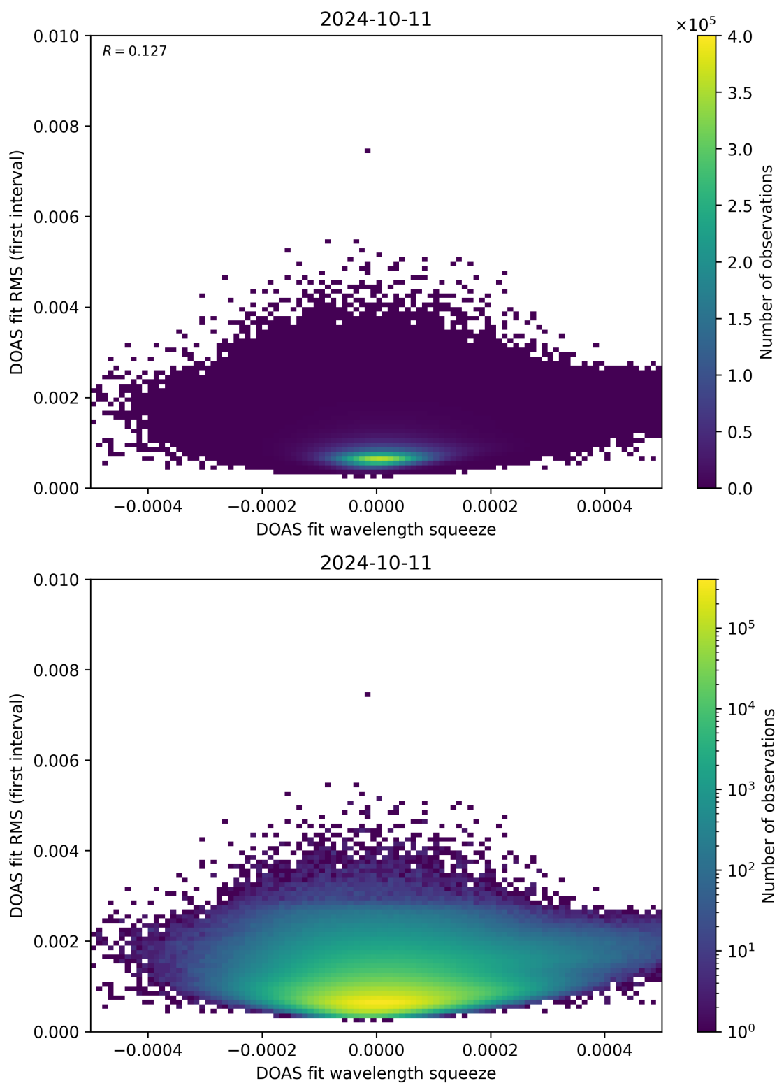
Figure 68: Scatter density plot of “DOAS fit wavelength squeeze” against “DOAS fit RMS (first interval)” for 2024-10-10 to 2024-10-12.
