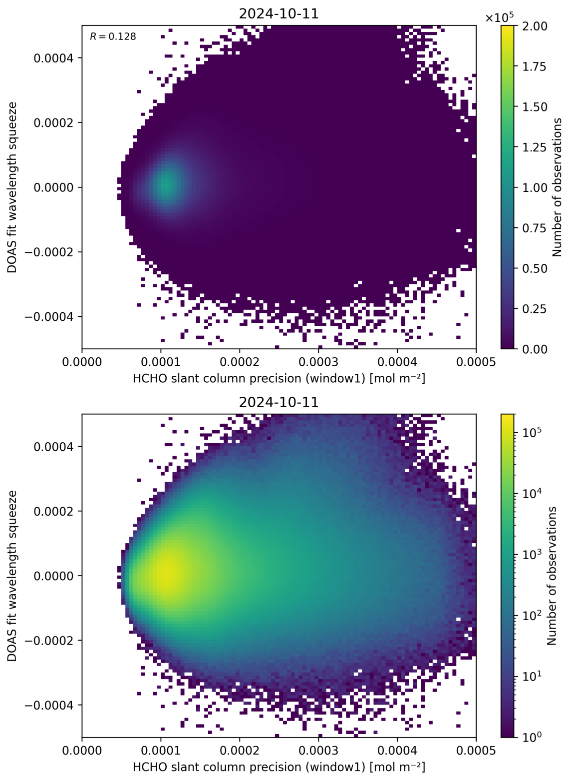
Figure 90: Scatter density plot of “HCHO slant column precision (window1)” against “DOAS fit wavelength squeeze” for 2024-10-10 to 2024-10-12.
