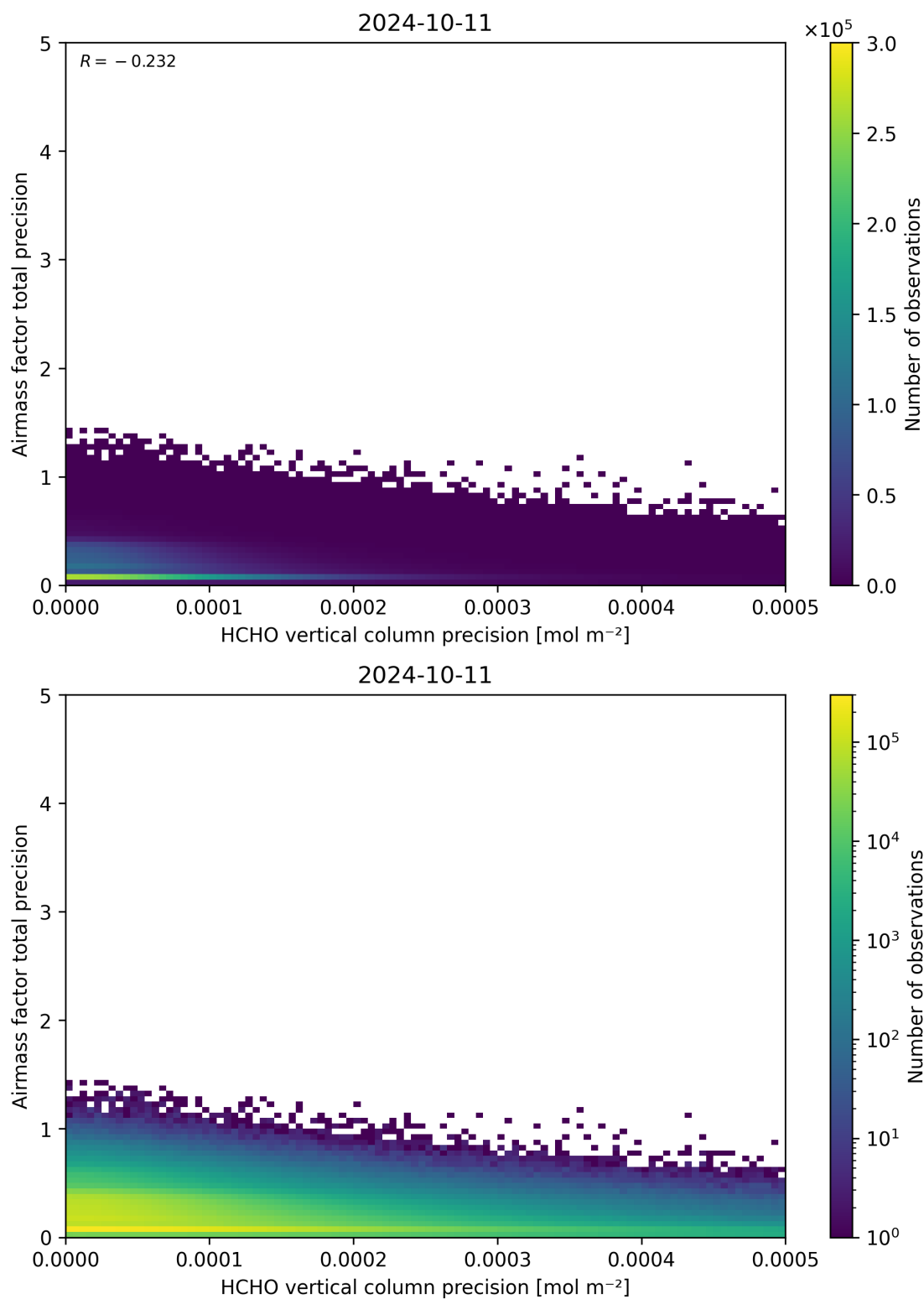
Figure 145: Scatter density plot of “HCHO vertical column precision” against “Airmass factor total precision” for 2024-10-10 to 2024-10-12.
