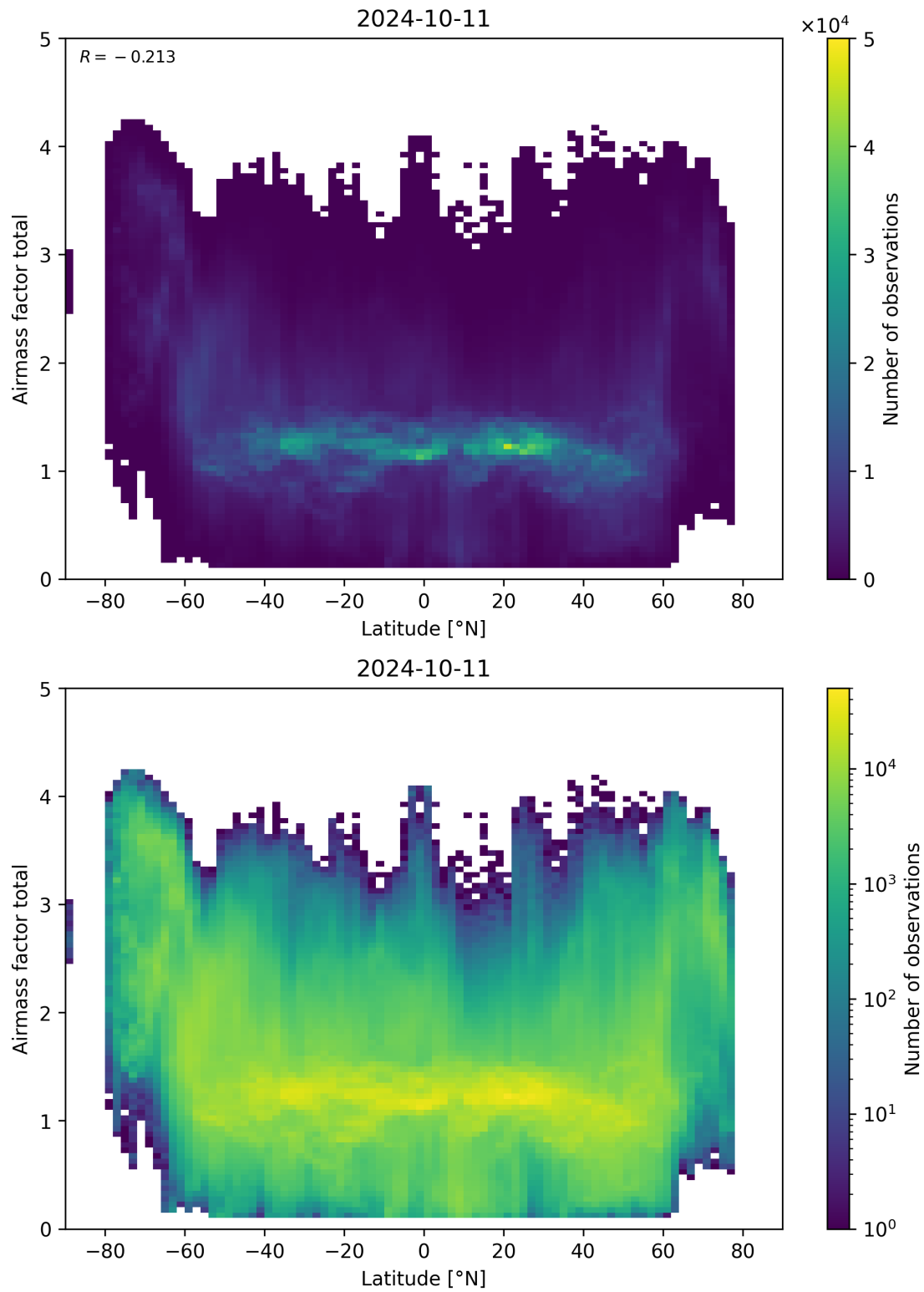
Figure 161: Scatter density plot of “Latitude” against “Airmass factor total” for 2024-10-10 to 2024-10-12.
