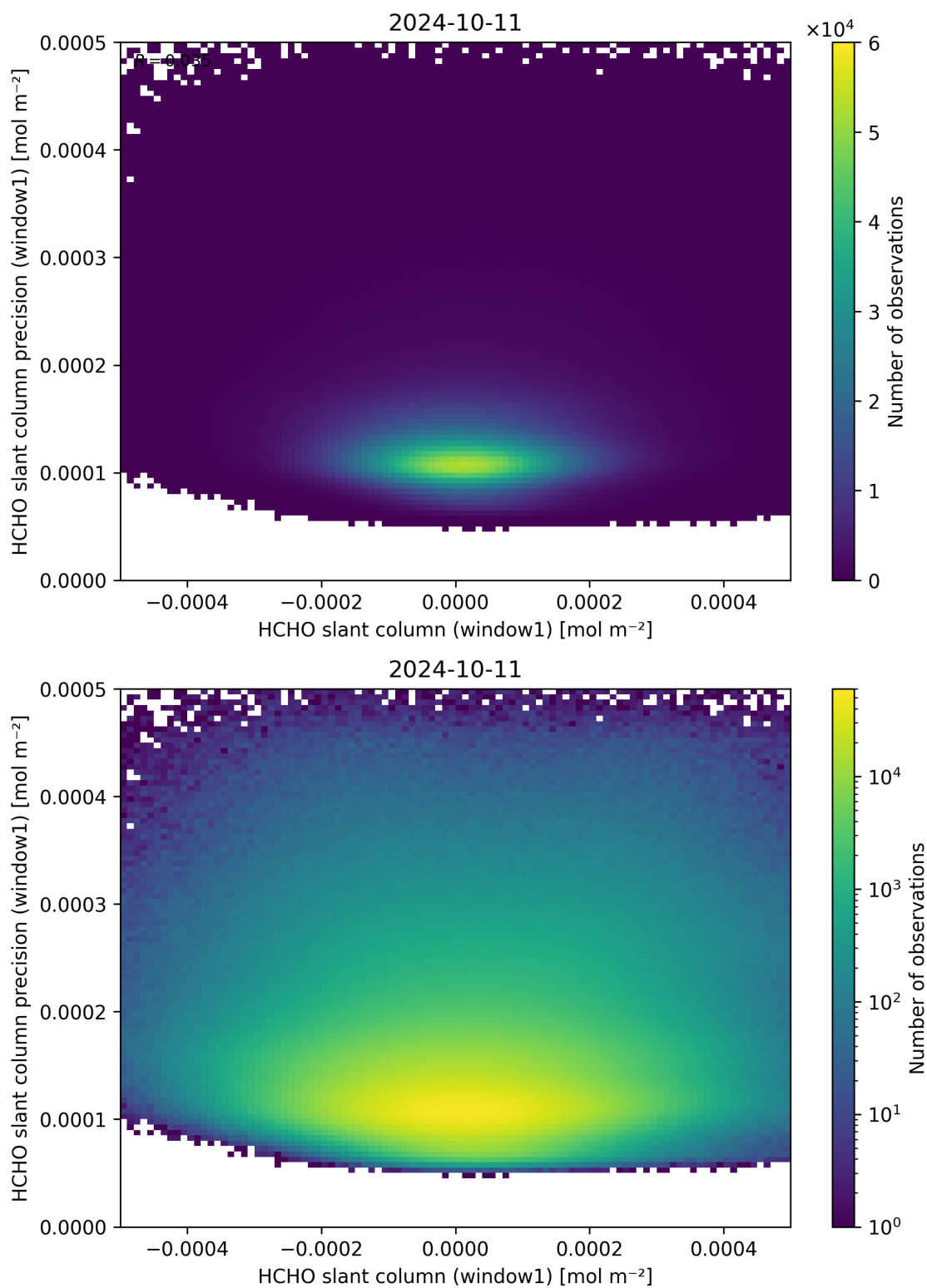
Figure 84: Scatter density plot of “HCHO slant column (window1)” against “HCHO slant column precision (window1)” for 2024-10-10 to 2024-10-12.
