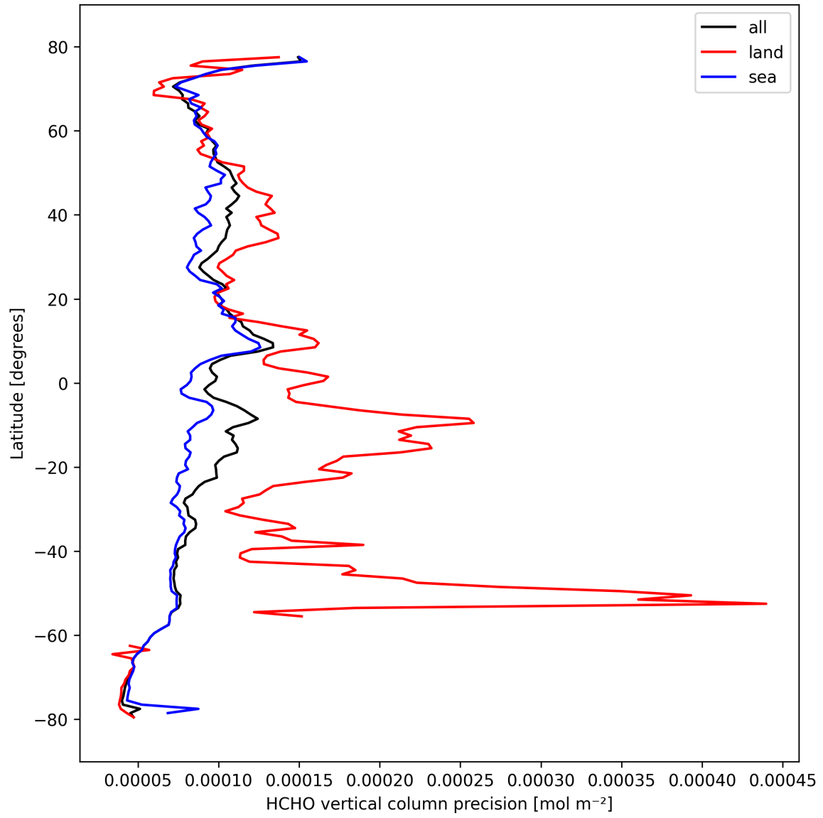
Figure 22: Zonal average of “HCHO vertical column precision” for 2024-10-10 to 2024-10-12.
