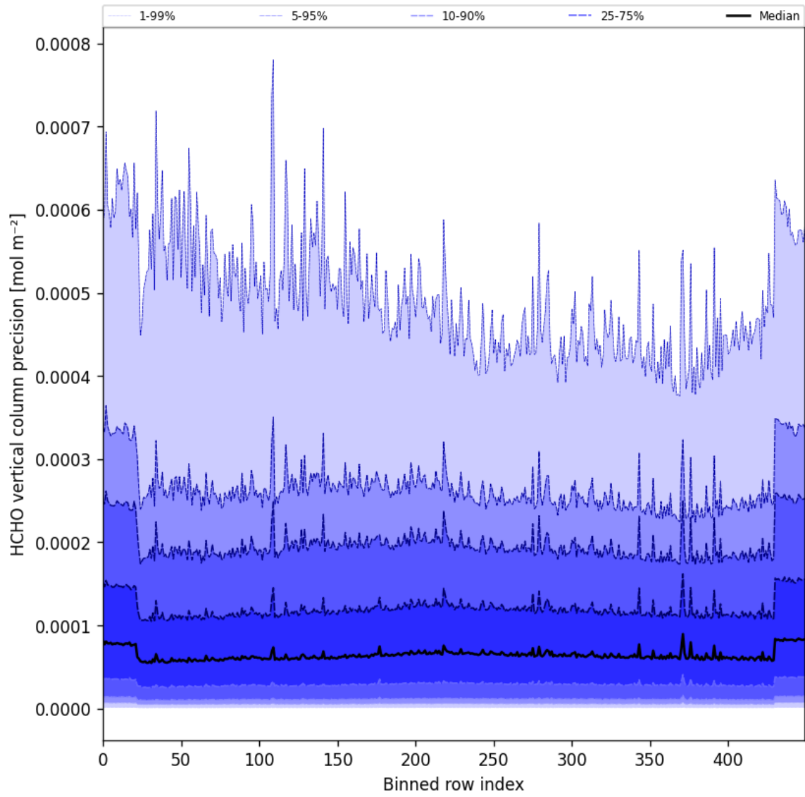
Figure 50: Along track statistics of “HCHO vertical column precision” for 2024-10-10 to 2024-10-12
