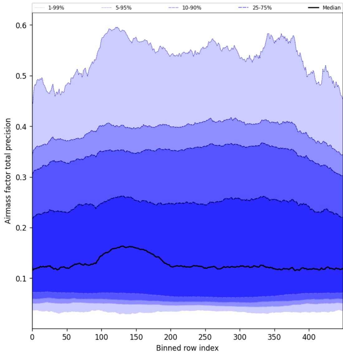
Figure 55: Along track statistics of “Airmass factor total precision” for 2024-10-10 to 2024-10-12
