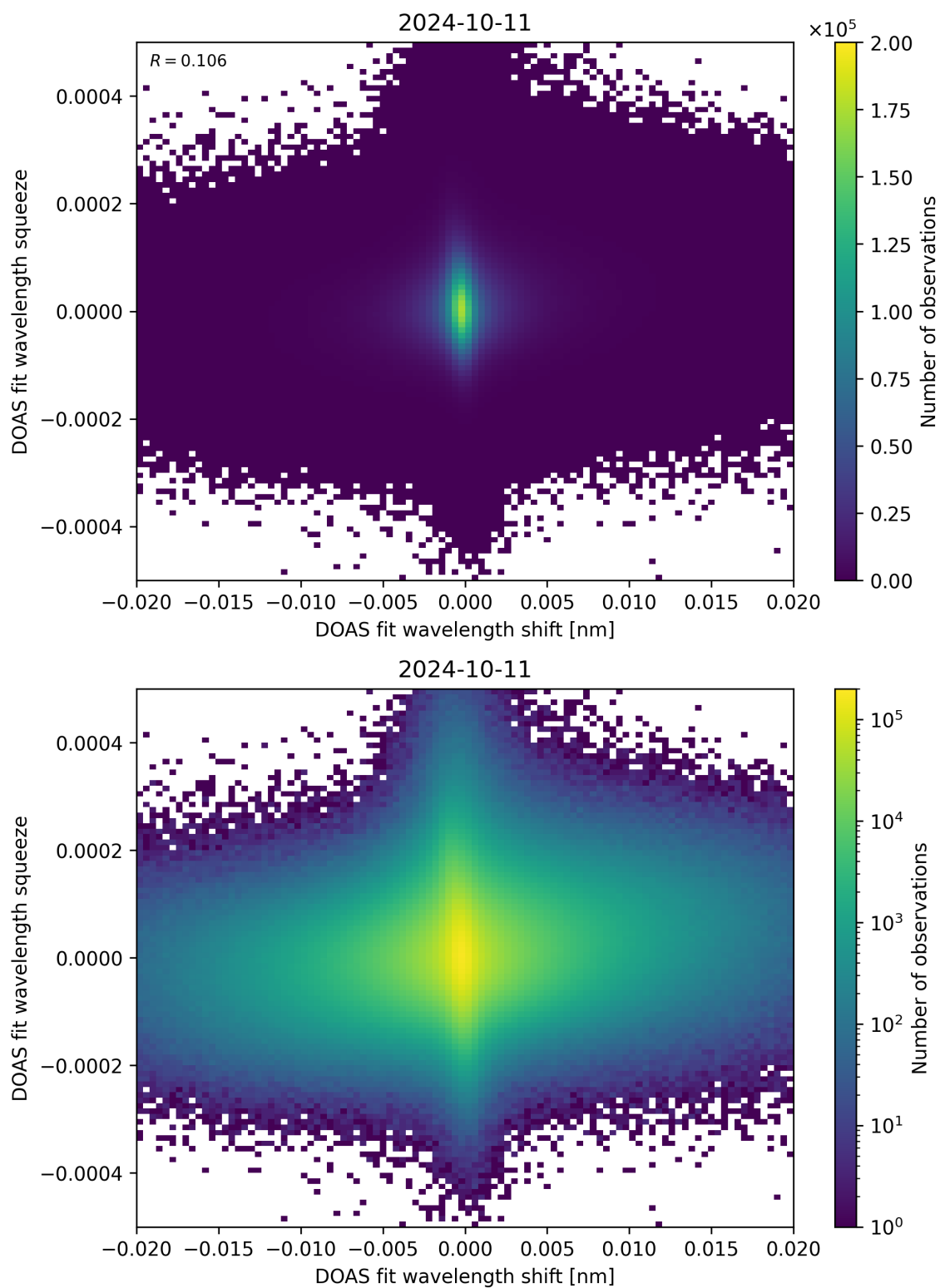
Figure 65: Scatter density plot of “DOAS fit wavelength shift” against “DOAS fit wavelength squeeze” for 2024-10-10 to 2024-10-12.
