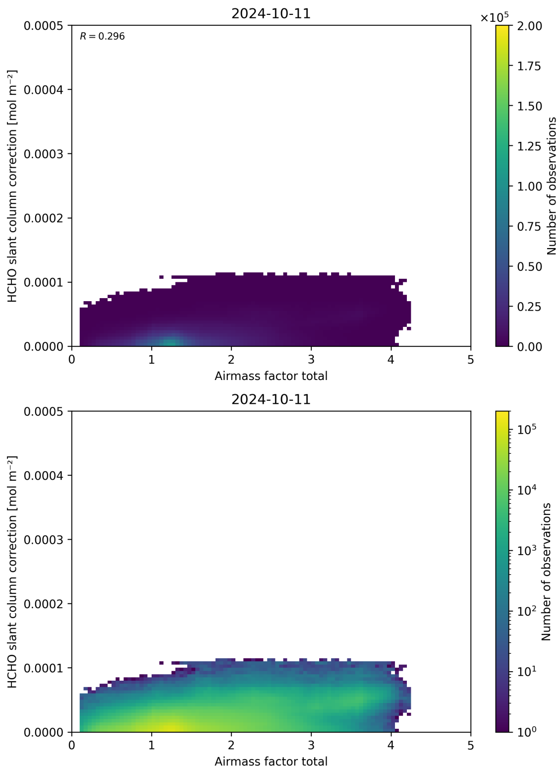
Figure 102: Scatter density plot of “Airmass factor total” against “HCHO slant column correction” for 2024-10-10 to 2024-10-12.
