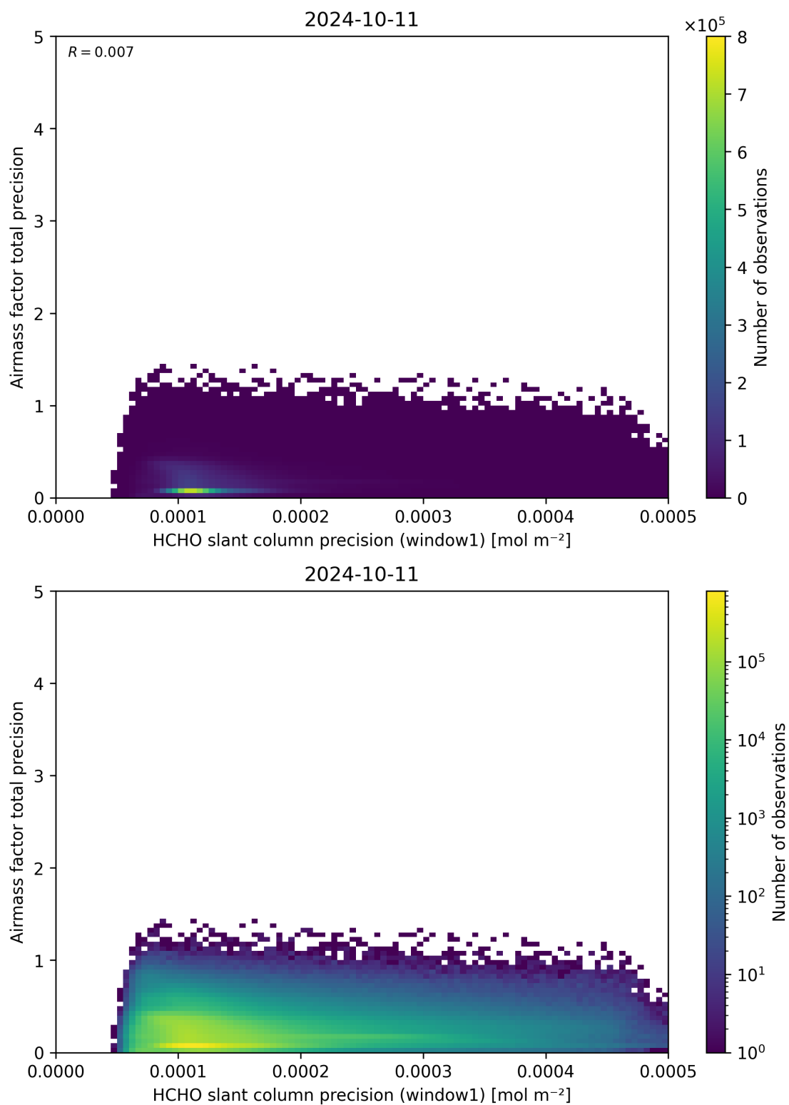
Figure 95: Scatter density plot of “HCHO slant column precision (window1)” against “Airmass factor total precision” for 2024-10-10 to 2024-10-12.
