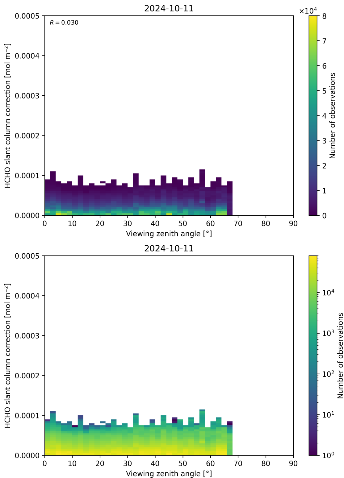
Figure 187: Scatter density plot of “Viewing zenith angle” against “HCHO slant column correction” for 2024-10-10 to 2024-10-12.
