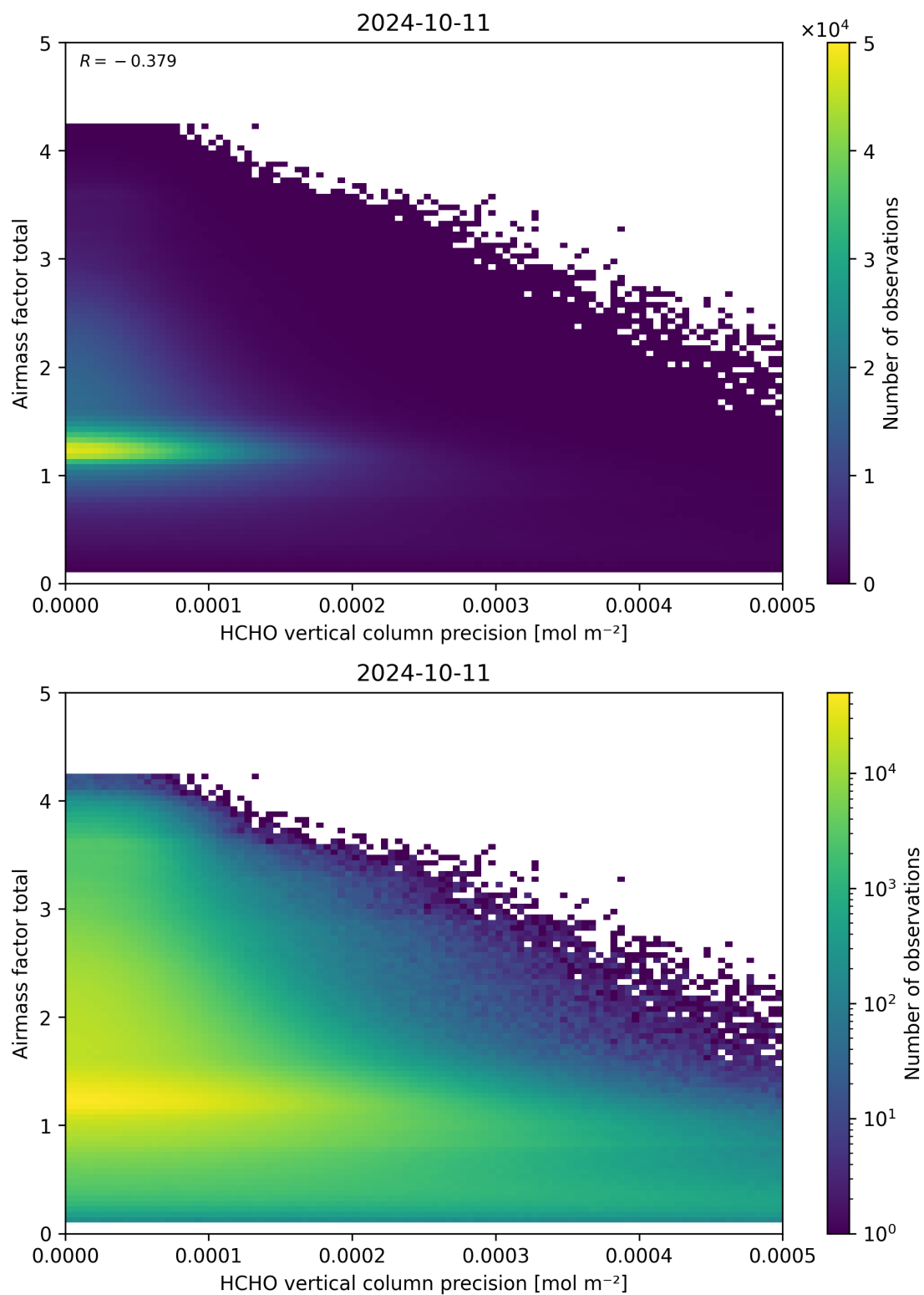
Figure 144: Scatter density plot of “HCHO vertical column precision” against “Airmass factor total” for 2024-10-10 to 2024-10-12.
