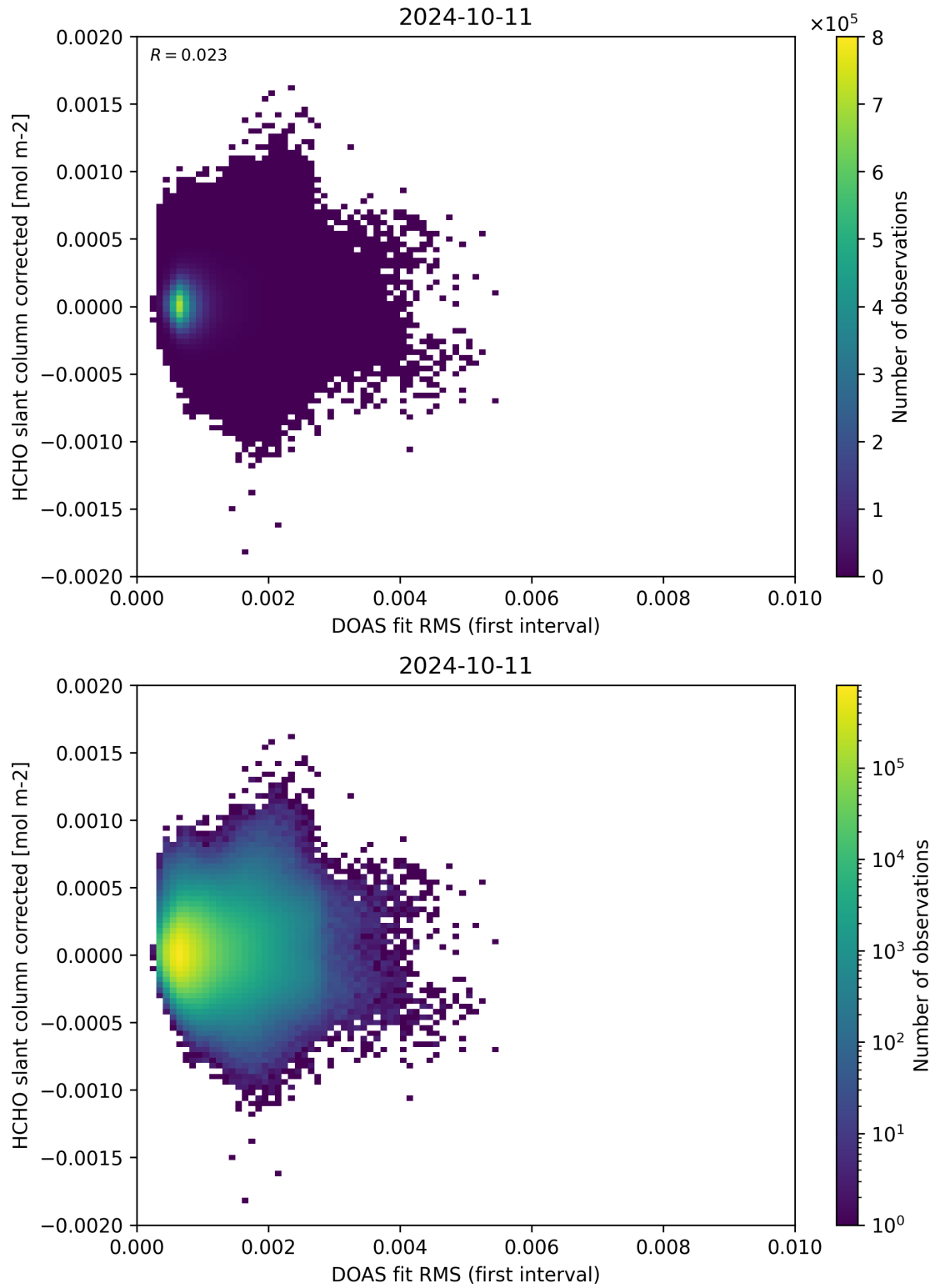
Figure 62: Scatter density plot of “DOAS fit RMS (first interval)” against “HCHO slant column corrected” for 2024-10-10 to 2024-10-12.
