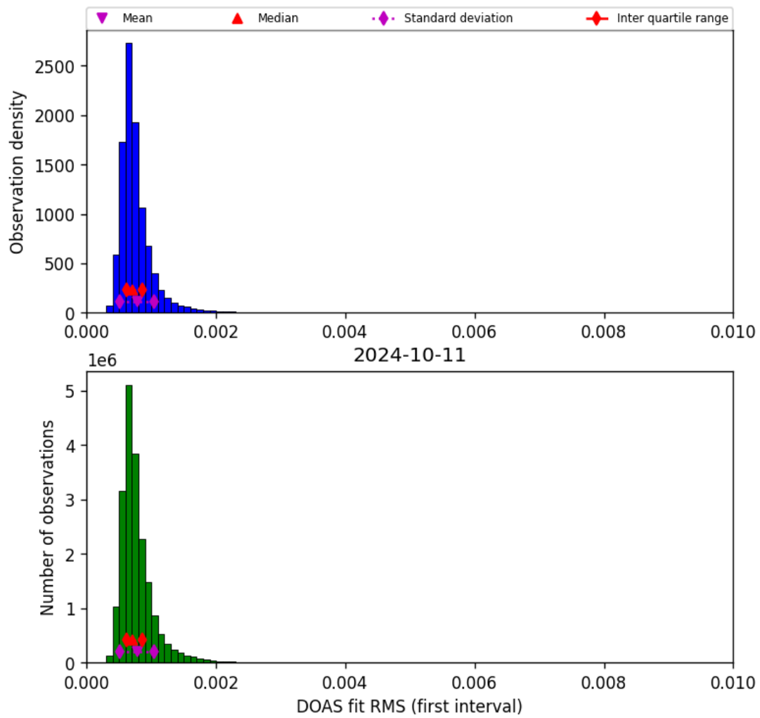
Figure 46: Histogram of “DOAS fit RMS (first interval)” for 2024-10-10 to 2024-10-12
