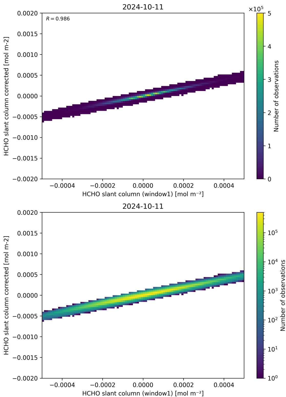
Figure 82: Scatter density plot of “HCHO slant column (window1)” against “HCHO slant column corrected” for 2024-10-10 to 2024-10-12.
