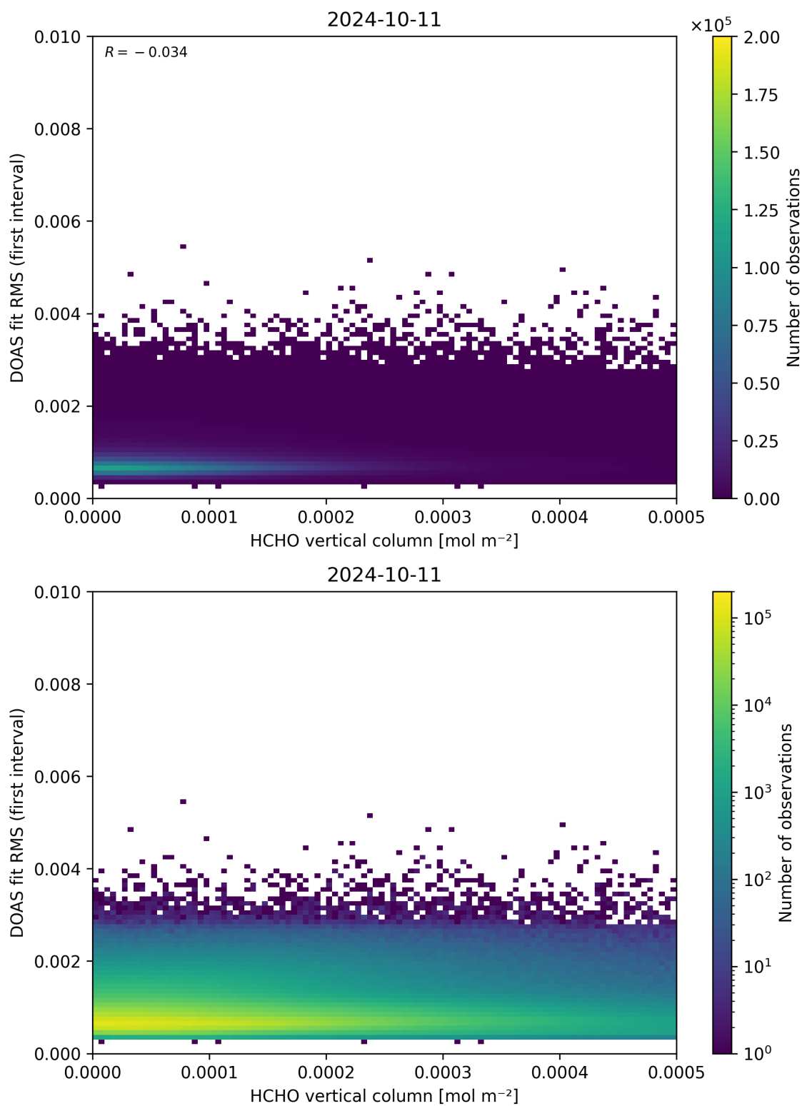
Figure 123: Scatter density plot of “HCHO vertical column” against “DOAS fit RMS (first interval)” for 2024-10-10 to 2024-10-12.
