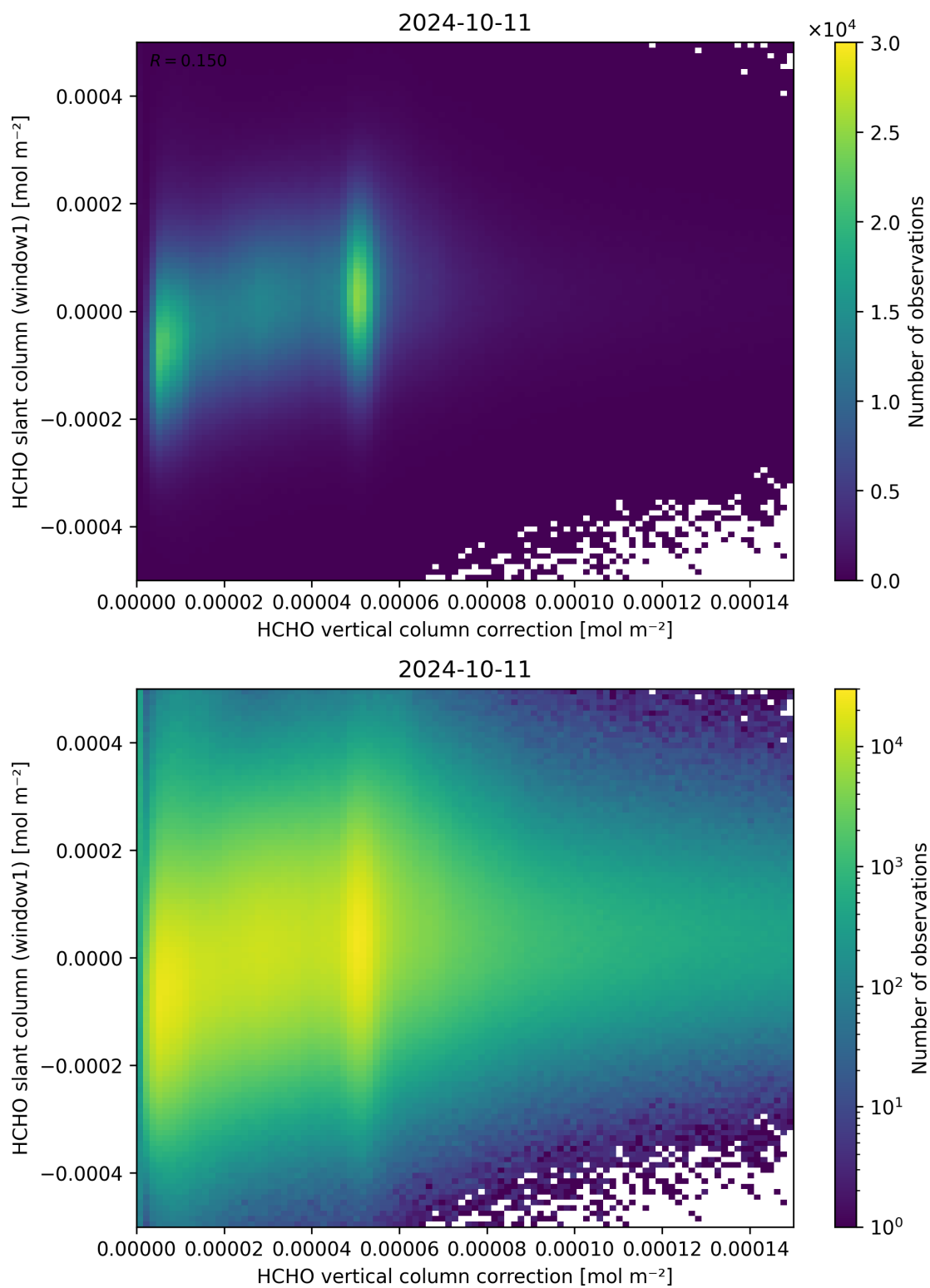
Figure 118: Scatter density plot of “HCHO vertical column correction” against “HCHO slant column (window1)” for 2024-10-10 to 2024-10-12.
