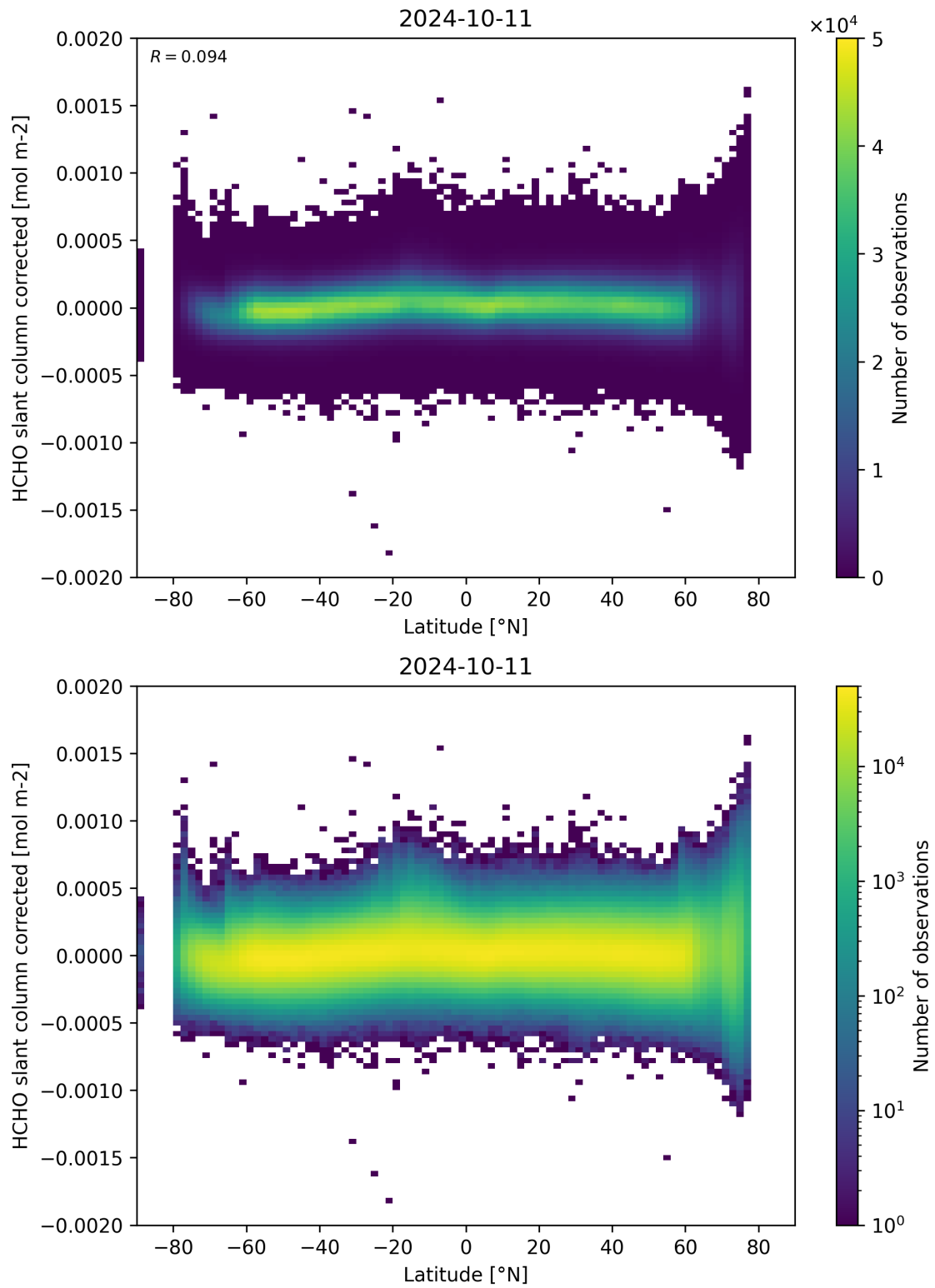
Figure 157: Scatter density plot of “Latitude” against “HCHO slant column corrected” for 2024-10-10 to 2024-10-12.
