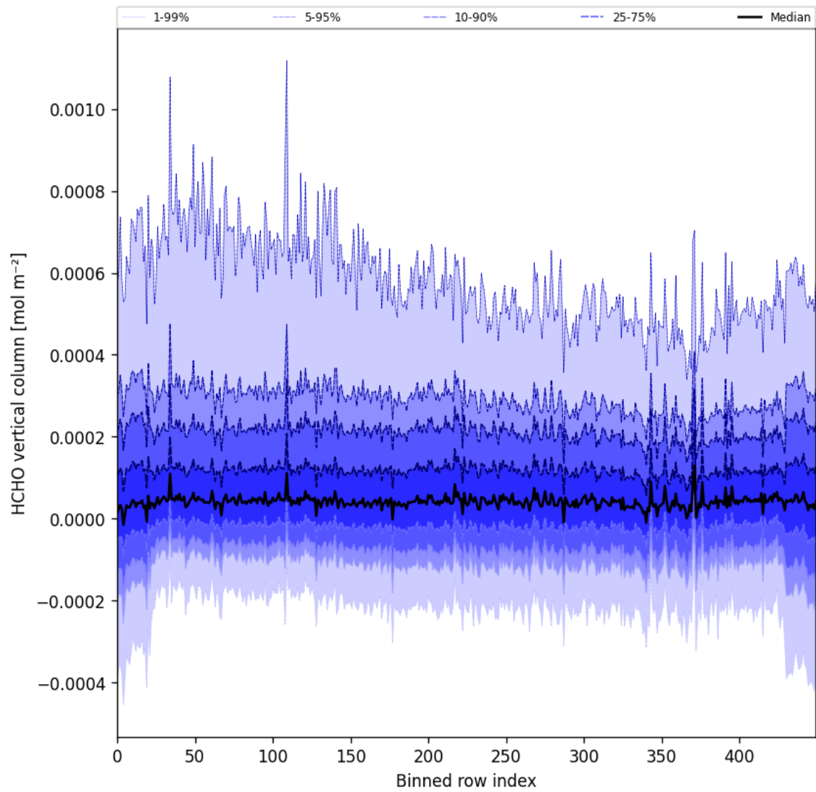
Figure 49: Along track statistics of “HCHO vertical column” for 2024-10-10 to 2024-10-12
