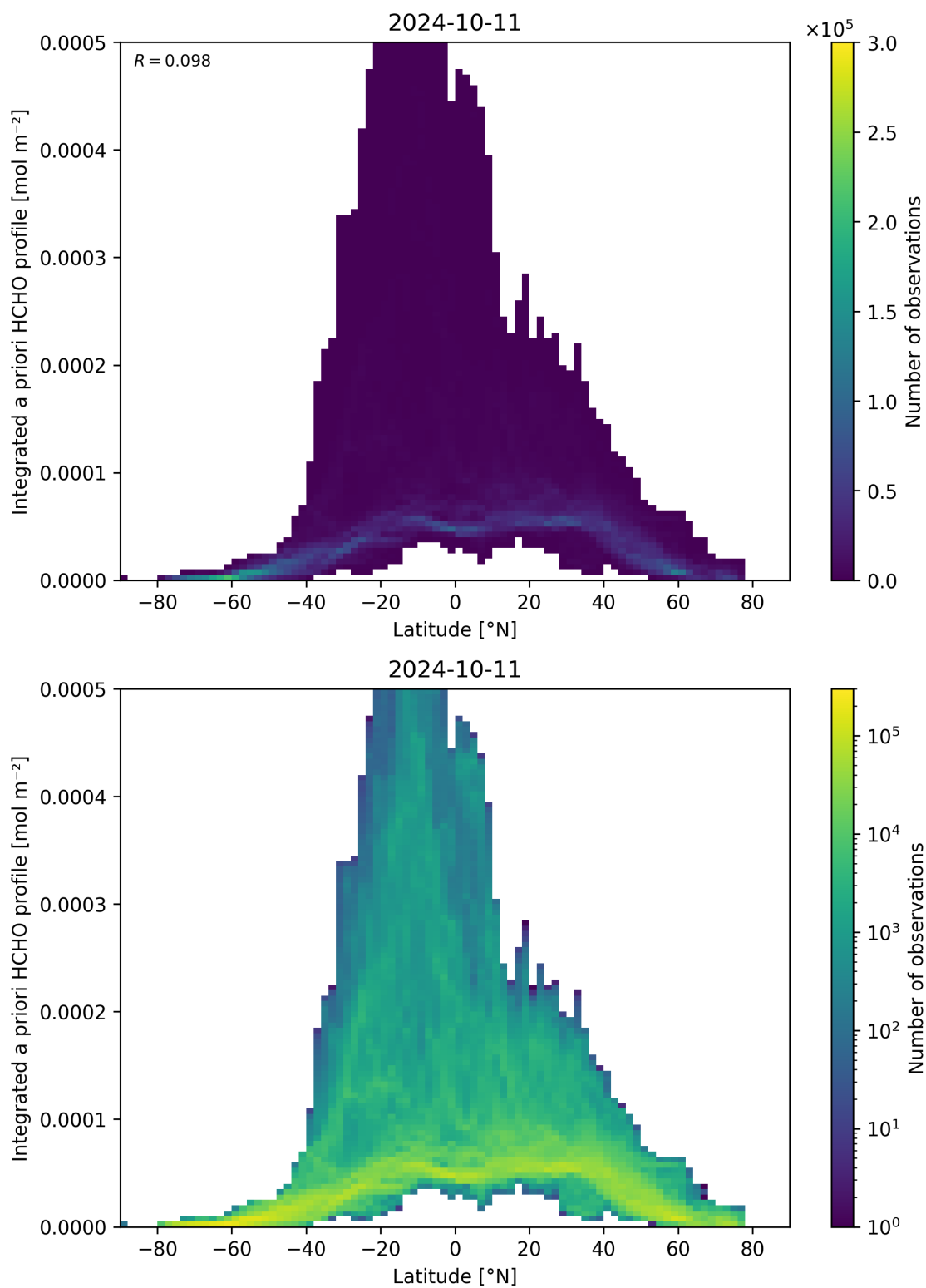
Figure 166: Scatter density plot of “Latitude” against “Integrated a priori HCHO profile” for 2024-10-10 to 2024-10-12.
