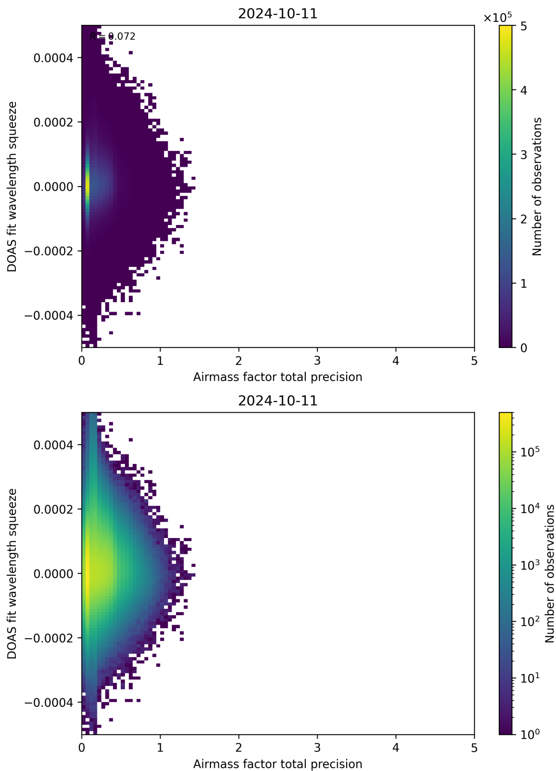
Figure 107: Scatter density plot of “Airmass factor total precision” against “DOAS fit wavelength squeeze” for 2024-10-10 to 2024-10-12.
