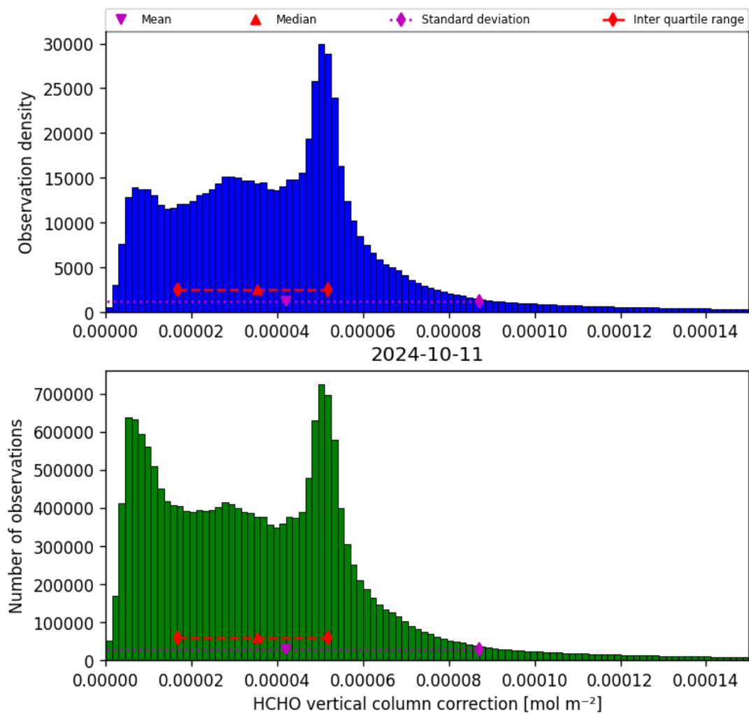
Figure 37: Histogram of “HCHO vertical column correction” for 2024-10-10 to 2024-10-12
