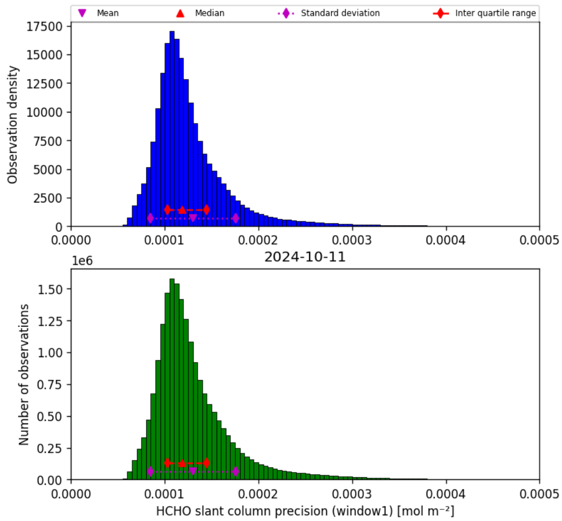
Figure 39: Histogram of “HCHO slant column precision (window1)” for 2024-10-10 to 2024-10-12
