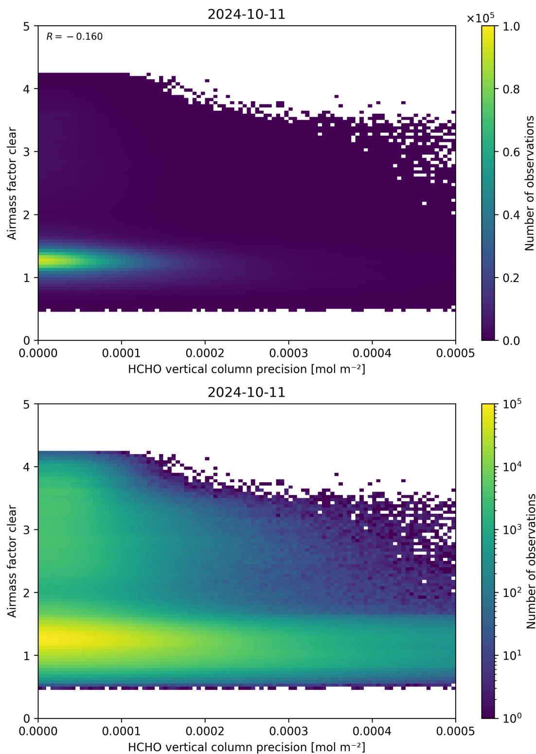
Figure 139: Scatter density plot of “HCHO vertical column precision” against “Airmass factor clear” for 2024-10-10 to 2024-10-12.
