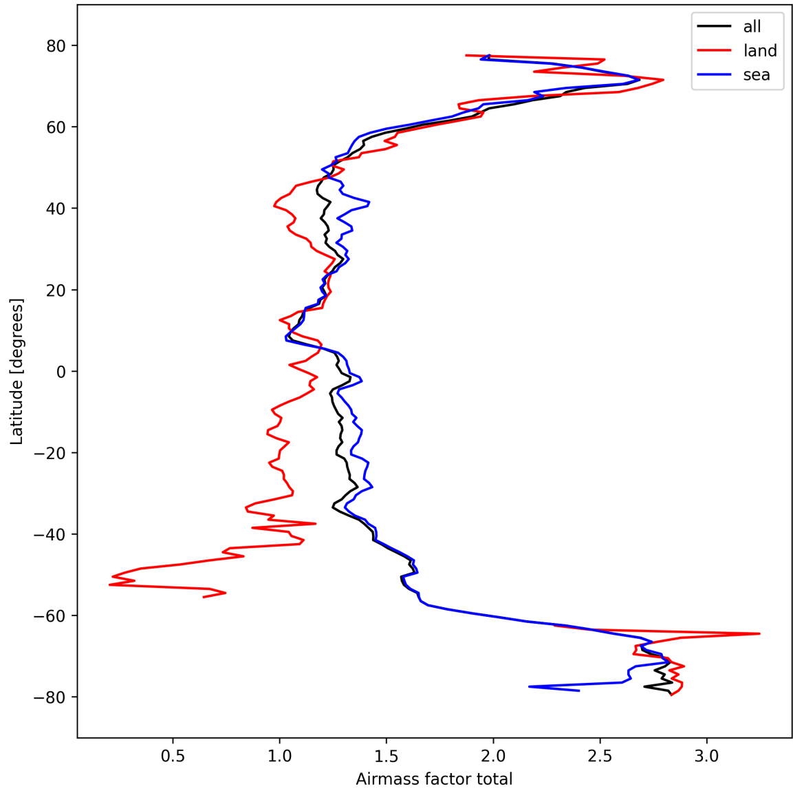
Figure 26: Zonal average of “Airmass factor total” for 2024-10-10 to 2024-10-12.
