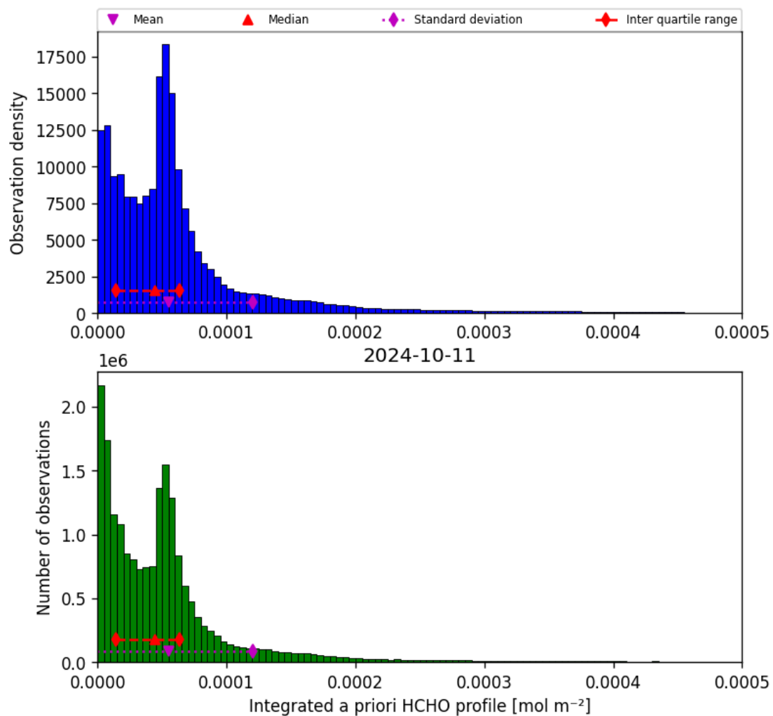
Figure 43: Histogram of “Integrated a priori HCHO profile” for 2024-10-10 to 2024-10-12
