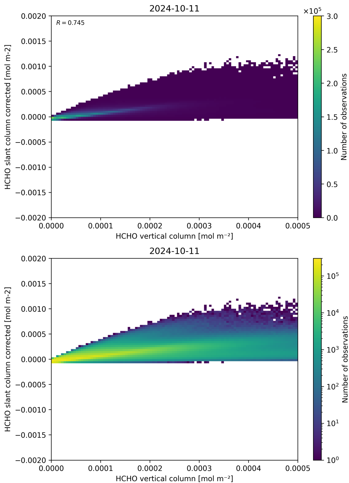
Figure 127: Scatter density plot of “HCHO vertical column” against “HCHO slant column corrected” for 2024-10-10 to 2024-10-12.
