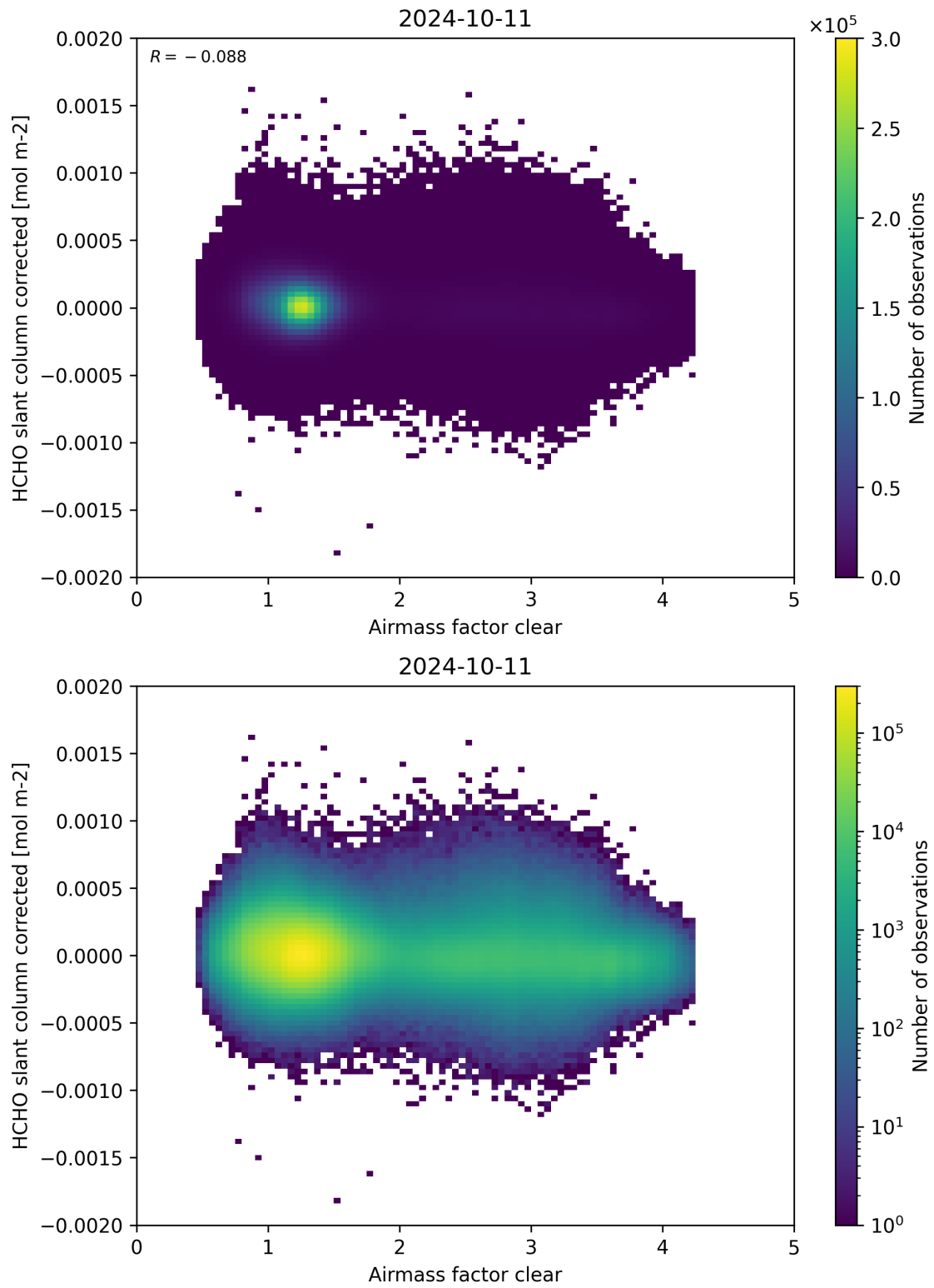
Figure 74: Scatter density plot of “Airmass factor clear” against “HCHO slant column corrected” for 2024-10-10 to 2024-10-12.
