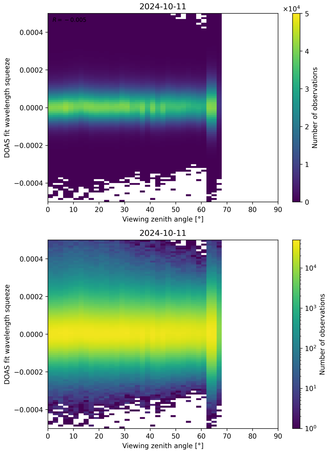
Figure 184: Scatter density plot of “Viewing zenith angle” against “DOAS fit wavelength squeeze” for 2024-10-10 to 2024-10-12.
