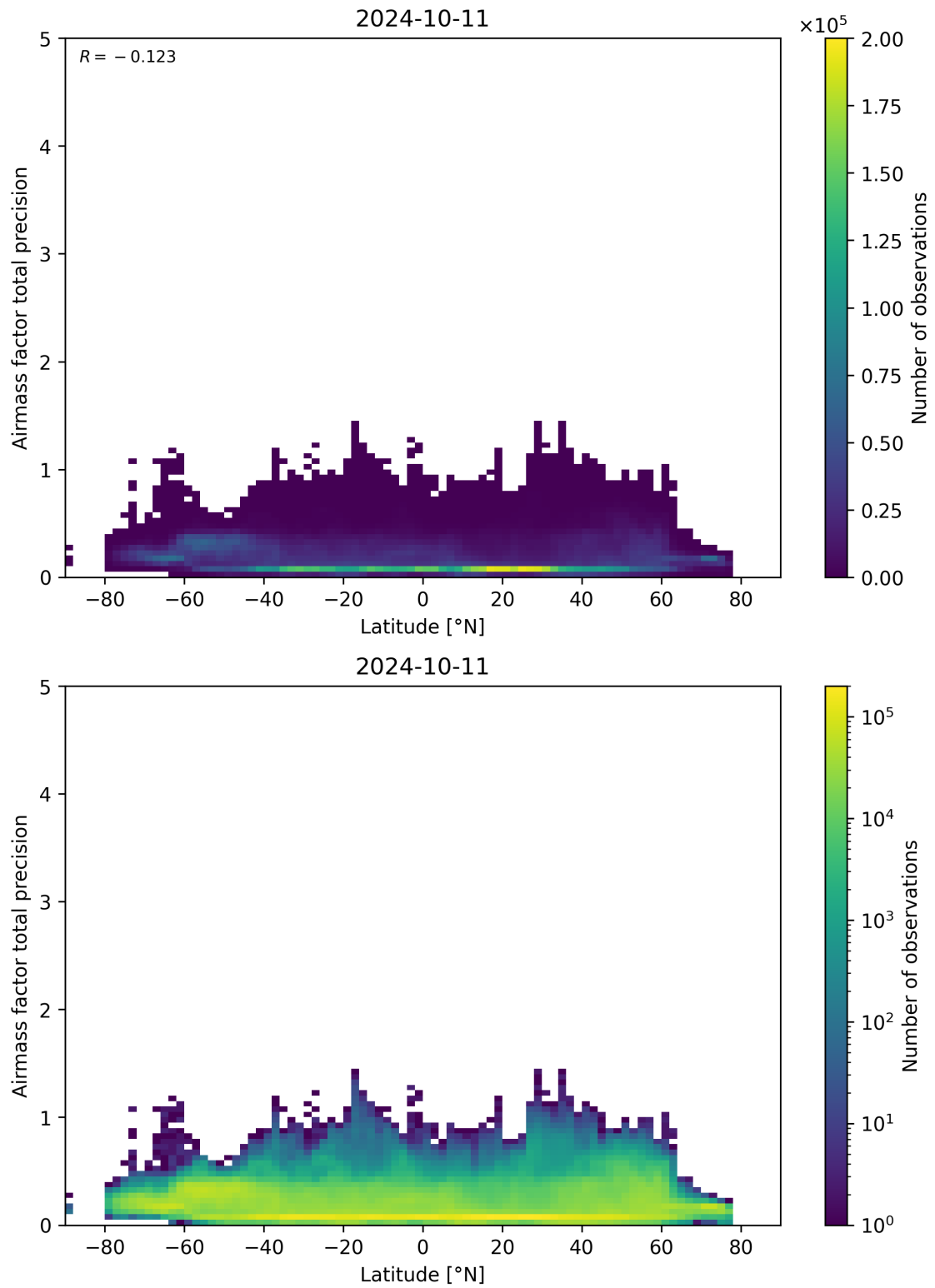
Figure 162: Scatter density plot of “Latitude” against “Airmass factor total precision” for 2024-10-10 to 2024-10-12.
