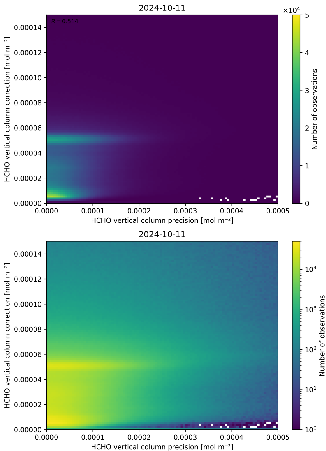
Figure 146: Scatter density plot of “HCHO vertical column precision” against “HCHO vertical column correction” for 2024-10-10 to 2024-10-12.
