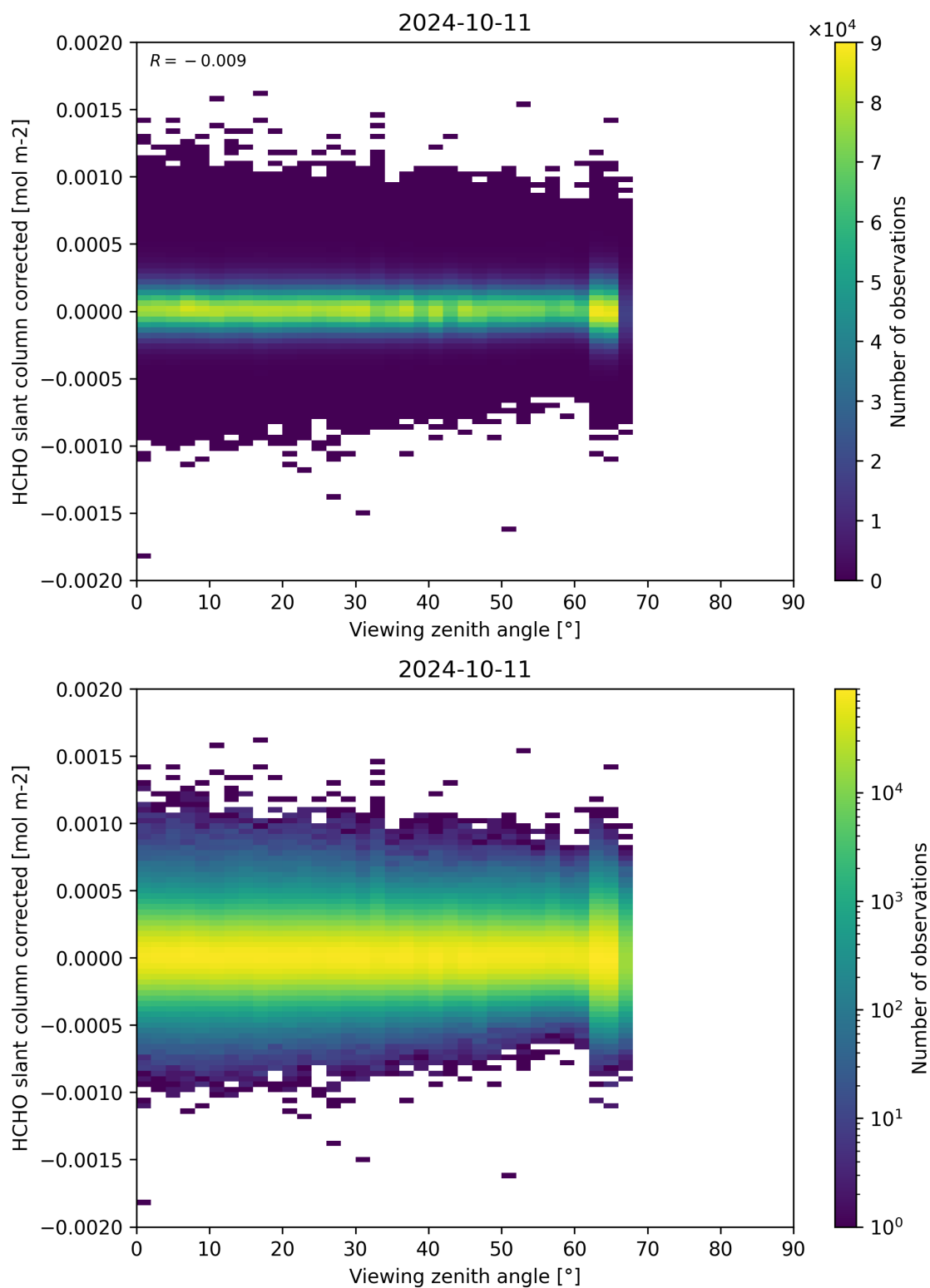
Figure 186: Scatter density plot of “Viewing zenith angle” against “HCHO slant column corrected” for 2024-10-10 to 2024-10-12.
