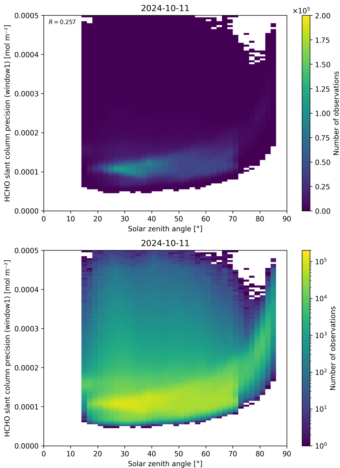
Figure 174: Scatter density plot of “Solar zenith angle” against “HCHO slant column precision (window1)” for 2024-10-10 to 2024-10-12.
