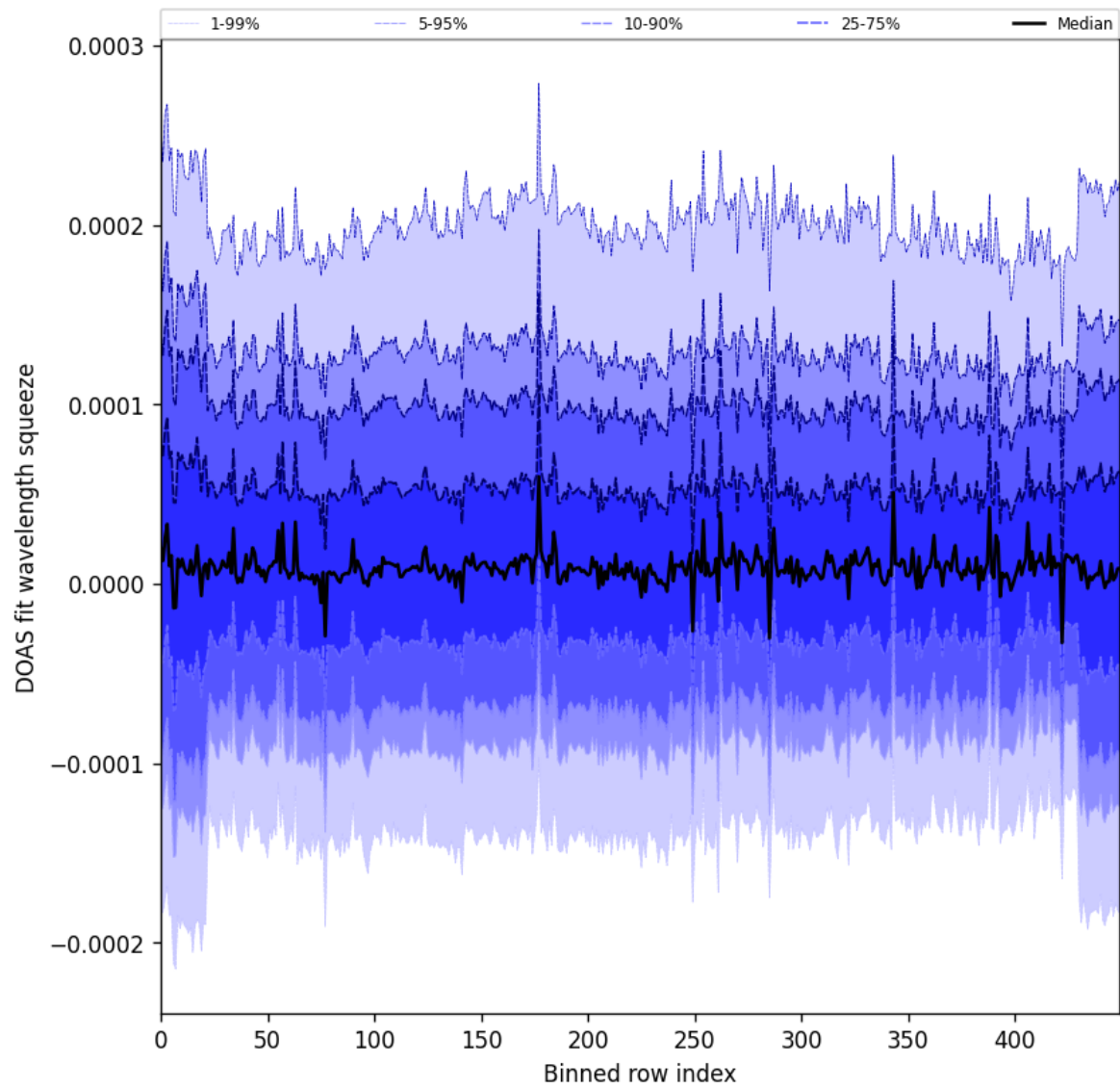
Figure 59: Along track statistics of “DOAS fit wavelength squeeze” for 2024-10-10 to 2024-10-12
