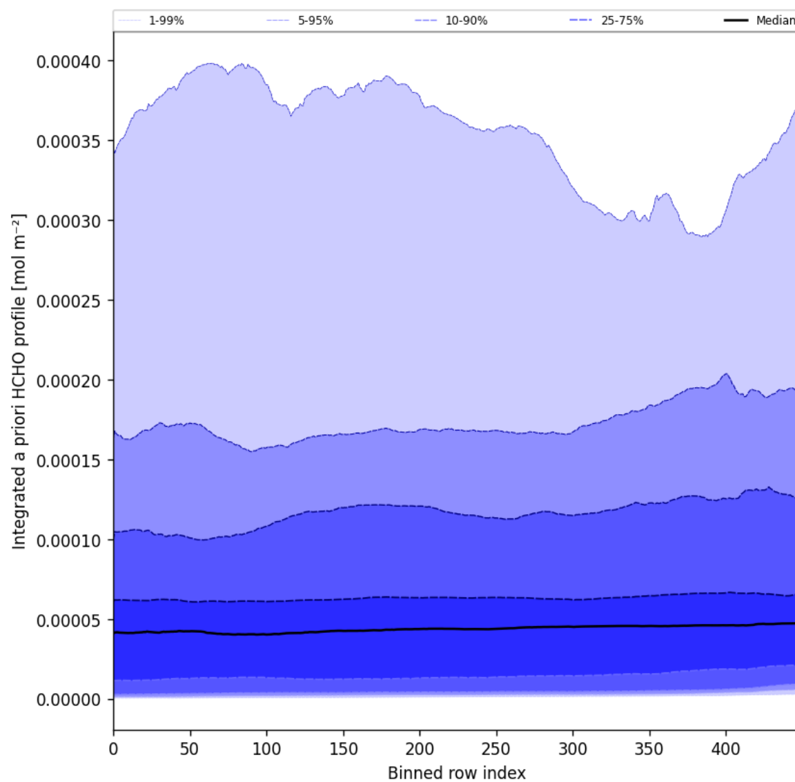
Figure 57: Along track statistics of “Integrated a priori HCHO profile” for 2024-10-10 to 2024-10-12
