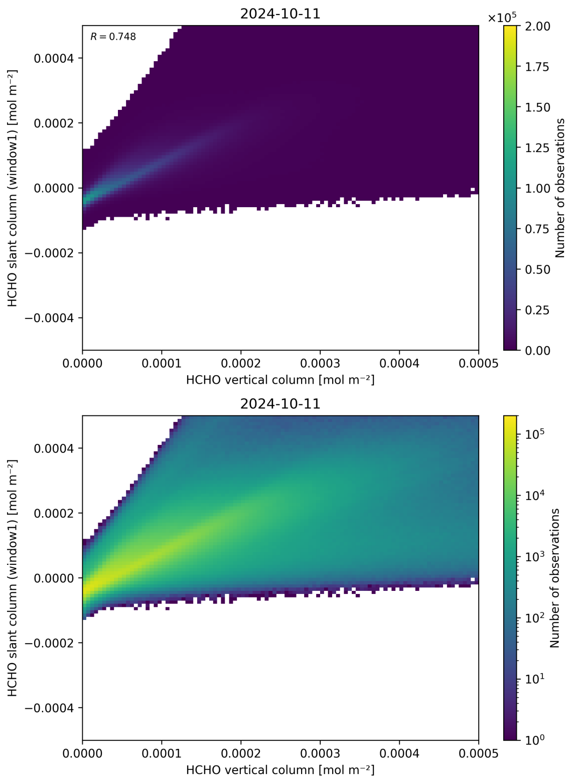
Figure 129: Scatter density plot of “HCHO vertical column” against “HCHO slant column (window1)” for 2024-10-10 to 2024-10-12.
