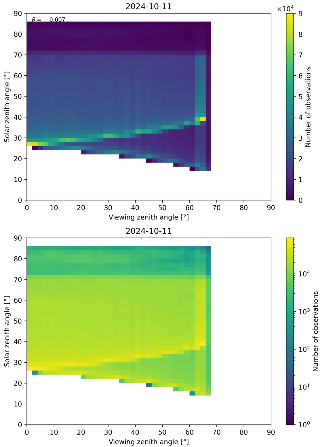
Figure 197: Scatter density plot of “Viewing zenith angle” against “Solar zenith angle” for 2024-10-10 to 2024-10-12.
