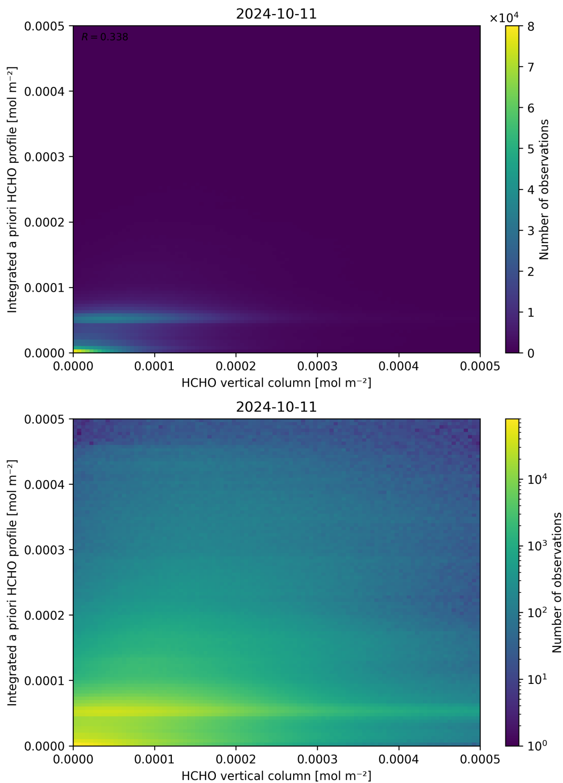
Figure 135: Scatter density plot of “HCHO vertical column” against “Integrated a priori HCHO profile” for 2024-10-10 to 2024-10-12.
