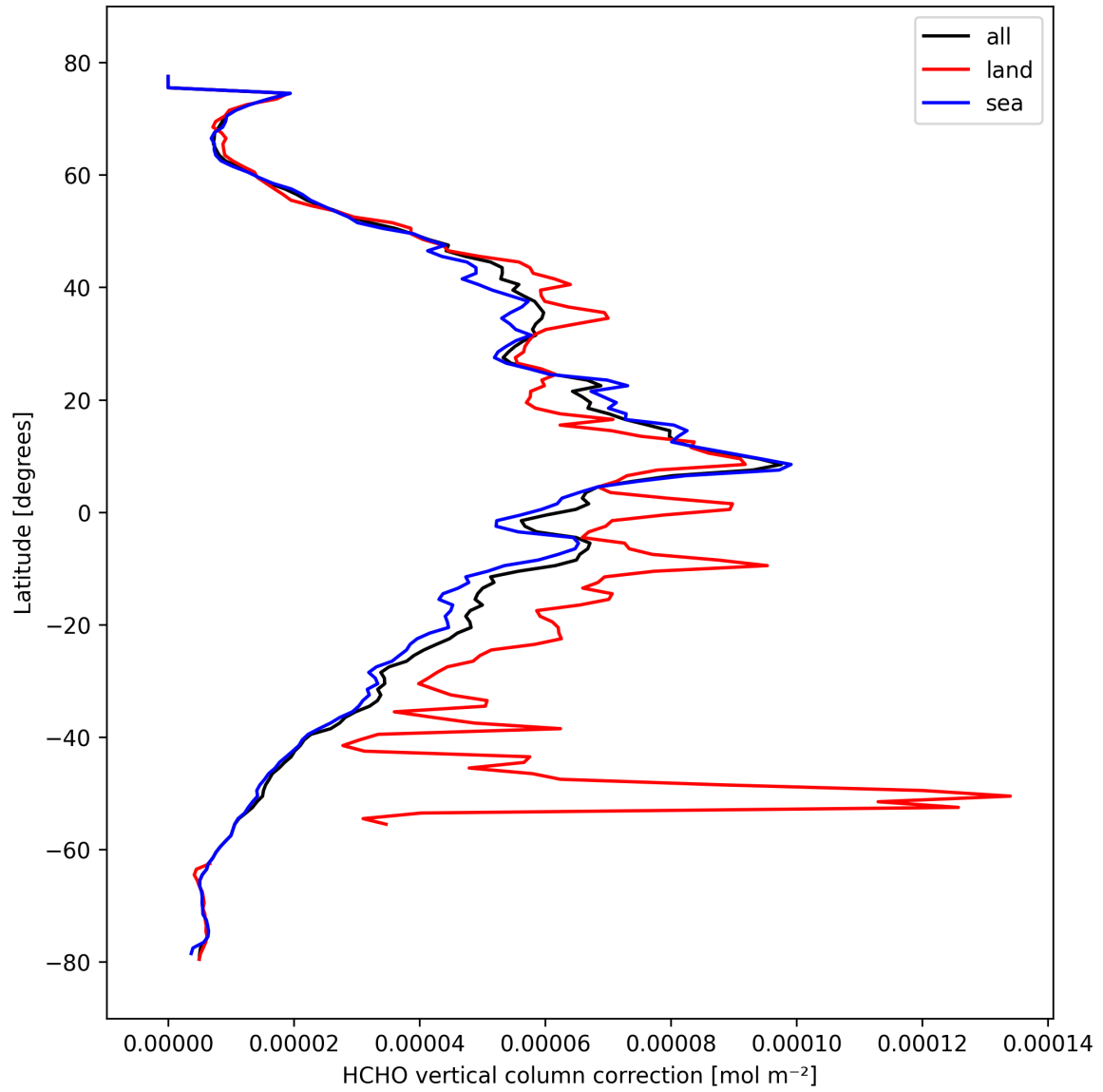
Figure 23: Zonal average of “HCHO vertical column correction” for 2024-10-10 to 2024-10-12.
