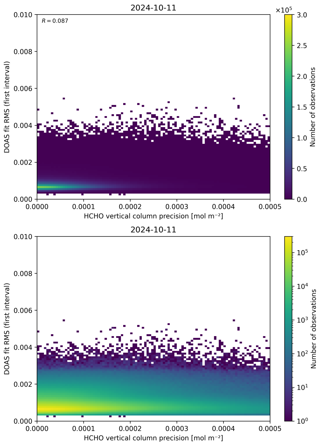
Figure 136: Scatter density plot of “HCHO vertical column precision” against “DOAS fit RMS (first interval)” for 2024-10-10 to 2024-10-12.
