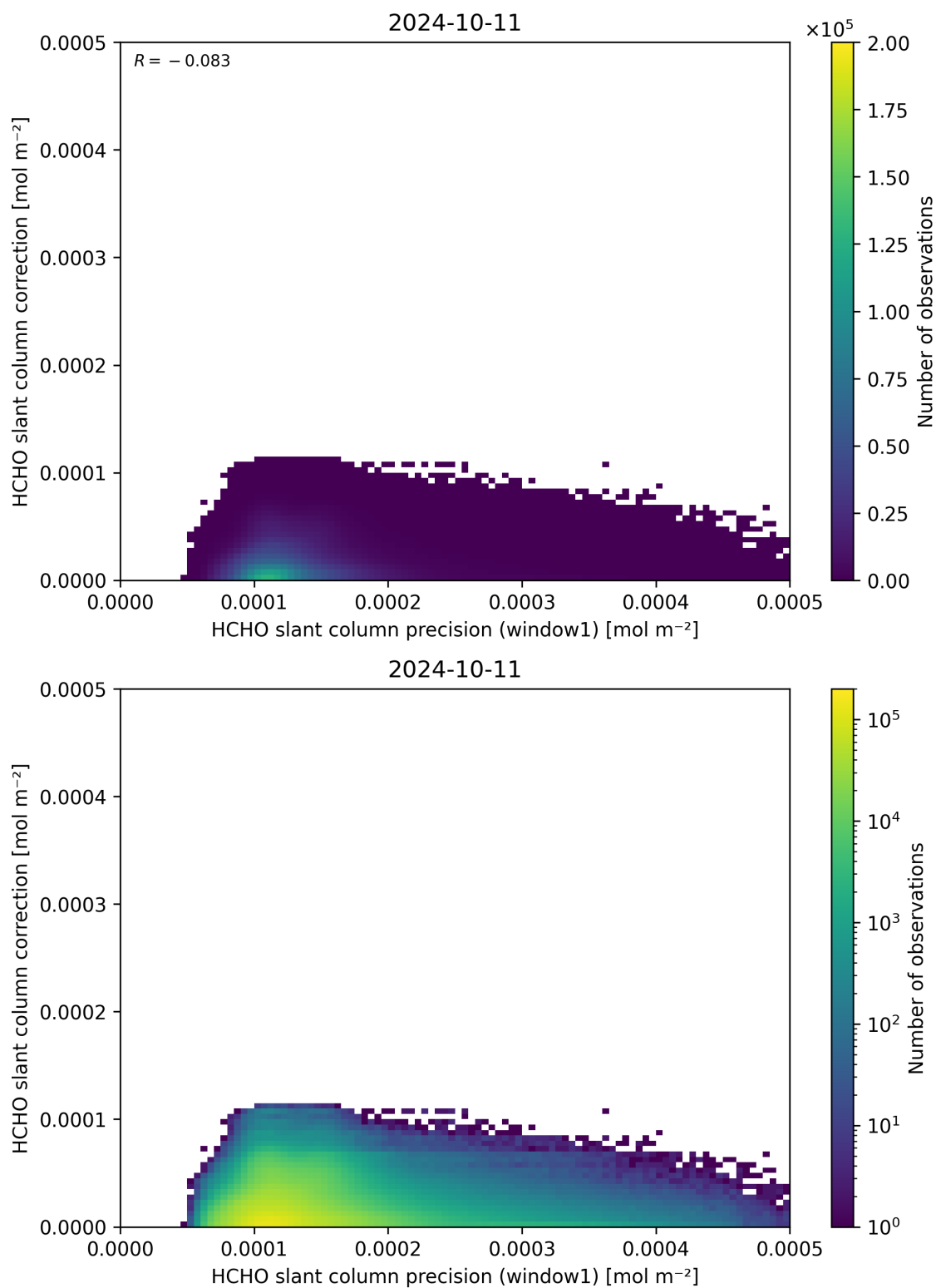
Figure 93: Scatter density plot of “HCHO slant column precision (window1)” against “HCHO slant column correction” for 2024-10-10 to 2024-10-12.
