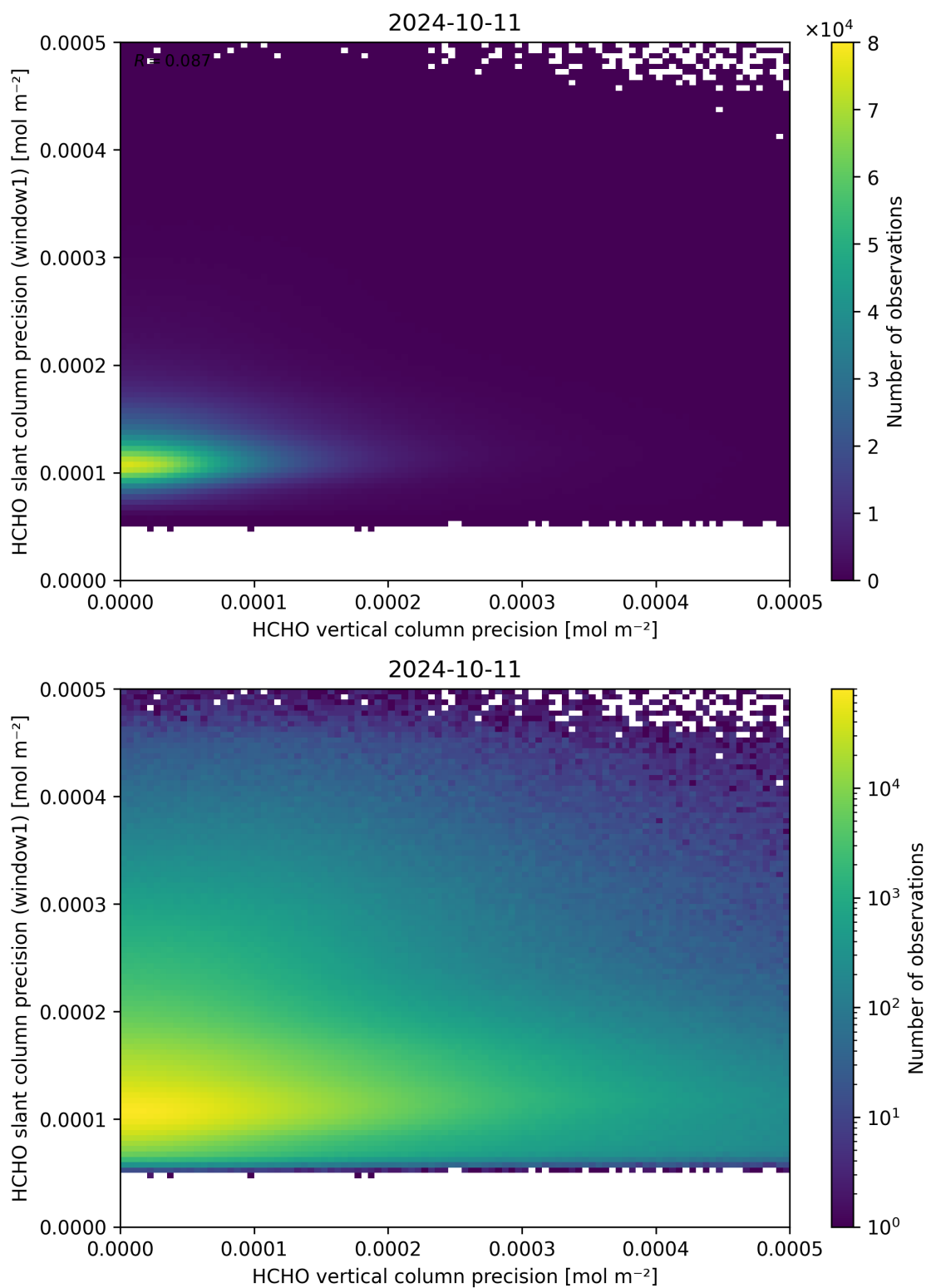
Figure 143: Scatter density plot of “HCHO vertical column precision” against “HCHO slant column precision (window1)” for 2024-10-10 to 2024-10-12.
