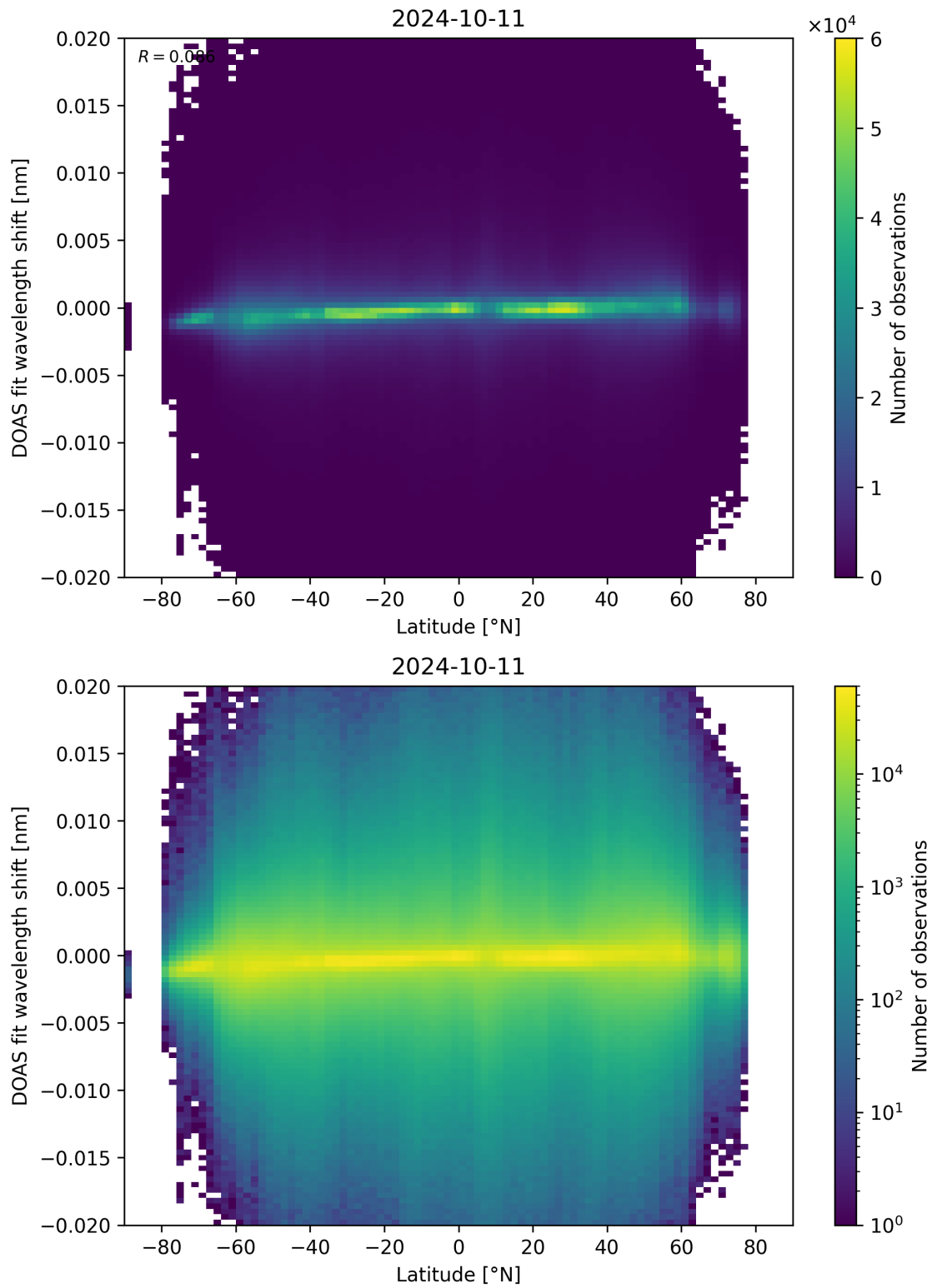
Figure 154: Scatter density plot of “Latitude” against “DOAS fit wavelength shift” for 2024-10-10 to 2024-10-12.
