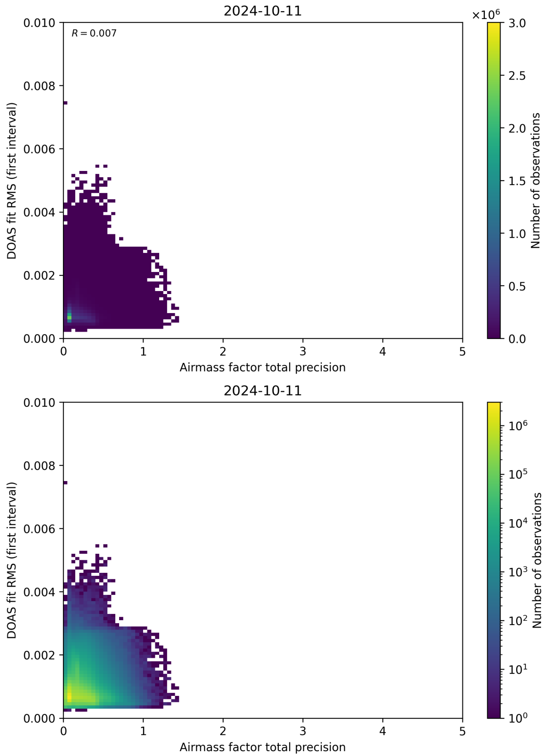
Figure 105: Scatter density plot of “Airmass factor total precision” against “DOAS fit RMS (first interval)” for 2024-10-10 to 2024-10-12.
