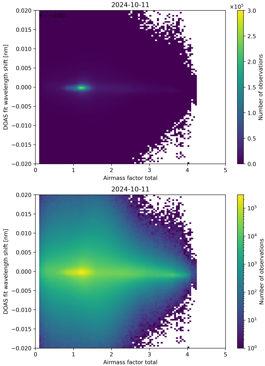
Figure 98: Scatter density plot of “Airmass factor total” against “DOAS fit wavelength shift” for 2024-10-10 to 2024-10-12.
