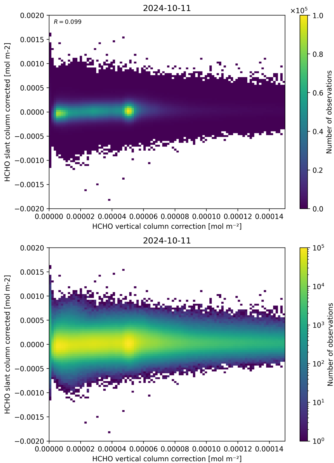
Figure 116: Scatter density plot of “HCHO vertical column correction” against “HCHO slant column corrected” for 2024-10-10 to 2024-10-12.
