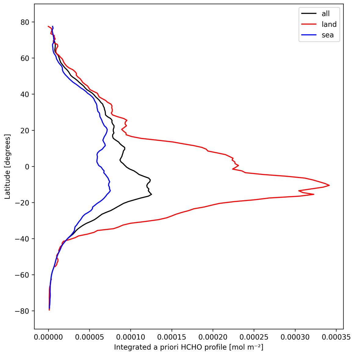
Figure 29: Zonal average of “Integrated a priori HCHO profile” for 2024-10-10 to 2024-10-12.
