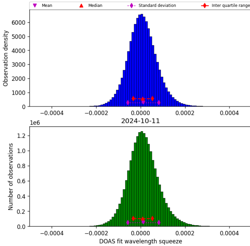
Figure 45: Histogram of “DOAS fit wavelength squeeze” for 2024-10-10 to 2024-10-12
