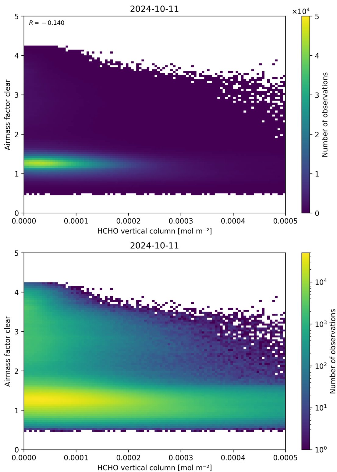
Figure 126: Scatter density plot of “HCHO vertical column” against “Airmass factor clear” for 2024-10-10 to 2024-10-12.
