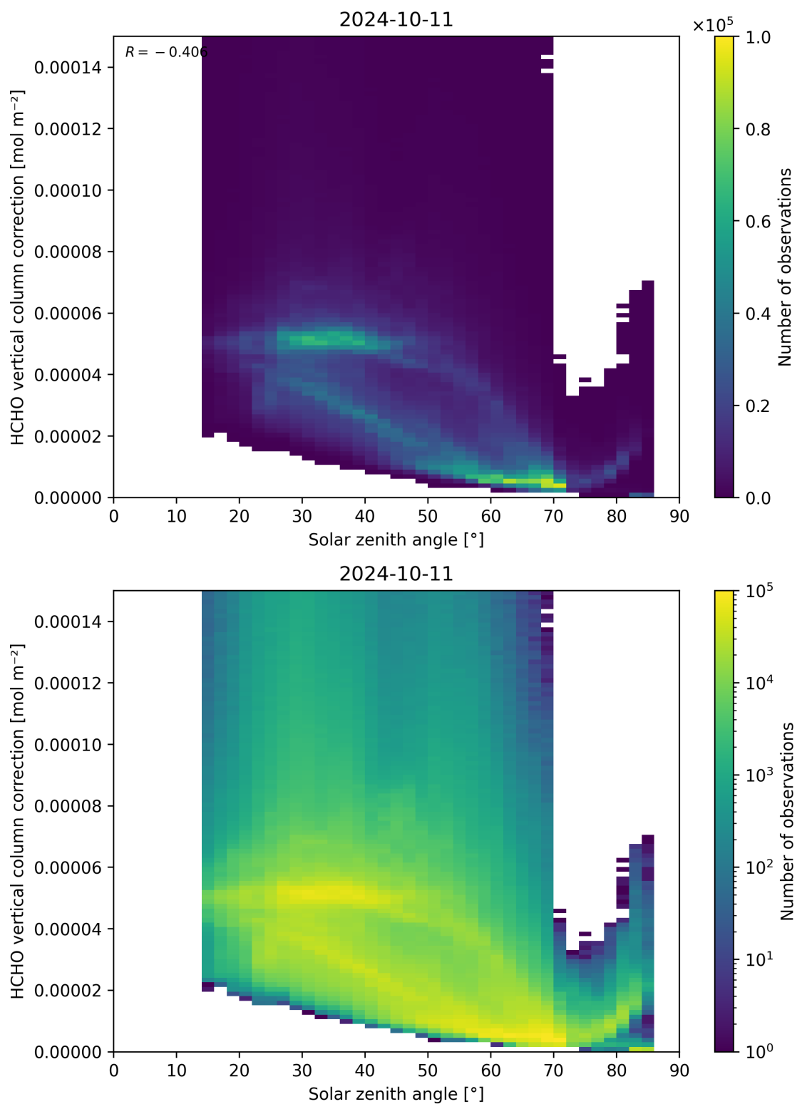
Figure 178: Scatter density plot of “Solar zenith angle” against “HCHO vertical column correction” for 2024-10-10 to 2024-10-12.
