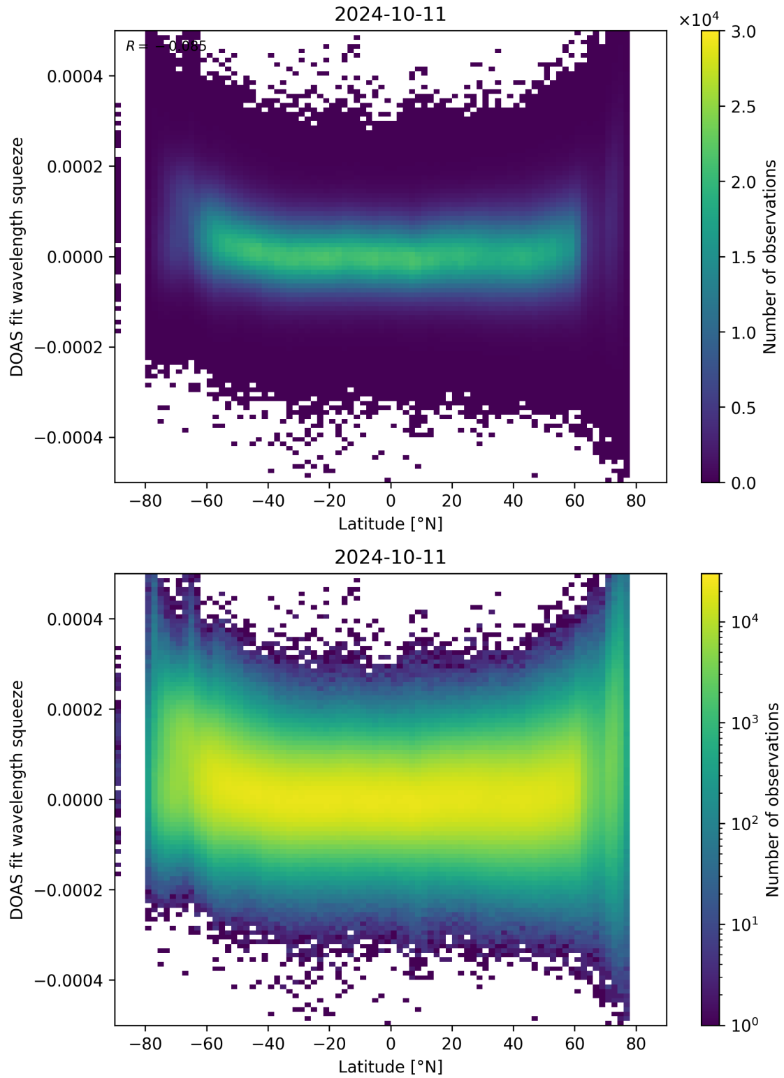
Figure 155: Scatter density plot of “Latitude” against “DOAS fit wavelength squeeze” for 2024-10-10 to 2024-10-12.
