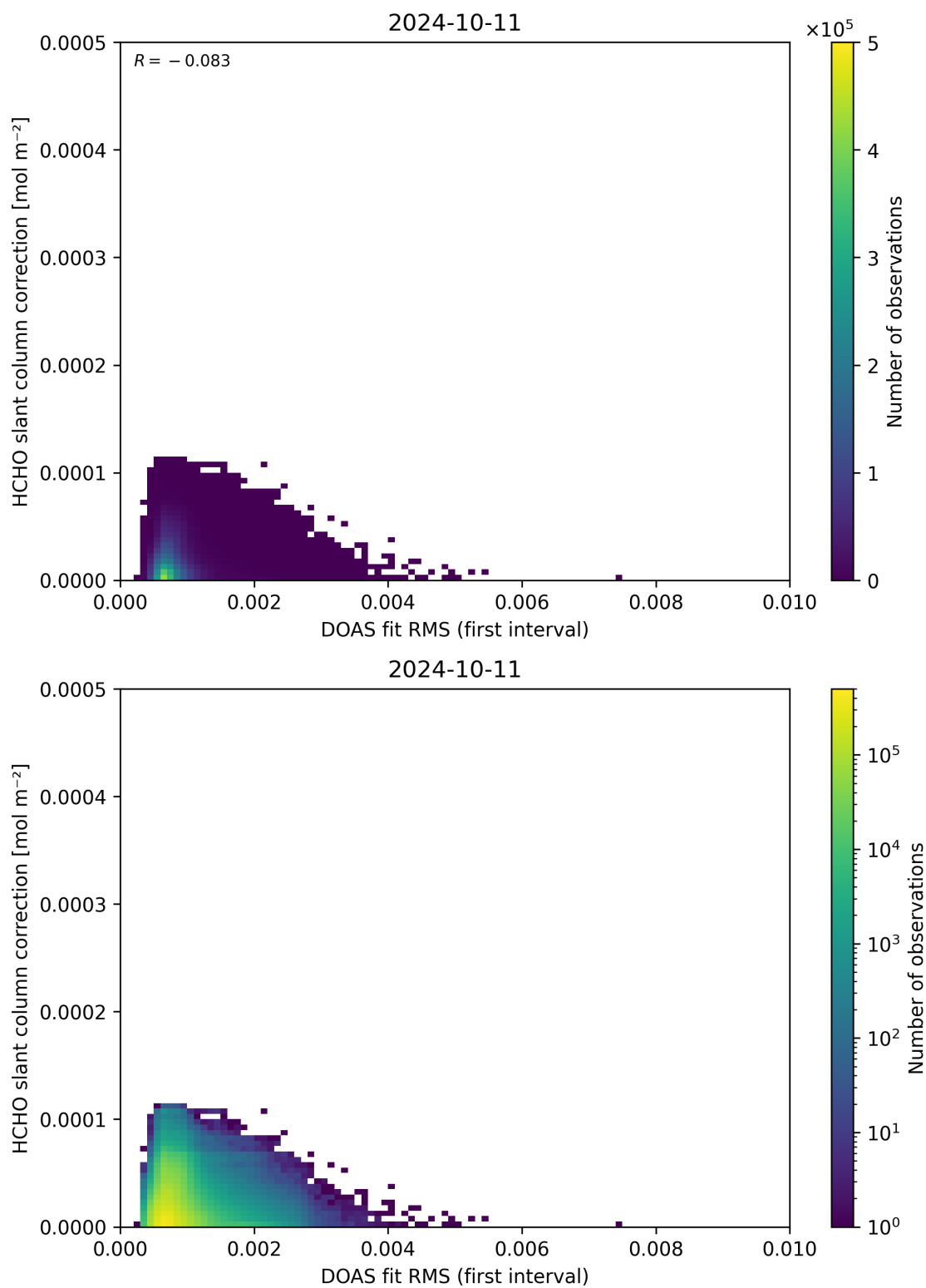
Figure 63: Scatter density plot of “DOAS fit RMS (first interval)” against “HCHO slant column correction” for 2024-10-10 to 2024-10-12.
