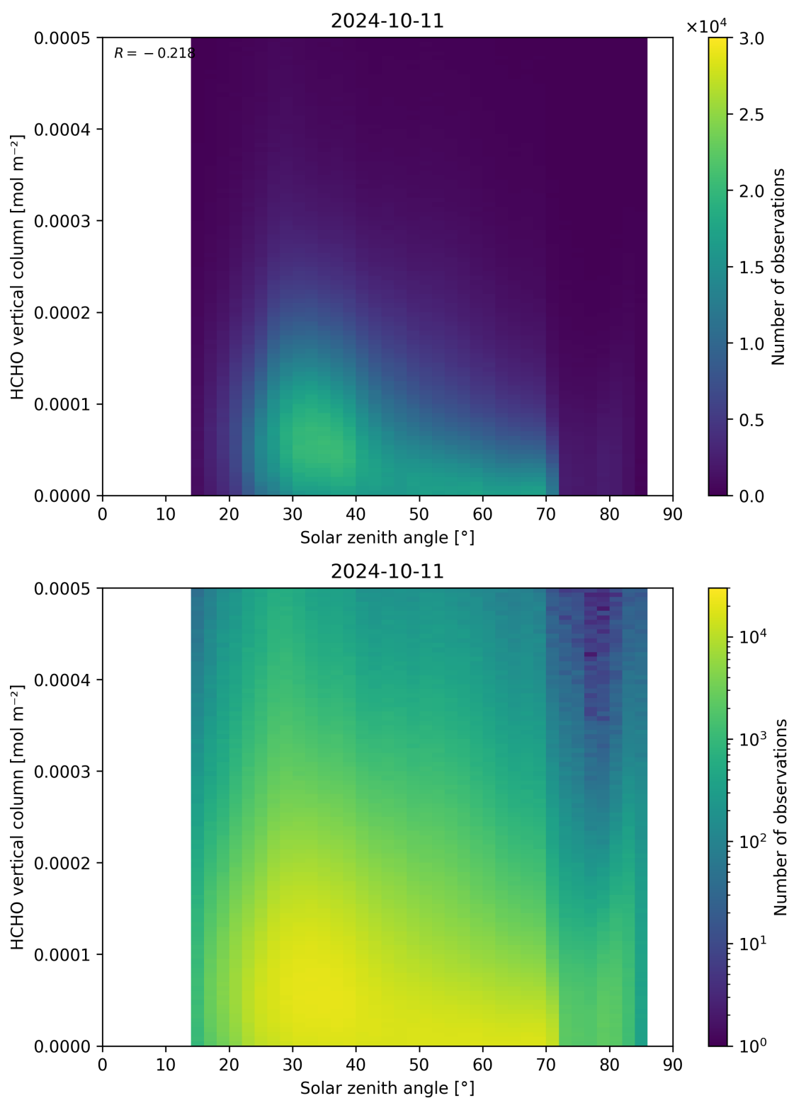
Figure 177: Scatter density plot of “Solar zenith angle” against “HCHO vertical column” for 2024-10-10 to 2024-10-12.
