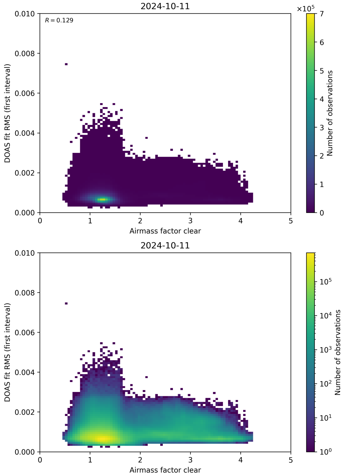
Figure 71: Scatter density plot of “Airmass factor clear” against “DOAS fit RMS (first interval)” for 2024-10-10 to 2024-10-12.
