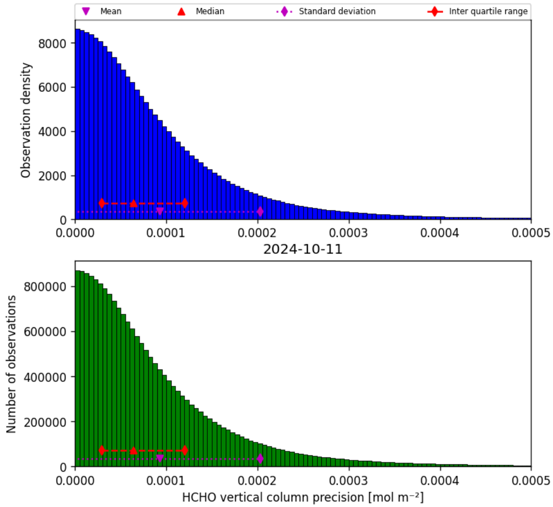
Figure 36: Histogram of “HCHO vertical column precision” for 2024-10-10 to 2024-10-12
