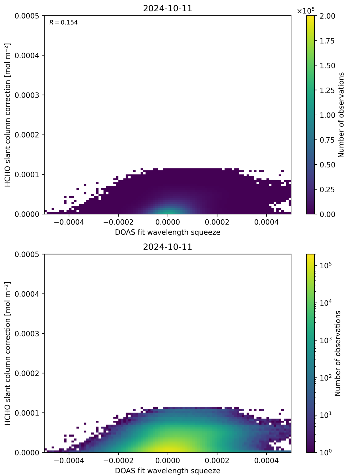
Figure 70: Scatter density plot of “DOAS fit wavelength squeeze” against “HCHO slant column correction” for 2024-10-10 to 2024-10-12.
