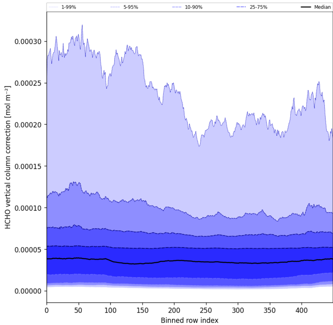
Figure 51: Along track statistics of “HCHO vertical column correction” for 2024-10-10 to 2024-10-12
