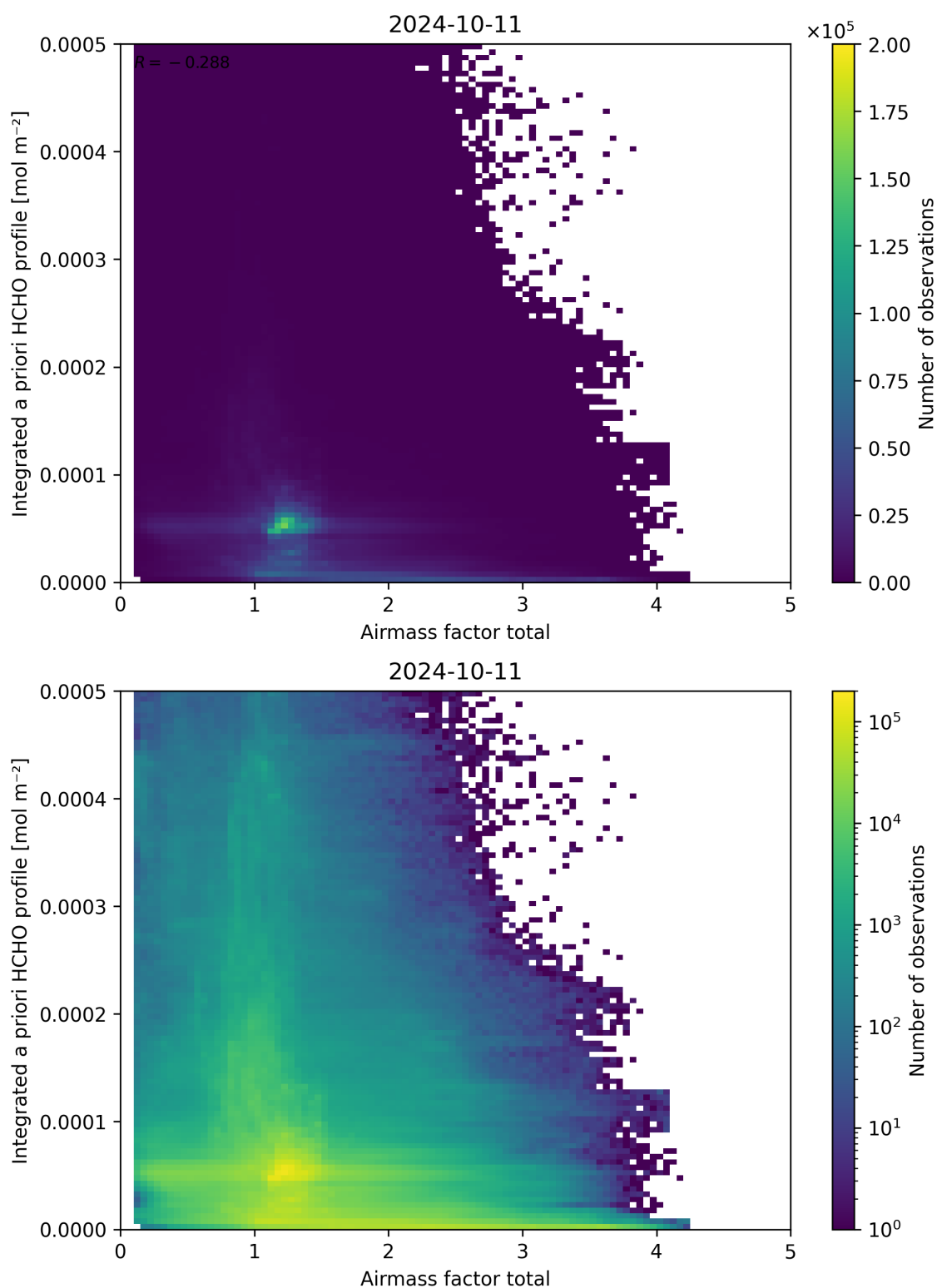
Figure 104: Scatter density plot of “Airmass factor total” against “Integrated a priori HCHO profile” for 2024-10-10 to 2024-10-12.
