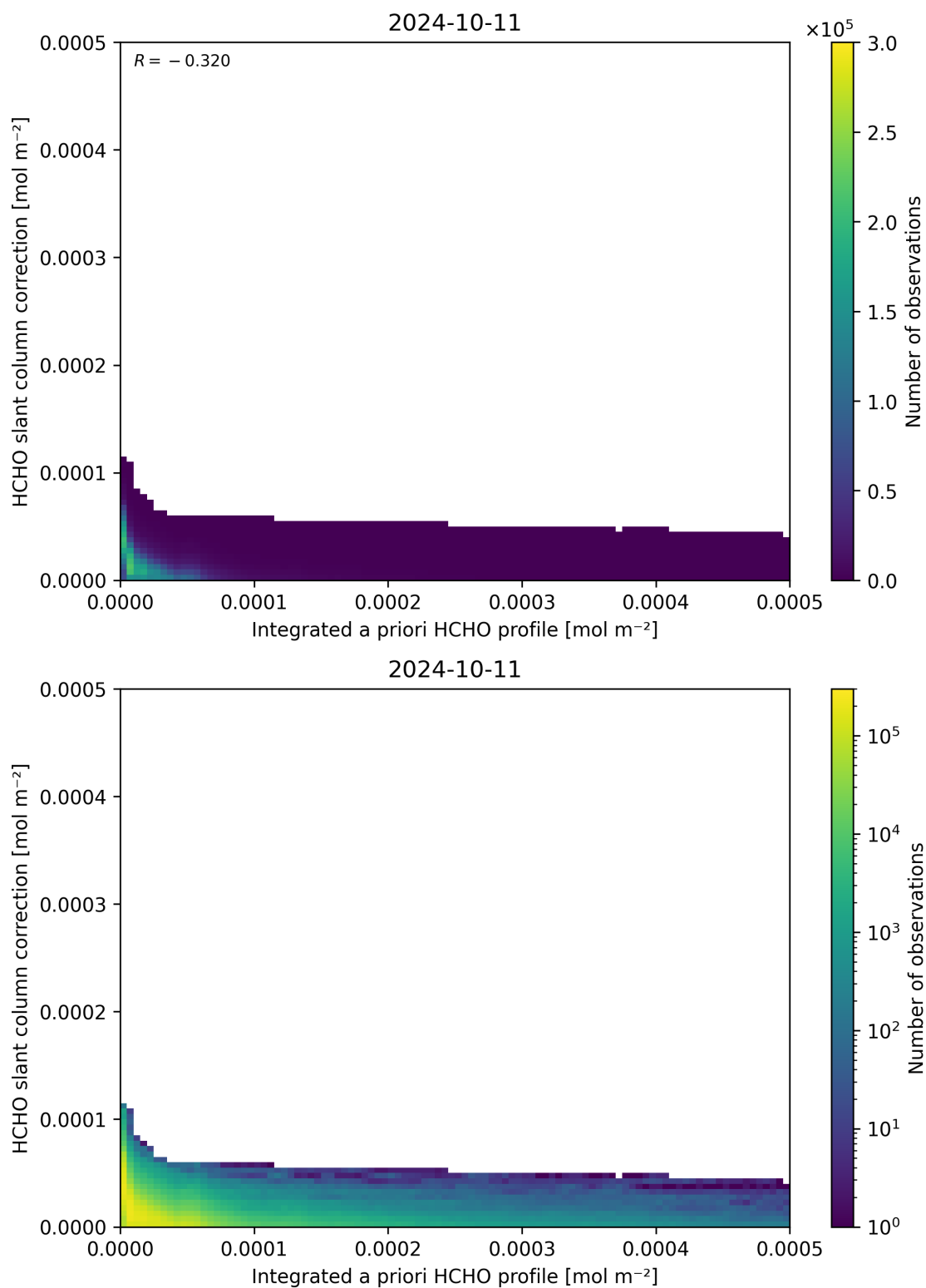
Figure 152: Scatter density plot of “Integrated a priori HCHO profile” against “HCHO slant column correction” for 2024-10-10 to 2024-10-12.
