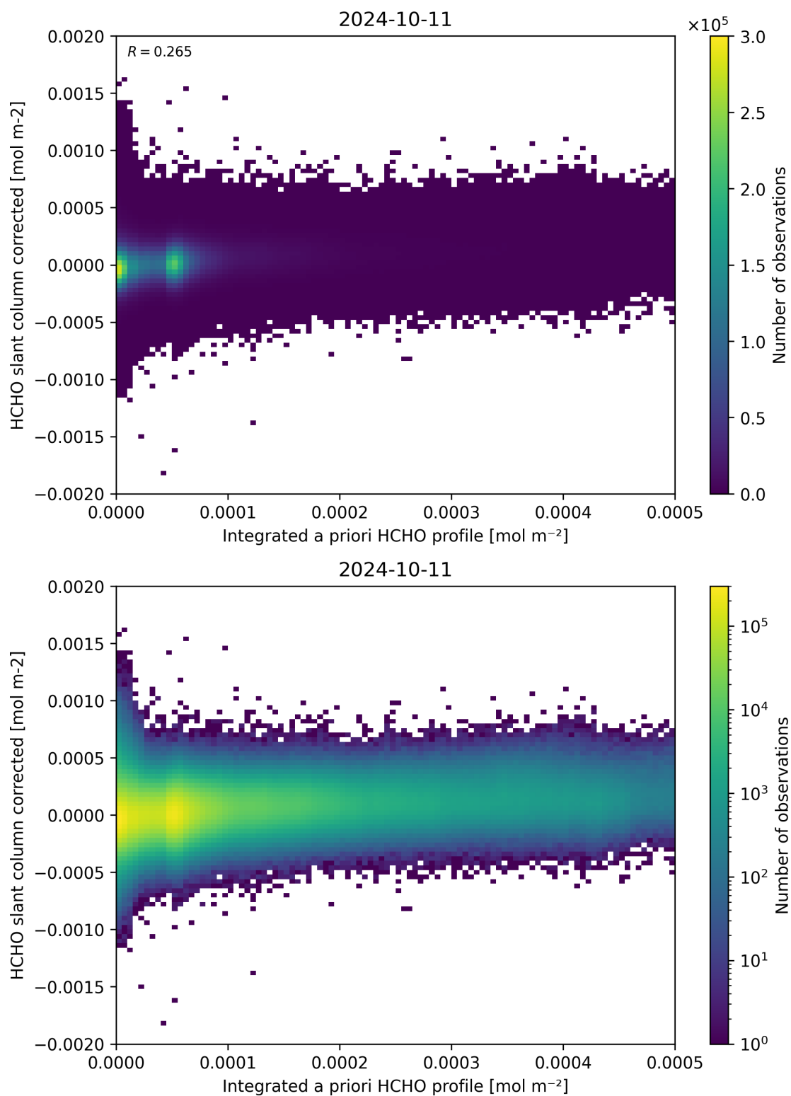
Figure 151: Scatter density plot of “Integrated a priori HCHO profile” against “HCHO slant column corrected” for 2024-10-10 to 2024-10-12.
