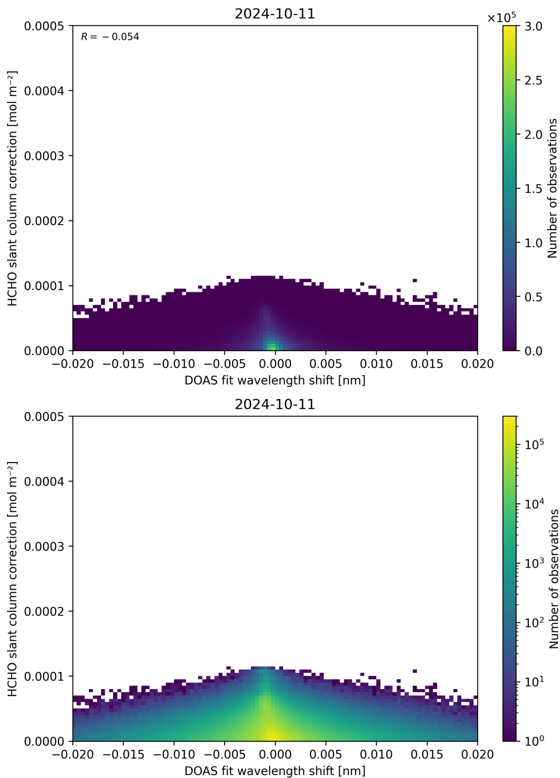
Figure 67: Scatter density plot of “DOAS fit wavelength shift” against “HCHO slant column correction” for 2024-10-10 to 2024-10-12.
