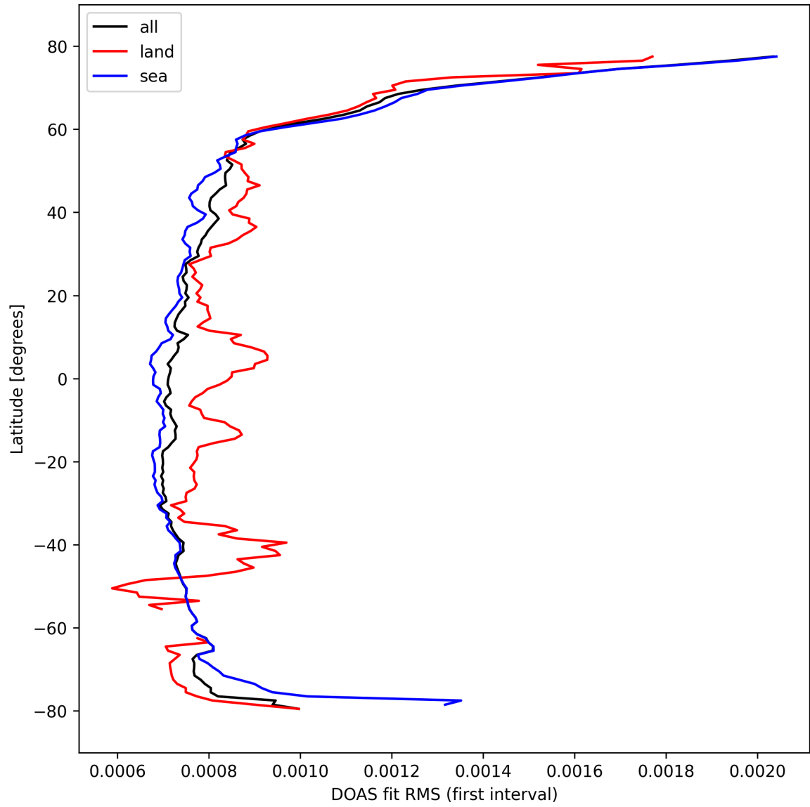
Figure 32: Zonal average of “DOAS fit RMS (first interval)” for 2024-10-10 to 2024-10-12.
