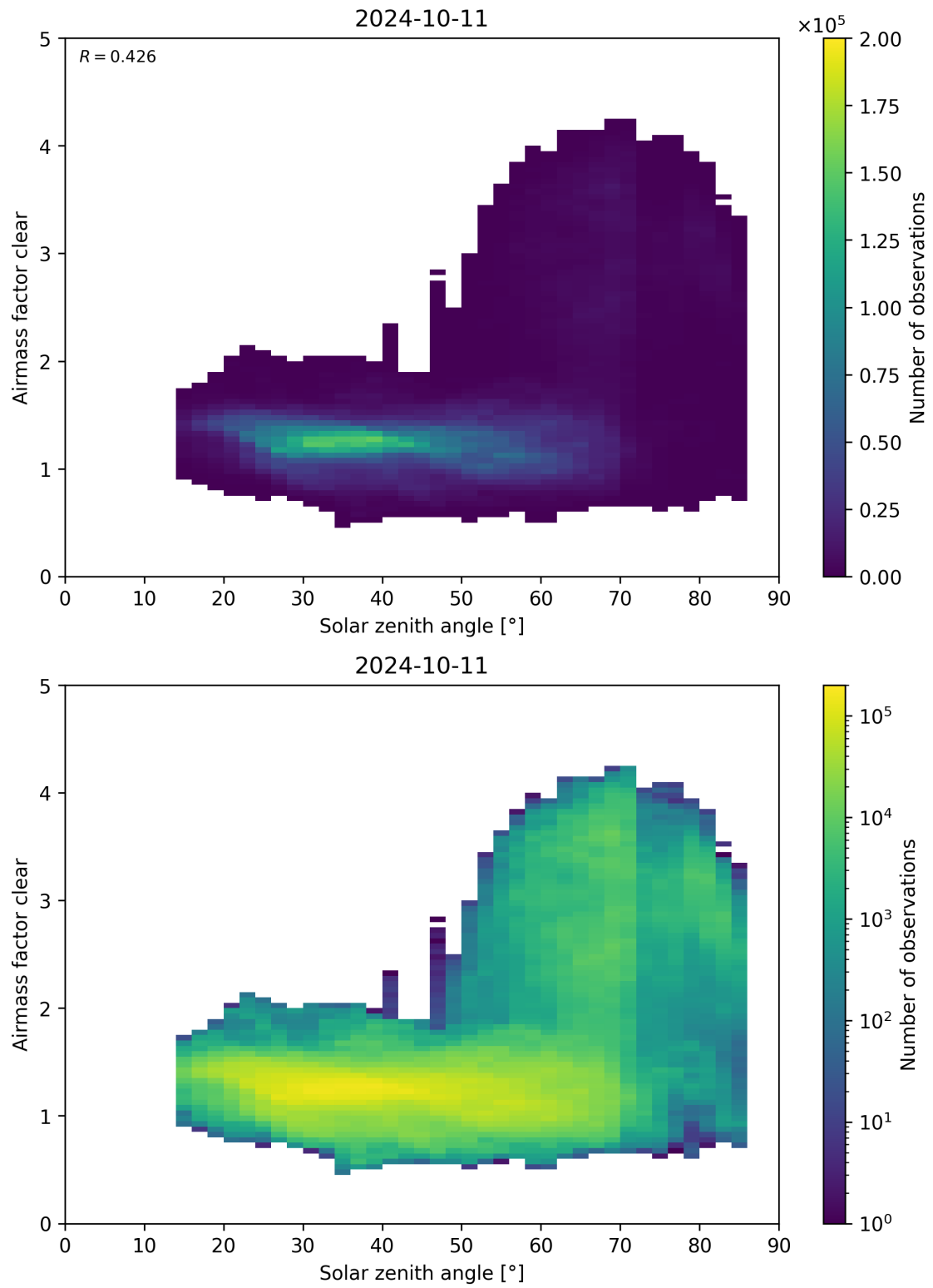
Figure 170: Scatter density plot of “Solar zenith angle” against “Airmass factor clear” for 2024-10-10 to 2024-10-12.
