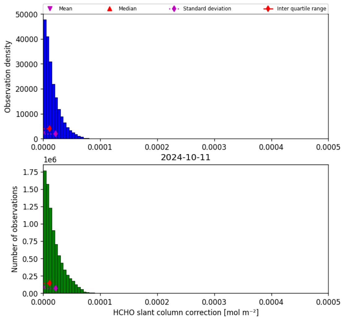
Figure 47: Histogram of “HCHO slant column correction” for 2024-10-10 to 2024-10-12
