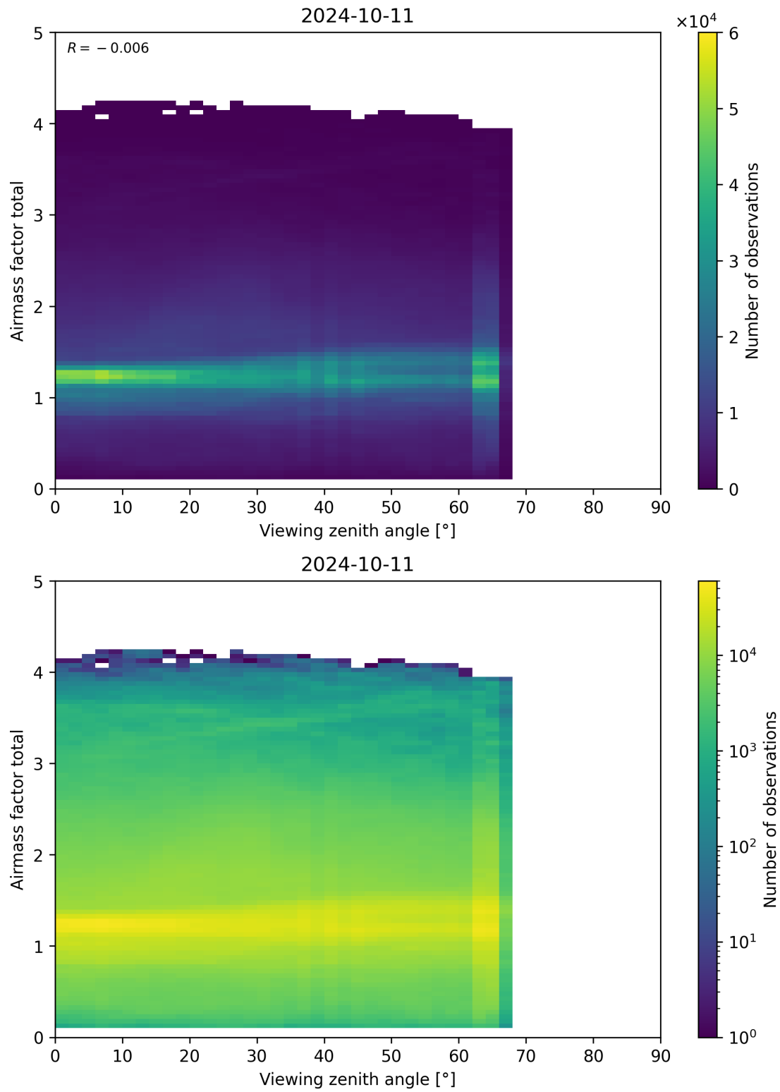
Figure 190: Scatter density plot of “Viewing zenith angle” against “Airmass factor total” for 2024-10-10 to 2024-10-12.
