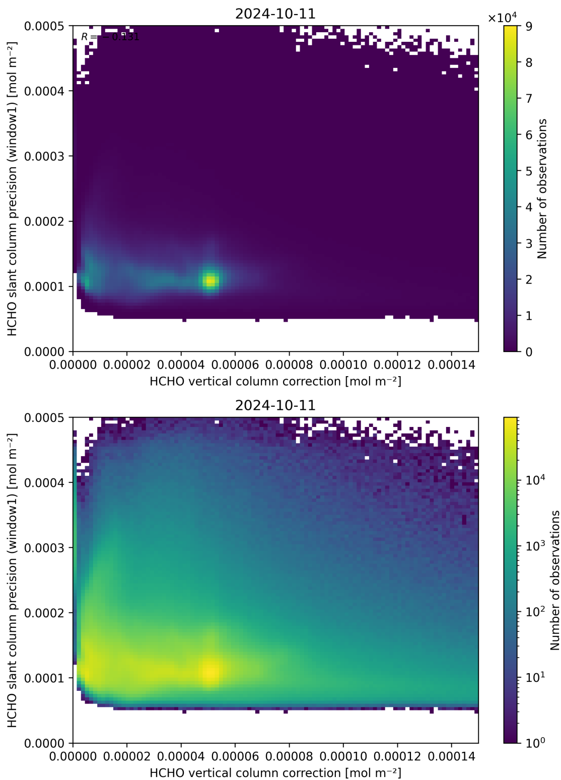
Figure 119: Scatter density plot of “HCHO vertical column correction” against “HCHO slant column precision (window1)” for 2024-10-10 to 2024-10-12.
