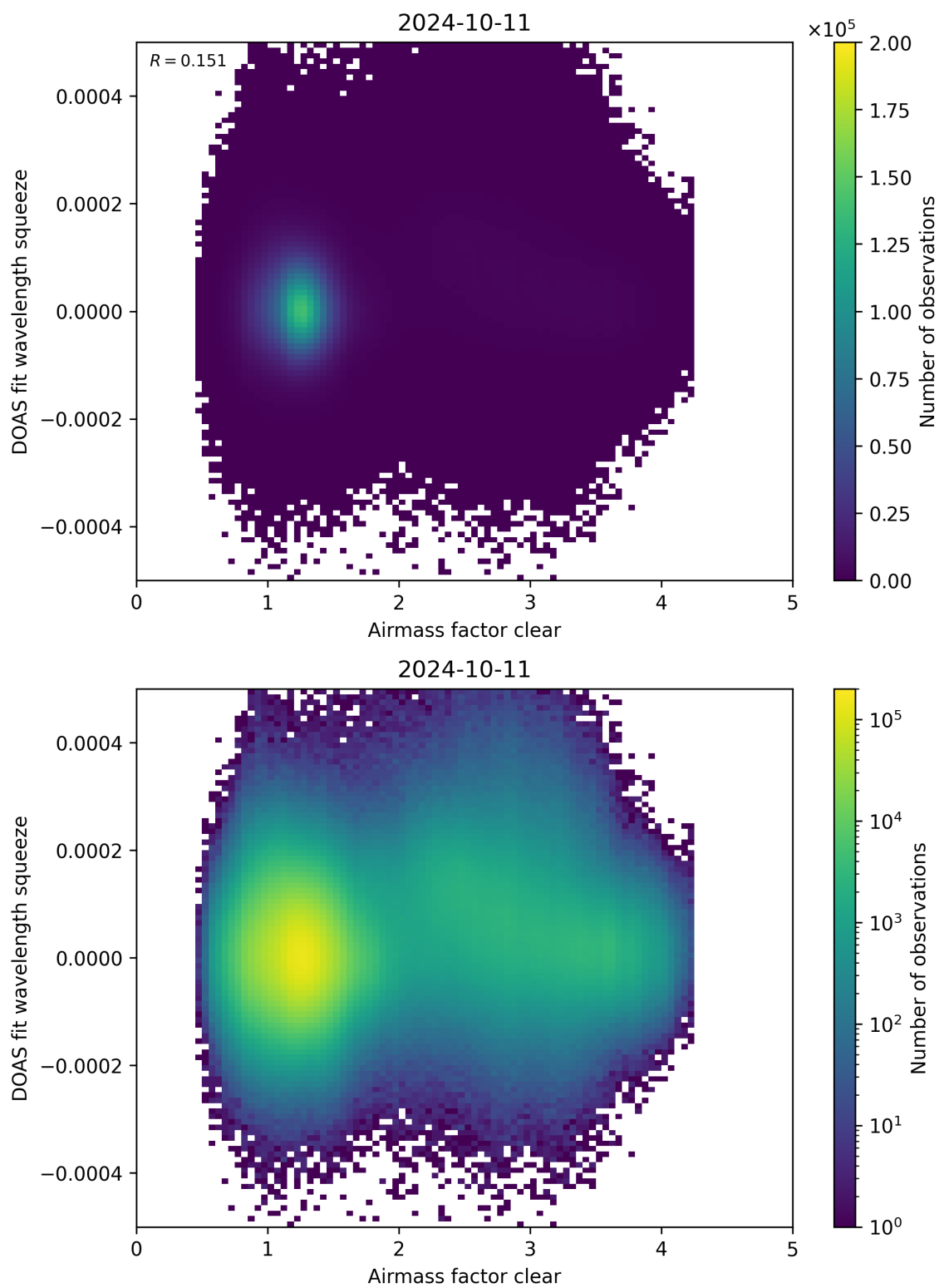
Figure 73: Scatter density plot of “Airmass factor clear” against “DOAS fit wavelength squeeze” for 2024-10-10 to 2024-10-12.
