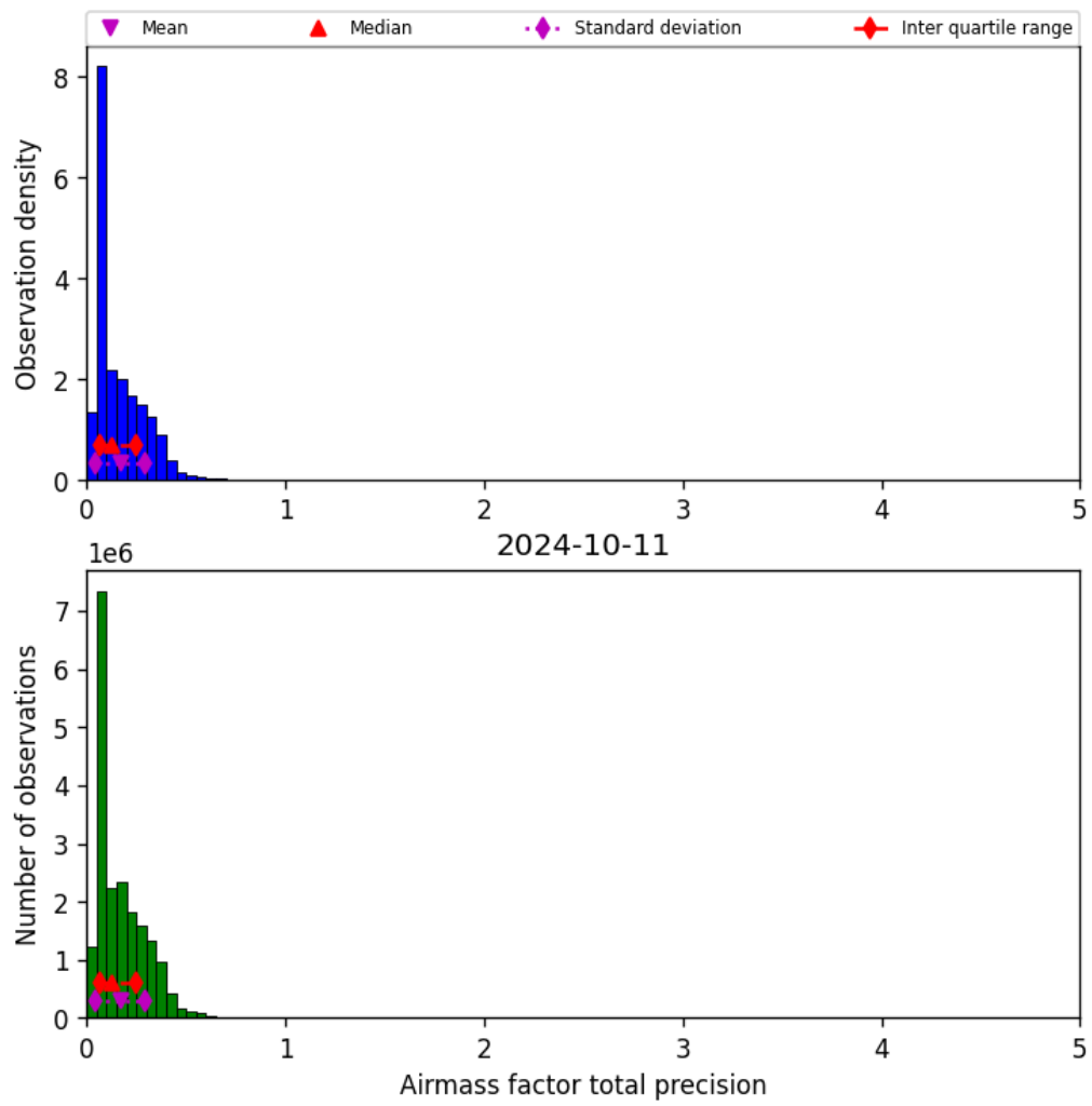
Figure 41: Histogram of “Airmass factor total precision” for 2024-10-10 to 2024-10-12
