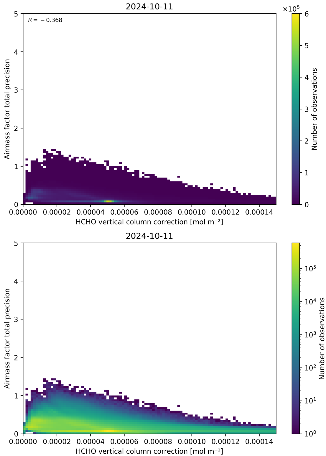
Figure 121: Scatter density plot of “HCHO vertical column correction” against “Airmass factor total precision” for 2024-10-10 to 2024-10-12.
