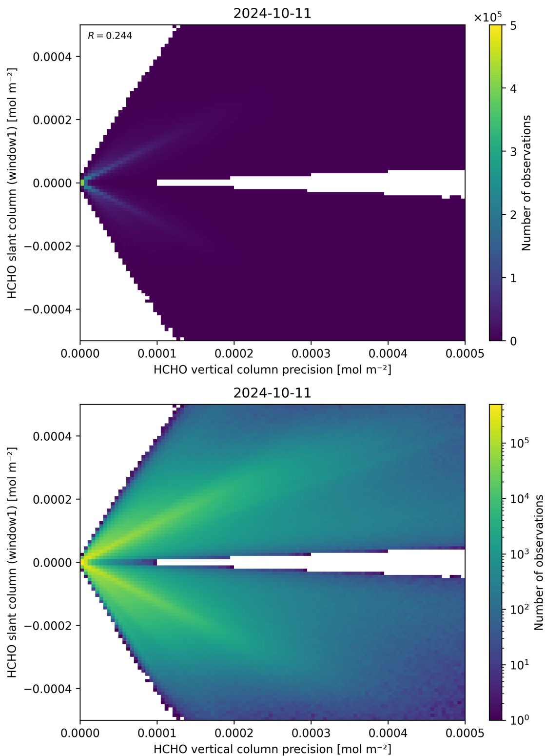
Figure 142: Scatter density plot of “HCHO vertical column precision” against “HCHO slant column (window1)” for 2024-10-10 to 2024-10-12.
