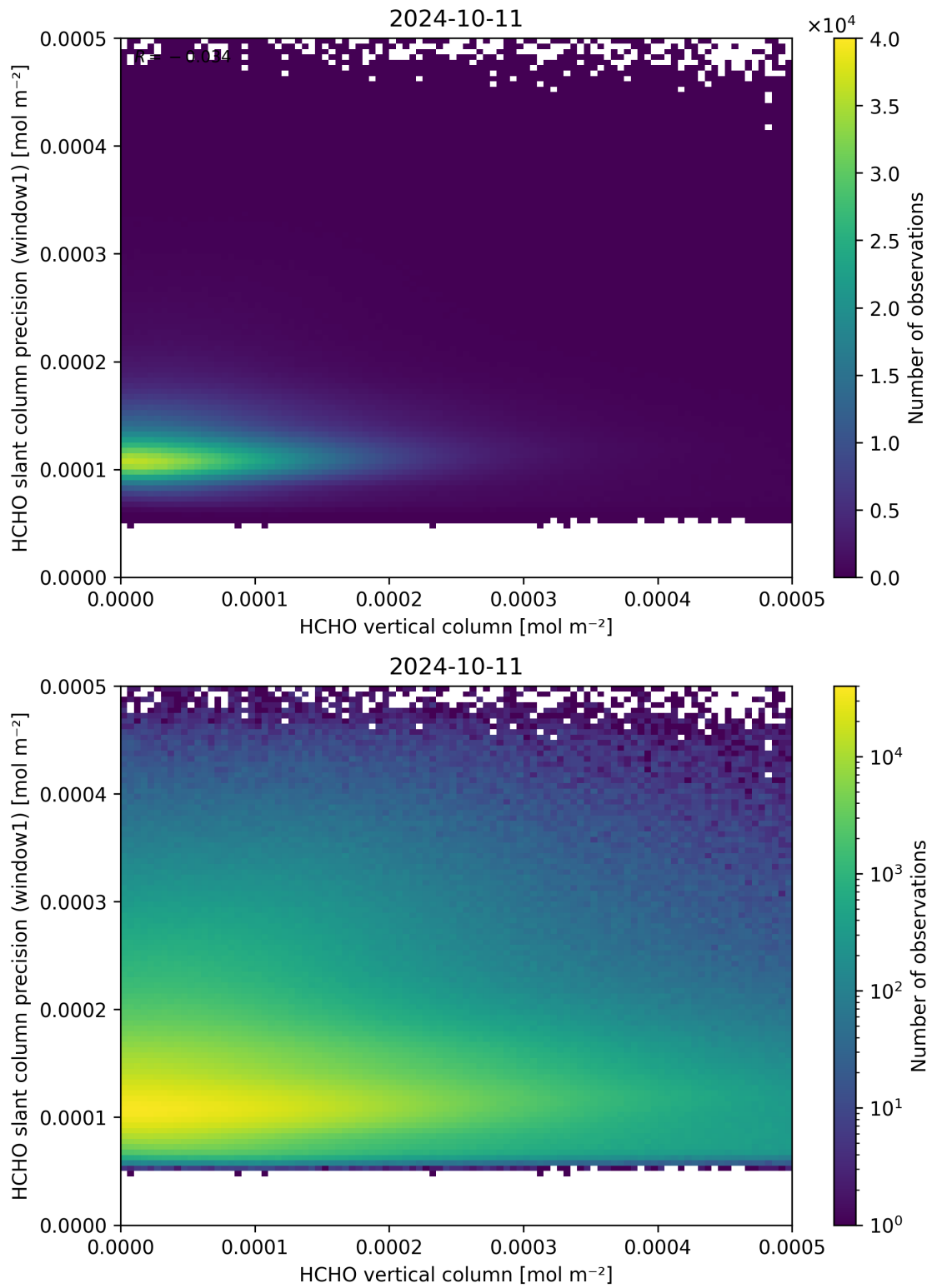
Figure 130: Scatter density plot of “HCHO vertical column” against “HCHO slant column precision (window1)” for 2024-10-10 to 2024-10-12.
