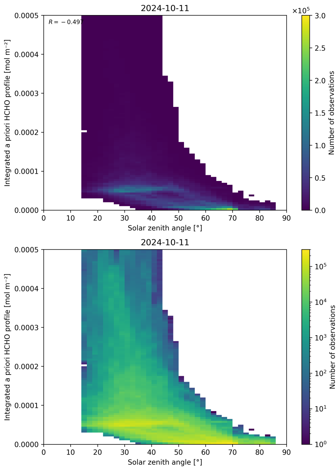
Figure 180: Scatter density plot of “Solar zenith angle” against “Integrated a priori HCHO profile” for 2024-10-10 to 2024-10-12.
