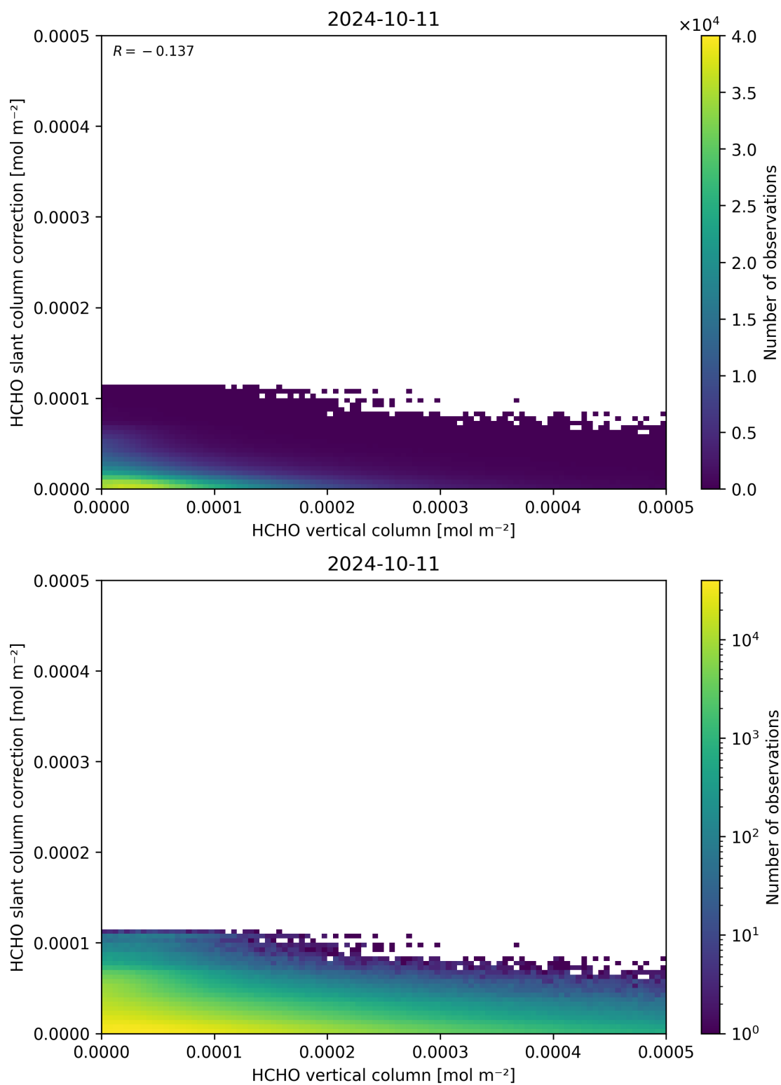
Figure 128: Scatter density plot of “HCHO vertical column” against “HCHO slant column correction” for 2024-10-10 to 2024-10-12.
