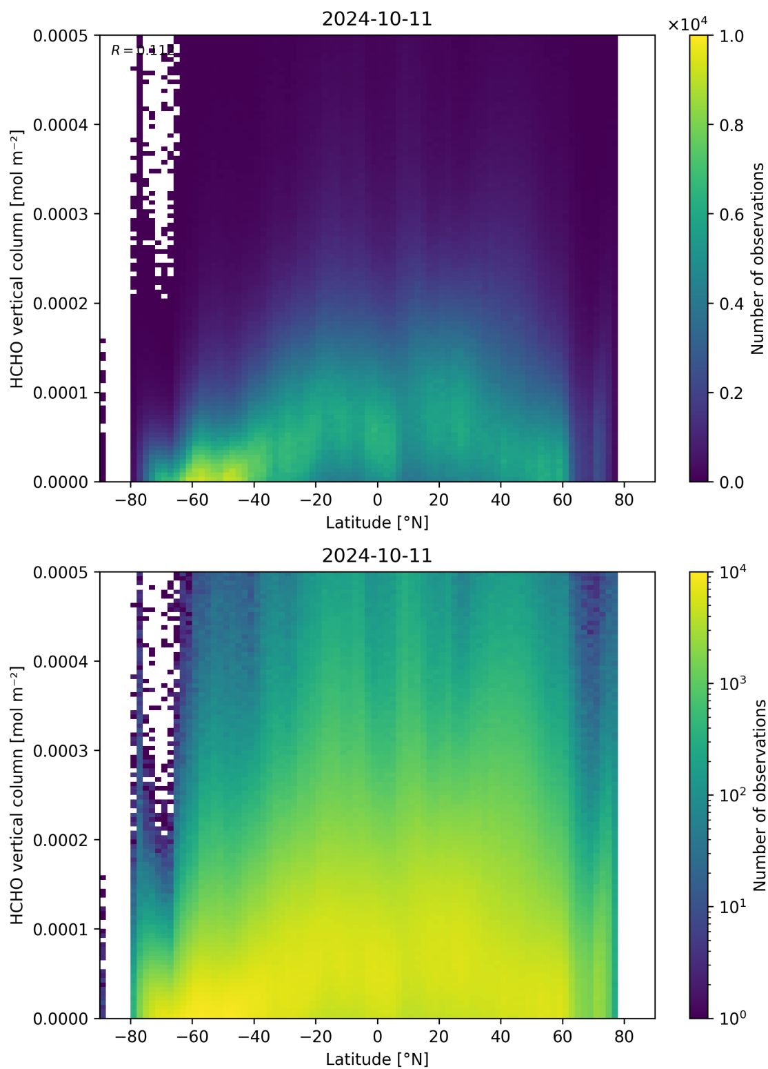
Figure 163: Scatter density plot of “Latitude” against “HCHO vertical column” for 2024-10-10 to 2024-10-12.
