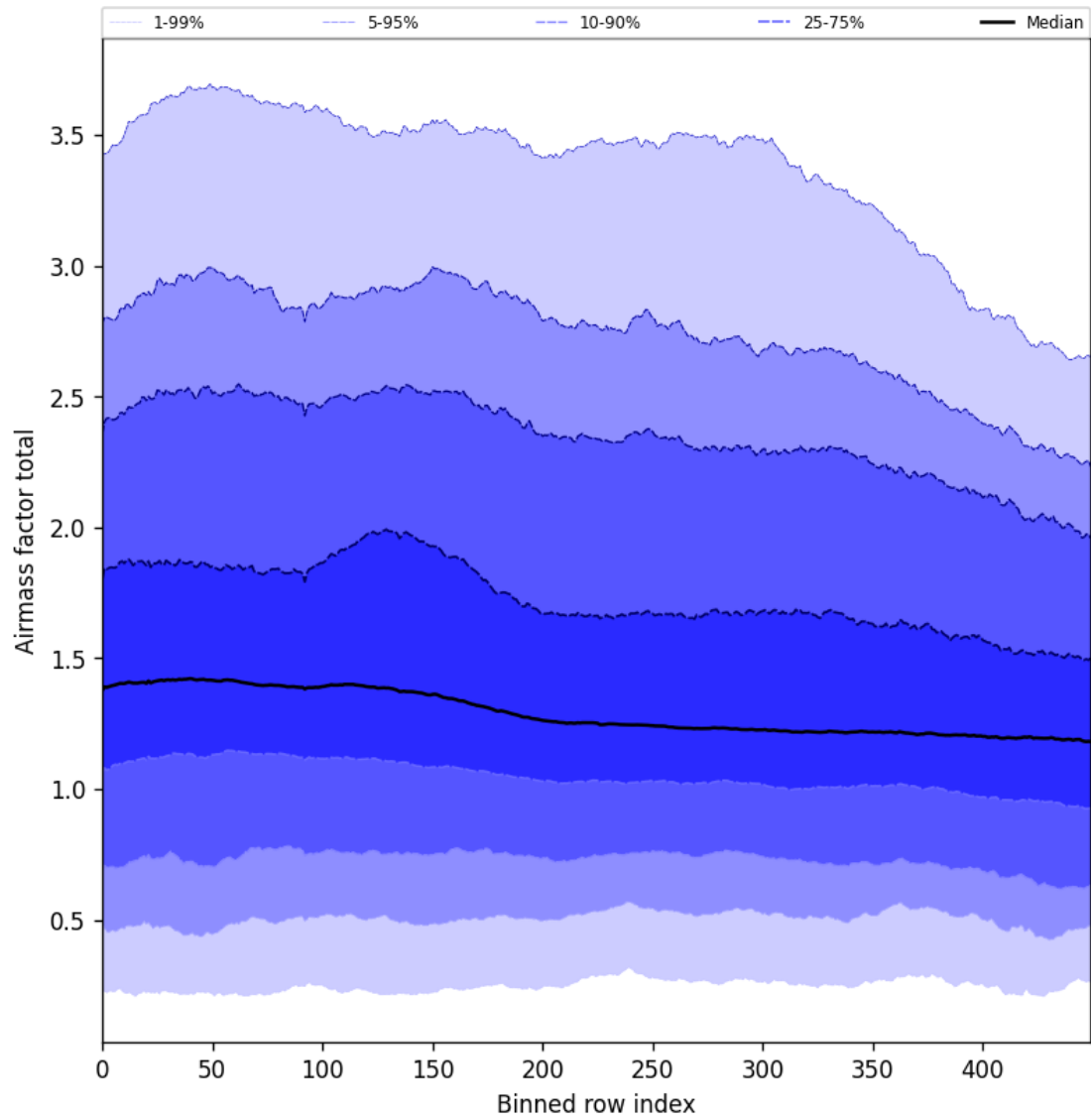
Figure 54: Along track statistics of “Airmass factor total” for 2024-10-10 to 2024-10-12
