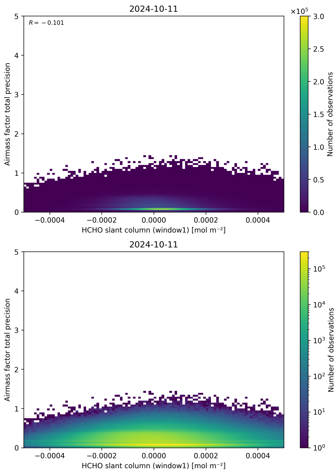
Figure 86: Scatter density plot of “HCHO slant column (window1)” against “Airmass factor total precision” for 2024-10-10 to 2024-10-12.
