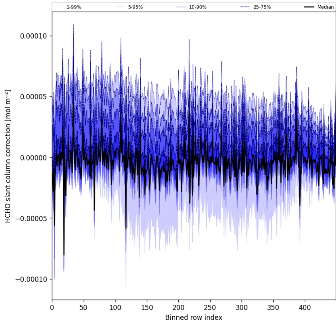
Figure 61: Along track statistics of “HCHO slant column correction” for 2024-10-10 to 2024-10-12
