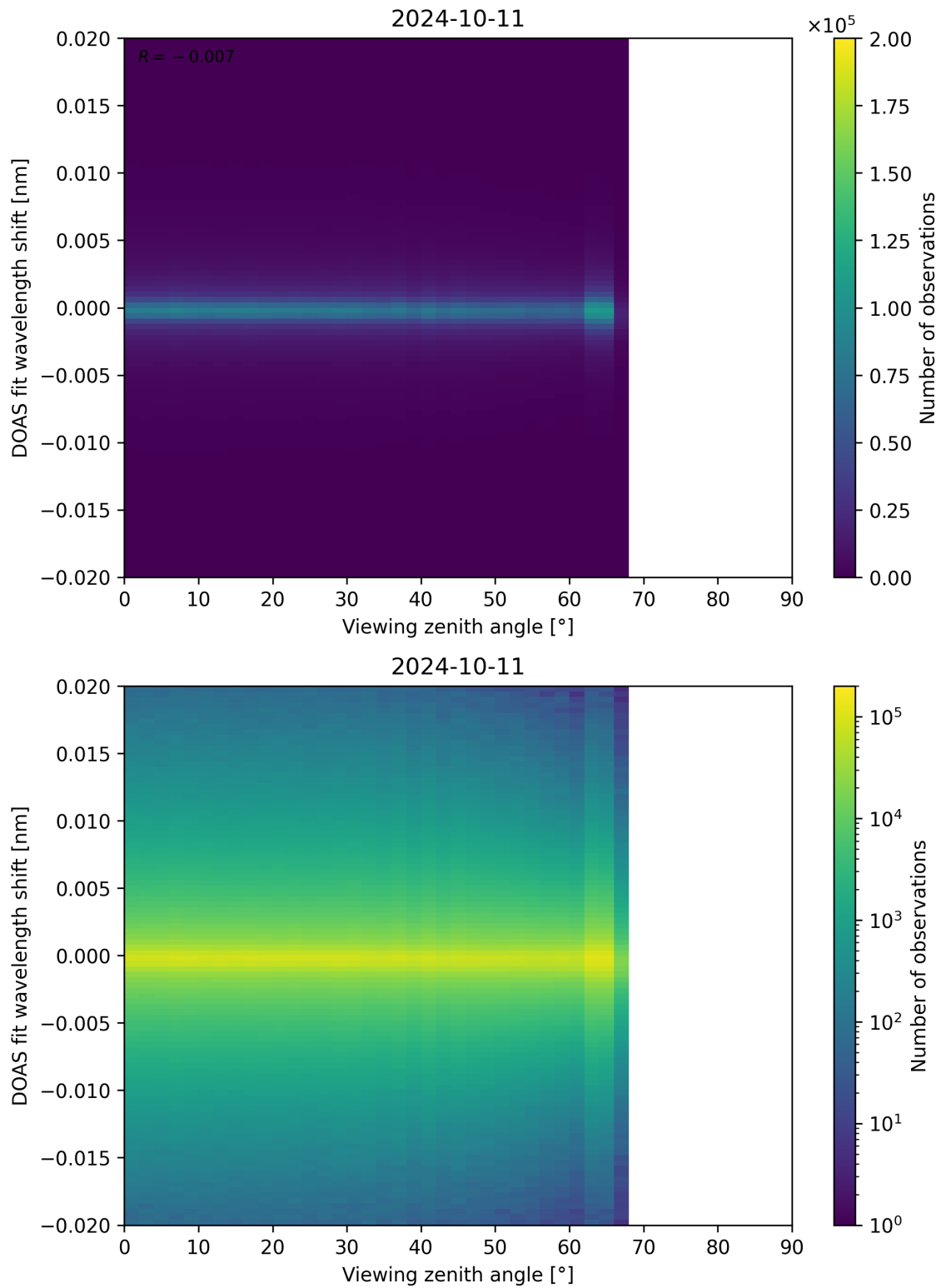
Figure 183: Scatter density plot of “Viewing zenith angle” against “DOAS fit wavelength shift” for 2024-10-10 to 2024-10-12.
