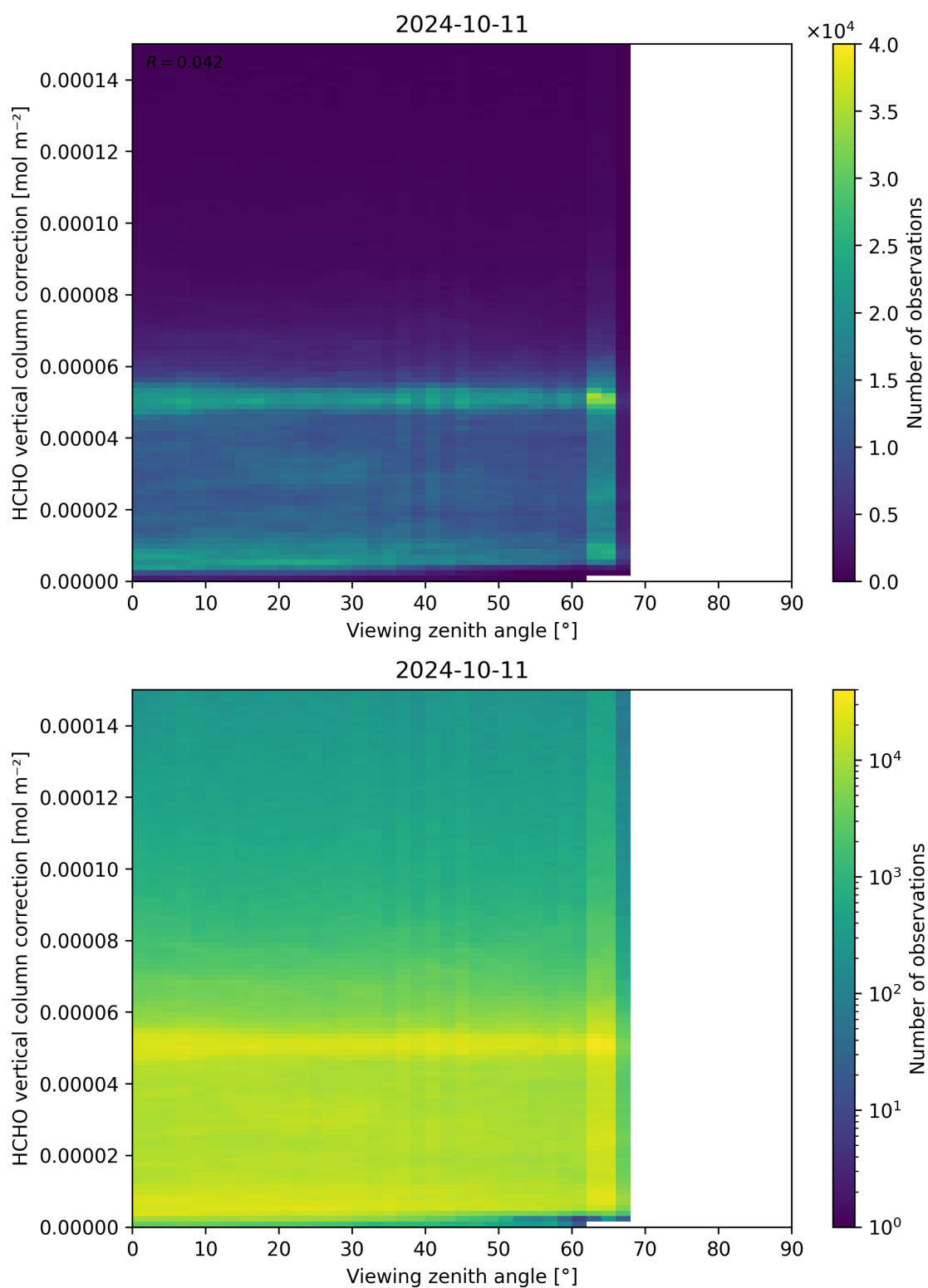
Figure 193: Scatter density plot of “Viewing zenith angle” against “HCHO vertical column correction” for 2024-10-10 to 2024-10-12.
