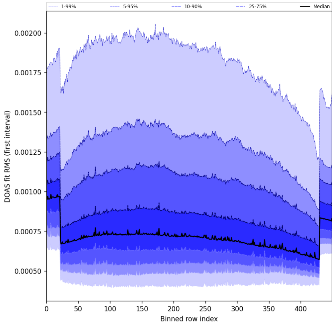
Figure 60: Along track statistics of “DOAS fit RMS (first interval)” for 2024-10-10 to 2024-10-12
