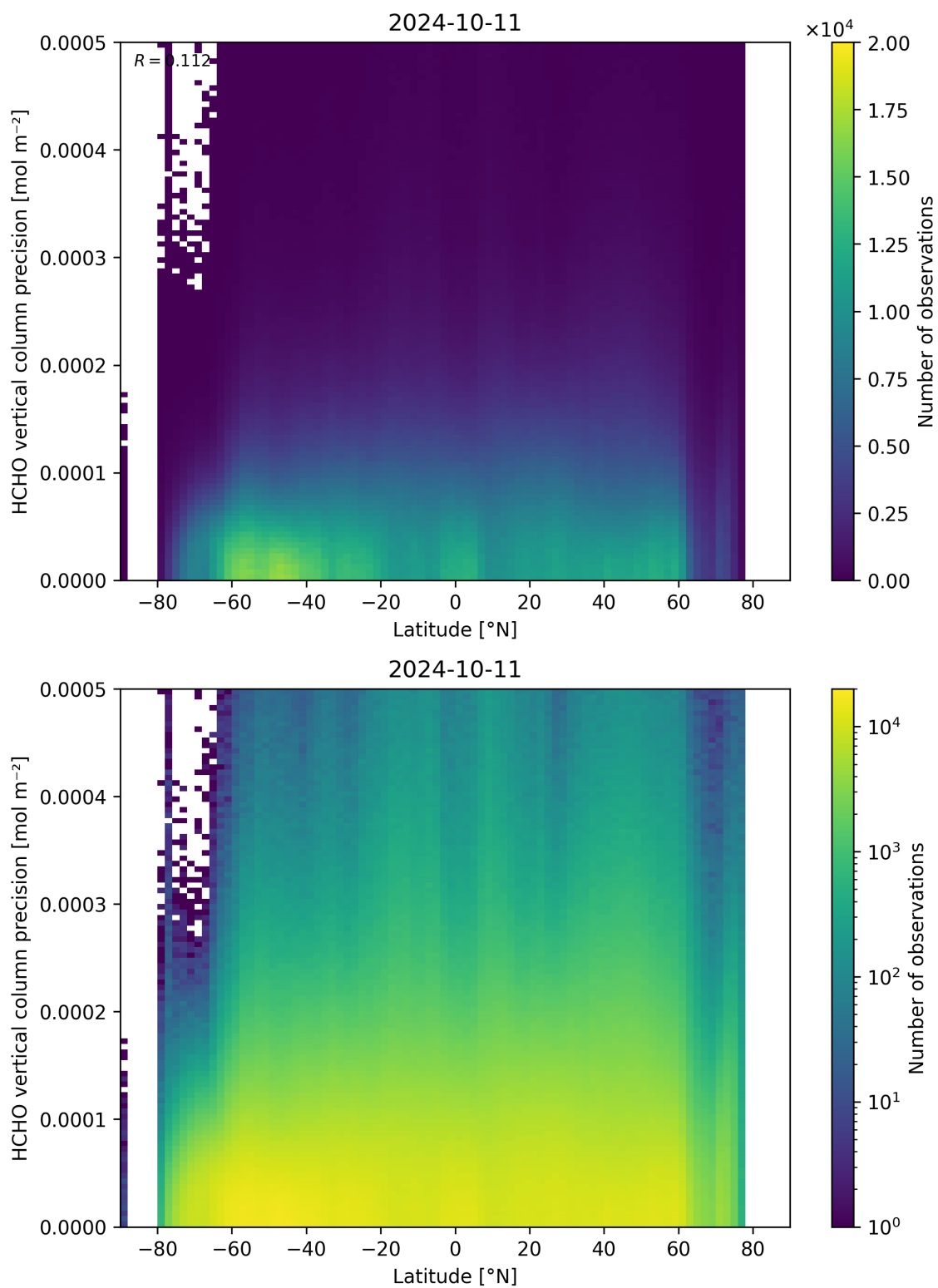
Figure 165: Scatter density plot of “Latitude” against “HCHO vertical column precision” for 2024-10-10 to 2024-10-12.
