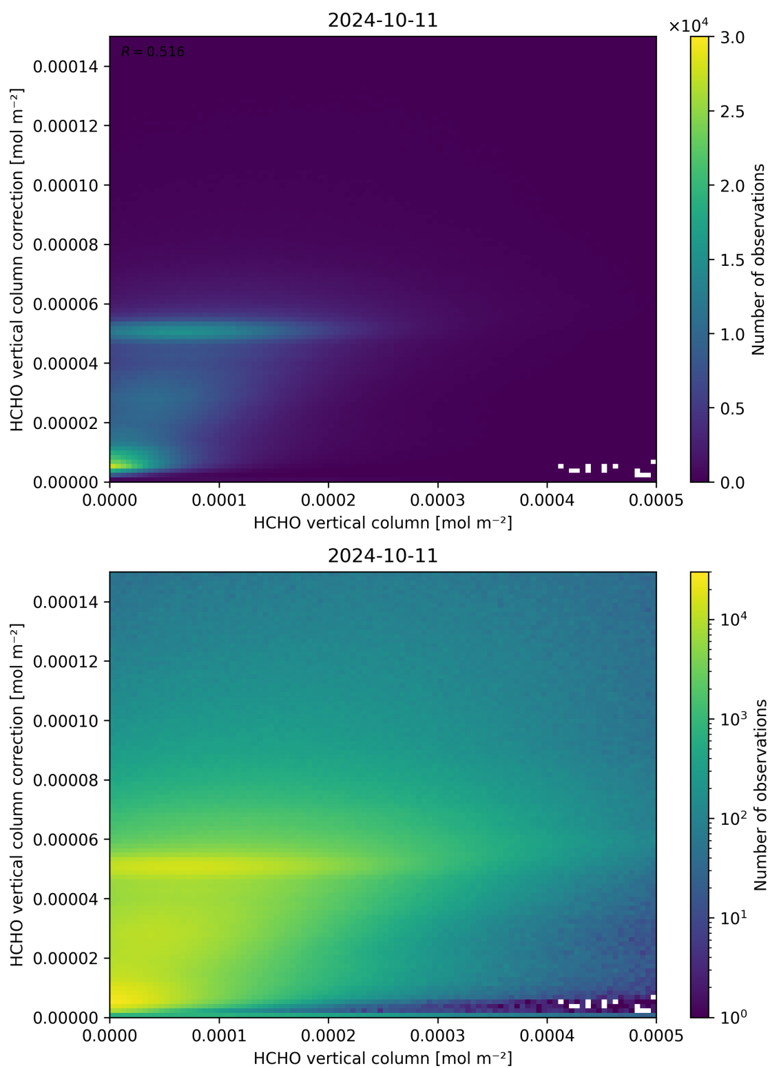
Figure 133: Scatter density plot of “HCHO vertical column” against “HCHO vertical column correction” for 2024-10-10 to 2024-10-12.
