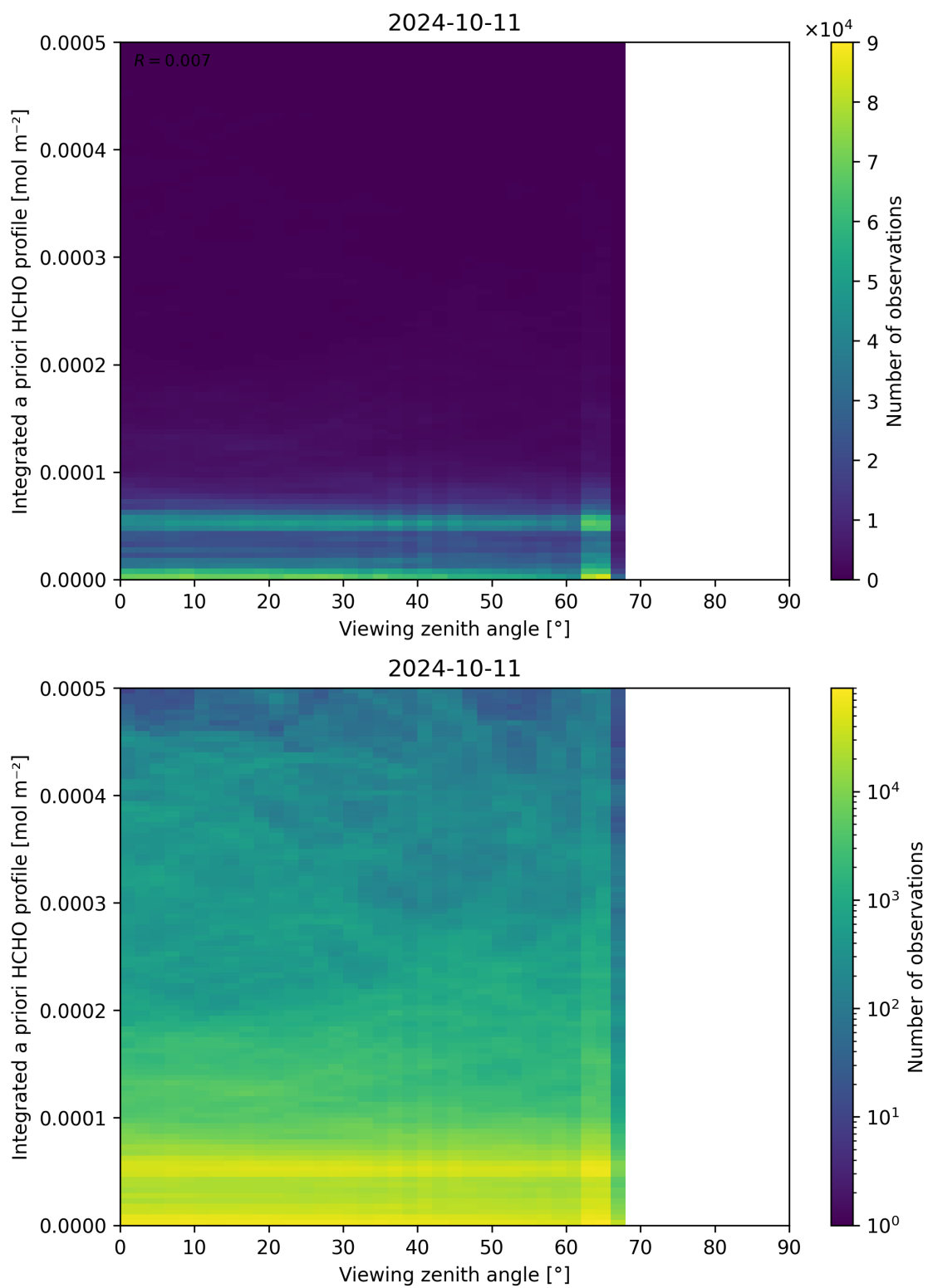
Figure 195: Scatter density plot of “Viewing zenith angle” against “Integrated a priori HCHO profile” for 2024-10-10 to 2024-10-12.
