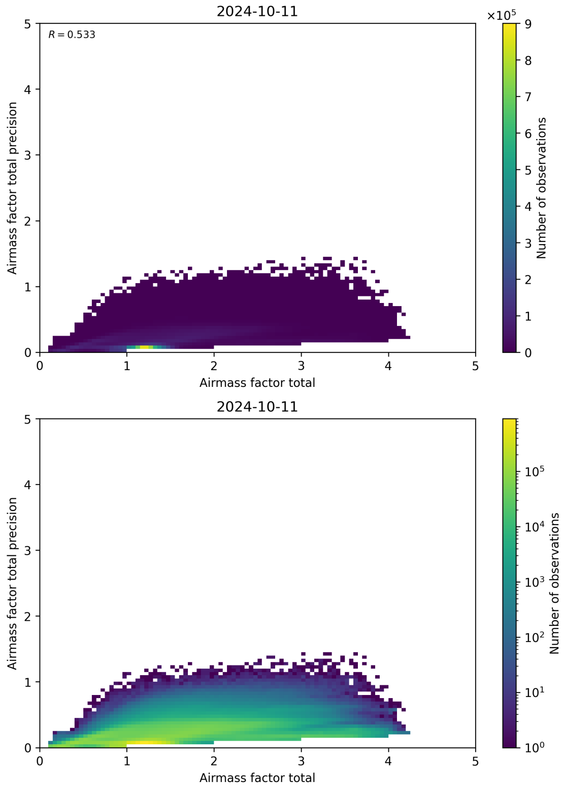
Figure 103: Scatter density plot of “Airmass factor total” against “Airmass factor total precision” for 2024-10-10 to 2024-10-12.
