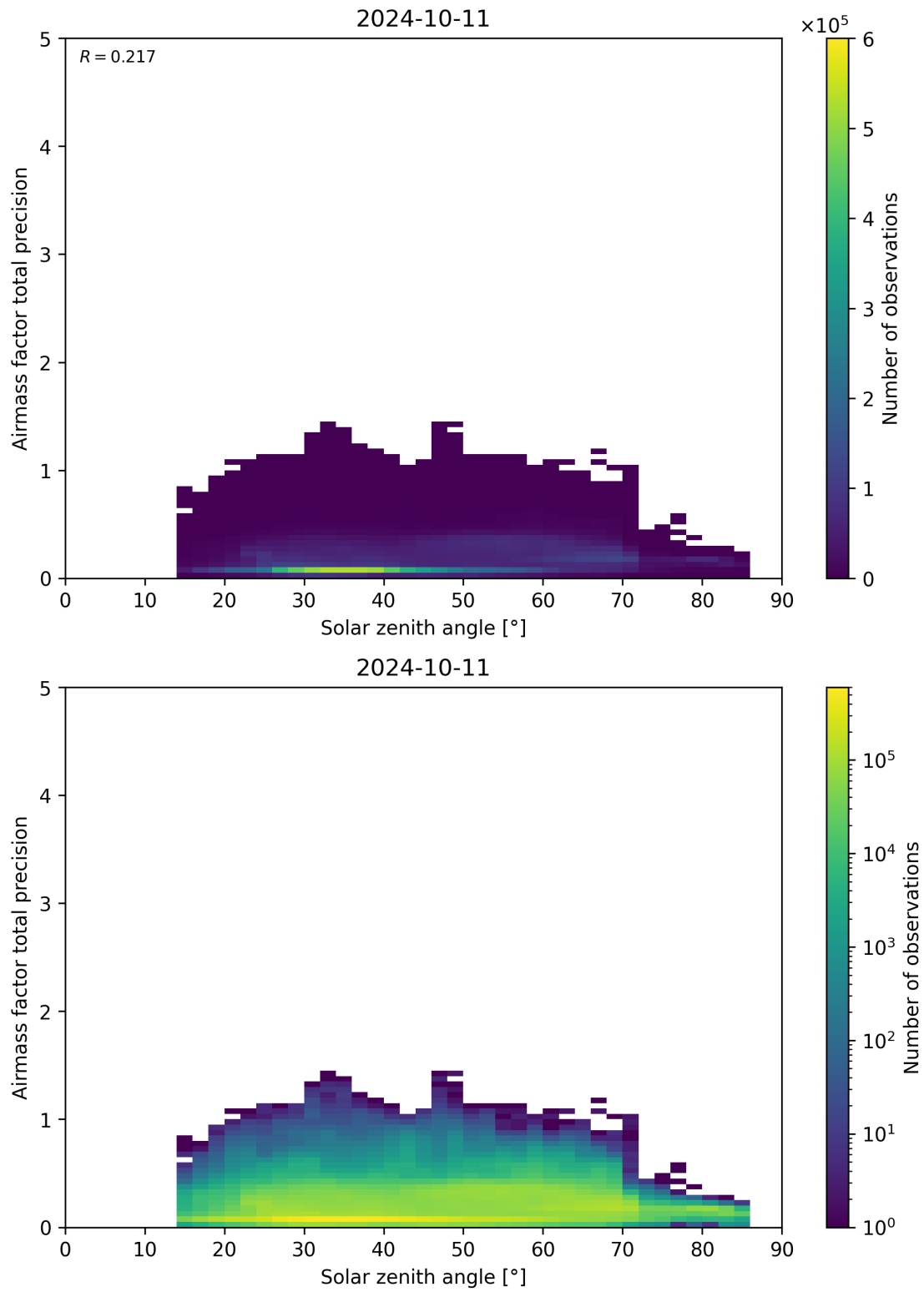
Figure 176: Scatter density plot of “Solar zenith angle” against “Airmass factor total precision” for 2024-10-10 to 2024-10-12.
