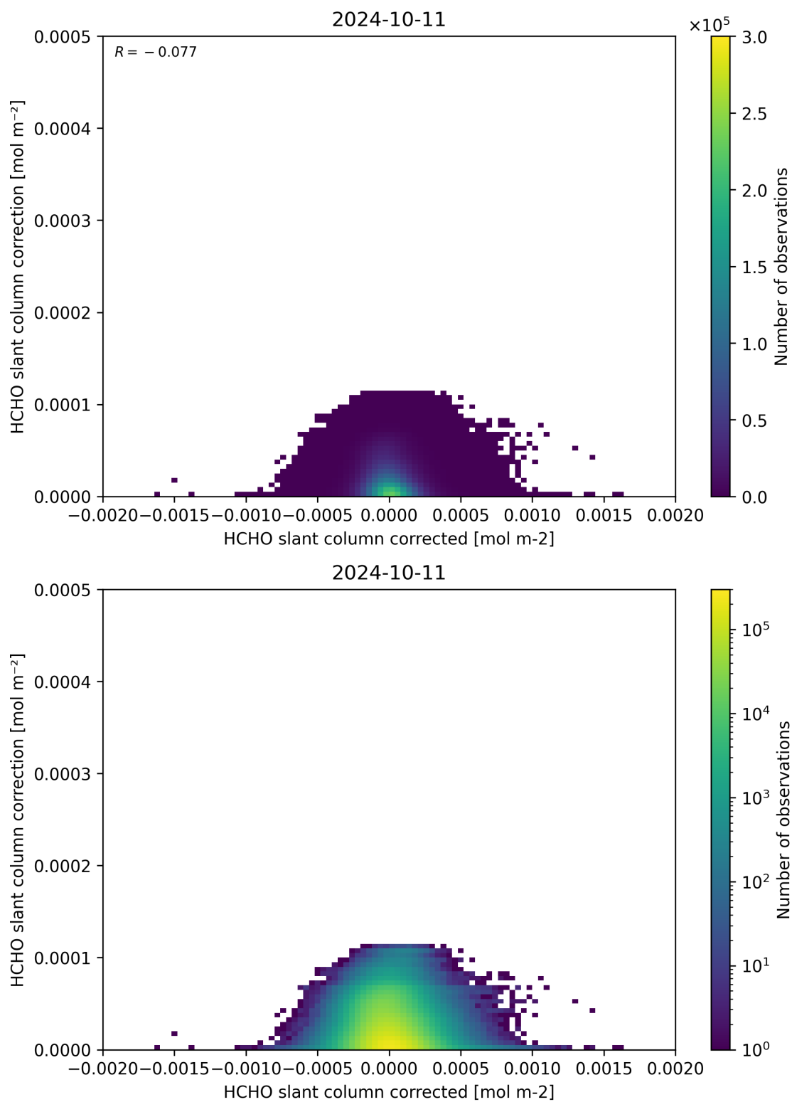
Figure 77: Scatter density plot of “HCHO slant column corrected” against “HCHO slant column correction” for 2024-10-10 to 2024-10-12.
