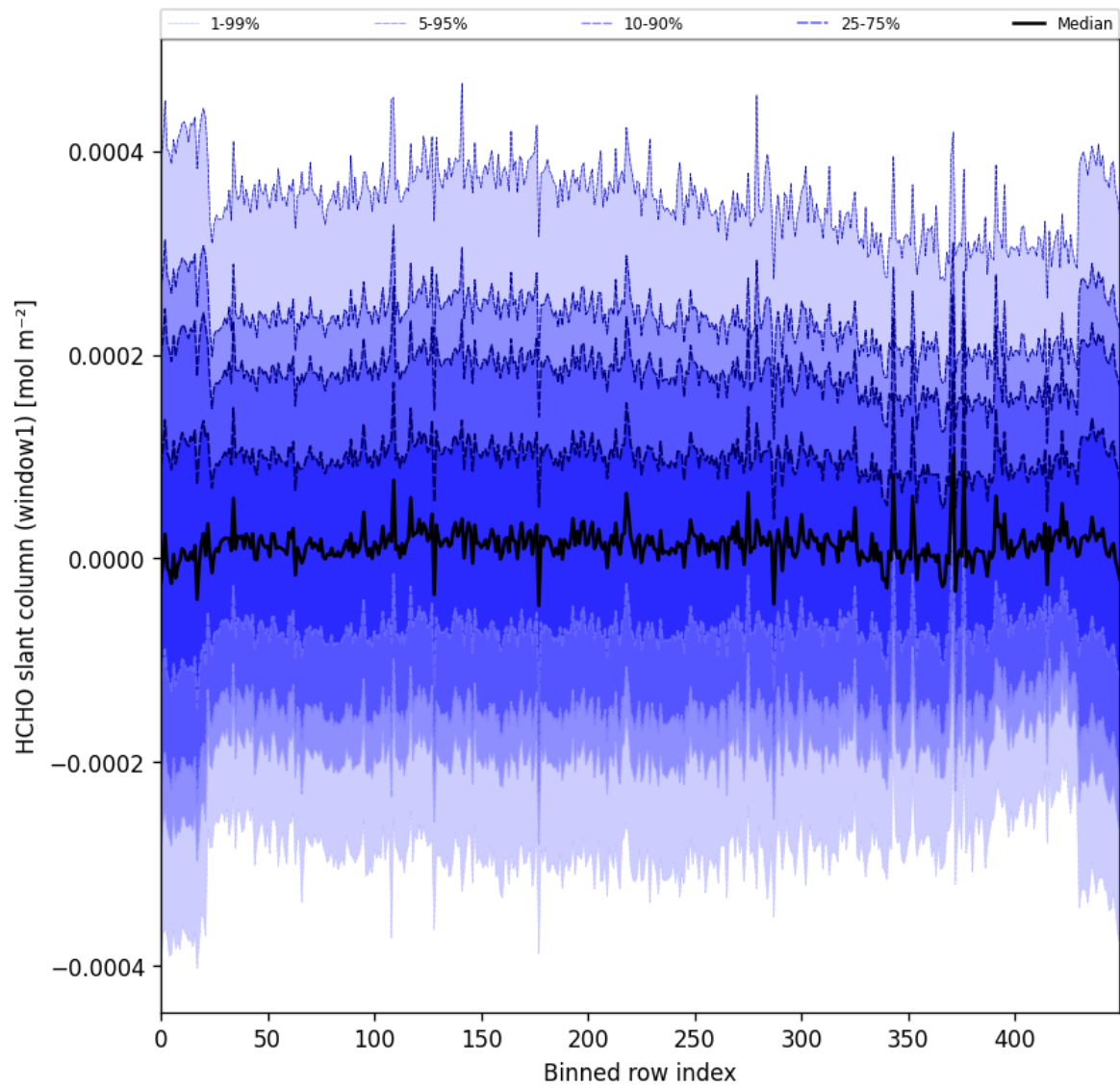
Figure 52: Along track statistics of “HCHO slant column (window1)” for 2024-10-10 to 2024-10-12
