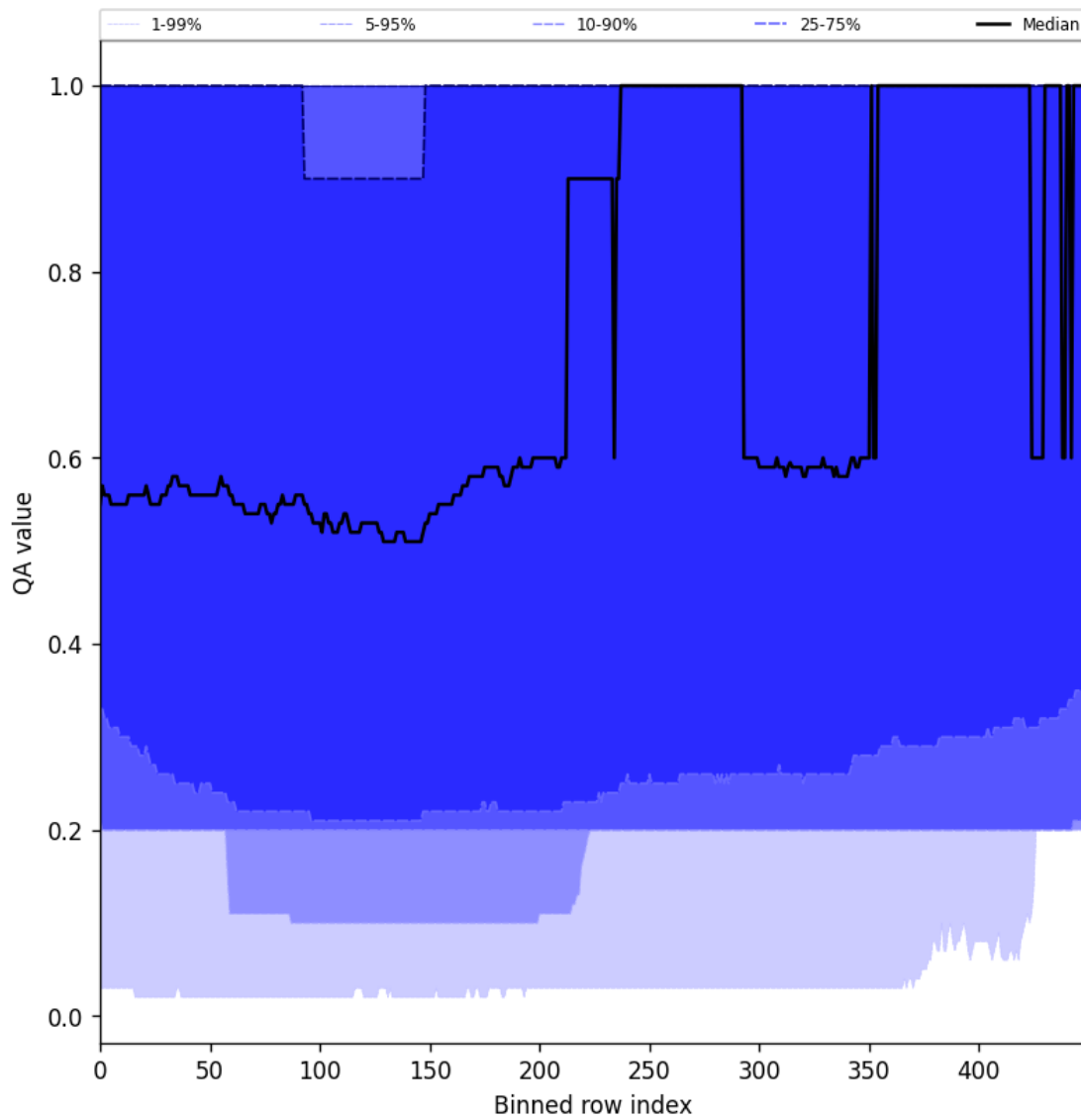
Figure 48: Along track statistics of “QA value” for 2024-10-10 to 2024-10-12
