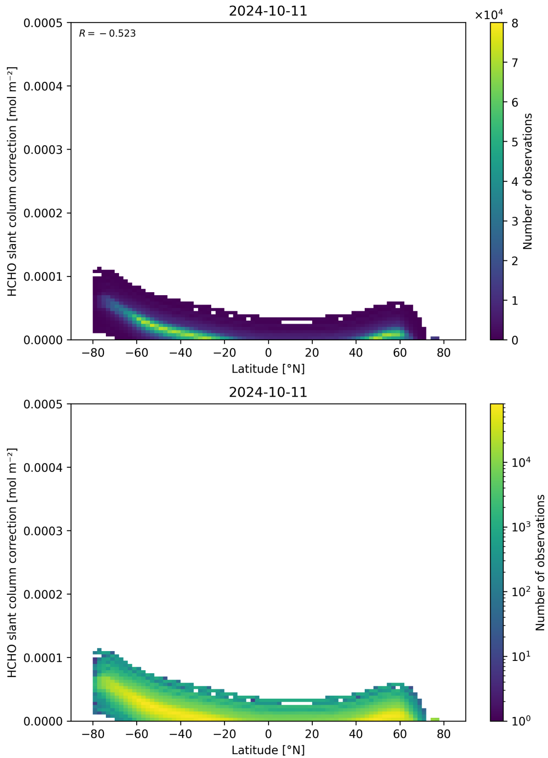
Figure 158: Scatter density plot of “Latitude” against “HCHO slant column correction” for 2024-10-10 to 2024-10-12.
