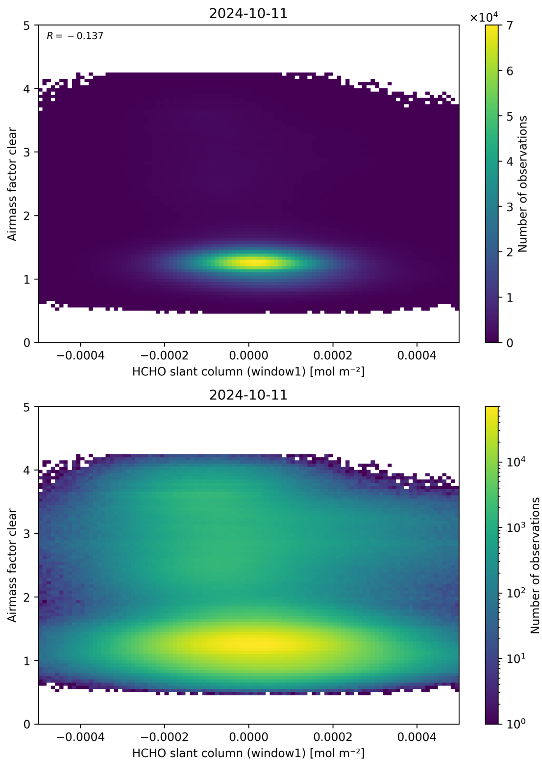
Figure 81: Scatter density plot of “HCHO slant column (window1)” against “Airmass factor clear” for 2024-10-10 to 2024-10-12.
