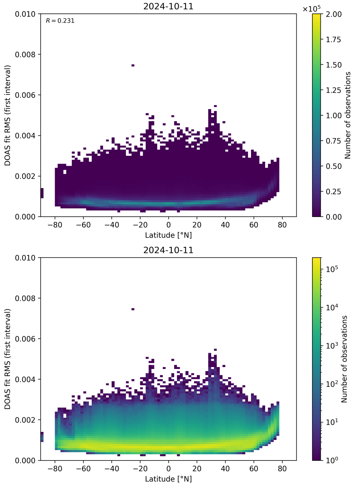
Figure 153: Scatter density plot of “Latitude” against “DOAS fit RMS (first interval)” for 2024-10-10 to 2024-10-12.
