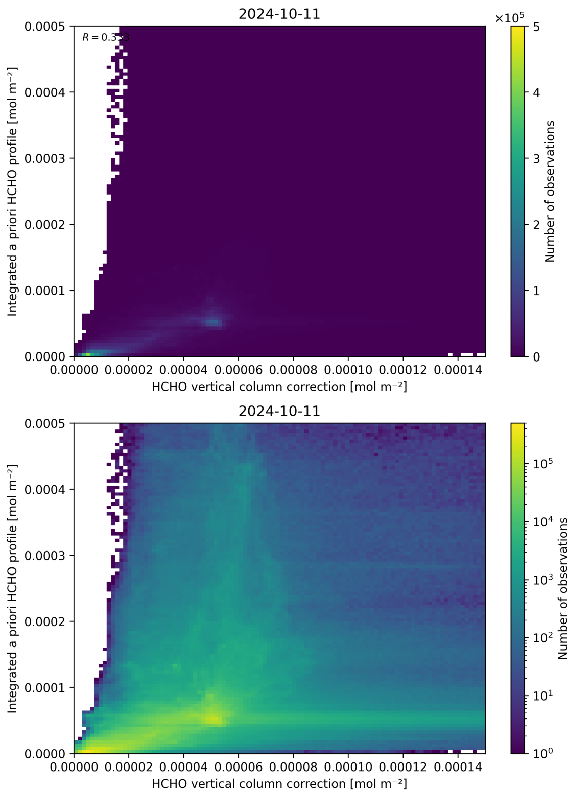
Figure 122: Scatter density plot of “HCHO vertical column correction” against “Integrated a priori HCHO profile” for 2024-10-10 to 2024-10-12.
