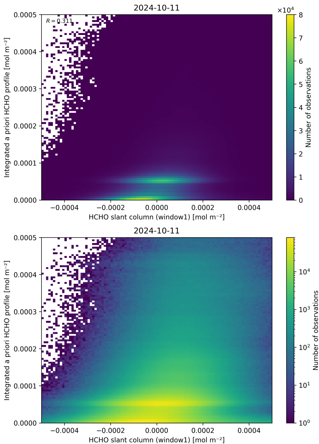
Figure 87: Scatter density plot of “HCHO slant column (window1)” against “Integrated a priori HCHO profile” for 2024-10-10 to 2024-10-12.
