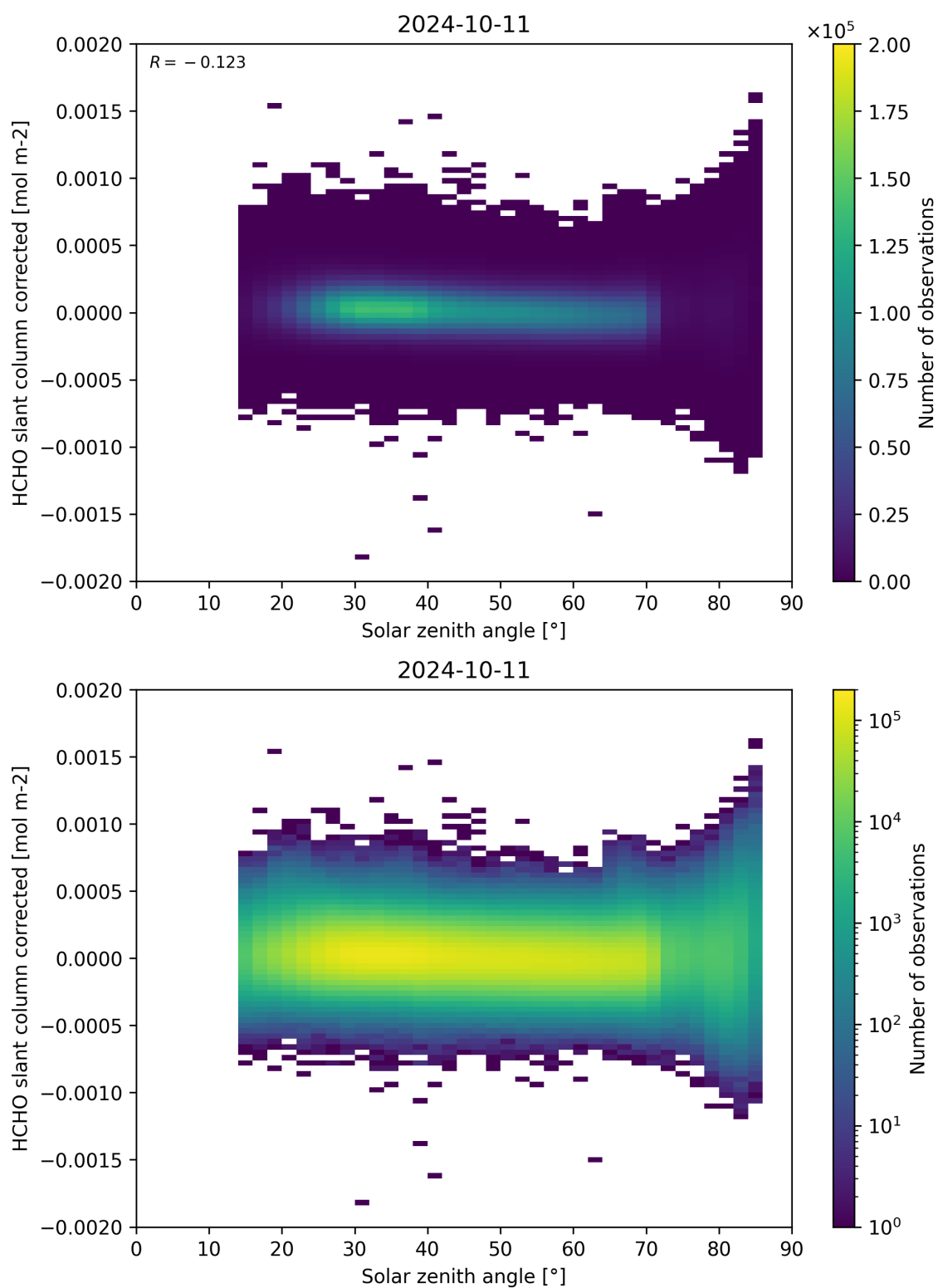
Figure 171: Scatter density plot of “Solar zenith angle” against “HCHO slant column corrected” for 2024-10-10 to 2024-10-12.
