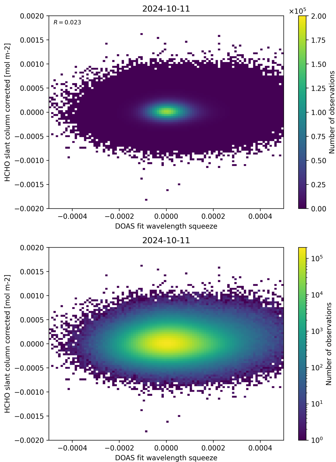
Figure 69: Scatter density plot of “DOAS fit wavelength squeeze” against “HCHO slant column corrected” for 2024-10-10 to 2024-10-12.
