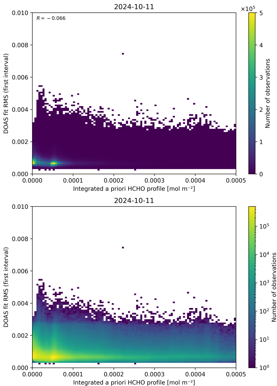
Figure 148: Scatter density plot of “Integrated a priori HCHO profile” against “DOAS fit RMS (first interval)” for 2024-10-10 to 2024-10-12.
