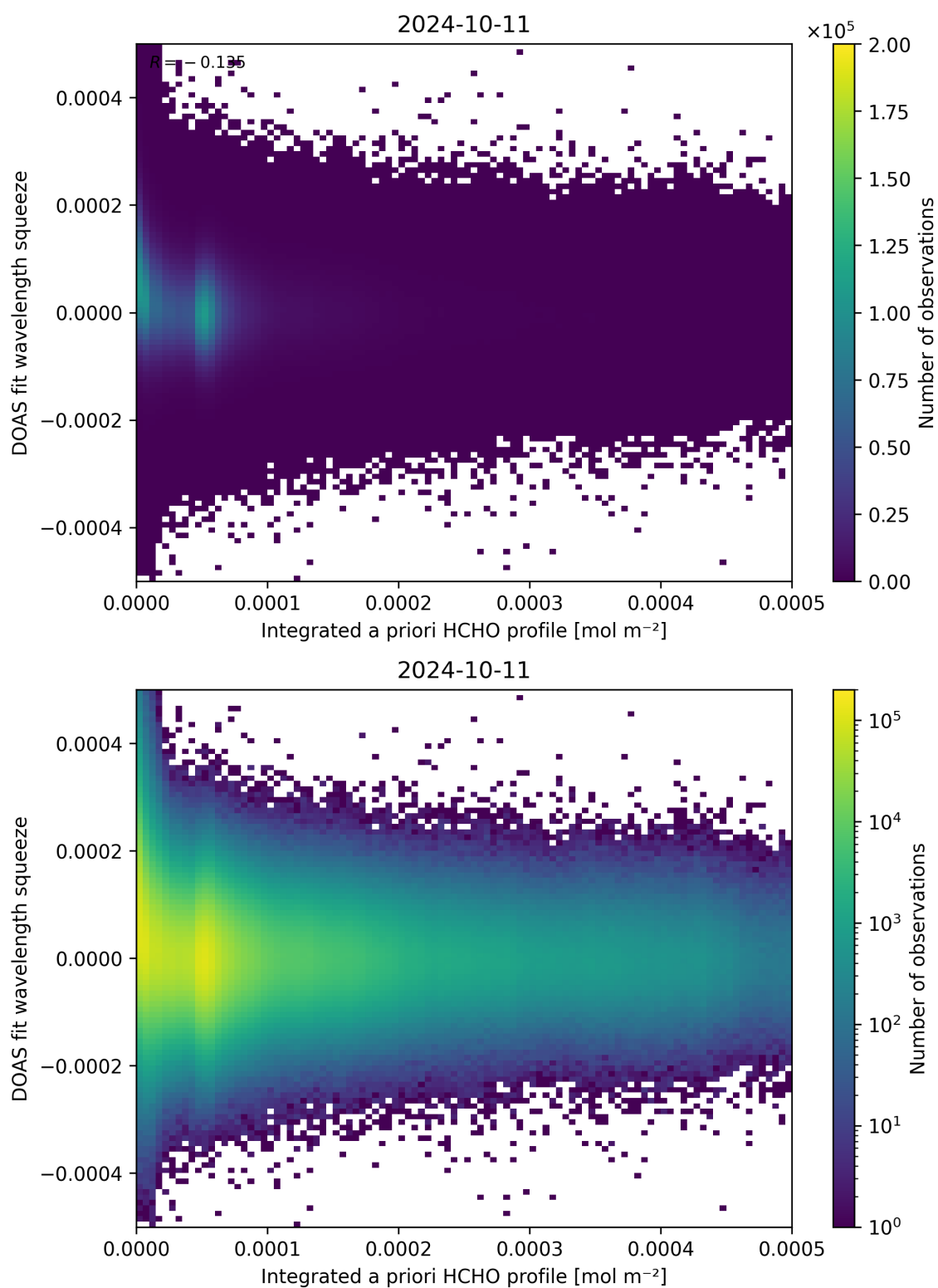
Figure 150: Scatter density plot of “Integrated a priori HCHO profile” against “DOAS fit wavelength squeeze” for 2024-10-10 to 2024-10-12.
