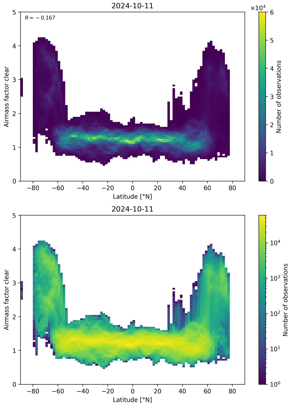
Figure 156: Scatter density plot of “Latitude” against “Airmass factor clear” for 2024-10-10 to 2024-10-12.
