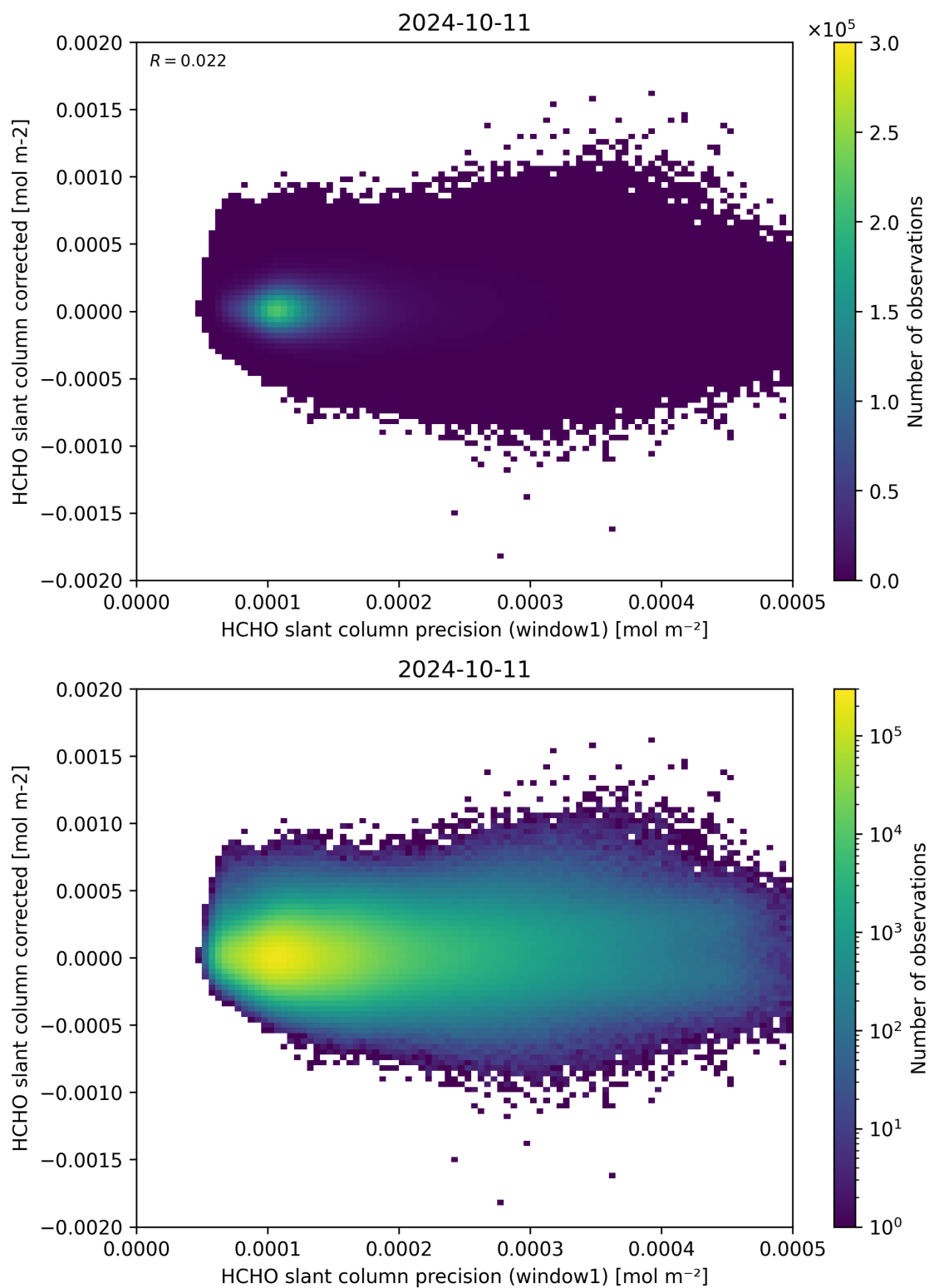
Figure 92: Scatter density plot of “HCHO slant column precision (window1)” against “HCHO slant column corrected” for 2024-10-10 to 2024-10-12.
