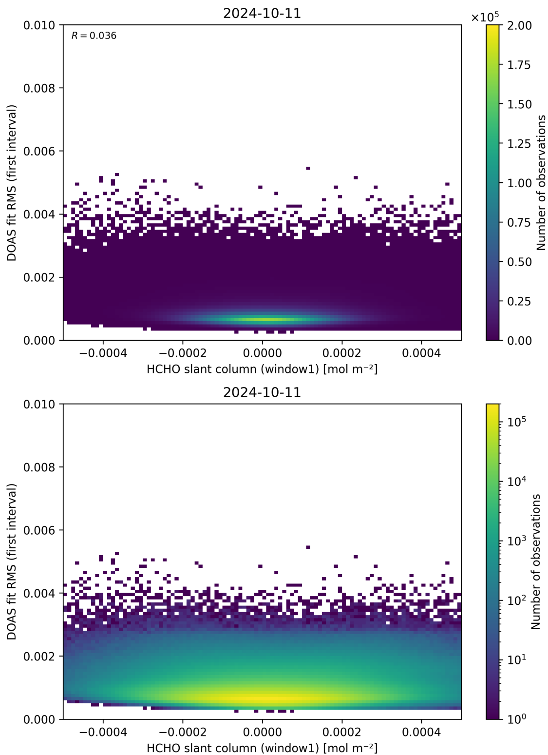
Figure 78: Scatter density plot of “HCHO slant column (window1)” against “DOAS fit RMS (first interval)” for 2024-10-10 to 2024-10-12.
