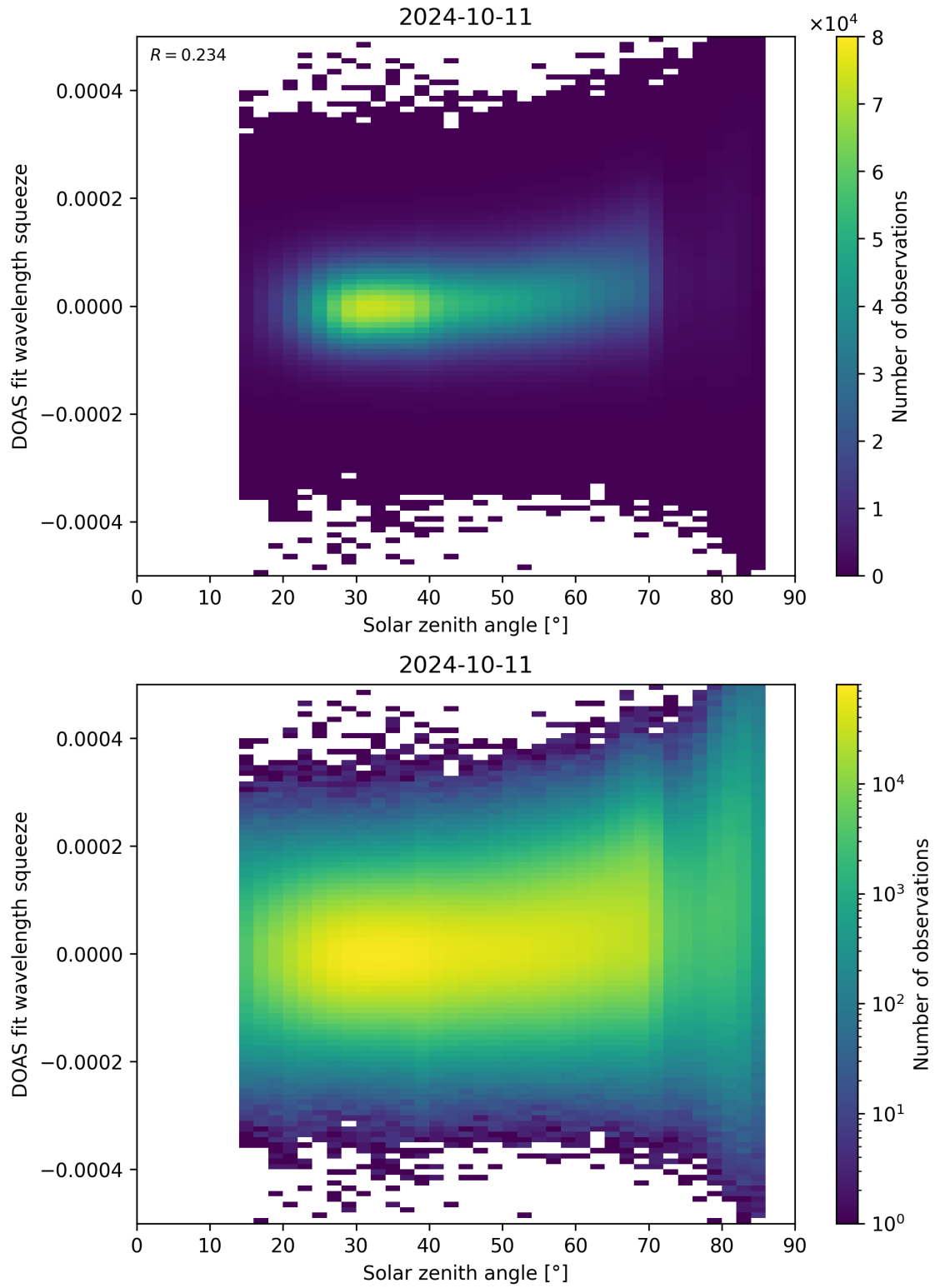
Figure 169: Scatter density plot of “Solar zenith angle” against “DOAS fit wavelength squeeze” for 2024-10-10 to 2024-10-12.
