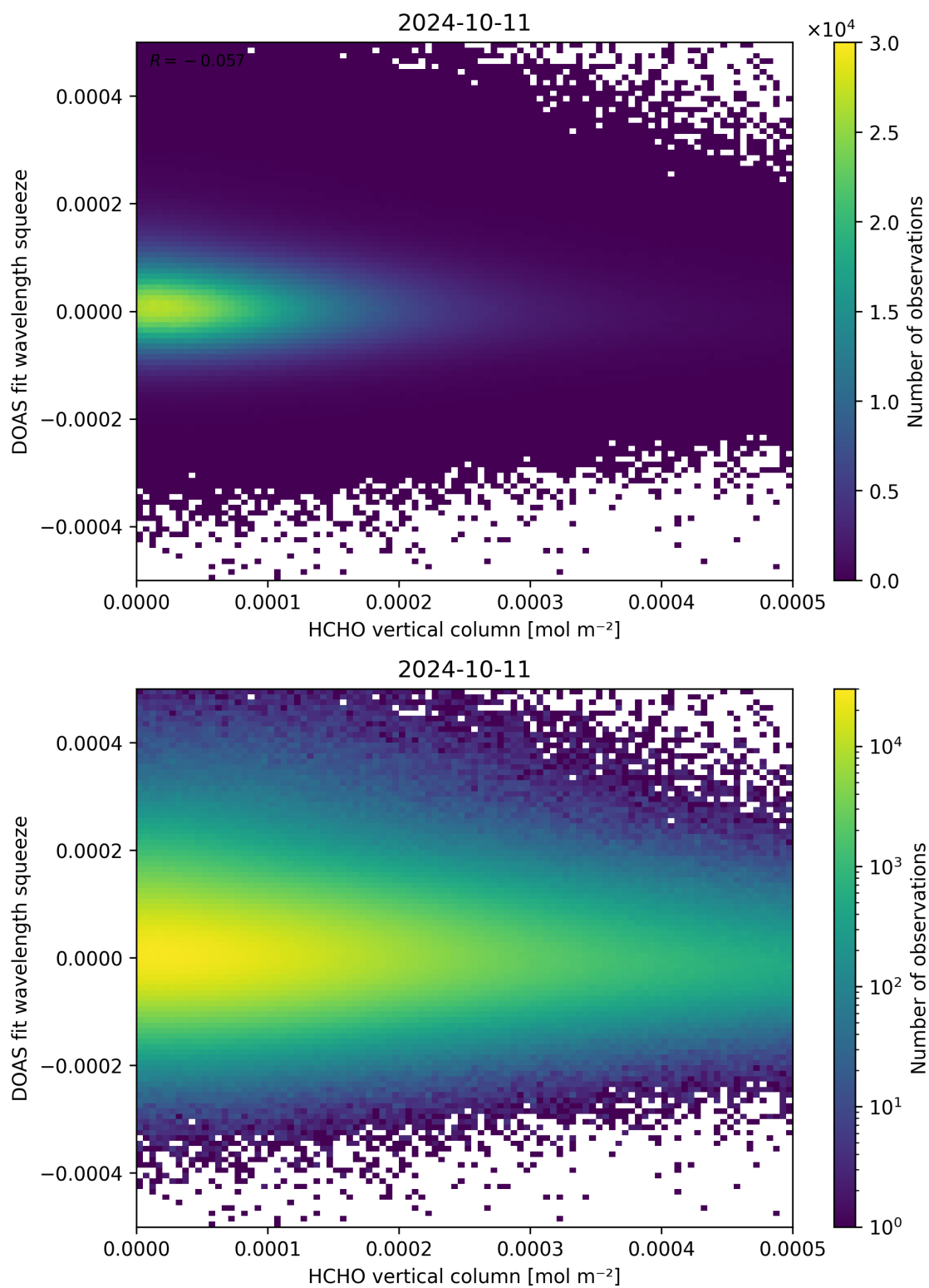
Figure 125: Scatter density plot of “HCHO vertical column” against “DOAS fit wavelength squeeze” for 2024-10-10 to 2024-10-12.
