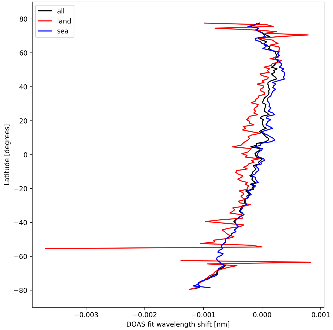
Figure 30: Zonal average of “DOAS fit wavelength shift” for 2024-10-10 to 2024-10-12.
