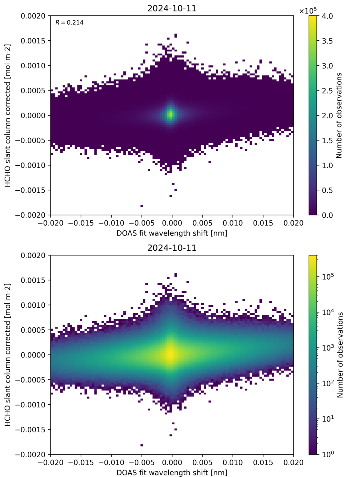
Figure 66: Scatter density plot of “DOAS fit wavelength shift” against “HCHO slant column corrected” for 2024-10-10 to 2024-10-12.
