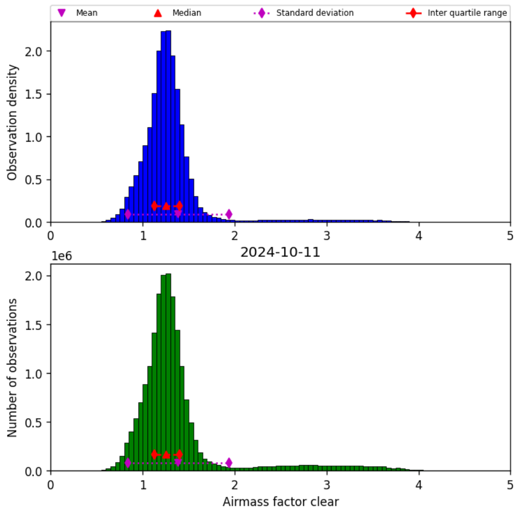
Figure 42: Histogram of “Airmass factor clear” for 2024-10-10 to 2024-10-12
