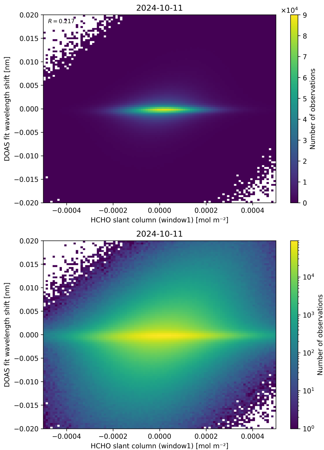
Figure 79: Scatter density plot of “HCHO slant column (window1)” against “DOAS fit wavelength shift” for 2024-10-10 to 2024-10-12.
