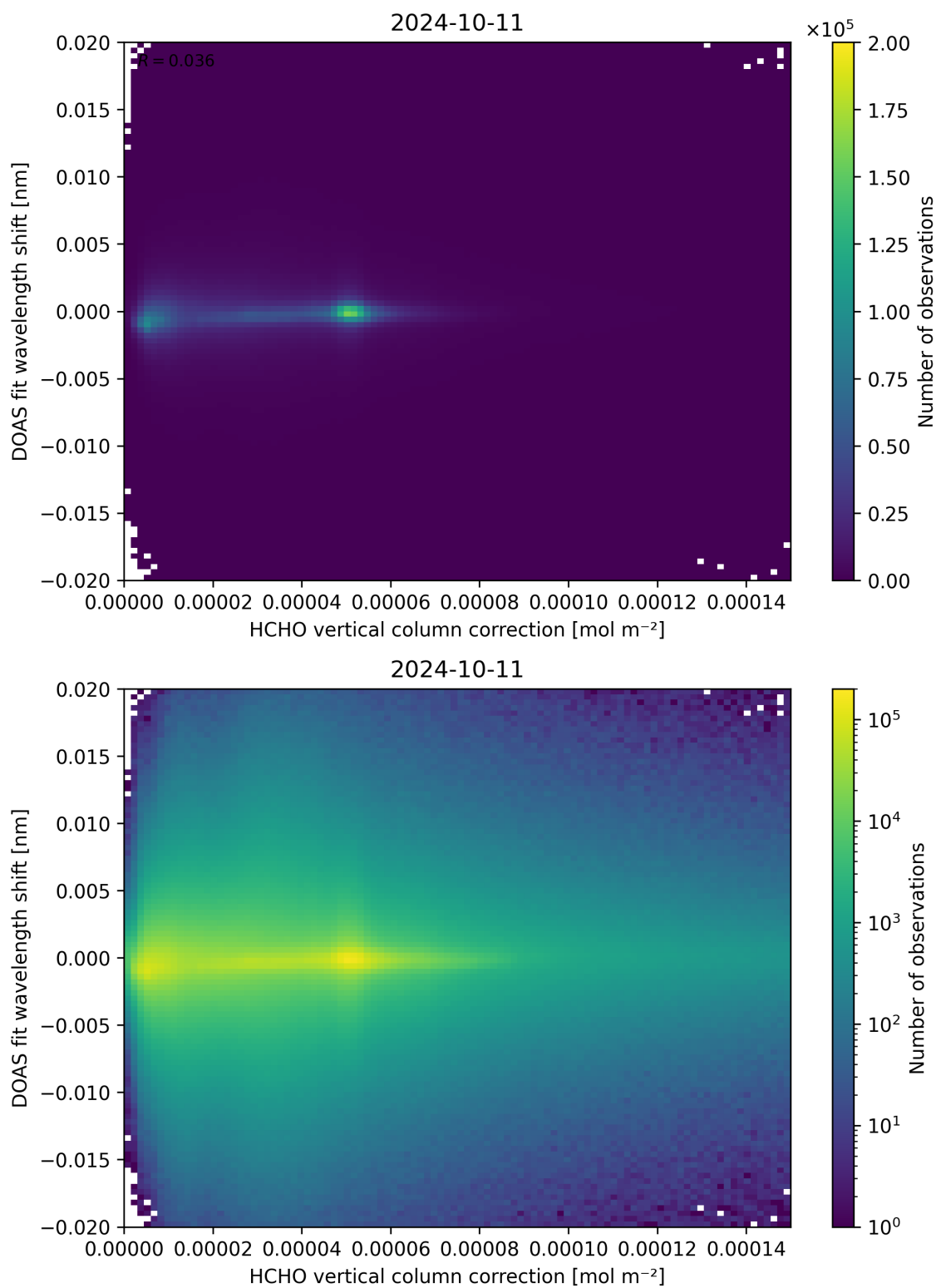
Figure 113: Scatter density plot of “HCHO vertical column correction” against “DOAS fit wavelength shift” for 2024-10-10 to 2024-10-12.
