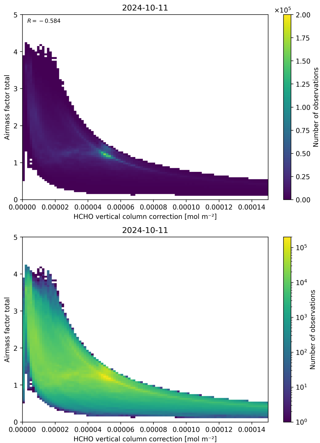
Figure 120: Scatter density plot of “HCHO vertical column correction” against “Airmass factor total” for 2024-10-10 to 2024-10-12.
