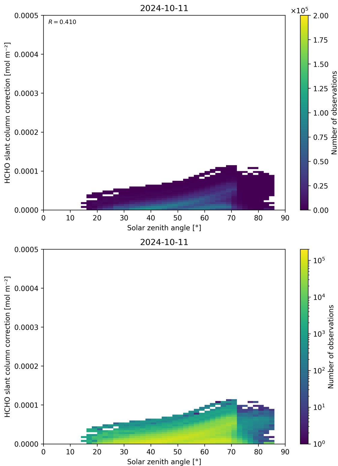
Figure 172: Scatter density plot of “Solar zenith angle” against “HCHO slant column correction” for 2024-10-10 to 2024-10-12.
