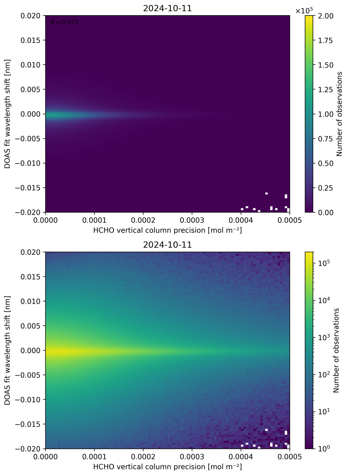
Figure 137: Scatter density plot of “HCHO vertical column precision” against “DOAS fit wavelength shift” for 2024-10-10 to 2024-10-12.
