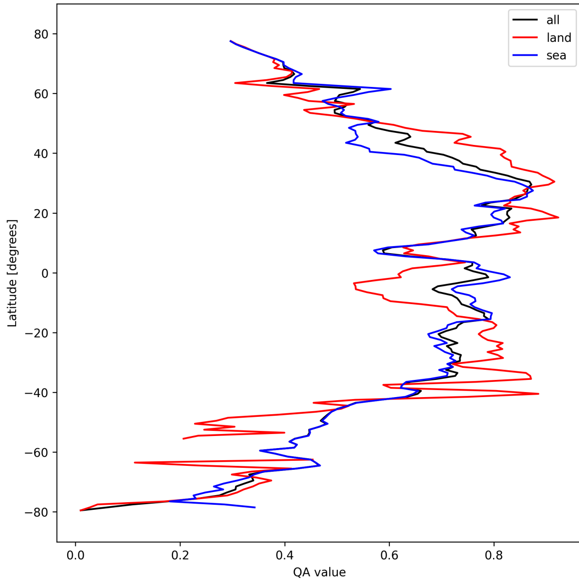
Figure 20: Zonal average of “QA value” for 2024-10-10 to 2024-10-12.
