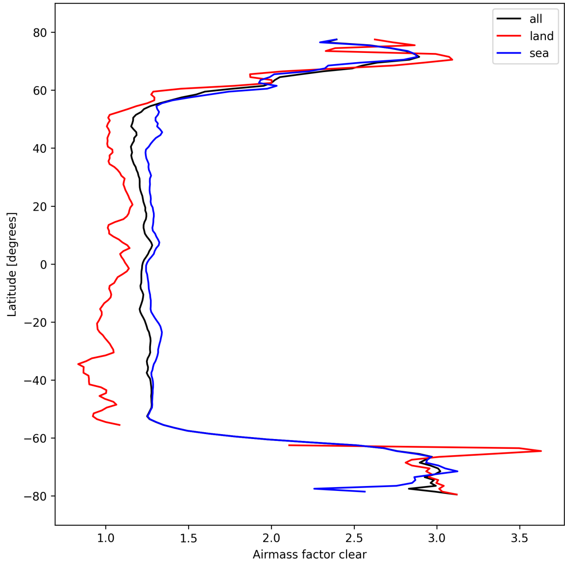
Figure 28: Zonal average of “Airmass factor clear” for 2024-10-10 to 2024-10-12.
