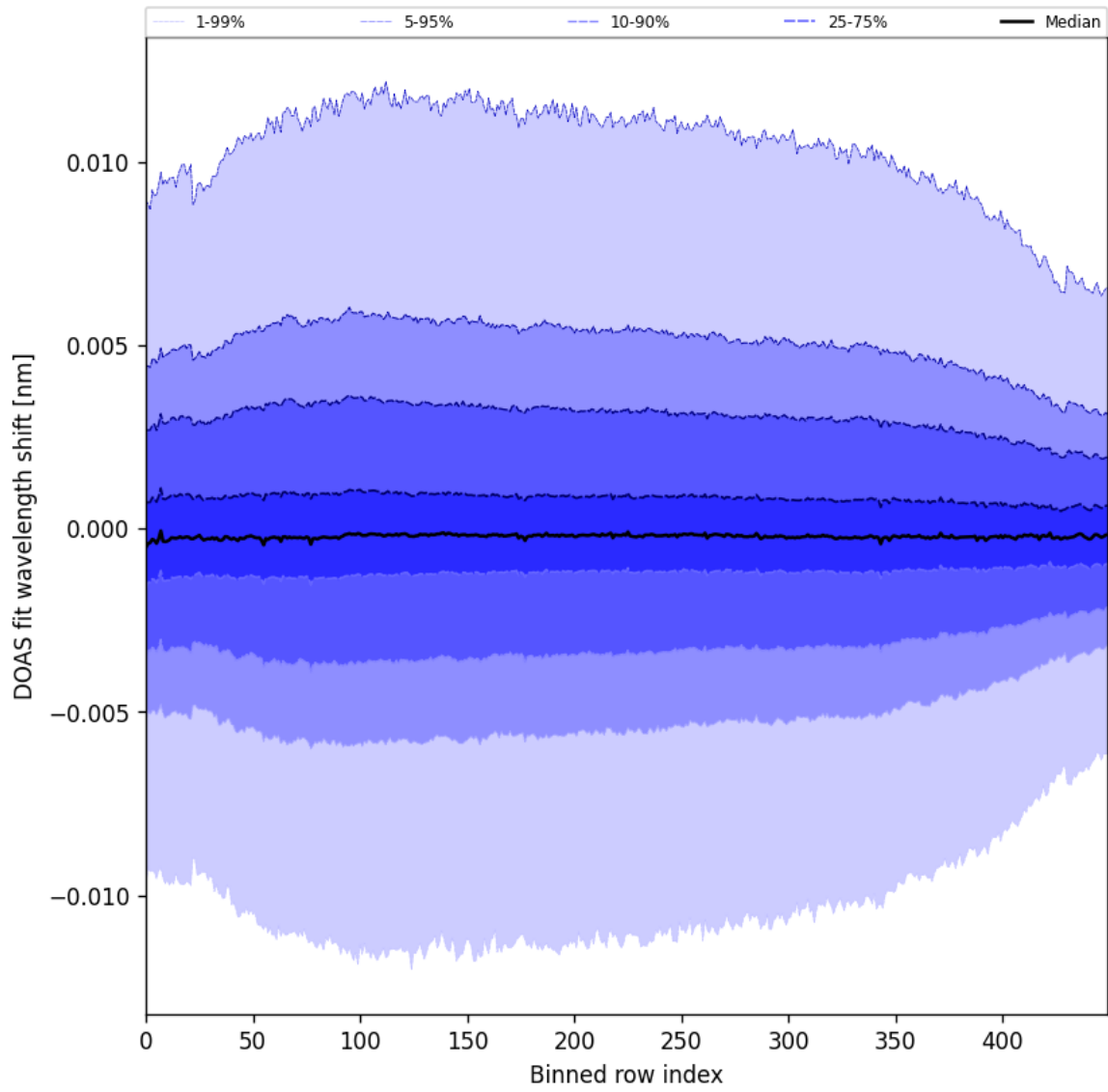
Figure 58: Along track statistics of “DOAS fit wavelength shift” for 2024-10-10 to 2024-10-12
