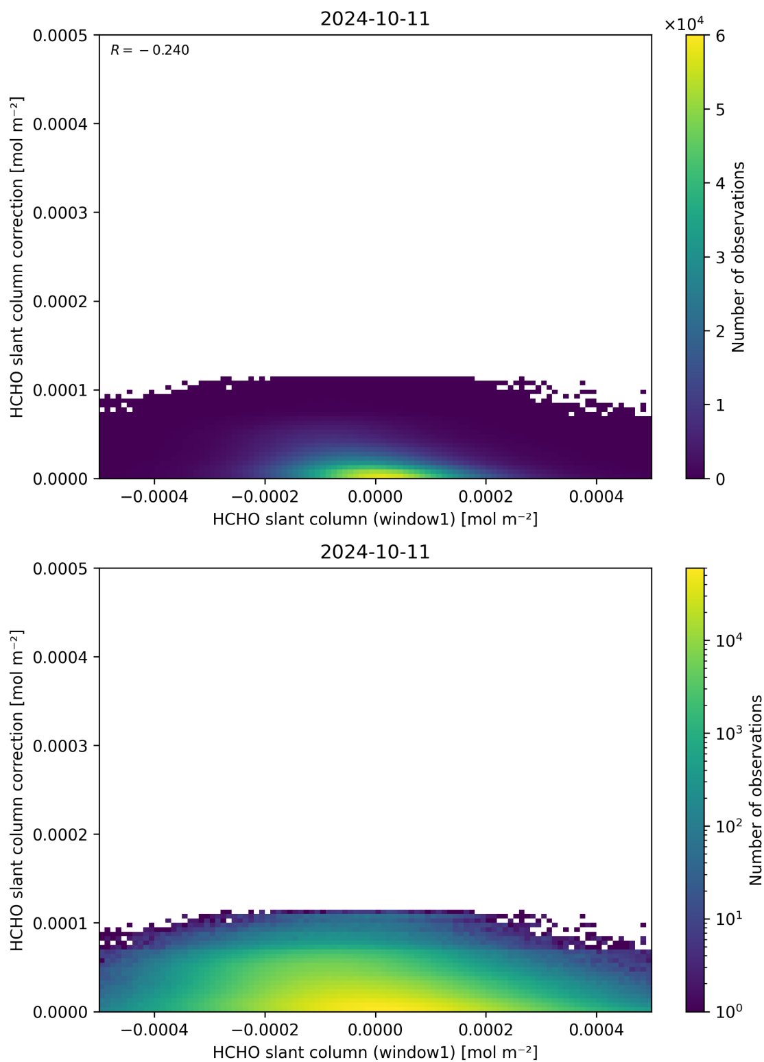
Figure 83: Scatter density plot of “HCHO slant column (window1)” against “HCHO slant column correction” for 2024-10-10 to 2024-10-12.
