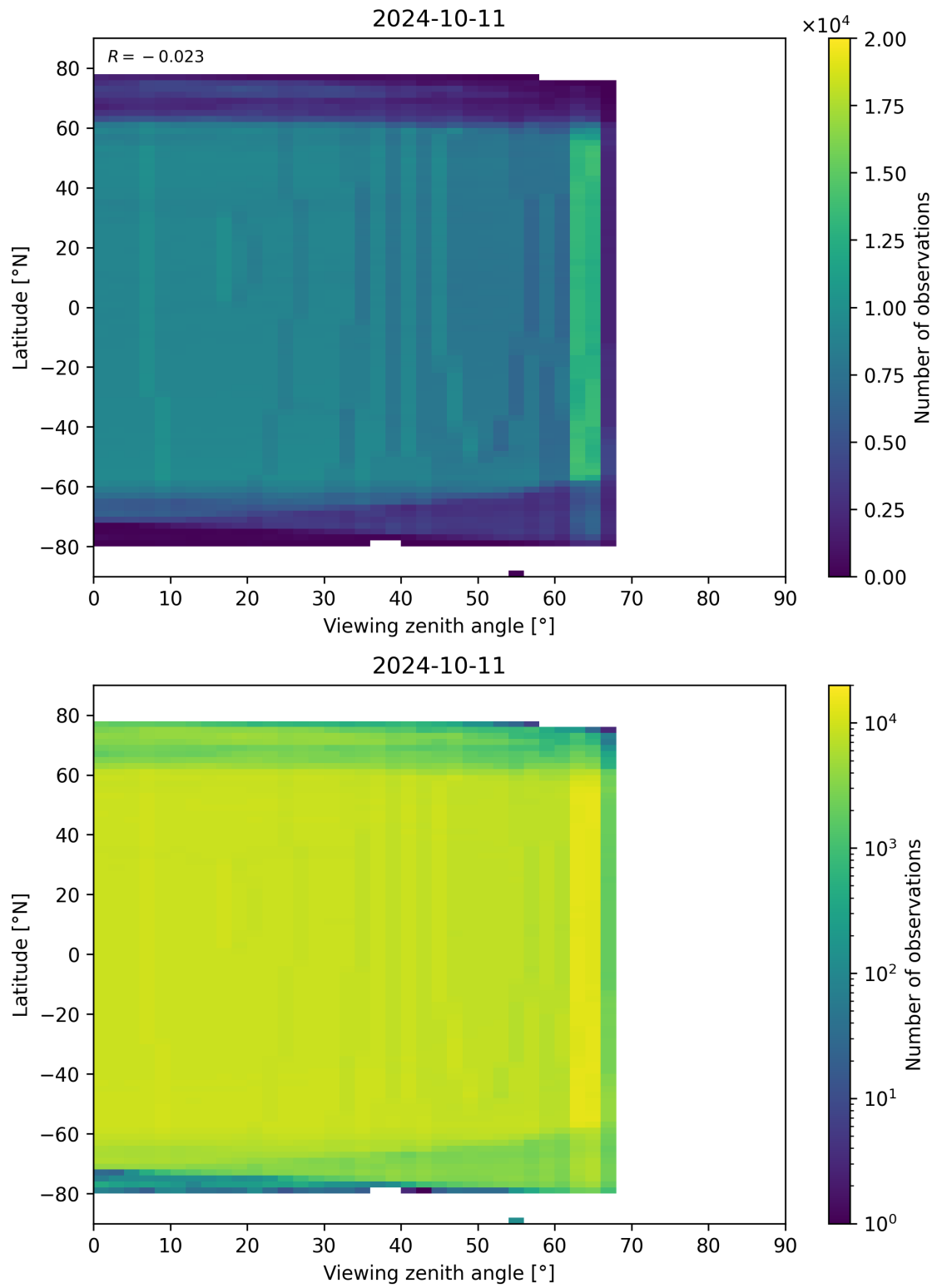
Figure 196: Scatter density plot of “Viewing zenith angle” against “Latitude” for 2024-10-10 to 2024-10-12.
