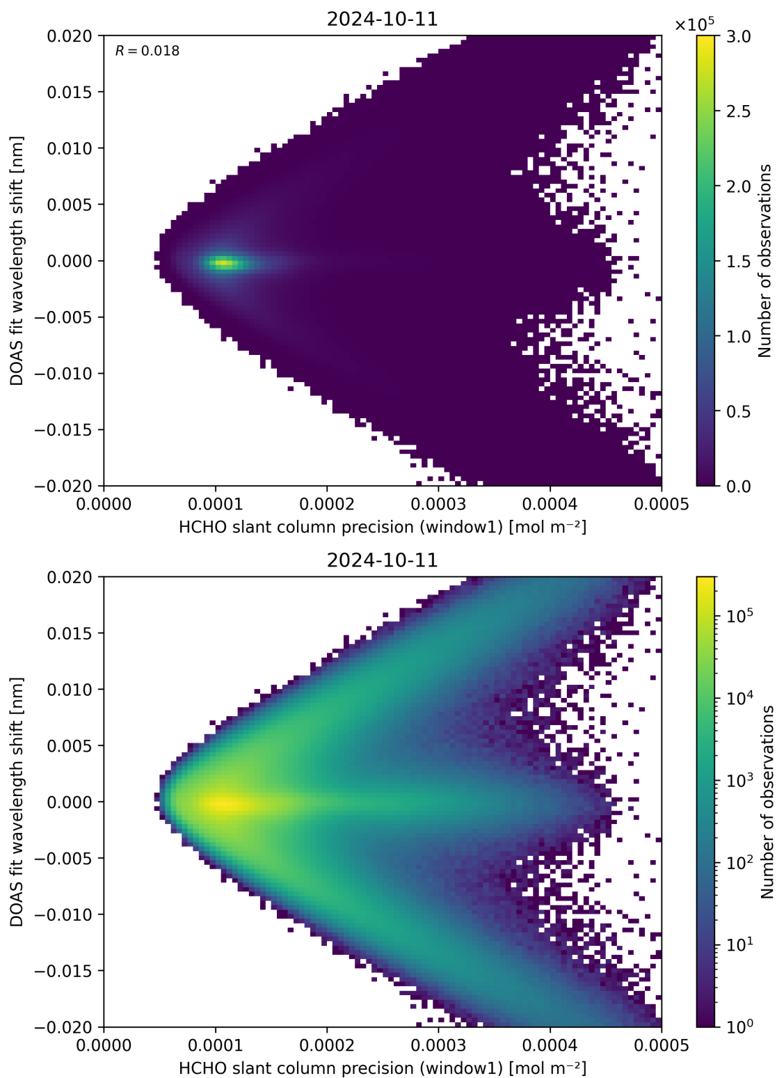
Figure 89: Scatter density plot of “HCHO slant column precision (window1)” against “DOAS fit wavelength shift” for 2024-10-10 to 2024-10-12.
