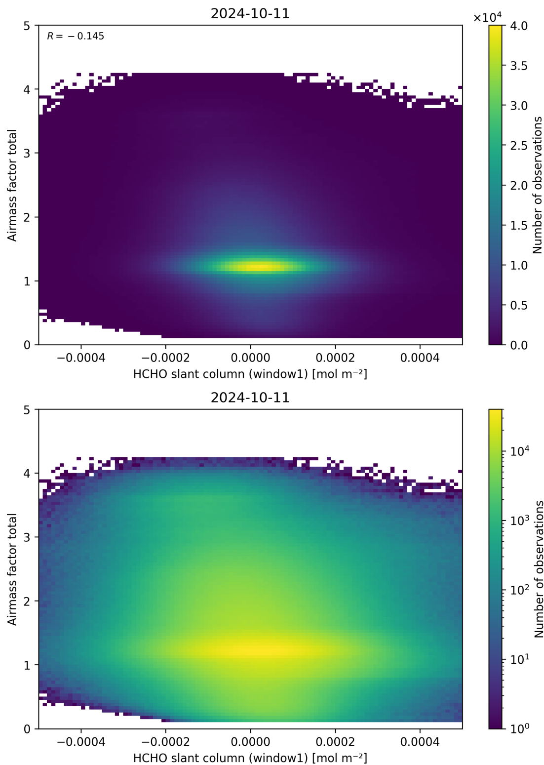
Figure 85: Scatter density plot of “HCHO slant column (window1)” against “Airmass factor total” for 2024-10-10 to 2024-10-12.
