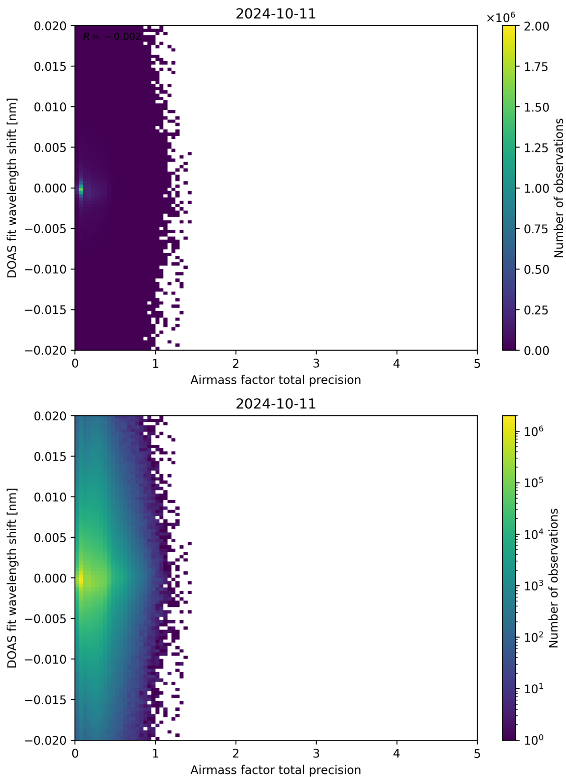
Figure 106: Scatter density plot of “Airmass factor total precision” against “DOAS fit wavelength shift” for 2024-10-10 to 2024-10-12.
