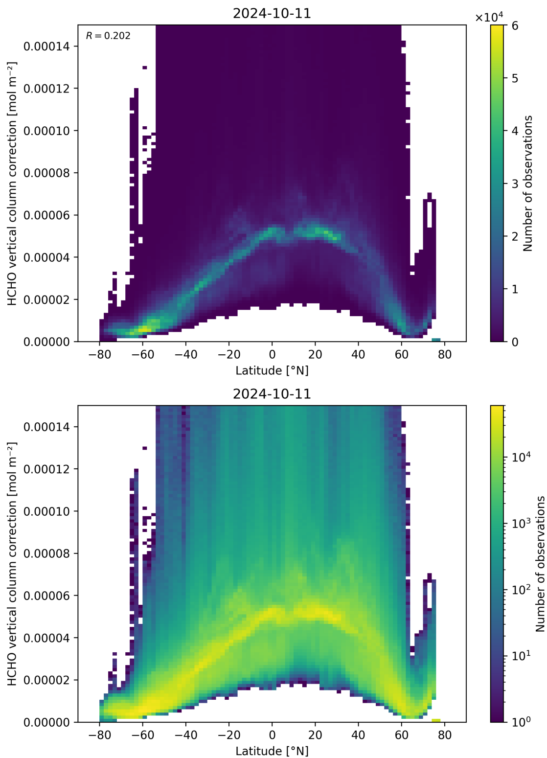
Figure 164: Scatter density plot of “Latitude” against “HCHO vertical column correction” for 2024-10-10 to 2024-10-12.
