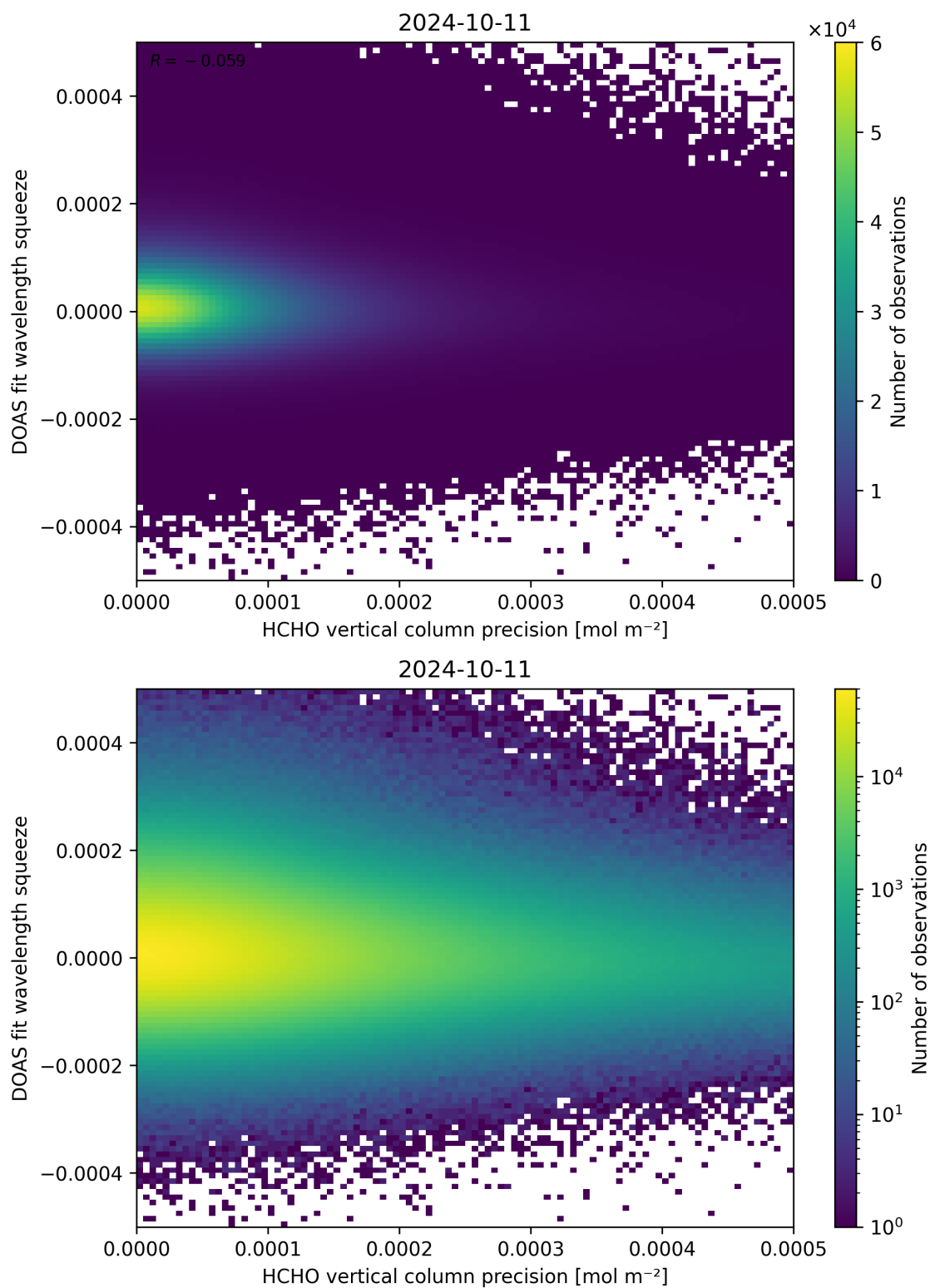
Figure 138: Scatter density plot of “HCHO vertical column precision” against “DOAS fit wavelength squeeze” for 2024-10-10 to 2024-10-12.
