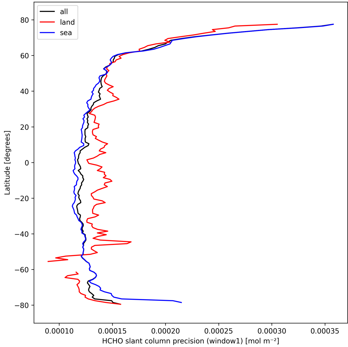
Figure 25: Zonal average of “HCHO slant column precision (window1)” for 2024-10-11 to 2024-10-13.
