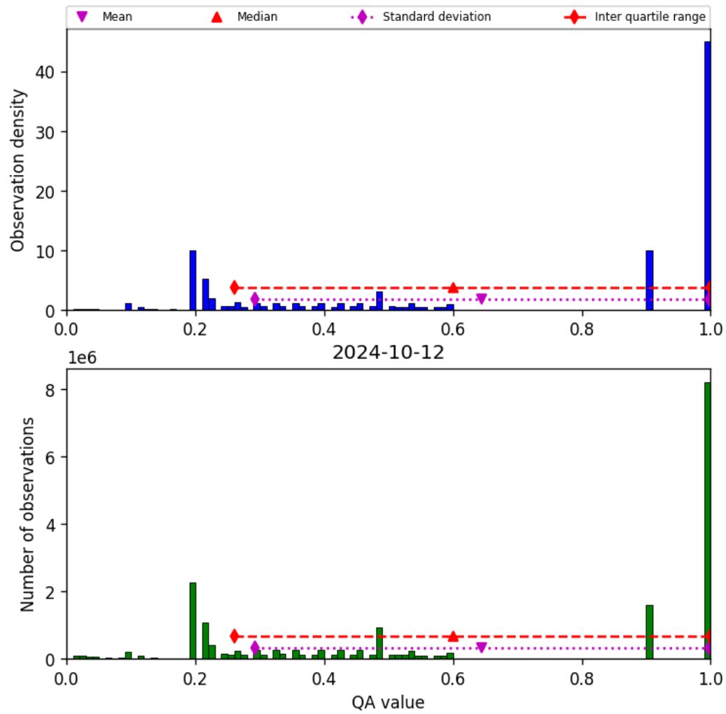
Figure 34: Histogram of “QA value” for 2024-10-11 to 2024-10-13
