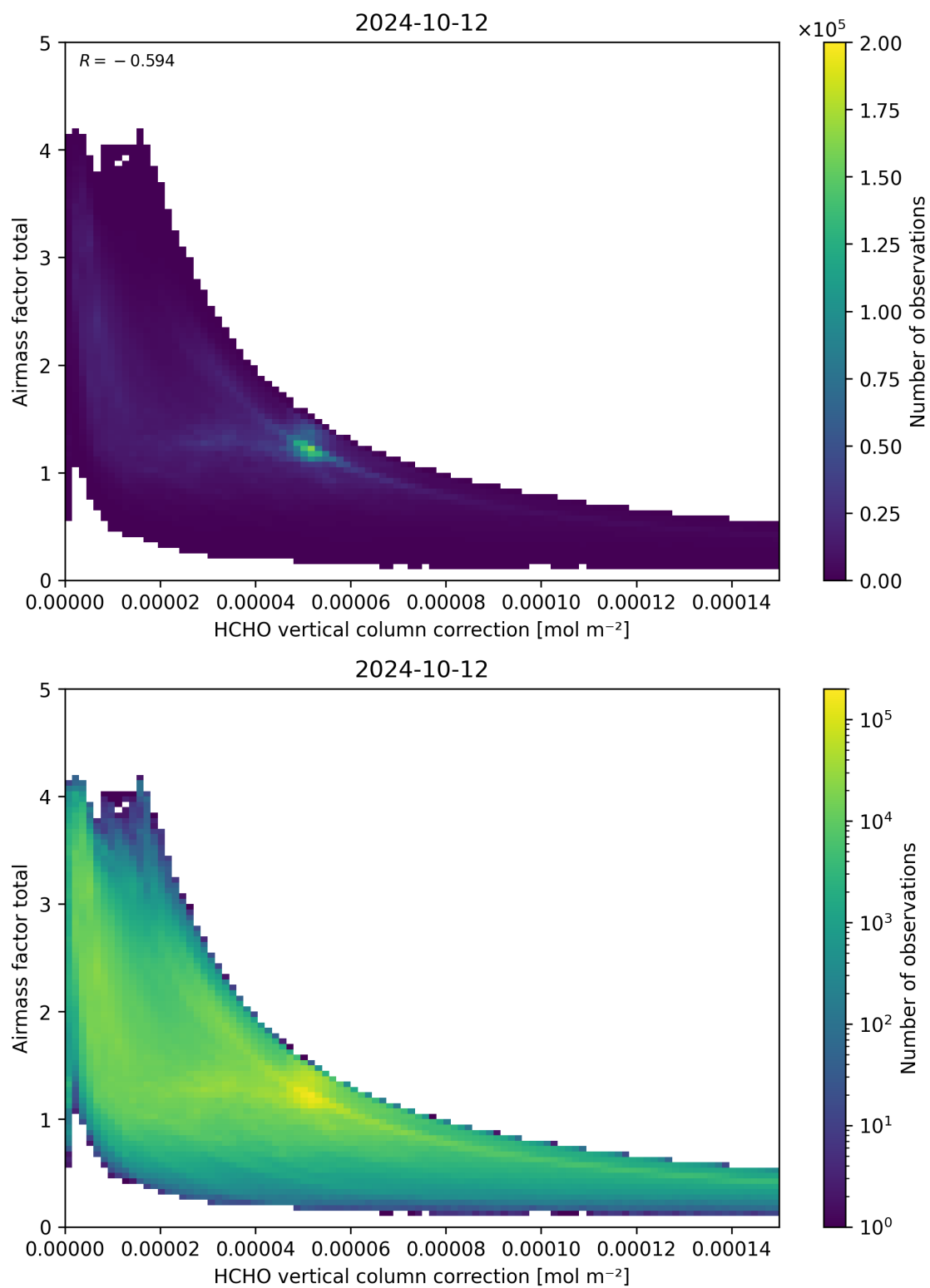
Figure 120: Scatter density plot of “HCHO vertical column correction” against “Airmass factor total” for 2024-10-11 to 2024-10-13.
