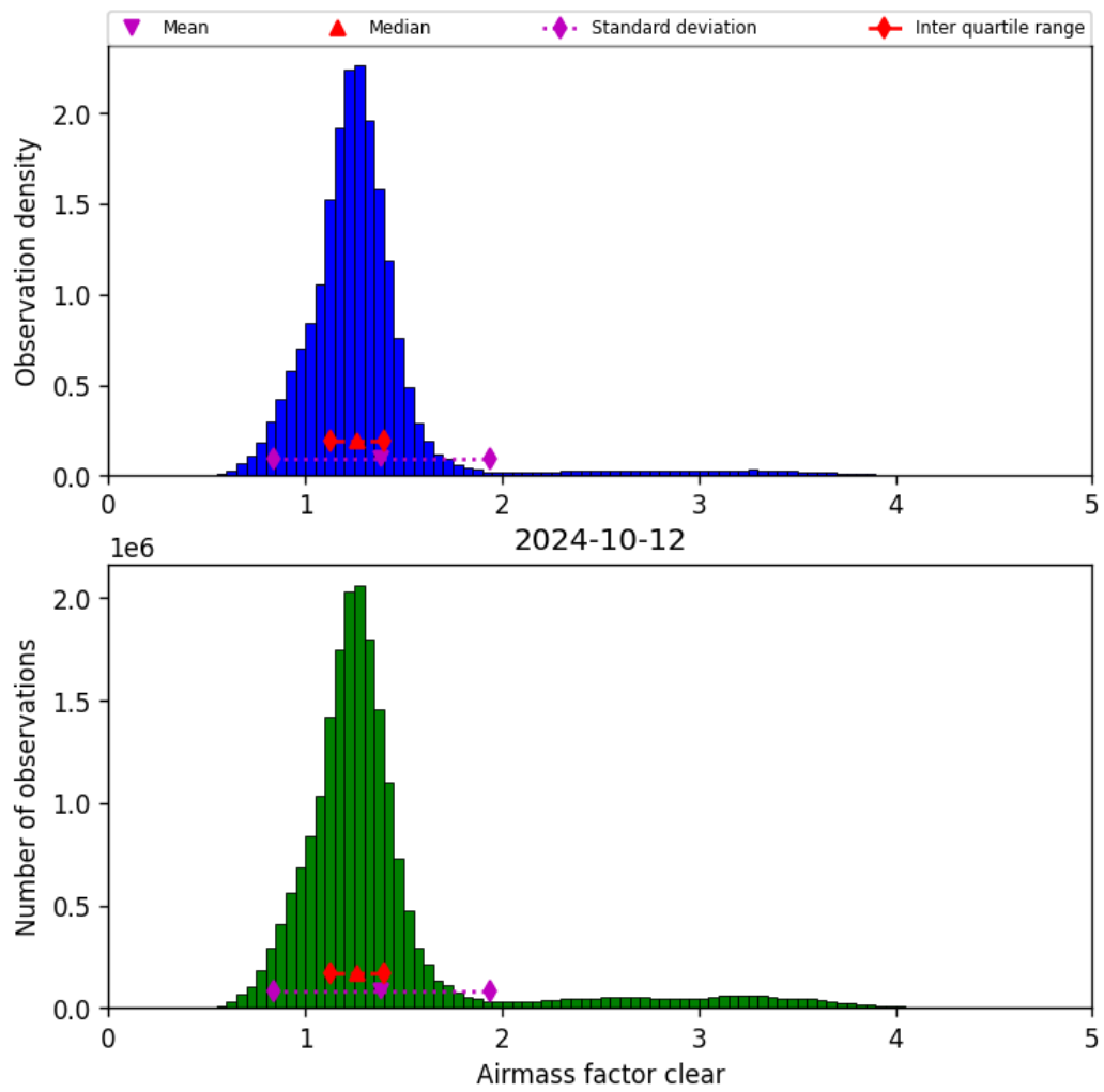
Figure 42: Histogram of “Airmass factor clear” for 2024-10-11 to 2024-10-13
