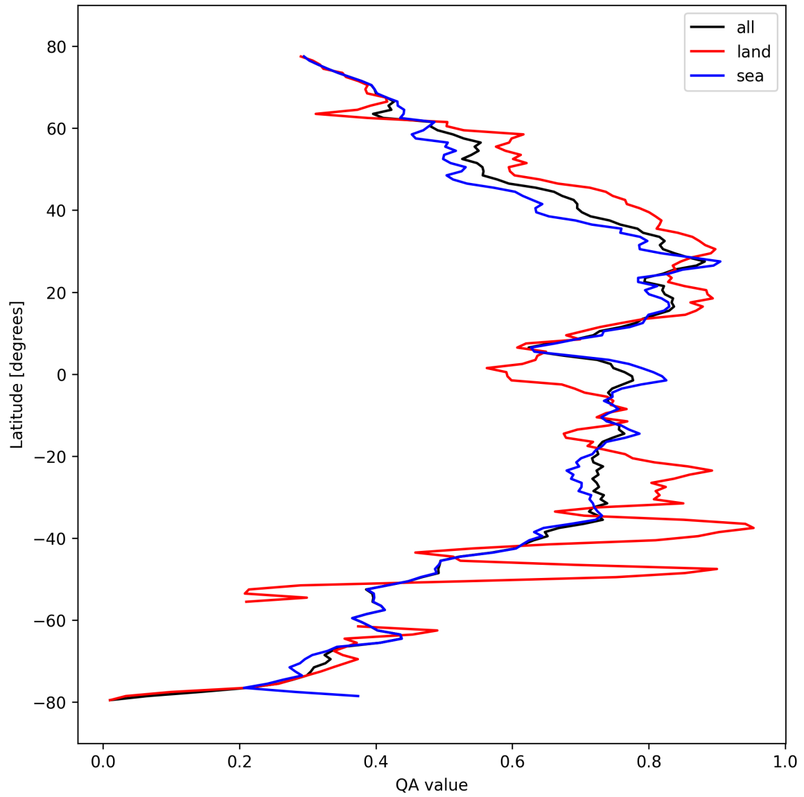
Figure 20: Zonal average of “QA value” for 2024-10-11 to 2024-10-13.
