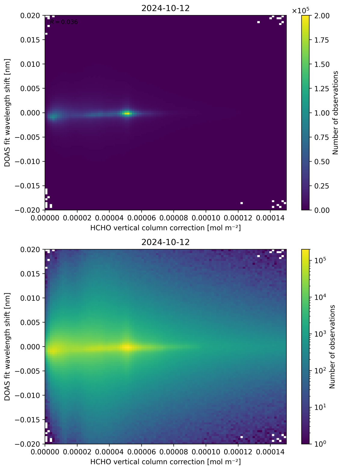
Figure 113: Scatter density plot of “HCHO vertical column correction” against “DOAS fit wavelength shift” for 2024-10-11 to 2024-10-13.
