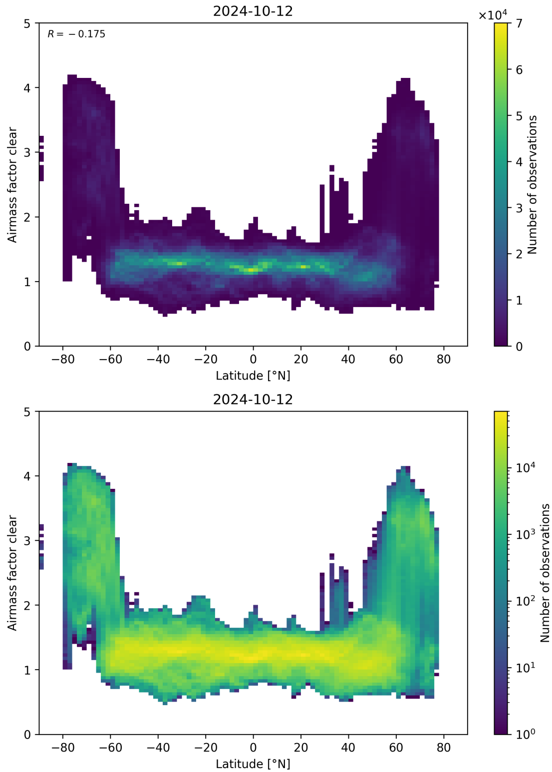
Figure 156: Scatter density plot of “Latitude” against “Airmass factor clear” for 2024-10-11 to 2024-10-13.
