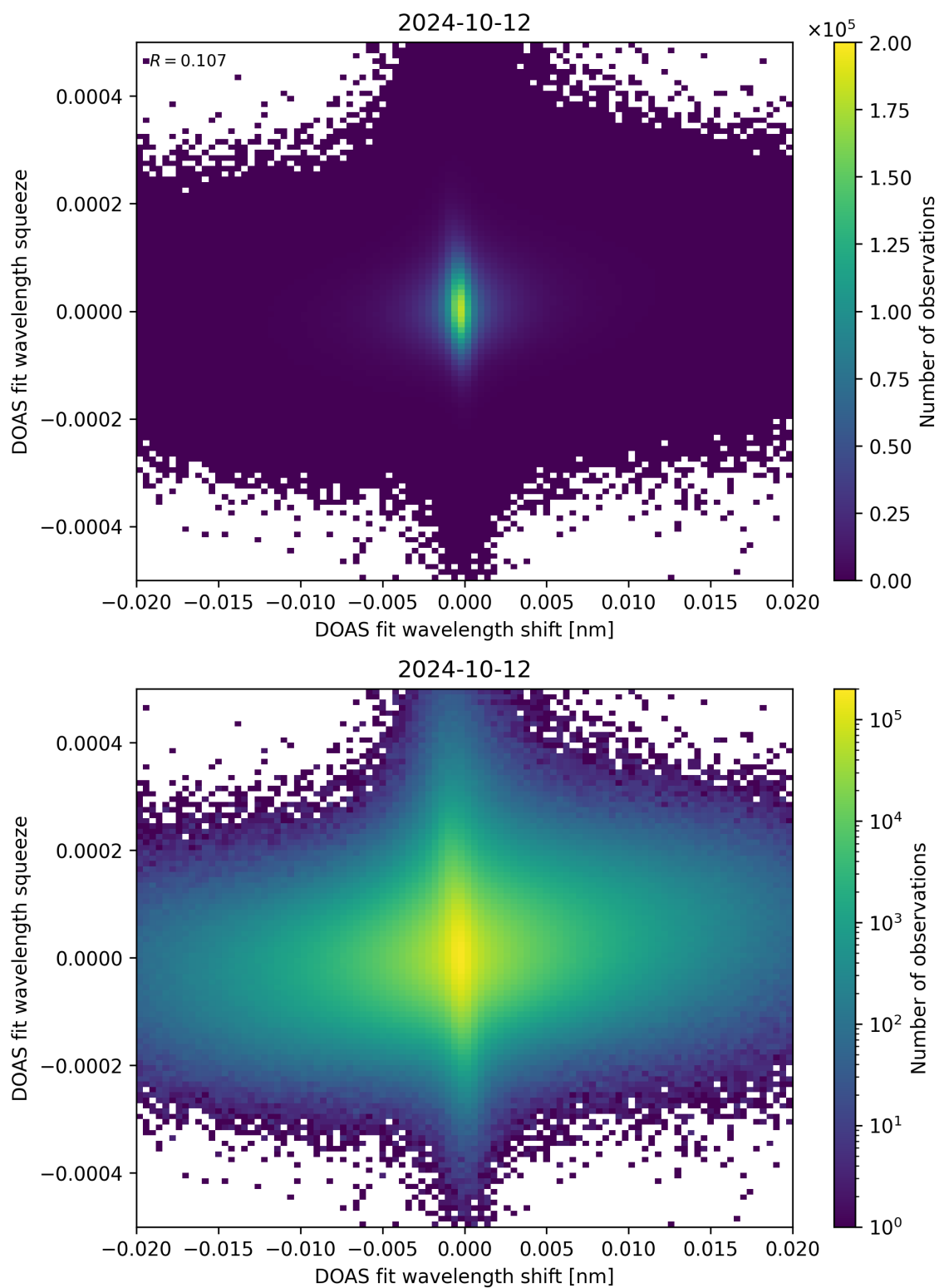
Figure 65: Scatter density plot of “DOAS fit wavelength shift” against “DOAS fit wavelength squeeze” for 2024-10-11 to 2024-10-13.
