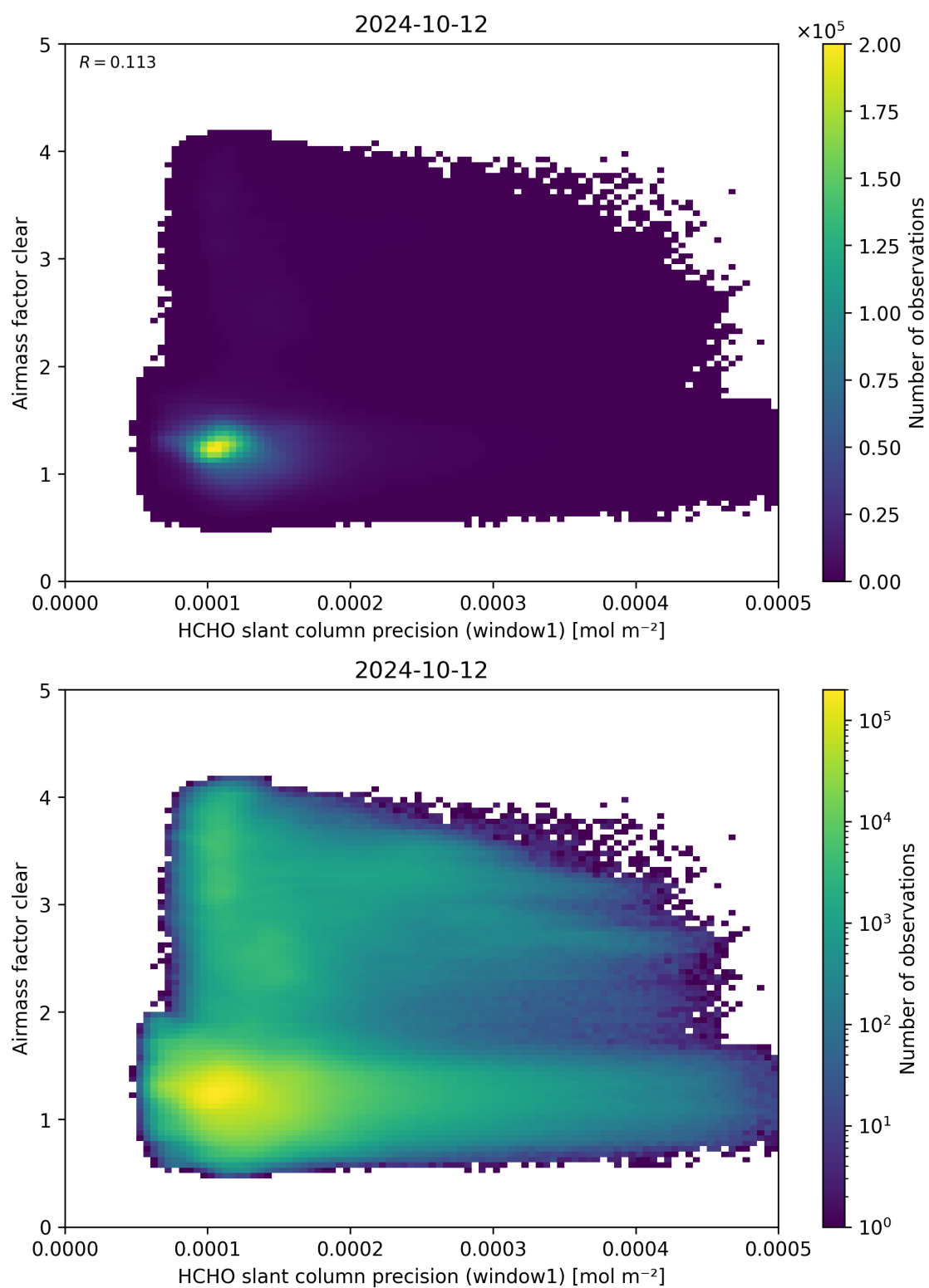
Figure 91: Scatter density plot of “HCHO slant column precision (window1)” against “Airmass factor clear” for 2024-10-11 to 2024-10-13.
