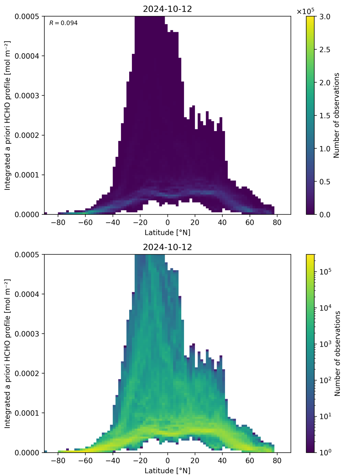
Figure 166: Scatter density plot of “Latitude” against “Integrated a priori HCHO profile” for 2024-10-11 to 2024-10-13.
