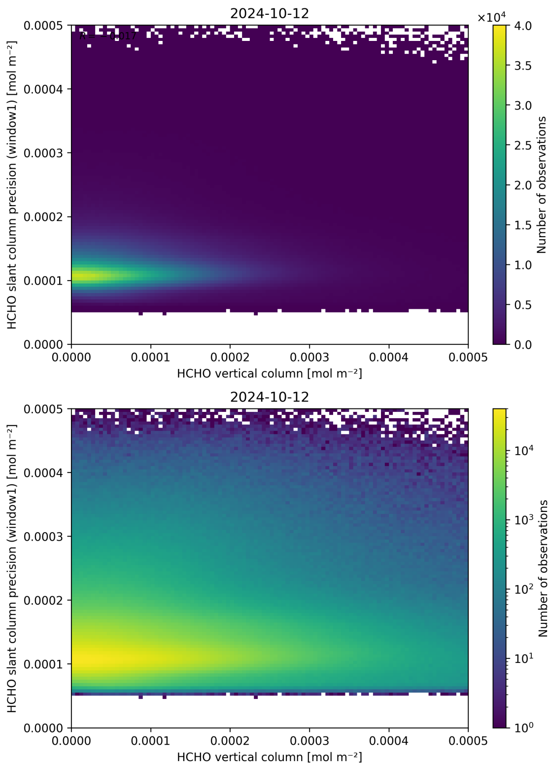
Figure 130: Scatter density plot of “HCHO vertical column” against “HCHO slant column precision (window1)” for 2024-10-11 to 2024-10-13.
