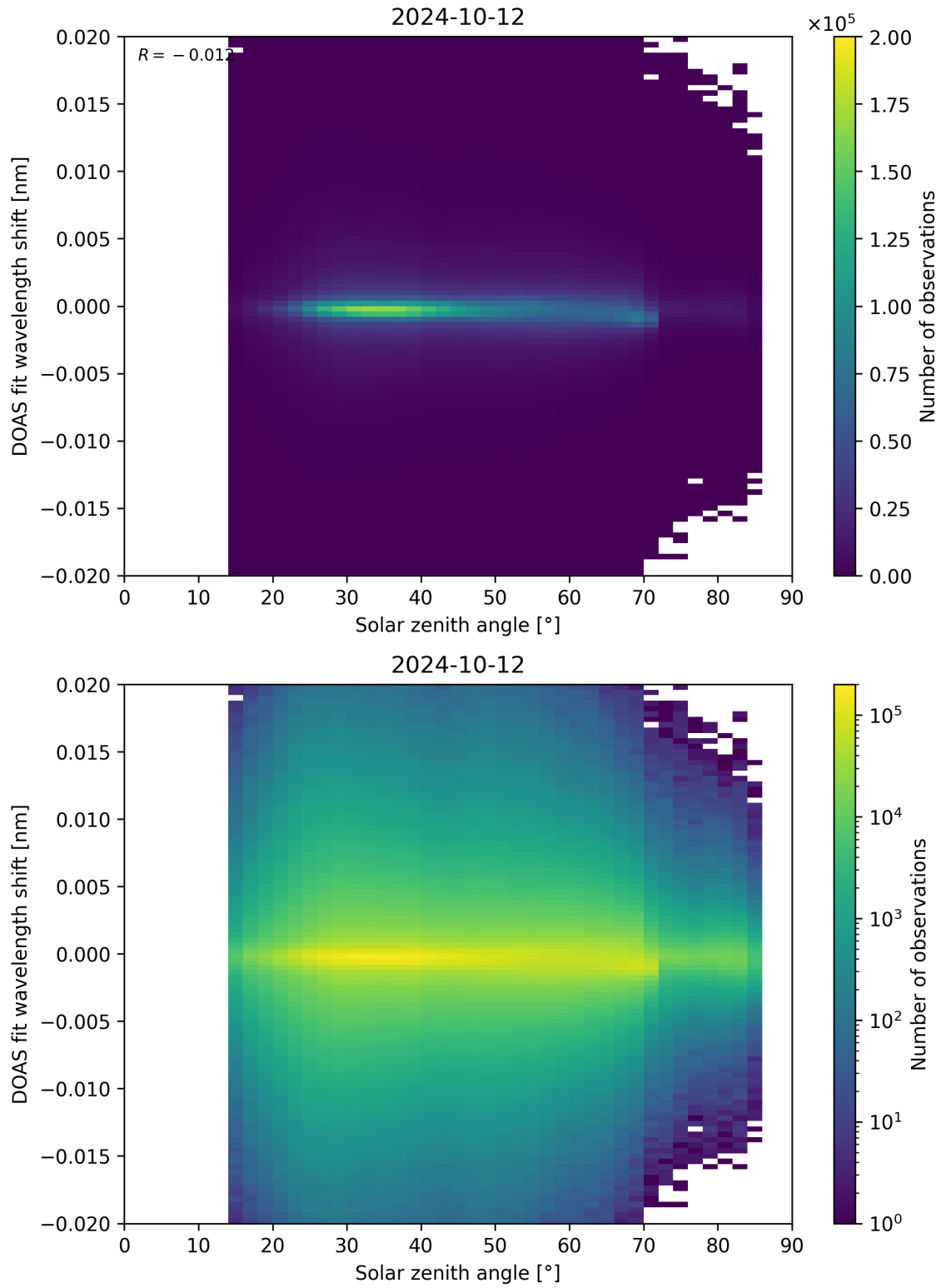
Figure 168: Scatter density plot of “Solar zenith angle” against “DOAS fit wavelength shift” for 2024-10-11 to 2024-10-13.
