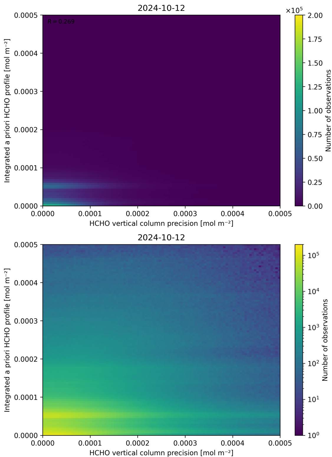
Figure 147: Scatter density plot of “HCHO vertical column precision” against “Integrated a priori HCHO profile” for 2024-10-11 to 2024-10-13.
