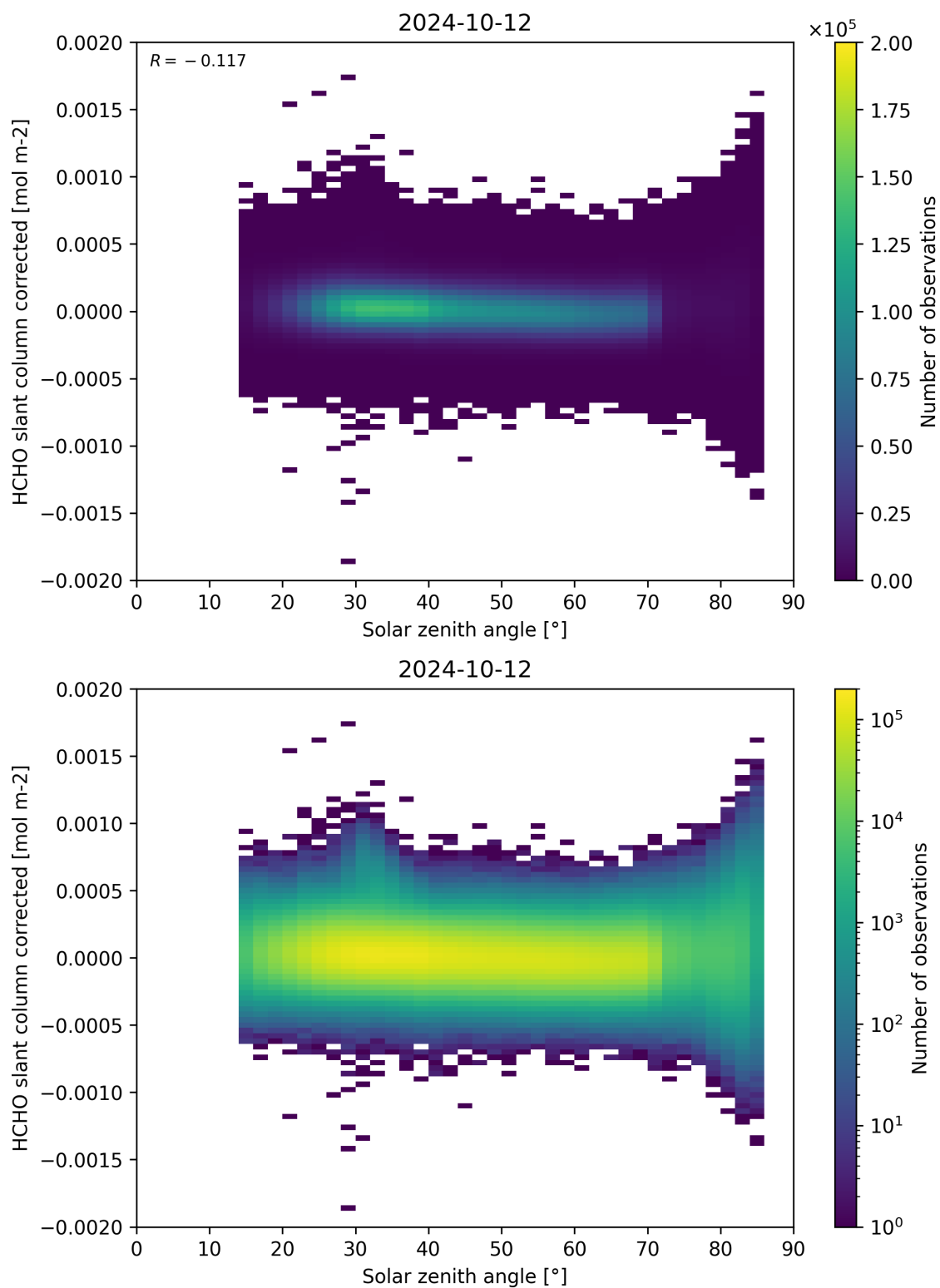
Figure 171: Scatter density plot of “Solar zenith angle” against “HCHO slant column corrected” for 2024-10-11 to 2024-10-13.
