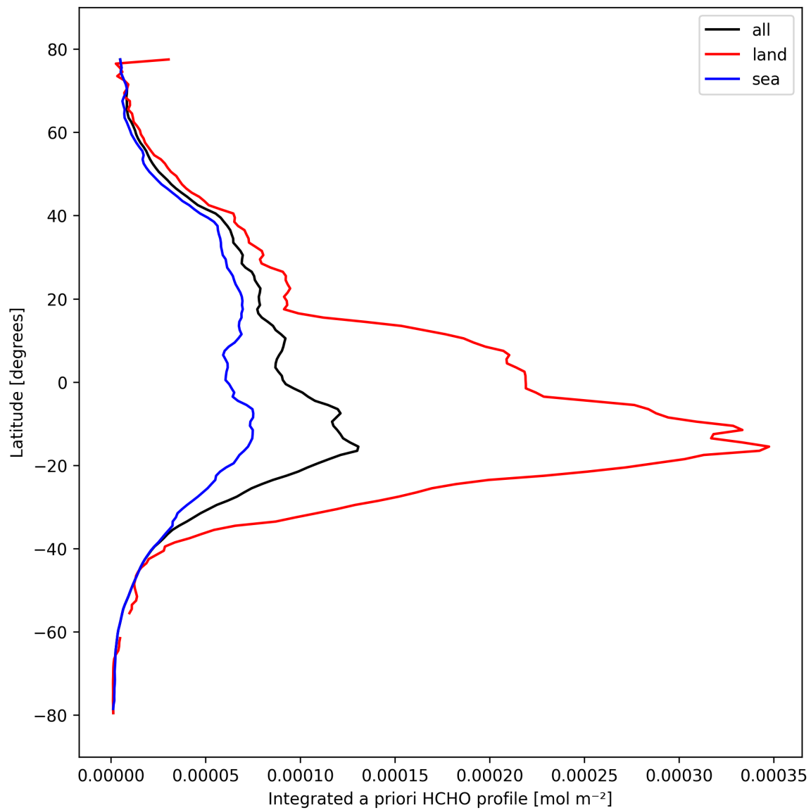
Figure 29: Zonal average of “Integrated a priori HCHO profile” for 2024-10-11 to 2024-10-13.
