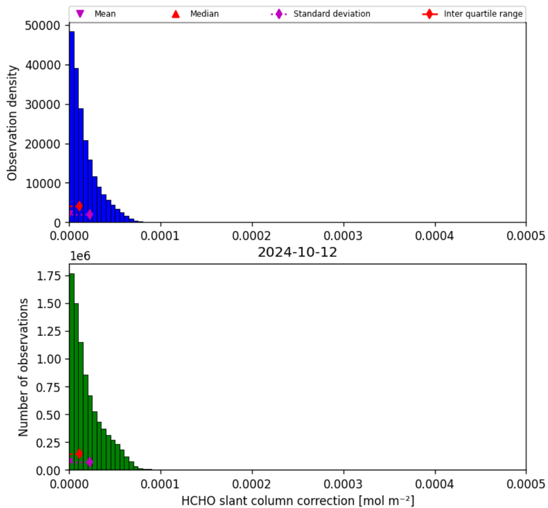
Figure 47: Histogram of “HCHO slant column correction” for 2024-10-11 to 2024-10-13
