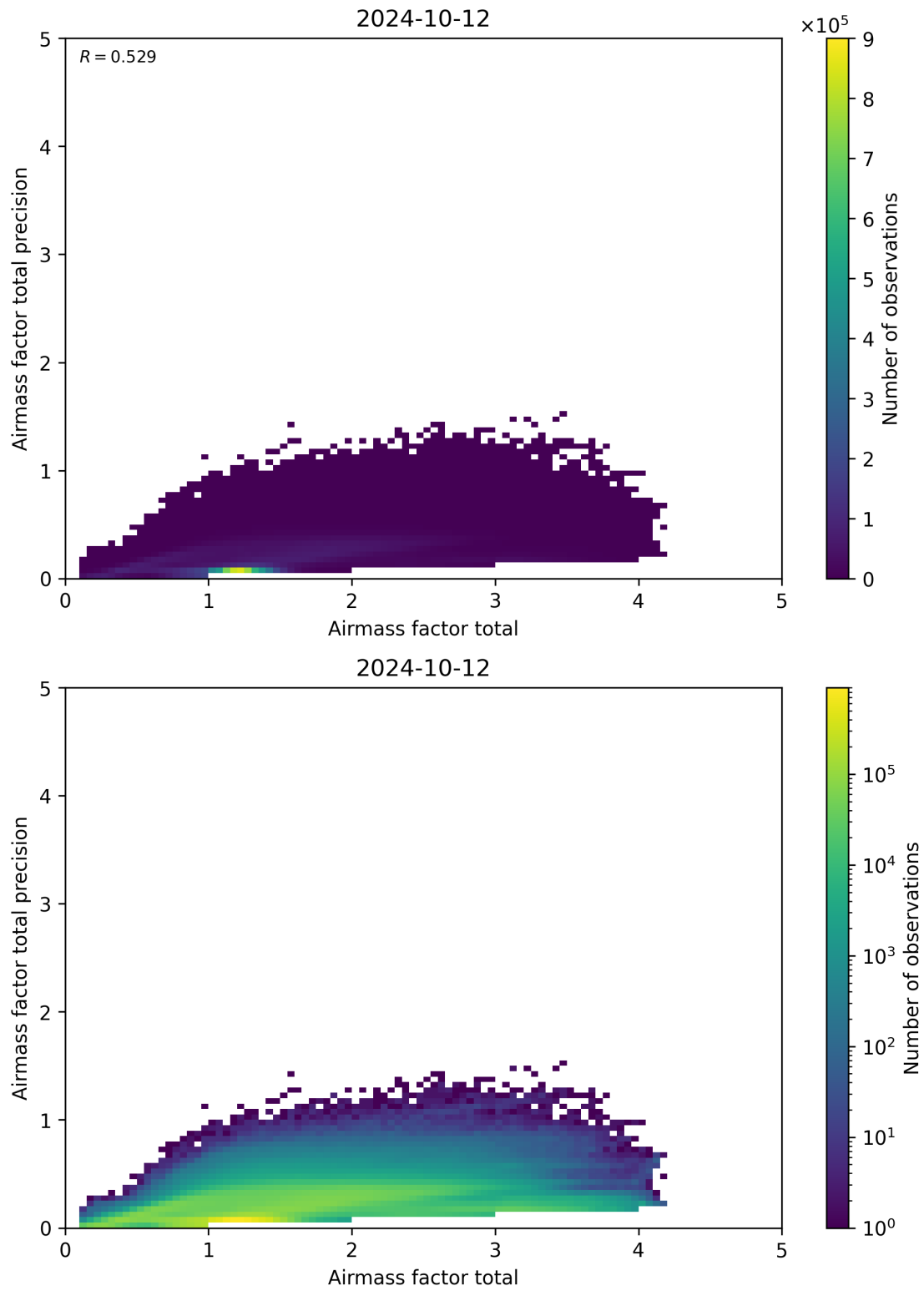
Figure 103: Scatter density plot of “Airmass factor total” against “Airmass factor total precision” for 2024-10-11 to 2024-10-13.
