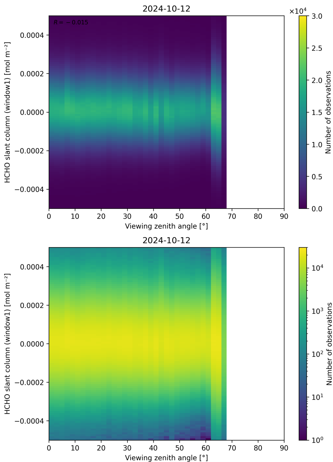
Figure 188: Scatter density plot of “Viewing zenith angle” against “HCHO slant column (window1)” for 2024-10-11 to 2024-10-13.
