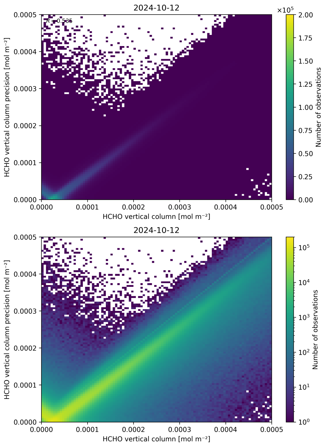
Figure 134: Scatter density plot of “HCHO vertical column” against “HCHO vertical column precision” for 2024-10-11 to 2024-10-13.
