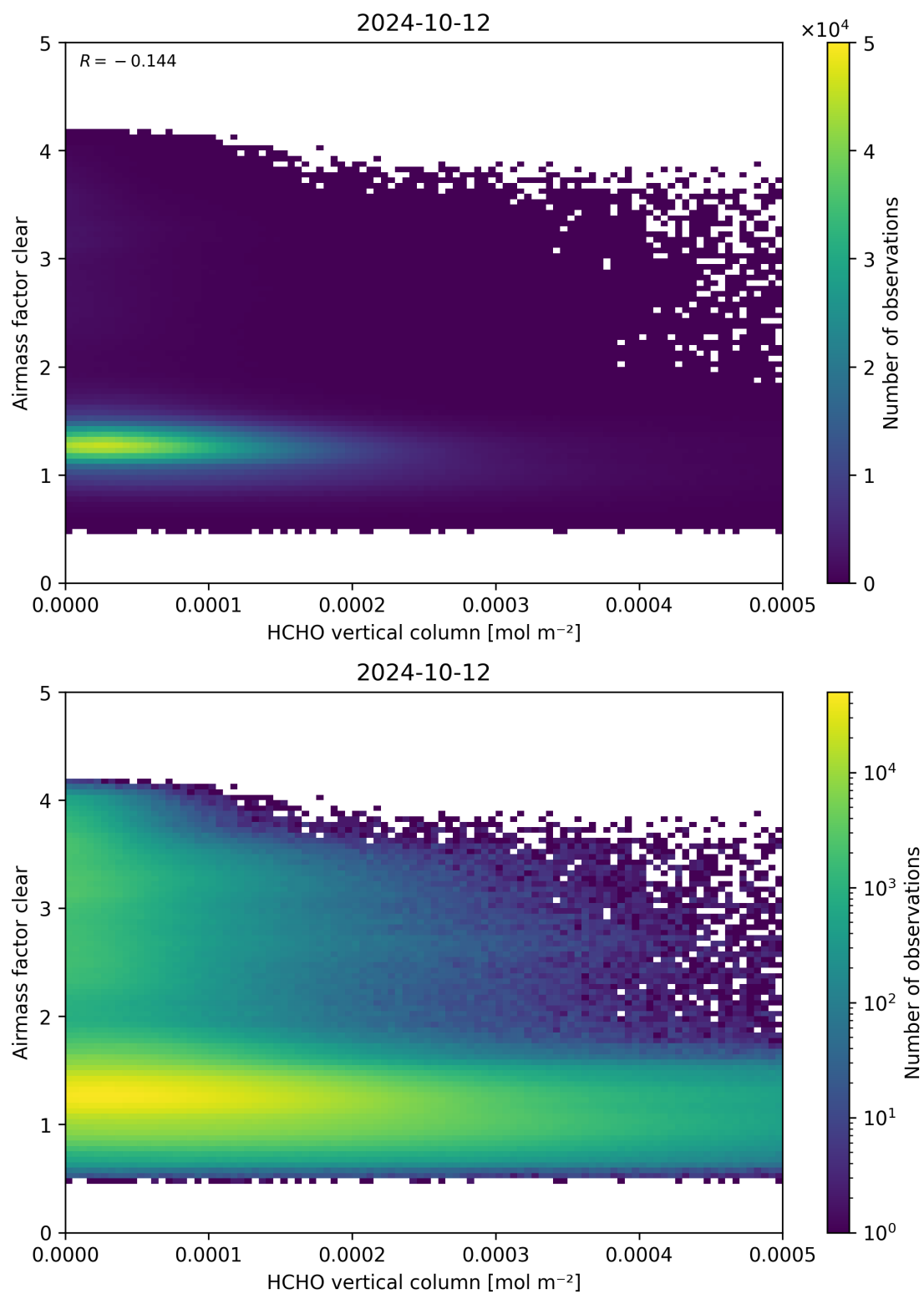
Figure 126: Scatter density plot of “HCHO vertical column” against “Airmass factor clear” for 2024-10-11 to 2024-10-13.
