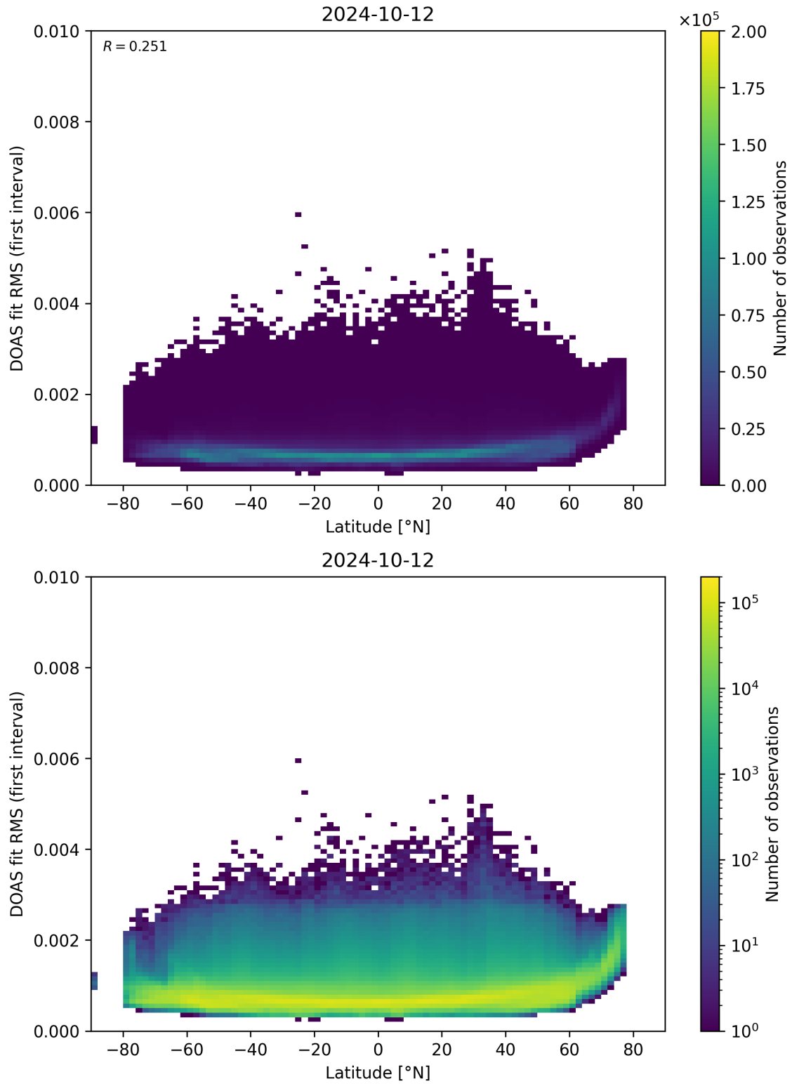
Figure 153: Scatter density plot of “Latitude” against “DOAS fit RMS (first interval)” for 2024-10-11 to 2024-10-13.
