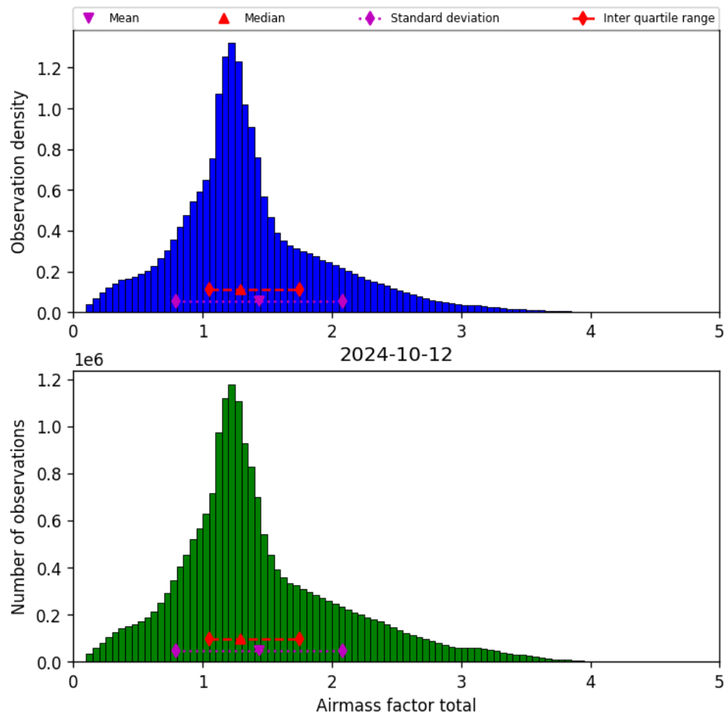
Figure 40: Histogram of “Airmass factor total” for 2024-10-11 to 2024-10-13
