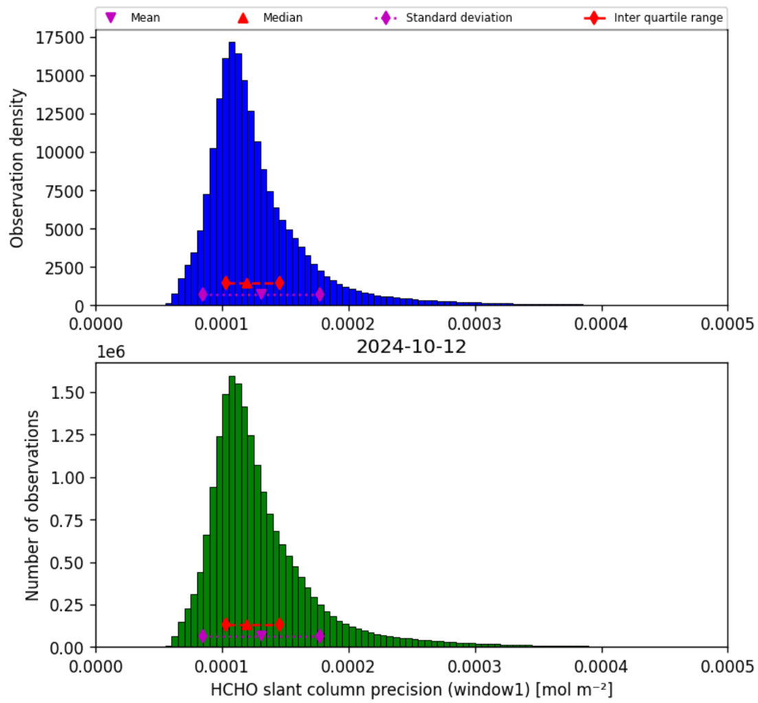
Figure 39: Histogram of “HCHO slant column precision (window1)” for 2024-10-11 to 2024-10-13
