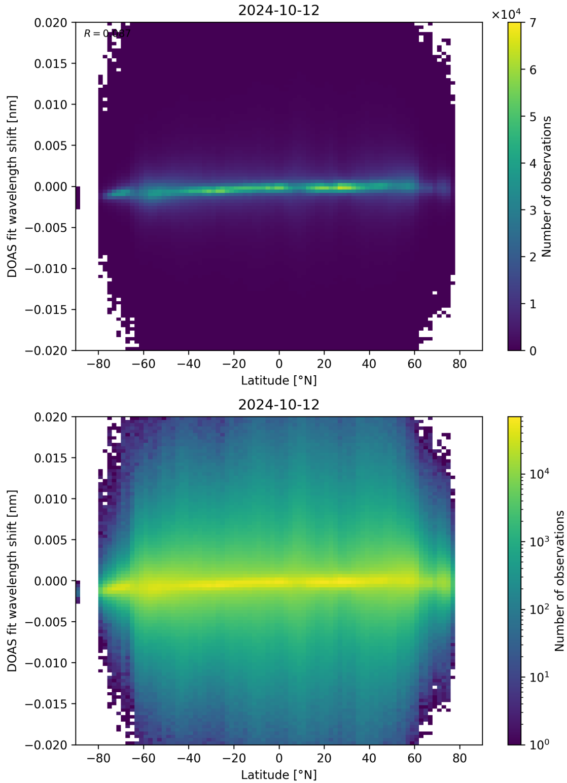
Figure 154: Scatter density plot of “Latitude” against “DOAS fit wavelength shift” for 2024-10-11 to 2024-10-13.
