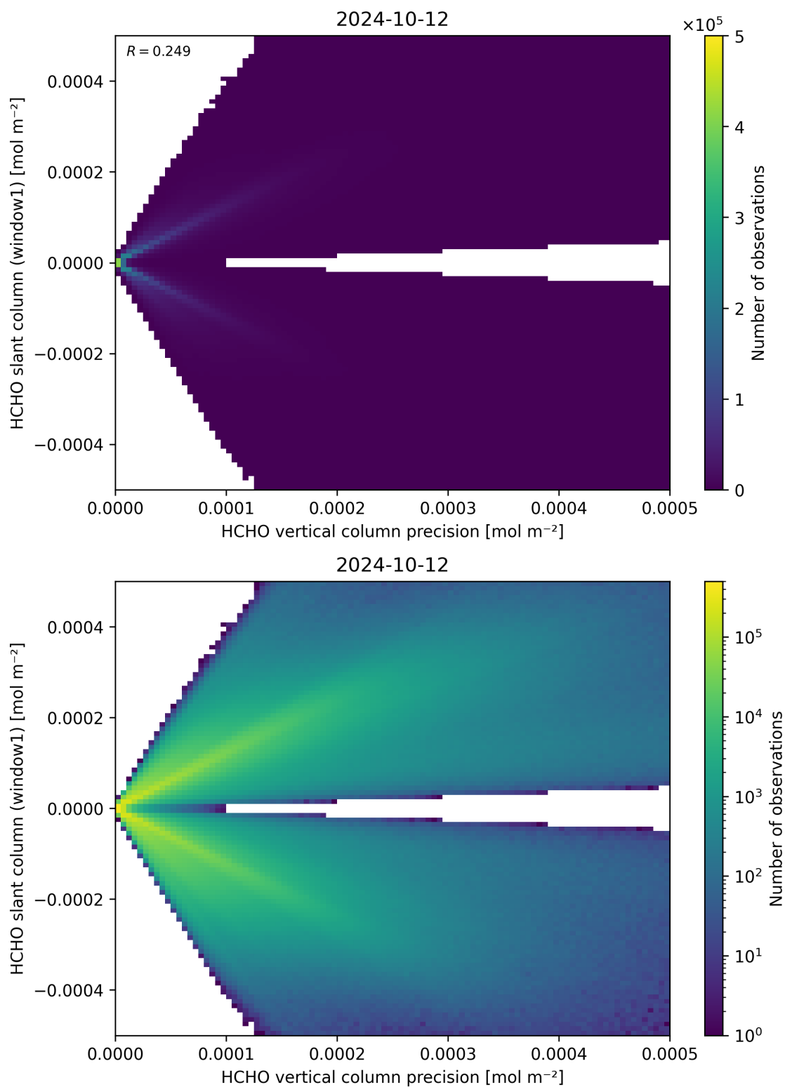
Figure 142: Scatter density plot of “HCHO vertical column precision” against “HCHO slant column (window1)” for 2024-10-11 to 2024-10-13.
