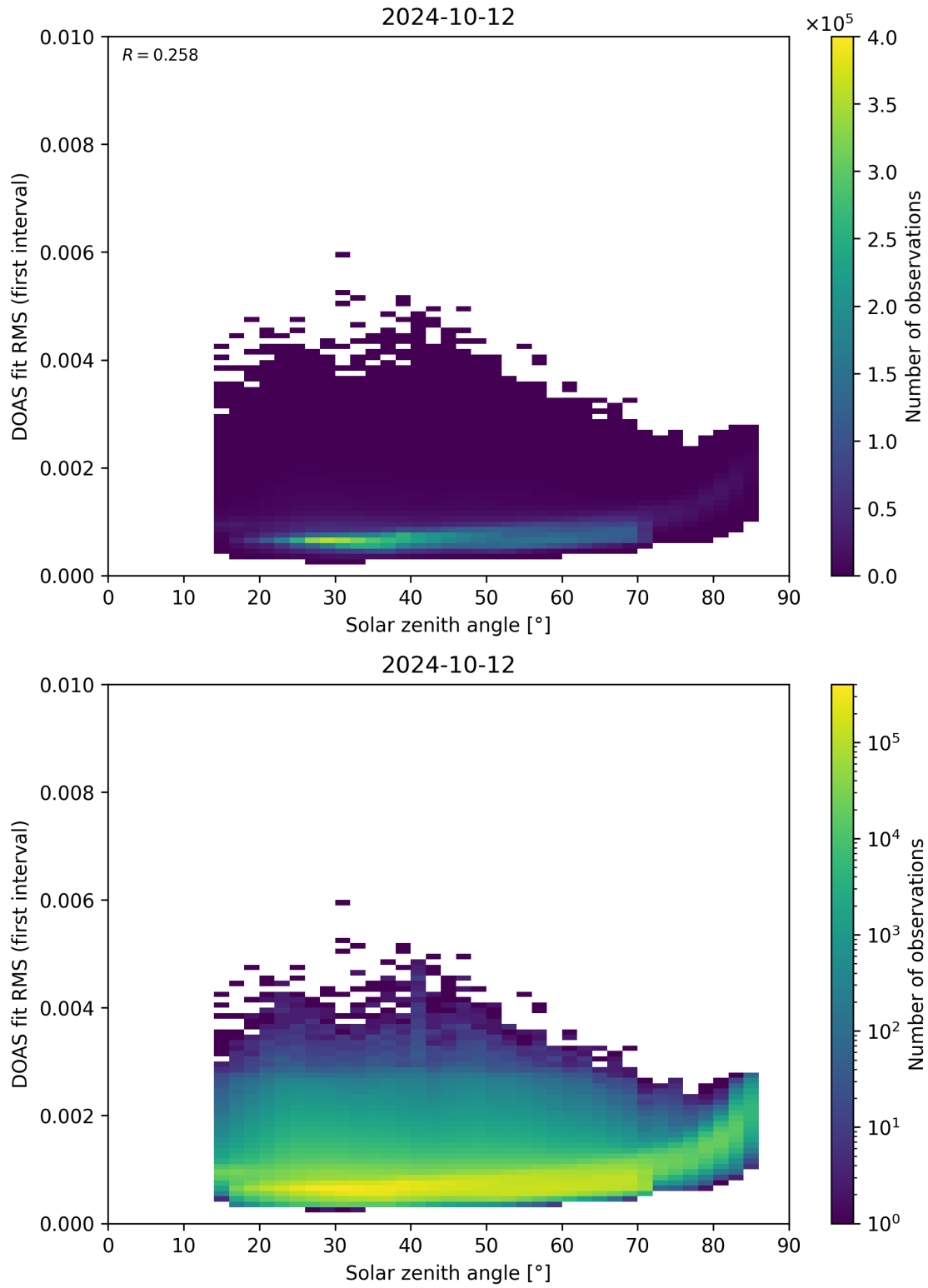
Figure 167: Scatter density plot of “Solar zenith angle” against “DOAS fit RMS (first interval)” for 2024-10-11 to 2024-10-13.
