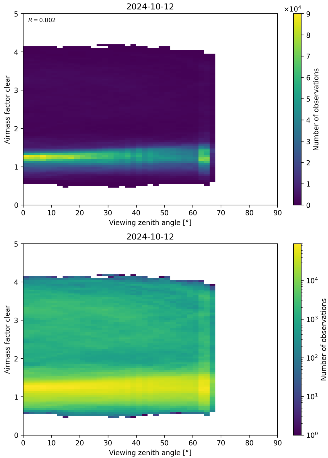
Figure 185: Scatter density plot of “Viewing zenith angle” against “Airmass factor clear” for 2024-10-11 to 2024-10-13.
