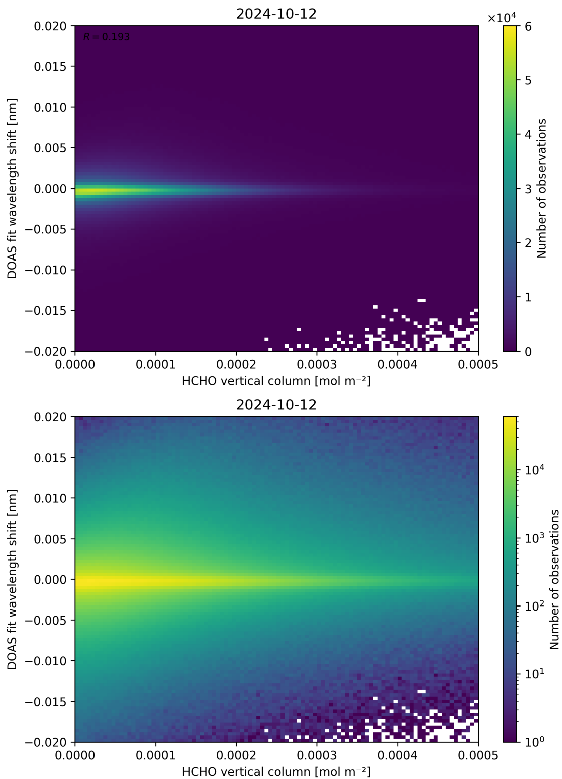
Figure 124: Scatter density plot of “HCHO vertical column” against “DOAS fit wavelength shift” for 2024-10-11 to 2024-10-13.
