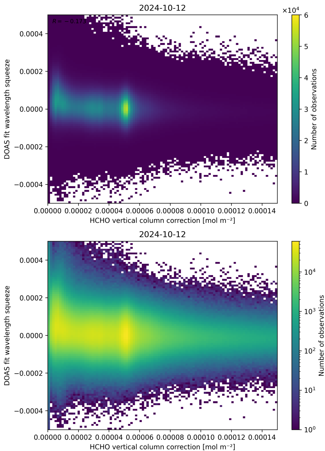
Figure 114: Scatter density plot of “HCHO vertical column correction” against “DOAS fit wavelength squeeze” for 2024-10-11 to 2024-10-13.
