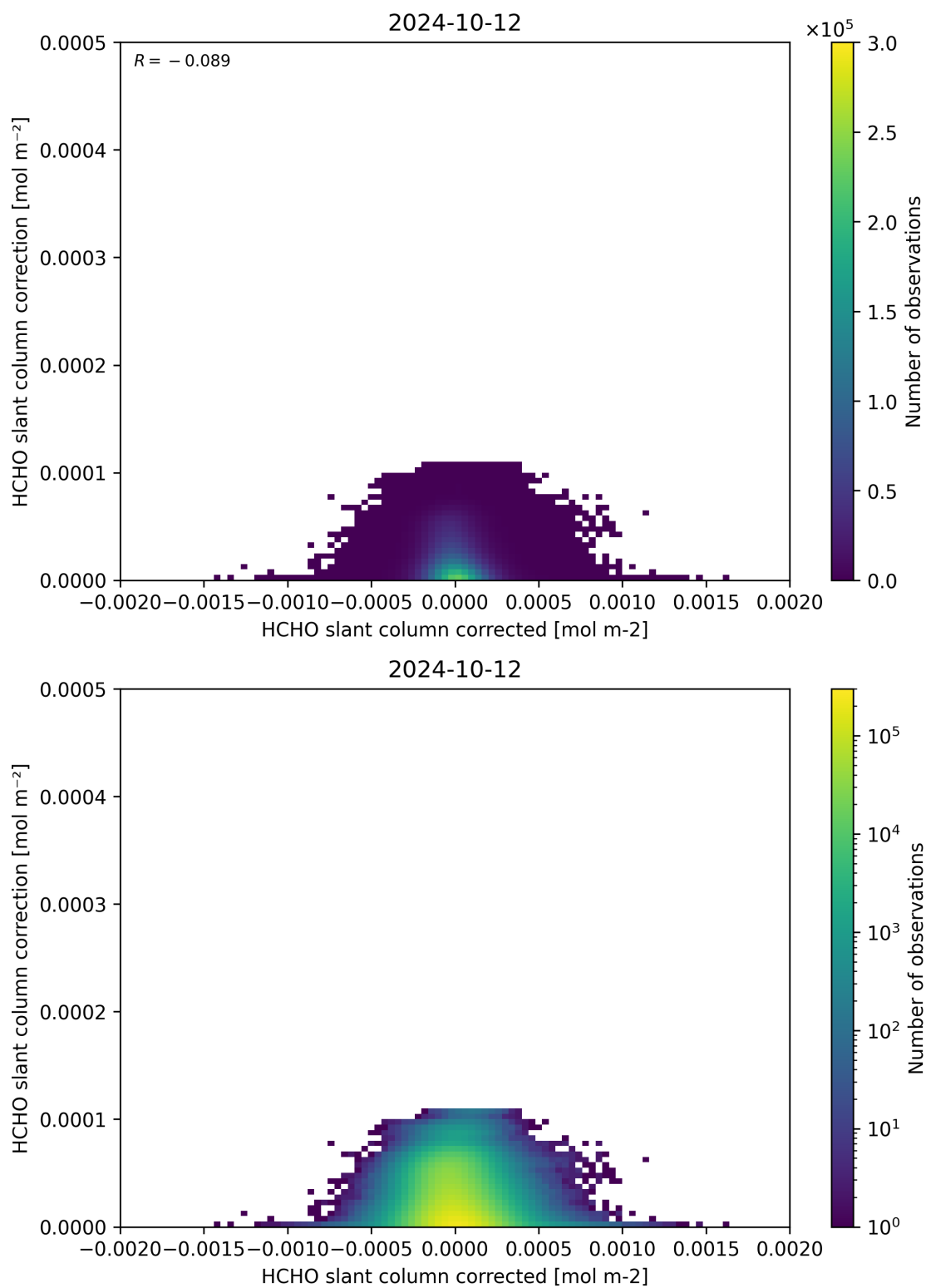
Figure 77: Scatter density plot of “HCHO slant column corrected” against “HCHO slant column correction” for 2024-10-11 to 2024-10-13.
