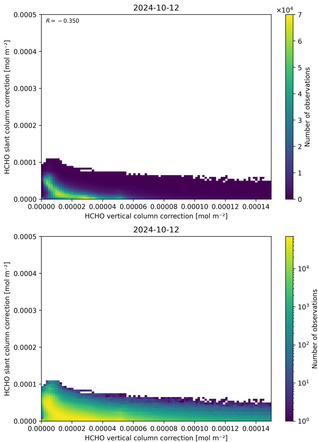
Figure 117: Scatter density plot of “HCHO vertical column correction” against “HCHO slant column correction” for 2024-10-11 to 2024-10-13.
