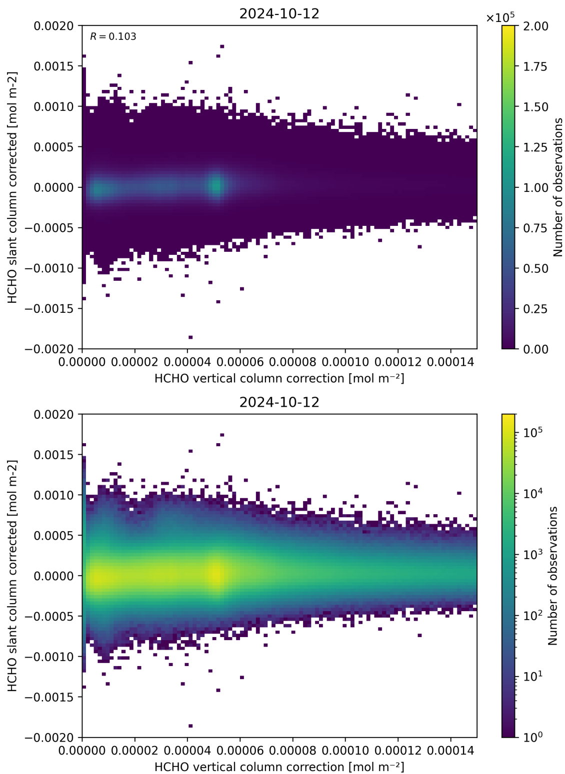
Figure 116: Scatter density plot of “HCHO vertical column correction” against “HCHO slant column corrected” for 2024-10-11 to 2024-10-13.
