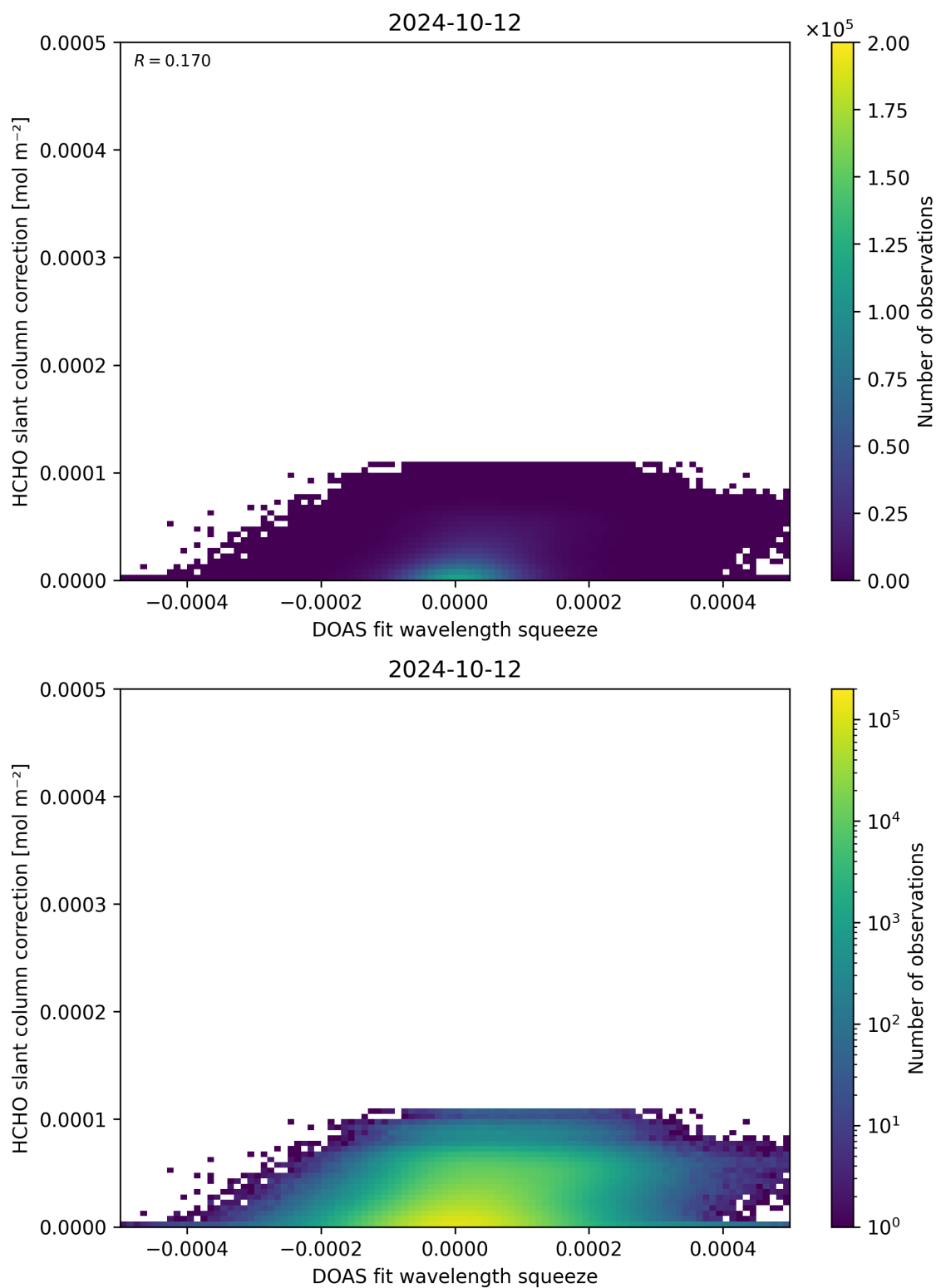
Figure 70: Scatter density plot of “DOAS fit wavelength squeeze” against “HCHO slant column correction” for 2024-10-11 to 2024-10-13.
