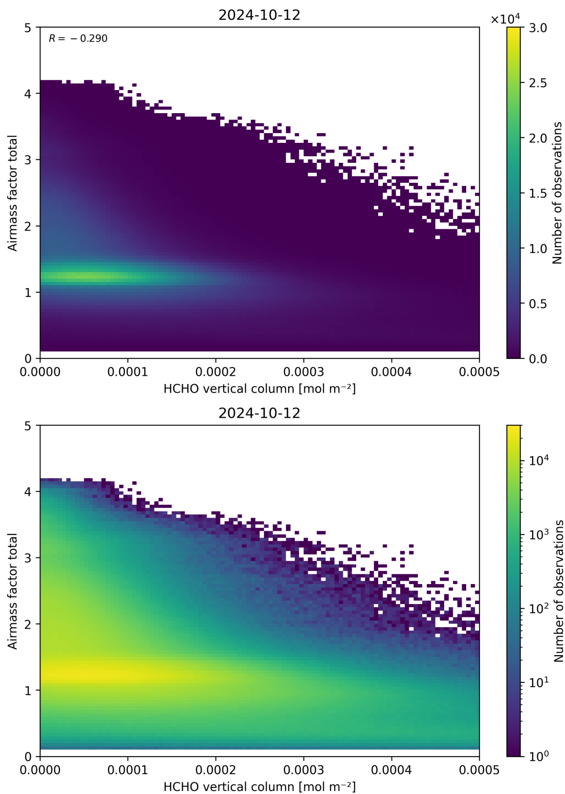
Figure 131: Scatter density plot of “HCHO vertical column” against “Airmass factor total” for 2024-10-11 to 2024-10-13.
