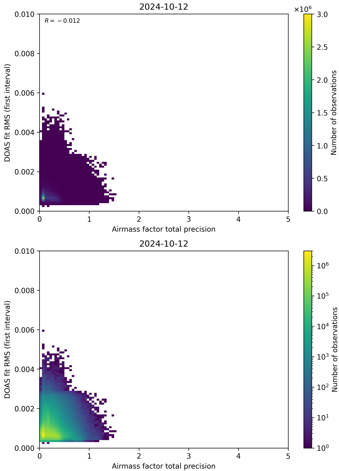
Figure 105: Scatter density plot of “Airmass factor total precision” against “DOAS fit RMS (first interval)” for 2024-10-11 to 2024-10-13.
