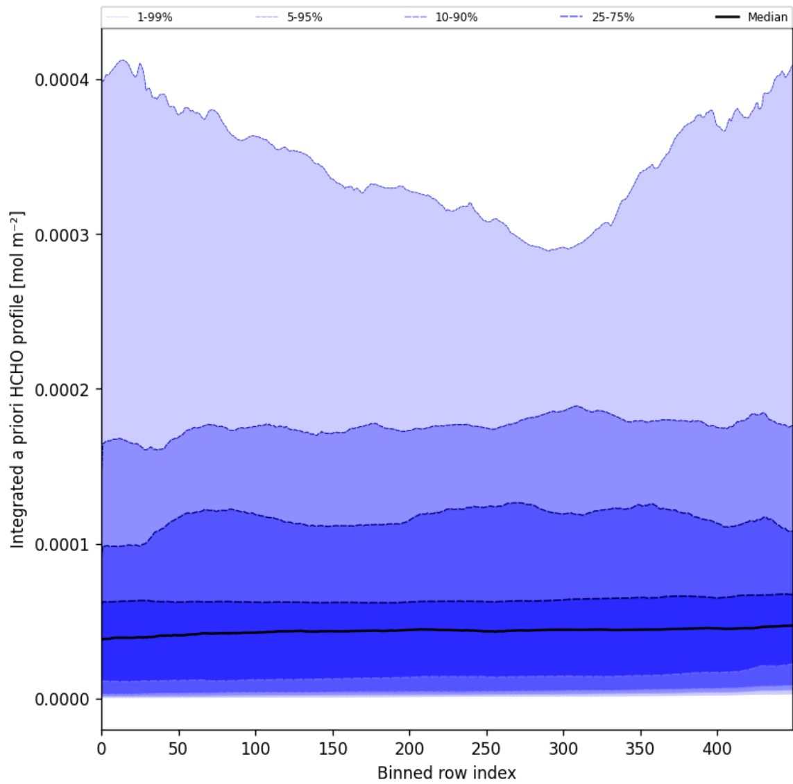
Figure 57: Along track statistics of “Integrated a priori HCHO profile” for 2024-10-11 to 2024-10-13
