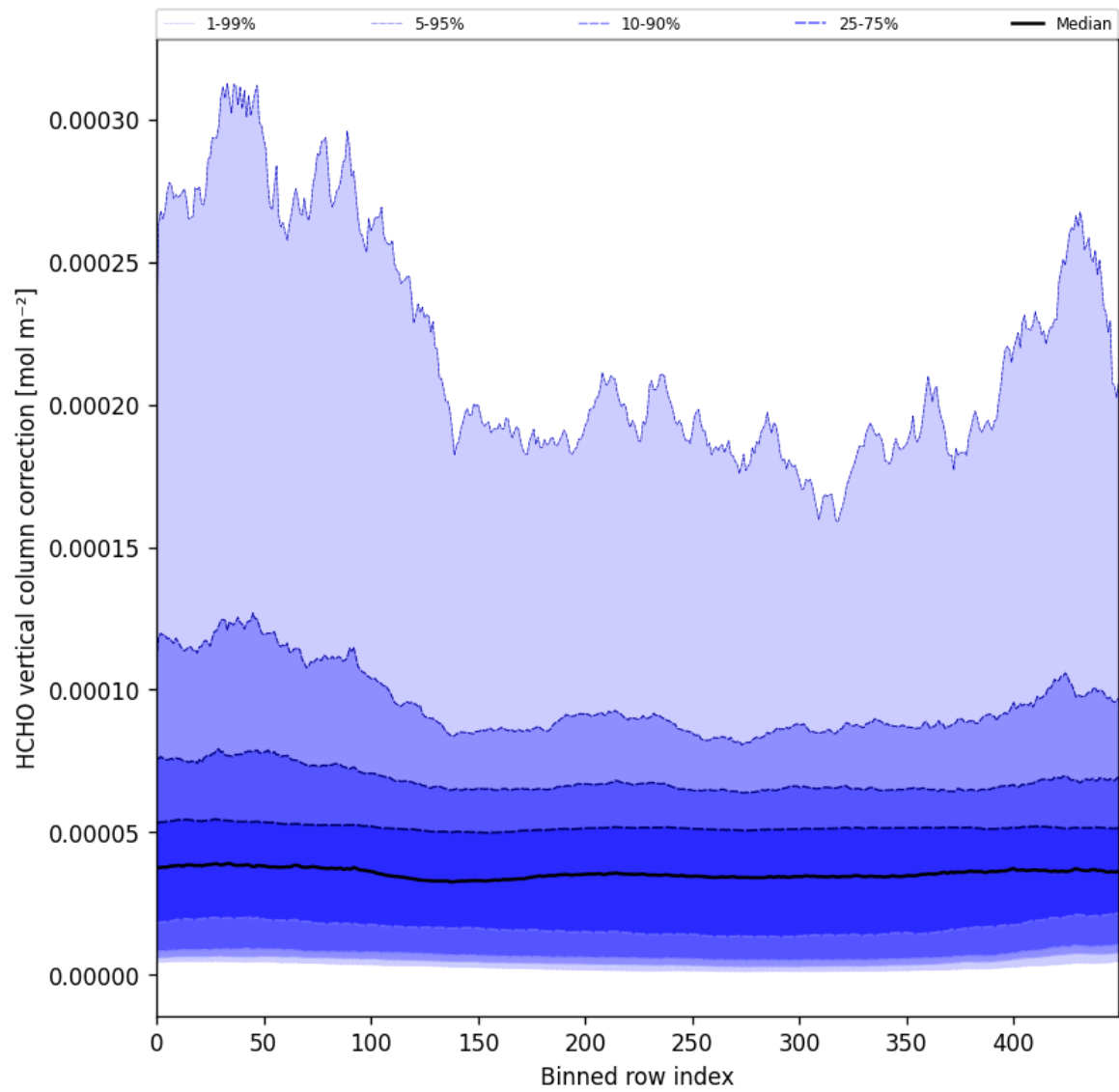
Figure 51: Along track statistics of “HCHO vertical column correction” for 2024-10-11 to 2024-10-13
