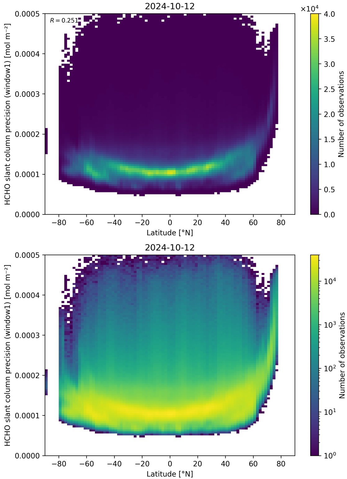
Figure 160: Scatter density plot of “Latitude” against “HCHO slant column precision (window1)” for 2024-10-11 to 2024-10-13.
