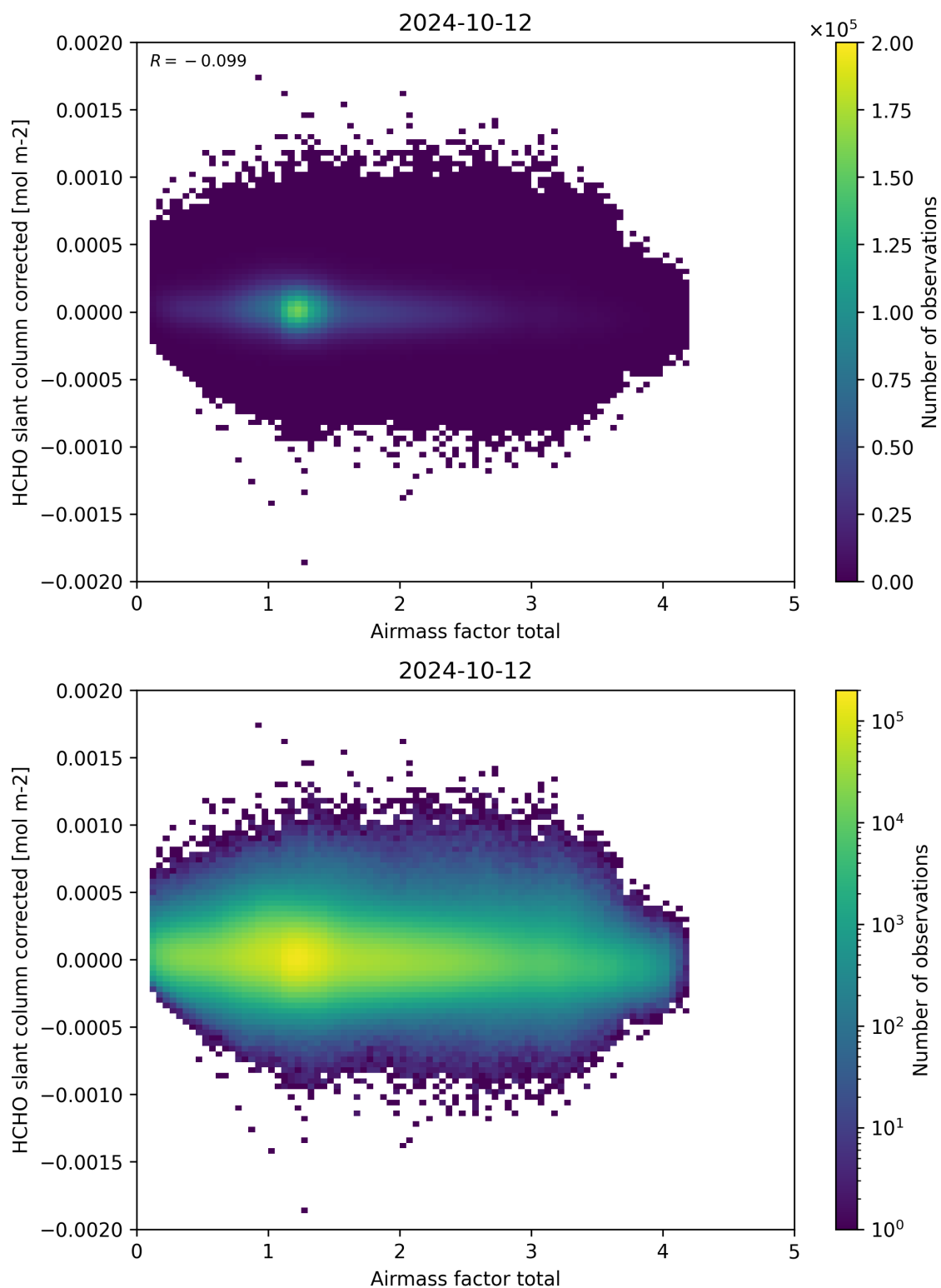
Figure 101: Scatter density plot of “Airmass factor total” against “HCHO slant column corrected” for 2024-10-11 to 2024-10-13.
