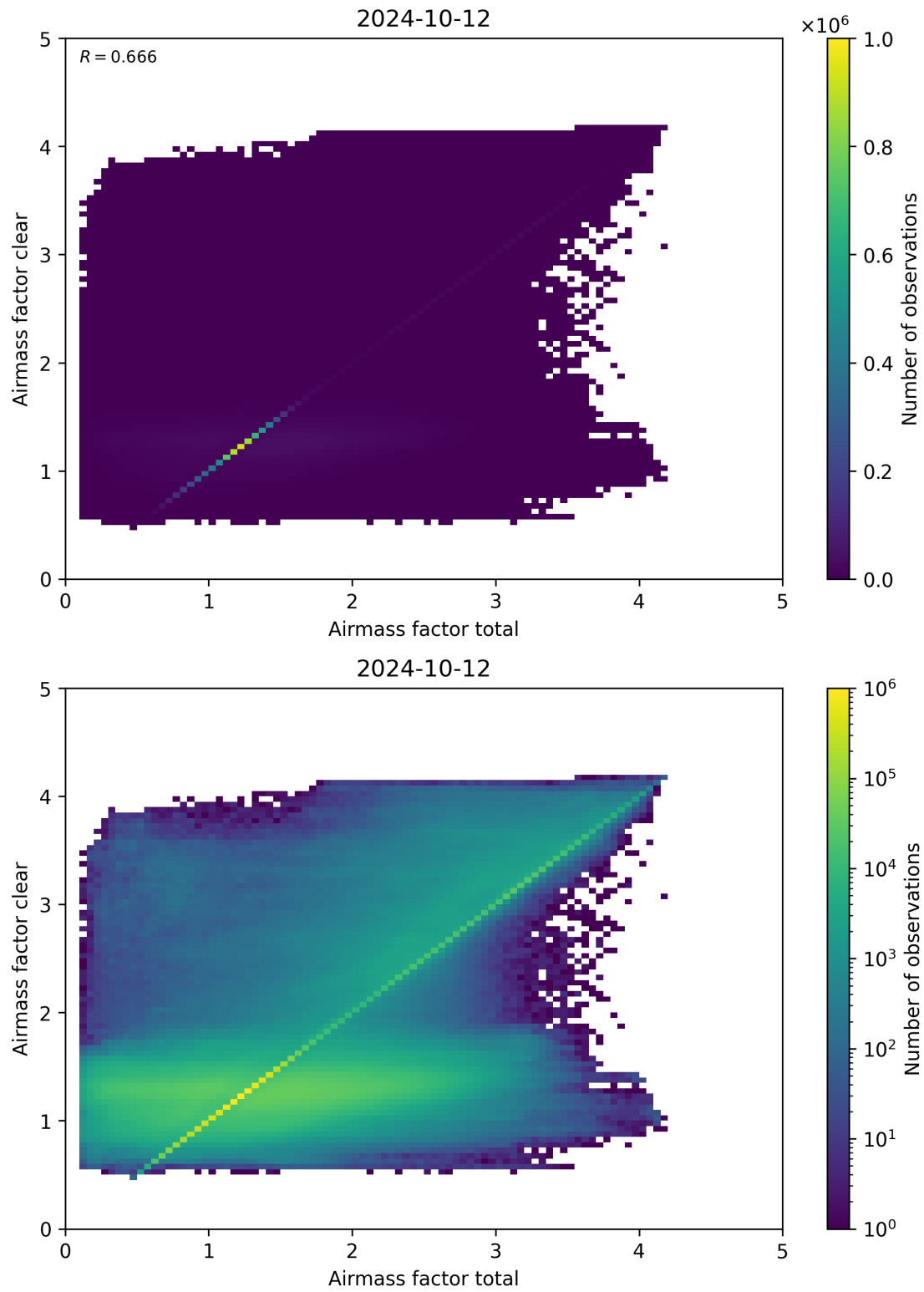
Figure 100: Scatter density plot of “Airmass factor total” against “Airmass factor clear” for 2024-10-11 to 2024-10-13.
