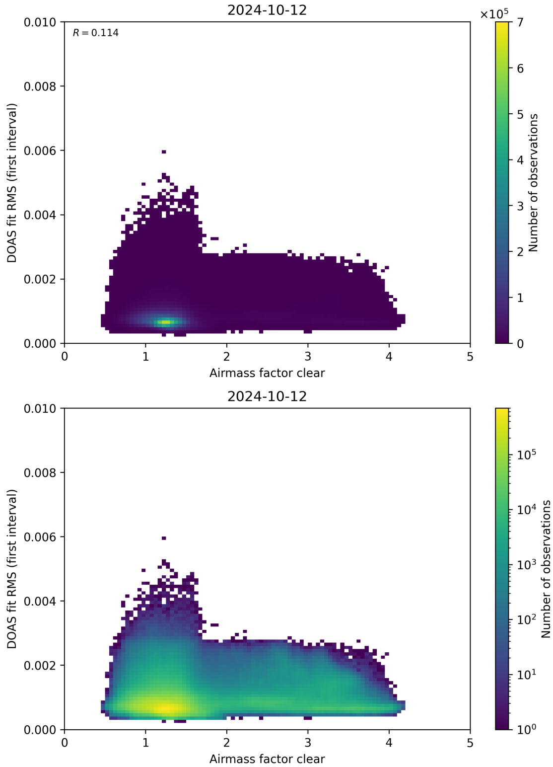
Figure 71: Scatter density plot of “Airmass factor clear” against “DOAS fit RMS (first interval)” for 2024-10-11 to 2024-10-13.
