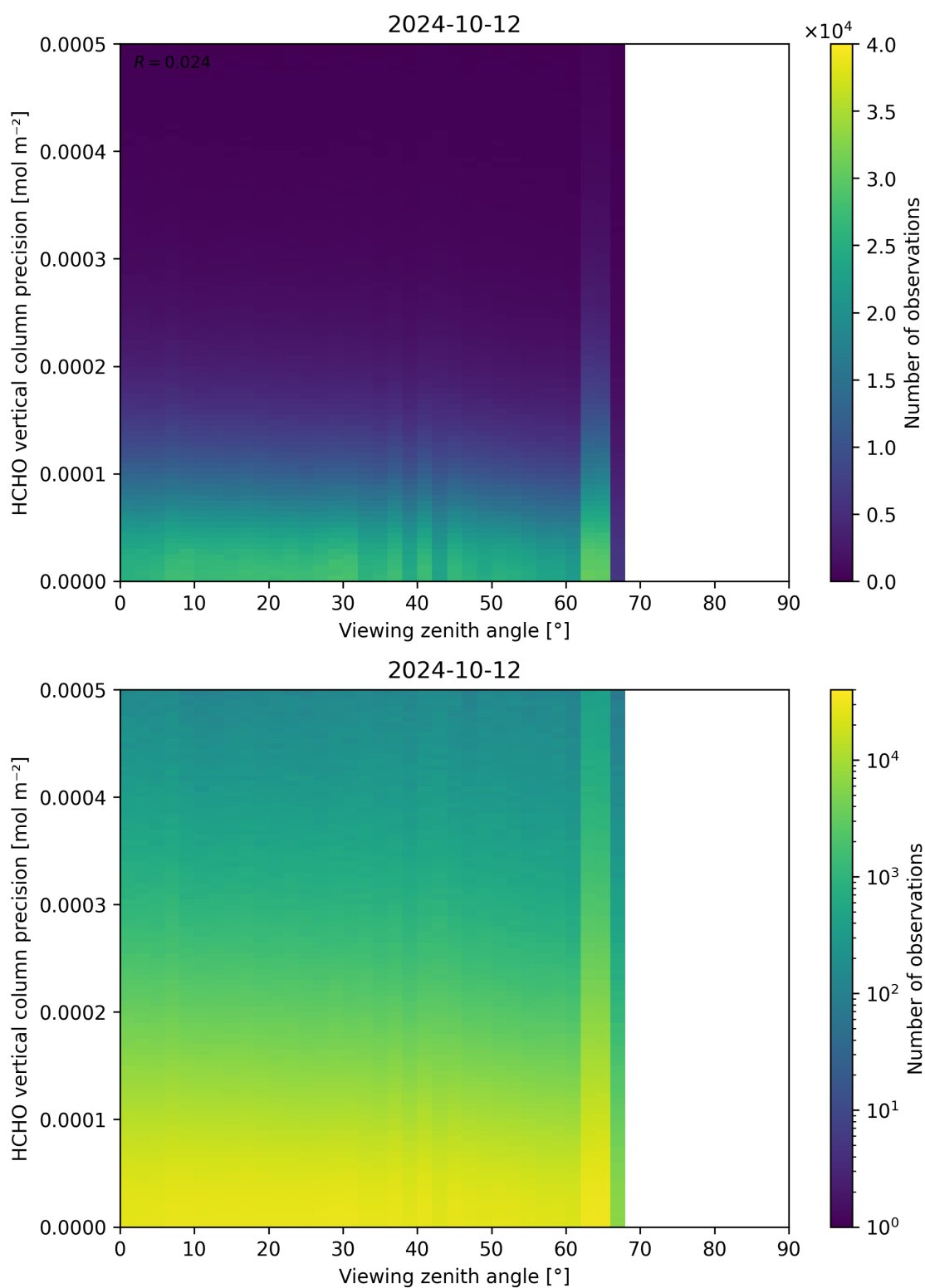
Figure 194: Scatter density plot of “Viewing zenith angle” against “HCHO vertical column precision” for 2024-10-11 to 2024-10-13.
