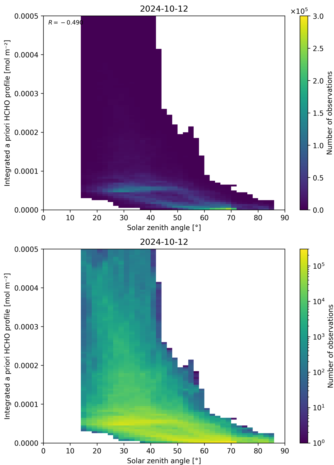
Figure 180: Scatter density plot of “Solar zenith angle” against “Integrated a priori HCHO profile” for 2024-10-11 to 2024-10-13.
