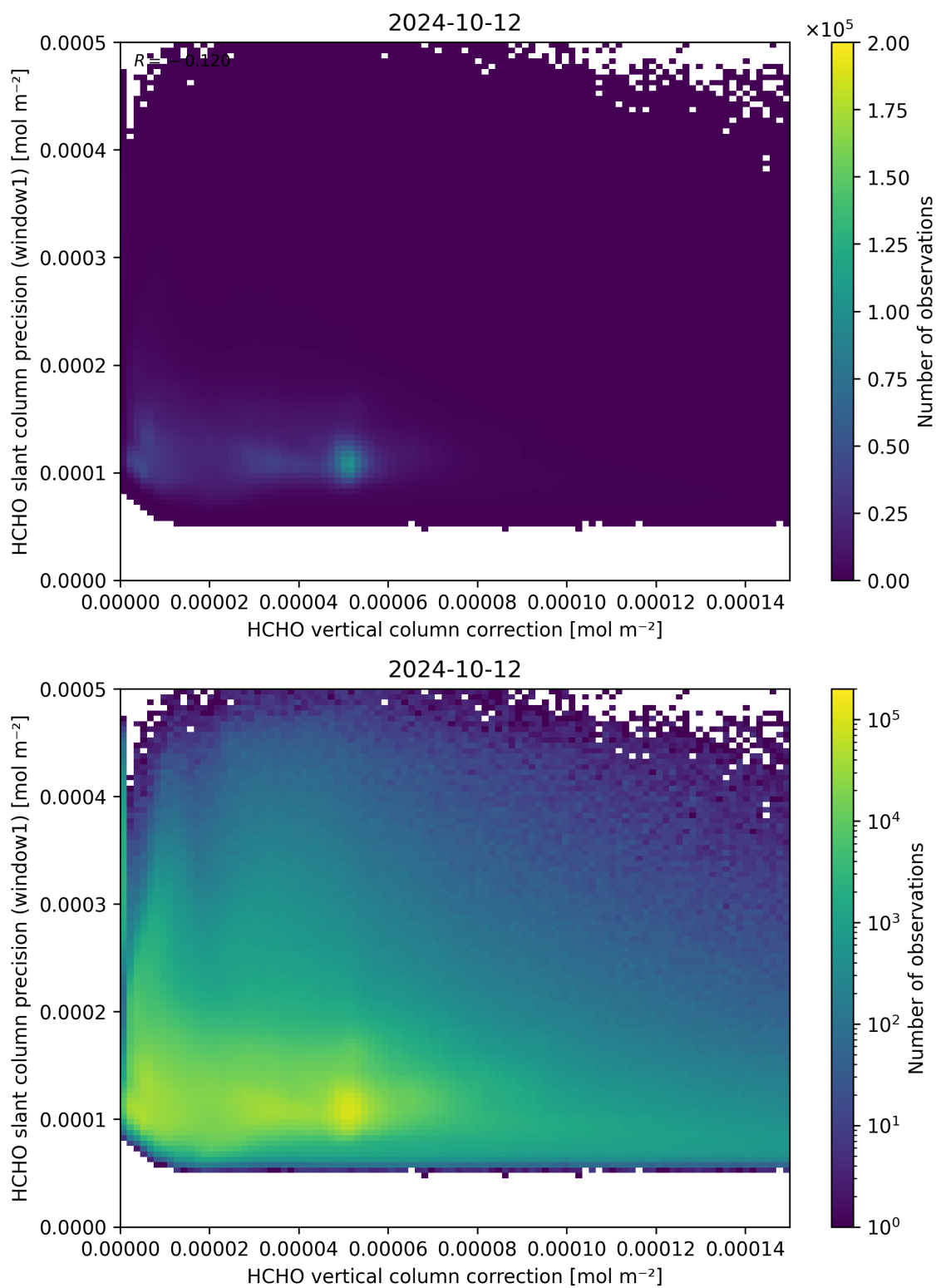
Figure 119: Scatter density plot of “HCHO vertical column correction” against “HCHO slant column precision (window1)” for 2024-10-11 to 2024-10-13.
