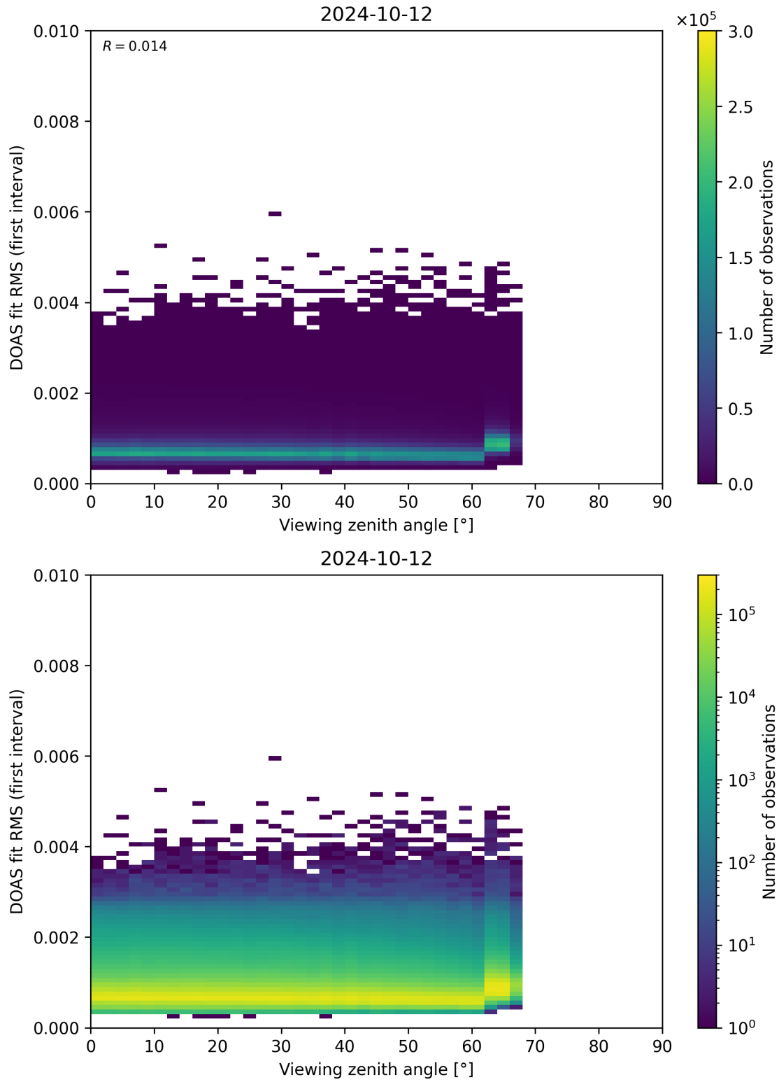
Figure 182: Scatter density plot of “Viewing zenith angle” against “DOAS fit RMS (first interval)” for 2024-10-11 to 2024-10-13.
