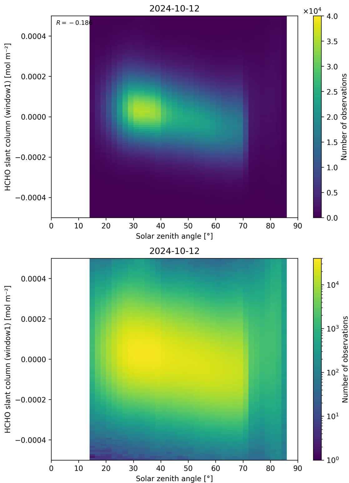
Figure 173: Scatter density plot of “Solar zenith angle” against “HCHO slant column (window1)” for 2024-10-11 to 2024-10-13.
