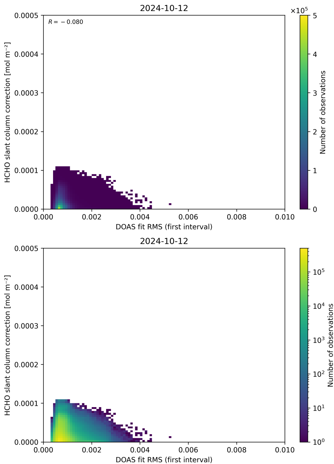
Figure 63: Scatter density plot of “DOAS fit RMS (first interval)” against “HCHO slant column correction” for 2024-10-11 to 2024-10-13.
