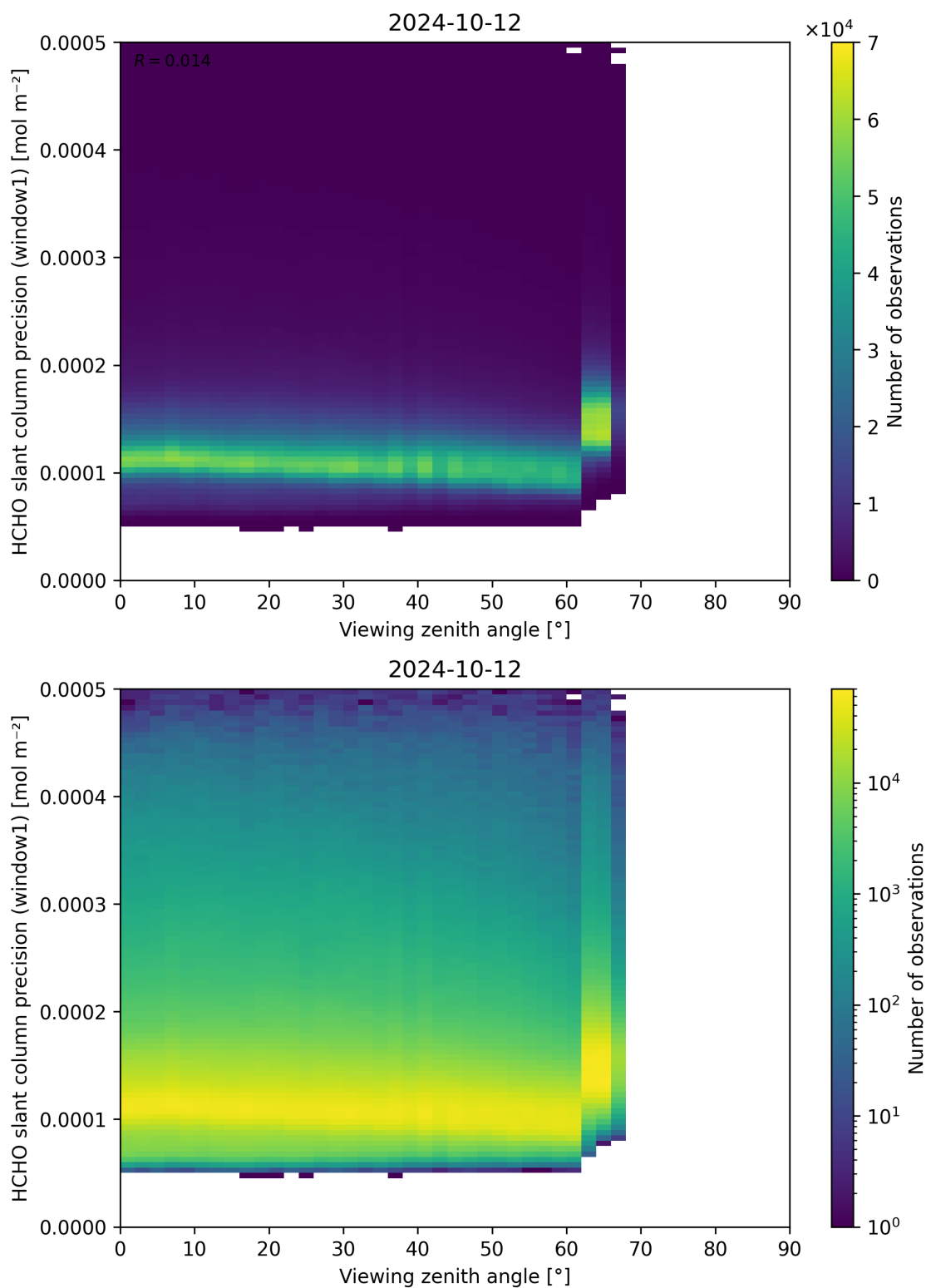
Figure 189: Scatter density plot of “Viewing zenith angle” against “HCHO slant column precision (window1)” for 2024-10-11 to 2024-10-13.
