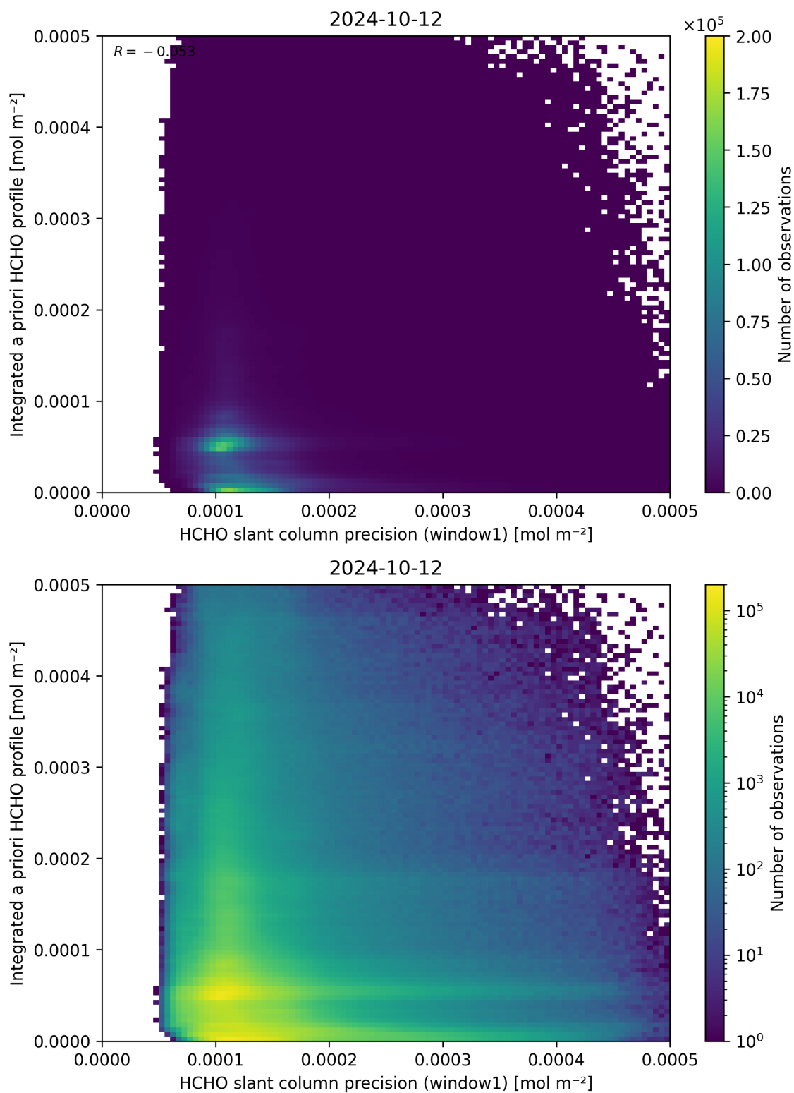
Figure 96: Scatter density plot of “HCHO slant column precision (window1)” against “Integrated a priori HCHO profile” for 2024-10-11 to 2024-10-13.
