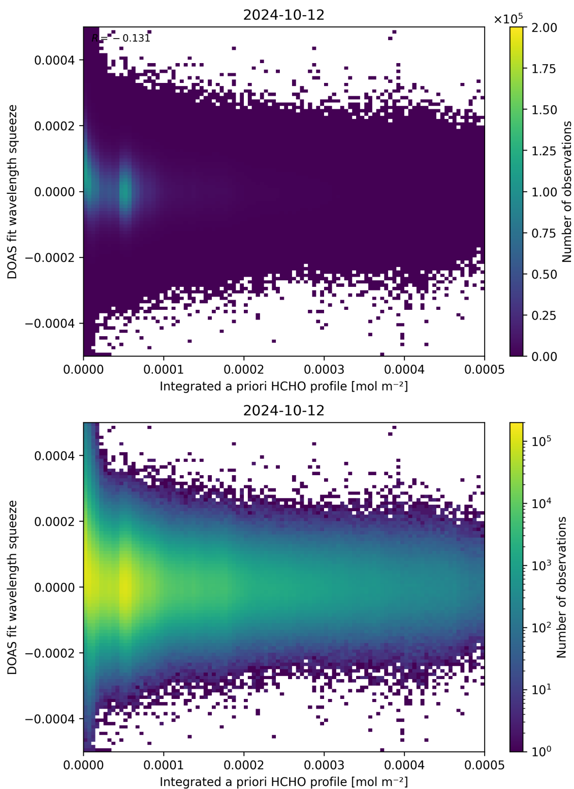
Figure 150: Scatter density plot of “Integrated a priori HCHO profile” against “DOAS fit wavelength squeeze” for 2024-10-11 to 2024-10-13.
