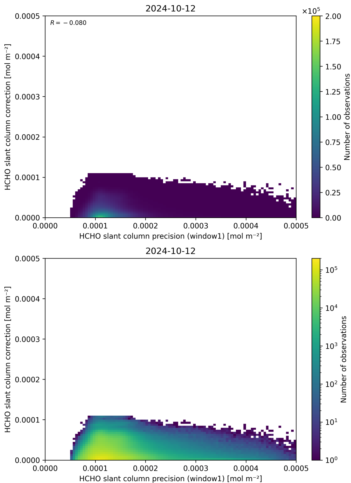
Figure 93: Scatter density plot of “HCHO slant column precision (window1)” against “HCHO slant column correction” for 2024-10-11 to 2024-10-13.
