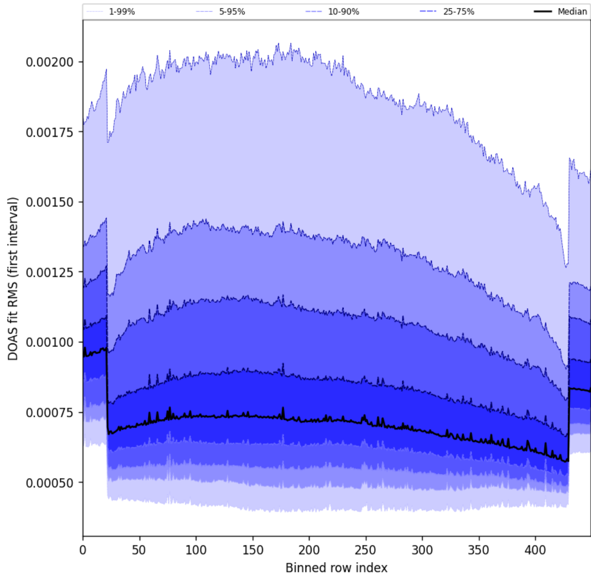
Figure 60: Along track statistics of “DOAS fit RMS (first interval)” for 2024-10-11 to 2024-10-13
