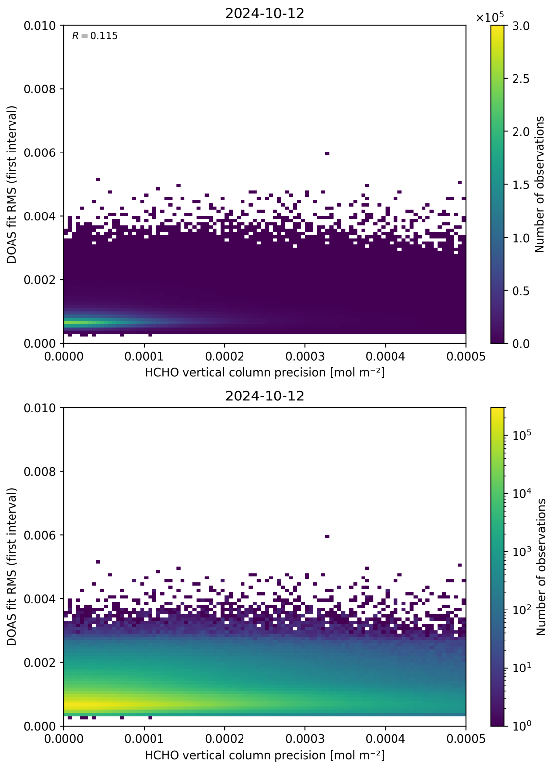
Figure 136: Scatter density plot of “HCHO vertical column precision” against “DOAS fit RMS (first interval)” for 2024-10-11 to 2024-10-13.
