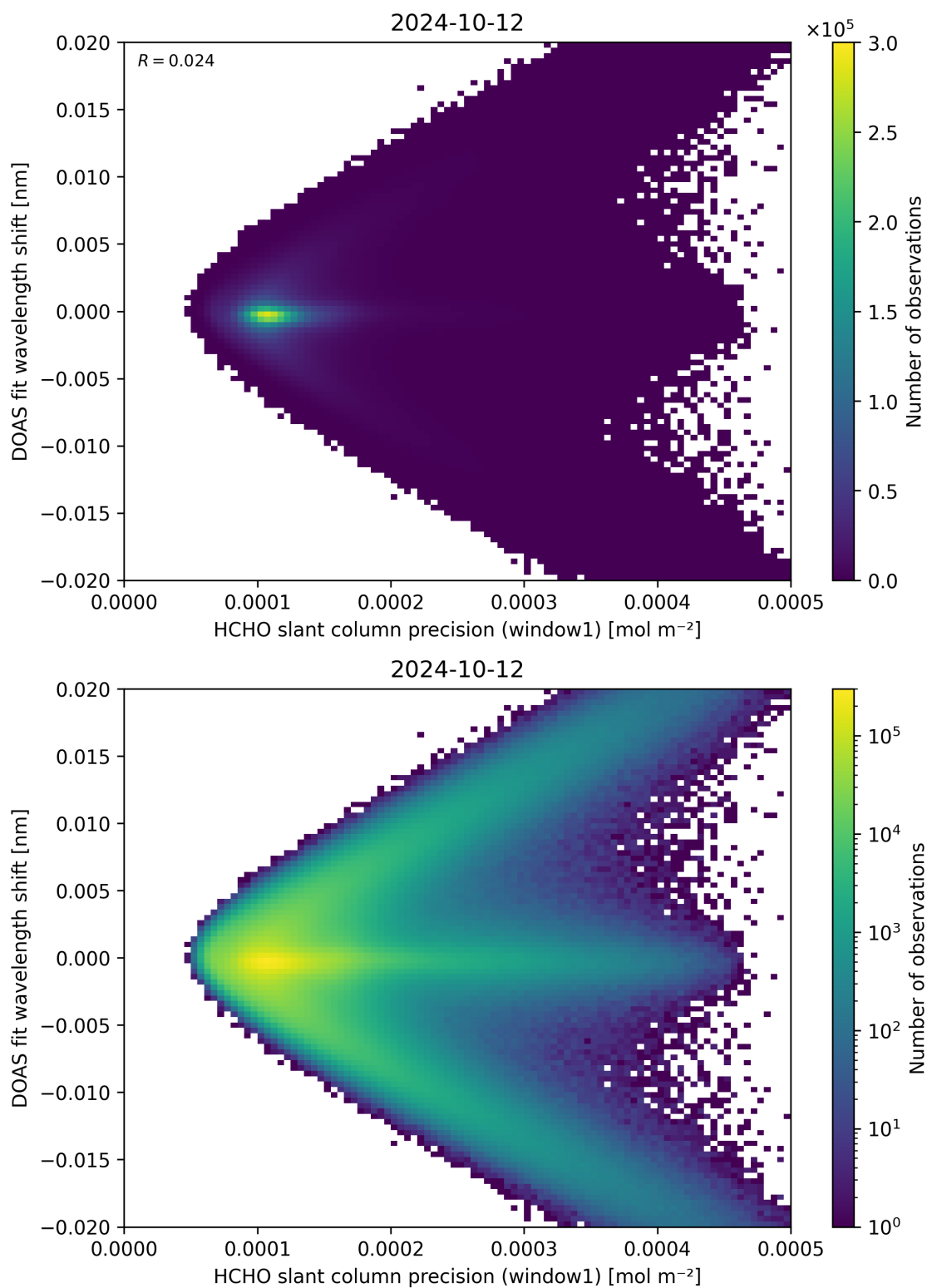
Figure 89: Scatter density plot of “HCHO slant column precision (window1)” against “DOAS fit wavelength shift” for 2024-10-11 to 2024-10-13.
