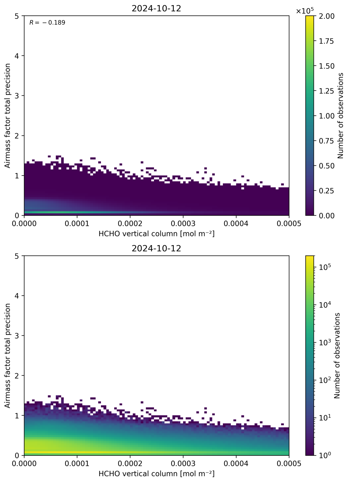
Figure 132: Scatter density plot of “HCHO vertical column” against “Airmass factor total precision” for 2024-10-11 to 2024-10-13.
