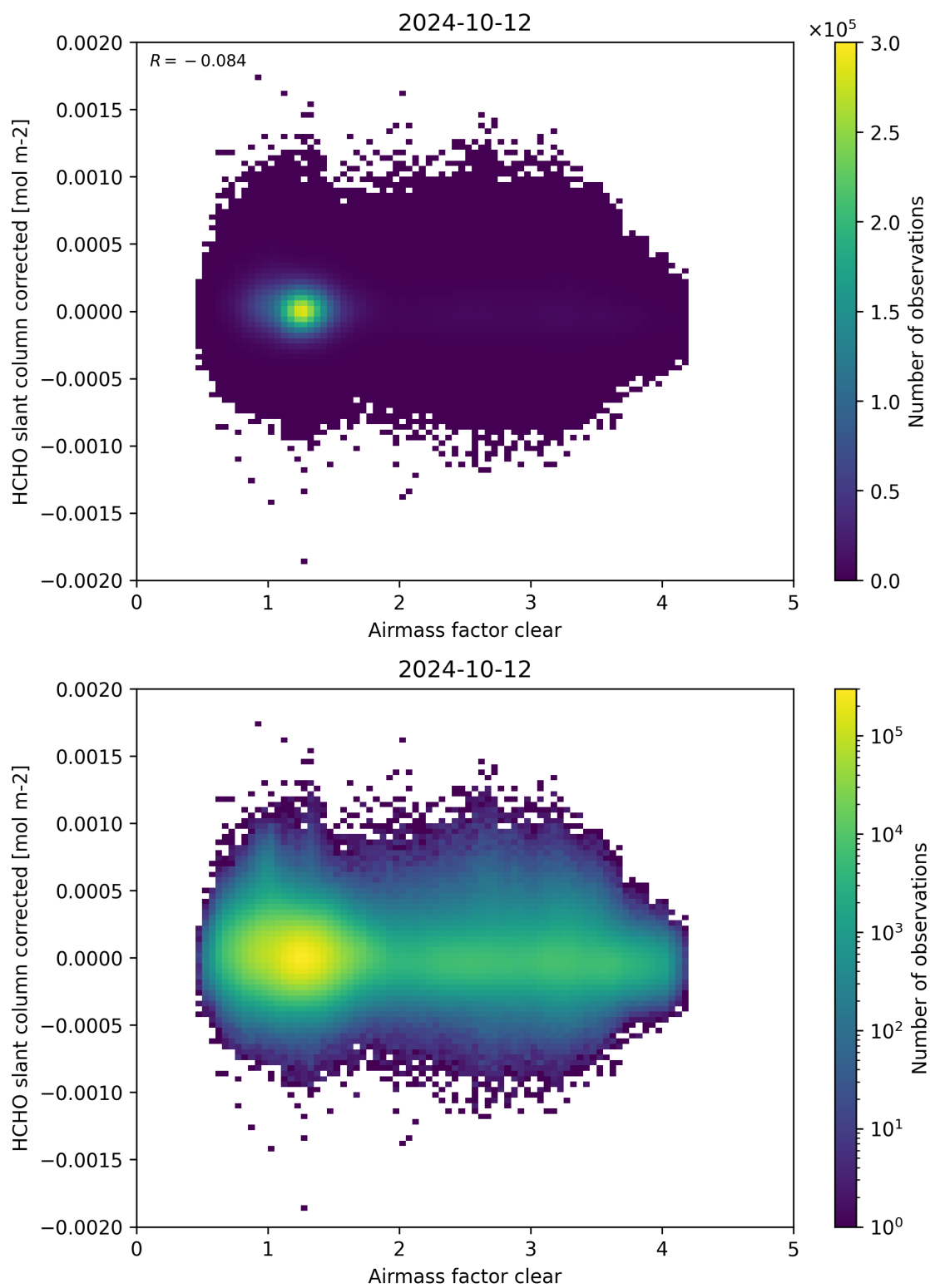
Figure 74: Scatter density plot of “Airmass factor clear” against “HCHO slant column corrected” for 2024-10-11 to 2024-10-13.
