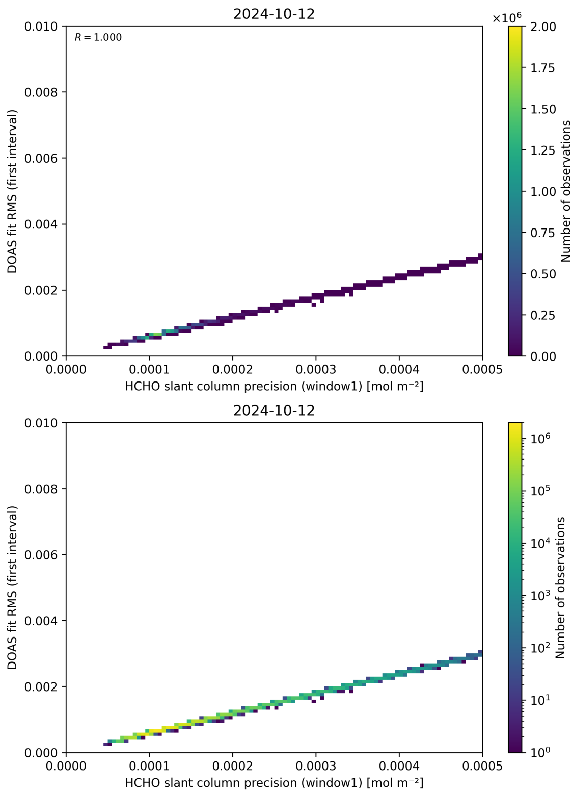
Figure 88: Scatter density plot of “HCHO slant column precision (window1)” against “DOAS fit RMS (first interval)” for 2024-10-11 to 2024-10-13.
