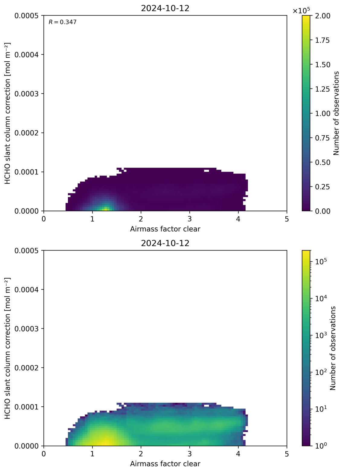
Figure 75: Scatter density plot of “Airmass factor clear” against “HCHO slant column correction” for 2024-10-11 to 2024-10-13.
