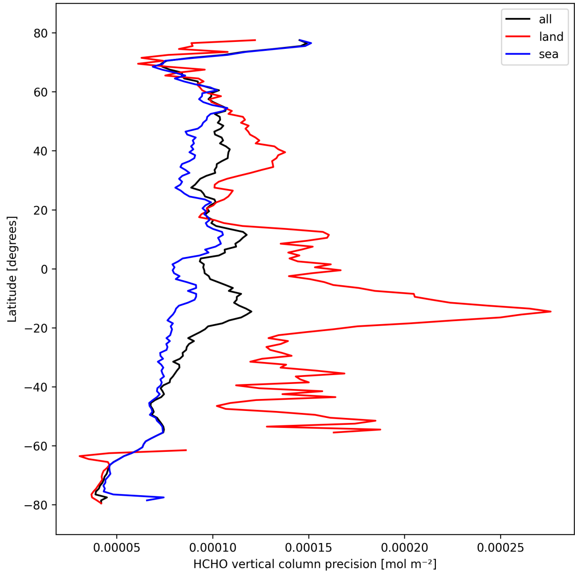
Figure 22: Zonal average of “HCHO vertical column precision” for 2024-10-11 to 2024-10-13.
