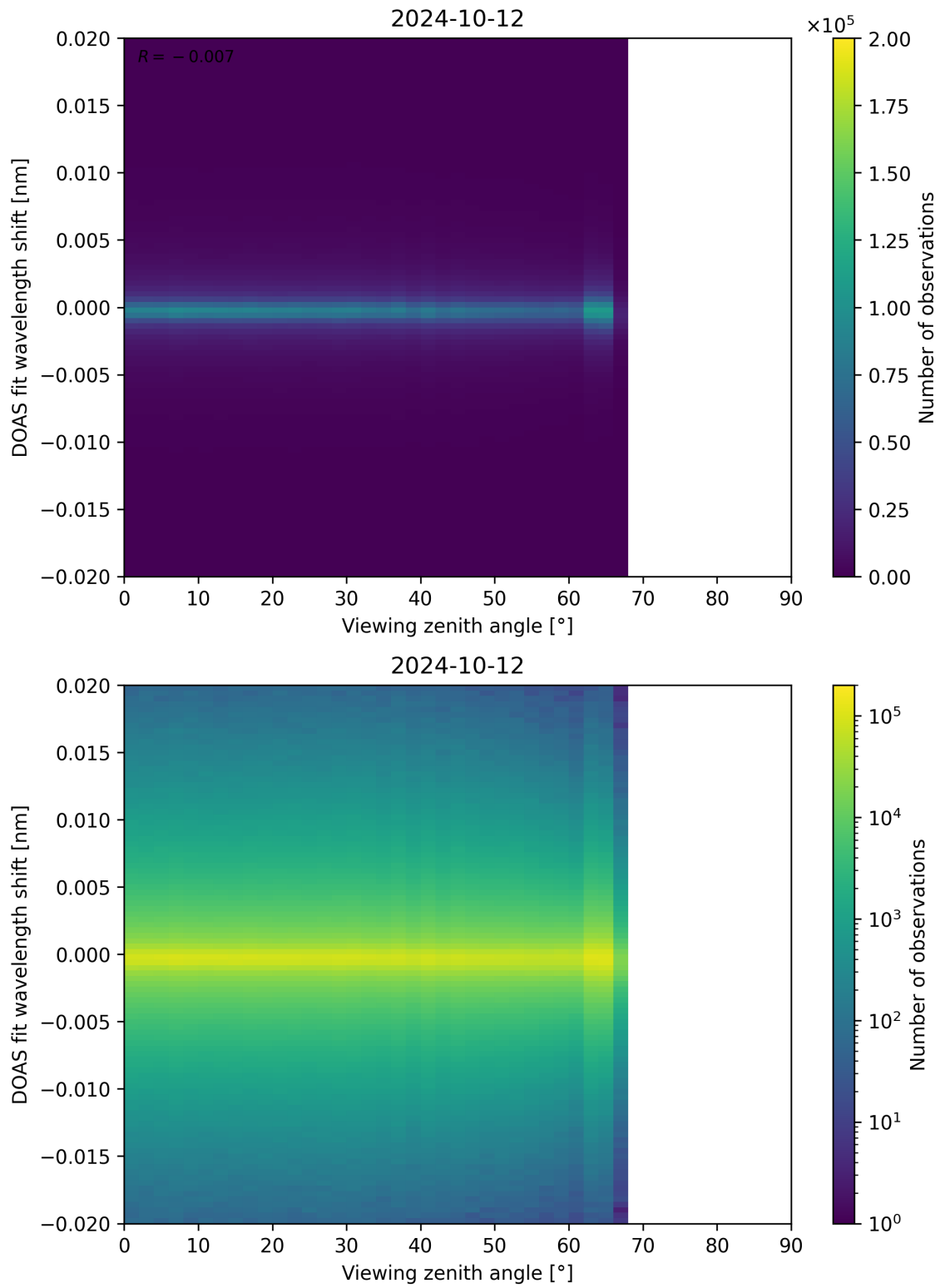
Figure 183: Scatter density plot of “Viewing zenith angle” against “DOAS fit wavelength shift” for 2024-10-11 to 2024-10-13.
