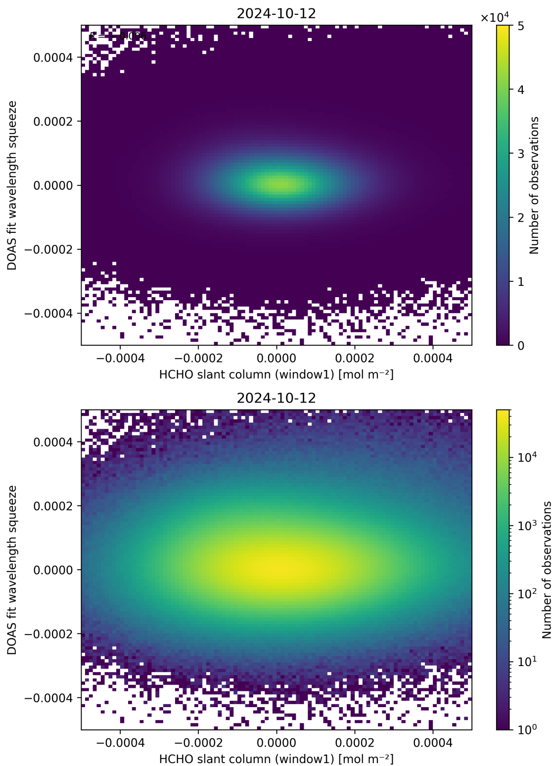
Figure 80: Scatter density plot of “HCHO slant column (window1)” against “DOAS fit wavelength squeeze” for 2024-10-11 to 2024-10-13.
