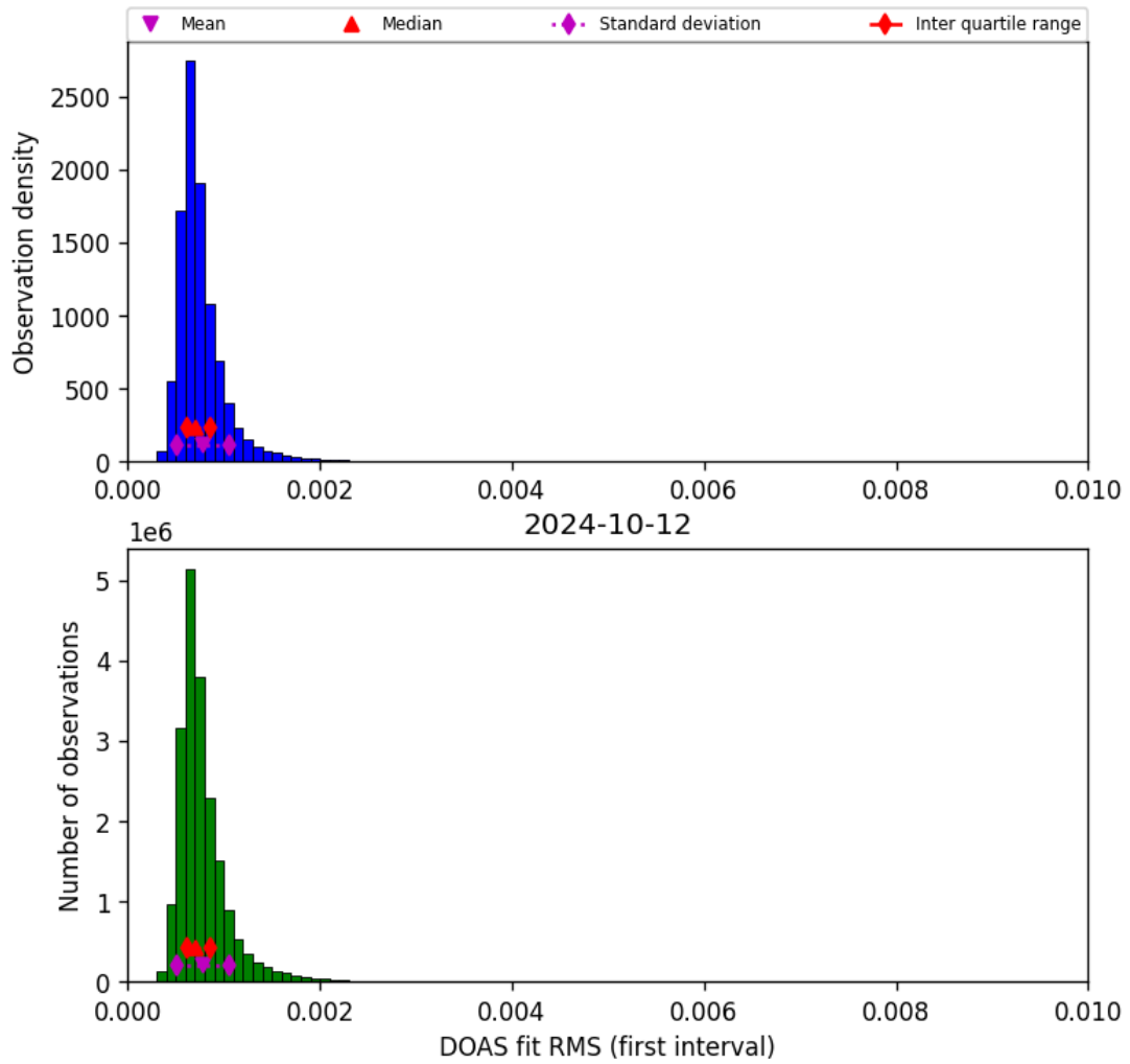
Figure 46: Histogram of “DOAS fit RMS (first interval)” for 2024-10-11 to 2024-10-13
