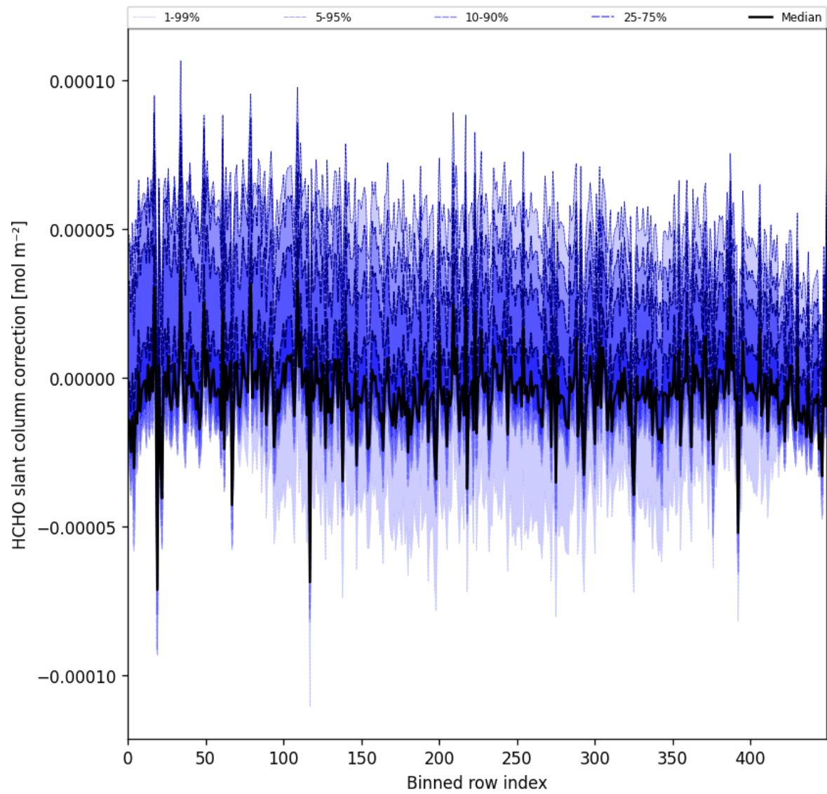
Figure 61: Along track statistics of “HCHO slant column correction” for 2024-10-11 to 2024-10-13
