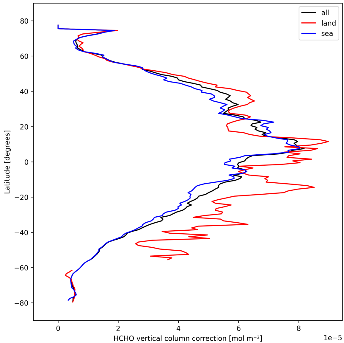
Figure 23: Zonal average of “HCHO vertical column correction” for 2024-10-11 to 2024-10-13.
