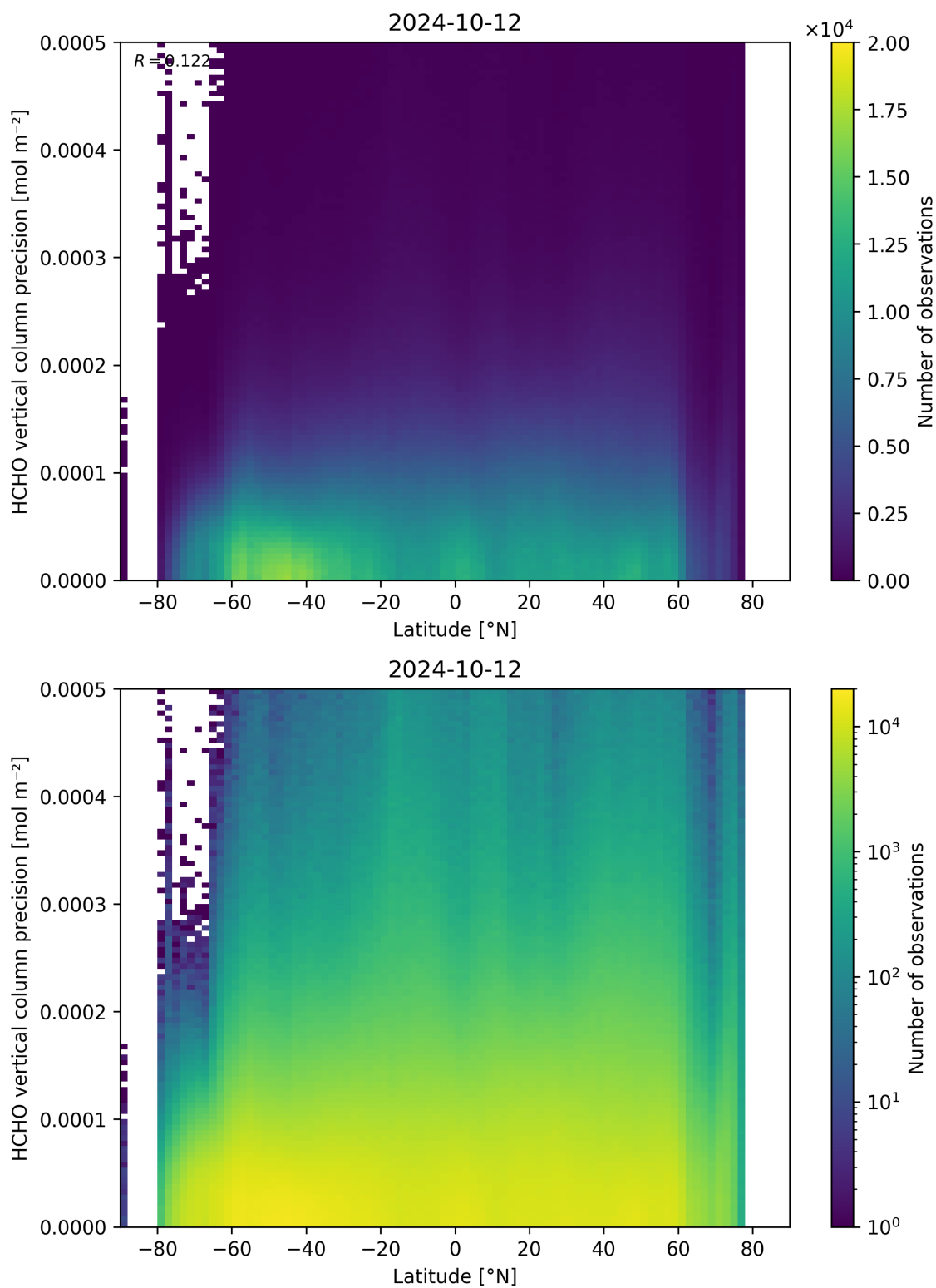
Figure 165: Scatter density plot of “Latitude” against “HCHO vertical column precision” for 2024-10-11 to 2024-10-13.
