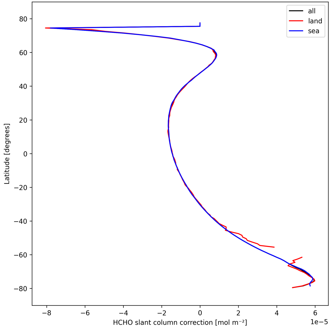
Figure 33: Zonal average of “HCHO slant column correction” for 2024-10-11 to 2024-10-13.
