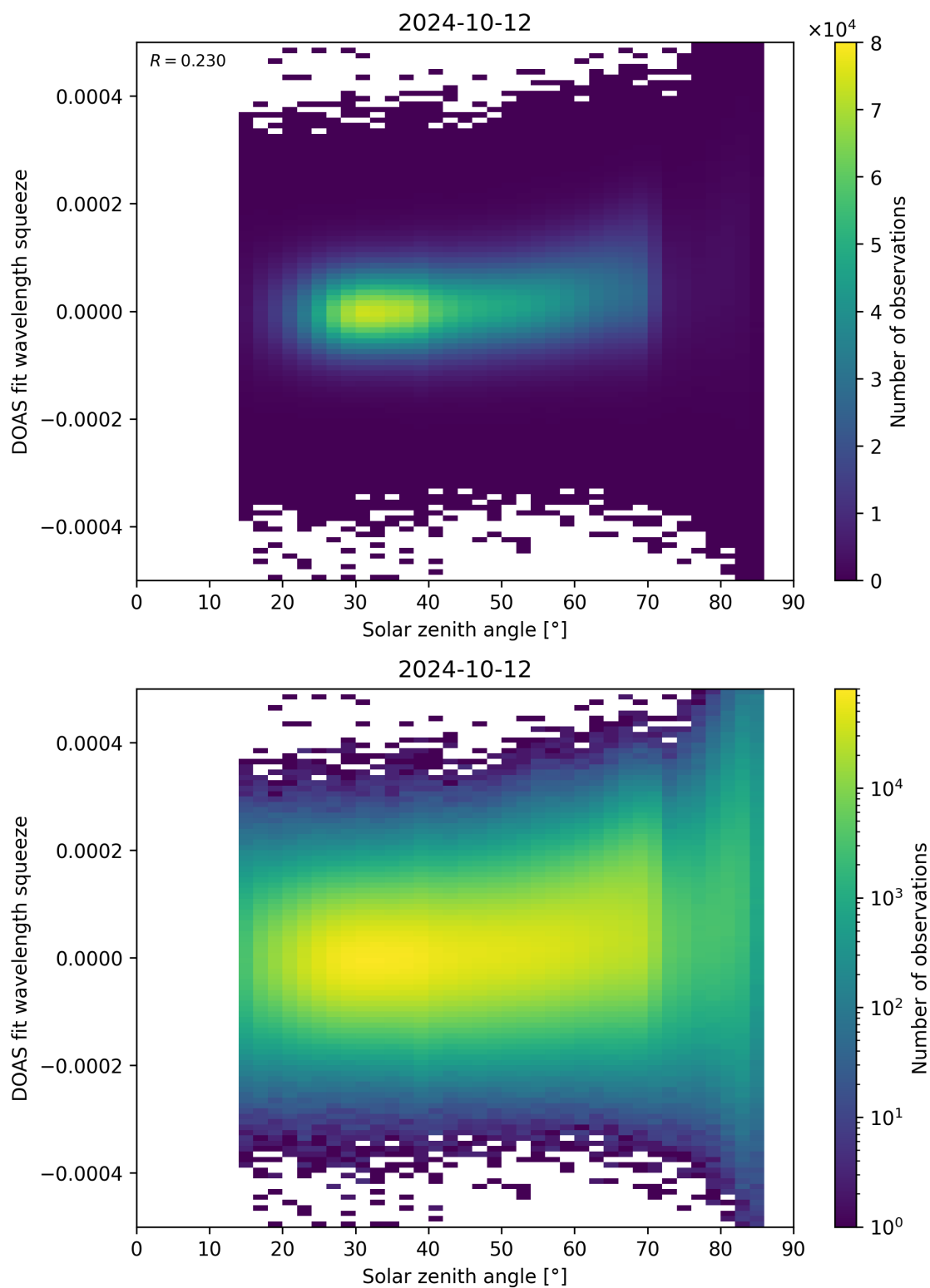
Figure 169: Scatter density plot of “Solar zenith angle” against “DOAS fit wavelength squeeze” for 2024-10-11 to 2024-10-13.
