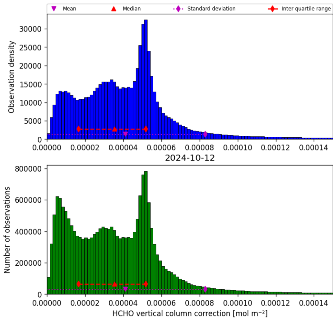
Figure 37: Histogram of “HCHO vertical column correction” for 2024-10-11 to 2024-10-13
