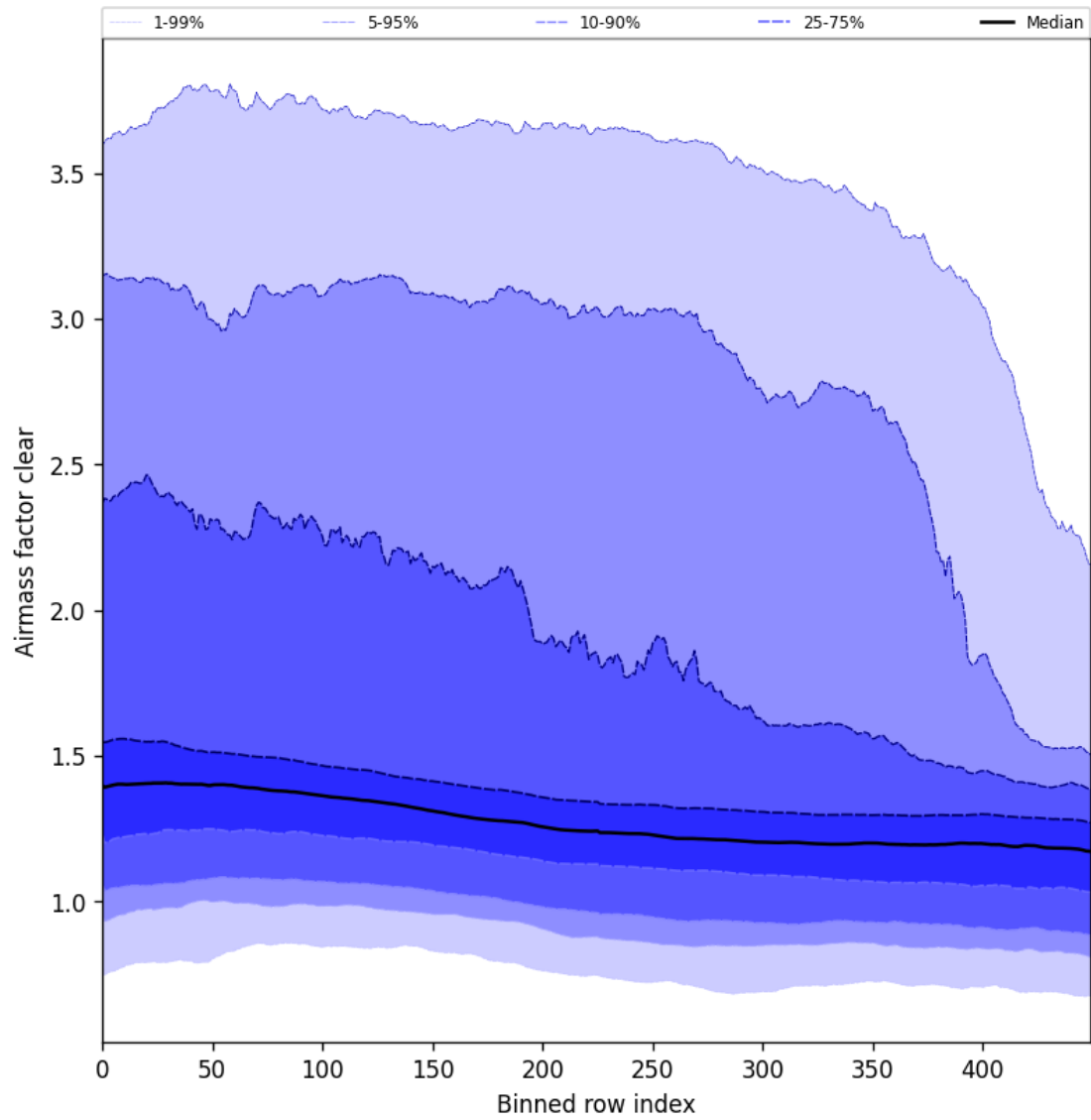
Figure 56: Along track statistics of “Airmass factor clear” for 2024-10-11 to 2024-10-13
