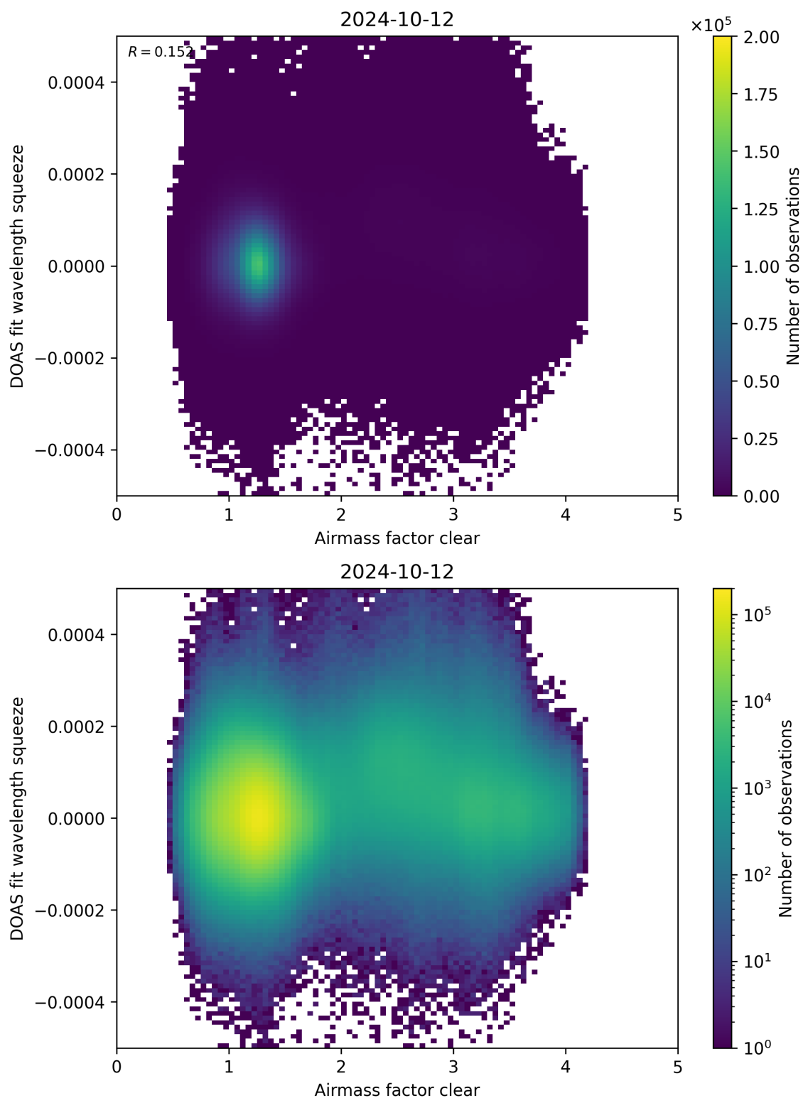
Figure 73: Scatter density plot of “Airmass factor clear” against “DOAS fit wavelength squeeze” for 2024-10-11 to 2024-10-13.
