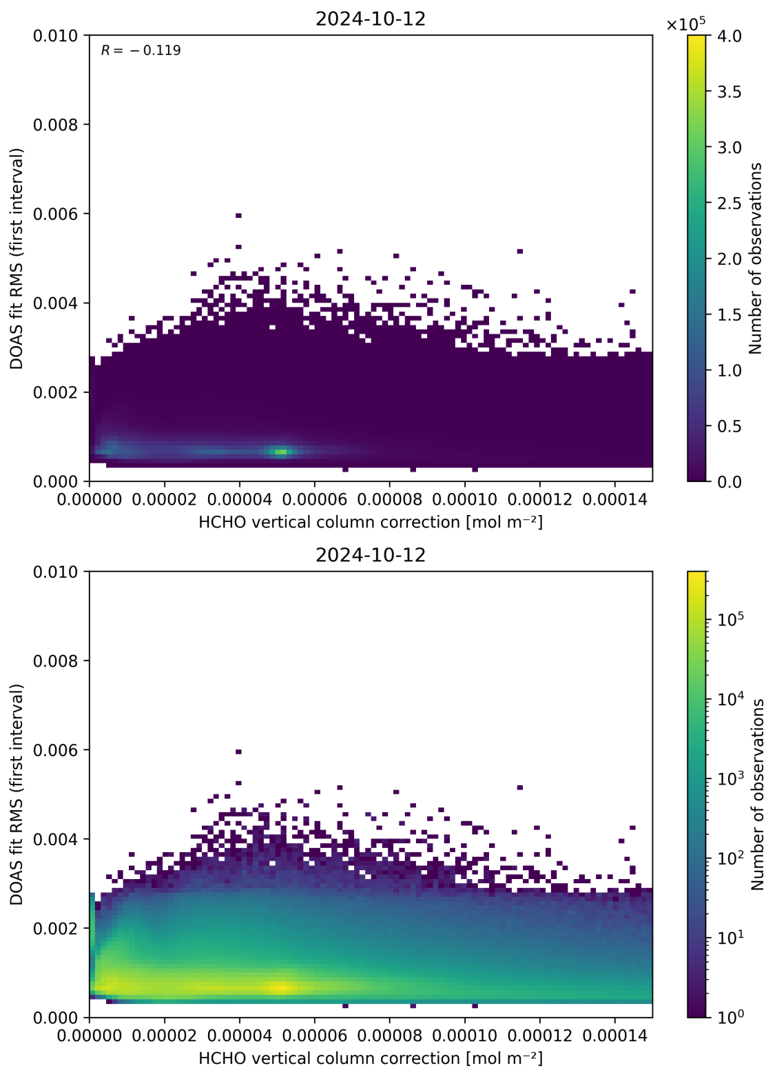
Figure 112: Scatter density plot of “HCHO vertical column correction” against “DOAS fit RMS (first interval)” for 2024-10-11 to 2024-10-13.
