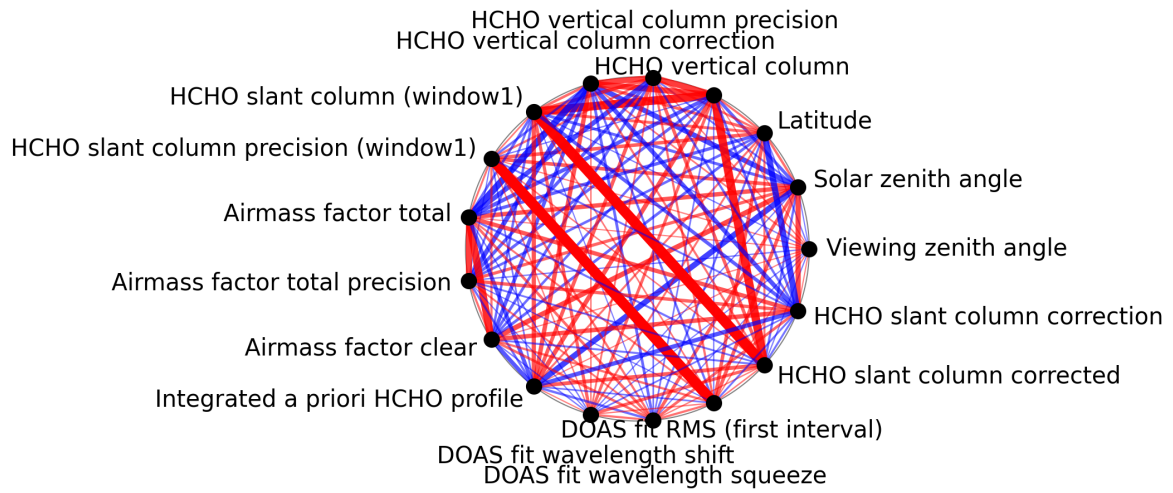
Figure 1: Map of correlation graph for 2024-10-11 to 2024-10-13.
