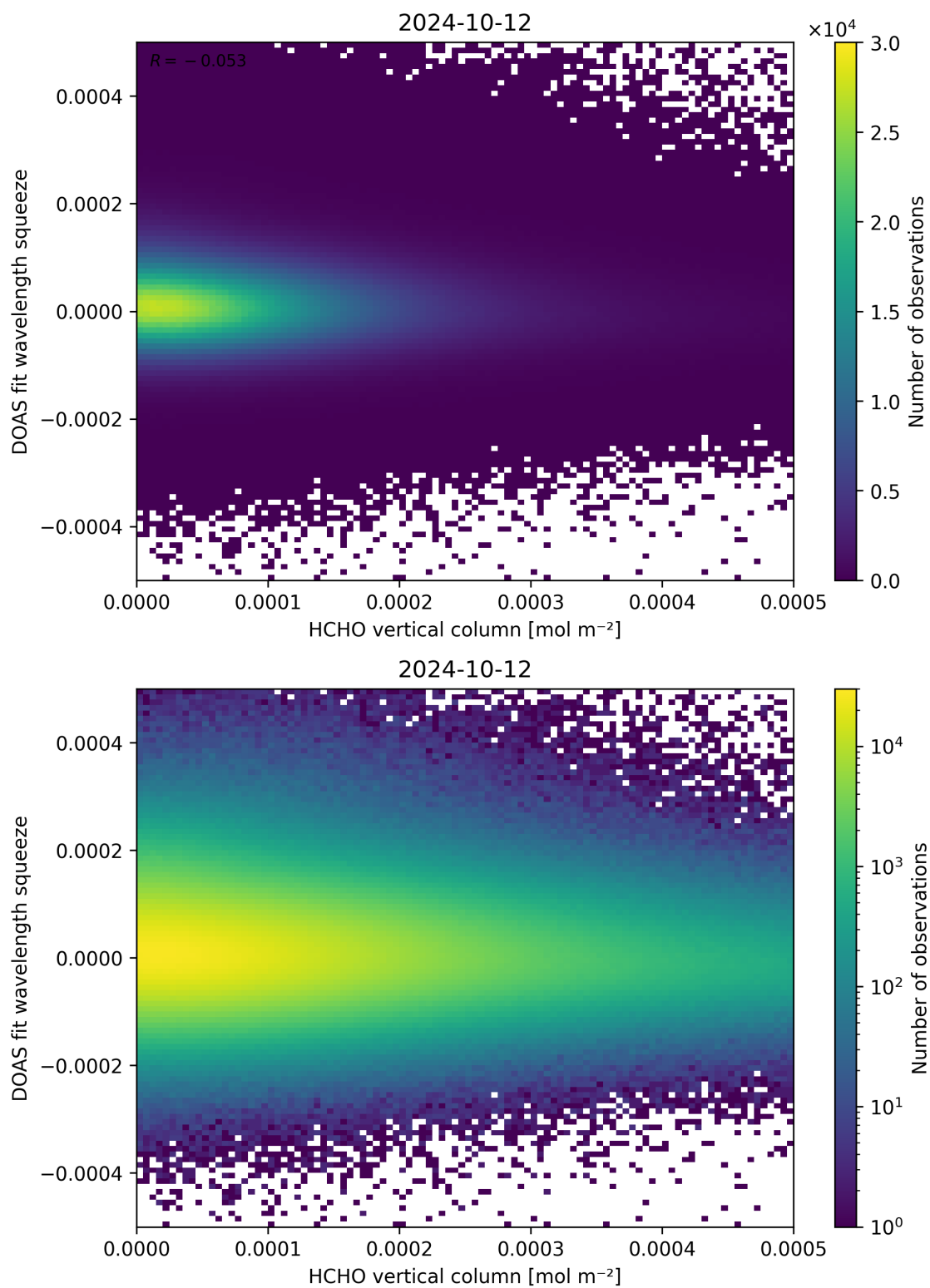
Figure 125: Scatter density plot of “HCHO vertical column” against “DOAS fit wavelength squeeze” for 2024-10-11 to 2024-10-13.
