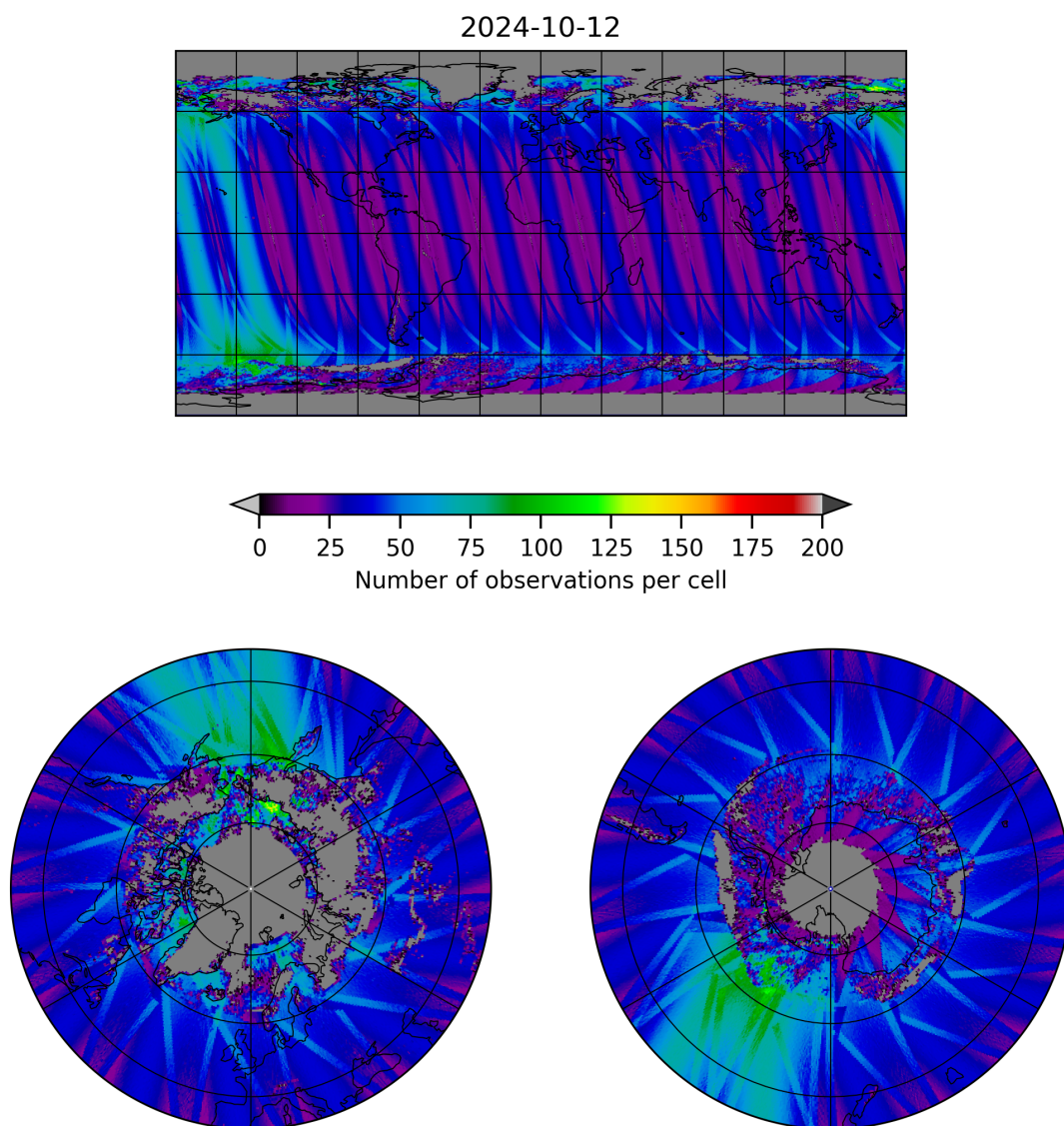
Figure 19: Map of the number of observations for 2024-10-11 to 2024-10-13
