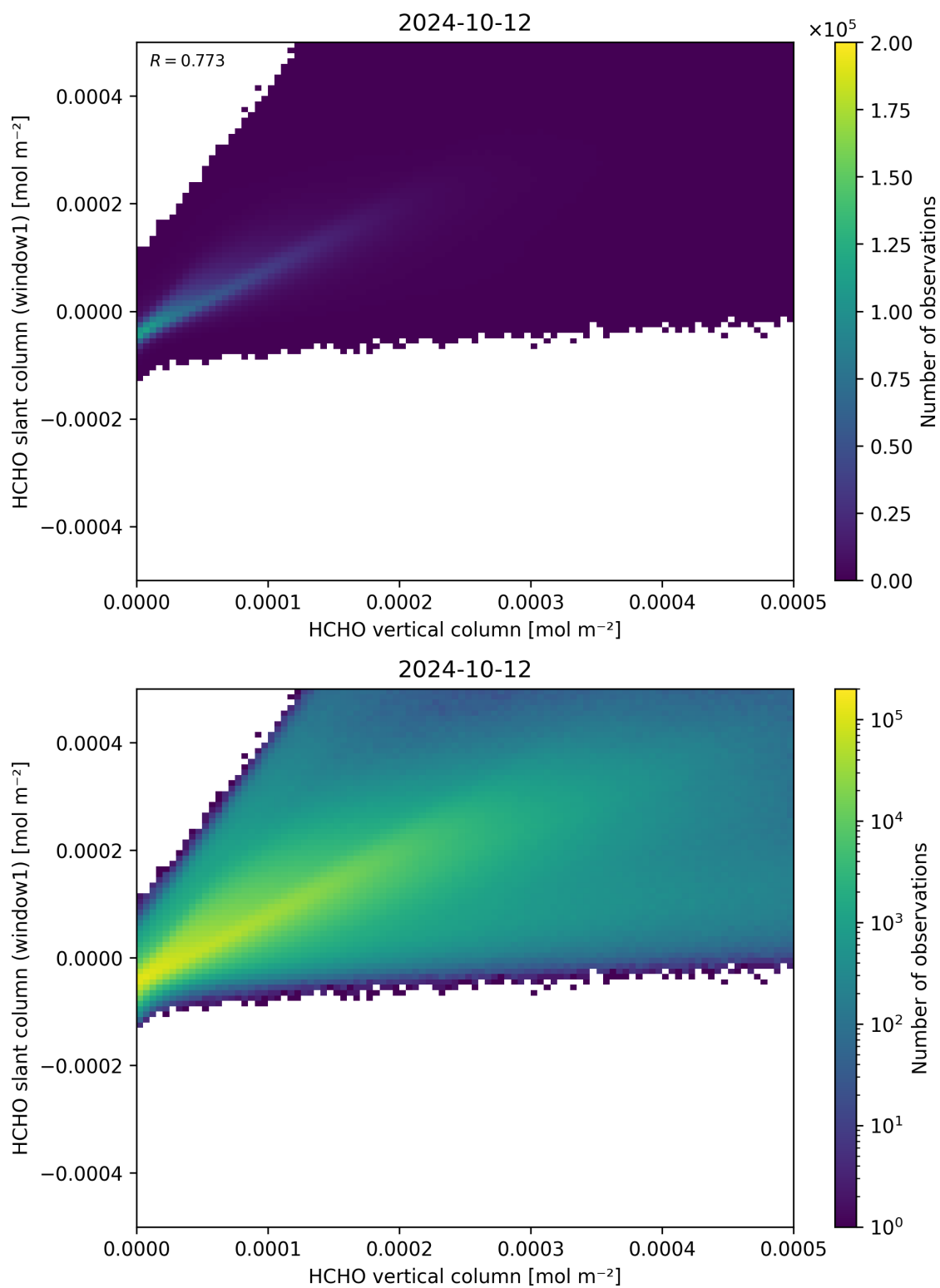
Figure 129: Scatter density plot of “HCHO vertical column” against “HCHO slant column (window1)” for 2024-10-11 to 2024-10-13.
