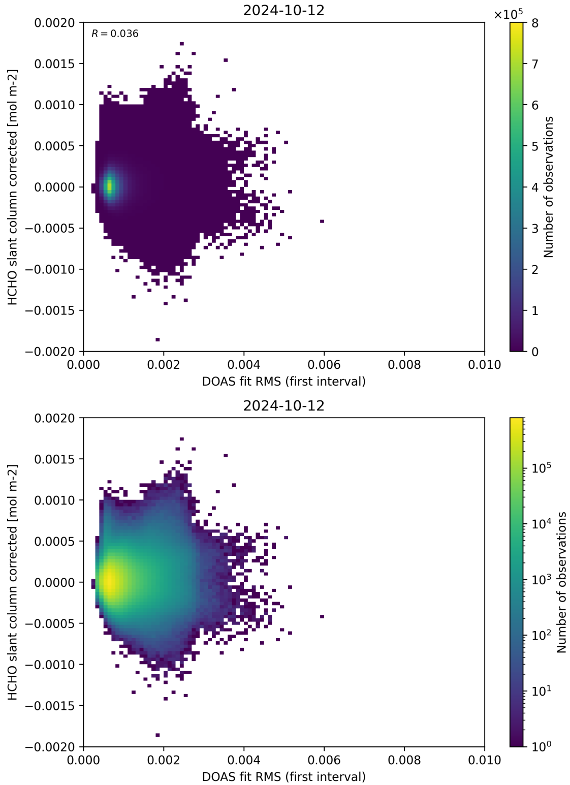
Figure 62: Scatter density plot of “DOAS fit RMS (first interval)” against “HCHO slant column corrected” for 2024-10-11 to 2024-10-13.
