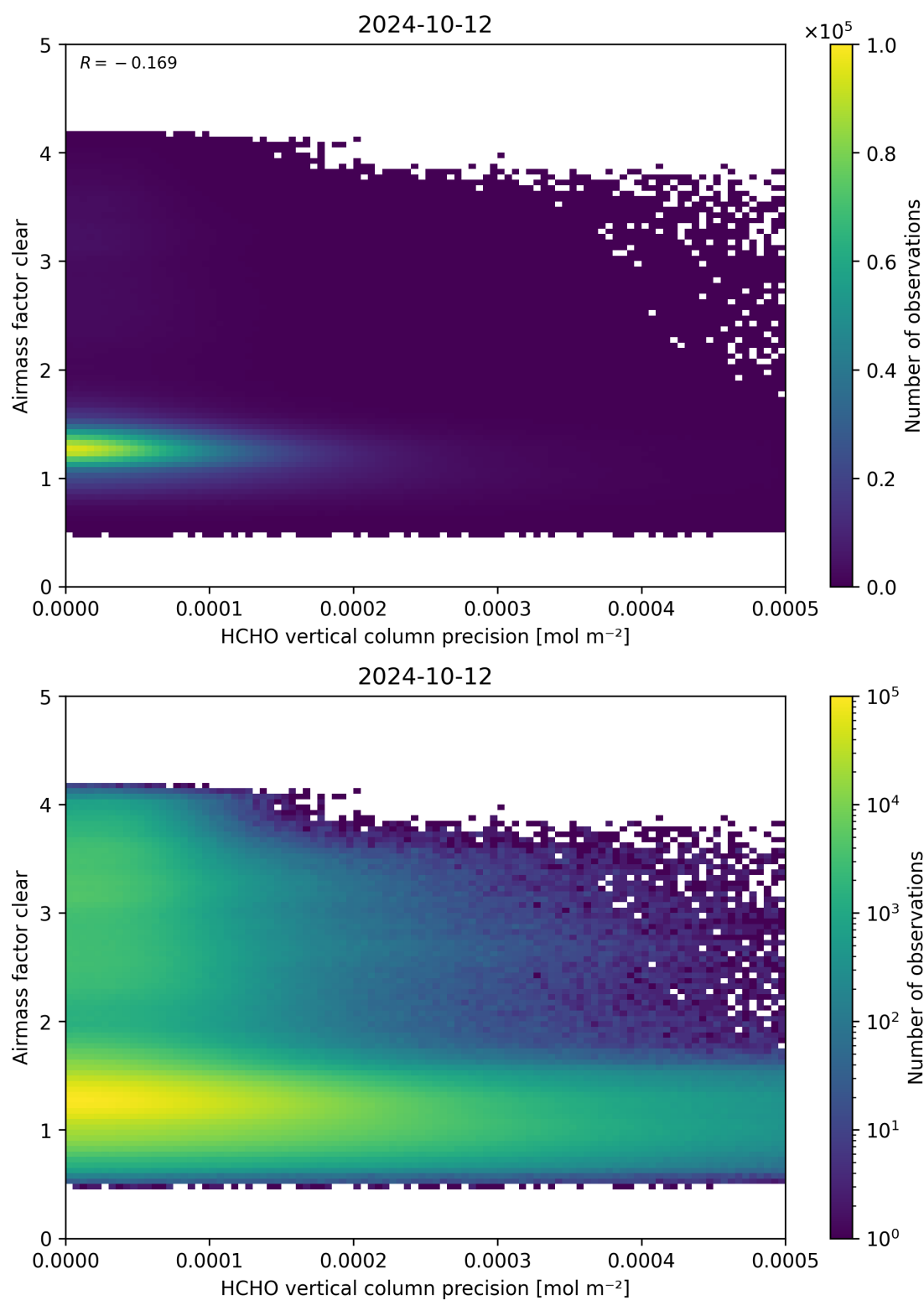
Figure 139: Scatter density plot of “HCHO vertical column precision” against “Airmass factor clear” for 2024-10-11 to 2024-10-13.
