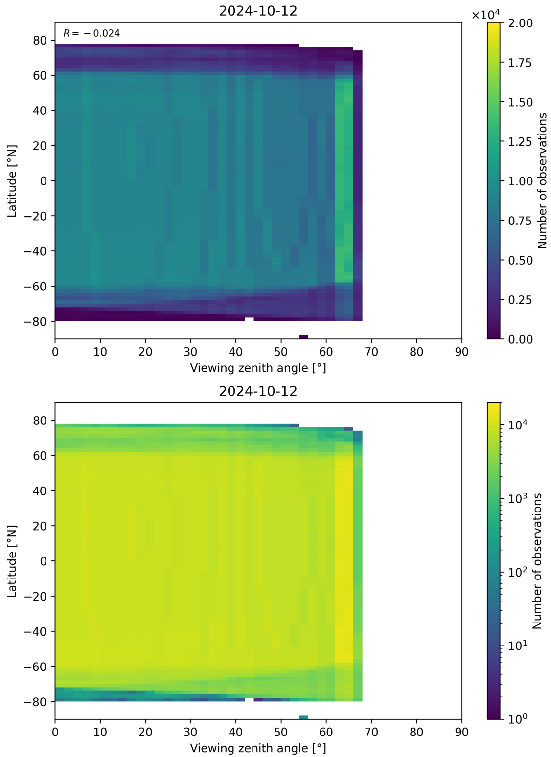
Figure 196: Scatter density plot of “Viewing zenith angle” against “Latitude” for 2024-10-11 to 2024-10-13.
