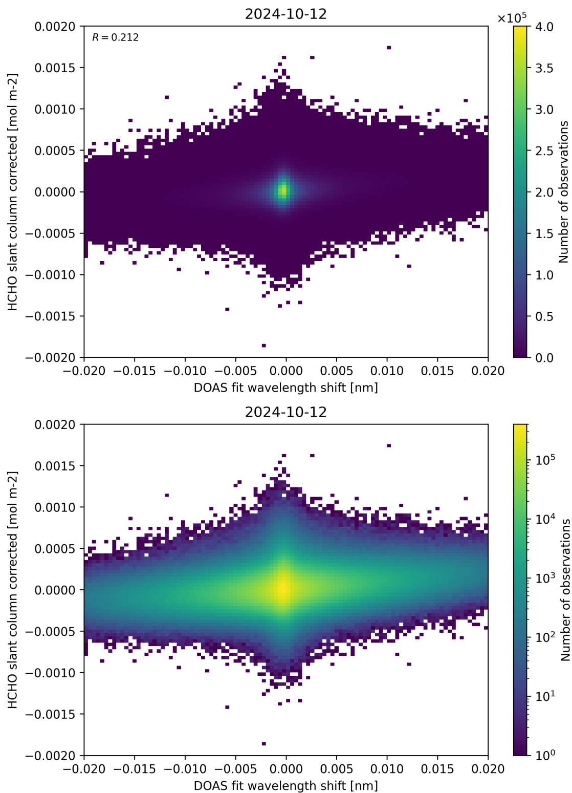
Figure 66: Scatter density plot of “DOAS fit wavelength shift” against “HCHO slant column corrected” for 2024-10-11 to 2024-10-13.
