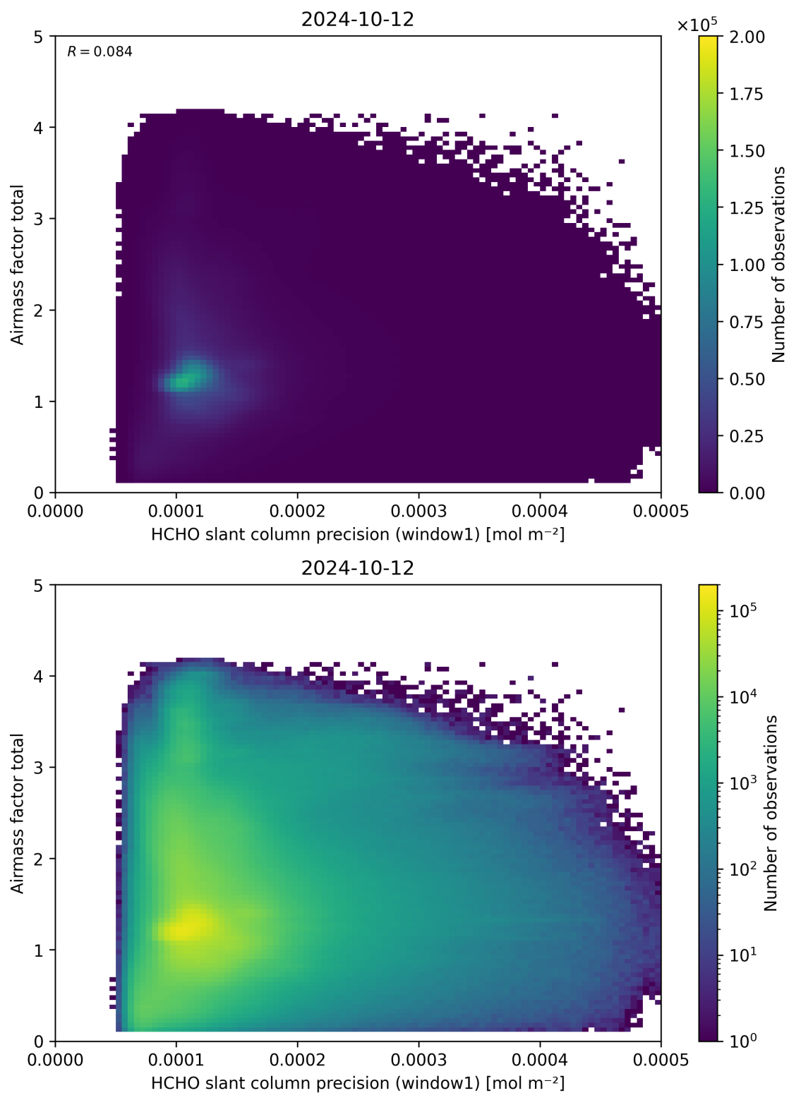
Figure 94: Scatter density plot of “HCHO slant column precision (window1)” against “Airmass factor total” for 2024-10-11 to 2024-10-13.
