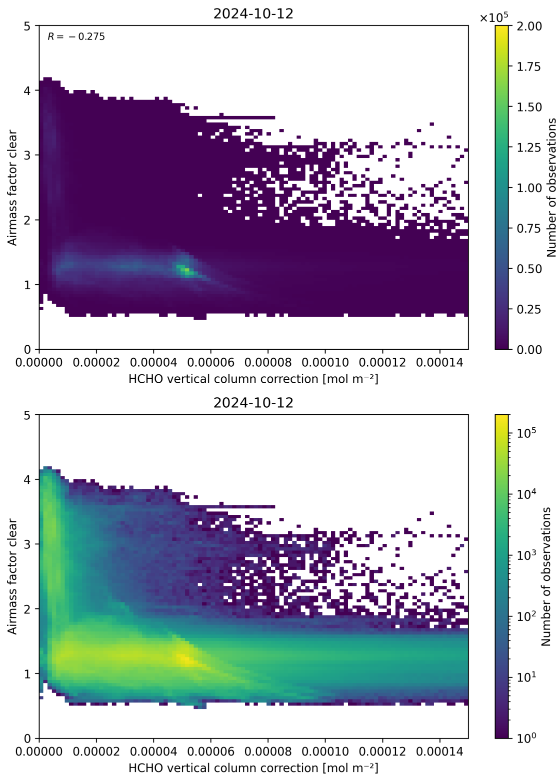
Figure 115: Scatter density plot of “HCHO vertical column correction” against “Airmass factor clear” for 2024-10-11 to 2024-10-13.
