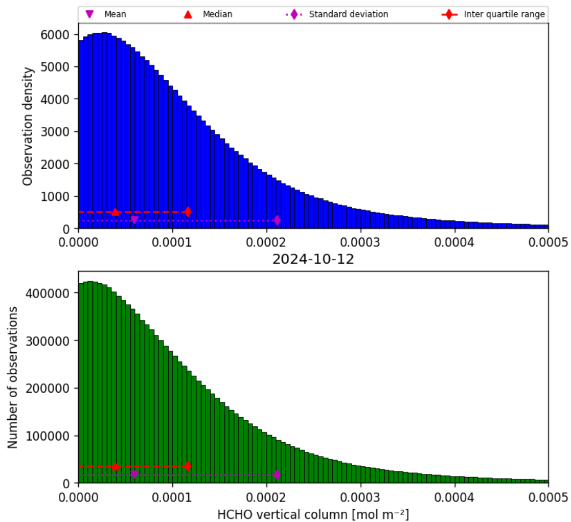
Figure 35: Histogram of “HCHO vertical column” for 2024-10-11 to 2024-10-13
