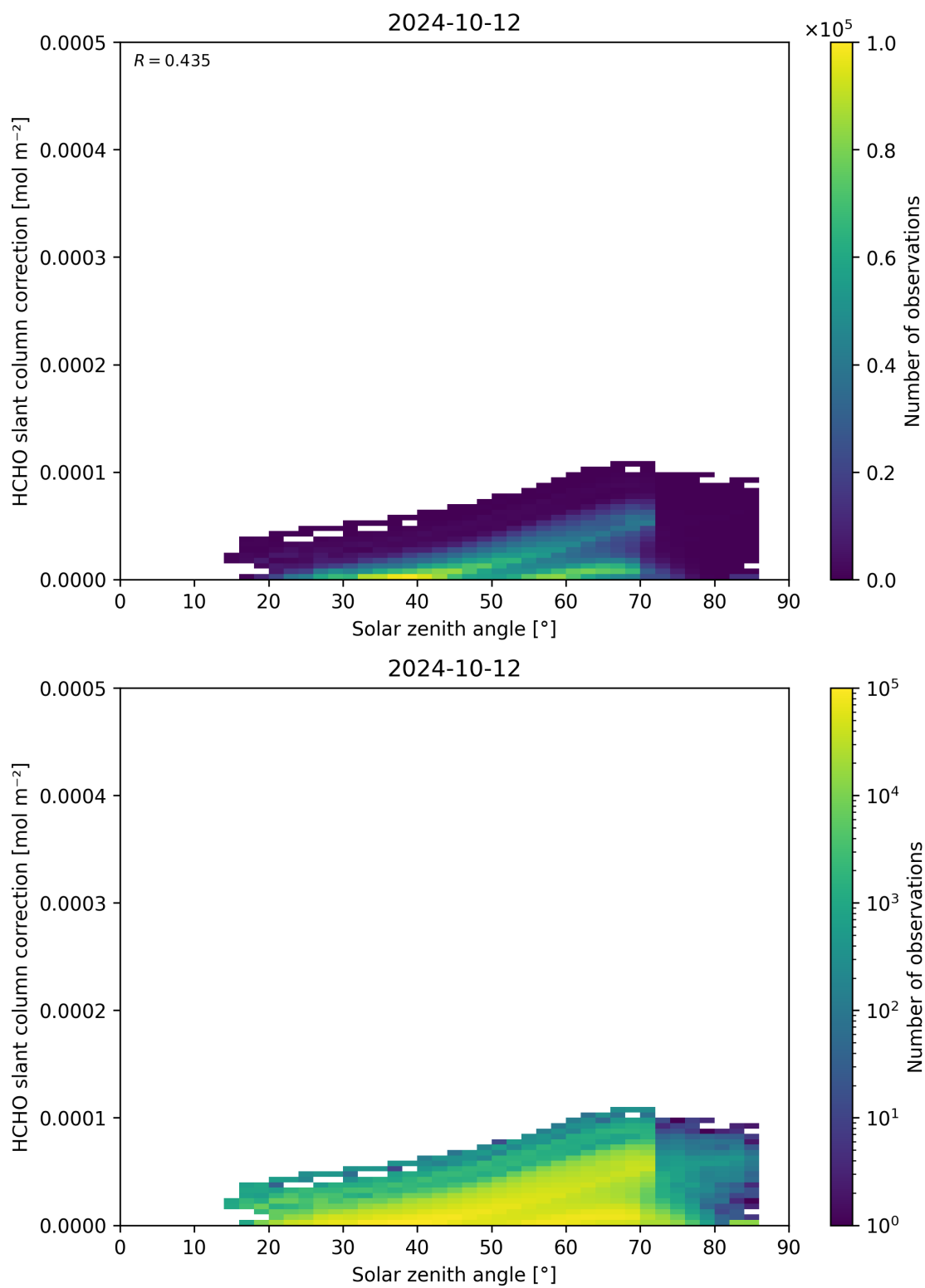
Figure 172: Scatter density plot of “Solar zenith angle” against “HCHO slant column correction” for 2024-10-11 to 2024-10-13.
