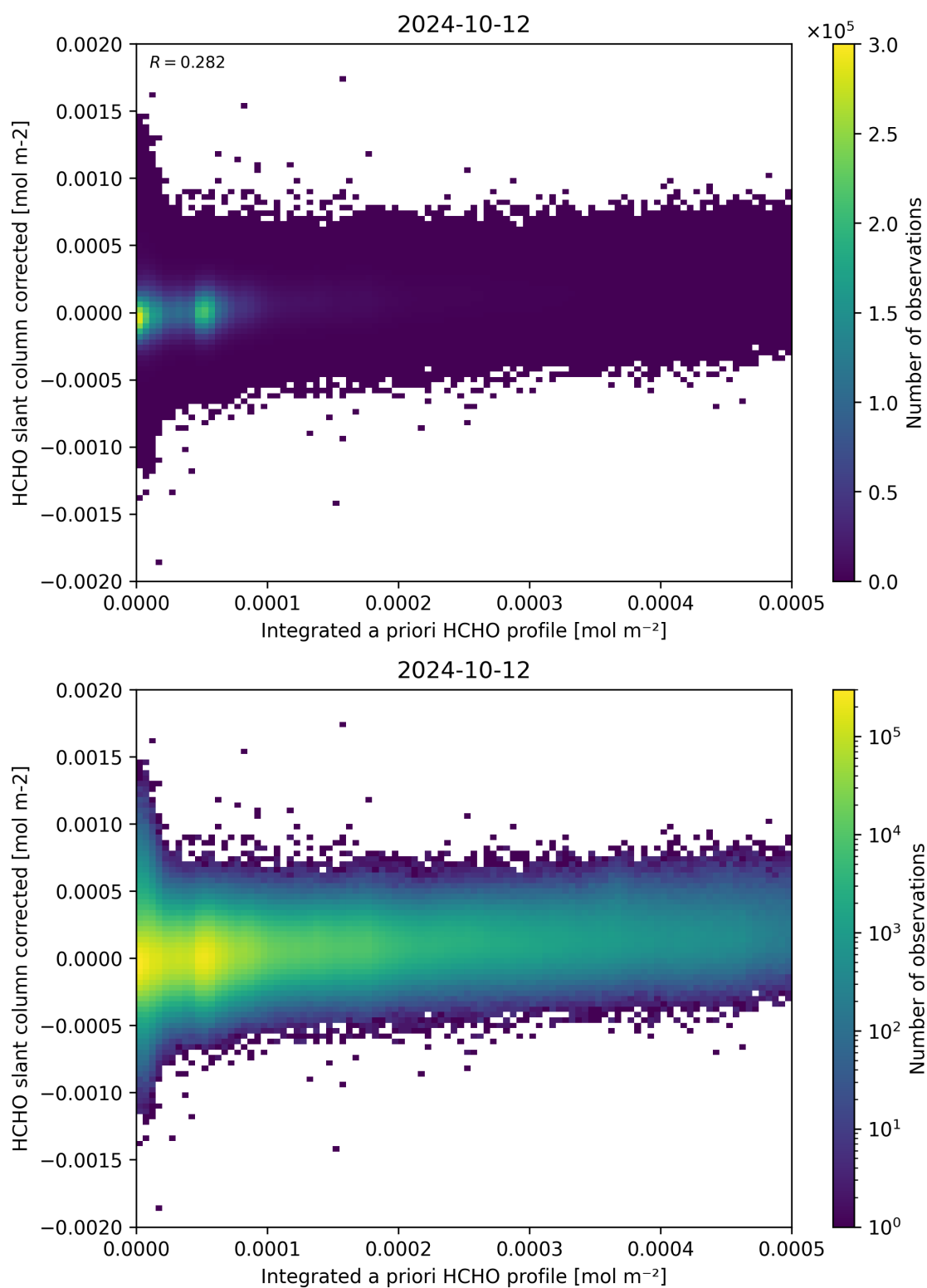
Figure 151: Scatter density plot of “Integrated a priori HCHO profile” against “HCHO slant column corrected” for 2024-10-11 to 2024-10-13.
