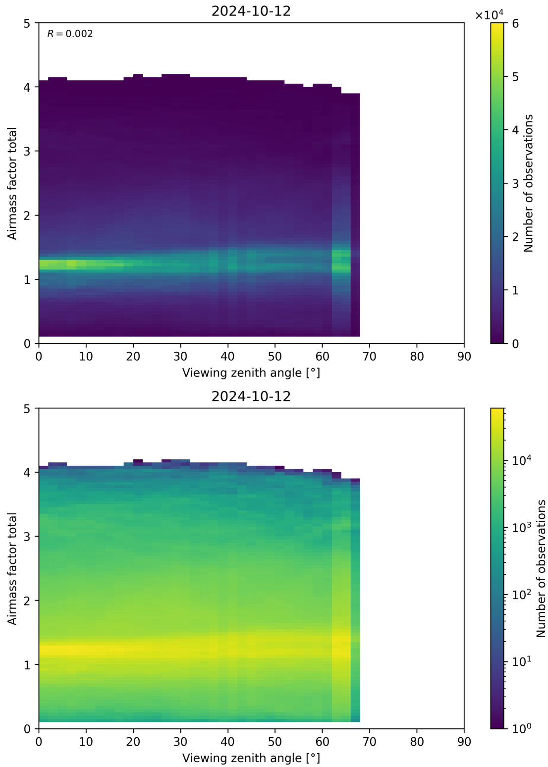
Figure 190: Scatter density plot of “Viewing zenith angle” against “Airmass factor total” for 2024-10-11 to 2024-10-13.
