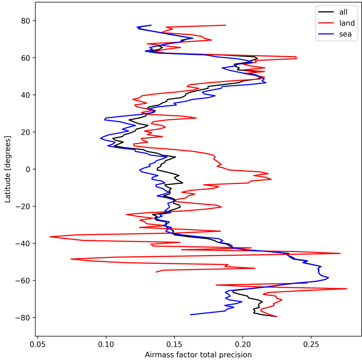
Figure 27: Zonal average of “Airmass factor total precision” for 2024-10-11 to 2024-10-13.
