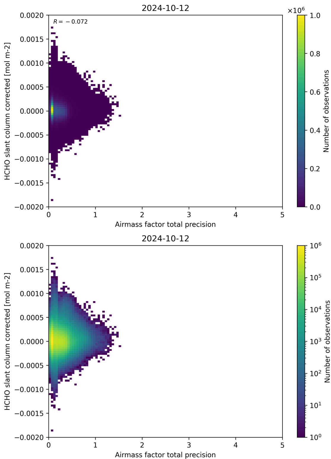
Figure 109: Scatter density plot of “Airmass factor total precision” against “HCHO slant column corrected” for 2024-10-11 to 2024-10-13.
