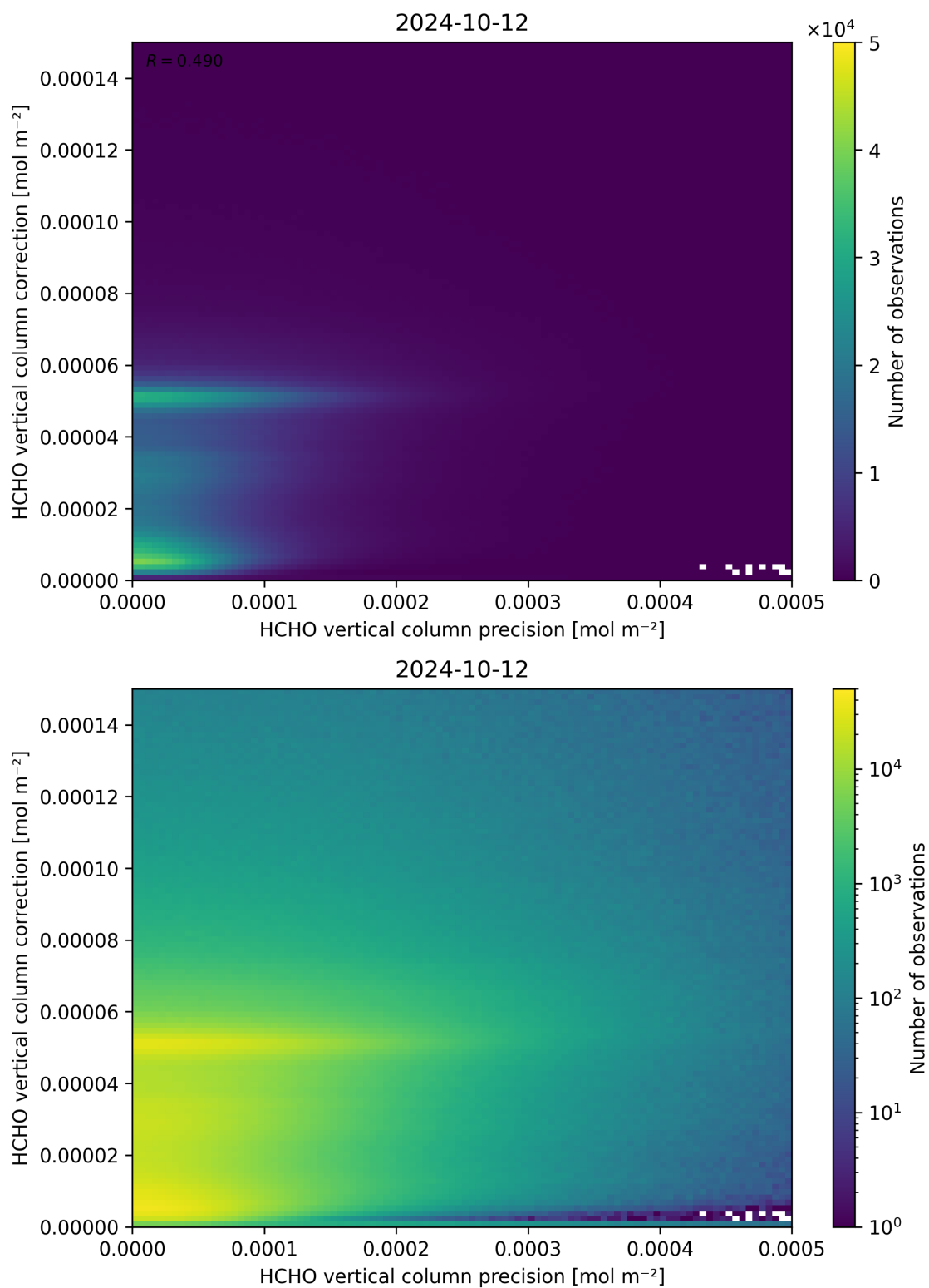
Figure 146: Scatter density plot of “HCHO vertical column precision” against “HCHO vertical column correction” for 2024-10-11 to 2024-10-13.
