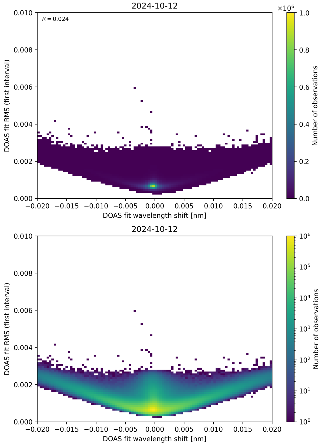
Figure 64: Scatter density plot of “DOAS fit wavelength shift” against “DOAS fit RMS (first interval)” for 2024-10-11 to 2024-10-13.
