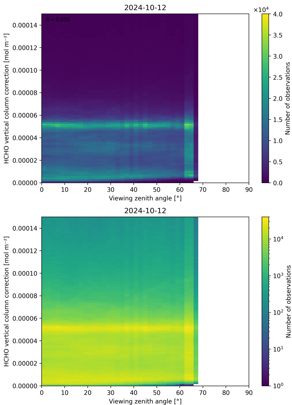
Figure 193: Scatter density plot of “Viewing zenith angle” against “HCHO vertical column correction” for 2024-10-11 to 2024-10-13.
