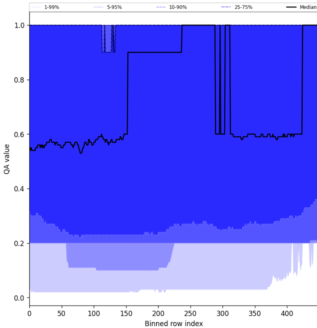
Figure 48: Along track statistics of “QA value” for 2024-10-11 to 2024-10-13
