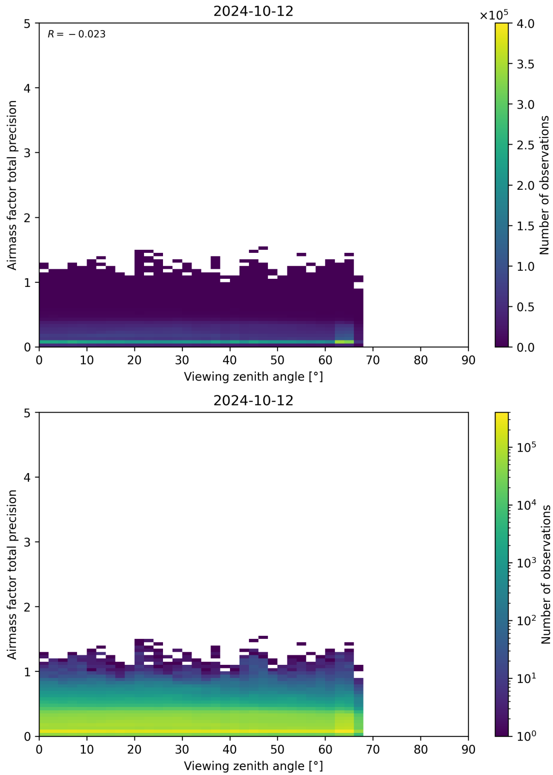
Figure 191: Scatter density plot of “Viewing zenith angle” against “Airmass factor total precision” for 2024-10-11 to 2024-10-13.
