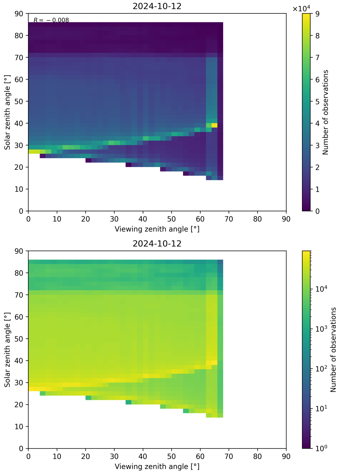
Figure 197: Scatter density plot of “Viewing zenith angle” against “Solar zenith angle” for 2024-10-11 to 2024-10-13.
