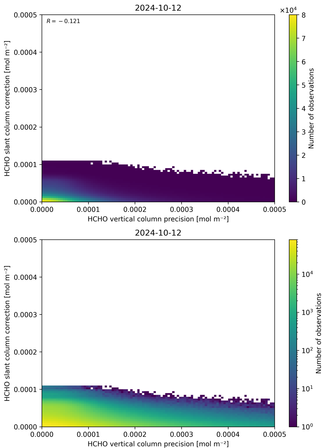
Figure 141: Scatter density plot of “HCHO vertical column precision” against “HCHO slant column correction” for 2024-10-11 to 2024-10-13.
