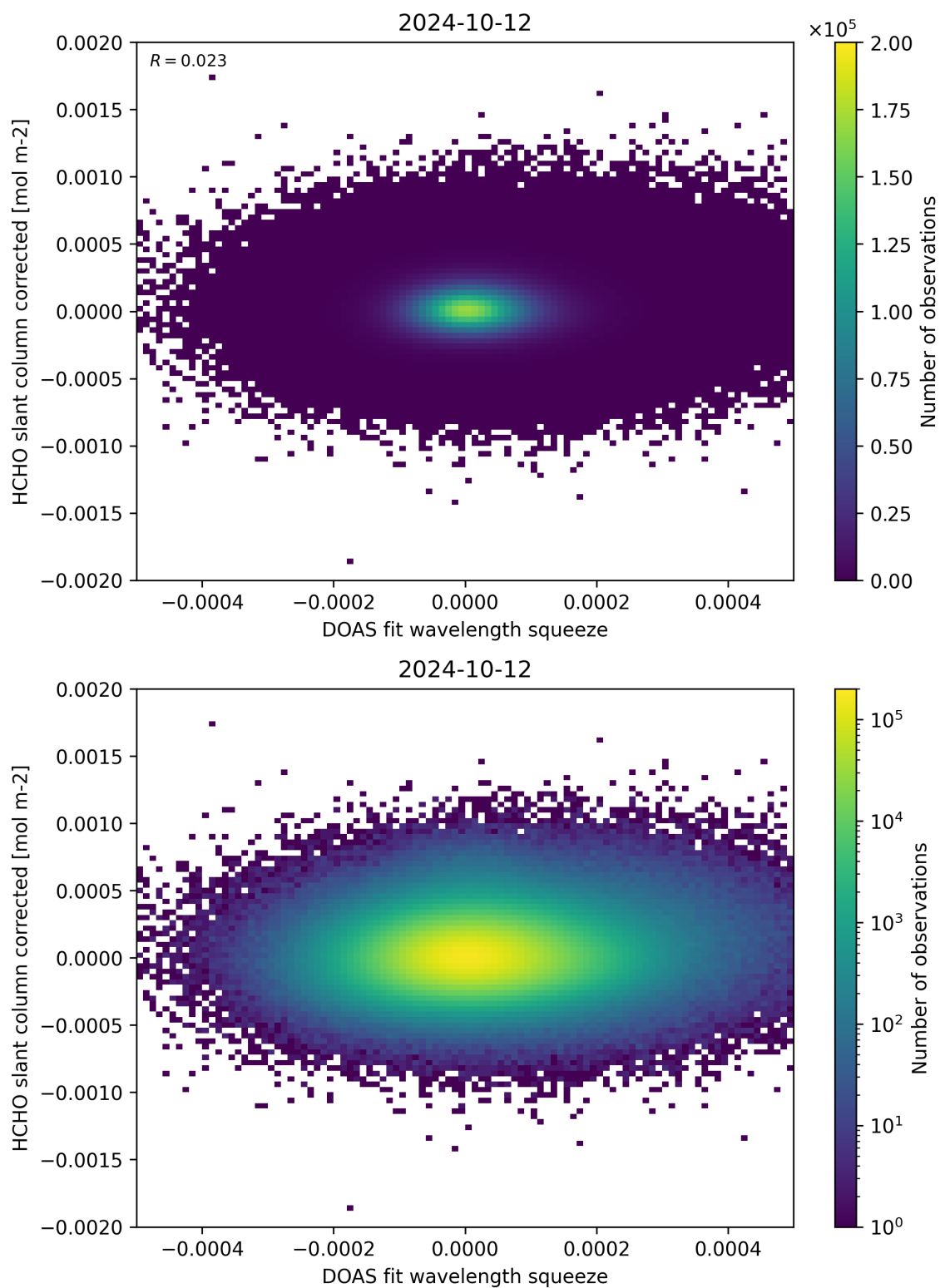
Figure 69: Scatter density plot of “DOAS fit wavelength squeeze” against “HCHO slant column corrected” for 2024-10-11 to 2024-10-13.
