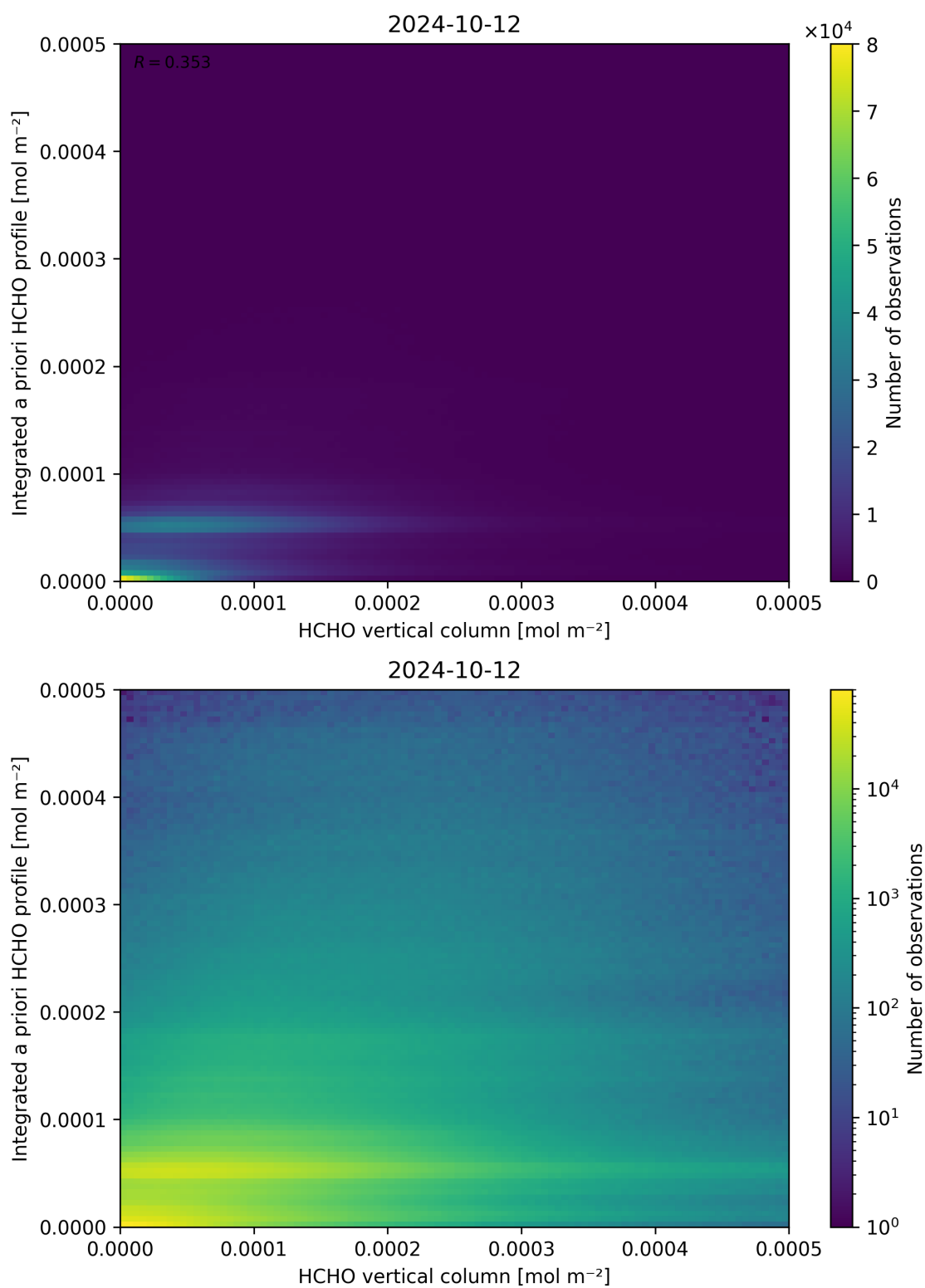
Figure 135: Scatter density plot of “HCHO vertical column” against “Integrated a priori HCHO profile” for 2024-10-11 to 2024-10-13.
