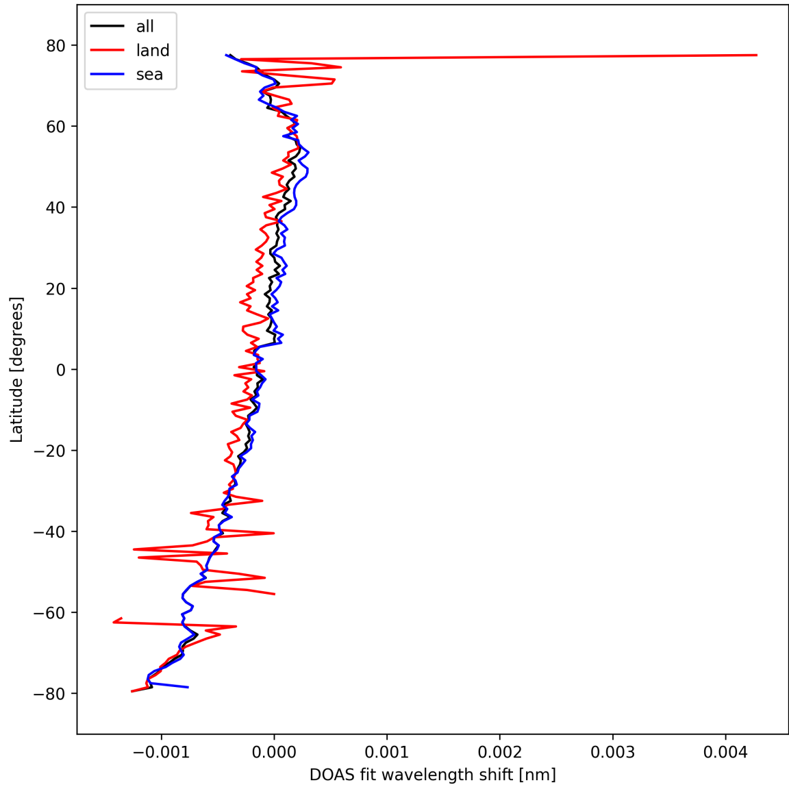
Figure 30: Zonal average of “DOAS fit wavelength shift” for 2024-10-11 to 2024-10-13.
