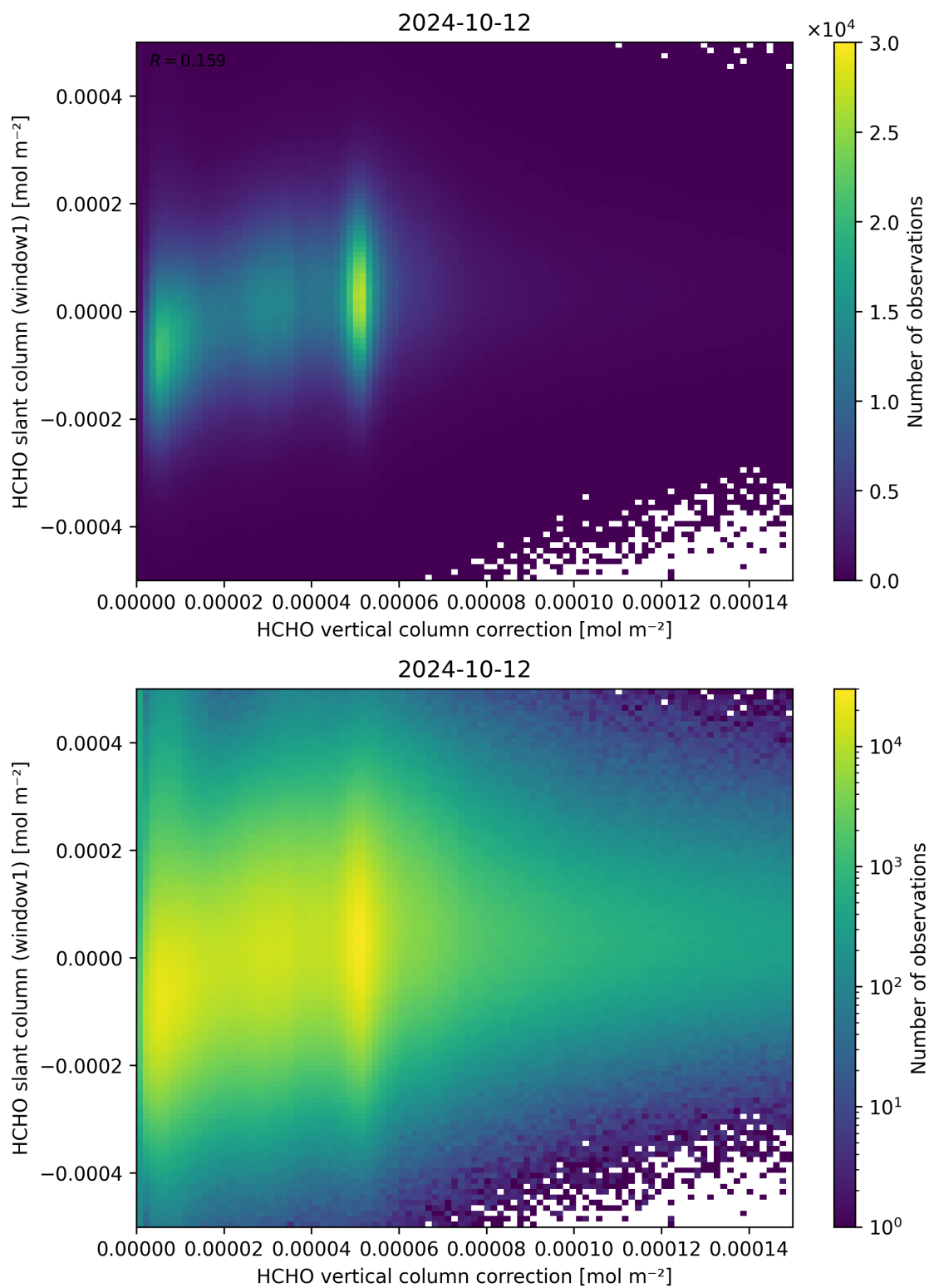
Figure 118: Scatter density plot of “HCHO vertical column correction” against “HCHO slant column (window1)” for 2024-10-11 to 2024-10-13.
