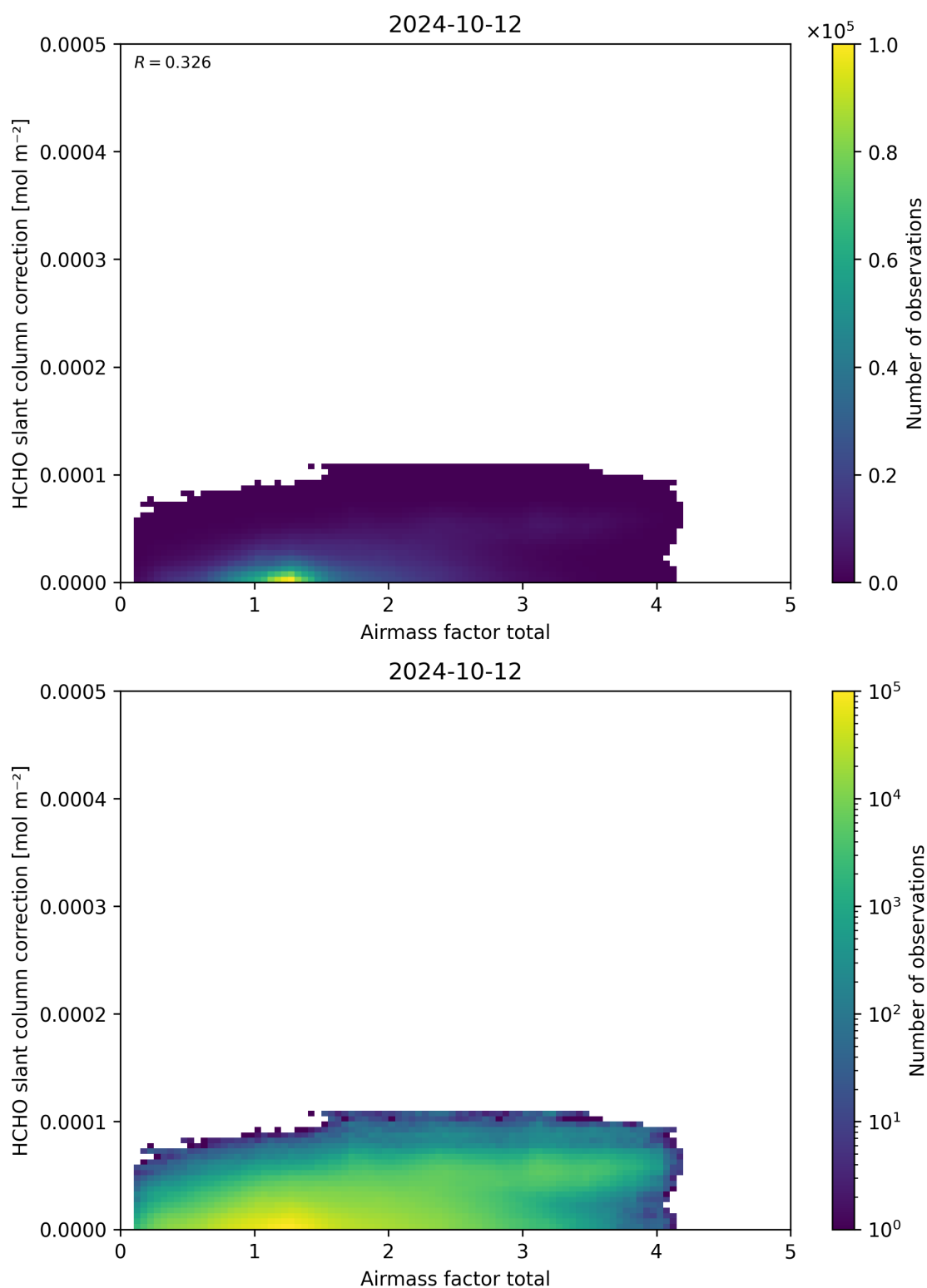
Figure 102: Scatter density plot of “Airmass factor total” against “HCHO slant column correction” for 2024-10-11 to 2024-10-13.
