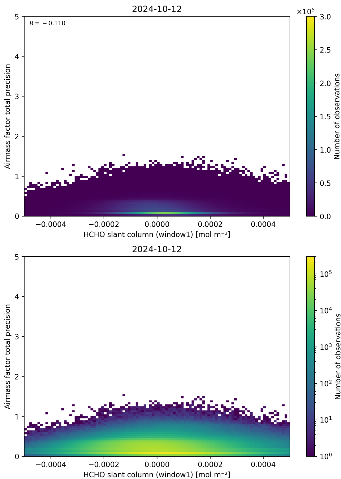
Figure 86: Scatter density plot of “HCHO slant column (window1)” against “Airmass factor total precision” for 2024-10-11 to 2024-10-13.
