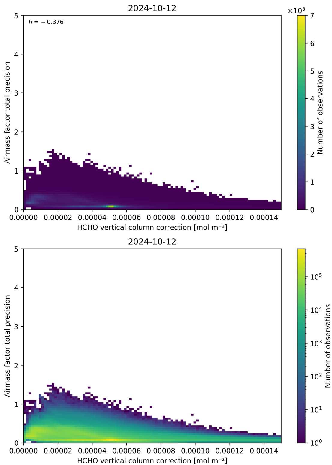
Figure 121: Scatter density plot of “HCHO vertical column correction” against “Airmass factor total precision” for 2024-10-11 to 2024-10-13.
