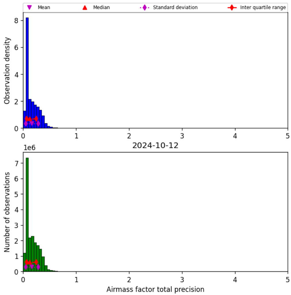
Figure 41: Histogram of “Airmass factor total precision” for 2024-10-11 to 2024-10-13
