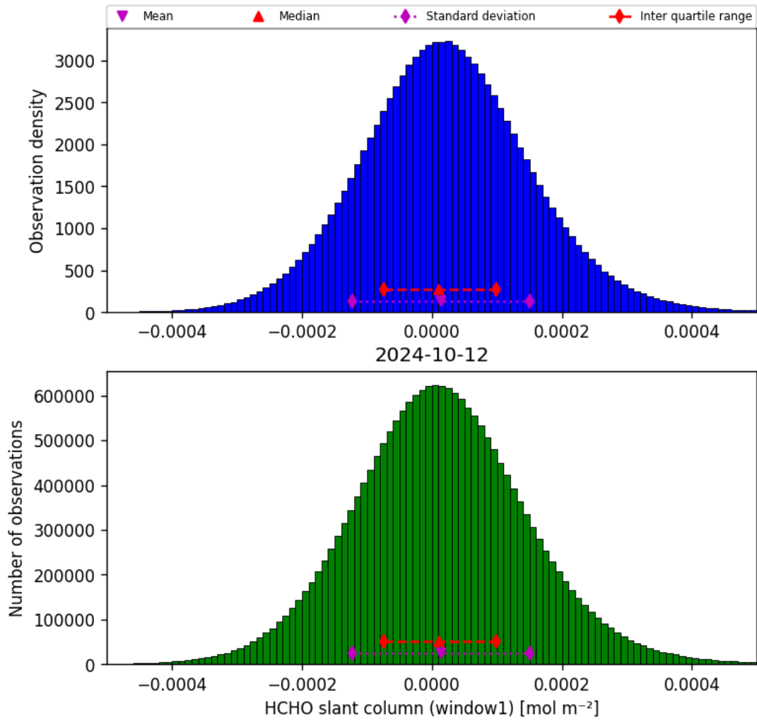
Figure 38: Histogram of “HCHO slant column (window1)” for 2024-10-11 to 2024-10-13
