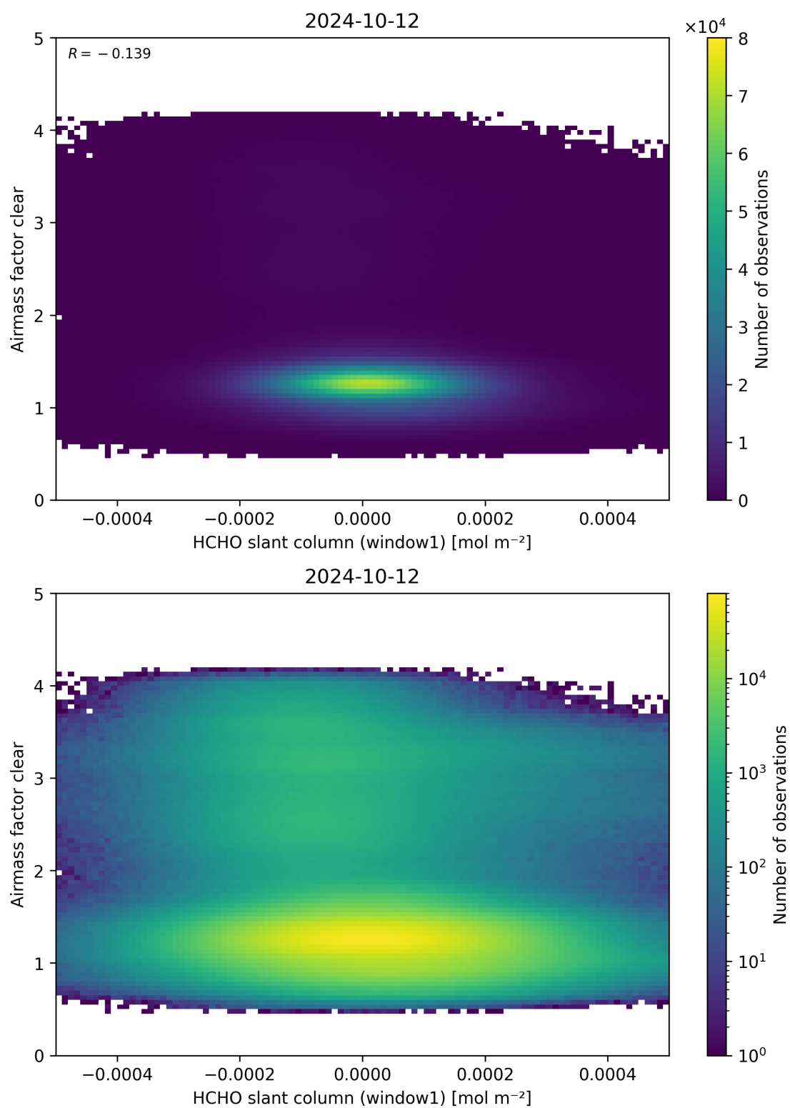
Figure 81: Scatter density plot of “HCHO slant column (window1)” against “Airmass factor clear” for 2024-10-11 to 2024-10-13.
