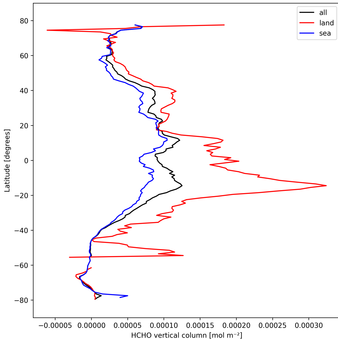
Figure 21: Zonal average of “HCHO vertical column” for 2024-10-11 to 2024-10-13.
