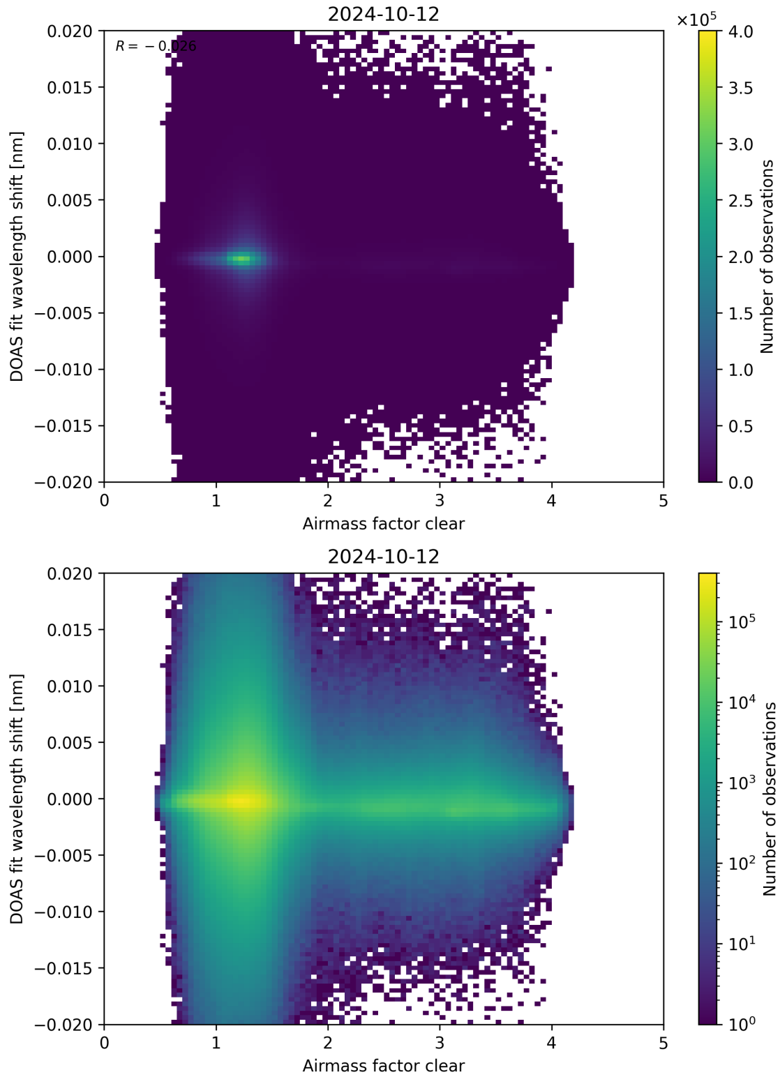
Figure 72: Scatter density plot of “Airmass factor clear” against “DOAS fit wavelength shift” for 2024-10-11 to 2024-10-13.
