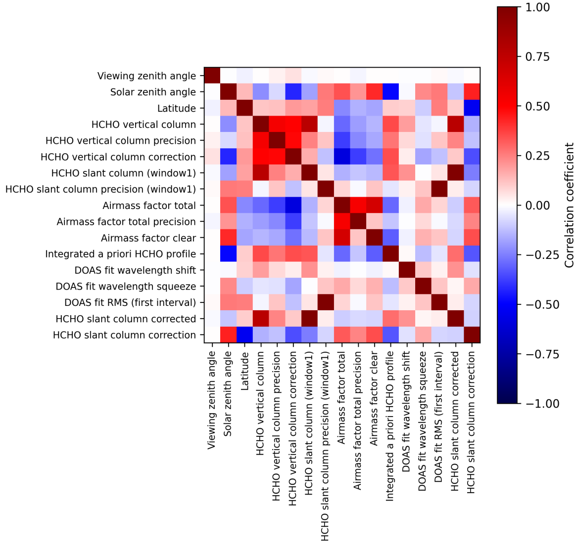
Figure 2: Map of correlation matrix for 2024-10-11 to 2024-10-13.
