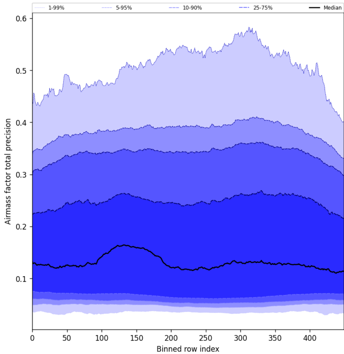
Figure 55: Along track statistics of “Airmass factor total precision” for 2024-10-11 to 2024-10-13
