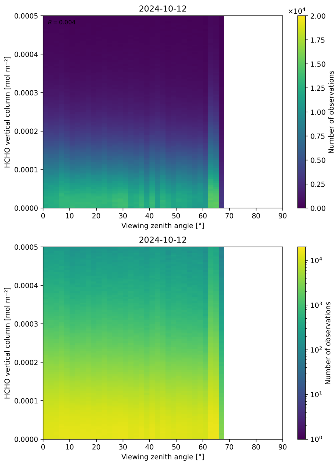
Figure 192: Scatter density plot of “Viewing zenith angle” against “HCHO vertical column” for 2024-10-11 to 2024-10-13.
