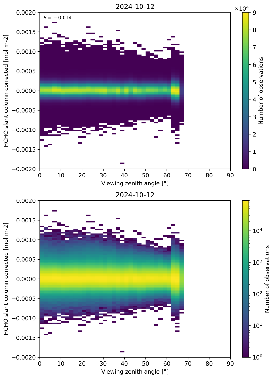
Figure 186: Scatter density plot of “Viewing zenith angle” against “HCHO slant column corrected” for 2024-10-11 to 2024-10-13.
