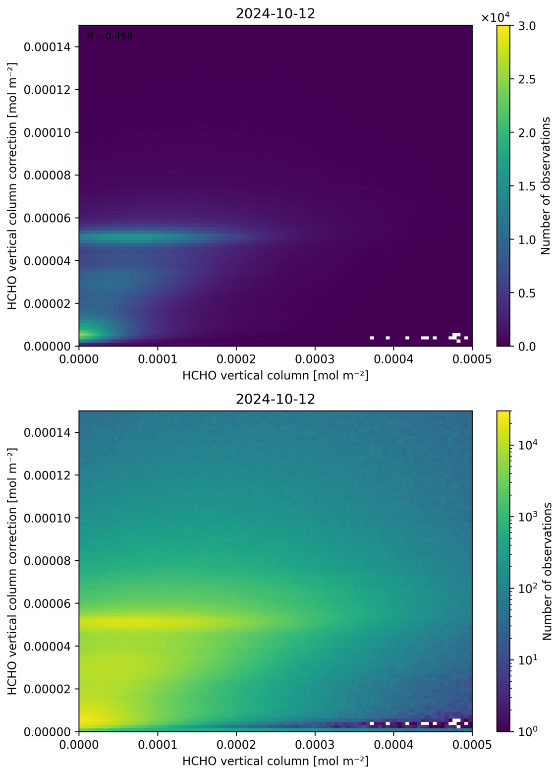
Figure 133: Scatter density plot of “HCHO vertical column” against “HCHO vertical column correction” for 2024-10-11 to 2024-10-13.
