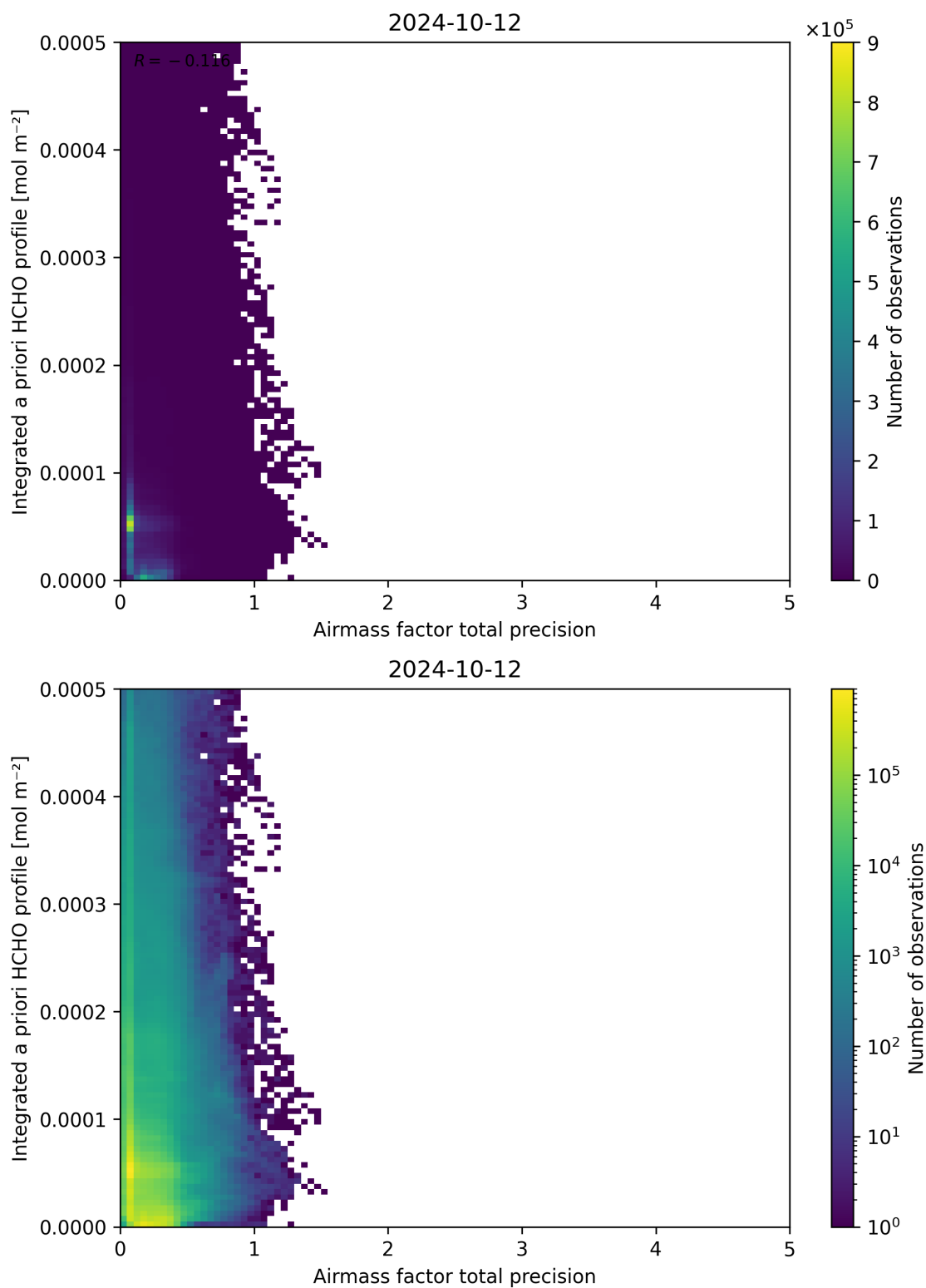
Figure 111: Scatter density plot of “Airmass factor total precision” against “Integrated a priori HCHO profile” for 2024-10-11 to 2024-10-13.
