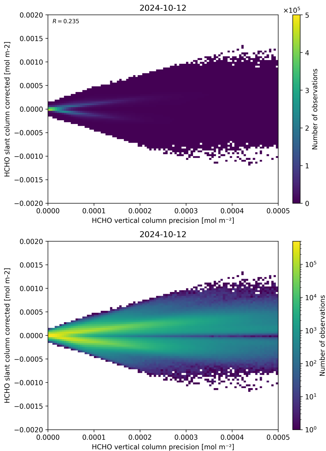
Figure 140: Scatter density plot of “HCHO vertical column precision” against “HCHO slant column corrected” for 2024-10-11 to 2024-10-13.
