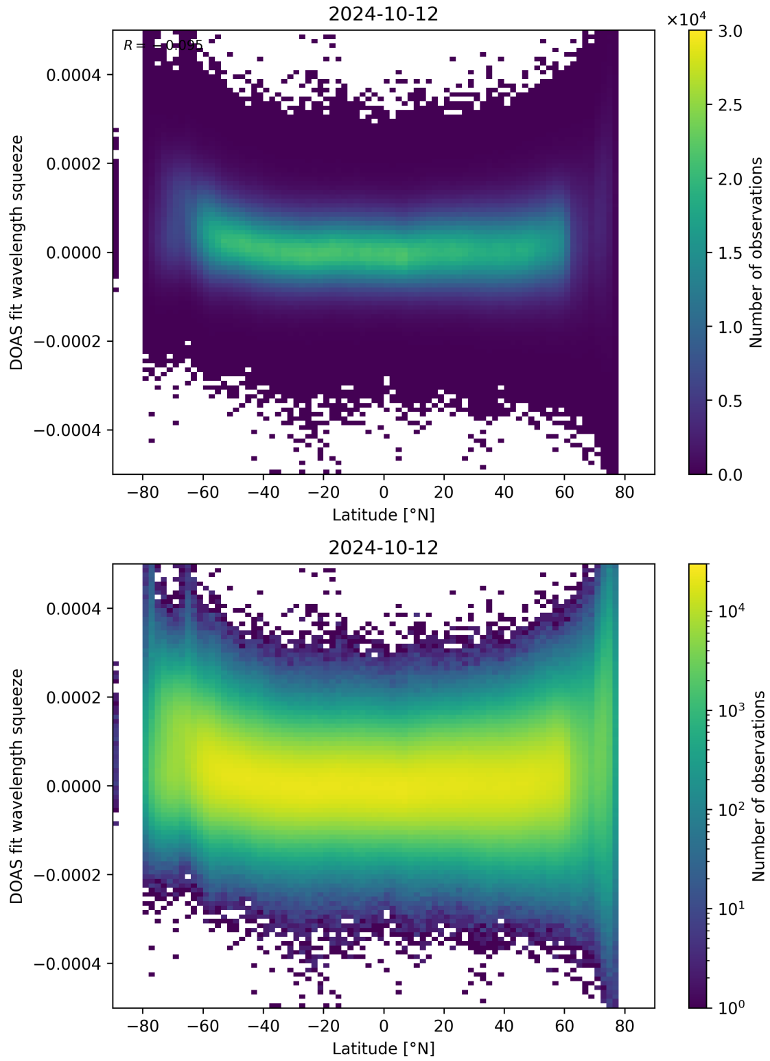
Figure 155: Scatter density plot of “Latitude” against “DOAS fit wavelength squeeze” for 2024-10-11 to 2024-10-13.
