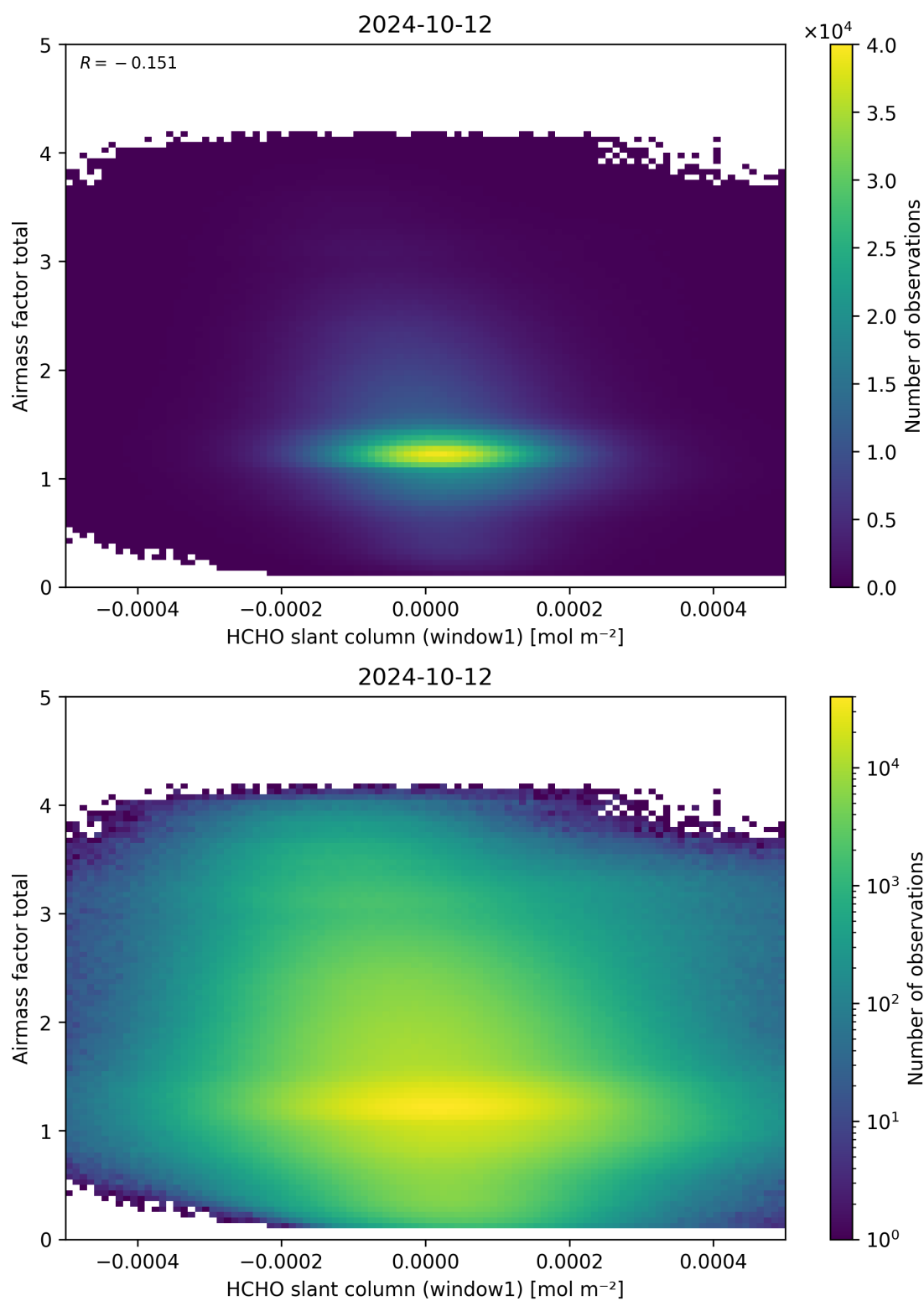
Figure 85: Scatter density plot of “HCHO slant column (window1)” against “Airmass factor total” for 2024-10-11 to 2024-10-13.
