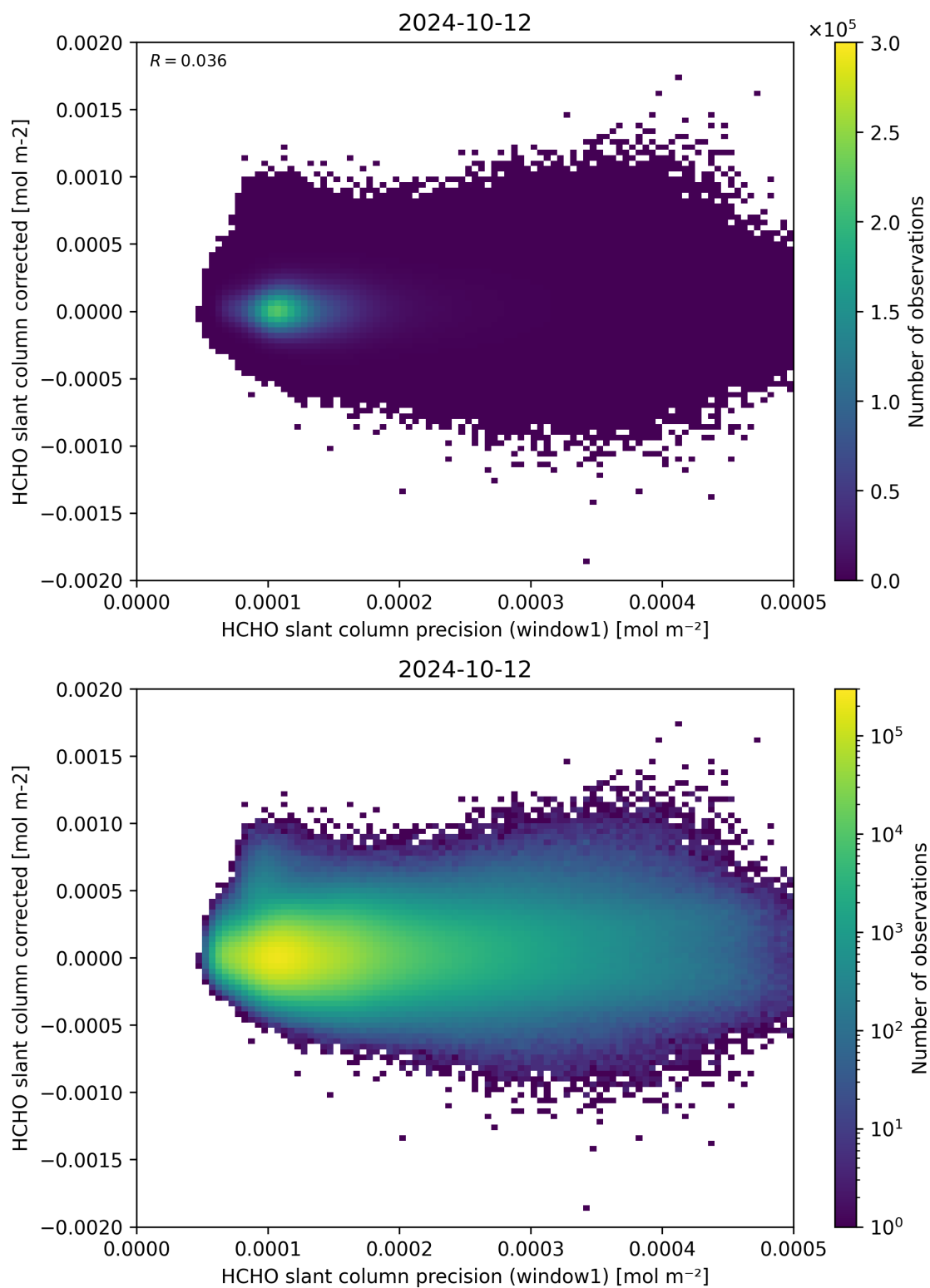
Figure 92: Scatter density plot of “HCHO slant column precision (window1)” against “HCHO slant column corrected” for 2024-10-11 to 2024-10-13.
