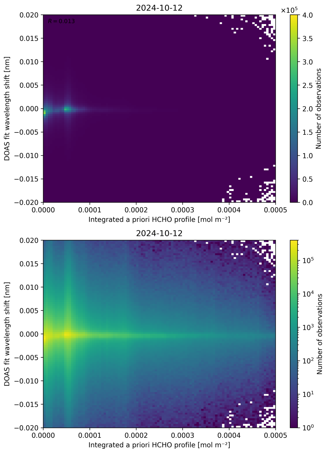
Figure 149: Scatter density plot of “Integrated a priori HCHO profile” against “DOAS fit wavelength shift” for 2024-10-11 to 2024-10-13.
