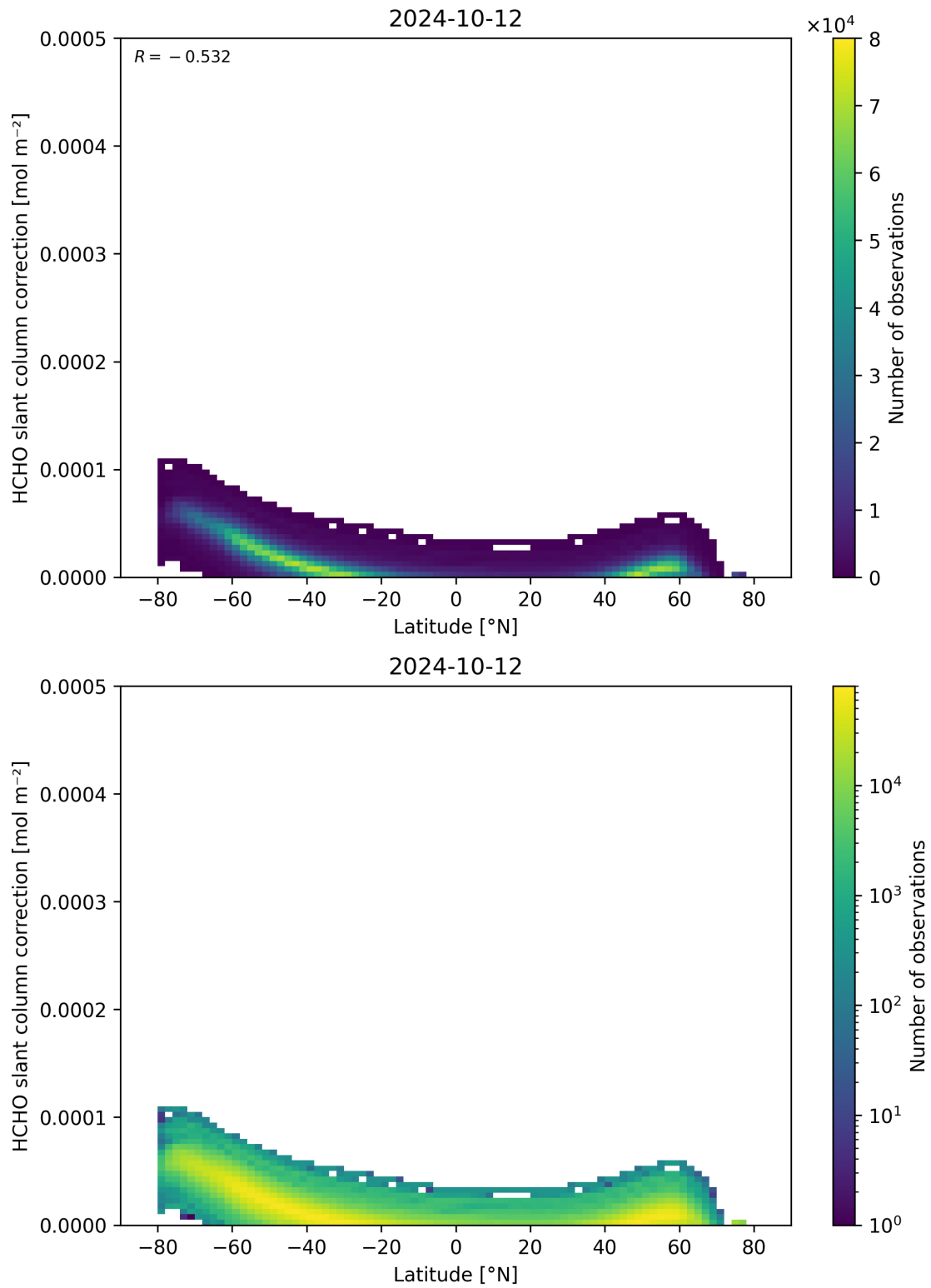
Figure 158: Scatter density plot of “Latitude” against “HCHO slant column correction” for 2024-10-11 to 2024-10-13.
