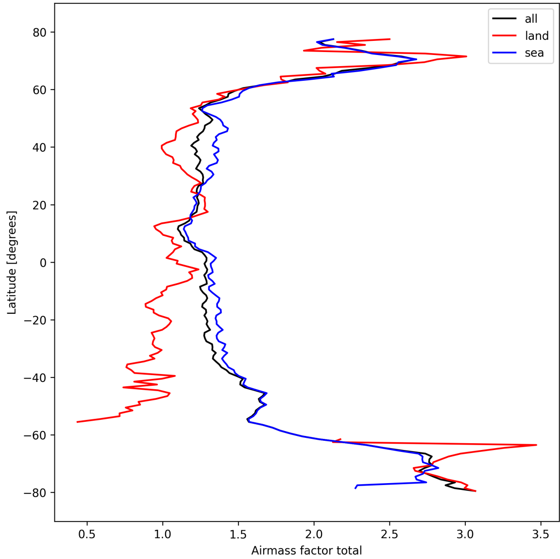
Figure 26: Zonal average of “Airmass factor total” for 2024-10-11 to 2024-10-13.
