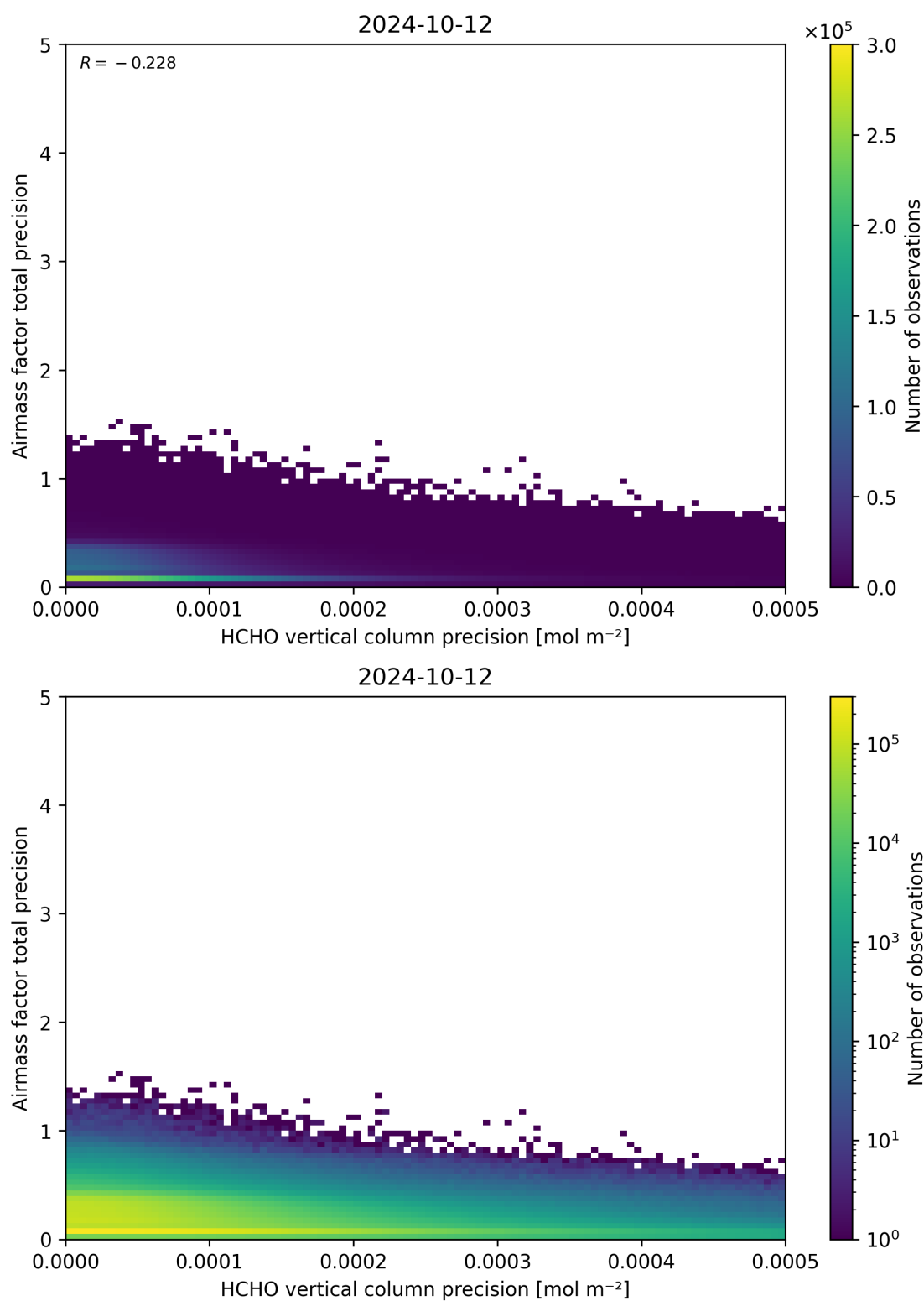
Figure 145: Scatter density plot of “HCHO vertical column precision” against “Airmass factor total precision” for 2024-10-11 to 2024-10-13.
