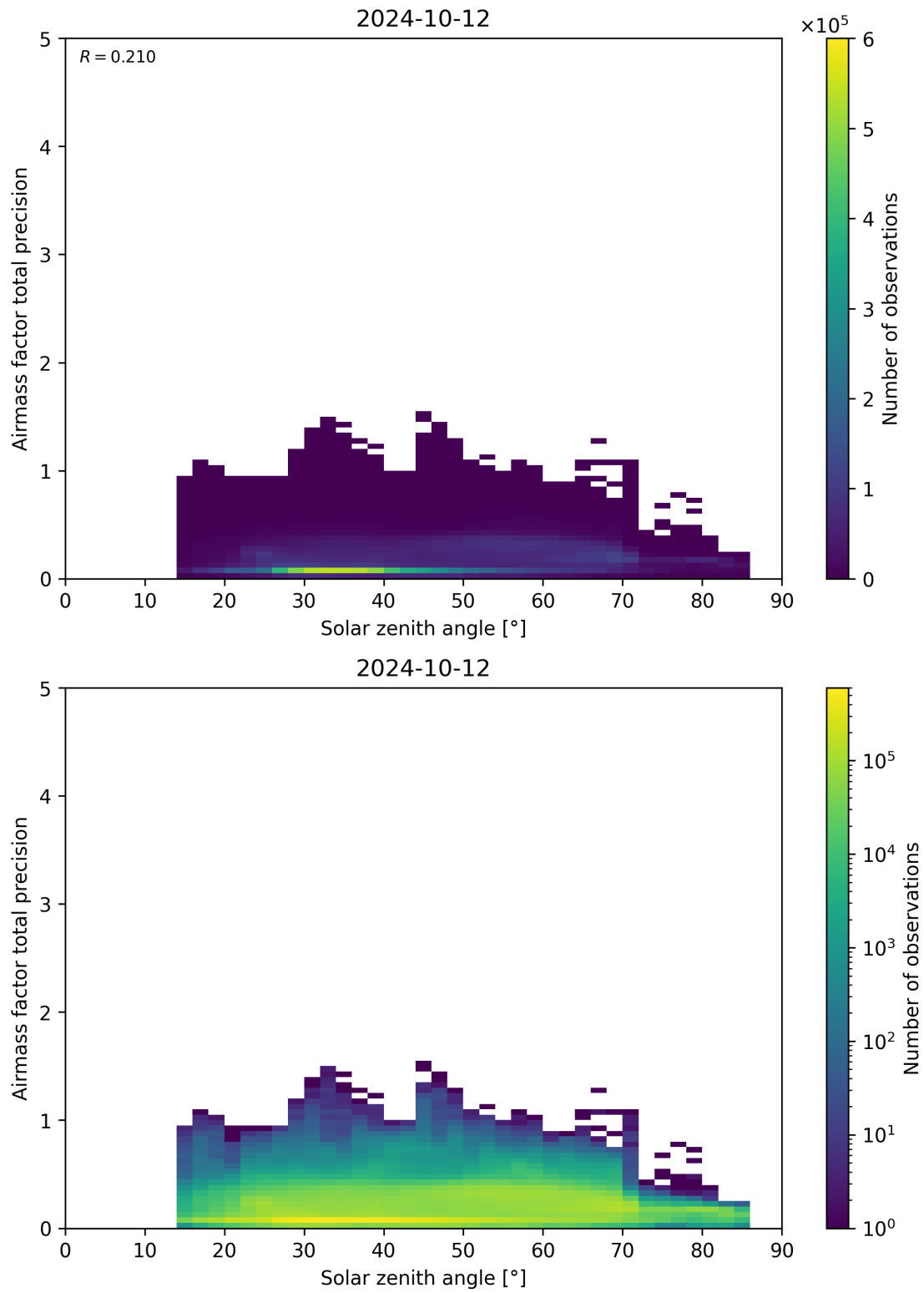
Figure 176: Scatter density plot of “Solar zenith angle” against “Airmass factor total precision” for 2024-10-11 to 2024-10-13.
