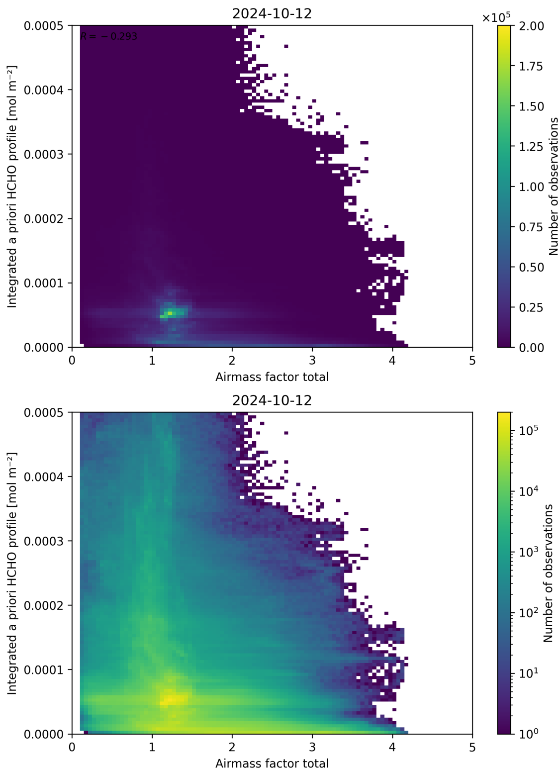
Figure 104: Scatter density plot of “Airmass factor total” against “Integrated a priori HCHO profile” for 2024-10-11 to 2024-10-13.
