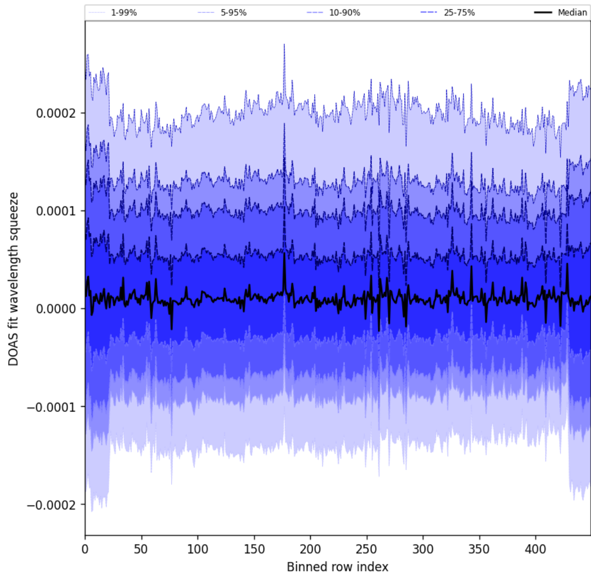
Figure 59: Along track statistics of “DOAS fit wavelength squeeze” for 2024-10-11 to 2024-10-13
