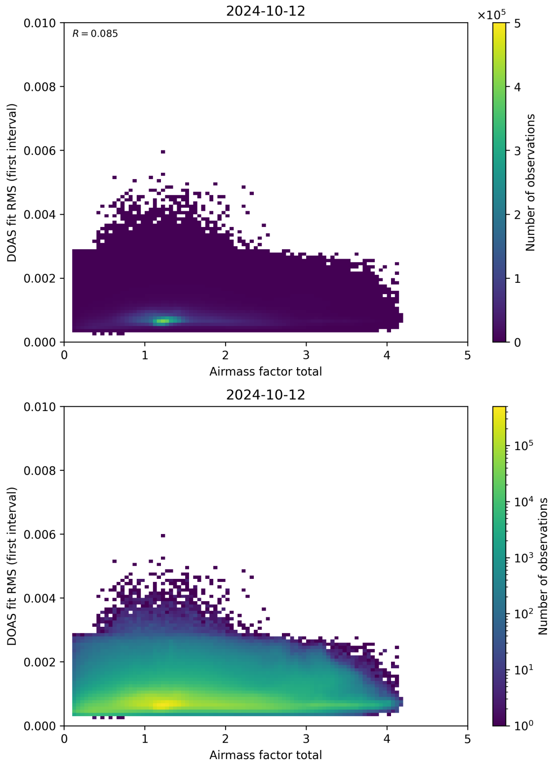
Figure 97: Scatter density plot of “Airmass factor total” against “DOAS fit RMS (first interval)” for 2024-10-11 to 2024-10-13.
