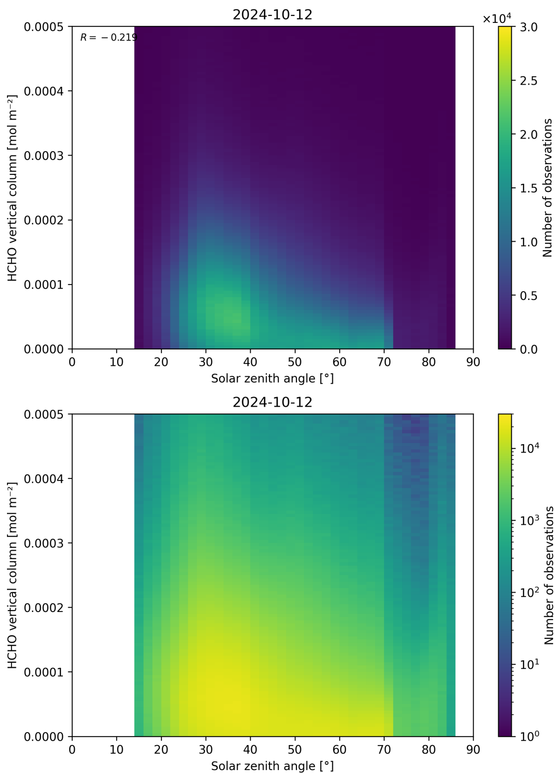
Figure 177: Scatter density plot of “Solar zenith angle” against “HCHO vertical column” for 2024-10-11 to 2024-10-13.
