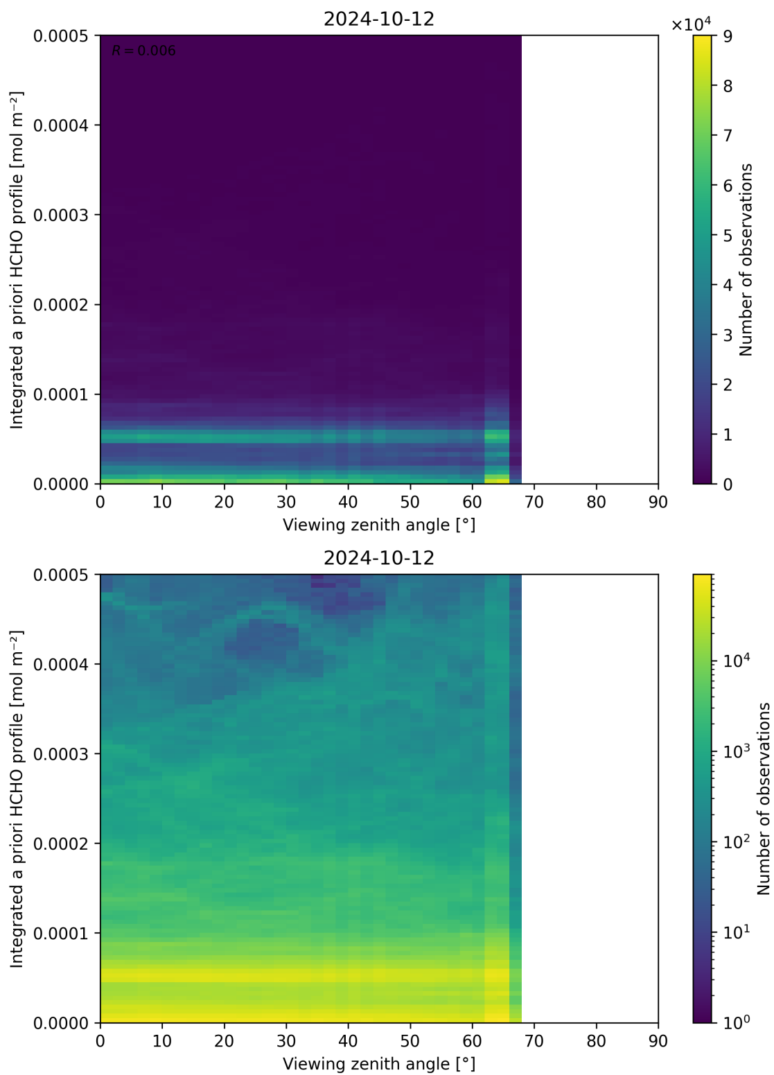
Figure 195: Scatter density plot of “Viewing zenith angle” against “Integrated a priori HCHO profile” for 2024-10-11 to 2024-10-13.
