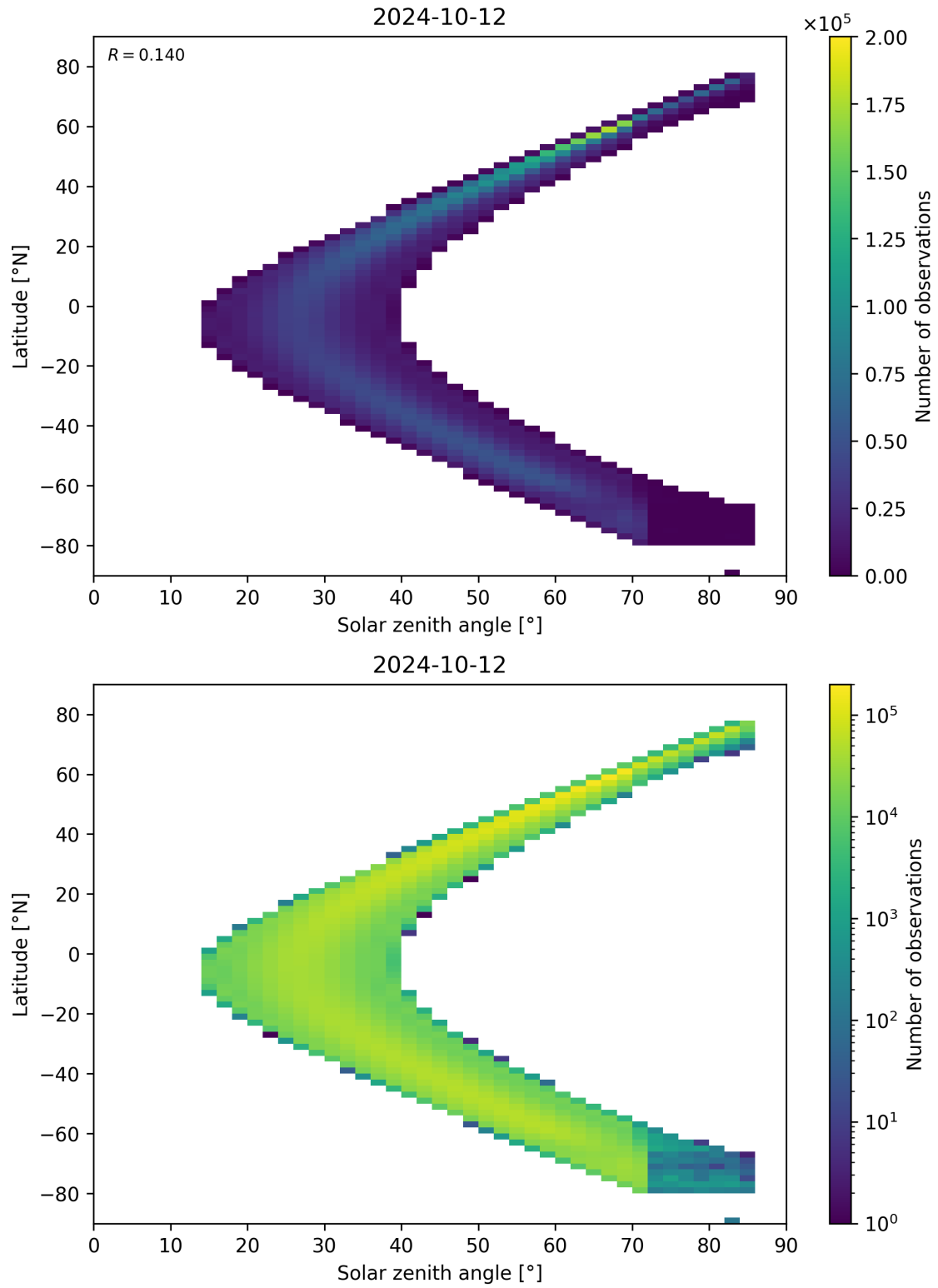
Figure 181: Scatter density plot of “Solar zenith angle” against “Latitude” for 2024-10-11 to 2024-10-13.
