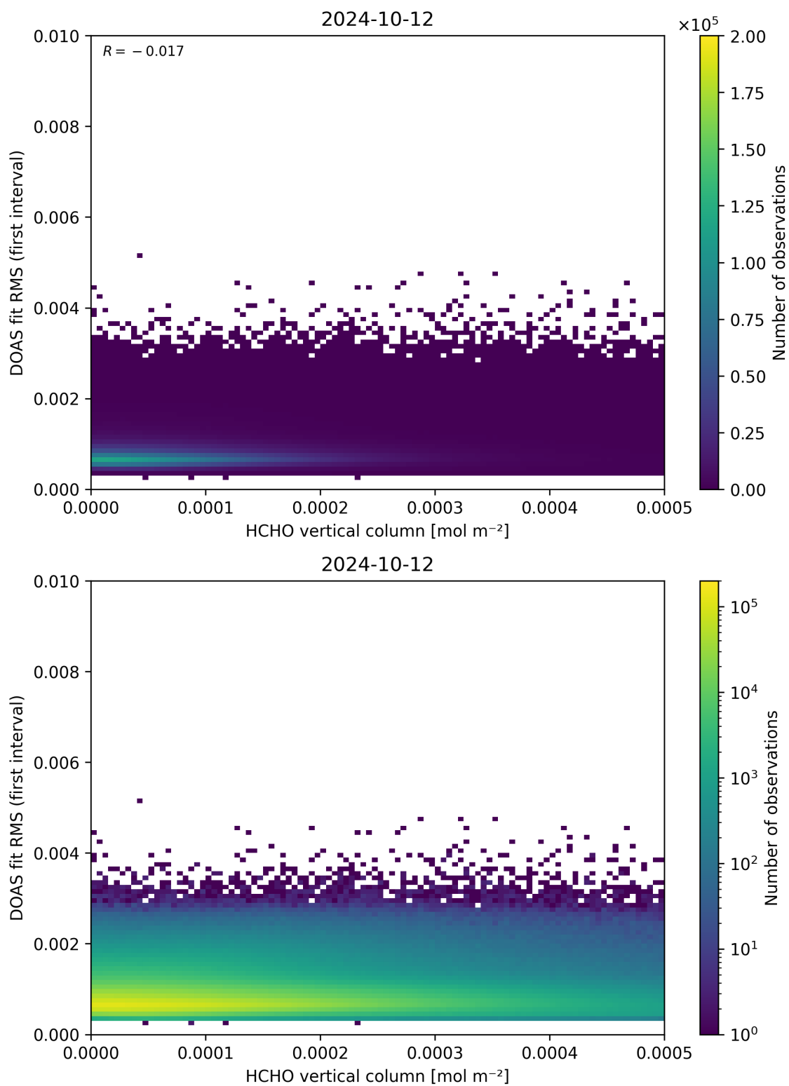
Figure 123: Scatter density plot of “HCHO vertical column” against “DOAS fit RMS (first interval)” for 2024-10-11 to 2024-10-13.
