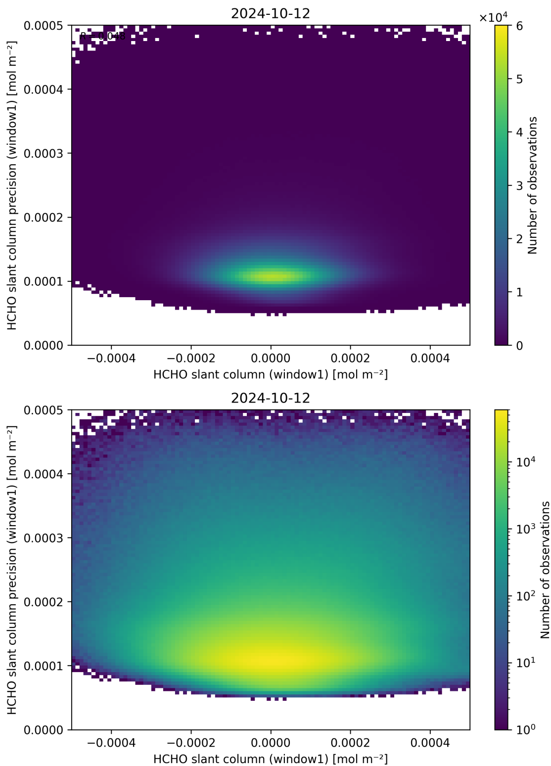
Figure 84: Scatter density plot of “HCHO slant column (window1)” against “HCHO slant column precision (window1)” for 2024-10-11 to 2024-10-13.
