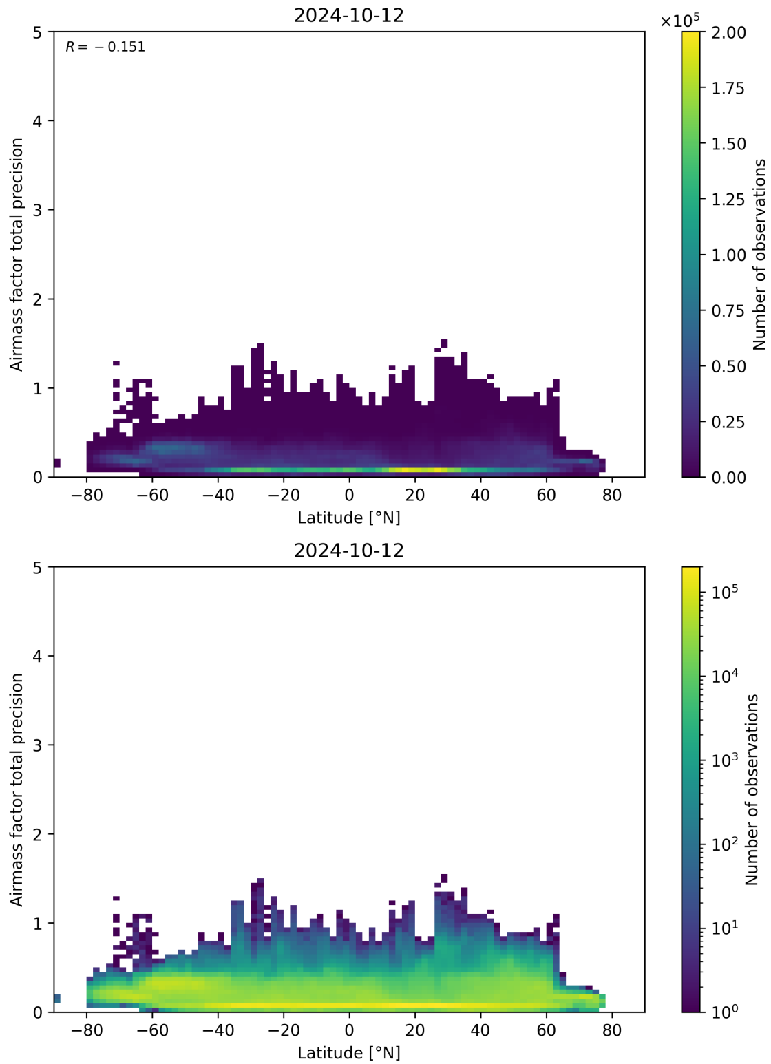
Figure 162: Scatter density plot of “Latitude” against “Airmass factor total precision” for 2024-10-11 to 2024-10-13.
