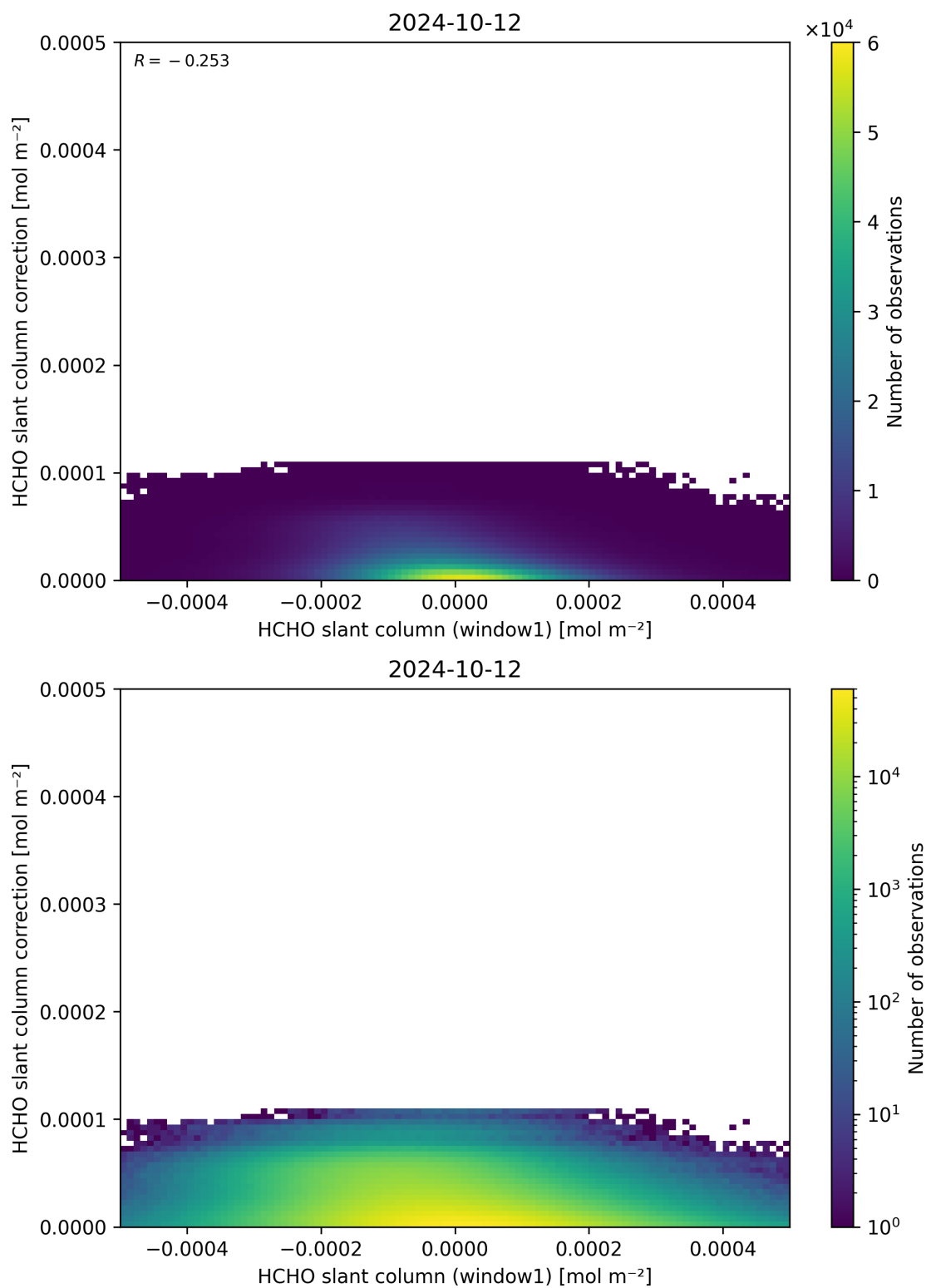
Figure 83: Scatter density plot of “HCHO slant column (window1)” against “HCHO slant column correction” for 2024-10-11 to 2024-10-13.
