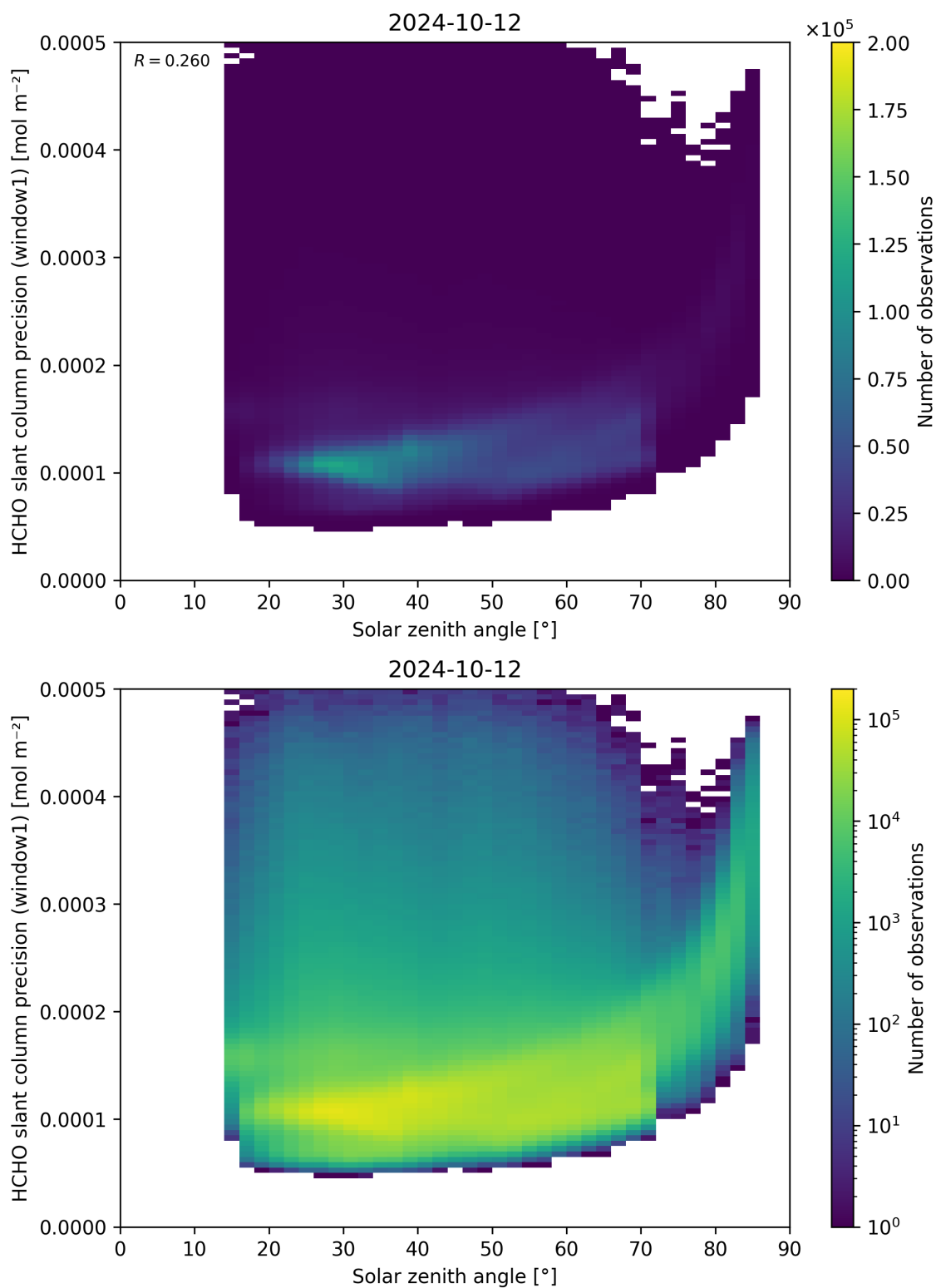
Figure 174: Scatter density plot of “Solar zenith angle” against “HCHO slant column precision (window1)” for 2024-10-11 to 2024-10-13.
