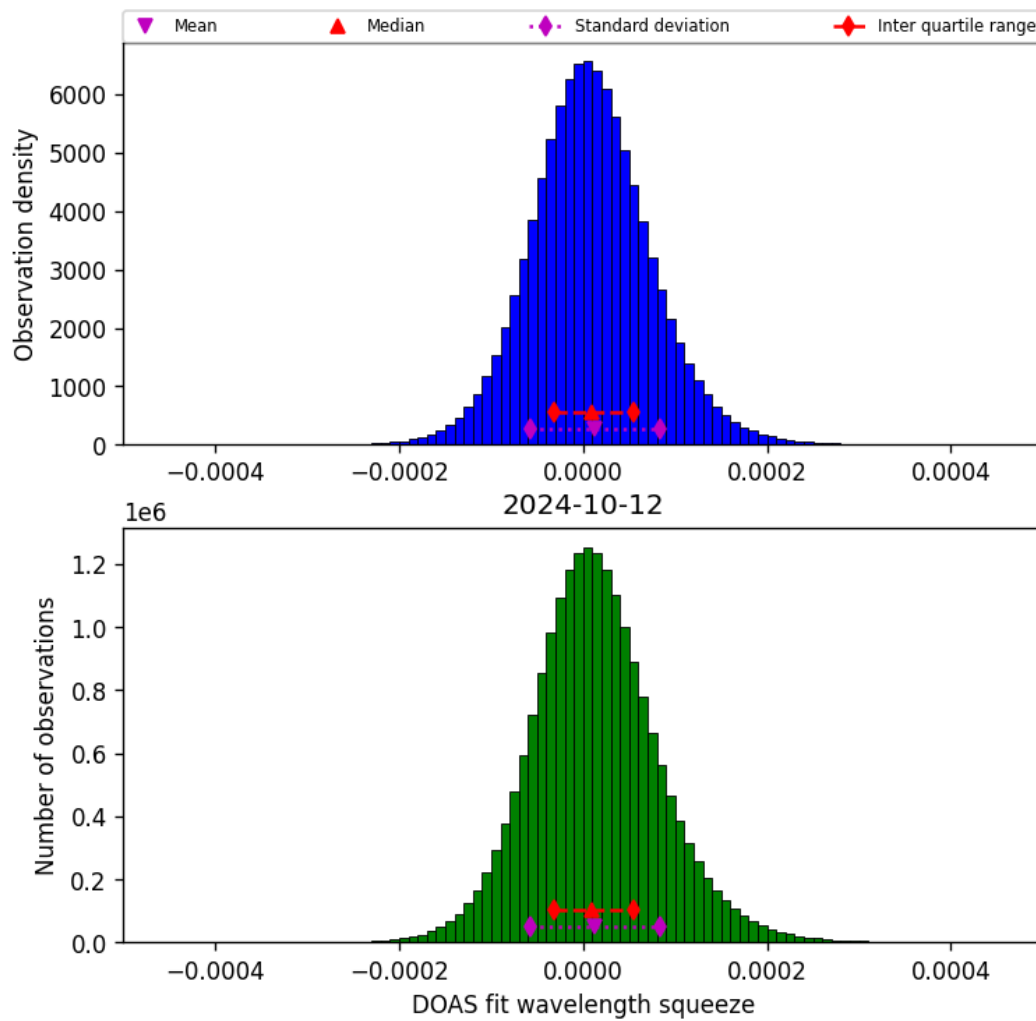
Figure 45: Histogram of “DOAS fit wavelength squeeze” for 2024-10-11 to 2024-10-13
