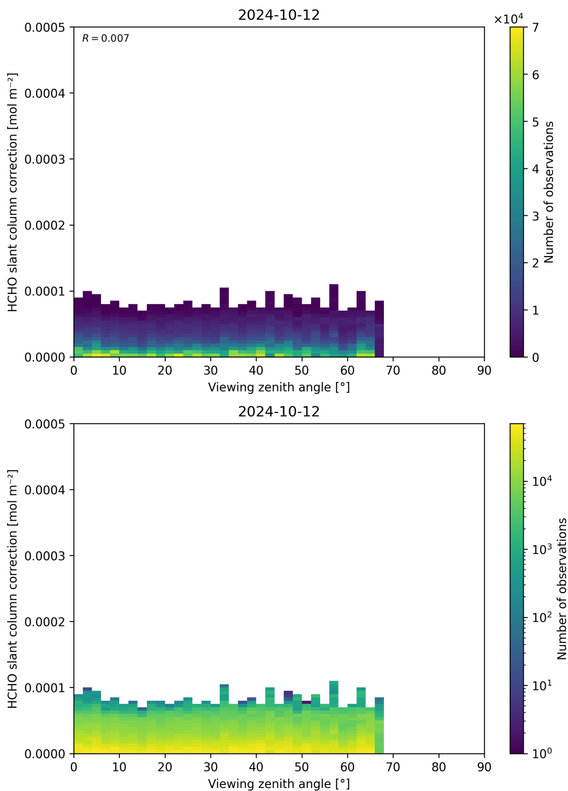
Figure 187: Scatter density plot of “Viewing zenith angle” against “HCHO slant column correction” for 2024-10-11 to 2024-10-13.
