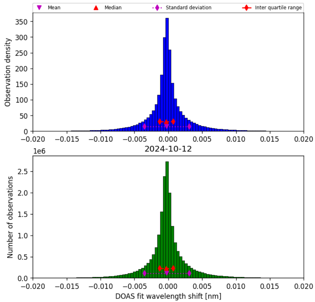
Figure 44: Histogram of “DOAS fit wavelength shift” for 2024-10-11 to 2024-10-13
