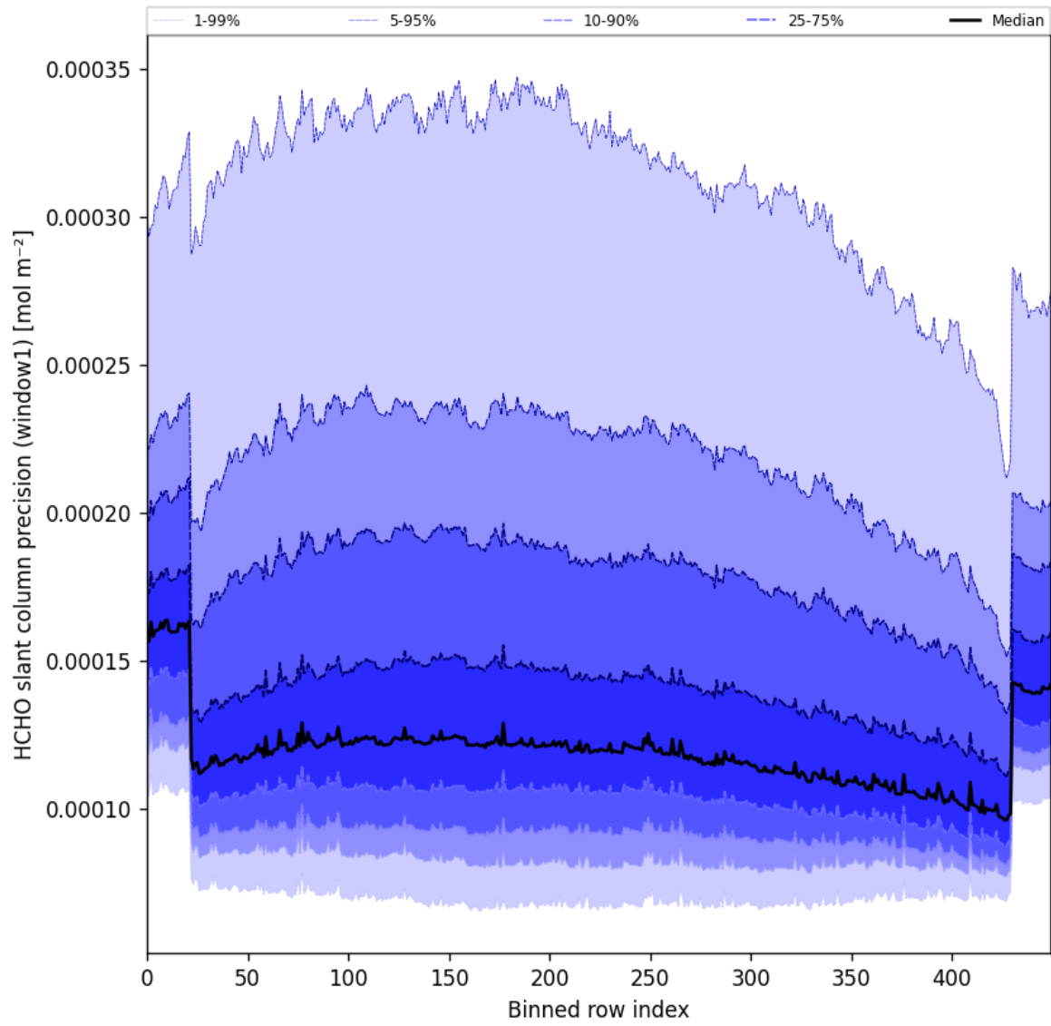
Figure 53: Along track statistics of “HCHO slant column precision (window1)” for 2024-10-11 to 2024-10-13
