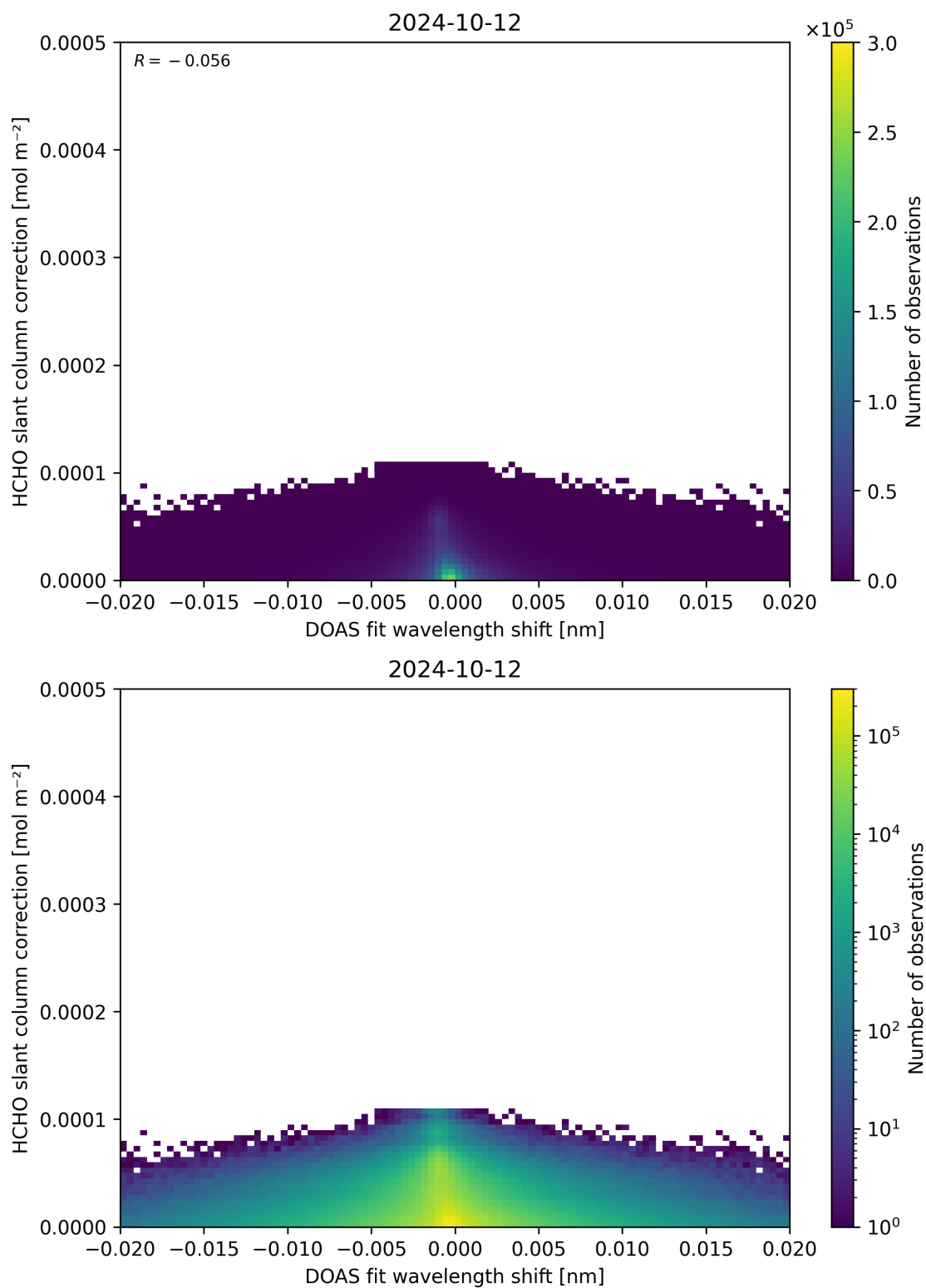
Figure 67: Scatter density plot of “DOAS fit wavelength shift” against “HCHO slant column correction” for 2024-10-11 to 2024-10-13.
