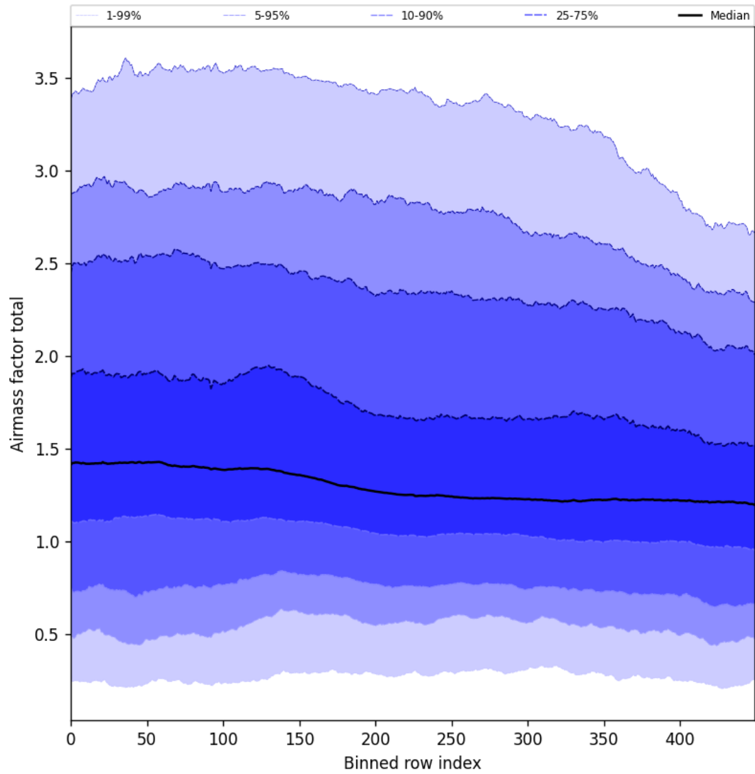
Figure 54: Along track statistics of “Airmass factor total” for 2024-10-11 to 2024-10-13
