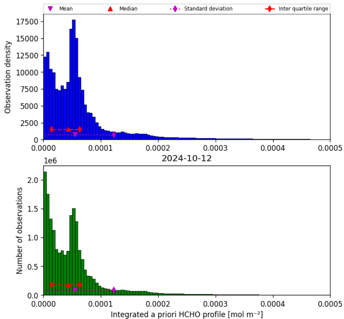
Figure 43: Histogram of “Integrated a priori HCHO profile” for 2024-10-11 to 2024-10-13
