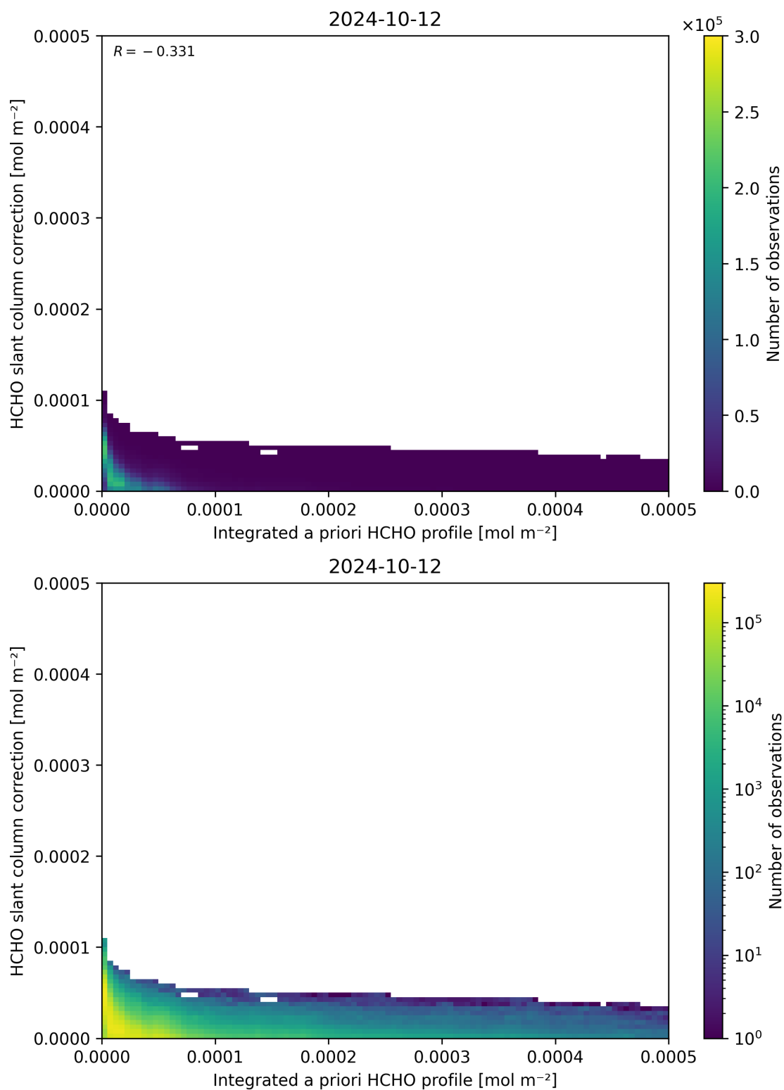
Figure 152: Scatter density plot of “Integrated a priori HCHO profile” against “HCHO slant column correction” for 2024-10-11 to 2024-10-13.
