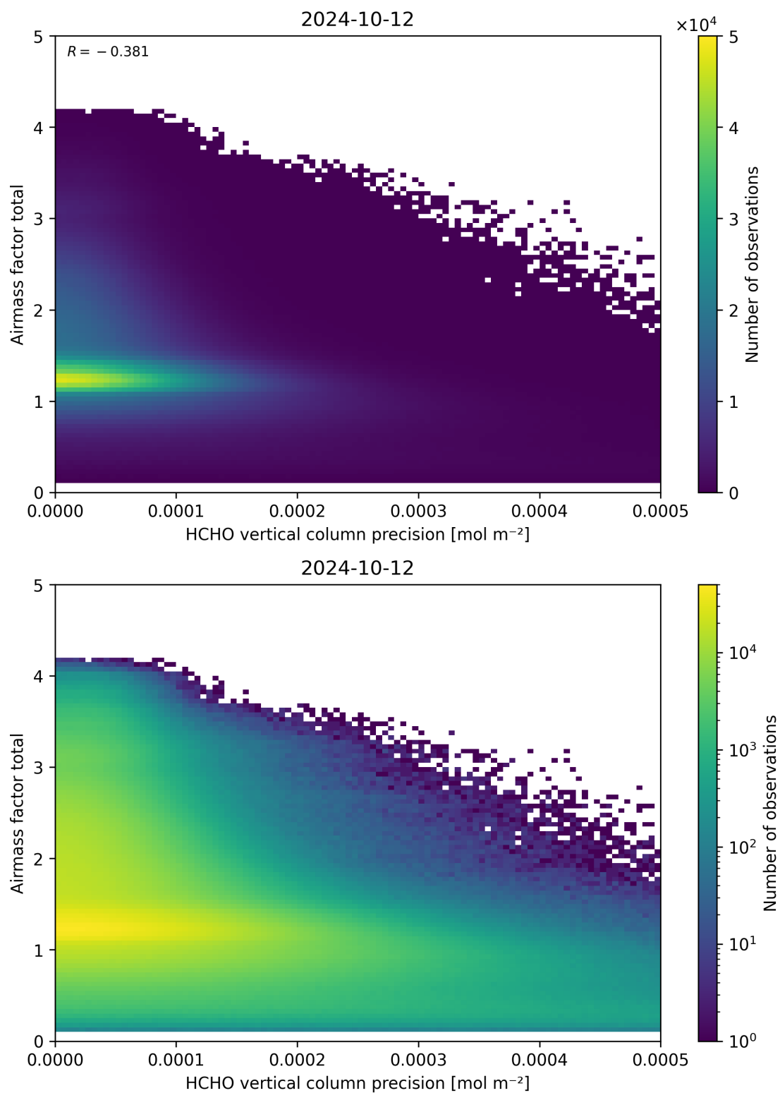
Figure 144: Scatter density plot of “HCHO vertical column precision” against “Airmass factor total” for 2024-10-11 to 2024-10-13.
