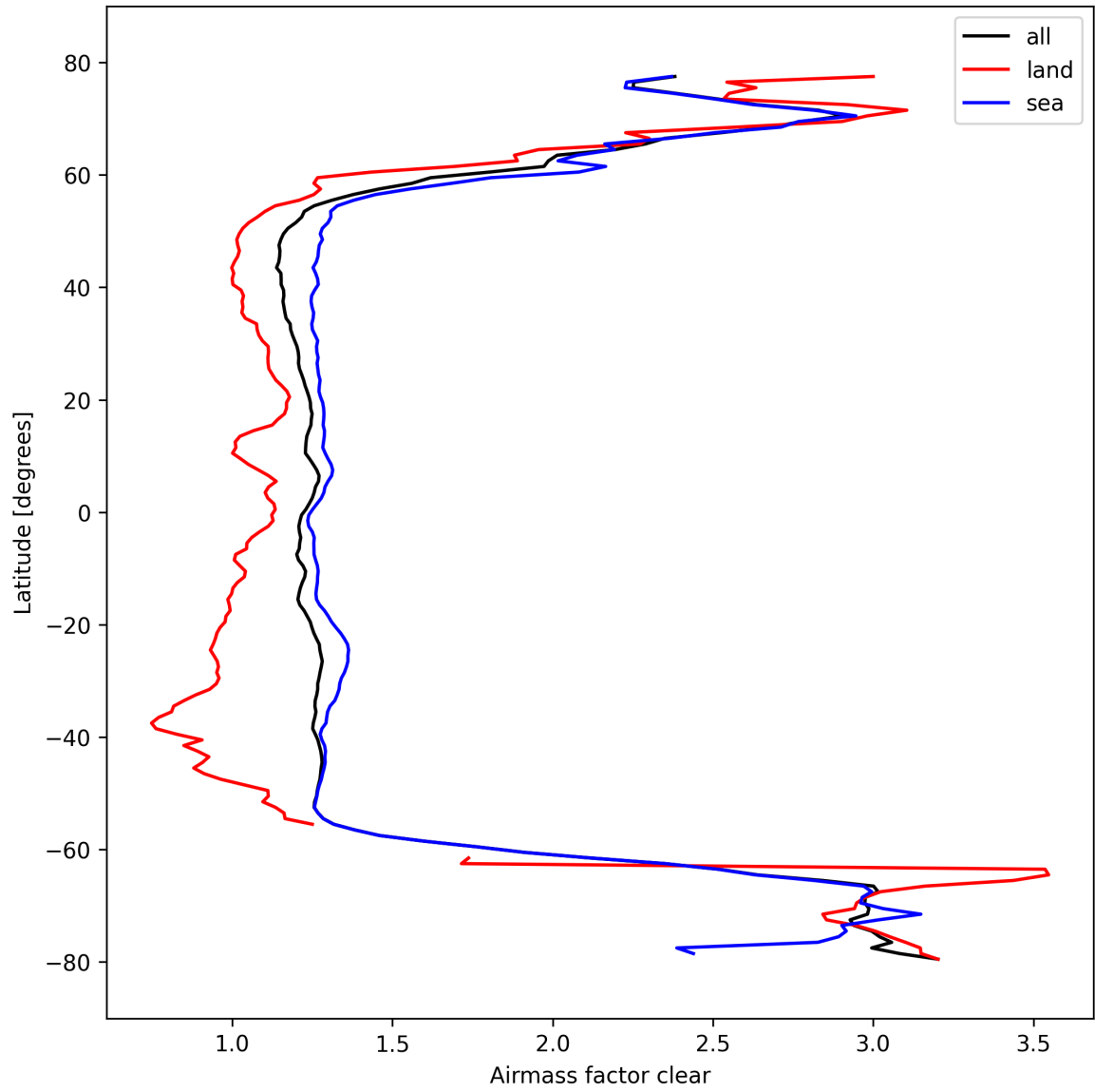
Figure 28: Zonal average of “Airmass factor clear” for 2024-10-11 to 2024-10-13.
