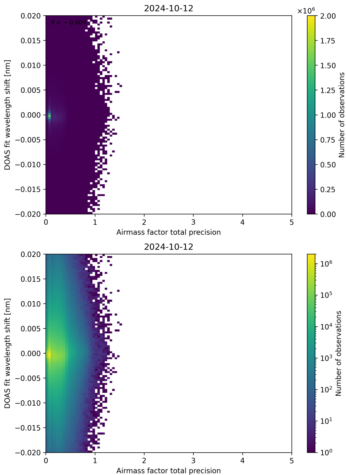
Figure 106: Scatter density plot of “Airmass factor total precision” against “DOAS fit wavelength shift” for 2024-10-11 to 2024-10-13.
