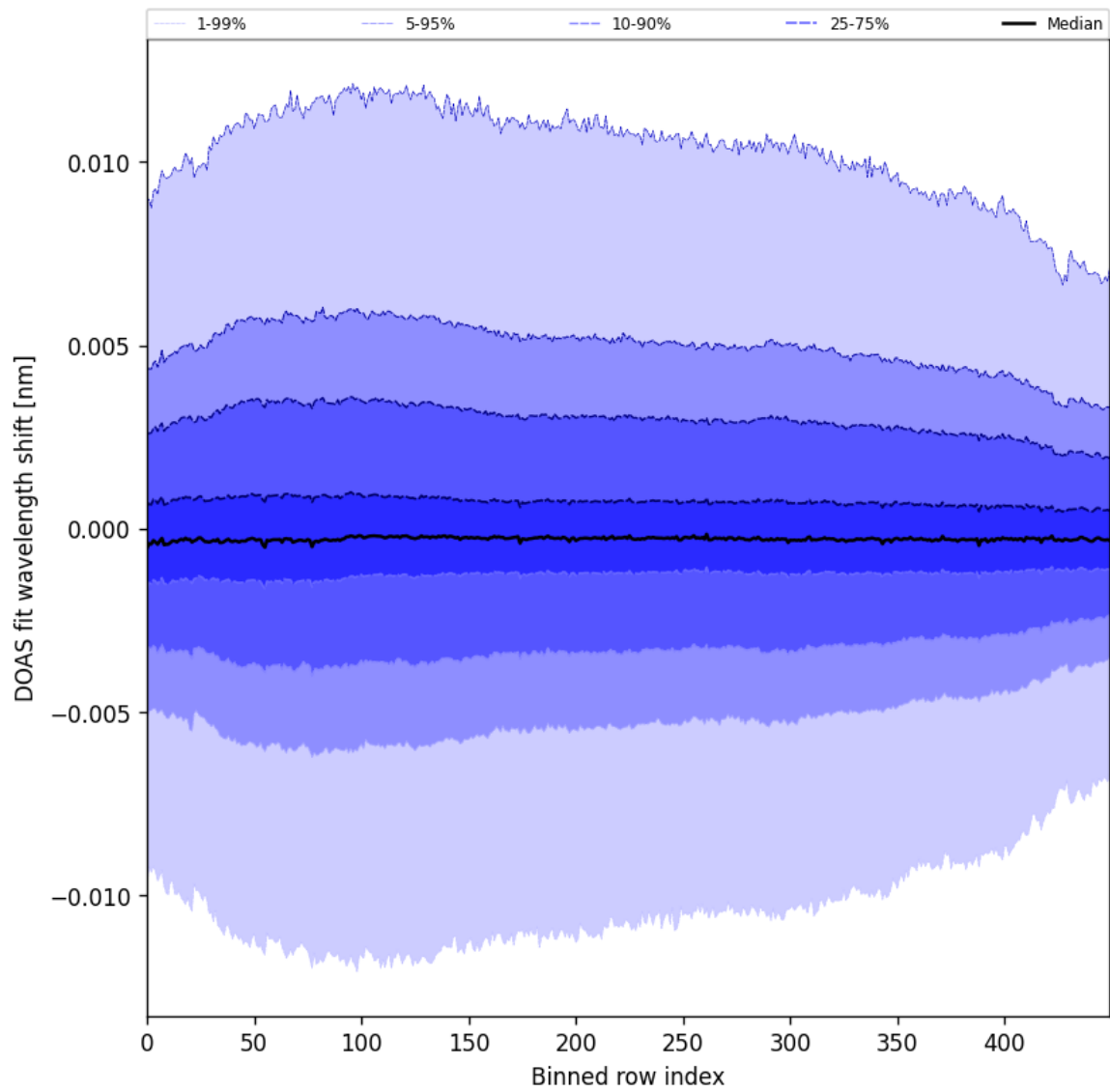
Figure 58: Along track statistics of “DOAS fit wavelength shift” for 2024-10-11 to 2024-10-13
