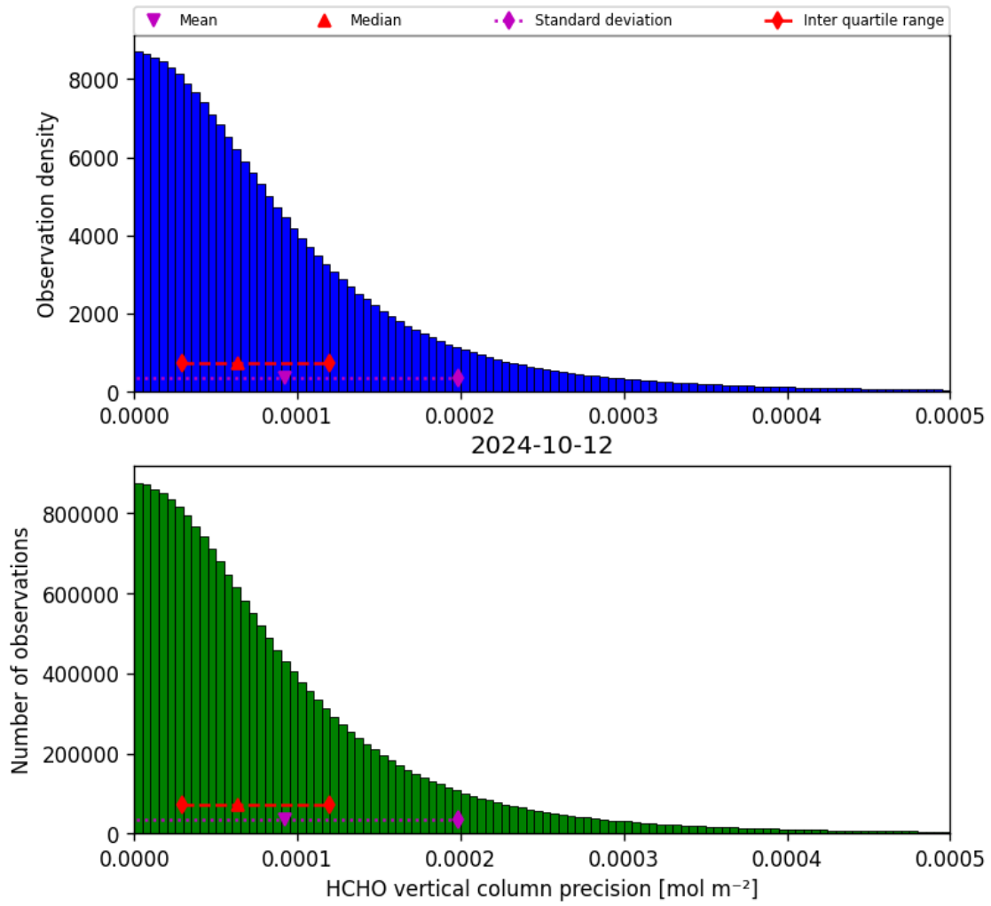
Figure 36: Histogram of “HCHO vertical column precision” for 2024-10-11 to 2024-10-13
