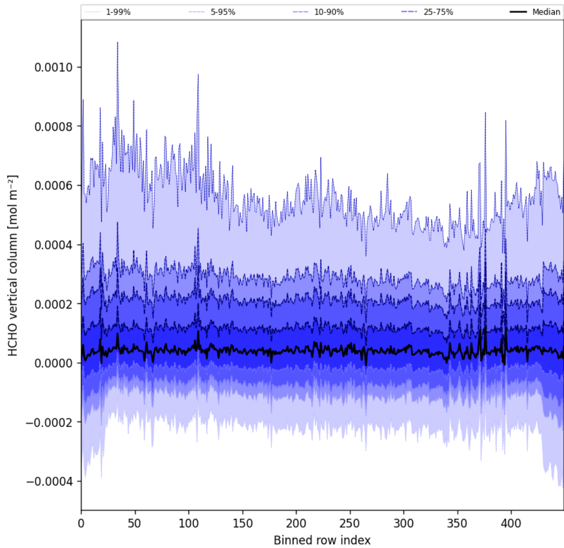
Figure 49: Along track statistics of “HCHO vertical column” for 2024-10-11 to 2024-10-13
