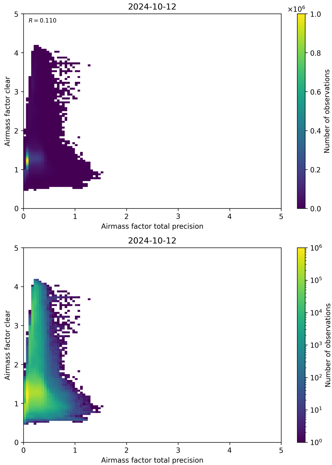
Figure 108: Scatter density plot of “Airmass factor total precision” against “Airmass factor clear” for 2024-10-11 to 2024-10-13.
