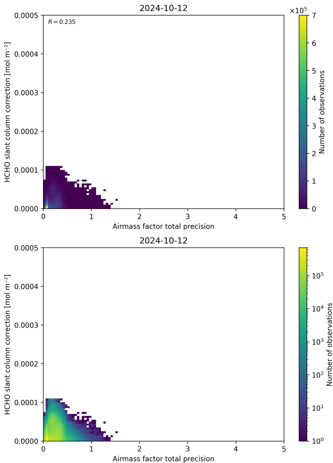
Figure 110: Scatter density plot of “Airmass factor total precision” against “HCHO slant column correction” for 2024-10-11 to 2024-10-13.
