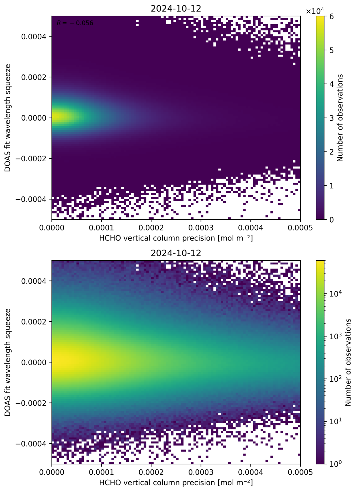
Figure 138: Scatter density plot of “HCHO vertical column precision” against “DOAS fit wavelength squeeze” for 2024-10-11 to 2024-10-13.
