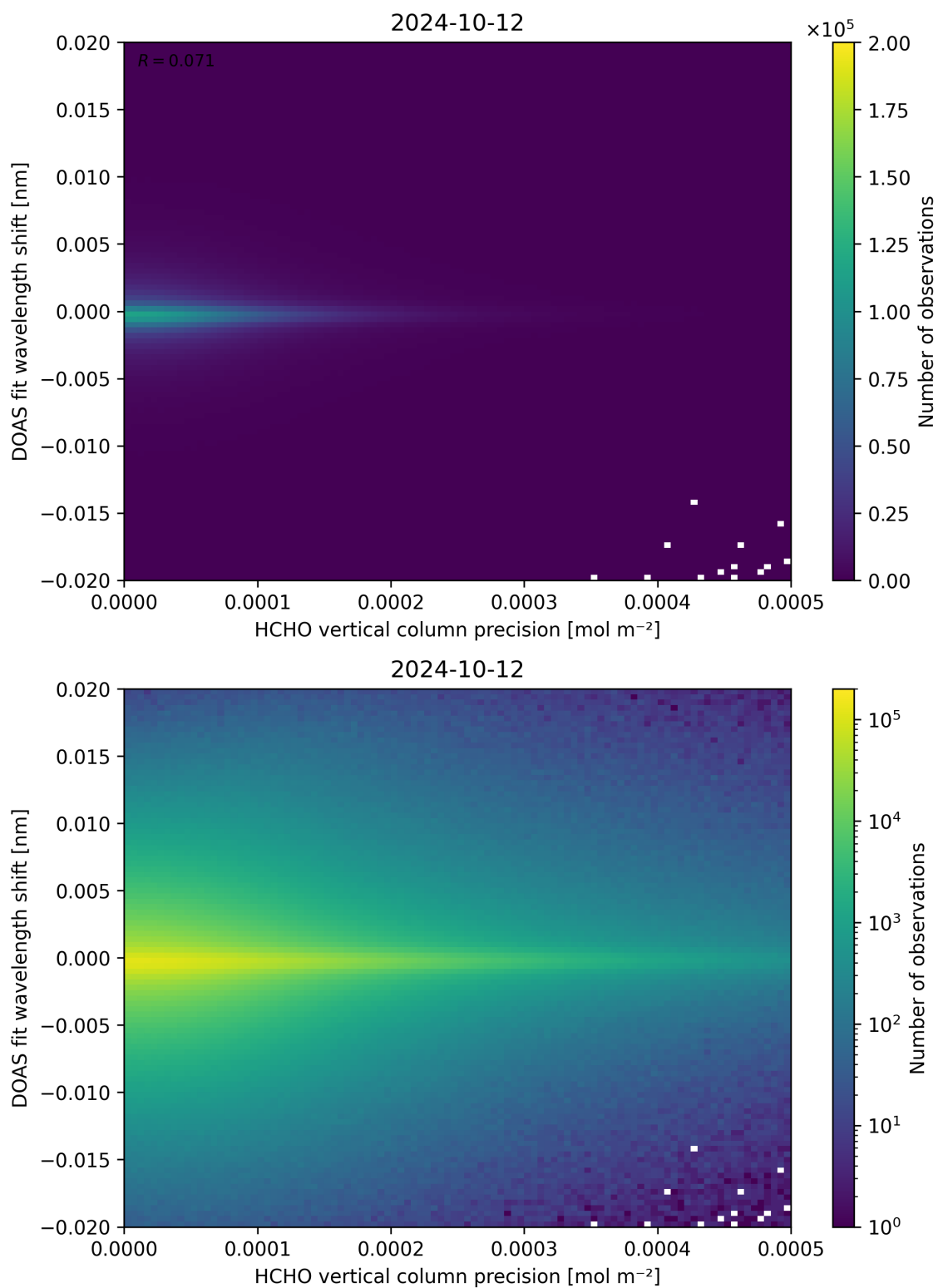
Figure 137: Scatter density plot of “HCHO vertical column precision” against “DOAS fit wavelength shift” for 2024-10-11 to 2024-10-13.
