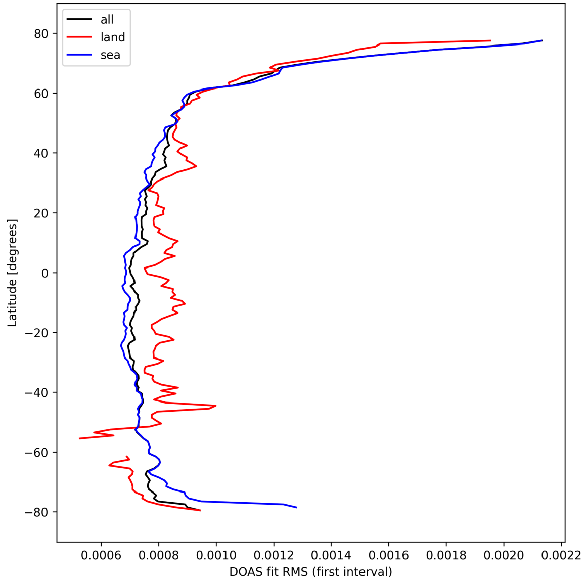
Figure 32: Zonal average of “DOAS fit RMS (first interval)” for 2024-10-11 to 2024-10-13.
