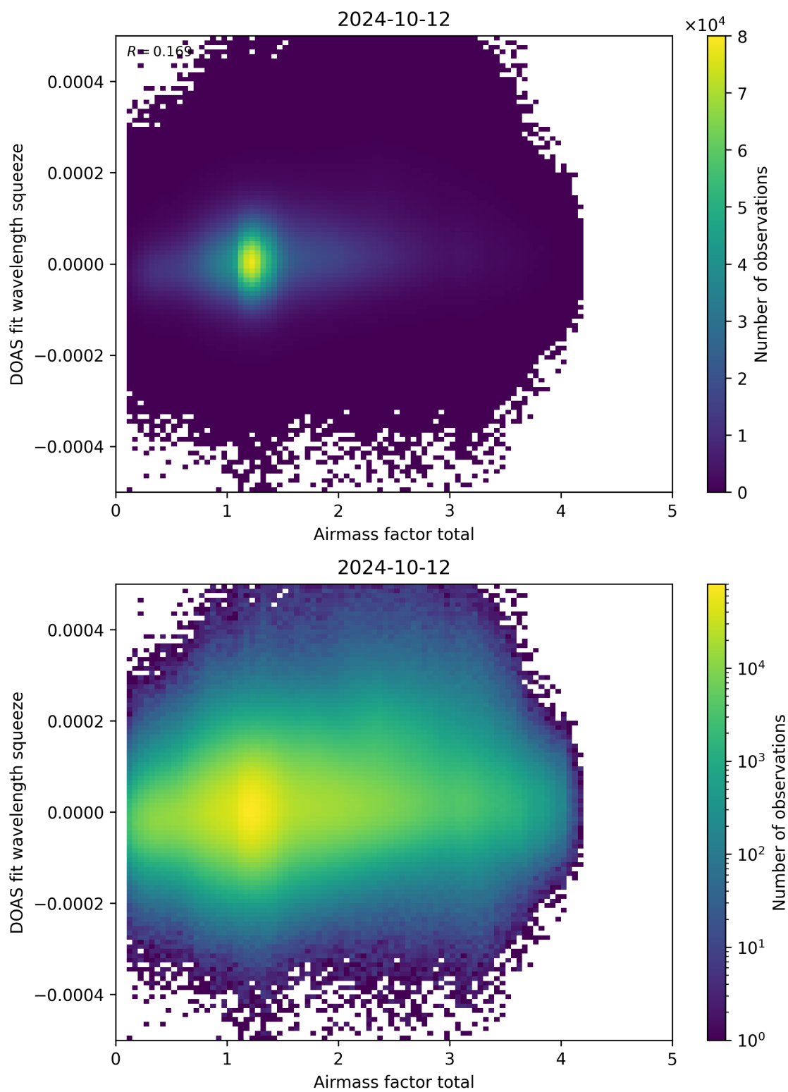
Figure 99: Scatter density plot of “Airmass factor total” against “DOAS fit wavelength squeeze” for 2024-10-11 to 2024-10-13.
