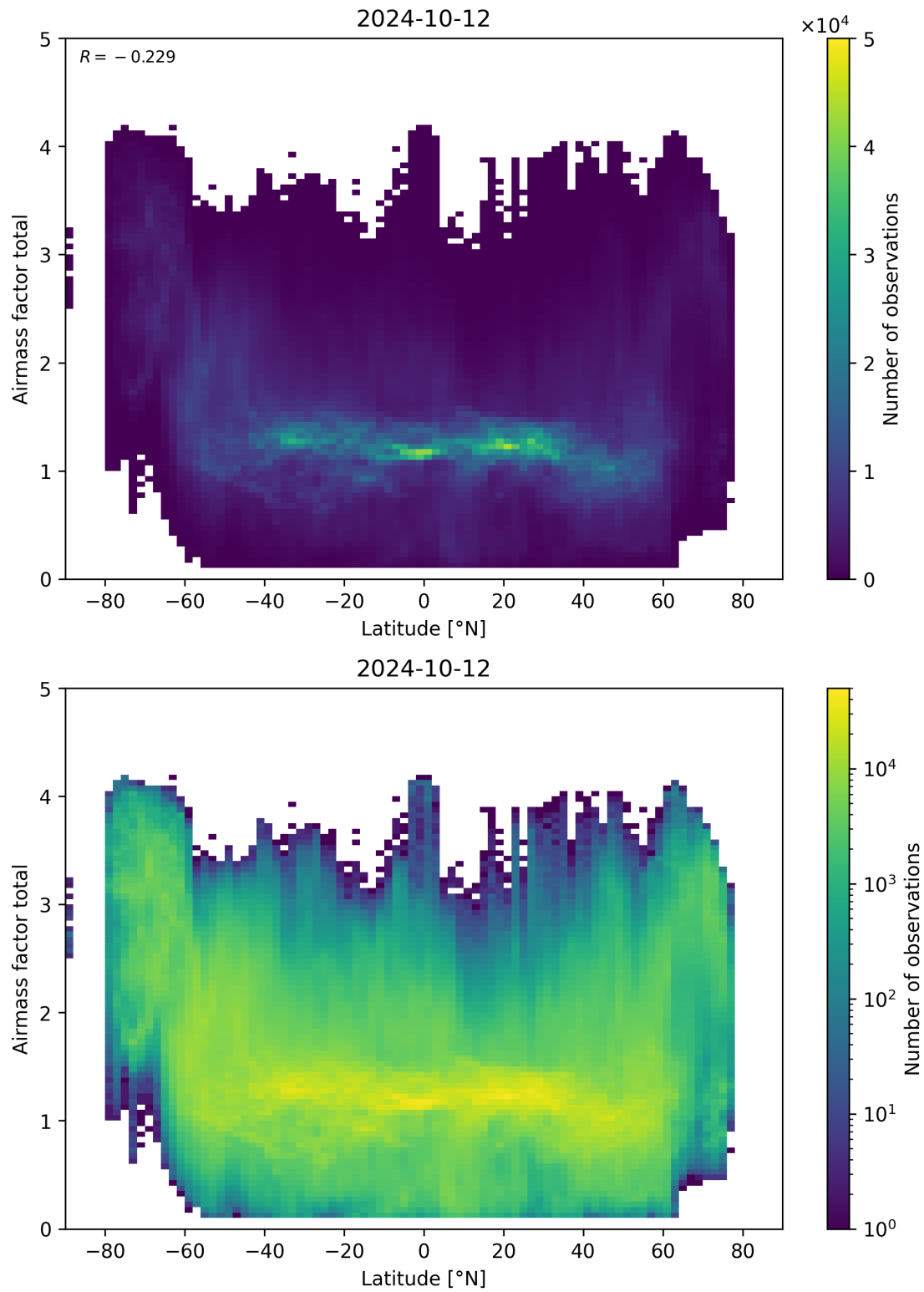
Figure 161: Scatter density plot of “Latitude” against “Airmass factor total” for 2024-10-11 to 2024-10-13.
