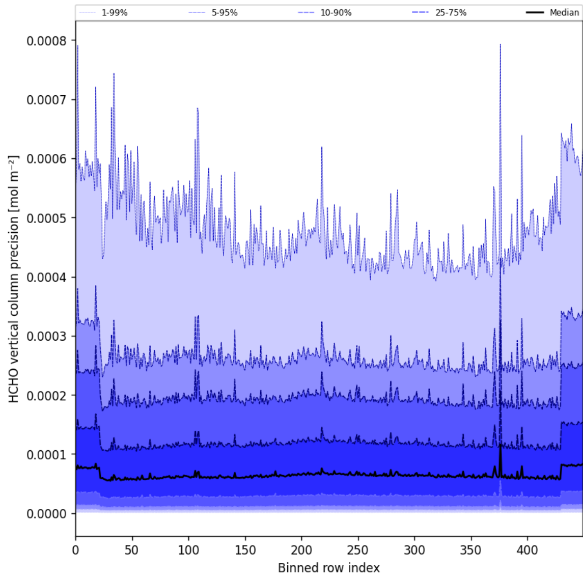
Figure 50: Along track statistics of “HCHO vertical column precision” for 2024-10-11 to 2024-10-13
