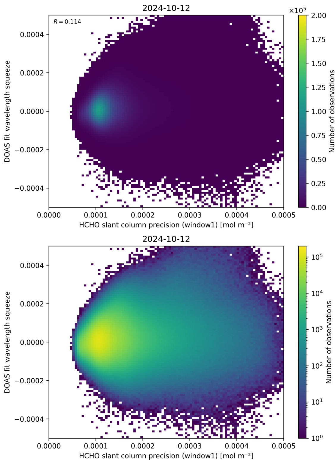
Figure 90: Scatter density plot of “HCHO slant column precision (window1)” against “DOAS fit wavelength squeeze” for 2024-10-11 to 2024-10-13.
