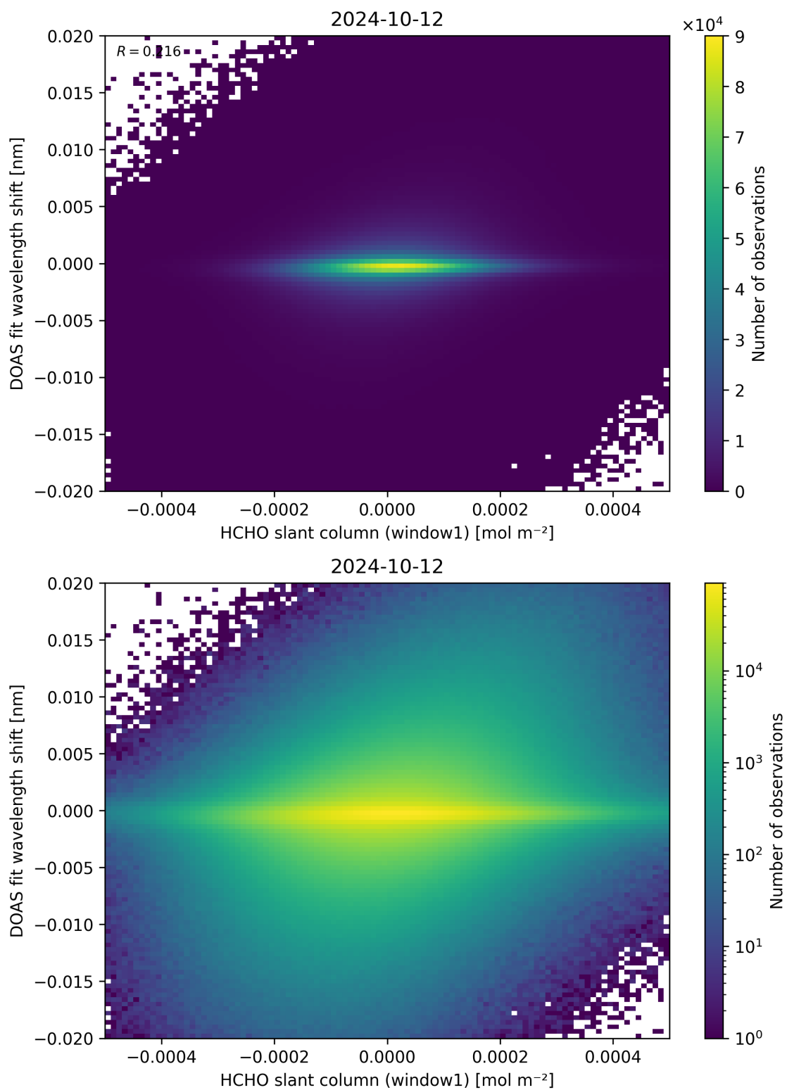
Figure 79: Scatter density plot of “HCHO slant column (window1)” against “DOAS fit wavelength shift” for 2024-10-11 to 2024-10-13.
