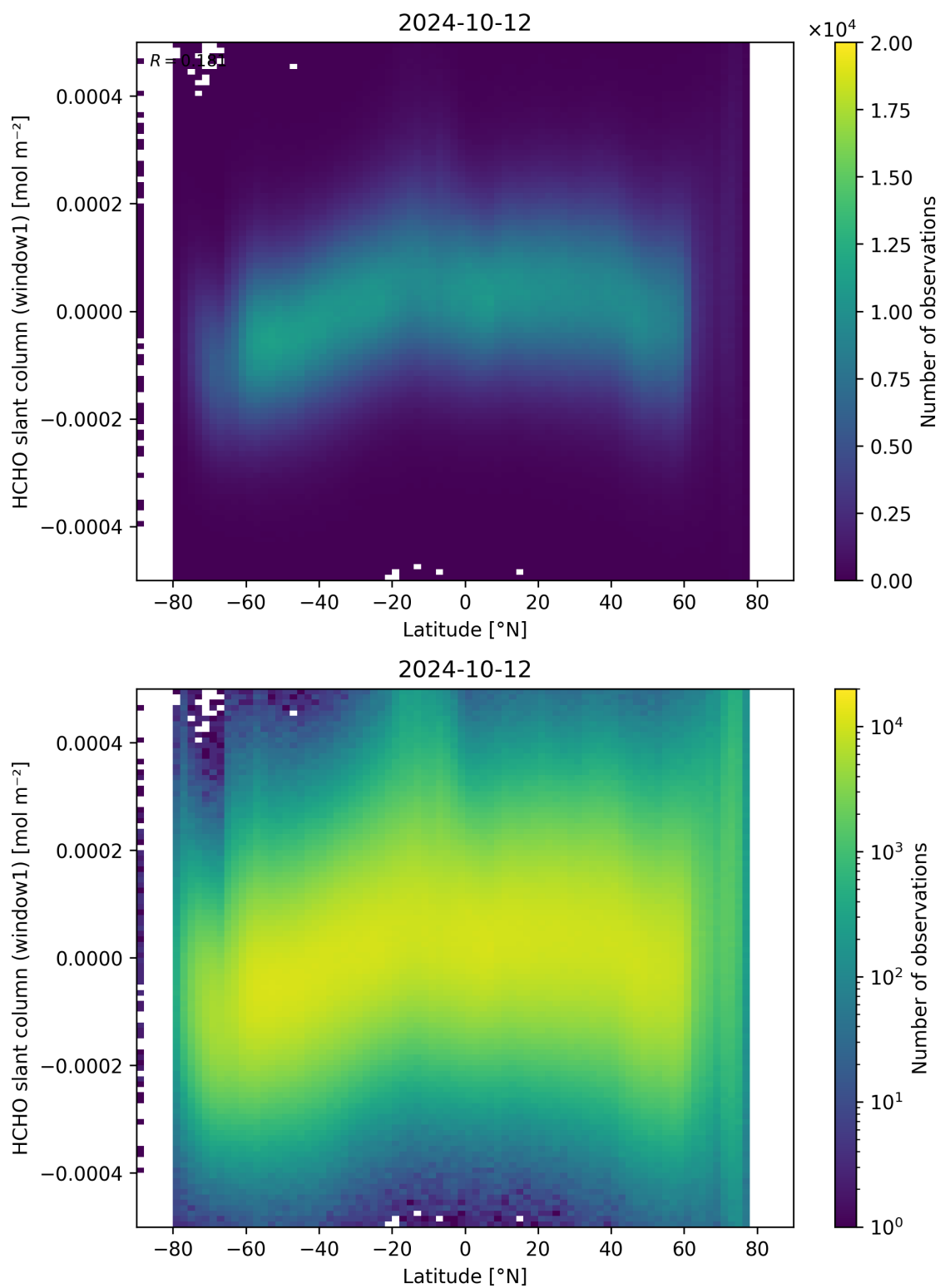
Figure 159: Scatter density plot of “Latitude” against “HCHO slant column (window1)” for 2024-10-11 to 2024-10-13.
