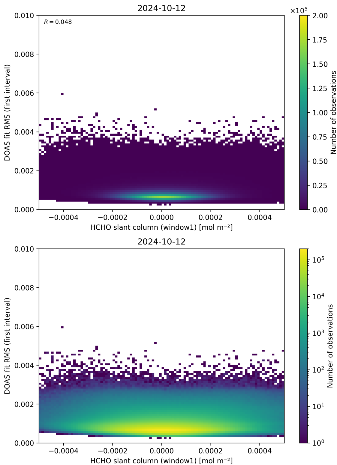
Figure 78: Scatter density plot of “HCHO slant column (window1)” against “DOAS fit RMS (first interval)” for 2024-10-11 to 2024-10-13.
