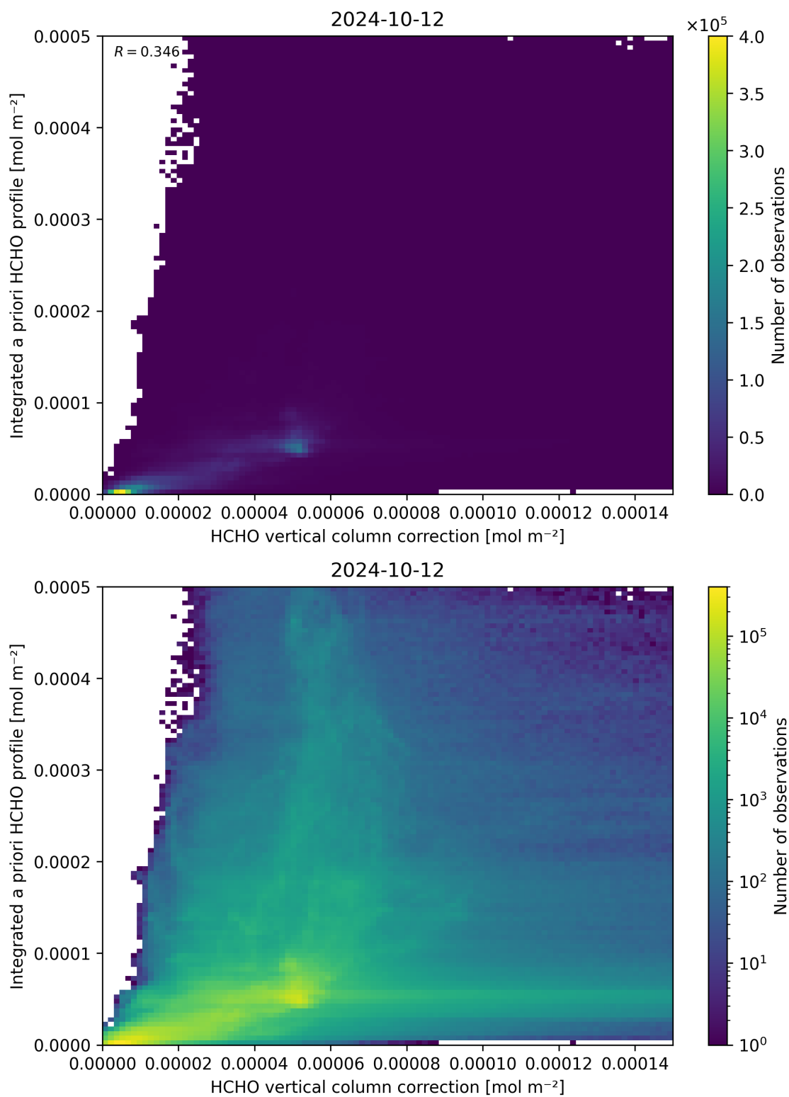
Figure 122: Scatter density plot of “HCHO vertical column correction” against “Integrated a priori HCHO profile” for 2024-10-11 to 2024-10-13.
