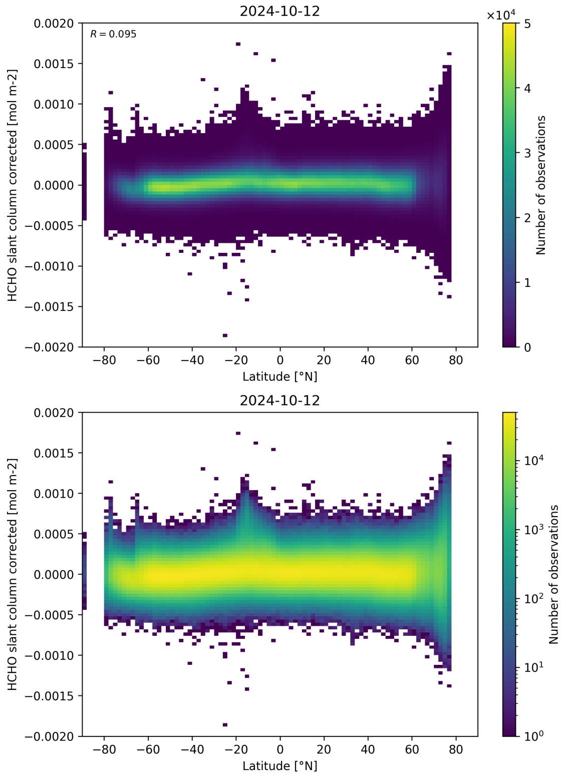
Figure 157: Scatter density plot of “Latitude” against “HCHO slant column corrected” for 2024-10-11 to 2024-10-13.
