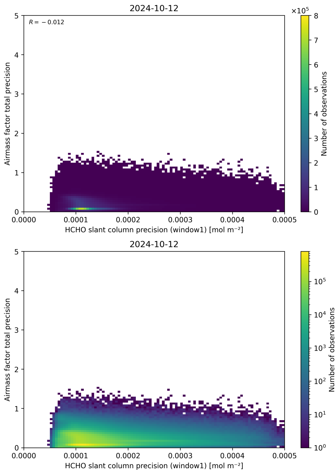
Figure 95: Scatter density plot of “HCHO slant column precision (window1)” against “Airmass factor total precision” for 2024-10-11 to 2024-10-13.
