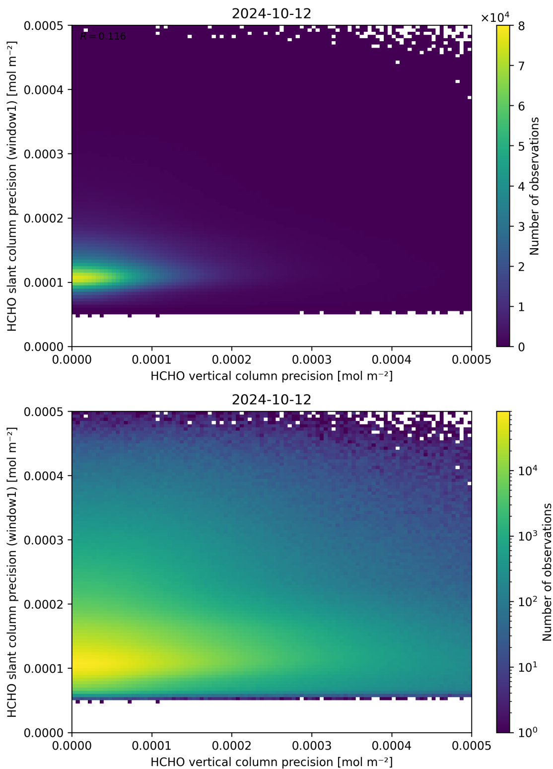
Figure 143: Scatter density plot of “HCHO vertical column precision” against “HCHO slant column precision (window1)” for 2024-10-11 to 2024-10-13.
