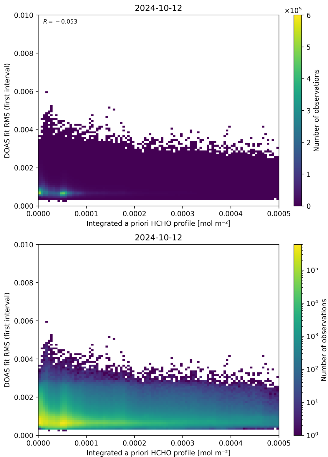
Figure 148: Scatter density plot of “Integrated a priori HCHO profile” against “DOAS fit RMS (first interval)” for 2024-10-11 to 2024-10-13.
