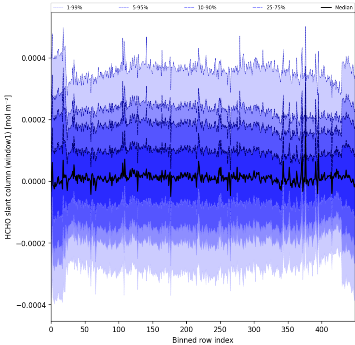
Figure 52: Along track statistics of “HCHO slant column (window1)” for 2024-10-11 to 2024-10-13
