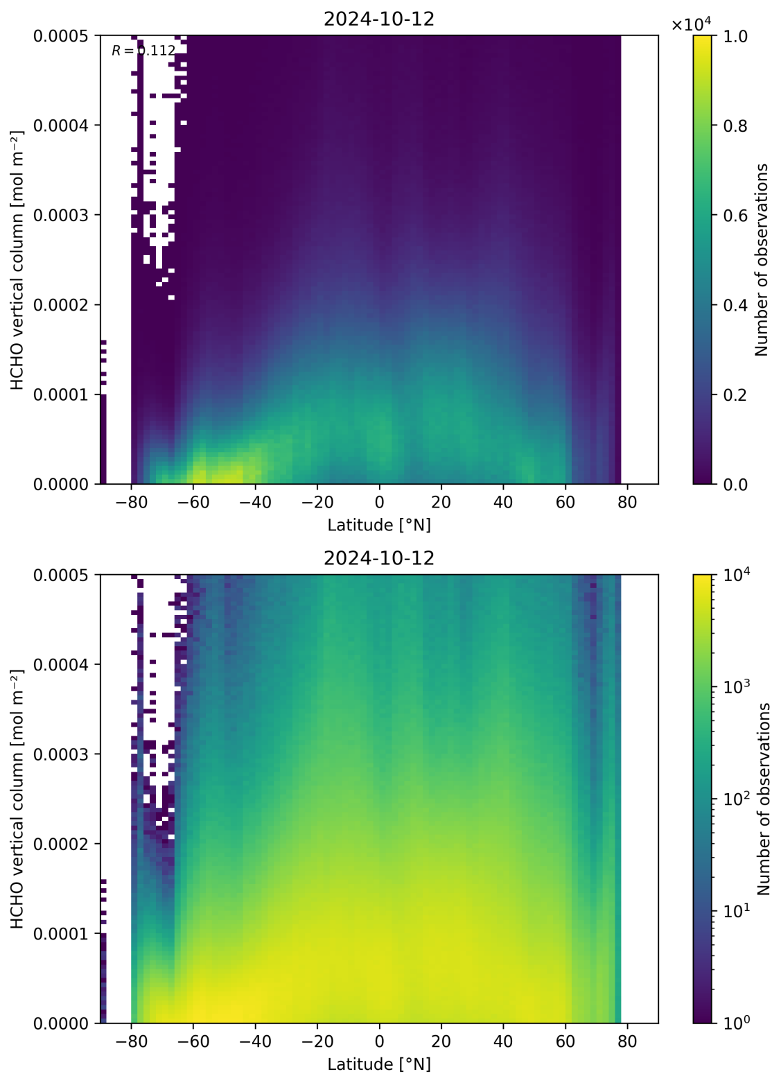
Figure 163: Scatter density plot of “Latitude” against “HCHO vertical column” for 2024-10-11 to 2024-10-13.
