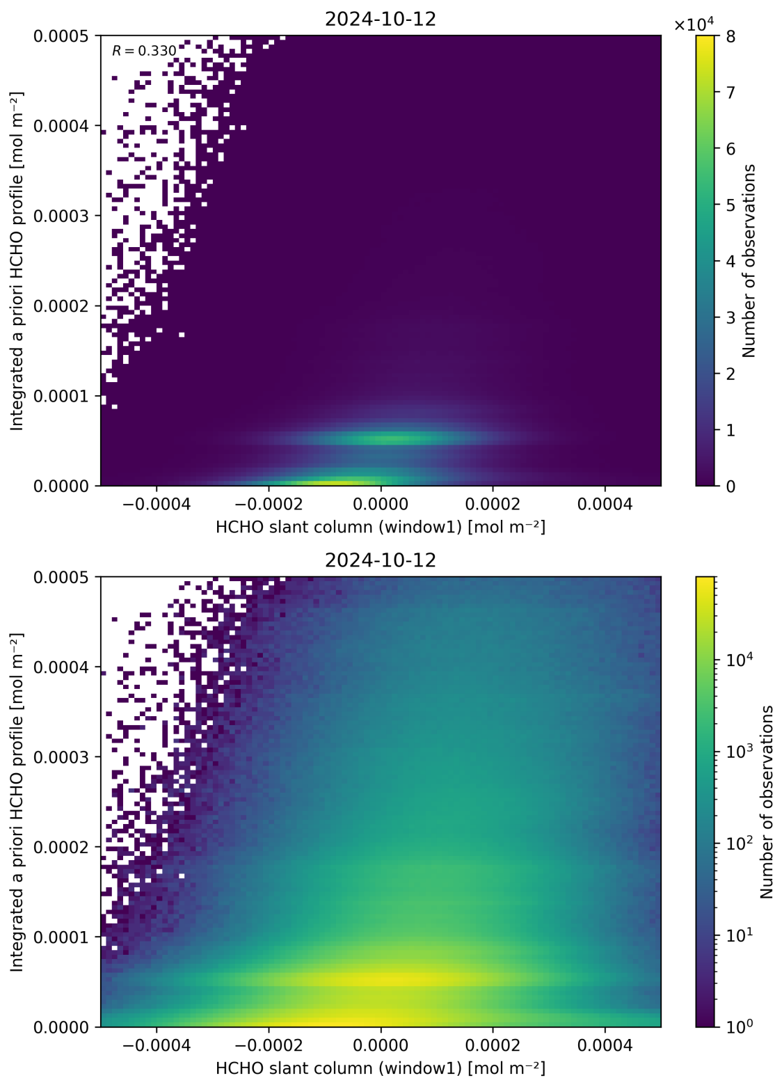
Figure 87: Scatter density plot of “HCHO slant column (window1)” against “Integrated a priori HCHO profile” for 2024-10-11 to 2024-10-13.
