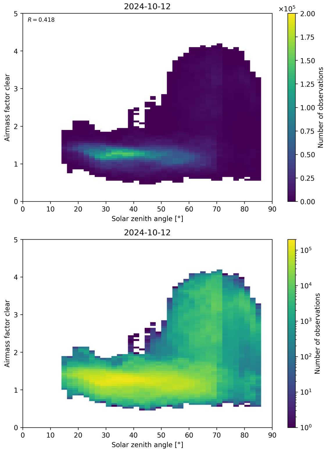
Figure 170: Scatter density plot of “Solar zenith angle” against “Airmass factor clear” for 2024-10-11 to 2024-10-13.
