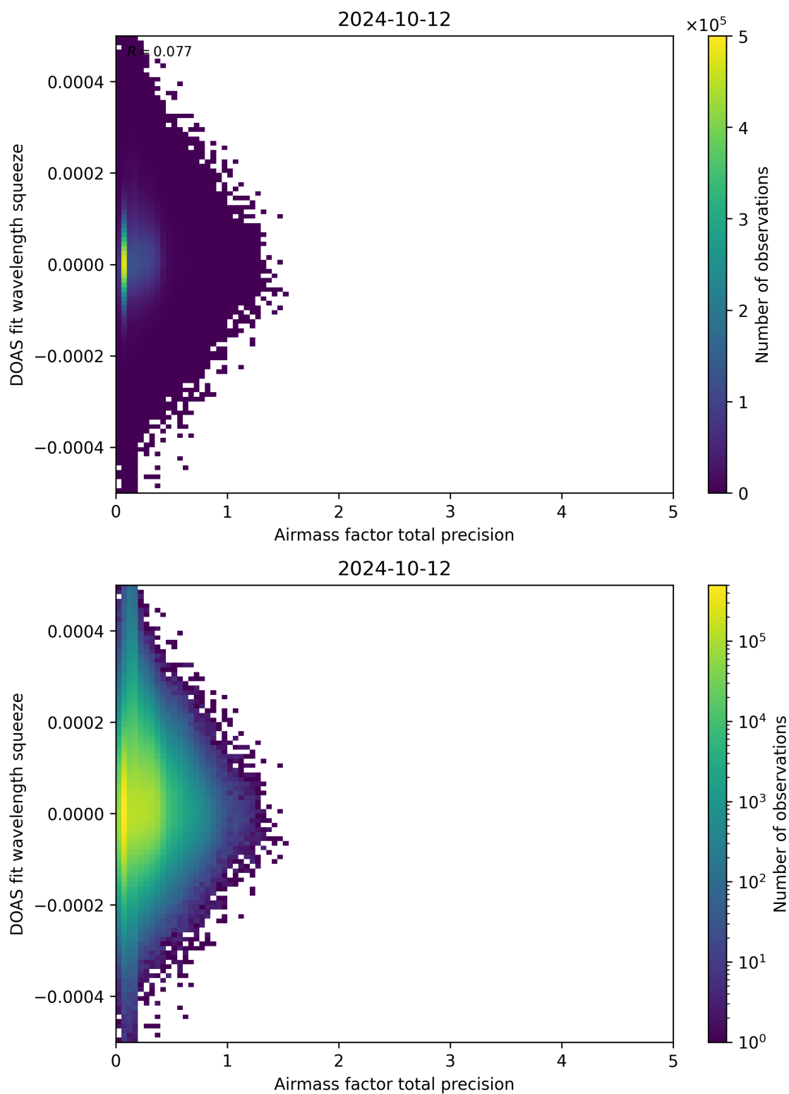
Figure 107: Scatter density plot of “Airmass factor total precision” against “DOAS fit wavelength squeeze” for 2024-10-11 to 2024-10-13.
