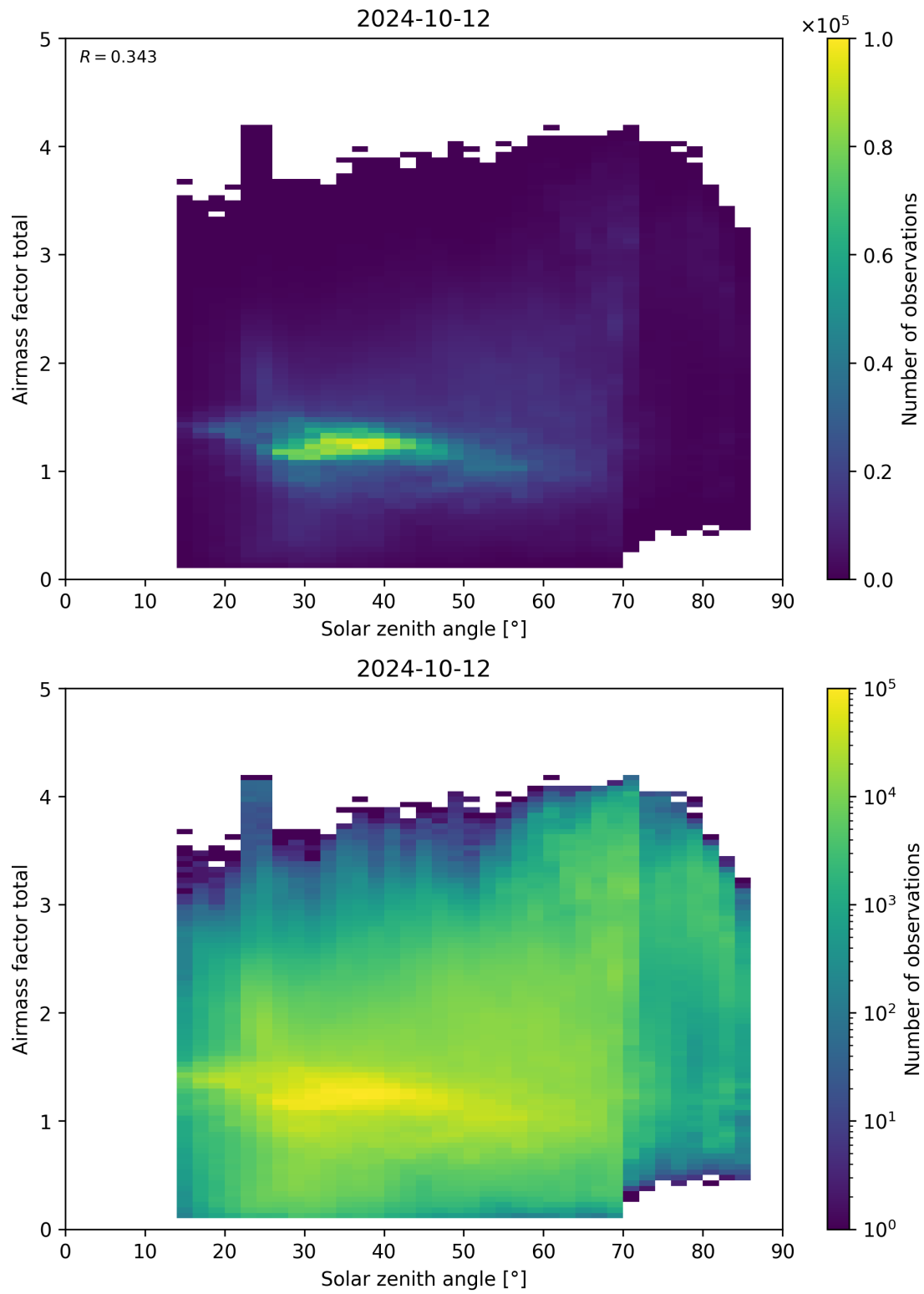
Figure 175: Scatter density plot of “Solar zenith angle” against “Airmass factor total” for 2024-10-11 to 2024-10-13.
