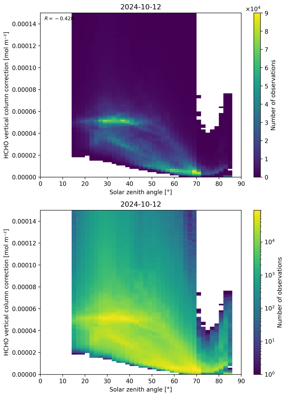
Figure 178: Scatter density plot of “Solar zenith angle” against “HCHO vertical column correction” for 2024-10-11 to 2024-10-13.
