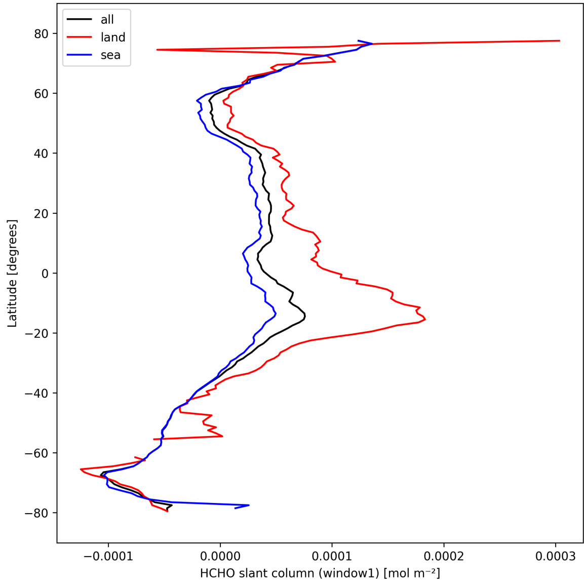
Figure 24: Zonal average of “HCHO slant column (window1)” for 2024-10-11 to 2024-10-13.
