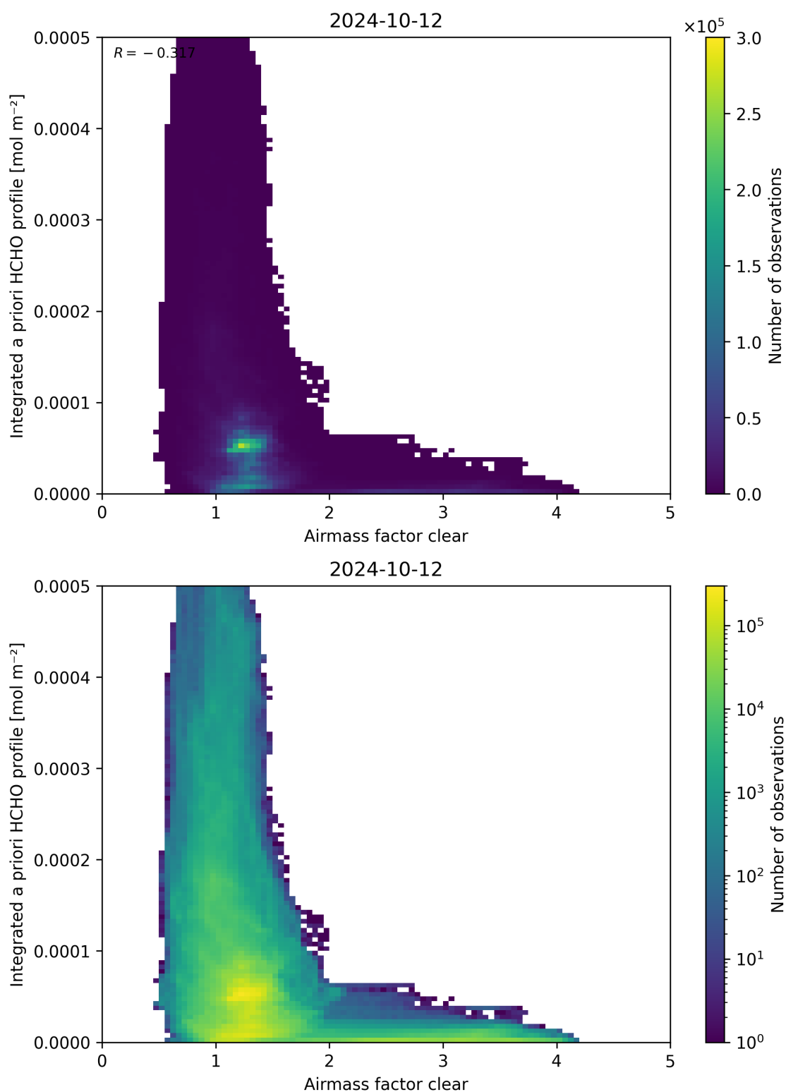
Figure 76: Scatter density plot of “Airmass factor clear” against “Integrated a priori HCHO profile” for 2024-10-11 to 2024-10-13.
