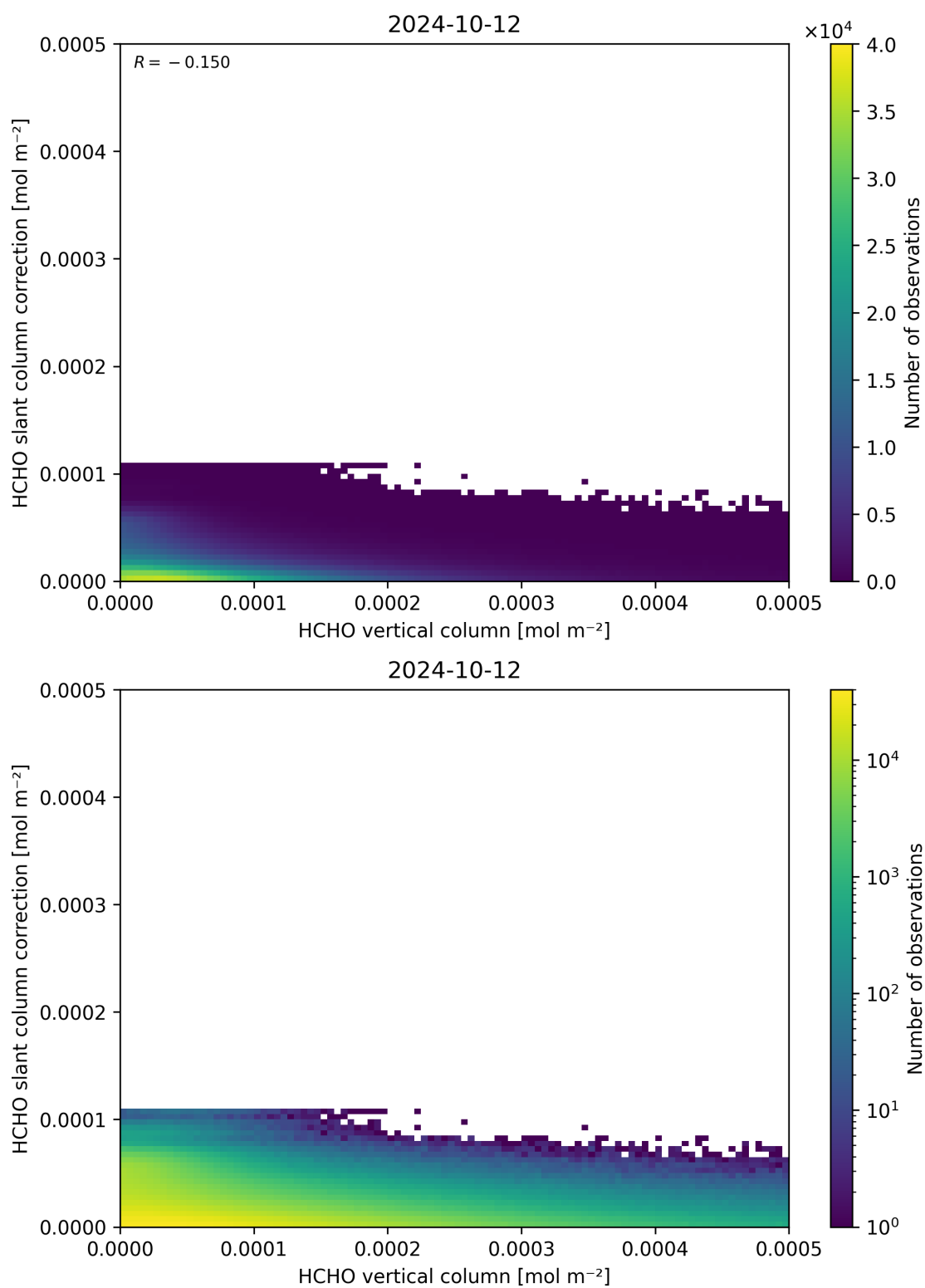
Figure 128: Scatter density plot of “HCHO vertical column” against “HCHO slant column correction” for 2024-10-11 to 2024-10-13.
