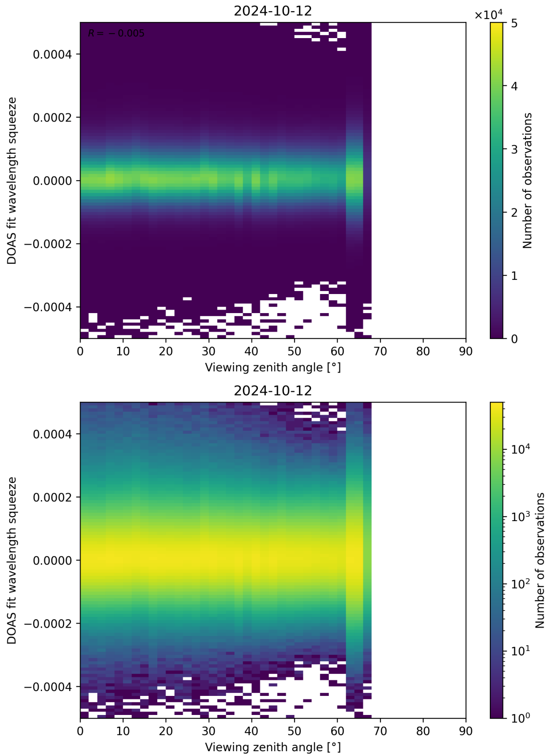
Figure 184: Scatter density plot of “Viewing zenith angle” against “DOAS fit wavelength squeeze” for 2024-10-11 to 2024-10-13.
