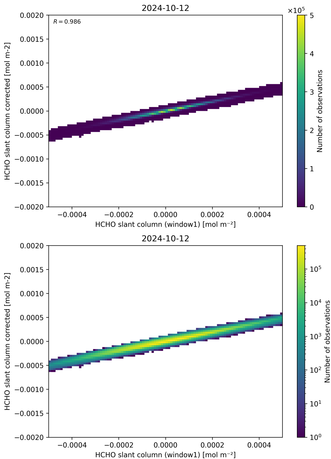
Figure 82: Scatter density plot of “HCHO slant column (window1)” against “HCHO slant column corrected” for 2024-10-11 to 2024-10-13.
