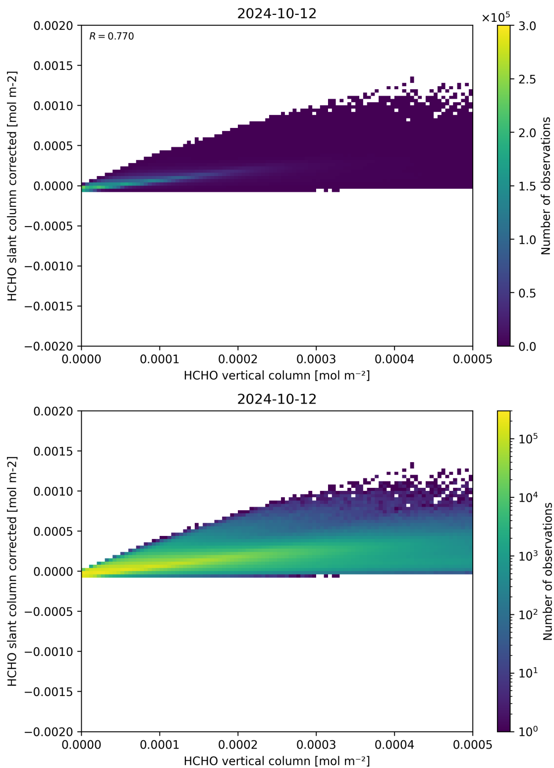
Figure 127: Scatter density plot of “HCHO vertical column” against “HCHO slant column corrected” for 2024-10-11 to 2024-10-13.
