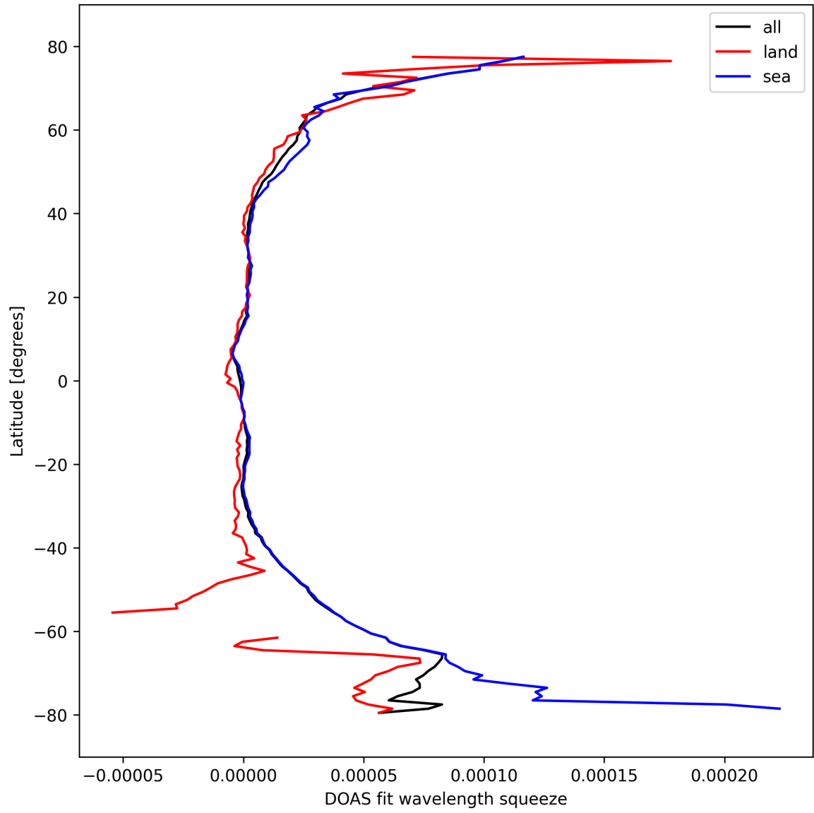
Figure 31: Zonal average of “DOAS fit wavelength squeeze” for 2024-10-11 to 2024-10-13.
