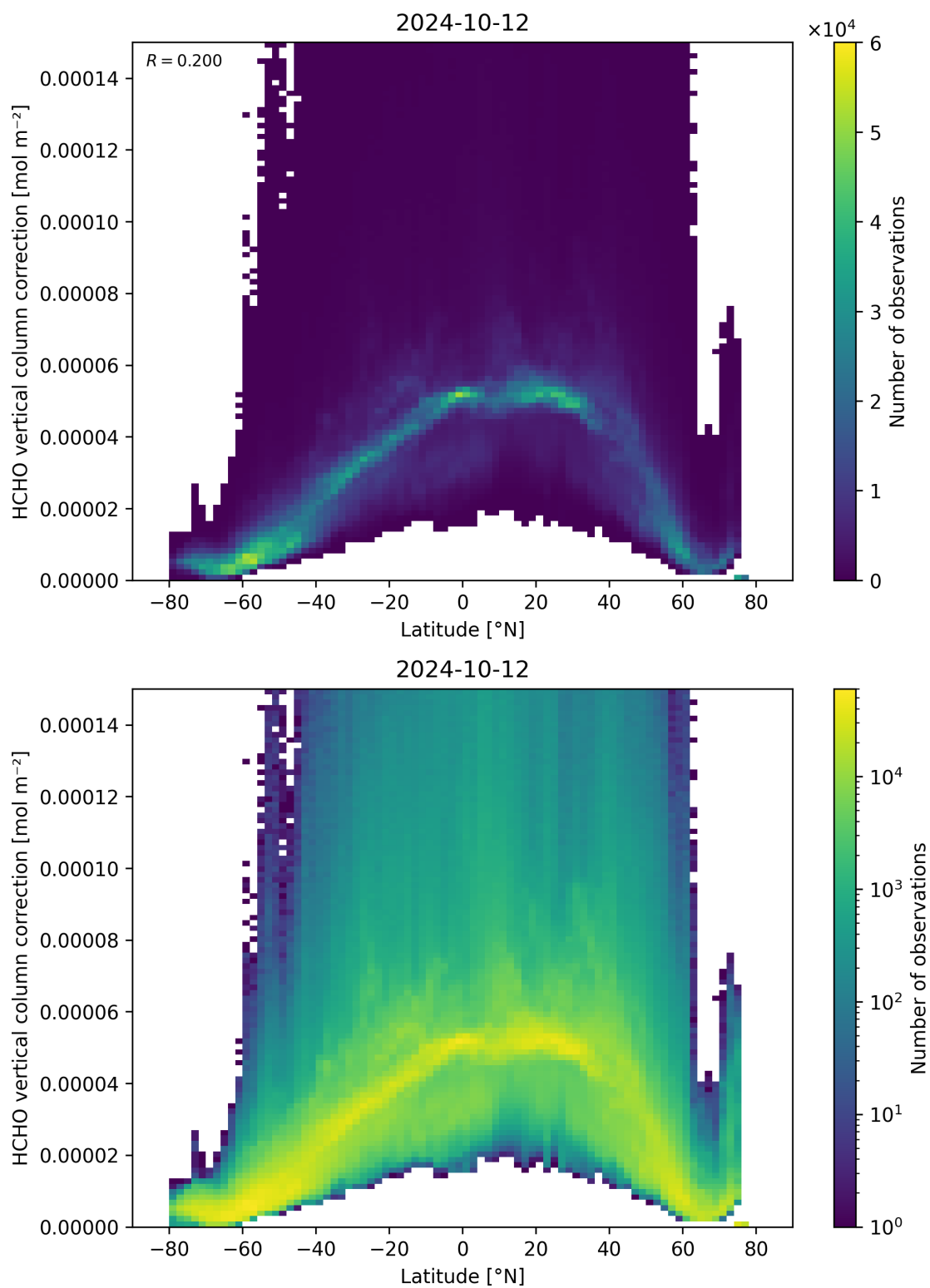
Figure 164: Scatter density plot of “Latitude” against “HCHO vertical column correction” for 2024-10-11 to 2024-10-13.
