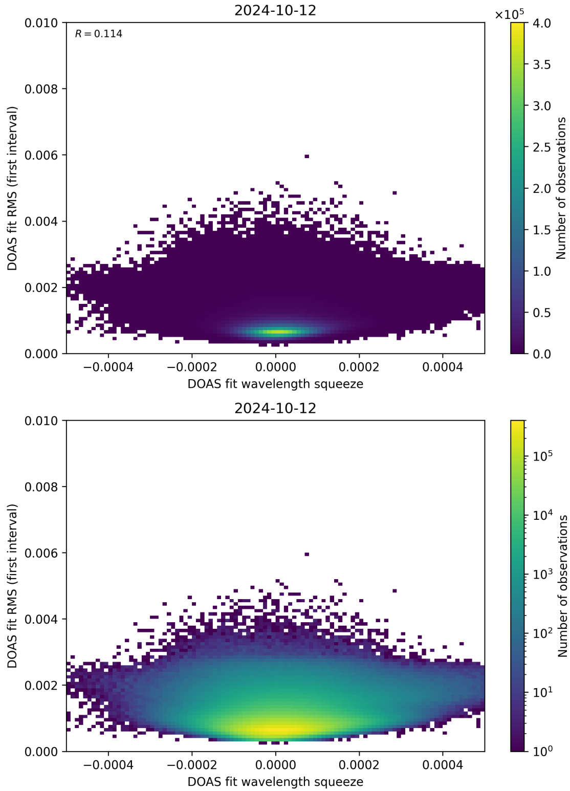
Figure 68: Scatter density plot of “DOAS fit wavelength squeeze” against “DOAS fit RMS (first interval)” for 2024-10-11 to 2024-10-13.
