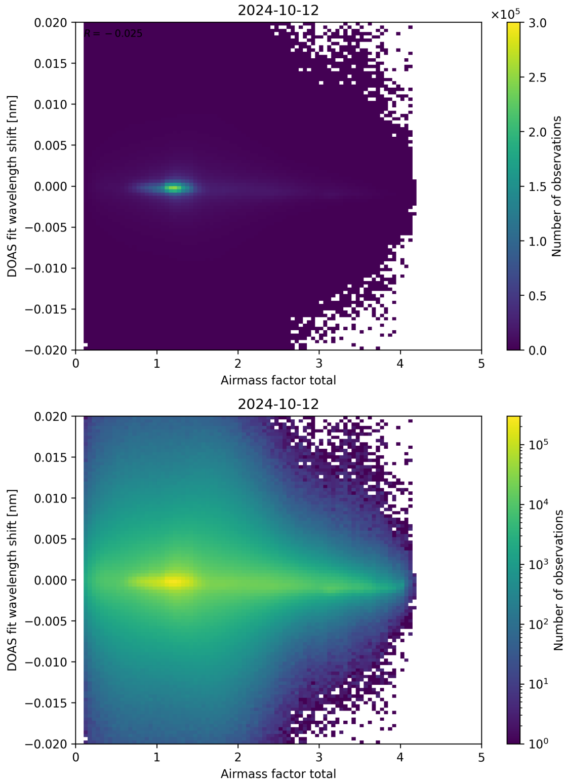
Figure 98: Scatter density plot of “Airmass factor total” against “DOAS fit wavelength shift” for 2024-10-11 to 2024-10-13.
