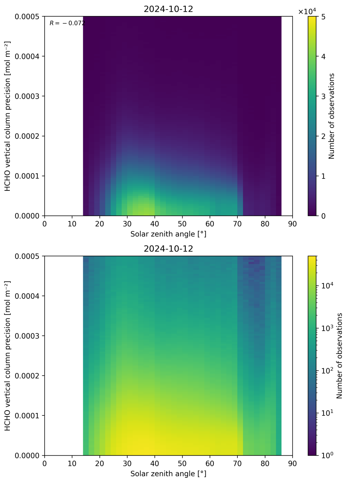
Figure 179: Scatter density plot of “Solar zenith angle” against “HCHO vertical column precision” for 2024-10-11 to 2024-10-13.
