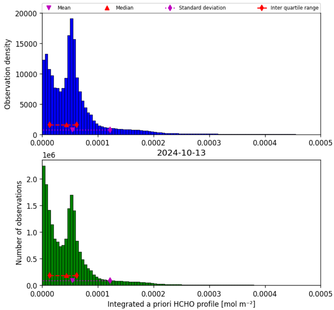
Figure 43: Histogram of “Integrated a priori HCHO profile” for 2024-10-12 to 2024-10-14
