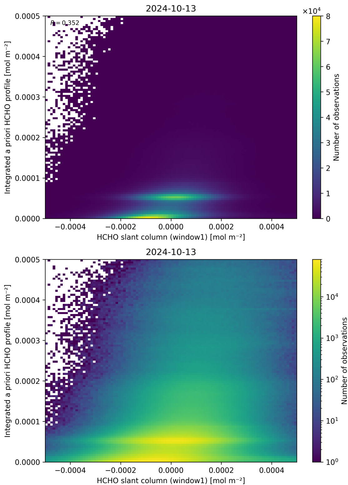
Figure 87: Scatter density plot of “HCHO slant column (window1)” against “Integrated a priori HCHO profile” for 2024-10-12 to 2024-10-14.
