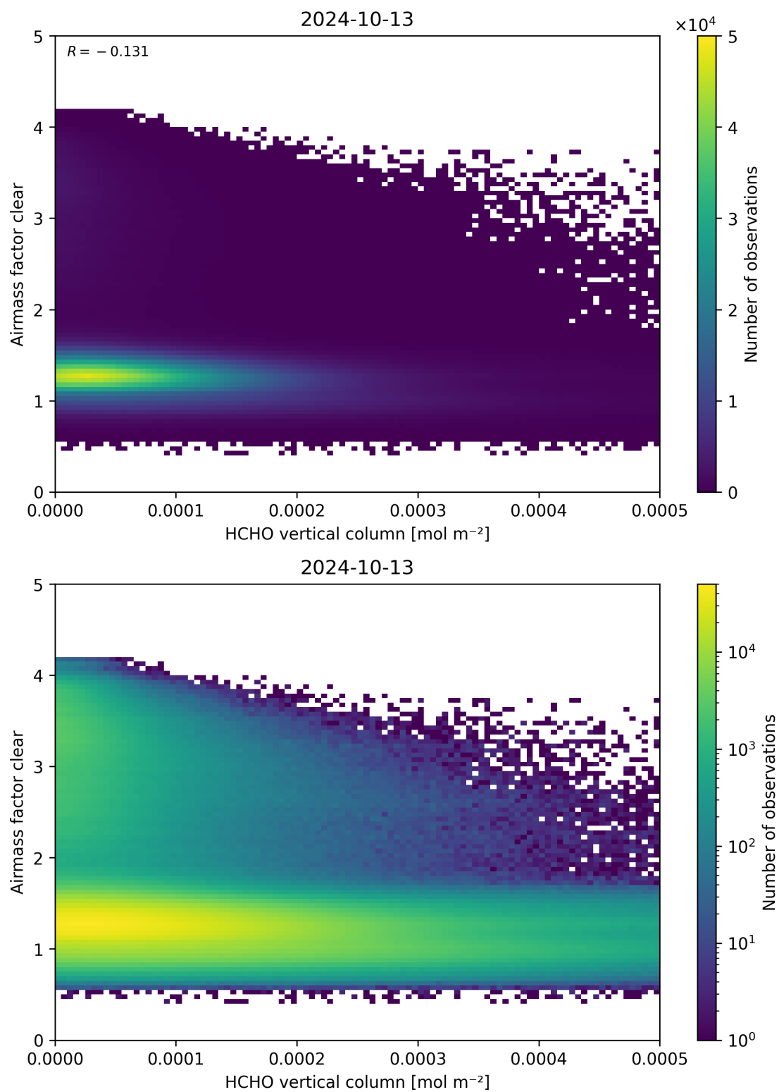
Figure 126: Scatter density plot of “HCHO vertical column” against “Airmass factor clear” for 2024-10-12 to 2024-10-14.
