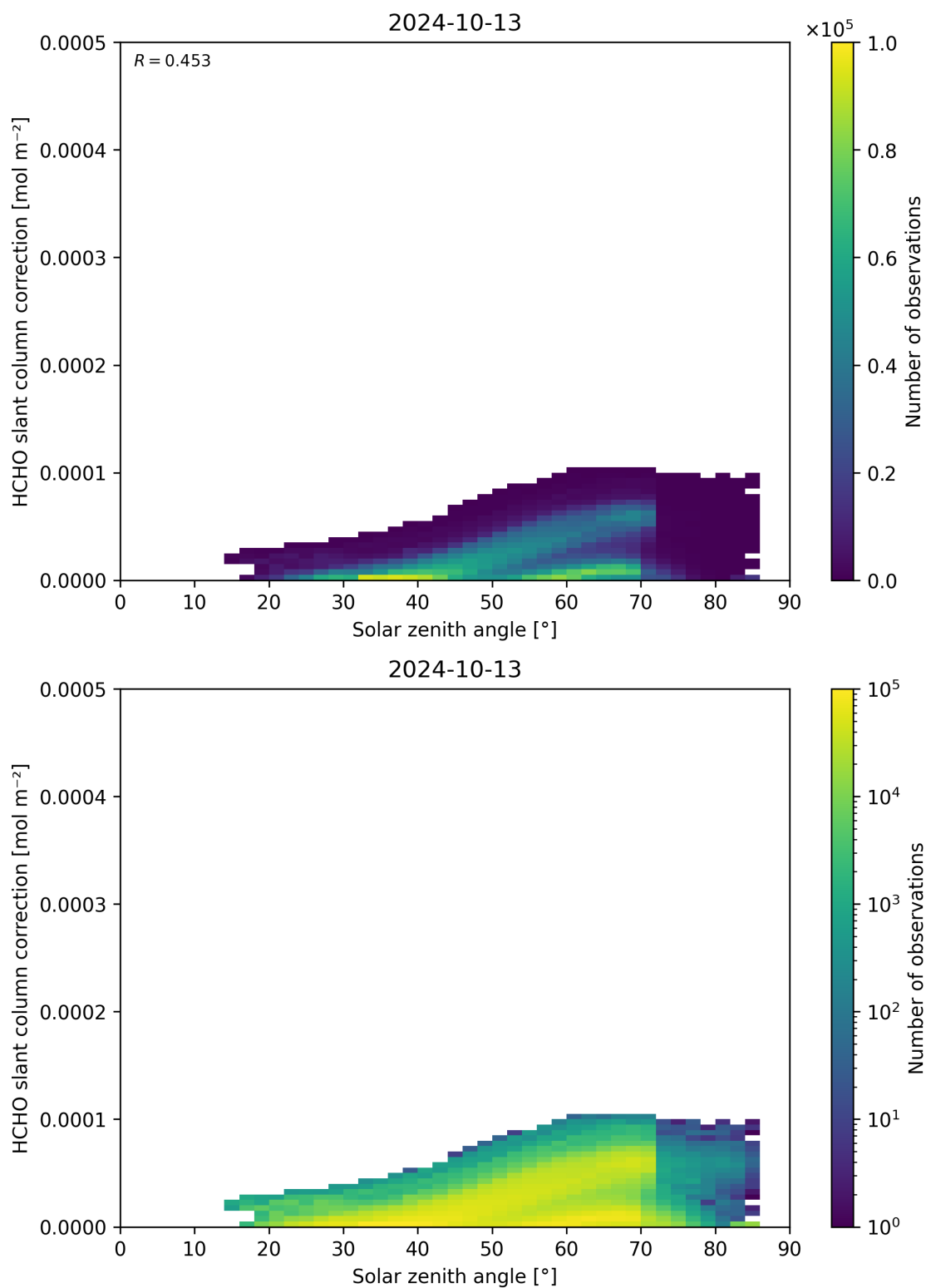
Figure 172: Scatter density plot of “Solar zenith angle” against “HCHO slant column correction” for 2024-10-12 to 2024-10-14.
