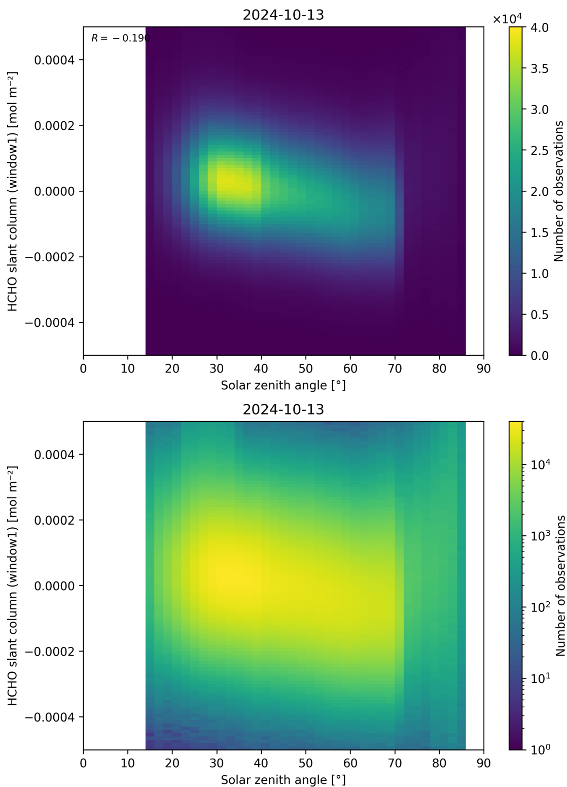
Figure 173: Scatter density plot of “Solar zenith angle” against “HCHO slant column (window1)” for 2024-10-12 to 2024-10-14.
