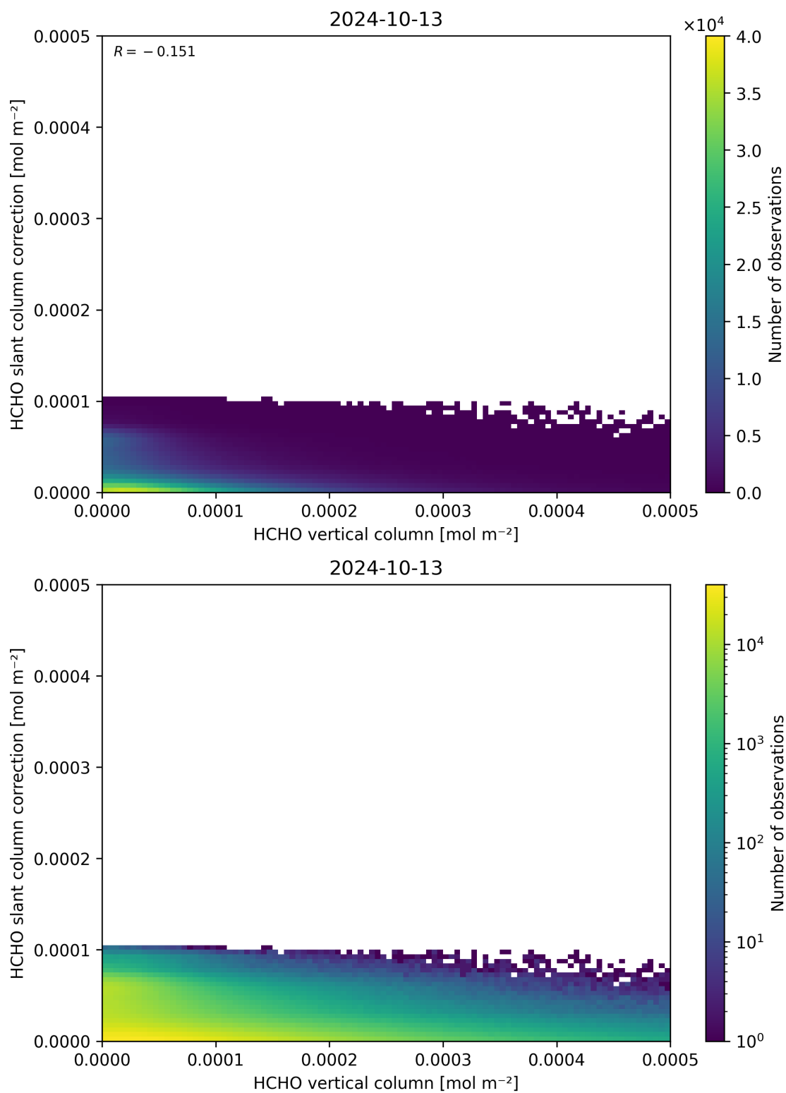
Figure 128: Scatter density plot of “HCHO vertical column” against “HCHO slant column correction” for 2024-10-12 to 2024-10-14.
