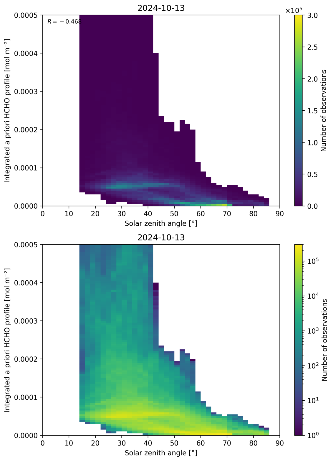
Figure 180: Scatter density plot of “Solar zenith angle” against “Integrated a priori HCHO profile” for 2024-10-12 to 2024-10-14.
