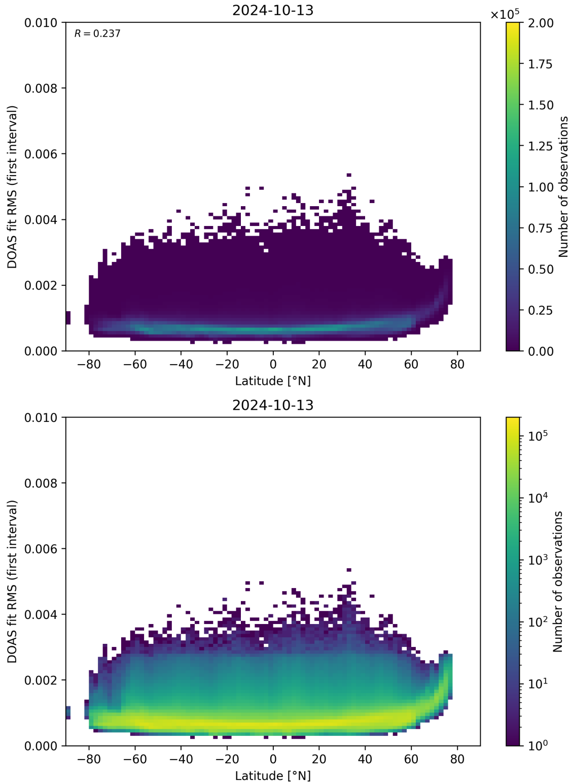
Figure 153: Scatter density plot of “Latitude” against “DOAS fit RMS (first interval)” for 2024-10-12 to 2024-10-14.
