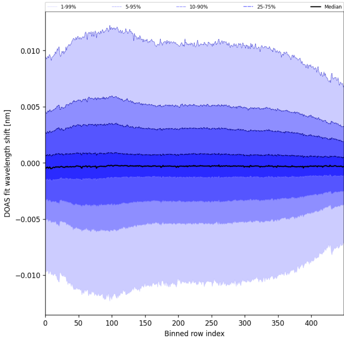
Figure 58: Along track statistics of “DOAS fit wavelength shift” for 2024-10-12 to 2024-10-14
