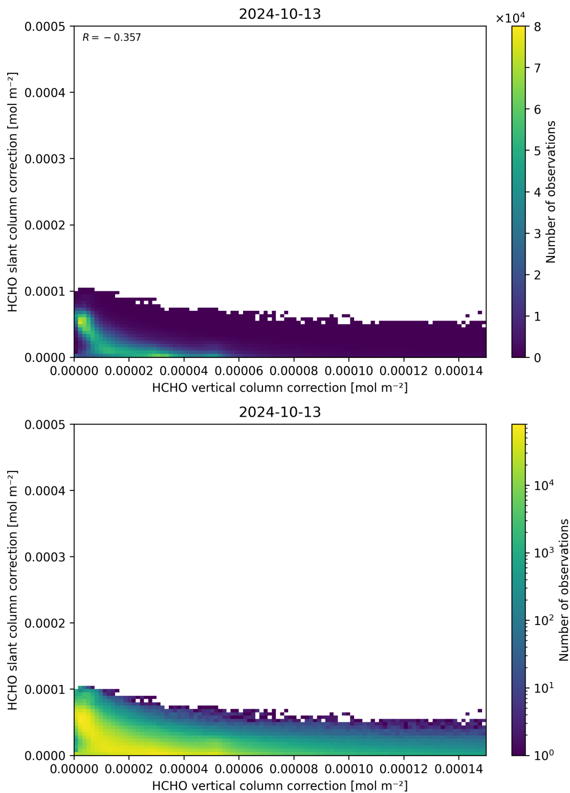
Figure 117: Scatter density plot of “HCHO vertical column correction” against “HCHO slant column correction” for 2024-10-12 to 2024-10-14.
