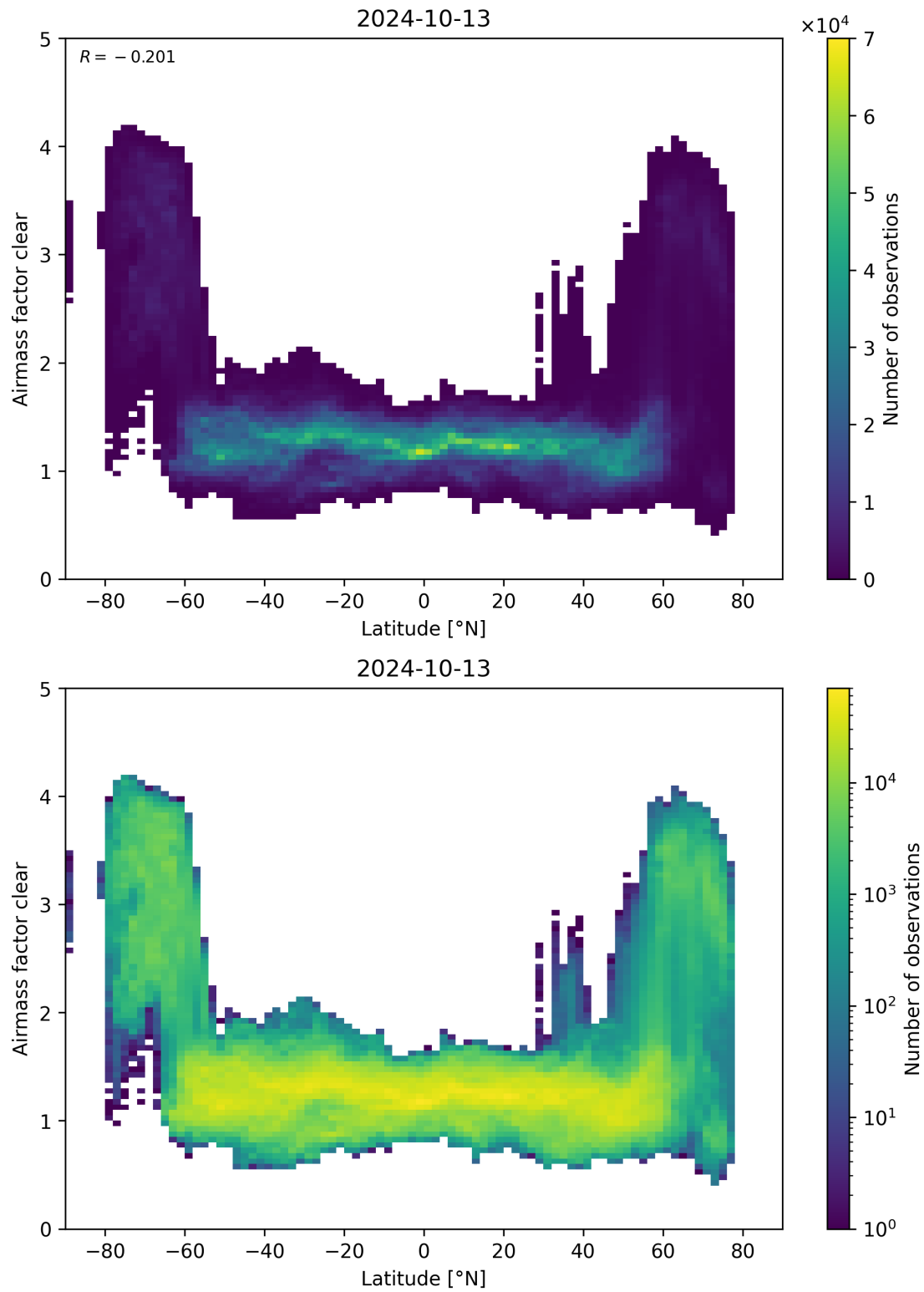
Figure 156: Scatter density plot of “Latitude” against “Airmass factor clear” for 2024-10-12 to 2024-10-14.
