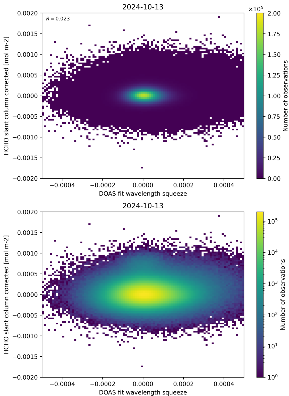
Figure 69: Scatter density plot of “DOAS fit wavelength squeeze” against “HCHO slant column corrected” for 2024-10-12 to 2024-10-14.
