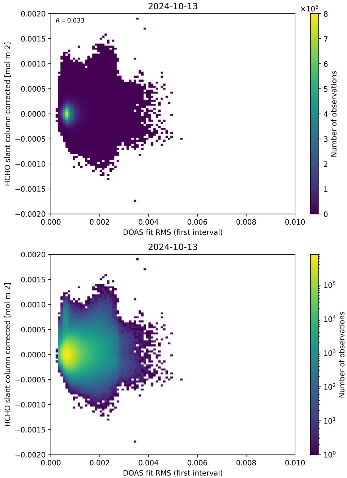
Figure 62: Scatter density plot of “DOAS fit RMS (first interval)” against “HCHO slant column corrected” for 2024-10-12 to 2024-10-14.
