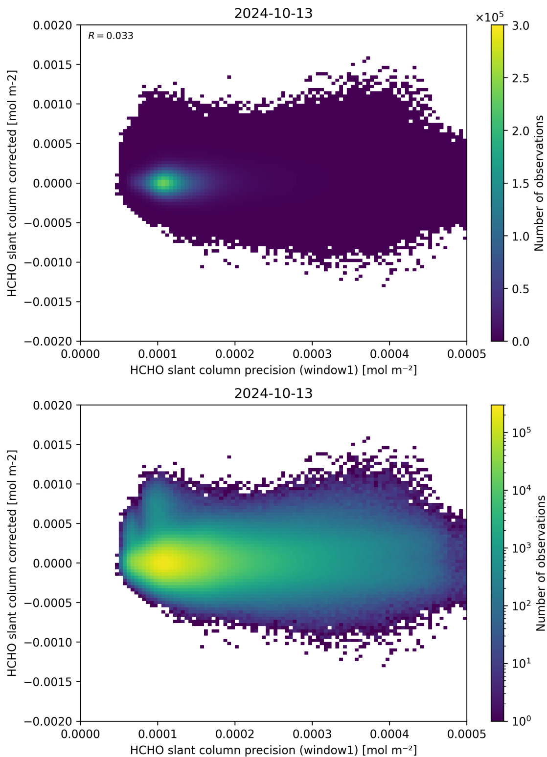
Figure 92: Scatter density plot of “HCHO slant column precision (window1)” against “HCHO slant column corrected” for 2024-10-12 to 2024-10-14.
