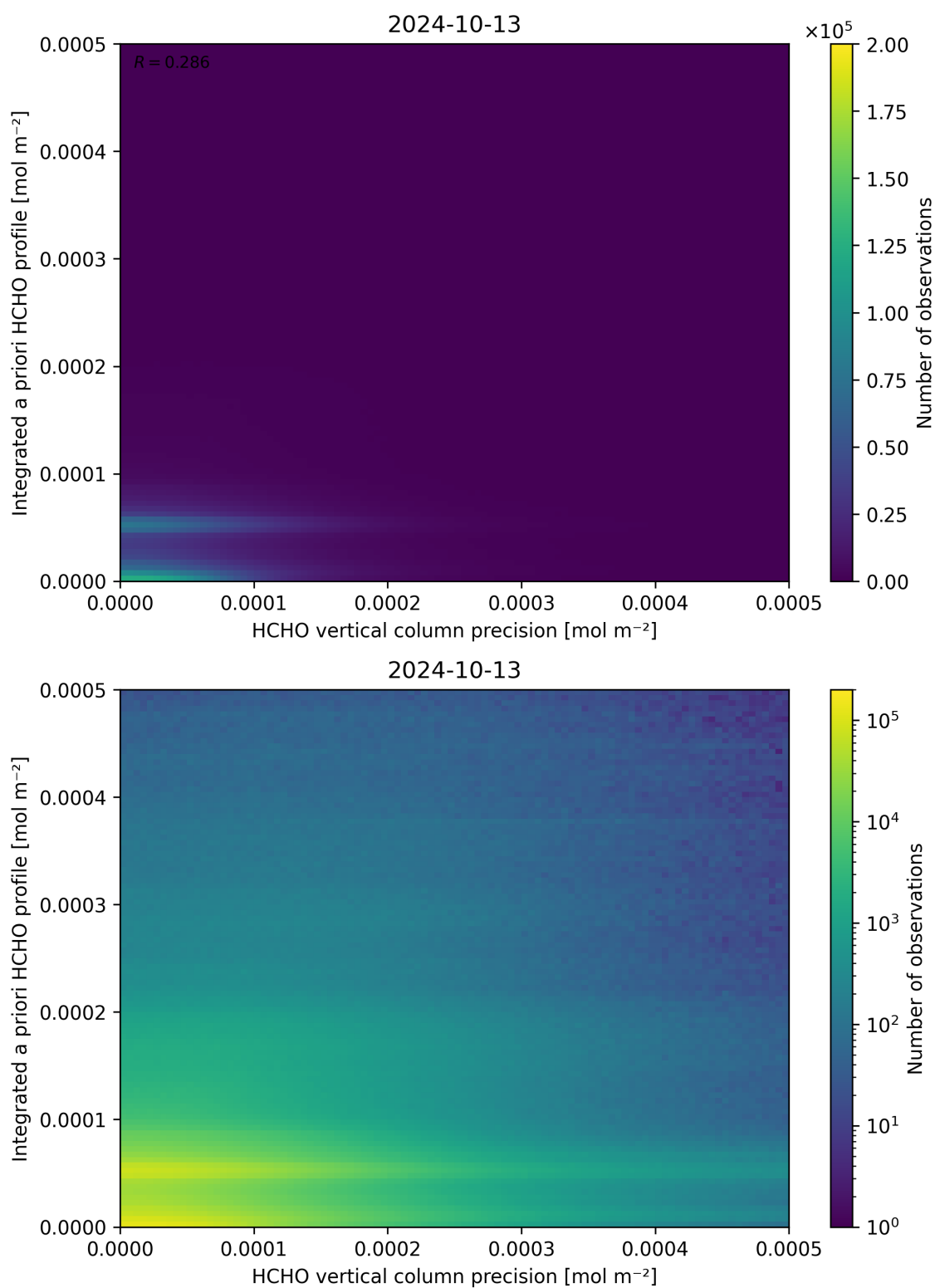
Figure 147: Scatter density plot of “HCHO vertical column precision” against “Integrated a priori HCHO profile” for 2024-10-12 to 2024-10-14.
