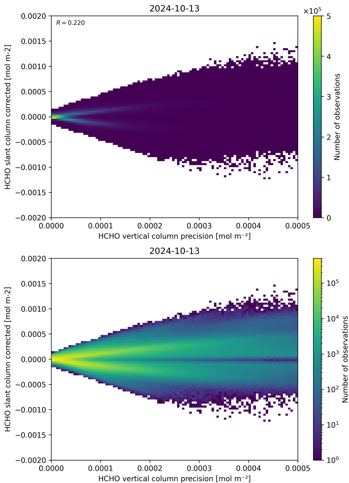
Figure 140: Scatter density plot of “HCHO vertical column precision” against “HCHO slant column corrected” for 2024-10-12 to 2024-10-14.
