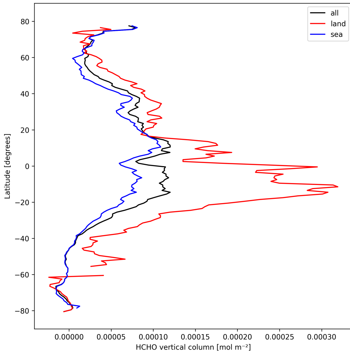
Figure 21: Zonal average of “HCHO vertical column” for 2024-10-12 to 2024-10-14.
