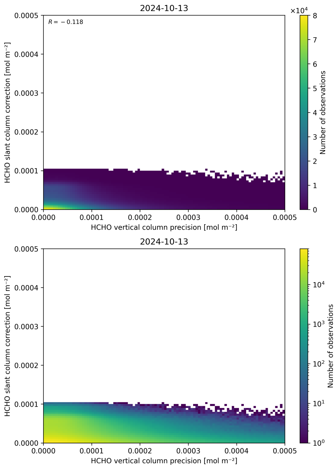
Figure 141: Scatter density plot of “HCHO vertical column precision” against “HCHO slant column correction” for 2024-10-12 to 2024-10-14.
