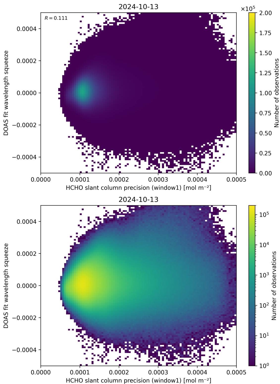
Figure 90: Scatter density plot of “HCHO slant column precision (window1)” against “DOAS fit wavelength squeeze” for 2024-10-12 to 2024-10-14.
