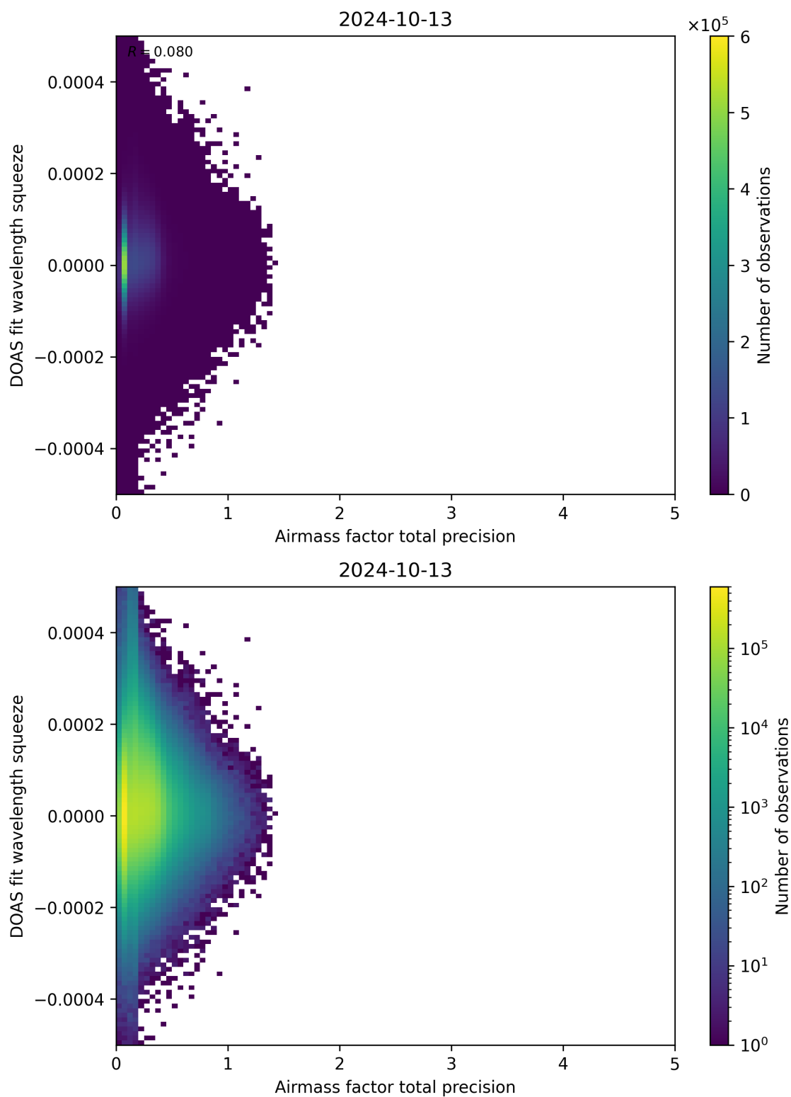
Figure 107: Scatter density plot of “Airmass factor total precision” against “DOAS fit wavelength squeeze” for 2024-10-12 to 2024-10-14.
