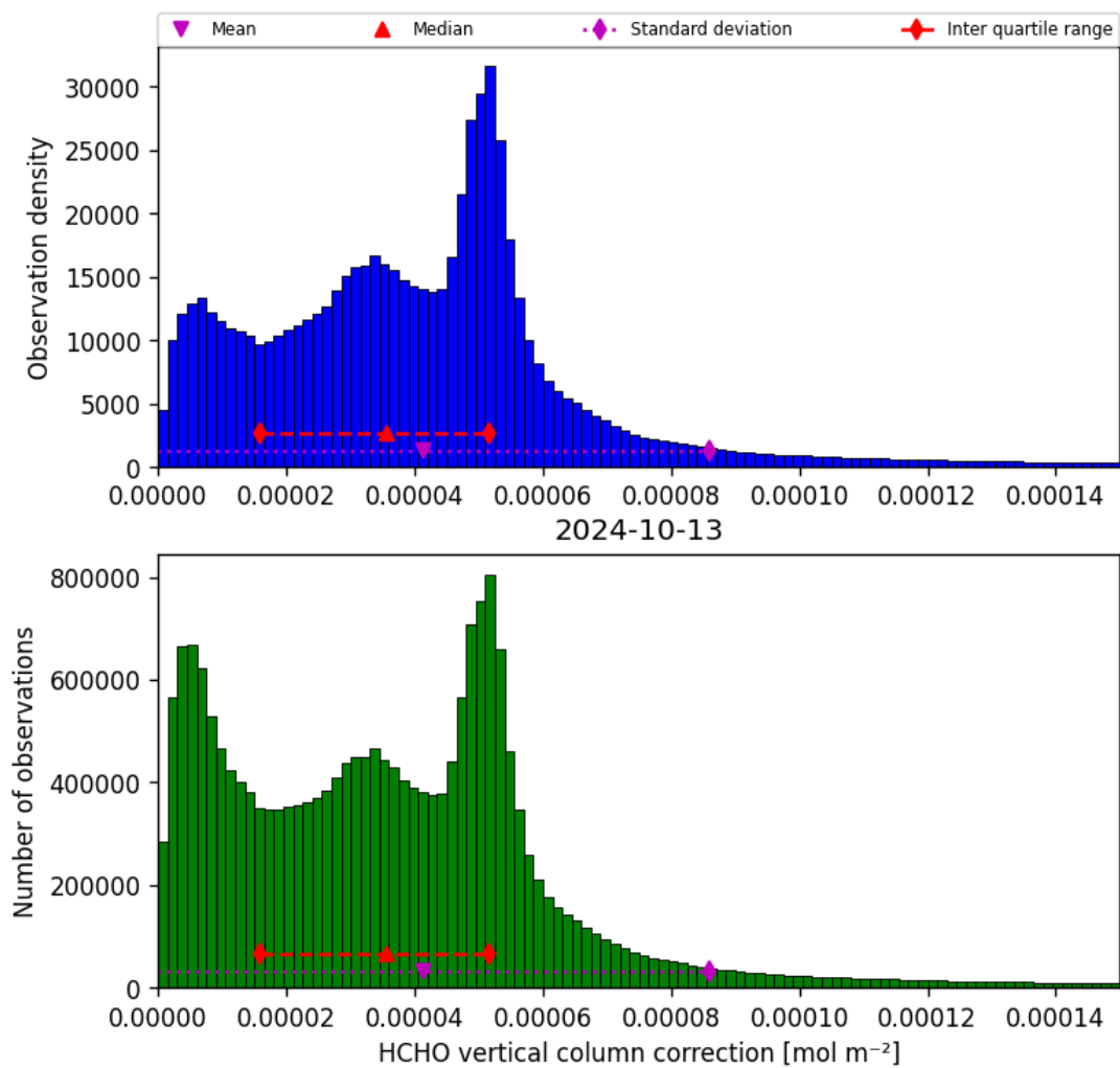
Figure 37: Histogram of “HCHO vertical column correction” for 2024-10-12 to 2024-10-14
