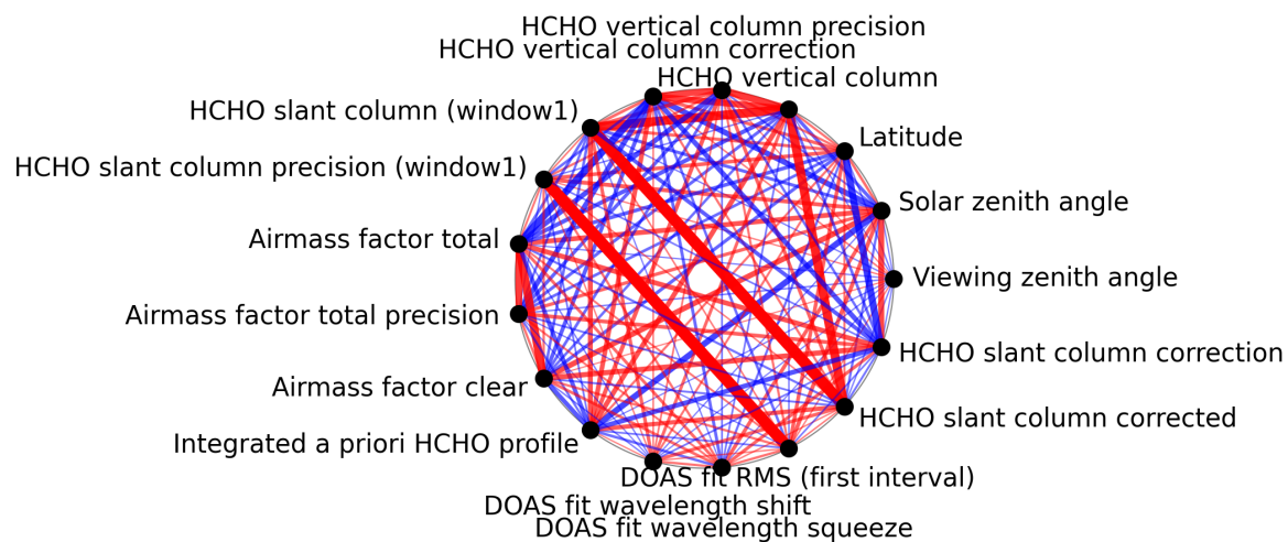
Figure 1: Map of correlation graph for 2024-10-12 to 2024-10-14.
