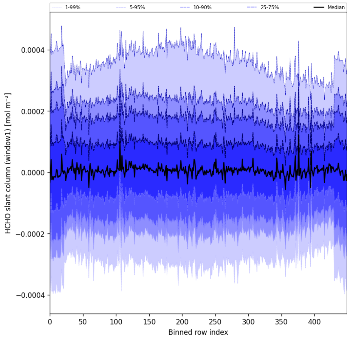
Figure 52: Along track statistics of “HCHO slant column (window1)” for 2024-10-12 to 2024-10-14
