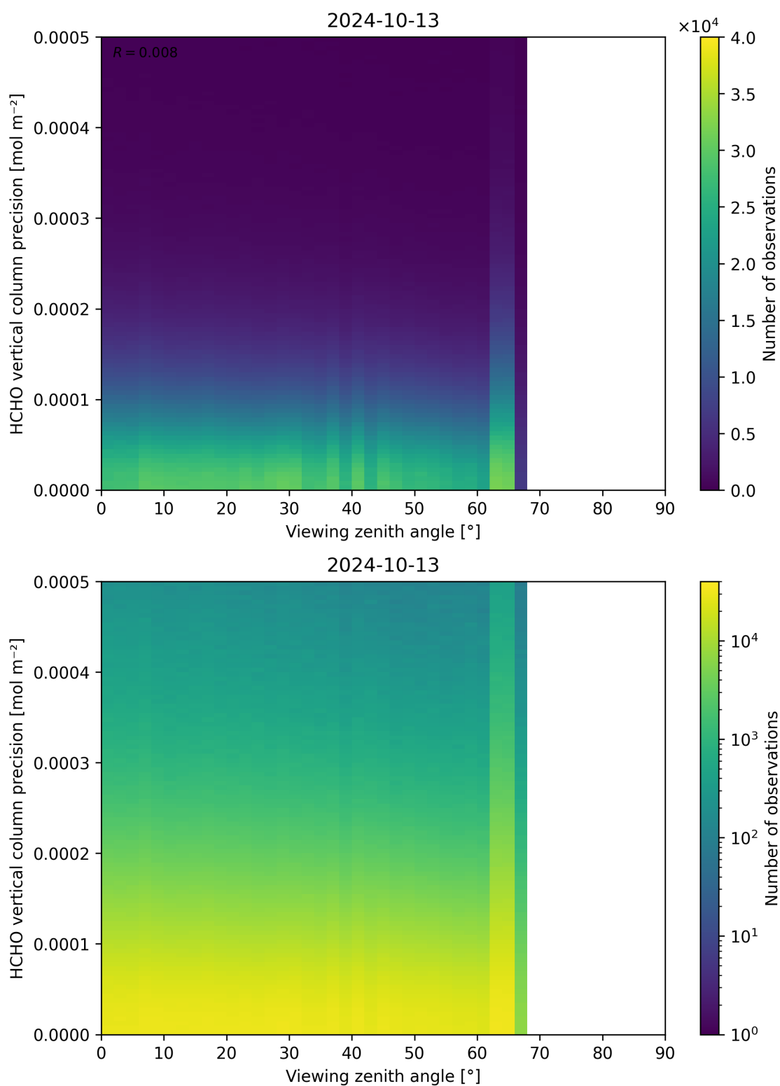
Figure 194: Scatter density plot of “Viewing zenith angle” against “HCHO vertical column precision” for 2024-10-12 to 2024-10-14.
