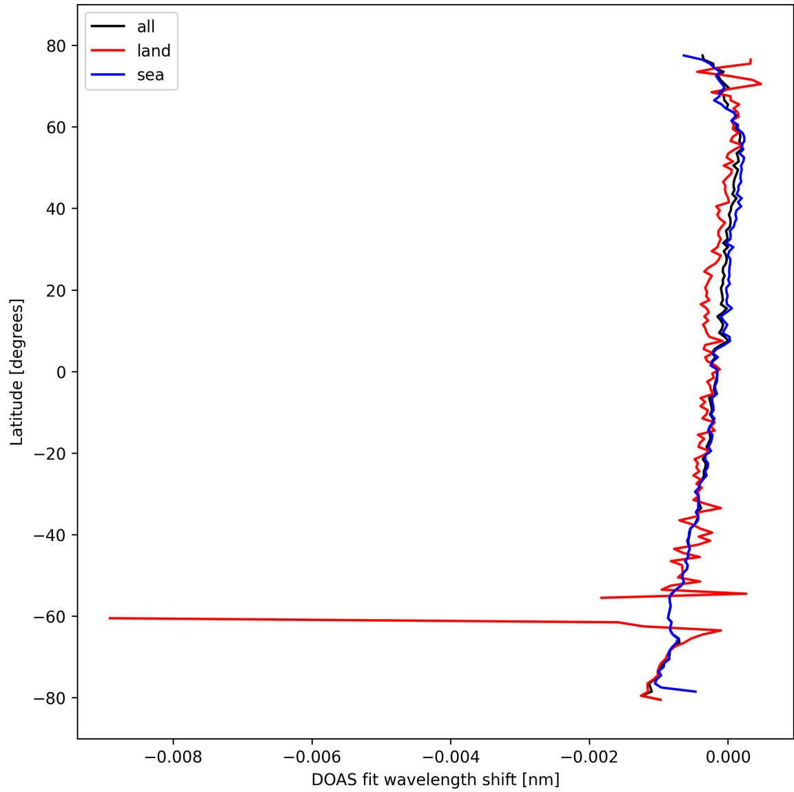
Figure 30: Zonal average of “DOAS fit wavelength shift” for 2024-10-12 to 2024-10-14.
