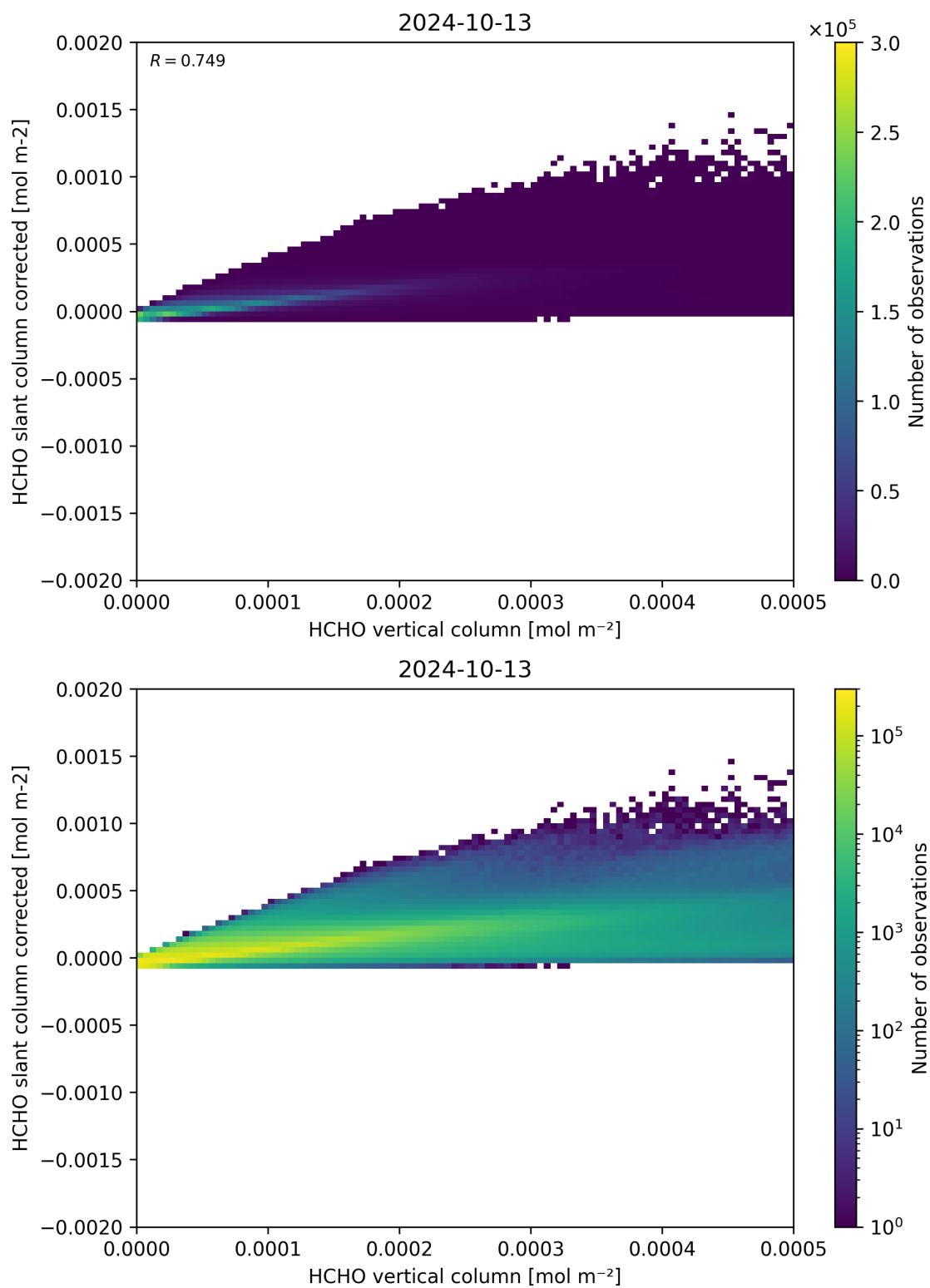
Figure 127: Scatter density plot of “HCHO vertical column” against “HCHO slant column corrected” for 2024-10-12 to 2024-10-14.
