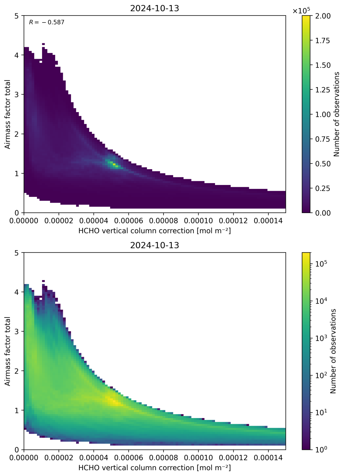
Figure 120: Scatter density plot of “HCHO vertical column correction” against “Airmass factor total” for 2024-10-12 to 2024-10-14.
