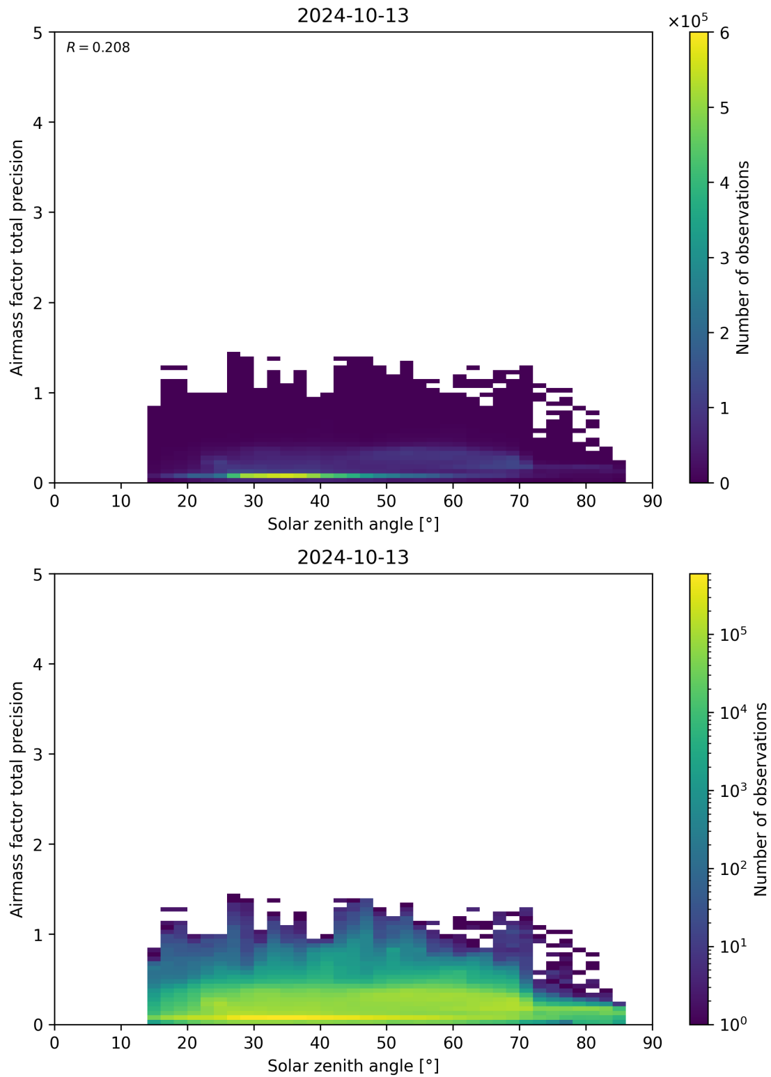
Figure 176: Scatter density plot of “Solar zenith angle” against “Airmass factor total precision” for 2024-10-12 to 2024-10-14.
