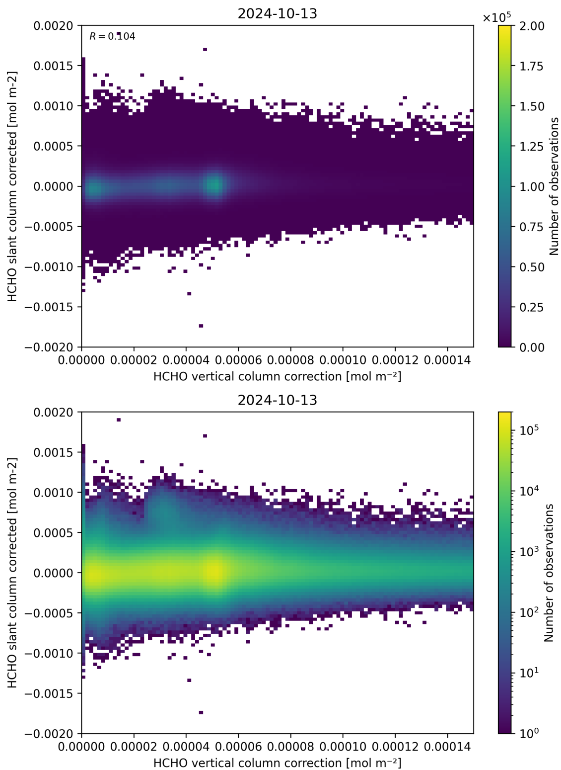
Figure 116: Scatter density plot of “HCHO vertical column correction” against “HCHO slant column corrected” for 2024-10-12 to 2024-10-14.
