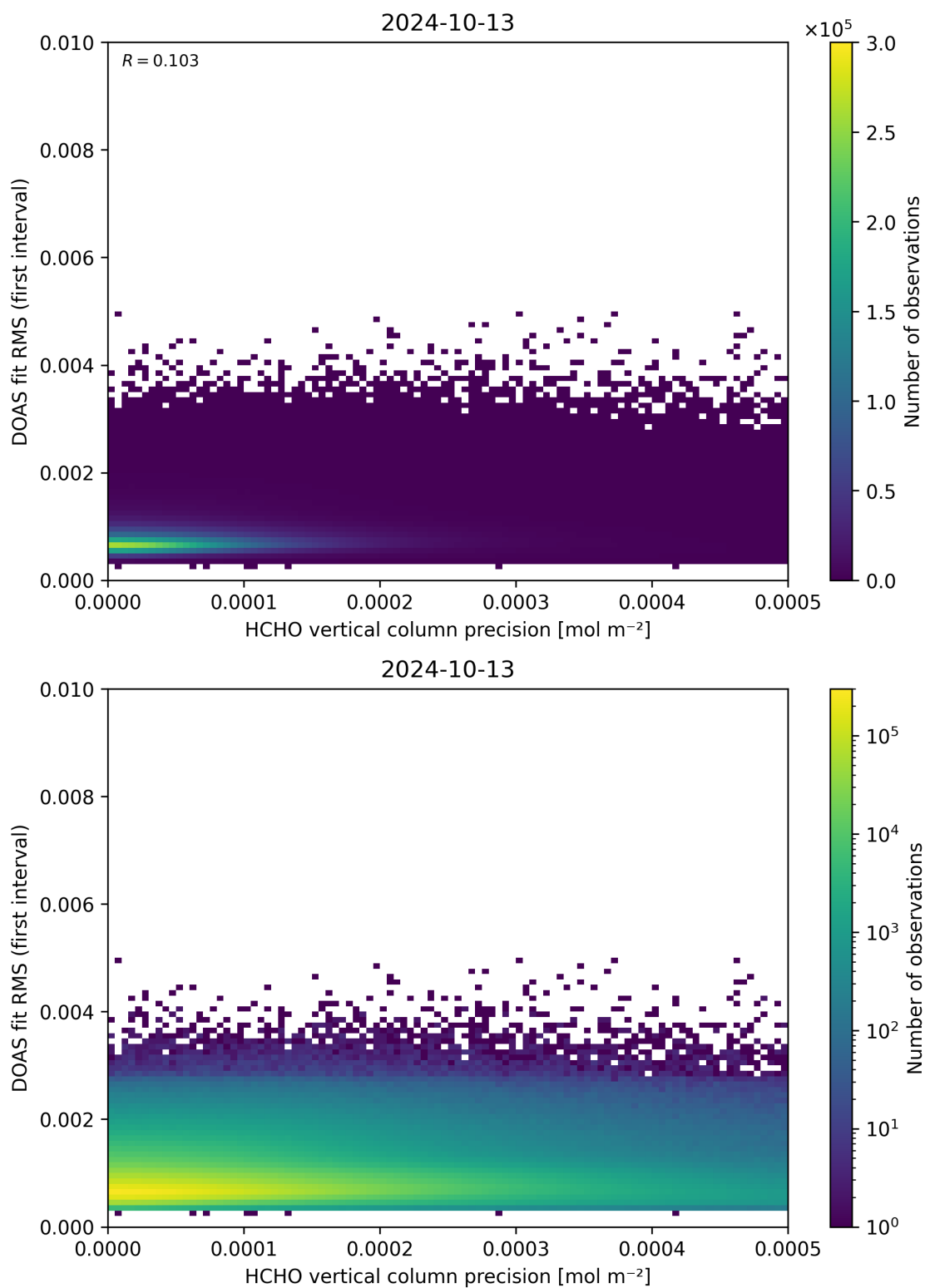
Figure 136: Scatter density plot of “HCHO vertical column precision” against “DOAS fit RMS (first interval)” for 2024-10-12 to 2024-10-14.
