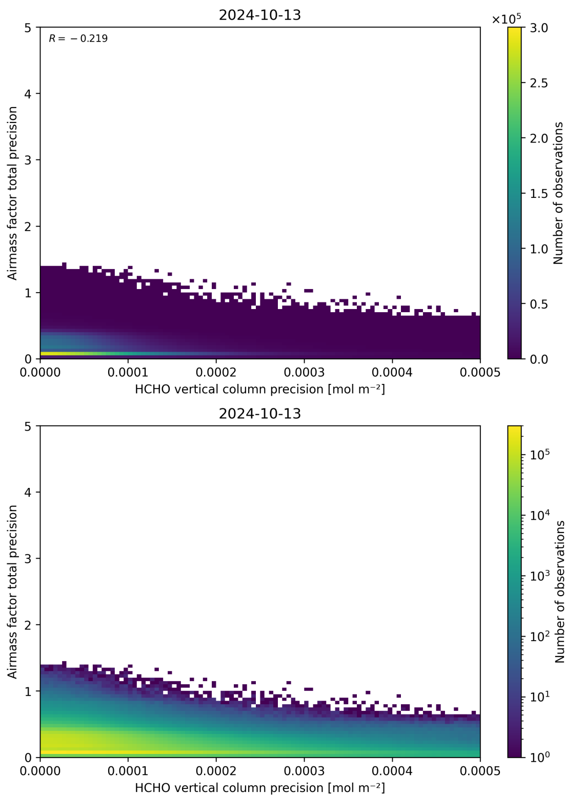
Figure 145: Scatter density plot of “HCHO vertical column precision” against “Airmass factor total precision” for 2024-10-12 to 2024-10-14.
