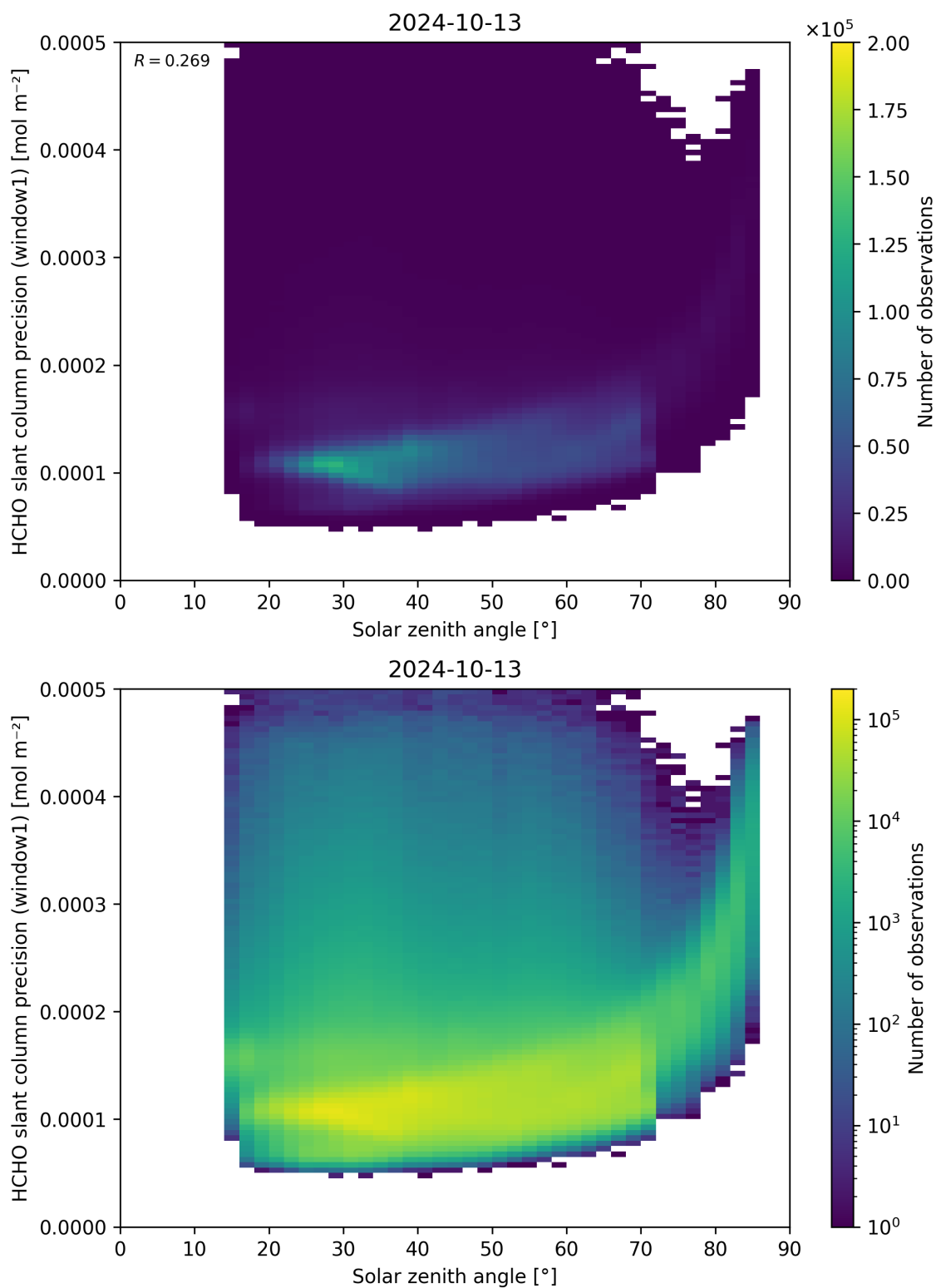
Figure 174: Scatter density plot of “Solar zenith angle” against “HCHO slant column precision (window1)” for 2024-10-12 to 2024-10-14.
