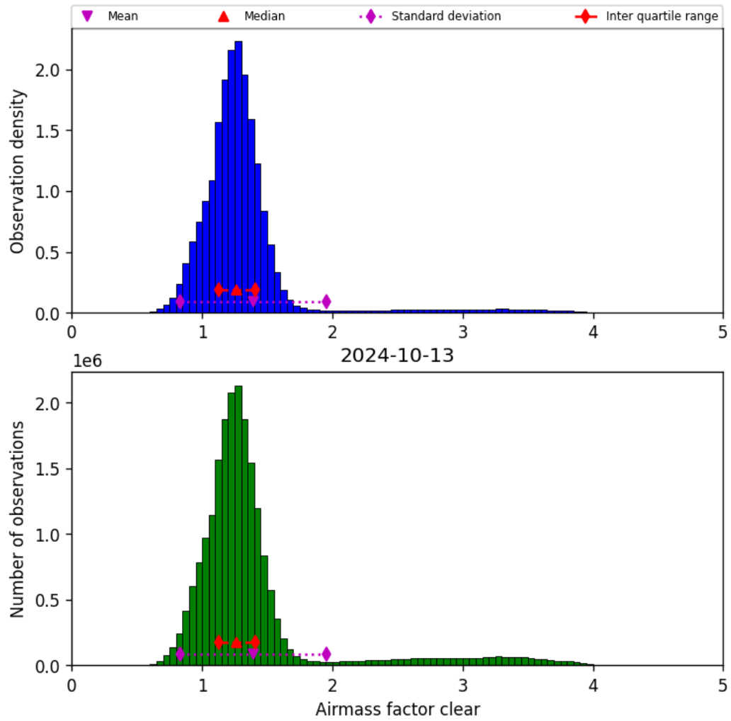
Figure 42: Histogram of “Airmass factor clear” for 2024-10-12 to 2024-10-14
