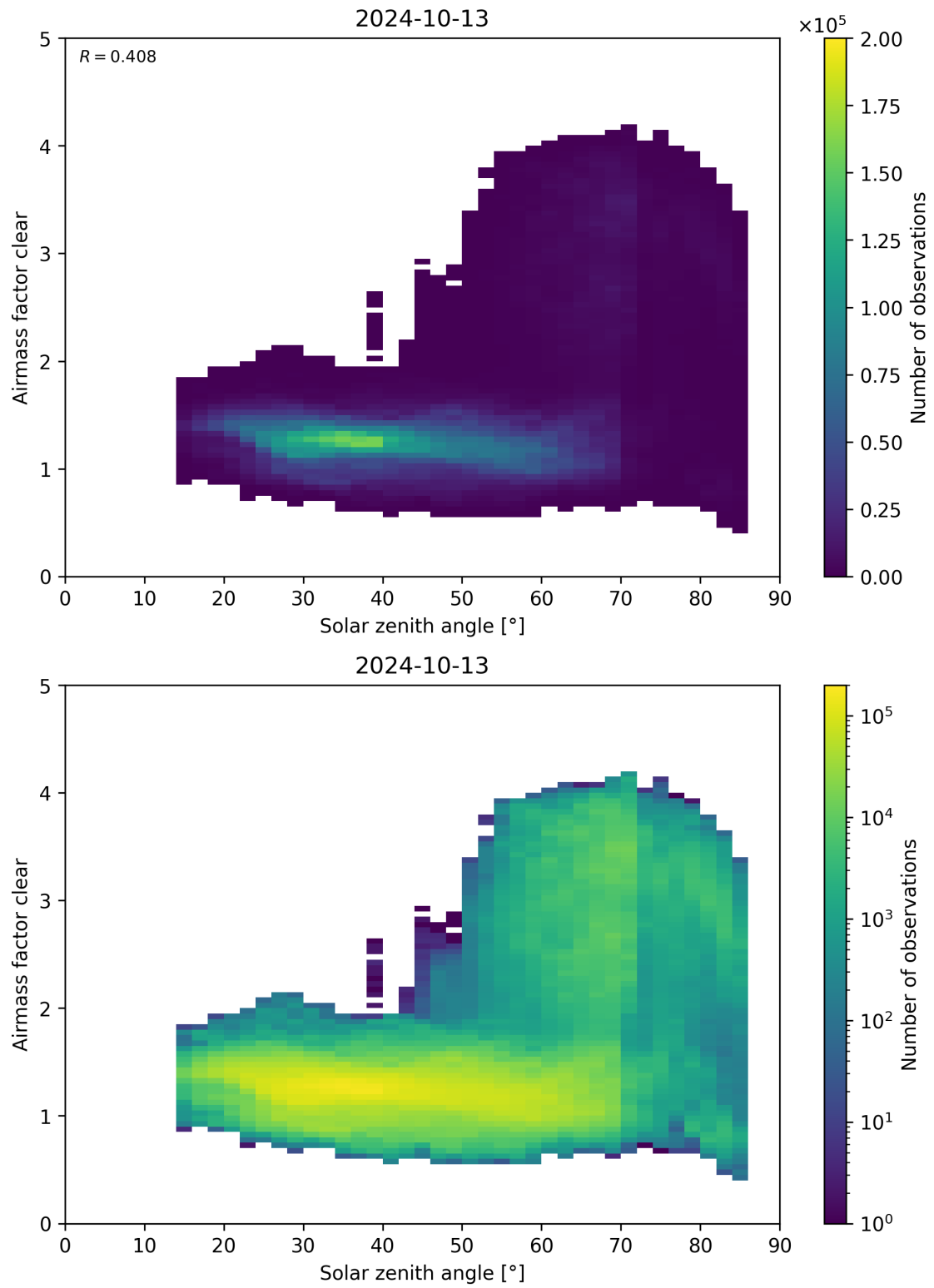
Figure 170: Scatter density plot of “Solar zenith angle” against “Airmass factor clear” for 2024-10-12 to 2024-10-14.
