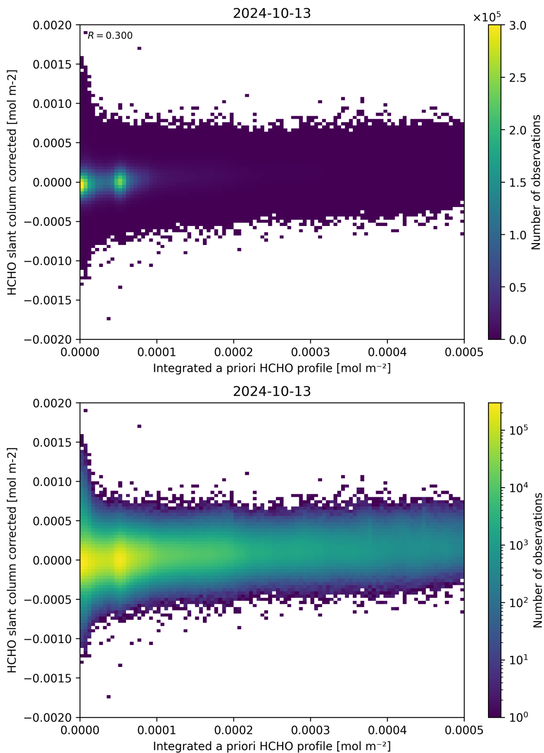
Figure 151: Scatter density plot of “Integrated a priori HCHO profile” against “HCHO slant column corrected” for 2024-10-12 to 2024-10-14.
