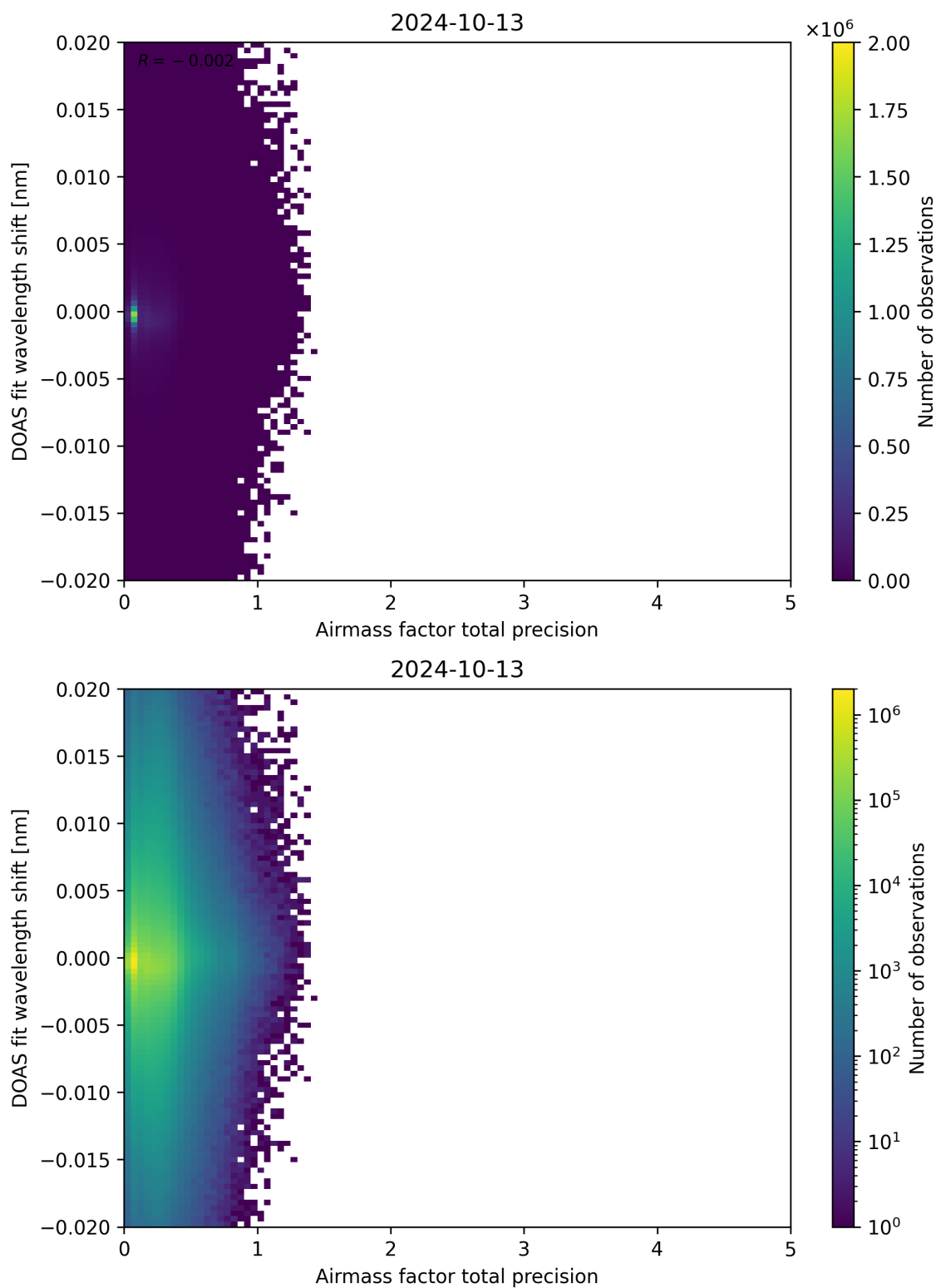
Figure 106: Scatter density plot of “Airmass factor total precision” against “DOAS fit wavelength shift” for 2024-10-12 to 2024-10-14.
