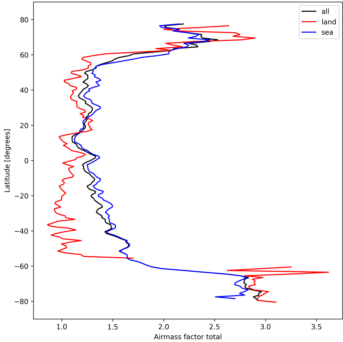
Figure 26: Zonal average of “Airmass factor total” for 2024-10-12 to 2024-10-14.
