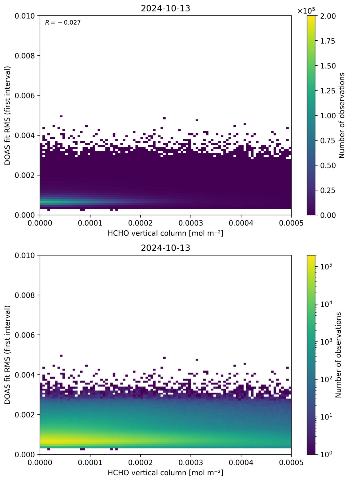
Figure 123: Scatter density plot of “HCHO vertical column” against “DOAS fit RMS (first interval)” for 2024-10-12 to 2024-10-14.
