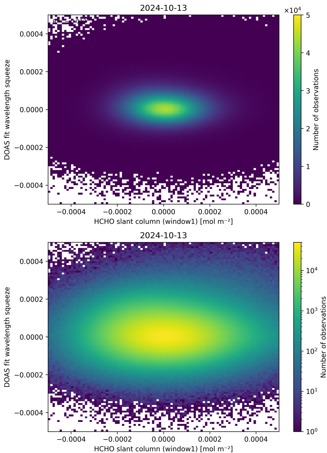
Figure 80: Scatter density plot of “HCHO slant column (window1)” against “DOAS fit wavelength squeeze” for 2024-10-12 to 2024-10-14.
