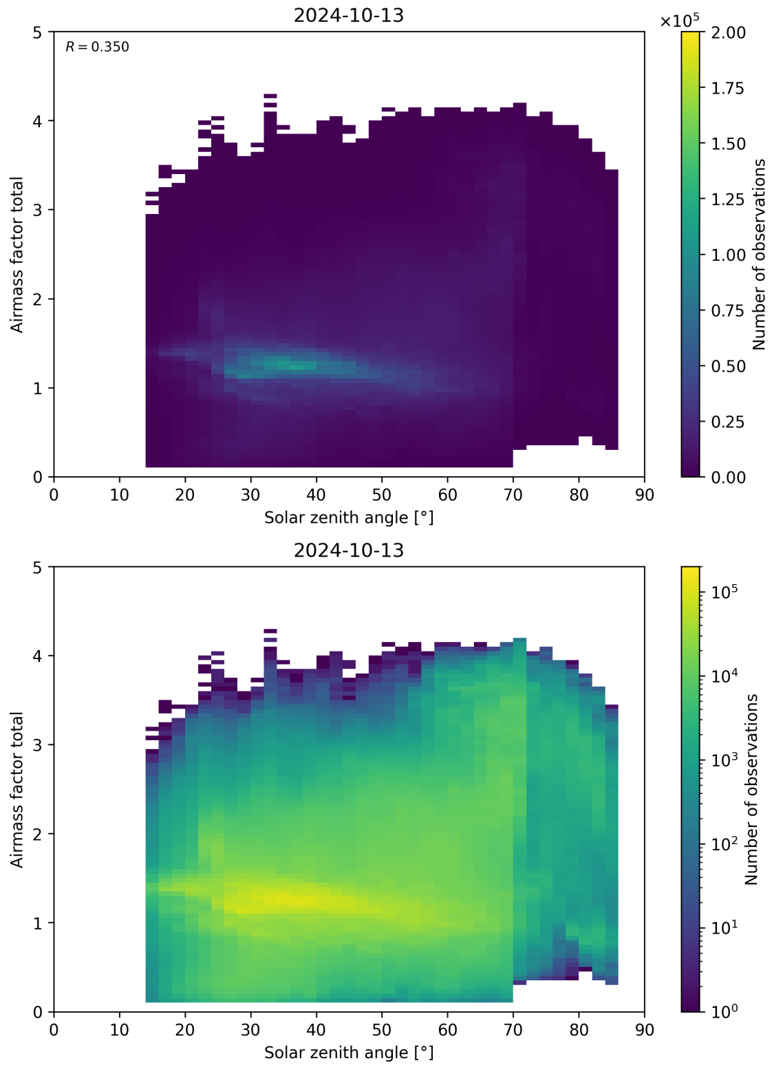
Figure 175: Scatter density plot of “Solar zenith angle” against “Airmass factor total” for 2024-10-12 to 2024-10-14.
