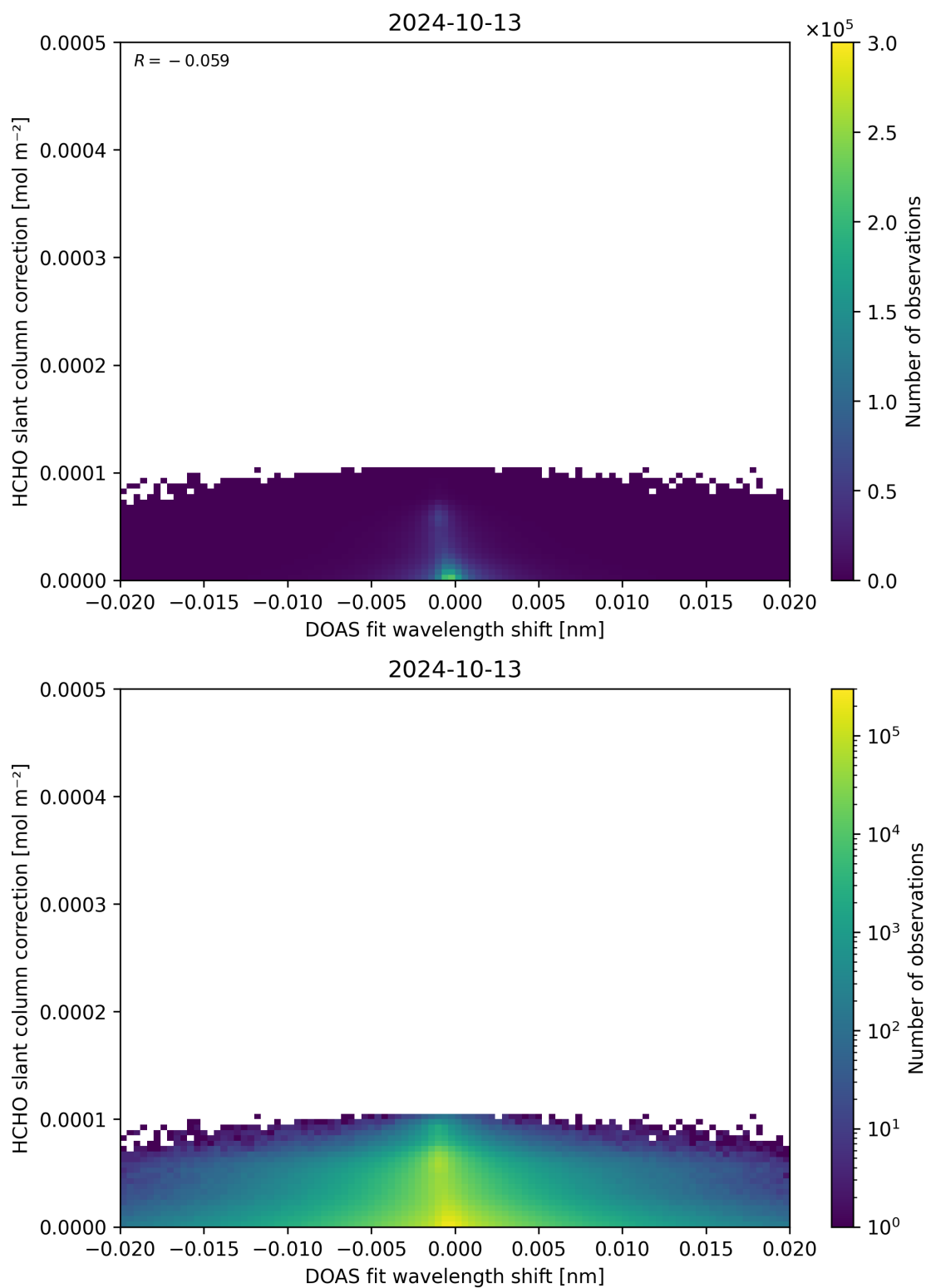
Figure 67: Scatter density plot of “DOAS fit wavelength shift” against “HCHO slant column correction” for 2024-10-12 to 2024-10-14.
