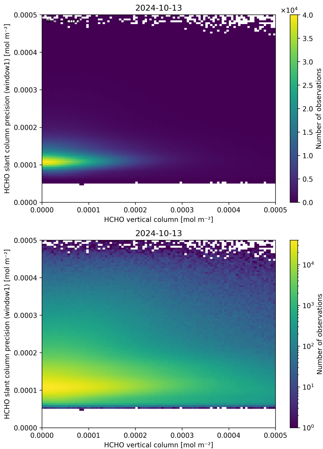
Figure 130: Scatter density plot of “HCHO vertical column” against “HCHO slant column precision (window1)” for 2024-10-12 to 2024-10-14.
