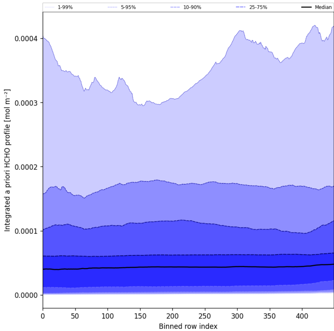
Figure 57: Along track statistics of "Integrated a priori HCHO profile" for 2024-10-12 to 2024-10-14
