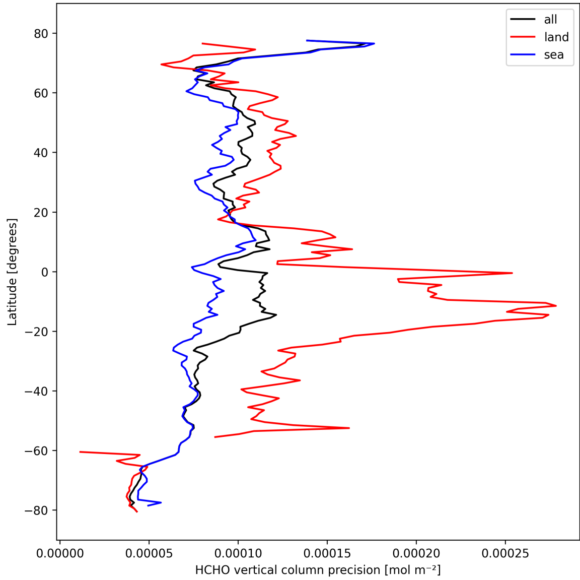
Figure 22: Zonal average of “HCHO vertical column precision” for 2024-10-12 to 2024-10-14.
