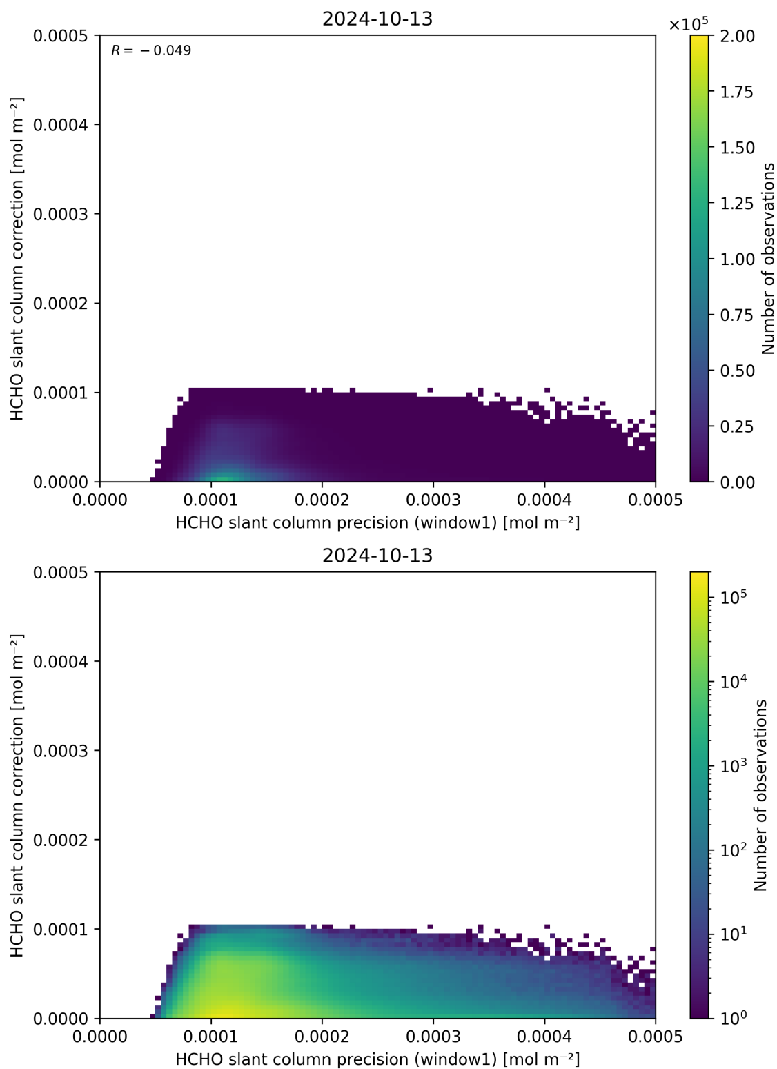
Figure 93: Scatter density plot of “HCHO slant column precision (window1)” against “HCHO slant column correction” for 2024-10-12 to 2024-10-14.
