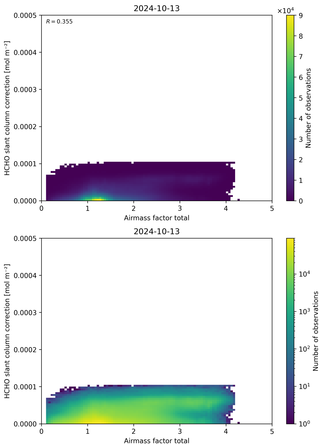
Figure 102: Scatter density plot of “Airmass factor total” against “HCHO slant column correction” for 2024-10-12 to 2024-10-14.
