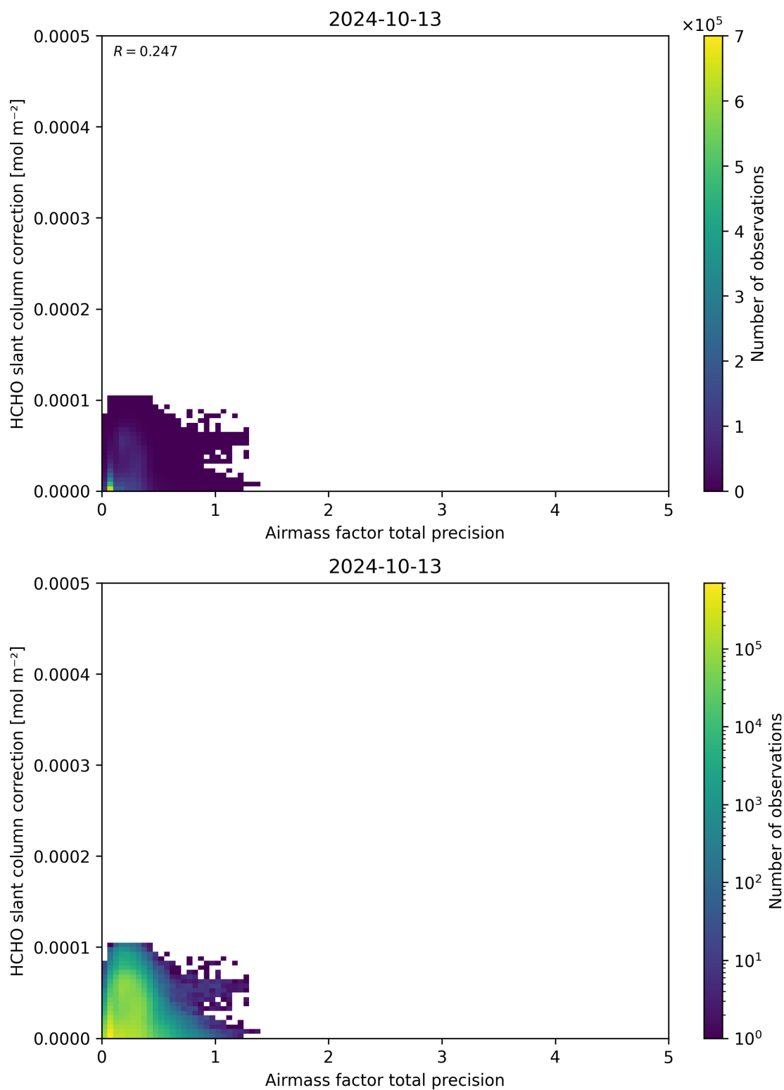
Figure 110: Scatter density plot of “Airmass factor total precision” against “HCHO slant column correction” for 2024-10-12 to 2024-10-14.
