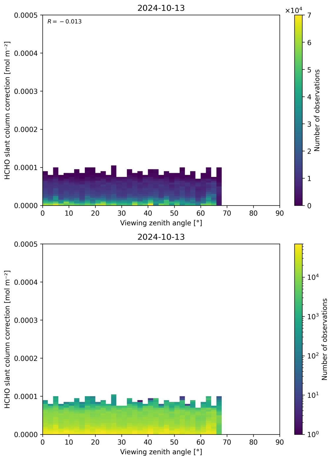
Figure 187: Scatter density plot of “Viewing zenith angle” against “HCHO slant column correction” for 2024-10-12 to 2024-10-14.
