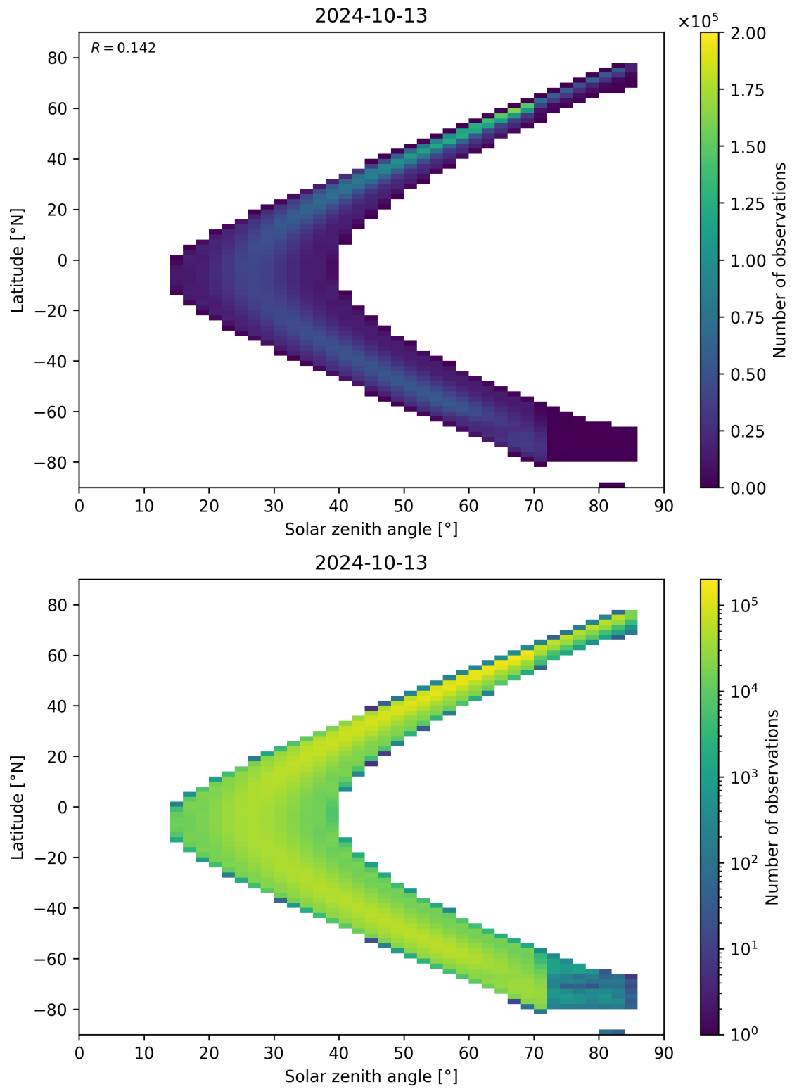
Figure 181: Scatter density plot of “Solar zenith angle” against “Latitude” for 2024-10-12 to 2024-10-14.
