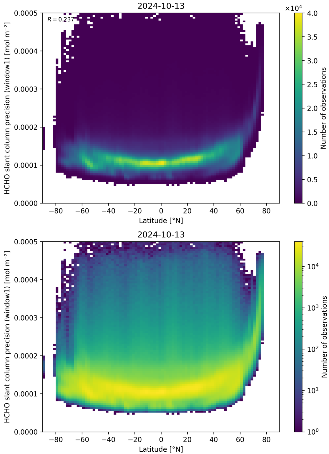
Figure 160: Scatter density plot of “Latitude” against “HCHO slant column precision (window1)” for 2024-10-12 to 2024-10-14.
