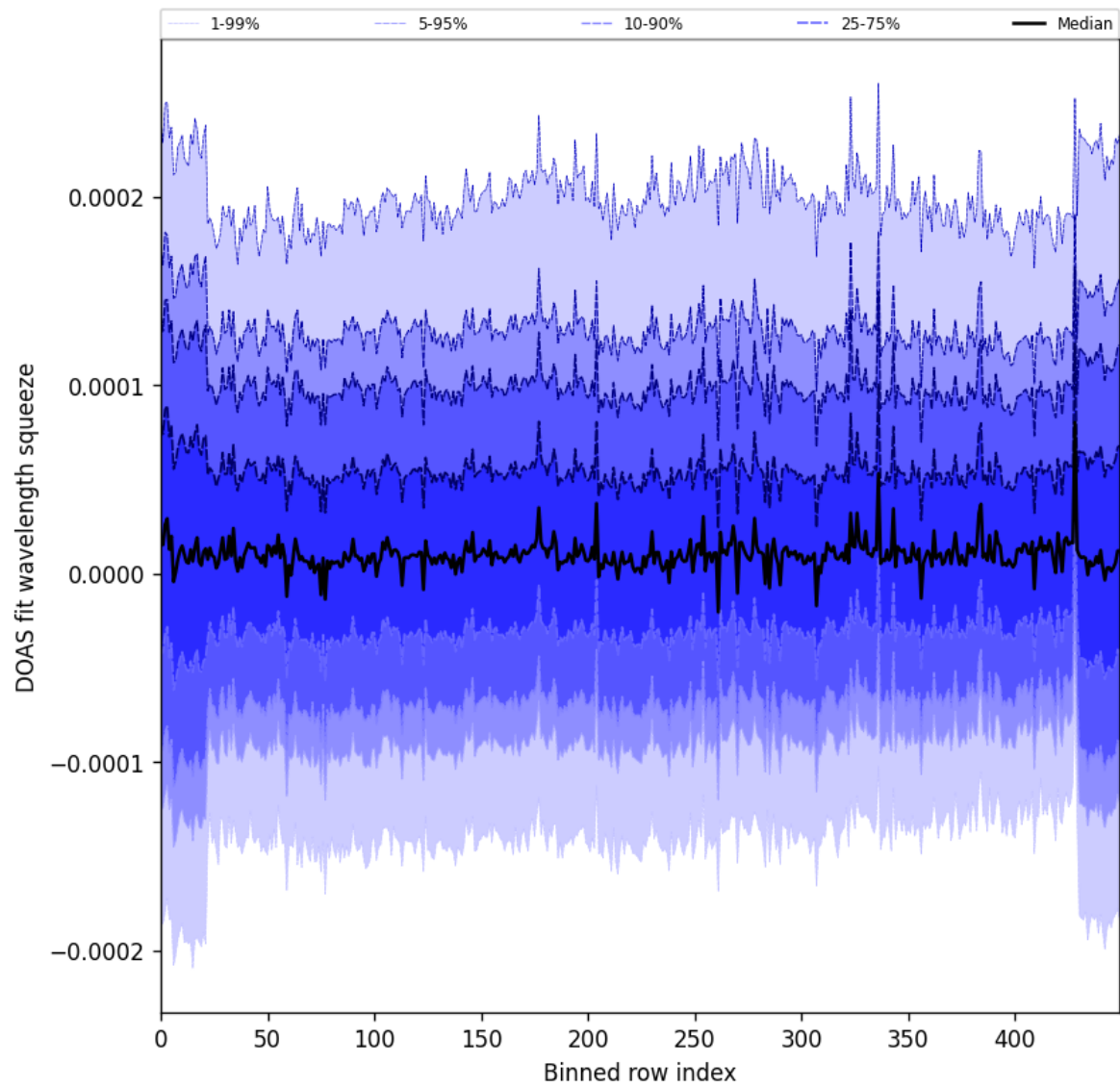
Figure 59: Along track statistics of “DOAS fit wavelength squeeze” for 2024-10-12 to 2024-10-14
