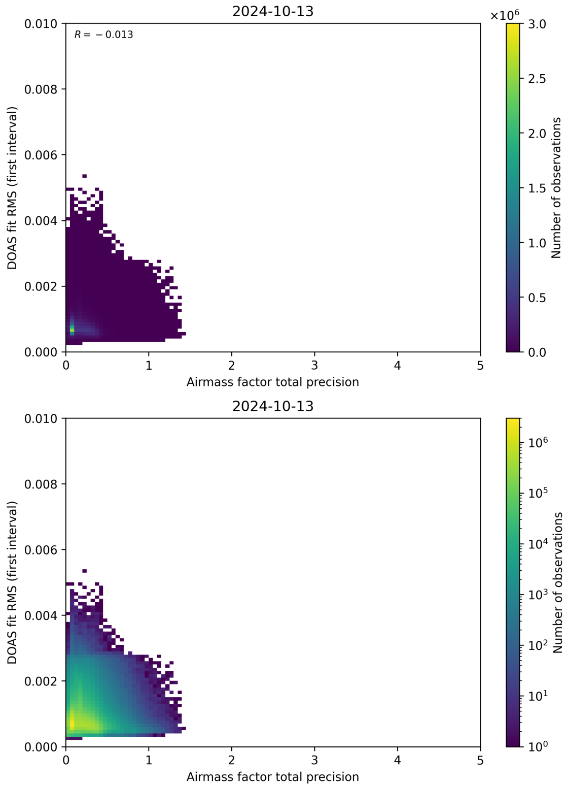
Figure 105: Scatter density plot of “Airmass factor total precision” against “DOAS fit RMS (first interval)” for 2024-10-12 to 2024-10-14.
