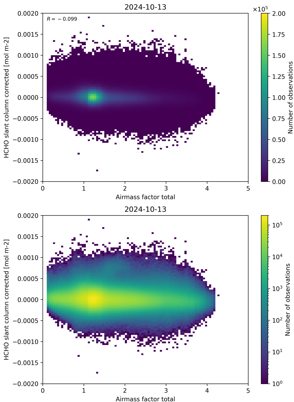
Figure 101: Scatter density plot of “Airmass factor total” against “HCHO slant column corrected” for 2024-10-12 to 2024-10-14.
