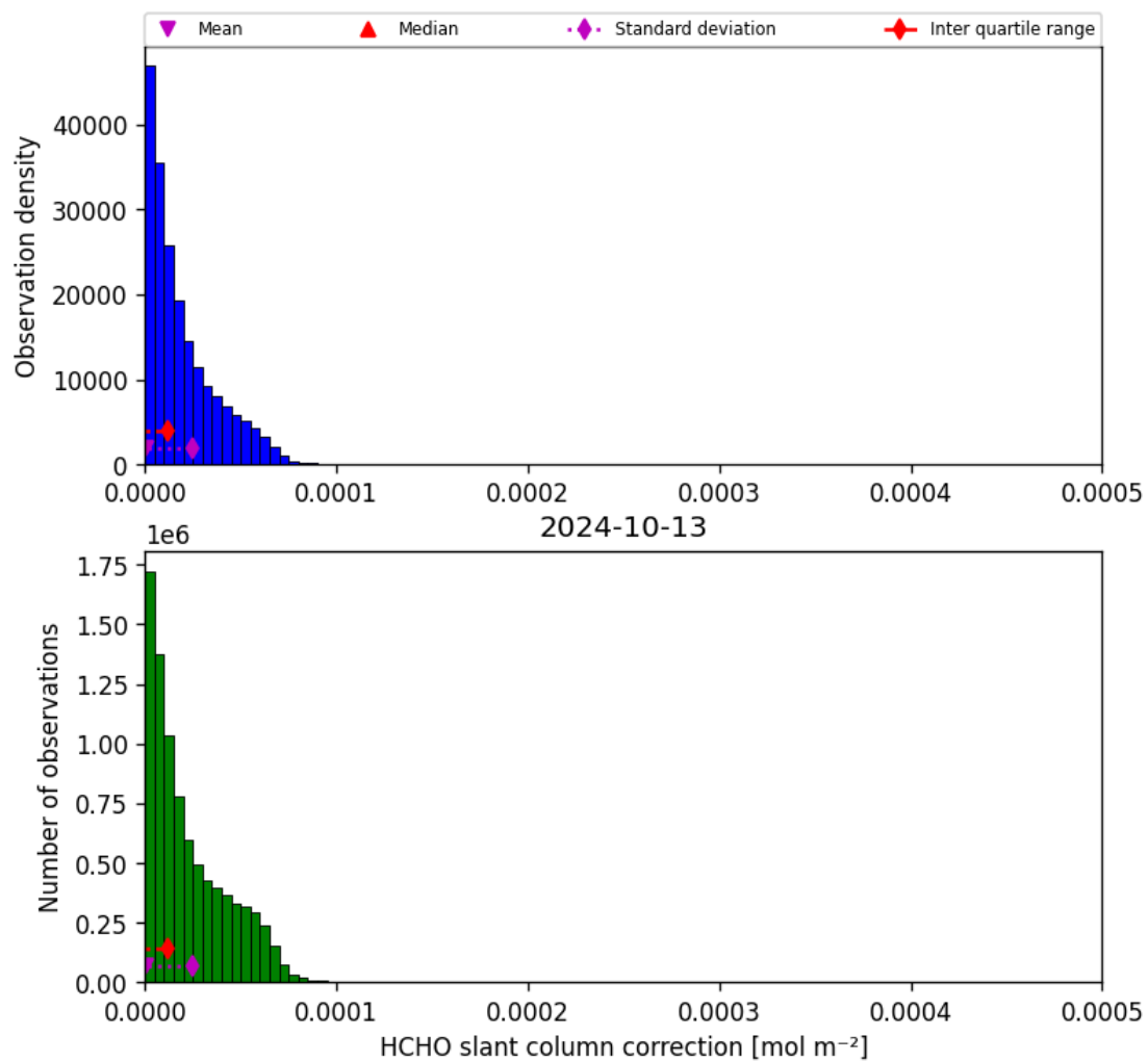
Figure 47: Histogram of “HCHO slant column correction” for 2024-10-12 to 2024-10-14
