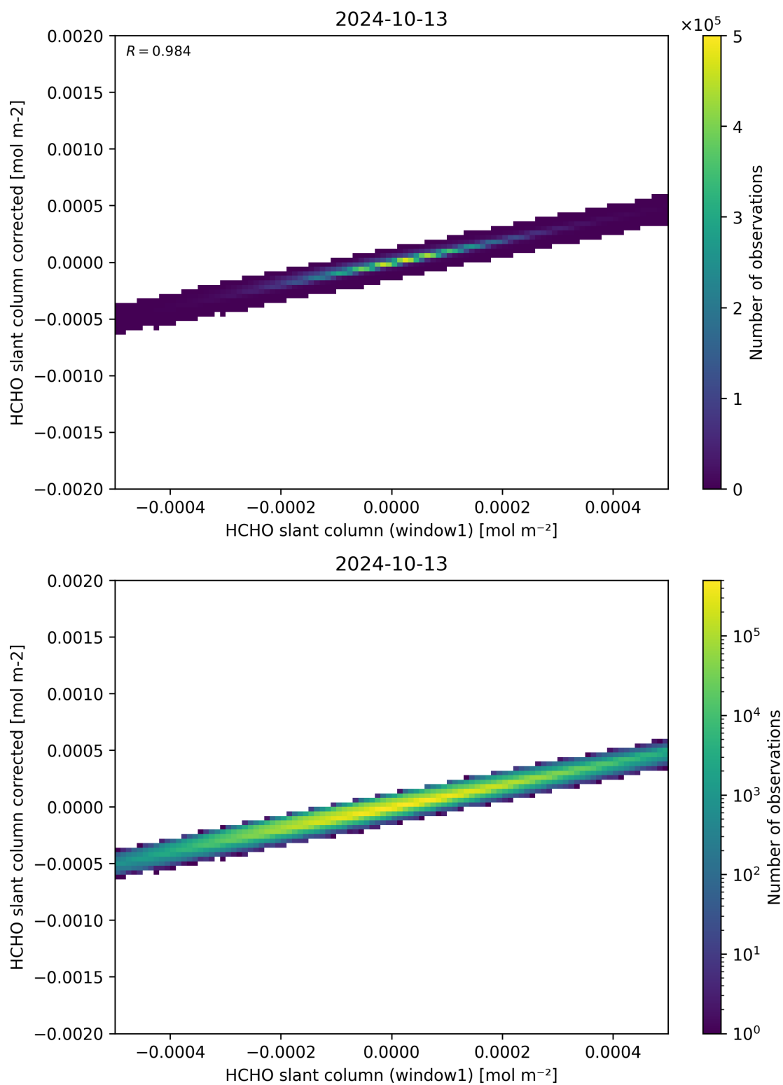
Figure 82: Scatter density plot of “HCHO slant column (window1)” against “HCHO slant column corrected” for 2024-10-12 to 2024-10-14.
