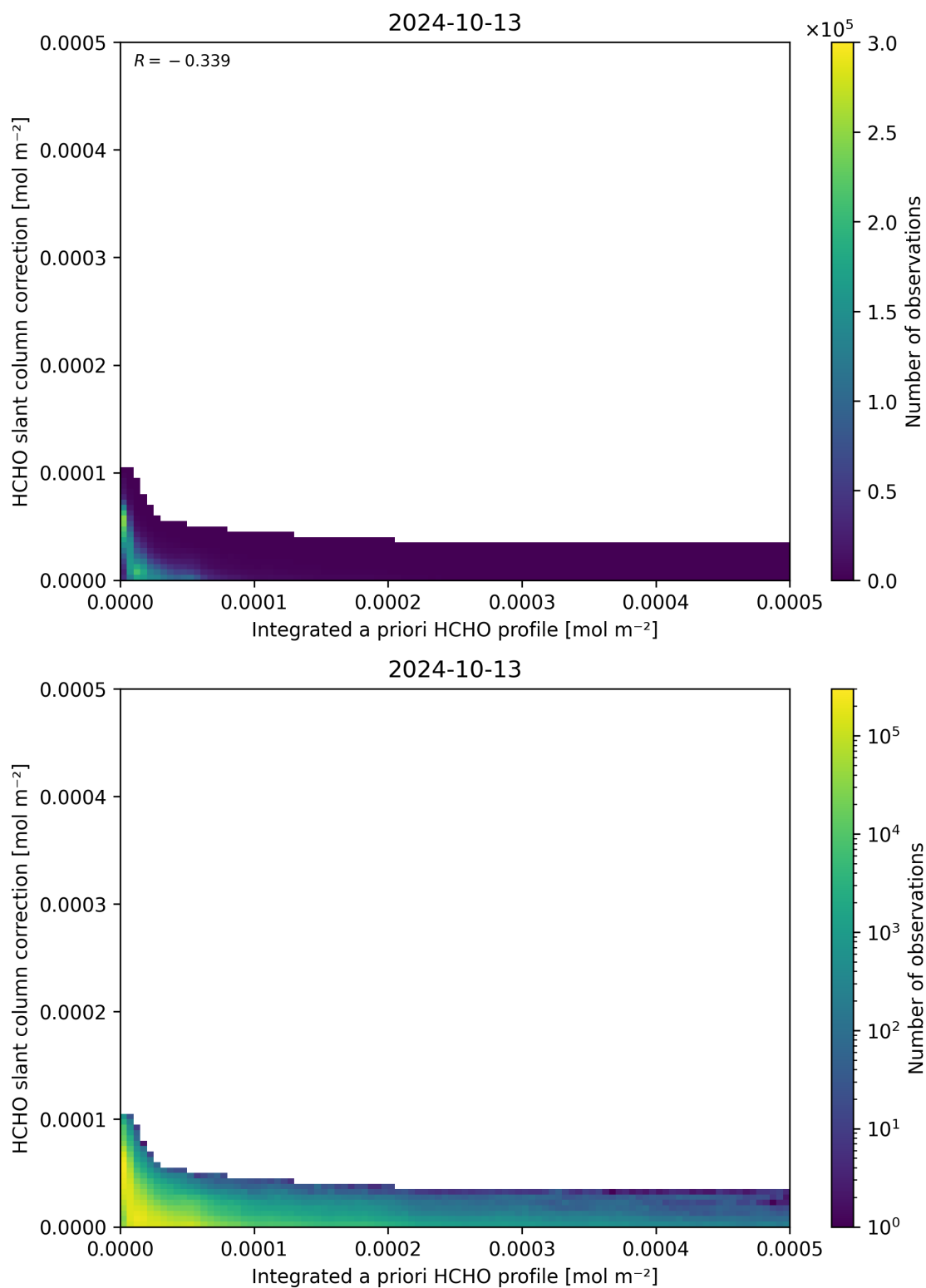
Figure 152: Scatter density plot of “Integrated a priori HCHO profile” against “HCHO slant column correction” for 2024-10-12 to 2024-10-14.
