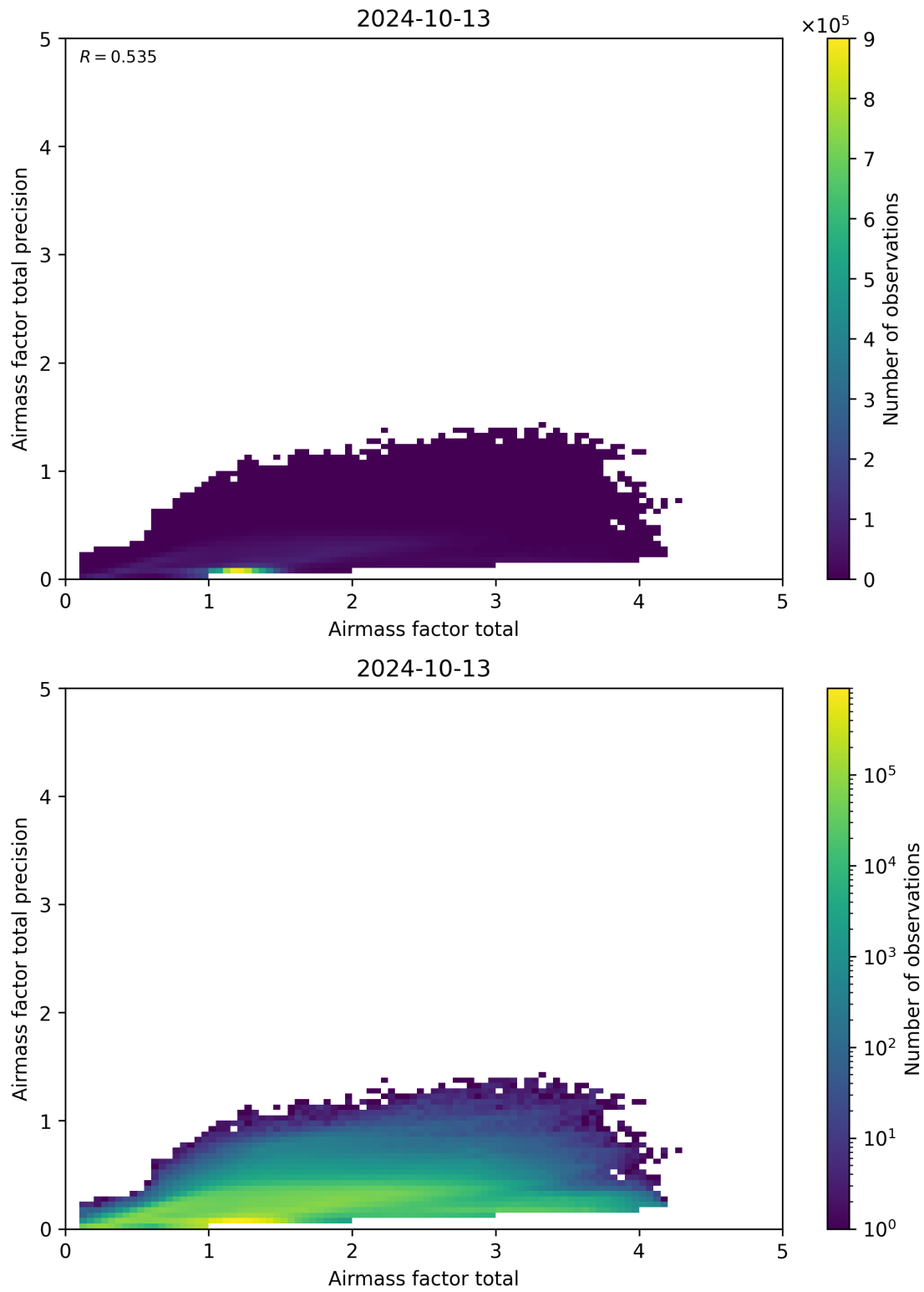
Figure 103: Scatter density plot of “Airmass factor total” against “Airmass factor total precision” for 2024-10-12 to 2024-10-14.
