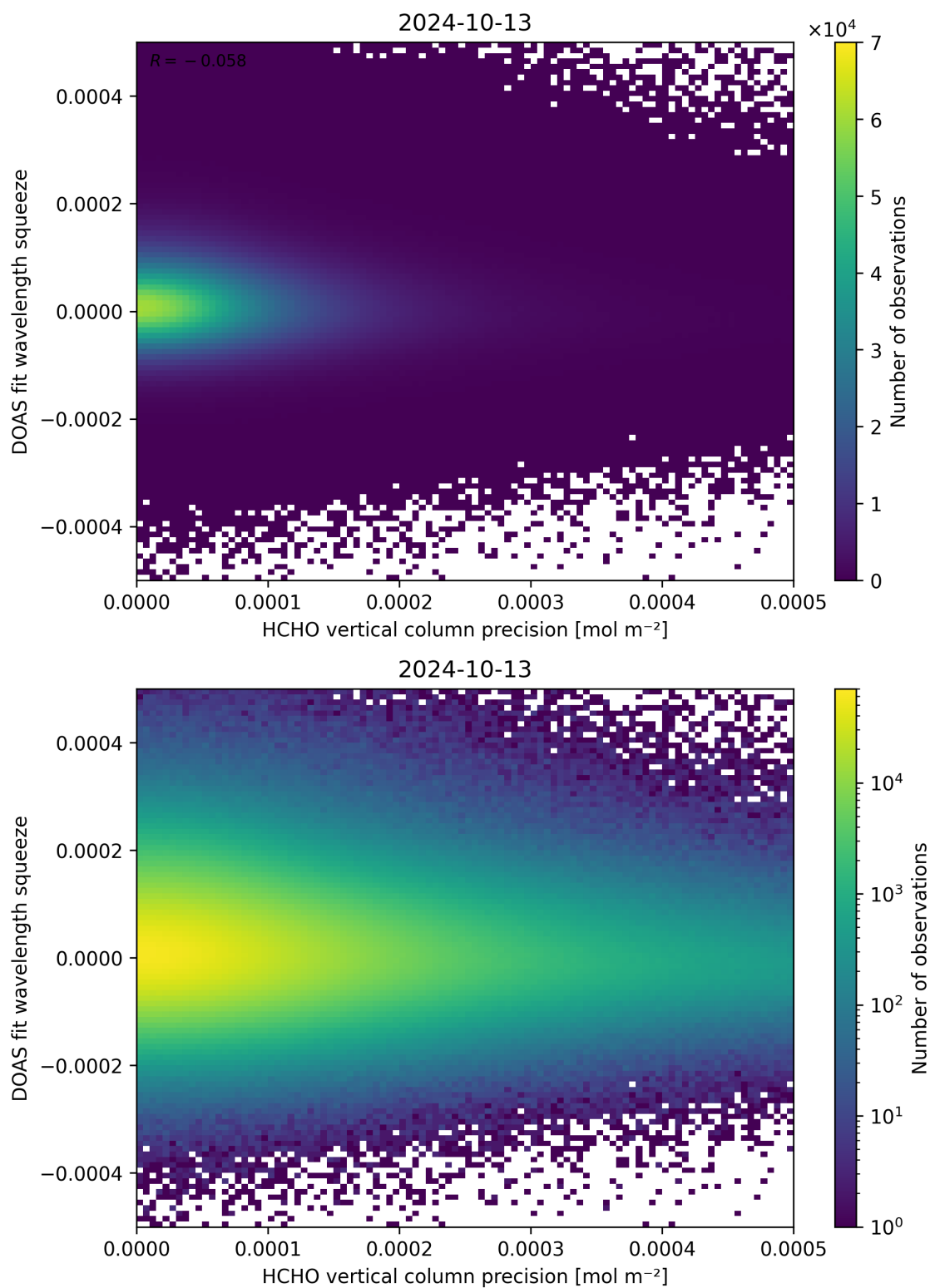
Figure 138: Scatter density plot of “HCHO vertical column precision” against “DOAS fit wavelength squeeze” for 2024-10-12 to 2024-10-14.
