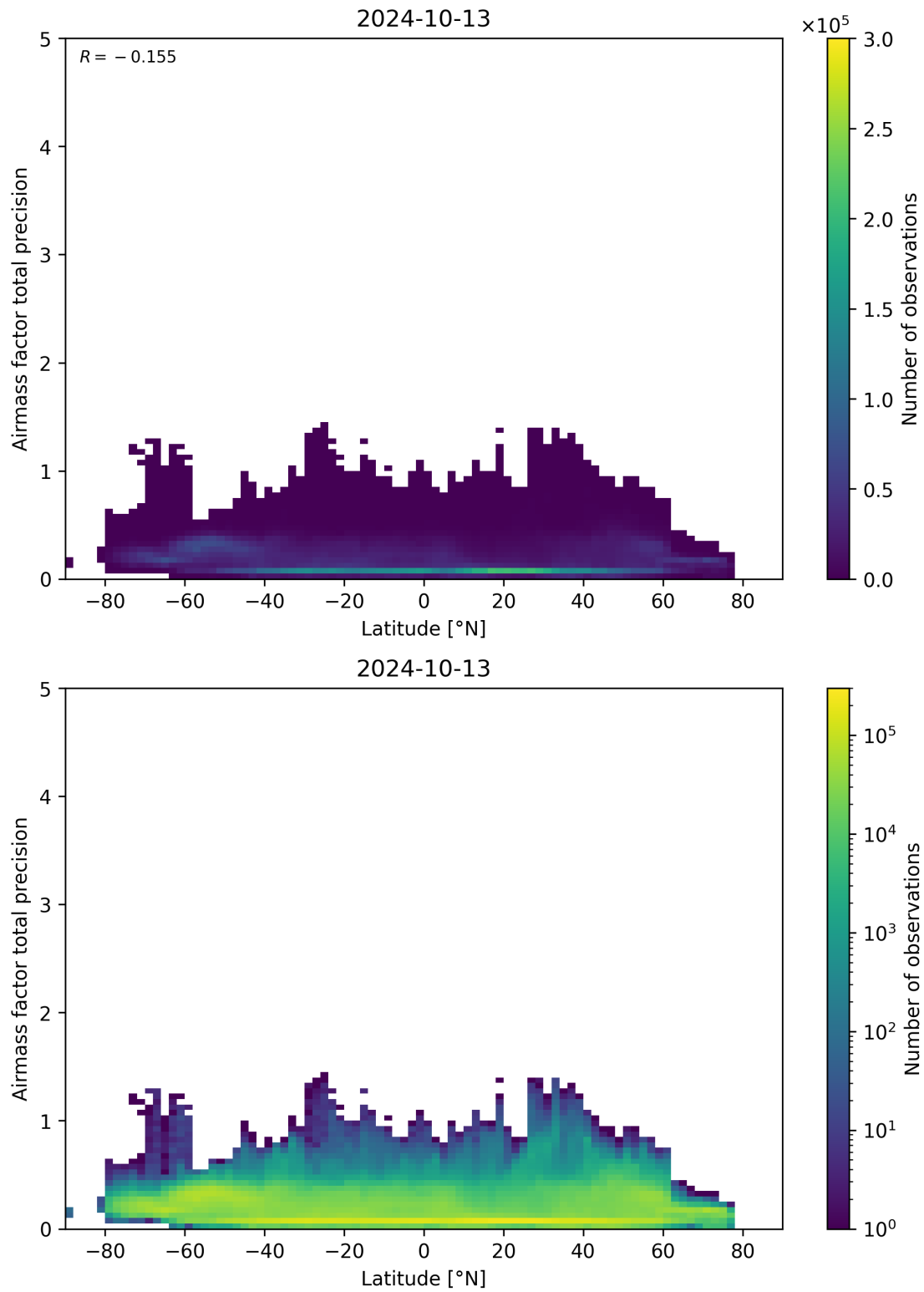
Figure 162: Scatter density plot of “Latitude” against “Airmass factor total precision” for 2024-10-12 to 2024-10-14.
