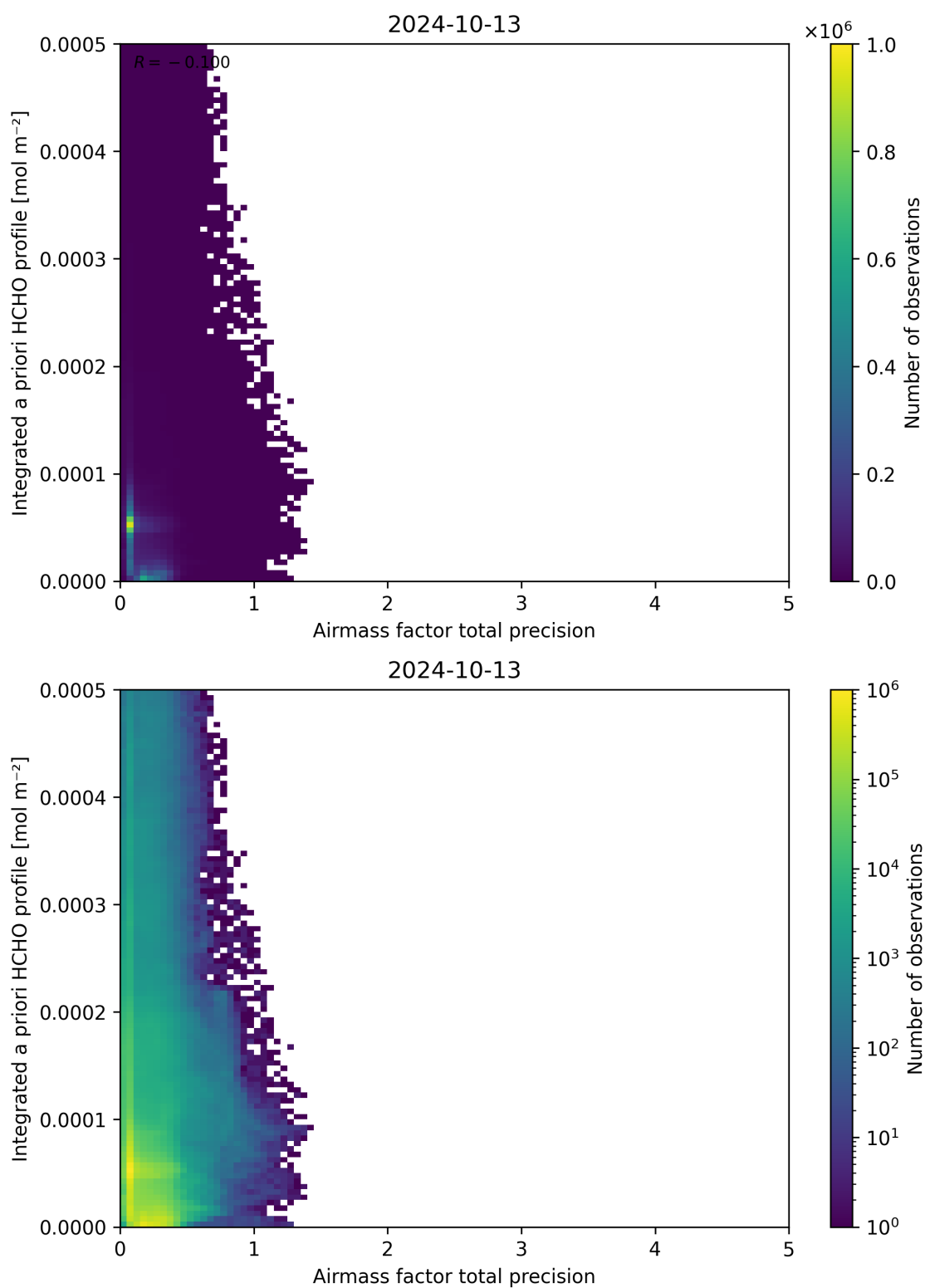
Figure 111: Scatter density plot of “Airmass factor total precision” against “Integrated a priori HCHO profile” for 2024-10-12 to 2024-10-14.
