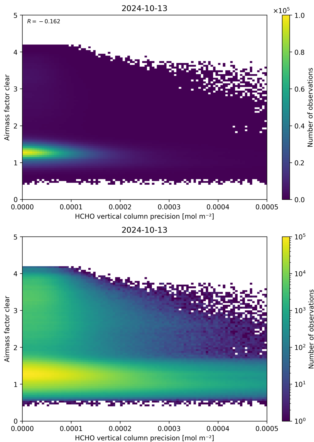
Figure 139: Scatter density plot of “HCHO vertical column precision” against “Airmass factor clear” for 2024-10-12 to 2024-10-14.
