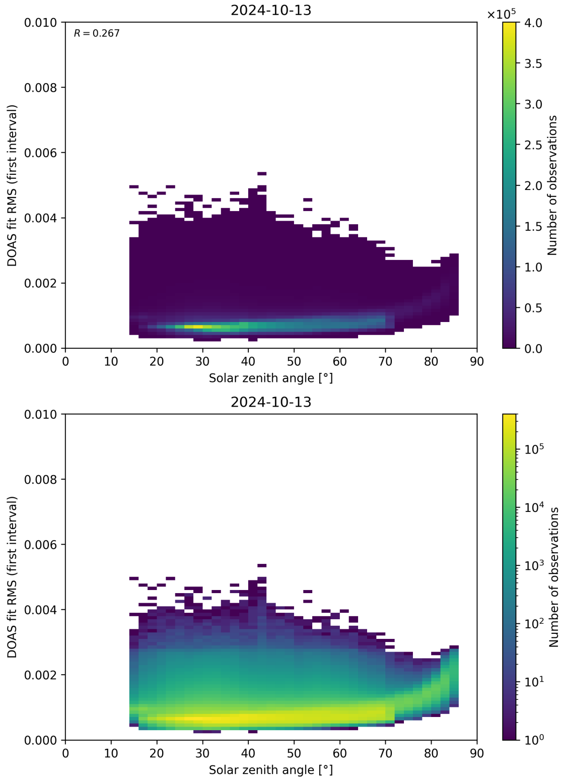
Figure 167: Scatter density plot of “Solar zenith angle” against “DOAS fit RMS (first interval)” for 2024-10-12 to 2024-10-14.
