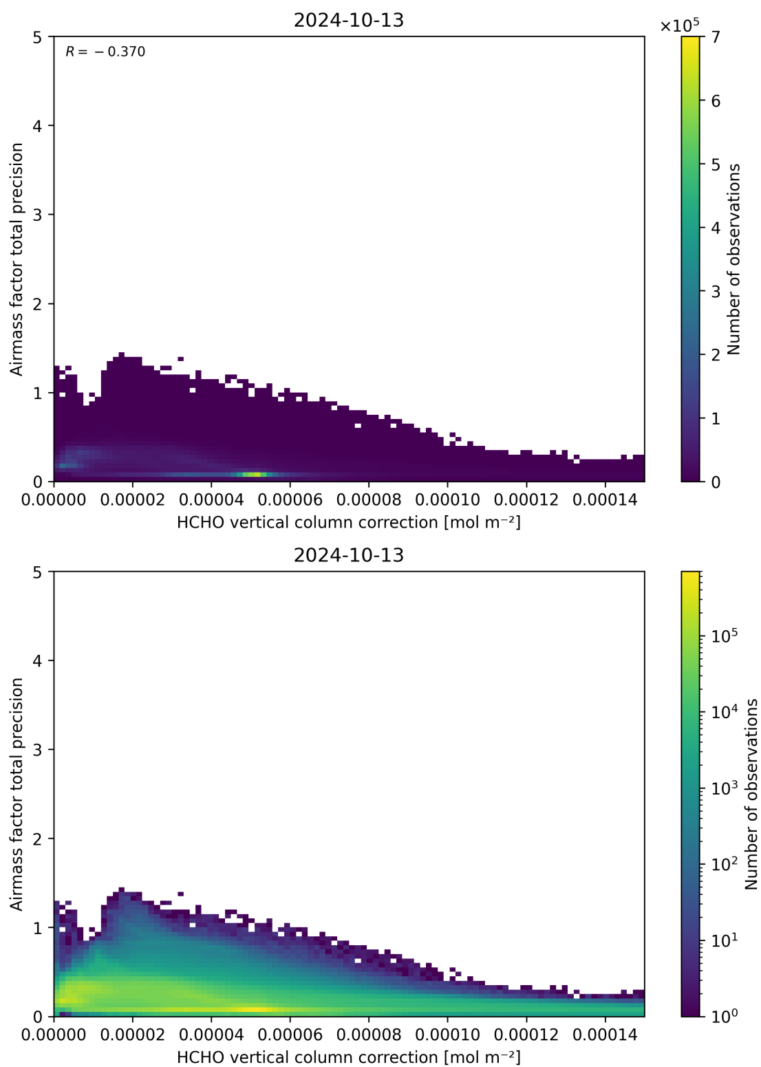
Figure 121: Scatter density plot of “HCHO vertical column correction” against “Airmass factor total precision” for 2024-10-12 to 2024-10-14.
