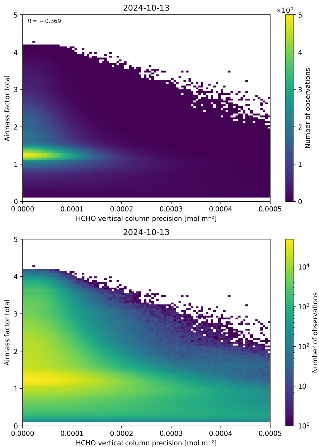
Figure 144: Scatter density plot of “HCHO vertical column precision” against “Airmass factor total” for 2024-10-12 to 2024-10-14.
