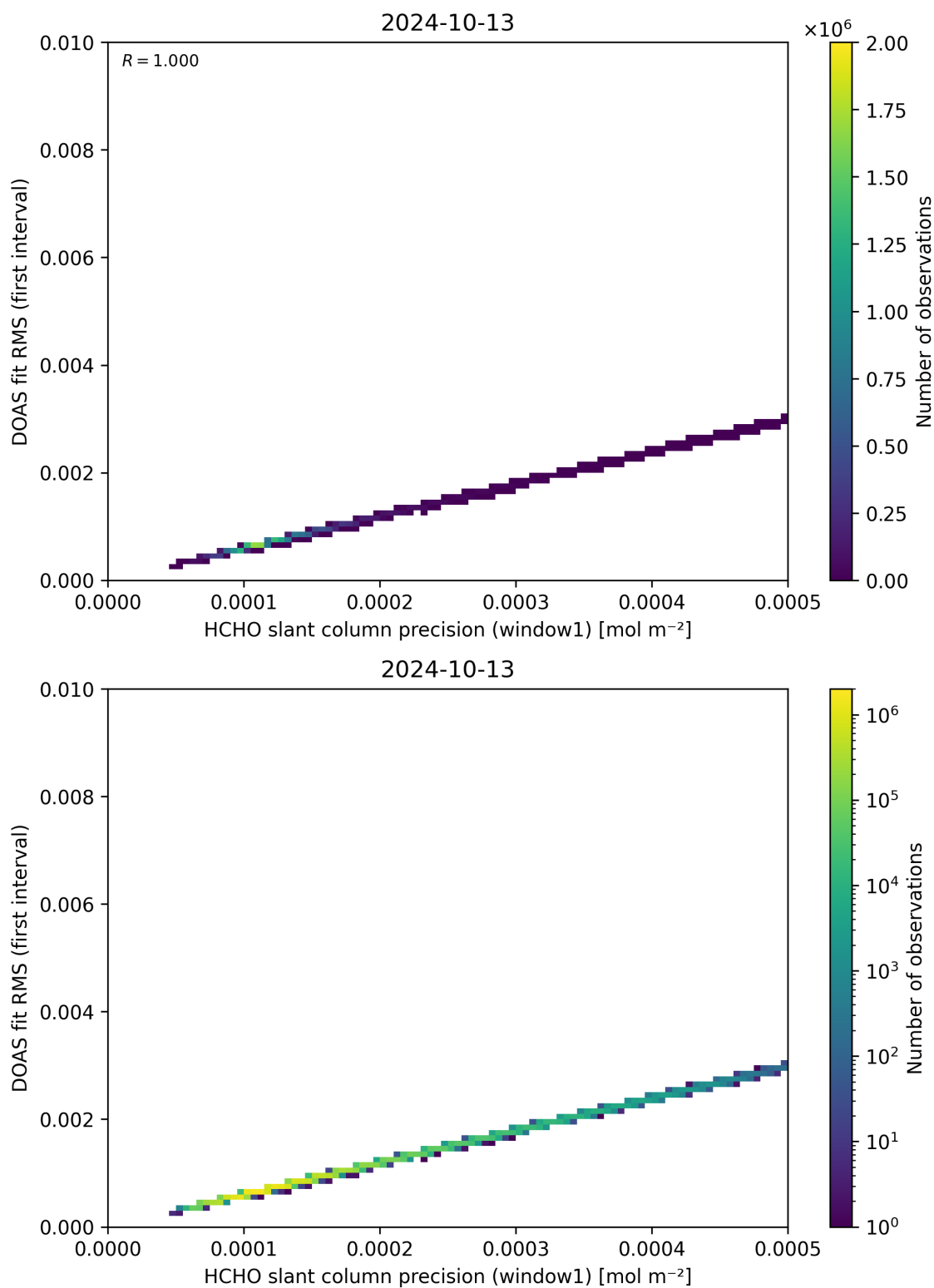
Figure 88: Scatter density plot of “HCHO slant column precision (window1)” against “DOAS fit RMS (first interval)” for 2024-10-12 to 2024-10-14.
