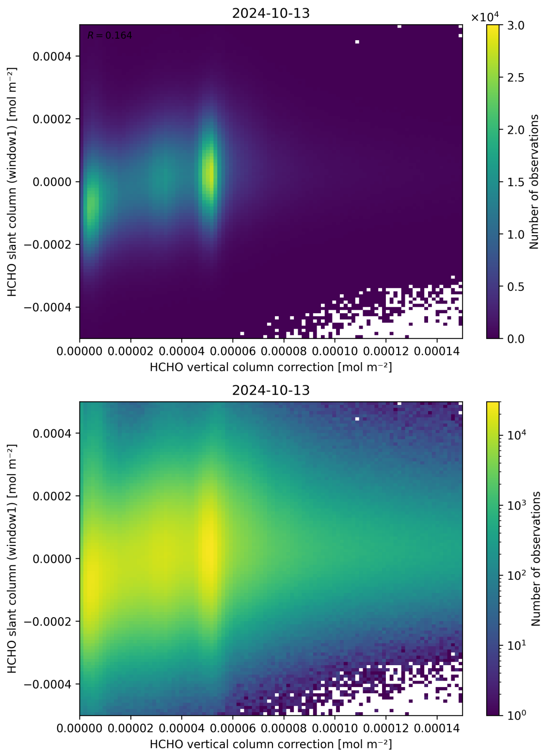
Figure 118: Scatter density plot of “HCHO vertical column correction” against “HCHO slant column (window1)” for 2024-10-12 to 2024-10-14.
