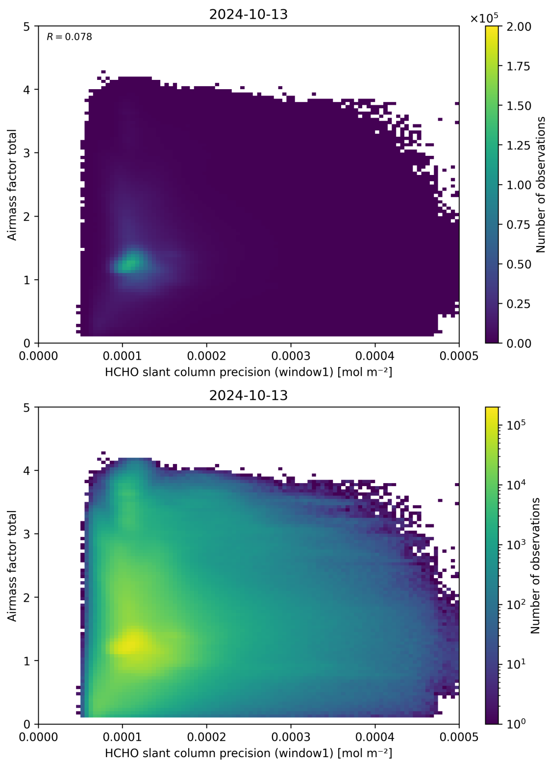
Figure 94: Scatter density plot of “HCHO slant column precision (window1)” against “Airmass factor total” for 2024-10-12 to 2024-10-14.
