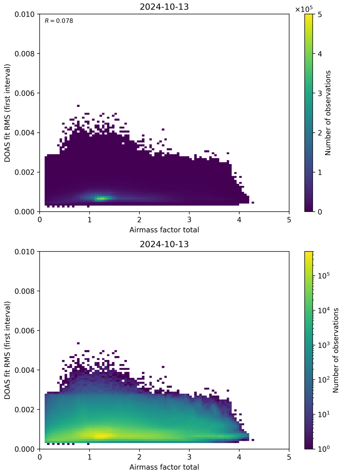
Figure 97: Scatter density plot of “Airmass factor total” against “DOAS fit RMS (first interval)” for 2024-10-12 to 2024-10-14.
