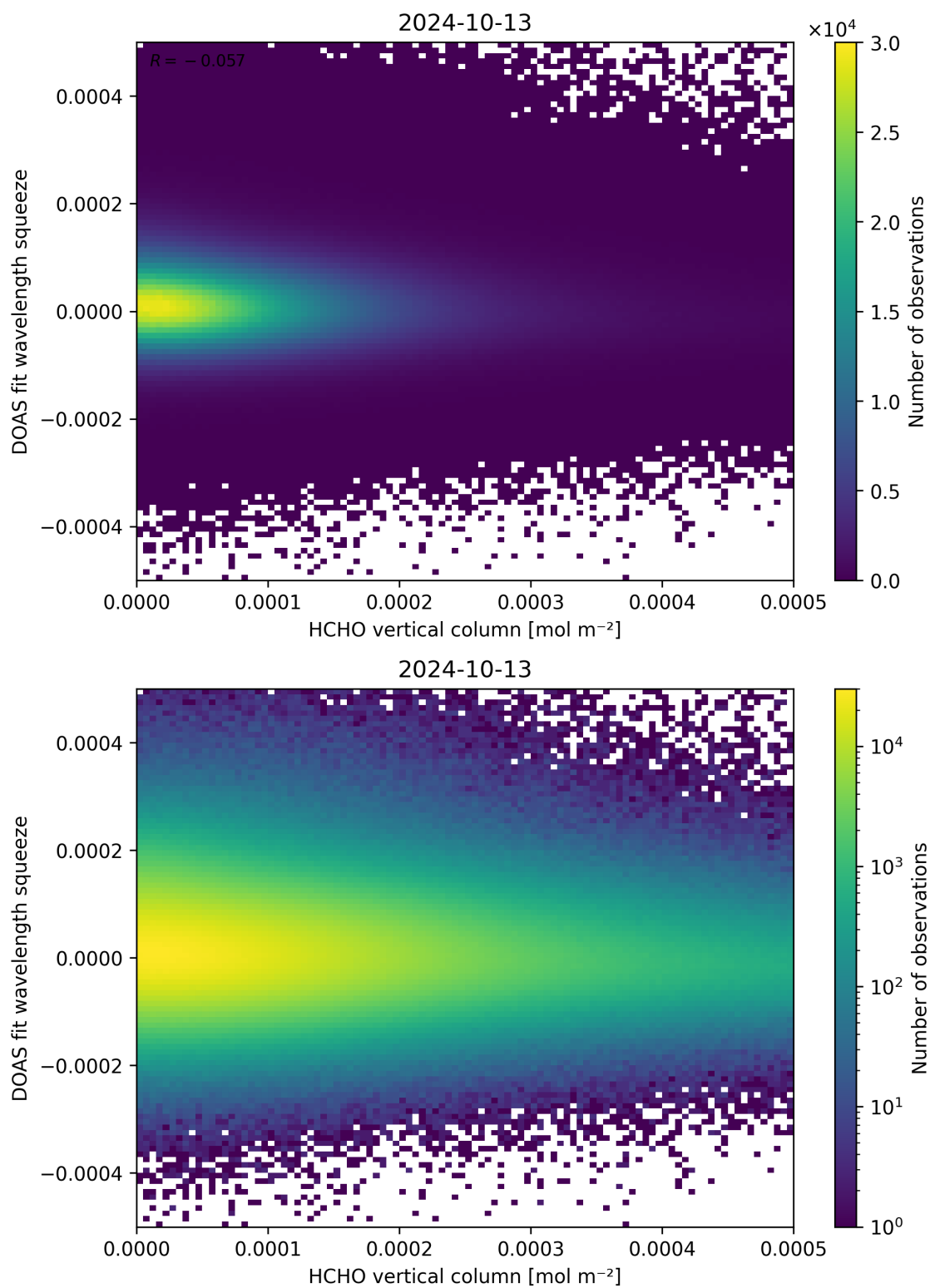
Figure 125: Scatter density plot of “HCHO vertical column” against “DOAS fit wavelength squeeze” for 2024-10-12 to 2024-10-14.
