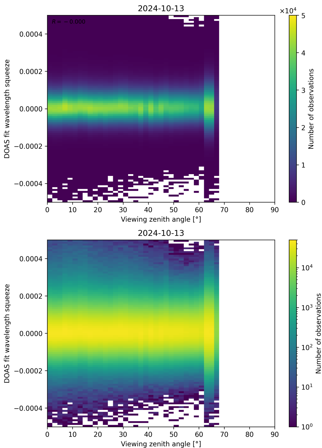
Figure 184: Scatter density plot of “Viewing zenith angle” against “DOAS fit wavelength squeeze” for 2024-10-12 to 2024-10-14.
