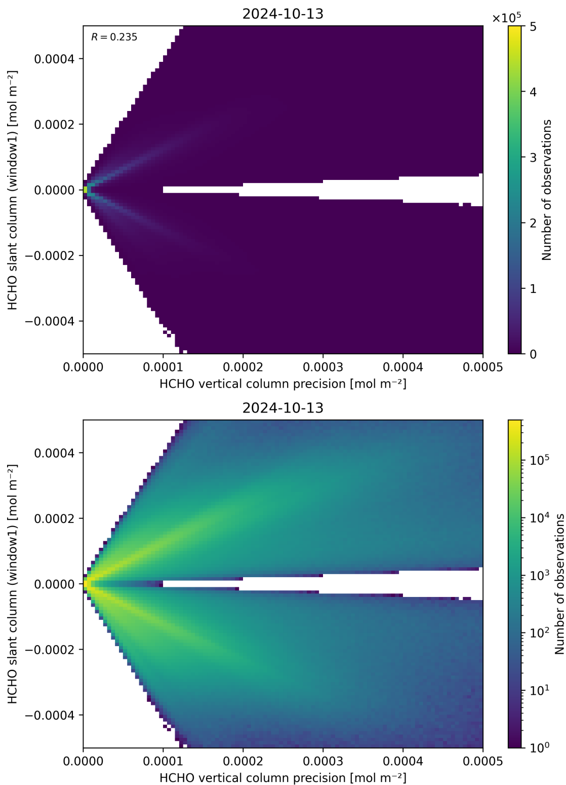
Figure 142: Scatter density plot of “HCHO vertical column precision” against “HCHO slant column (window1)” for 2024-10-12 to 2024-10-14.
