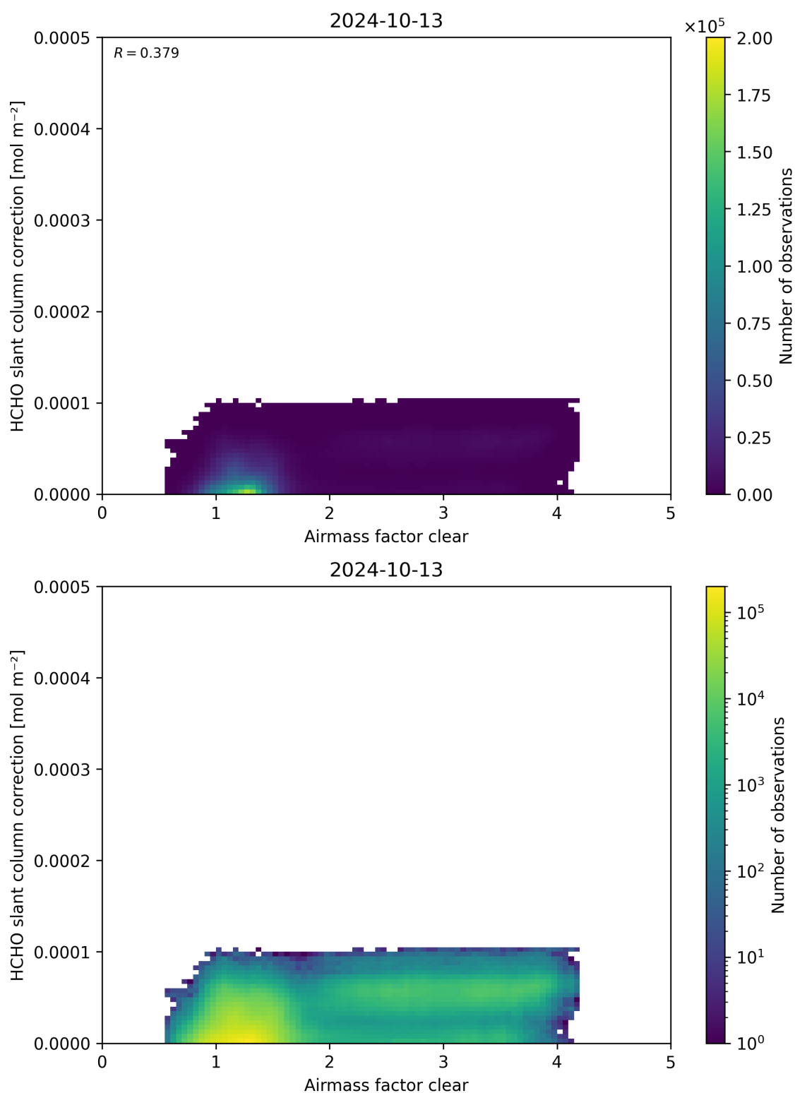
Figure 75: Scatter density plot of “Airmass factor clear” against “HCHO slant column correction” for 2024-10-12 to 2024-10-14.
