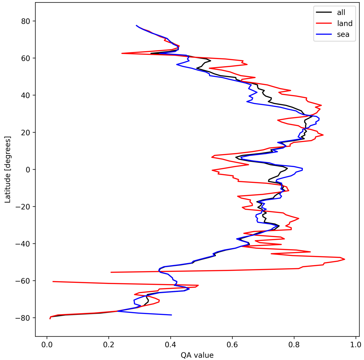
Figure 20: Zonal average of “QA value” for 2024-10-12 to 2024-10-14.
