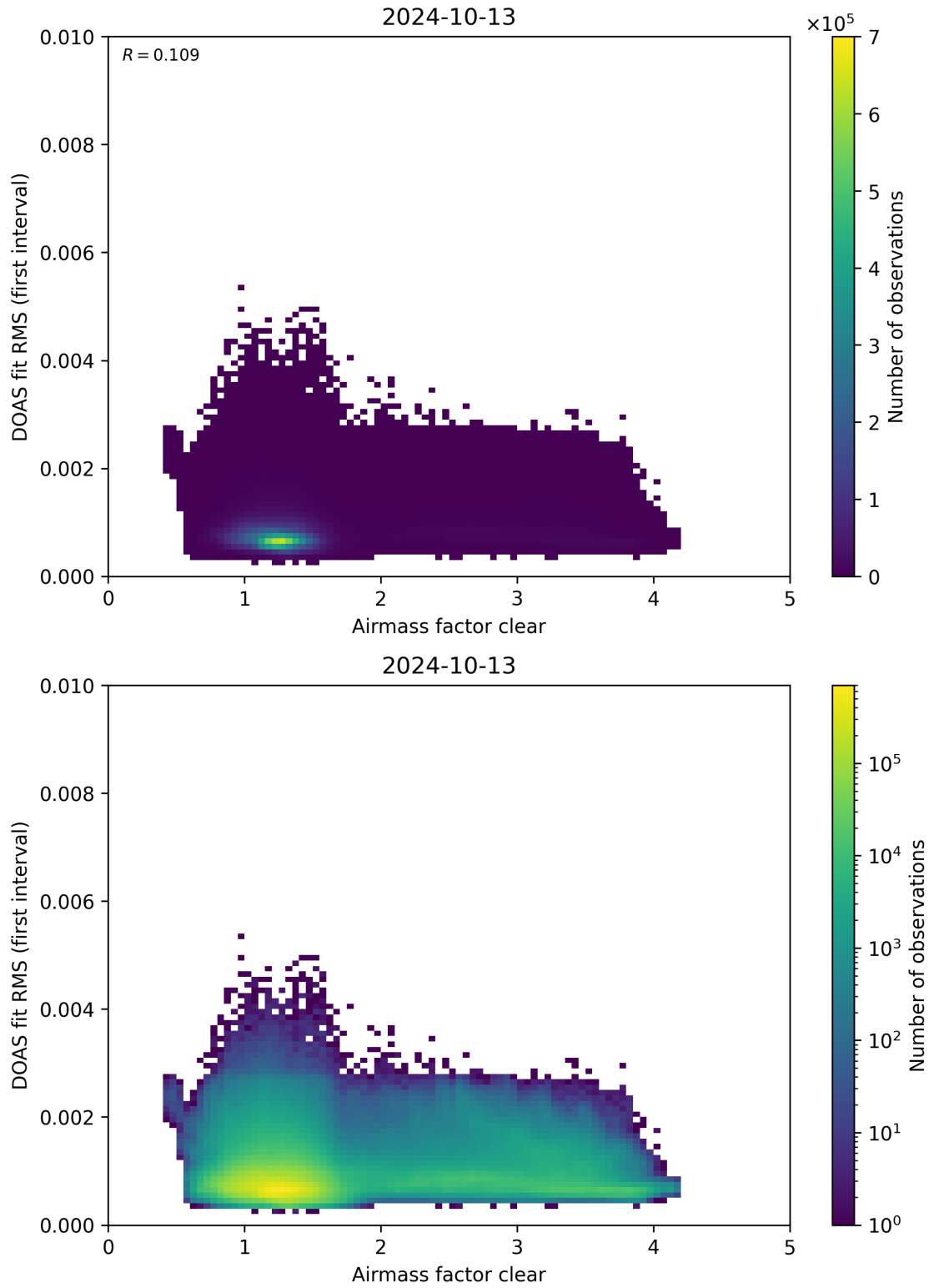
Figure 71: Scatter density plot of “Airmass factor clear” against “DOAS fit RMS (first interval)” for 2024-10-12 to 2024-10-14.
