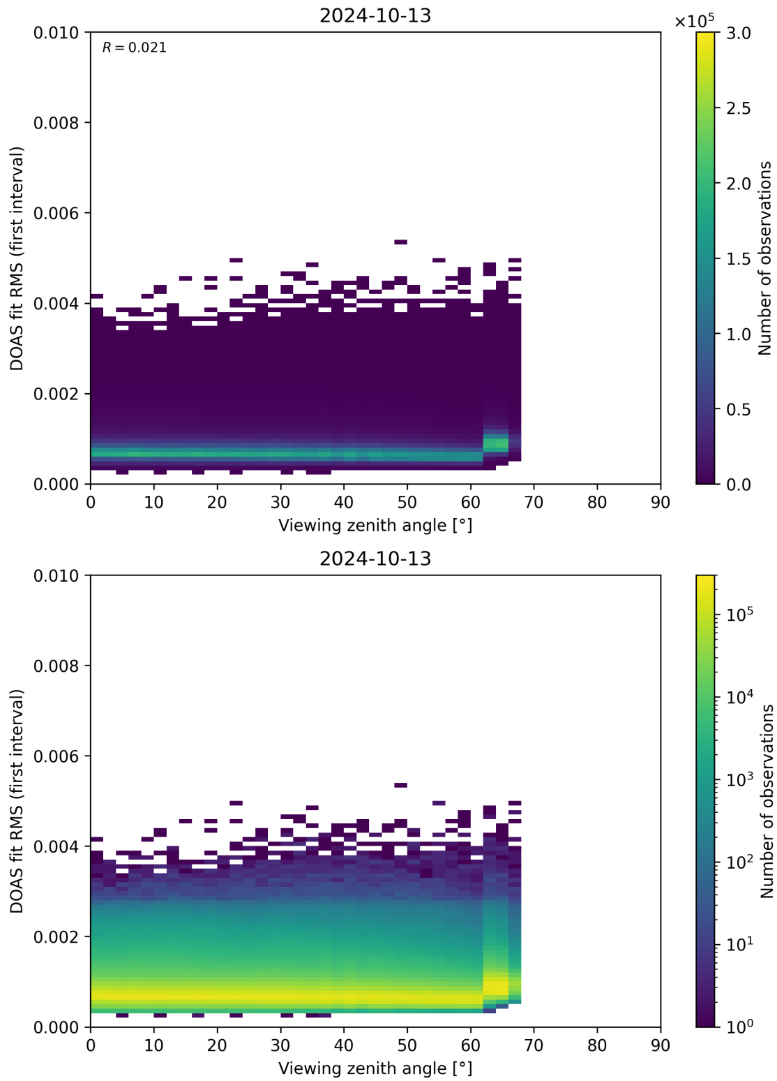
Figure 182: Scatter density plot of “Viewing zenith angle” against “DOAS fit RMS (first interval)” for 2024-10-12 to 2024-10-14.
