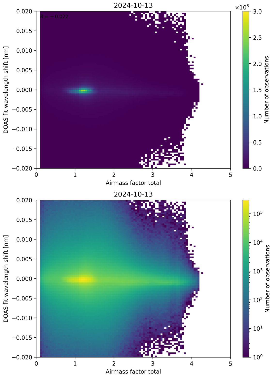
Figure 98: Scatter density plot of “Airmass factor total” against “DOAS fit wavelength shift” for 2024-10-12 to 2024-10-14.
