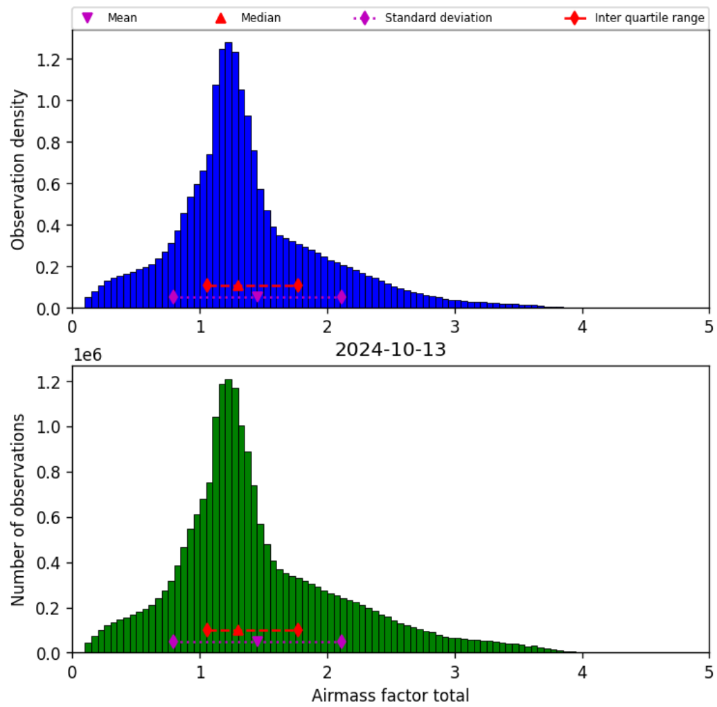
Figure 40: Histogram of “Airmass factor total” for 2024-10-12 to 2024-10-14
