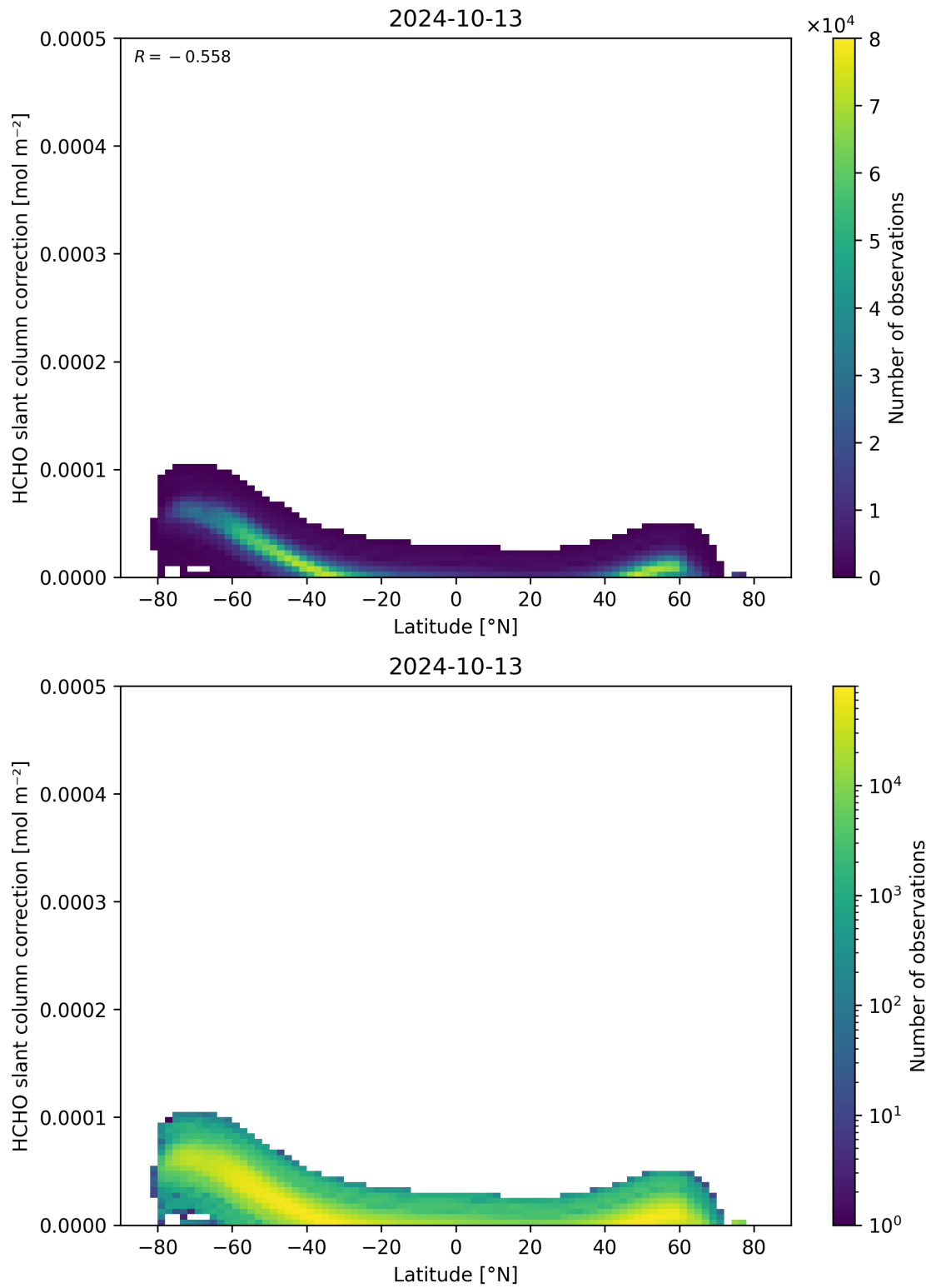
Figure 158: Scatter density plot of “Latitude” against “HCHO slant column correction” for 2024-10-12 to 2024-10-14.
