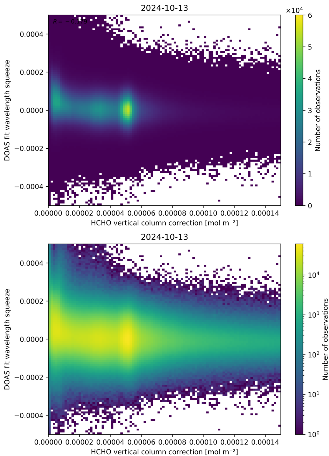
Figure 114: Scatter density plot of “HCHO vertical column correction” against “DOAS fit wavelength squeeze” for 2024-10-12 to 2024-10-14.
