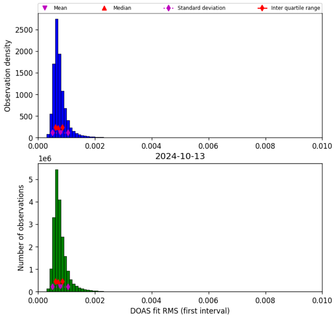
Figure 46: Histogram of “DOAS fit RMS (first interval)” for 2024-10-12 to 2024-10-14
