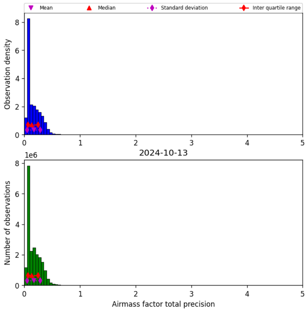
Figure 41: Histogram of “Airmass factor total precision” for 2024-10-12 to 2024-10-14
