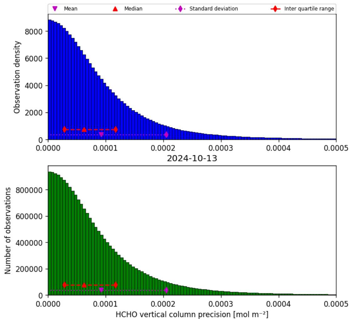
Figure 36: Histogram of “HCHO vertical column precision” for 2024-10-12 to 2024-10-14
