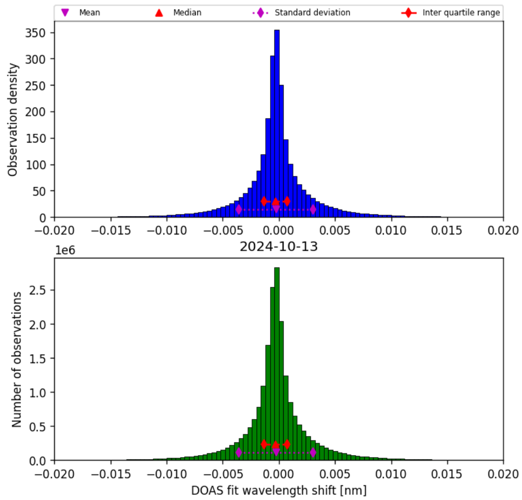
Figure 44: Histogram of “DOAS fit wavelength shift” for 2024-10-12 to 2024-10-14
