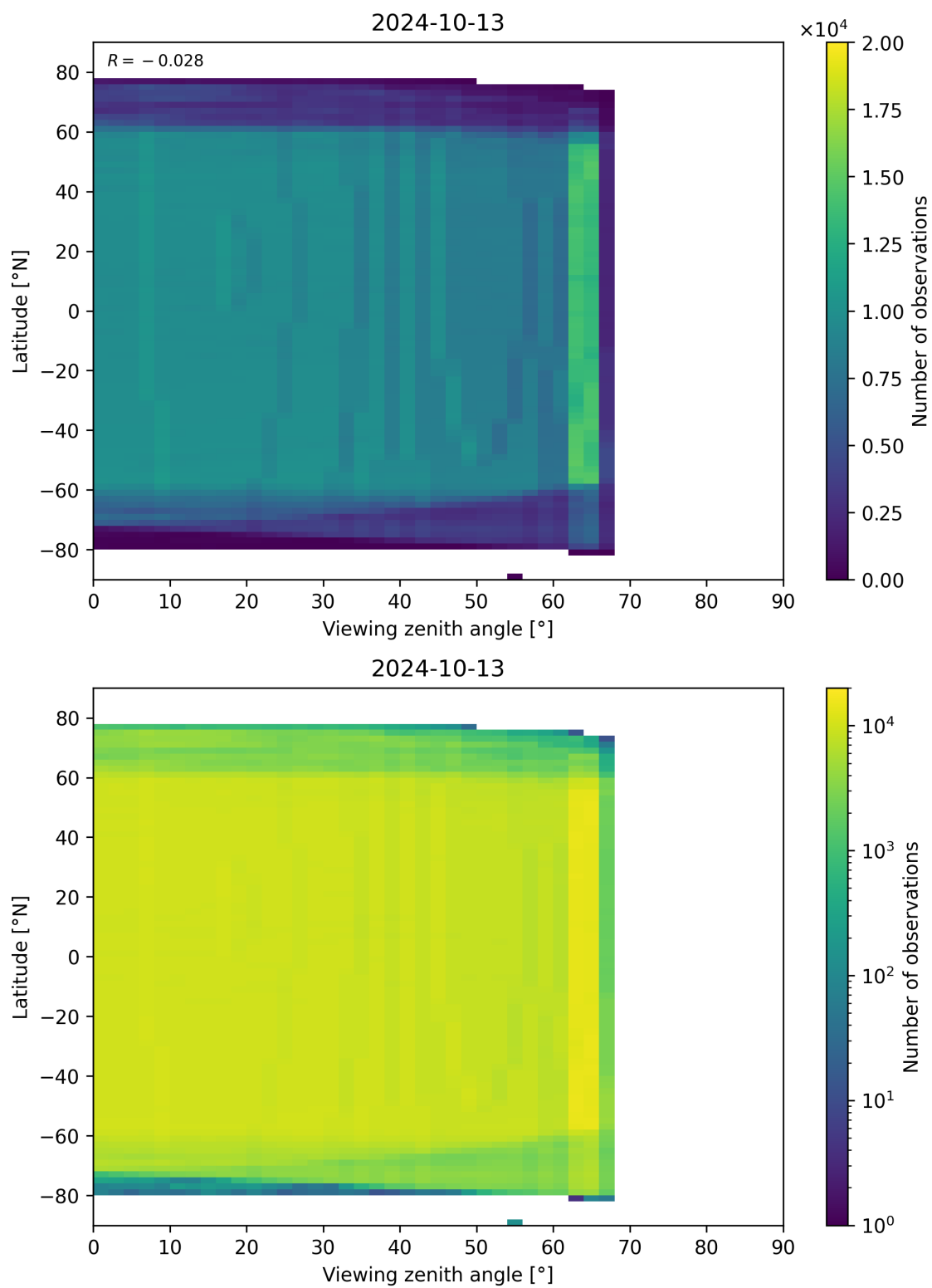
Figure 196: Scatter density plot of “Viewing zenith angle” against “Latitude” for 2024-10-12 to 2024-10-14.
