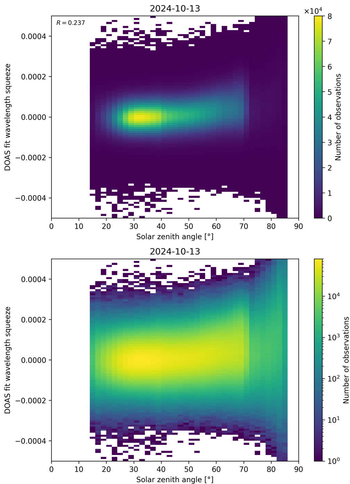
Figure 169: Scatter density plot of “Solar zenith angle” against “DOAS fit wavelength squeeze” for 2024-10-12 to 2024-10-14.
