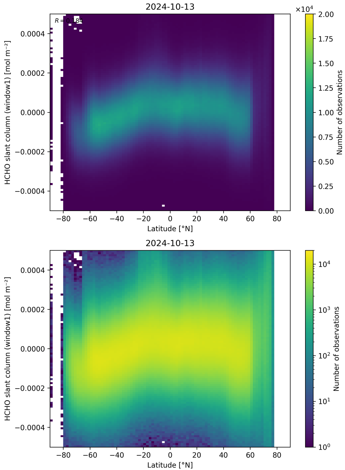
Figure 159: Scatter density plot of “Latitude” against “HCHO slant column (window1)” for 2024-10-12 to 2024-10-14.
