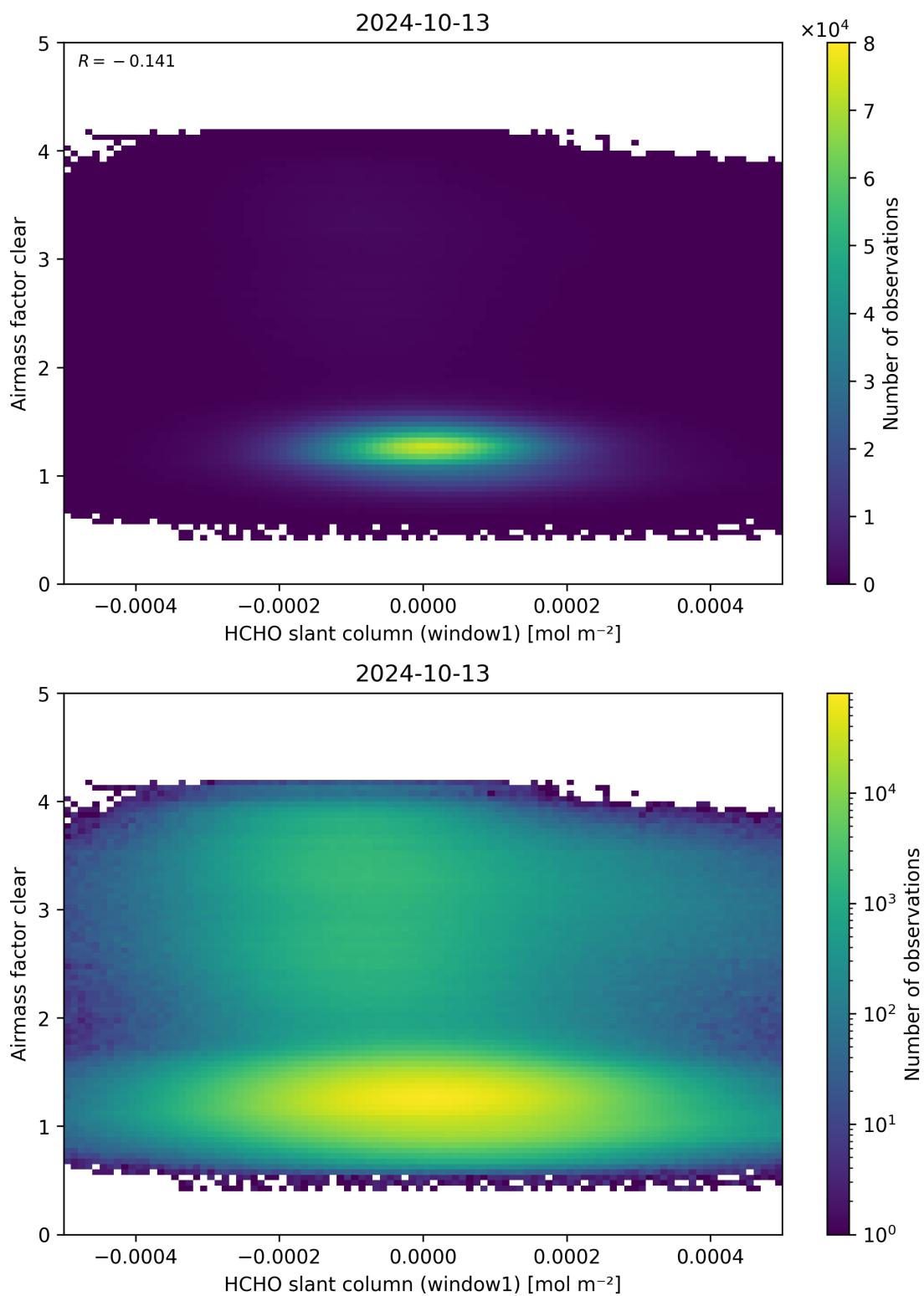
Figure 81: Scatter density plot of “HCHO slant column (window1)” against “Airmass factor clear” for 2024-10-12 to 2024-10-14.
