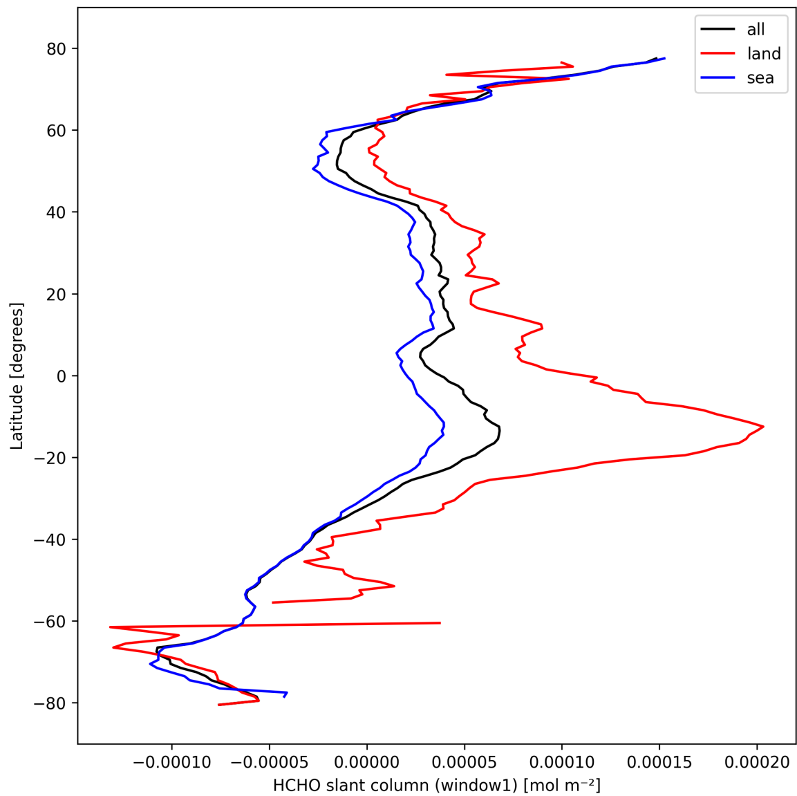
Figure 24: Zonal average of “HCHO slant column (window1)” for 2024-10-12 to 2024-10-14.
