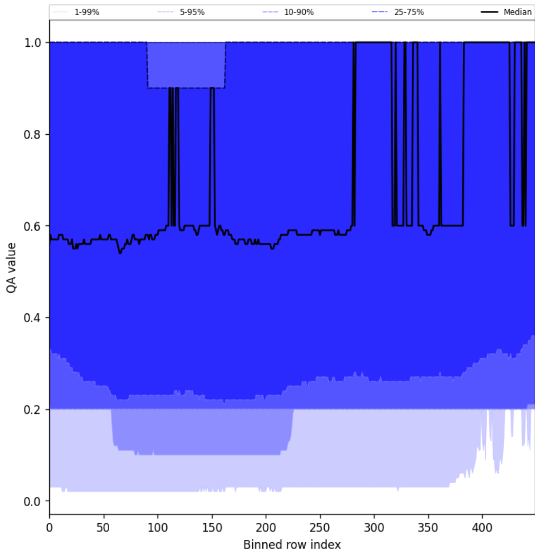
Figure 48: Along track statistics of “QA value” for 2024-10-12 to 2024-10-14
