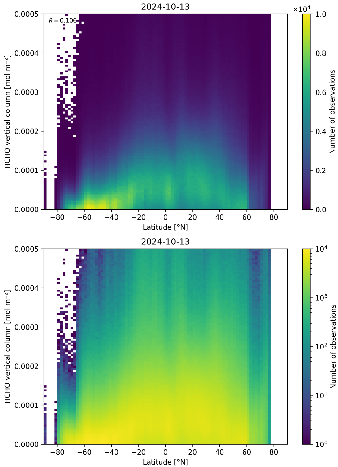
Figure 163: Scatter density plot of “Latitude” against “HCHO vertical column” for 2024-10-12 to 2024-10-14.
