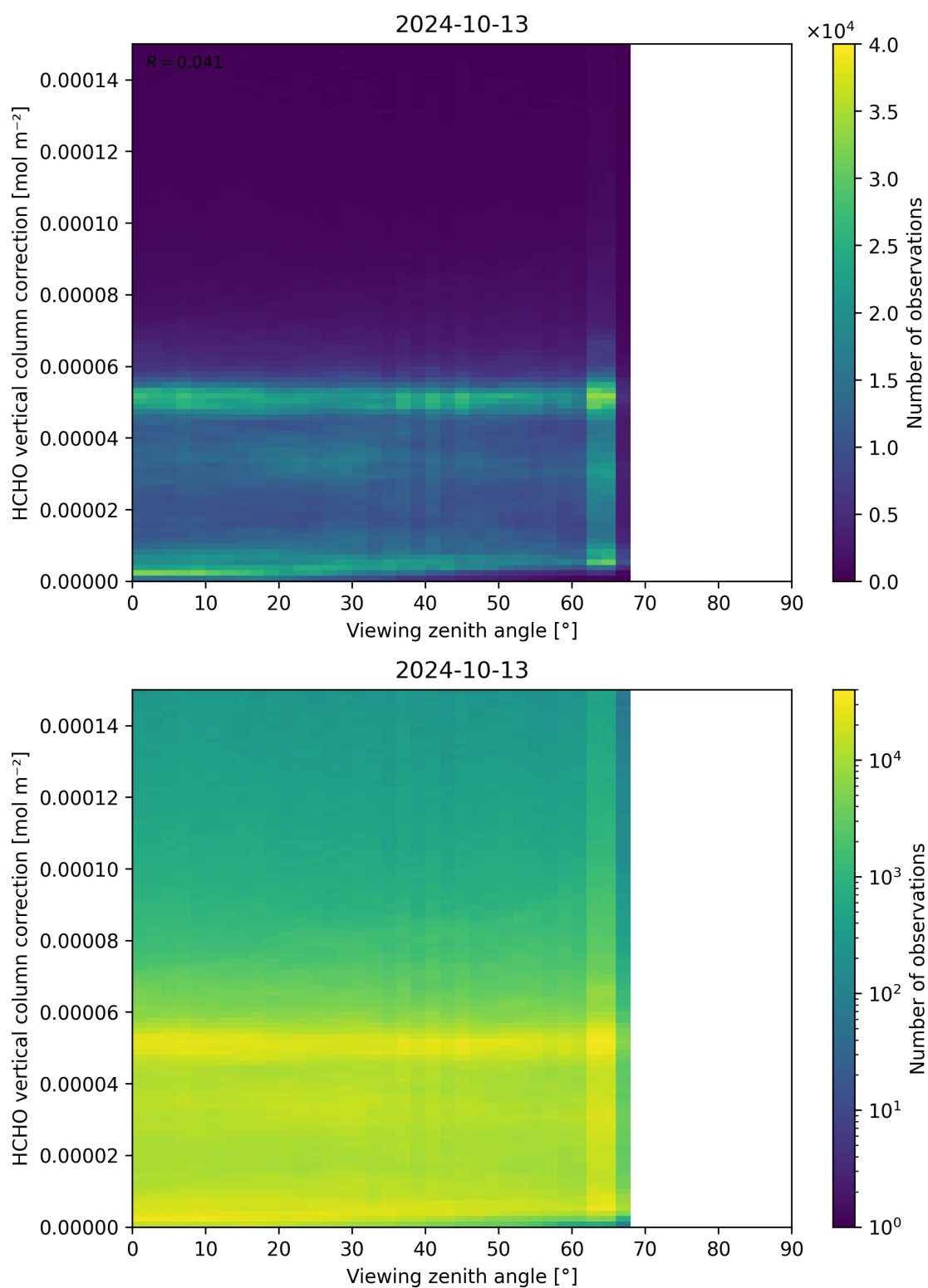
Figure 193: Scatter density plot of “Viewing zenith angle” against “HCHO vertical column correction” for 2024-10-12 to 2024-10-14.
