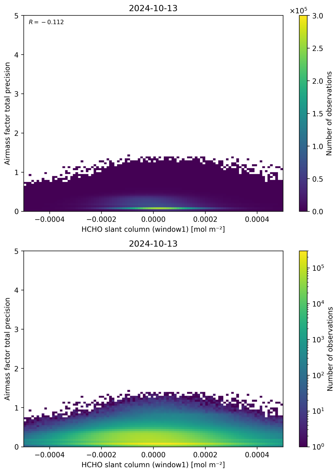
Figure 86: Scatter density plot of “HCHO slant column (window1)” against “Airmass factor total precision” for 2024-10-12 to 2024-10-14.
