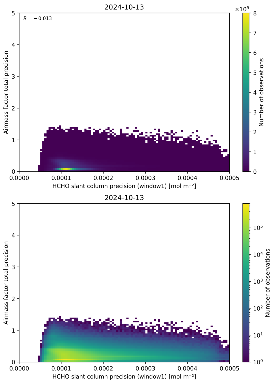
Figure 95: Scatter density plot of “HCHO slant column precision (window1)” against “Airmass factor total precision” for 2024-10-12 to 2024-10-14.
