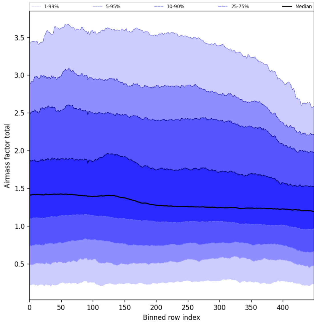
Figure 54: Along track statistics of “Airmass factor total” for 2024-10-12 to 2024-10-14
