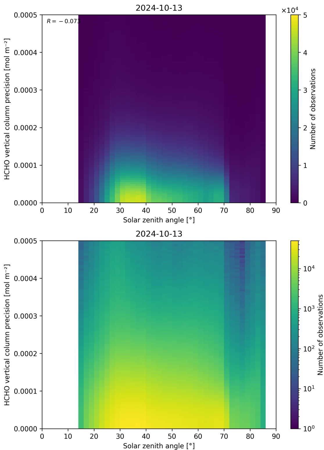
Figure 179: Scatter density plot of “Solar zenith angle” against “HCHO vertical column precision” for 2024-10-12 to 2024-10-14.
