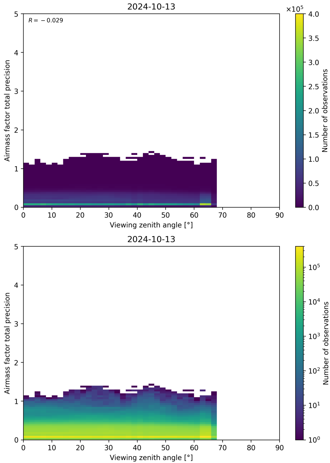
Figure 191: Scatter density plot of “Viewing zenith angle” against “Airmass factor total precision” for 2024-10-12 to 2024-10-14.
