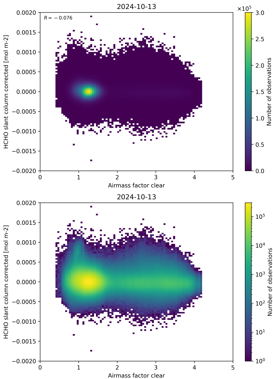
Figure 74: Scatter density plot of “Airmass factor clear” against “HCHO slant column corrected” for 2024-10-12 to 2024-10-14.
