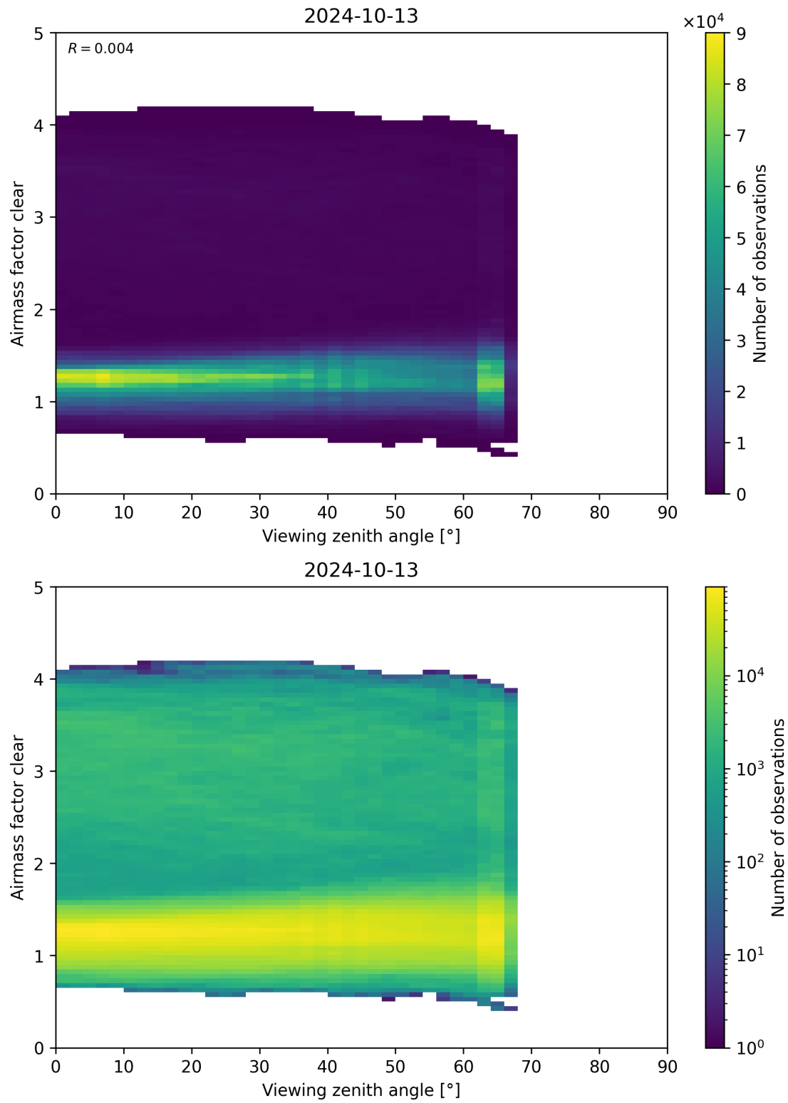
Figure 185: Scatter density plot of “Viewing zenith angle” against “Airmass factor clear” for 2024-10-12 to 2024-10-14.
