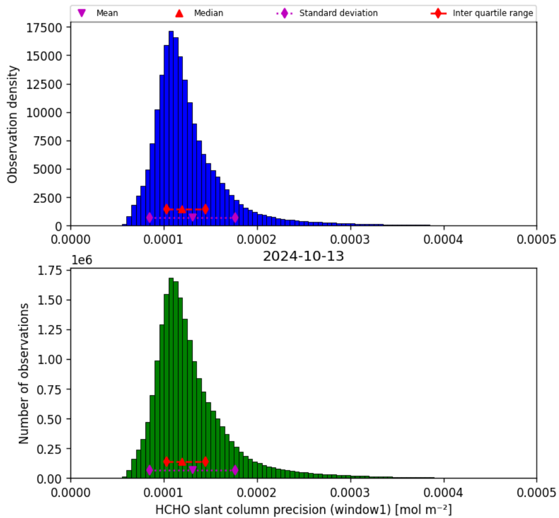
Figure 39: Histogram of “HCHO slant column precision (window1)” for 2024-10-12 to 2024-10-14
