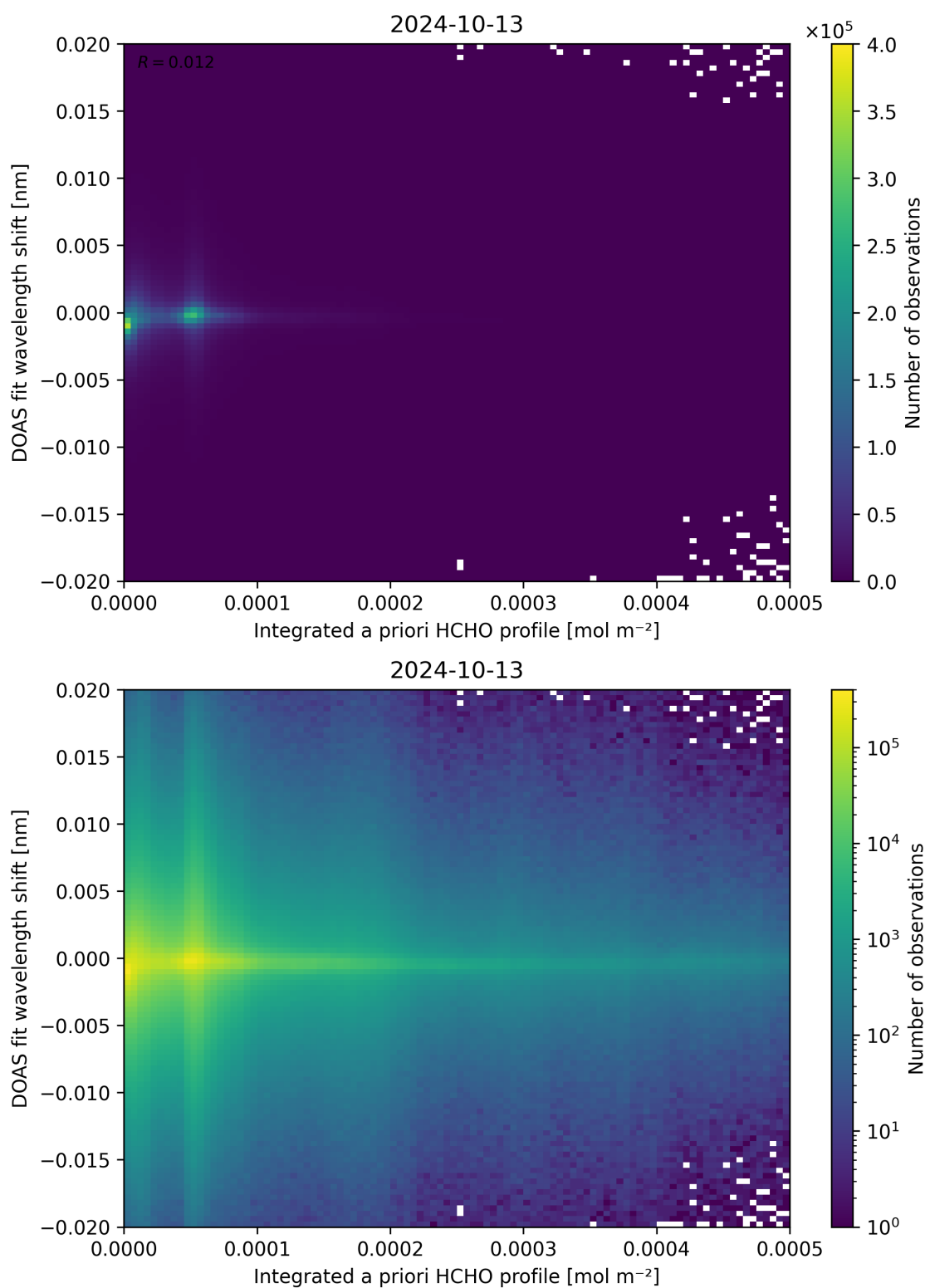
Figure 149: Scatter density plot of “Integrated a priori HCHO profile” against “DOAS fit wavelength shift” for 2024-10-12 to 2024-10-14.
