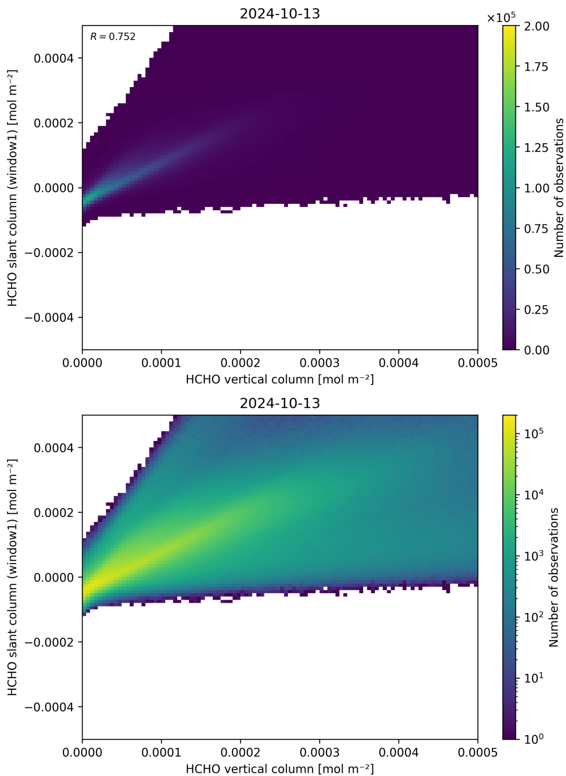
Figure 129: Scatter density plot of “HCHO vertical column” against “HCHO slant column (window1)” for 2024-10-12 to 2024-10-14.
