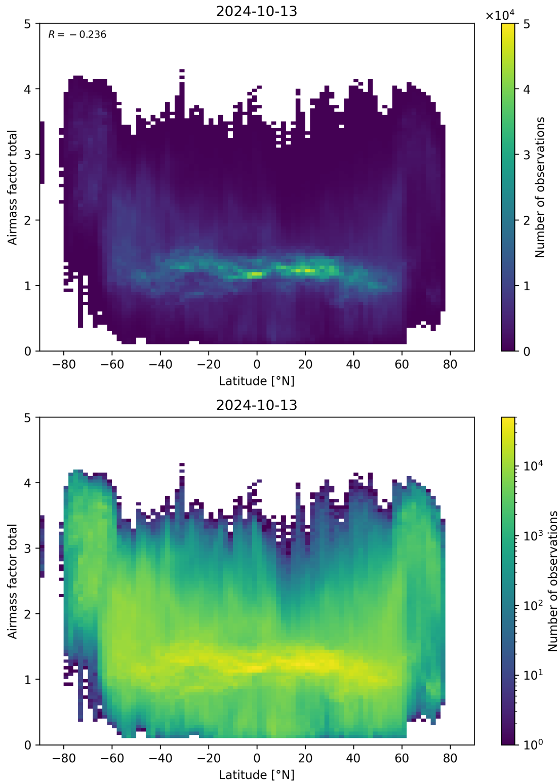
Figure 161: Scatter density plot of “Latitude” against “Airmass factor total” for 2024-10-12 to 2024-10-14.
