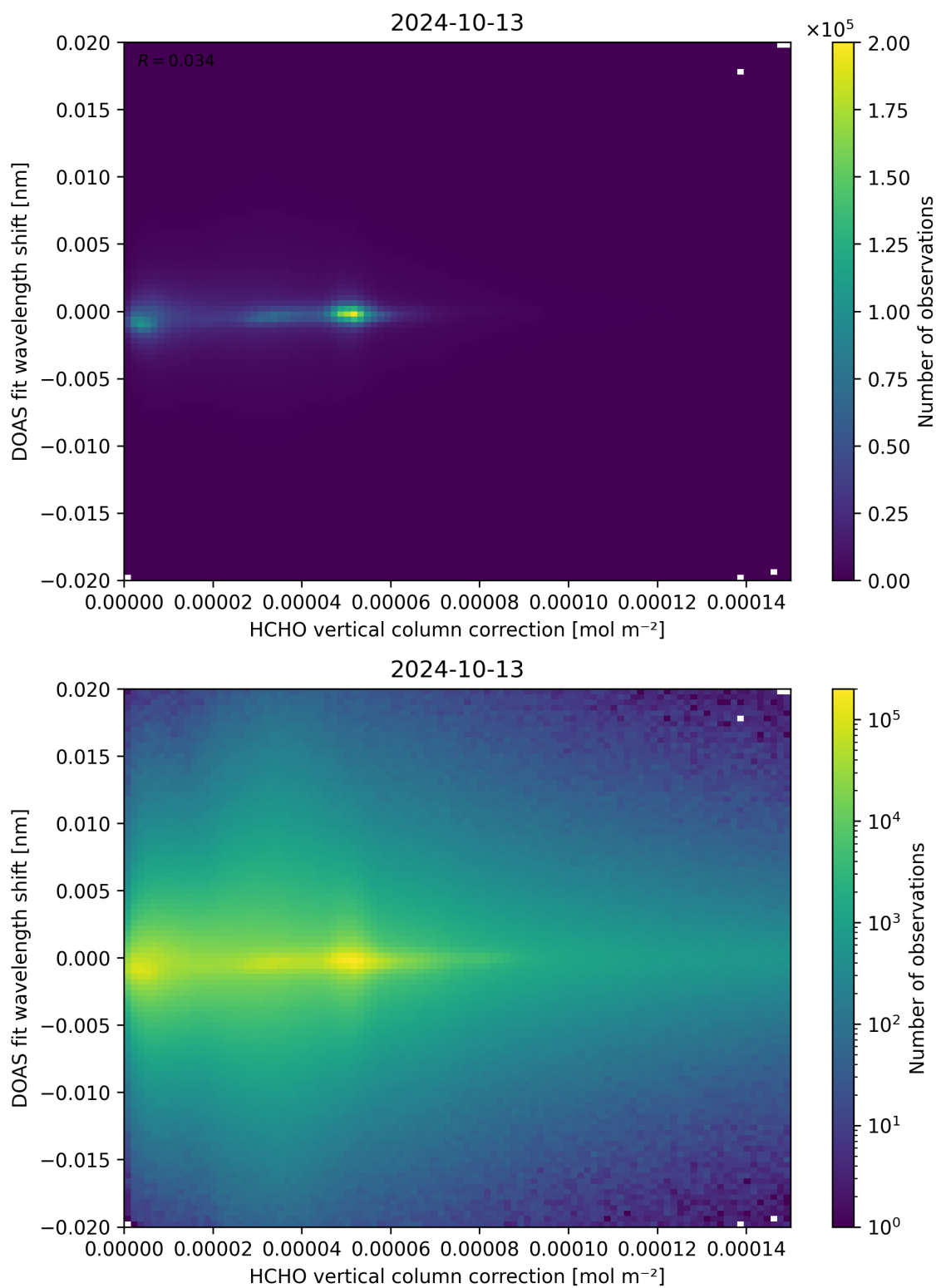
Figure 113: Scatter density plot of “HCHO vertical column correction” against “DOAS fit wavelength shift” for 2024-10-12 to 2024-10-14.
