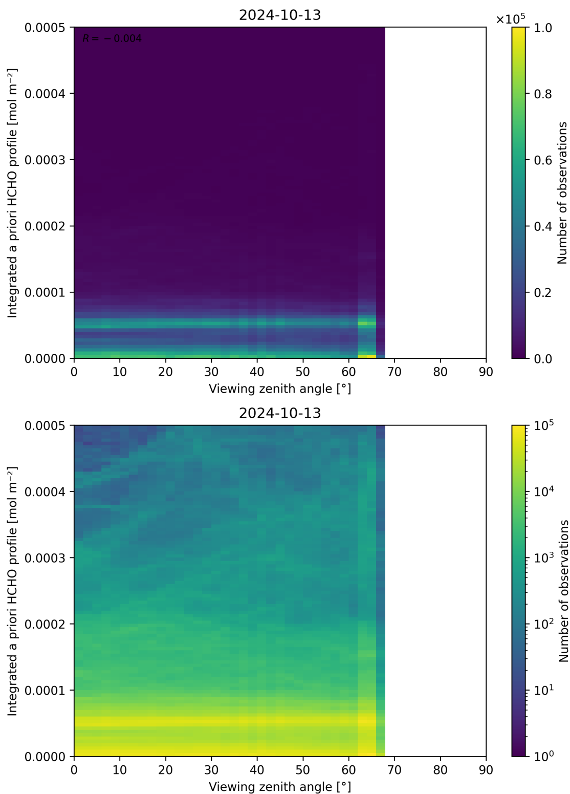
Figure 195: Scatter density plot of “Viewing zenith angle” against “Integrated a priori HCHO profile” for 2024-10-12 to 2024-10-14.
