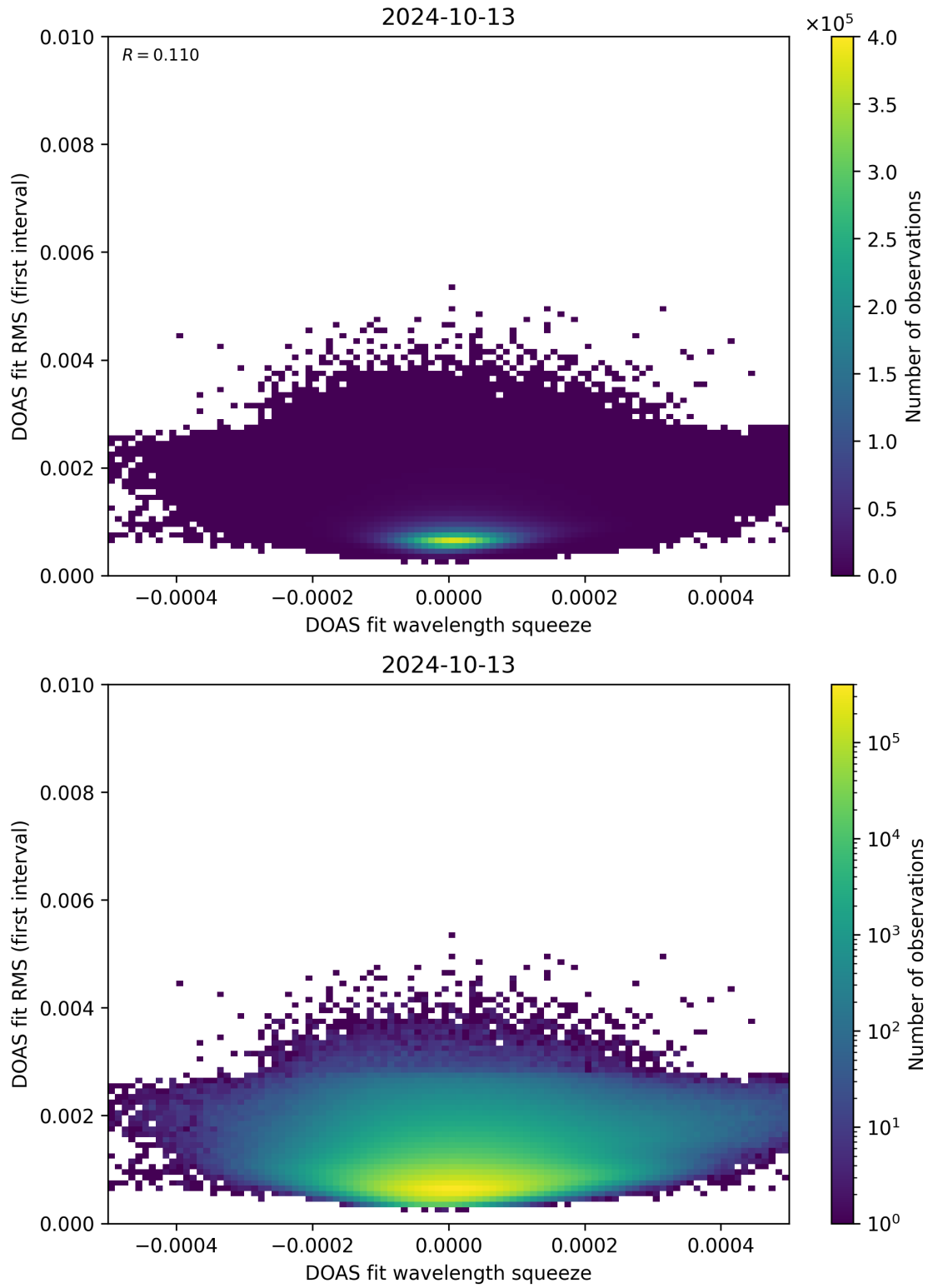
Figure 68: Scatter density plot of “DOAS fit wavelength squeeze” against “DOAS fit RMS (first interval)” for 2024-10-12 to 2024-10-14.
