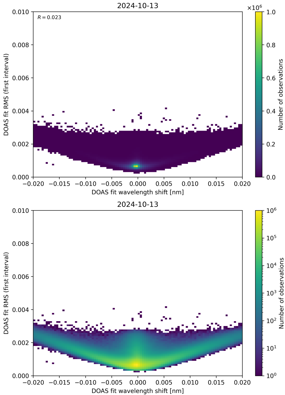
Figure 64: Scatter density plot of “DOAS fit wavelength shift” against “DOAS fit RMS (first interval)” for 2024-10-12 to 2024-10-14.
