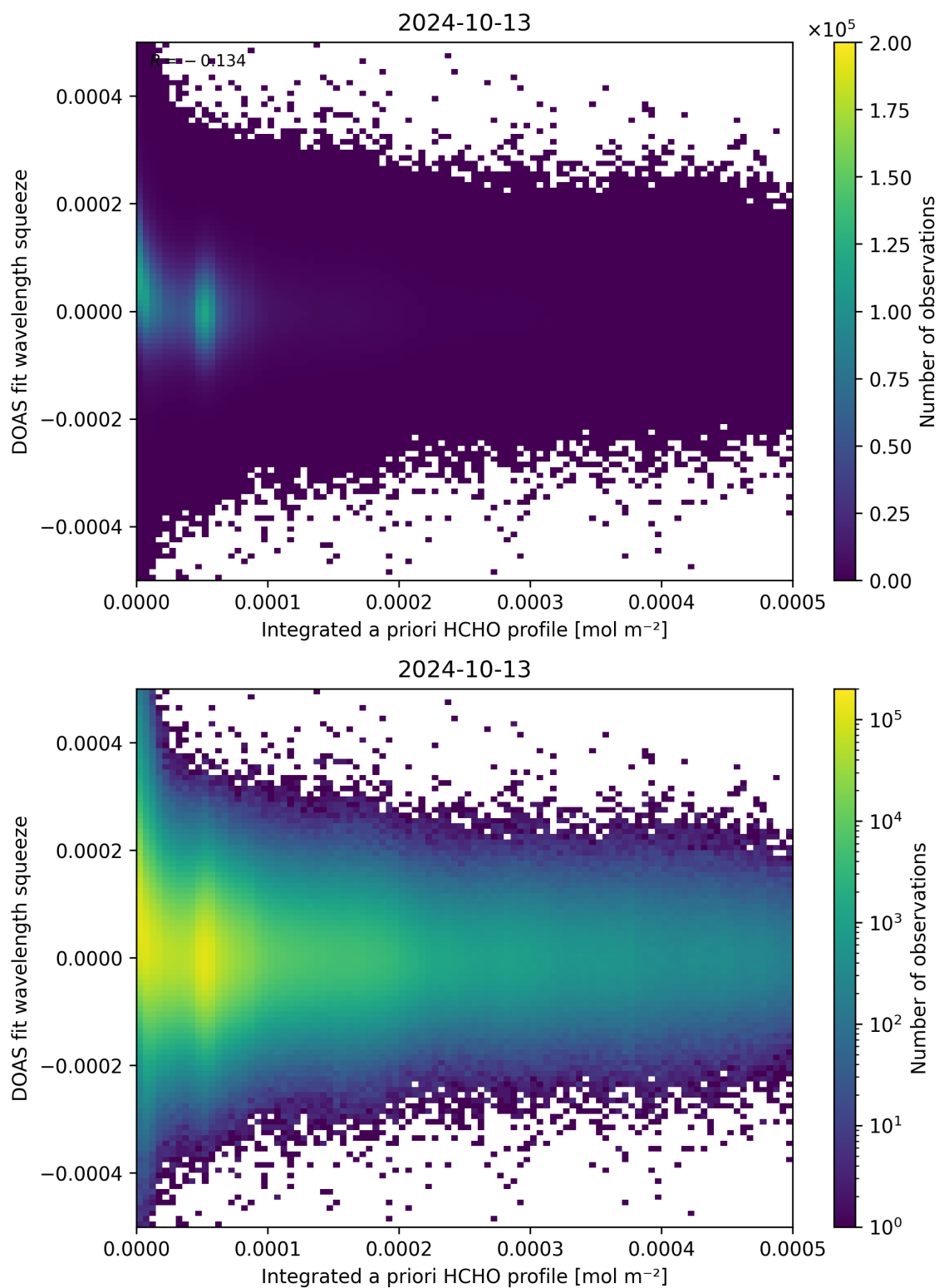
Figure 150: Scatter density plot of “Integrated a priori HCHO profile” against “DOAS fit wavelength squeeze” for 2024-10-12 to 2024-10-14.
