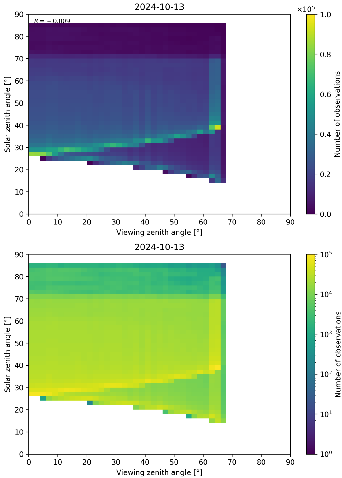
Figure 197: Scatter density plot of “Viewing zenith angle” against “Solar zenith angle” for 2024-10-12 to 2024-10-14.
