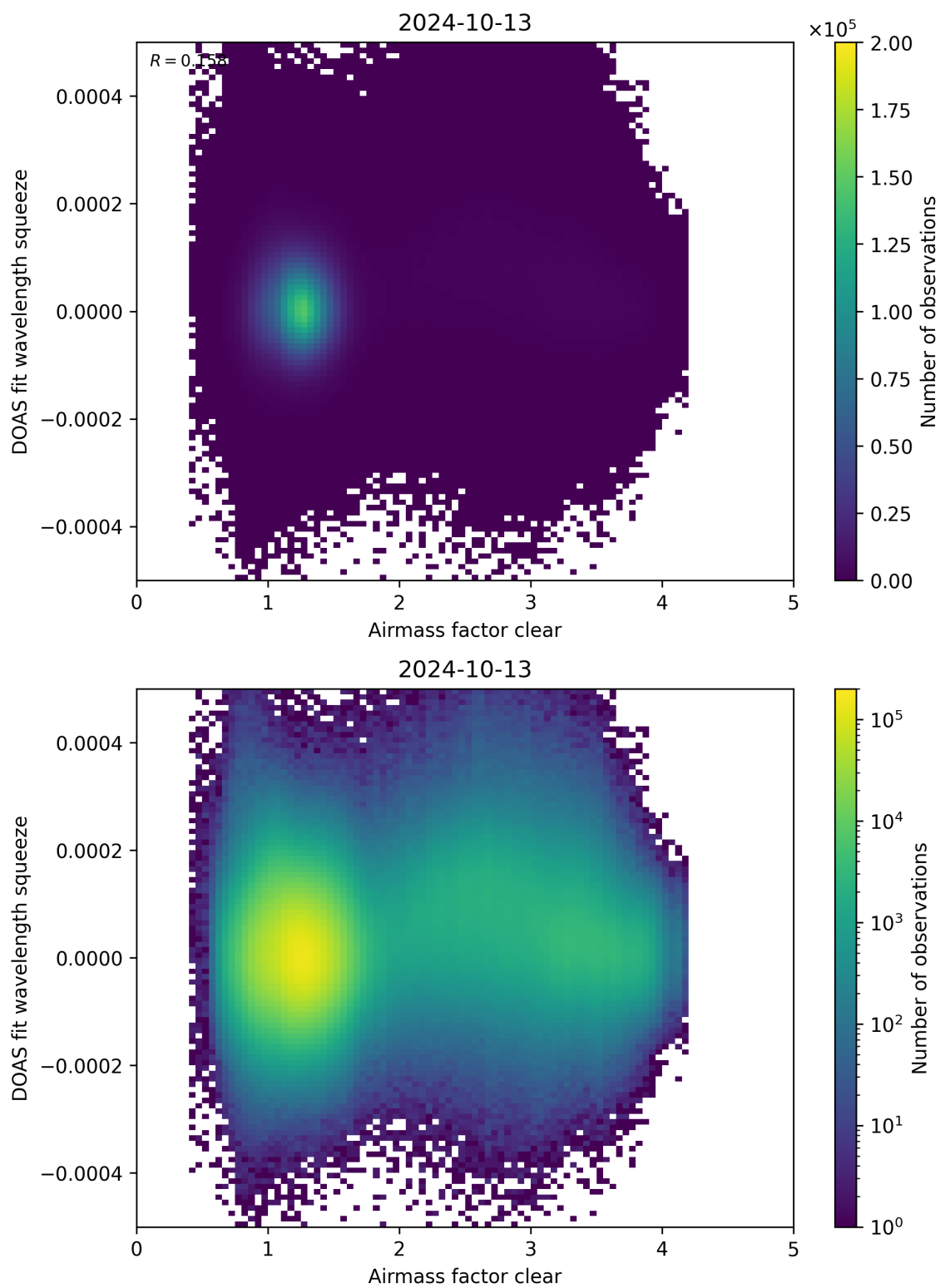
Figure 73: Scatter density plot of “Airmass factor clear” against “DOAS fit wavelength squeeze” for 2024-10-12 to 2024-10-14.
