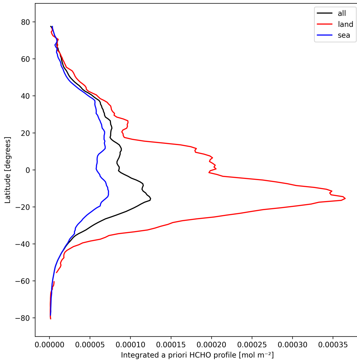
Figure 29: Zonal average of “Integrated a priori HCHO profile” for 2024-10-12 to 2024-10-14.
