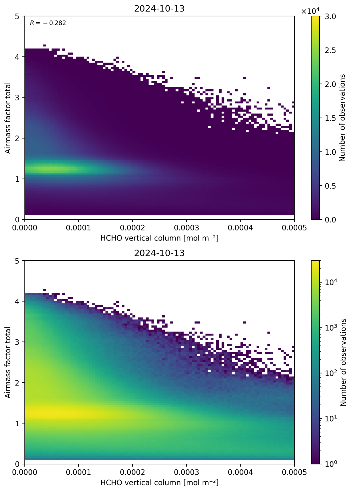
Figure 131: Scatter density plot of “HCHO vertical column” against “Airmass factor total” for 2024-10-12 to 2024-10-14.
