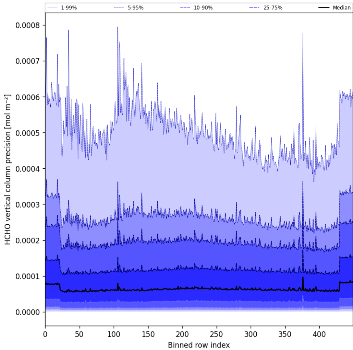
Figure 50: Along track statistics of “HCHO vertical column precision” for 2024-10-12 to 2024-10-14
