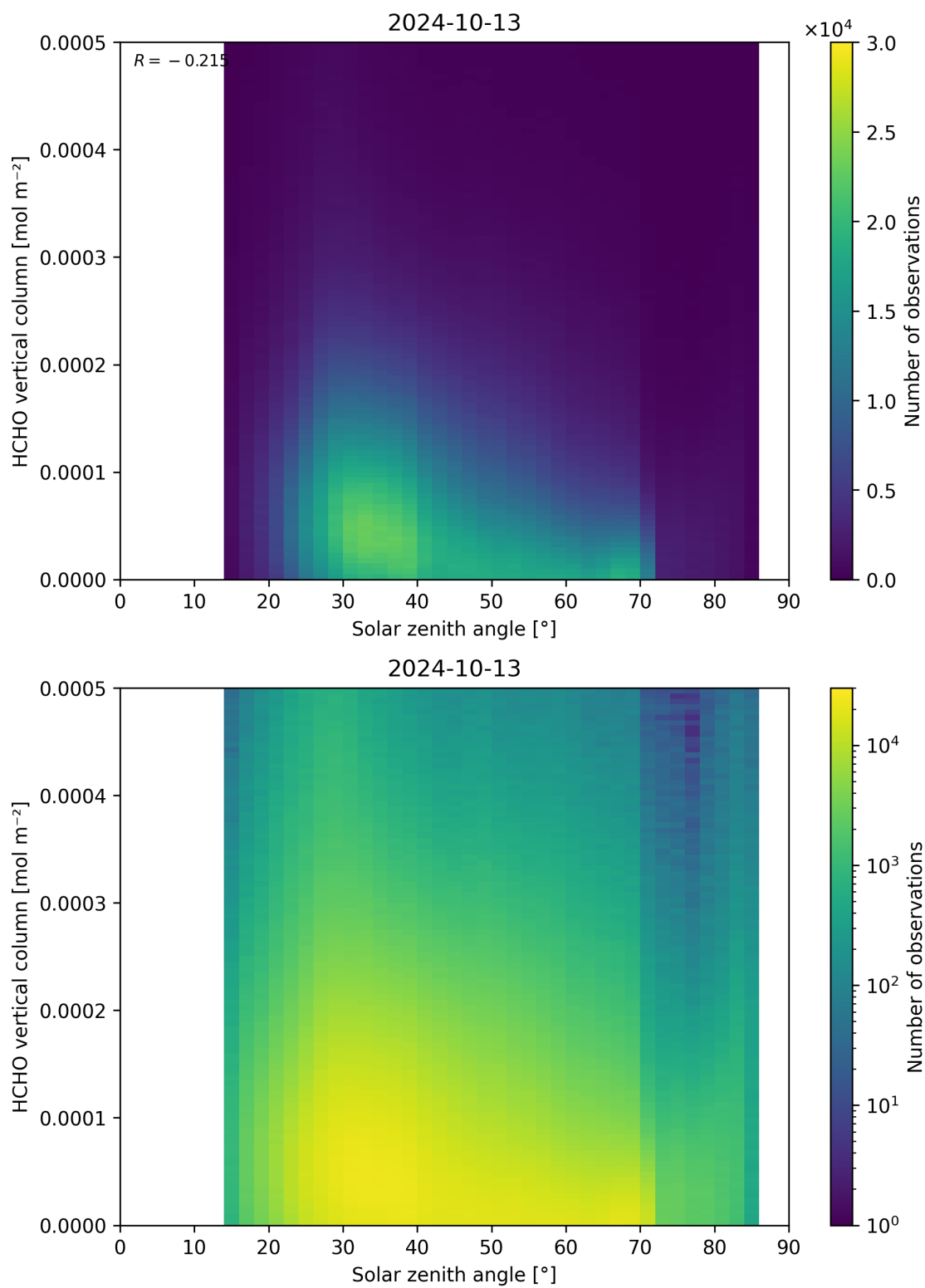
Figure 177: Scatter density plot of “Solar zenith angle” against “HCHO vertical column” for 2024-10-12 to 2024-10-14.
