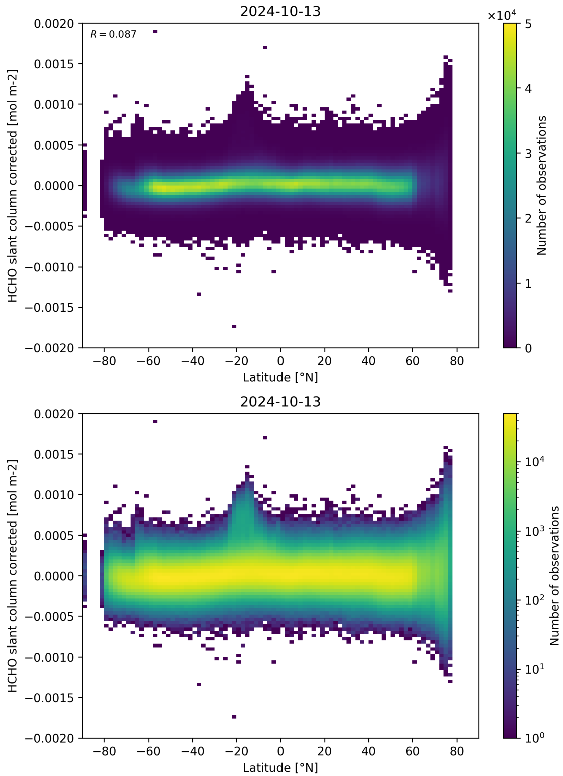
Figure 157: Scatter density plot of “Latitude” against “HCHO slant column corrected” for 2024-10-12 to 2024-10-14.
