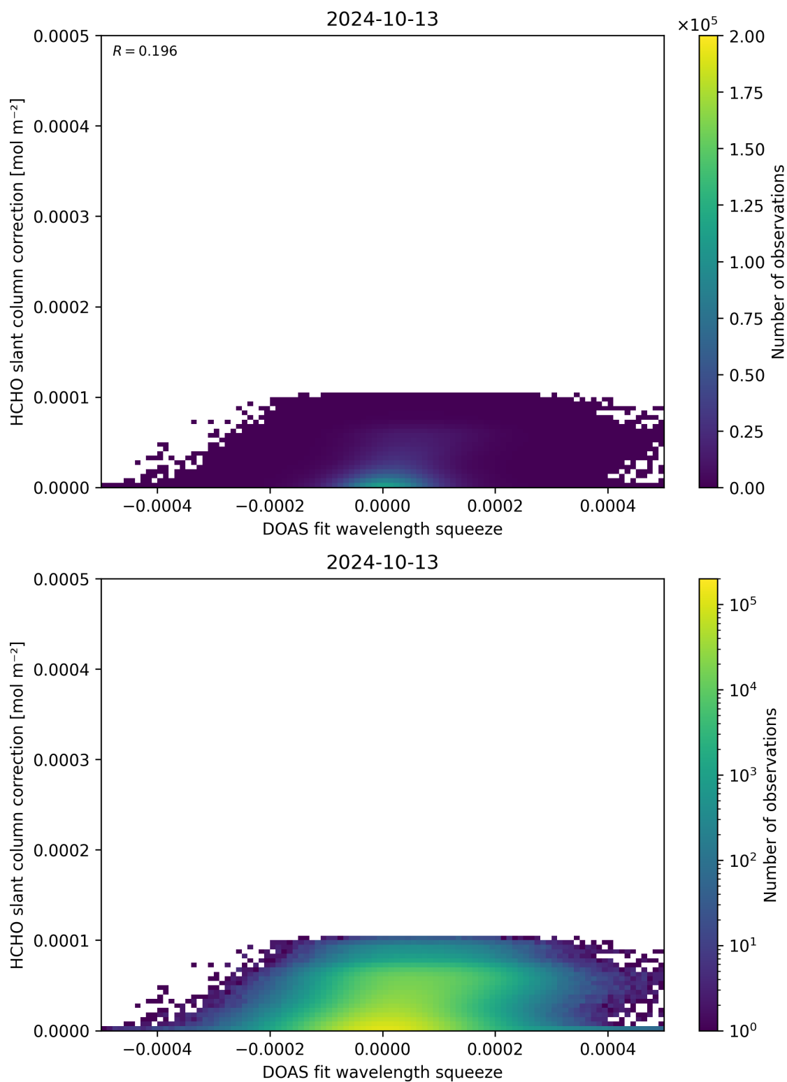
Figure 70: Scatter density plot of “DOAS fit wavelength squeeze” against “HCHO slant column correction” for 2024-10-12 to 2024-10-14.
