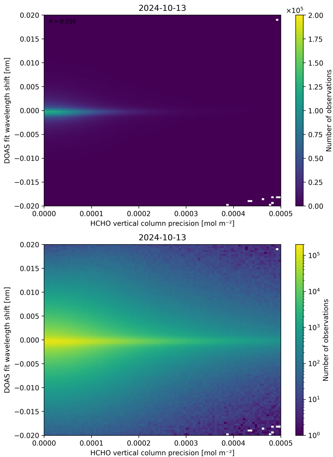
Figure 137: Scatter density plot of “HCHO vertical column precision” against “DOAS fit wavelength shift” for 2024-10-12 to 2024-10-14.
