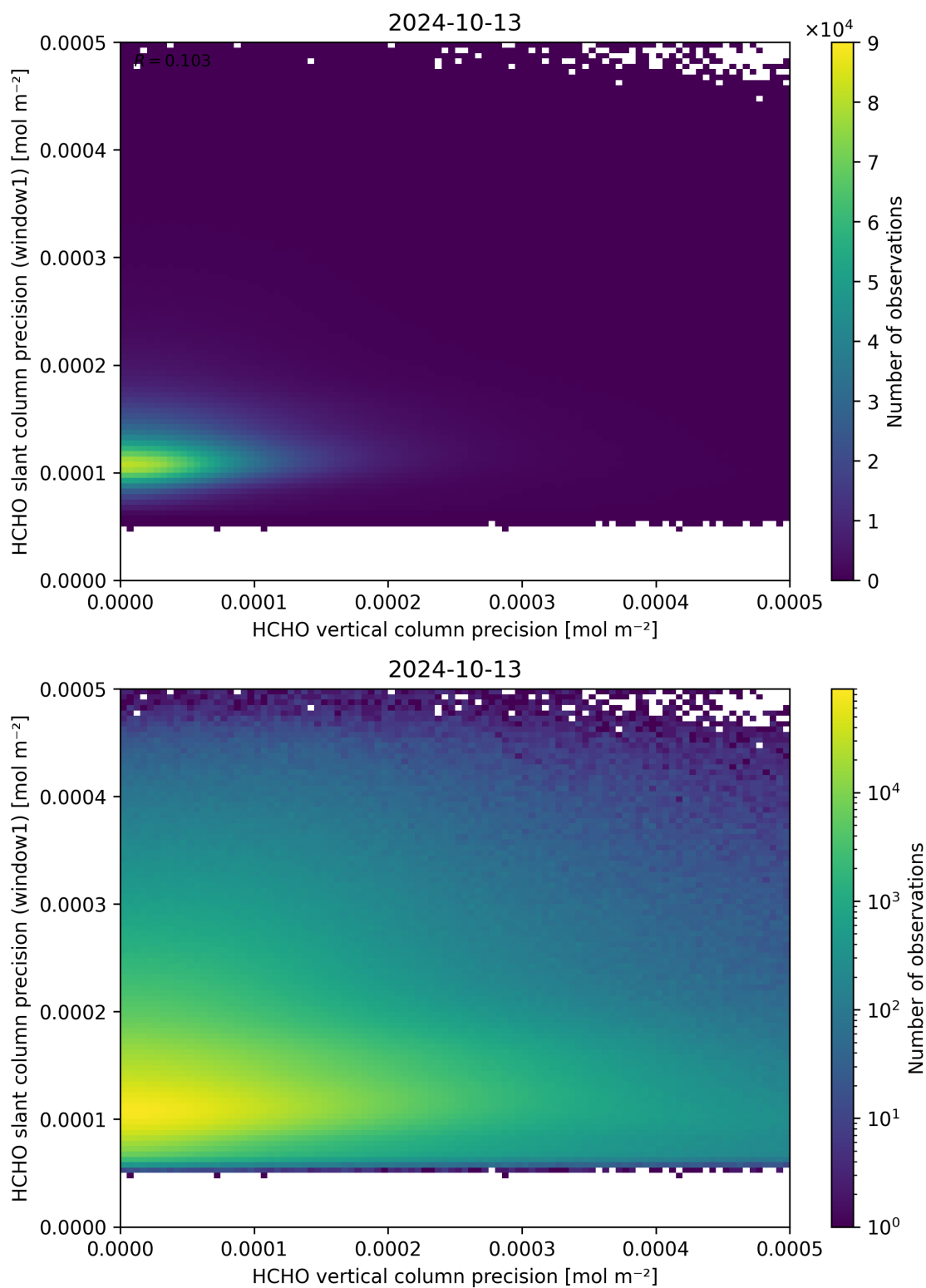
Figure 143: Scatter density plot of “HCHO vertical column precision” against “HCHO slant column precision (window1)” for 2024-10-12 to 2024-10-14.
