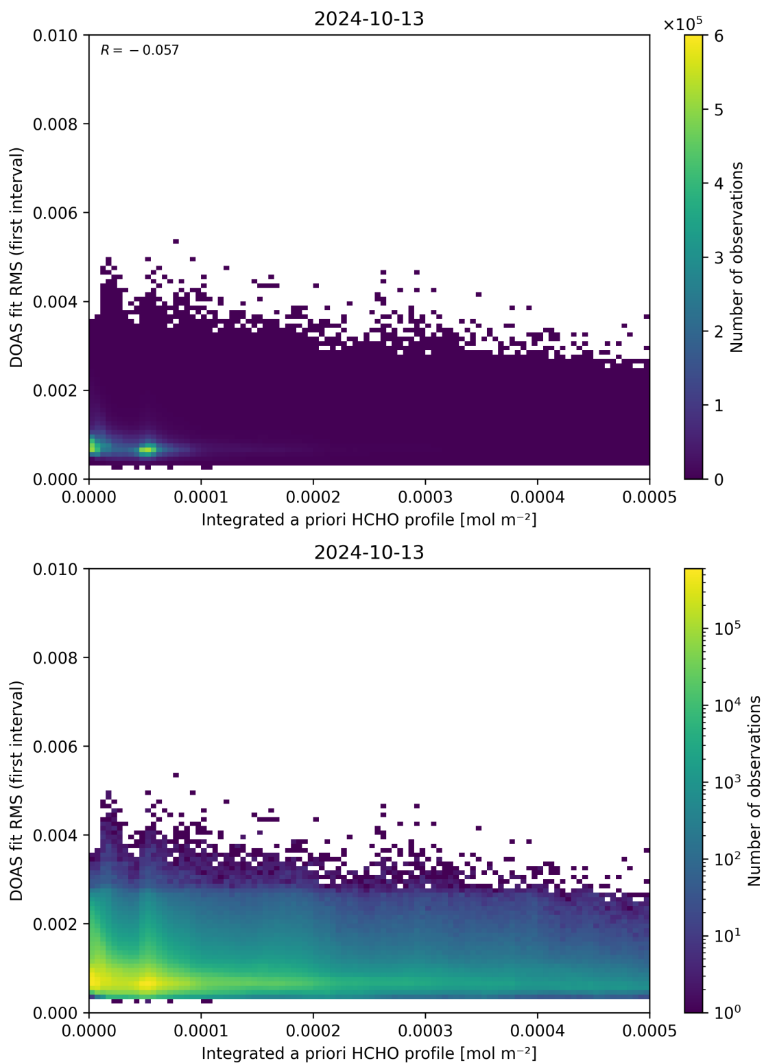
Figure 148: Scatter density plot of “Integrated a priori HCHO profile” against “DOAS fit RMS (first interval)” for 2024-10-12 to 2024-10-14.
