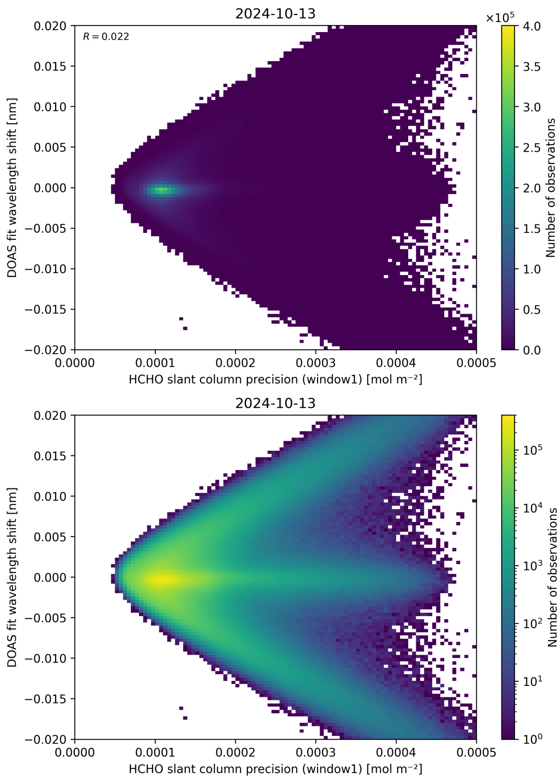
Figure 89: Scatter density plot of “HCHO slant column precision (window1)” against “DOAS fit wavelength shift” for 2024-10-12 to 2024-10-14.
