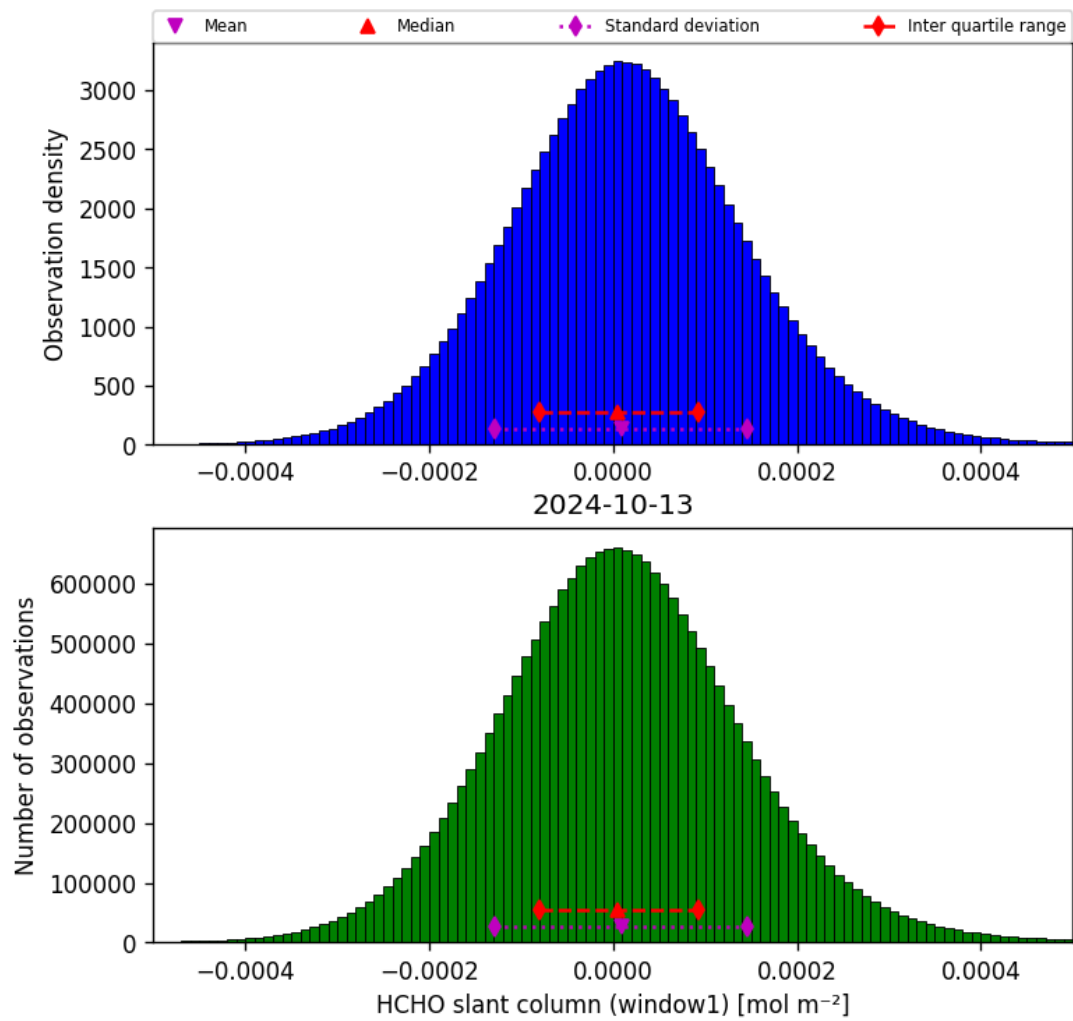
Figure 38: Histogram of “HCHO slant column (window1)” for 2024-10-12 to 2024-10-14
