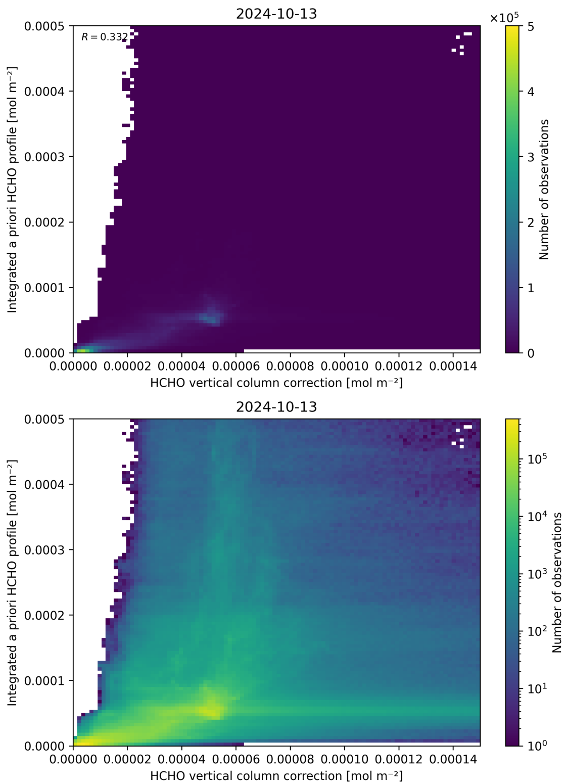
Figure 122: Scatter density plot of “HCHO vertical column correction” against “Integrated a priori HCHO profile” for 2024-10-12 to 2024-10-14.
