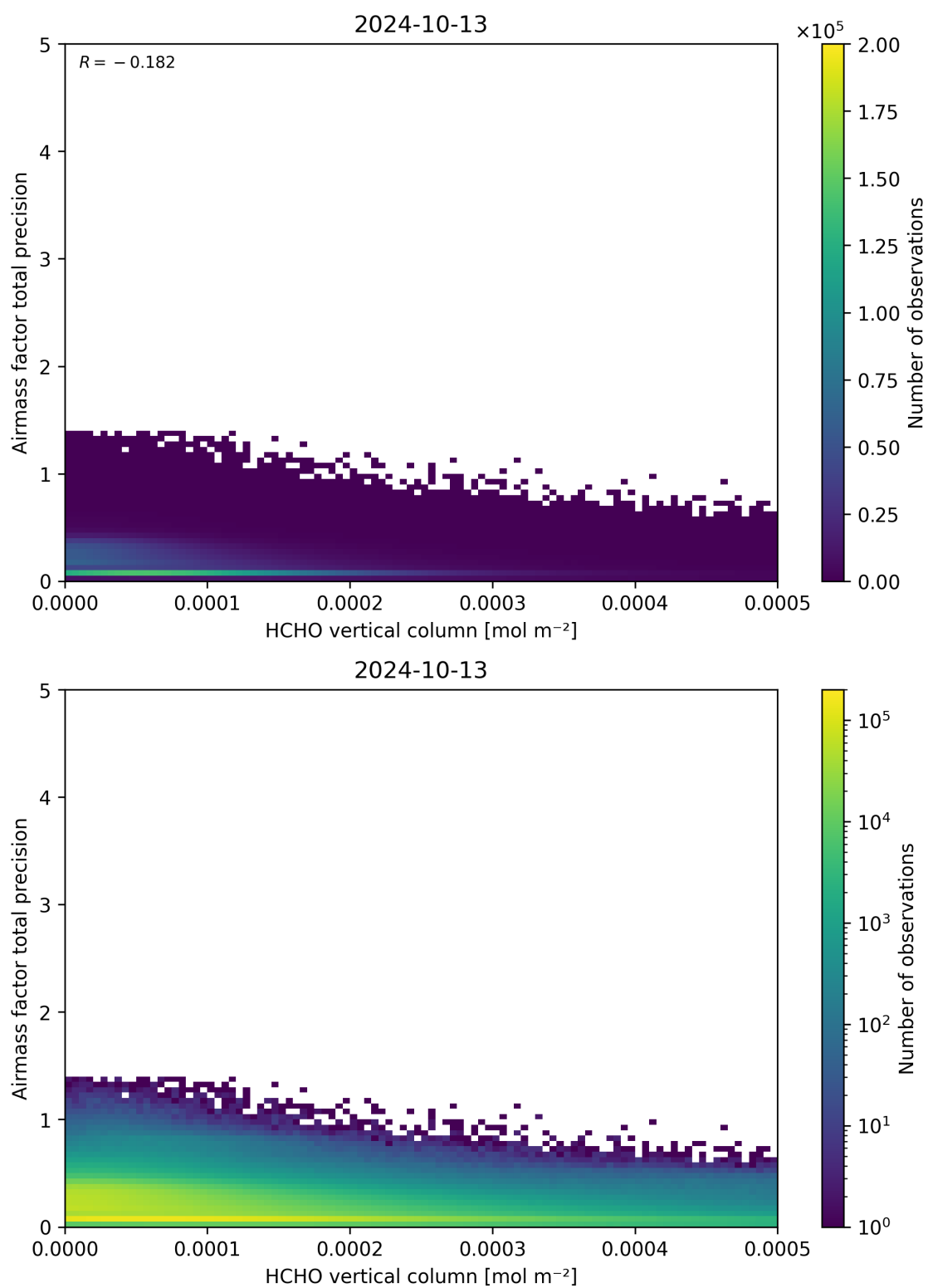
Figure 132: Scatter density plot of “HCHO vertical column” against “Airmass factor total precision” for 2024-10-12 to 2024-10-14.
