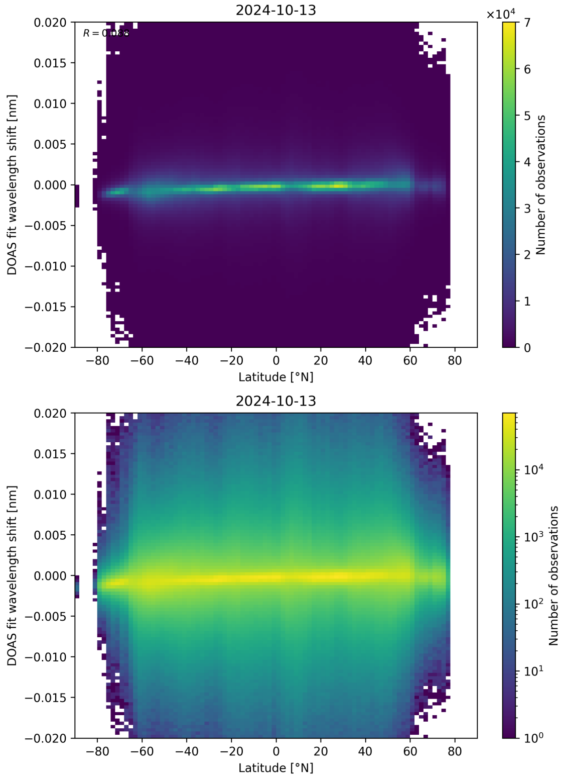
Figure 154: Scatter density plot of “Latitude” against “DOAS fit wavelength shift” for 2024-10-12 to 2024-10-14.
