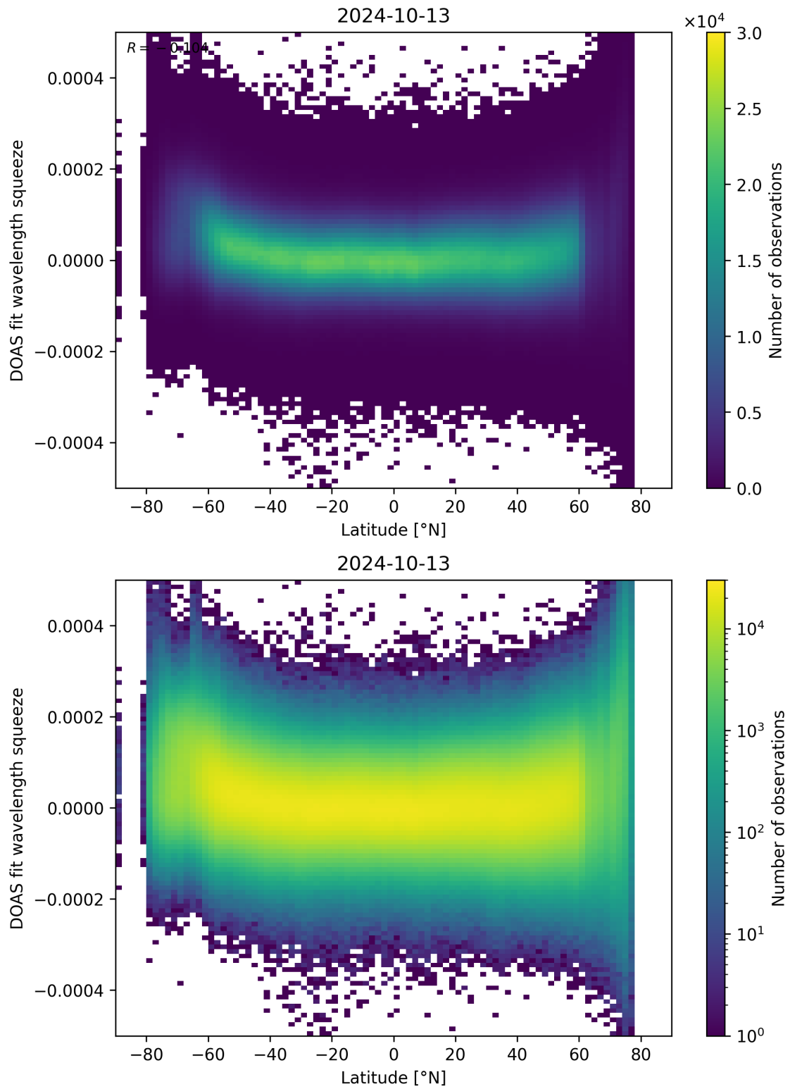
Figure 155: Scatter density plot of “Latitude” against “DOAS fit wavelength squeeze” for 2024-10-12 to 2024-10-14.
