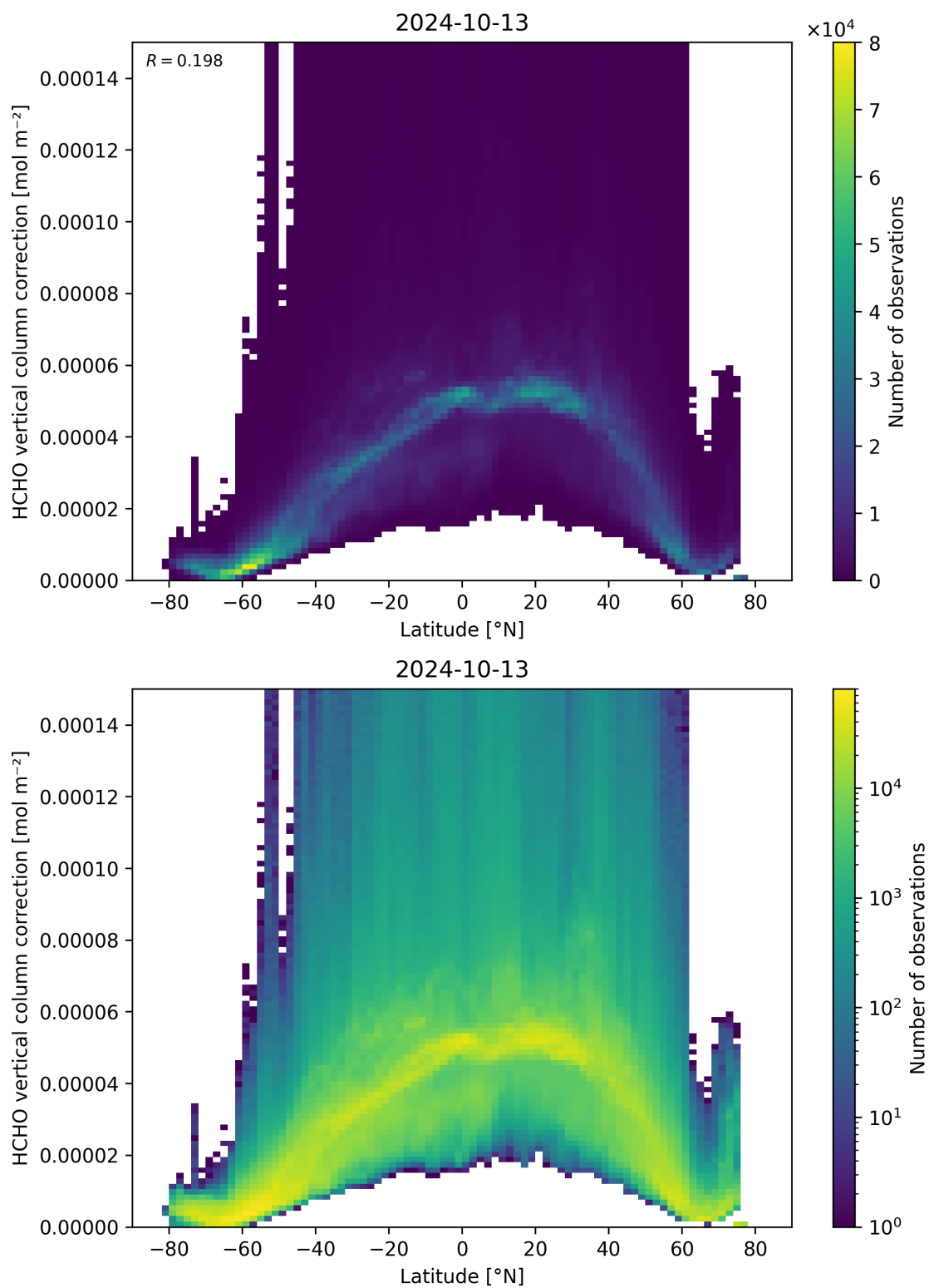
Figure 164: Scatter density plot of “Latitude” against “HCHO vertical column correction” for 2024-10-12 to 2024-10-14.
