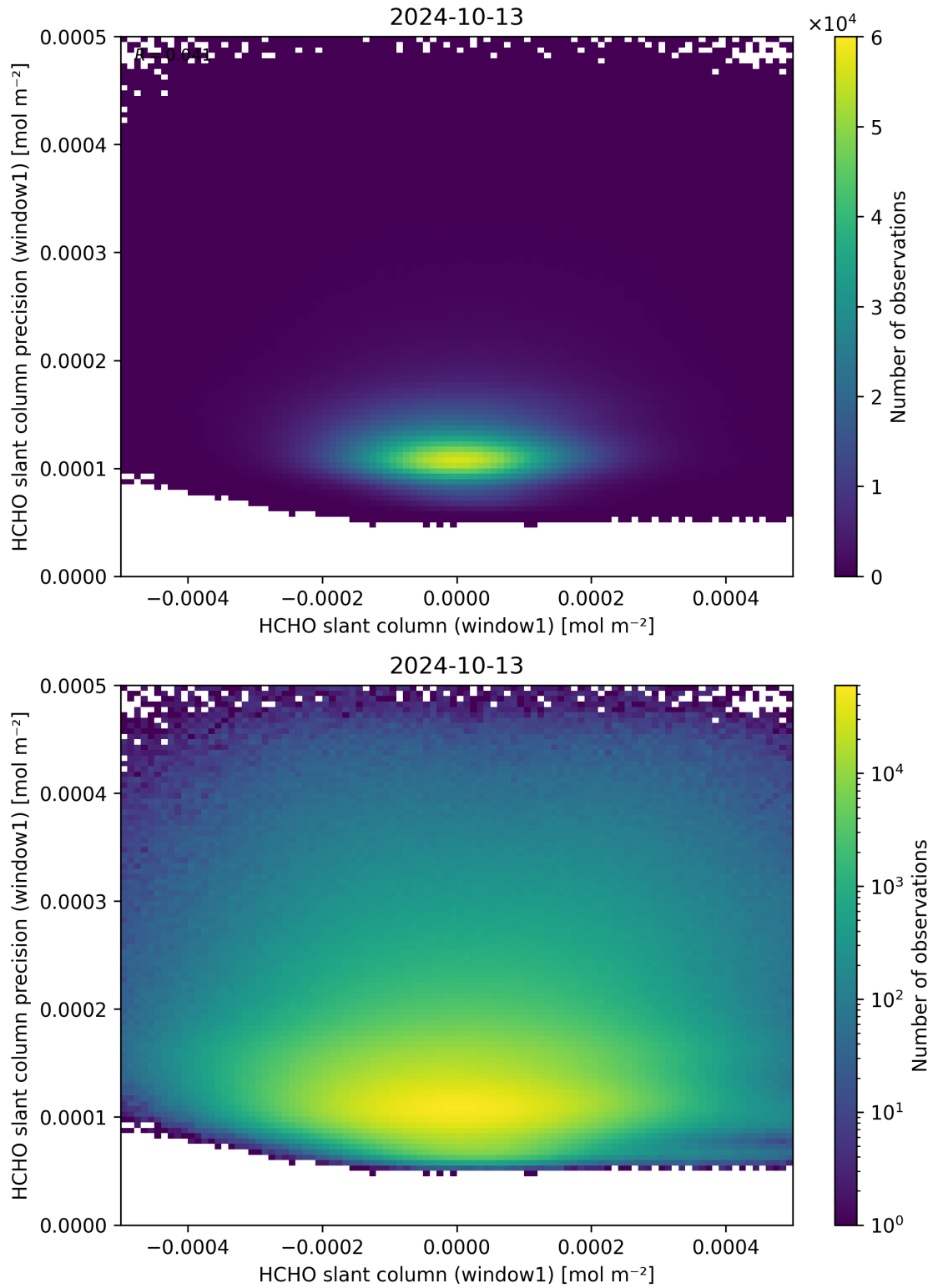
Figure 84: Scatter density plot of “HCHO slant column (window1)” against “HCHO slant column precision (window1)” for 2024-10-12 to 2024-10-14.
