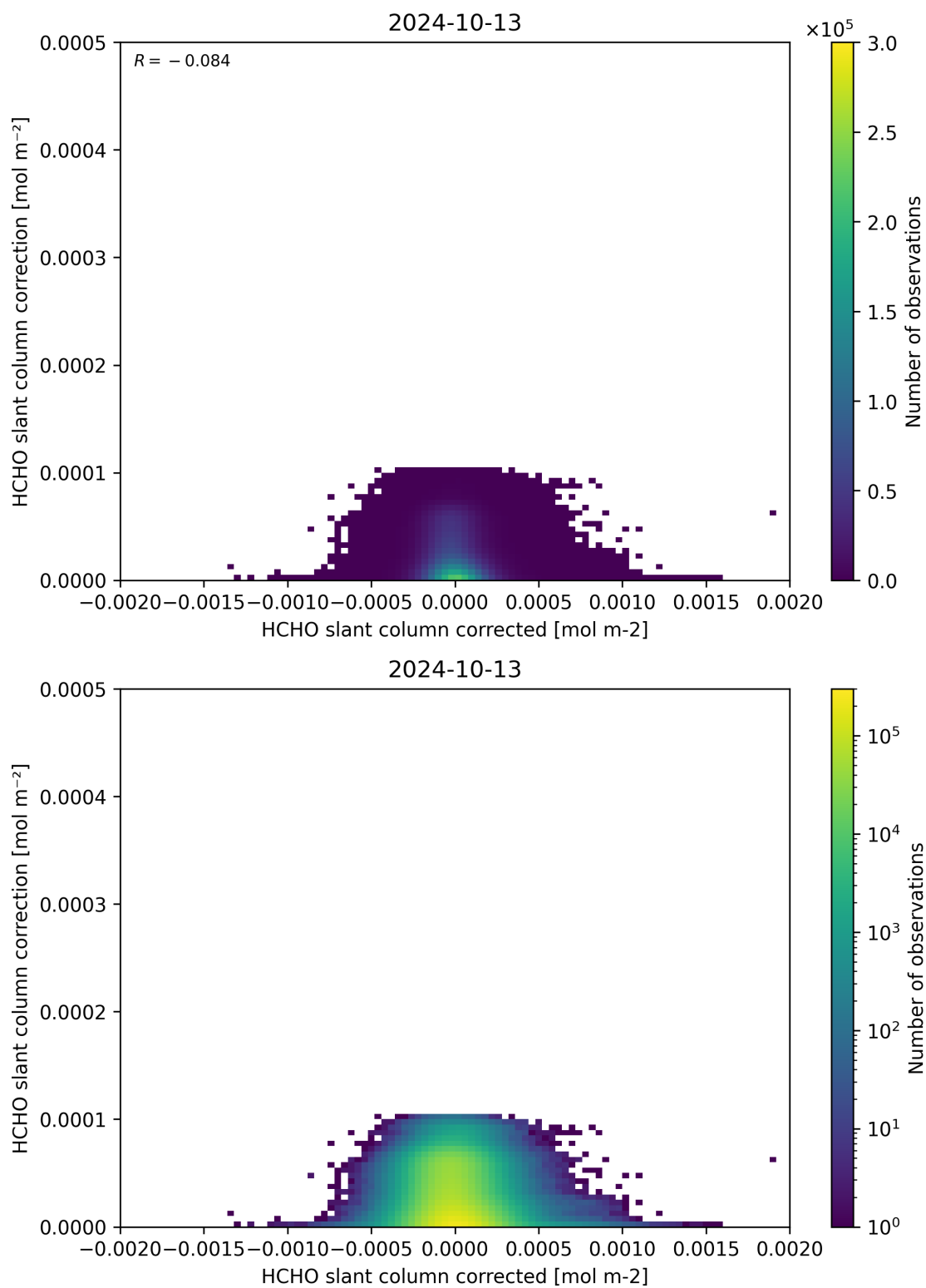
Figure 77: Scatter density plot of “HCHO slant column corrected” against “HCHO slant column correction” for 2024-10-12 to 2024-10-14.
