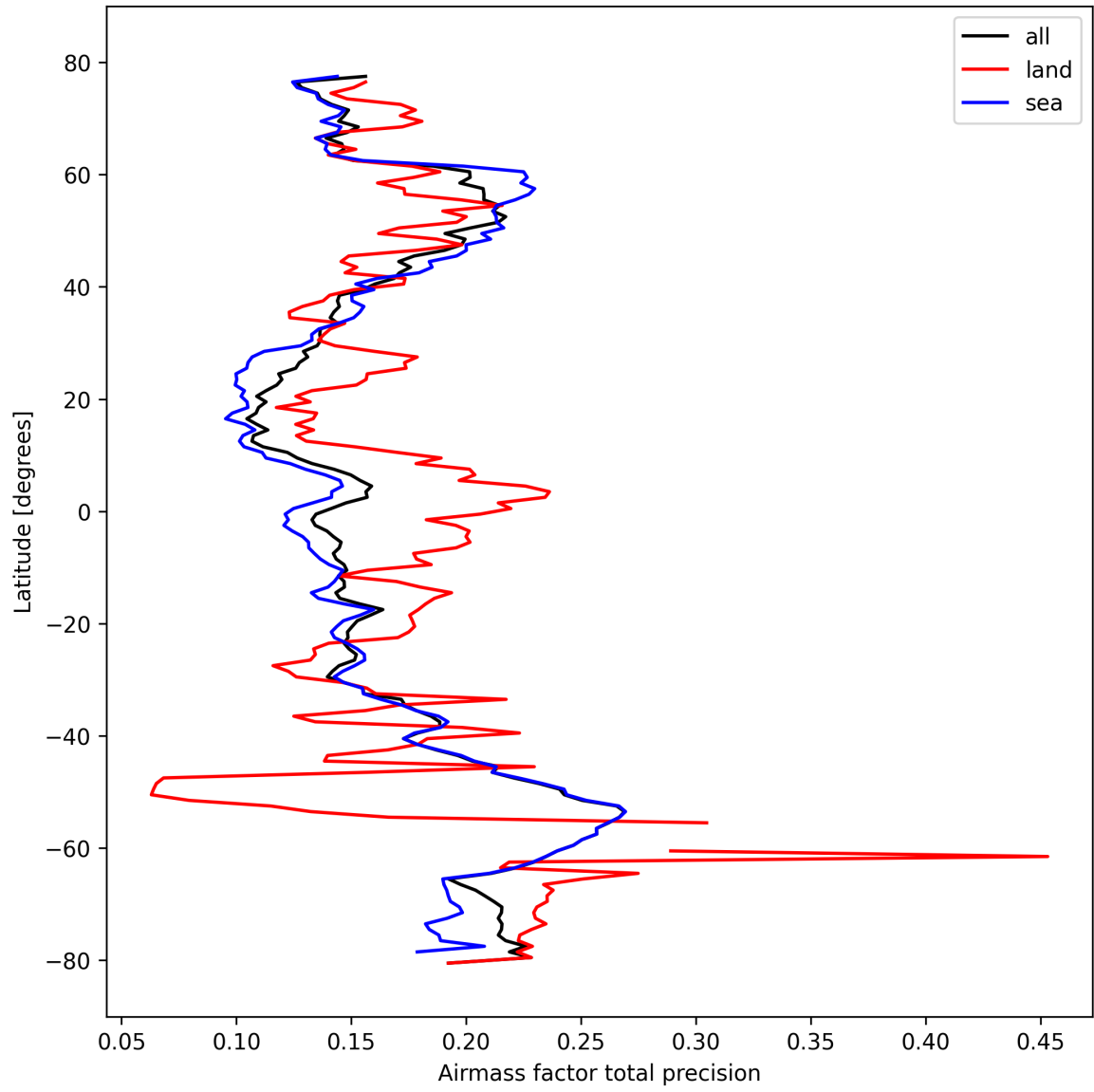
Figure 27: Zonal average of “Airmass factor total precision” for 2024-10-12 to 2024-10-14.
