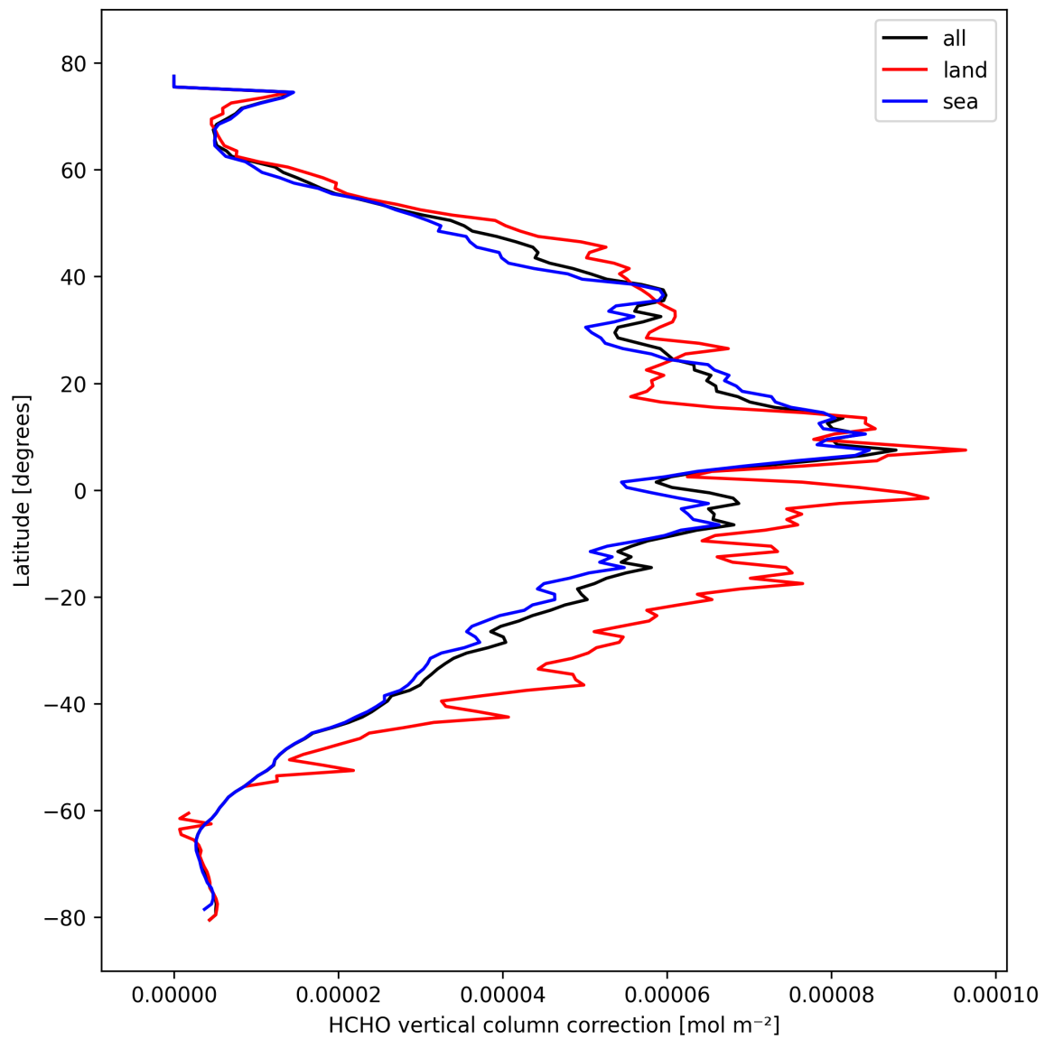
Figure 23: Zonal average of “HCHO vertical column correction” for 2024-10-12 to 2024-10-14.
