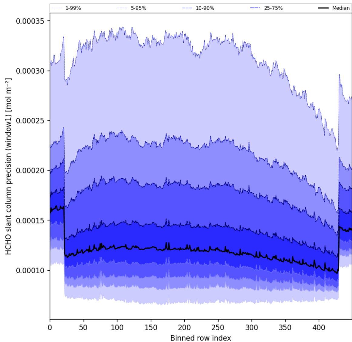
Figure 53: Along track statistics of “HCHO slant column precision (window1)” for 2024-10-12 to 2024-10-14
