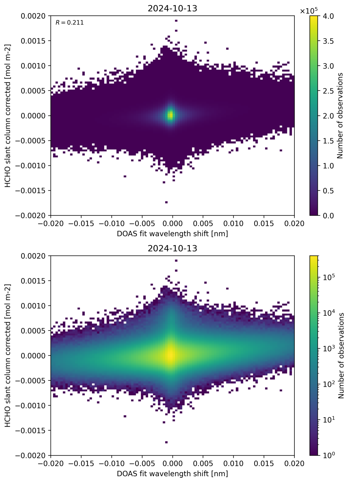
Figure 66: Scatter density plot of “DOAS fit wavelength shift” against “HCHO slant column corrected” for 2024-10-12 to 2024-10-14.
