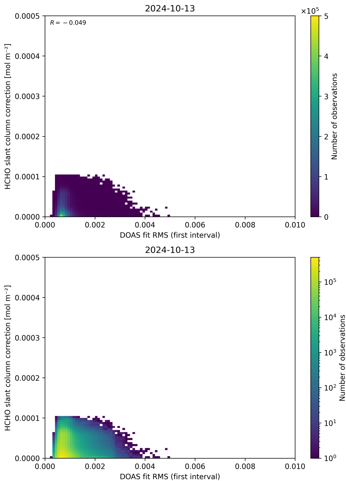
Figure 63: Scatter density plot of “DOAS fit RMS (first interval)” against “HCHO slant column correction” for 2024-10-12 to 2024-10-14.
