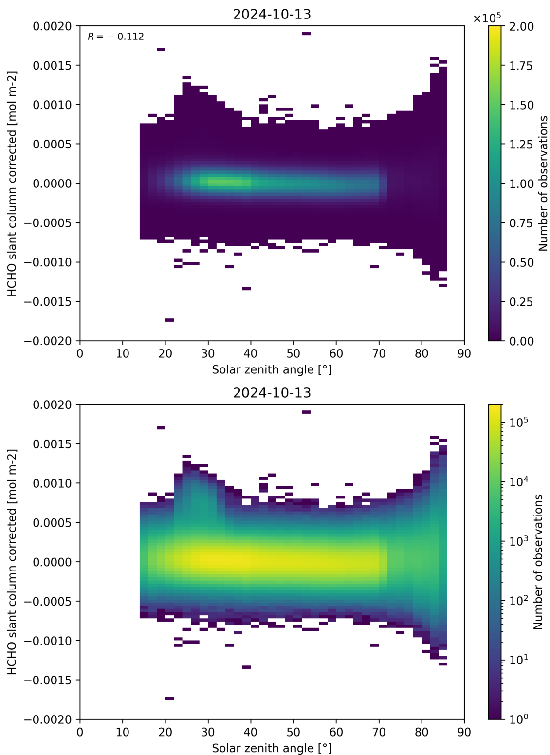
Figure 171: Scatter density plot of “Solar zenith angle” against “HCHO slant column corrected” for 2024-10-12 to 2024-10-14.
