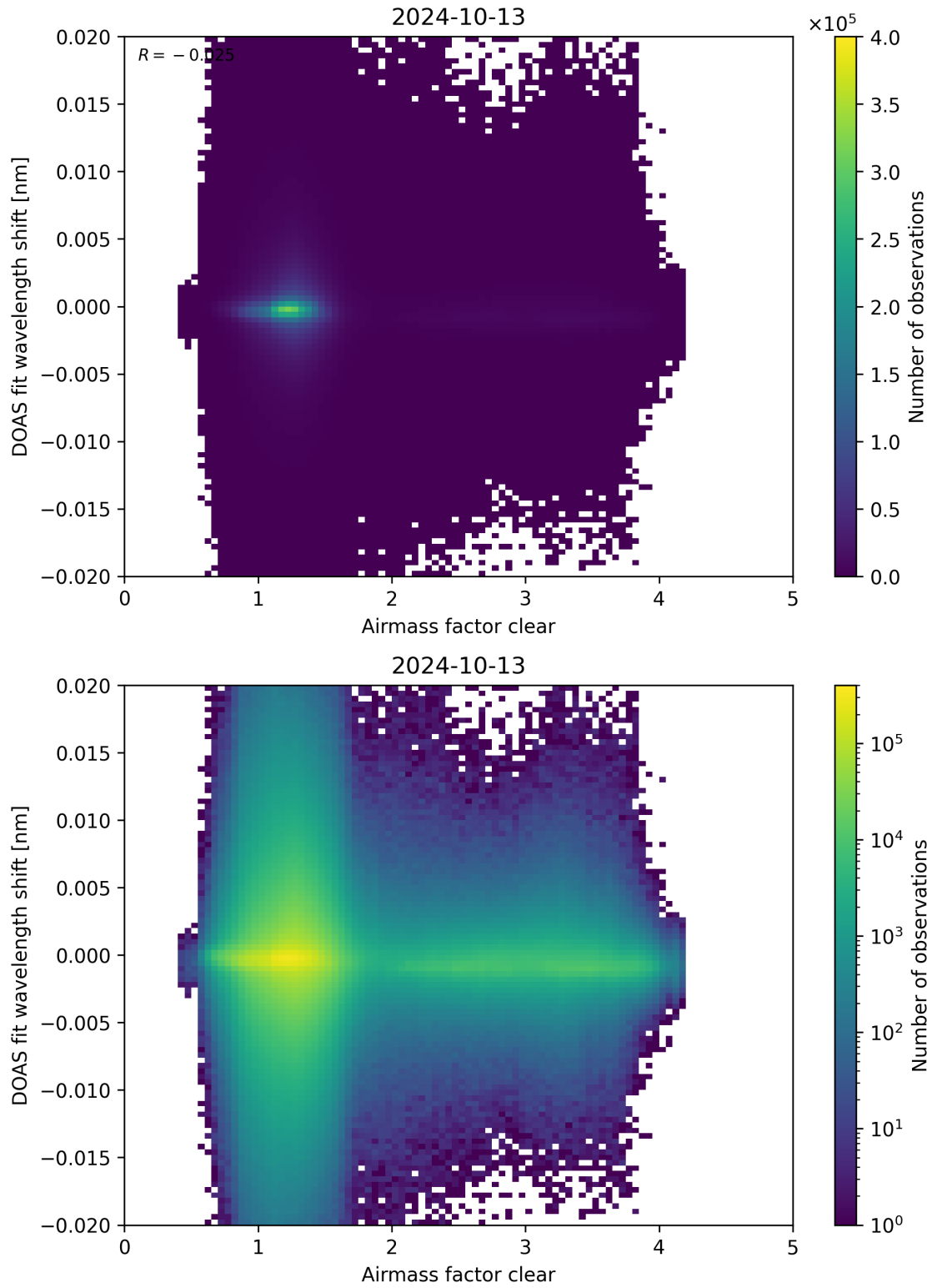
Figure 72: Scatter density plot of “Airmass factor clear” against “DOAS fit wavelength shift” for 2024-10-12 to 2024-10-14.
