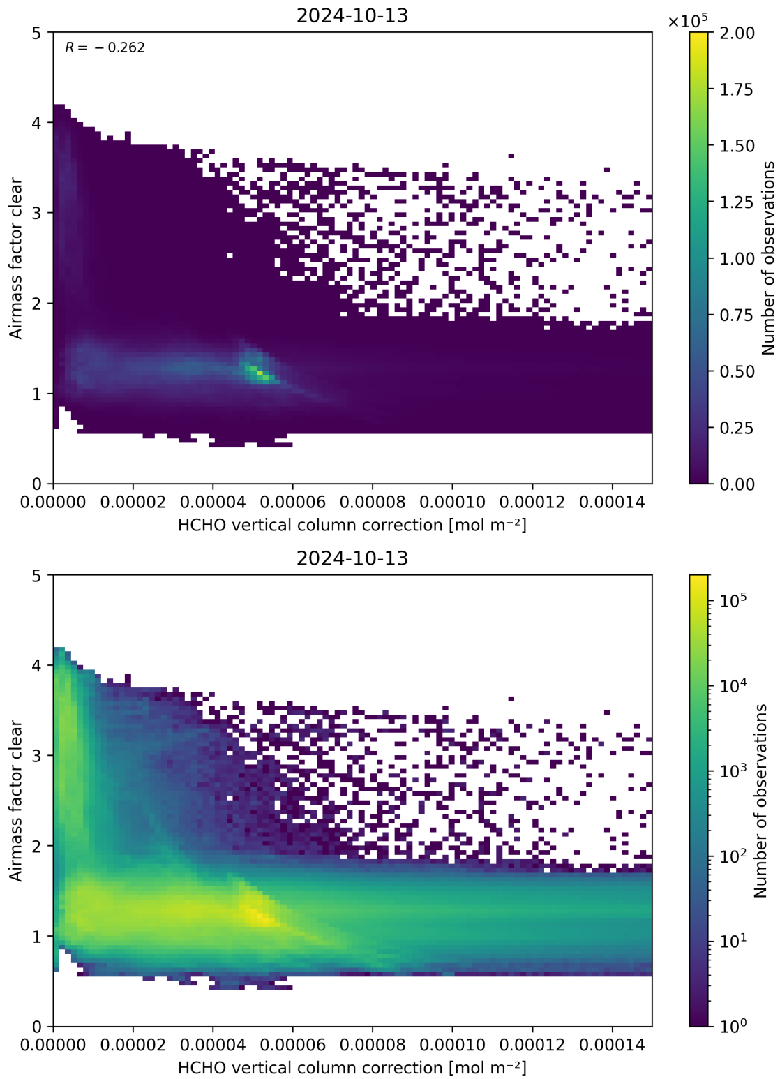
Figure 115: Scatter density plot of “HCHO vertical column correction” against “Airmass factor clear” for 2024-10-12 to 2024-10-14.
