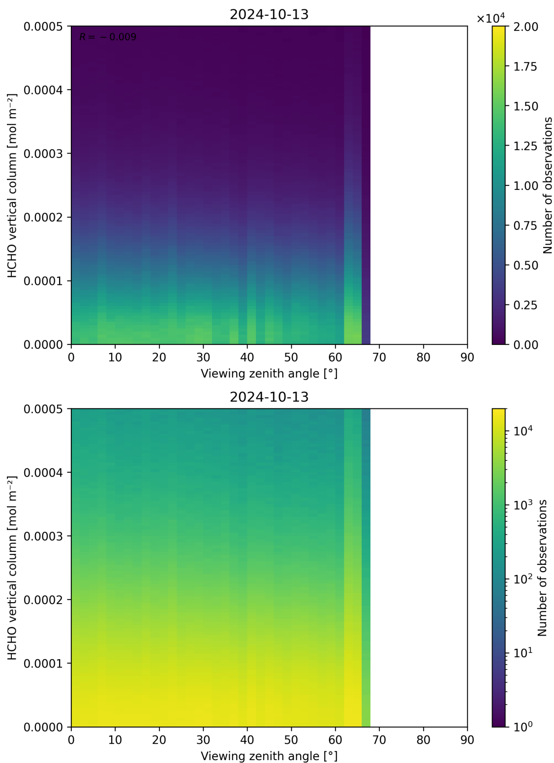
Figure 192: Scatter density plot of “Viewing zenith angle” against “HCHO vertical column” for 2024-10-12 to 2024-10-14.
