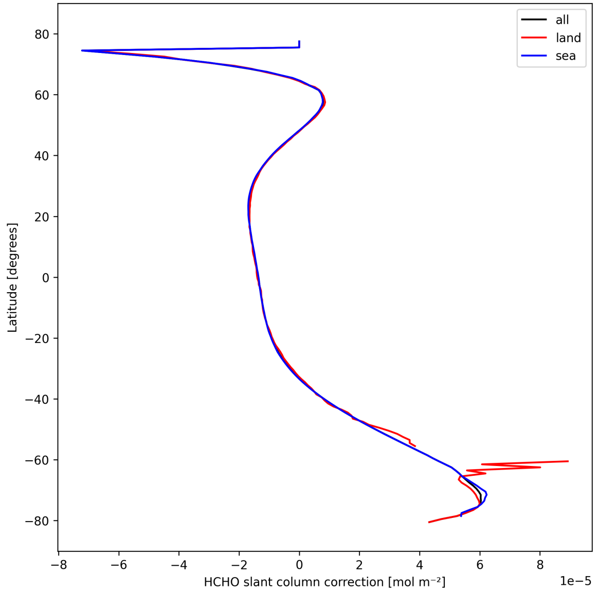
Figure 33: Zonal average of “HCHO slant column correction” for 2024-10-12 to 2024-10-14.
