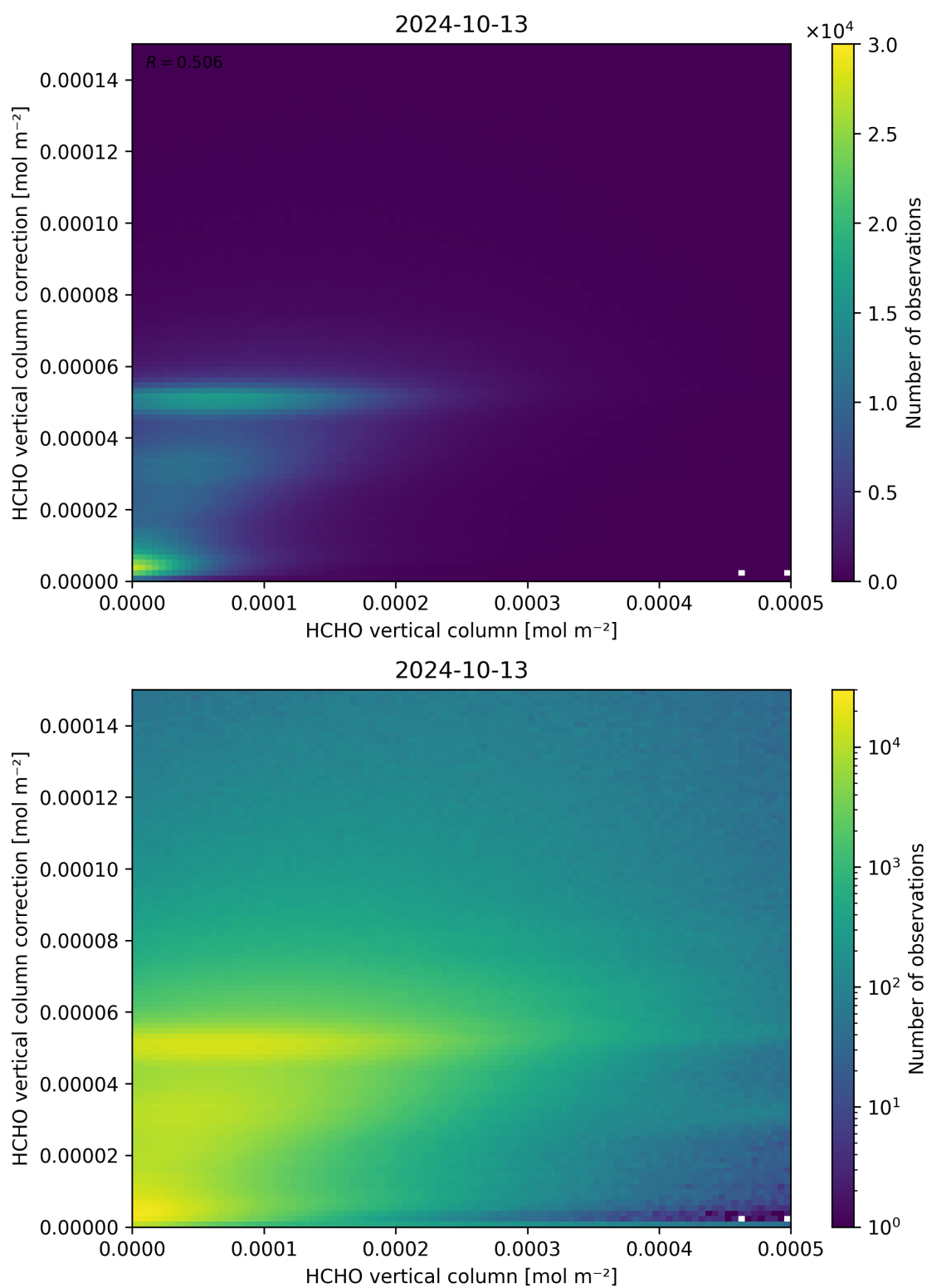
Figure 133: Scatter density plot of “HCHO vertical column” against “HCHO vertical column correction” for 2024-10-12 to 2024-10-14.
