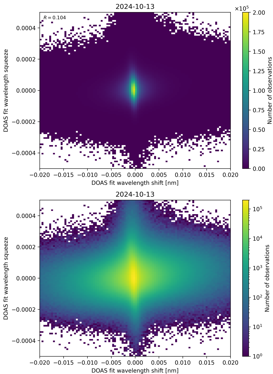
Figure 65: Scatter density plot of “DOAS fit wavelength shift” against “DOAS fit wavelength squeeze” for 2024-10-12 to 2024-10-14.
