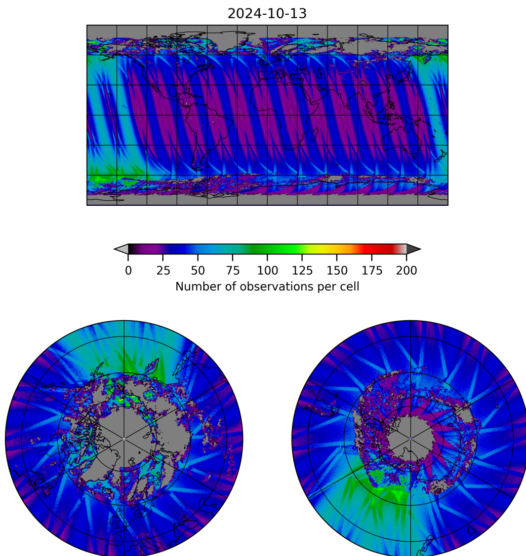
Figure 19: Map of the number of observations for 2024-10-12 to 2024-10-14
