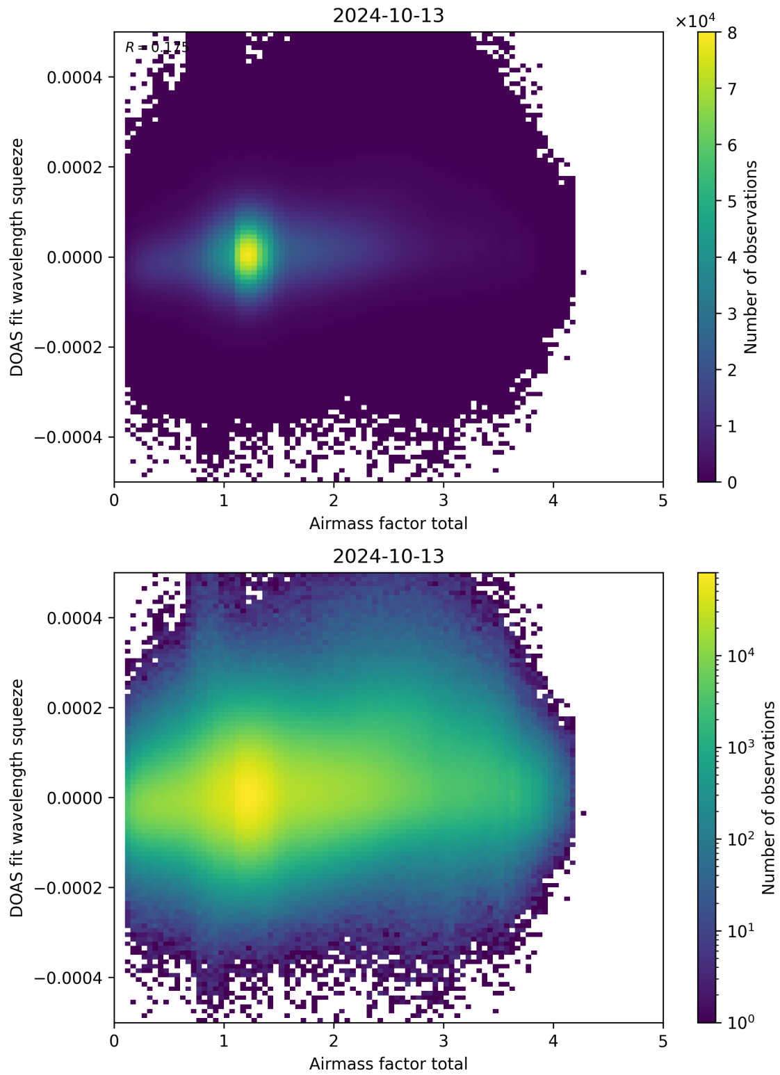
Figure 99: Scatter density plot of “Airmass factor total” against “DOAS fit wavelength squeeze” for 2024-10-12 to 2024-10-14.
