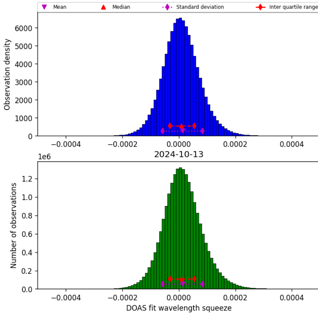
Figure 45: Histogram of “DOAS fit wavelength squeeze” for 2024-10-12 to 2024-10-14
