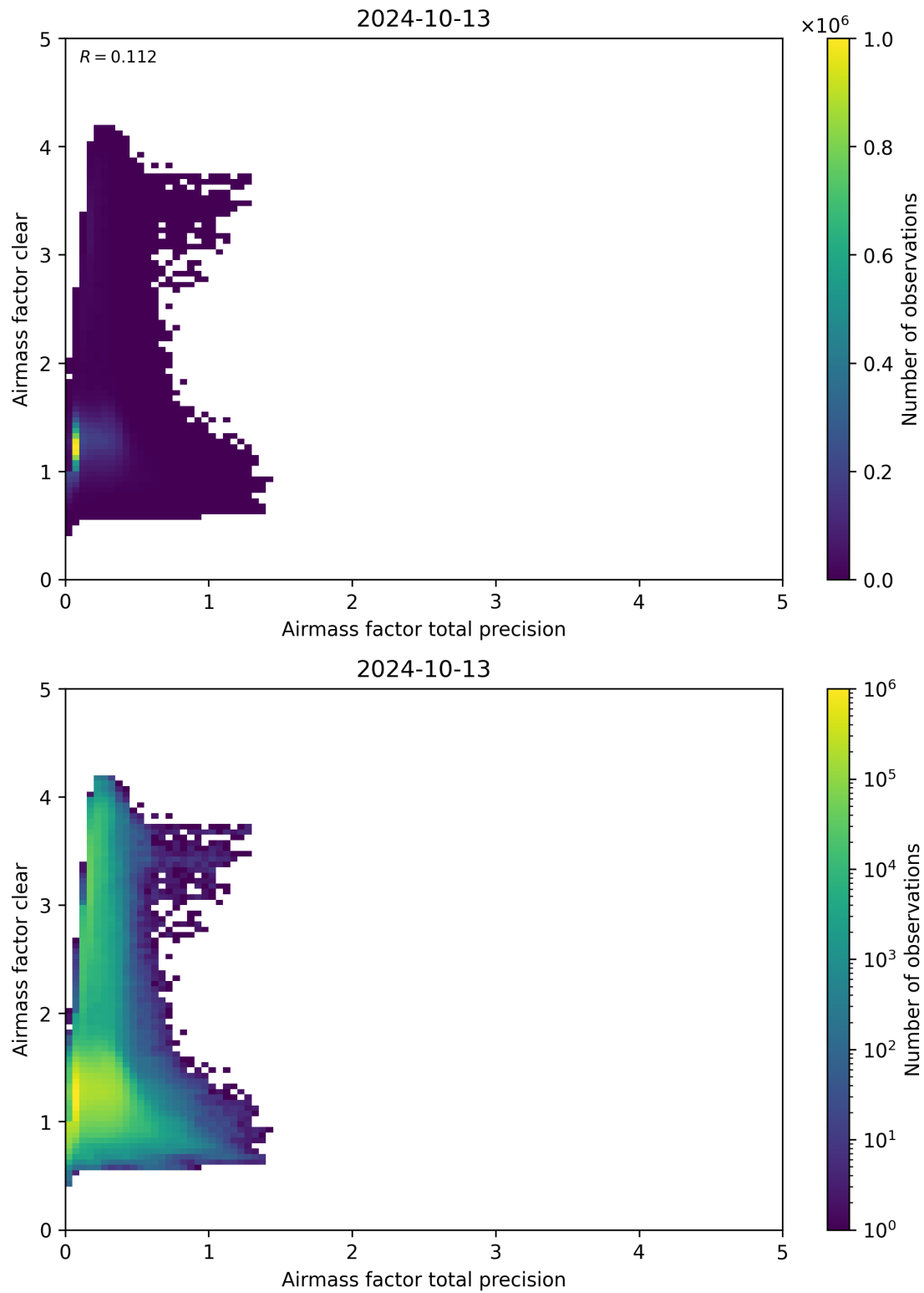
Figure 108: Scatter density plot of “Airmass factor total precision” against “Airmass factor clear” for 2024-10-12 to 2024-10-14.
