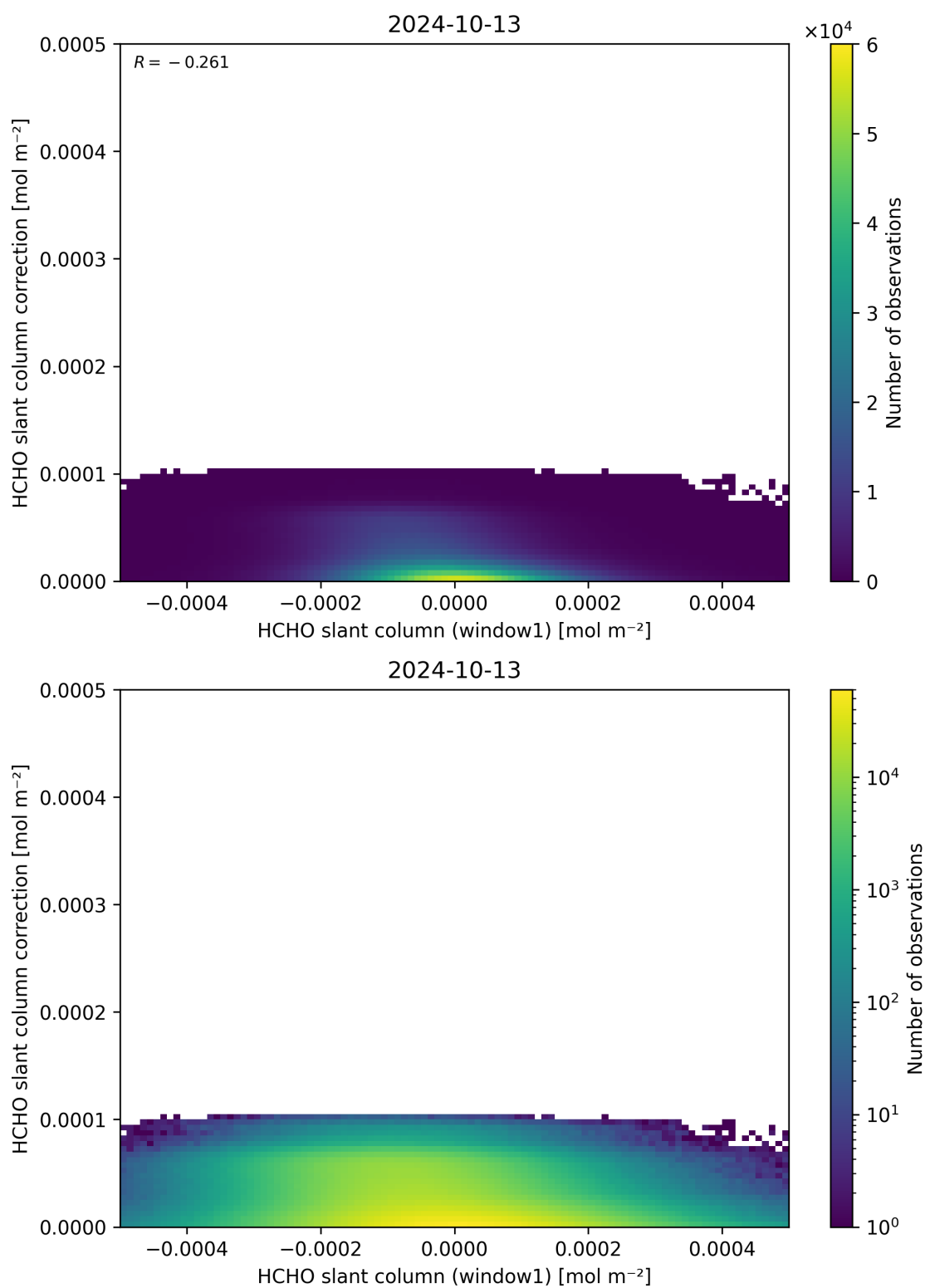
Figure 83: Scatter density plot of “HCHO slant column (window1)” against “HCHO slant column correction” for 2024-10-12 to 2024-10-14.
