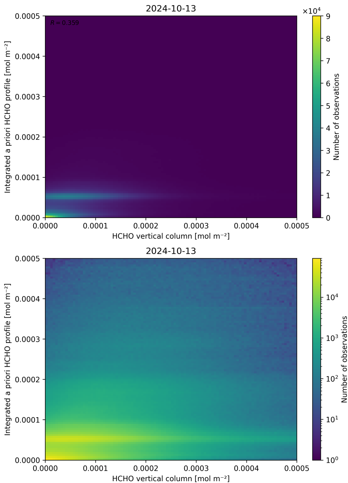
Figure 135: Scatter density plot of “HCHO vertical column” against “Integrated a priori HCHO profile” for 2024-10-12 to 2024-10-14.
