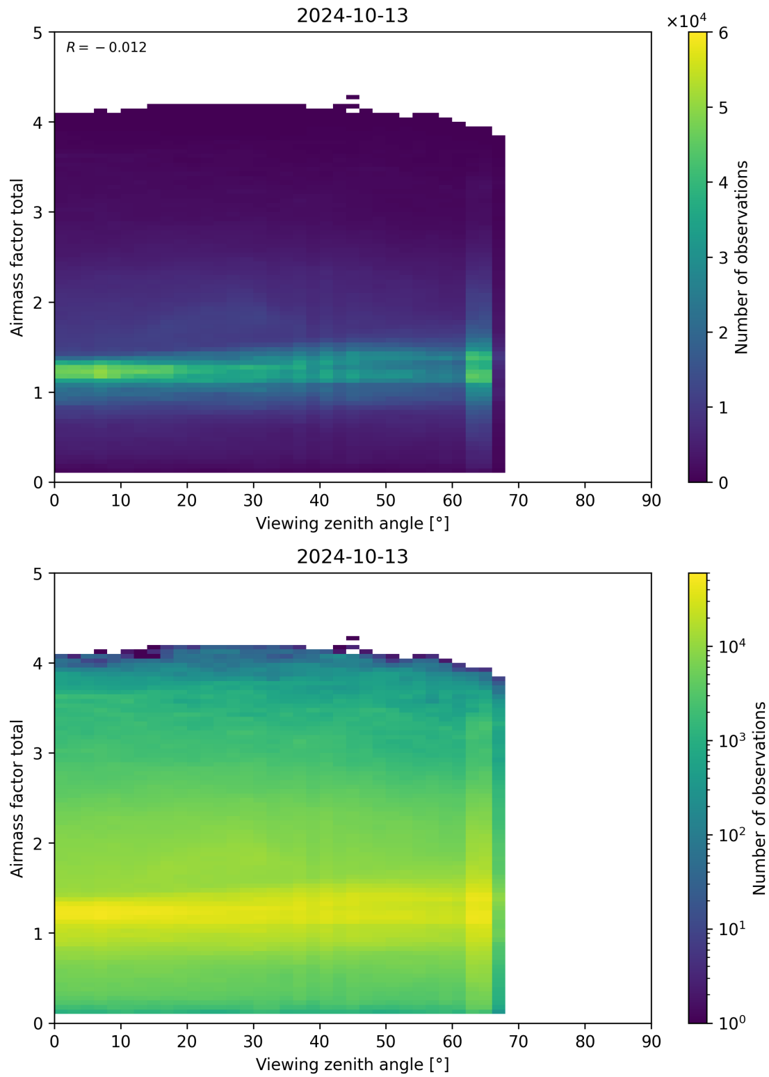
Figure 190: Scatter density plot of “Viewing zenith angle” against “Airmass factor total” for 2024-10-12 to 2024-10-14.
