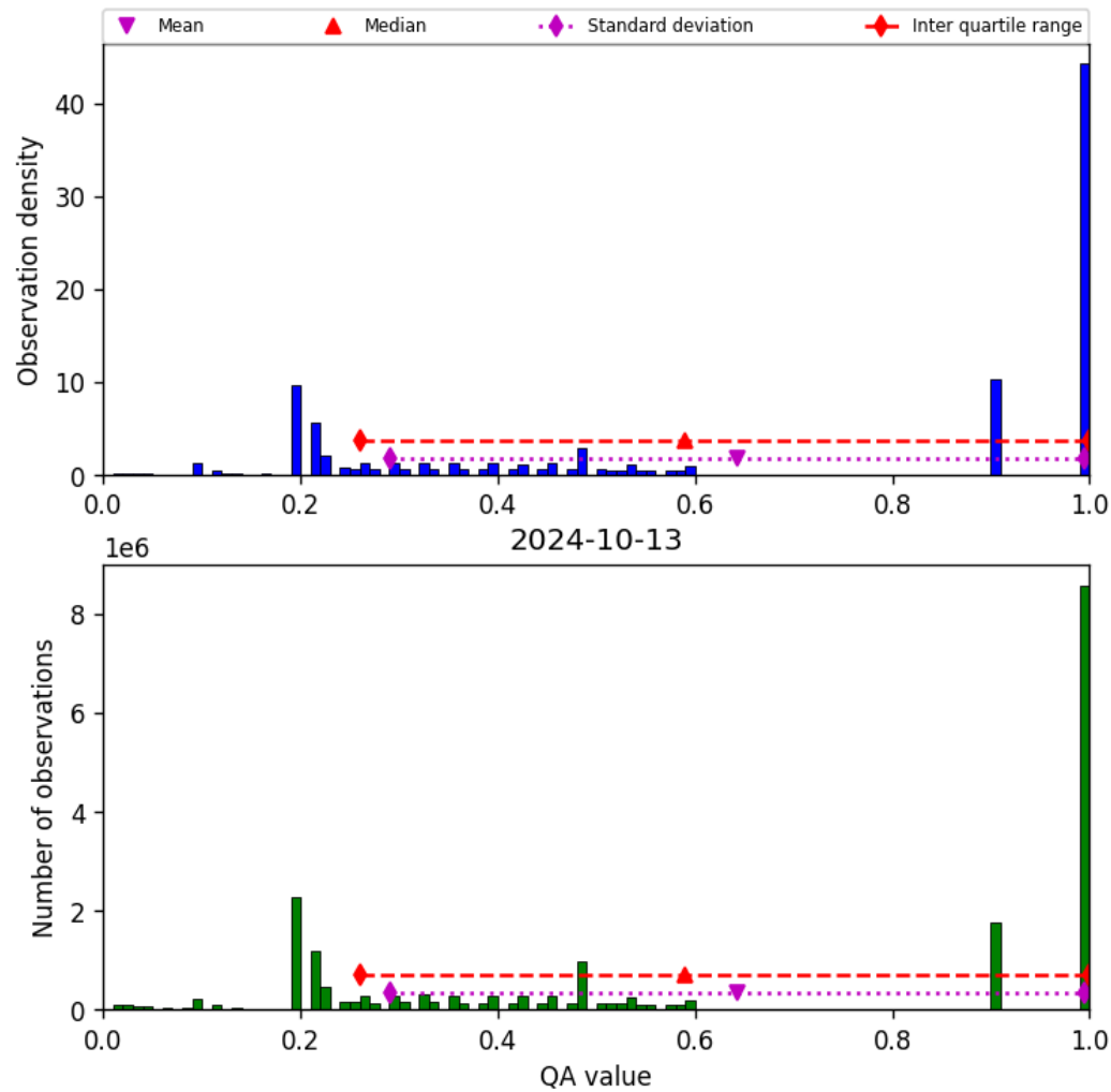
Figure 34: Histogram of “QA value” for 2024-10-12 to 2024-10-14
