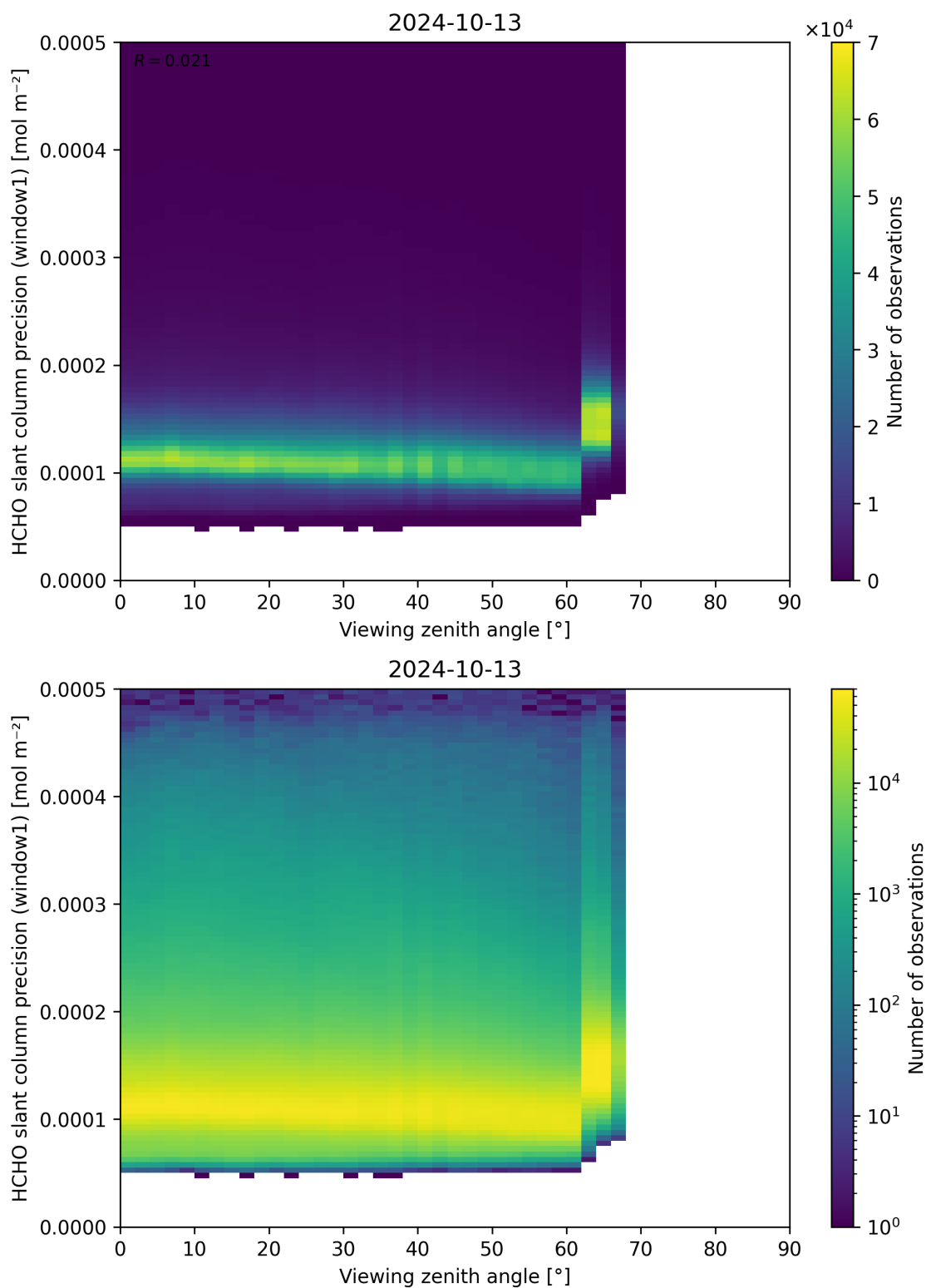
Figure 189: Scatter density plot of “Viewing zenith angle” against “HCHO slant column precision (window1)” for 2024-10-12 to 2024-10-14.
