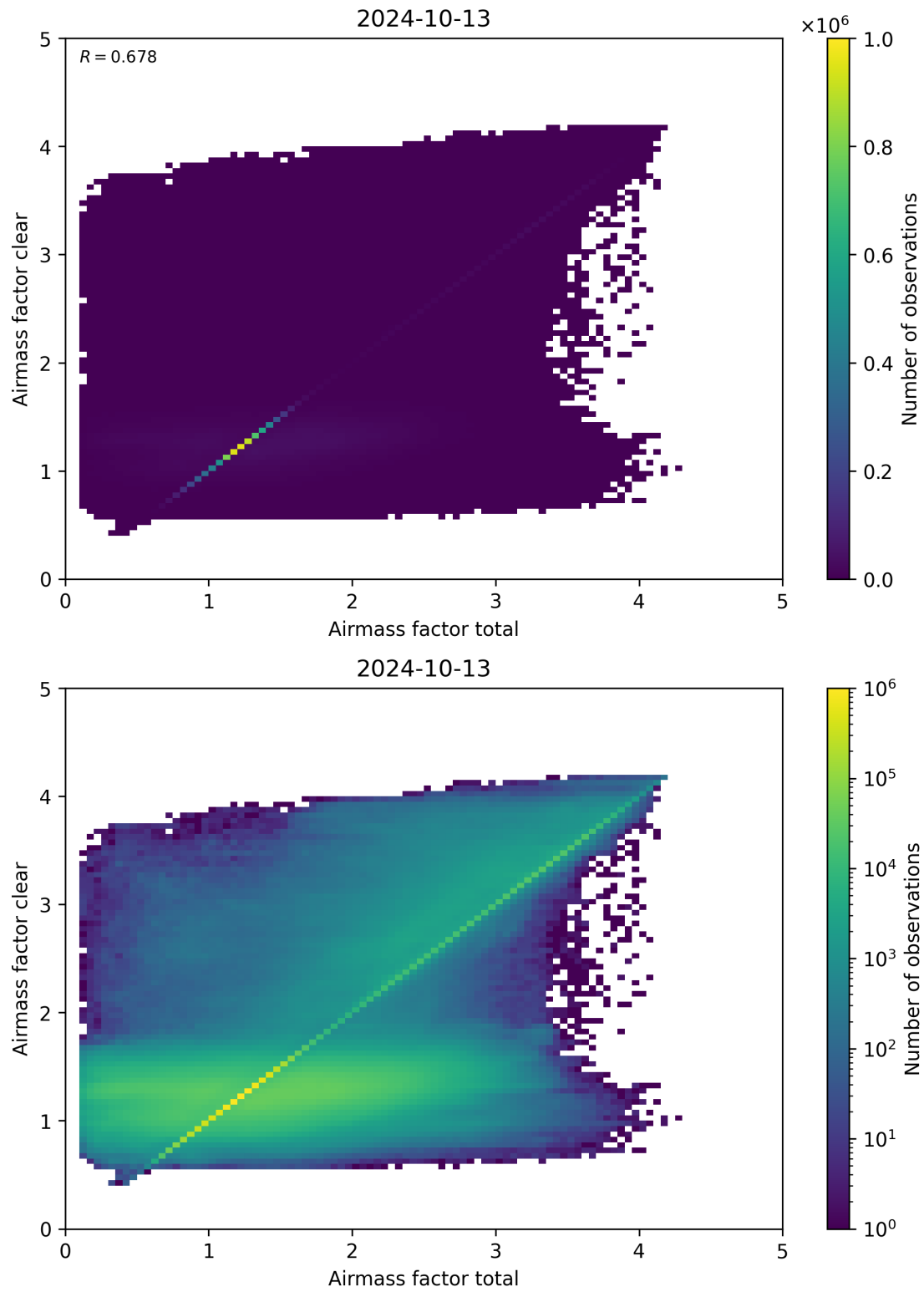
Figure 100: Scatter density plot of “Airmass factor total” against “Airmass factor clear” for 2024-10-12 to 2024-10-14.
