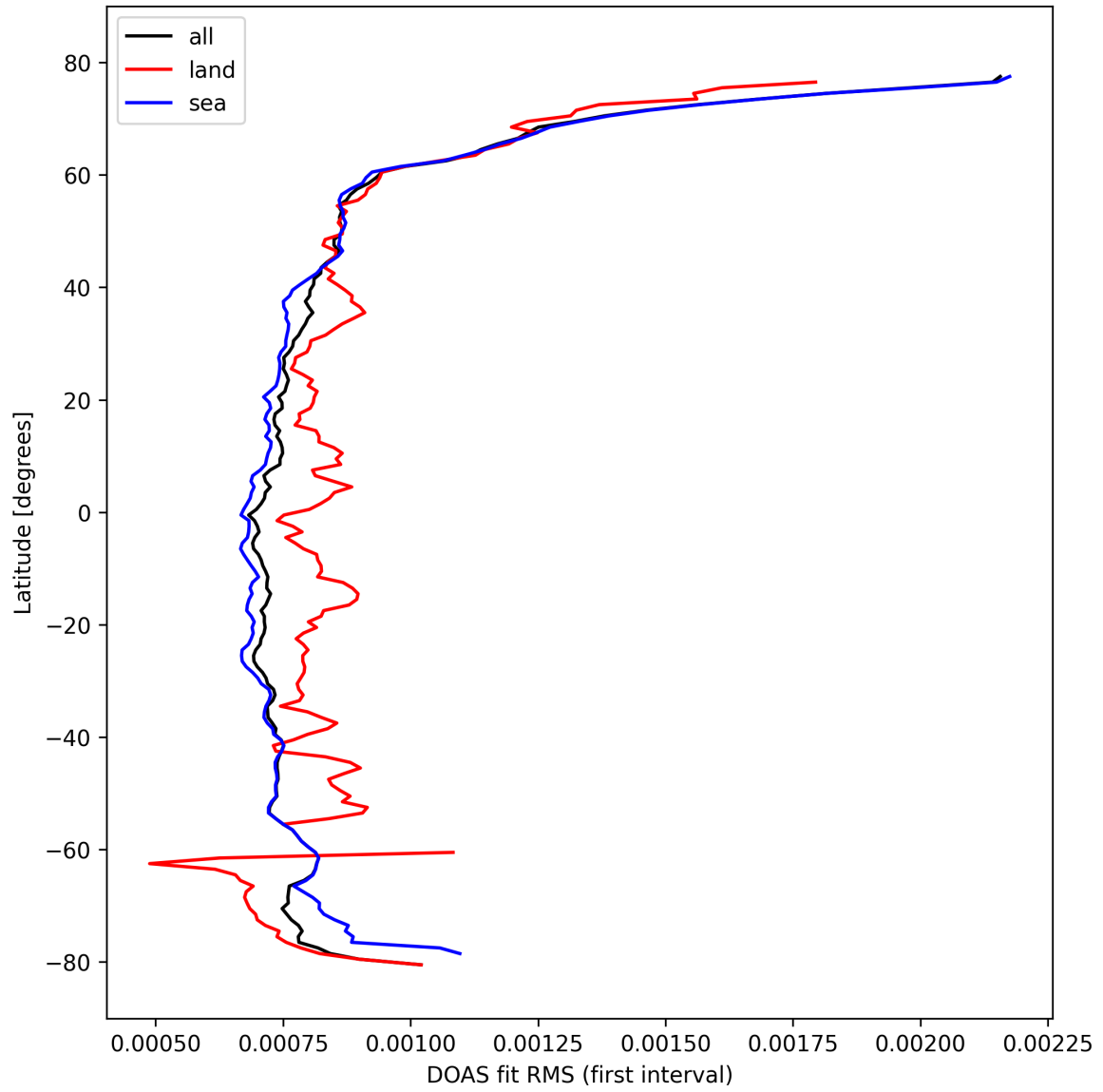
Figure 32: Zonal average of “DOAS fit RMS (first interval)” for 2024-10-12 to 2024-10-14.
