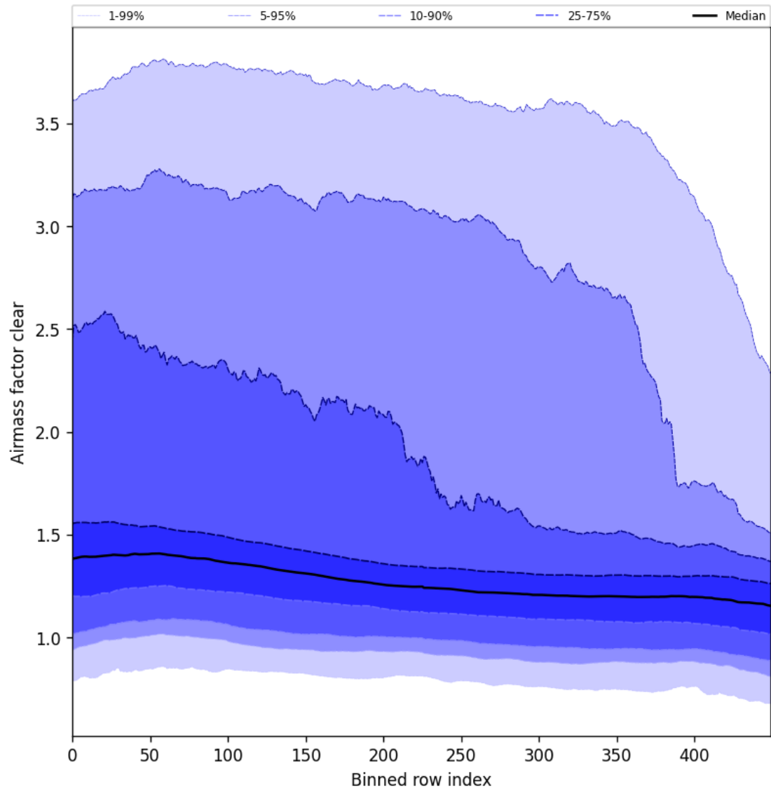
Figure 56: Along track statistics of “Airmass factor clear” for 2024-10-12 to 2024-10-14
