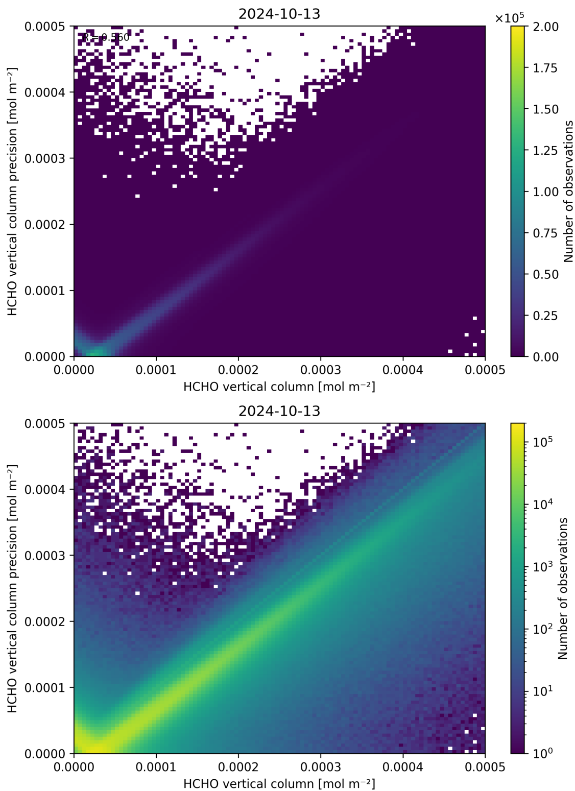
Figure 134: Scatter density plot of “HCHO vertical column” against “HCHO vertical column precision” for 2024-10-12 to 2024-10-14.
