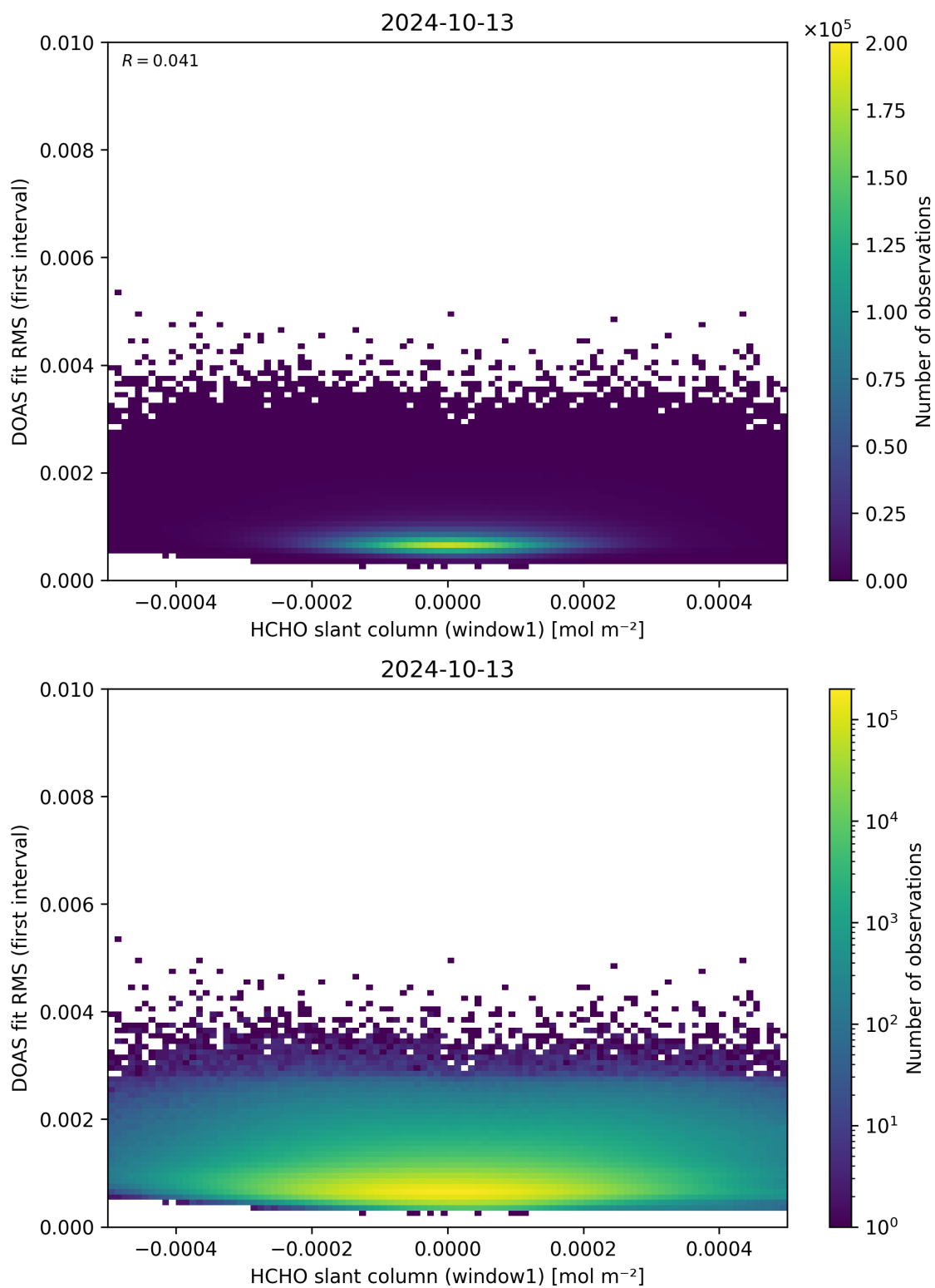
Figure 78: Scatter density plot of “HCHO slant column (window1)” against “DOAS fit RMS (first interval)” for 2024-10-12 to 2024-10-14.
