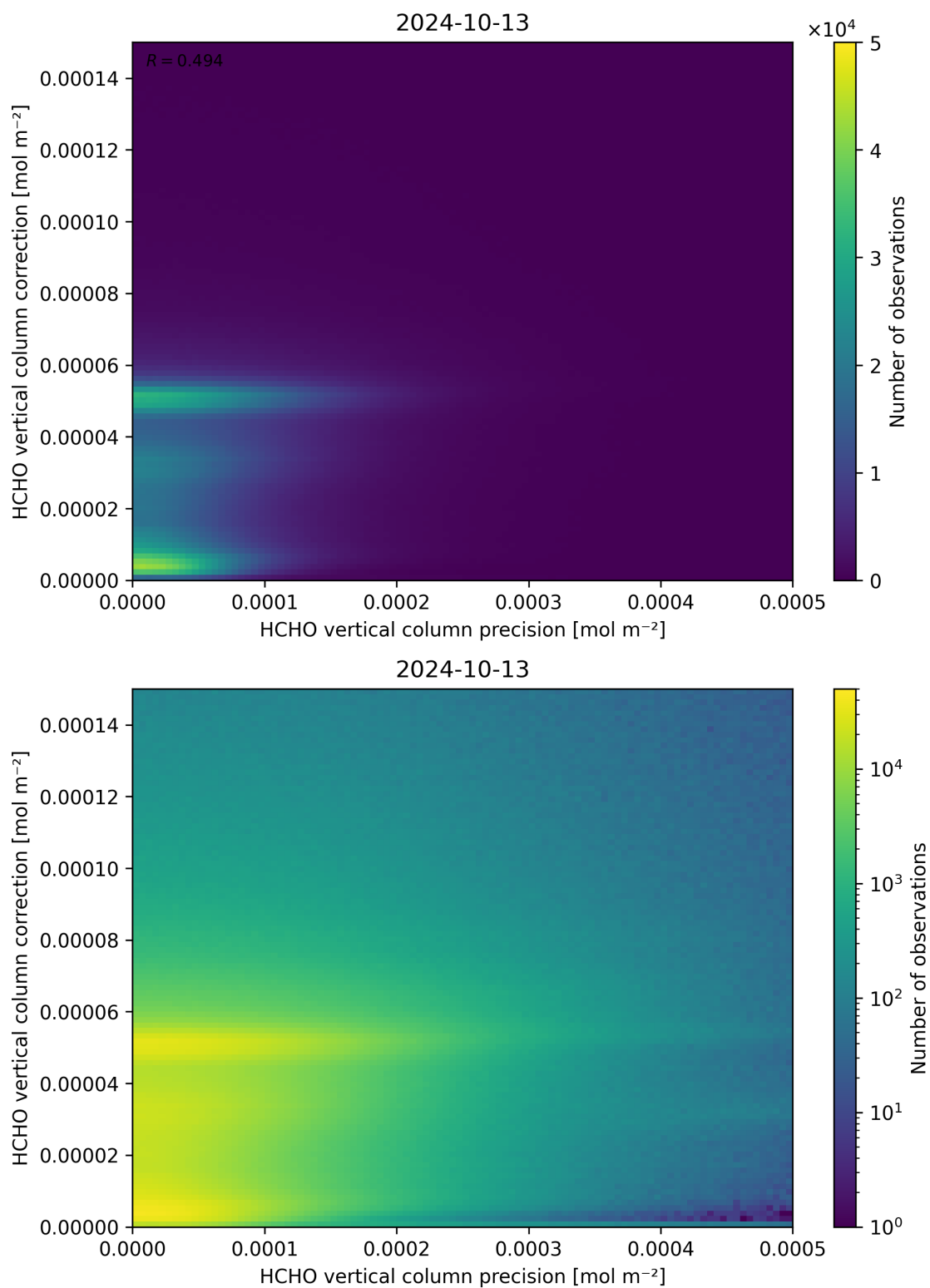
Figure 146: Scatter density plot of “HCHO vertical column precision” against “HCHO vertical column correction” for 2024-10-12 to 2024-10-14.
