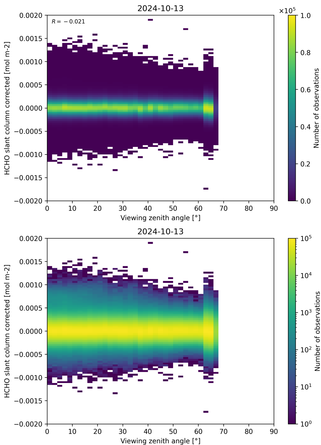
Figure 186: Scatter density plot of “Viewing zenith angle” against “HCHO slant column corrected” for 2024-10-12 to 2024-10-14.
