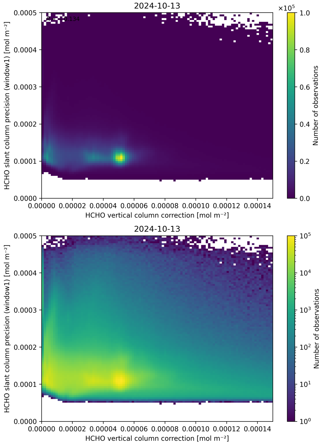
Figure 119: Scatter density plot of “HCHO vertical column correction” against “HCHO slant column precision (window1)” for 2024-10-12 to 2024-10-14.
