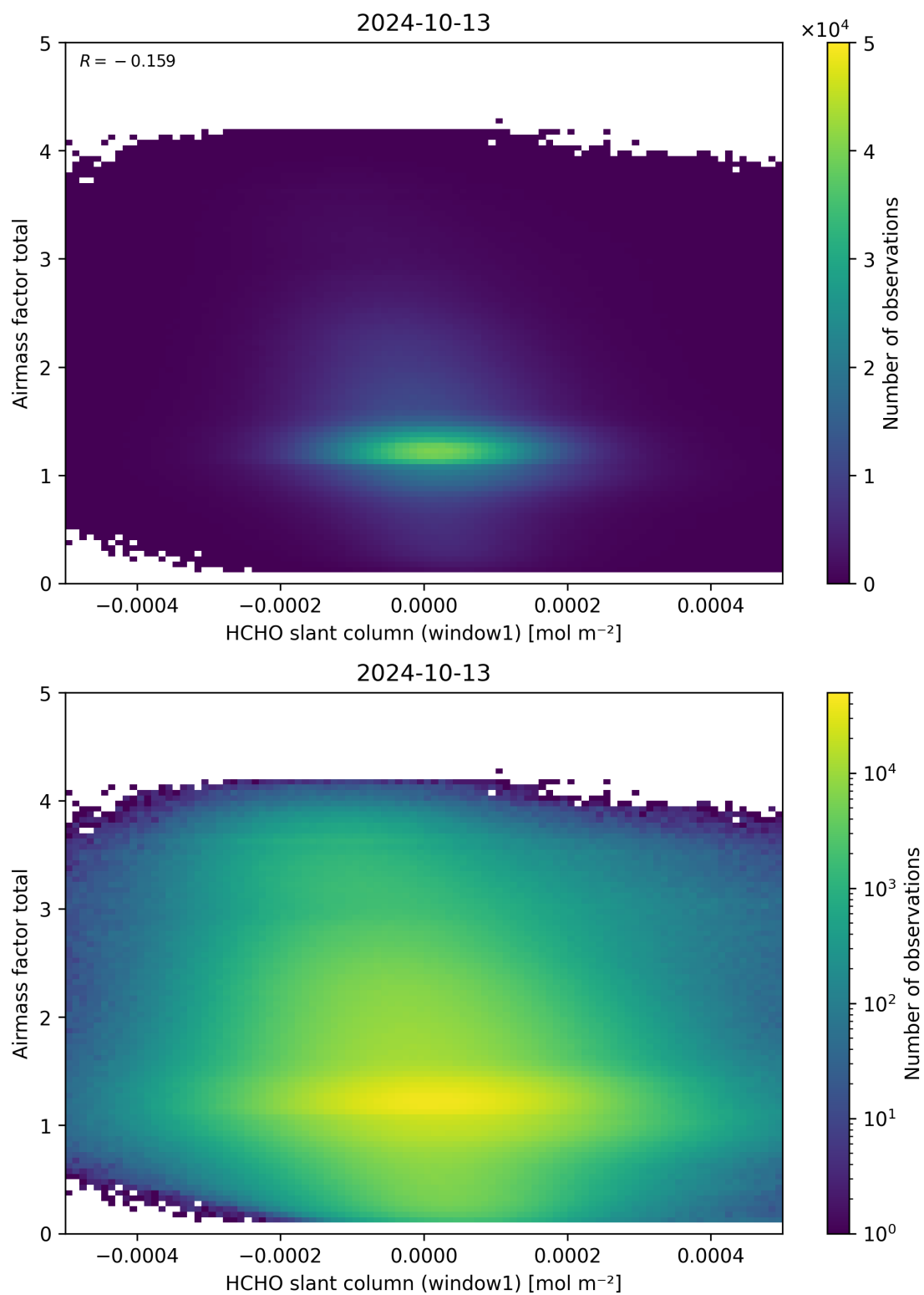
Figure 85: Scatter density plot of “HCHO slant column (window1)” against “Airmass factor total” for 2024-10-12 to 2024-10-14.
