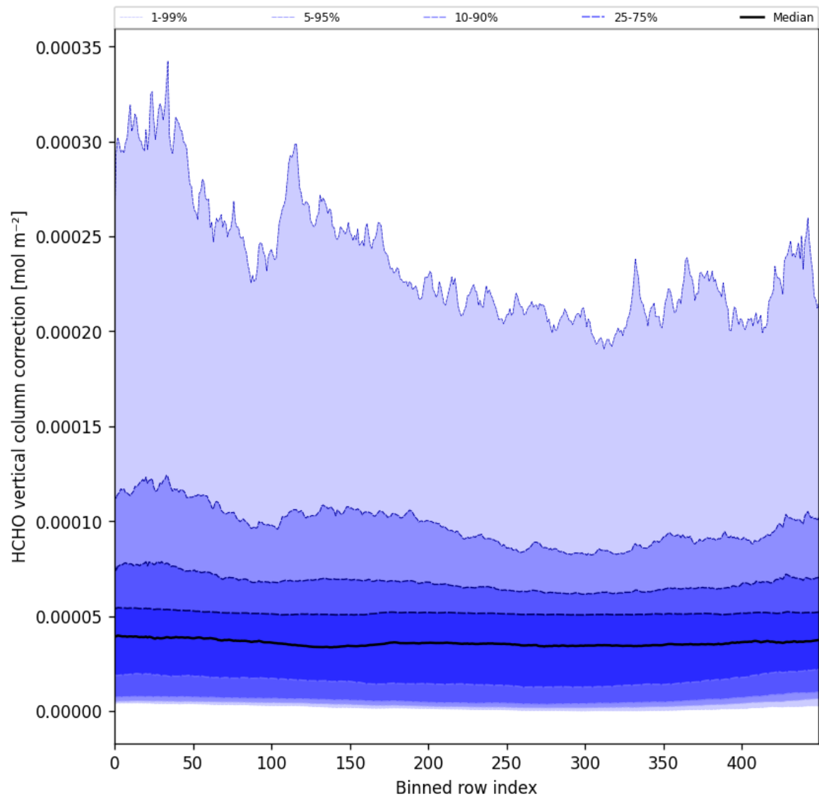
Figure 51: Along track statistics of “HCHO vertical column correction” for 2024-10-12 to 2024-10-14
