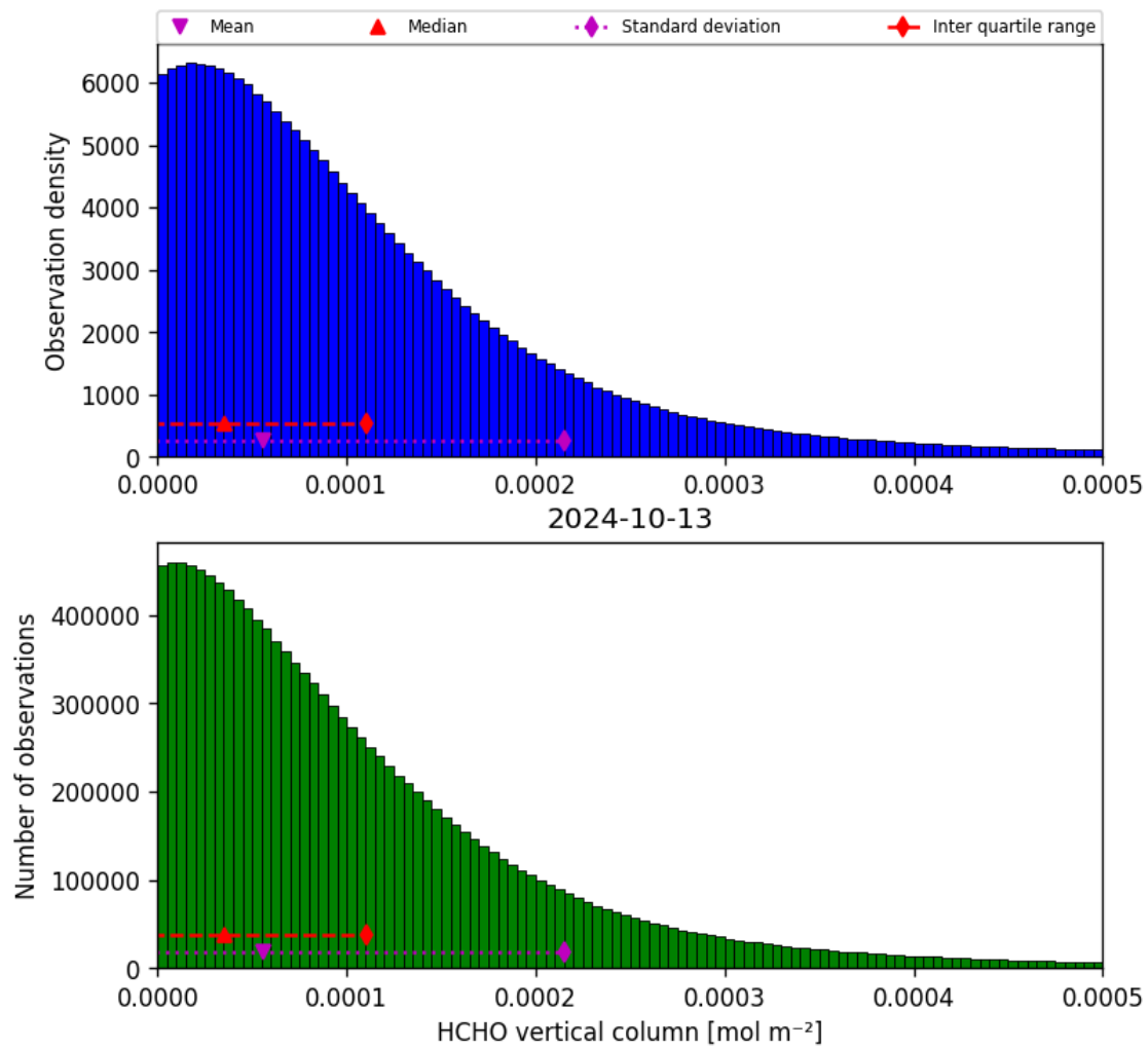
Figure 35: Histogram of “HCHO vertical column” for 2024-10-12 to 2024-10-14
