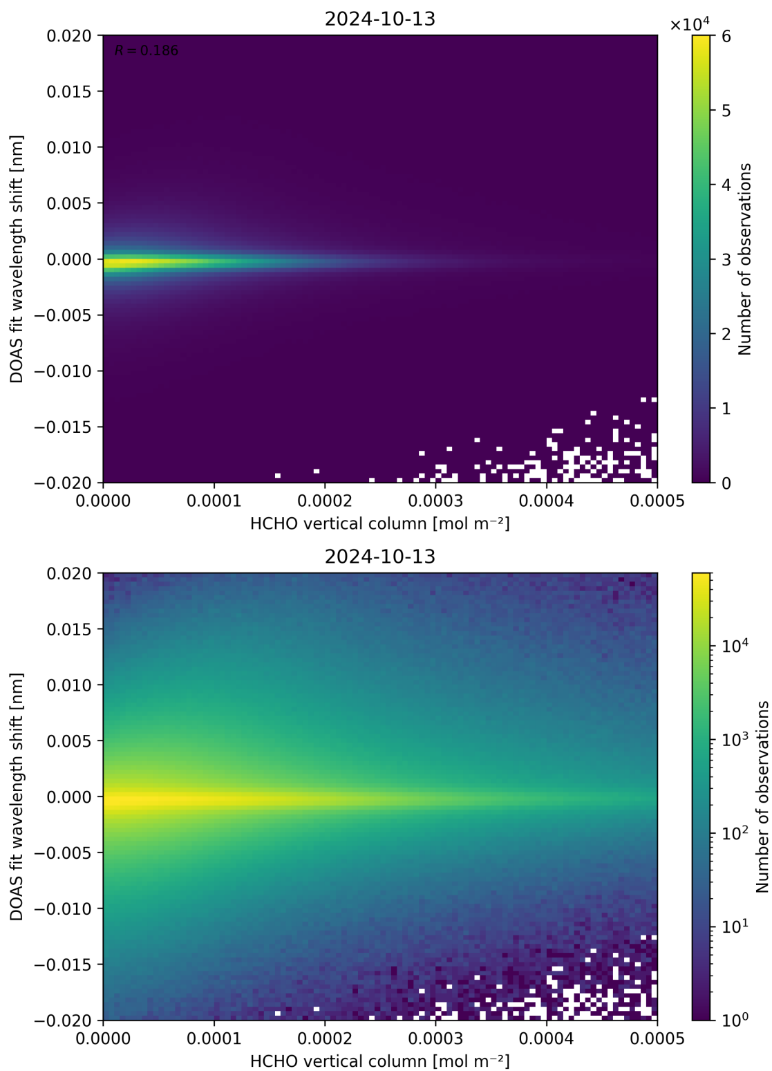
Figure 124: Scatter density plot of “HCHO vertical column” against “DOAS fit wavelength shift” for 2024-10-12 to 2024-10-14.
