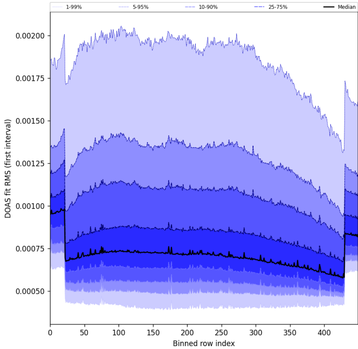
Figure 60: Along track statistics of “DOAS fit RMS (first interval)” for 2024-10-12 to 2024-10-14
