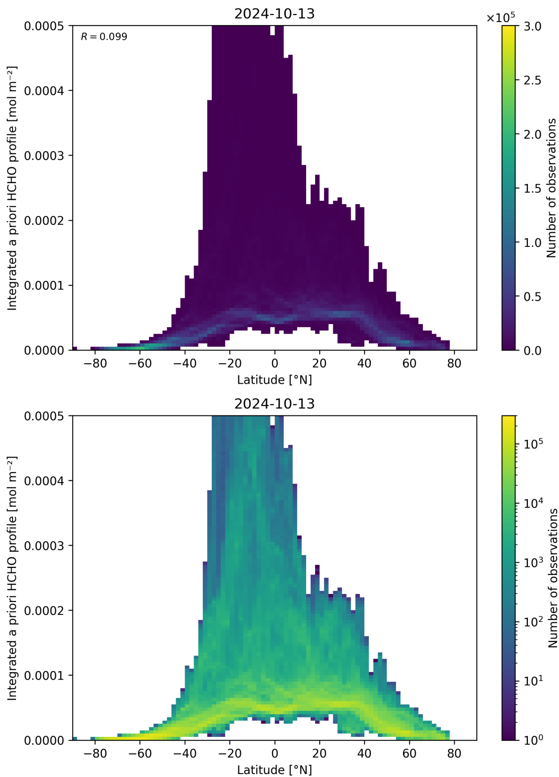
Figure 166: Scatter density plot of “Latitude” against “Integrated a priori HCHO profile” for 2024-10-12 to 2024-10-14.
