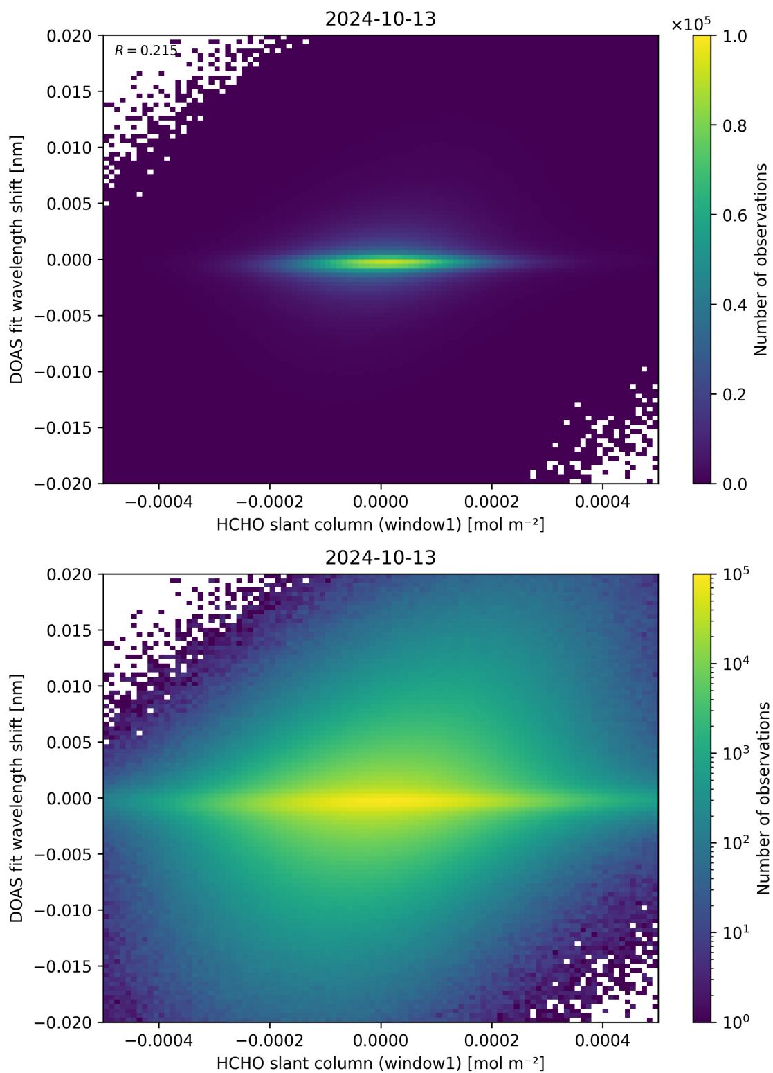
Figure 79: Scatter density plot of “HCHO slant column (window1)” against “DOAS fit wavelength shift” for 2024-10-12 to 2024-10-14.
