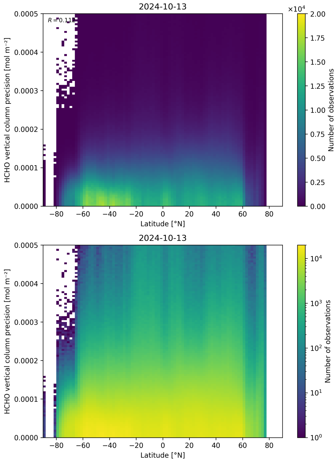
Figure 165: Scatter density plot of “Latitude” against “HCHO vertical column precision” for 2024-10-12 to 2024-10-14.
