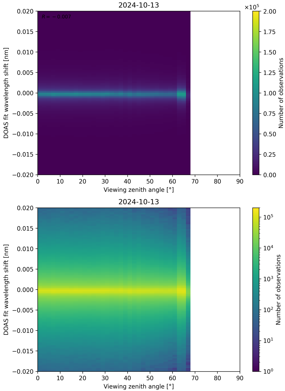
Figure 183: Scatter density plot of “Viewing zenith angle” against “DOAS fit wavelength shift” for 2024-10-12 to 2024-10-14.
