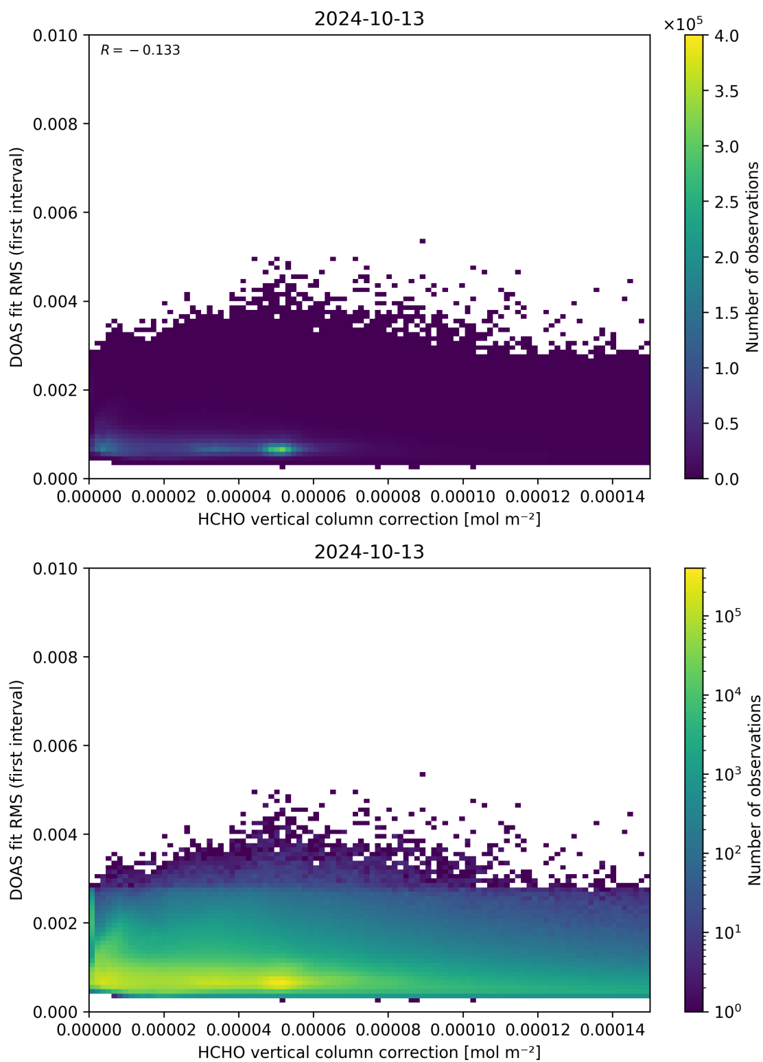
Figure 112: Scatter density plot of “HCHO vertical column correction” against “DOAS fit RMS (first interval)” for 2024-10-12 to 2024-10-14.
