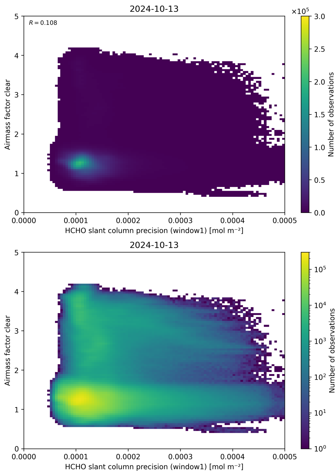
Figure 91: Scatter density plot of “HCHO slant column precision (window1)” against “Airmass factor clear” for 2024-10-12 to 2024-10-14.
