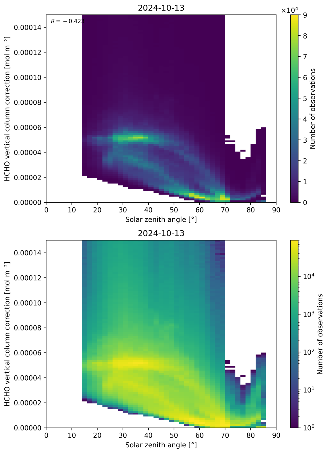
Figure 178: Scatter density plot of “Solar zenith angle” against “HCHO vertical column correction” for 2024-10-12 to 2024-10-14.
