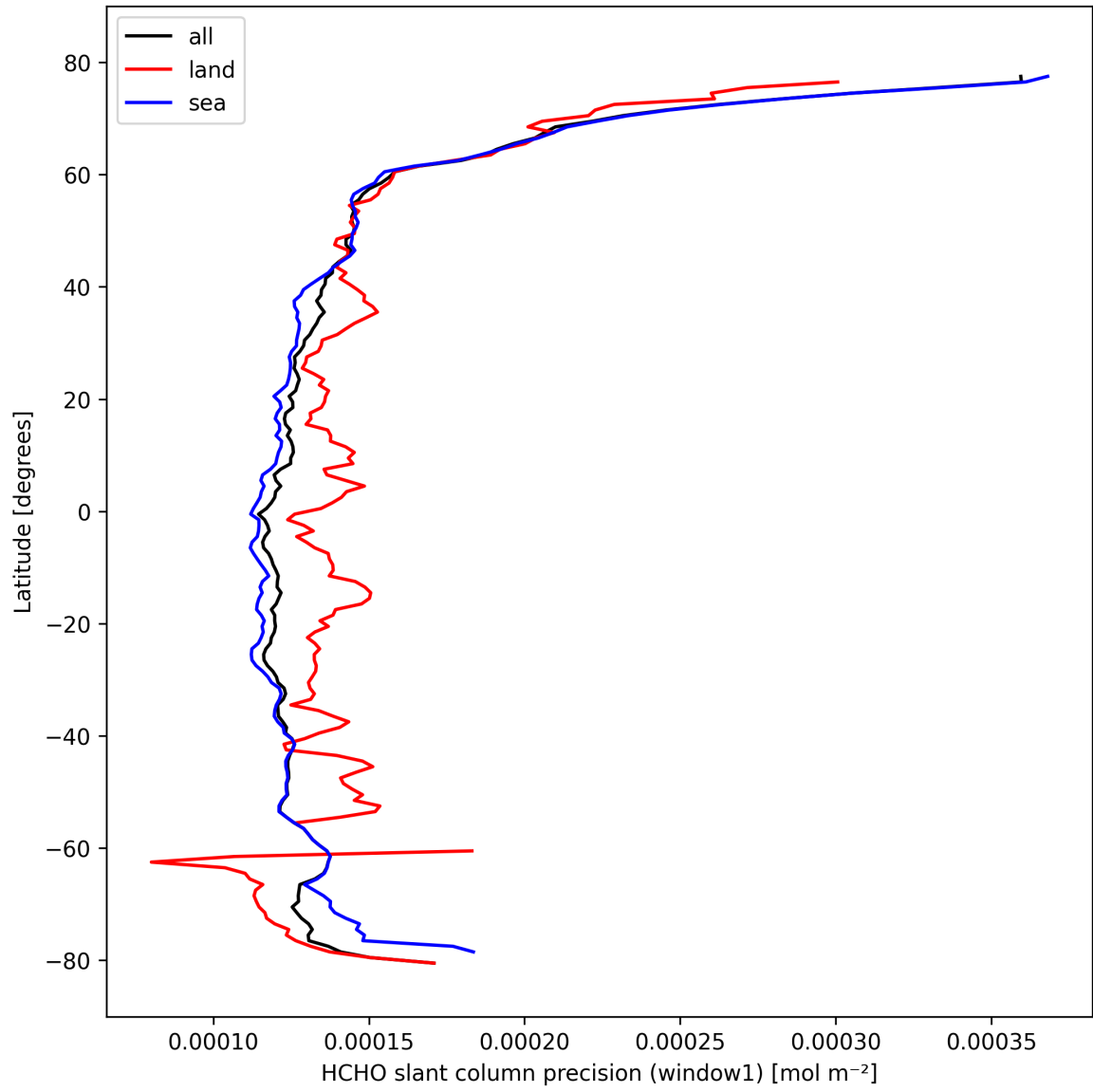
Figure 25: Zonal average of “HCHO slant column precision (window1)” for 2024-10-12 to 2024-10-14.
