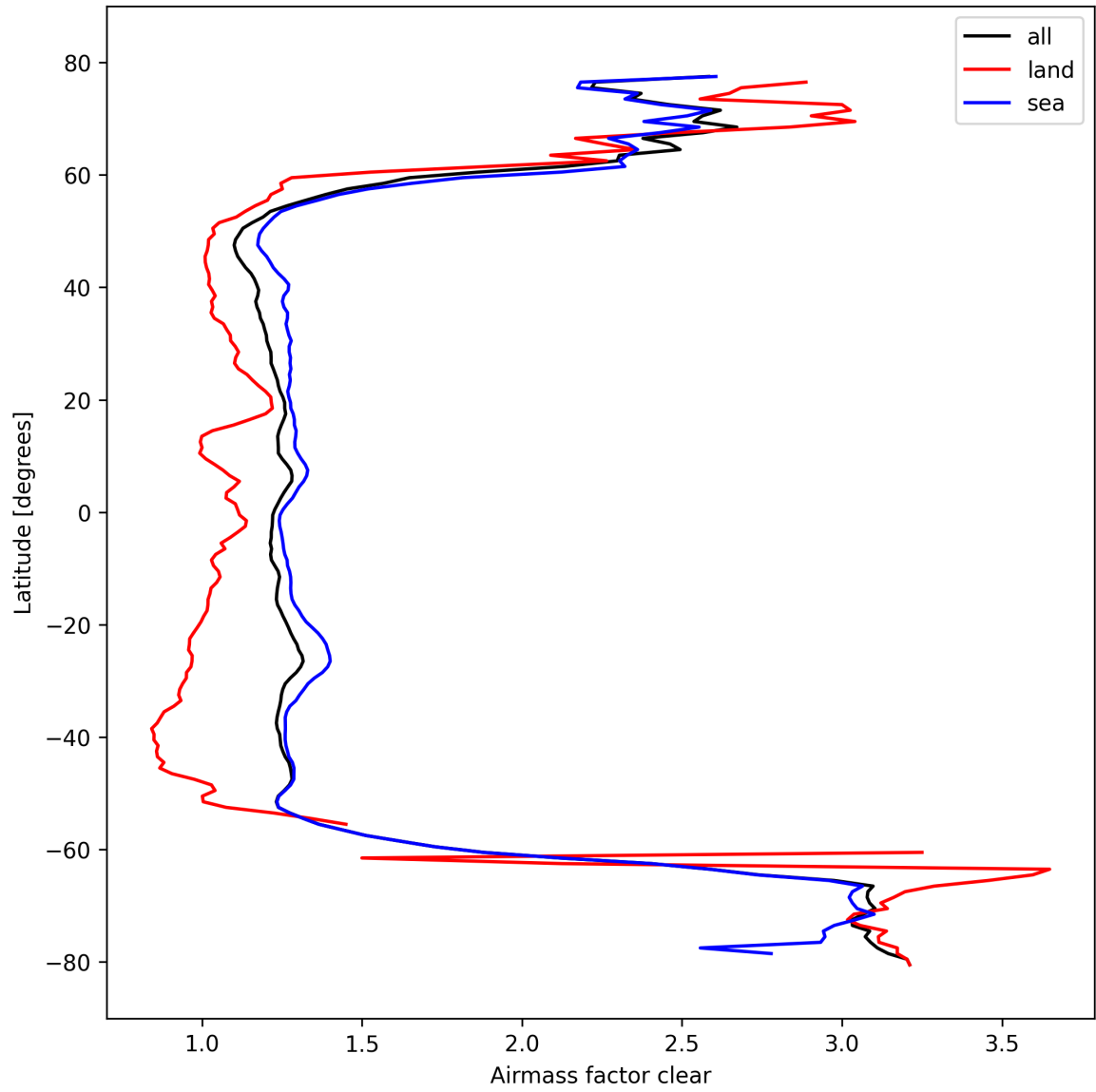
Figure 28: Zonal average of “Airmass factor clear” for 2024-10-12 to 2024-10-14.
