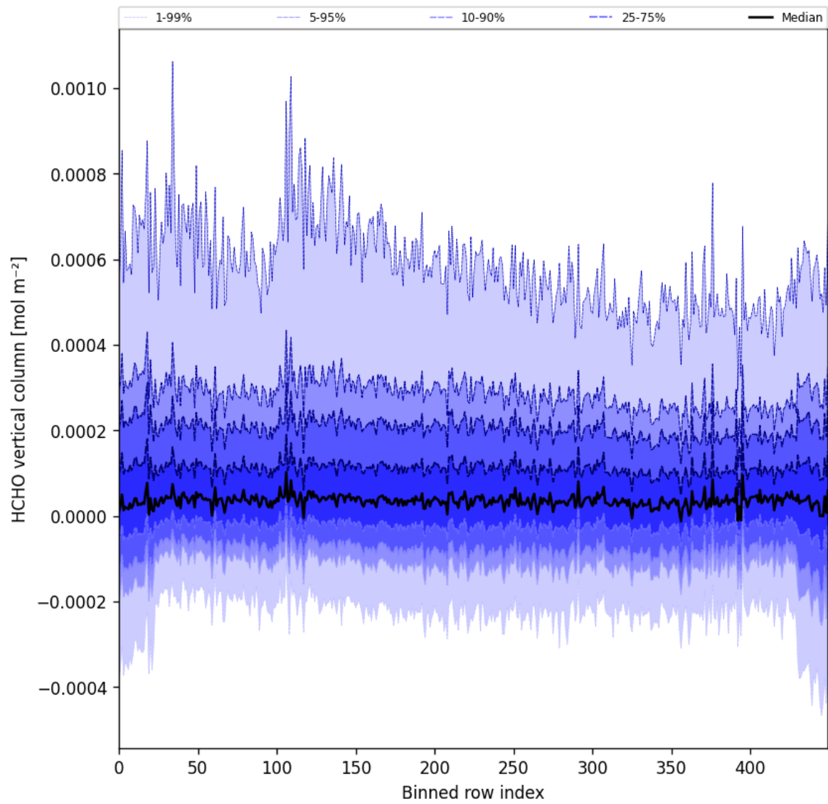
Figure 49: Along track statistics of “HCHO vertical column” for 2024-10-12 to 2024-10-14
