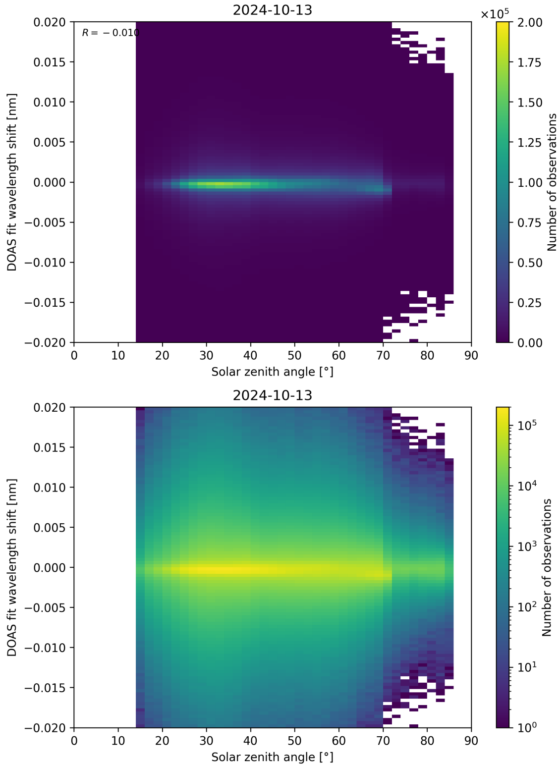
Figure 168: Scatter density plot of “Solar zenith angle” against “DOAS fit wavelength shift” for 2024-10-12 to 2024-10-14.
