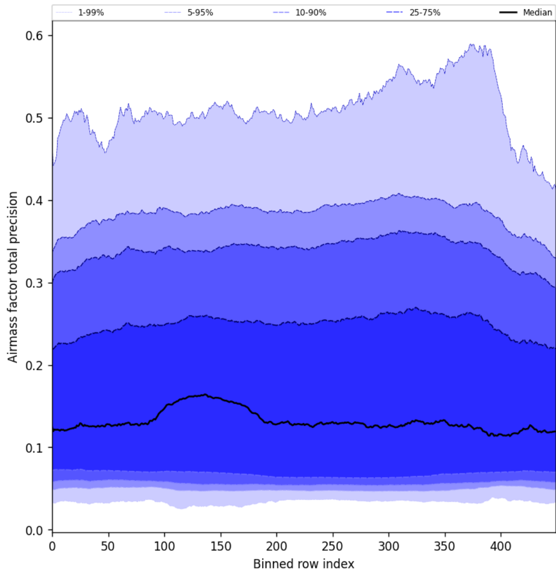
Figure 55: Along track statistics of “Airmass factor total precision” for 2024-10-12 to 2024-10-14
