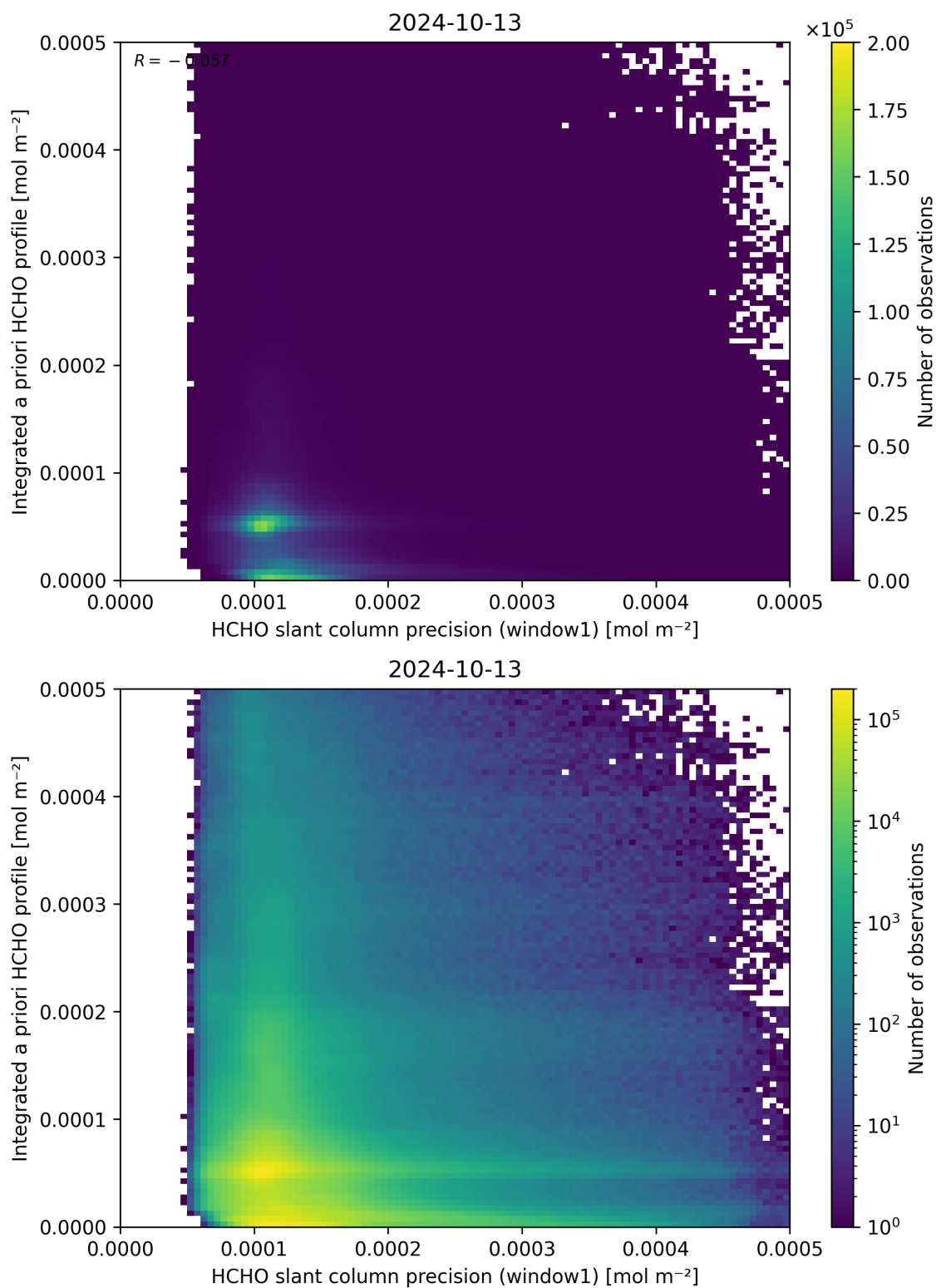
Figure 96: Scatter density plot of “HCHO slant column precision (window1)” against “Integrated a priori HCHO profile” for 2024-10-12 to 2024-10-14.
