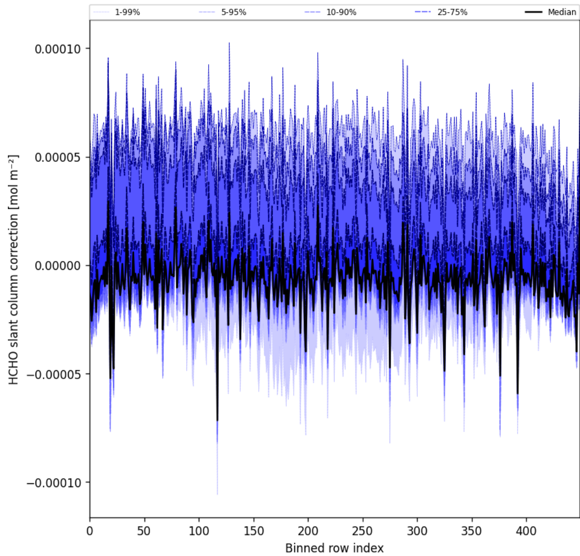
Figure 61: Along track statistics of “HCHO slant column correction” for 2024-10-12 to 2024-10-14
