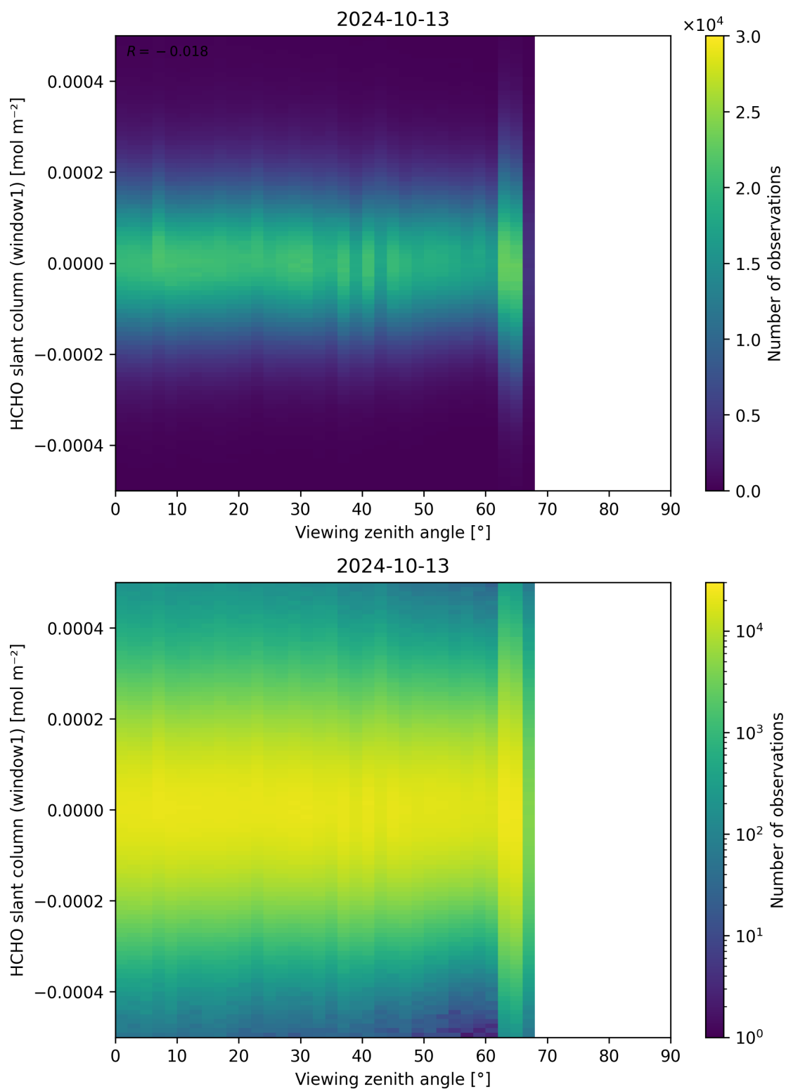
Figure 188: Scatter density plot of “Viewing zenith angle” against “HCHO slant column (window1)” for 2024-10-12 to 2024-10-14.
