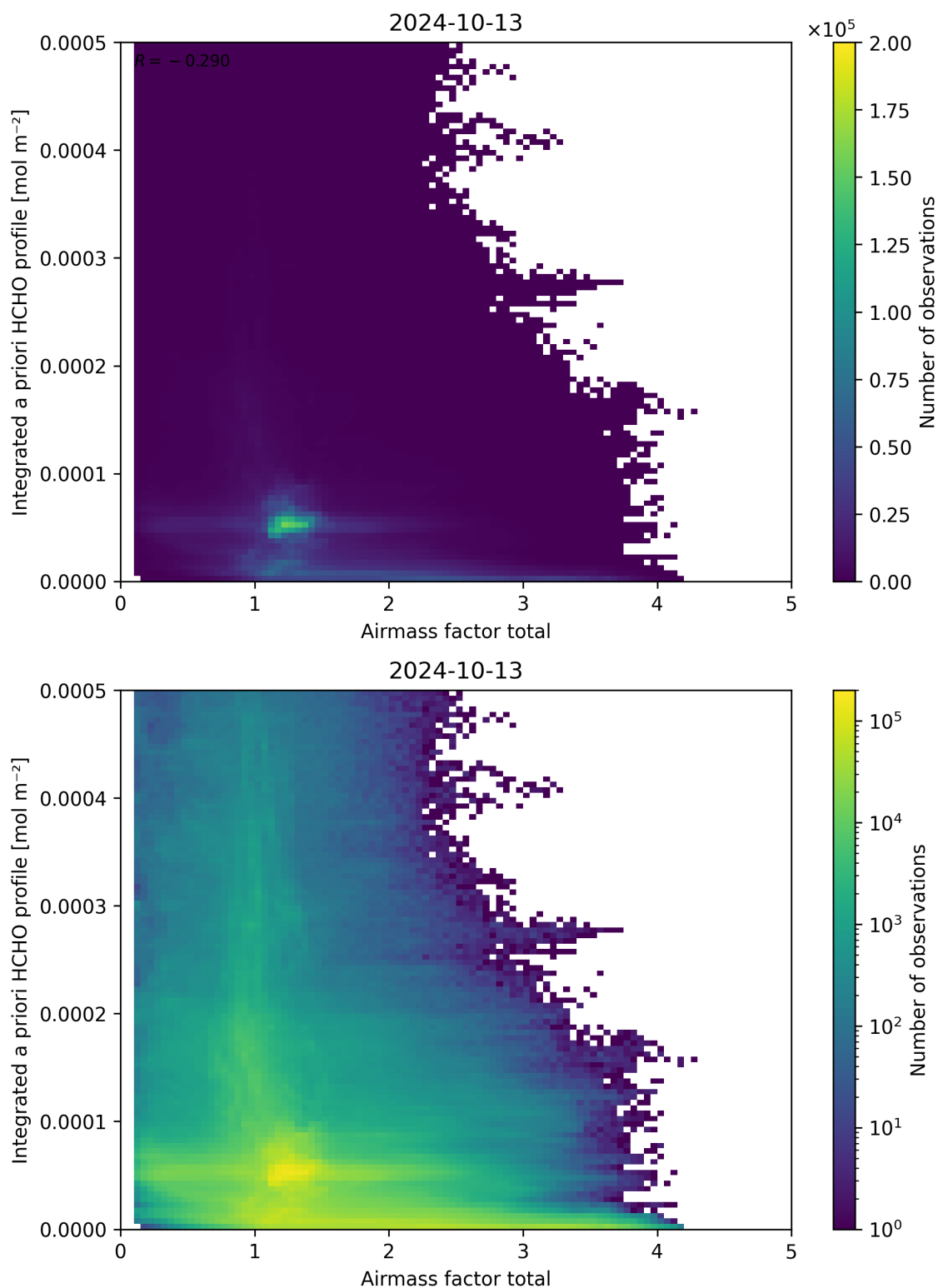
Figure 104: Scatter density plot of “Airmass factor total” against “Integrated a priori HCHO profile” for 2024-10-12 to 2024-10-14.
