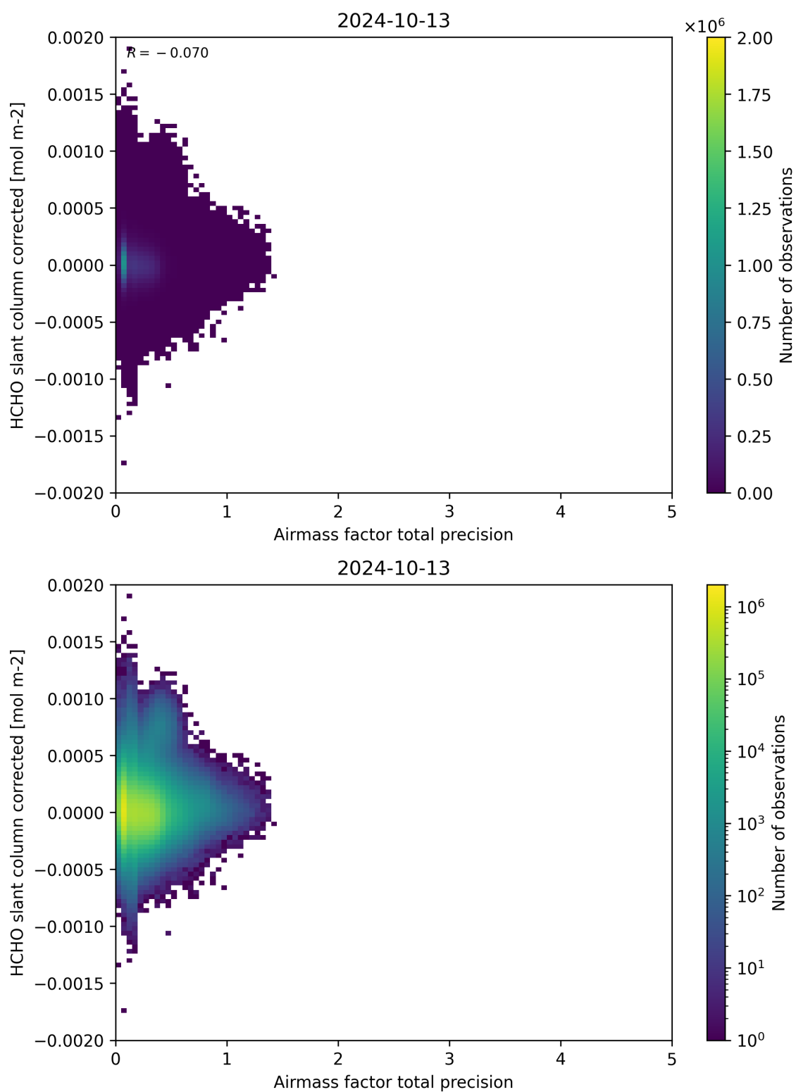
Figure 109: Scatter density plot of “Airmass factor total precision” against “HCHO slant column corrected” for 2024-10-12 to 2024-10-14.
