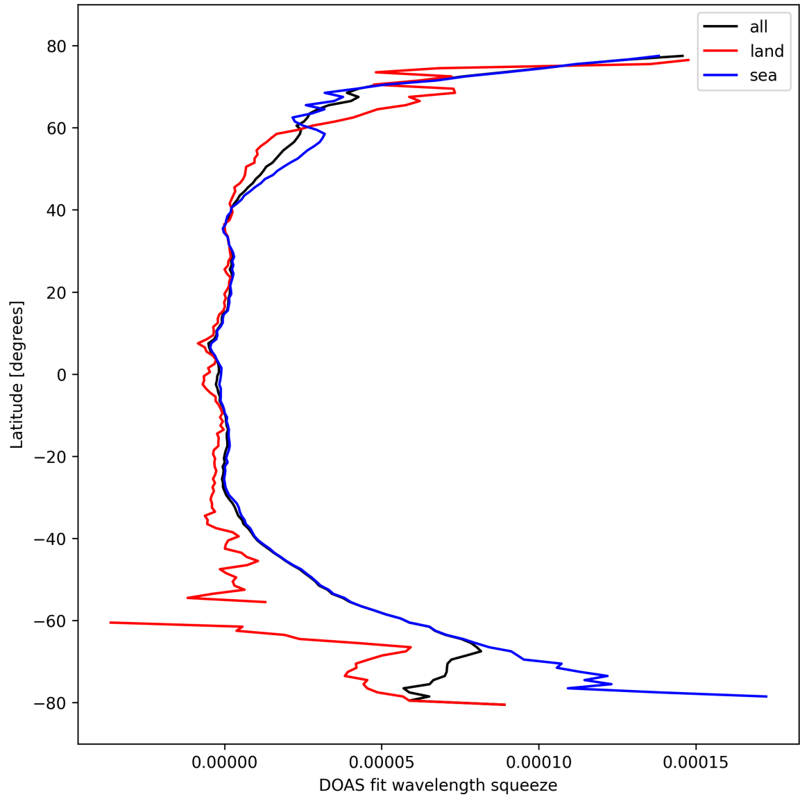
Figure 31: Zonal average of “DOAS fit wavelength squeeze” for 2024-10-12 to 2024-10-14.
