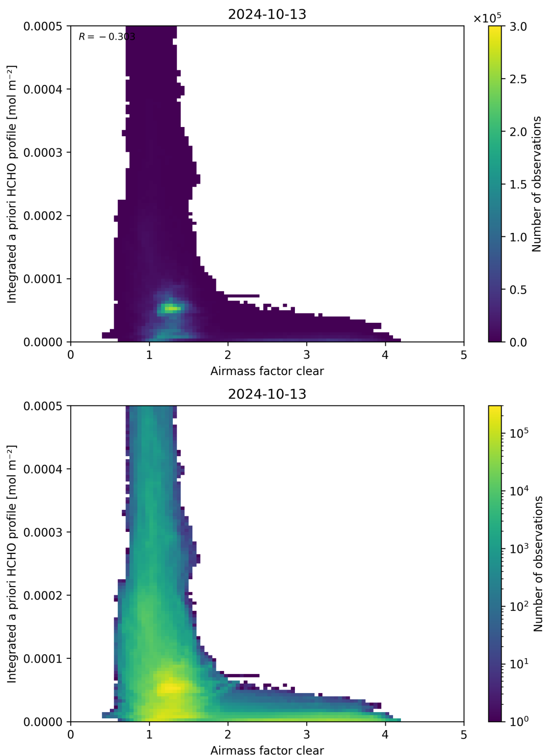
Figure 76: Scatter density plot of “Airmass factor clear” against “Integrated a priori HCHO profile” for 2024-10-12 to 2024-10-14.
