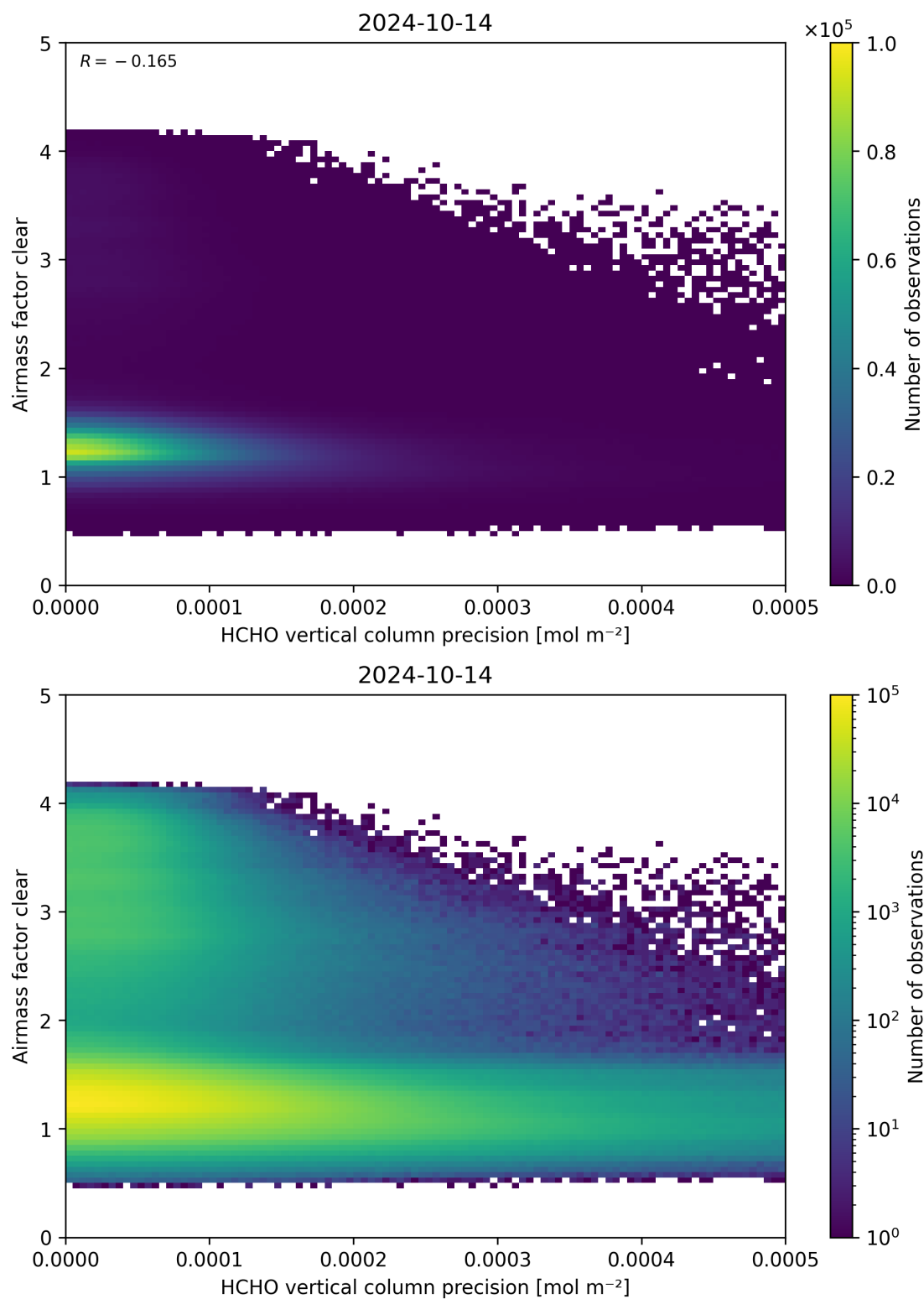
Figure 139: Scatter density plot of “HCHO vertical column precision” against “Airmass factor clear” for 2024-10-14 to 2024-10-15.
