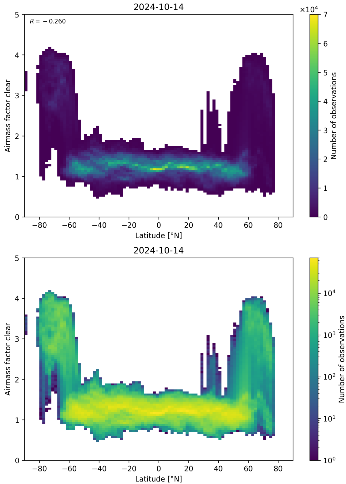
Figure 156: Scatter density plot of “Latitude” against “Airmass factor clear” for 2024-10-14 to 2024-10-15.
