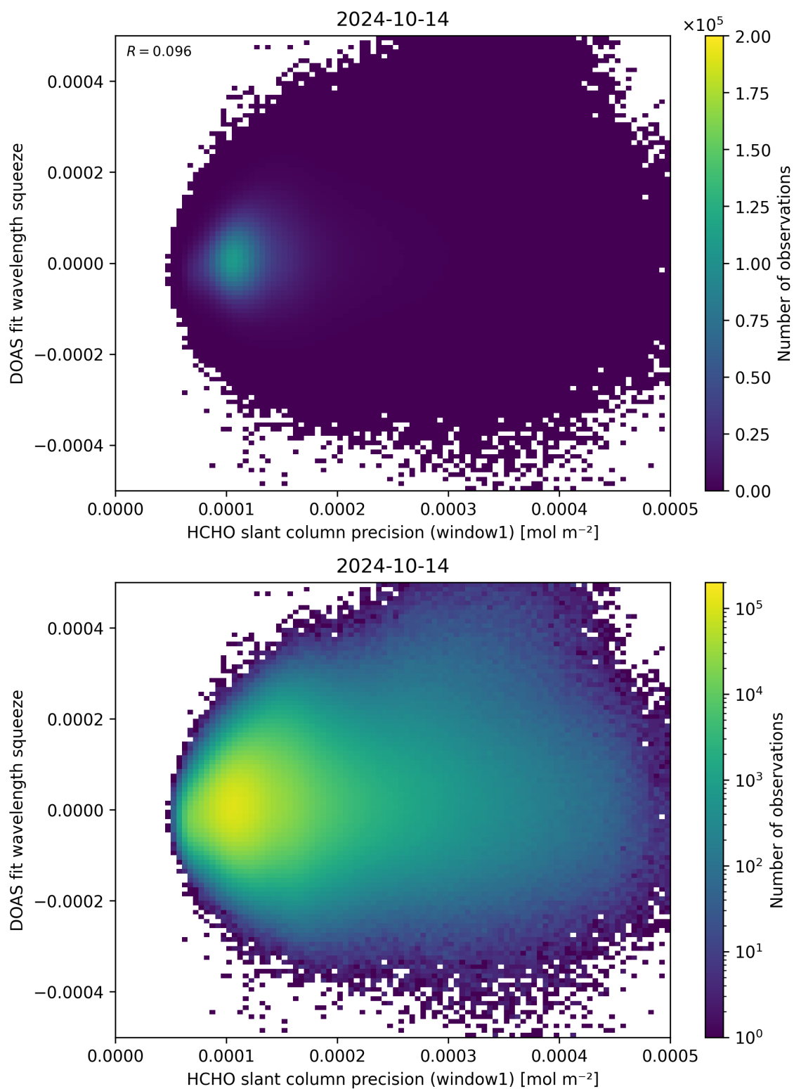
Figure 90: Scatter density plot of “HCHO slant column precision (window1)” against “DOAS fit wavelength squeeze” for 2024-10-14 to 2024-10-15.
