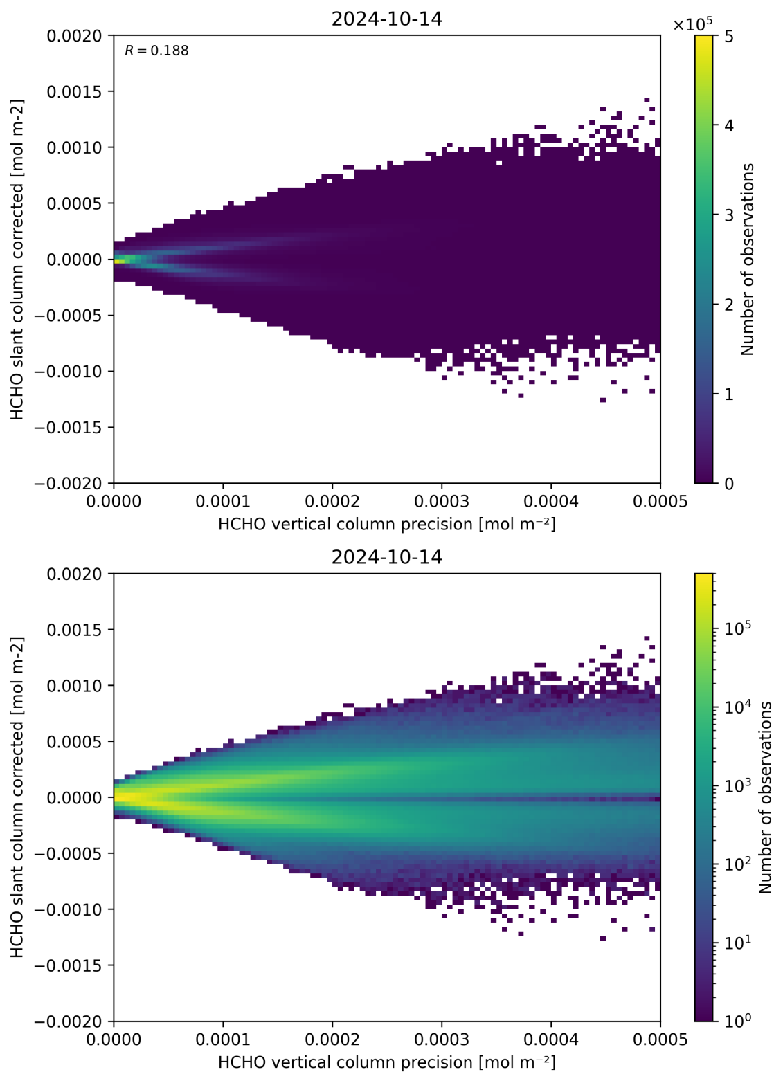
Figure 140: Scatter density plot of “HCHO vertical column precision” against “HCHO slant column corrected” for 2024-10-14 to 2024-10-15.
