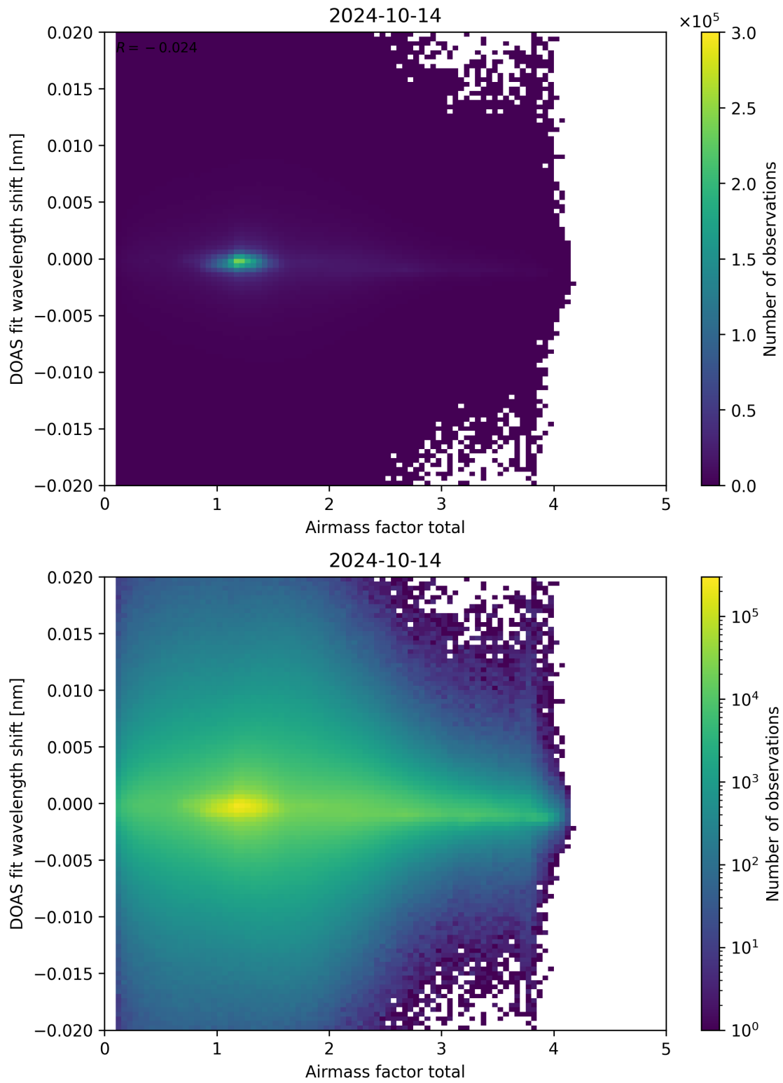
Figure 98: Scatter density plot of “Airmass factor total” against “DOAS fit wavelength shift” for 2024-10-14 to 2024-10-15.
