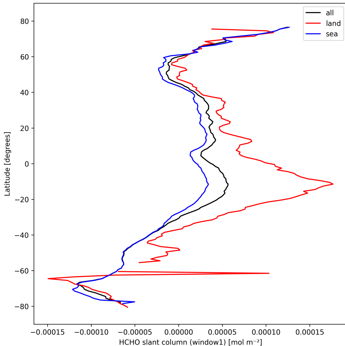
Figure 24: Zonal average of “HCHO slant column (window1)” for 2024-10-14 to 2024-10-15.
