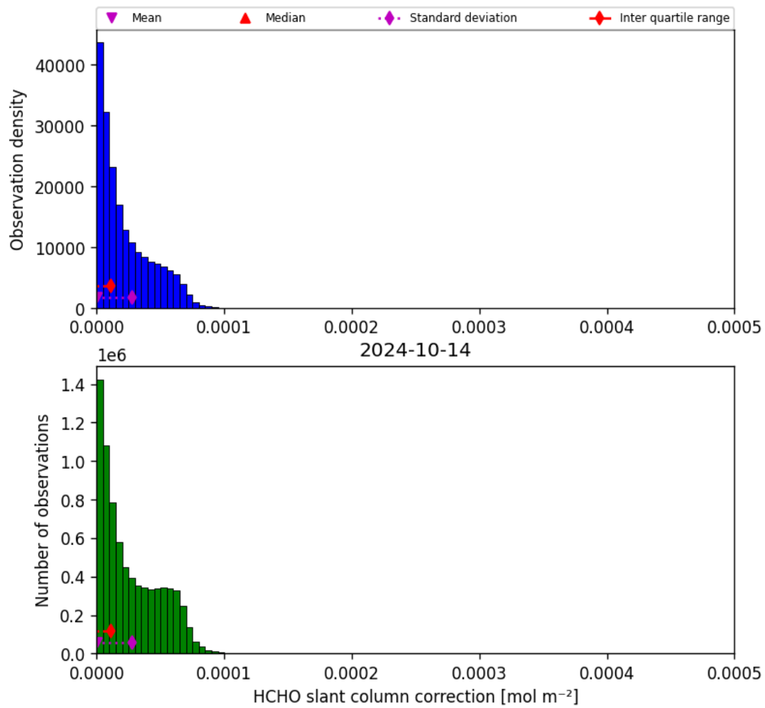
Figure 47: Histogram of “HCHO slant column correction” for 2024-10-14 to 2024-10-15
