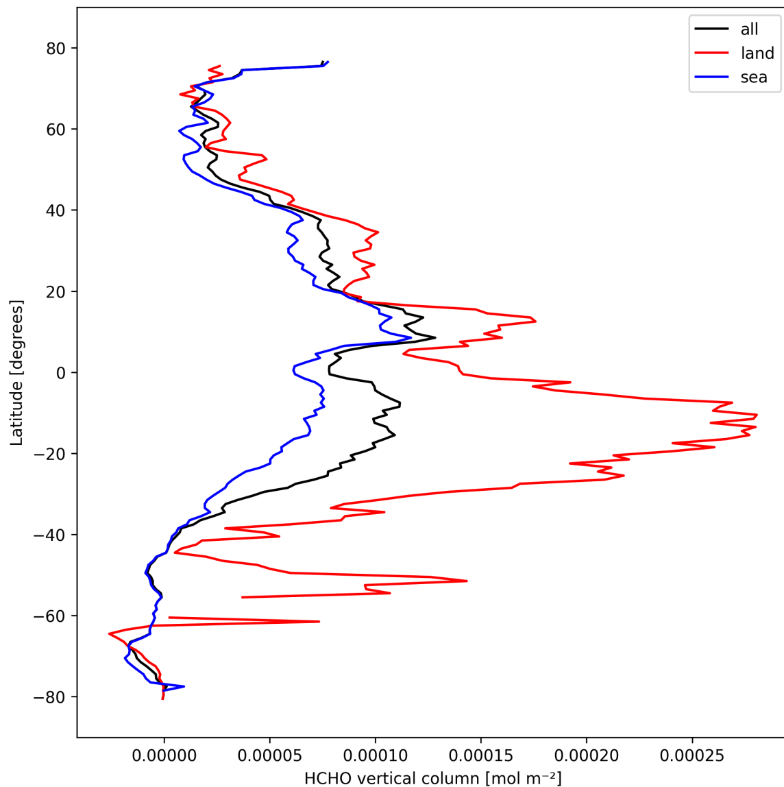
Figure 21: Zonal average of “HCHO vertical column” for 2024-10-14 to 2024-10-15.
