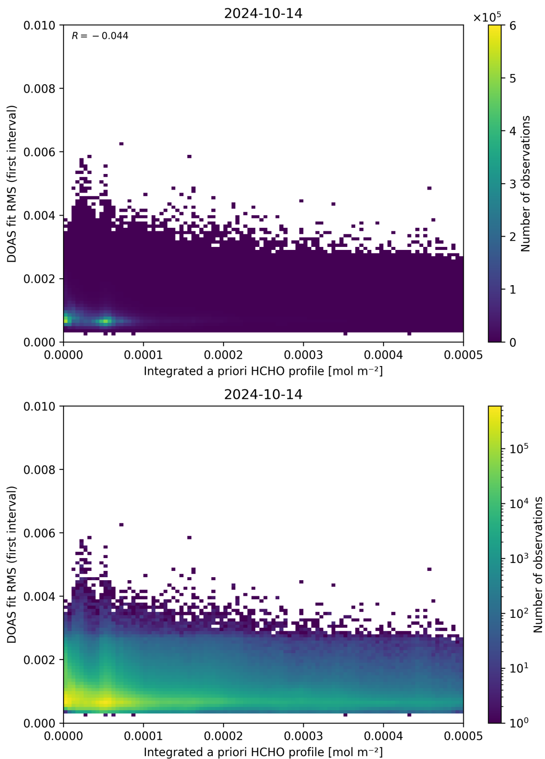
Figure 148: Scatter density plot of “Integrated a priori HCHO profile” against “DOAS fit RMS (first interval)” for 2024-10-14 to 2024-10-15.
