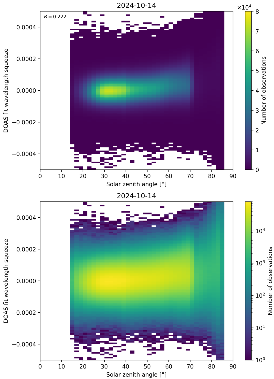
Figure 169: Scatter density plot of “Solar zenith angle” against “DOAS fit wavelength squeeze” for 2024-10-14 to 2024-10-15.
