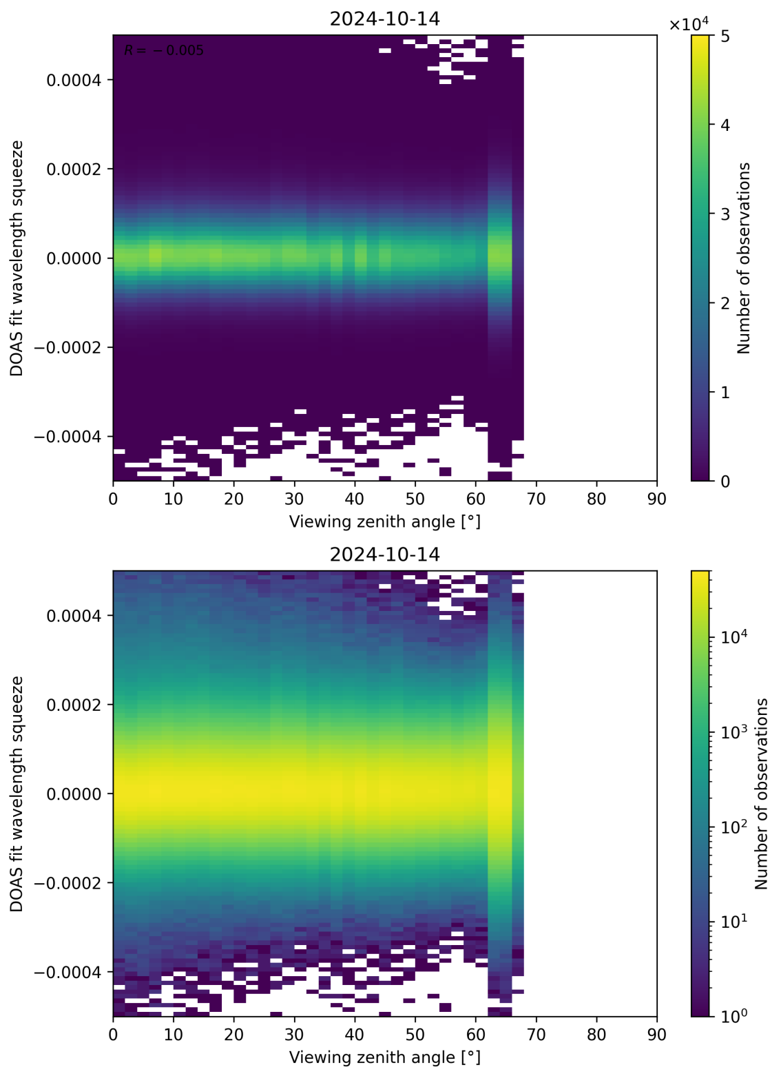
Figure 184: Scatter density plot of “Viewing zenith angle” against “DOAS fit wavelength squeeze” for 2024-10-14 to 2024-10-15.
