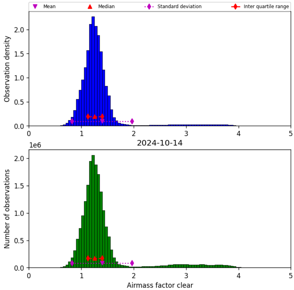
Figure 42: Histogram of “Airmass factor clear” for 2024-10-14 to 2024-10-15
