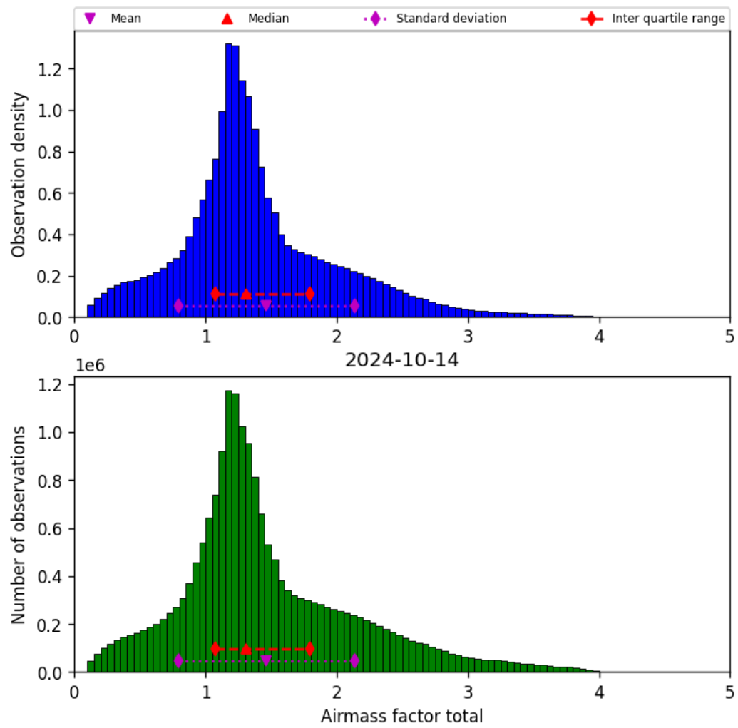
Figure 40: Histogram of “Airmass factor total” for 2024-10-14 to 2024-10-15
