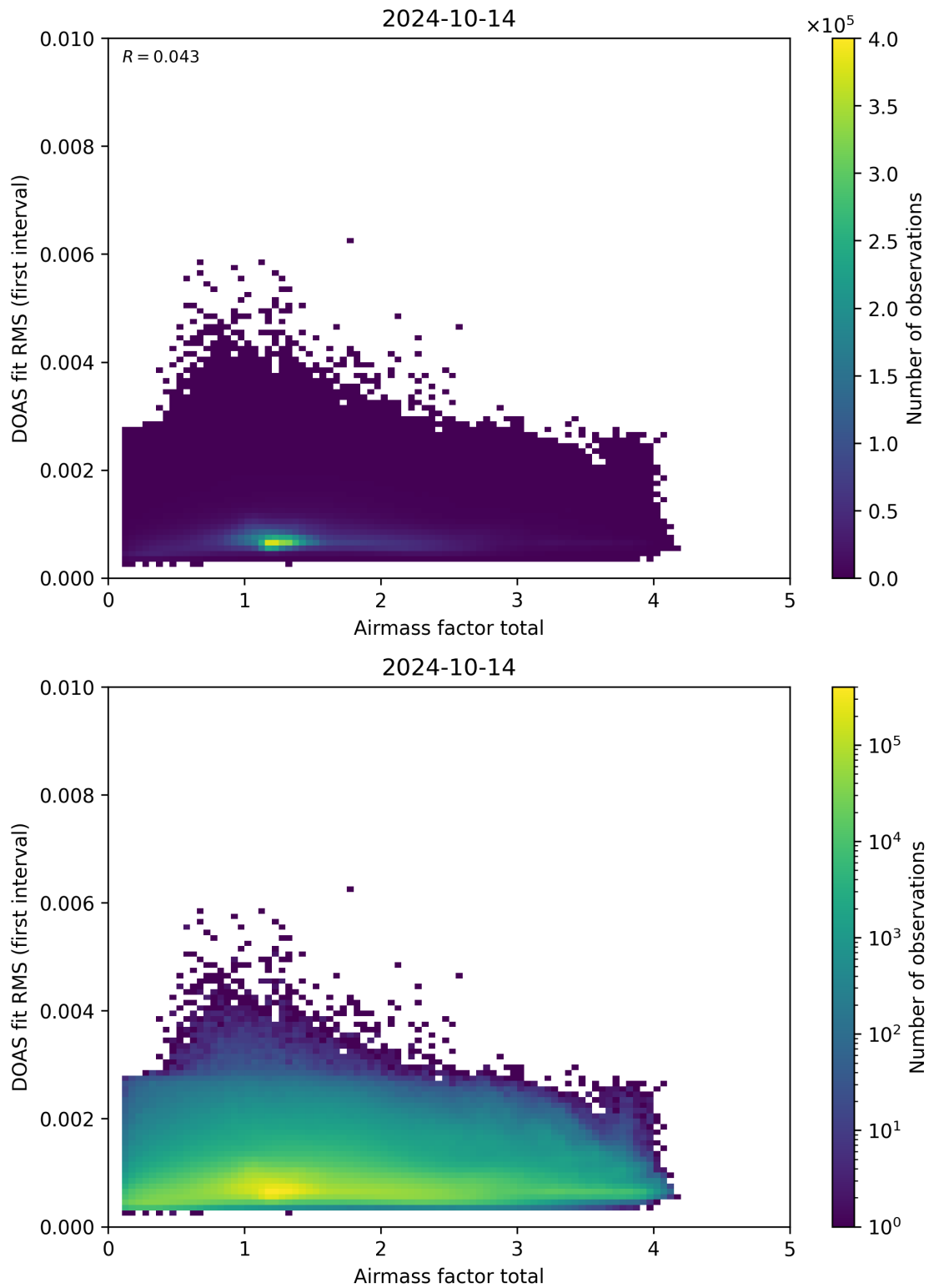
Figure 97: Scatter density plot of “Airmass factor total” against “DOAS fit RMS (first interval)” for 2024-10-14 to 2024-10-15.
