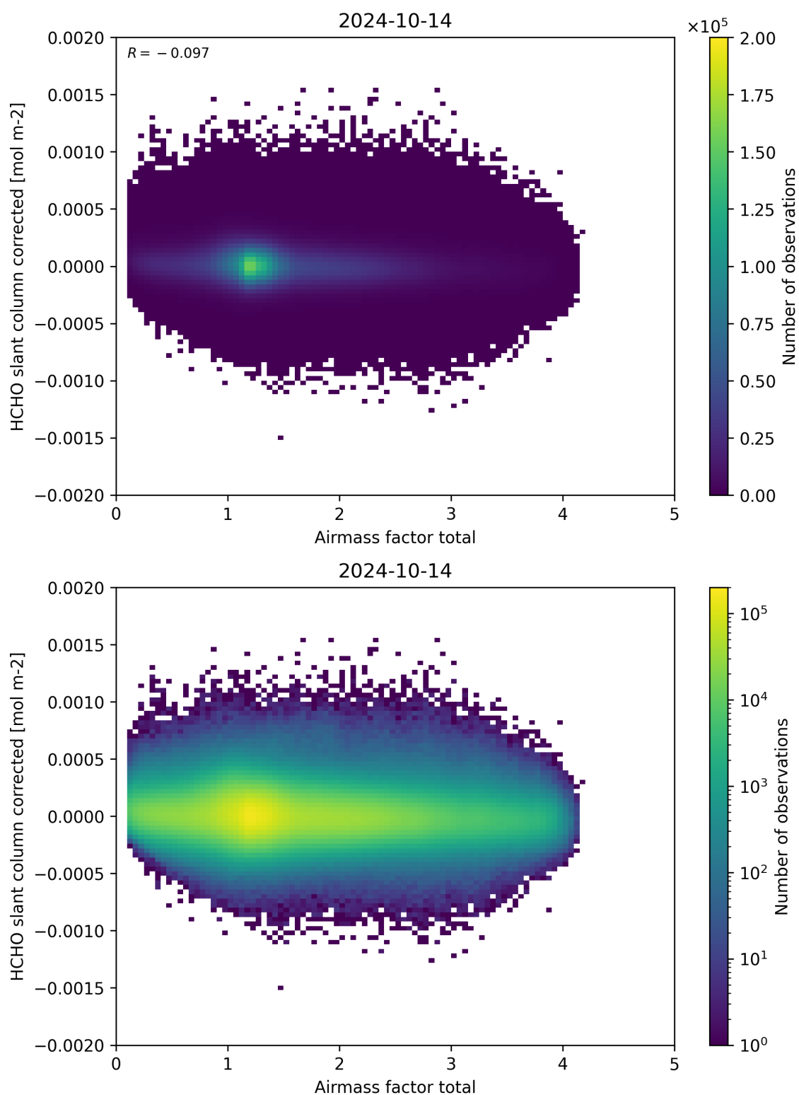
Figure 101: Scatter density plot of “Airmass factor total” against “HCHO slant column corrected” for 2024-10-14 to 2024-10-15.
