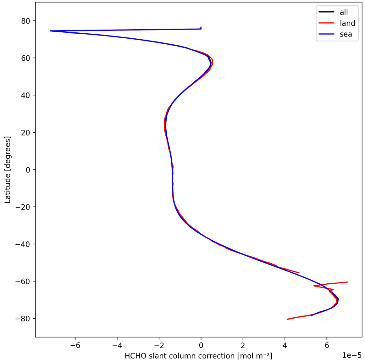
Figure 33: Zonal average of “HCHO slant column correction” for 2024-10-14 to 2024-10-15.
