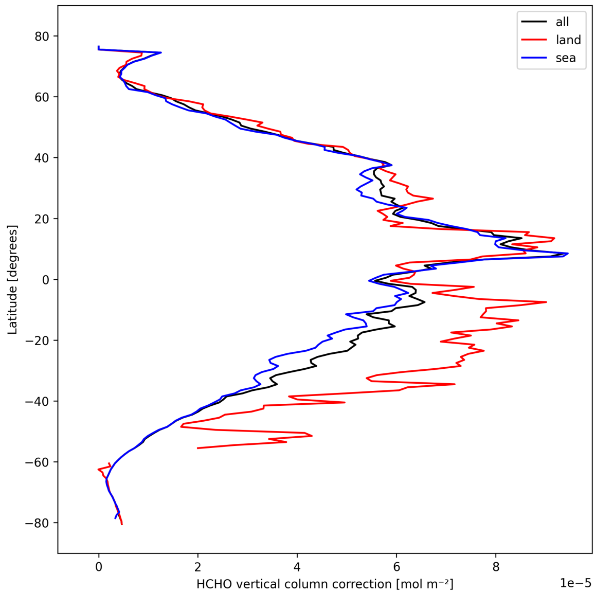
Figure 23: Zonal average of “HCHO vertical column correction” for 2024-10-14 to 2024-10-15.
