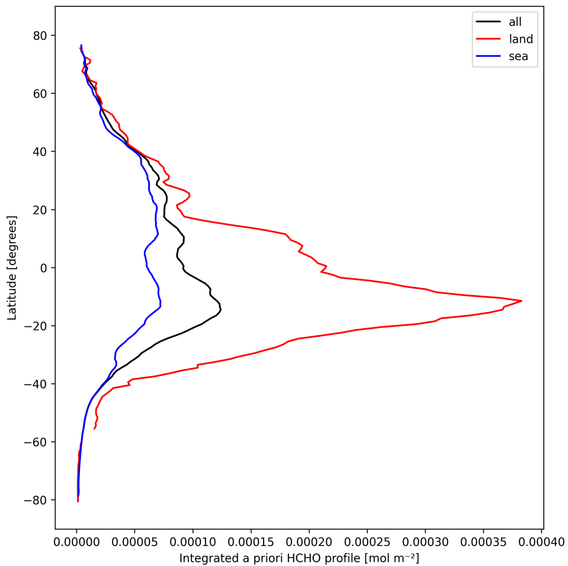
Figure 29: Zonal average of “Integrated a priori HCHO profile” for 2024-10-14 to 2024-10-15.
