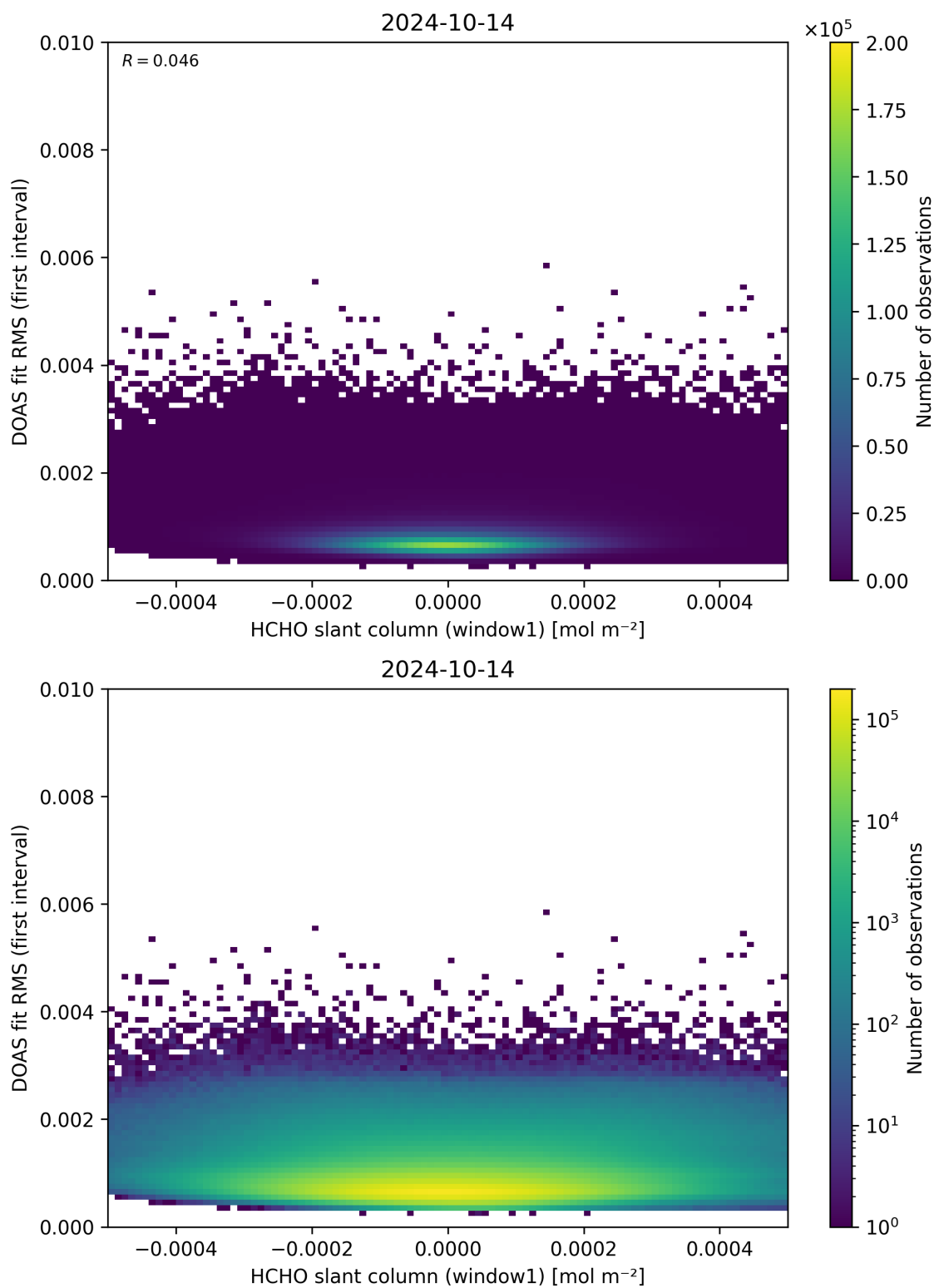
Figure 78: Scatter density plot of “HCHO slant column (window1)” against “DOAS fit RMS (first interval)” for 2024-10-14 to 2024-10-15.
