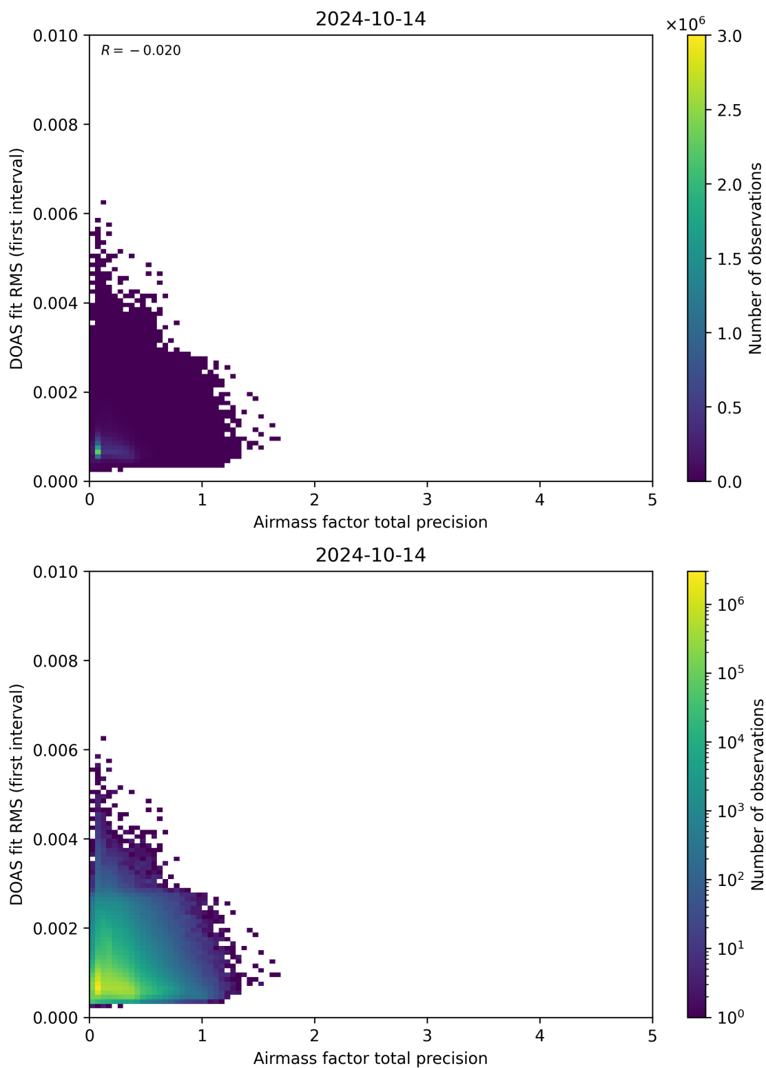
Figure 105: Scatter density plot of “Airmass factor total precision” against “DOAS fit RMS (first interval)” for 2024-10-14 to 2024-10-15.
