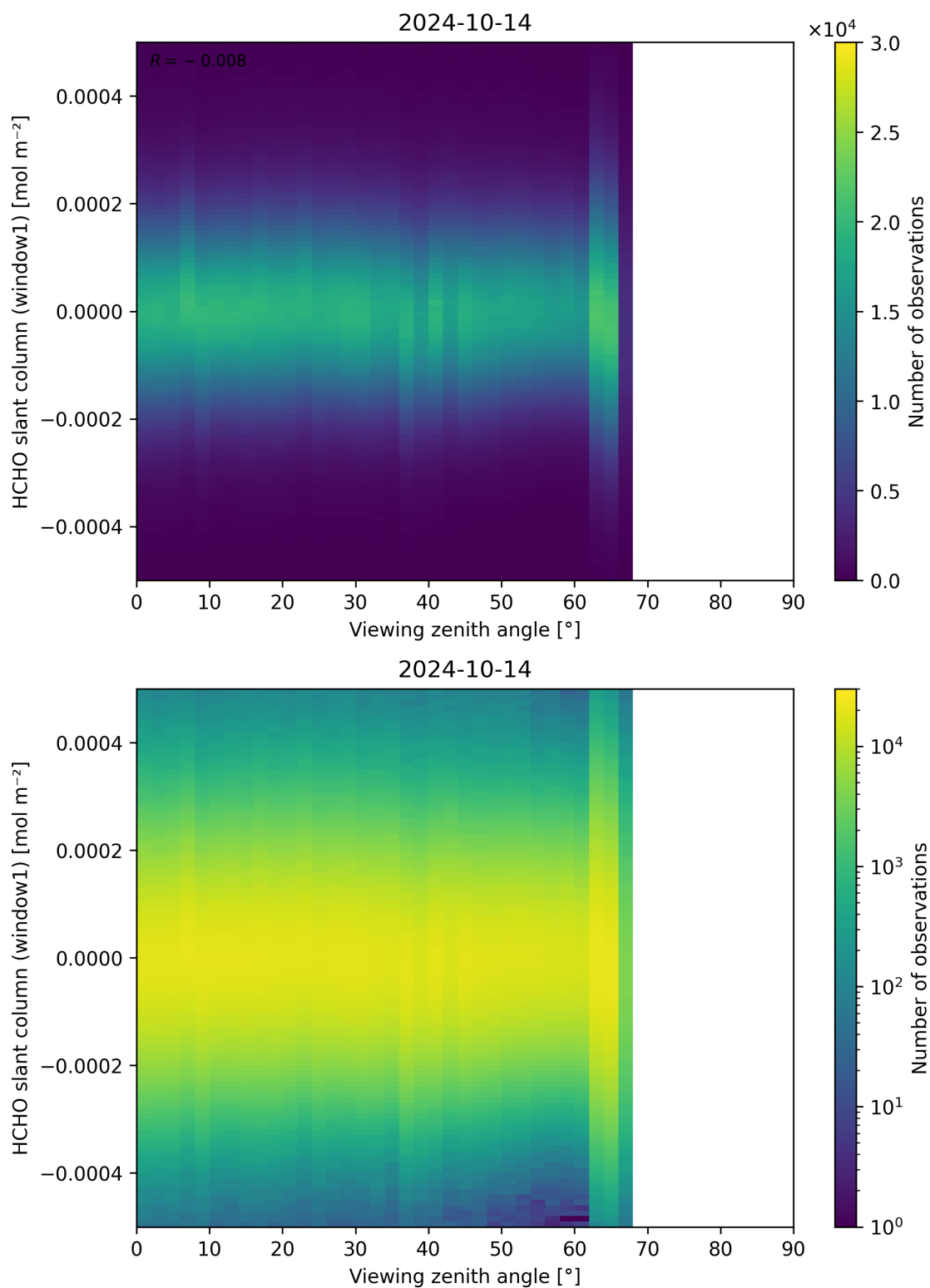
Figure 188: Scatter density plot of “Viewing zenith angle” against “HCHO slant column (window1)” for 2024-10-14 to 2024-10-15.
