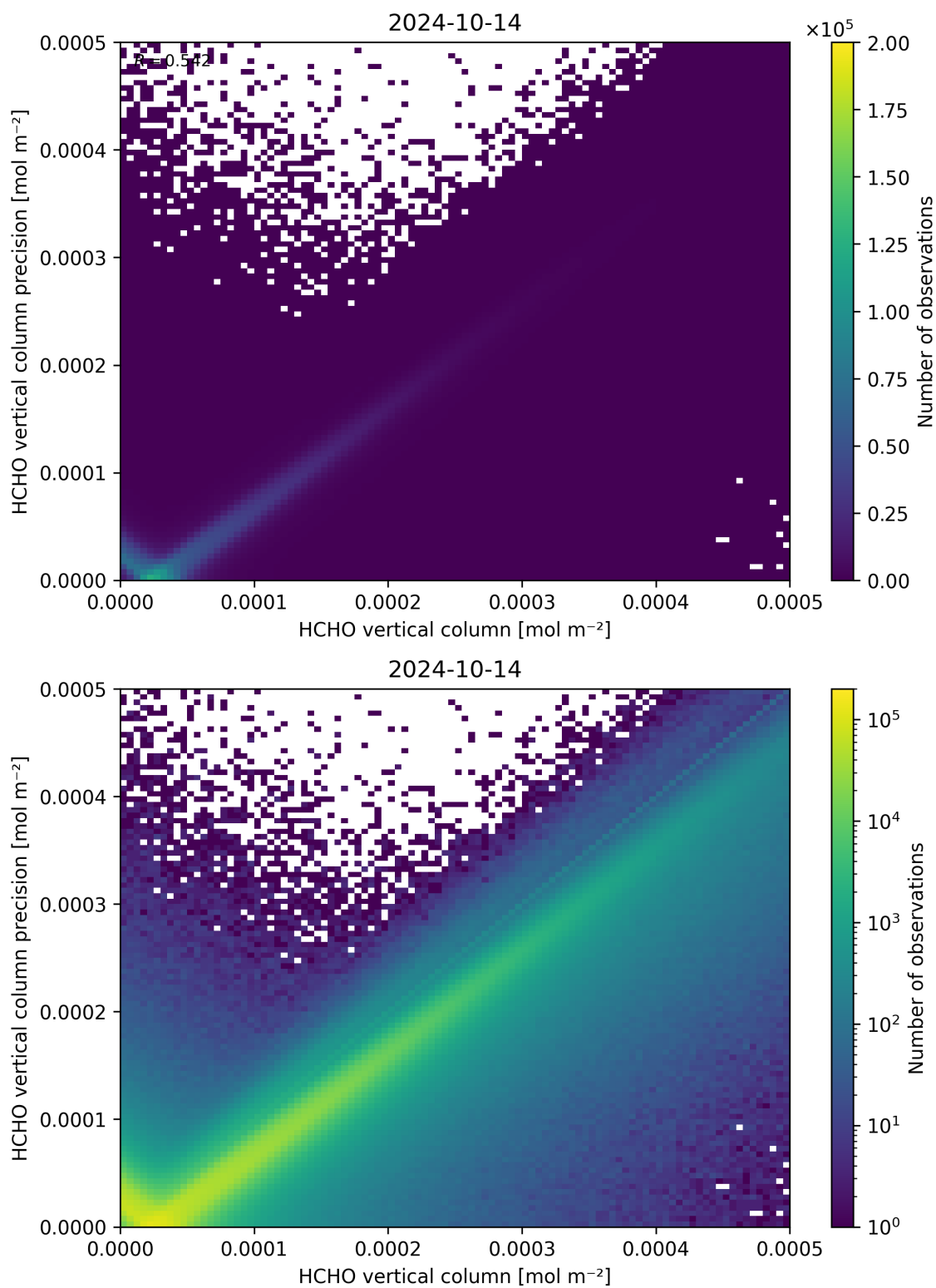
Figure 134: Scatter density plot of “HCHO vertical column” against “HCHO vertical column precision” for 2024-10-14 to 2024-10-15.
