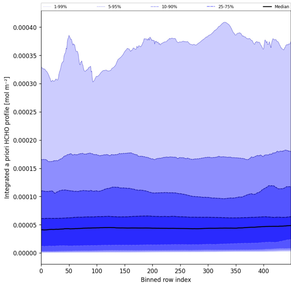
Figure 57: Along track statistics of “Integrated a priori HCHO profile” for 2024-10-14 to 2024-10-15
