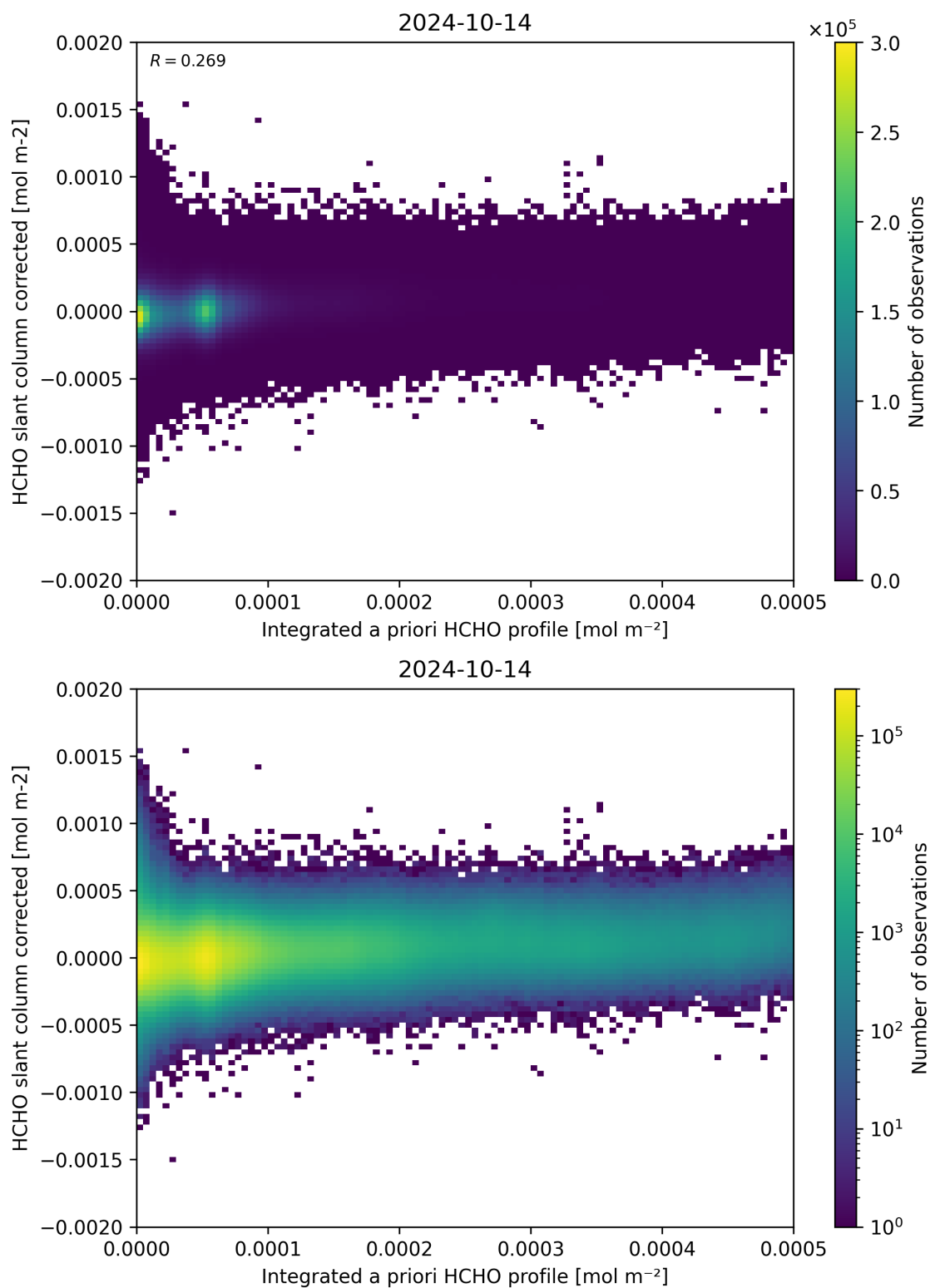
Figure 151: Scatter density plot of “Integrated a priori HCHO profile” against “HCHO slant column corrected” for 2024-10-14 to 2024-10-15.
