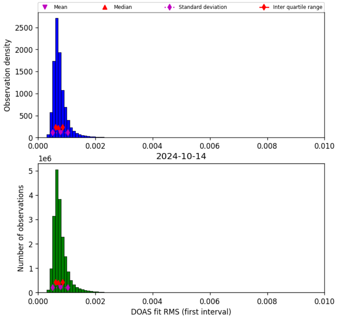
Figure 46: Histogram of “DOAS fit RMS (first interval)” for 2024-10-14 to 2024-10-15
