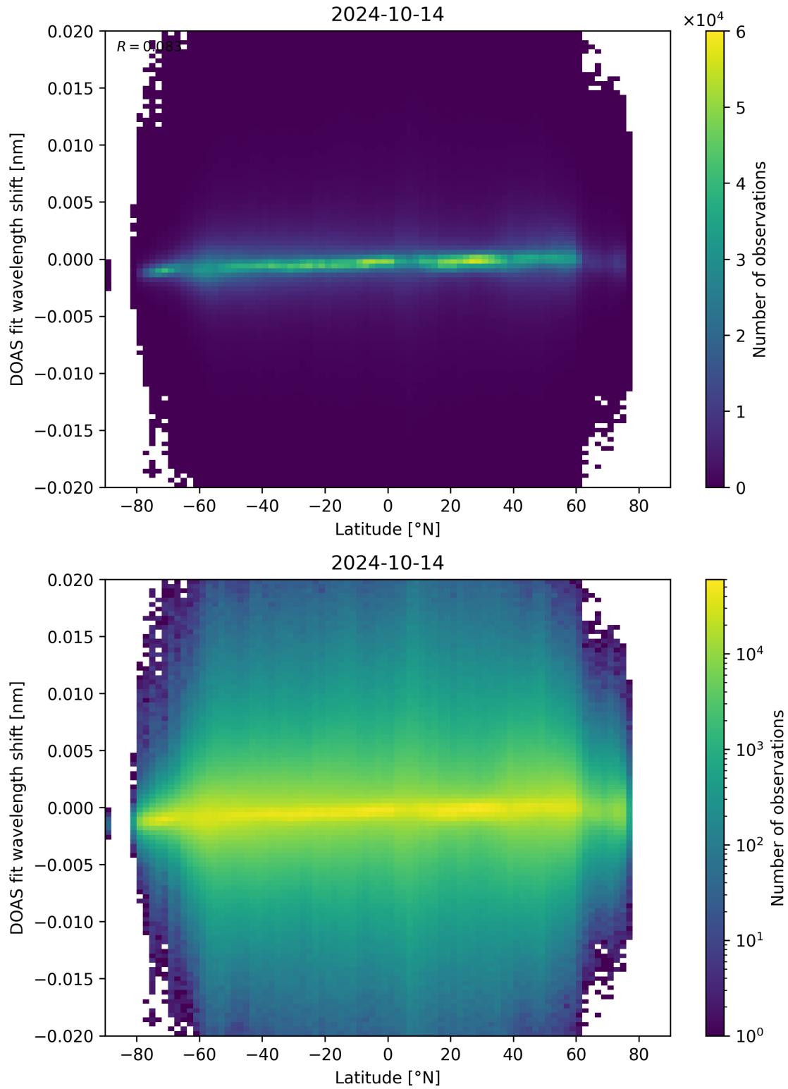
Figure 154: Scatter density plot of “Latitude” against “DOAS fit wavelength shift” for 2024-10-14 to 2024-10-15.
