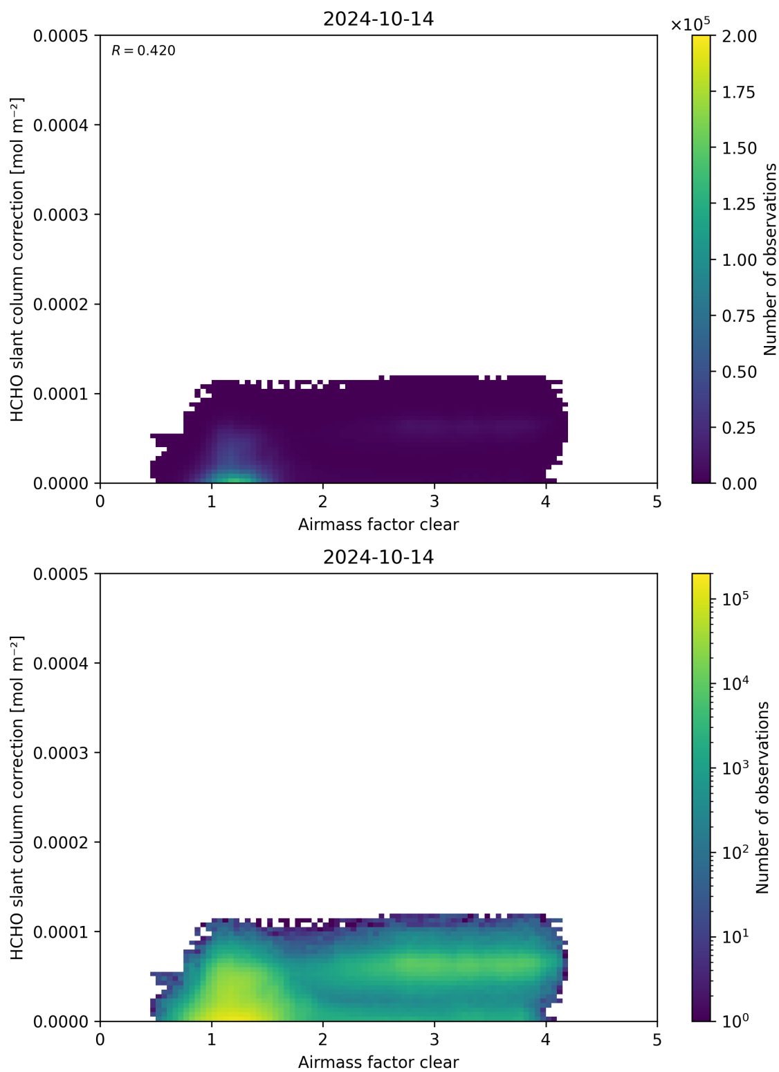
Figure 75: Scatter density plot of “Airmass factor clear” against “HCHO slant column correction” for 2024-10-14 to 2024-10-15.
