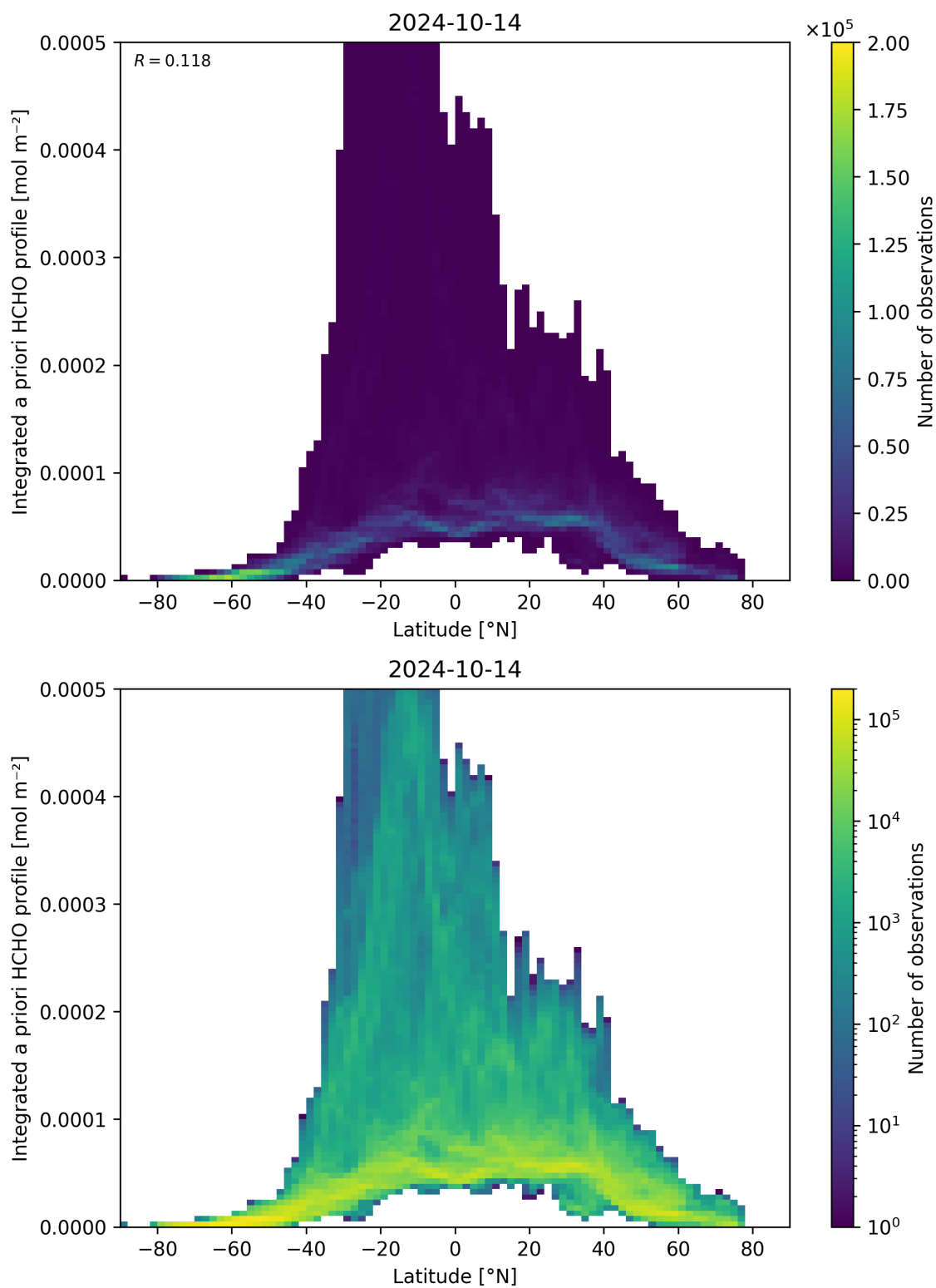
Figure 166: Scatter density plot of “Latitude” against “Integrated a priori HCHO profile” for 2024-10-14 to 2024-10-15.
