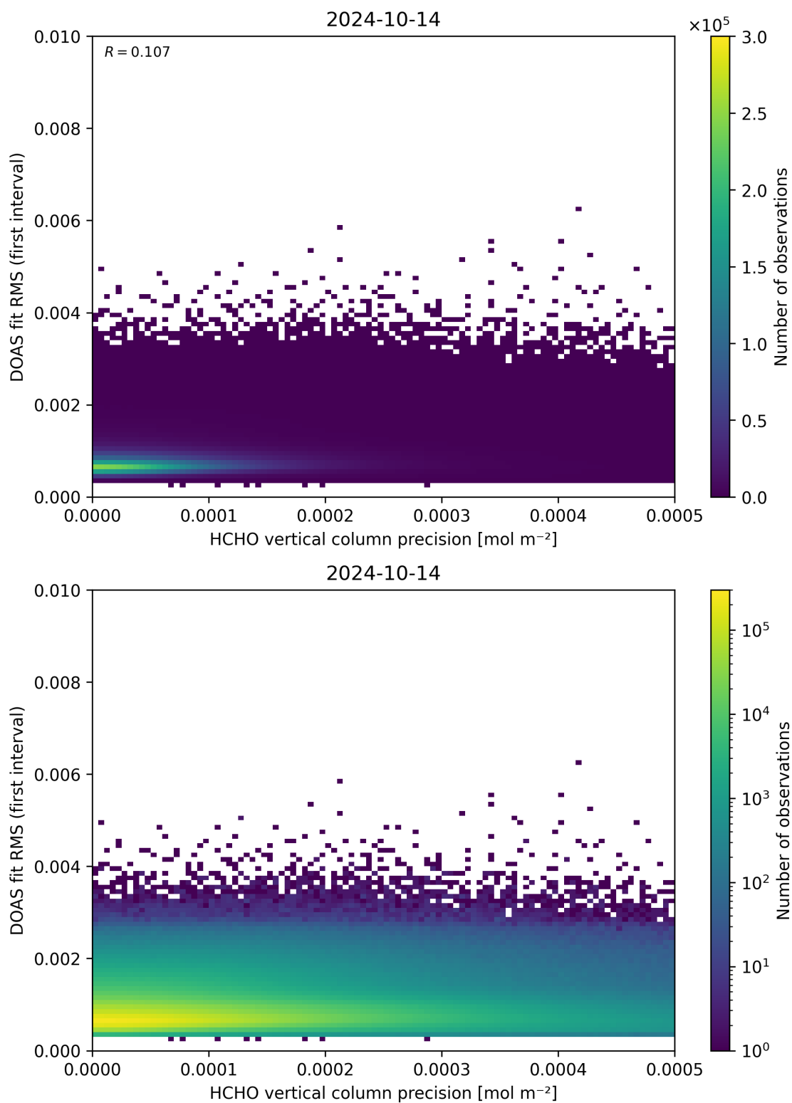
Figure 136: Scatter density plot of “HCHO vertical column precision” against “DOAS fit RMS (first interval)” for 2024-10-14 to 2024-10-15.
