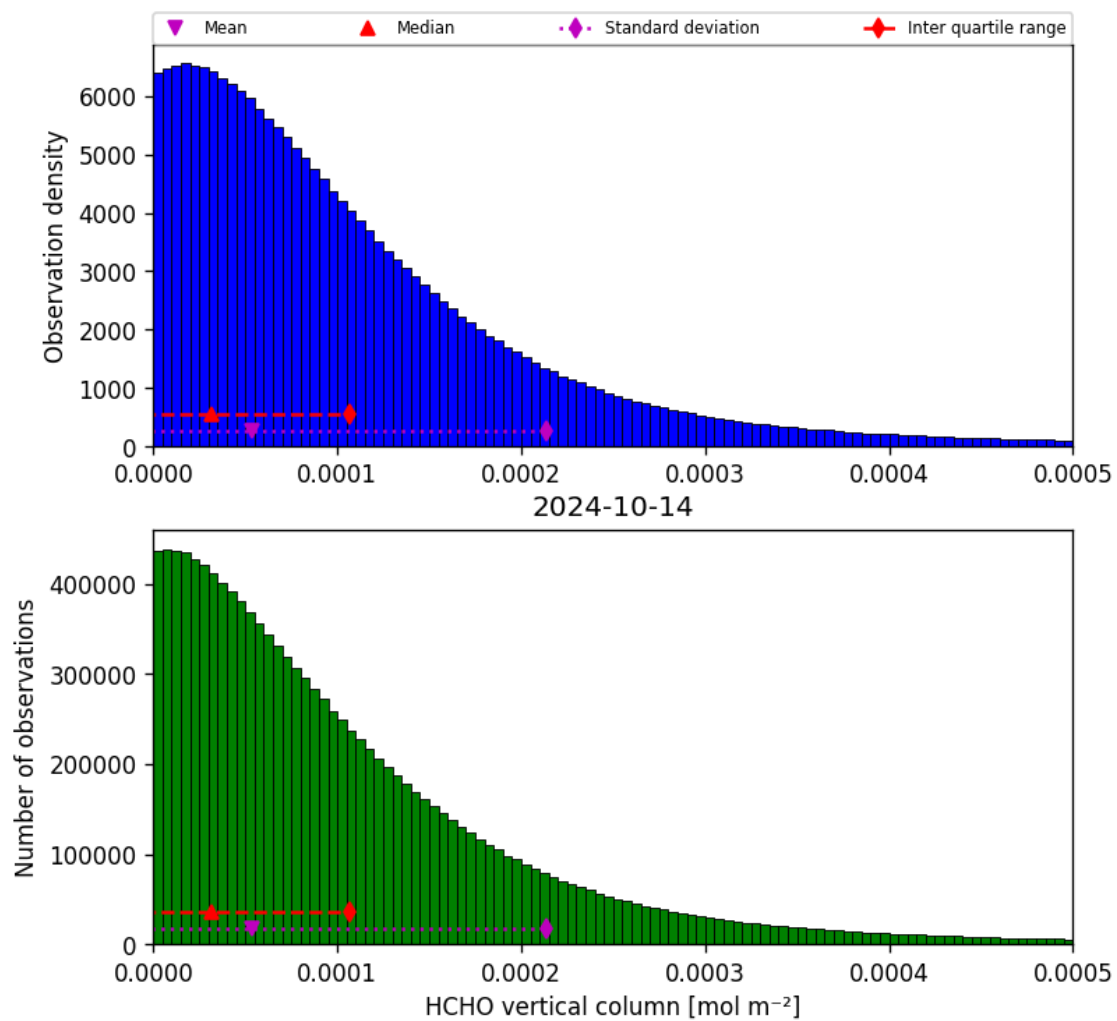
Figure 35: Histogram of “HCHO vertical column” for 2024-10-14 to 2024-10-15
