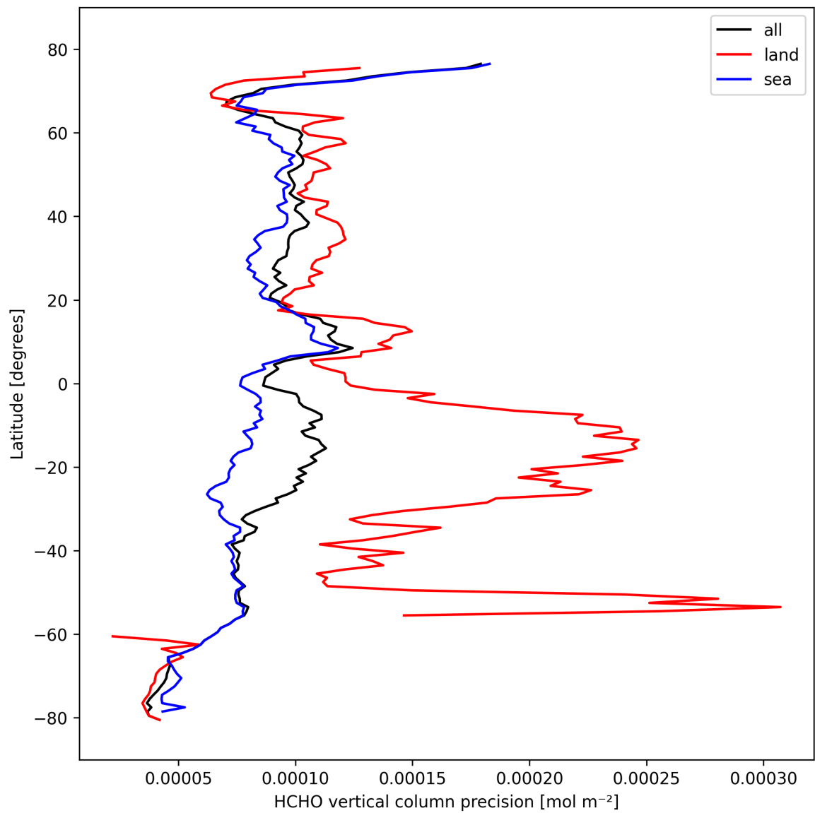
Figure 22: Zonal average of “HCHO vertical column precision” for 2024-10-14 to 2024-10-15.
