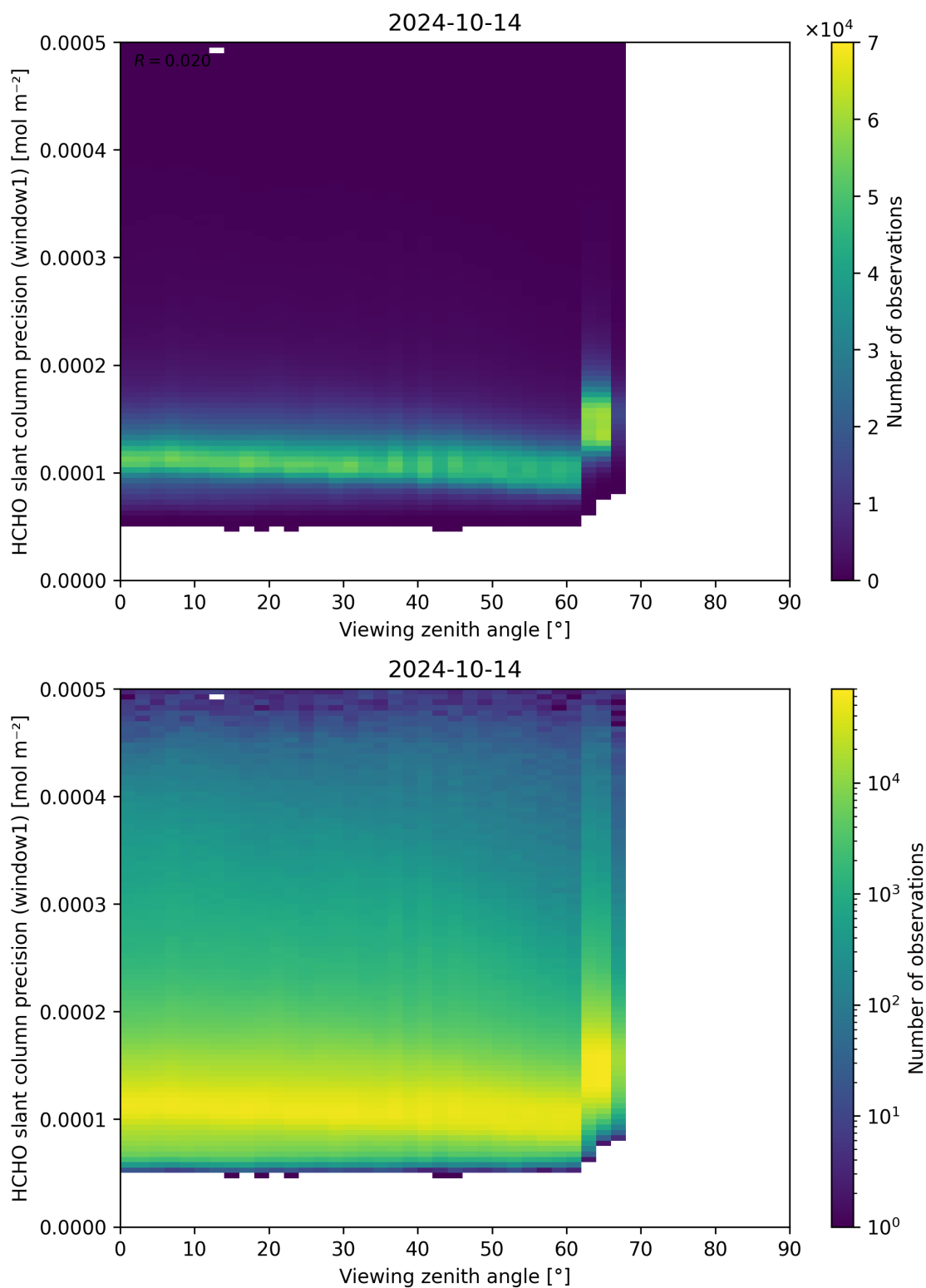
Figure 189: Scatter density plot of “Viewing zenith angle” against “HCHO slant column precision (window1)” for 2024-10-14 to 2024-10-15.
