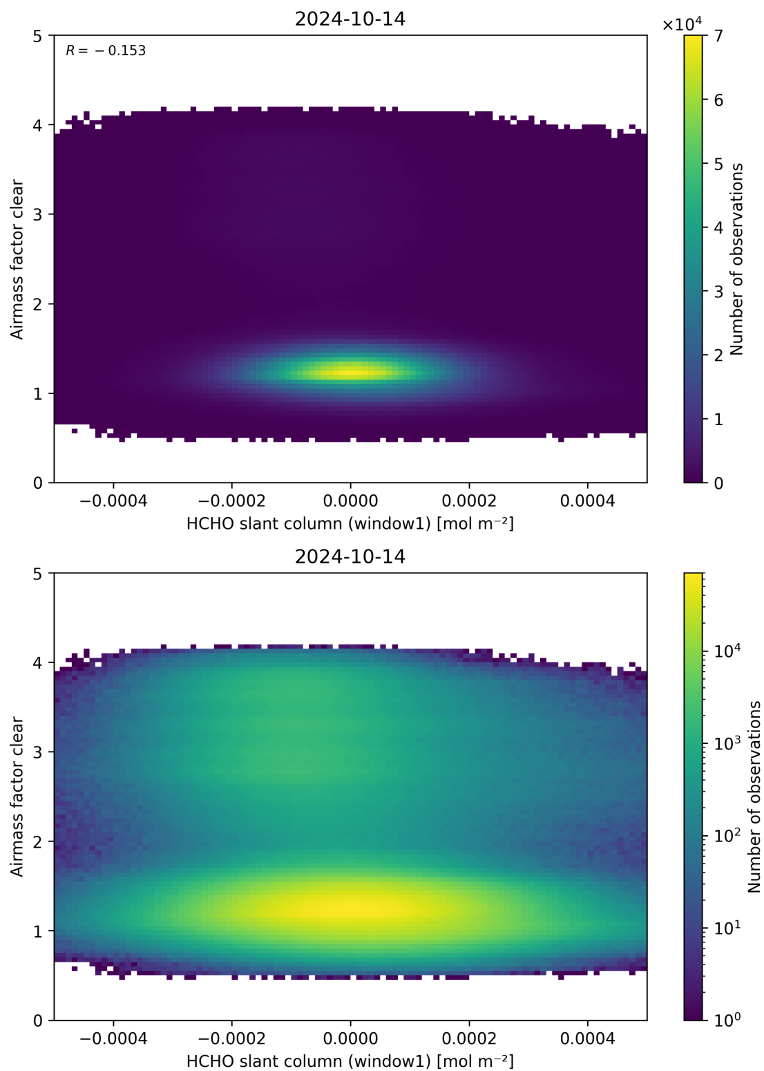
Figure 81: Scatter density plot of “HCHO slant column (window1)” against “Airmass factor clear” for 2024-10-14 to 2024-10-15.
