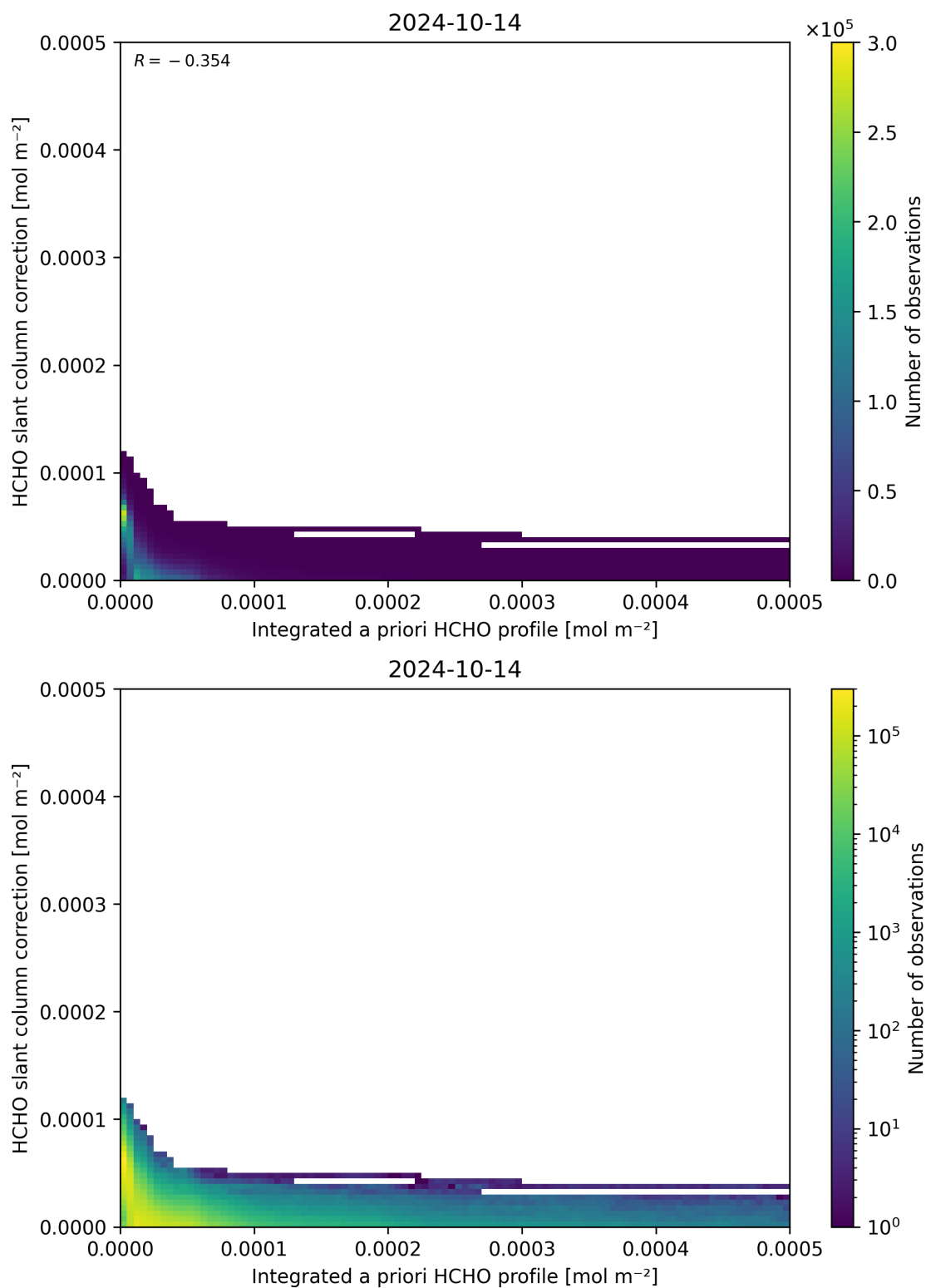
Figure 152: Scatter density plot of “Integrated a priori HCHO profile” against “HCHO slant column correction” for 2024-10-14 to 2024-10-15.
