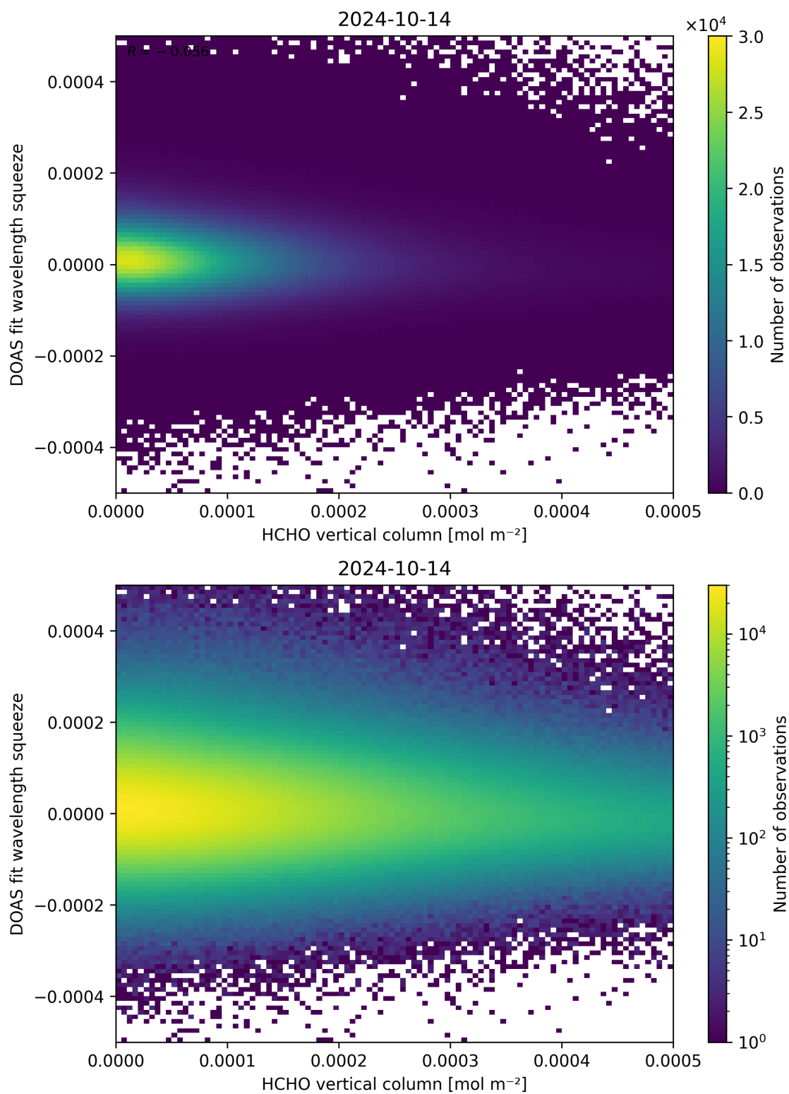
Figure 125: Scatter density plot of “HCHO vertical column” against “DOAS fit wavelength squeeze” for 2024-10-14 to 2024-10-15.
