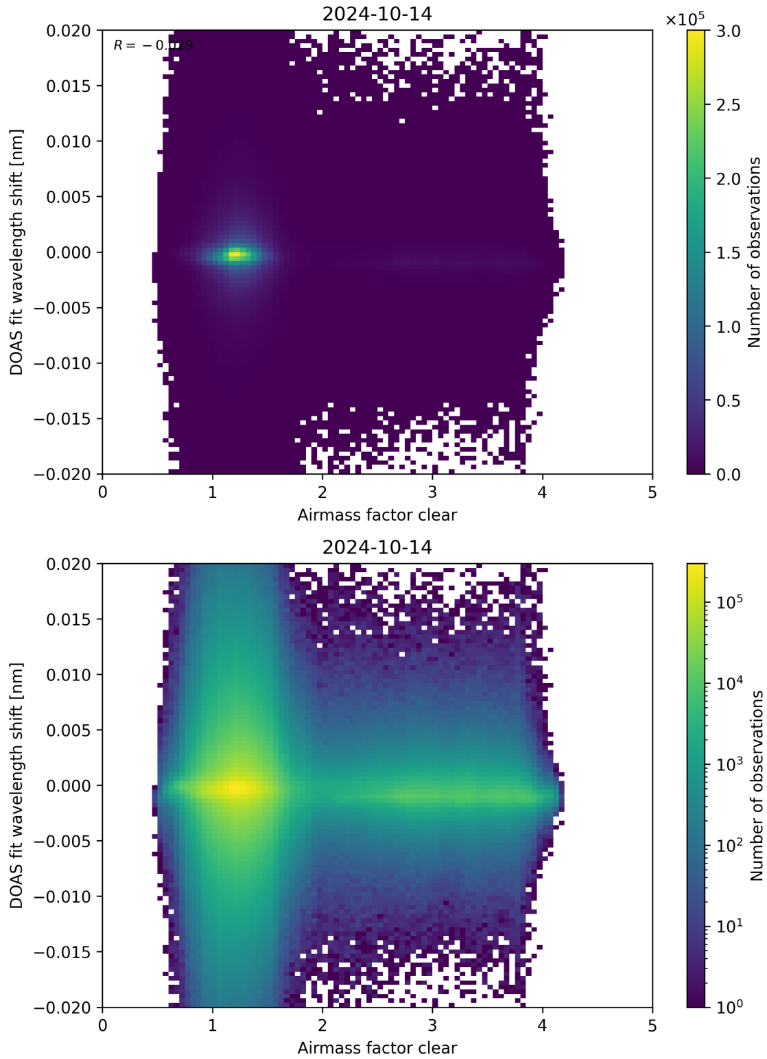
Figure 72: Scatter density plot of “Airmass factor clear” against “DOAS fit wavelength shift” for 2024-10-14 to 2024-10-15.
