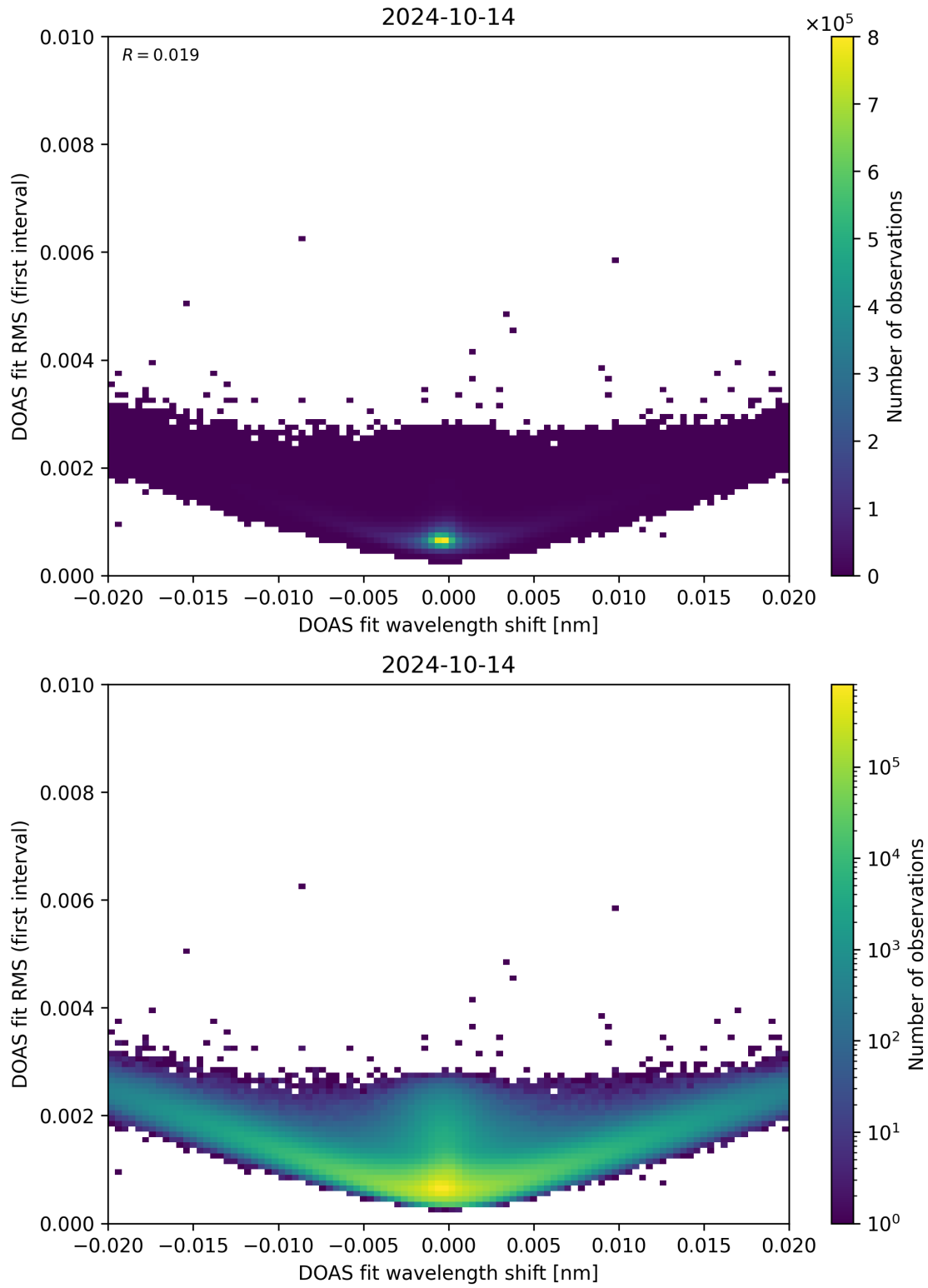
Figure 64: Scatter density plot of “DOAS fit wavelength shift” against “DOAS fit RMS (first interval)” for 2024-10-14 to 2024-10-15.
