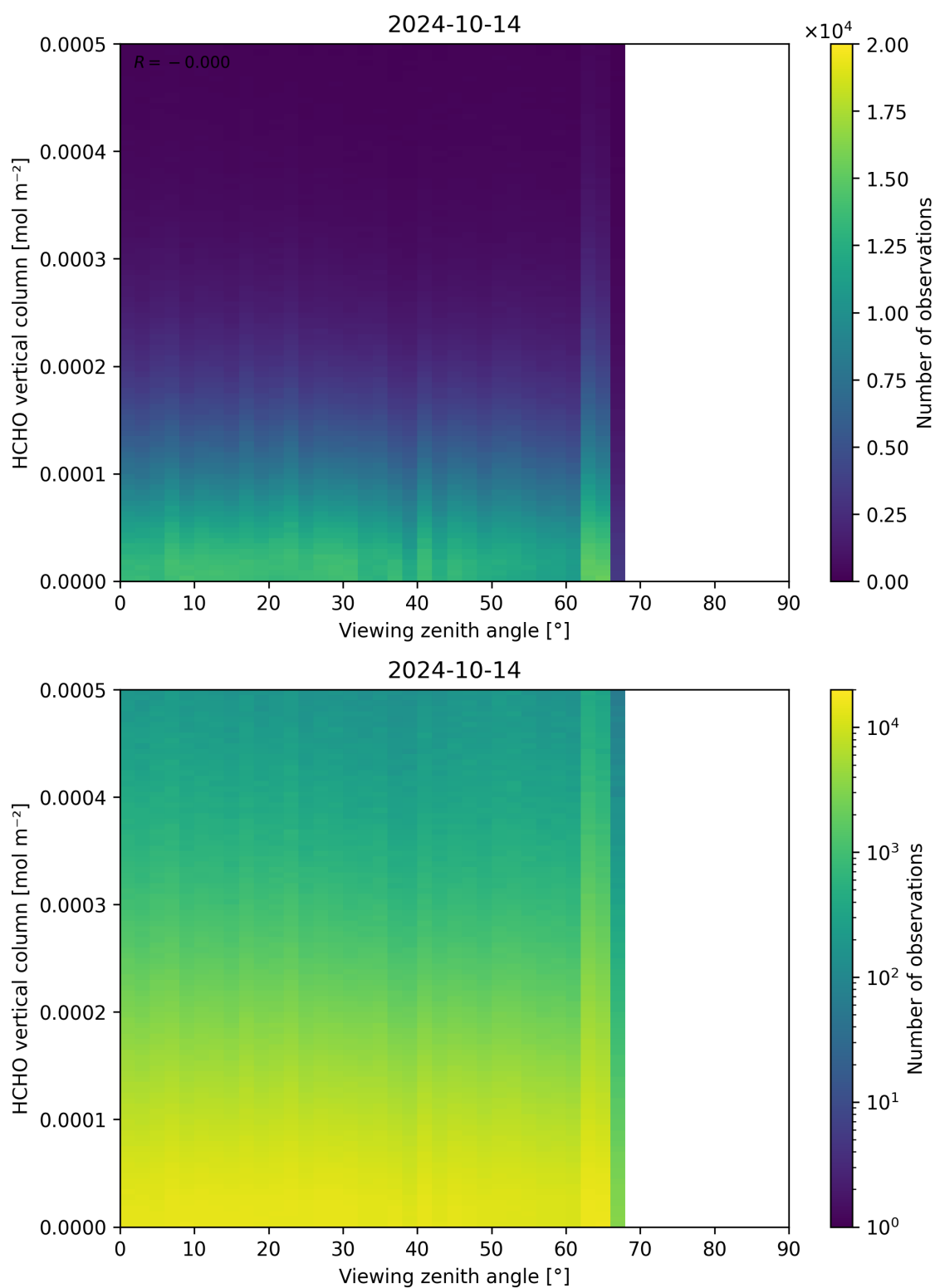
Figure 192: Scatter density plot of “Viewing zenith angle” against “HCHO vertical column” for 2024-10-14 to 2024-10-15.
