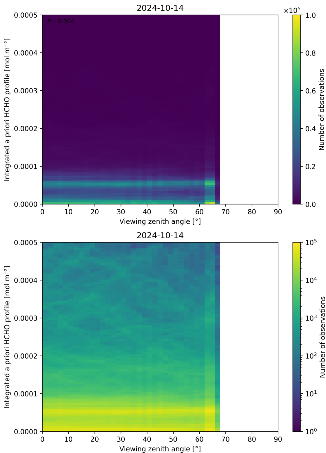
Figure 195: Scatter density plot of “Viewing zenith angle” against “Integrated a priori HCHO profile” for 2024-10-14 to 2024-10-15.
