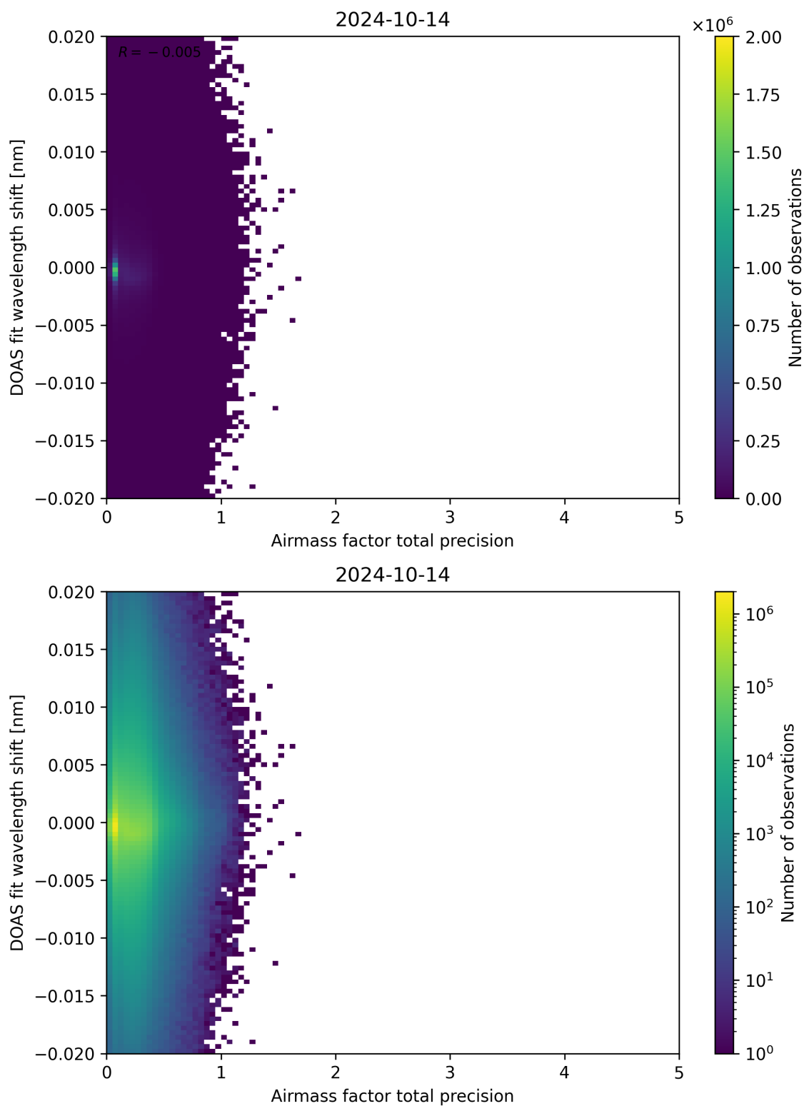
Figure 106: Scatter density plot of “Airmass factor total precision” against “DOAS fit wavelength shift” for 2024-10-14 to 2024-10-15.
