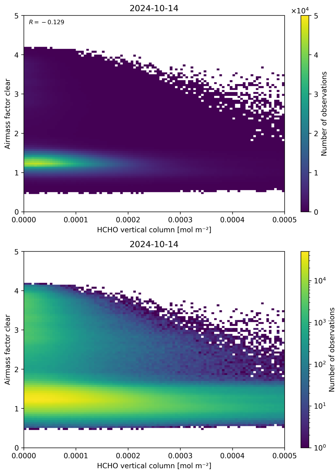
Figure 126: Scatter density plot of “HCHO vertical column” against “Airmass factor clear” for 2024-10-14 to 2024-10-15.
