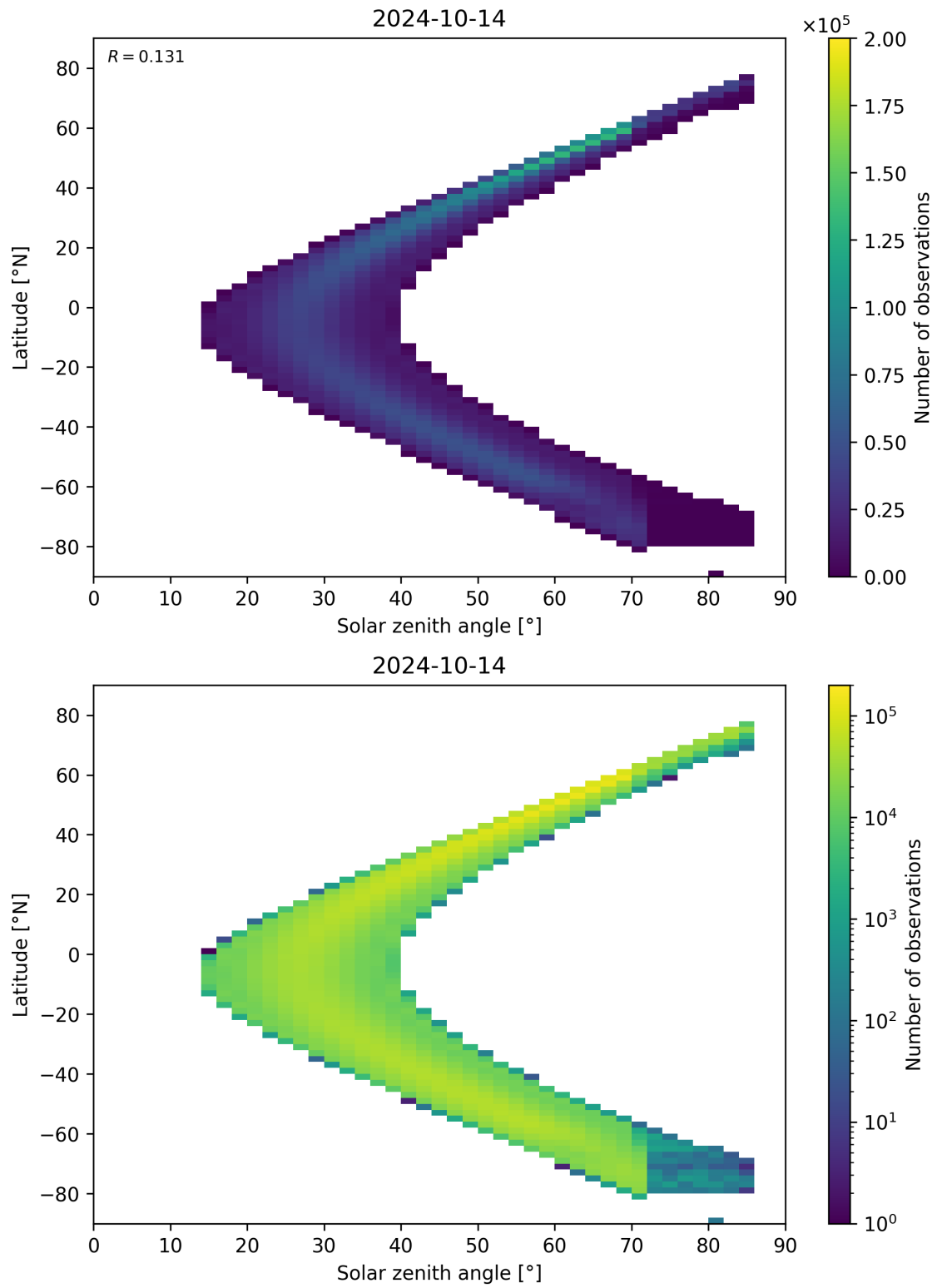
Figure 181: Scatter density plot of “Solar zenith angle” against “Latitude” for 2024-10-14 to 2024-10-15.
