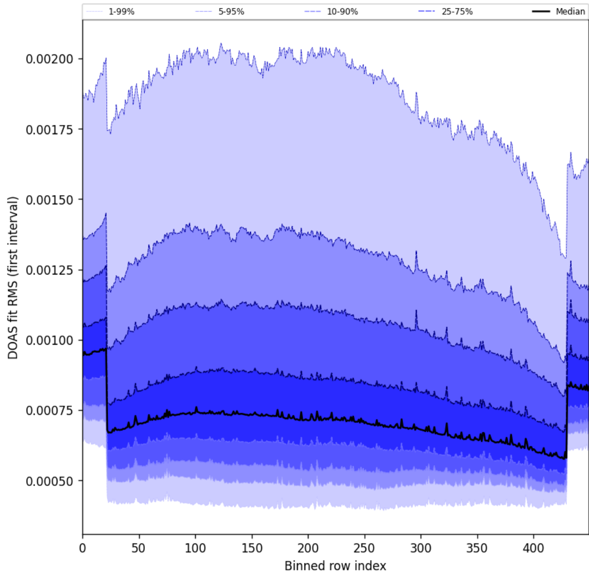
Figure 60: Along track statistics of “DOAS fit RMS (first interval)” for 2024-10-14 to 2024-10-15
