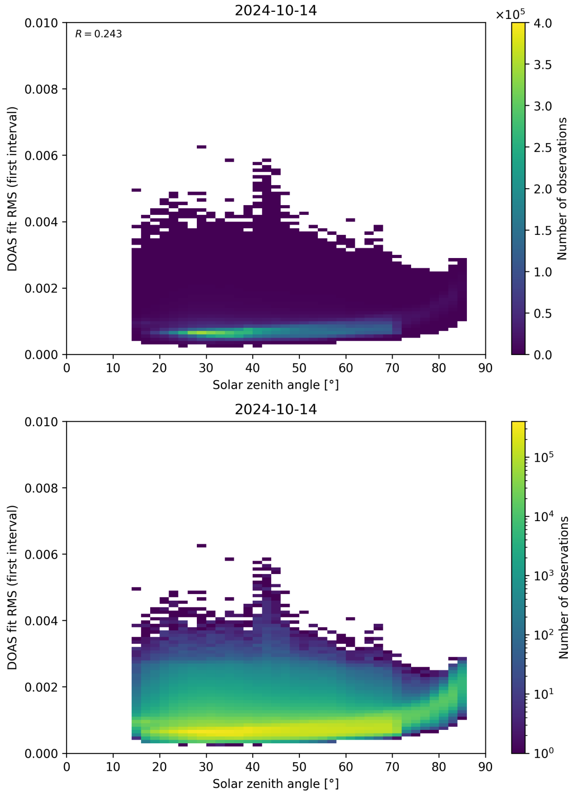
Figure 167: Scatter density plot of “Solar zenith angle” against “DOAS fit RMS (first interval)” for 2024-10-14 to 2024-10-15.
