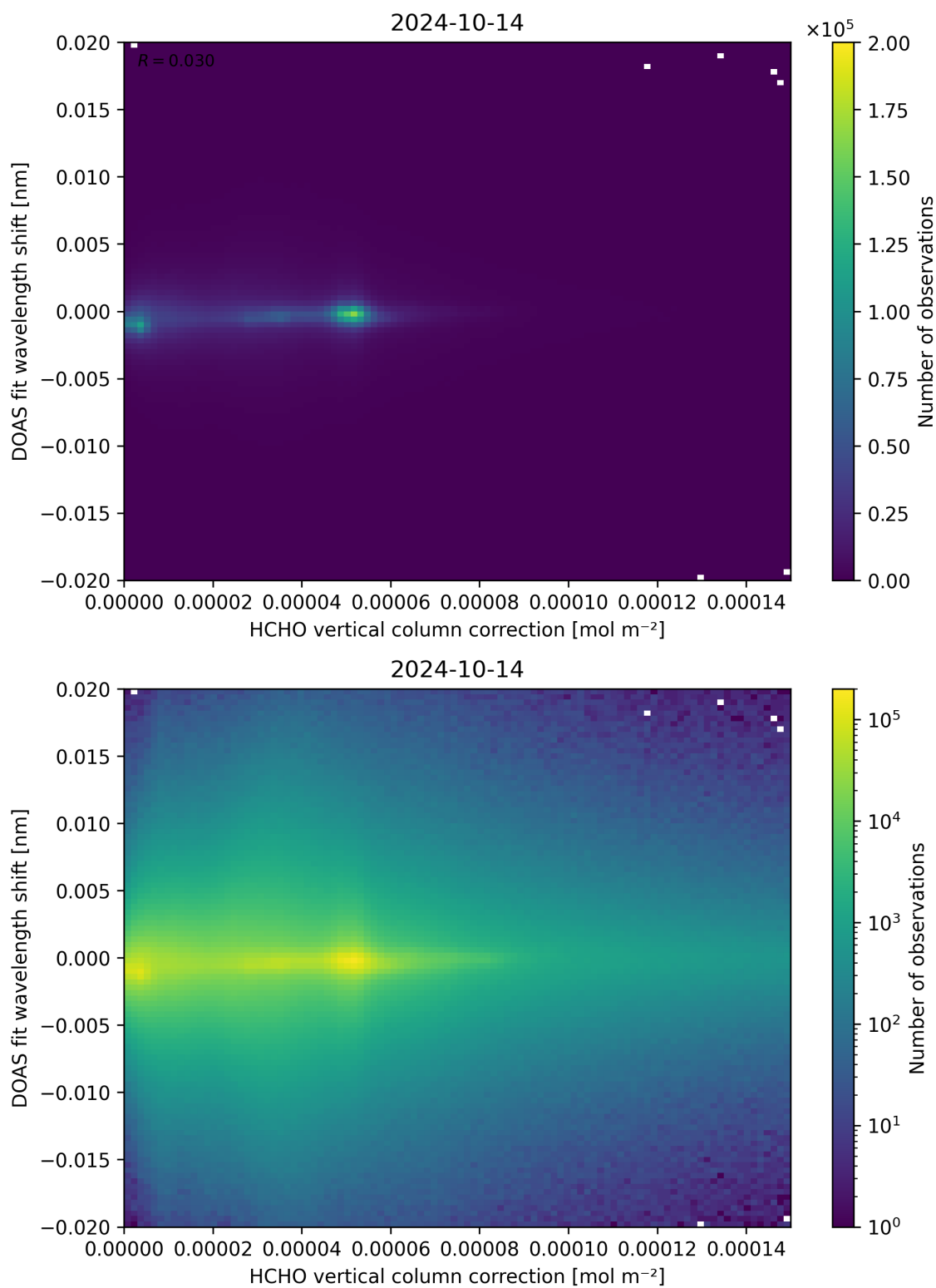
Figure 113: Scatter density plot of “HCHO vertical column correction” against “DOAS fit wavelength shift” for 2024-10-14 to 2024-10-15.
