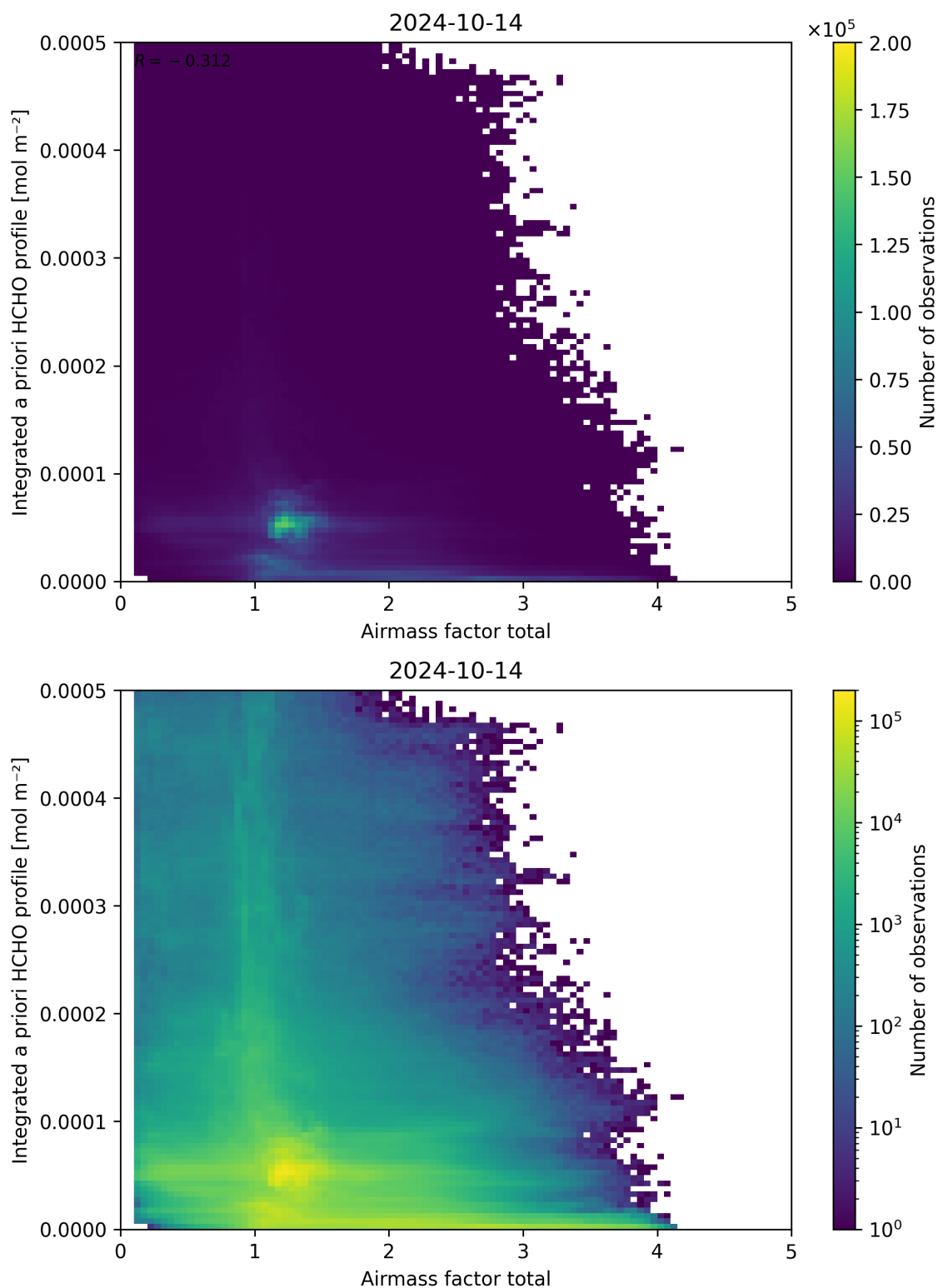
Figure 104: Scatter density plot of “Airmass factor total” against “Integrated a priori HCHO profile” for 2024-10-14 to 2024-10-15.
