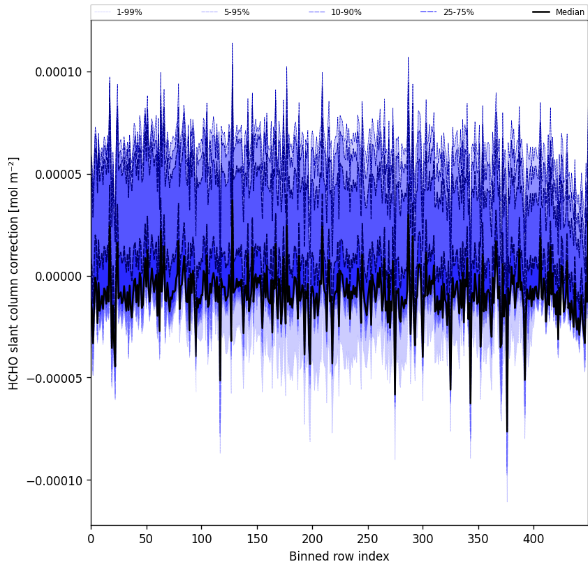
Figure 61: Along track statistics of “HCHO slant column correction” for 2024-10-14 to 2024-10-15
