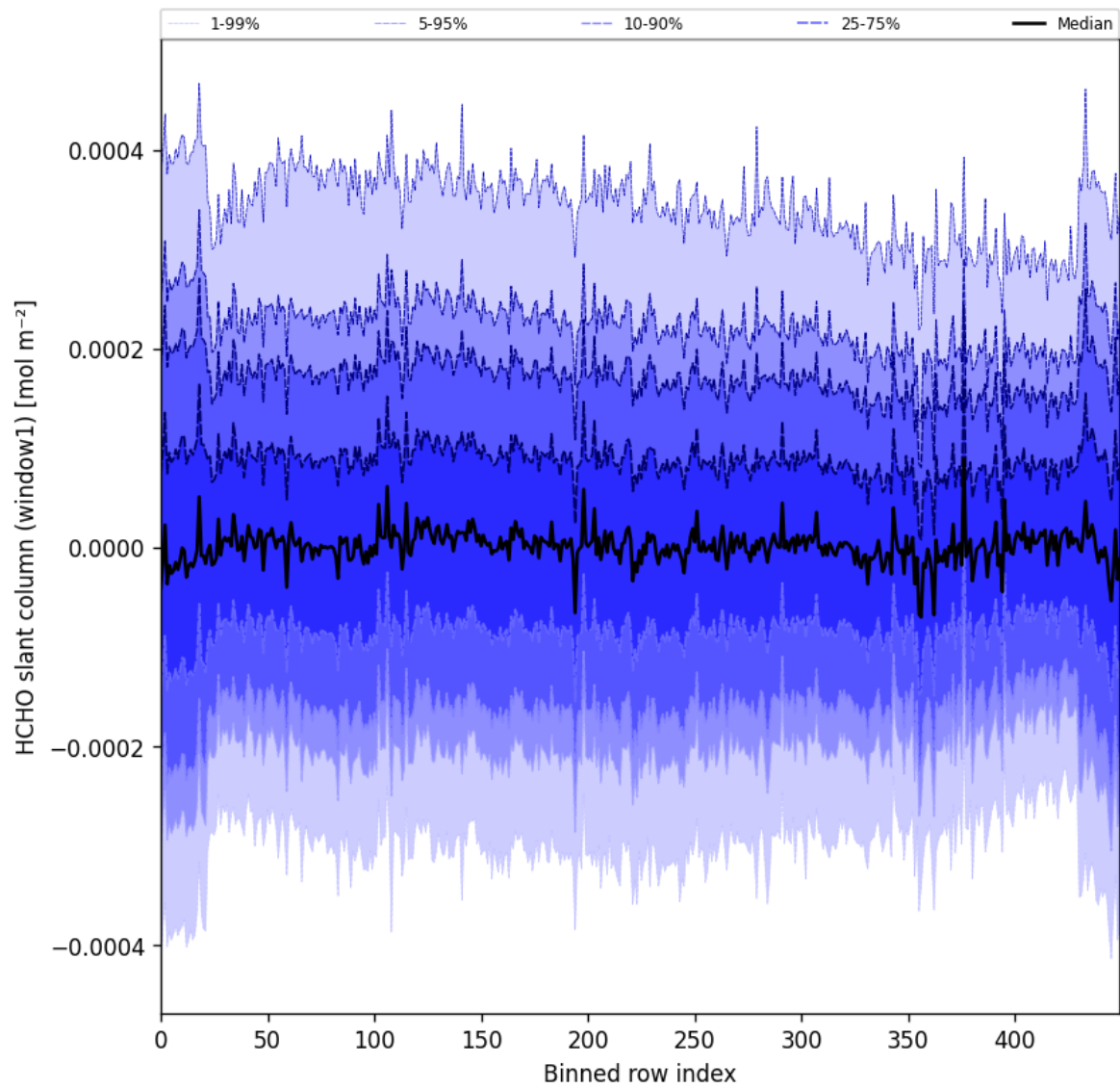
Figure 52: Along track statistics of “HCHO slant column (window1)” for 2024-10-14 to 2024-10-15
