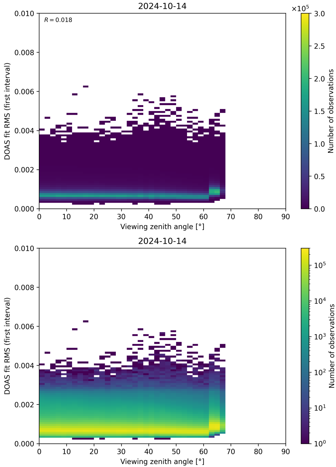
Figure 182: Scatter density plot of “Viewing zenith angle” against “DOAS fit RMS (first interval)” for 2024-10-14 to 2024-10-15.
