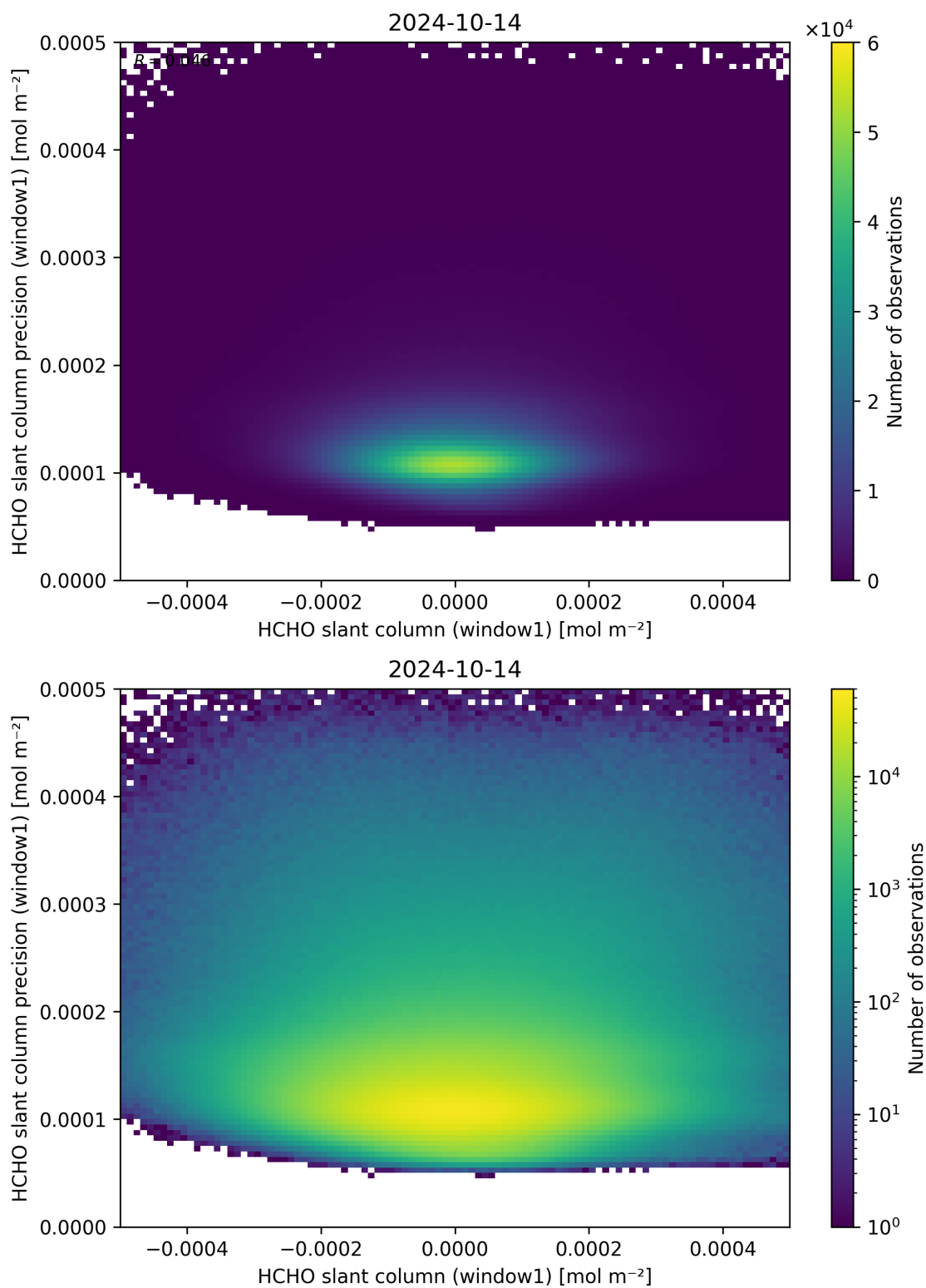
Figure 84: Scatter density plot of “HCHO slant column (window1)” against “HCHO slant column precision (window1)” for 2024-10-14 to 2024-10-15.
