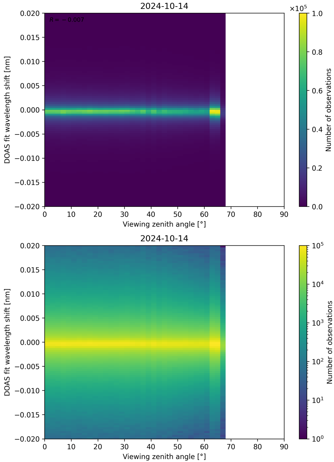
Figure 183: Scatter density plot of “Viewing zenith angle” against “DOAS fit wavelength shift” for 2024-10-14 to 2024-10-15.
