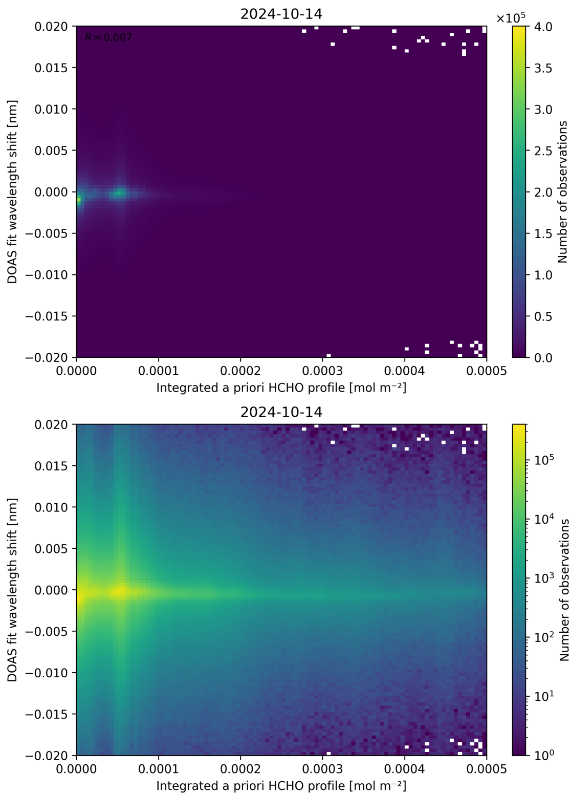
Figure 149: Scatter density plot of “Integrated a priori HCHO profile” against “DOAS fit wavelength shift” for 2024-10-14 to 2024-10-15.
