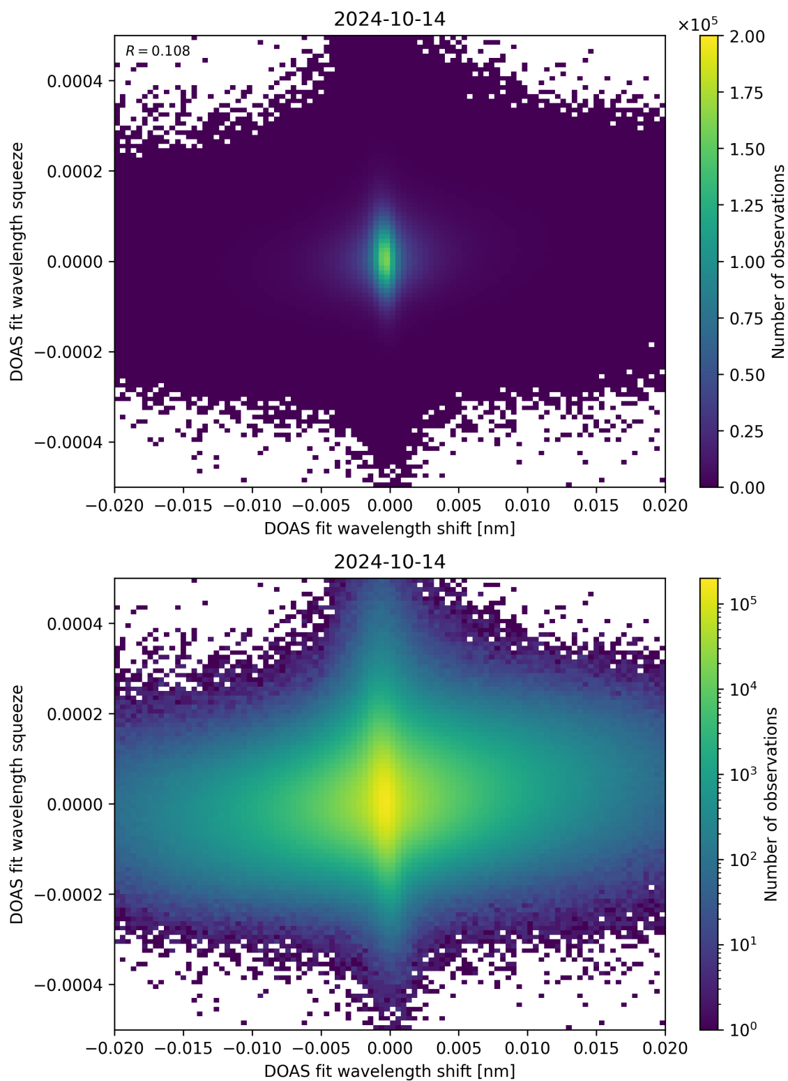
Figure 65: Scatter density plot of “DOAS fit wavelength shift” against “DOAS fit wavelength squeeze” for 2024-10-14 to 2024-10-15.
