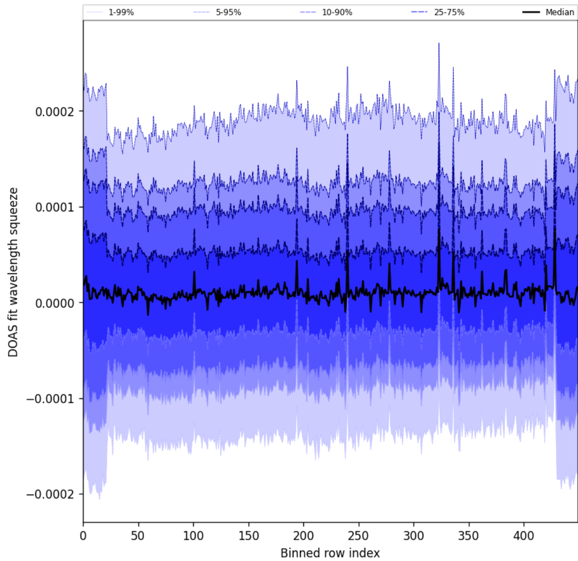
Figure 59: Along track statistics of “DOAS fit wavelength squeeze” for 2024-10-14 to 2024-10-15
