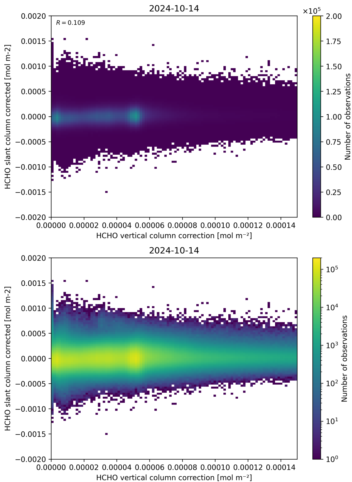
Figure 116: Scatter density plot of “HCHO vertical column correction” against “HCHO slant column corrected” for 2024-10-14 to 2024-10-15.
