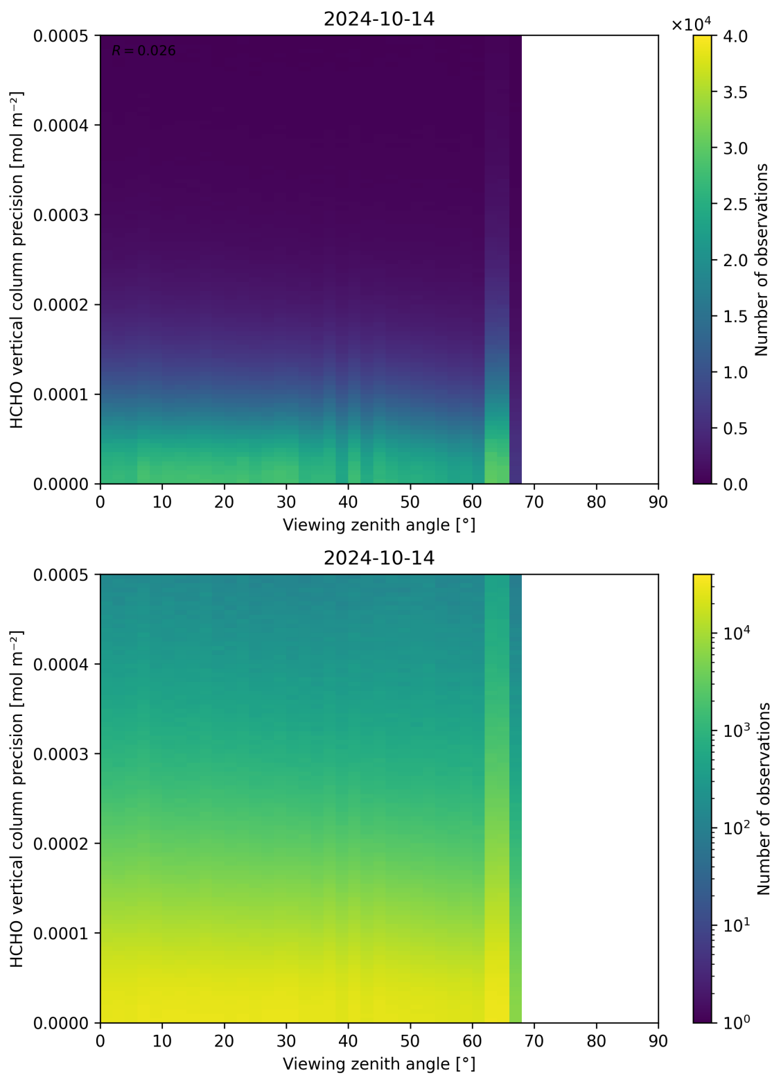
Figure 194: Scatter density plot of “Viewing zenith angle” against “HCHO vertical column precision” for 2024-10-14 to 2024-10-15.
