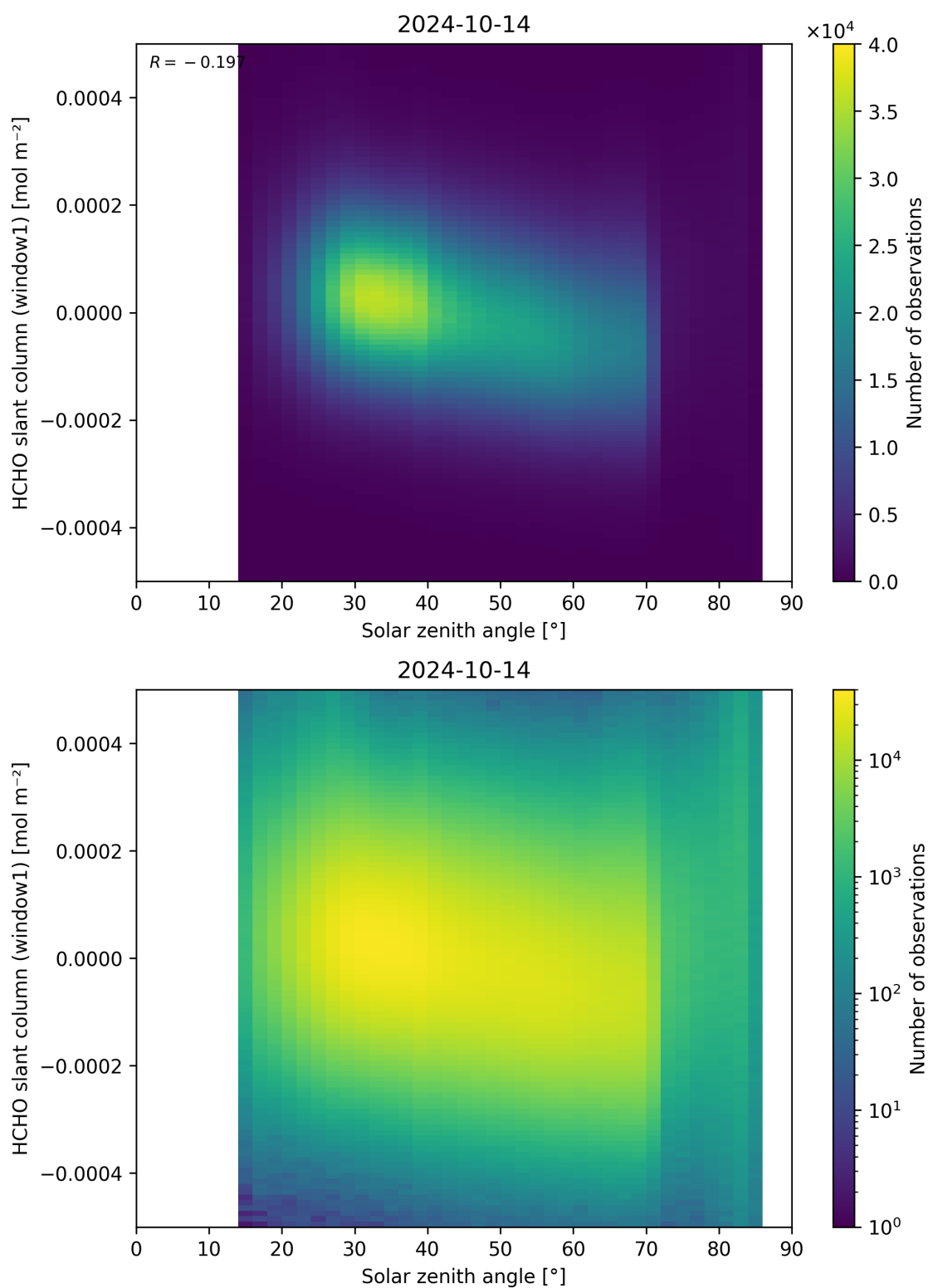
Figure 173: Scatter density plot of “Solar zenith angle” against “HCHO slant column (window1)” for 2024-10-14 to 2024-10-15.
