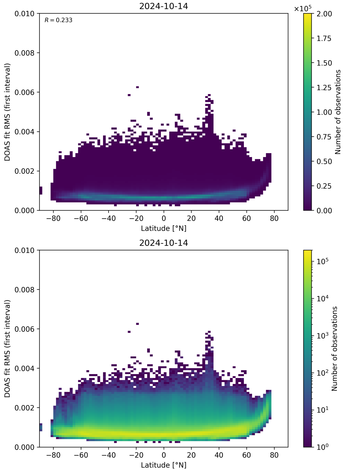
Figure 153: Scatter density plot of “Latitude” against “DOAS fit RMS (first interval)” for 2024-10-14 to 2024-10-15.
