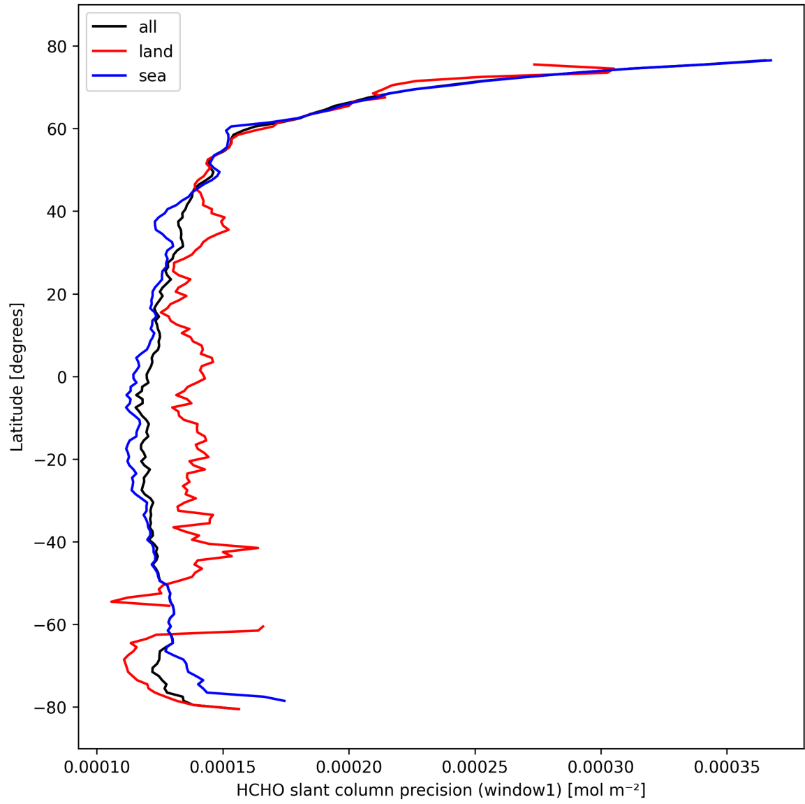
Figure 25: Zonal average of “HCHO slant column precision (window1)” for 2024-10-14 to 2024-10-15.
