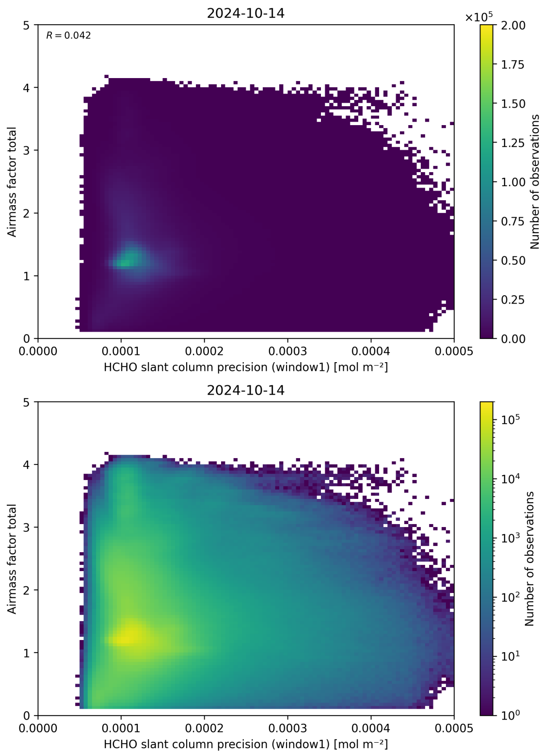
Figure 94: Scatter density plot of “HCHO slant column precision (window1)” against “Airmass factor total” for 2024-10-14 to 2024-10-15.
