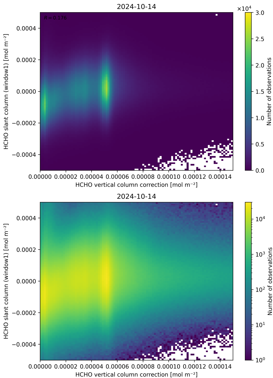
Figure 118: Scatter density plot of “HCHO vertical column correction” against “HCHO slant column (window1)” for 2024-10-14 to 2024-10-15.
