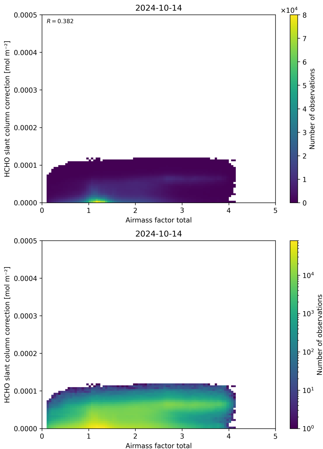
Figure 102: Scatter density plot of “Airmass factor total” against “HCHO slant column correction” for 2024-10-14 to 2024-10-15.
