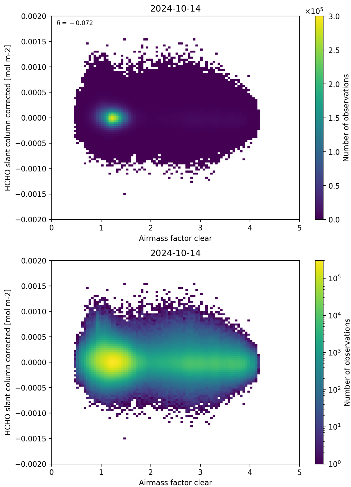
Figure 74: Scatter density plot of “Airmass factor clear” against “HCHO slant column corrected” for 2024-10-14 to 2024-10-15.
