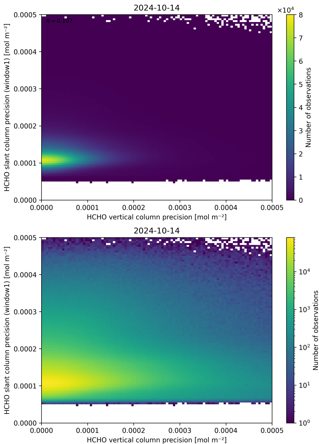
Figure 143: Scatter density plot of “HCHO vertical column precision” against “HCHO slant column precision (window1)” for 2024-10-14 to 2024-10-15.
