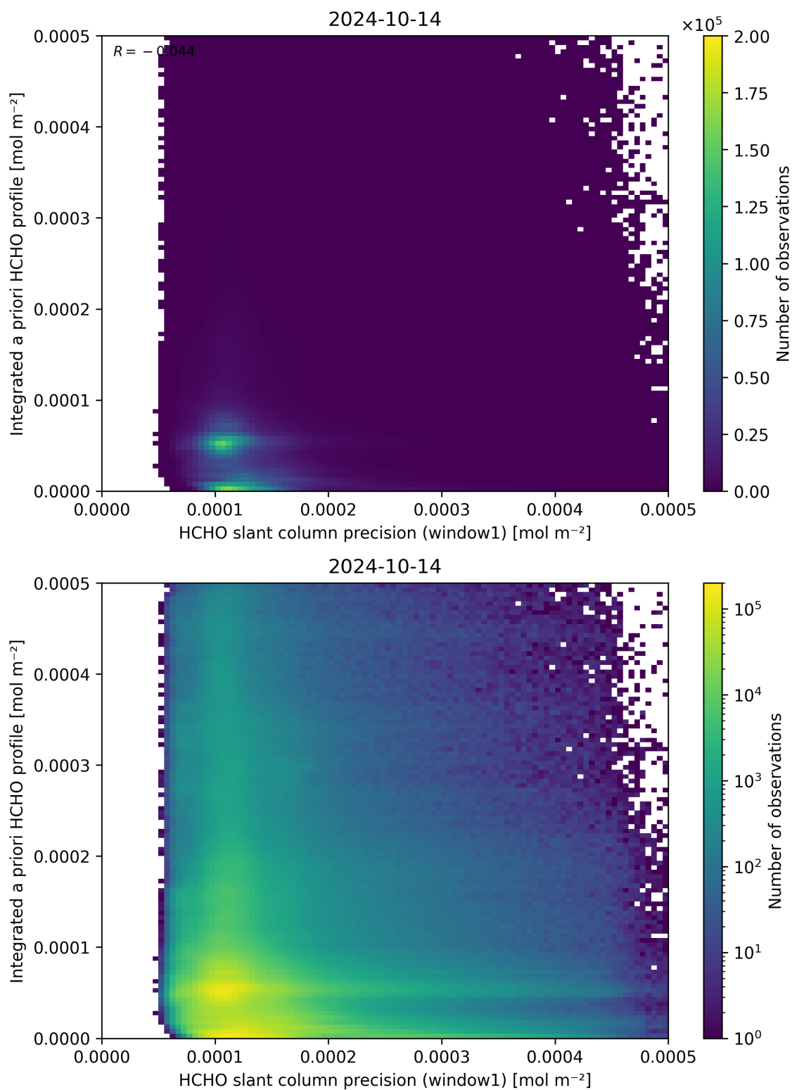
Figure 96: Scatter density plot of “HCHO slant column precision (window1)” against “Integrated a priori HCHO profile” for 2024-10-14 to 2024-10-15.
