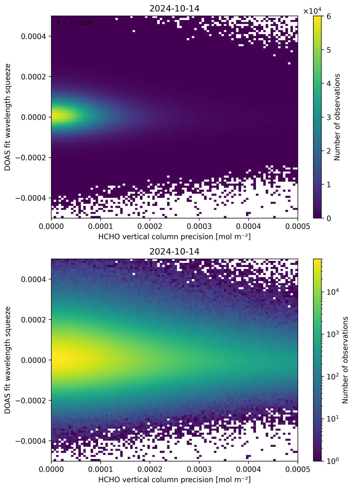
Figure 138: Scatter density plot of “HCHO vertical column precision” against “DOAS fit wavelength squeeze” for 2024-10-14 to 2024-10-15.
