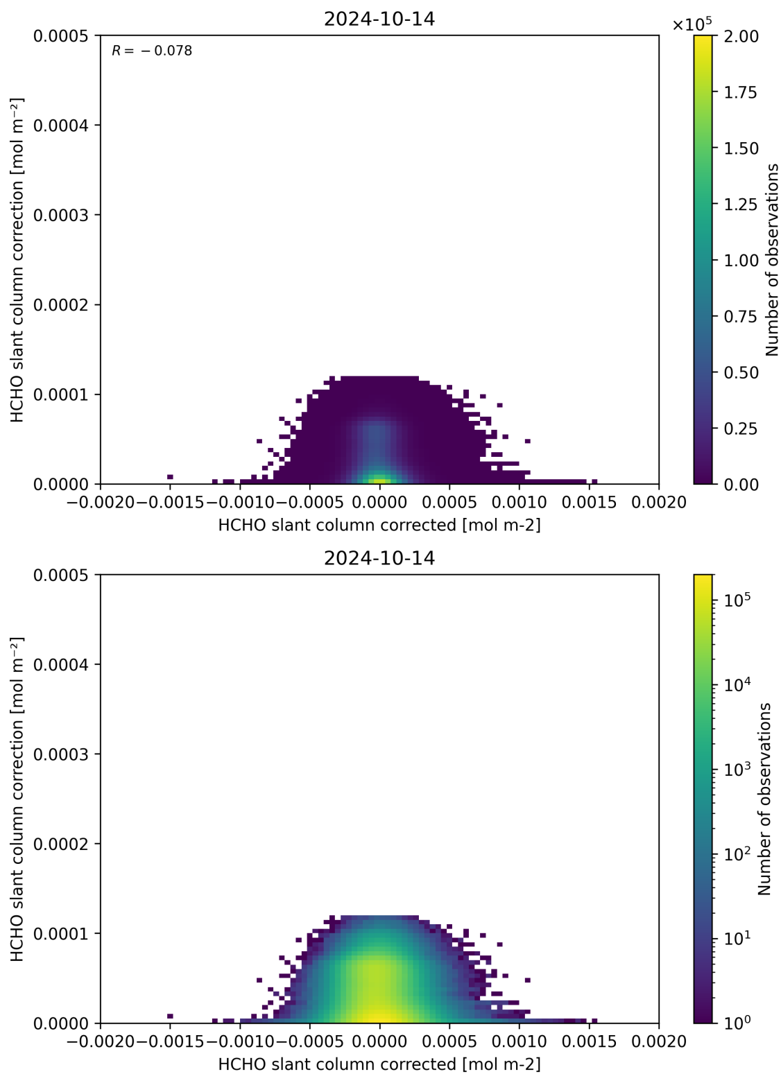
Figure 77: Scatter density plot of “HCHO slant column corrected” against “HCHO slant column correction” for 2024-10-14 to 2024-10-15.
