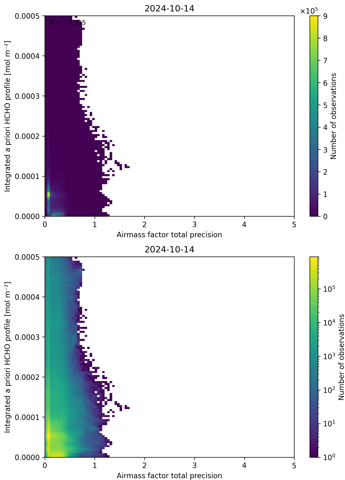
Figure 111: Scatter density plot of “Airmass factor total precision” against “Integrated a priori HCHO profile” for 2024-10-14 to 2024-10-15.
