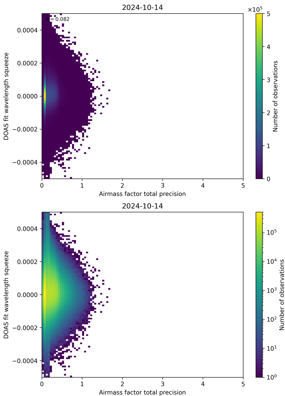
Figure 107: Scatter density plot of “Airmass factor total precision” against “DOAS fit wavelength squeeze” for 2024-10-14 to 2024-10-15.
