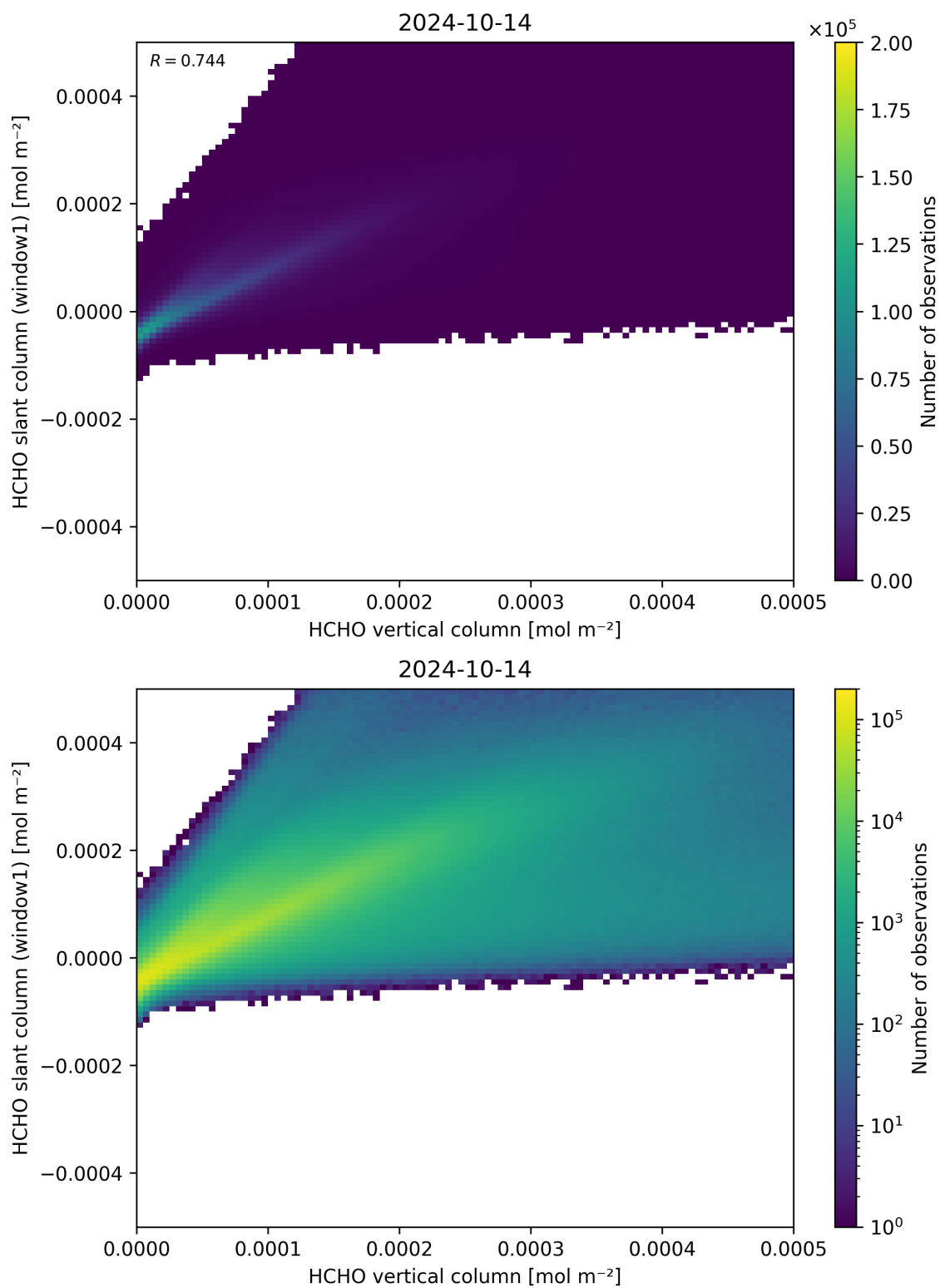
Figure 129: Scatter density plot of “HCHO vertical column” against “HCHO slant column (window1)” for 2024-10-14 to 2024-10-15.
