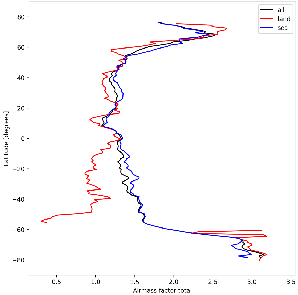
Figure 26: Zonal average of “Airmass factor total” for 2024-10-14 to 2024-10-15.
