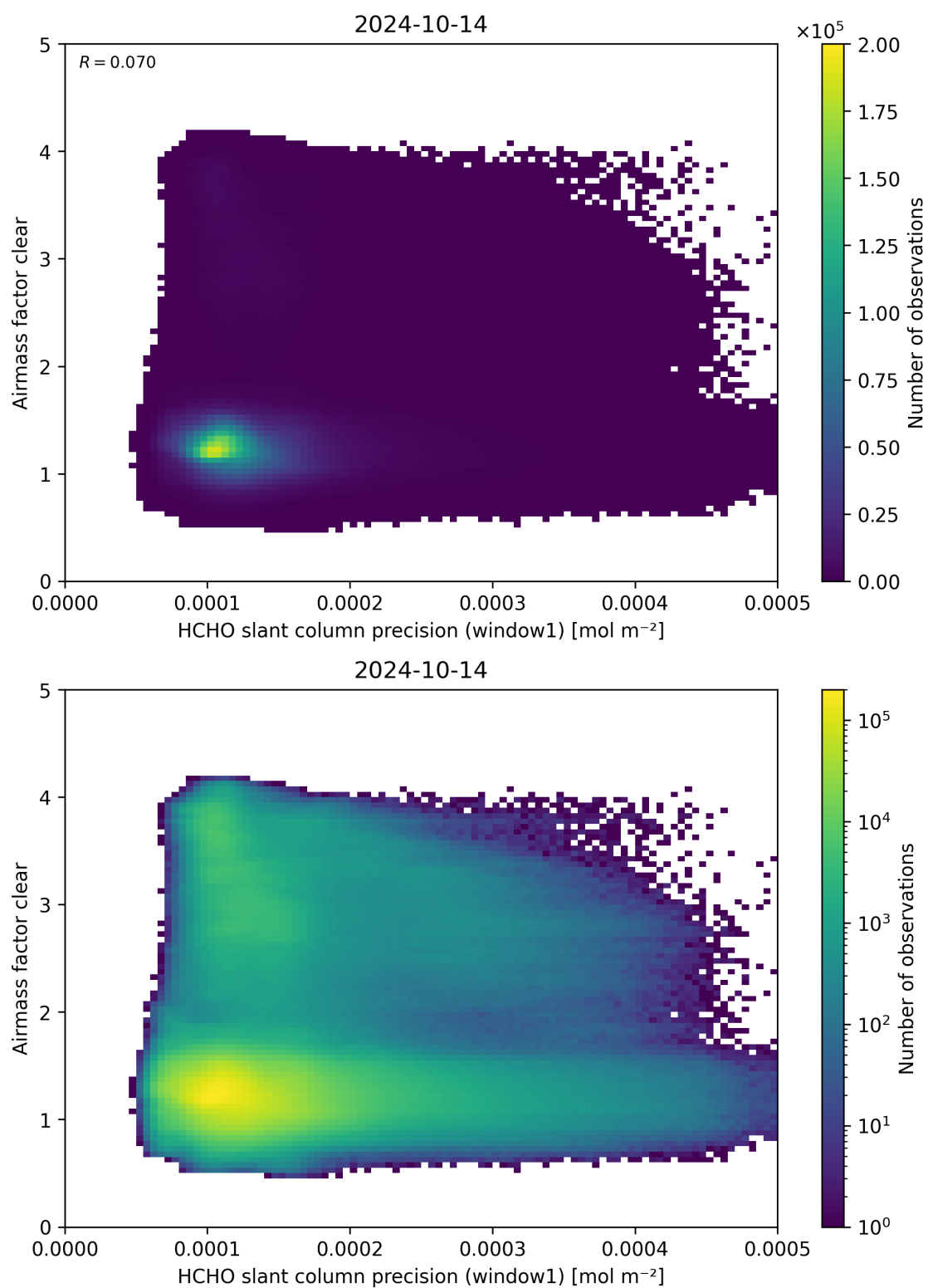
Figure 91: Scatter density plot of “HCHO slant column precision (window1)” against “Airmass factor clear” for 2024-10-14 to 2024-10-15.
