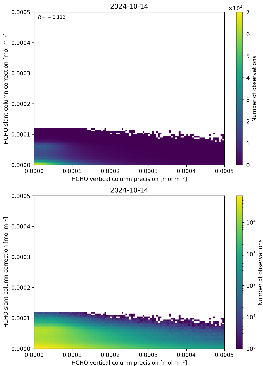
Figure 141: Scatter density plot of “HCHO vertical column precision” against “HCHO slant column correction” for 2024-10-14 to 2024-10-15.
