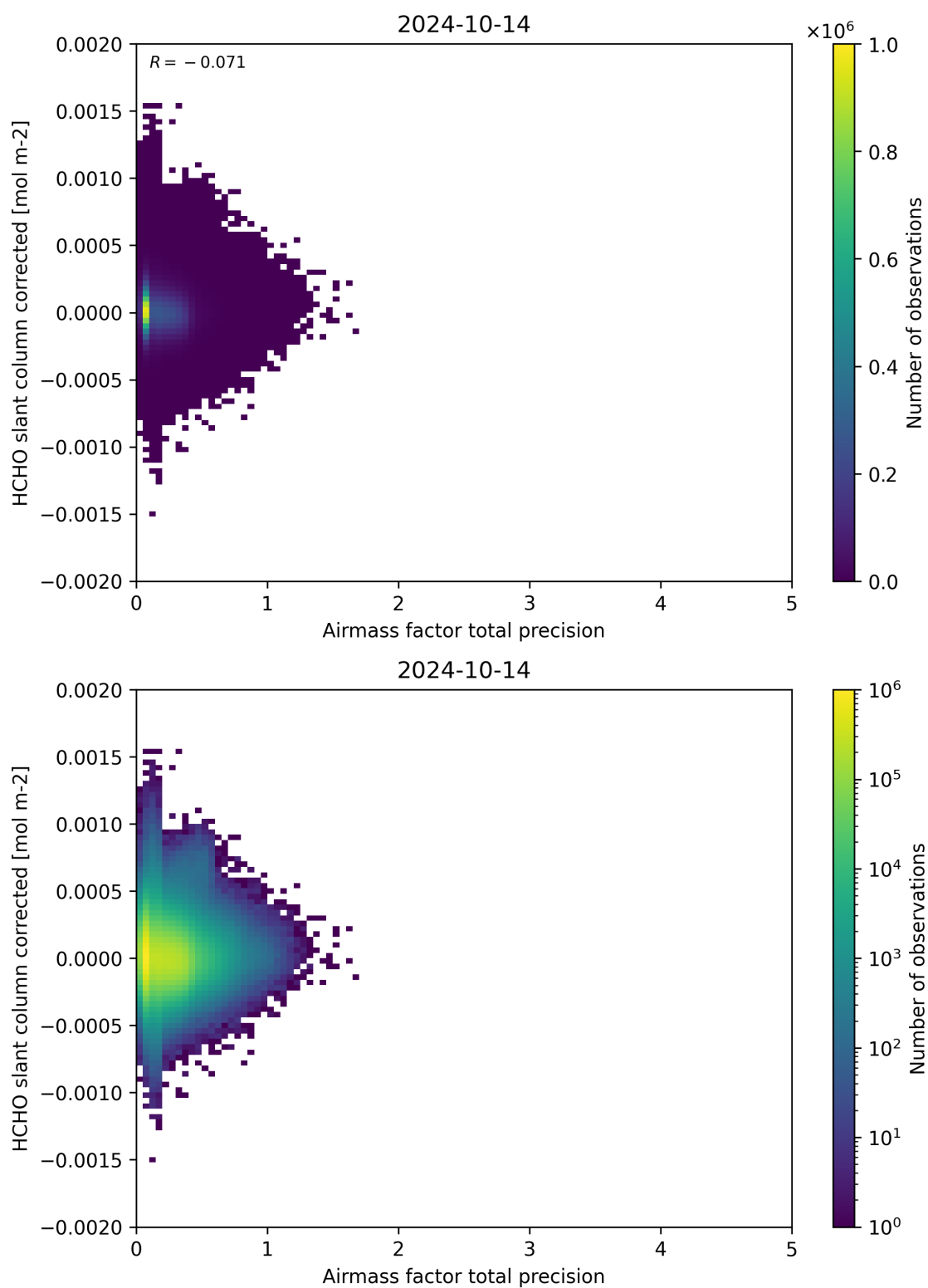
Figure 109: Scatter density plot of “Airmass factor total precision” against “HCHO slant column corrected” for 2024-10-14 to 2024-10-15.
