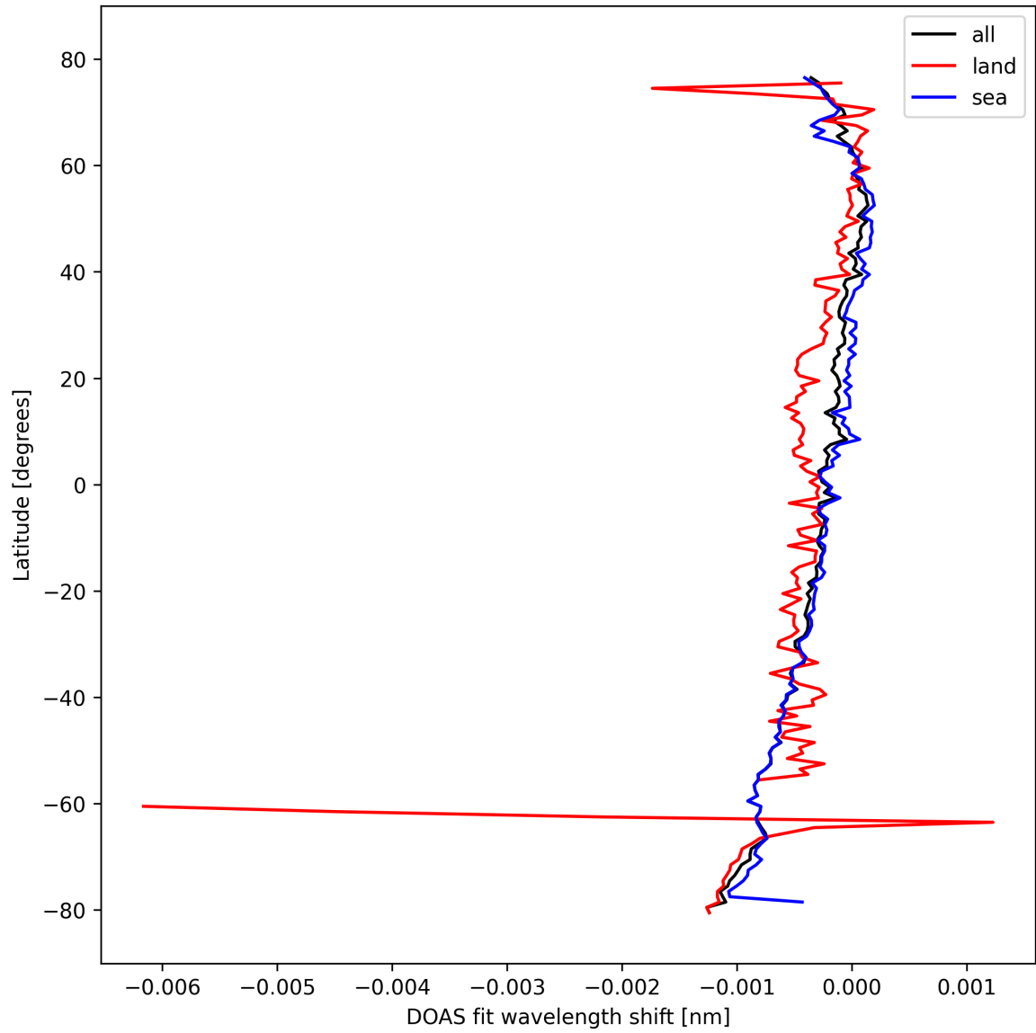
Figure 30: Zonal average of "DOAS fit wavelength shift" for 2024-10-14 to 2024-10-15.
