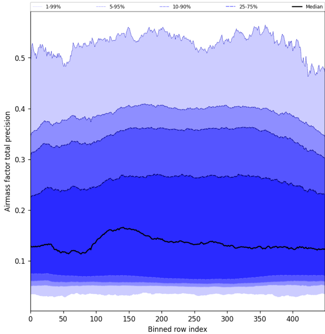
Figure 55: Along track statistics of “Airmass factor total precision” for 2024-10-14 to 2024-10-15
