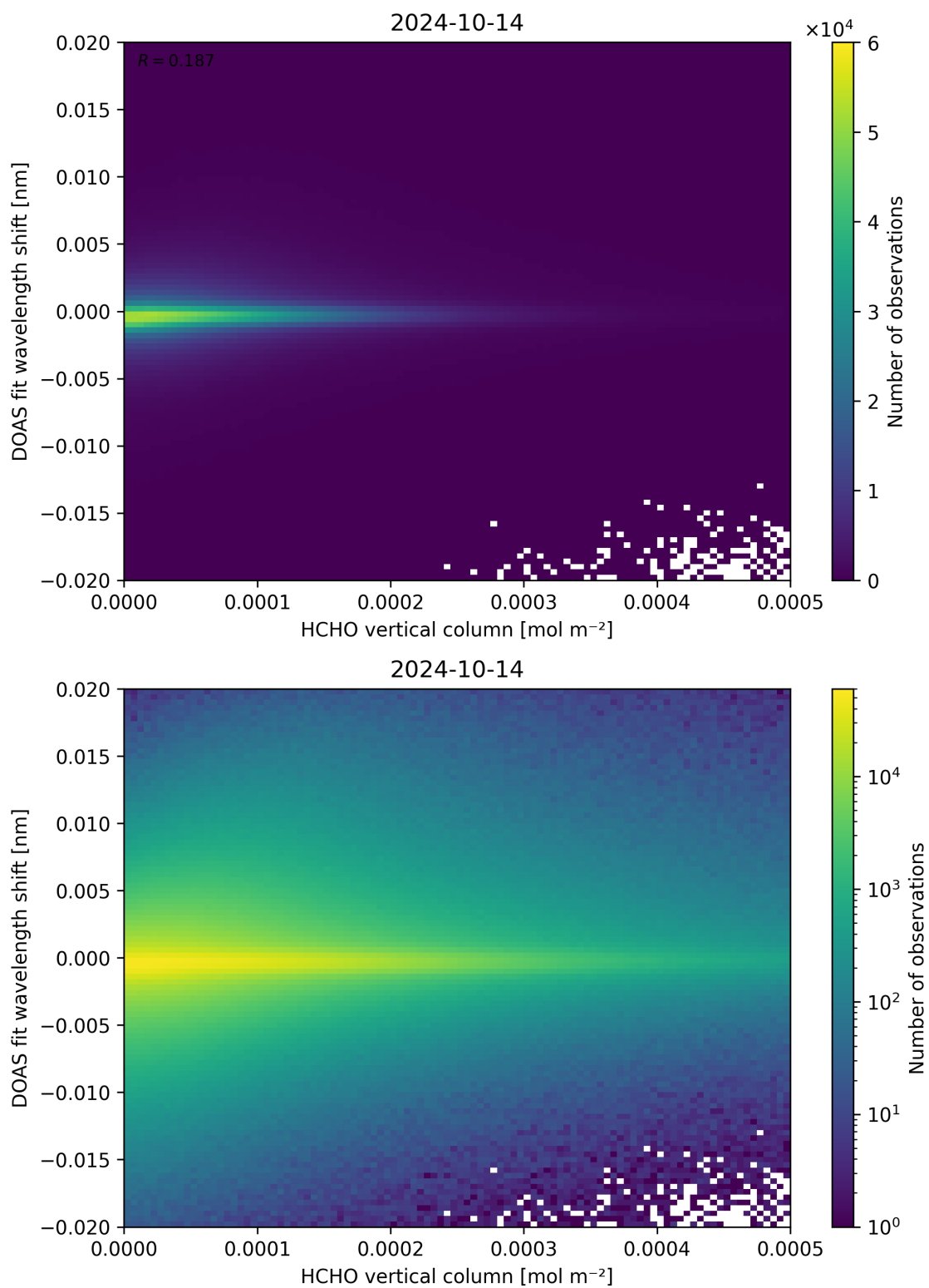
Figure 124: Scatter density plot of “HCHO vertical column” against “DOAS fit wavelength shift” for 2024-10-14 to 2024-10-15.
