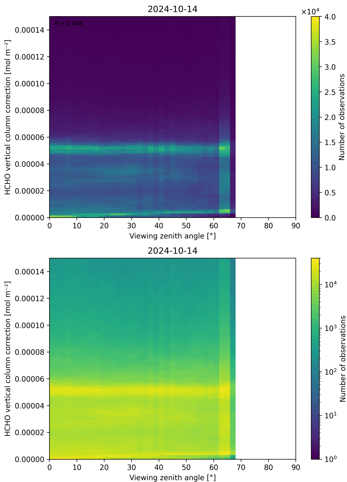
Figure 193: Scatter density plot of “Viewing zenith angle” against “HCHO vertical column correction” for 2024-10-14 to 2024-10-15.
