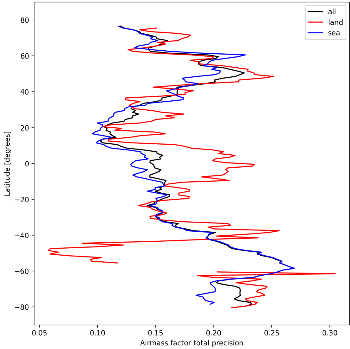
Figure 27: Zonal average of “Airmass factor total precision” for 2024-10-14 to 2024-10-15.
