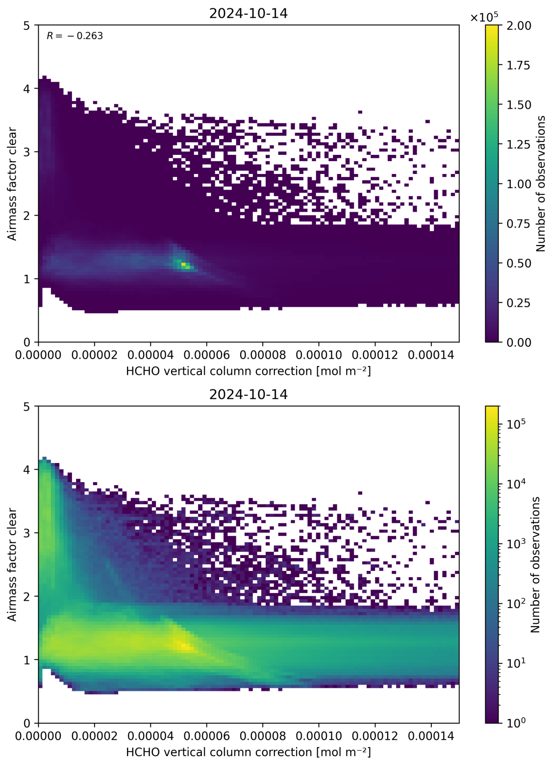
Figure 115: Scatter density plot of “HCHO vertical column correction” against “Airmass factor clear” for 2024-10-14 to 2024-10-15.
