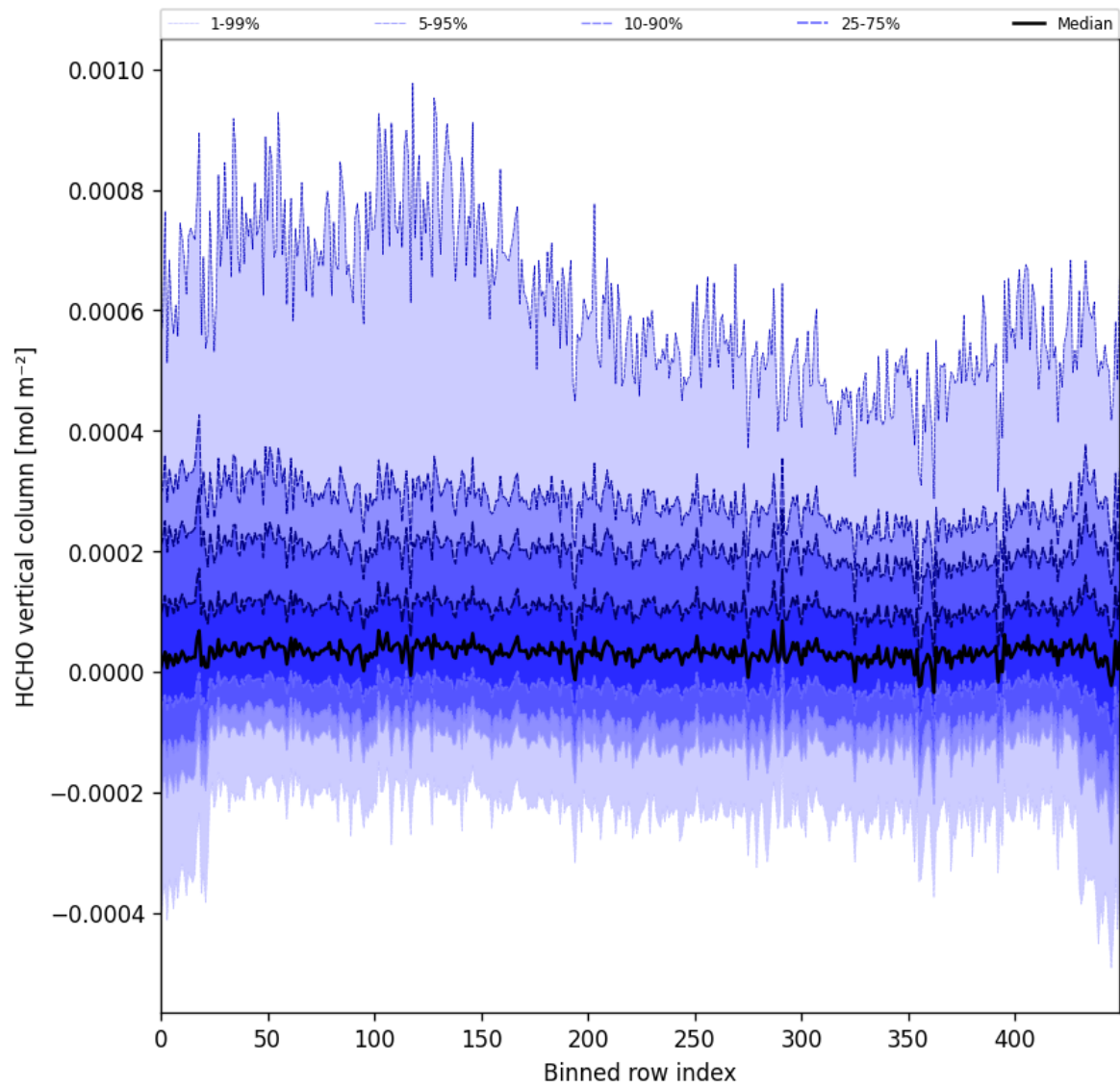
Figure 49: Along track statistics of “HCHO vertical column” for 2024-10-14 to 2024-10-15
