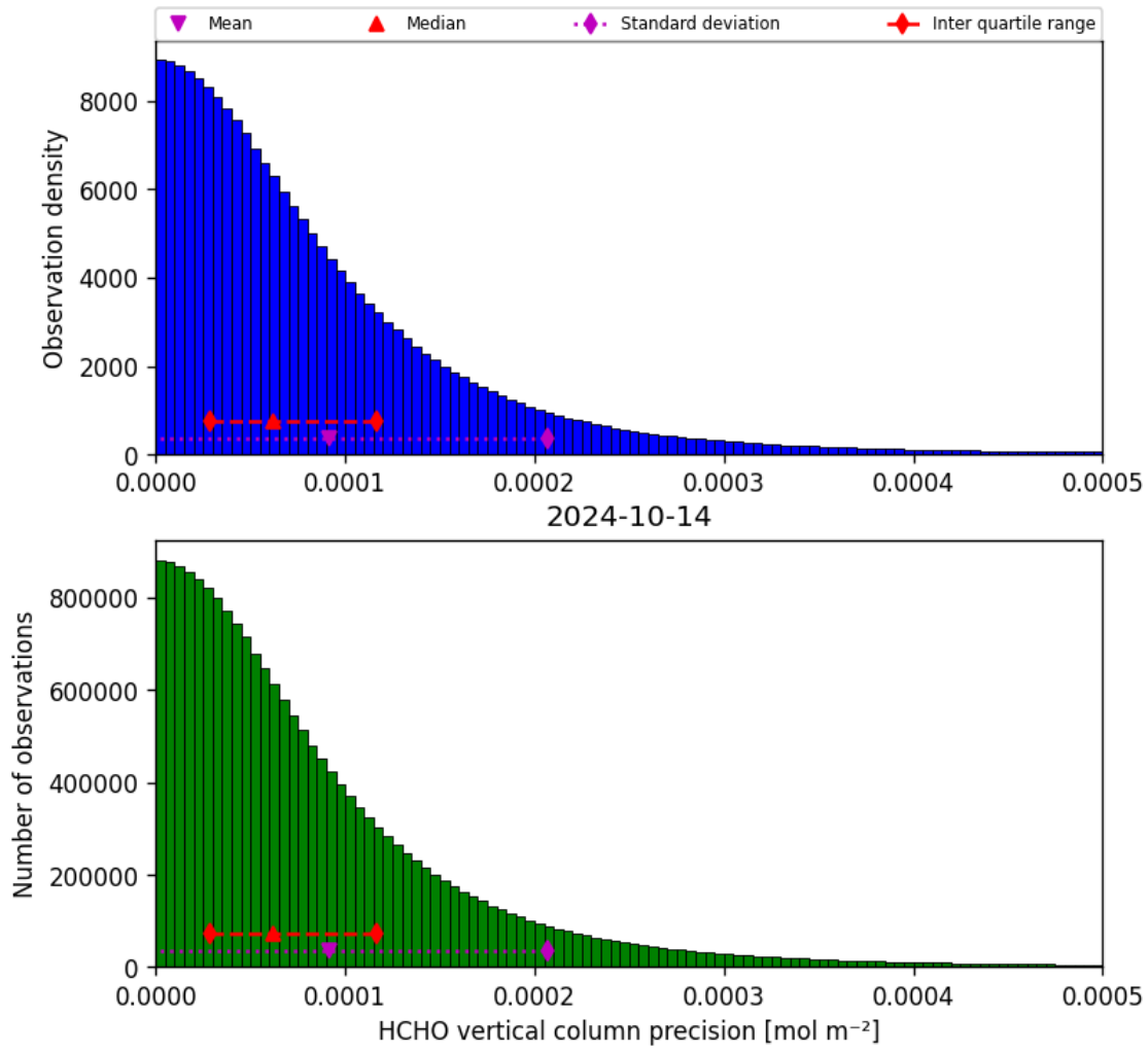
Figure 36: Histogram of “HCHO vertical column precision” for 2024-10-14 to 2024-10-15
