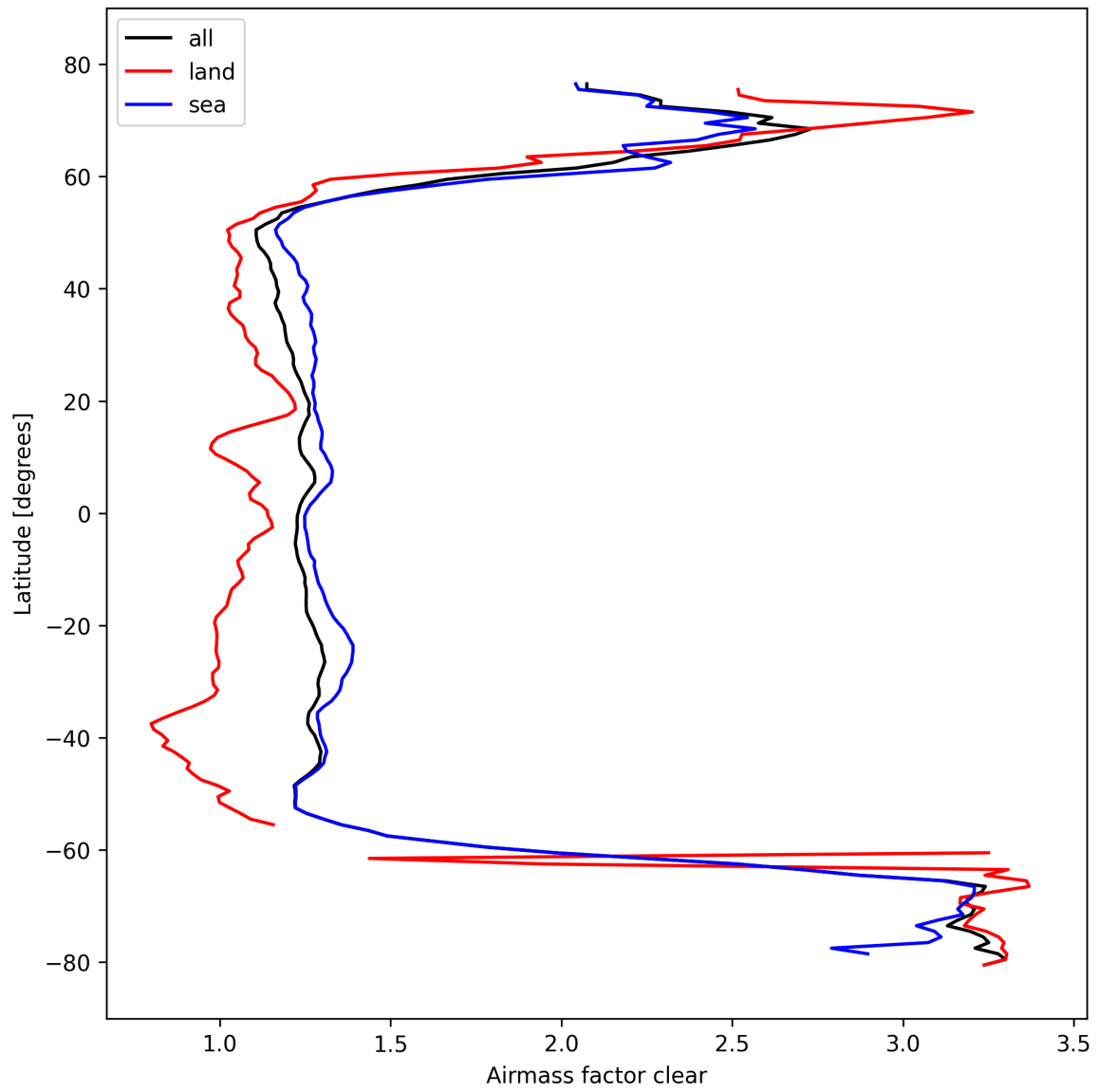
Figure 28: Zonal average of “Airmass factor clear” for 2024-10-14 to 2024-10-15.
