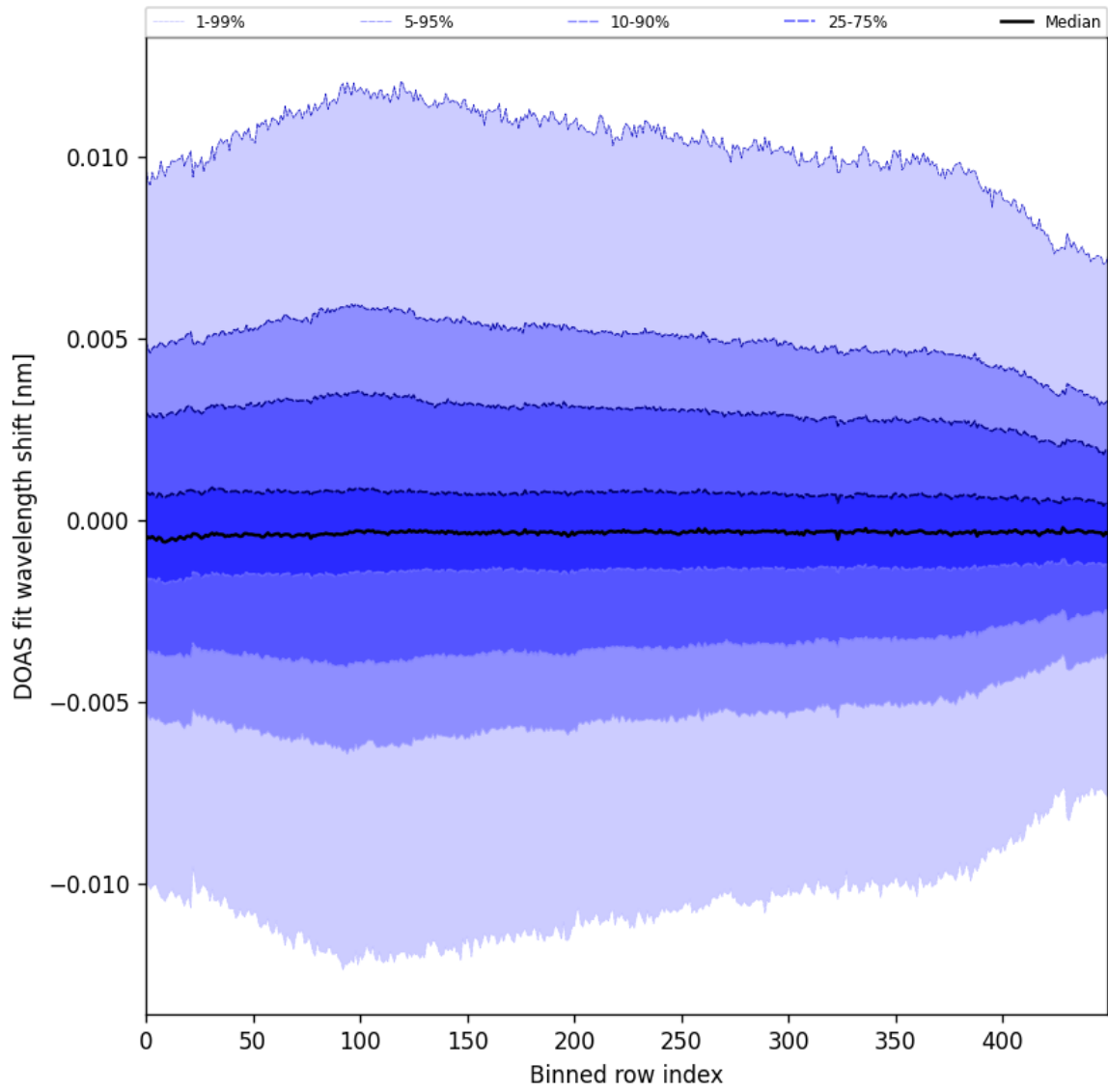
Figure 58: Along track statistics of “DOAS fit wavelength shift” for 2024-10-14 to 2024-10-15
