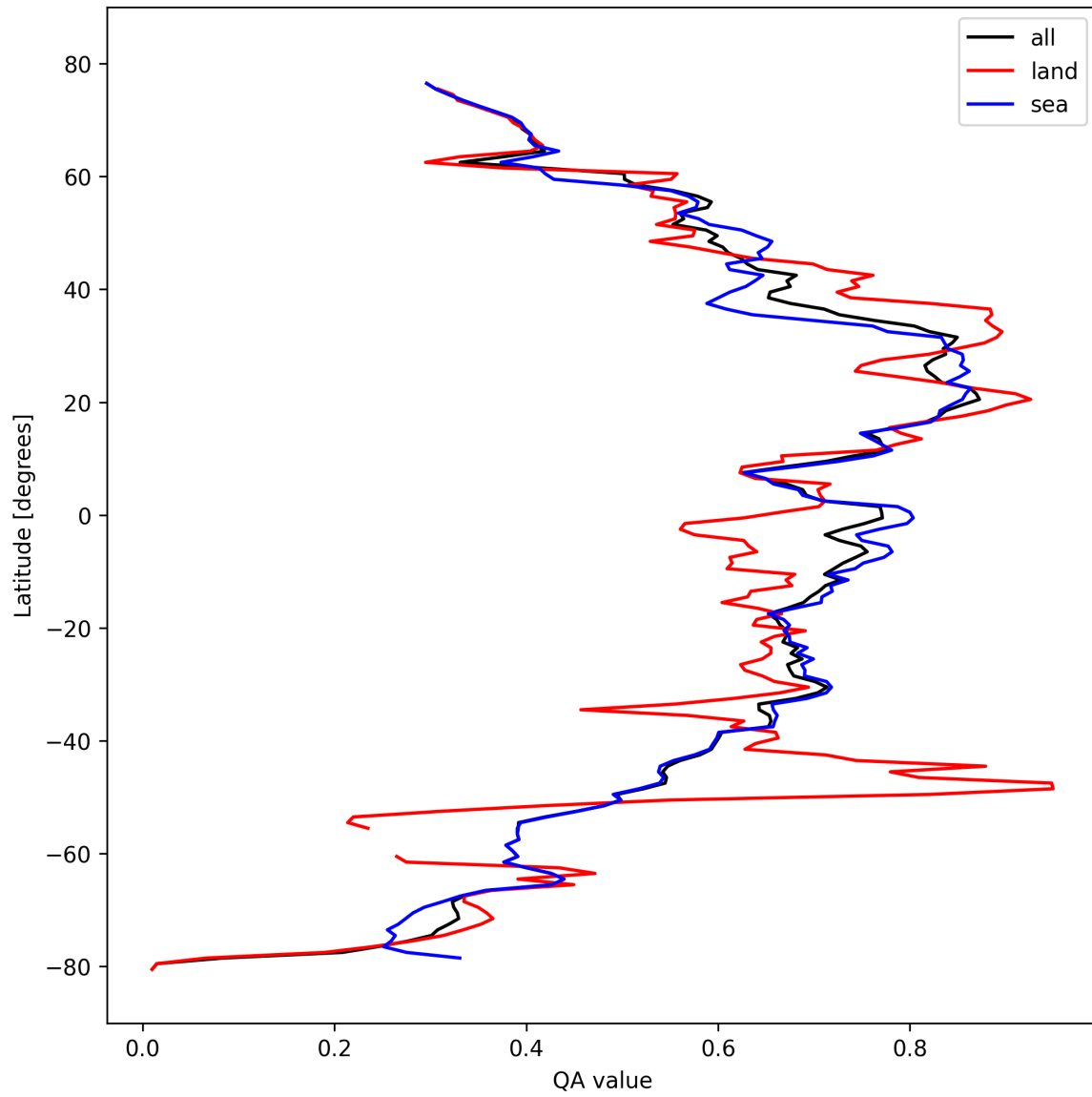
Figure 20: Zonal average of “QA value” for 2024-10-14 to 2024-10-15.
