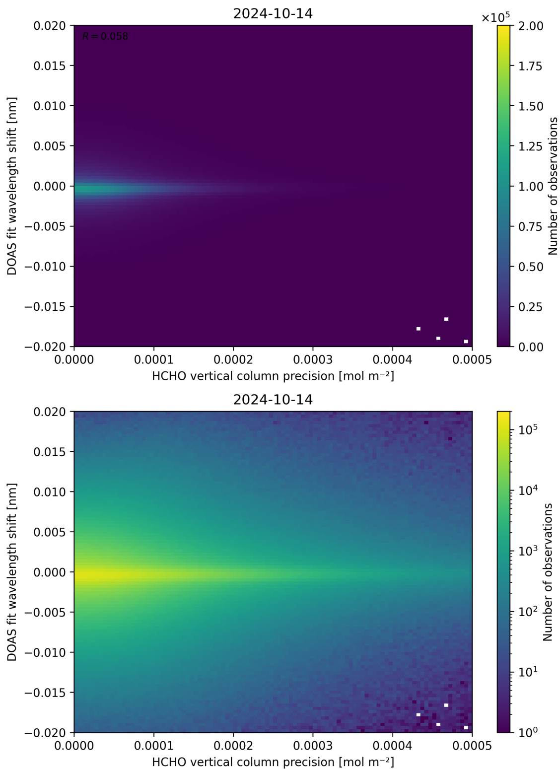
Figure 137: Scatter density plot of “HCHO vertical column precision” against “DOAS fit wavelength shift” for 2024-10-14 to 2024-10-15.
