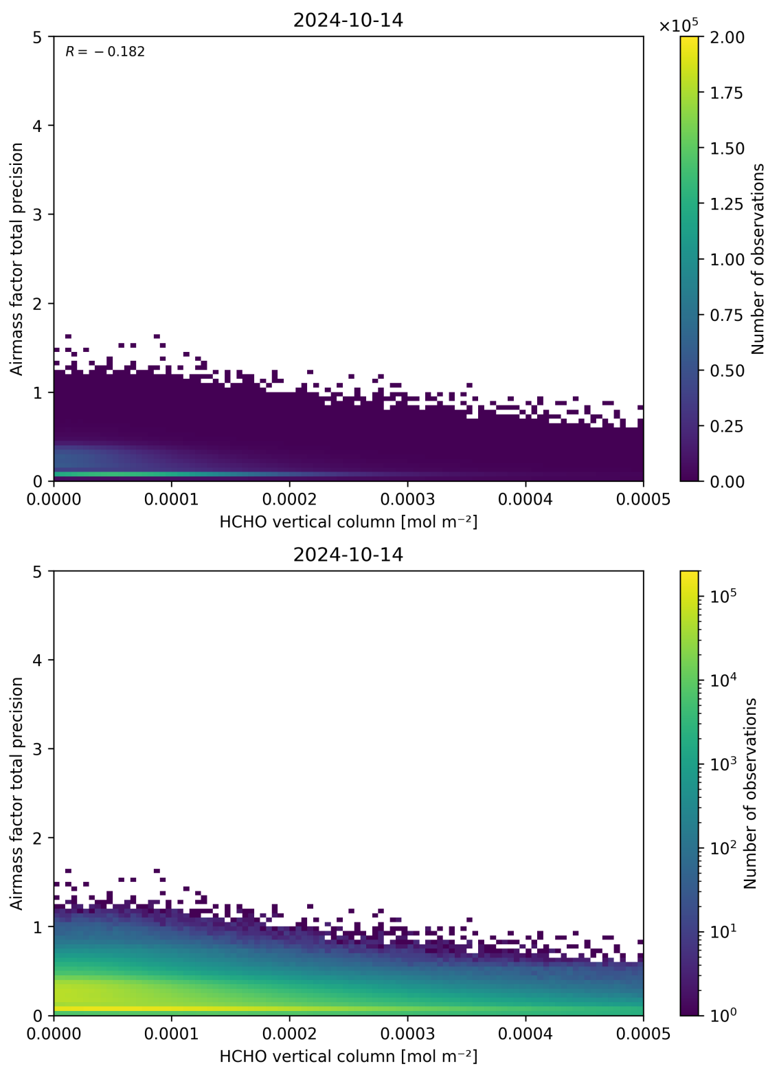
Figure 132: Scatter density plot of “HCHO vertical column” against “Airmass factor total precision” for 2024-10-14 to 2024-10-15.
