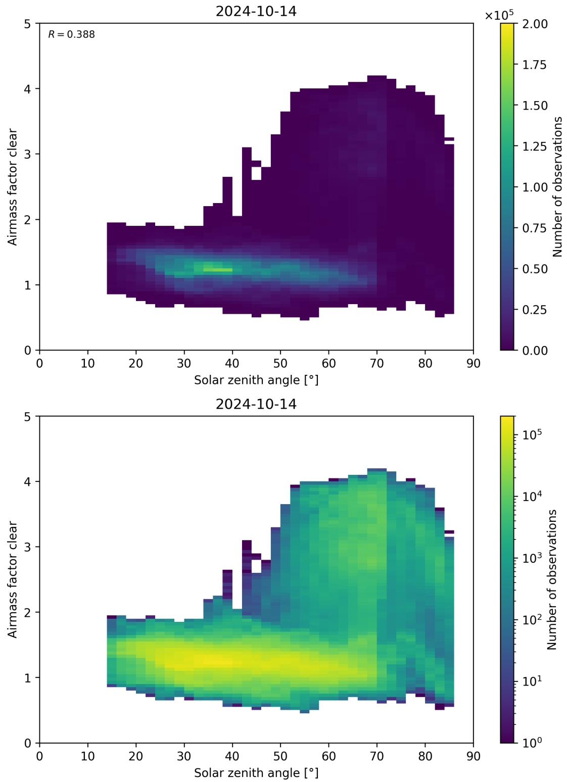
Figure 170: Scatter density plot of “Solar zenith angle” against “Airmass factor clear” for 2024-10-14 to 2024-10-15.
