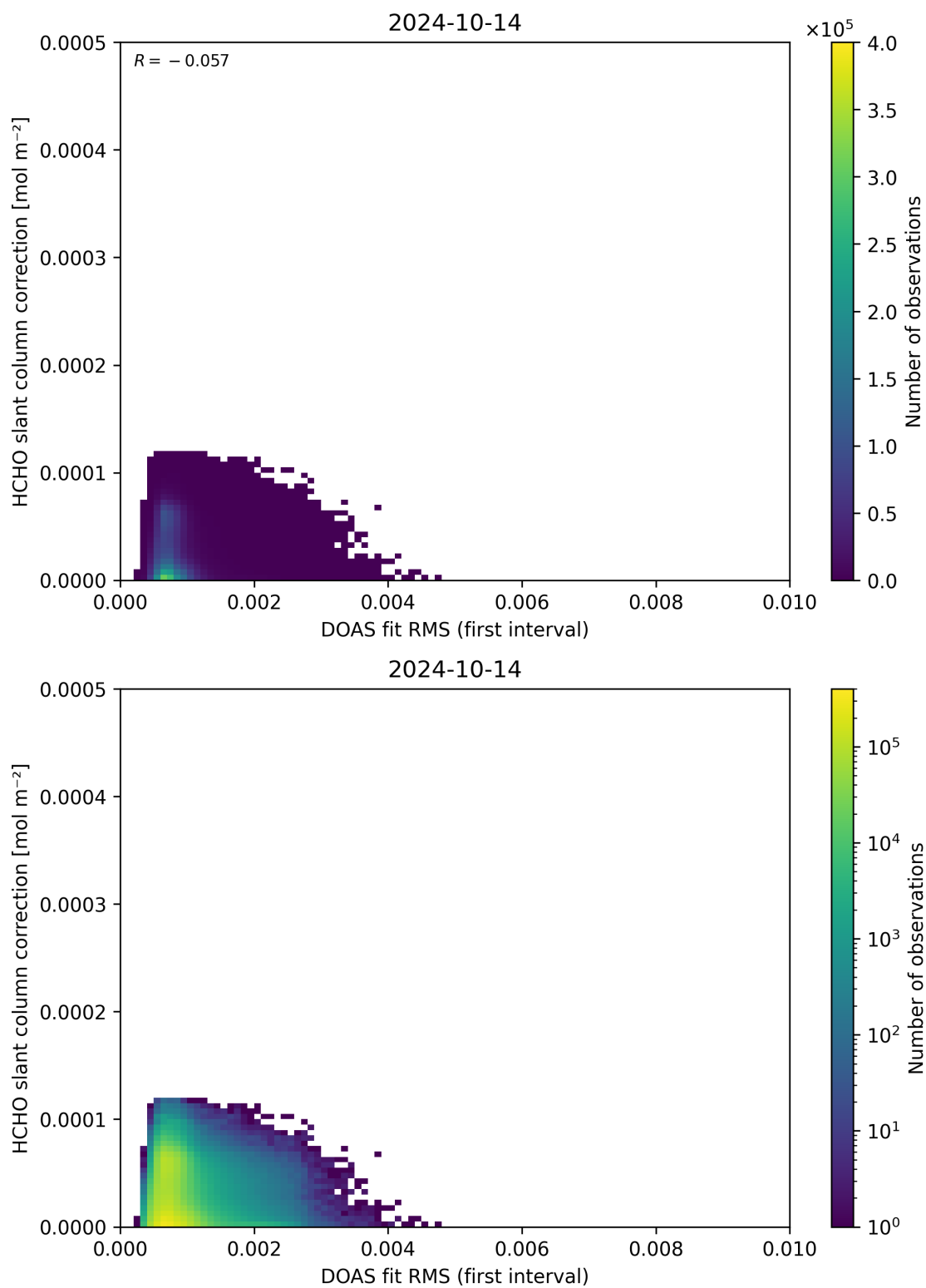
Figure 63: Scatter density plot of “DOAS fit RMS (first interval)” against “HCHO slant column correction” for 2024-10-14 to 2024-10-15.
