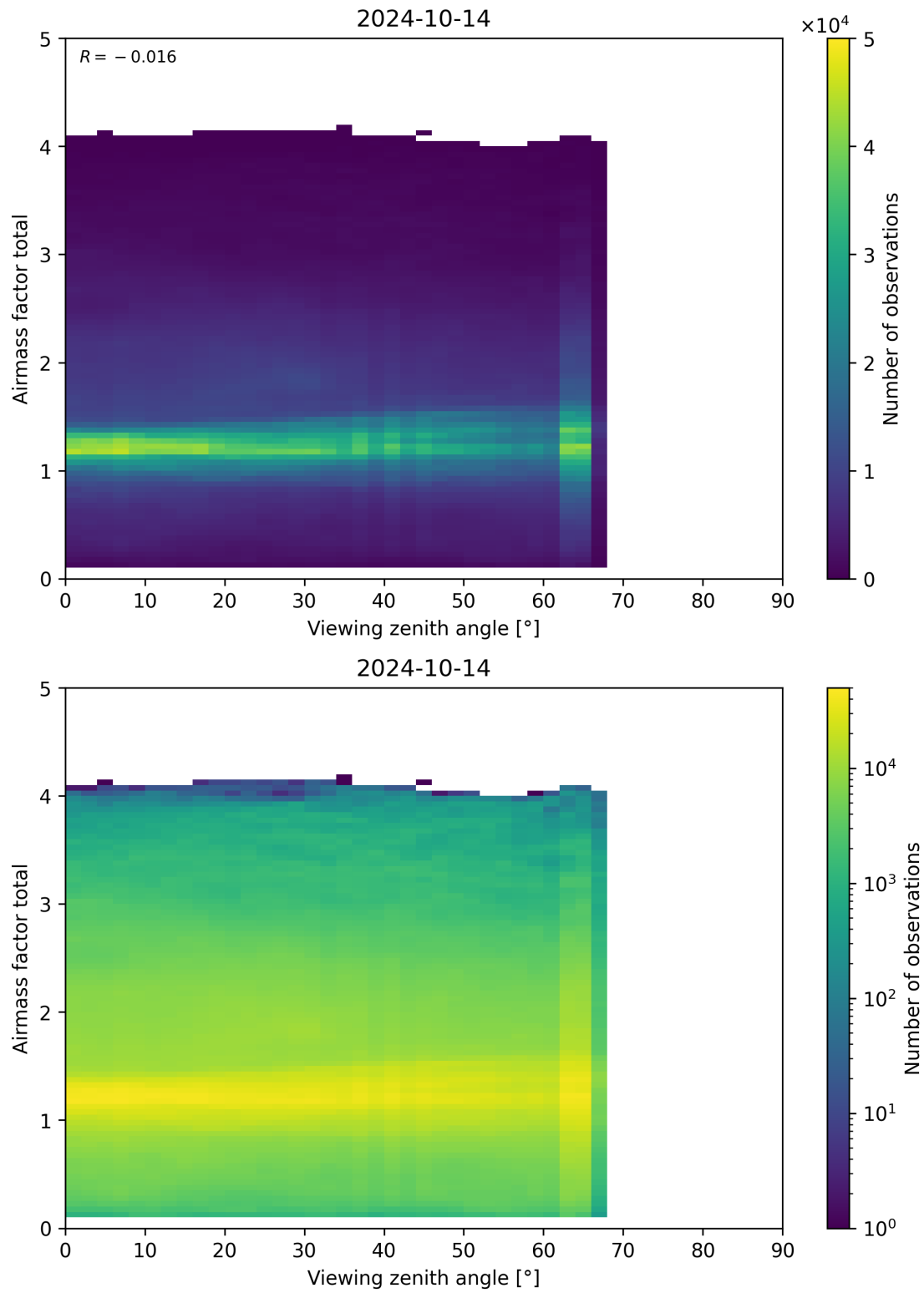
Figure 190: Scatter density plot of “Viewing zenith angle” against “Airmass factor total” for 2024-10-14 to 2024-10-15.
