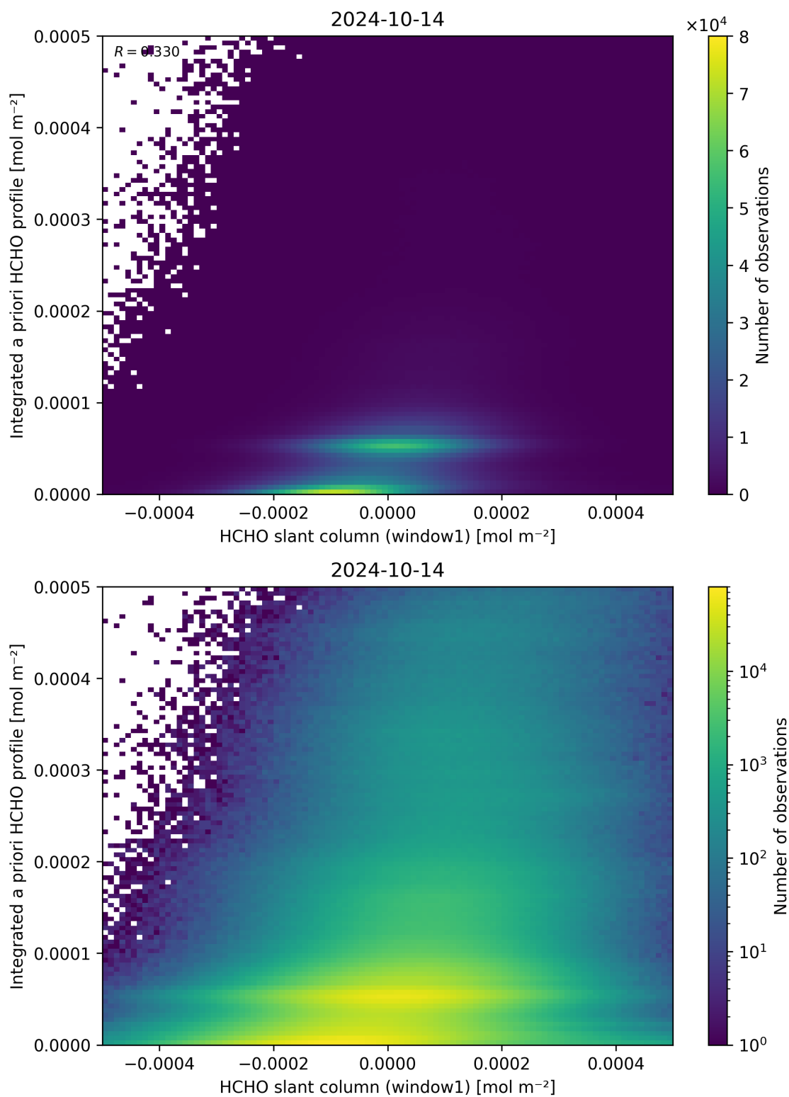
Figure 87: Scatter density plot of “HCHO slant column (window1)” against “Integrated a priori HCHO profile” for 2024-10-14 to 2024-10-15.
