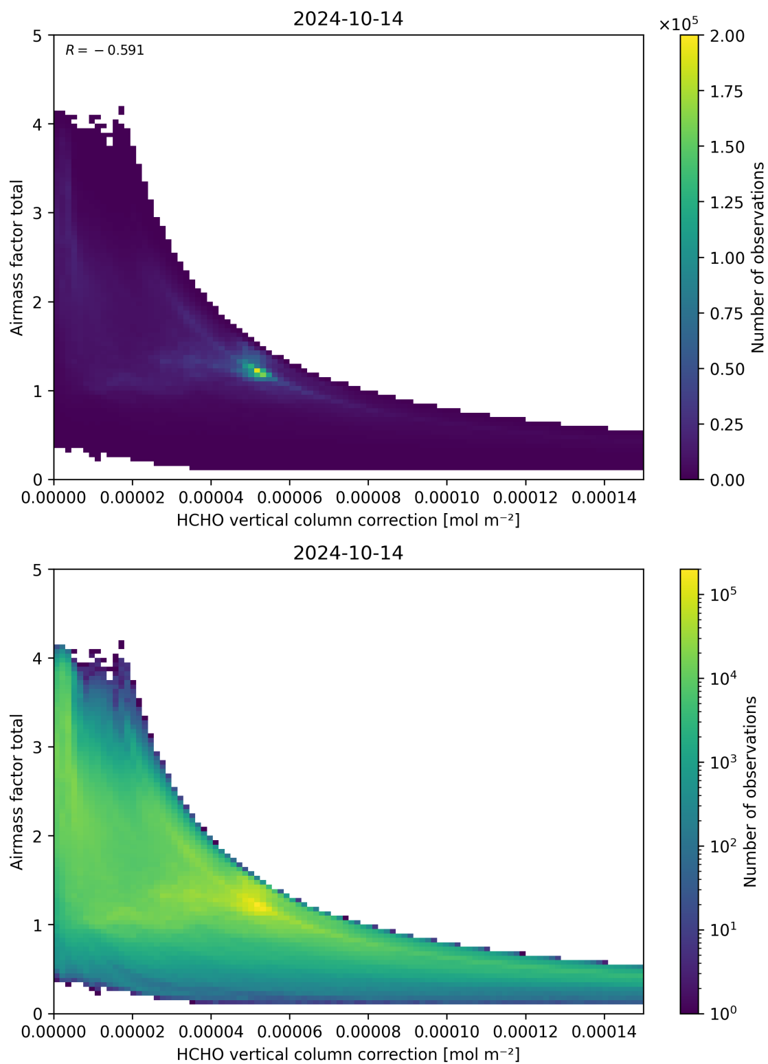
Figure 120: Scatter density plot of “HCHO vertical column correction” against “Airmass factor total” for 2024-10-14 to 2024-10-15.
