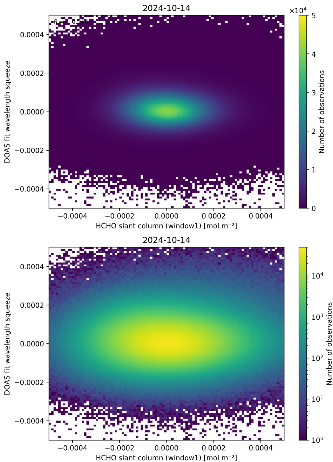
Figure 80: Scatter density plot of “HCHO slant column (window1)” against “DOAS fit wavelength squeeze” for 2024-10-14 to 2024-10-15.
