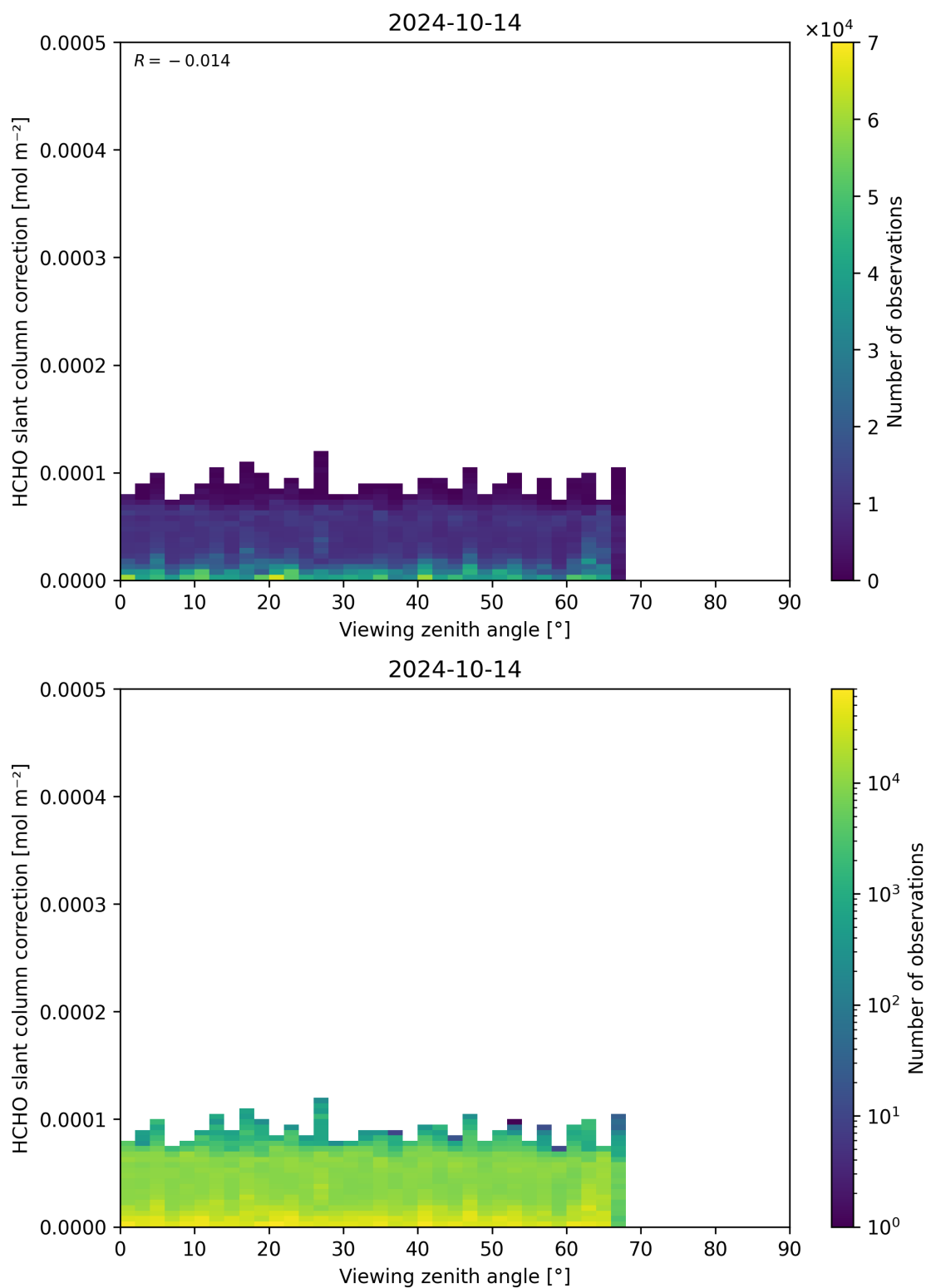
Figure 187: Scatter density plot of “Viewing zenith angle” against “HCHO slant column correction” for 2024-10-14 to 2024-10-15.
