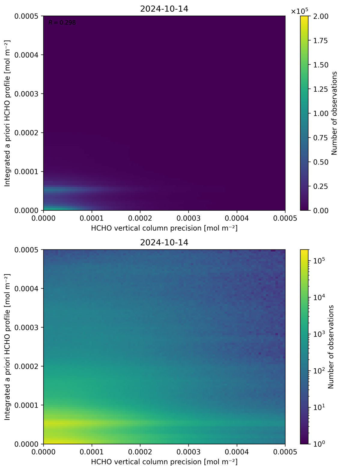
Figure 147: Scatter density plot of “HCHO vertical column precision” against “Integrated a priori HCHO profile” for 2024-10-14 to 2024-10-15.
