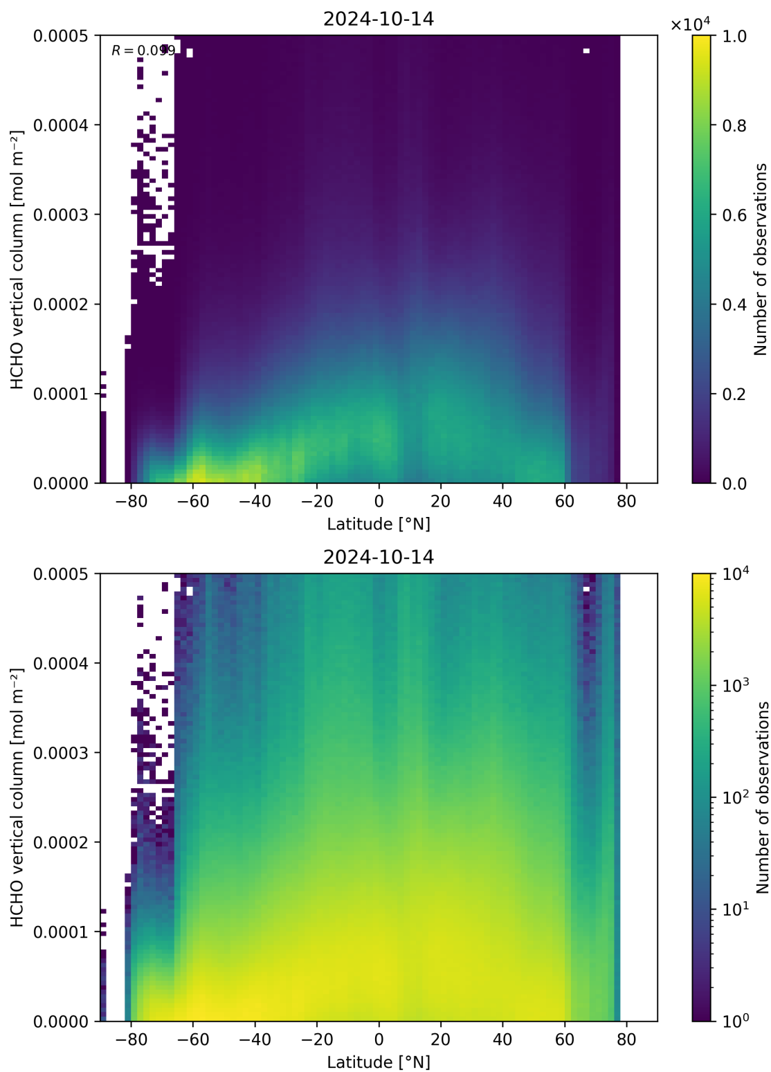
Figure 163: Scatter density plot of “Latitude” against “HCHO vertical column” for 2024-10-14 to 2024-10-15.
