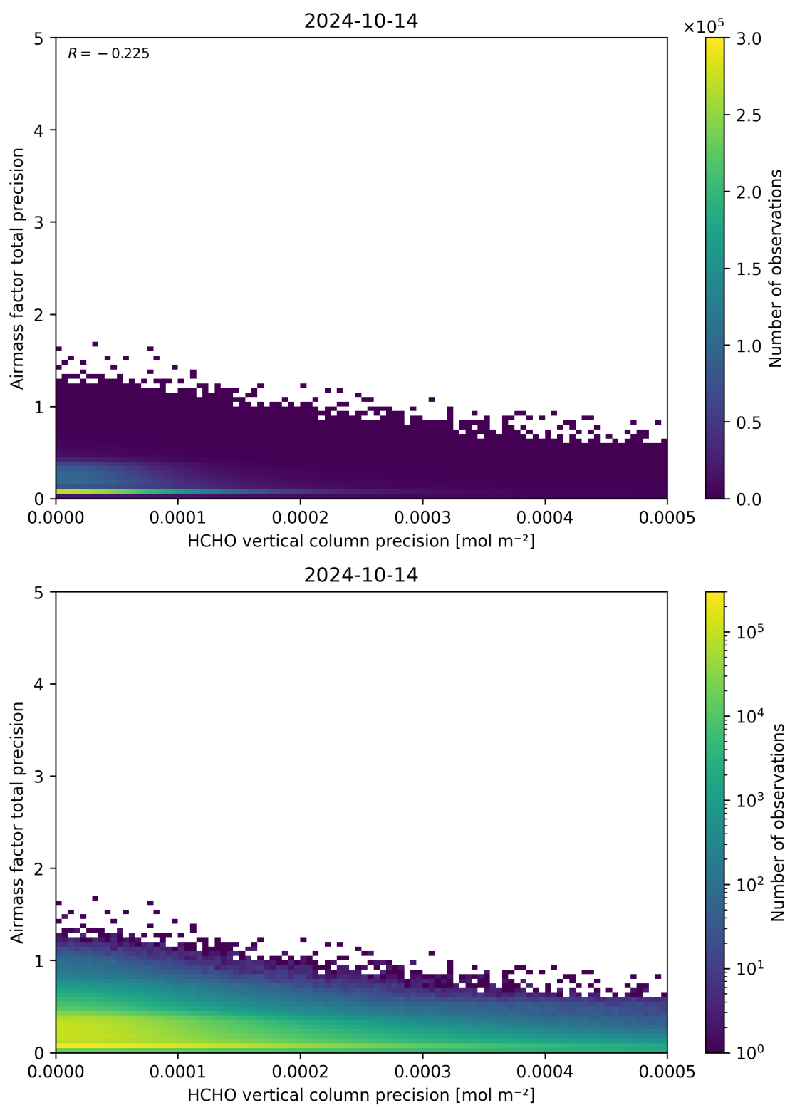
Figure 145: Scatter density plot of “HCHO vertical column precision” against “Airmass factor total precision” for 2024-10-14 to 2024-10-15.
