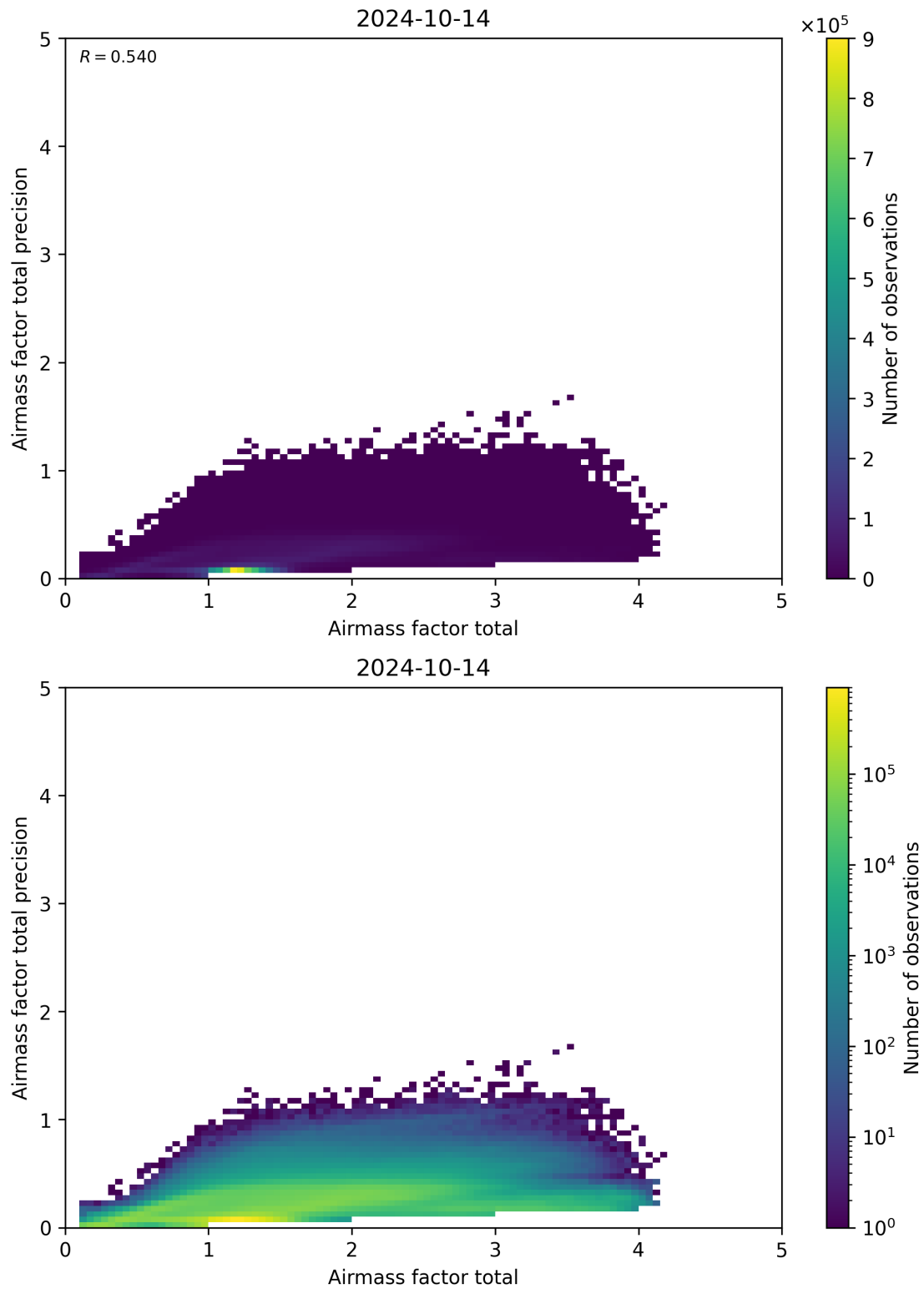
Figure 103: Scatter density plot of “Airmass factor total” against “Airmass factor total precision” for 2024-10-14 to 2024-10-15.
