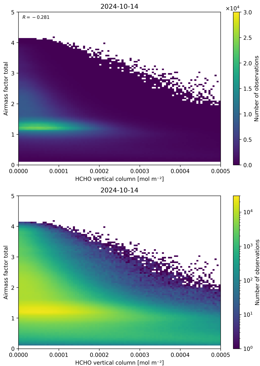
Figure 131: Scatter density plot of “HCHO vertical column” against “Airmass factor total” for 2024-10-14 to 2024-10-15.
