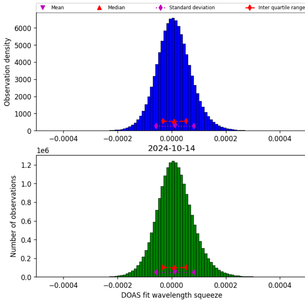
Figure 45: Histogram of “DOAS fit wavelength squeeze” for 2024-10-14 to 2024-10-15
