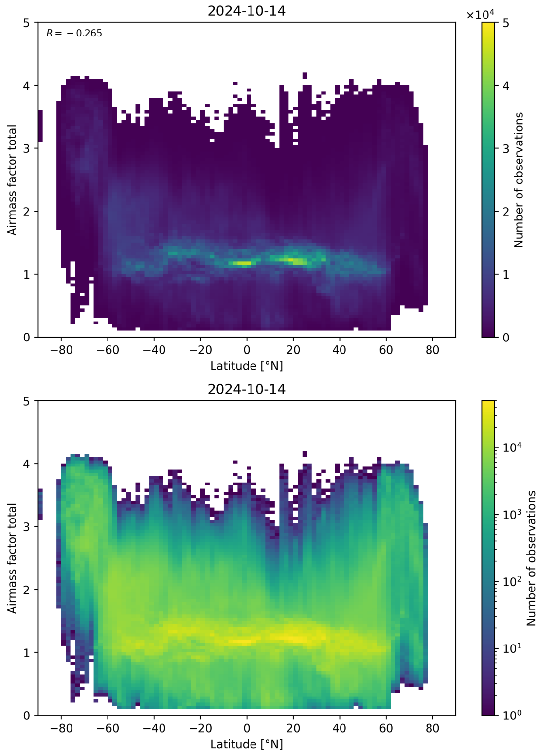
Figure 161: Scatter density plot of “Latitude” against “Airmass factor total” for 2024-10-14 to 2024-10-15.
