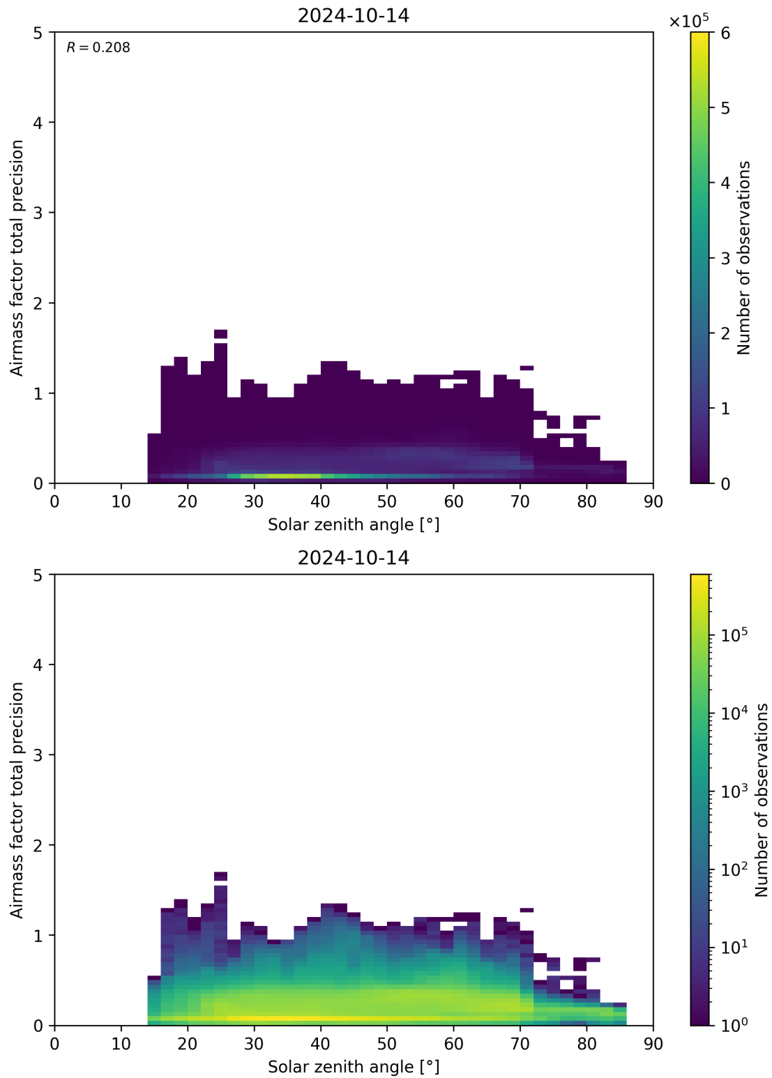
Figure 176: Scatter density plot of “Solar zenith angle” against “Airmass factor total precision” for 2024-10-14 to 2024-10-15.
