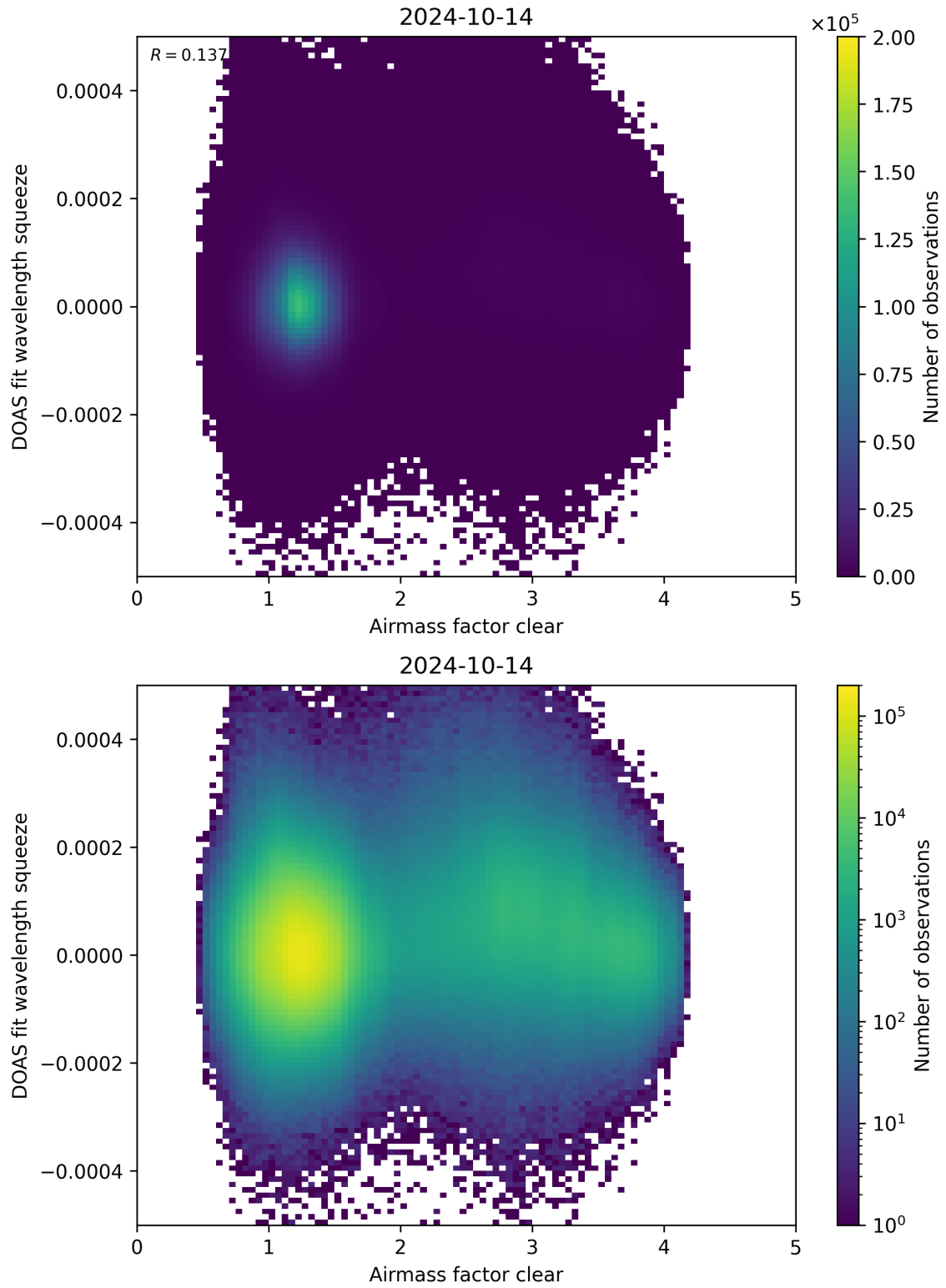
Figure 73: Scatter density plot of “Airmass factor clear” against “DOAS fit wavelength squeeze” for 2024-10-14 to 2024-10-15.
