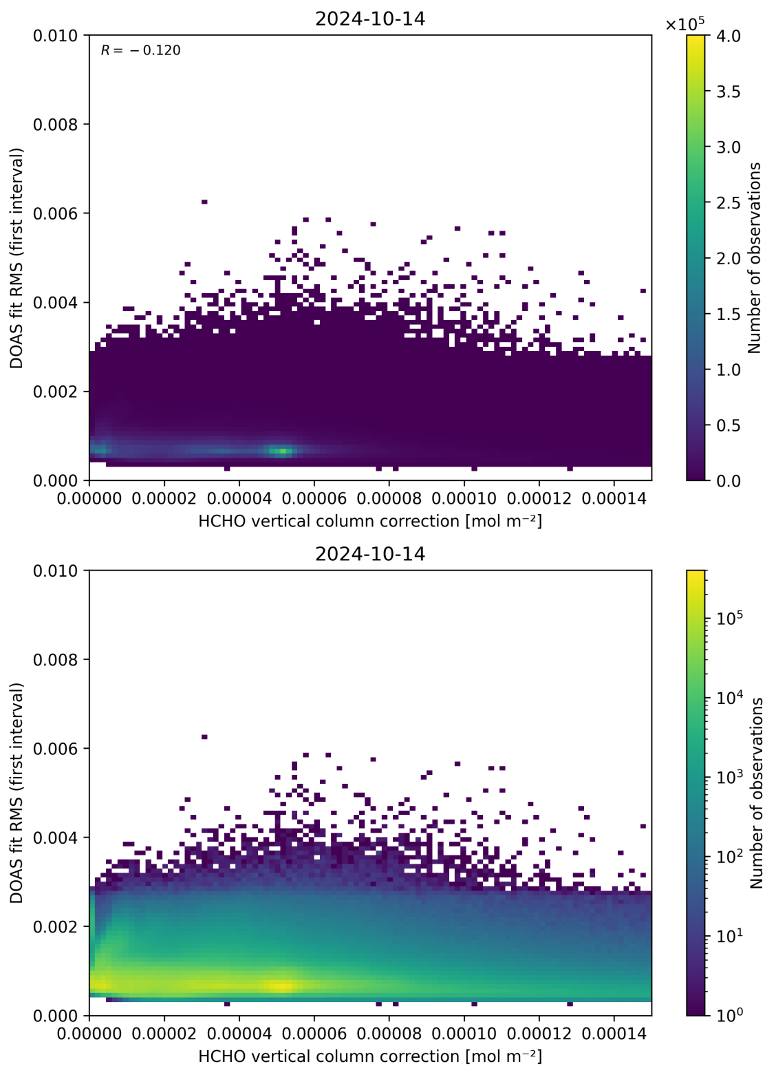
Figure 112: Scatter density plot of “HCHO vertical column correction” against “DOAS fit RMS (first interval)” for 2024-10-14 to 2024-10-15.
