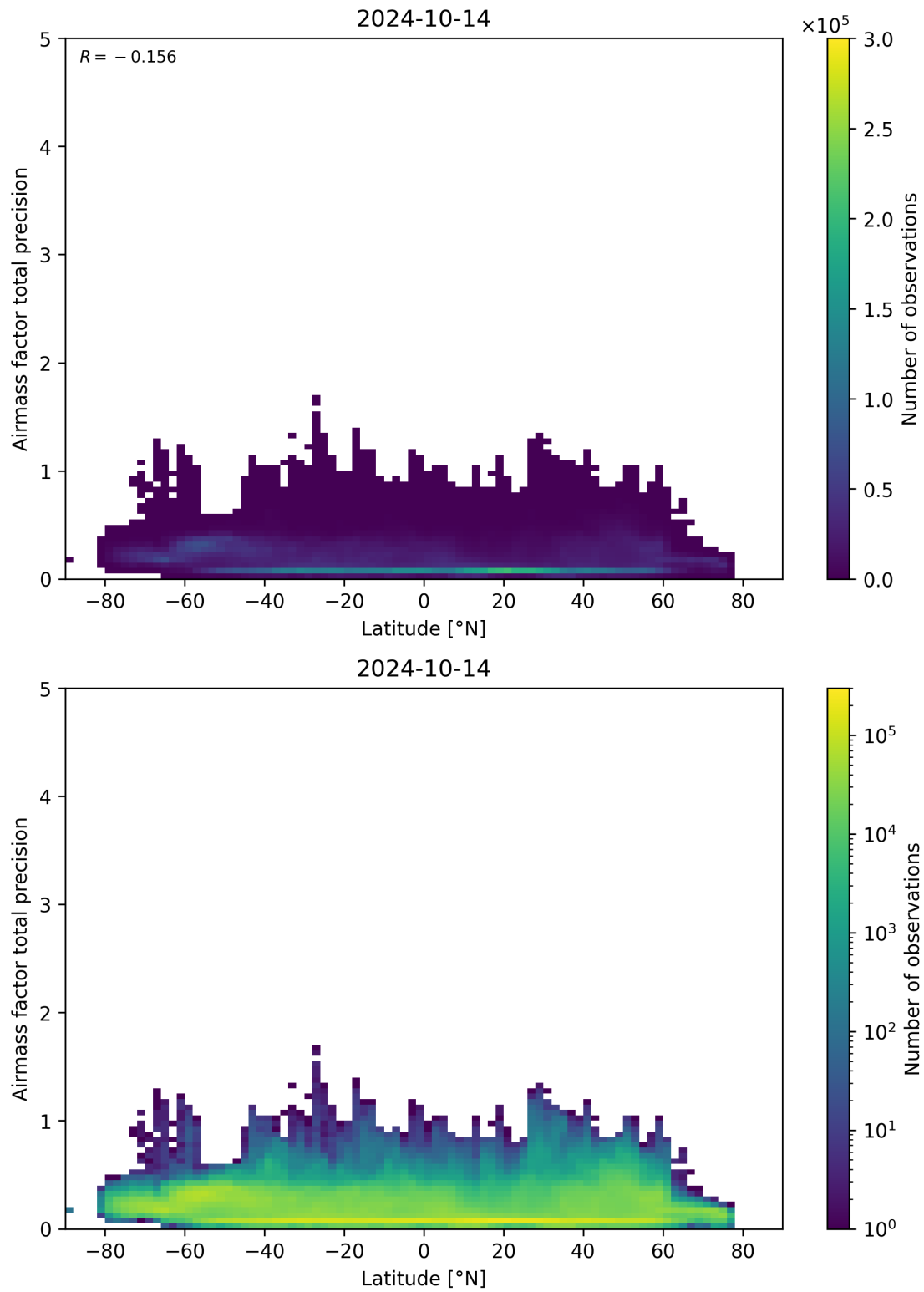
Figure 162: Scatter density plot of “Latitude” against “Airmass factor total precision” for 2024-10-14 to 2024-10-15.
