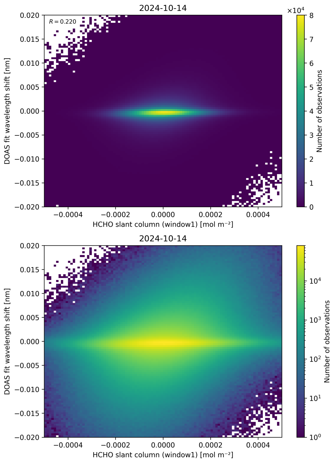
Figure 79: Scatter density plot of “HCHO slant column (window1)” against “DOAS fit wavelength shift” for 2024-10-14 to 2024-10-15.
