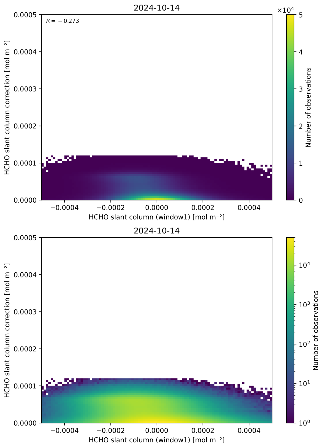
Figure 83: Scatter density plot of “HCHO slant column (window1)” against “HCHO slant column correction” for 2024-10-14 to 2024-10-15.
