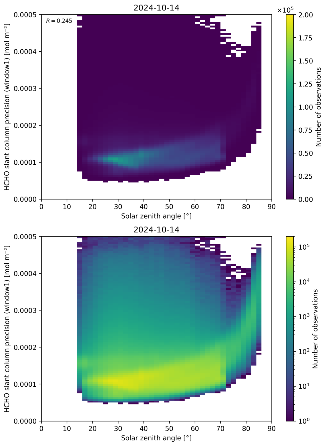
Figure 174: Scatter density plot of “Solar zenith angle” against “HCHO slant column precision (window1)” for 2024-10-14 to 2024-10-15.
