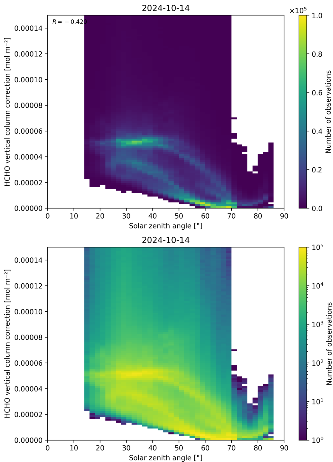
Figure 178: Scatter density plot of “Solar zenith angle” against “HCHO vertical column correction” for 2024-10-14 to 2024-10-15.
