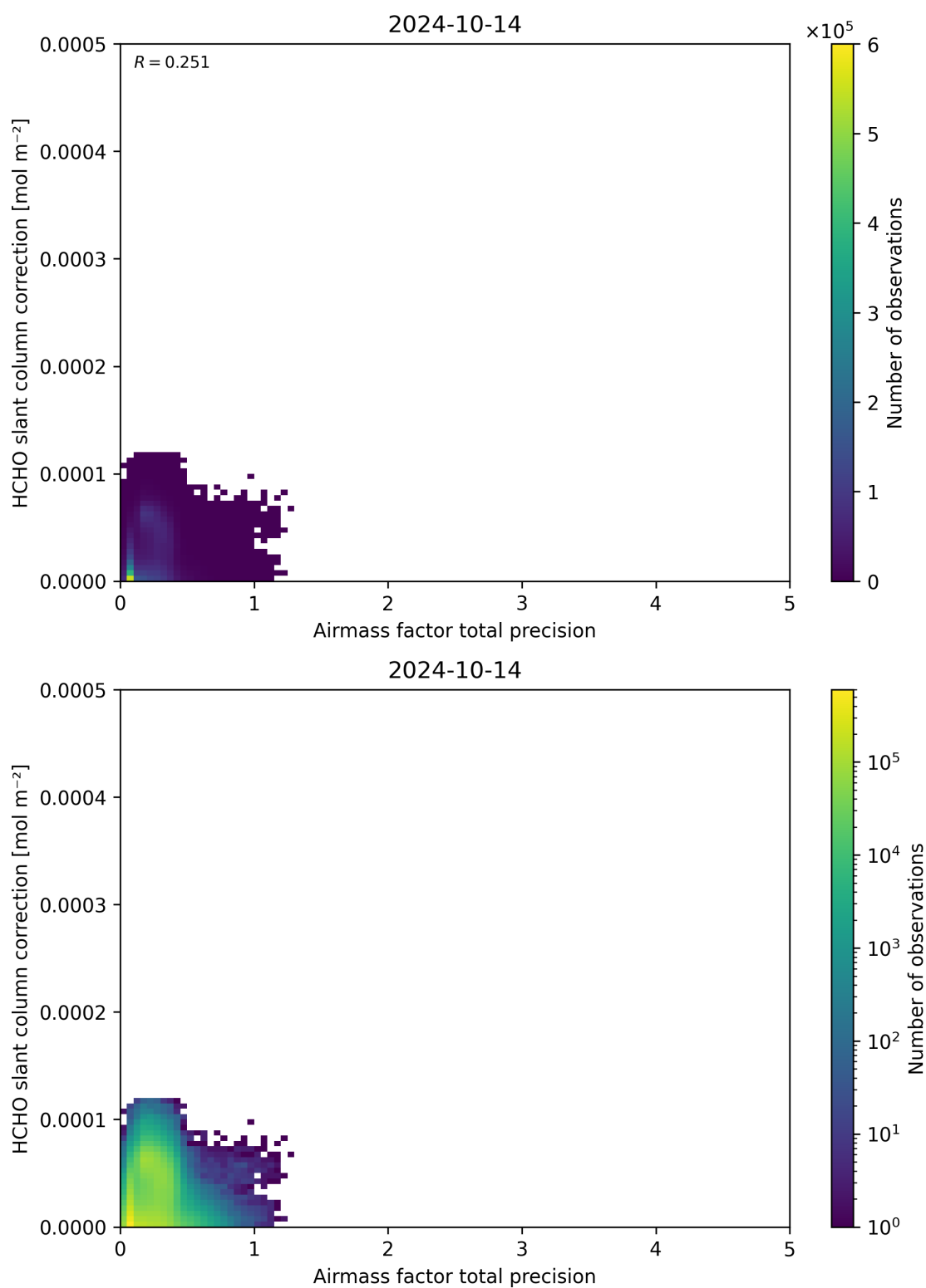
Figure 110: Scatter density plot of “Airmass factor total precision” against “HCHO slant column correction” for 2024-10-14 to 2024-10-15.
