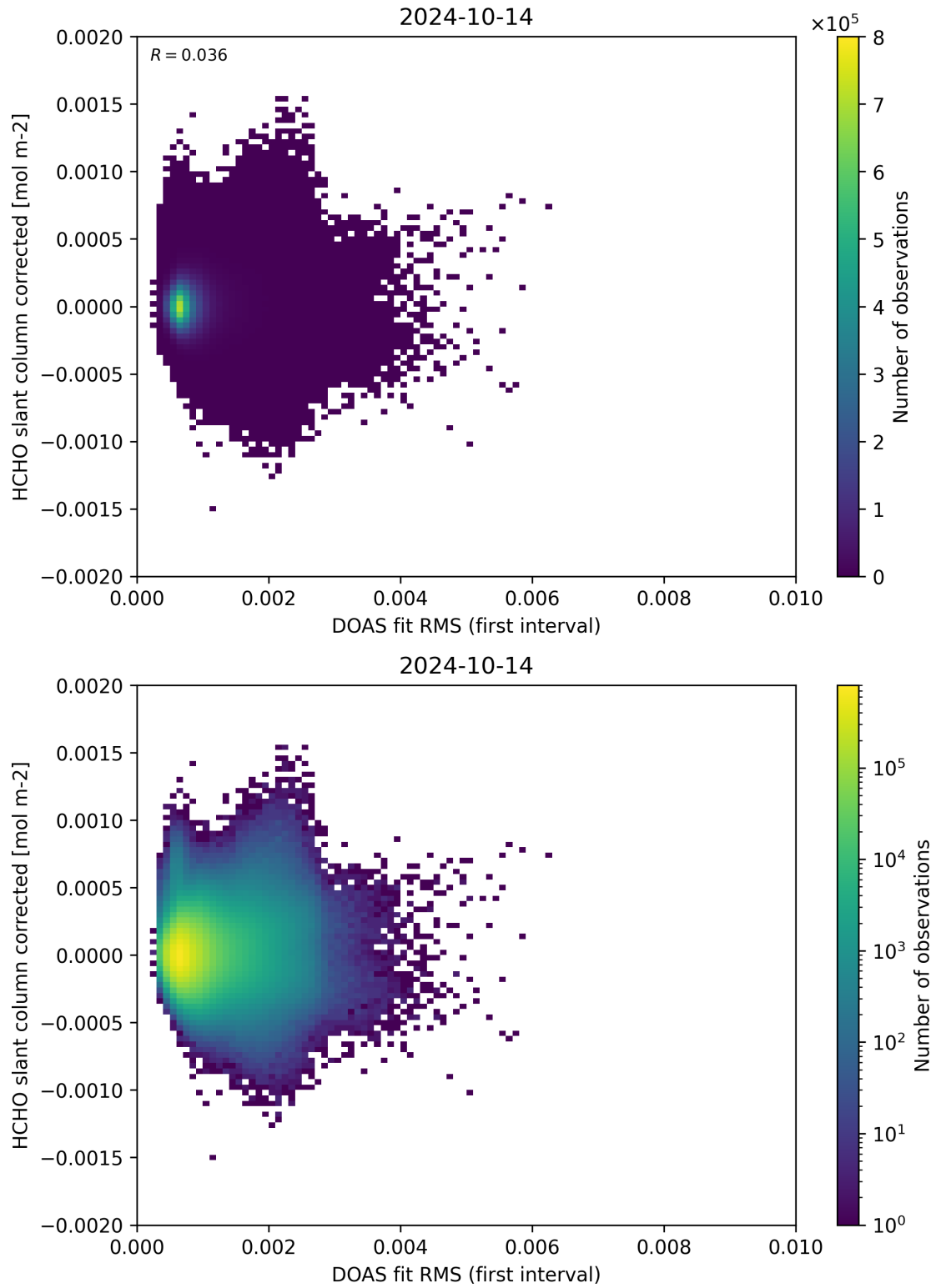
Figure 62: Scatter density plot of “DOAS fit RMS (first interval)” against “HCHO slant column corrected” for 2024-10-14 to 2024-10-15.
