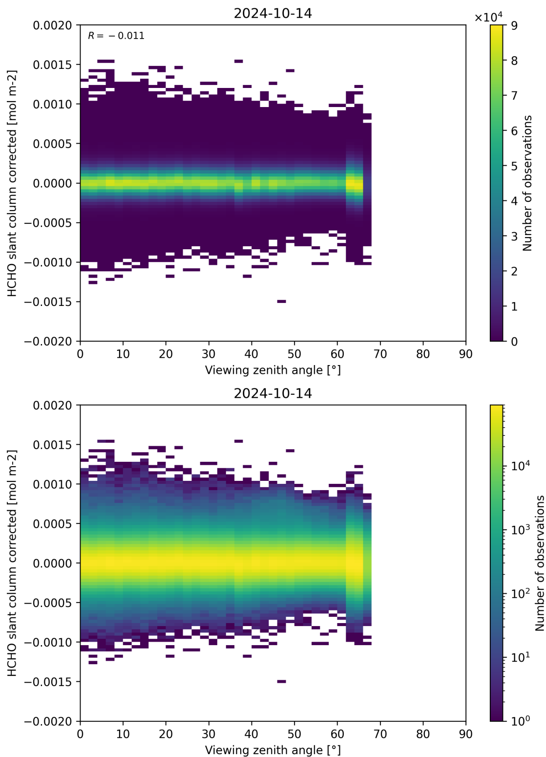
Figure 186: Scatter density plot of “Viewing zenith angle” against “HCHO slant column corrected” for 2024-10-14 to 2024-10-15.
