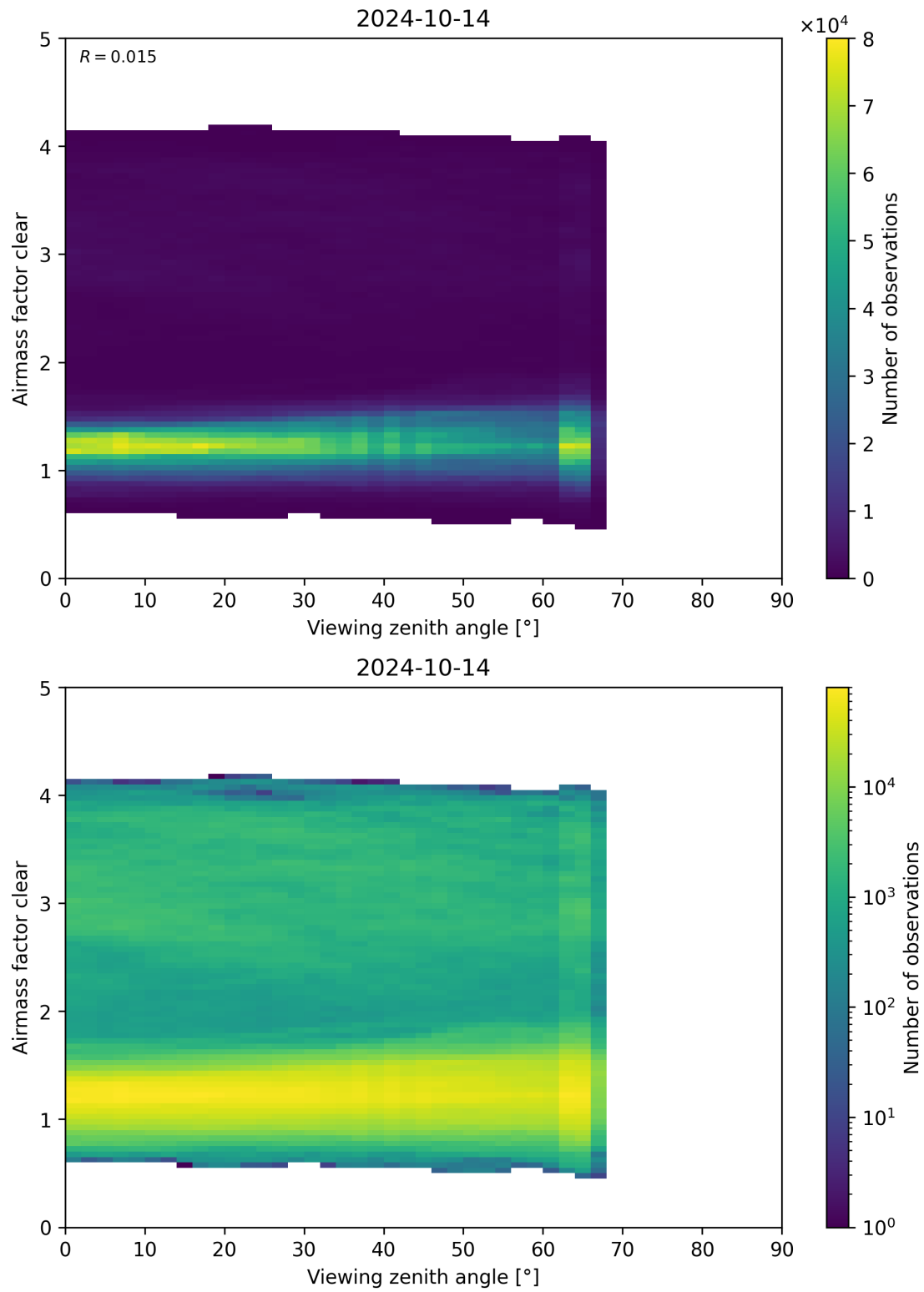
Figure 185: Scatter density plot of “Viewing zenith angle” against “Airmass factor clear” for 2024-10-14 to 2024-10-15.
