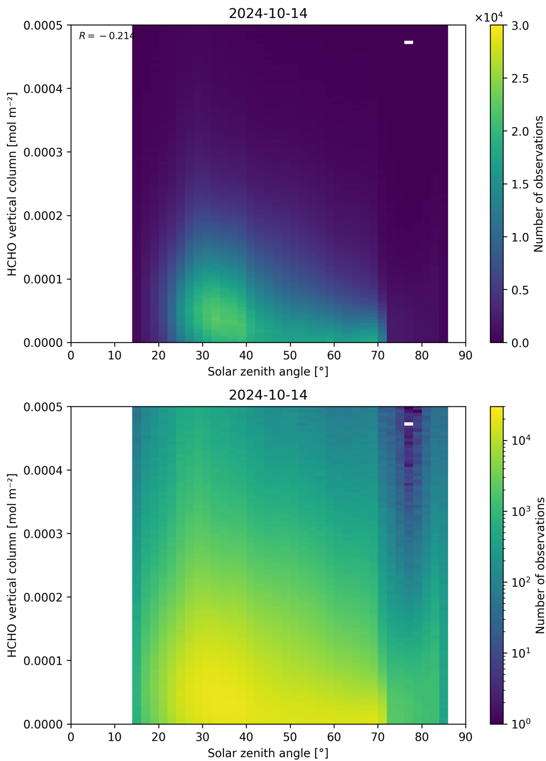
Figure 177: Scatter density plot of “Solar zenith angle” against “HCHO vertical column” for 2024-10-14 to 2024-10-15.
