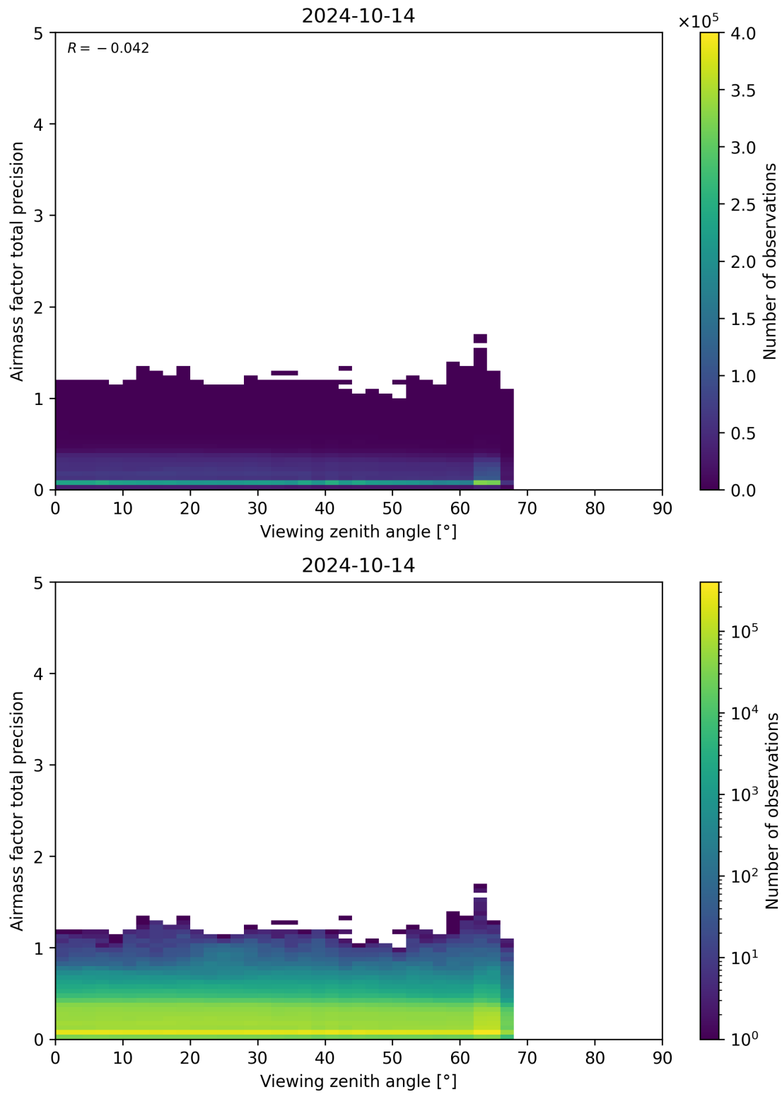
Figure 191: Scatter density plot of “Viewing zenith angle” against “Airmass factor total precision” for 2024-10-14 to 2024-10-15.
