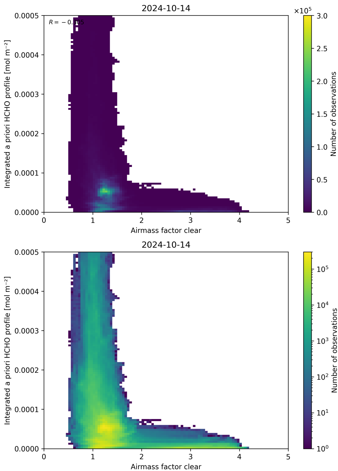
Figure 76: Scatter density plot of “Airmass factor clear” against “Integrated a priori HCHO profile” for 2024-10-14 to 2024-10-15.
