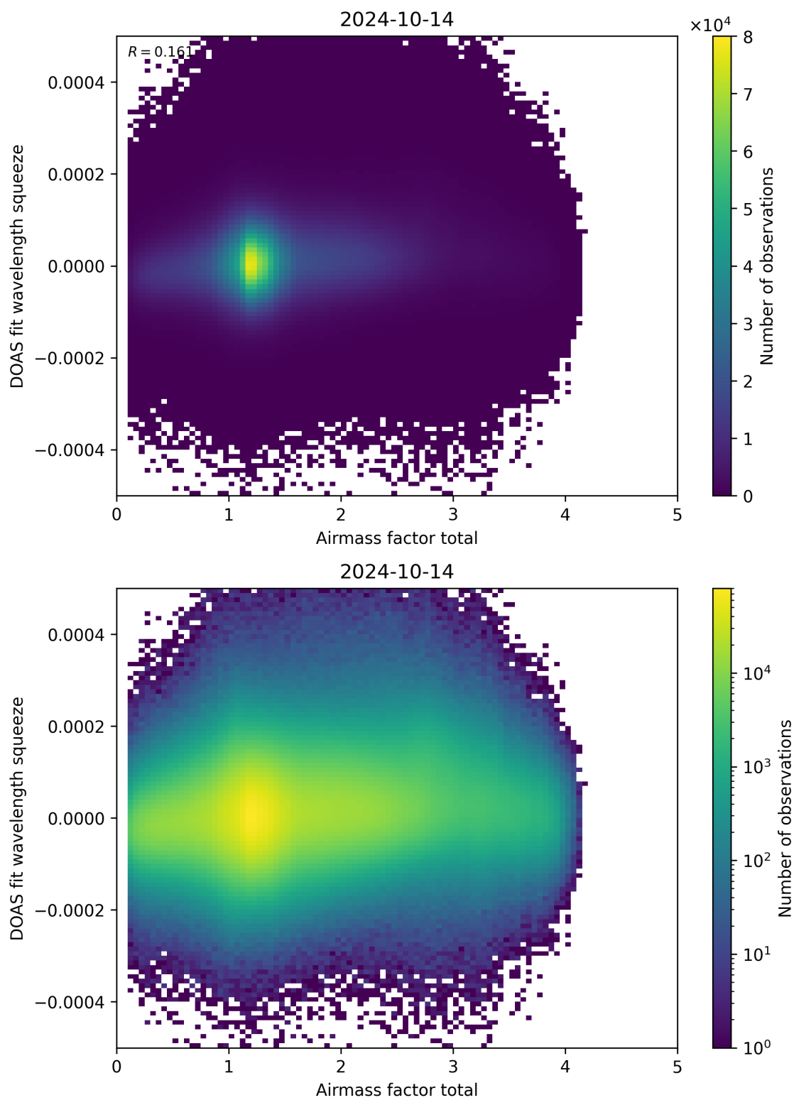
Figure 99: Scatter density plot of “Airmass factor total” against “DOAS fit wavelength squeeze” for 2024-10-14 to 2024-10-15.
