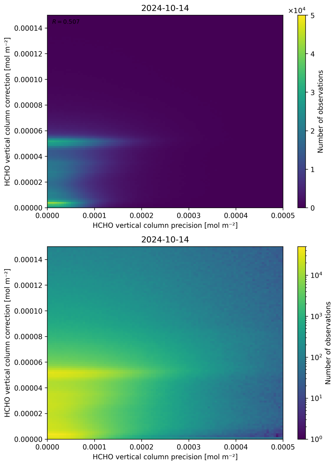
Figure 146: Scatter density plot of “HCHO vertical column precision” against “HCHO vertical column correction” for 2024-10-14 to 2024-10-15.
