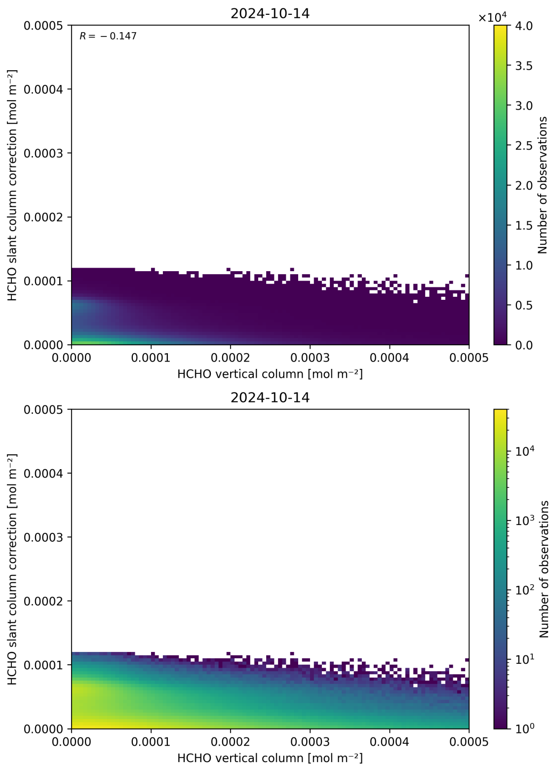
Figure 128: Scatter density plot of “HCHO vertical column” against “HCHO slant column correction” for 2024-10-14 to 2024-10-15.
