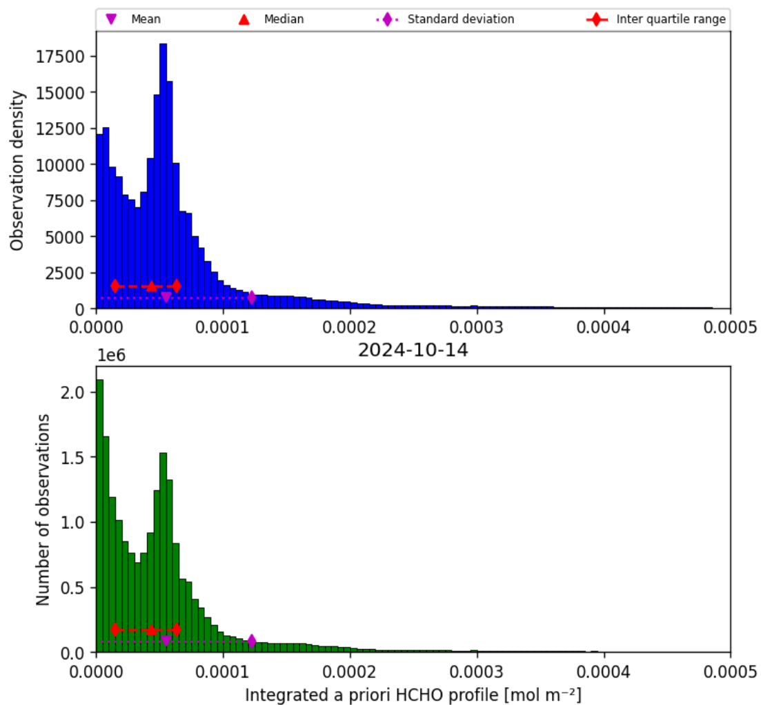
Figure 43: Histogram of “Integrated a priori HCHO profile” for 2024-10-14 to 2024-10-15
