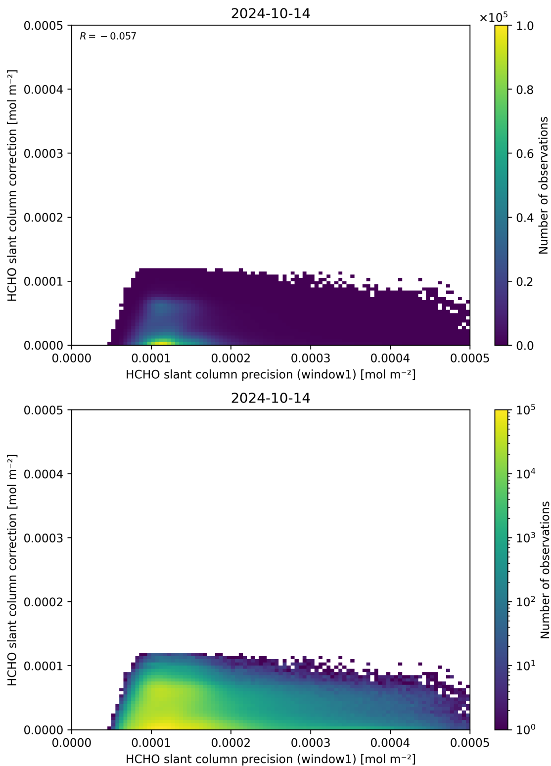
Figure 93: Scatter density plot of “HCHO slant column precision (window1)” against “HCHO slant column correction” for 2024-10-14 to 2024-10-15.
