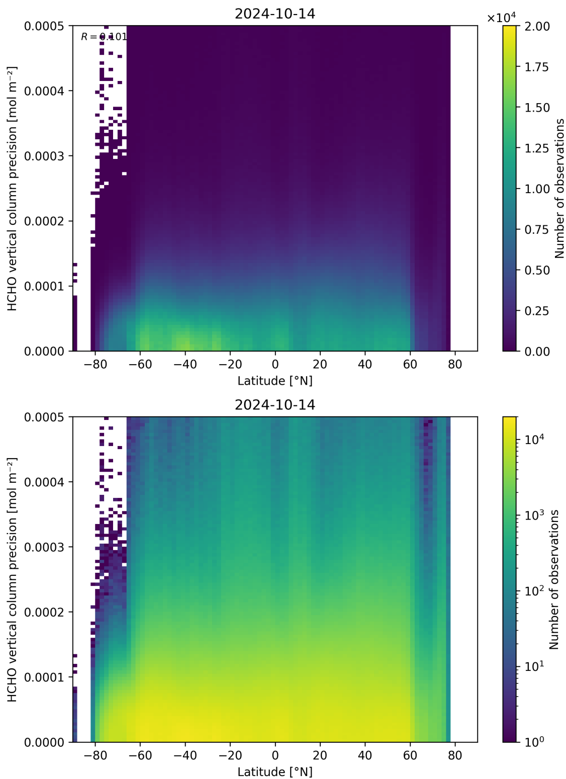
Figure 165: Scatter density plot of “Latitude” against “HCHO vertical column precision” for 2024-10-14 to 2024-10-15.
