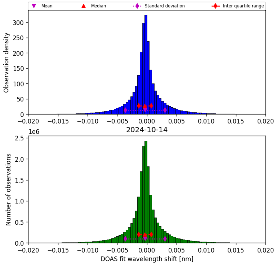
Figure 44: Histogram of “DOAS fit wavelength shift” for 2024-10-14 to 2024-10-15
