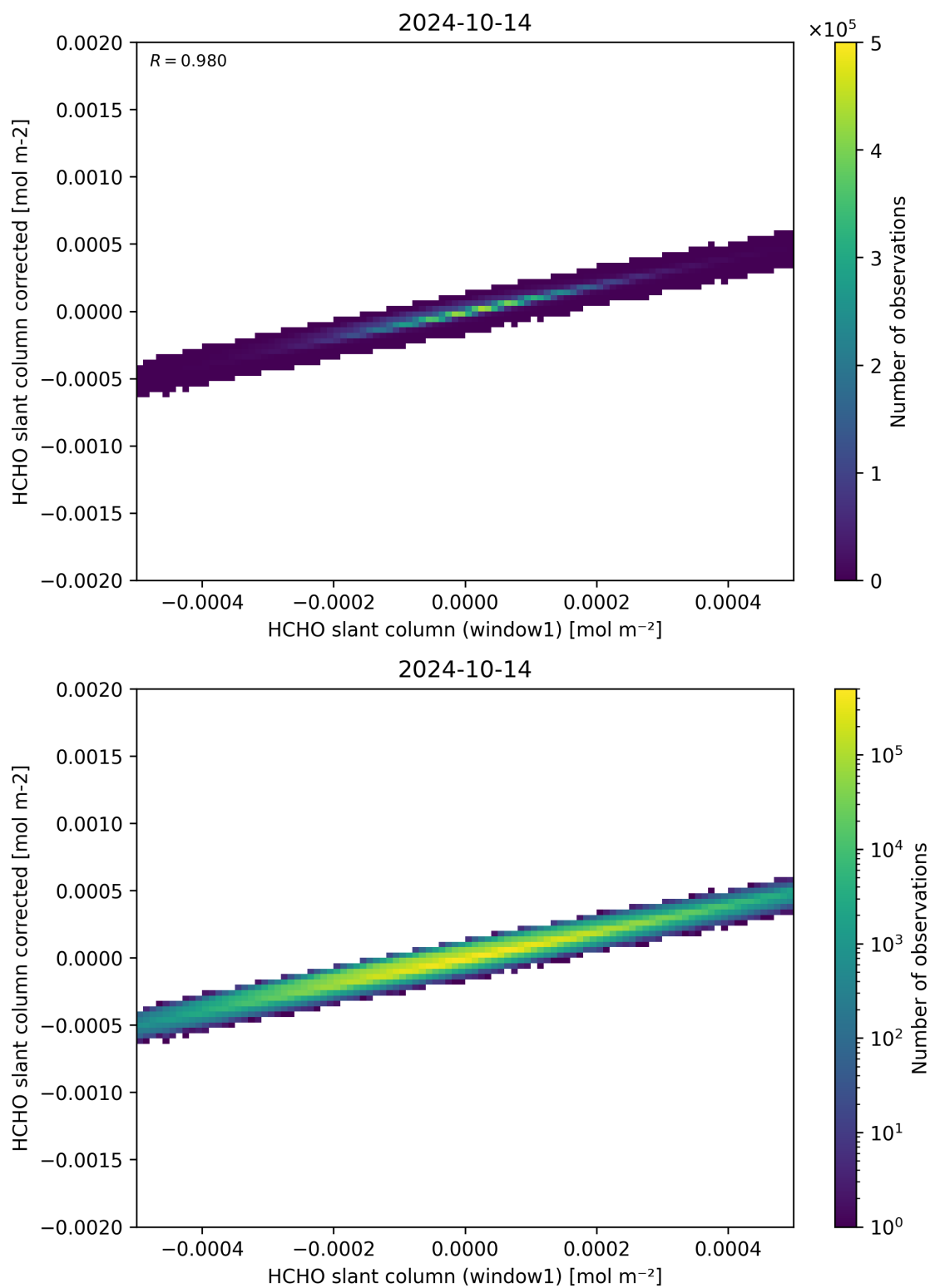
Figure 82: Scatter density plot of “HCHO slant column (window1)” against “HCHO slant column corrected” for 2024-10-14 to 2024-10-15.
