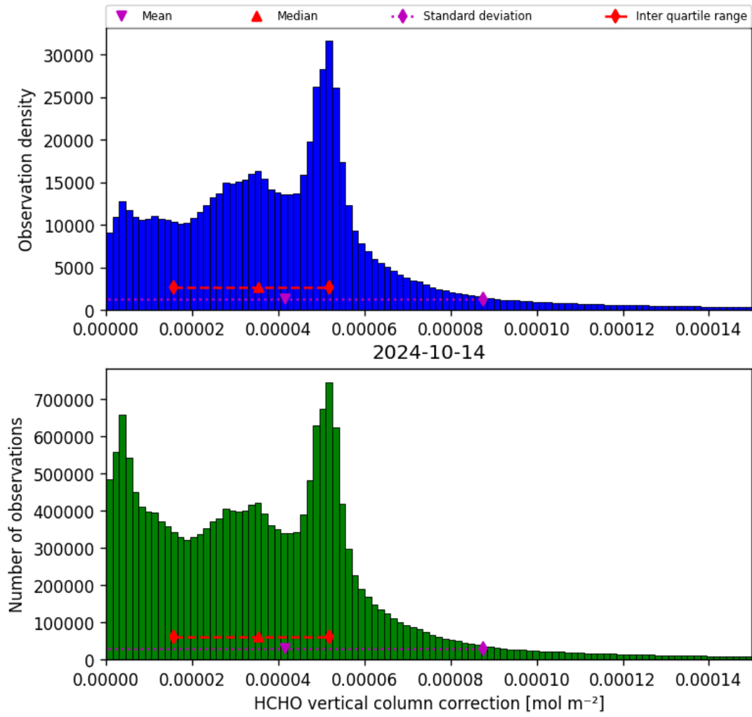
Figure 37: Histogram of “HCHO vertical column correction” for 2024-10-14 to 2024-10-15
