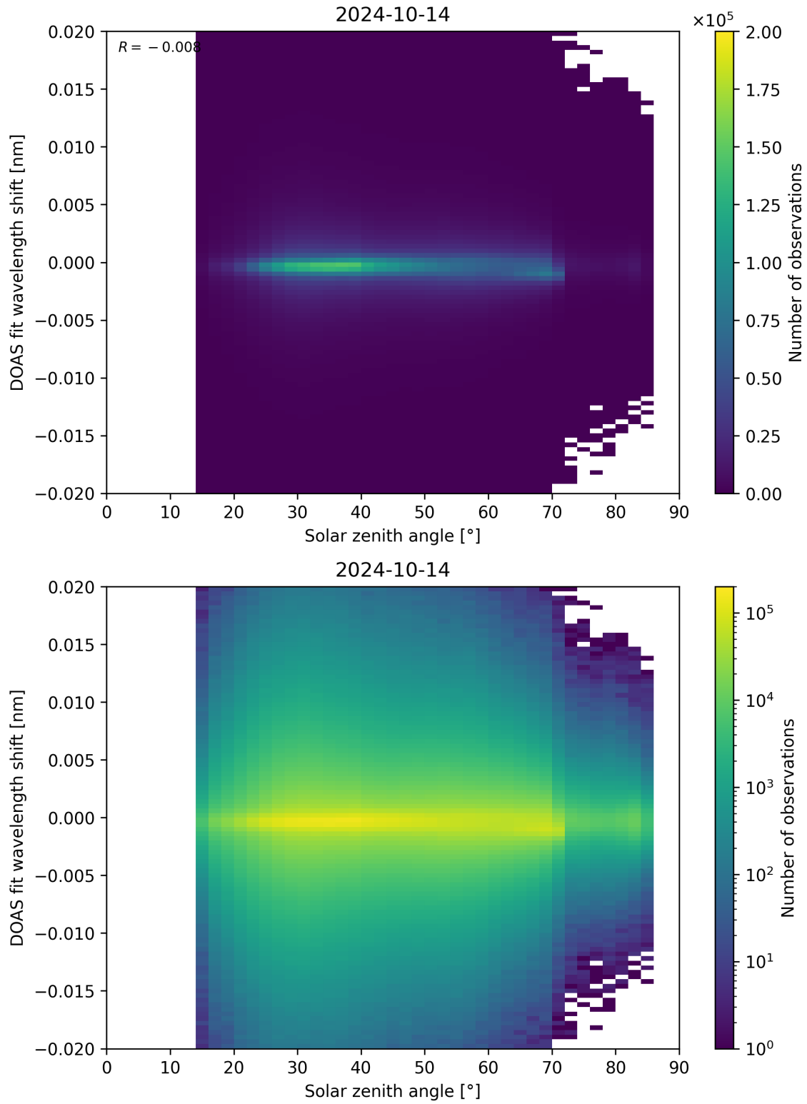
Figure 168: Scatter density plot of “Solar zenith angle” against “DOAS fit wavelength shift” for 2024-10-14 to 2024-10-15.
