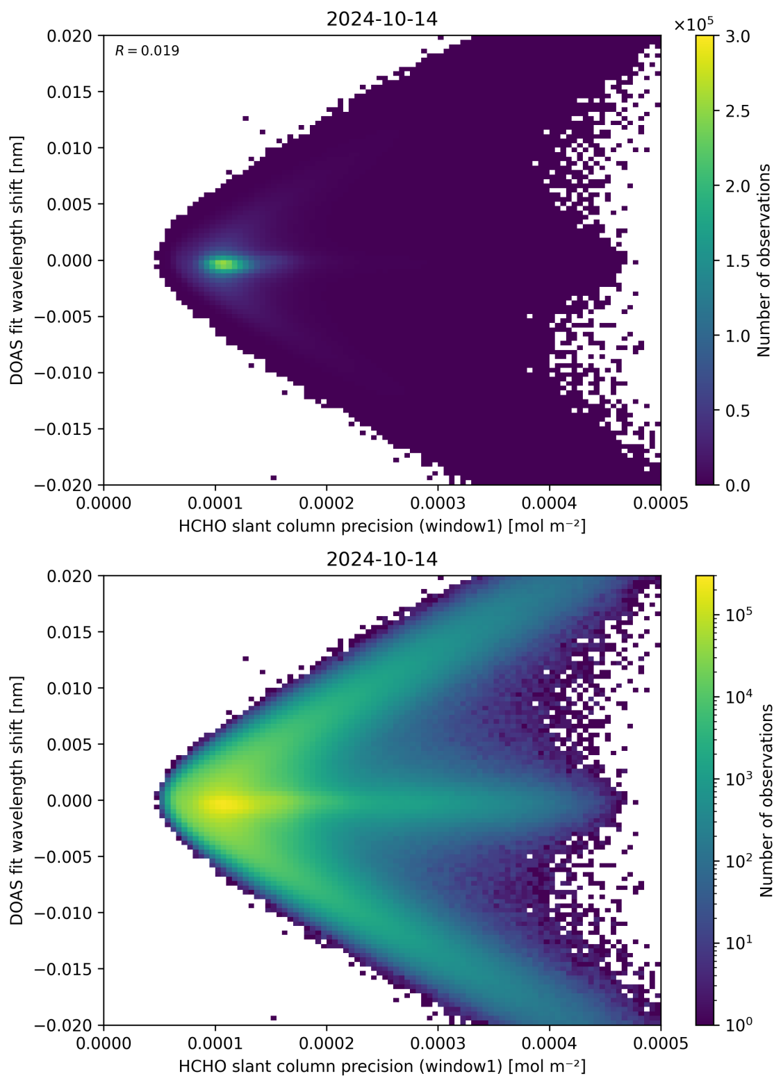
Figure 89: Scatter density plot of “HCHO slant column precision (window1)” against “DOAS fit wavelength shift” for 2024-10-14 to 2024-10-15.
