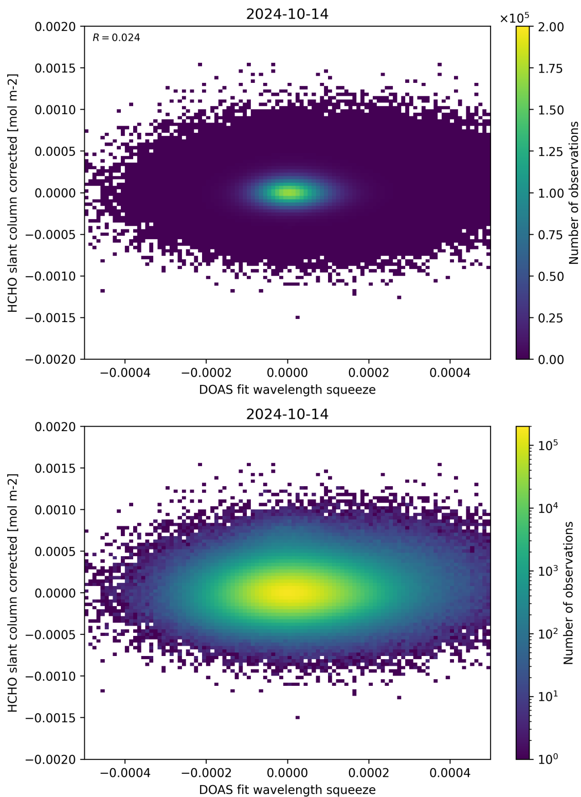
Figure 69: Scatter density plot of “DOAS fit wavelength squeeze” against “HCHO slant column corrected” for 2024-10-14 to 2024-10-15.
