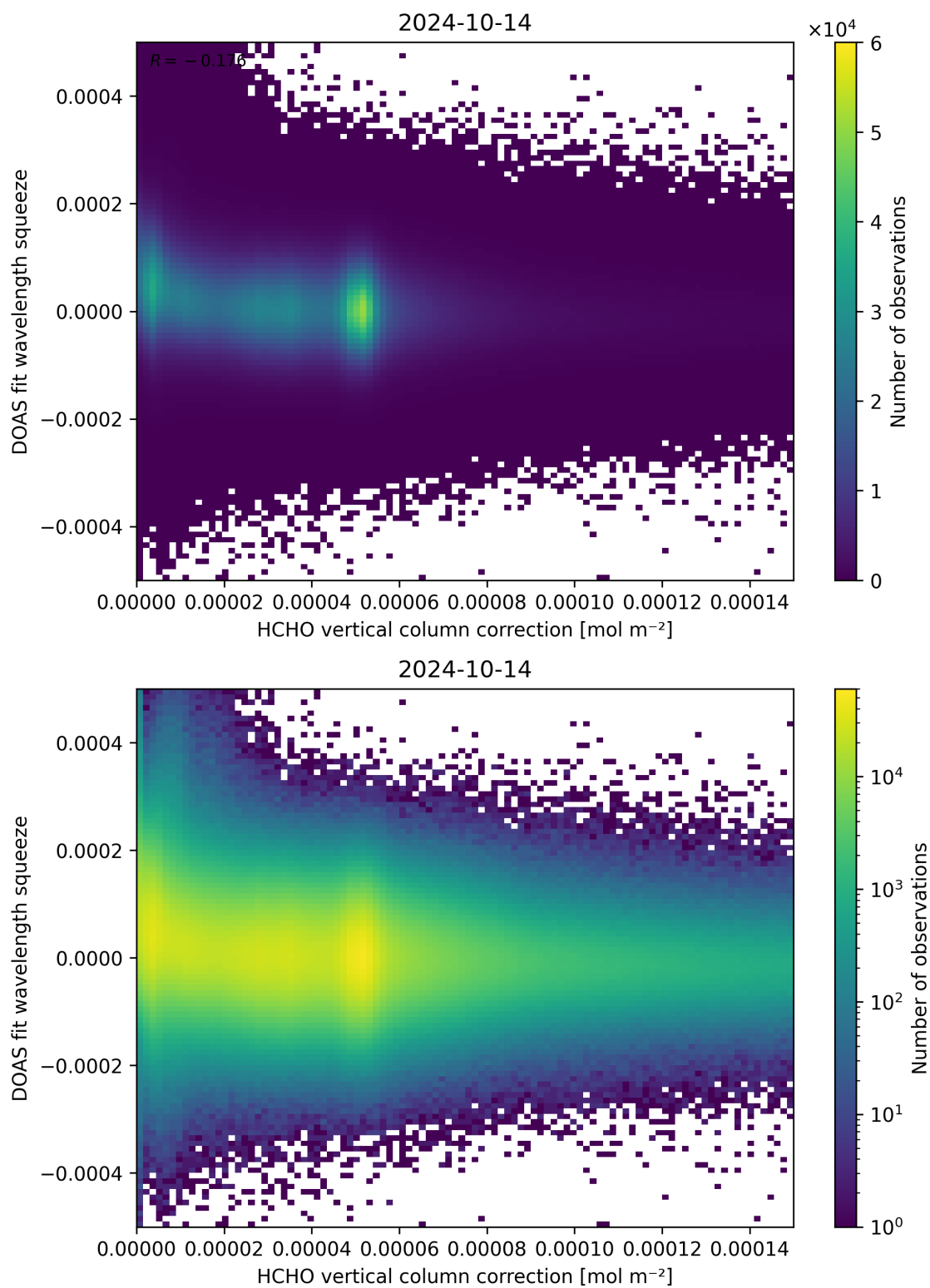
Figure 114: Scatter density plot of “HCHO vertical column correction” against “DOAS fit wavelength squeeze” for 2024-10-14 to 2024-10-15.
