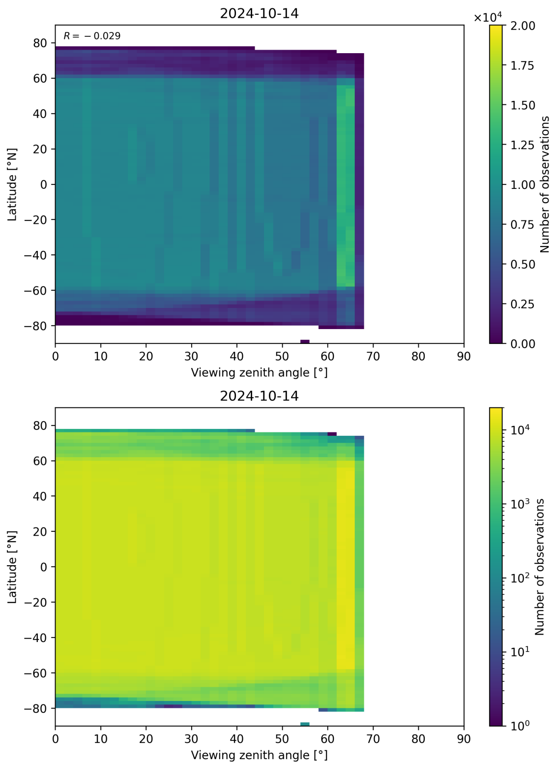
Figure 196: Scatter density plot of “Viewing zenith angle” against “Latitude” for 2024-10-14 to 2024-10-15.
