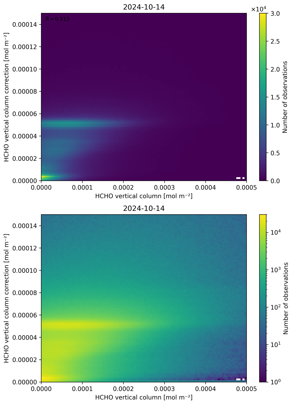
Figure 133: Scatter density plot of “HCHO vertical column” against “HCHO vertical column correction” for 2024-10-14 to 2024-10-15.
