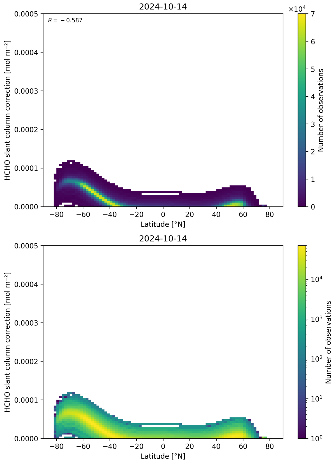
Figure 158: Scatter density plot of “Latitude” against “HCHO slant column correction” for 2024-10-14 to 2024-10-15.
