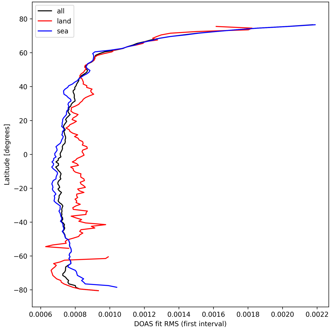
Figure 32: Zonal average of “DOAS fit RMS (first interval)” for 2024-10-14 to 2024-10-15.
