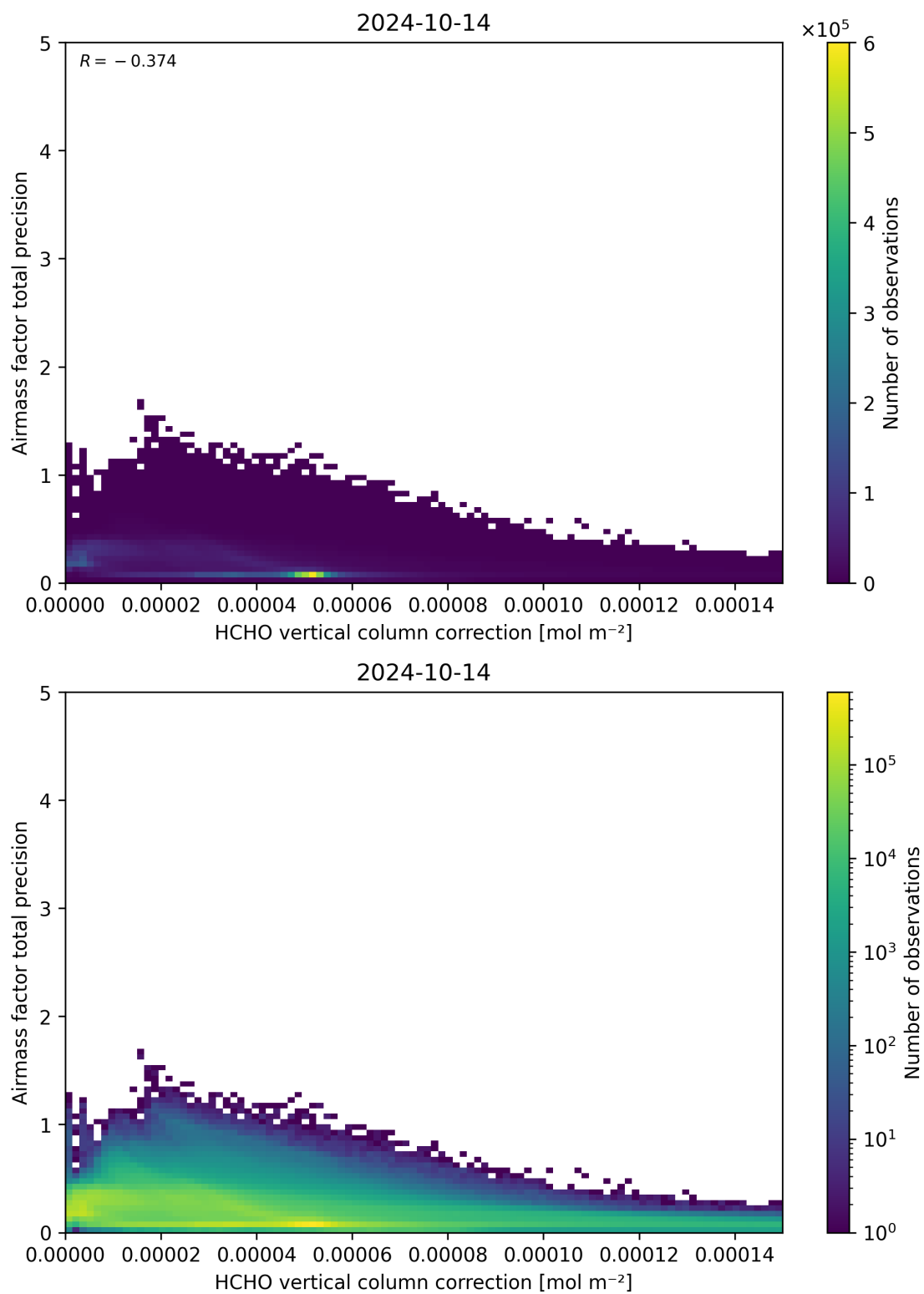
Figure 121: Scatter density plot of “HCHO vertical column correction” against “Airmass factor total precision” for 2024-10-14 to 2024-10-15.
