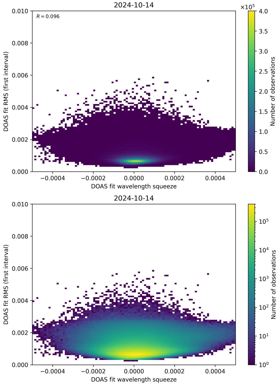
Figure 68: Scatter density plot of “DOAS fit wavelength squeeze” against “DOAS fit RMS (first interval)” for 2024-10-14 to 2024-10-15.
