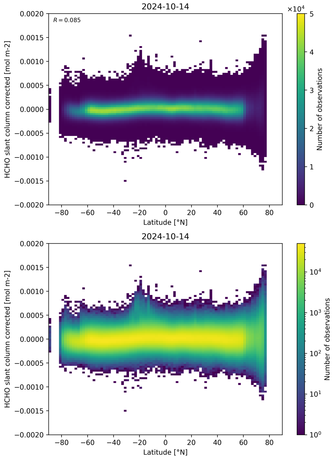
Figure 157: Scatter density plot of “Latitude” against “HCHO slant column corrected” for 2024-10-14 to 2024-10-15.
