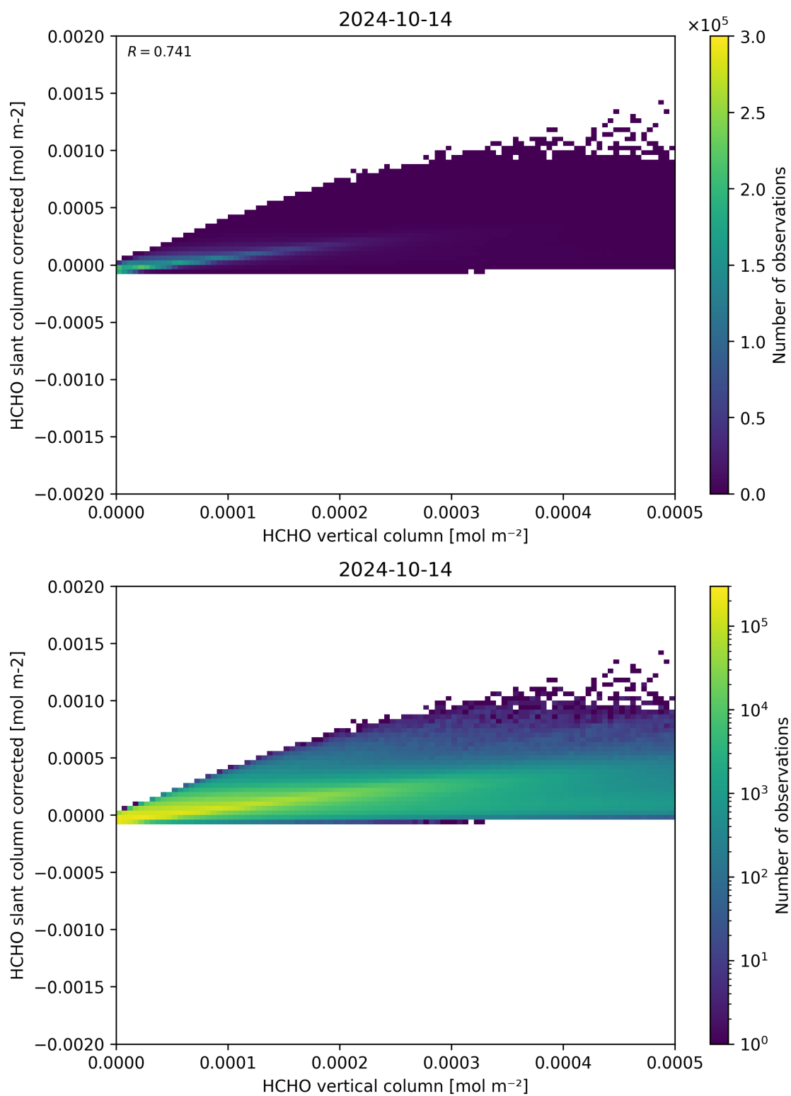
Figure 127: Scatter density plot of “HCHO vertical column” against “HCHO slant column corrected” for 2024-10-14 to 2024-10-15.
