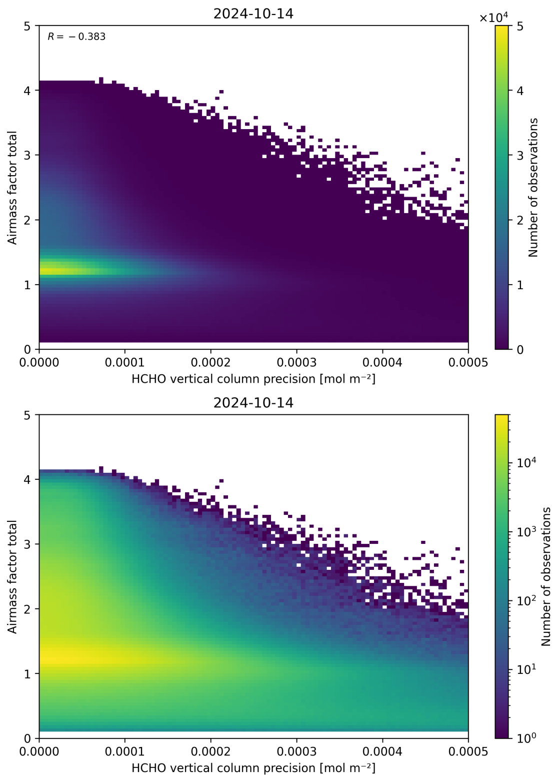
Figure 144: Scatter density plot of “HCHO vertical column precision” against “Airmass factor total” for 2024-10-14 to 2024-10-15.
