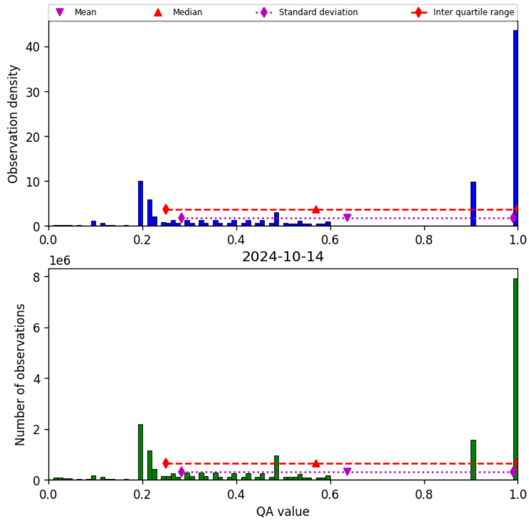
Figure 34: Histogram of “QA value” for 2024-10-14 to 2024-10-15
