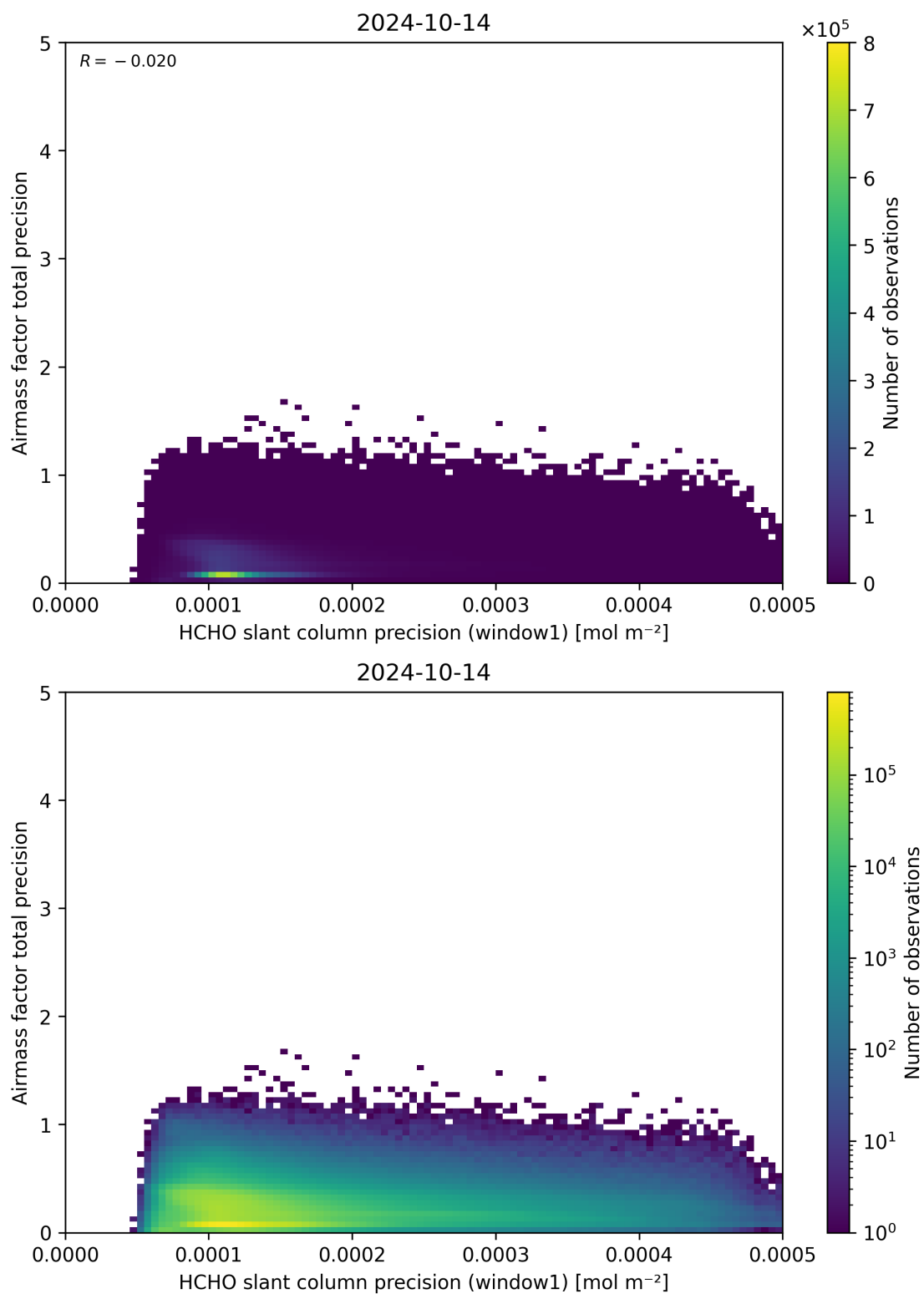
Figure 95: Scatter density plot of “HCHO slant column precision (window1)” against “Airmass factor total precision” for 2024-10-14 to 2024-10-15.
