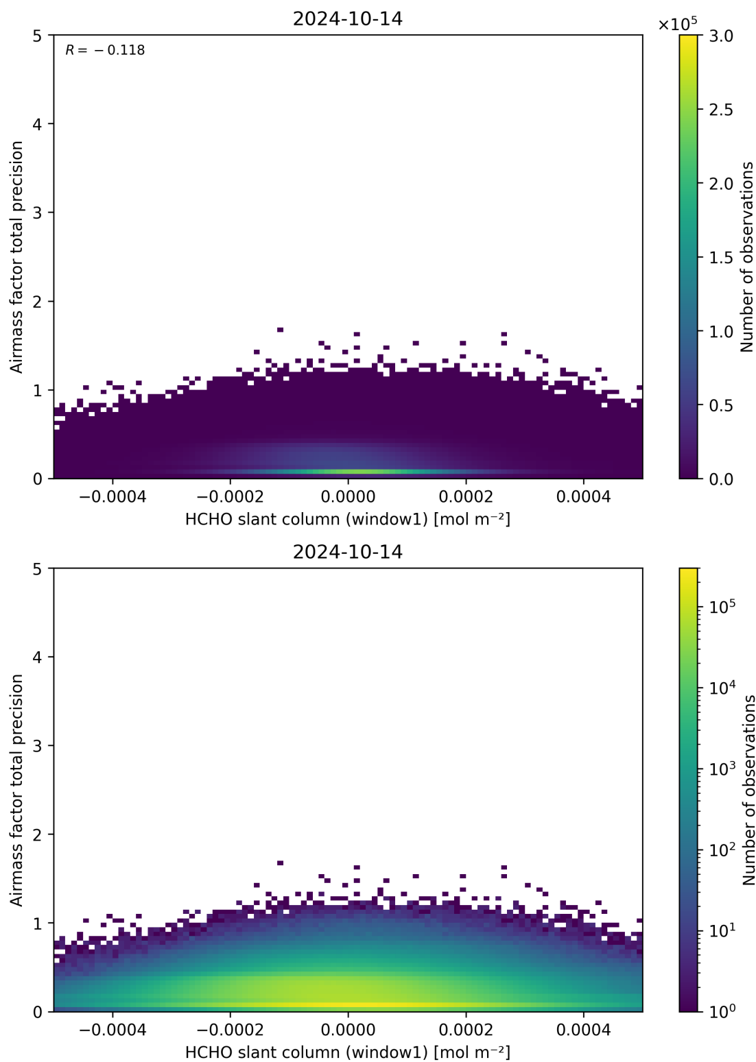
Figure 86: Scatter density plot of “HCHO slant column (window1)” against “Airmass factor total precision” for 2024-10-14 to 2024-10-15.
