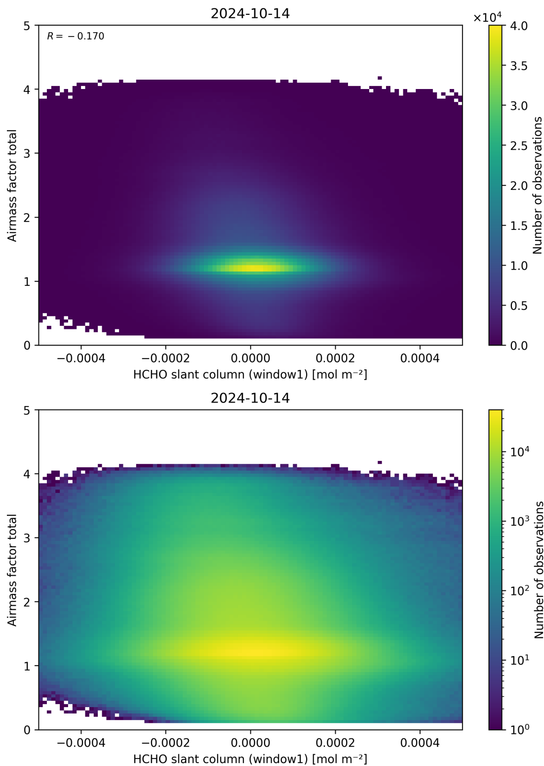
Figure 85: Scatter density plot of “HCHO slant column (window1)” against “Airmass factor total” for 2024-10-14 to 2024-10-15.
