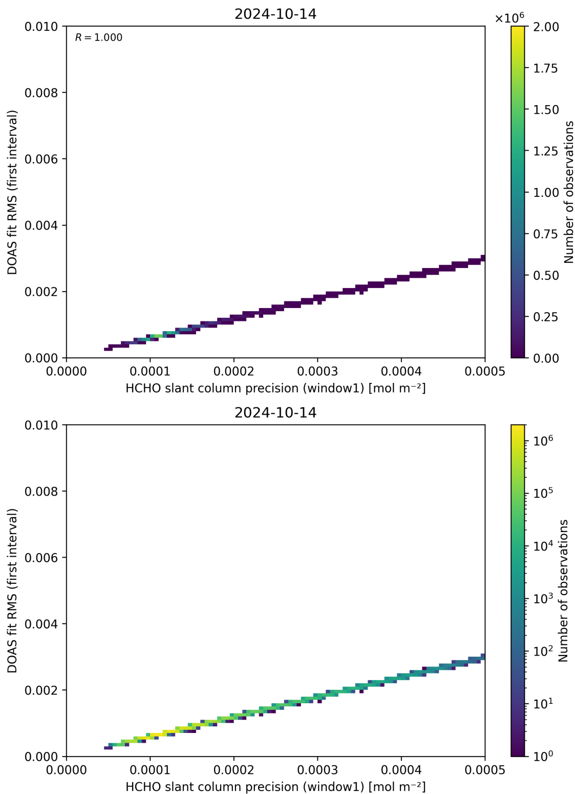
Figure 88: Scatter density plot of “HCHO slant column precision (window1)” against “DOAS fit RMS (first interval)” for 2024-10-14 to 2024-10-15.
