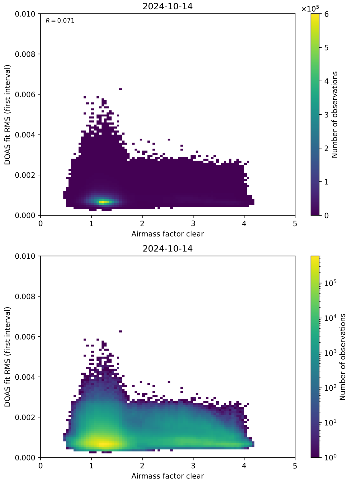
Figure 71: Scatter density plot of “Airmass factor clear” against “DOAS fit RMS (first interval)” for 2024-10-14 to 2024-10-15.
