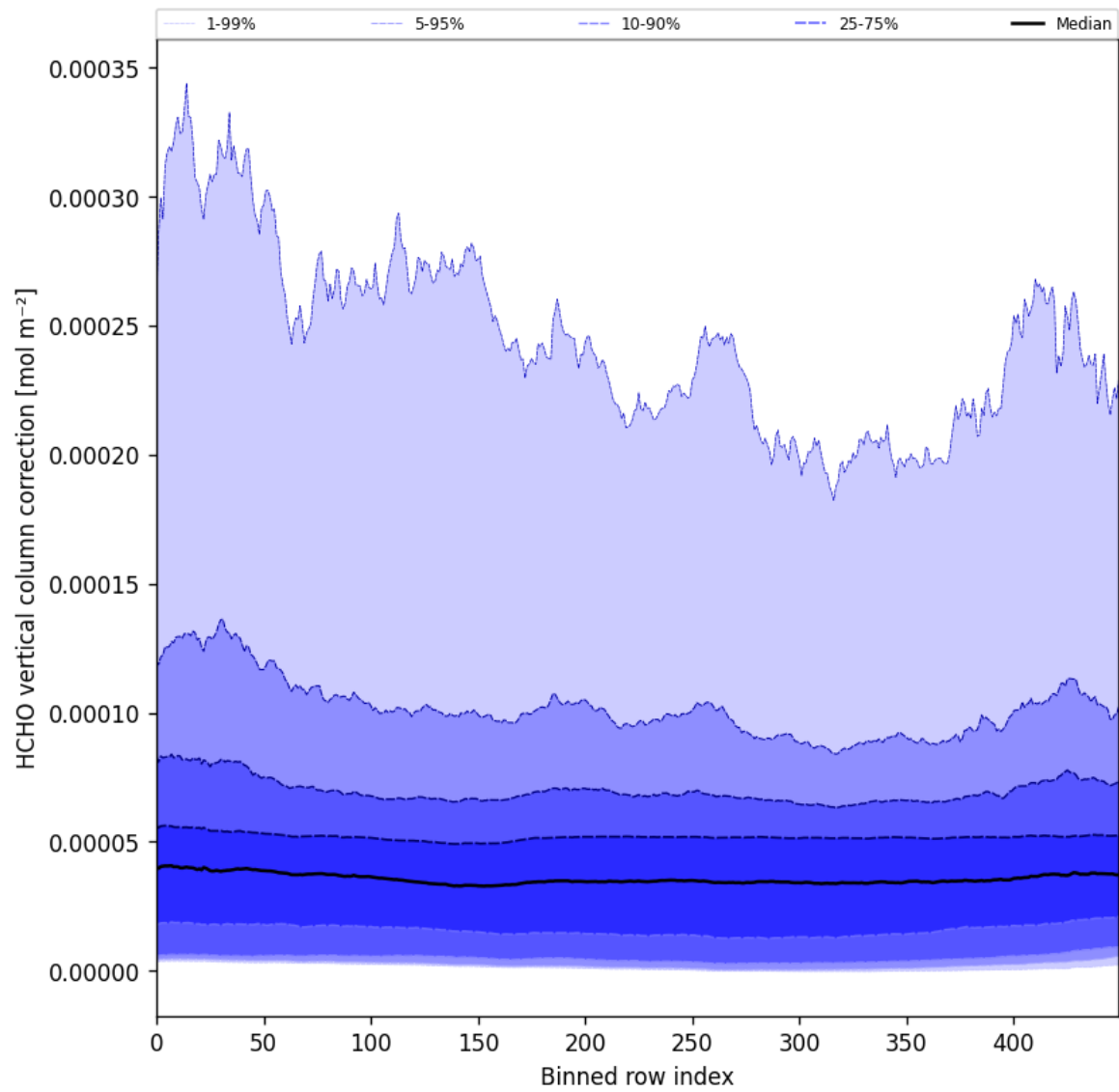
Figure 51: Along track statistics of “HCHO vertical column correction” for 2024-10-14 to 2024-10-15
