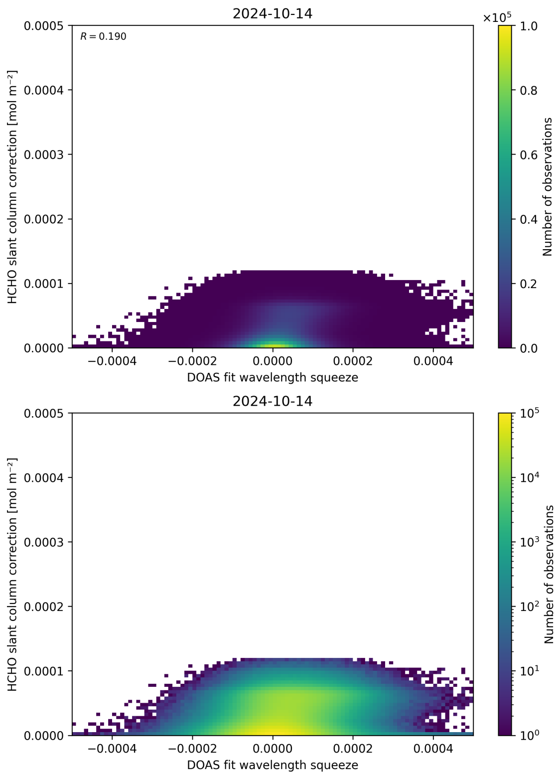
Figure 70: Scatter density plot of “DOAS fit wavelength squeeze” against “HCHO slant column correction” for 2024-10-14 to 2024-10-15.
