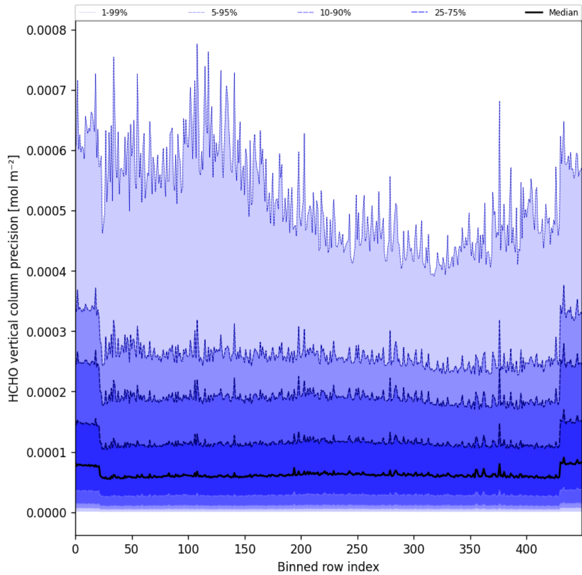
Figure 50: Along track statistics of “HCHO vertical column precision” for 2024-10-14 to 2024-10-15
