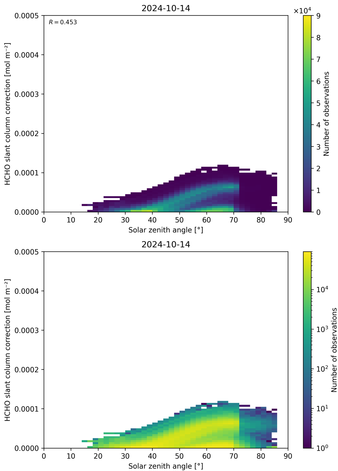
Figure 172: Scatter density plot of “Solar zenith angle” against “HCHO slant column correction” for 2024-10-14 to 2024-10-15.
