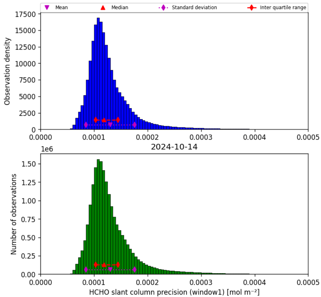
Figure 39: Histogram of “HCHO slant column precision (window1)” for 2024-10-14 to 2024-10-15
