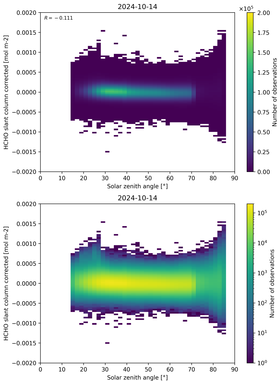
Figure 171: Scatter density plot of “Solar zenith angle” against “HCHO slant column corrected” for 2024-10-14 to 2024-10-15.
