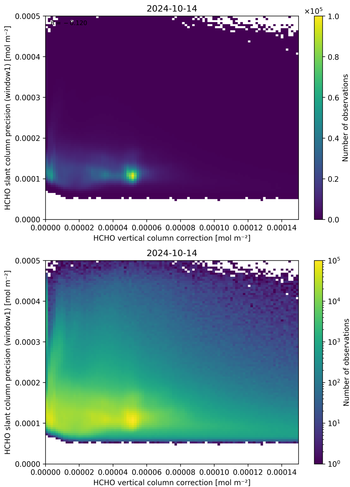
Figure 119: Scatter density plot of “HCHO vertical column correction” against “HCHO slant column precision (window1)” for 2024-10-14 to 2024-10-15.
