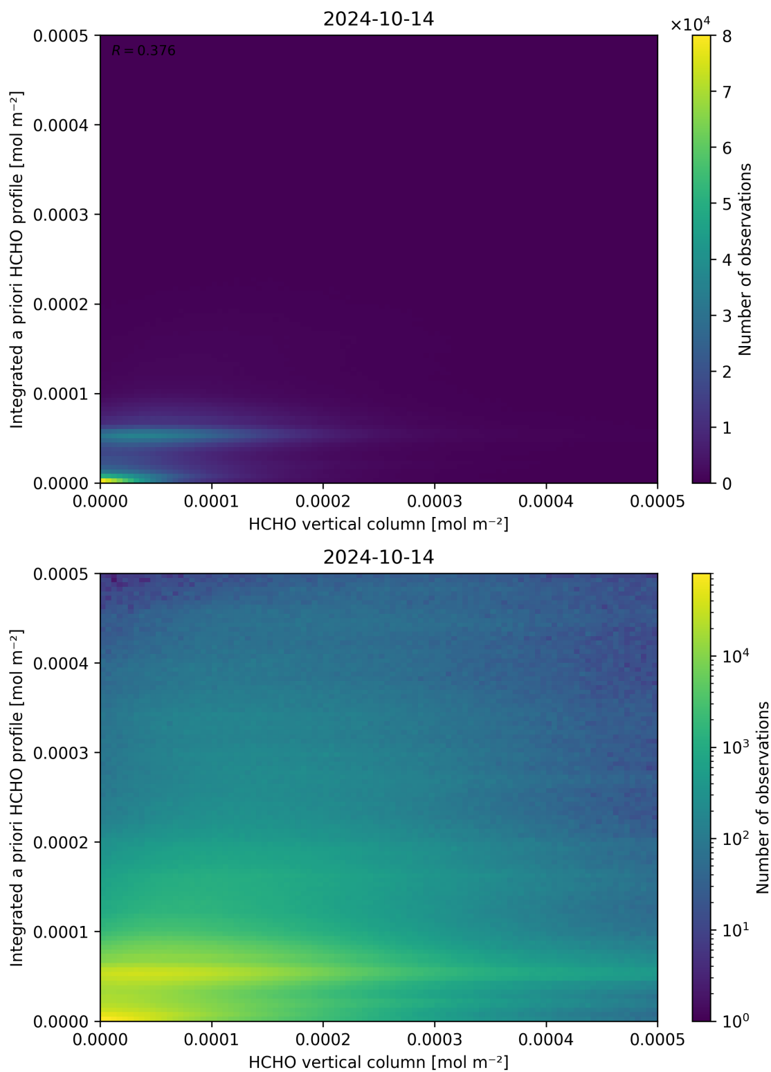
Figure 135: Scatter density plot of “HCHO vertical column” against “Integrated a priori HCHO profile” for 2024-10-14 to 2024-10-15.
