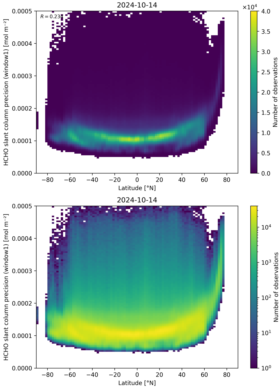
Figure 160: Scatter density plot of “Latitude” against “HCHO slant column precision (window1)” for 2024-10-14 to 2024-10-15.
