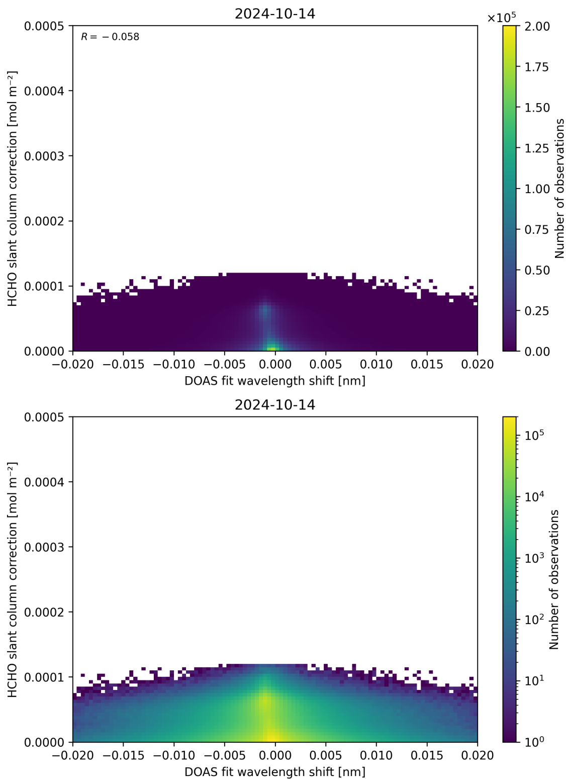
Figure 67: Scatter density plot of “DOAS fit wavelength shift” against “HCHO slant column correction” for 2024-10-14 to 2024-10-15.
