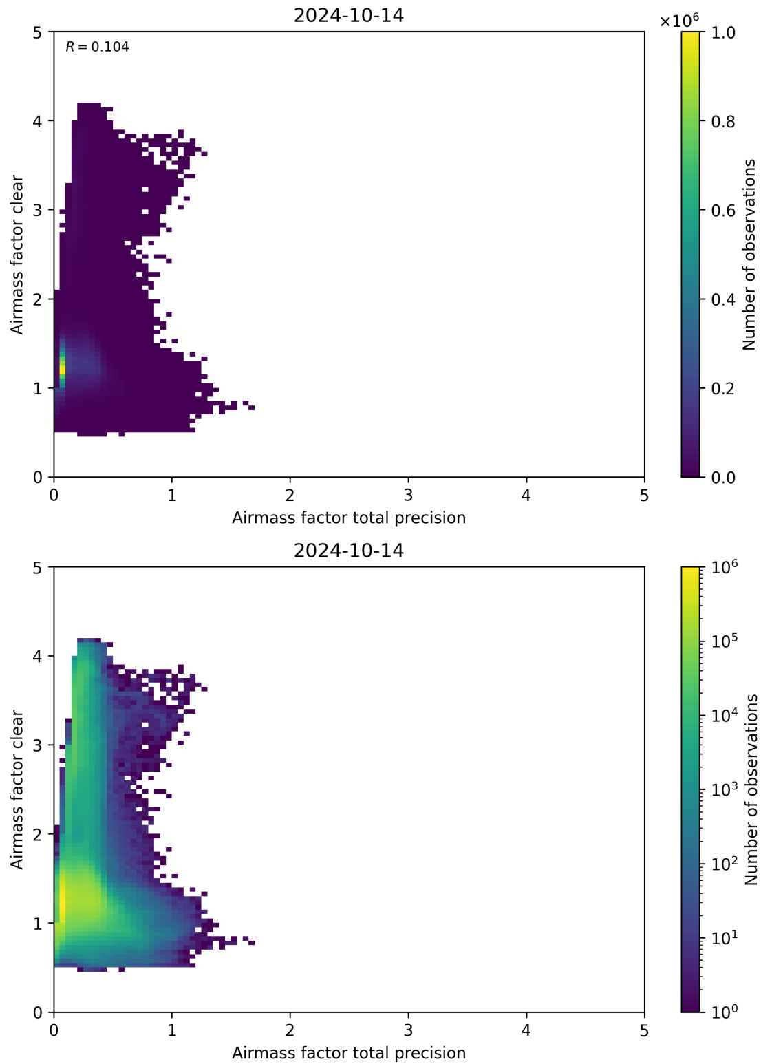
Figure 108: Scatter density plot of “Airmass factor total precision” against “Airmass factor clear” for 2024-10-14 to 2024-10-15.
