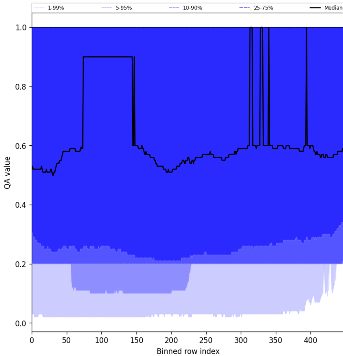
Figure 48: Along track statistics of “QA value” for 2024-10-14 to 2024-10-15
