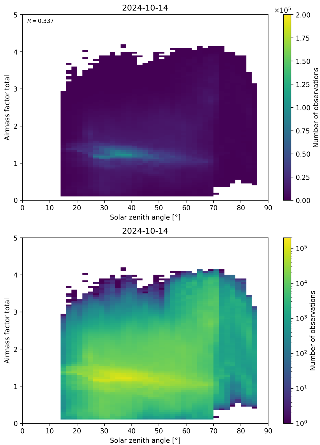
Figure 175: Scatter density plot of “Solar zenith angle” against “Airmass factor total” for 2024-10-14 to 2024-10-15.
