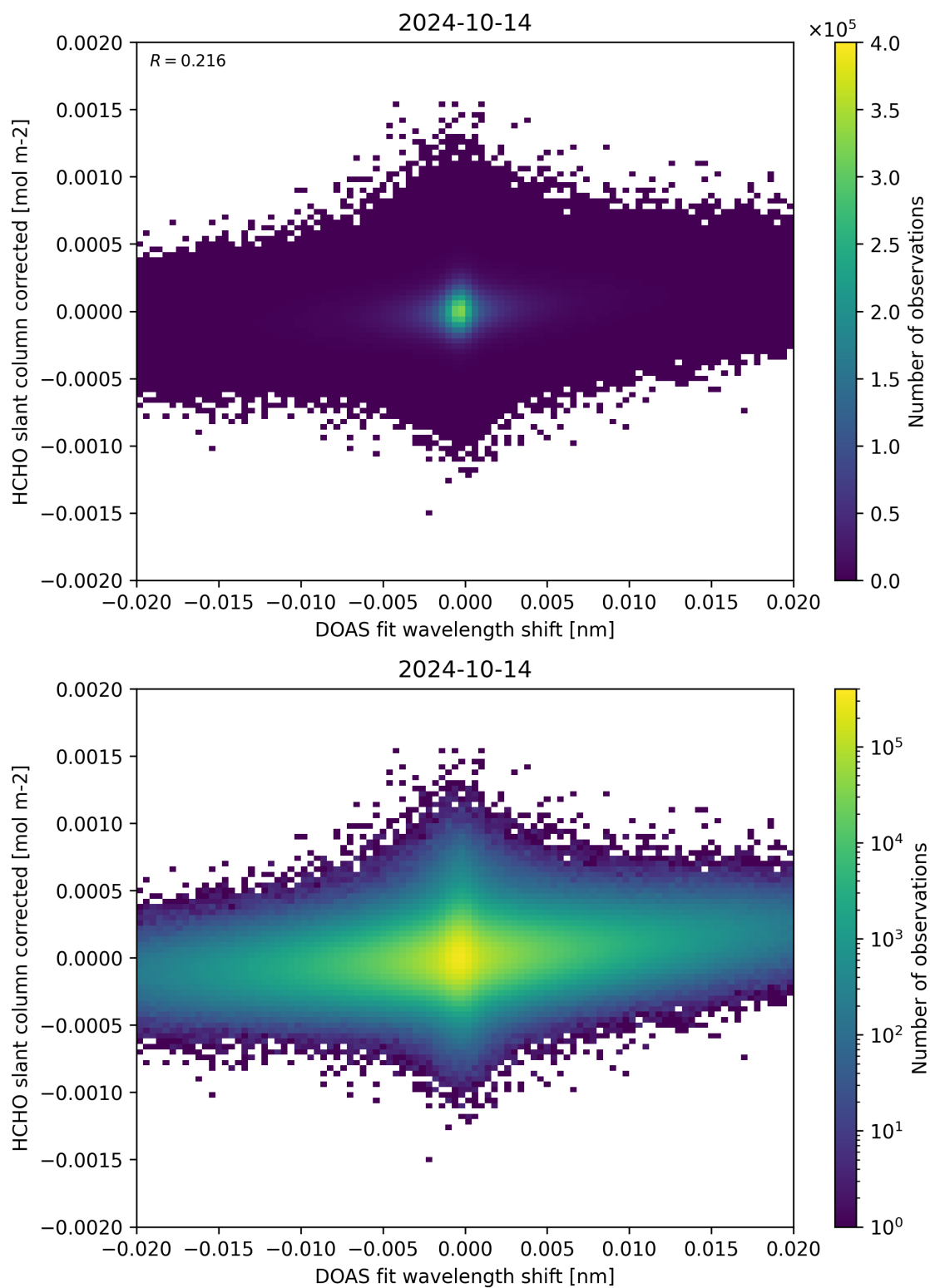
Figure 66: Scatter density plot of “DOAS fit wavelength shift” against “HCHO slant column corrected” for 2024-10-14 to 2024-10-15.
