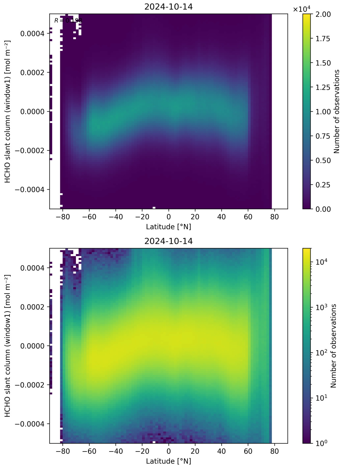
Figure 159: Scatter density plot of “Latitude” against “HCHO slant column (window1)” for 2024-10-14 to 2024-10-15.
