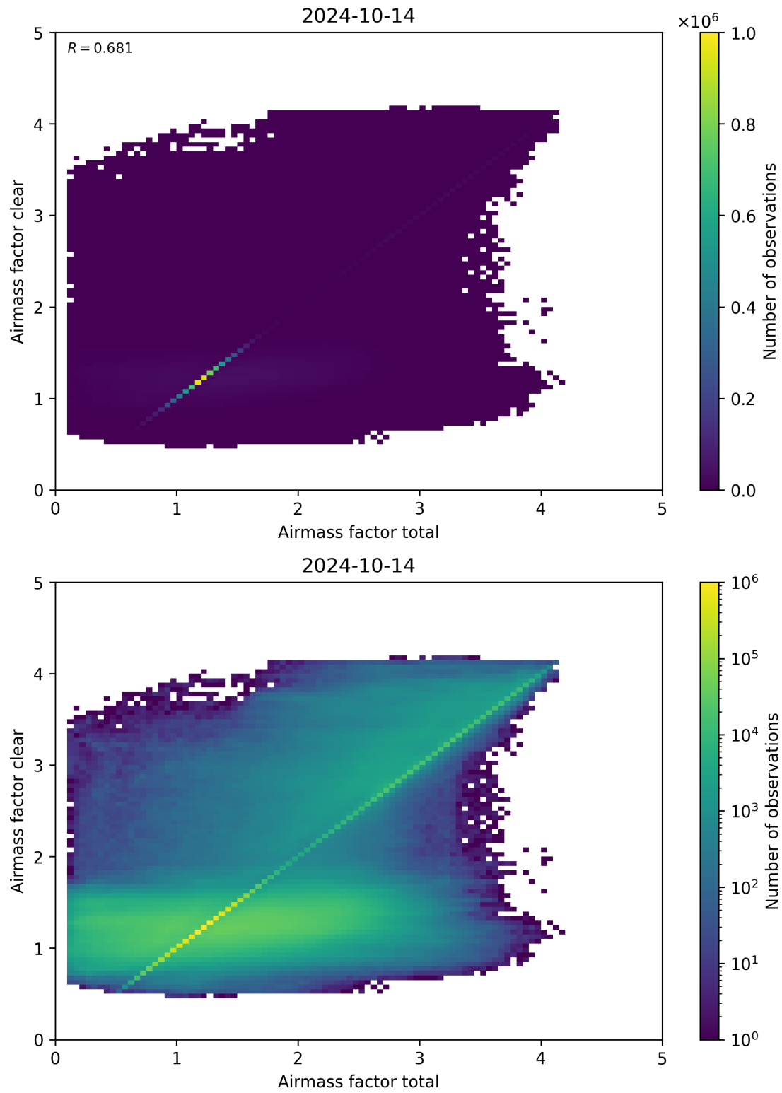
Figure 100: Scatter density plot of “Airmass factor total” against “Airmass factor clear” for 2024-10-14 to 2024-10-15.
