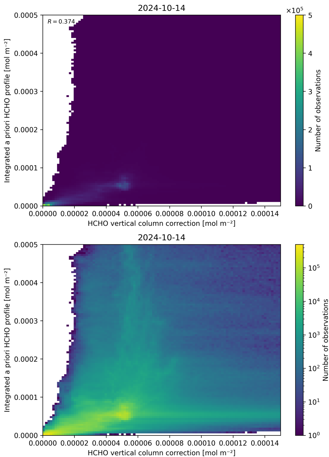
Figure 122: Scatter density plot of “HCHO vertical column correction” against “Integrated a priori HCHO profile” for 2024-10-14 to 2024-10-15.
