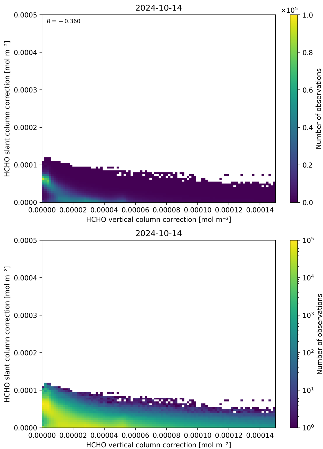
Figure 117: Scatter density plot of “HCHO vertical column correction” against “HCHO slant column correction” for 2024-10-14 to 2024-10-15.
