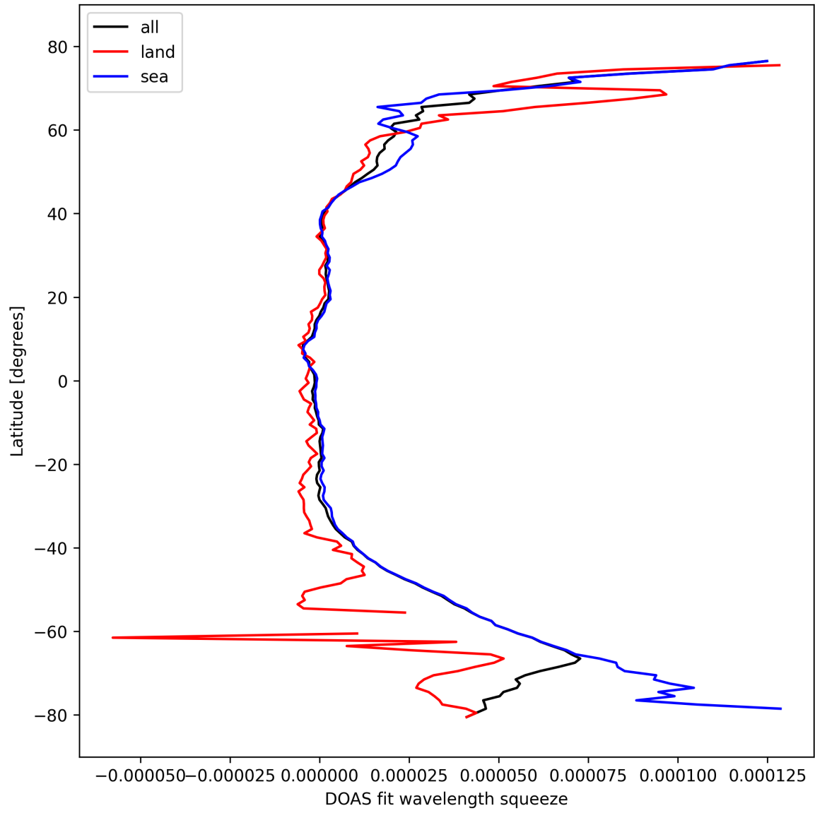
Figure 31: Zonal average of “DOAS fit wavelength squeeze” for 2024-10-14 to 2024-10-15.
