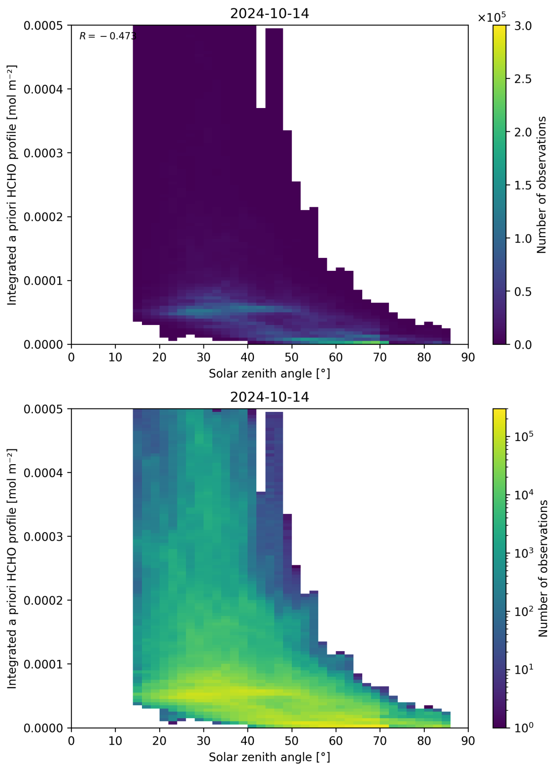
Figure 180: Scatter density plot of “Solar zenith angle” against “Integrated a priori HCHO profile” for 2024-10-14 to 2024-10-15.
