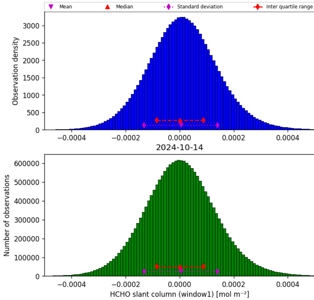
Figure 38: Histogram of “HCHO slant column (window1)” for 2024-10-14 to 2024-10-15
