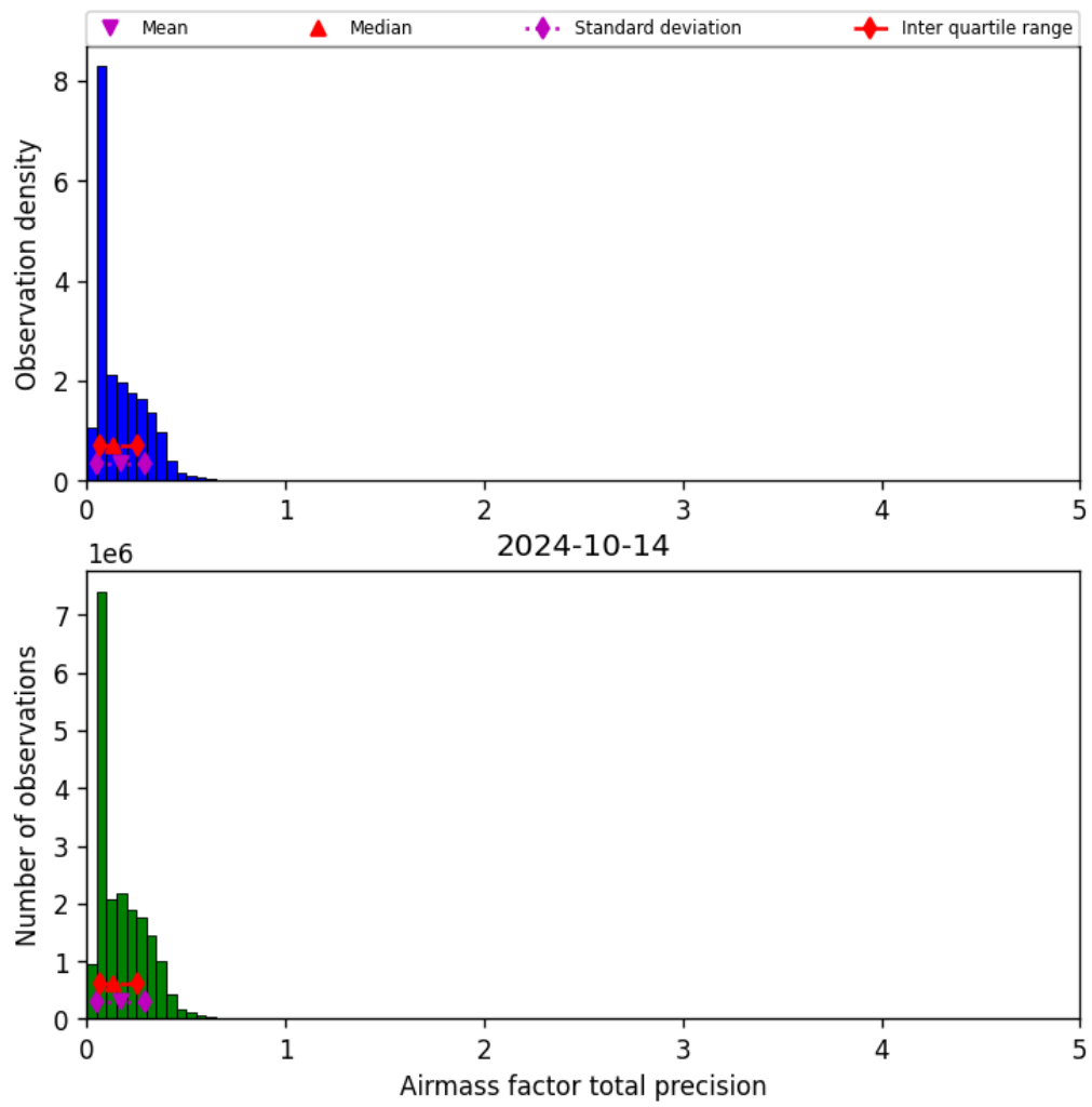
Figure 41: Histogram of “Airmass factor total precision” for 2024-10-14 to 2024-10-15
