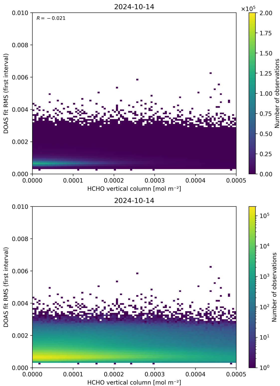
Figure 123: Scatter density plot of “HCHO vertical column” against “DOAS fit RMS (first interval)” for 2024-10-14 to 2024-10-15.
