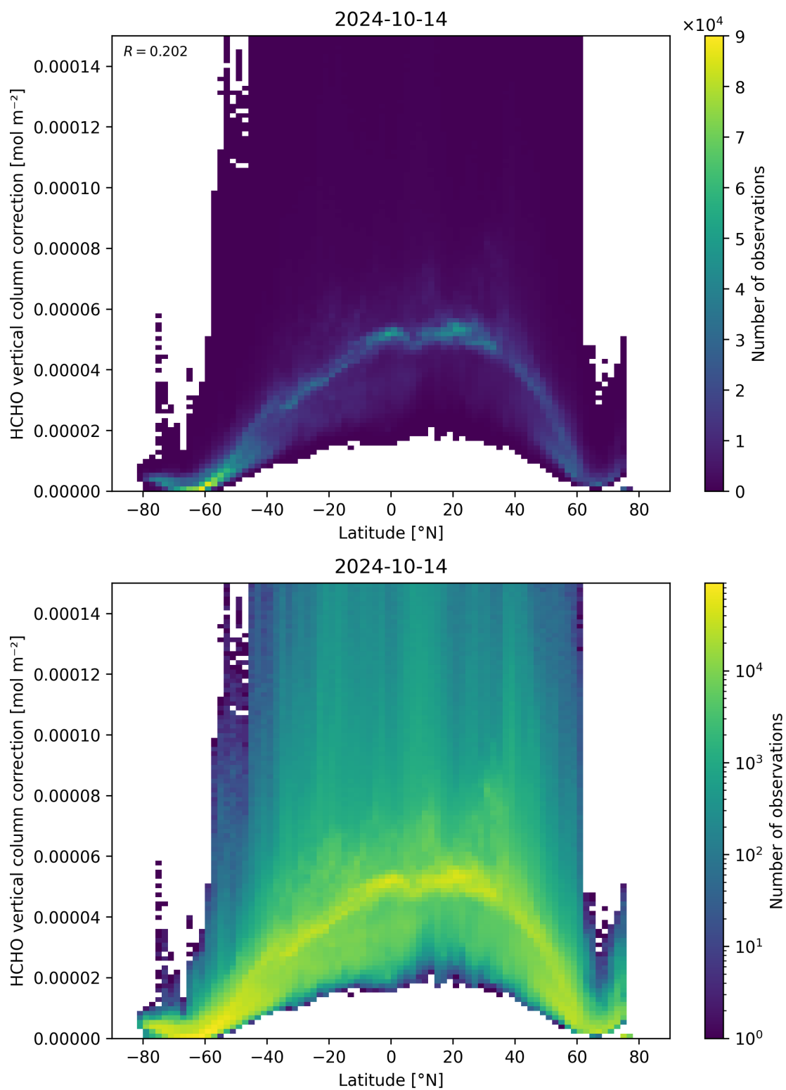
Figure 164: Scatter density plot of “Latitude” against “HCHO vertical column correction” for 2024-10-14 to 2024-10-15.
