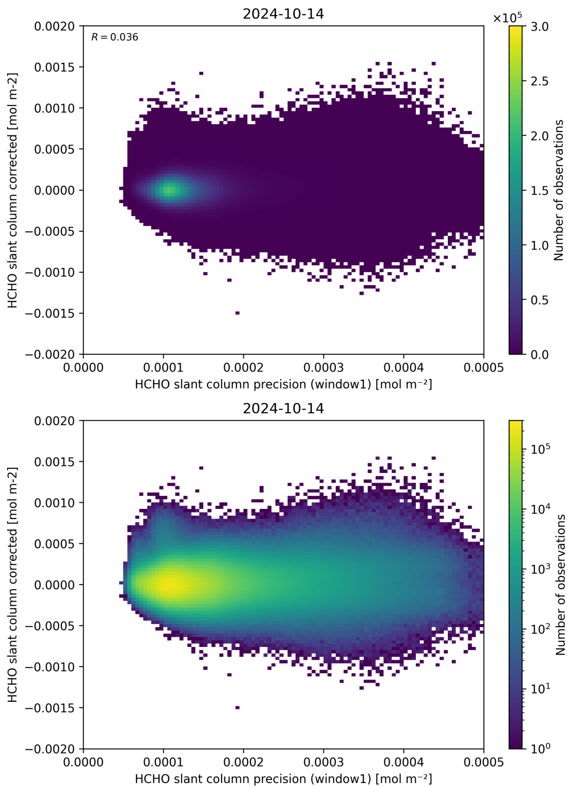
Figure 92: Scatter density plot of “HCHO slant column precision (window1)” against “HCHO slant column corrected” for 2024-10-14 to 2024-10-15.
