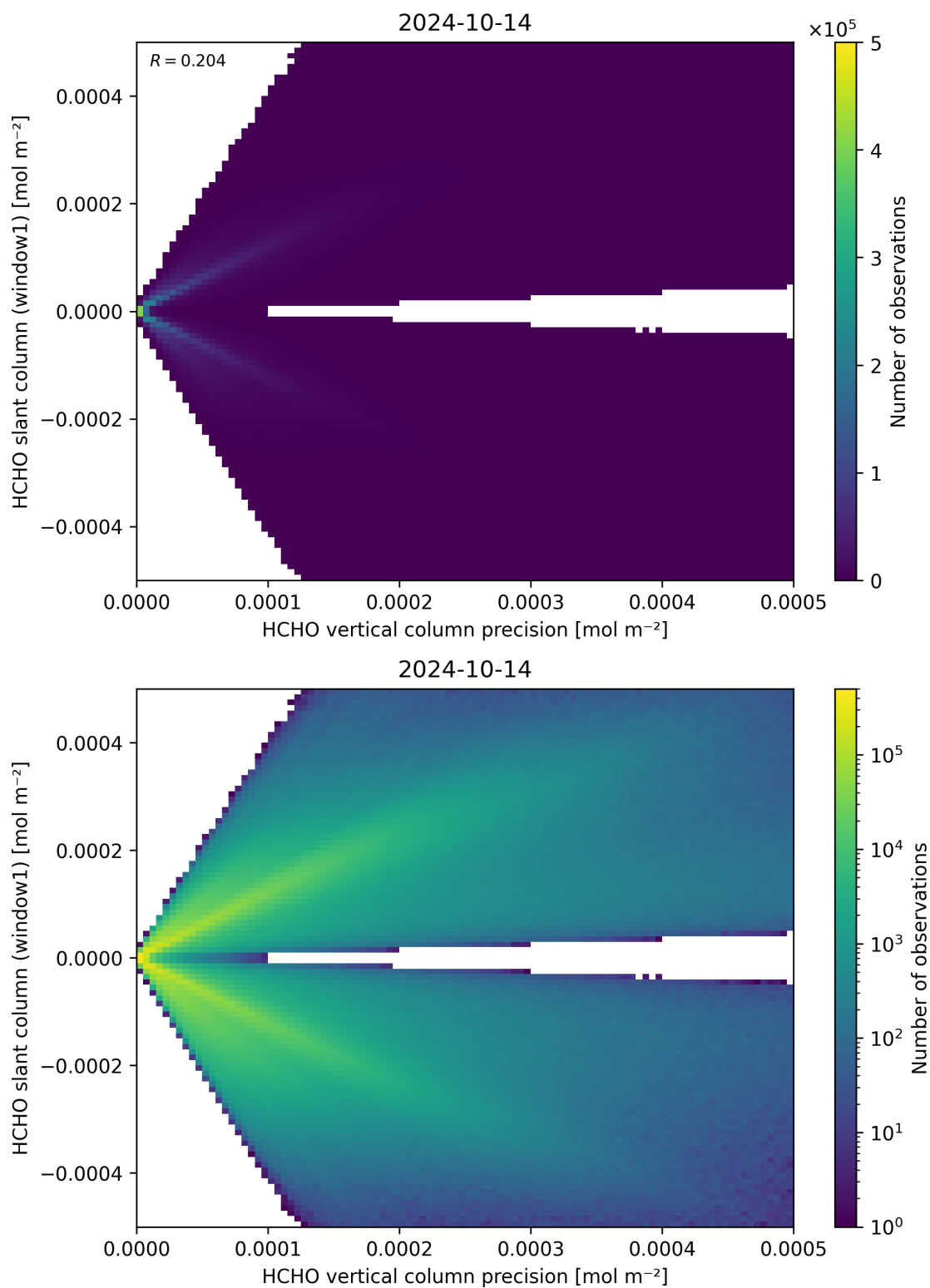
Figure 142: Scatter density plot of “HCHO vertical column precision” against “HCHO slant column (window1)” for 2024-10-14 to 2024-10-15.
