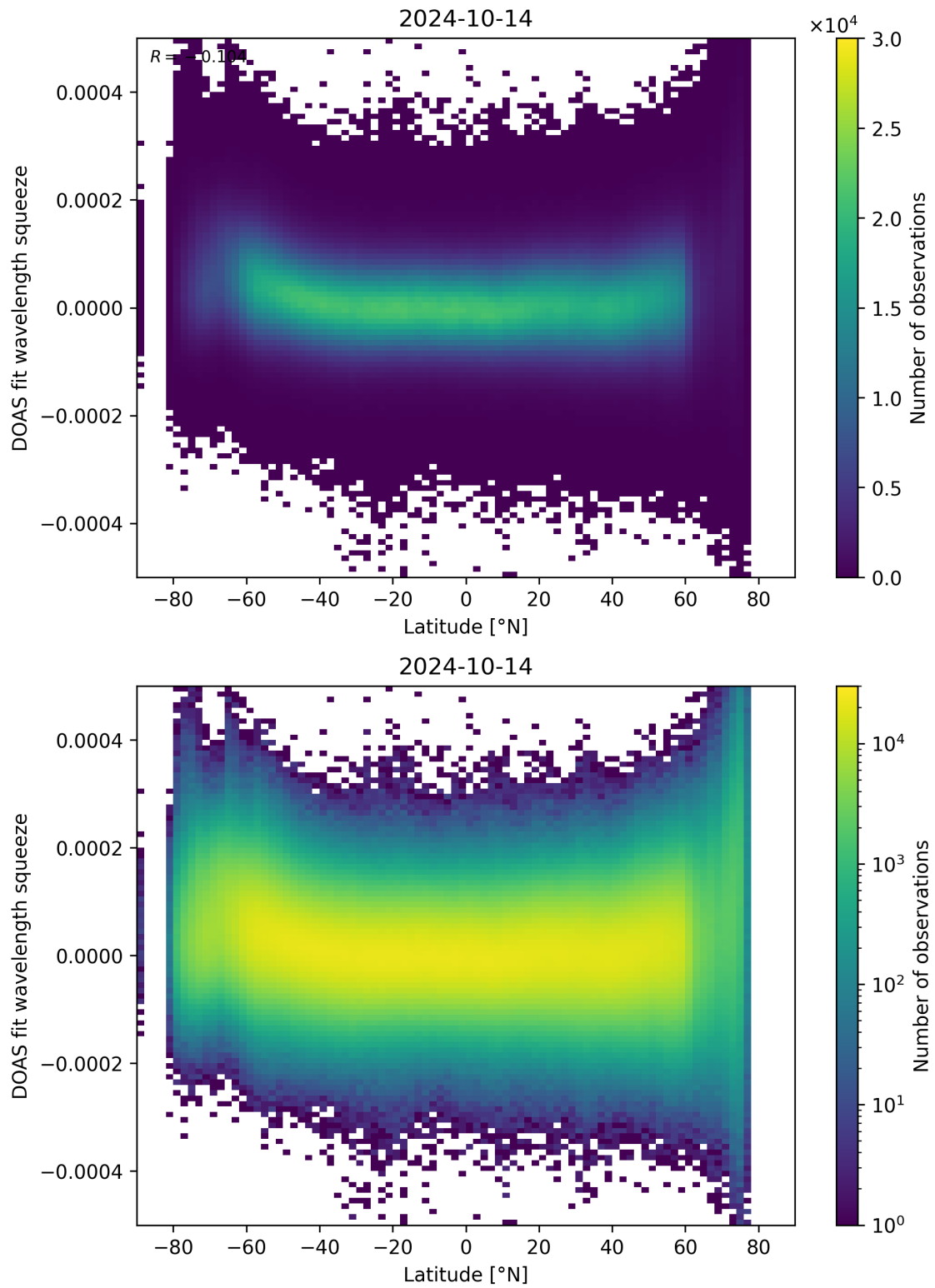
Figure 155: Scatter density plot of “Latitude” against “DOAS fit wavelength squeeze” for 2024-10-14 to 2024-10-15.
