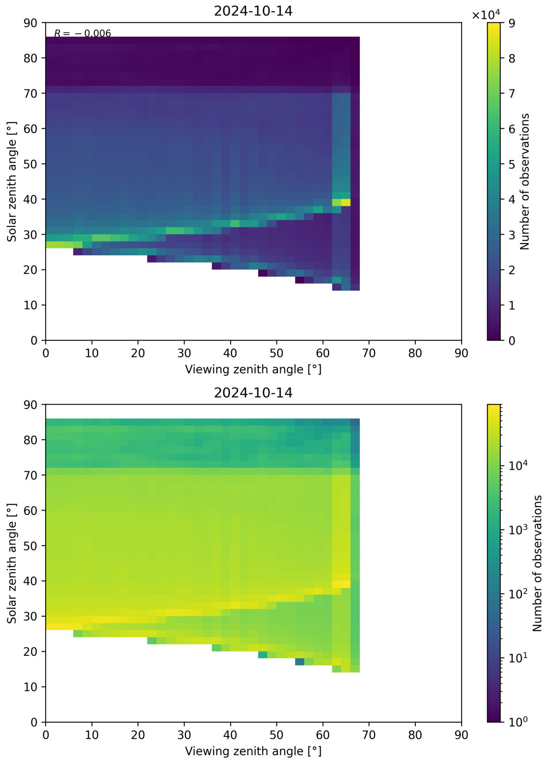
Figure 197: Scatter density plot of “Viewing zenith angle” against “Solar zenith angle” for 2024-10-14 to 2024-10-15.
