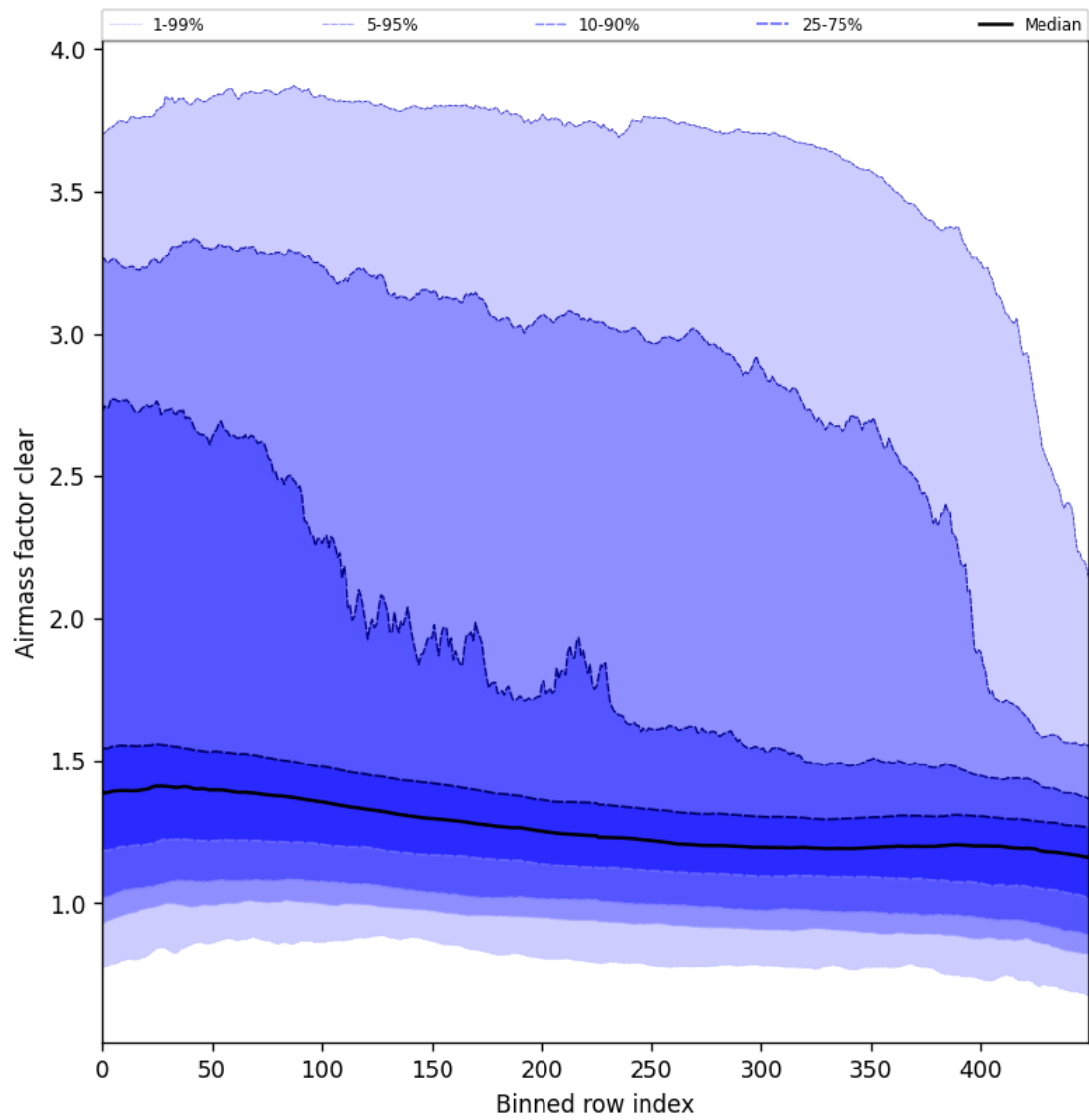
Figure 56: Along track statistics of “Airmass factor clear” for 2024-10-14 to 2024-10-15
