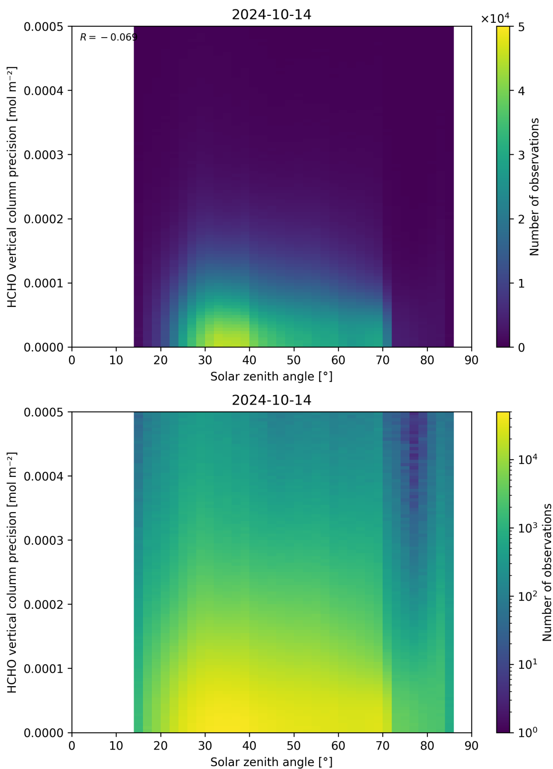
Figure 179: Scatter density plot of “Solar zenith angle” against “HCHO vertical column precision” for 2024-10-14 to 2024-10-15.
