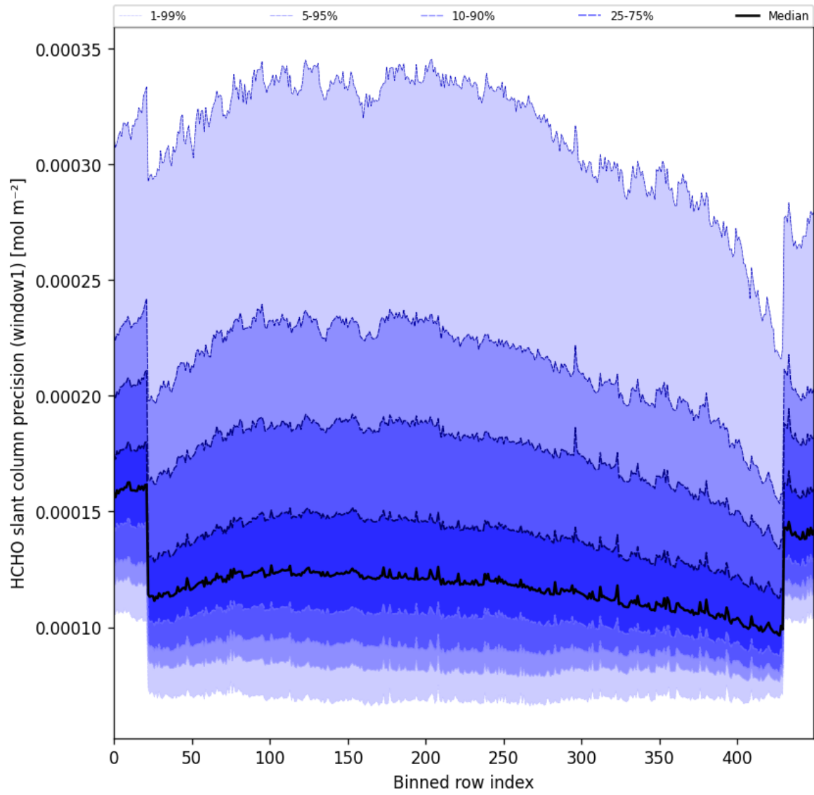
Figure 53: Along track statistics of “HCHO slant column precision (window1)” for 2024-10-14 to 2024-10-15
