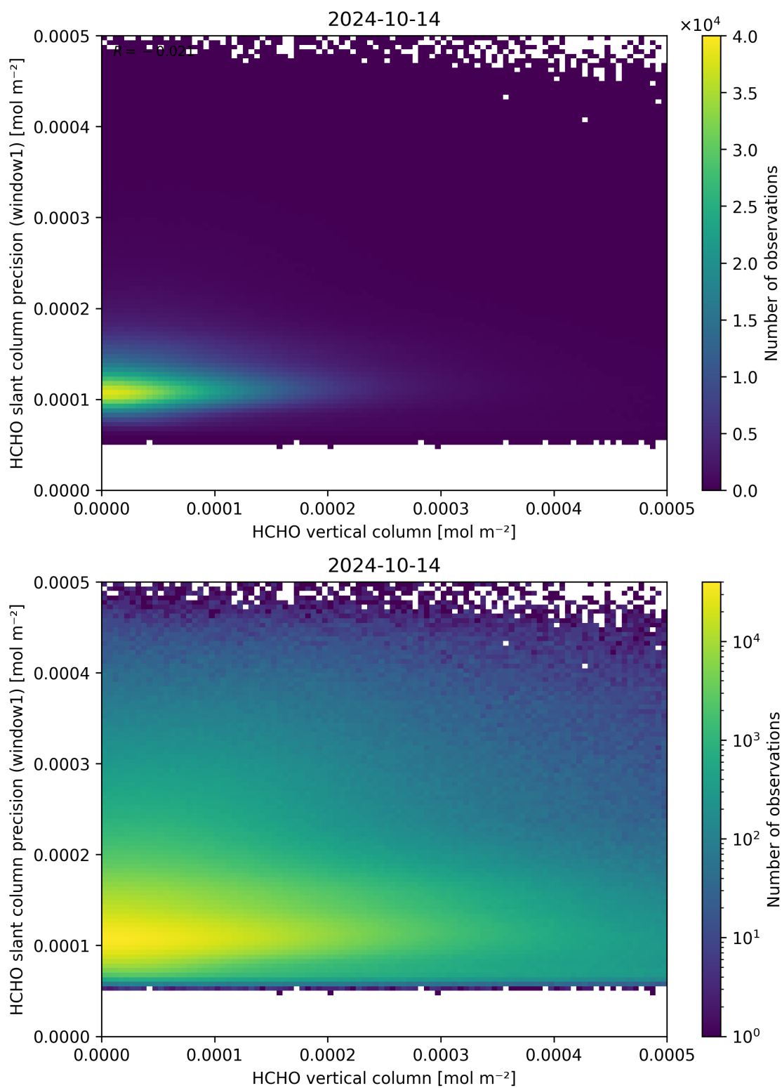
Figure 130: Scatter density plot of “HCHO vertical column” against “HCHO slant column precision (window1)” for 2024-10-14 to 2024-10-15.
