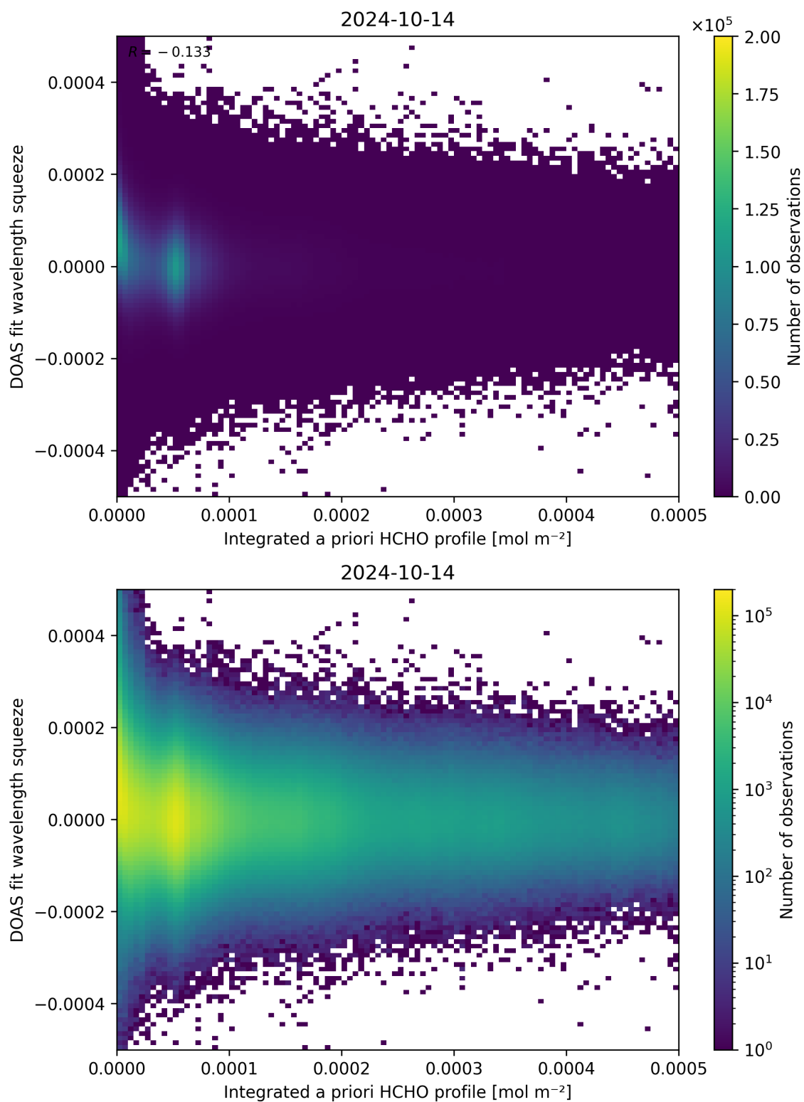
Figure 150: Scatter density plot of “Integrated a priori HCHO profile” against “DOAS fit wavelength squeeze” for 2024-10-14 to 2024-10-15.
