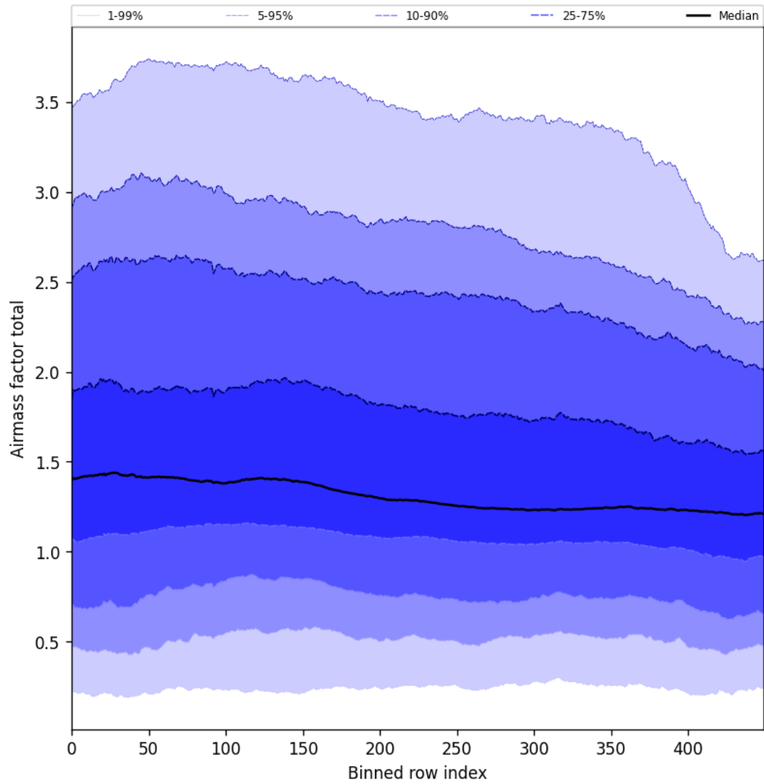
Figure 54: Along track statistics of “Airmass factor total” for 2024-10-14 to 2024-10-15
