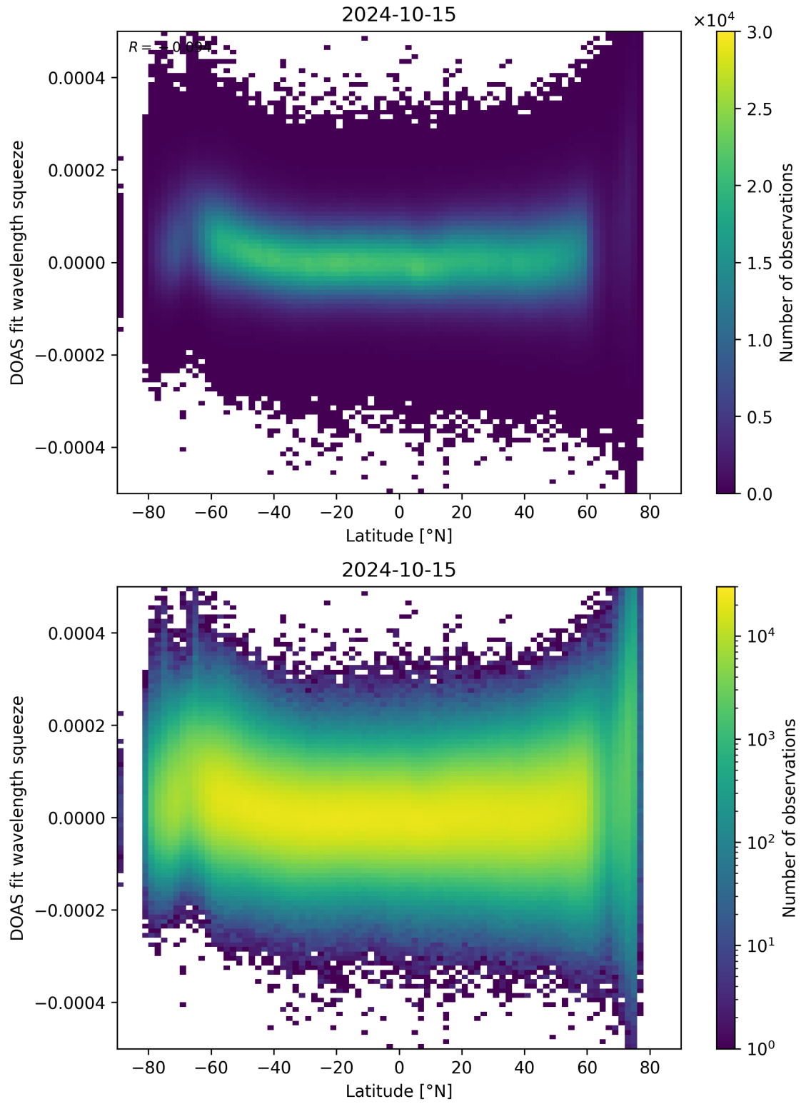
Figure 155: Scatter density plot of “Latitude” against “DOAS fit wavelength squeeze” for 2024-10-14 to 2024-10-16.
