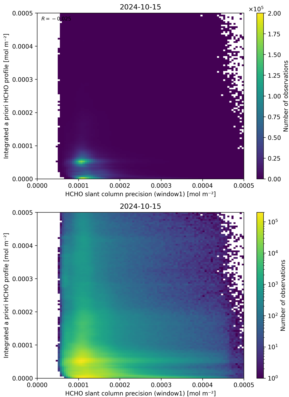
Figure 96: Scatter density plot of “HCHO slant column precision (window1)” against “Integrated a priori HCHO profile” for 2024-10-14 to 2024-10-16.
