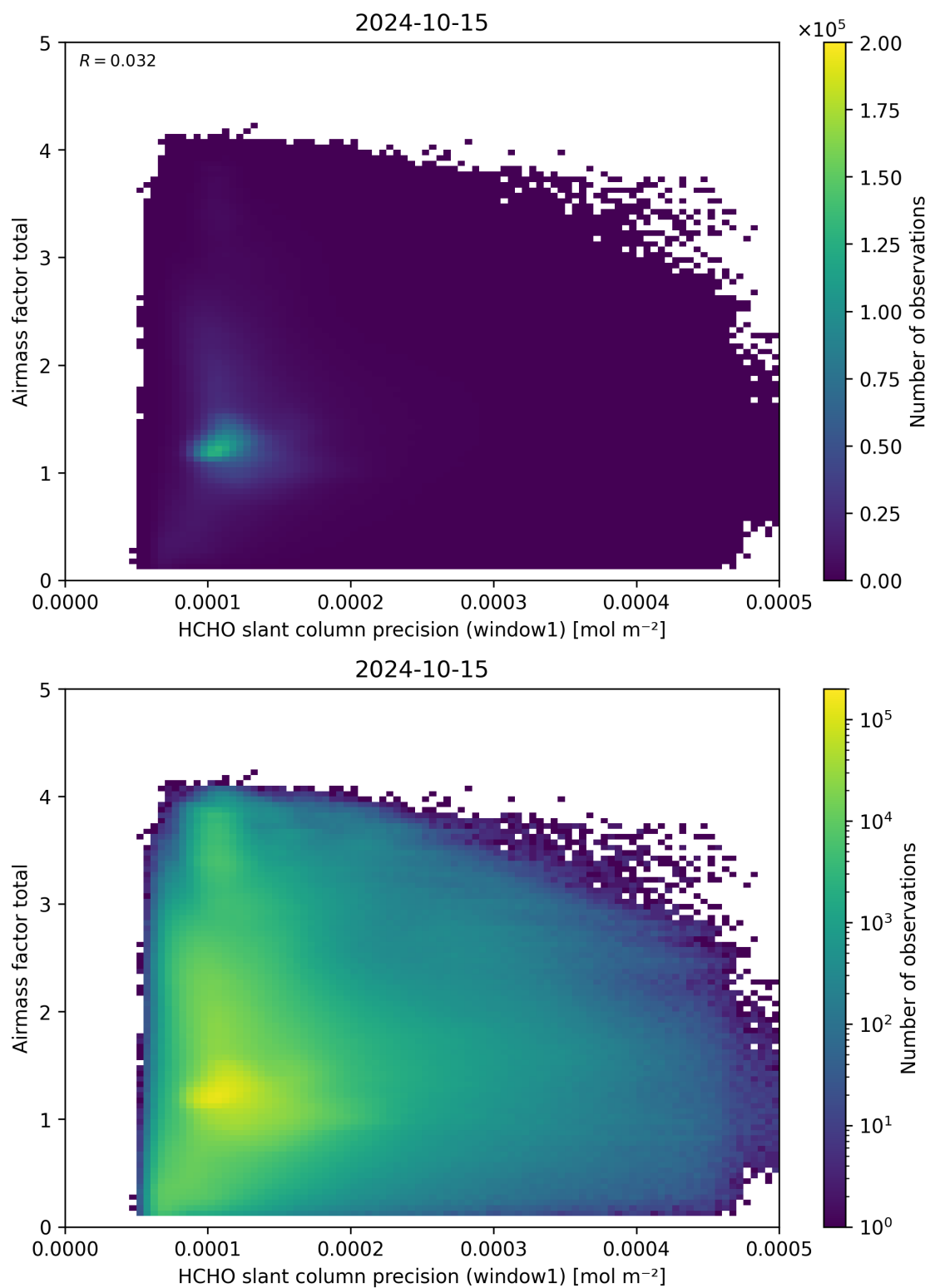
Figure 94: Scatter density plot of “HCHO slant column precision (window1)” against “Airmass factor total” for 2024-10-14 to 2024-10-16.
