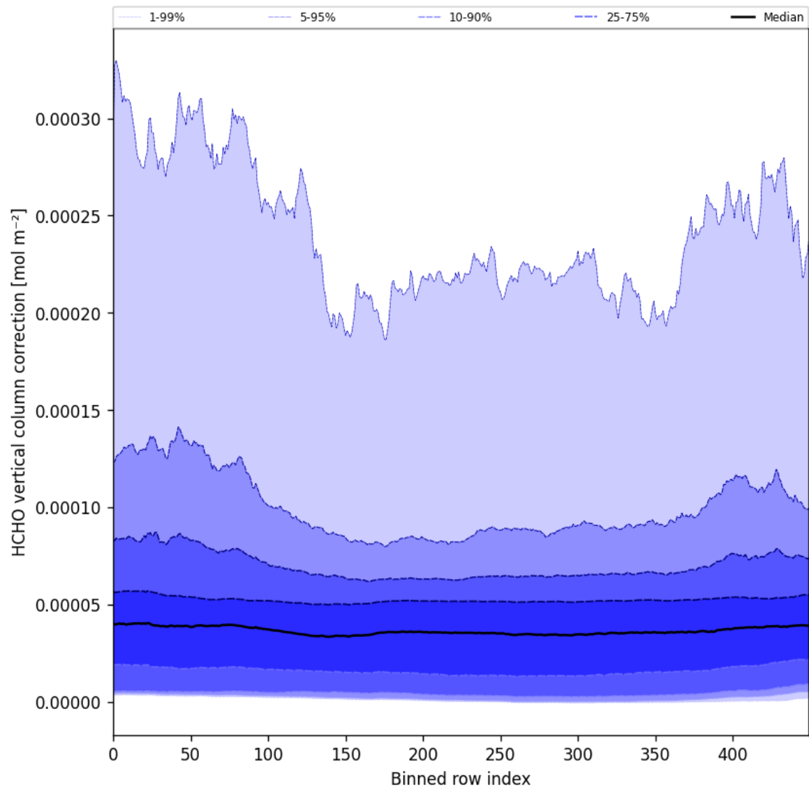
Figure 51: Along track statistics of “HCHO vertical column correction” for 2024-10-14 to 2024-10-16
