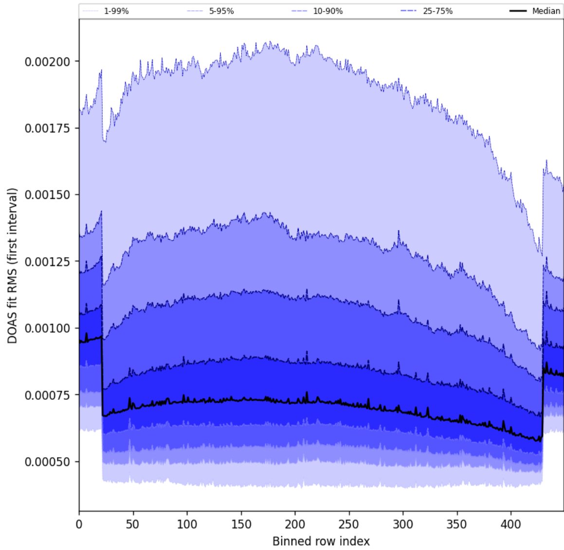
Figure 60: Along track statistics of “DOAS fit RMS (first interval)” for 2024-10-14 to 2024-10-16
