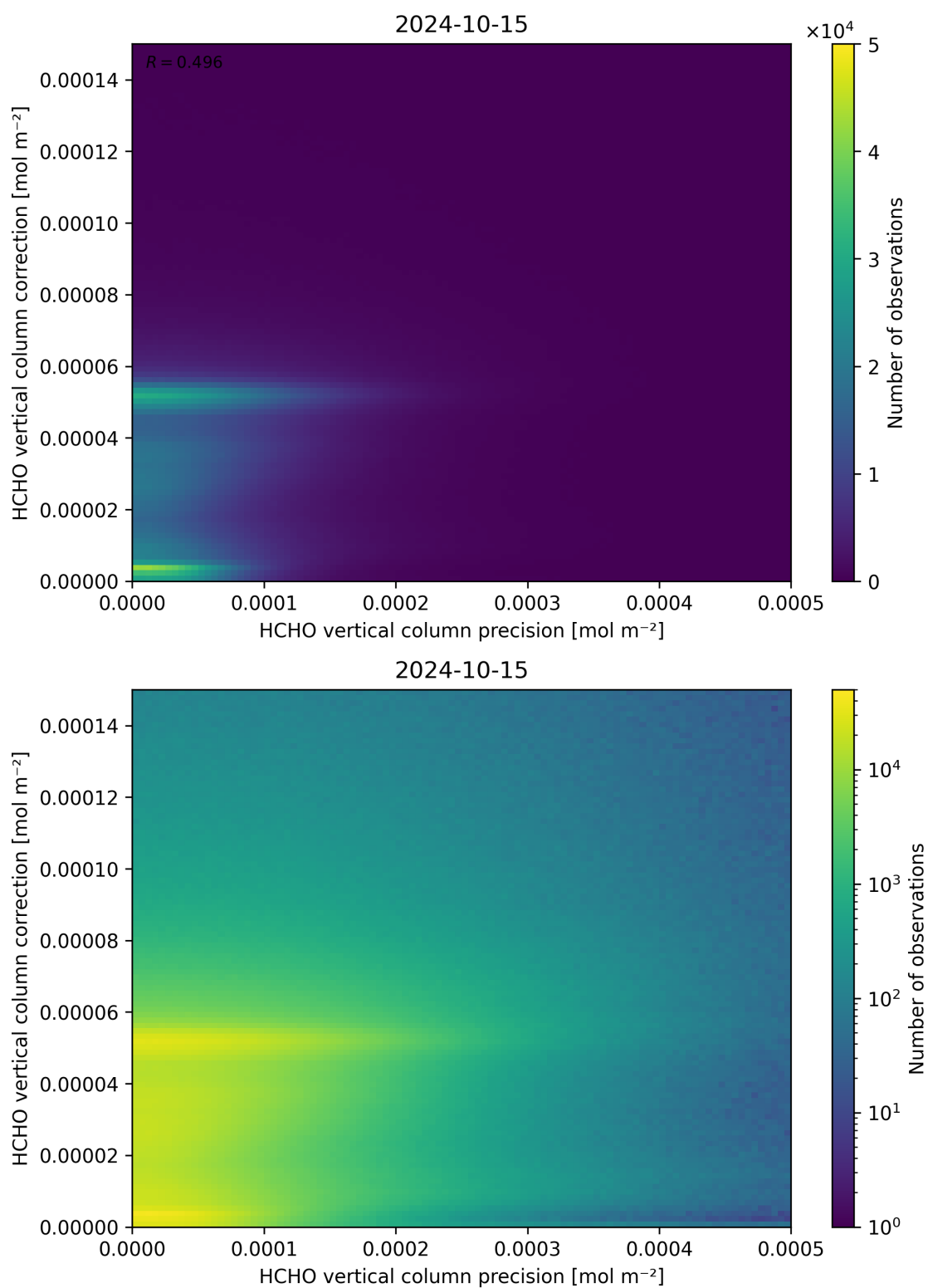
Figure 146: Scatter density plot of “HCHO vertical column precision” against “HCHO vertical column correction” for 2024-10-14 to 2024-10-16.
