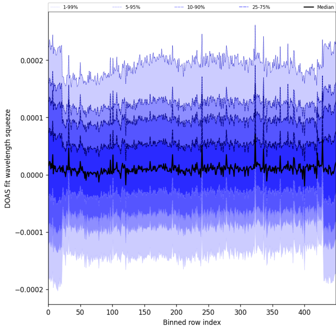
Figure 59: Along track statistics of “DOAS fit wavelength squeeze” for 2024-10-14 to 2024-10-16
