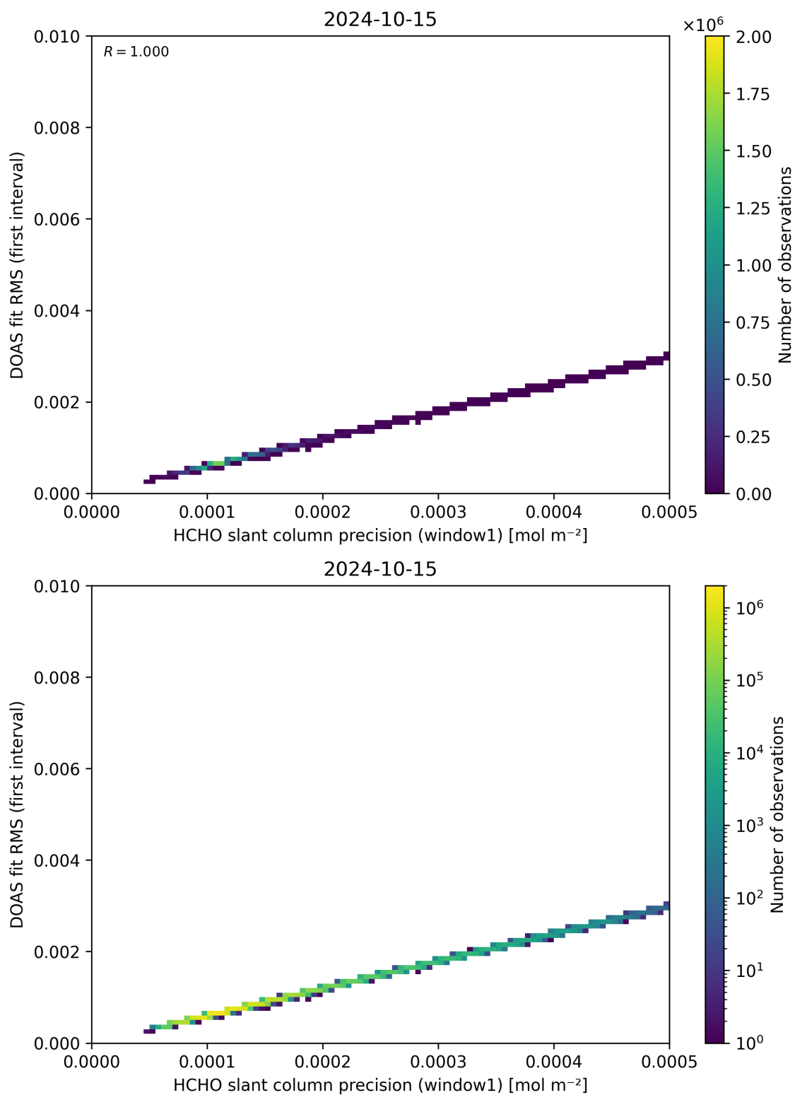
Figure 88: Scatter density plot of “HCHO slant column precision (window1)” against “DOAS fit RMS (first interval)” for 2024-10-14 to 2024-10-16.
