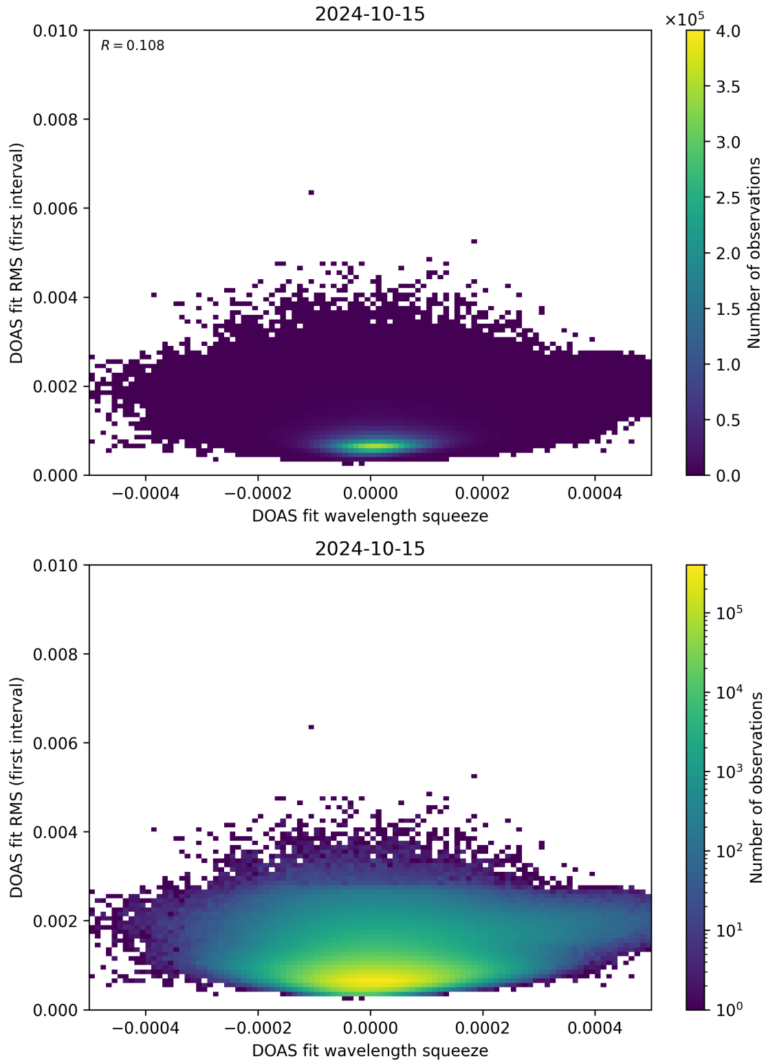
Figure 68: Scatter density plot of “DOAS fit wavelength squeeze” against “DOAS fit RMS (first interval)” for 2024-10-14 to 2024-10-16.
