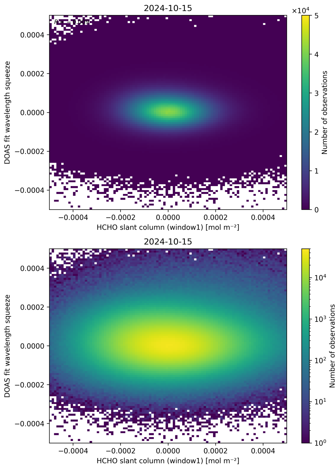
Figure 80: Scatter density plot of “HCHO slant column (window1)” against “DOAS fit wavelength squeeze” for 2024-10-14 to 2024-10-16.
