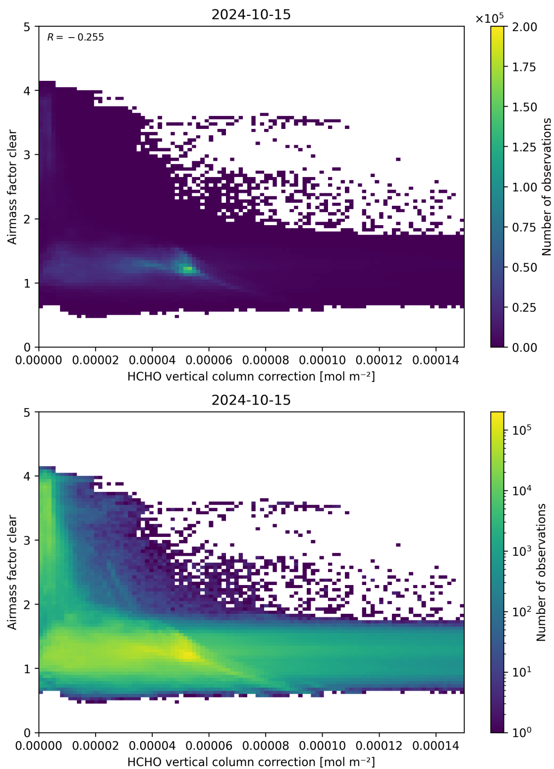
Figure 115: Scatter density plot of “HCHO vertical column correction” against “Airmass factor clear” for 2024-10-14 to 2024-10-16.
