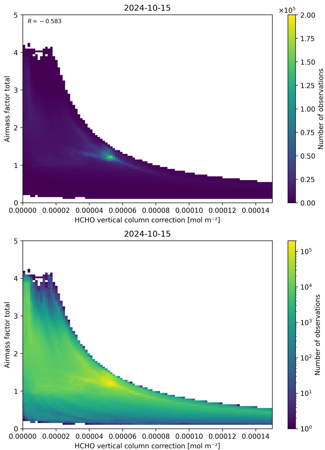
Figure 120: Scatter density plot of “HCHO vertical column correction” against “Airmass factor total” for 2024-10-14 to 2024-10-16.
