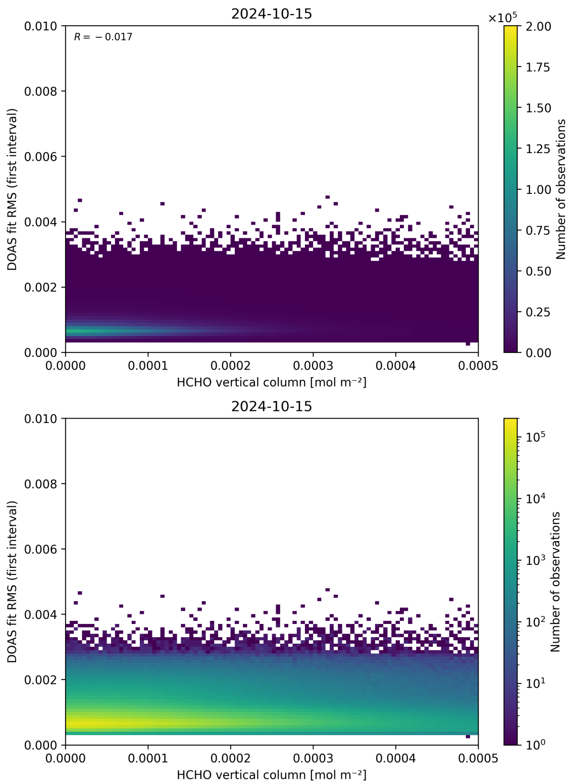
Figure 123: Scatter density plot of “HCHO vertical column” against “DOAS fit RMS (first interval)” for 2024-10-14 to 2024-10-16.
