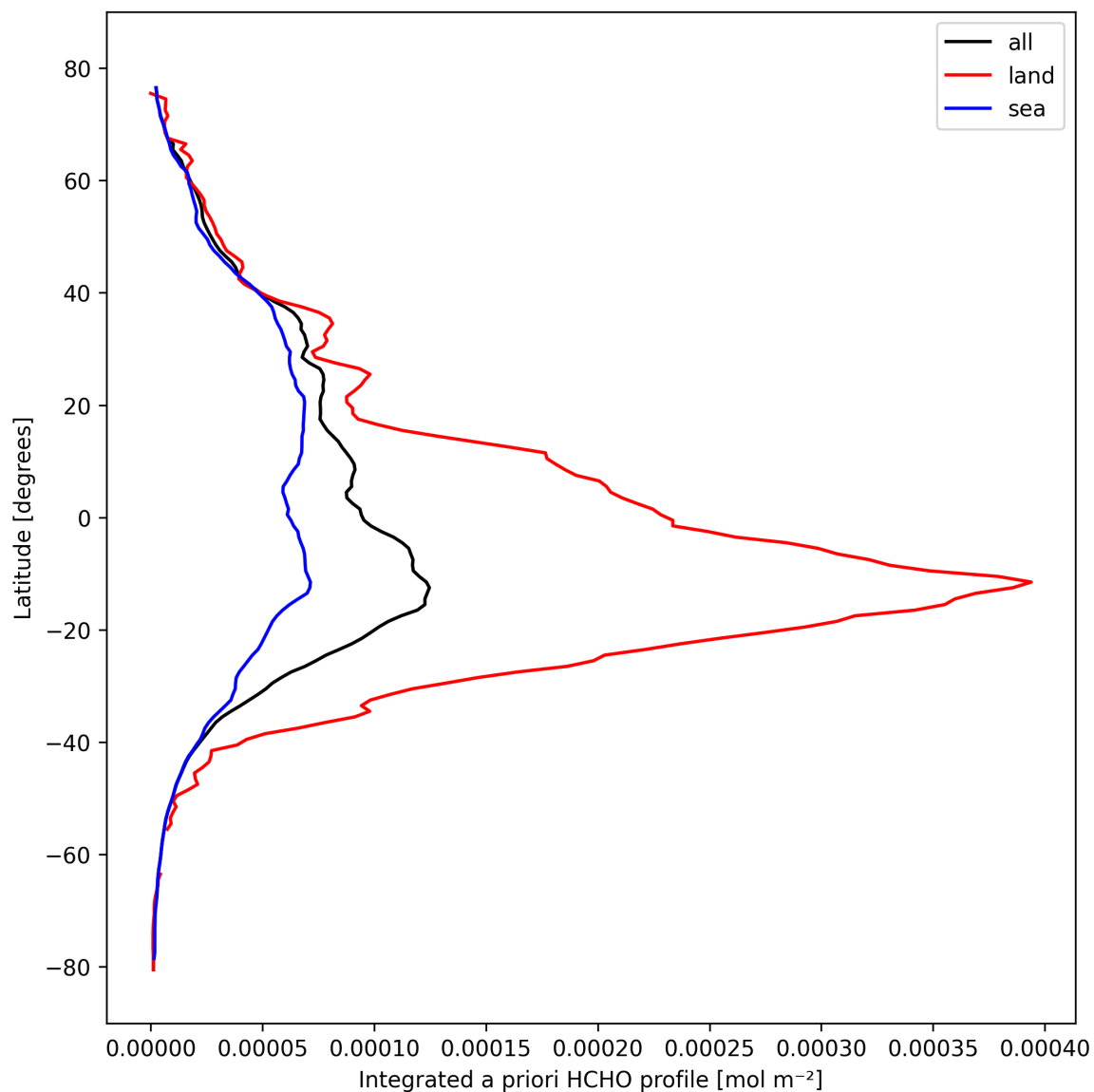
Figure 29: Zonal average of “Integrated a priori HCHO profile” for 2024-10-14 to 2024-10-16.
