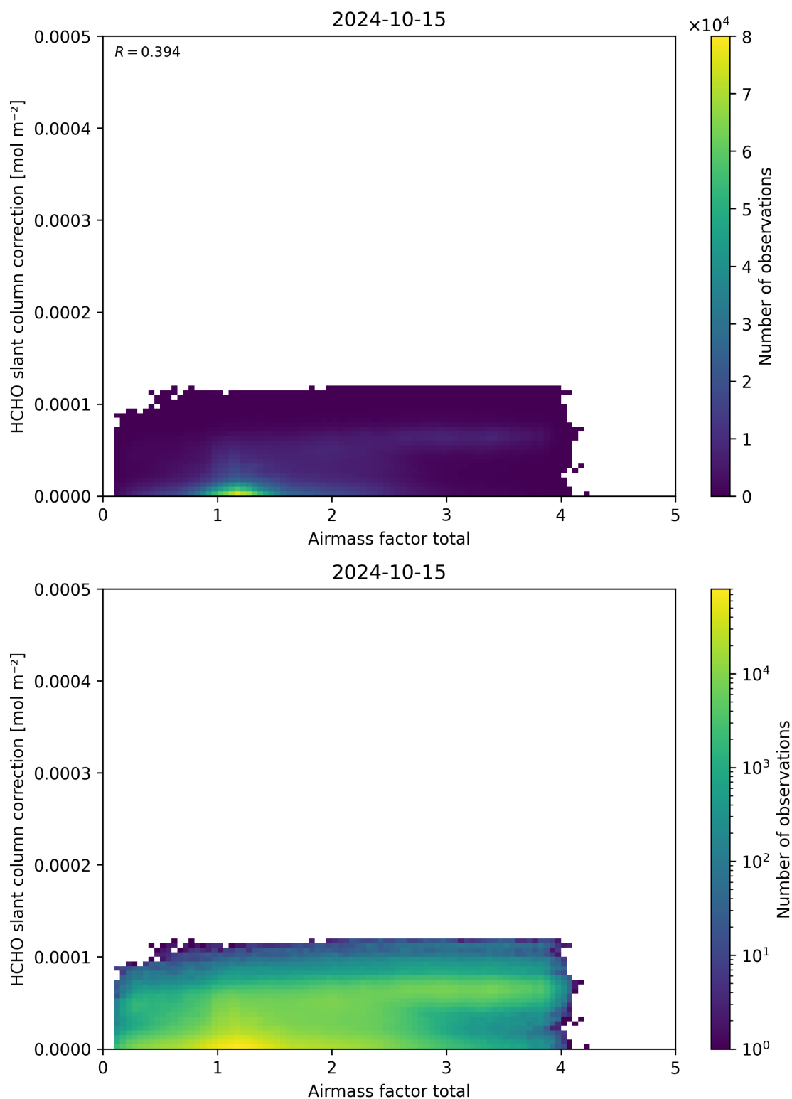
Figure 102: Scatter density plot of “Airmass factor total” against “HCHO slant column correction” for 2024-10-14 to 2024-10-16.
