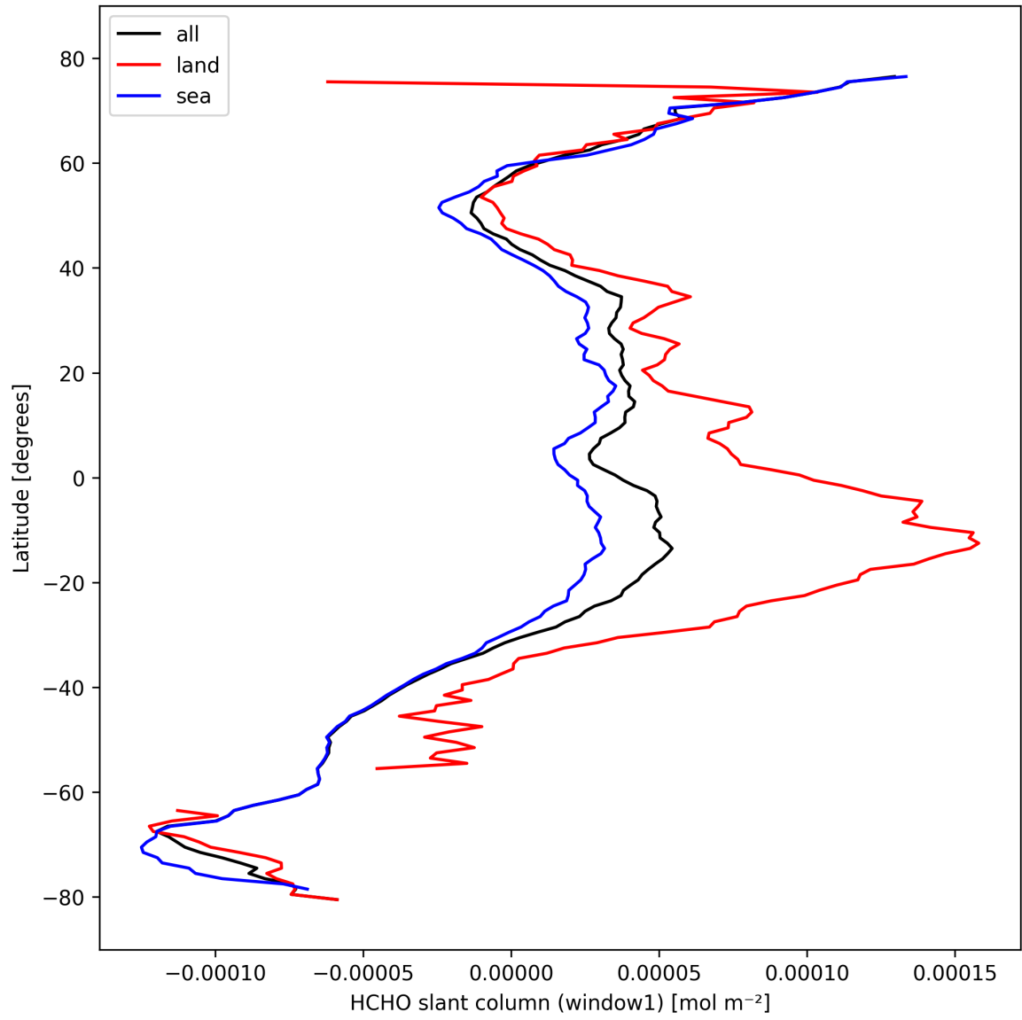
Figure 24: Zonal average of “HCHO slant column (window1)” for 2024-10-14 to 2024-10-16.
