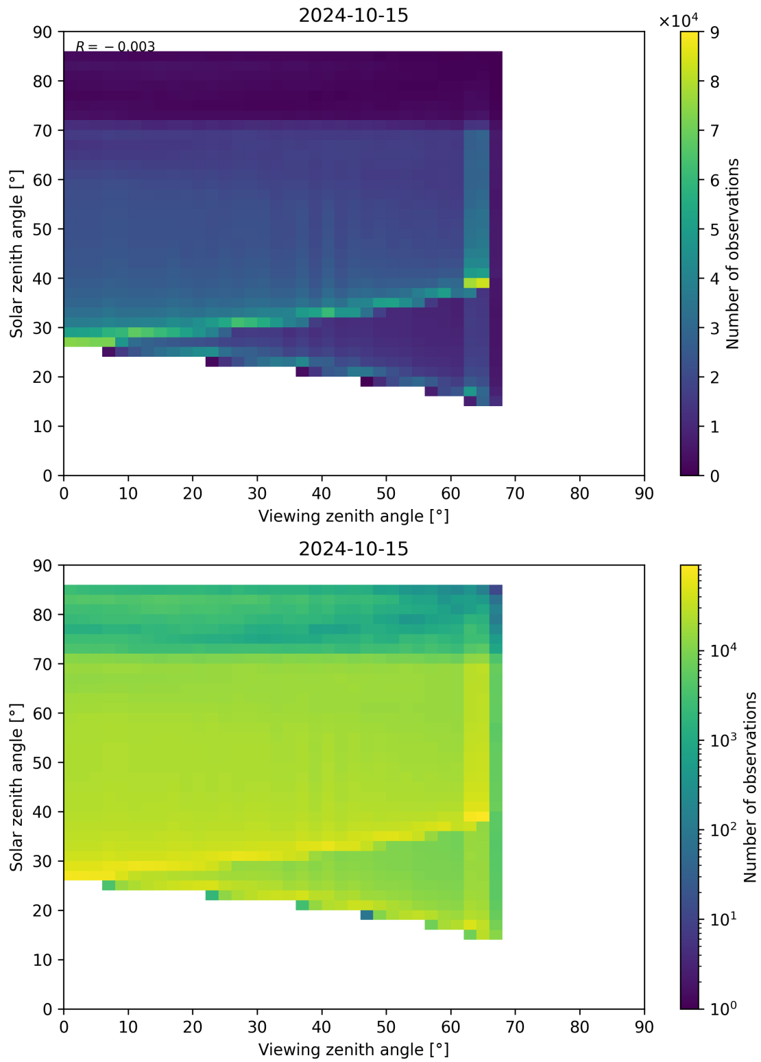
Figure 197: Scatter density plot of “Viewing zenith angle” against “Solar zenith angle” for 2024-10-14 to 2024-10-16.
