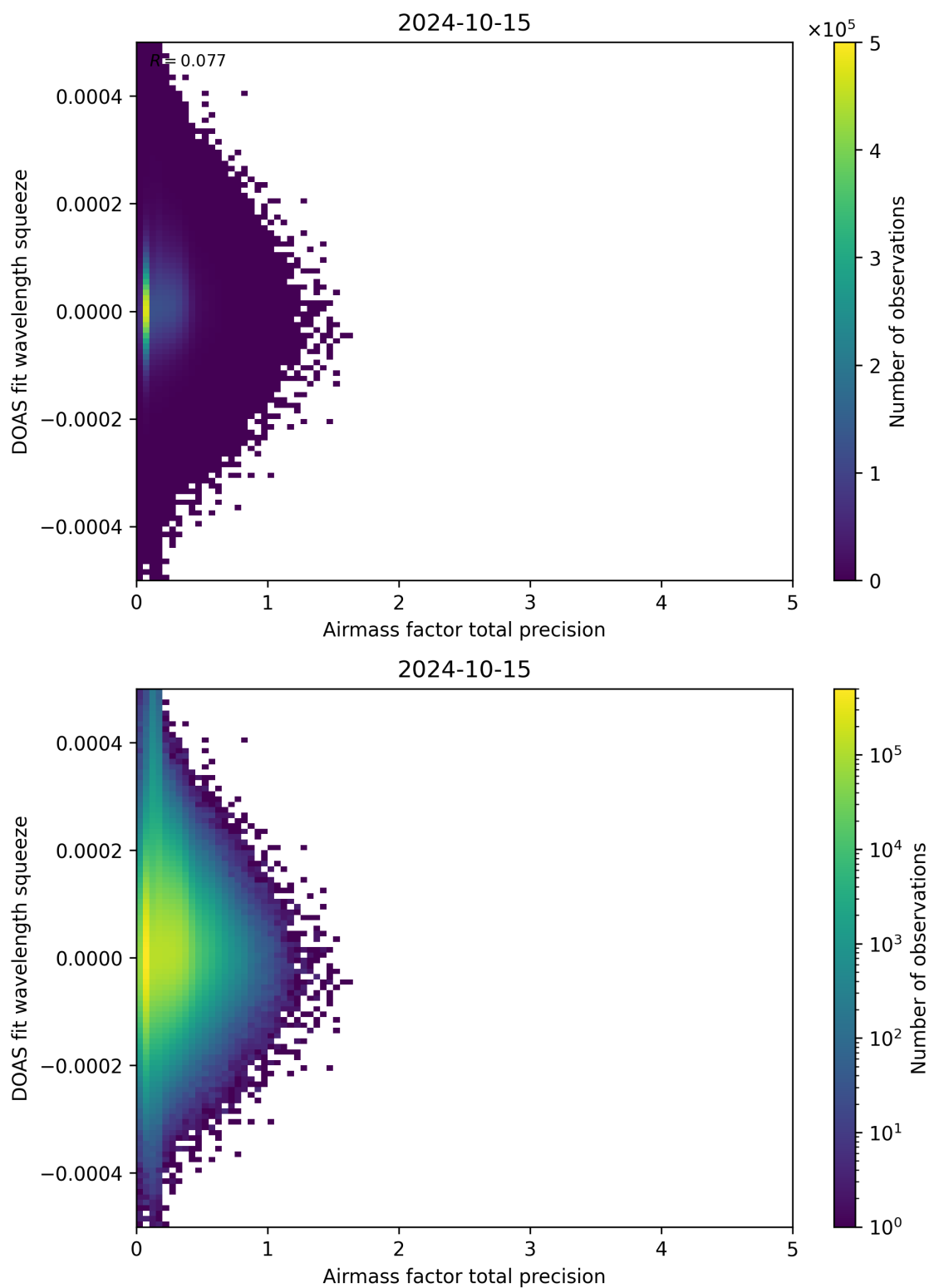
Figure 107: Scatter density plot of “Airmass factor total precision” against “DOAS fit wavelength squeeze” for 2024-10-14 to 2024-10-16.
