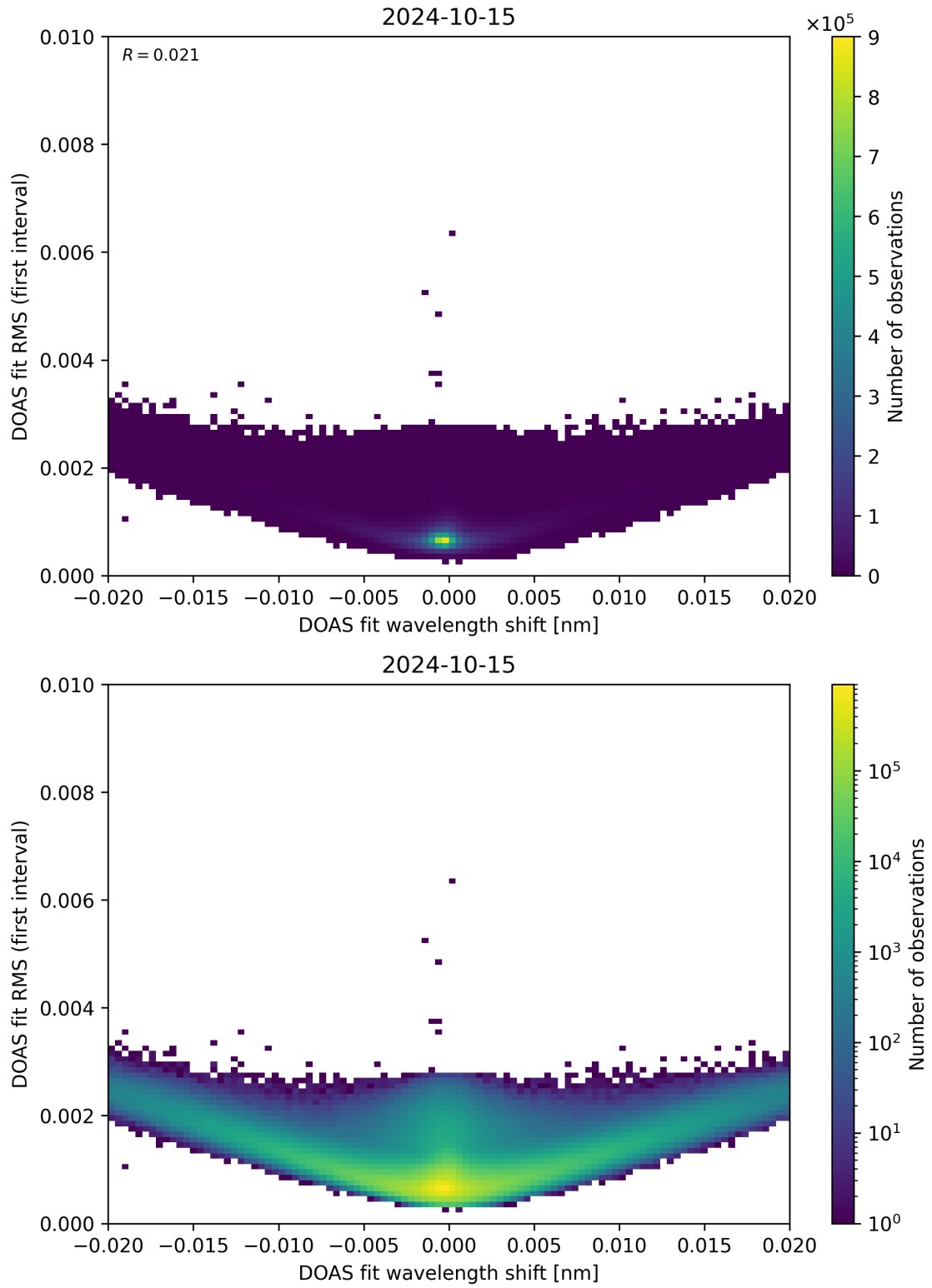
Figure 64: Scatter density plot of “DOAS fit wavelength shift” against “DOAS fit RMS (first interval)” for 2024-10-14 to 2024-10-16.
