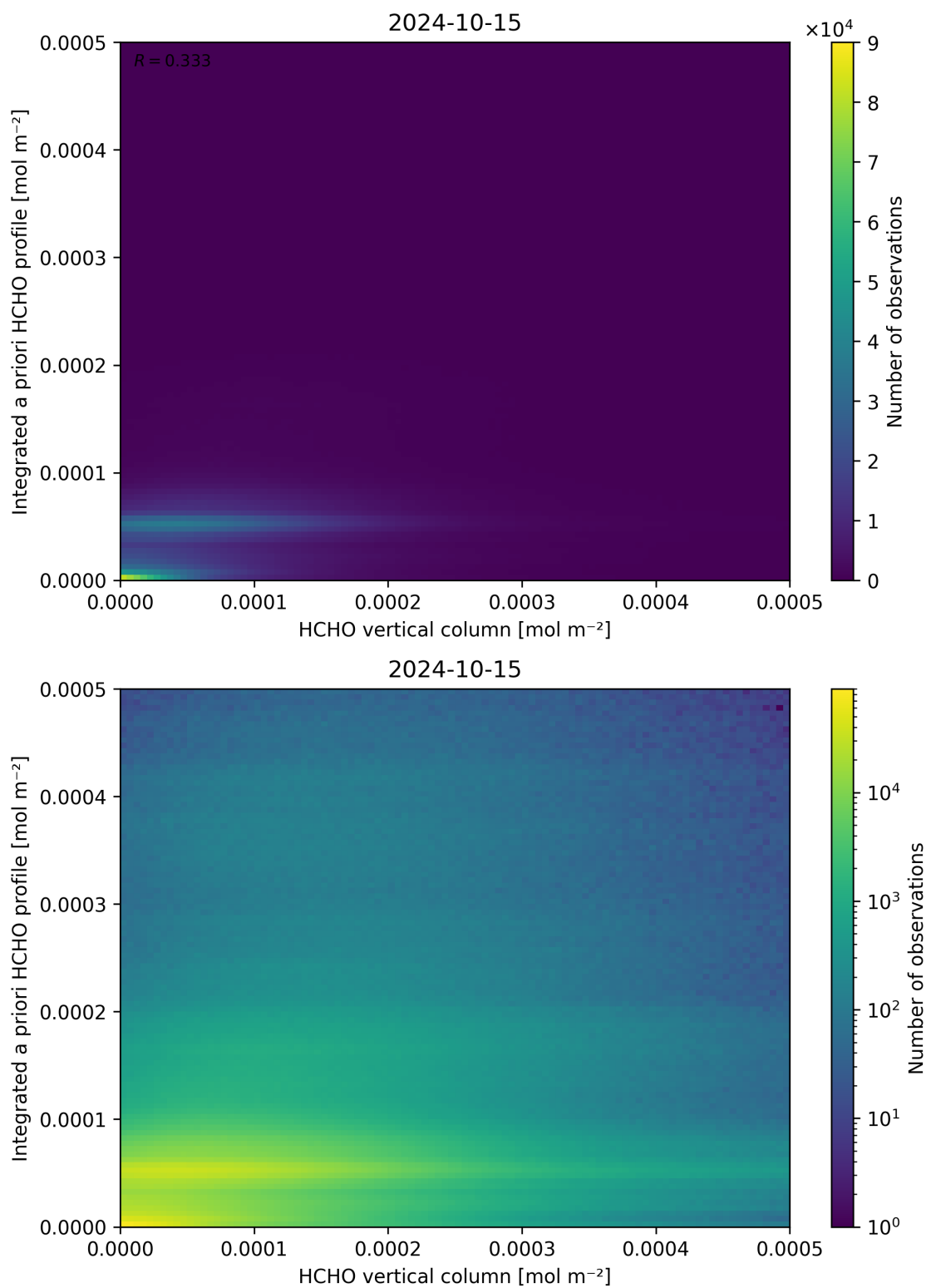
Figure 135: Scatter density plot of “HCHO vertical column” against “Integrated a priori HCHO profile” for 2024-10-14 to 2024-10-16.
