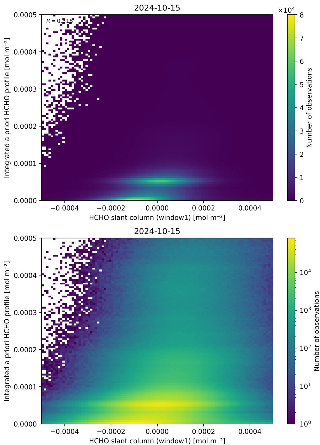
Figure 87: Scatter density plot of “HCHO slant column (window1)” against “Integrated a priori HCHO profile” for 2024-10-14 to 2024-10-16.
