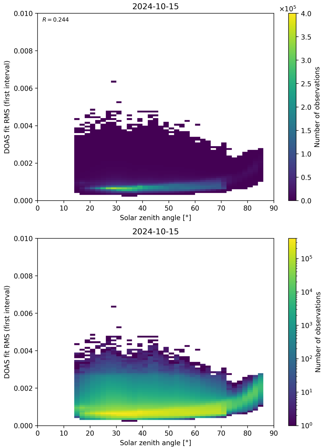
Figure 167: Scatter density plot of “Solar zenith angle” against “DOAS fit RMS (first interval)” for 2024-10-14 to 2024-10-16.
