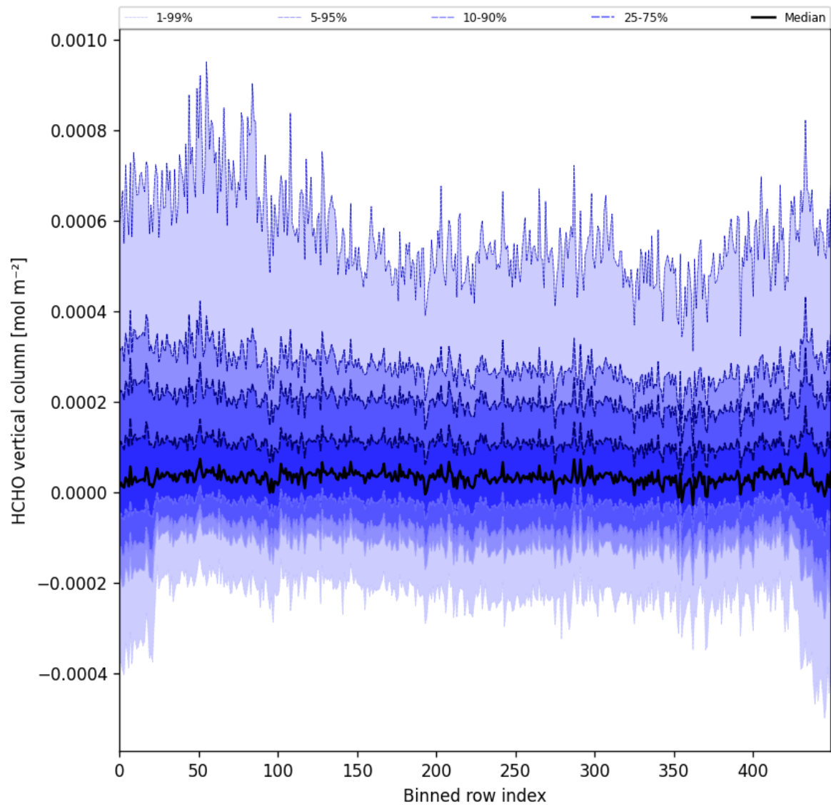
Figure 49: Along track statistics of “HCHO vertical column” for 2024-10-14 to 2024-10-16
