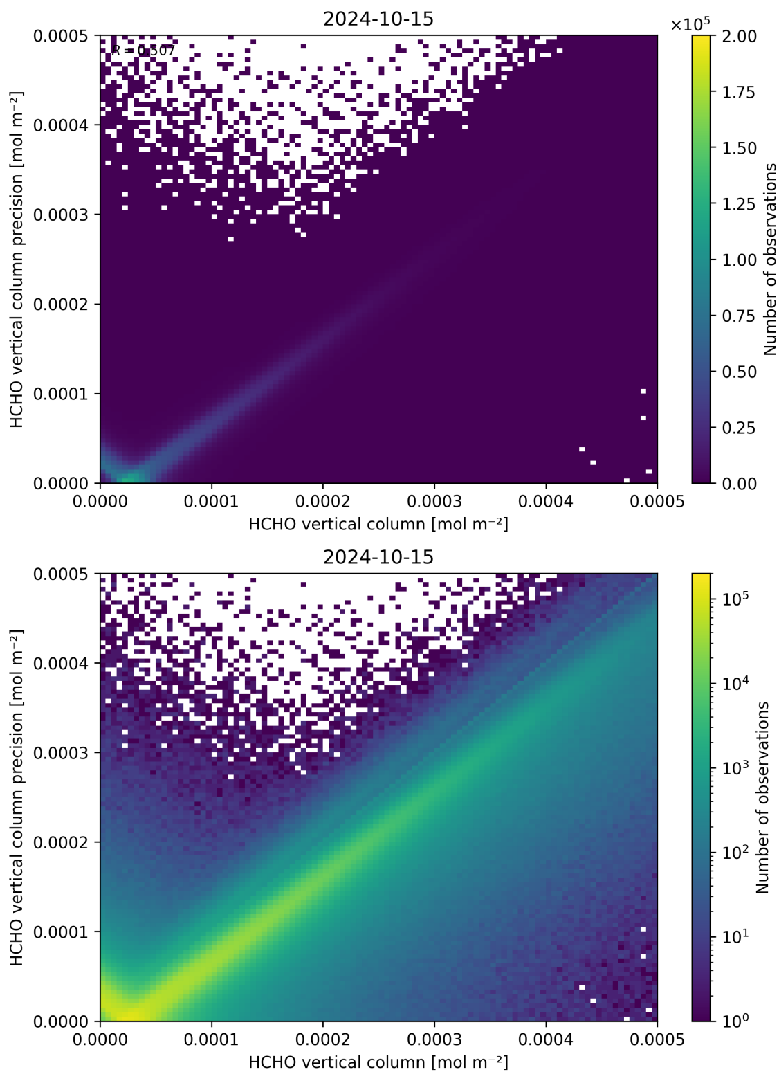
Figure 134: Scatter density plot of “HCHO vertical column” against “HCHO vertical column precision” for 2024-10-14 to 2024-10-16.
