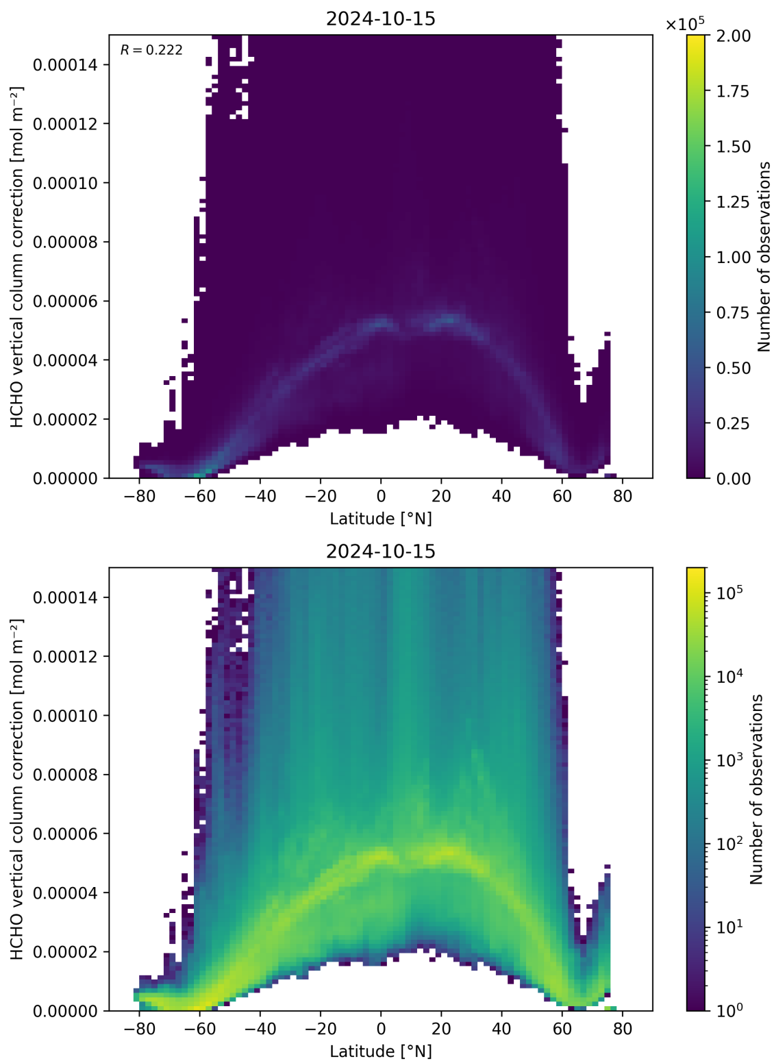
Figure 164: Scatter density plot of “Latitude” against “HCHO vertical column correction” for 2024-10-14 to 2024-10-16.
