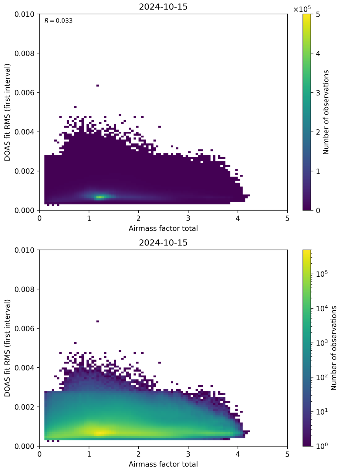
Figure 97: Scatter density plot of “Airmass factor total” against “DOAS fit RMS (first interval)” for 2024-10-14 to 2024-10-16.
