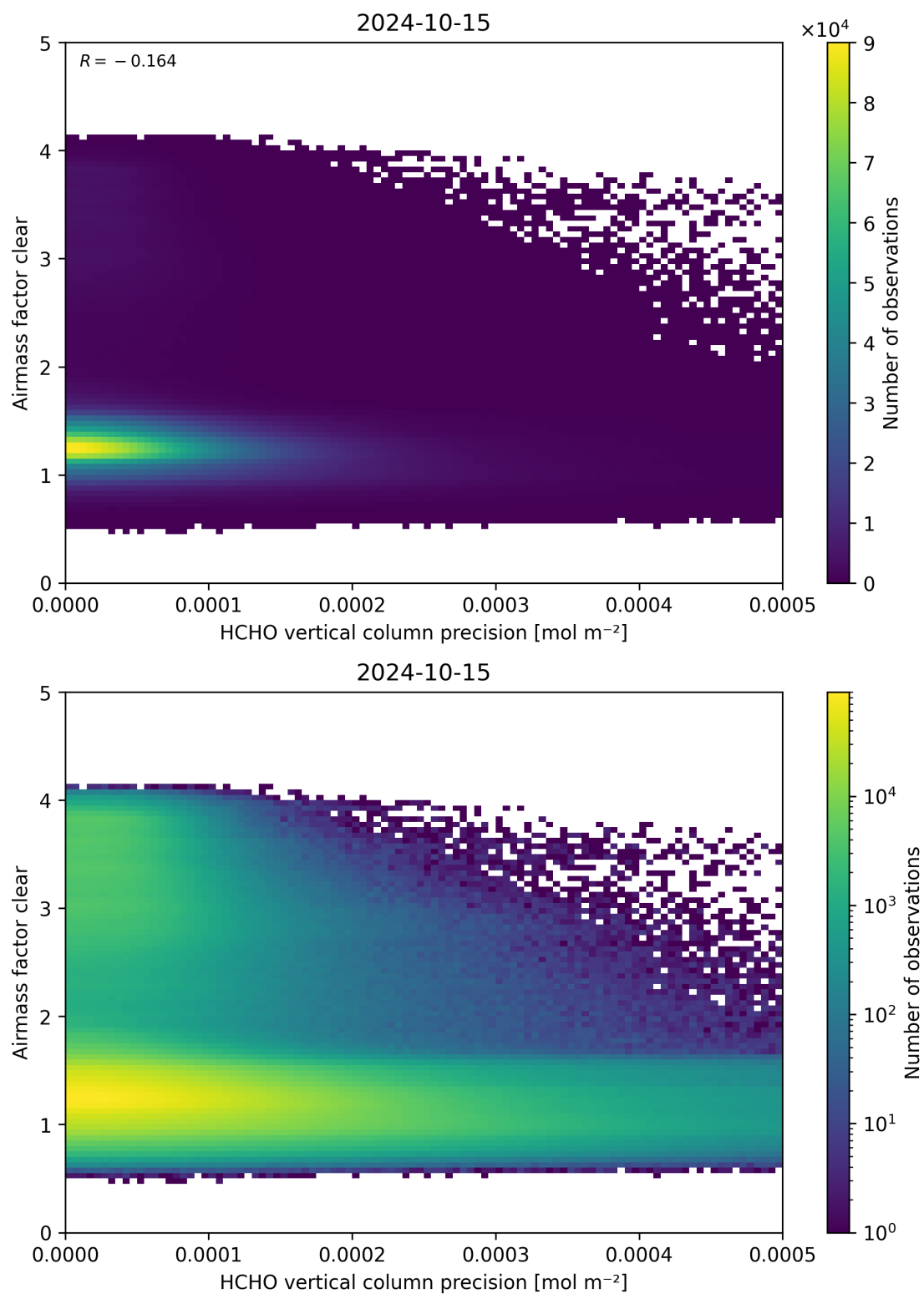
Figure 139: Scatter density plot of “HCHO vertical column precision” against “Airmass factor clear” for 2024-10-14 to 2024-10-16.
