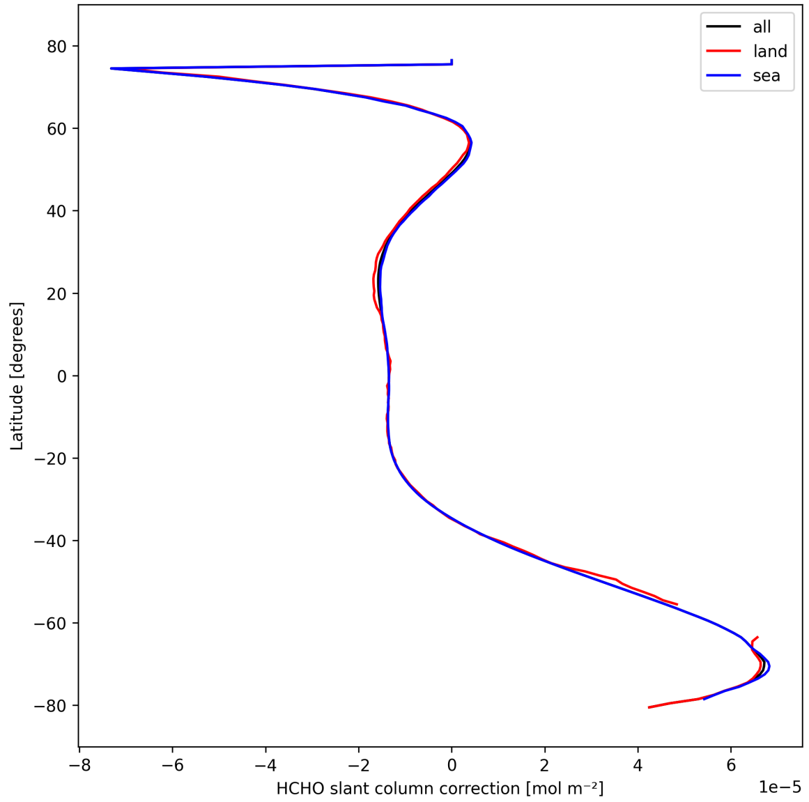
Figure 33: Zonal average of "HCHO slant column correction" for 2024-10-14 to 2024-10-16.
