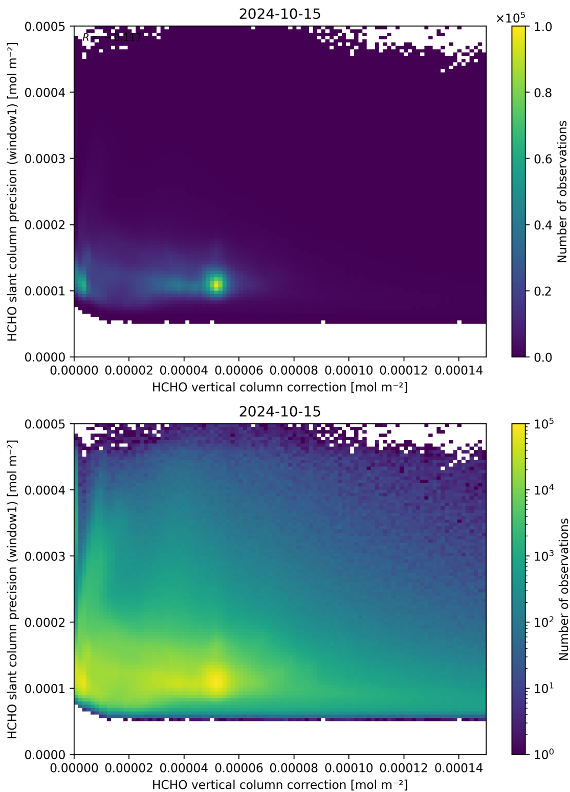
Figure 119: Scatter density plot of “HCHO vertical column correction” against “HCHO slant column precision (window1)” for 2024-10-14 to 2024-10-16.
