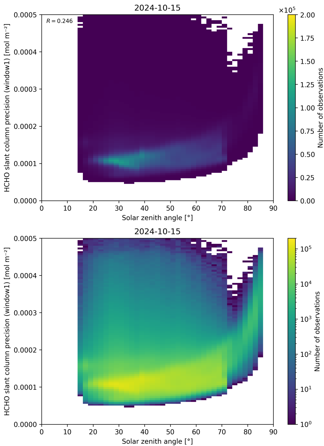
Figure 174: Scatter density plot of “Solar zenith angle” against “HCHO slant column precision (window1)” for 2024-10-14 to 2024-10-16.
