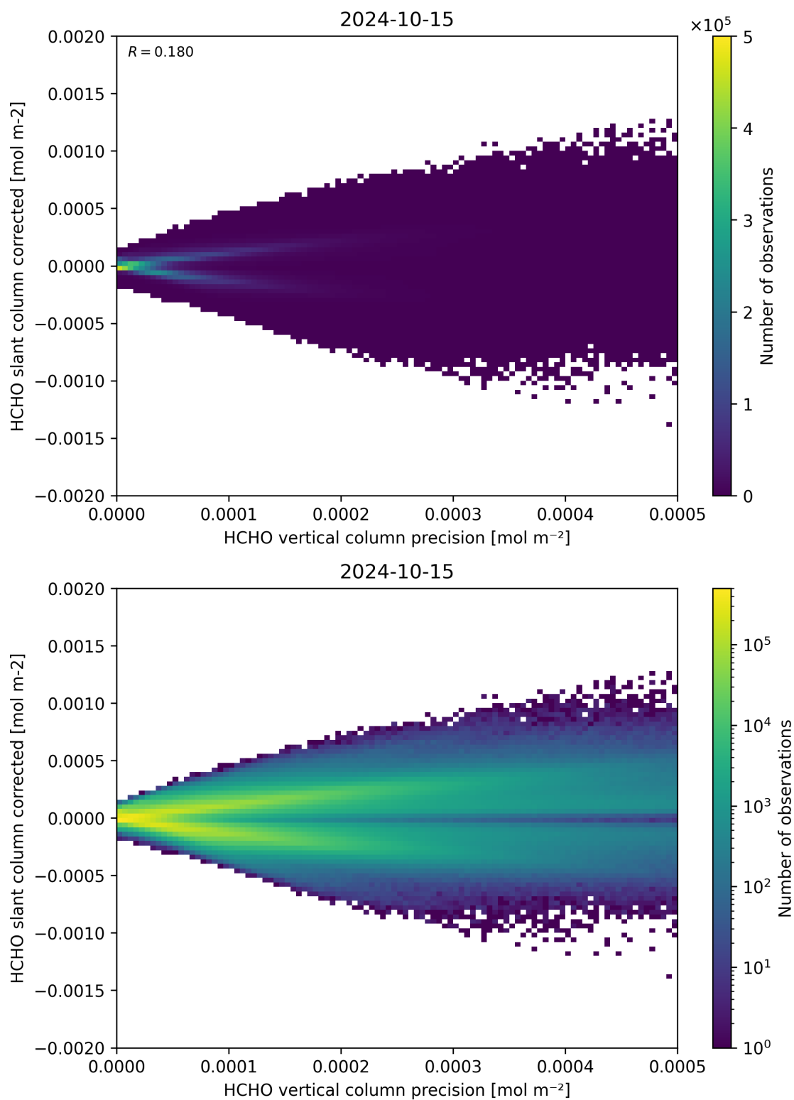
Figure 140: Scatter density plot of “HCHO vertical column precision” against “HCHO slant column corrected” for 2024-10-14 to 2024-10-16.
