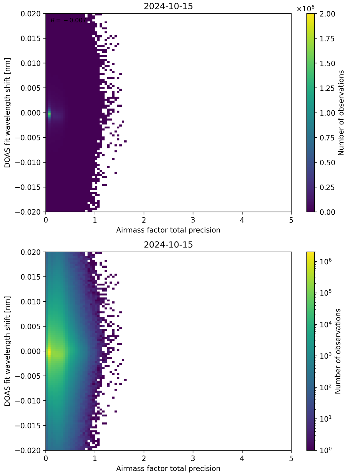
Figure 106: Scatter density plot of “Airmass factor total precision” against “DOAS fit wavelength shift” for 2024-10-14 to 2024-10-16.
