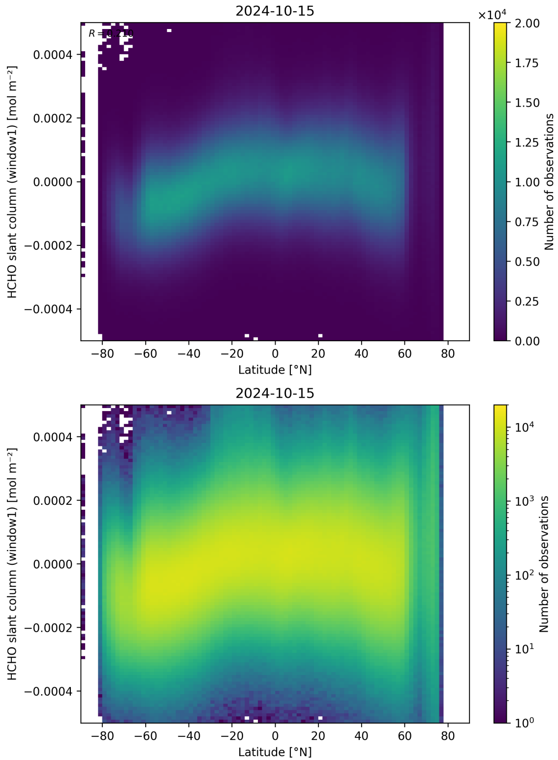
Figure 159: Scatter density plot of “Latitude” against “HCHO slant column (window1)” for 2024-10-14 to 2024-10-16.
