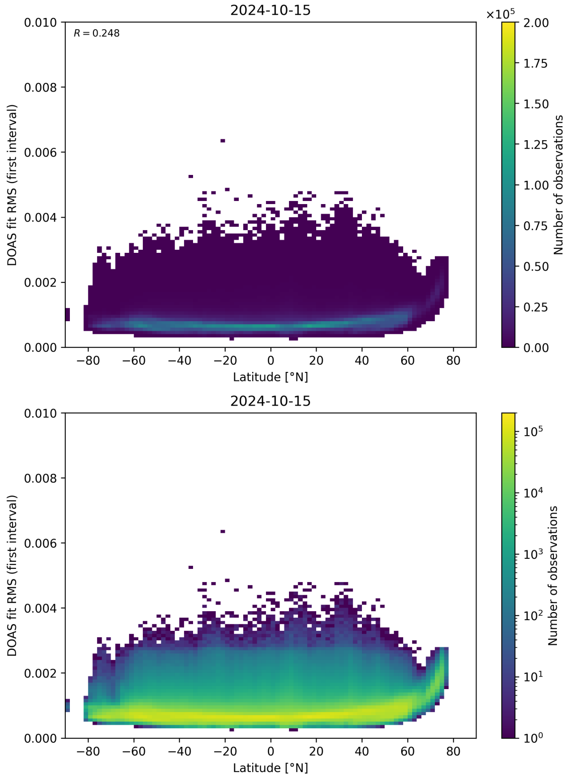
Figure 153: Scatter density plot of “Latitude” against “DOAS fit RMS (first interval)” for 2024-10-14 to 2024-10-16.
