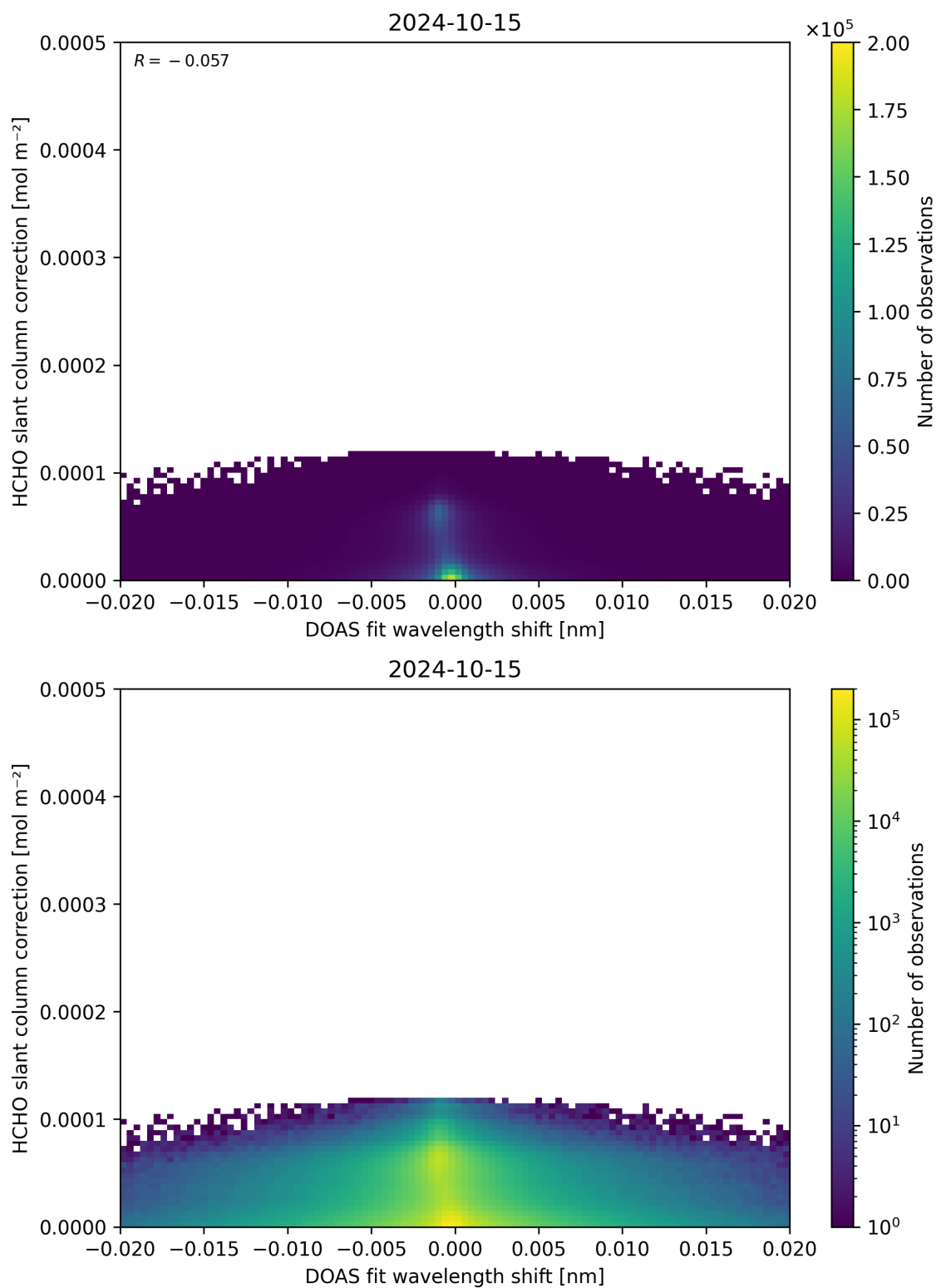
Figure 67: Scatter density plot of “DOAS fit wavelength shift” against “HCHO slant column correction” for 2024-10-14 to 2024-10-16.
