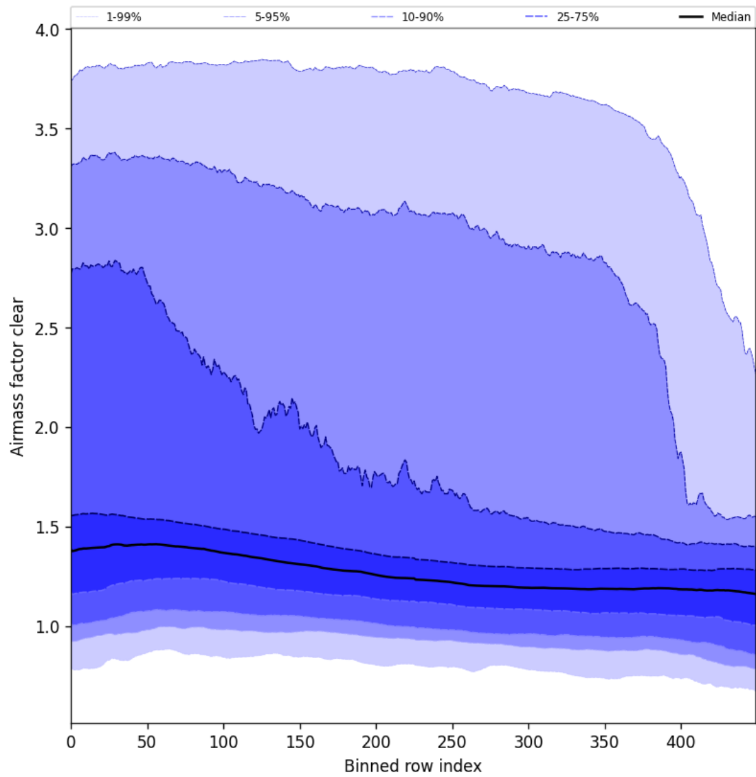
Figure 56: Along track statistics of “Airmass factor clear” for 2024-10-14 to 2024-10-16
