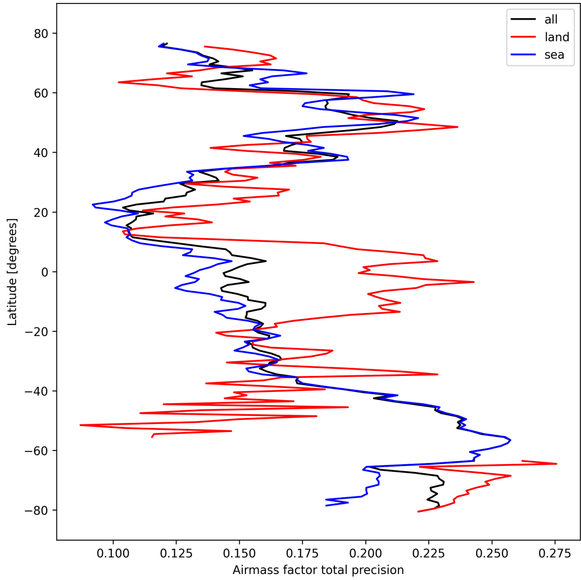
Figure 27: Zonal average of “Airmass factor total precision” for 2024-10-14 to 2024-10-16.
