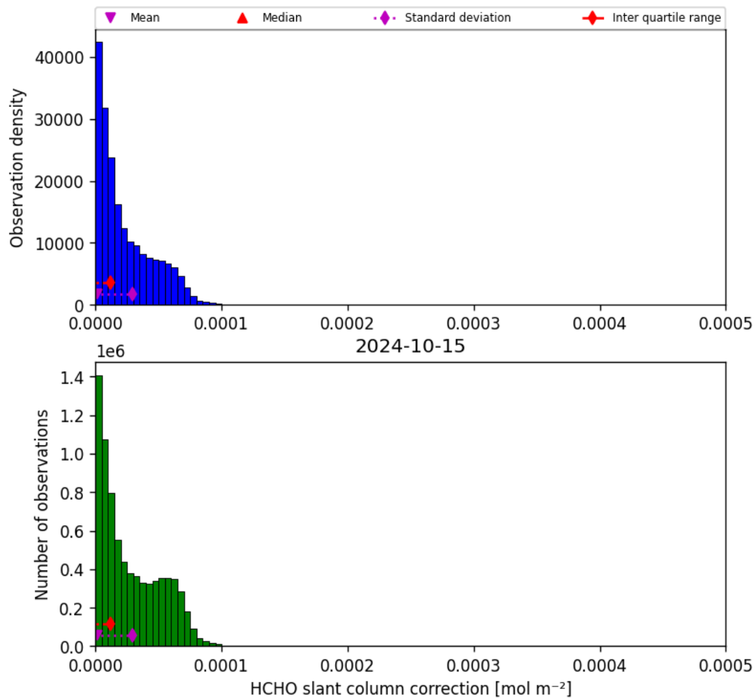
Figure 47: Histogram of “HCHO slant column correction” for 2024-10-14 to 2024-10-16
