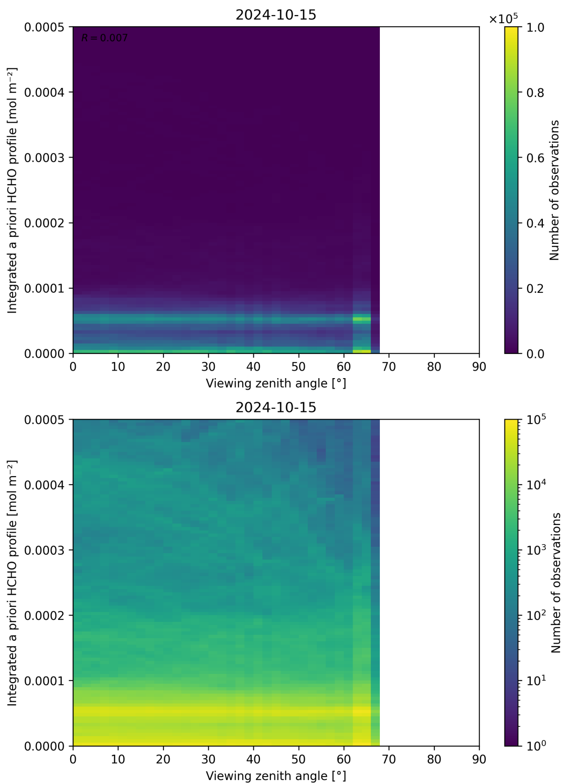
Figure 195: Scatter density plot of “Viewing zenith angle” against “Integrated a priori HCHO profile” for 2024-10-14 to 2024-10-16.
