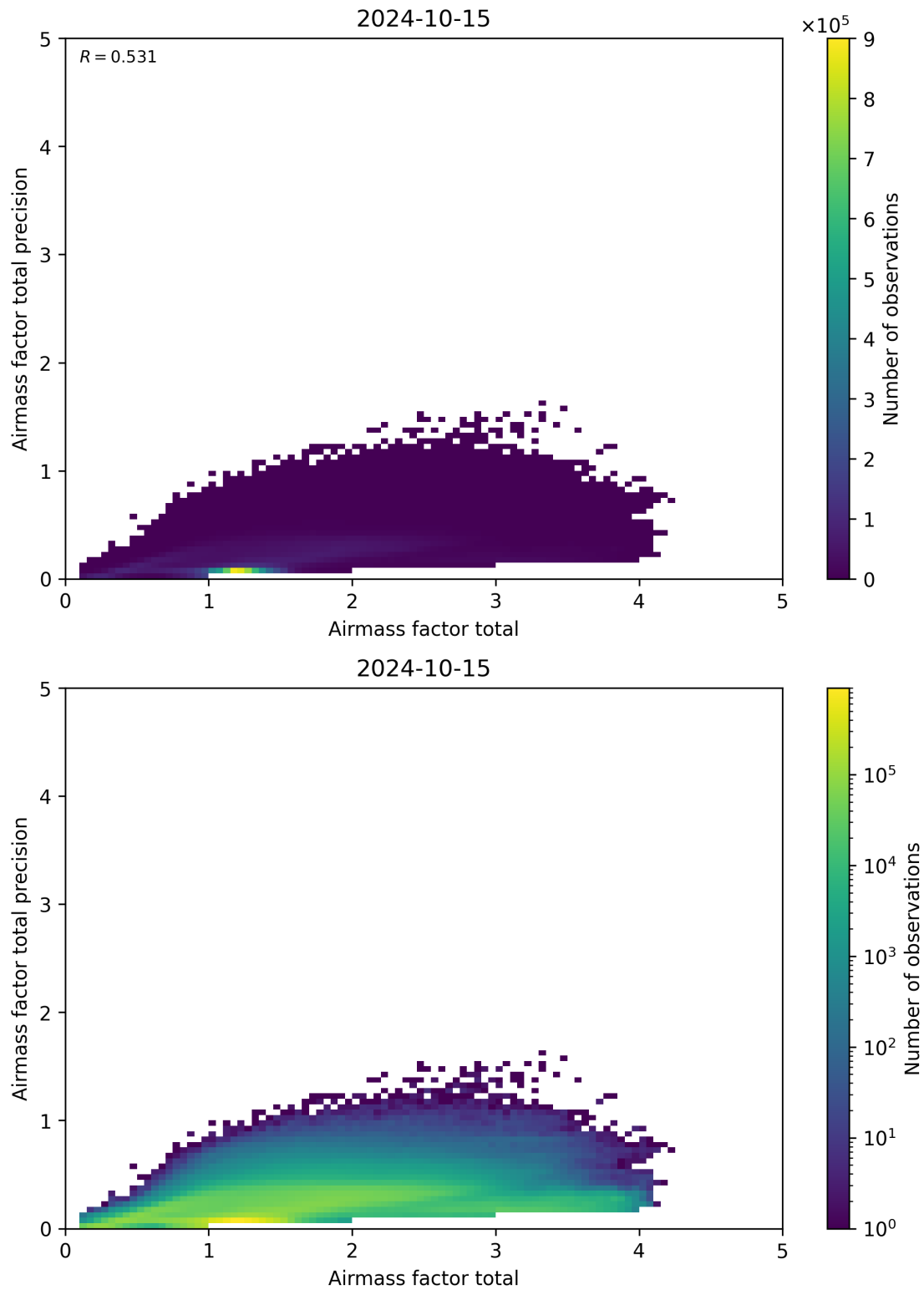
Figure 103: Scatter density plot of “Airmass factor total” against “Airmass factor total precision” for 2024-10-14 to 2024-10-16.
