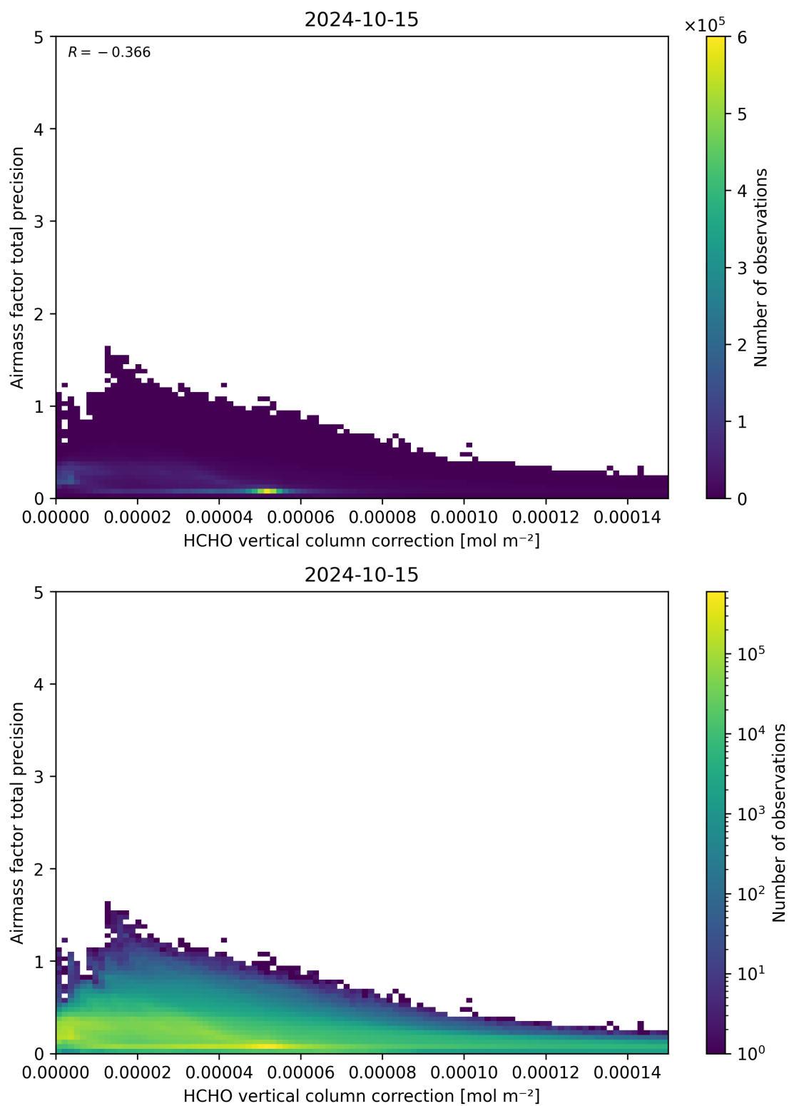
Figure 121: Scatter density plot of “HCHO vertical column correction” against “Airmass factor total precision” for 2024-10-14 to 2024-10-16.
