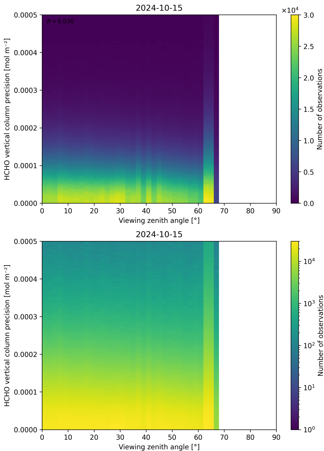
Figure 194: Scatter density plot of “Viewing zenith angle” against “HCHO vertical column precision” for 2024-10-14 to 2024-10-16.
