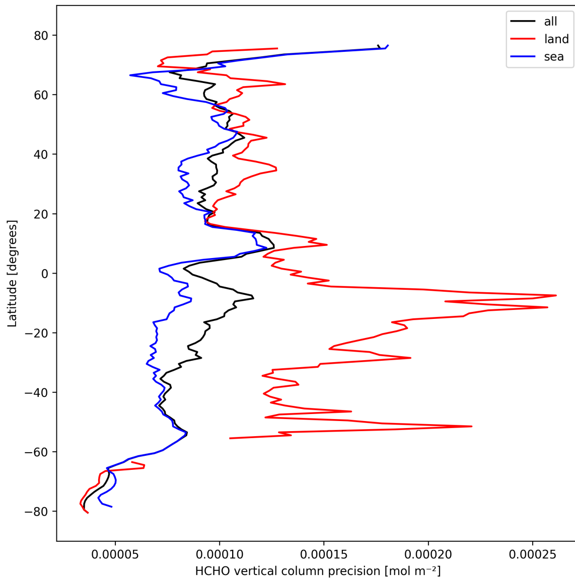
Figure 22: Zonal average of “HCHO vertical column precision” for 2024-10-14 to 2024-10-16.
