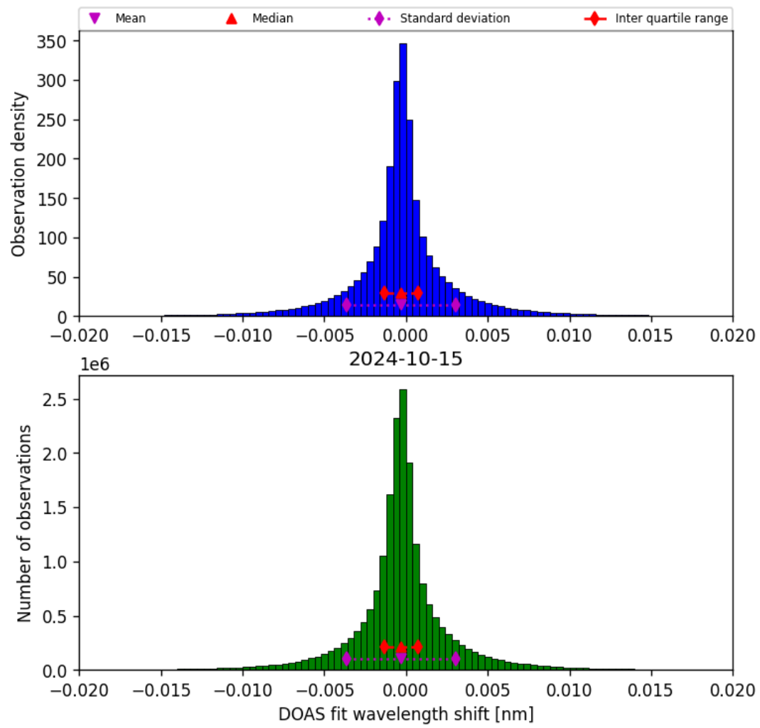
Figure 44: Histogram of “DOAS fit wavelength shift” for 2024-10-14 to 2024-10-16
