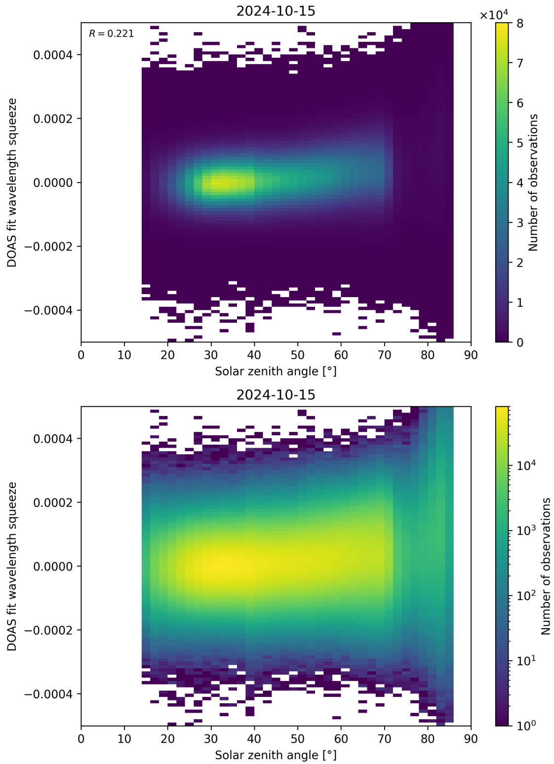
Figure 169: Scatter density plot of “Solar zenith angle” against “DOAS fit wavelength squeeze” for 2024-10-14 to 2024-10-16.
