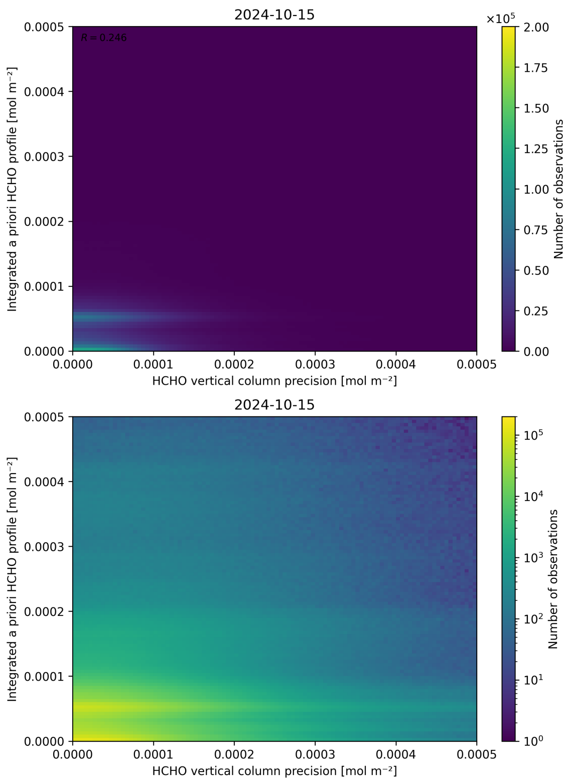
Figure 147: Scatter density plot of “HCHO vertical column precision” against “Integrated a priori HCHO profile” for 2024-10-14 to 2024-10-16.
