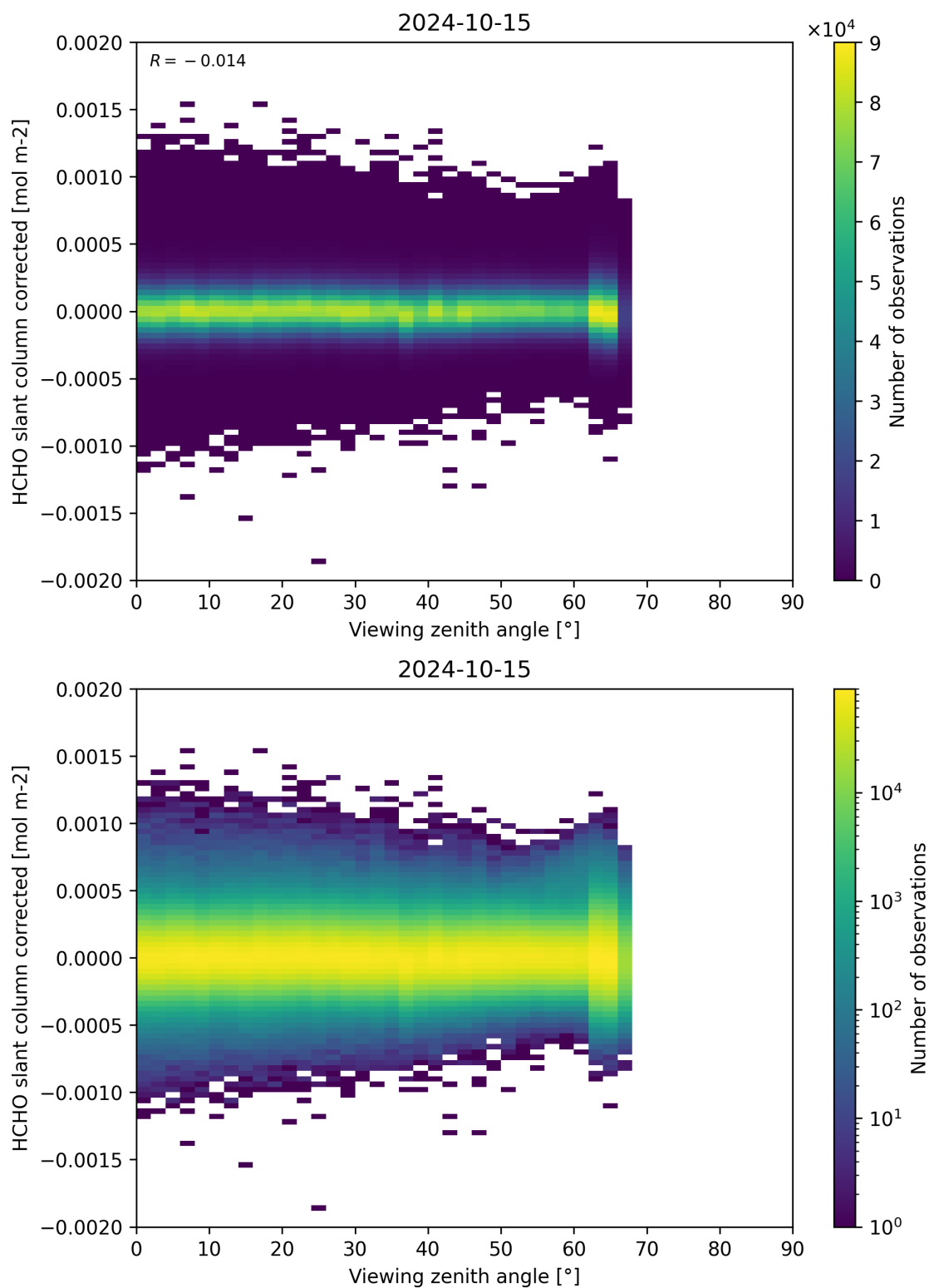
Figure 186: Scatter density plot of “Viewing zenith angle” against “HCHO slant column corrected” for 2024-10-14 to 2024-10-16.
