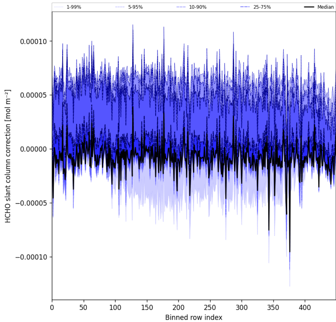
Figure 61: Along track statistics of “HCHO slant column correction” for 2024-10-14 to 2024-10-16
