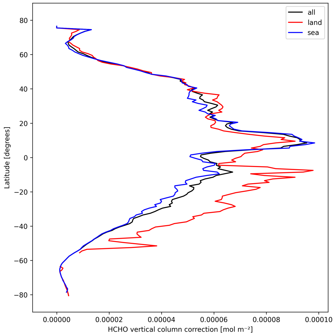
Figure 23: Zonal average of “HCHO vertical column correction” for 2024-10-14 to 2024-10-16.
