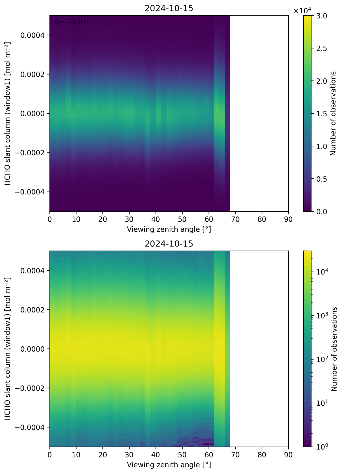
Figure 188: Scatter density plot of “Viewing zenith angle” against “HCHO slant column (window1)” for 2024-10-14 to 2024-10-16.
