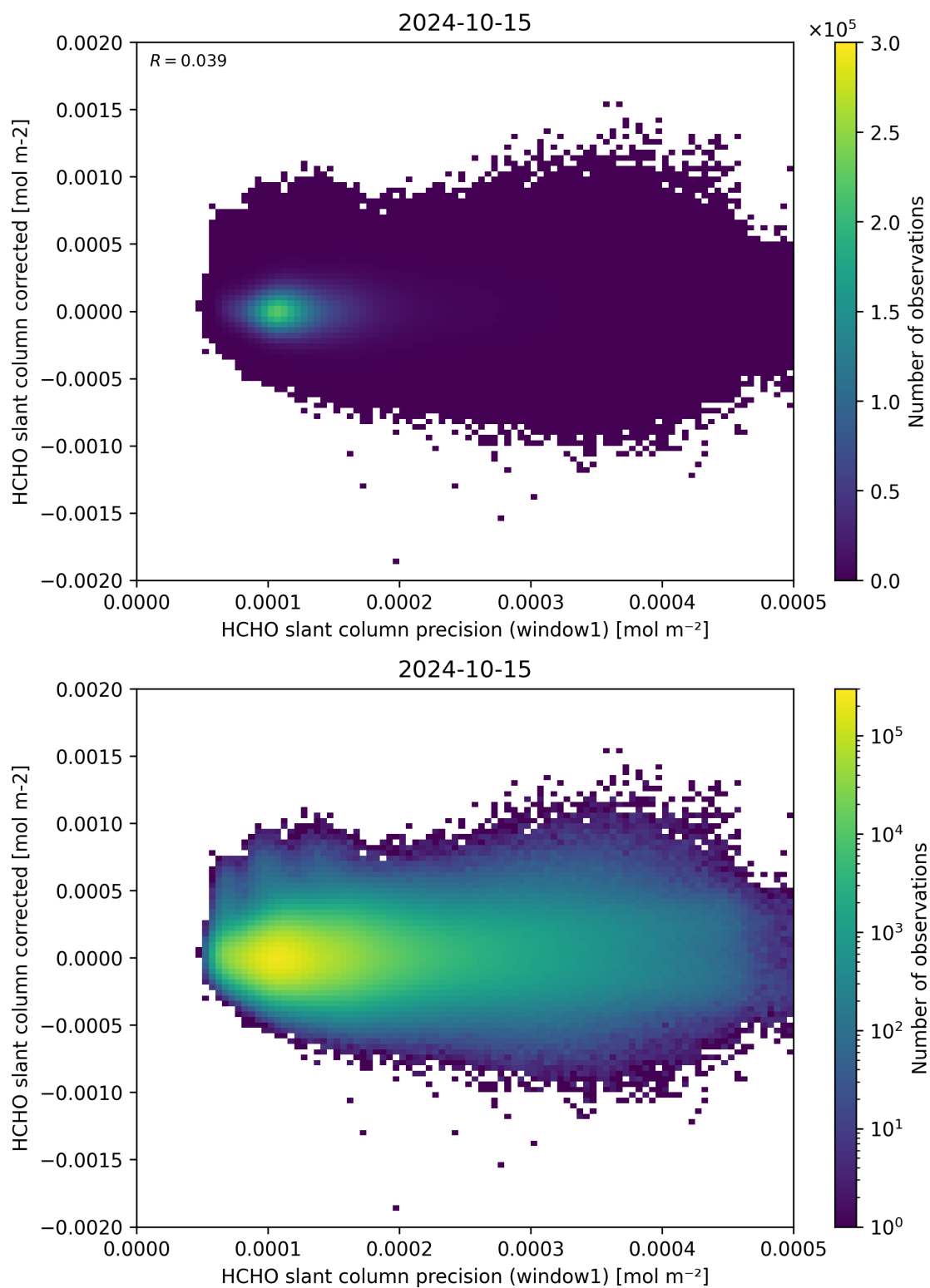
Figure 92: Scatter density plot of “HCHO slant column precision (window1)” against “HCHO slant column corrected” for 2024-10-14 to 2024-10-16.
