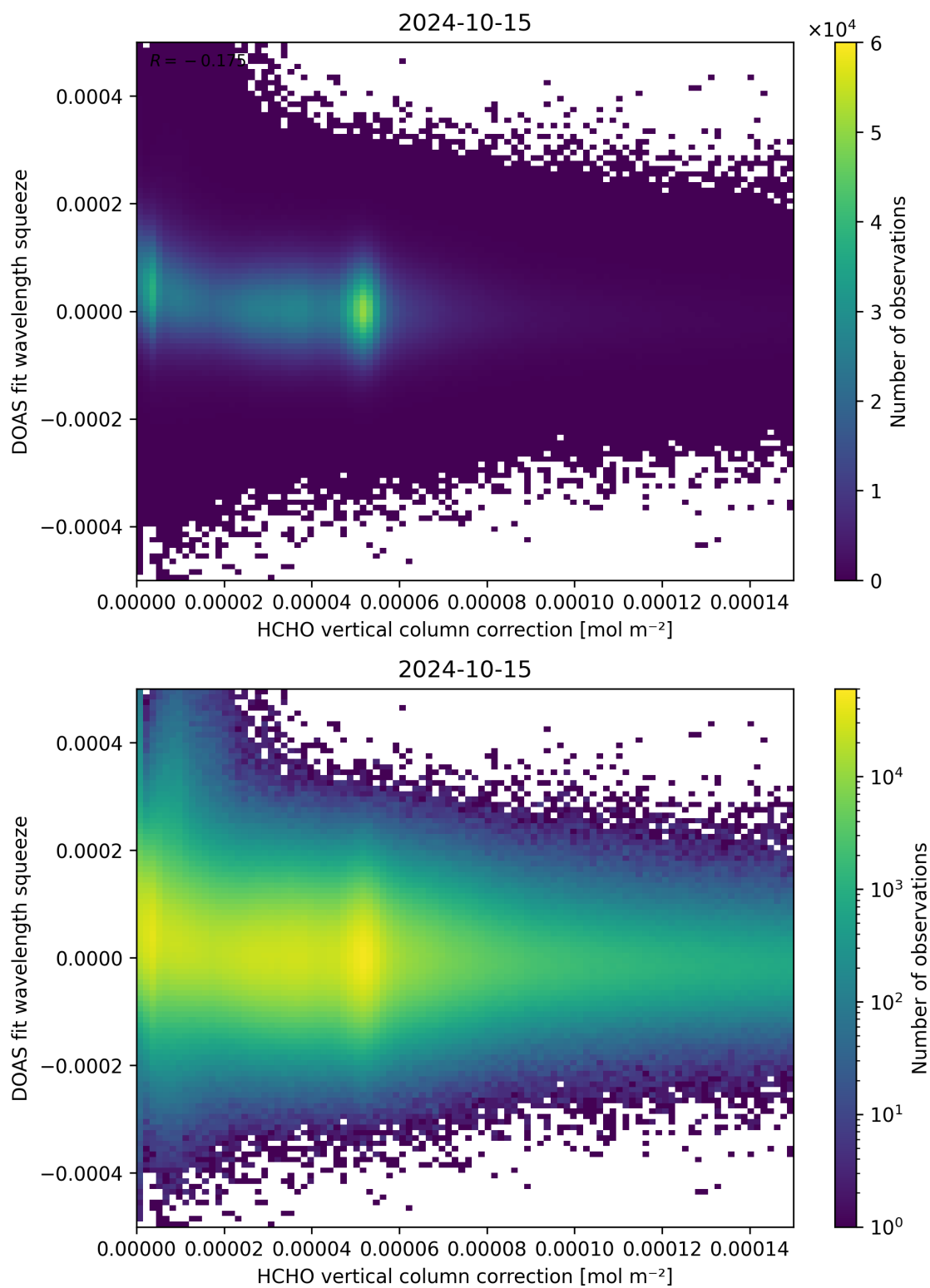
Figure 114: Scatter density plot of “HCHO vertical column correction” against “DOAS fit wavelength squeeze” for 2024-10-14 to 2024-10-16.
