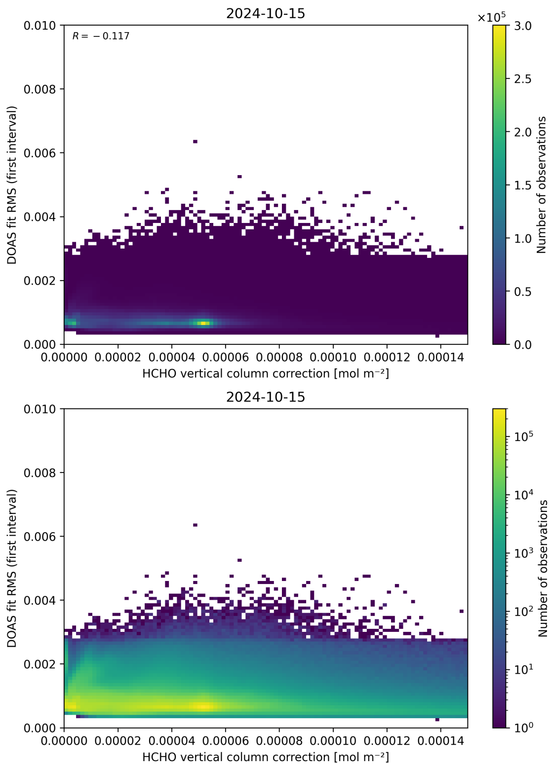
Figure 112: Scatter density plot of “HCHO vertical column correction” against “DOAS fit RMS (first interval)” for 2024-10-14 to 2024-10-16.
