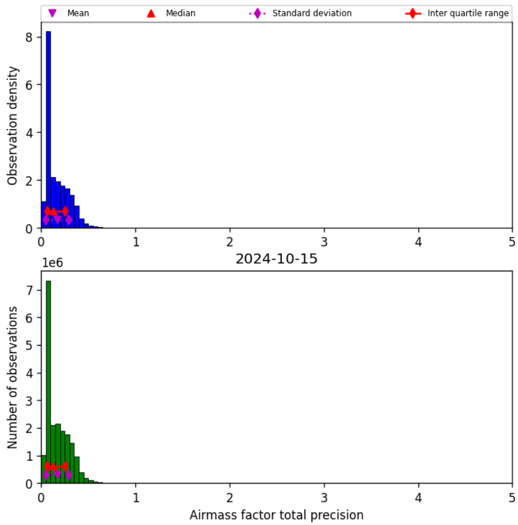
Figure 41: Histogram of “Airmass factor total precision” for 2024-10-14 to 2024-10-16
