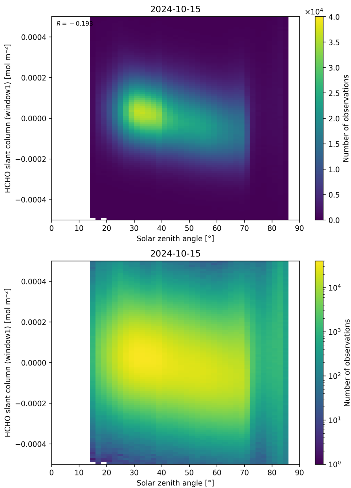
Figure 173: Scatter density plot of “Solar zenith angle” against “HCHO slant column (window1)” for 2024-10-14 to 2024-10-16.
