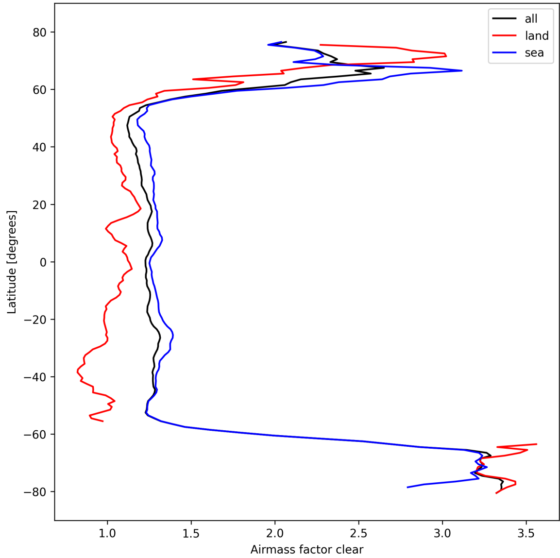
Figure 28: Zonal average of “Airmass factor clear” for 2024-10-14 to 2024-10-16.
