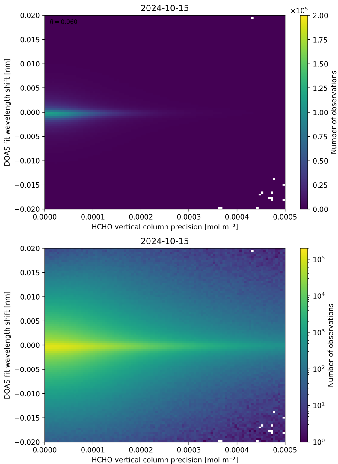
Figure 137: Scatter density plot of “HCHO vertical column precision” against “DOAS fit wavelength shift” for 2024-10-14 to 2024-10-16.
