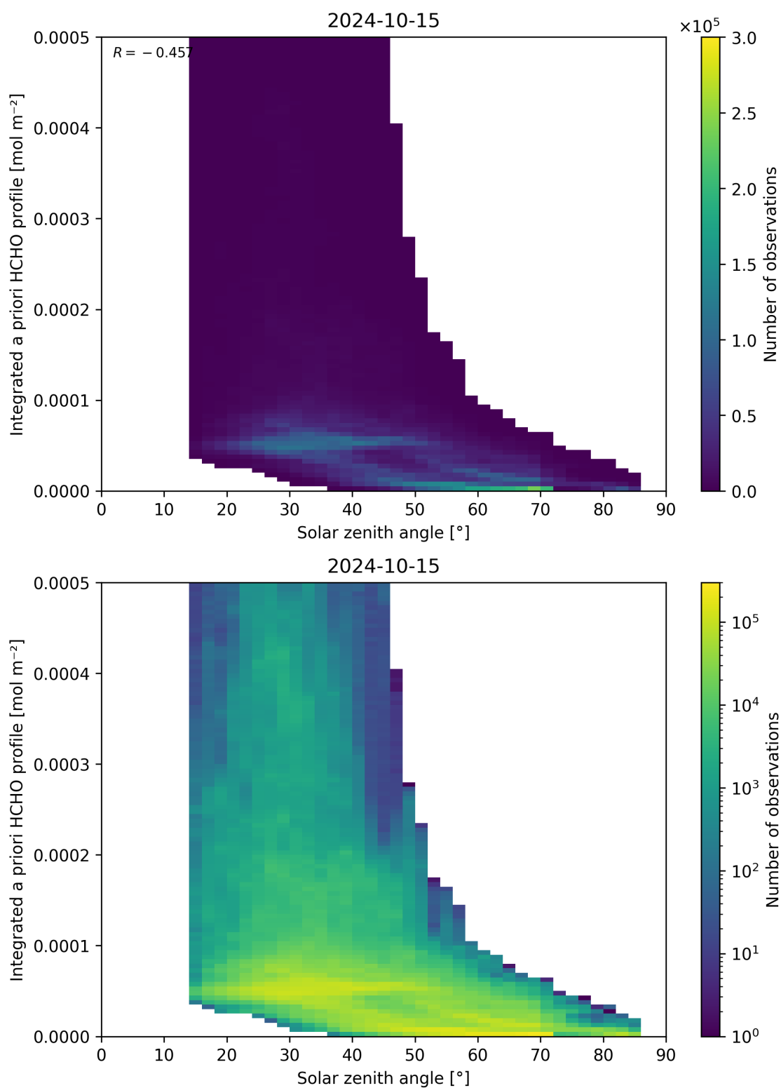
Figure 180: Scatter density plot of “Solar zenith angle” against “Integrated a priori HCHO profile” for 2024-10-14 to 2024-10-16.
