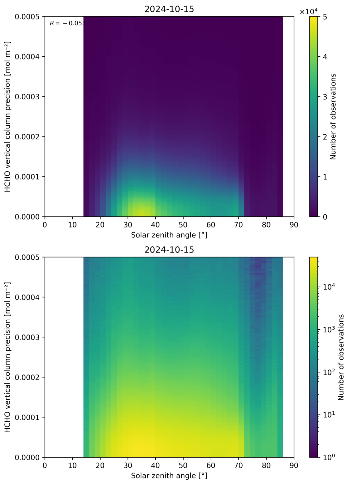
Figure 179: Scatter density plot of “Solar zenith angle” against “HCHO vertical column precision” for 2024-10-14 to 2024-10-16.
