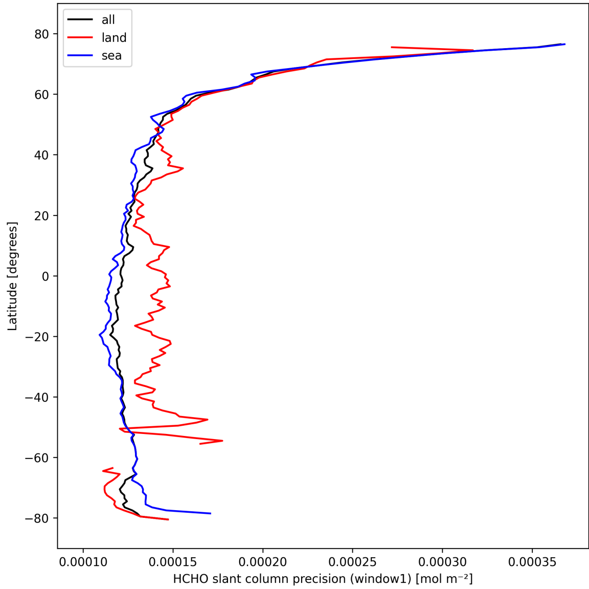
Figure 25: Zonal average of "HCHO slant column precision (window1)" for 2024-10-14 to 2024-10-16.
