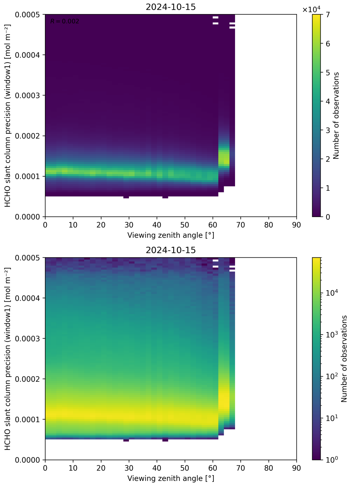
Figure 189: Scatter density plot of “Viewing zenith angle” against “HCHO slant column precision (window1)” for 2024-10-14 to 2024-10-16.
