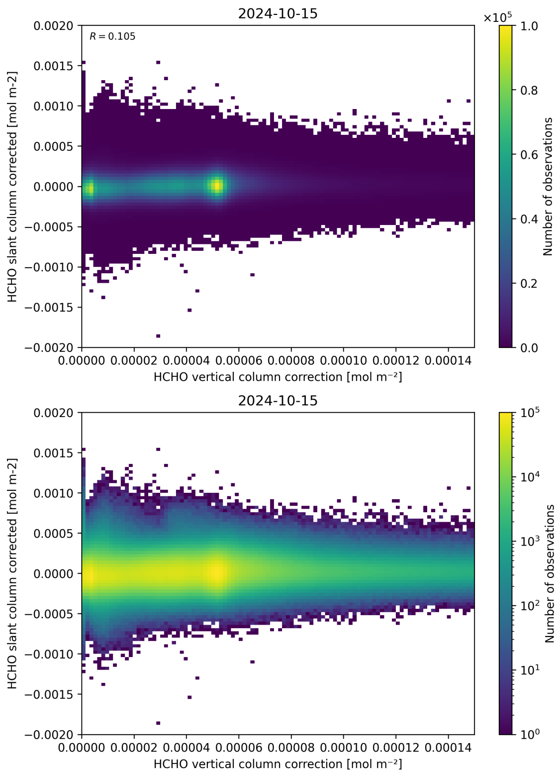
Figure 116: Scatter density plot of “HCHO vertical column correction” against “HCHO slant column corrected” for 2024-10-14 to 2024-10-16.
