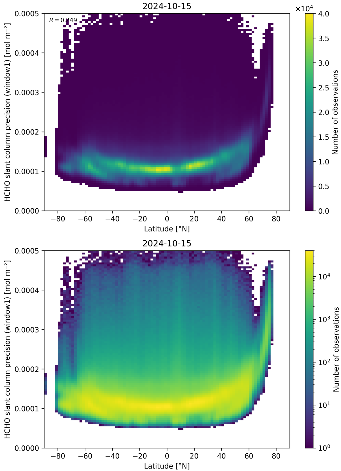
Figure 160: Scatter density plot of “Latitude” against “HCHO slant column precision (window1)” for 2024-10-14 to 2024-10-16.
