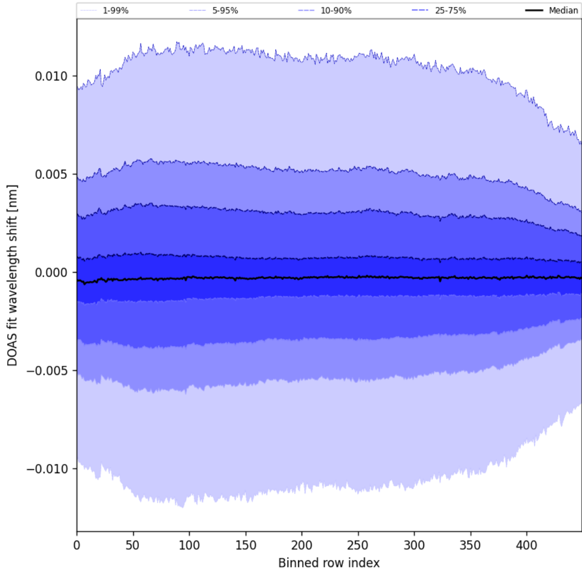
Figure 58: Along track statistics of “DOAS fit wavelength shift” for 2024-10-14 to 2024-10-16
