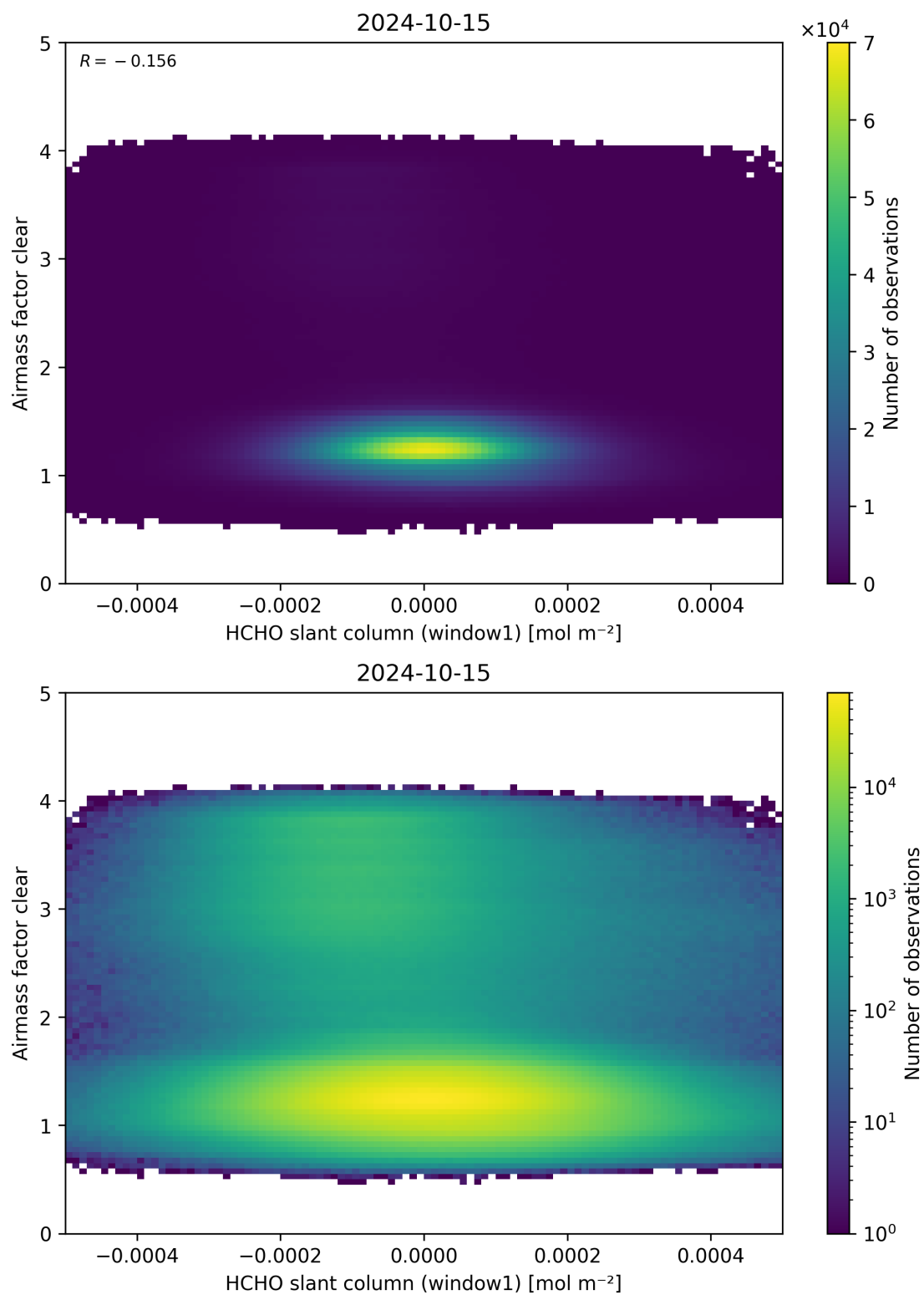
Figure 81: Scatter density plot of “HCHO slant column (window1)” against “Airmass factor clear” for 2024-10-14 to 2024-10-16.
