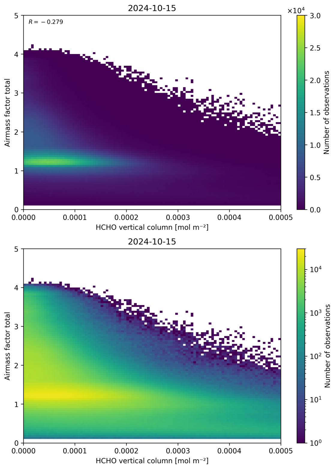
Figure 131: Scatter density plot of “HCHO vertical column” against “Airmass factor total” for 2024-10-14 to 2024-10-16.
