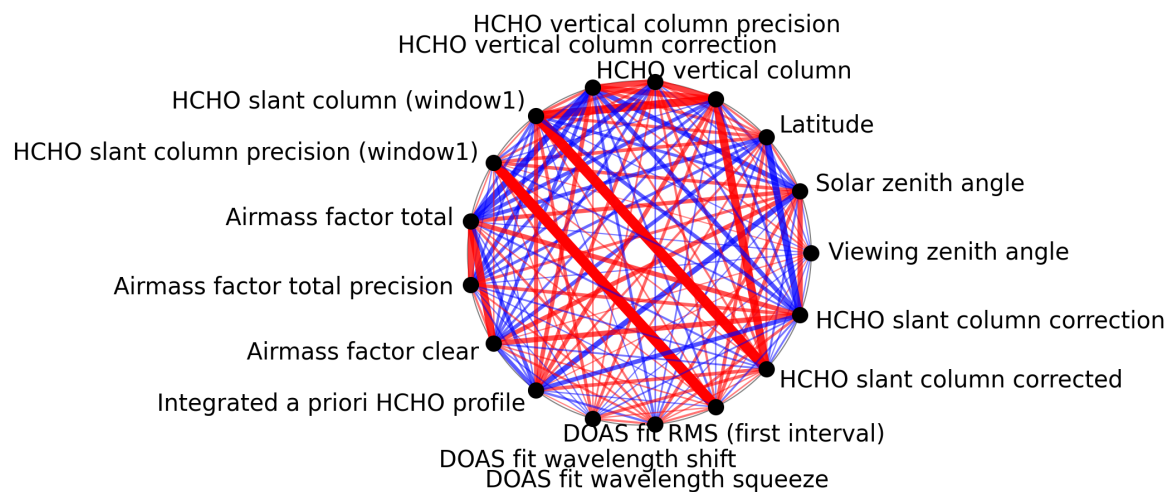
Figure 1: Map of correlation graph for 2024-10-14 to 2024-10-16.
