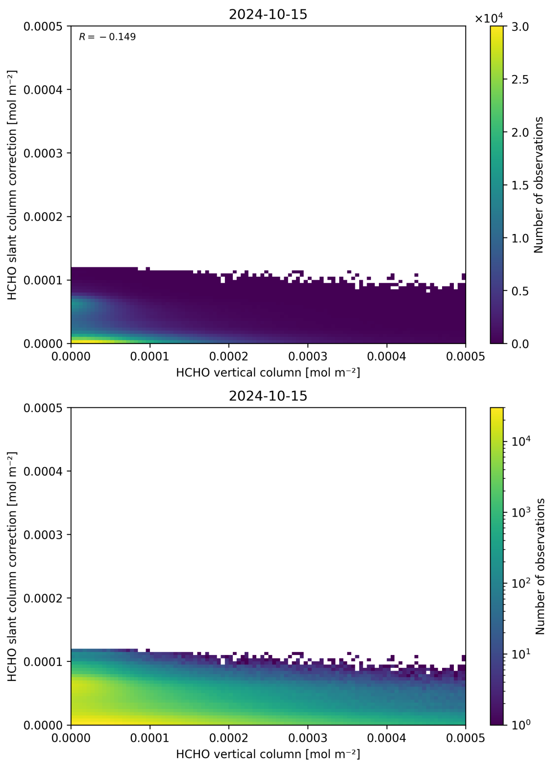
Figure 128: Scatter density plot of “HCHO vertical column” against “HCHO slant column correction” for 2024-10-14 to 2024-10-16.
