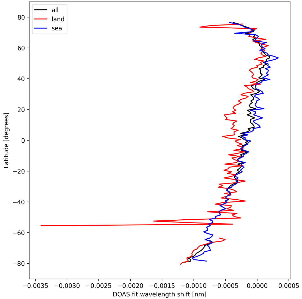
Figure 30: Zonal average of “DOAS fit wavelength shift” for 2024-10-14 to 2024-10-16.
