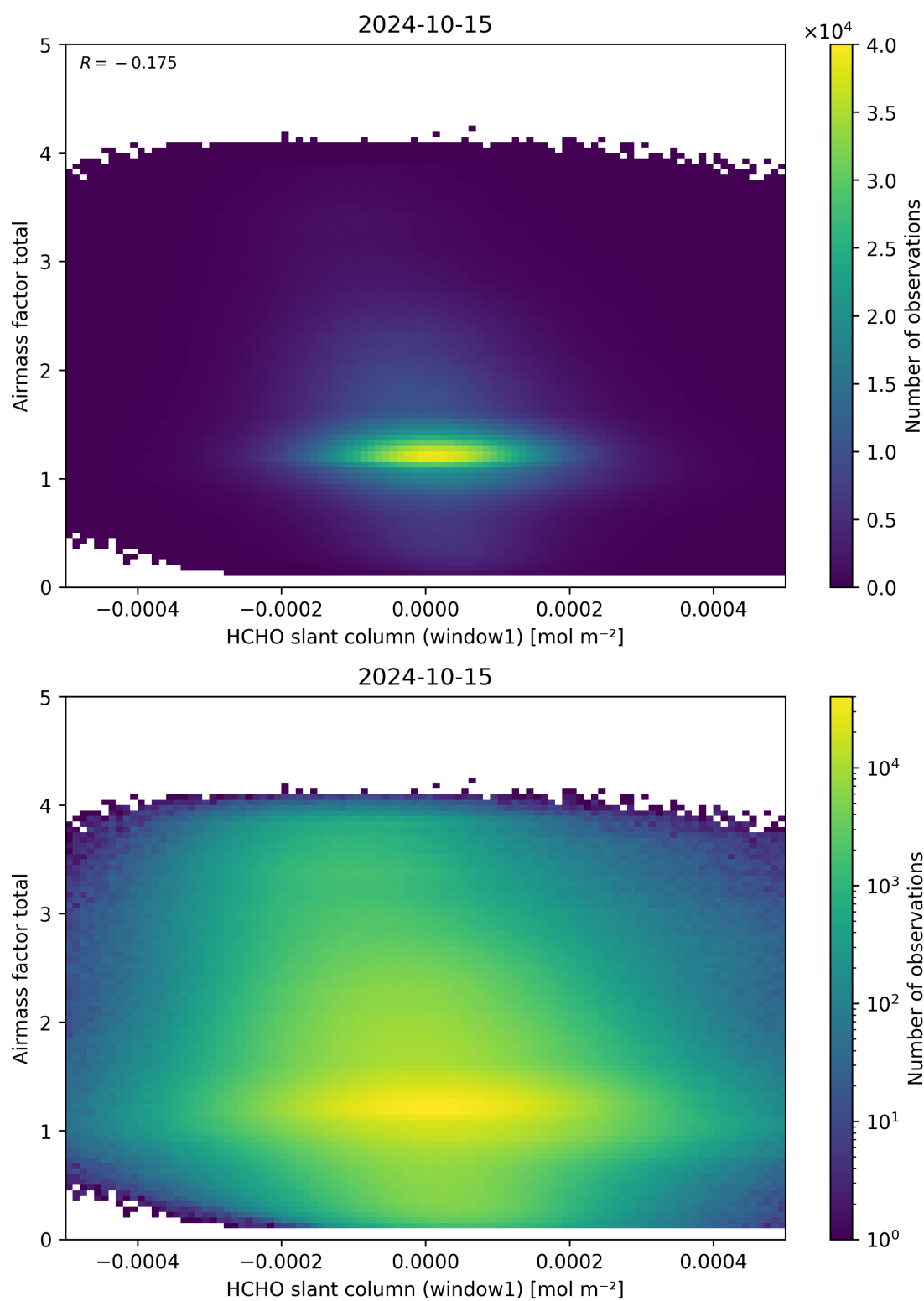
Figure 85: Scatter density plot of “HCHO slant column (window1)” against “Airmass factor total” for 2024-10-14 to 2024-10-16.
