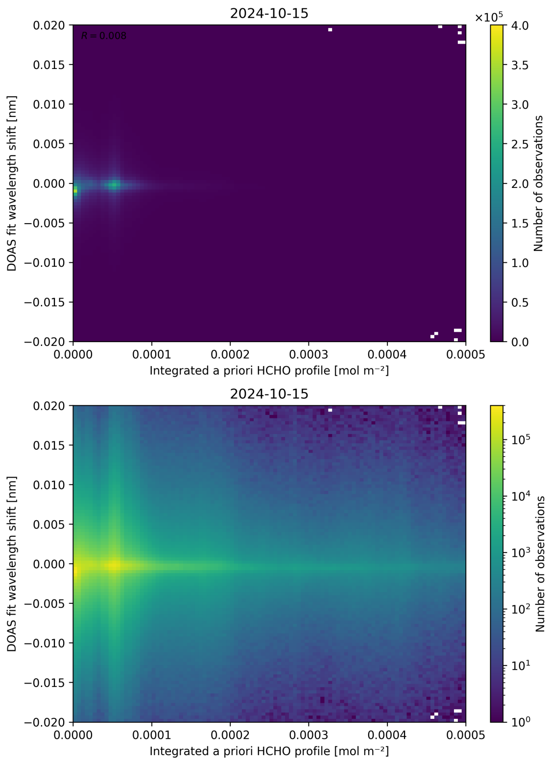
Figure 149: Scatter density plot of “Integrated a priori HCHO profile” against “DOAS fit wavelength shift” for 2024-10-14 to 2024-10-16.
