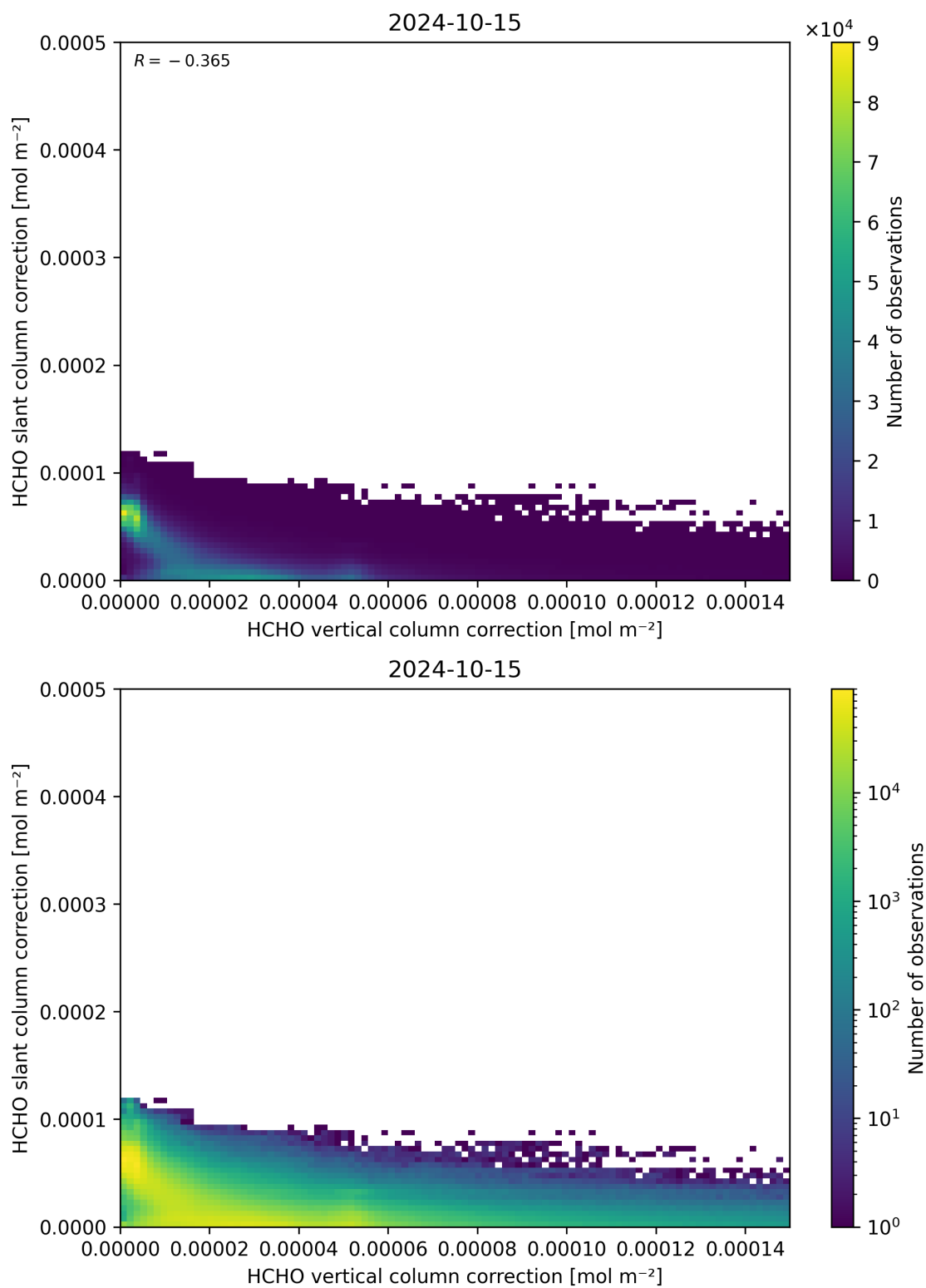
Figure 117: Scatter density plot of “HCHO vertical column correction” against “HCHO slant column correction” for 2024-10-14 to 2024-10-16.
