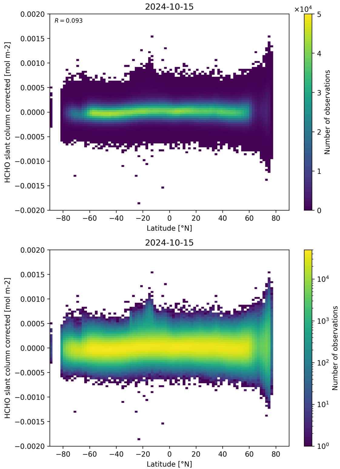
Figure 157: Scatter density plot of “Latitude” against “HCHO slant column corrected” for 2024-10-14 to 2024-10-16.
