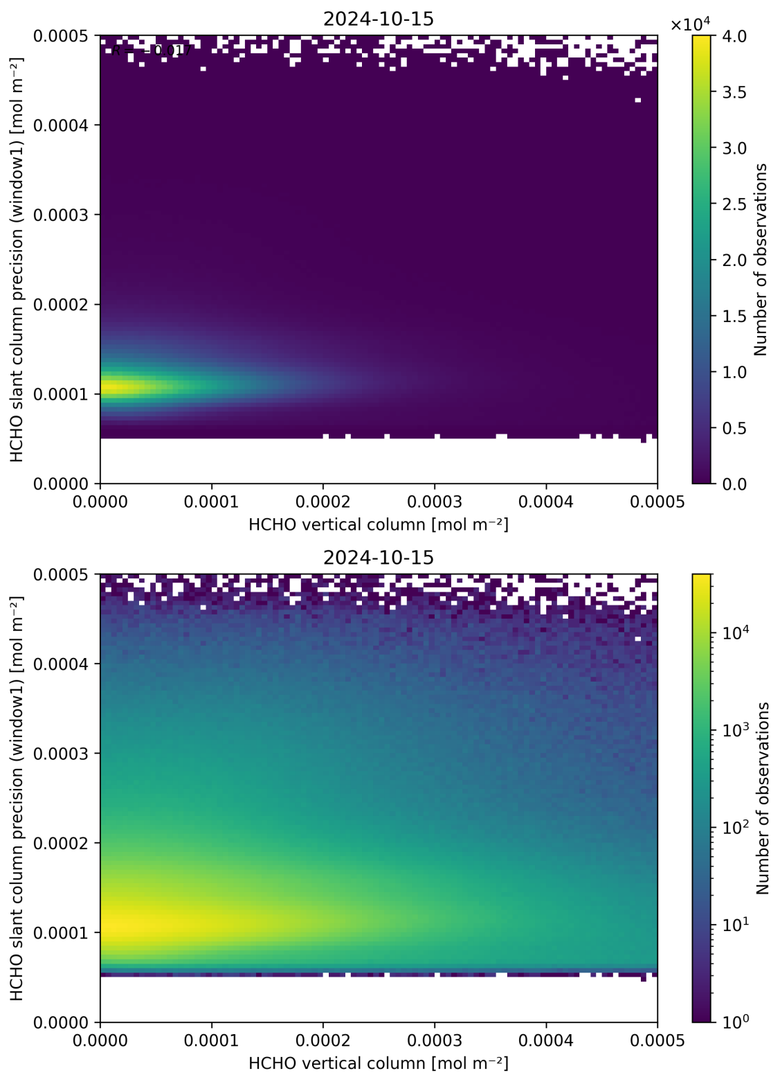
Figure 130: Scatter density plot of “HCHO vertical column” against “HCHO slant column precision (window1)” for 2024-10-14 to 2024-10-16.
