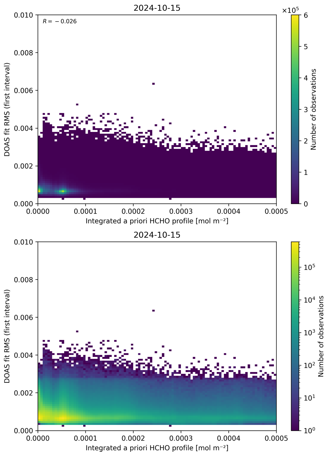
Figure 148: Scatter density plot of “Integrated a priori HCHO profile” against “DOAS fit RMS (first interval)” for 2024-10-14 to 2024-10-16.
