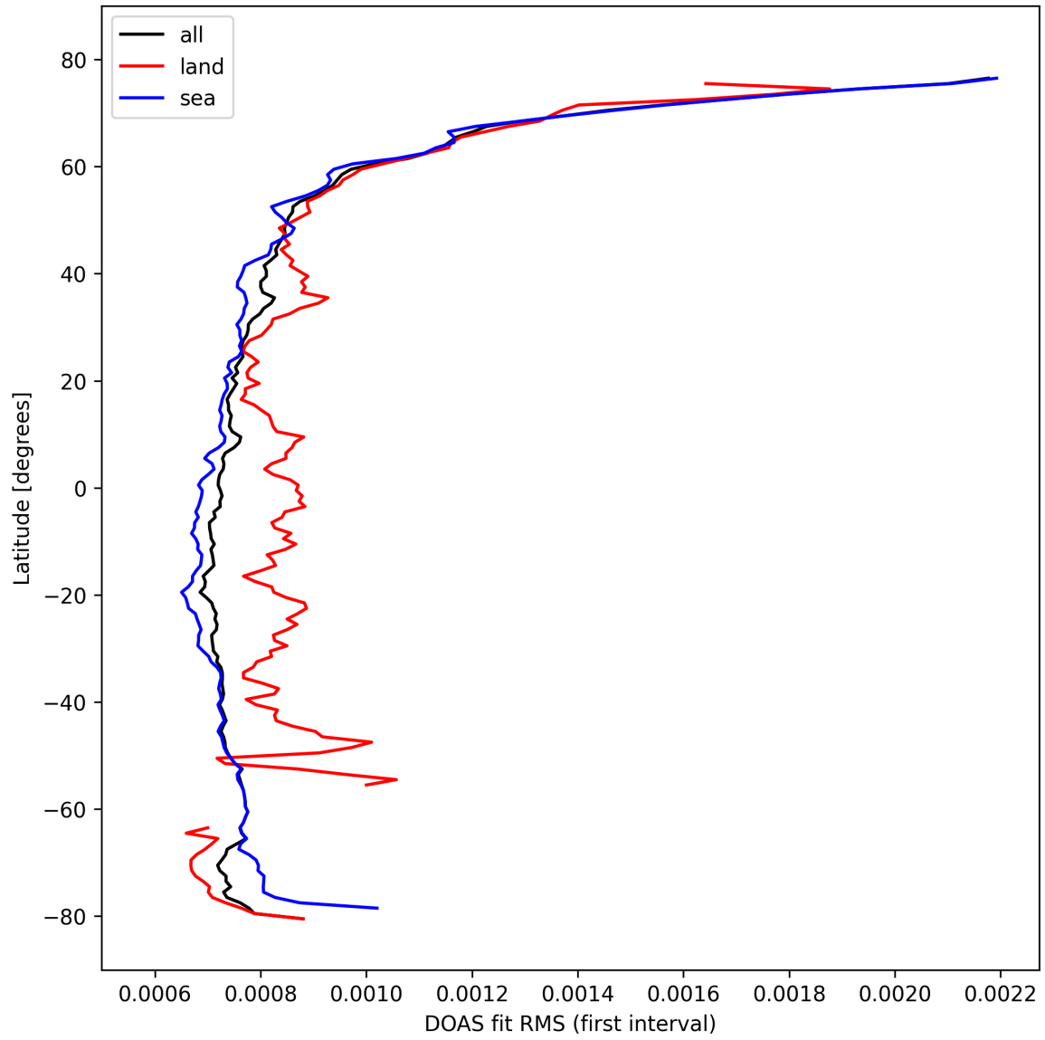
Figure 32: Zonal average of “DOAS fit RMS (first interval)” for 2024-10-14 to 2024-10-16.
