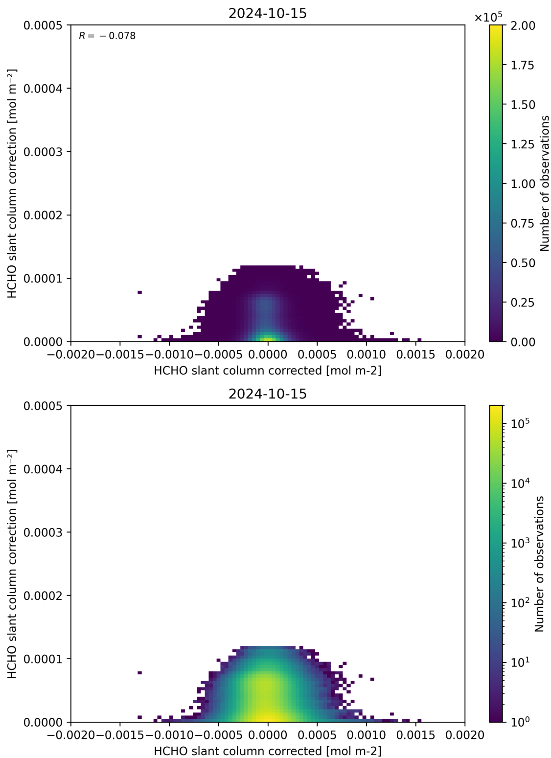
Figure 77: Scatter density plot of “HCHO slant column corrected” against “HCHO slant column correction” for 2024-10-14 to 2024-10-16.
