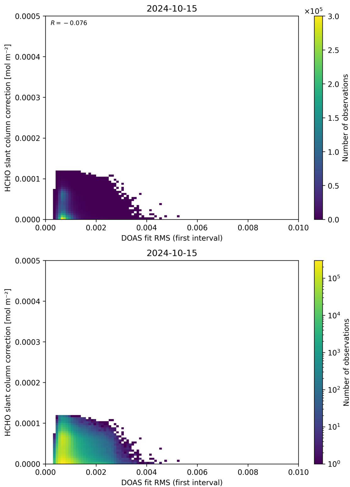
Figure 63: Scatter density plot of “DOAS fit RMS (first interval)” against “HCHO slant column correction” for 2024-10-14 to 2024-10-16.
