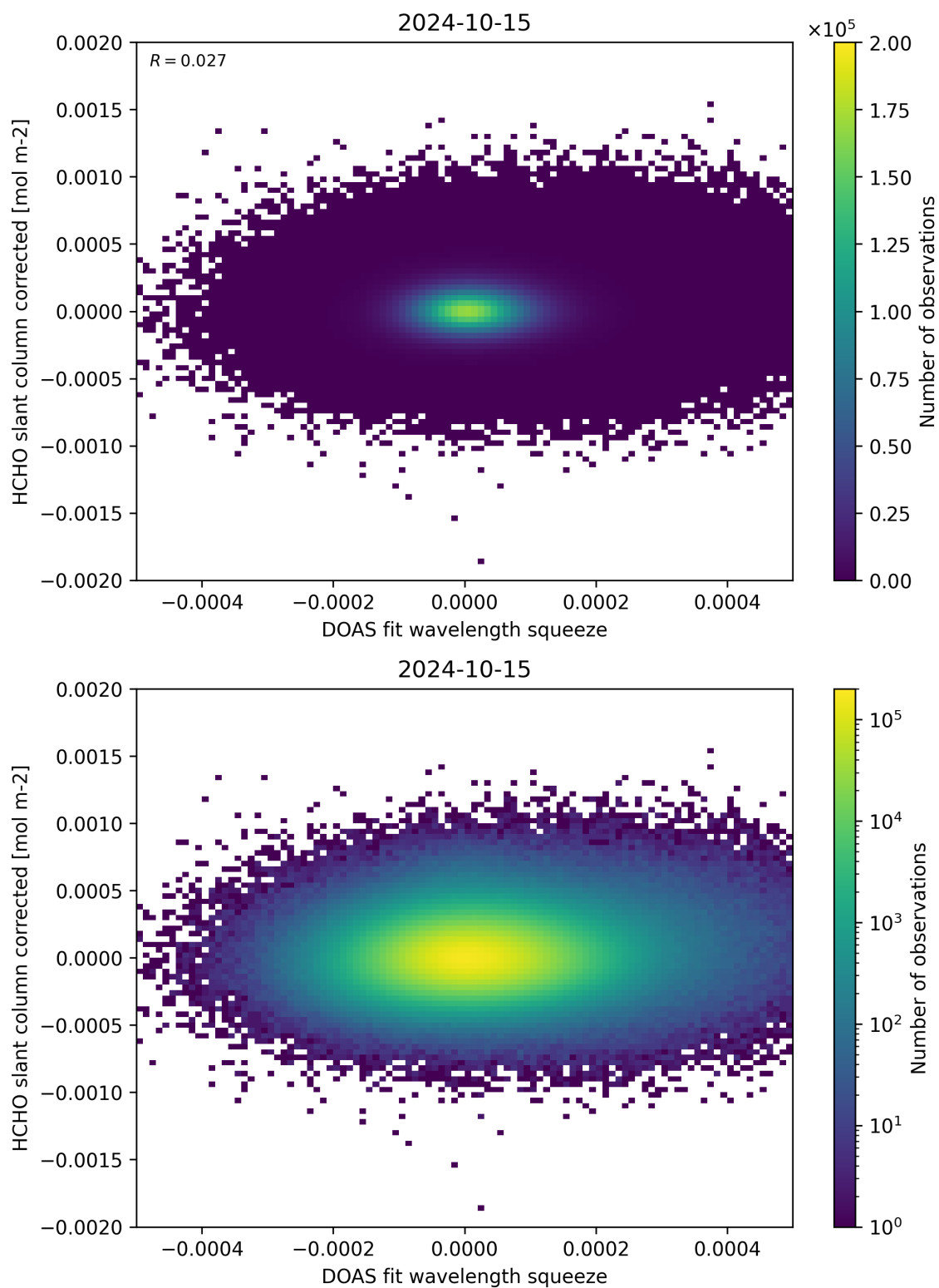
Figure 69: Scatter density plot of “DOAS fit wavelength squeeze” against “HCHO slant column corrected” for 2024-10-14 to 2024-10-16.
