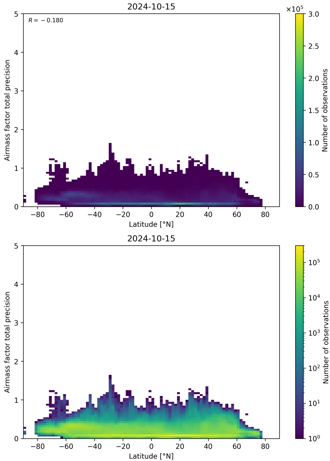
Figure 162: Scatter density plot of “Latitude” against “Airmass factor total precision” for 2024-10-14 to 2024-10-16.
