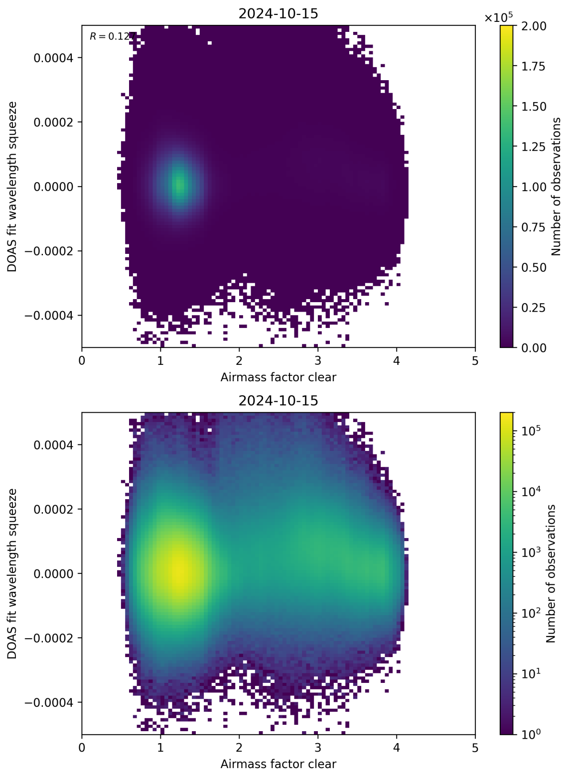
Figure 73: Scatter density plot of “Airmass factor clear” against “DOAS fit wavelength squeeze” for 2024-10-14 to 2024-10-16.
