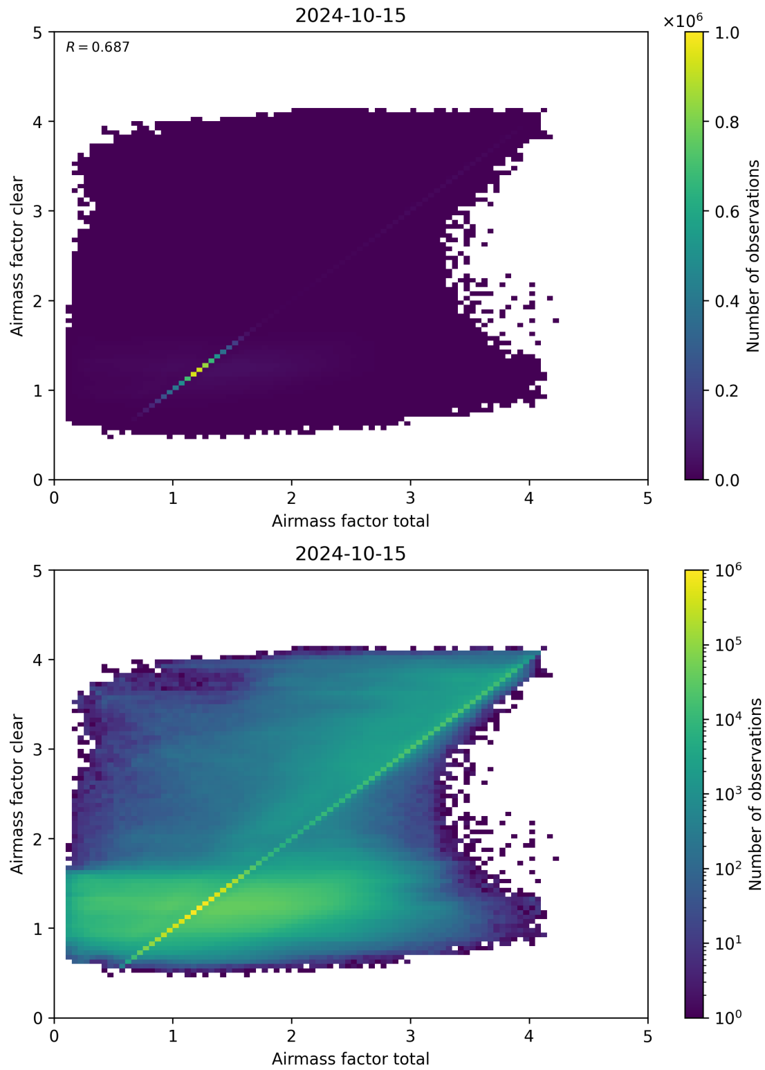
Figure 100: Scatter density plot of “Airmass factor total” against “Airmass factor clear” for 2024-10-14 to 2024-10-16.
