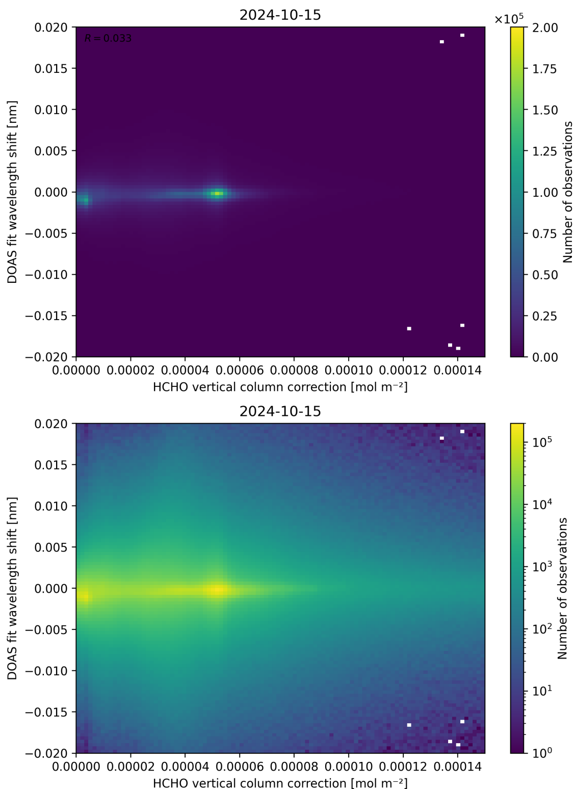
Figure 113: Scatter density plot of “HCHO vertical column correction” against “DOAS fit wavelength shift” for 2024-10-14 to 2024-10-16.
