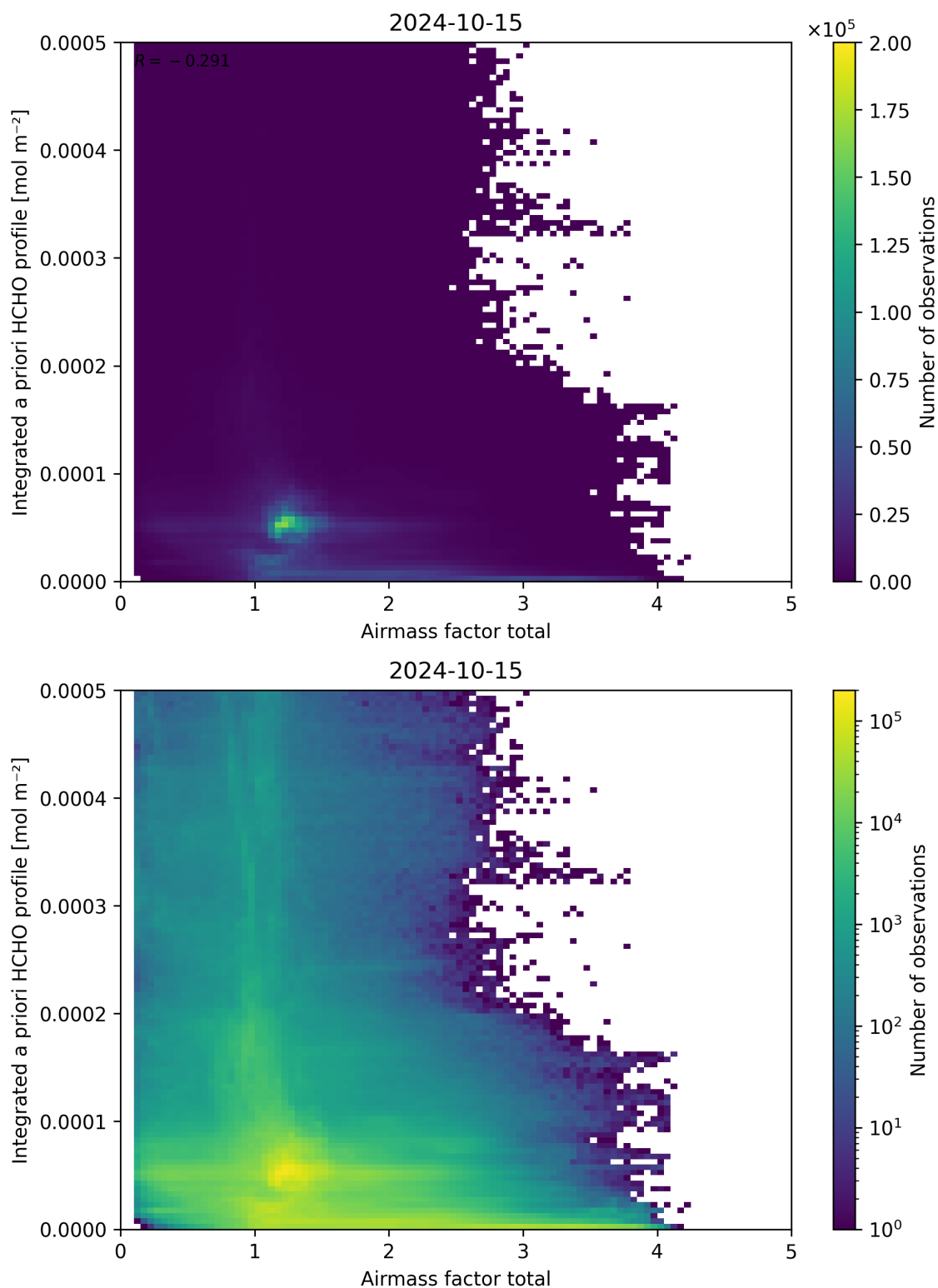
Figure 104: Scatter density plot of “Airmass factor total” against “Integrated a priori HCHO profile” for 2024-10-14 to 2024-10-16.
