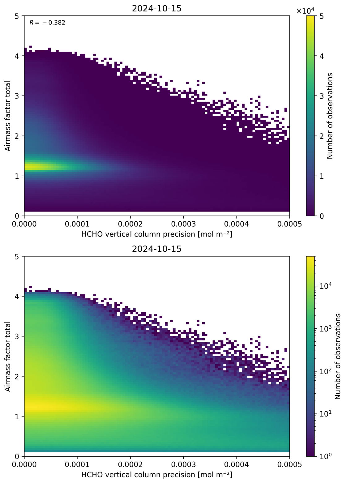
Figure 144: Scatter density plot of “HCHO vertical column precision” against “Airmass factor total” for 2024-10-14 to 2024-10-16.
