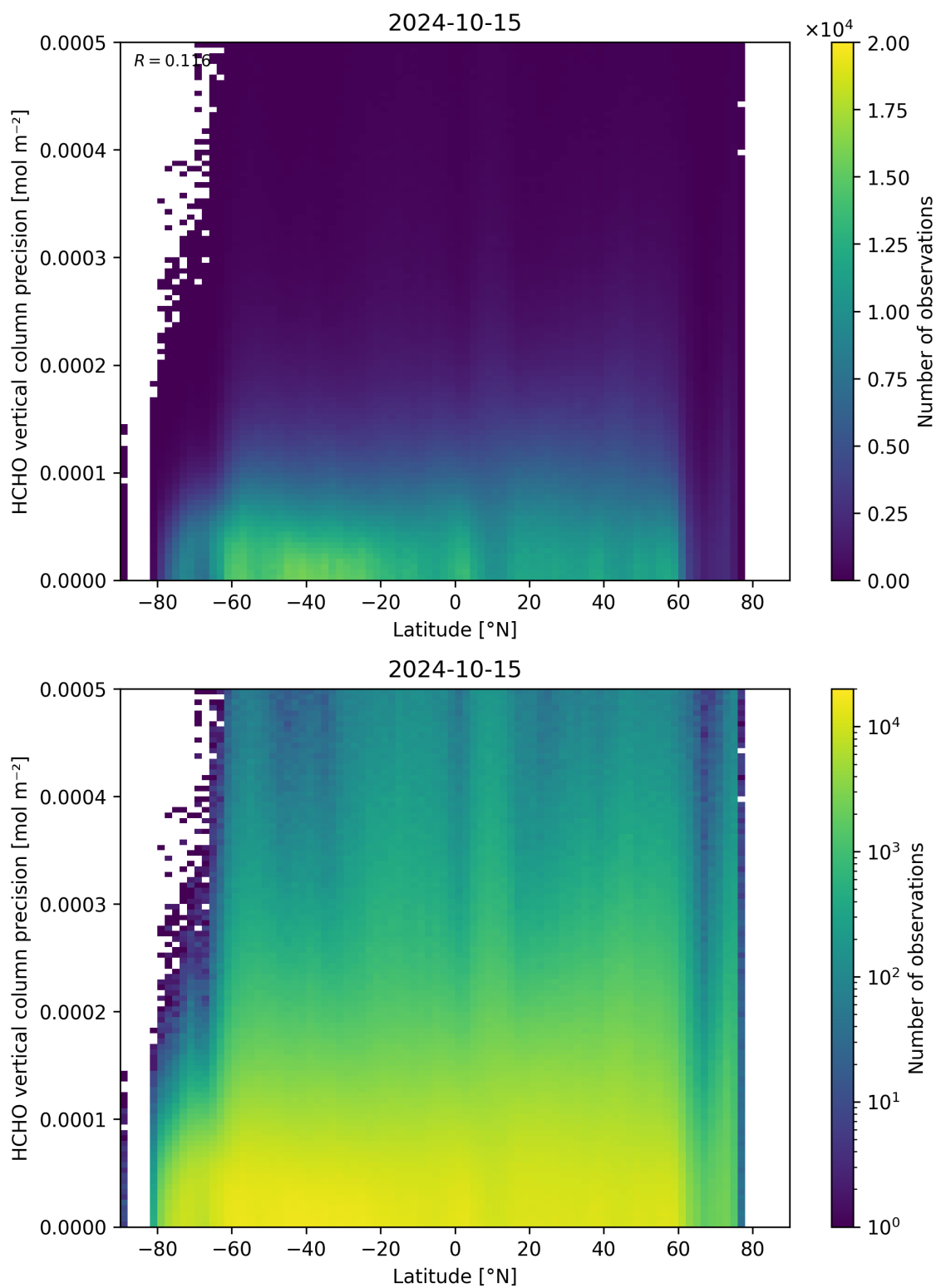
Figure 165: Scatter density plot of “Latitude” against “HCHO vertical column precision” for 2024-10-14 to 2024-10-16.
