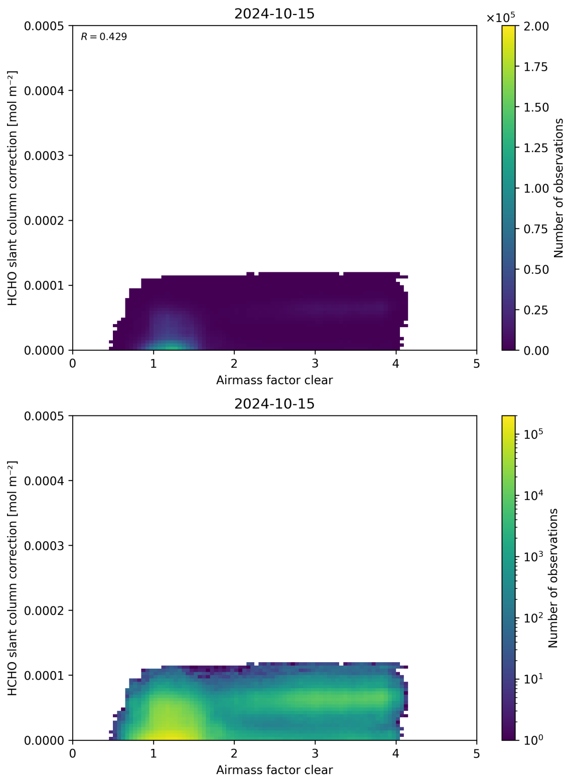
Figure 75: Scatter density plot of “Airmass factor clear” against “HCHO slant column correction” for 2024-10-14 to 2024-10-16.
