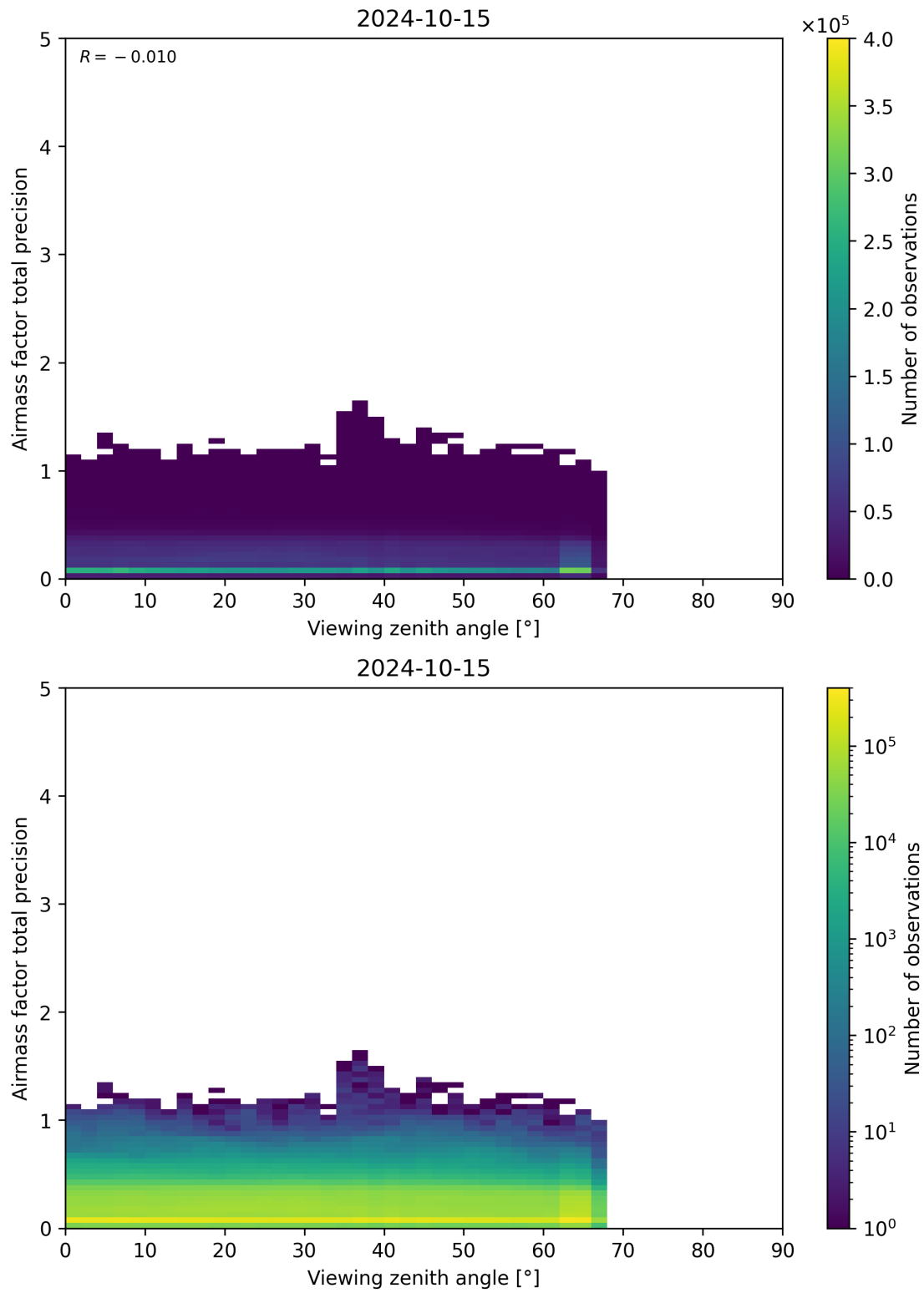
Figure 191: Scatter density plot of “Viewing zenith angle” against “Airmass factor total precision” for 2024-10-14 to 2024-10-16.
