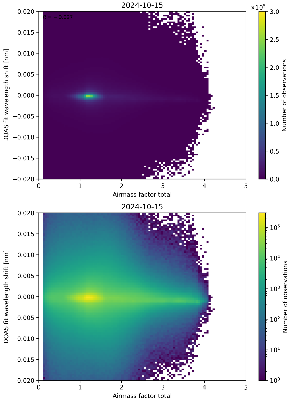
Figure 98: Scatter density plot of “Airmass factor total” against “DOAS fit wavelength shift” for 2024-10-14 to 2024-10-16.
