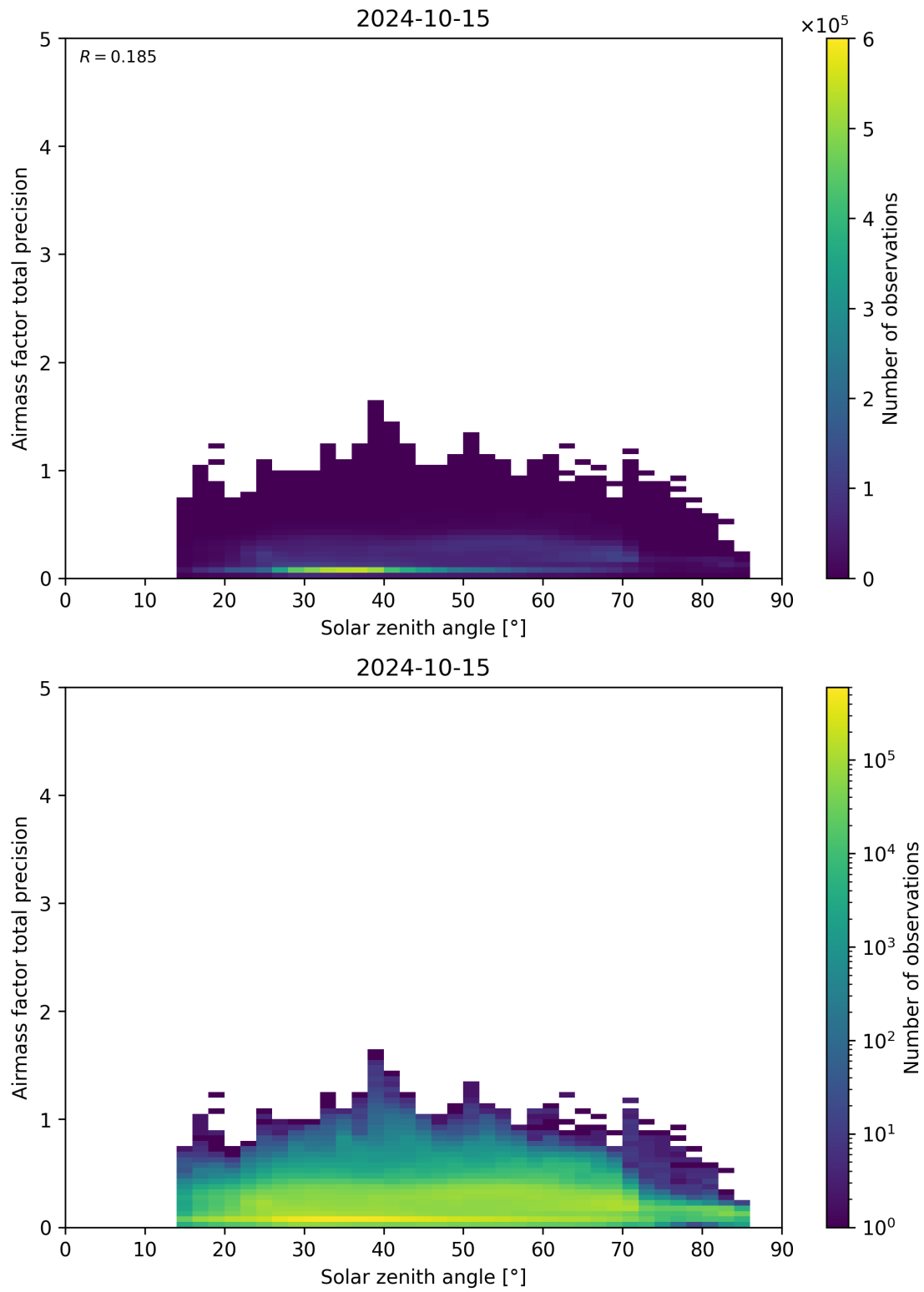
Figure 176: Scatter density plot of “Solar zenith angle” against “Airmass factor total precision” for 2024-10-14 to 2024-10-16.
