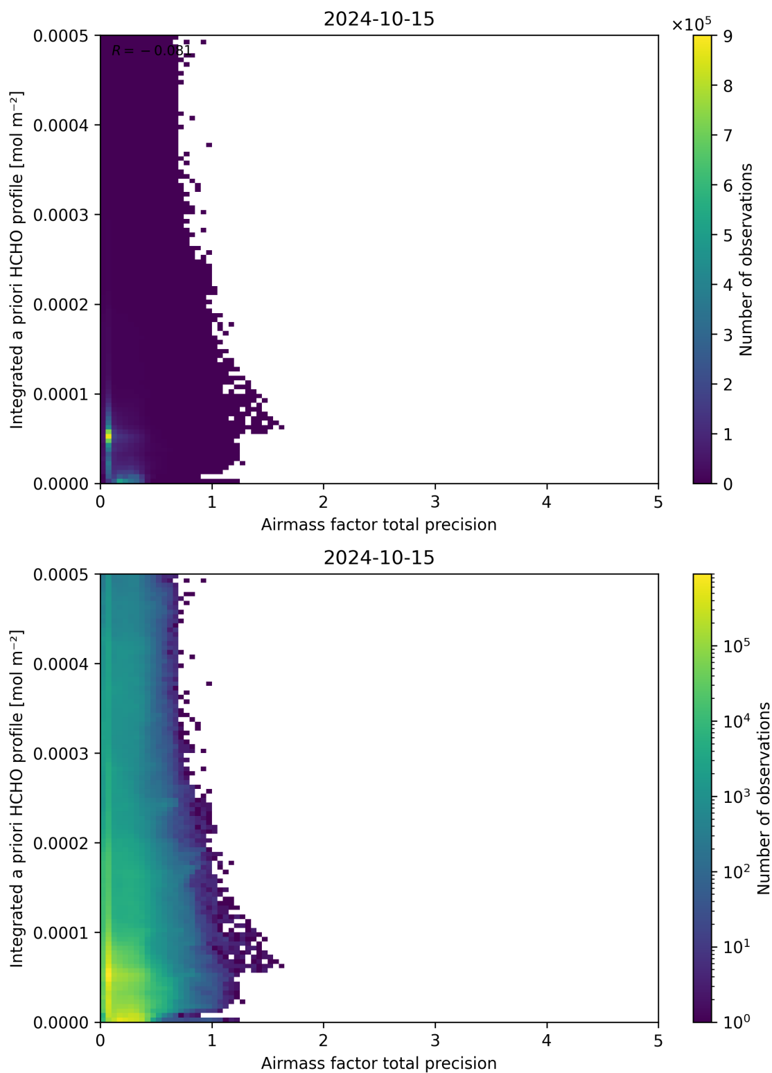
Figure 111: Scatter density plot of “Airmass factor total precision” against “Integrated a priori HCHO profile” for 2024-10-14 to 2024-10-16.
