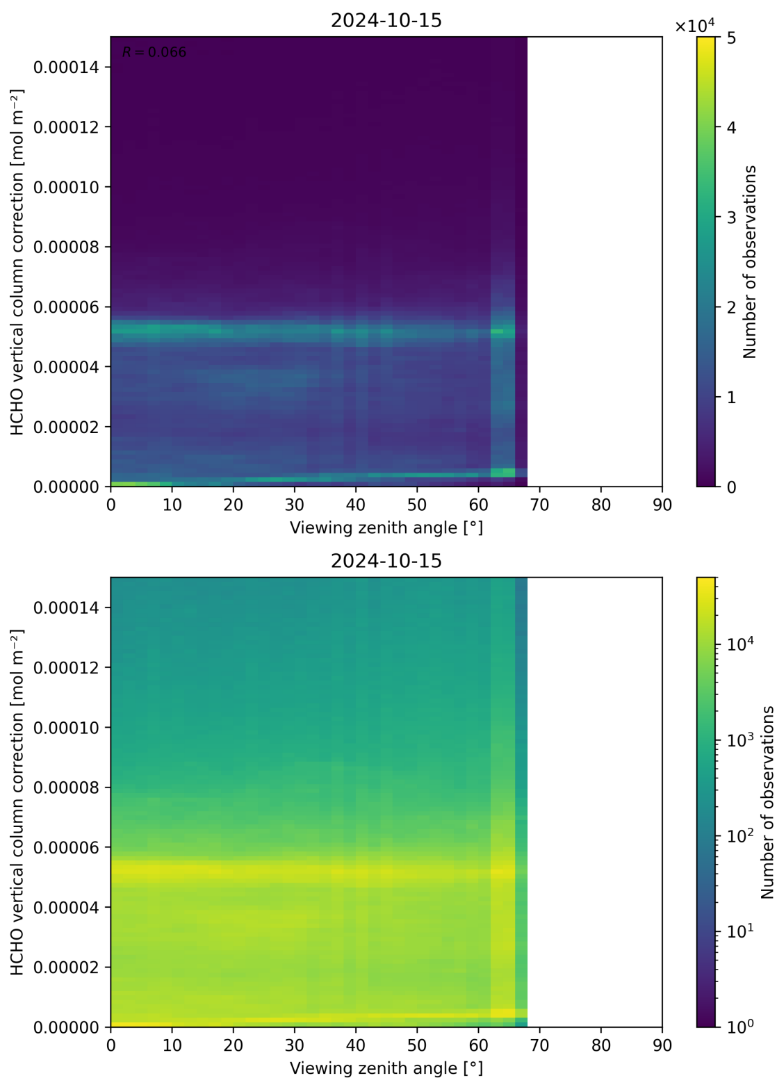
Figure 193: Scatter density plot of “Viewing zenith angle” against “HCHO vertical column correction” for 2024-10-14 to 2024-10-16.
