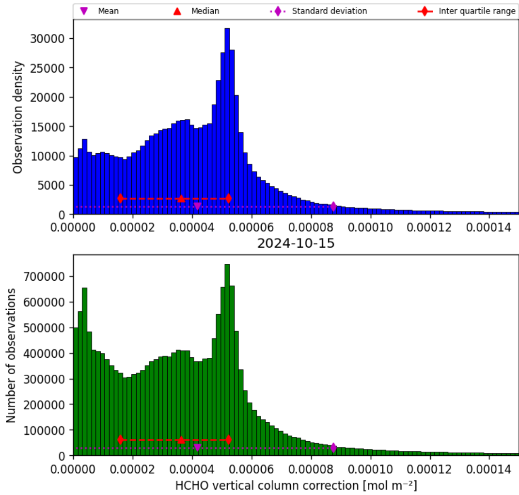
Figure 37: Histogram of “HCHO vertical column correction” for 2024-10-14 to 2024-10-16
