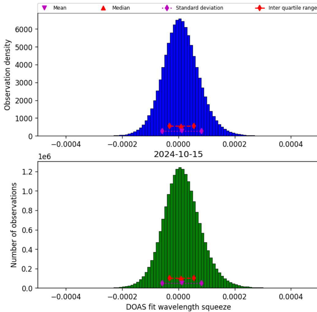
Figure 45: Histogram of “DOAS fit wavelength squeeze” for 2024-10-14 to 2024-10-16
