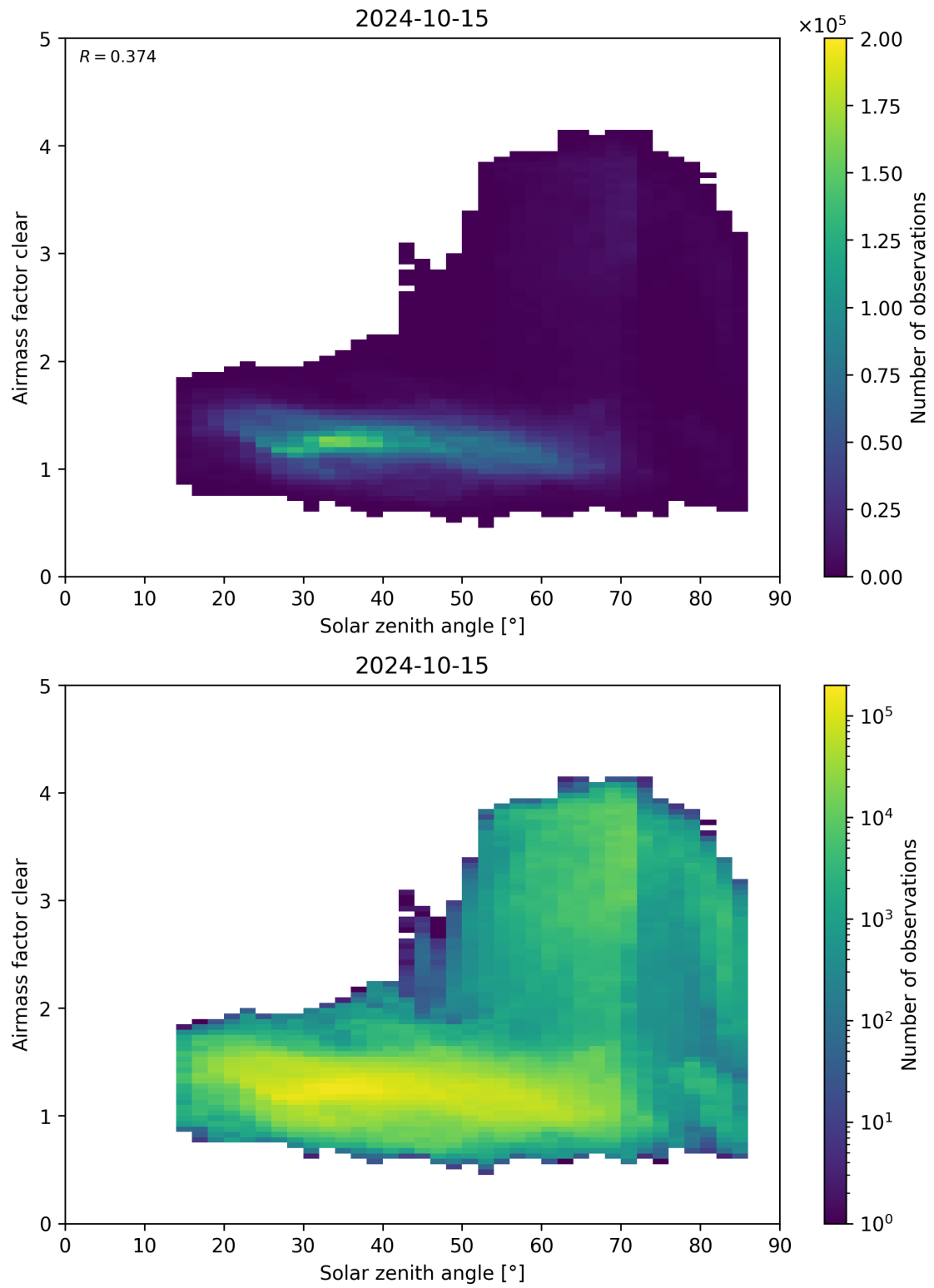
Figure 170: Scatter density plot of “Solar zenith angle” against “Airmass factor clear” for 2024-10-14 to 2024-10-16.
