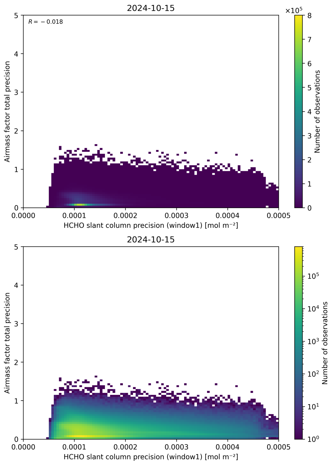
Figure 95: Scatter density plot of “HCHO slant column precision (window1)” against “Airmass factor total precision” for 2024-10-14 to 2024-10-16.
