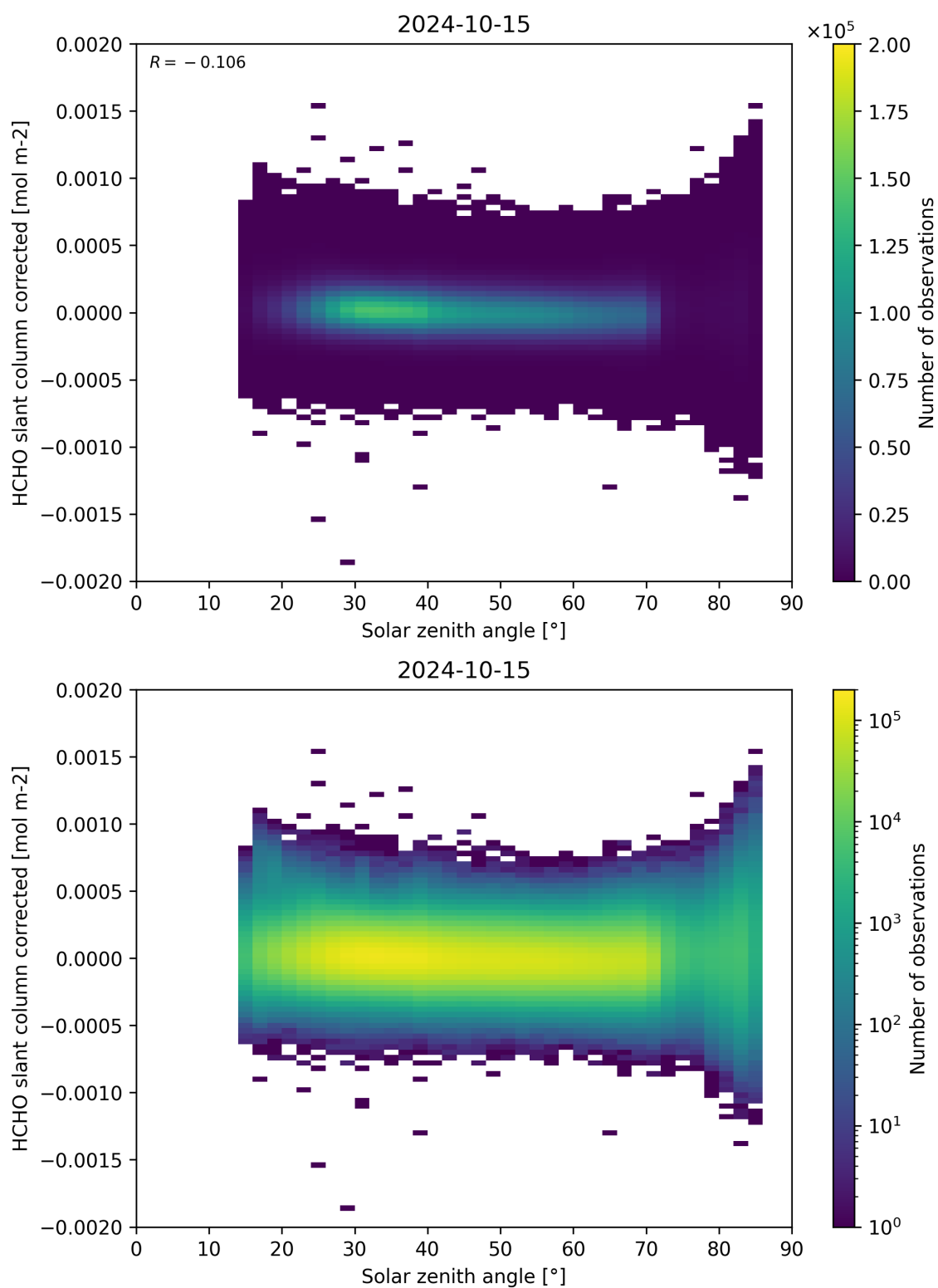
Figure 171: Scatter density plot of “Solar zenith angle” against “HCHO slant column corrected” for 2024-10-14 to 2024-10-16.
