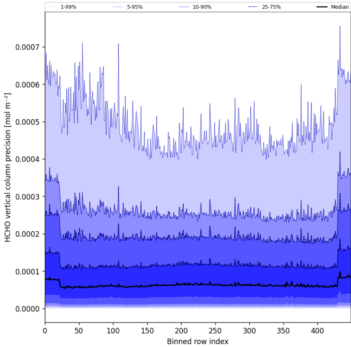
Figure 50: Along track statistics of “HCHO vertical column precision” for 2024-10-14 to 2024-10-16
