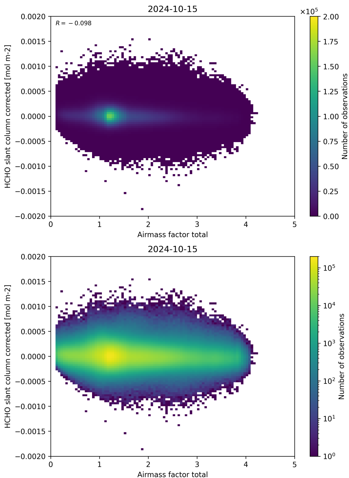
Figure 101: Scatter density plot of “Airmass factor total” against “HCHO slant column corrected” for 2024-10-14 to 2024-10-16.
