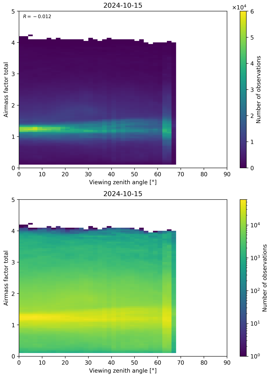
Figure 190: Scatter density plot of “Viewing zenith angle” against “Airmass factor total” for 2024-10-14 to 2024-10-16.
