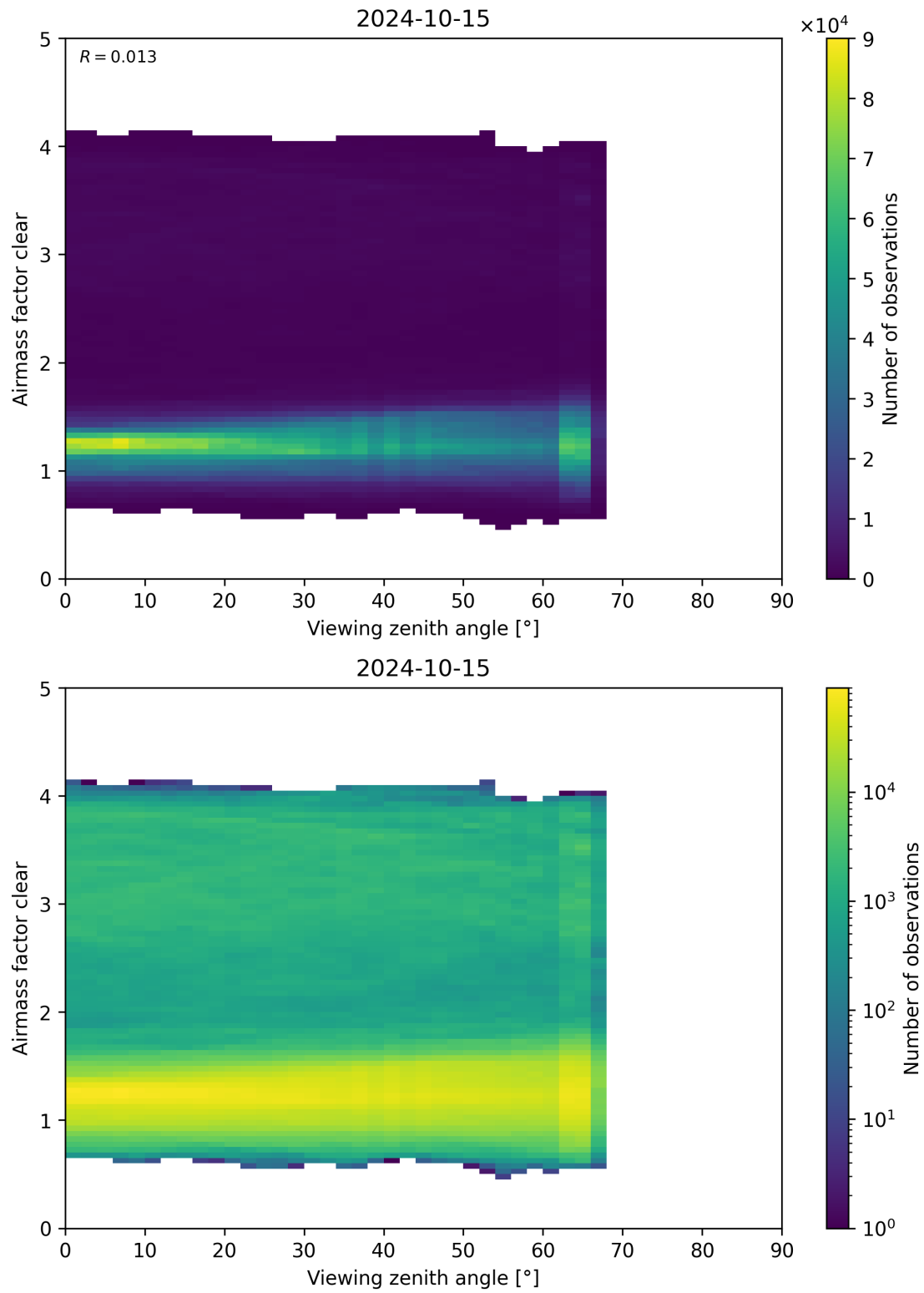
Figure 185: Scatter density plot of “Viewing zenith angle” against “Airmass factor clear” for 2024-10-14 to 2024-10-16.
