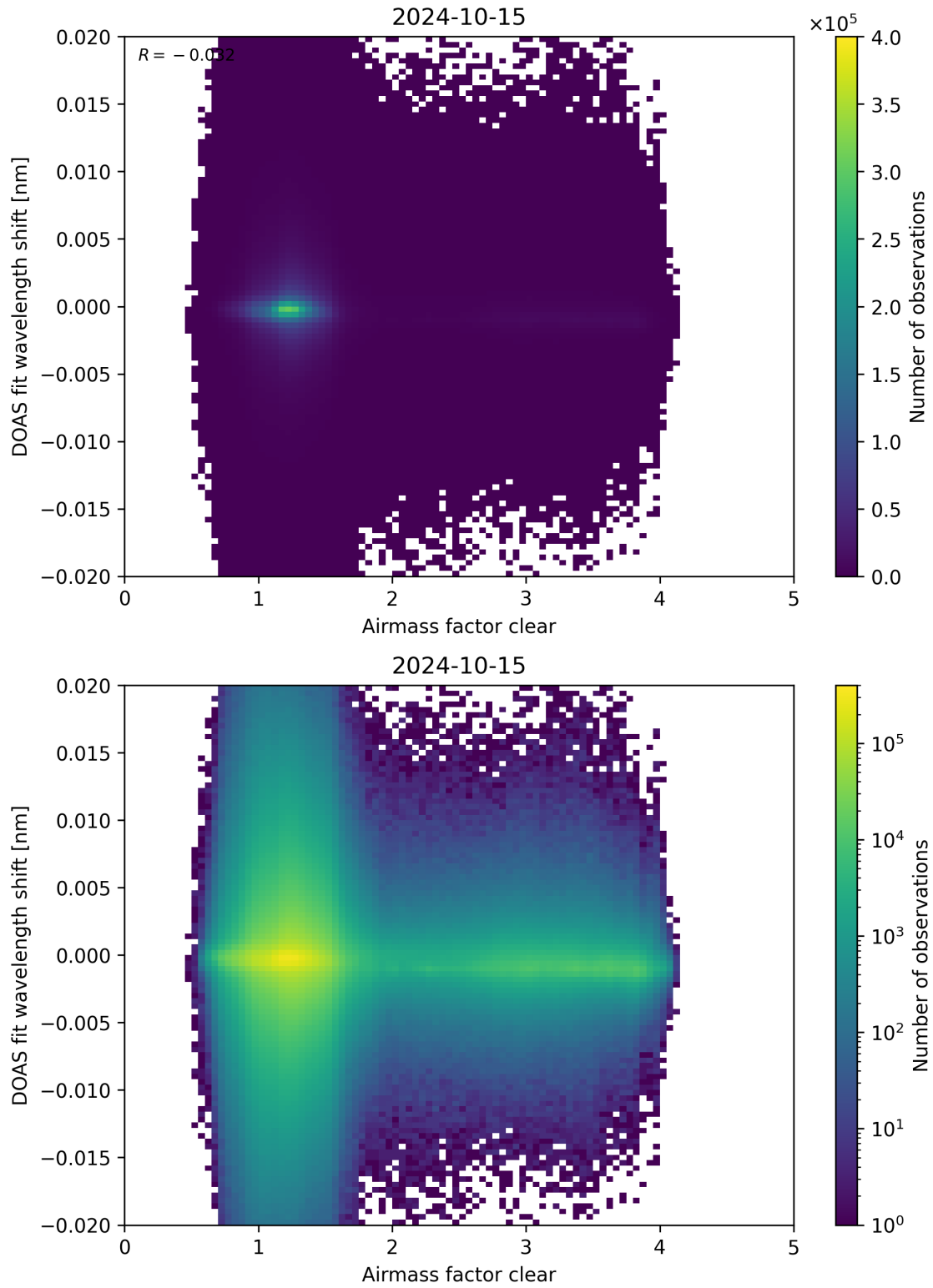
Figure 72: Scatter density plot of “Airmass factor clear” against “DOAS fit wavelength shift” for 2024-10-14 to 2024-10-16.
