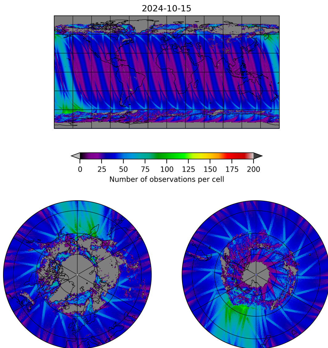
Figure 19: Map of the number of observations for 2024-10-14 to 2024-10-16
