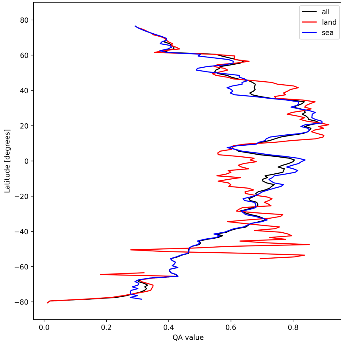
Figure 20: Zonal average of “QA value” for 2024-10-14 to 2024-10-16.
