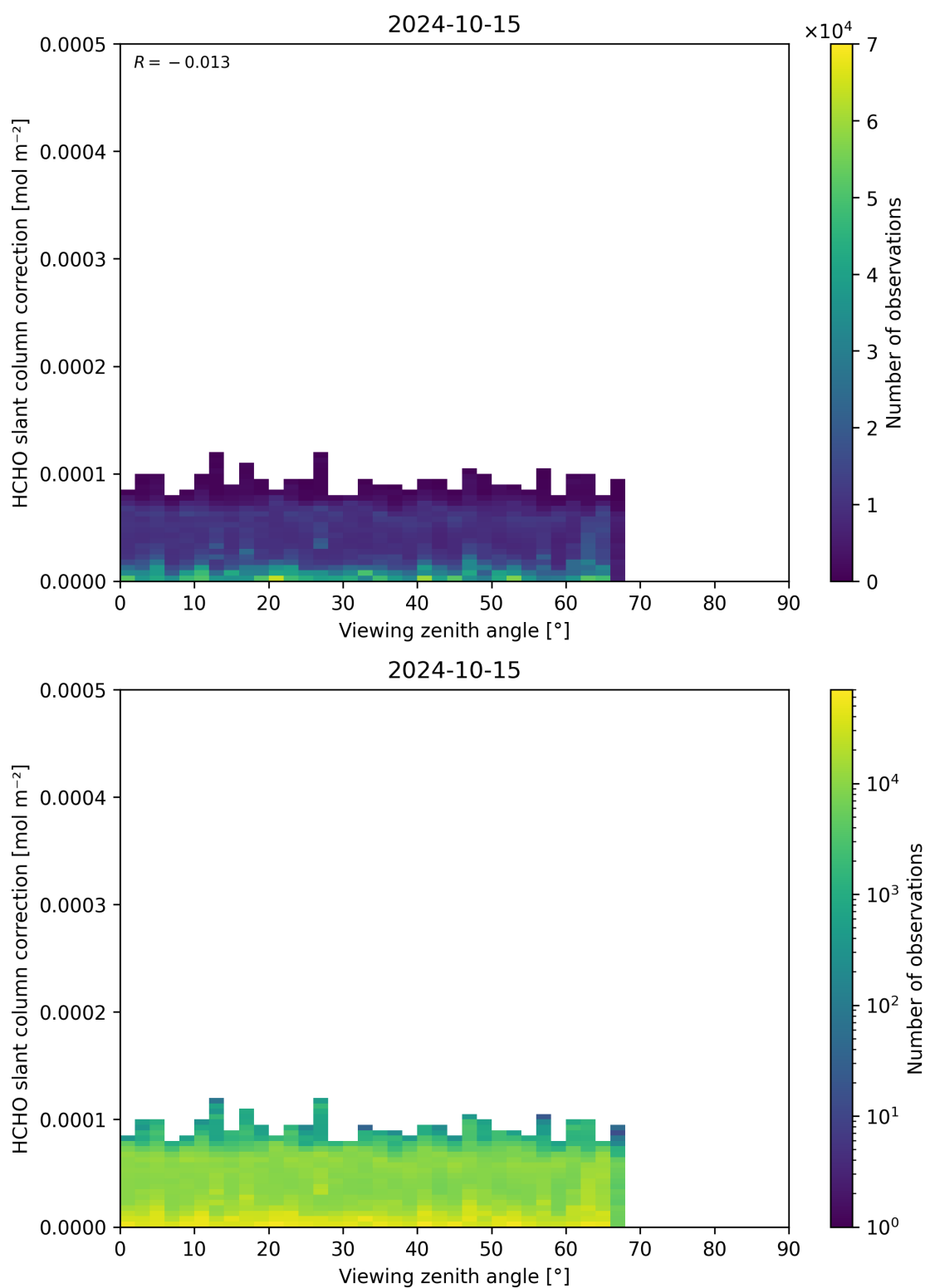
Figure 187: Scatter density plot of “Viewing zenith angle” against “HCHO slant column correction” for 2024-10-14 to 2024-10-16.
