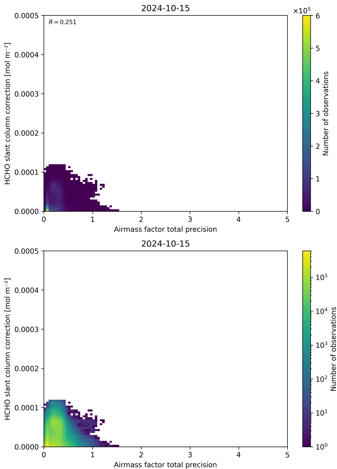
Figure 110: Scatter density plot of “Airmass factor total precision” against “HCHO slant column correction” for 2024-10-14 to 2024-10-16.
