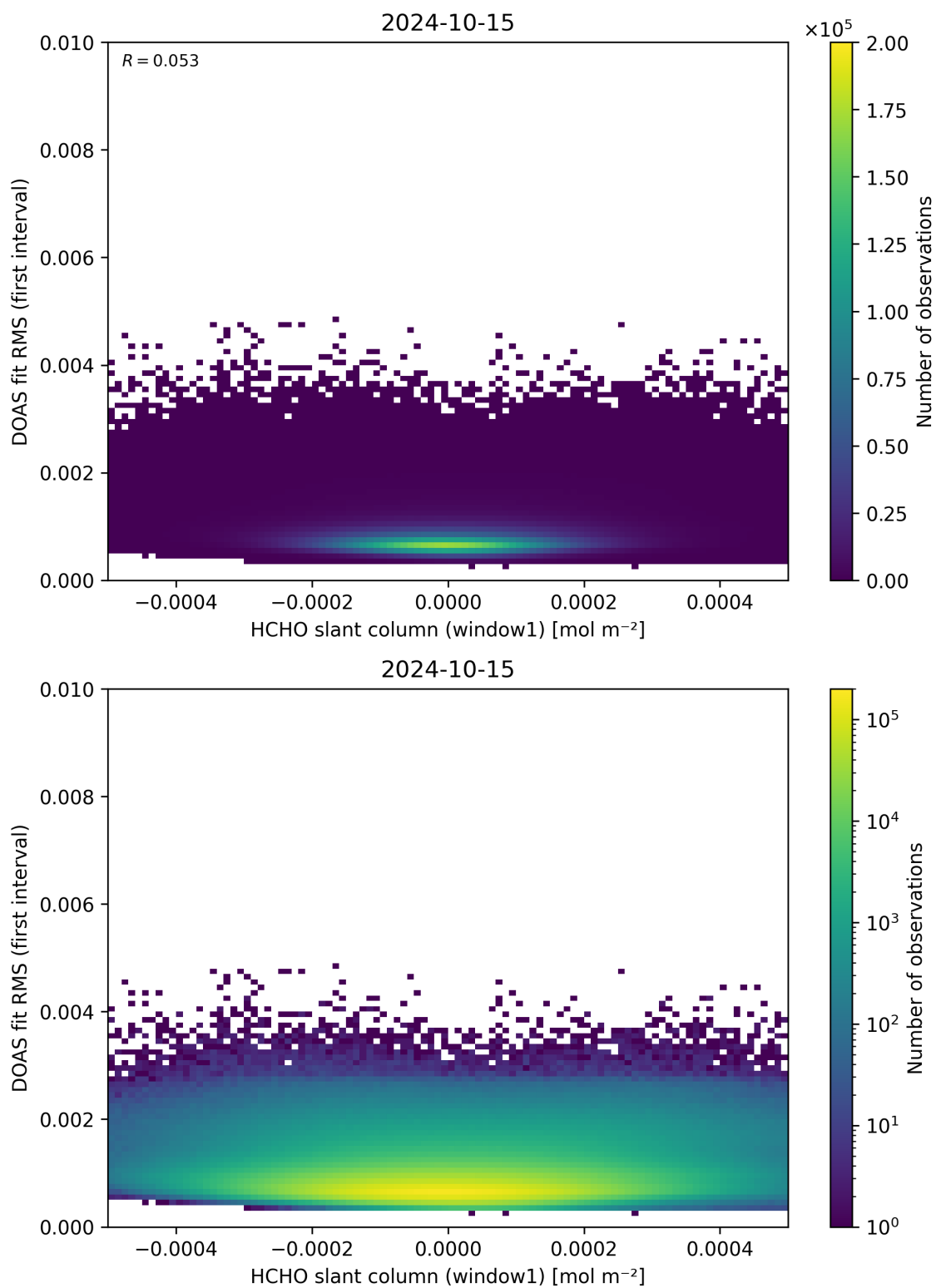
Figure 78: Scatter density plot of “HCHO slant column (window1)” against “DOAS fit RMS (first interval)” for 2024-10-14 to 2024-10-16.
