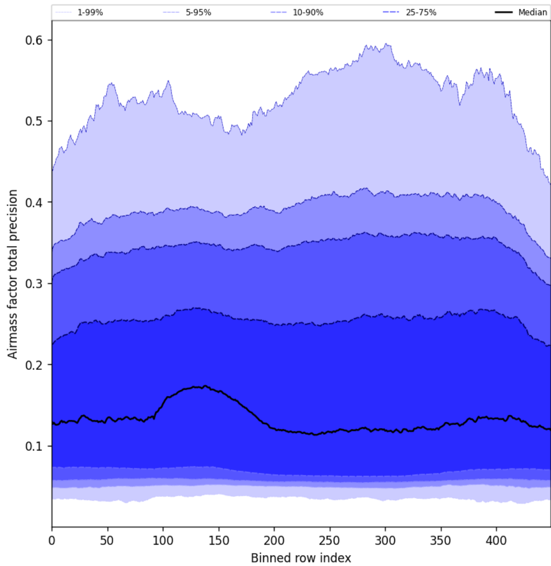
Figure 55: Along track statistics of “Airmass factor total precision” for 2024-10-14 to 2024-10-16
