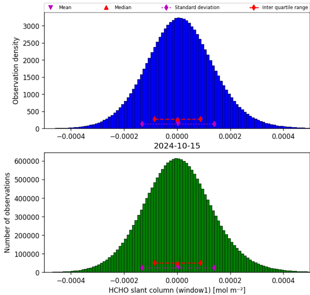
Figure 38: Histogram of “HCHO slant column (window1)” for 2024-10-14 to 2024-10-16
