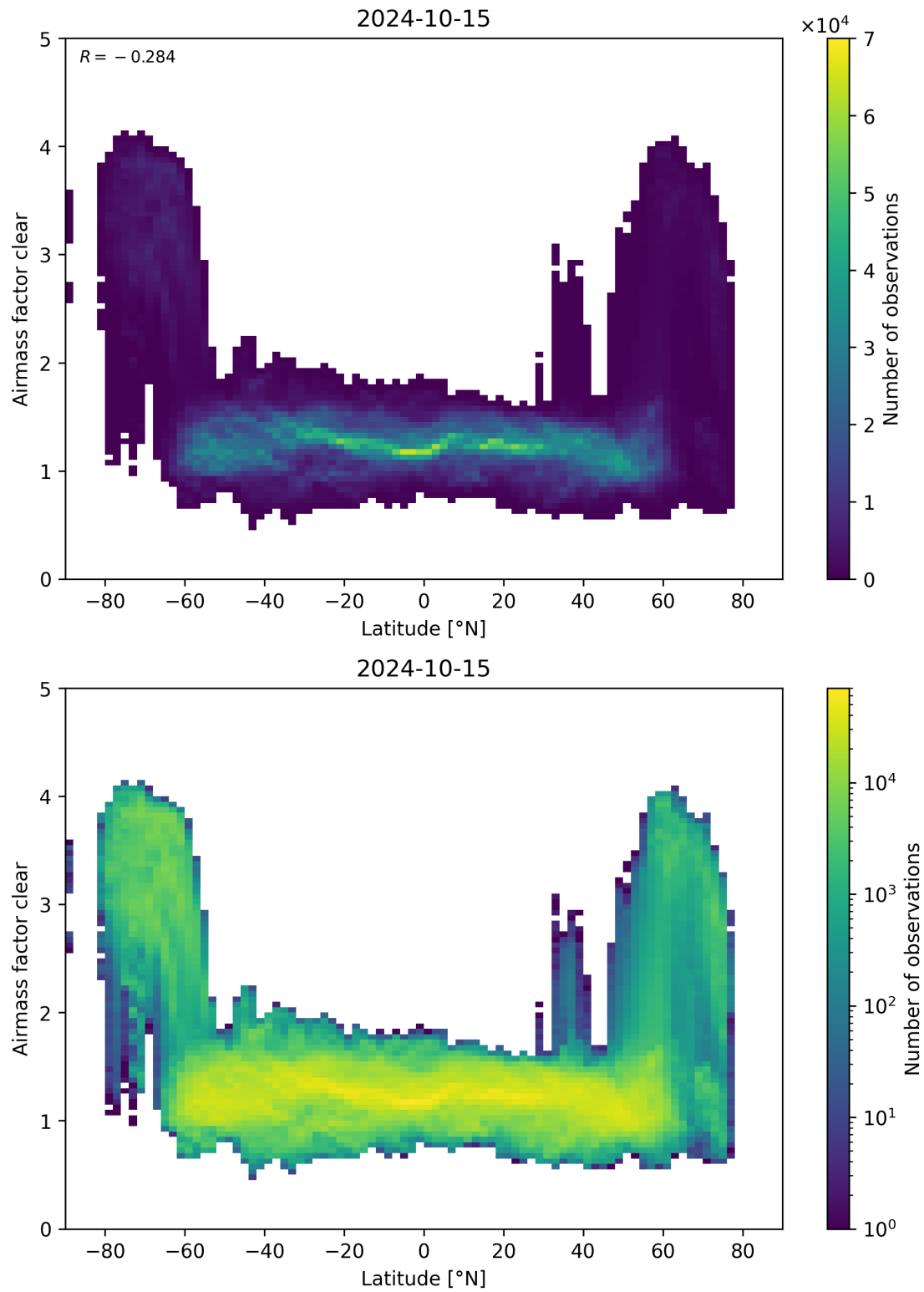
Figure 156: Scatter density plot of “Latitude” against “Airmass factor clear” for 2024-10-14 to 2024-10-16.
