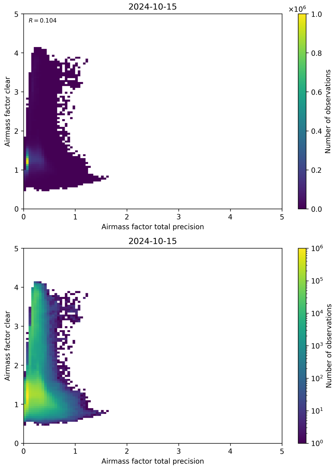
Figure 108: Scatter density plot of “Airmass factor total precision” against “Airmass factor clear” for 2024-10-14 to 2024-10-16.
