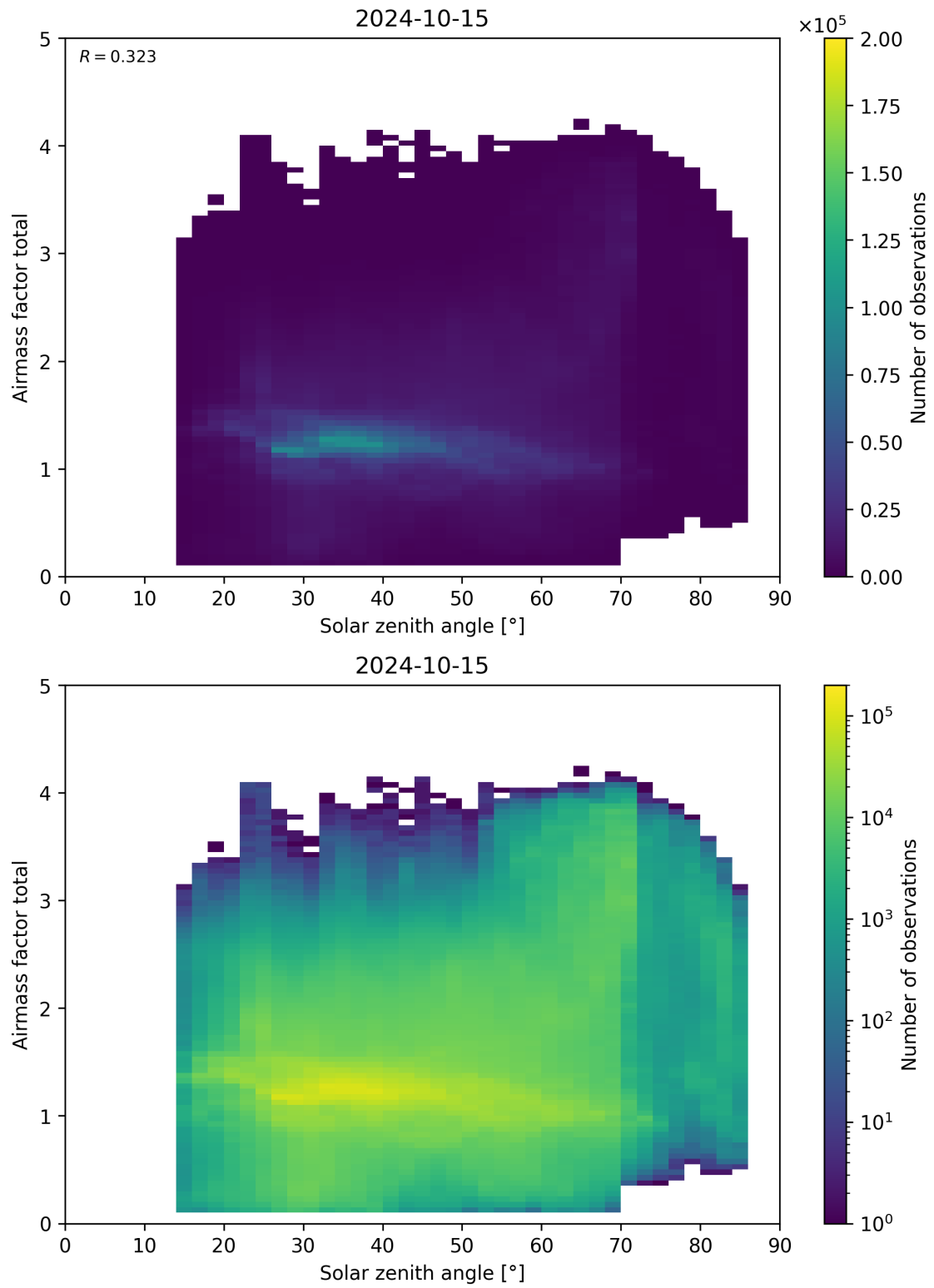
Figure 175: Scatter density plot of “Solar zenith angle” against “Airmass factor total” for 2024-10-14 to 2024-10-16.
