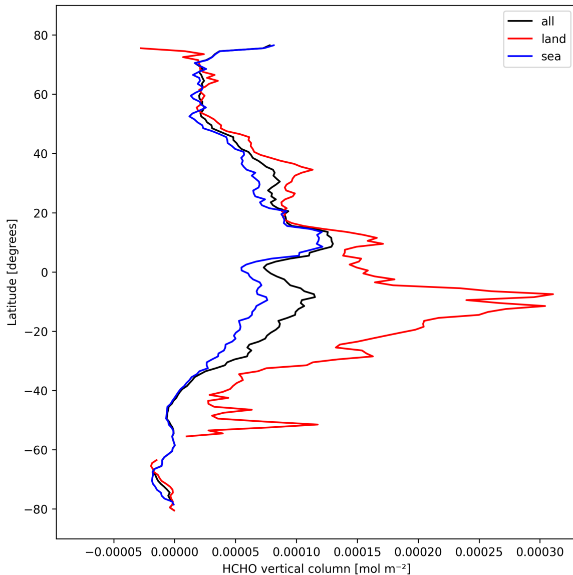
Figure 21: Zonal average of “HCHO vertical column” for 2024-10-14 to 2024-10-16.
