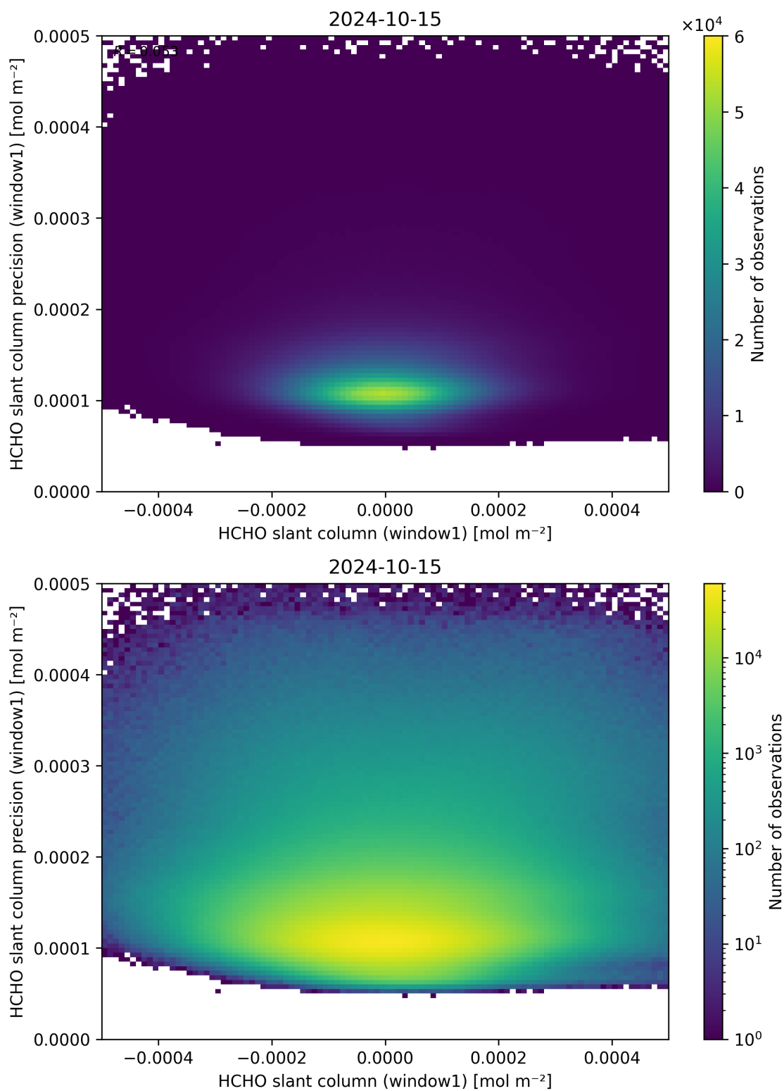
Figure 84: Scatter density plot of “HCHO slant column (window1)” against “HCHO slant column precision (window1)” for 2024-10-14 to 2024-10-16.
