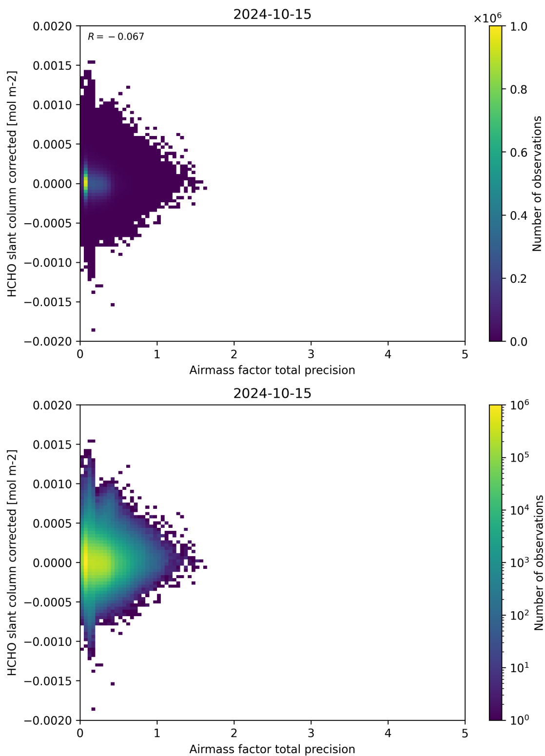
Figure 109: Scatter density plot of “Airmass factor total precision” against “HCHO slant column corrected” for 2024-10-14 to 2024-10-16.
