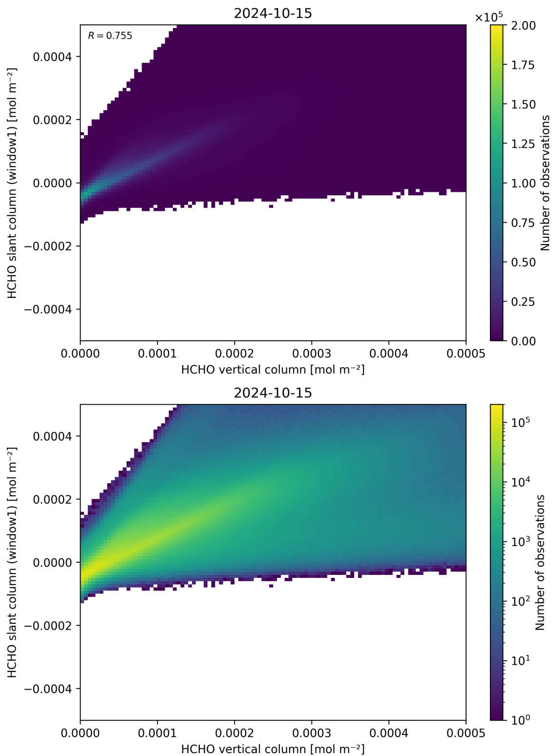
Figure 129: Scatter density plot of “HCHO vertical column” against “HCHO slant column (window1)” for 2024-10-14 to 2024-10-16.
