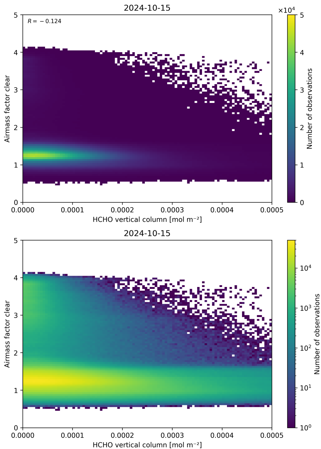
Figure 126: Scatter density plot of “HCHO vertical column” against “Airmass factor clear” for 2024-10-14 to 2024-10-16.
