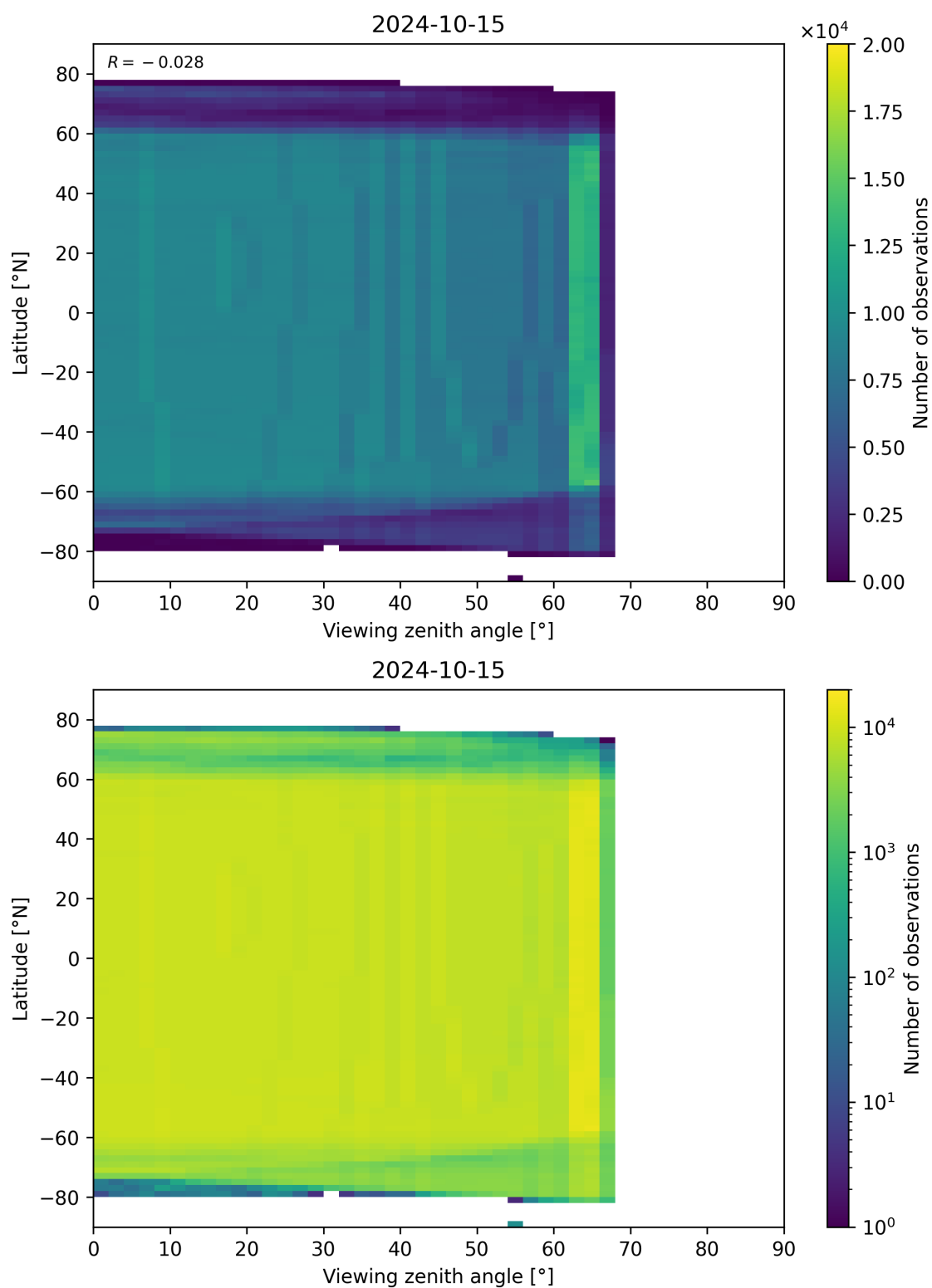
Figure 196: Scatter density plot of “Viewing zenith angle” against “Latitude” for 2024-10-14 to 2024-10-16.
