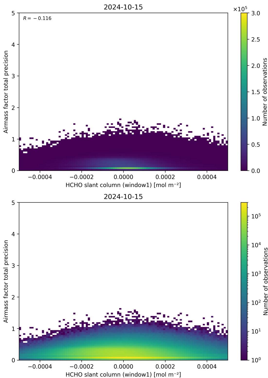
Figure 86: Scatter density plot of “HCHO slant column (window1)” against “Airmass factor total precision” for 2024-10-14 to 2024-10-16.
