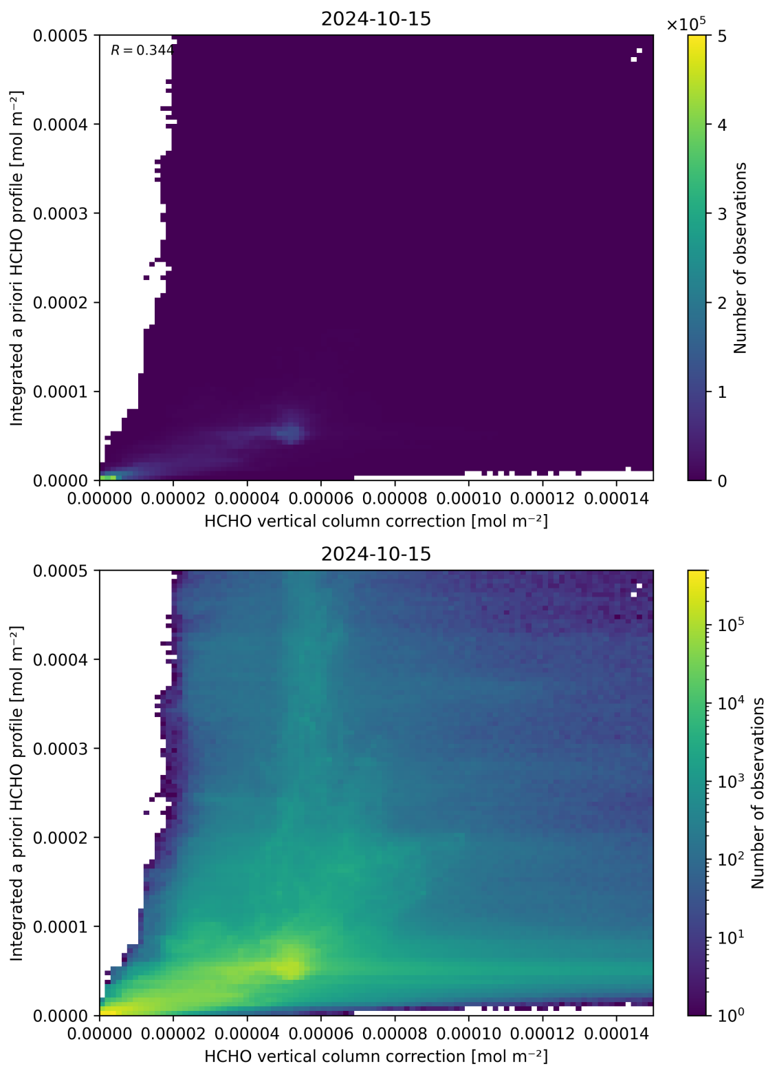
Figure 122: Scatter density plot of “HCHO vertical column correction” against “Integrated a priori HCHO profile” for 2024-10-14 to 2024-10-16.
