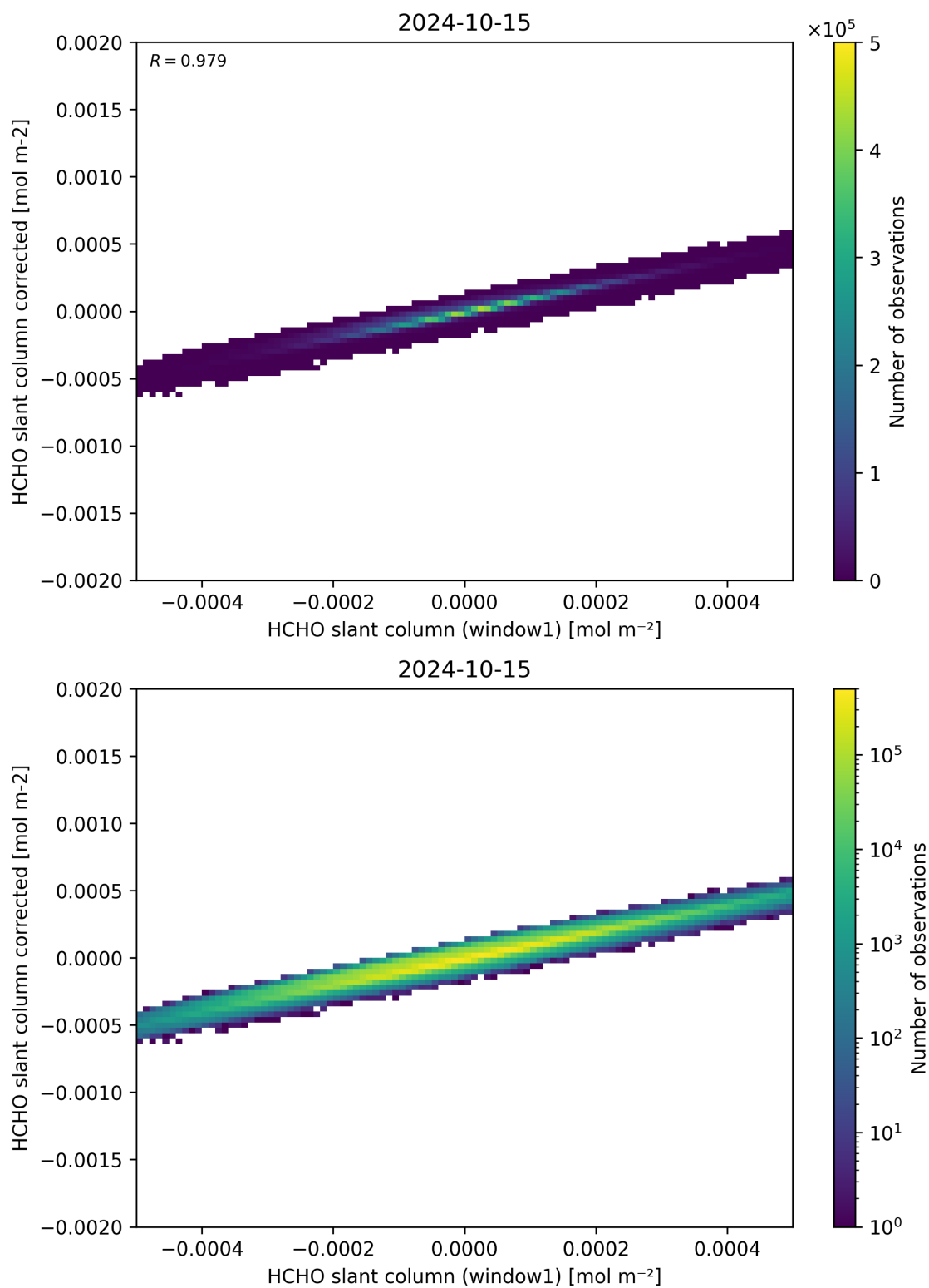
Figure 82: Scatter density plot of “HCHO slant column (window1)” against “HCHO slant column corrected” for 2024-10-14 to 2024-10-16.
