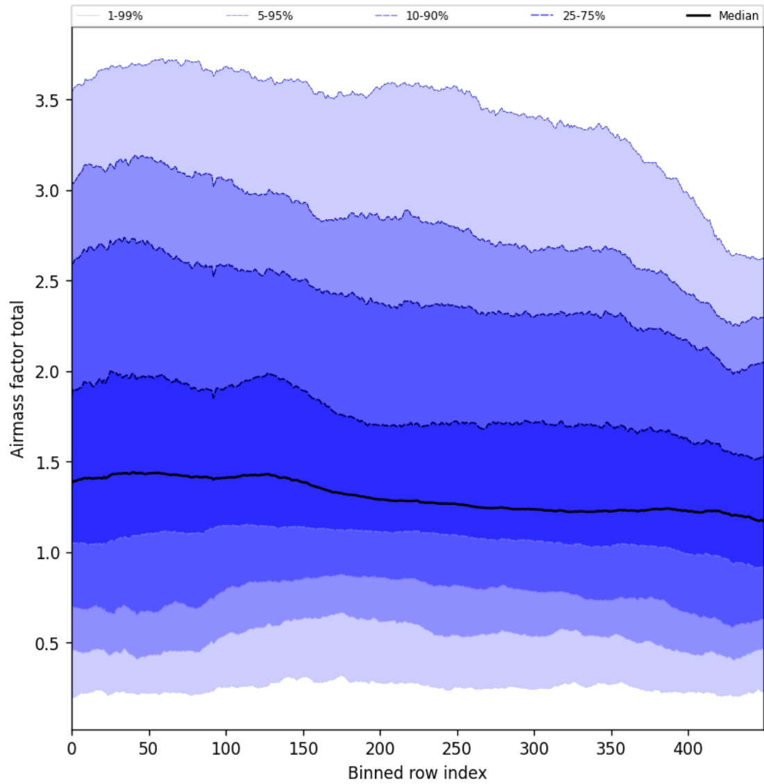
Figure 54: Along track statistics of “Airmass factor total” for 2024-10-14 to 2024-10-16
