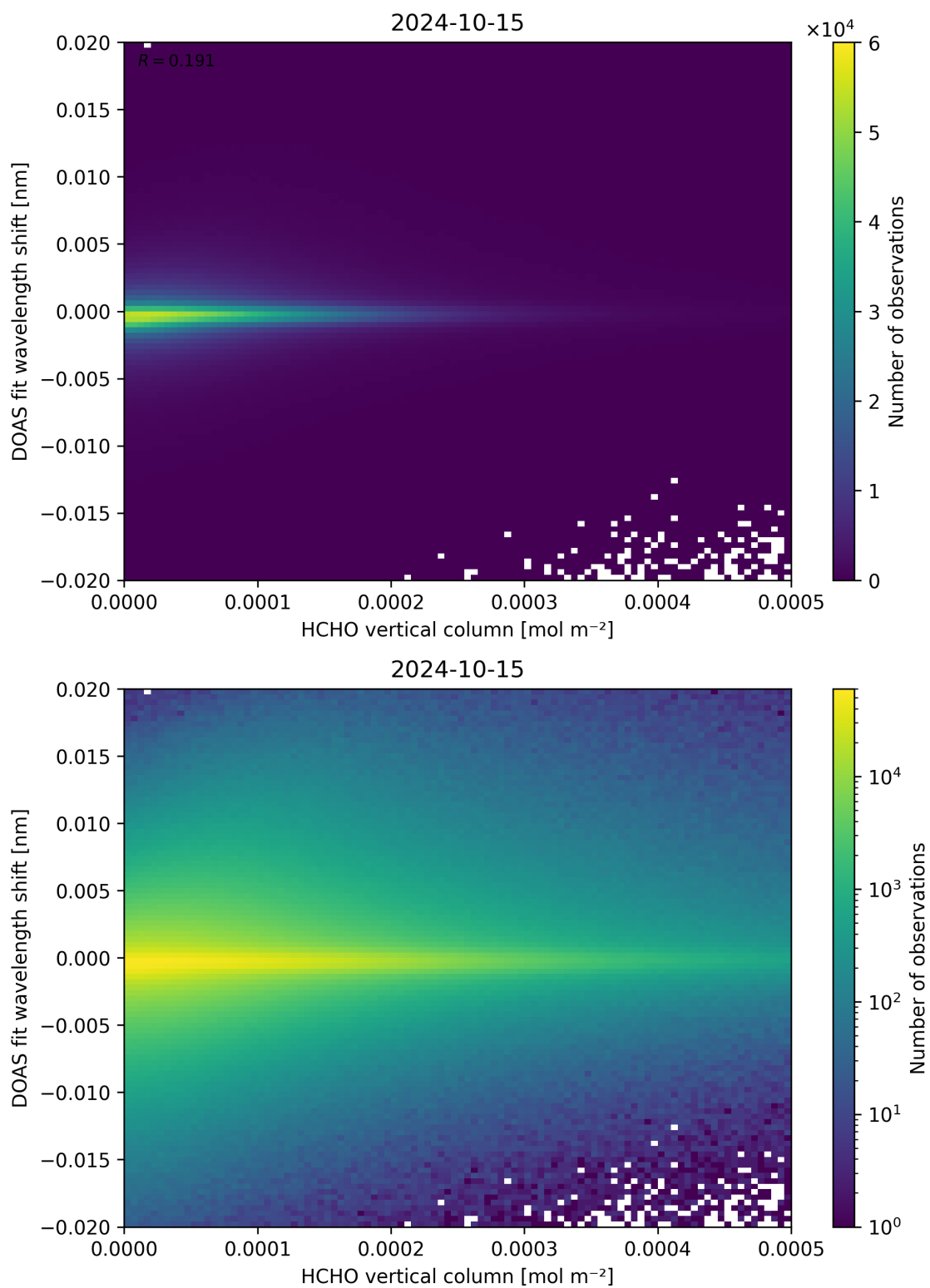
Figure 124: Scatter density plot of “HCHO vertical column” against “DOAS fit wavelength shift” for 2024-10-14 to 2024-10-16.
