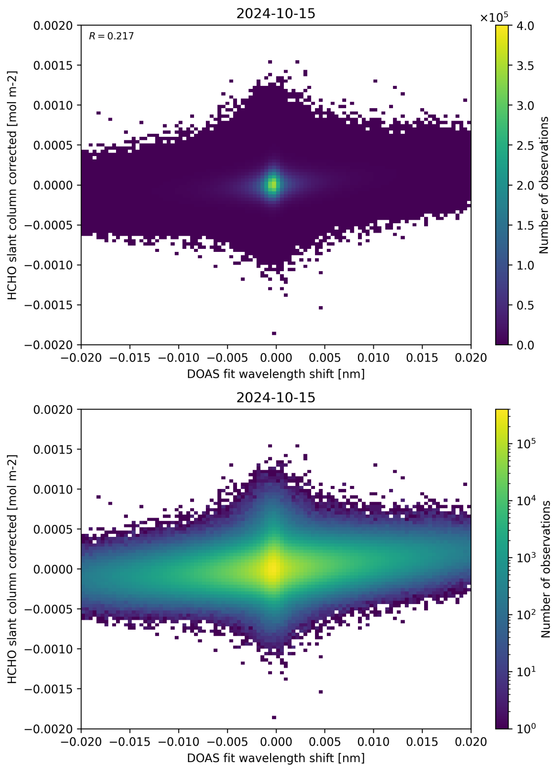
Figure 66: Scatter density plot of “DOAS fit wavelength shift” against “HCHO slant column corrected” for 2024-10-14 to 2024-10-16.
