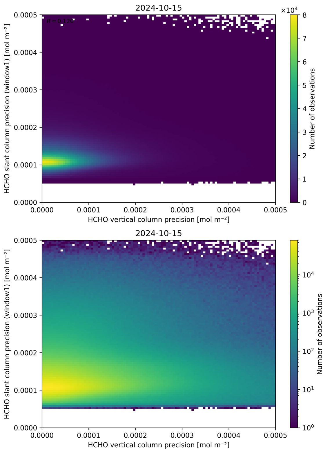
Figure 143: Scatter density plot of “HCHO vertical column precision” against “HCHO slant column precision (window1)” for 2024-10-14 to 2024-10-16.
