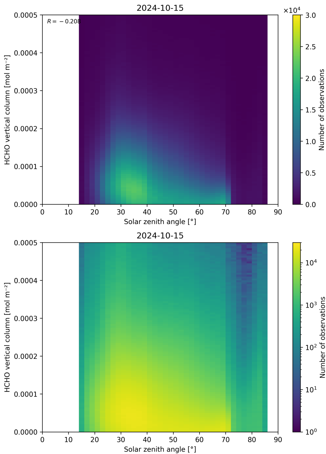
Figure 177: Scatter density plot of “Solar zenith angle” against “HCHO vertical column” for 2024-10-14 to 2024-10-16.
