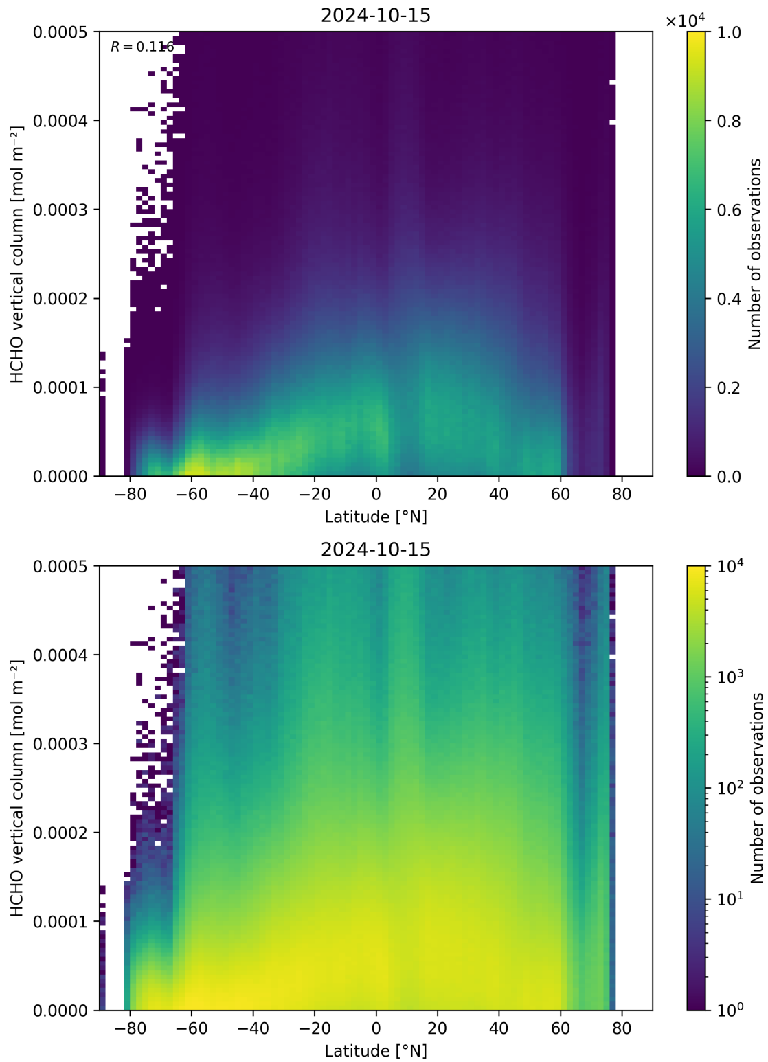
Figure 163: Scatter density plot of “Latitude” against “HCHO vertical column” for 2024-10-14 to 2024-10-16.
