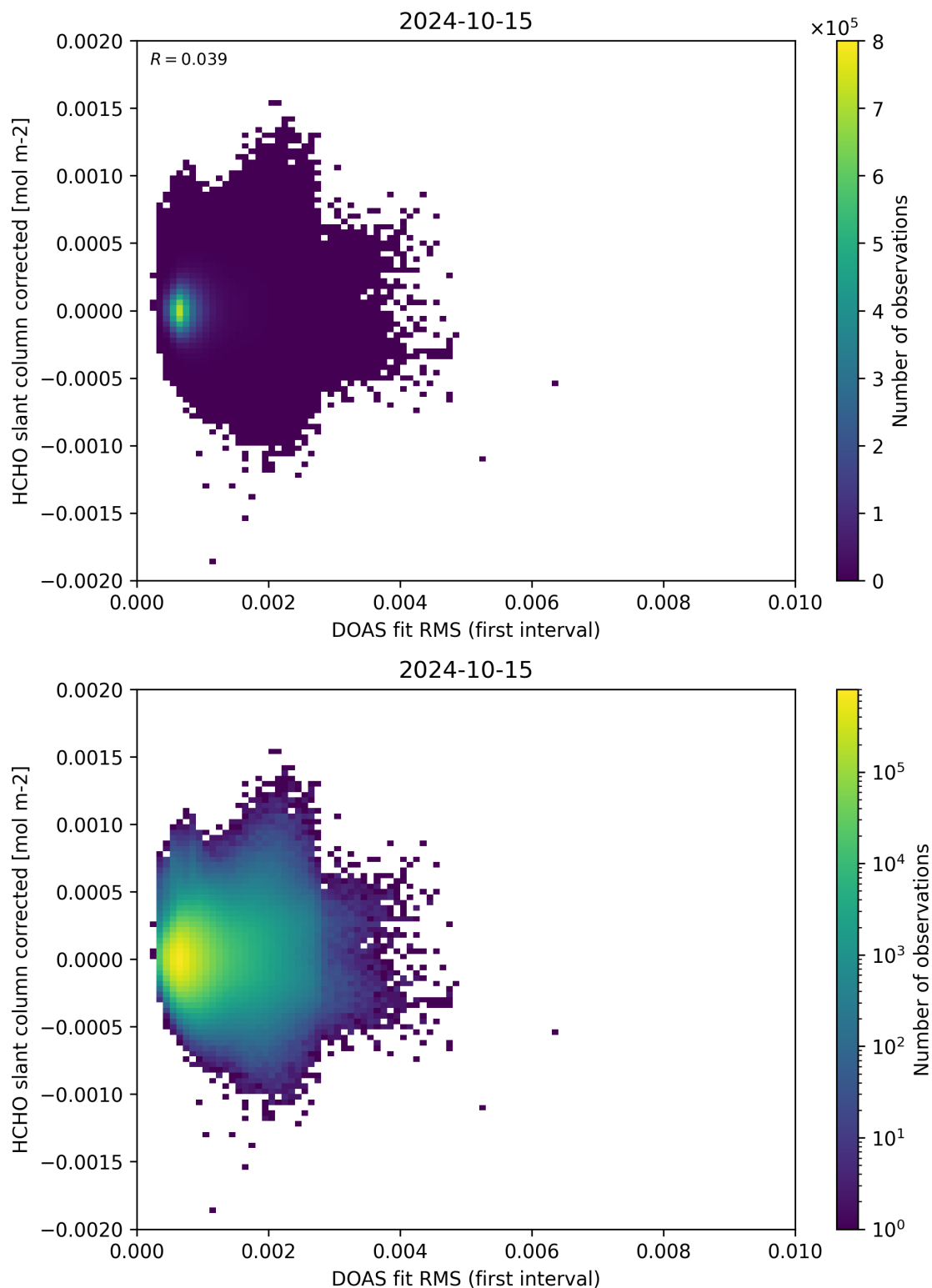
Figure 62: Scatter density plot of “DOAS fit RMS (first interval)” against “HCHO slant column corrected” for 2024-10-14 to 2024-10-16.
