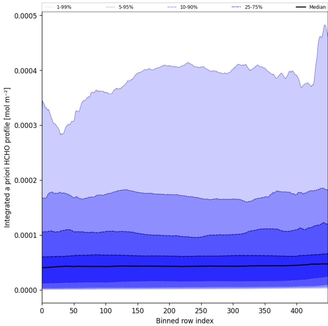
Figure 57: Along track statistics of “Integrated a priori HCHO profile” for 2024-10-14 to 2024-10-16
