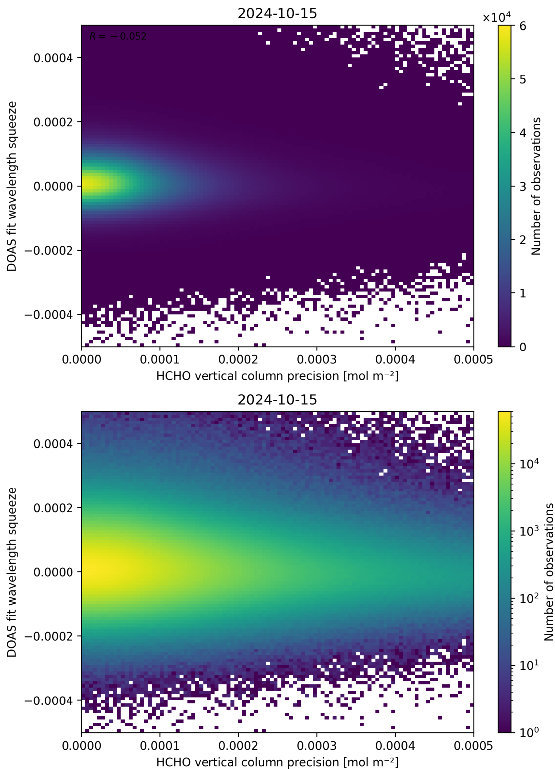
Figure 138: Scatter density plot of “HCHO vertical column precision” against “DOAS fit wavelength squeeze” for 2024-10-14 to 2024-10-16.
