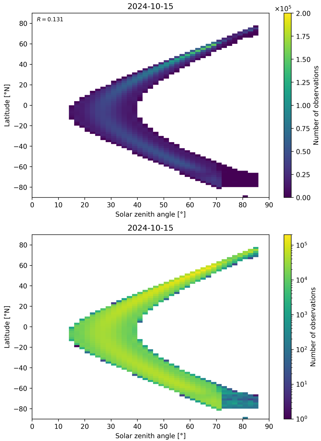
Figure 181: Scatter density plot of “Solar zenith angle” against “Latitude” for 2024-10-14 to 2024-10-16.
