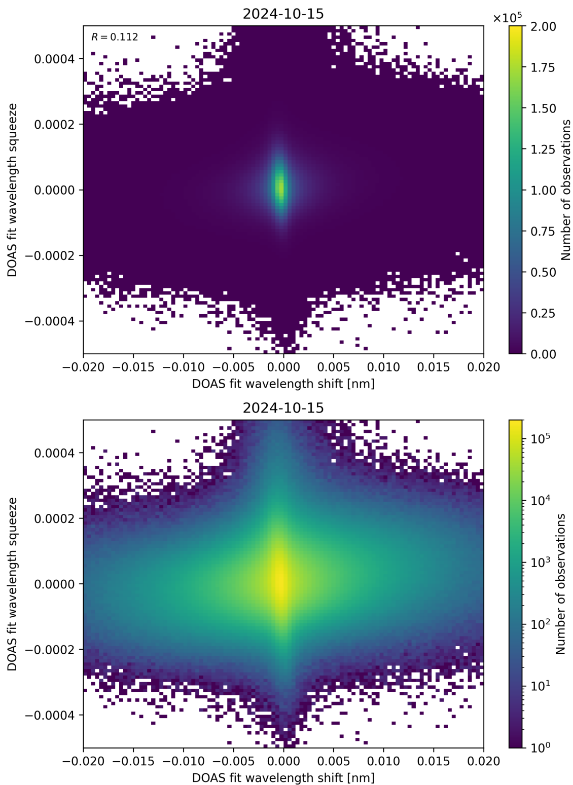
Figure 65: Scatter density plot of “DOAS fit wavelength shift” against “DOAS fit wavelength squeeze” for 2024-10-14 to 2024-10-16.
