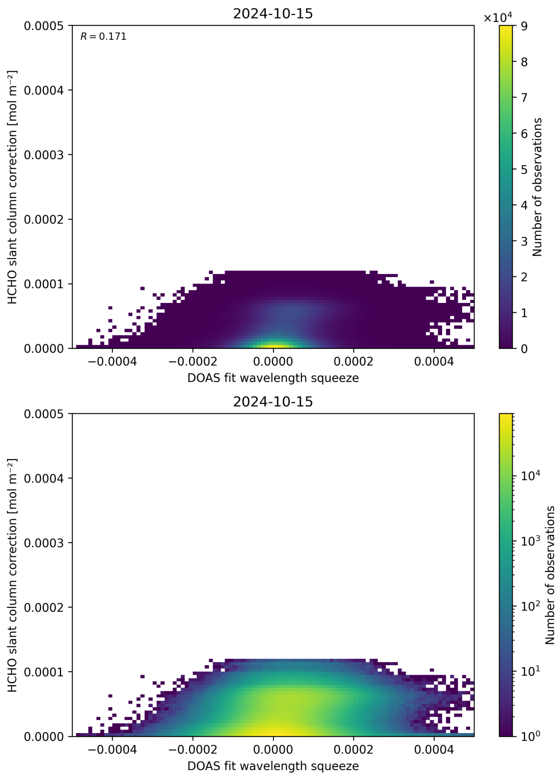
Figure 70: Scatter density plot of “DOAS fit wavelength squeeze” against “HCHO slant column correction” for 2024-10-14 to 2024-10-16.
