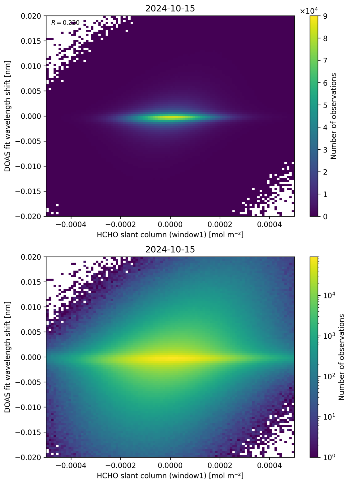
Figure 79: Scatter density plot of “HCHO slant column (window1)” against “DOAS fit wavelength shift” for 2024-10-14 to 2024-10-16.
