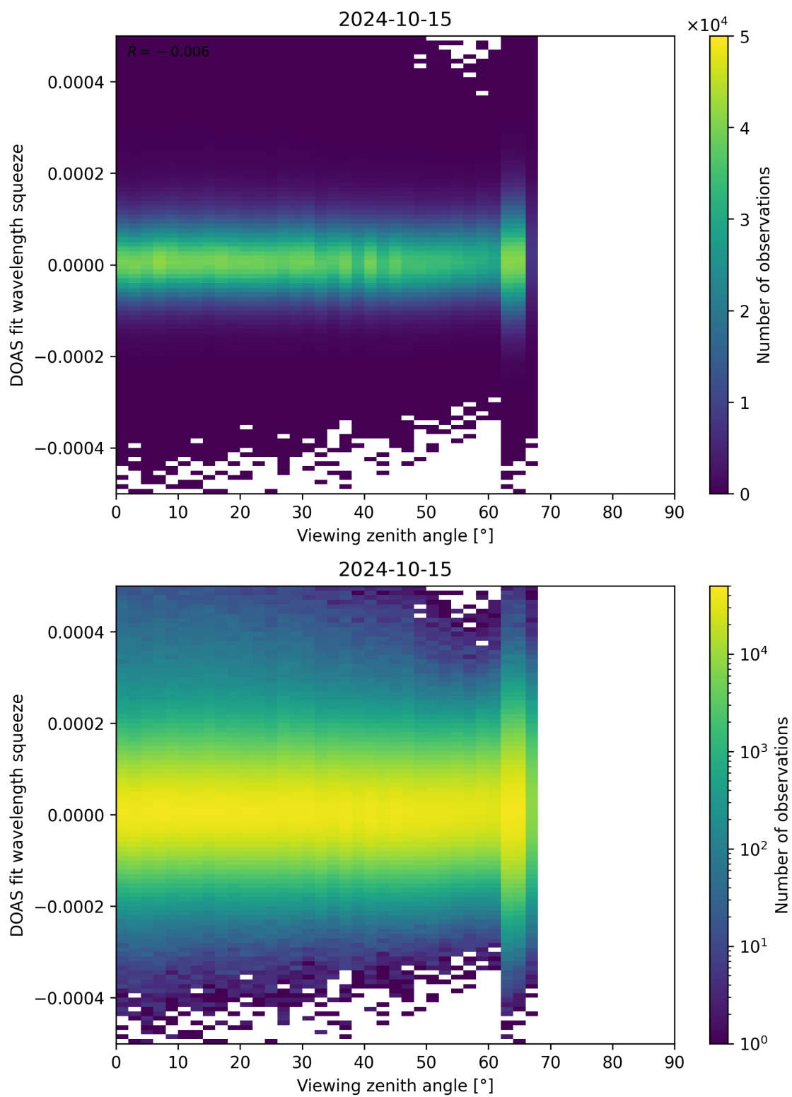
Figure 184: Scatter density plot of “Viewing zenith angle” against “DOAS fit wavelength squeeze” for 2024-10-14 to 2024-10-16.
