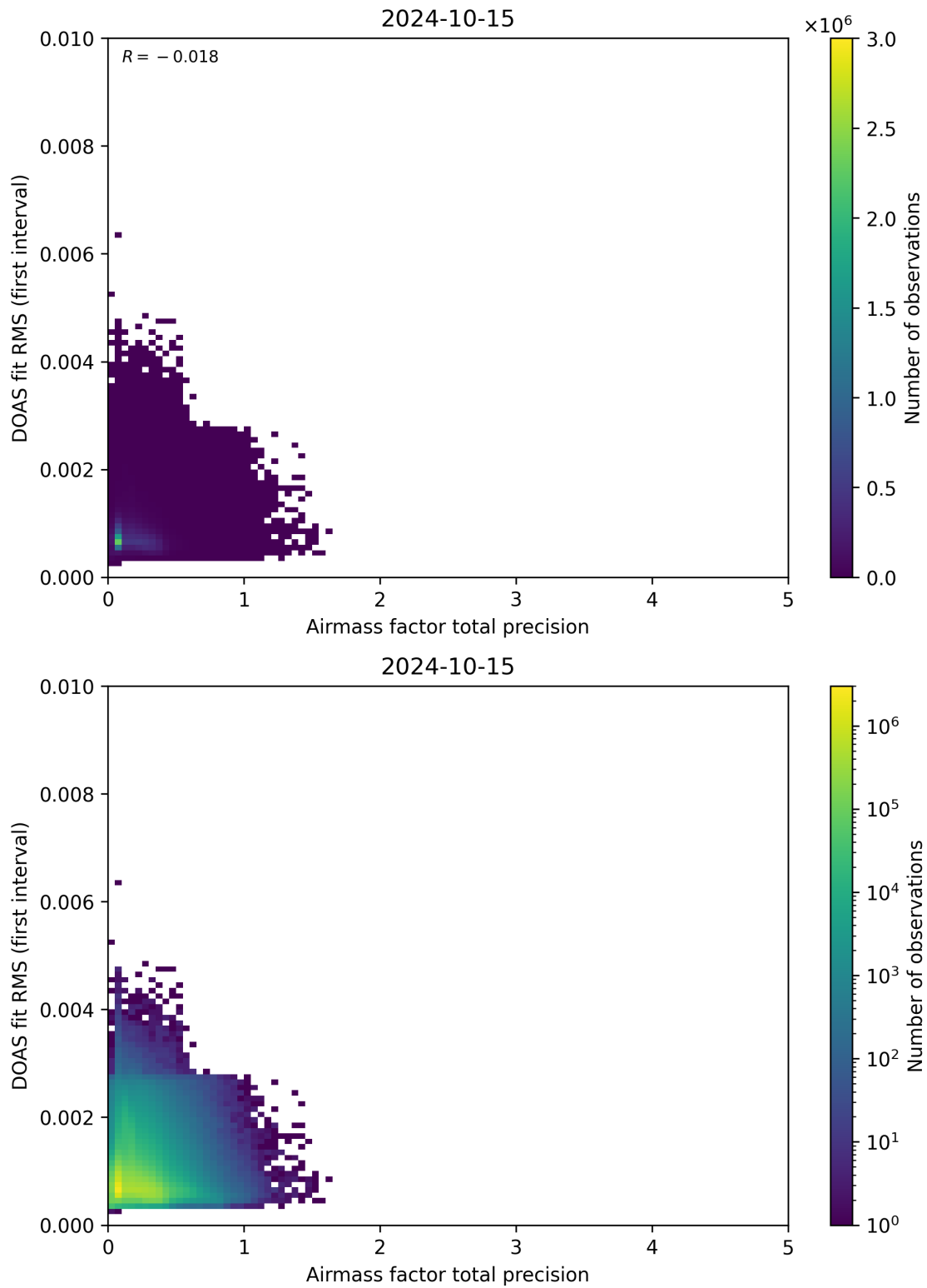
Figure 105: Scatter density plot of “Airmass factor total precision” against “DOAS fit RMS (first interval)” for 2024-10-14 to 2024-10-16.
