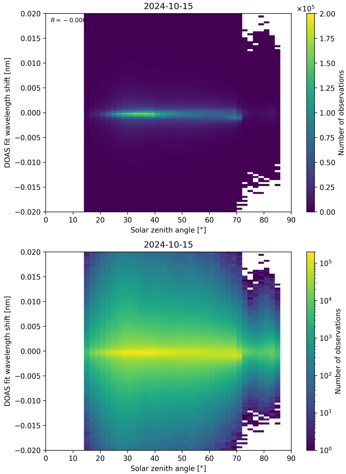
Figure 168: Scatter density plot of “Solar zenith angle” against “DOAS fit wavelength shift” for 2024-10-14 to 2024-10-16.
