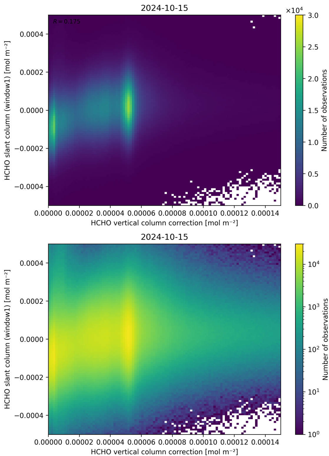
Figure 118: Scatter density plot of “HCHO vertical column correction” against “HCHO slant column (window1)” for 2024-10-14 to 2024-10-16.
