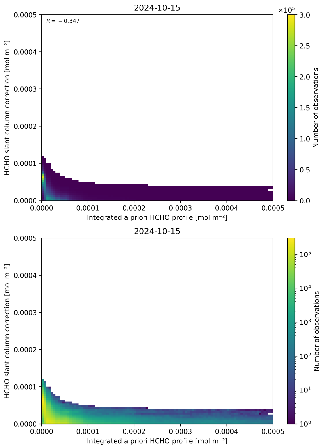
Figure 152: Scatter density plot of “Integrated a priori HCHO profile” against “HCHO slant column correction” for 2024-10-14 to 2024-10-16.
