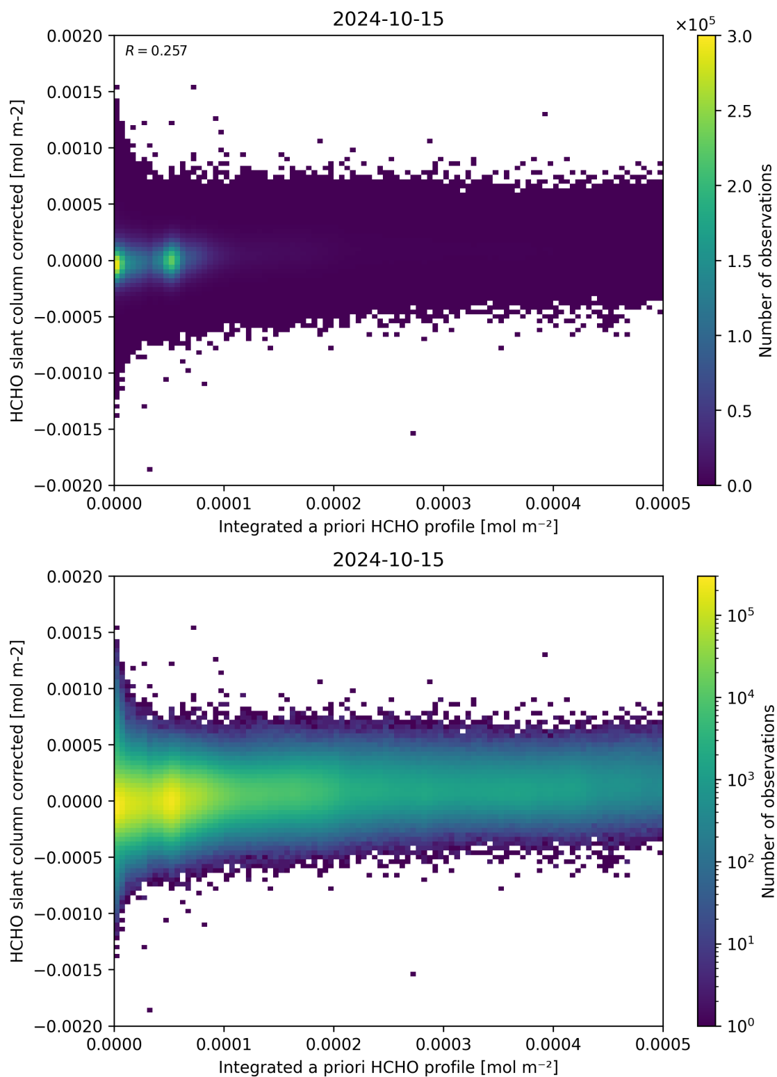
Figure 151: Scatter density plot of “Integrated a priori HCHO profile” against “HCHO slant column corrected” for 2024-10-14 to 2024-10-16.
