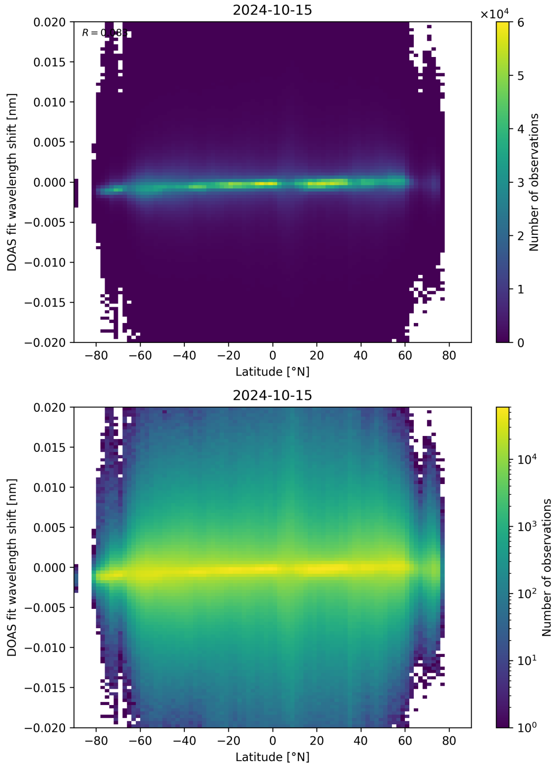
Figure 154: Scatter density plot of “Latitude” against “DOAS fit wavelength shift” for 2024-10-14 to 2024-10-16.
