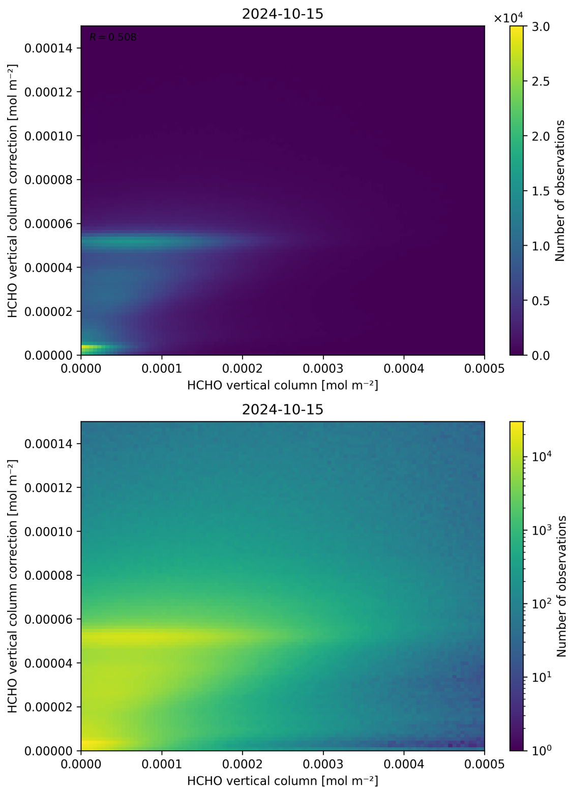
Figure 133: Scatter density plot of “HCHO vertical column” against “HCHO vertical column correction” for 2024-10-14 to 2024-10-16.
