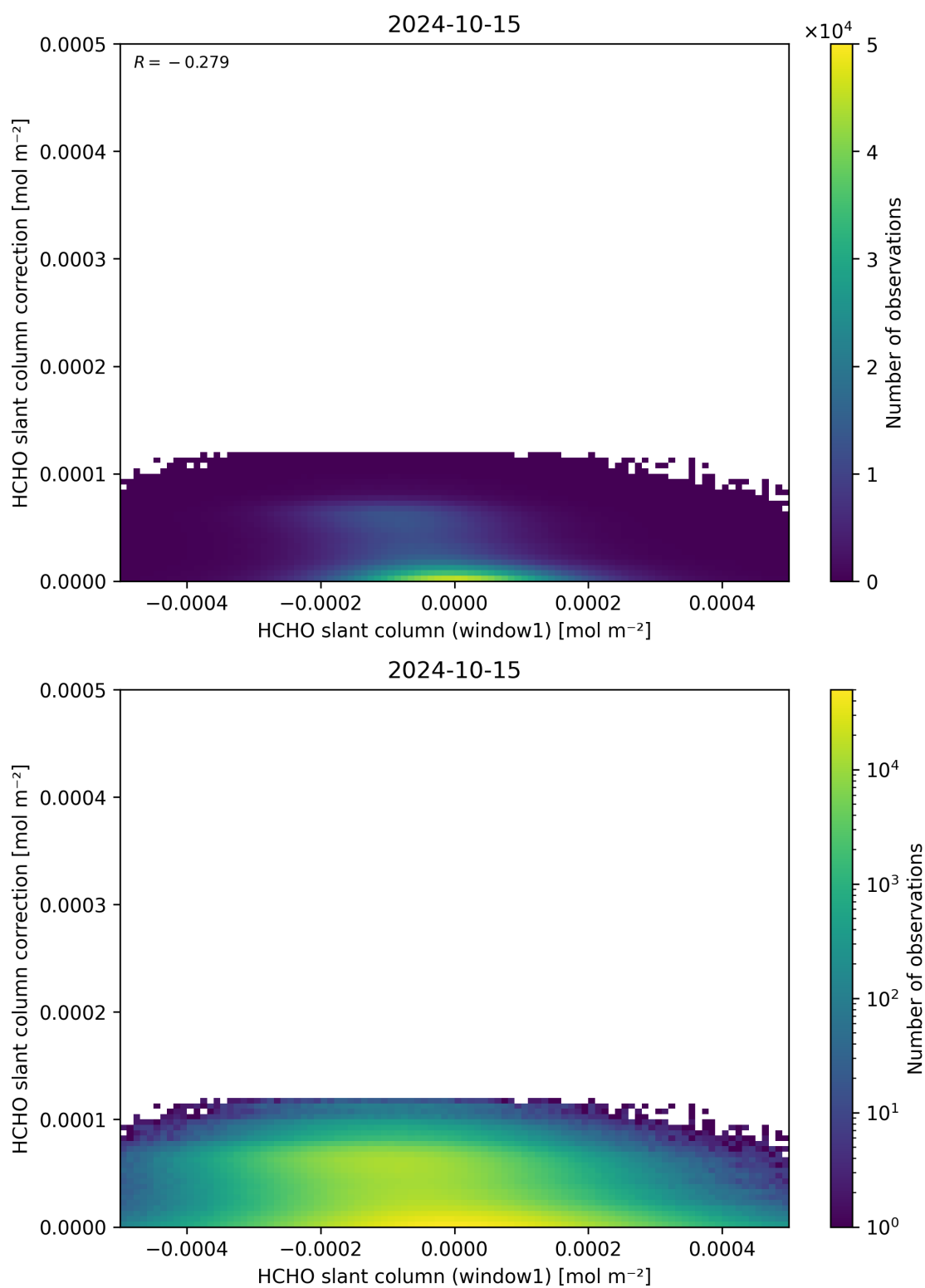
Figure 83: Scatter density plot of “HCHO slant column (window1)” against “HCHO slant column correction” for 2024-10-14 to 2024-10-16.
