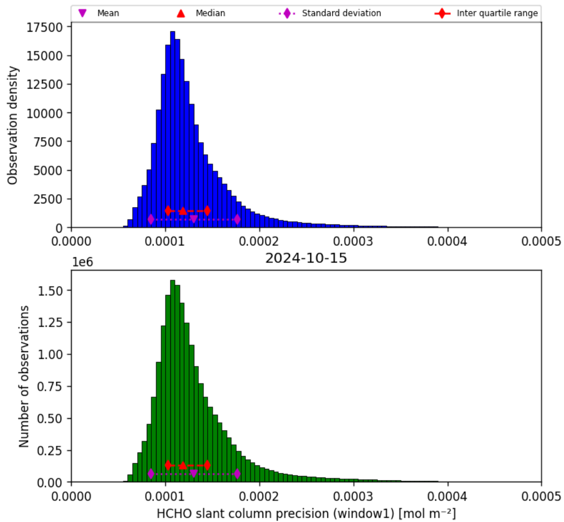
Figure 39: Histogram of “HCHO slant column precision (window1)” for 2024-10-14 to 2024-10-16
