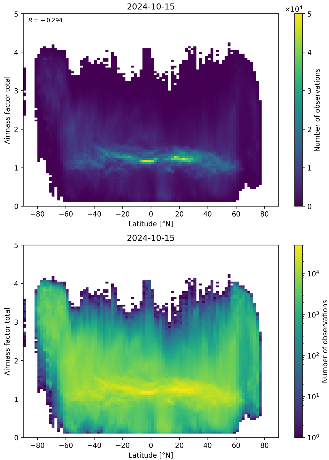
Figure 161: Scatter density plot of “Latitude” against “Airmass factor total” for 2024-10-14 to 2024-10-16.
