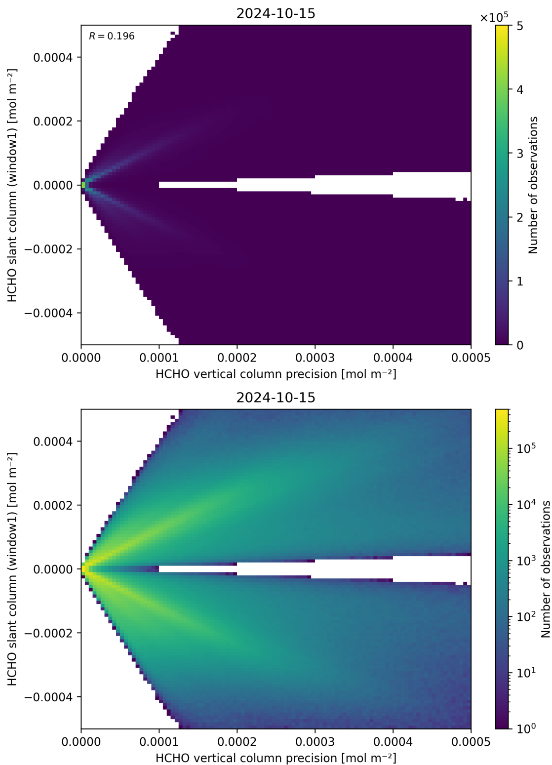
Figure 142: Scatter density plot of “HCHO vertical column precision” against “HCHO slant column (window1)” for 2024-10-14 to 2024-10-16.
