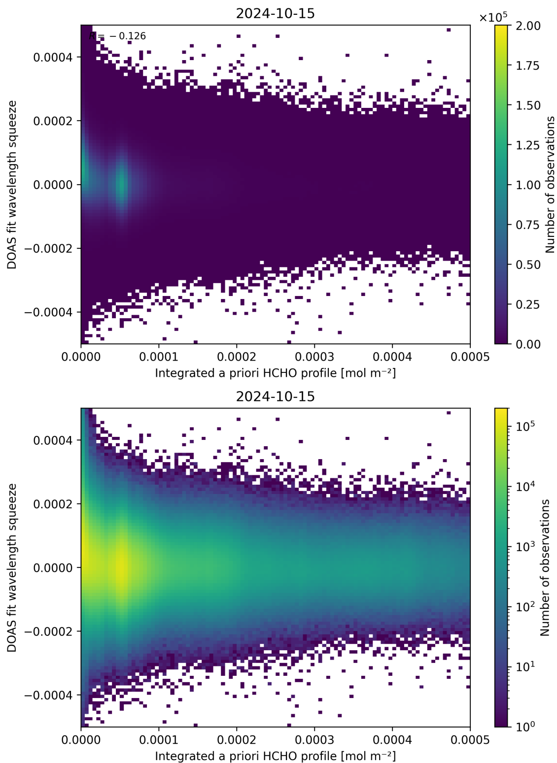
Figure 150: Scatter density plot of “Integrated a priori HCHO profile” against “DOAS fit wavelength squeeze” for 2024-10-14 to 2024-10-16.
