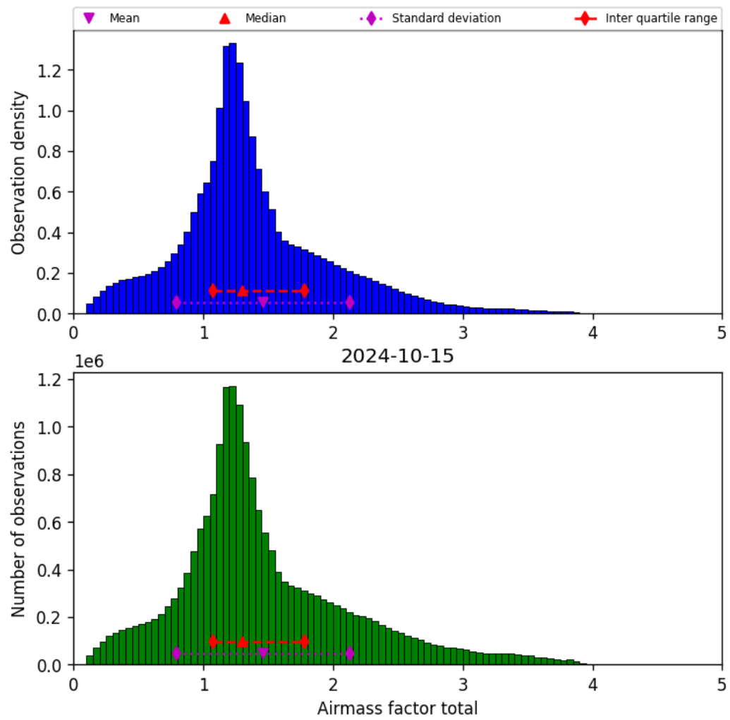
Figure 40: Histogram of “Airmass factor total” for 2024-10-14 to 2024-10-16
