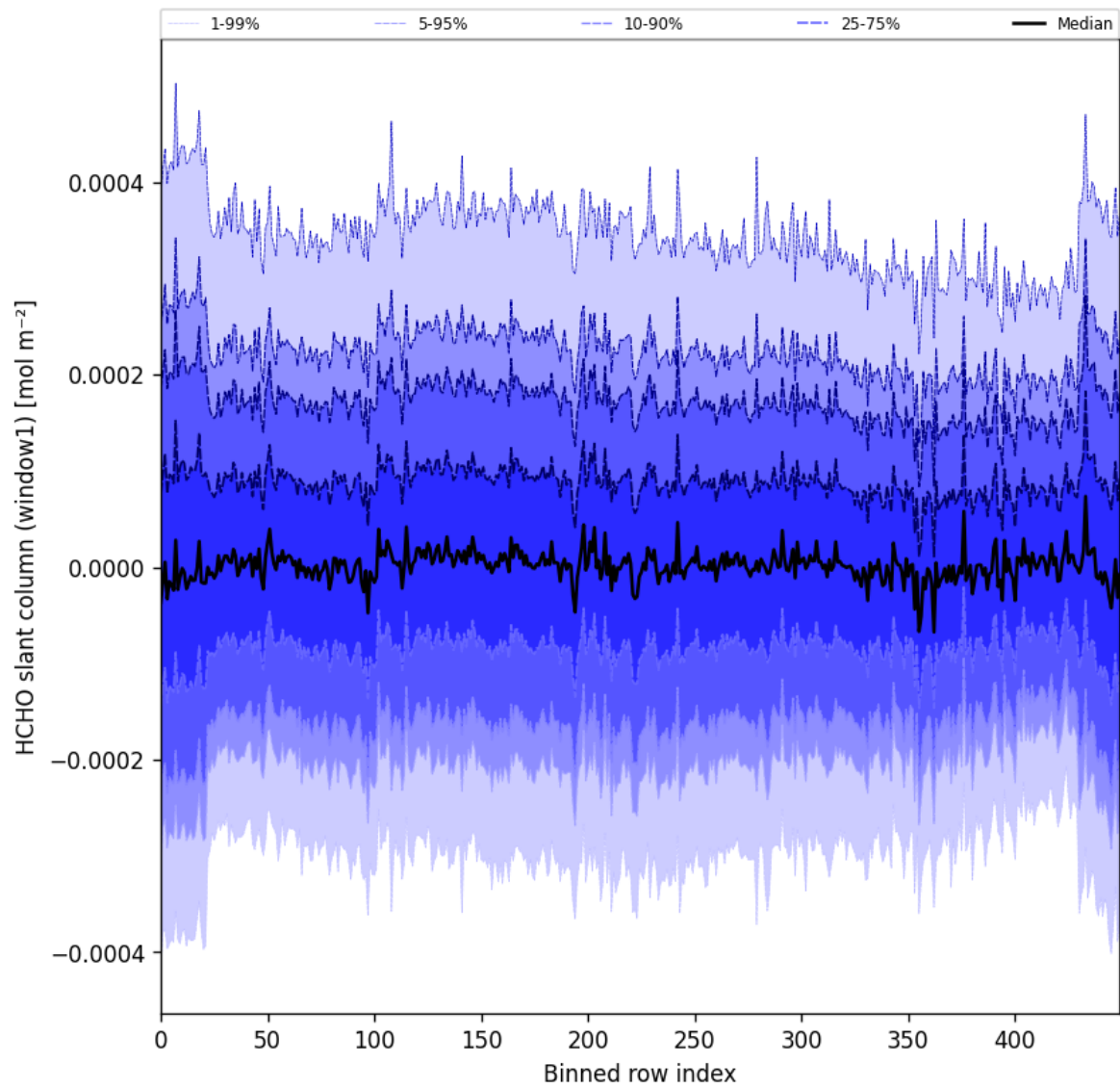
Figure 52: Along track statistics of “HCHO slant column (window1)” for 2024-10-14 to 2024-10-16
