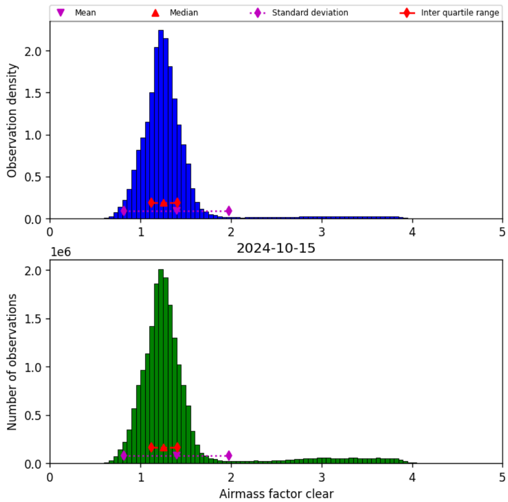
Figure 42: Histogram of “Airmass factor clear” for 2024-10-14 to 2024-10-16
