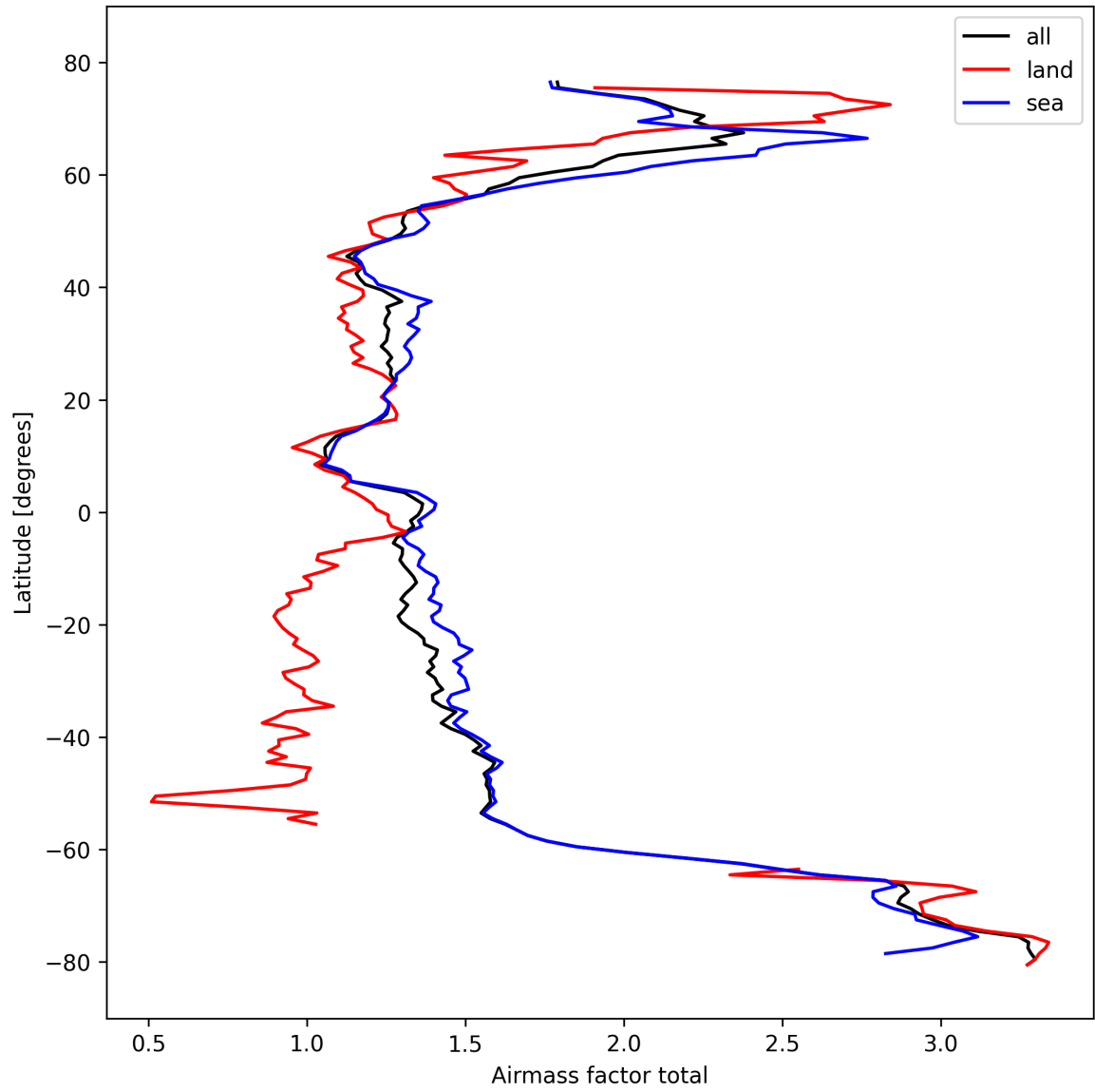
Figure 26: Zonal average of “Airmass factor total” for 2024-10-14 to 2024-10-16.
