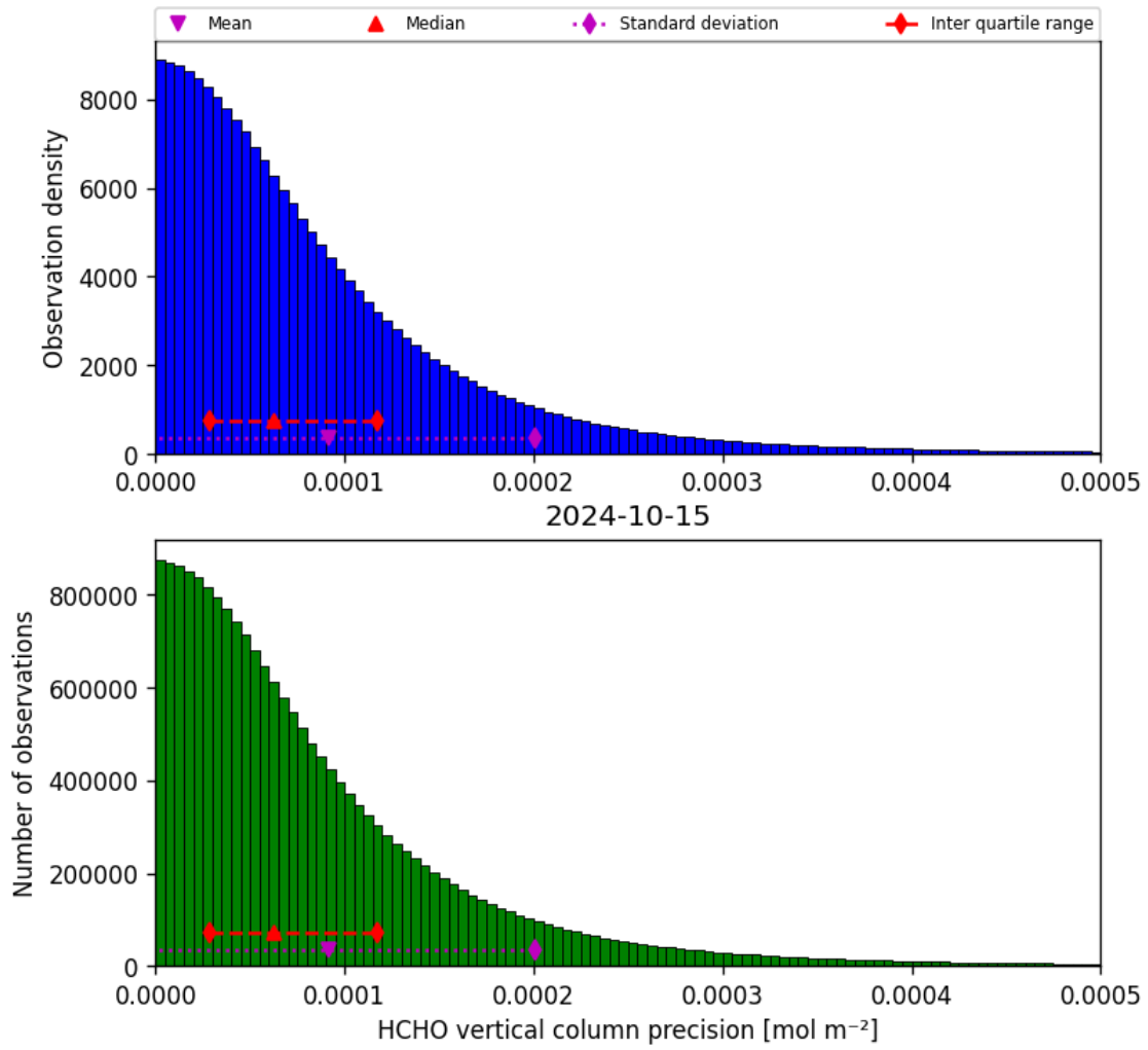
Figure 36: Histogram of “HCHO vertical column precision” for 2024-10-14 to 2024-10-16
