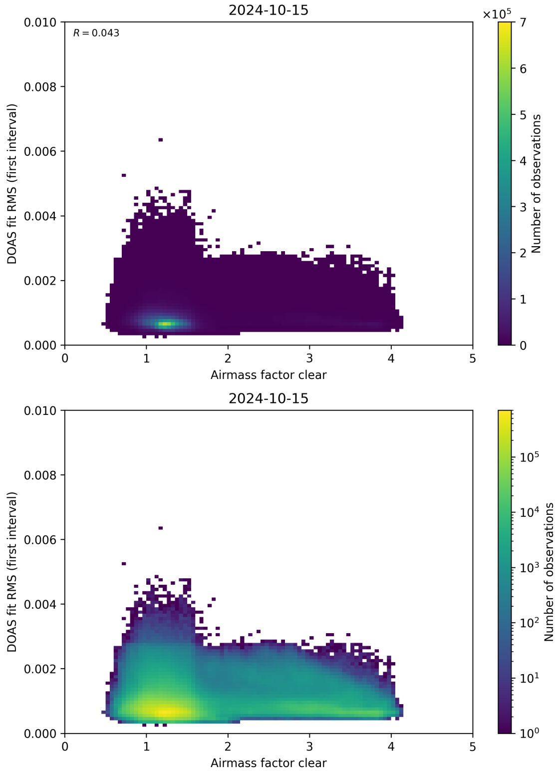
Figure 71: Scatter density plot of “Airmass factor clear” against “DOAS fit RMS (first interval)” for 2024-10-14 to 2024-10-16.
