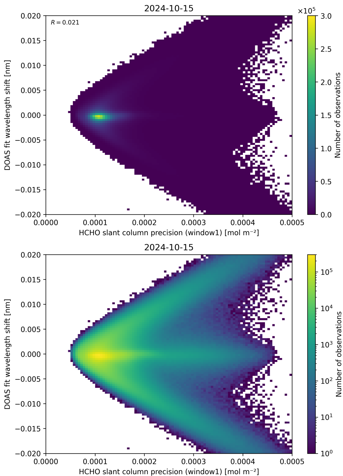
Figure 89: Scatter density plot of “HCHO slant column precision (window1)” against “DOAS fit wavelength shift” for 2024-10-14 to 2024-10-16.
