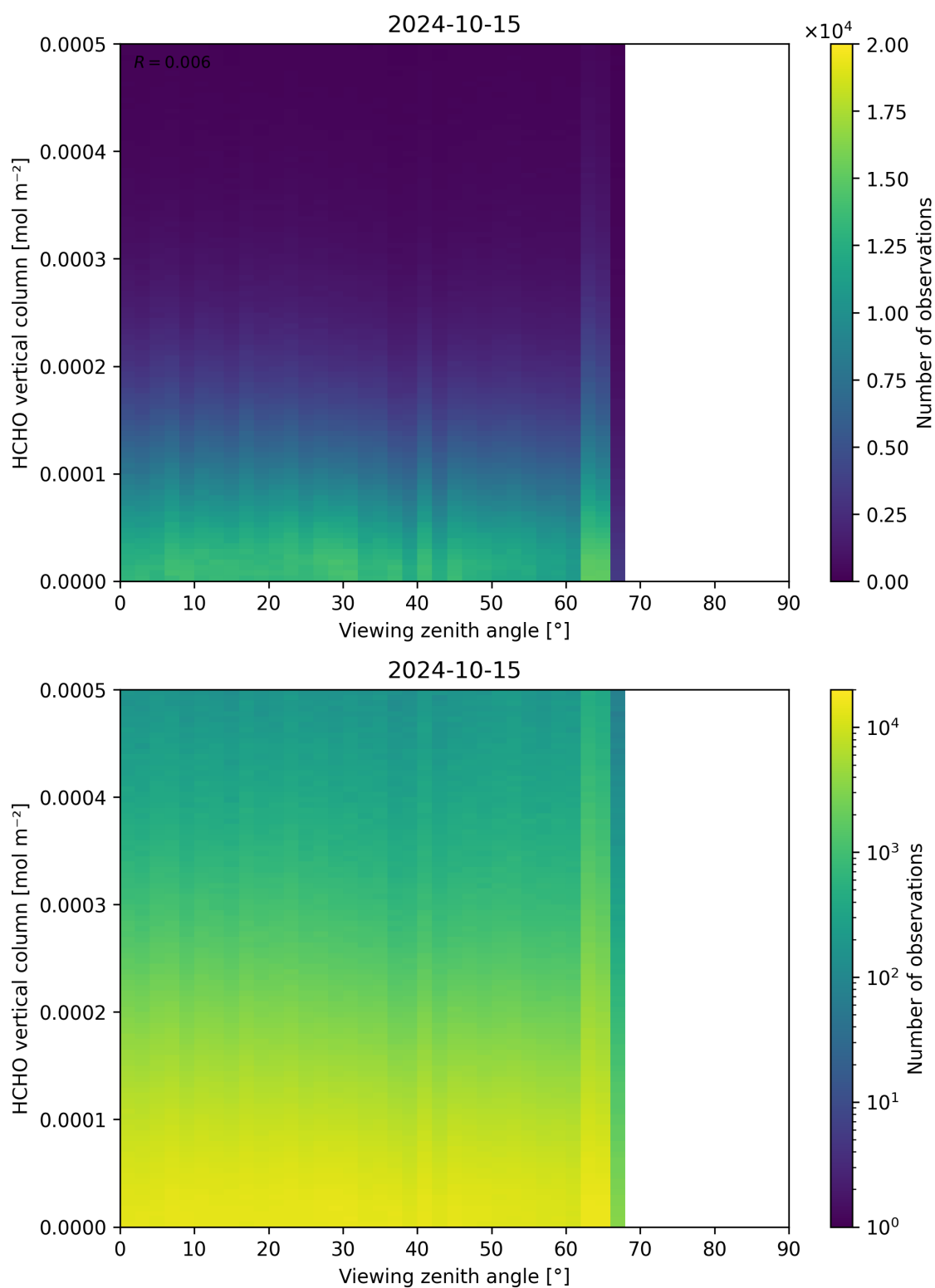
Figure 192: Scatter density plot of “Viewing zenith angle” against “HCHO vertical column” for 2024-10-14 to 2024-10-16.
