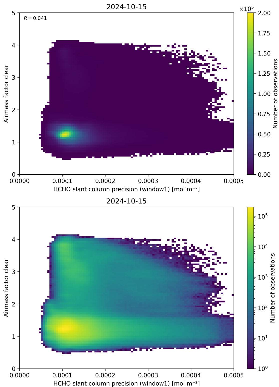
Figure 91: Scatter density plot of “HCHO slant column precision (window1)” against “Airmass factor clear” for 2024-10-14 to 2024-10-16.
