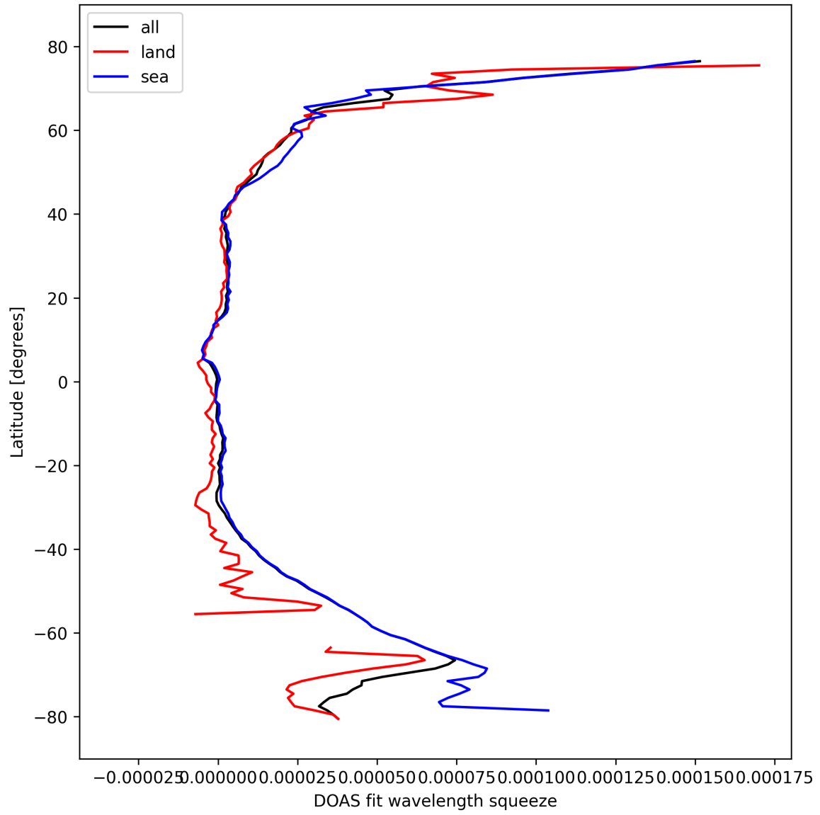
Figure 31: Zonal average of “DOAS fit wavelength squeeze” for 2024-10-14 to 2024-10-16.
