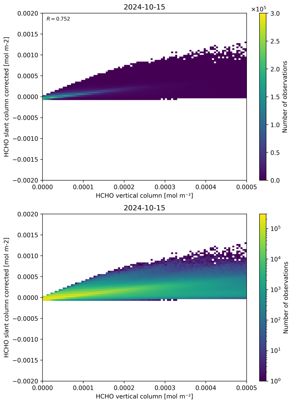
Figure 127: Scatter density plot of “HCHO vertical column” against “HCHO slant column corrected” for 2024-10-14 to 2024-10-16.
