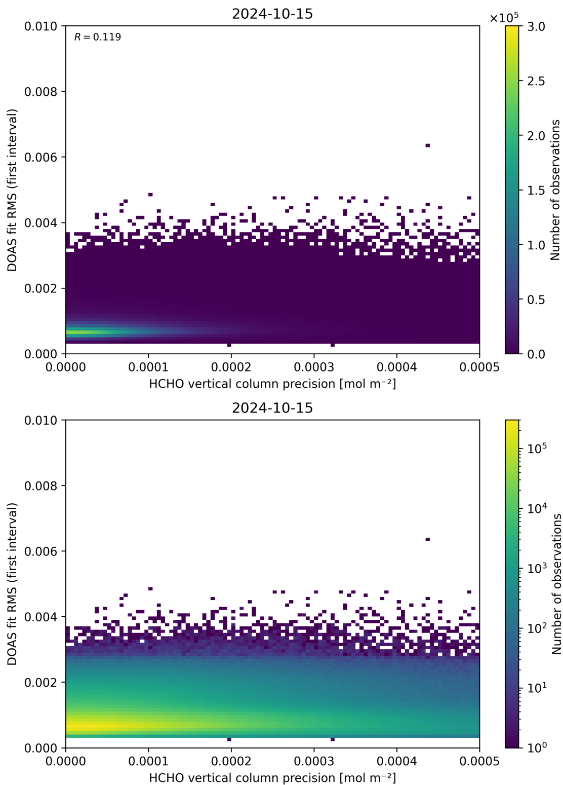
Figure 136: Scatter density plot of “HCHO vertical column precision” against “DOAS fit RMS (first interval)” for 2024-10-14 to 2024-10-16.
