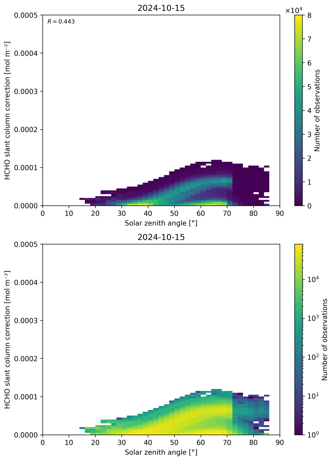
Figure 172: Scatter density plot of “Solar zenith angle” against “HCHO slant column correction” for 2024-10-14 to 2024-10-16.
