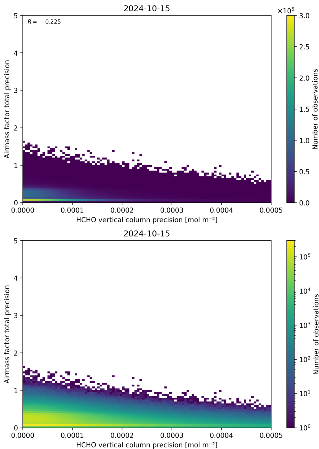
Figure 145: Scatter density plot of “HCHO vertical column precision” against “Airmass factor total precision” for 2024-10-14 to 2024-10-16.
