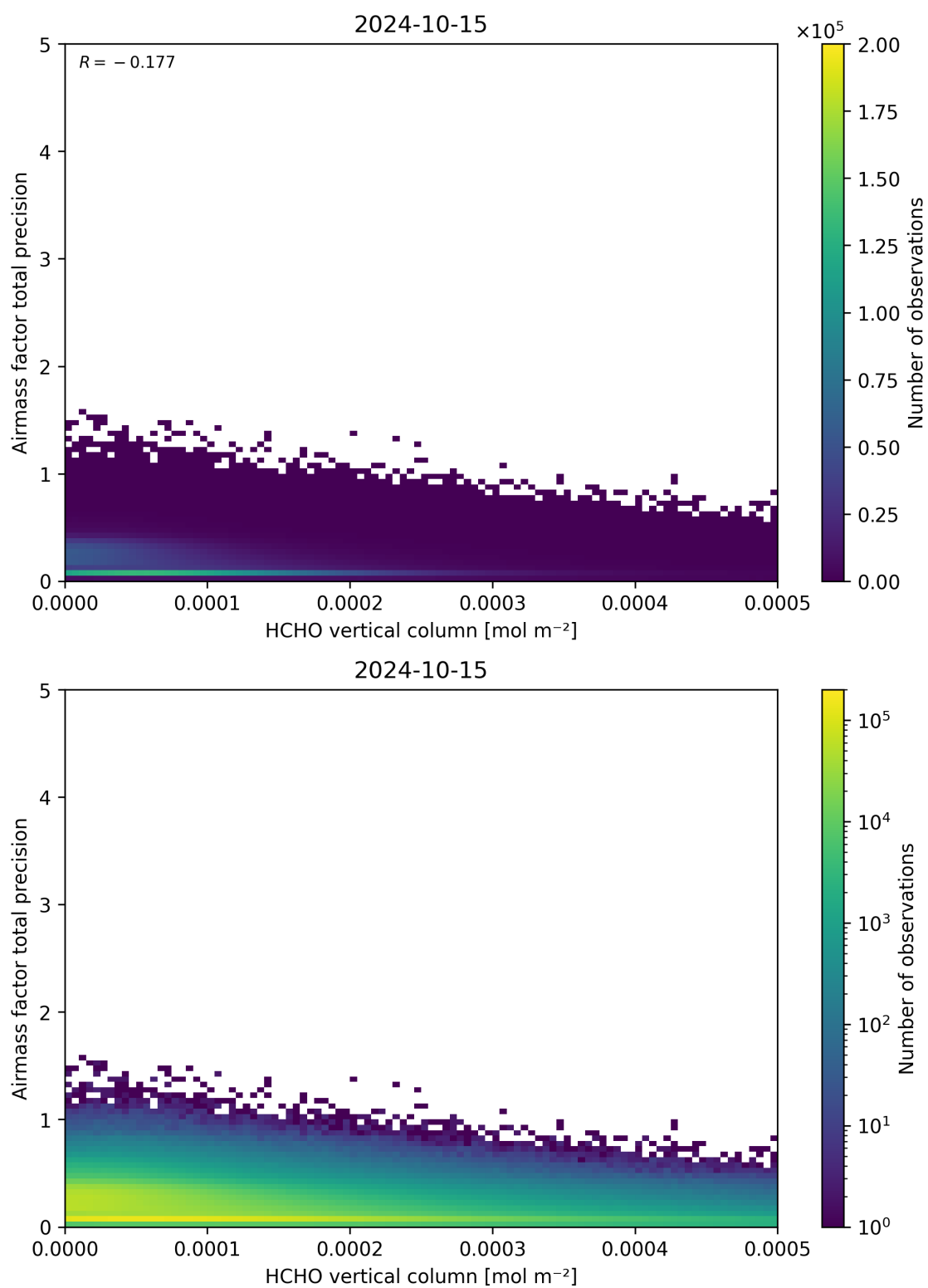
Figure 132: Scatter density plot of “HCHO vertical column” against “Airmass factor total precision” for 2024-10-14 to 2024-10-16.
