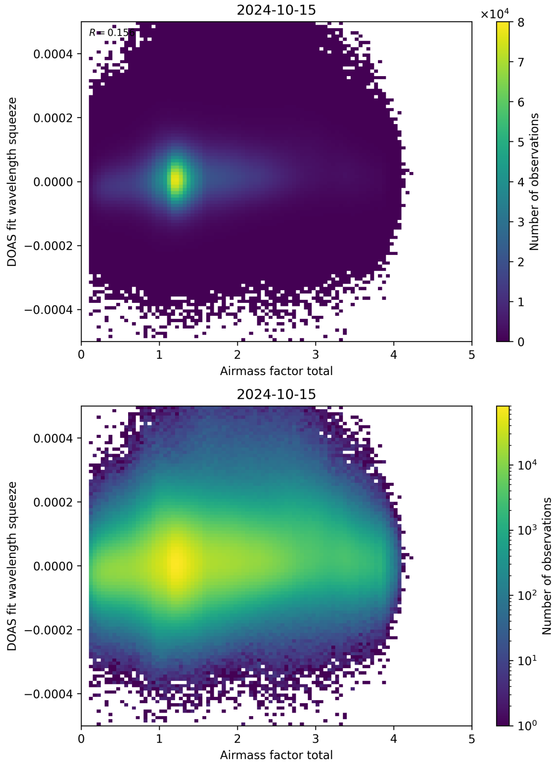
Figure 99: Scatter density plot of “Airmass factor total” against “DOAS fit wavelength squeeze” for 2024-10-14 to 2024-10-16.
