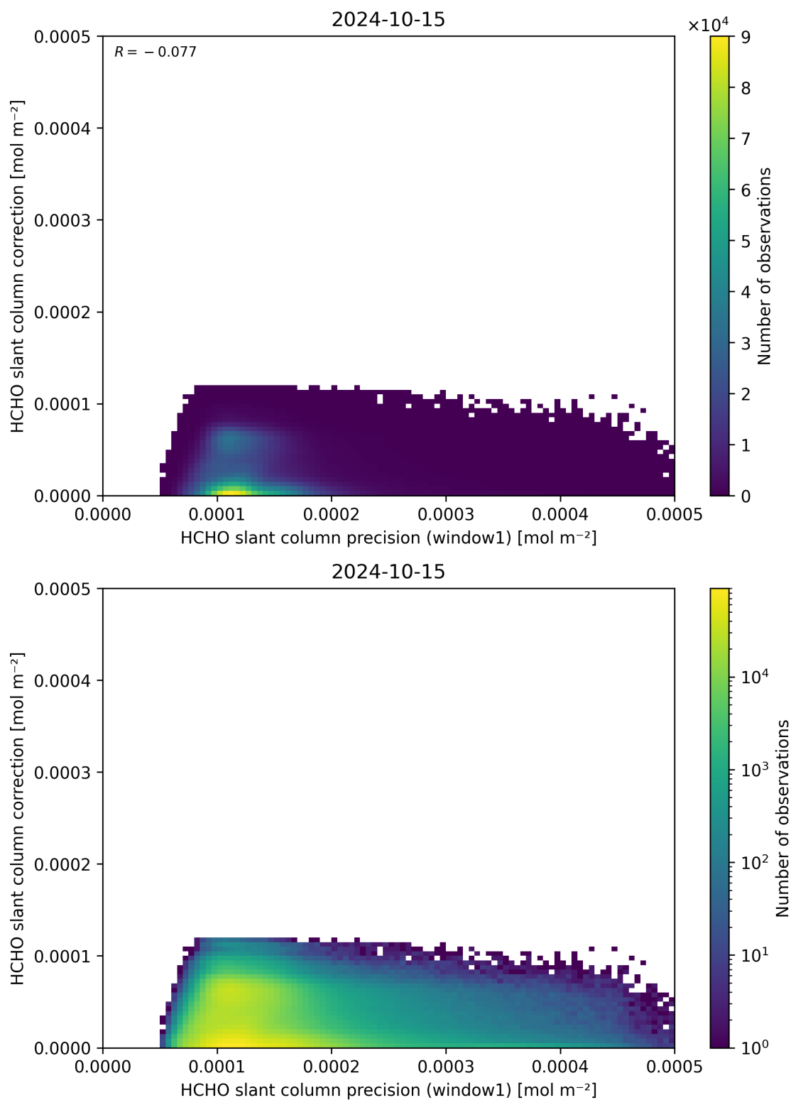
Figure 93: Scatter density plot of “HCHO slant column precision (window1)” against “HCHO slant column correction” for 2024-10-14 to 2024-10-16.
