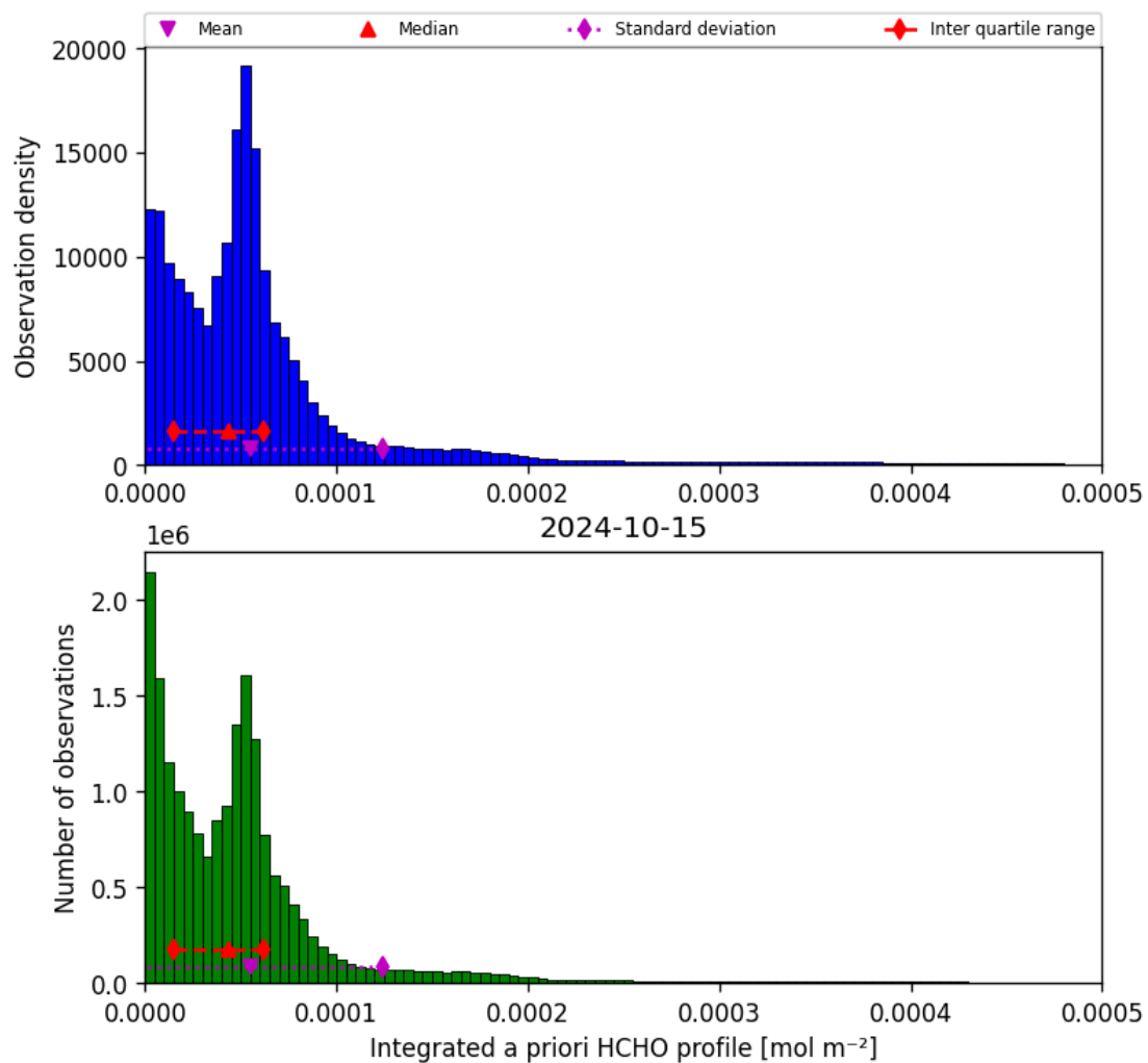
Figure 43: Histogram of “Integrated a priori HCHO profile” for 2024-10-14 to 2024-10-16
