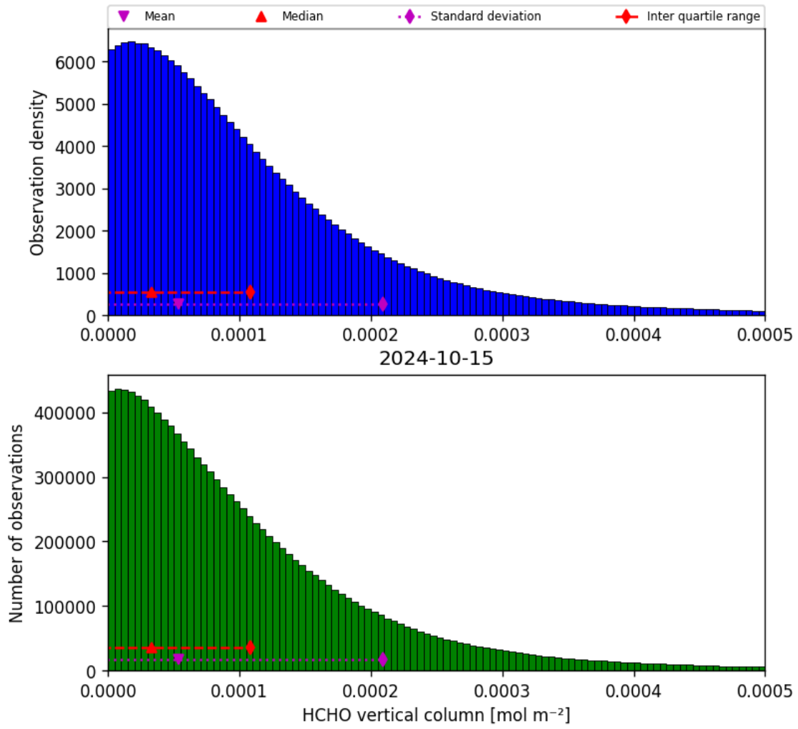
Figure 35: Histogram of “HCHO vertical column” for 2024-10-14 to 2024-10-16
