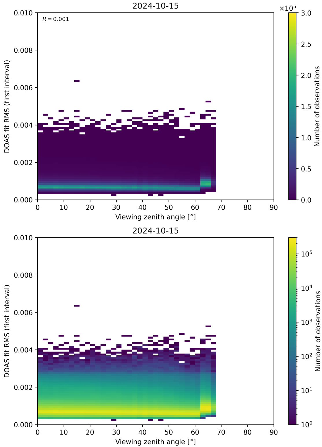
Figure 182: Scatter density plot of “Viewing zenith angle” against “DOAS fit RMS (first interval)” for 2024-10-14 to 2024-10-16.
