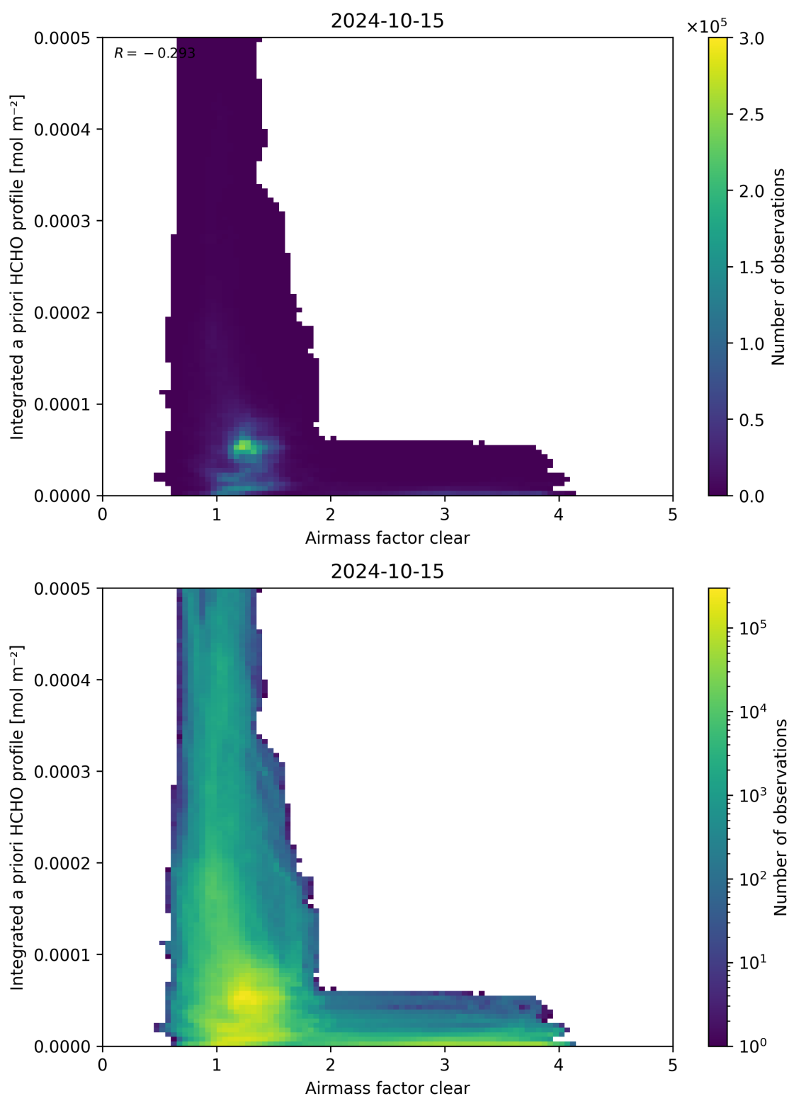
Figure 76: Scatter density plot of “Airmass factor clear” against “Integrated a priori HCHO profile” for 2024-10-14 to 2024-10-16.
