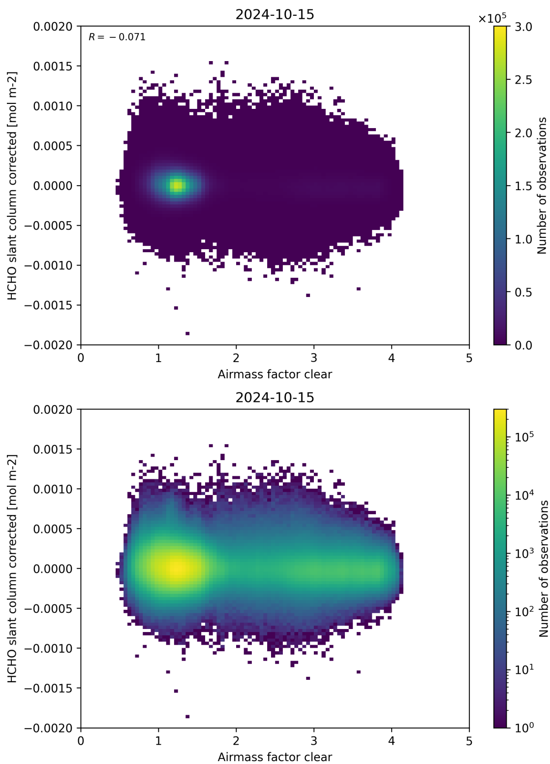
Figure 74: Scatter density plot of “Airmass factor clear” against “HCHO slant column corrected” for 2024-10-14 to 2024-10-16.
