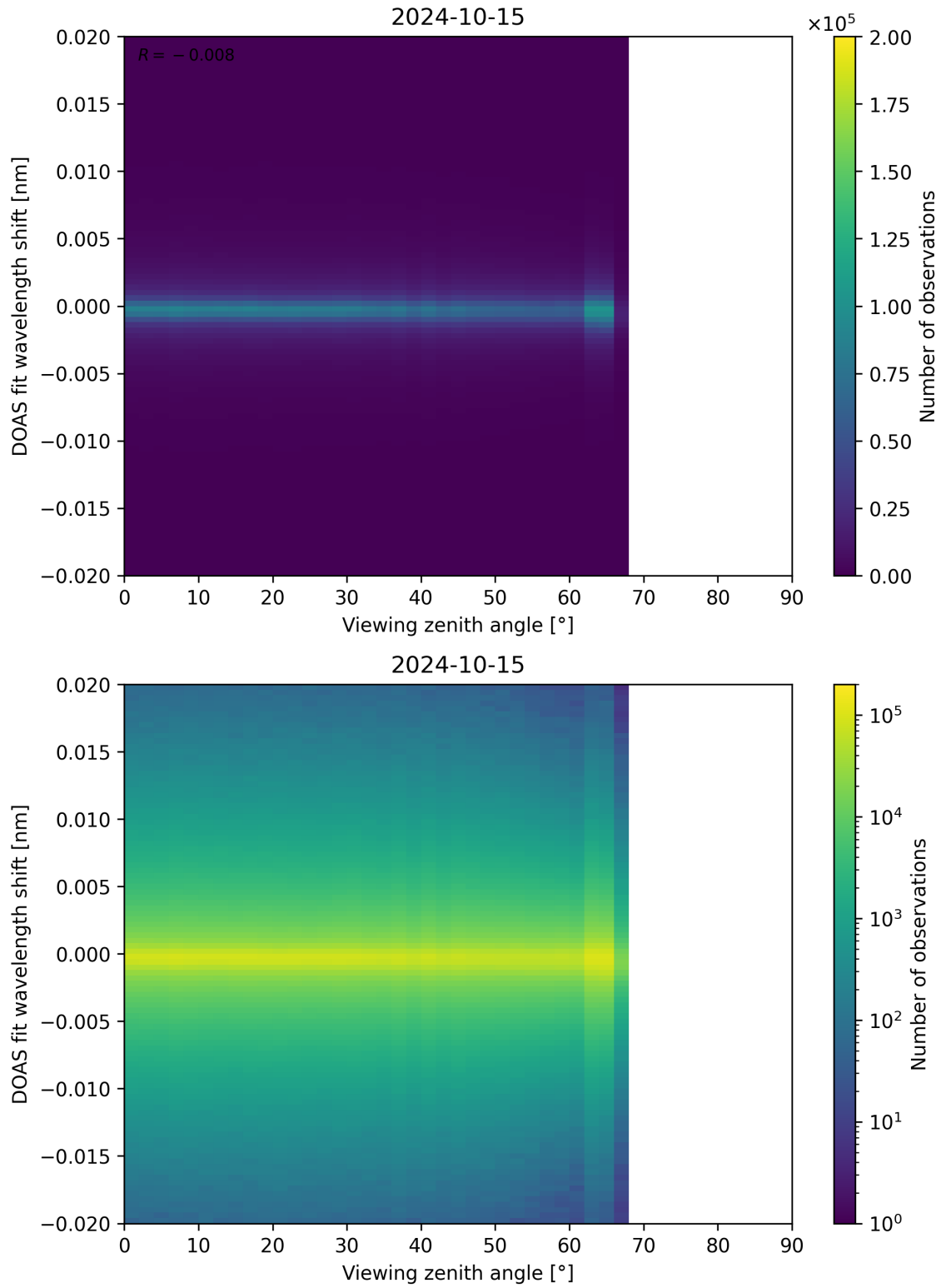
Figure 183: Scatter density plot of “Viewing zenith angle” against “DOAS fit wavelength shift” for 2024-10-14 to 2024-10-16.
