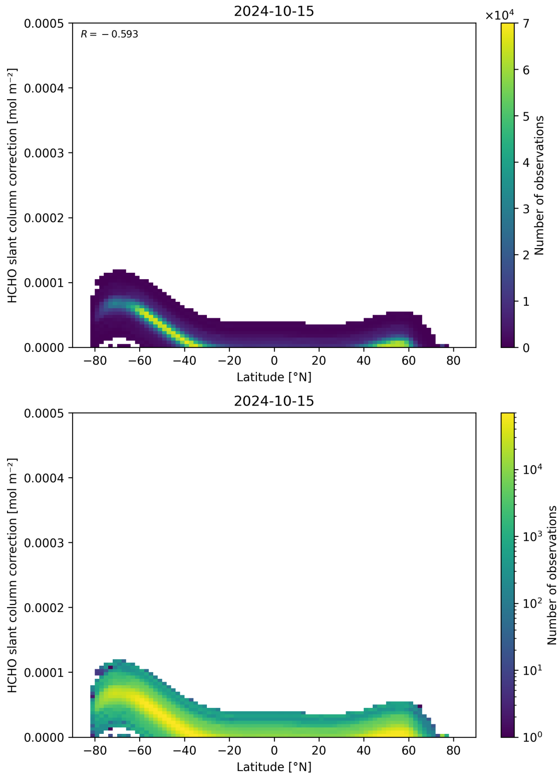
Figure 158: Scatter density plot of “Latitude” against “HCHO slant column correction” for 2024-10-14 to 2024-10-16.
