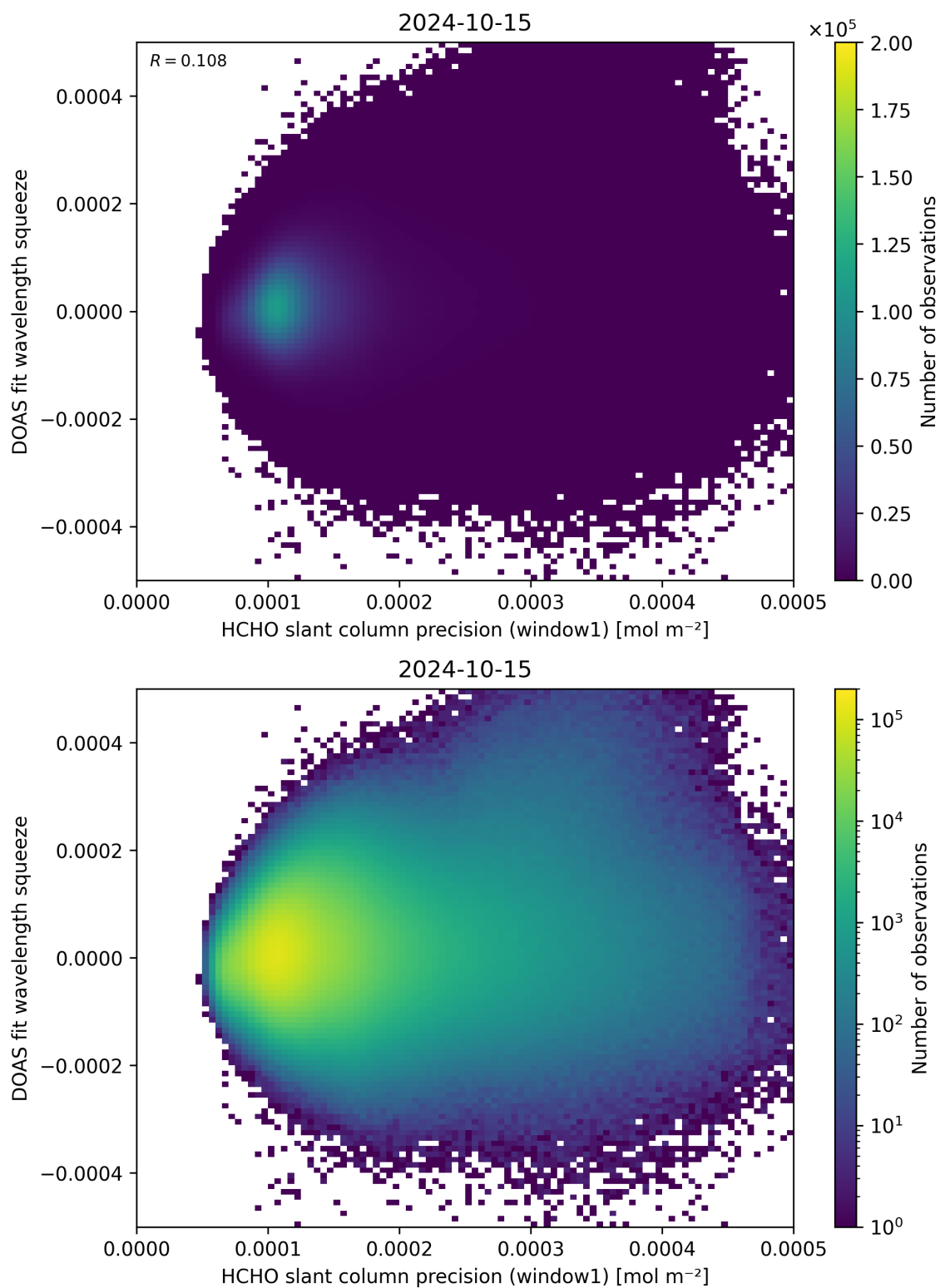
Figure 90: Scatter density plot of “HCHO slant column precision (window1)” against “DOAS fit wavelength squeeze” for 2024-10-14 to 2024-10-16.
