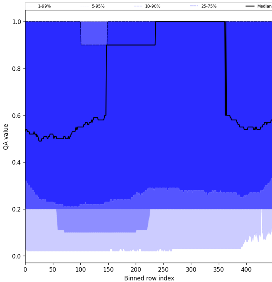
Figure 48: Along track statistics of “QA value” for 2024-10-14 to 2024-10-16
