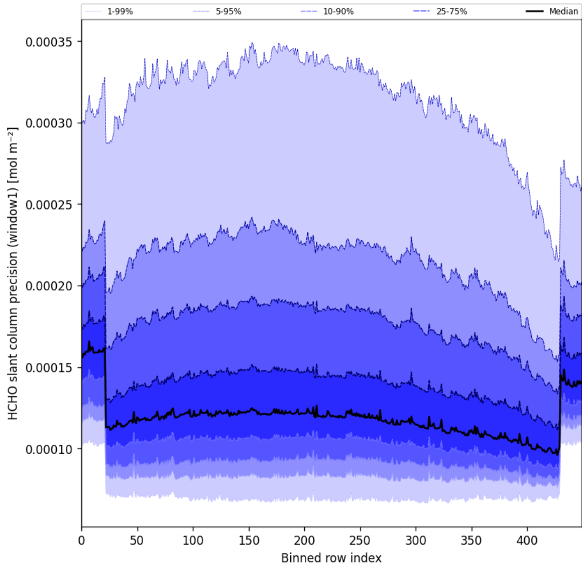
Figure 53: Along track statistics of "HCHO slant column precision (window1)" for 2024-10-14 to 2024-10-16
