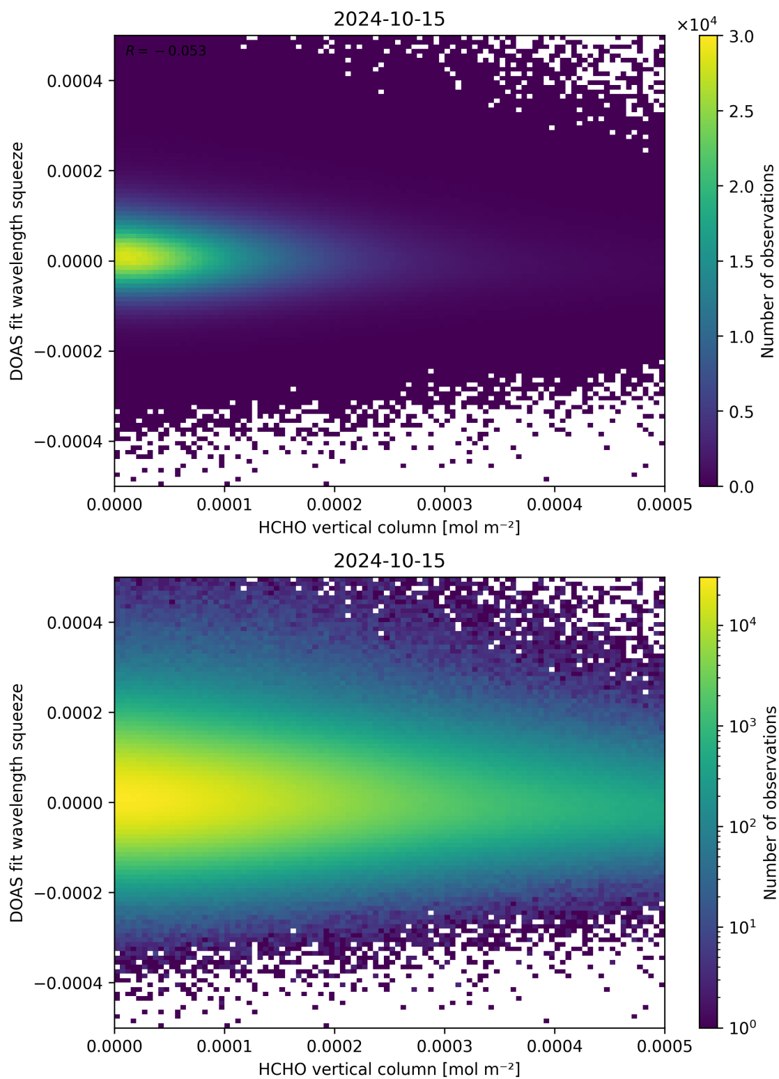
Figure 125: Scatter density plot of “HCHO vertical column” against “DOAS fit wavelength squeeze” for 2024-10-14 to 2024-10-16.
