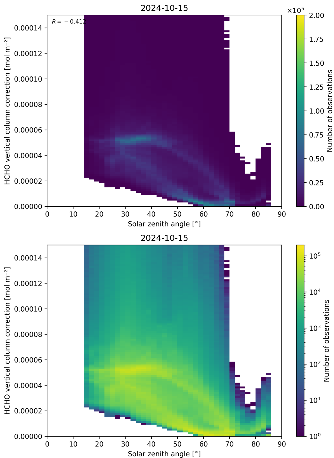
Figure 178: Scatter density plot of “Solar zenith angle” against “HCHO vertical column correction” for 2024-10-14 to 2024-10-16.
