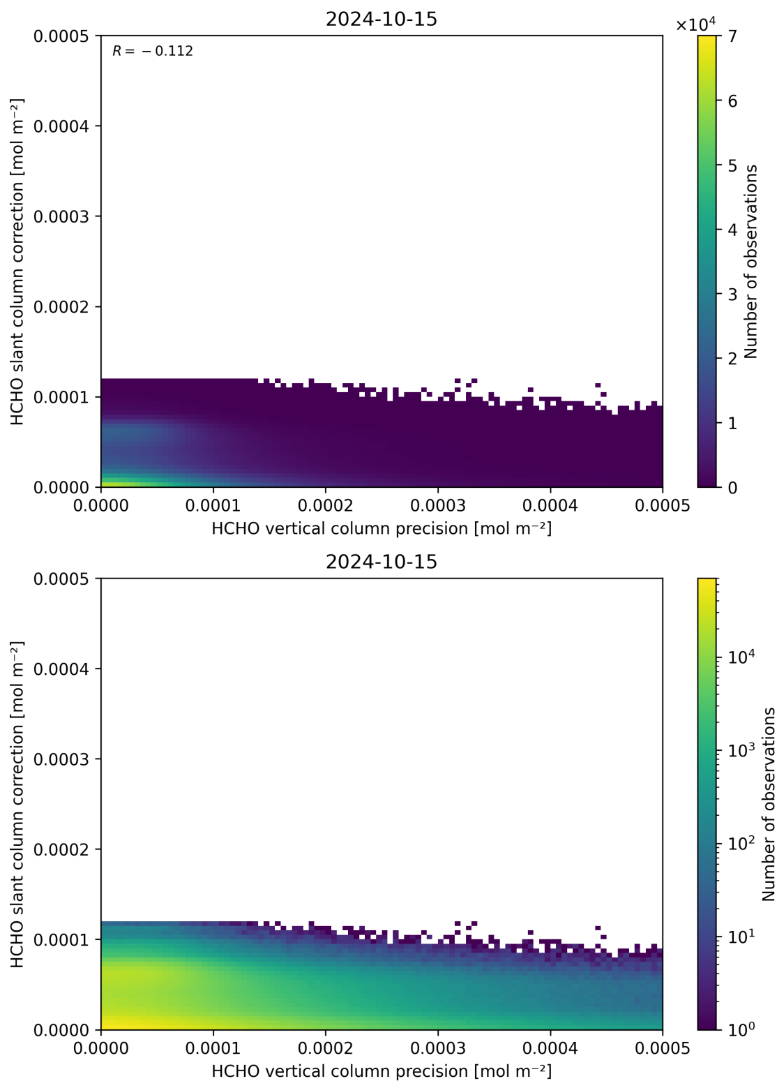
Figure 141: Scatter density plot of “HCHO vertical column precision” against “HCHO slant column correction” for 2024-10-14 to 2024-10-16.
