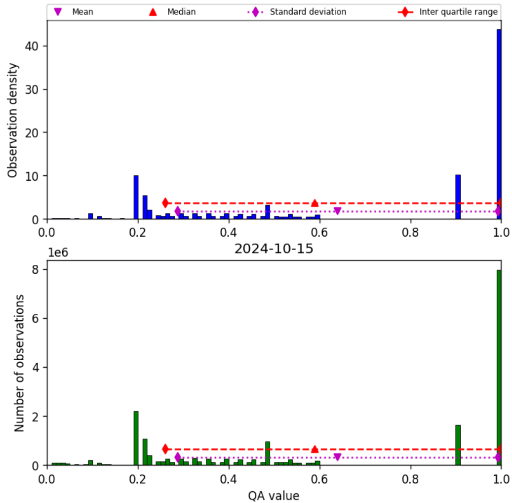
Figure 34: Histogram of “QA value” for 2024-10-14 to 2024-10-16
