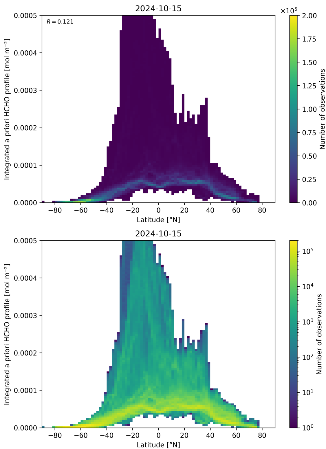
Figure 166: Scatter density plot of “Latitude” against “Integrated a priori HCHO profile” for 2024-10-14 to 2024-10-16.
