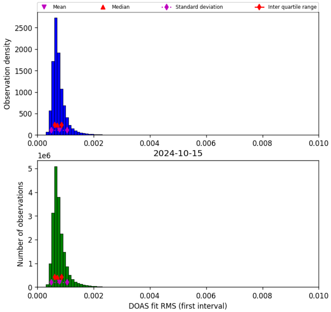
Figure 46: Histogram of “DOAS fit RMS (first interval)” for 2024-10-14 to 2024-10-16
