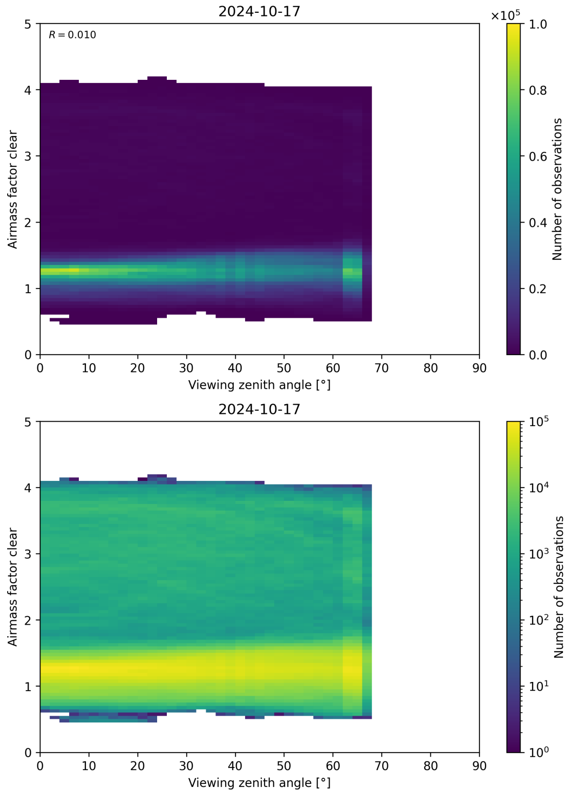
Figure 185: Scatter density plot of “Viewing zenith angle” against “Airmass factor clear” for 2024-10-16 to 2024-10-18.
