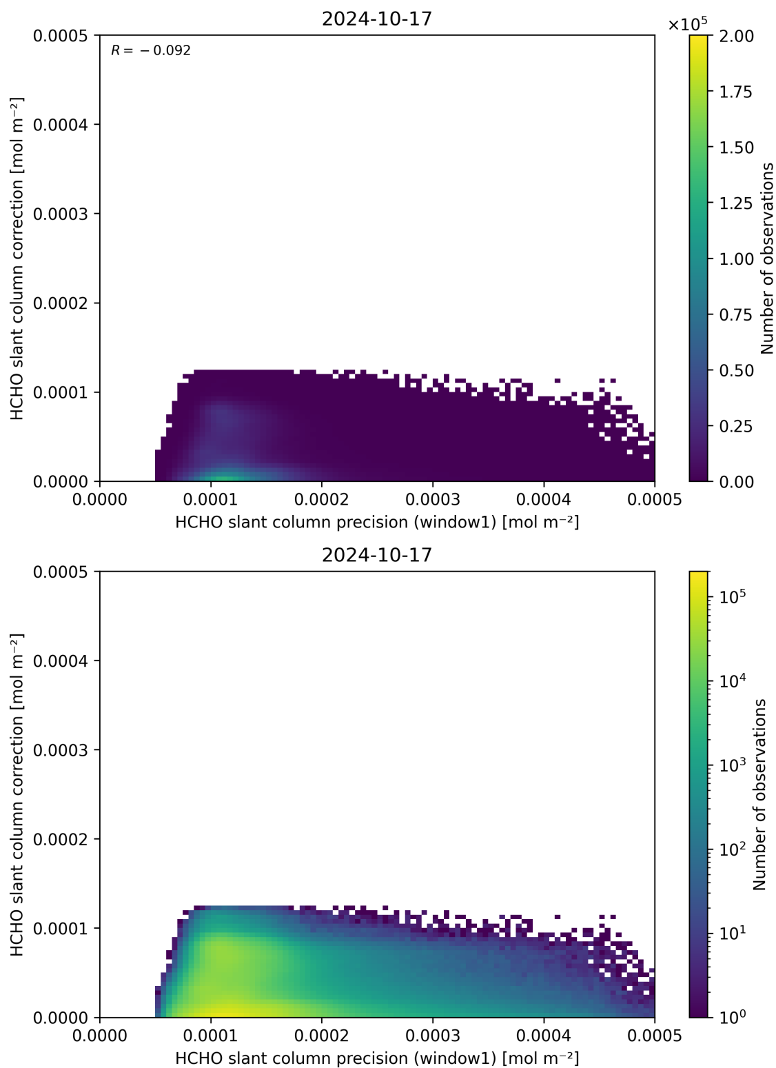
Figure 93: Scatter density plot of “HCHO slant column precision (window1)” against “HCHO slant column correction” for 2024-10-16 to 2024-10-18.
