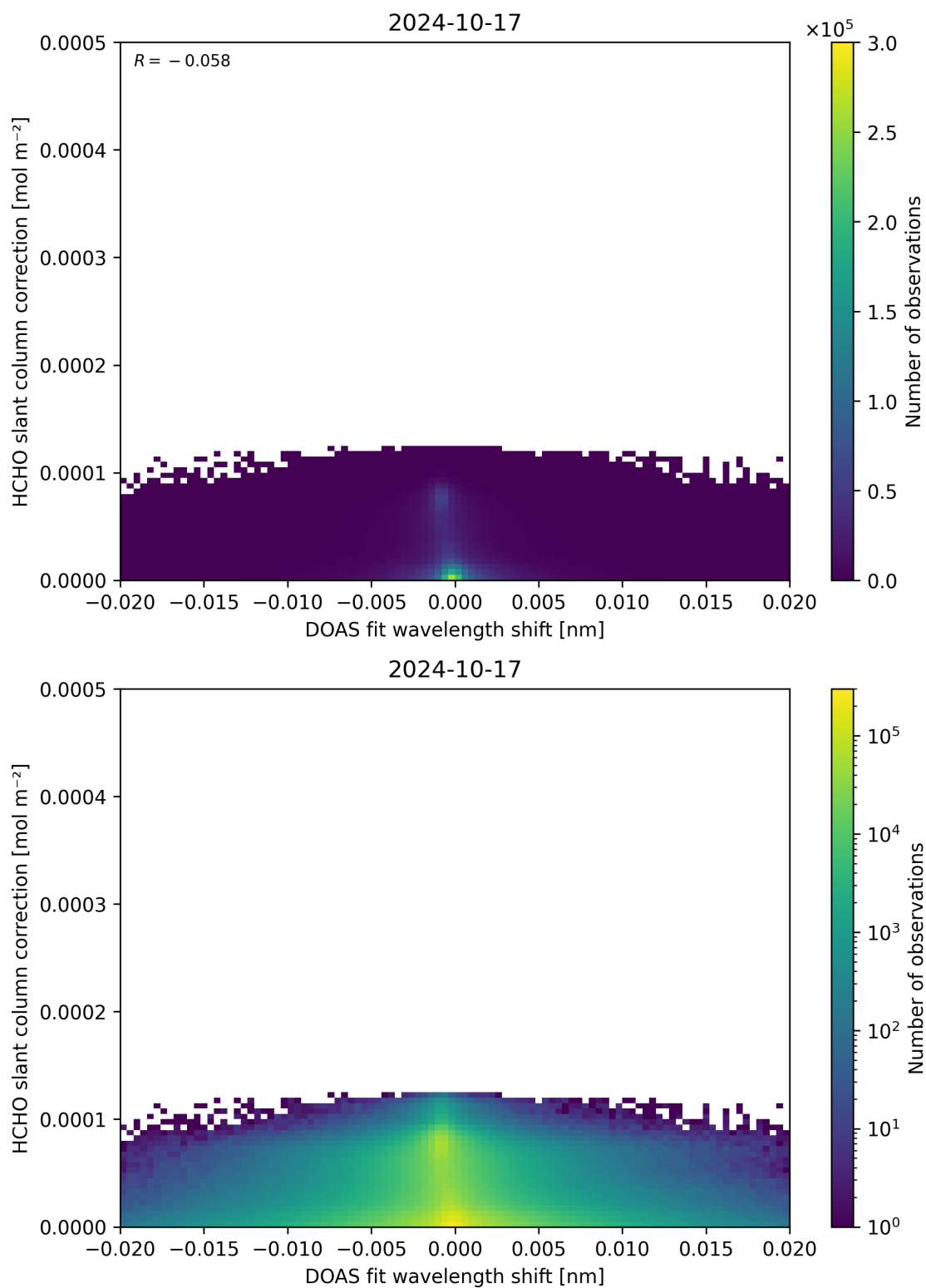
Figure 67: Scatter density plot of “DOAS fit wavelength shift” against “HCHO slant column correction” for 2024-10-16 to 2024-10-18.
