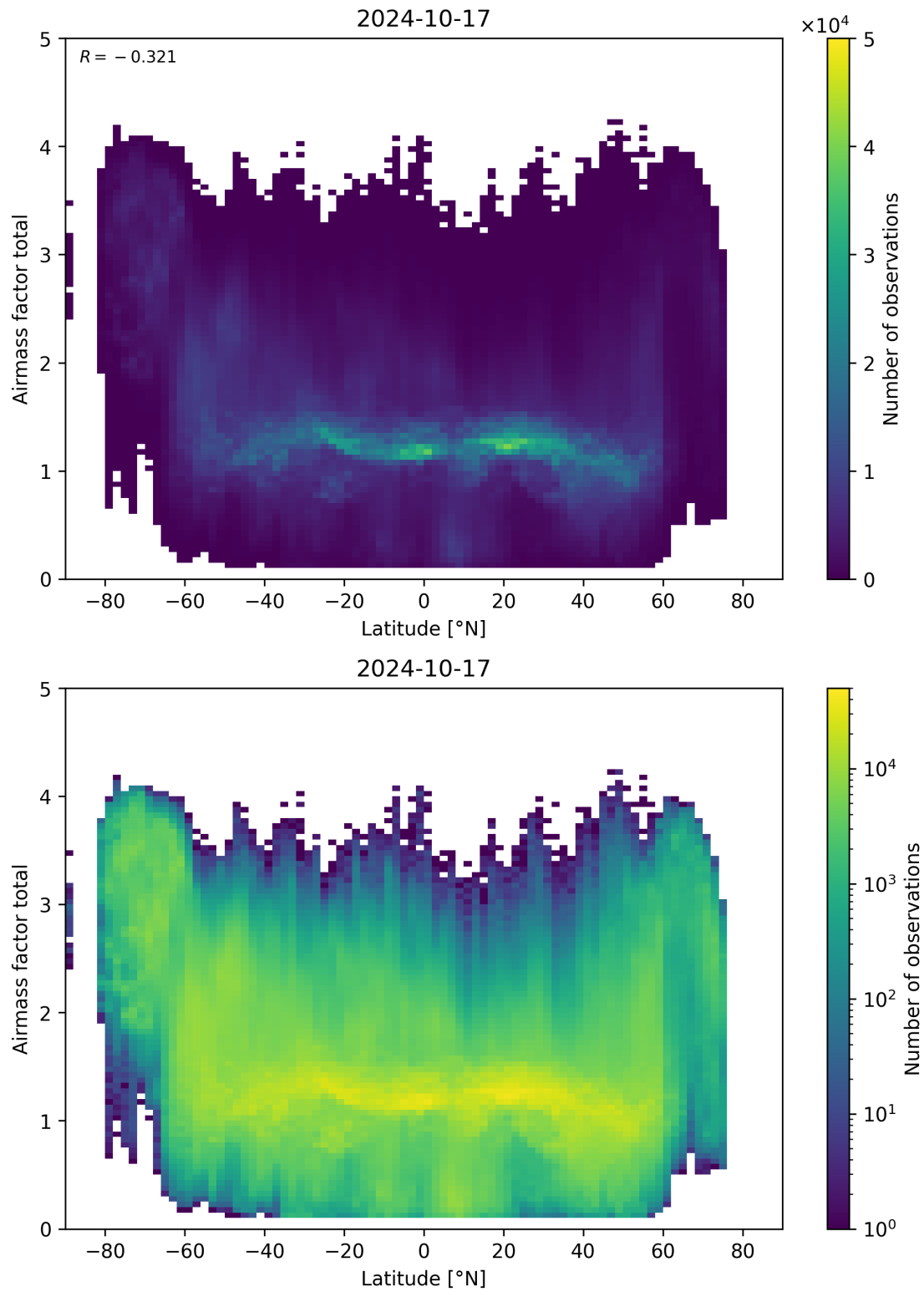
Figure 161: Scatter density plot of “Latitude” against “Airmass factor total” for 2024-10-16 to 2024-10-18.
