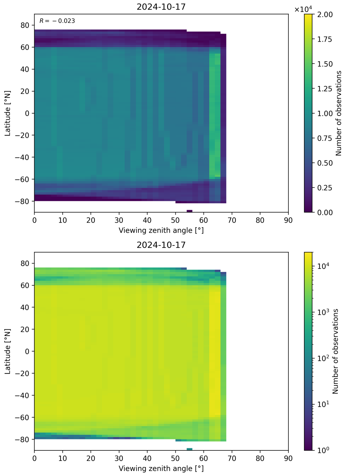
Figure 196: Scatter density plot of “Viewing zenith angle” against “Latitude” for 2024-10-16 to 2024-10-18.
