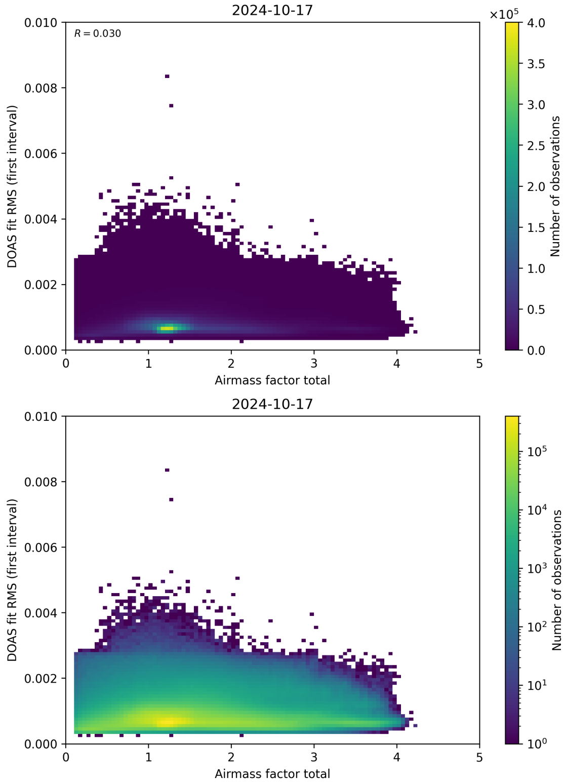
Figure 97: Scatter density plot of “Airmass factor total” against “DOAS fit RMS (first interval)” for 2024-10-16 to 2024-10-18.
