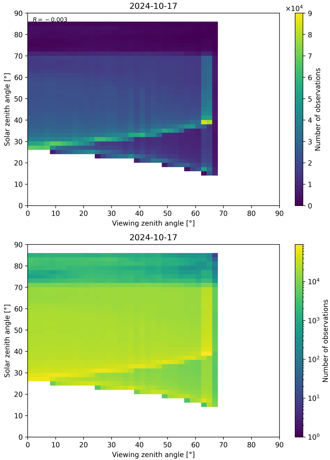
Figure 197: Scatter density plot of “Viewing zenith angle” against “Solar zenith angle” for 2024-10-16 to 2024-10-18.
