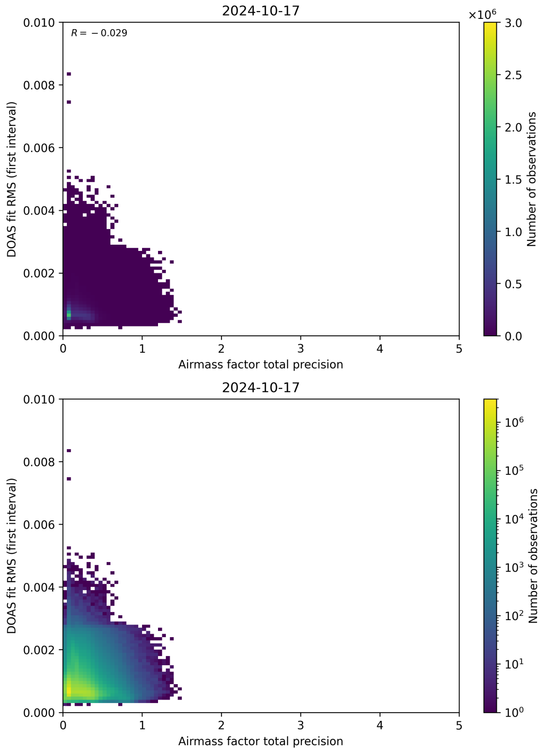
Figure 105: Scatter density plot of “Airmass factor total precision” against “DOAS fit RMS (first interval)” for 2024-10-16 to 2024-10-18.
