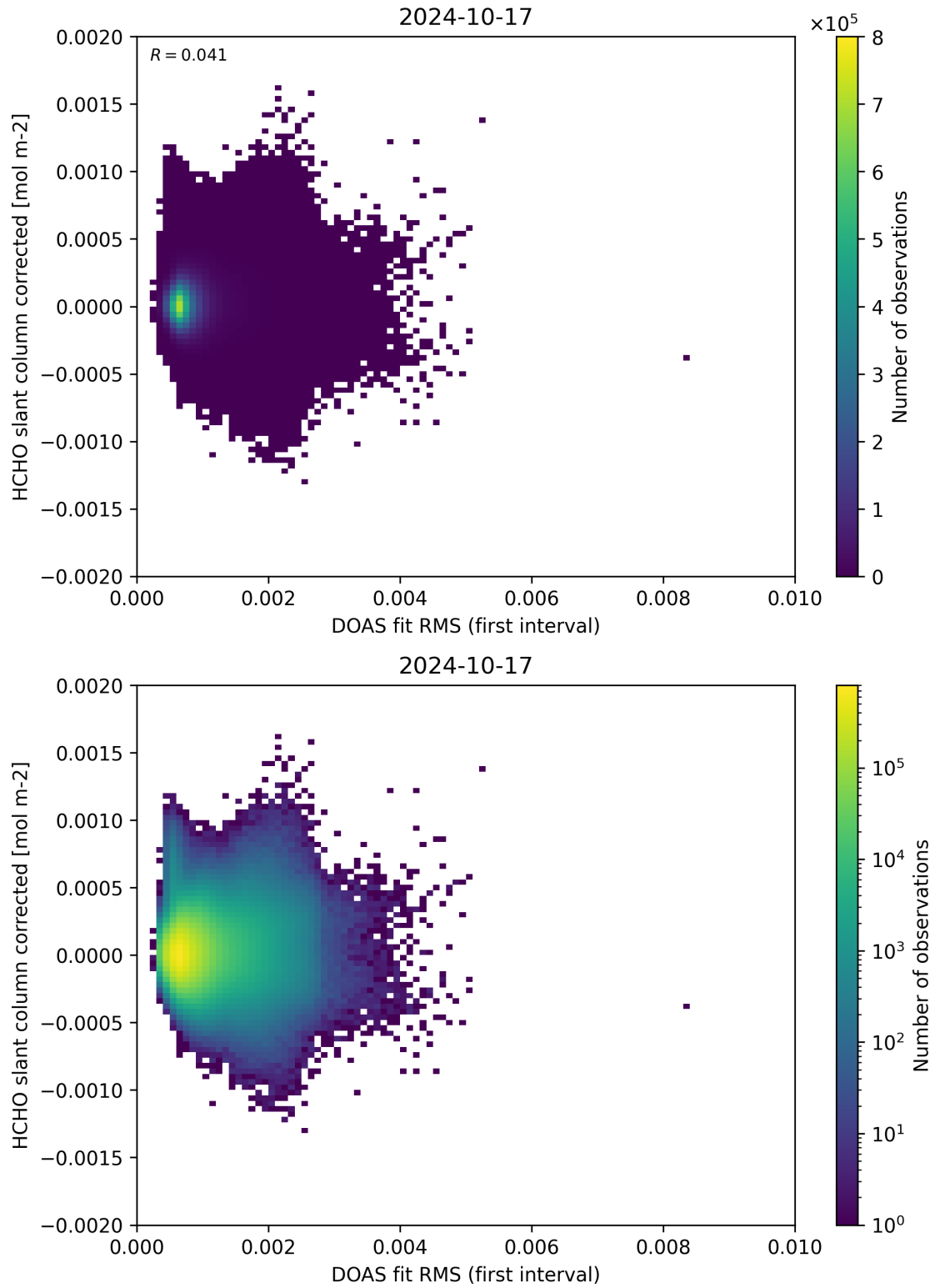
Figure 62: Scatter density plot of “DOAS fit RMS (first interval)” against “HCHO slant column corrected” for 2024-10-16 to 2024-10-18.
