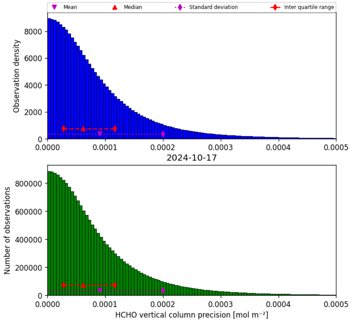
Figure 36: Histogram of “HCHO vertical column precision” for 2024-10-16 to 2024-10-18
