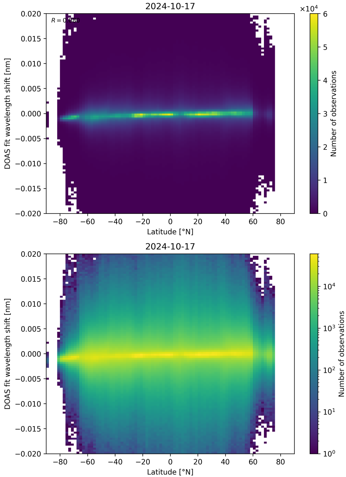
Figure 154: Scatter density plot of “Latitude” against “DOAS fit wavelength shift” for 2024-10-16 to 2024-10-18.
