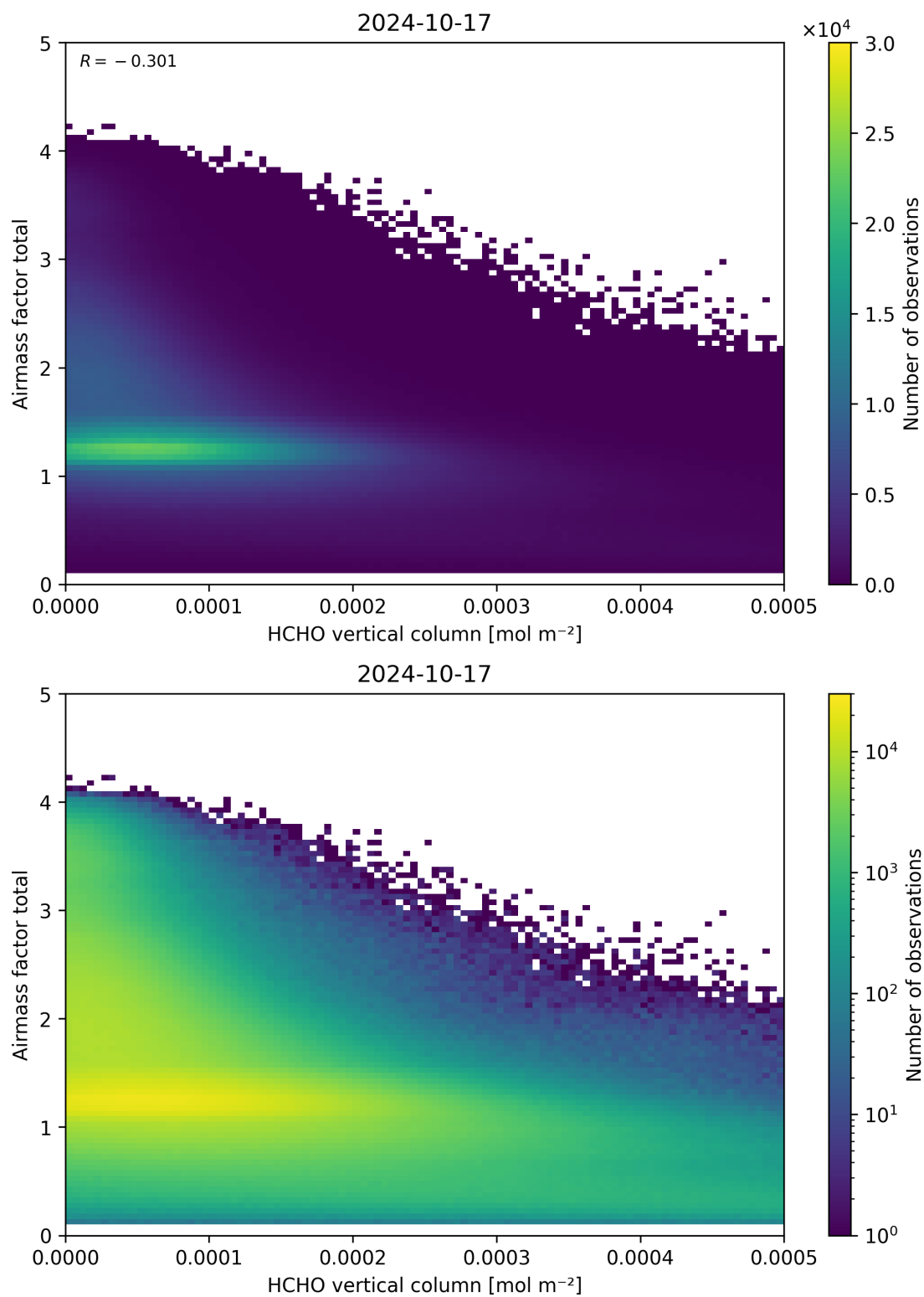
Figure 131: Scatter density plot of “HCHO vertical column” against “Airmass factor total” for 2024-10-16 to 2024-10-18.
