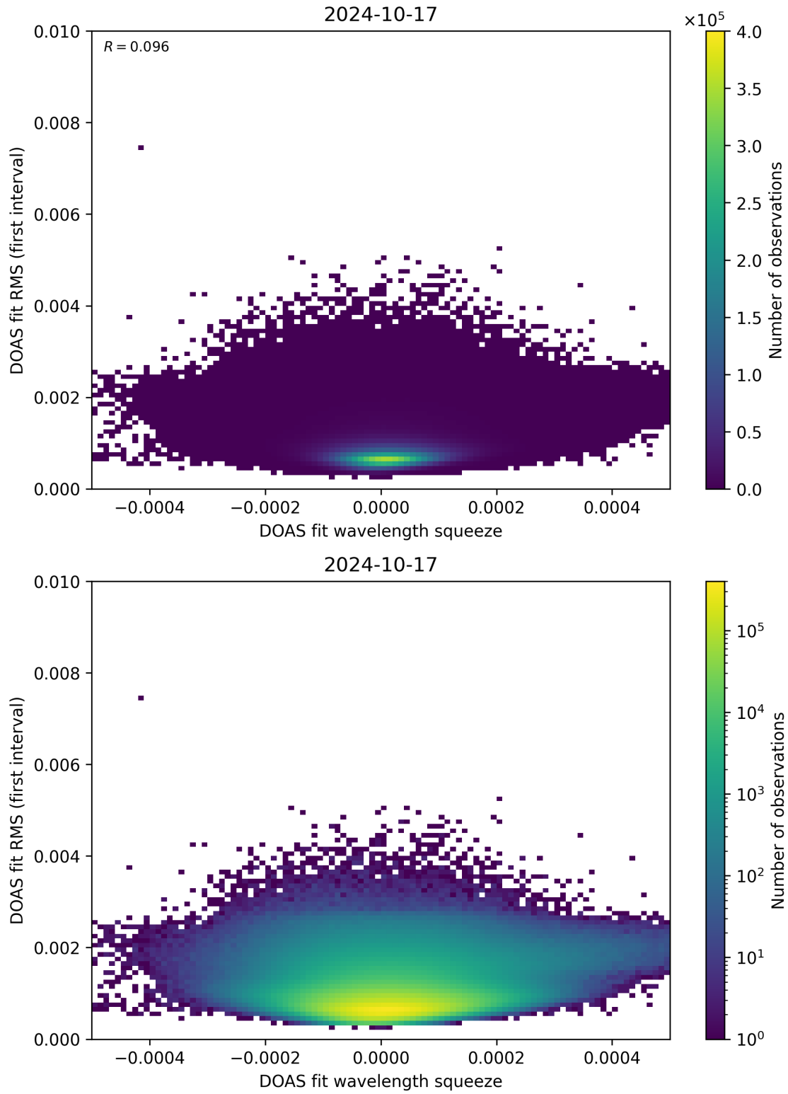
Figure 68: Scatter density plot of “DOAS fit wavelength squeeze” against “DOAS fit RMS (first interval)” for 2024-10-16 to 2024-10-18.
