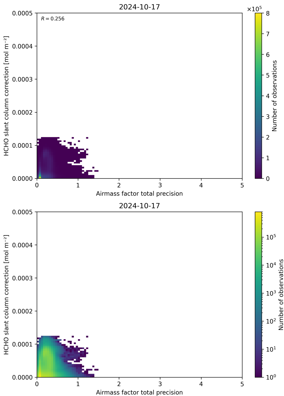
Figure 110: Scatter density plot of “Airmass factor total precision” against “HCHO slant column correction” for 2024-10-16 to 2024-10-18.
