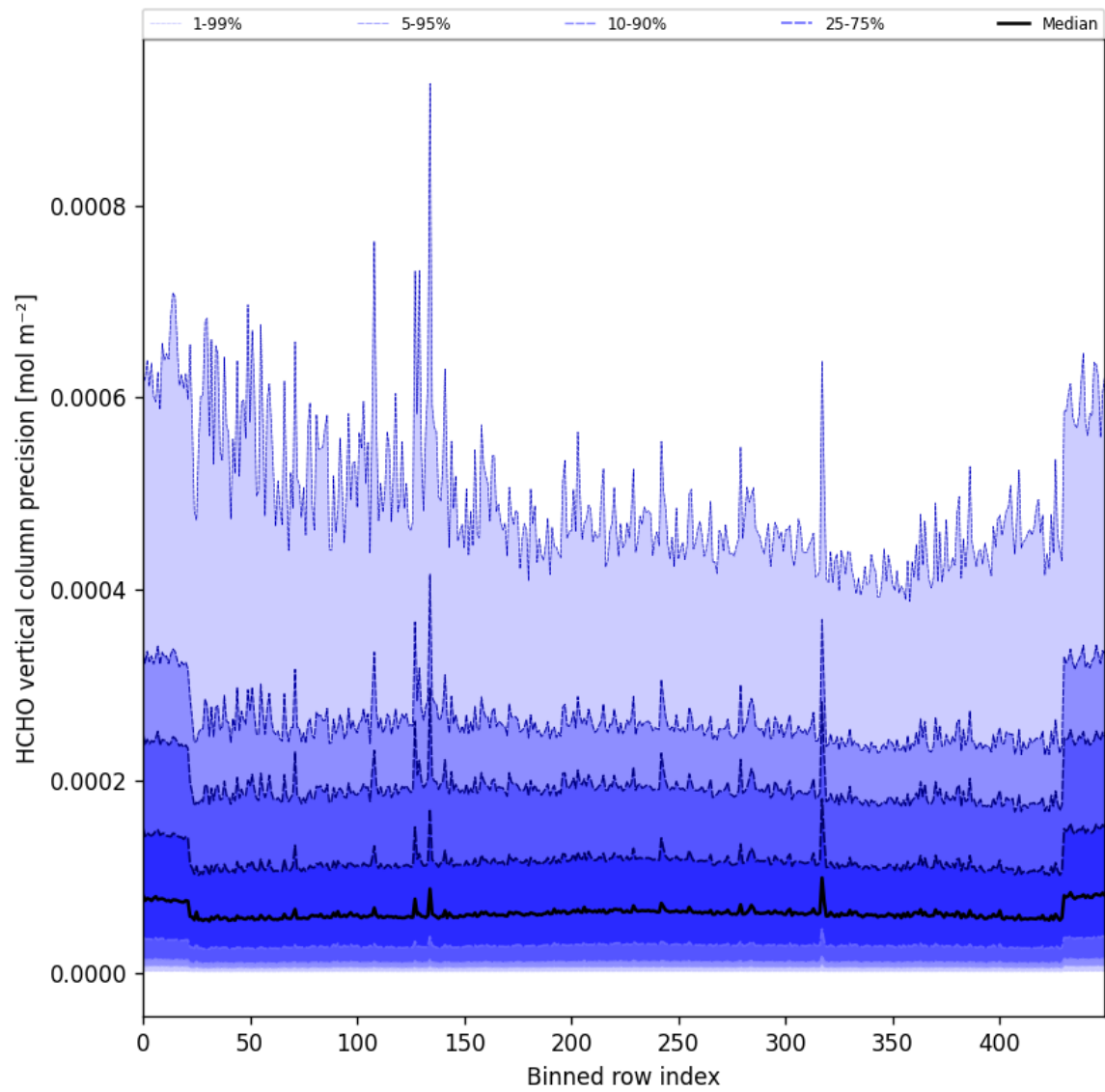
Figure 50: Along track statistics of “HCHO vertical column precision” for 2024-10-16 to 2024-10-18
