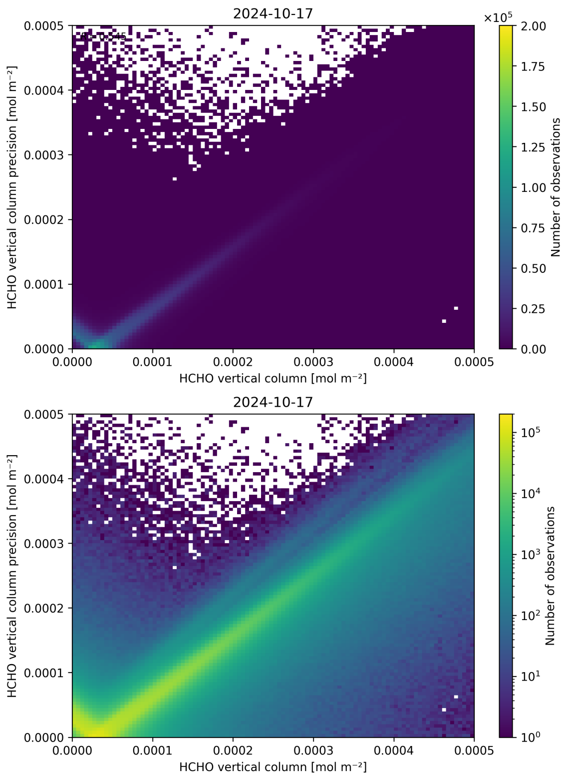
Figure 134: Scatter density plot of “HCHO vertical column” against “HCHO vertical column precision” for 2024-10-16 to 2024-10-18.
