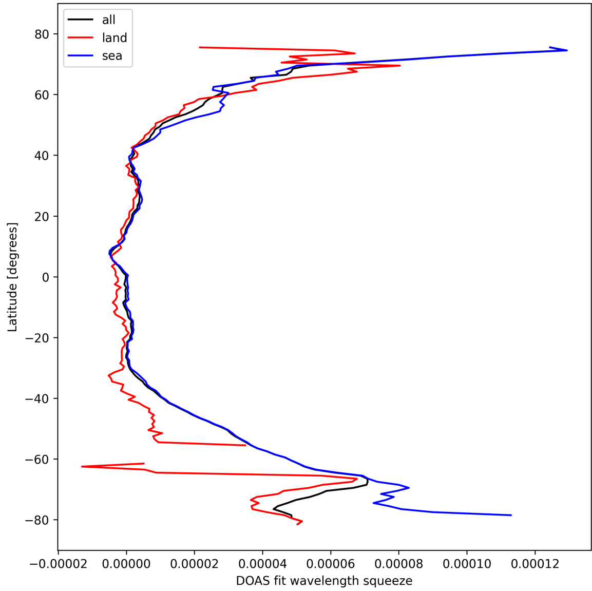
Figure 31: Zonal average of “DOAS fit wavelength squeeze” for 2024-10-16 to 2024-10-18.
