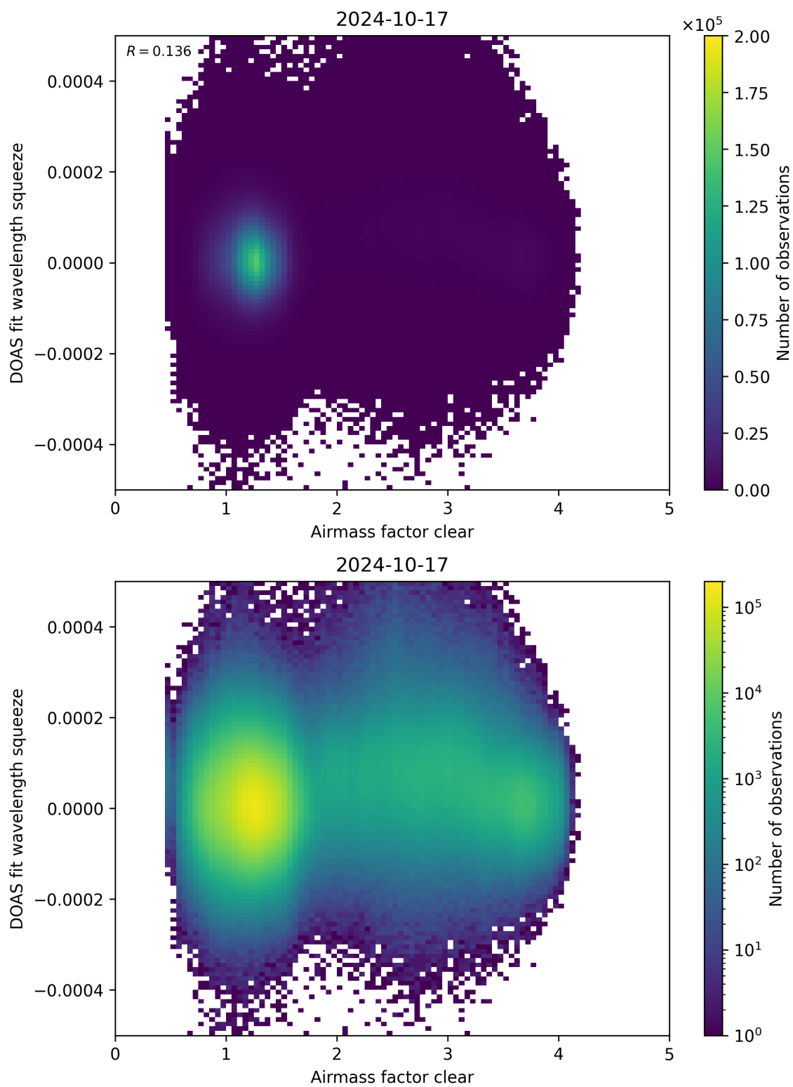
Figure 73: Scatter density plot of “Airmass factor clear” against “DOAS fit wavelength squeeze” for 2024-10-16 to 2024-10-18.
