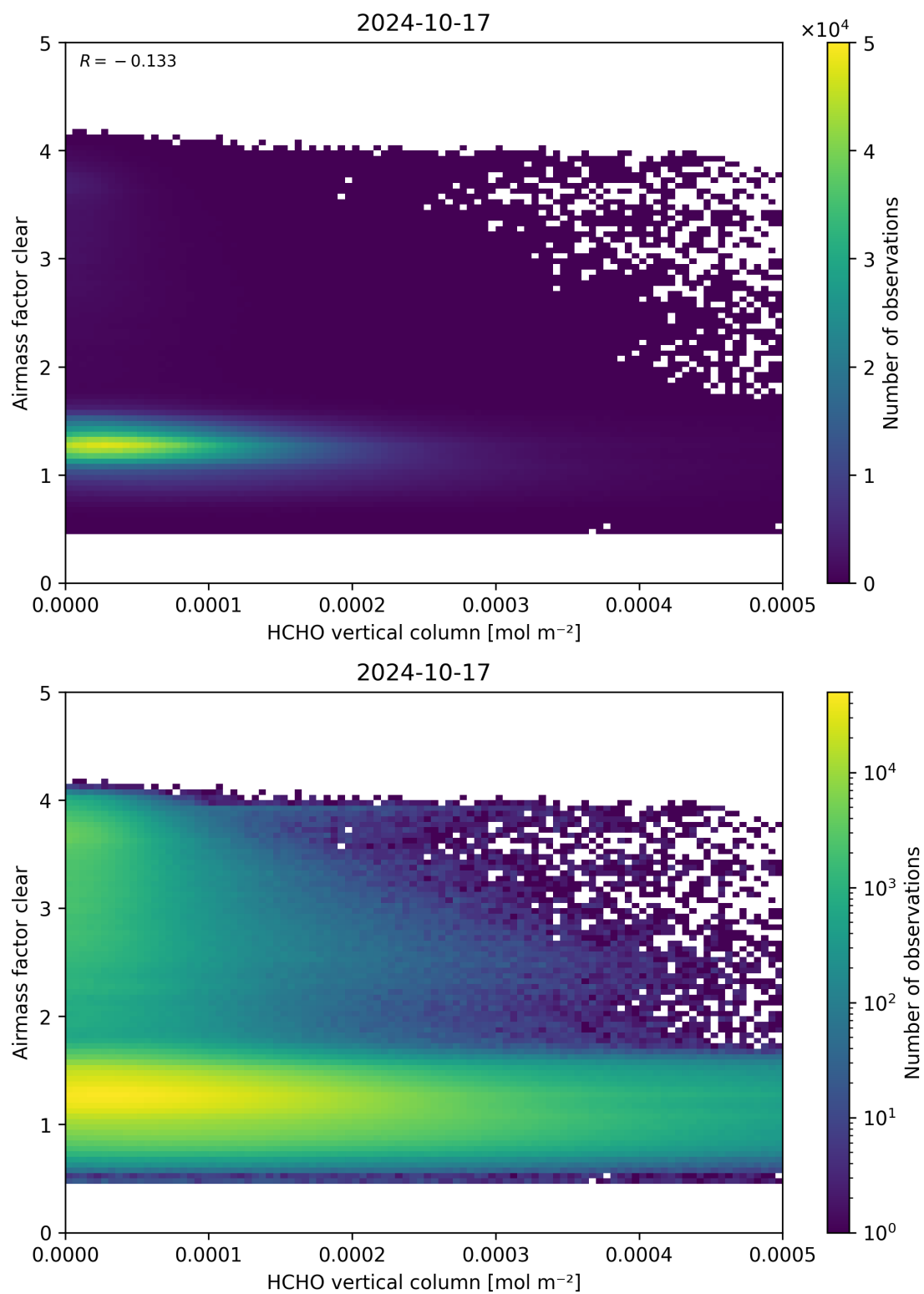
Figure 126: Scatter density plot of “HCHO vertical column” against “Airmass factor clear” for 2024-10-16 to 2024-10-18.
