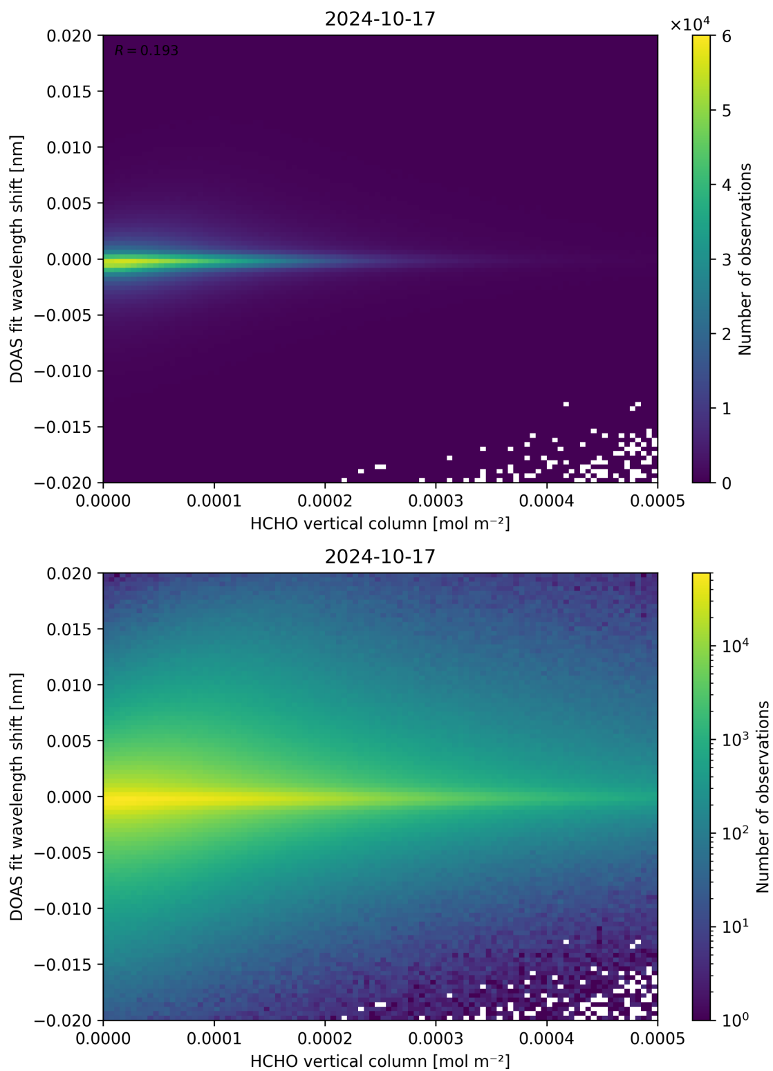
Figure 124: Scatter density plot of “HCHO vertical column” against “DOAS fit wavelength shift” for 2024-10-16 to 2024-10-18.
