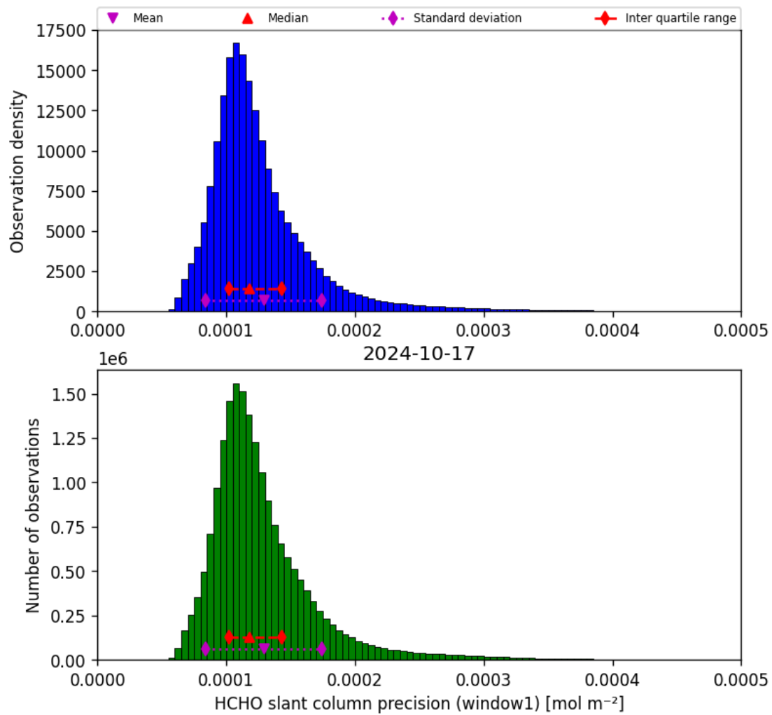
Figure 39: Histogram of “HCHO slant column precision (window1)” for 2024-10-16 to 2024-10-18
