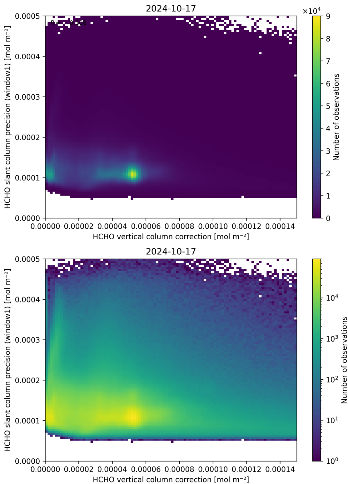
Figure 119: Scatter density plot of “HCHO vertical column correction” against “HCHO slant column precision (window1)” for 2024-10-16 to 2024-10-18.
