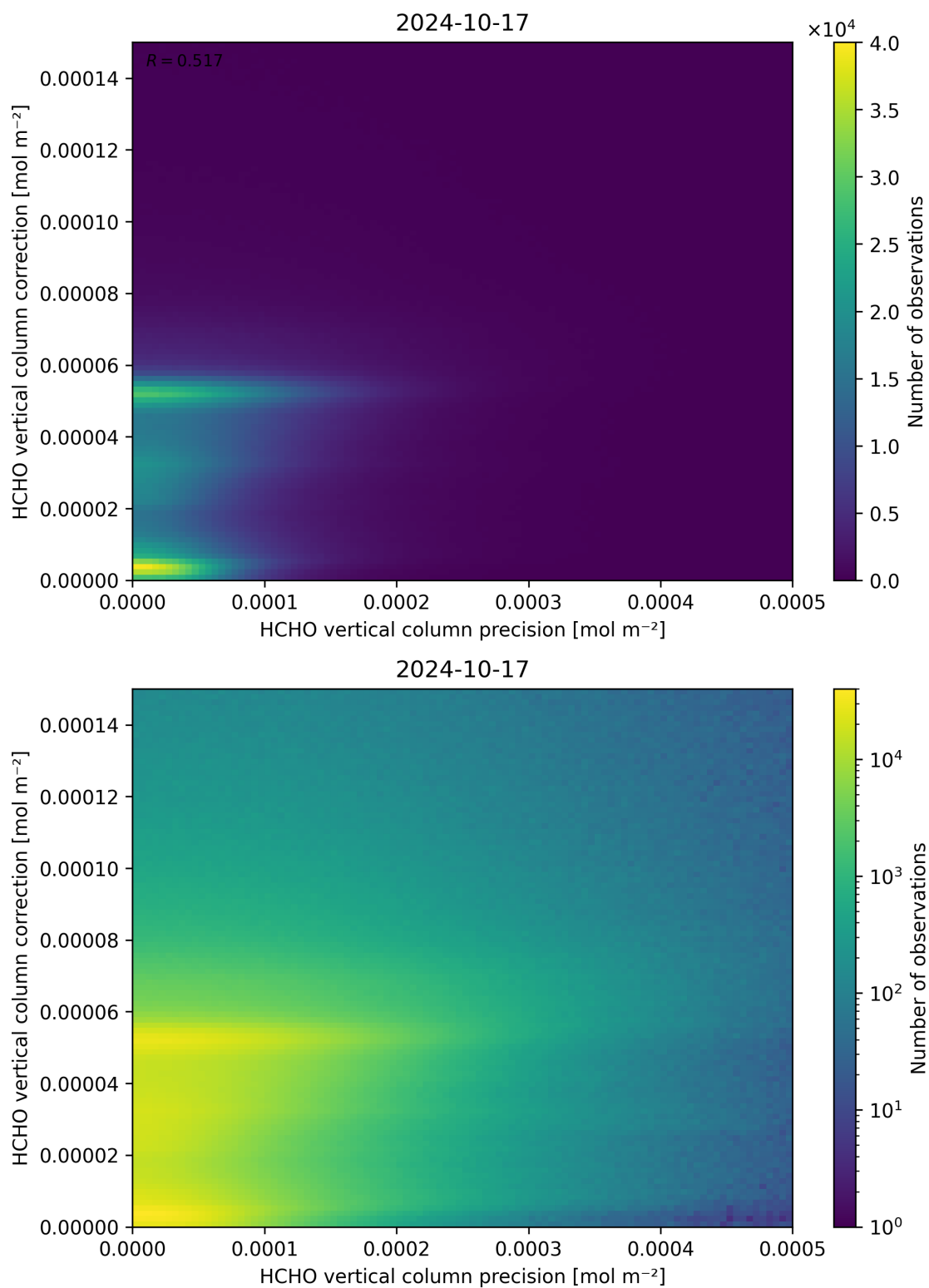
Figure 146: Scatter density plot of “HCHO vertical column precision” against “HCHO vertical column correction” for 2024-10-16 to 2024-10-18.
