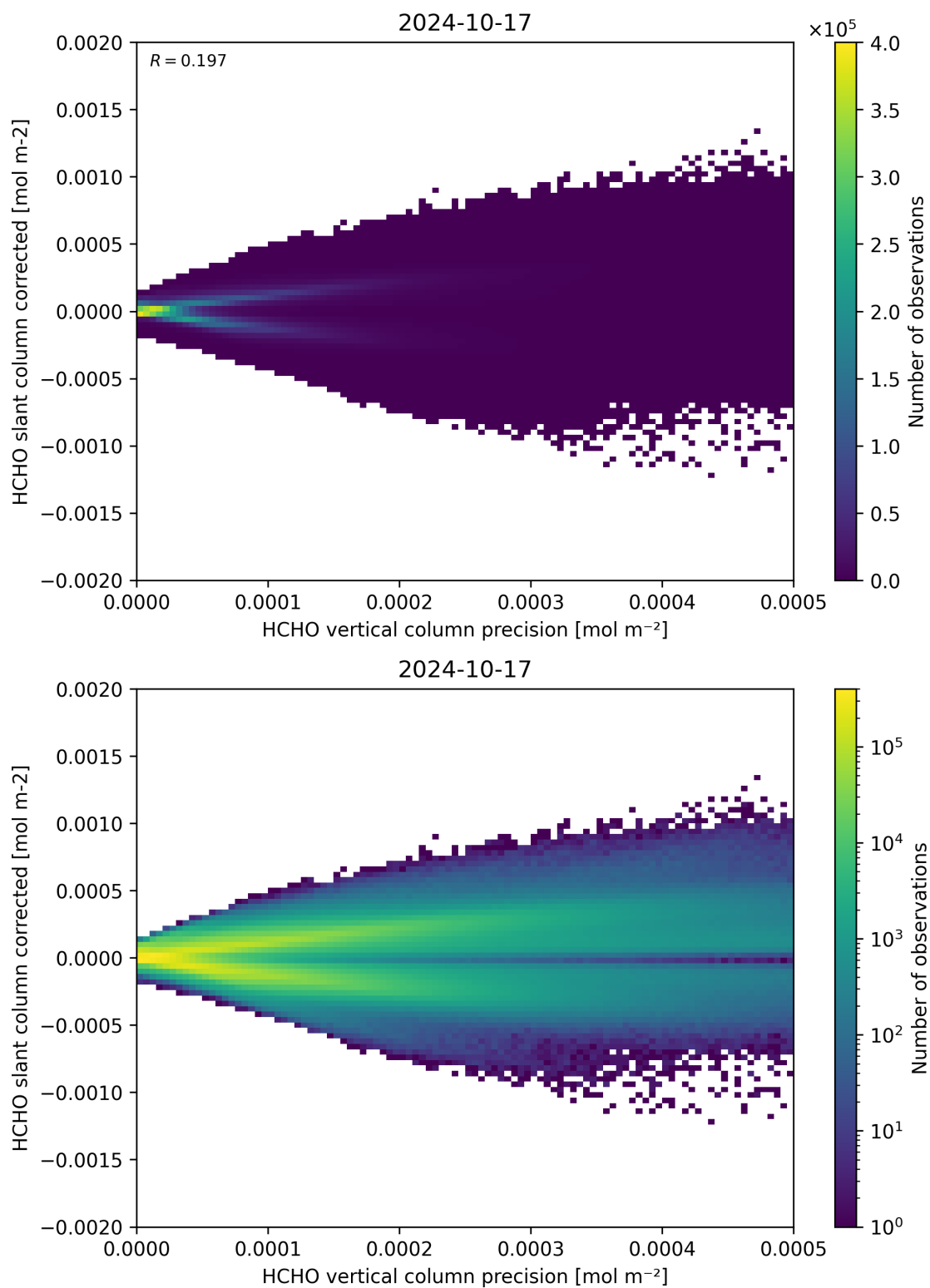
Figure 140: Scatter density plot of “HCHO vertical column precision” against “HCHO slant column corrected” for 2024-10-16 to 2024-10-18.
