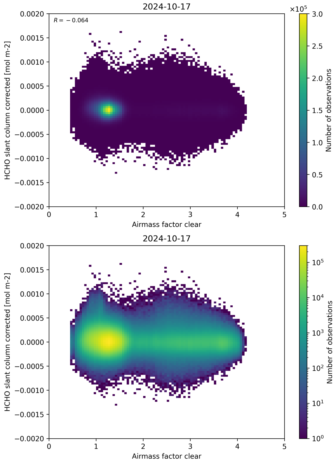
Figure 74: Scatter density plot of “Airmass factor clear” against “HCHO slant column corrected” for 2024-10-16 to 2024-10-18.
