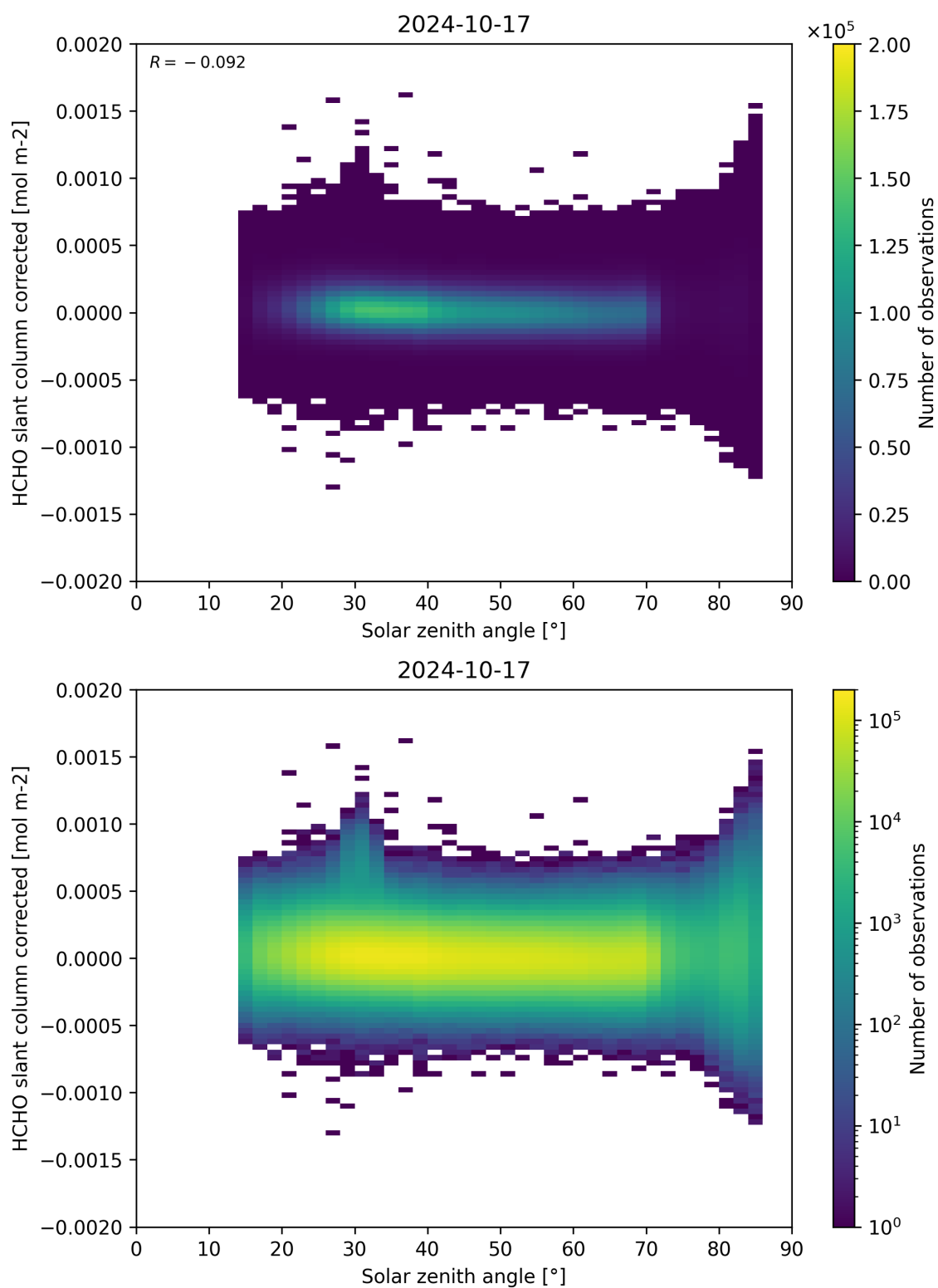
Figure 171: Scatter density plot of “Solar zenith angle” against “HCHO slant column corrected” for 2024-10-16 to 2024-10-18.
