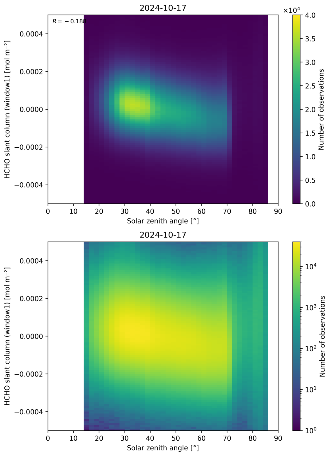
Figure 173: Scatter density plot of “Solar zenith angle” against “HCHO slant column (window1)” for 2024-10-16 to 2024-10-18.
