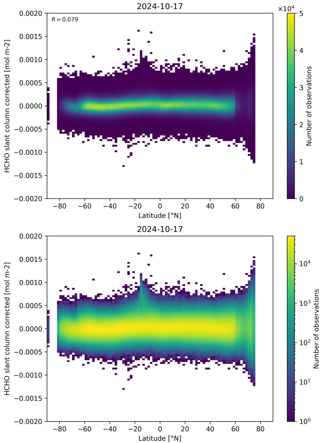
Figure 157: Scatter density plot of “Latitude” against “HCHO slant column corrected” for 2024-10-16 to 2024-10-18.
