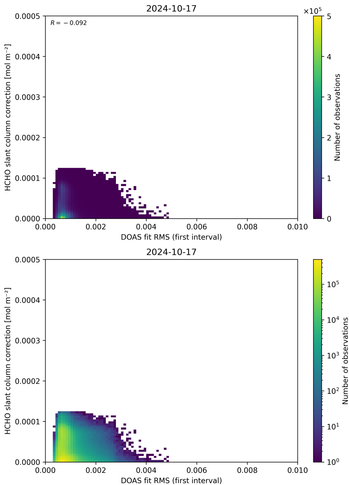
Figure 63: Scatter density plot of “DOAS fit RMS (first interval)” against “HCHO slant column correction” for 2024-10-16 to 2024-10-18.
