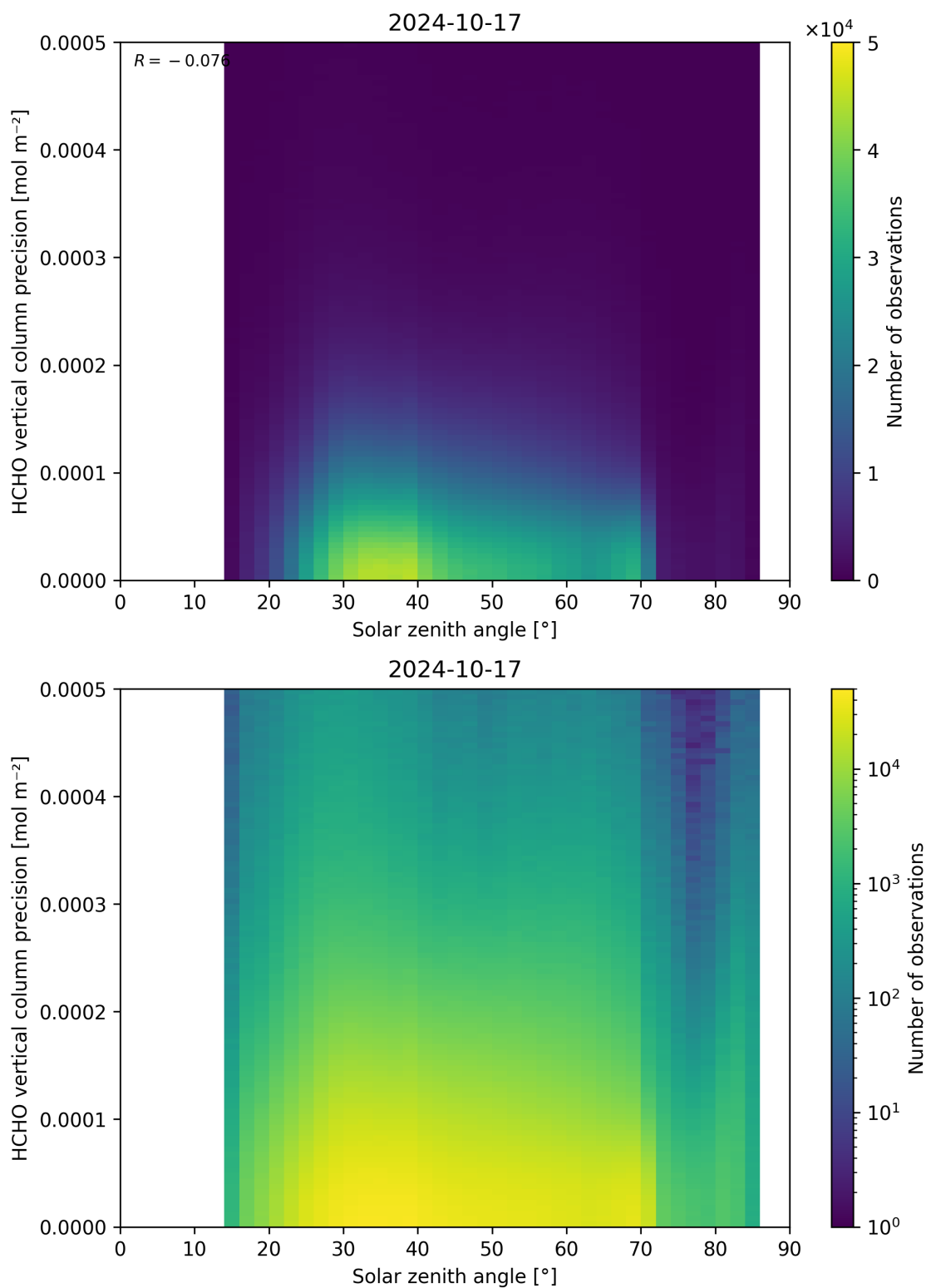
Figure 179: Scatter density plot of “Solar zenith angle” against “HCHO vertical column precision” for 2024-10-16 to 2024-10-18.
