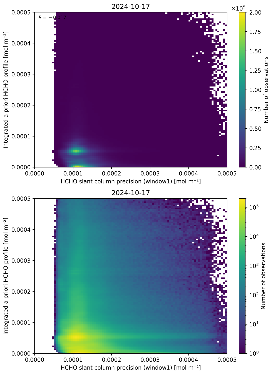
Figure 96: Scatter density plot of “HCHO slant column precision (window1)” against “Integrated a priori HCHO profile” for 2024-10-16 to 2024-10-18.
