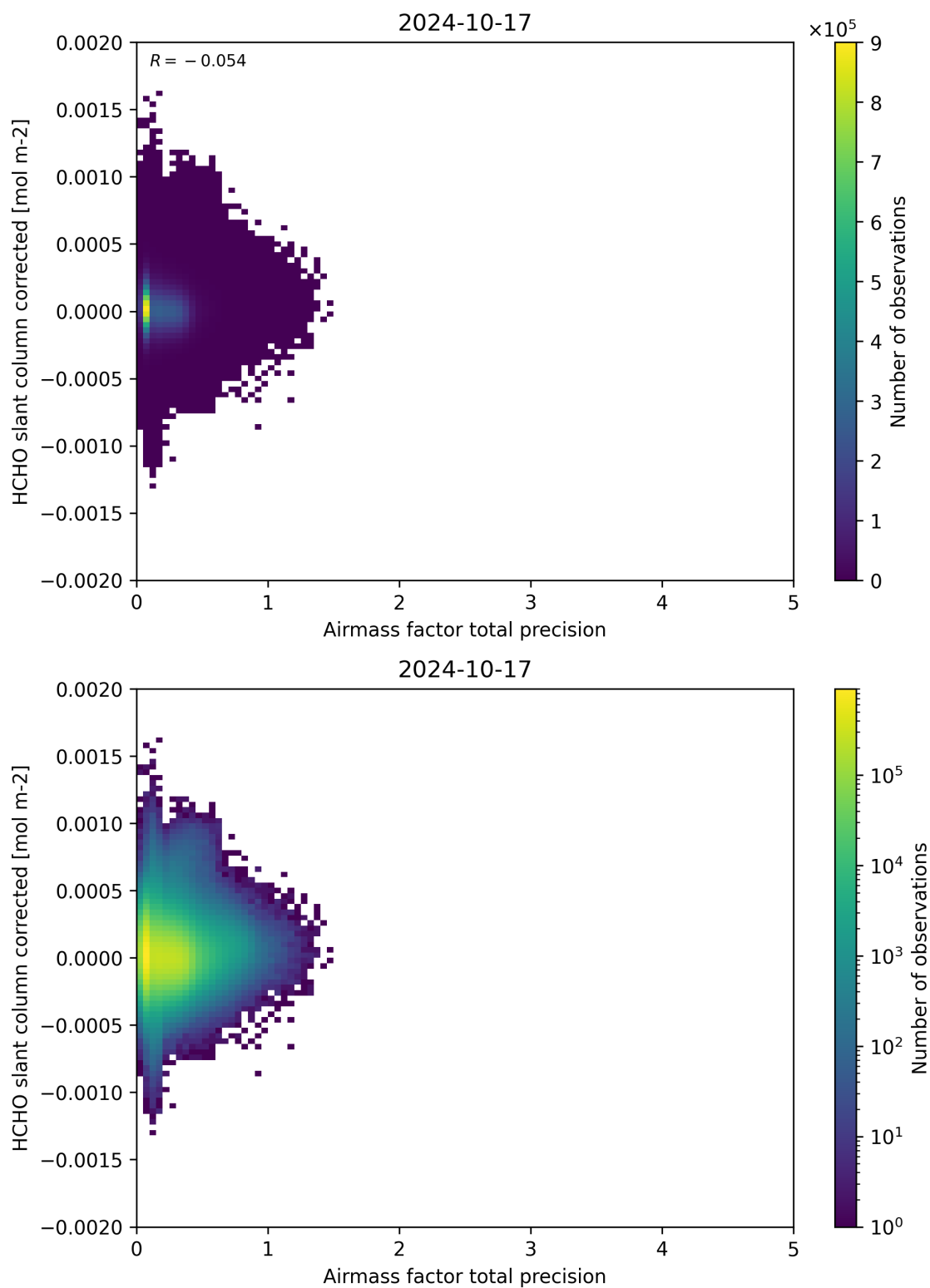
Figure 109: Scatter density plot of “Airmass factor total precision” against “HCHO slant column corrected” for 2024-10-16 to 2024-10-18.
