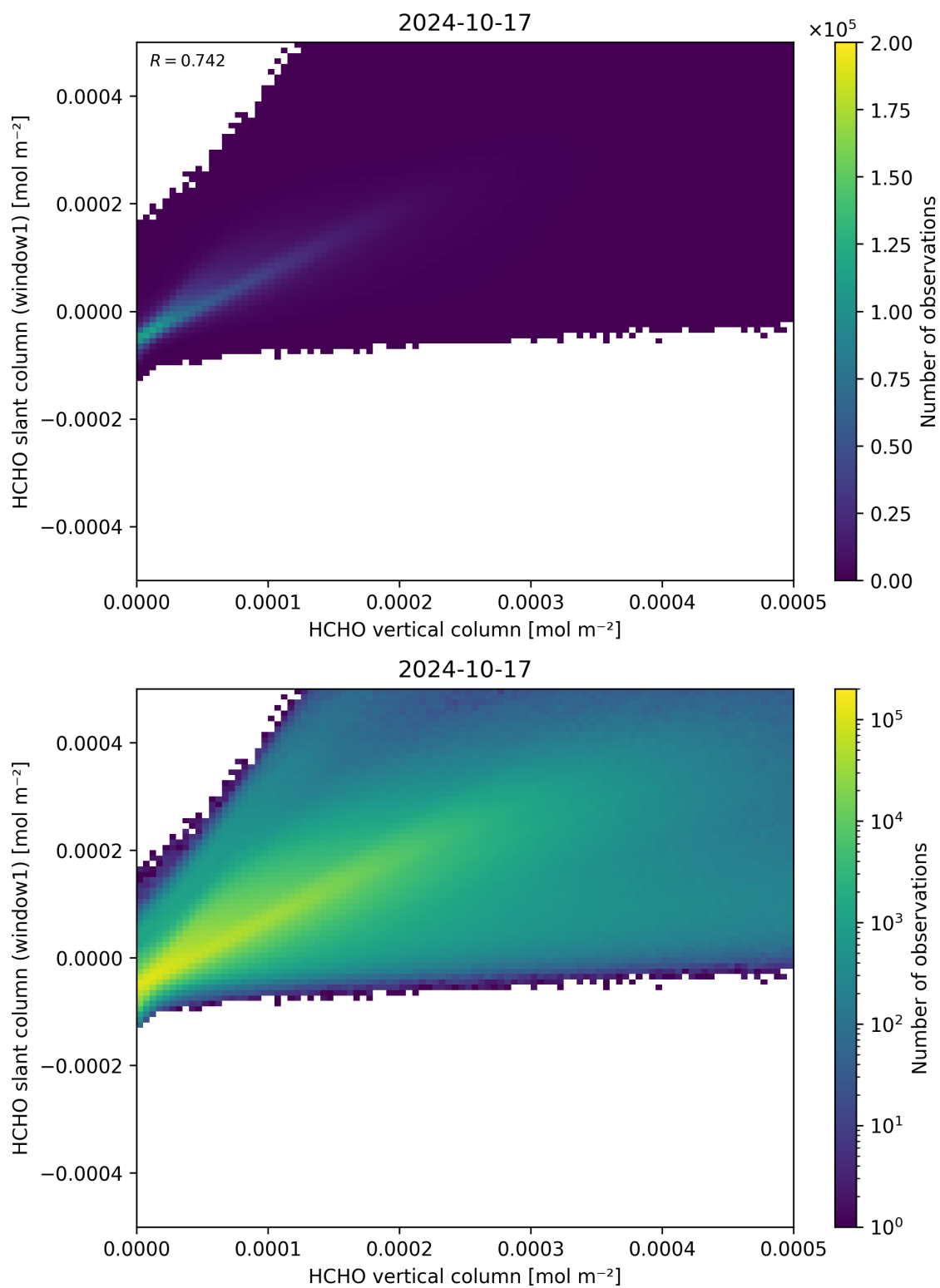
Figure 129: Scatter density plot of “HCHO vertical column” against “HCHO slant column (window1)” for 2024-10-16 to 2024-10-18.
