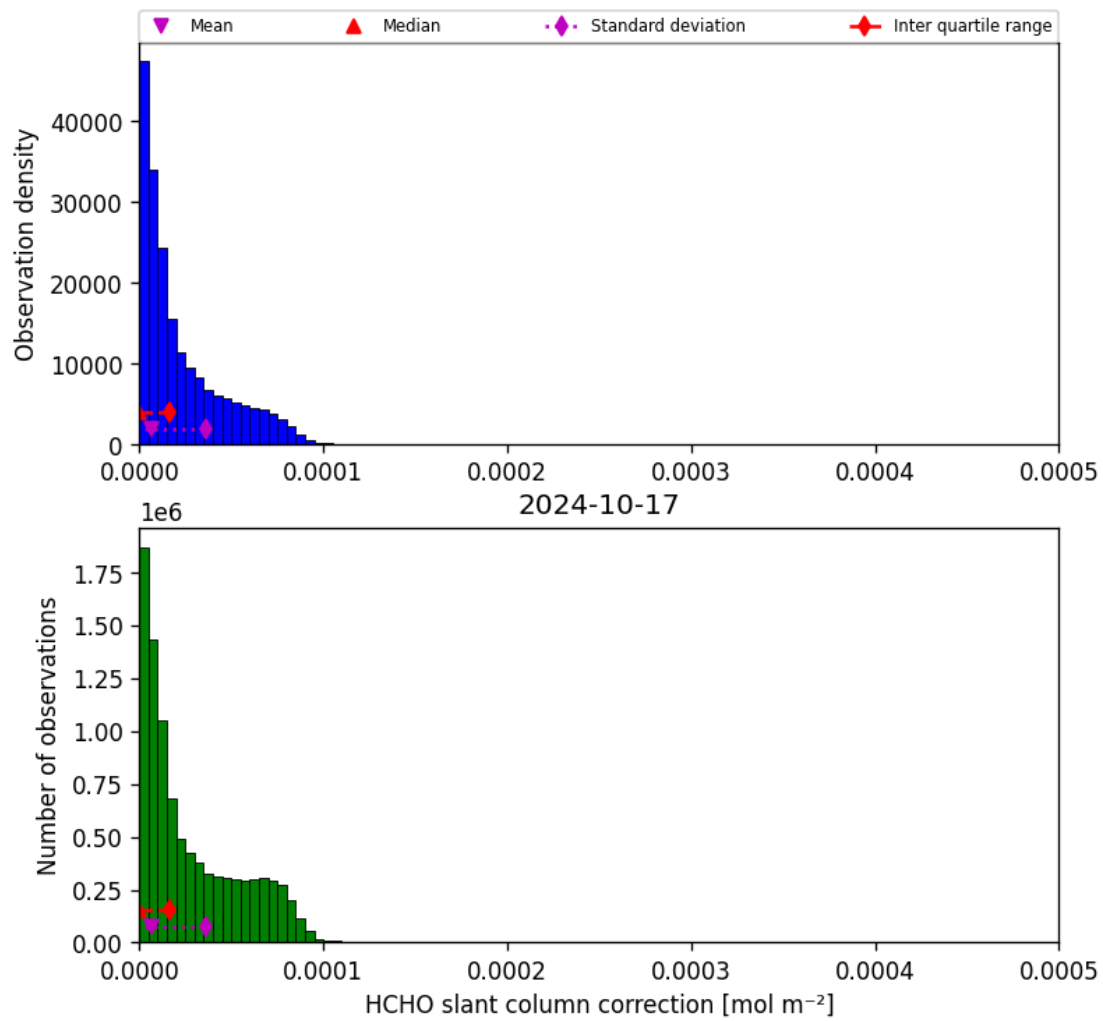
Figure 47: Histogram of “HCHO slant column correction” for 2024-10-16 to 2024-10-18
