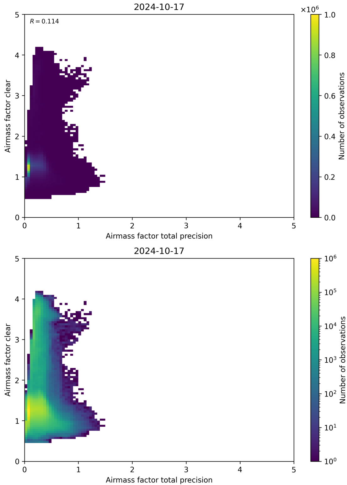
Figure 108: Scatter density plot of “Airmass factor total precision” against “Airmass factor clear” for 2024-10-16 to 2024-10-18.
