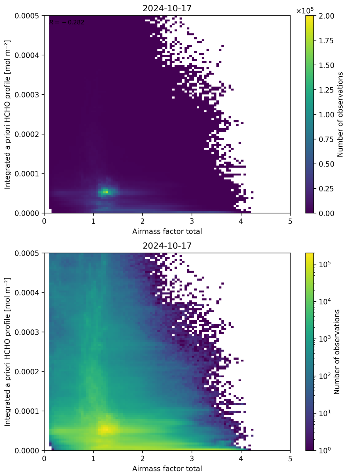
Figure 104: Scatter density plot of “Airmass factor total” against “Integrated a priori HCHO profile” for 2024-10-16 to 2024-10-18.
