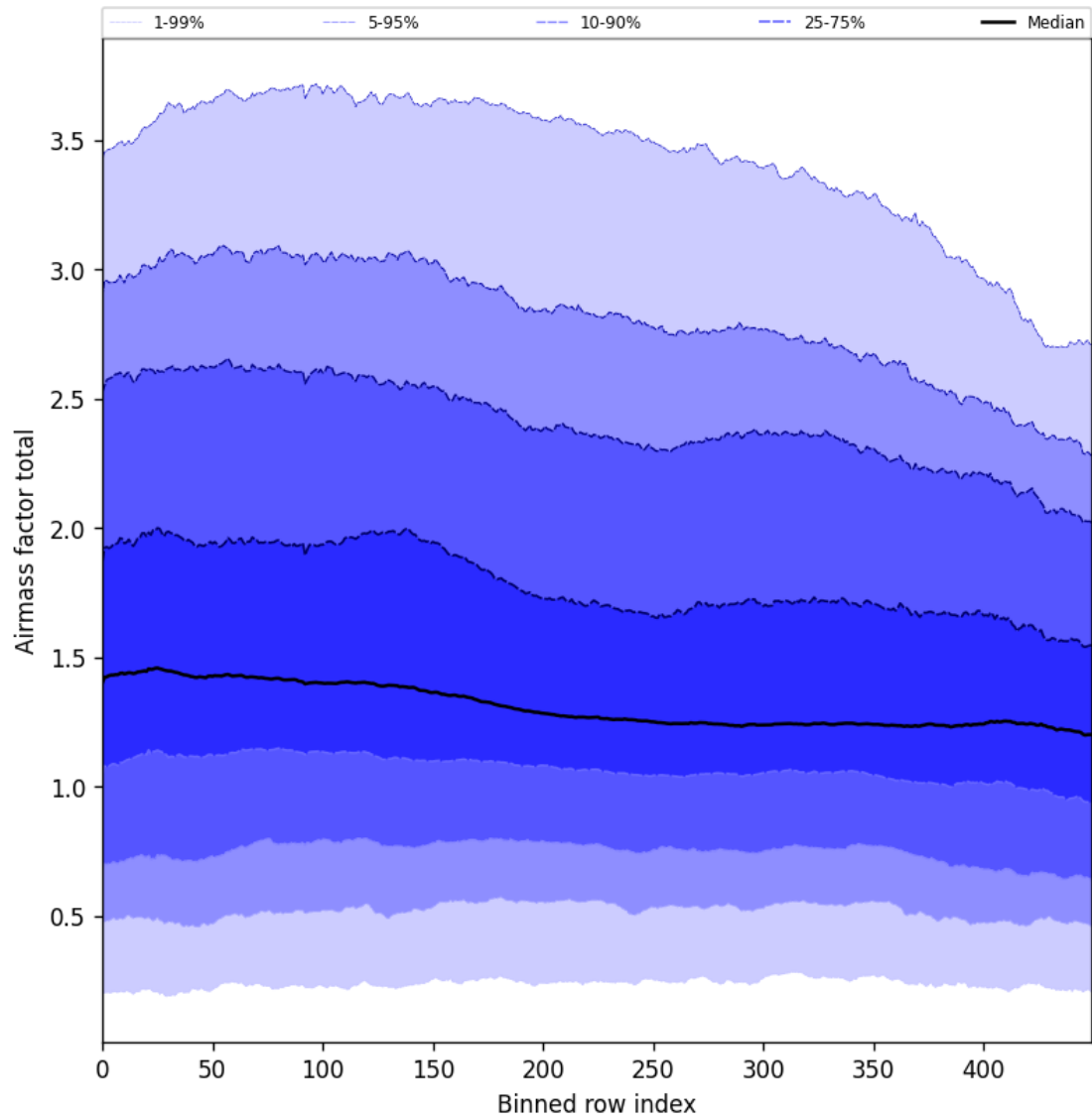
Figure 54: Along track statistics of “Airmass factor total” for 2024-10-16 to 2024-10-18
