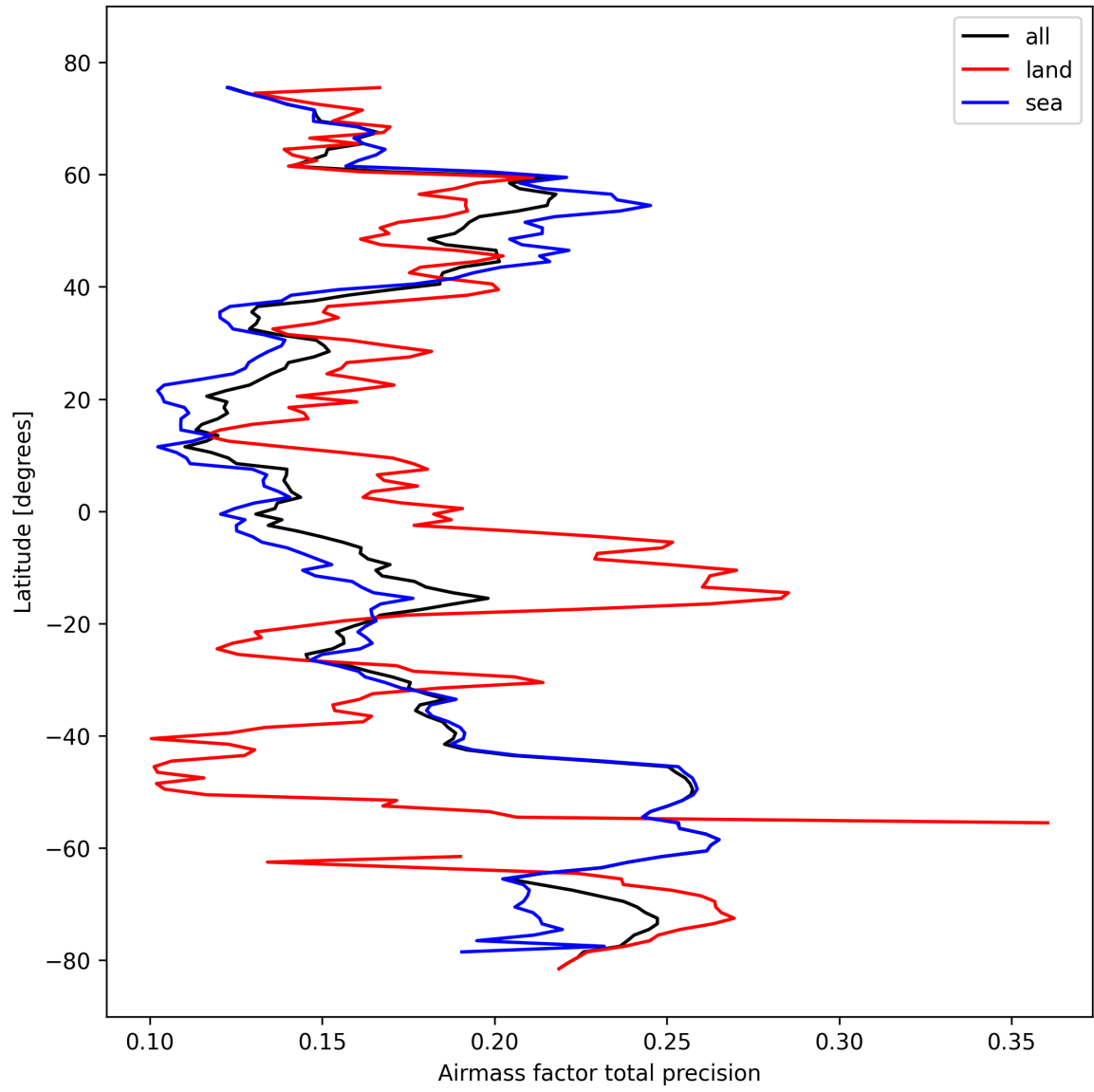
Figure 27: Zonal average of “Airmass factor total precision” for 2024-10-16 to 2024-10-18.
