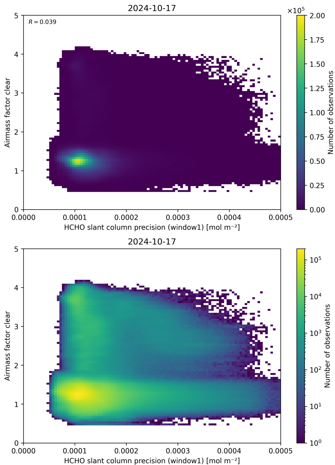
Figure 91: Scatter density plot of “HCHO slant column precision (window1)” against “Airmass factor clear” for 2024-10-16 to 2024-10-18.
