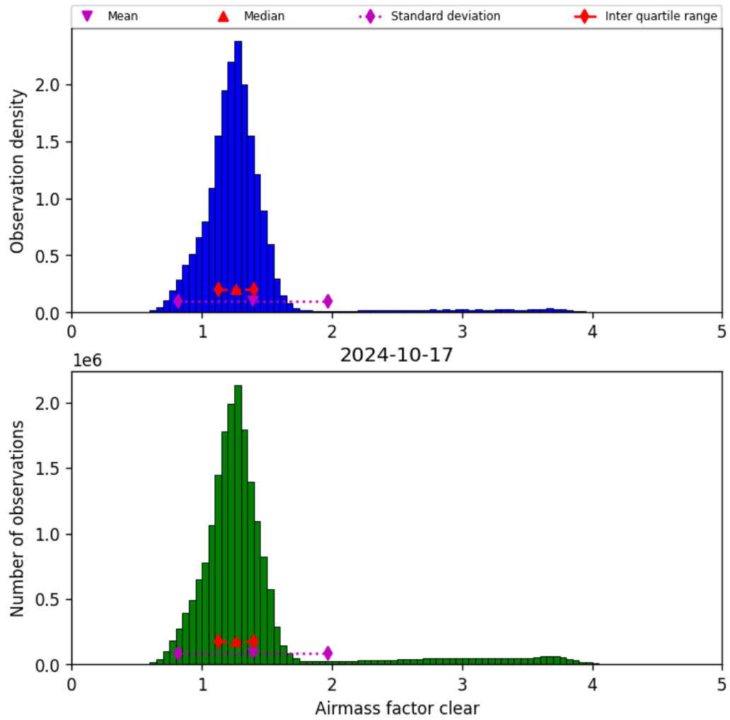
Figure 42: Histogram of “Airmass factor clear” for 2024-10-16 to 2024-10-18
