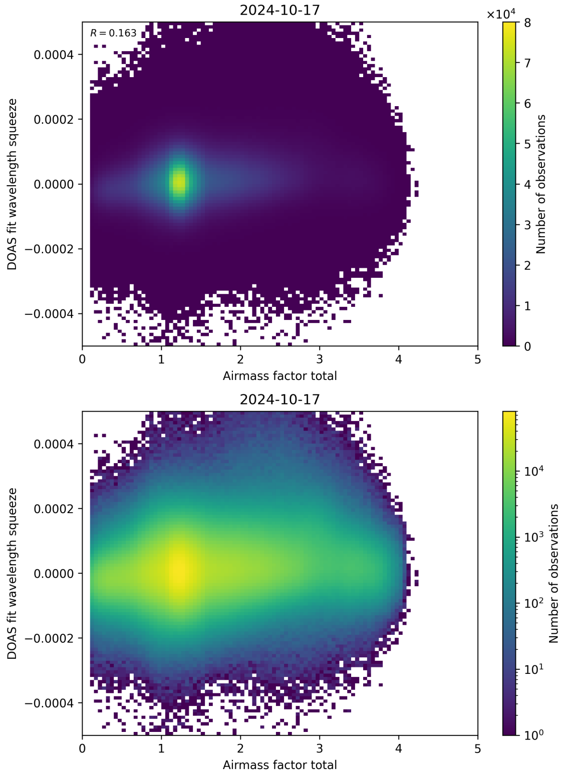
Figure 99: Scatter density plot of “Airmass factor total” against “DOAS fit wavelength squeeze” for 2024-10-16 to 2024-10-18.
