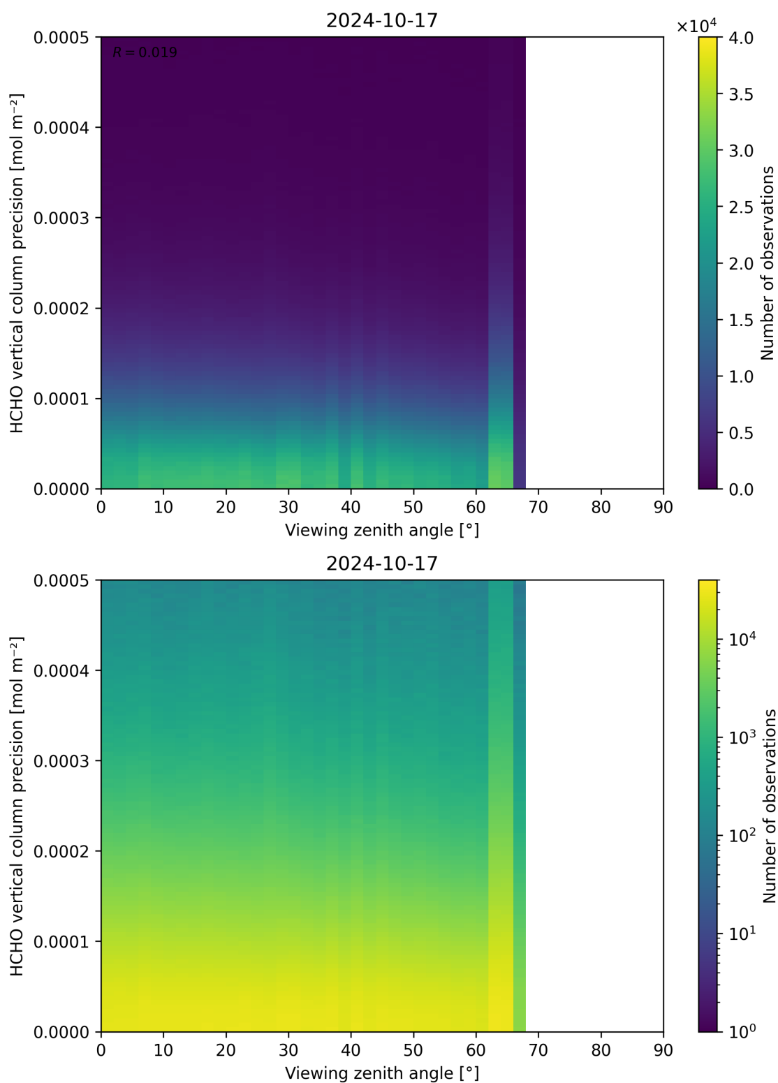
Figure 194: Scatter density plot of “Viewing zenith angle” against “HCHO vertical column precision” for 2024-10-16 to 2024-10-18.
