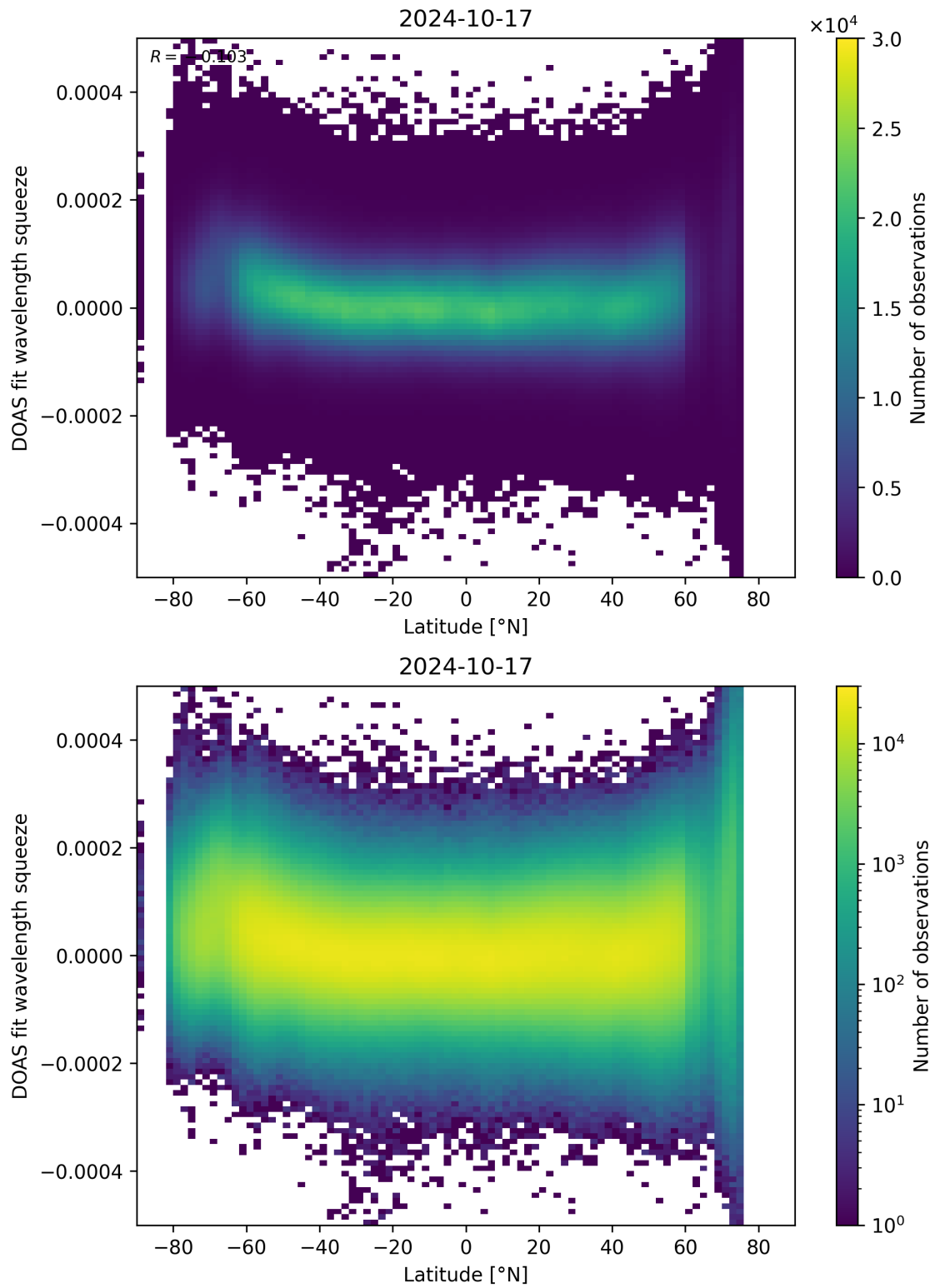
Figure 155: Scatter density plot of “Latitude” against “DOAS fit wavelength squeeze” for 2024-10-16 to 2024-10-18.
