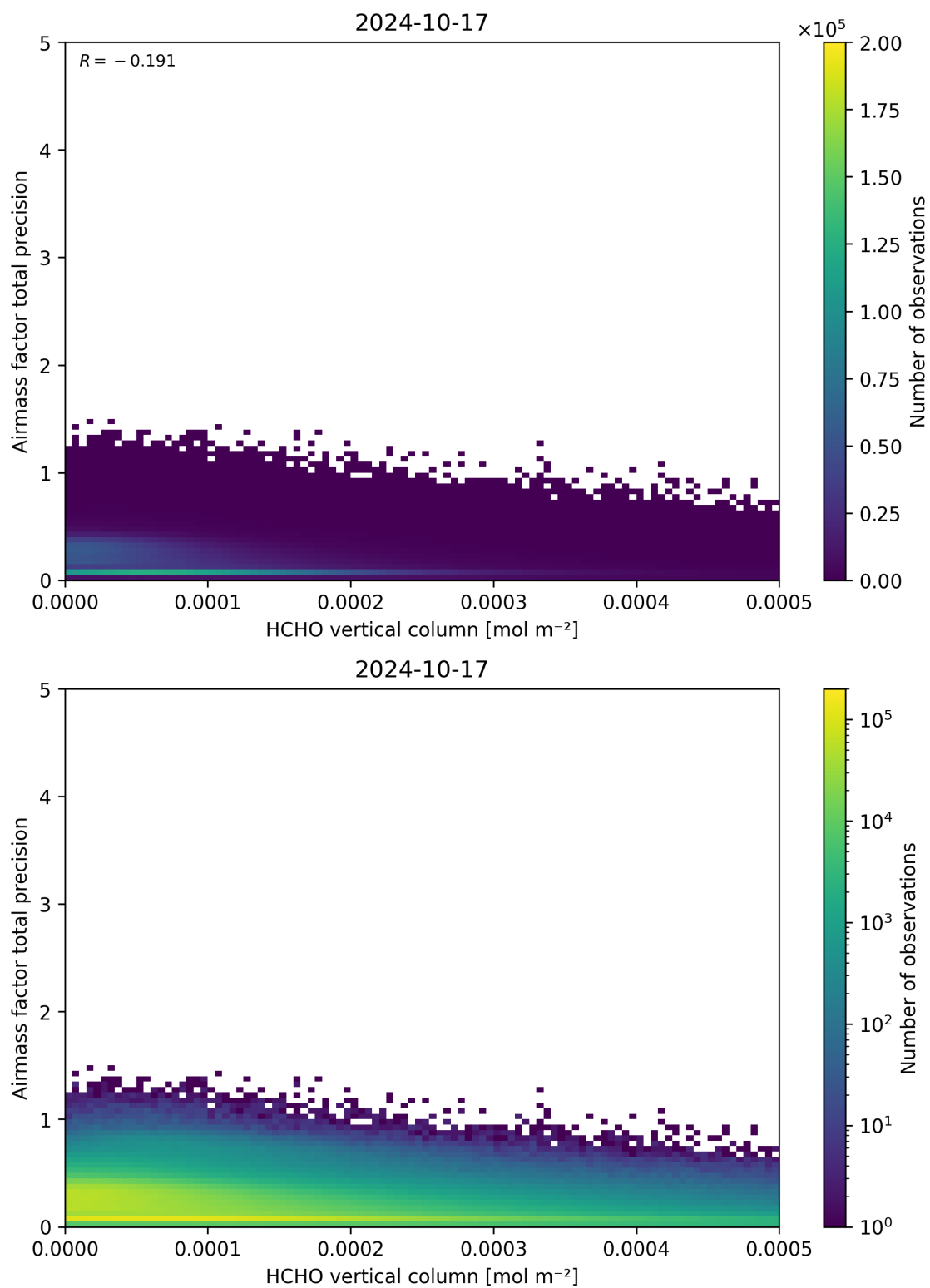
Figure 132: Scatter density plot of “HCHO vertical column” against “Airmass factor total precision” for 2024-10-16 to 2024-10-18.
