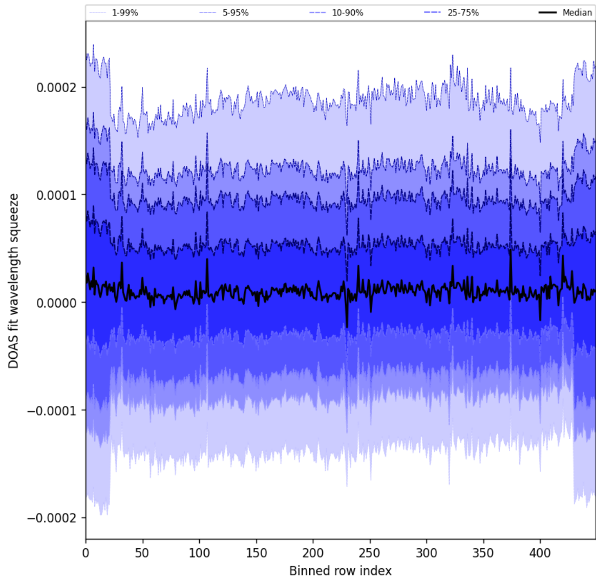
Figure 59: Along track statistics of “DOAS fit wavelength squeeze” for 2024-10-16 to 2024-10-18
