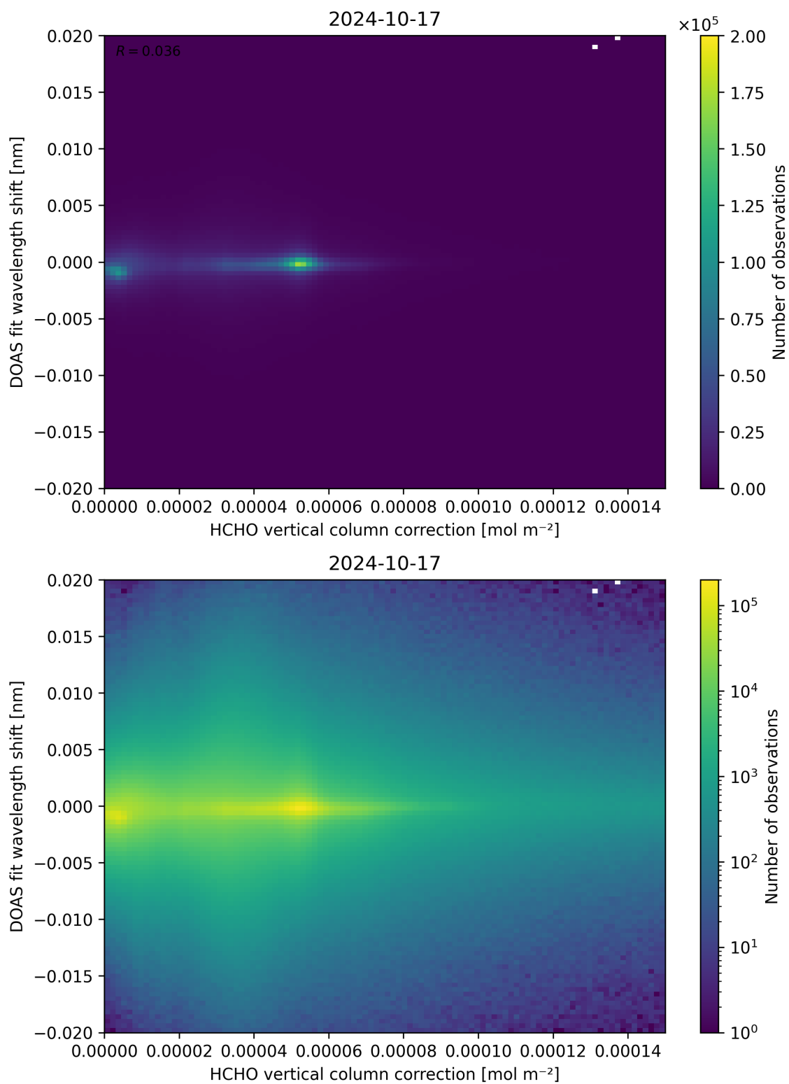
Figure 113: Scatter density plot of “HCHO vertical column correction” against “DOAS fit wavelength shift” for 2024-10-16 to 2024-10-18.
