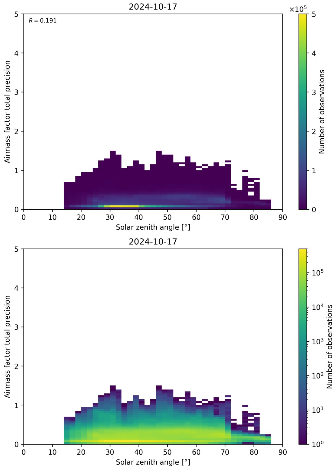
Figure 176: Scatter density plot of “Solar zenith angle” against “Airmass factor total precision” for 2024-10-16 to 2024-10-18.
