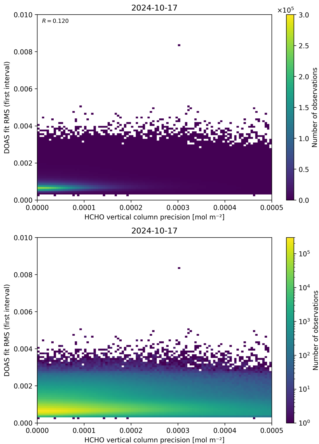
Figure 136: Scatter density plot of “HCHO vertical column precision” against “DOAS fit RMS (first interval)” for 2024-10-16 to 2024-10-18.
