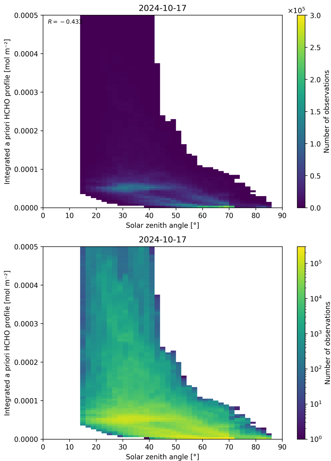
Figure 180: Scatter density plot of “Solar zenith angle” against “Integrated a priori HCHO profile” for 2024-10-16 to 2024-10-18.
