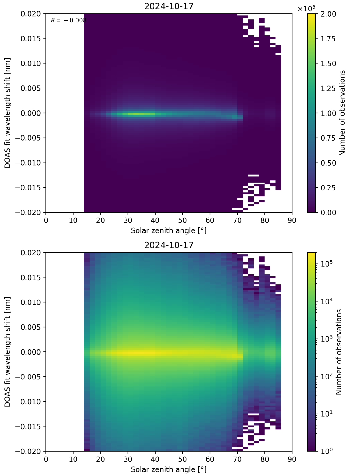
Figure 168: Scatter density plot of “Solar zenith angle” against “DOAS fit wavelength shift” for 2024-10-16 to 2024-10-18.
