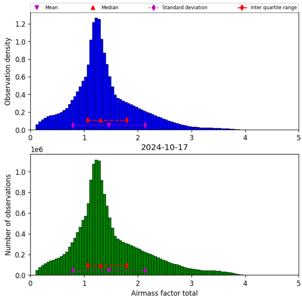
Figure 40: Histogram of "Airmass factor total" for 2024-10-16 to 2024-10-18
