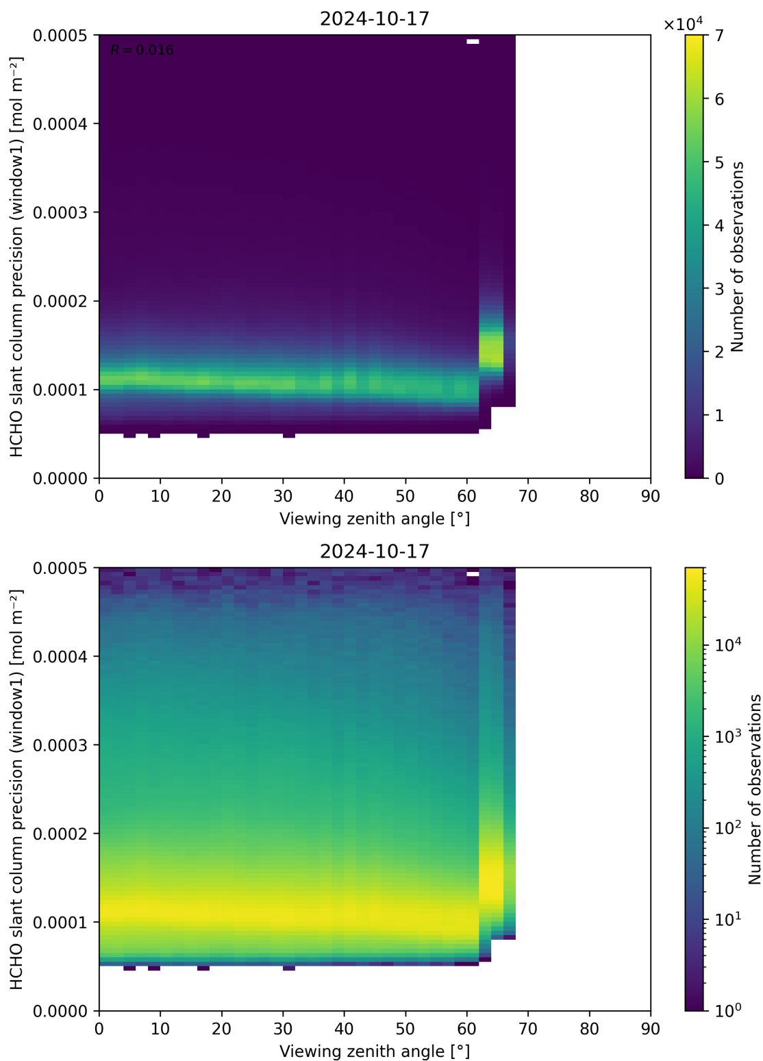
Figure 189: Scatter density plot of “Viewing zenith angle” against “HCHO slant column precision (window1)” for 2024-10-16 to 2024-10-18.
