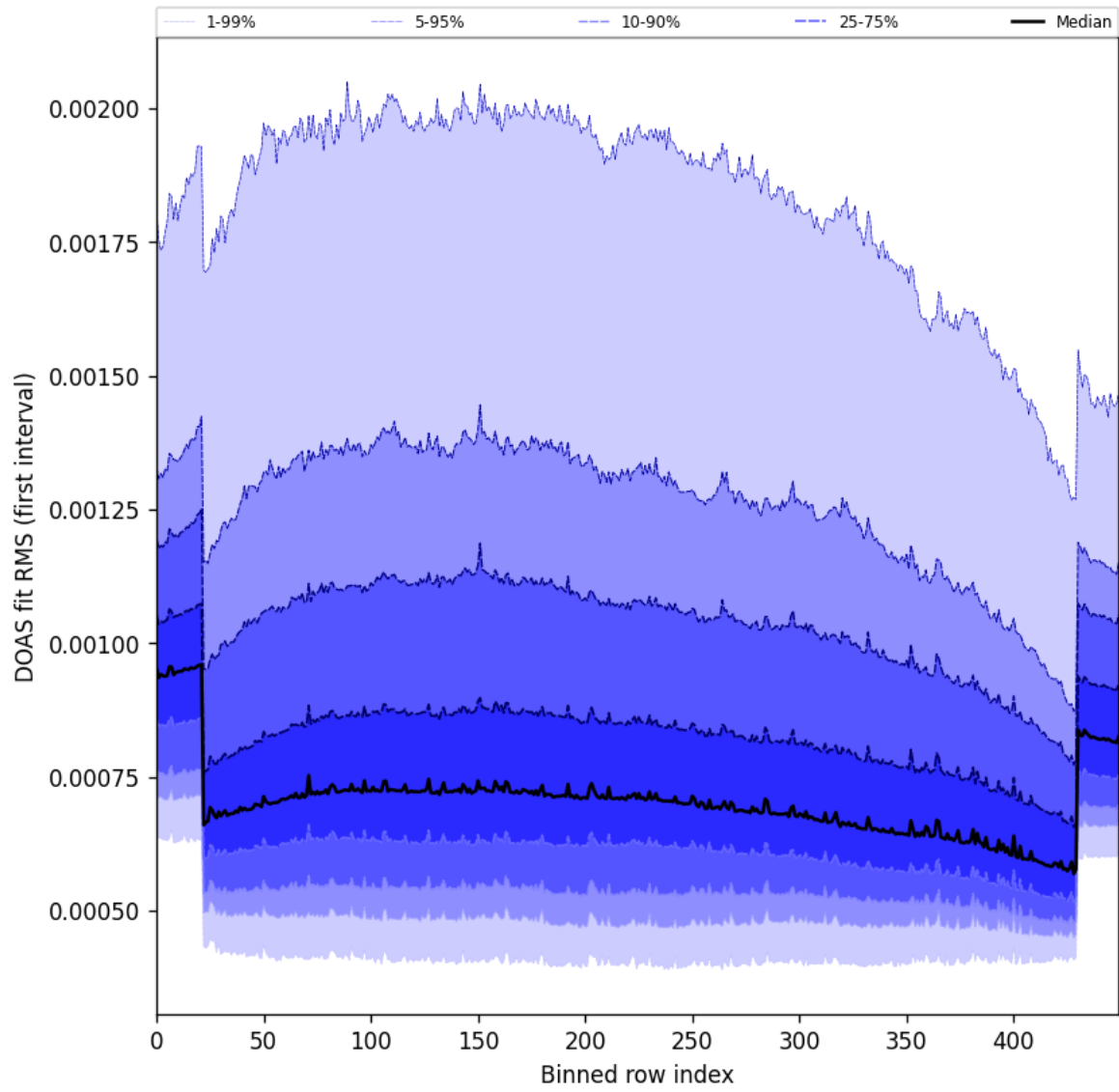
Figure 60: Along track statistics of “DOAS fit RMS (first interval)” for 2024-10-16 to 2024-10-18
