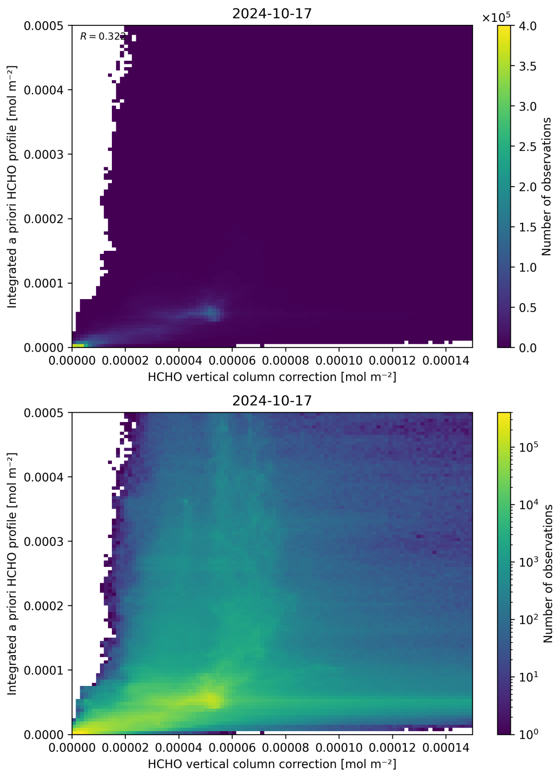
Figure 122: Scatter density plot of “HCHO vertical column correction” against “Integrated a priori HCHO profile” for 2024-10-16 to 2024-10-18.
