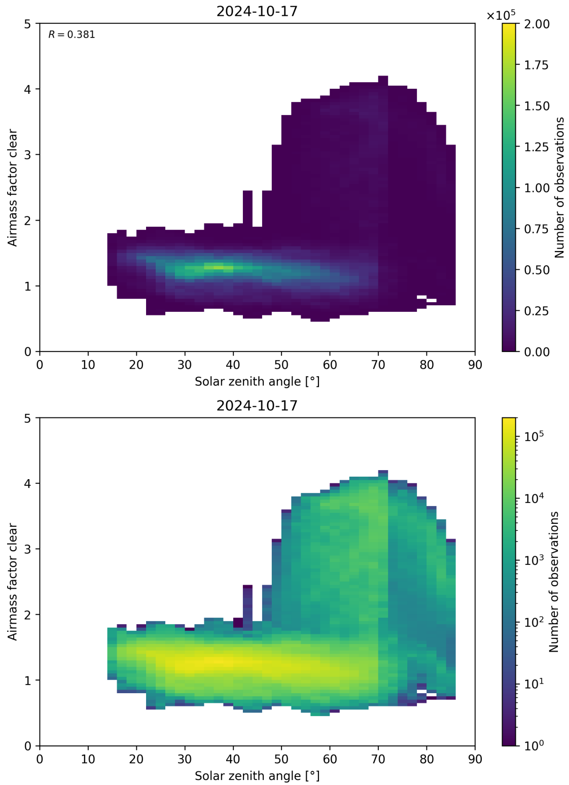
Figure 170: Scatter density plot of “Solar zenith angle” against “Airmass factor clear” for 2024-10-16 to 2024-10-18.
