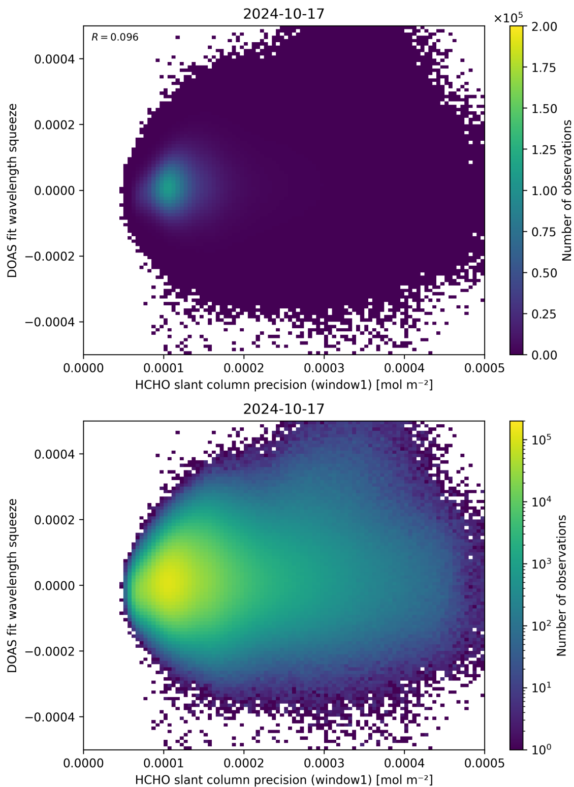
Figure 90: Scatter density plot of “HCHO slant column precision (window1)” against “DOAS fit wavelength squeeze” for 2024-10-16 to 2024-10-18.
