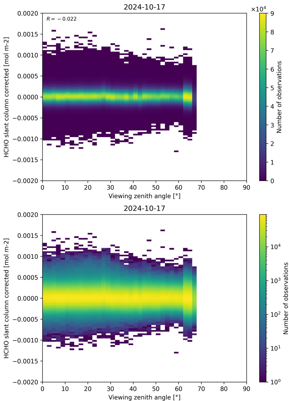
Figure 186: Scatter density plot of “Viewing zenith angle” against “HCHO slant column corrected” for 2024-10-16 to 2024-10-18.
