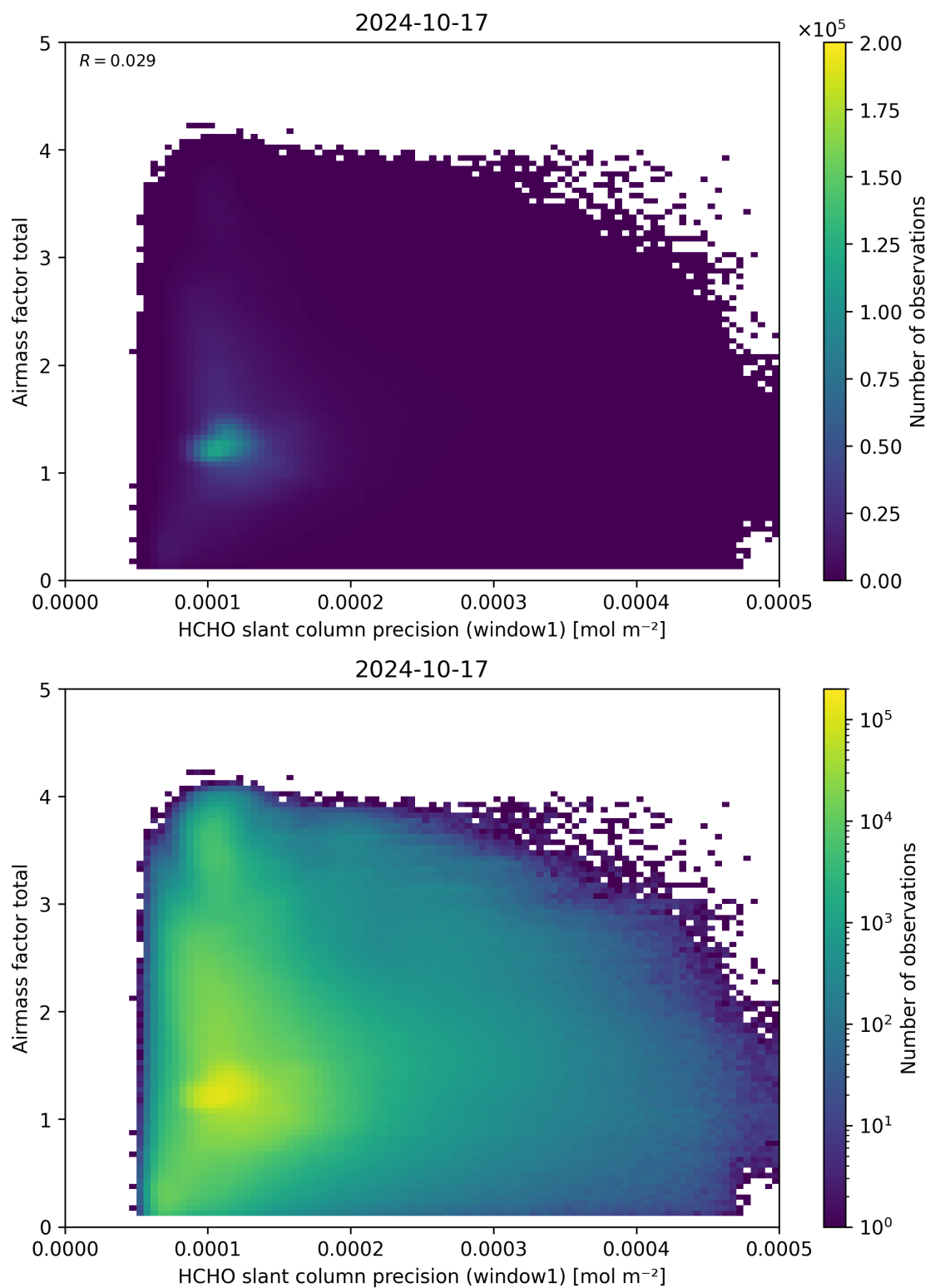
Figure 94: Scatter density plot of “HCHO slant column precision (window1)” against “Airmass factor total” for 2024-10-16 to 2024-10-18.
