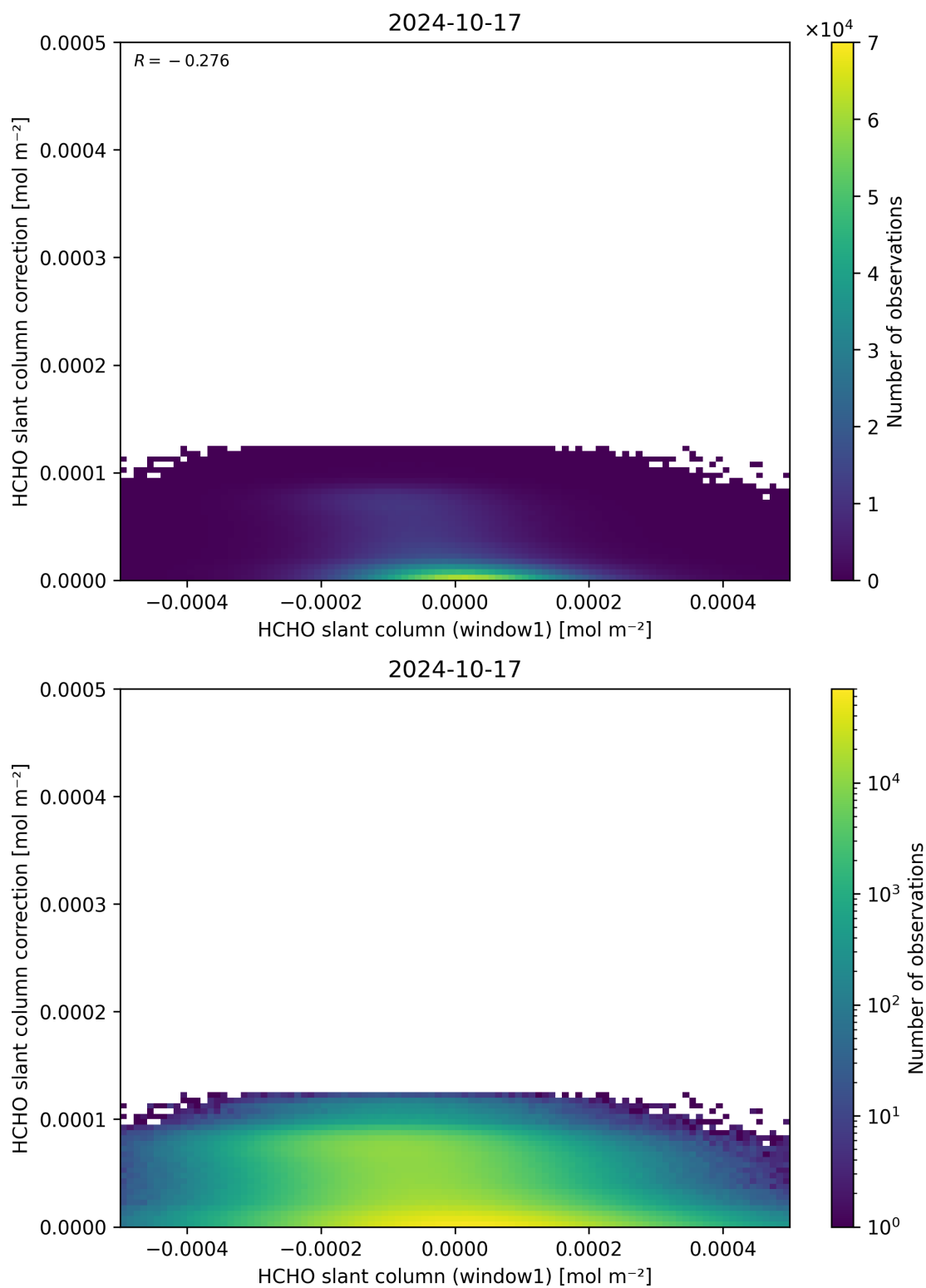
Figure 83: Scatter density plot of “HCHO slant column (window1)” against “HCHO slant column correction” for 2024-10-16 to 2024-10-18.
