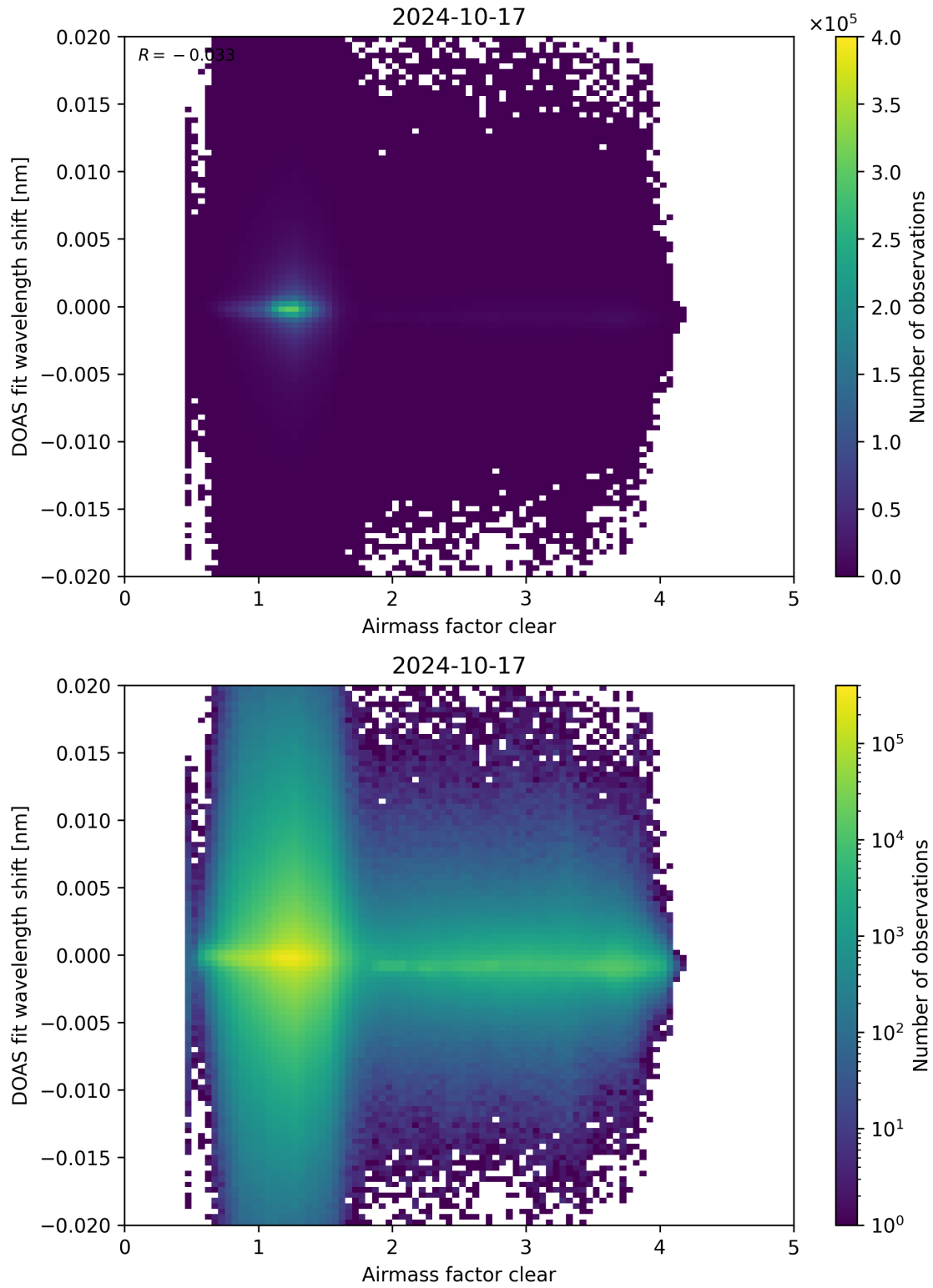
Figure 72: Scatter density plot of “Airmass factor clear” against “DOAS fit wavelength shift” for 2024-10-16 to 2024-10-18.
