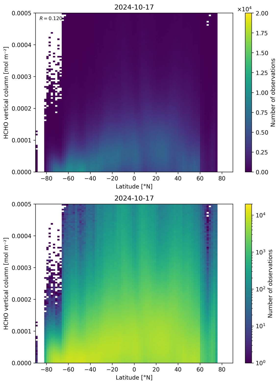
Figure 163: Scatter density plot of “Latitude” against “HCHO vertical column” for 2024-10-16 to 2024-10-18.
