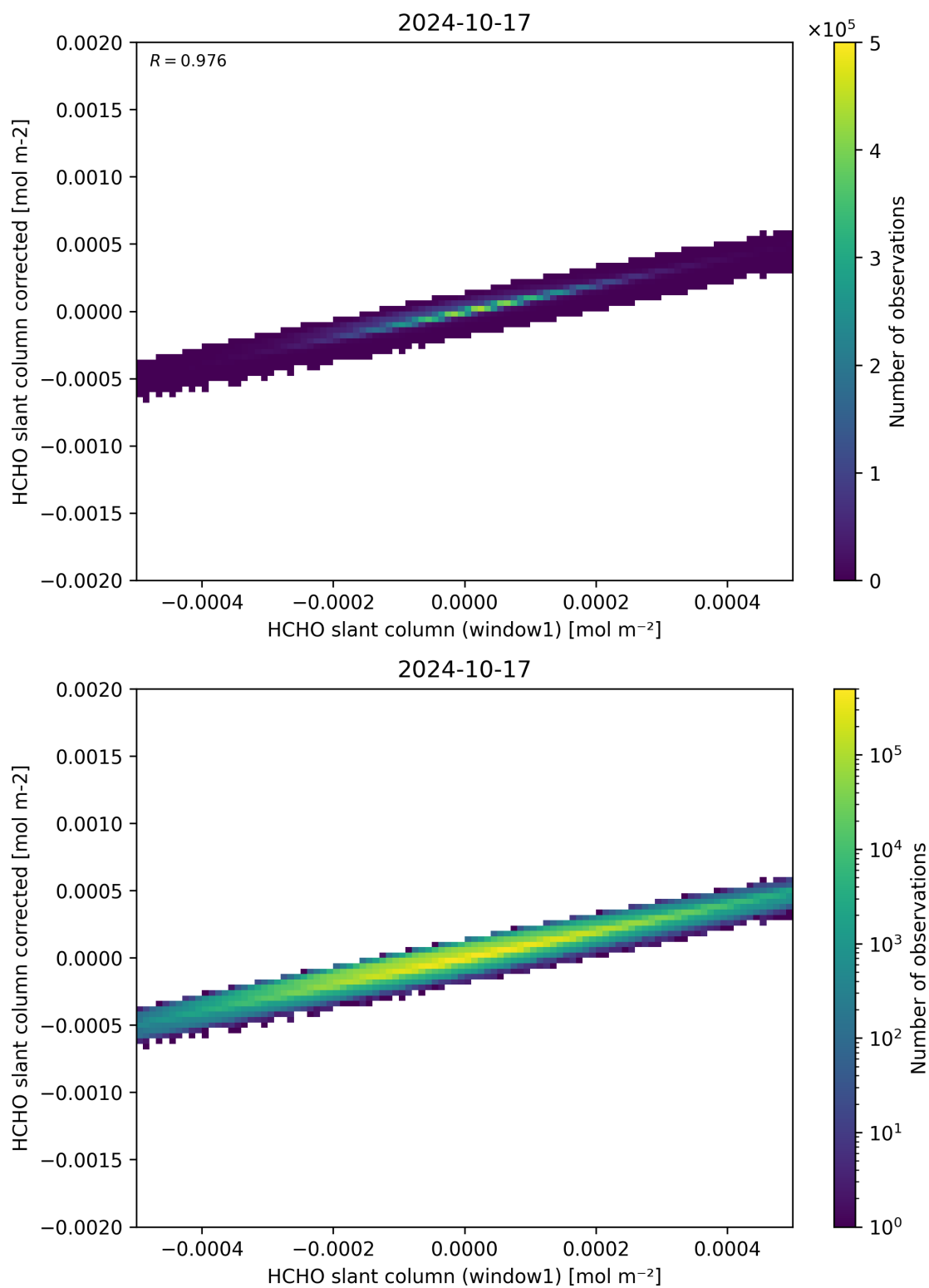
Figure 82: Scatter density plot of “HCHO slant column (window1)” against “HCHO slant column corrected” for 2024-10-16 to 2024-10-18.
