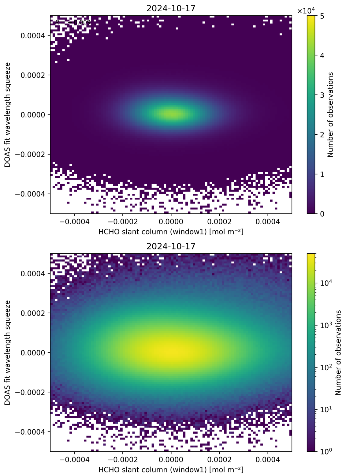
Figure 80: Scatter density plot of “HCHO slant column (window1)” against “DOAS fit wavelength squeeze” for 2024-10-16 to 2024-10-18.
