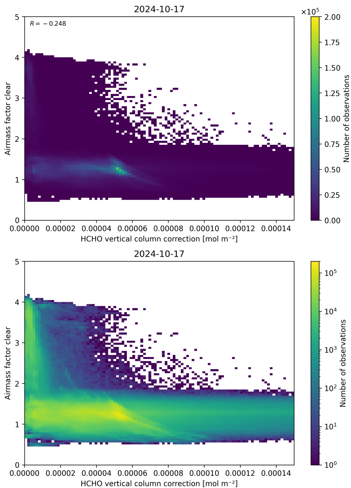
Figure 115: Scatter density plot of “HCHO vertical column correction” against “Airmass factor clear” for 2024-10-16 to 2024-10-18.
