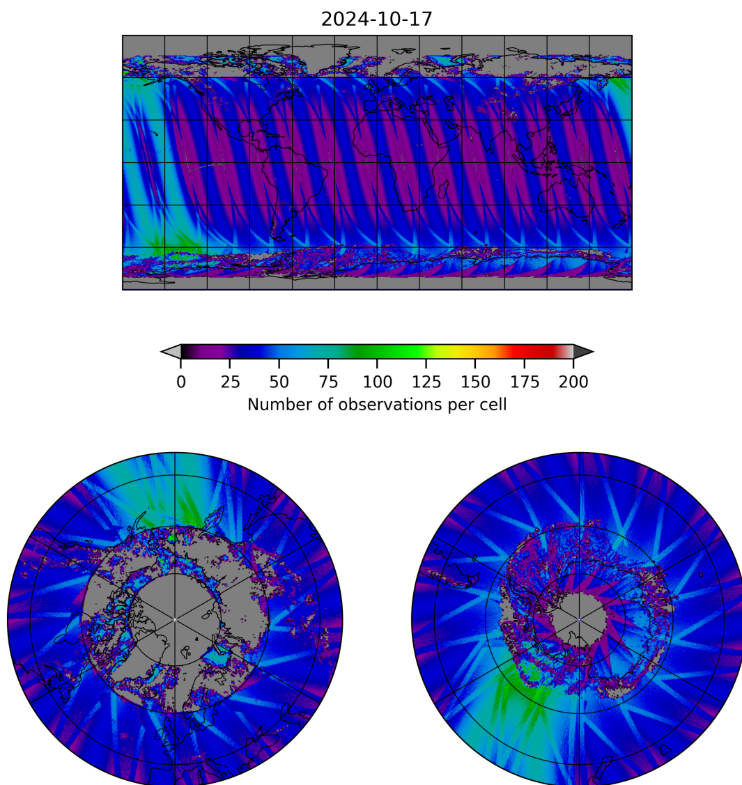
Figure 19: Map of the number of observations for 2024-10-16 to 2024-10-18
