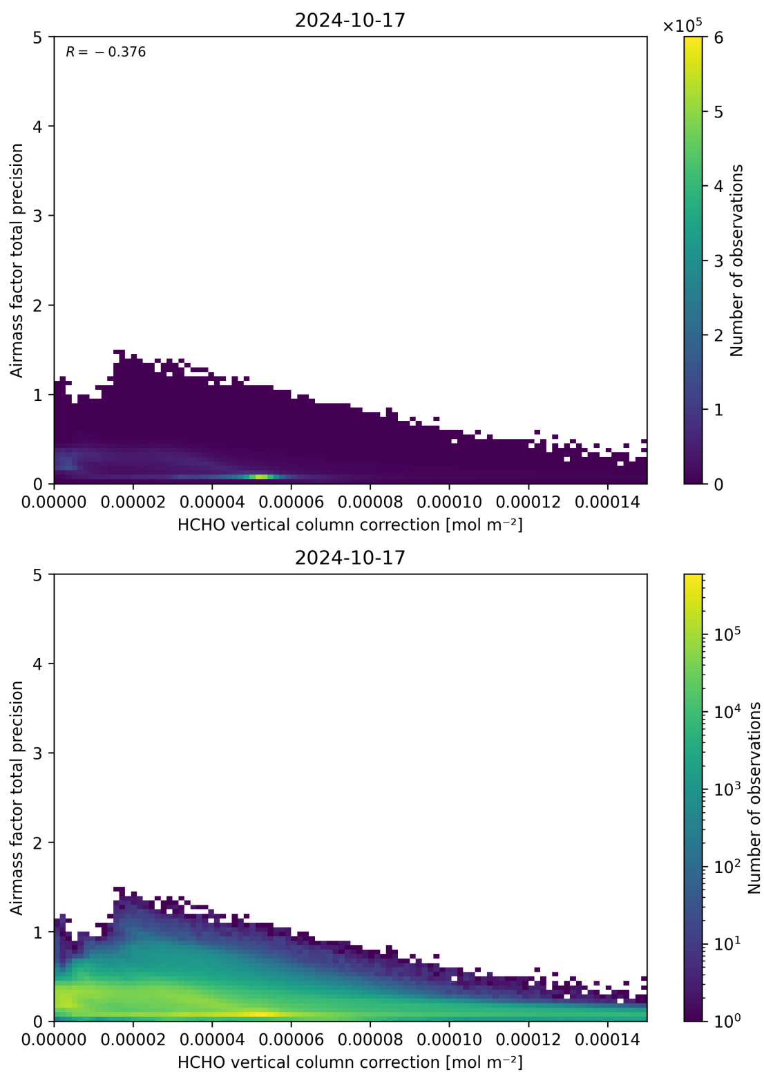
Figure 121: Scatter density plot of “HCHO vertical column correction” against “Airmass factor total precision” for 2024-10-16 to 2024-10-18.
