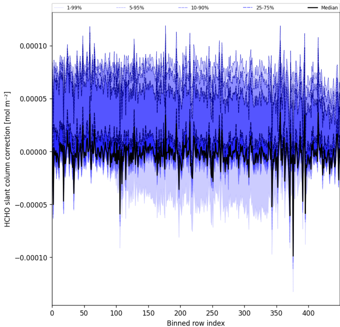
Figure 61: Along track statistics of “HCHO slant column correction” for 2024-10-16 to 2024-10-18
