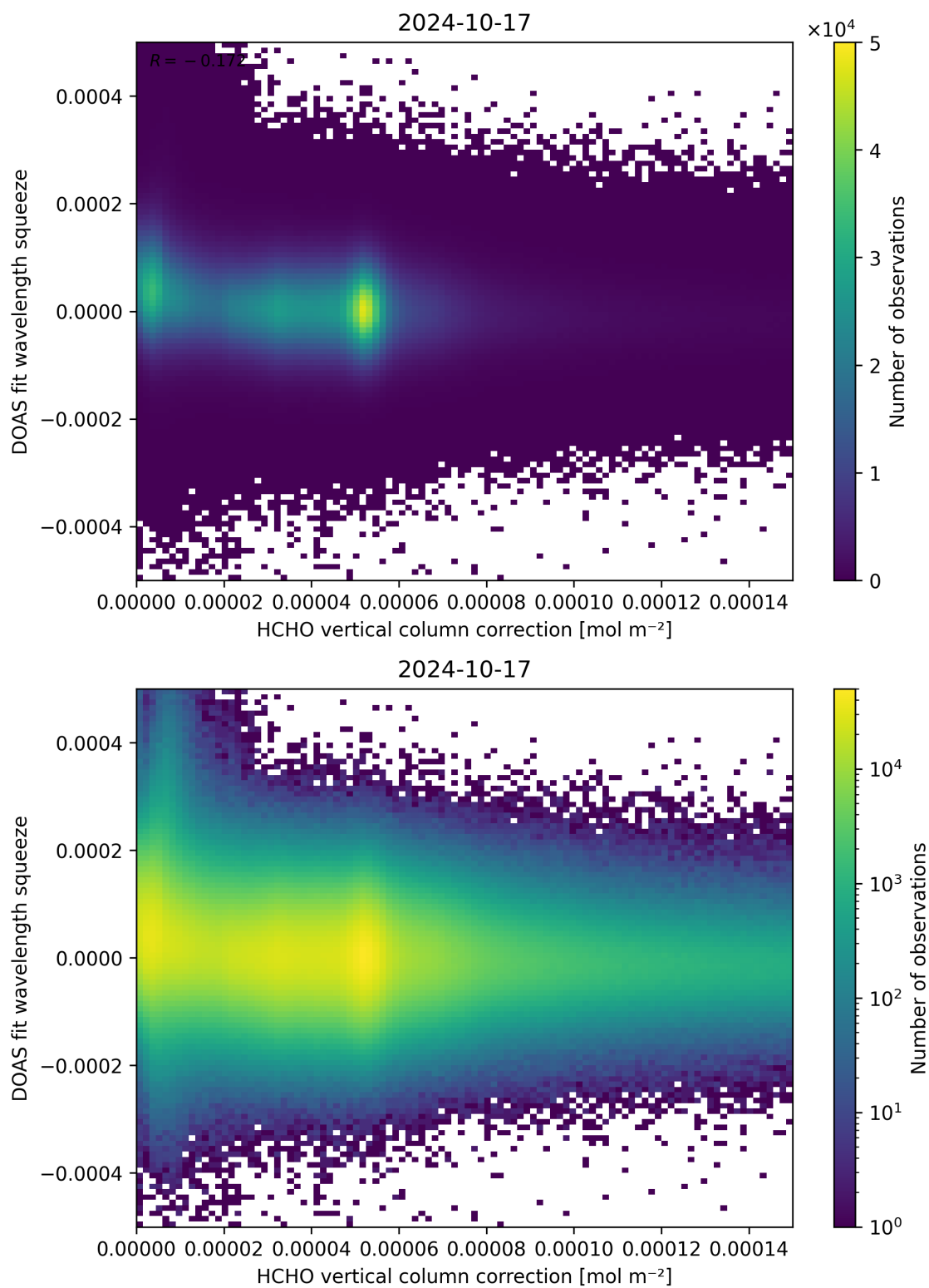
Figure 114: Scatter density plot of “HCHO vertical column correction” against “DOAS fit wavelength squeeze” for 2024-10-16 to 2024-10-18.
