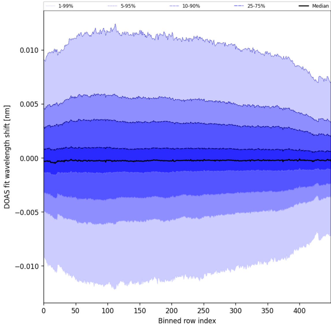
Figure 58: Along track statistics of “DOAS fit wavelength shift” for 2024-10-16 to 2024-10-18
