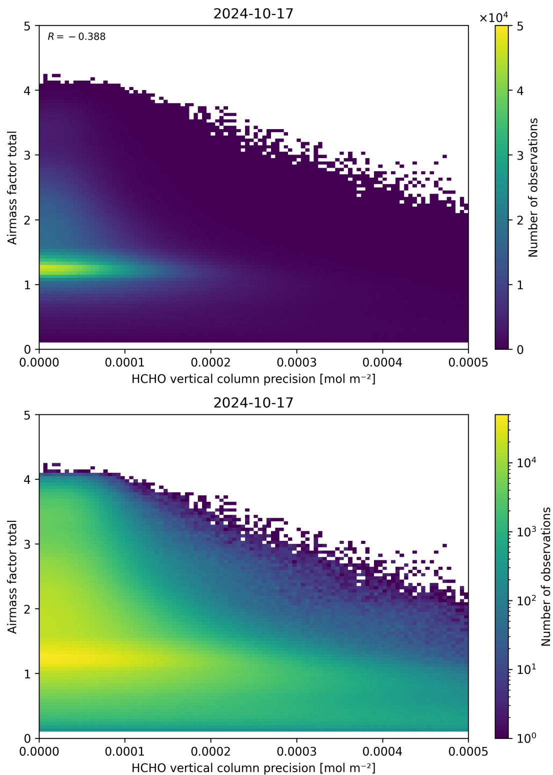
Figure 144: Scatter density plot of “HCHO vertical column precision” against “Airmass factor total” for 2024-10-16 to 2024-10-18.
