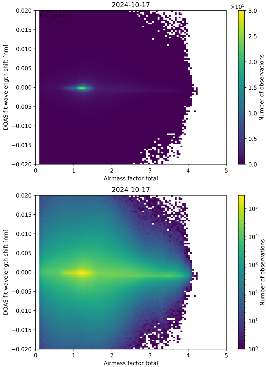
Figure 98: Scatter density plot of “Airmass factor total” against “DOAS fit wavelength shift” for 2024-10-16 to 2024-10-18.
