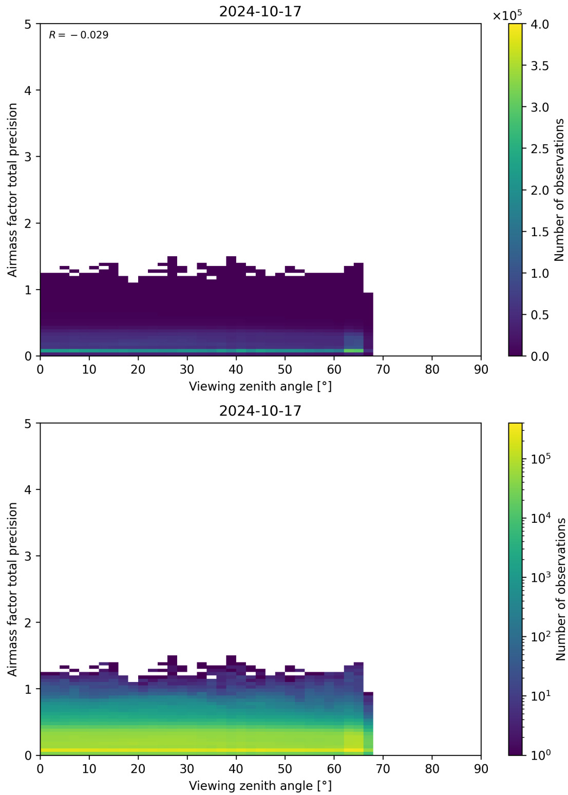
Figure 191: Scatter density plot of “Viewing zenith angle” against “Airmass factor total precision” for 2024-10-16 to 2024-10-18.
