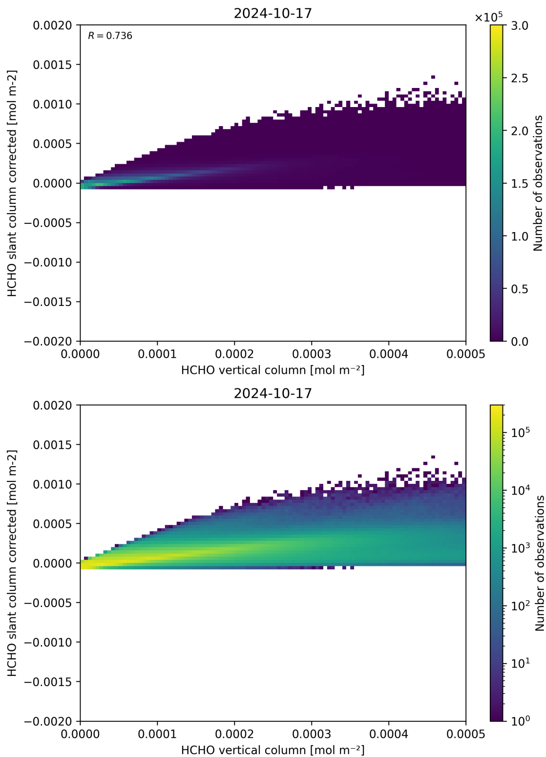
Figure 127: Scatter density plot of “HCHO vertical column” against “HCHO slant column corrected” for 2024-10-16 to 2024-10-18.
