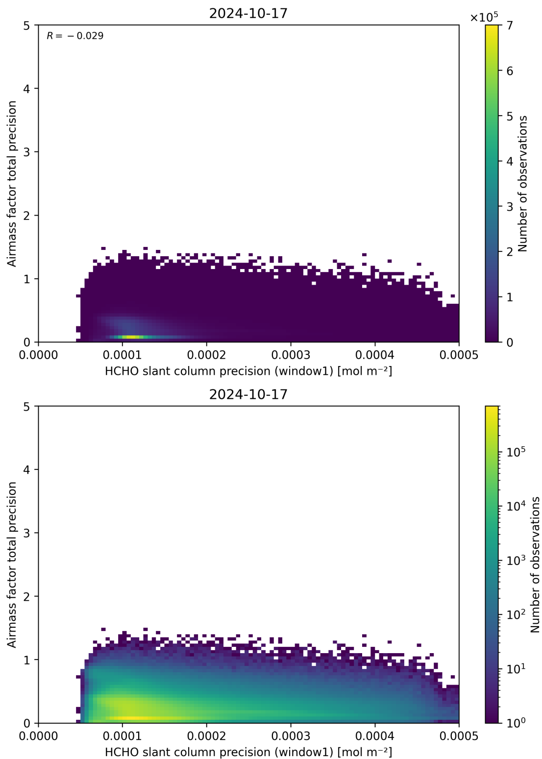
Figure 95: Scatter density plot of “HCHO slant column precision (window1)” against “Airmass factor total precision” for 2024-10-16 to 2024-10-18.
