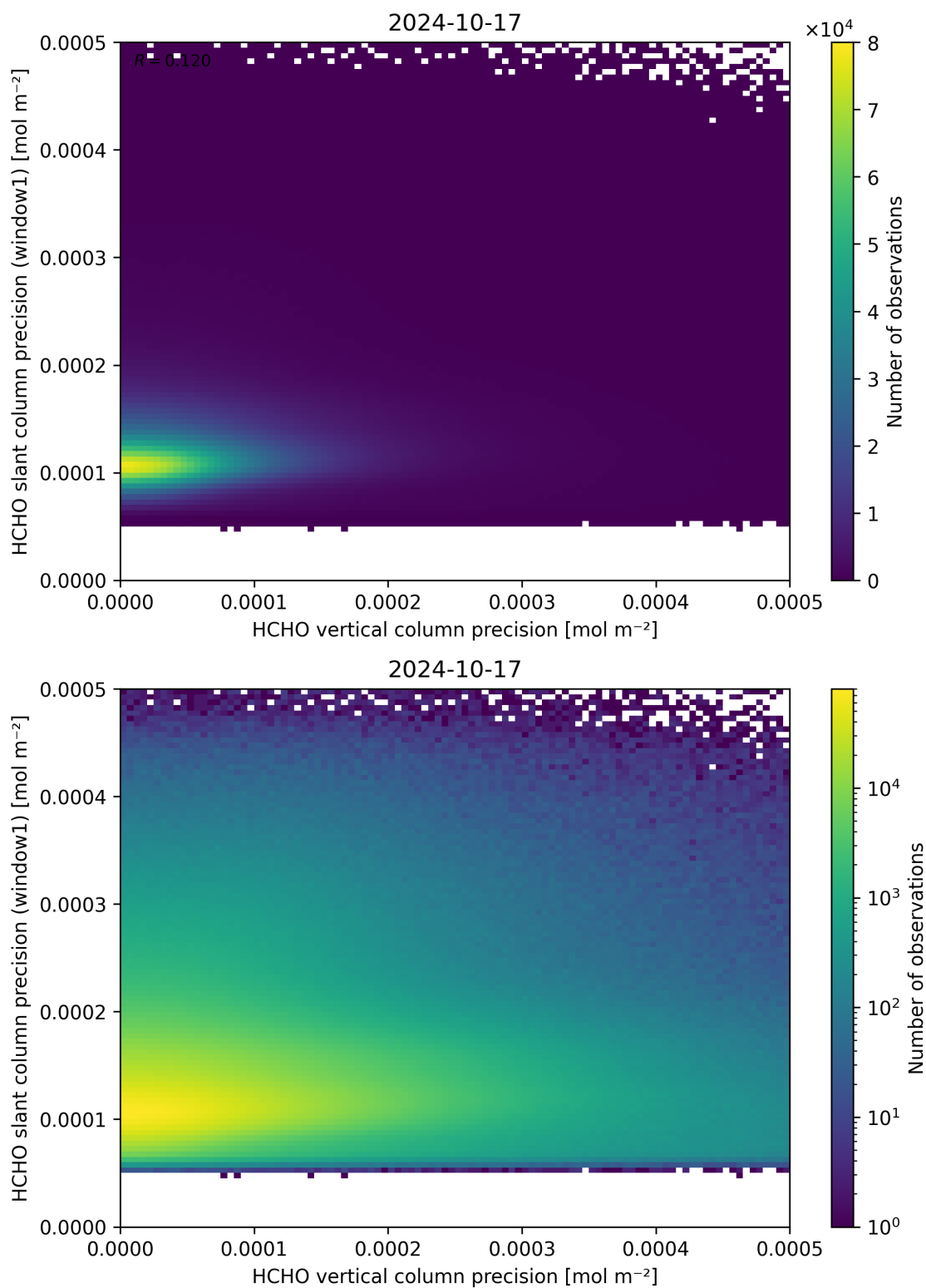
Figure 143: Scatter density plot of “HCHO vertical column precision” against “HCHO slant column precision (window1)” for 2024-10-16 to 2024-10-18.
