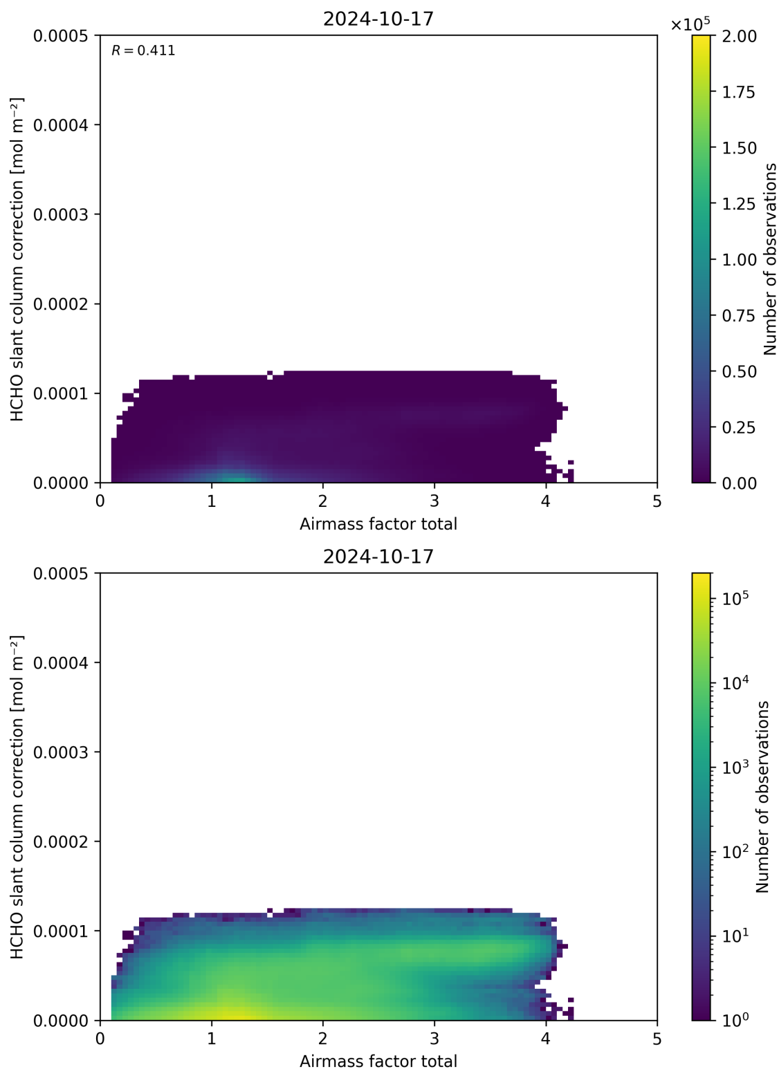
Figure 102: Scatter density plot of “Airmass factor total” against “HCHO slant column correction” for 2024-10-16 to 2024-10-18.
