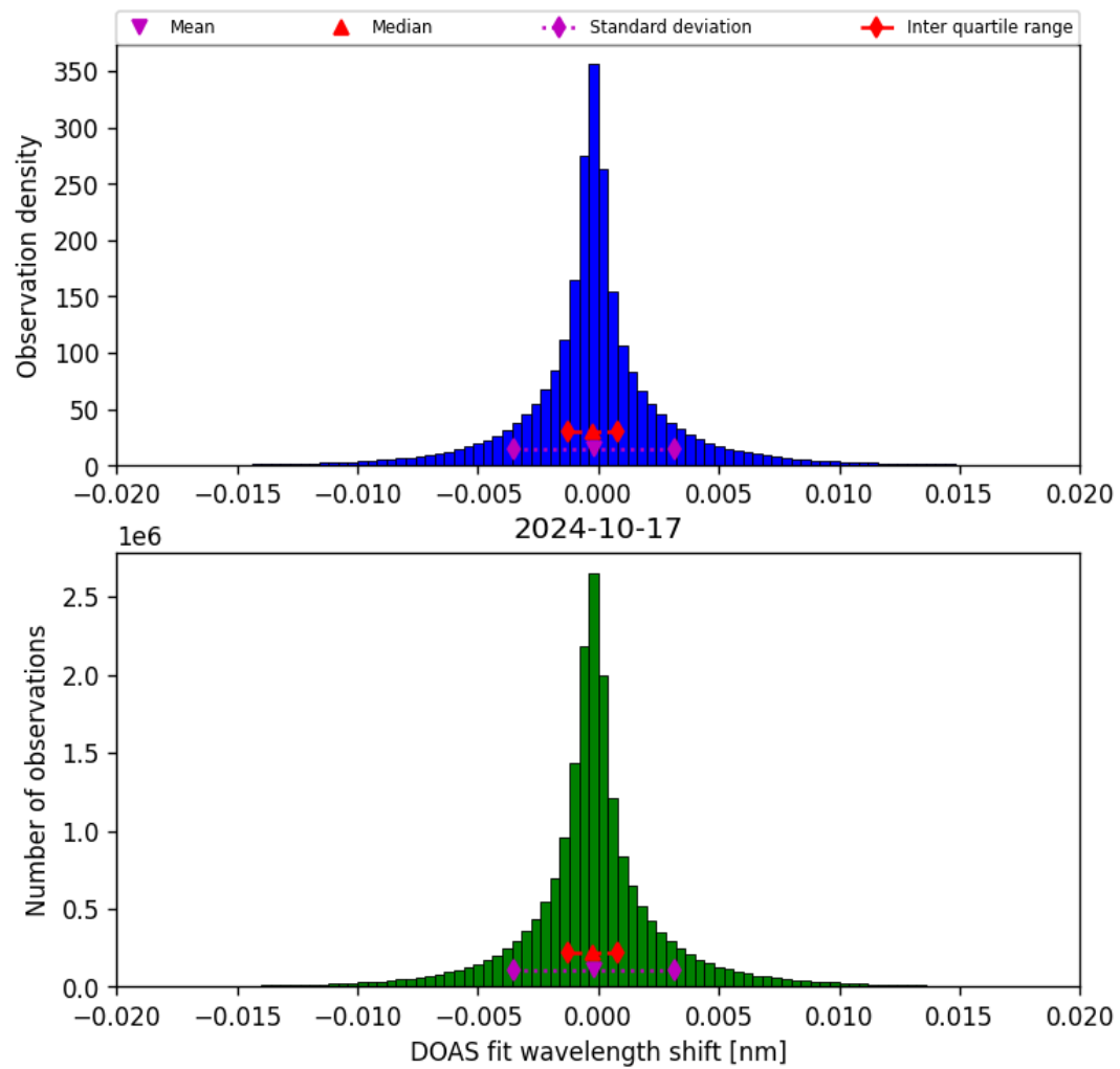
Figure 44: Histogram of “DOAS fit wavelength shift” for 2024-10-16 to 2024-10-18
