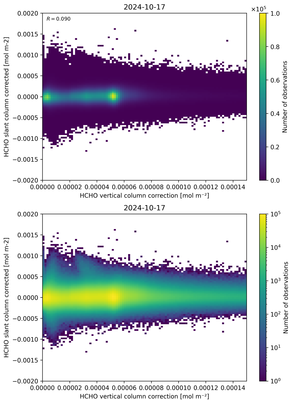
Figure 116: Scatter density plot of “HCHO vertical column correction” against “HCHO slant column corrected” for 2024-10-16 to 2024-10-18.
