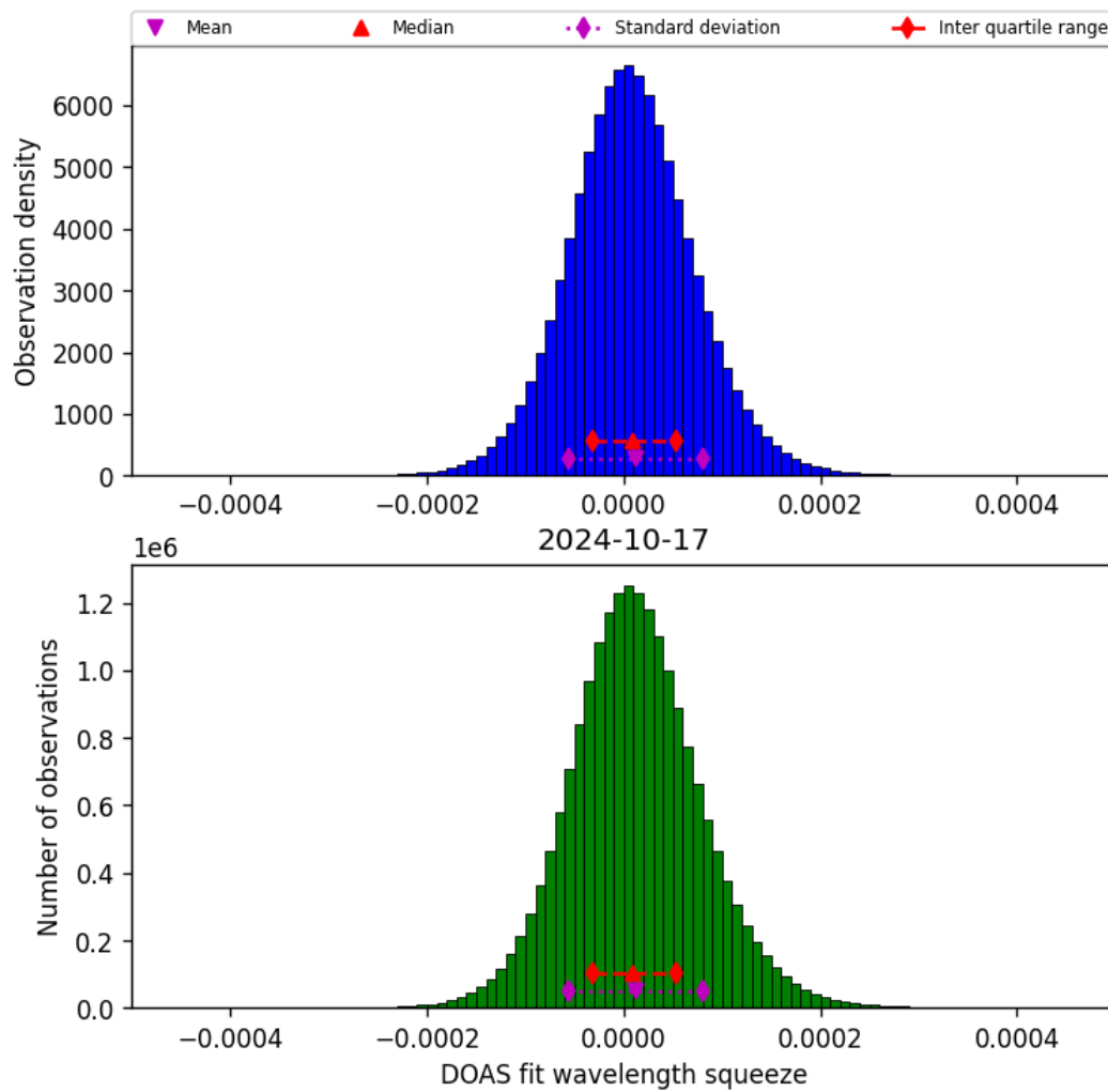
Figure 45: Histogram of “DOAS fit wavelength squeeze” for 2024-10-16 to 2024-10-18
