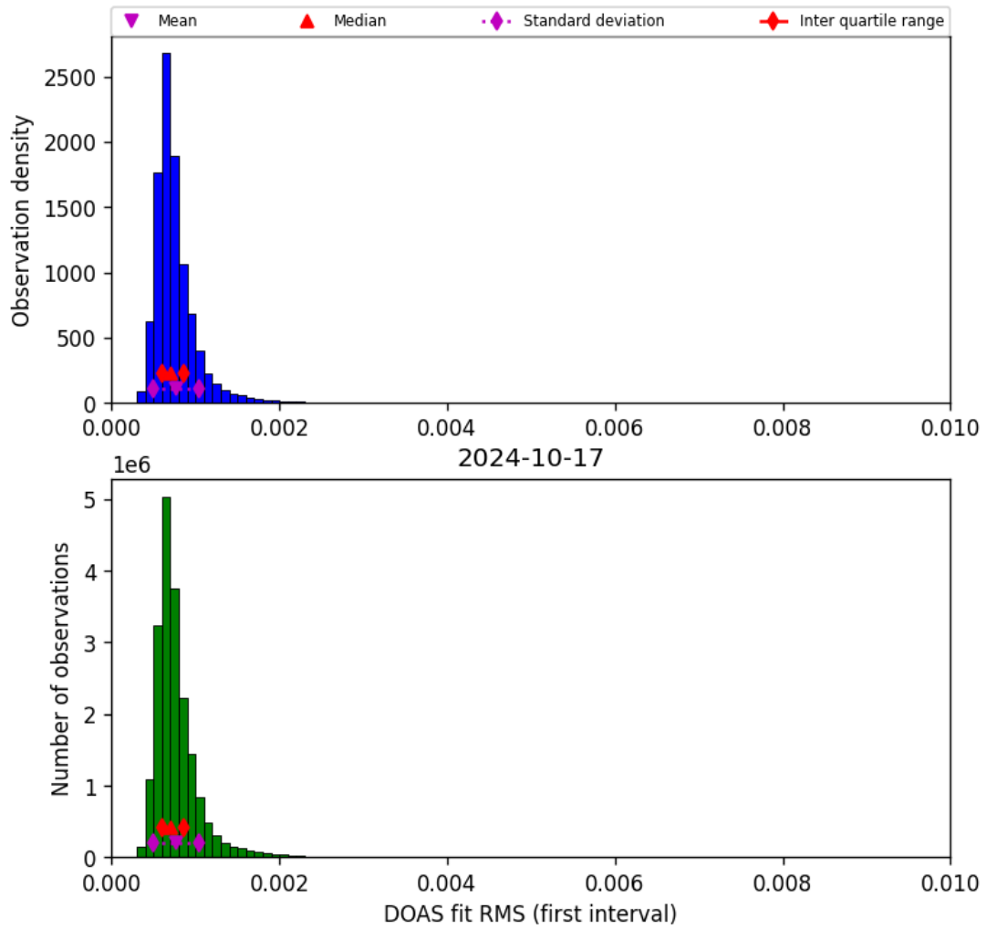
Figure 46: Histogram of “DOAS fit RMS (first interval)” for 2024-10-16 to 2024-10-18
