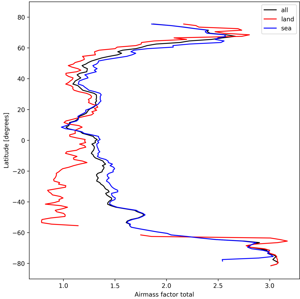
Figure 26: Zonal average of “Airmass factor total” for 2024-10-16 to 2024-10-18.
