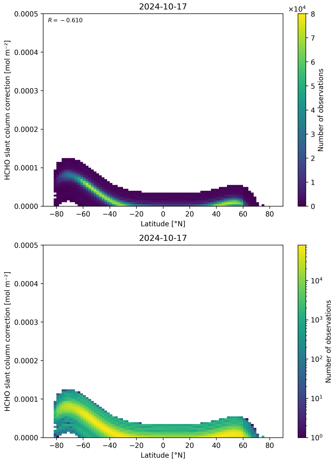
Figure 158: Scatter density plot of “Latitude” against “HCHO slant column correction” for 2024-10-16 to 2024-10-18.
