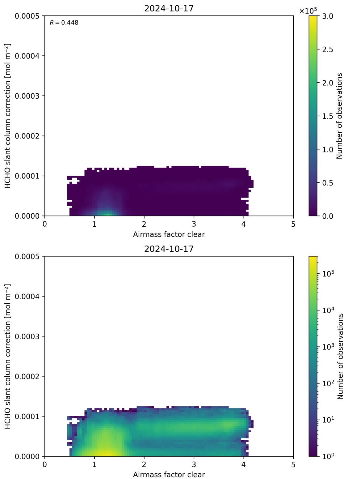
Figure 75: Scatter density plot of “Airmass factor clear” against “HCHO slant column correction” for 2024-10-16 to 2024-10-18.
