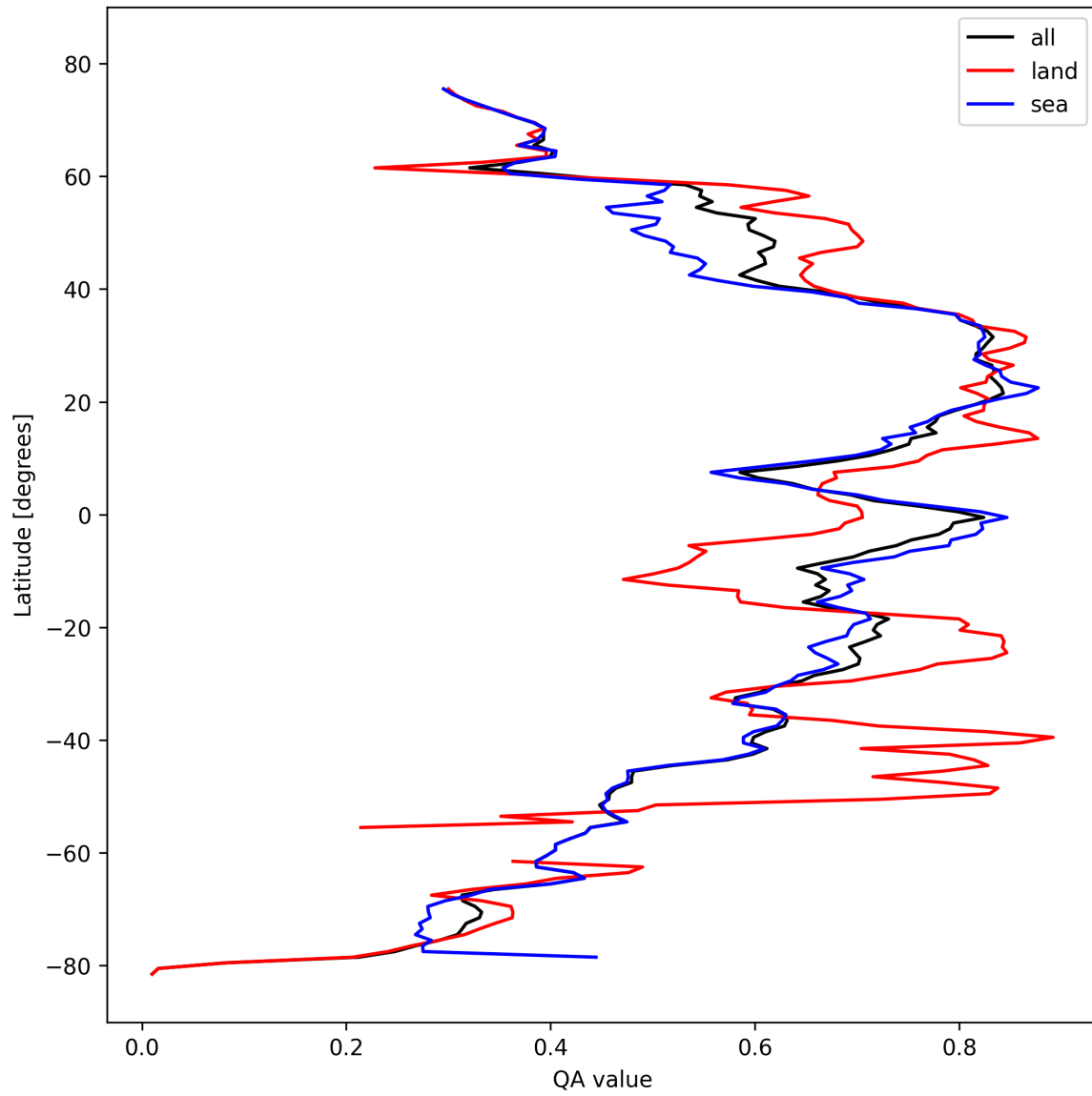
Figure 20: Zonal average of “QA value” for 2024-10-16 to 2024-10-18.
