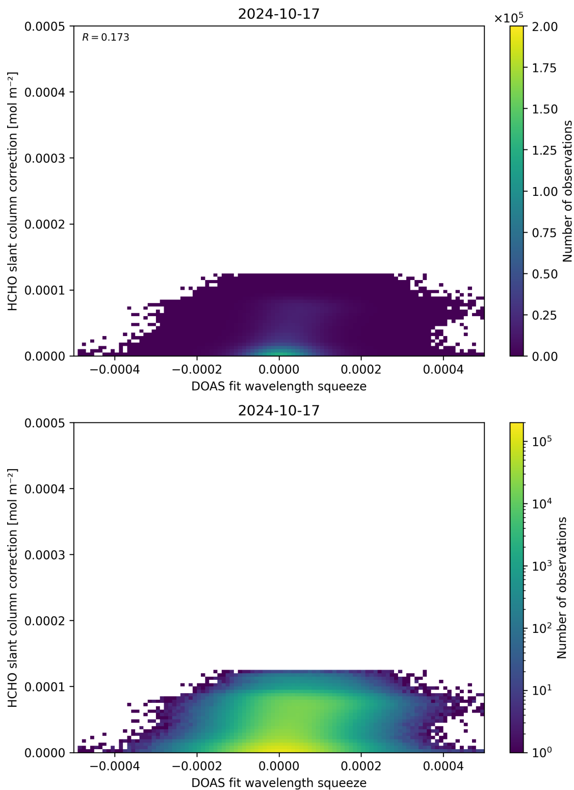
Figure 70: Scatter density plot of “DOAS fit wavelength squeeze” against “HCHO slant column correction” for 2024-10-16 to 2024-10-18.
