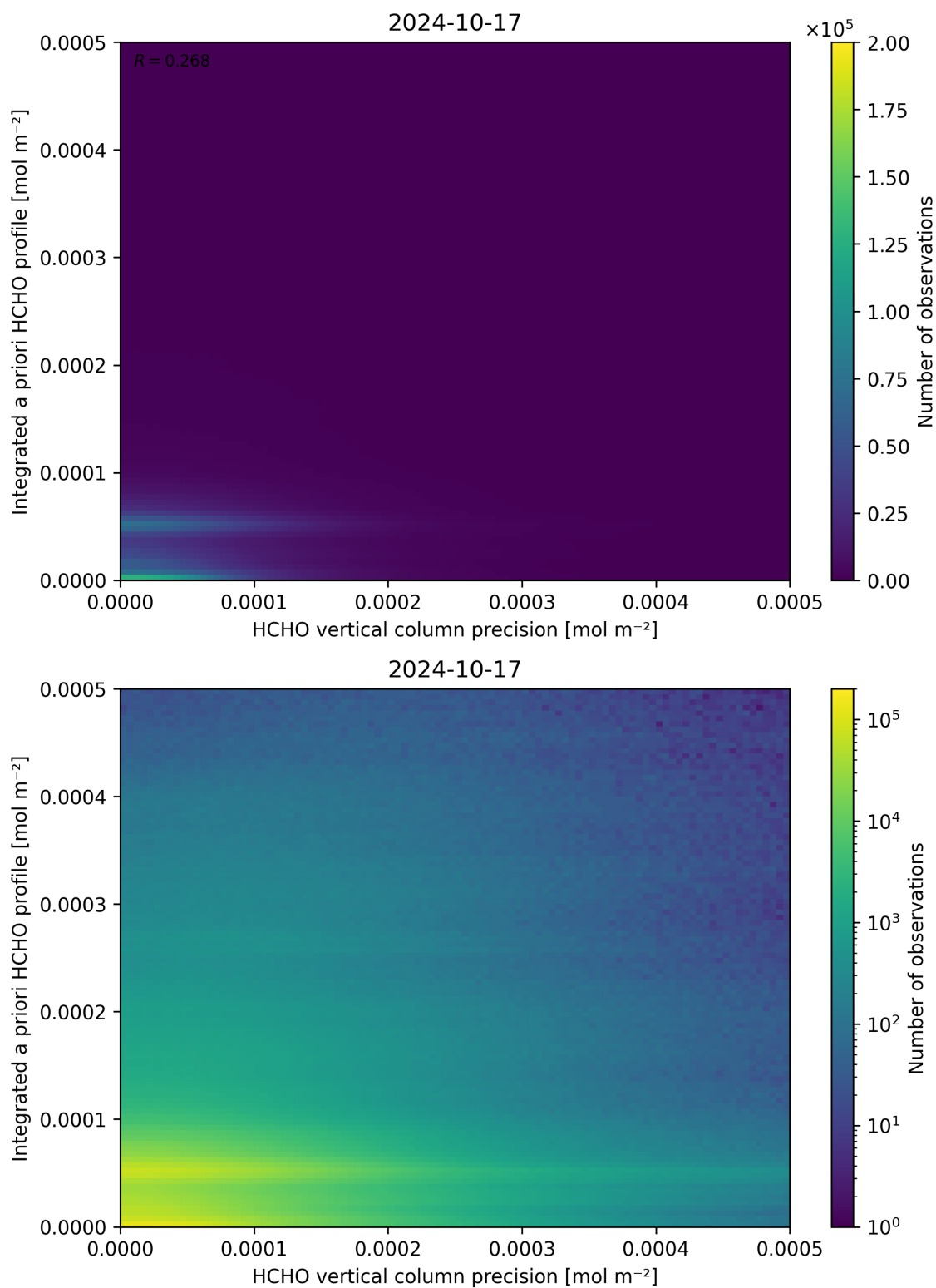
Figure 147: Scatter density plot of “HCHO vertical column precision” against “Integrated a priori HCHO profile” for 2024-10-16 to 2024-10-18.
