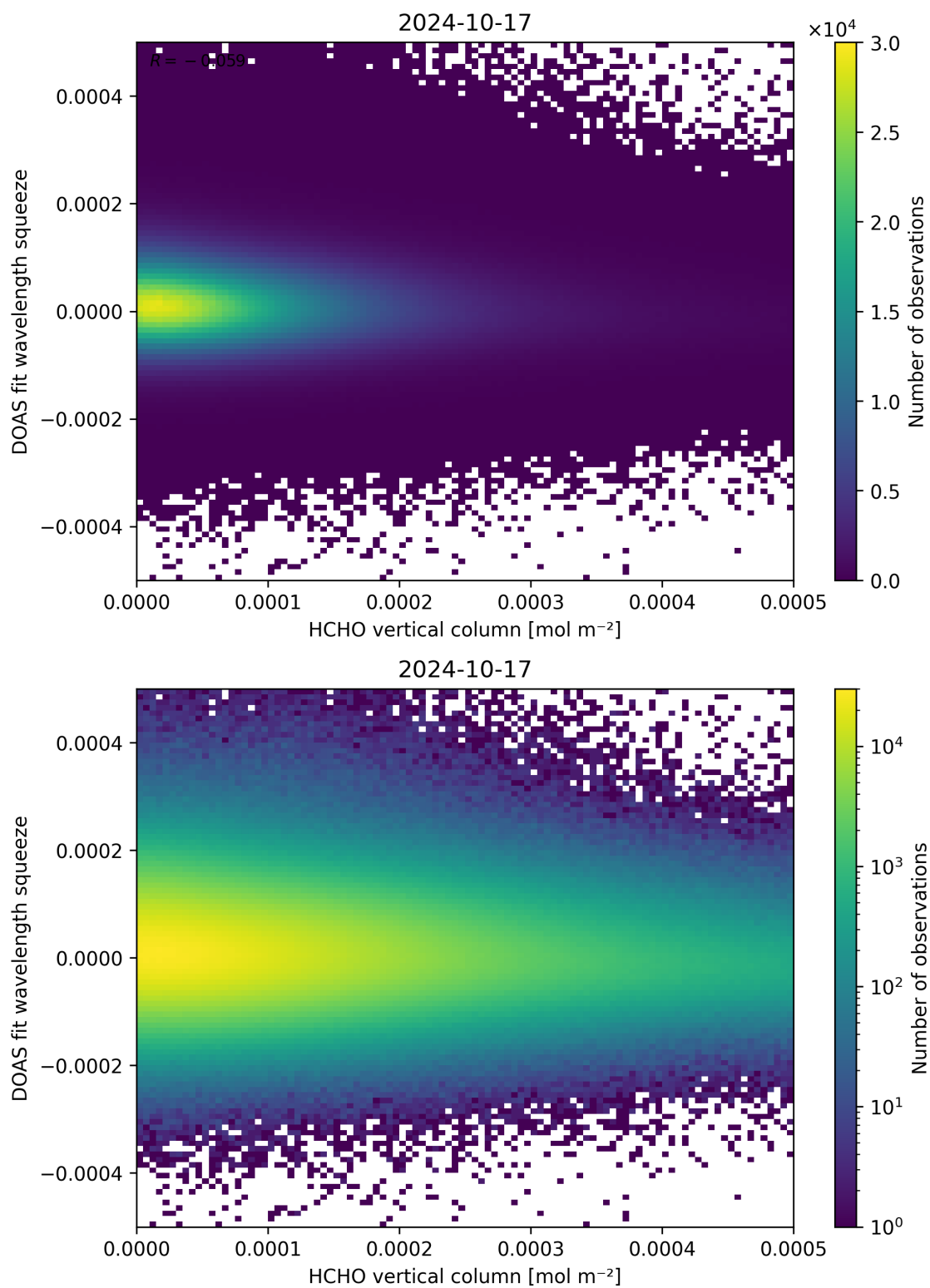
Figure 125: Scatter density plot of “HCHO vertical column” against “DOAS fit wavelength squeeze” for 2024-10-16 to 2024-10-18.
