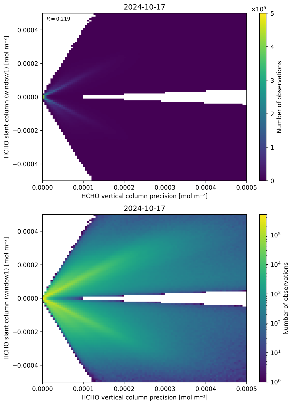
Figure 142: Scatter density plot of “HCHO vertical column precision” against “HCHO slant column (window1)” for 2024-10-16 to 2024-10-18.
