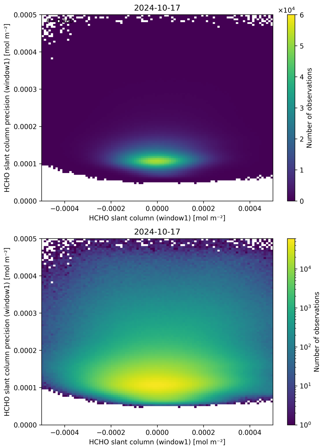
Figure 84: Scatter density plot of “HCHO slant column (window1)” against “HCHO slant column precision (window1)” for 2024-10-16 to 2024-10-18.
