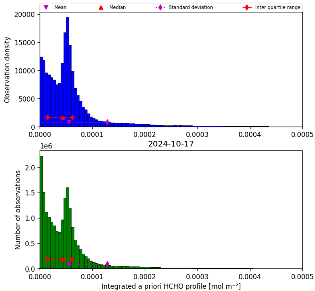
Figure 43: Histogram of “Integrated a priori HCHO profile” for 2024-10-16 to 2024-10-18
