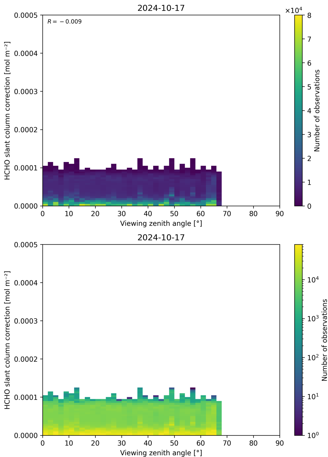
Figure 187: Scatter density plot of “Viewing zenith angle” against “HCHO slant column correction” for 2024-10-16 to 2024-10-18.
