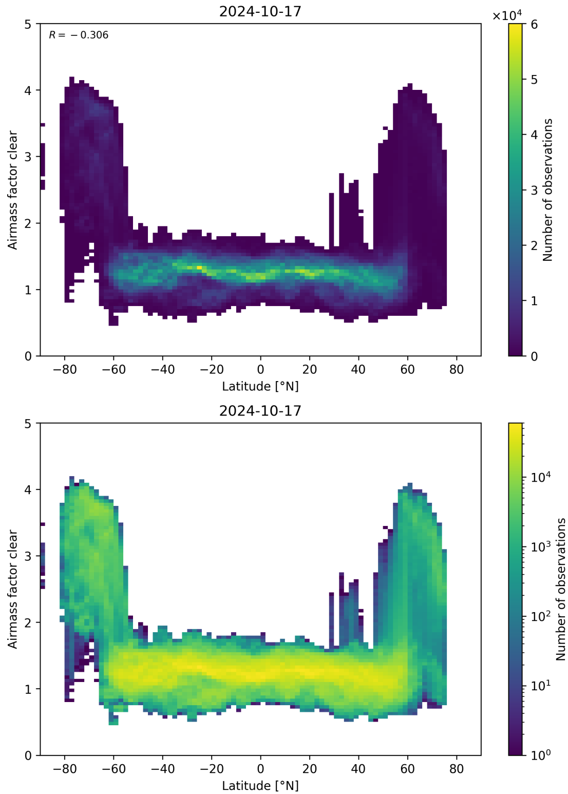
Figure 156: Scatter density plot of “Latitude” against “Airmass factor clear” for 2024-10-16 to 2024-10-18.
