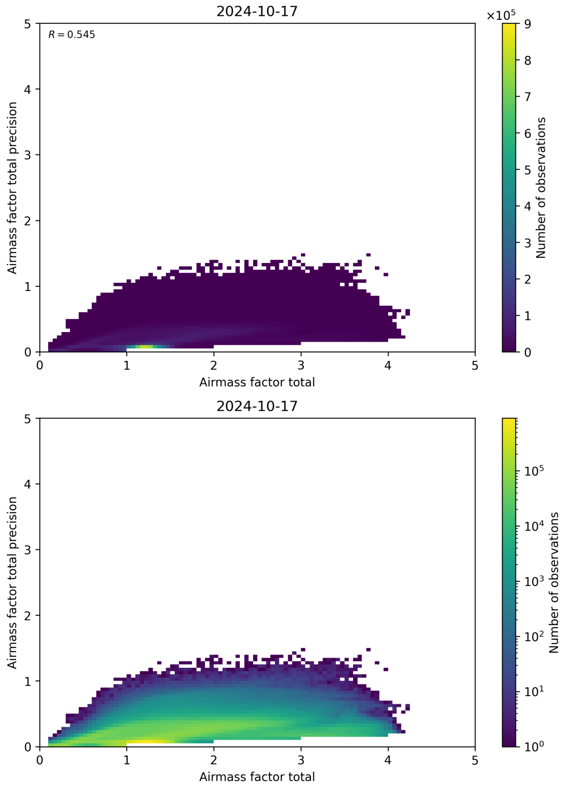
Figure 103: Scatter density plot of “Airmass factor total” against “Airmass factor total precision” for 2024-10-16 to 2024-10-18.
