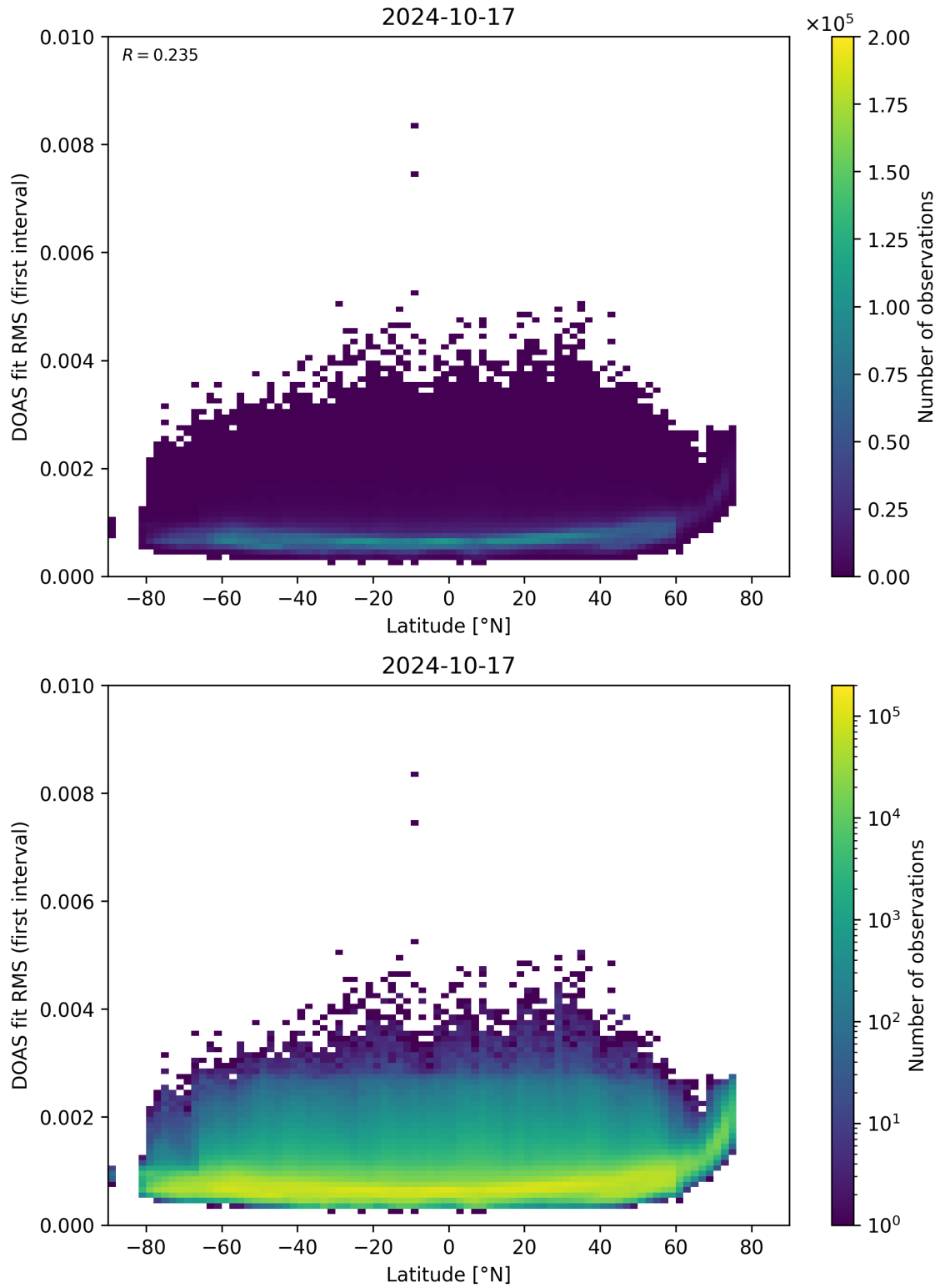
Figure 153: Scatter density plot of “Latitude” against “DOAS fit RMS (first interval)” for 2024-10-16 to 2024-10-18.
