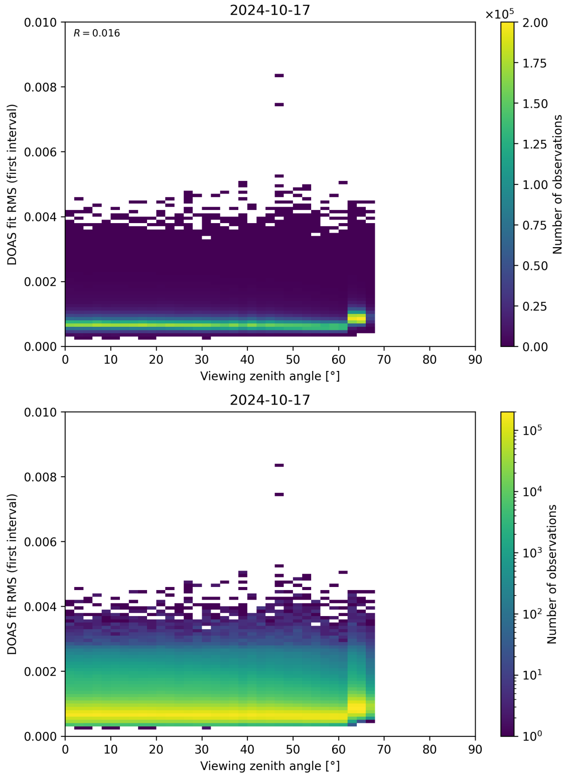
Figure 182: Scatter density plot of “Viewing zenith angle” against “DOAS fit RMS (first interval)” for 2024-10-16 to 2024-10-18.
