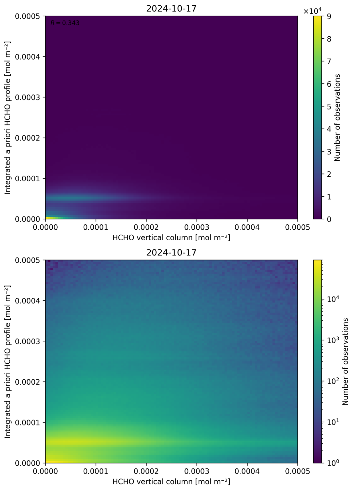
Figure 135: Scatter density plot of “HCHO vertical column” against “Integrated a priori HCHO profile” for 2024-10-16 to 2024-10-18.
