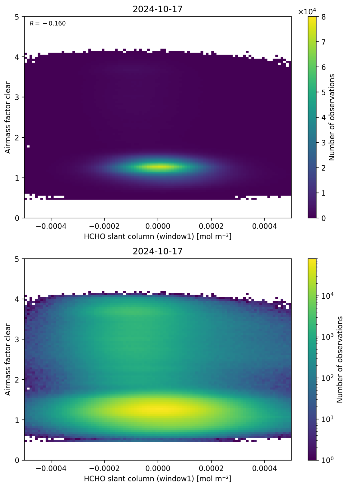
Figure 81: Scatter density plot of “HCHO slant column (window1)” against “Airmass factor clear” for 2024-10-16 to 2024-10-18.
