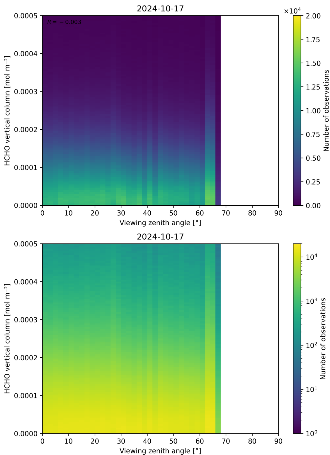
Figure 192: Scatter density plot of “Viewing zenith angle” against “HCHO vertical column” for 2024-10-16 to 2024-10-18.
