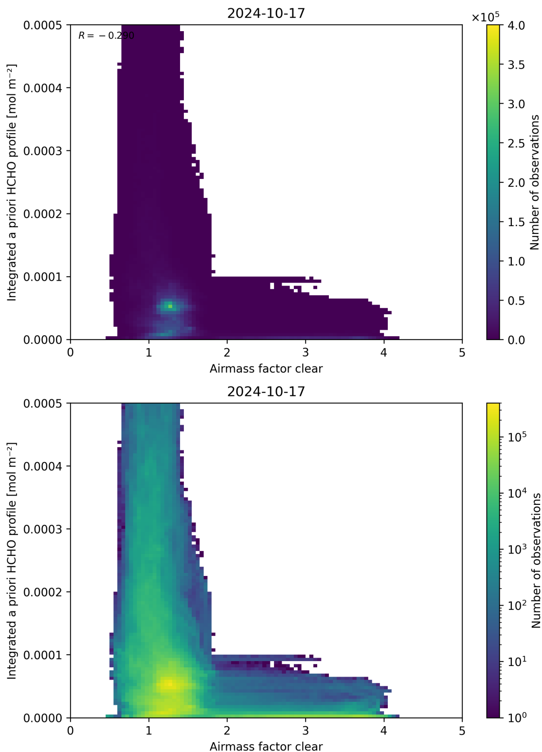
Figure 76: Scatter density plot of “Airmass factor clear” against “Integrated a priori HCHO profile” for 2024-10-16 to 2024-10-18.
