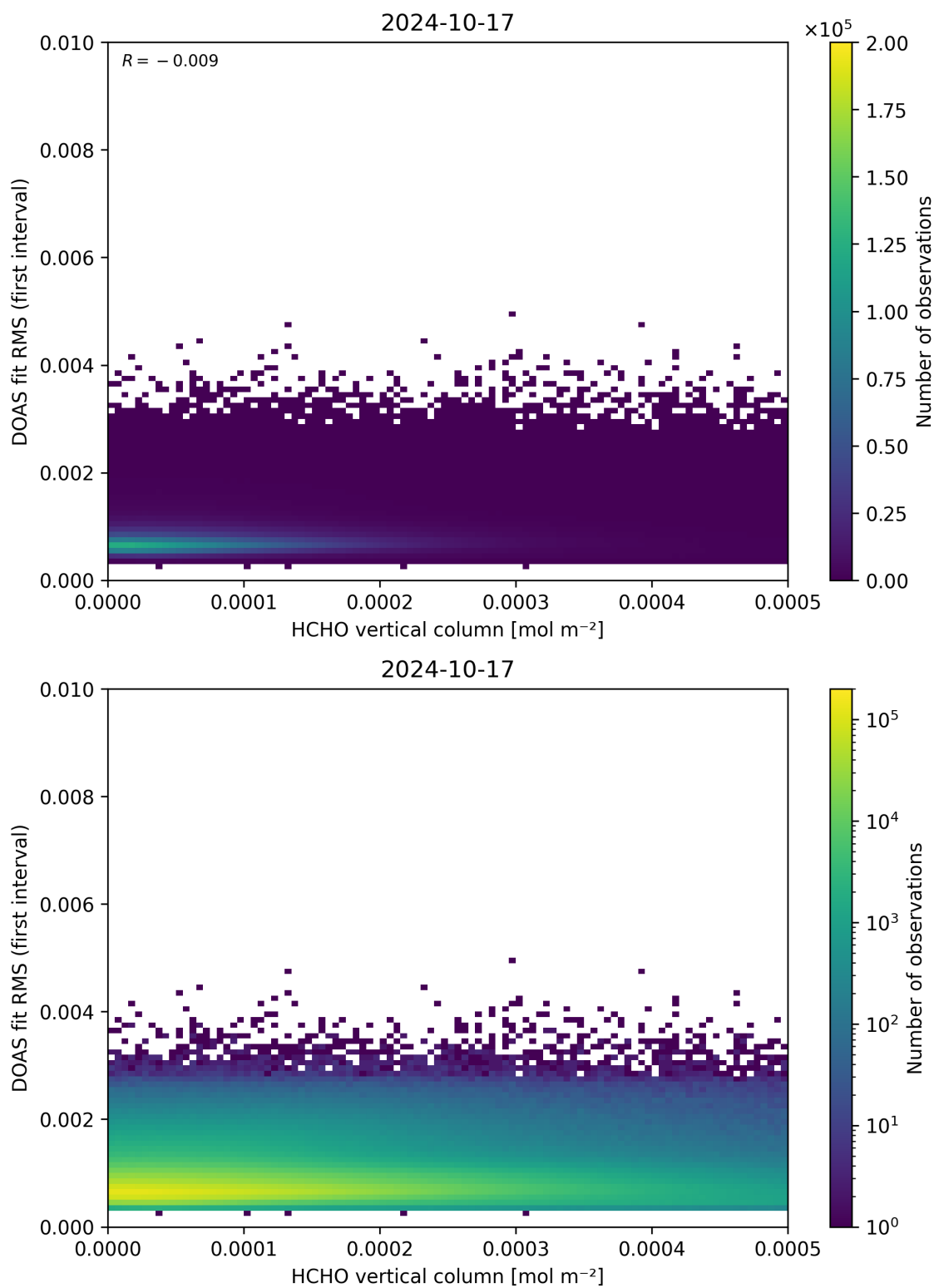
Figure 123: Scatter density plot of “HCHO vertical column” against “DOAS fit RMS (first interval)” for 2024-10-16 to 2024-10-18.
