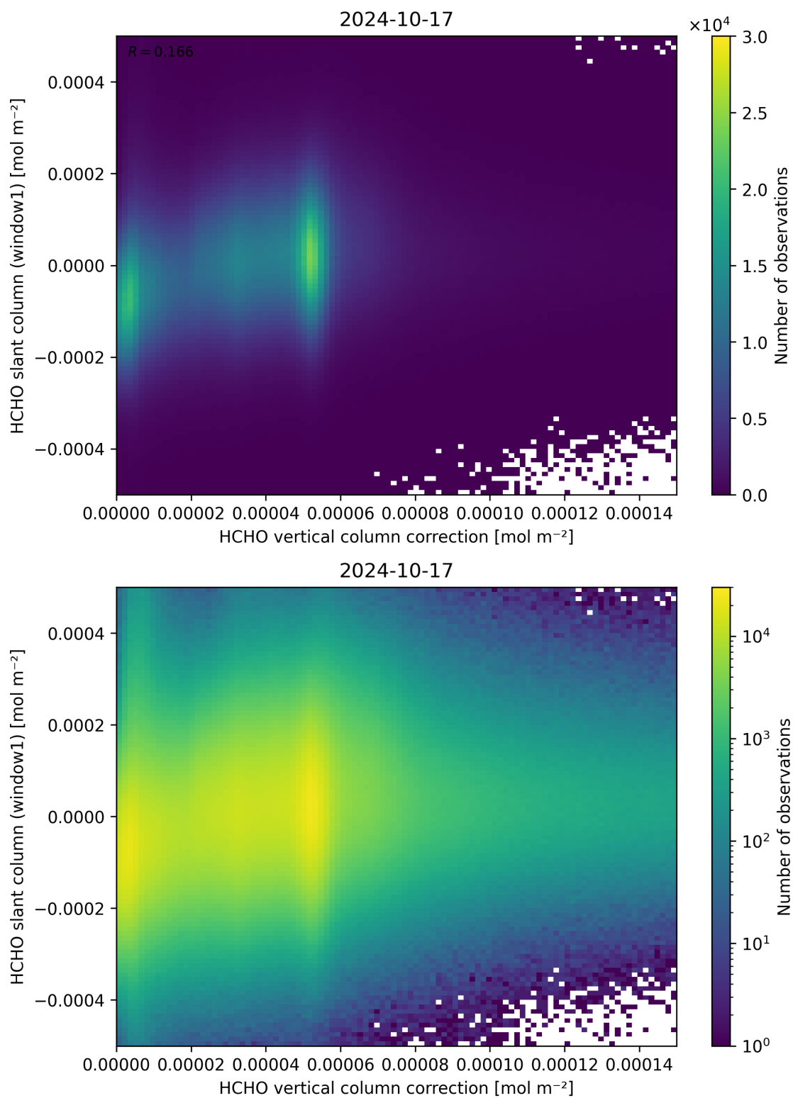
Figure 118: Scatter density plot of “HCHO vertical column correction” against “HCHO slant column (window1)” for 2024-10-16 to 2024-10-18.
