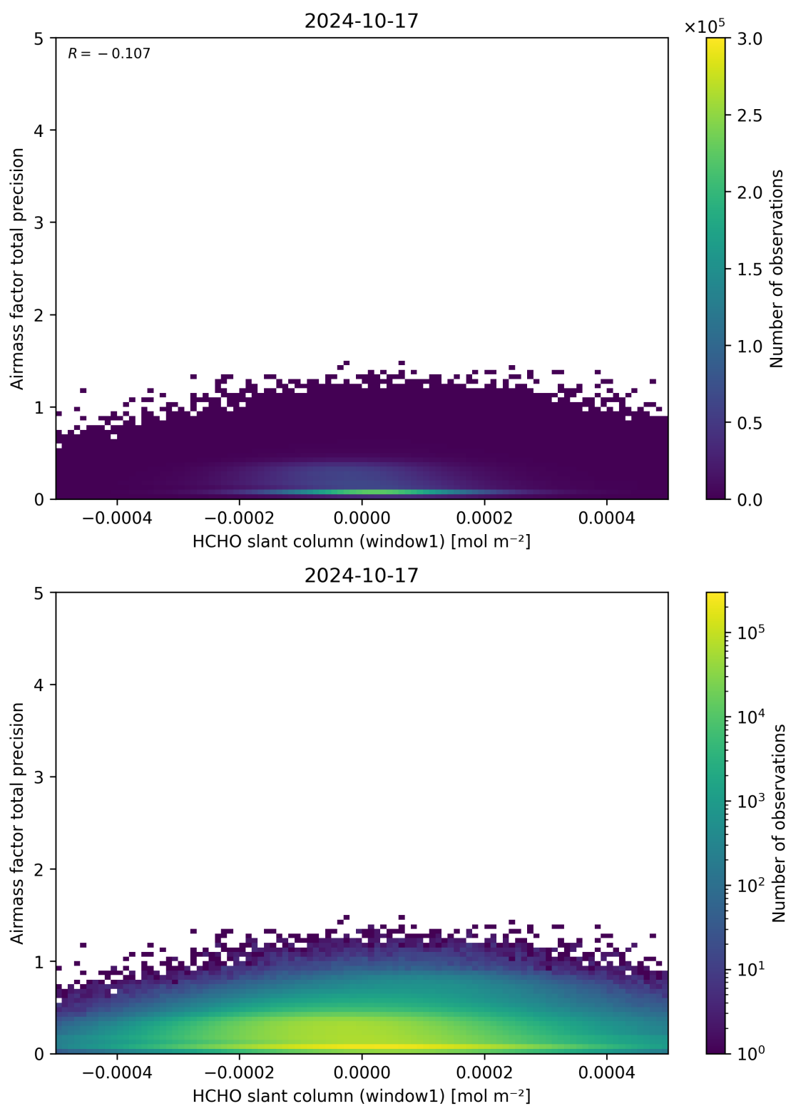
Figure 86: Scatter density plot of “HCHO slant column (window1)” against “Airmass factor total precision” for 2024-10-16 to 2024-10-18.
