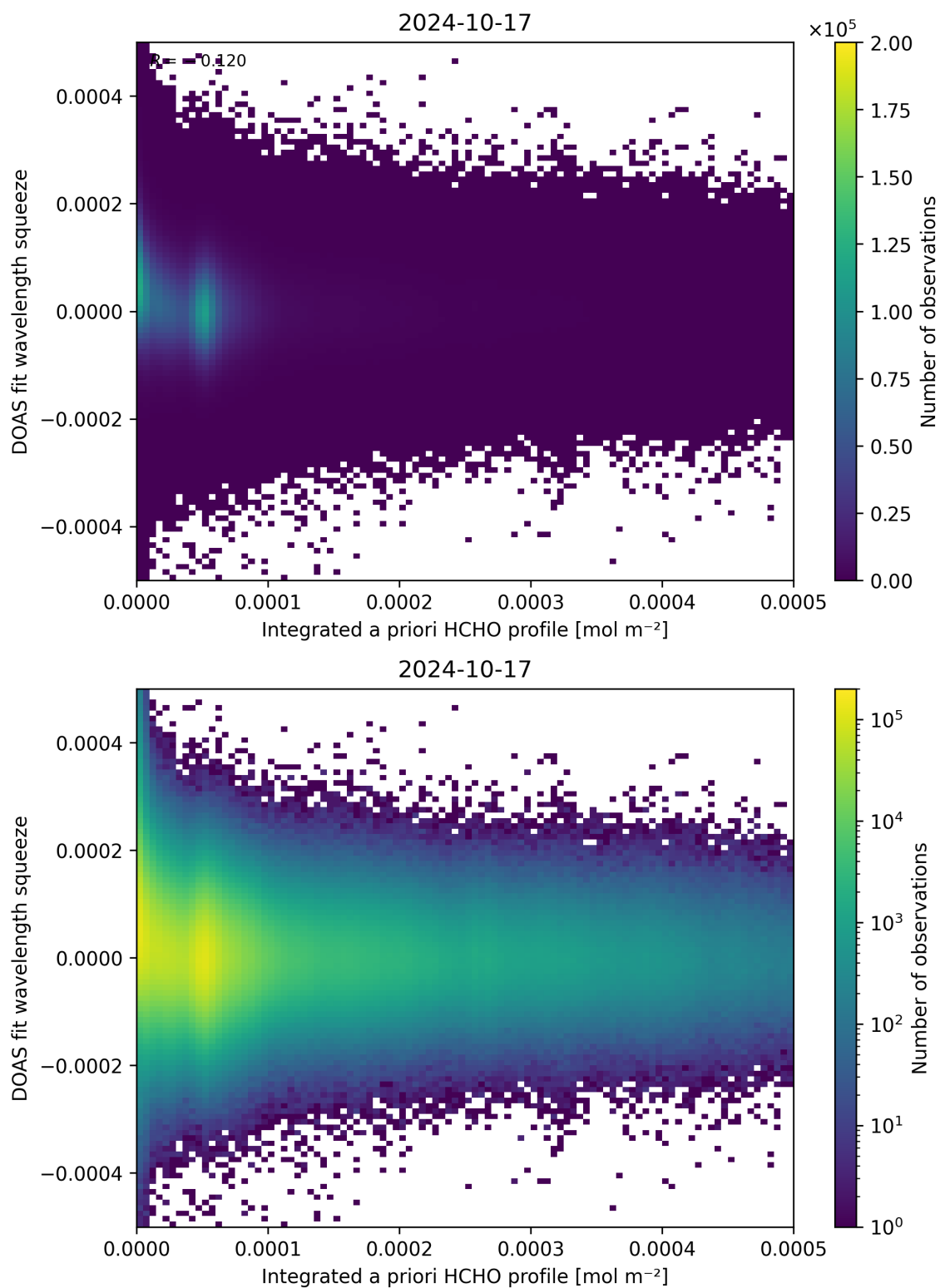
Figure 150: Scatter density plot of “Integrated a priori HCHO profile” against “DOAS fit wavelength squeeze” for 2024-10-16 to 2024-10-18.
