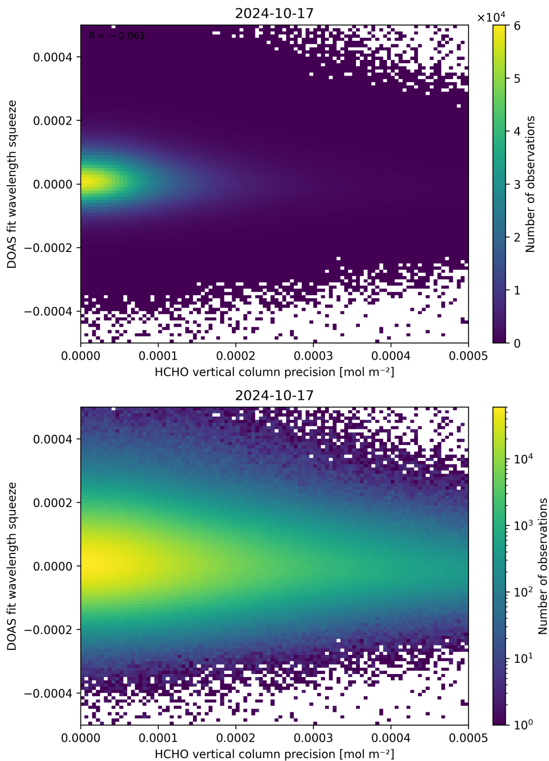
Figure 138: Scatter density plot of “HCHO vertical column precision” against “DOAS fit wavelength squeeze” for 2024-10-16 to 2024-10-18.
