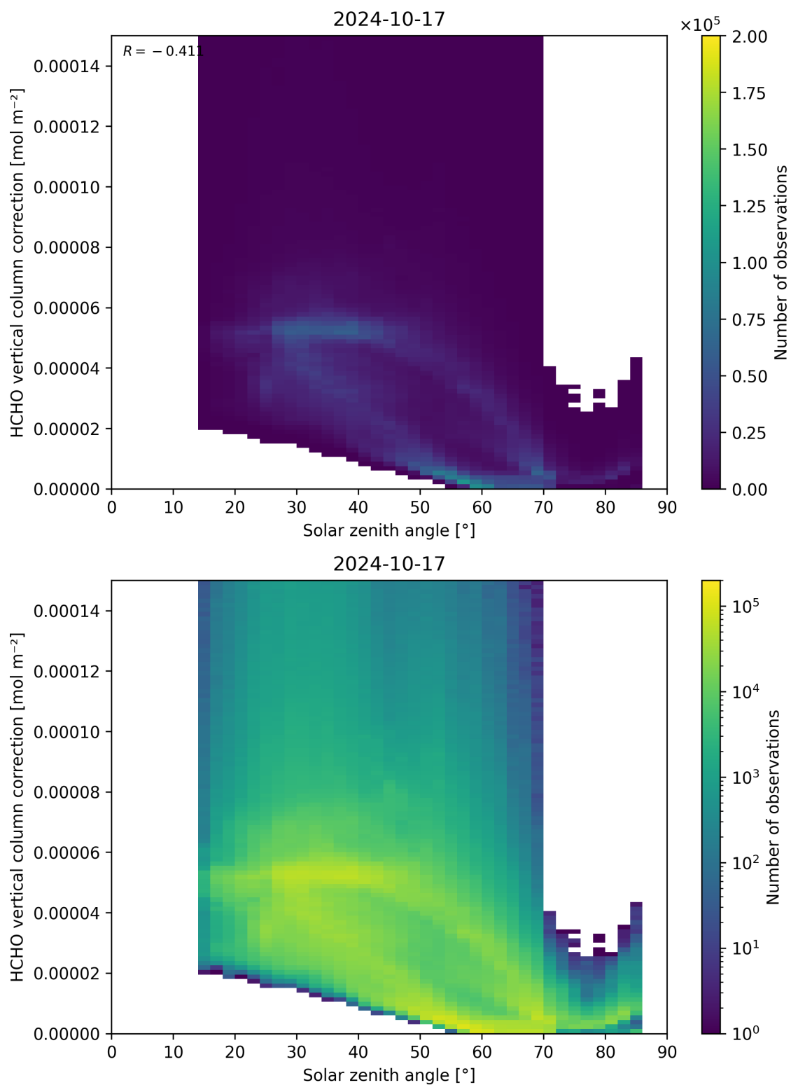
Figure 178: Scatter density plot of “Solar zenith angle” against “HCHO vertical column correction” for 2024-10-16 to 2024-10-18.
