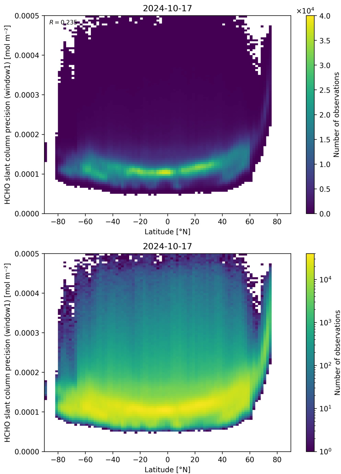
Figure 160: Scatter density plot of “Latitude” against “HCHO slant column precision (window1)” for 2024-10-16 to 2024-10-18.
