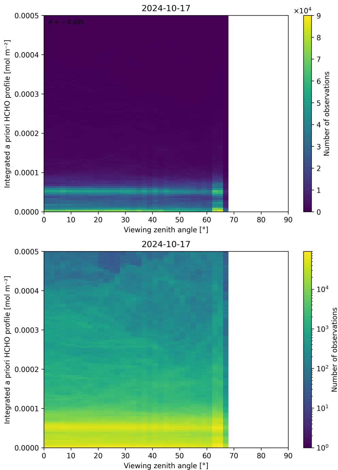
Figure 195: Scatter density plot of “Viewing zenith angle” against “Integrated a priori HCHO profile” for 2024-10-16 to 2024-10-18.
