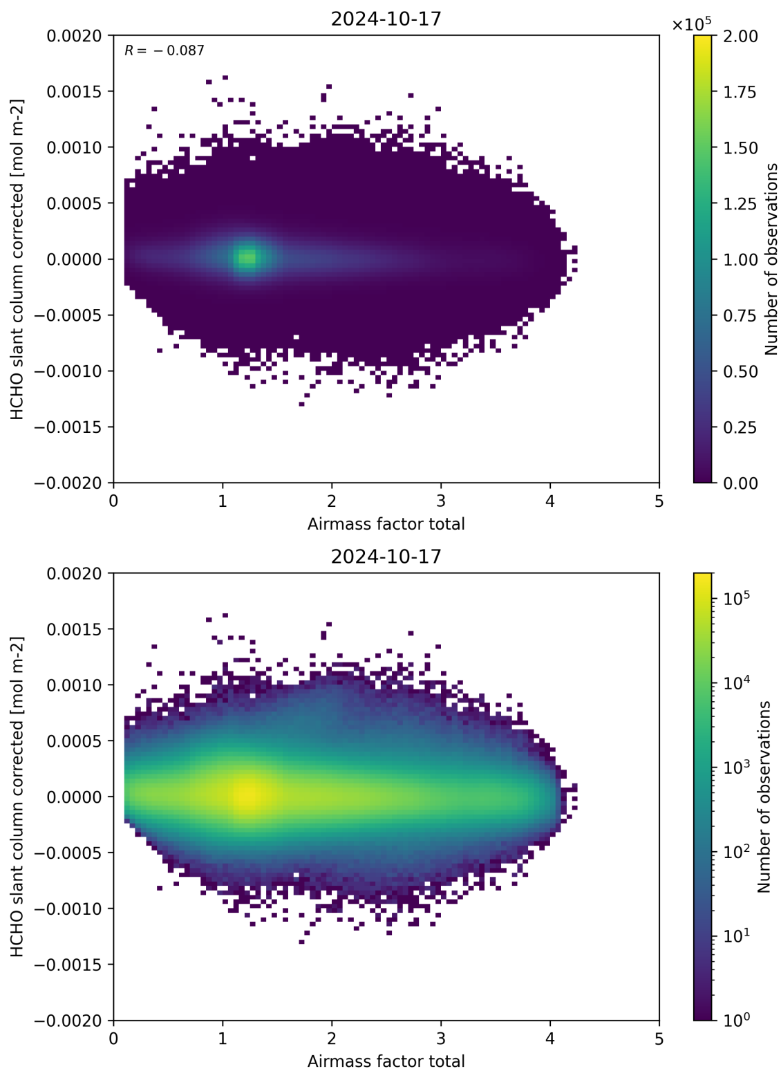
Figure 101: Scatter density plot of “Airmass factor total” against “HCHO slant column corrected” for 2024-10-16 to 2024-10-18.
