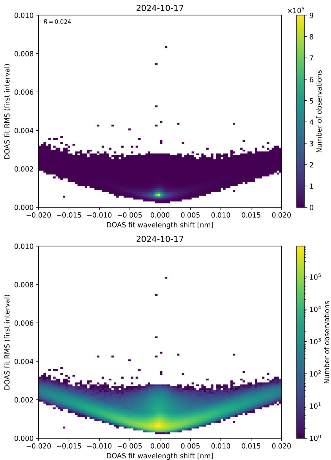
Figure 64: Scatter density plot of “DOAS fit wavelength shift” against “DOAS fit RMS (first interval)” for 2024-10-16 to 2024-10-18.
