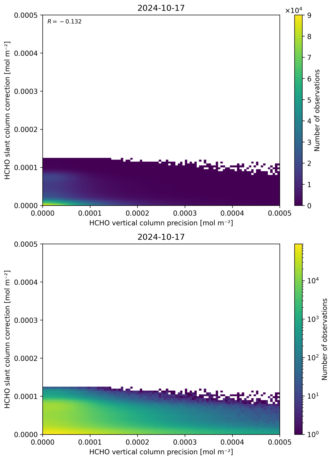
Figure 141: Scatter density plot of “HCHO vertical column precision” against “HCHO slant column correction” for 2024-10-16 to 2024-10-18.
