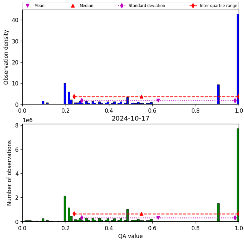
Figure 34: Histogram of “QA value” for 2024-10-16 to 2024-10-18
