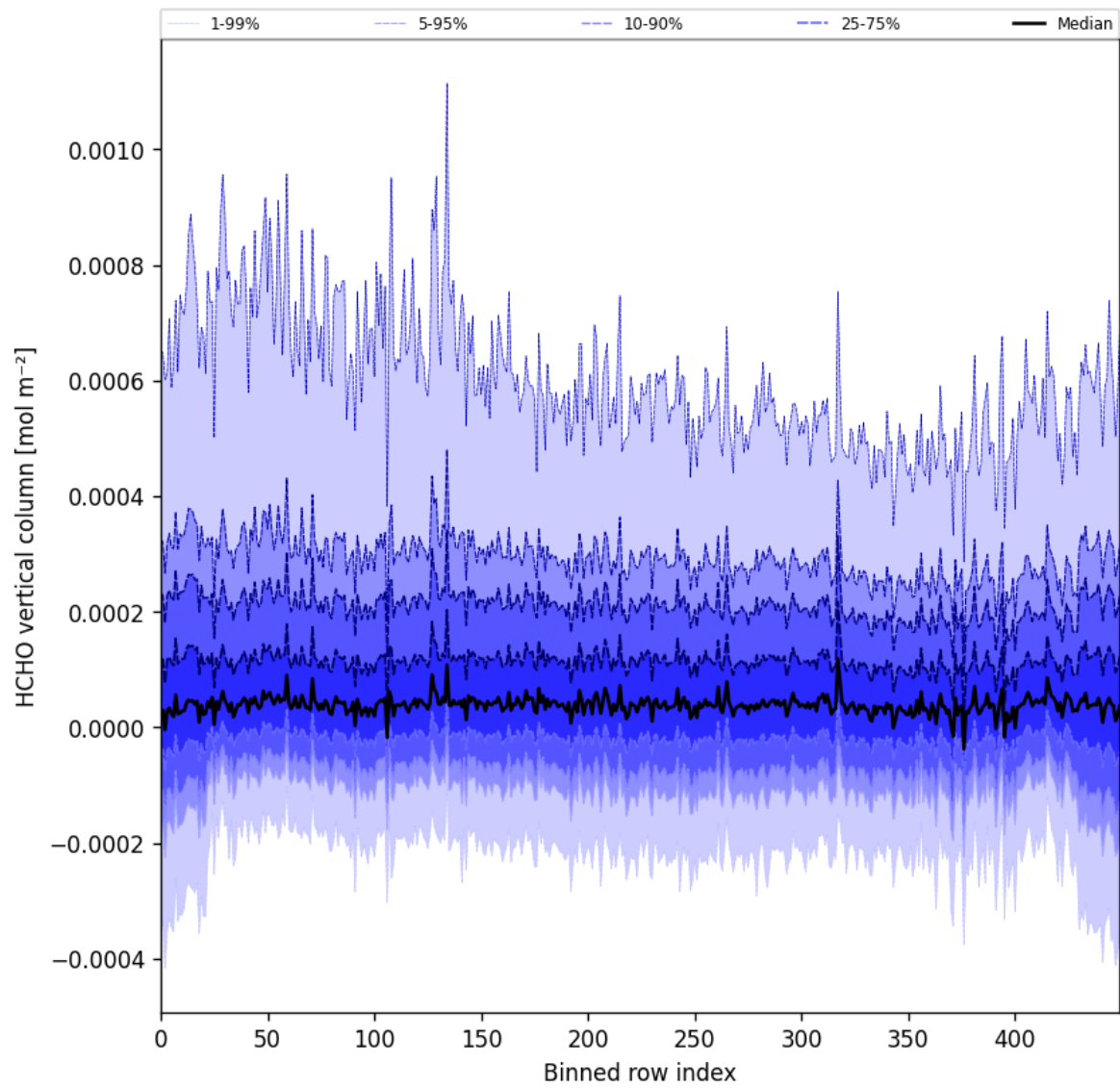
Figure 49: Along track statistics of “HCHO vertical column” for 2024-10-16 to 2024-10-18
