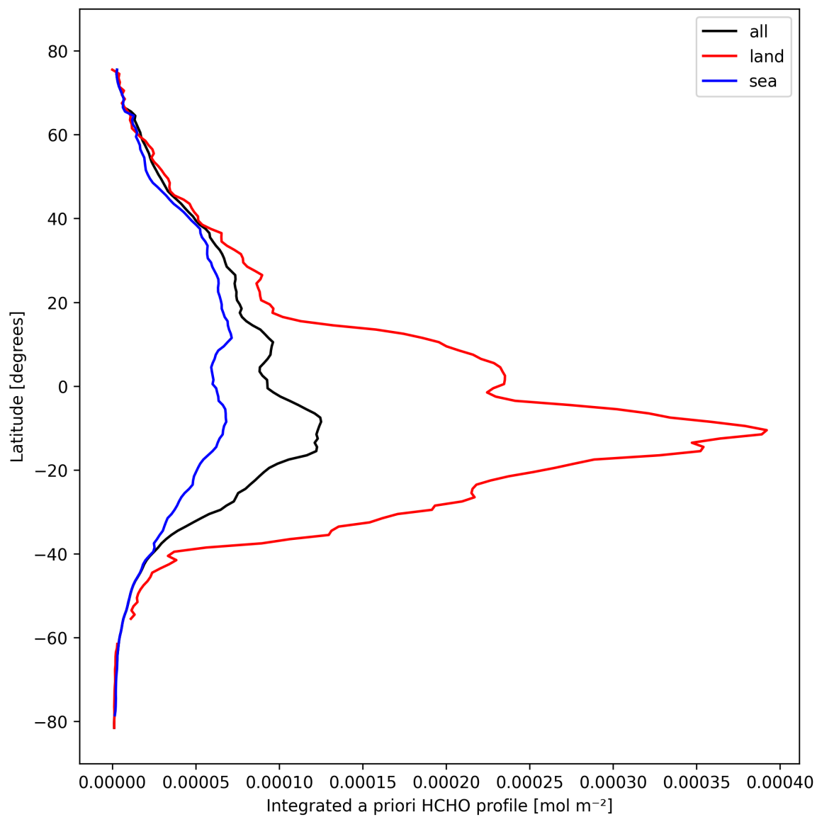
Figure 29: Zonal average of “Integrated a priori HCHO profile” for 2024-10-16 to 2024-10-18.
