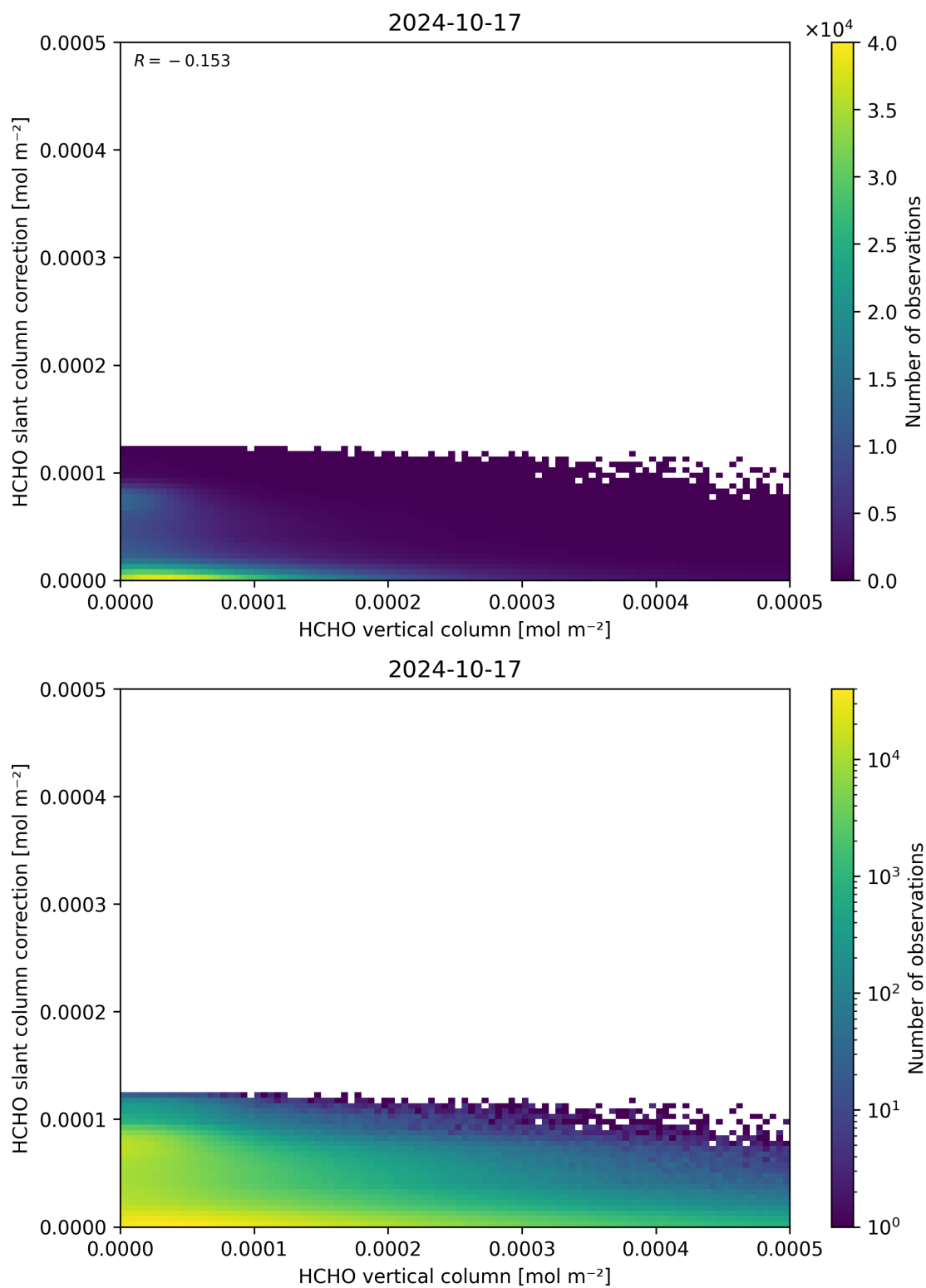
Figure 128: Scatter density plot of “HCHO vertical column” against “HCHO slant column correction” for 2024-10-16 to 2024-10-18.
