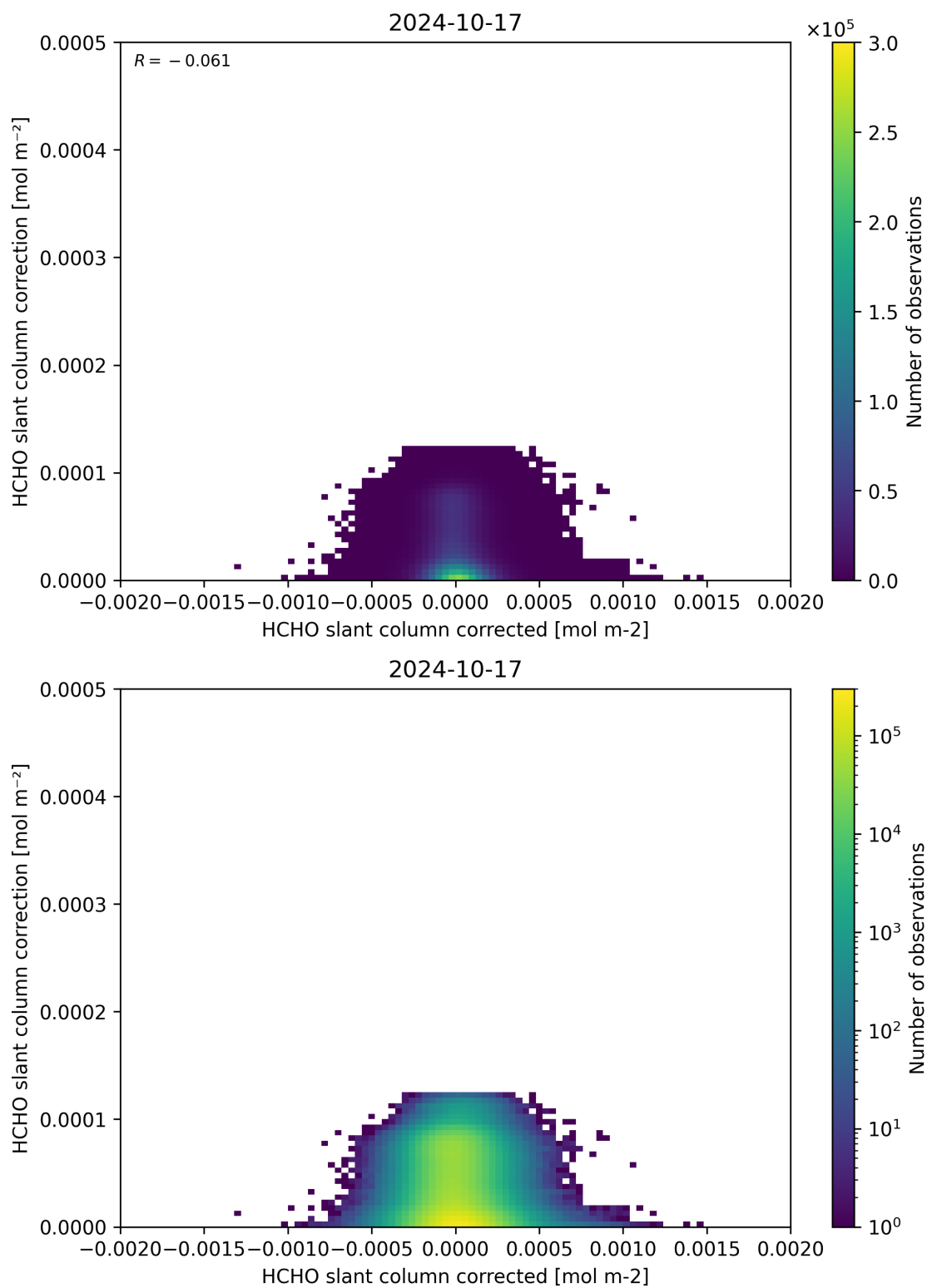
Figure 77: Scatter density plot of “HCHO slant column corrected” against “HCHO slant column correction” for 2024-10-16 to 2024-10-18.
