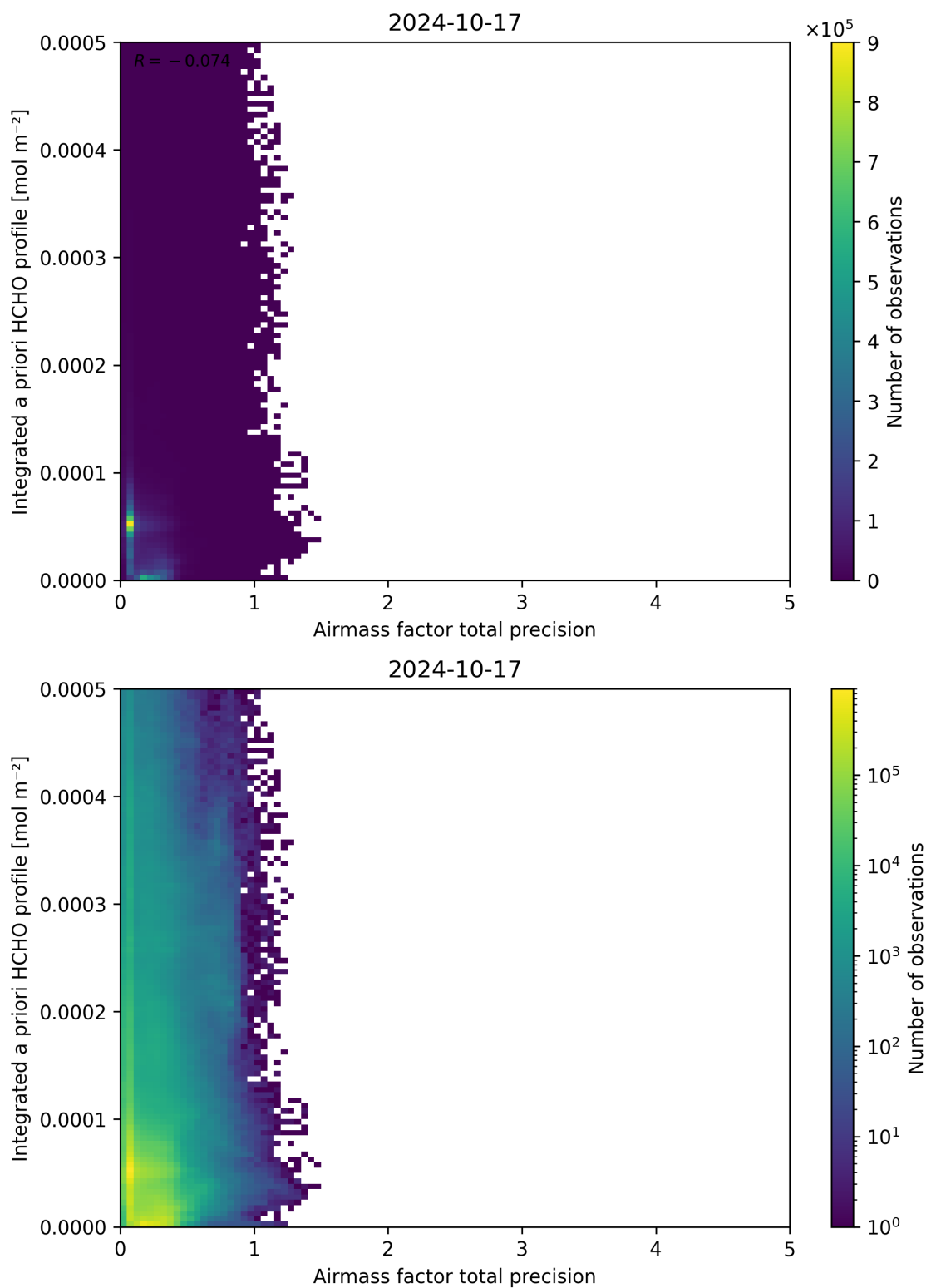
Figure 111: Scatter density plot of “Airmass factor total precision” against “Integrated a priori HCHO profile” for 2024-10-16 to 2024-10-18.
