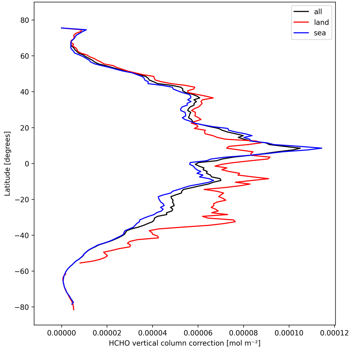
Figure 23: Zonal average of “HCHO vertical column correction” for 2024-10-16 to 2024-10-18.
