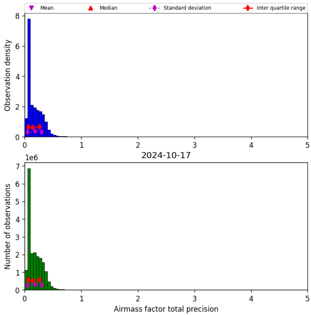
Figure 41: Histogram of “Airmass factor total precision” for 2024-10-16 to 2024-10-18
