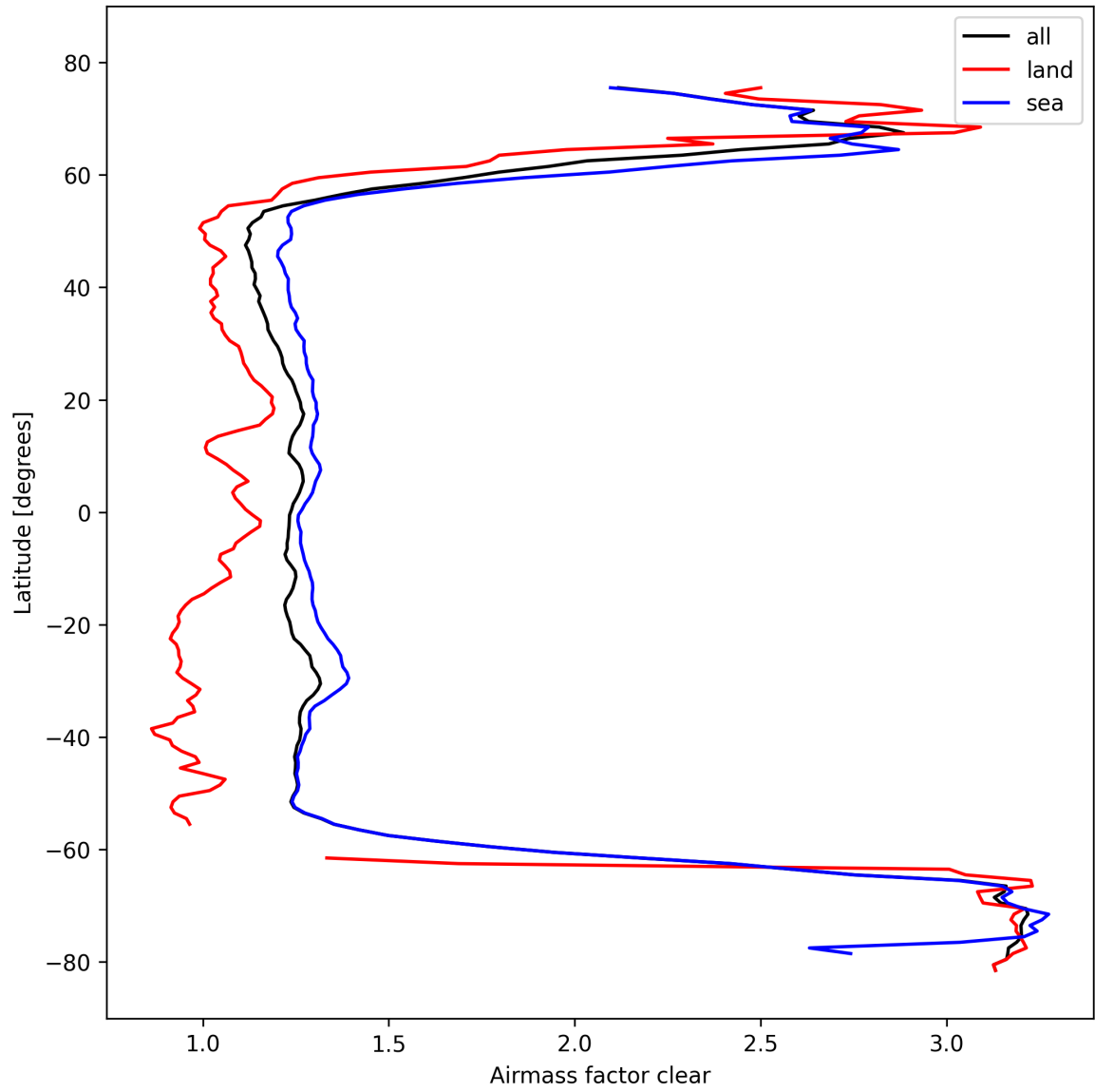
Figure 28: Zonal average of “Airmass factor clear” for 2024-10-16 to 2024-10-18.
