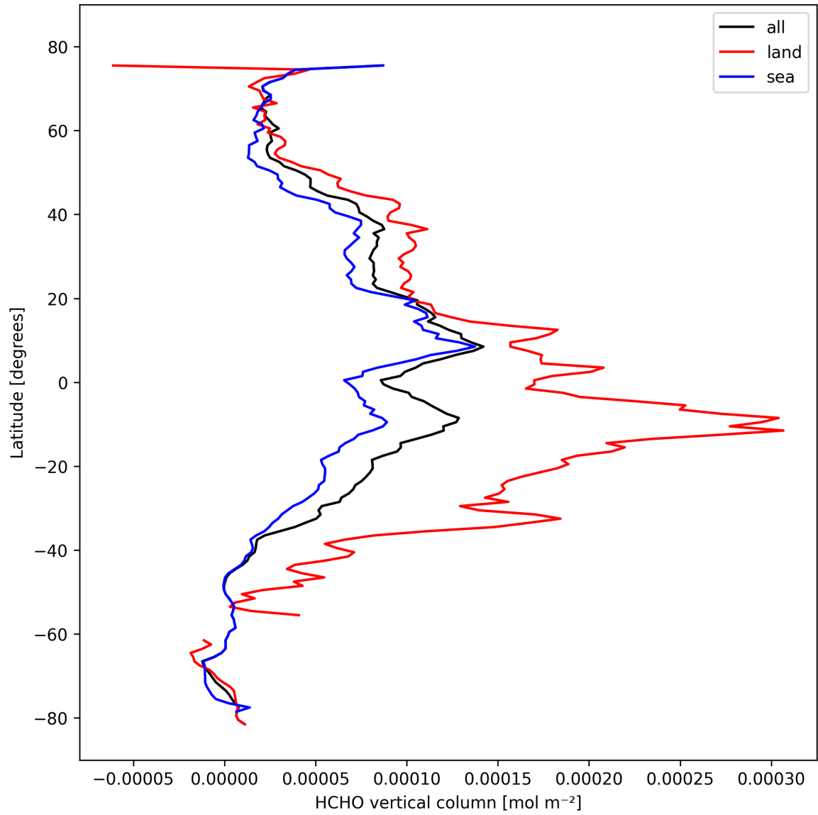
Figure 21: Zonal average of “HCHO vertical column” for 2024-10-16 to 2024-10-18.
