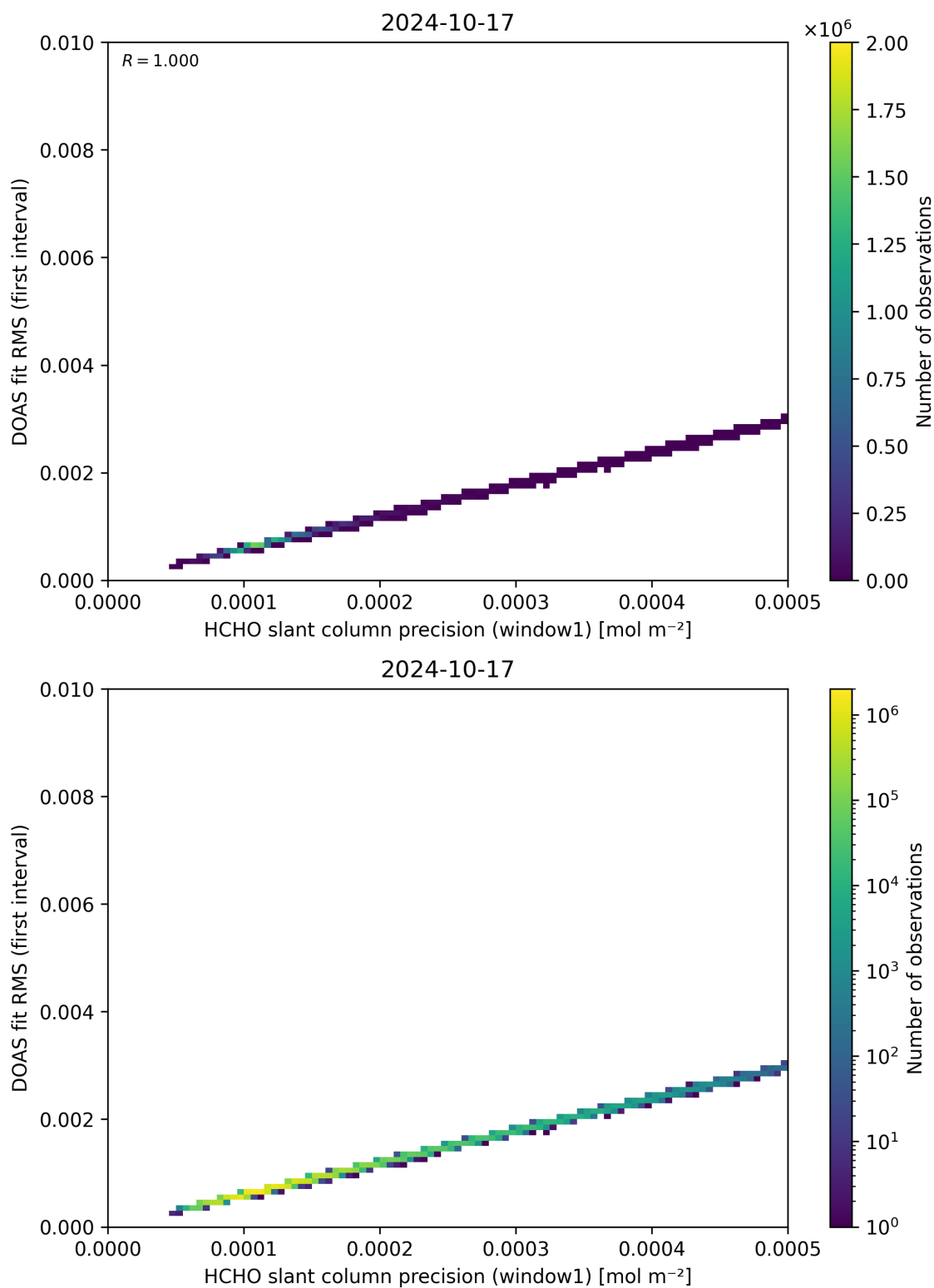
Figure 88: Scatter density plot of “HCHO slant column precision (window1)” against “DOAS fit RMS (first interval)” for 2024-10-16 to 2024-10-18.
