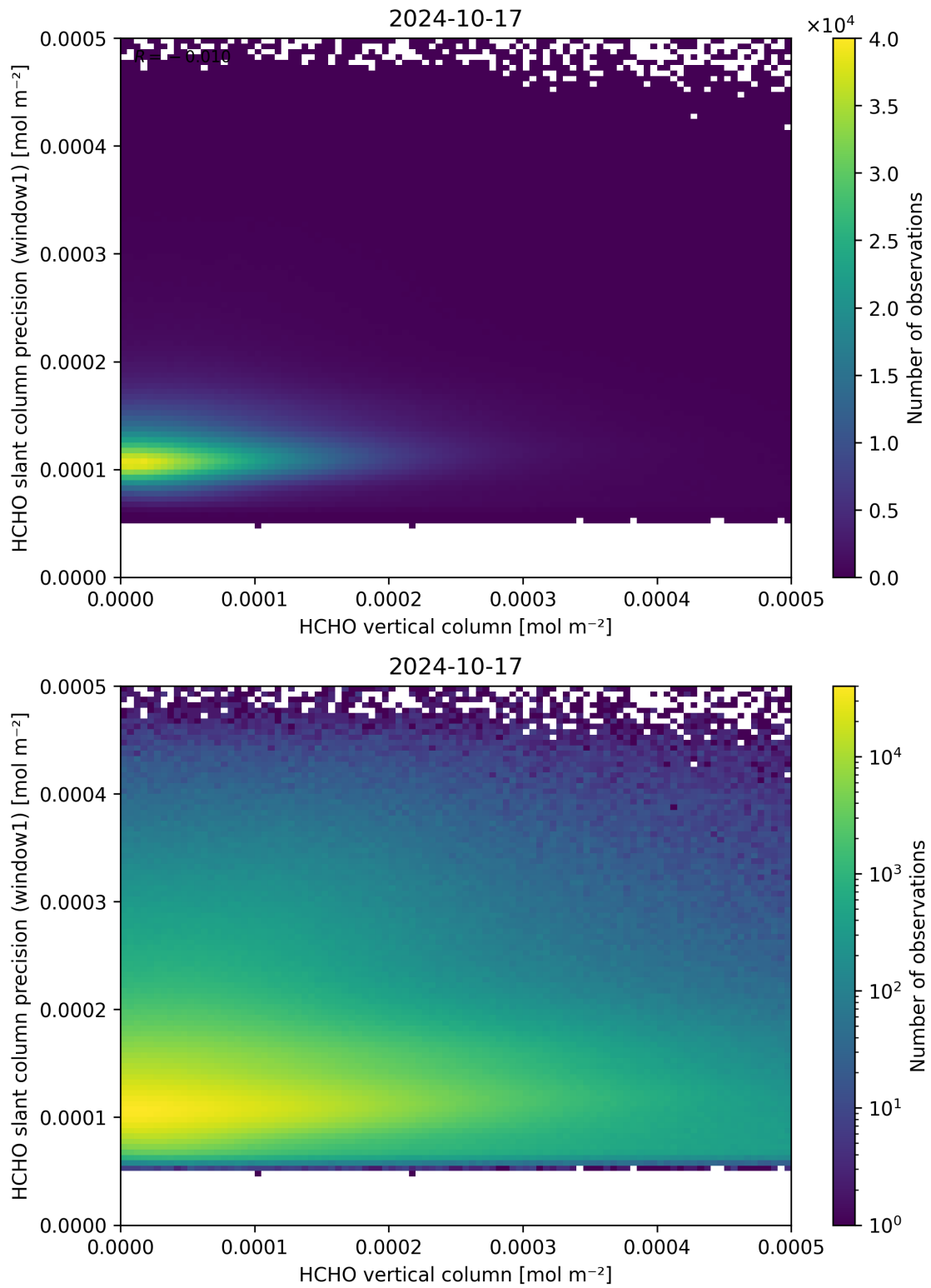
Figure 130: Scatter density plot of “HCHO vertical column” against “HCHO slant column precision (window1)” for 2024-10-16 to 2024-10-18.
