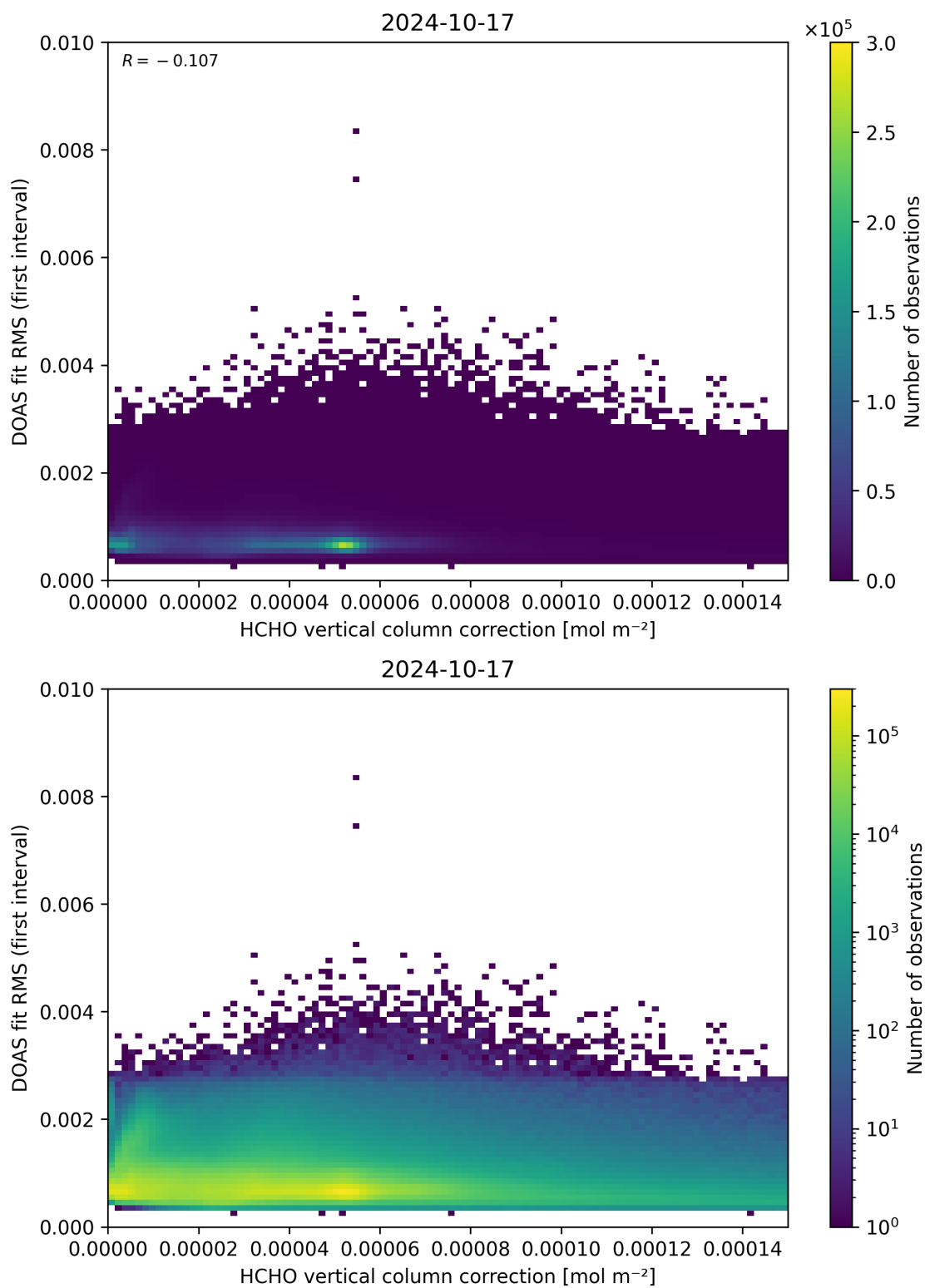
Figure 112: Scatter density plot of “HCHO vertical column correction” against “DOAS fit RMS (first interval)” for 2024-10-16 to 2024-10-18.
