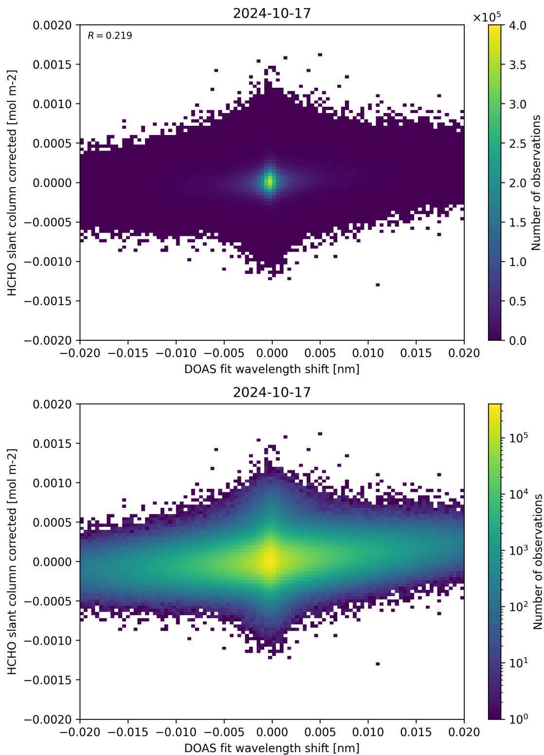
Figure 66: Scatter density plot of “DOAS fit wavelength shift” against “HCHO slant column corrected” for 2024-10-16 to 2024-10-18.
