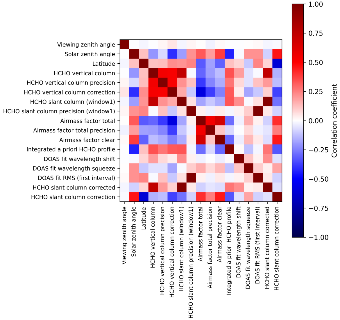
Figure 2: Map of correlation matrix for 2024-10-16 to 2024-10-18.
