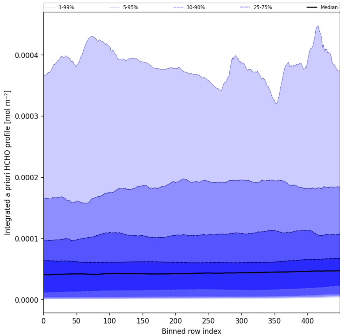
Figure 57: Along track statistics of “Integrated a priori HCHO profile” for 2024-10-16 to 2024-10-18
