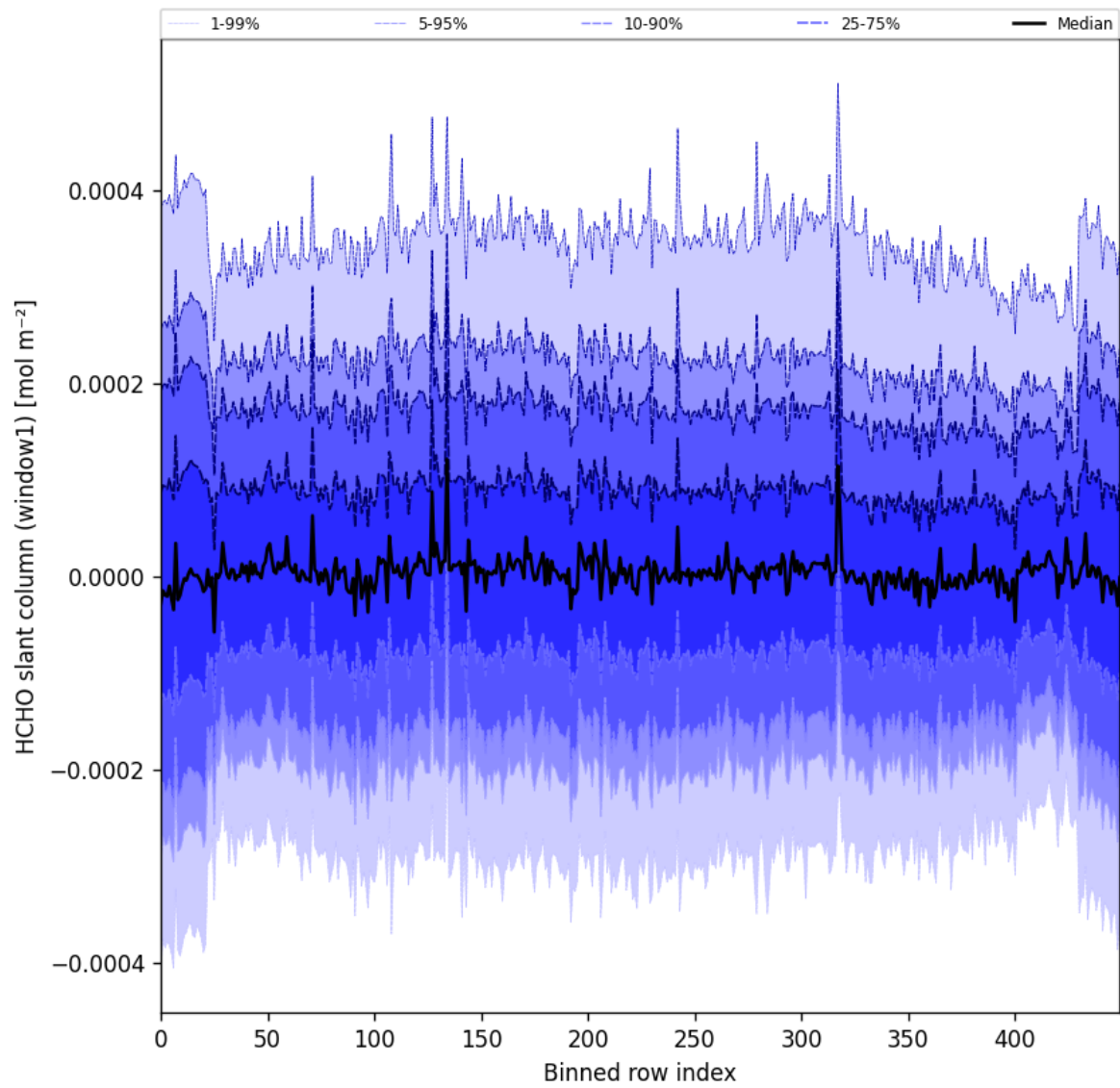
Figure 52: Along track statistics of “HCHO slant column (window1)” for 2024-10-16 to 2024-10-18
