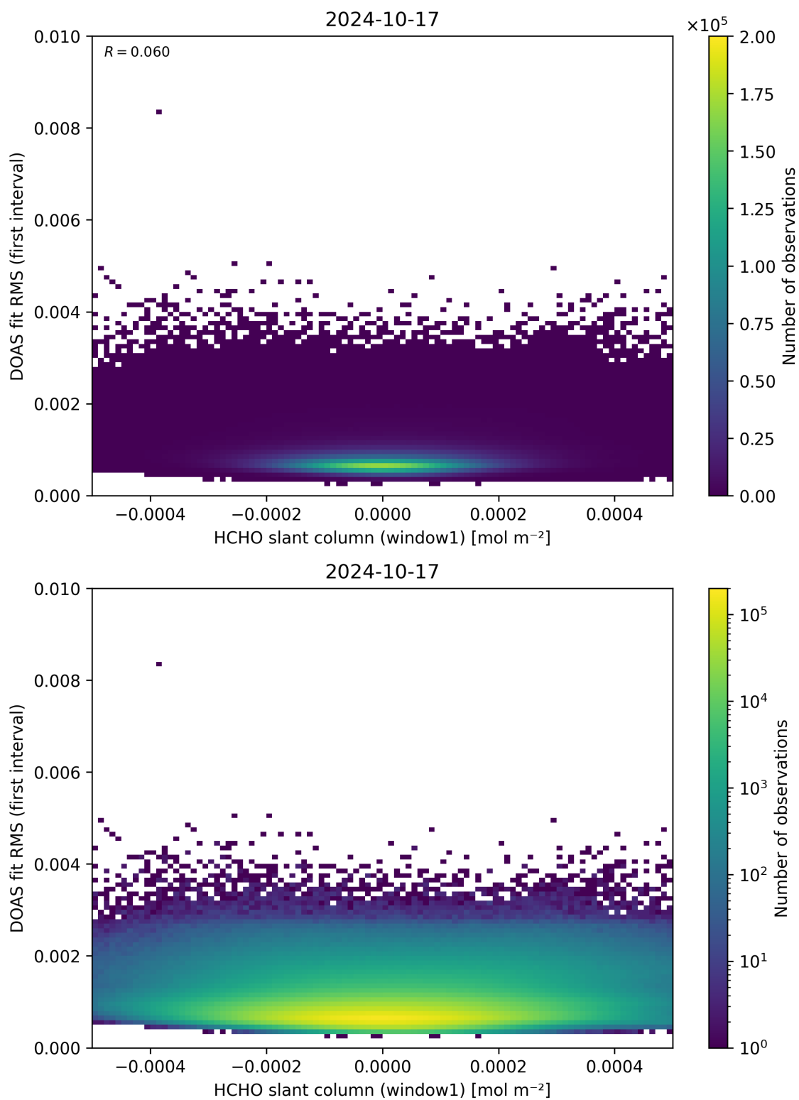
Figure 78: Scatter density plot of “HCHO slant column (window1)” against “DOAS fit RMS (first interval)” for 2024-10-16 to 2024-10-18.
