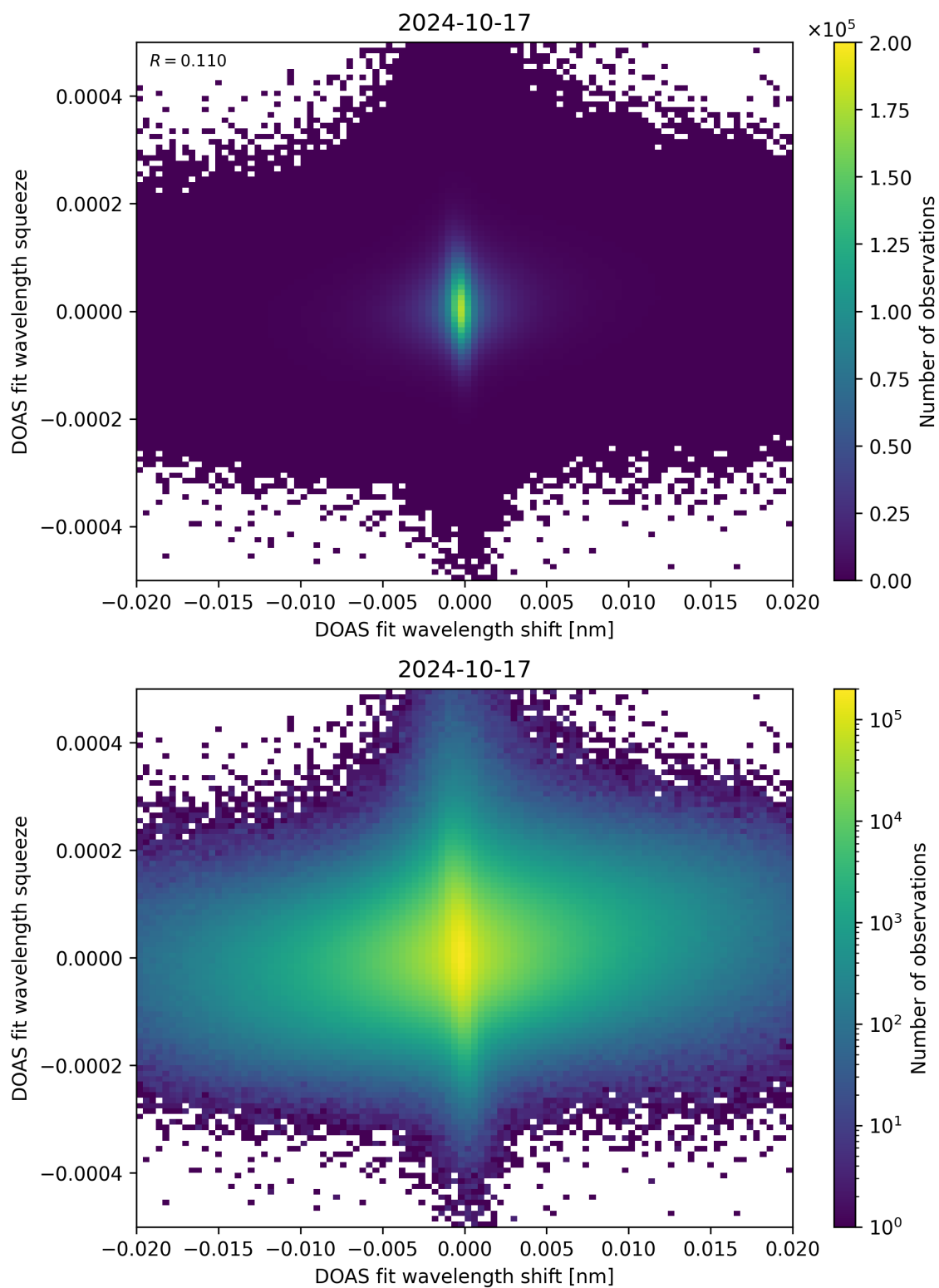
Figure 65: Scatter density plot of “DOAS fit wavelength shift” against “DOAS fit wavelength squeeze” for 2024-10-16 to 2024-10-18.
