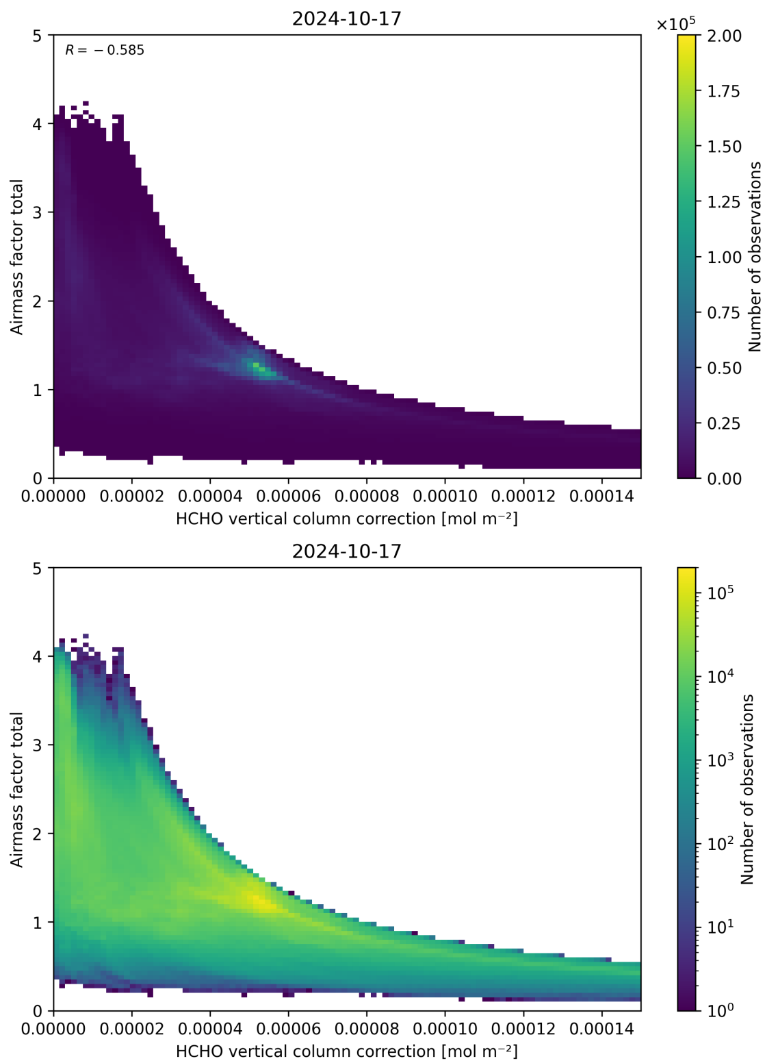
Figure 120: Scatter density plot of “HCHO vertical column correction” against “Airmass factor total” for 2024-10-16 to 2024-10-18.
