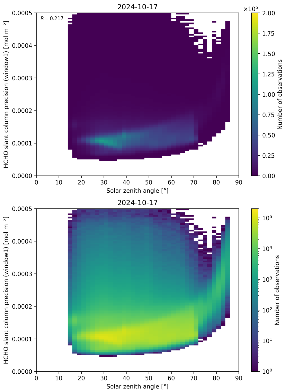
Figure 174: Scatter density plot of “Solar zenith angle” against “HCHO slant column precision (window1)” for 2024-10-16 to 2024-10-18.
