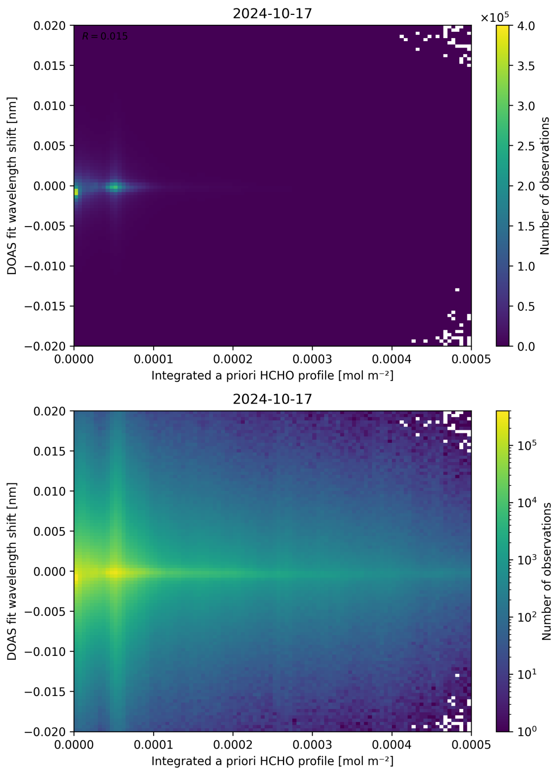
Figure 149: Scatter density plot of “Integrated a priori HCHO profile” against “DOAS fit wavelength shift” for 2024-10-16 to 2024-10-18.
