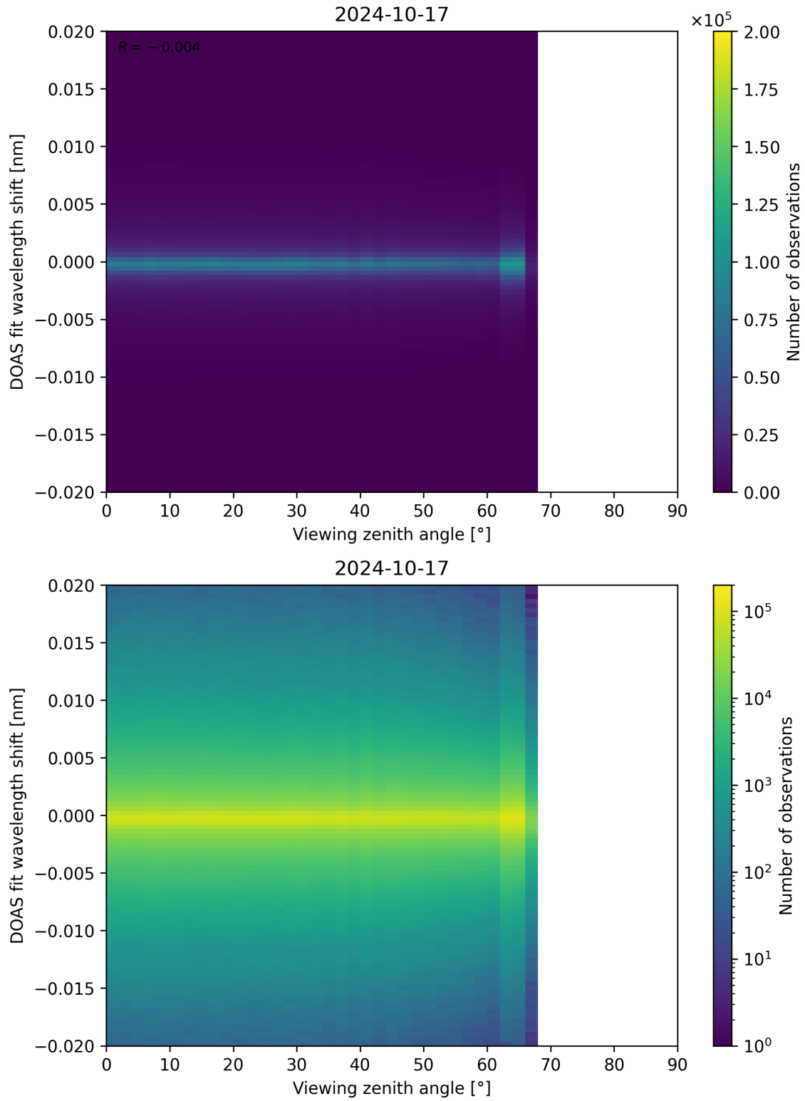
Figure 183: Scatter density plot of “Viewing zenith angle” against “DOAS fit wavelength shift” for 2024-10-16 to 2024-10-18.
