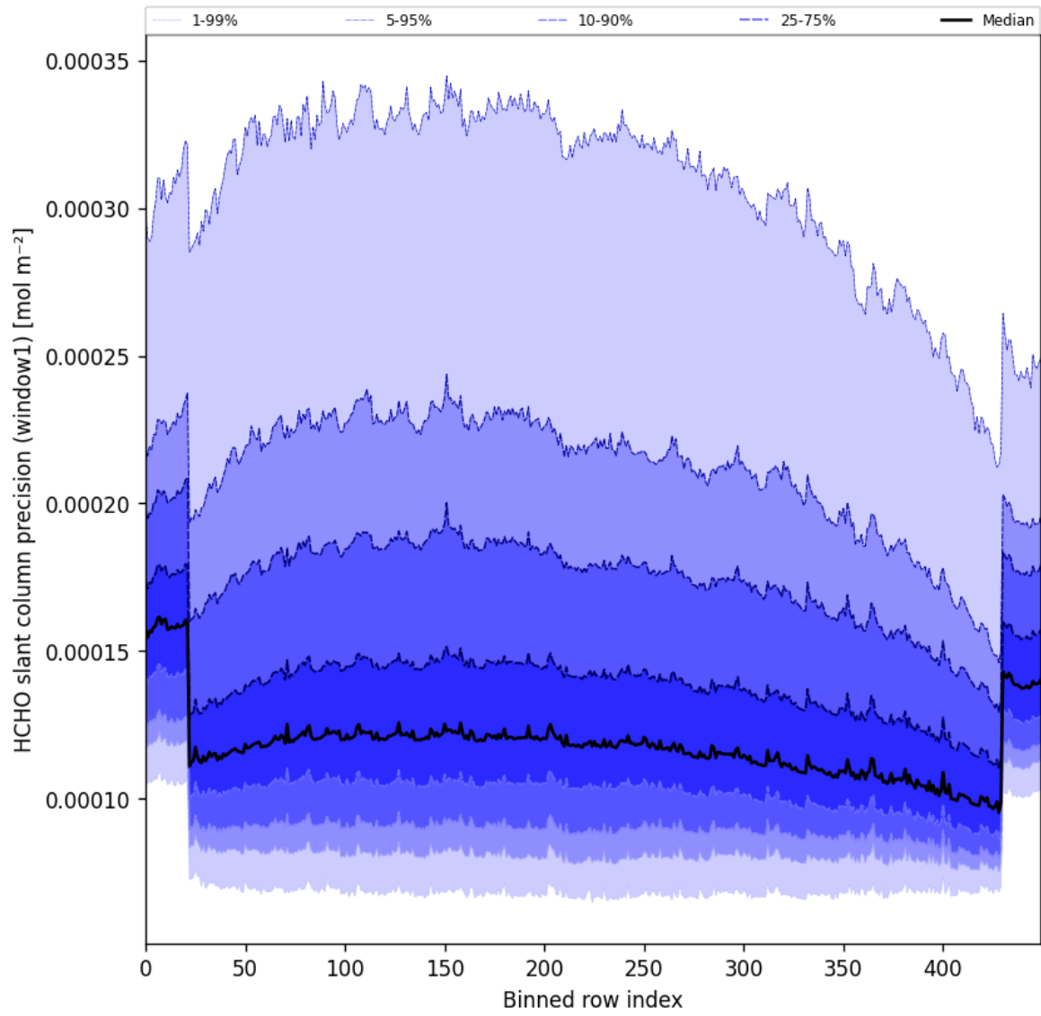
Figure 53: Along track statistics of “HCHO slant column precision (window1)” for 2024-10-16 to 2024-10-18
