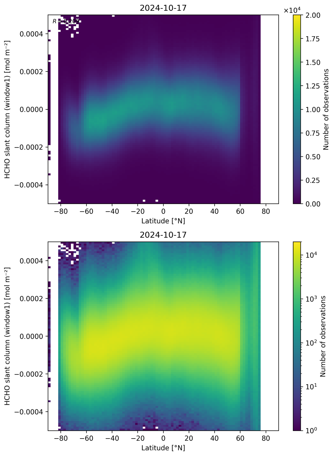
Figure 159: Scatter density plot of “Latitude” against “HCHO slant column (window1)” for 2024-10-16 to 2024-10-18.
