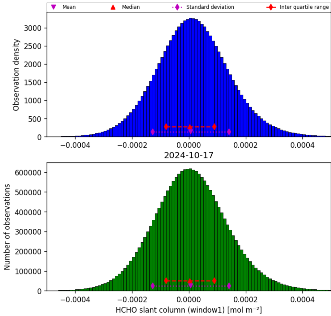
Figure 38: Histogram of “HCHO slant column (window1)” for 2024-10-16 to 2024-10-18
