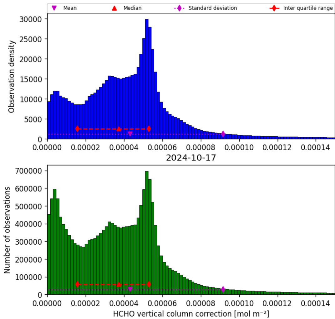
Figure 37: Histogram of “HCHO vertical column correction” for 2024-10-16 to 2024-10-18
