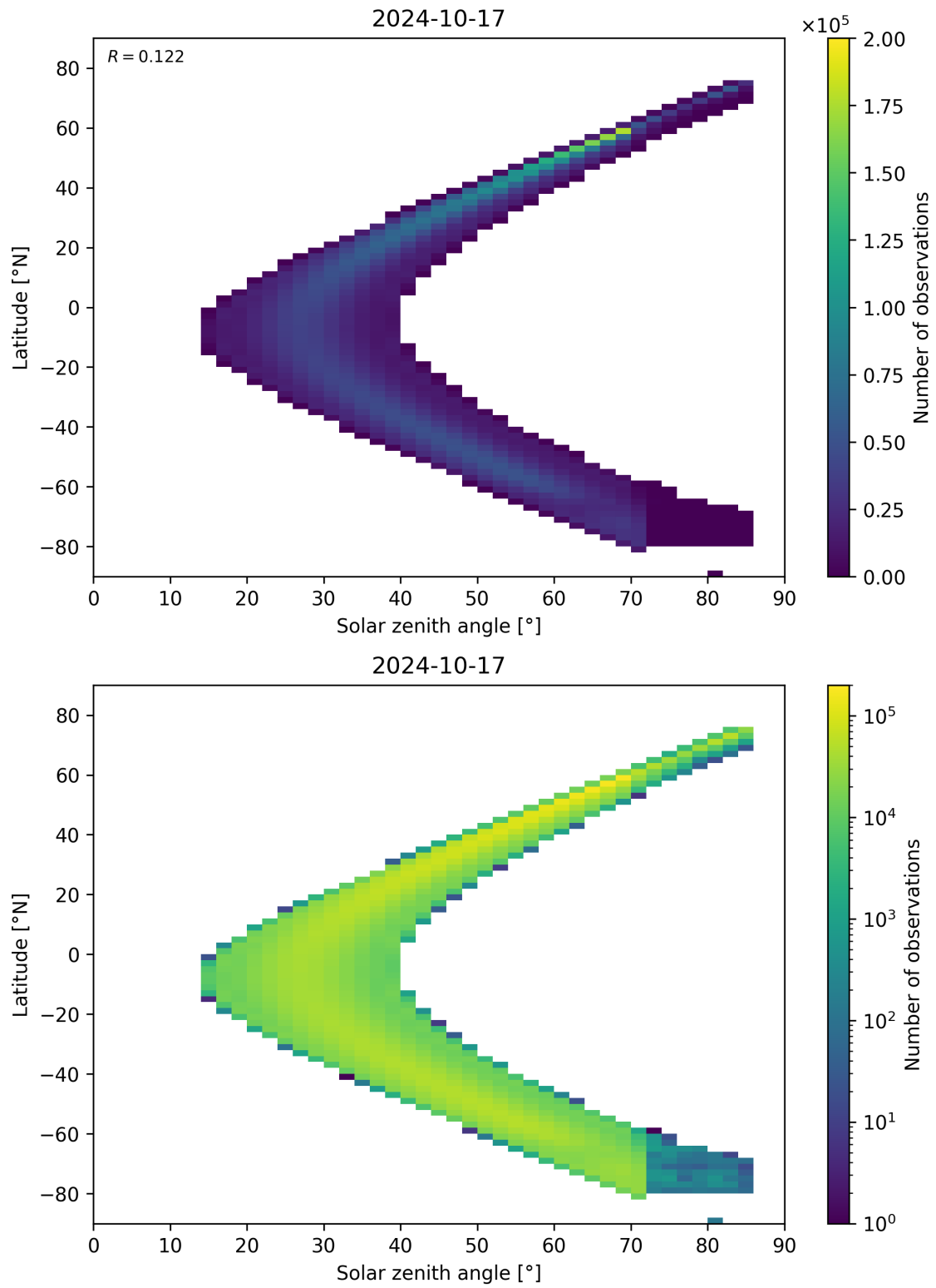
Figure 181: Scatter density plot of “Solar zenith angle” against “Latitude” for 2024-10-16 to 2024-10-18.
