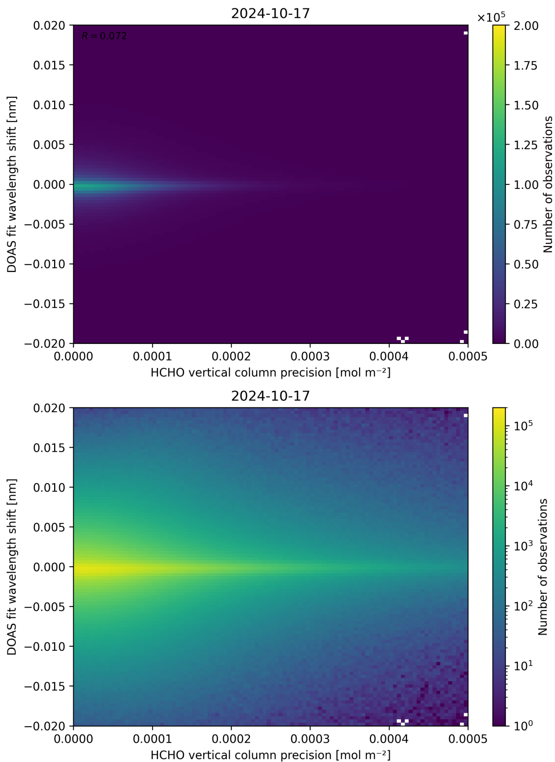
Figure 137: Scatter density plot of “HCHO vertical column precision” against “DOAS fit wavelength shift” for 2024-10-16 to 2024-10-18.
