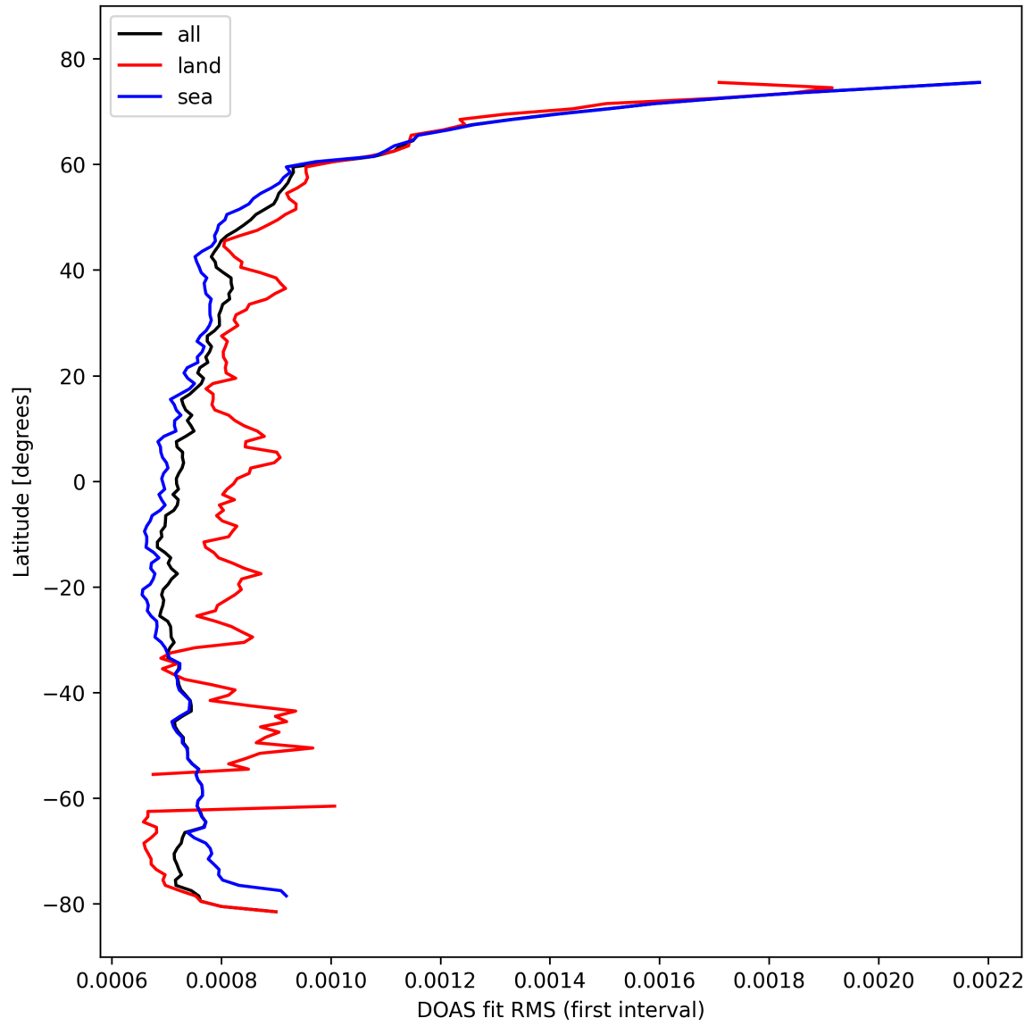
Figure 32: Zonal average of “DOAS fit RMS (first interval)” for 2024-10-16 to 2024-10-18.
