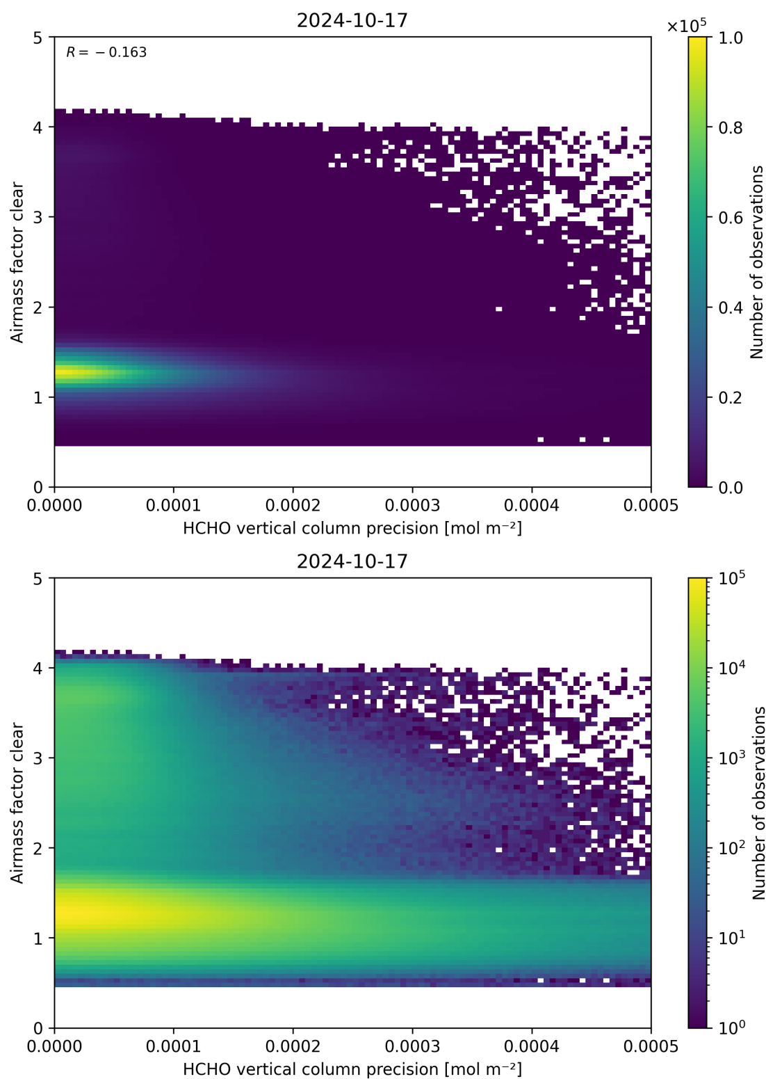
Figure 139: Scatter density plot of “HCHO vertical column precision” against “Airmass factor clear” for 2024-10-16 to 2024-10-18.
