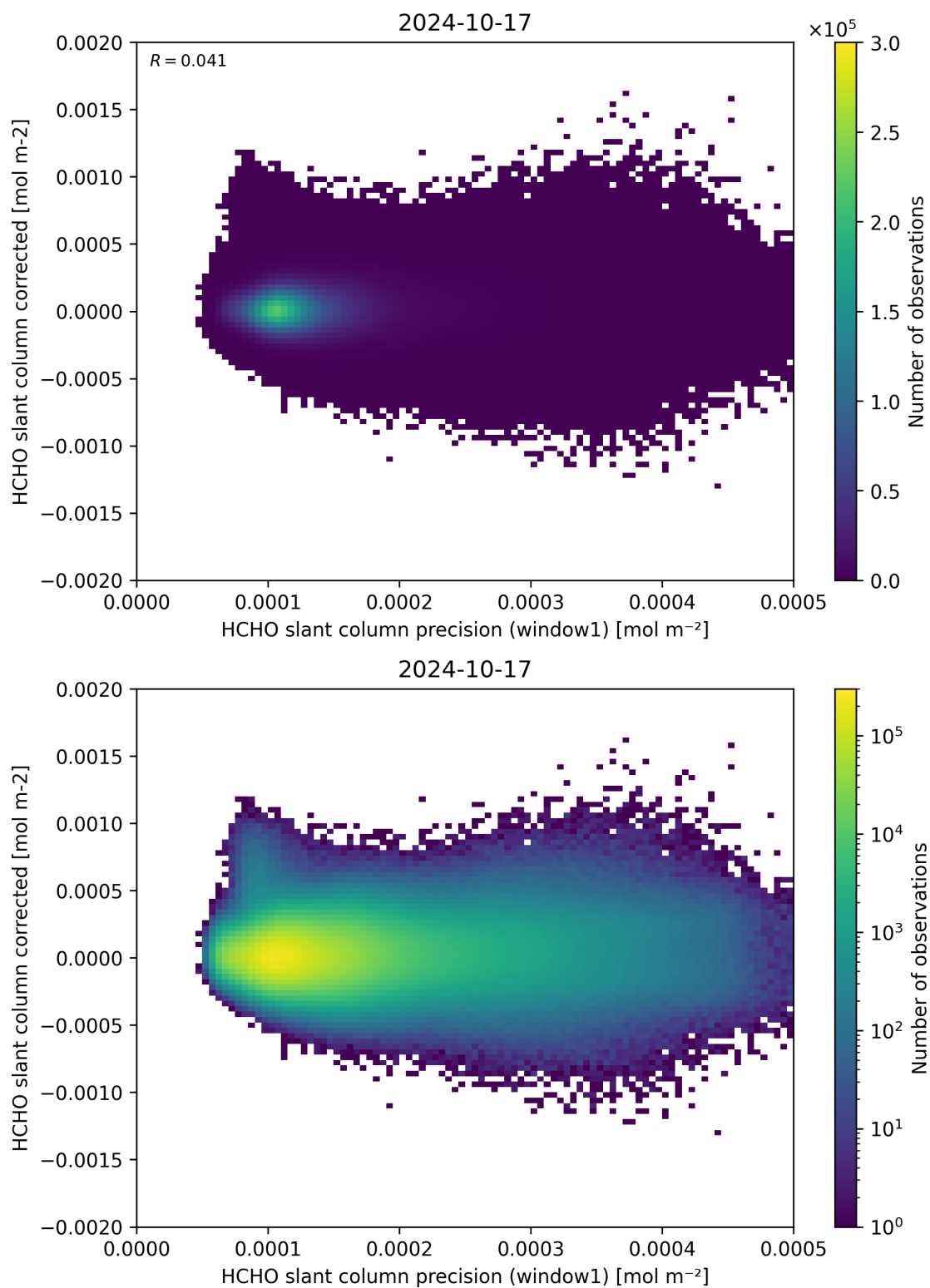
Figure 92: Scatter density plot of “HCHO slant column precision (window1)” against “HCHO slant column corrected” for 2024-10-16 to 2024-10-18.
