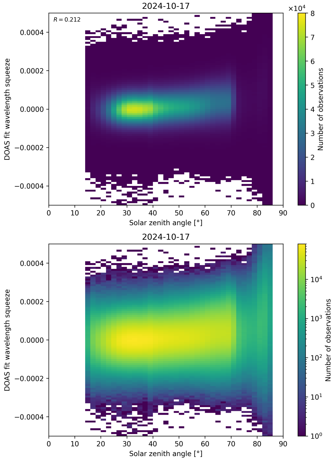
Figure 169: Scatter density plot of “Solar zenith angle” against “DOAS fit wavelength squeeze” for 2024-10-16 to 2024-10-18.
