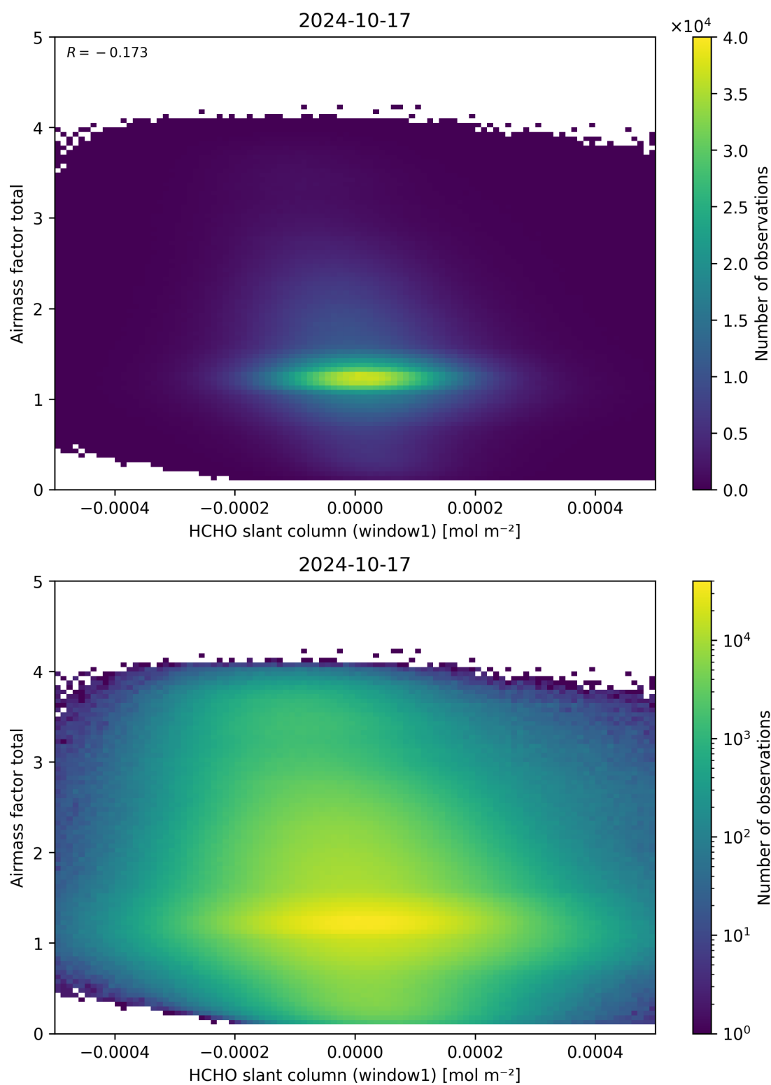
Figure 85: Scatter density plot of “HCHO slant column (window1)” against “Airmass factor total” for 2024-10-16 to 2024-10-18.
