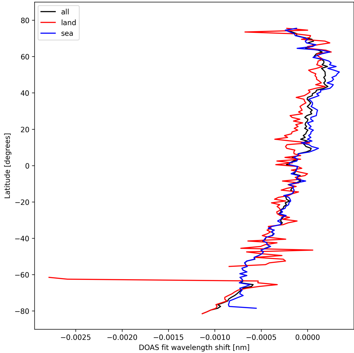
Figure 30: Zonal average of "DOAS fit wavelength shift" for 2024-10-16 to 2024-10-18.
