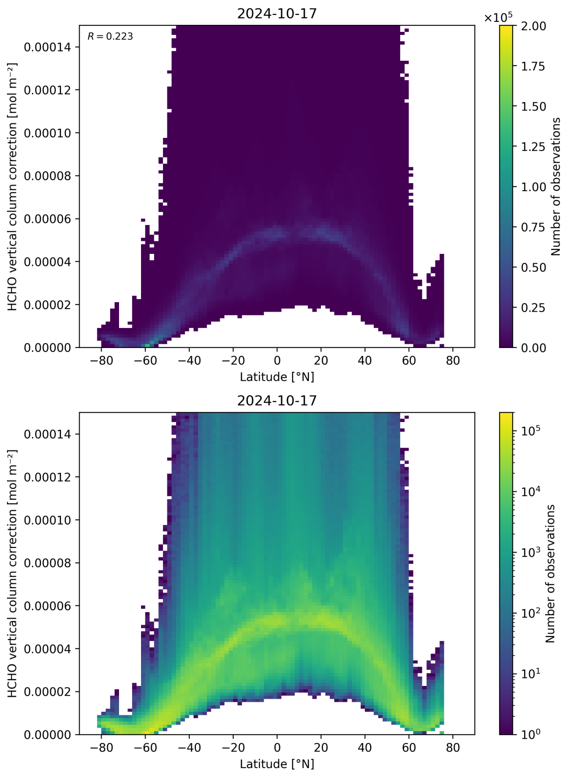
Figure 164: Scatter density plot of “Latitude” against “HCHO vertical column correction” for 2024-10-16 to 2024-10-18.
