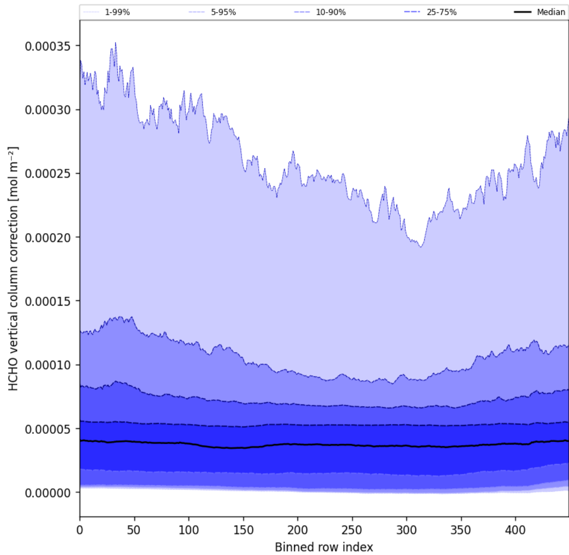
Figure 51: Along track statistics of “HCHO vertical column correction” for 2024-10-16 to 2024-10-18
