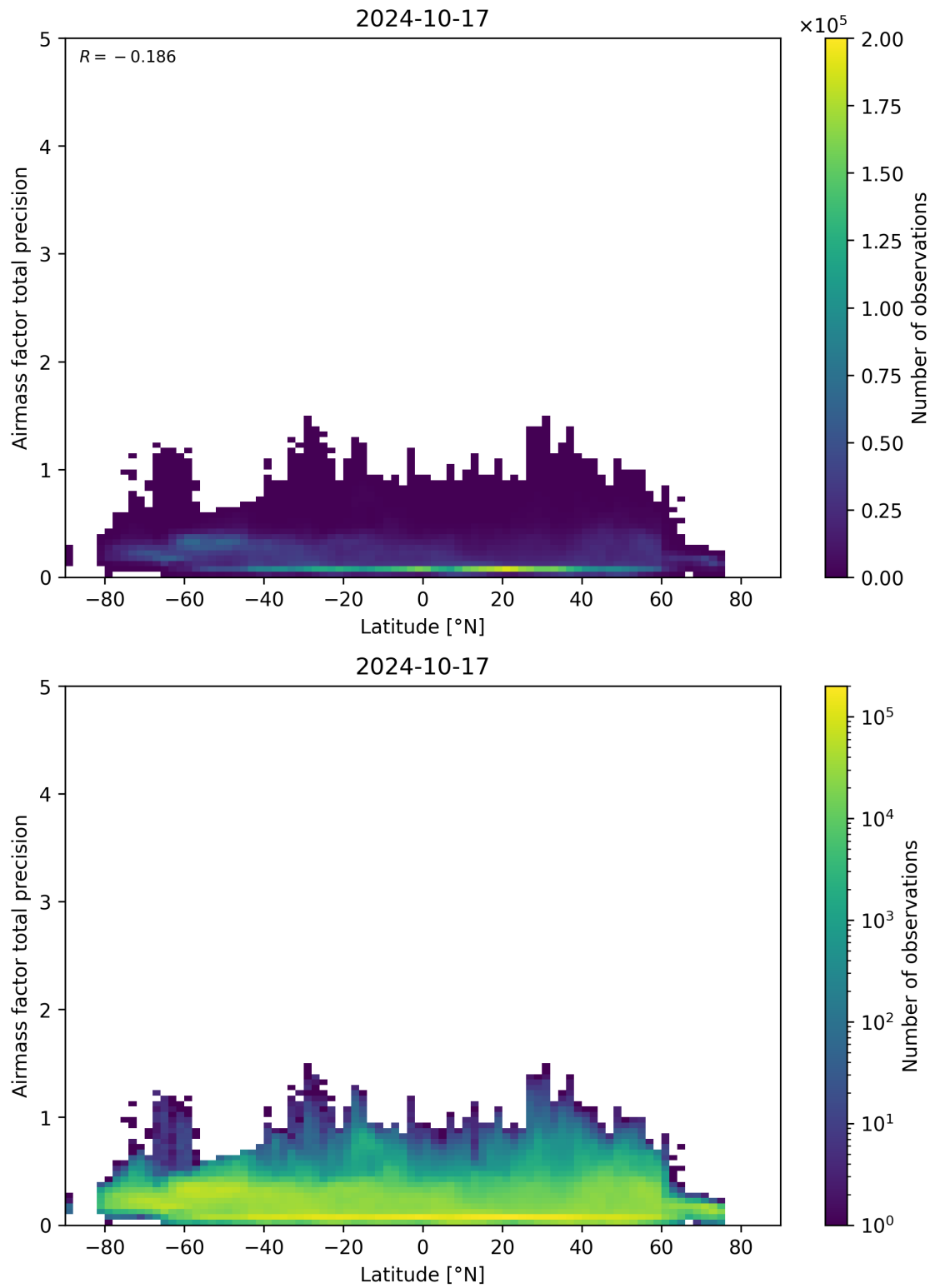
Figure 162: Scatter density plot of “Latitude” against “Airmass factor total precision” for 2024-10-16 to 2024-10-18.
