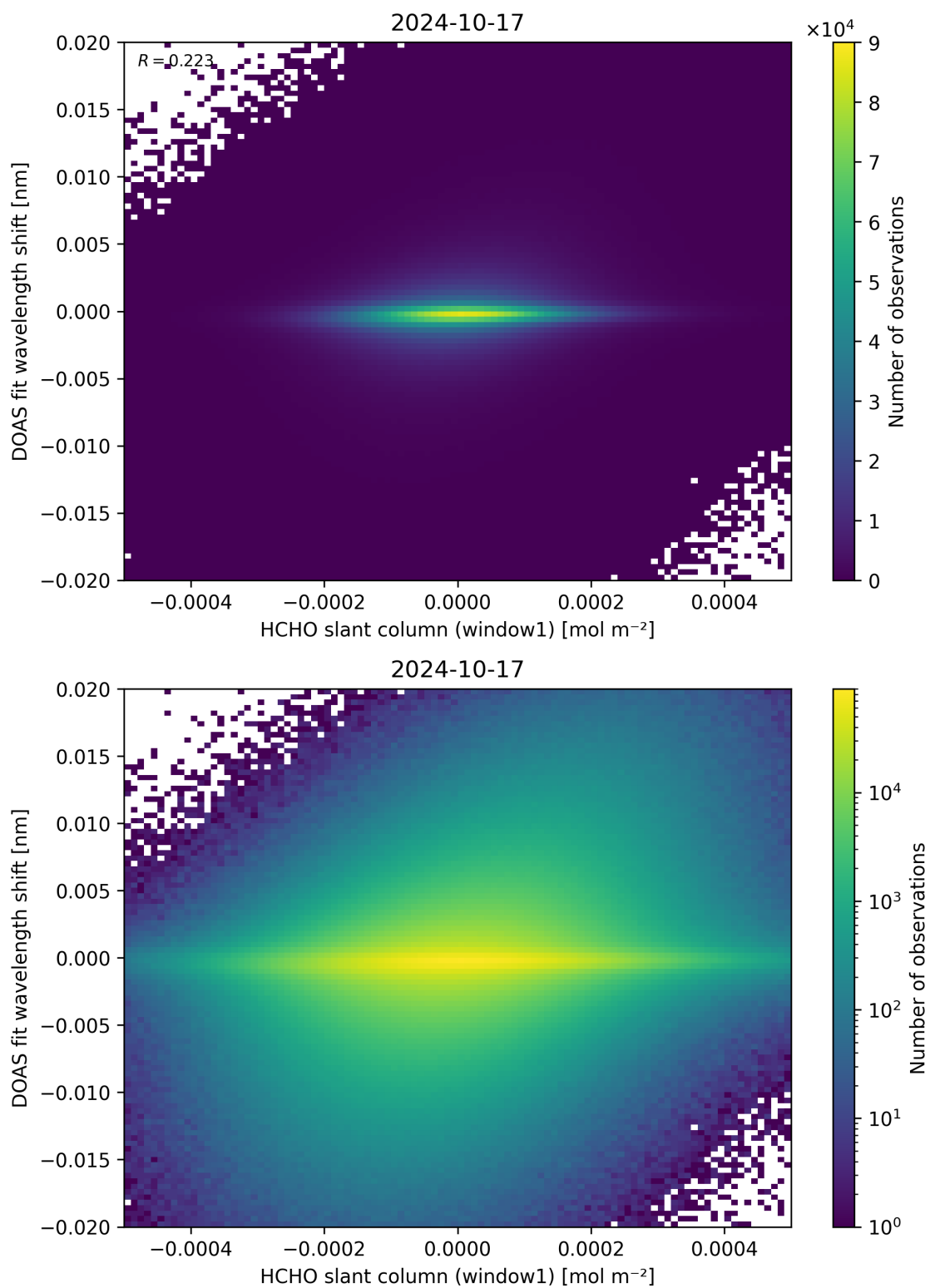
Figure 79: Scatter density plot of “HCHO slant column (window1)” against “DOAS fit wavelength shift” for 2024-10-16 to 2024-10-18.
