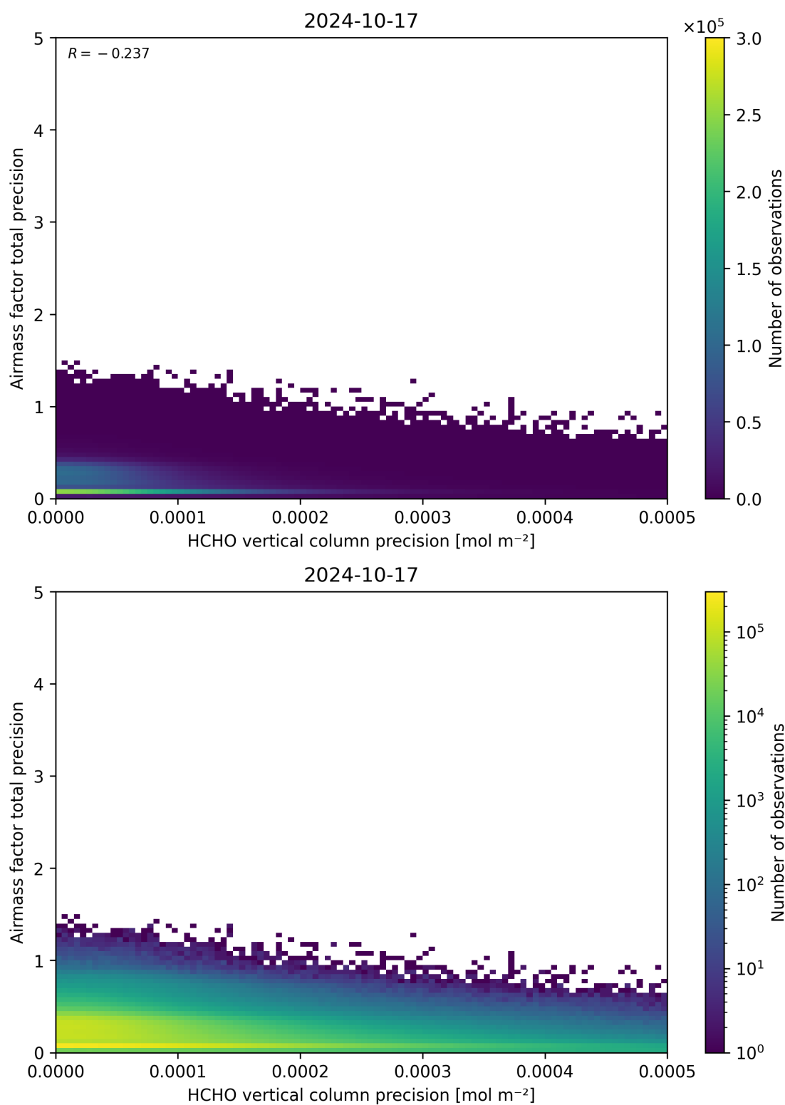
Figure 145: Scatter density plot of “HCHO vertical column precision” against “Airmass factor total precision” for 2024-10-16 to 2024-10-18.
