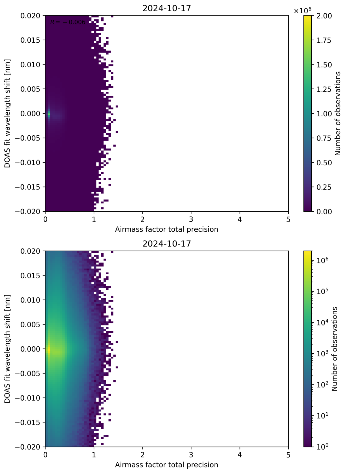
Figure 106: Scatter density plot of “Airmass factor total precision” against “DOAS fit wavelength shift” for 2024-10-16 to 2024-10-18.
