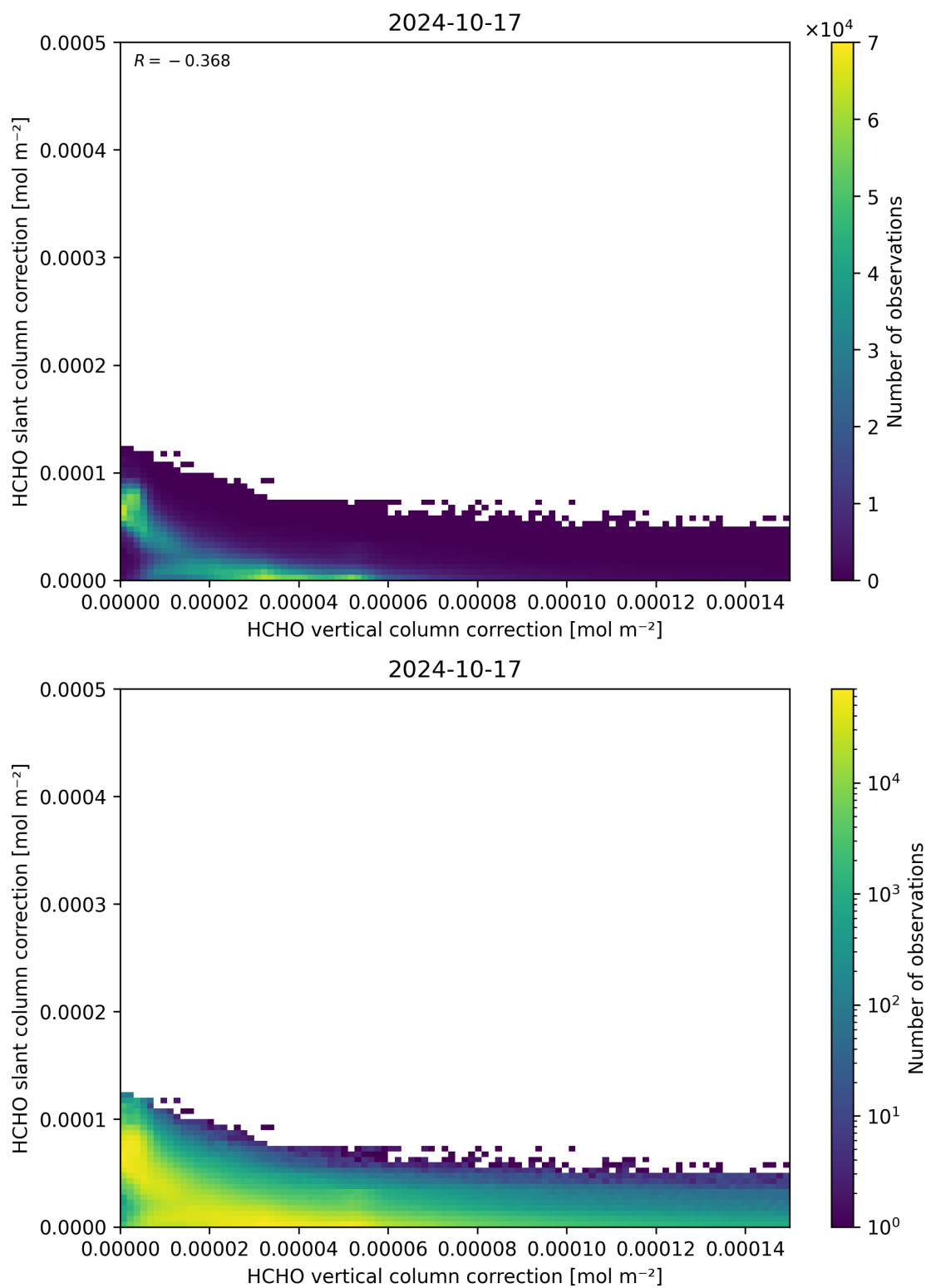
Figure 117: Scatter density plot of “HCHO vertical column correction” against “HCHO slant column correction” for 2024-10-16 to 2024-10-18.
