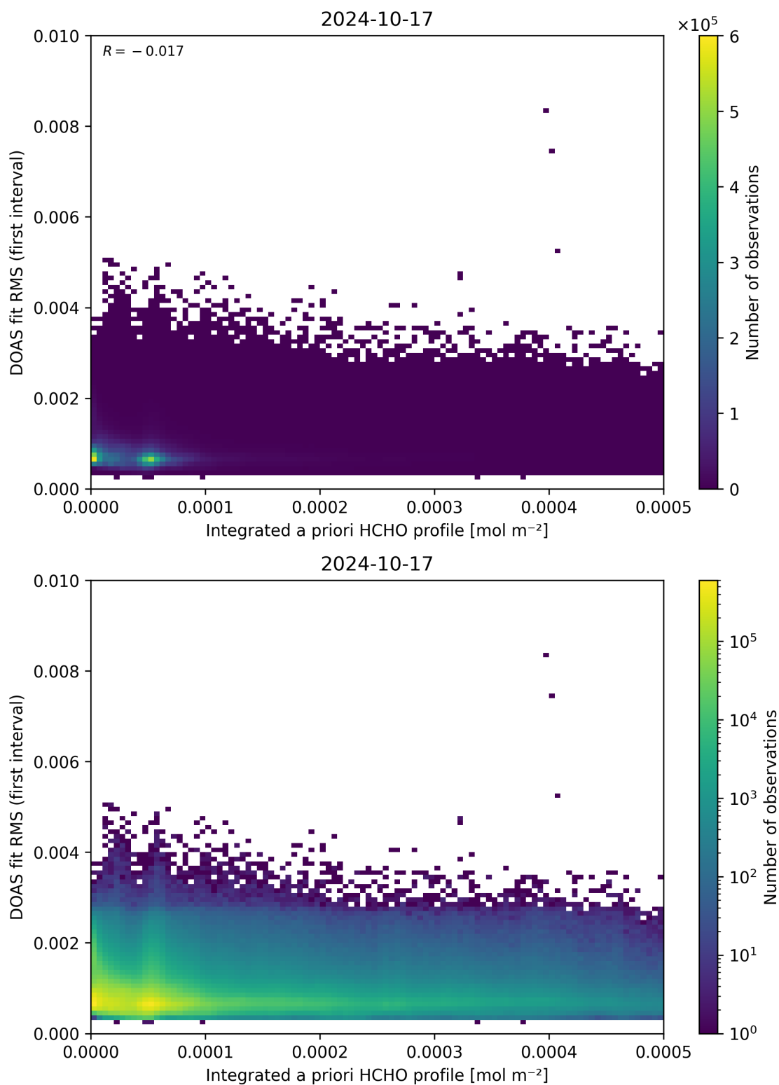
Figure 148: Scatter density plot of “Integrated a priori HCHO profile” against “DOAS fit RMS (first interval)” for 2024-10-16 to 2024-10-18.
