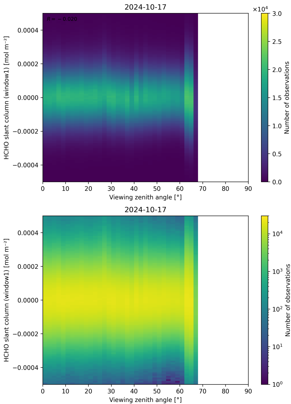
Figure 188: Scatter density plot of “Viewing zenith angle” against “HCHO slant column (window1)” for 2024-10-16 to 2024-10-18.
