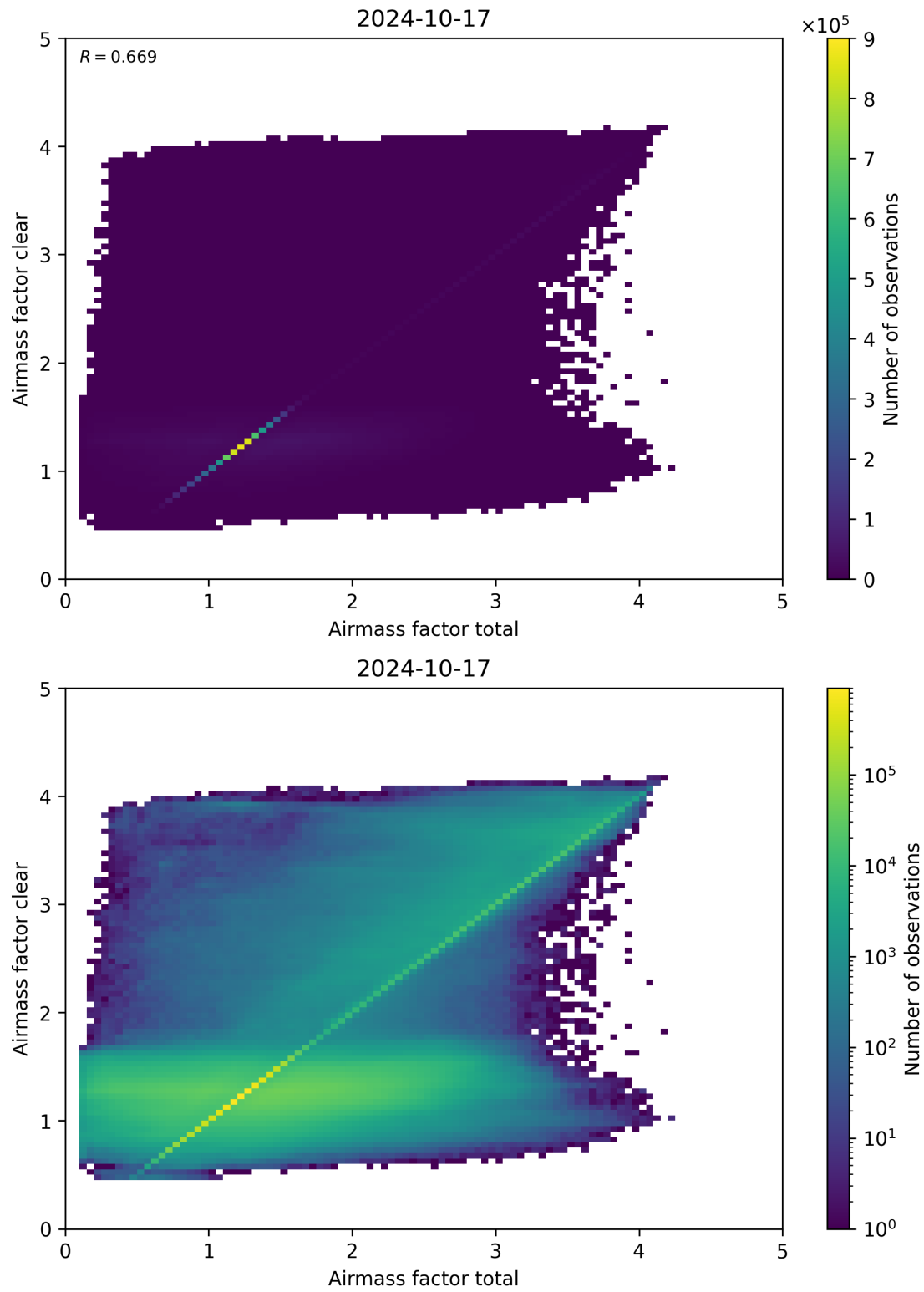
Figure 100: Scatter density plot of “Airmass factor total” against “Airmass factor clear” for 2024-10-16 to 2024-10-18.
