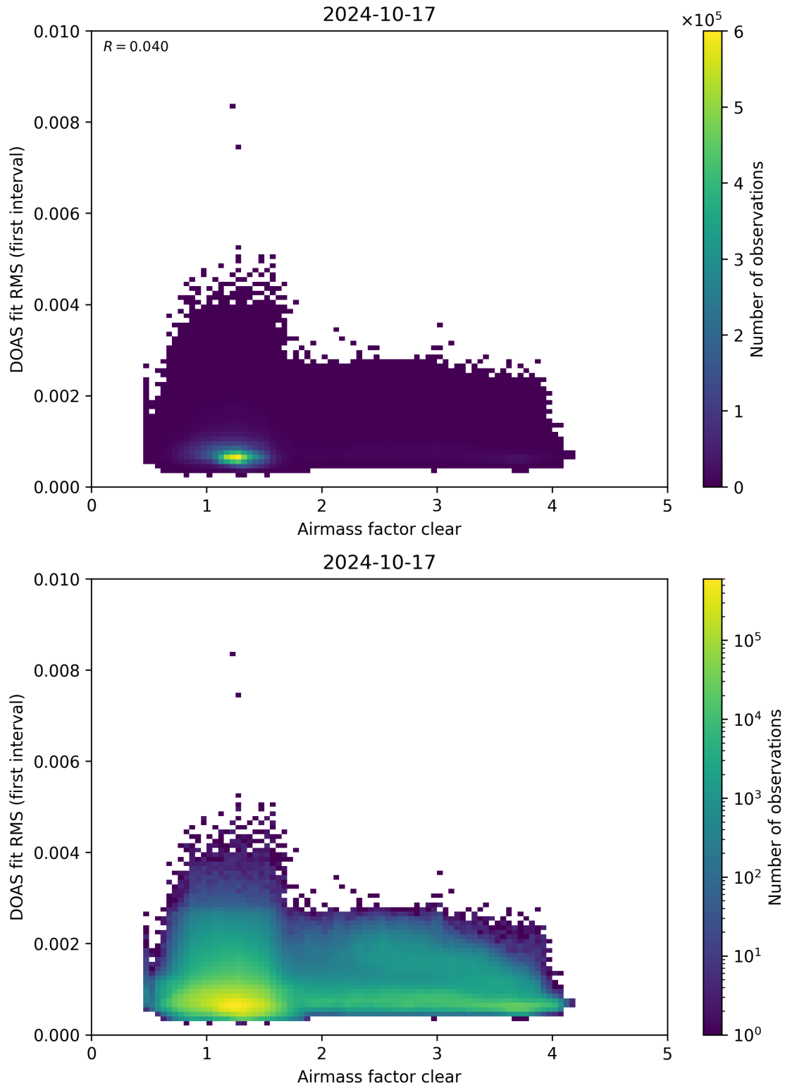
Figure 71: Scatter density plot of “Airmass factor clear” against “DOAS fit RMS (first interval)” for 2024-10-16 to 2024-10-18.
