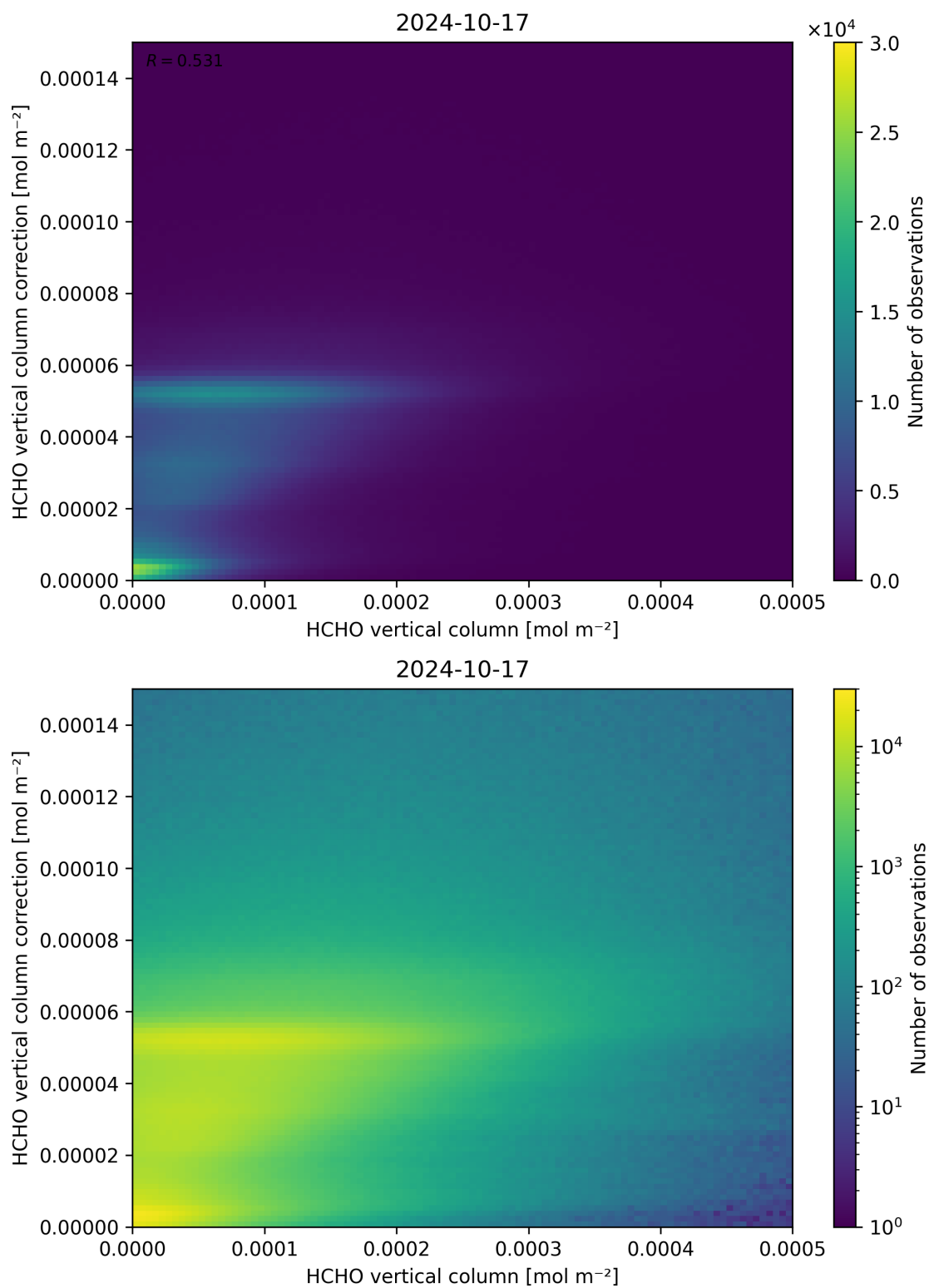
Figure 133: Scatter density plot of “HCHO vertical column” against “HCHO vertical column correction” for 2024-10-16 to 2024-10-18.
