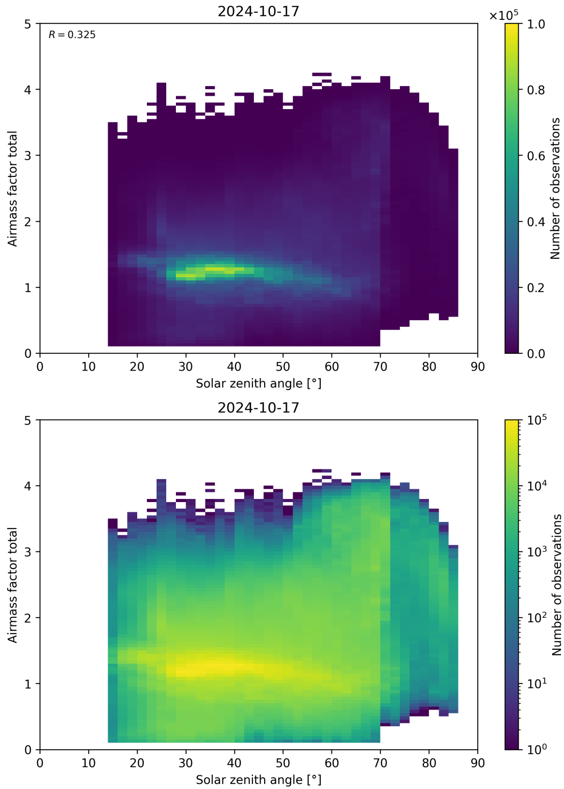
Figure 175: Scatter density plot of “Solar zenith angle” against “Airmass factor total” for 2024-10-16 to 2024-10-18.
