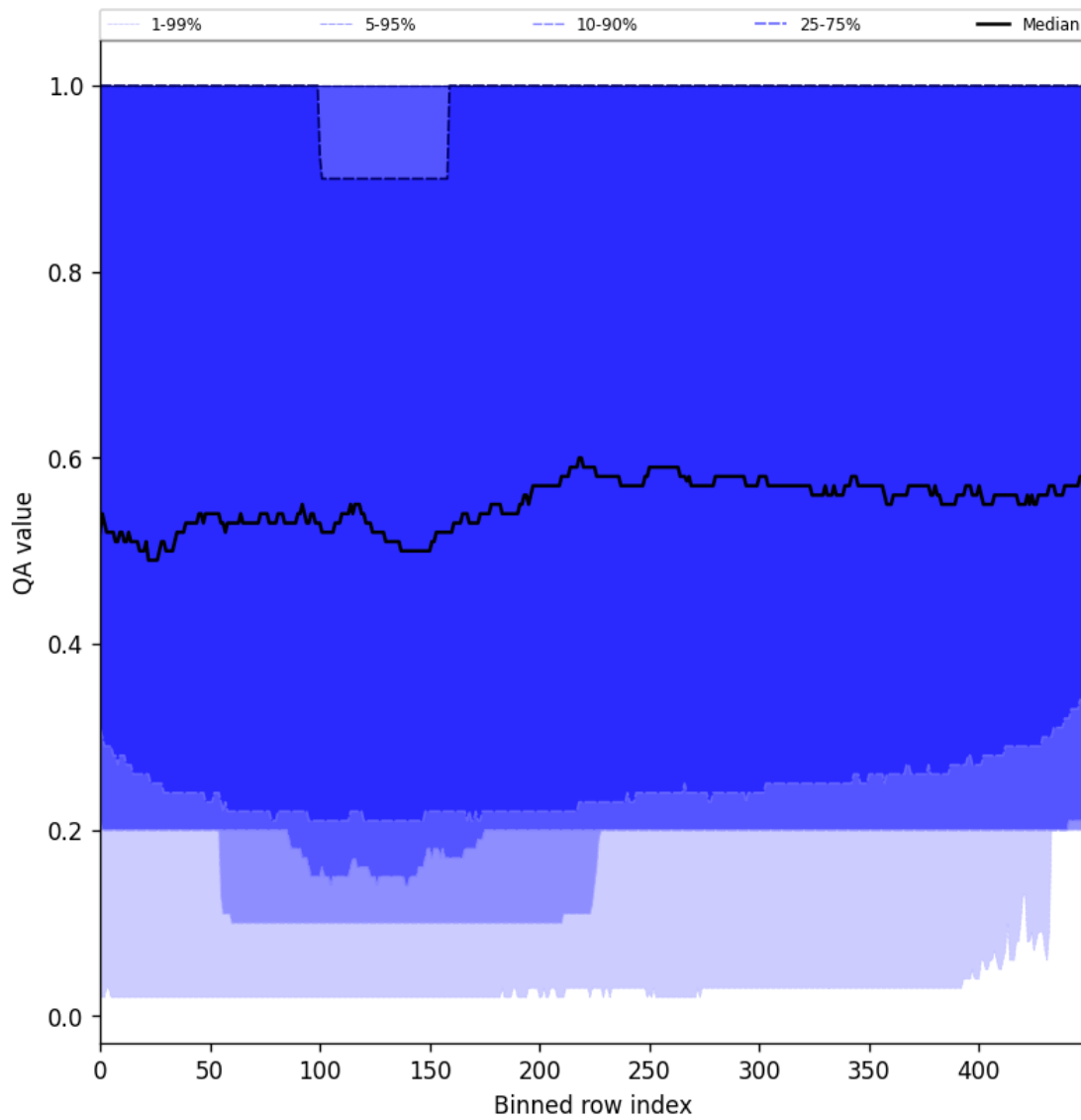
Figure 48: Along track statistics of “QA value” for 2024-10-16 to 2024-10-18
