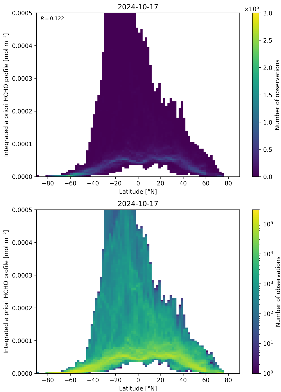
Figure 166: Scatter density plot of “Latitude” against “Integrated a priori HCHO profile” for 2024-10-16 to 2024-10-18.
