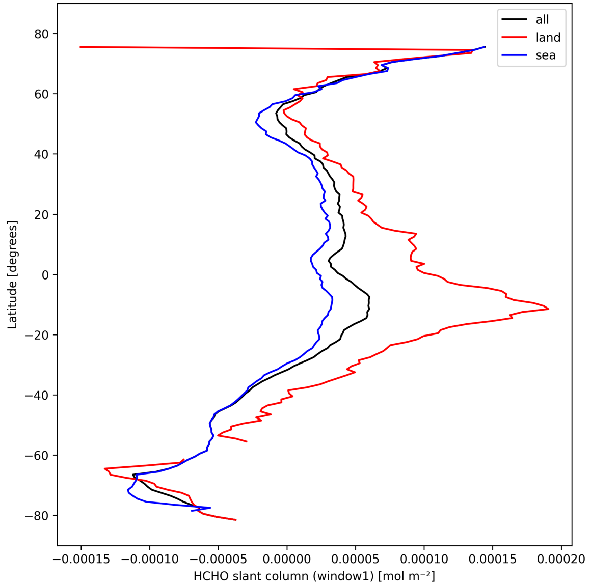
Figure 24: Zonal average of “HCHO slant column (window1)” for 2024-10-16 to 2024-10-18.
