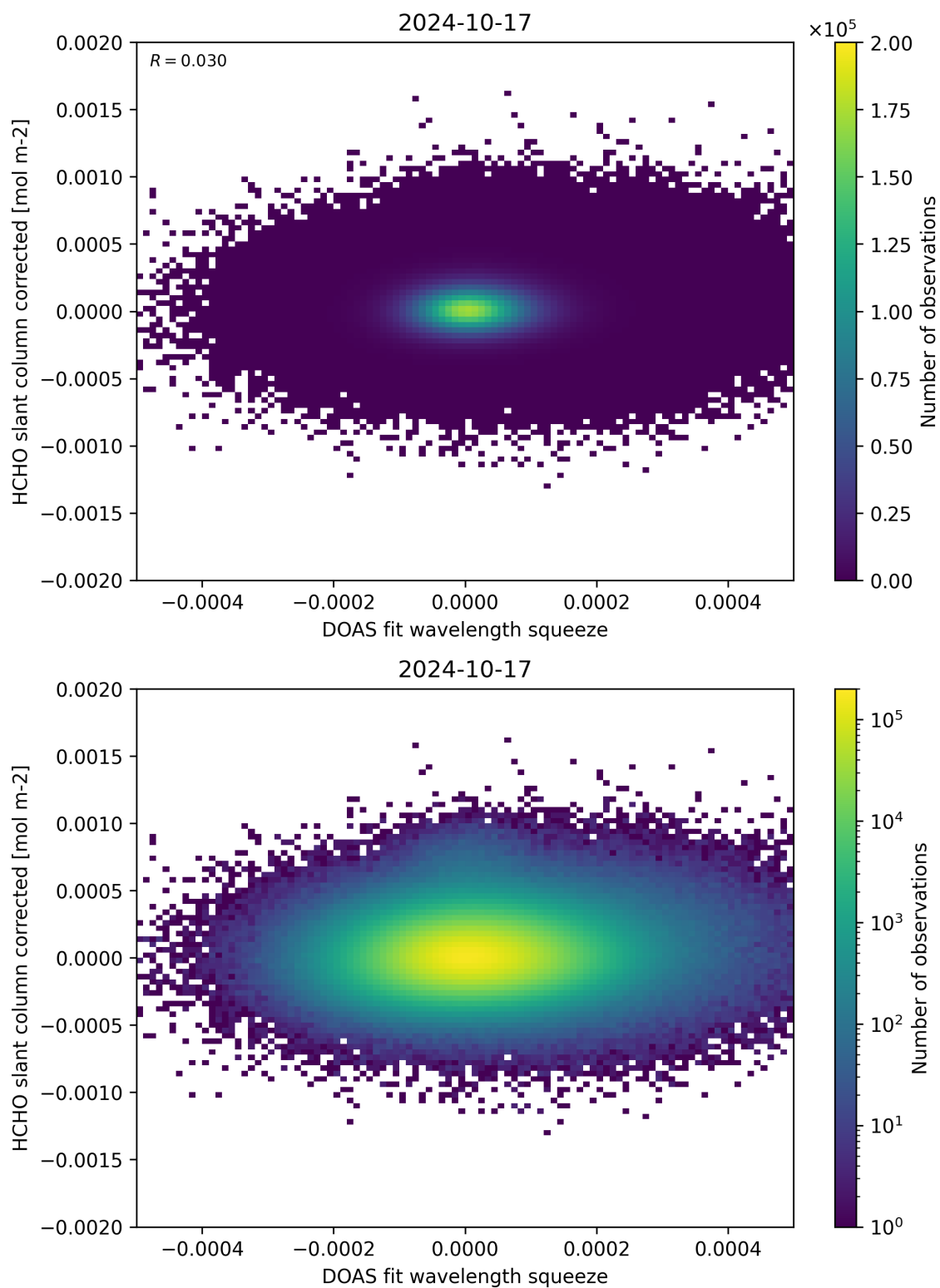
Figure 69: Scatter density plot of “DOAS fit wavelength squeeze” against “HCHO slant column corrected” for 2024-10-16 to 2024-10-18.
