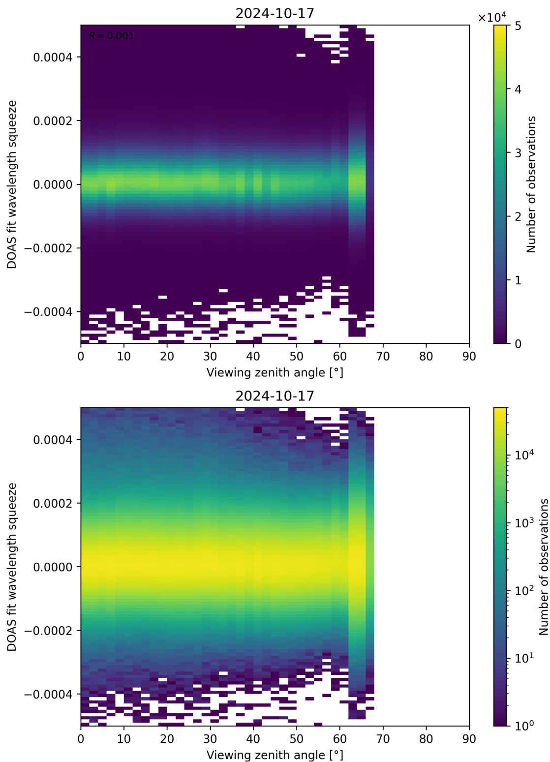
Figure 184: Scatter density plot of “Viewing zenith angle” against “DOAS fit wavelength squeeze” for 2024-10-16 to 2024-10-18.
