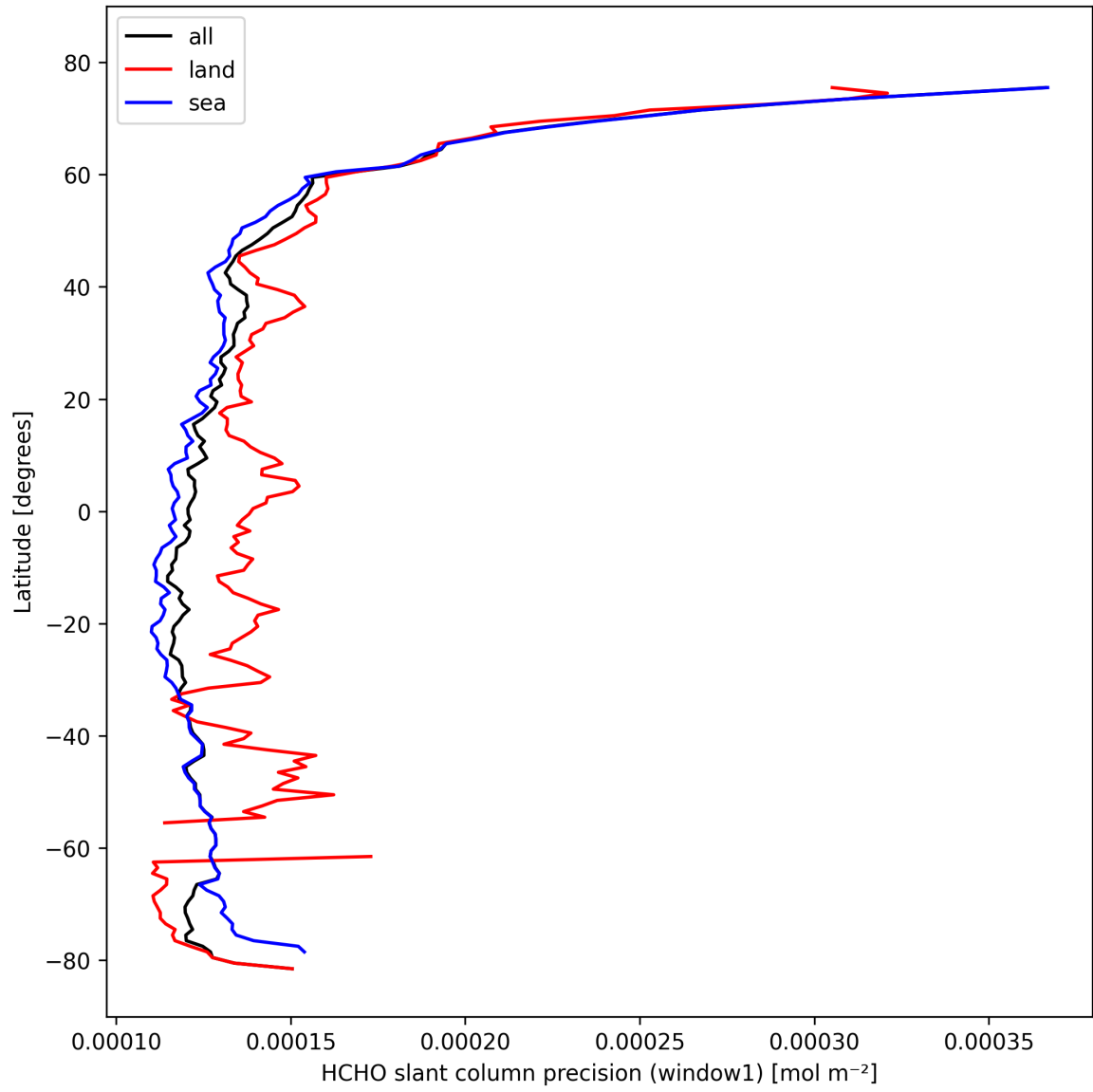
Figure 25: Zonal average of "HCHO slant column precision (window1)" for 2024-10-16 to 2024-10-18.
