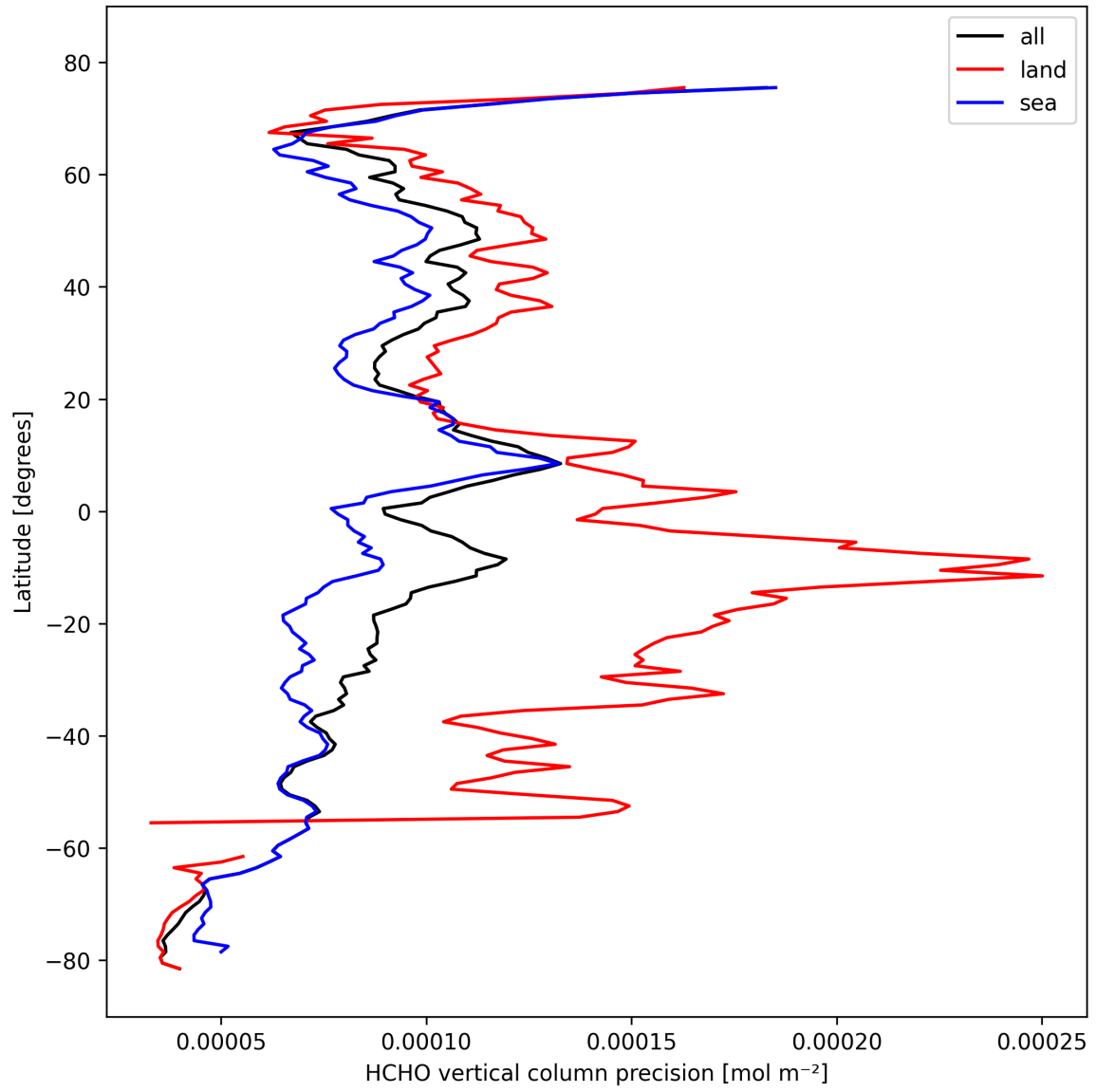
Figure 22: Zonal average of “HCHO vertical column precision” for 2024-10-16 to 2024-10-18.
