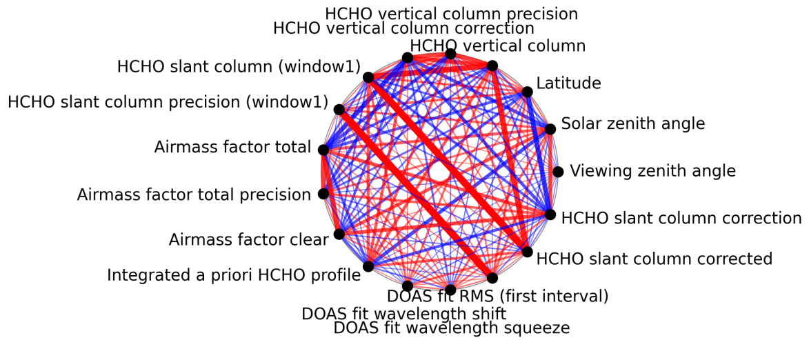
Figure 1: Map of correlation graph for 2024-10-16 to 2024-10-18.
