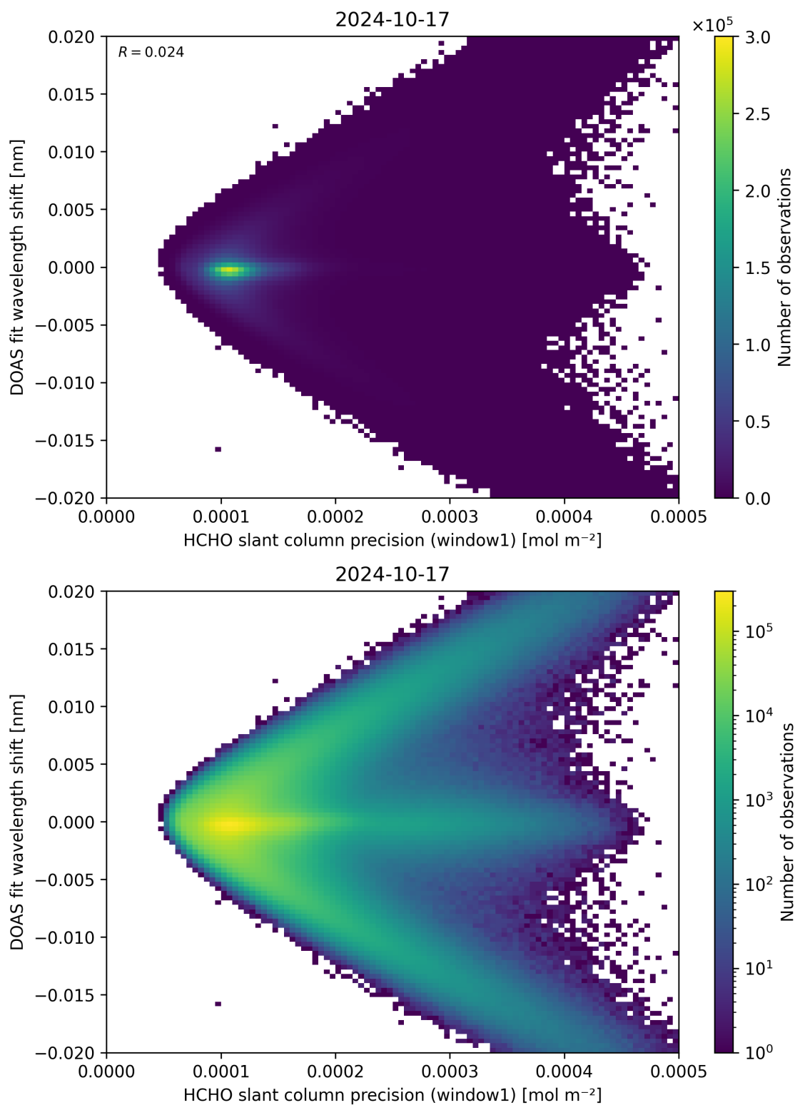
Figure 89: Scatter density plot of “HCHO slant column precision (window1)” against “DOAS fit wavelength shift” for 2024-10-16 to 2024-10-18.
