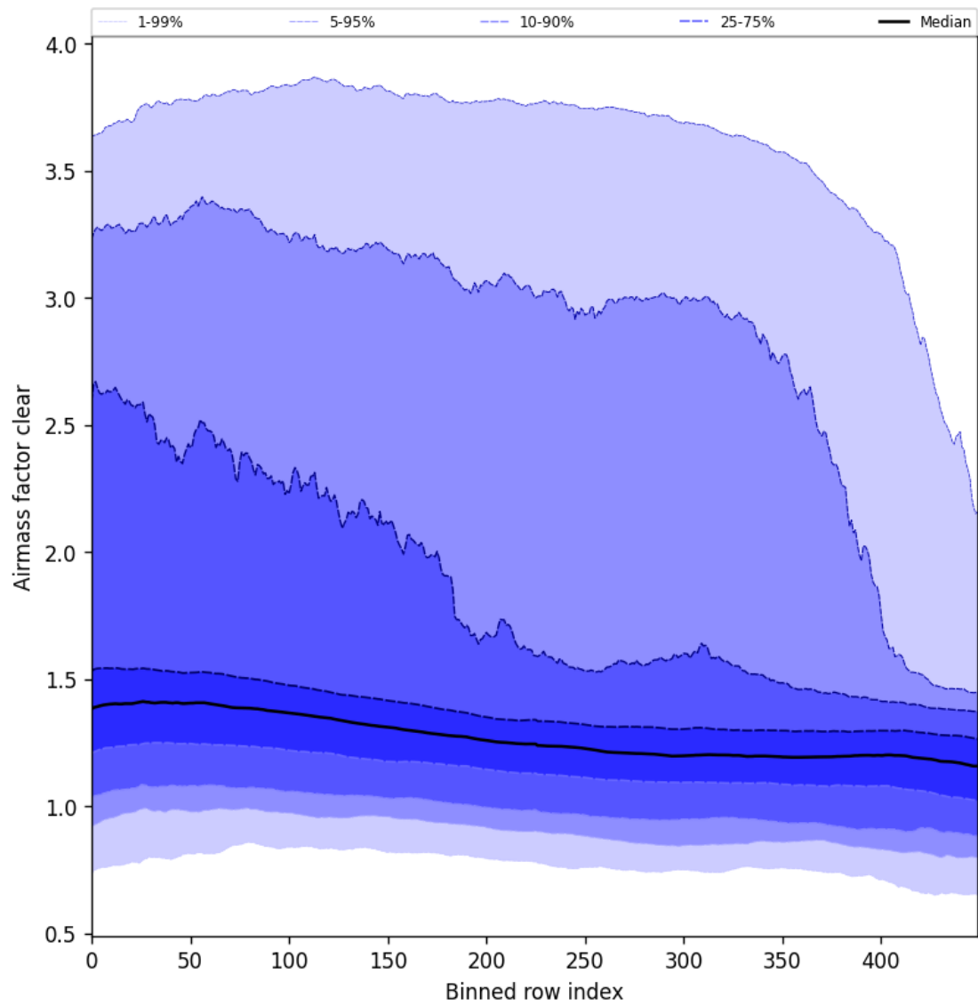
Figure 56: Along track statistics of “Airmass factor clear” for 2024-10-16 to 2024-10-18
