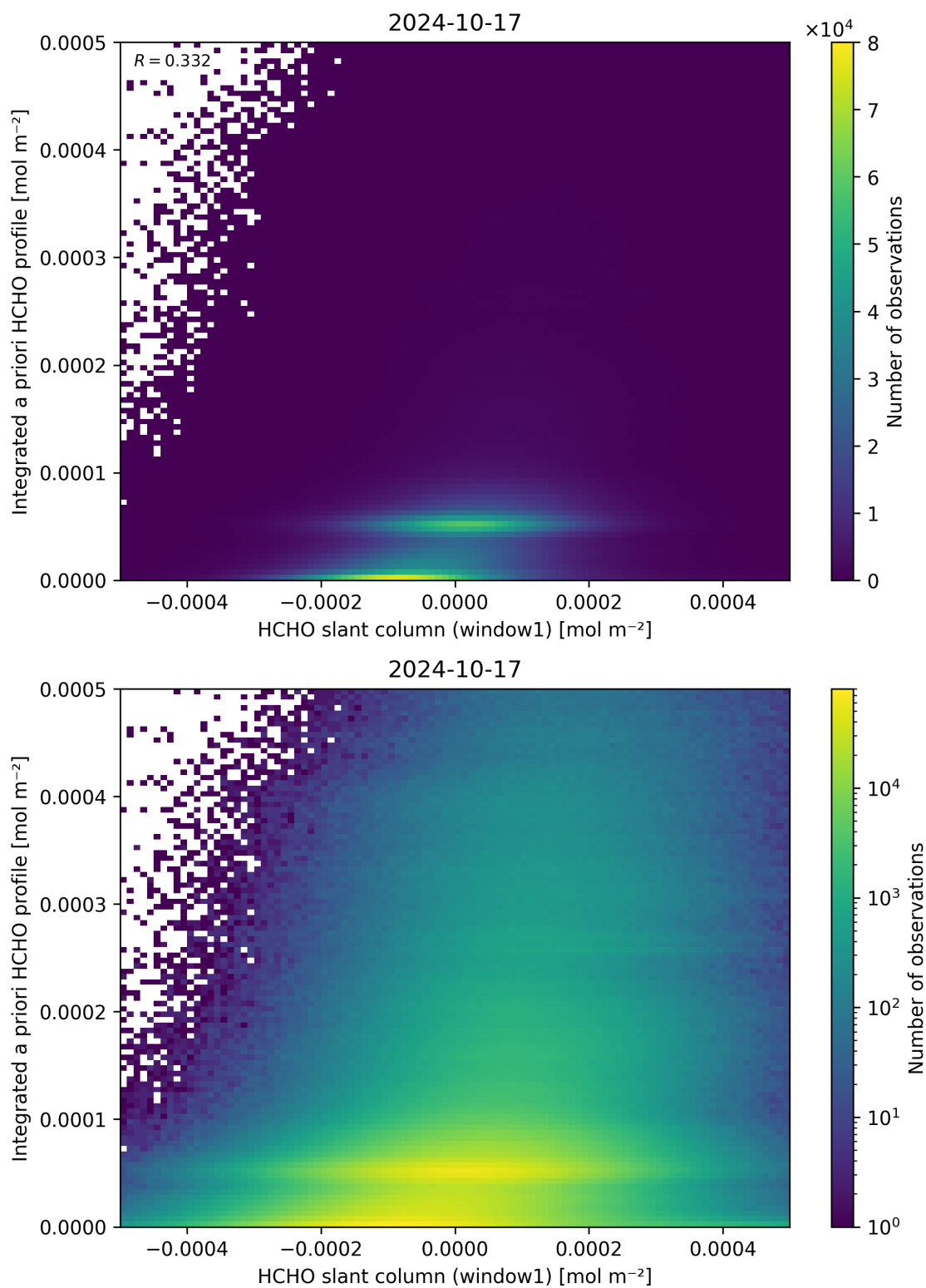
Figure 87: Scatter density plot of “HCHO slant column (window1)” against “Integrated a priori HCHO profile” for 2024-10-16 to 2024-10-18.
