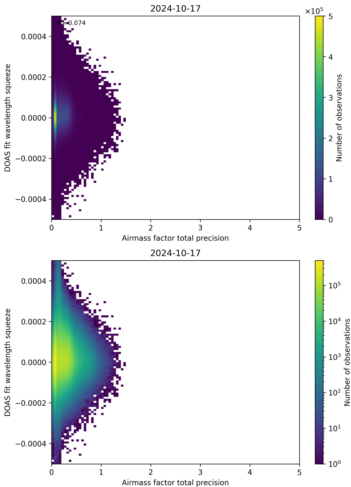
Figure 107: Scatter density plot of “Airmass factor total precision” against “DOAS fit wavelength squeeze” for 2024-10-16 to 2024-10-18.
