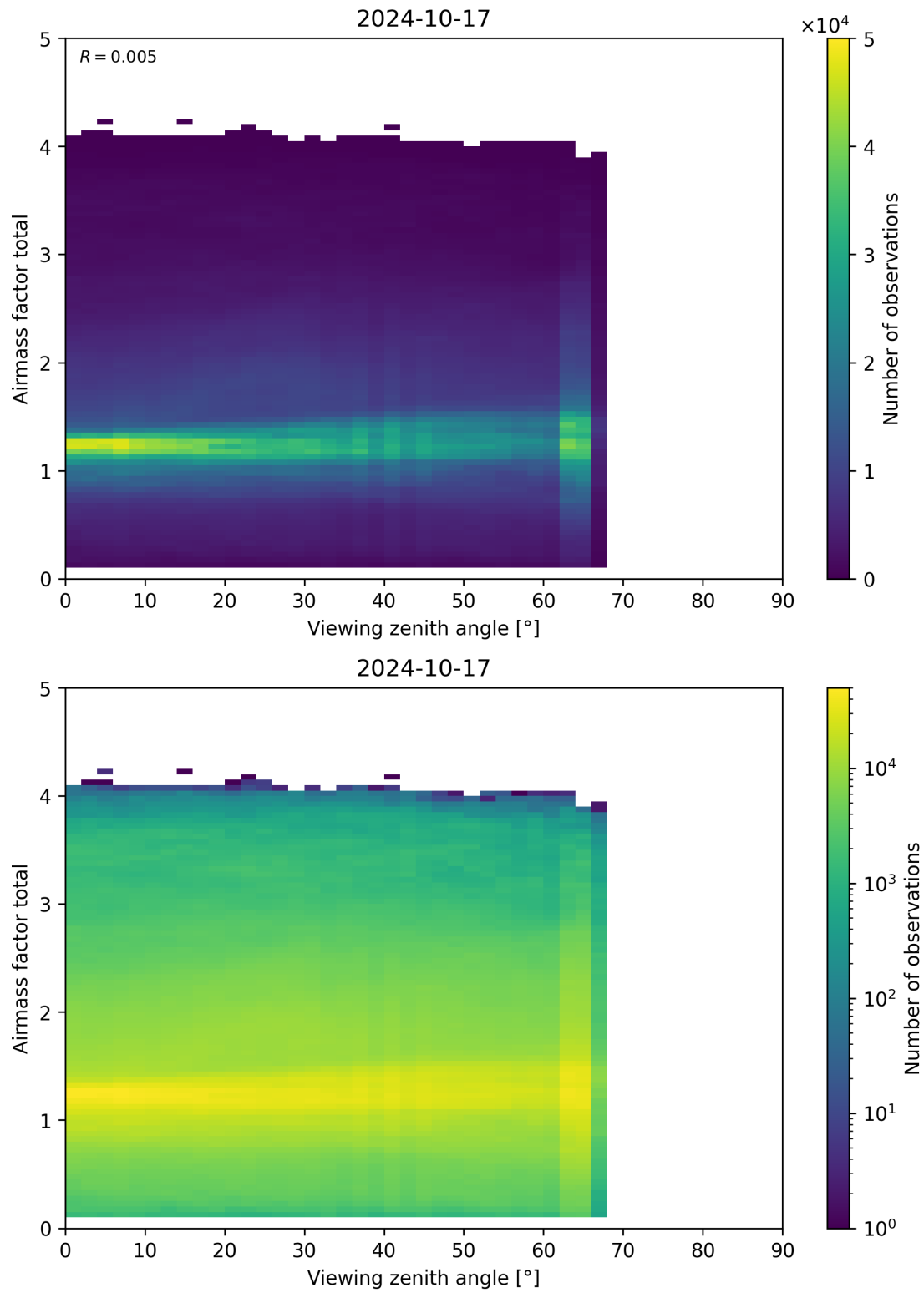
Figure 190: Scatter density plot of “Viewing zenith angle” against “Airmass factor total” for 2024-10-16 to 2024-10-18.
