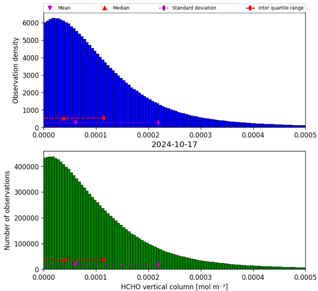
Figure 35: Histogram of “HCHO vertical column” for 2024-10-16 to 2024-10-18
