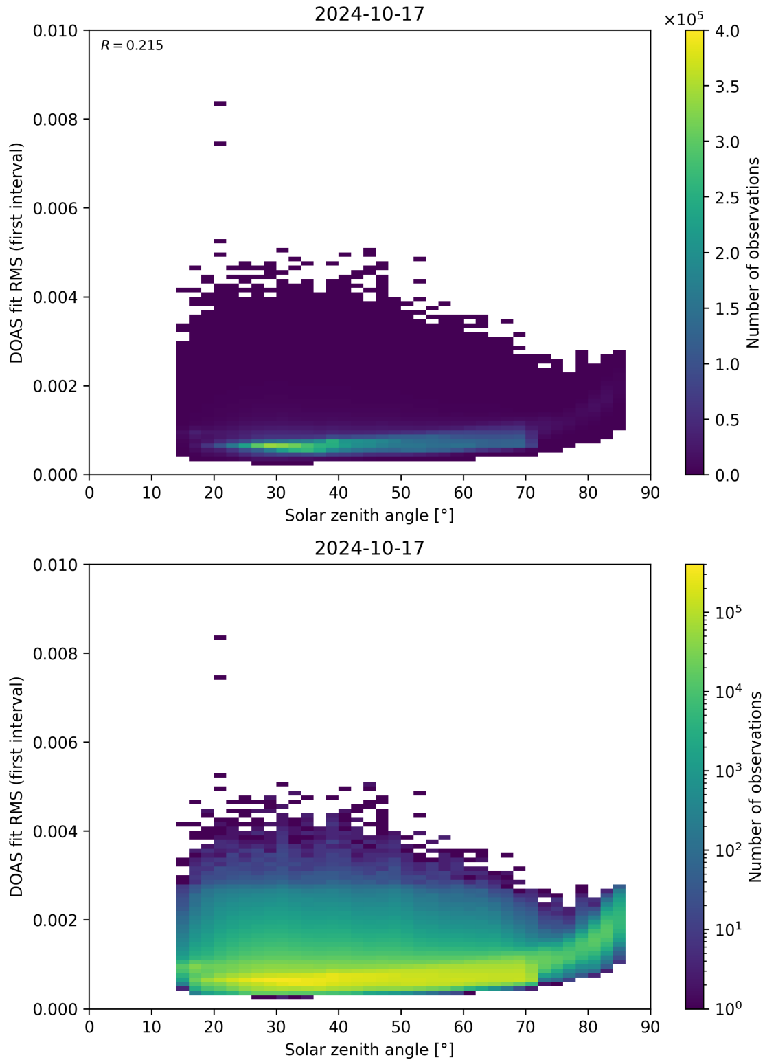
Figure 167: Scatter density plot of “Solar zenith angle” against “DOAS fit RMS (first interval)” for 2024-10-16 to 2024-10-18.
