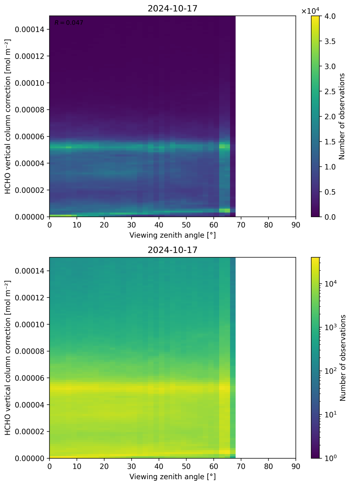
Figure 193: Scatter density plot of “Viewing zenith angle” against “HCHO vertical column correction” for 2024-10-16 to 2024-10-18.
