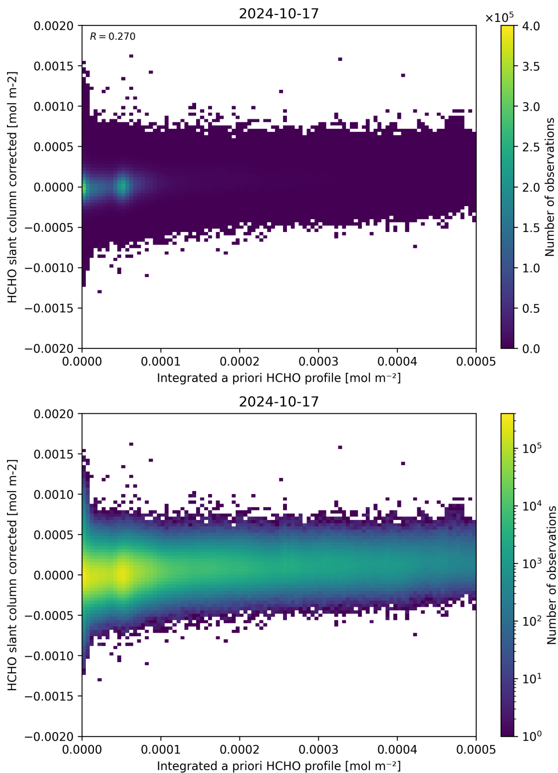
Figure 151: Scatter density plot of “Integrated a priori HCHO profile” against “HCHO slant column corrected” for 2024-10-16 to 2024-10-18.
