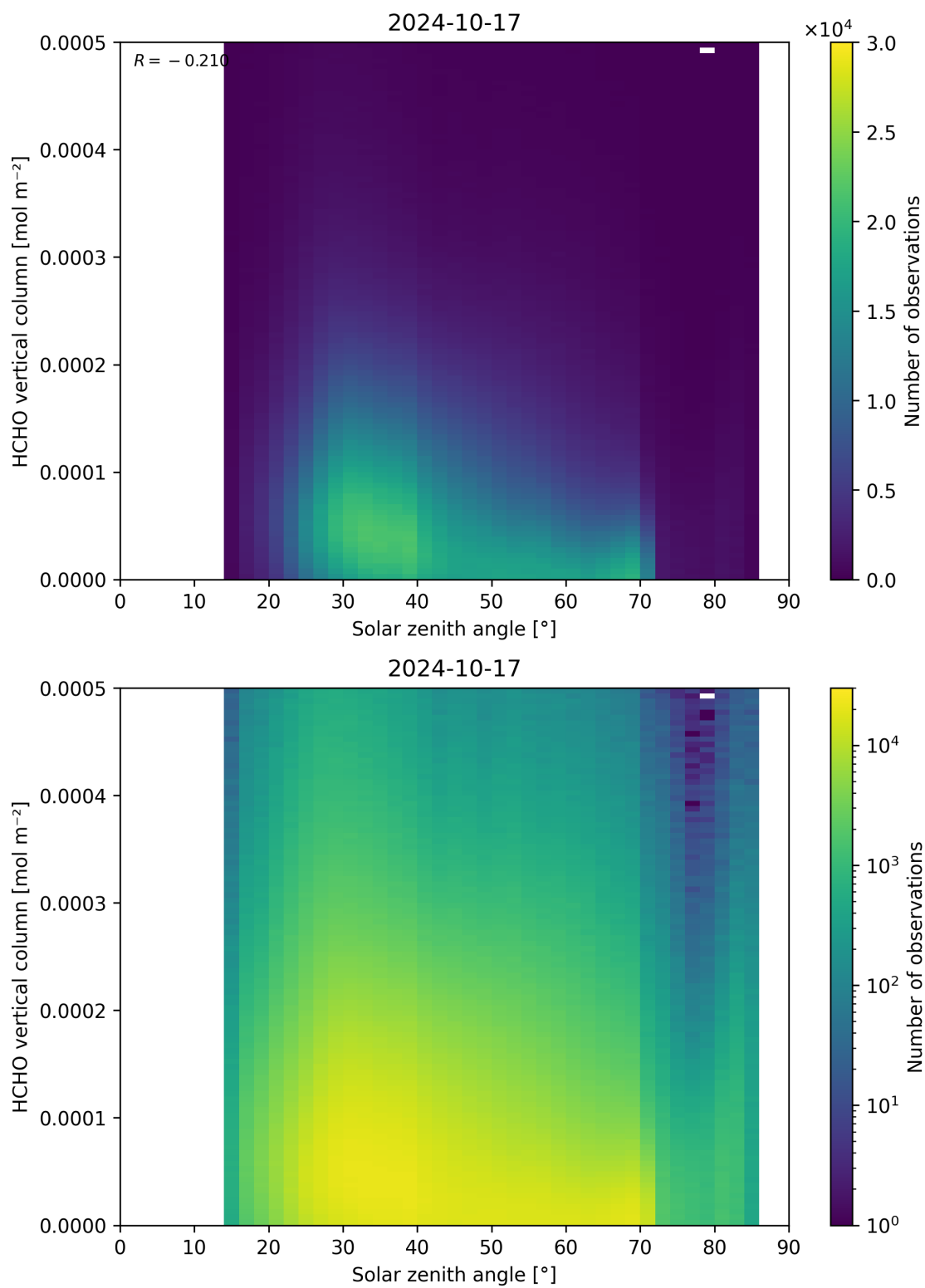
Figure 177: Scatter density plot of “Solar zenith angle” against “HCHO vertical column” for 2024-10-16 to 2024-10-18.
