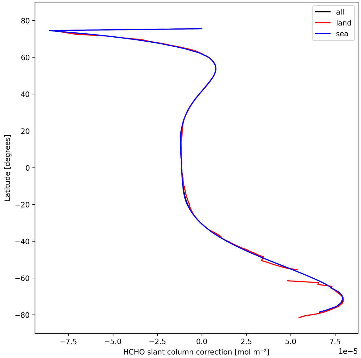
Figure 33: Zonal average of “HCHO slant column correction” for 2024-10-16 to 2024-10-18.
