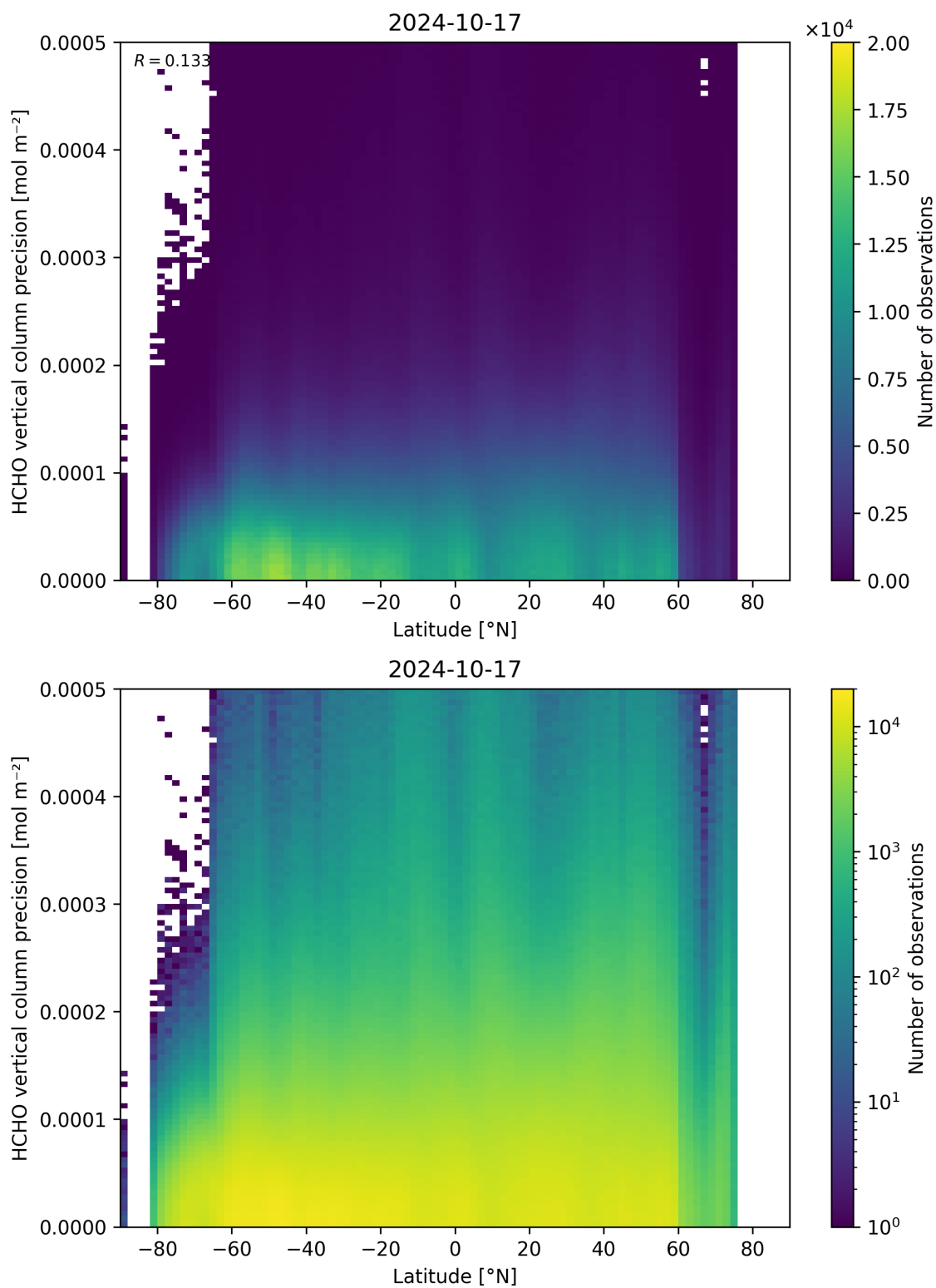
Figure 165: Scatter density plot of “Latitude” against “HCHO vertical column precision” for 2024-10-16 to 2024-10-18.
