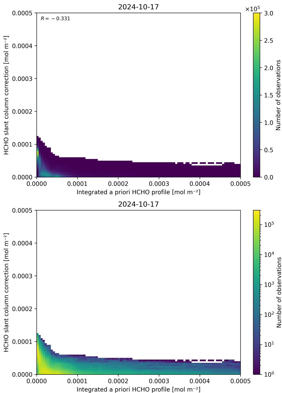
Figure 152: Scatter density plot of “Integrated a priori HCHO profile” against “HCHO slant column correction” for 2024-10-16 to 2024-10-18.
