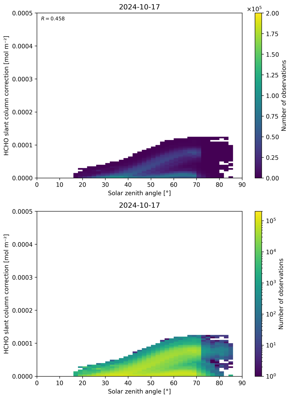
Figure 172: Scatter density plot of “Solar zenith angle” against “HCHO slant column correction” for 2024-10-16 to 2024-10-18.
