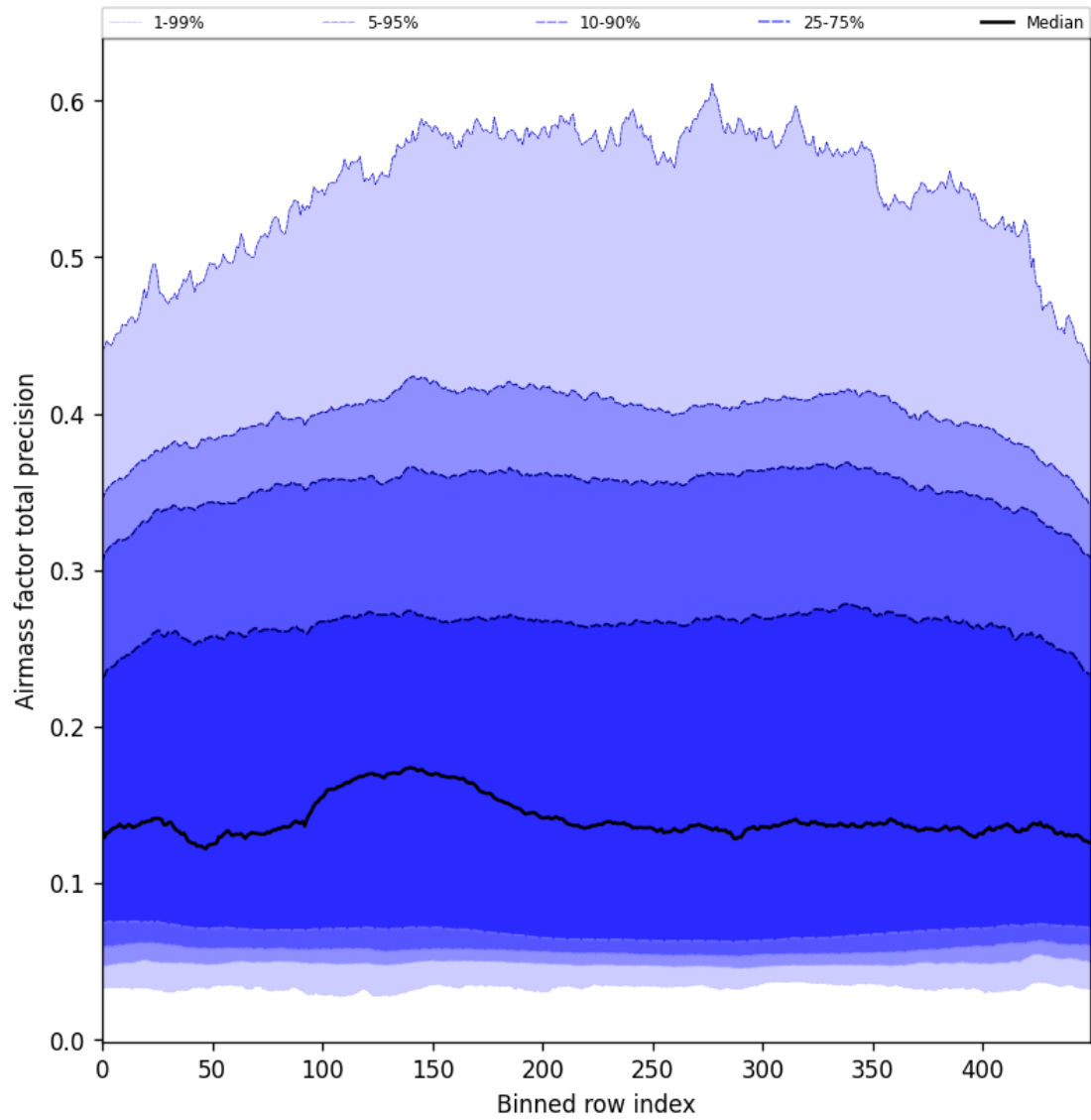
Figure 55: Along track statistics of “Airmass factor total precision” for 2024-10-16 to 2024-10-18
