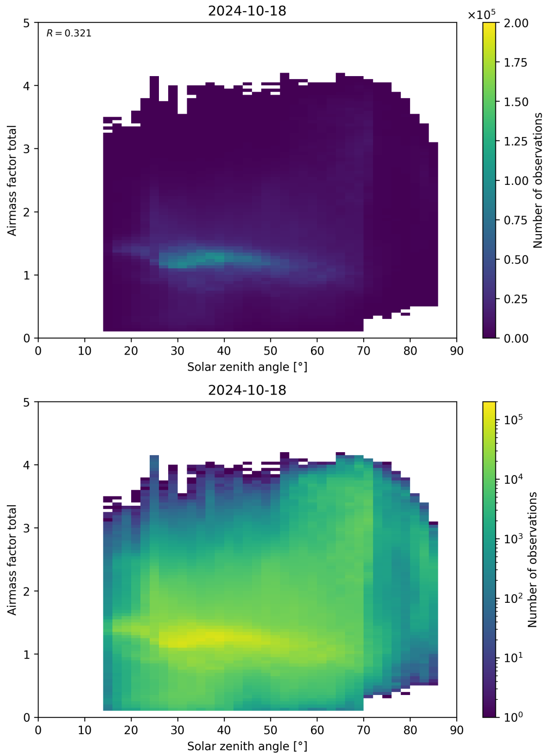
Figure 175: Scatter density plot of “Solar zenith angle” against “Airmass factor total” for 2024-10-17 to 2024-10-19.
