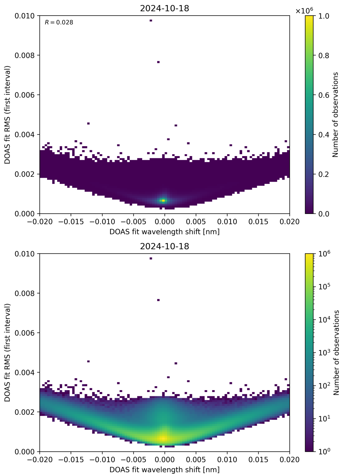
Figure 64: Scatter density plot of “DOAS fit wavelength shift” against “DOAS fit RMS (first interval)” for 2024-10-17 to 2024-10-19.
