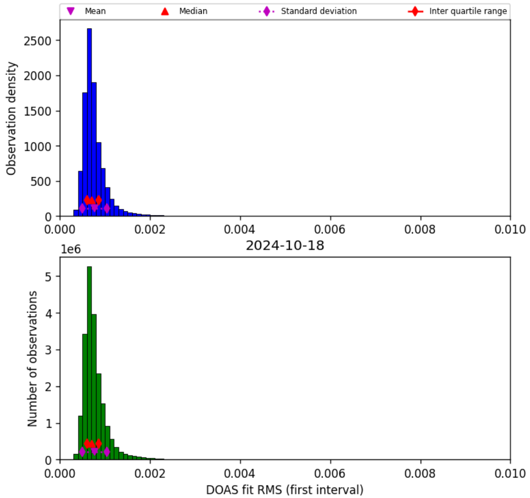
Figure 46: Histogram of “DOAS fit RMS (first interval)” for 2024-10-17 to 2024-10-19
