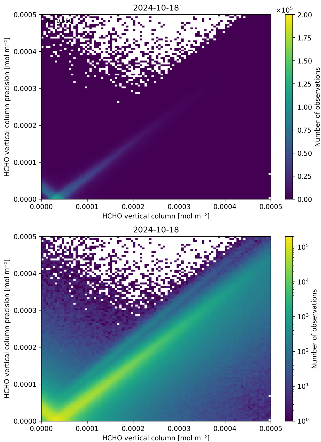
Figure 134: Scatter density plot of “HCHO vertical column” against “HCHO vertical column precision” for 2024-10-17 to 2024-10-19.
