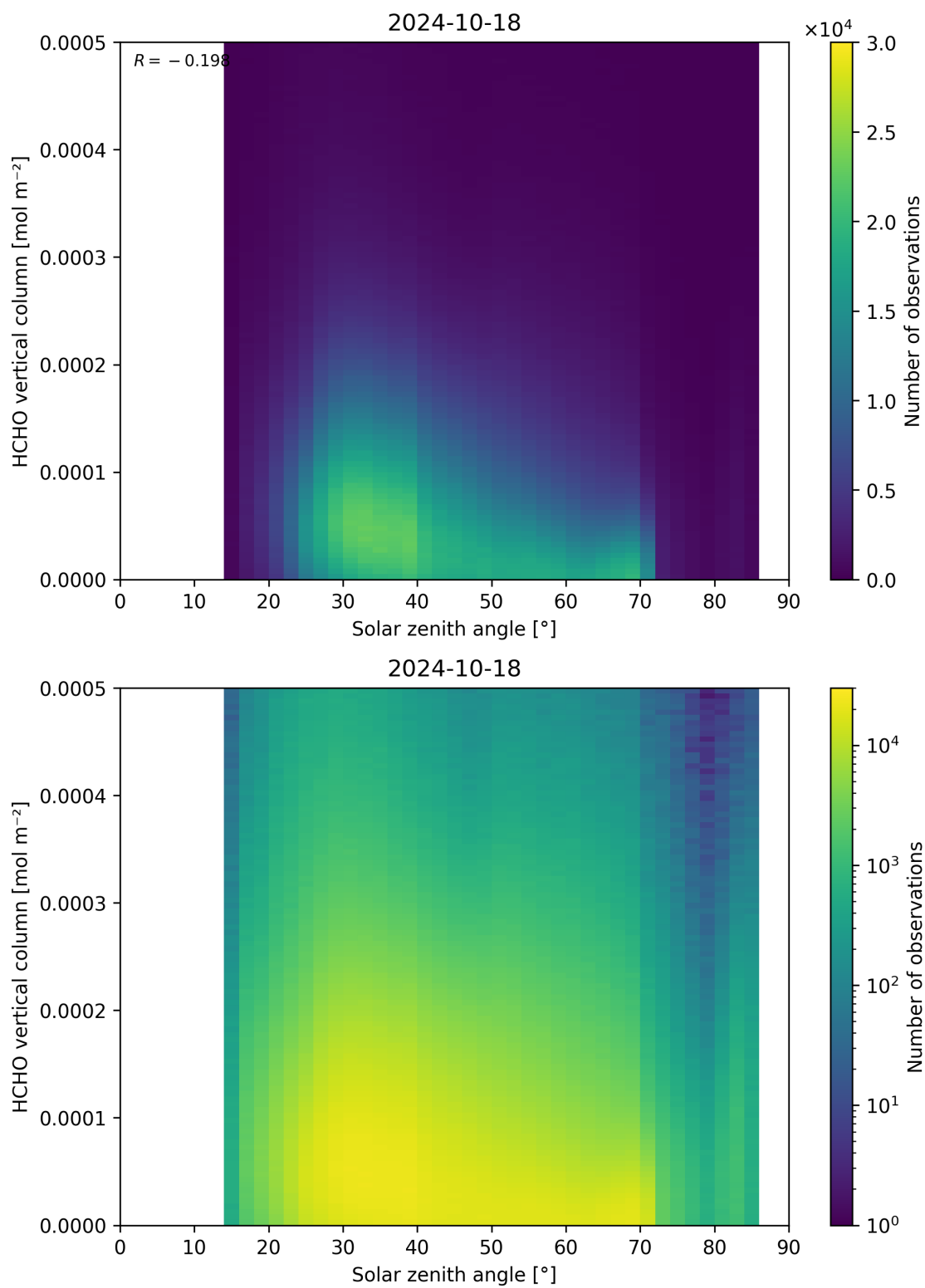
Figure 177: Scatter density plot of “Solar zenith angle” against “HCHO vertical column” for 2024-10-17 to 2024-10-19.
