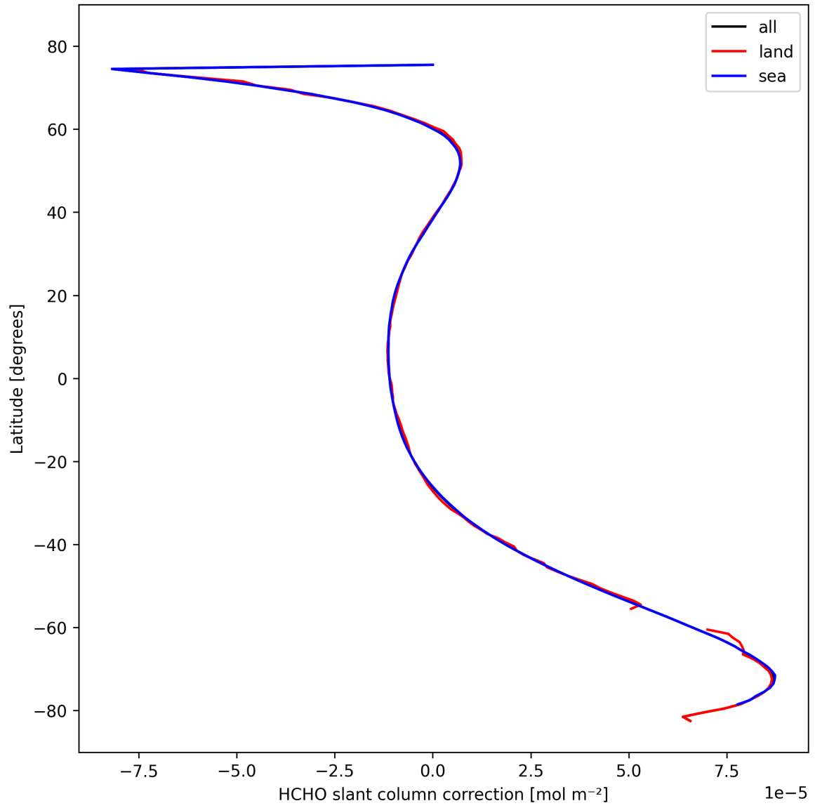
Figure 33: Zonal average of “HCHO slant column correction” for 2024-10-17 to 2024-10-19.
