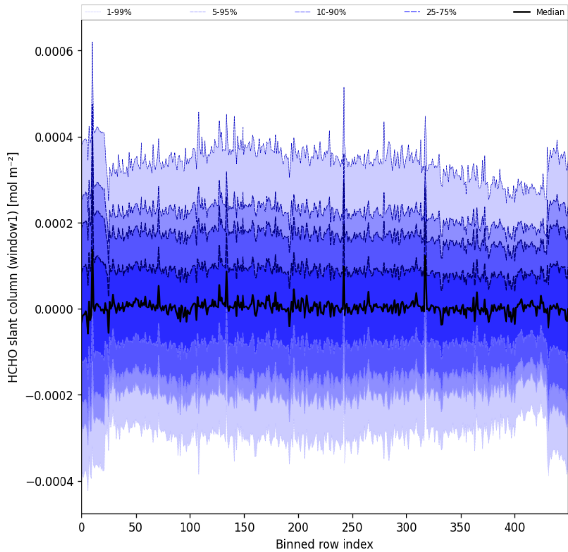
Figure 52: Along track statistics of “HCHO slant column (window1)” for 2024-10-17 to 2024-10-19
