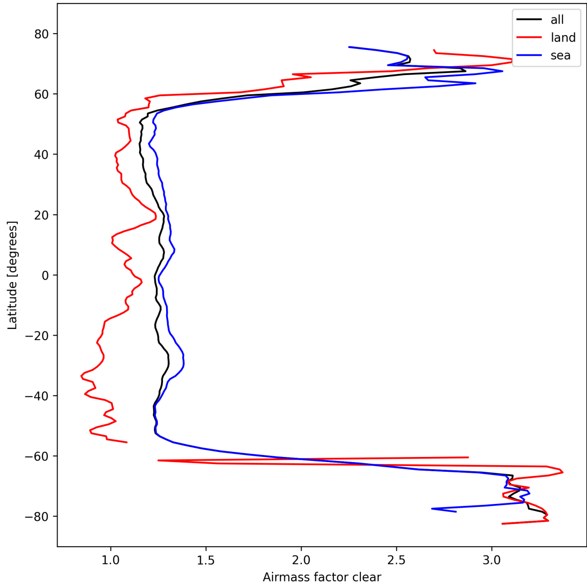
Figure 28: Zonal average of “Airmass factor clear” for 2024-10-17 to 2024-10-19.
