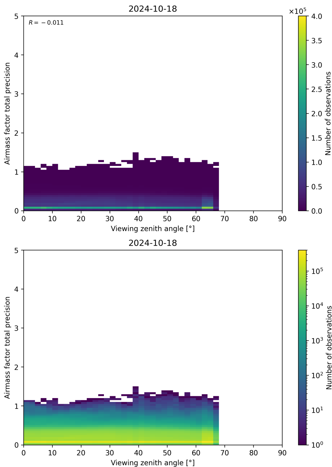
Figure 191: Scatter density plot of “Viewing zenith angle” against “Airmass factor total precision” for 2024-10-17 to 2024-10-19.
