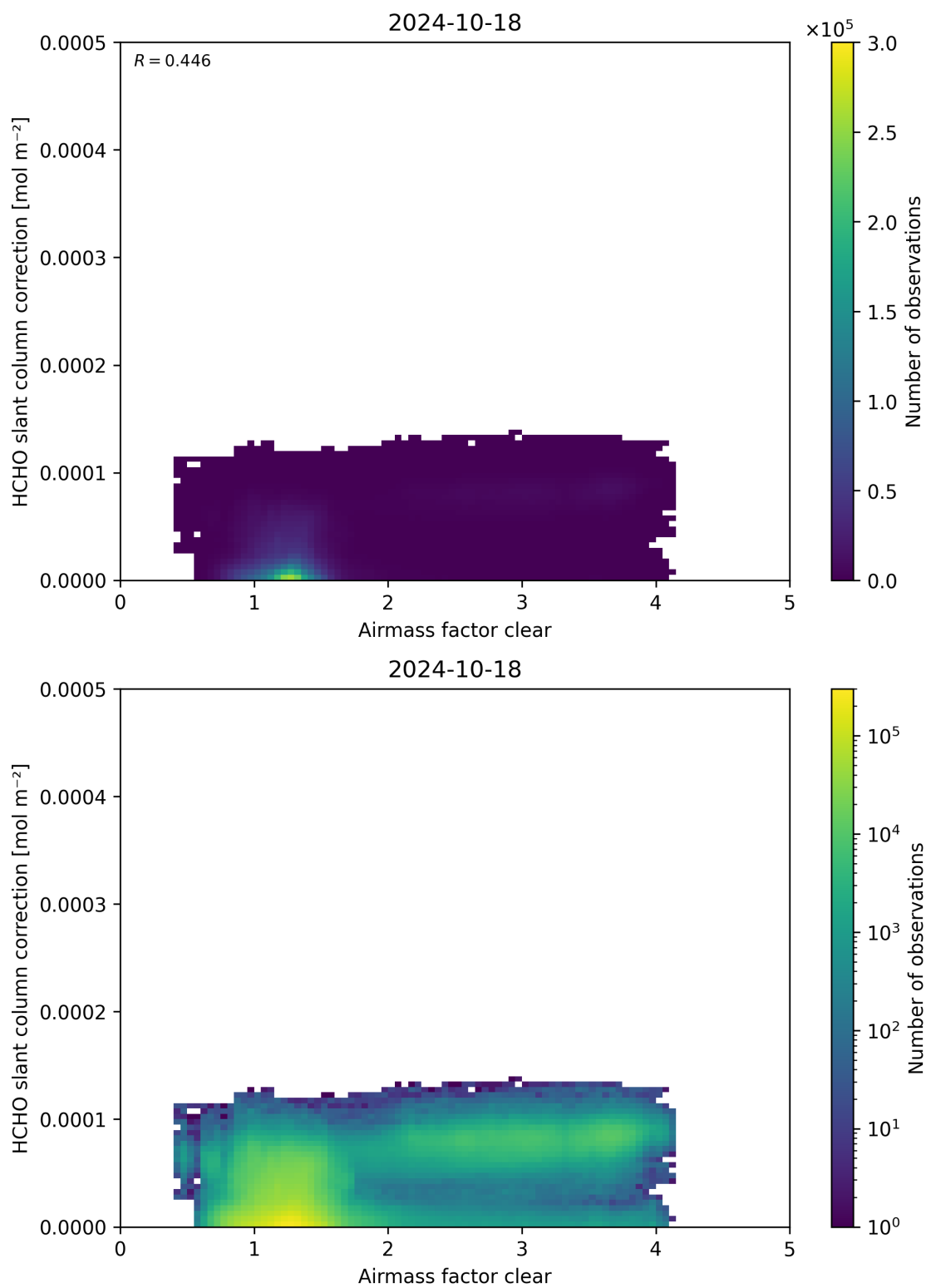
Figure 75: Scatter density plot of “Airmass factor clear” against “HCHO slant column correction” for 2024-10-17 to 2024-10-19.
