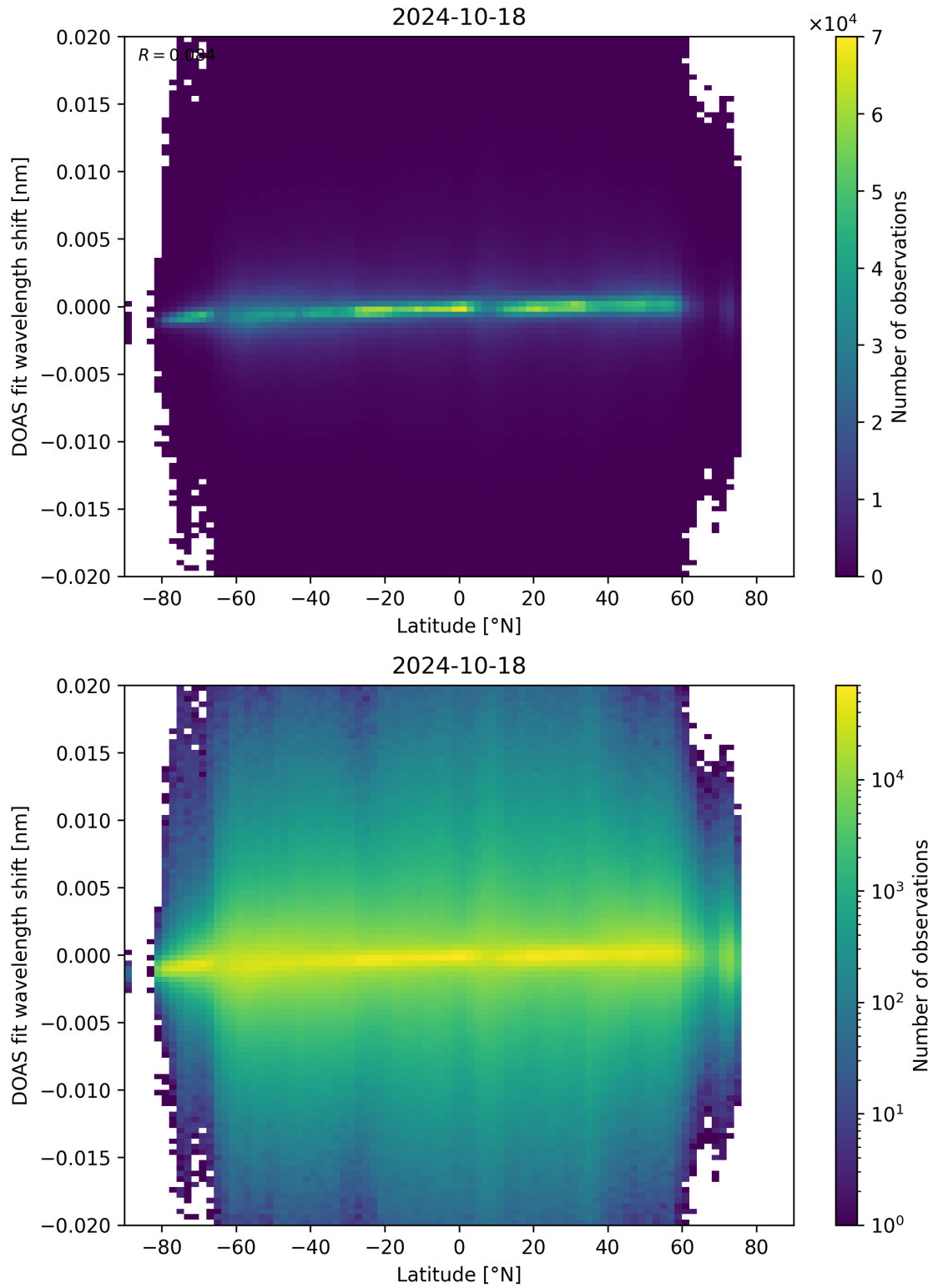
Figure 154: Scatter density plot of “Latitude” against “DOAS fit wavelength shift” for 2024-10-17 to 2024-10-19.
