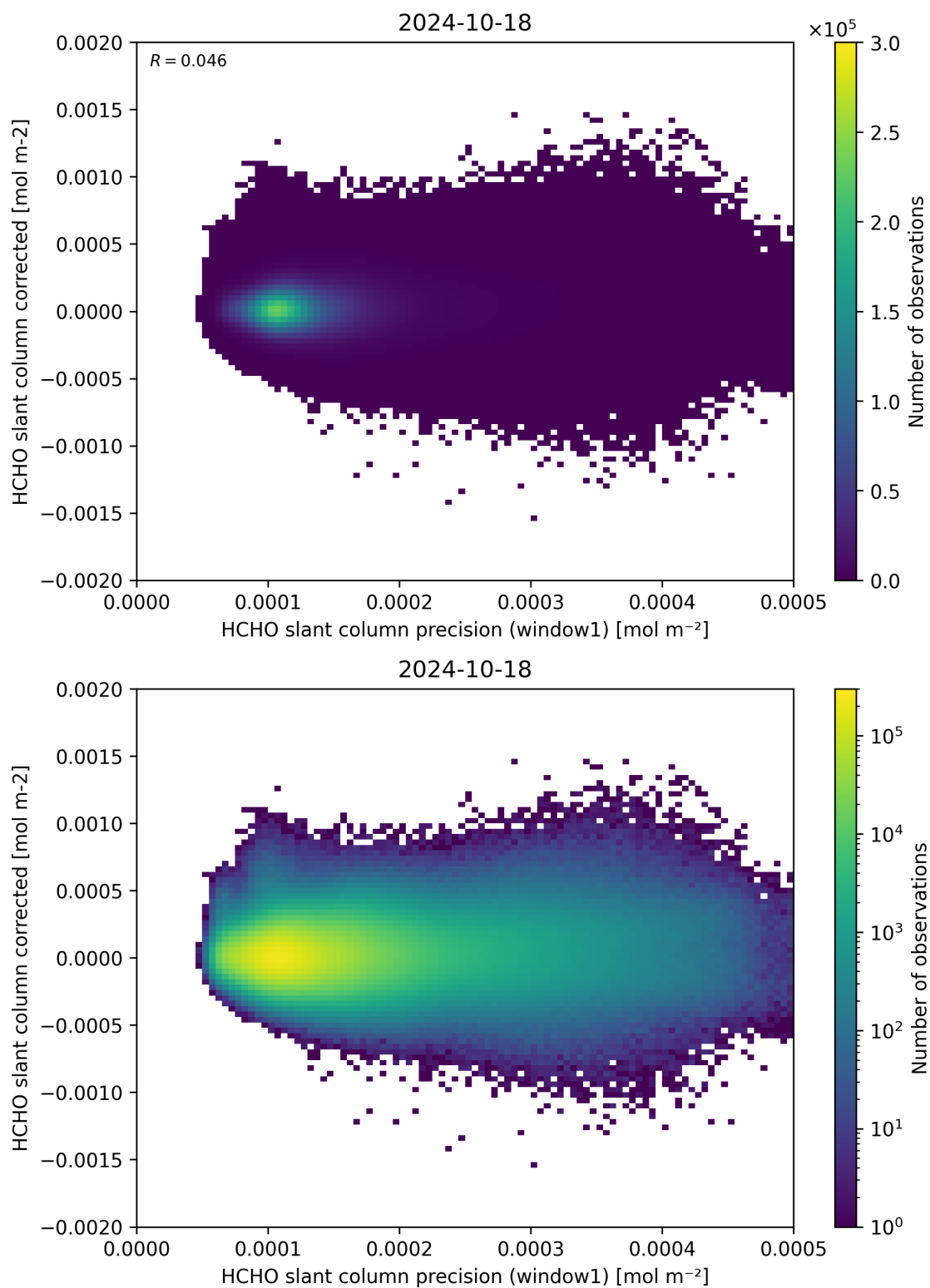
Figure 92: Scatter density plot of “HCHO slant column precision (window1)” against “HCHO slant column corrected” for 2024-10-17 to 2024-10-19.
