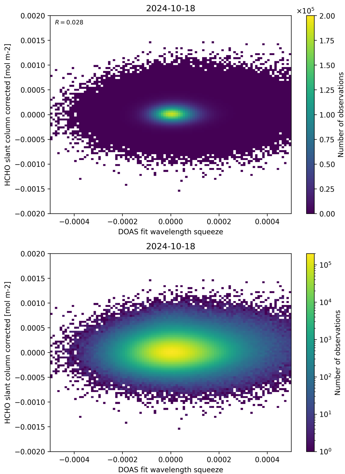
Figure 69: Scatter density plot of “DOAS fit wavelength squeeze” against “HCHO slant column corrected” for 2024-10-17 to 2024-10-19.
