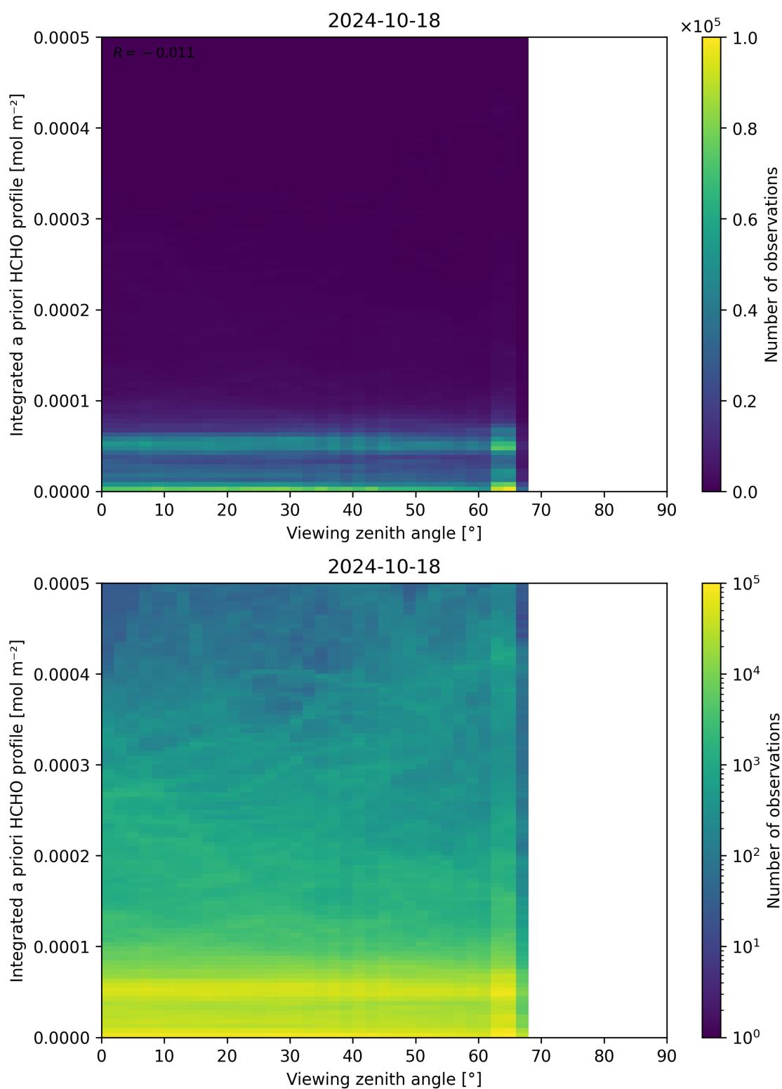
Figure 195: Scatter density plot of “Viewing zenith angle” against “Integrated a priori HCHO profile” for 2024-10-17 to 2024-10-19.
