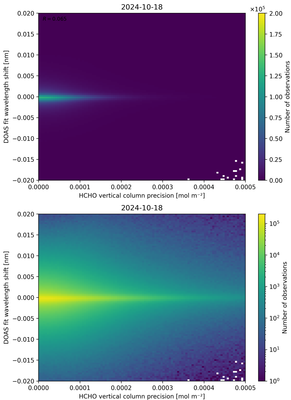
Figure 137: Scatter density plot of “HCHO vertical column precision” against “DOAS fit wavelength shift” for 2024-10-17 to 2024-10-19.
