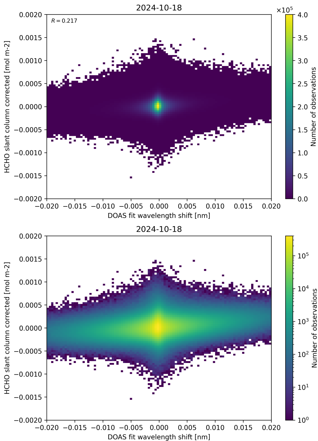
Figure 66: Scatter density plot of “DOAS fit wavelength shift” against “HCHO slant column corrected” for 2024-10-17 to 2024-10-19.
