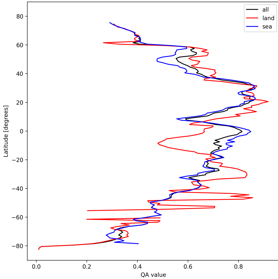
Figure 20: Zonal average of “QA value” for 2024-10-17 to 2024-10-19.
