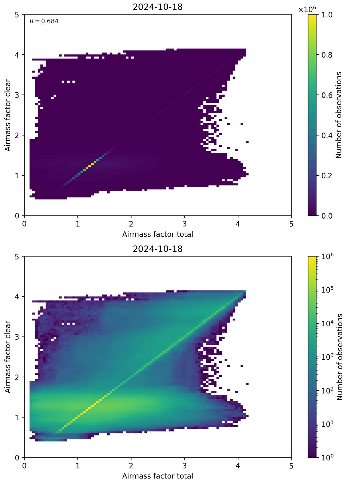
Figure 100: Scatter density plot of “Airmass factor total” against “Airmass factor clear” for 2024-10-17 to 2024-10-19.
