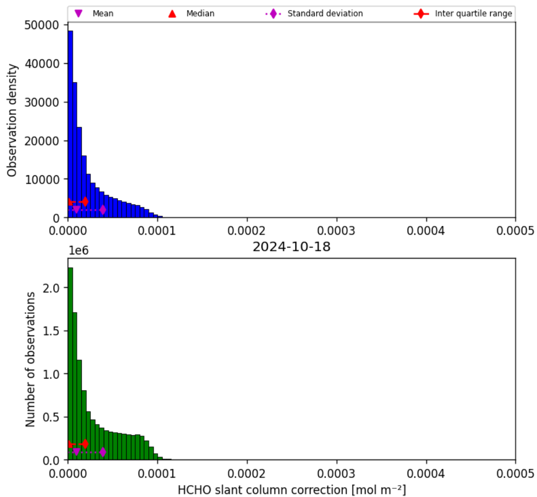
Figure 47: Histogram of “HCHO slant column correction” for 2024-10-17 to 2024-10-19
