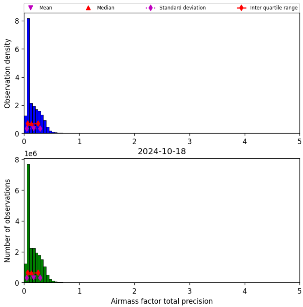
Figure 41: Histogram of “Airmass factor total precision” for 2024-10-17 to 2024-10-19
