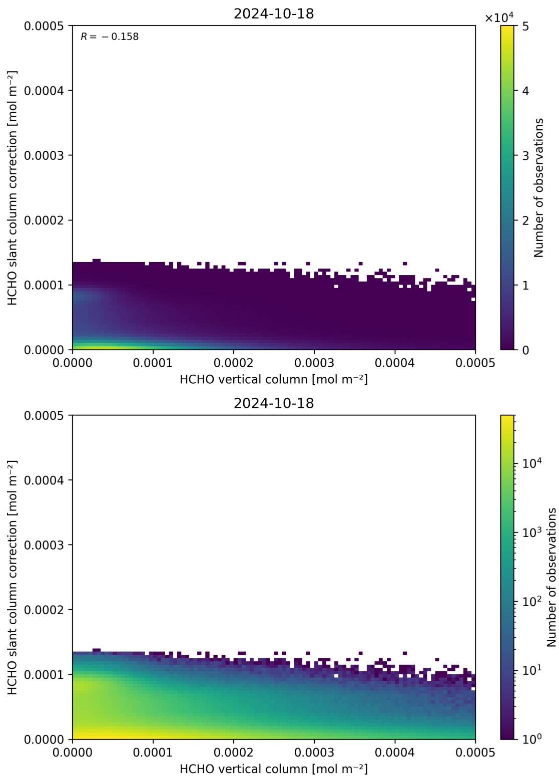
Figure 128: Scatter density plot of “HCHO vertical column” against “HCHO slant column correction” for 2024-10-17 to 2024-10-19.
