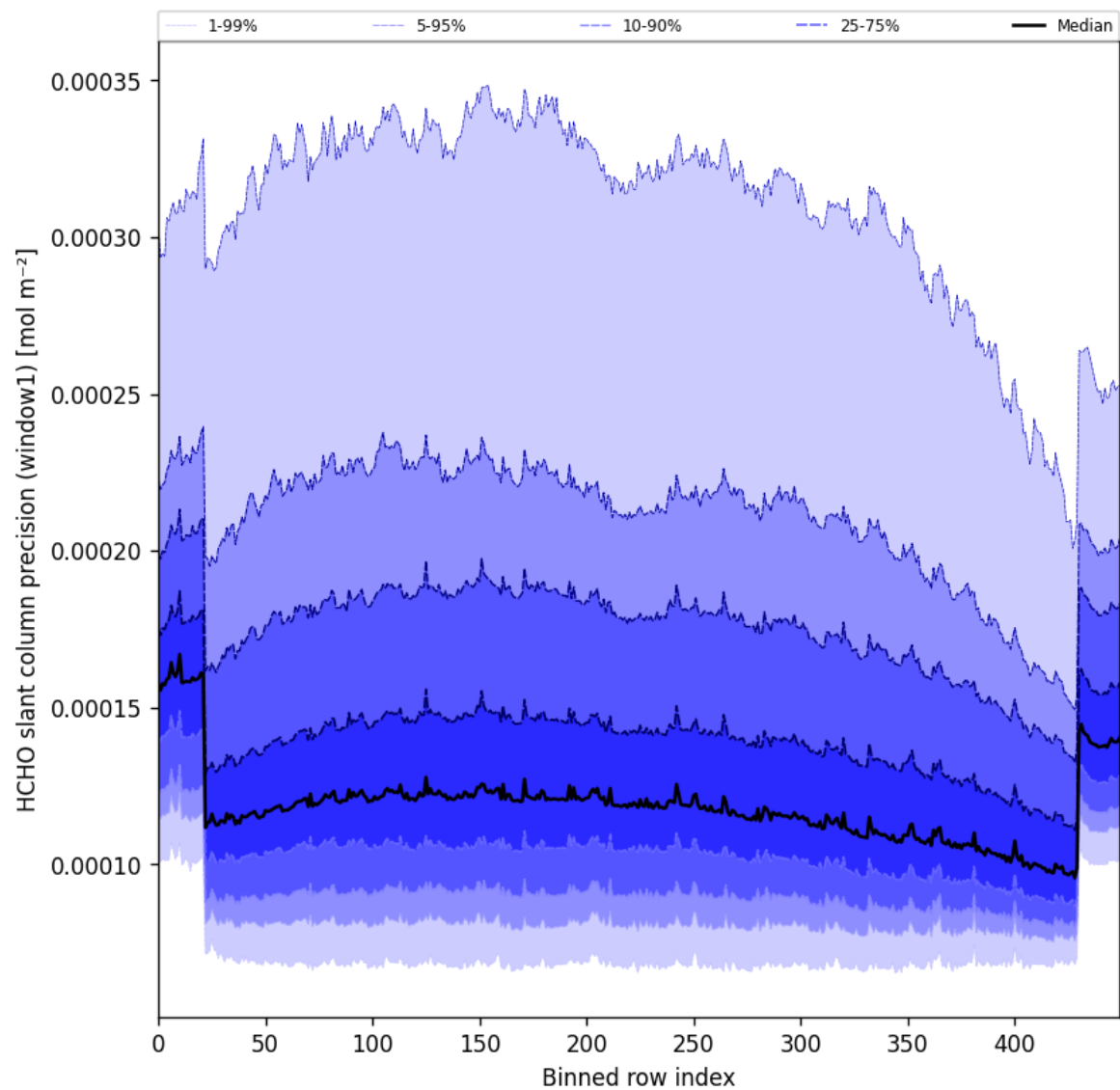
Figure 53: Along track statistics of “HCHO slant column precision (window1)” for 2024-10-17 to 2024-10-19
