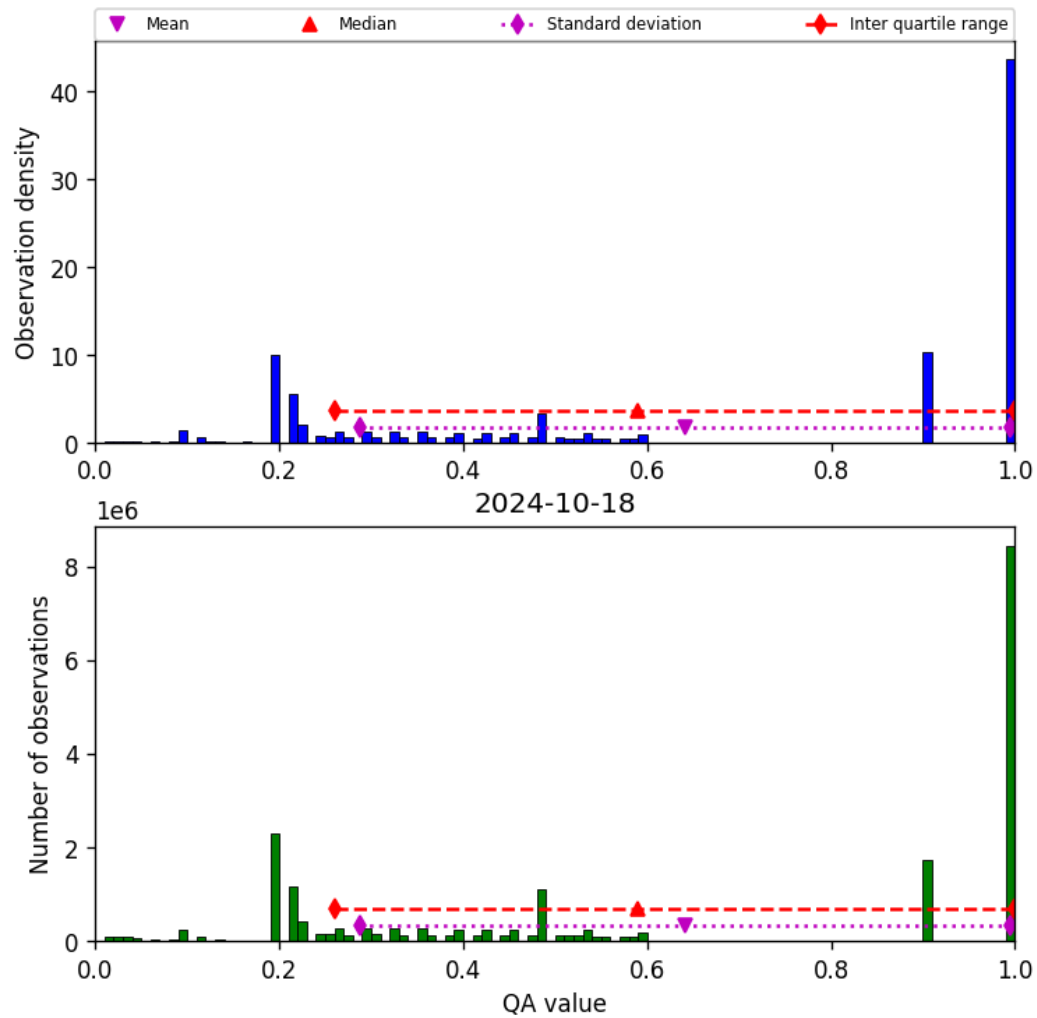
Figure 34: Histogram of “QA value” for 2024-10-17 to 2024-10-19
