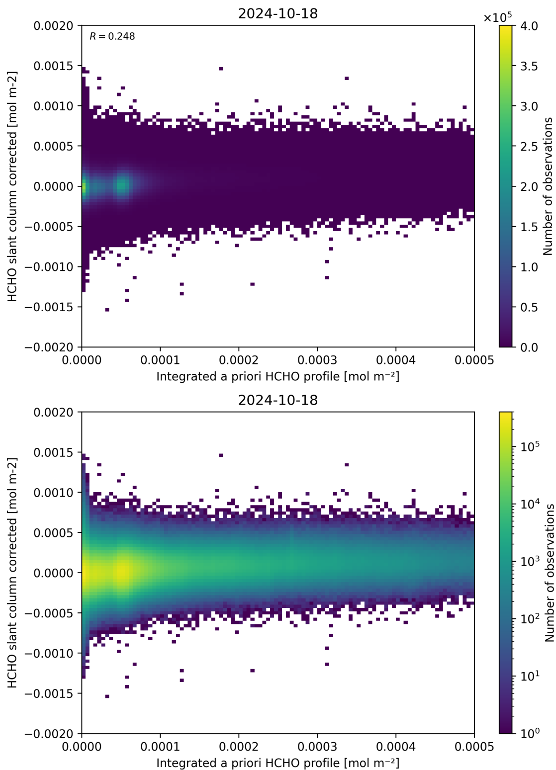
Figure 151: Scatter density plot of “Integrated a priori HCHO profile” against “HCHO slant column corrected” for 2024-10-17 to 2024-10-19.
