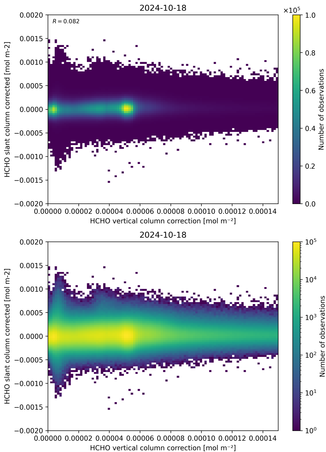
Figure 116: Scatter density plot of “HCHO vertical column correction” against “HCHO slant column corrected” for 2024-10-17 to 2024-10-19.
