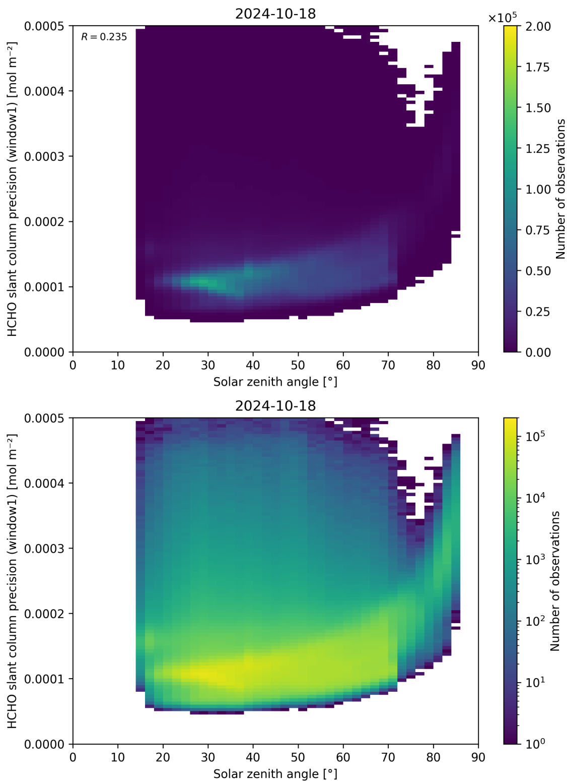
Figure 174: Scatter density plot of “Solar zenith angle” against “HCHO slant column precision (window1)” for 2024-10-17 to 2024-10-19.
