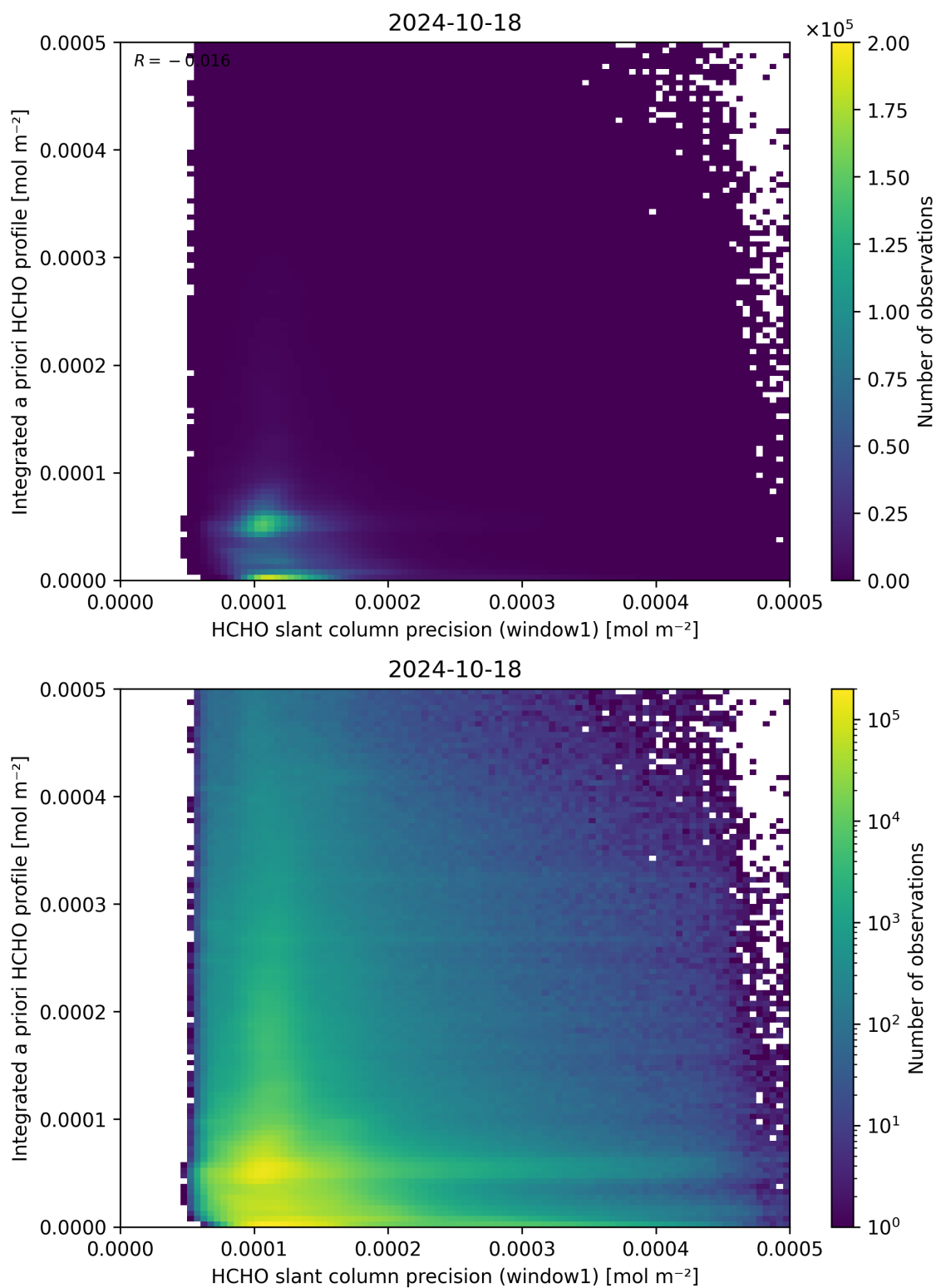
Figure 96: Scatter density plot of “HCHO slant column precision (window1)” against “Integrated a priori HCHO profile” for 2024-10-17 to 2024-10-19.
