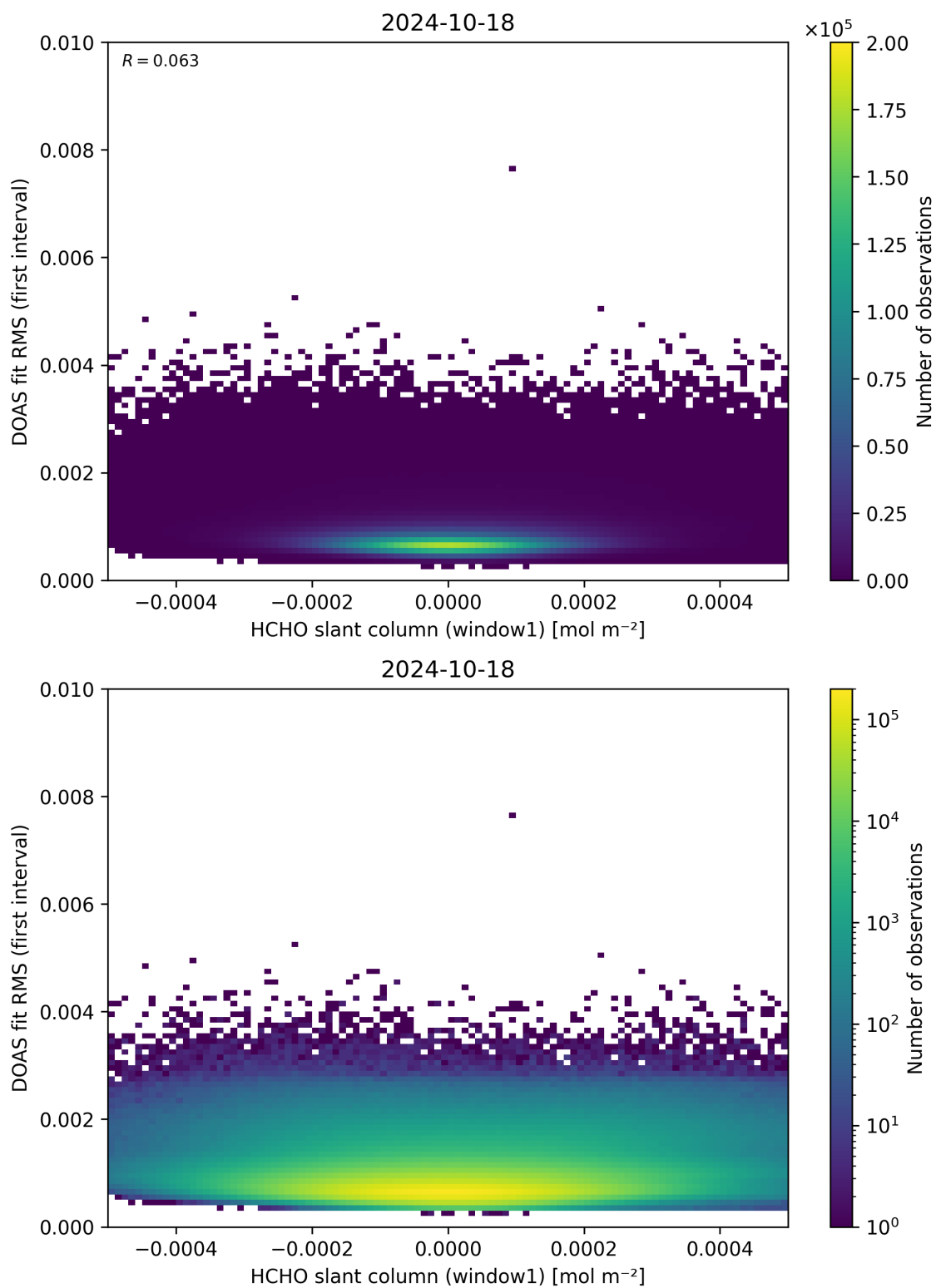
Figure 78: Scatter density plot of “HCHO slant column (window1)” against “DOAS fit RMS (first interval)” for 2024-10-17 to 2024-10-19.
