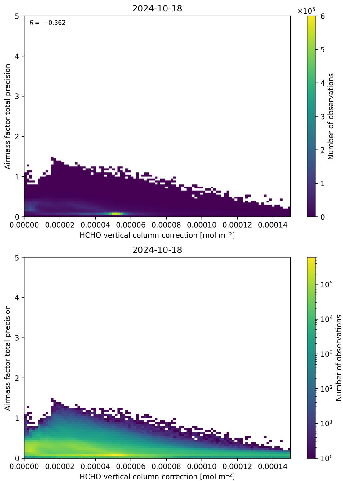
Figure 121: Scatter density plot of “HCHO vertical column correction” against “Airmass factor total precision” for 2024-10-17 to 2024-10-19.
