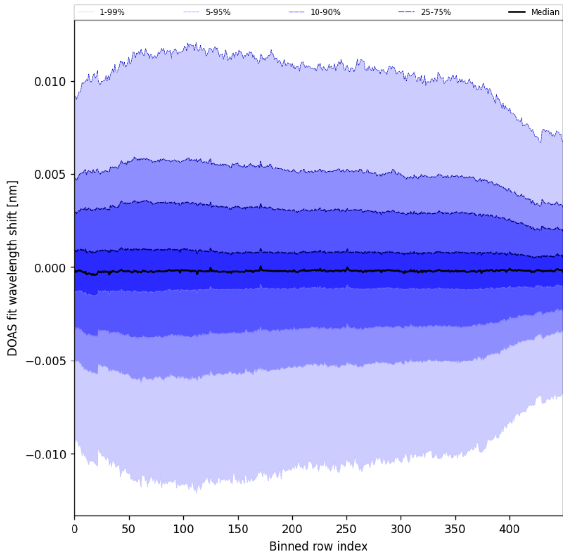
Figure 58: Along track statistics of “DOAS fit wavelength shift” for 2024-10-17 to 2024-10-19
