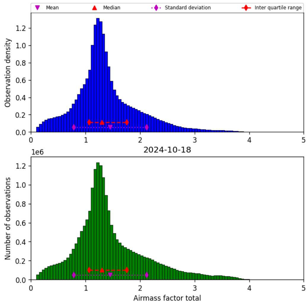
Figure 40: Histogram of “Airmass factor total” for 2024-10-17 to 2024-10-19
