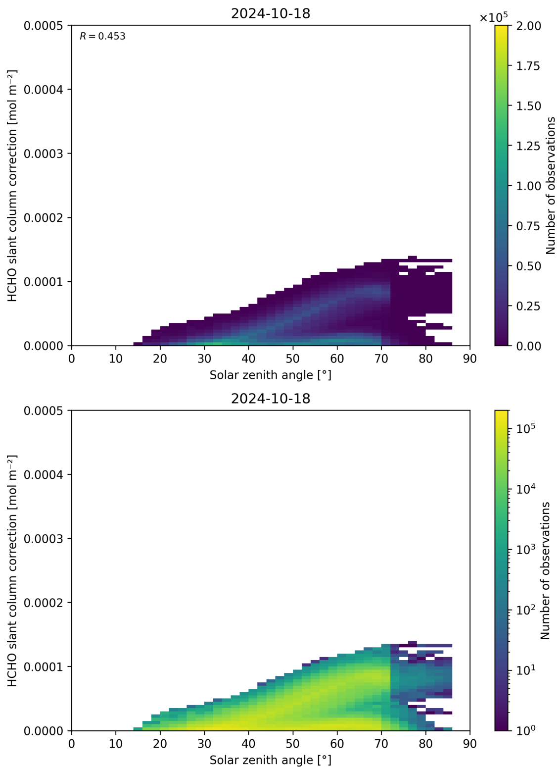
Figure 172: Scatter density plot of “Solar zenith angle” against “HCHO slant column correction” for 2024-10-17 to 2024-10-19.
