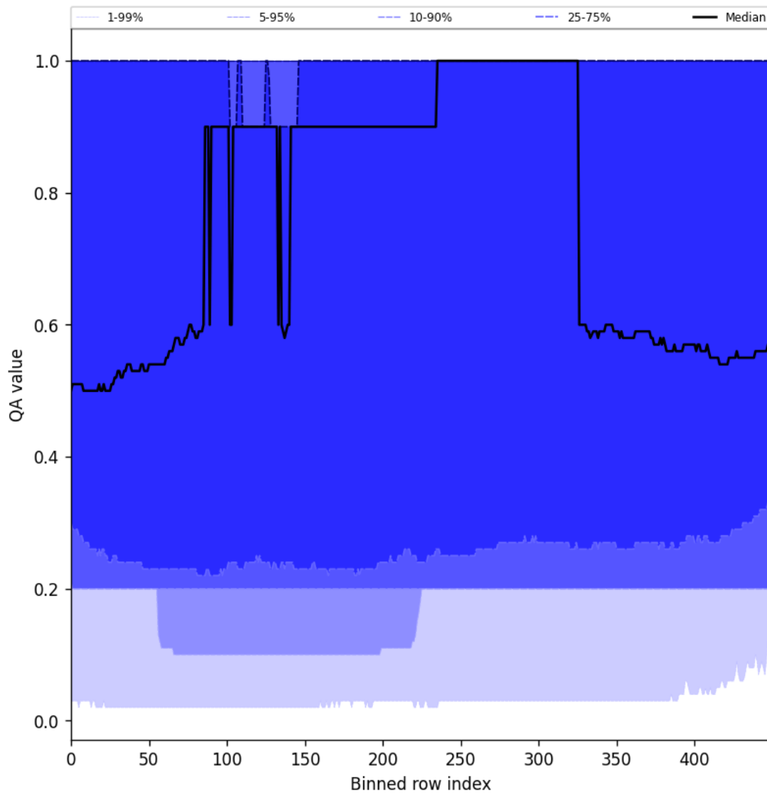
Figure 48: Along track statistics of “QA value” for 2024-10-17 to 2024-10-19
