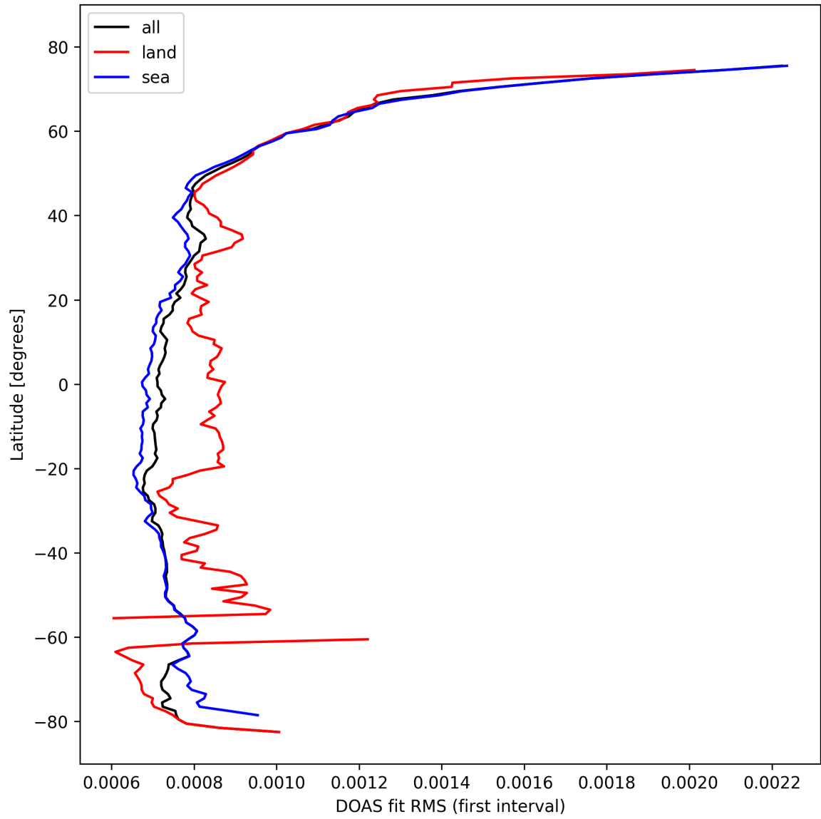
Figure 32: Zonal average of “DOAS fit RMS (first interval)” for 2024-10-17 to 2024-10-19.
