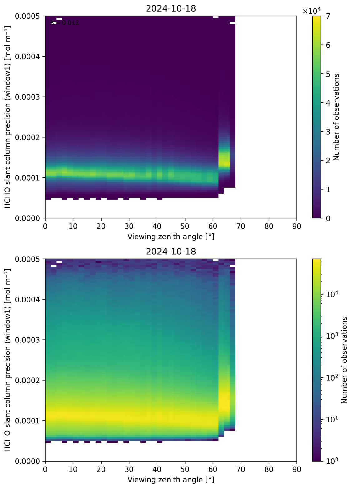
Figure 189: Scatter density plot of “Viewing zenith angle” against “HCHO slant column precision (window1)” for 2024-10-17 to 2024-10-19.
