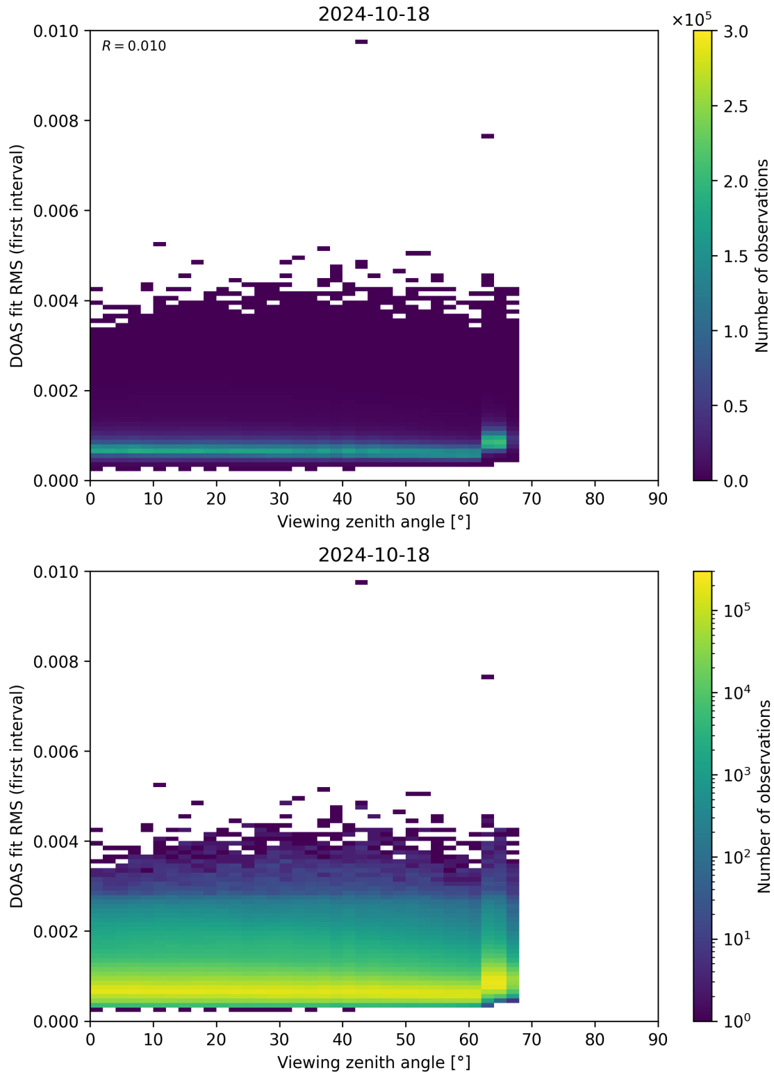
Figure 182: Scatter density plot of “Viewing zenith angle” against “DOAS fit RMS (first interval)” for 2024-10-17 to 2024-10-19.
