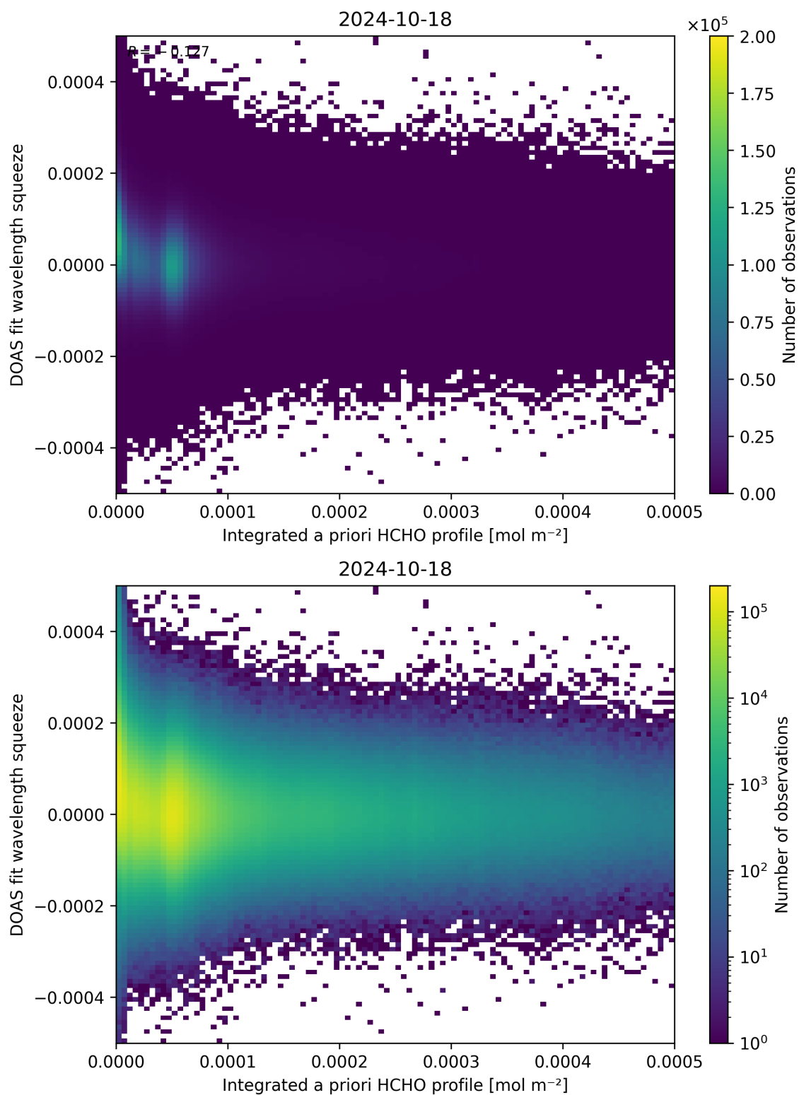
Figure 150: Scatter density plot of “Integrated a priori HCHO profile” against “DOAS fit wavelength squeeze” for 2024-10-17 to 2024-10-19.
