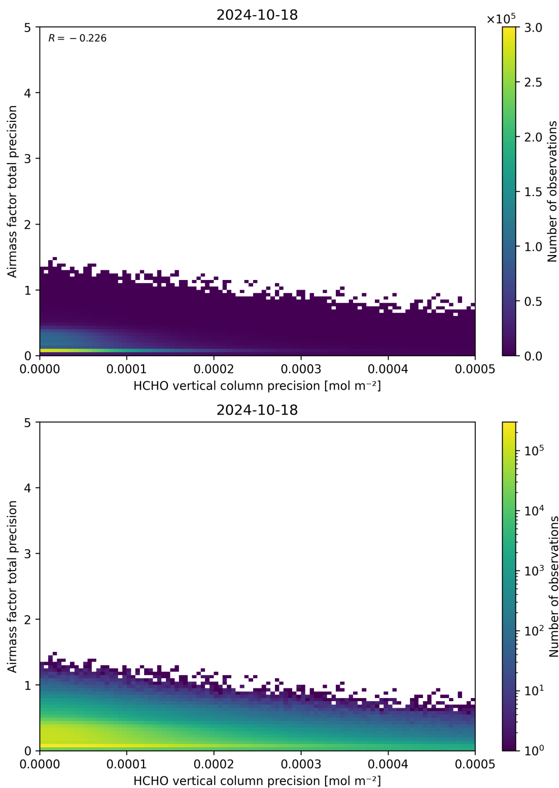
Figure 145: Scatter density plot of “HCHO vertical column precision” against “Airmass factor total precision” for 2024-10-17 to 2024-10-19.
