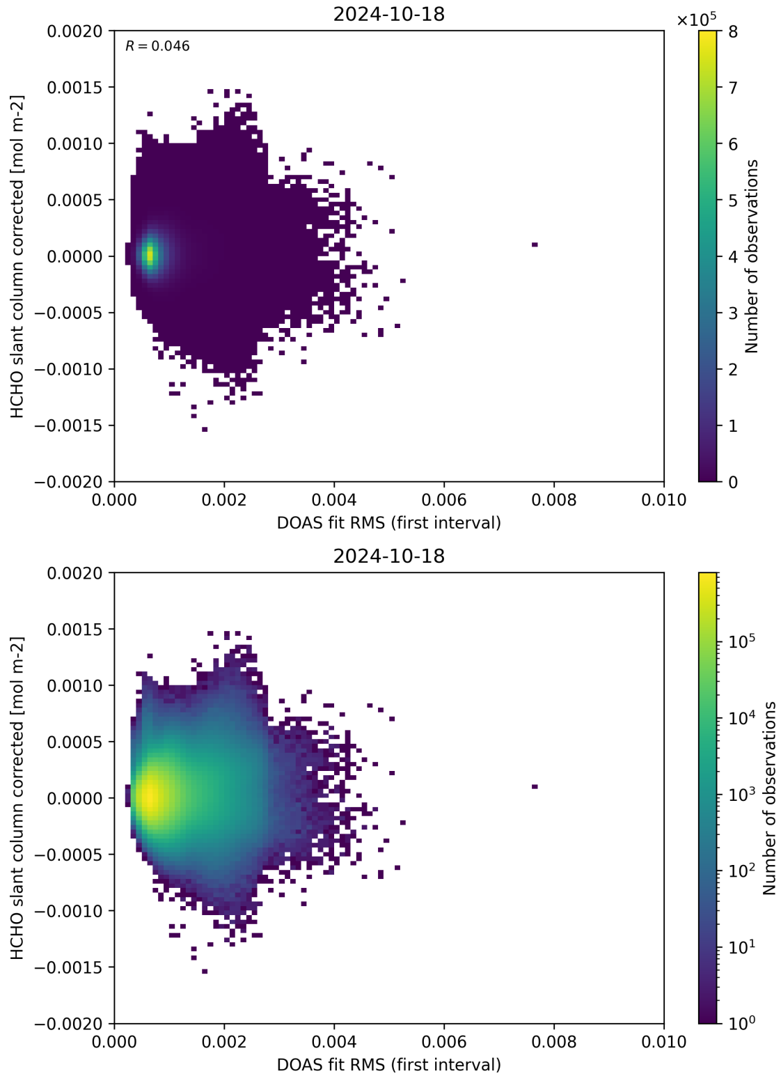
Figure 62: Scatter density plot of “DOAS fit RMS (first interval)” against “HCHO slant column corrected” for 2024-10-17 to 2024-10-19.
