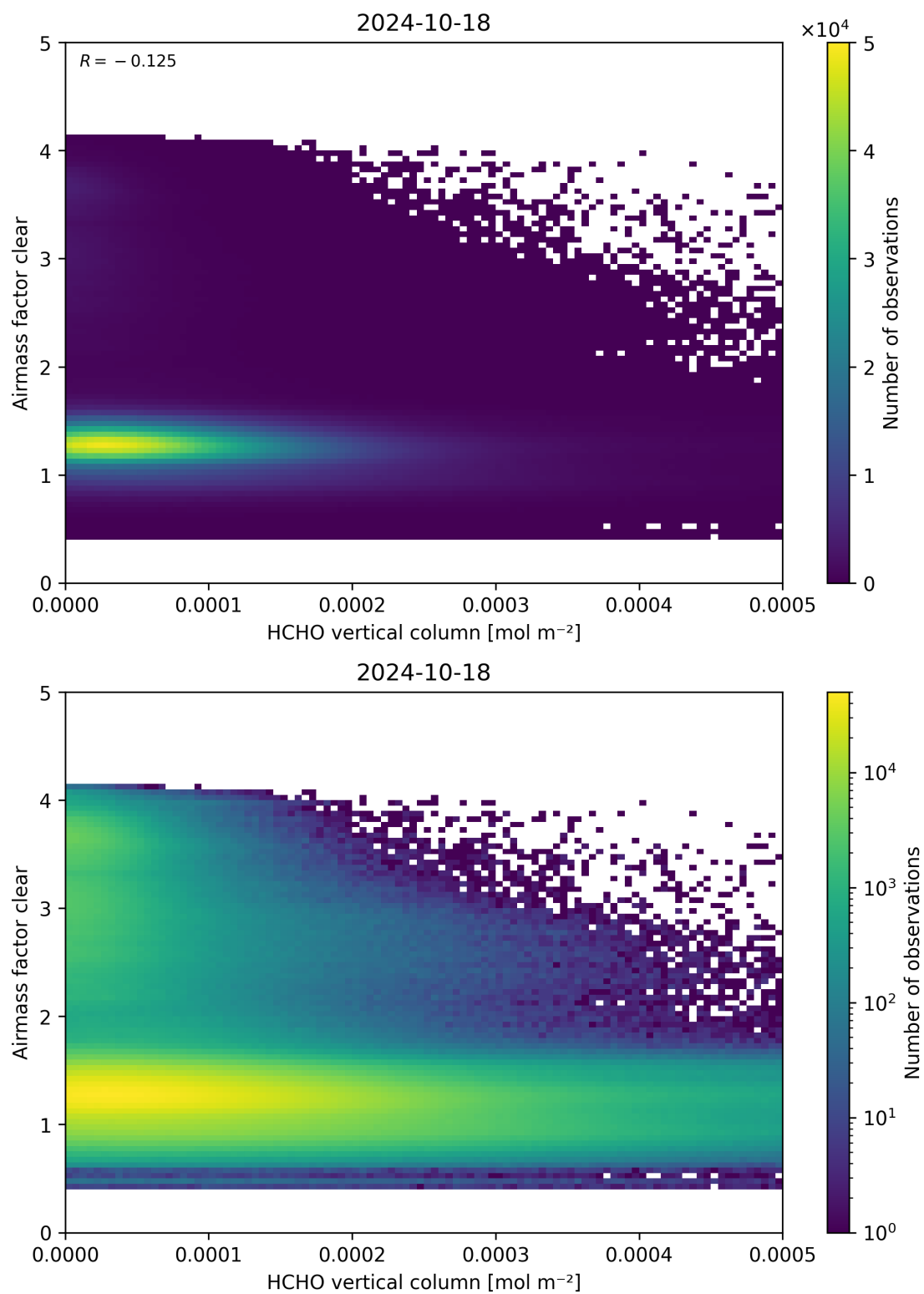
Figure 126: Scatter density plot of “HCHO vertical column” against “Airmass factor clear” for 2024-10-17 to 2024-10-19.
