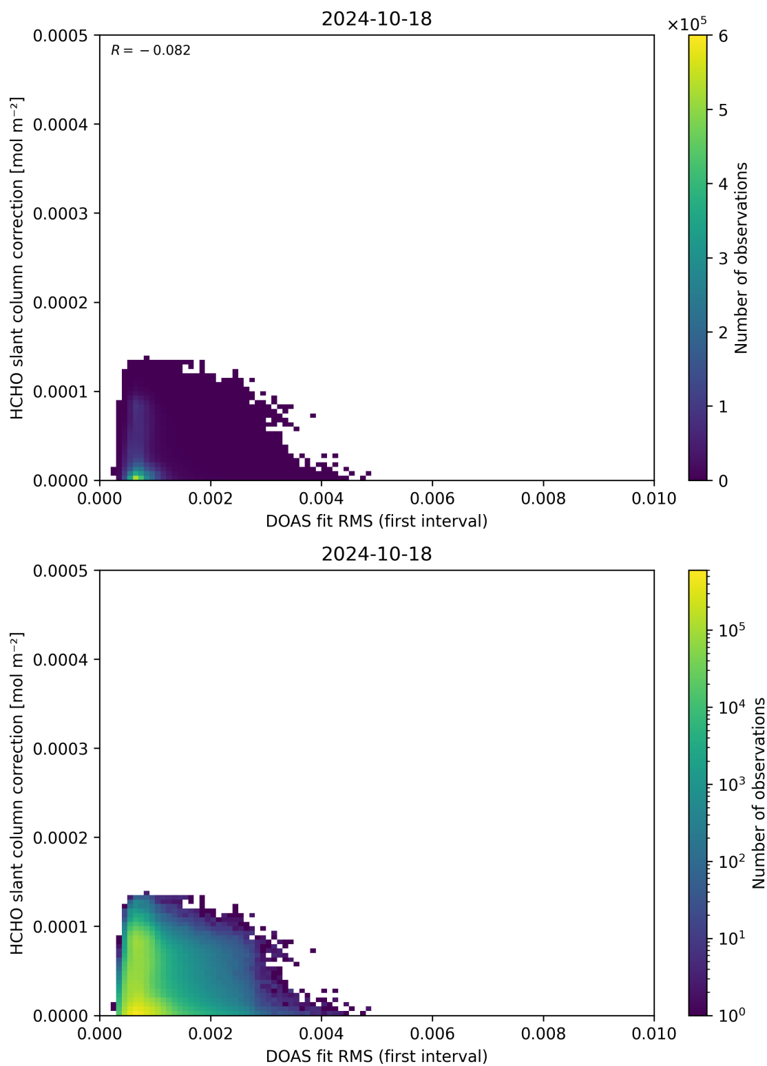
Figure 63: Scatter density plot of “DOAS fit RMS (first interval)” against “HCHO slant column correction” for 2024-10-17 to 2024-10-19.
