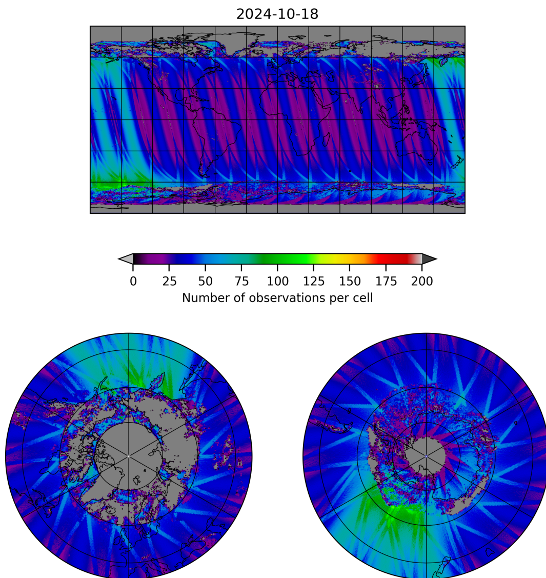
Figure 19: Map of the number of observations for 2024-10-17 to 2024-10-19
