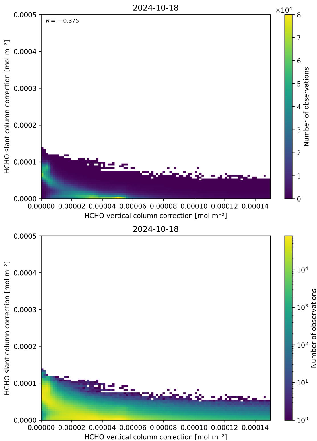
Figure 117: Scatter density plot of “HCHO vertical column correction” against “HCHO slant column correction” for 2024-10-17 to 2024-10-19.
