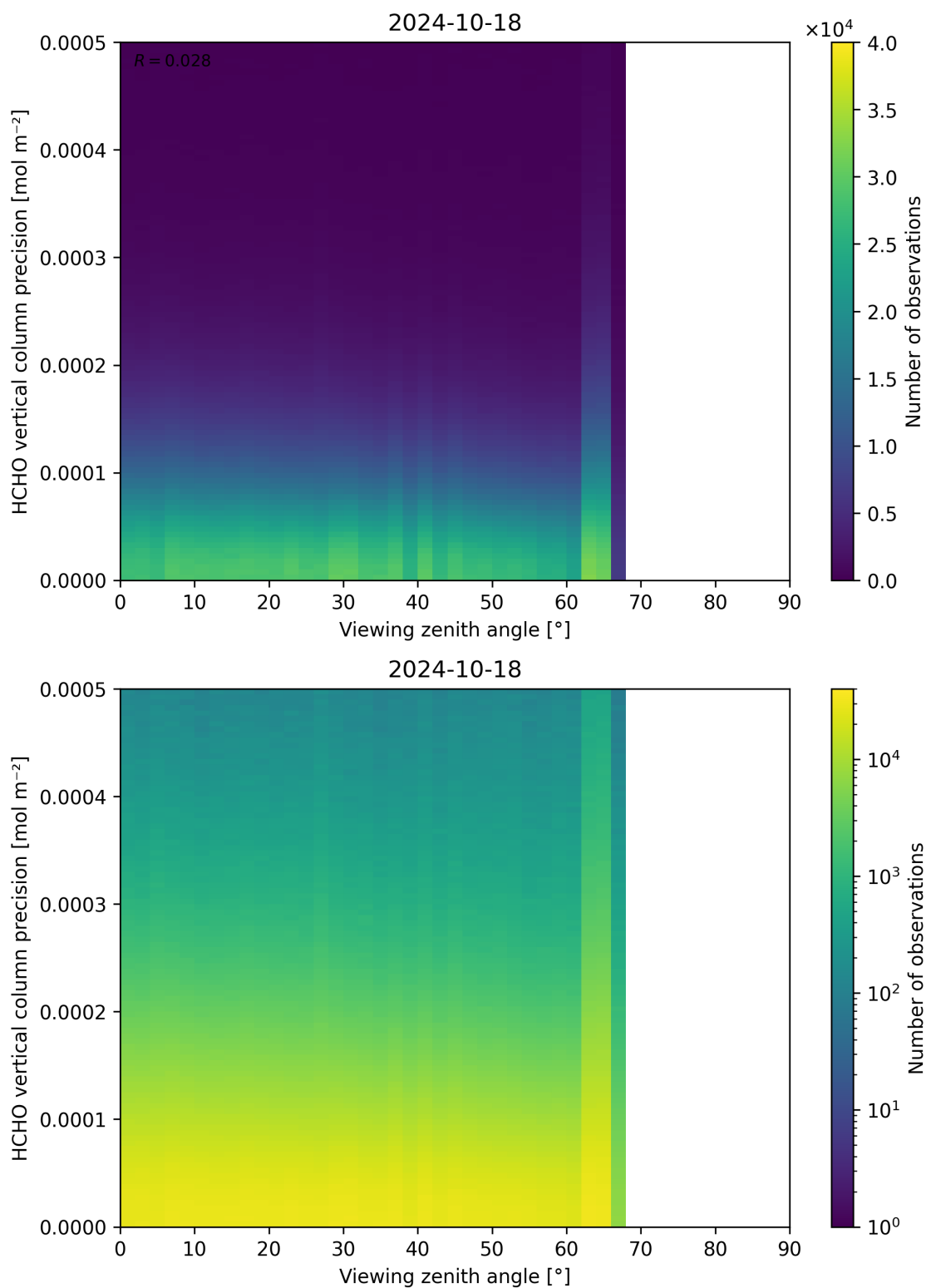
Figure 194: Scatter density plot of “Viewing zenith angle” against “HCHO vertical column precision” for 2024-10-17 to 2024-10-19.
