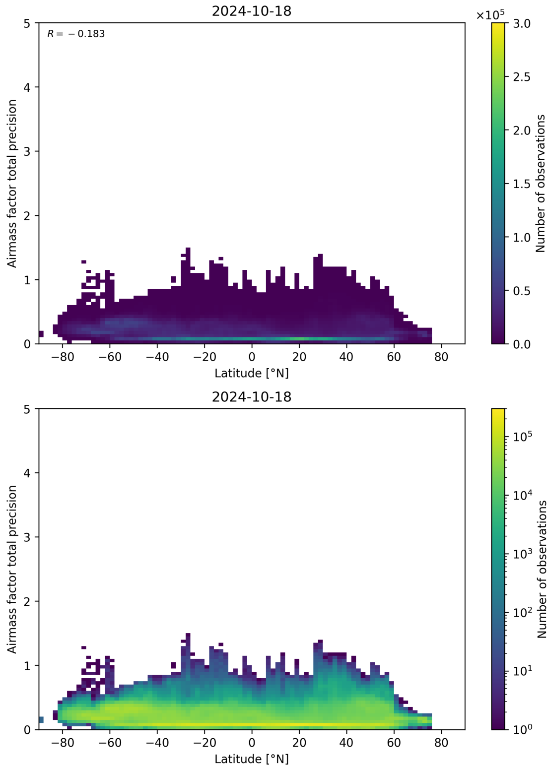
Figure 162: Scatter density plot of “Latitude” against “Airmass factor total precision” for 2024-10-17 to 2024-10-19.
