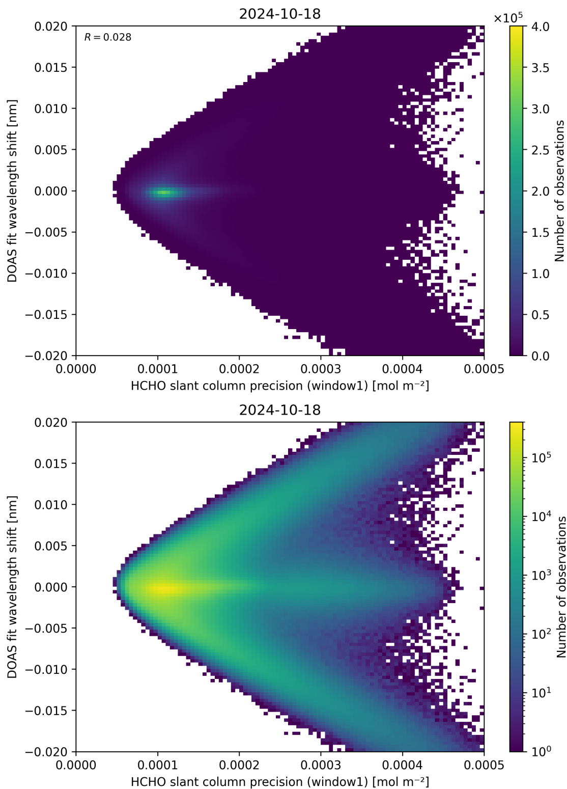
Figure 89: Scatter density plot of “HCHO slant column precision (window1)” against “DOAS fit wavelength shift” for 2024-10-17 to 2024-10-19.
