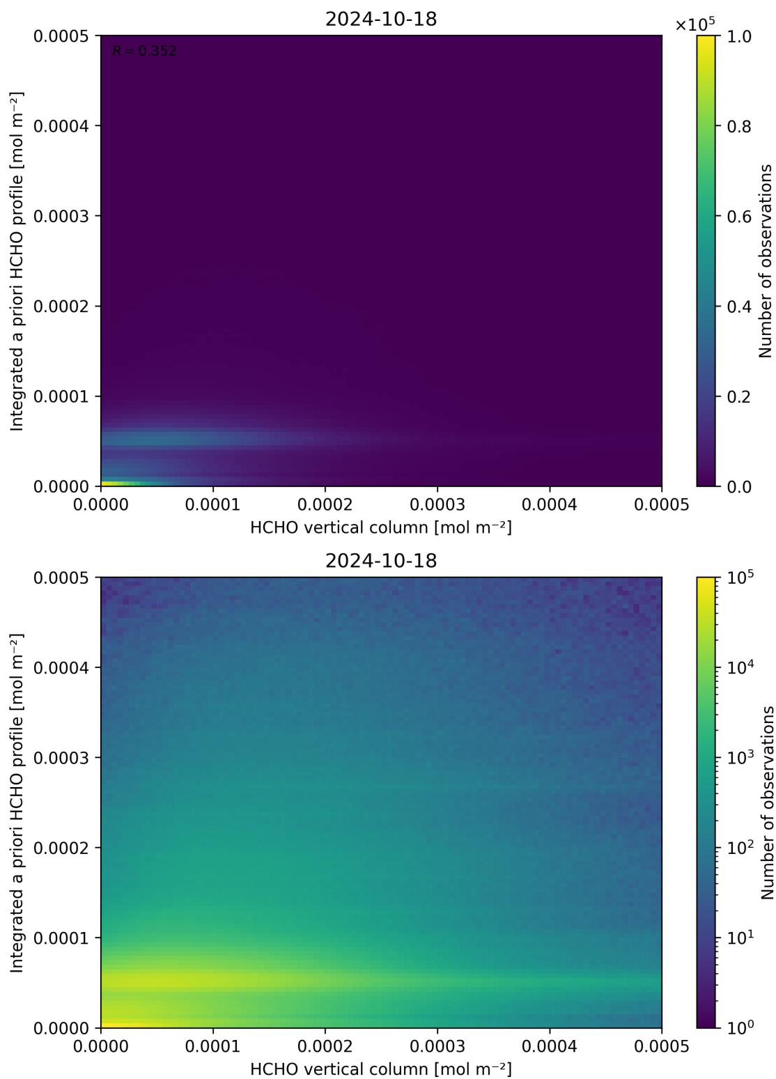
Figure 135: Scatter density plot of “HCHO vertical column” against “Integrated a priori HCHO profile” for 2024-10-17 to 2024-10-19.
