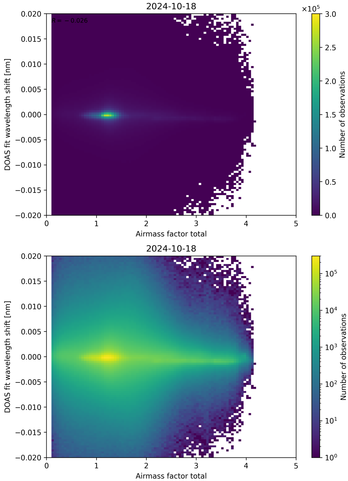
Figure 98: Scatter density plot of “Airmass factor total” against “DOAS fit wavelength shift” for 2024-10-17 to 2024-10-19.
