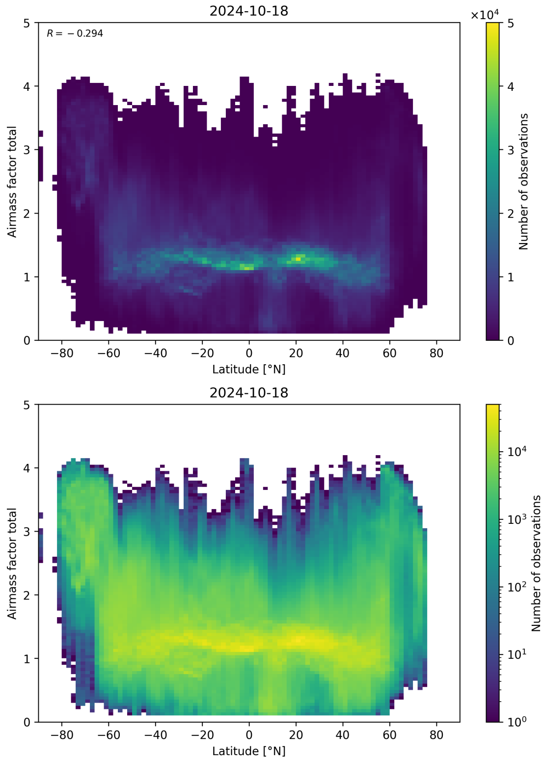
Figure 161: Scatter density plot of “Latitude” against “Airmass factor total” for 2024-10-17 to 2024-10-19.
