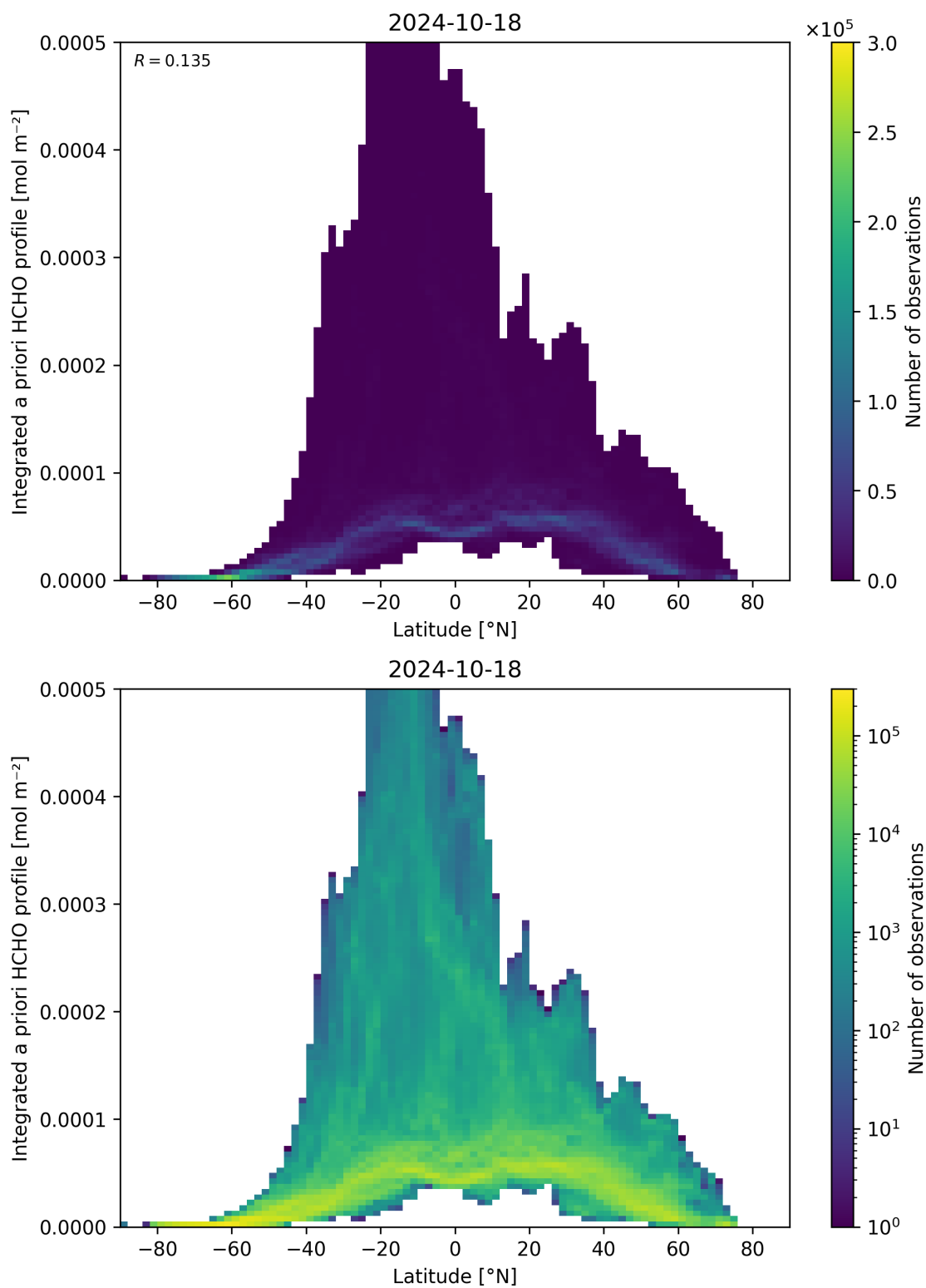
Figure 166: Scatter density plot of “Latitude” against “Integrated a priori HCHO profile” for 2024-10-17 to 2024-10-19.
