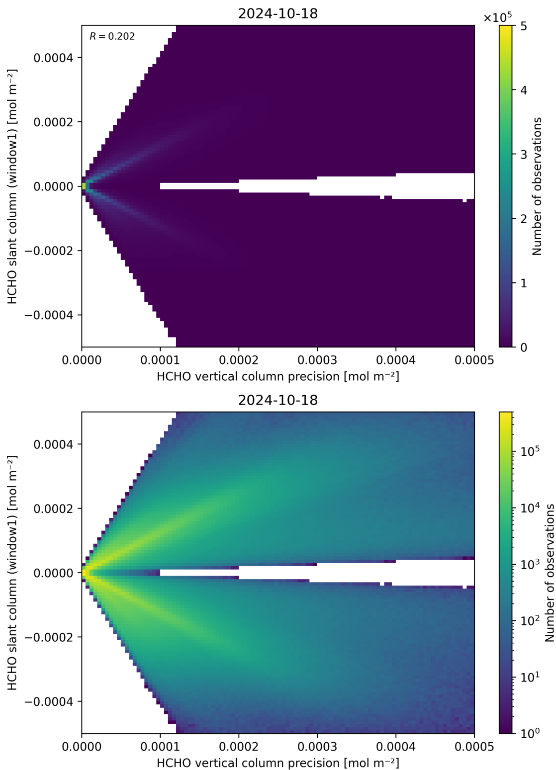
Figure 142: Scatter density plot of “HCHO vertical column precision” against “HCHO slant column (window1)” for 2024-10-17 to 2024-10-19.
