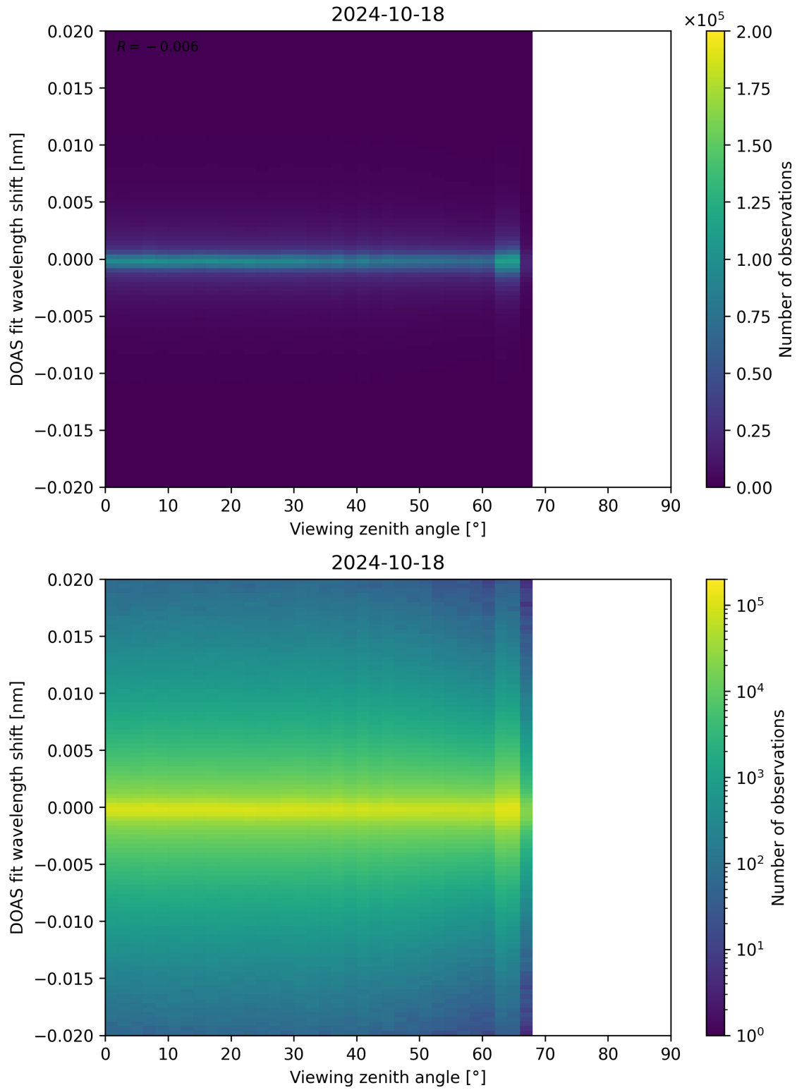
Figure 183: Scatter density plot of “Viewing zenith angle” against “DOAS fit wavelength shift” for 2024-10-17 to 2024-10-19.
