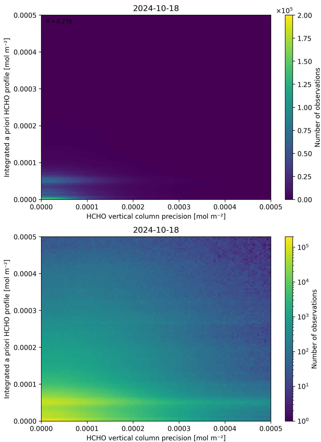
Figure 147: Scatter density plot of “HCHO vertical column precision” against “Integrated a priori HCHO profile” for 2024-10-17 to 2024-10-19.
