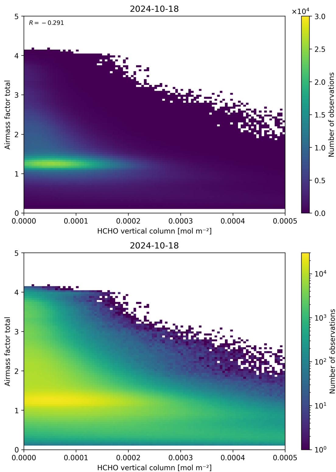
Figure 131: Scatter density plot of “HCHO vertical column” against “Airmass factor total” for 2024-10-17 to 2024-10-19.
