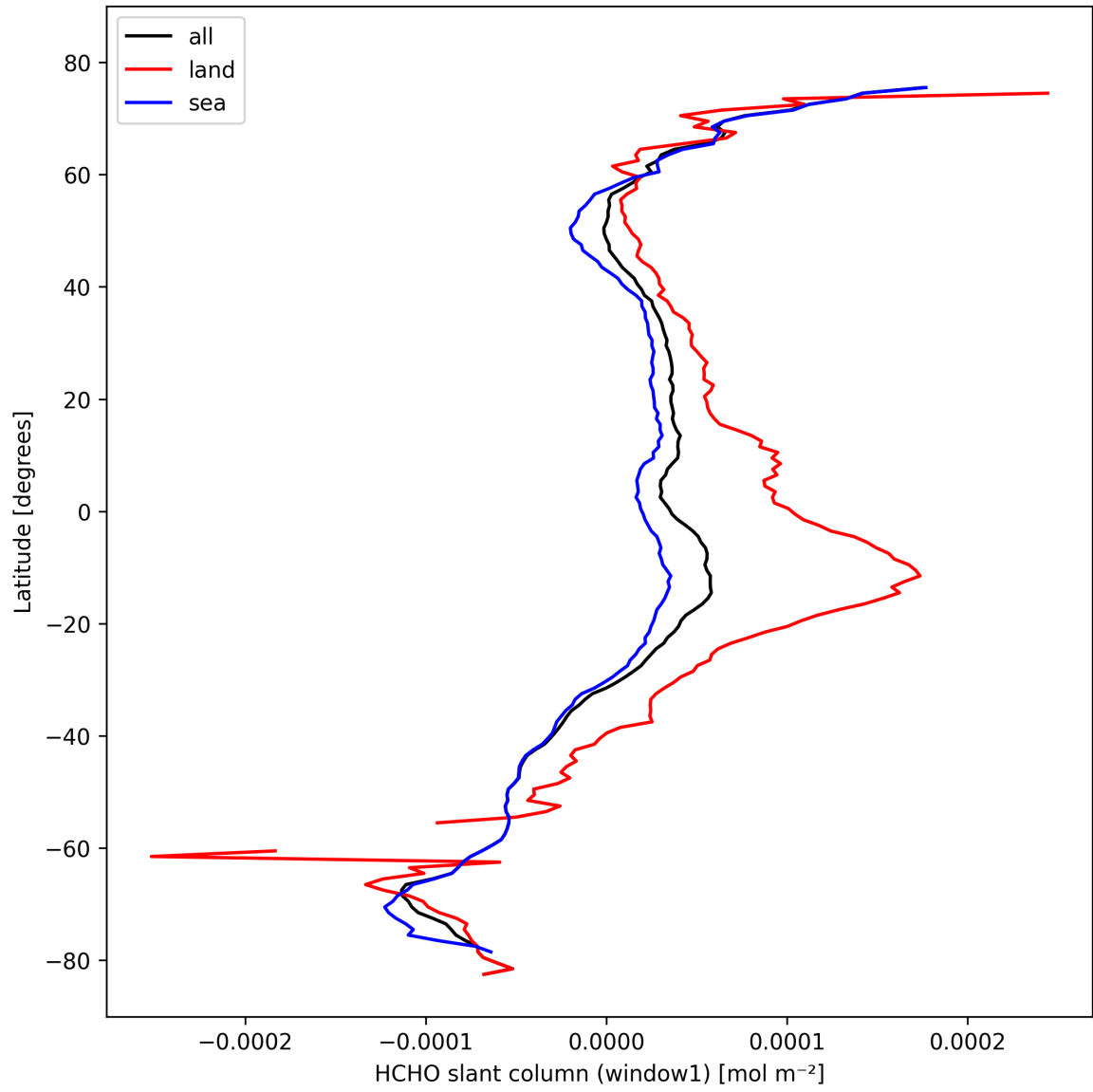
Figure 24: Zonal average of “HCHO slant column (window1)” for 2024-10-17 to 2024-10-19.
