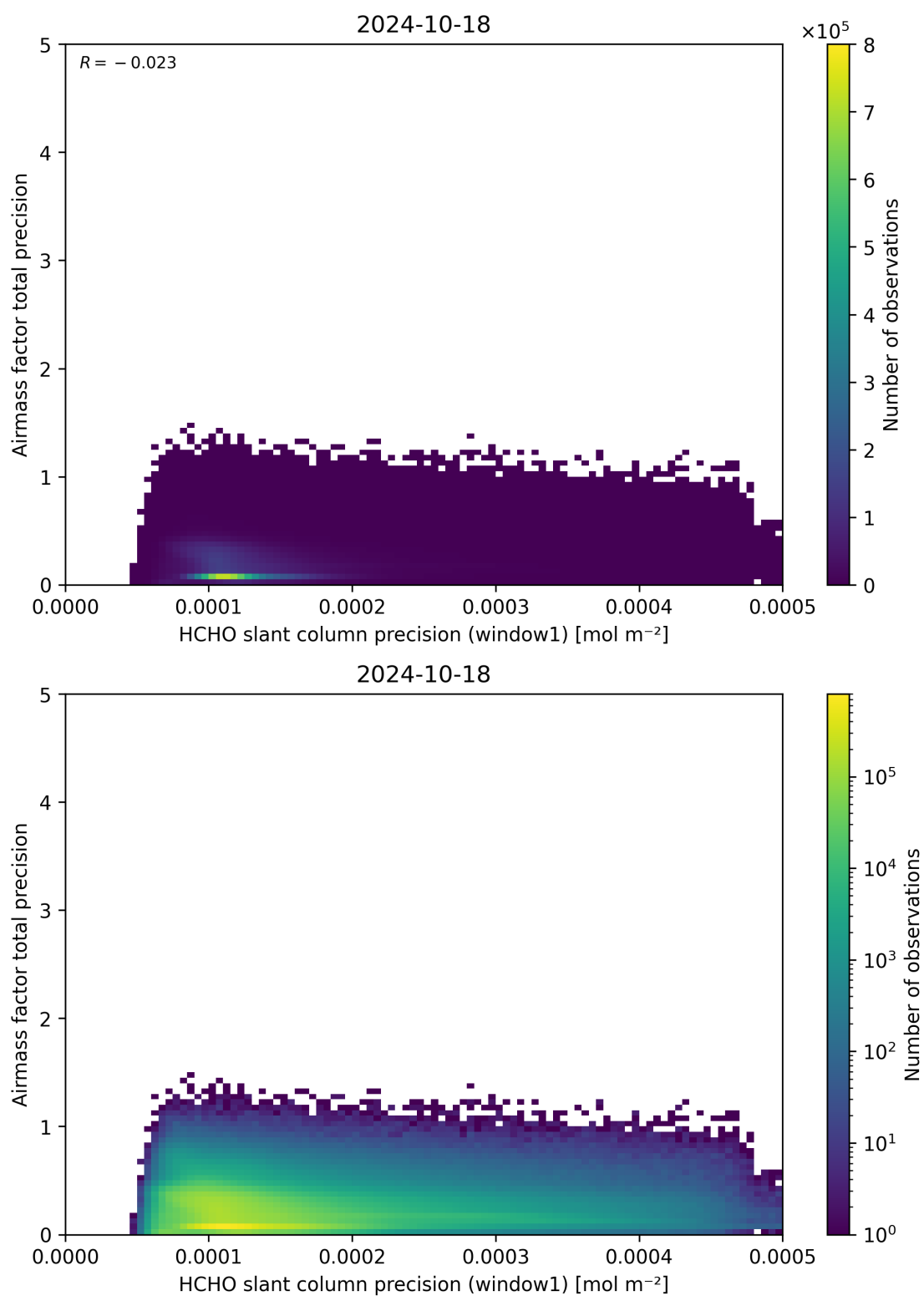
Figure 95: Scatter density plot of “HCHO slant column precision (window1)” against “Airmass factor total precision” for 2024-10-17 to 2024-10-19.
