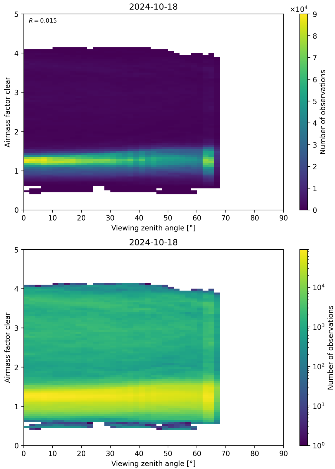
Figure 185: Scatter density plot of “Viewing zenith angle” against “Airmass factor clear” for 2024-10-17 to 2024-10-19.
