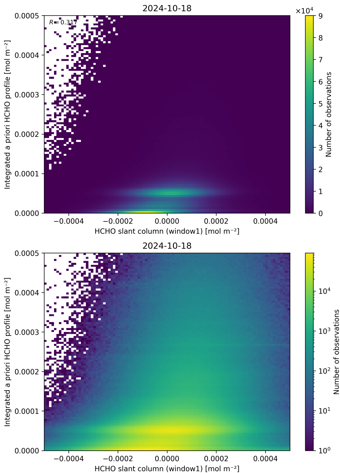
Figure 87: Scatter density plot of “HCHO slant column (window1)” against “Integrated a priori HCHO profile” for 2024-10-17 to 2024-10-19.
