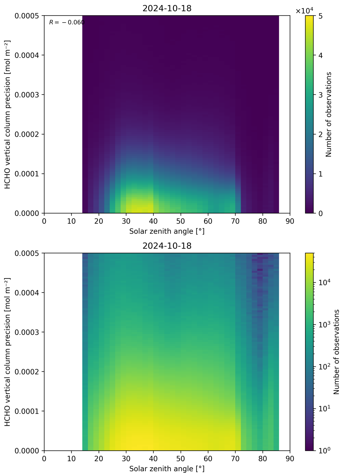
Figure 179: Scatter density plot of “Solar zenith angle” against “HCHO vertical column precision” for 2024-10-17 to 2024-10-19.
