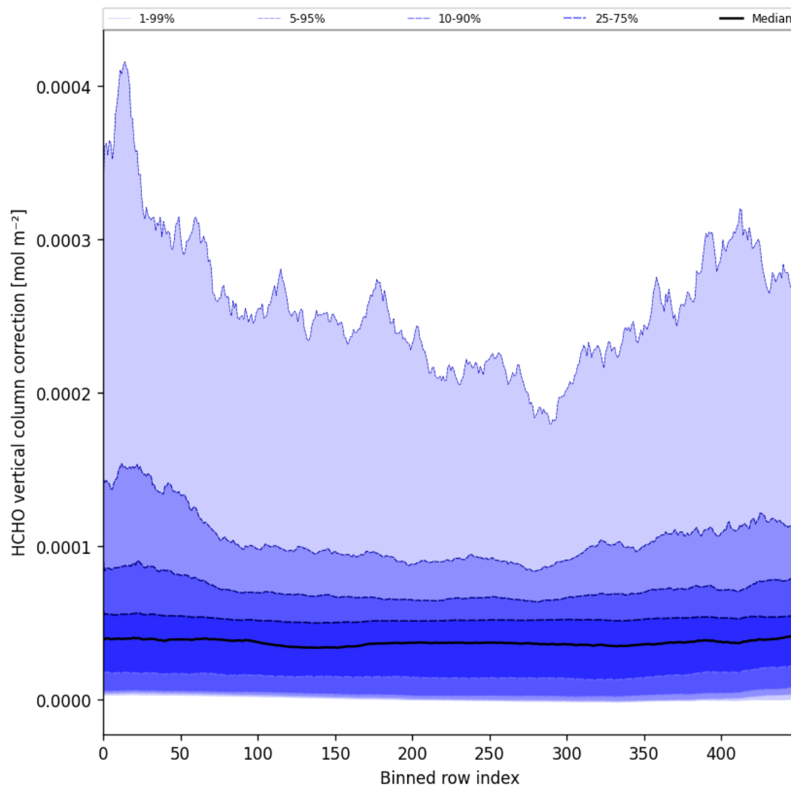
Figure 51: Along track statistics of “HCHO vertical column correction” for 2024-10-17 to 2024-10-19
