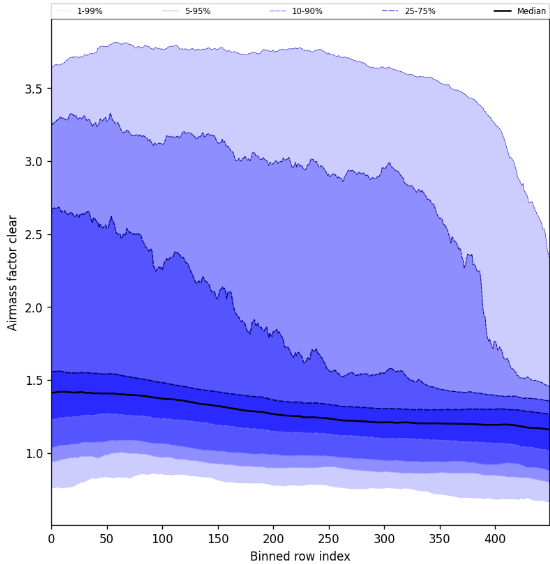
Figure 56: Along track statistics of “Airmass factor clear” for 2024-10-17 to 2024-10-19
