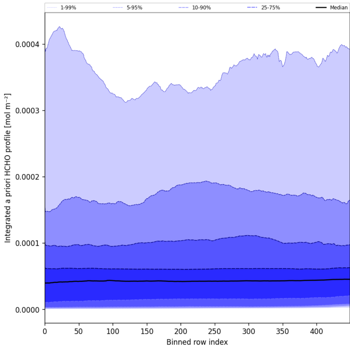
Figure 57: Along track statistics of “Integrated a priori HCHO profile” for 2024-10-17 to 2024-10-19
