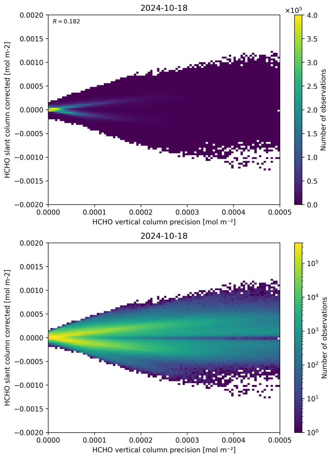
Figure 140: Scatter density plot of “HCHO vertical column precision” against “HCHO slant column corrected” for 2024-10-17 to 2024-10-19.
