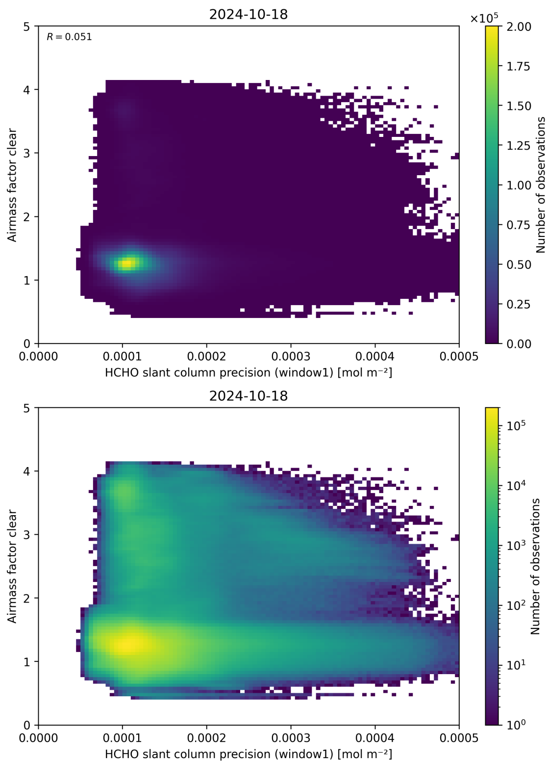
Figure 91: Scatter density plot of “HCHO slant column precision (window1)” against “Airmass factor clear” for 2024-10-17 to 2024-10-19.
