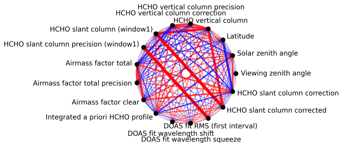
Figure 1: Map of correlation graph for 2024-10-17 to 2024-10-19.
