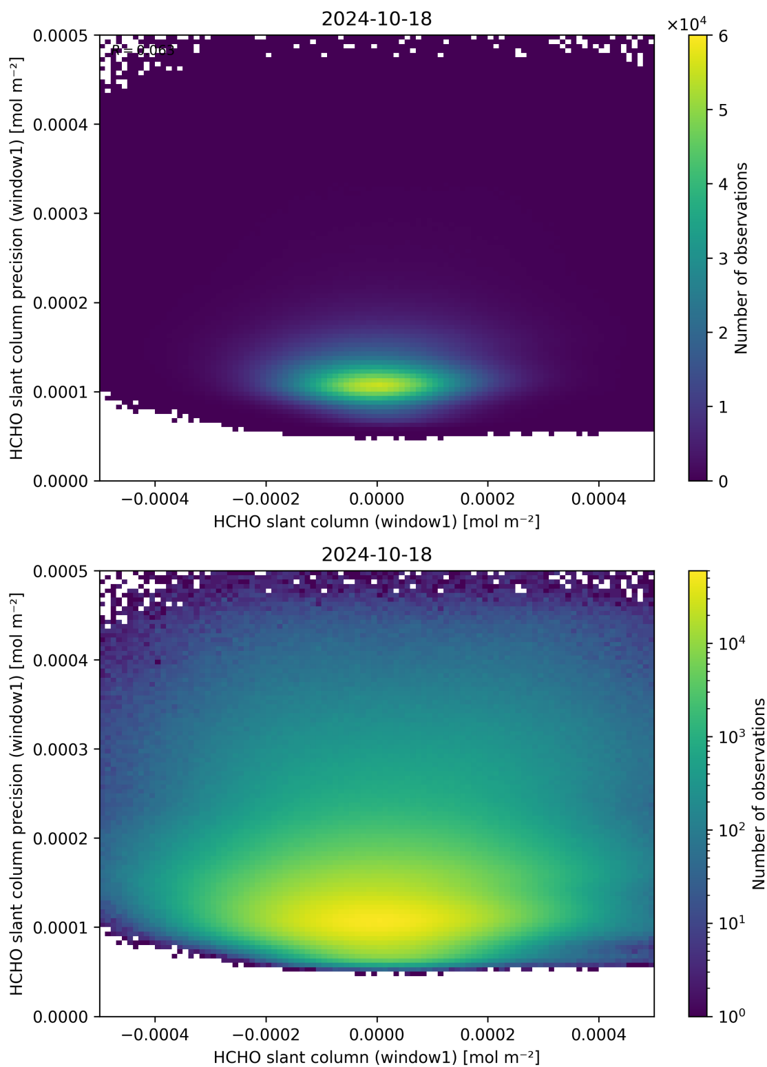
Figure 84: Scatter density plot of “HCHO slant column (window1)” against “HCHO slant column precision (window1)” for 2024-10-17 to 2024-10-19.
