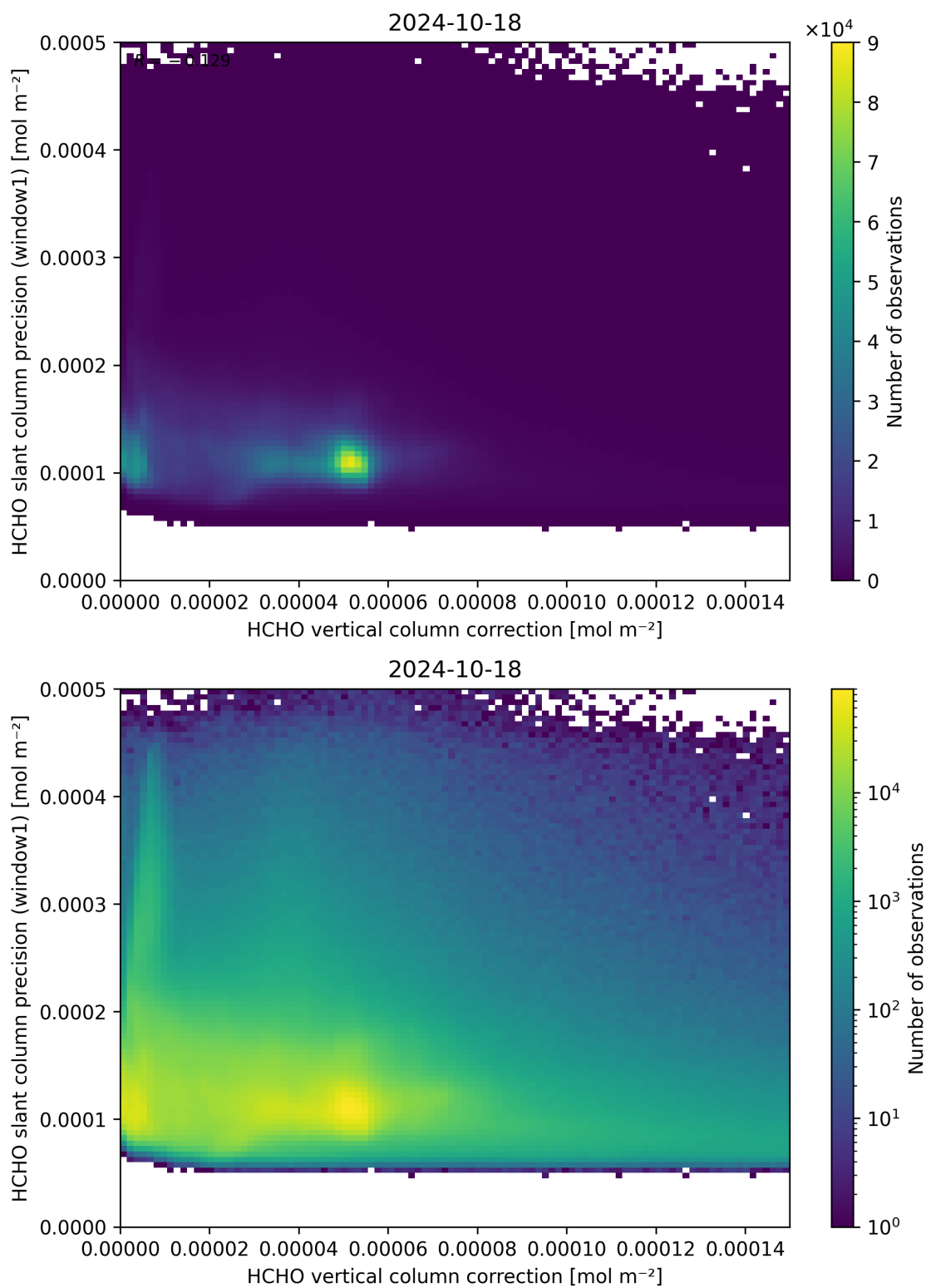
Figure 119: Scatter density plot of “HCHO vertical column correction” against “HCHO slant column precision (window1)” for 2024-10-17 to 2024-10-19.
