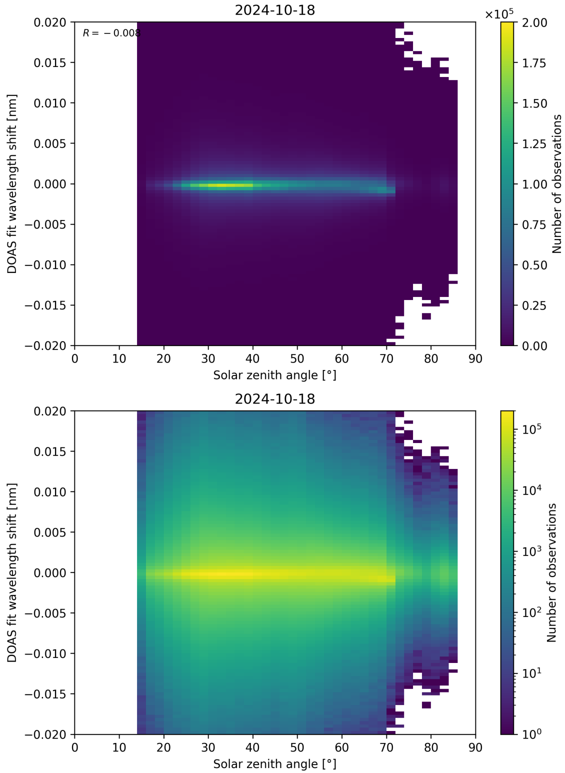
Figure 168: Scatter density plot of “Solar zenith angle” against “DOAS fit wavelength shift” for 2024-10-17 to 2024-10-19.
