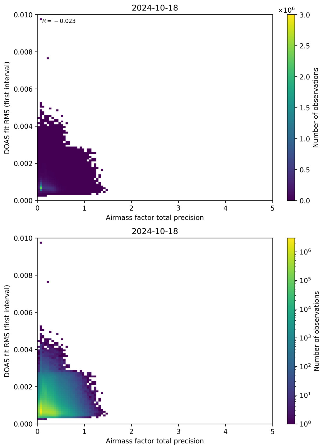
Figure 105: Scatter density plot of “Airmass factor total precision” against “DOAS fit RMS (first interval)” for 2024-10-17 to 2024-10-19.
