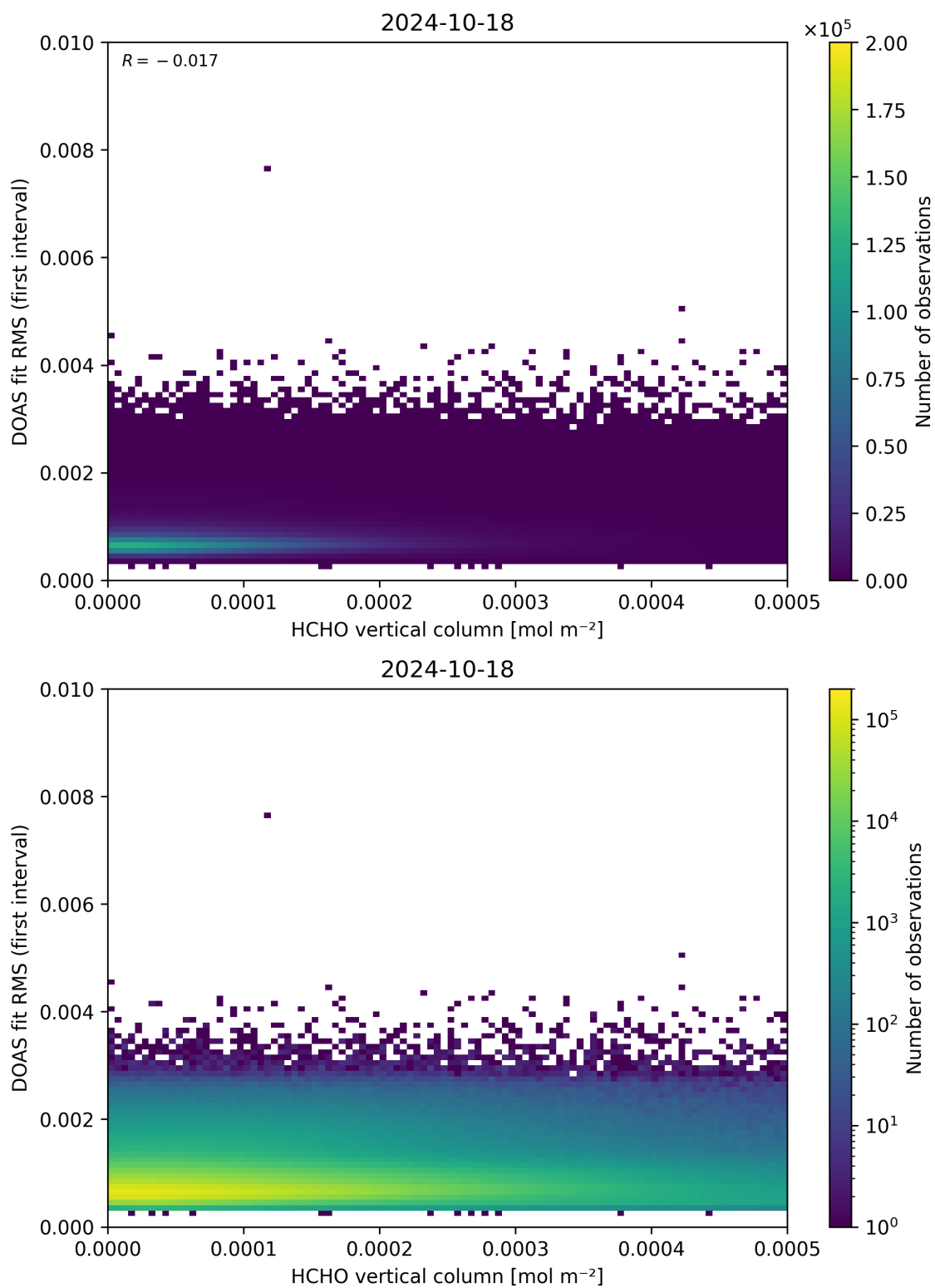
Figure 123: Scatter density plot of “HCHO vertical column” against “DOAS fit RMS (first interval)” for 2024-10-17 to 2024-10-19.
