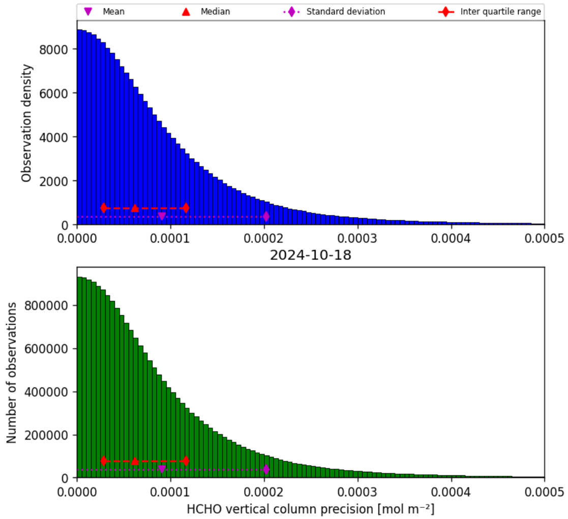
Figure 36: Histogram of “HCHO vertical column precision” for 2024-10-17 to 2024-10-19
