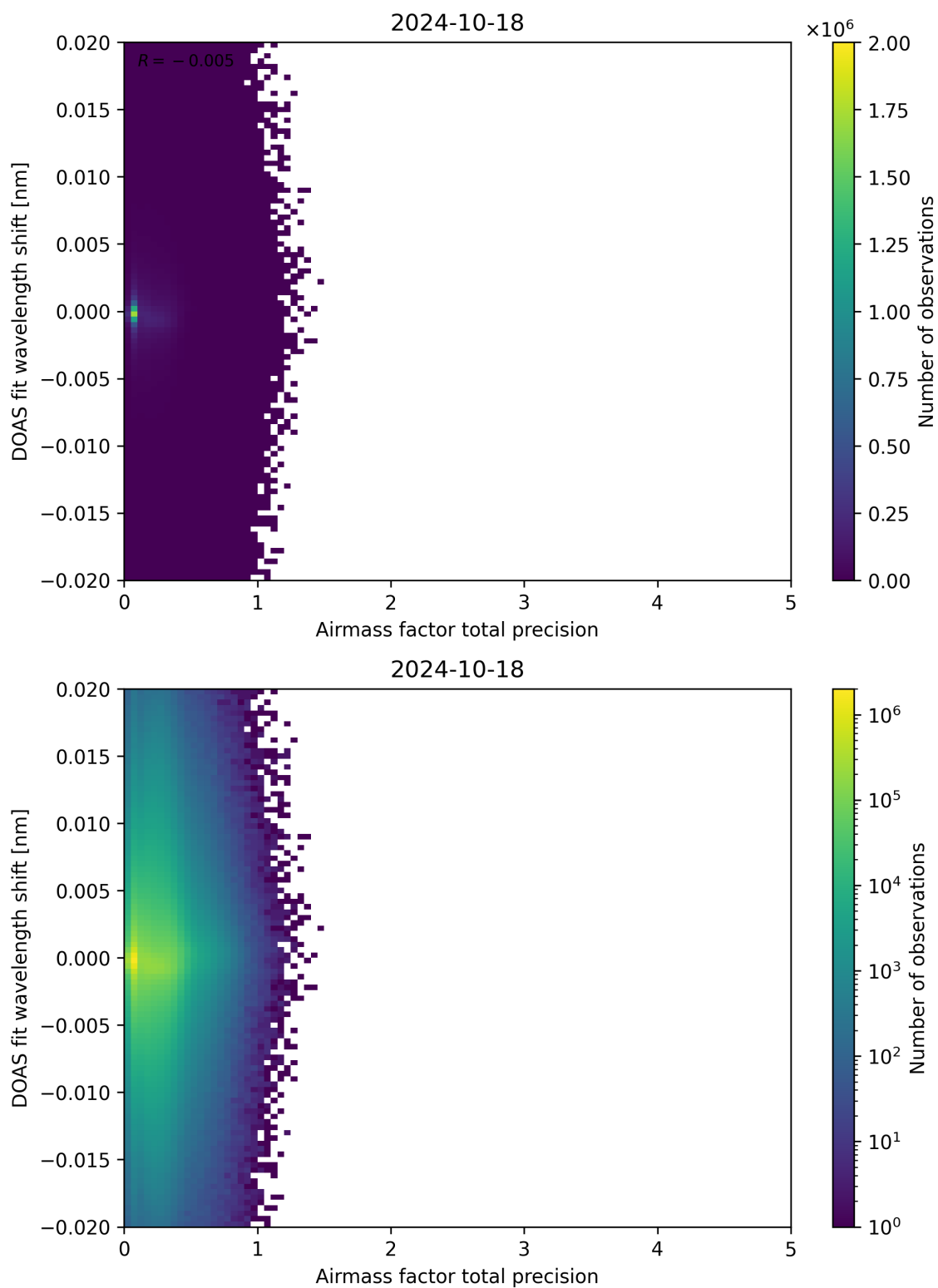
Figure 106: Scatter density plot of “Airmass factor total precision” against “DOAS fit wavelength shift” for 2024-10-17 to 2024-10-19.
