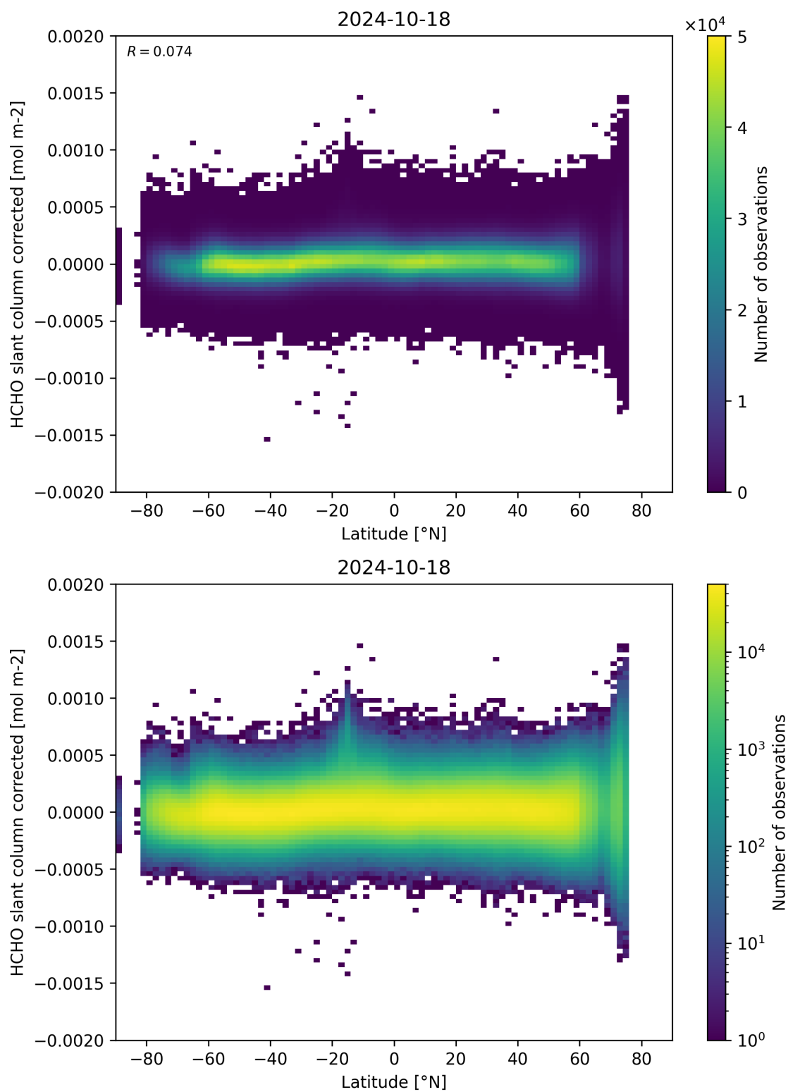
Figure 157: Scatter density plot of “Latitude” against “HCHO slant column corrected” for 2024-10-17 to 2024-10-19.
