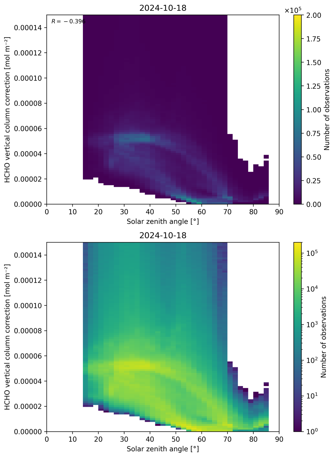
Figure 178: Scatter density plot of “Solar zenith angle” against “HCHO vertical column correction” for 2024-10-17 to 2024-10-19.
