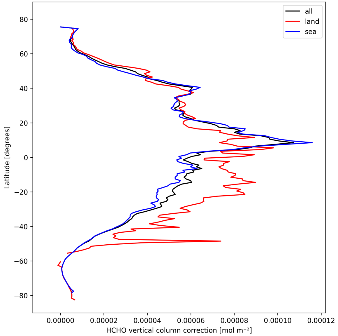
Figure 23: Zonal average of “HCHO vertical column correction” for 2024-10-17 to 2024-10-19.
