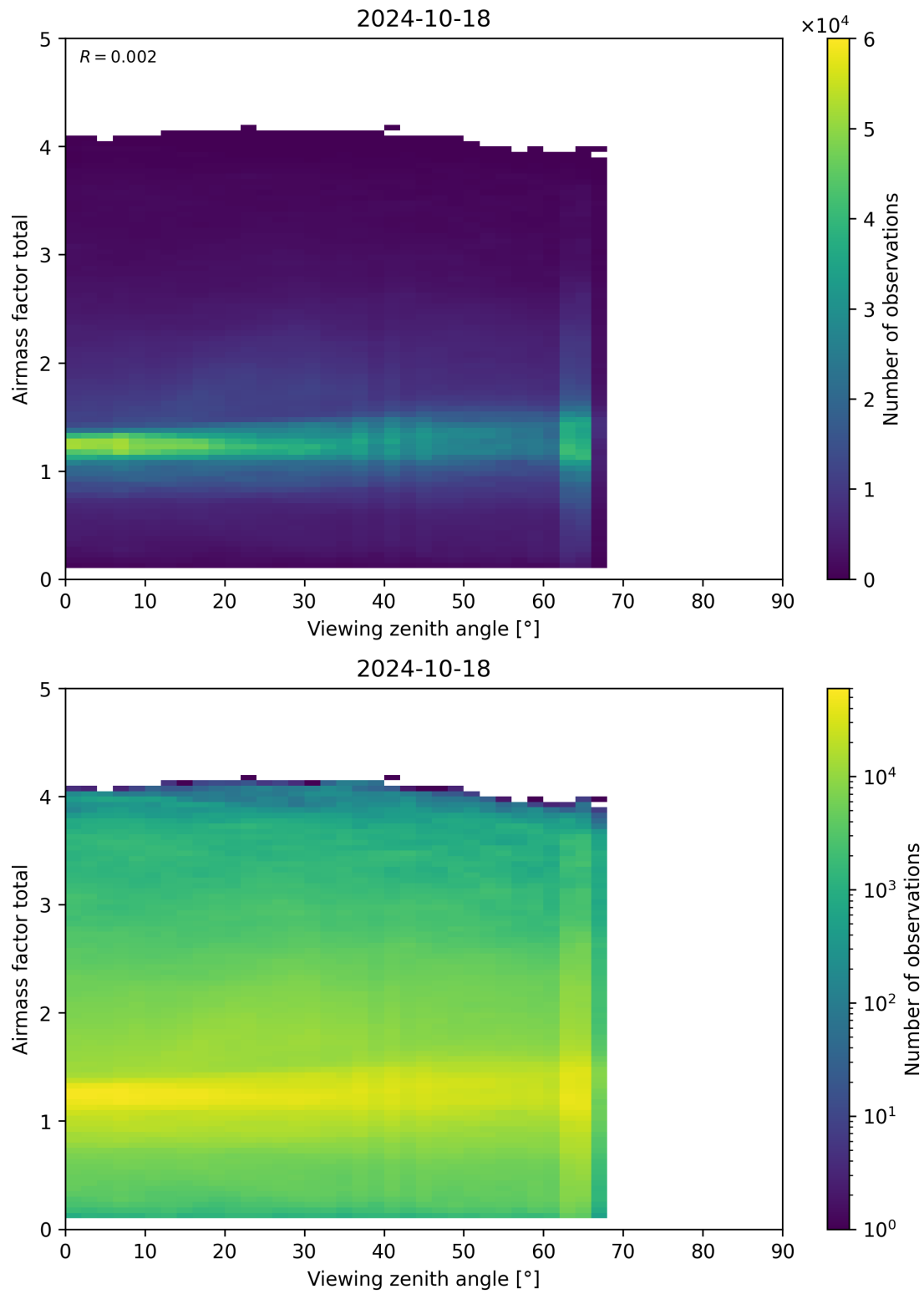
Figure 190: Scatter density plot of “Viewing zenith angle” against “Airmass factor total” for 2024-10-17 to 2024-10-19.
