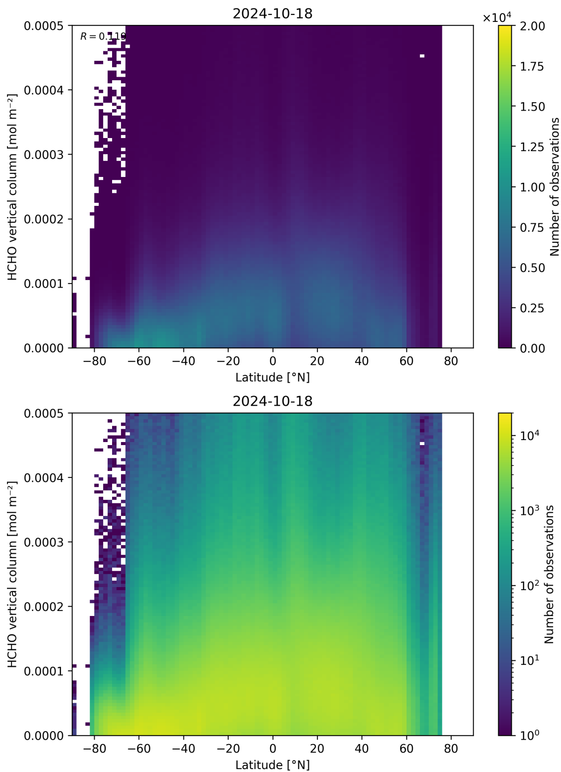
Figure 163: Scatter density plot of “Latitude” against “HCHO vertical column” for 2024-10-17 to 2024-10-19.
