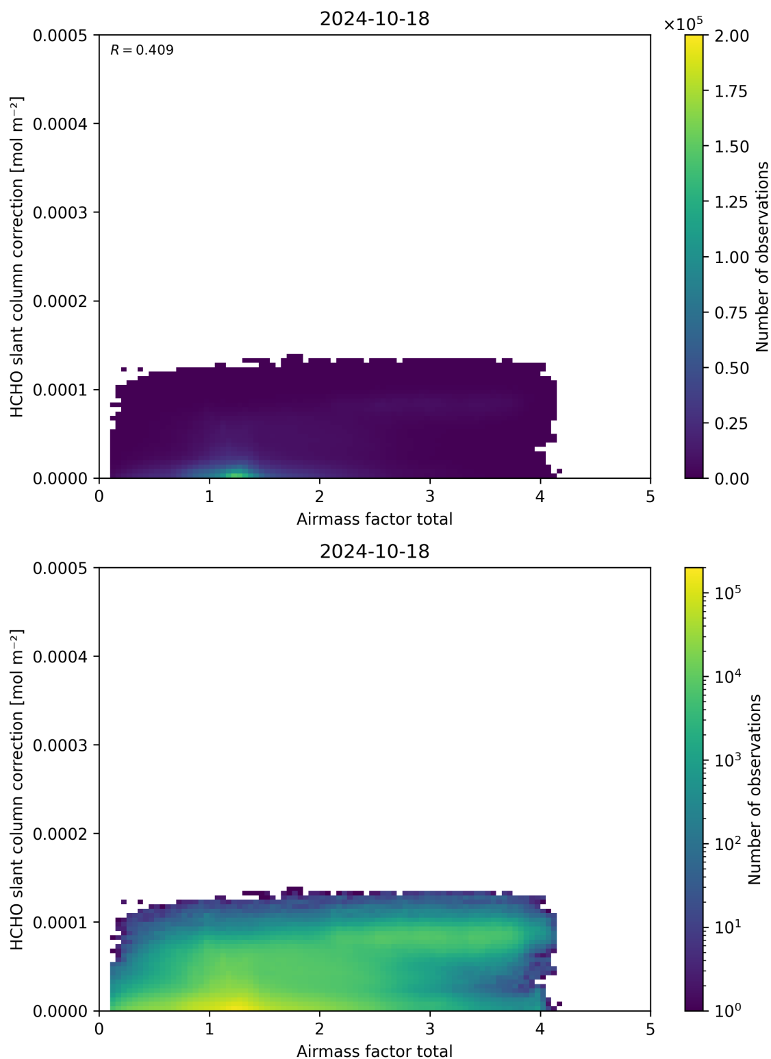
Figure 102: Scatter density plot of “Airmass factor total” against “HCHO slant column correction” for 2024-10-17 to 2024-10-19.
