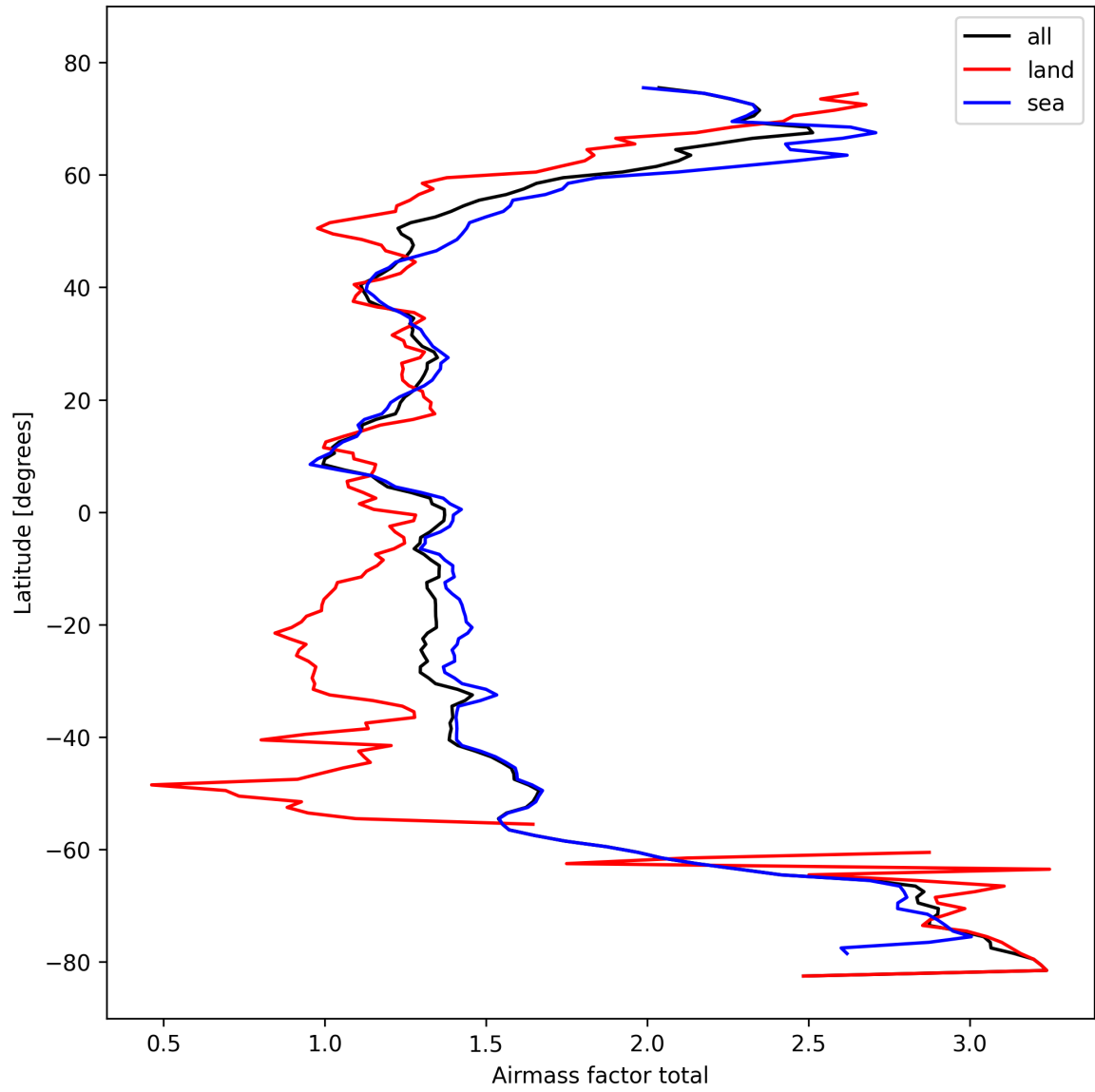
Figure 26: Zonal average of “Airmass factor total” for 2024-10-17 to 2024-10-19.
