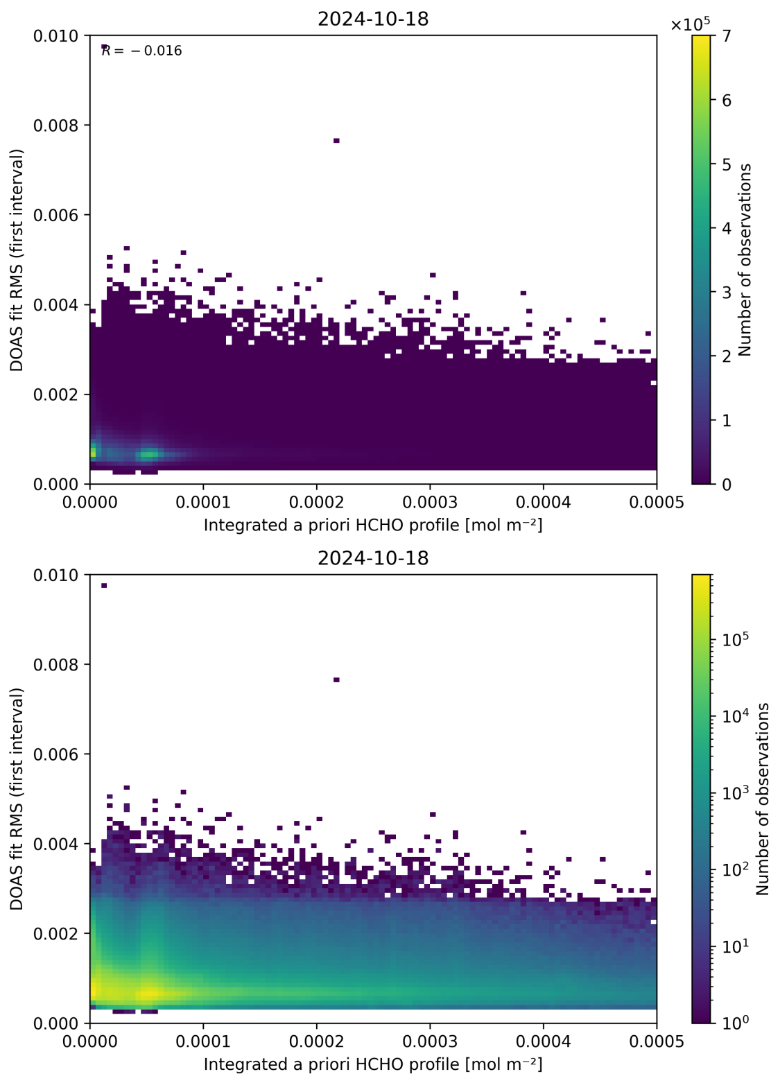
Figure 148: Scatter density plot of “Integrated a priori HCHO profile” against “DOAS fit RMS (first interval)” for 2024-10-17 to 2024-10-19.
