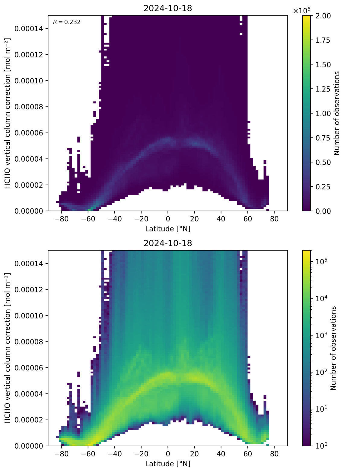
Figure 164: Scatter density plot of “Latitude” against “HCHO vertical column correction” for 2024-10-17 to 2024-10-19.
