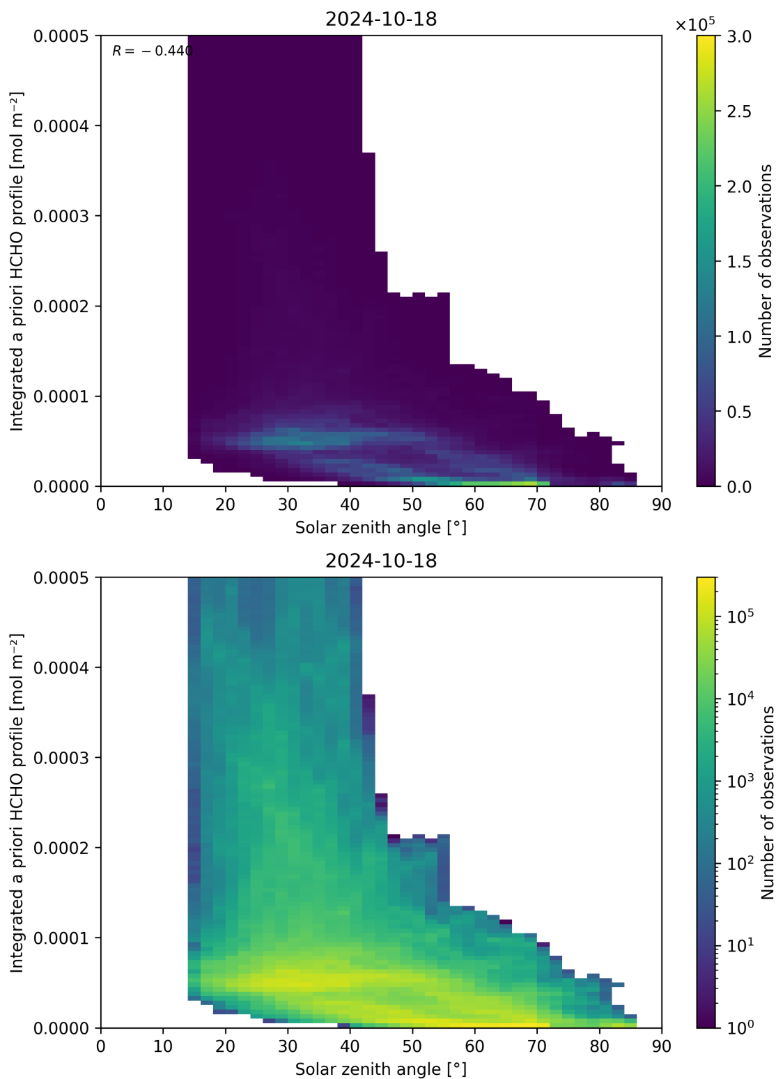
Figure 180: Scatter density plot of “Solar zenith angle” against “Integrated a priori HCHO profile” for 2024-10-17 to 2024-10-19.
