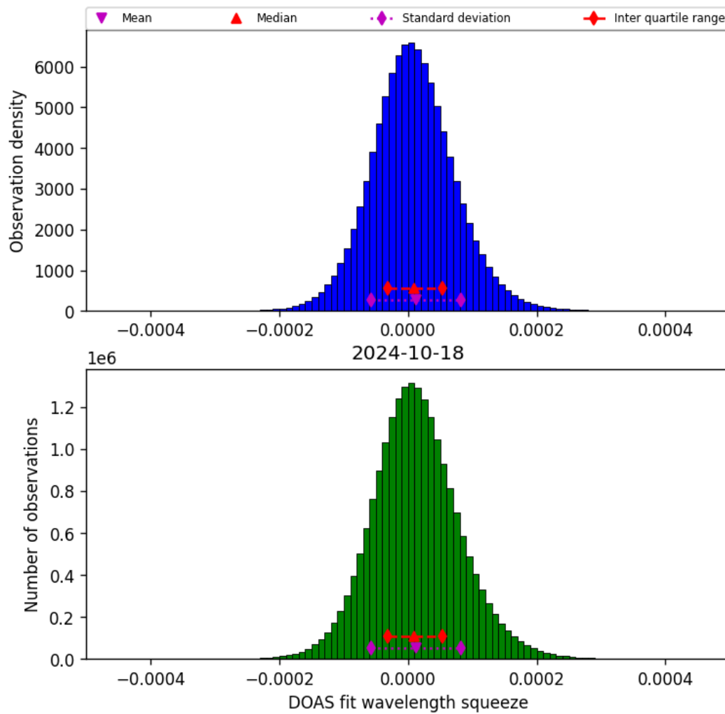
Figure 45: Histogram of “DOAS fit wavelength squeeze” for 2024-10-17 to 2024-10-19
