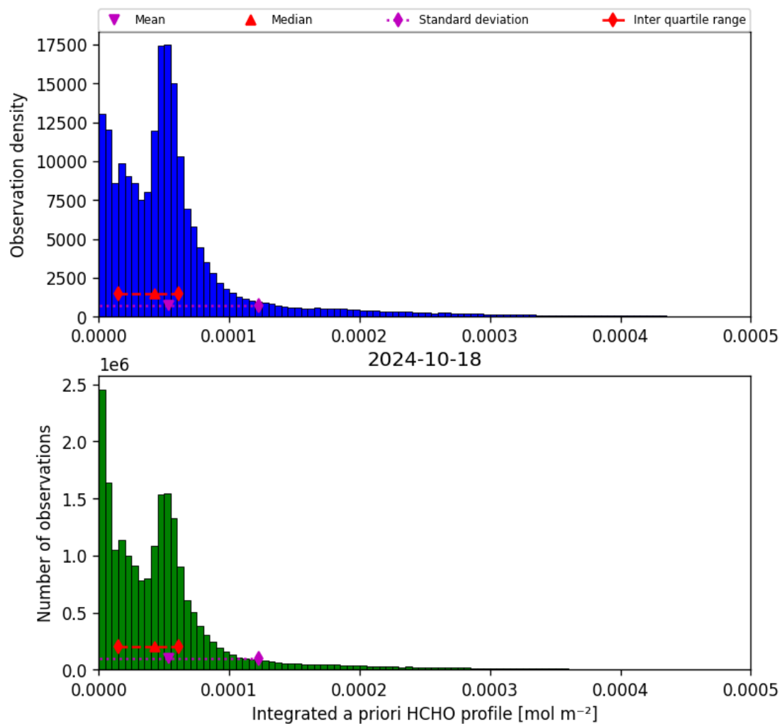
Figure 43: Histogram of “Integrated a priori HCHO profile” for 2024-10-17 to 2024-10-19
