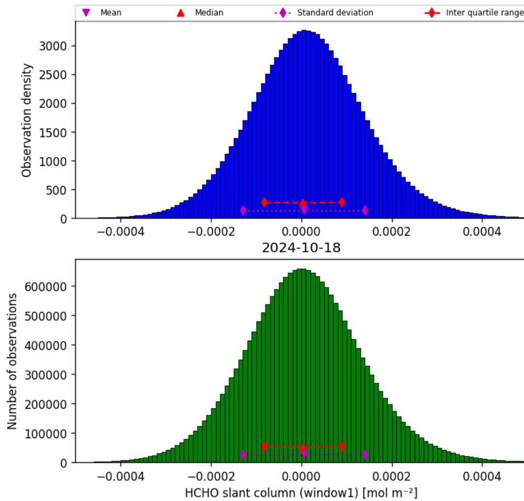
Figure 38: Histogram of “HCHO slant column (window1)” for 2024-10-17 to 2024-10-19
