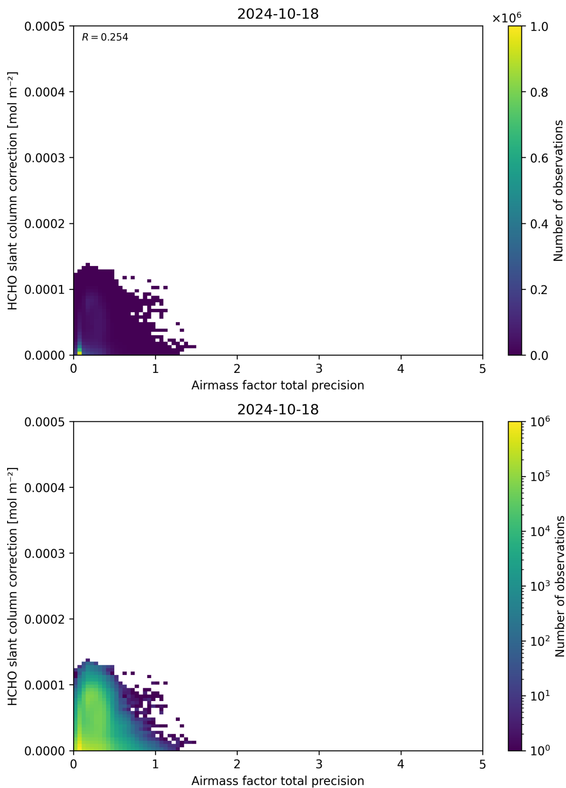
Figure 110: Scatter density plot of “Airmass factor total precision” against “HCHO slant column correction” for 2024-10-17 to 2024-10-19.
