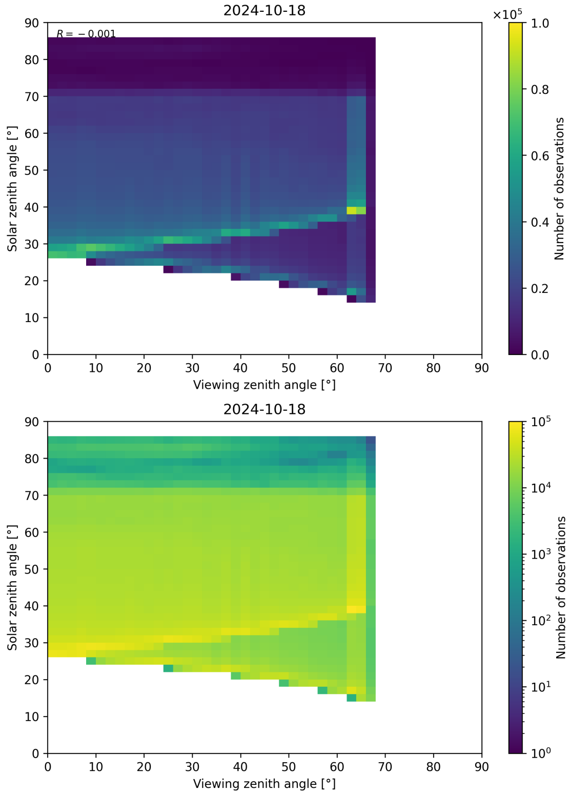
Figure 197: Scatter density plot of “Viewing zenith angle” against “Solar zenith angle” for 2024-10-17 to 2024-10-19.
