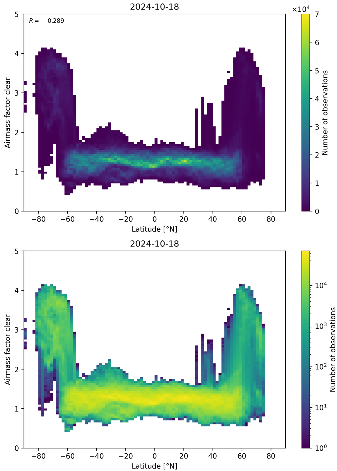
Figure 156: Scatter density plot of “Latitude” against “Airmass factor clear” for 2024-10-17 to 2024-10-19.
