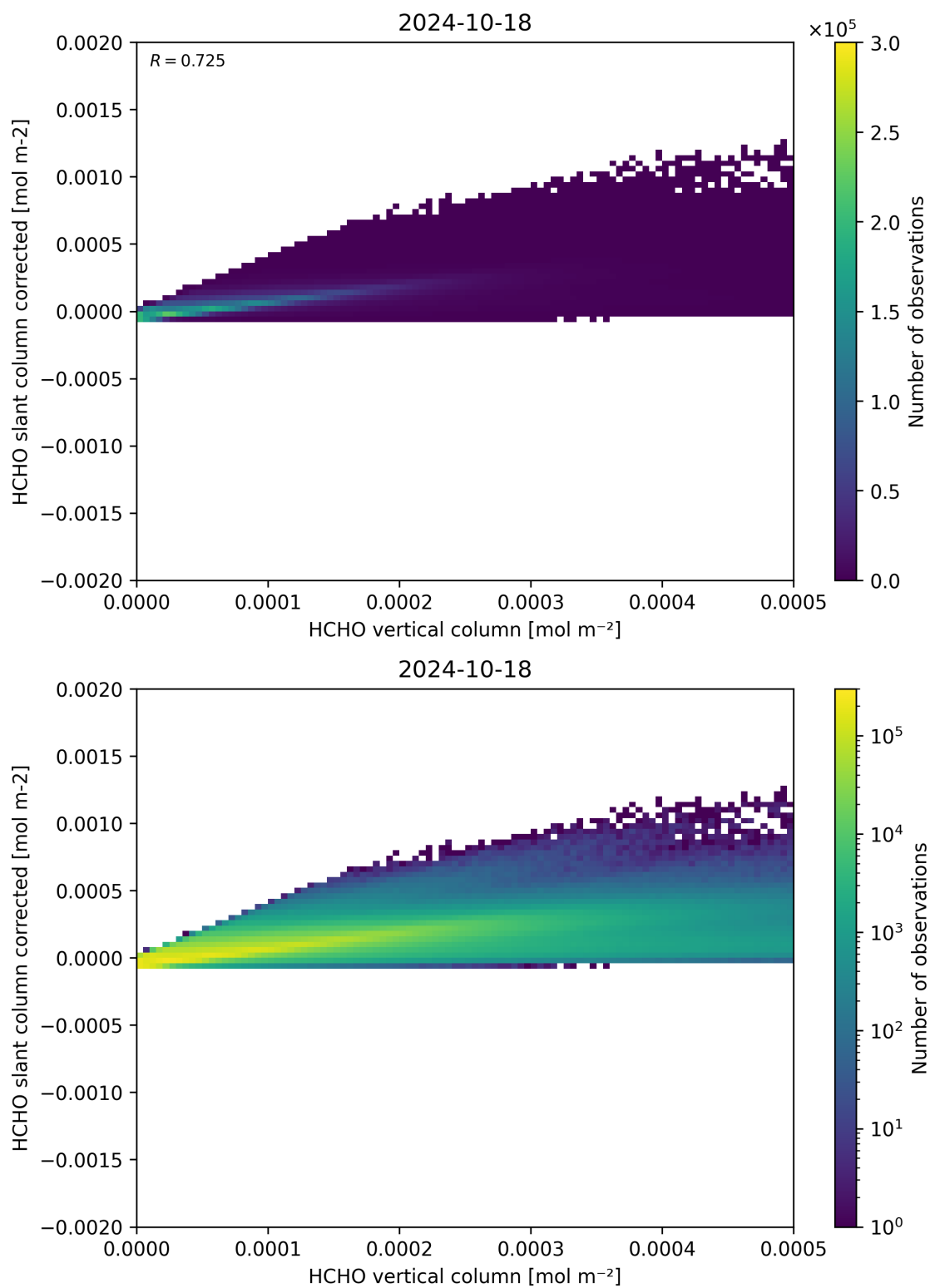
Figure 127: Scatter density plot of “HCHO vertical column” against “HCHO slant column corrected” for 2024-10-17 to 2024-10-19.
