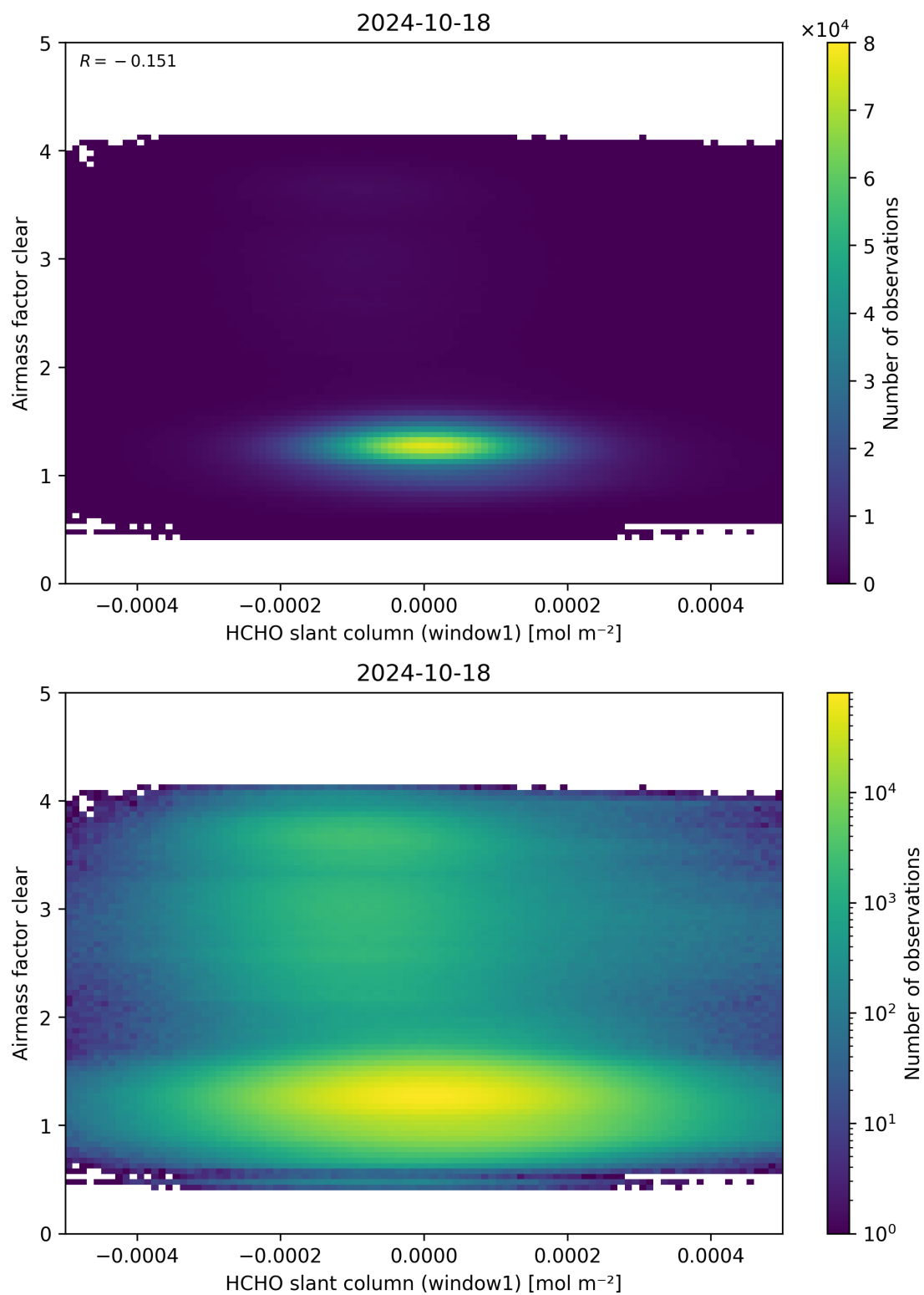
Figure 81: Scatter density plot of “HCHO slant column (window1)” against “Airmass factor clear” for 2024-10-17 to 2024-10-19.
