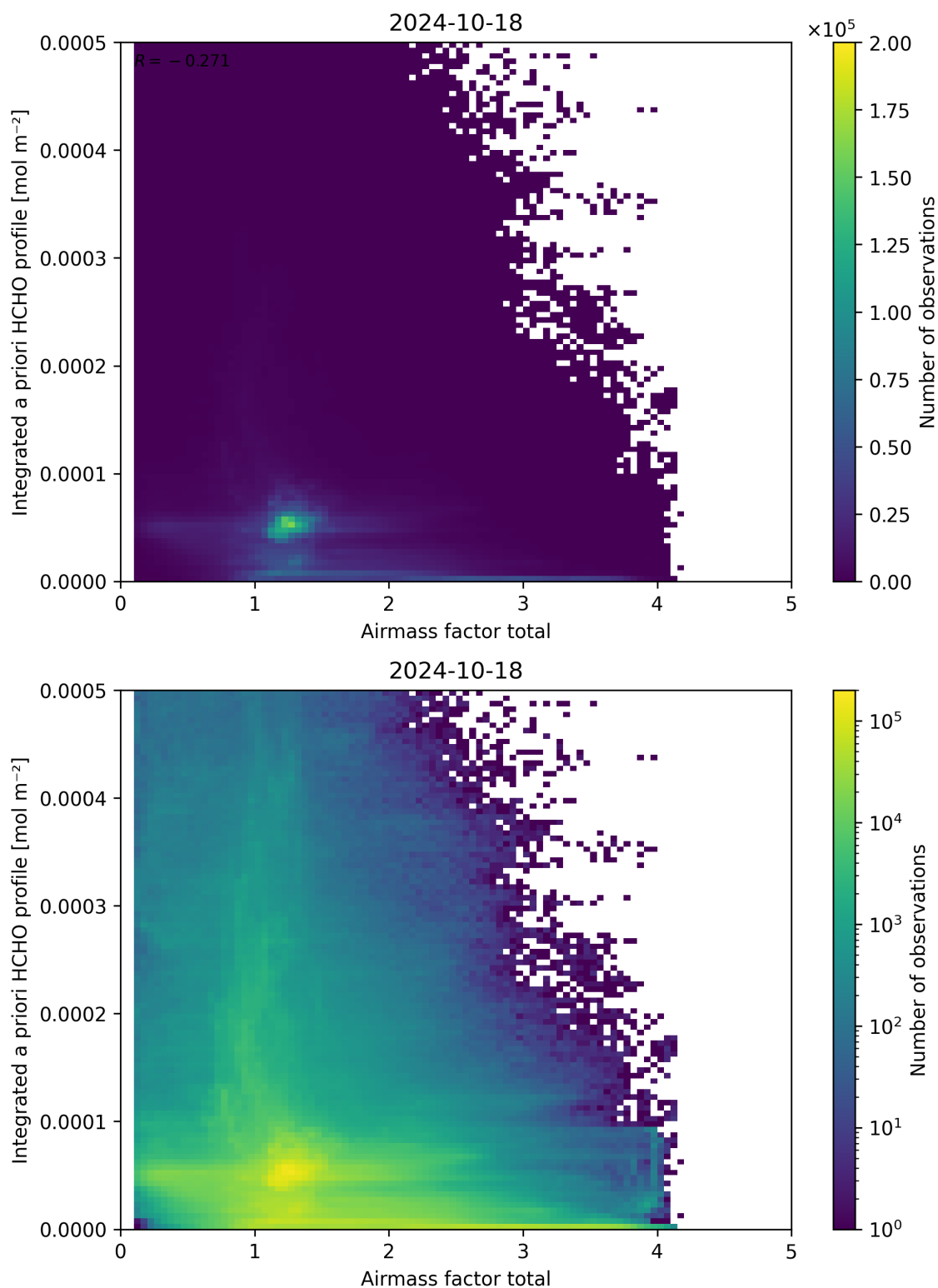
Figure 104: Scatter density plot of “Airmass factor total” against “Integrated a priori HCHO profile” for 2024-10-17 to 2024-10-19.
