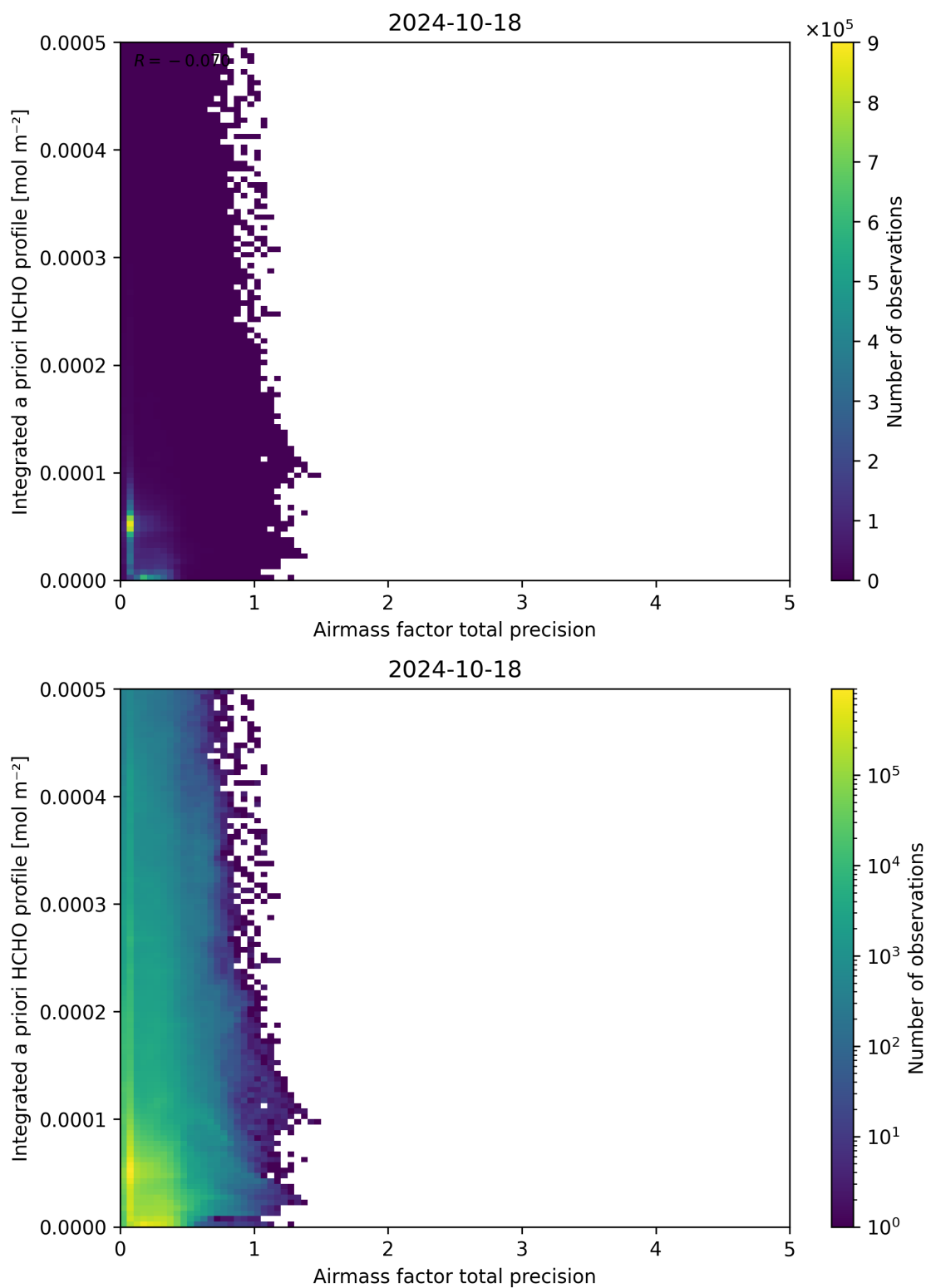
Figure 111: Scatter density plot of “Airmass factor total precision” against “Integrated a priori HCHO profile” for 2024-10-17 to 2024-10-19.
