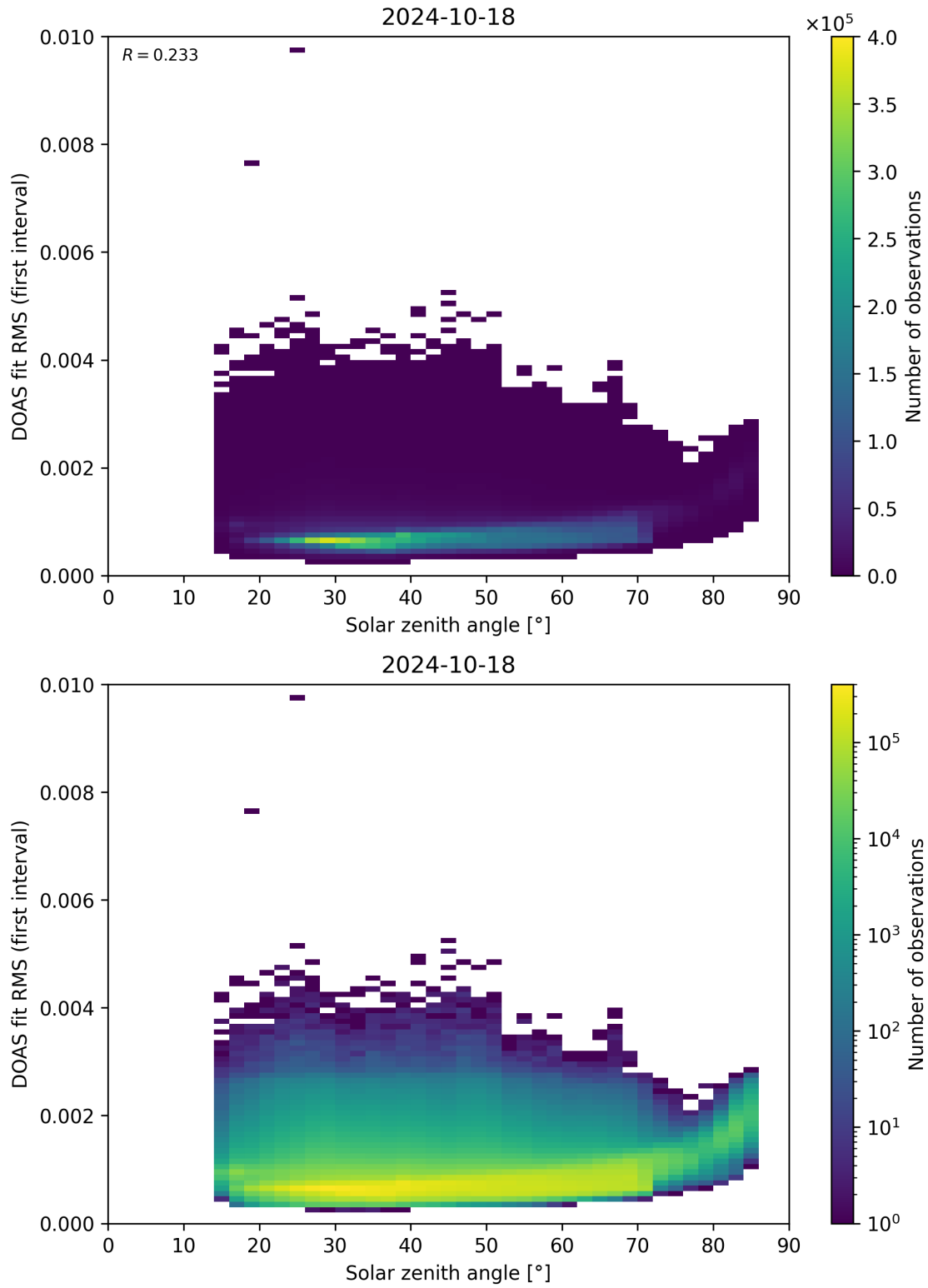
Figure 167: Scatter density plot of “Solar zenith angle” against “DOAS fit RMS (first interval)” for 2024-10-17 to 2024-10-19.
