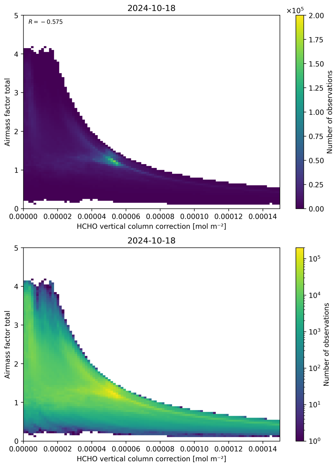
Figure 120: Scatter density plot of “HCHO vertical column correction” against “Airmass factor total” for 2024-10-17 to 2024-10-19.
