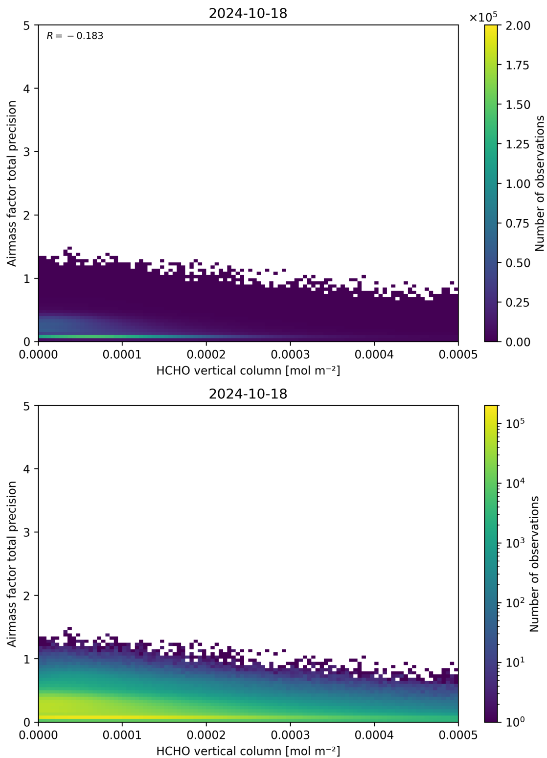
Figure 132: Scatter density plot of “HCHO vertical column” against “Airmass factor total precision” for 2024-10-17 to 2024-10-19.
