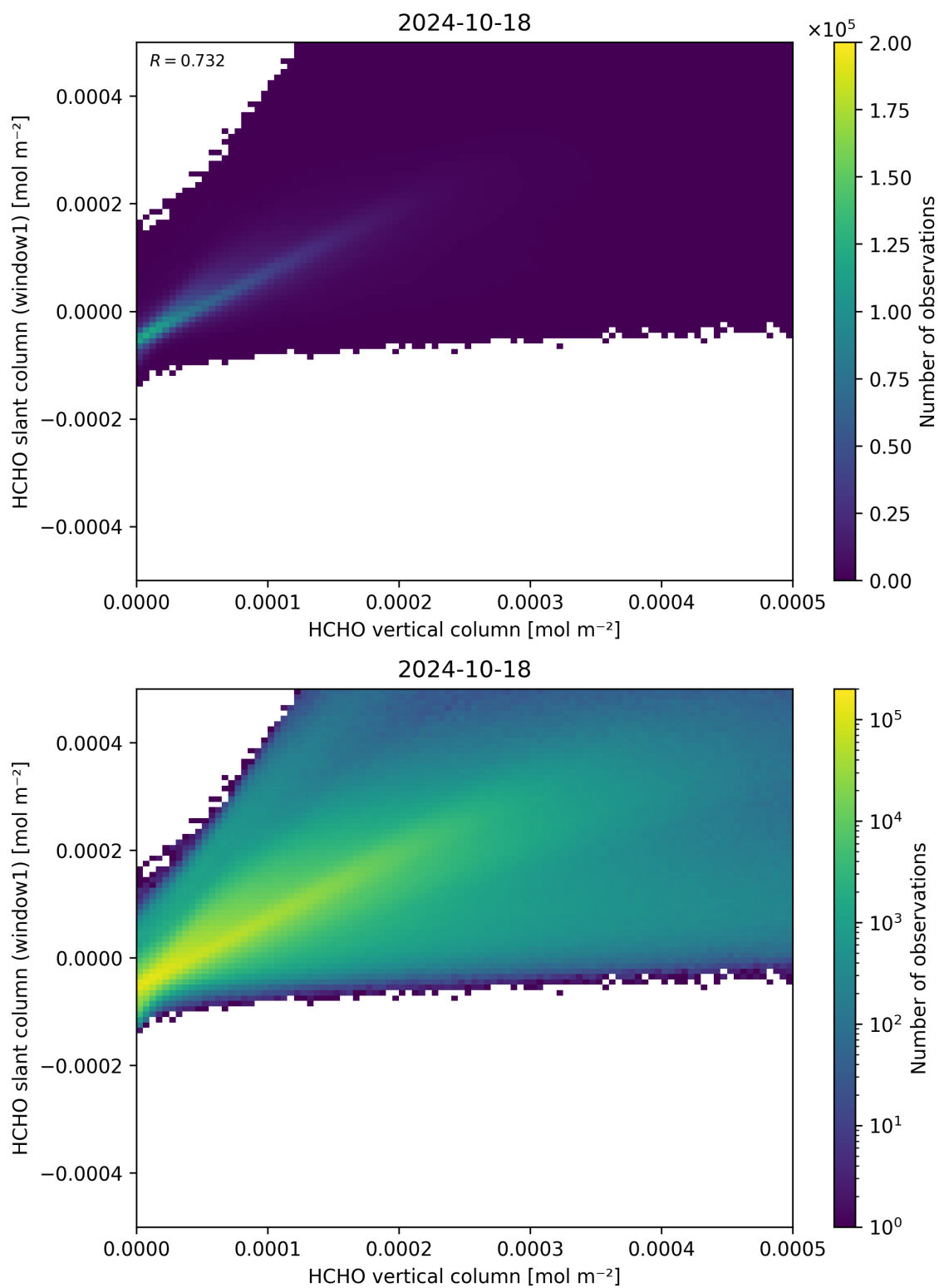
Figure 129: Scatter density plot of “HCHO vertical column” against “HCHO slant column (window1)” for 2024-10-17 to 2024-10-19.
