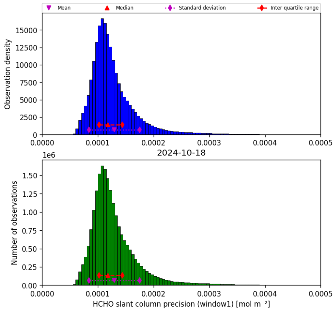
Figure 39: Histogram of “HCHO slant column precision (window1)” for 2024-10-17 to 2024-10-19
