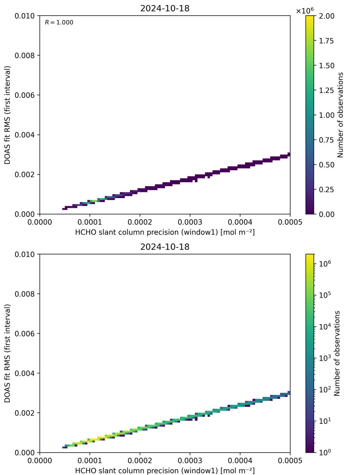
Figure 88: Scatter density plot of “HCHO slant column precision (window1)” against “DOAS fit RMS (first interval)” for 2024-10-17 to 2024-10-19.
