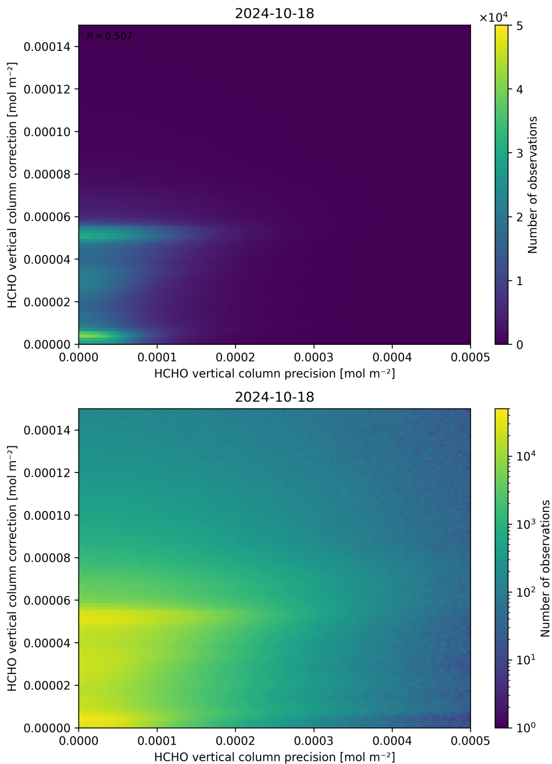
Figure 146: Scatter density plot of “HCHO vertical column precision” against “HCHO vertical column correction” for 2024-10-17 to 2024-10-19.
