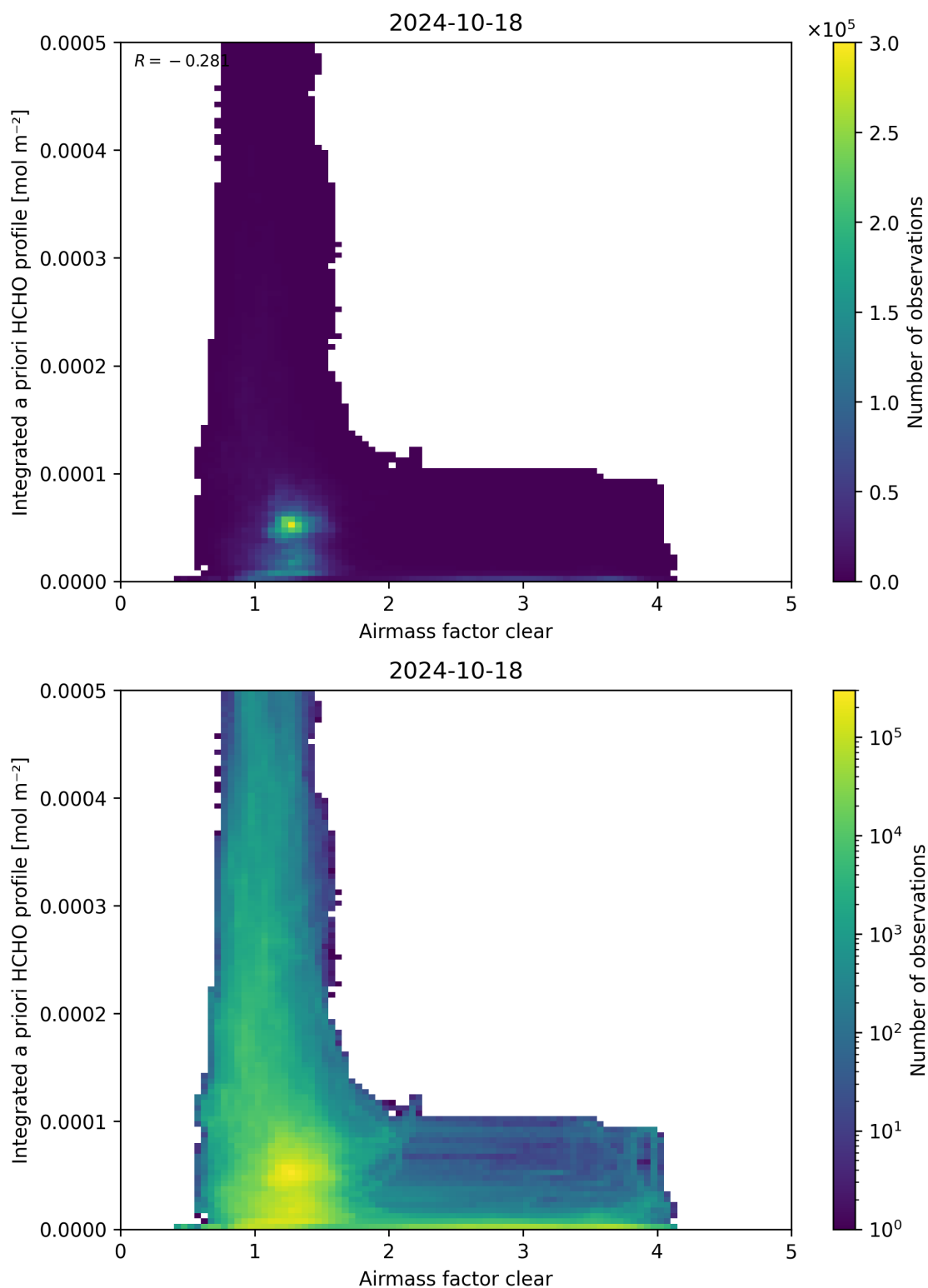
Figure 76: Scatter density plot of “Airmass factor clear” against “Integrated a priori HCHO profile” for 2024-10-17 to 2024-10-19.
