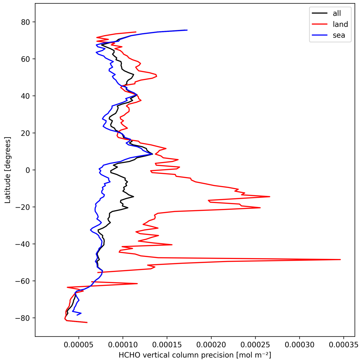
Figure 22: Zonal average of “HCHO vertical column precision” for 2024-10-17 to 2024-10-19.
