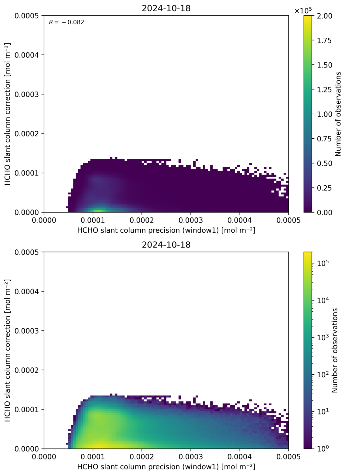
Figure 93: Scatter density plot of “HCHO slant column precision (window1)” against “HCHO slant column correction” for 2024-10-17 to 2024-10-19.
