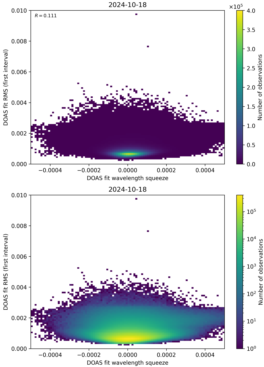
Figure 68: Scatter density plot of “DOAS fit wavelength squeeze” against “DOAS fit RMS (first interval)” for 2024-10-17 to 2024-10-19.
