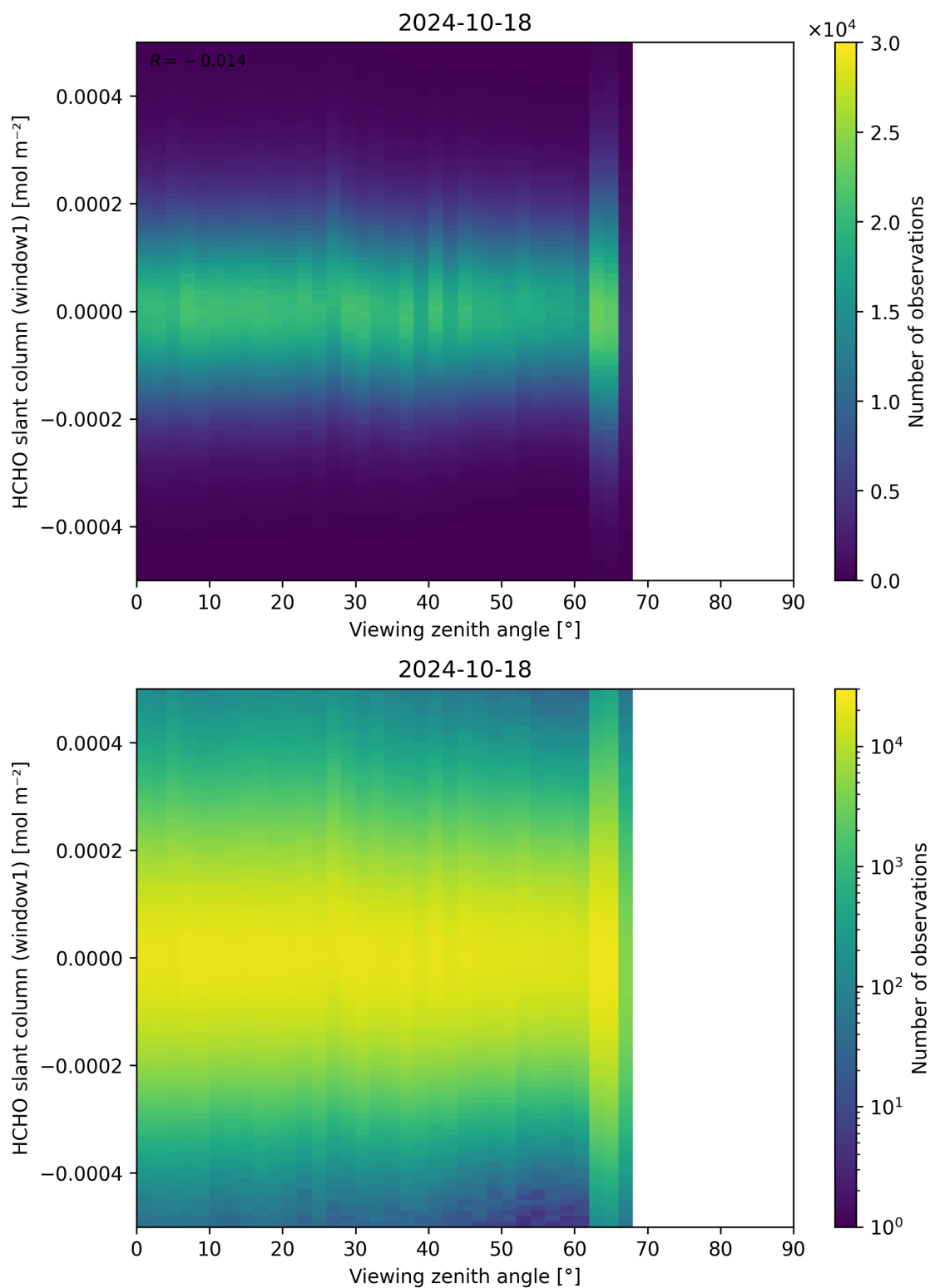
Figure 188: Scatter density plot of “Viewing zenith angle” against “HCHO slant column (window1)” for 2024-10-17 to 2024-10-19.
