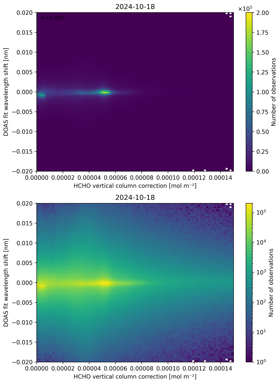
Figure 113: Scatter density plot of “HCHO vertical column correction” against “DOAS fit wavelength shift” for 2024-10-17 to 2024-10-19.
