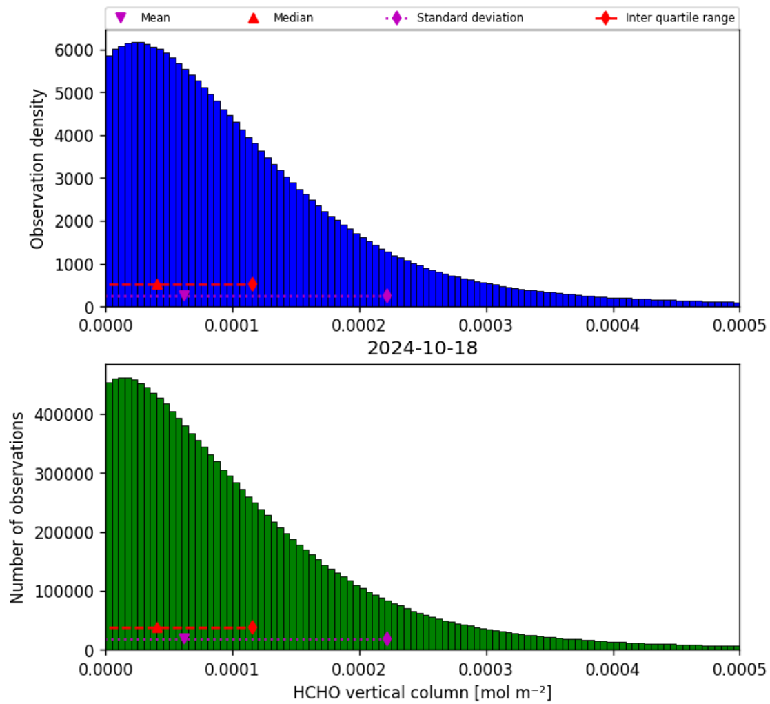
Figure 35: Histogram of “HCHO vertical column” for 2024-10-17 to 2024-10-19
