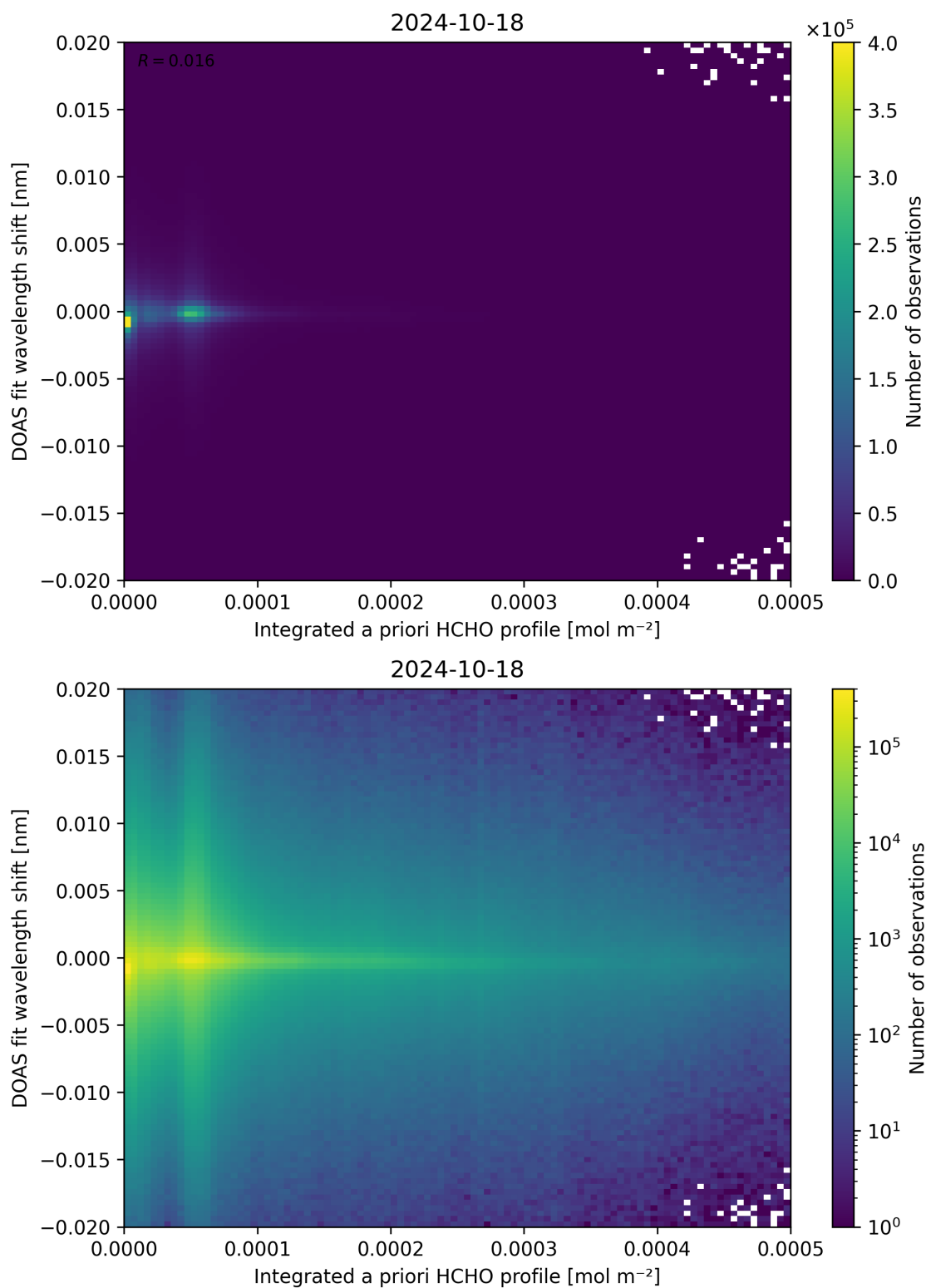
Figure 149: Scatter density plot of “Integrated a priori HCHO profile” against “DOAS fit wavelength shift” for 2024-10-17 to 2024-10-19.
