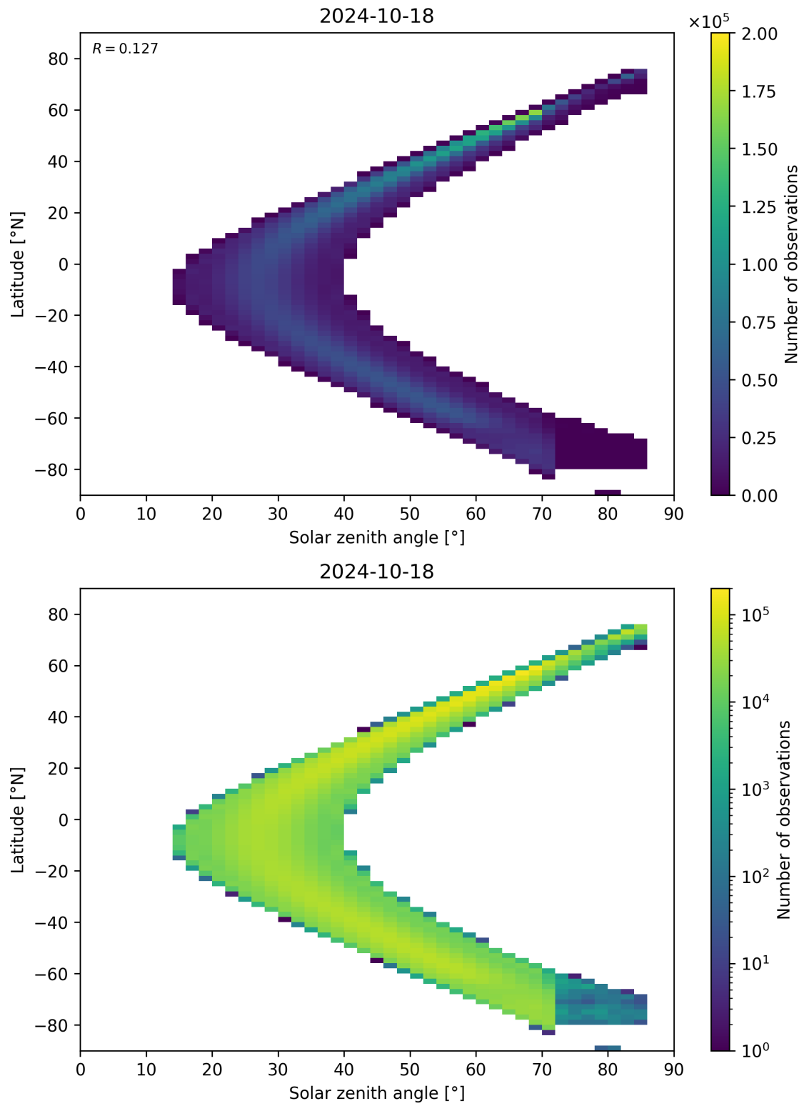
Figure 181: Scatter density plot of “Solar zenith angle” against “Latitude” for 2024-10-17 to 2024-10-19.
