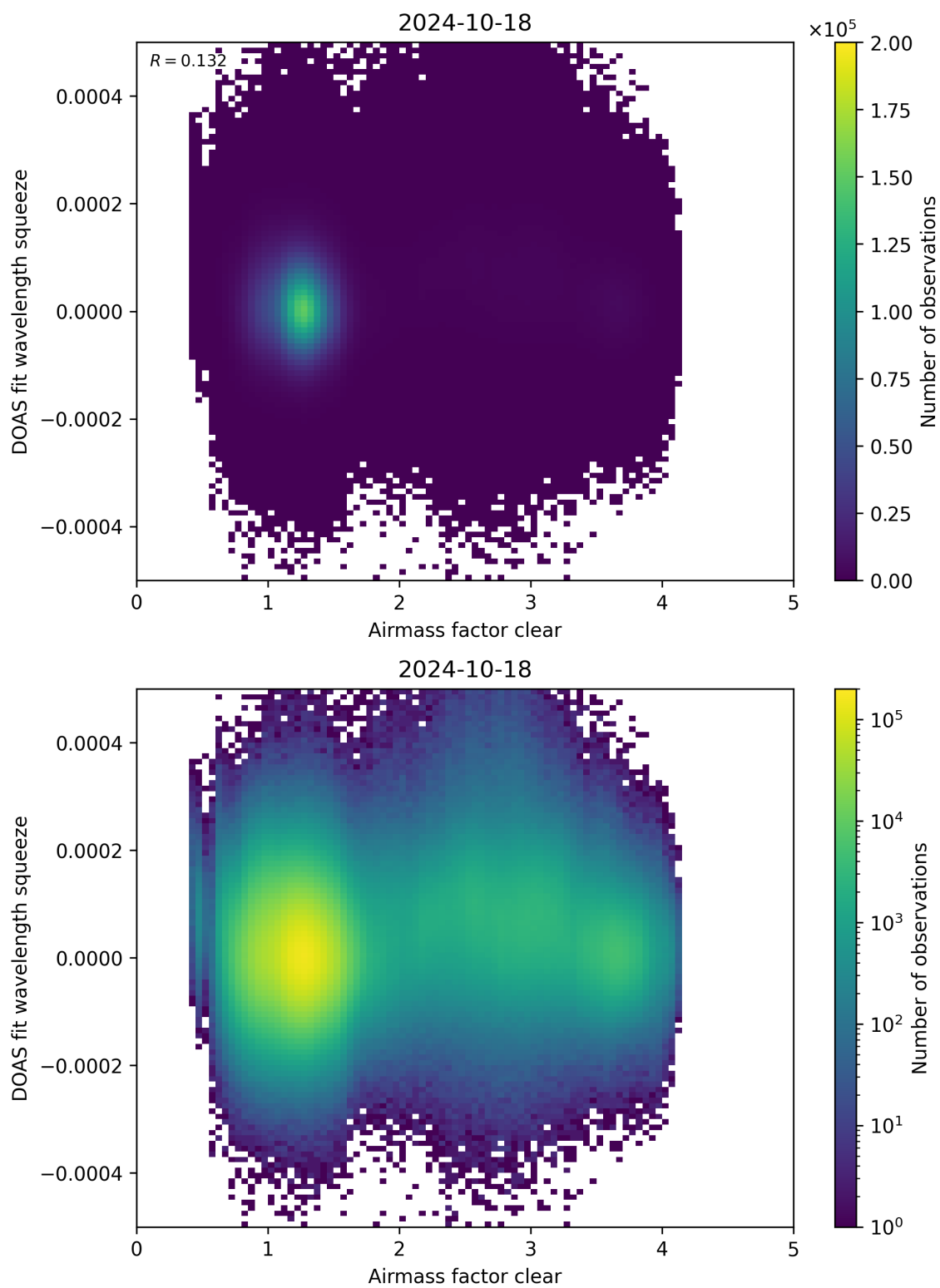
Figure 73: Scatter density plot of “Airmass factor clear” against “DOAS fit wavelength squeeze” for 2024-10-17 to 2024-10-19.
