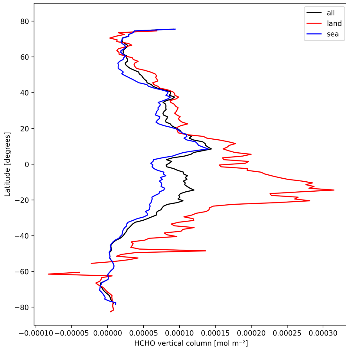
Figure 21: Zonal average of “HCHO vertical column” for 2024-10-17 to 2024-10-19.
