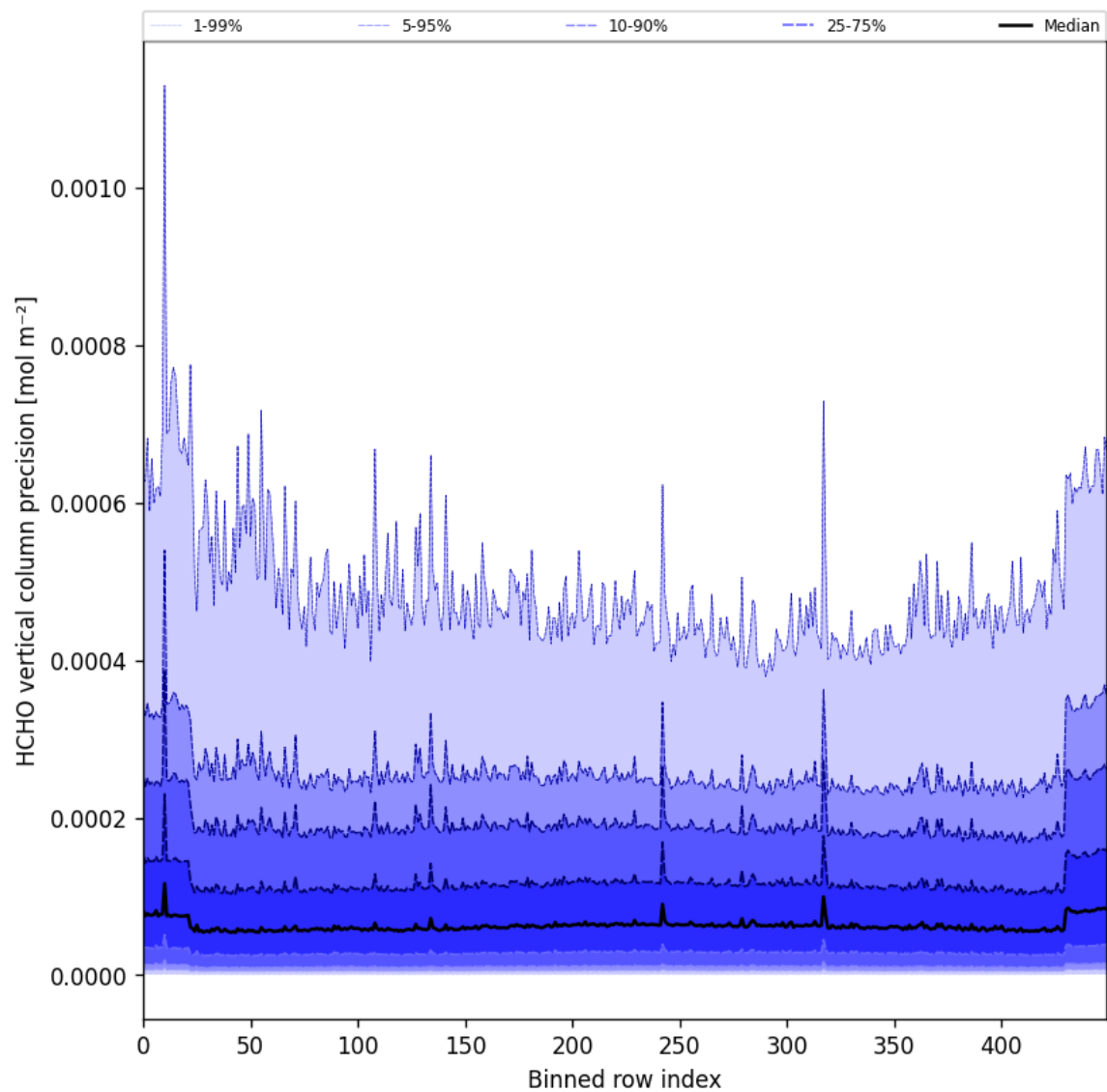
Figure 50: Along track statistics of “HCHO vertical column precision” for 2024-10-17 to 2024-10-19
