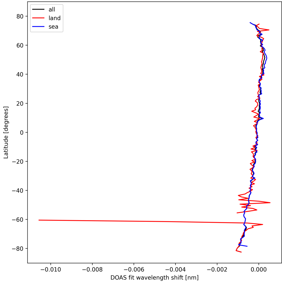
Figure 30: Zonal average of “DOAS fit wavelength shift” for 2024-10-17 to 2024-10-19.
