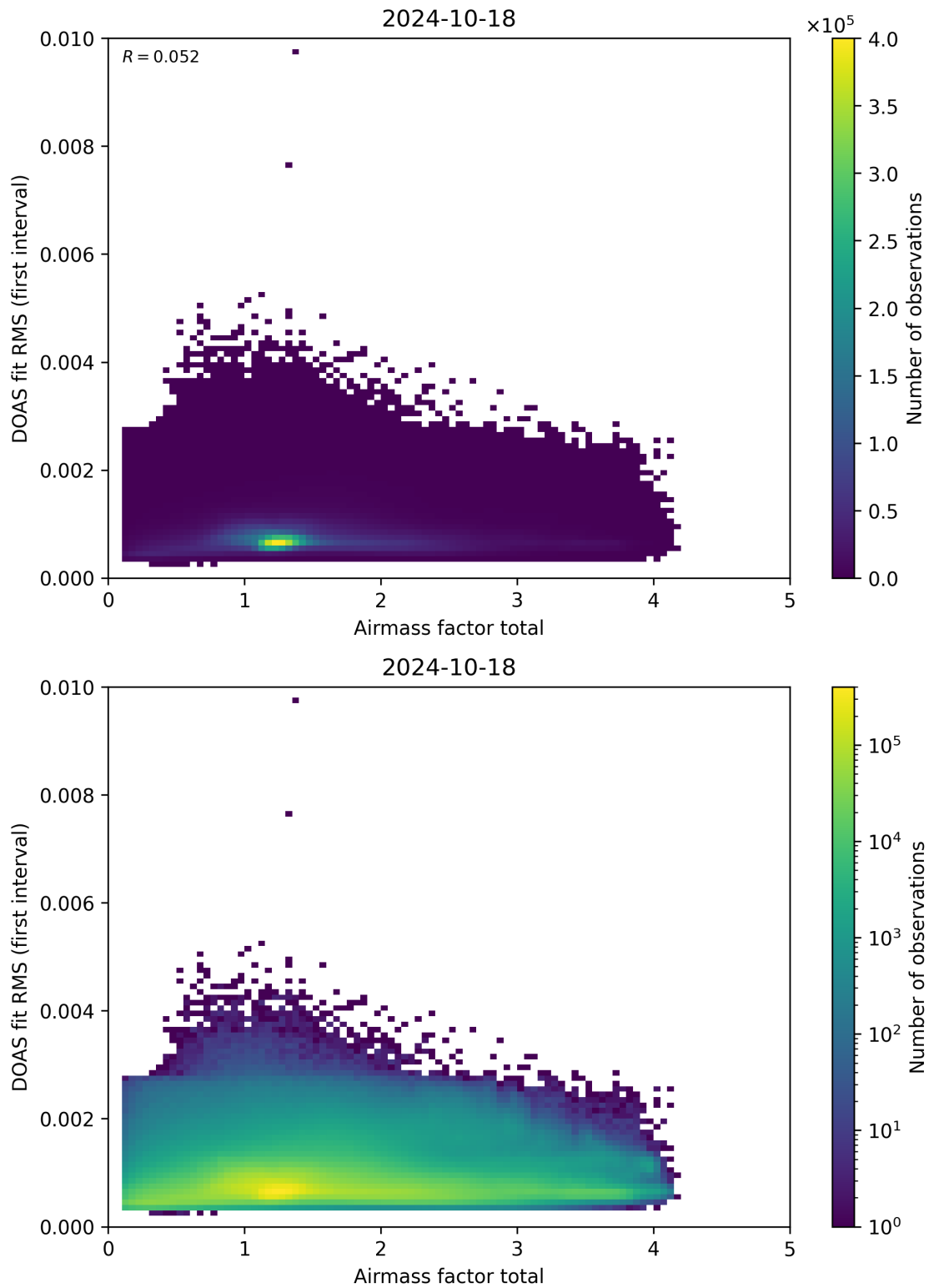
Figure 97: Scatter density plot of “Airmass factor total” against “DOAS fit RMS (first interval)” for 2024-10-17 to 2024-10-19.
