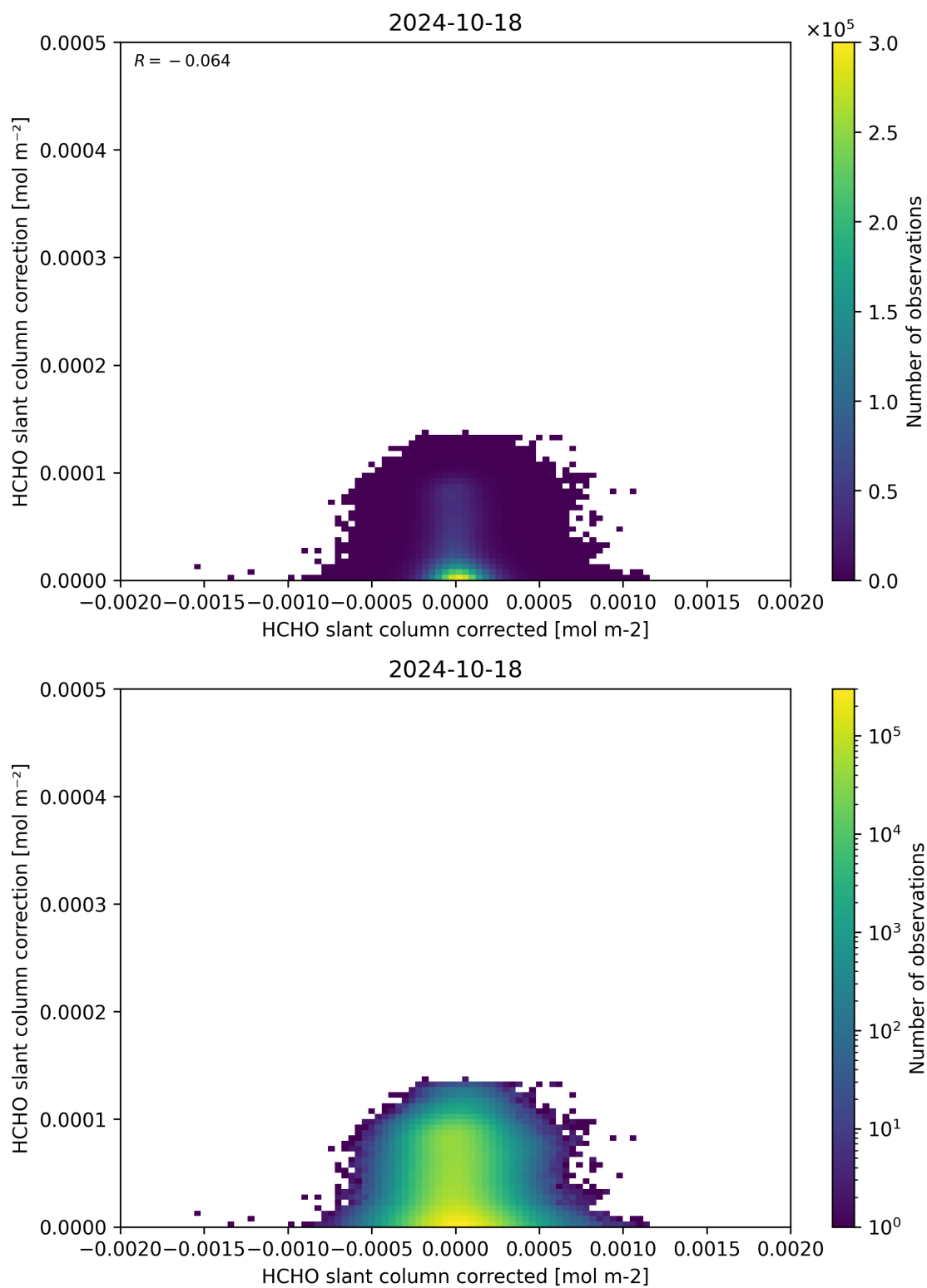
Figure 77: Scatter density plot of “HCHO slant column corrected” against “HCHO slant column correction” for 2024-10-17 to 2024-10-19.
