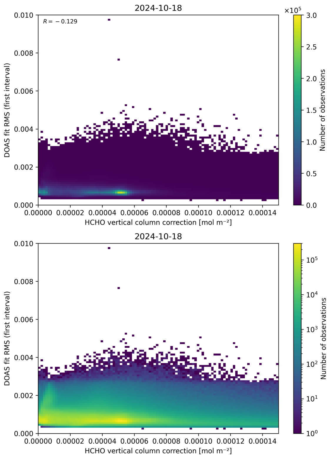
Figure 112: Scatter density plot of “HCHO vertical column correction” against “DOAS fit RMS (first interval)” for 2024-10-17 to 2024-10-19.
