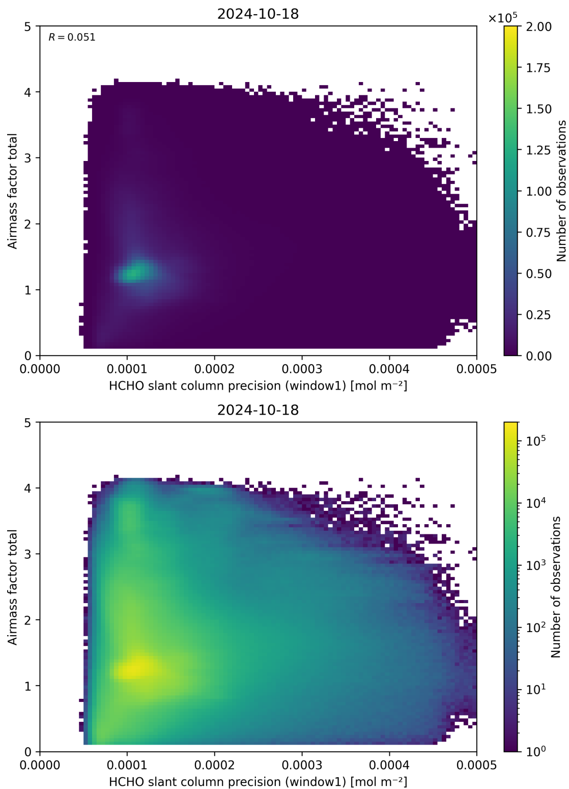
Figure 94: Scatter density plot of “HCHO slant column precision (window1)” against “Airmass factor total” for 2024-10-17 to 2024-10-19.
