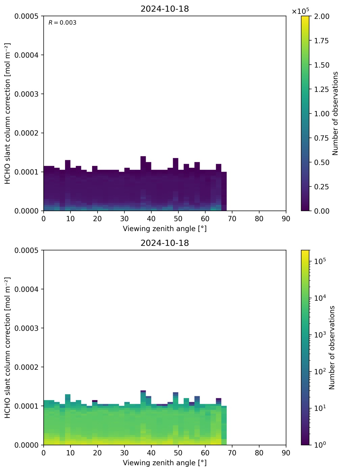
Figure 187: Scatter density plot of “Viewing zenith angle” against “HCHO slant column correction” for 2024-10-17 to 2024-10-19.
