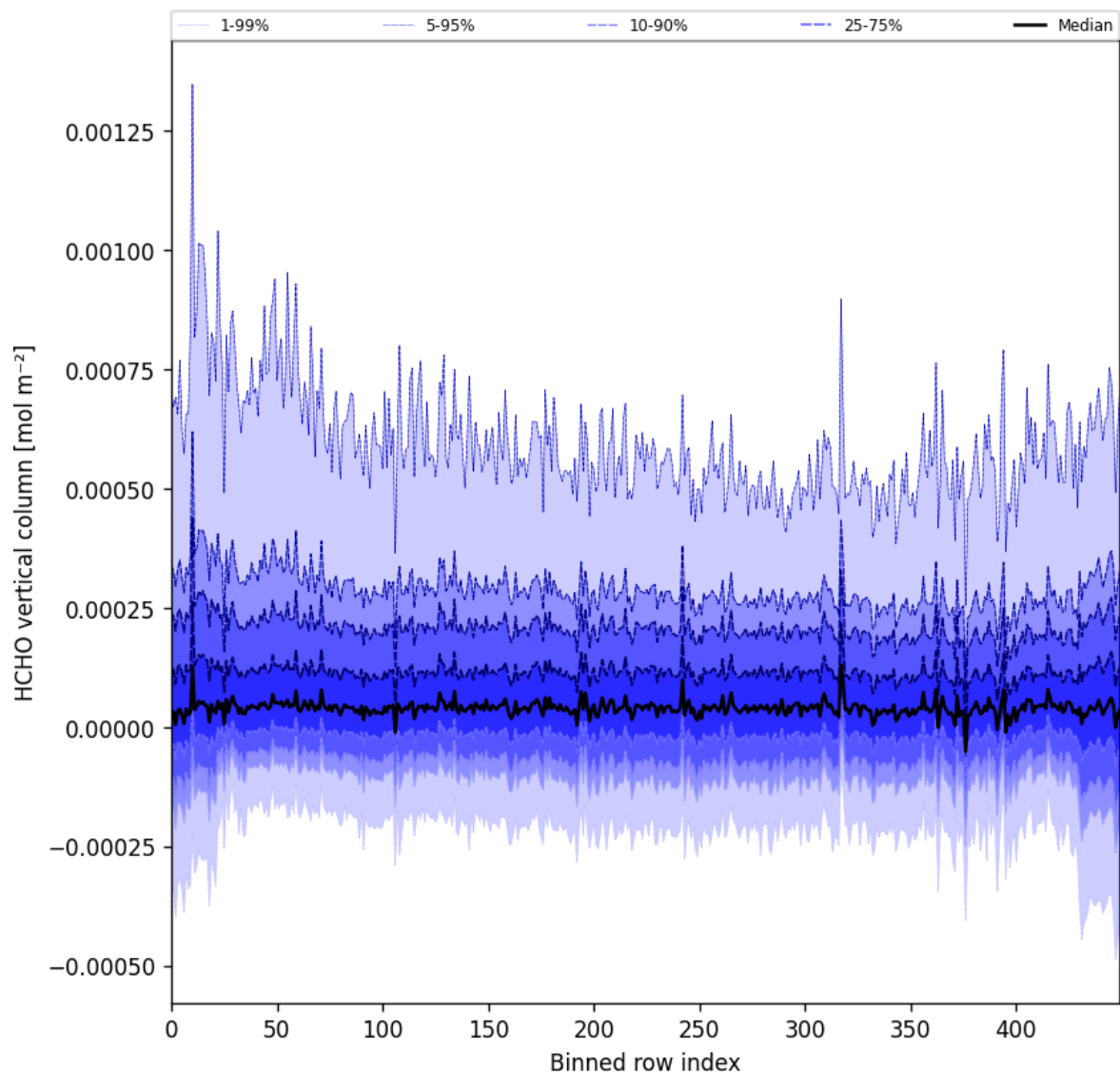
Figure 49: Along track statistics of “HCHO vertical column” for 2024-10-17 to 2024-10-19
