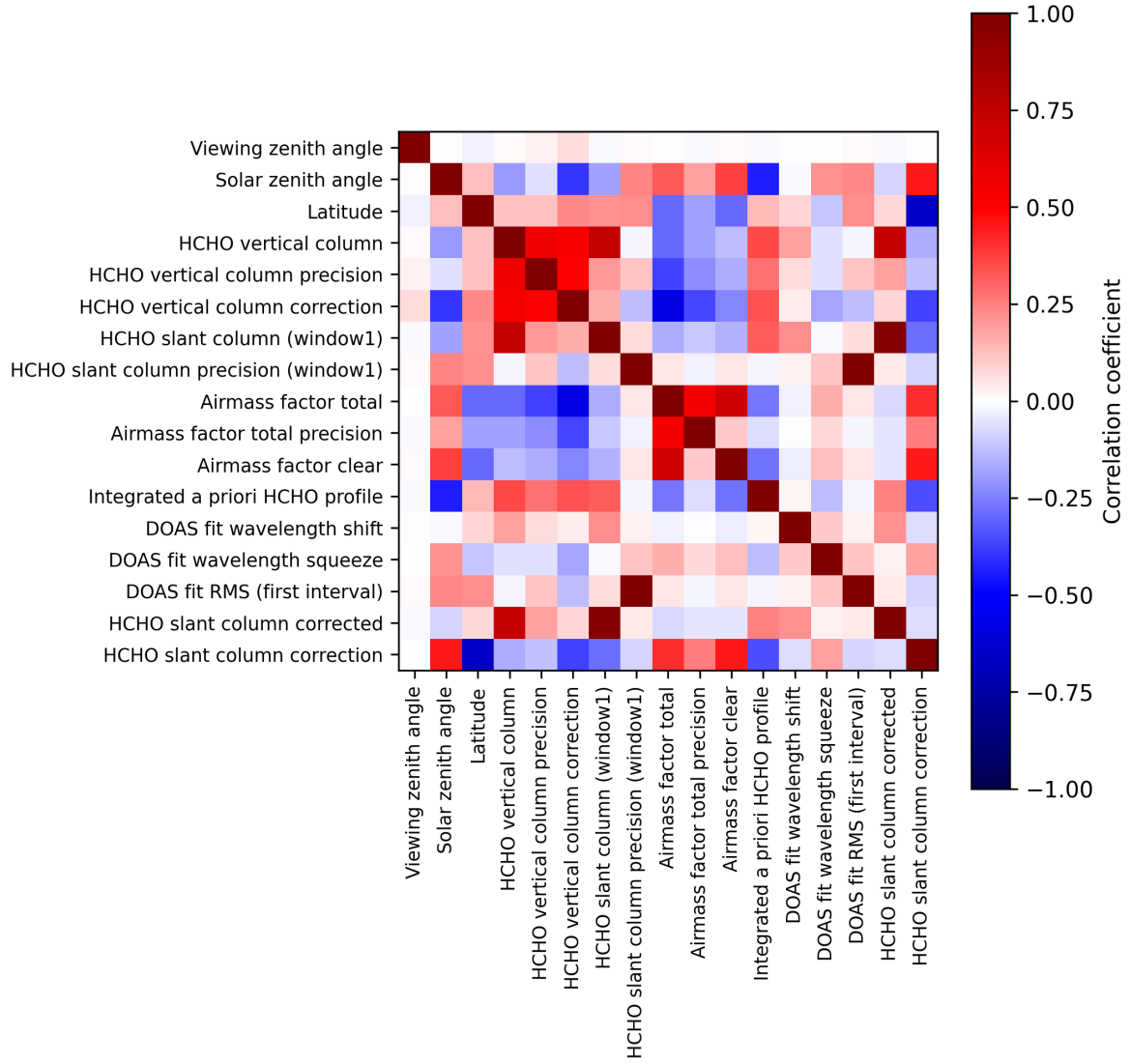
Figure 2: Map of correlation matrix for 2024-10-17 to 2024-10-19.
