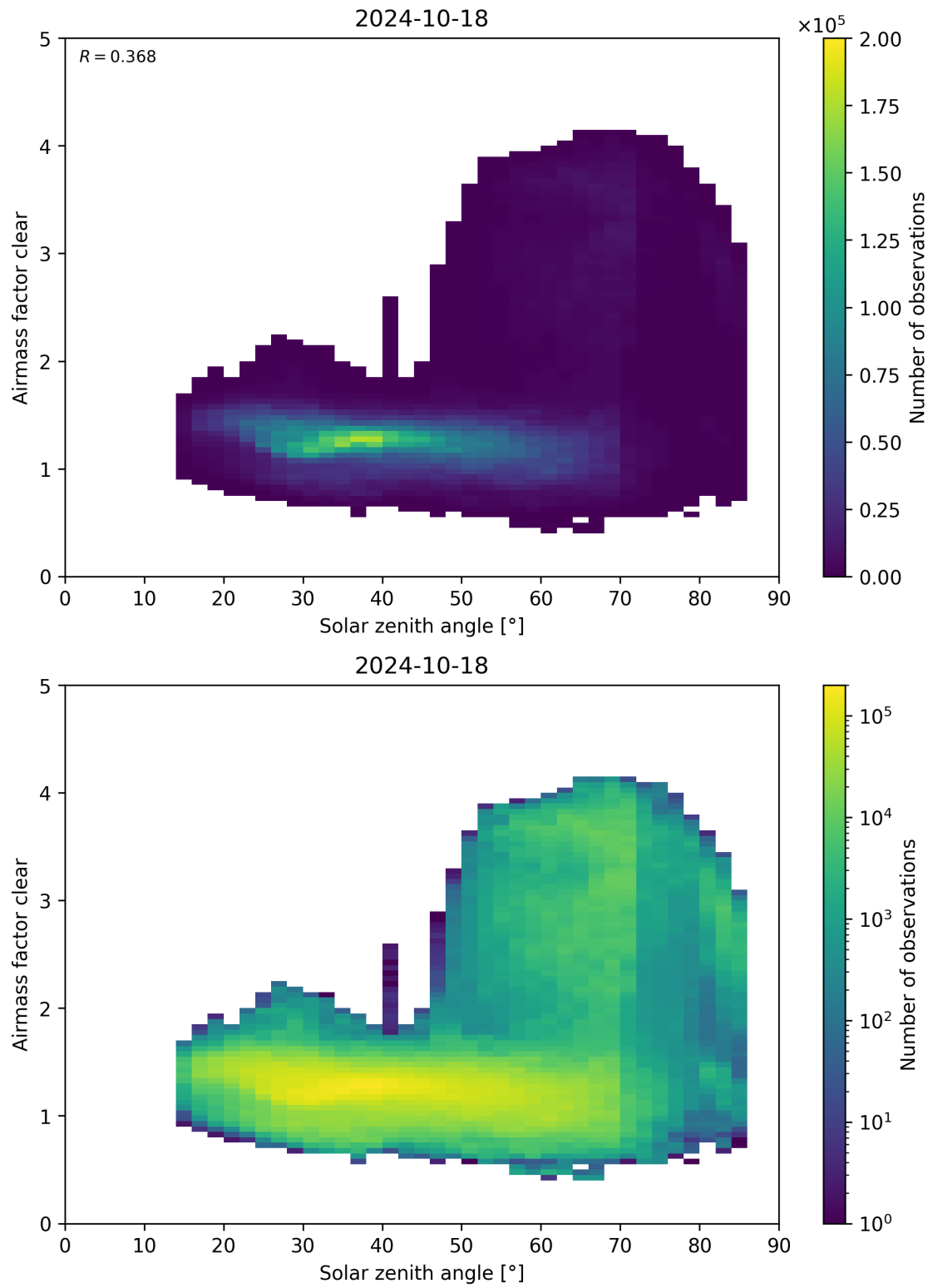
Figure 170: Scatter density plot of “Solar zenith angle” against “Airmass factor clear” for 2024-10-17 to 2024-10-19.
