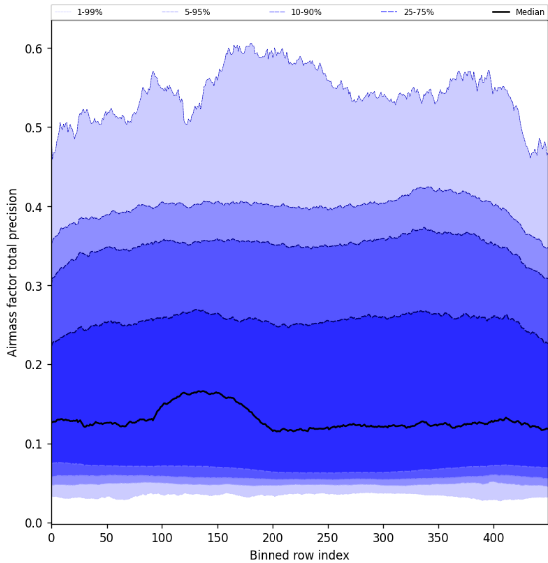
Figure 55: Along track statistics of “Airmass factor total precision” for 2024-10-17 to 2024-10-19
