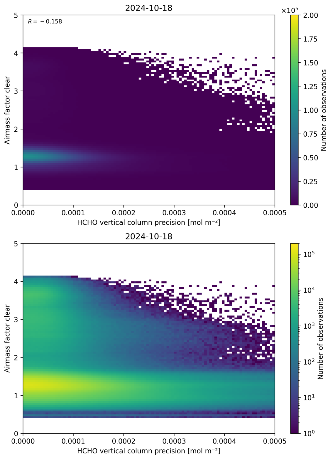
Figure 139: Scatter density plot of “HCHO vertical column precision” against “Airmass factor clear” for 2024-10-17 to 2024-10-19.
