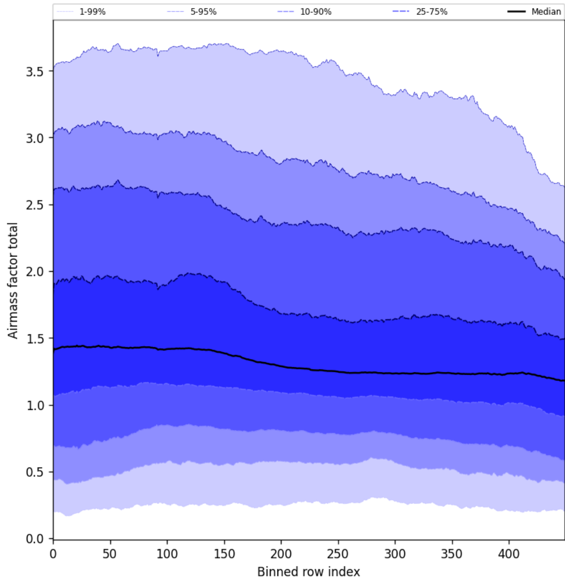
Figure 54: Along track statistics of “Airmass factor total” for 2024-10-17 to 2024-10-19
