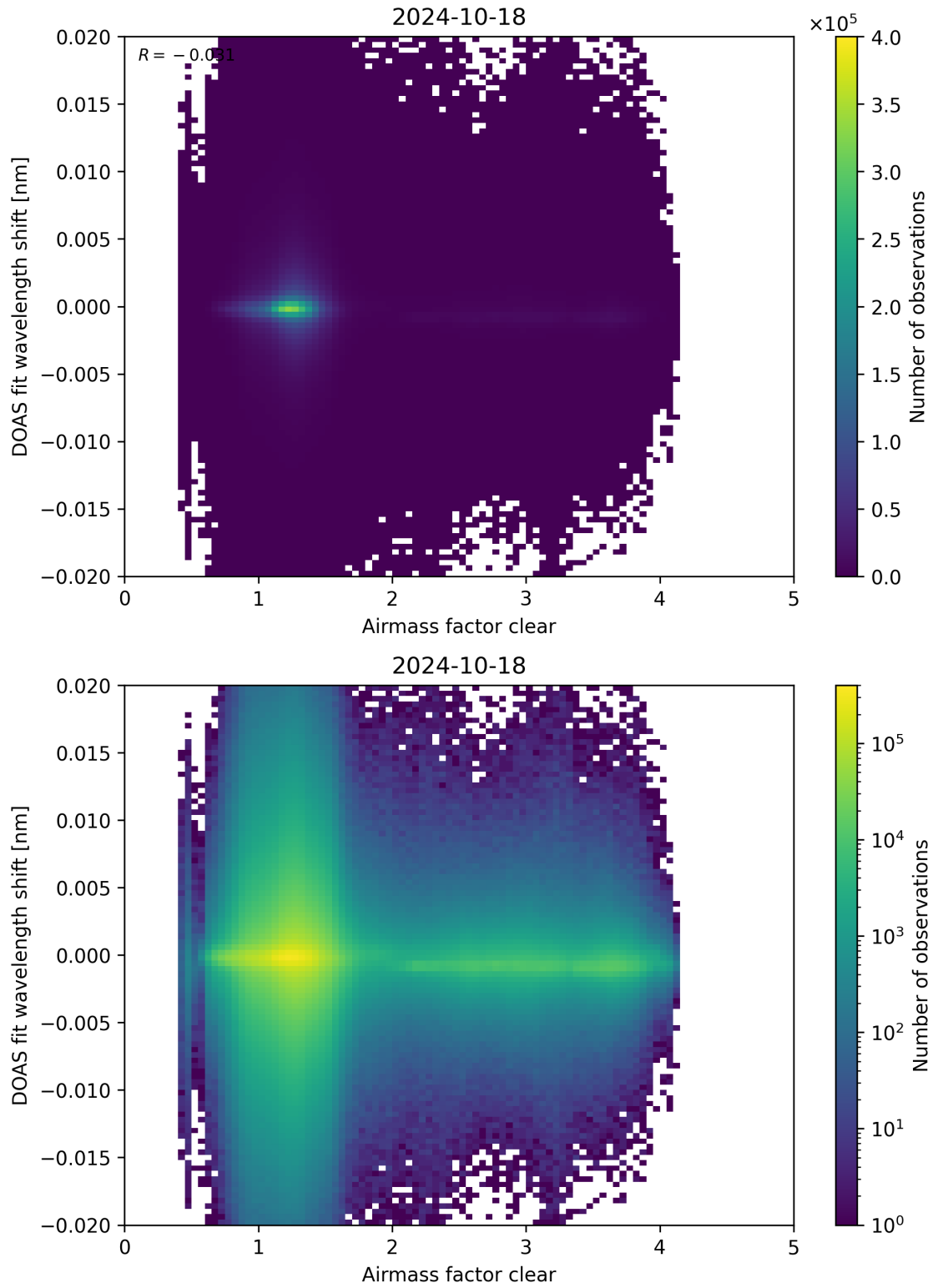
Figure 72: Scatter density plot of “Airmass factor clear” against “DOAS fit wavelength shift” for 2024-10-17 to 2024-10-19.
