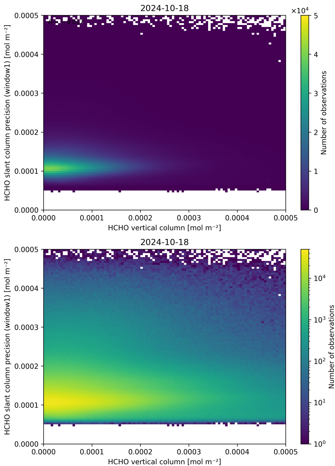
Figure 130: Scatter density plot of “HCHO vertical column” against “HCHO slant column precision (window1)” for 2024-10-17 to 2024-10-19.
