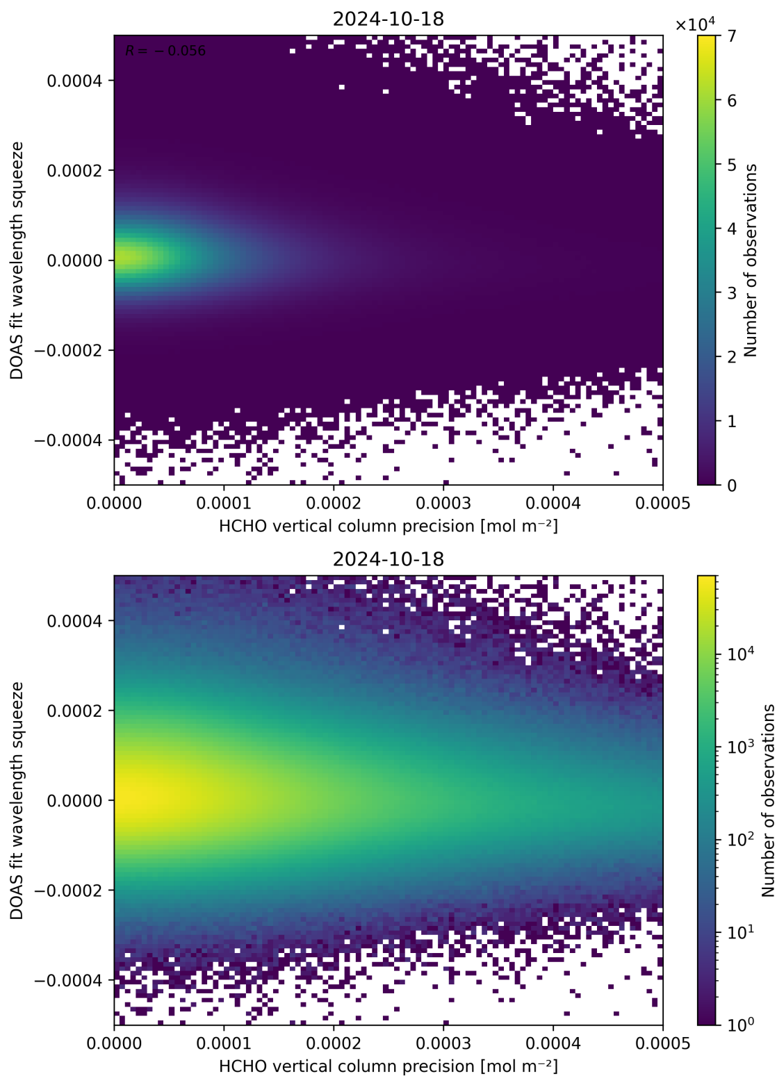
Figure 138: Scatter density plot of “HCHO vertical column precision” against “DOAS fit wavelength squeeze” for 2024-10-17 to 2024-10-19.
