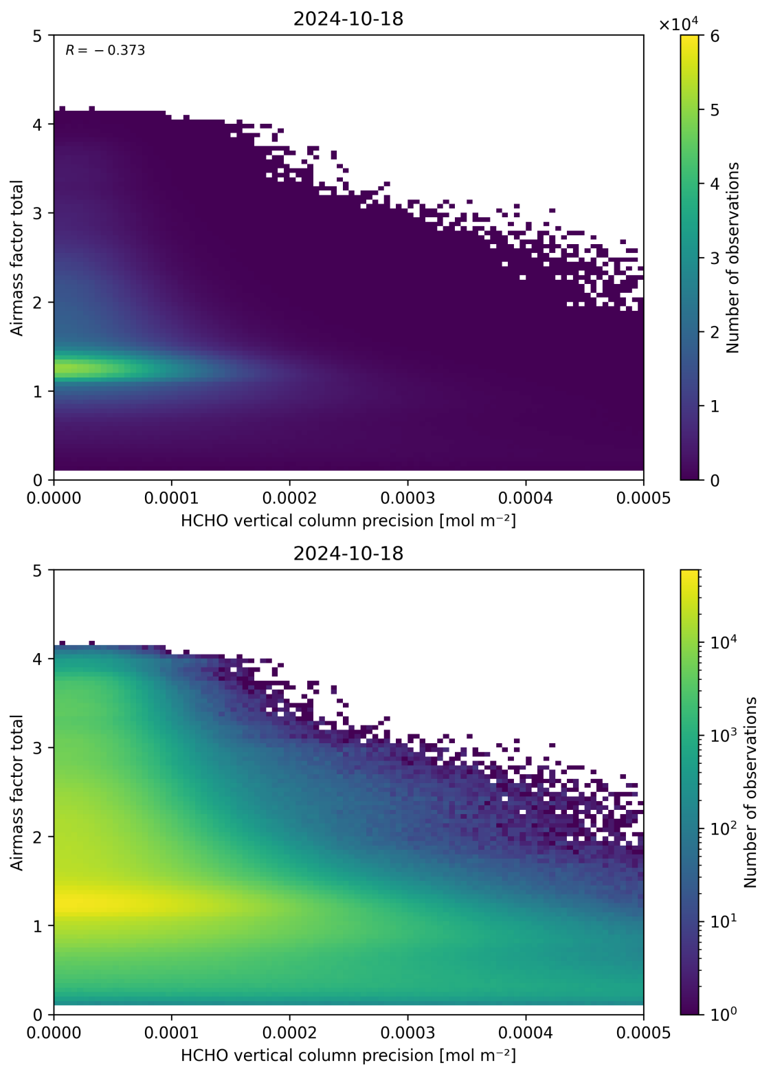
Figure 144: Scatter density plot of “HCHO vertical column precision” against “Airmass factor total” for 2024-10-17 to 2024-10-19.
