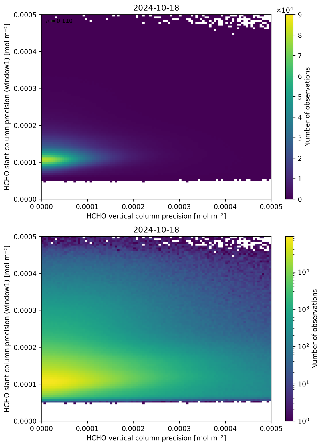
Figure 143: Scatter density plot of “HCHO vertical column precision” against “HCHO slant column precision (window1)” for 2024-10-17 to 2024-10-19.
