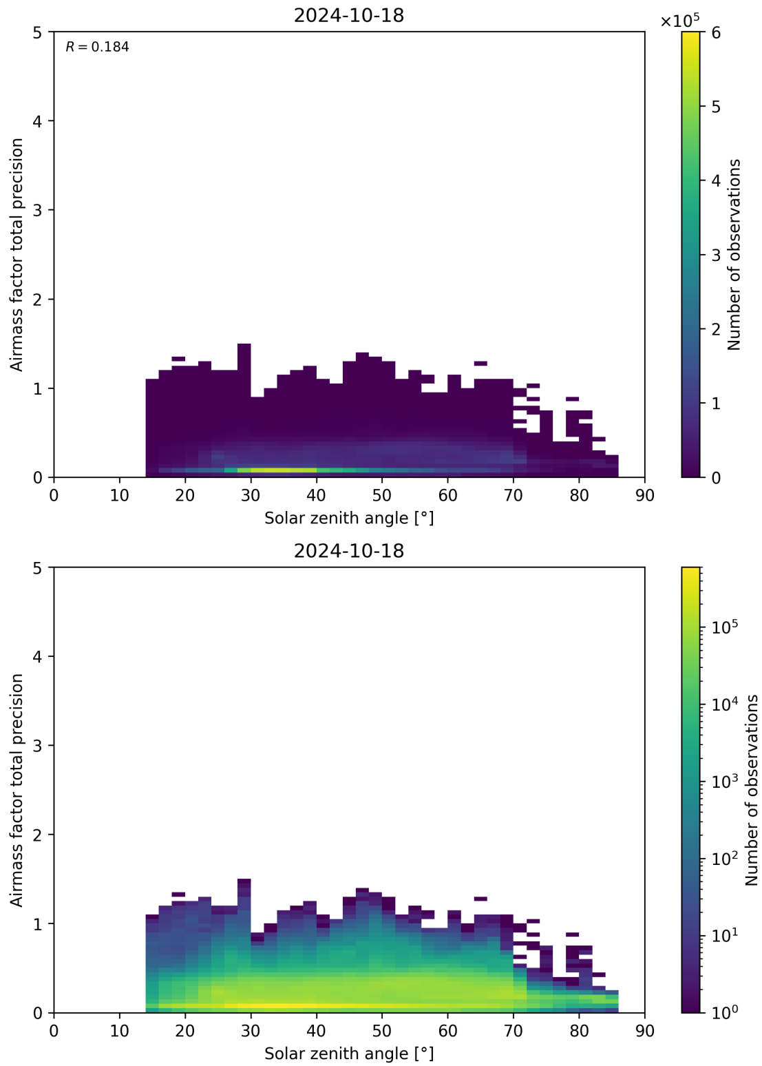
Figure 176: Scatter density plot of “Solar zenith angle” against “Airmass factor total precision” for 2024-10-17 to 2024-10-19.
