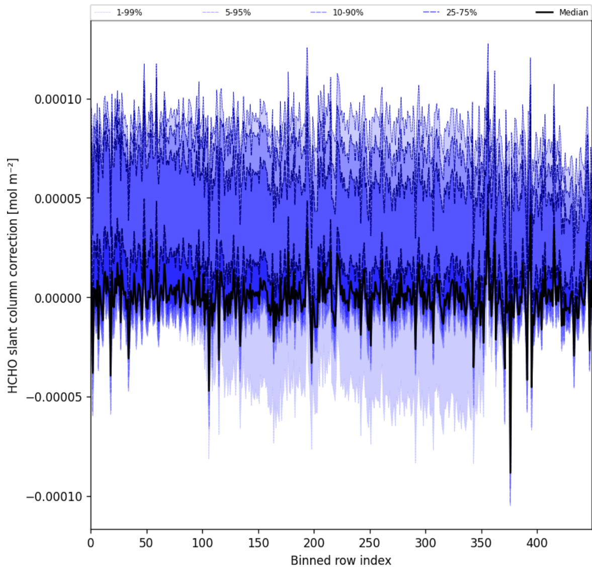
Figure 61: Along track statistics of “HCHO slant column correction” for 2024-10-17 to 2024-10-19
