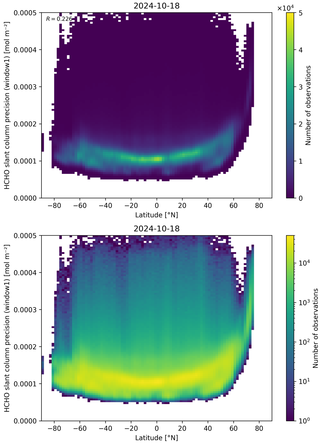
Figure 160: Scatter density plot of “Latitude” against “HCHO slant column precision (window1)” for 2024-10-17 to 2024-10-19.
