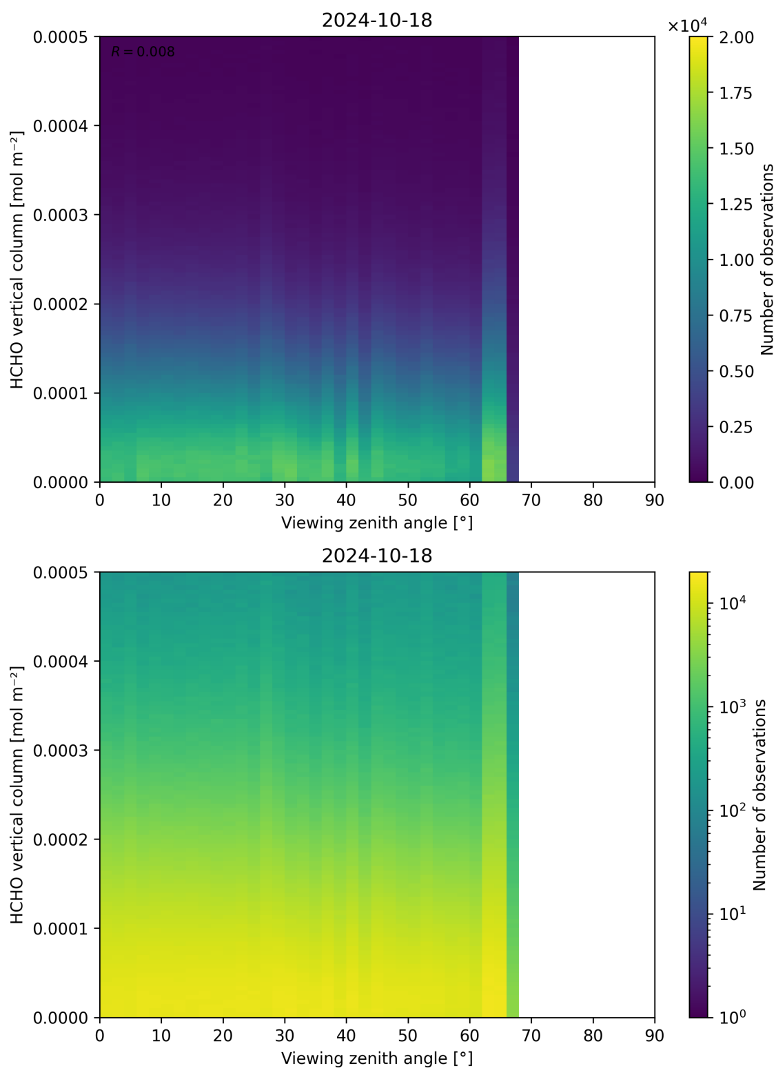
Figure 192: Scatter density plot of “Viewing zenith angle” against “HCHO vertical column” for 2024-10-17 to 2024-10-19.
