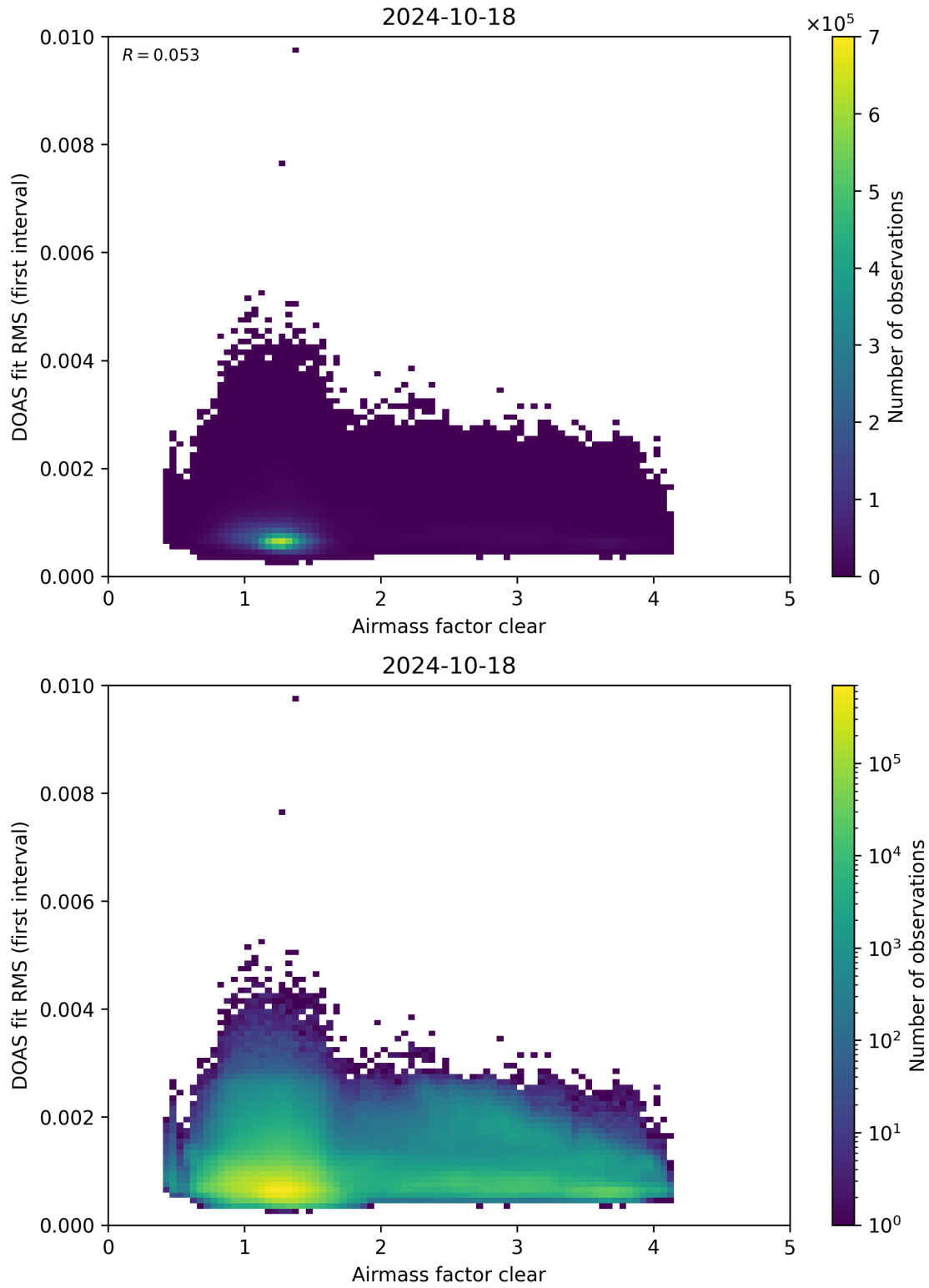
Figure 71: Scatter density plot of “Airmass factor clear” against “DOAS fit RMS (first interval)” for 2024-10-17 to 2024-10-19.
