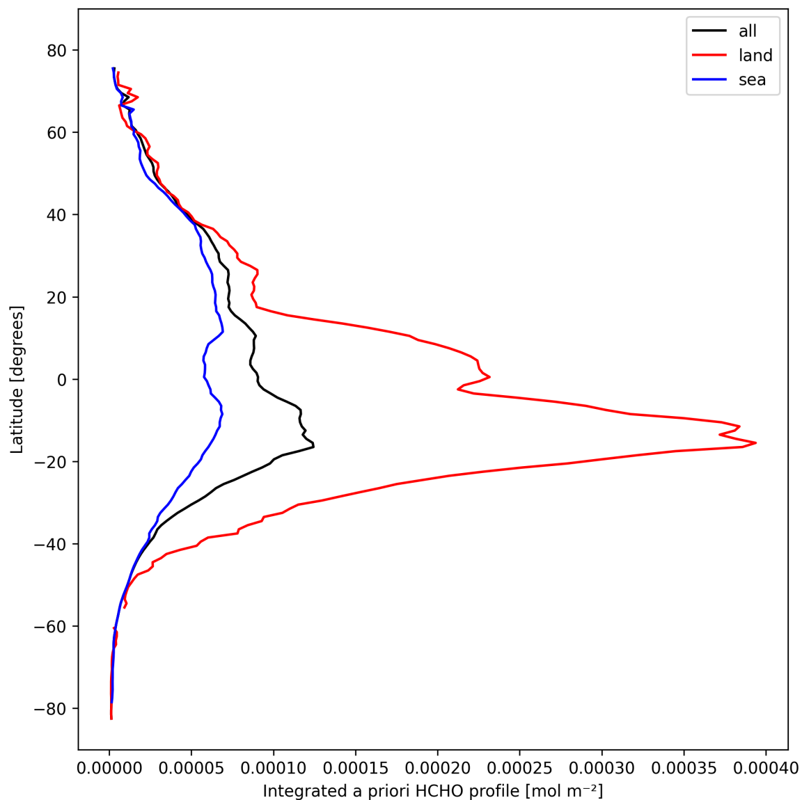
Figure 29: Zonal average of “Integrated a priori HCHO profile” for 2024-10-17 to 2024-10-19.
