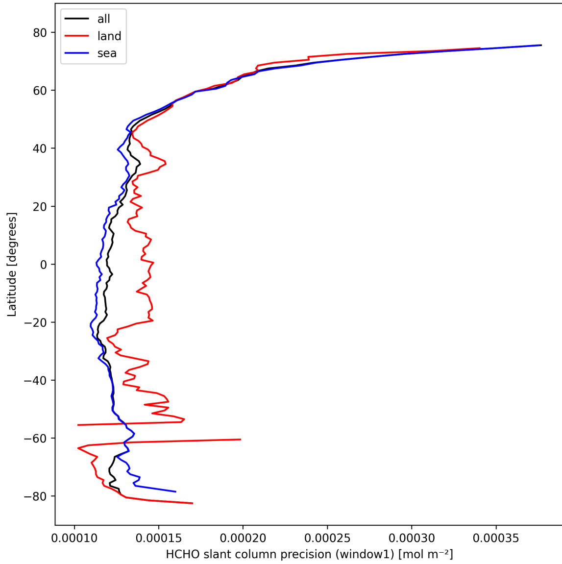
Figure 25: Zonal average of "HCHO slant column precision (window1)" for 2024-10-17 to 2024-10-19.
