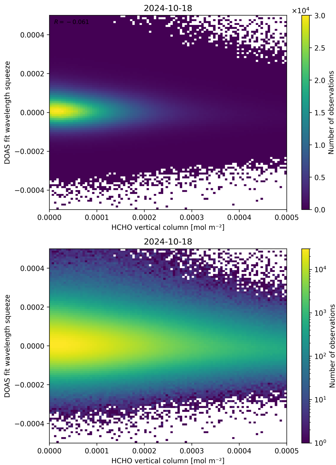
Figure 125: Scatter density plot of “HCHO vertical column” against “DOAS fit wavelength squeeze” for 2024-10-17 to 2024-10-19.
