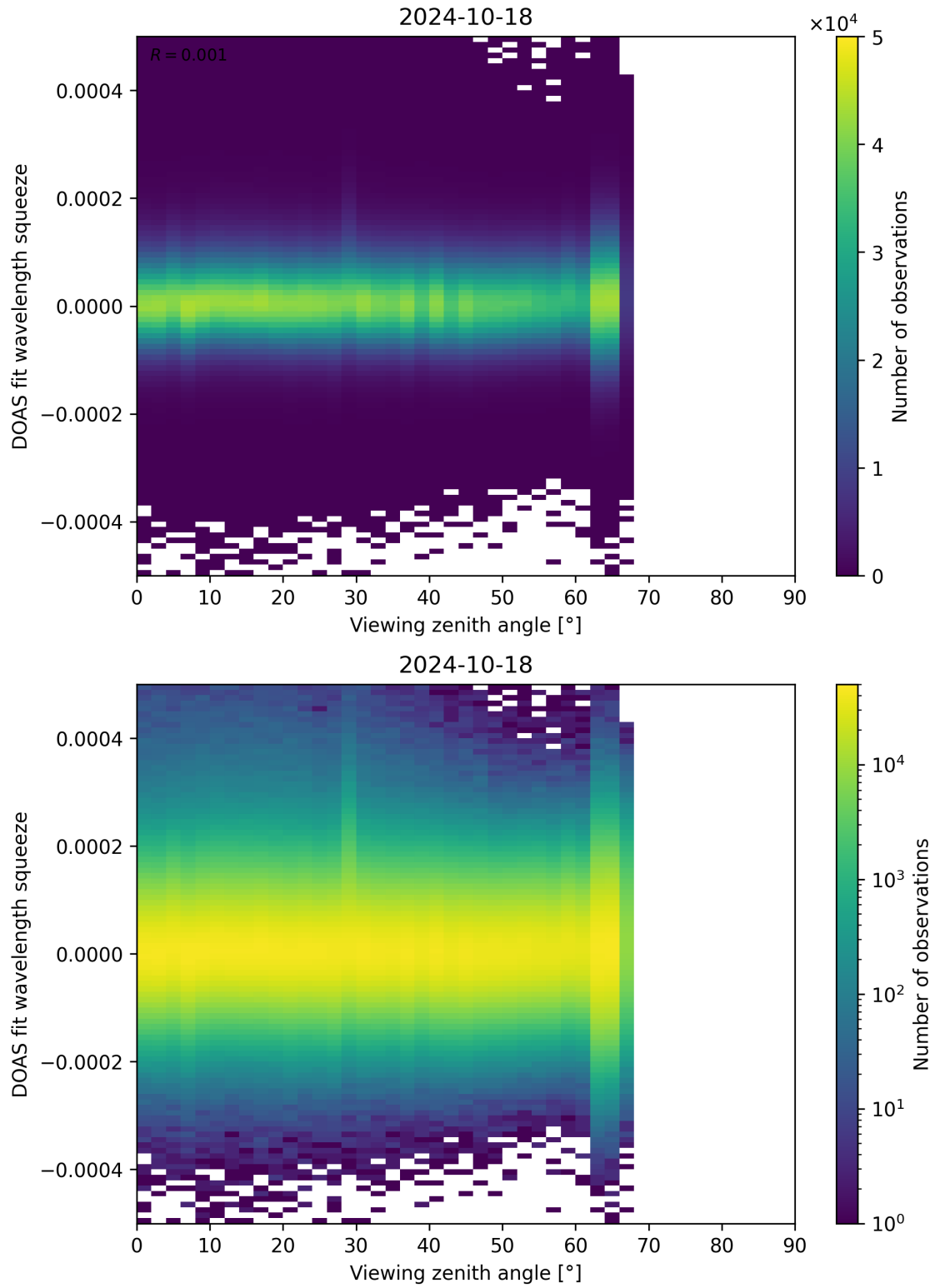
Figure 184: Scatter density plot of “Viewing zenith angle” against “DOAS fit wavelength squeeze” for 2024-10-17 to 2024-10-19.
