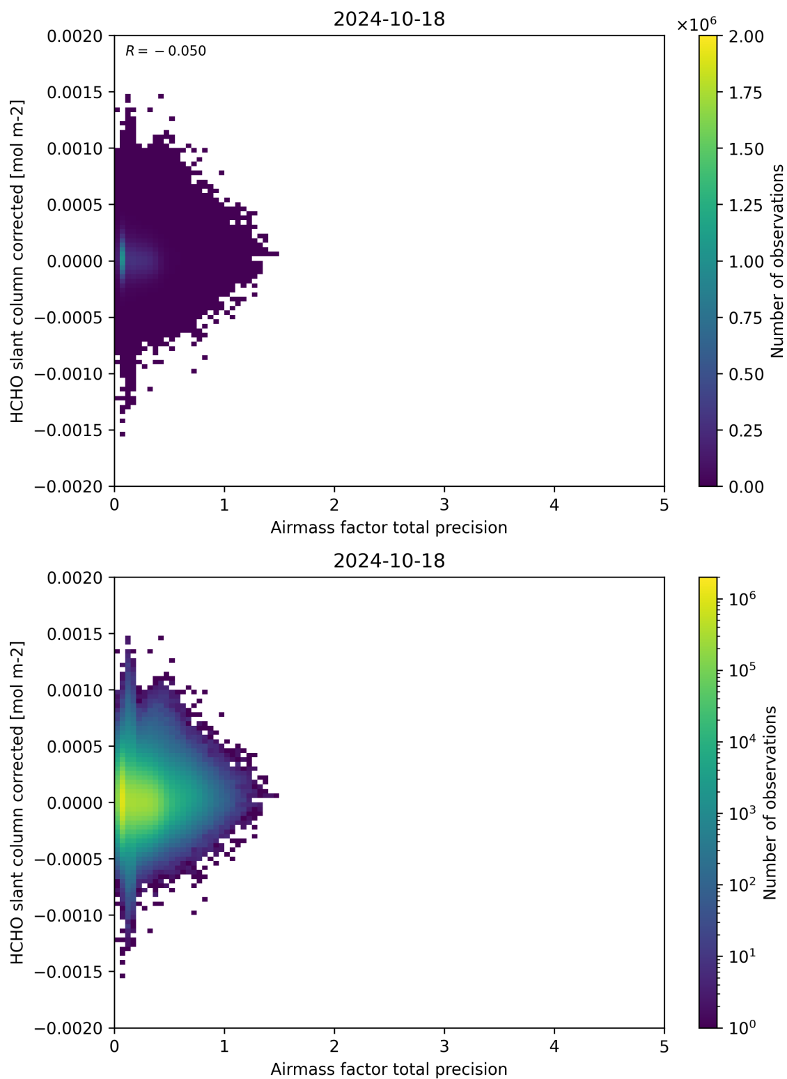
Figure 109: Scatter density plot of “Airmass factor total precision” against “HCHO slant column corrected” for 2024-10-17 to 2024-10-19.
