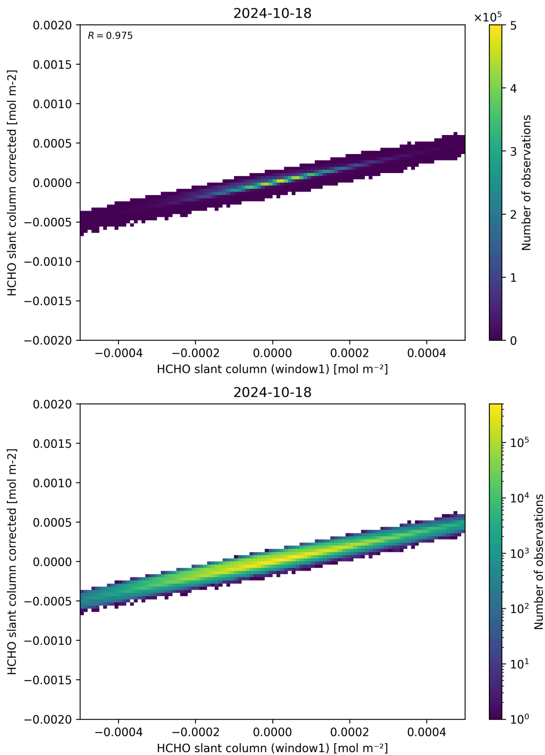
Figure 82: Scatter density plot of “HCHO slant column (window1)” against “HCHO slant column corrected” for 2024-10-17 to 2024-10-19.
