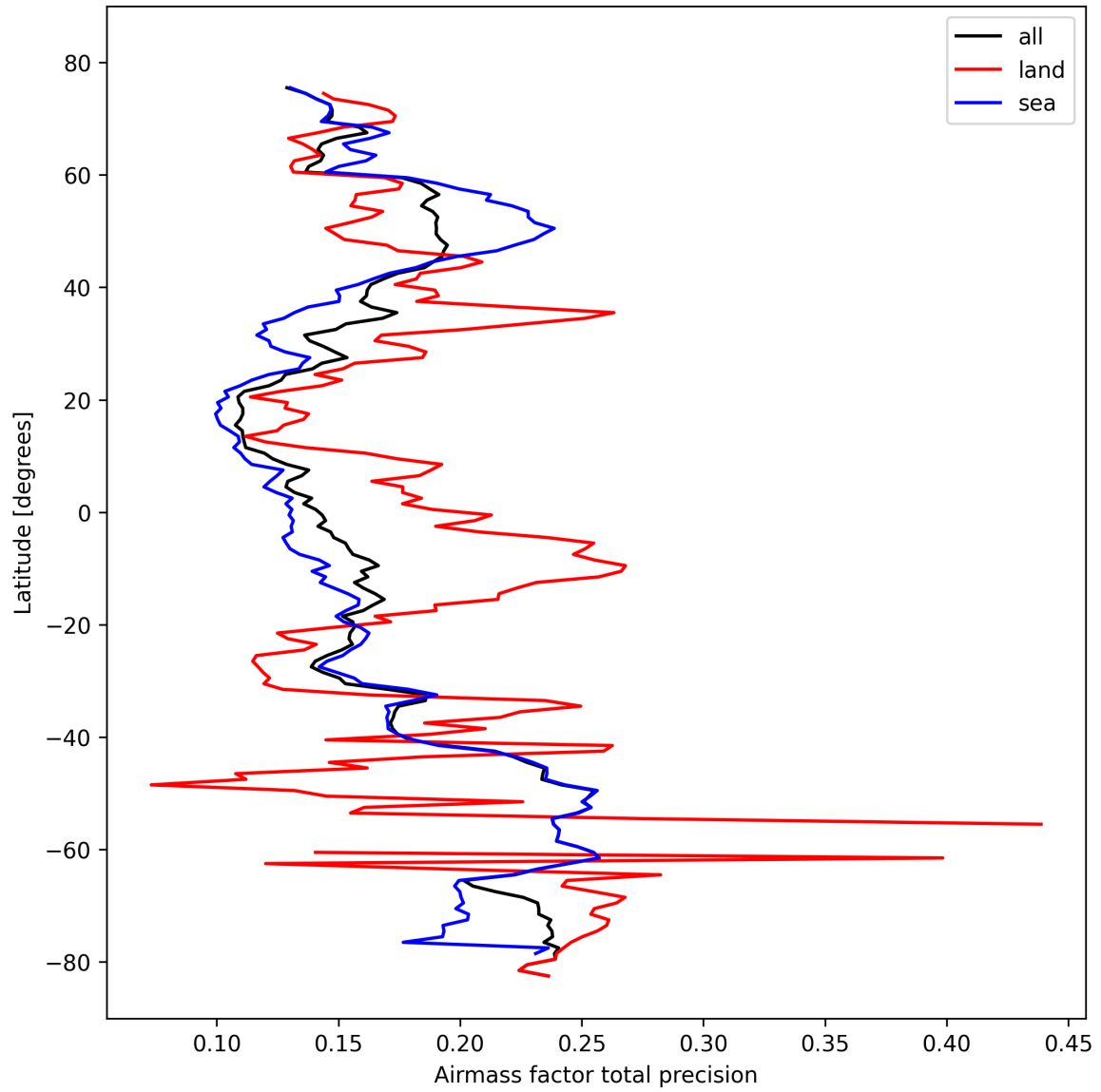
Figure 27: Zonal average of “Airmass factor total precision” for 2024-10-17 to 2024-10-19.
