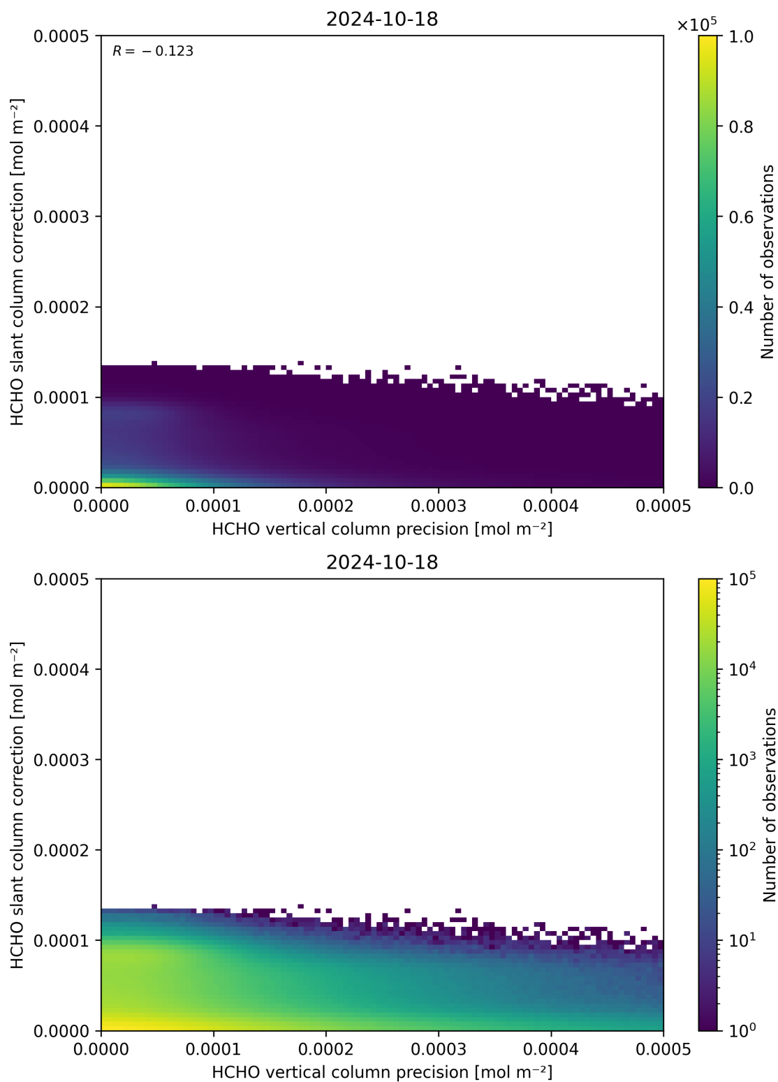
Figure 141: Scatter density plot of “HCHO vertical column precision” against “HCHO slant column correction” for 2024-10-17 to 2024-10-19.
