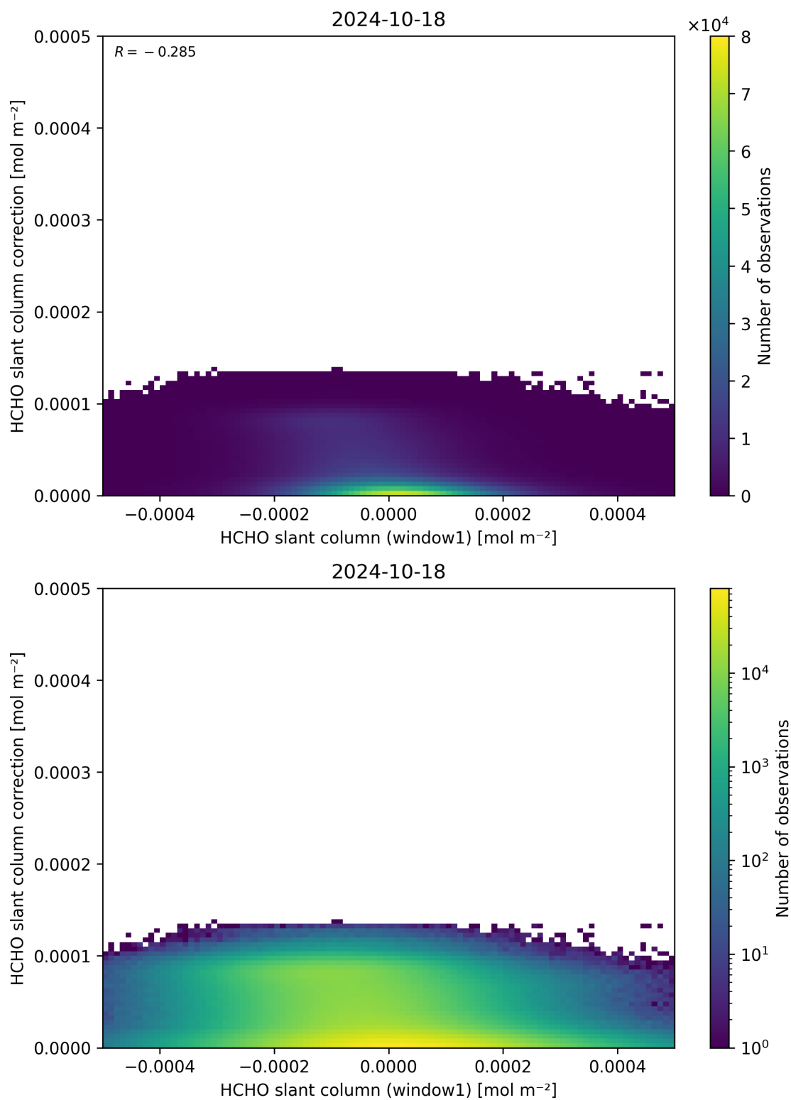
Figure 83: Scatter density plot of “HCHO slant column (window1)” against “HCHO slant column correction” for 2024-10-17 to 2024-10-19.
