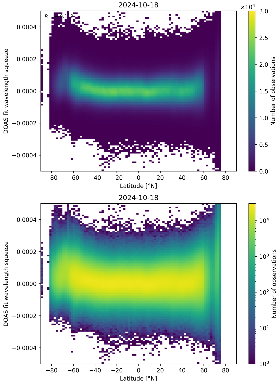
Figure 155: Scatter density plot of “Latitude” against “DOAS fit wavelength squeeze” for 2024-10-17 to 2024-10-19.
