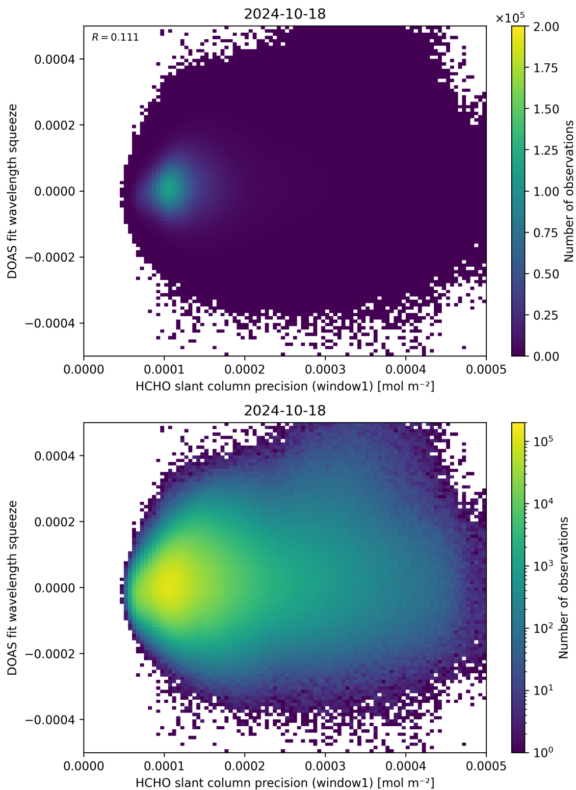
Figure 90: Scatter density plot of “HCHO slant column precision (window1)” against “DOAS fit wavelength squeeze” for 2024-10-17 to 2024-10-19.
