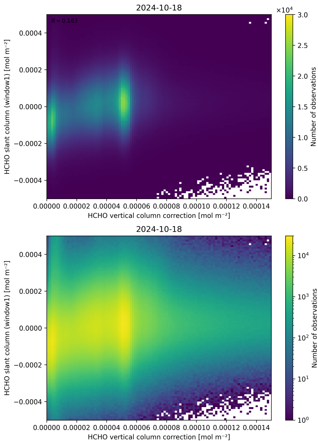
Figure 118: Scatter density plot of “HCHO vertical column correction” against “HCHO slant column (window1)” for 2024-10-17 to 2024-10-19.
