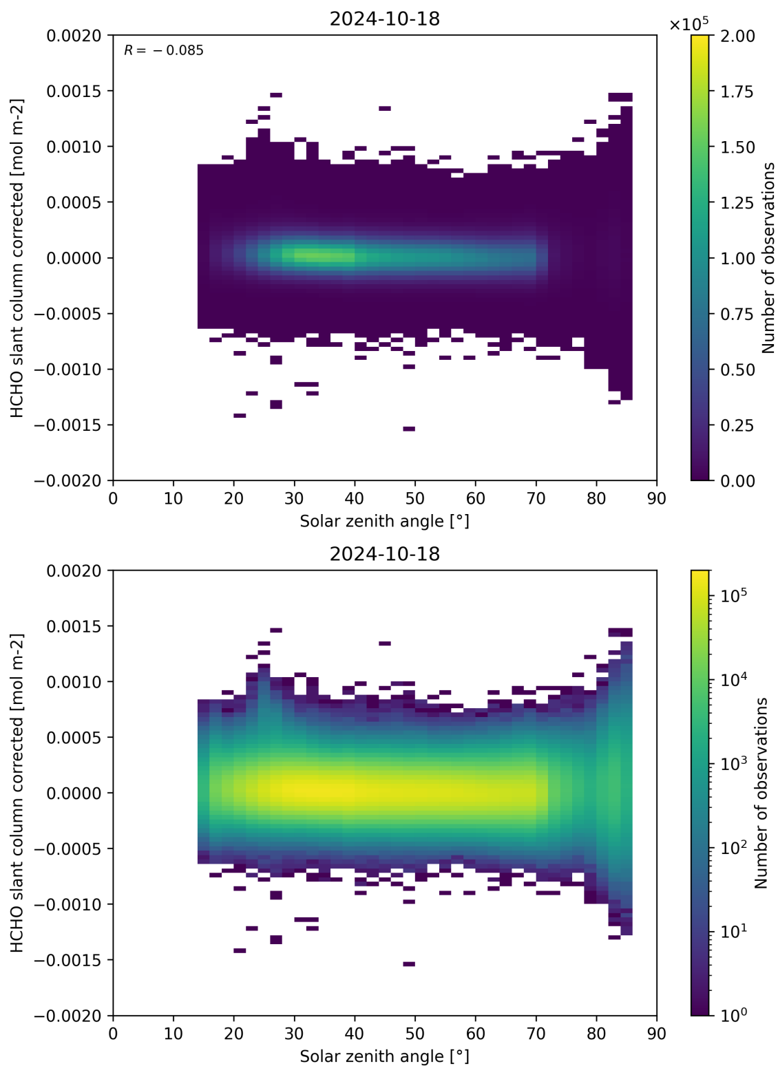
Figure 171: Scatter density plot of “Solar zenith angle” against “HCHO slant column corrected” for 2024-10-17 to 2024-10-19.
