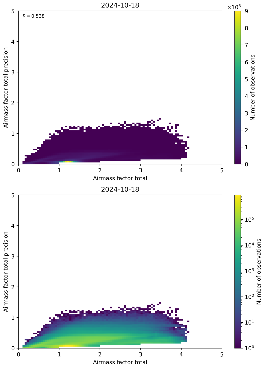
Figure 103: Scatter density plot of “Airmass factor total” against “Airmass factor total precision” for 2024-10-17 to 2024-10-19.
