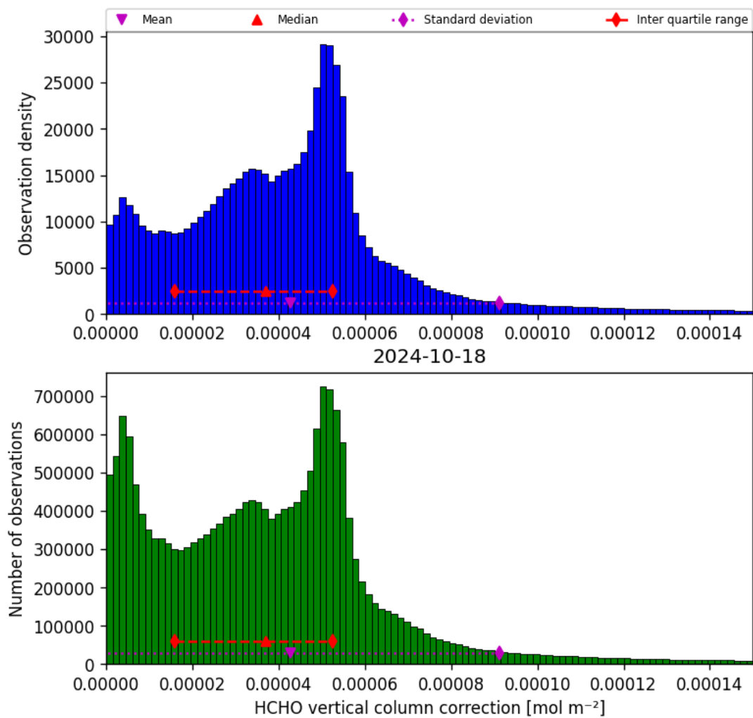
Figure 37: Histogram of “HCHO vertical column correction” for 2024-10-17 to 2024-10-19
