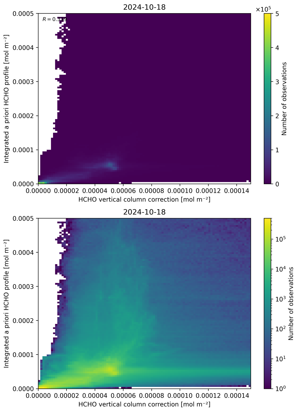
Figure 122: Scatter density plot of “HCHO vertical column correction” against “Integrated a priori HCHO profile” for 2024-10-17 to 2024-10-19.
