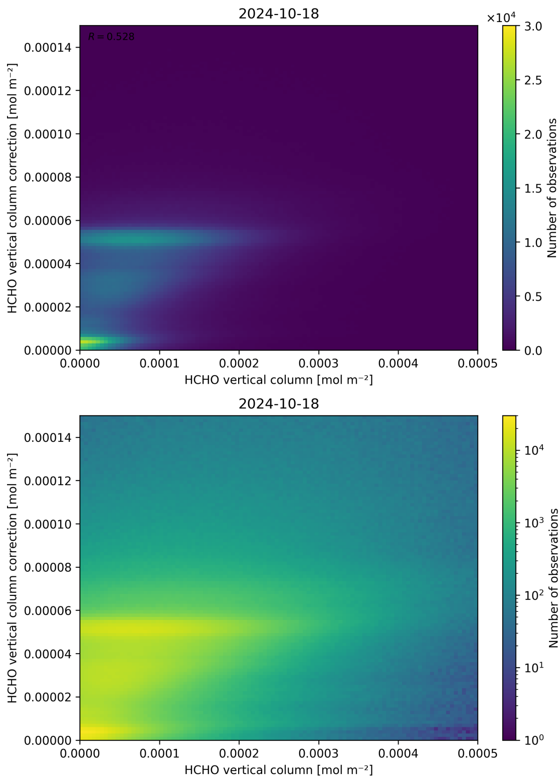
Figure 133: Scatter density plot of “HCHO vertical column” against “HCHO vertical column correction” for 2024-10-17 to 2024-10-19.
