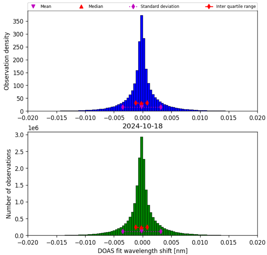
Figure 44: Histogram of “DOAS fit wavelength shift” for 2024-10-17 to 2024-10-19
