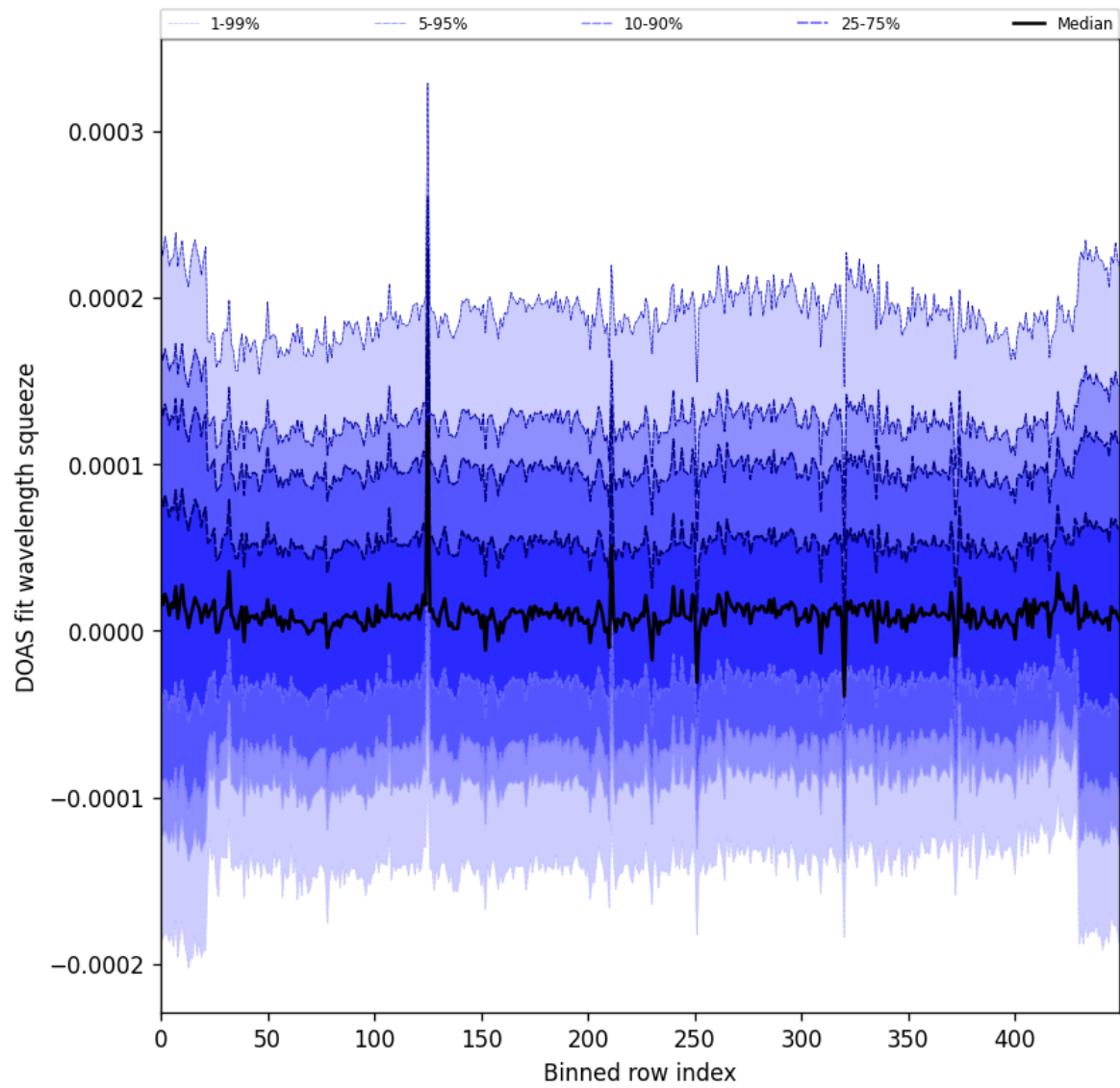
Figure 59: Along track statistics of “DOAS fit wavelength squeeze” for 2024-10-17 to 2024-10-19
