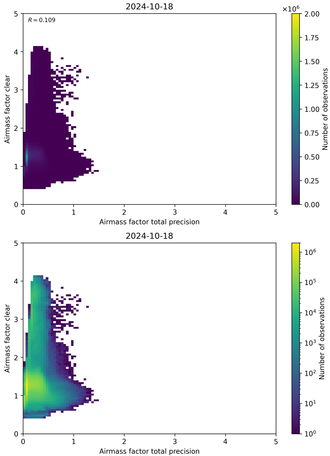
Figure 108: Scatter density plot of “Airmass factor total precision” against “Airmass factor clear” for 2024-10-17 to 2024-10-19.
