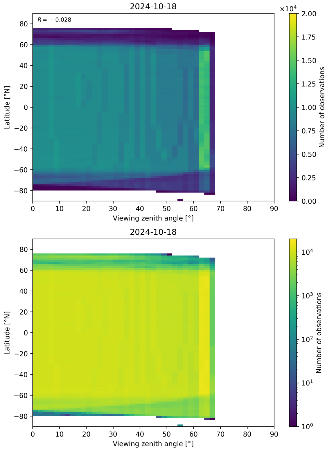
Figure 196: Scatter density plot of “Viewing zenith angle” against “Latitude” for 2024-10-17 to 2024-10-19.
