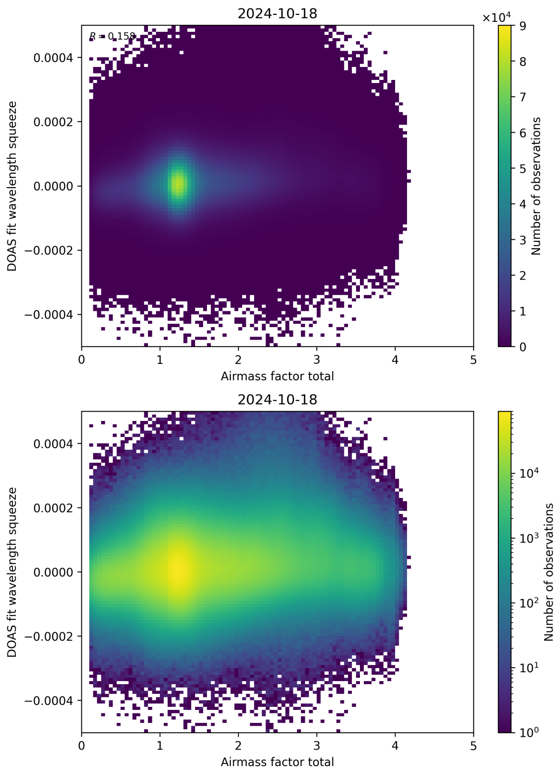
Figure 99: Scatter density plot of “Airmass factor total” against “DOAS fit wavelength squeeze” for 2024-10-17 to 2024-10-19.
