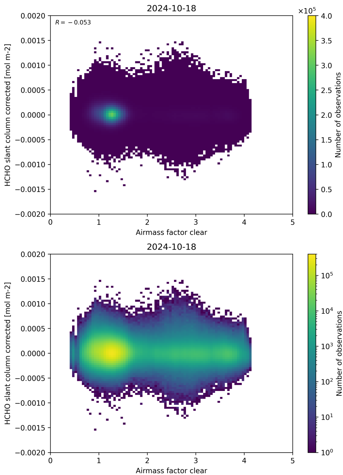
Figure 74: Scatter density plot of “Airmass factor clear” against “HCHO slant column corrected” for 2024-10-17 to 2024-10-19.
