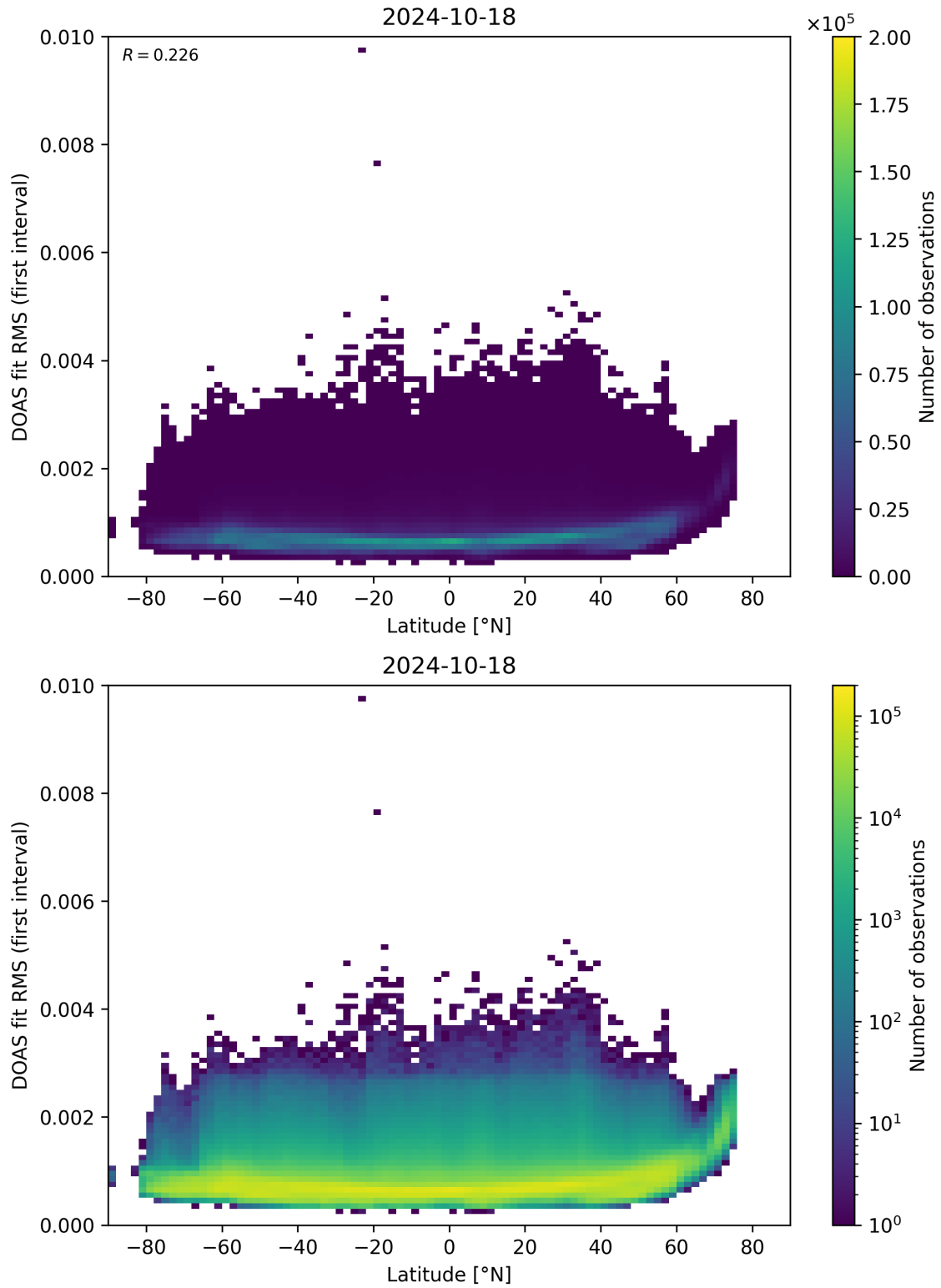
Figure 153: Scatter density plot of “Latitude” against “DOAS fit RMS (first interval)” for 2024-10-17 to 2024-10-19.
