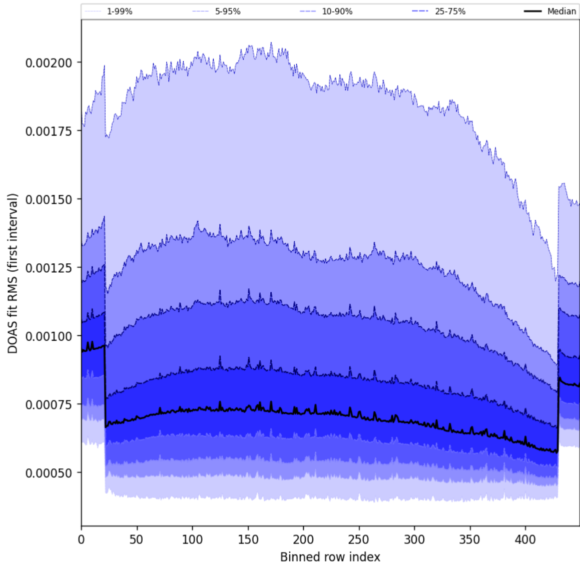
Figure 60: Along track statistics of “DOAS fit RMS (first interval)” for 2024-10-17 to 2024-10-19
