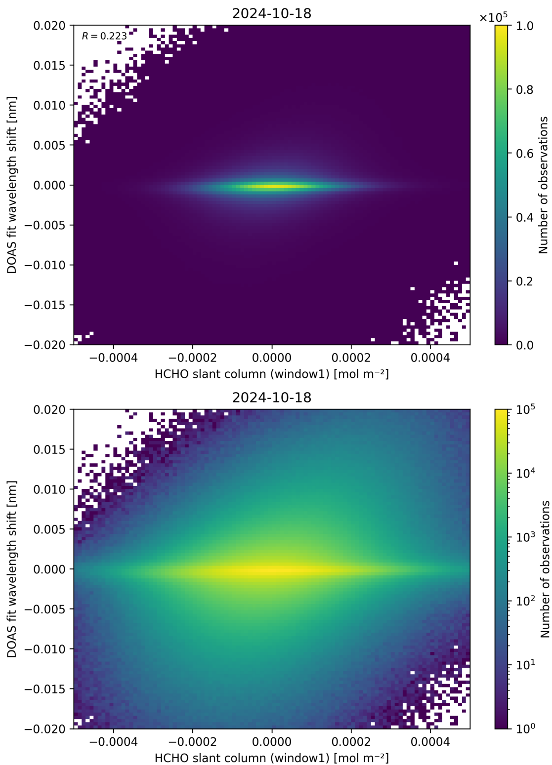
Figure 79: Scatter density plot of “HCHO slant column (window1)” against “DOAS fit wavelength shift” for 2024-10-17 to 2024-10-19.
