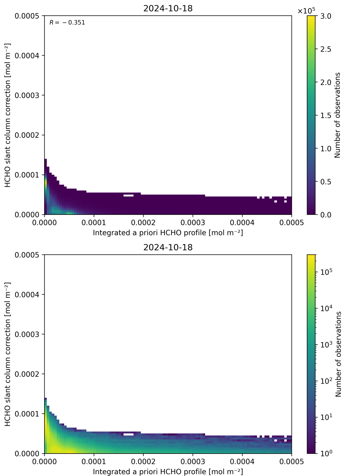
Figure 152: Scatter density plot of “Integrated a priori HCHO profile” against “HCHO slant column correction” for 2024-10-17 to 2024-10-19.
