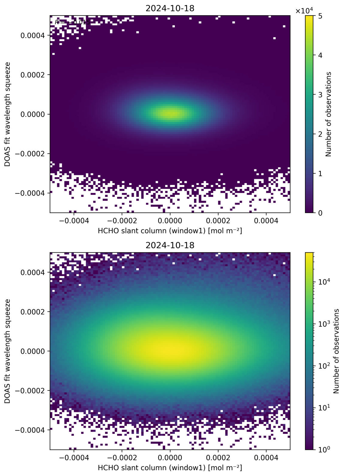
Figure 80: Scatter density plot of “HCHO slant column (window1)” against “DOAS fit wavelength squeeze” for 2024-10-17 to 2024-10-19.
