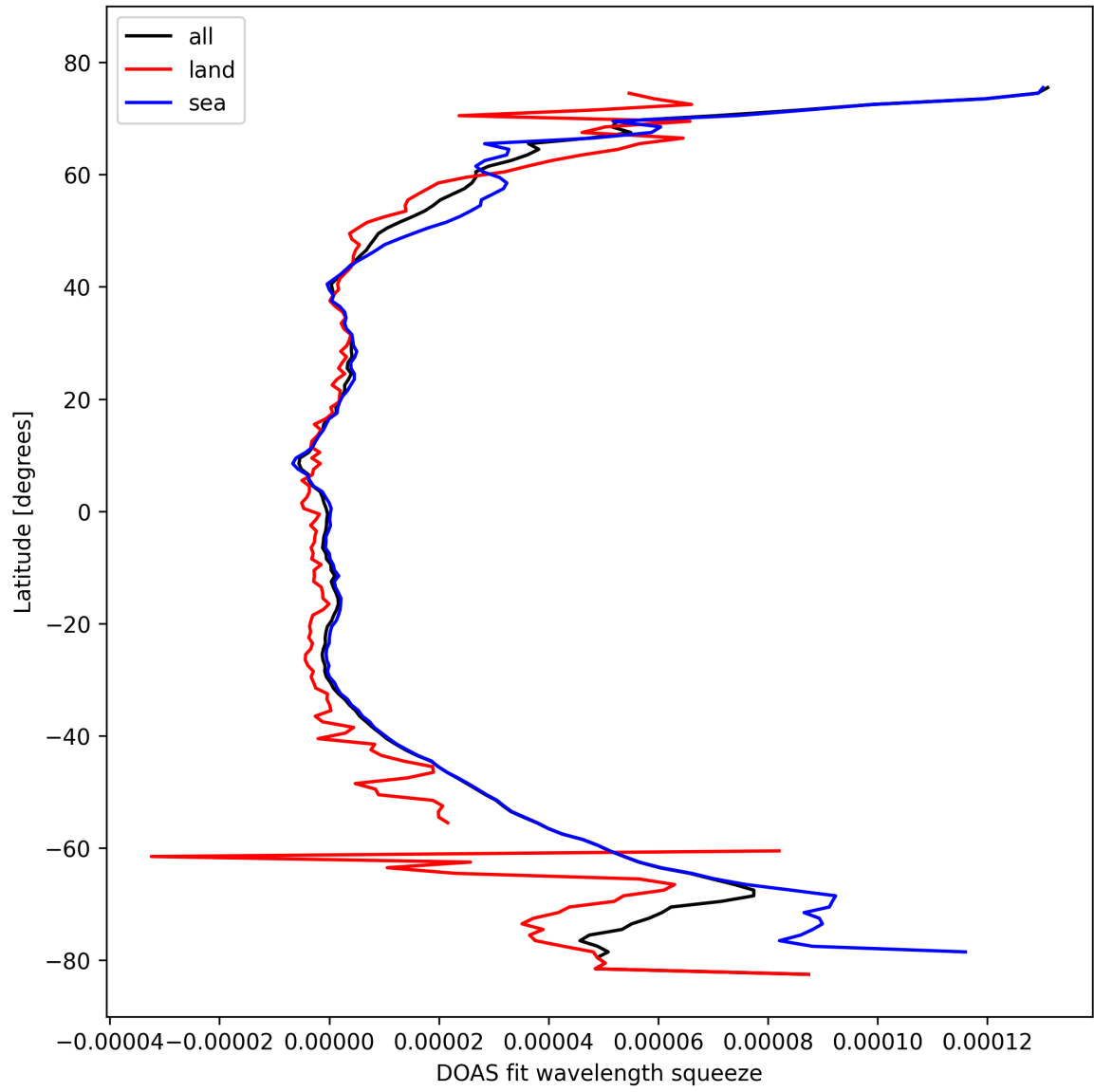
Figure 31: Zonal average of “DOAS fit wavelength squeeze” for 2024-10-17 to 2024-10-19.
