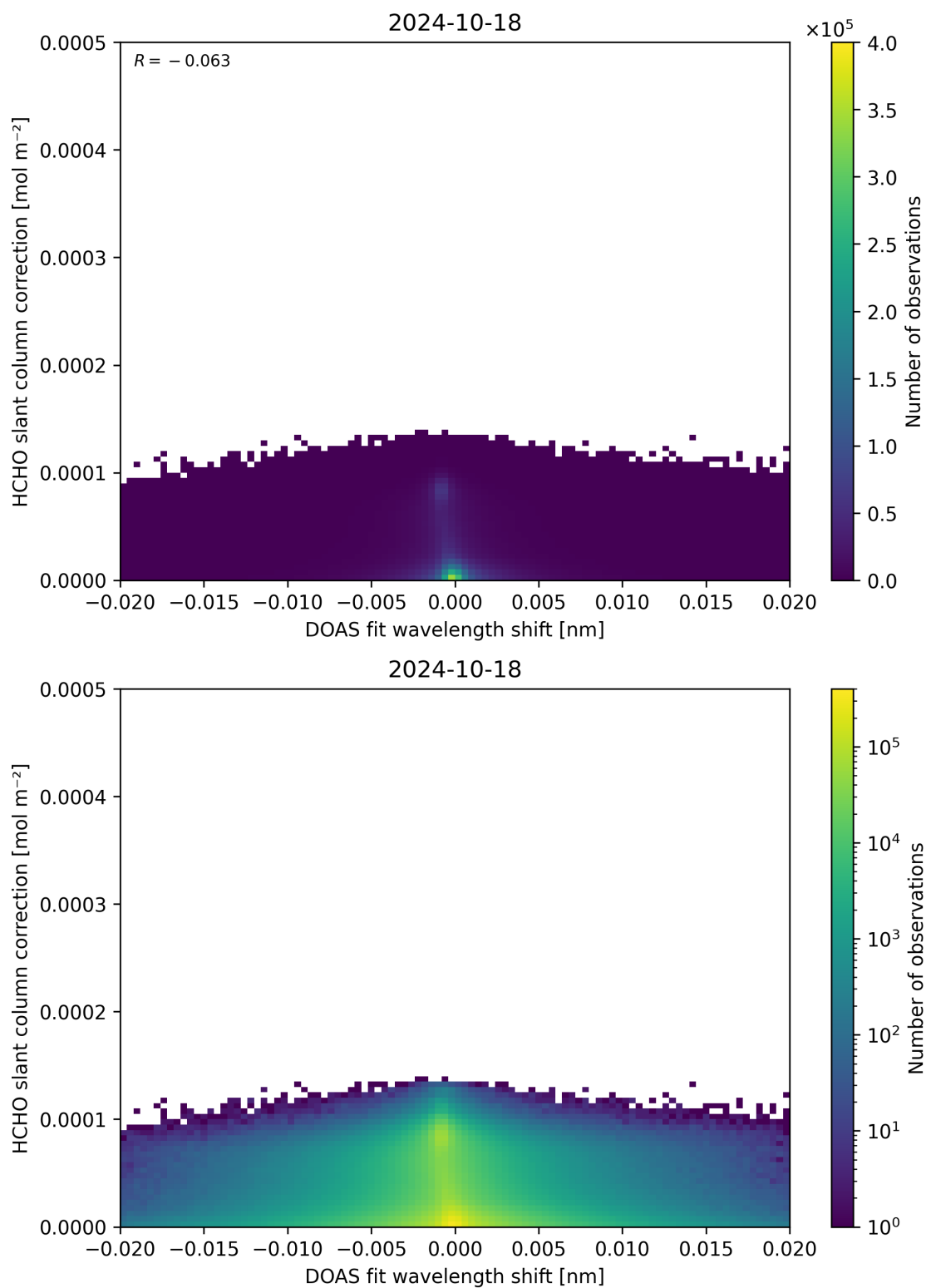
Figure 67: Scatter density plot of “DOAS fit wavelength shift” against “HCHO slant column correction” for 2024-10-17 to 2024-10-19.
