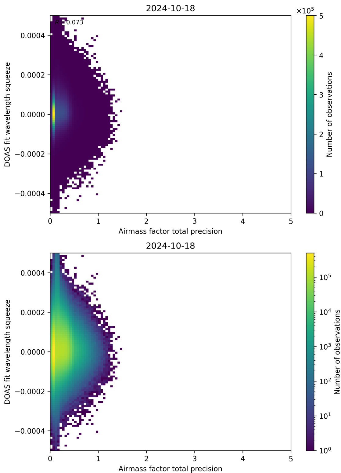
Figure 107: Scatter density plot of “Airmass factor total precision” against “DOAS fit wavelength squeeze” for 2024-10-17 to 2024-10-19.
