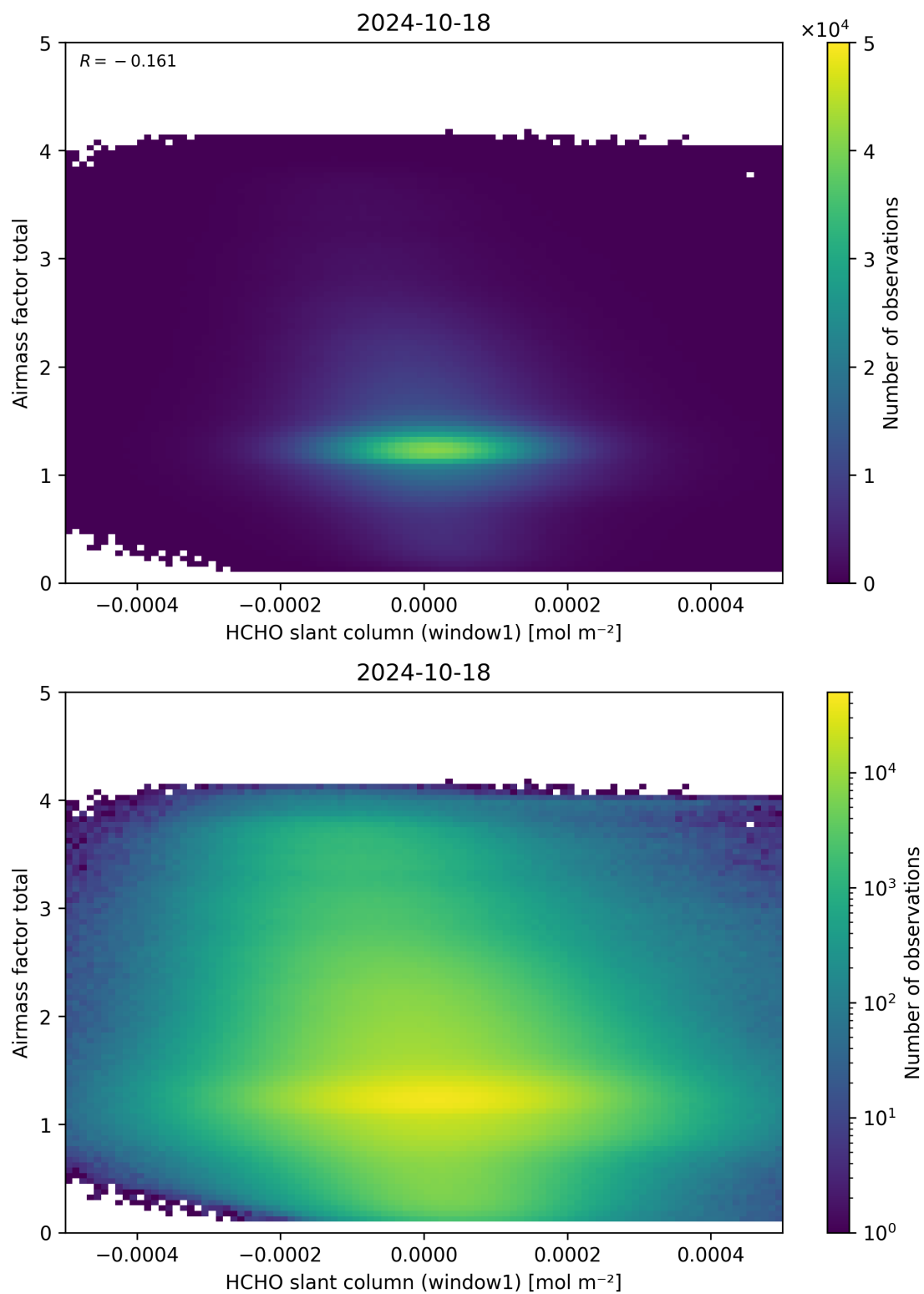
Figure 85: Scatter density plot of “HCHO slant column (window1)” against “Airmass factor total” for 2024-10-17 to 2024-10-19.
