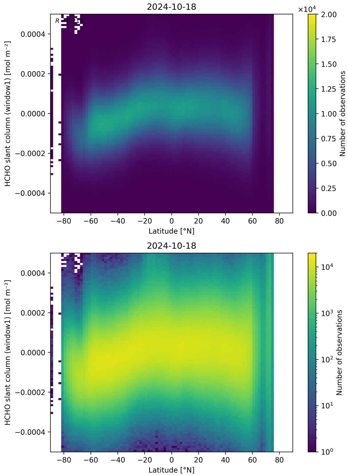
Figure 159: Scatter density plot of “Latitude” against “HCHO slant column (window1)” for 2024-10-17 to 2024-10-19.
