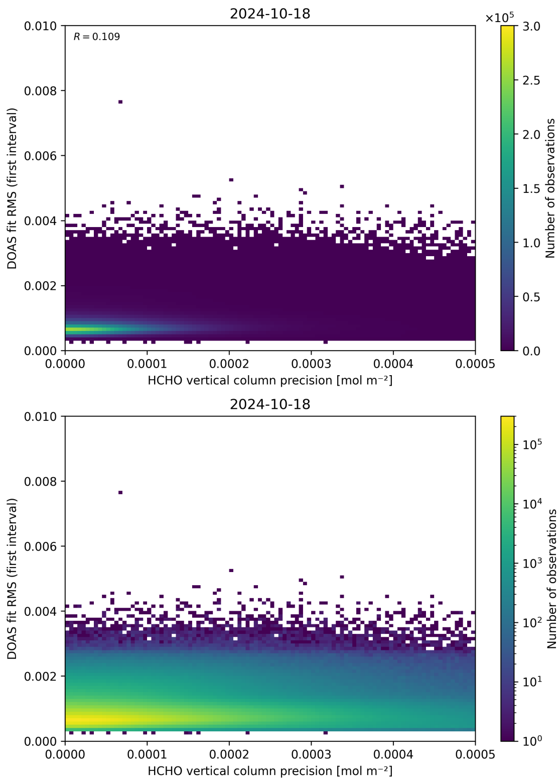
Figure 136: Scatter density plot of “HCHO vertical column precision” against “DOAS fit RMS (first interval)” for 2024-10-17 to 2024-10-19.
