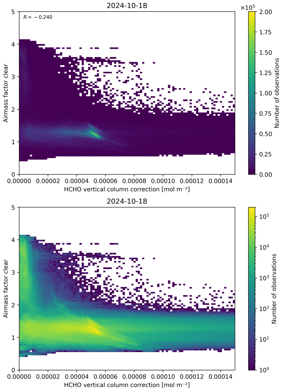
Figure 115: Scatter density plot of “HCHO vertical column correction” against “Airmass factor clear” for 2024-10-17 to 2024-10-19.
