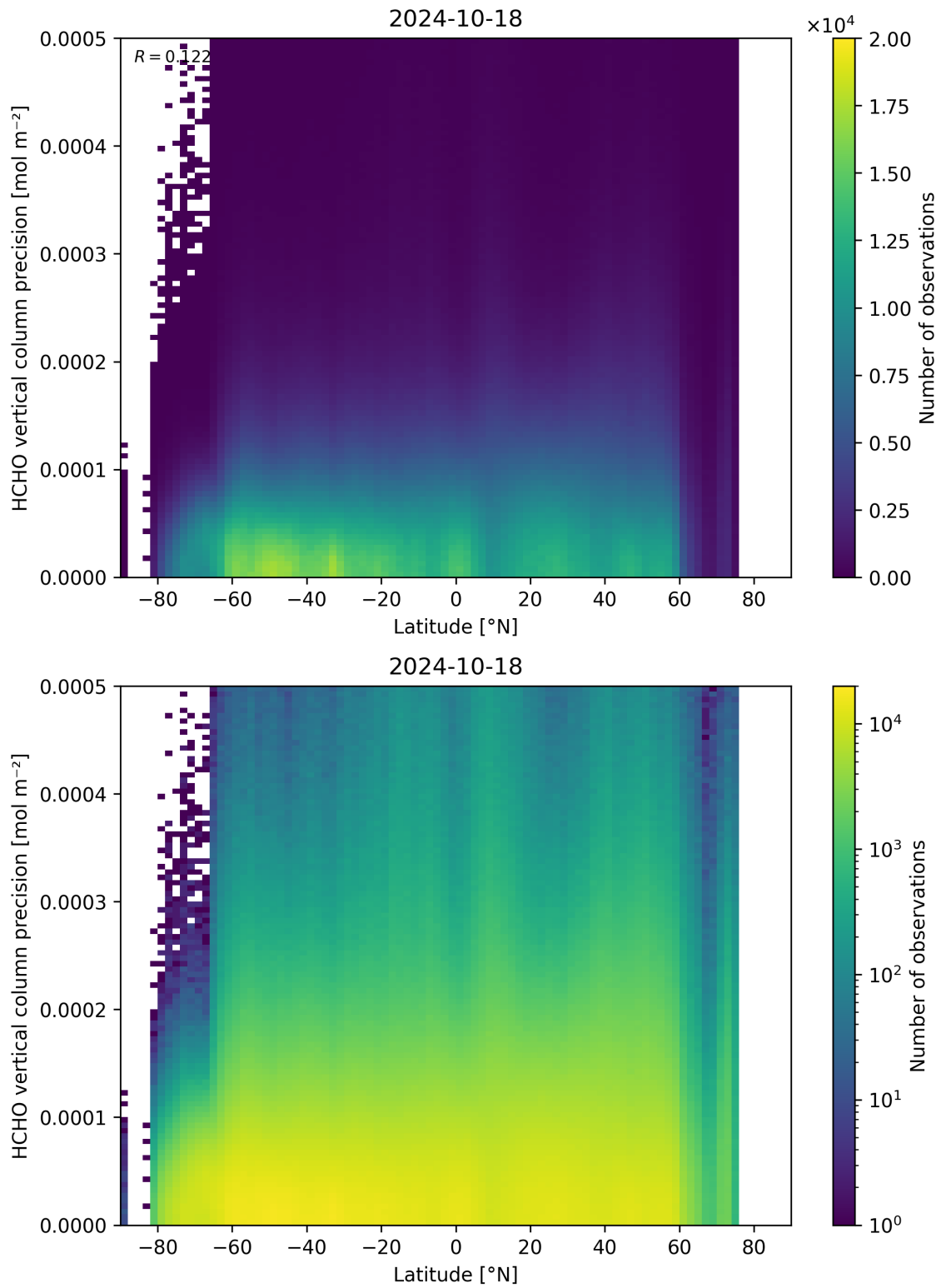
Figure 165: Scatter density plot of “Latitude” against “HCHO vertical column precision” for 2024-10-17 to 2024-10-19.
