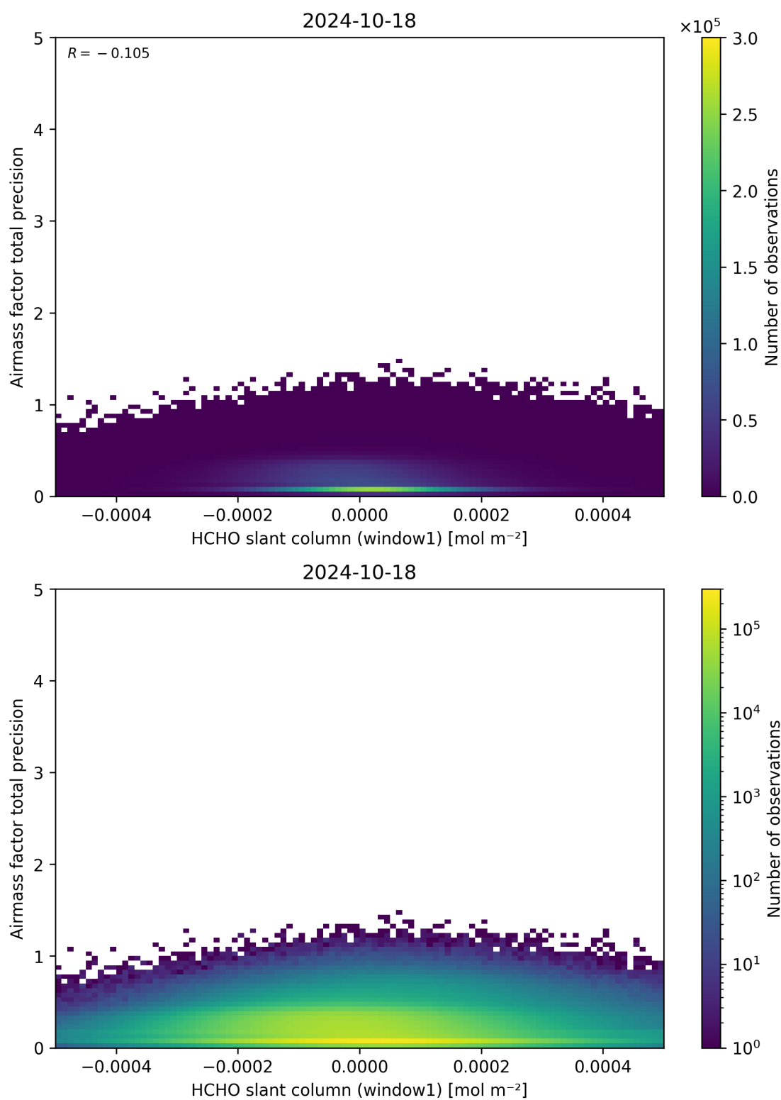
Figure 86: Scatter density plot of “HCHO slant column (window1)” against “Airmass factor total precision” for 2024-10-17 to 2024-10-19.
