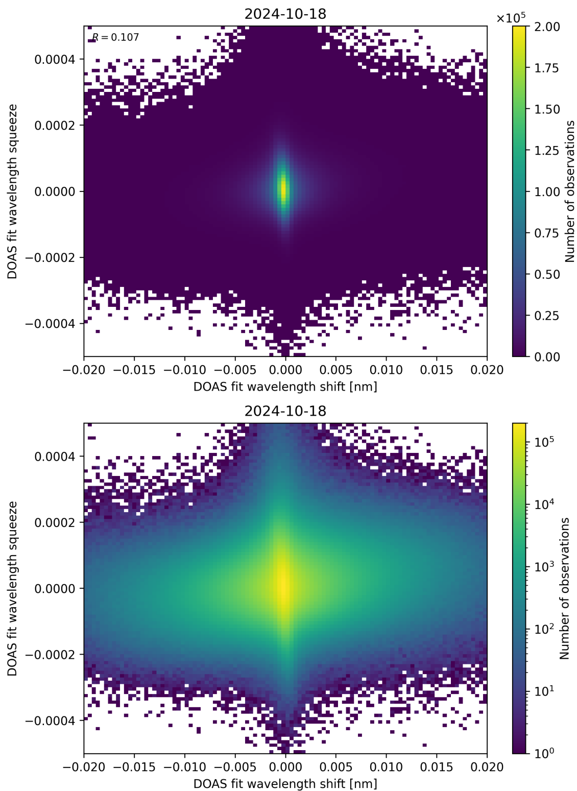
Figure 65: Scatter density plot of “DOAS fit wavelength shift” against “DOAS fit wavelength squeeze” for 2024-10-17 to 2024-10-19.
