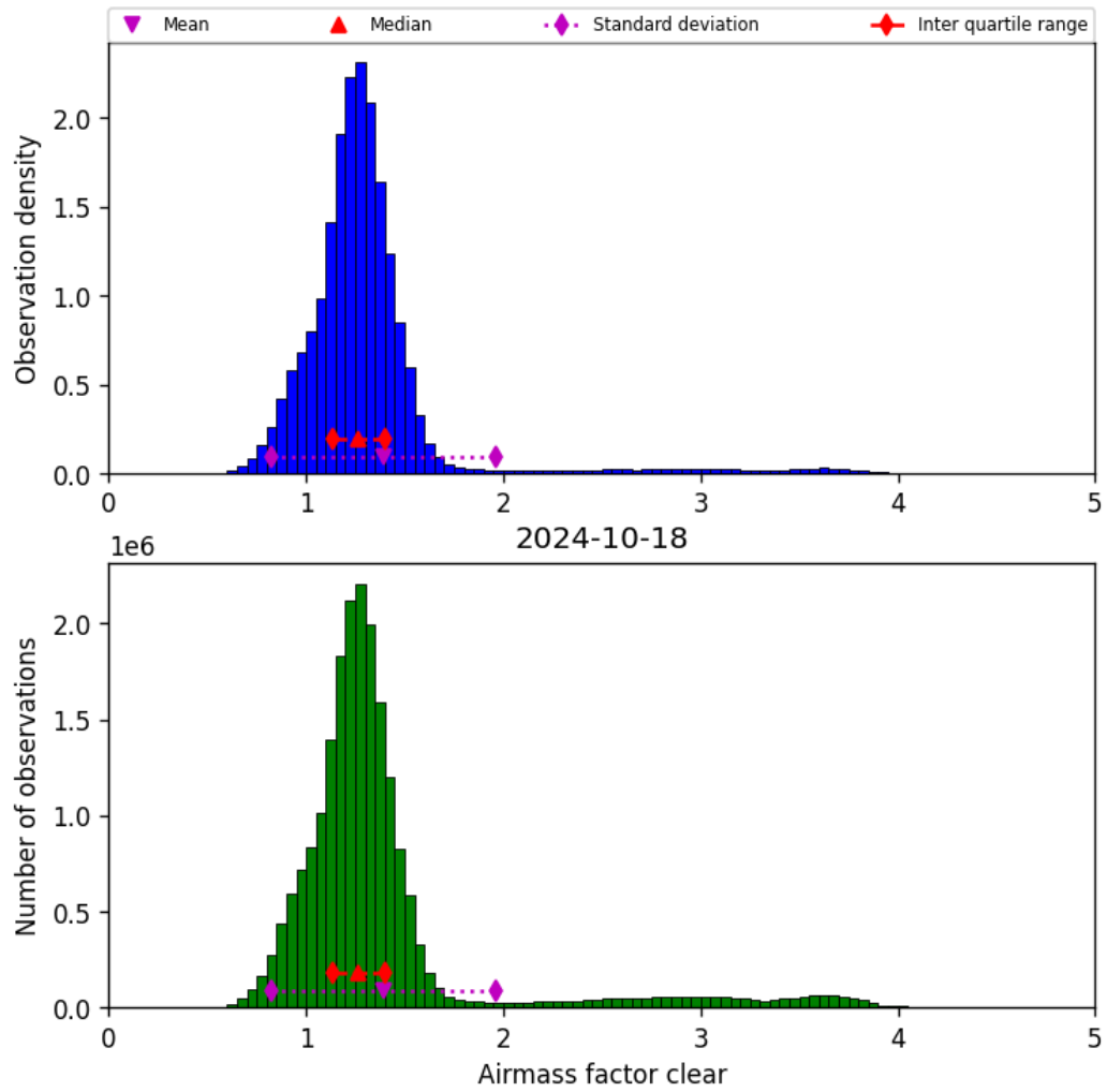
Figure 42: Histogram of “Airmass factor clear” for 2024-10-17 to 2024-10-19
