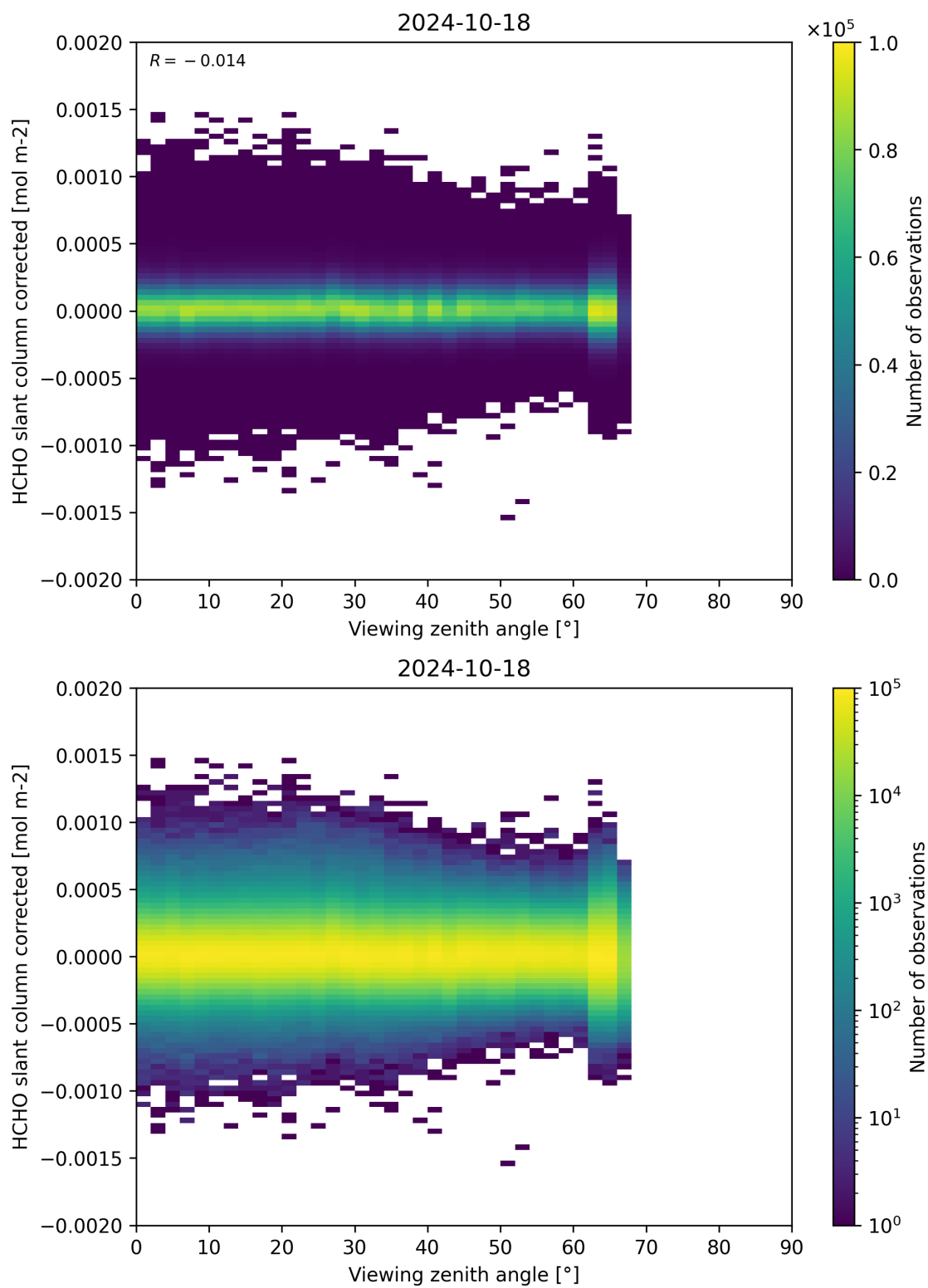
Figure 186: Scatter density plot of “Viewing zenith angle” against “HCHO slant column corrected” for 2024-10-17 to 2024-10-19.
