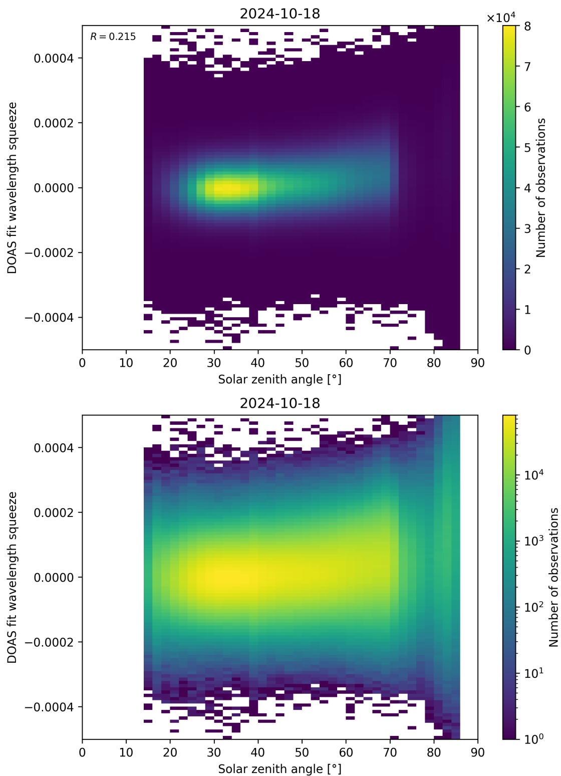
Figure 169: Scatter density plot of “Solar zenith angle” against “DOAS fit wavelength squeeze” for 2024-10-17 to 2024-10-19.
