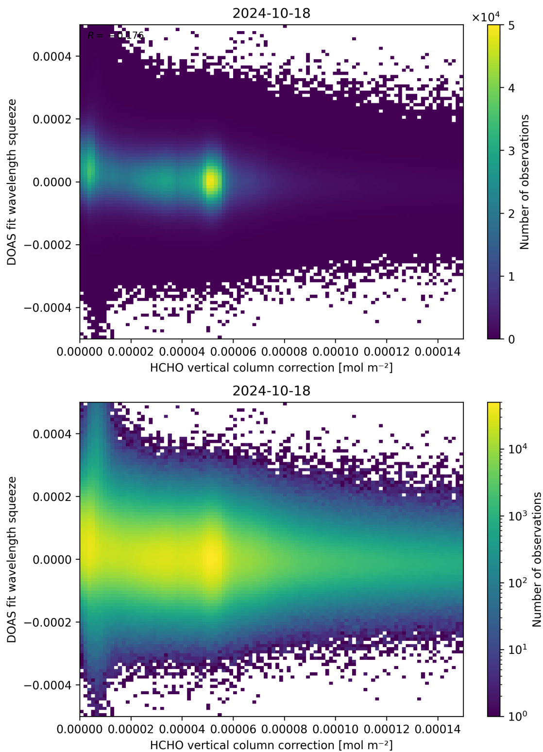
Figure 114: Scatter density plot of “HCHO vertical column correction” against “DOAS fit wavelength squeeze” for 2024-10-17 to 2024-10-19.
