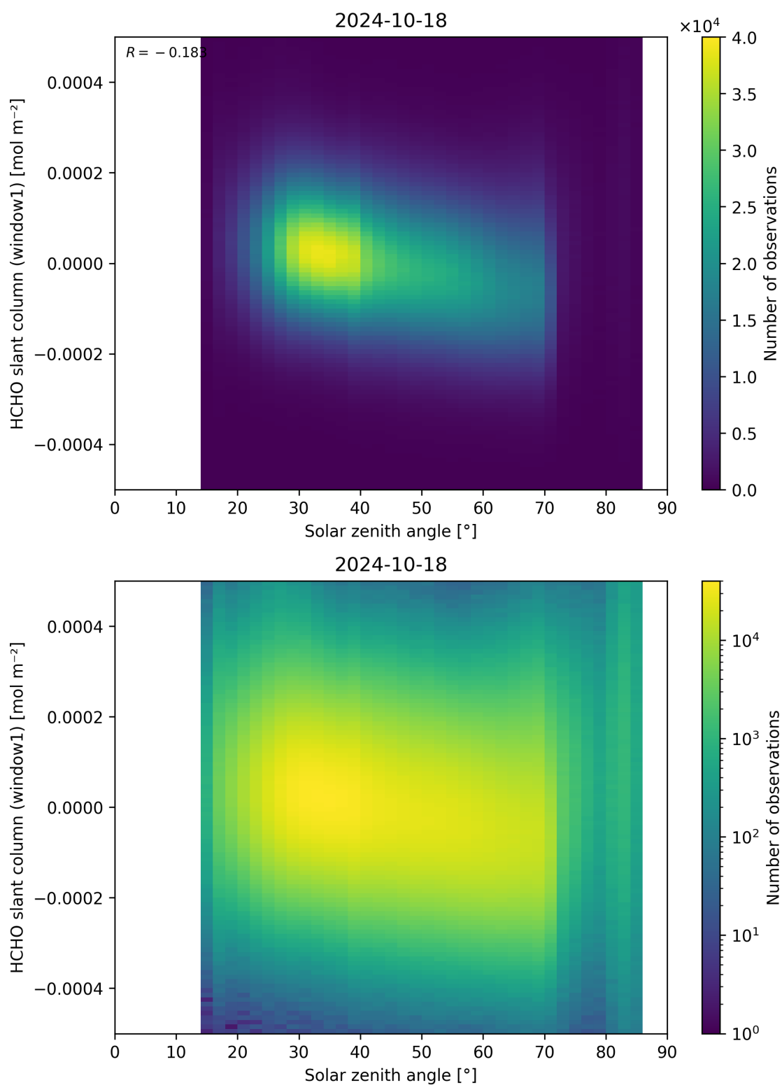
Figure 173: Scatter density plot of “Solar zenith angle” against “HCHO slant column (window1)” for 2024-10-17 to 2024-10-19.
