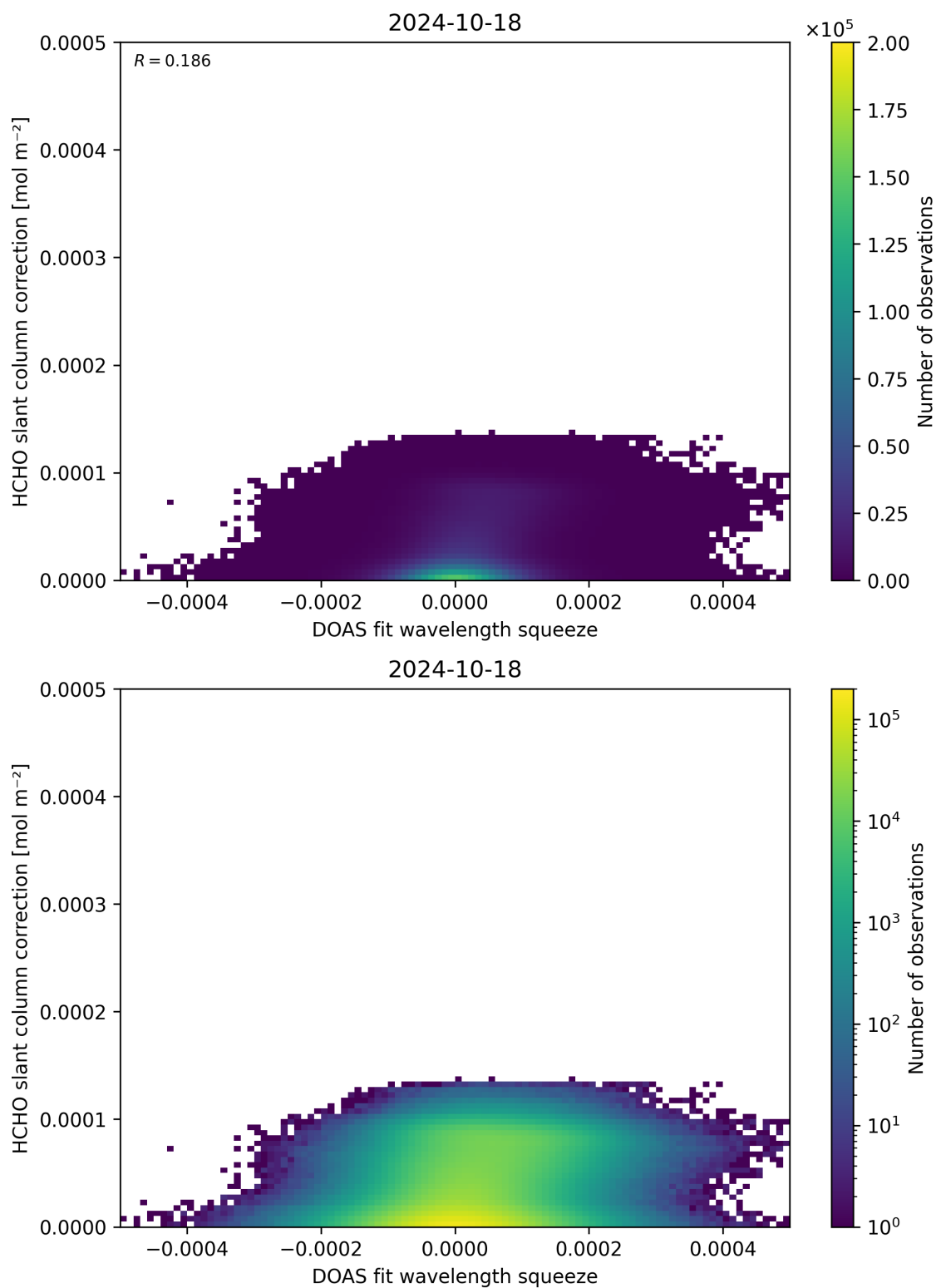
Figure 70: Scatter density plot of “DOAS fit wavelength squeeze” against “HCHO slant column correction” for 2024-10-17 to 2024-10-19.
