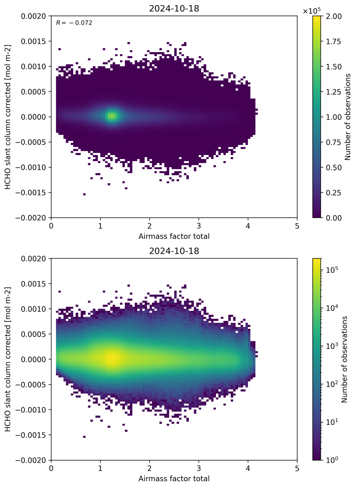
Figure 101: Scatter density plot of “Airmass factor total” against “HCHO slant column corrected” for 2024-10-17 to 2024-10-19.
