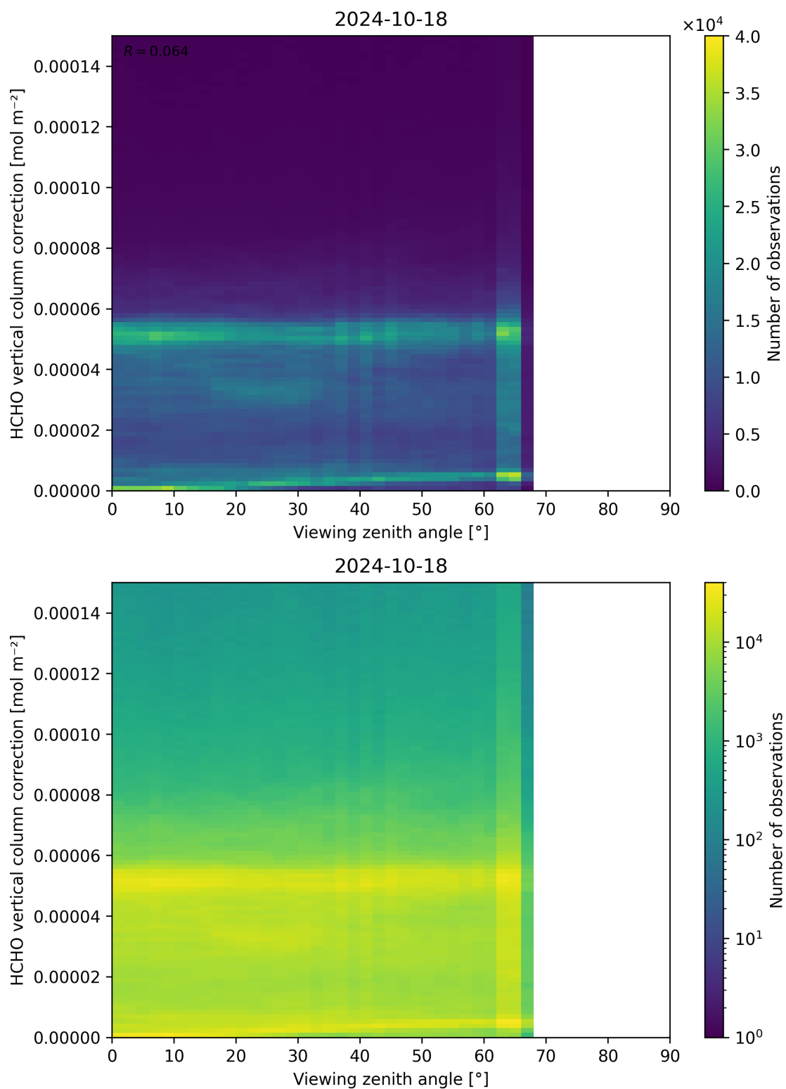
Figure 193: Scatter density plot of “Viewing zenith angle” against “HCHO vertical column correction” for 2024-10-17 to 2024-10-19.
