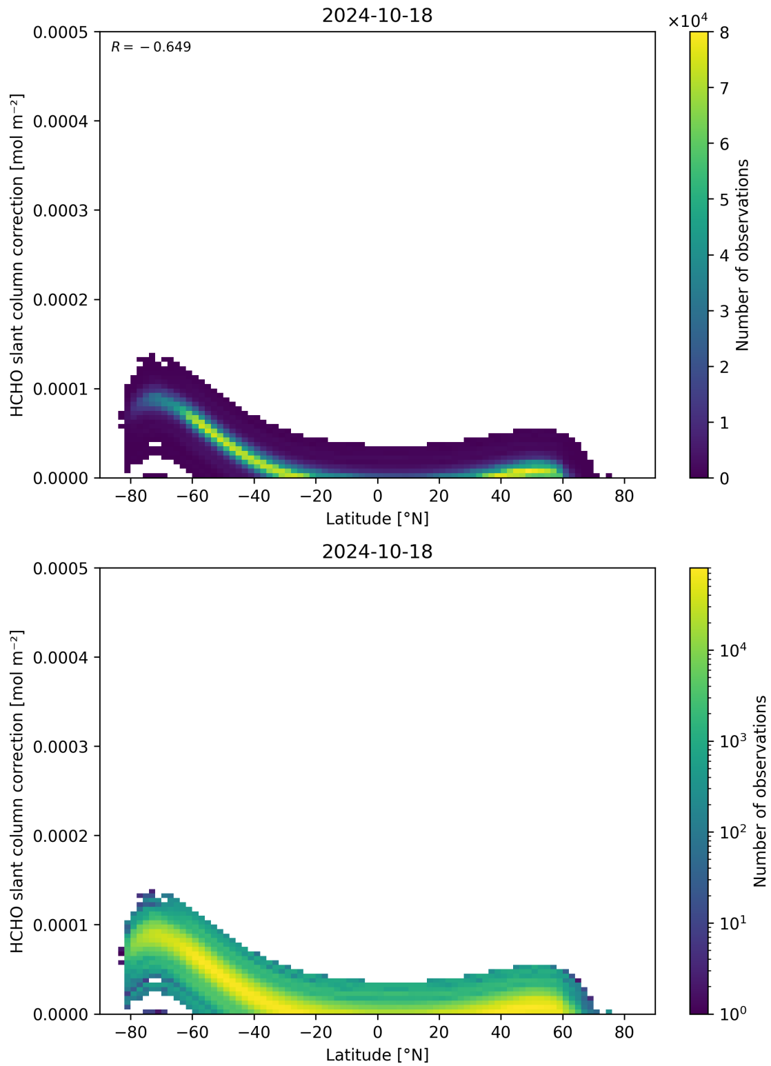
Figure 158: Scatter density plot of “Latitude” against “HCHO slant column correction” for 2024-10-17 to 2024-10-19.
