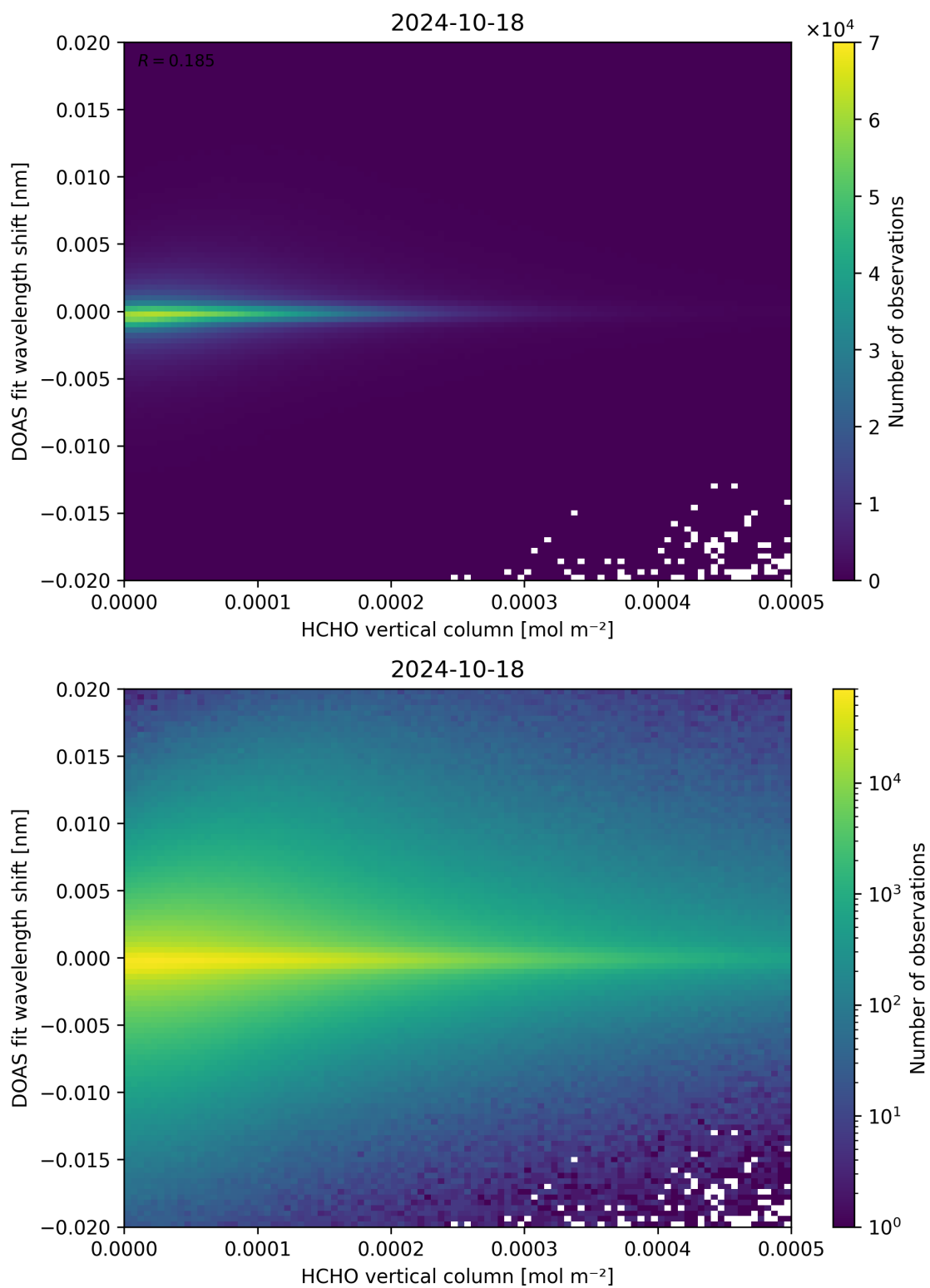
Figure 124: Scatter density plot of “HCHO vertical column” against “DOAS fit wavelength shift” for 2024-10-17 to 2024-10-19.
