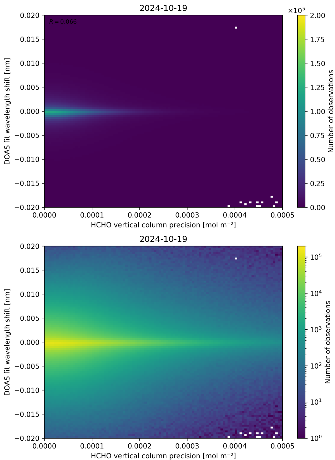
Figure 137: Scatter density plot of “HCHO vertical column precision” against “DOAS fit wavelength shift” for 2024-10-19 to 2024-10-20.
