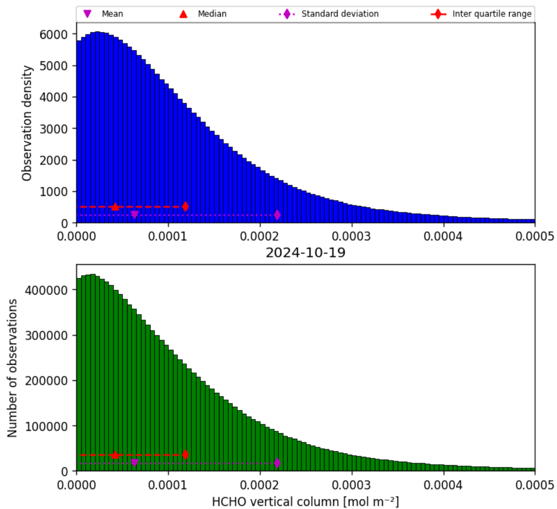
Figure 35: Histogram of “HCHO vertical column” for 2024-10-19 to 2024-10-20
