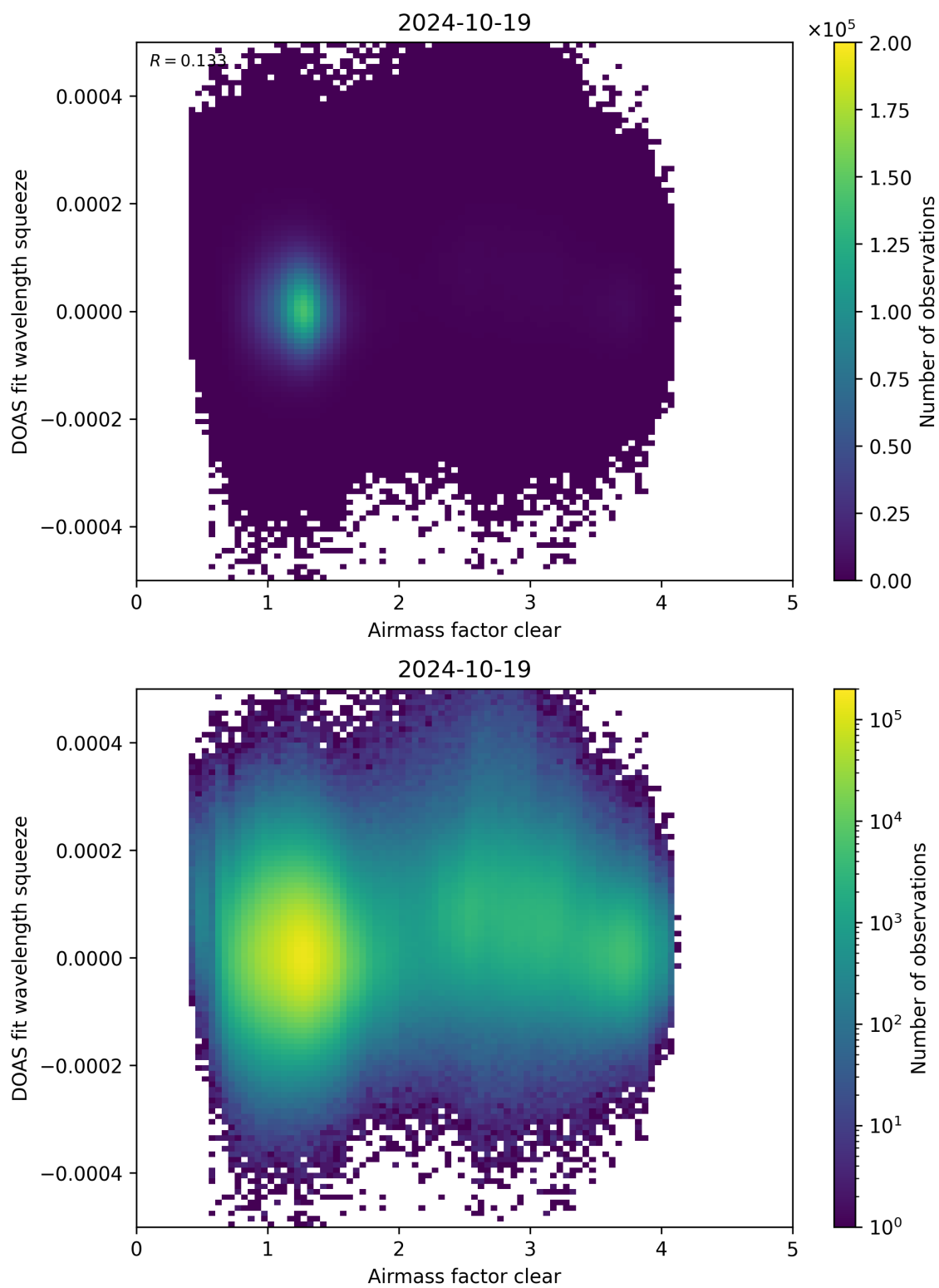
Figure 73: Scatter density plot of “Airmass factor clear” against “DOAS fit wavelength squeeze” for 2024-10-19 to 2024-10-20.
