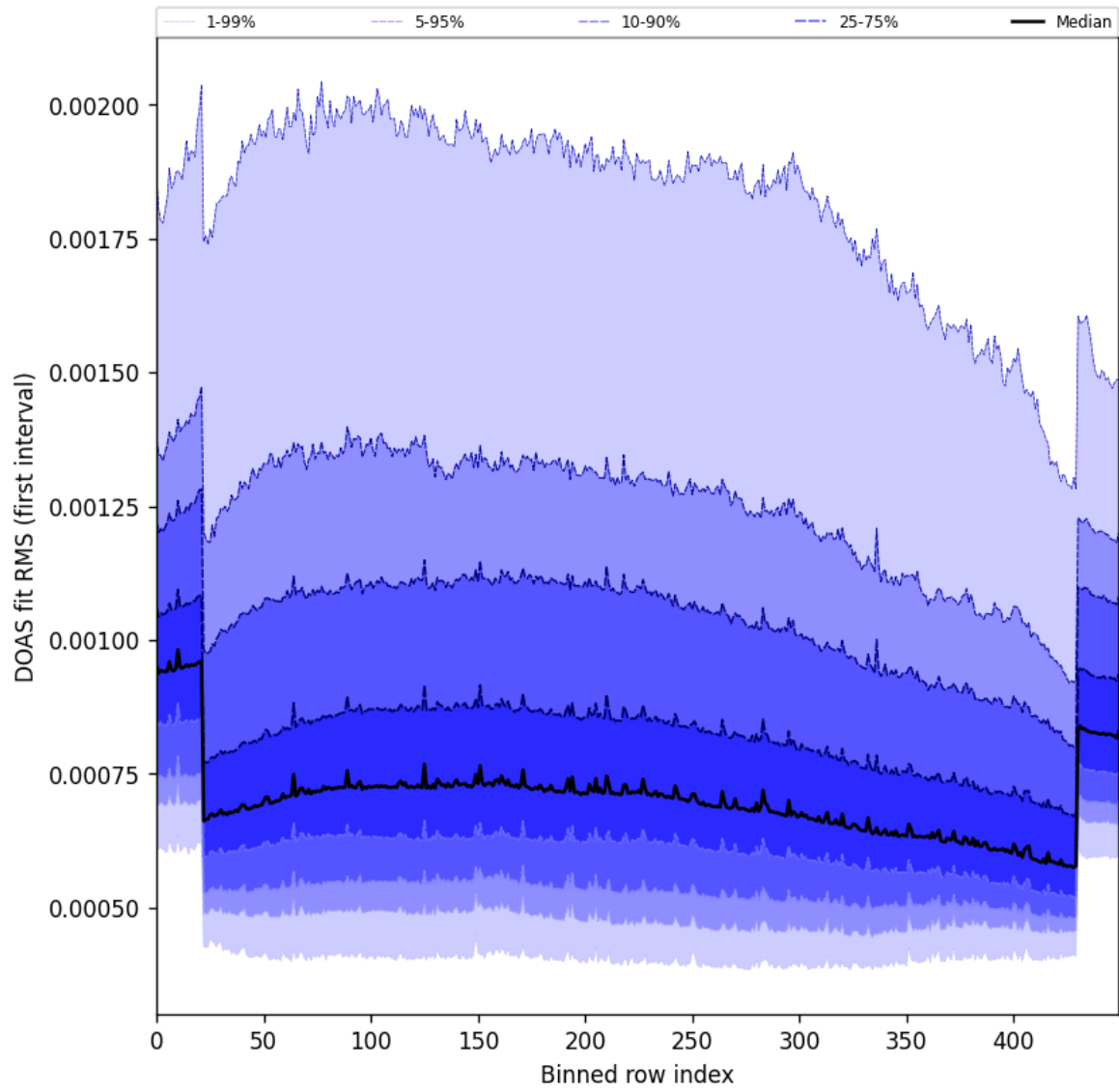
Figure 60: Along track statistics of “DOAS fit RMS (first interval)” for 2024-10-19 to 2024-10-20
