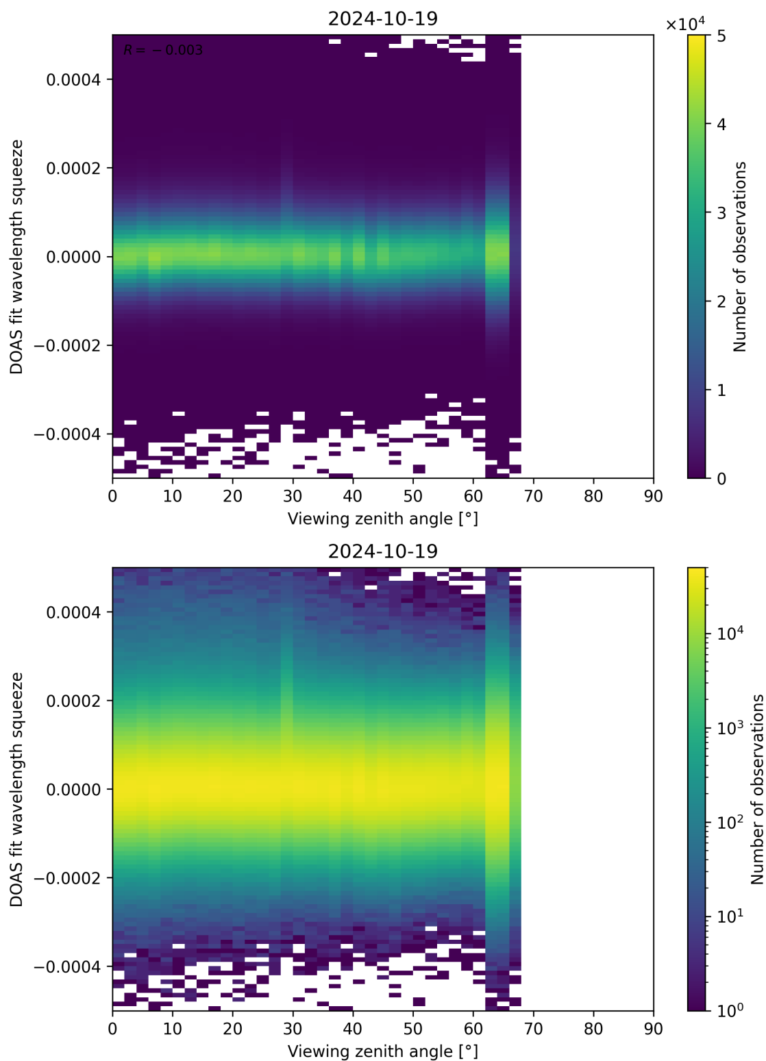
Figure 184: Scatter density plot of “Viewing zenith angle” against “DOAS fit wavelength squeeze” for 2024-10-19 to 2024-10-20.
