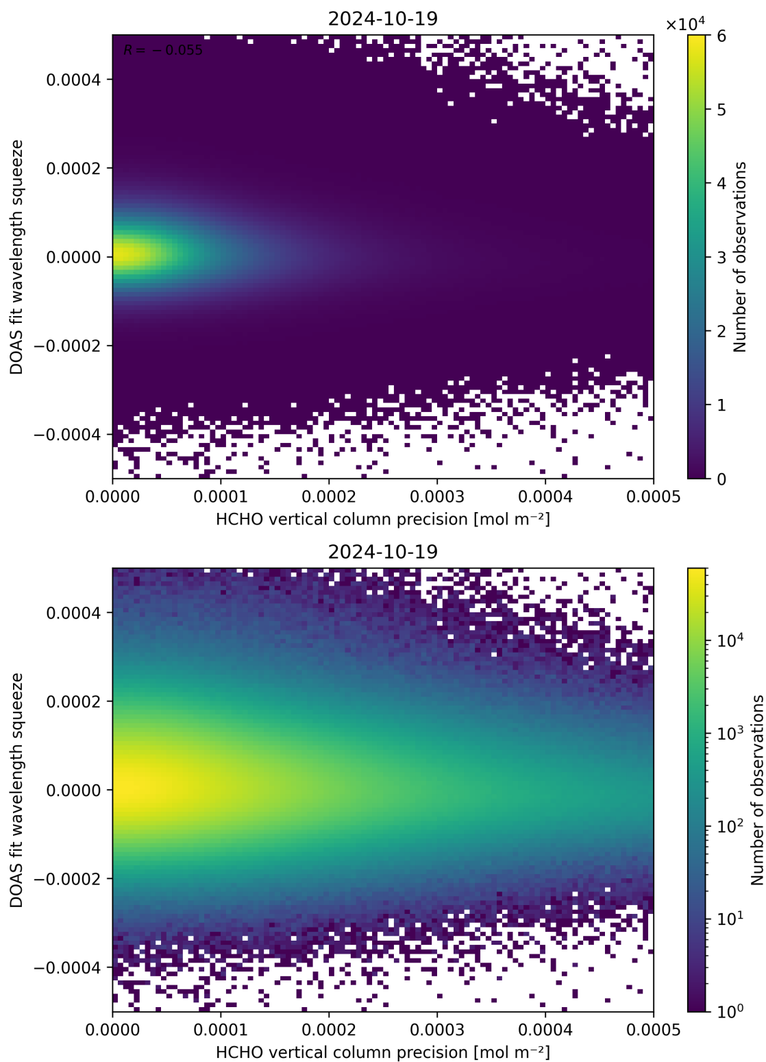
Figure 138: Scatter density plot of “HCHO vertical column precision” against “DOAS fit wavelength squeeze” for 2024-10-19 to 2024-10-20.
