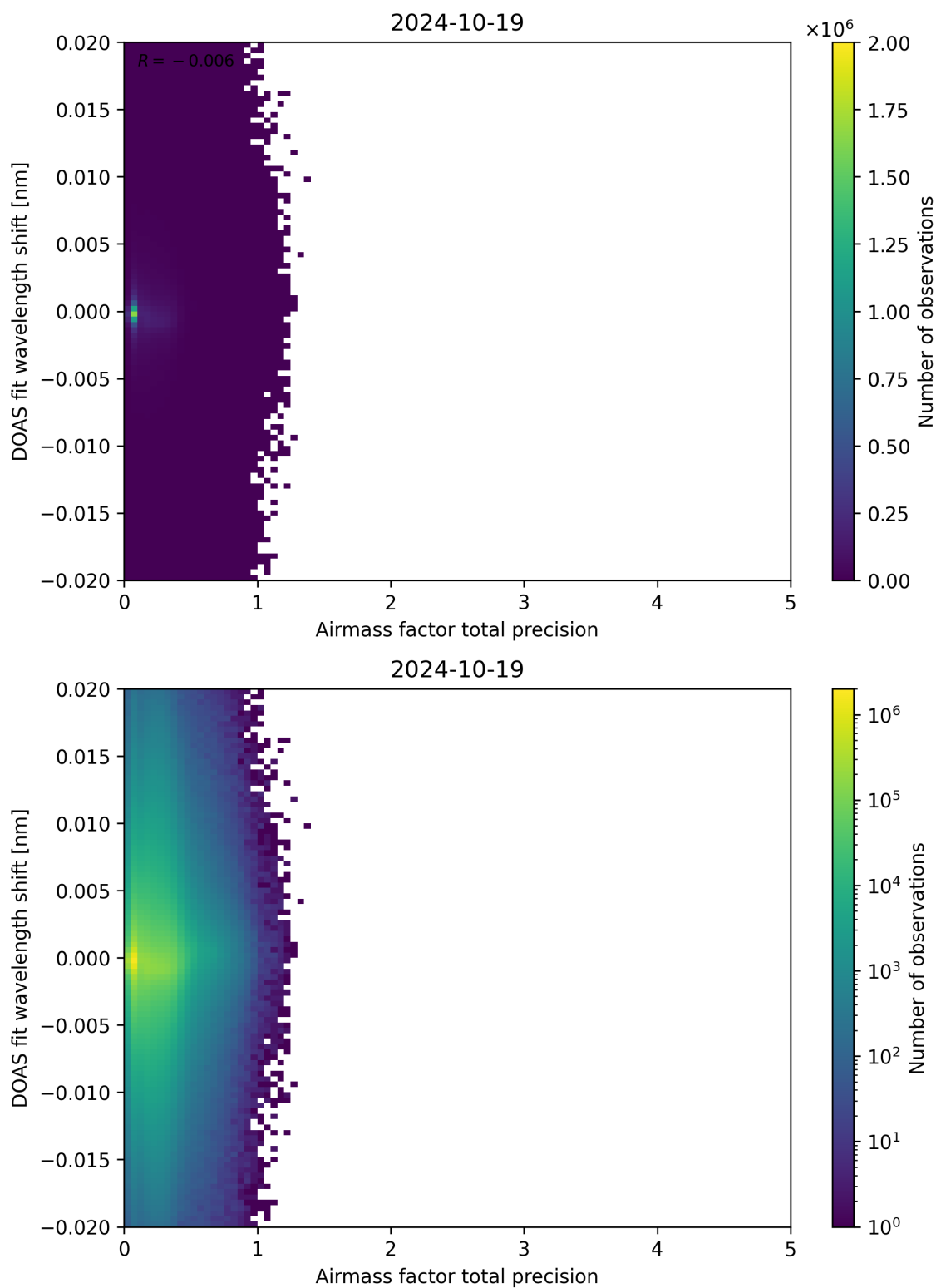
Figure 106: Scatter density plot of “Airmass factor total precision” against “DOAS fit wavelength shift” for 2024-10-19 to 2024-10-20.
