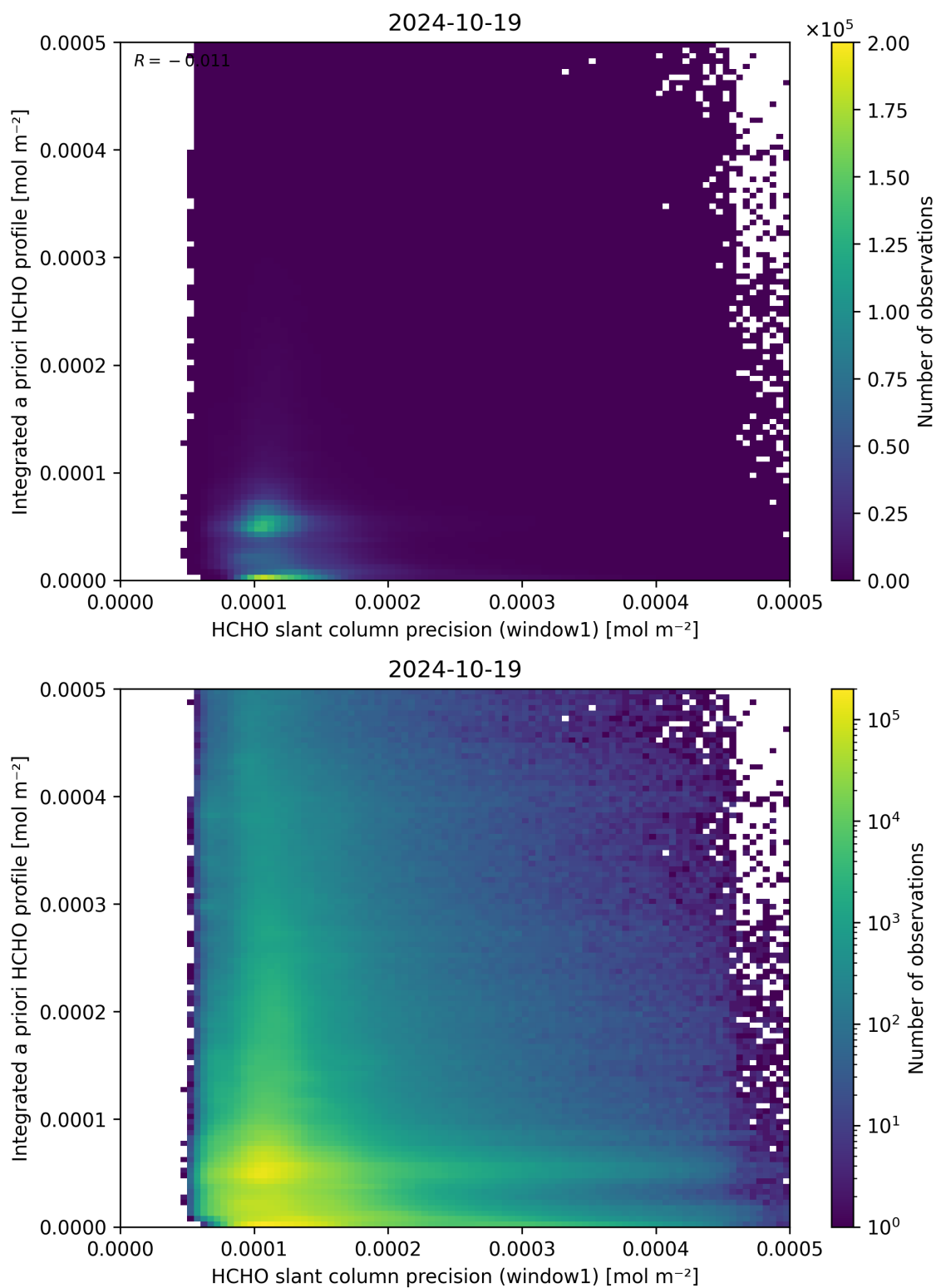
Figure 96: Scatter density plot of “HCHO slant column precision (window1)” against “Integrated a priori HCHO profile” for 2024-10-19 to 2024-10-20.
