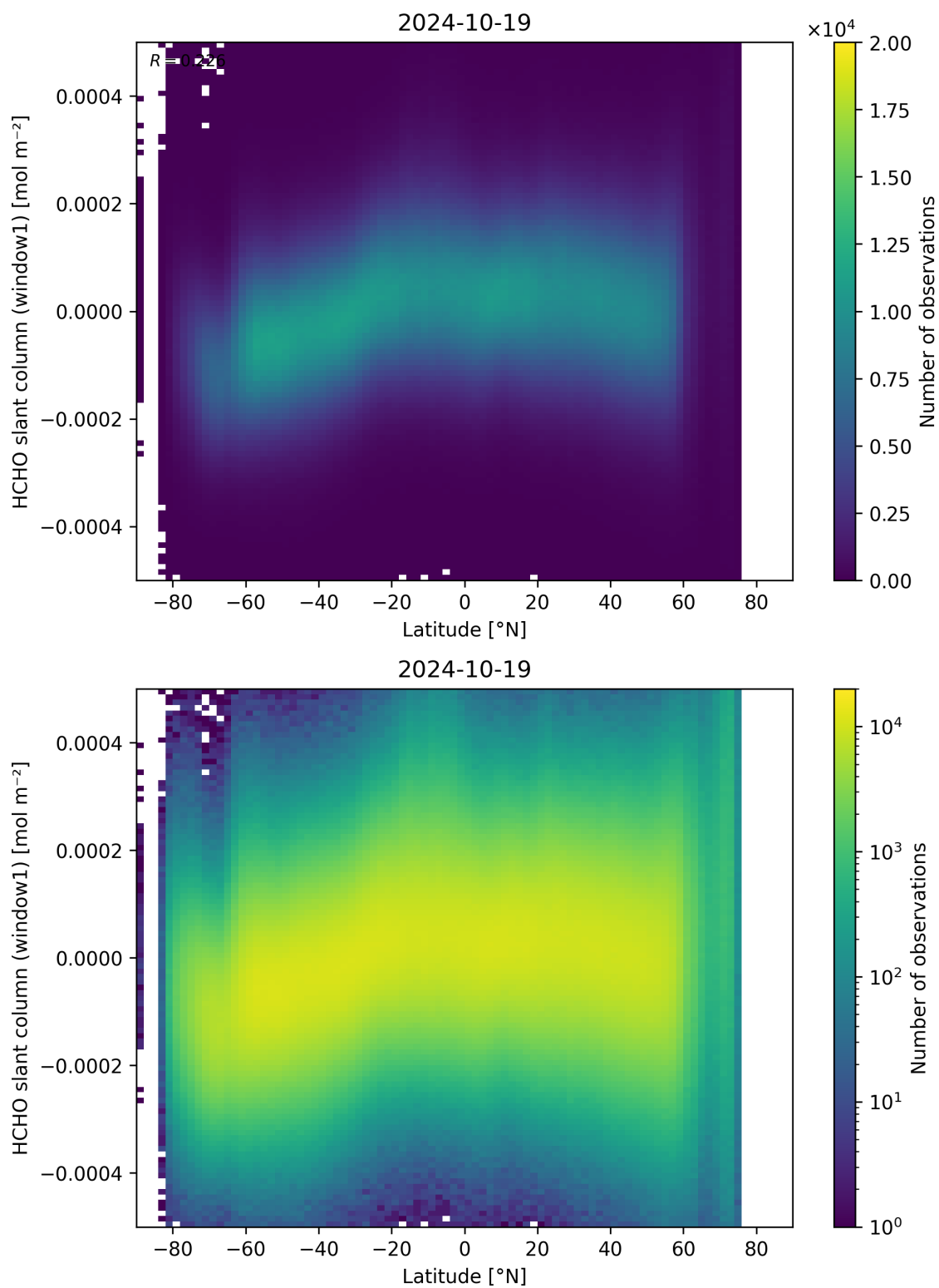
Figure 159: Scatter density plot of “Latitude” against “HCHO slant column (window1)” for 2024-10-19 to 2024-10-20.
