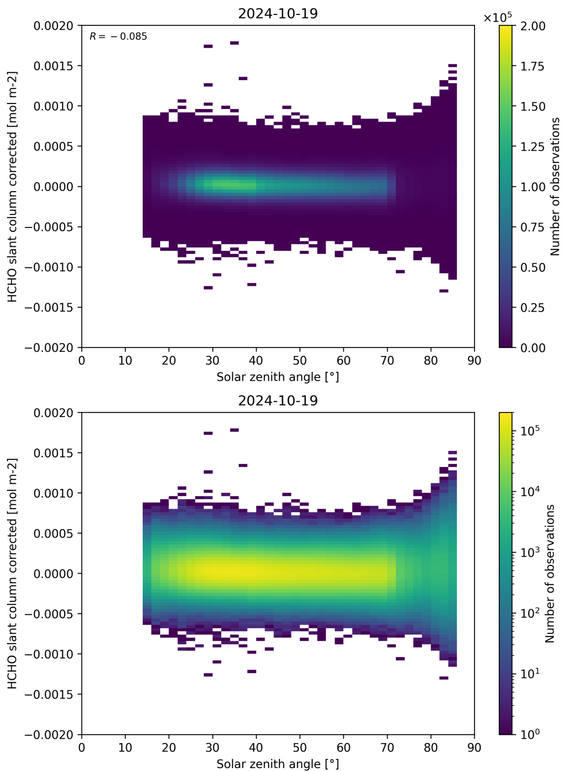
Figure 171: Scatter density plot of “Solar zenith angle” against “HCHO slant column corrected” for 2024-10-19 to 2024-10-20.
