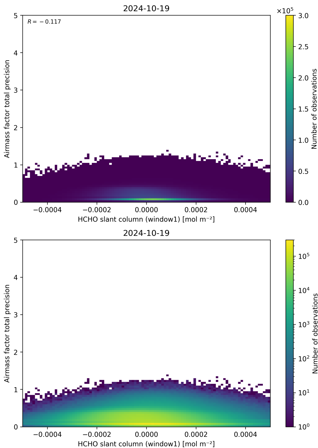
Figure 86: Scatter density plot of “HCHO slant column (window1)” against “Airmass factor total precision” for 2024-10-19 to 2024-10-20.
