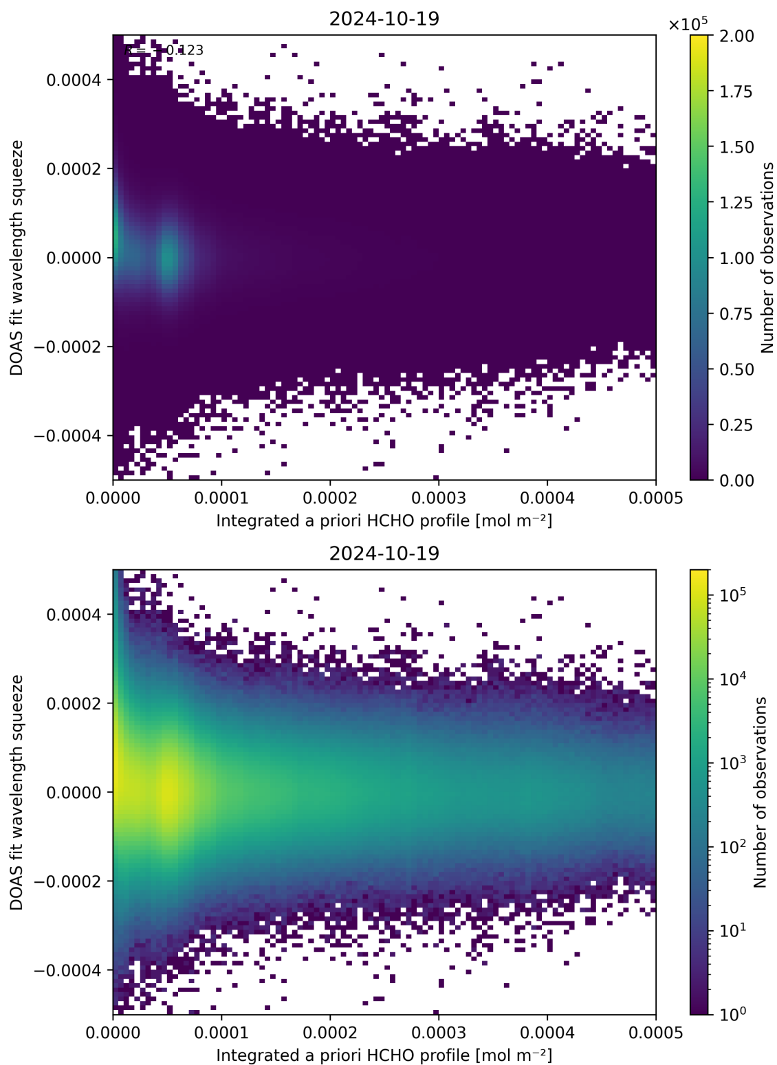
Figure 150: Scatter density plot of “Integrated a priori HCHO profile” against “DOAS fit wavelength squeeze” for 2024-10-19 to 2024-10-20.
