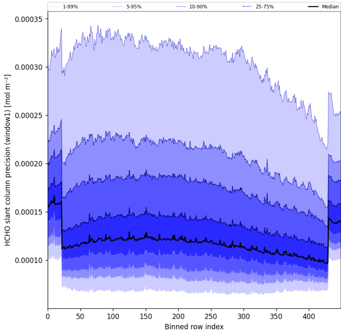
Figure 53: Along track statistics of “HCHO slant column precision (window1)” for 2024-10-19 to 2024-10-20
