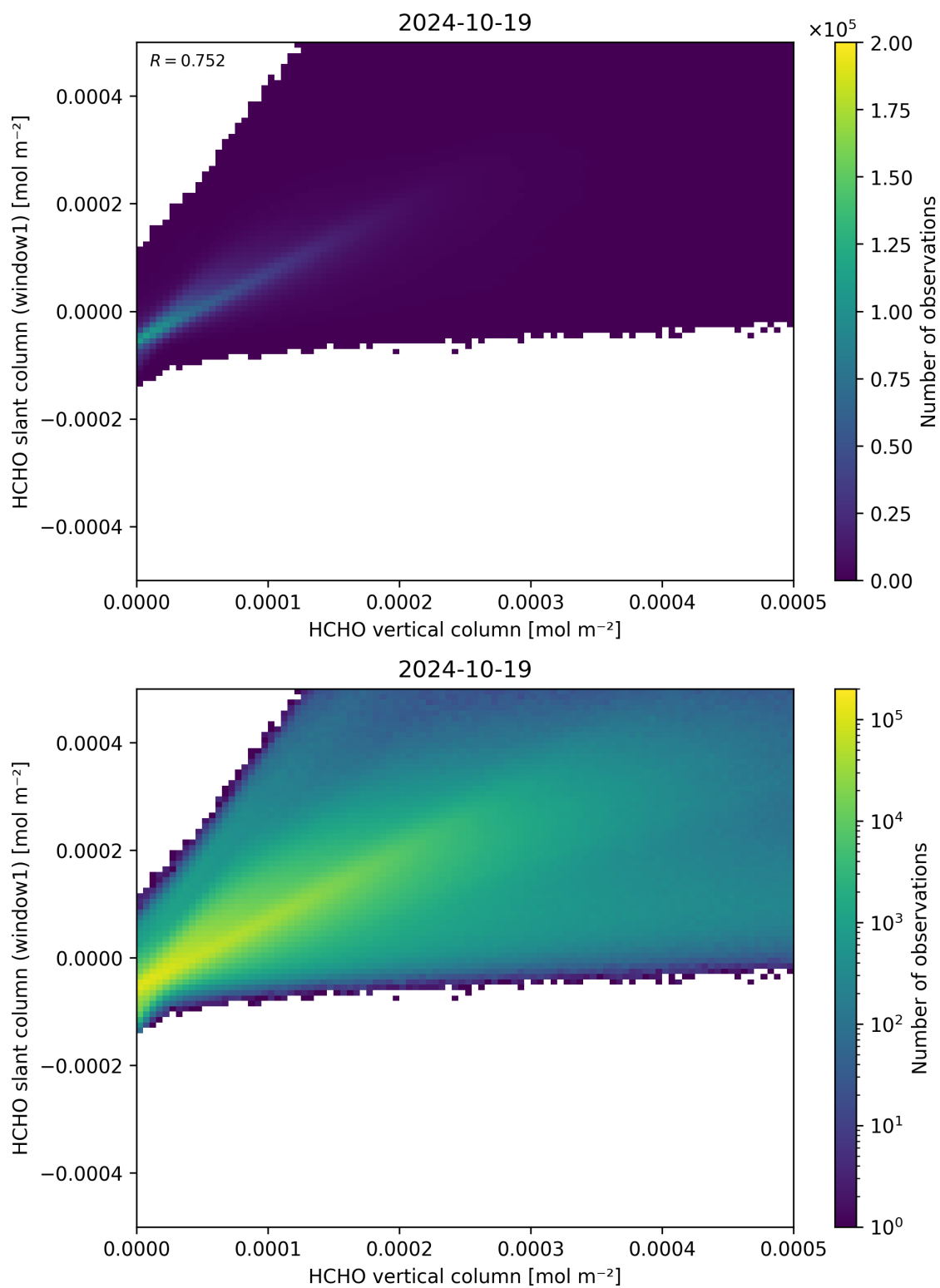
Figure 129: Scatter density plot of “HCHO vertical column” against “HCHO slant column (window1)” for 2024-10-19 to 2024-10-20.
