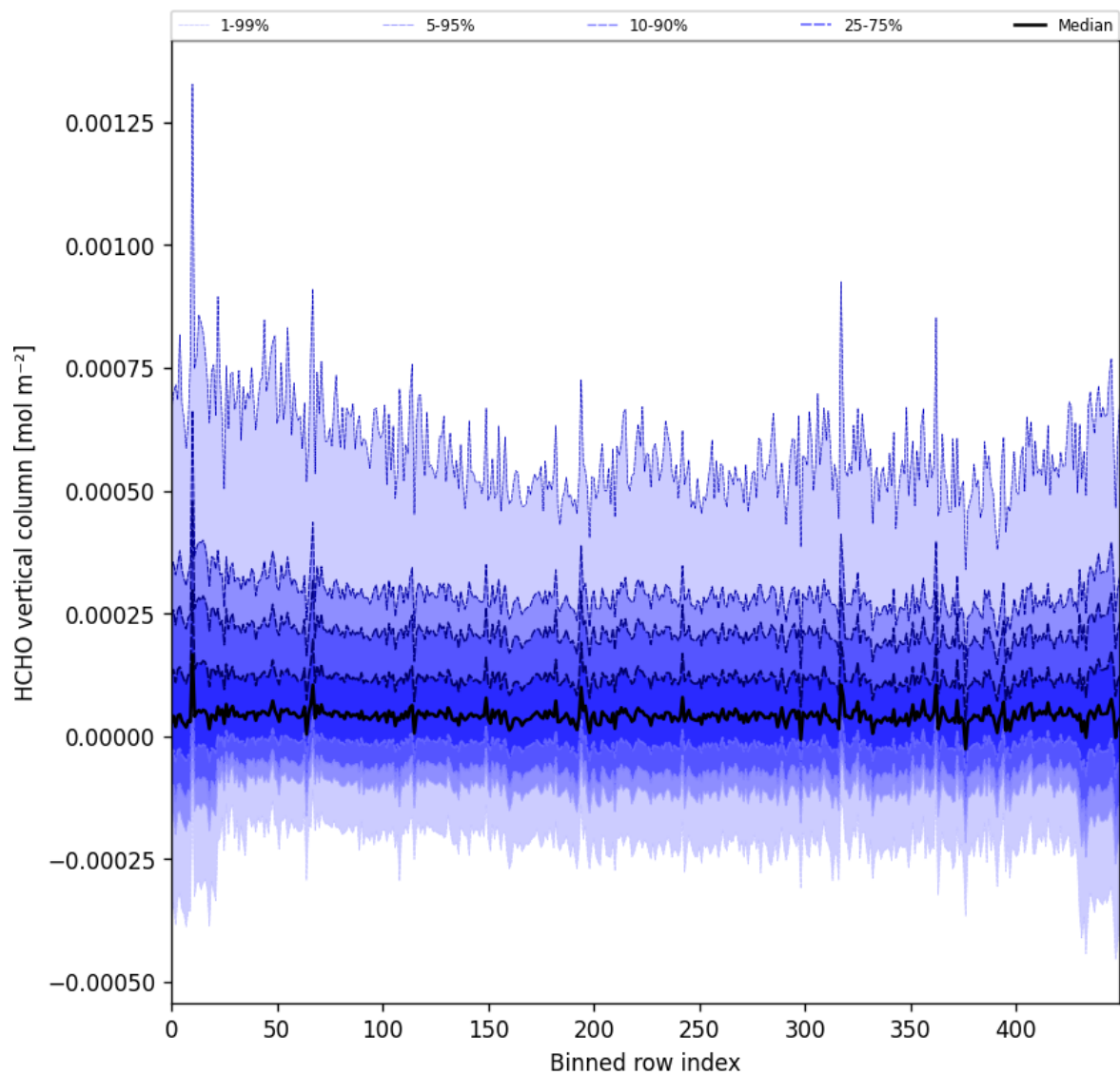
Figure 49: Along track statistics of “HCHO vertical column” for 2024-10-19 to 2024-10-20
