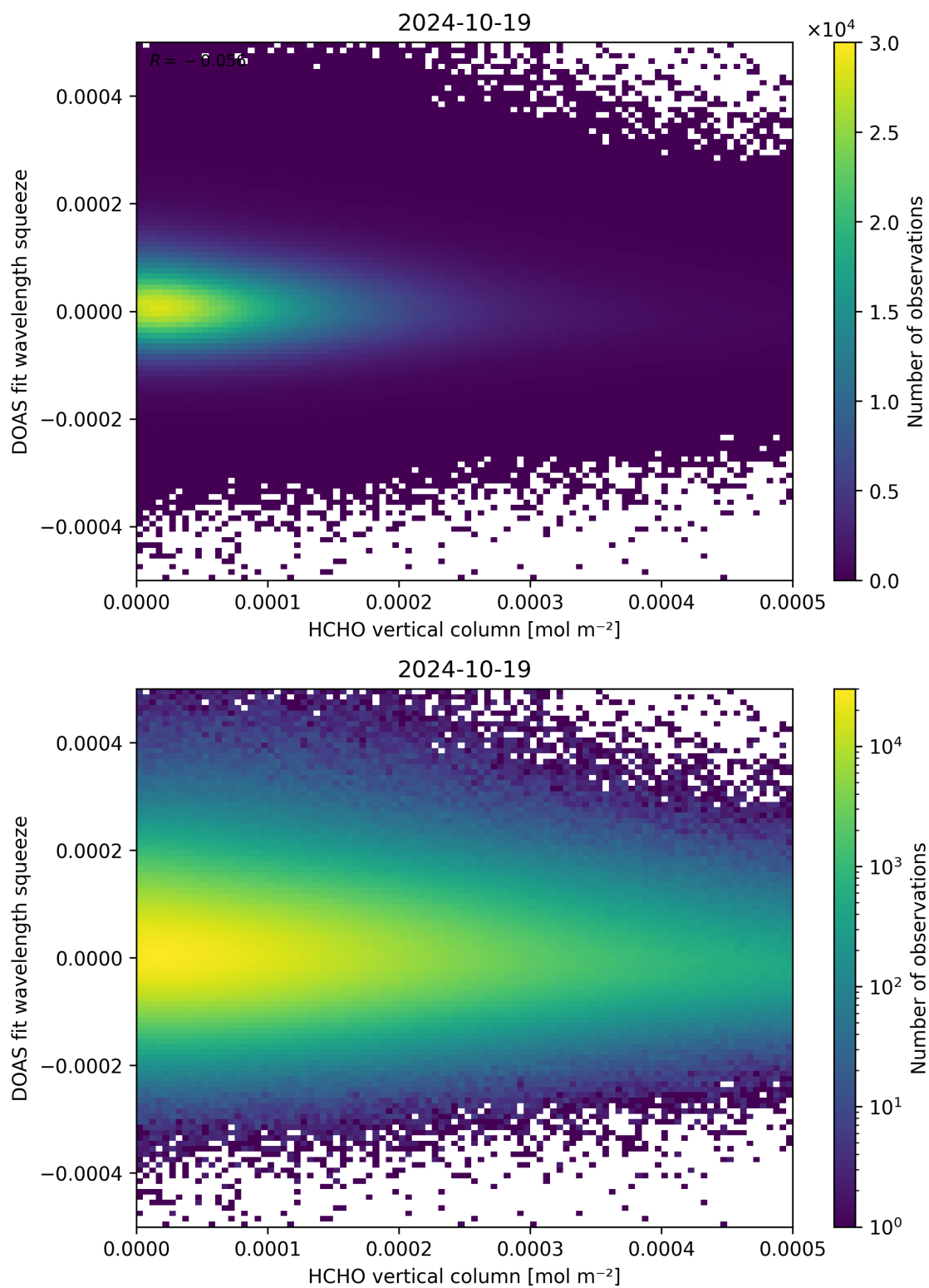
Figure 125: Scatter density plot of “HCHO vertical column” against “DOAS fit wavelength squeeze” for 2024-10-19 to 2024-10-20.
