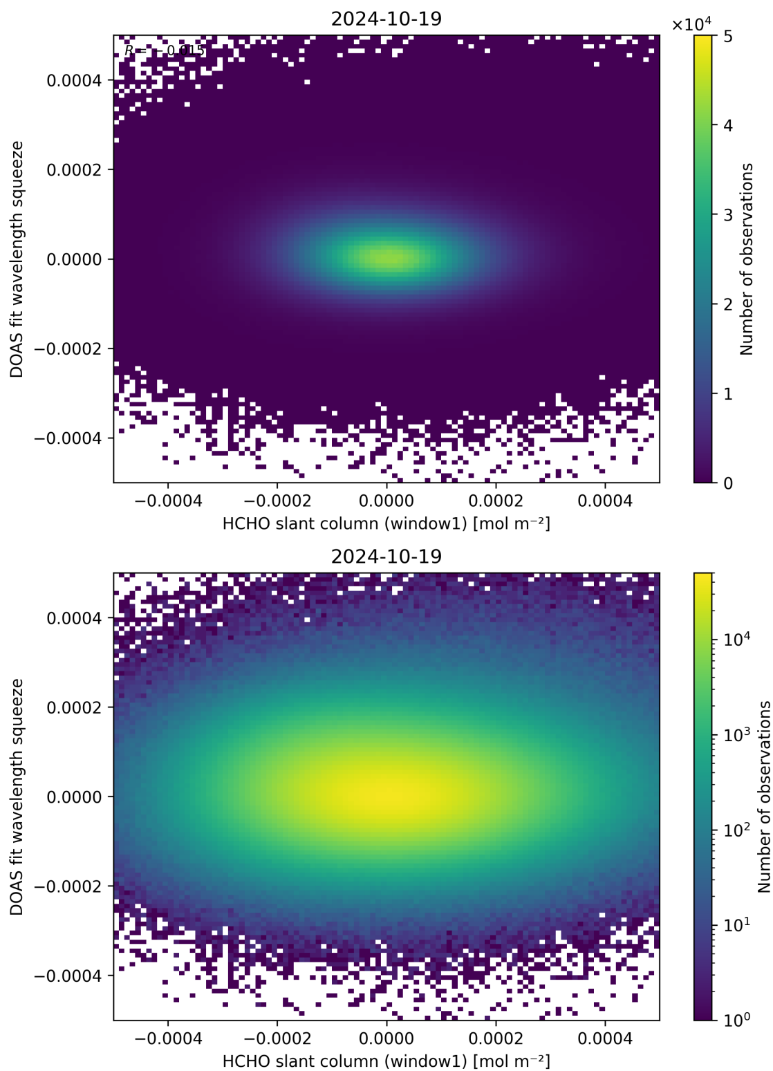
Figure 80: Scatter density plot of “HCHO slant column (window1)” against “DOAS fit wavelength squeeze” for 2024-10-19 to 2024-10-20.
