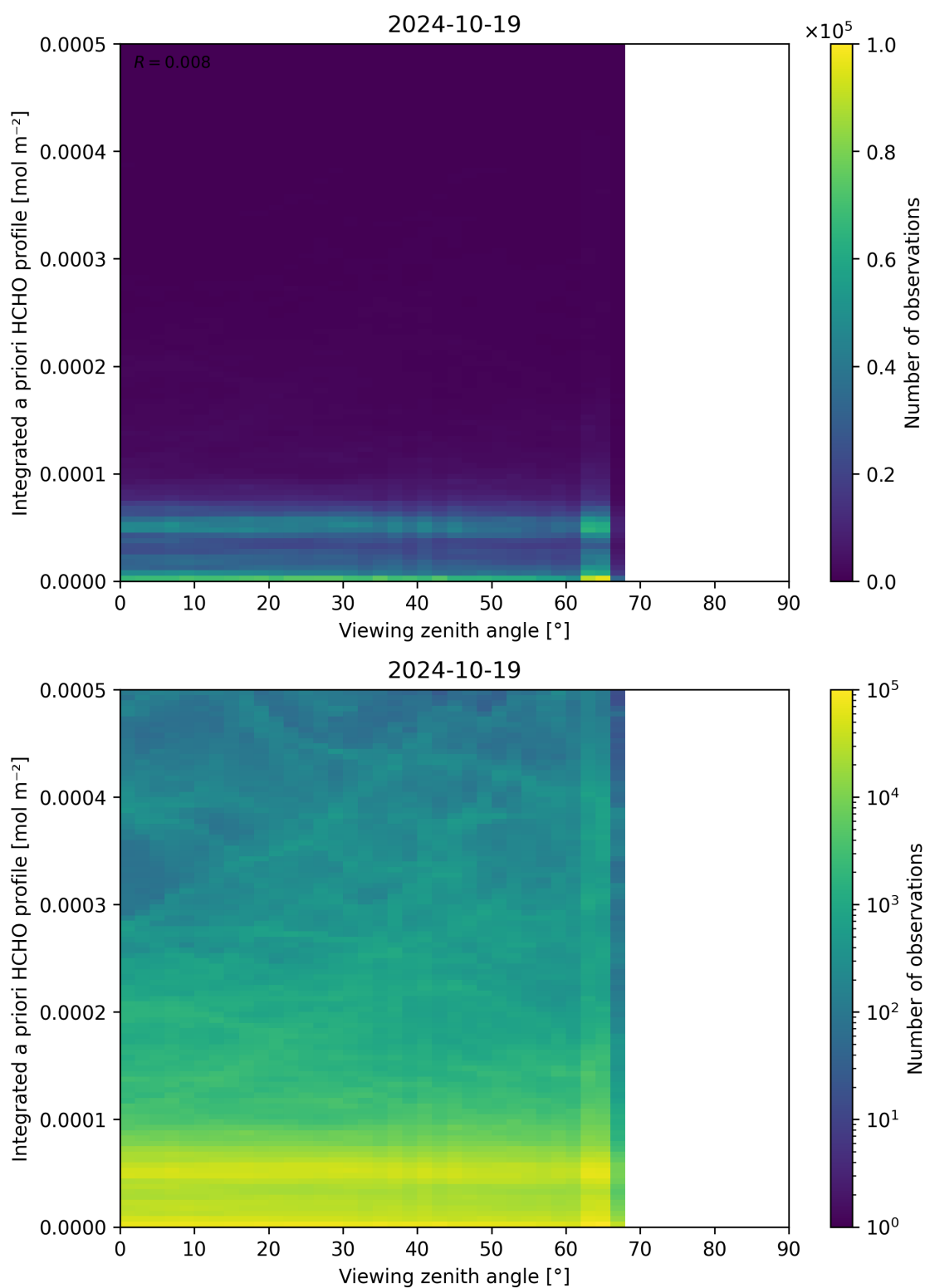
Figure 195: Scatter density plot of “Viewing zenith angle” against “Integrated a priori HCHO profile” for 2024-10-19 to 2024-10-20.
