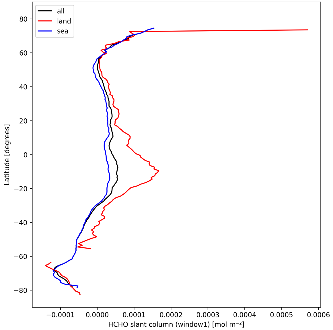
Figure 24: Zonal average of “HCHO slant column (window1)” for 2024-10-19 to 2024-10-20.
