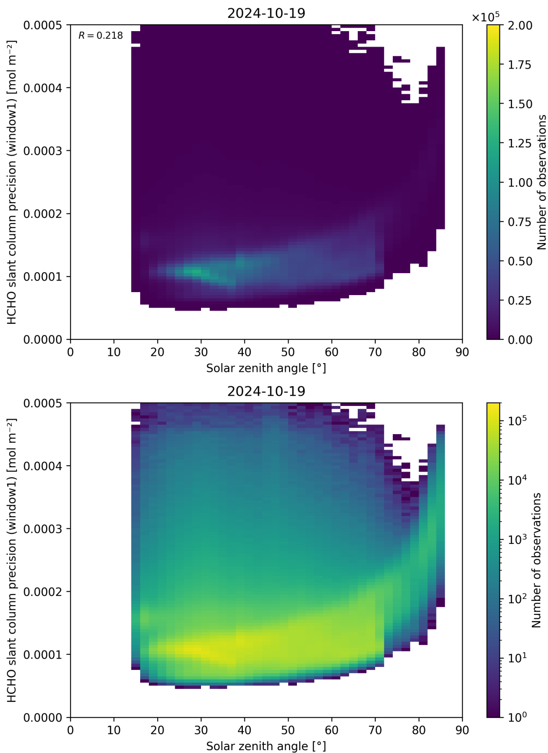
Figure 174: Scatter density plot of “Solar zenith angle” against “HCHO slant column precision (window1)” for 2024-10-19 to 2024-10-20.
