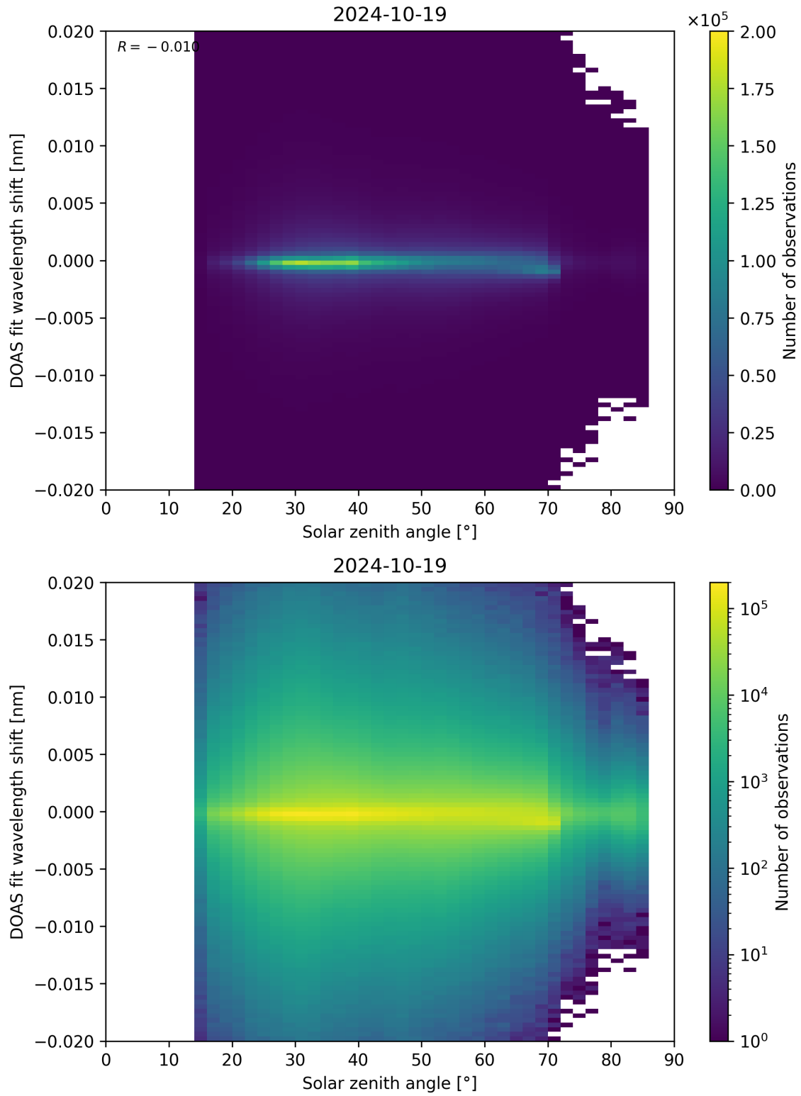
Figure 168: Scatter density plot of “Solar zenith angle” against “DOAS fit wavelength shift” for 2024-10-19 to 2024-10-20.
