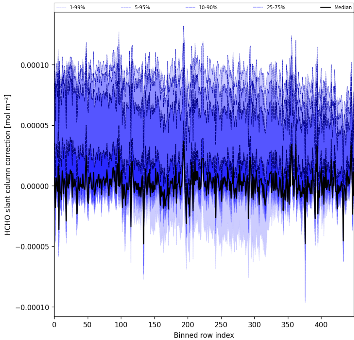
Figure 61: Along track statistics of “HCHO slant column correction” for 2024-10-19 to 2024-10-20
