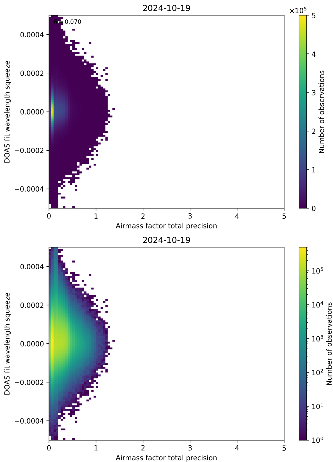
Figure 107: Scatter density plot of “Airmass factor total precision” against “DOAS fit wavelength squeeze” for 2024-10-19 to 2024-10-20.
