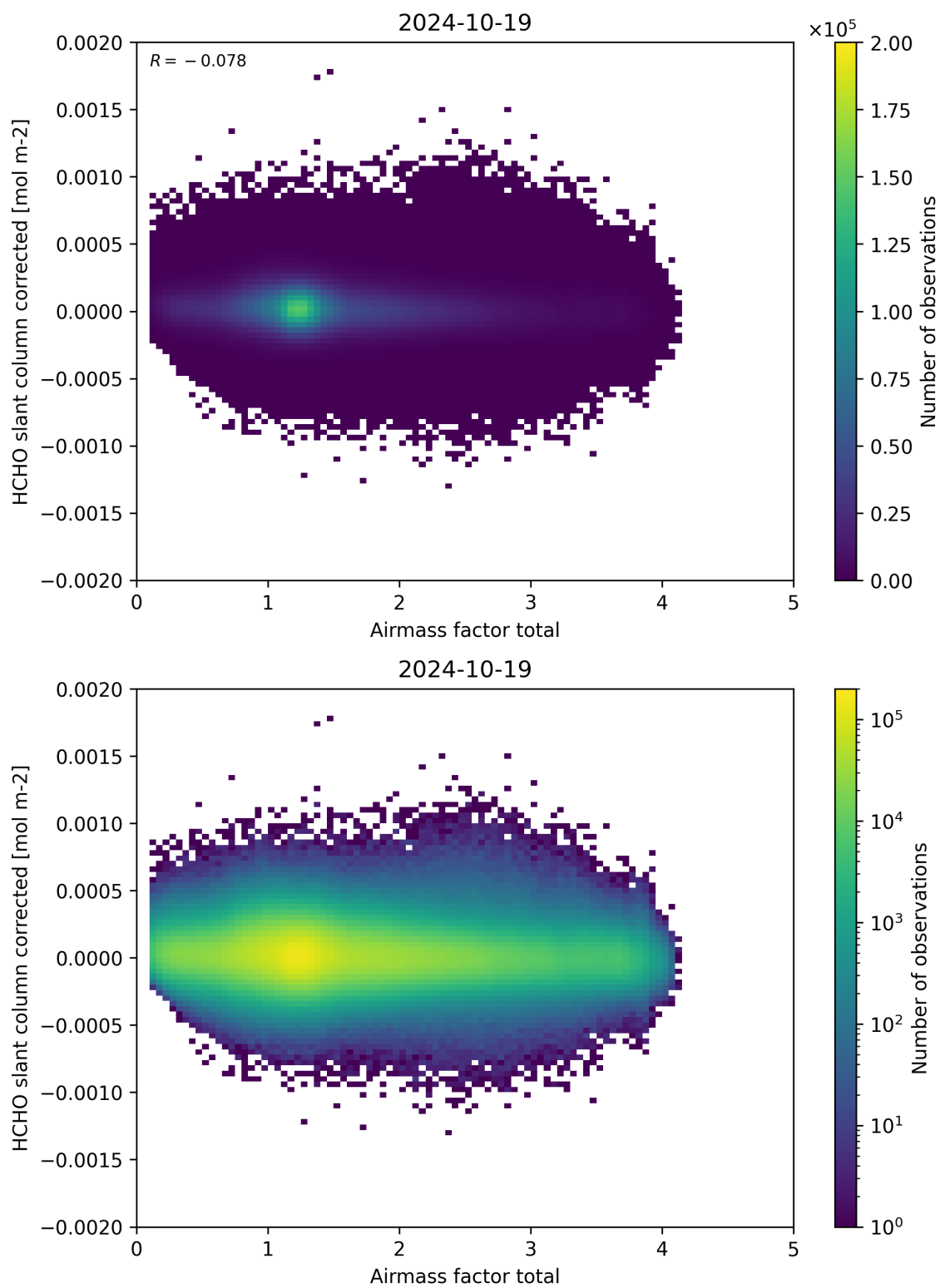
Figure 101: Scatter density plot of “Airmass factor total” against “HCHO slant column corrected” for 2024-10-19 to 2024-10-20.
