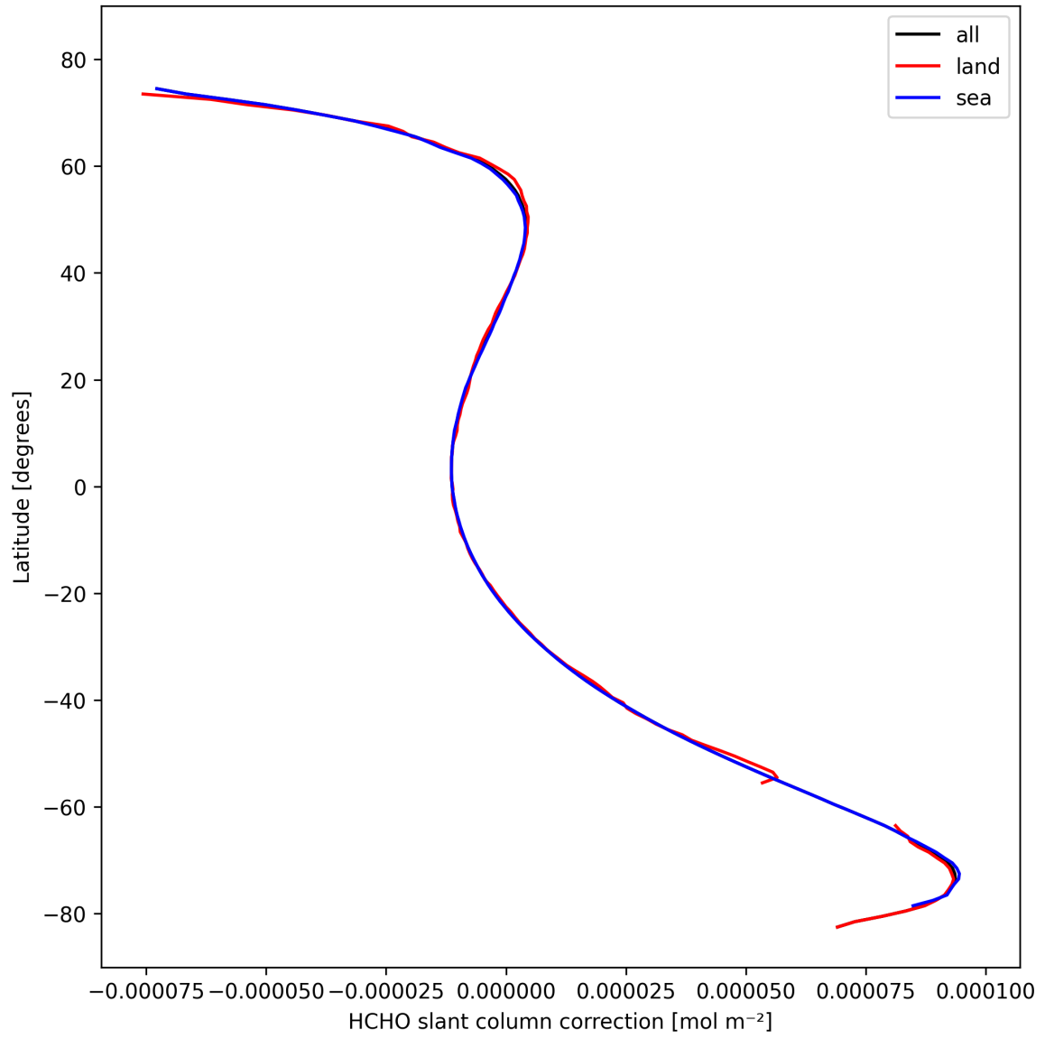
Figure 33: Zonal average of “HCHO slant column correction” for 2024-10-19 to 2024-10-20.
