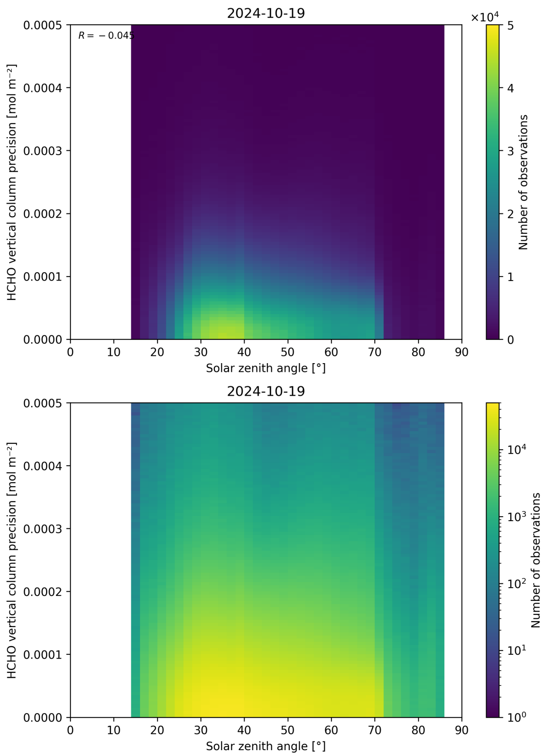
Figure 179: Scatter density plot of “Solar zenith angle” against “HCHO vertical column precision” for 2024-10-19 to 2024-10-20.
