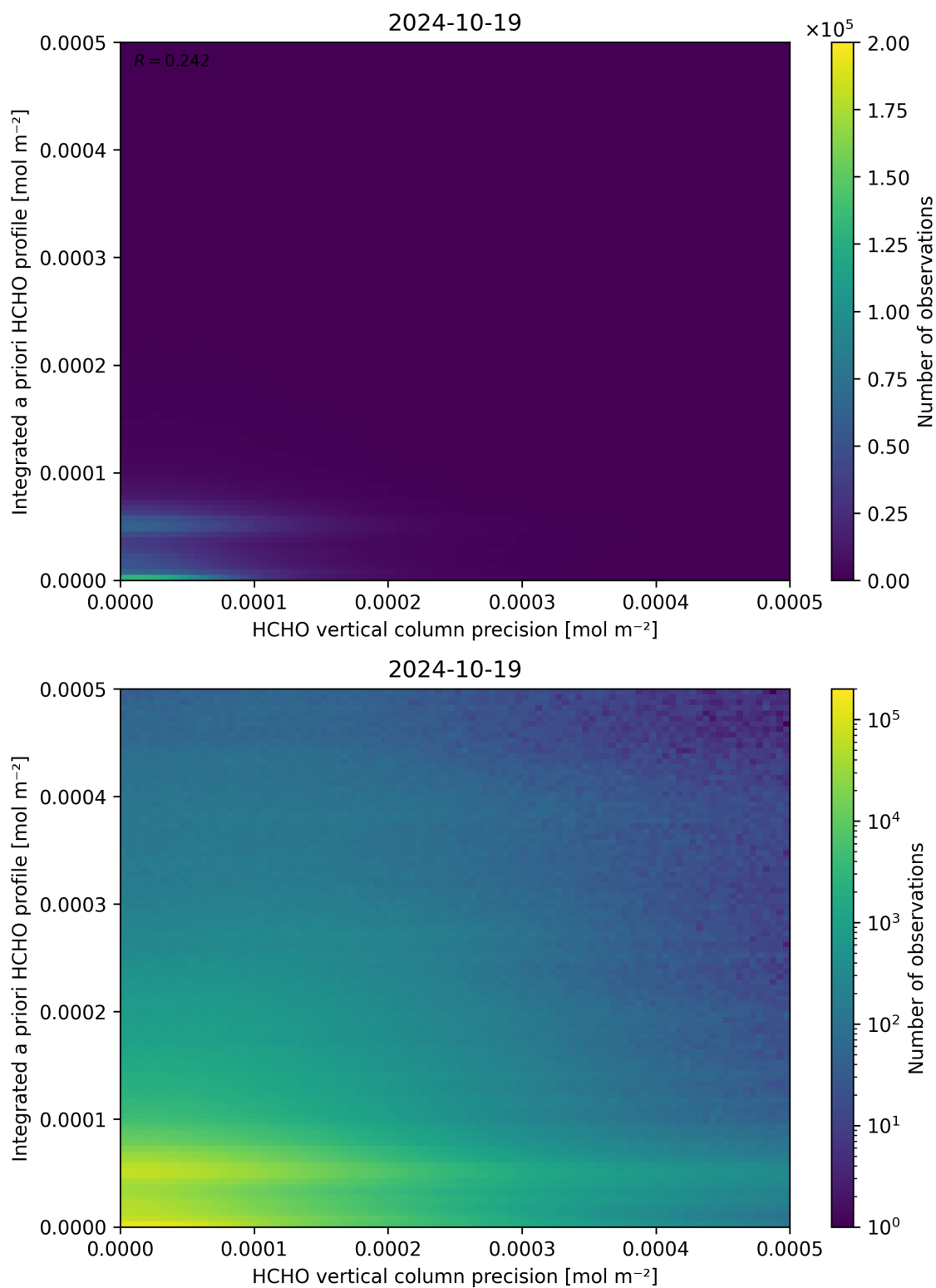
Figure 147: Scatter density plot of “HCHO vertical column precision” against “Integrated a priori HCHO profile” for 2024-10-19 to 2024-10-20.
