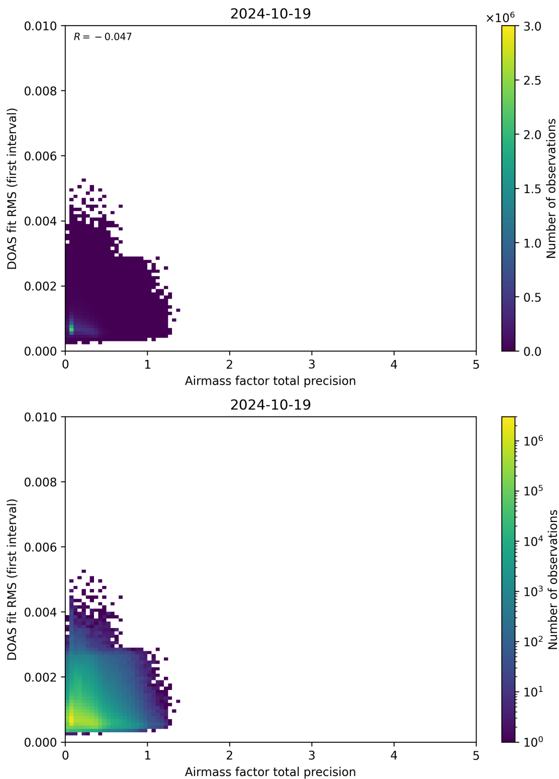
Figure 105: Scatter density plot of “Airmass factor total precision” against “DOAS fit RMS (first interval)” for 2024-10-19 to 2024-10-20.
