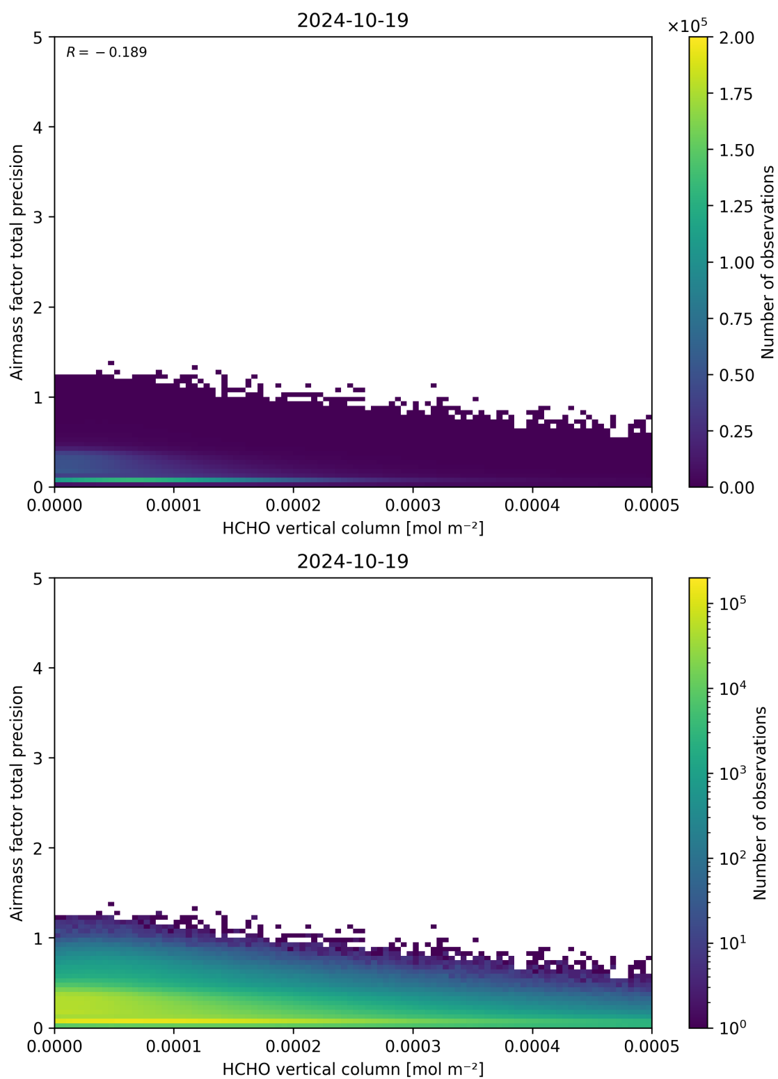
Figure 132: Scatter density plot of “HCHO vertical column” against “Airmass factor total precision” for 2024-10-19 to 2024-10-20.
