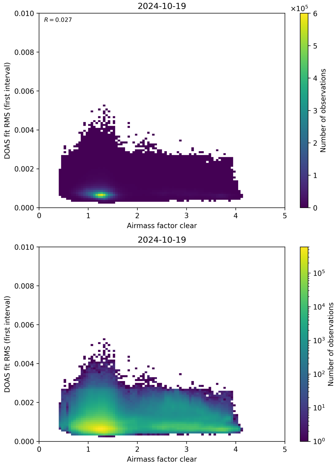
Figure 71: Scatter density plot of “Airmass factor clear” against “DOAS fit RMS (first interval)” for 2024-10-19 to 2024-10-20.
