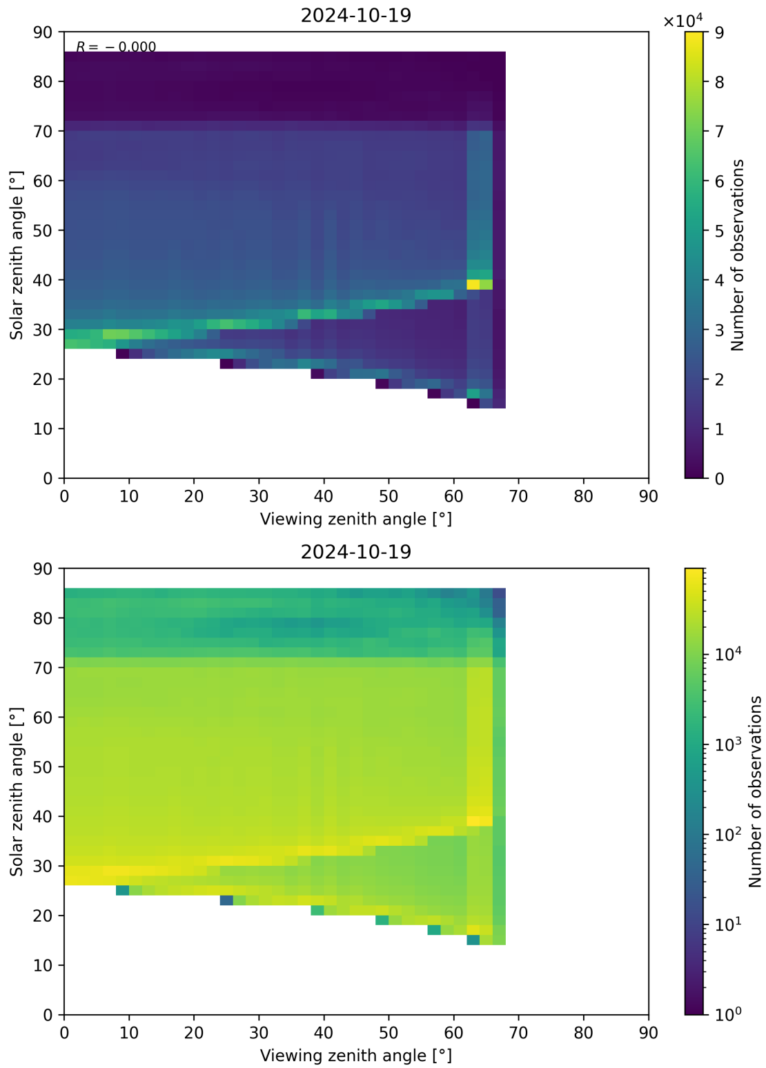
Figure 197: Scatter density plot of “Viewing zenith angle” against “Solar zenith angle” for 2024-10-19 to 2024-10-20.
