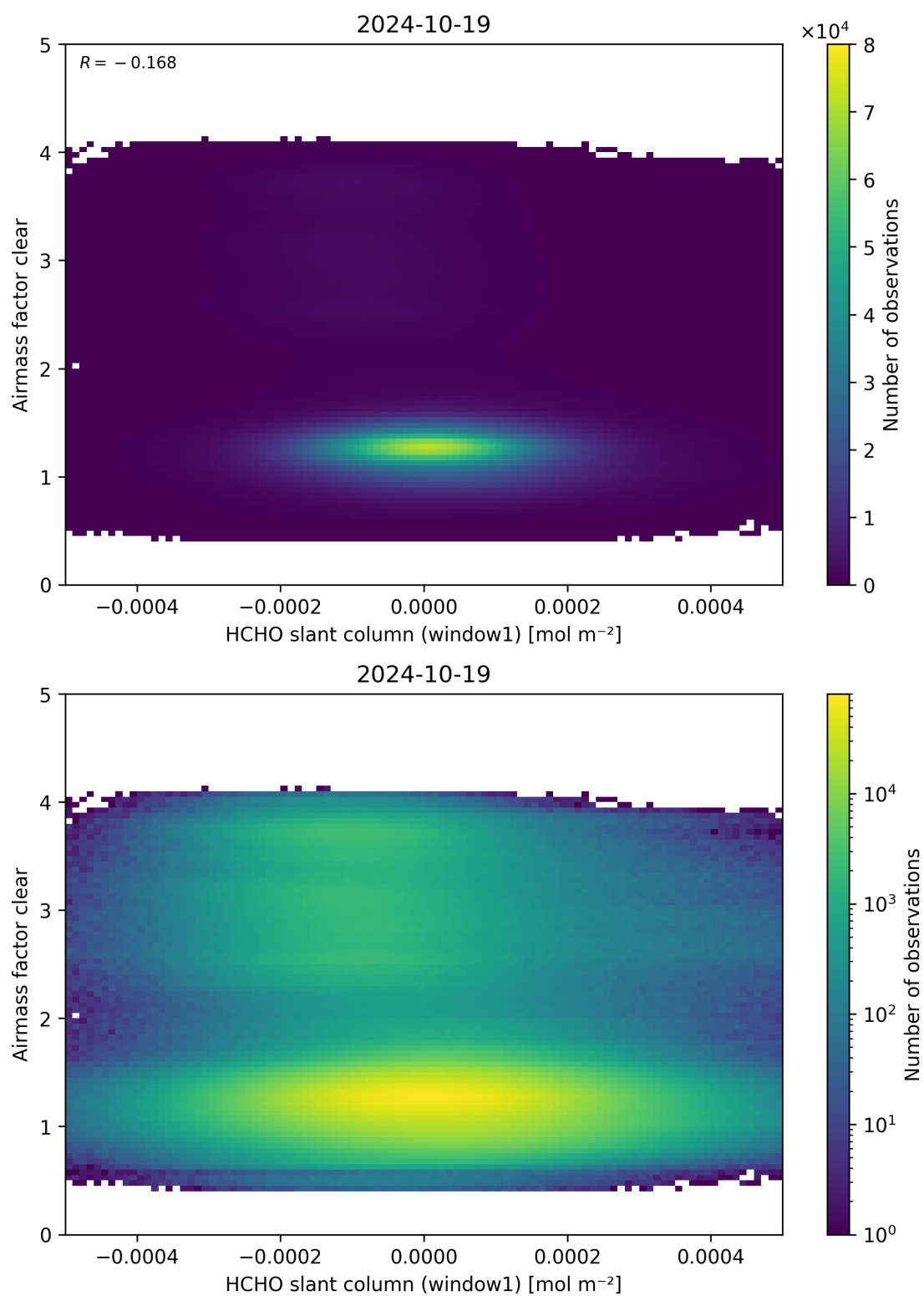
Figure 81: Scatter density plot of “HCHO slant column (window1)” against “Airmass factor clear” for 2024-10-19 to 2024-10-20.
