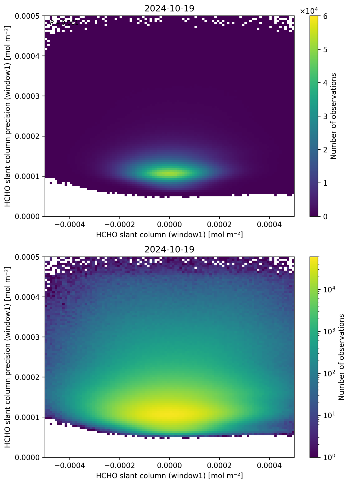
Figure 84: Scatter density plot of “HCHO slant column (window1)” against “HCHO slant column precision (window1)” for 2024-10-19 to 2024-10-20.
