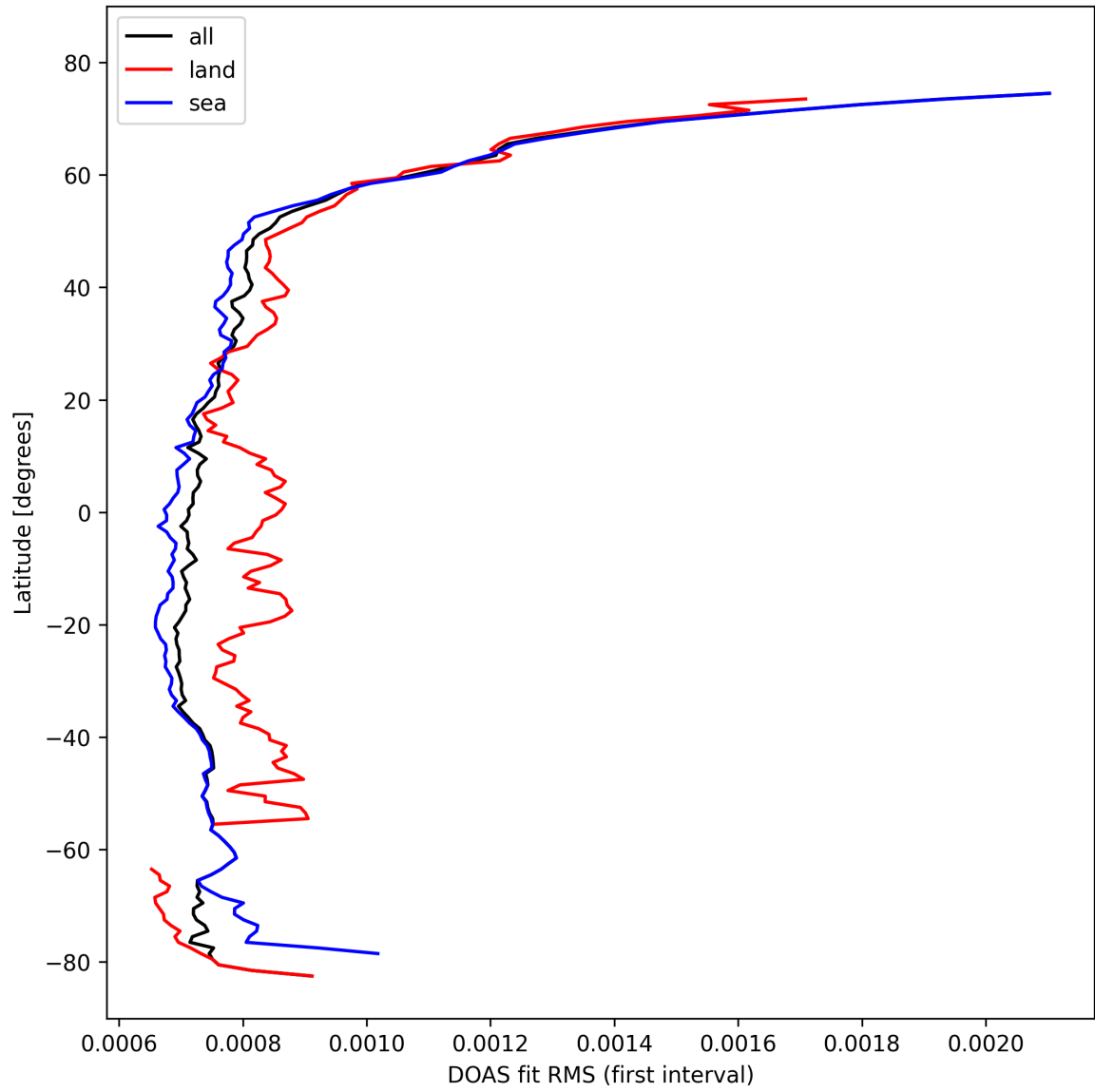
Figure 32: Zonal average of “DOAS fit RMS (first interval)” for 2024-10-19 to 2024-10-20.
