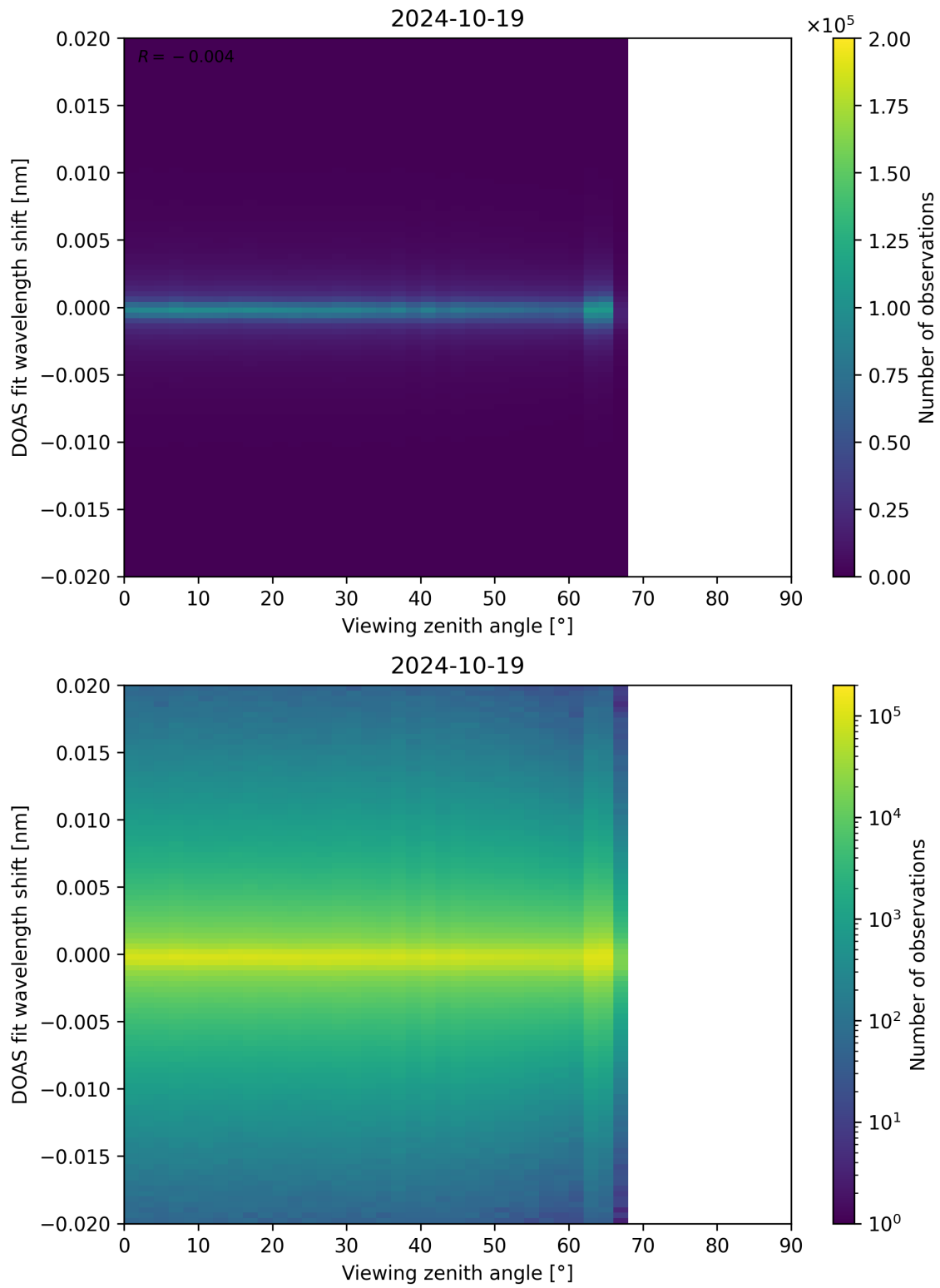
Figure 183: Scatter density plot of “Viewing zenith angle” against “DOAS fit wavelength shift” for 2024-10-19 to 2024-10-20.
