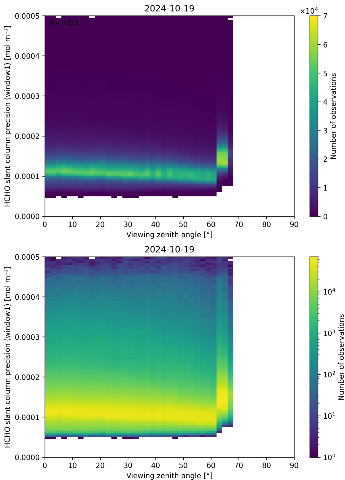
Figure 189: Scatter density plot of “Viewing zenith angle” against “HCHO slant column precision (window1)” for 2024-10-19 to 2024-10-20.
