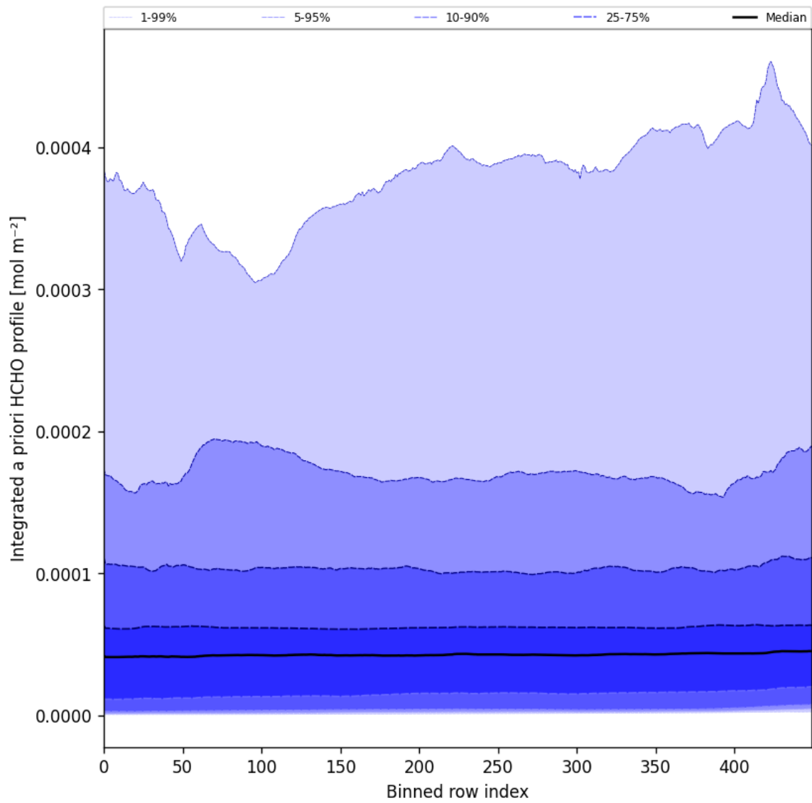
Figure 57: Along track statistics of "Integrated a priori HCHO profile" for 2024-10-19 to 2024-10-20
