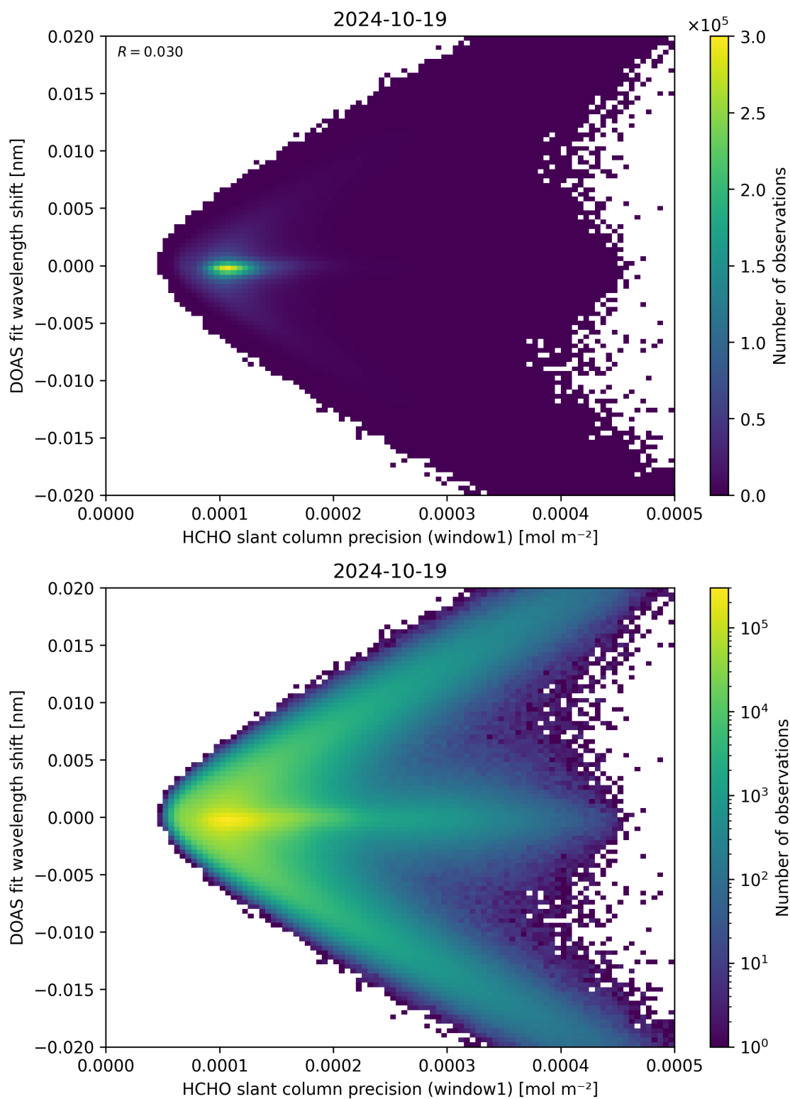
Figure 89: Scatter density plot of “HCHO slant column precision (window1)” against “DOAS fit wavelength shift” for 2024-10-19 to 2024-10-20.
