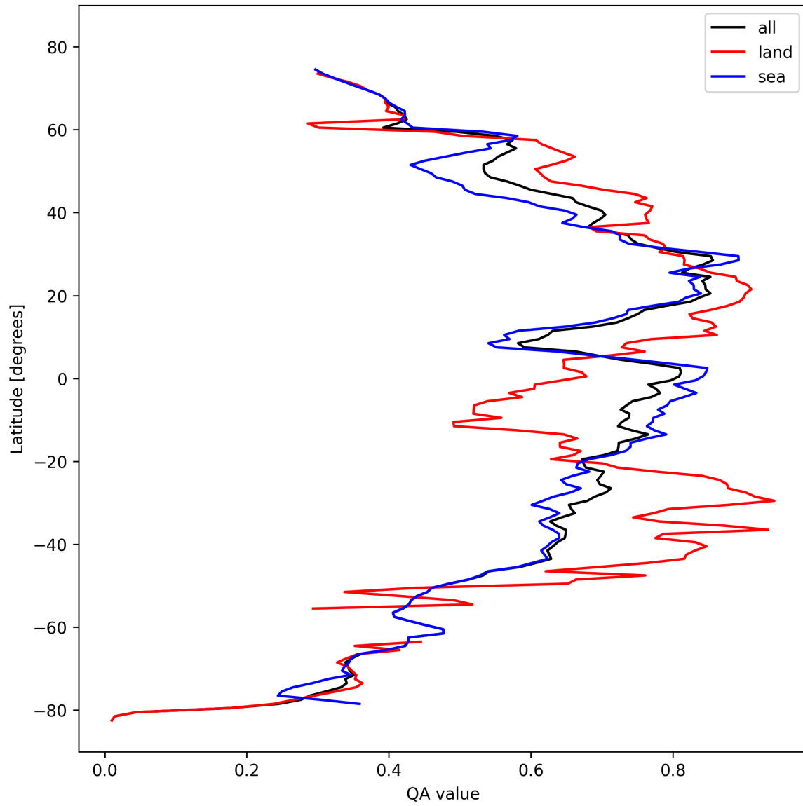
Figure 20: Zonal average of “QA value” for 2024-10-19 to 2024-10-20.
