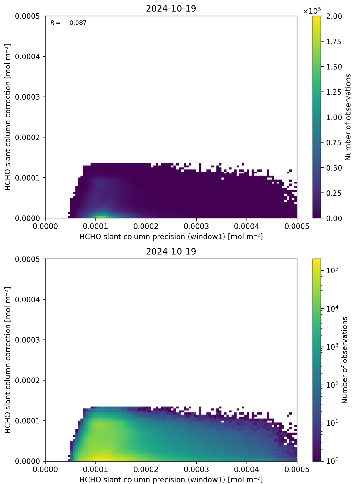
Figure 93: Scatter density plot of “HCHO slant column precision (window1)” against “HCHO slant column correction” for 2024-10-19 to 2024-10-20.
