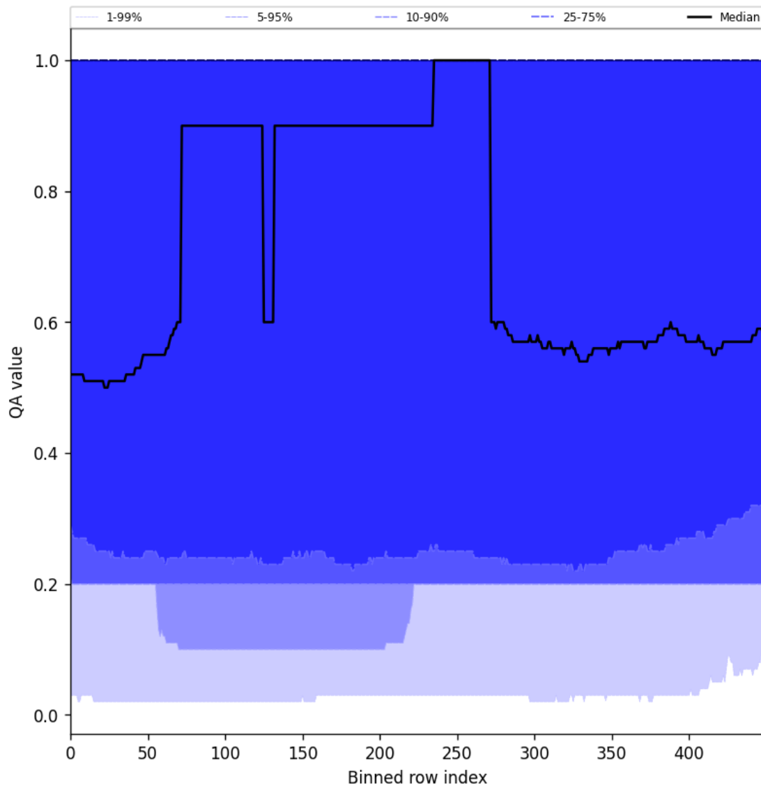
Figure 48: Along track statistics of “QA value” for 2024-10-19 to 2024-10-20
