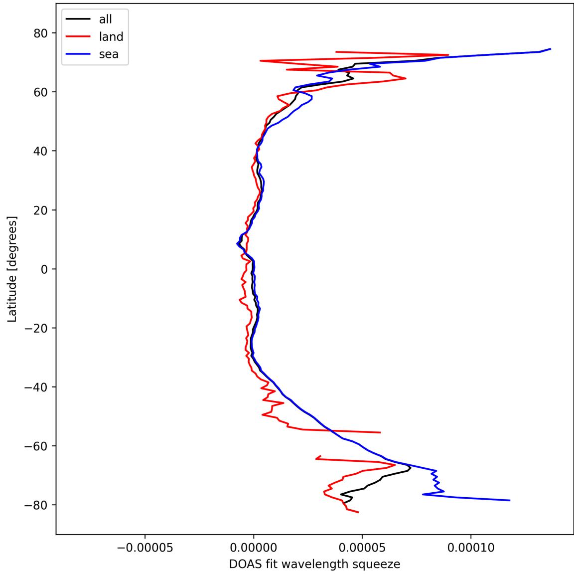
Figure 31: Zonal average of “DOAS fit wavelength squeeze” for 2024-10-19 to 2024-10-20.
