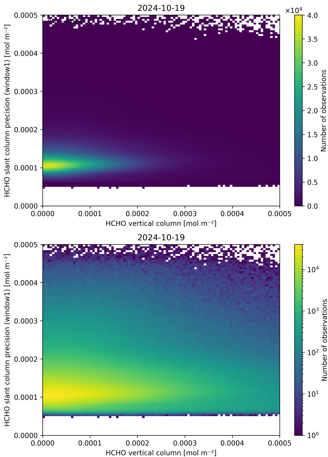
Figure 130: Scatter density plot of “HCHO vertical column” against “HCHO slant column precision (window1)” for 2024-10-19 to 2024-10-20.
