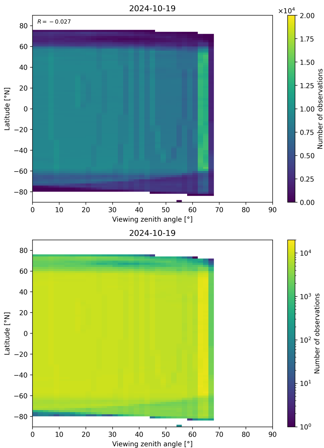
Figure 196: Scatter density plot of “Viewing zenith angle” against “Latitude” for 2024-10-19 to 2024-10-20.
