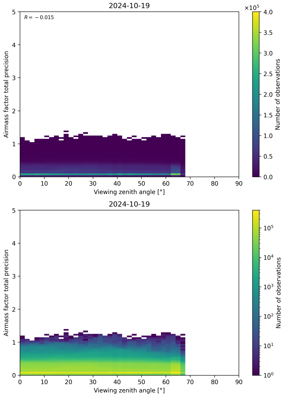
Figure 191: Scatter density plot of “Viewing zenith angle” against “Airmass factor total precision” for 2024-10-19 to 2024-10-20.
