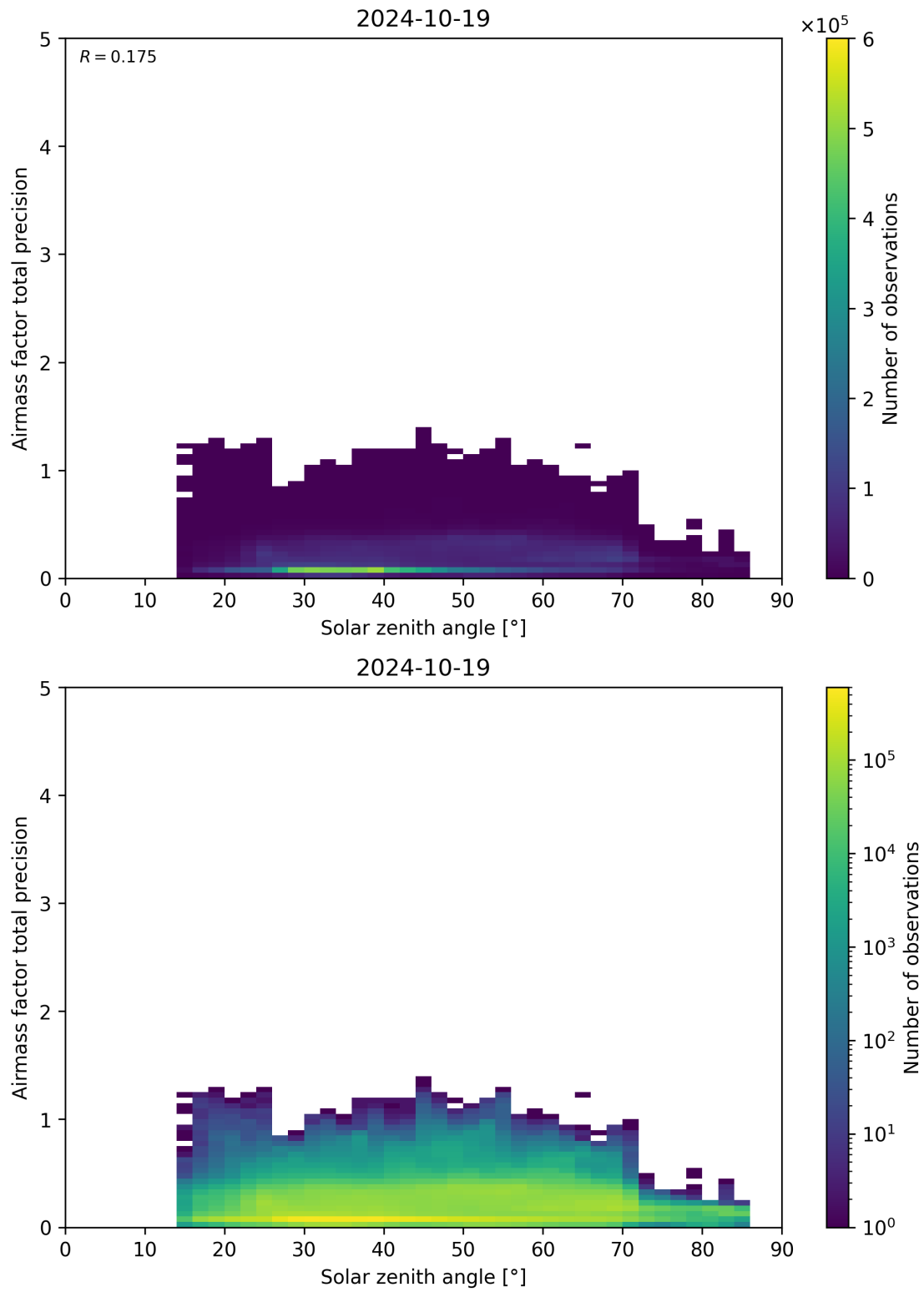
Figure 176: Scatter density plot of “Solar zenith angle” against “Airmass factor total precision” for 2024-10-19 to 2024-10-20.
