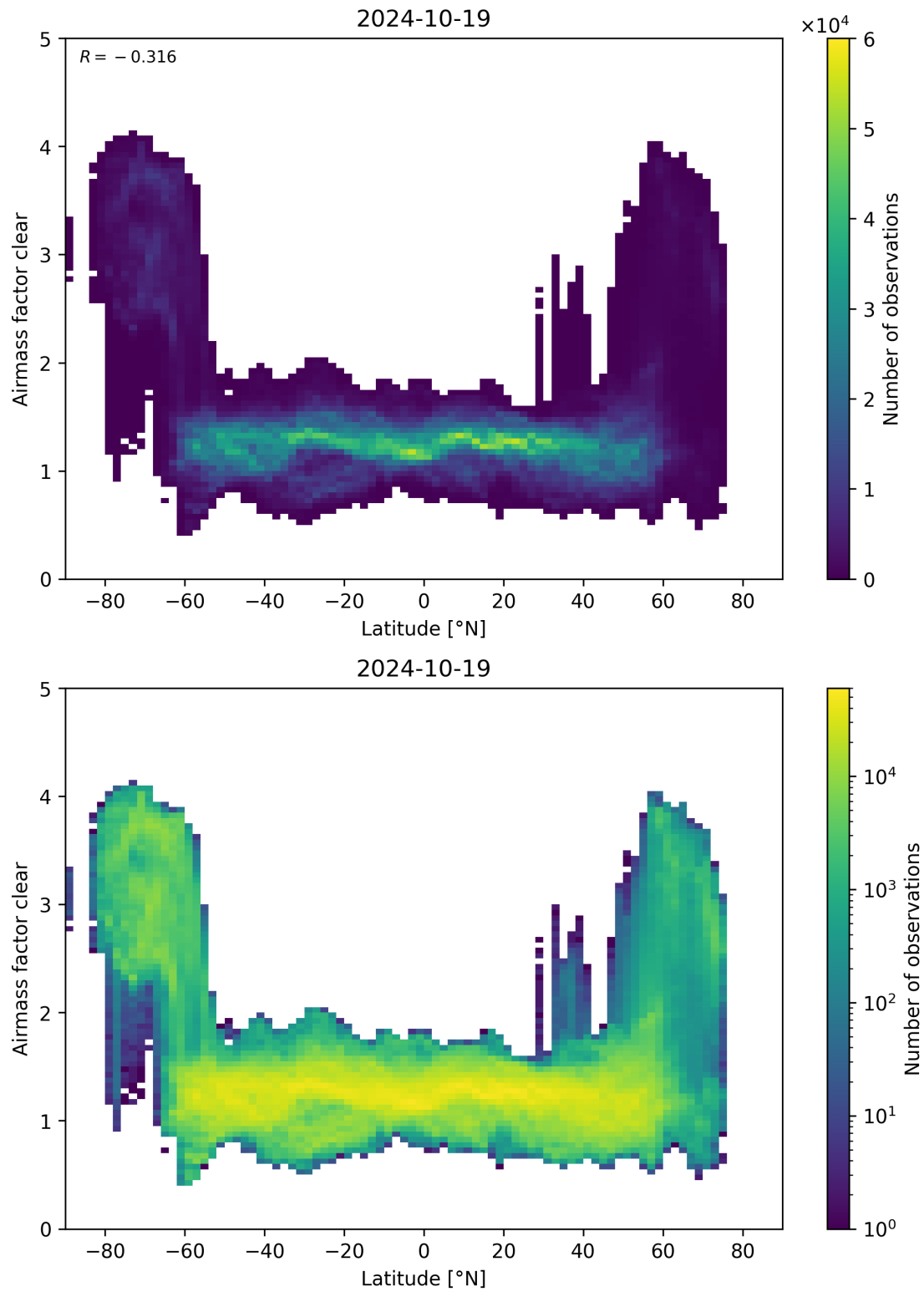
Figure 156: Scatter density plot of “Latitude” against “Airmass factor clear” for 2024-10-19 to 2024-10-20.
