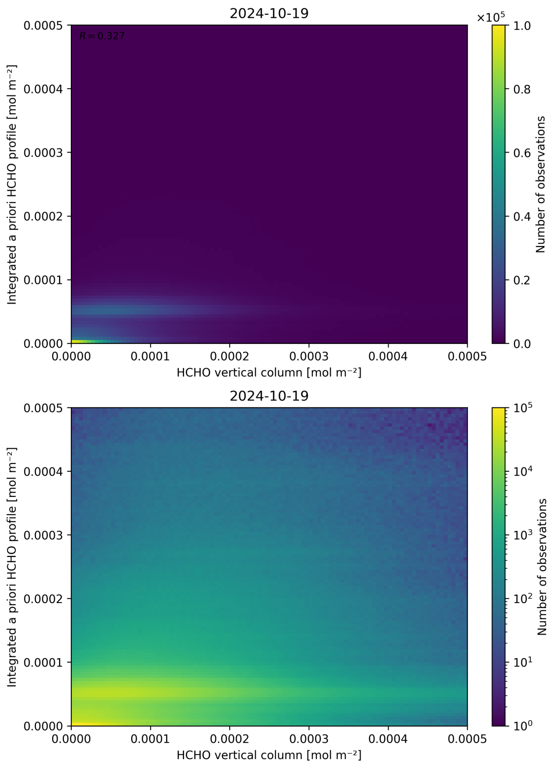
Figure 135: Scatter density plot of “HCHO vertical column” against “Integrated a priori HCHO profile” for 2024-10-19 to 2024-10-20.
