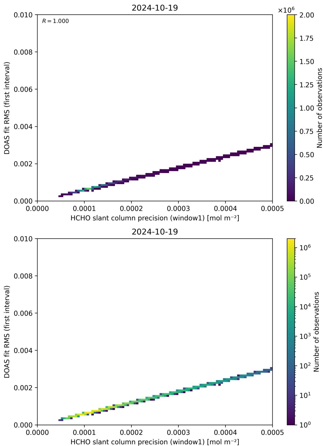
Figure 88: Scatter density plot of “HCHO slant column precision (window1)” against “DOAS fit RMS (first interval)” for 2024-10-19 to 2024-10-20.
