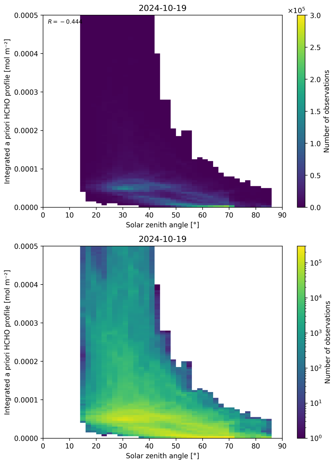
Figure 180: Scatter density plot of “Solar zenith angle” against “Integrated a priori HCHO profile” for 2024-10-19 to 2024-10-20.
