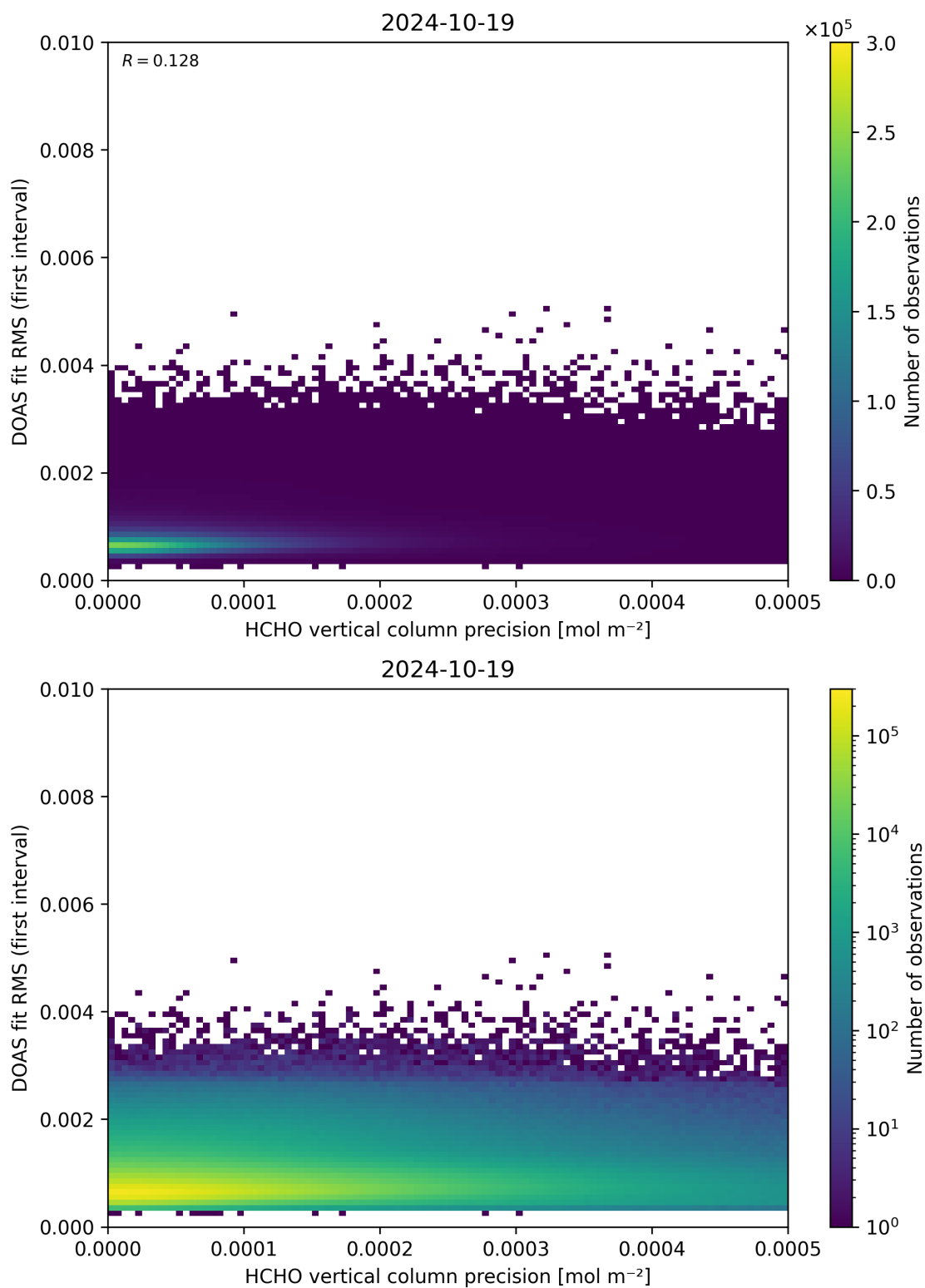
Figure 136: Scatter density plot of “HCHO vertical column precision” against “DOAS fit RMS (first interval)” for 2024-10-19 to 2024-10-20.
