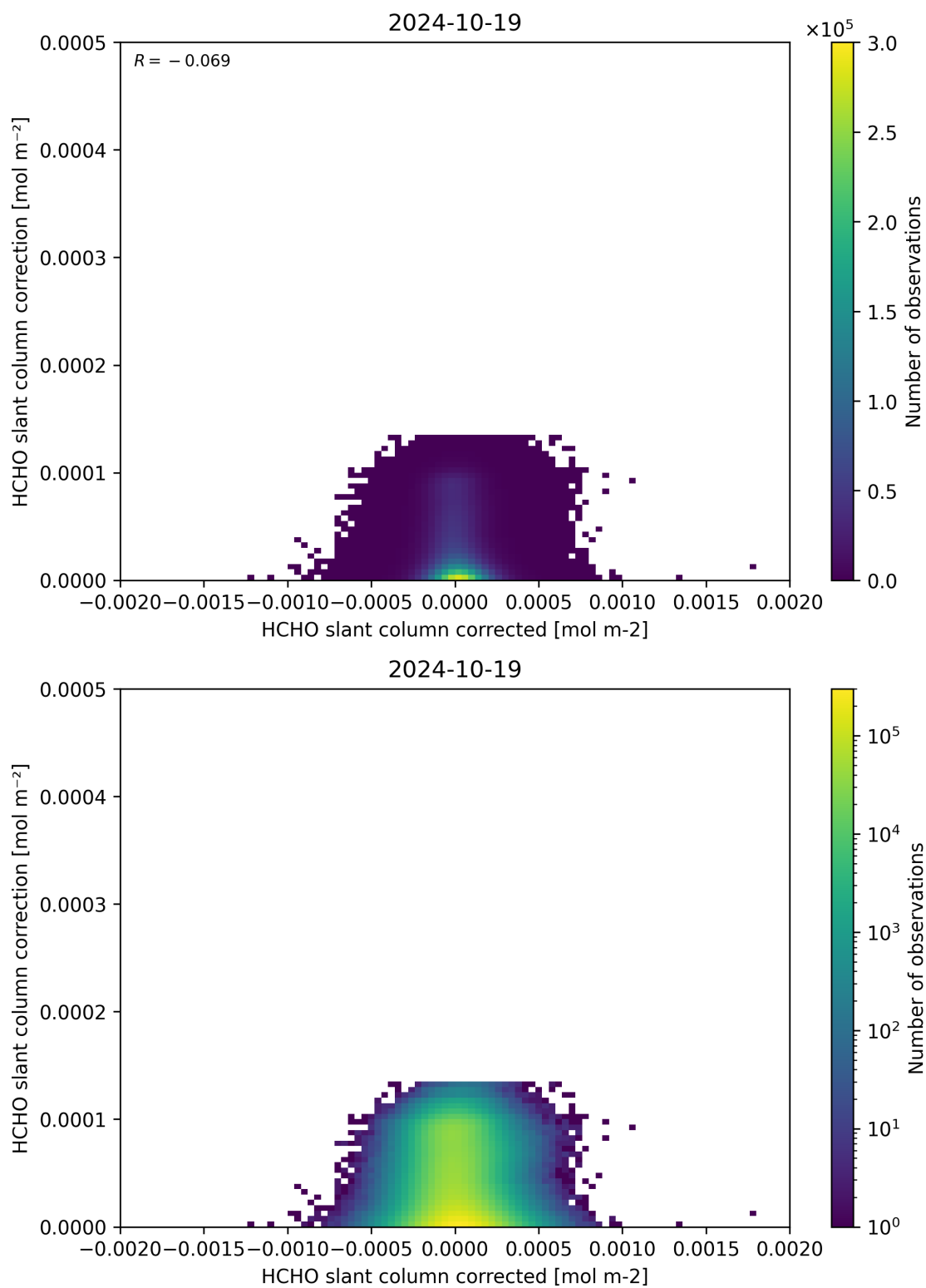
Figure 77: Scatter density plot of “HCHO slant column corrected” against “HCHO slant column correction” for 2024-10-19 to 2024-10-20.
