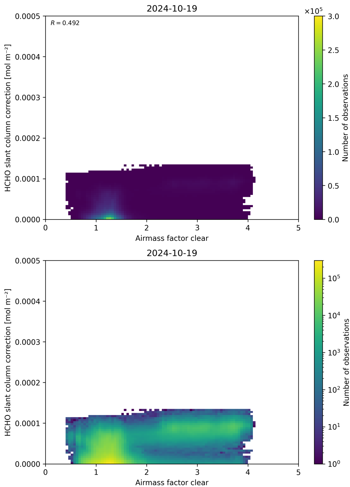
Figure 75: Scatter density plot of “Airmass factor clear” against “HCHO slant column correction” for 2024-10-19 to 2024-10-20.
