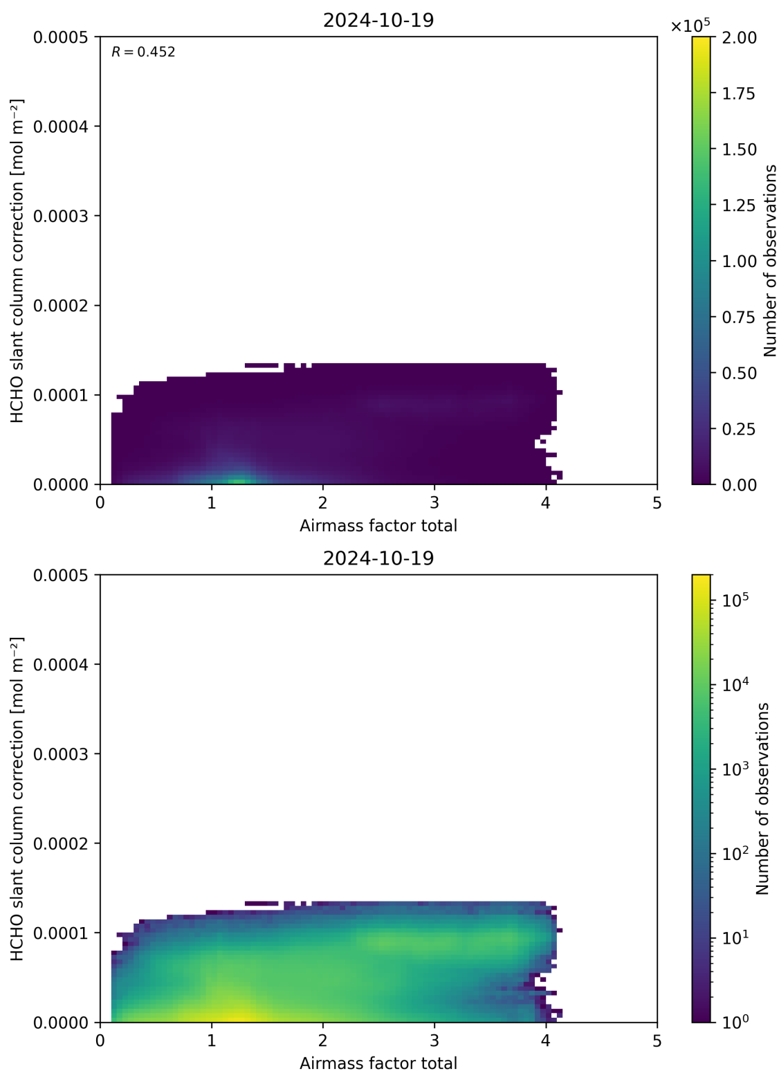
Figure 102: Scatter density plot of “Airmass factor total” against “HCHO slant column correction” for 2024-10-19 to 2024-10-20.
