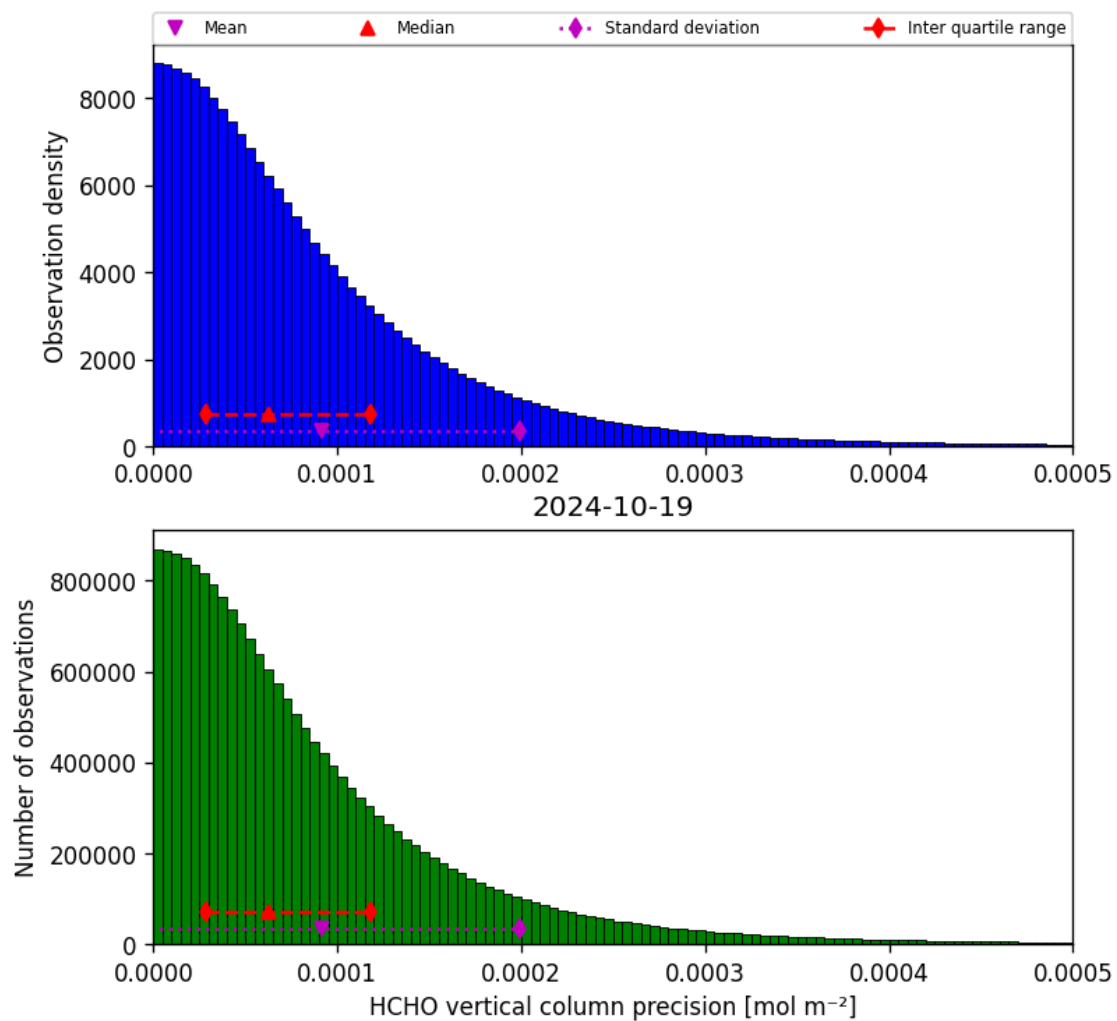
Figure 36: Histogram of “HCHO vertical column precision” for 2024-10-19 to 2024-10-20
