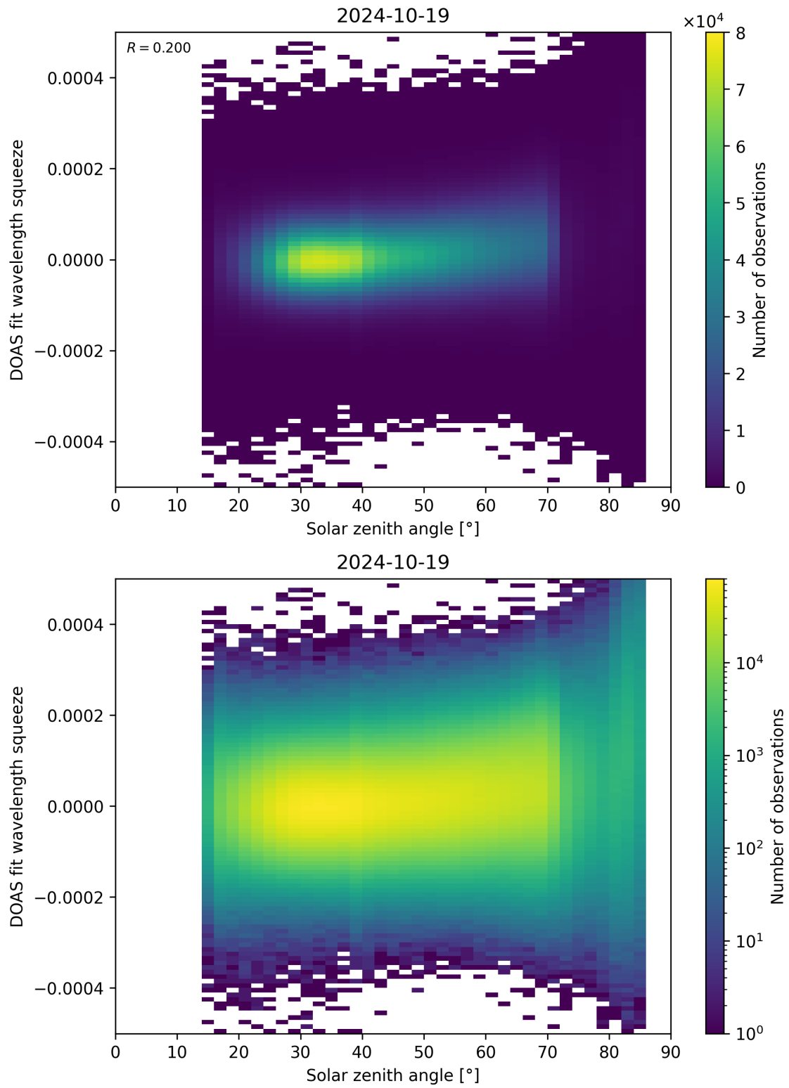
Figure 169: Scatter density plot of “Solar zenith angle” against “DOAS fit wavelength squeeze” for 2024-10-19 to 2024-10-20.
