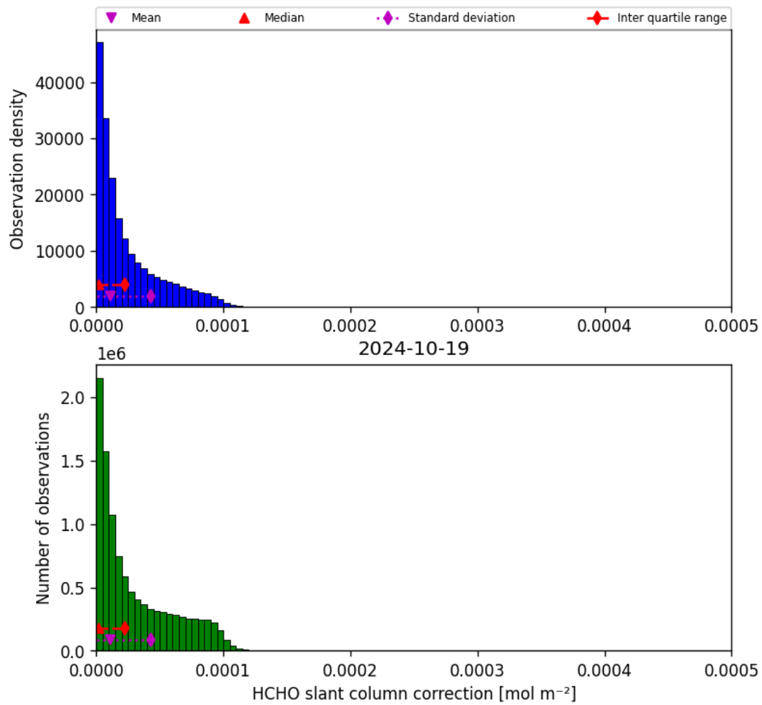
Figure 47: Histogram of “HCHO slant column correction” for 2024-10-19 to 2024-10-20
