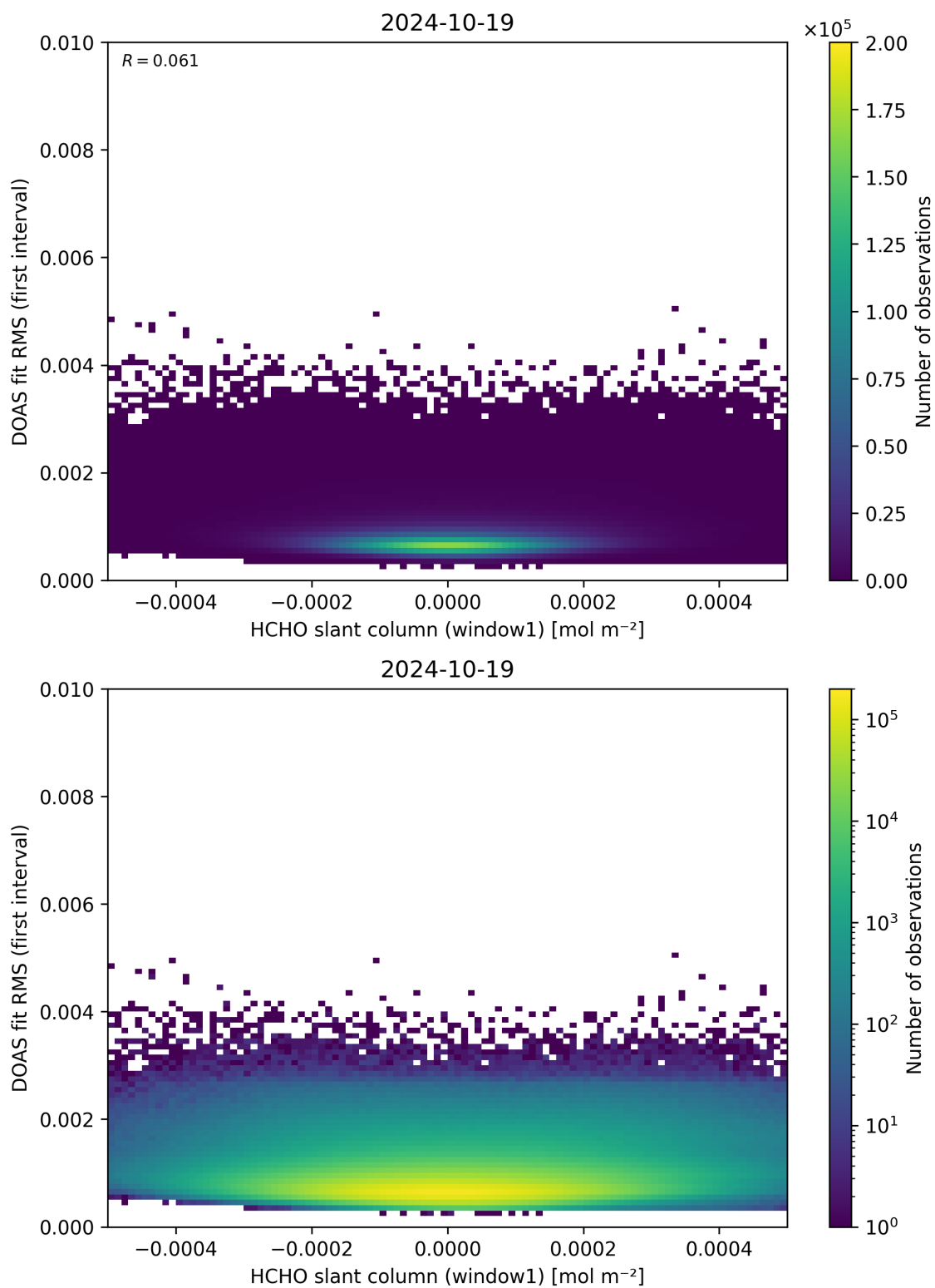
Figure 78: Scatter density plot of “HCHO slant column (window1)” against “DOAS fit RMS (first interval)” for 2024-10-19 to 2024-10-20.
