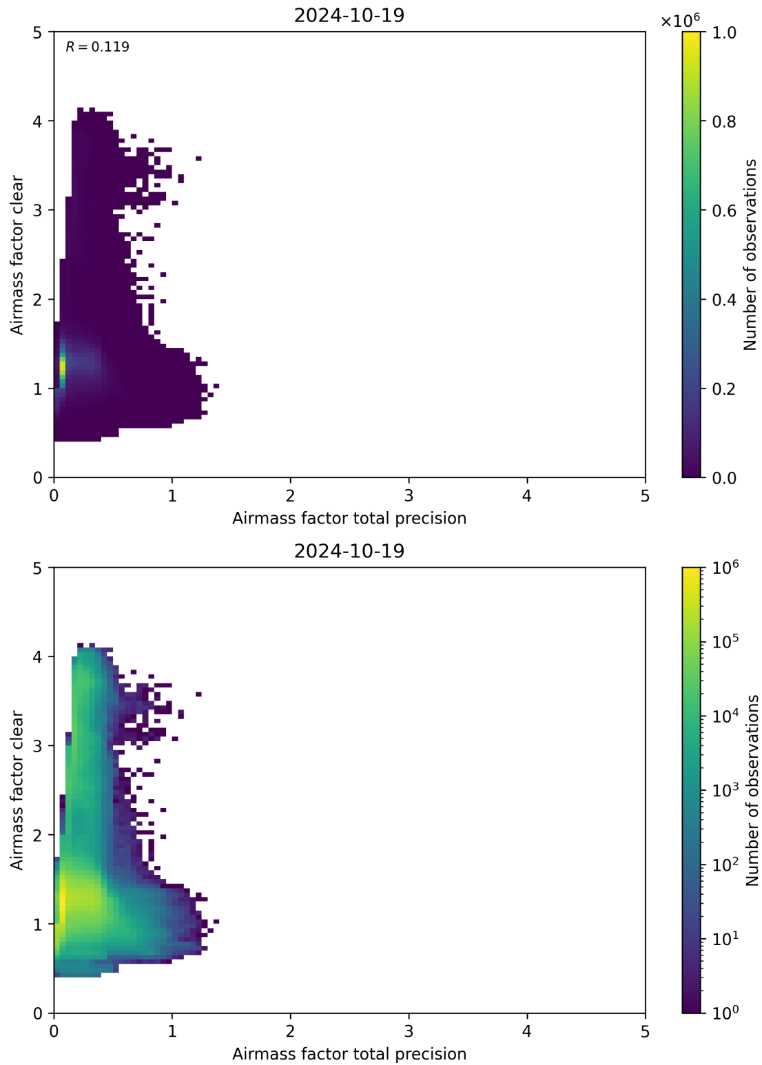
Figure 108: Scatter density plot of “Airmass factor total precision” against “Airmass factor clear” for 2024-10-19 to 2024-10-20.
