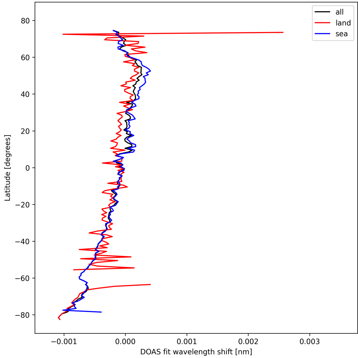
Figure 30: Zonal average of "DOAS fit wavelength shift" for 2024-10-19 to 2024-10-20.
