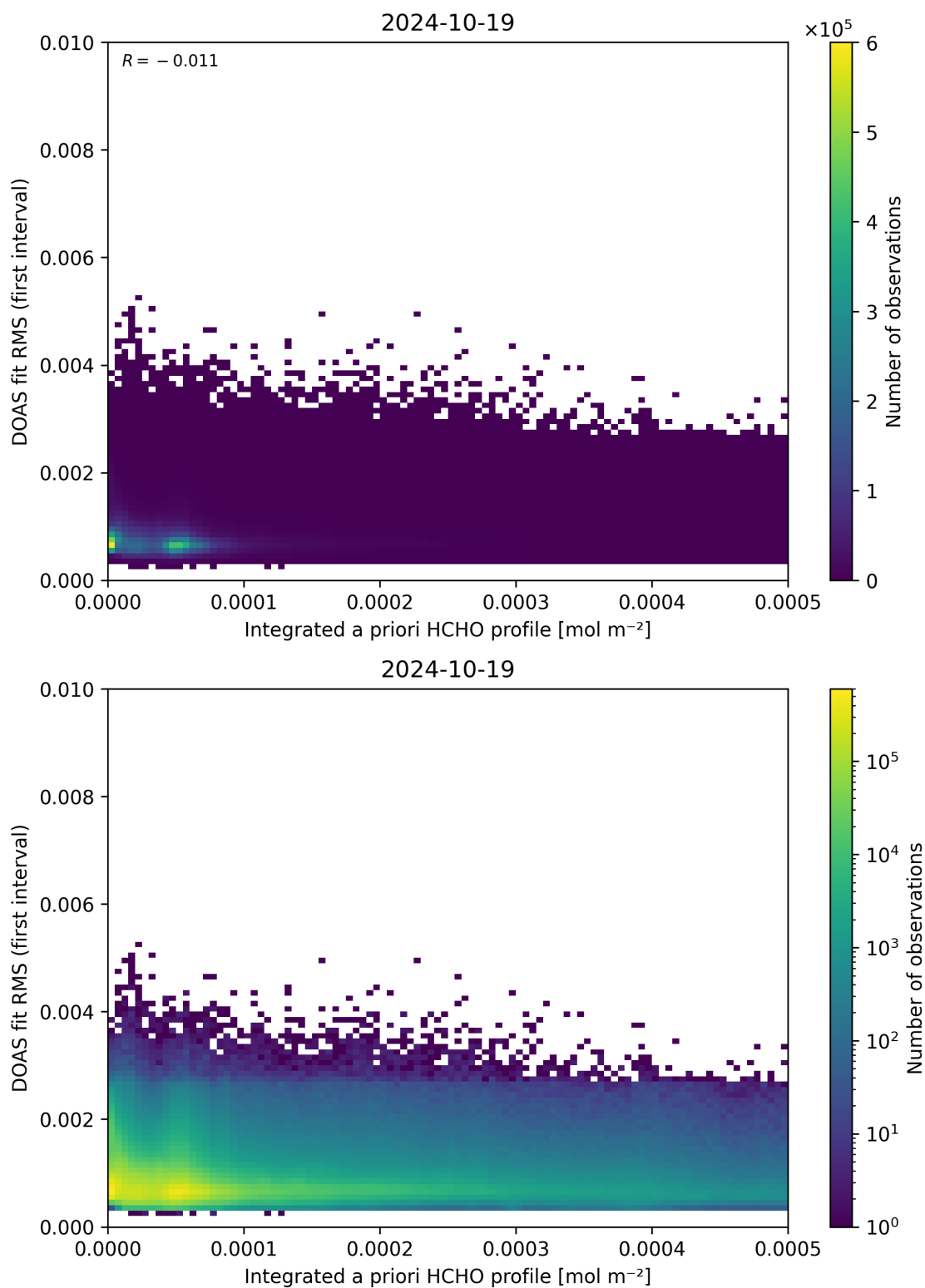
Figure 148: Scatter density plot of “Integrated a priori HCHO profile” against “DOAS fit RMS (first interval)” for 2024-10-19 to 2024-10-20.
