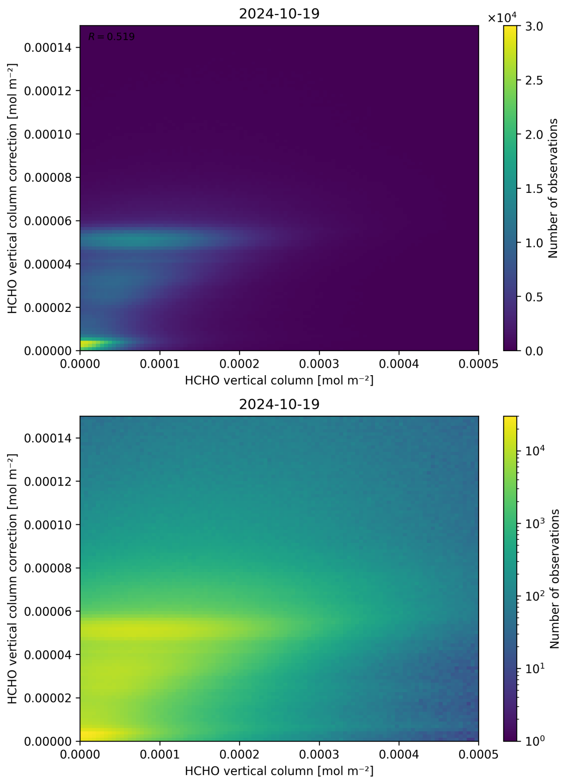
Figure 133: Scatter density plot of “HCHO vertical column” against “HCHO vertical column correction” for 2024-10-19 to 2024-10-20.
