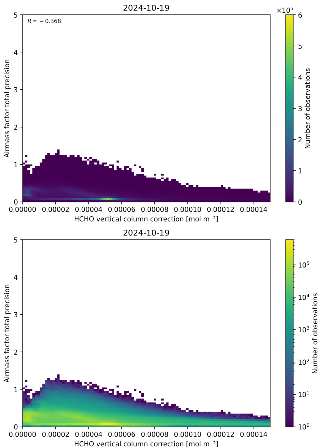
Figure 121: Scatter density plot of “HCHO vertical column correction” against “Airmass factor total precision” for 2024-10-19 to 2024-10-20.
