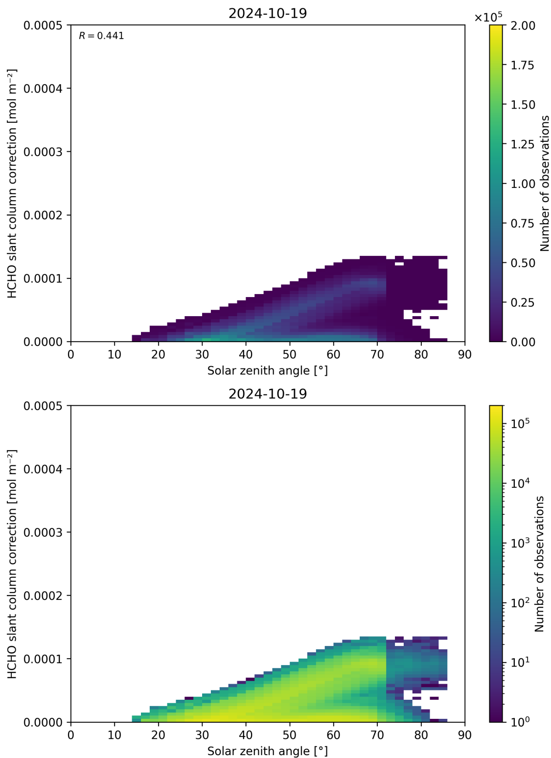
Figure 172: Scatter density plot of “Solar zenith angle” against “HCHO slant column correction” for 2024-10-19 to 2024-10-20.
