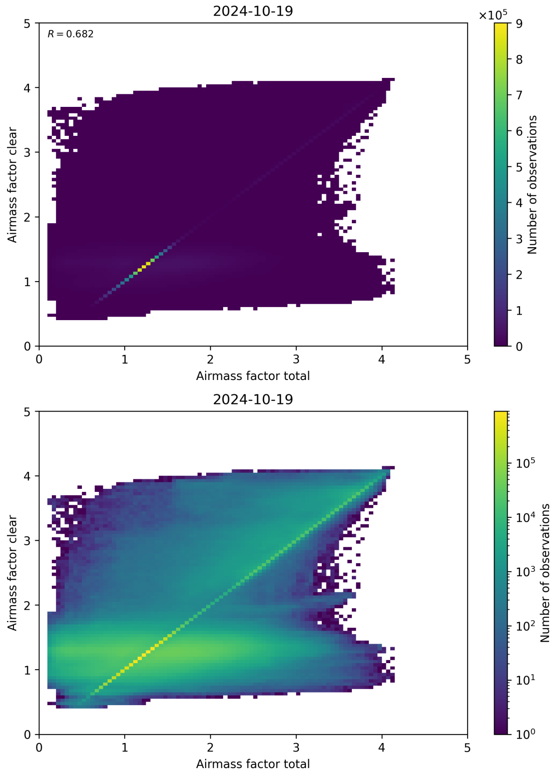
Figure 100: Scatter density plot of “Airmass factor total” against “Airmass factor clear” for 2024-10-19 to 2024-10-20.
