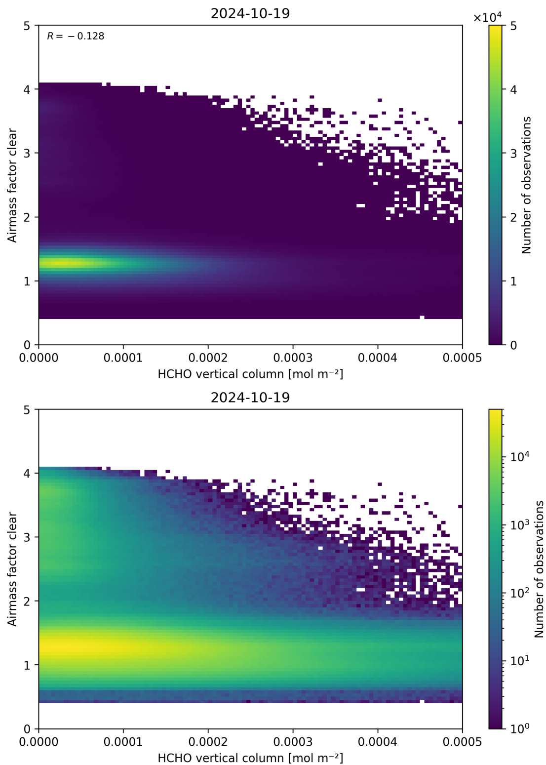
Figure 126: Scatter density plot of “HCHO vertical column” against “Airmass factor clear” for 2024-10-19 to 2024-10-20.
