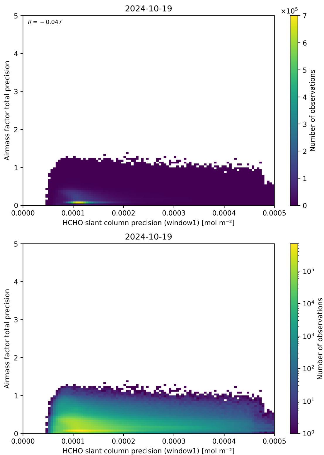
Figure 95: Scatter density plot of “HCHO slant column precision (window1)” against “Airmass factor total precision” for 2024-10-19 to 2024-10-20.
