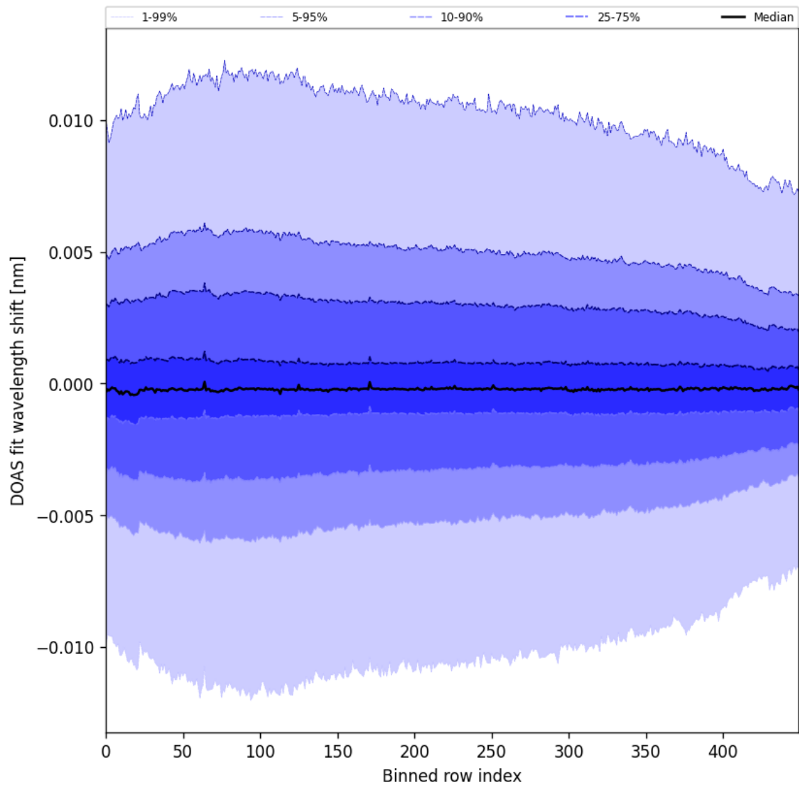
Figure 58: Along track statistics of “DOAS fit wavelength shift” for 2024-10-19 to 2024-10-20
