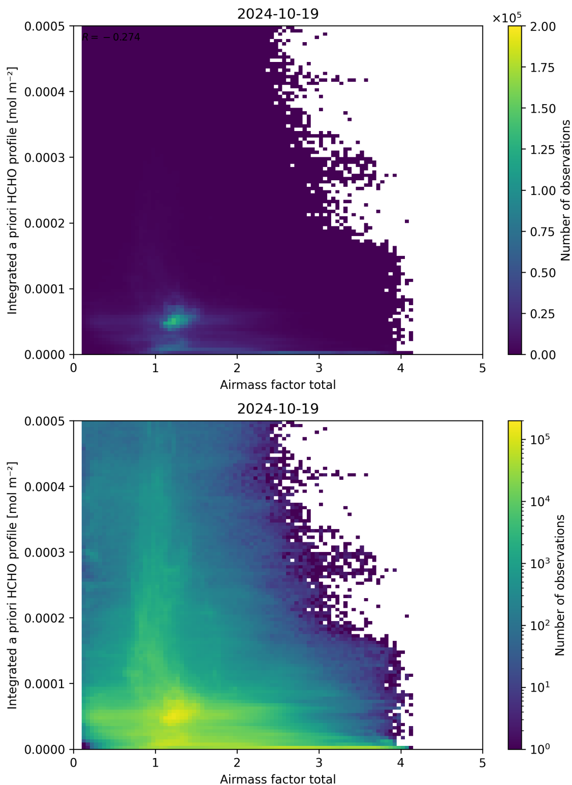
Figure 104: Scatter density plot of “Airmass factor total” against “Integrated a priori HCHO profile” for 2024-10-19 to 2024-10-20.
