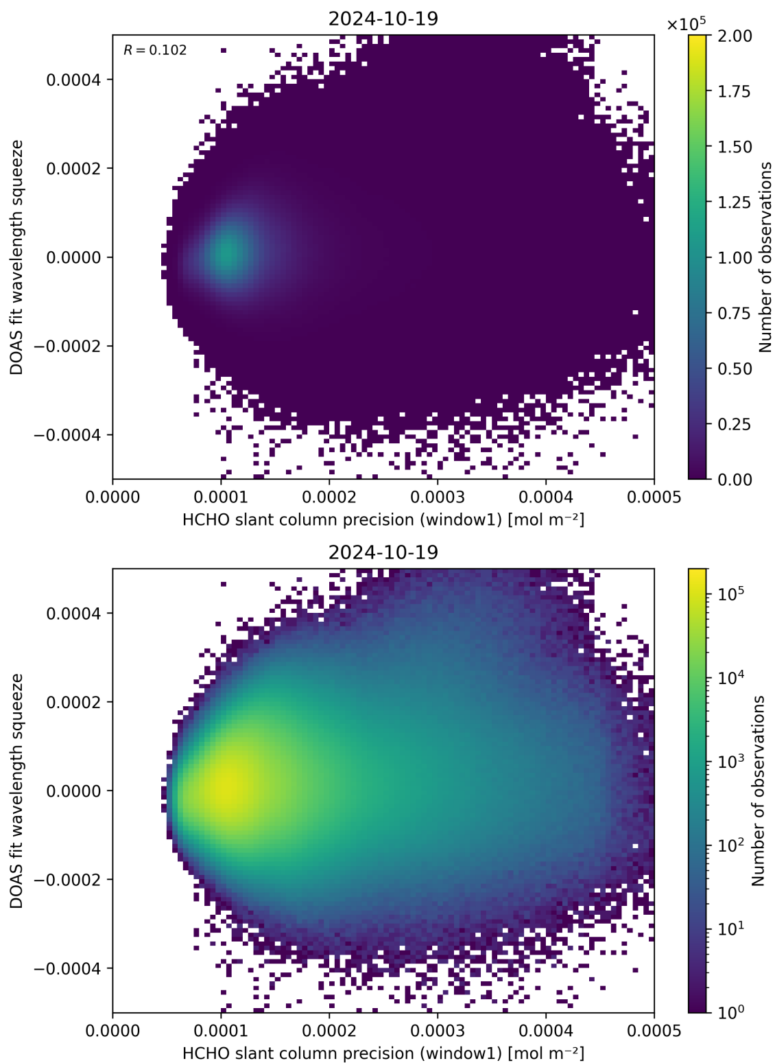
Figure 90: Scatter density plot of “HCHO slant column precision (window1)” against “DOAS fit wavelength squeeze” for 2024-10-19 to 2024-10-20.
