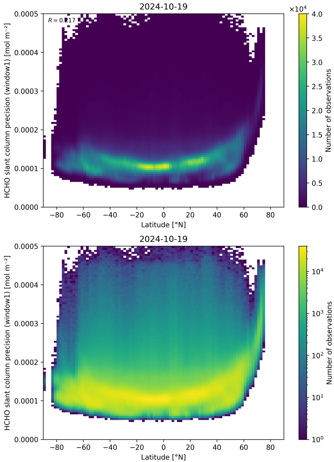
Figure 160: Scatter density plot of “Latitude” against “HCHO slant column precision (window1)” for 2024-10-19 to 2024-10-20.
