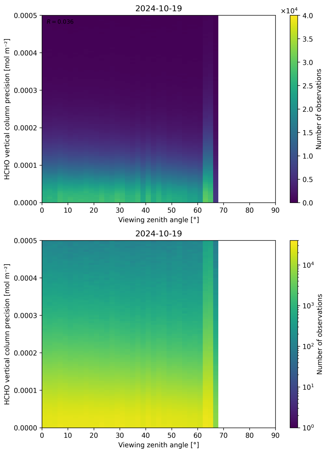
Figure 194: Scatter density plot of “Viewing zenith angle” against “HCHO vertical column precision” for 2024-10-19 to 2024-10-20.
