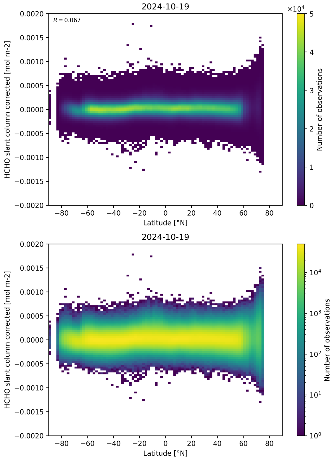
Figure 157: Scatter density plot of “Latitude” against “HCHO slant column corrected” for 2024-10-19 to 2024-10-20.
