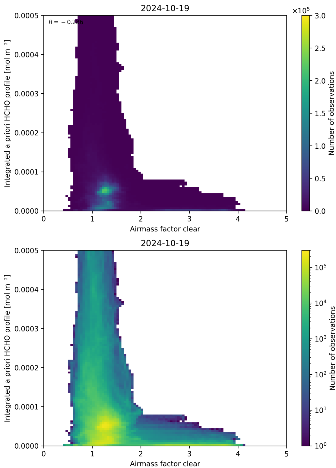
Figure 76: Scatter density plot of “Airmass factor clear” against “Integrated a priori HCHO profile” for 2024-10-19 to 2024-10-20.
