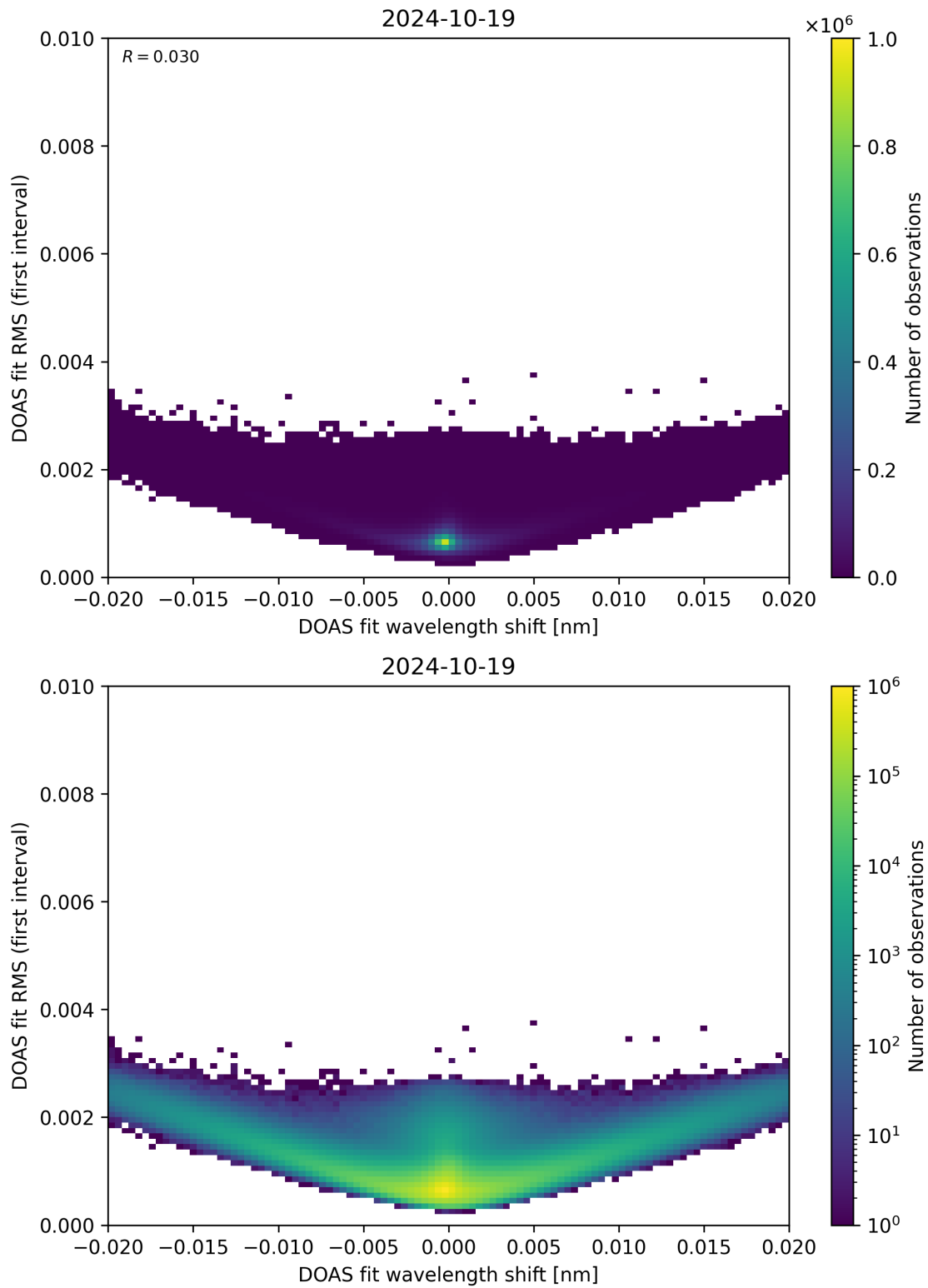
Figure 64: Scatter density plot of “DOAS fit wavelength shift” against “DOAS fit RMS (first interval)” for 2024-10-19 to 2024-10-20.
