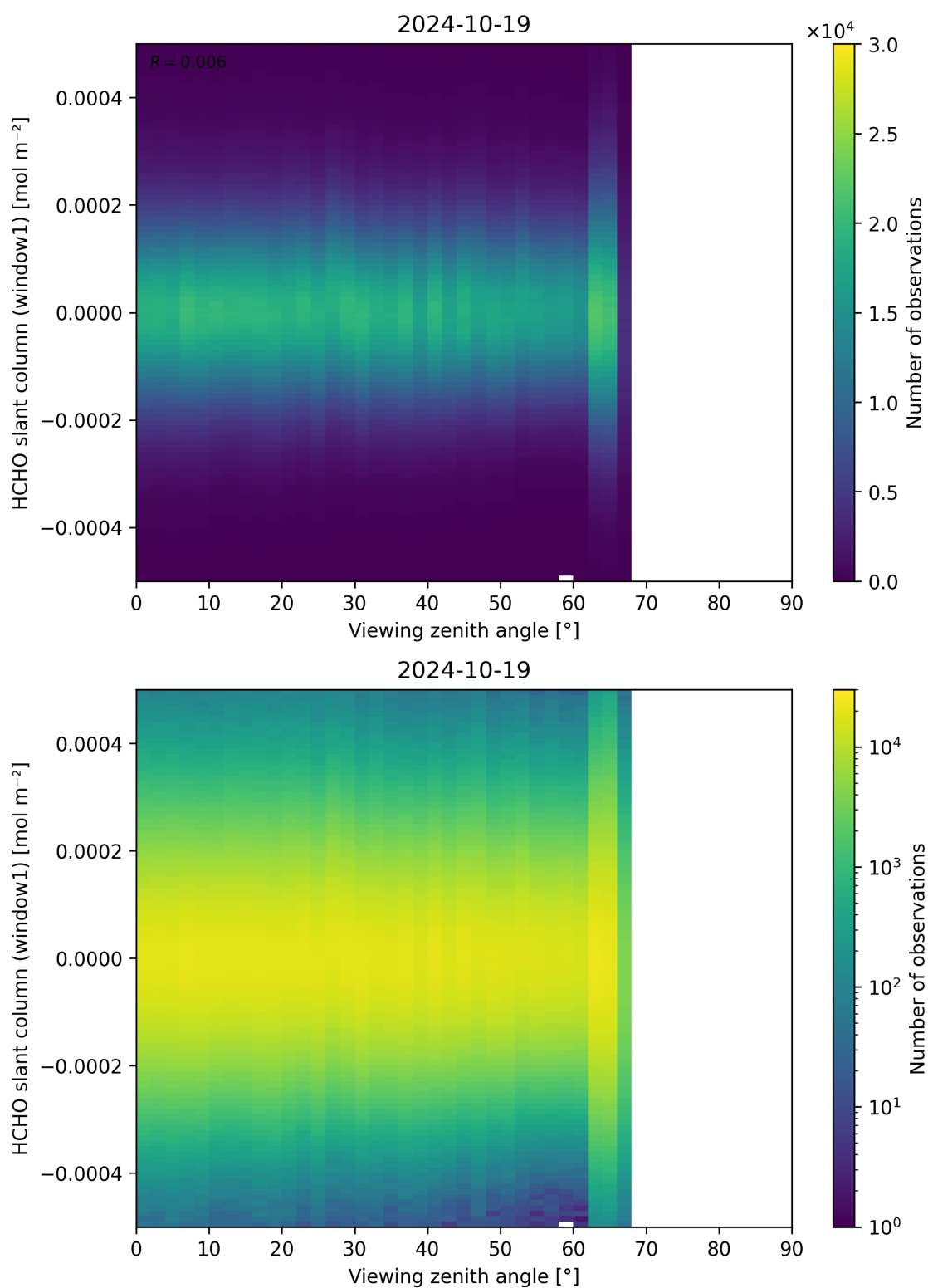
Figure 188: Scatter density plot of “Viewing zenith angle” against “HCHO slant column (window1)” for 2024-10-19 to 2024-10-20.
