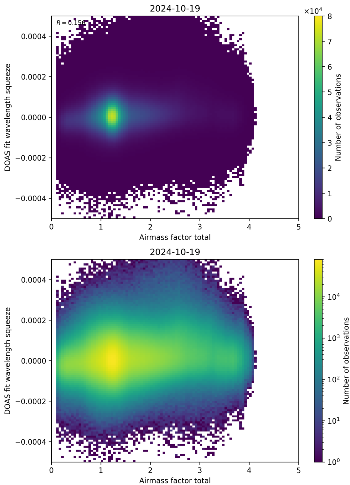
Figure 99: Scatter density plot of “Airmass factor total” against “DOAS fit wavelength squeeze” for 2024-10-19 to 2024-10-20.
