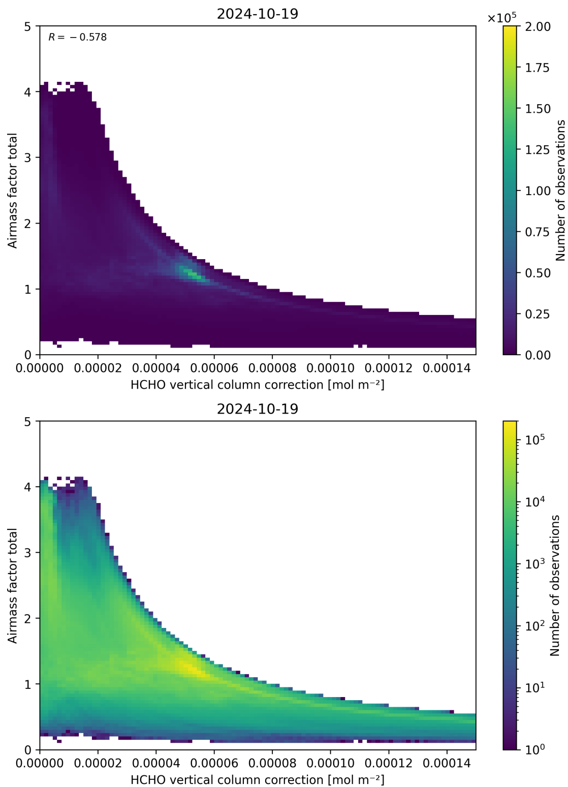
Figure 120: Scatter density plot of “HCHO vertical column correction” against “Airmass factor total” for 2024-10-19 to 2024-10-20.
