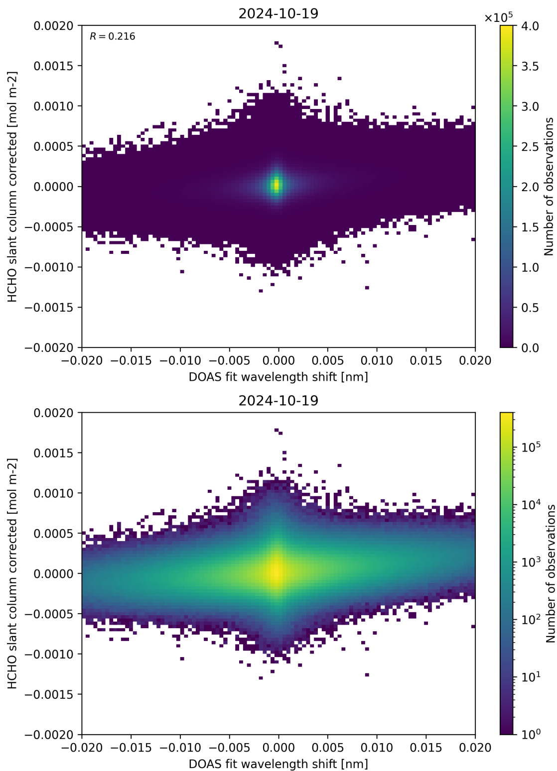
Figure 66: Scatter density plot of “DOAS fit wavelength shift” against “HCHO slant column corrected” for 2024-10-19 to 2024-10-20.
