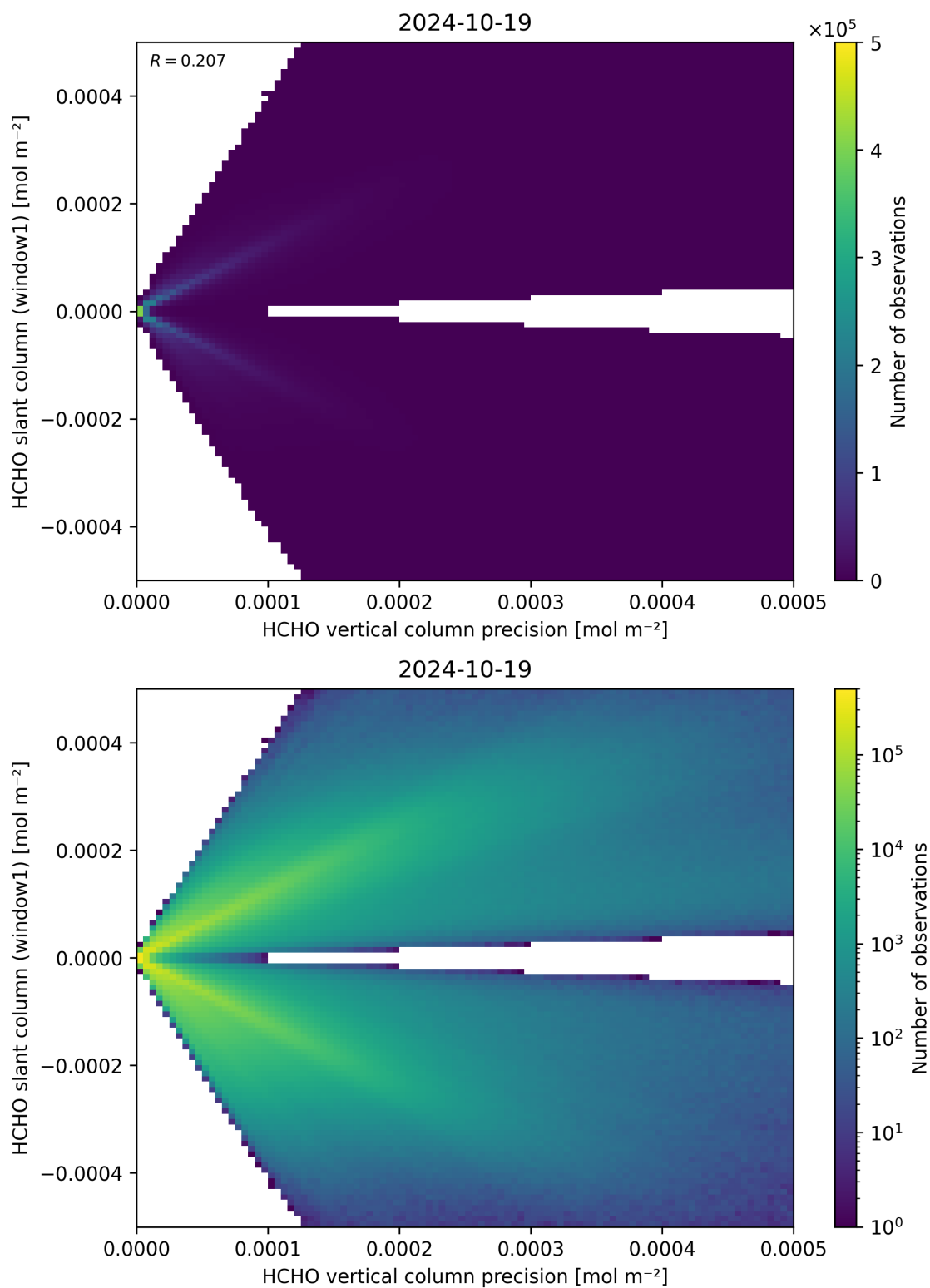
Figure 142: Scatter density plot of “HCHO vertical column precision” against “HCHO slant column (window1)” for 2024-10-19 to 2024-10-20.
