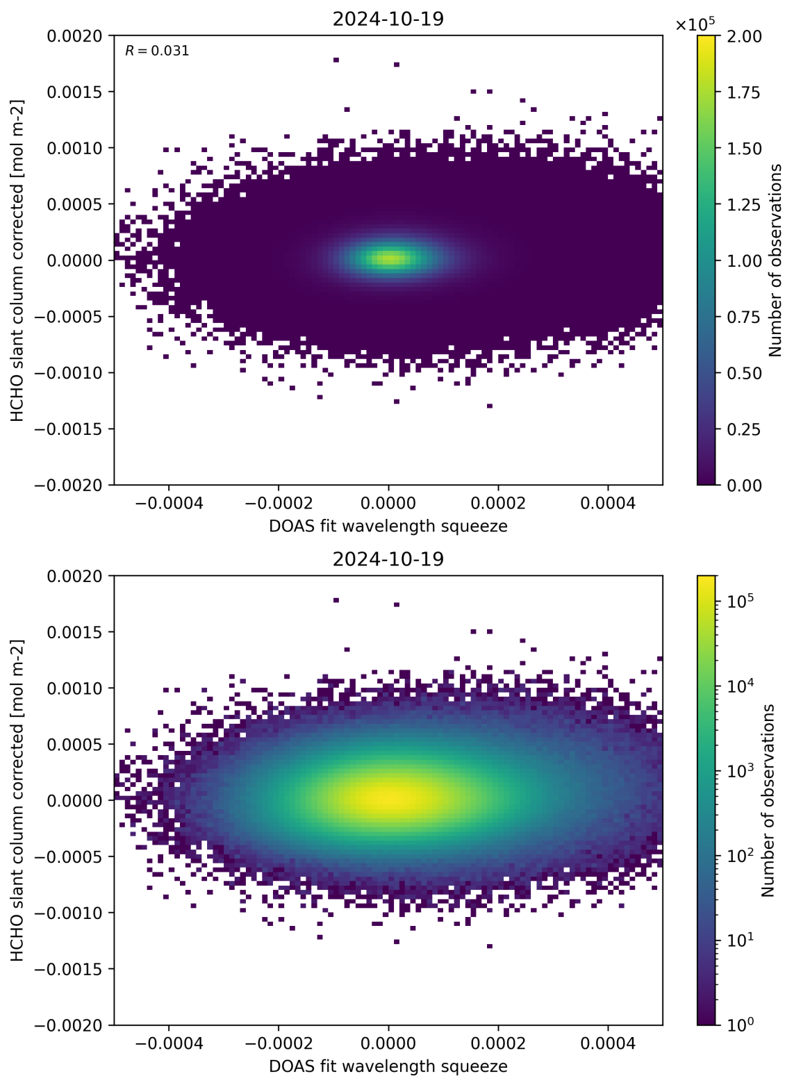
Figure 69: Scatter density plot of “DOAS fit wavelength squeeze” against “HCHO slant column corrected” for 2024-10-19 to 2024-10-20.
