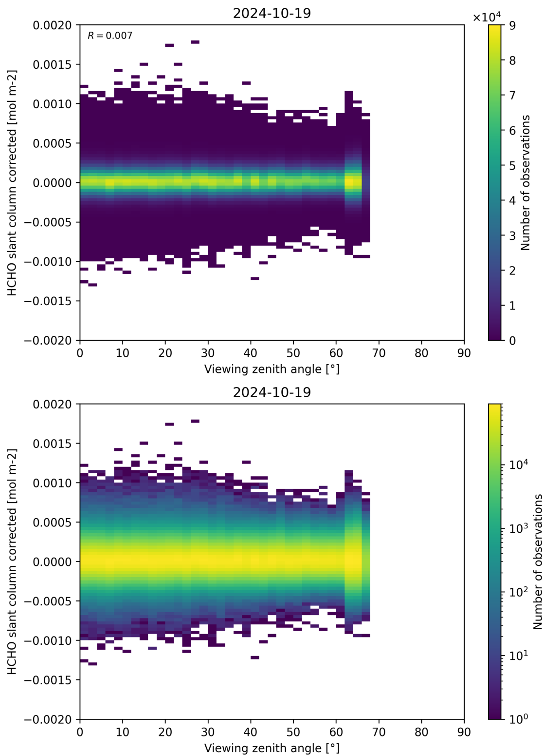
Figure 186: Scatter density plot of “Viewing zenith angle” against “HCHO slant column corrected” for 2024-10-19 to 2024-10-20.
