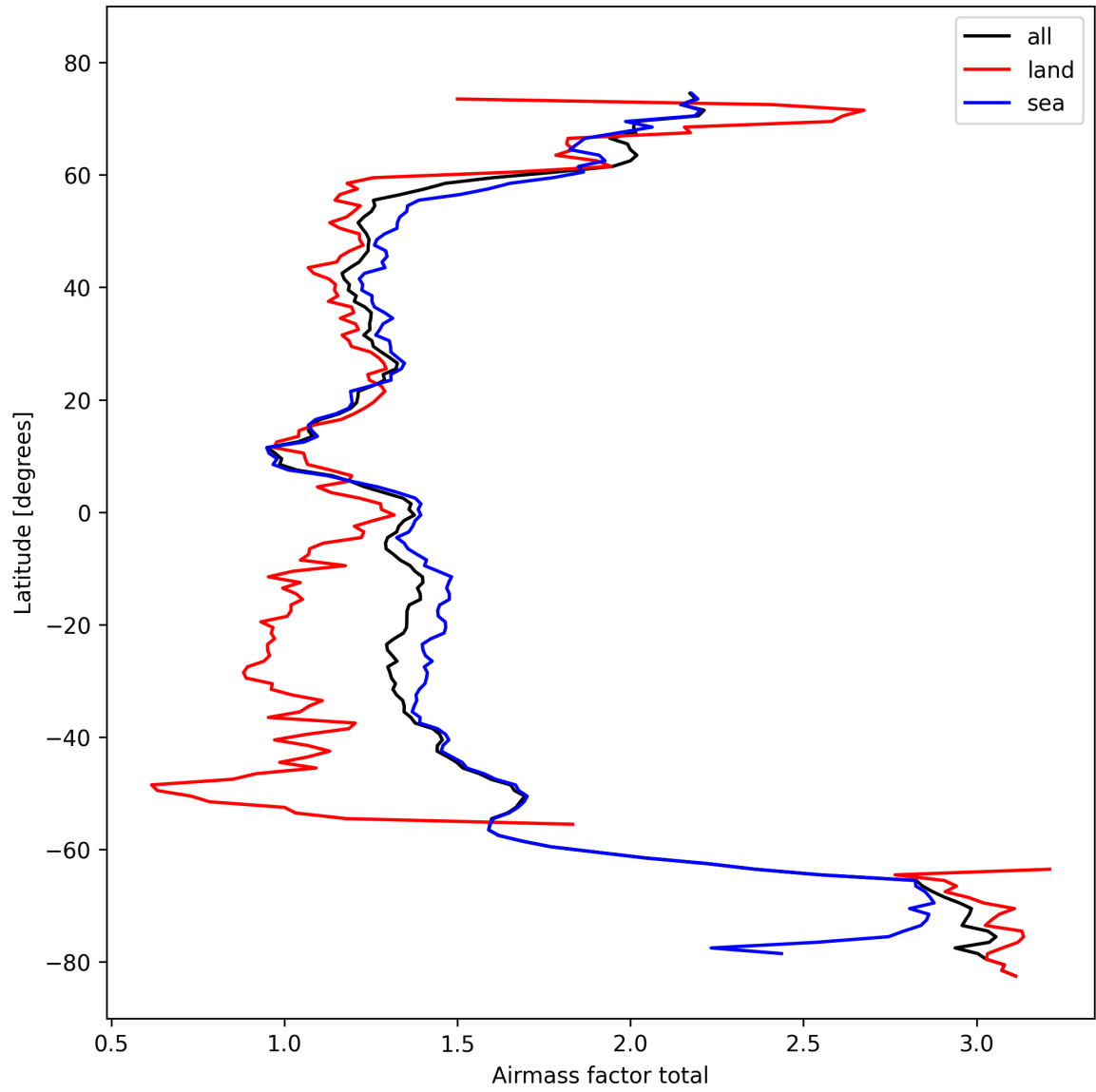
Figure 26: Zonal average of “Airmass factor total” for 2024-10-19 to 2024-10-20.
