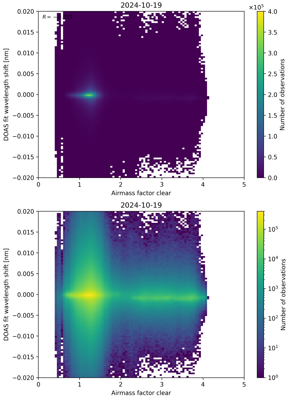
Figure 72: Scatter density plot of “Airmass factor clear” against “DOAS fit wavelength shift” for 2024-10-19 to 2024-10-20.
