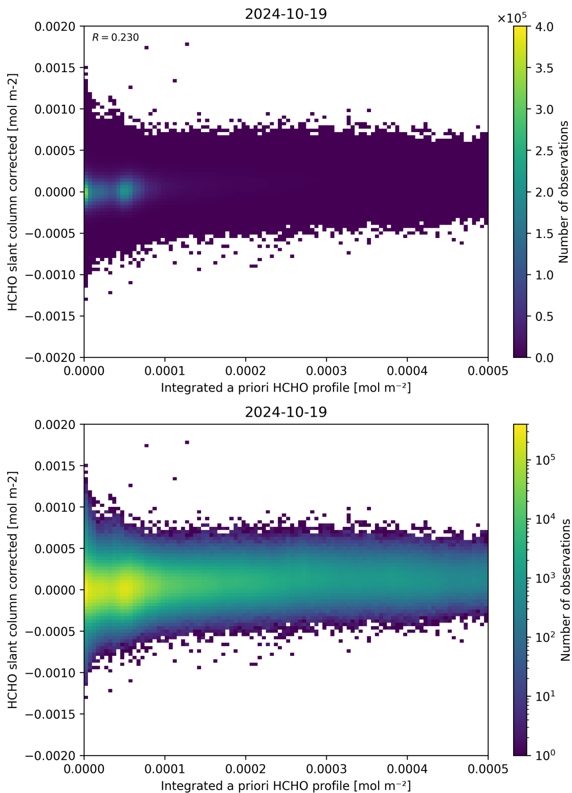
Figure 151: Scatter density plot of “Integrated a priori HCHO profile” against “HCHO slant column corrected” for 2024-10-19 to 2024-10-20.
