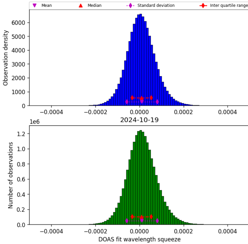
Figure 45: Histogram of “DOAS fit wavelength squeeze” for 2024-10-19 to 2024-10-20
