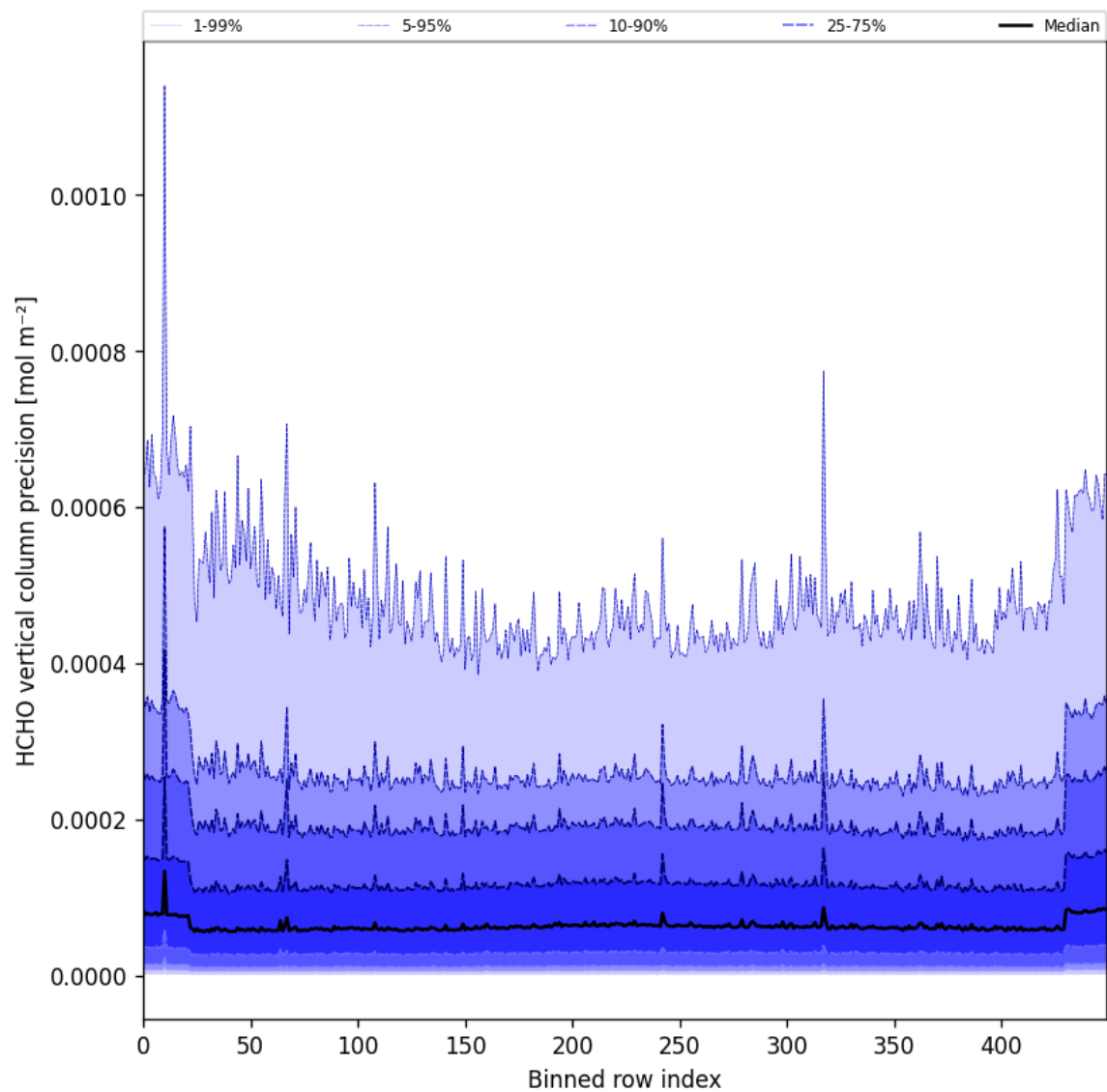
Figure 50: Along track statistics of “HCHO vertical column precision” for 2024-10-19 to 2024-10-20
