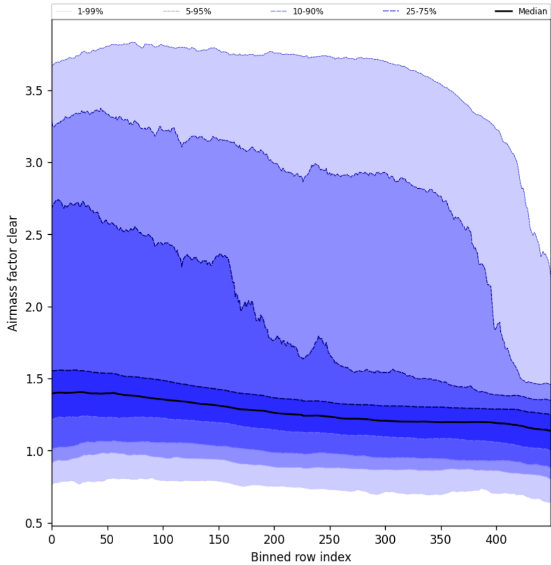
Figure 56: Along track statistics of “Airmass factor clear” for 2024-10-19 to 2024-10-20
