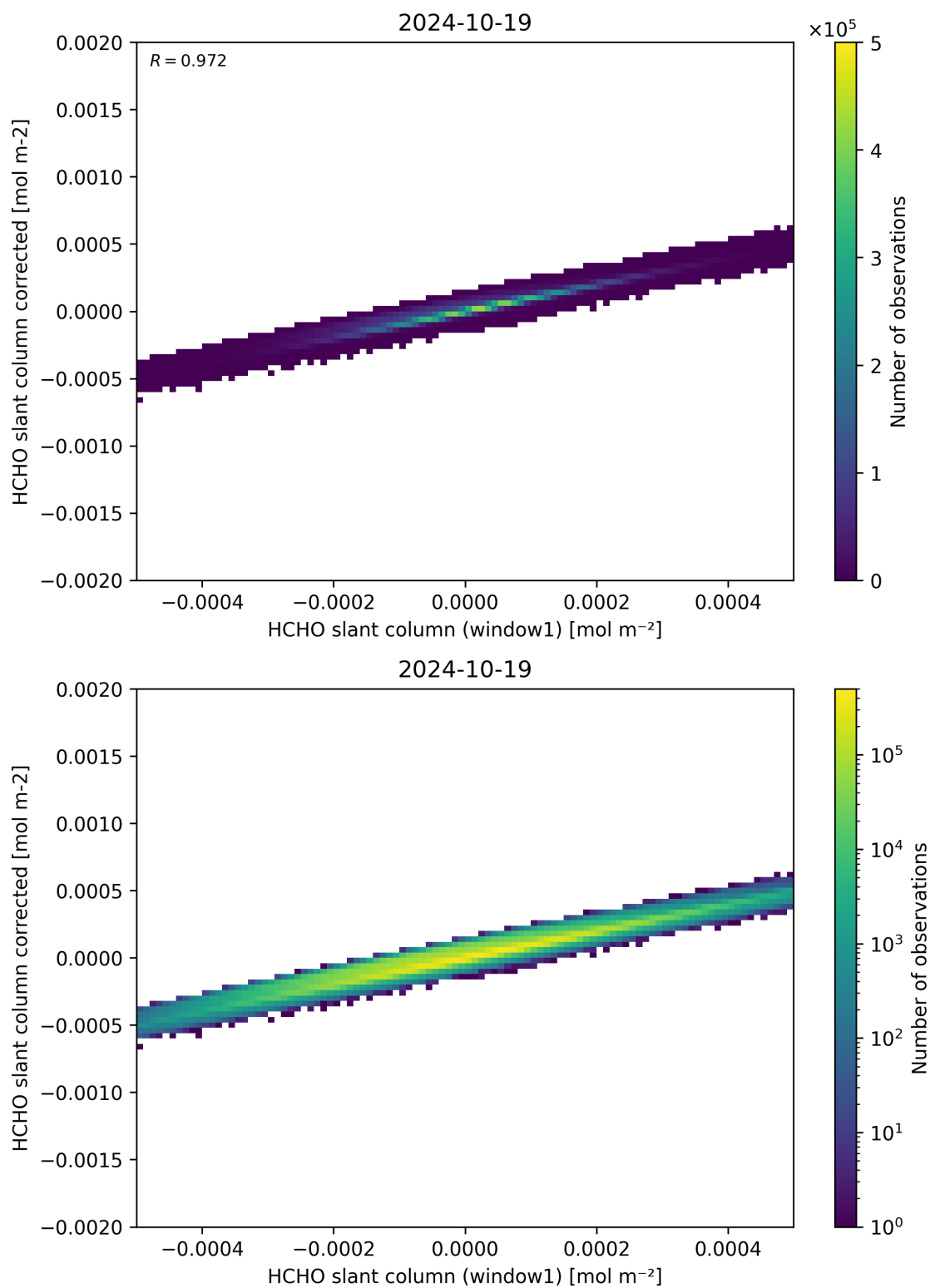
Figure 82: Scatter density plot of “HCHO slant column (window1)” against “HCHO slant column corrected” for 2024-10-19 to 2024-10-20.
