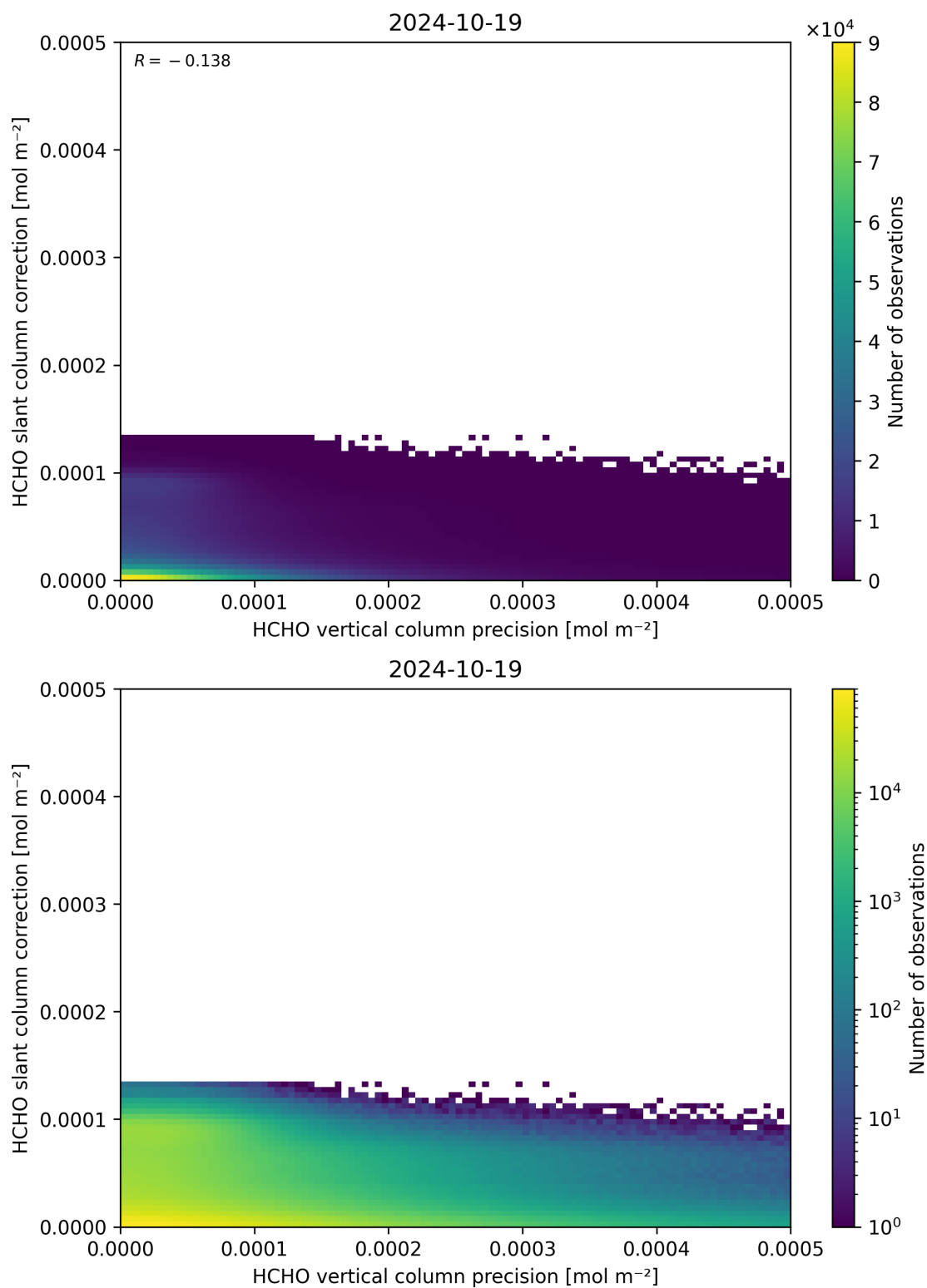
Figure 141: Scatter density plot of “HCHO vertical column precision” against “HCHO slant column correction” for 2024-10-19 to 2024-10-20.
