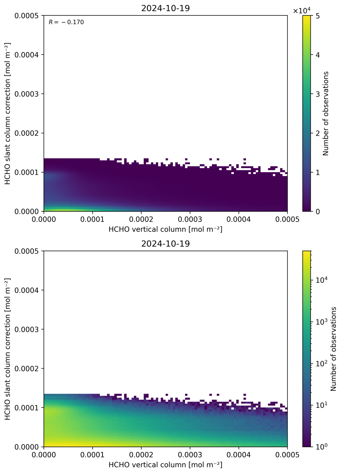
Figure 128: Scatter density plot of “HCHO vertical column” against “HCHO slant column correction” for 2024-10-19 to 2024-10-20.
