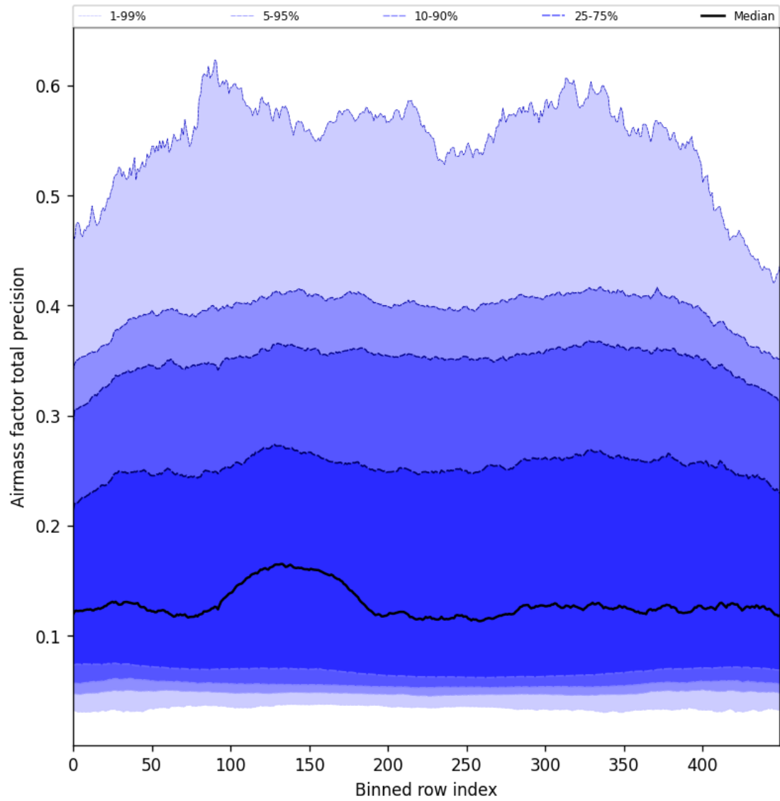
Figure 55: Along track statistics of “Airmass factor total precision” for 2024-10-19 to 2024-10-20
