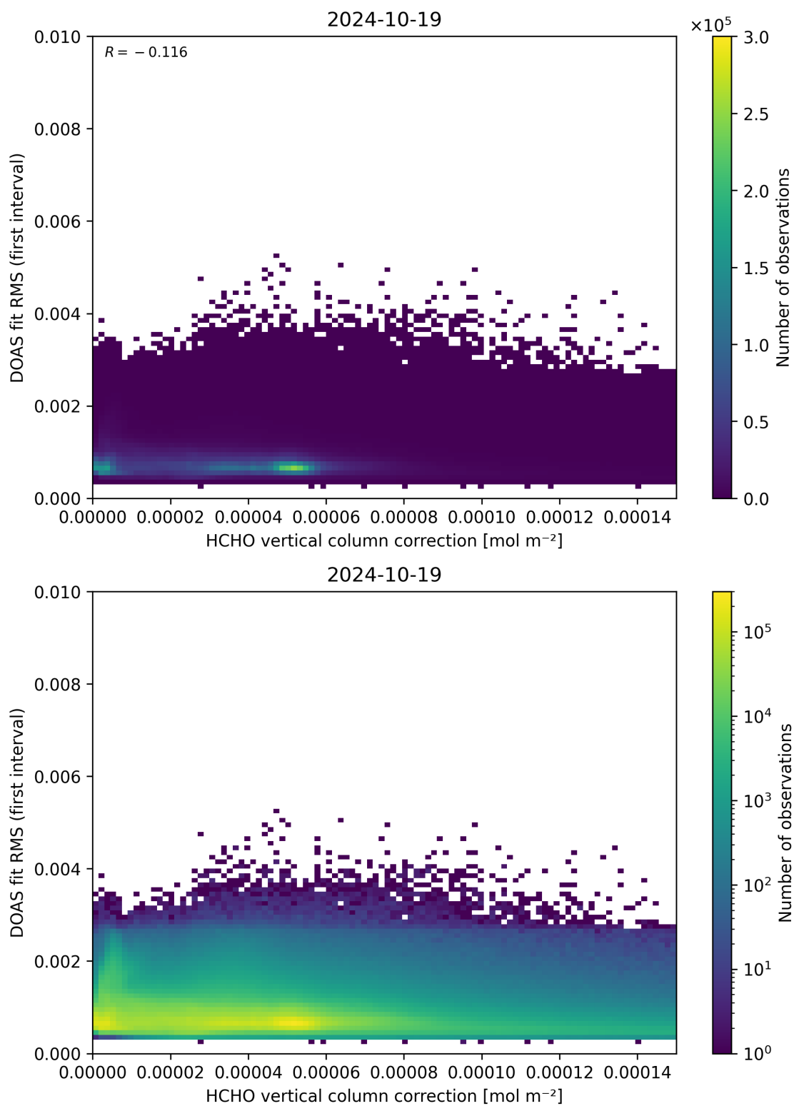
Figure 112: Scatter density plot of “HCHO vertical column correction” against “DOAS fit RMS (first interval)” for 2024-10-19 to 2024-10-20.
