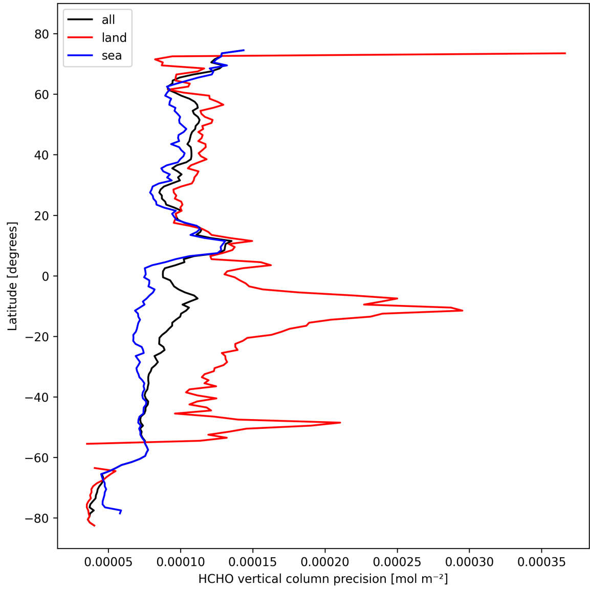
Figure 22: Zonal average of “HCHO vertical column precision” for 2024-10-19 to 2024-10-20.
