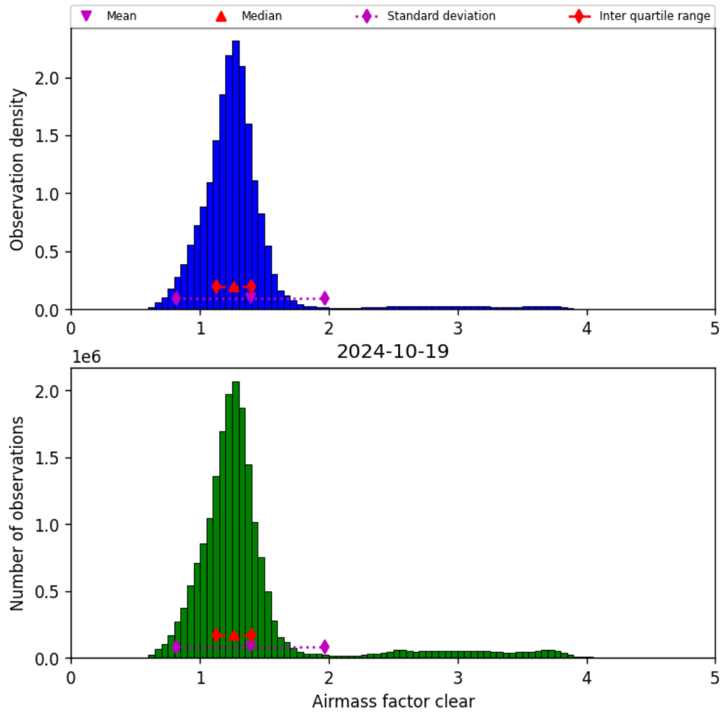
Figure 42: Histogram of “Airmass factor clear” for 2024-10-19 to 2024-10-20
