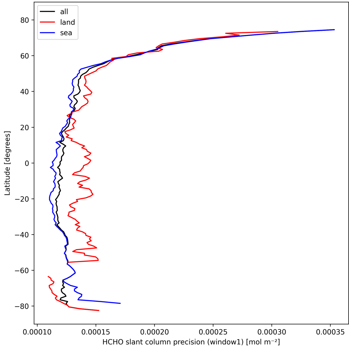
Figure 25: Zonal average of “HCHO slant column precision (window1)” for 2024-10-19 to 2024-10-20.
