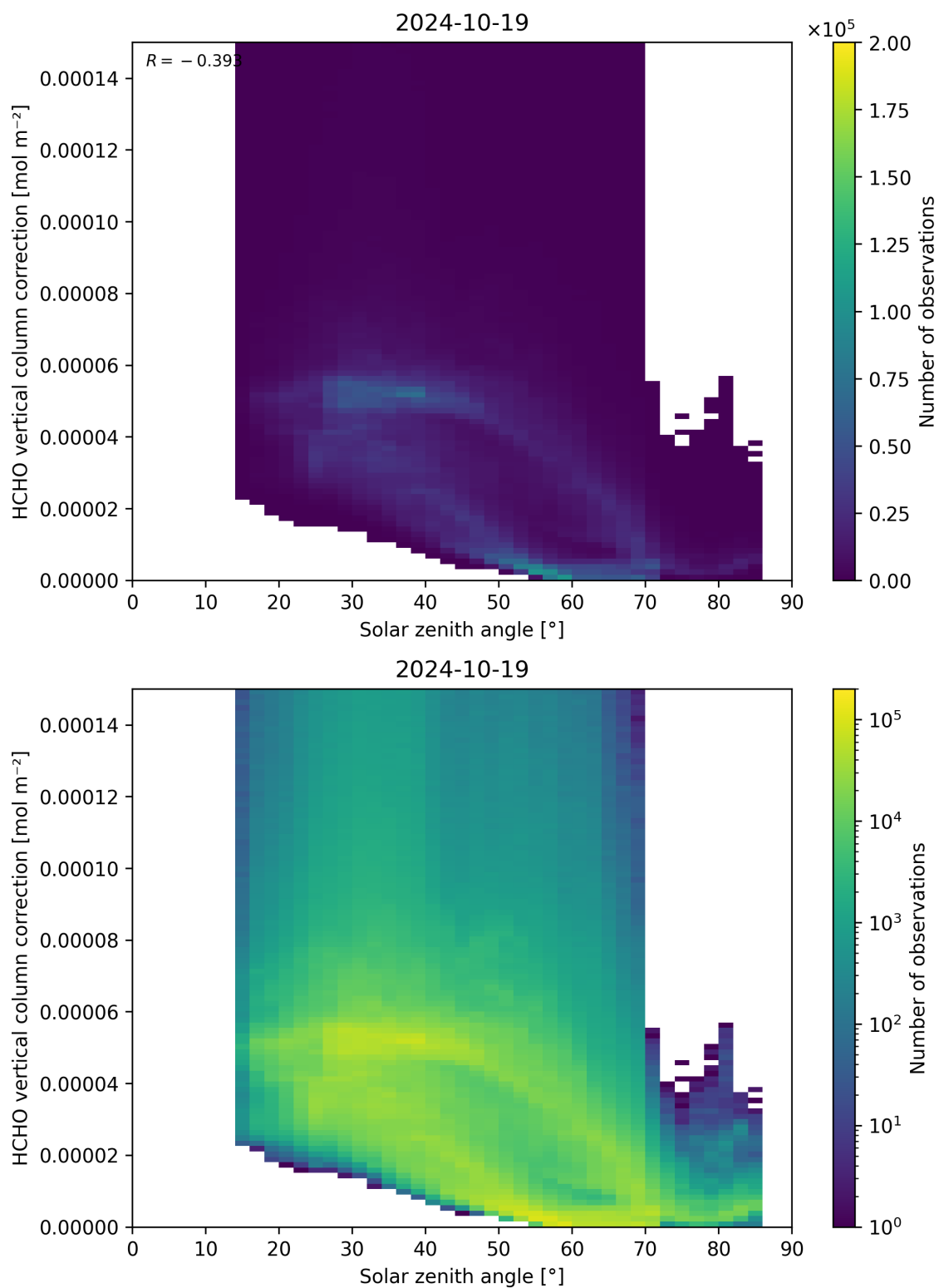
Figure 178: Scatter density plot of “Solar zenith angle” against “HCHO vertical column correction” for 2024-10-19 to 2024-10-20.
