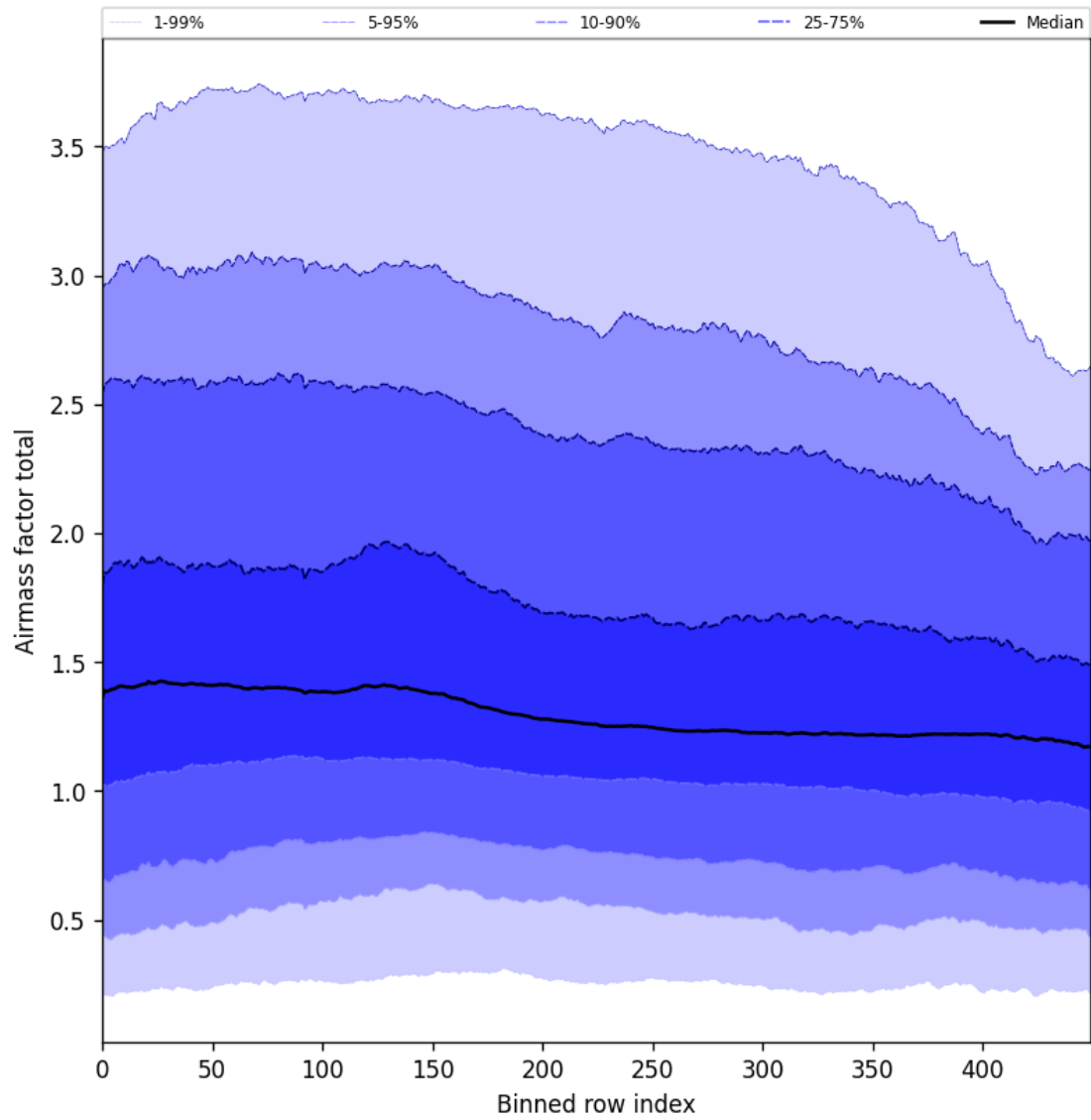
Figure 54: Along track statistics of “Airmass factor total” for 2024-10-19 to 2024-10-20
