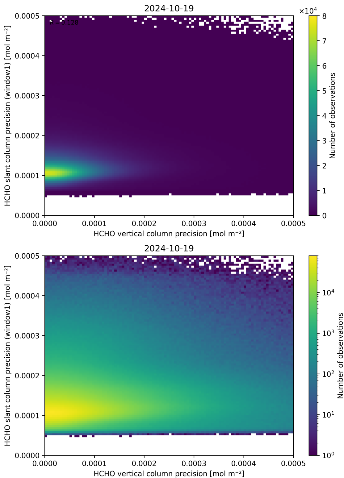
Figure 143: Scatter density plot of “HCHO vertical column precision” against “HCHO slant column precision (window1)” for 2024-10-19 to 2024-10-20.
