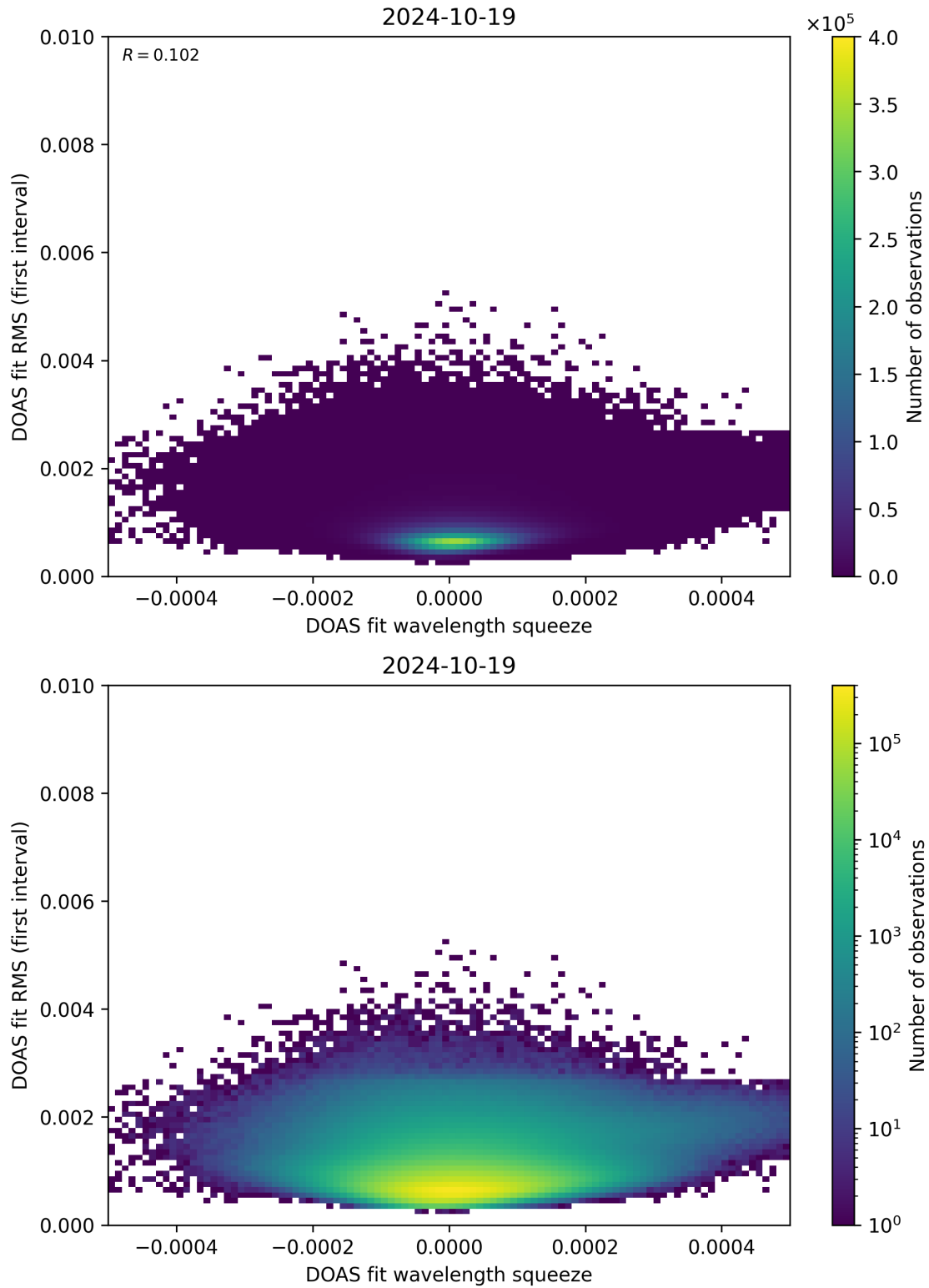
Figure 68: Scatter density plot of “DOAS fit wavelength squeeze” against “DOAS fit RMS (first interval)” for 2024-10-19 to 2024-10-20.
