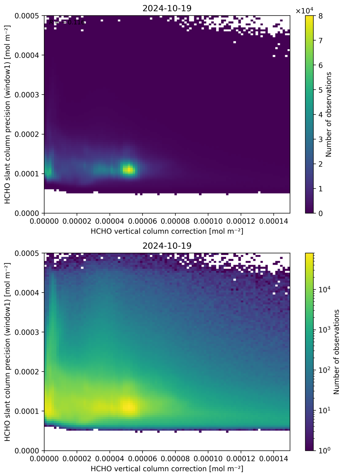
Figure 119: Scatter density plot of “HCHO vertical column correction” against “HCHO slant column precision (window1)” for 2024-10-19 to 2024-10-20.
