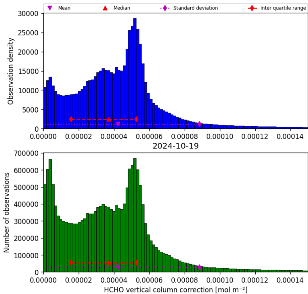
Figure 37: Histogram of “HCHO vertical column correction” for 2024-10-19 to 2024-10-20
