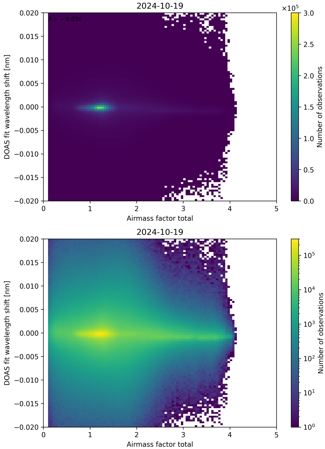
Figure 98: Scatter density plot of “Airmass factor total” against “DOAS fit wavelength shift” for 2024-10-19 to 2024-10-20.
