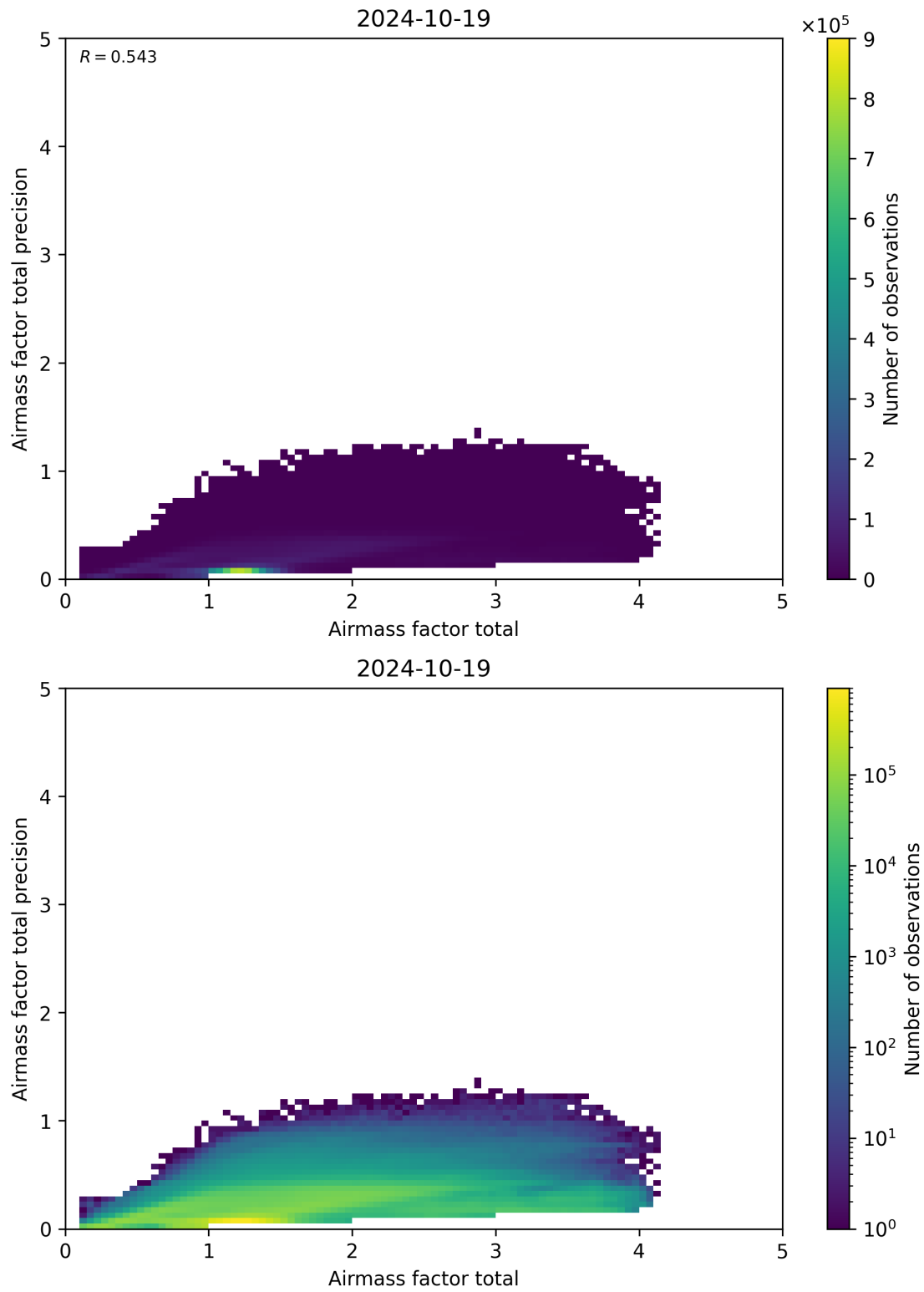
Figure 103: Scatter density plot of “Airmass factor total” against “Airmass factor total precision” for 2024-10-19 to 2024-10-20.
