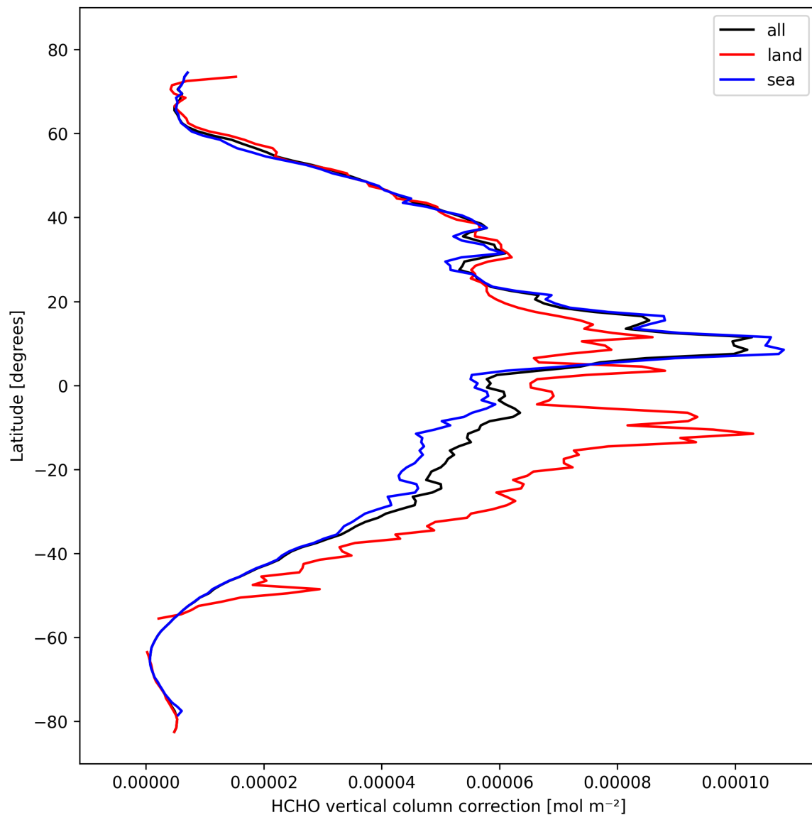
Figure 23: Zonal average of “HCHO vertical column correction” for 2024-10-19 to 2024-10-20.
