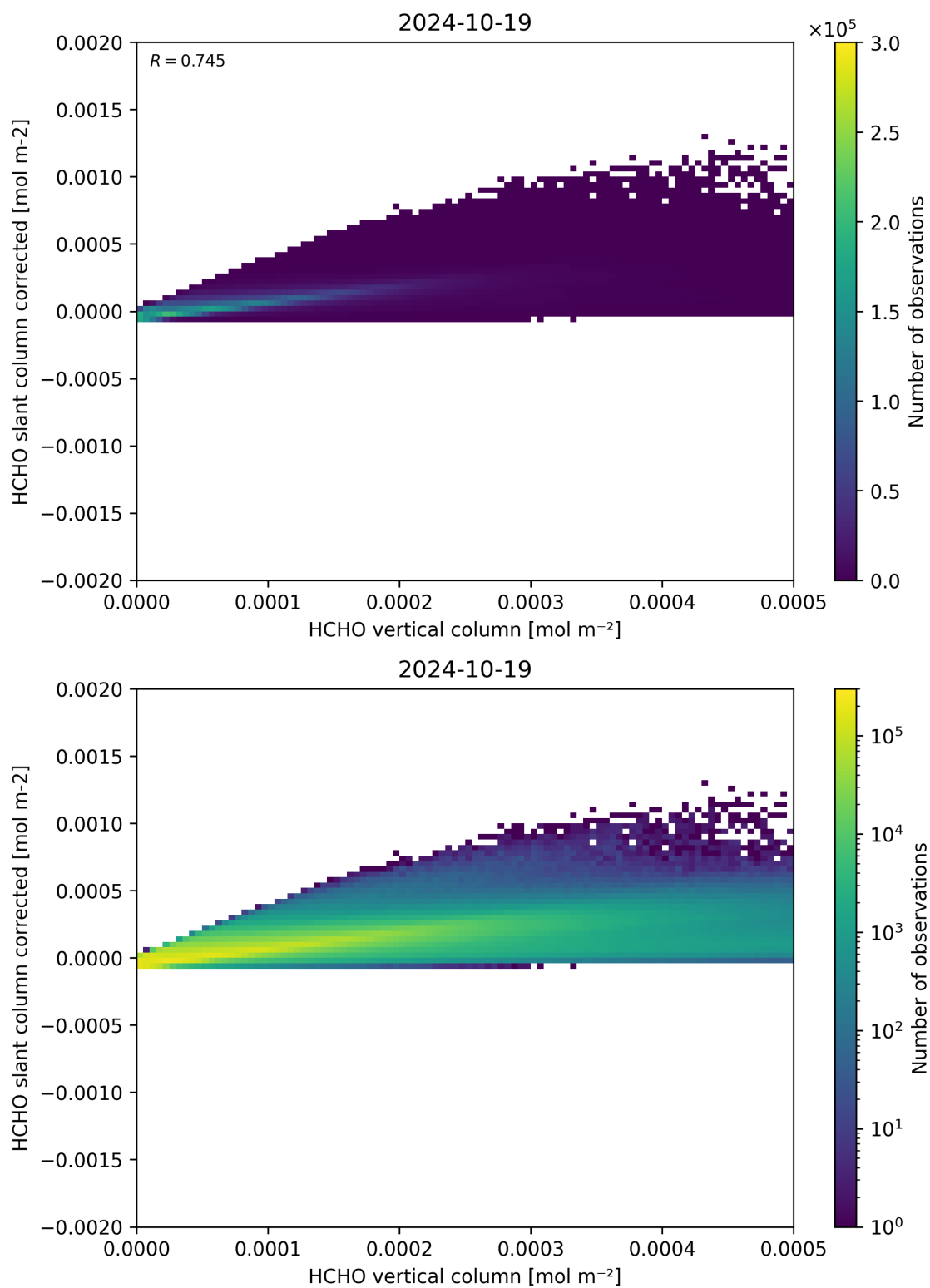
Figure 127: Scatter density plot of “HCHO vertical column” against “HCHO slant column corrected” for 2024-10-19 to 2024-10-20.
