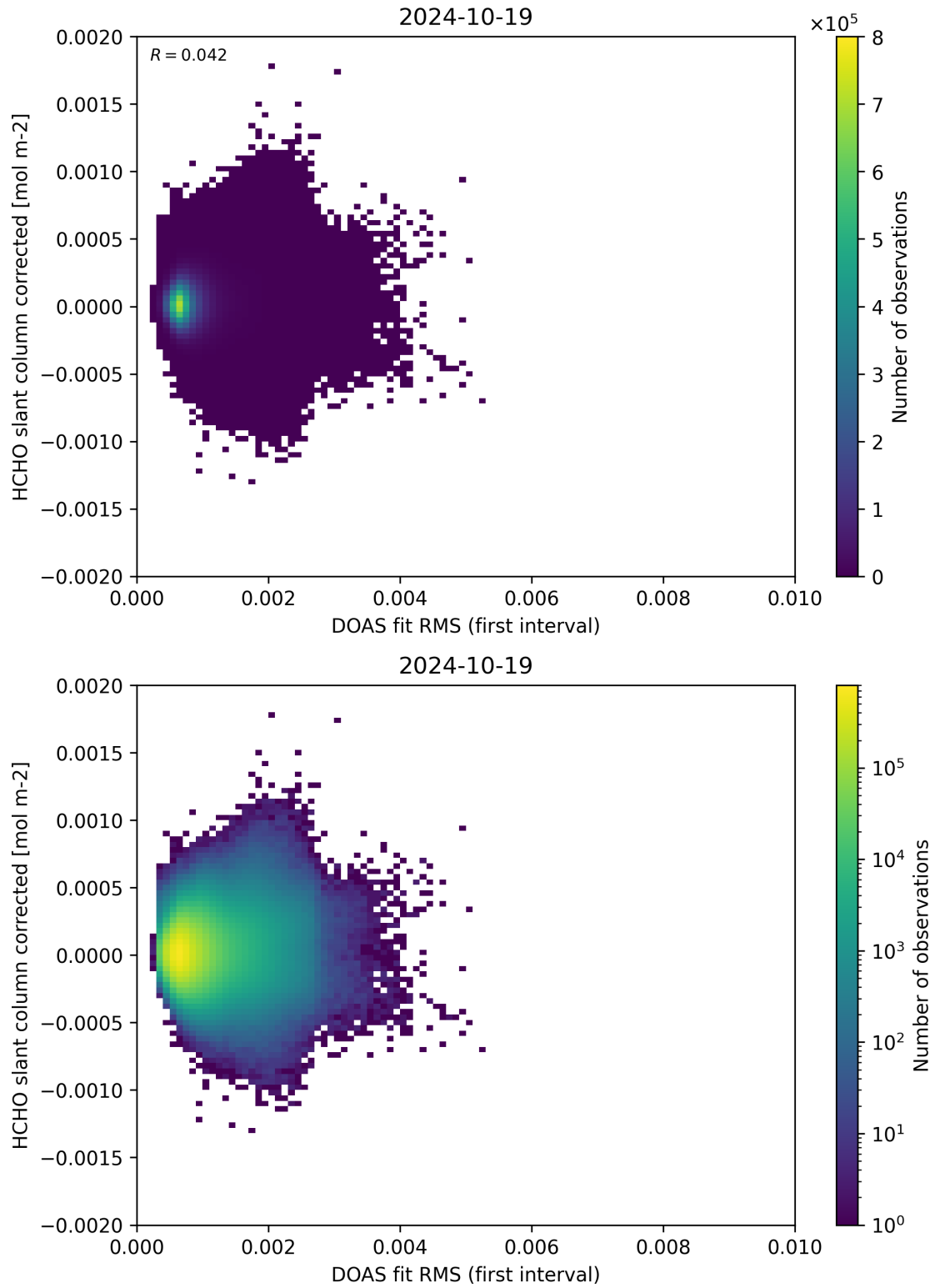
Figure 62: Scatter density plot of “DOAS fit RMS (first interval)” against “HCHO slant column corrected” for 2024-10-19 to 2024-10-20.
