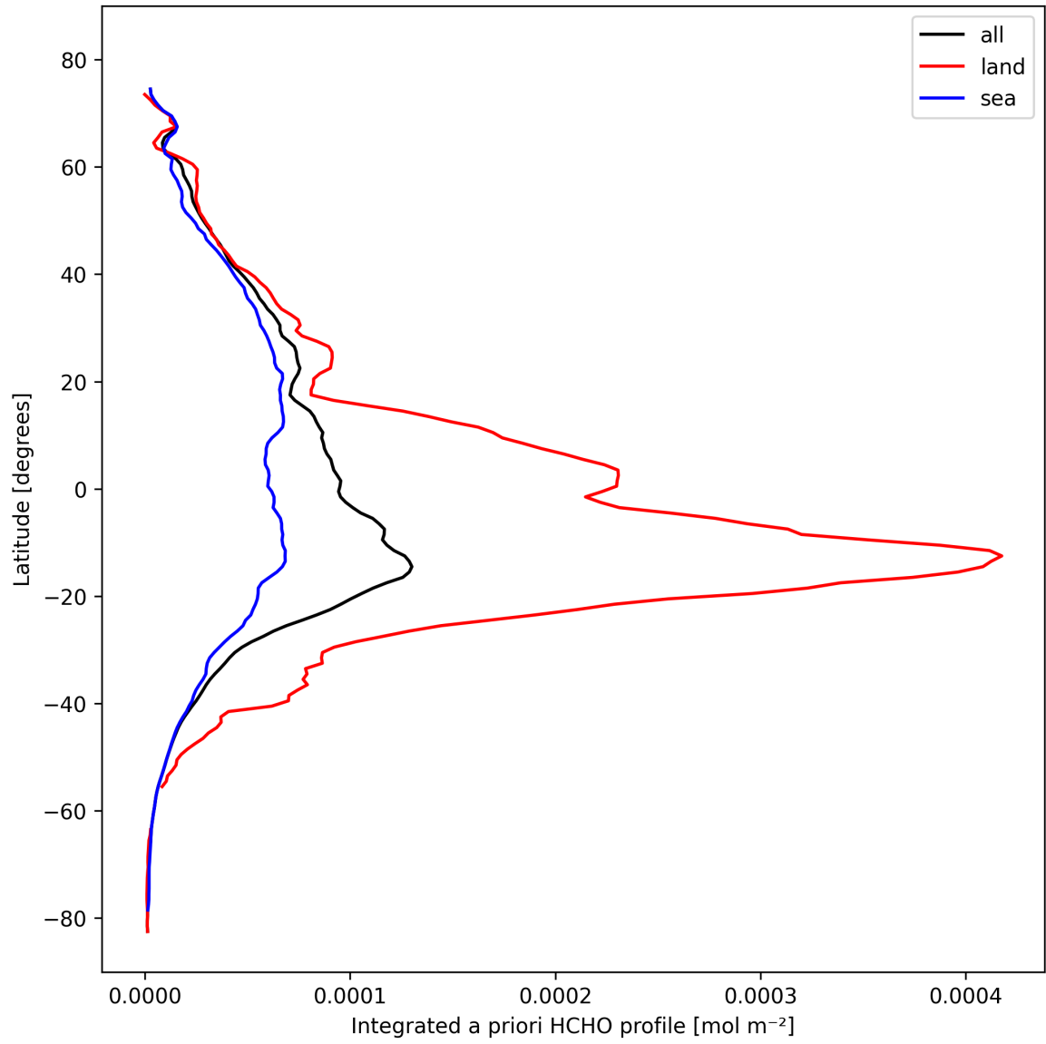
Figure 29: Zonal average of “Integrated a priori HCHO profile” for 2024-10-19 to 2024-10-20.
