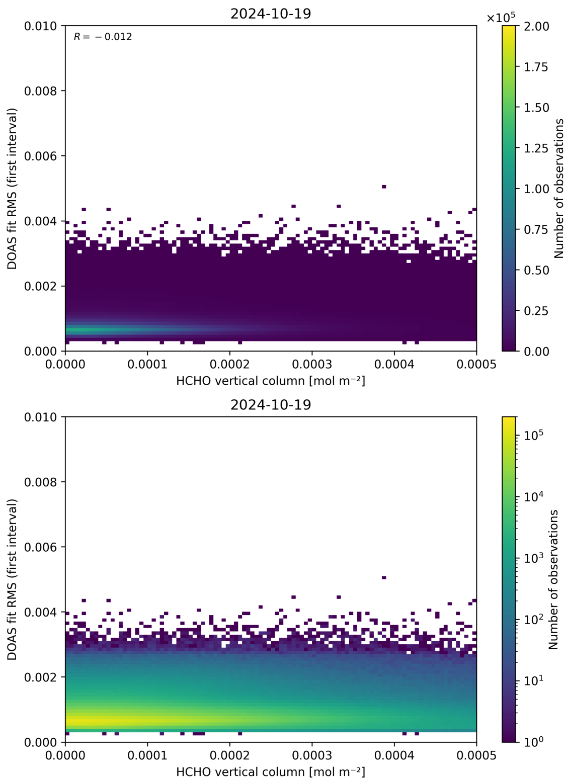
Figure 123: Scatter density plot of “HCHO vertical column” against “DOAS fit RMS (first interval)” for 2024-10-19 to 2024-10-20.
