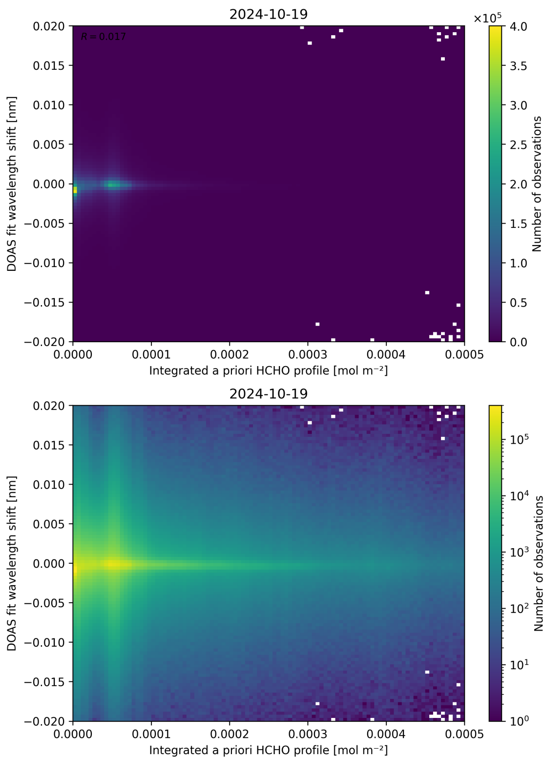
Figure 149: Scatter density plot of “Integrated a priori HCHO profile” against “DOAS fit wavelength shift” for 2024-10-19 to 2024-10-20.
