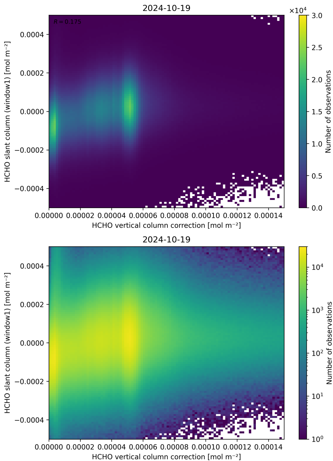
Figure 118: Scatter density plot of “HCHO vertical column correction” against “HCHO slant column (window1)” for 2024-10-19 to 2024-10-20.
