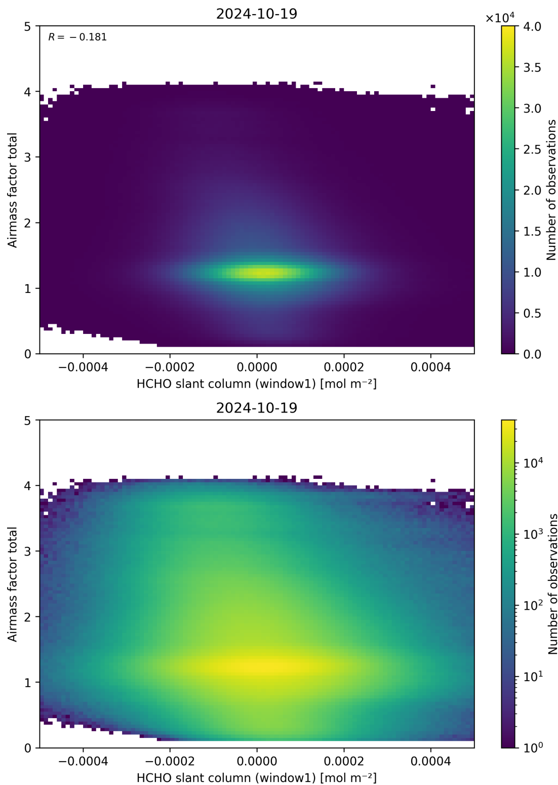
Figure 85: Scatter density plot of “HCHO slant column (window1)” against “Airmass factor total” for 2024-10-19 to 2024-10-20.
