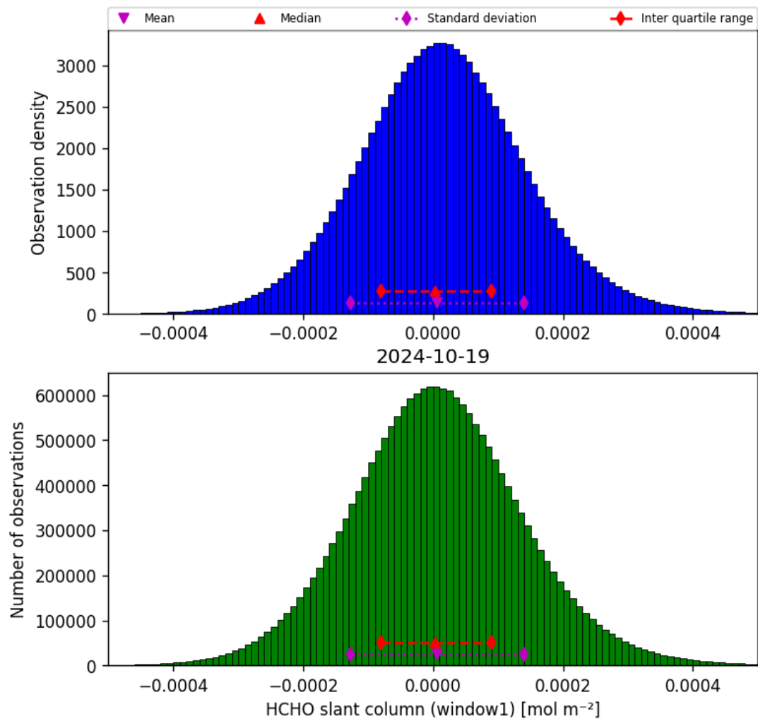
Figure 38: Histogram of “HCHO slant column (window1)” for 2024-10-19 to 2024-10-20
