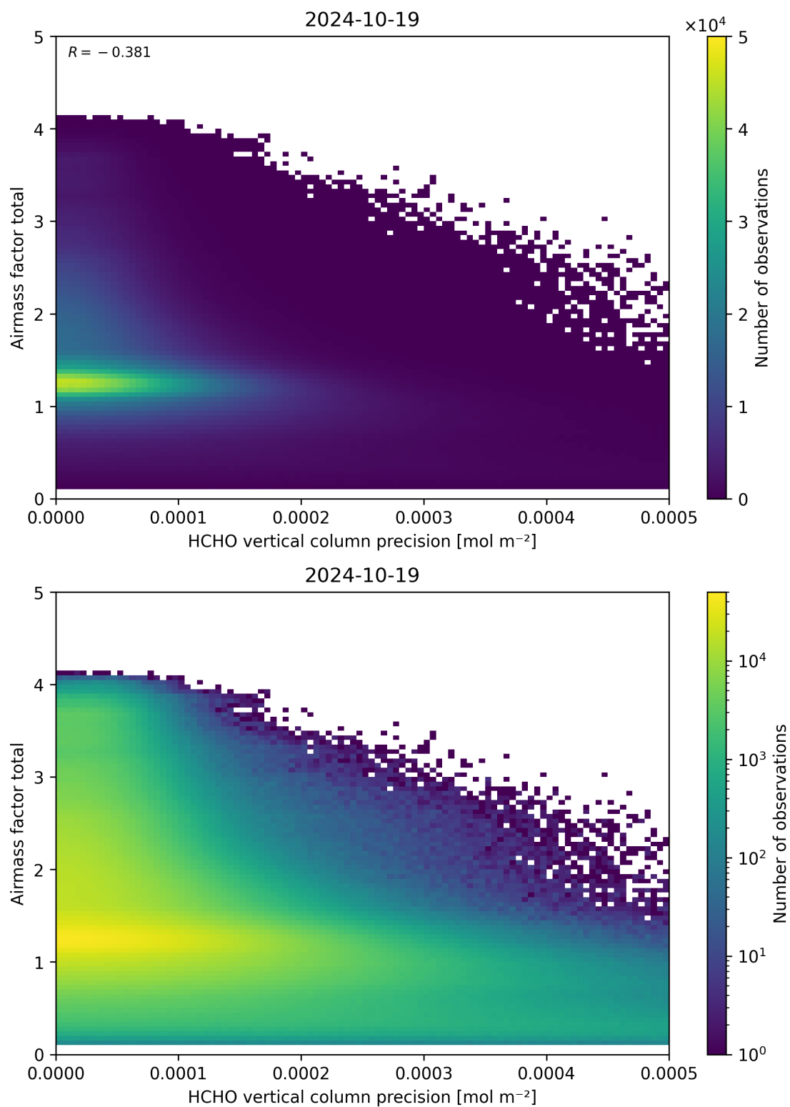
Figure 144: Scatter density plot of “HCHO vertical column precision” against “Airmass factor total” for 2024-10-19 to 2024-10-20.
