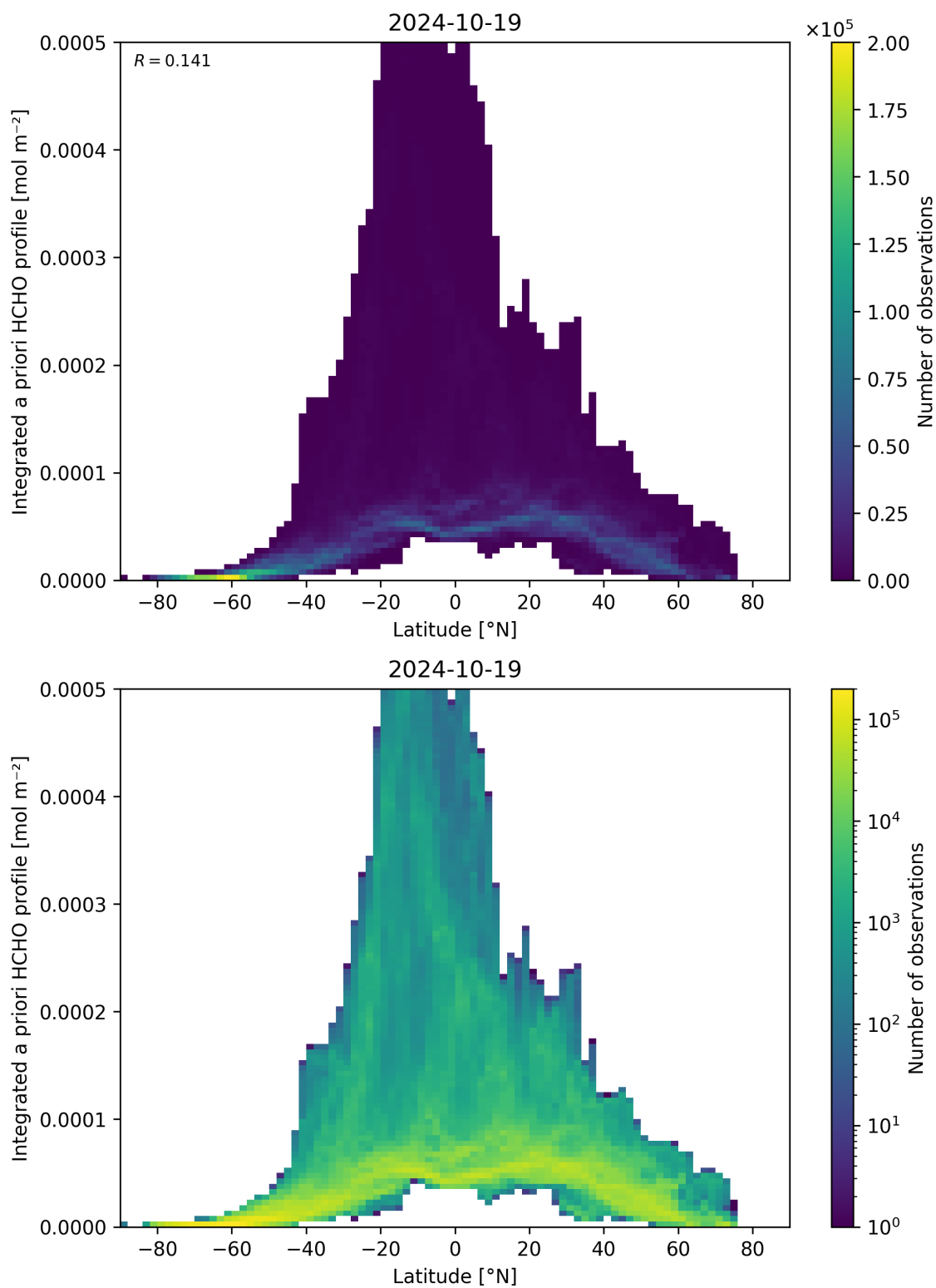
Figure 166: Scatter density plot of “Latitude” against “Integrated a priori HCHO profile” for 2024-10-19 to 2024-10-20.
