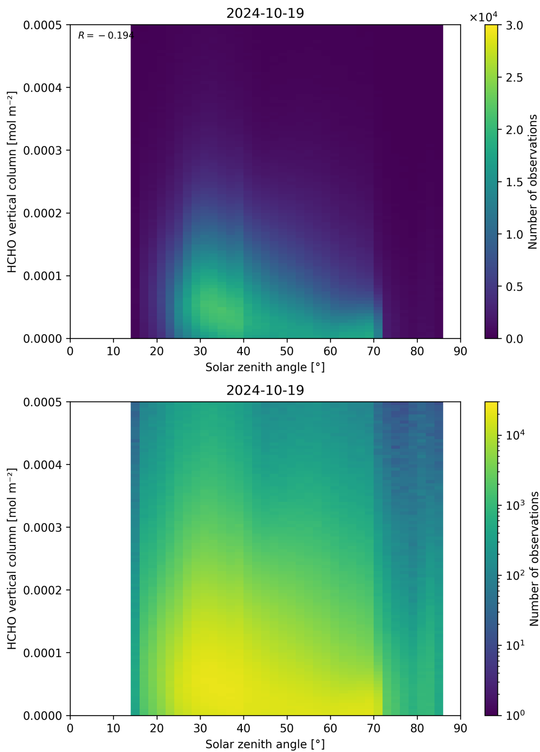
Figure 177: Scatter density plot of “Solar zenith angle” against “HCHO vertical column” for 2024-10-19 to 2024-10-20.
