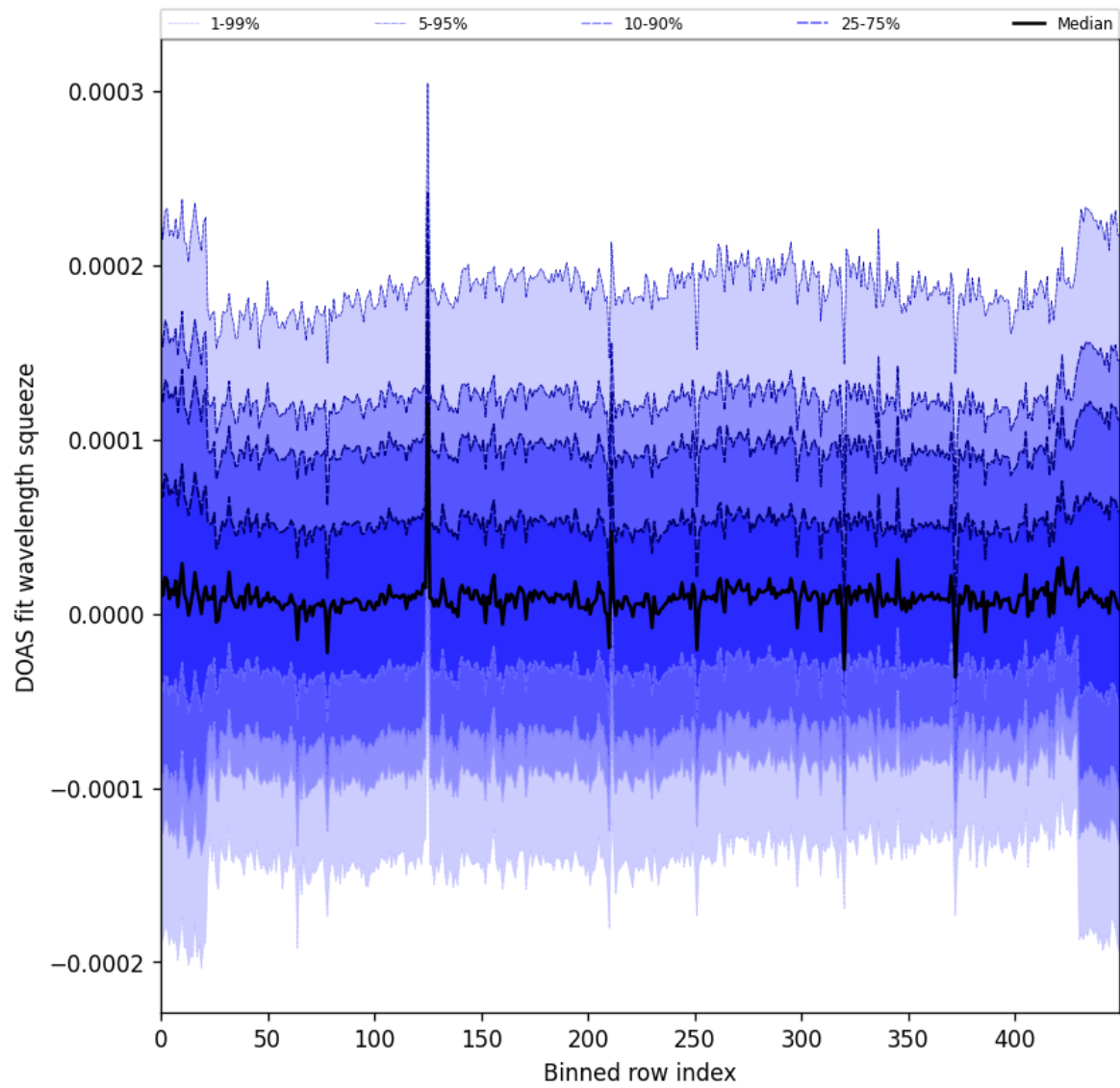
Figure 59: Along track statistics of “DOAS fit wavelength squeeze” for 2024-10-19 to 2024-10-20
