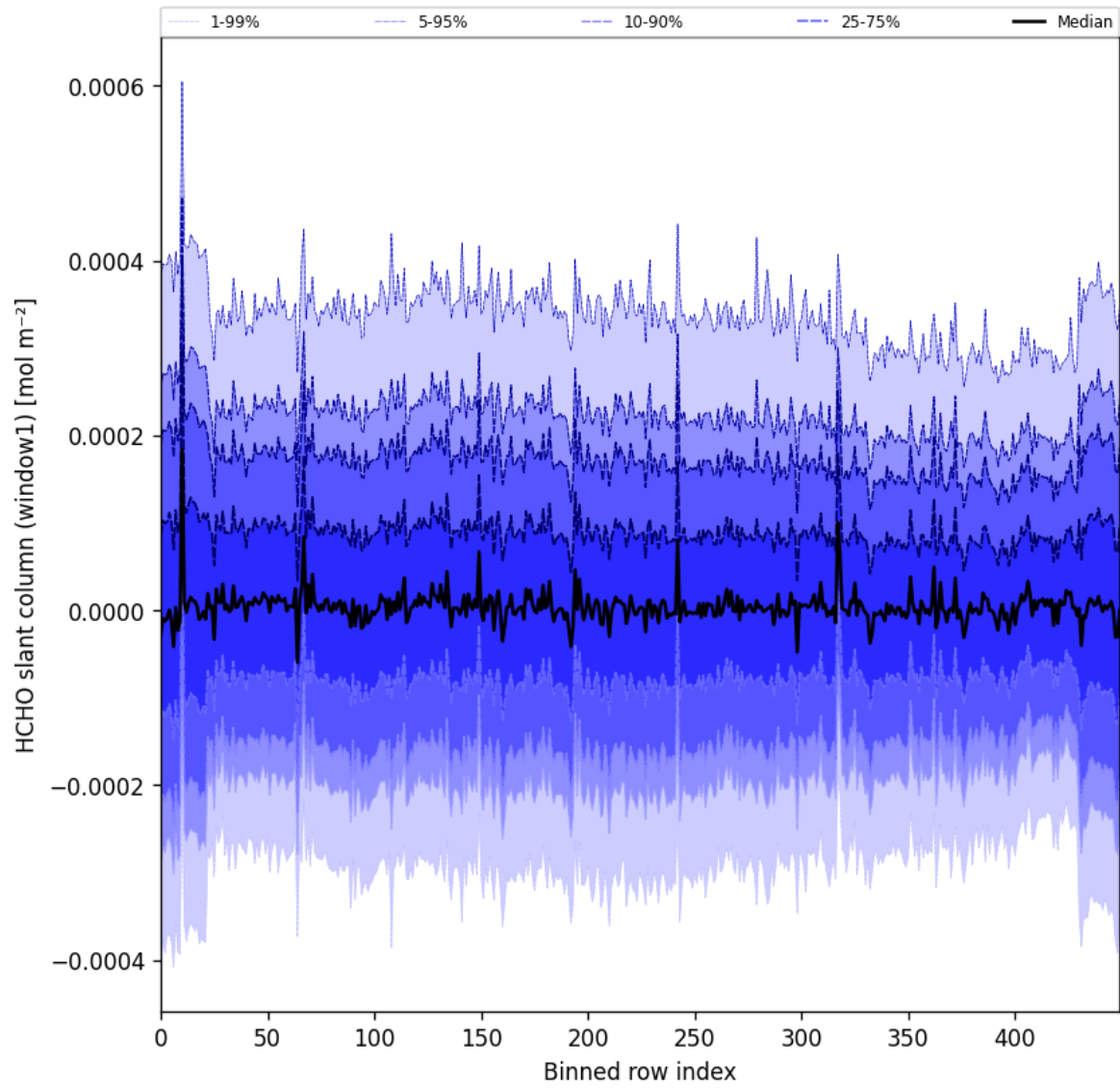
Figure 52: Along track statistics of “HCHO slant column (window1)” for 2024-10-19 to 2024-10-20
