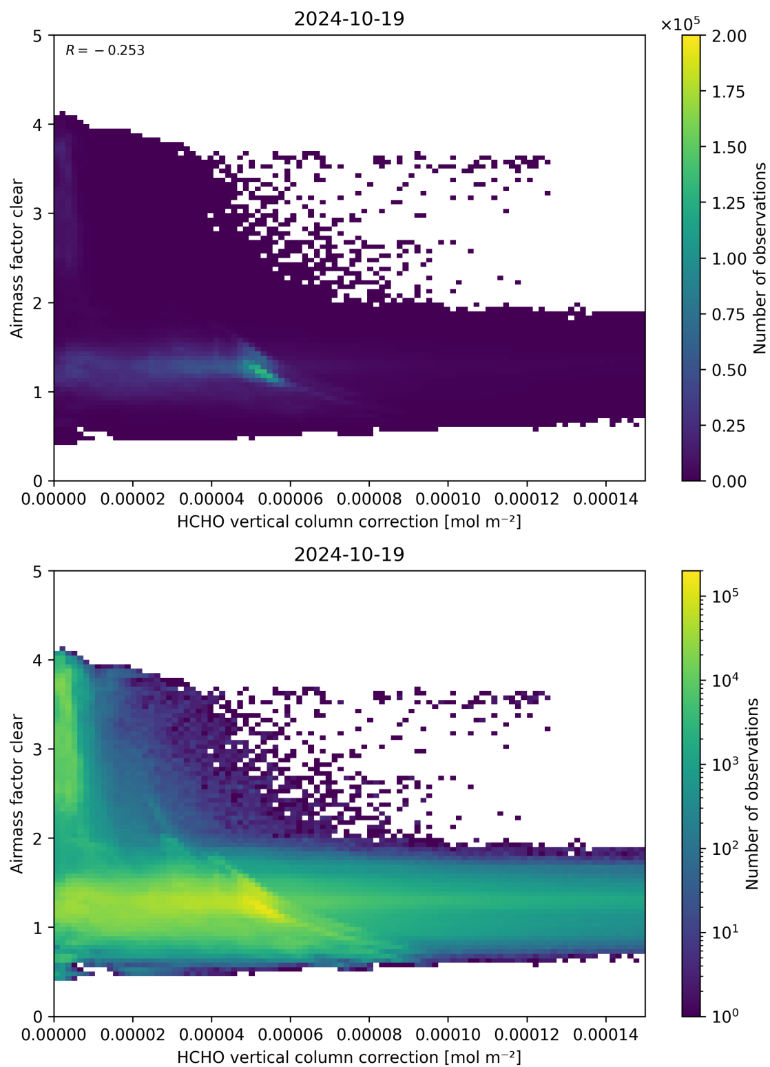
Figure 115: Scatter density plot of “HCHO vertical column correction” against “Airmass factor clear” for 2024-10-19 to 2024-10-20.
