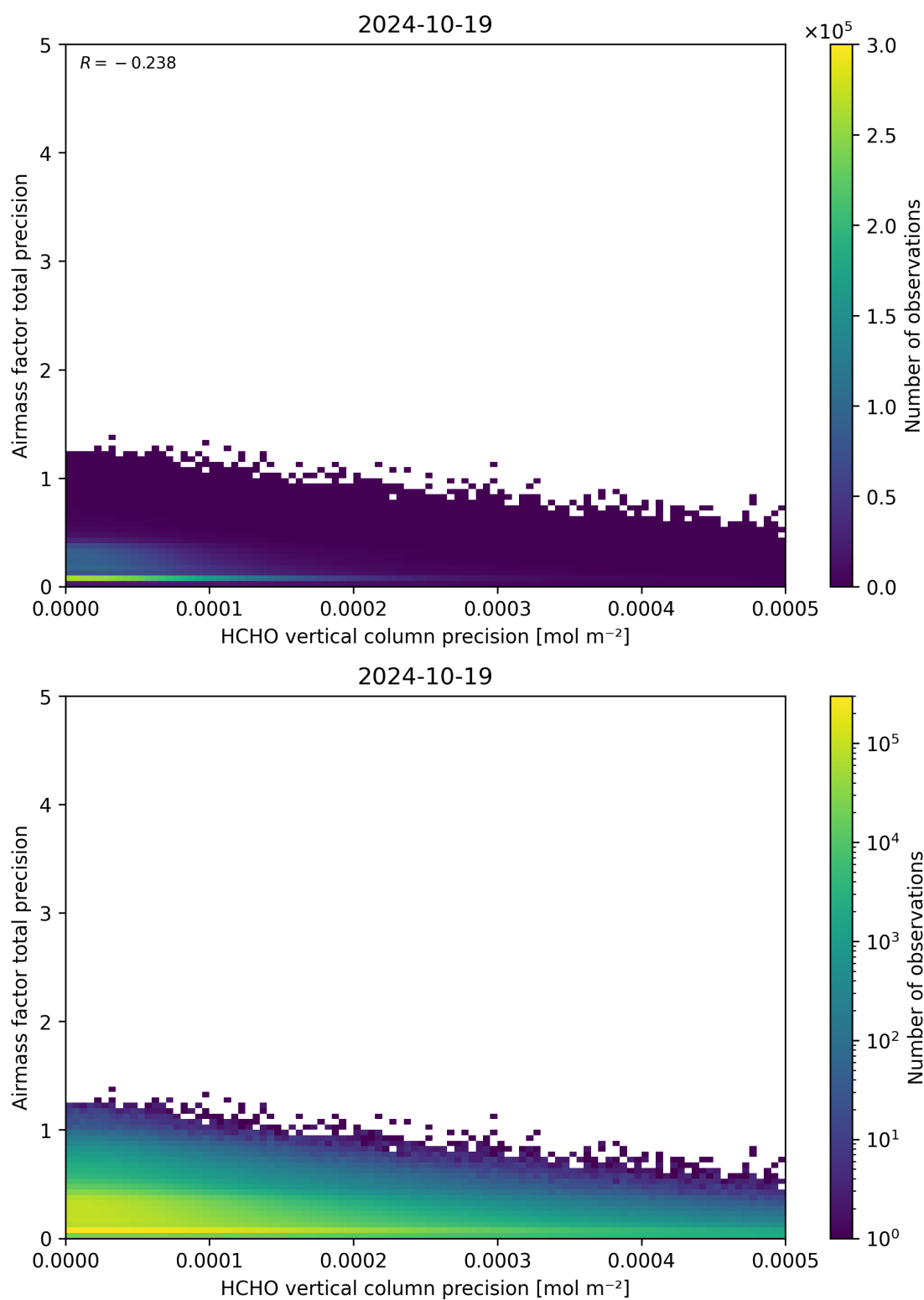
Figure 145: Scatter density plot of “HCHO vertical column precision” against “Airmass factor total precision” for 2024-10-19 to 2024-10-20.
