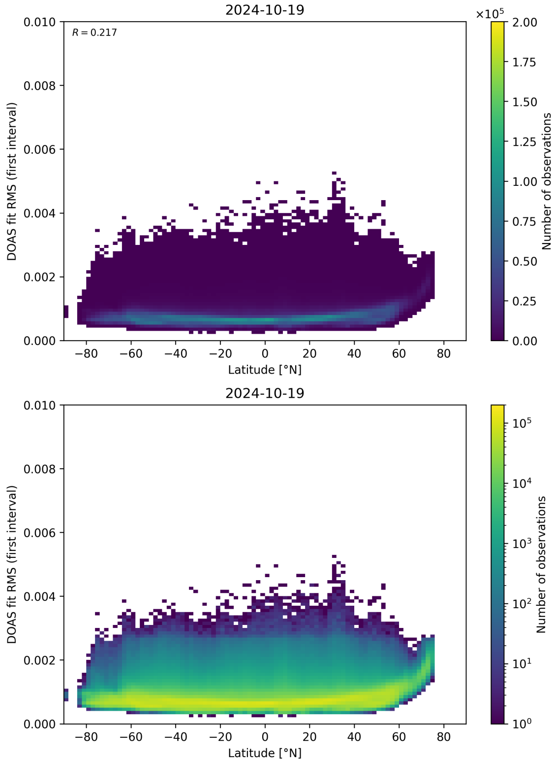
Figure 153: Scatter density plot of “Latitude” against “DOAS fit RMS (first interval)” for 2024-10-19 to 2024-10-20.
