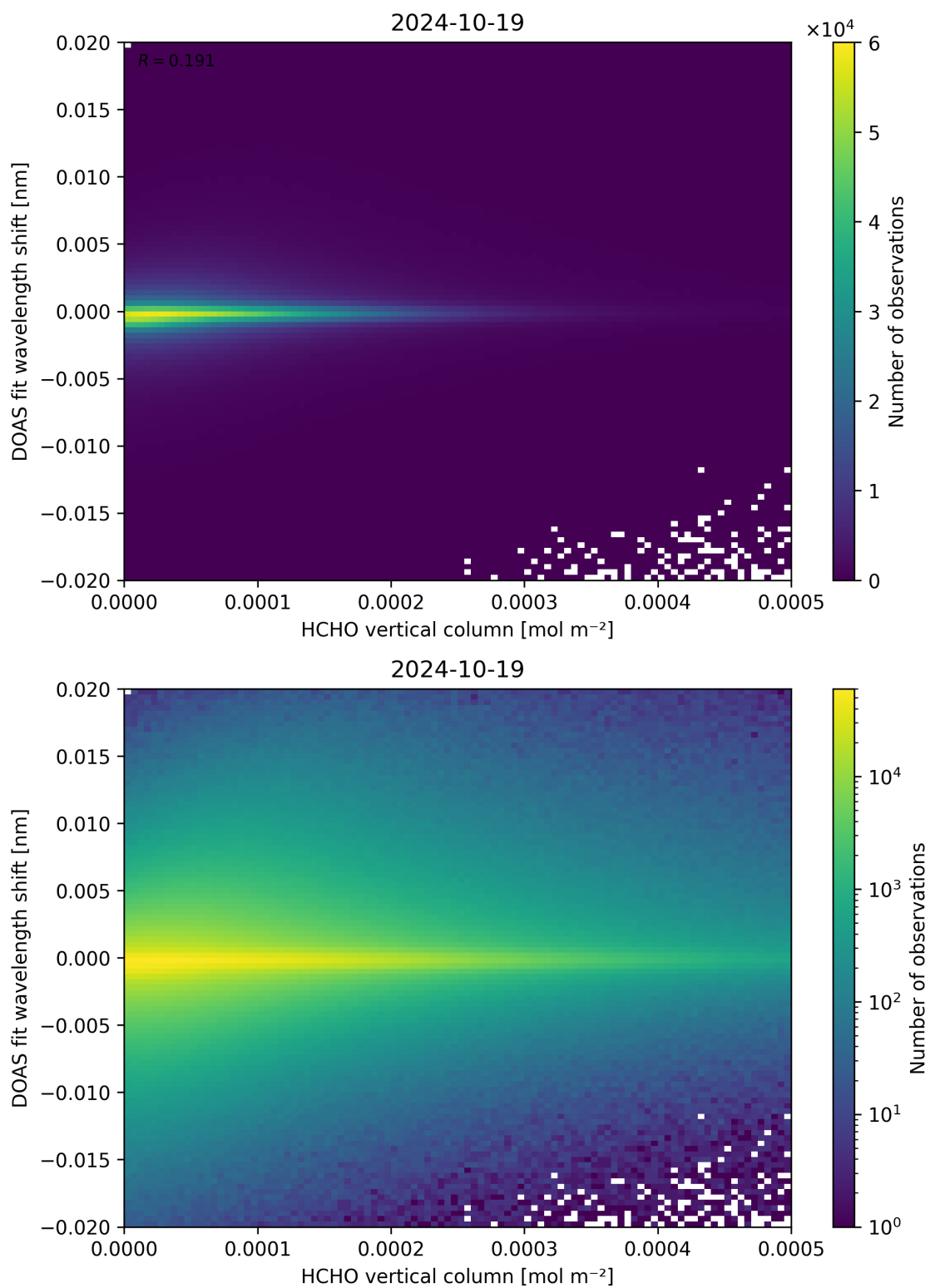
Figure 124: Scatter density plot of “HCHO vertical column” against “DOAS fit wavelength shift” for 2024-10-19 to 2024-10-20.
