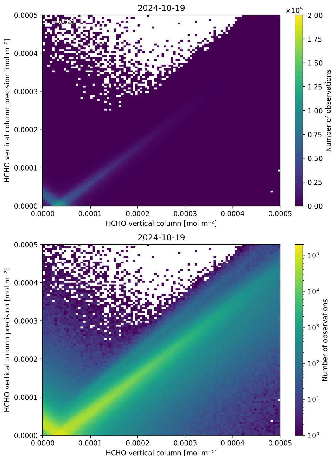
Figure 134: Scatter density plot of “HCHO vertical column” against “HCHO vertical column precision” for 2024-10-19 to 2024-10-20.
