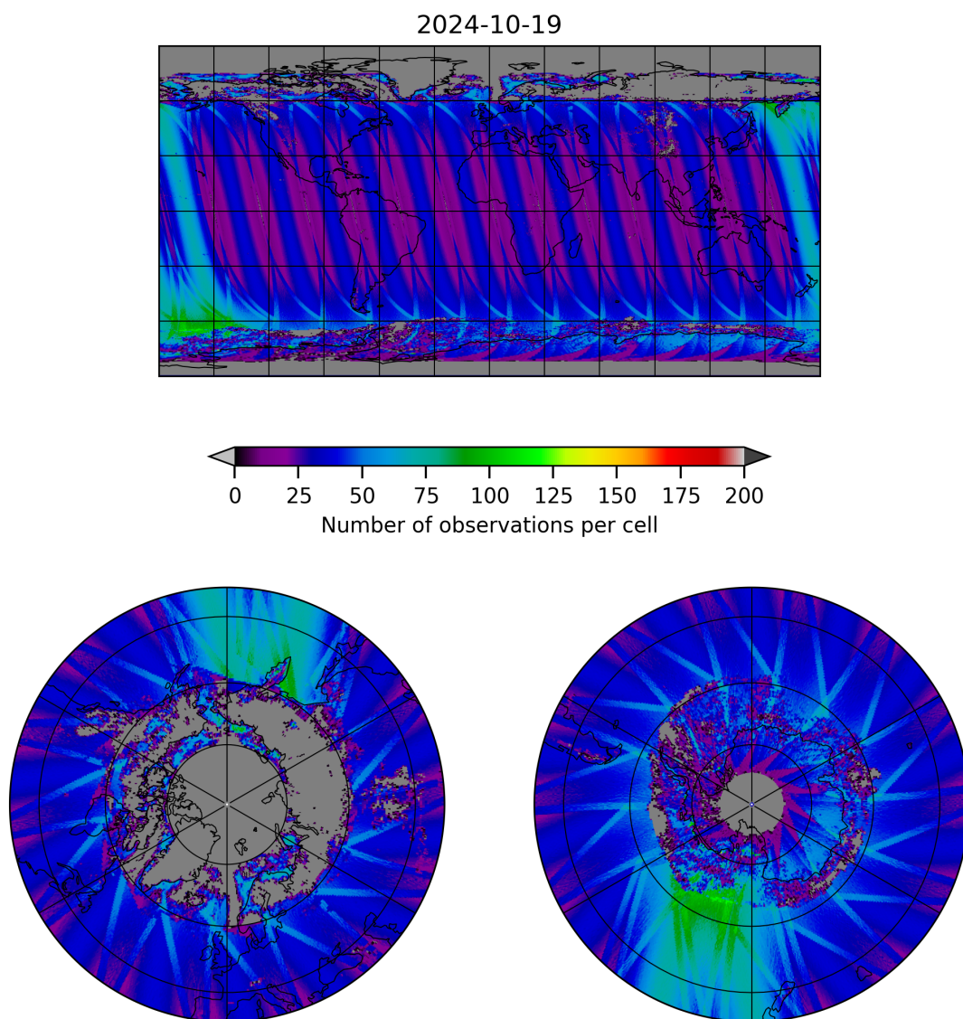
Figure 19: Map of the number of observations for 2024-10-19 to 2024-10-20
