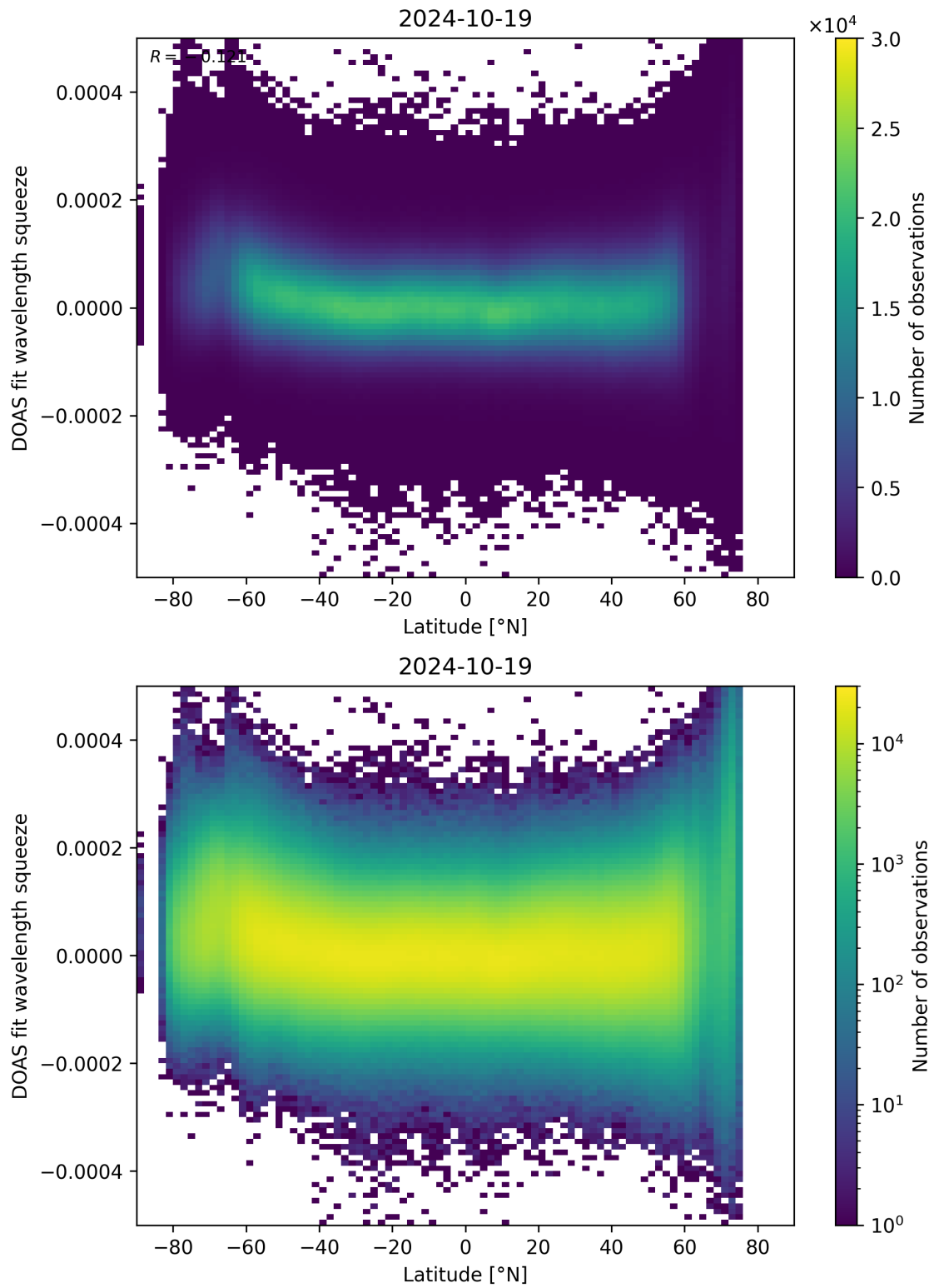
Figure 155: Scatter density plot of “Latitude” against “DOAS fit wavelength squeeze” for 2024-10-19 to 2024-10-20.
