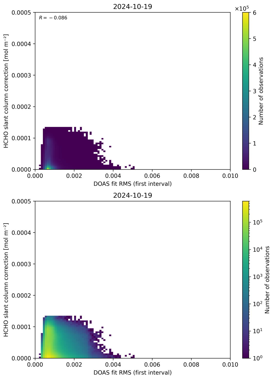
Figure 63: Scatter density plot of “DOAS fit RMS (first interval)” against “HCHO slant column correction” for 2024-10-19 to 2024-10-20.
