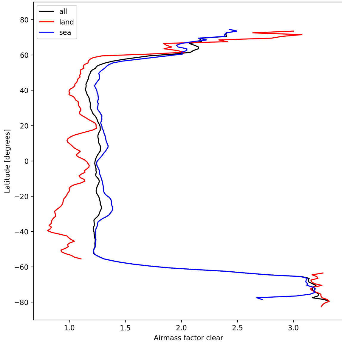
Figure 28: Zonal average of “Airmass factor clear” for 2024-10-19 to 2024-10-20.
