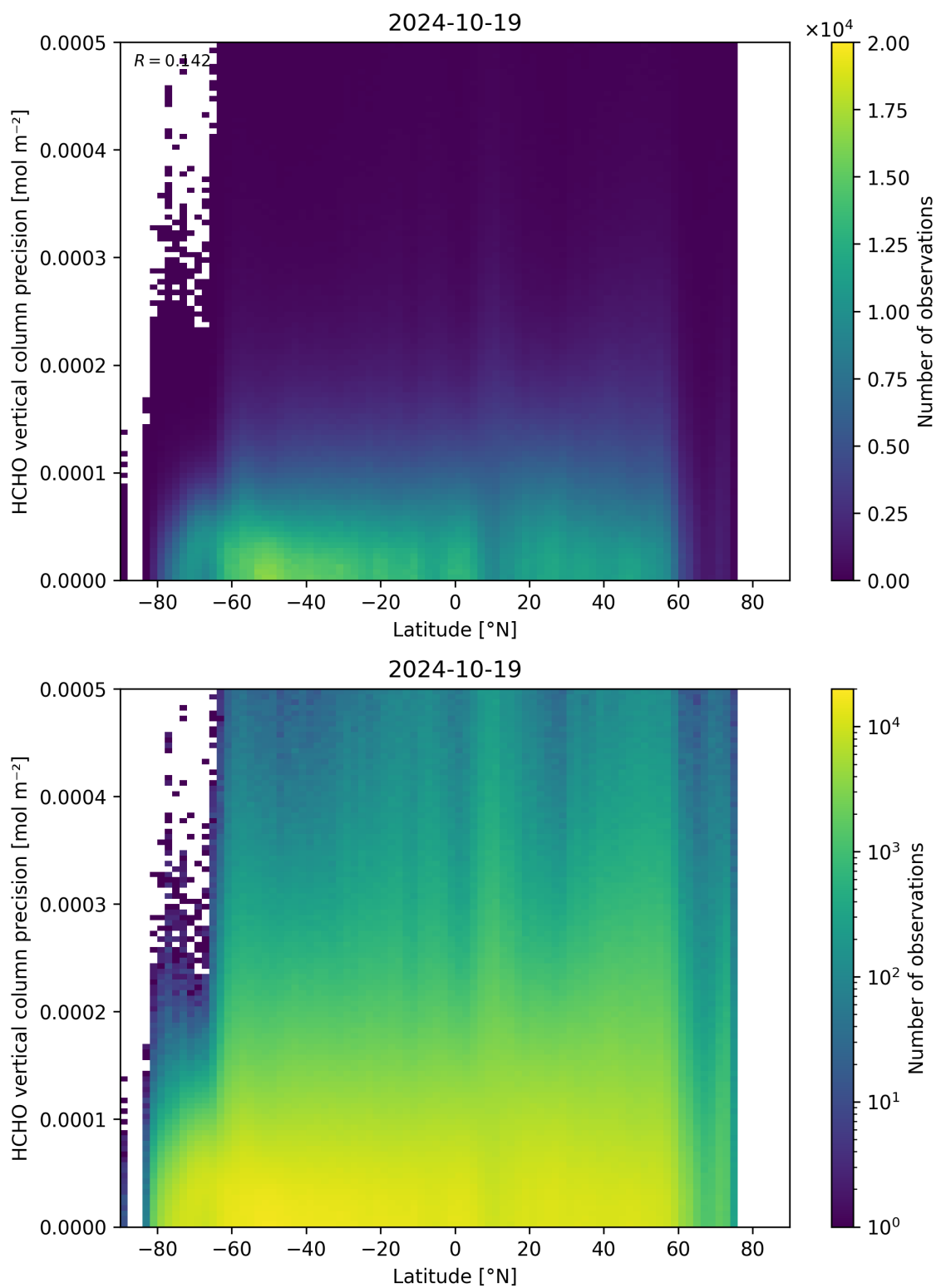
Figure 165: Scatter density plot of “Latitude” against “HCHO vertical column precision” for 2024-10-19 to 2024-10-20.
