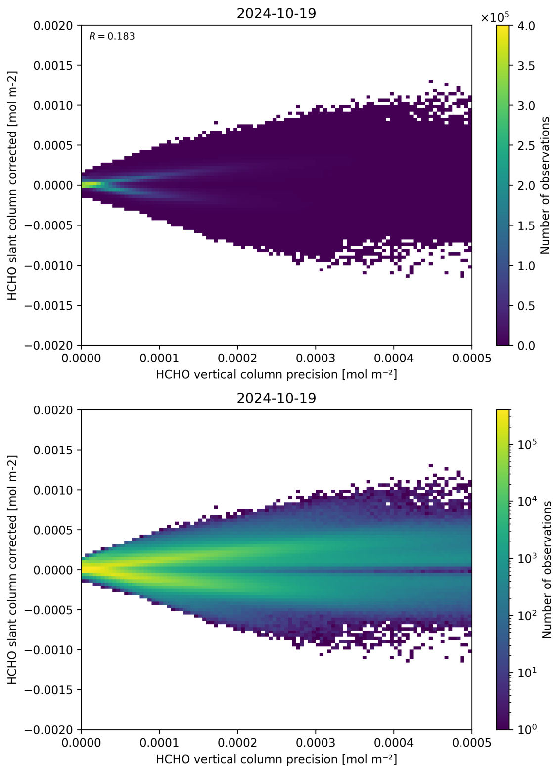
Figure 140: Scatter density plot of “HCHO vertical column precision” against “HCHO slant column corrected” for 2024-10-19 to 2024-10-20.
