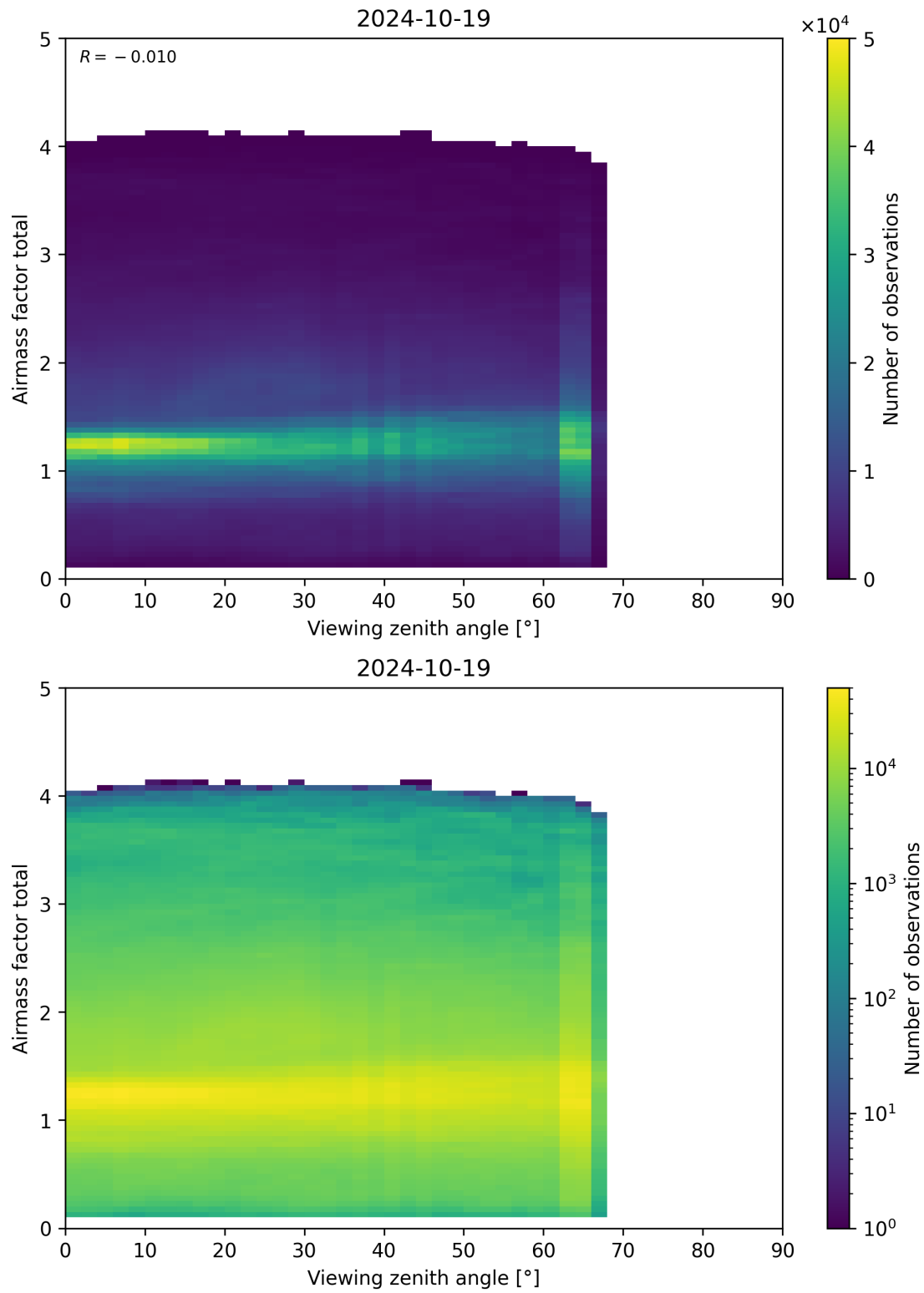
Figure 190: Scatter density plot of “Viewing zenith angle” against “Airmass factor total” for 2024-10-19 to 2024-10-20.
