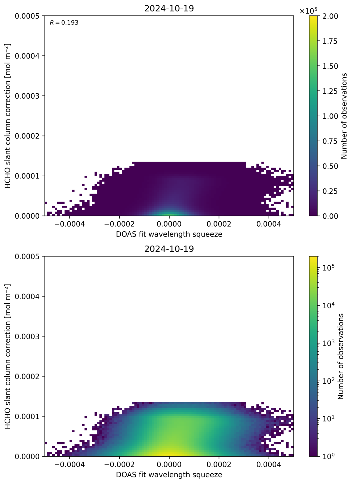
Figure 70: Scatter density plot of “DOAS fit wavelength squeeze” against “HCHO slant column correction” for 2024-10-19 to 2024-10-20.
