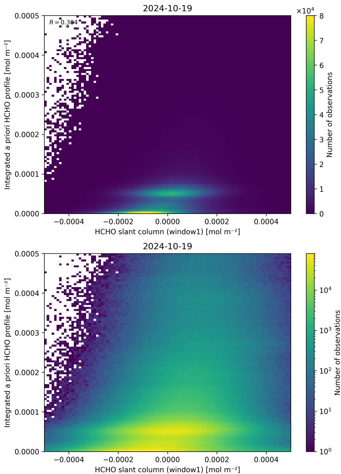
Figure 87: Scatter density plot of “HCHO slant column (window1)” against “Integrated a priori HCHO profile” for 2024-10-19 to 2024-10-20.
