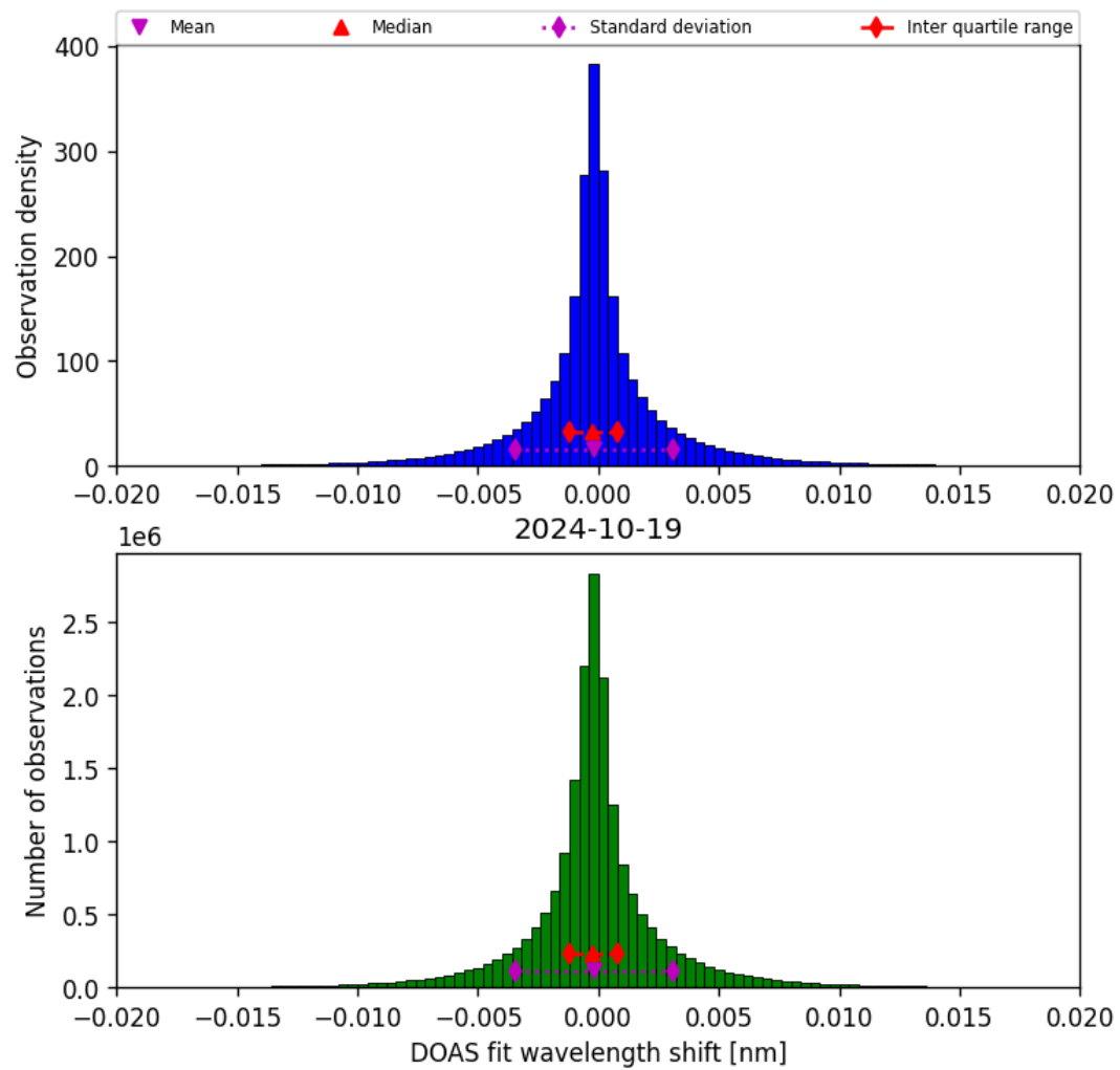
Figure 44: Histogram of “DOAS fit wavelength shift” for 2024-10-19 to 2024-10-20
