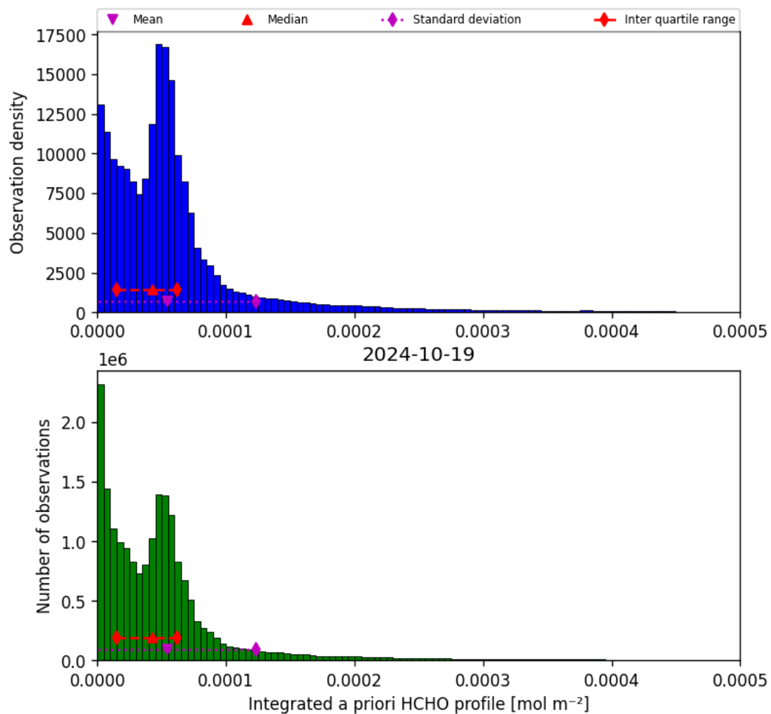
Figure 43: Histogram of “Integrated a priori HCHO profile” for 2024-10-19 to 2024-10-20
