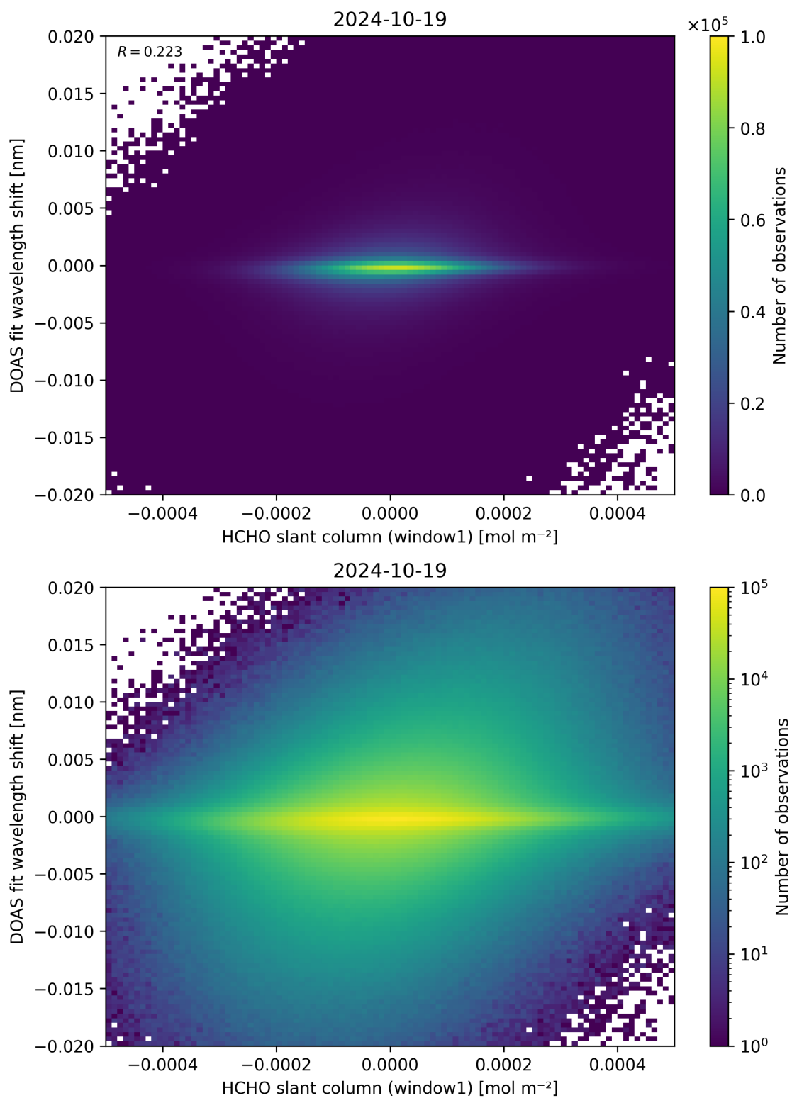
Figure 79: Scatter density plot of “HCHO slant column (window1)” against “DOAS fit wavelength shift” for 2024-10-19 to 2024-10-20.
