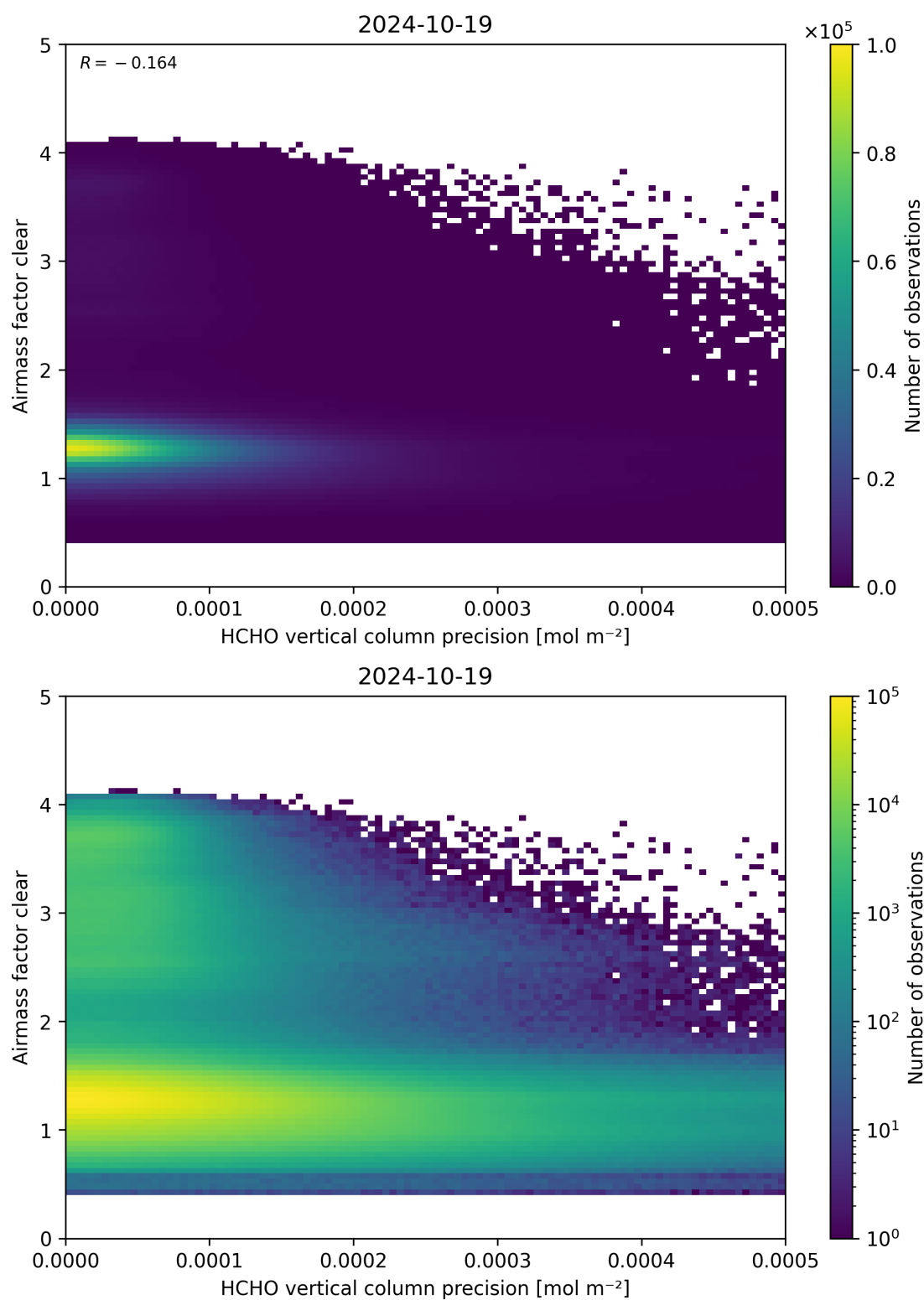
Figure 139: Scatter density plot of “HCHO vertical column precision” against “Airmass factor clear” for 2024-10-19 to 2024-10-20.
