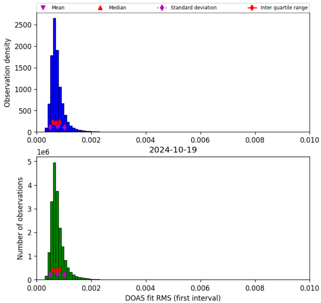
Figure 46: Histogram of “DOAS fit RMS (first interval)” for 2024-10-19 to 2024-10-20
