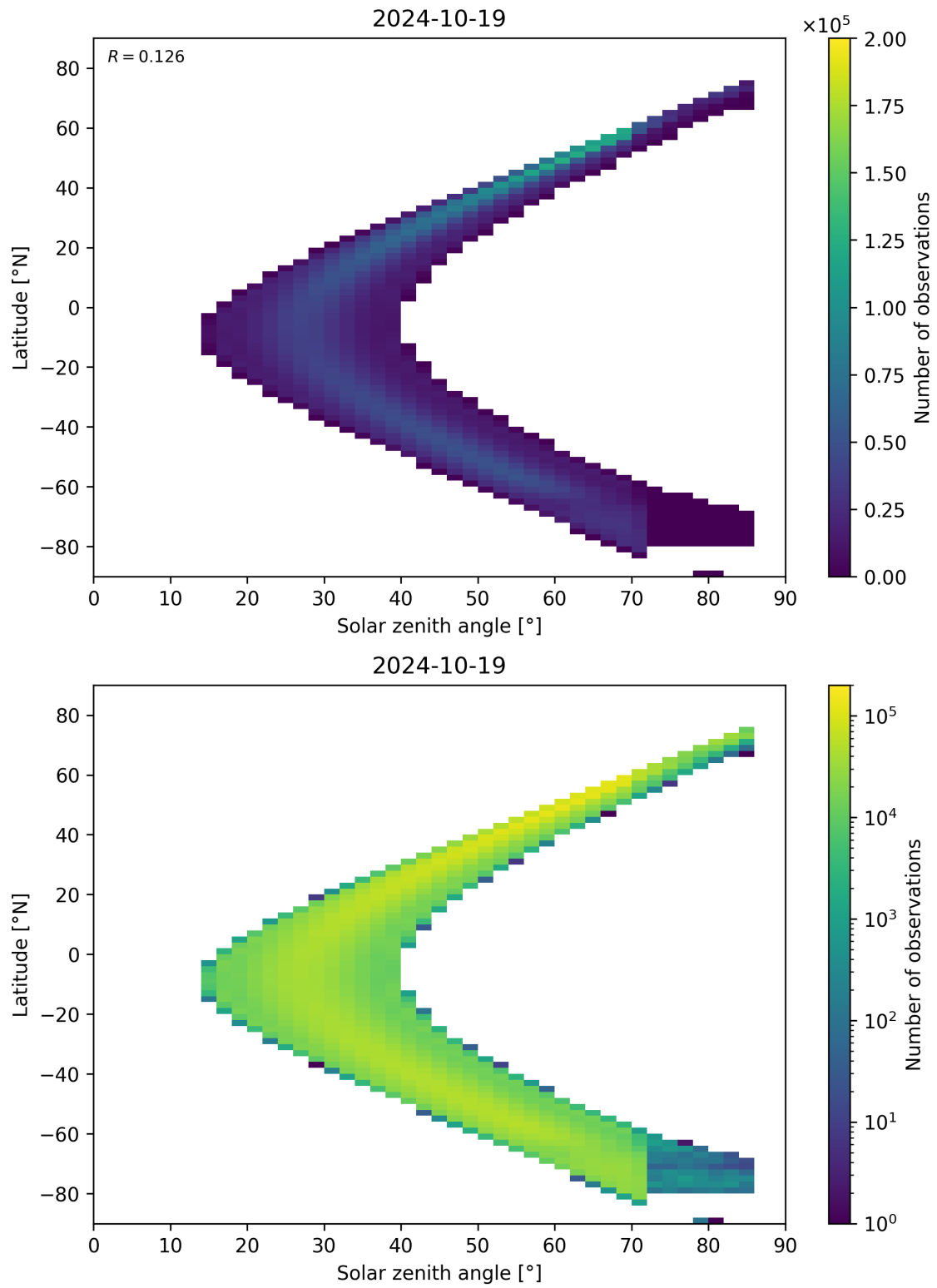
Figure 181: Scatter density plot of “Solar zenith angle” against “Latitude” for 2024-10-19 to 2024-10-20.
