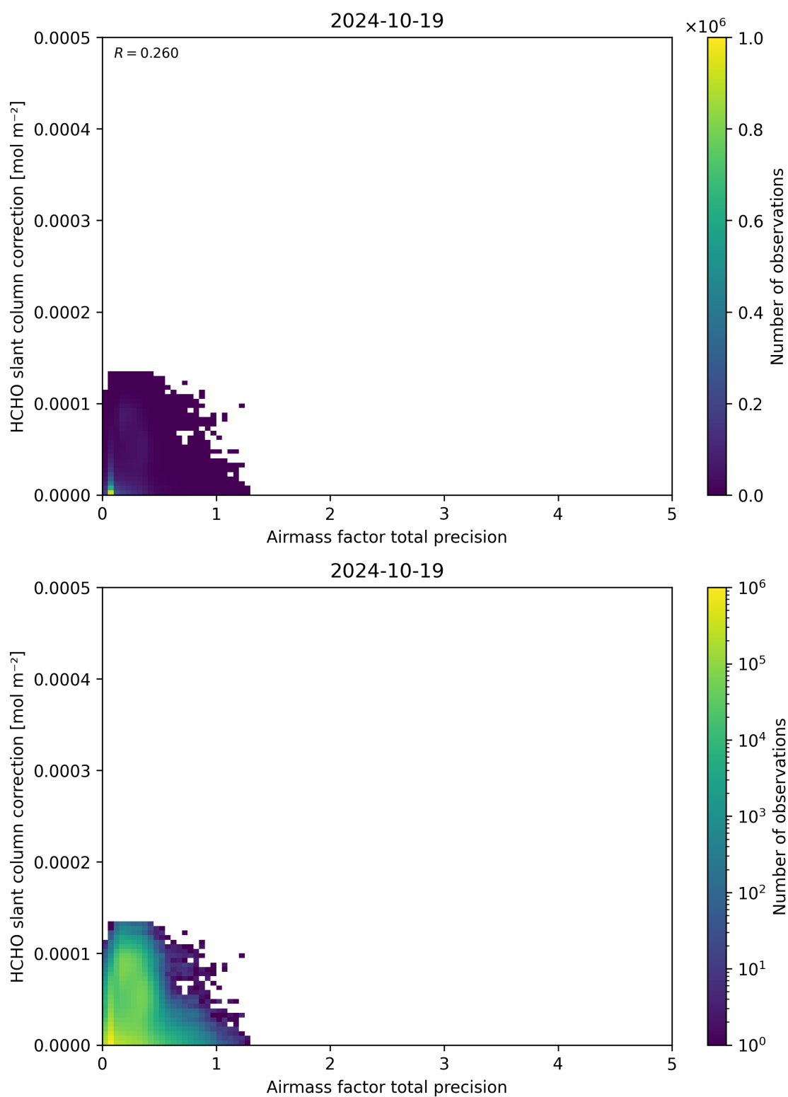
Figure 110: Scatter density plot of “Airmass factor total precision” against “HCHO slant column correction” for 2024-10-19 to 2024-10-20.
