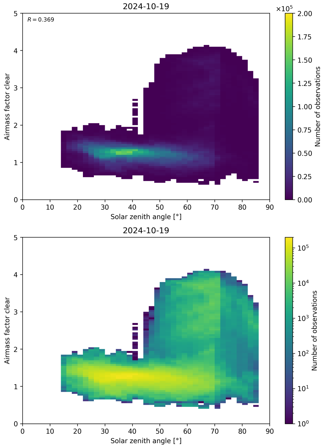
Figure 170: Scatter density plot of “Solar zenith angle” against “Airmass factor clear” for 2024-10-19 to 2024-10-20.
