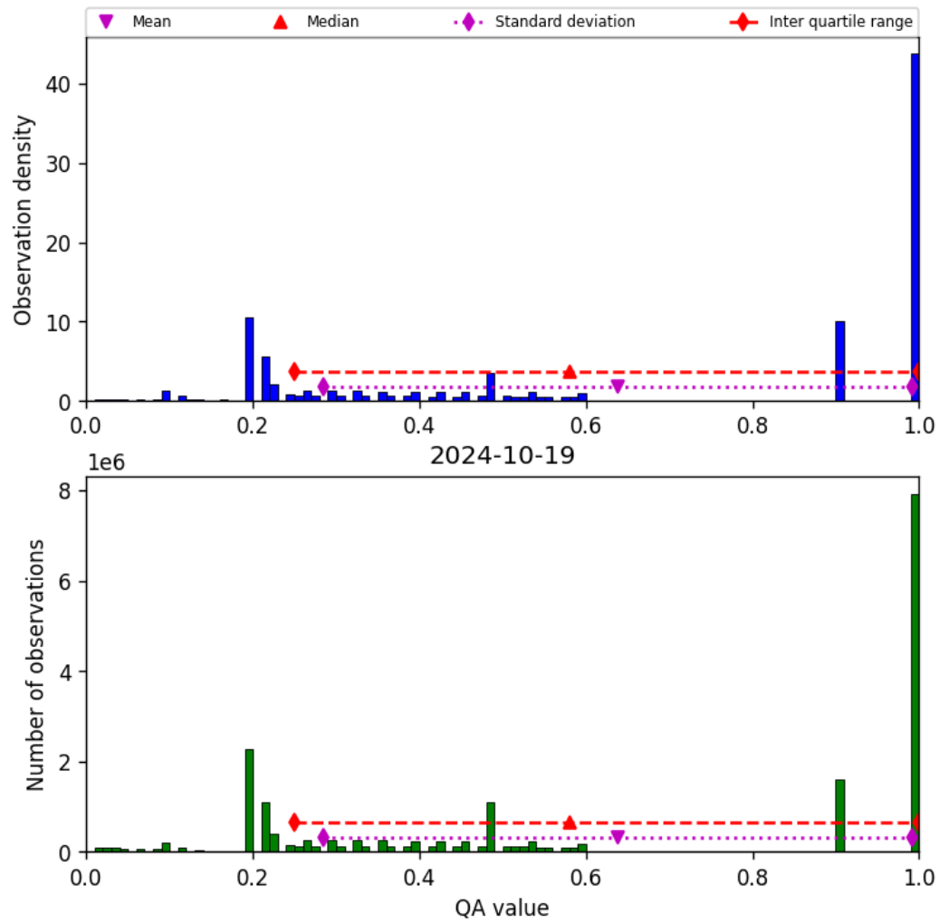
Figure 34: Histogram of “QA value” for 2024-10-19 to 2024-10-20
