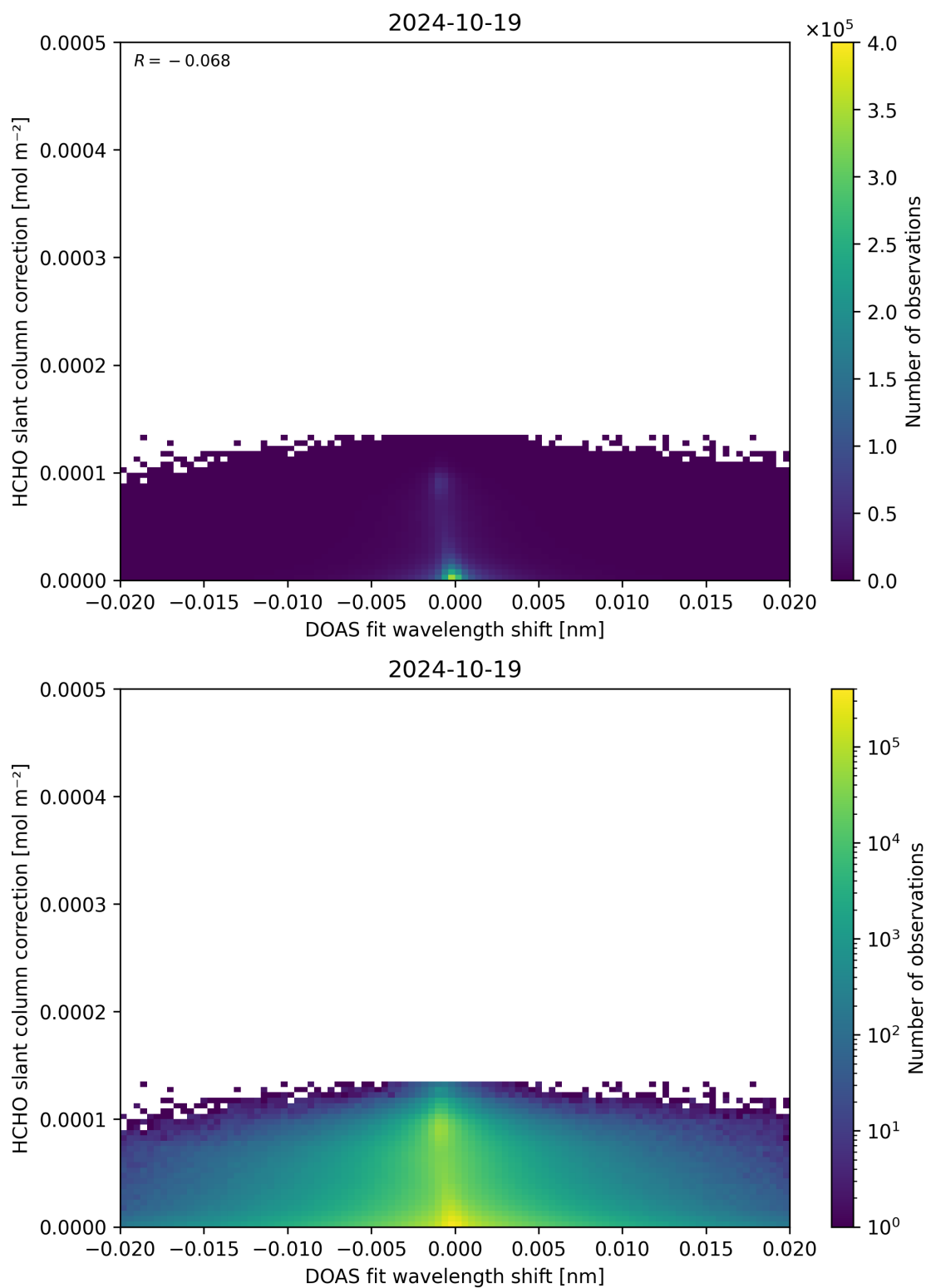
Figure 67: Scatter density plot of “DOAS fit wavelength shift” against “HCHO slant column correction” for 2024-10-19 to 2024-10-20.
