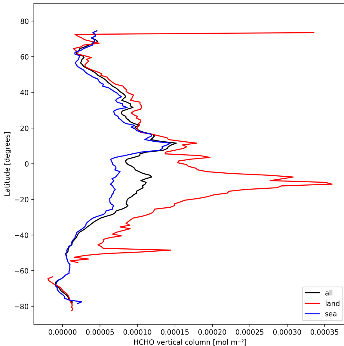
Figure 21: Zonal average of “HCHO vertical column” for 2024-10-19 to 2024-10-20.
