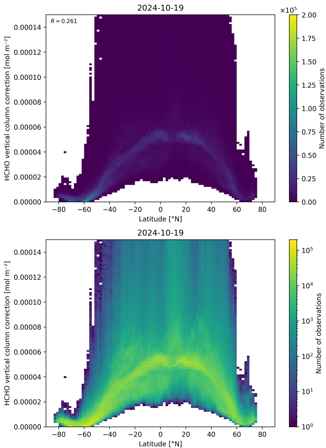
Figure 164: Scatter density plot of “Latitude” against “HCHO vertical column correction” for 2024-10-19 to 2024-10-20.
