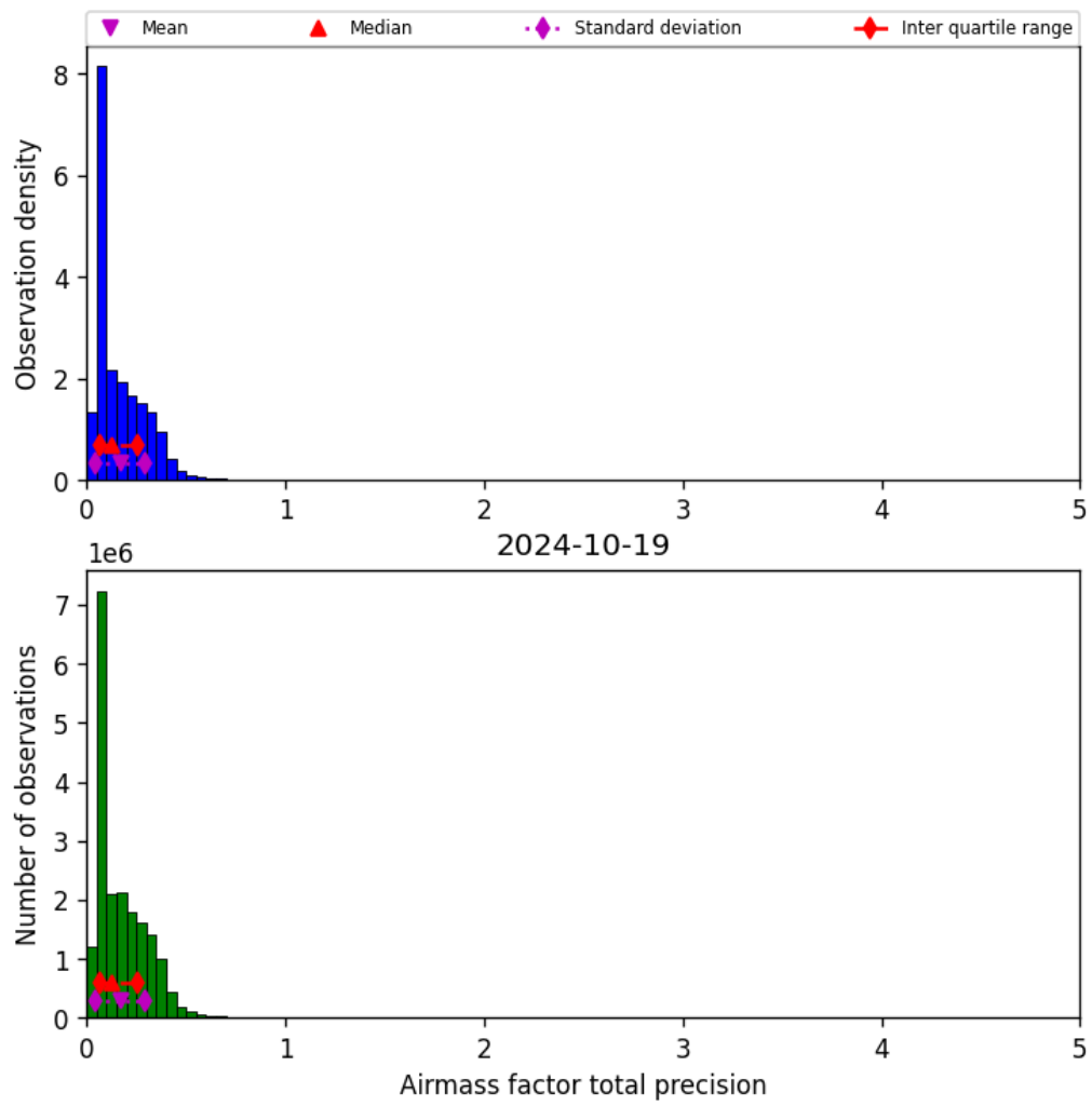
Figure 41: Histogram of “Airmass factor total precision” for 2024-10-19 to 2024-10-20
