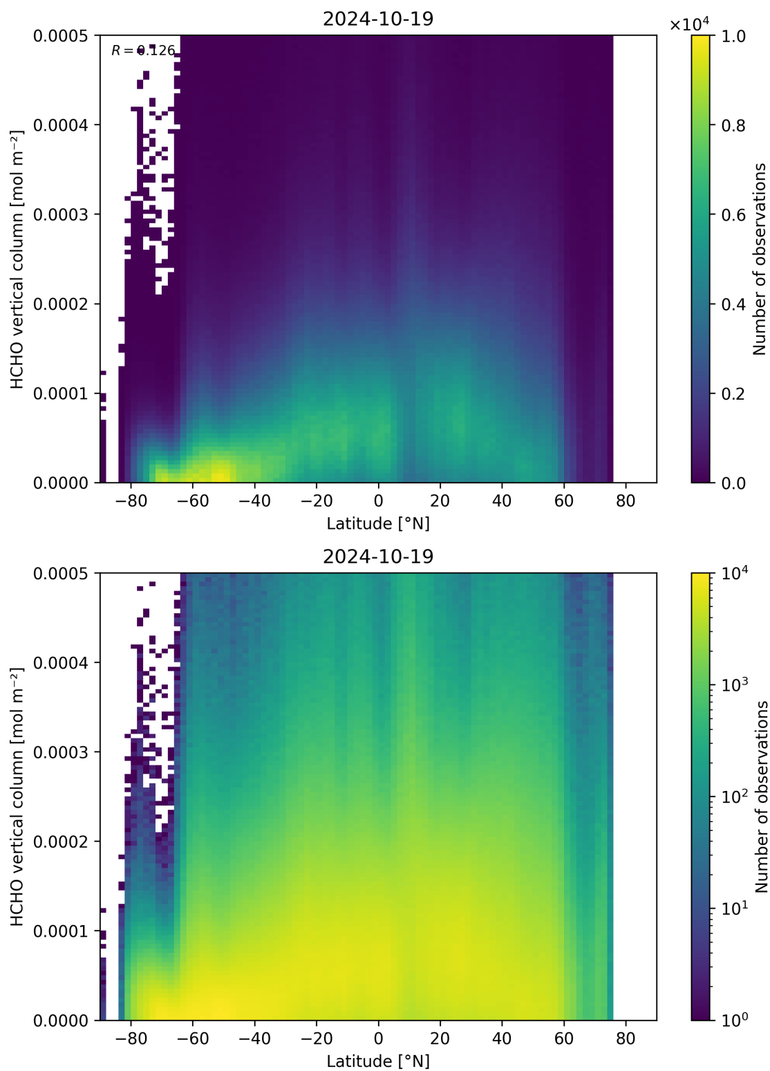
Figure 163: Scatter density plot of “Latitude” against “HCHO vertical column” for 2024-10-19 to 2024-10-20.
