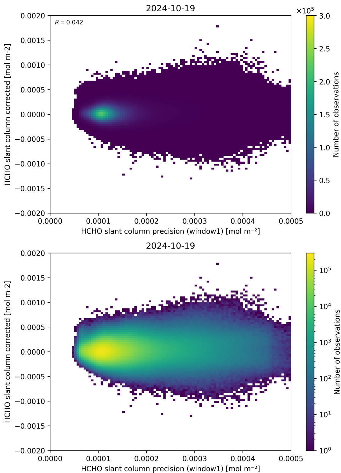
Figure 92: Scatter density plot of “HCHO slant column precision (window1)” against “HCHO slant column corrected” for 2024-10-19 to 2024-10-20.
