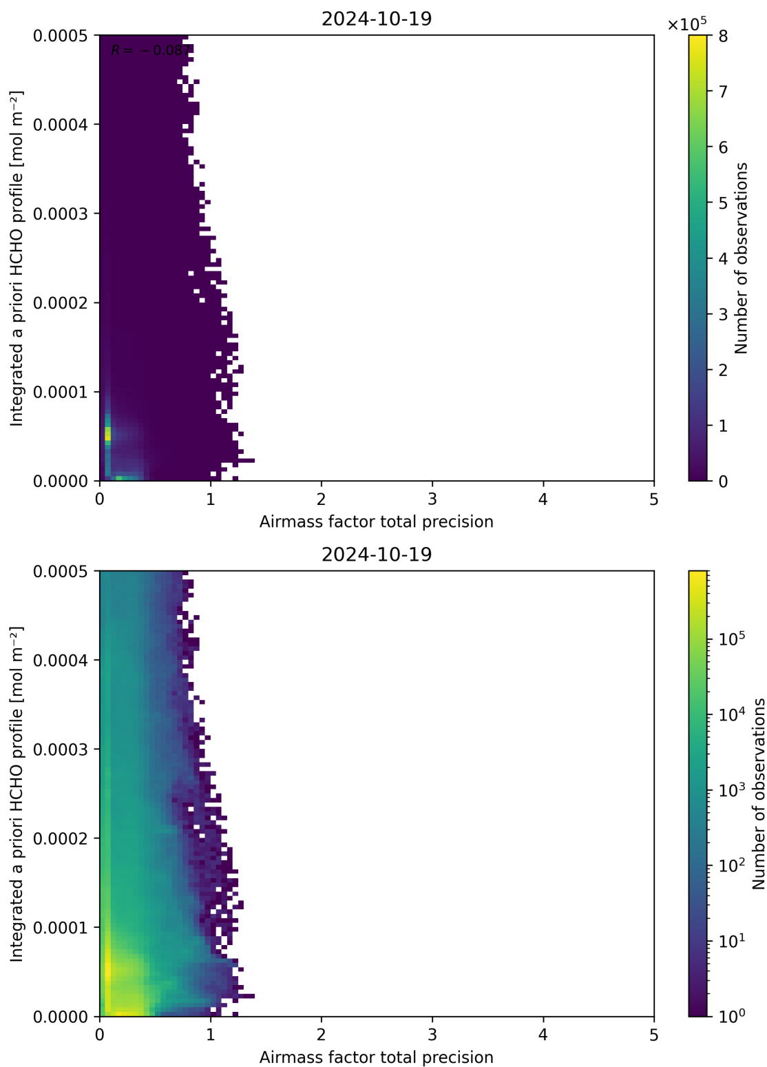
Figure 111: Scatter density plot of “Airmass factor total precision” against “Integrated a priori HCHO profile” for 2024-10-19 to 2024-10-20.
