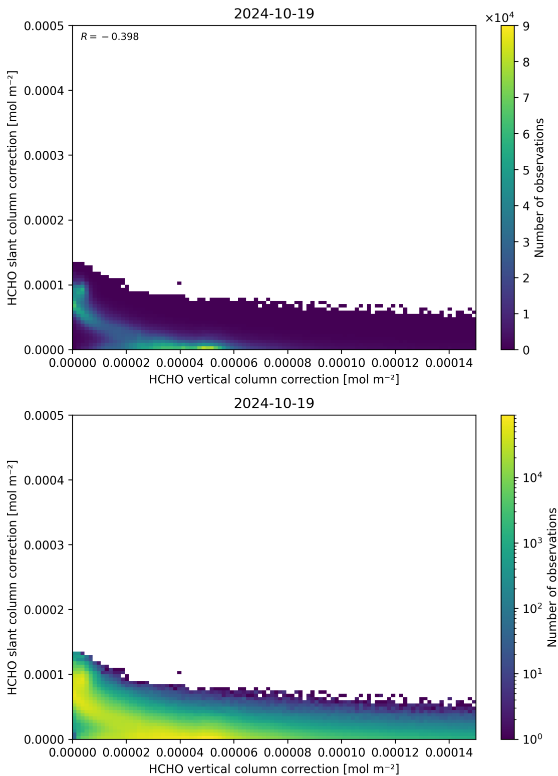
Figure 117: Scatter density plot of “HCHO vertical column correction” against “HCHO slant column correction” for 2024-10-19 to 2024-10-20.
