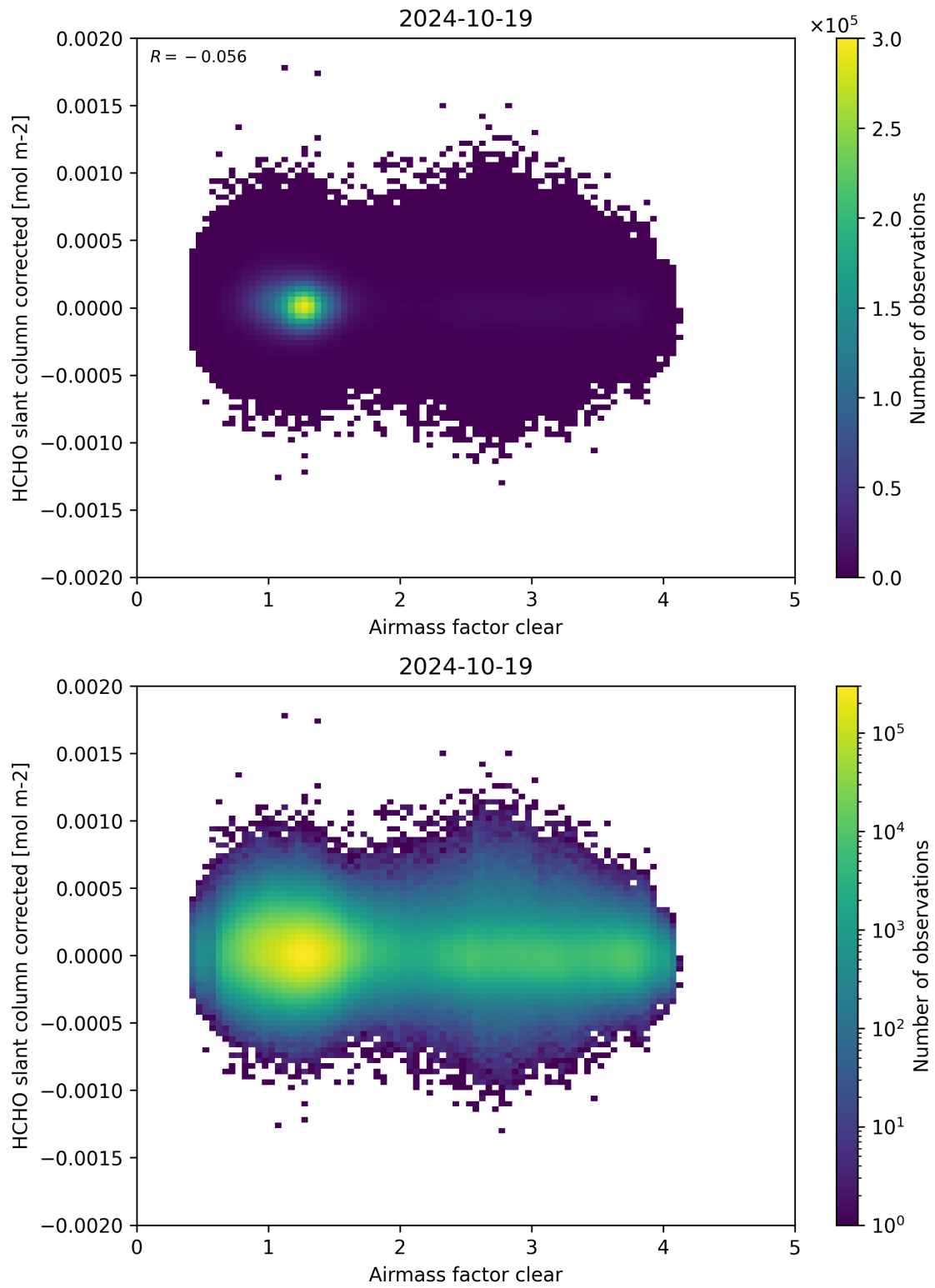
Figure 74: Scatter density plot of “Airmass factor clear” against “HCHO slant column corrected” for 2024-10-19 to 2024-10-20.
