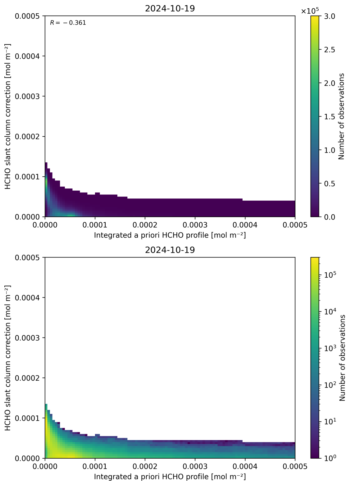
Figure 152: Scatter density plot of “Integrated a priori HCHO profile” against “HCHO slant column correction” for 2024-10-19 to 2024-10-20.
