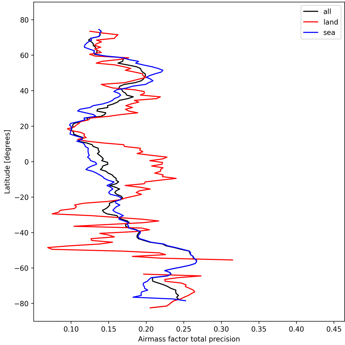
Figure 27: Zonal average of “Airmass factor total precision” for 2024-10-19 to 2024-10-20.
