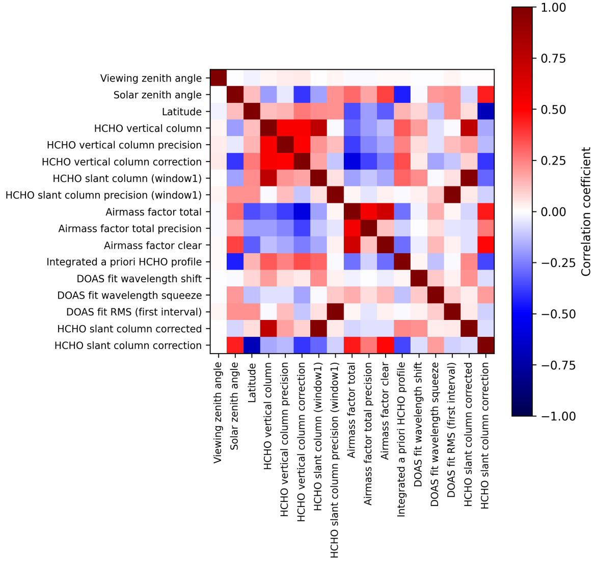
Figure 2: Map of correlation matrix for 2024-10-19 to 2024-10-20.
