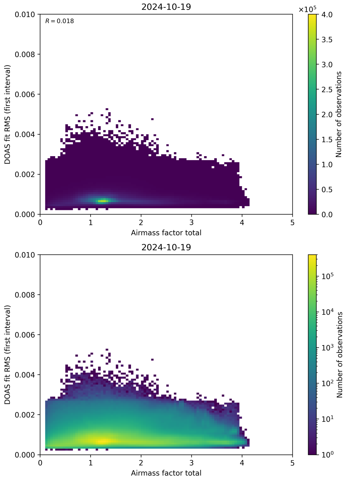
Figure 97: Scatter density plot of “Airmass factor total” against “DOAS fit RMS (first interval)” for 2024-10-19 to 2024-10-20.
