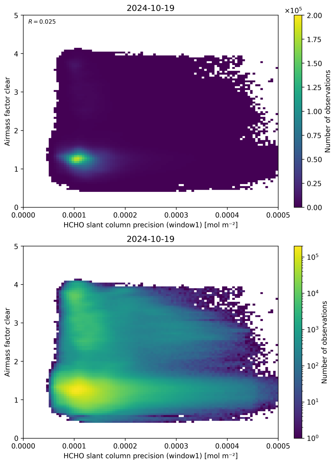
Figure 91: Scatter density plot of “HCHO slant column precision (window1)” against “Airmass factor clear” for 2024-10-19 to 2024-10-20.
