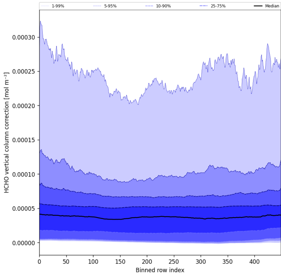
Figure 51: Along track statistics of “HCHO vertical column correction” for 2024-10-19 to 2024-10-20
