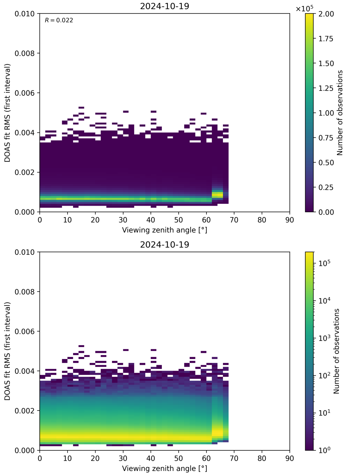
Figure 182: Scatter density plot of “Viewing zenith angle” against “DOAS fit RMS (first interval)” for 2024-10-19 to 2024-10-20.
