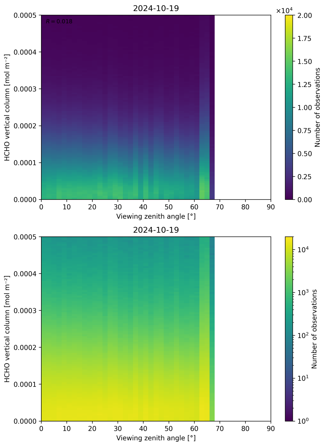
Figure 192: Scatter density plot of “Viewing zenith angle” against “HCHO vertical column” for 2024-10-19 to 2024-10-20.
