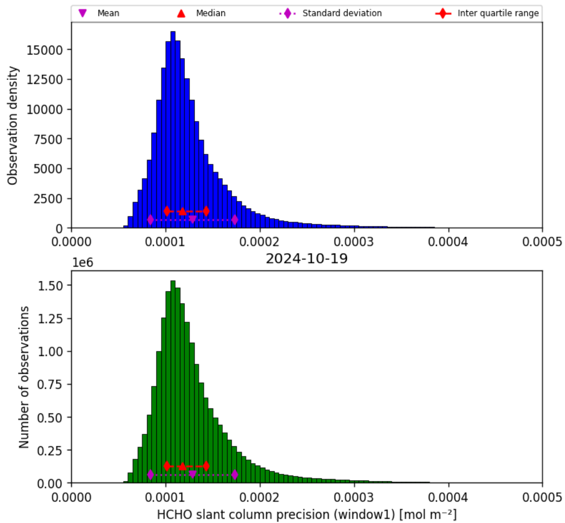
Figure 39: Histogram of “HCHO slant column precision (window1)” for 2024-10-19 to 2024-10-20
