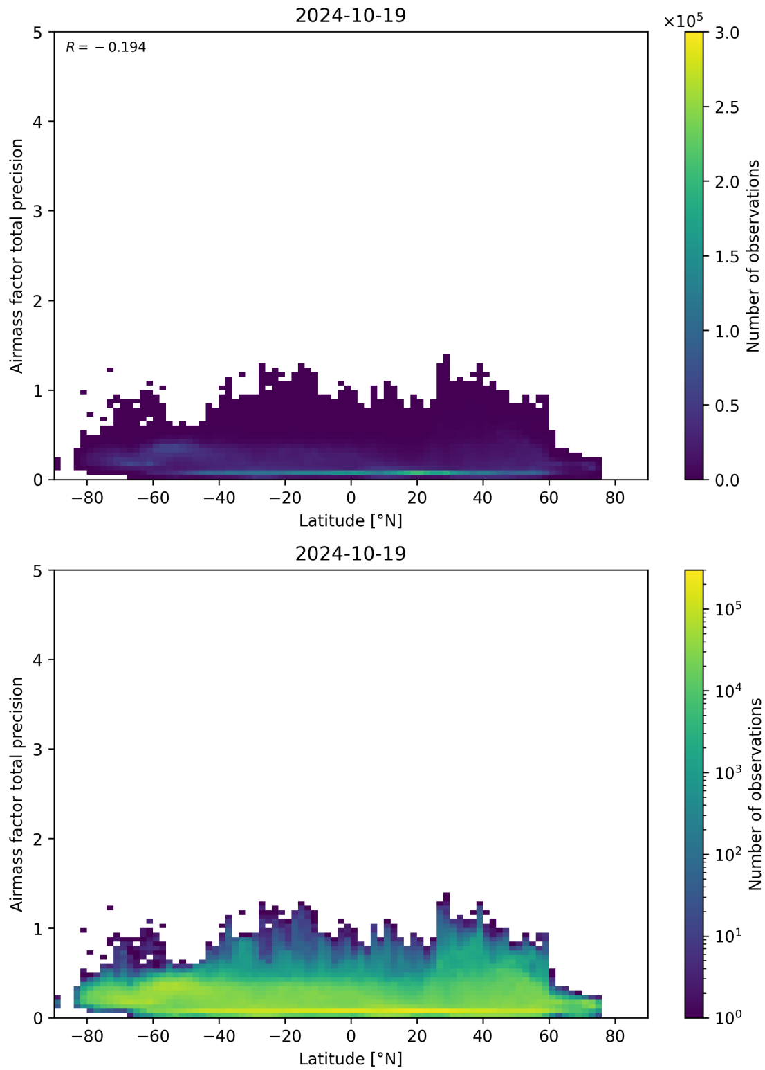
Figure 162: Scatter density plot of “Latitude” against “Airmass factor total precision” for 2024-10-19 to 2024-10-20.
