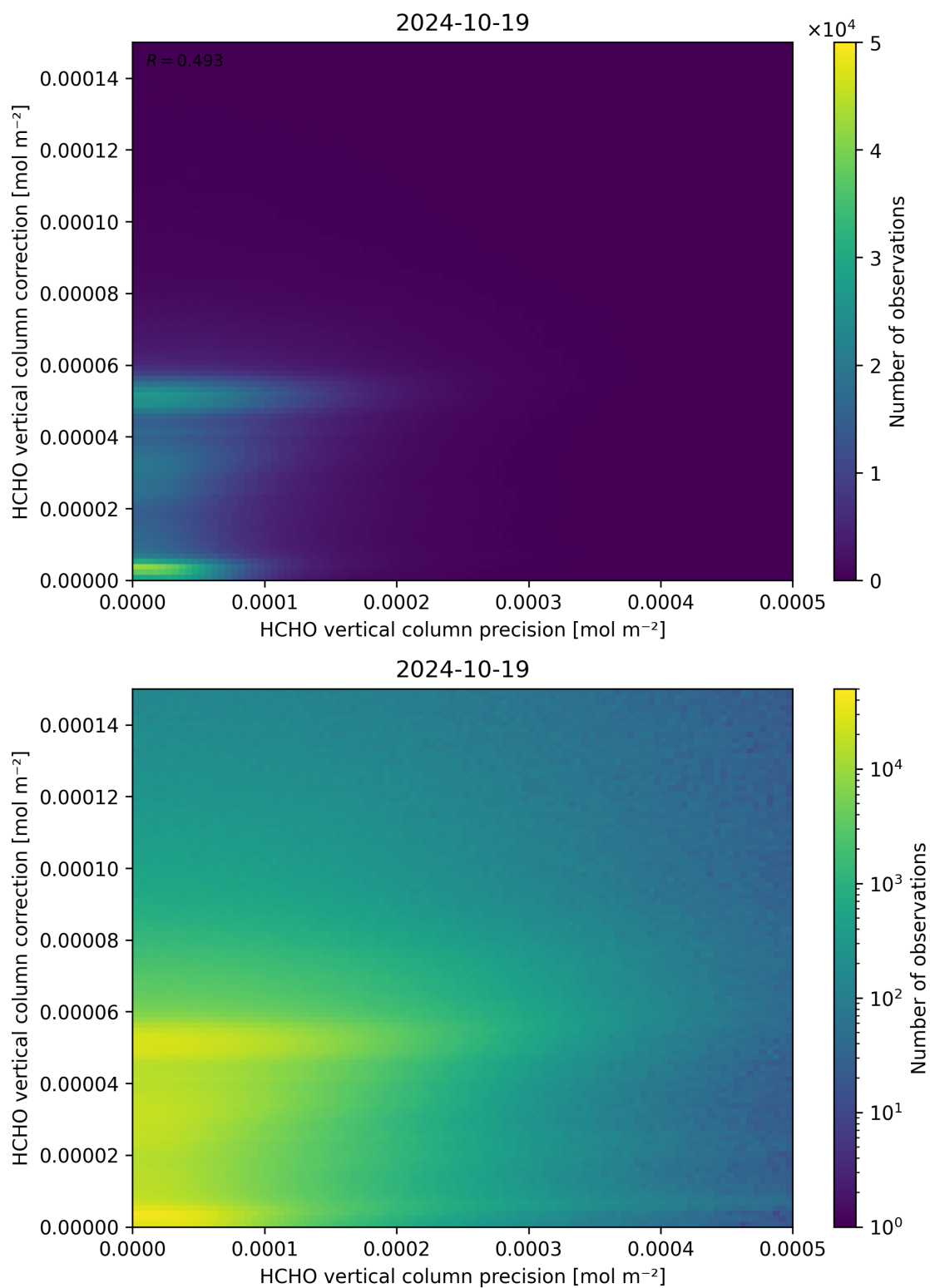
Figure 146: Scatter density plot of “HCHO vertical column precision” against “HCHO vertical column correction” for 2024-10-19 to 2024-10-20.
