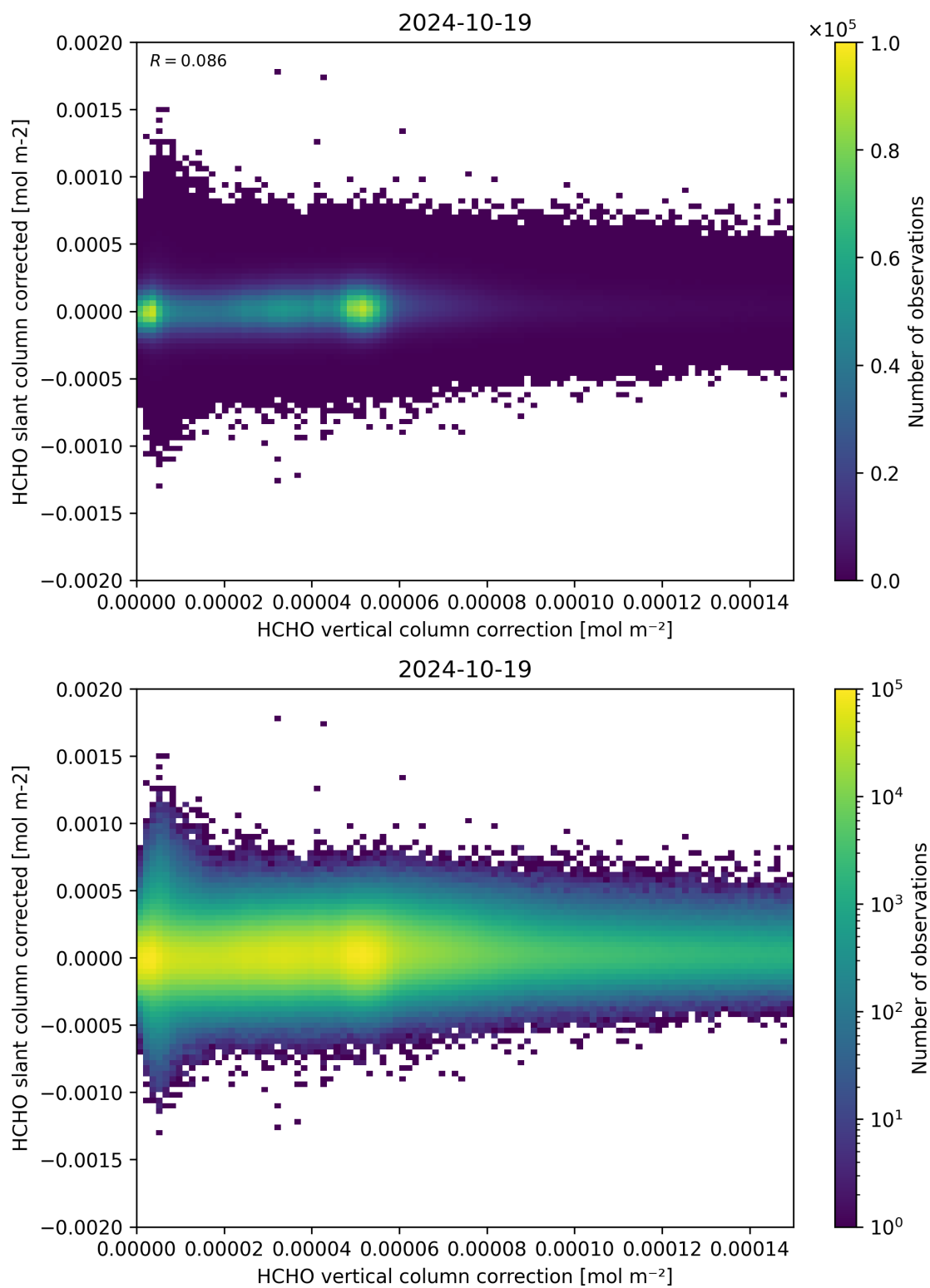
Figure 116: Scatter density plot of “HCHO vertical column correction” against “HCHO slant column corrected” for 2024-10-19 to 2024-10-20.
