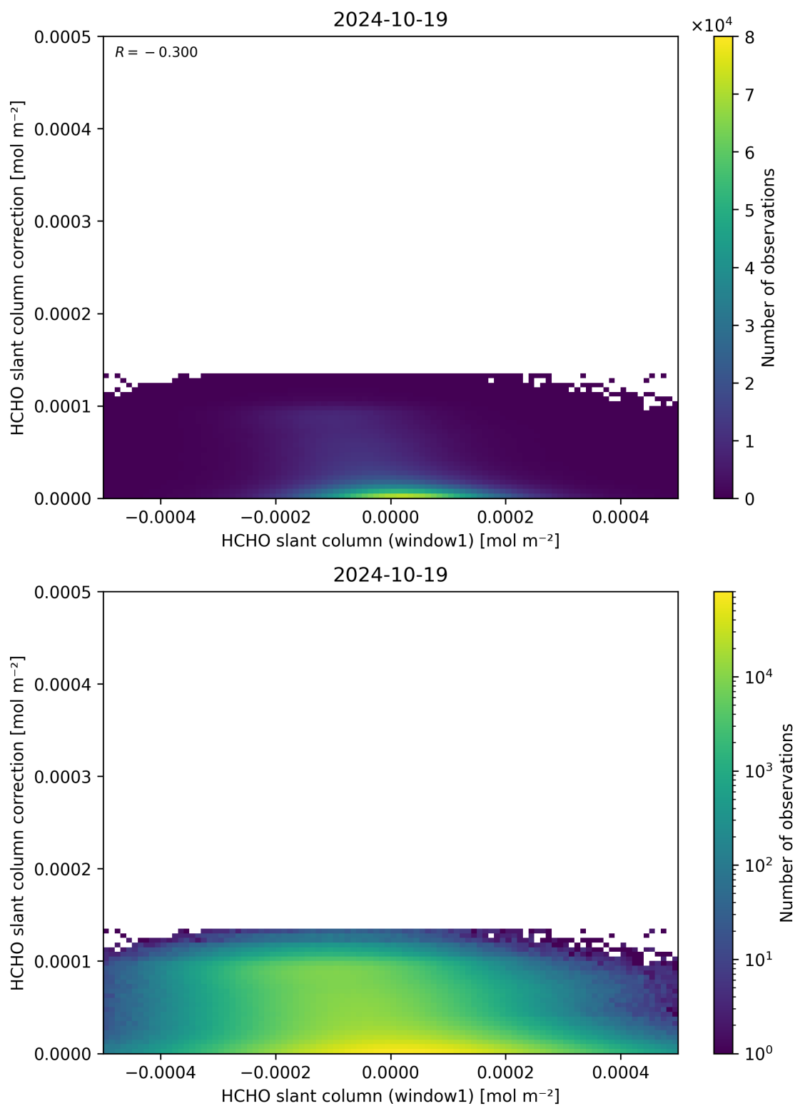
Figure 83: Scatter density plot of “HCHO slant column (window1)” against “HCHO slant column correction” for 2024-10-19 to 2024-10-20.
