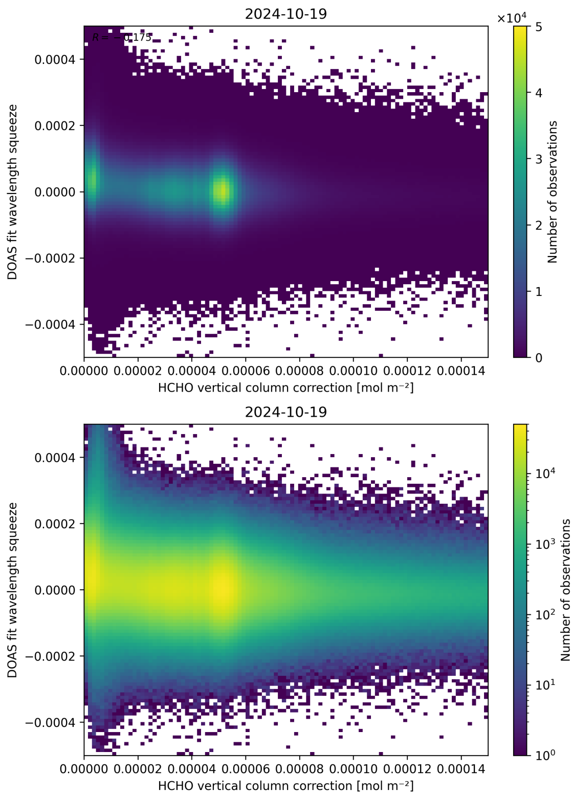
Figure 114: Scatter density plot of “HCHO vertical column correction” against “DOAS fit wavelength squeeze” for 2024-10-19 to 2024-10-20.
