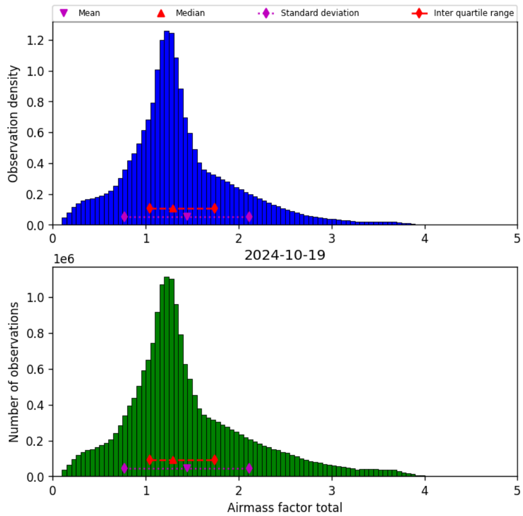
Figure 40: Histogram of “Airmass factor total” for 2024-10-19 to 2024-10-20
