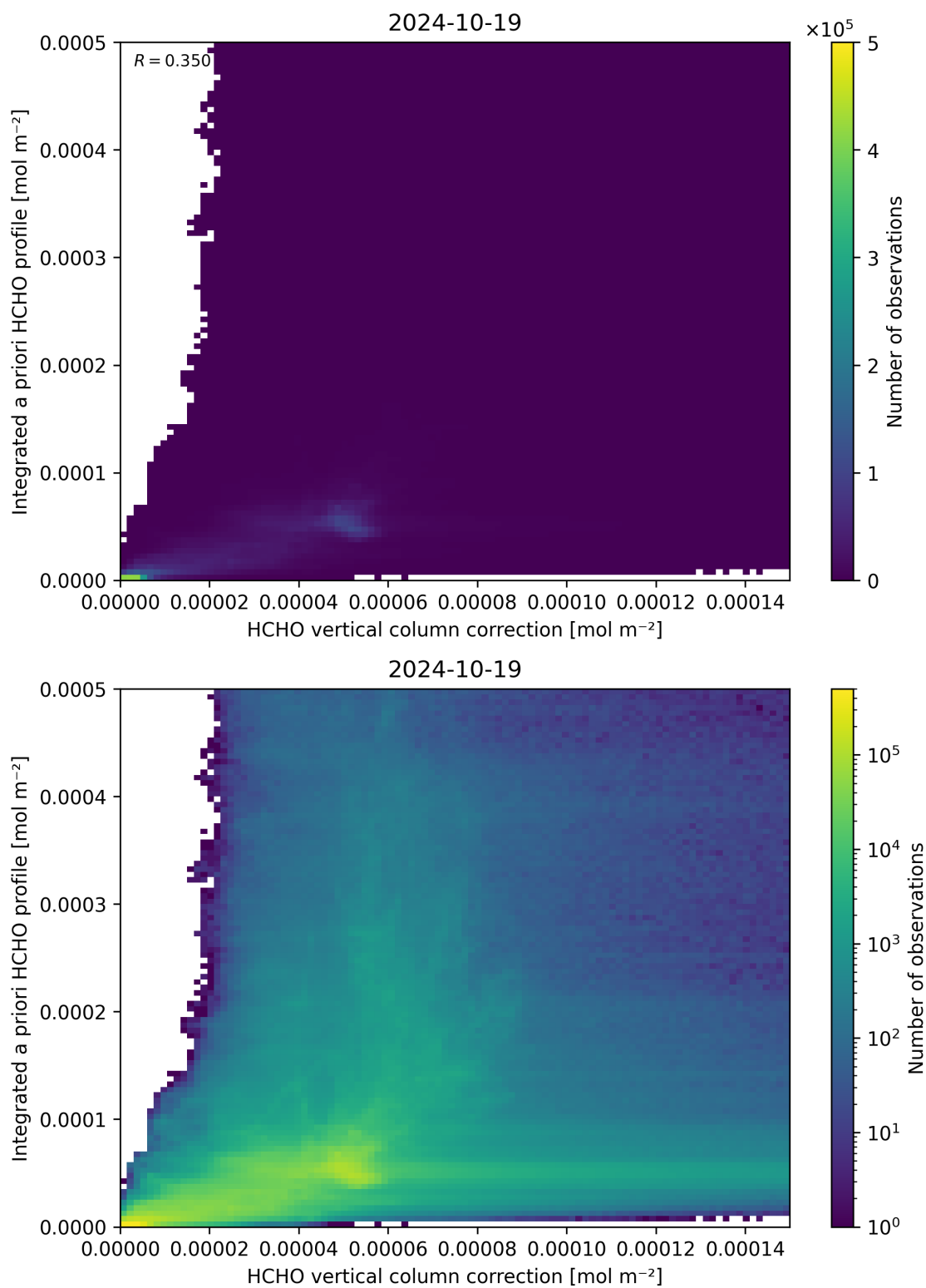
Figure 122: Scatter density plot of “HCHO vertical column correction” against “Integrated a priori HCHO profile” for 2024-10-19 to 2024-10-20.
