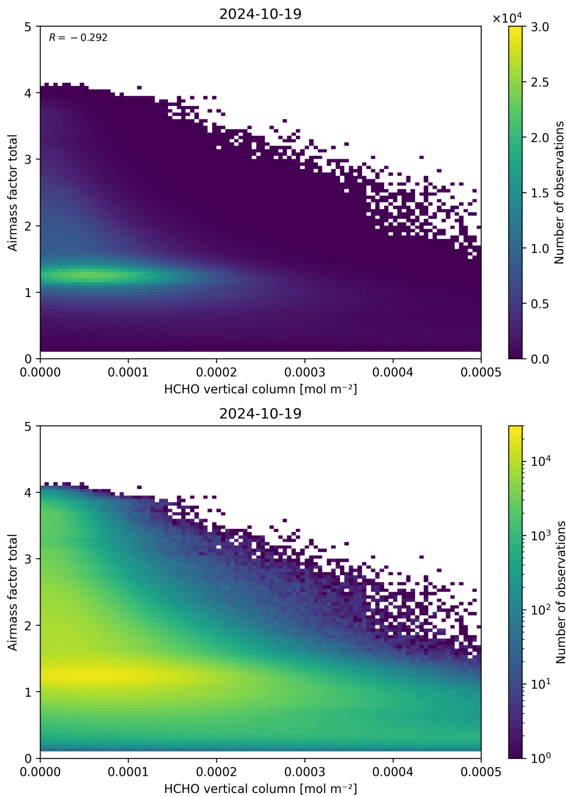
Figure 131: Scatter density plot of “HCHO vertical column” against “Airmass factor total” for 2024-10-19 to 2024-10-20.
