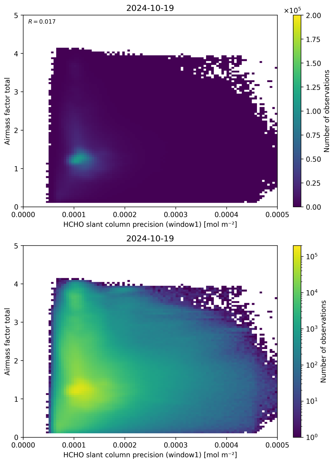
Figure 94: Scatter density plot of “HCHO slant column precision (window1)” against “Airmass factor total” for 2024-10-19 to 2024-10-20.
