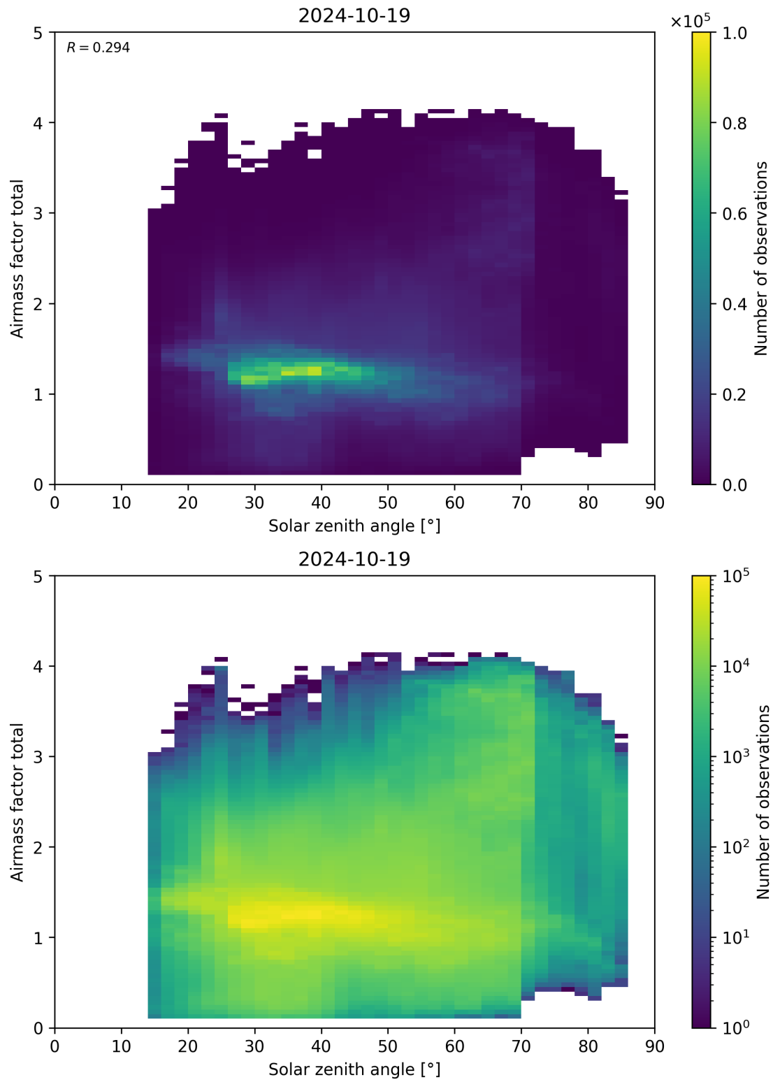
Figure 175: Scatter density plot of “Solar zenith angle” against “Airmass factor total” for 2024-10-19 to 2024-10-20.
