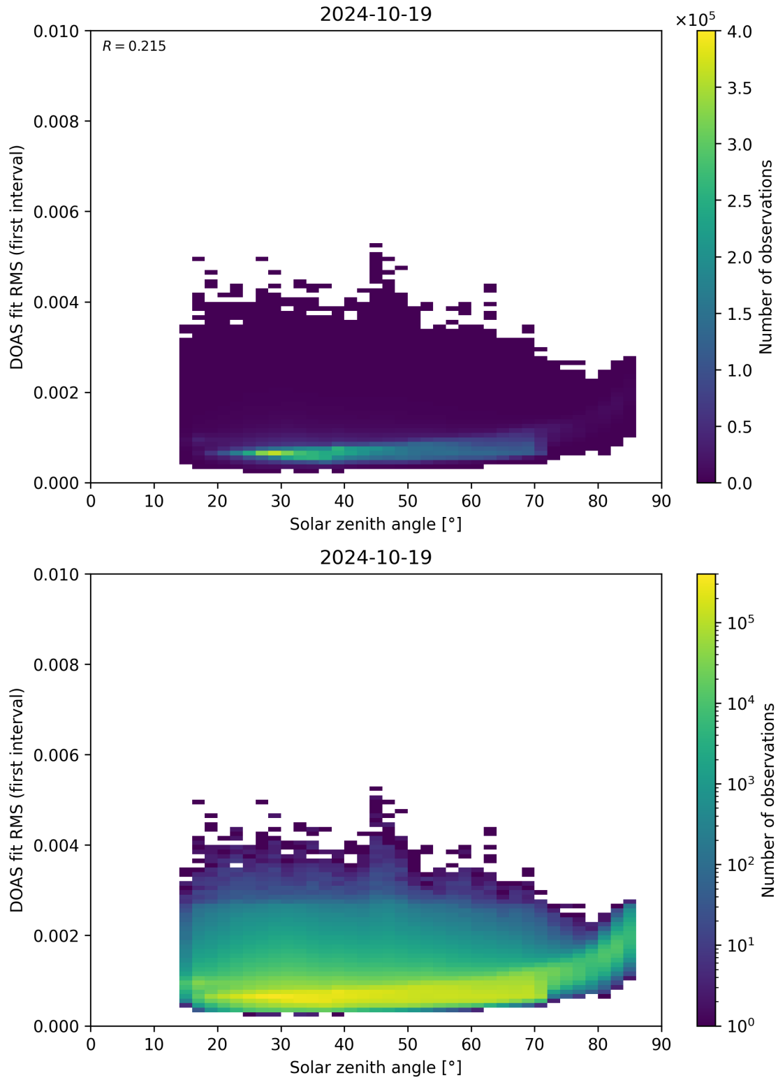
Figure 167: Scatter density plot of “Solar zenith angle” against “DOAS fit RMS (first interval)” for 2024-10-19 to 2024-10-20.
