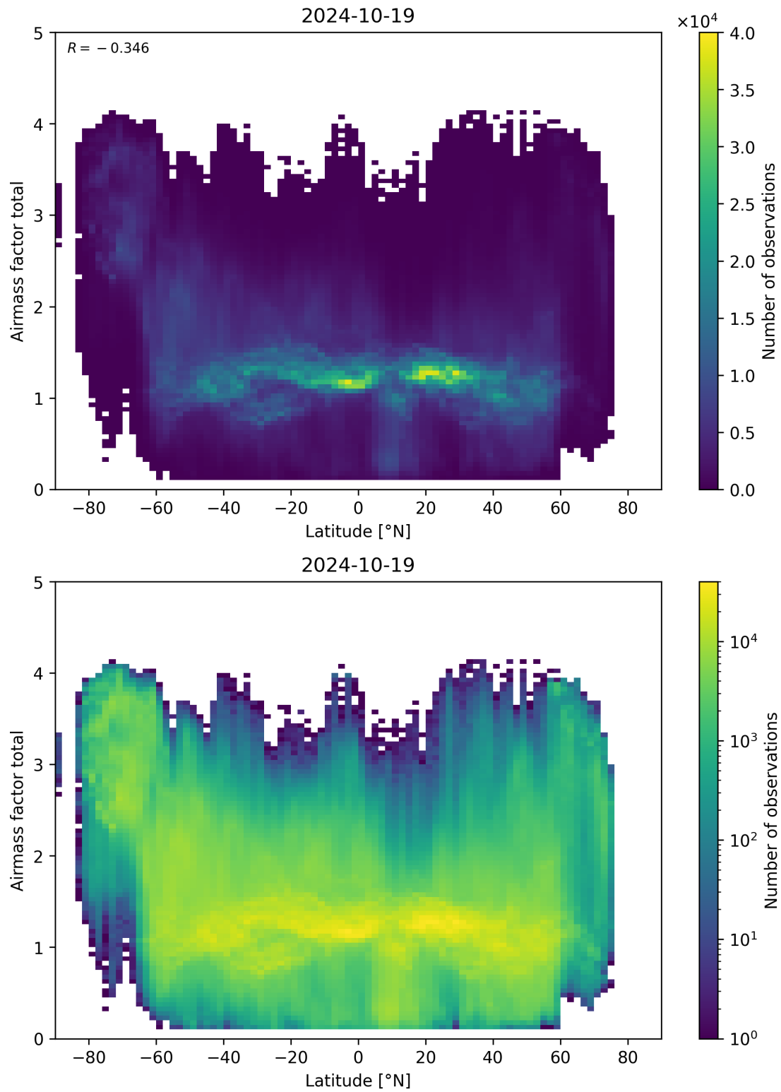
Figure 161: Scatter density plot of “Latitude” against “Airmass factor total” for 2024-10-19 to 2024-10-20.
