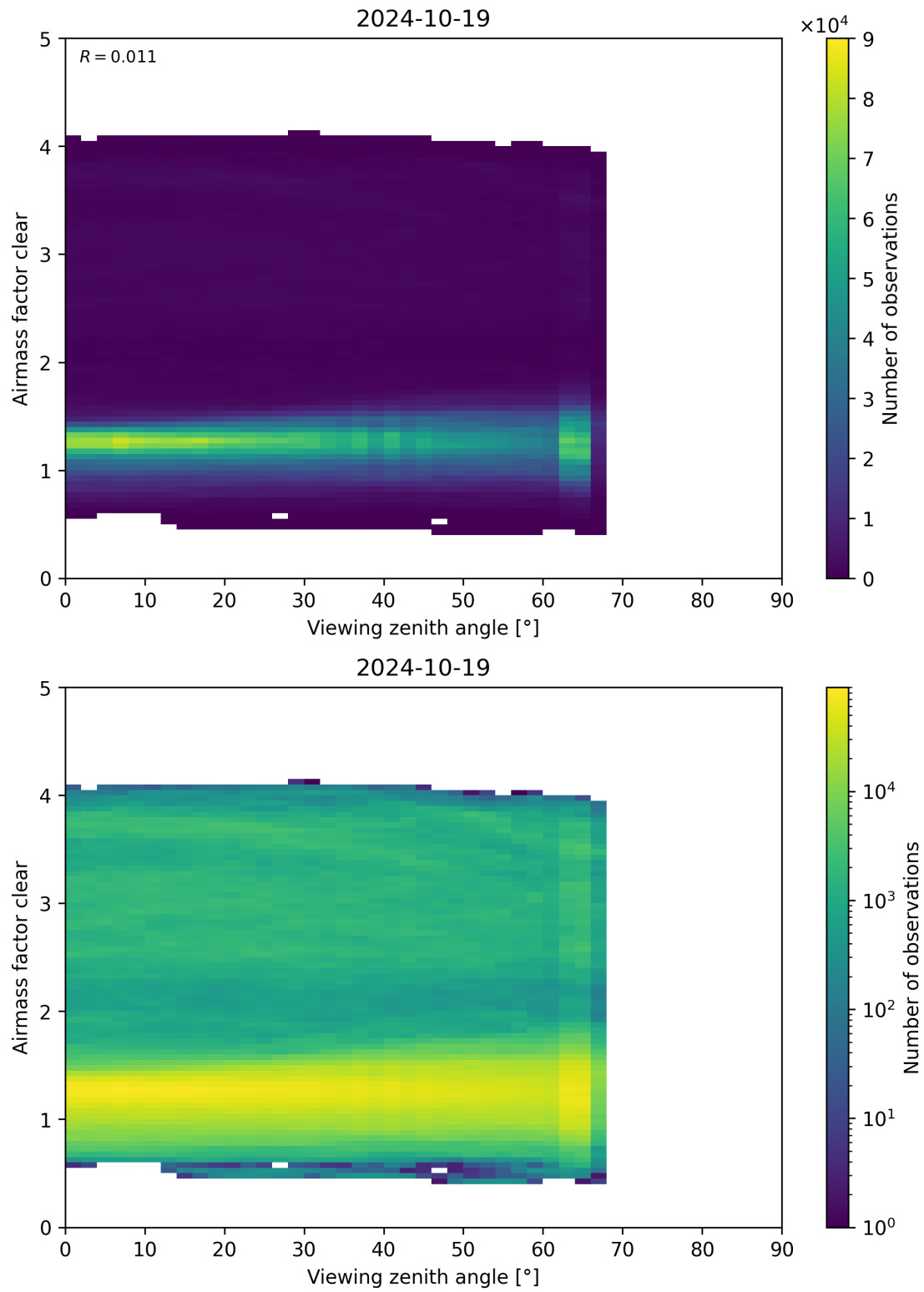
Figure 185: Scatter density plot of “Viewing zenith angle” against “Airmass factor clear” for 2024-10-19 to 2024-10-20.
