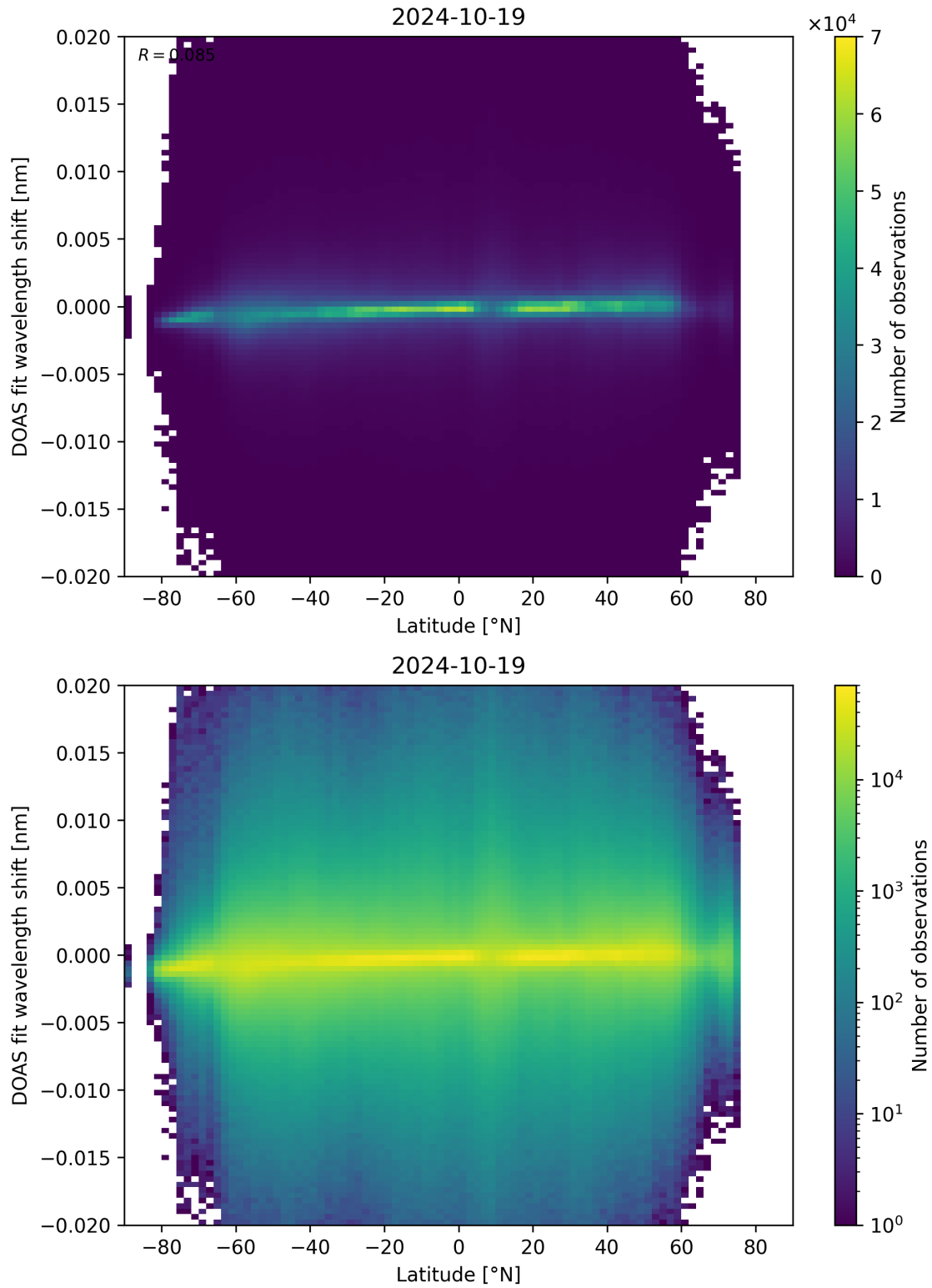
Figure 154: Scatter density plot of “Latitude” against “DOAS fit wavelength shift” for 2024-10-19 to 2024-10-20.
