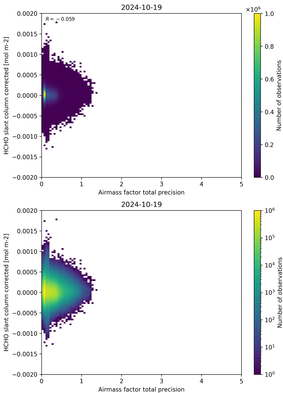
Figure 109: Scatter density plot of “Airmass factor total precision” against “HCHO slant column corrected” for 2024-10-19 to 2024-10-20.
