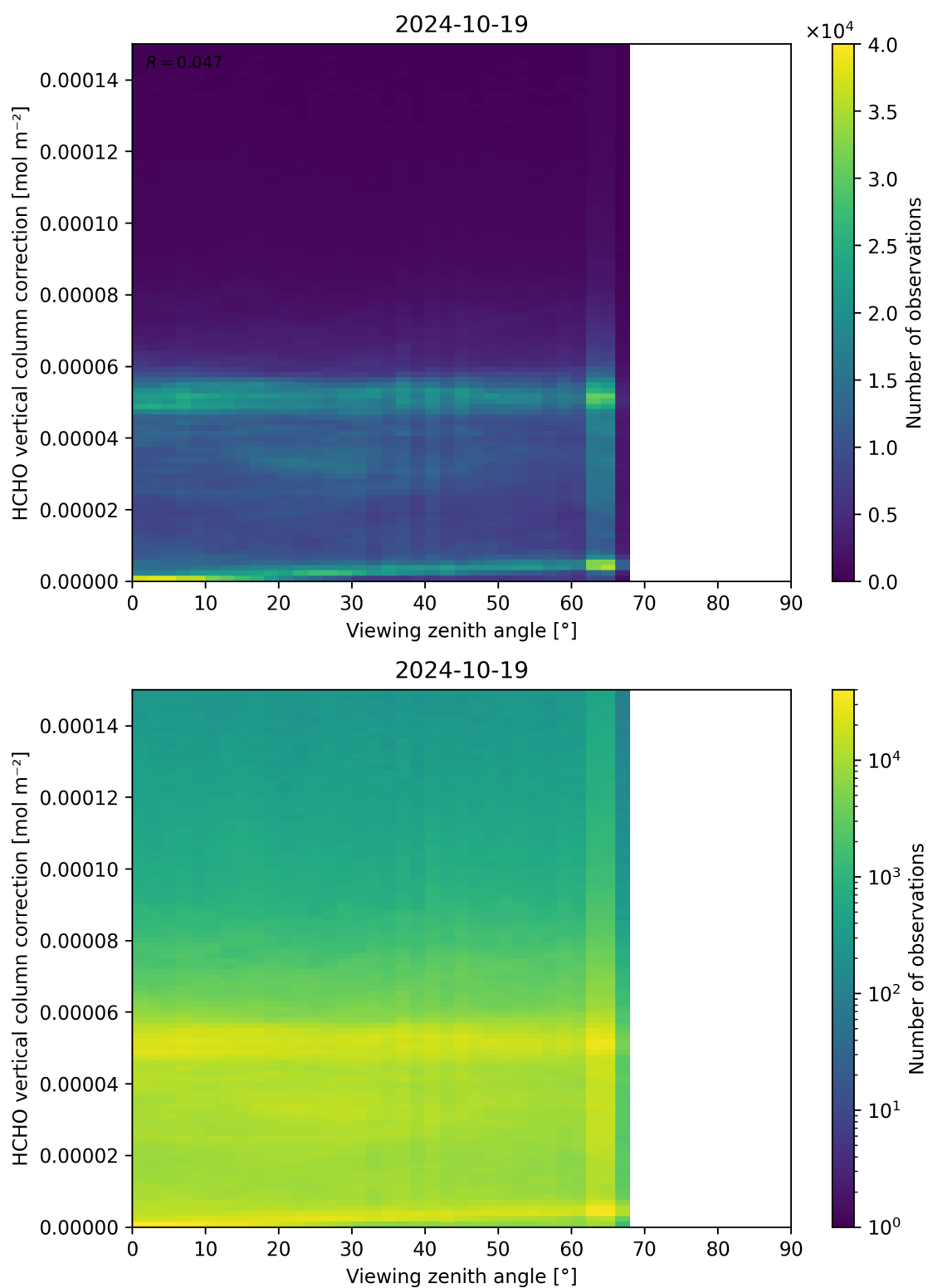
Figure 193: Scatter density plot of “Viewing zenith angle” against “HCHO vertical column correction” for 2024-10-19 to 2024-10-20.
