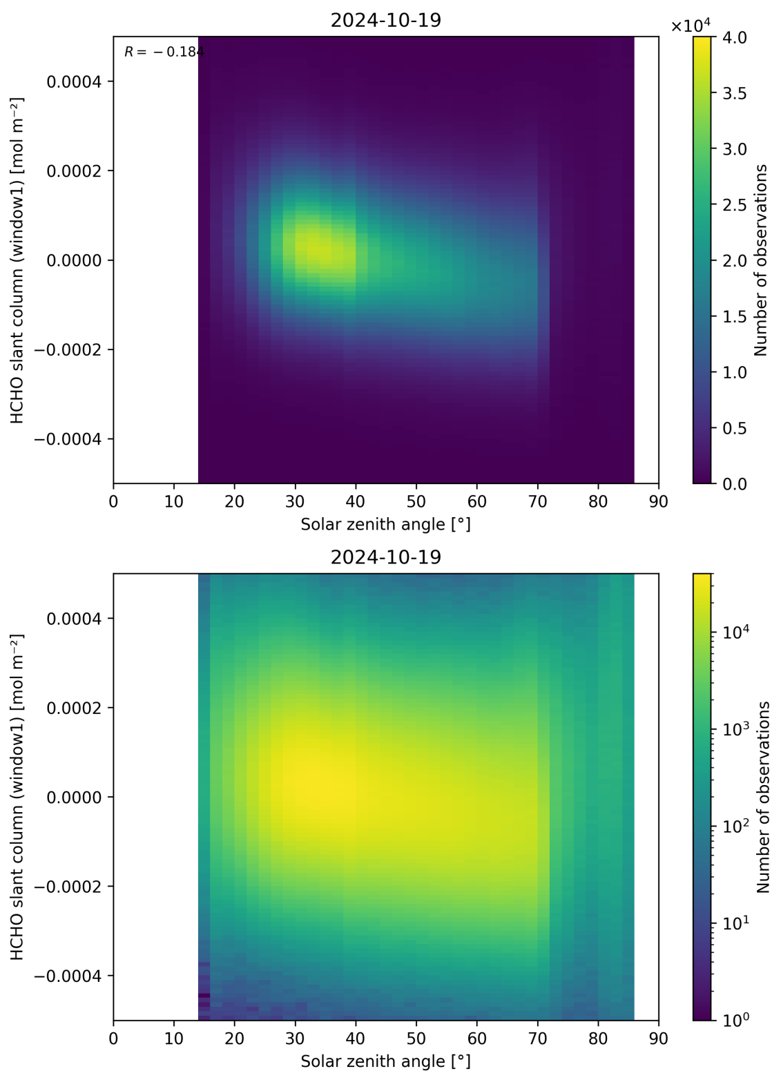
Figure 173: Scatter density plot of “Solar zenith angle” against “HCHO slant column (window1)” for 2024-10-19 to 2024-10-20.
