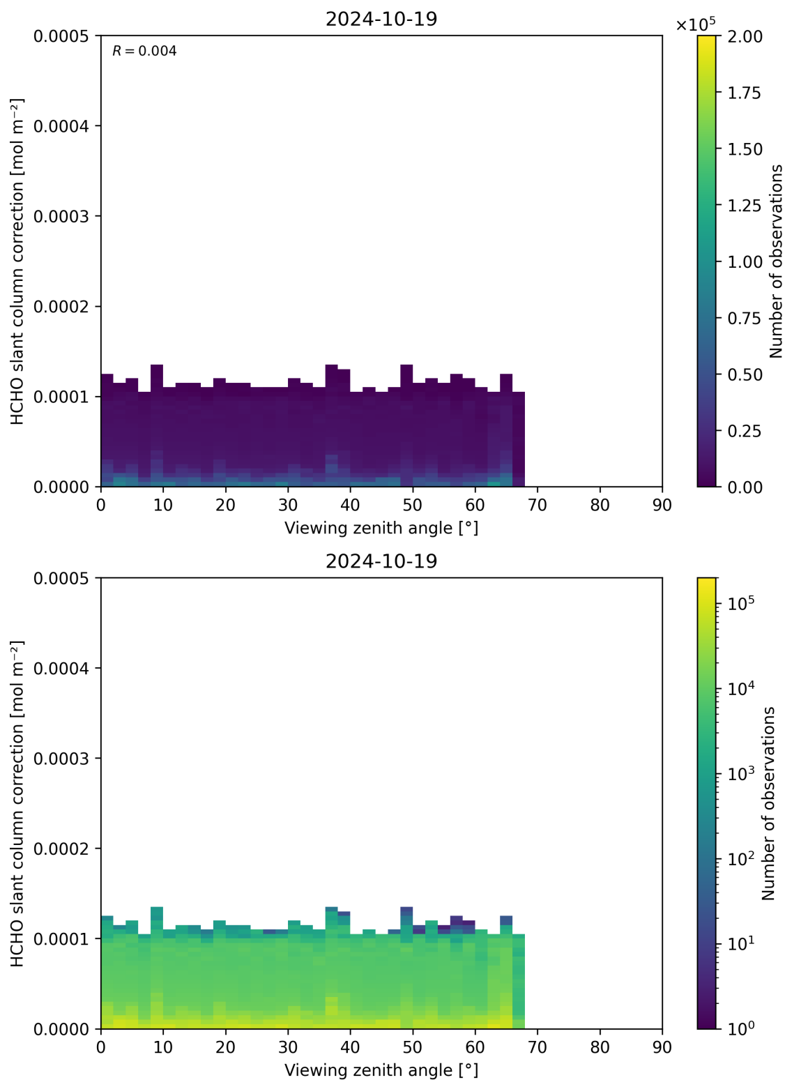
Figure 187: Scatter density plot of “Viewing zenith angle” against “HCHO slant column correction” for 2024-10-19 to 2024-10-20.
