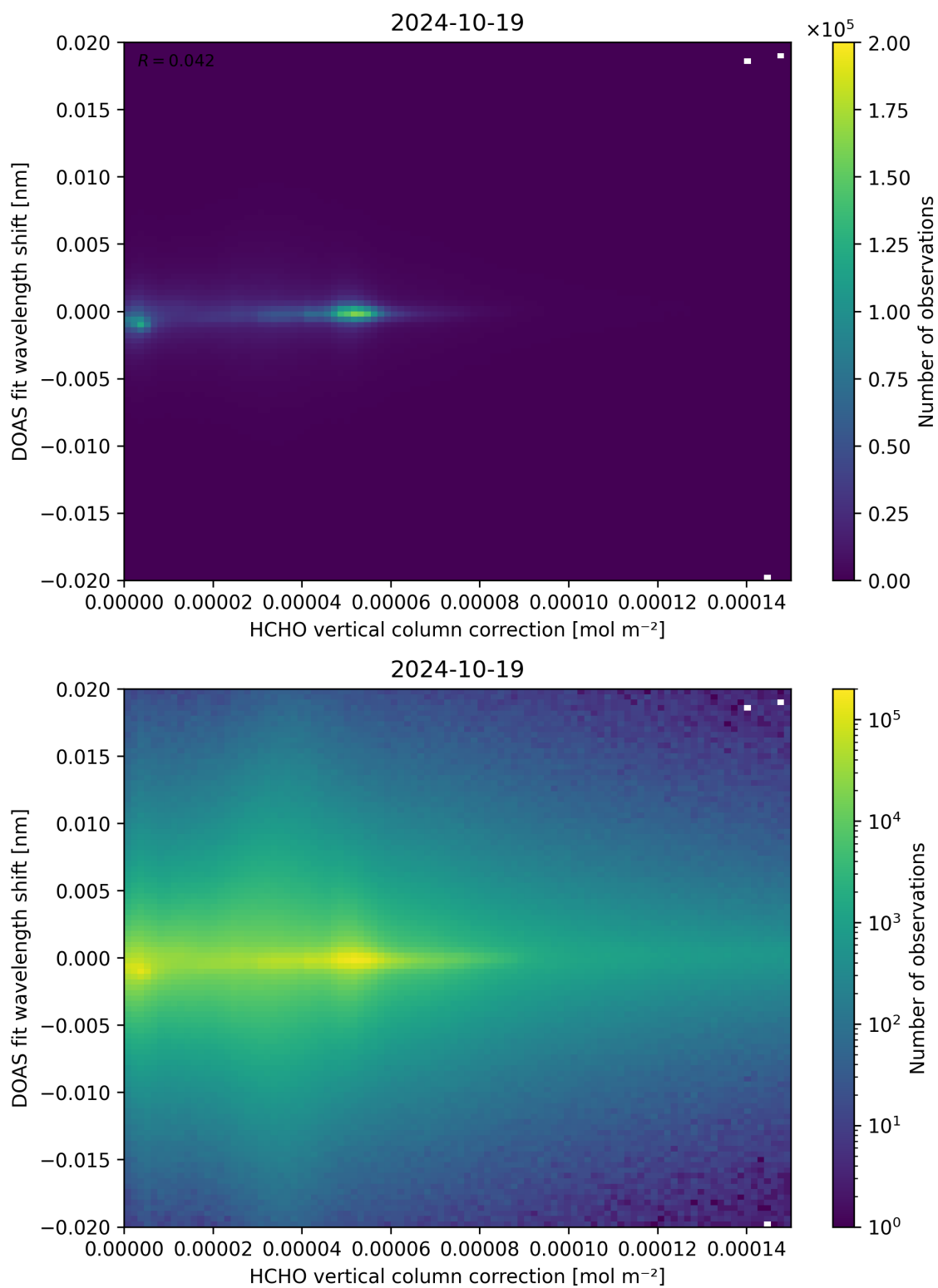
Figure 113: Scatter density plot of “HCHO vertical column correction” against “DOAS fit wavelength shift” for 2024-10-19 to 2024-10-20.
