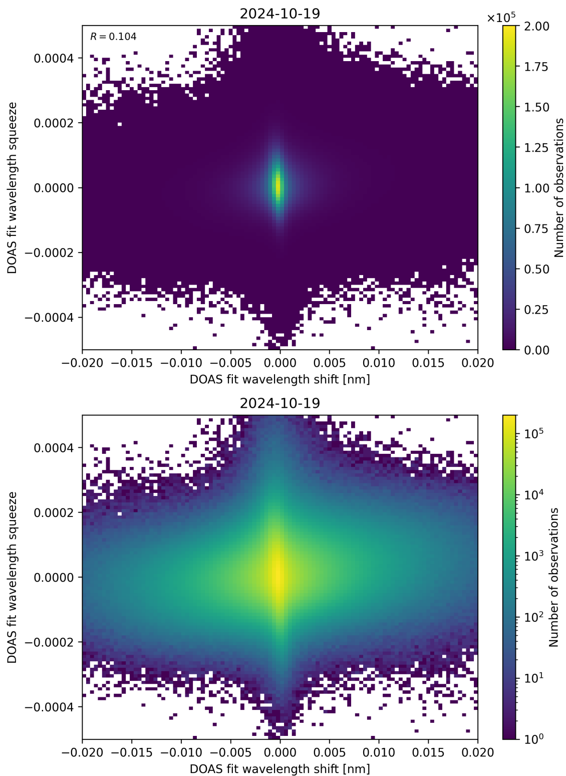
Figure 65: Scatter density plot of “DOAS fit wavelength shift” against “DOAS fit wavelength squeeze” for 2024-10-19 to 2024-10-20.
