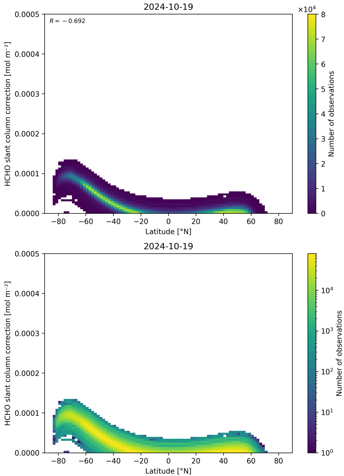
Figure 158: Scatter density plot of “Latitude” against “HCHO slant column correction” for 2024-10-19 to 2024-10-20.
