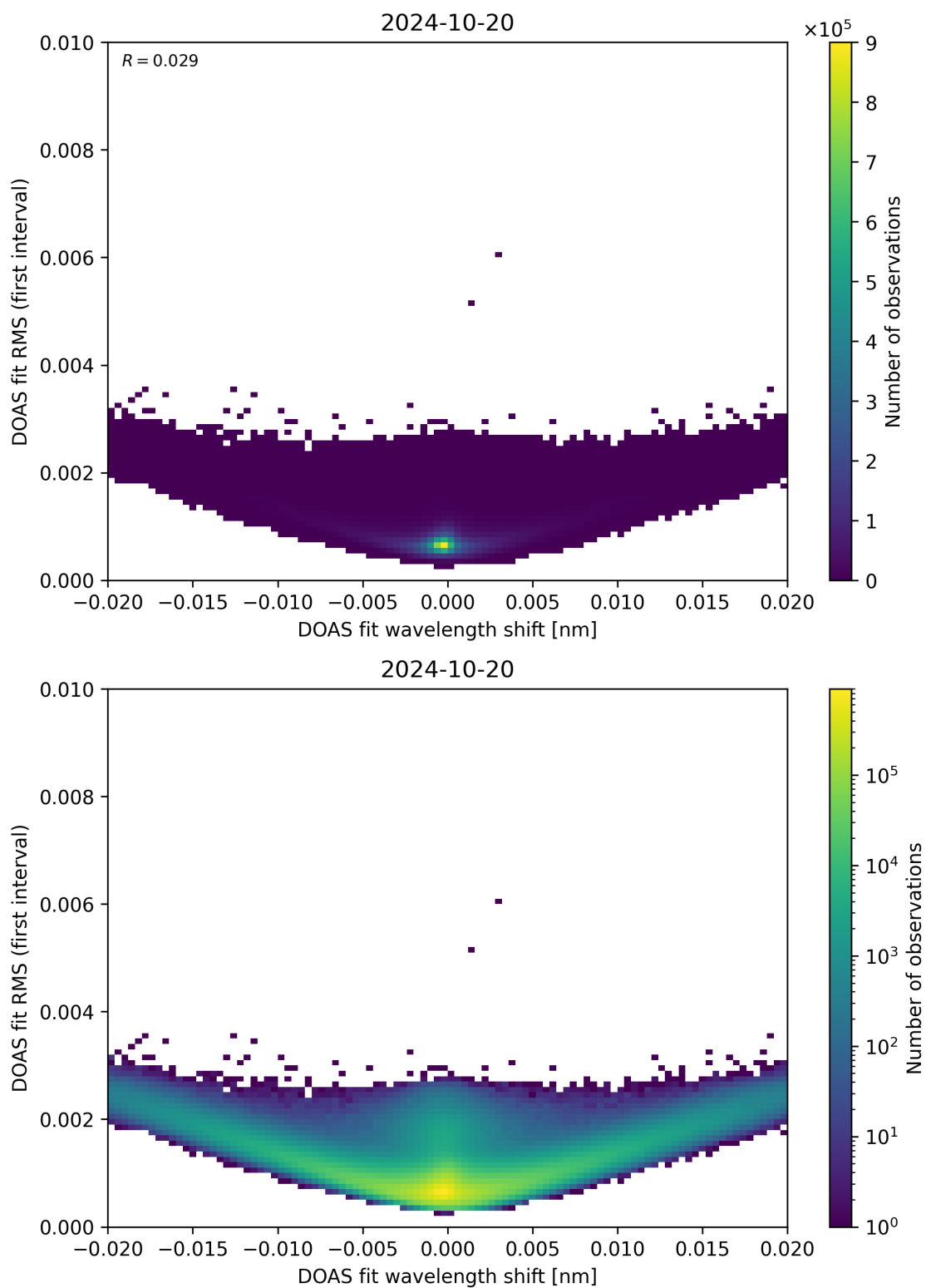
Figure 64: Scatter density plot of “DOAS fit wavelength shift” against “DOAS fit RMS (first interval)” for 2024-10-19 to 2024-10-21.
