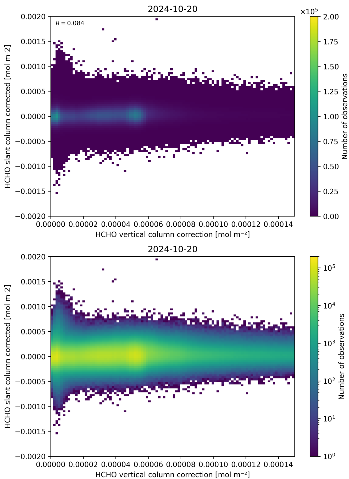
Figure 116: Scatter density plot of “HCHO vertical column correction” against “HCHO slant column corrected” for 2024-10-19 to 2024-10-21.
