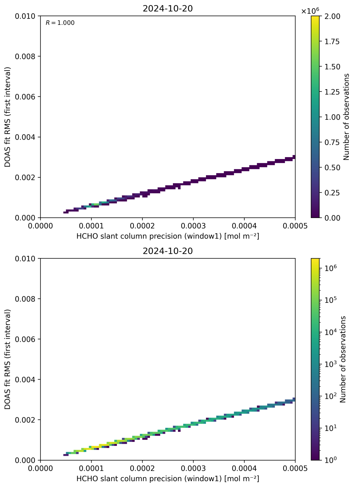
Figure 88: Scatter density plot of “HCHO slant column precision (window1)” against “DOAS fit RMS (first interval)” for 2024-10-19 to 2024-10-21.
