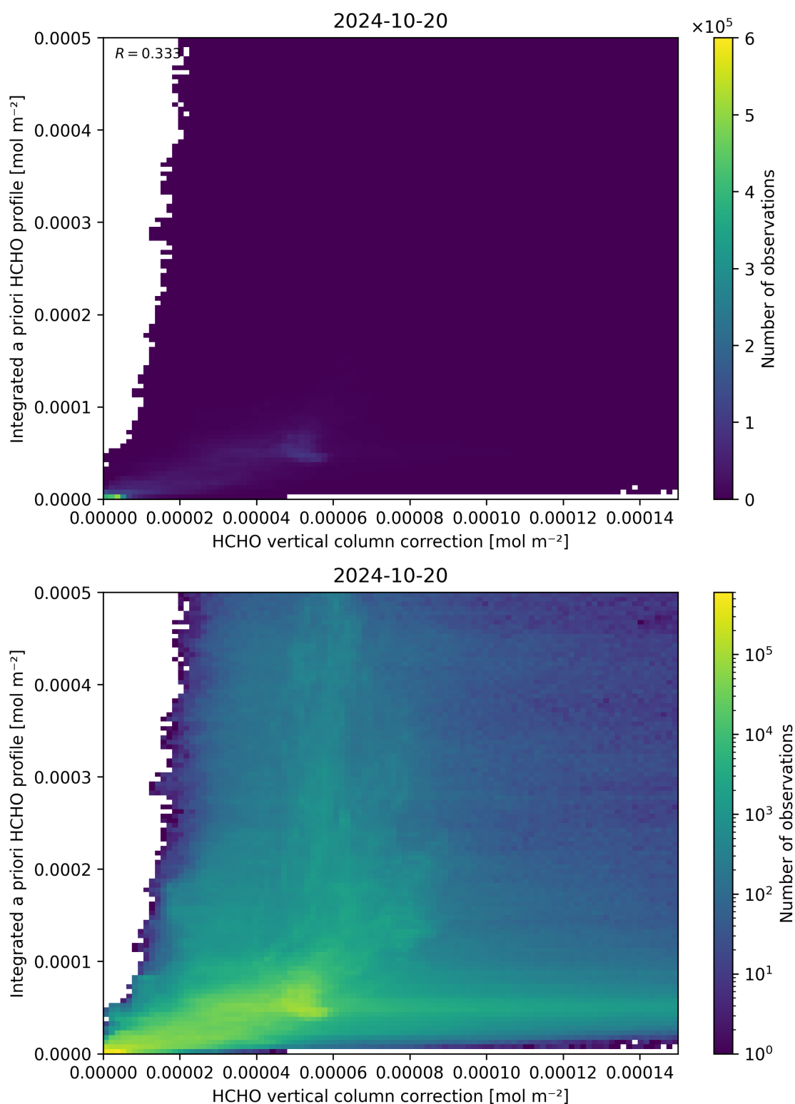
Figure 122: Scatter density plot of “HCHO vertical column correction” against “Integrated a priori HCHO profile” for 2024-10-19 to 2024-10-21.
