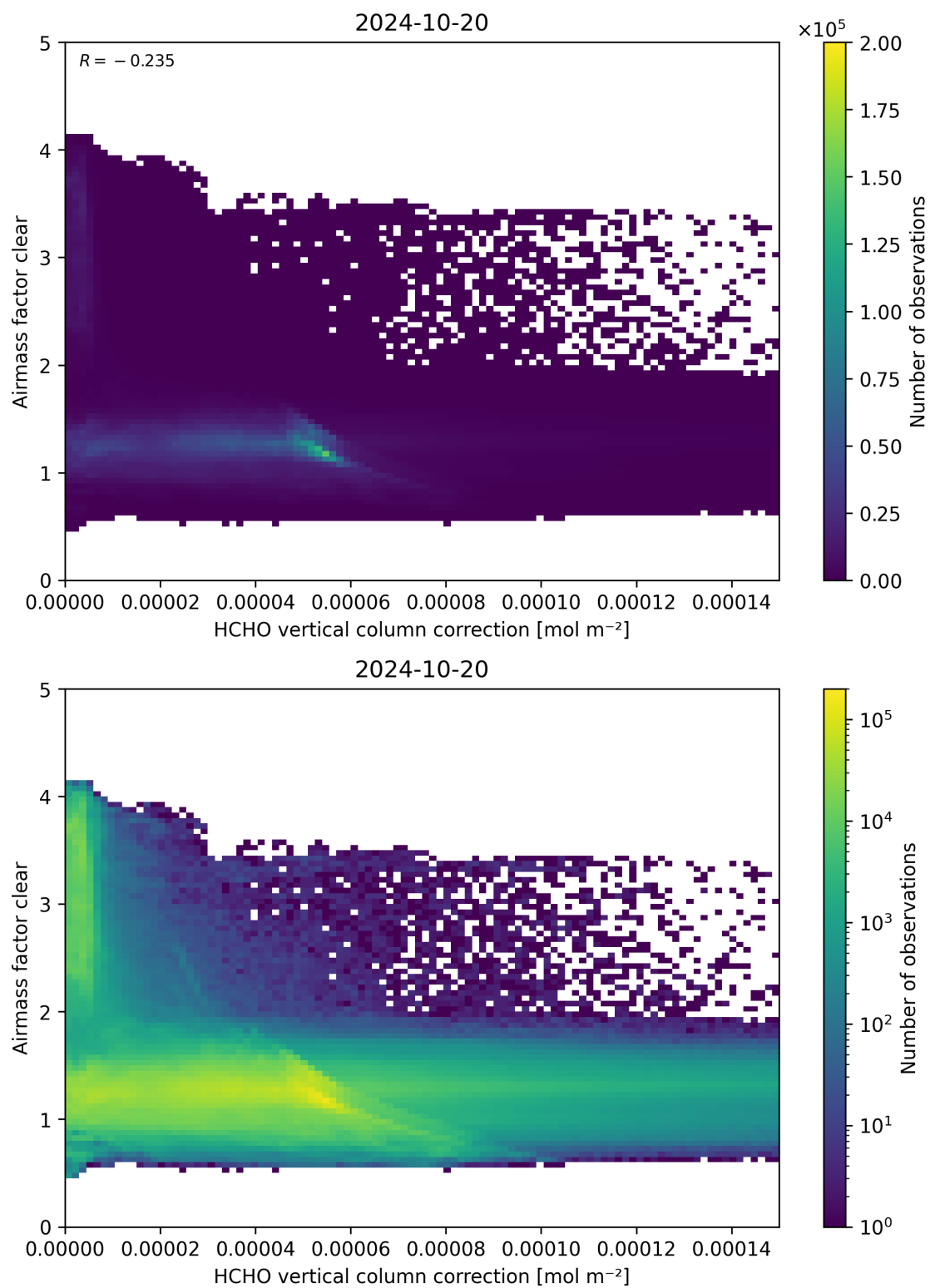
Figure 115: Scatter density plot of “HCHO vertical column correction” against “Airmass factor clear” for 2024-10-19 to 2024-10-21.
