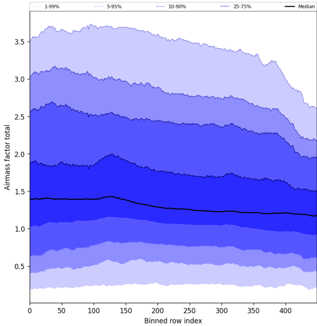
Figure 54: Along track statistics of “Airmass factor total” for 2024-10-19 to 2024-10-21
