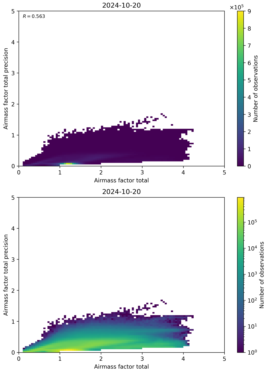
Figure 103: Scatter density plot of “Airmass factor total” against “Airmass factor total precision” for 2024-10-19 to 2024-10-21.
