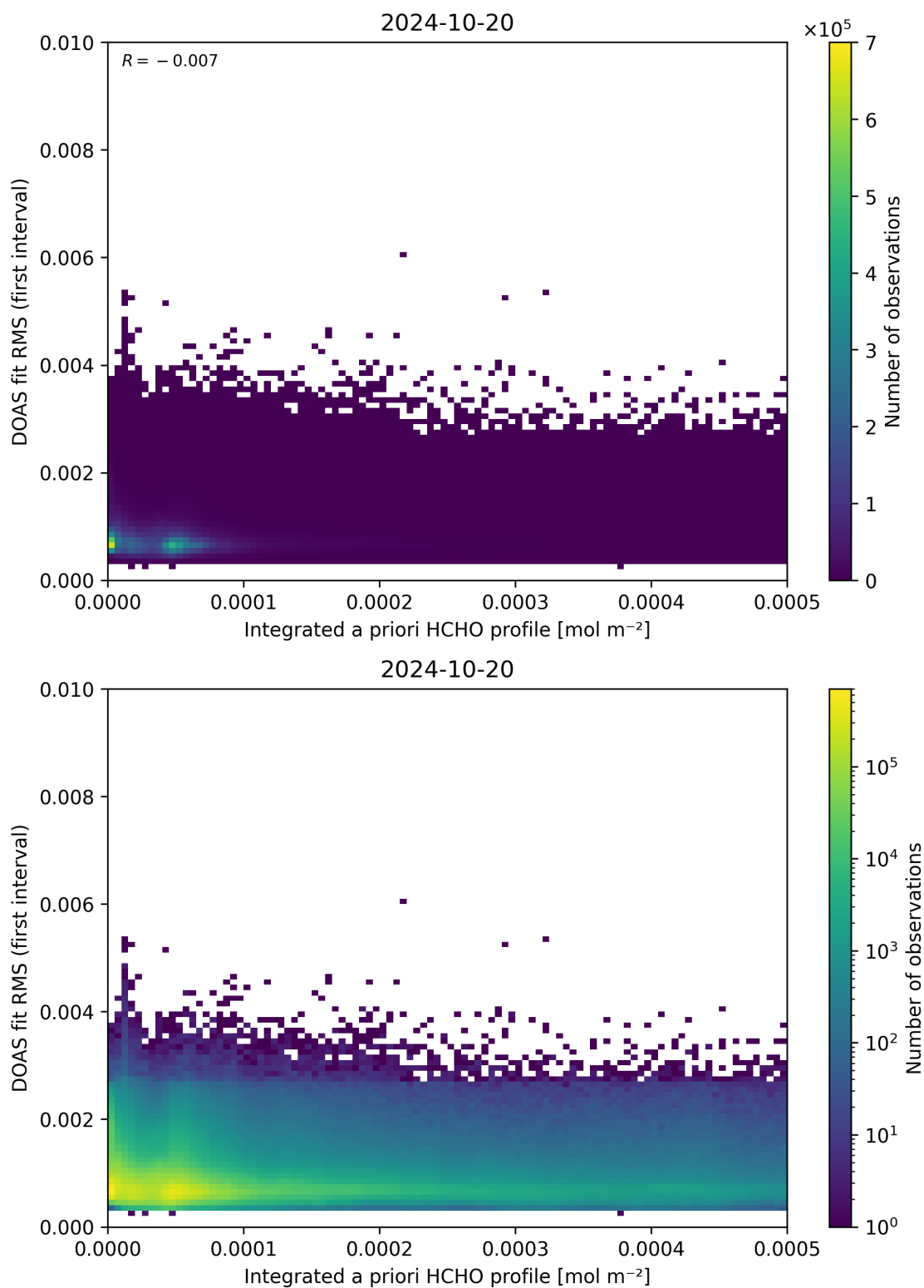
Figure 148: Scatter density plot of “Integrated a priori HCHO profile” against “DOAS fit RMS (first interval)” for 2024-10-19 to 2024-10-21.
