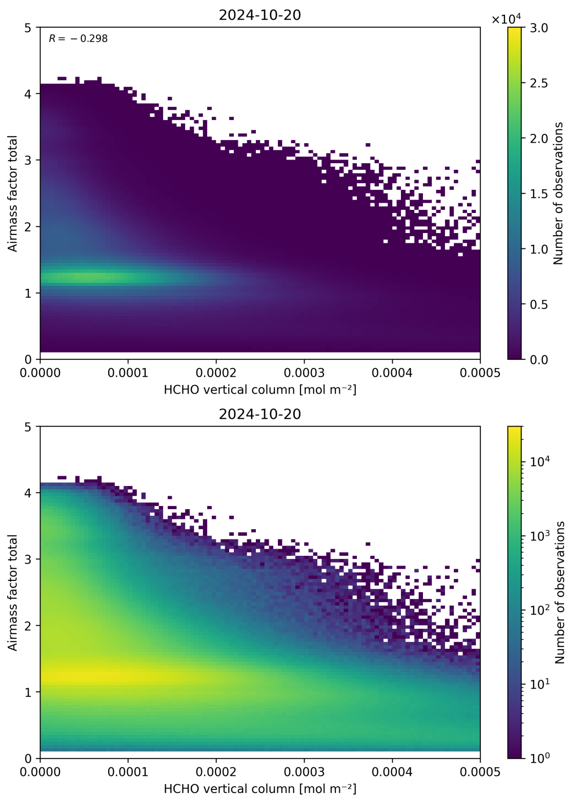
Figure 131: Scatter density plot of “HCHO vertical column” against “Airmass factor total” for 2024-10-19 to 2024-10-21.
