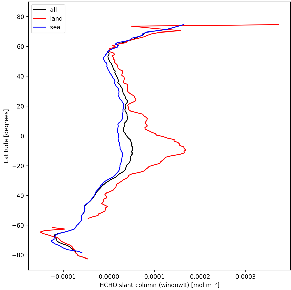
Figure 24: Zonal average of “HCHO slant column (window1)” for 2024-10-19 to 2024-10-21.
