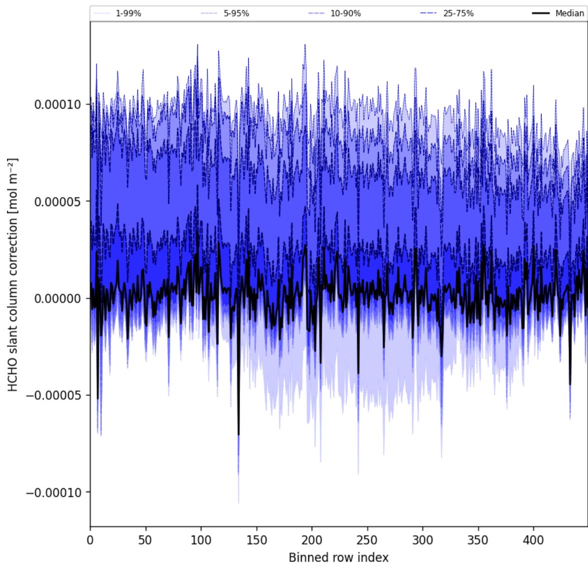
Figure 61: Along track statistics of “HCHO slant column correction” for 2024-10-19 to 2024-10-21
