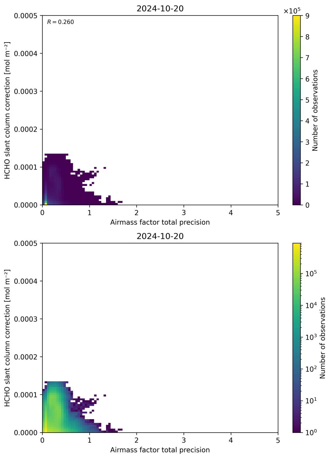
Figure 110: Scatter density plot of “Airmass factor total precision” against “HCHO slant column correction” for 2024-10-19 to 2024-10-21.
