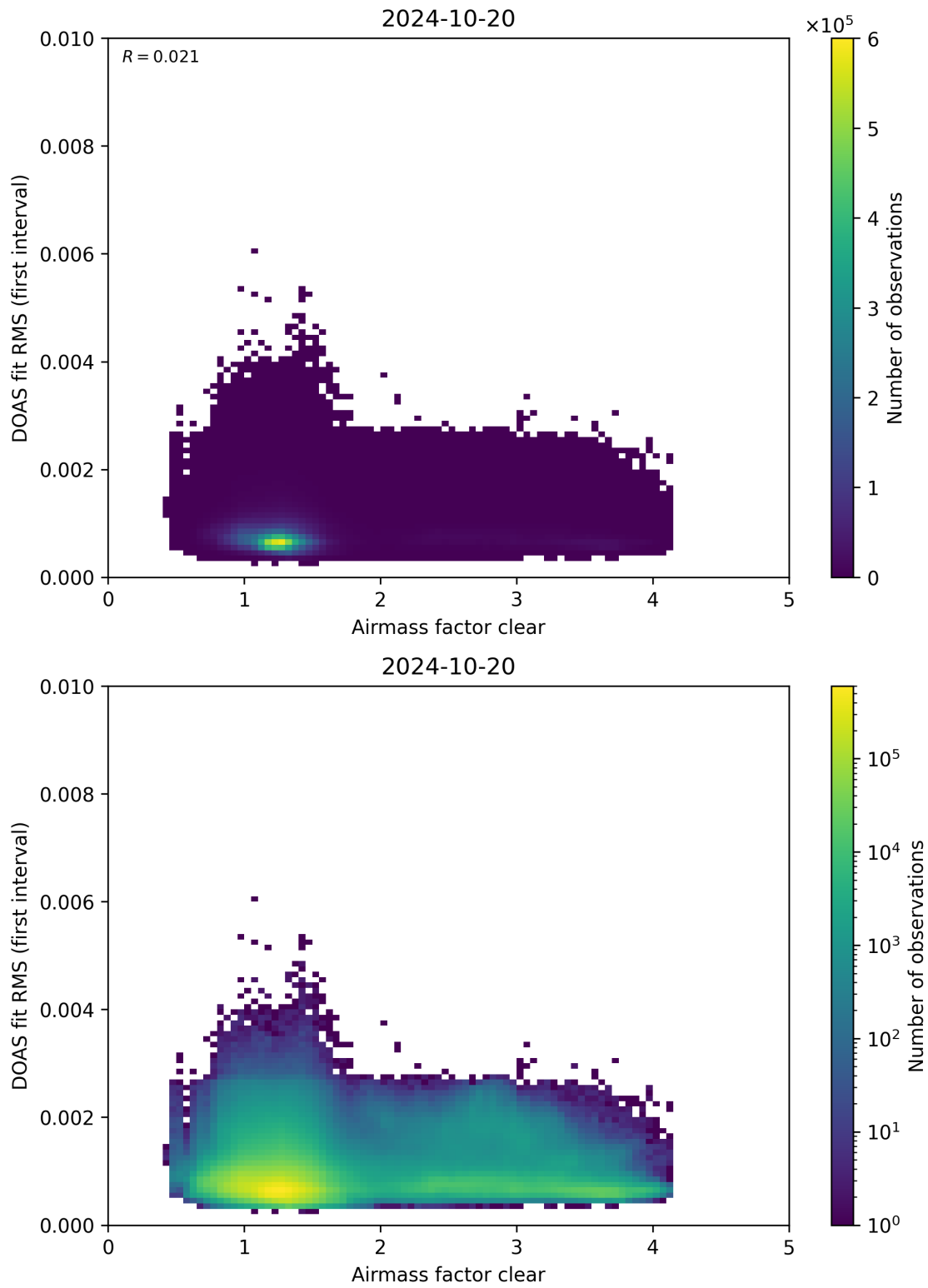
Figure 71: Scatter density plot of “Airmass factor clear” against “DOAS fit RMS (first interval)” for 2024-10-19 to 2024-10-21.
