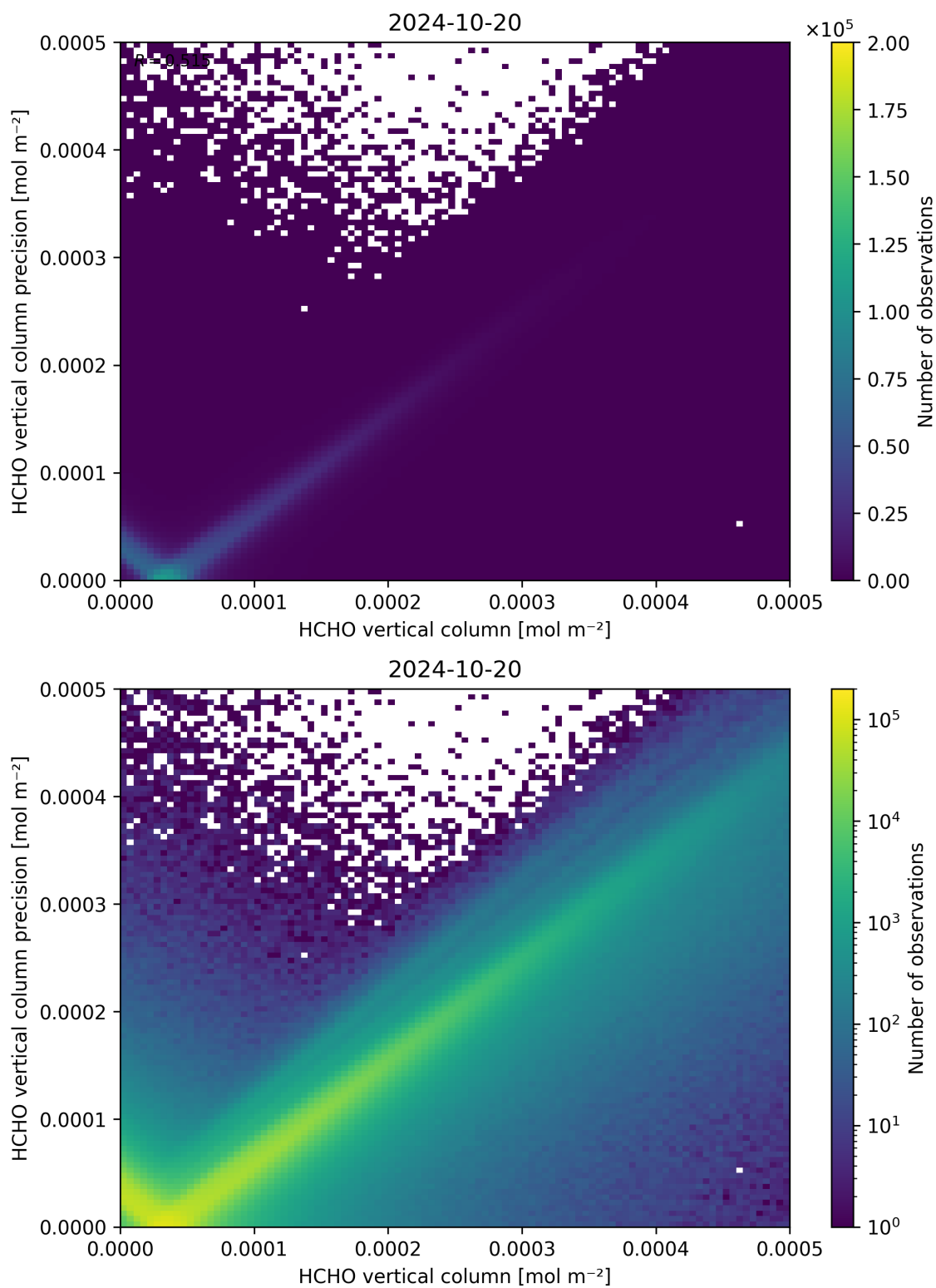
Figure 134: Scatter density plot of “HCHO vertical column” against “HCHO vertical column precision” for 2024-10-19 to 2024-10-21.
