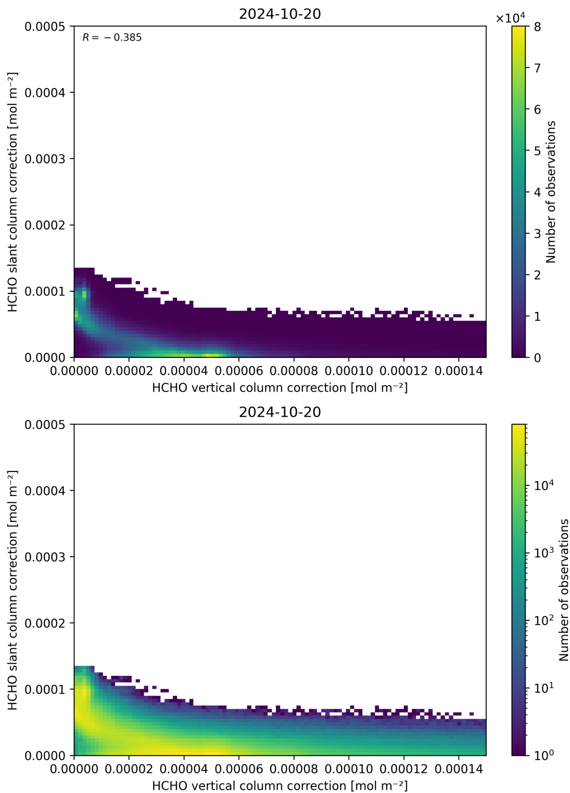
Figure 117: Scatter density plot of “HCHO vertical column correction” against “HCHO slant column correction” for 2024-10-19 to 2024-10-21.
