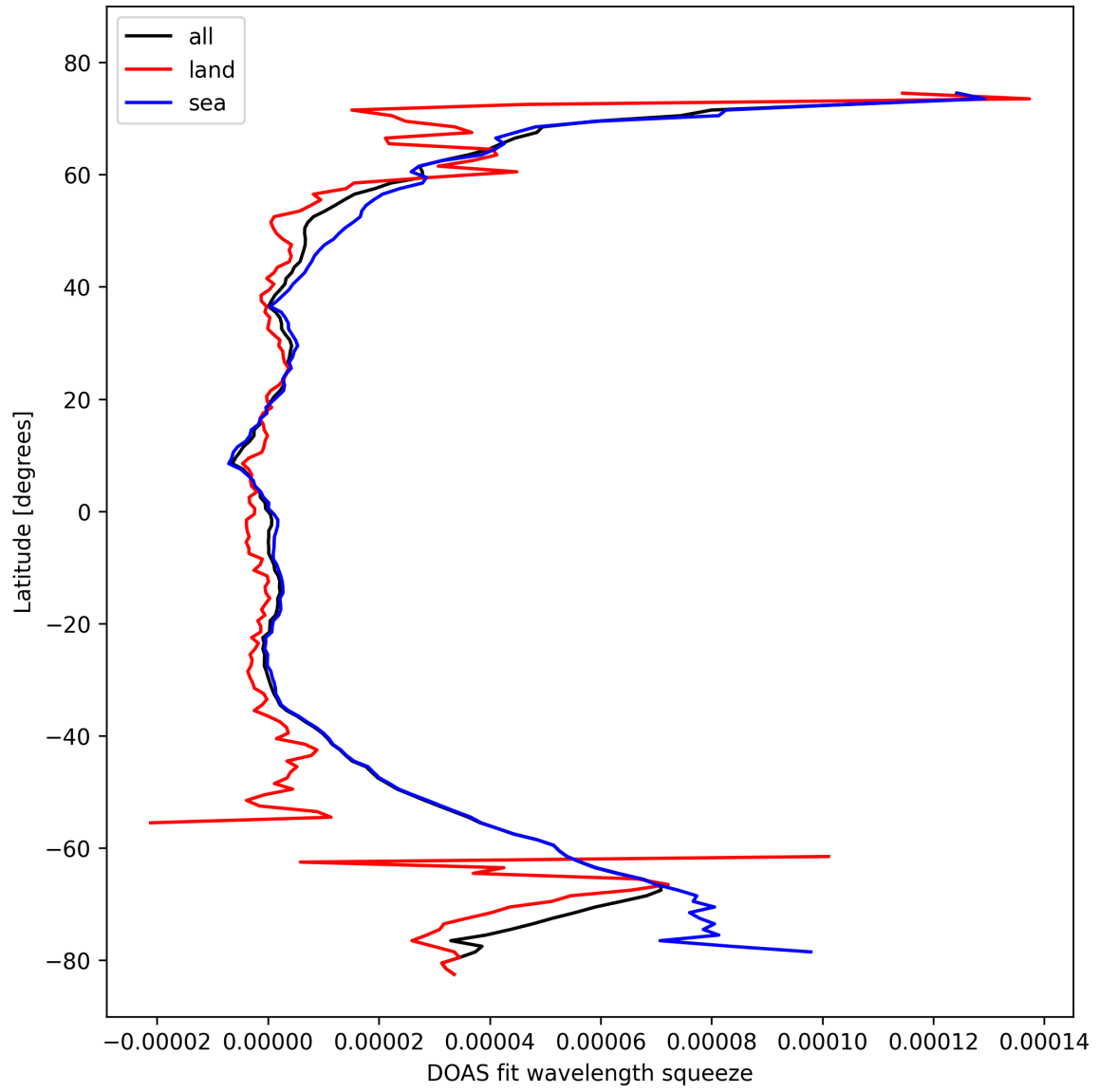
Figure 31: Zonal average of “DOAS fit wavelength squeeze” for 2024-10-19 to 2024-10-21.
