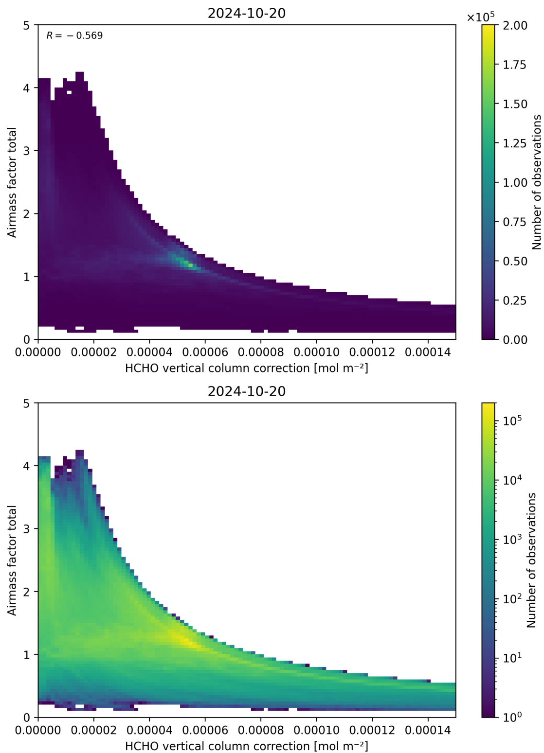
Figure 120: Scatter density plot of “HCHO vertical column correction” against “Airmass factor total” for 2024-10-19 to 2024-10-21.
