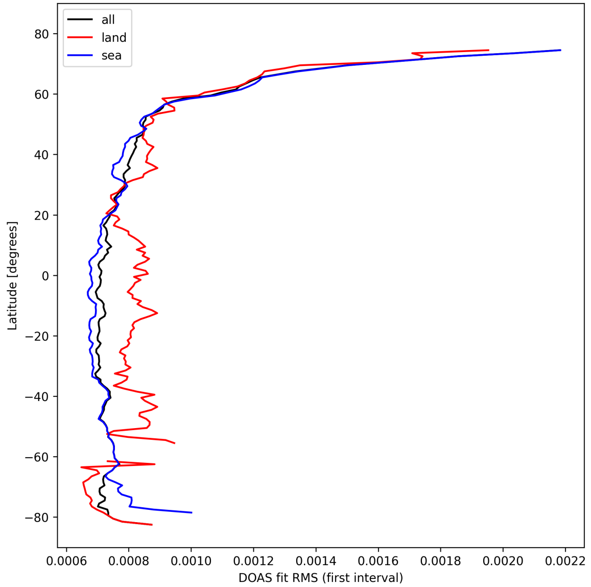
Figure 32: Zonal average of “DOAS fit RMS (first interval)” for 2024-10-19 to 2024-10-21.
