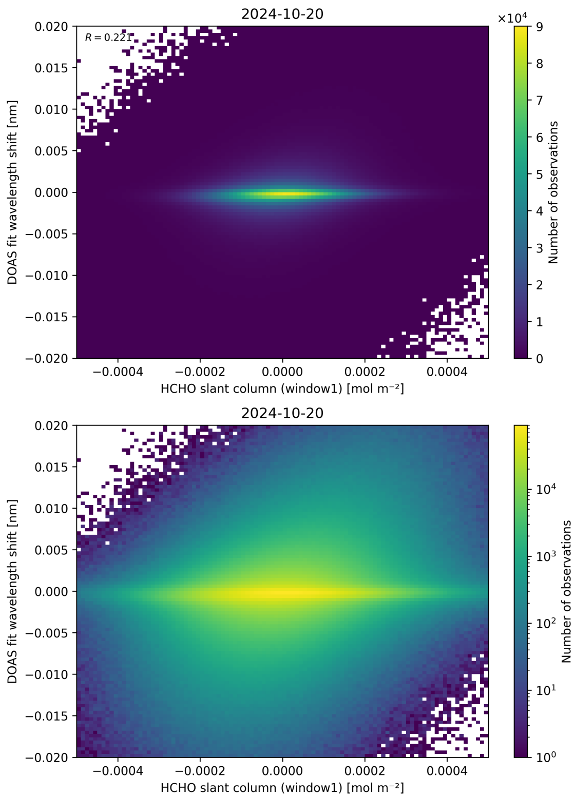
Figure 79: Scatter density plot of “HCHO slant column (window1)” against “DOAS fit wavelength shift” for 2024-10-19 to 2024-10-21.
