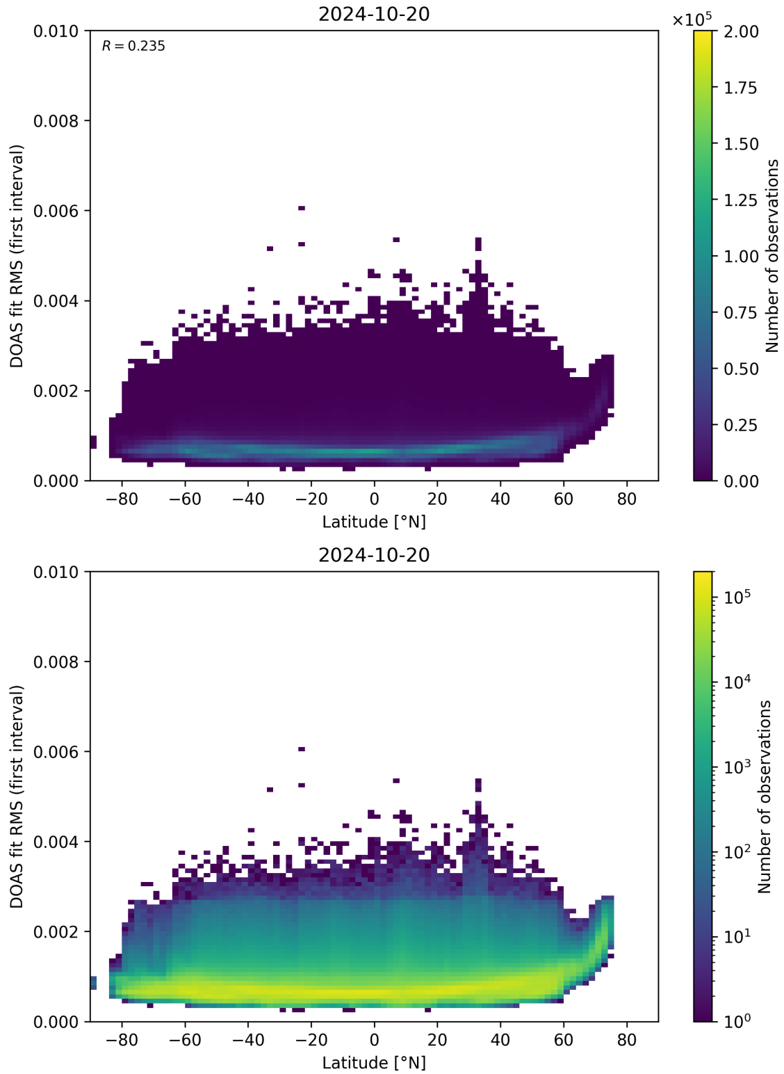
Figure 153: Scatter density plot of “Latitude” against “DOAS fit RMS (first interval)” for 2024-10-19 to 2024-10-21.
