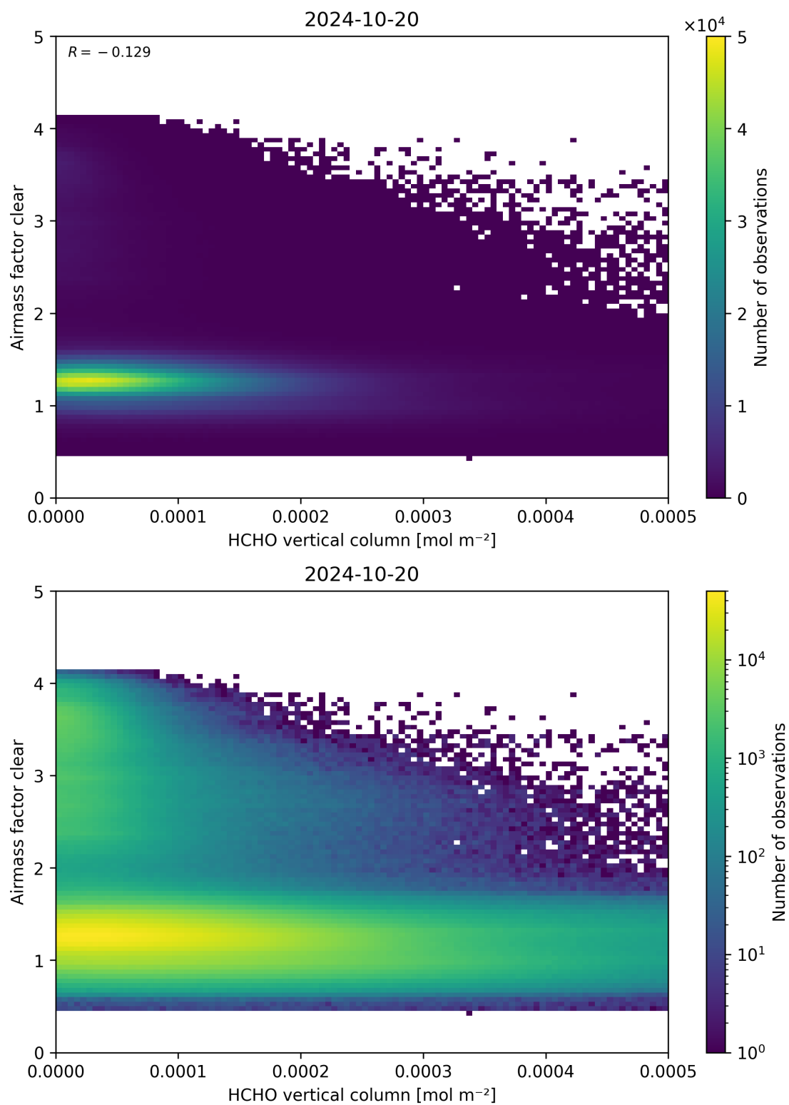
Figure 126: Scatter density plot of “HCHO vertical column” against “Airmass factor clear” for 2024-10-19 to 2024-10-21.
