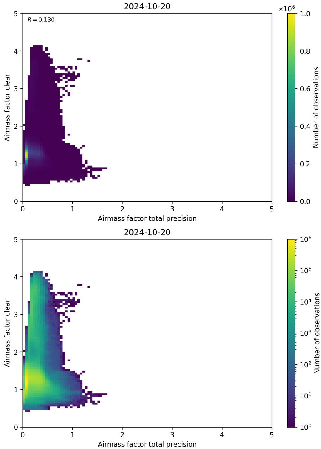
Figure 108: Scatter density plot of “Airmass factor total precision” against “Airmass factor clear” for 2024-10-19 to 2024-10-21.
