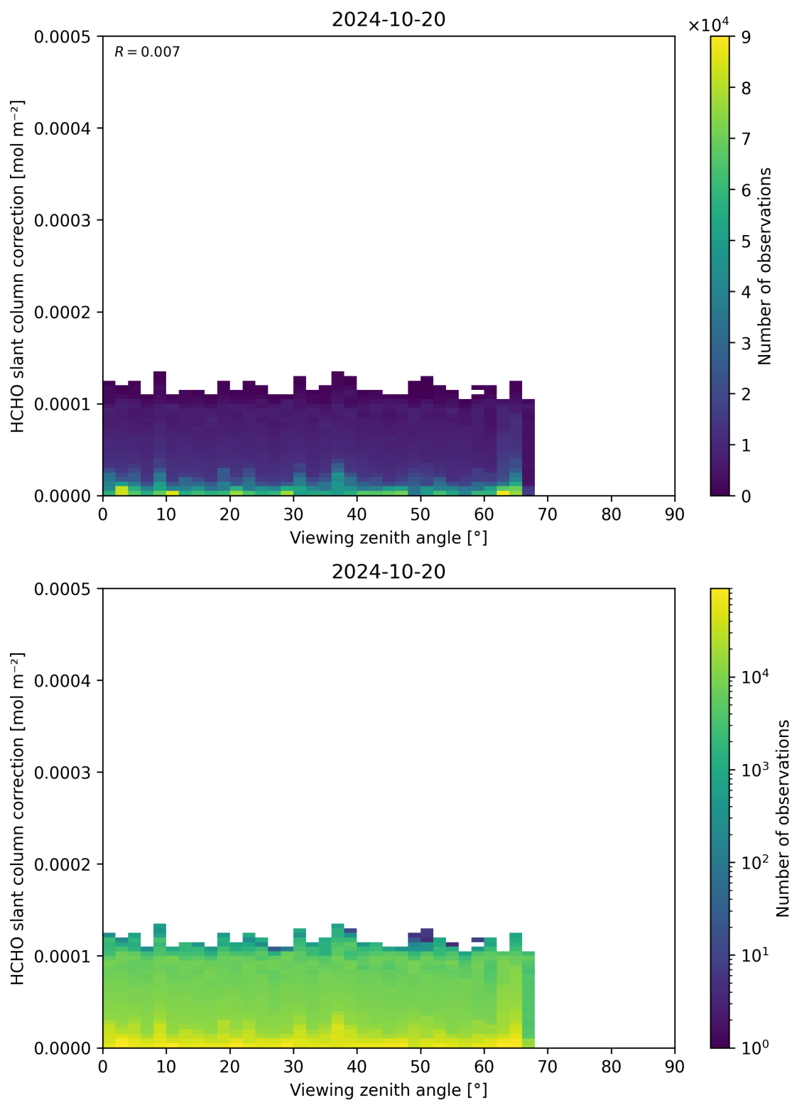
Figure 187: Scatter density plot of “Viewing zenith angle” against “HCHO slant column correction” for 2024-10-19 to 2024-10-21.
