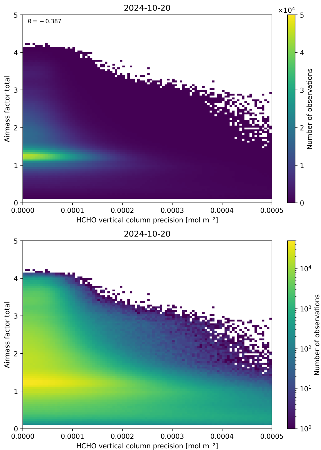
Figure 144: Scatter density plot of “HCHO vertical column precision” against “Airmass factor total” for 2024-10-19 to 2024-10-21.
