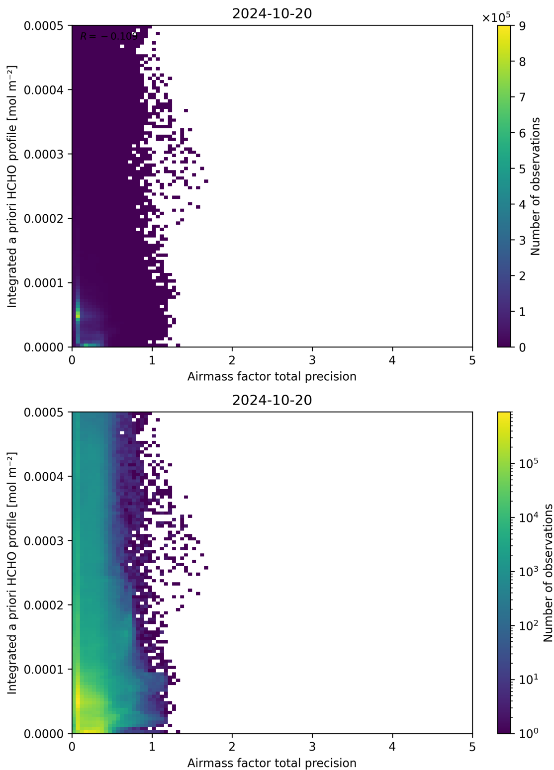
Figure 111: Scatter density plot of “Airmass factor total precision” against “Integrated a priori HCHO profile” for 2024-10-19 to 2024-10-21.
