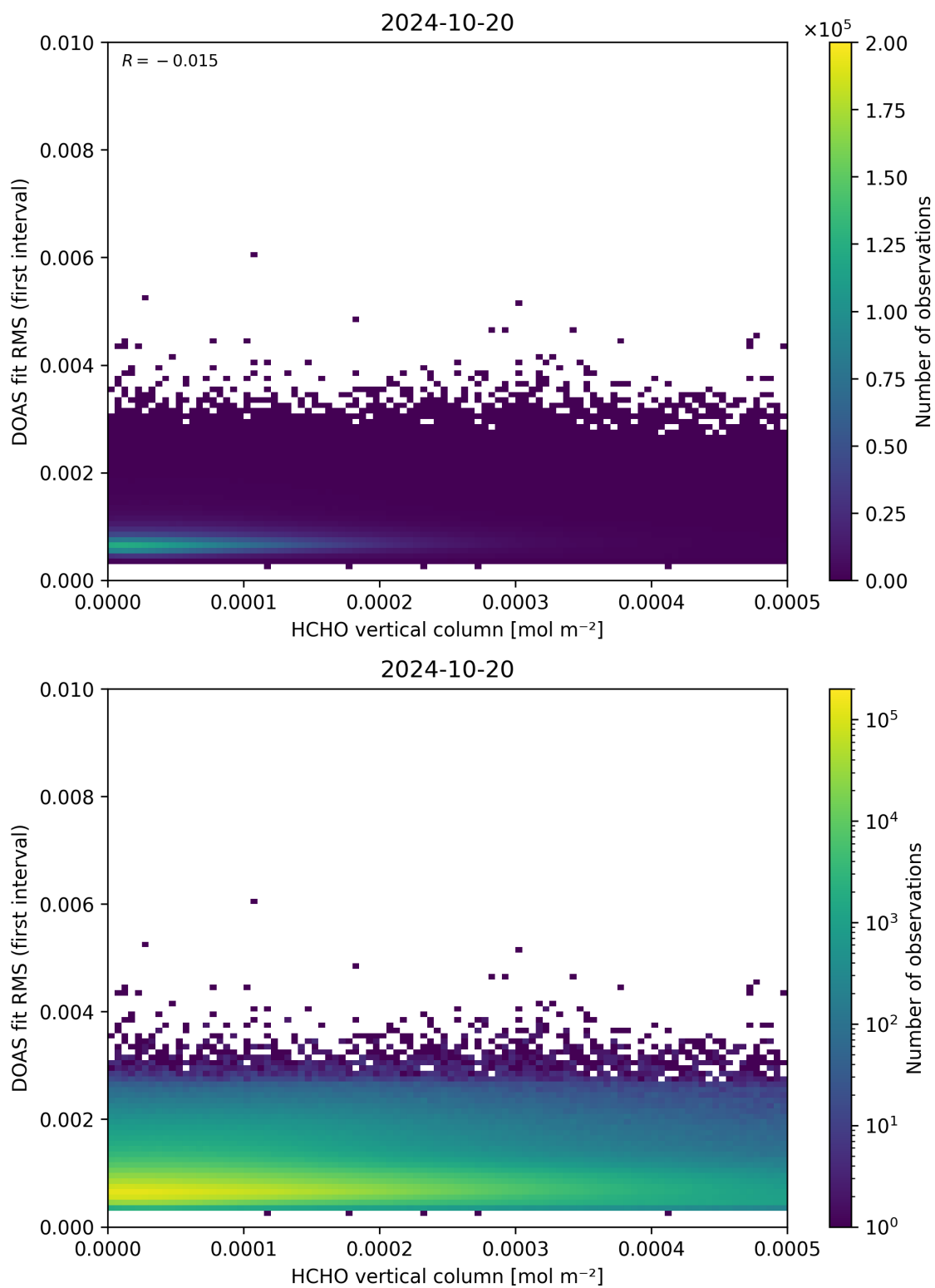
Figure 123: Scatter density plot of “HCHO vertical column” against “DOAS fit RMS (first interval)” for 2024-10-19 to 2024-10-21.
