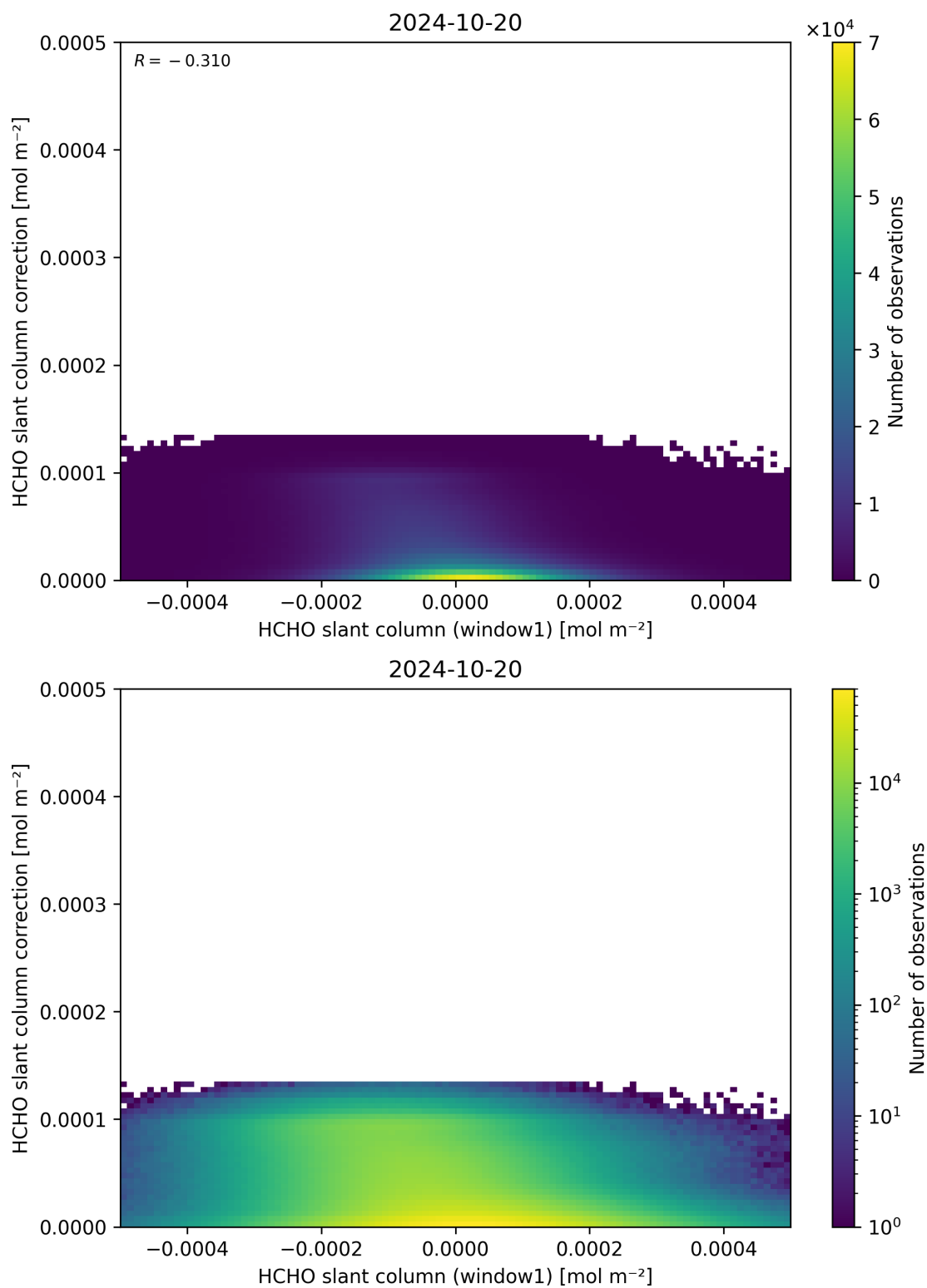
Figure 83: Scatter density plot of “HCHO slant column (window1)” against “HCHO slant column correction” for 2024-10-19 to 2024-10-21.
