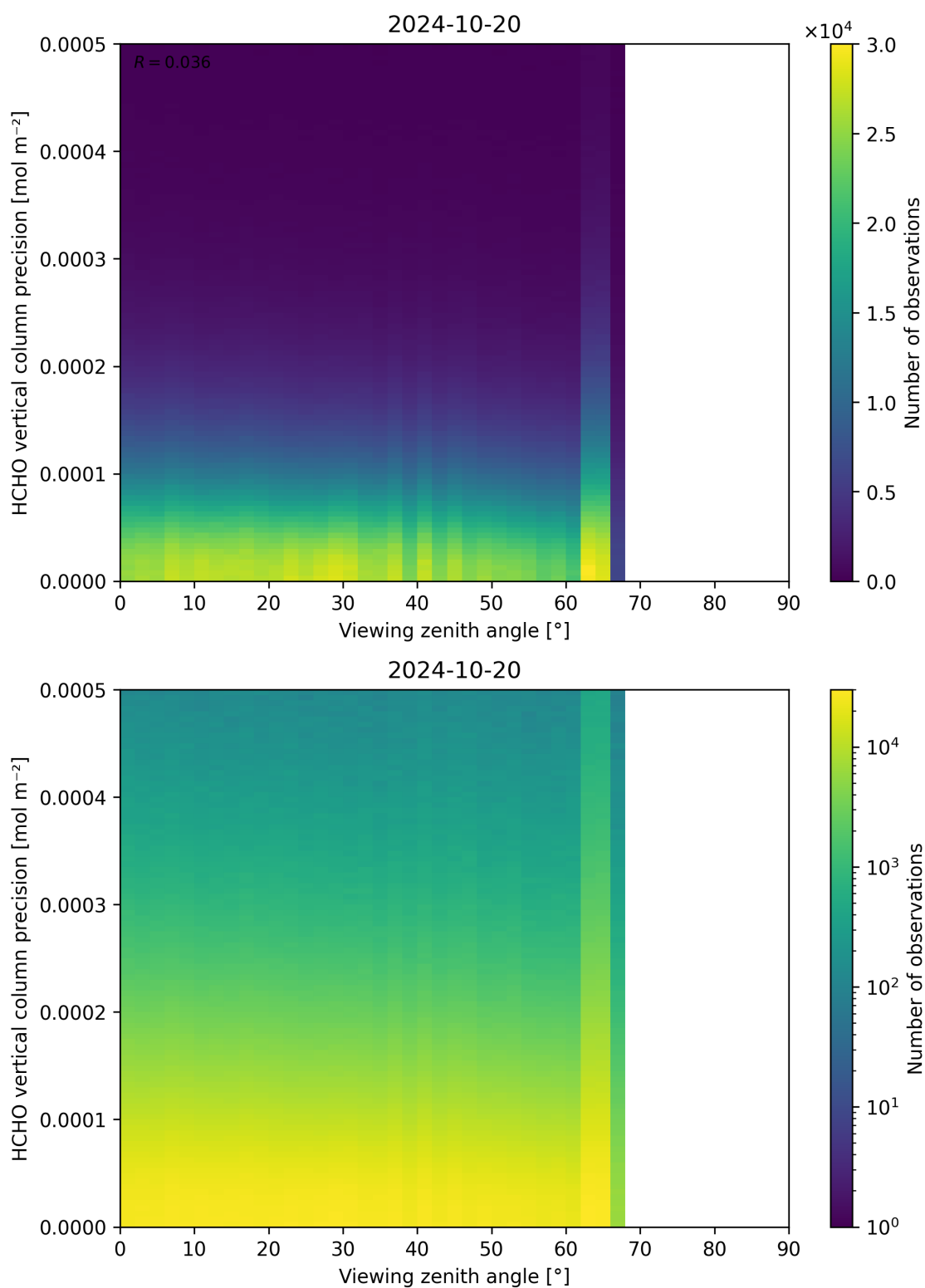
Figure 194: Scatter density plot of “Viewing zenith angle” against “HCHO vertical column precision” for 2024-10-19 to 2024-10-21.
