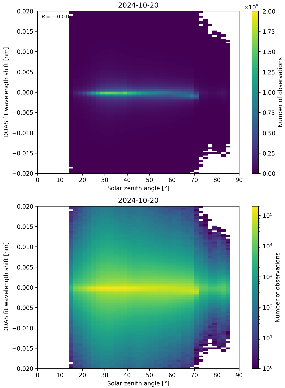
Figure 168: Scatter density plot of “Solar zenith angle” against “DOAS fit wavelength shift” for 2024-10-19 to 2024-10-21.
