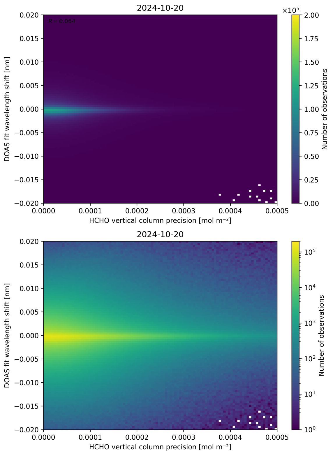
Figure 137: Scatter density plot of “HCHO vertical column precision” against “DOAS fit wavelength shift” for 2024-10-19 to 2024-10-21.
