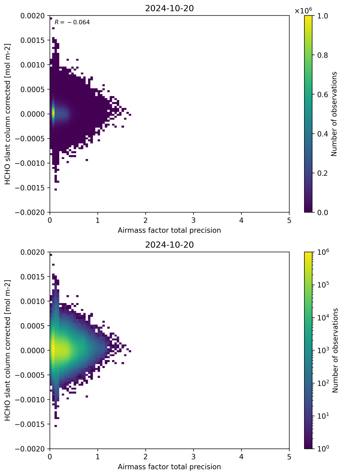
Figure 109: Scatter density plot of “Airmass factor total precision” against “HCHO slant column corrected” for 2024-10-19 to 2024-10-21.
