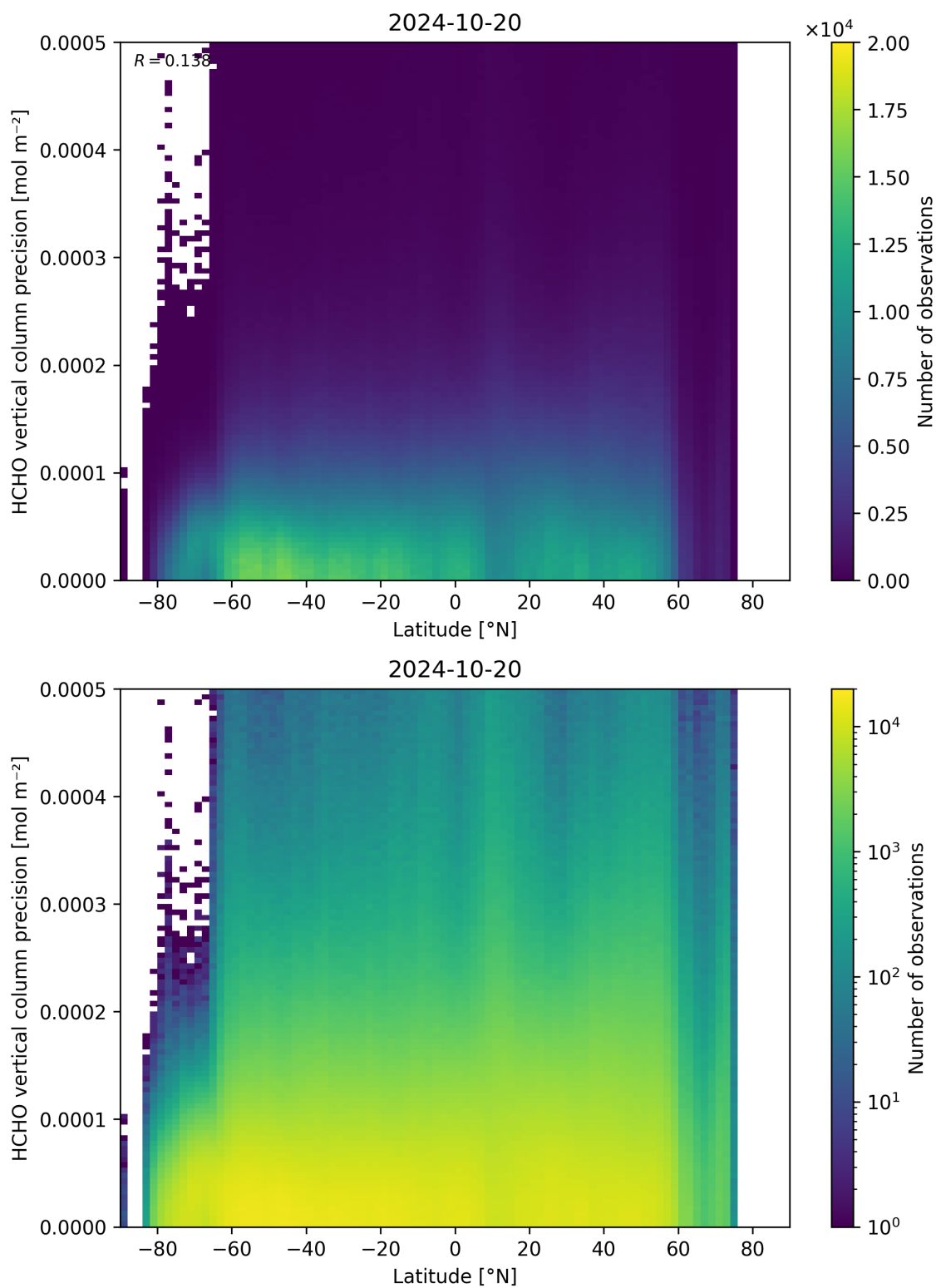
Figure 165: Scatter density plot of “Latitude” against “HCHO vertical column precision” for 2024-10-19 to 2024-10-21.
