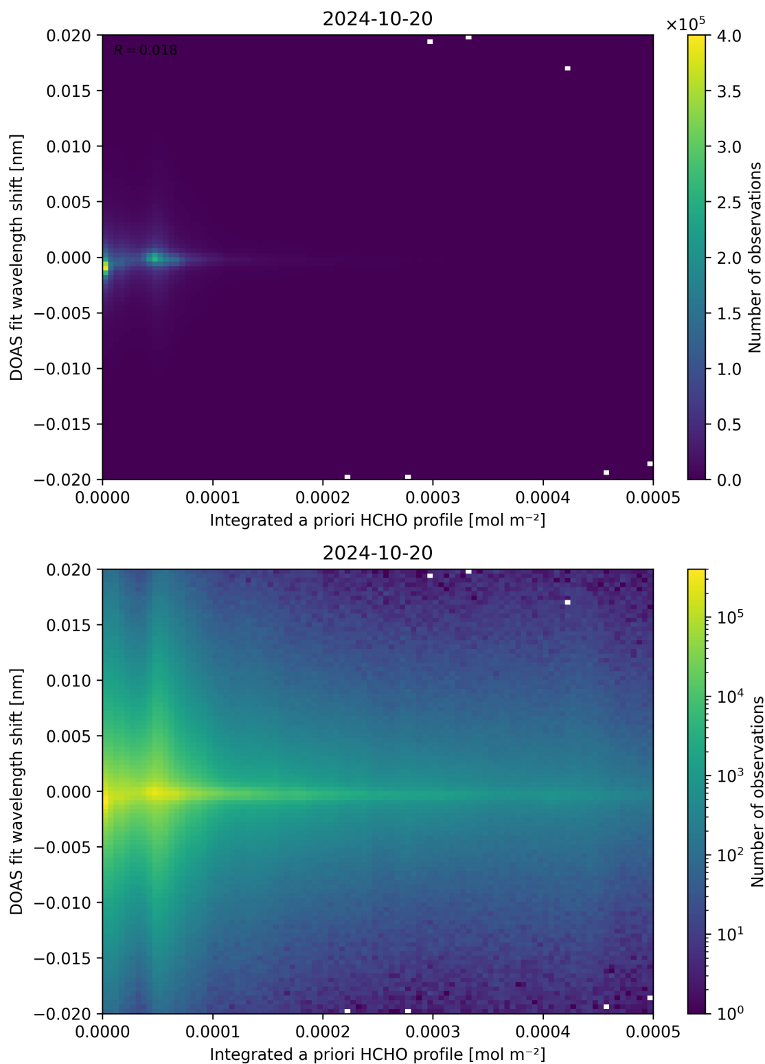
Figure 149: Scatter density plot of “Integrated a priori HCHO profile” against “DOAS fit wavelength shift” for 2024-10-19 to 2024-10-21.
