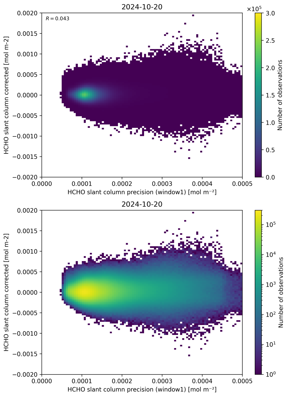
Figure 92: Scatter density plot of “HCHO slant column precision (window1)” against “HCHO slant column corrected” for 2024-10-19 to 2024-10-21.
