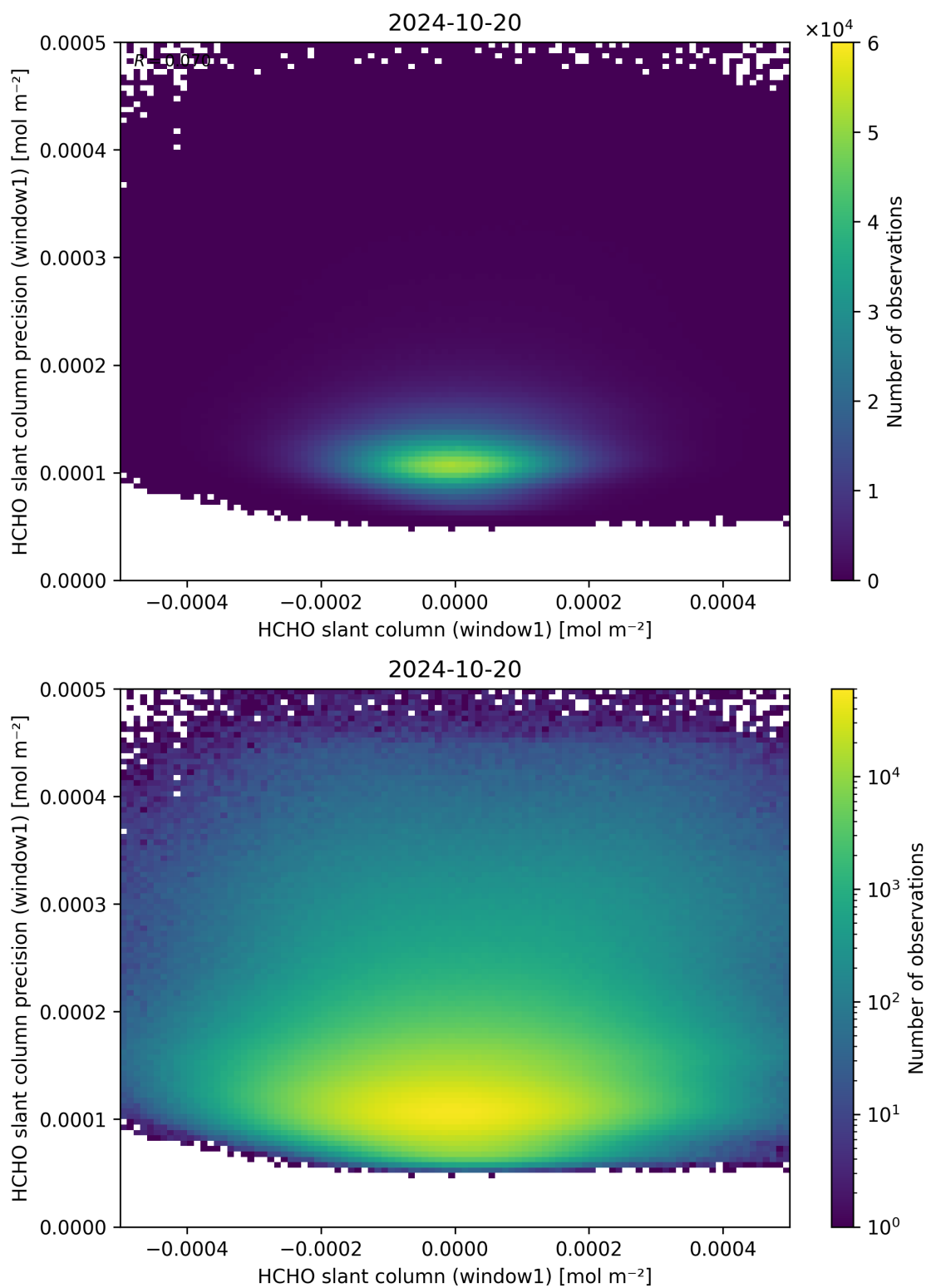
Figure 84: Scatter density plot of “HCHO slant column (window1)” against “HCHO slant column precision (window1)” for 2024-10-19 to 2024-10-21.
