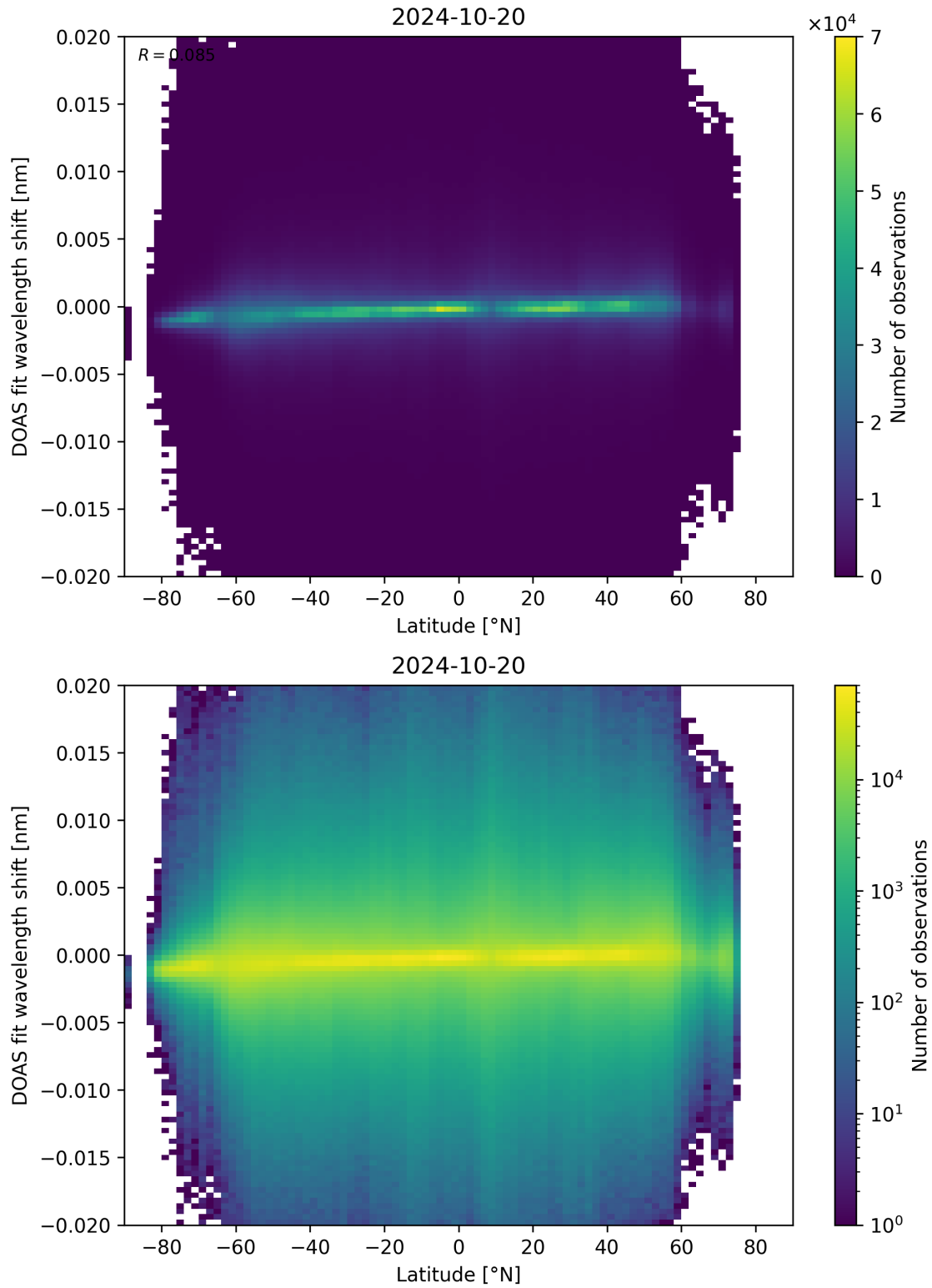
Figure 154: Scatter density plot of “Latitude” against “DOAS fit wavelength shift” for 2024-10-19 to 2024-10-21.
