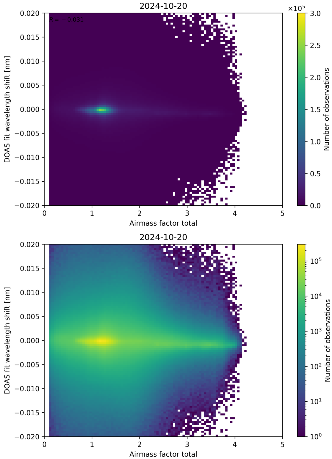
Figure 98: Scatter density plot of “Airmass factor total” against “DOAS fit wavelength shift” for 2024-10-19 to 2024-10-21.
