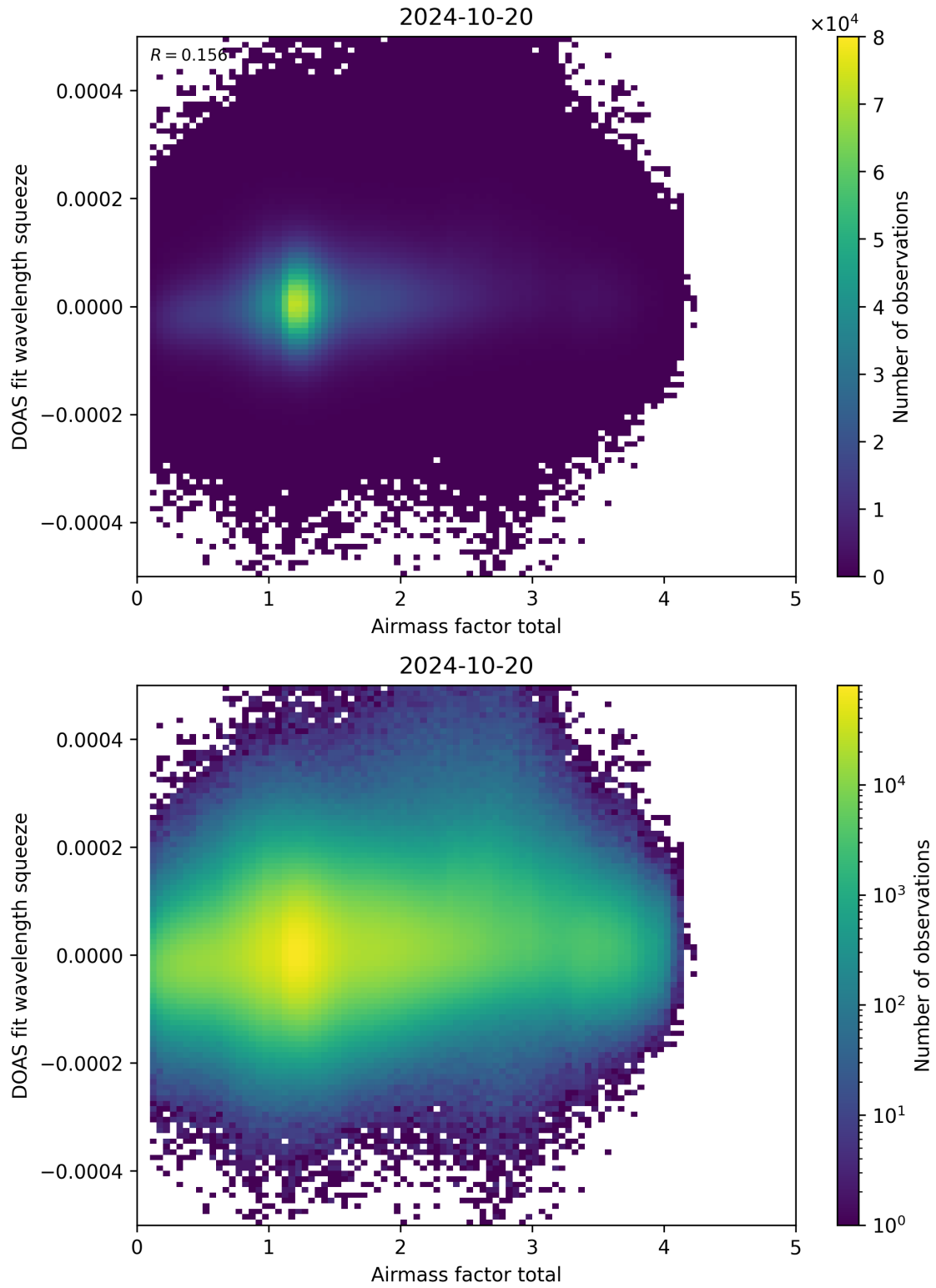
Figure 99: Scatter density plot of “Airmass factor total” against “DOAS fit wavelength squeeze” for 2024-10-19 to 2024-10-21.
