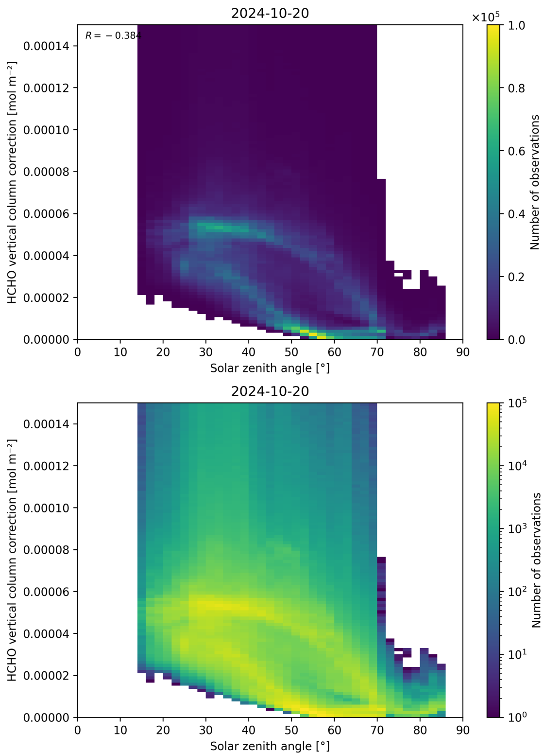
Figure 178: Scatter density plot of “Solar zenith angle” against “HCHO vertical column correction” for 2024-10-19 to 2024-10-21.
