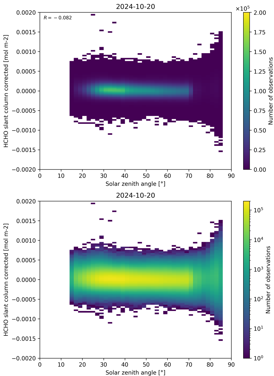
Figure 171: Scatter density plot of “Solar zenith angle” against “HCHO slant column corrected” for 2024-10-19 to 2024-10-21.
