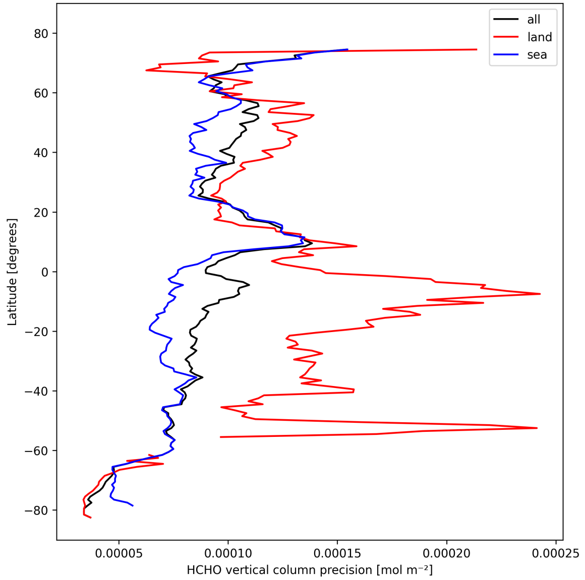
Figure 22: Zonal average of “HCHO vertical column precision” for 2024-10-19 to 2024-10-21.
