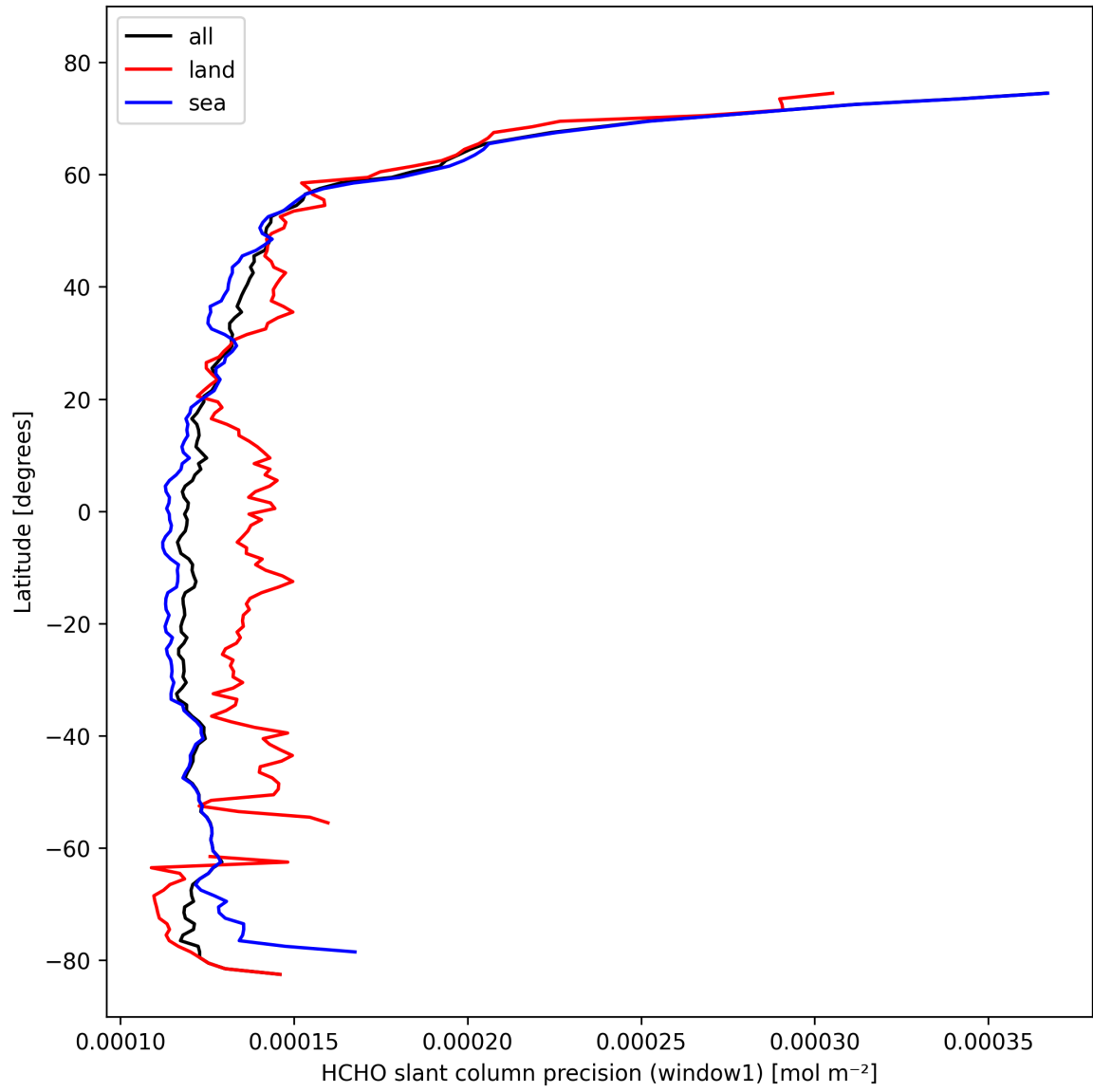
Figure 25: Zonal average of "HCHO slant column precision (window1)" for 2024-10-19 to 2024-10-21.
