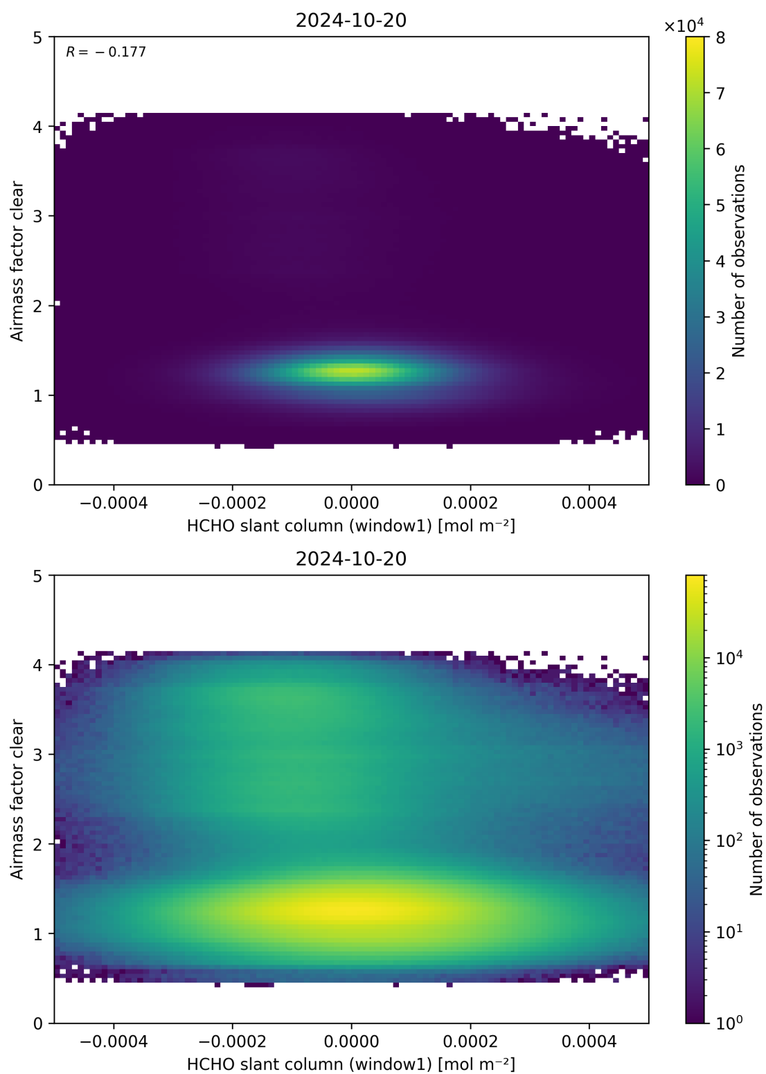
Figure 81: Scatter density plot of “HCHO slant column (window1)” against “Airmass factor clear” for 2024-10-19 to 2024-10-21.
