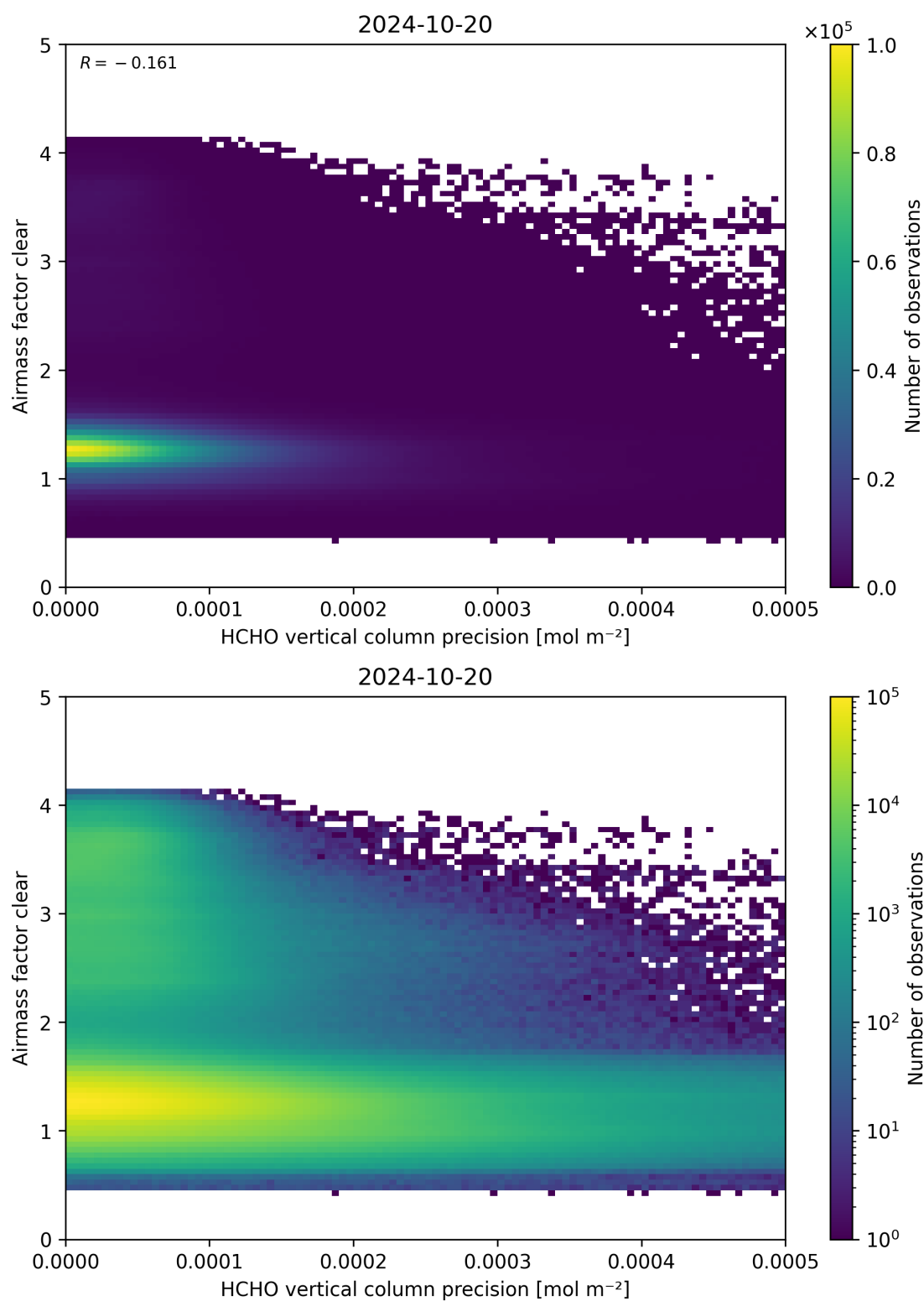
Figure 139: Scatter density plot of “HCHO vertical column precision” against “Airmass factor clear” for 2024-10-19 to 2024-10-21.
