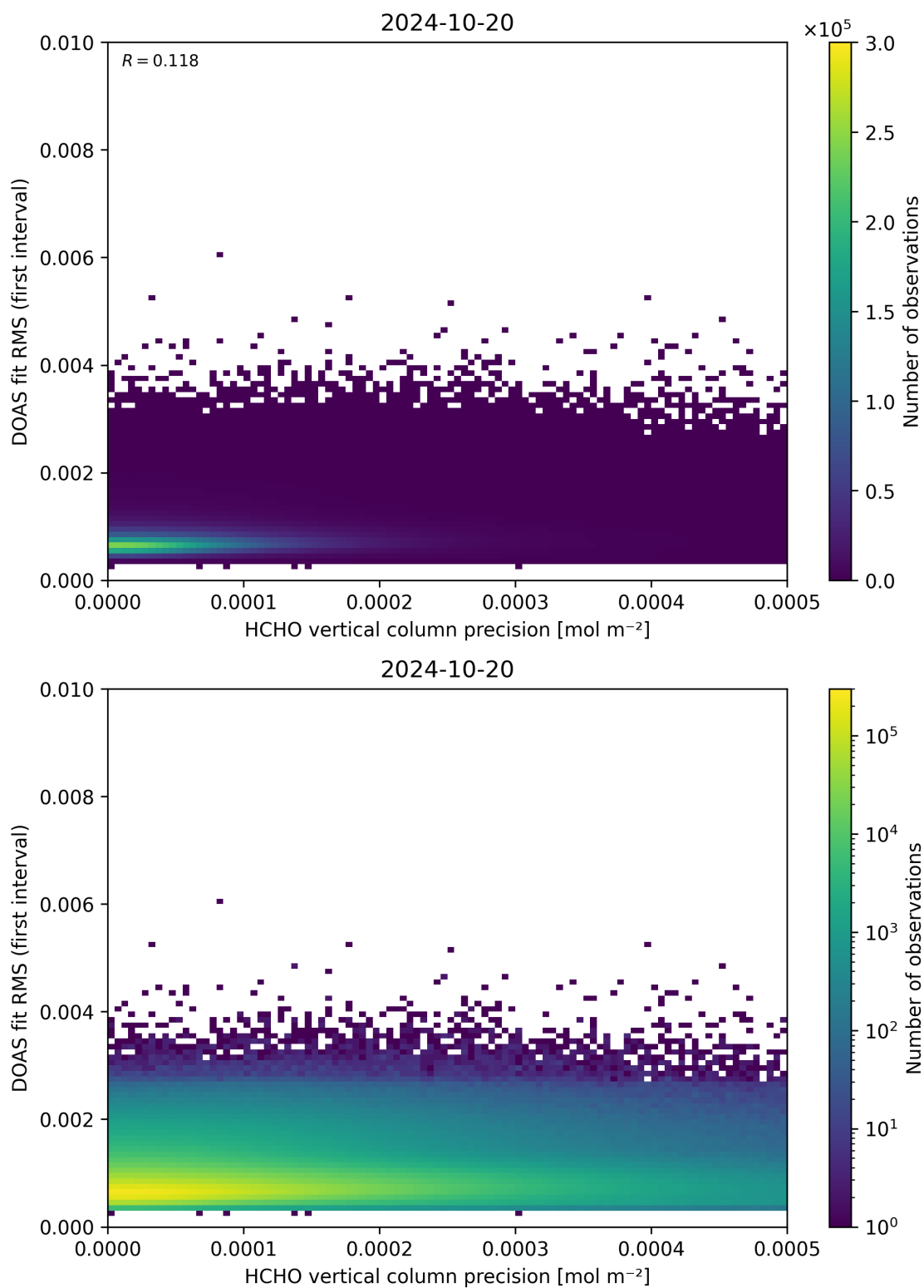
Figure 136: Scatter density plot of “HCHO vertical column precision” against “DOAS fit RMS (first interval)” for 2024-10-19 to 2024-10-21.
