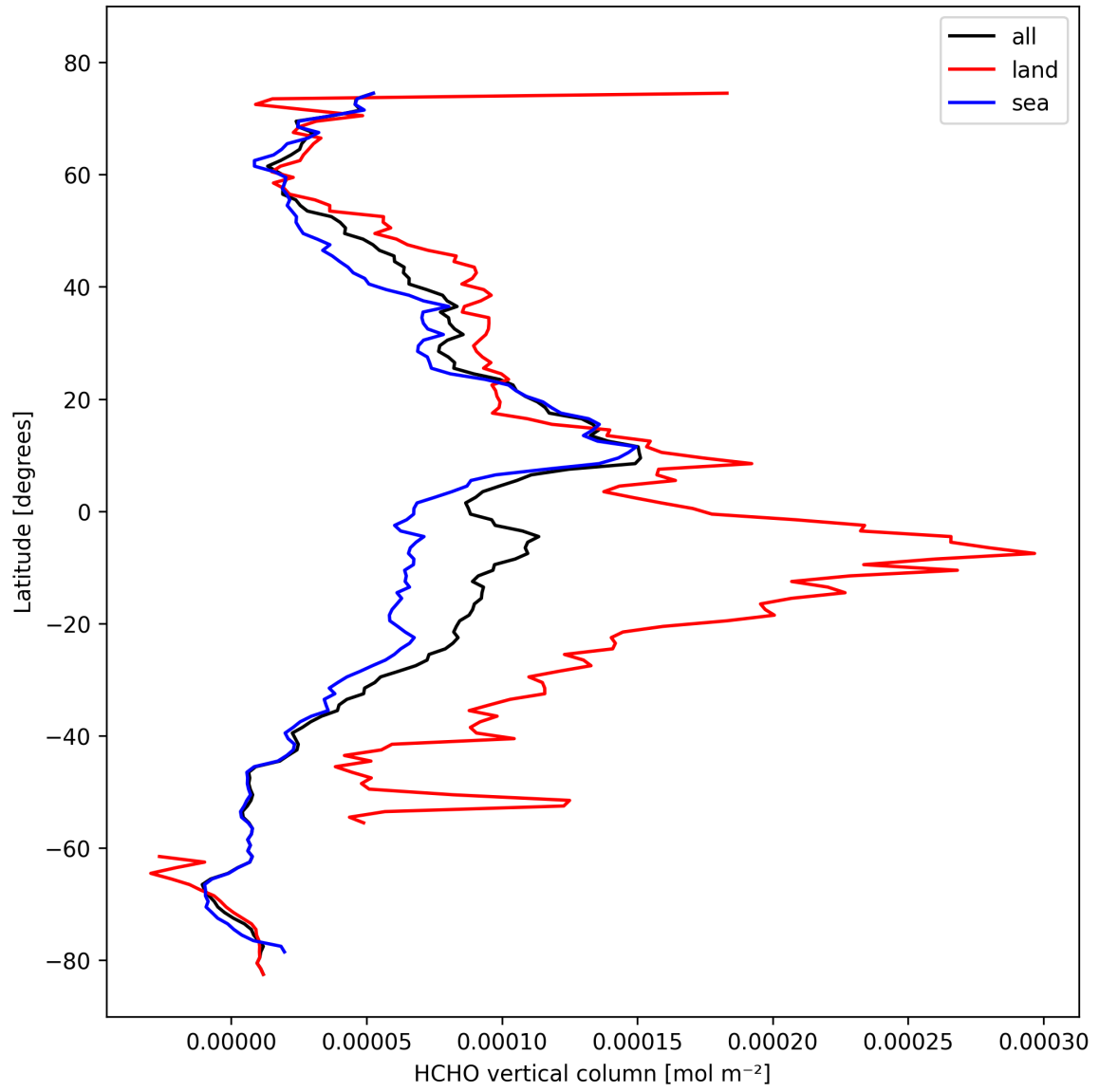
Figure 21: Zonal average of “HCHO vertical column” for 2024-10-19 to 2024-10-21.
