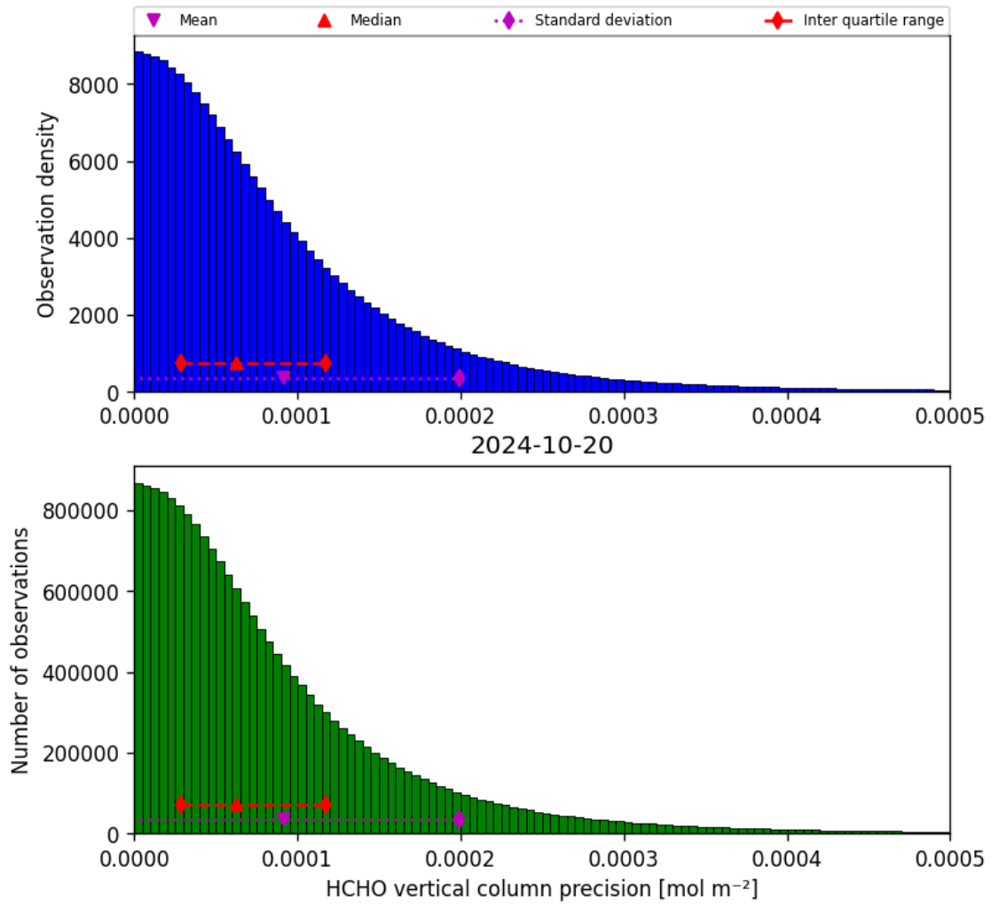
Figure 36: Histogram of “HCHO vertical column precision” for 2024-10-19 to 2024-10-21
