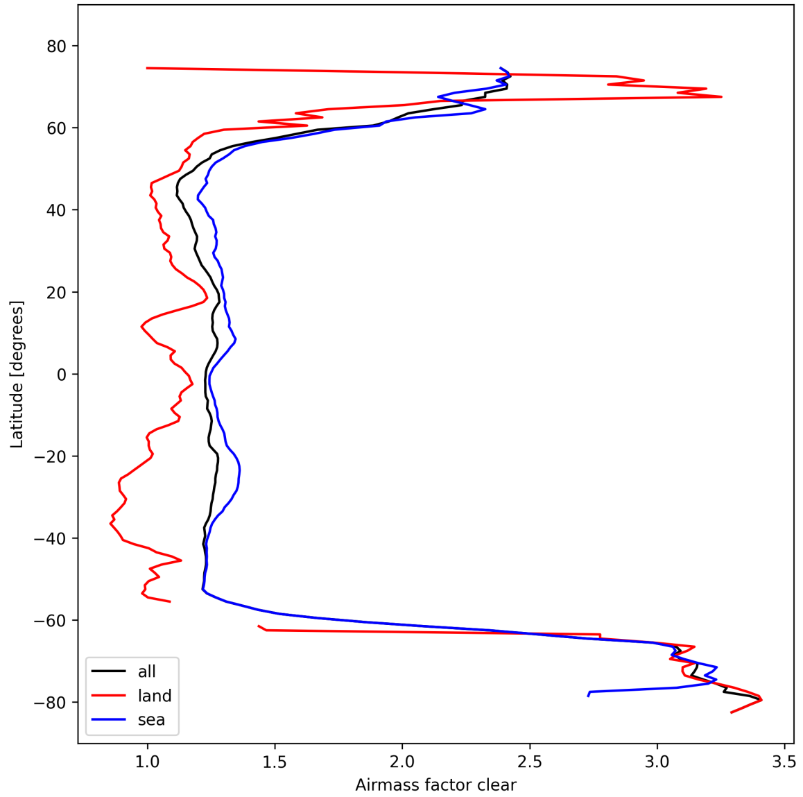
Figure 28: Zonal average of “Airmass factor clear” for 2024-10-19 to 2024-10-21.
