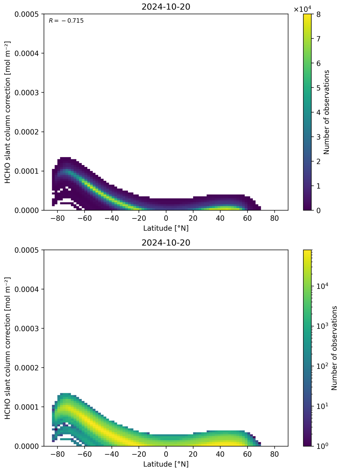
Figure 158: Scatter density plot of “Latitude” against “HCHO slant column correction” for 2024-10-19 to 2024-10-21.
