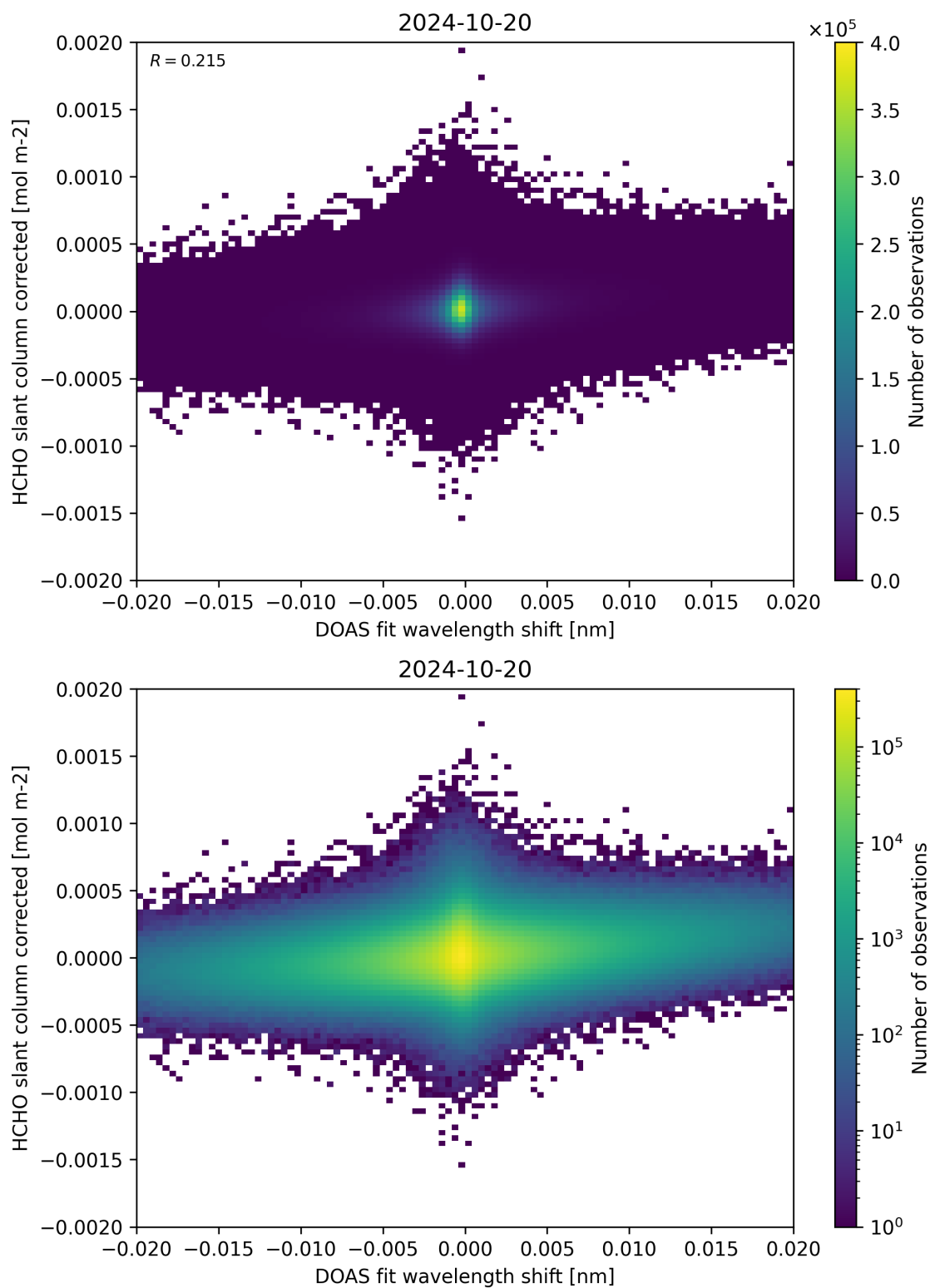
Figure 66: Scatter density plot of “DOAS fit wavelength shift” against “HCHO slant column corrected” for 2024-10-19 to 2024-10-21.
