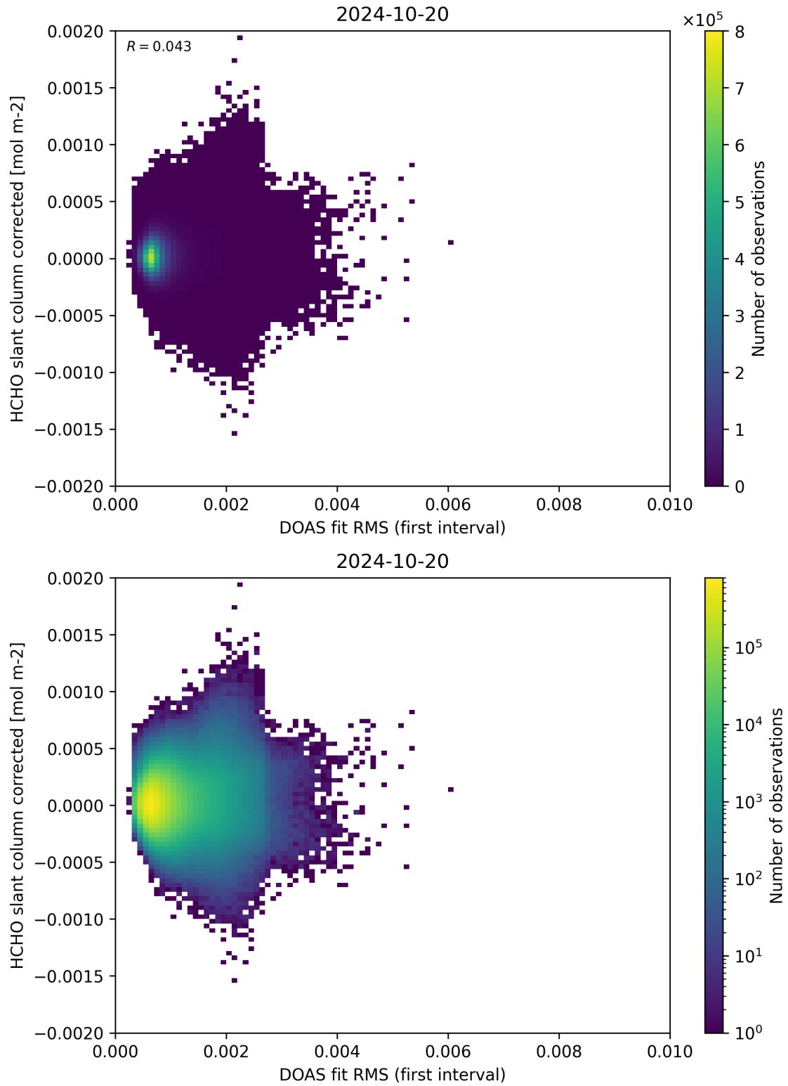
Figure 62: Scatter density plot of “DOAS fit RMS (first interval)” against “HCHO slant column corrected” for 2024-10-19 to 2024-10-21.
