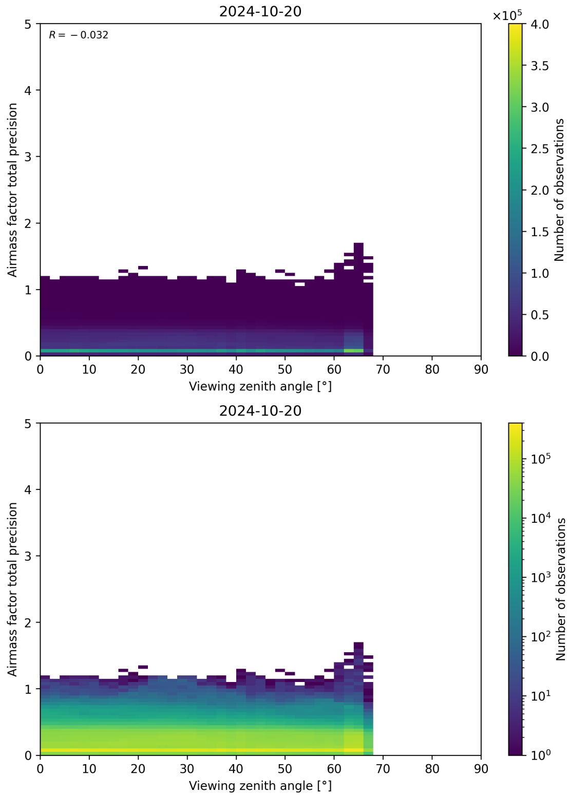
Figure 191: Scatter density plot of “Viewing zenith angle” against “Airmass factor total precision” for 2024-10-19 to 2024-10-21.
