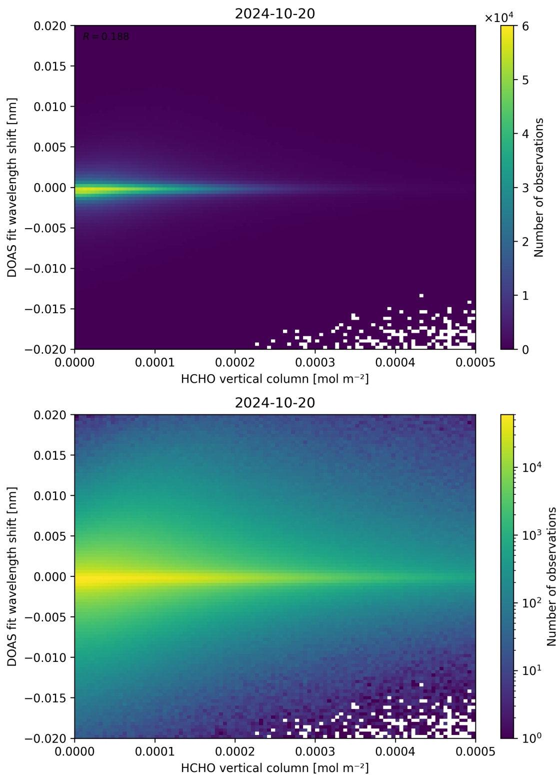
Figure 124: Scatter density plot of “HCHO vertical column” against “DOAS fit wavelength shift” for 2024-10-19 to 2024-10-21.
