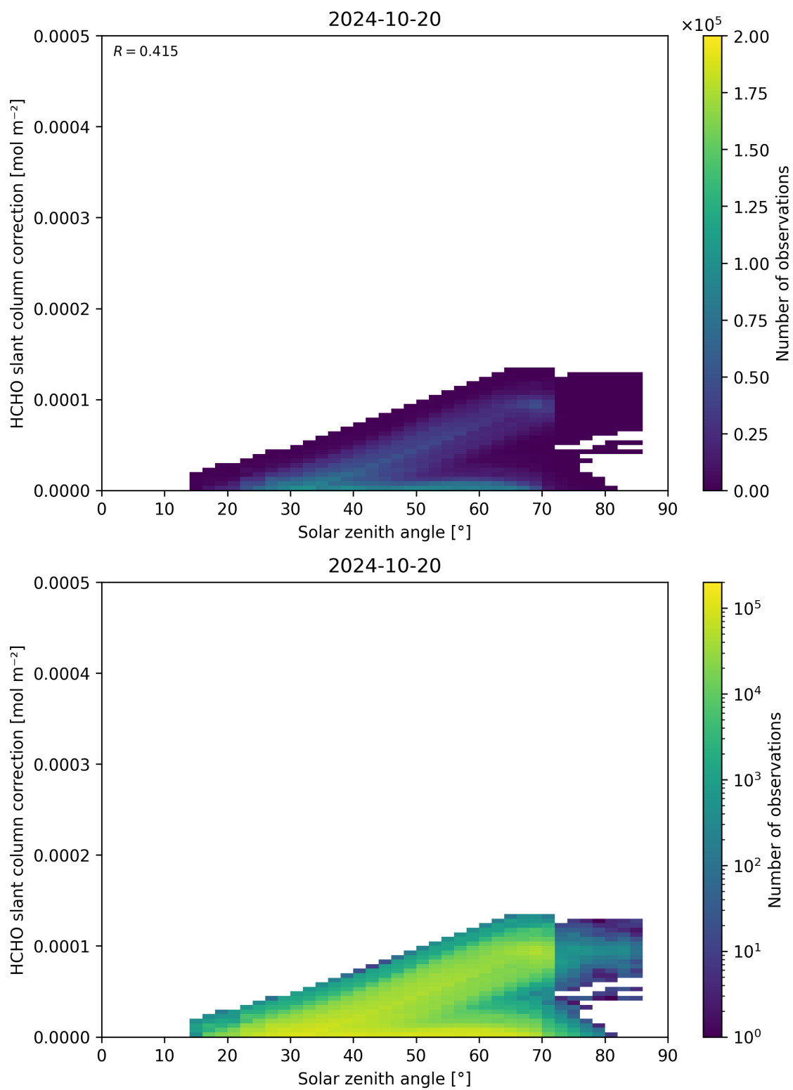
Figure 172: Scatter density plot of “Solar zenith angle” against “HCHO slant column correction” for 2024-10-19 to 2024-10-21.
