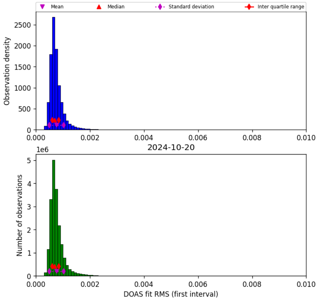
Figure 46: Histogram of “DOAS fit RMS (first interval)” for 2024-10-19 to 2024-10-21
