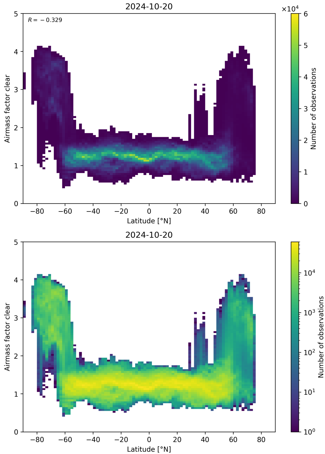
Figure 156: Scatter density plot of “Latitude” against “Airmass factor clear” for 2024-10-19 to 2024-10-21.
