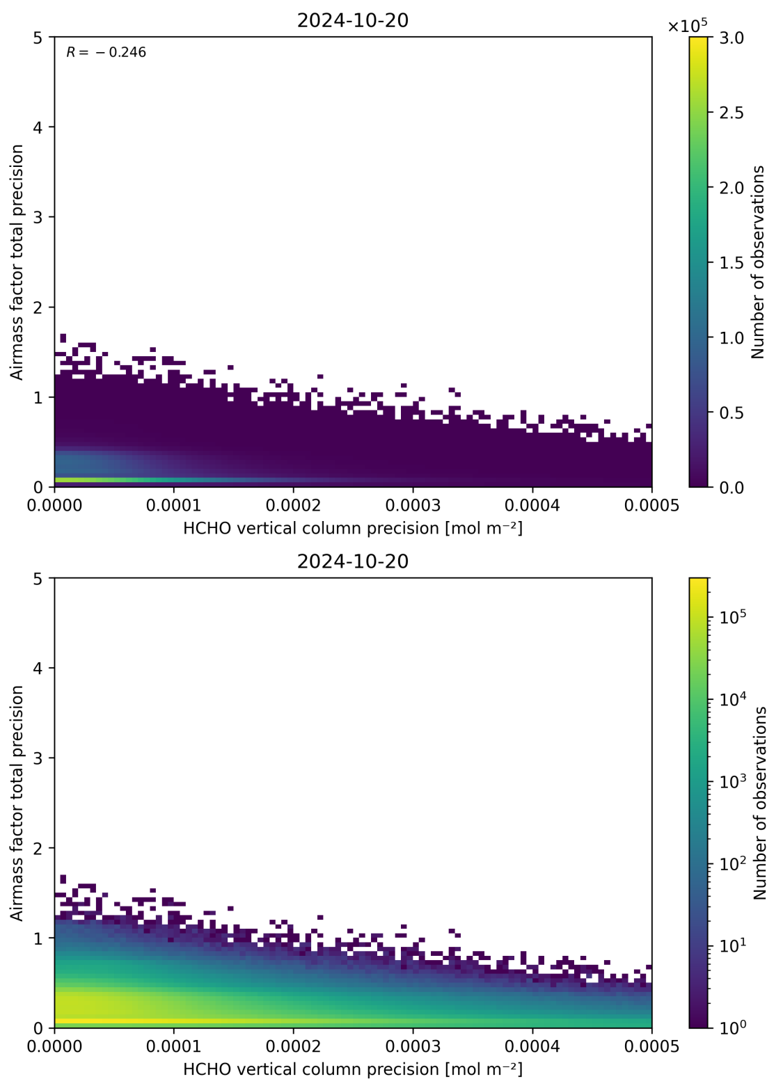
Figure 145: Scatter density plot of “HCHO vertical column precision” against “Airmass factor total precision” for 2024-10-19 to 2024-10-21.
