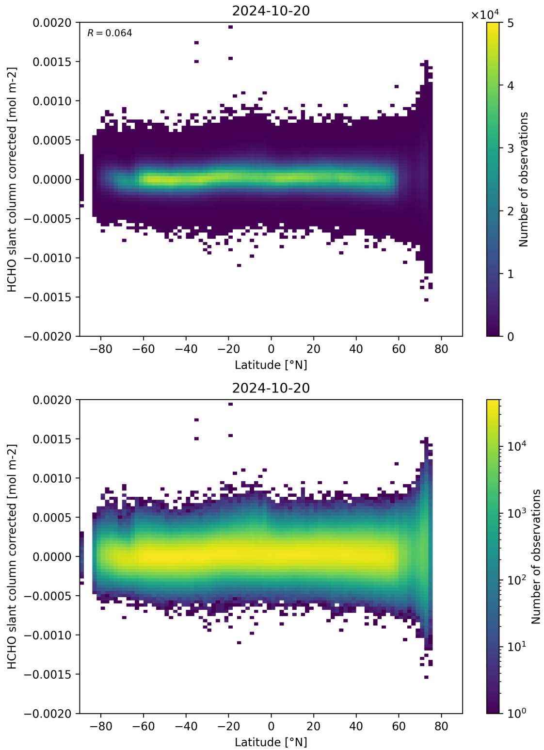
Figure 157: Scatter density plot of “Latitude” against “HCHO slant column corrected” for 2024-10-19 to 2024-10-21.
