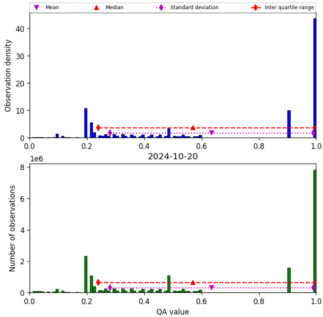
Figure 34: Histogram of “QA value” for 2024-10-19 to 2024-10-21
