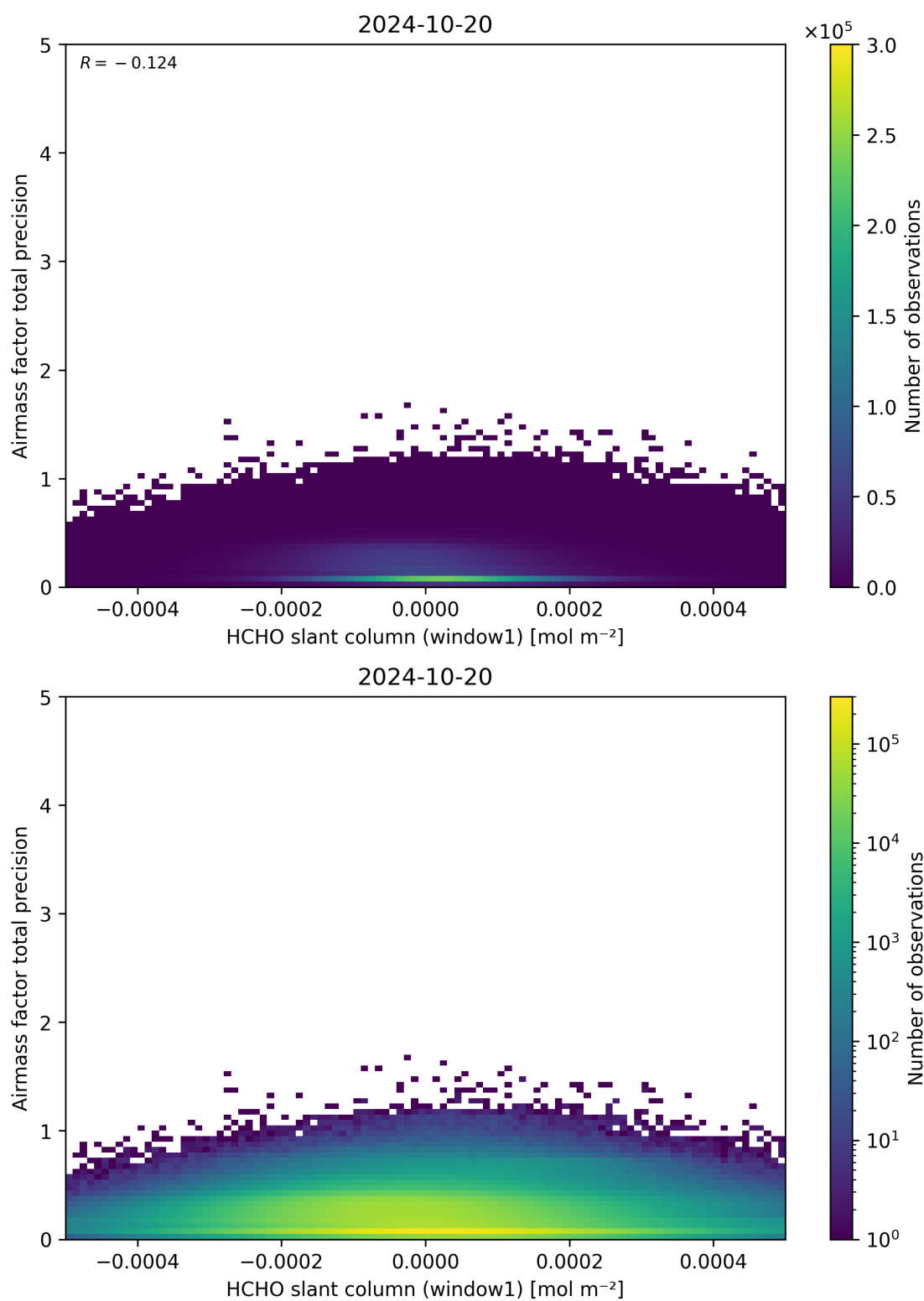
Figure 86: Scatter density plot of “HCHO slant column (window1)” against “Airmass factor total precision” for 2024-10-19 to 2024-10-21.
