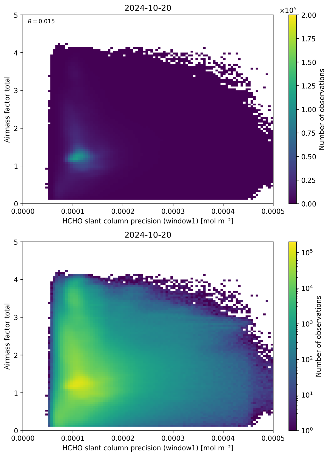
Figure 94: Scatter density plot of “HCHO slant column precision (window1)” against “Airmass factor total” for 2024-10-19 to 2024-10-21.
