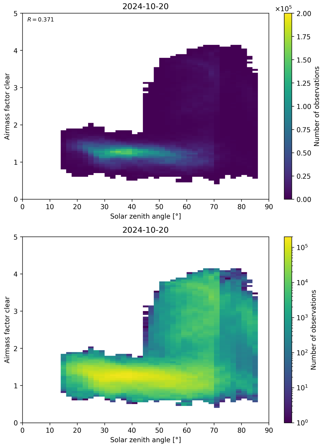
Figure 170: Scatter density plot of “Solar zenith angle” against “Airmass factor clear” for 2024-10-19 to 2024-10-21.
