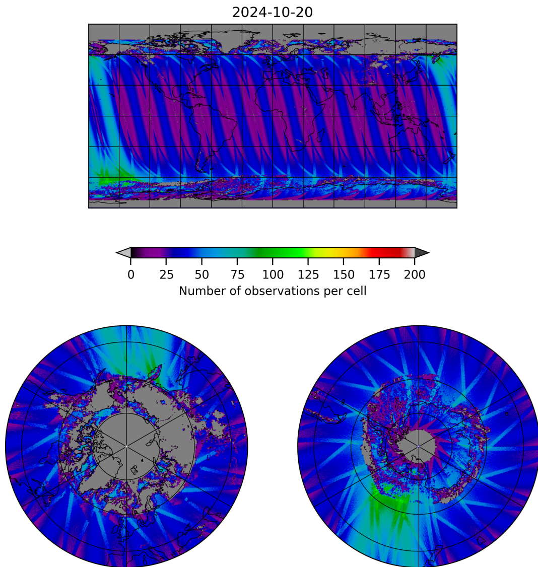
Figure 19: Map of the number of observations for 2024-10-19 to 2024-10-21
