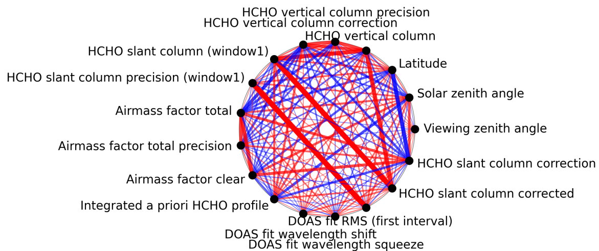
Figure 1: Map of correlation graph for 2024-10-19 to 2024-10-21.
