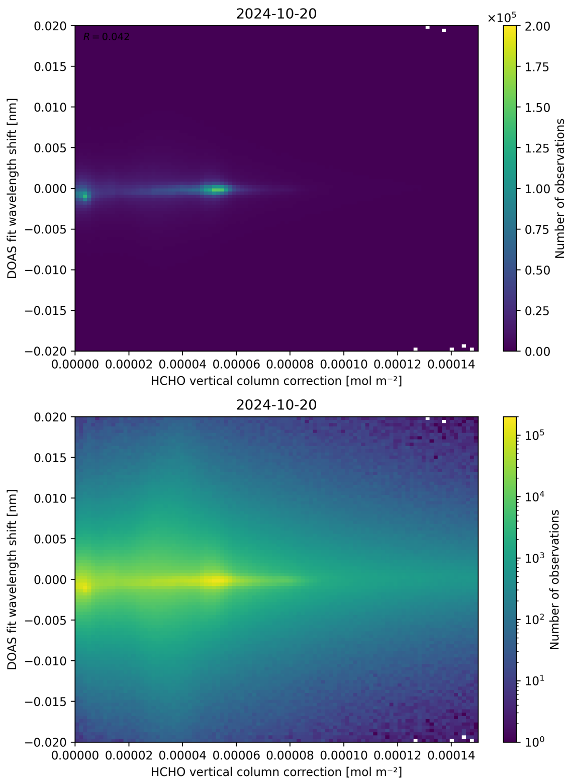
Figure 113: Scatter density plot of “HCHO vertical column correction” against “DOAS fit wavelength shift” for 2024-10-19 to 2024-10-21.
