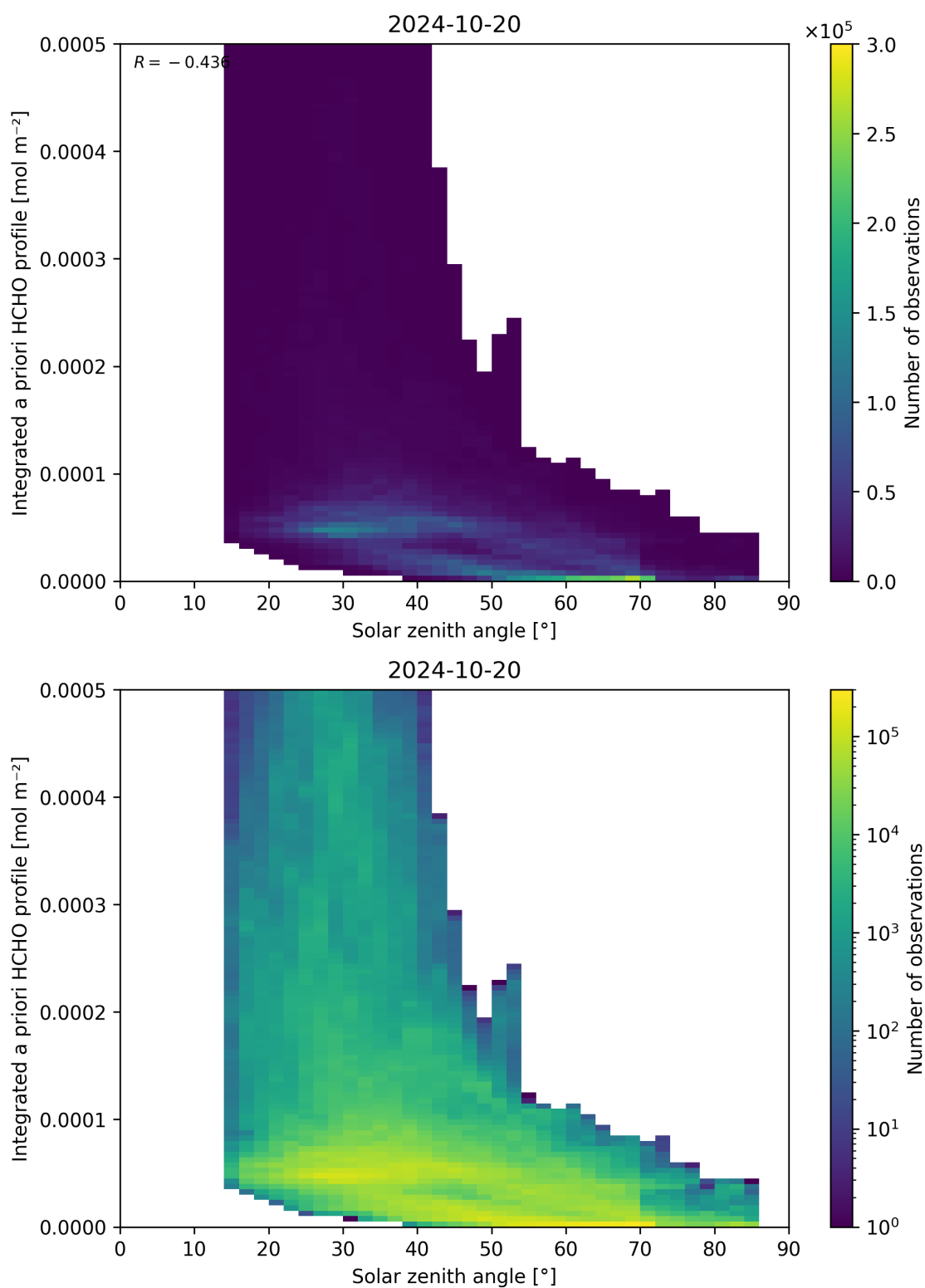
Figure 180: Scatter density plot of “Solar zenith angle” against “Integrated a priori HCHO profile” for 2024-10-19 to 2024-10-21.
