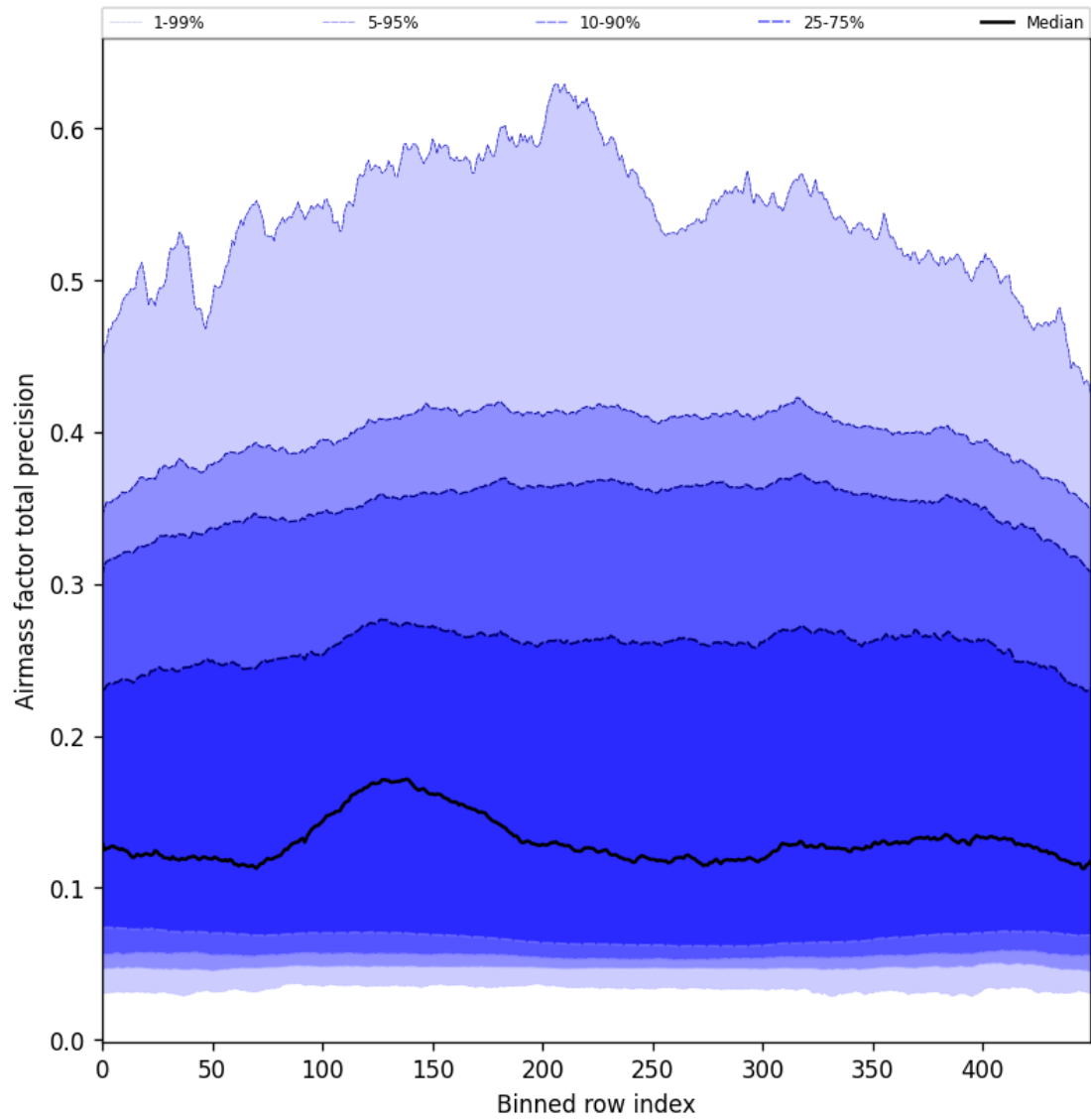
Figure 55: Along track statistics of “Airmass factor total precision” for 2024-10-19 to 2024-10-21
