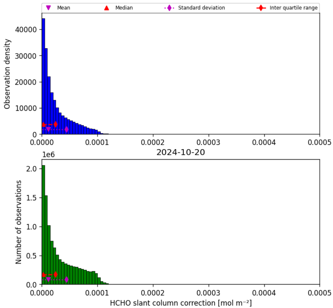
Figure 47: Histogram of “HCHO slant column correction” for 2024-10-19 to 2024-10-21
