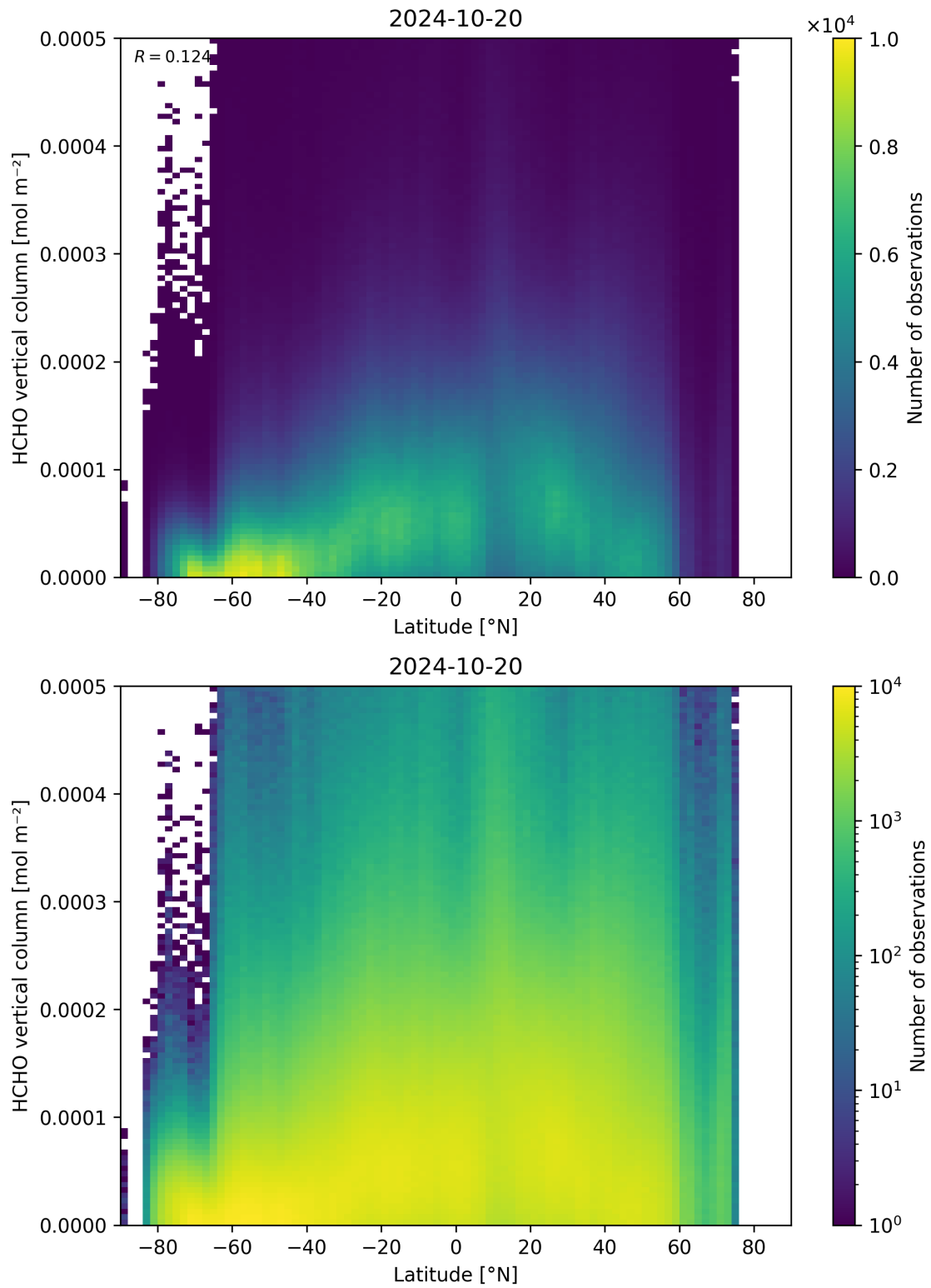
Figure 163: Scatter density plot of “Latitude” against “HCHO vertical column” for 2024-10-19 to 2024-10-21.
