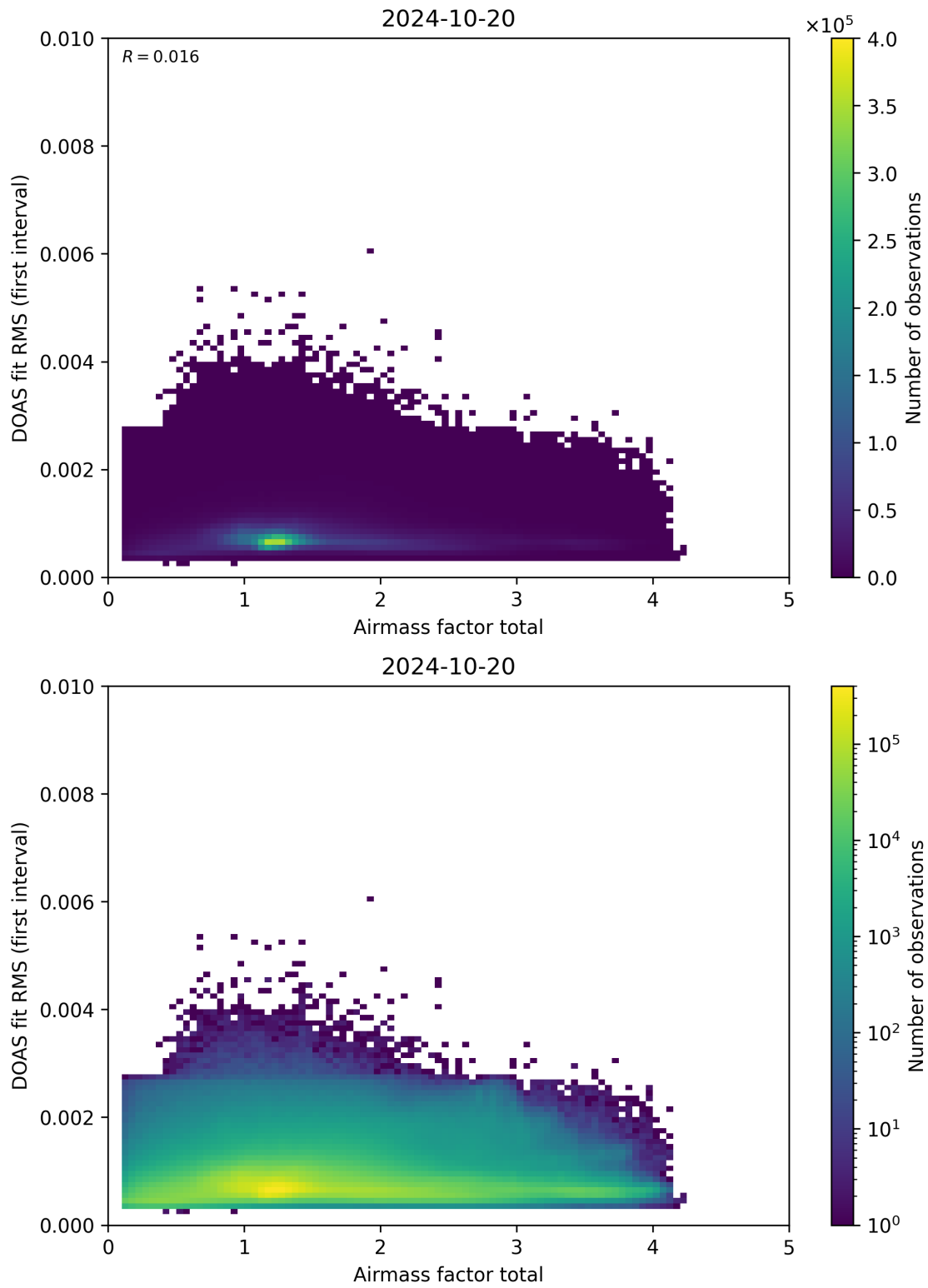
Figure 97: Scatter density plot of “Airmass factor total” against “DOAS fit RMS (first interval)” for 2024-10-19 to 2024-10-21.
