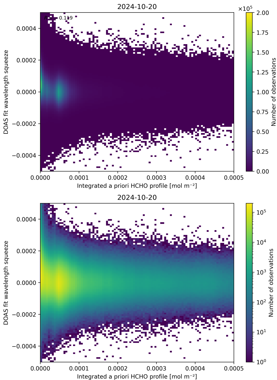
Figure 150: Scatter density plot of “Integrated a priori HCHO profile” against “DOAS fit wavelength squeeze” for 2024-10-19 to 2024-10-21.
