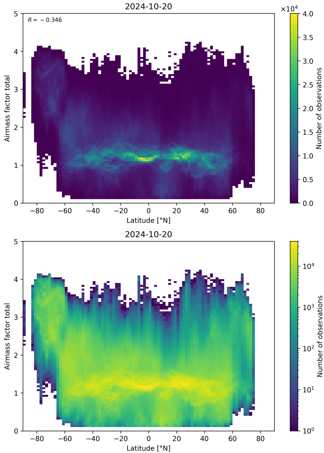
Figure 161: Scatter density plot of “Latitude” against “Airmass factor total” for 2024-10-19 to 2024-10-21.
