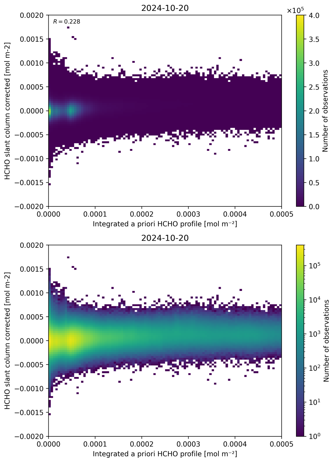
Figure 151: Scatter density plot of “Integrated a priori HCHO profile” against “HCHO slant column corrected” for 2024-10-19 to 2024-10-21.
