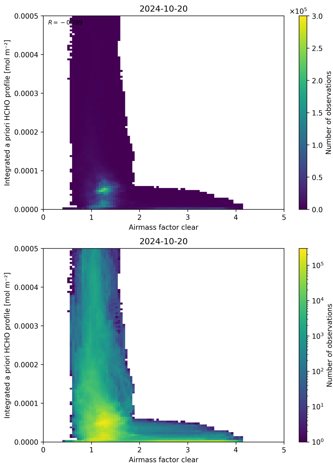
Figure 76: Scatter density plot of “Airmass factor clear” against “Integrated a priori HCHO profile” for 2024-10-19 to 2024-10-21.
