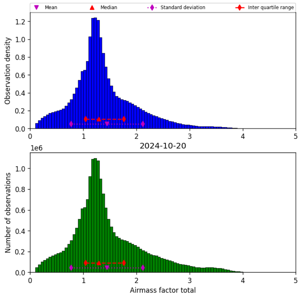
Figure 40: Histogram of “Airmass factor total” for 2024-10-19 to 2024-10-21
