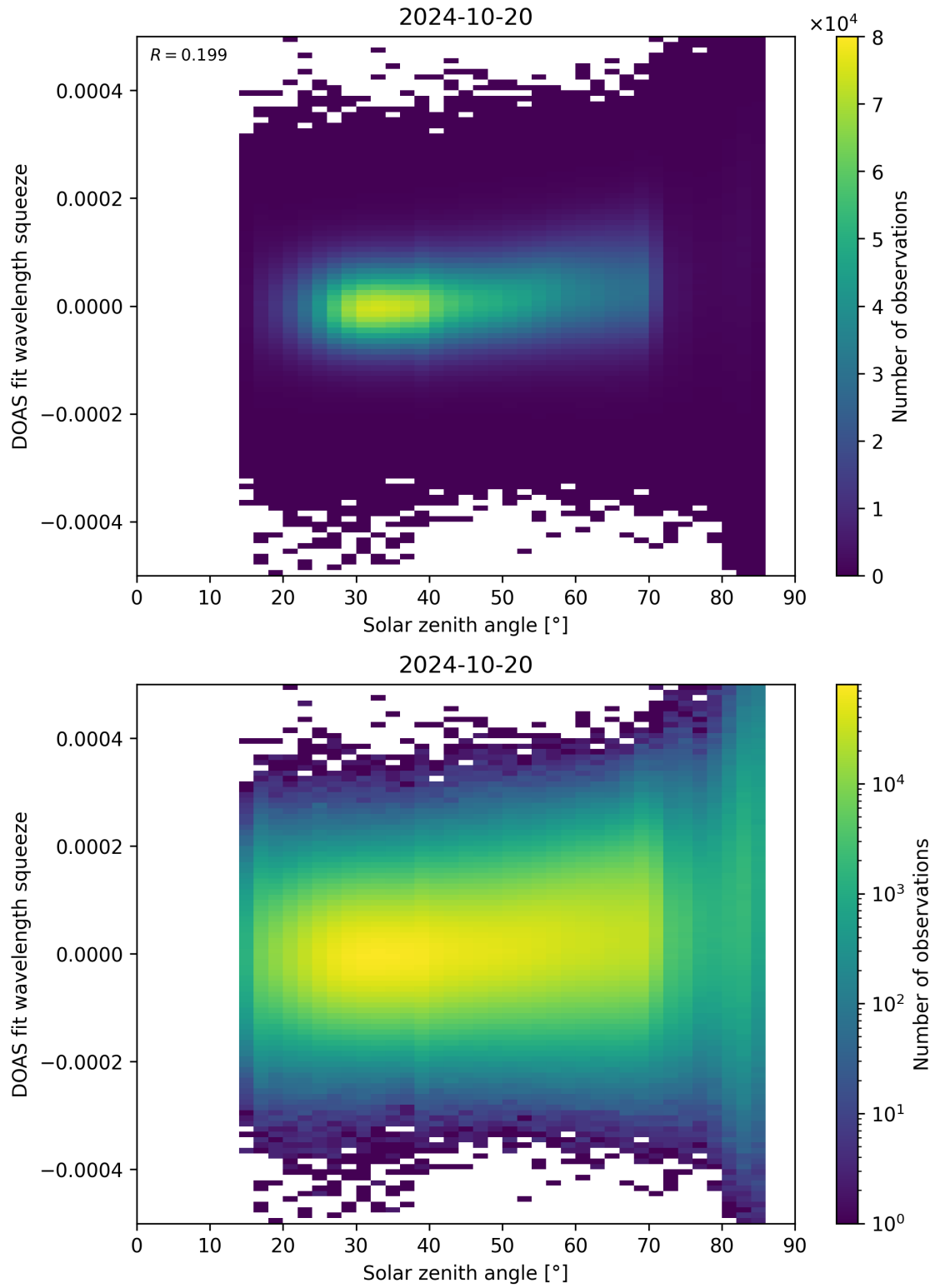
Figure 169: Scatter density plot of “Solar zenith angle” against “DOAS fit wavelength squeeze” for 2024-10-19 to 2024-10-21.
