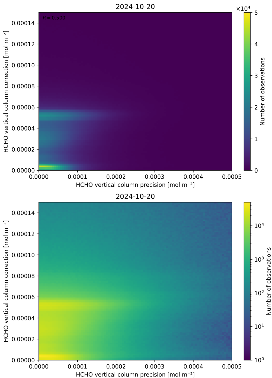
Figure 146: Scatter density plot of “HCHO vertical column precision” against “HCHO vertical column correction” for 2024-10-19 to 2024-10-21.
