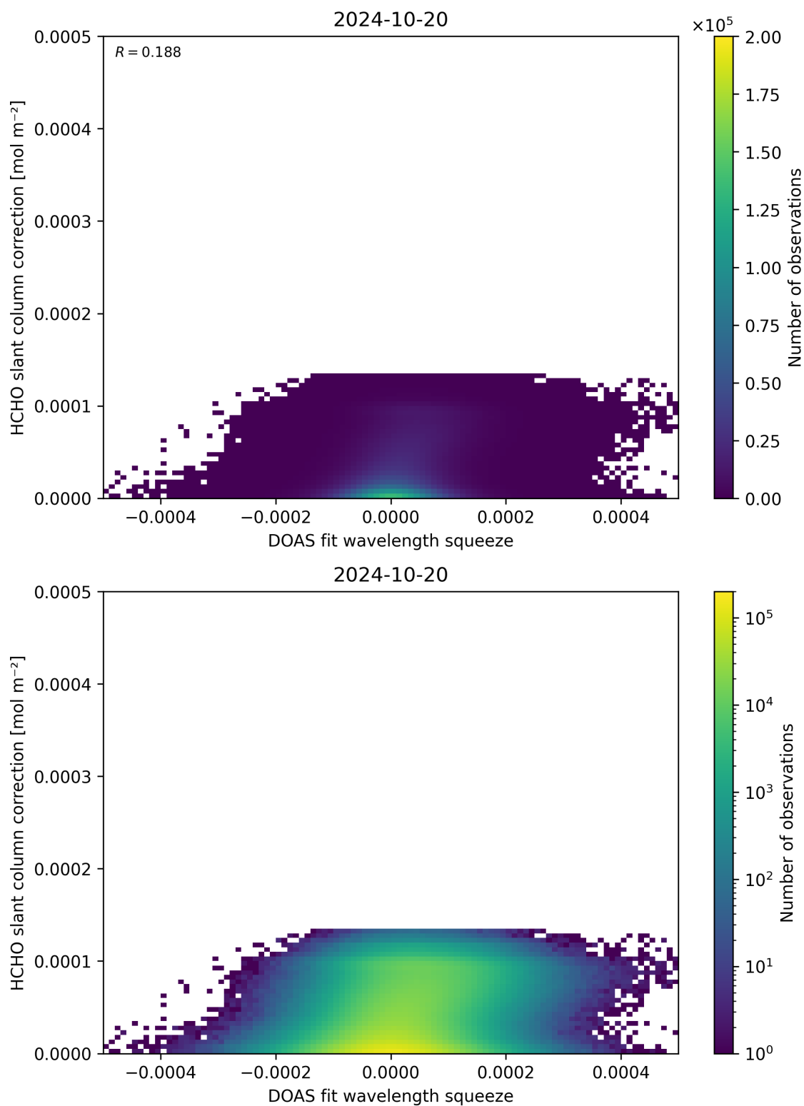
Figure 70: Scatter density plot of “DOAS fit wavelength squeeze” against “HCHO slant column correction” for 2024-10-19 to 2024-10-21.
