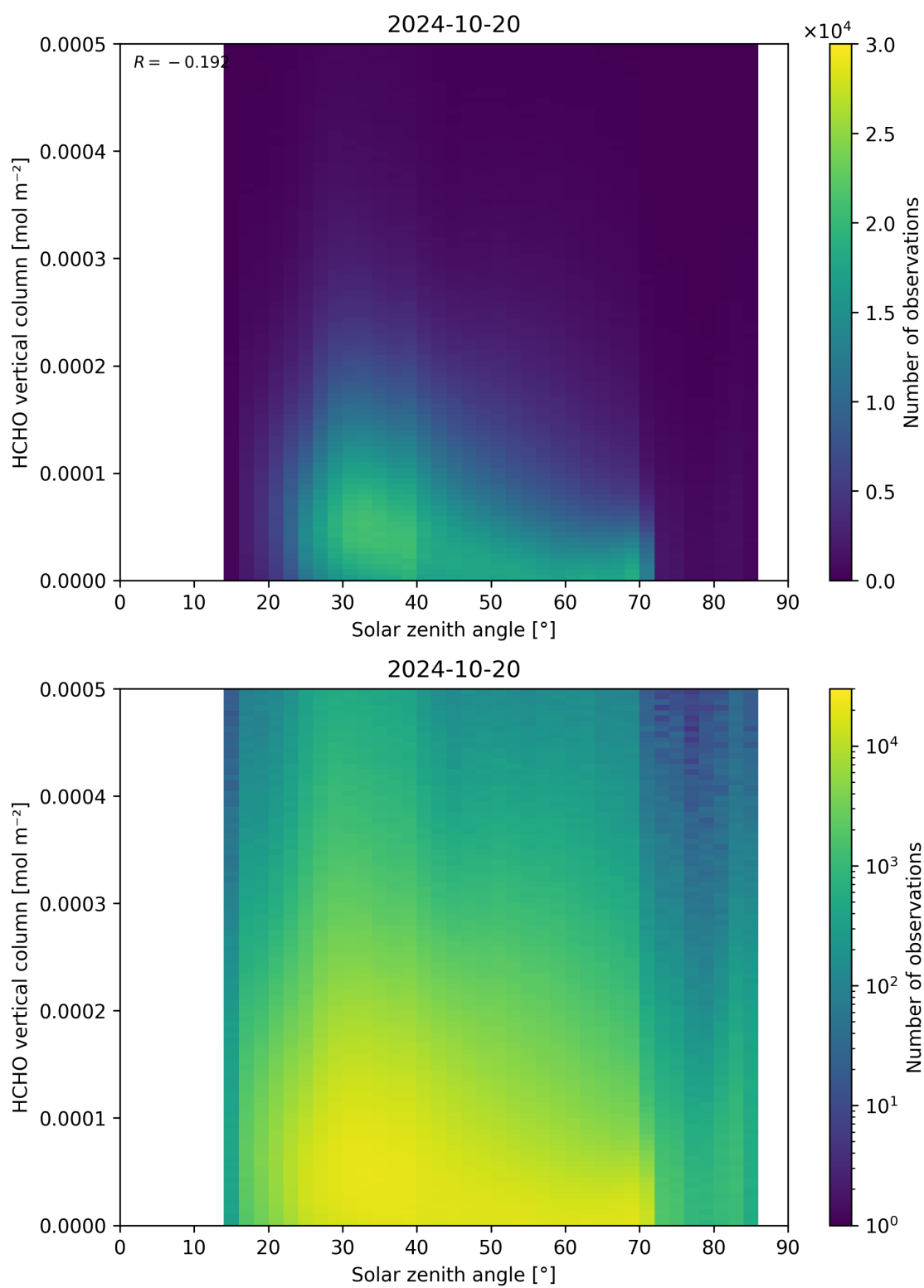
Figure 177: Scatter density plot of “Solar zenith angle” against “HCHO vertical column” for 2024-10-19 to 2024-10-21.
