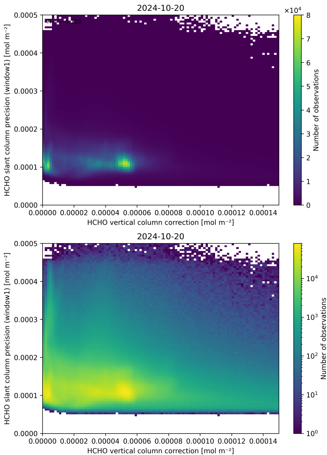
Figure 119: Scatter density plot of “HCHO vertical column correction” against “HCHO slant column precision (window1)” for 2024-10-19 to 2024-10-21.
