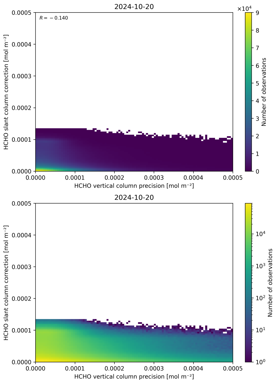
Figure 141: Scatter density plot of “HCHO vertical column precision” against “HCHO slant column correction” for 2024-10-19 to 2024-10-21.
