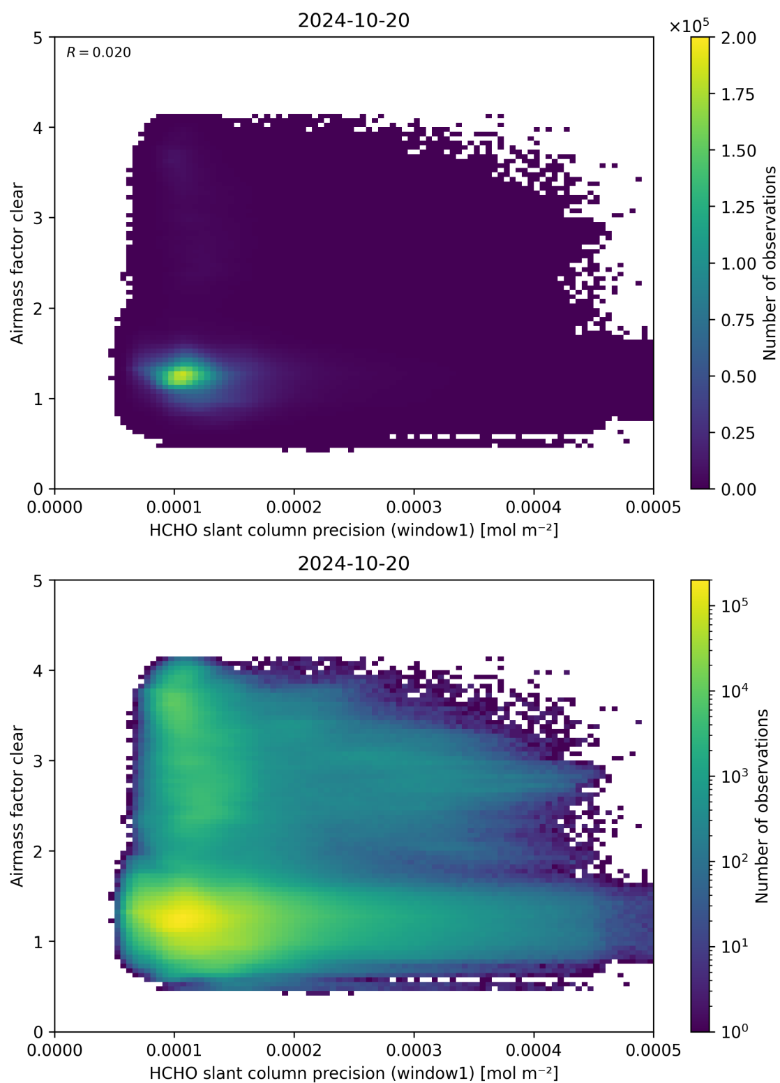
Figure 91: Scatter density plot of “HCHO slant column precision (window1)” against “Airmass factor clear” for 2024-10-19 to 2024-10-21.
