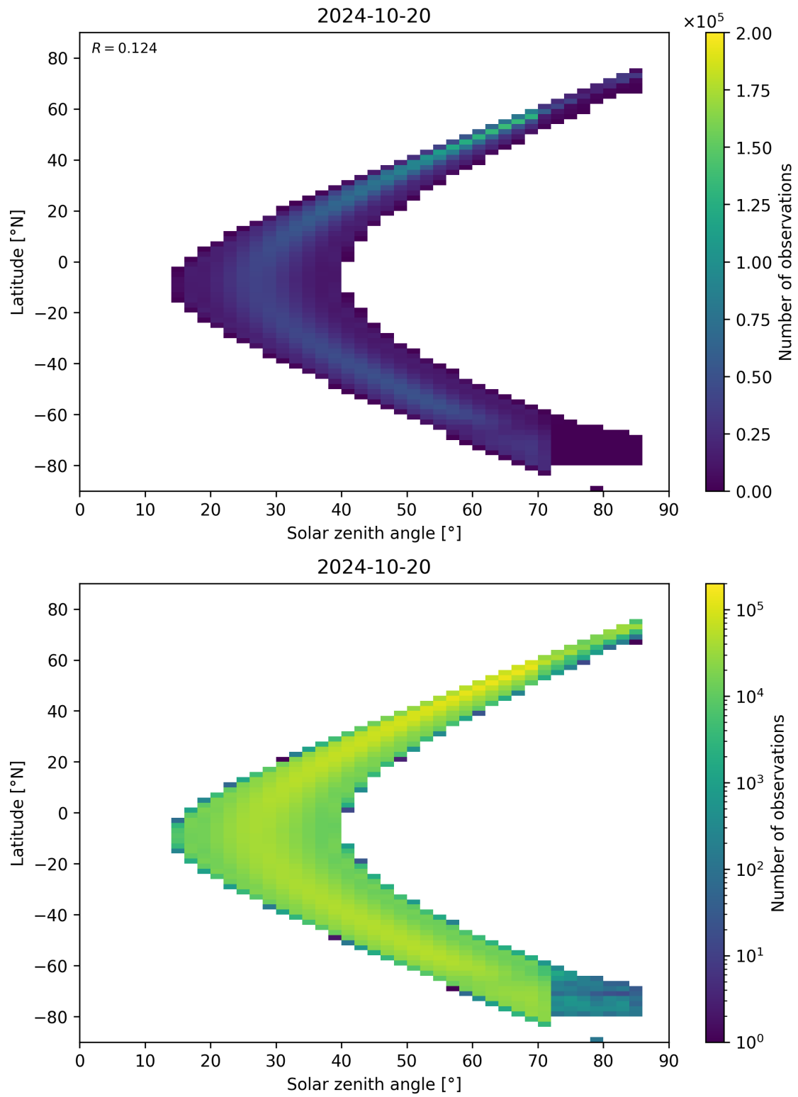
Figure 181: Scatter density plot of “Solar zenith angle” against “Latitude” for 2024-10-19 to 2024-10-21.
