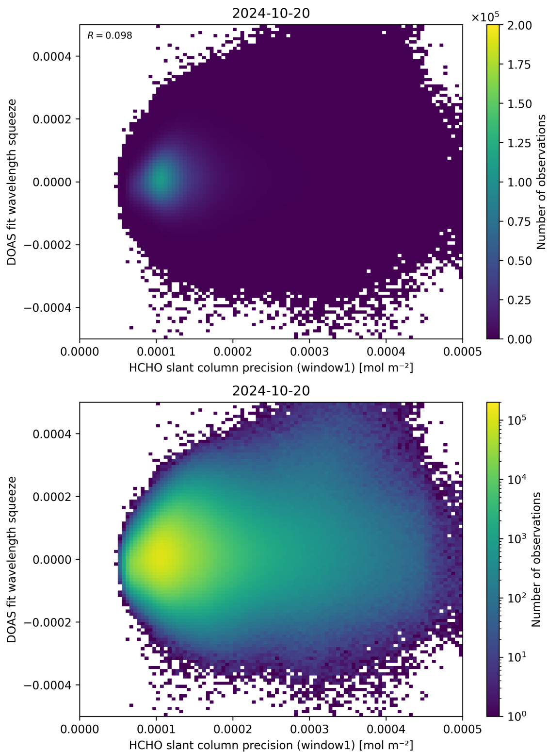
Figure 90: Scatter density plot of “HCHO slant column precision (window1)” against “DOAS fit wavelength squeeze” for 2024-10-19 to 2024-10-21.
