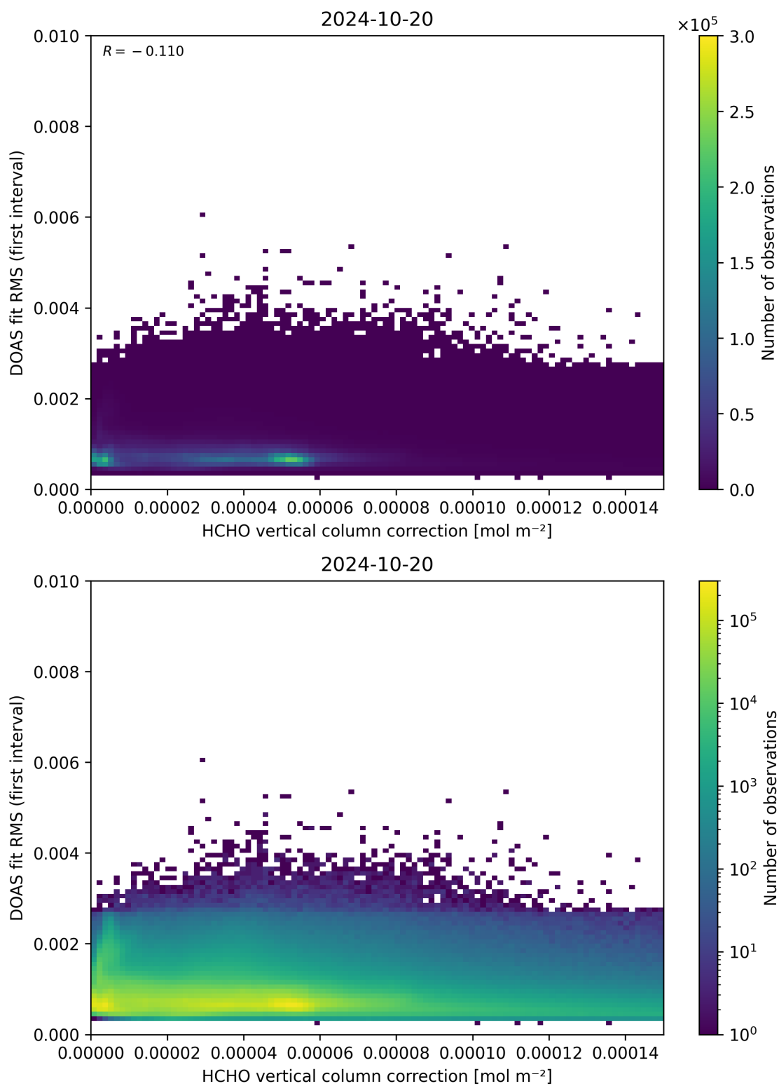
Figure 112: Scatter density plot of “HCHO vertical column correction” against “DOAS fit RMS (first interval)” for 2024-10-19 to 2024-10-21.
