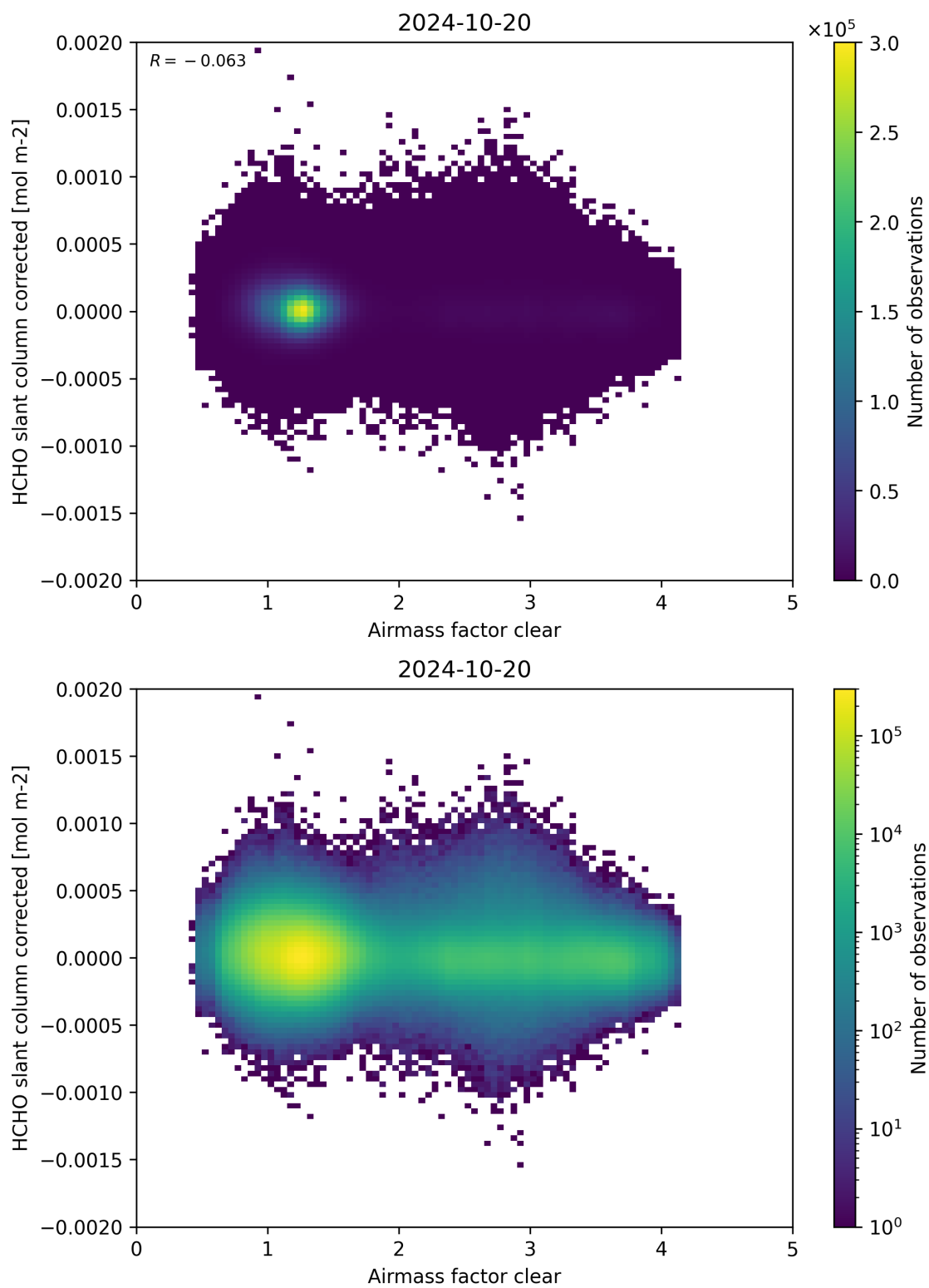
Figure 74: Scatter density plot of “Airmass factor clear” against “HCHO slant column corrected” for 2024-10-19 to 2024-10-21.
