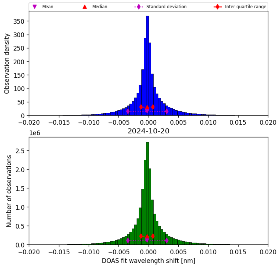
Figure 44: Histogram of “DOAS fit wavelength shift” for 2024-10-19 to 2024-10-21
