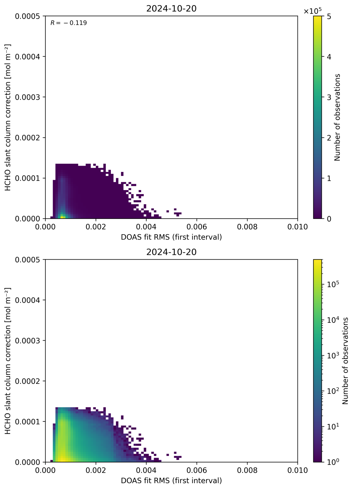
Figure 63: Scatter density plot of “DOAS fit RMS (first interval)” against “HCHO slant column correction” for 2024-10-19 to 2024-10-21.
