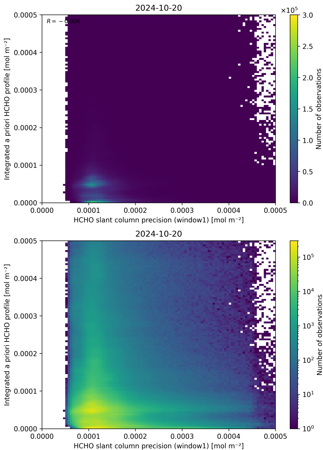
Figure 96: Scatter density plot of “HCHO slant column precision (window1)” against “Integrated a priori HCHO profile” for 2024-10-19 to 2024-10-21.
