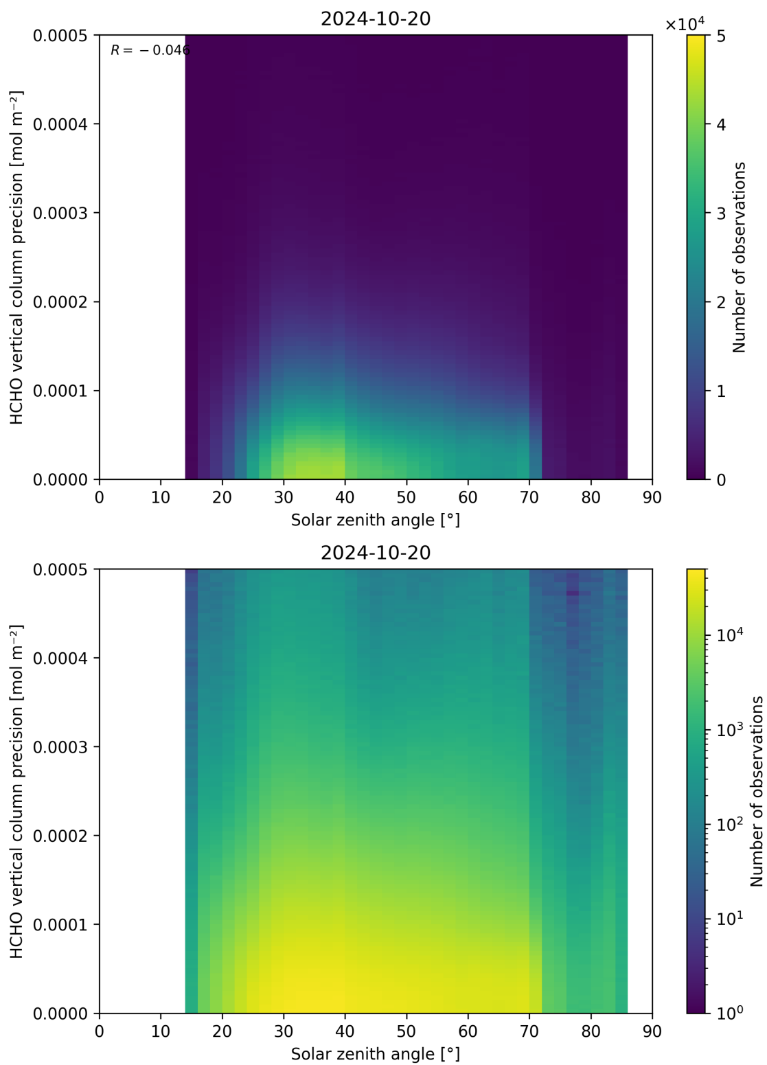
Figure 179: Scatter density plot of “Solar zenith angle” against “HCHO vertical column precision” for 2024-10-19 to 2024-10-21.
