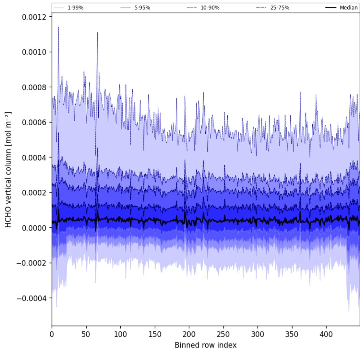
Figure 49: Along track statistics of “HCHO vertical column” for 2024-10-19 to 2024-10-21
