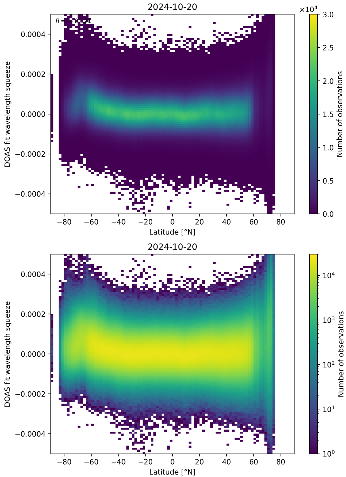
Figure 155: Scatter density plot of “Latitude” against “DOAS fit wavelength squeeze” for 2024-10-19 to 2024-10-21.
