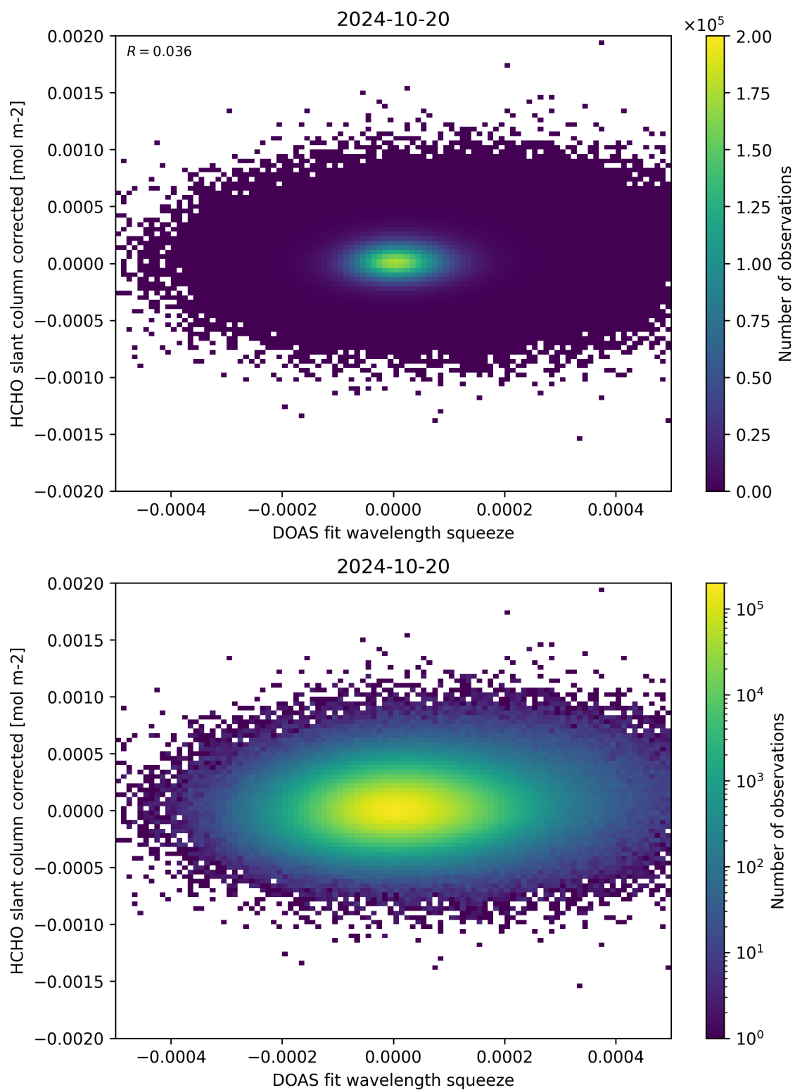
Figure 69: Scatter density plot of “DOAS fit wavelength squeeze” against “HCHO slant column corrected” for 2024-10-19 to 2024-10-21.
