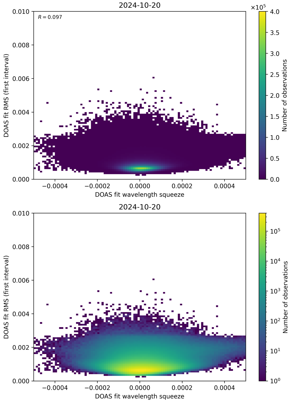
Figure 68: Scatter density plot of “DOAS fit wavelength squeeze” against “DOAS fit RMS (first interval)” for 2024-10-19 to 2024-10-21.
