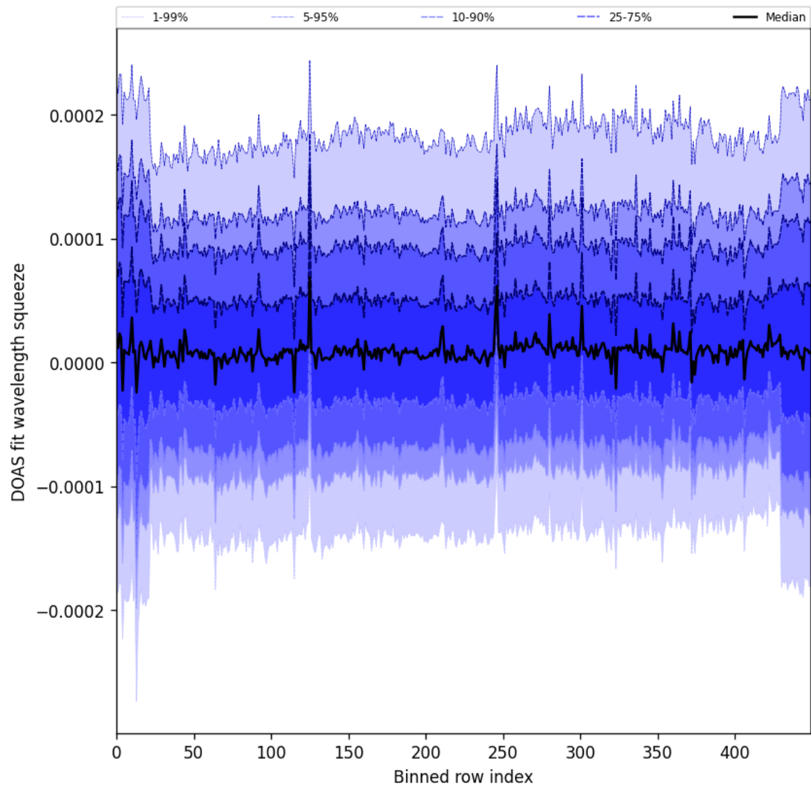
Figure 59: Along track statistics of “DOAS fit wavelength squeeze” for 2024-10-20 to 2024-10-22
