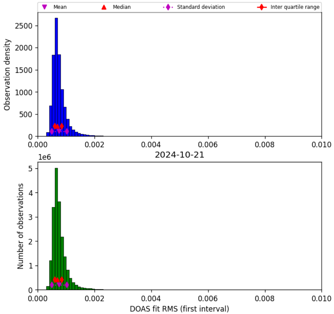
Figure 46: Histogram of “DOAS fit RMS (first interval)” for 2024-10-20 to 2024-10-22
