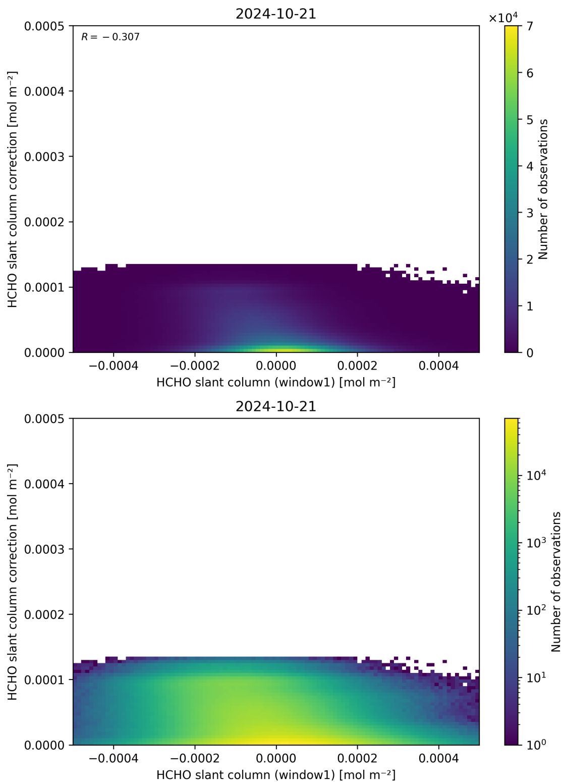
Figure 83: Scatter density plot of “HCHO slant column (window1)” against “HCHO slant column correction” for 2024-10-20 to 2024-10-22.
