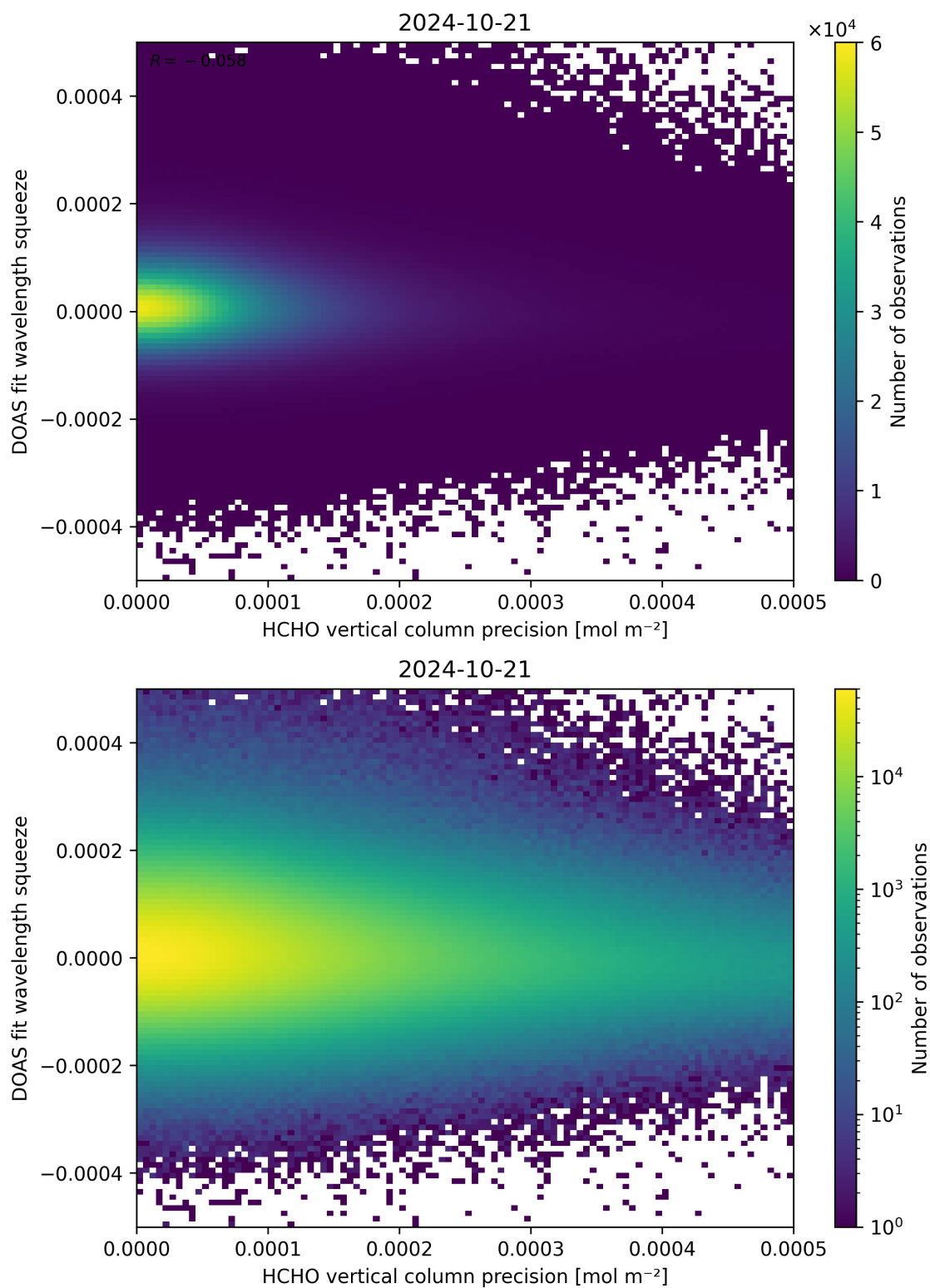
Figure 138: Scatter density plot of “HCHO vertical column precision” against “DOAS fit wavelength squeeze” for 2024-10-20 to 2024-10-22.
