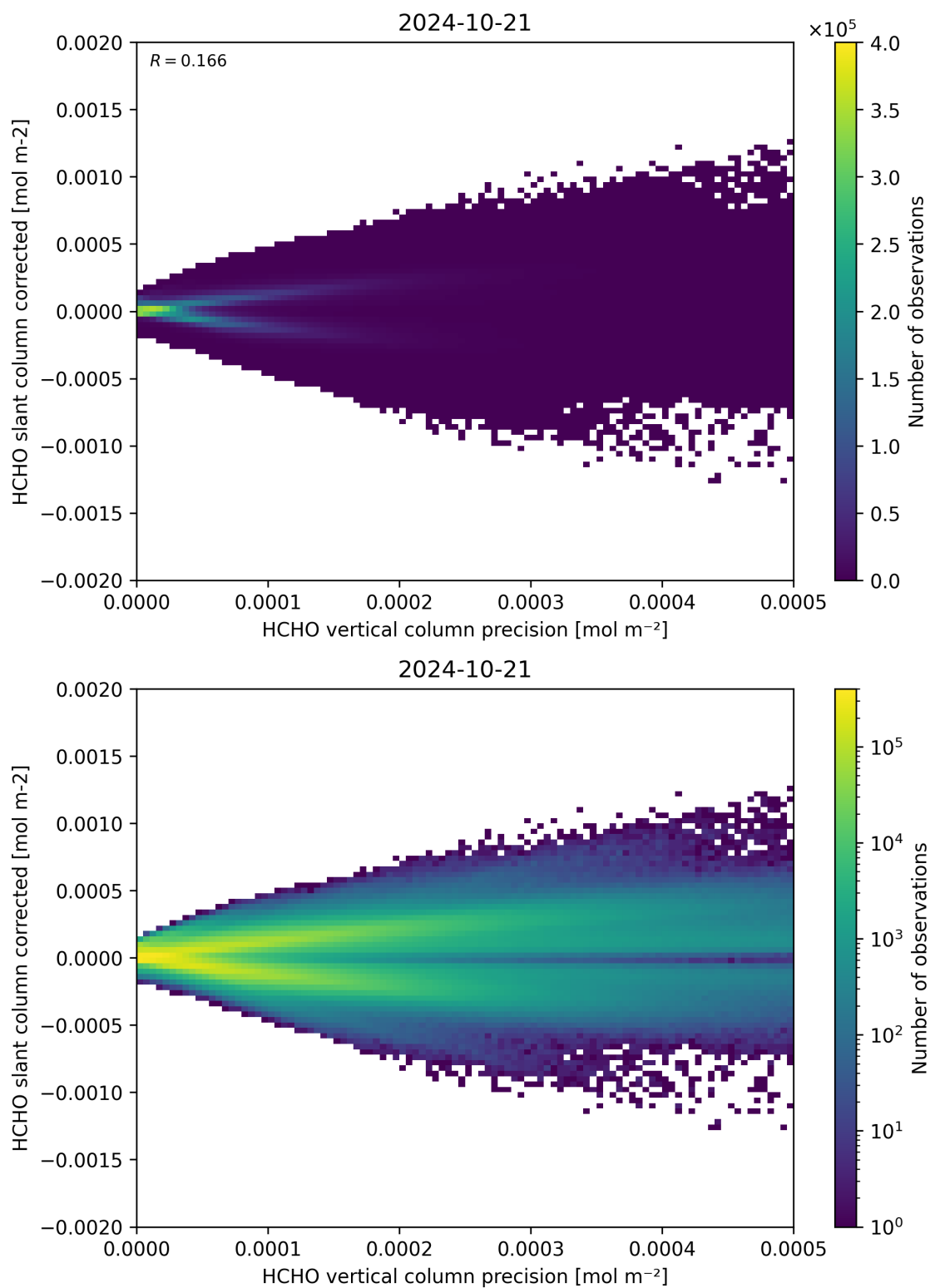
Figure 140: Scatter density plot of “HCHO vertical column precision” against “HCHO slant column corrected” for 2024-10-20 to 2024-10-22.
