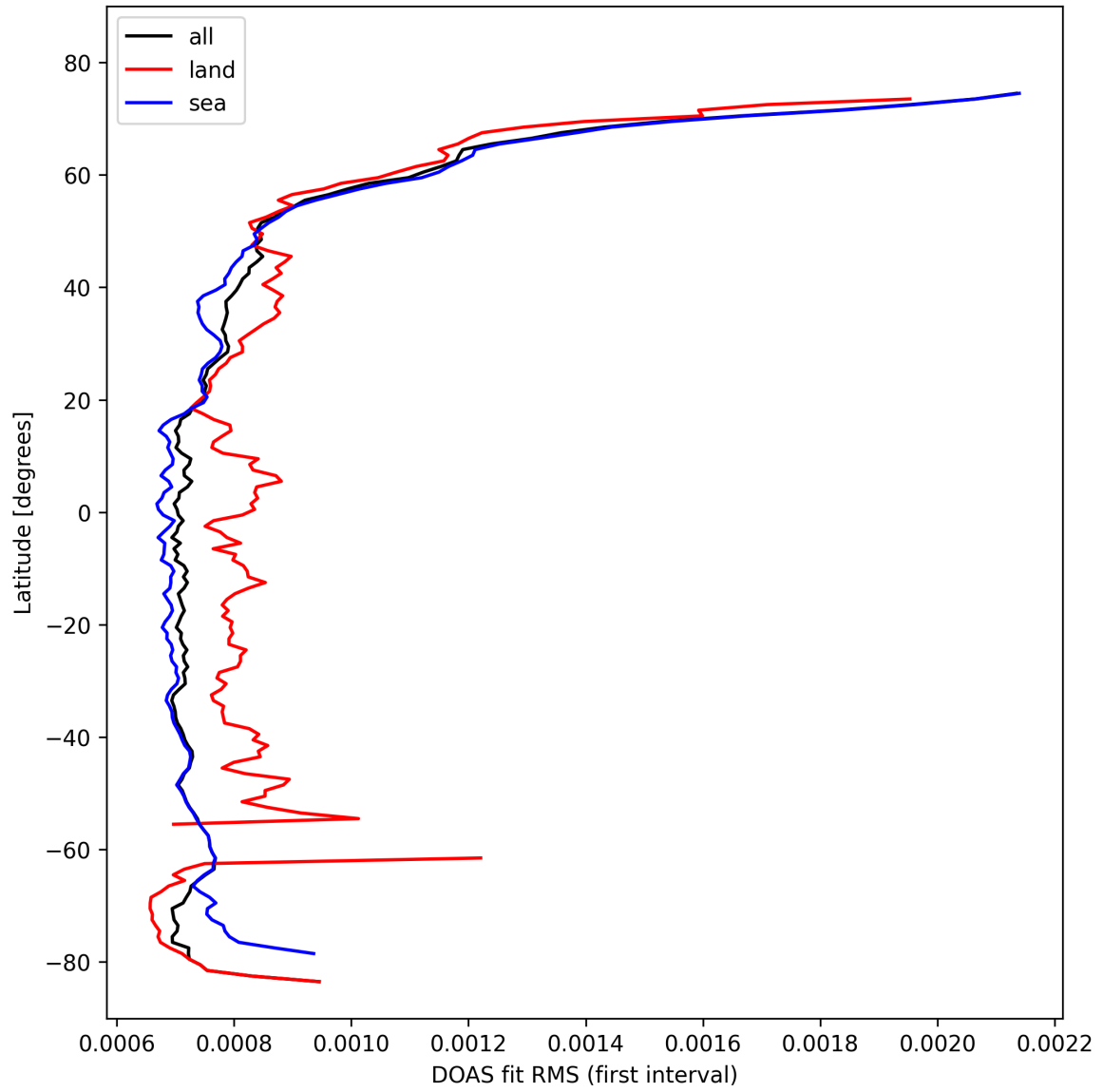
Figure 32: Zonal average of “DOAS fit RMS (first interval)” for 2024-10-20 to 2024-10-22.
