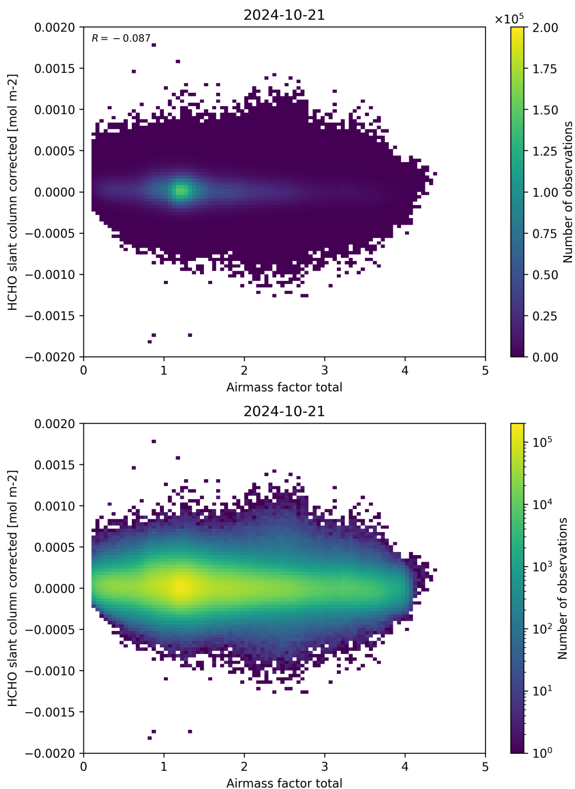
Figure 101: Scatter density plot of “Airmass factor total” against “HCHO slant column corrected” for 2024-10-20 to 2024-10-22.
