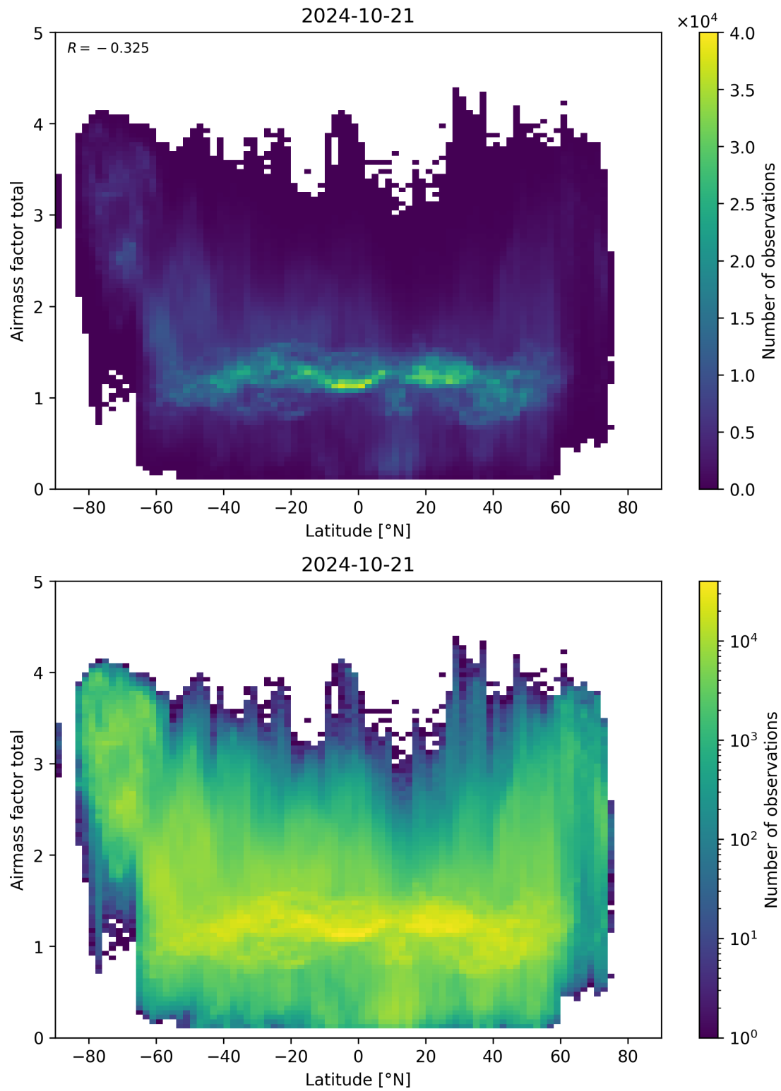
Figure 161: Scatter density plot of “Latitude” against “Airmass factor total” for 2024-10-20 to 2024-10-22.
