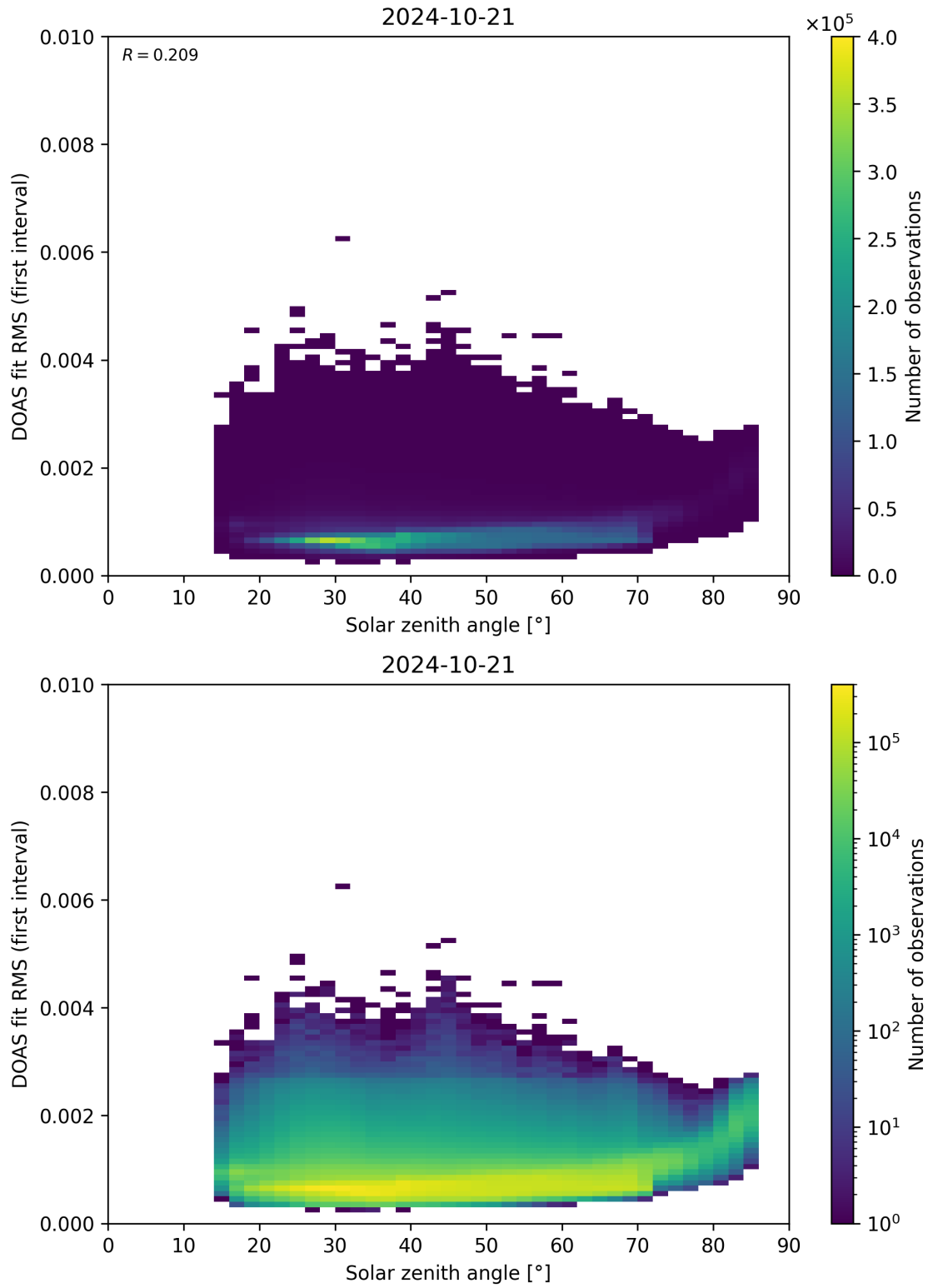
Figure 167: Scatter density plot of “Solar zenith angle” against “DOAS fit RMS (first interval)” for 2024-10-20 to 2024-10-22.
