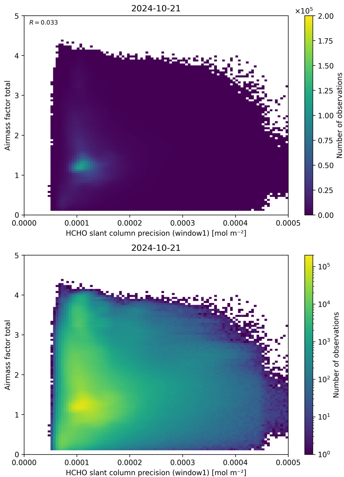
Figure 94: Scatter density plot of “HCHO slant column precision (window1)” against “Airmass factor total” for 2024-10-20 to 2024-10-22.
