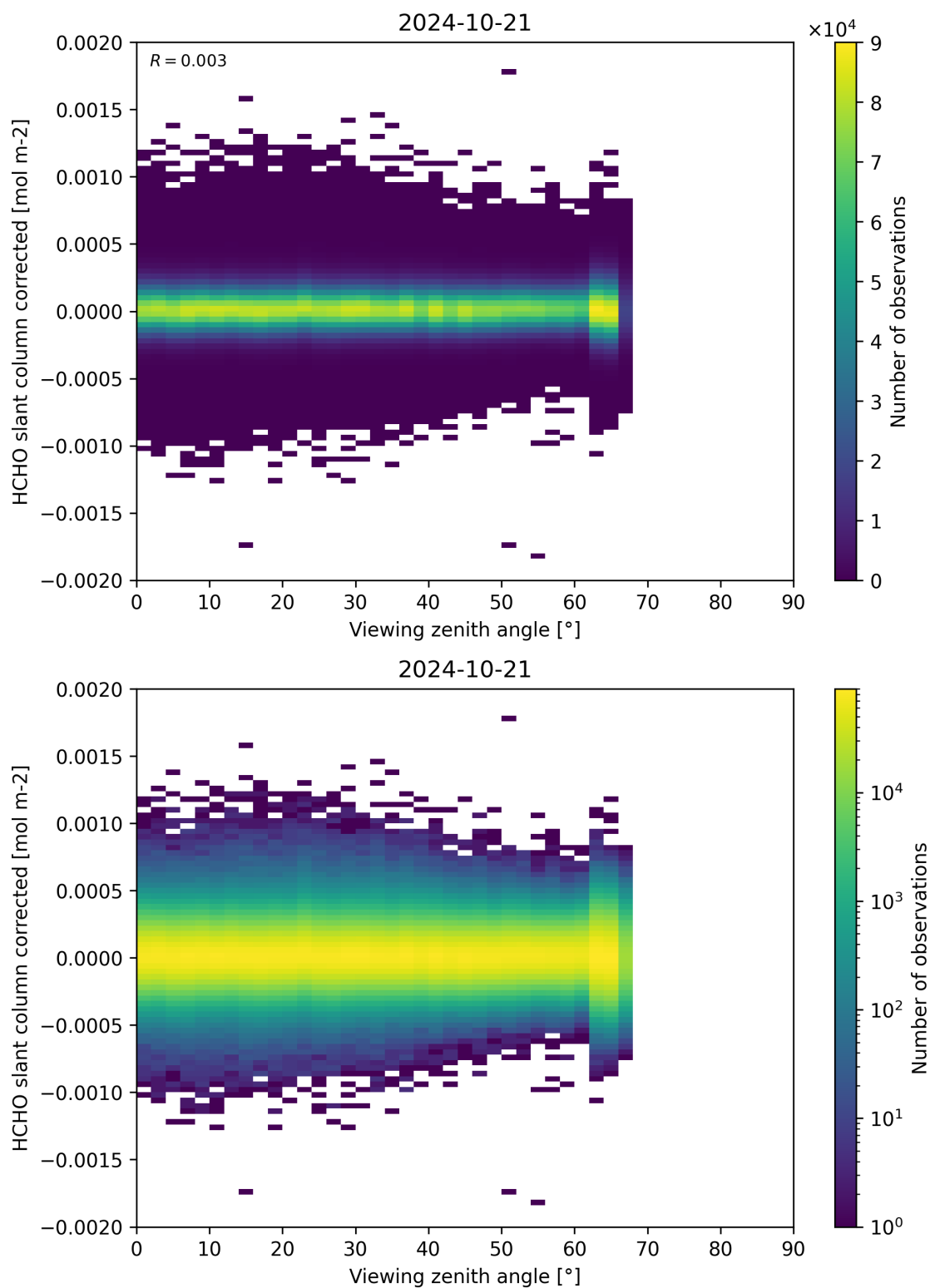
Figure 186: Scatter density plot of “Viewing zenith angle” against “HCHO slant column corrected” for 2024-10-20 to 2024-10-22.
