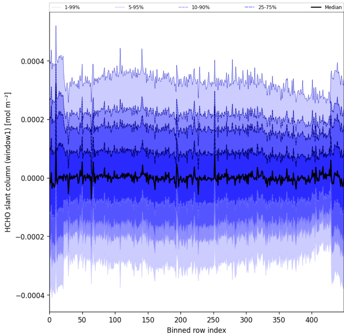
Figure 52: Along track statistics of “HCHO slant column (window1)” for 2024-10-20 to 2024-10-22
