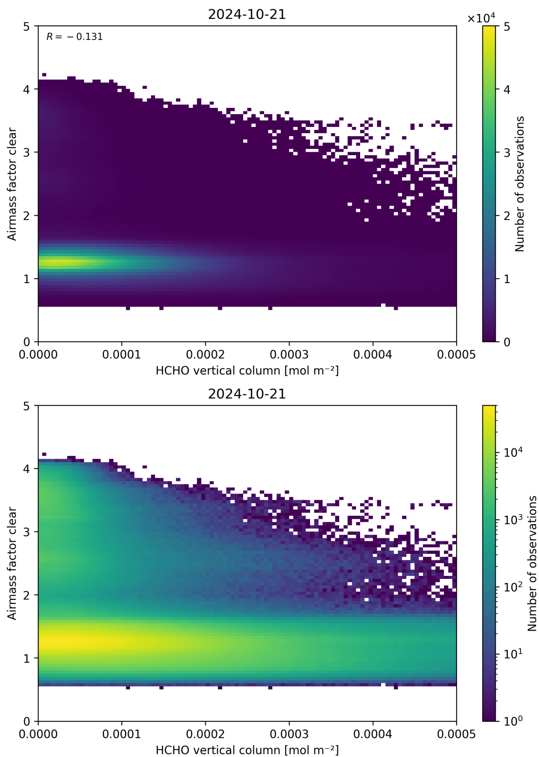
Figure 126: Scatter density plot of “HCHO vertical column” against “Airmass factor clear” for 2024-10-20 to 2024-10-22.
