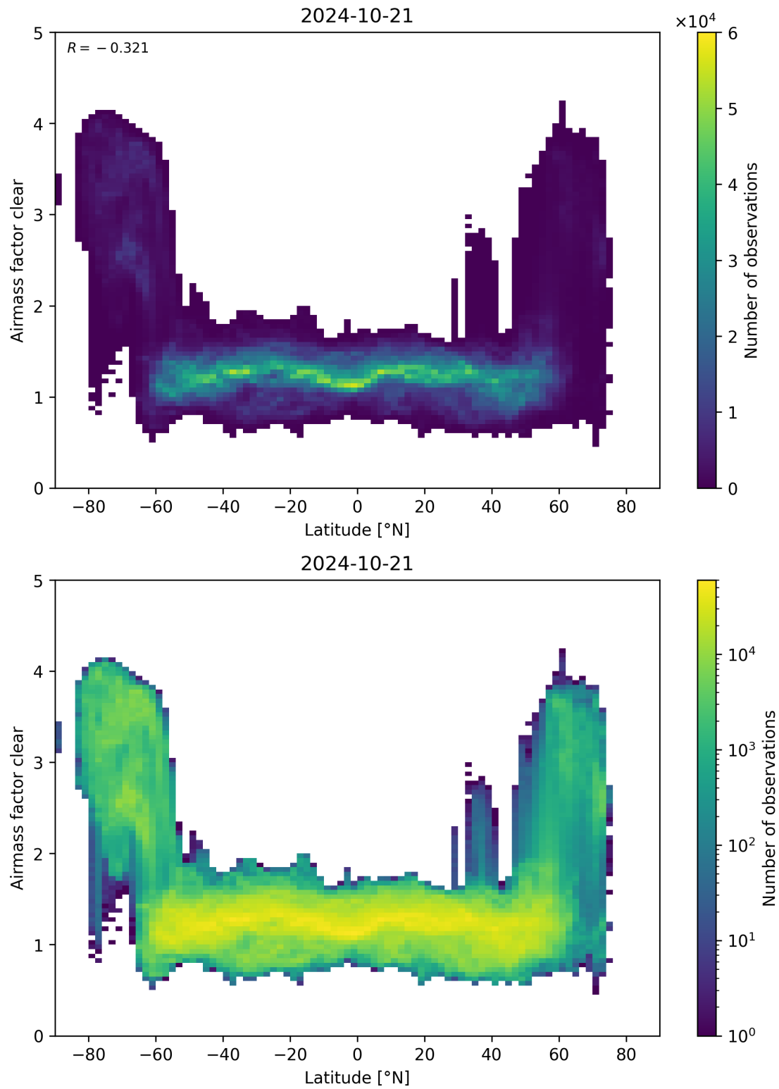
Figure 156: Scatter density plot of “Latitude” against “Airmass factor clear” for 2024-10-20 to 2024-10-22.
