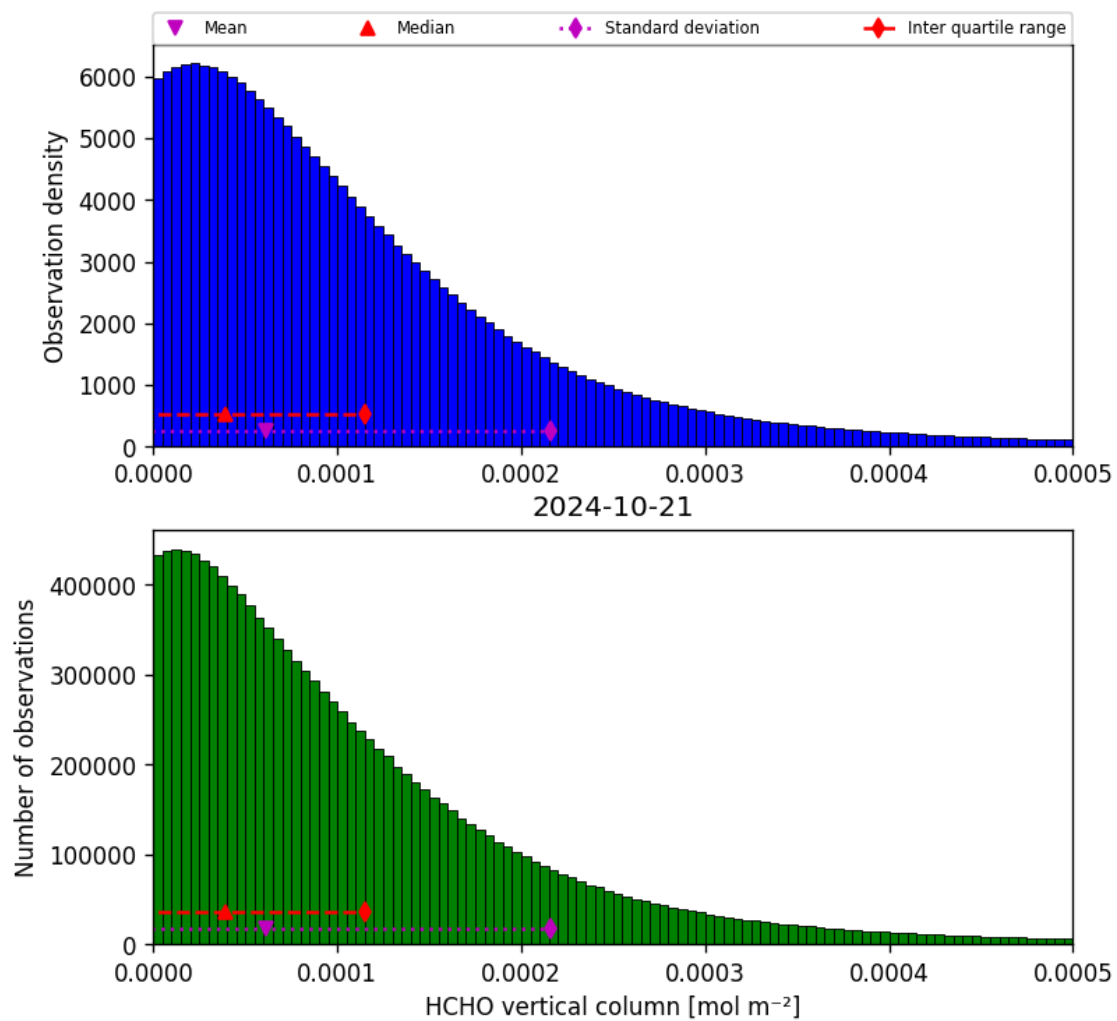
Figure 35: Histogram of “HCHO vertical column” for 2024-10-20 to 2024-10-22
