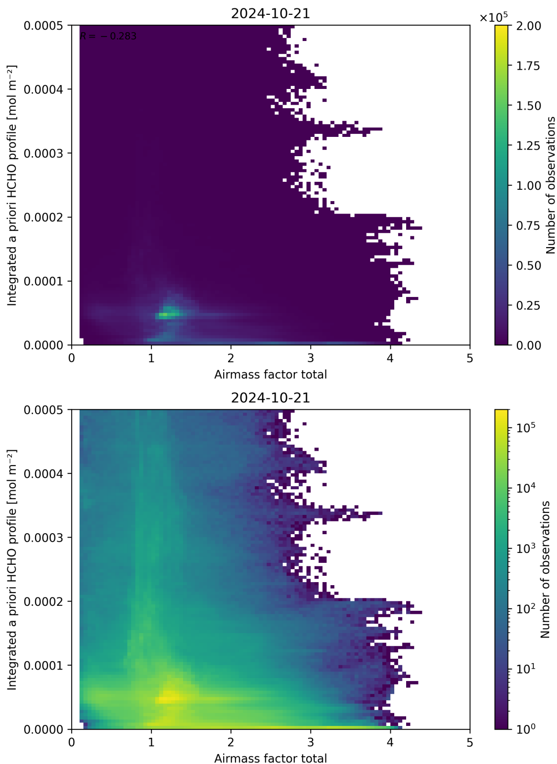
Figure 104: Scatter density plot of “Airmass factor total” against “Integrated a priori HCHO profile” for 2024-10-20 to 2024-10-22.
