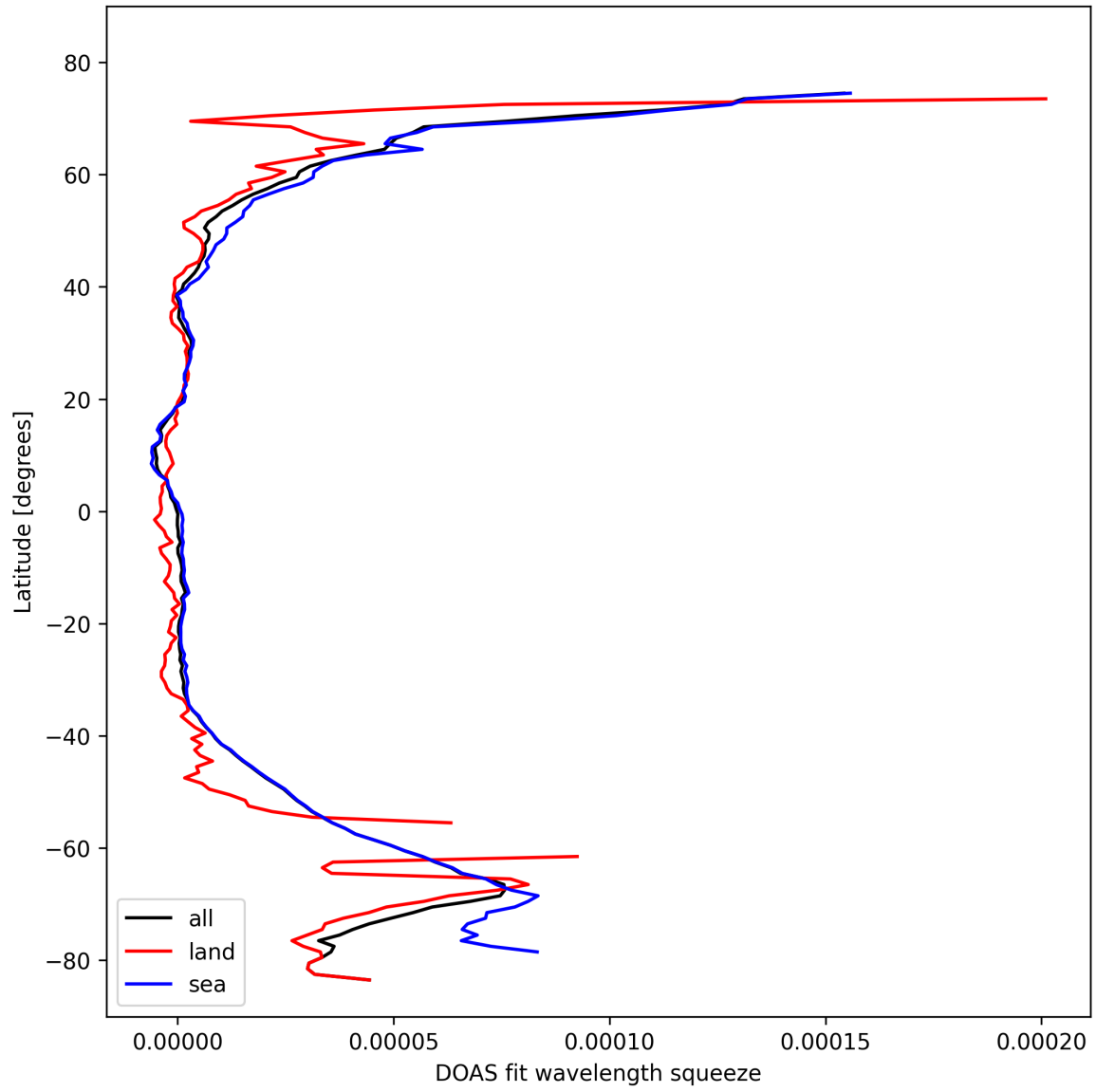
Figure 31: Zonal average of “DOAS fit wavelength squeeze” for 2024-10-20 to 2024-10-22.
