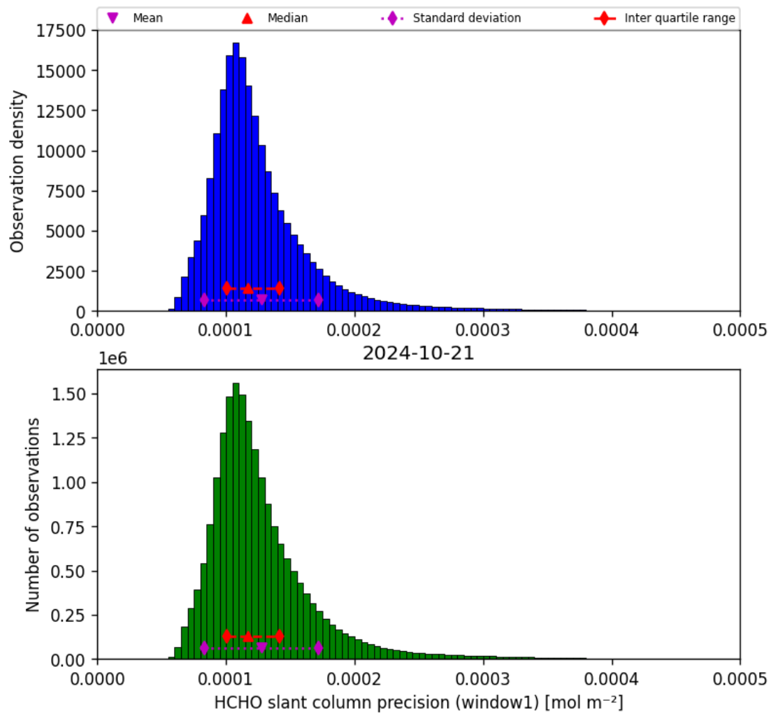
Figure 39: Histogram of “HCHO slant column precision (window1)” for 2024-10-20 to 2024-10-22
