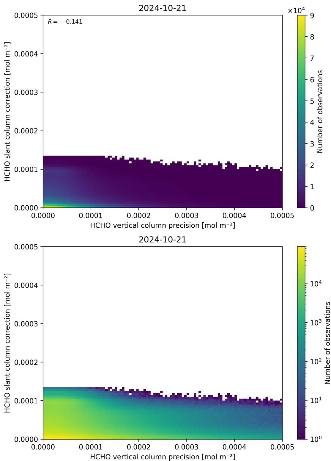
Figure 141: Scatter density plot of “HCHO vertical column precision” against “HCHO slant column correction” for 2024-10-20 to 2024-10-22.
