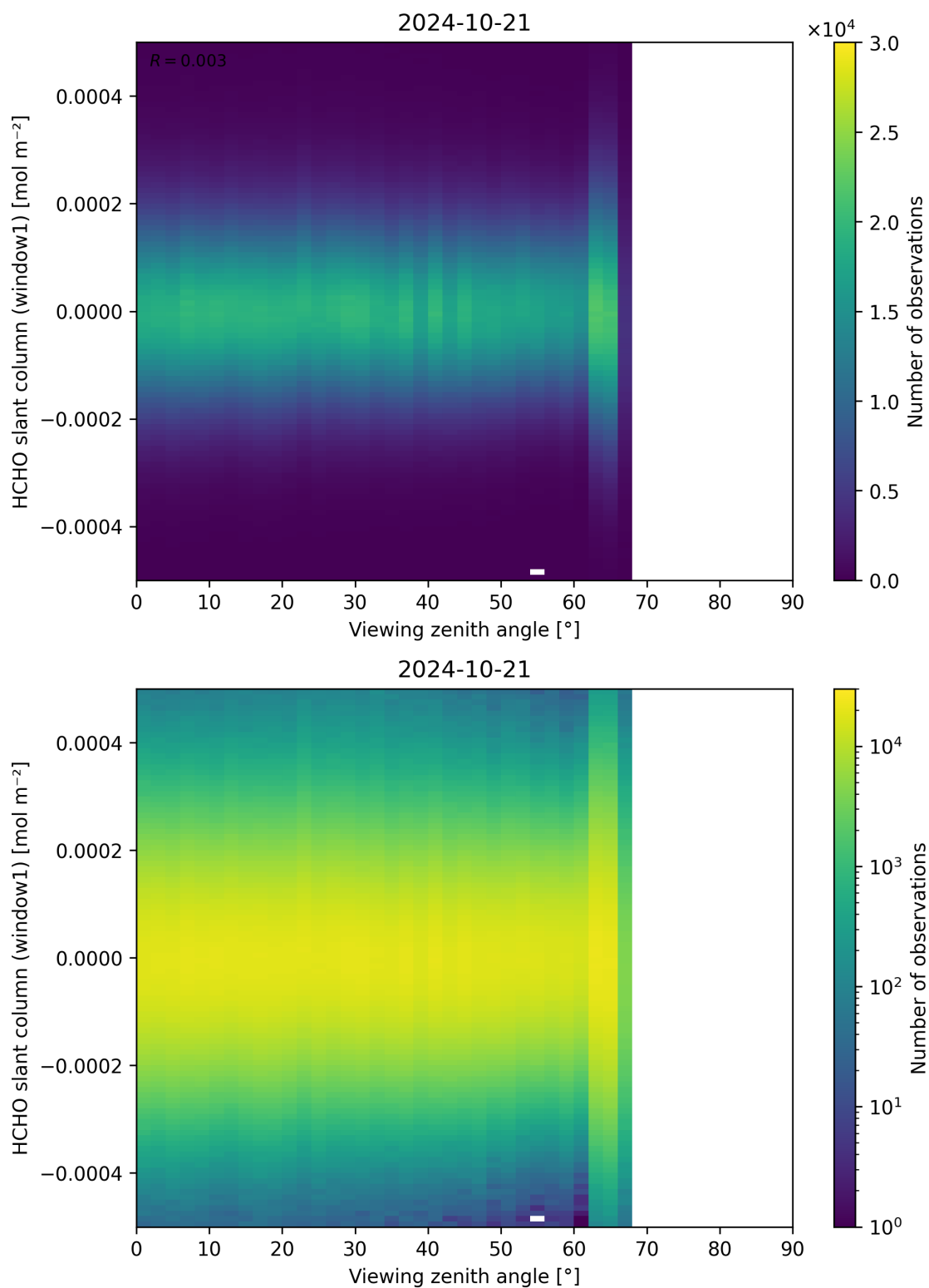
Figure 188: Scatter density plot of “Viewing zenith angle” against “HCHO slant column (window1)” for 2024-10-20 to 2024-10-22.
