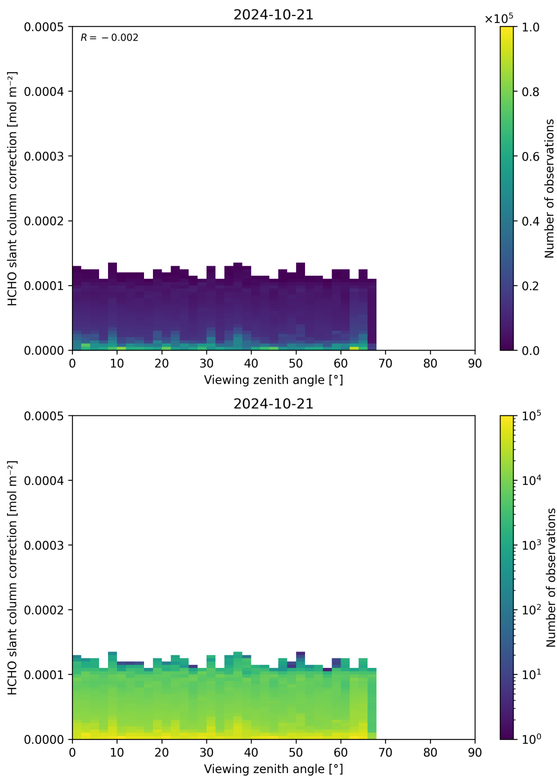
Figure 187: Scatter density plot of “Viewing zenith angle” against “HCHO slant column correction” for 2024-10-20 to 2024-10-22.
