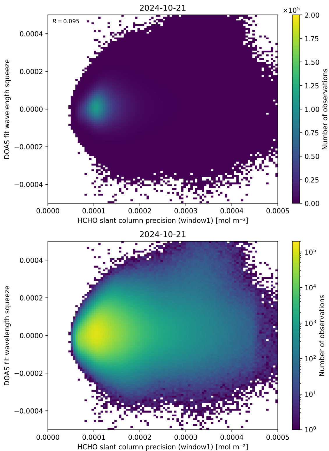
Figure 90: Scatter density plot of “HCHO slant column precision (window1)” against “DOAS fit wavelength squeeze” for 2024-10-20 to 2024-10-22.
