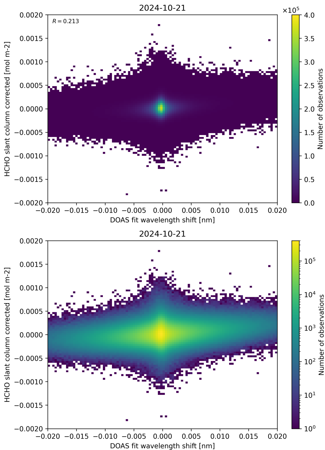
Figure 66: Scatter density plot of “DOAS fit wavelength shift” against “HCHO slant column corrected” for 2024-10-20 to 2024-10-22.
