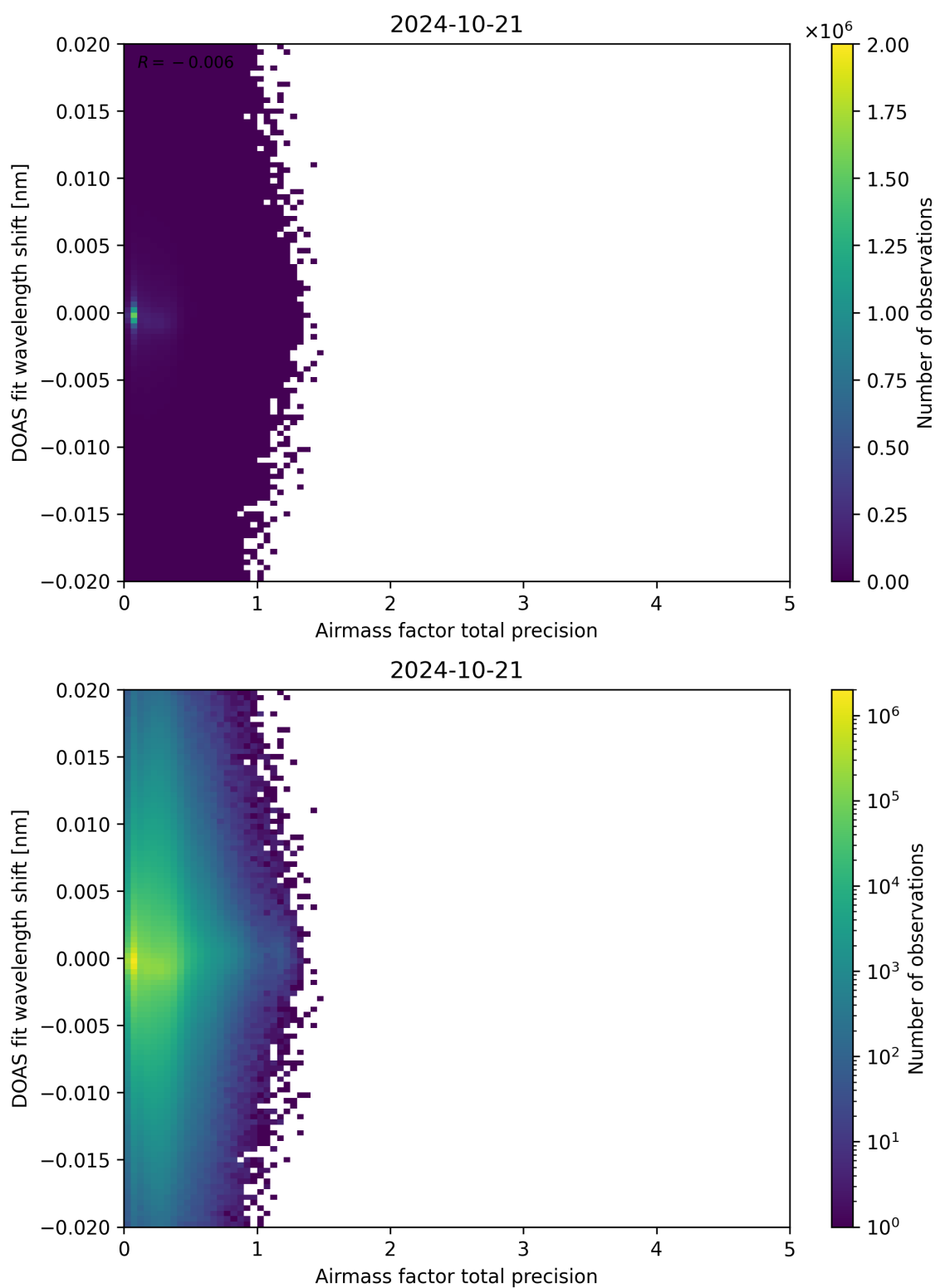
Figure 106: Scatter density plot of “Airmass factor total precision” against “DOAS fit wavelength shift” for 2024-10-20 to 2024-10-22.
