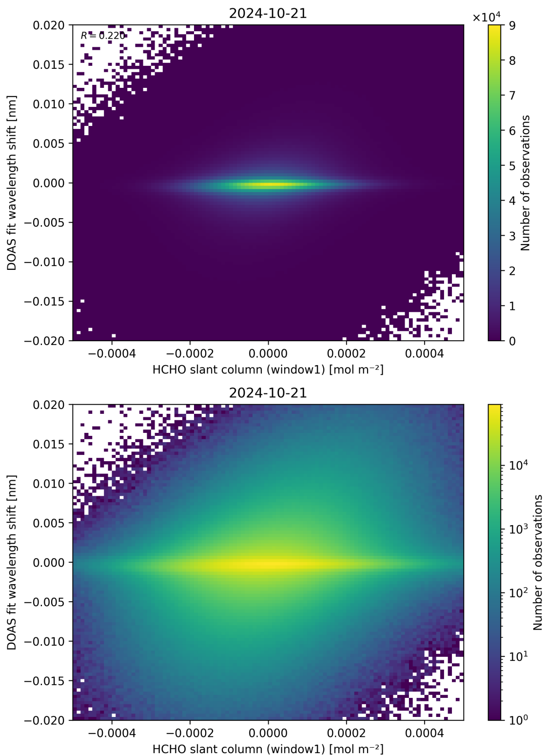
Figure 79: Scatter density plot of “HCHO slant column (window1)” against “DOAS fit wavelength shift” for 2024-10-20 to 2024-10-22.
