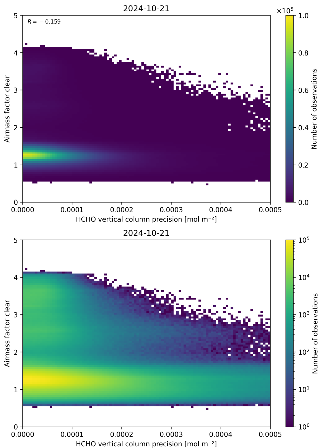
Figure 139: Scatter density plot of “HCHO vertical column precision” against “Airmass factor clear” for 2024-10-20 to 2024-10-22.
