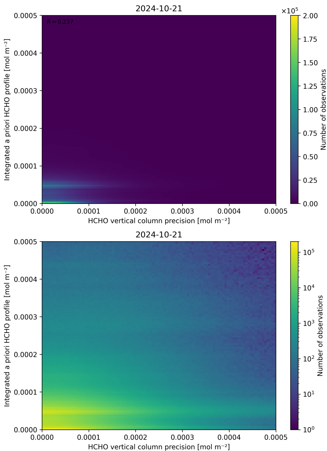
Figure 147: Scatter density plot of “HCHO vertical column precision” against “Integrated a priori HCHO profile” for 2024-10-20 to 2024-10-22.
