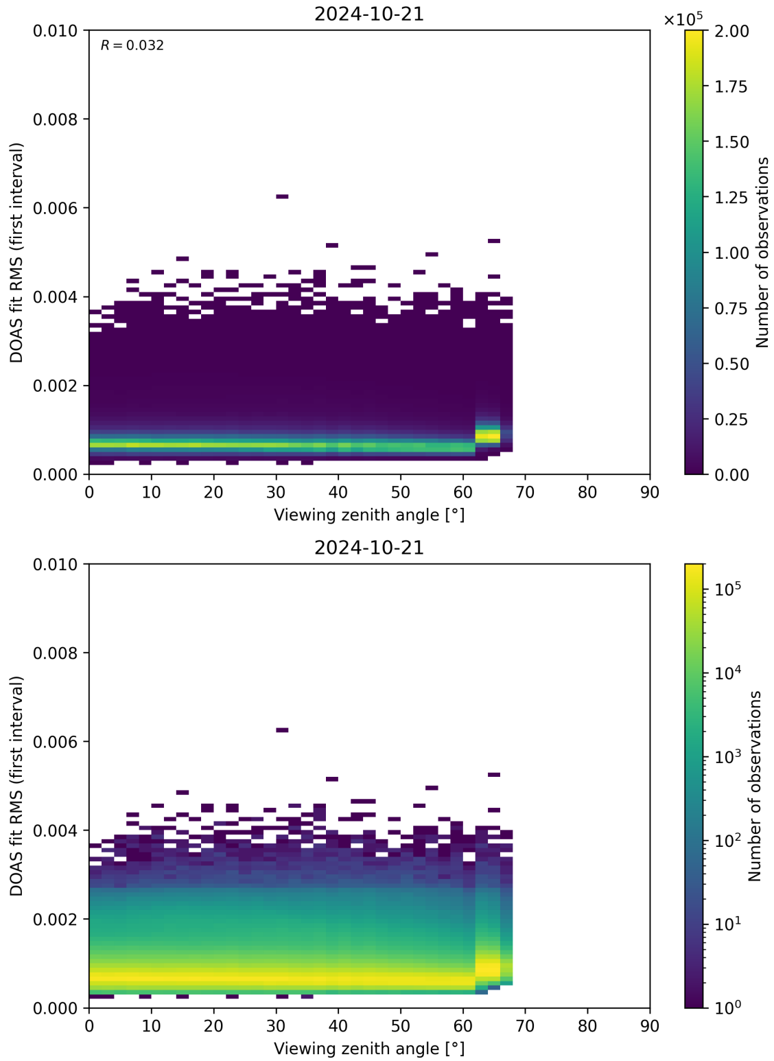
Figure 182: Scatter density plot of “Viewing zenith angle” against “DOAS fit RMS (first interval)” for 2024-10-20 to 2024-10-22.
