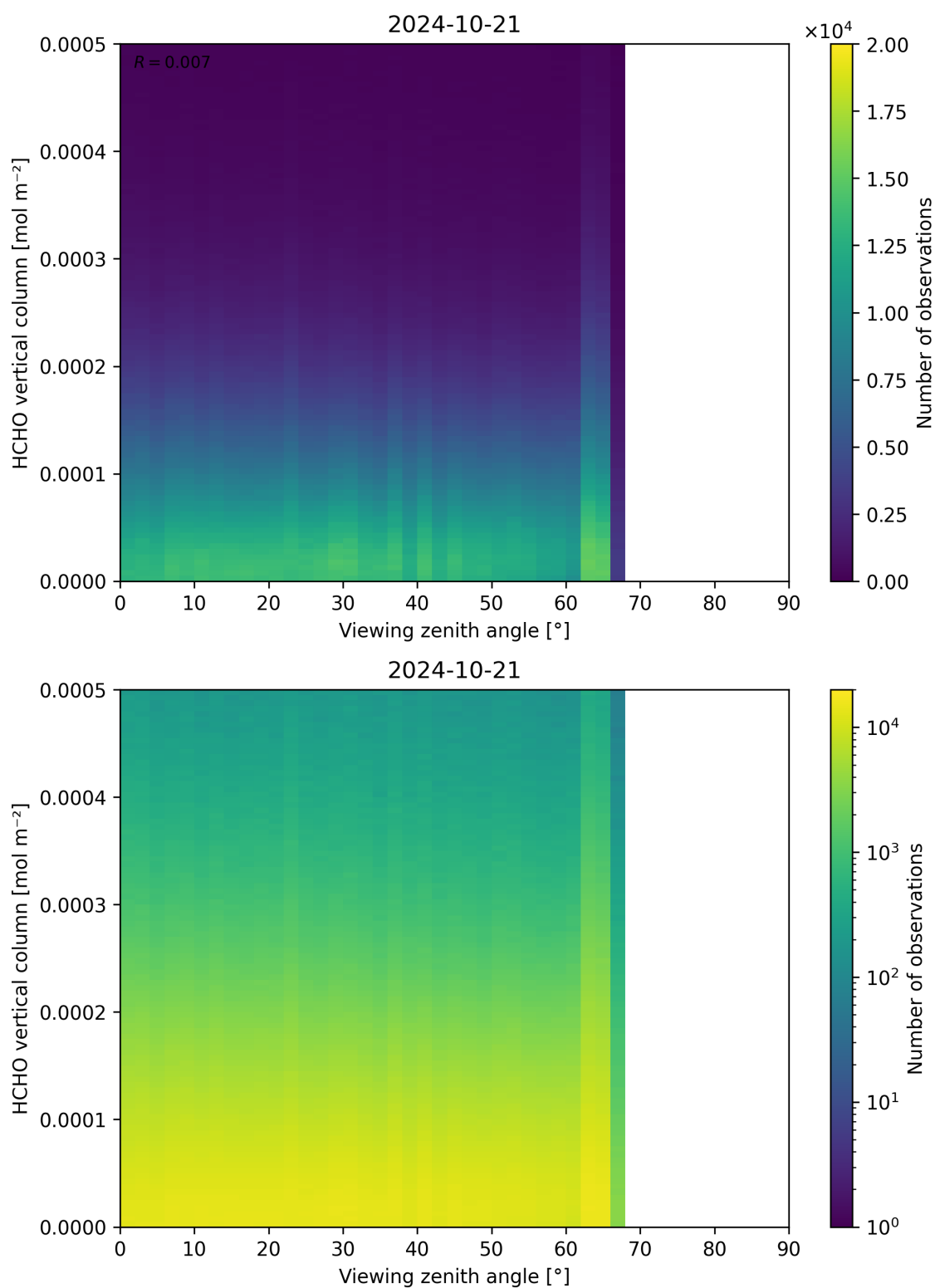
Figure 192: Scatter density plot of “Viewing zenith angle” against “HCHO vertical column” for 2024-10-20 to 2024-10-22.
