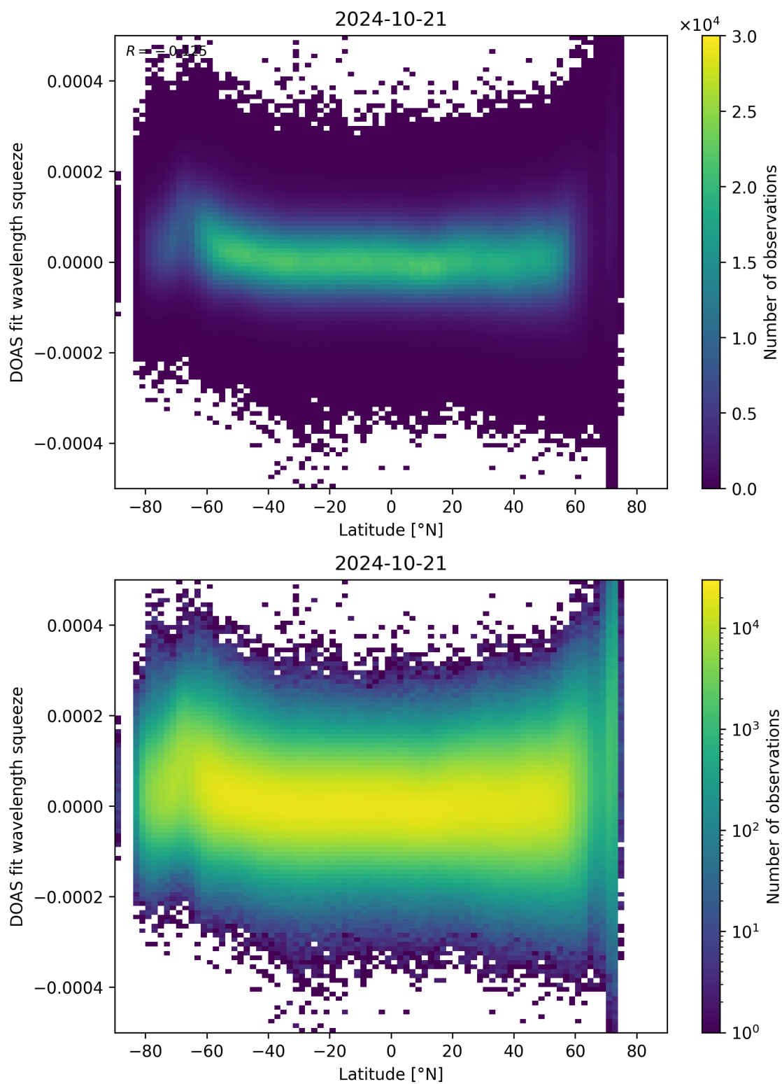
Figure 155: Scatter density plot of “Latitude” against “DOAS fit wavelength squeeze” for 2024-10-20 to 2024-10-22.
