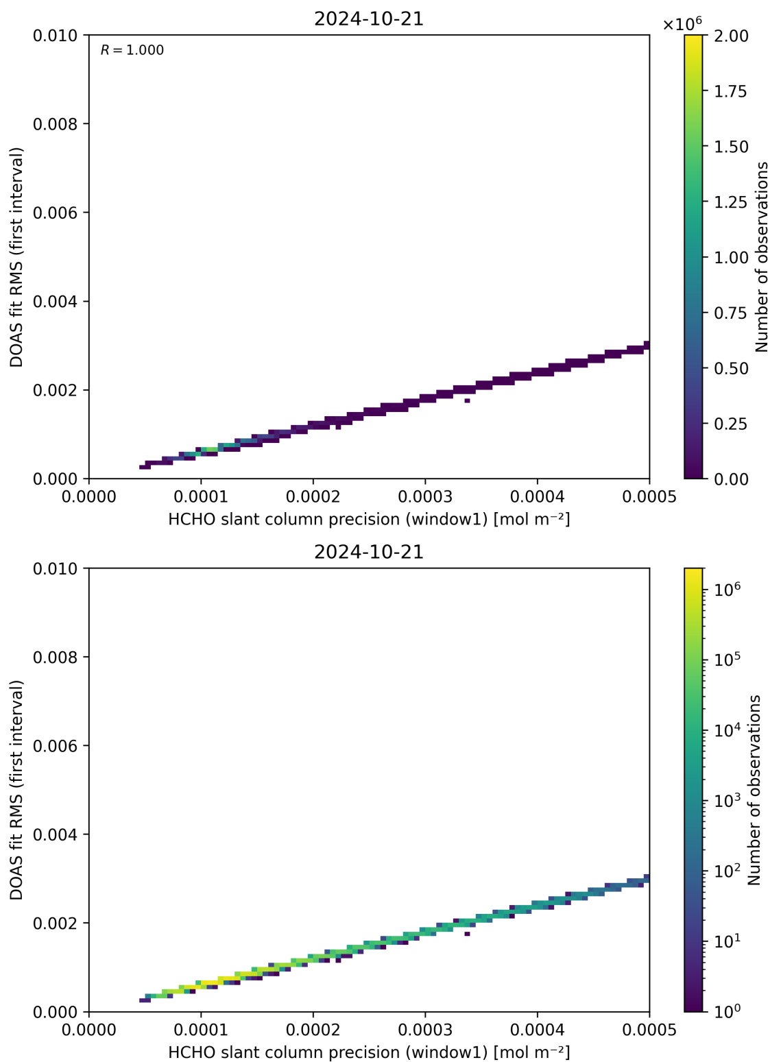
Figure 88: Scatter density plot of “HCHO slant column precision (window1)” against “DOAS fit RMS (first interval)” for 2024-10-20 to 2024-10-22.
