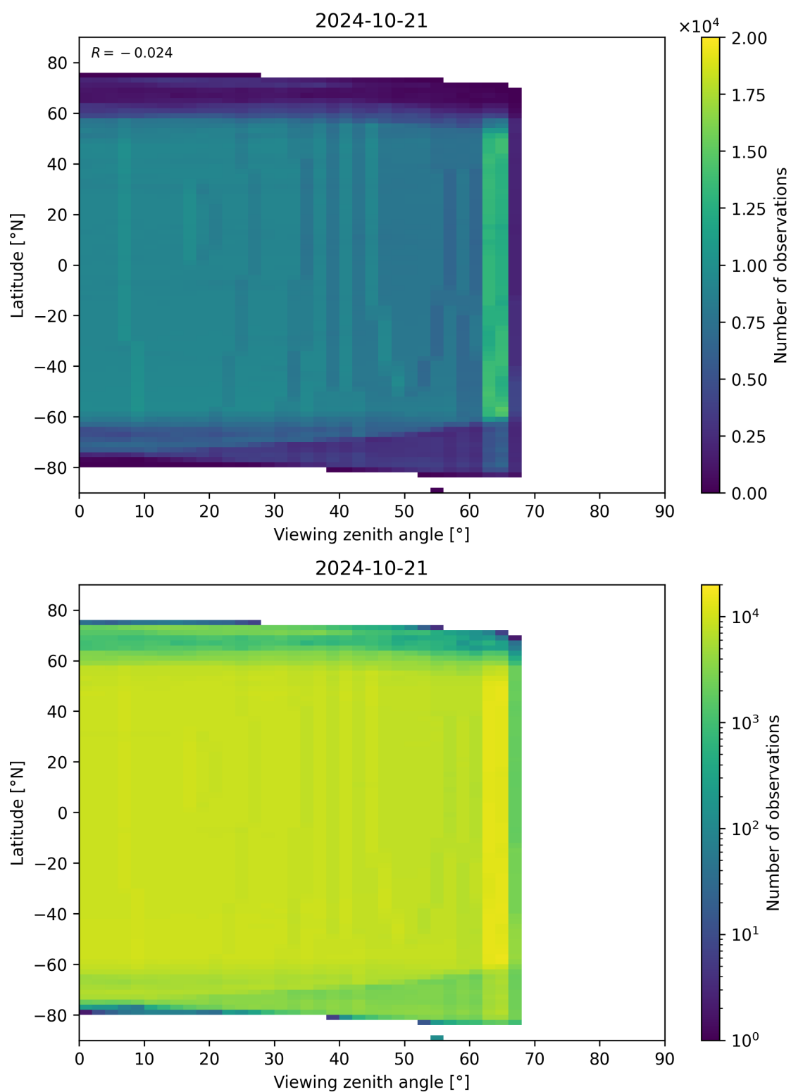
Figure 196: Scatter density plot of “Viewing zenith angle” against “Latitude” for 2024-10-20 to 2024-10-22.
