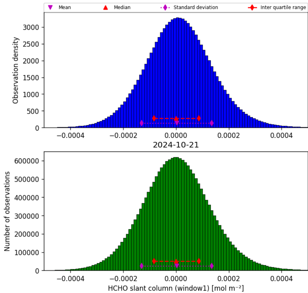
Figure 38: Histogram of “HCHO slant column (window1)” for 2024-10-20 to 2024-10-22
