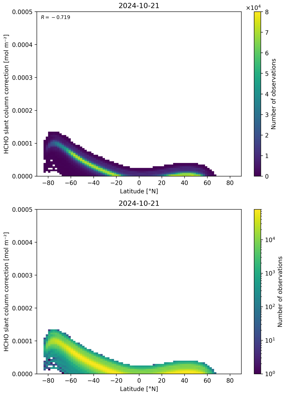
Figure 158: Scatter density plot of “Latitude” against “HCHO slant column correction” for 2024-10-20 to 2024-10-22.
