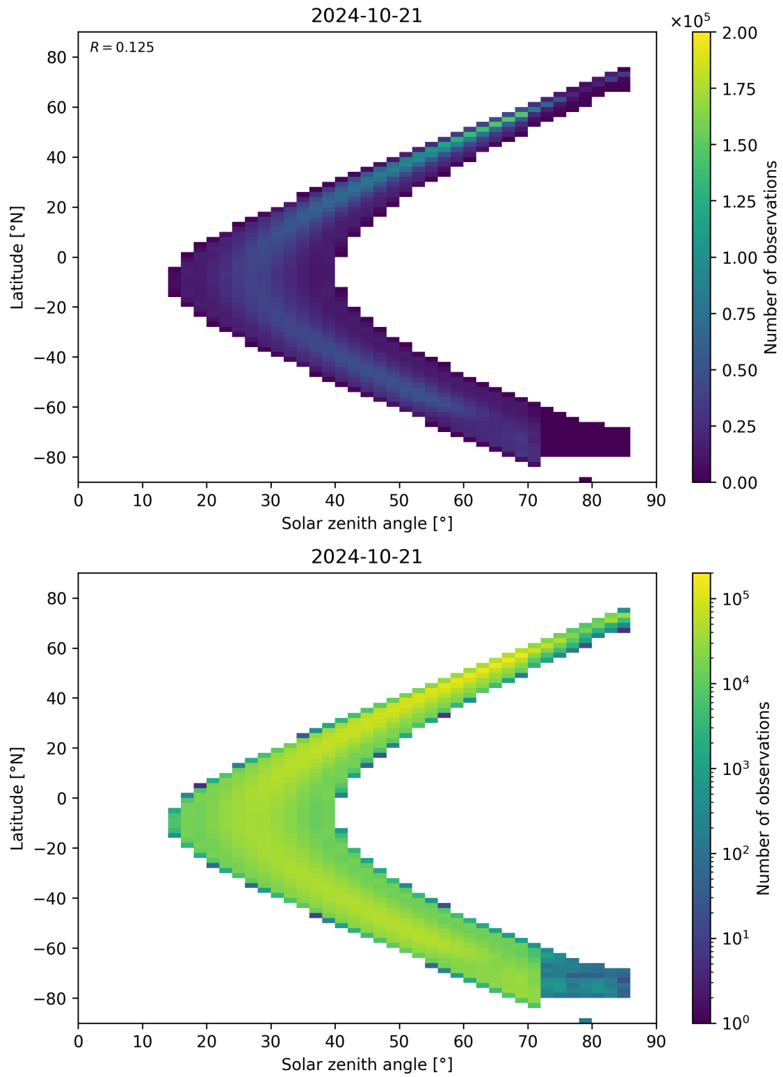
Figure 181: Scatter density plot of “Solar zenith angle” against “Latitude” for 2024-10-20 to 2024-10-22.
