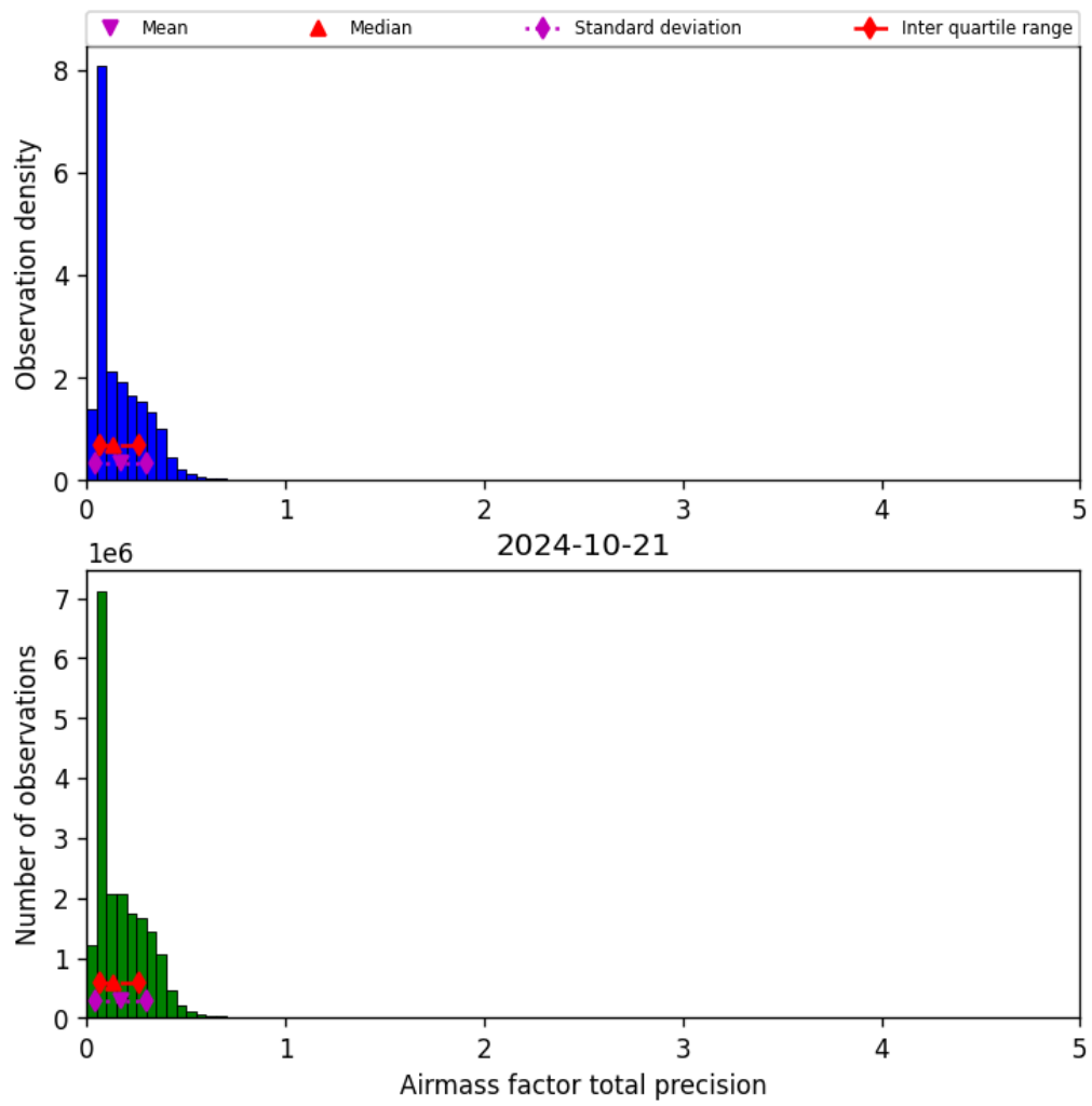
Figure 41: Histogram of “Airmass factor total precision” for 2024-10-20 to 2024-10-22
