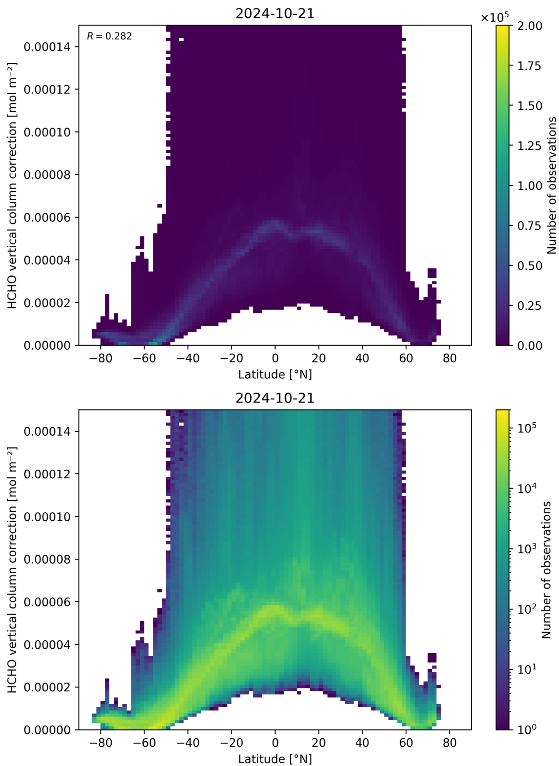
Figure 164: Scatter density plot of “Latitude” against “HCHO vertical column correction” for 2024-10-20 to 2024-10-22.
