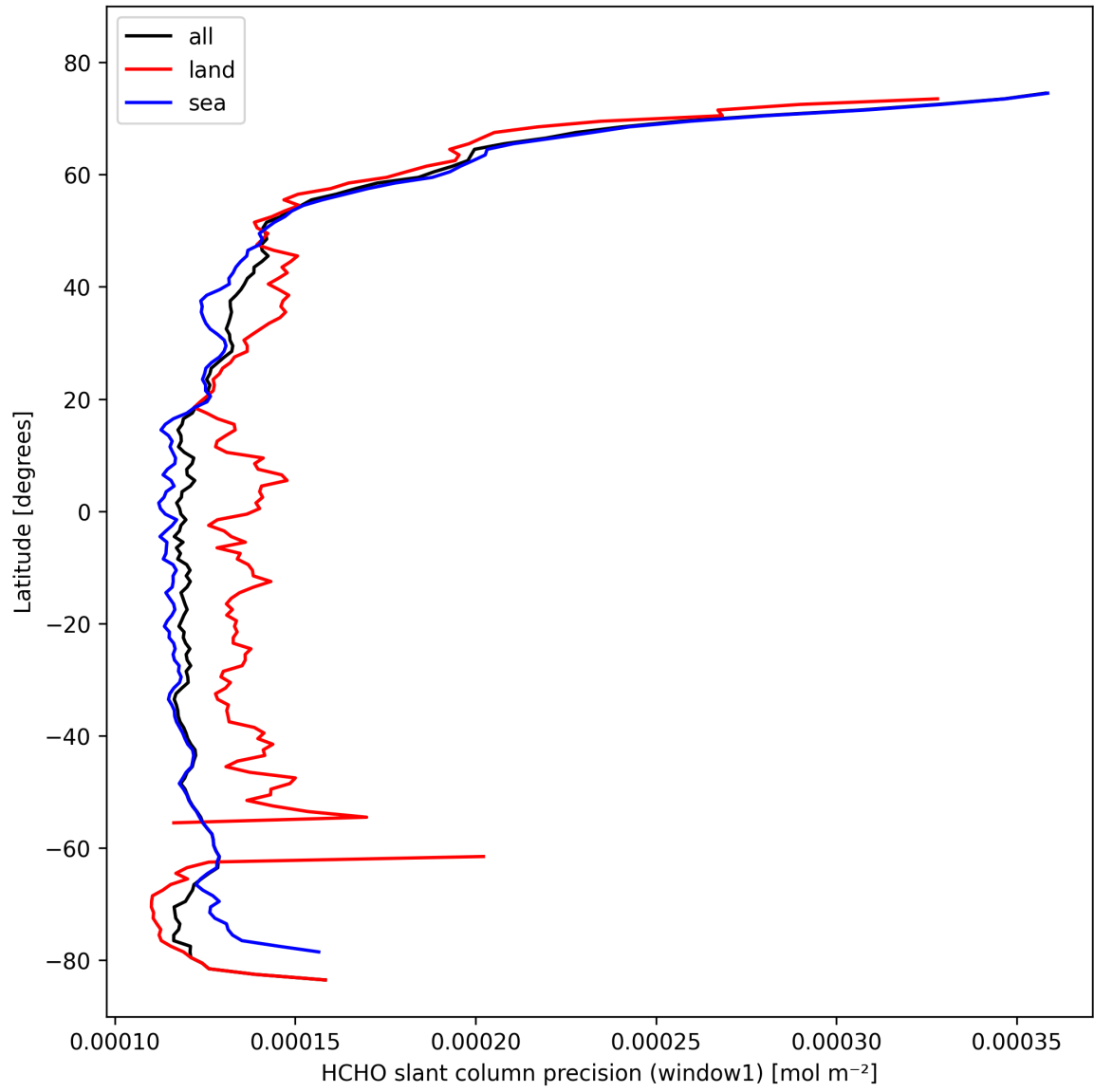
Figure 25: Zonal average of “HCHO slant column precision (window1)” for 2024-10-20 to 2024-10-22.
