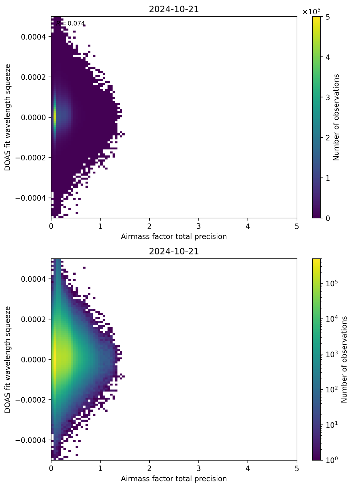
Figure 107: Scatter density plot of “Airmass factor total precision” against “DOAS fit wavelength squeeze” for 2024-10-20 to 2024-10-22.
