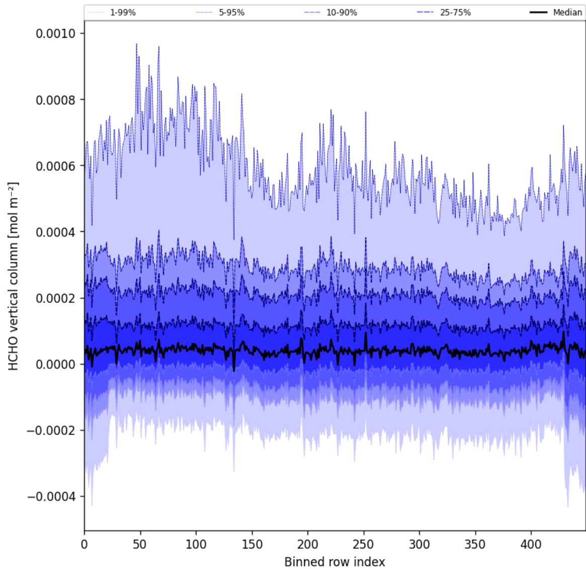
Figure 49: Along track statistics of “HCHO vertical column” for 2024-10-20 to 2024-10-22
