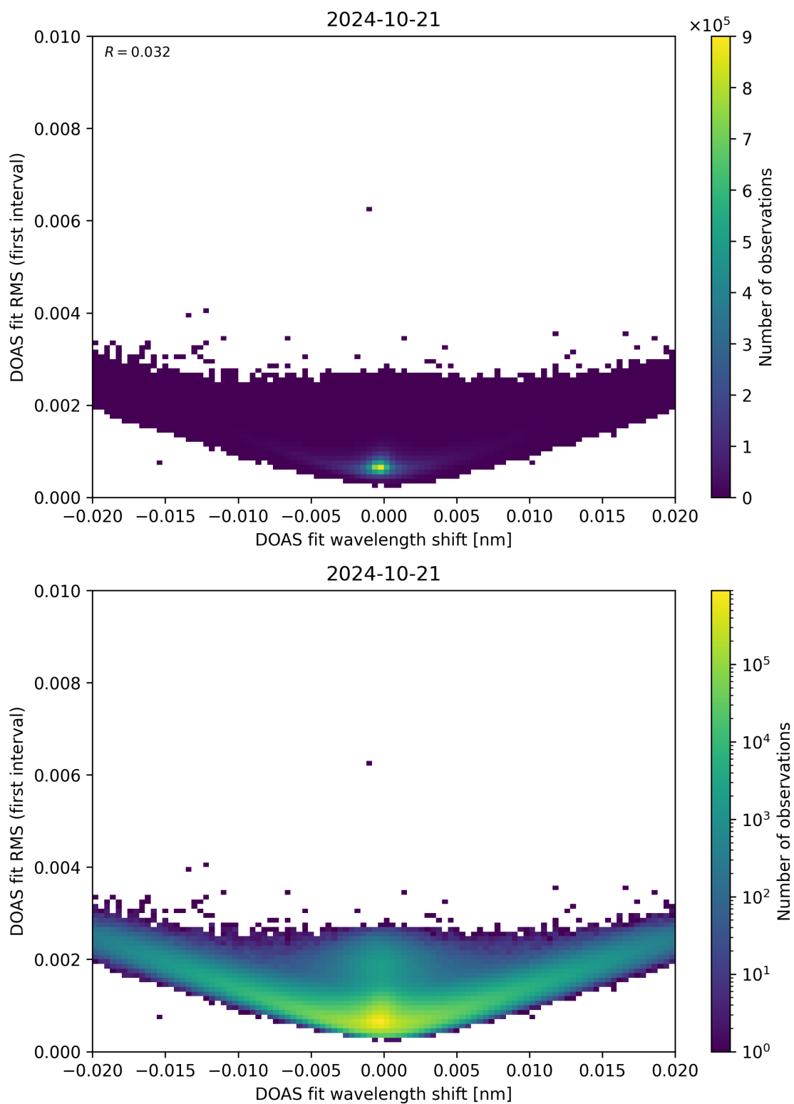
Figure 64: Scatter density plot of “DOAS fit wavelength shift” against “DOAS fit RMS (first interval)” for 2024-10-20 to 2024-10-22.
