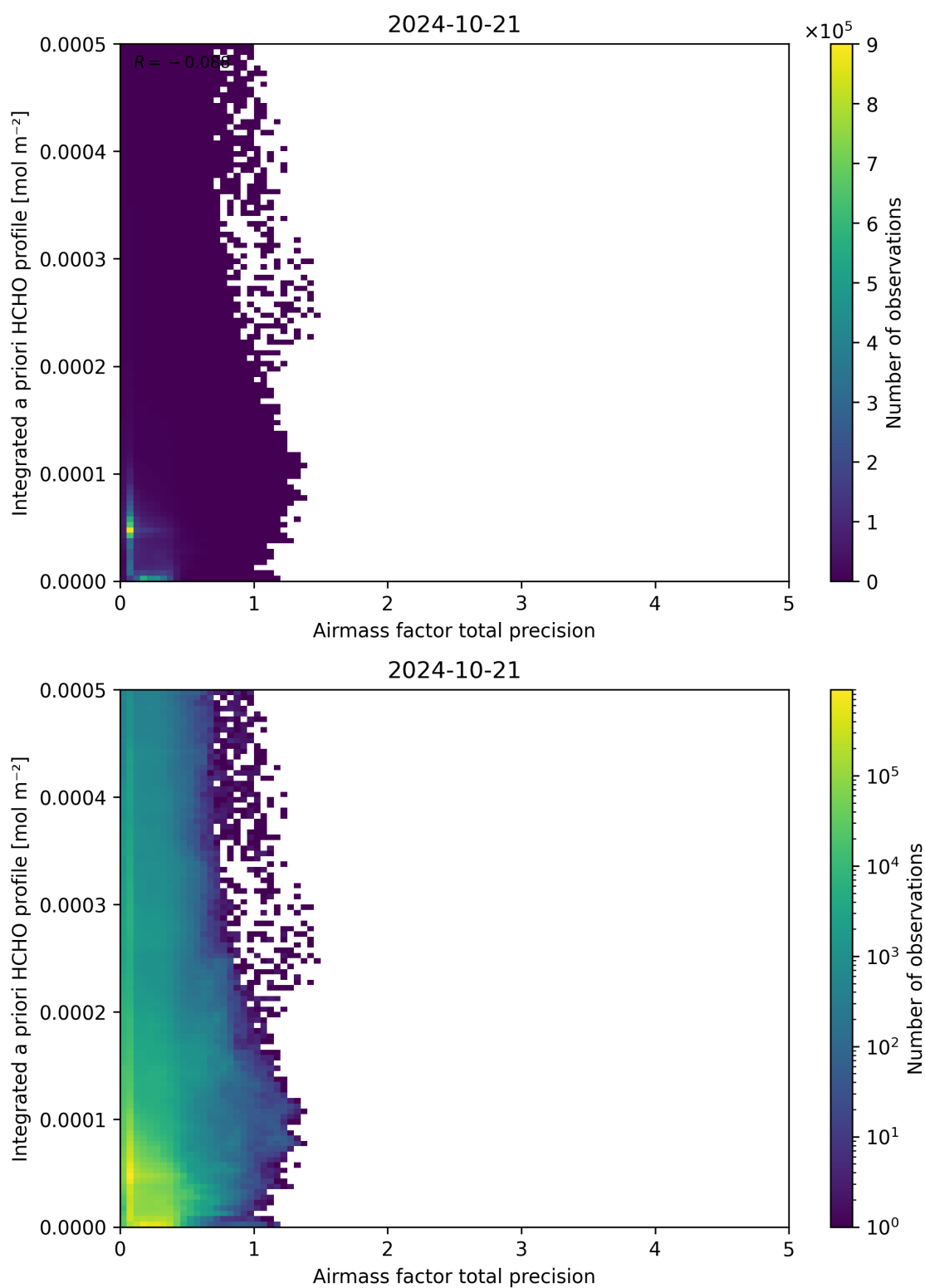
Figure 111: Scatter density plot of “Airmass factor total precision” against “Integrated a priori HCHO profile” for 2024-10-20 to 2024-10-22.
