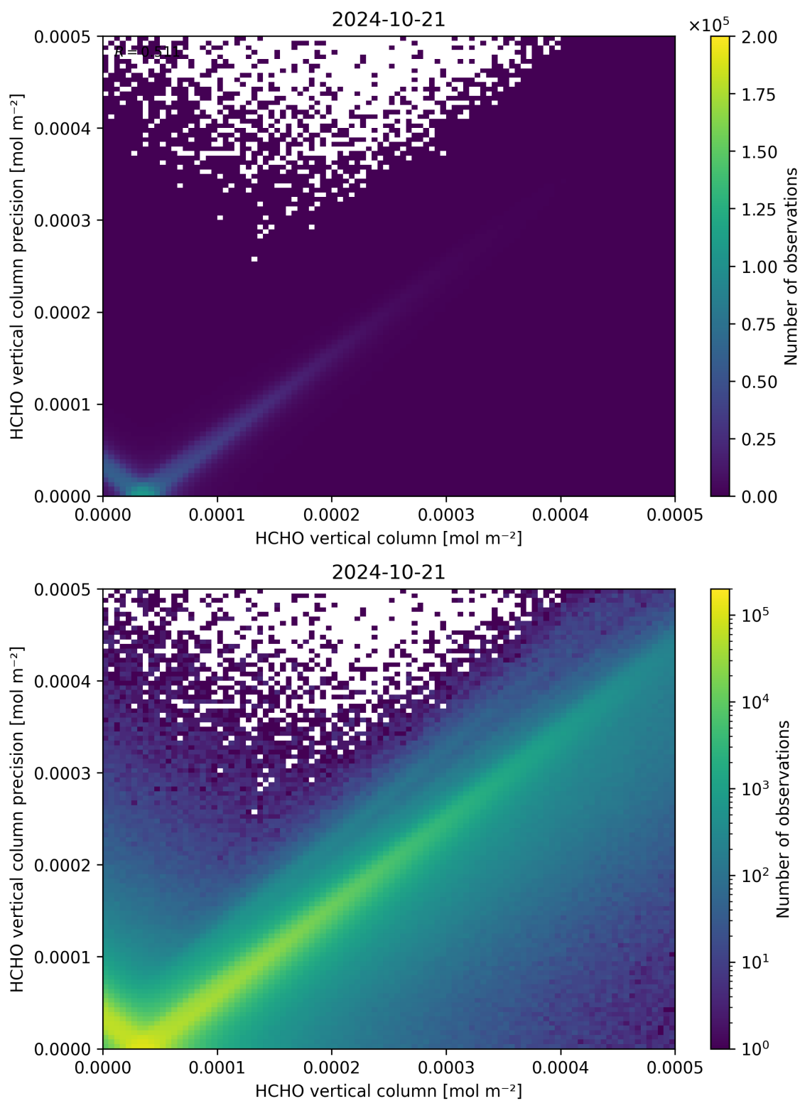
Figure 134: Scatter density plot of “HCHO vertical column” against “HCHO vertical column precision” for 2024-10-20 to 2024-10-22.
