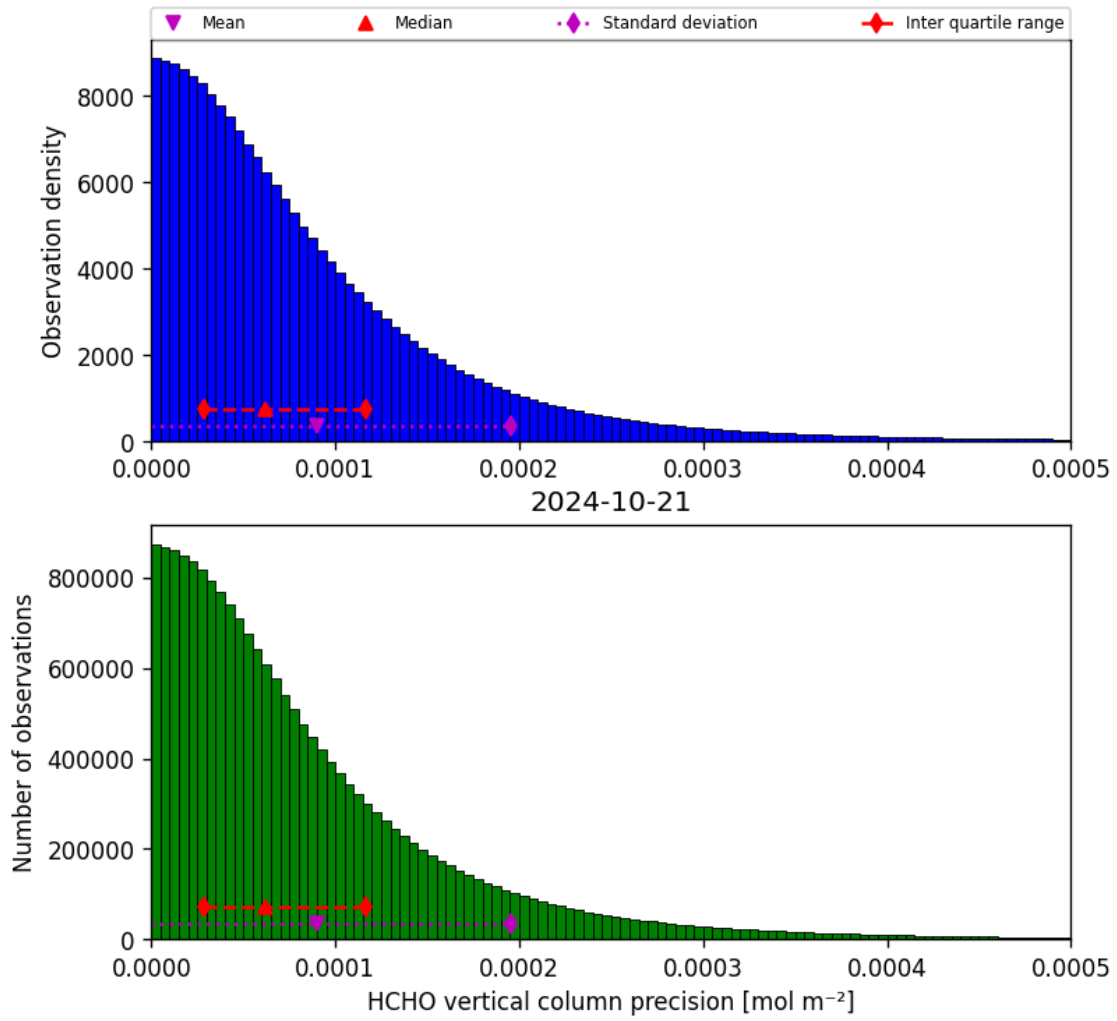
Figure 36: Histogram of “HCHO vertical column precision” for 2024-10-20 to 2024-10-22
