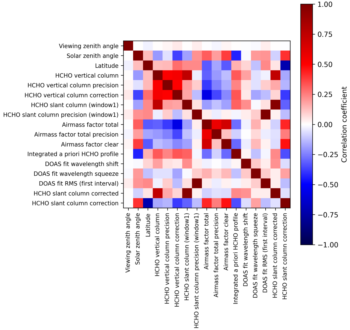
Figure 2: Map of correlation matrix for 2024-10-20 to 2024-10-22.
