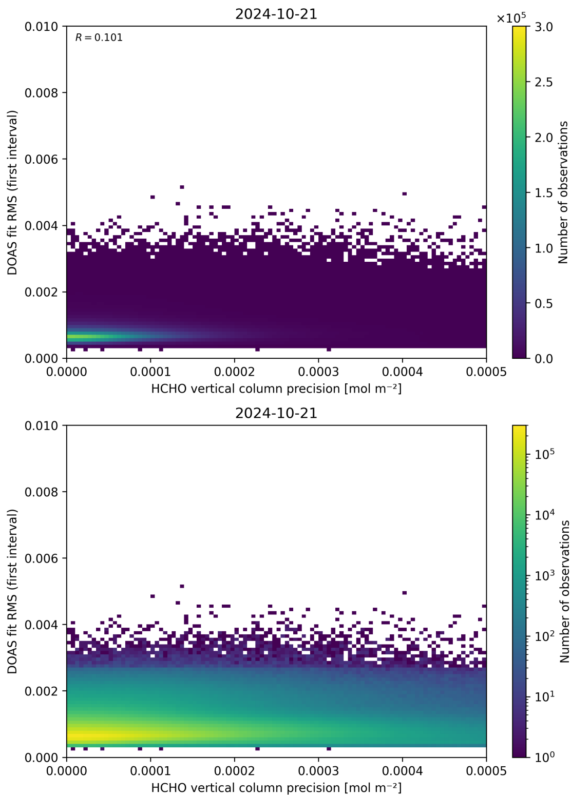
Figure 136: Scatter density plot of “HCHO vertical column precision” against “DOAS fit RMS (first interval)” for 2024-10-20 to 2024-10-22.
