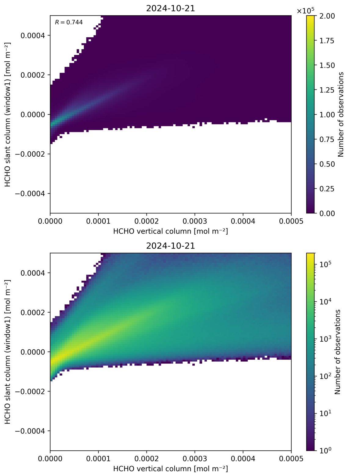
Figure 129: Scatter density plot of “HCHO vertical column” against “HCHO slant column (window1)” for 2024-10-20 to 2024-10-22.
