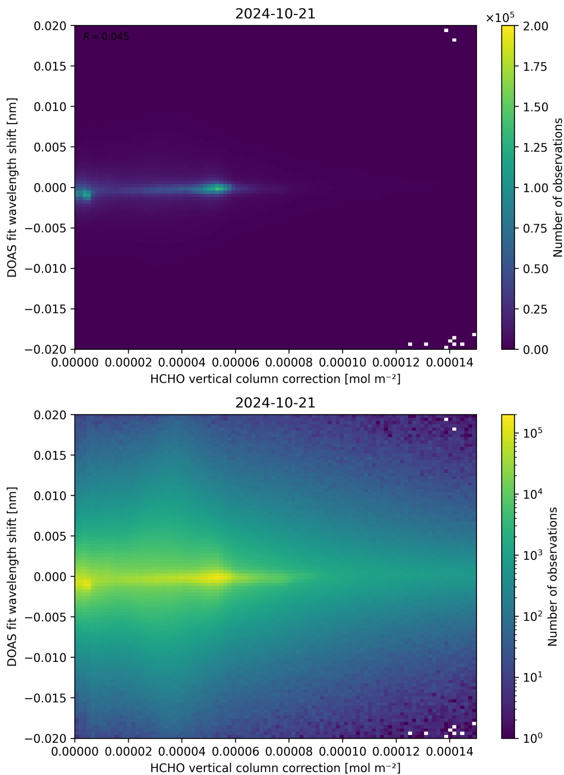
Figure 113: Scatter density plot of “HCHO vertical column correction” against “DOAS fit wavelength shift” for 2024-10-20 to 2024-10-22.
