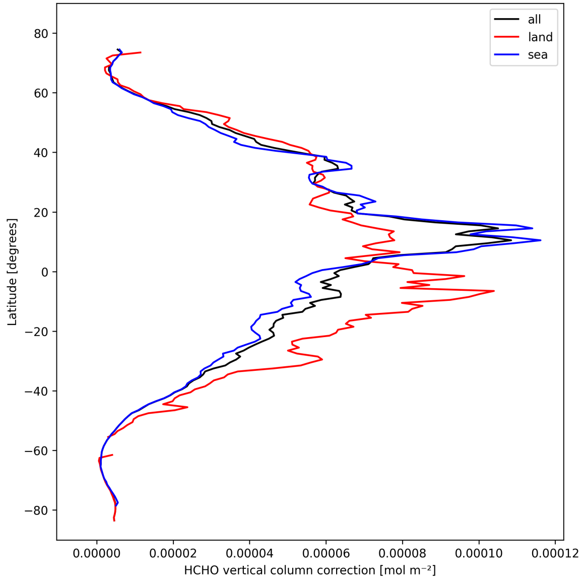
Figure 23: Zonal average of “HCHO vertical column correction” for 2024-10-20 to 2024-10-22.
