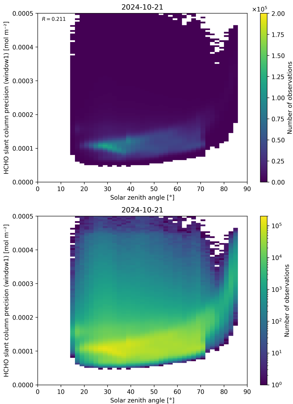
Figure 174: Scatter density plot of “Solar zenith angle” against “HCHO slant column precision (window1)” for 2024-10-20 to 2024-10-22.
