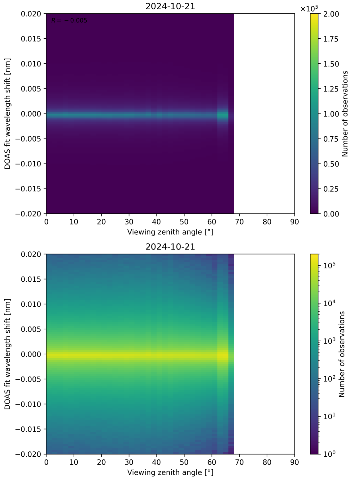
Figure 183: Scatter density plot of “Viewing zenith angle” against “DOAS fit wavelength shift” for 2024-10-20 to 2024-10-22.
