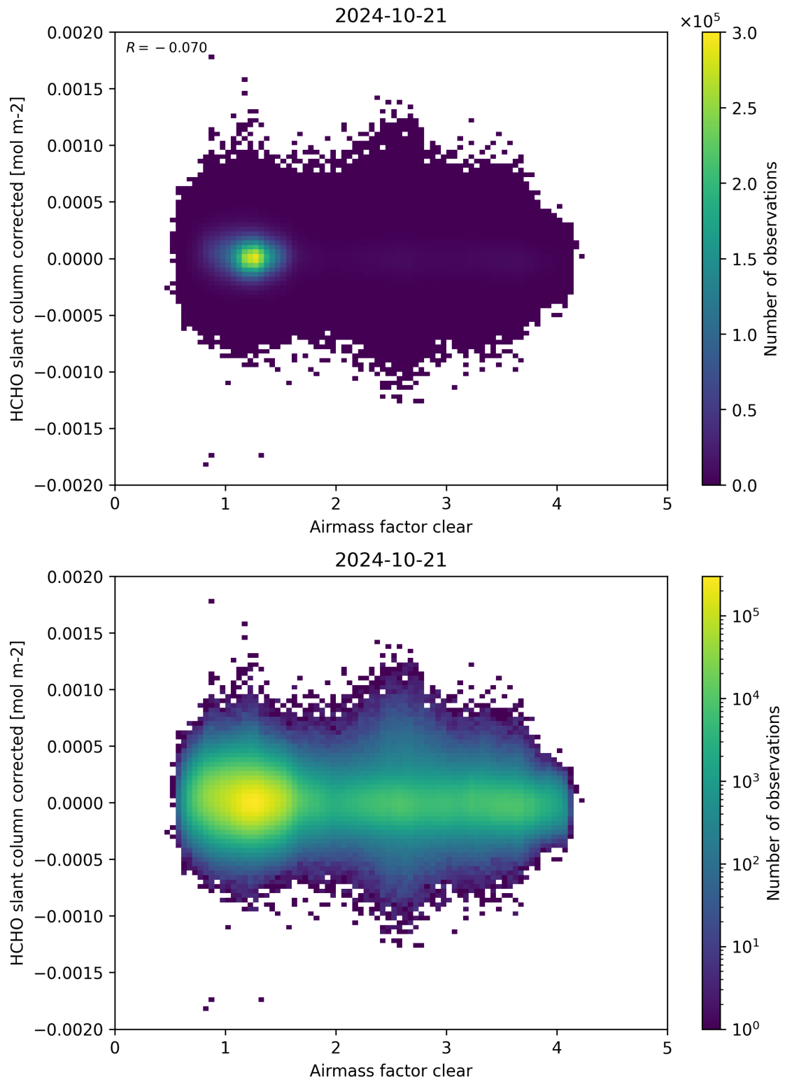
Figure 74: Scatter density plot of “Airmass factor clear” against “HCHO slant column corrected” for 2024-10-20 to 2024-10-22.
