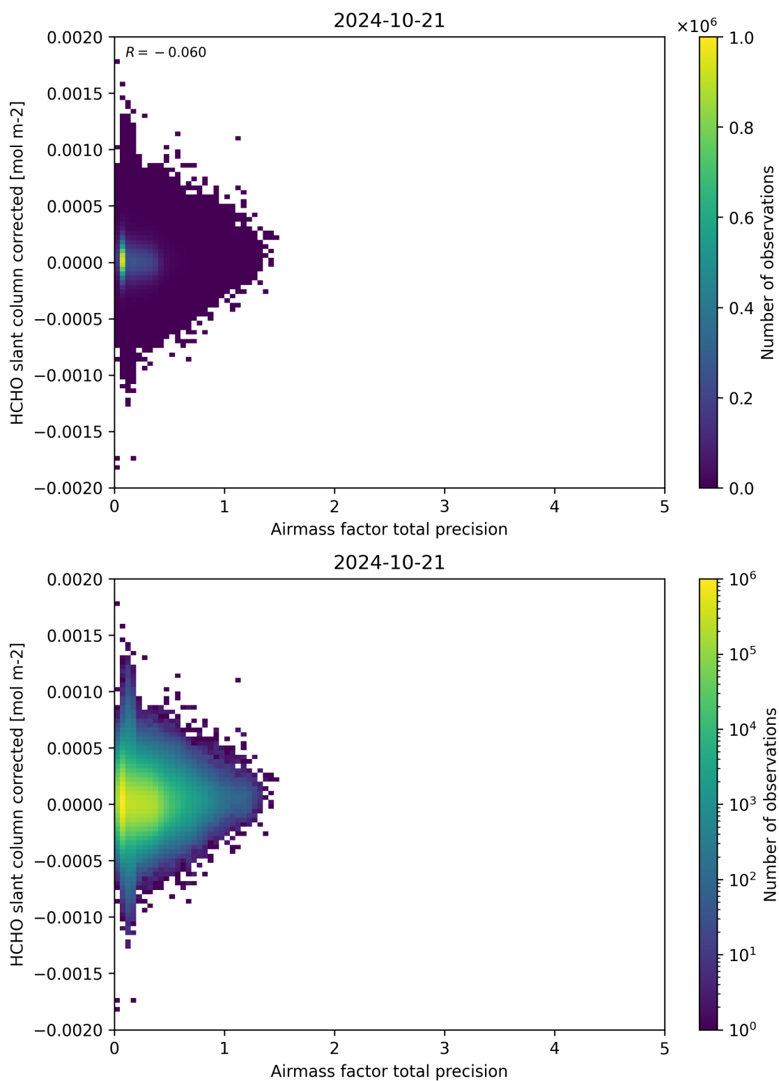
Figure 109: Scatter density plot of “Airmass factor total precision” against “HCHO slant column corrected” for 2024-10-20 to 2024-10-22.
