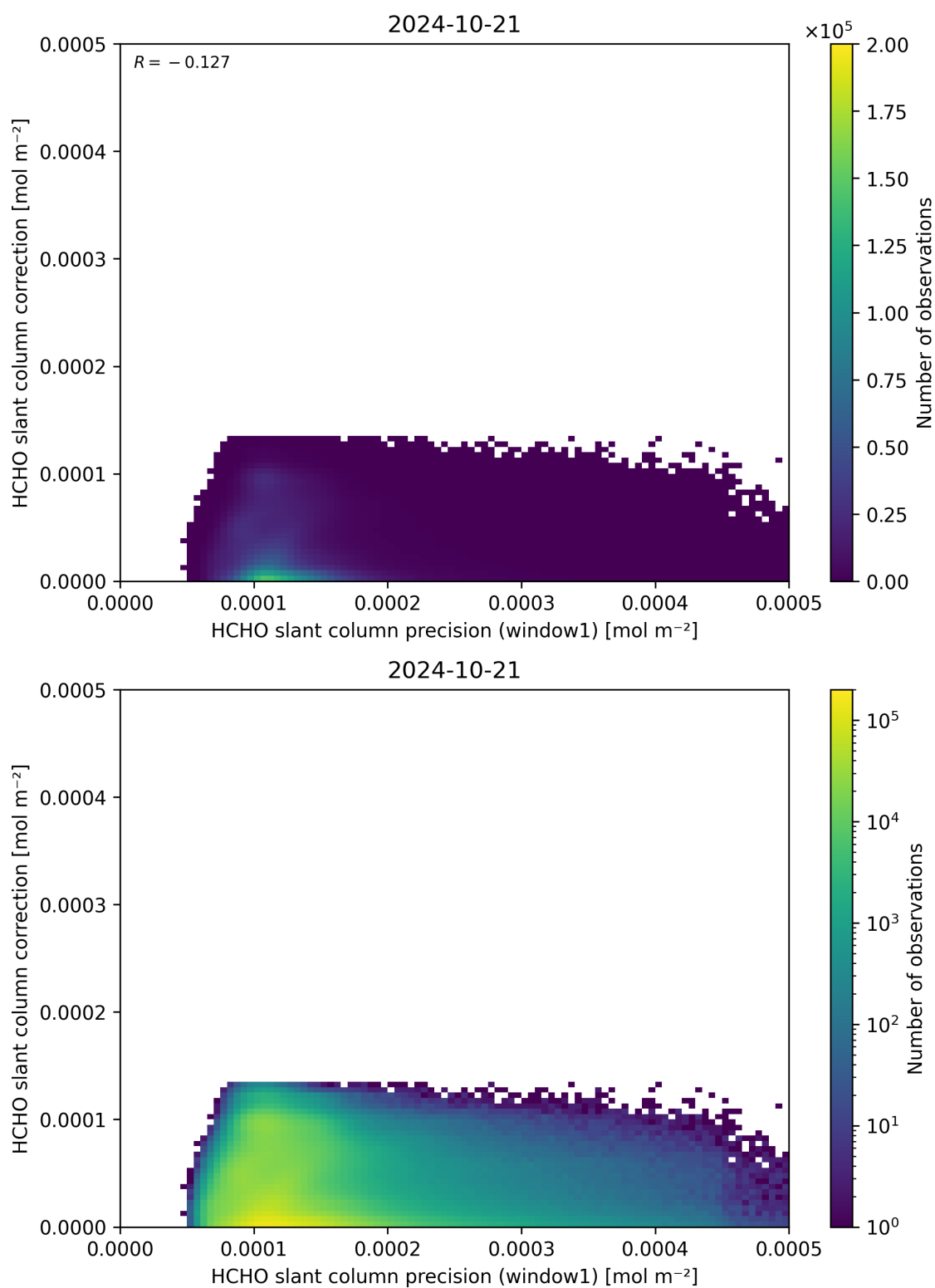
Figure 93: Scatter density plot of “HCHO slant column precision (window1)” against “HCHO slant column correction” for 2024-10-20 to 2024-10-22.
