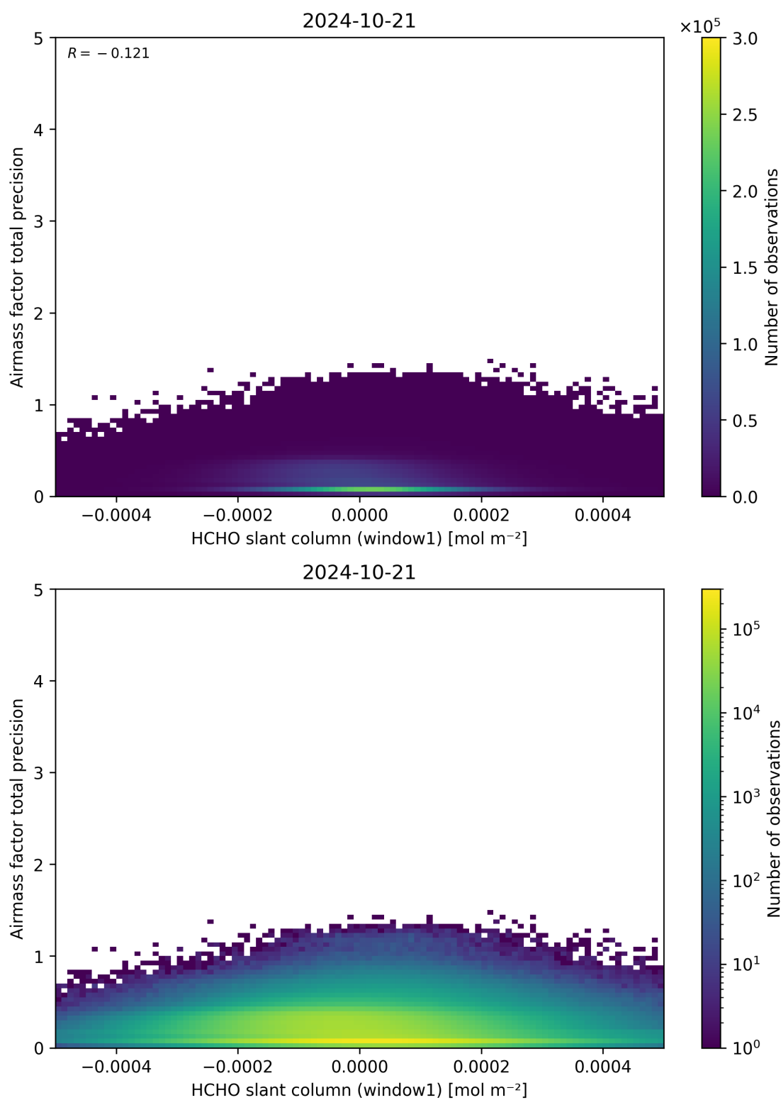
Figure 86: Scatter density plot of “HCHO slant column (window1)” against “Airmass factor total precision” for 2024-10-20 to 2024-10-22.
