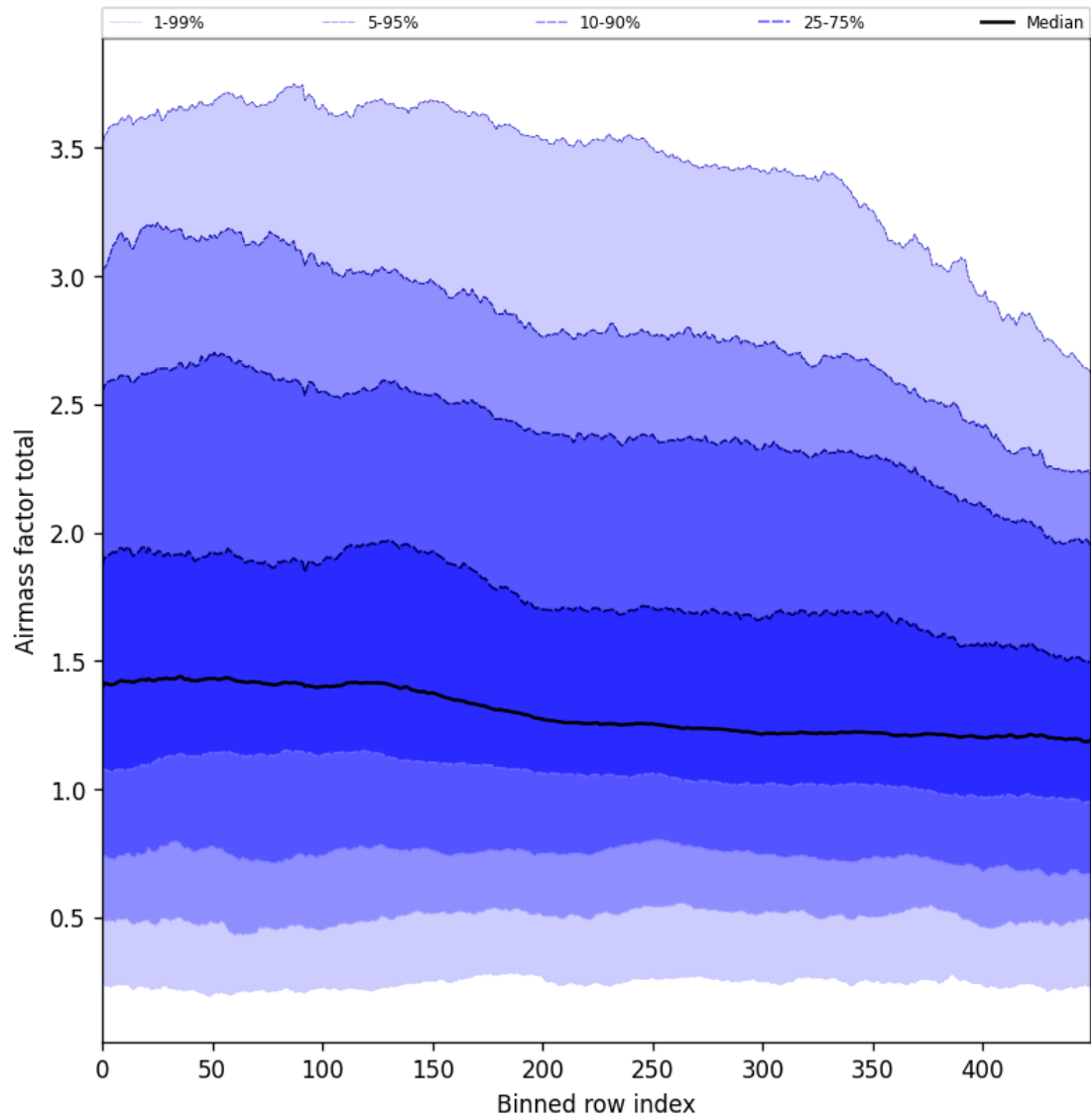
Figure 54: Along track statistics of “Airmass factor total” for 2024-10-20 to 2024-10-22
