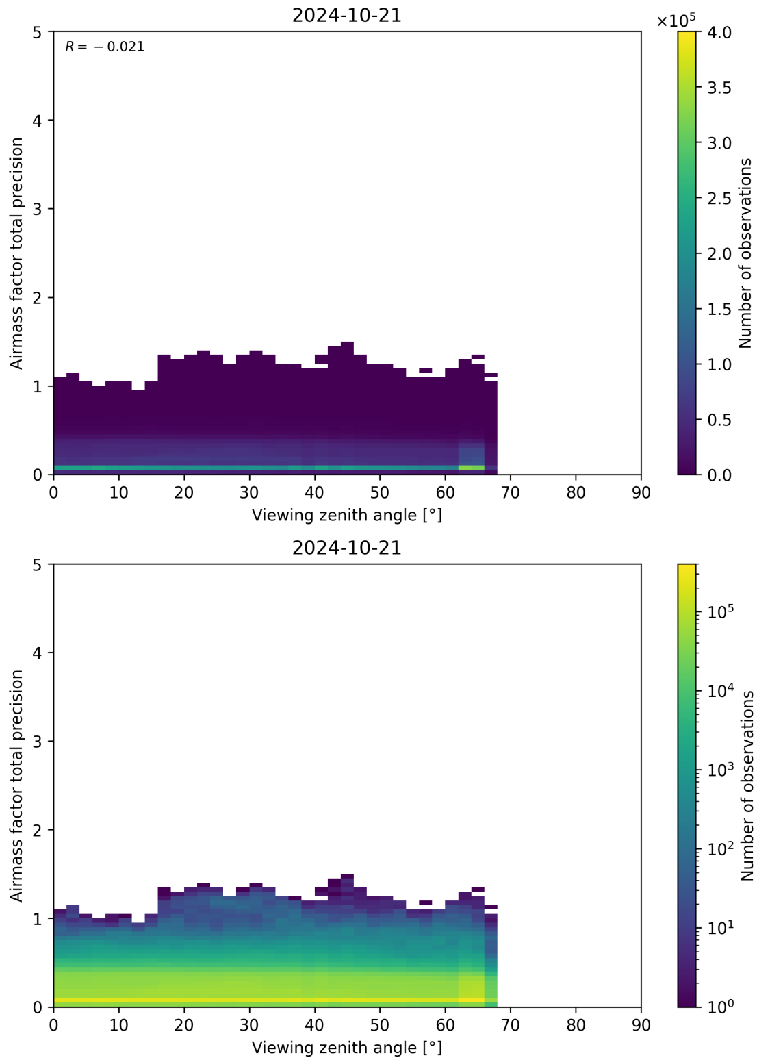
Figure 191: Scatter density plot of “Viewing zenith angle” against “Airmass factor total precision” for 2024-10-20 to 2024-10-22.
