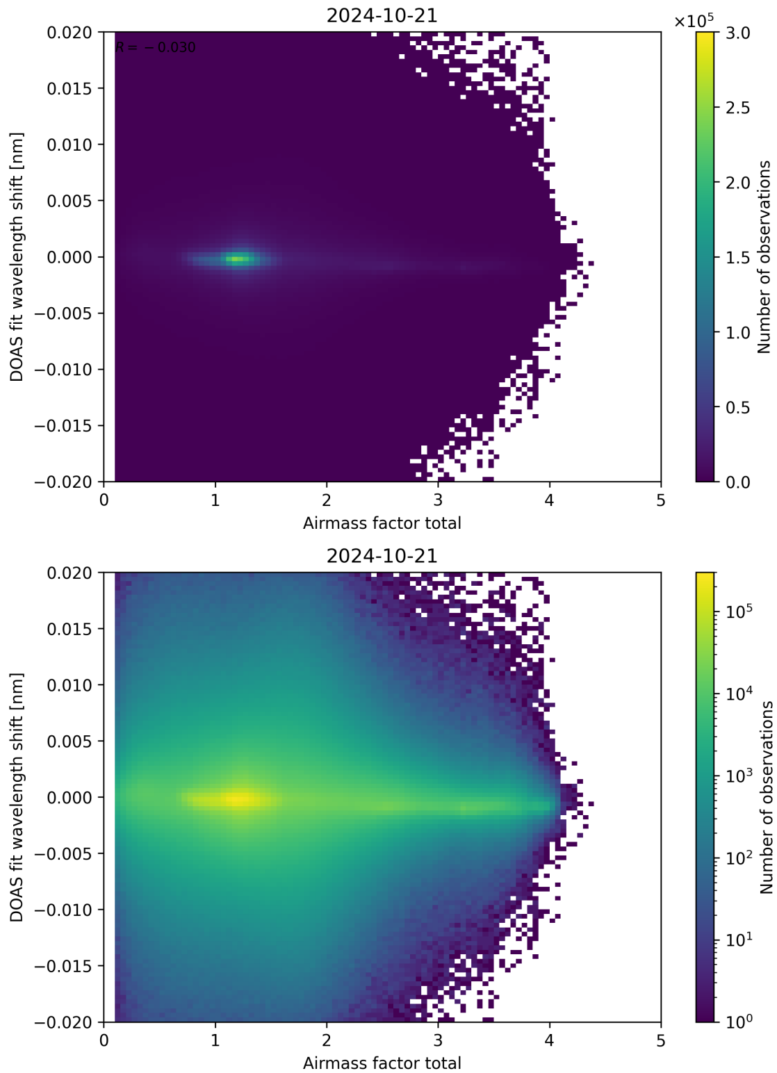
Figure 98: Scatter density plot of “Airmass factor total” against “DOAS fit wavelength shift” for 2024-10-20 to 2024-10-22.
