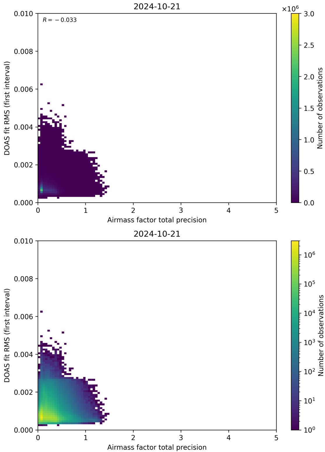
Figure 105: Scatter density plot of “Airmass factor total precision” against “DOAS fit RMS (first interval)” for 2024-10-20 to 2024-10-22.
