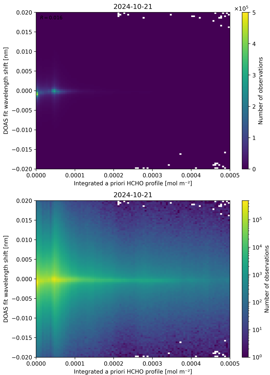
Figure 149: Scatter density plot of “Integrated a priori HCHO profile” against “DOAS fit wavelength shift” for 2024-10-20 to 2024-10-22.
