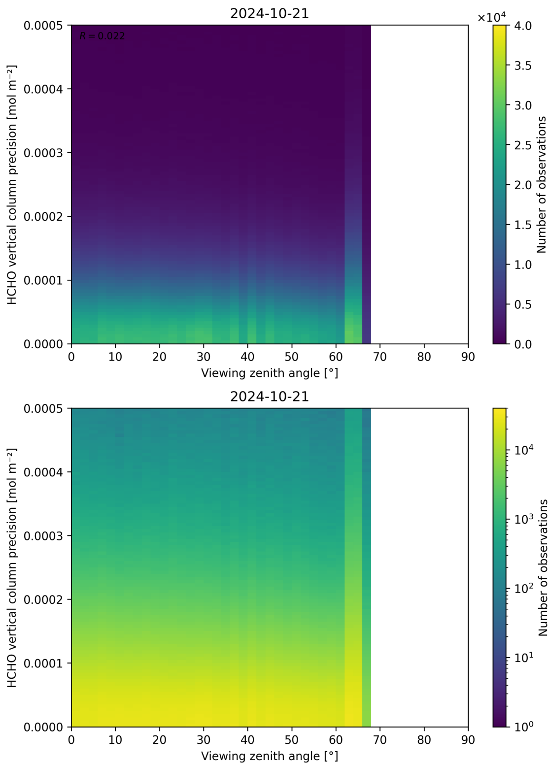
Figure 194: Scatter density plot of “Viewing zenith angle” against “HCHO vertical column precision” for 2024-10-20 to 2024-10-22.
