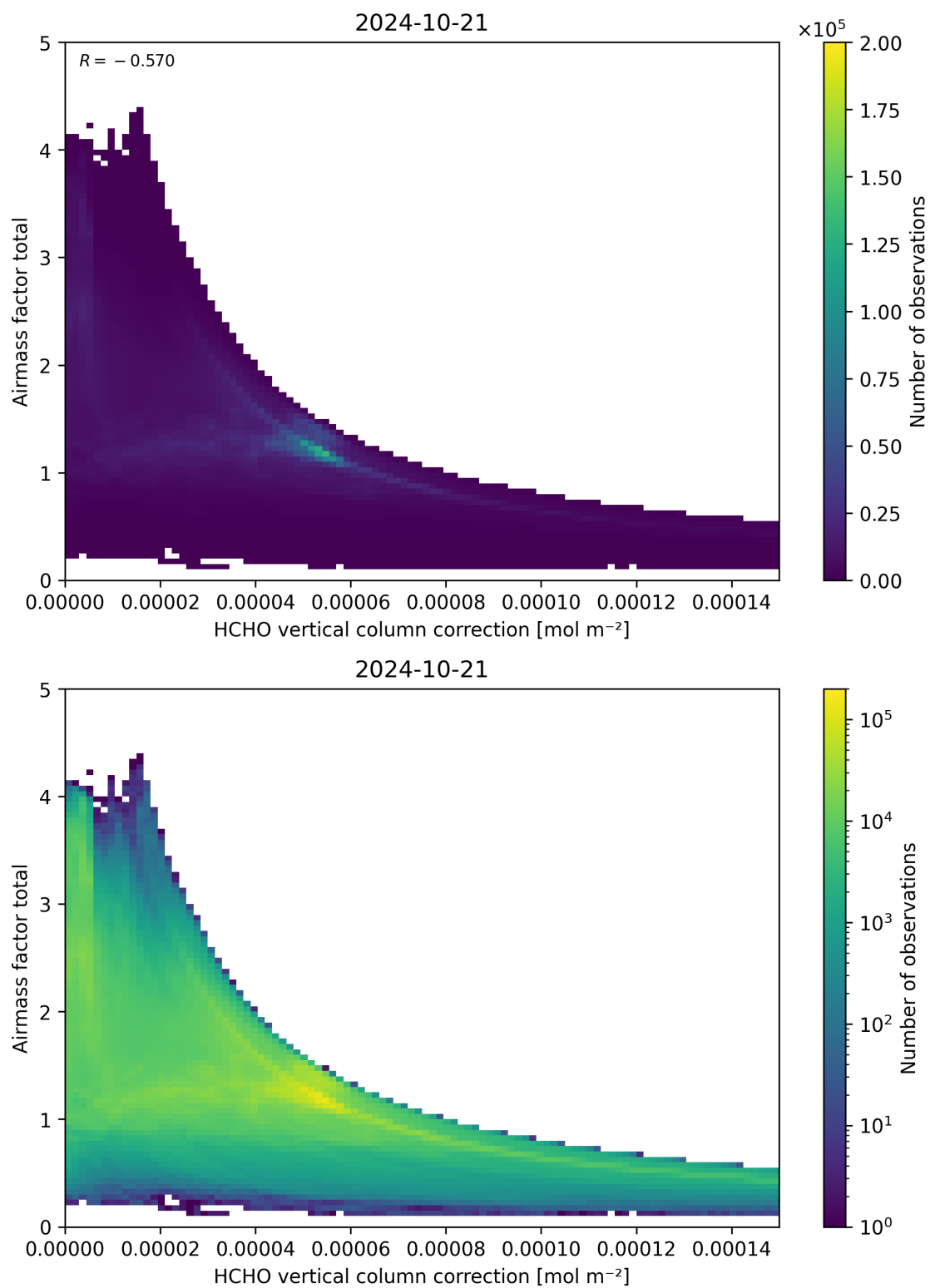
Figure 120: Scatter density plot of “HCHO vertical column correction” against “Airmass factor total” for 2024-10-20 to 2024-10-22.
