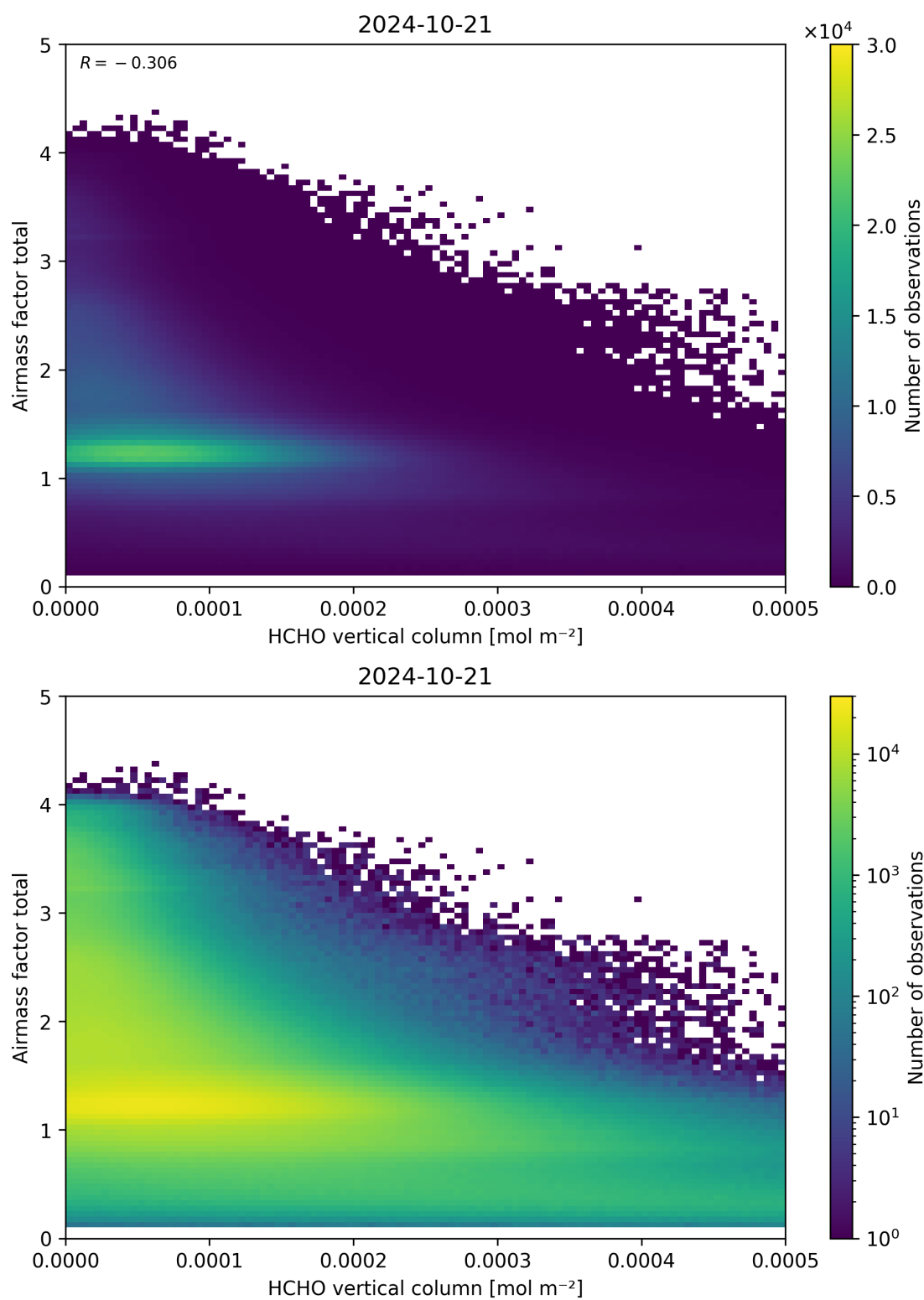
Figure 131: Scatter density plot of “HCHO vertical column” against “Airmass factor total” for 2024-10-20 to 2024-10-22.
