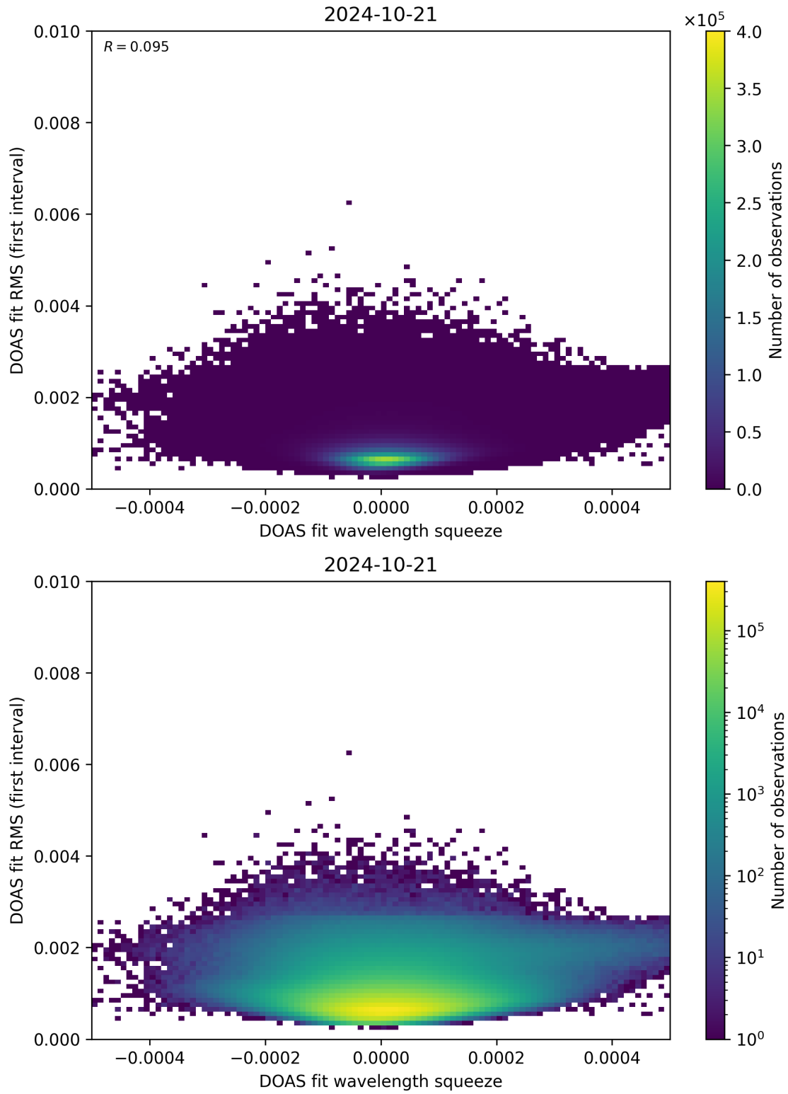
Figure 68: Scatter density plot of “DOAS fit wavelength squeeze” against “DOAS fit RMS (first interval)” for 2024-10-20 to 2024-10-22.
