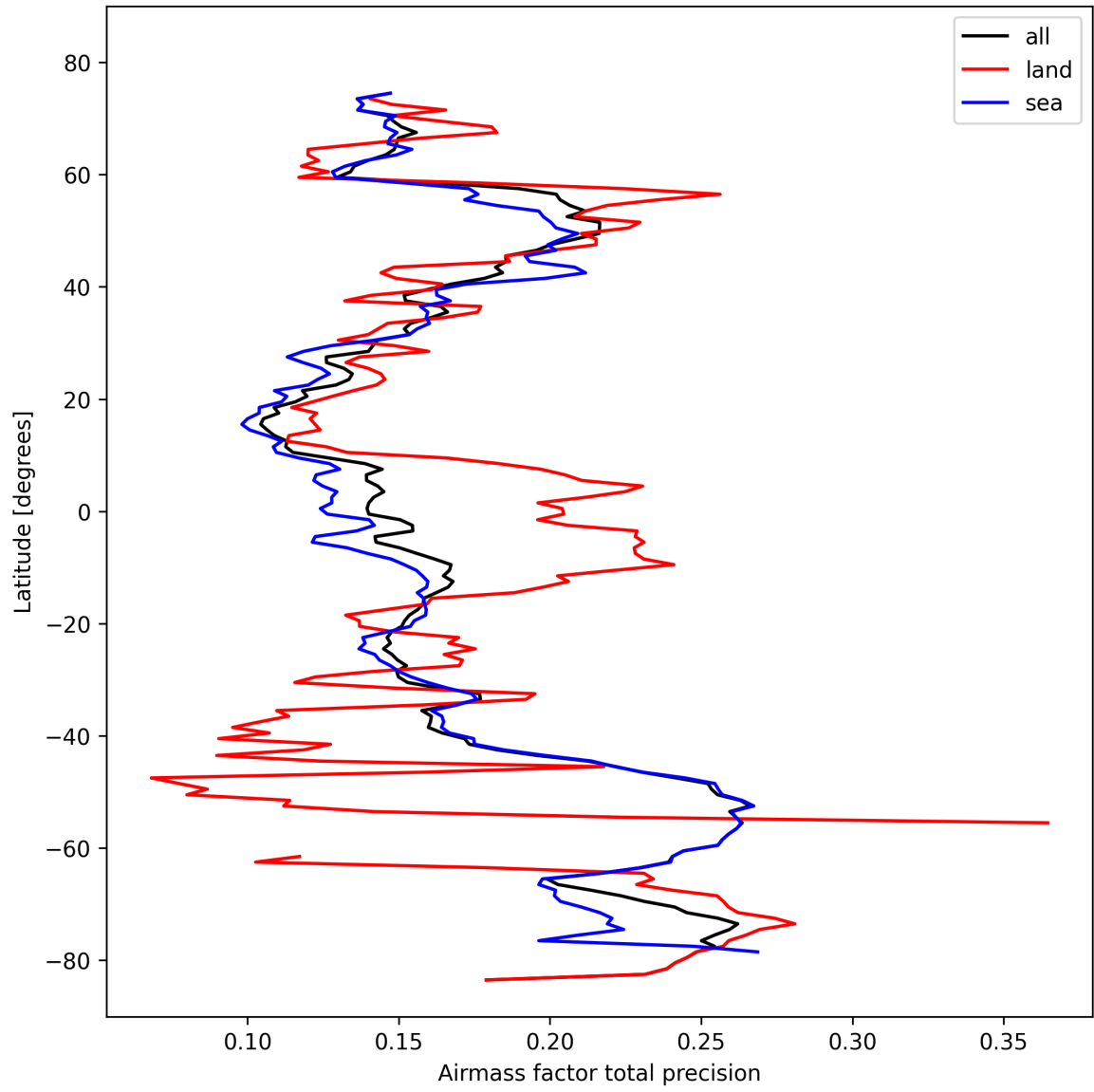
Figure 27: Zonal average of “Airmass factor total precision” for 2024-10-20 to 2024-10-22.
