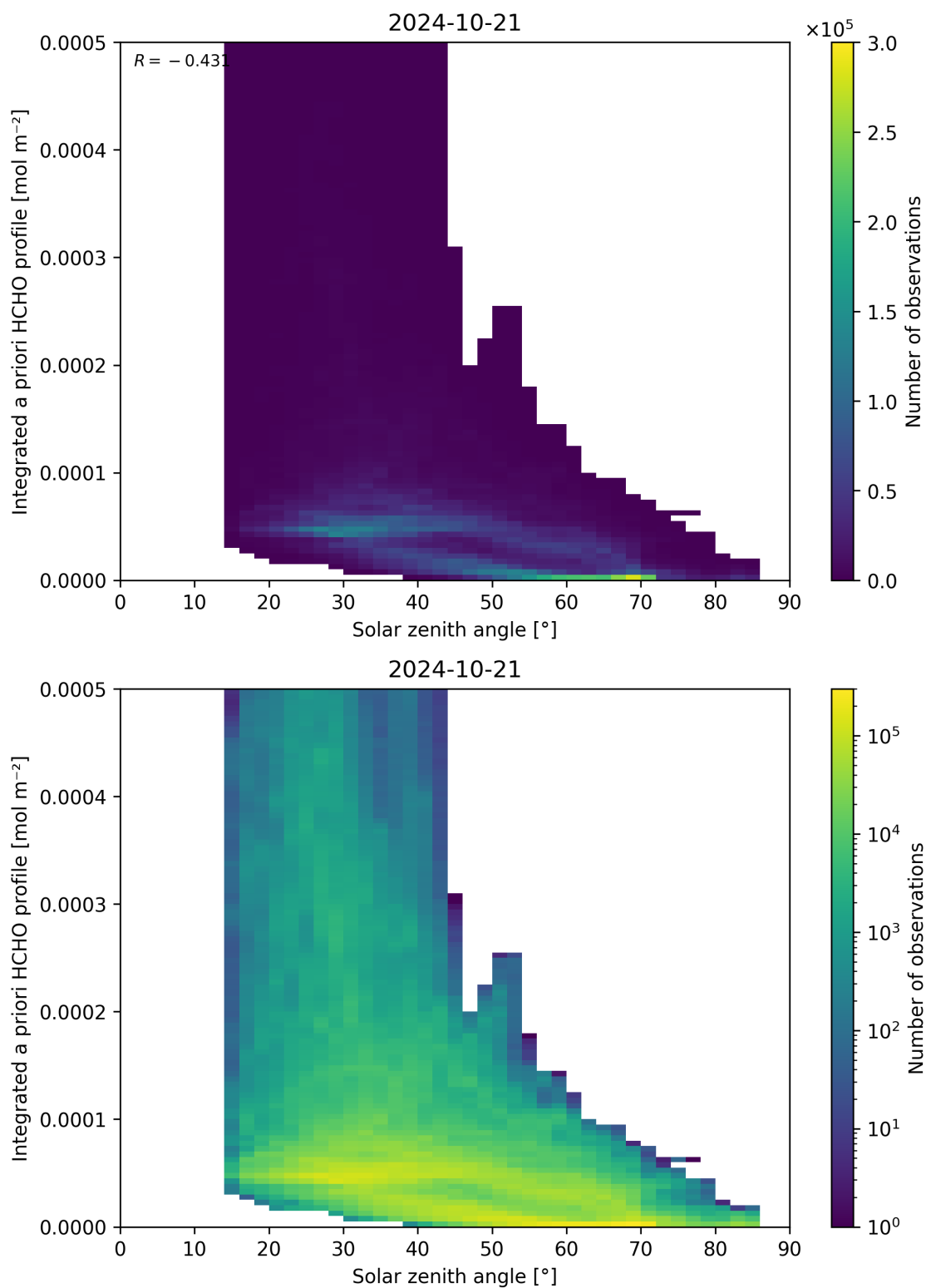
Figure 180: Scatter density plot of “Solar zenith angle” against “Integrated a priori HCHO profile” for 2024-10-20 to 2024-10-22.
