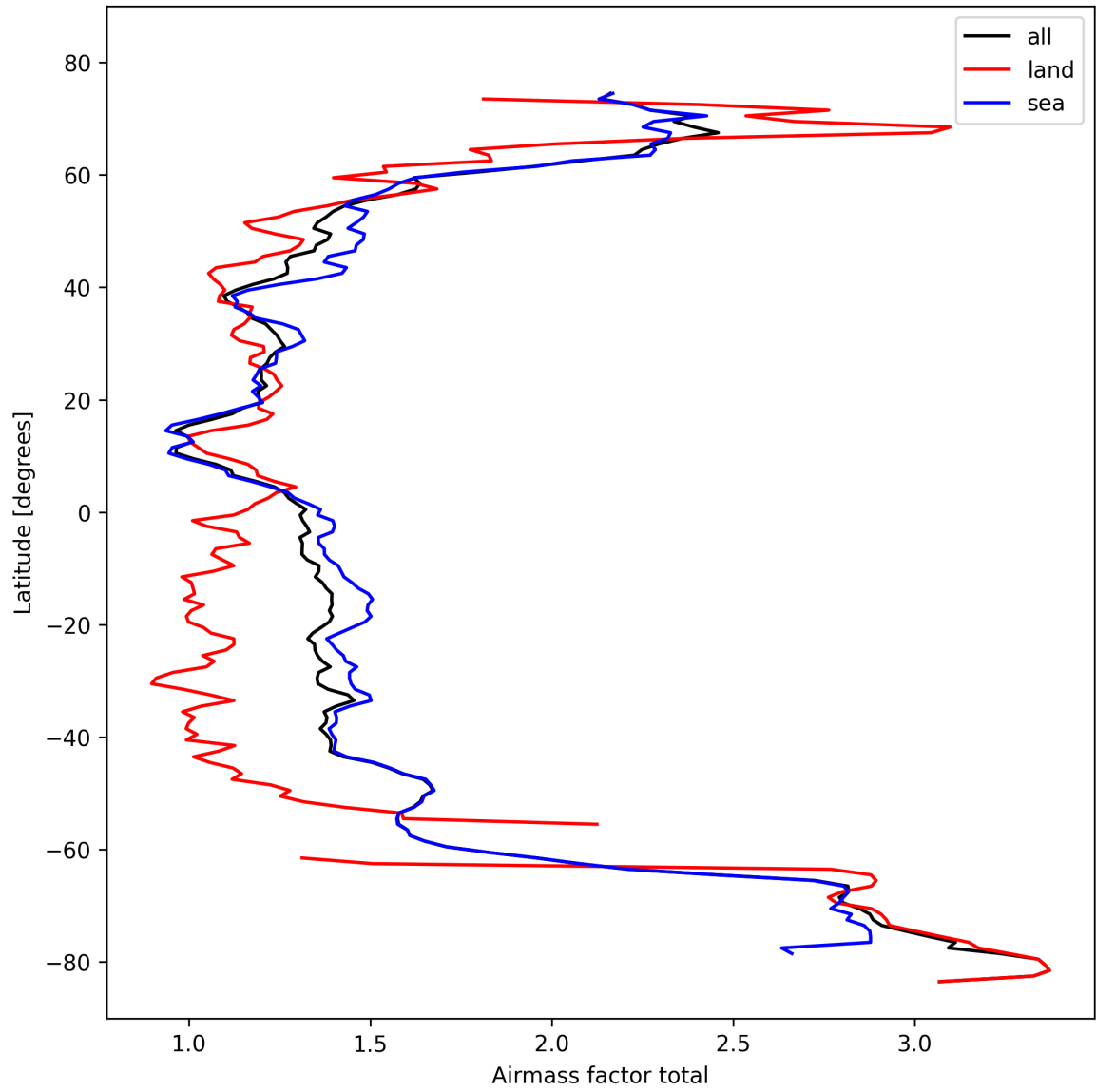
Figure 26: Zonal average of “Airmass factor total” for 2024-10-20 to 2024-10-22.
