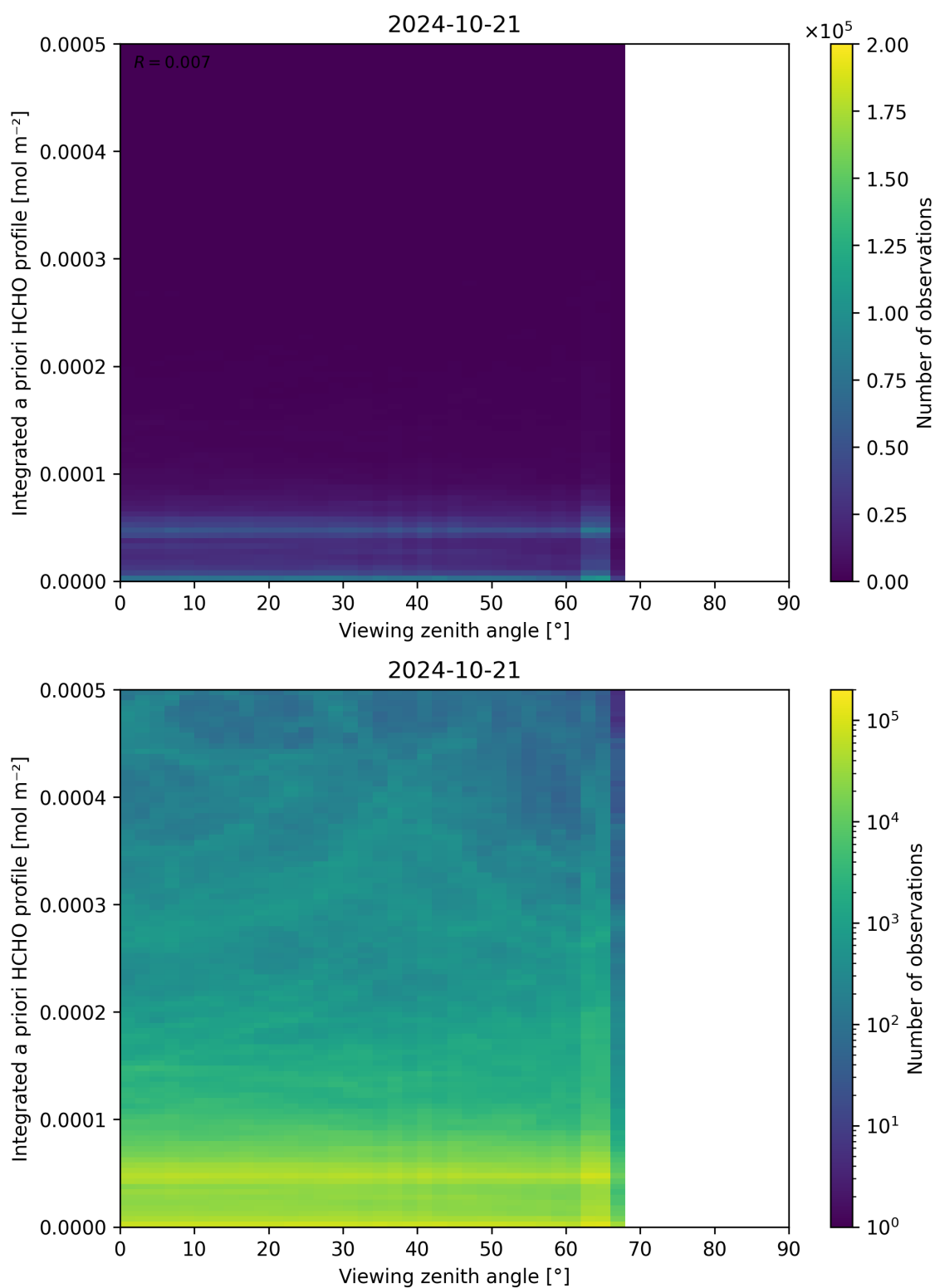
Figure 195: Scatter density plot of “Viewing zenith angle” against “Integrated a priori HCHO profile” for 2024-10-20 to 2024-10-22.
