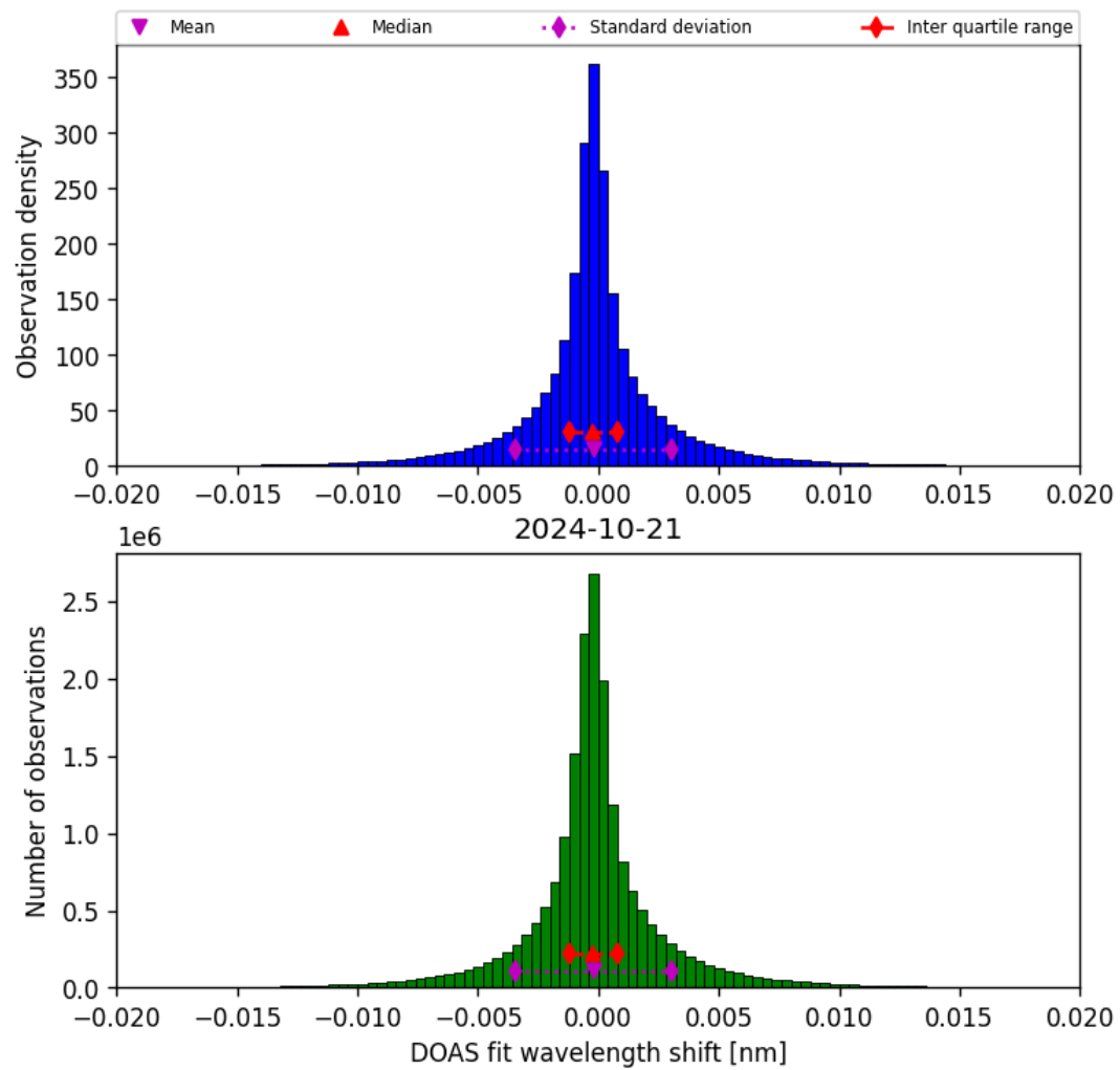
Figure 44: Histogram of “DOAS fit wavelength shift” for 2024-10-20 to 2024-10-22
