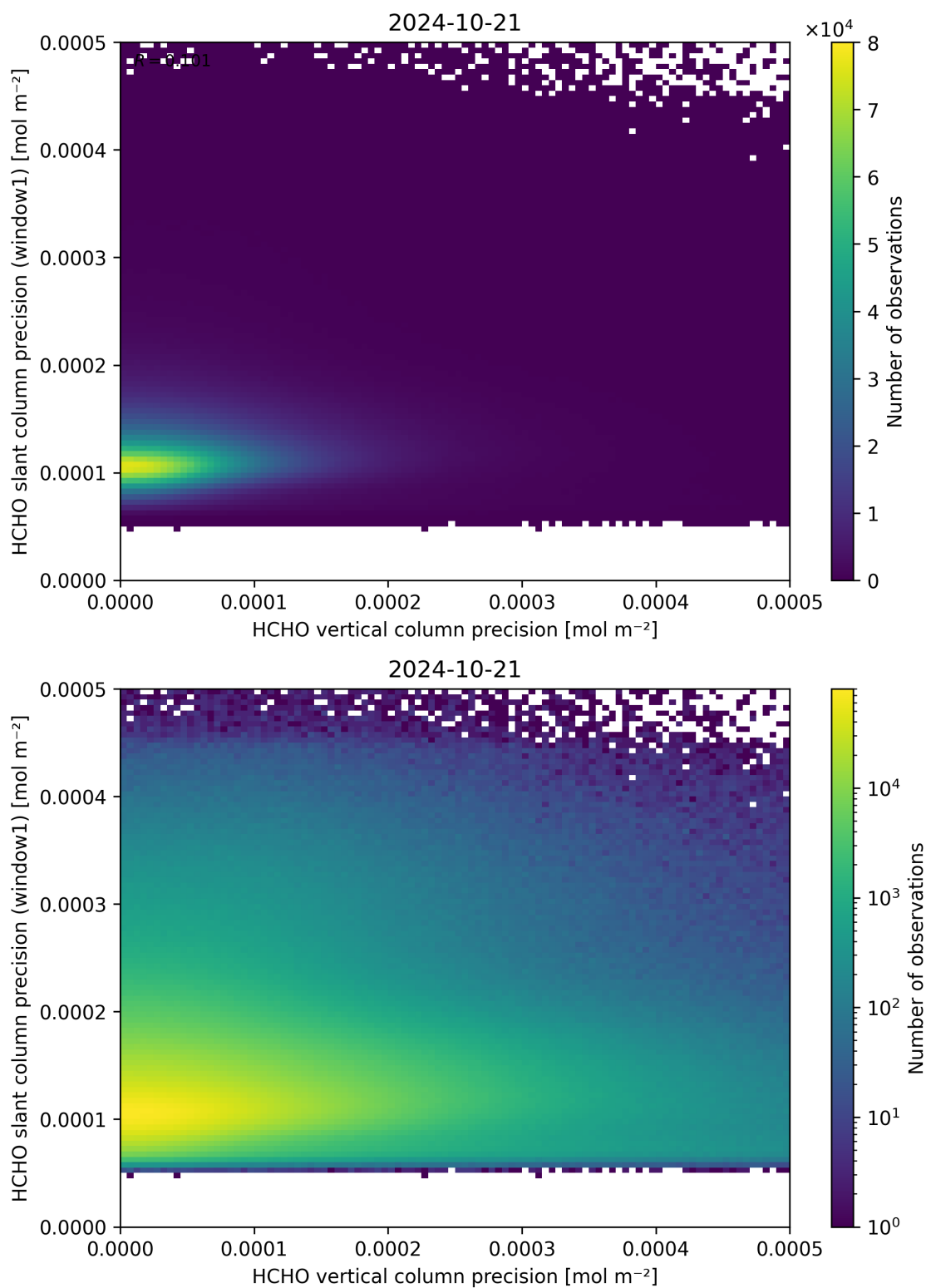
Figure 143: Scatter density plot of “HCHO vertical column precision” against “HCHO slant column precision (window1)” for 2024-10-20 to 2024-10-22.
