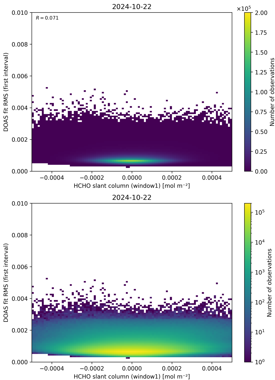
Figure 78: Scatter density plot of “HCHO slant column (window1)” against “DOAS fit RMS (first interval)” for 2024-10-21 to 2024-10-23.
