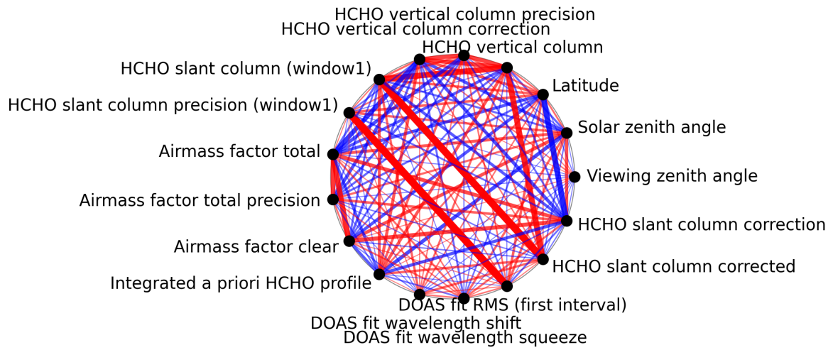
Figure 1: Map of correlation graph for 2024-10-21 to 2024-10-23.
