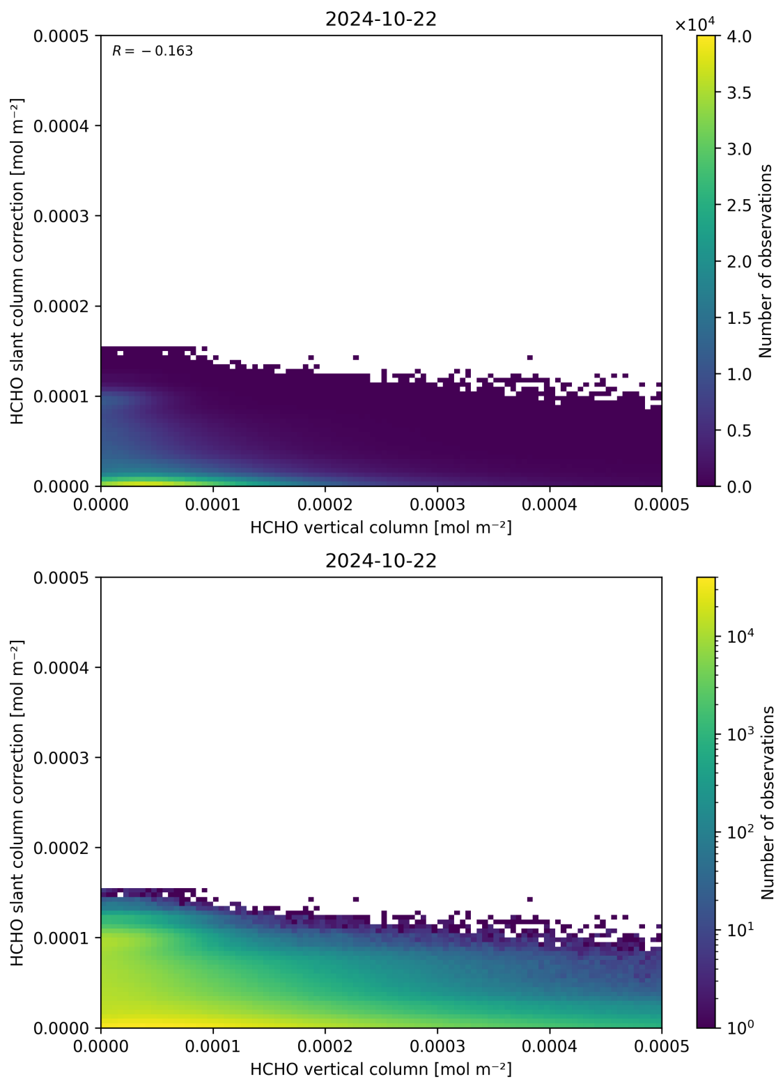
Figure 128: Scatter density plot of “HCHO vertical column” against “HCHO slant column correction” for 2024-10-21 to 2024-10-23.
