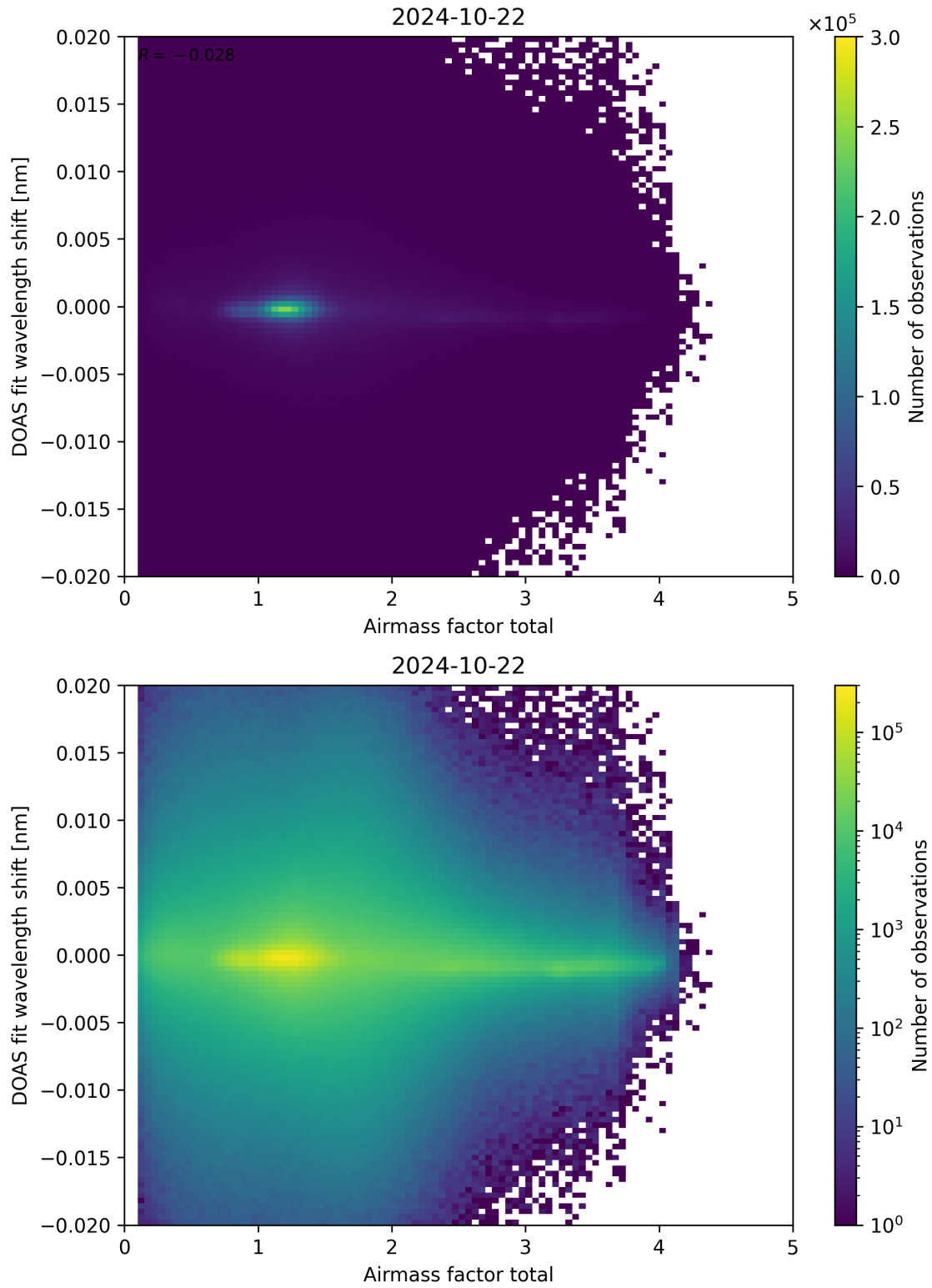
Figure 98: Scatter density plot of “Airmass factor total” against “DOAS fit wavelength shift” for 2024-10-21 to 2024-10-23.
