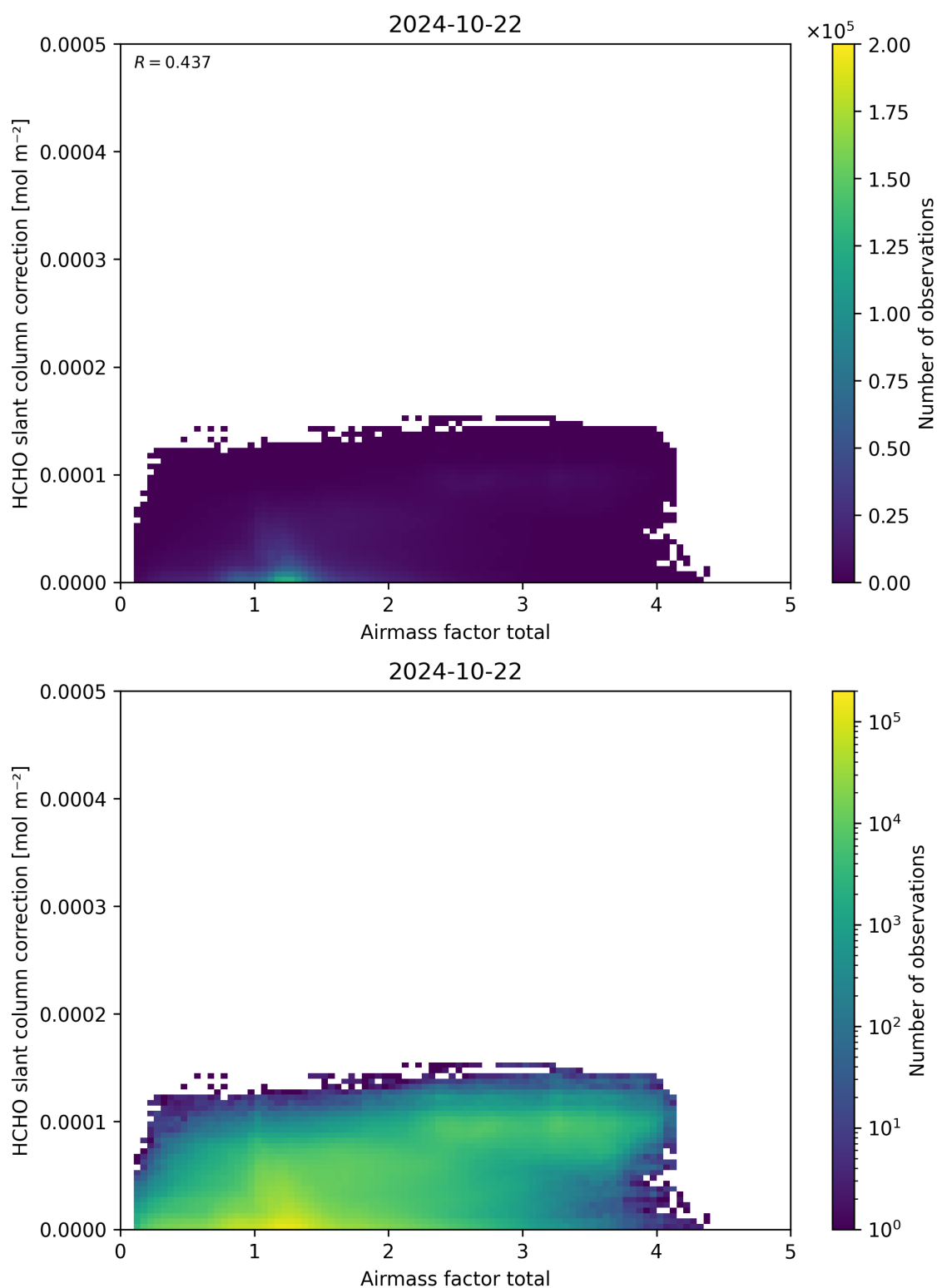
Figure 102: Scatter density plot of “Airmass factor total” against “HCHO slant column correction” for 2024-10-21 to 2024-10-23.
