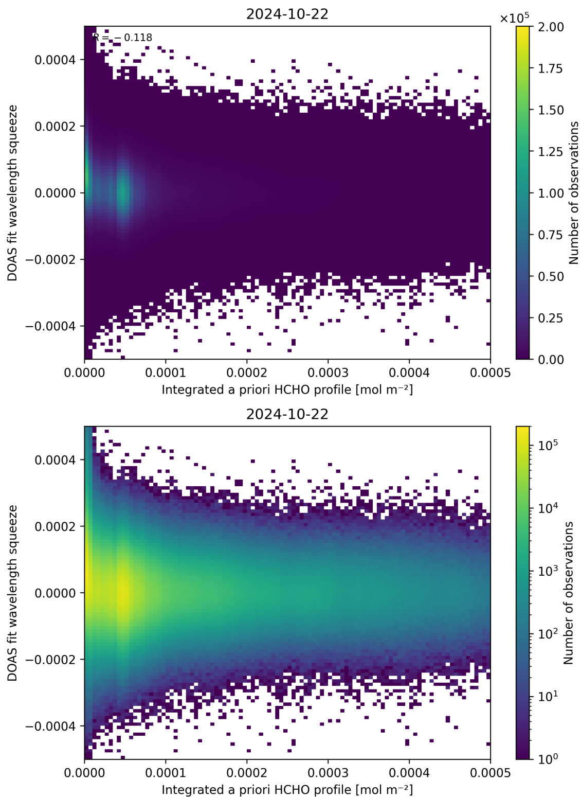
Figure 150: Scatter density plot of “Integrated a priori HCHO profile” against “DOAS fit wavelength squeeze” for 2024-10-21 to 2024-10-23.
