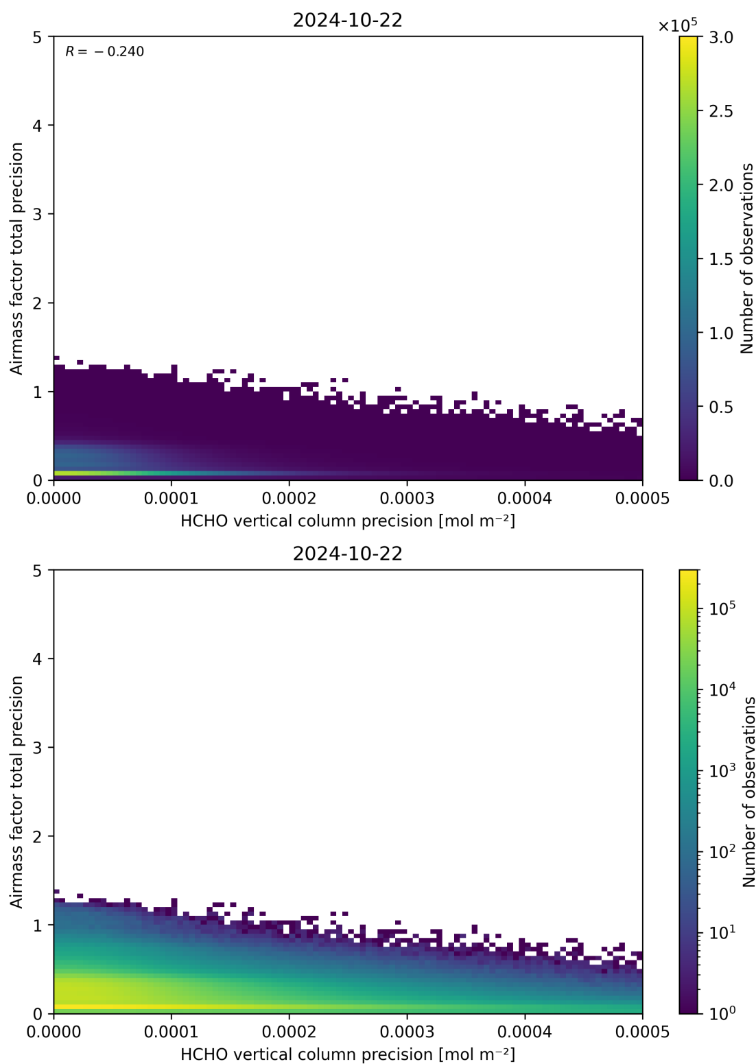
Figure 145: Scatter density plot of “HCHO vertical column precision” against “Airmass factor total precision” for 2024-10-21 to 2024-10-23.
