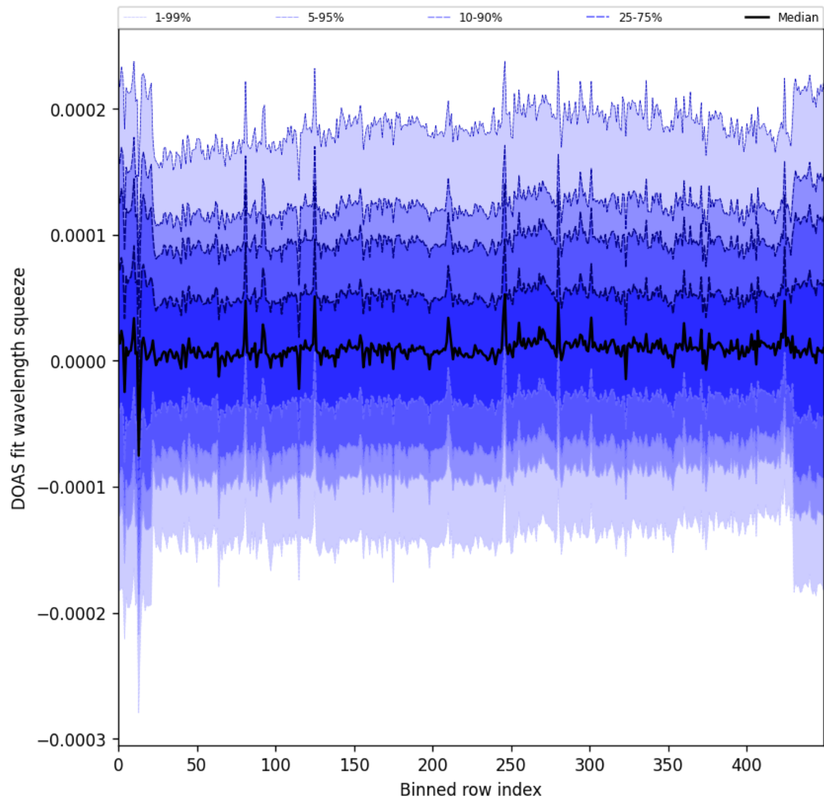
Figure 59: Along track statistics of “DOAS fit wavelength squeeze” for 2024-10-21 to 2024-10-23
