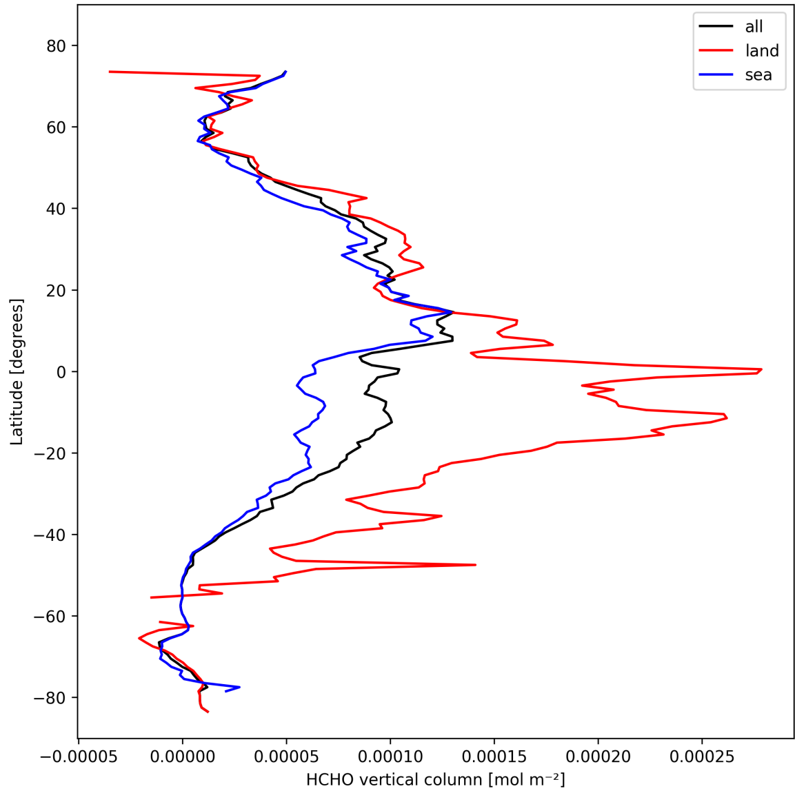
Figure 21: Zonal average of “HCHO vertical column” for 2024-10-21 to 2024-10-23.
