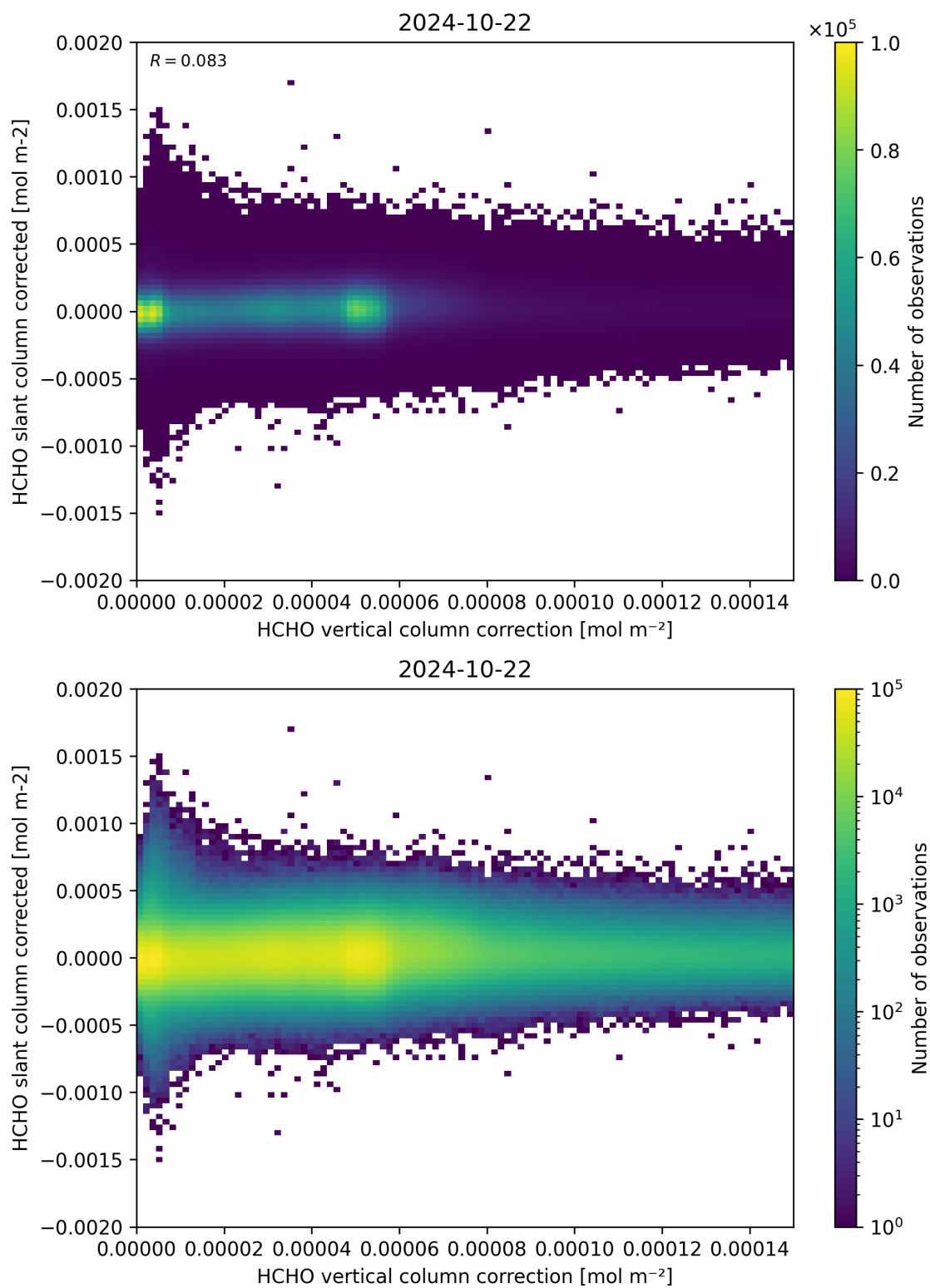
Figure 116: Scatter density plot of “HCHO vertical column correction” against “HCHO slant column corrected” for 2024-10-21 to 2024-10-23.
