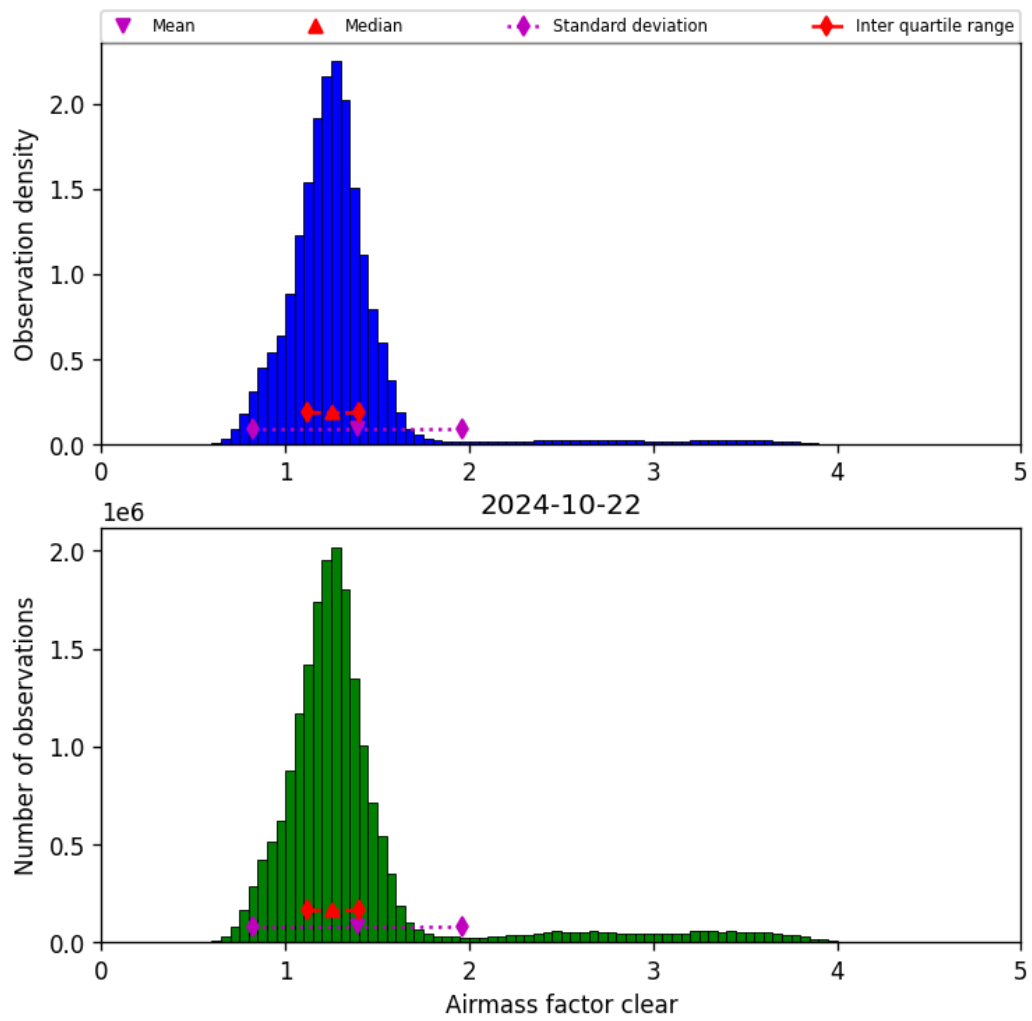
Figure 42: Histogram of “Airmass factor clear” for 2024-10-21 to 2024-10-23
