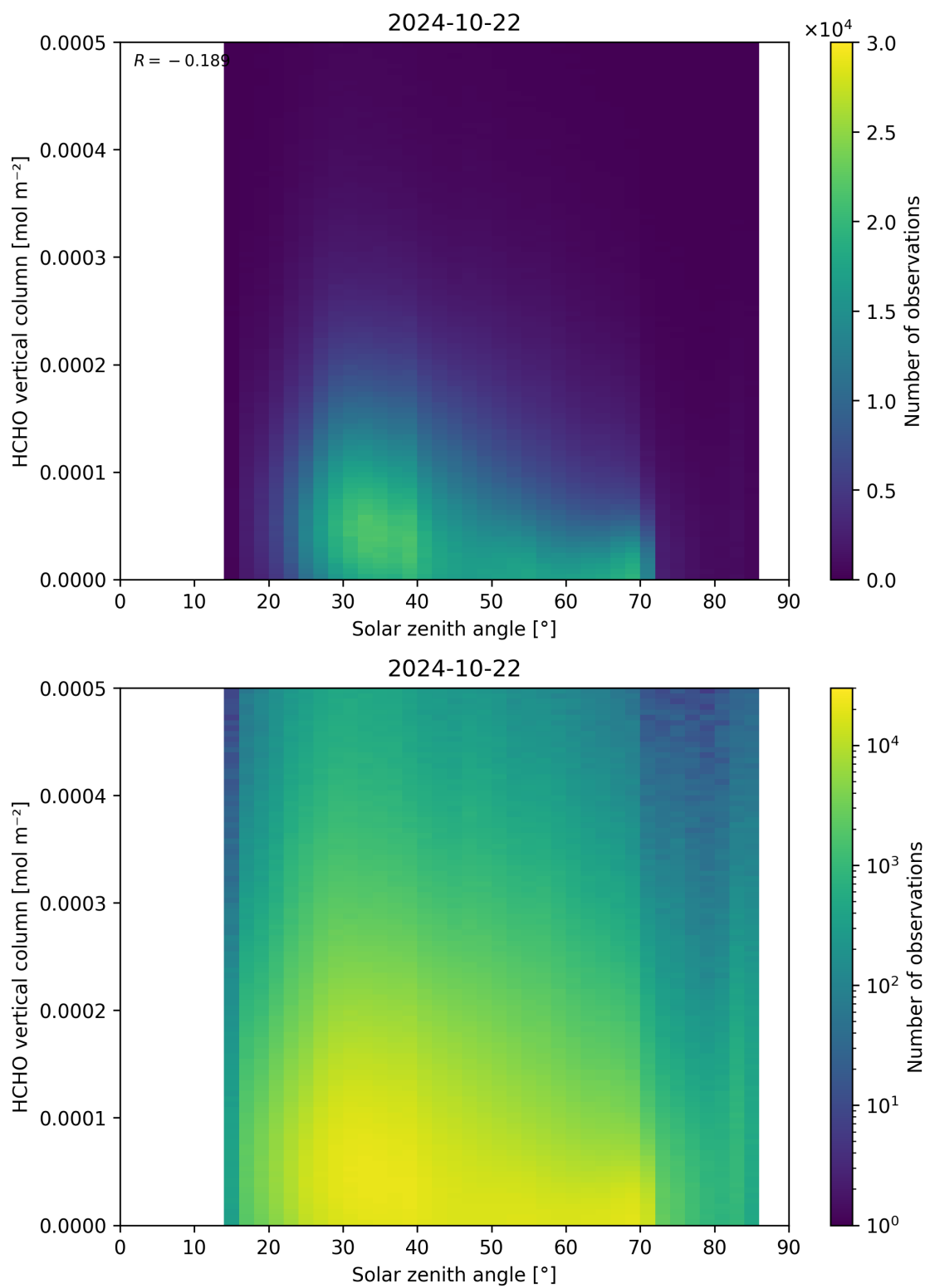
Figure 177: Scatter density plot of “Solar zenith angle” against “HCHO vertical column” for 2024-10-21 to 2024-10-23.
