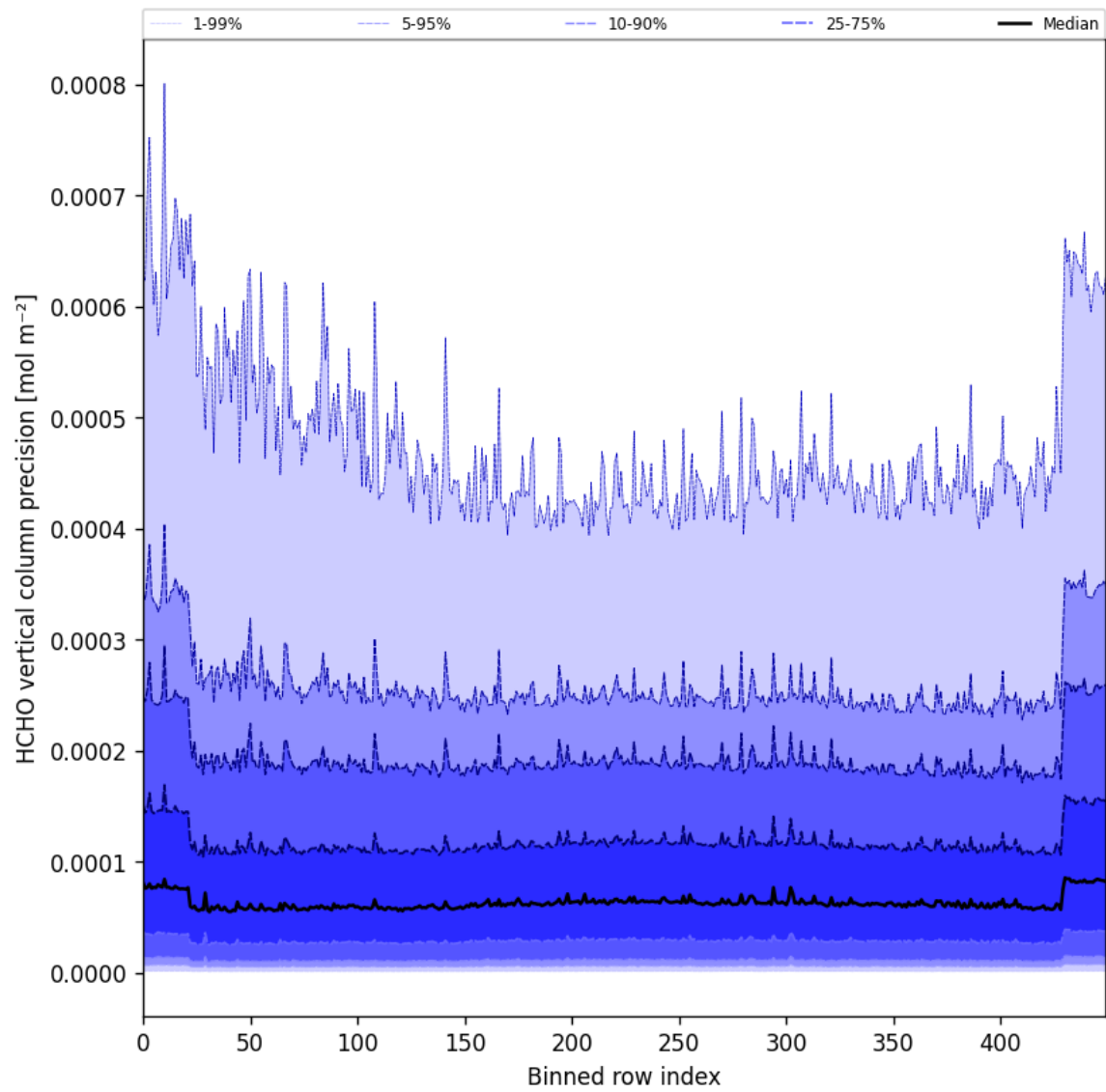
Figure 50: Along track statistics of "HCHO vertical column precision" for 2024-10-21 to 2024-10-23
