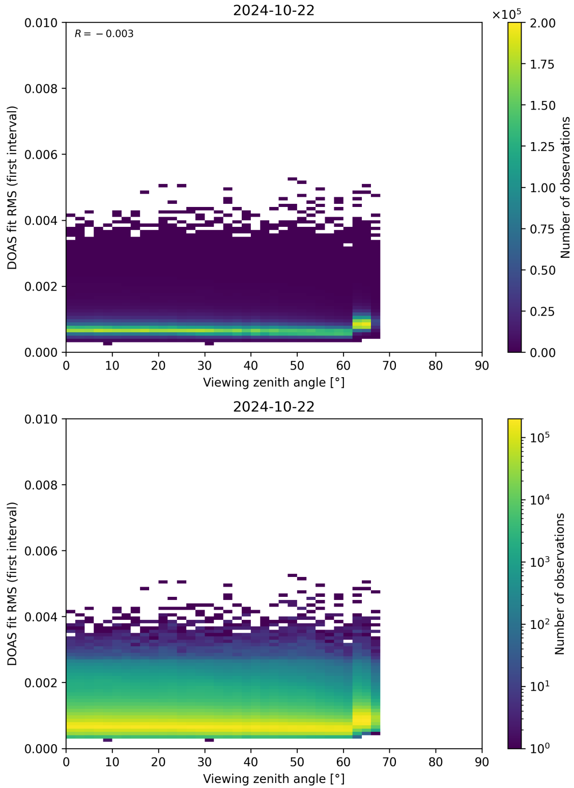
Figure 182: Scatter density plot of “Viewing zenith angle” against “DOAS fit RMS (first interval)” for 2024-10-21 to 2024-10-23.
