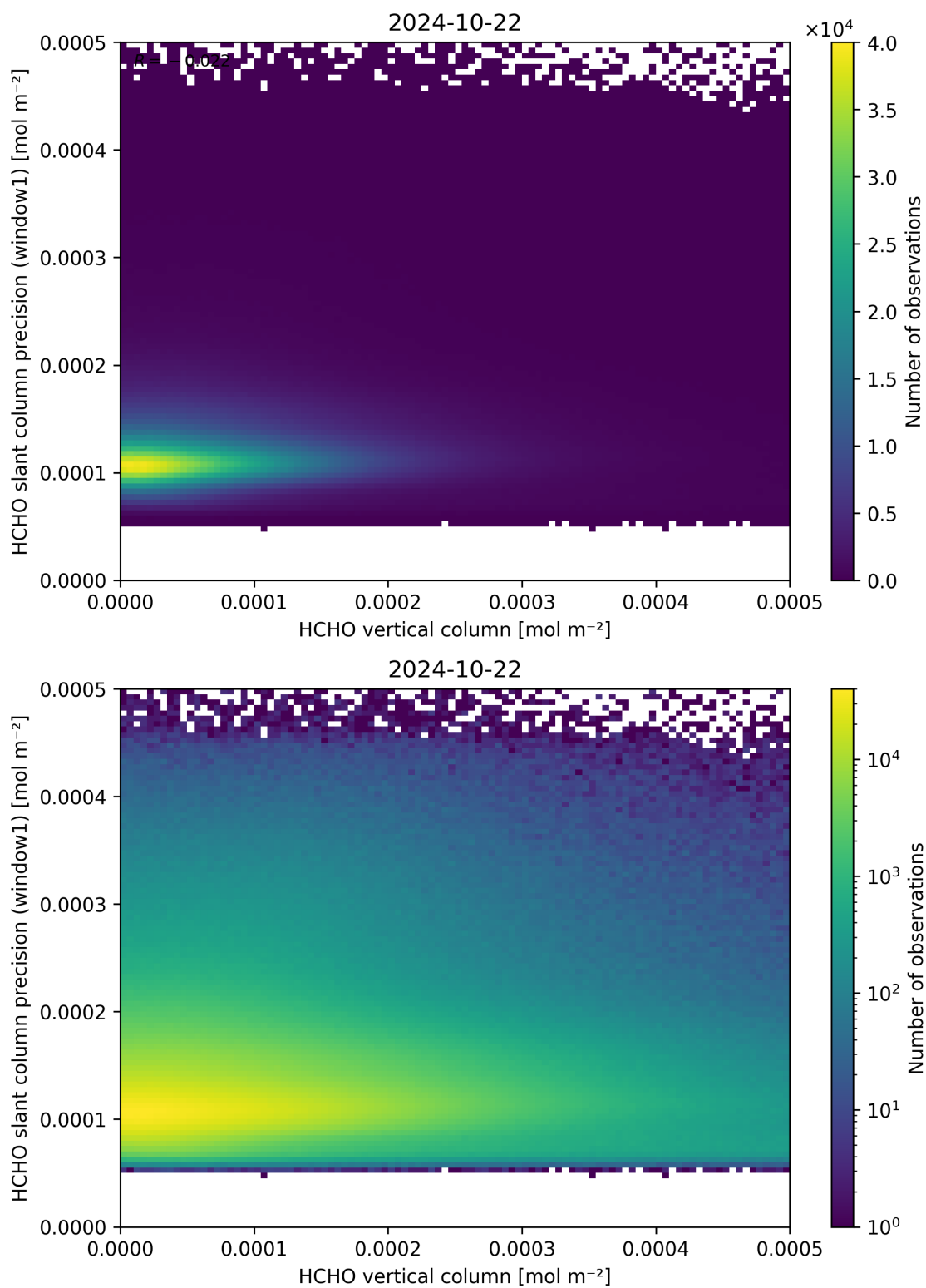
Figure 130: Scatter density plot of “HCHO vertical column” against “HCHO slant column precision (window1)” for 2024-10-21 to 2024-10-23.
