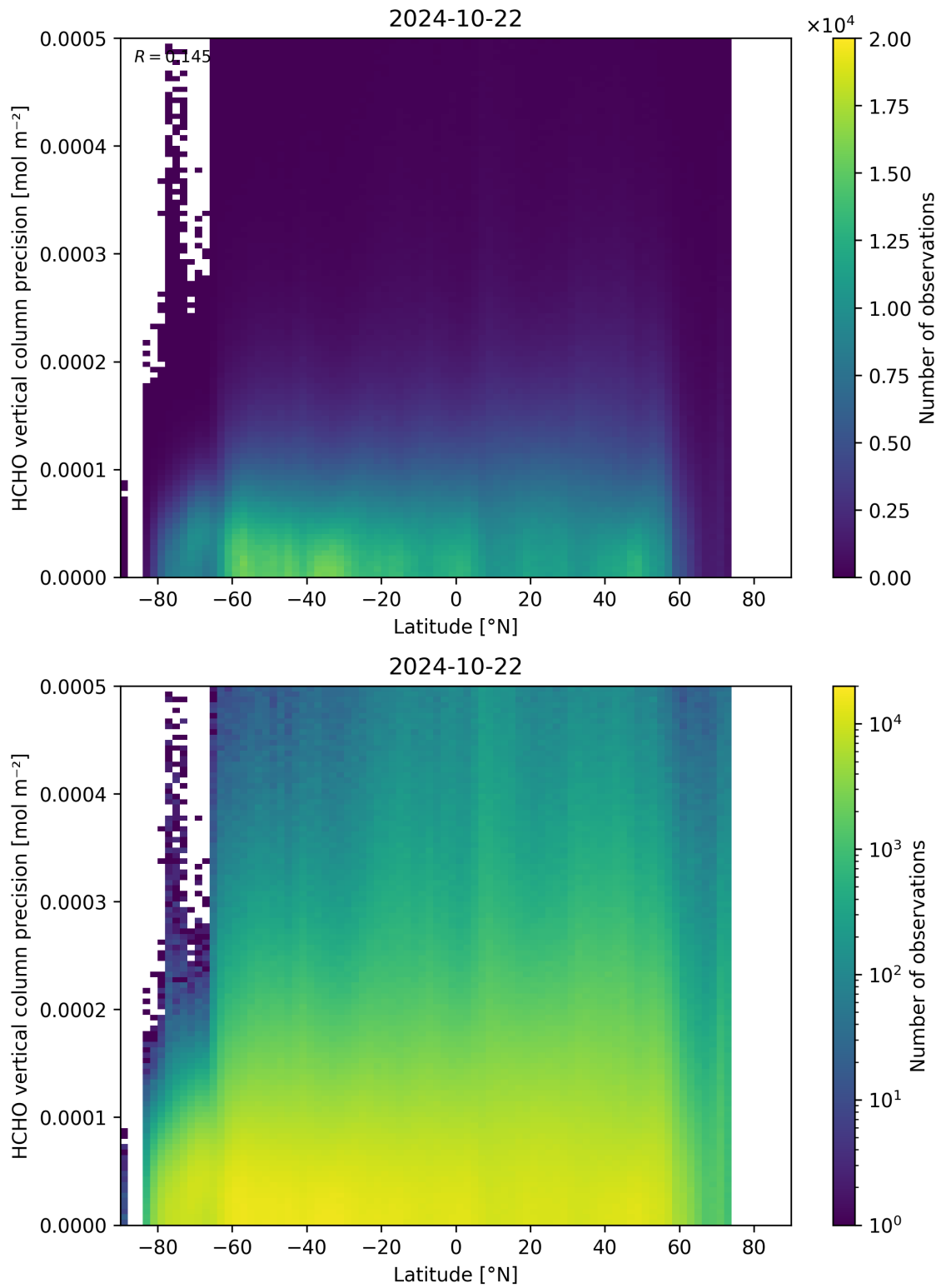
Figure 165: Scatter density plot of “Latitude” against “HCHO vertical column precision” for 2024-10-21 to 2024-10-23.
