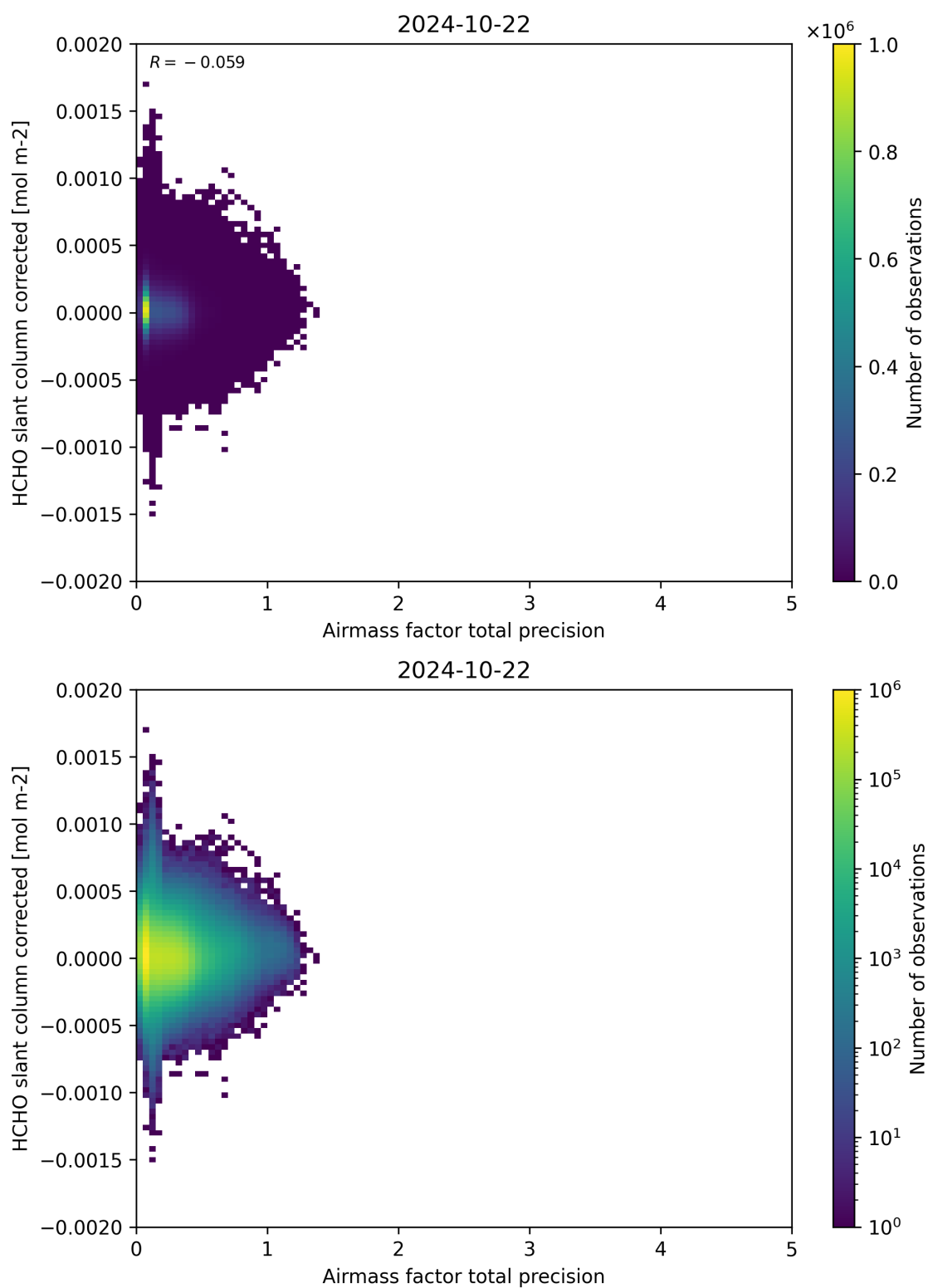
Figure 109: Scatter density plot of “Airmass factor total precision” against “HCHO slant column corrected” for 2024-10-21 to 2024-10-23.
