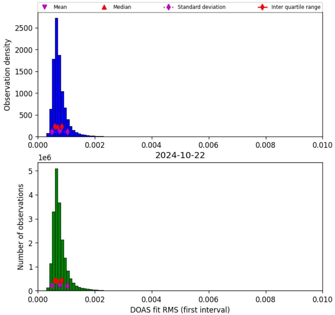
Figure 46: Histogram of “DOAS fit RMS (first interval)” for 2024-10-21 to 2024-10-23
