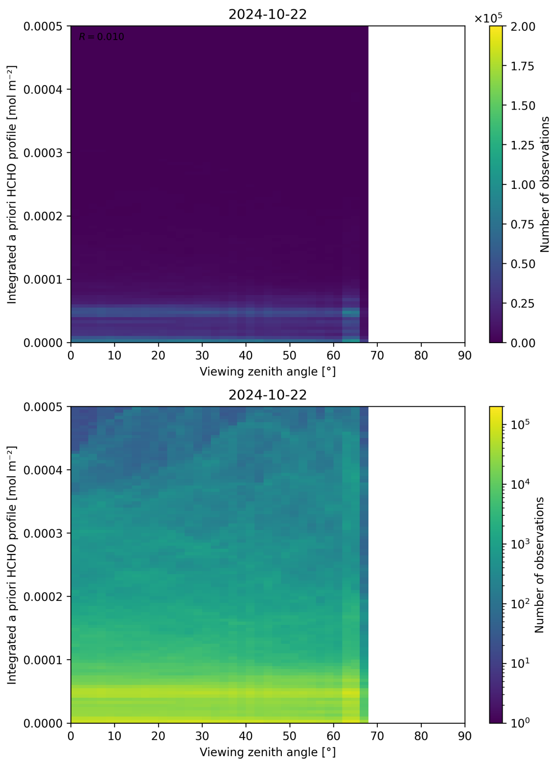
Figure 195: Scatter density plot of “Viewing zenith angle” against “Integrated a priori HCHO profile” for 2024-10-21 to 2024-10-23.
