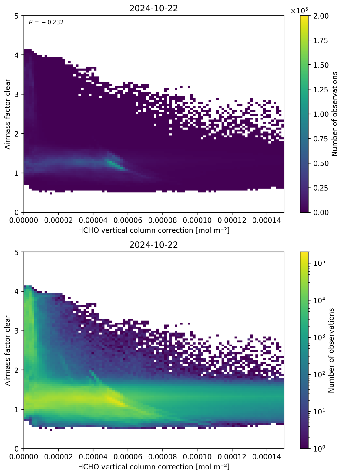
Figure 115: Scatter density plot of “HCHO vertical column correction” against “Airmass factor clear” for 2024-10-21 to 2024-10-23.
