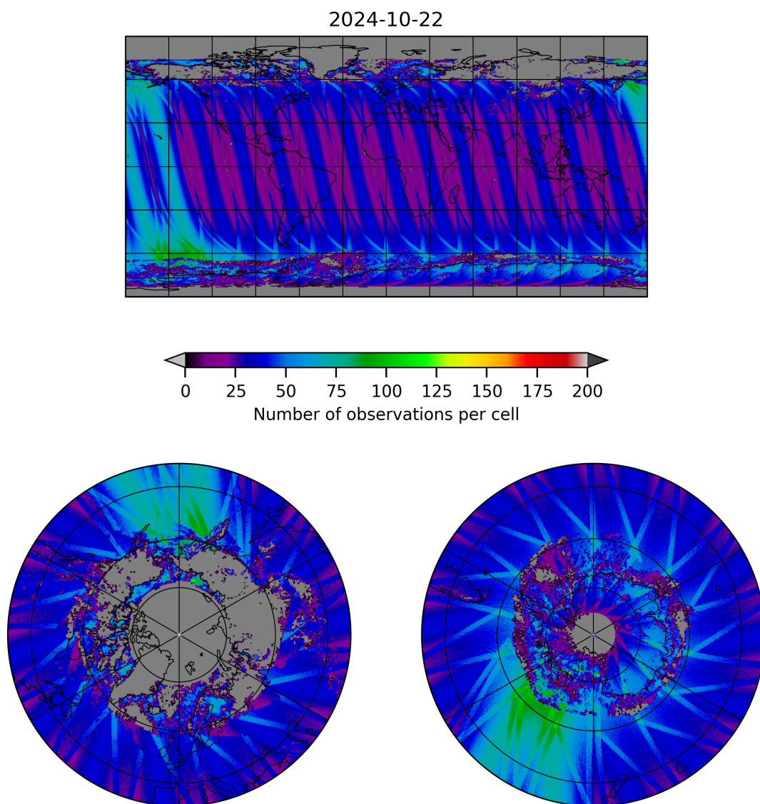
Figure 19: Map of the number of observations for 2024-10-21 to 2024-10-23
