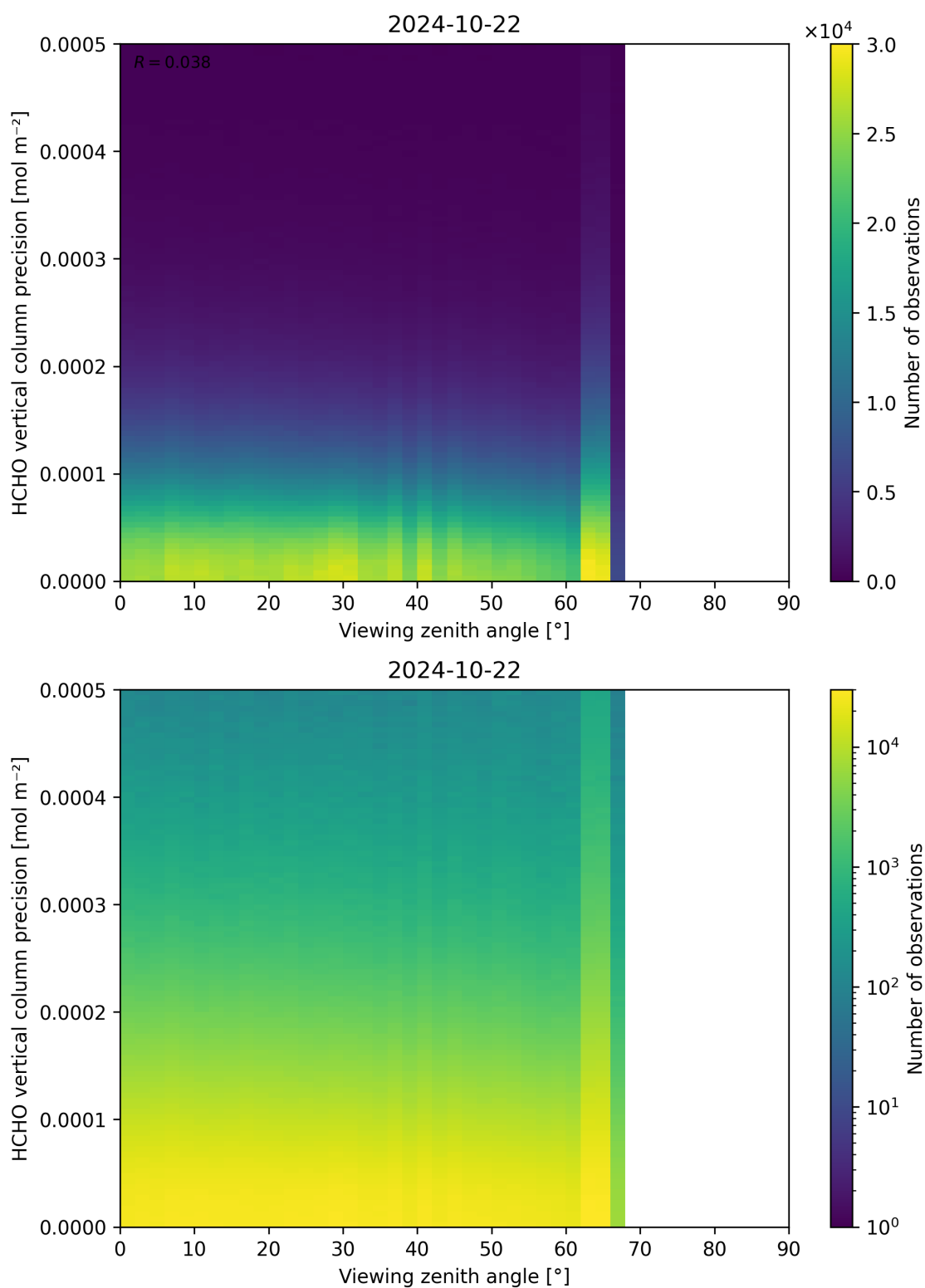
Figure 194: Scatter density plot of “Viewing zenith angle” against “HCHO vertical column precision” for 2024-10-21 to 2024-10-23.
