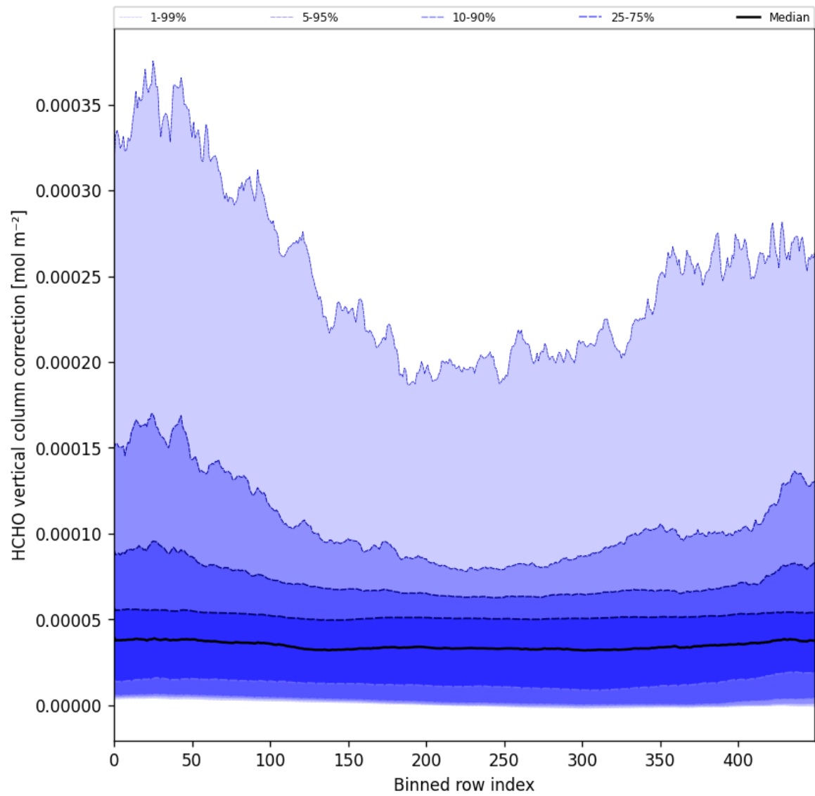
Figure 51: Along track statistics of “HCHO vertical column correction” for 2024-10-21 to 2024-10-23
