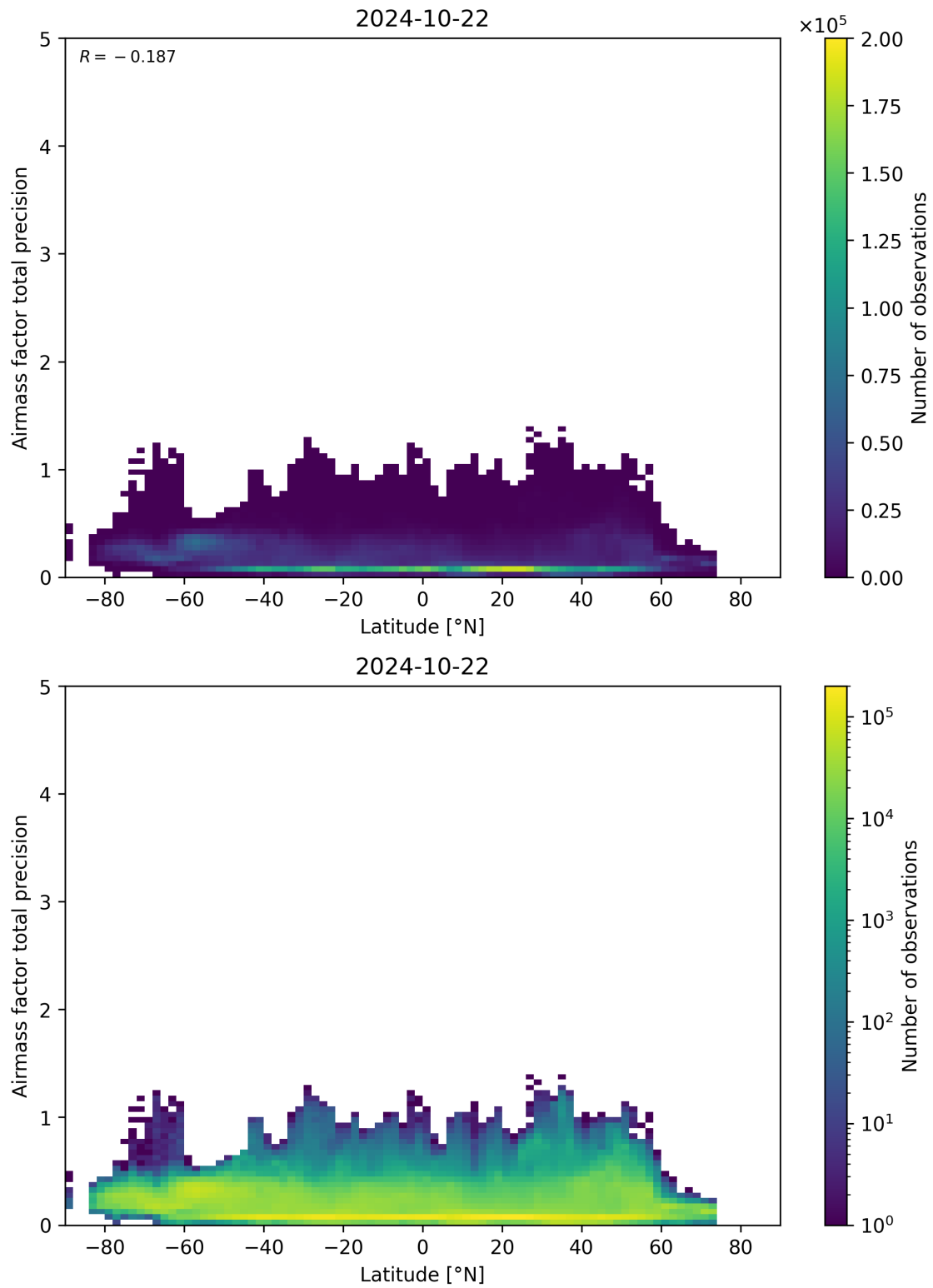
Figure 162: Scatter density plot of “Latitude” against “Airmass factor total precision” for 2024-10-21 to 2024-10-23.
