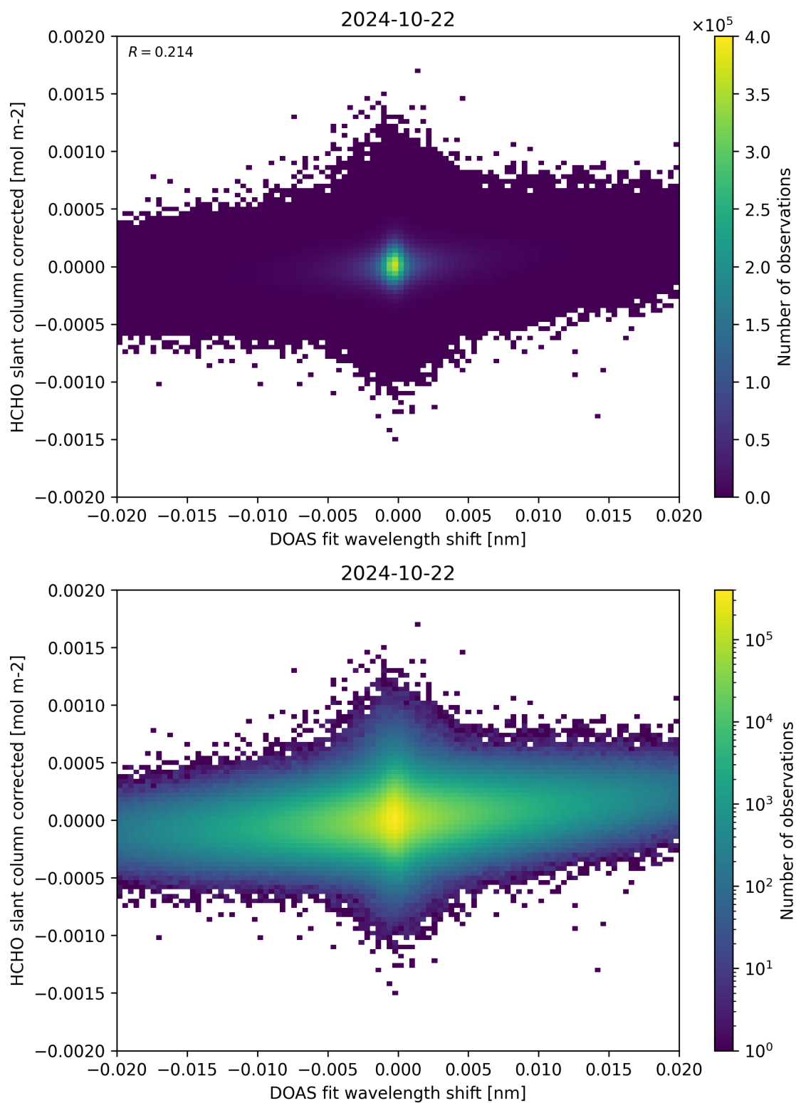
Figure 66: Scatter density plot of “DOAS fit wavelength shift” against “HCHO slant column corrected” for 2024-10-21 to 2024-10-23.
