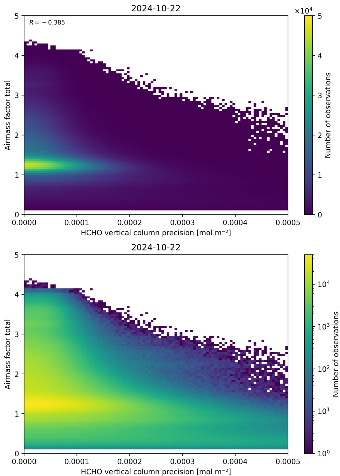
Figure 144: Scatter density plot of “HCHO vertical column precision” against “Airmass factor total” for 2024-10-21 to 2024-10-23.
