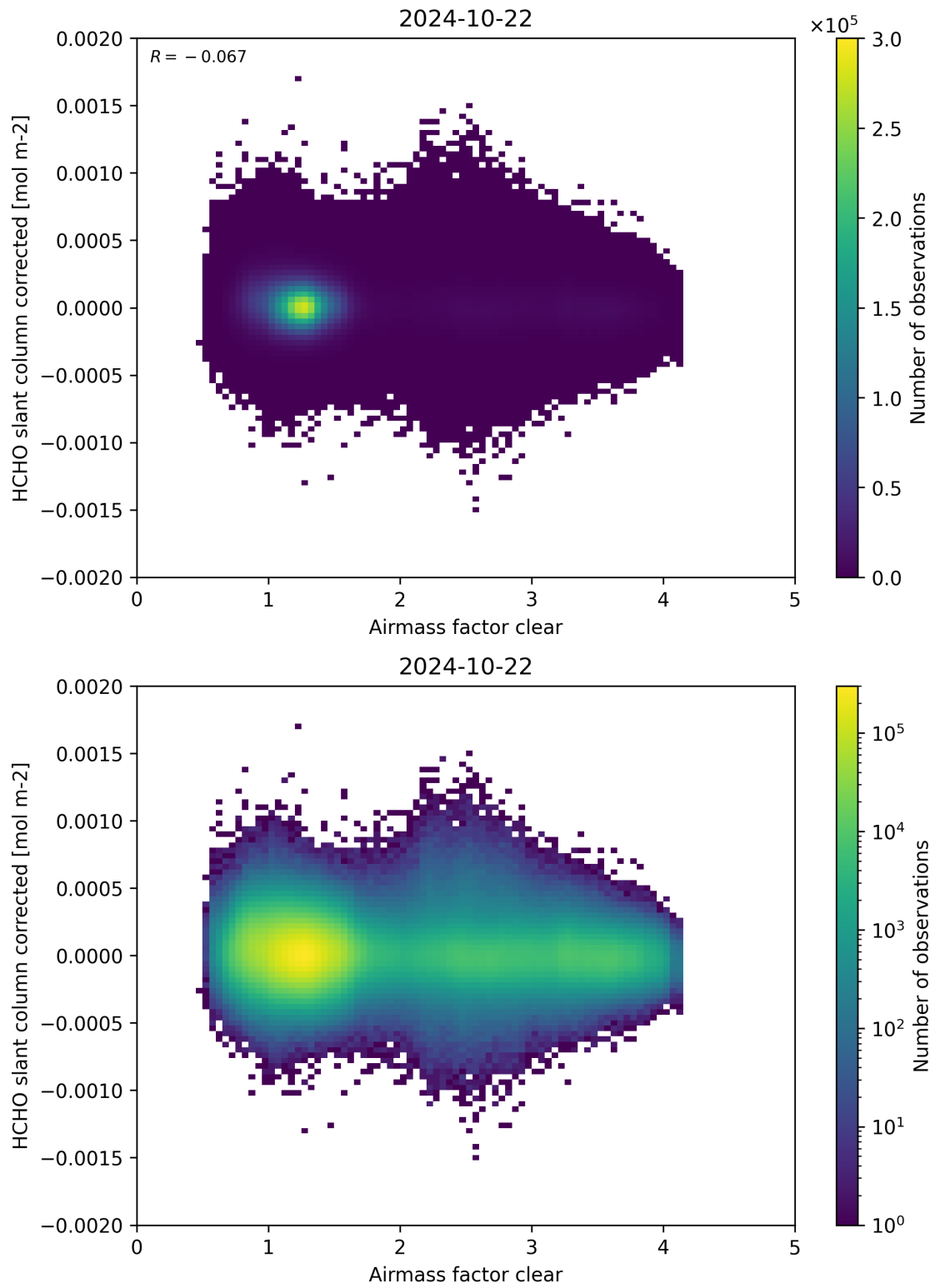
Figure 74: Scatter density plot of “Airmass factor clear” against “HCHO slant column corrected” for 2024-10-21 to 2024-10-23.
