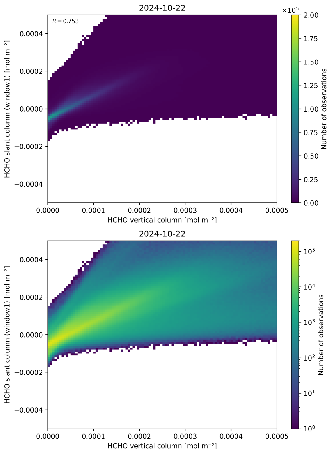
Figure 129: Scatter density plot of “HCHO vertical column” against “HCHO slant column (window1)” for 2024-10-21 to 2024-10-23.
