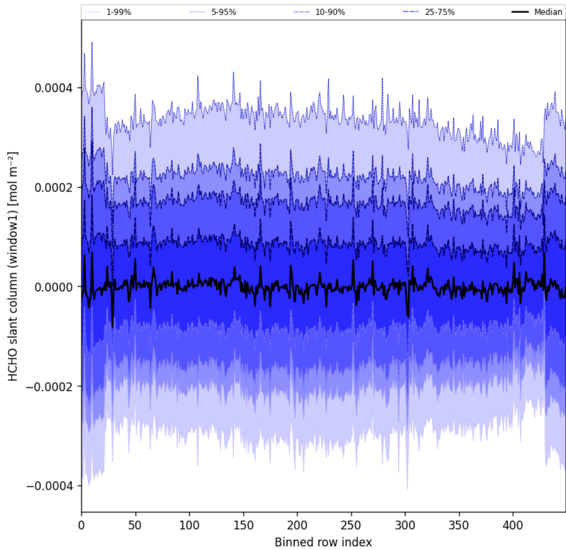
Figure 52: Along track statistics of “HCHO slant column (window1)” for 2024-10-21 to 2024-10-23
