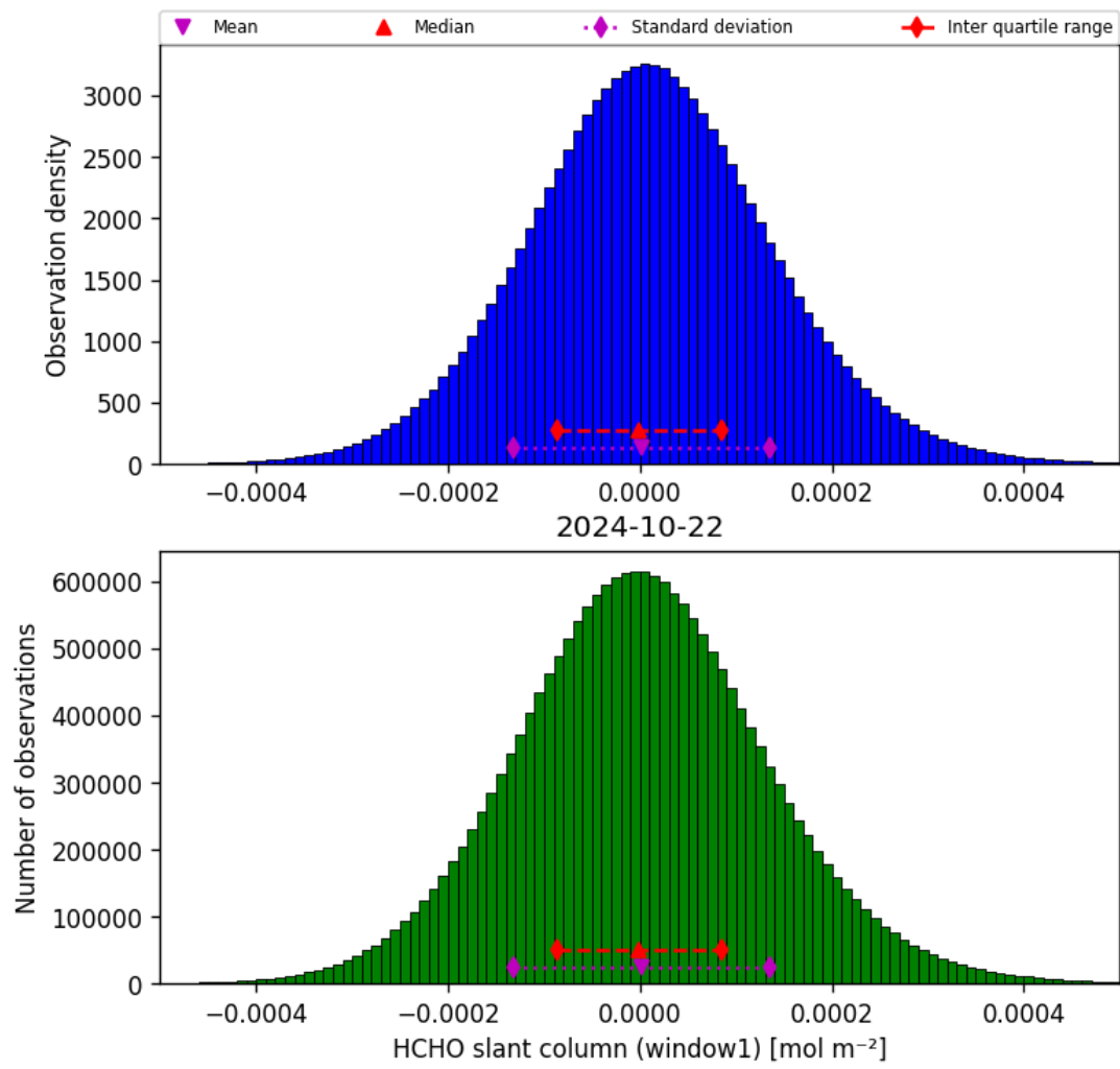
Figure 38: Histogram of “HCHO slant column (window1)” for 2024-10-21 to 2024-10-23
