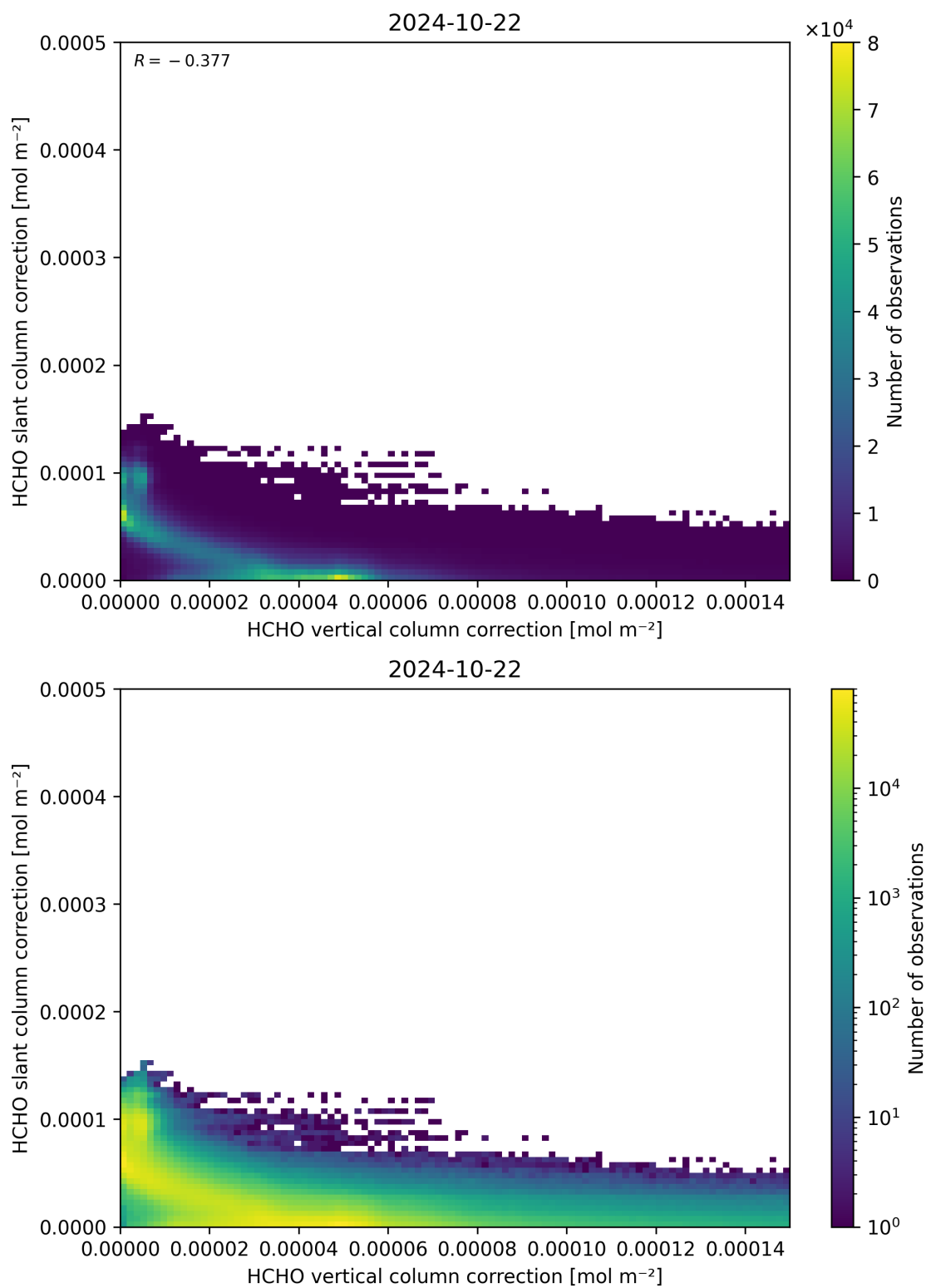
Figure 117: Scatter density plot of “HCHO vertical column correction” against “HCHO slant column correction” for 2024-10-21 to 2024-10-23.
