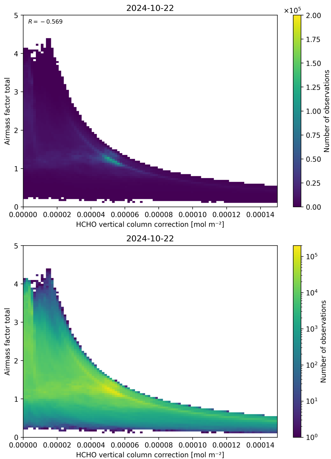
Figure 120: Scatter density plot of “HCHO vertical column correction” against “Airmass factor total” for 2024-10-21 to 2024-10-23.
