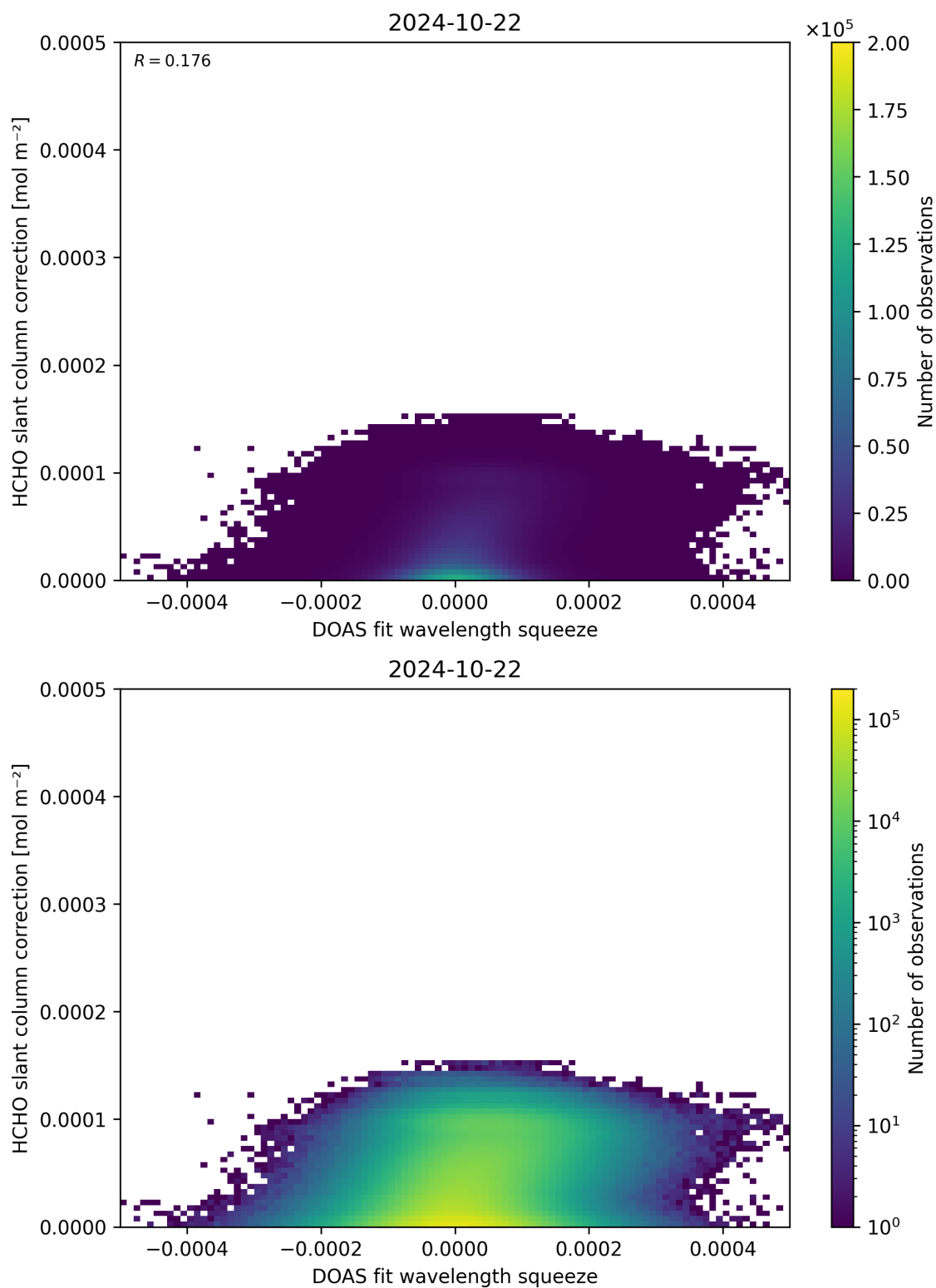
Figure 70: Scatter density plot of “DOAS fit wavelength squeeze” against “HCHO slant column correction” for 2024-10-21 to 2024-10-23.
