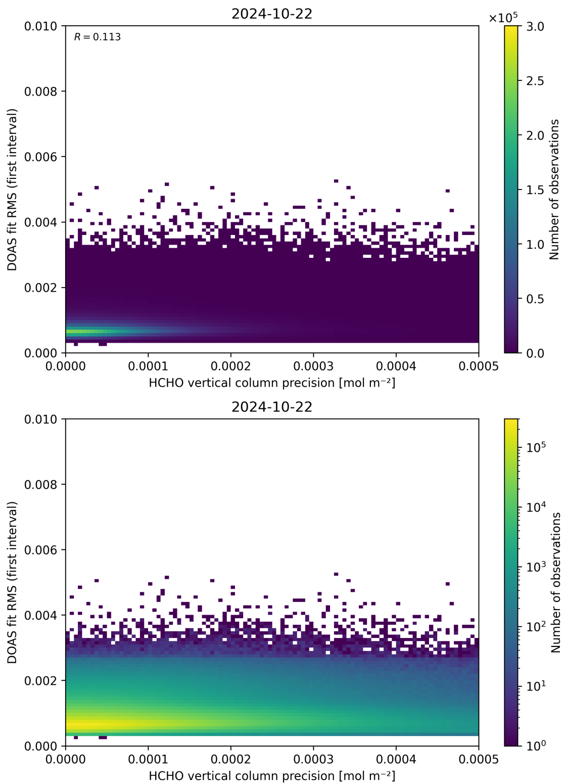
Figure 136: Scatter density plot of “HCHO vertical column precision” against “DOAS fit RMS (first interval)” for 2024-10-21 to 2024-10-23.
