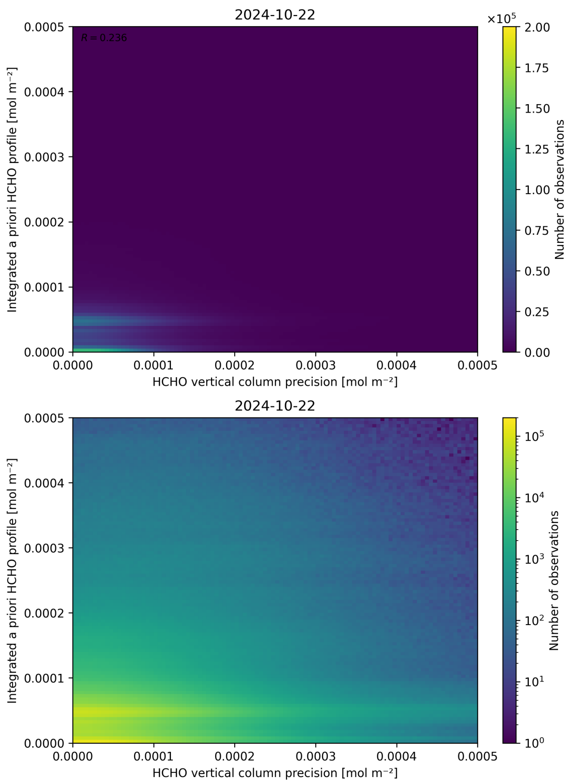
Figure 147: Scatter density plot of “HCHO vertical column precision” against “Integrated a priori HCHO profile” for 2024-10-21 to 2024-10-23.
