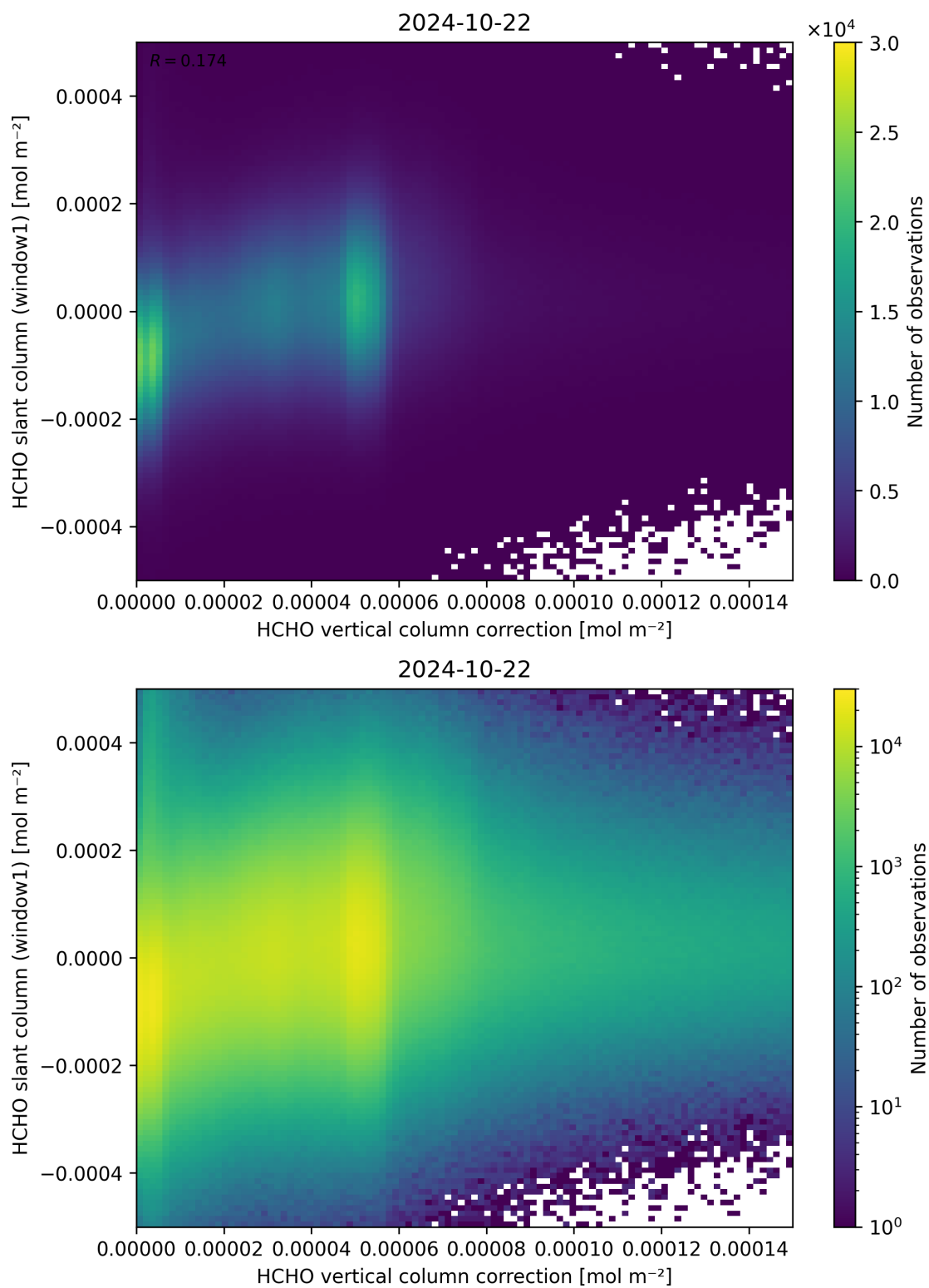
Figure 118: Scatter density plot of “HCHO vertical column correction” against “HCHO slant column (window1)” for 2024-10-21 to 2024-10-23.
