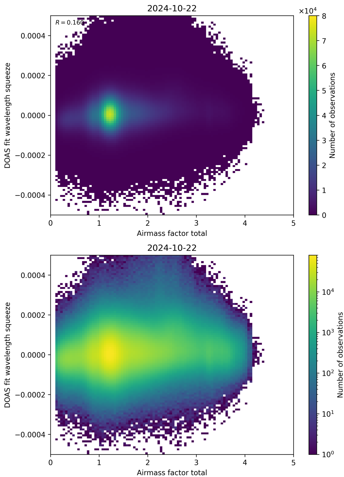
Figure 99: Scatter density plot of “Airmass factor total” against “DOAS fit wavelength squeeze” for 2024-10-21 to 2024-10-23.
