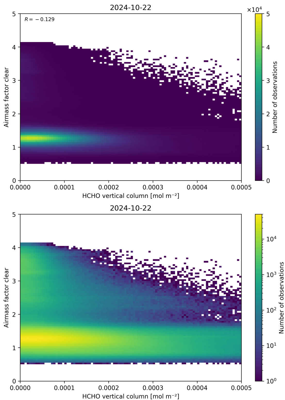
Figure 126: Scatter density plot of “HCHO vertical column” against “Airmass factor clear” for 2024-10-21 to 2024-10-23.
