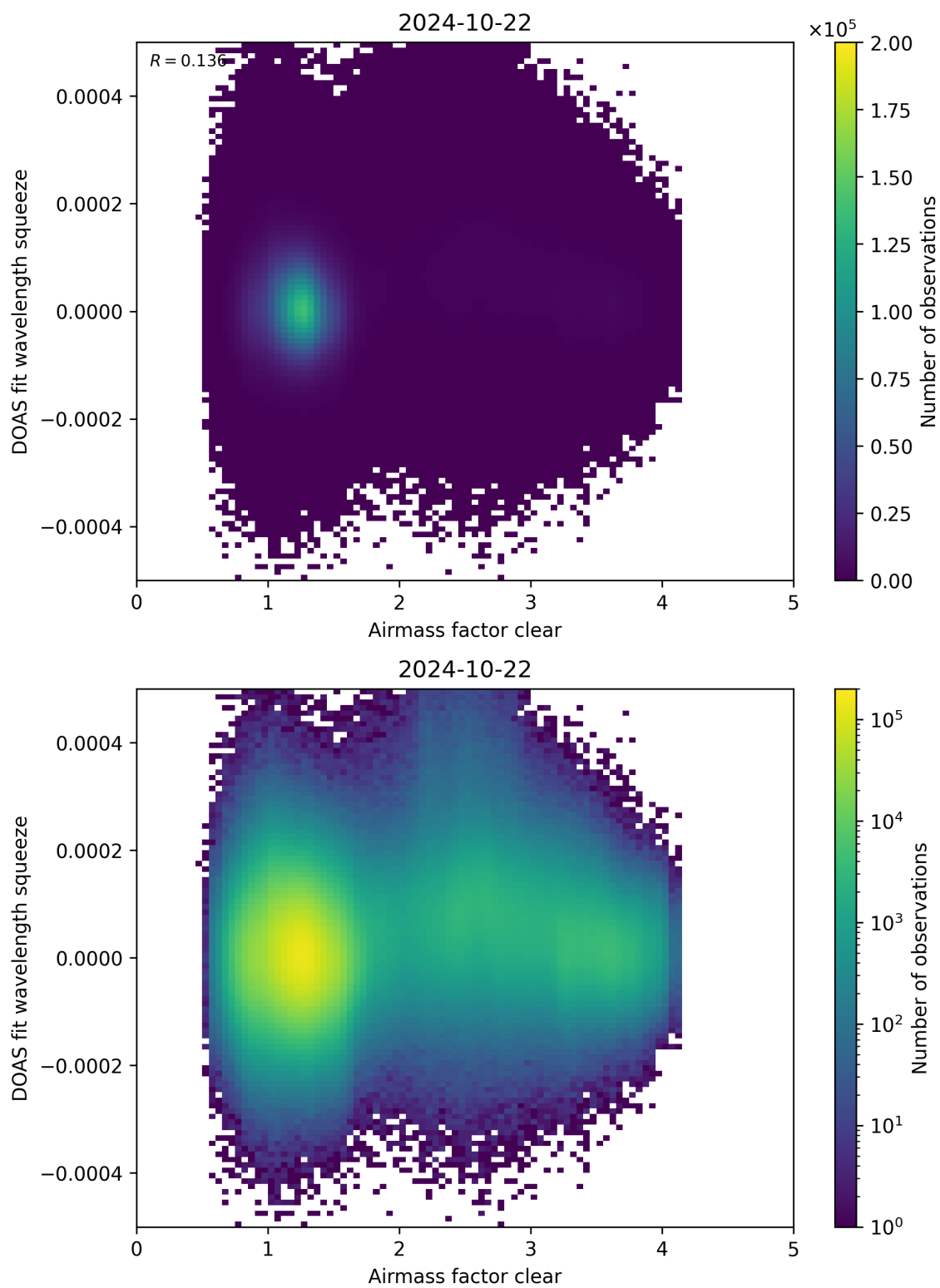
Figure 73: Scatter density plot of “Airmass factor clear” against “DOAS fit wavelength squeeze” for 2024-10-21 to 2024-10-23.
