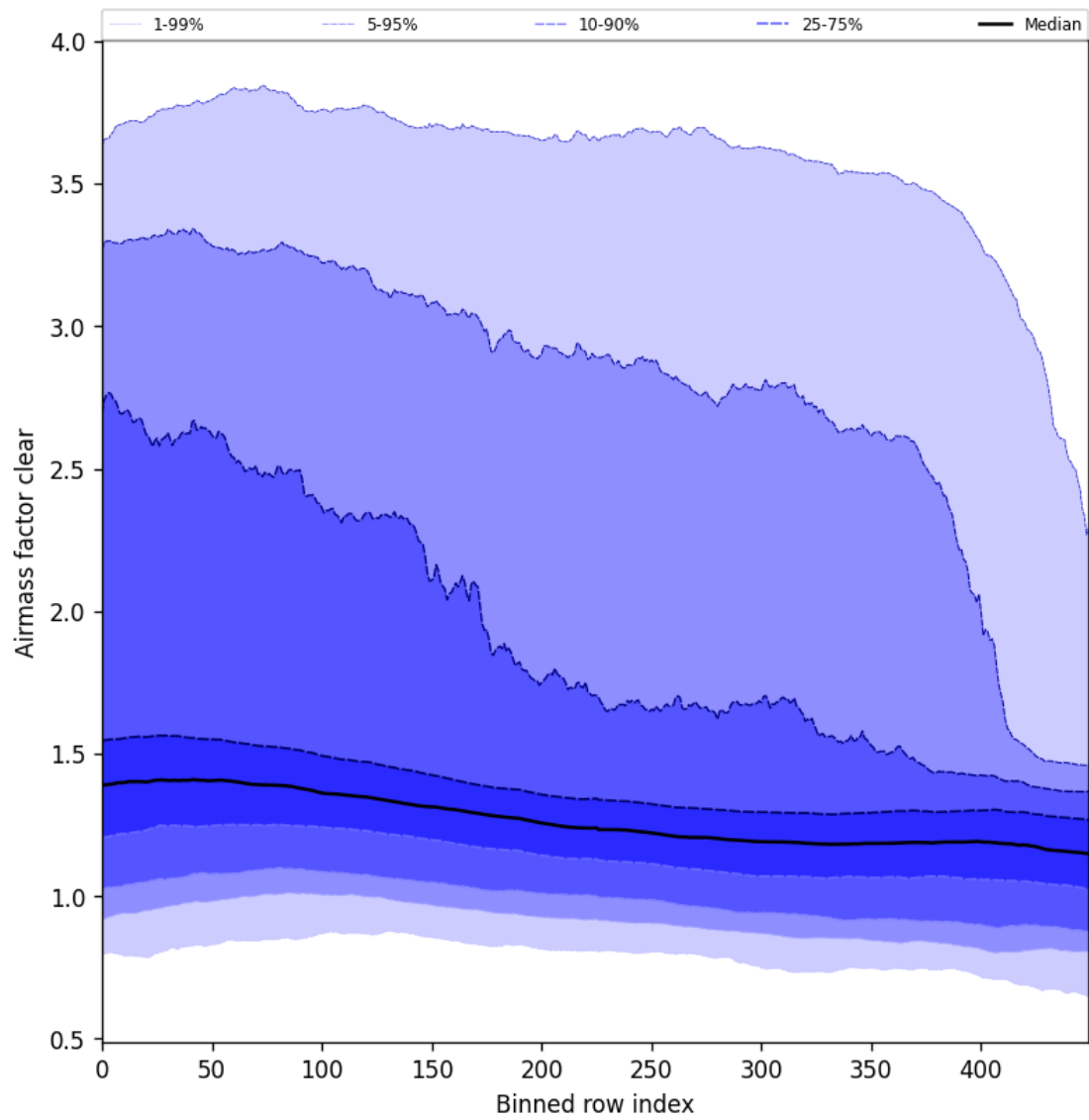
Figure 56: Along track statistics of “Airmass factor clear” for 2024-10-21 to 2024-10-23
