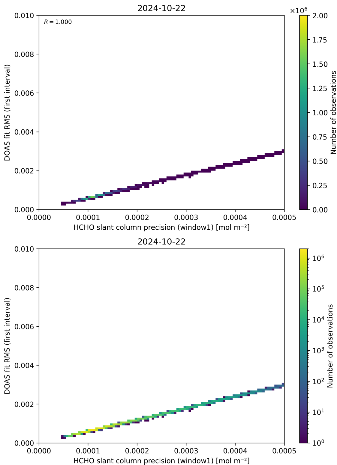
Figure 88: Scatter density plot of “HCHO slant column precision (window1)” against “DOAS fit RMS (first interval)” for 2024-10-21 to 2024-10-23.
