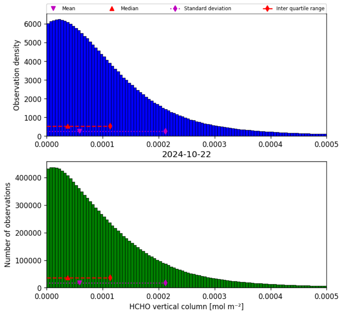
Figure 35: Histogram of “HCHO vertical column” for 2024-10-21 to 2024-10-23
