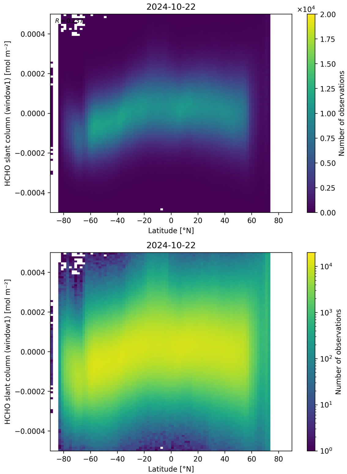
Figure 159: Scatter density plot of “Latitude” against “HCHO slant column (window1)” for 2024-10-21 to 2024-10-23.
