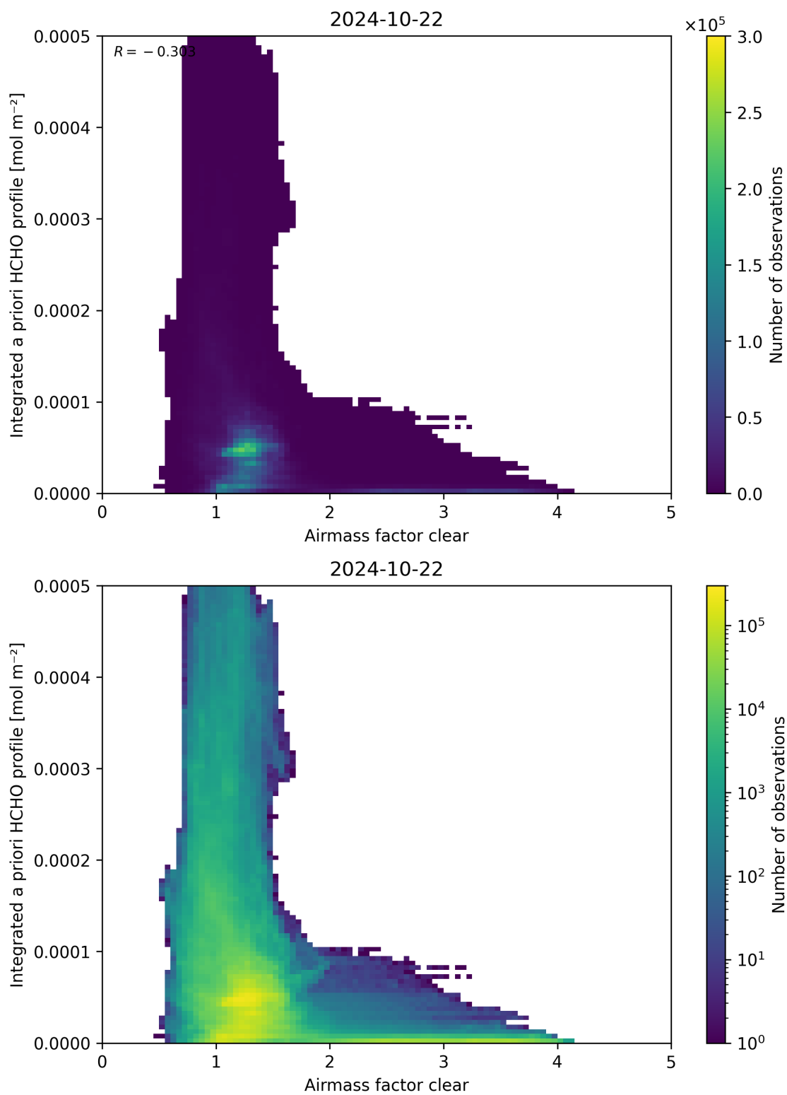
Figure 76: Scatter density plot of “Airmass factor clear” against “Integrated a priori HCHO profile” for 2024-10-21 to 2024-10-23.
