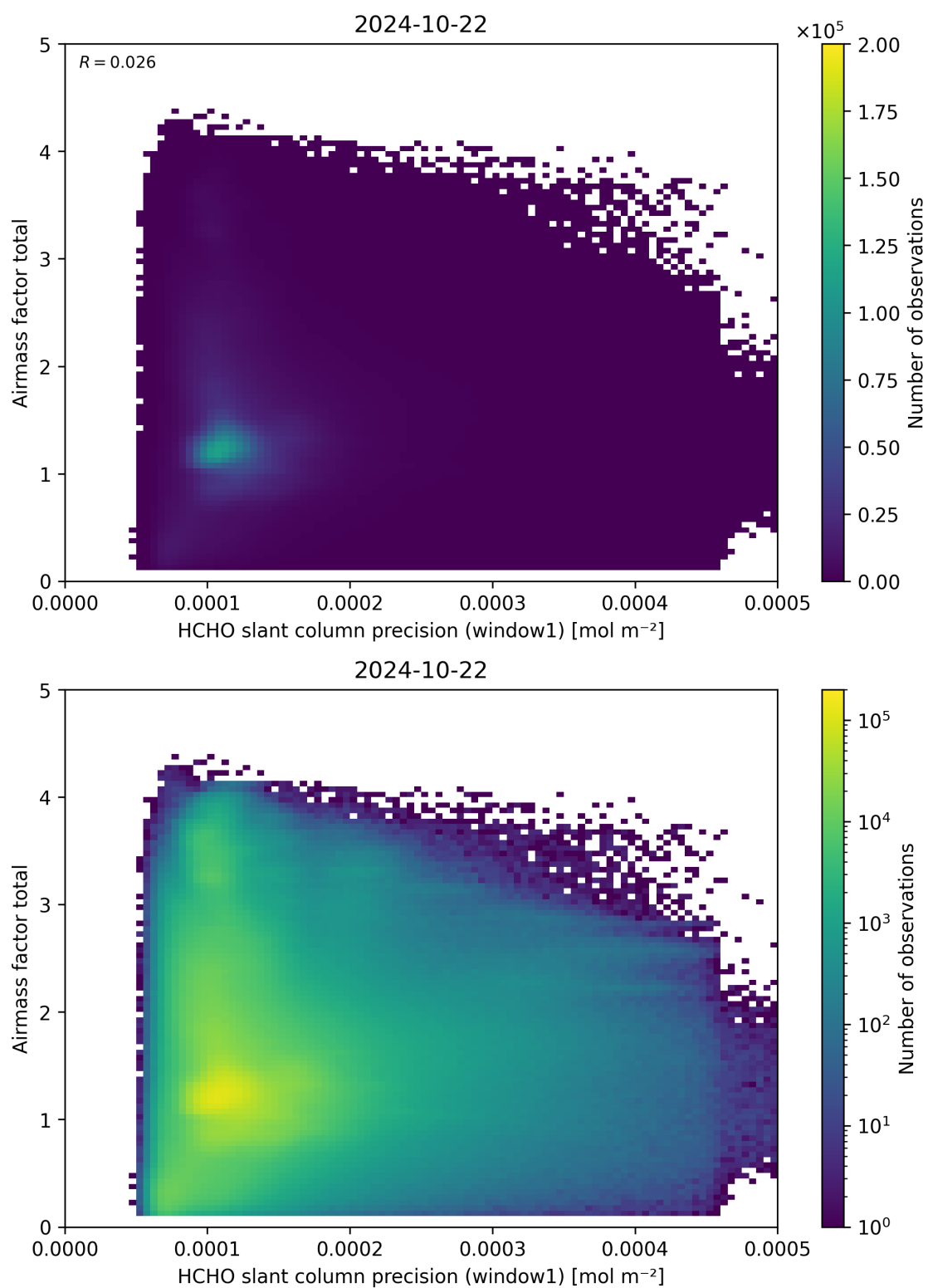
Figure 94: Scatter density plot of “HCHO slant column precision (window1)” against “Airmass factor total” for 2024-10-21 to 2024-10-23.
