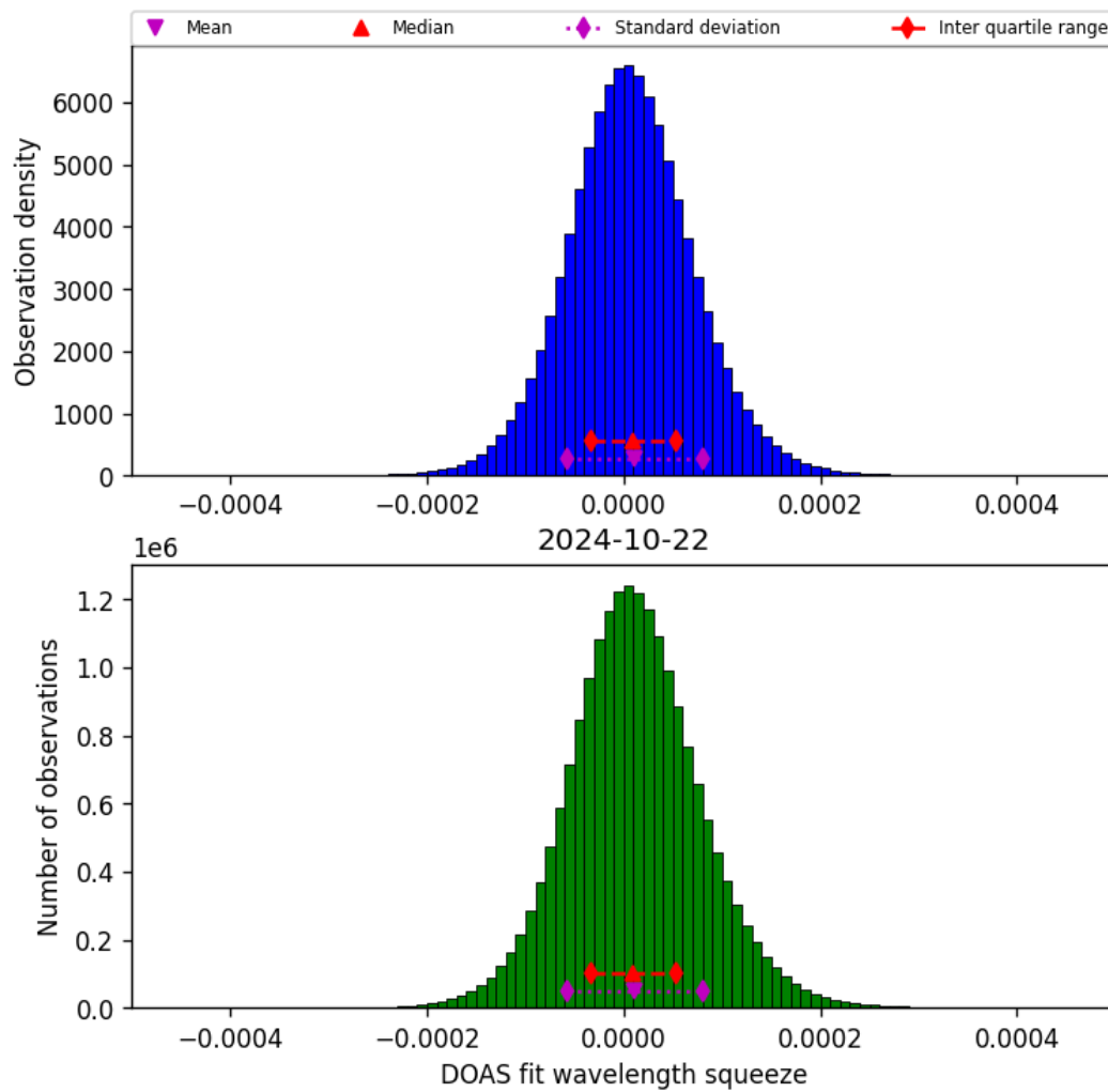
Figure 45: Histogram of “DOAS fit wavelength squeeze” for 2024-10-21 to 2024-10-23
