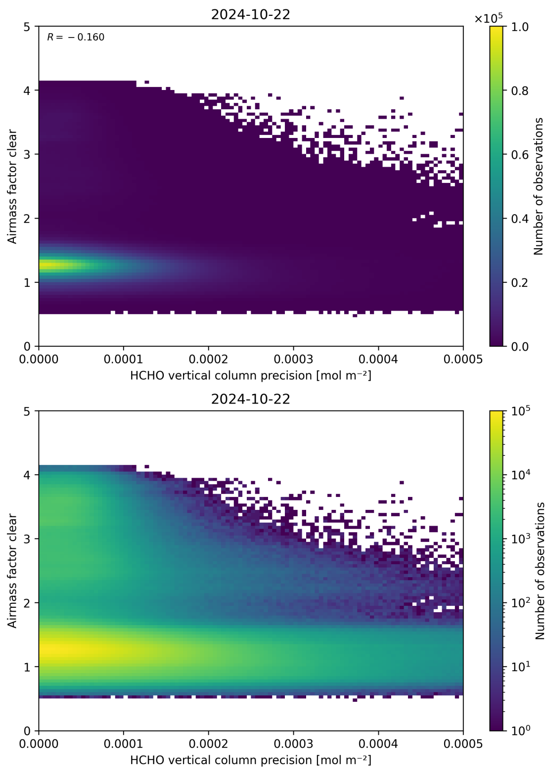
Figure 139: Scatter density plot of “HCHO vertical column precision” against “Airmass factor clear” for 2024-10-21 to 2024-10-23.
