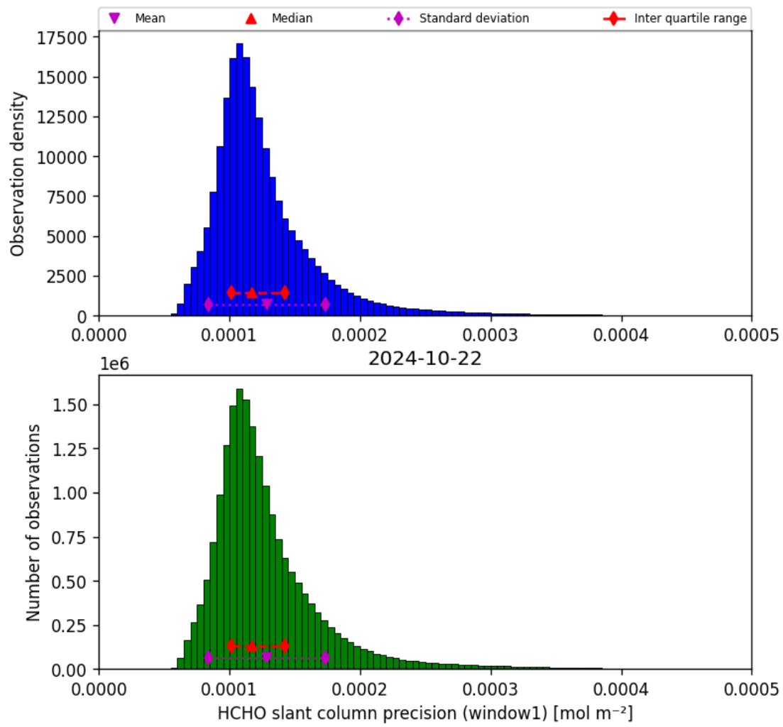
Figure 39: Histogram of “HCHO slant column precision (window1)” for 2024-10-21 to 2024-10-23
