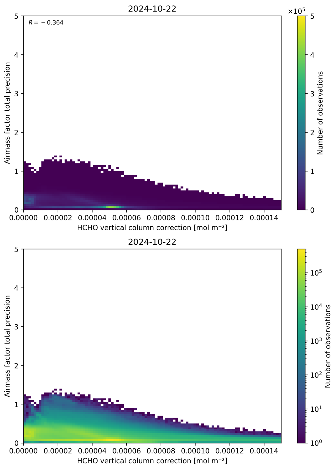
Figure 121: Scatter density plot of “HCHO vertical column correction” against “Airmass factor total precision” for 2024-10-21 to 2024-10-23.
