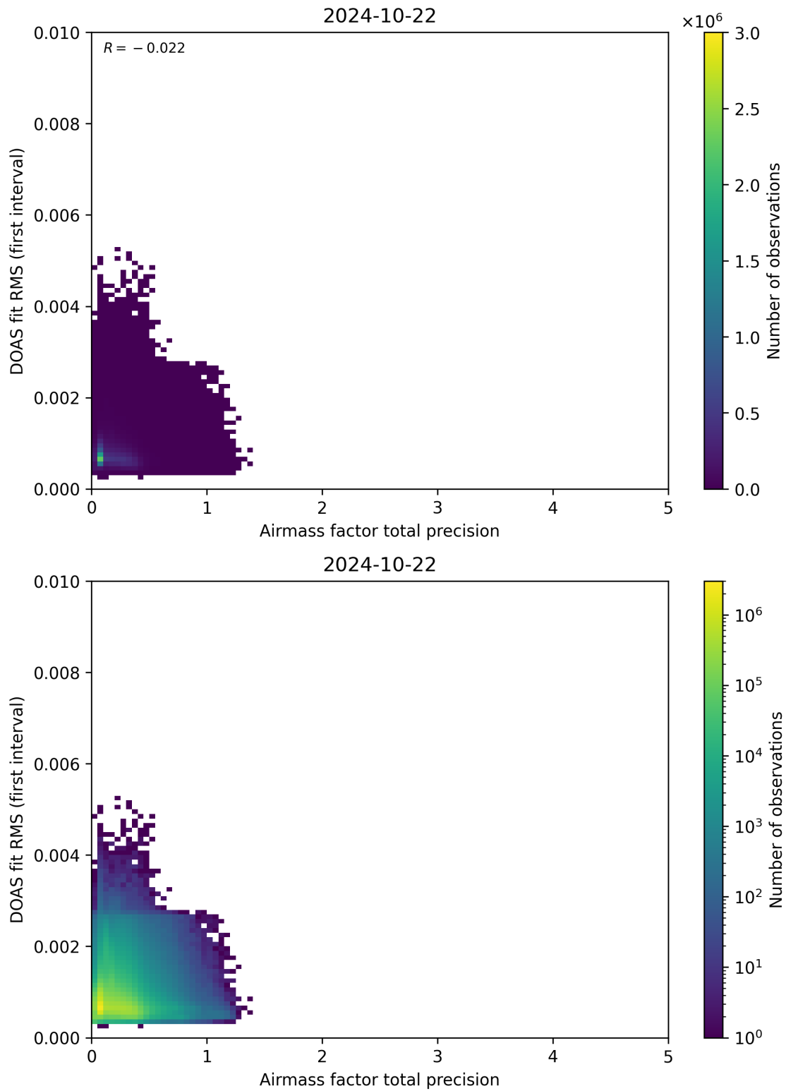
Figure 105: Scatter density plot of “Airmass factor total precision” against “DOAS fit RMS (first interval)” for 2024-10-21 to 2024-10-23.
