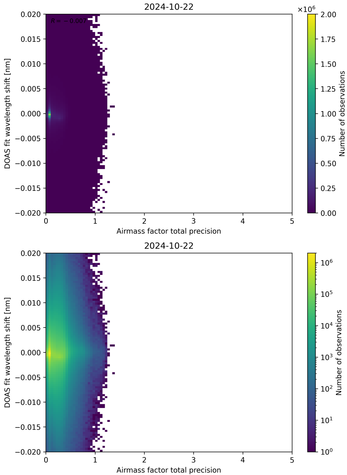
Figure 106: Scatter density plot of “Airmass factor total precision” against “DOAS fit wavelength shift” for 2024-10-21 to 2024-10-23.
