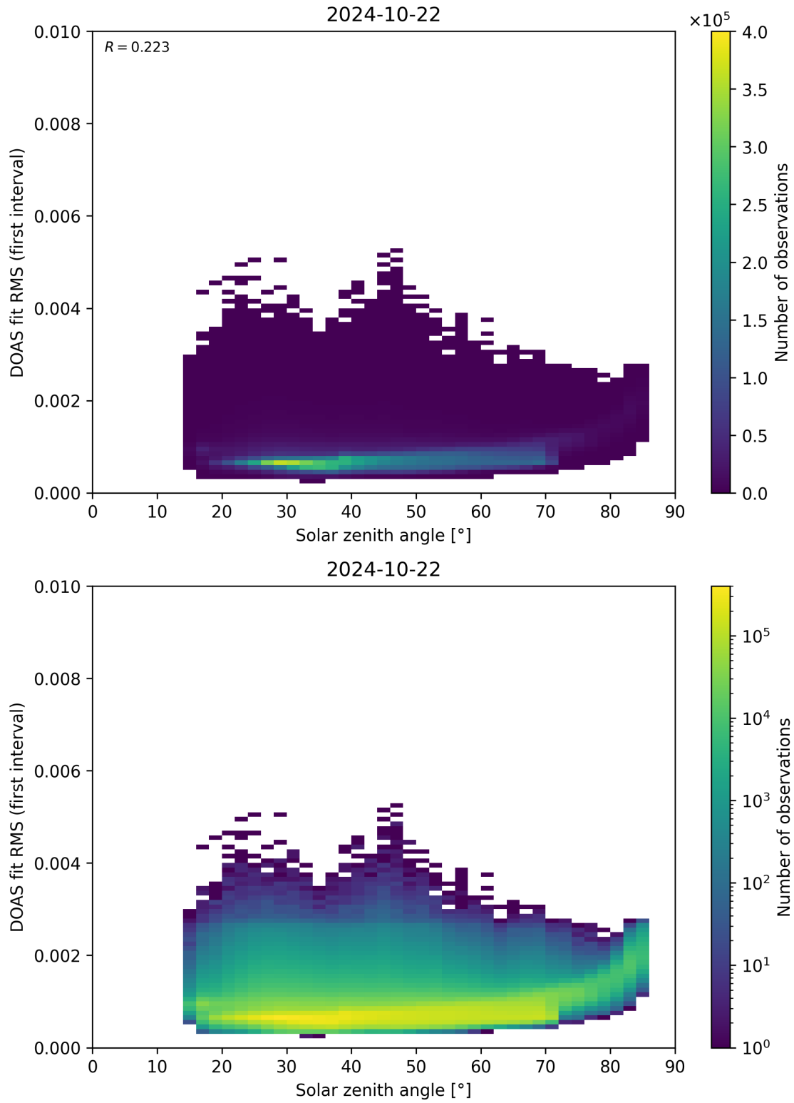
Figure 167: Scatter density plot of “Solar zenith angle” against “DOAS fit RMS (first interval)” for 2024-10-21 to 2024-10-23.
