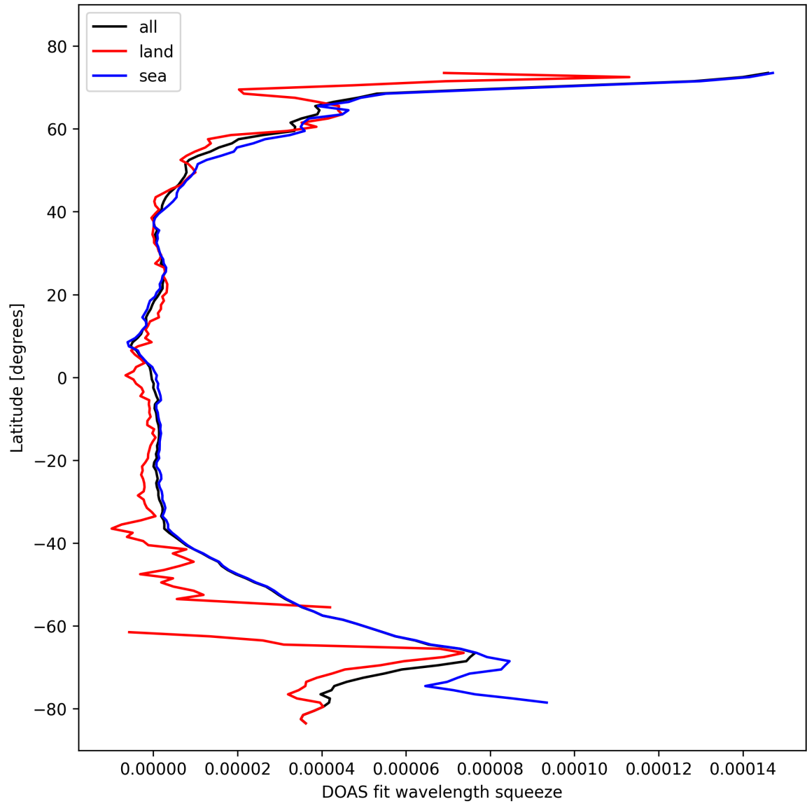
Figure 31: Zonal average of “DOAS fit wavelength squeeze” for 2024-10-21 to 2024-10-23.
