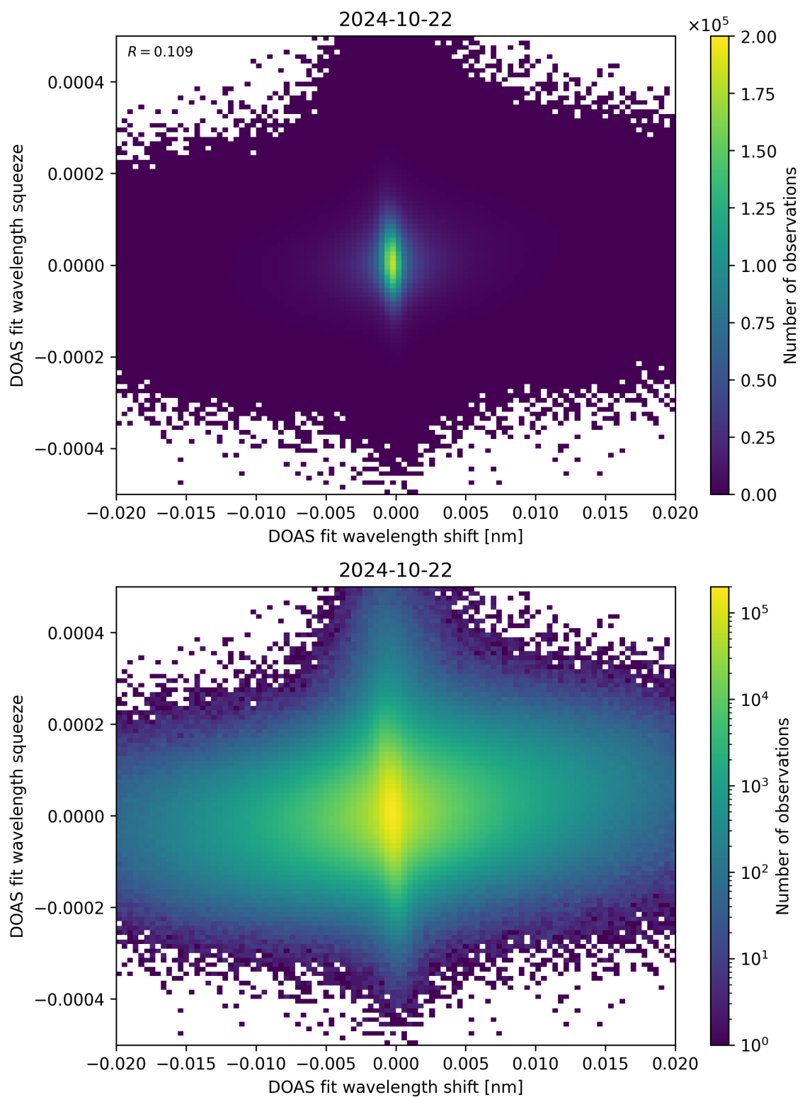
Figure 65: Scatter density plot of “DOAS fit wavelength shift” against “DOAS fit wavelength squeeze” for 2024-10-21 to 2024-10-23.
