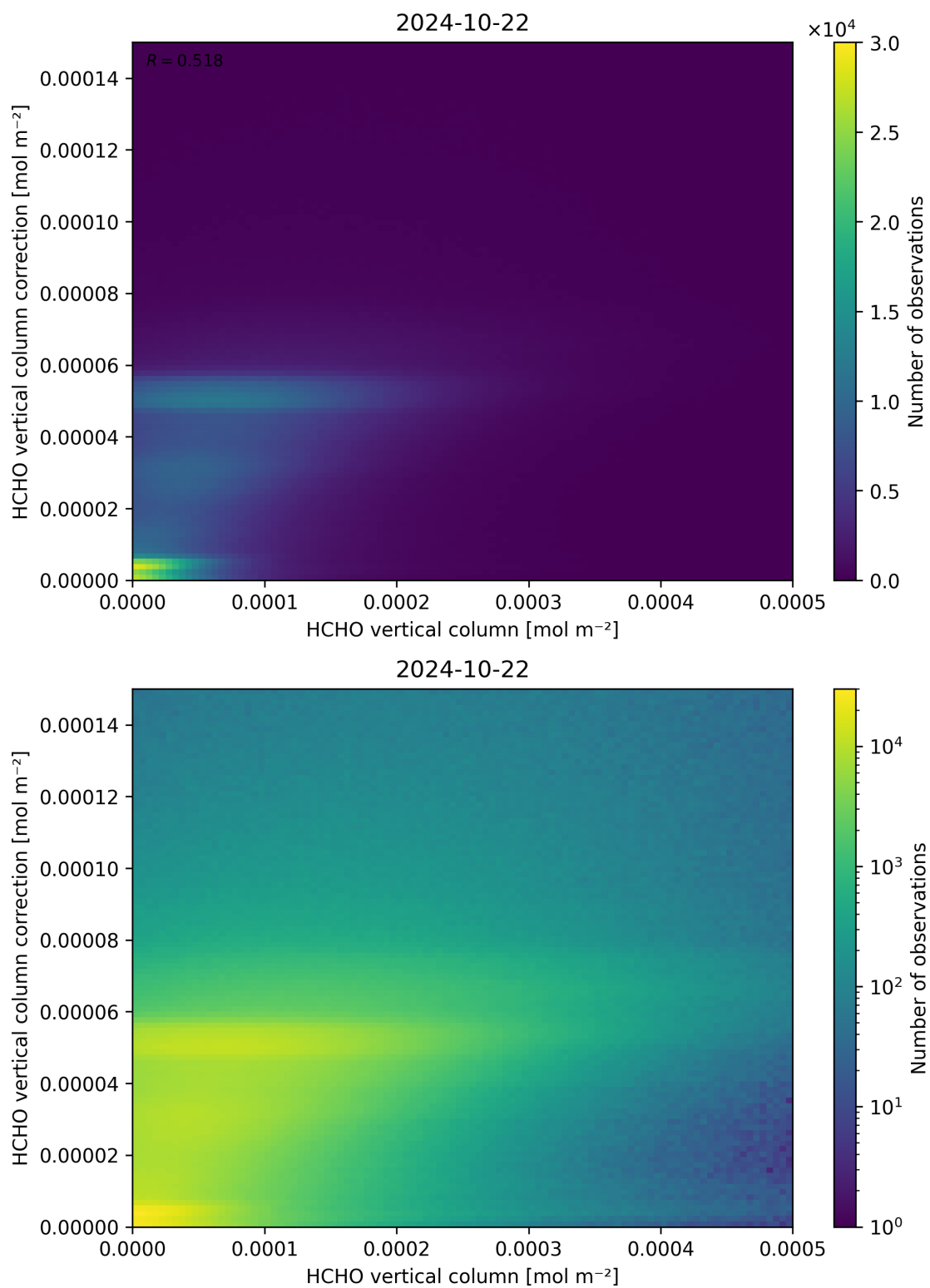
Figure 133: Scatter density plot of “HCHO vertical column” against “HCHO vertical column correction” for 2024-10-21 to 2024-10-23.
