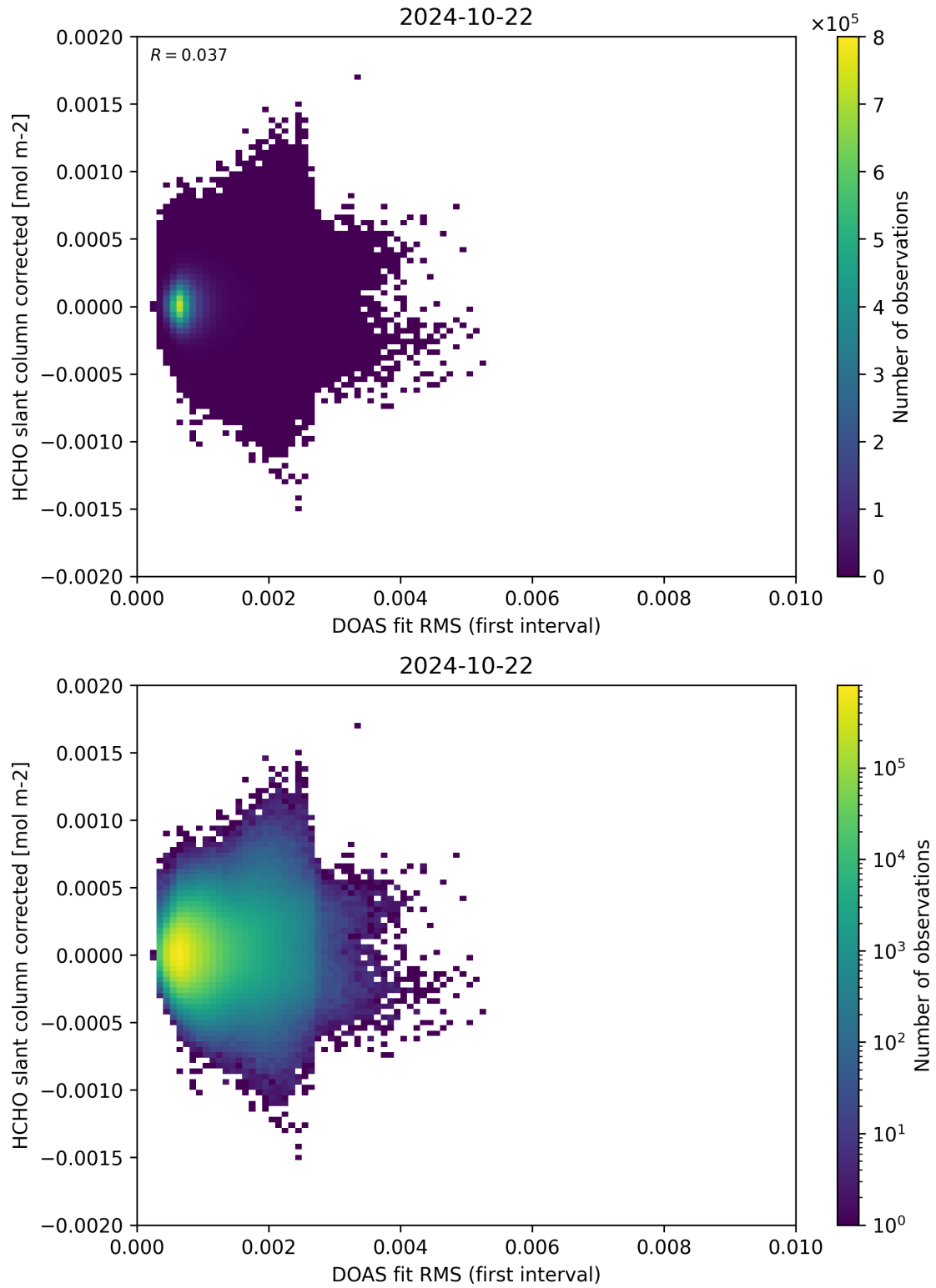
Figure 62: Scatter density plot of “DOAS fit RMS (first interval)” against “HCHO slant column corrected” for 2024-10-21 to 2024-10-23.
