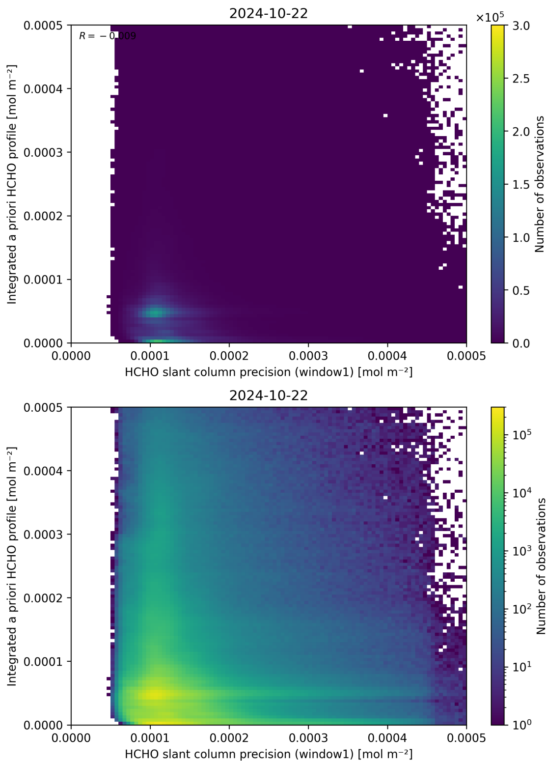
Figure 96: Scatter density plot of “HCHO slant column precision (window1)” against “Integrated a priori HCHO profile” for 2024-10-21 to 2024-10-23.
