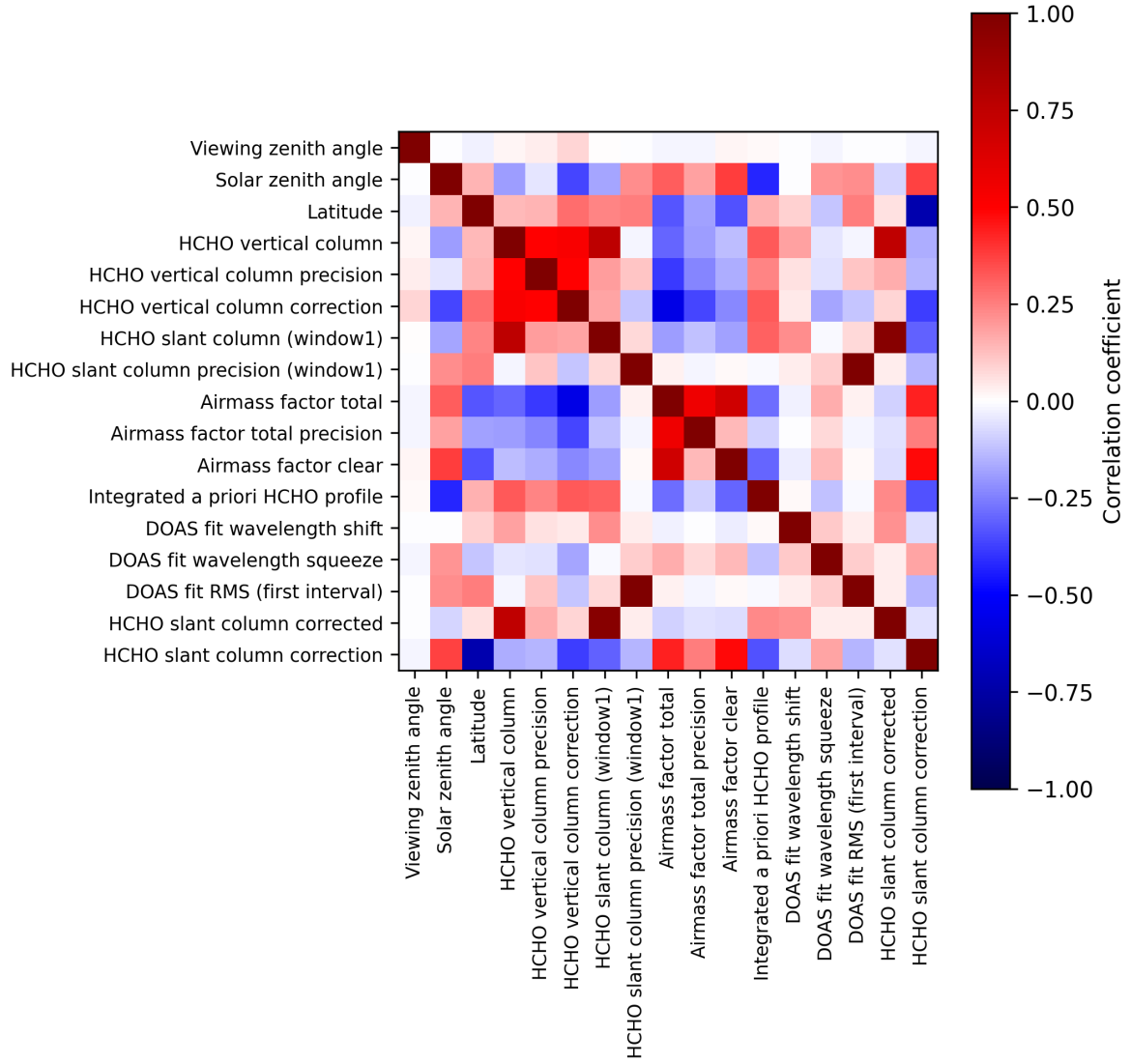
Figure 2: Map of correlation matrix for 2024-10-21 to 2024-10-23.
