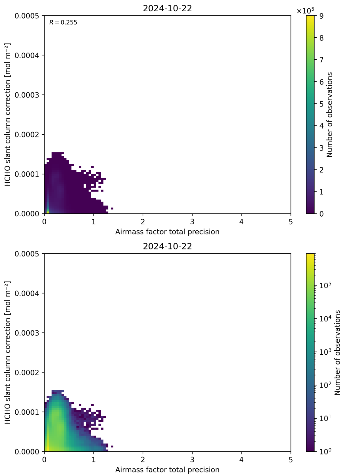
Figure 110: Scatter density plot of “Airmass factor total precision” against “HCHO slant column correction” for 2024-10-21 to 2024-10-23.
