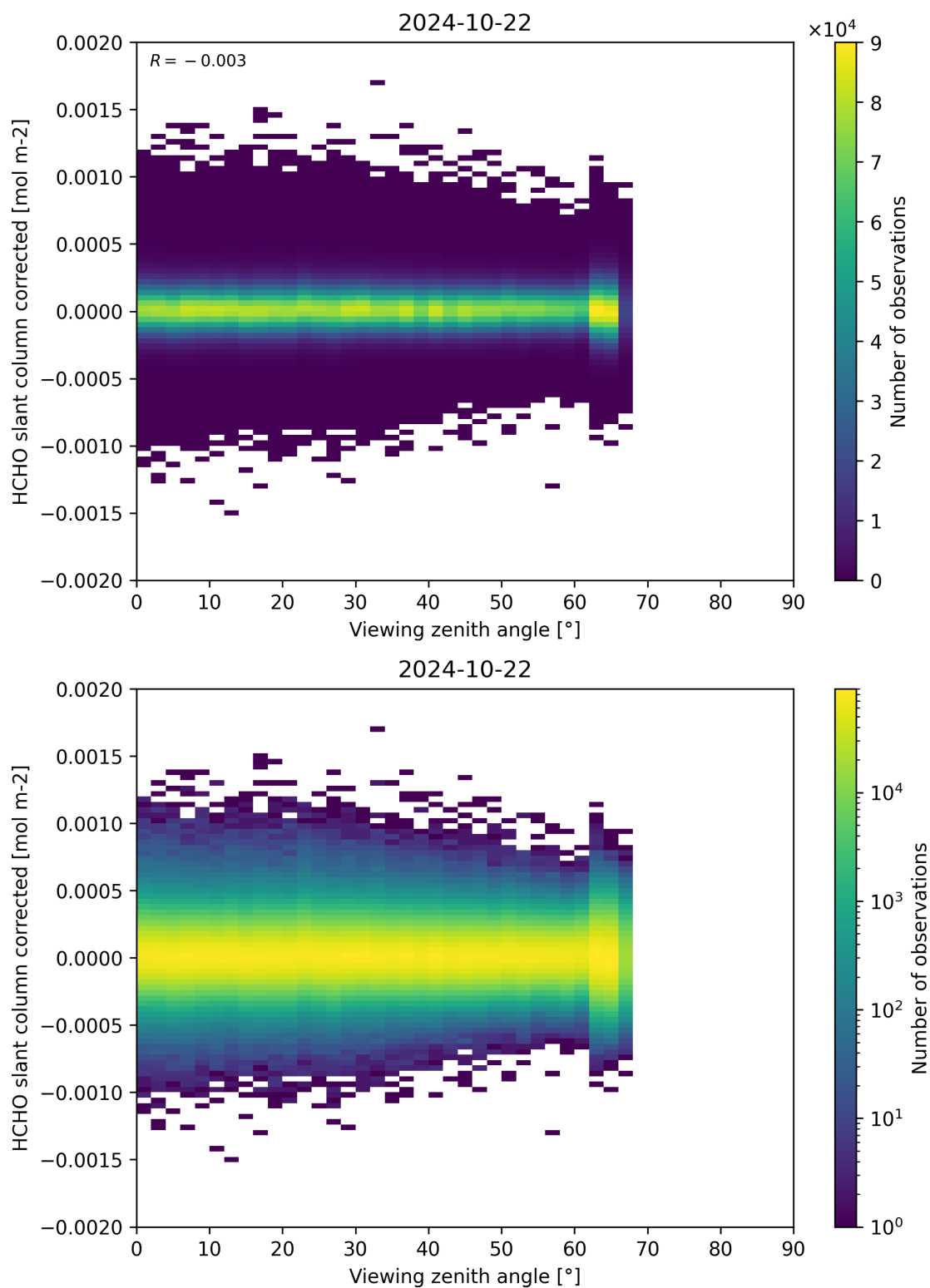
Figure 186: Scatter density plot of “Viewing zenith angle” against “HCHO slant column corrected” for 2024-10-21 to 2024-10-23.
