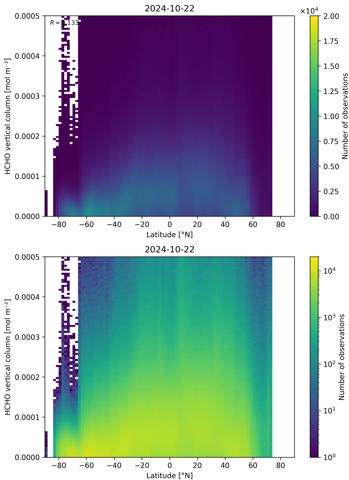
Figure 163: Scatter density plot of “Latitude” against “HCHO vertical column” for 2024-10-21 to 2024-10-23.
