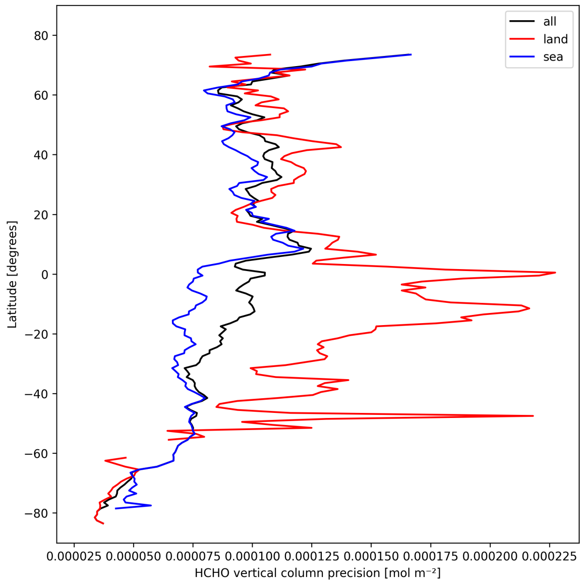
Figure 22: Zonal average of “HCHO vertical column precision” for 2024-10-21 to 2024-10-23.
