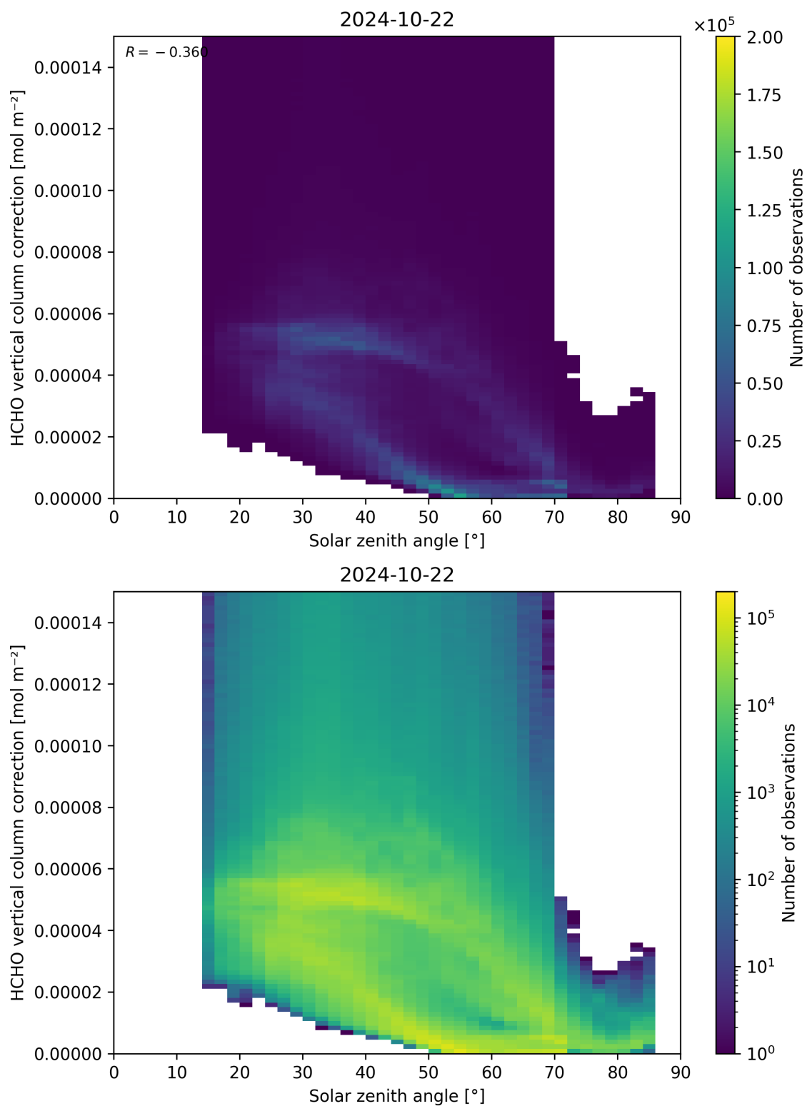
Figure 178: Scatter density plot of “Solar zenith angle” against “HCHO vertical column correction” for 2024-10-21 to 2024-10-23.
