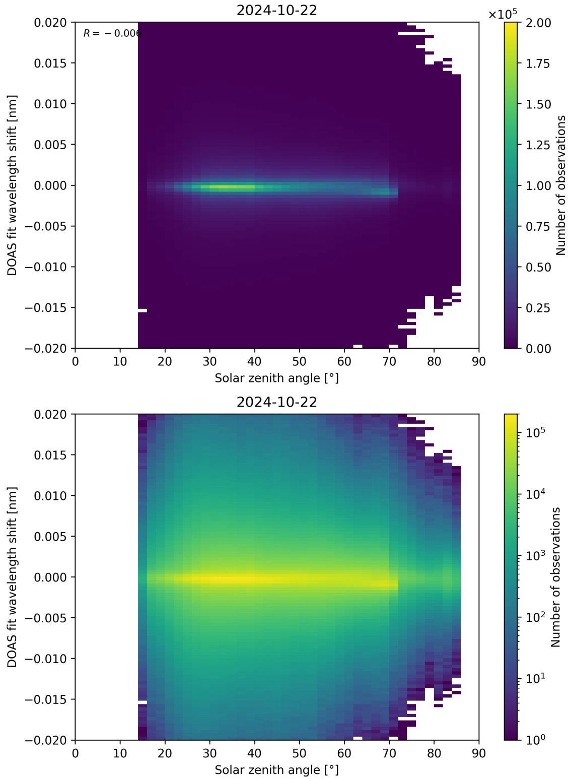
Figure 168: Scatter density plot of “Solar zenith angle” against “DOAS fit wavelength shift” for 2024-10-21 to 2024-10-23.
