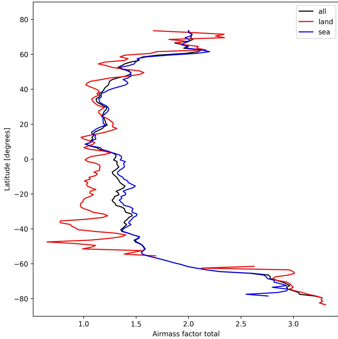
Figure 26: Zonal average of “Airmass factor total” for 2024-10-21 to 2024-10-23.
