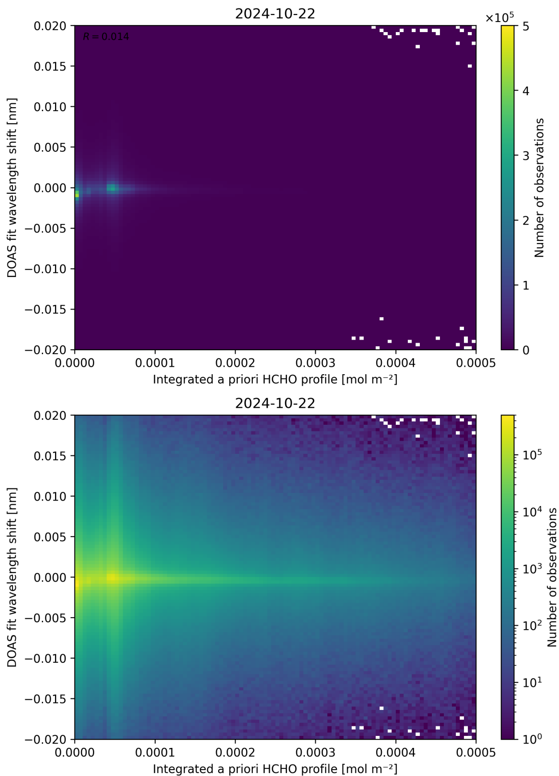
Figure 149: Scatter density plot of “Integrated a priori HCHO profile” against “DOAS fit wavelength shift” for 2024-10-21 to 2024-10-23.
