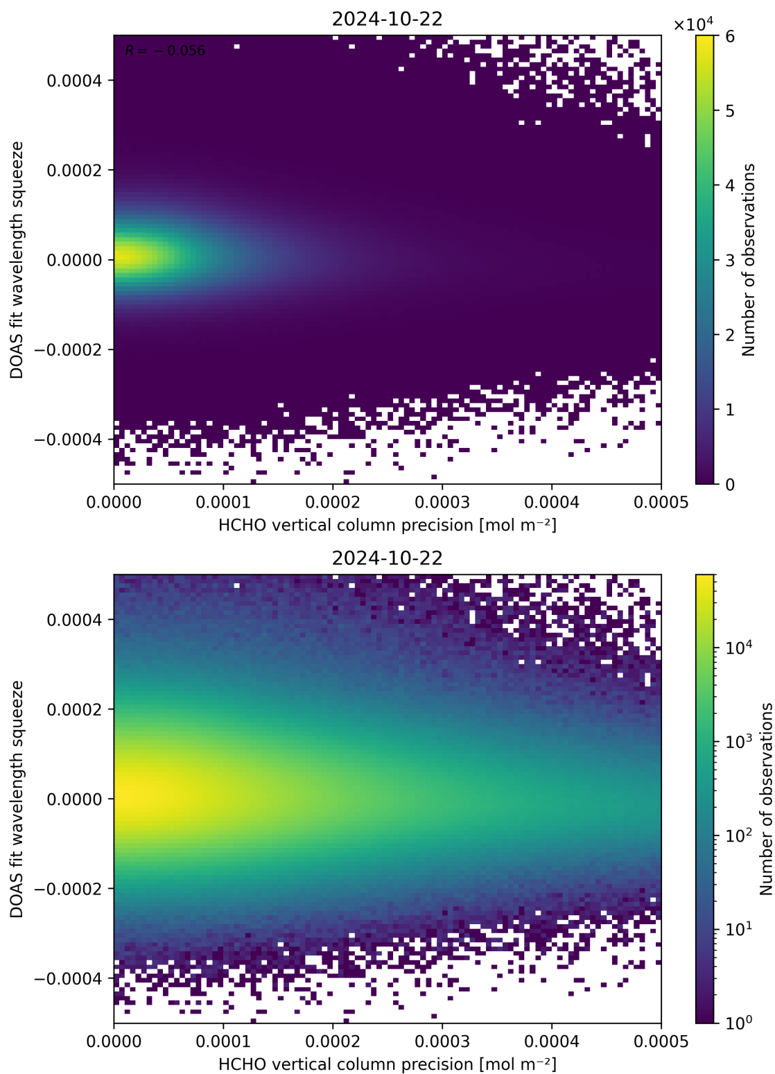
Figure 138: Scatter density plot of “HCHO vertical column precision” against “DOAS fit wavelength squeeze” for 2024-10-21 to 2024-10-23.
