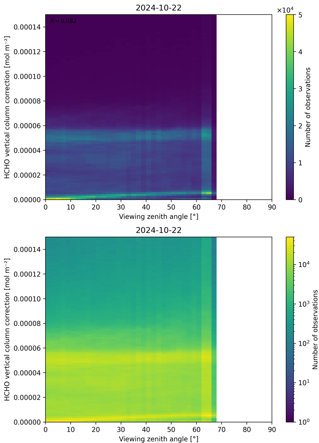
Figure 193: Scatter density plot of “Viewing zenith angle” against “HCHO vertical column correction” for 2024-10-21 to 2024-10-23.
