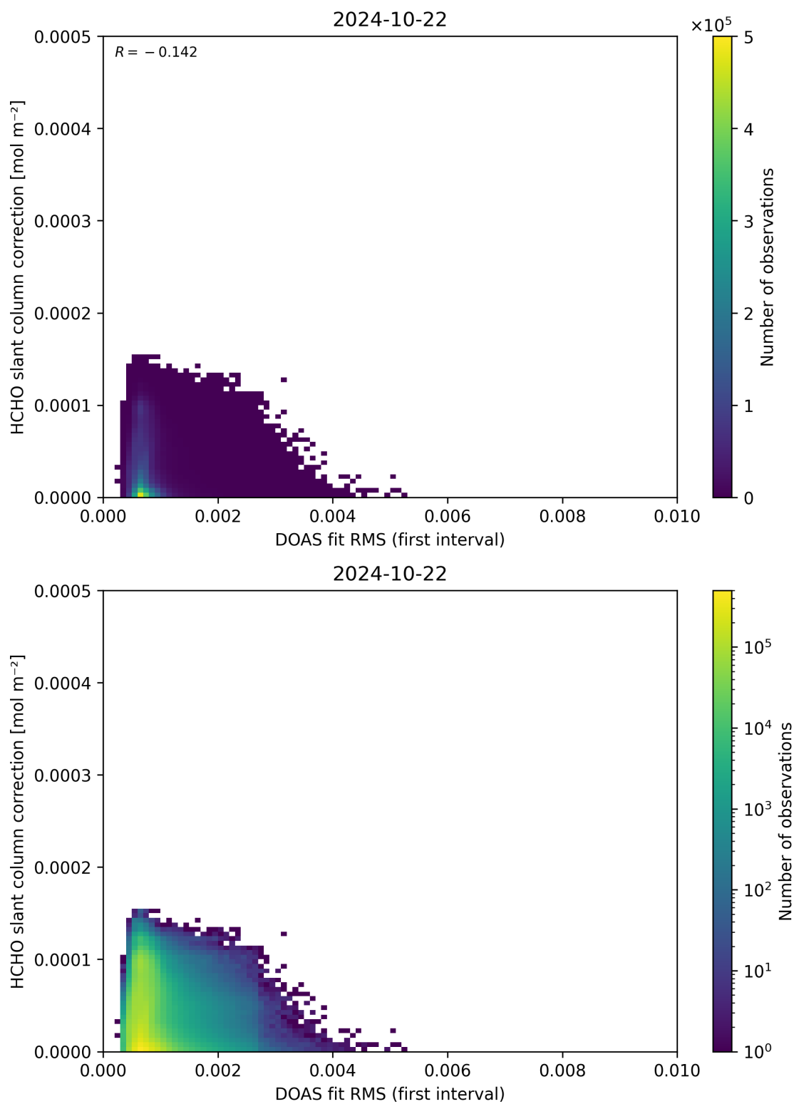
Figure 63: Scatter density plot of “DOAS fit RMS (first interval)” against “HCHO slant column correction” for 2024-10-21 to 2024-10-23.
