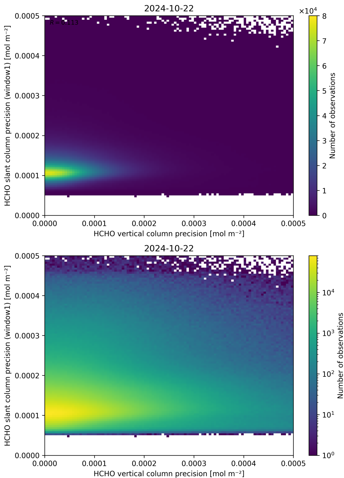
Figure 143: Scatter density plot of “HCHO vertical column precision” against “HCHO slant column precision (window1)” for 2024-10-21 to 2024-10-23.
