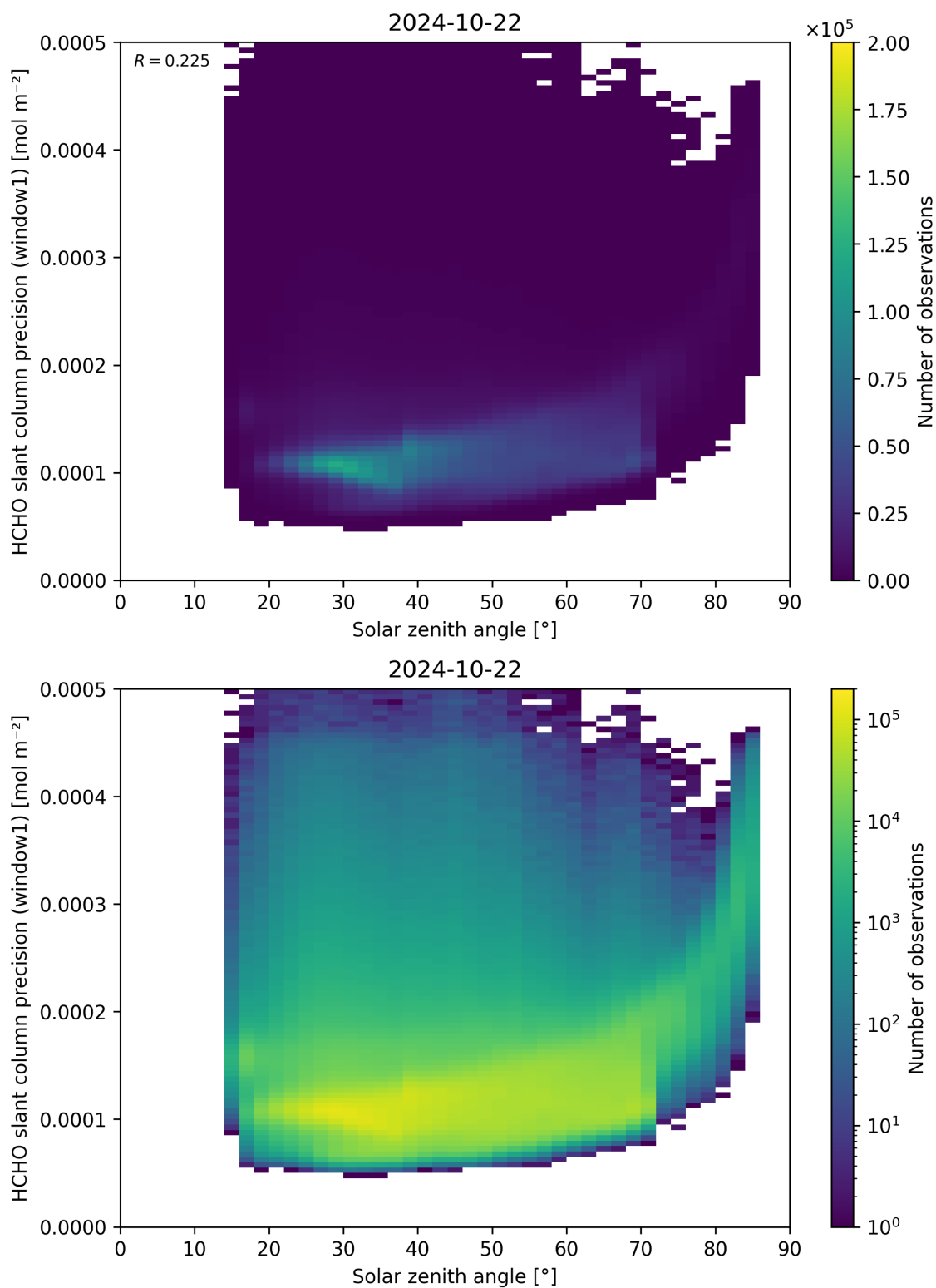
Figure 174: Scatter density plot of “Solar zenith angle” against “HCHO slant column precision (window1)” for 2024-10-21 to 2024-10-23.
