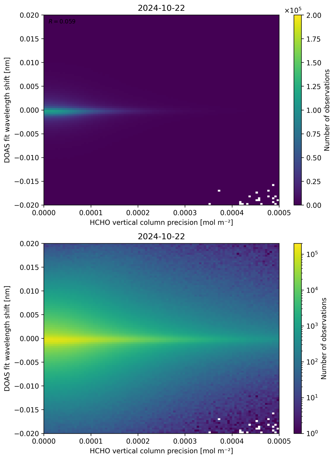
Figure 137: Scatter density plot of “HCHO vertical column precision” against “DOAS fit wavelength shift” for 2024-10-21 to 2024-10-23.
