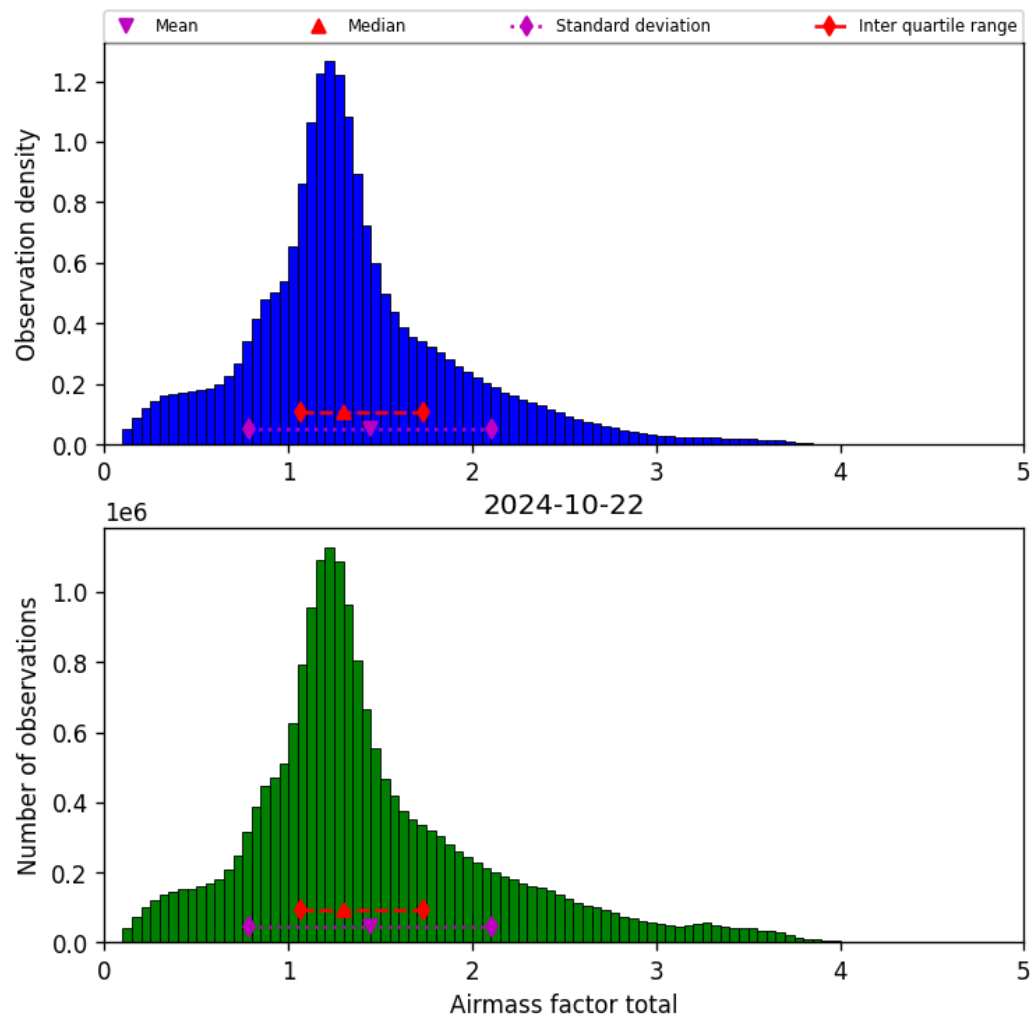
Figure 40: Histogram of “Airmass factor total” for 2024-10-21 to 2024-10-23
