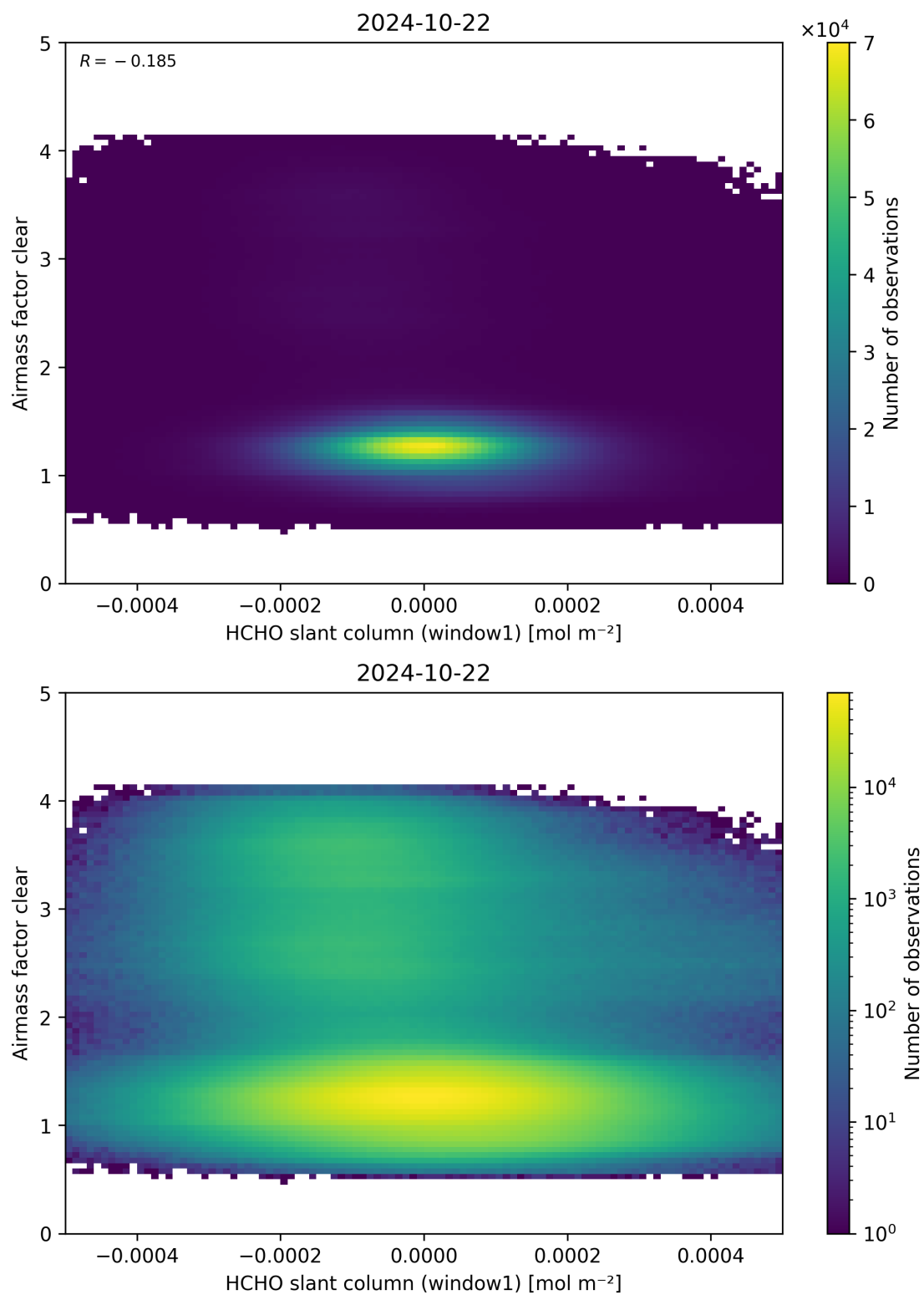
Figure 81: Scatter density plot of “HCHO slant column (window1)” against “Airmass factor clear” for 2024-10-21 to 2024-10-23.
