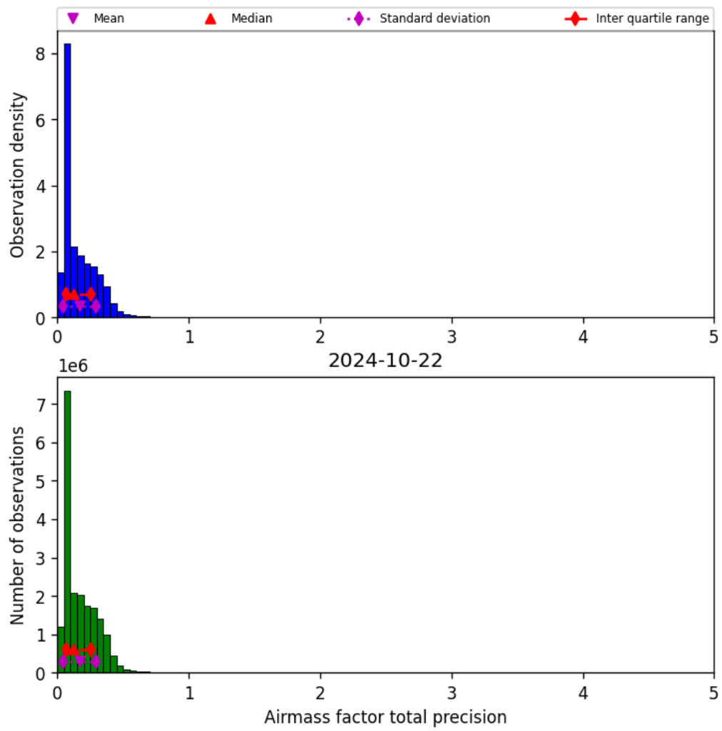
Figure 41: Histogram of “Airmass factor total precision” for 2024-10-21 to 2024-10-23
