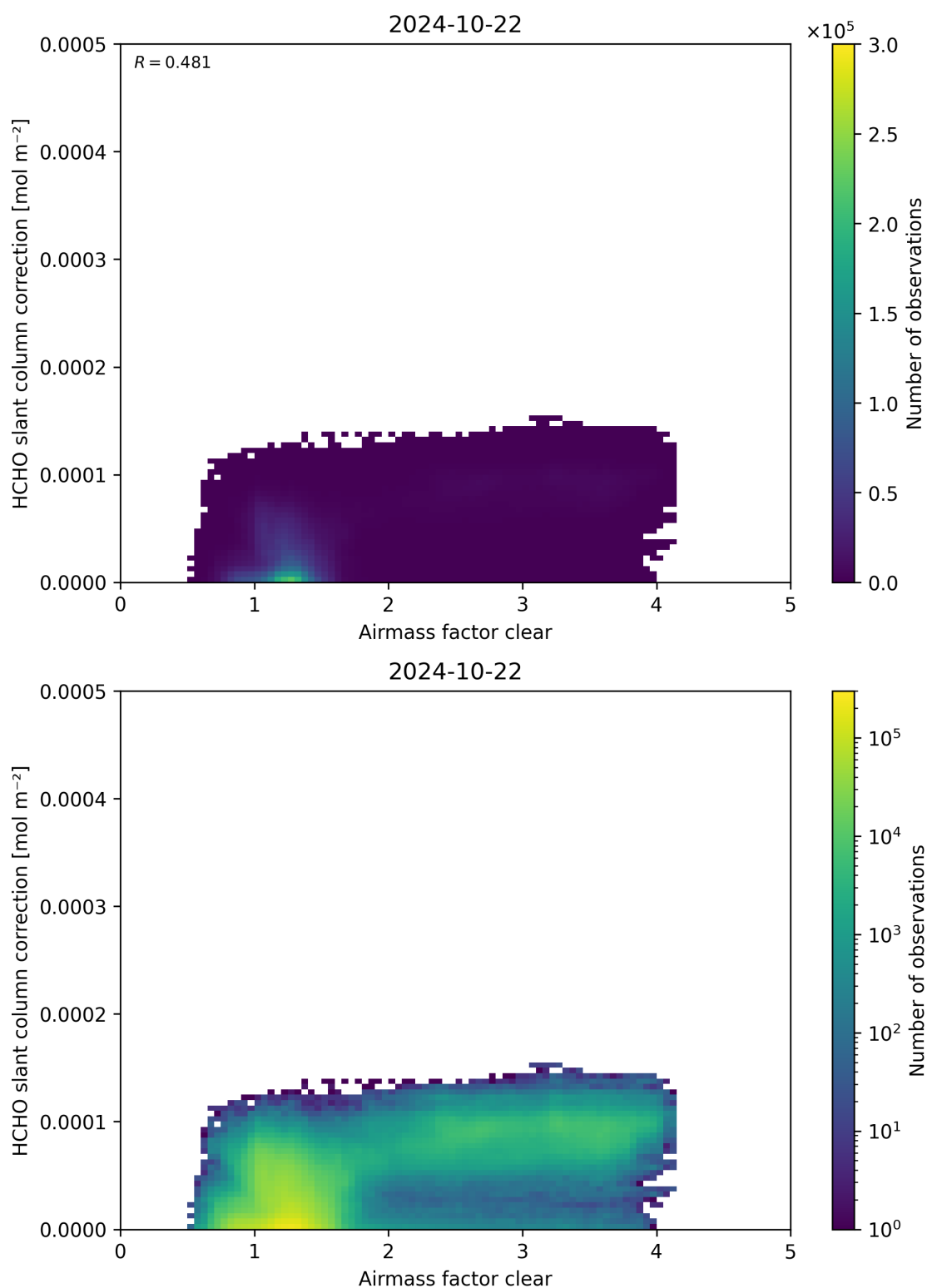
Figure 75: Scatter density plot of “Airmass factor clear” against “HCHO slant column correction” for 2024-10-21 to 2024-10-23.
