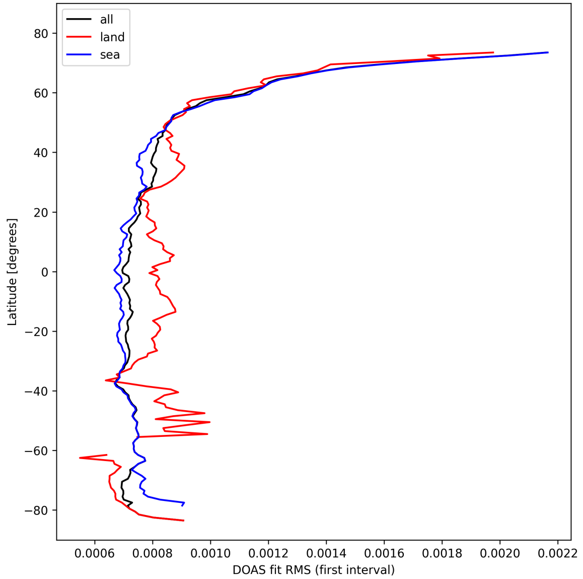
Figure 32: Zonal average of “DOAS fit RMS (first interval)” for 2024-10-21 to 2024-10-23.
