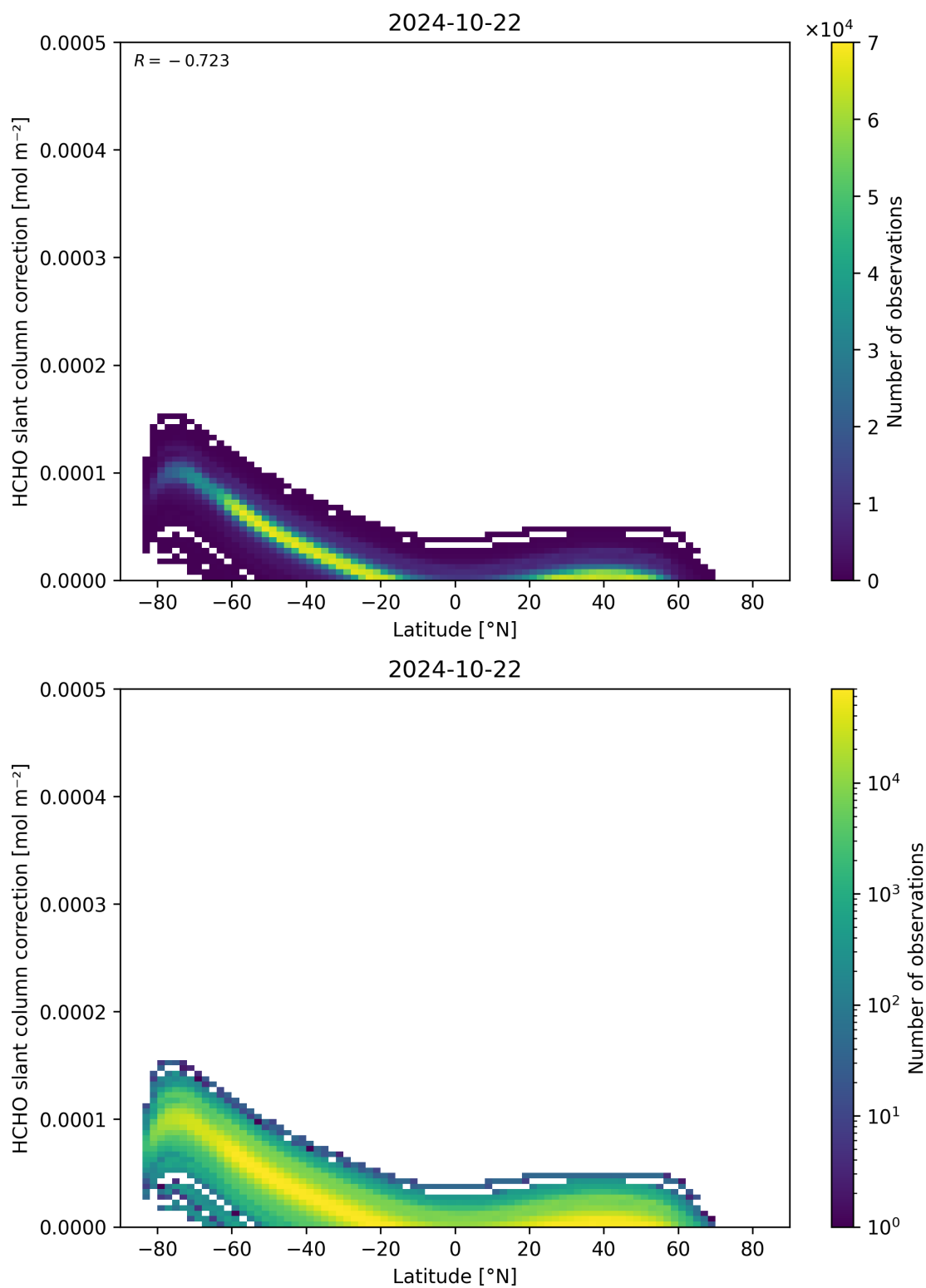
Figure 158: Scatter density plot of “Latitude” against “HCHO slant column correction” for 2024-10-21 to 2024-10-23.
