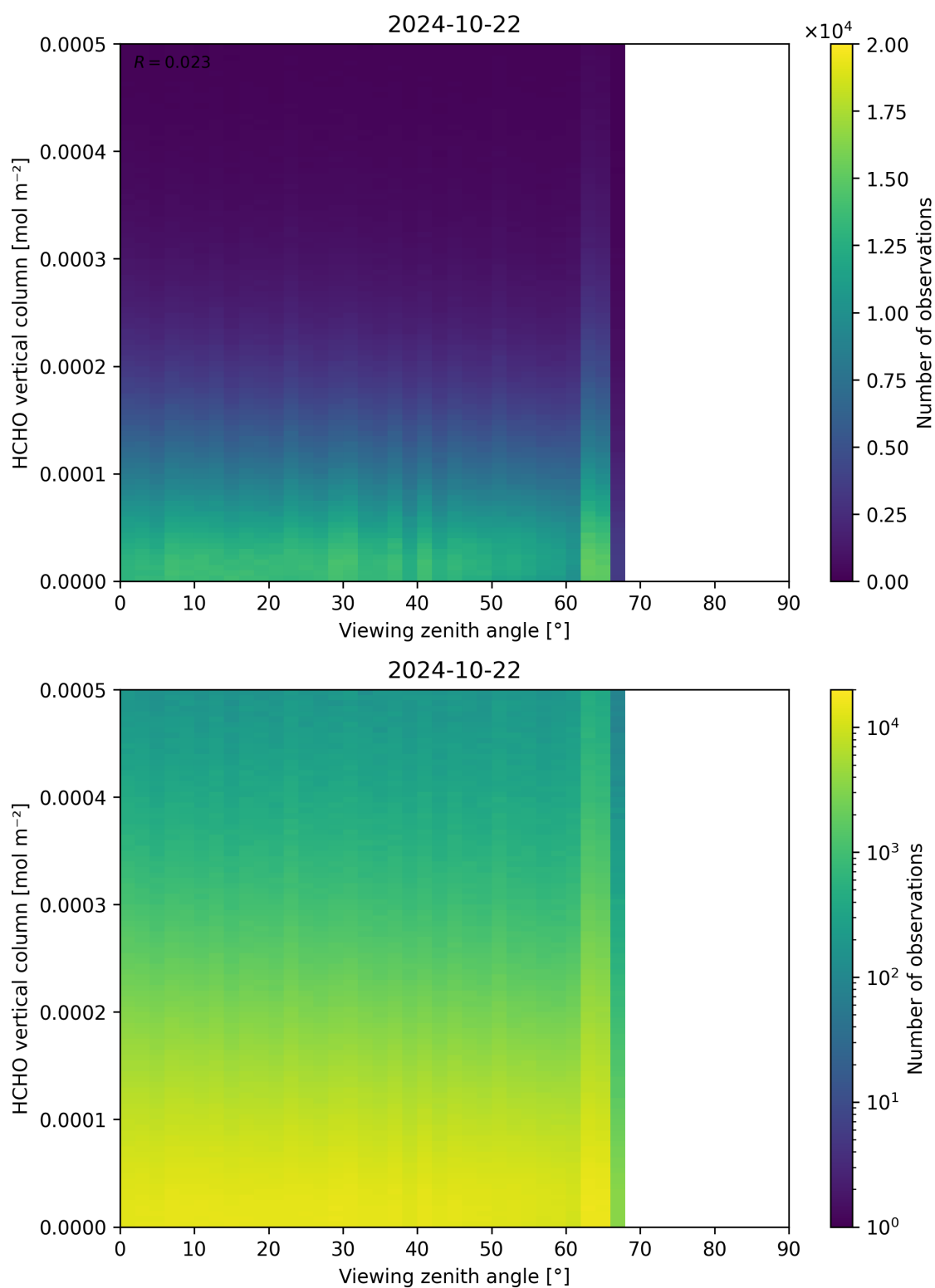
Figure 192: Scatter density plot of “Viewing zenith angle” against “HCHO vertical column” for 2024-10-21 to 2024-10-23.
