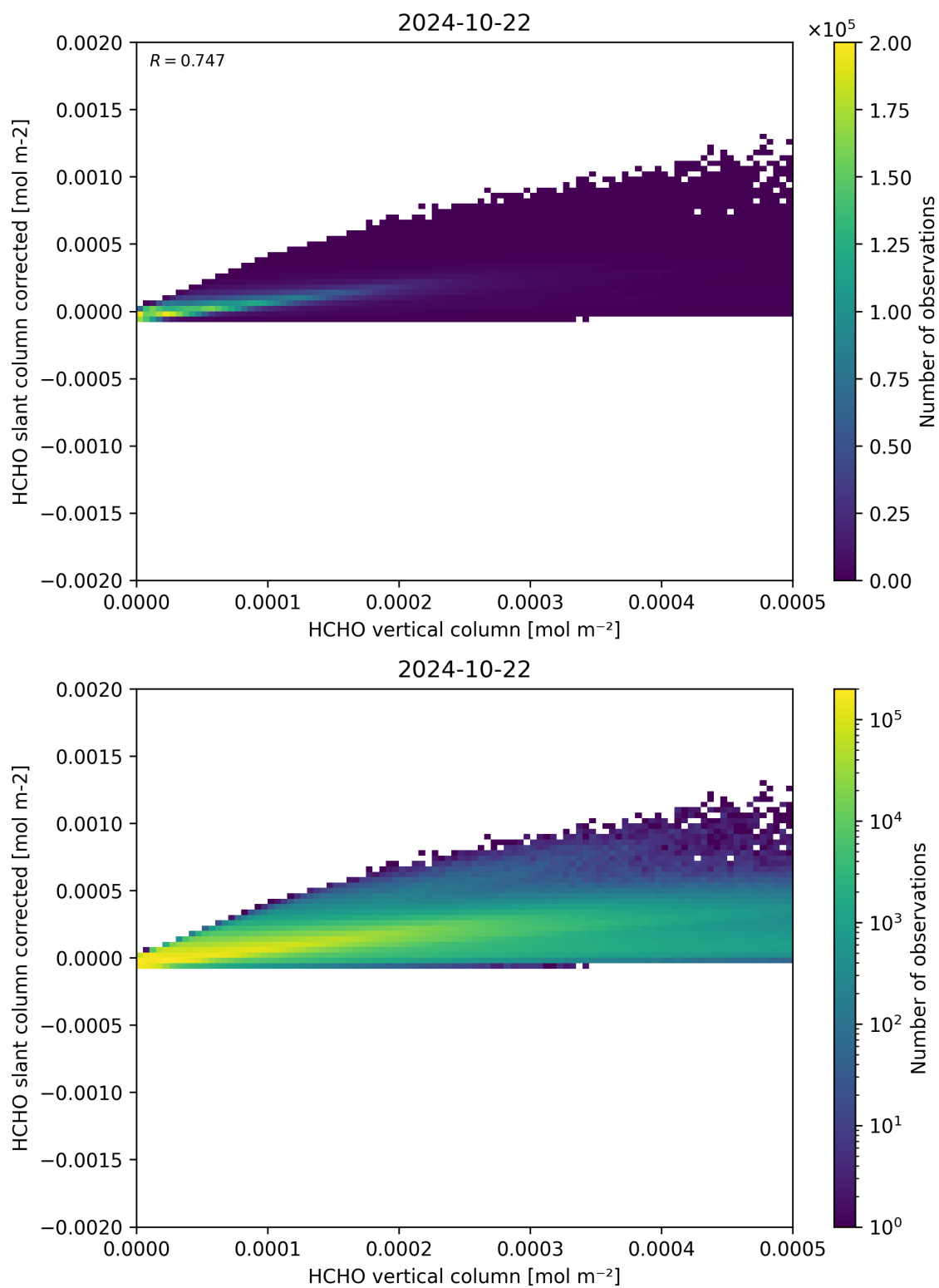
Figure 127: Scatter density plot of “HCHO vertical column” against “HCHO slant column corrected” for 2024-10-21 to 2024-10-23.
