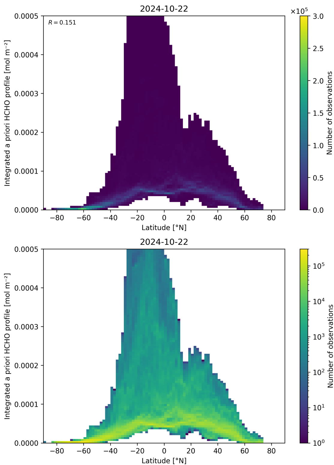
Figure 166: Scatter density plot of “Latitude” against “Integrated a priori HCHO profile” for 2024-10-21 to 2024-10-23.
