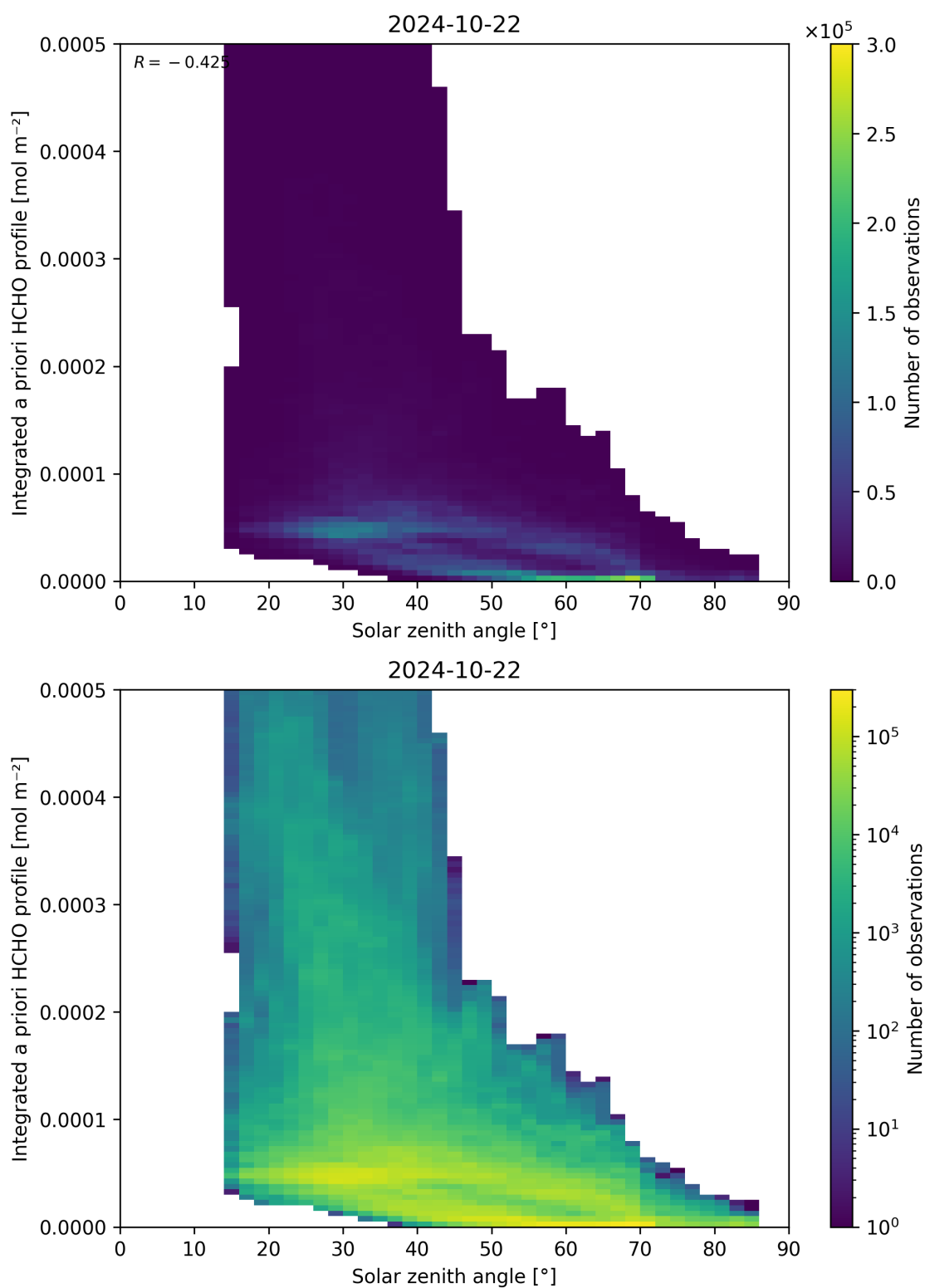
Figure 180: Scatter density plot of “Solar zenith angle” against “Integrated a priori HCHO profile” for 2024-10-21 to 2024-10-23.
