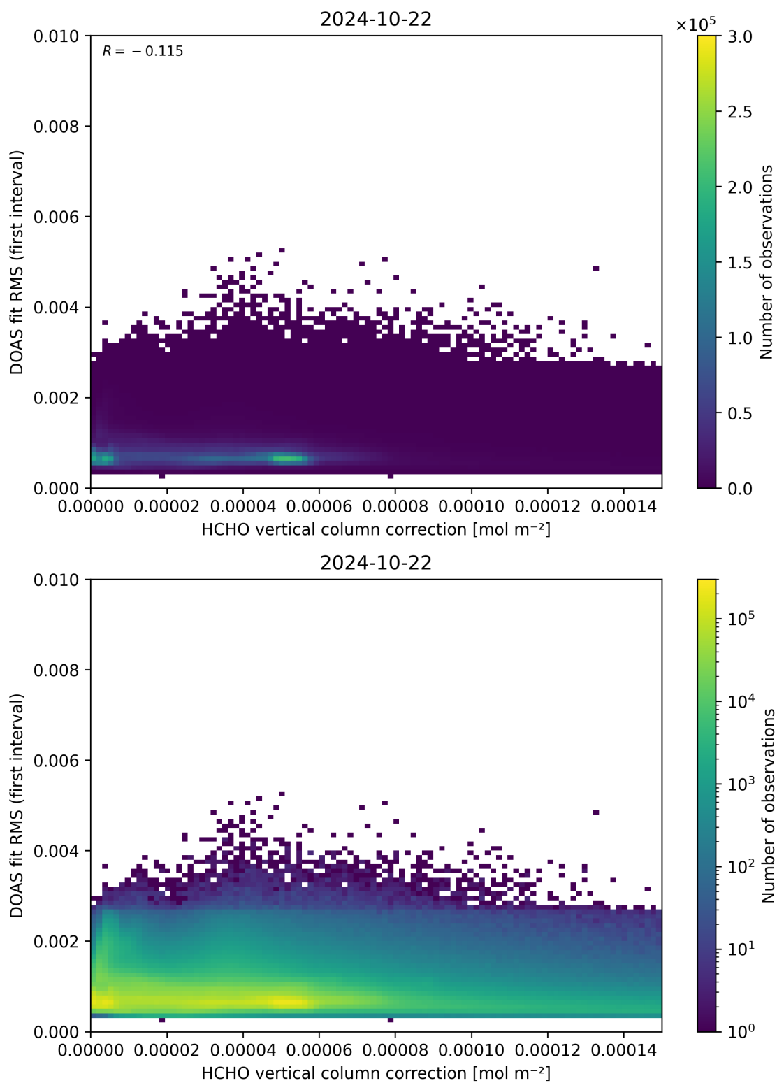
Figure 112: Scatter density plot of “HCHO vertical column correction” against “DOAS fit RMS (first interval)” for 2024-10-21 to 2024-10-23.
