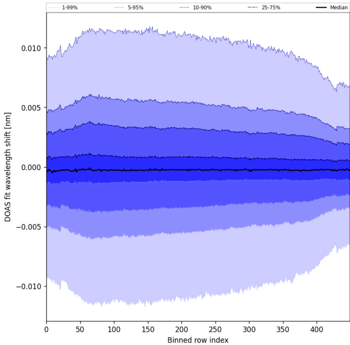
Figure 58: Along track statistics of “DOAS fit wavelength shift” for 2024-10-21 to 2024-10-23
