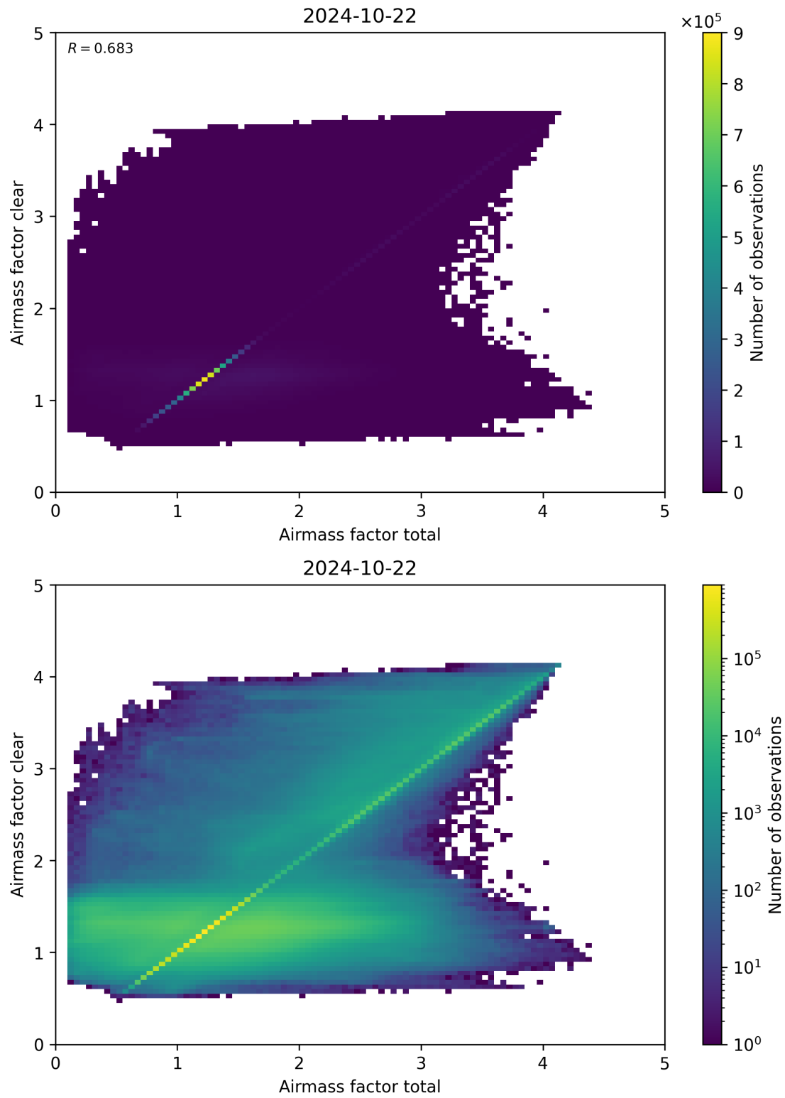
Figure 100: Scatter density plot of “Airmass factor total” against “Airmass factor clear” for 2024-10-21 to 2024-10-23.
