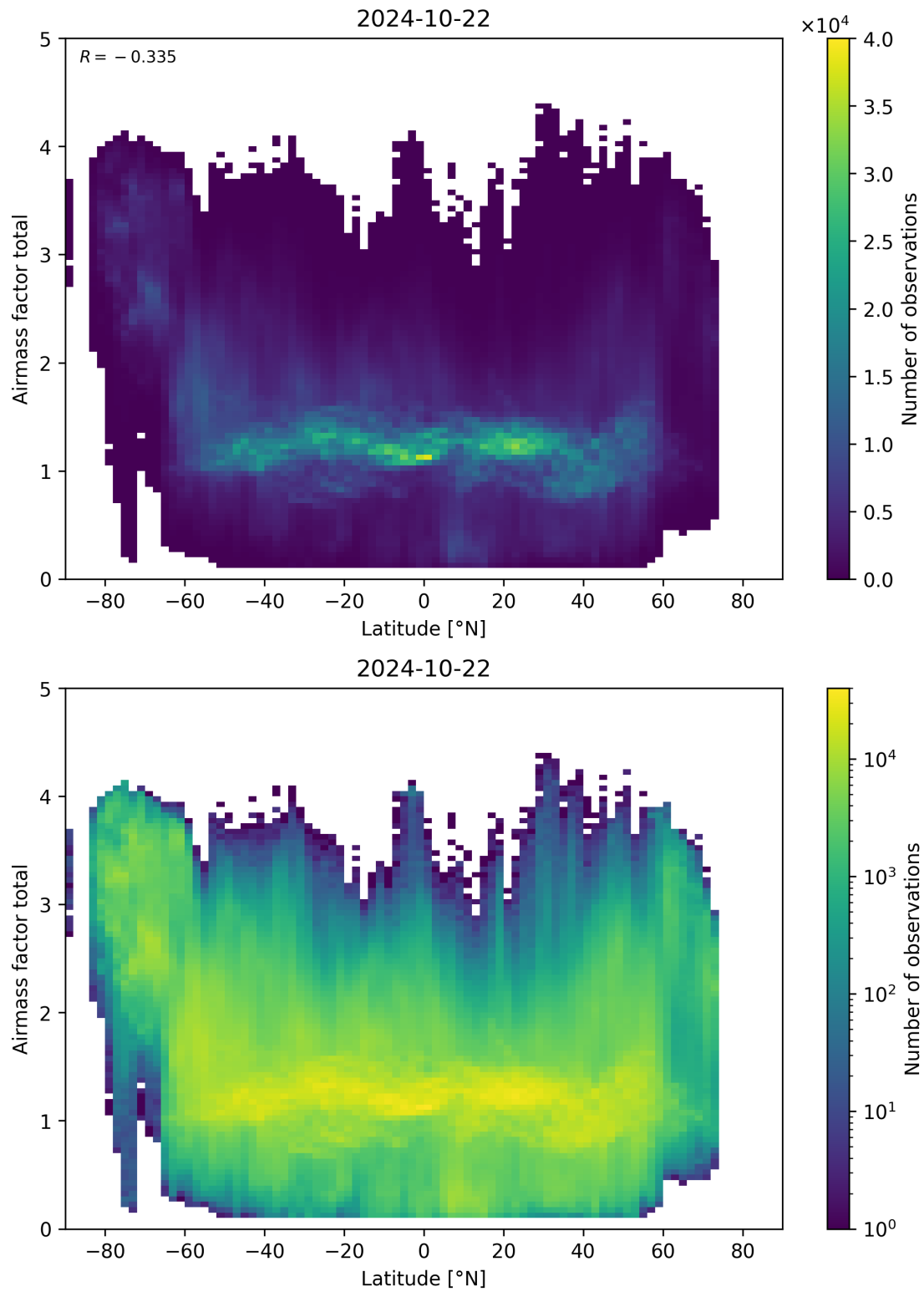
Figure 161: Scatter density plot of “Latitude” against “Airmass factor total” for 2024-10-21 to 2024-10-23.
