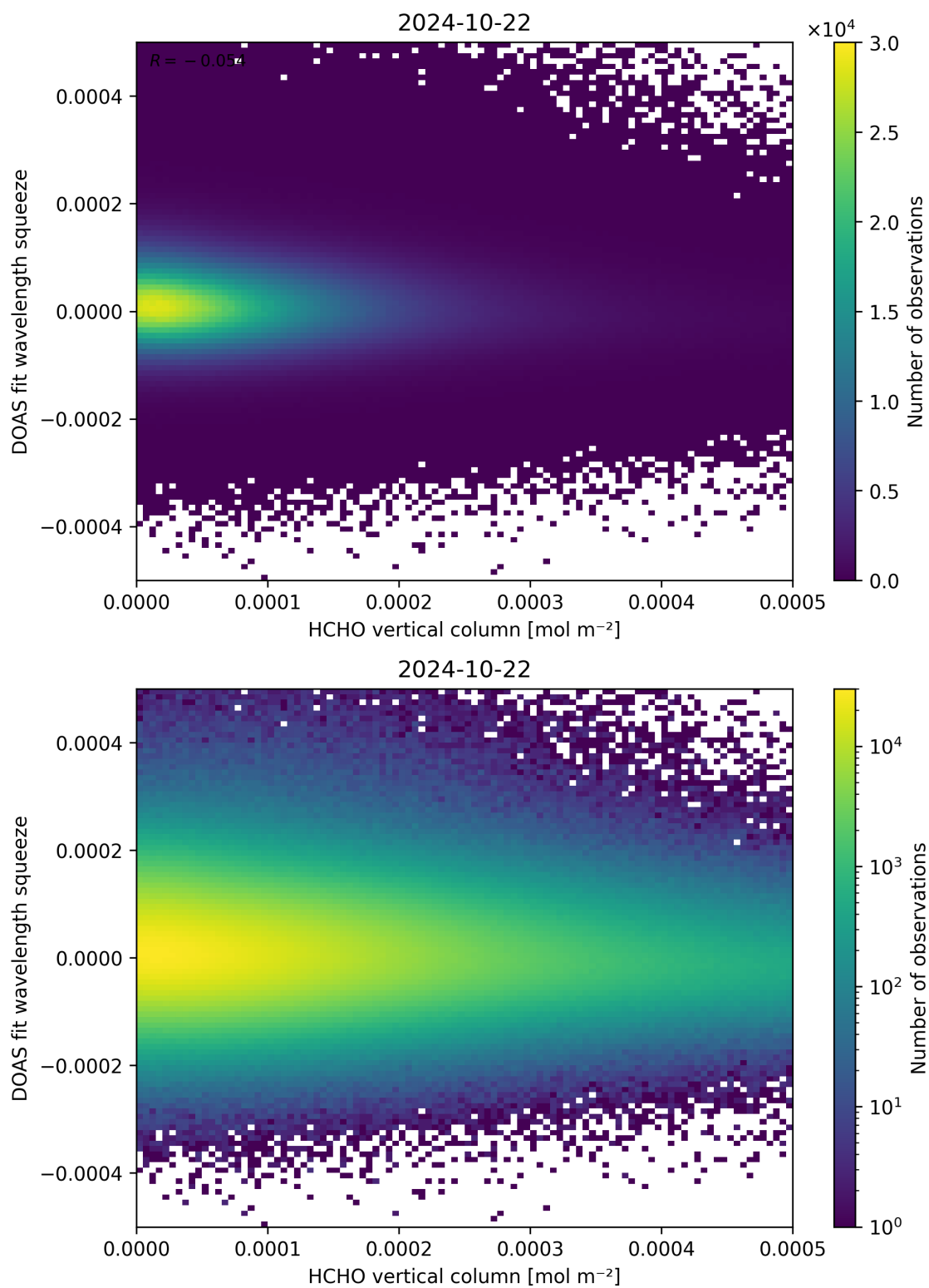
Figure 125: Scatter density plot of “HCHO vertical column” against “DOAS fit wavelength squeeze” for 2024-10-21 to 2024-10-23.
