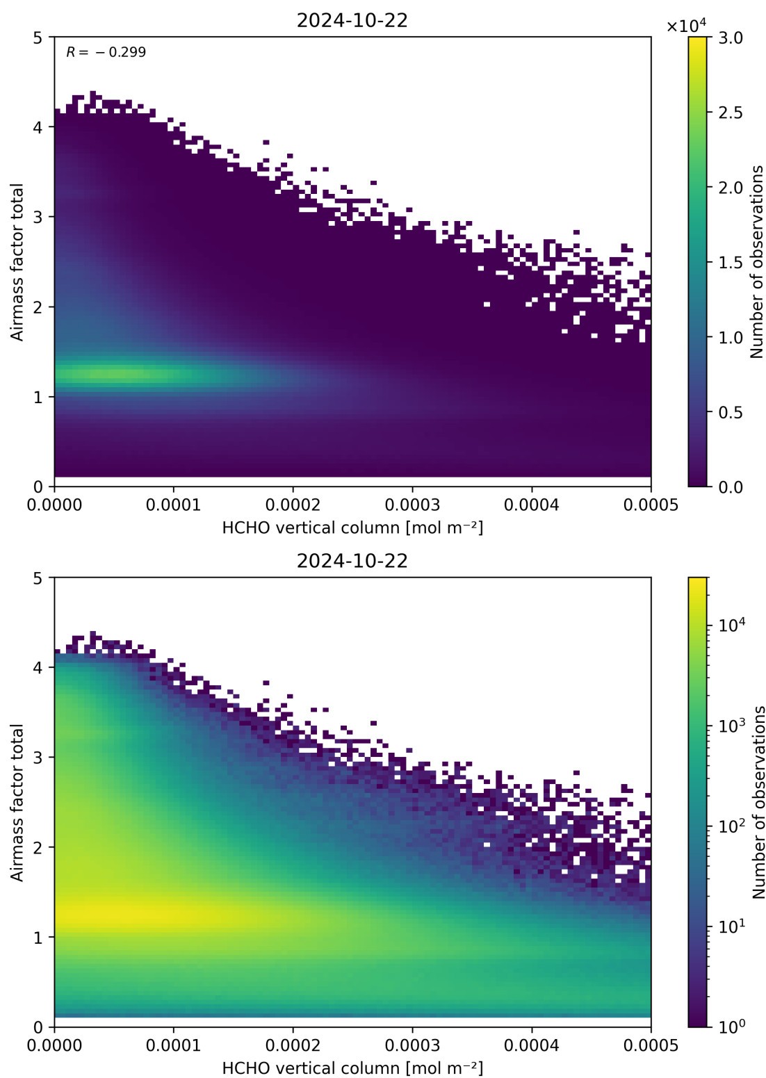
Figure 131: Scatter density plot of “HCHO vertical column” against “Airmass factor total” for 2024-10-21 to 2024-10-23.
