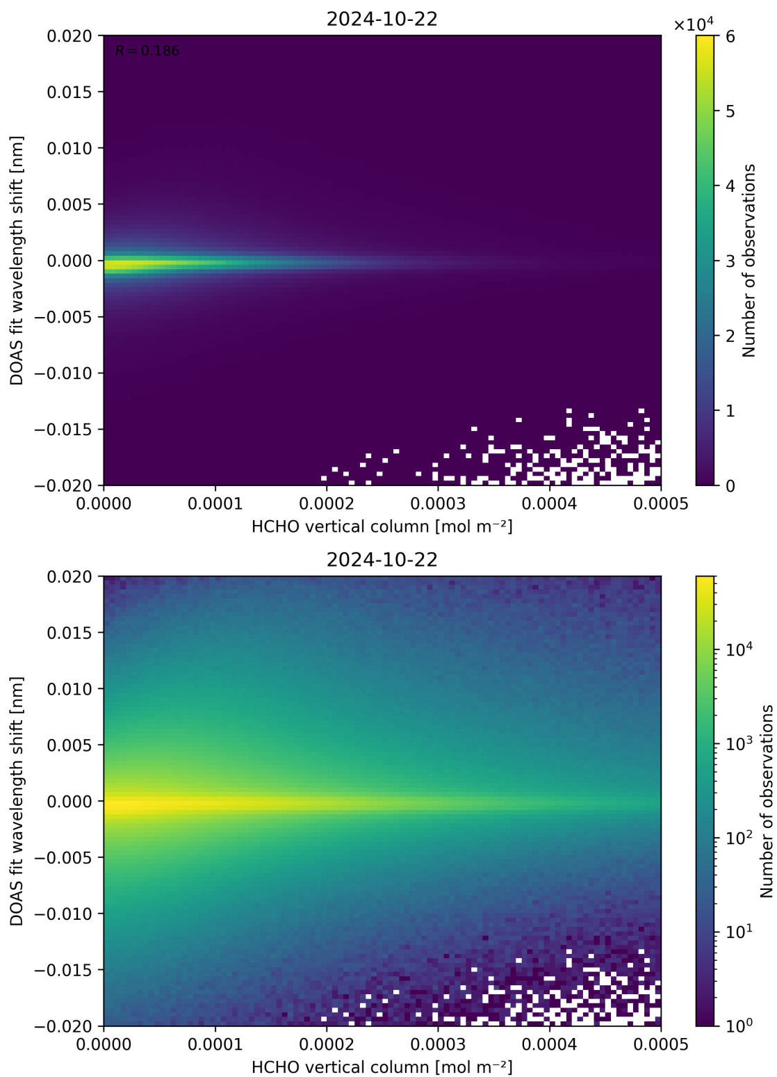
Figure 124: Scatter density plot of “HCHO vertical column” against “DOAS fit wavelength shift” for 2024-10-21 to 2024-10-23.
