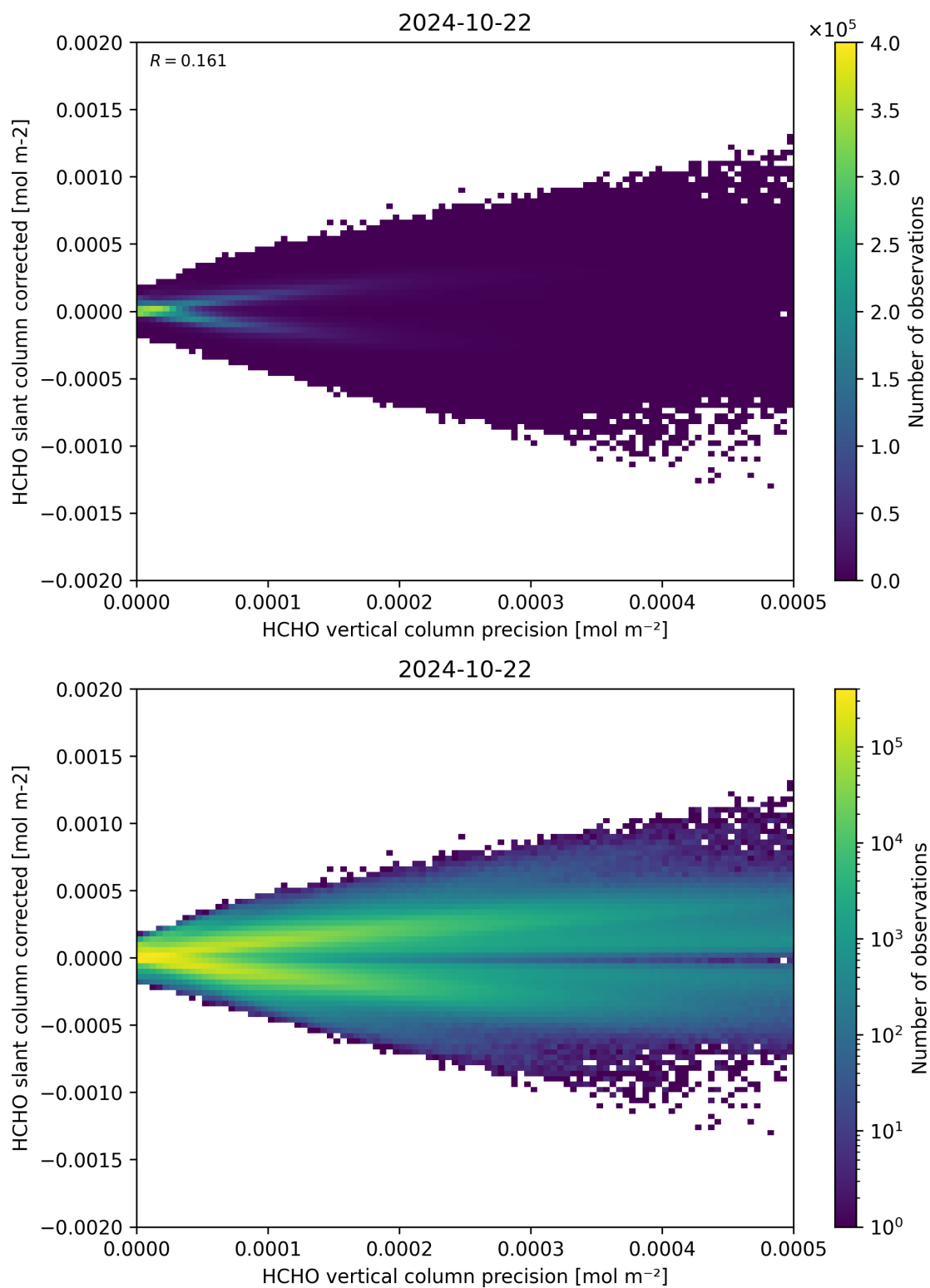
Figure 140: Scatter density plot of “HCHO vertical column precision” against “HCHO slant column corrected” for 2024-10-21 to 2024-10-23.
