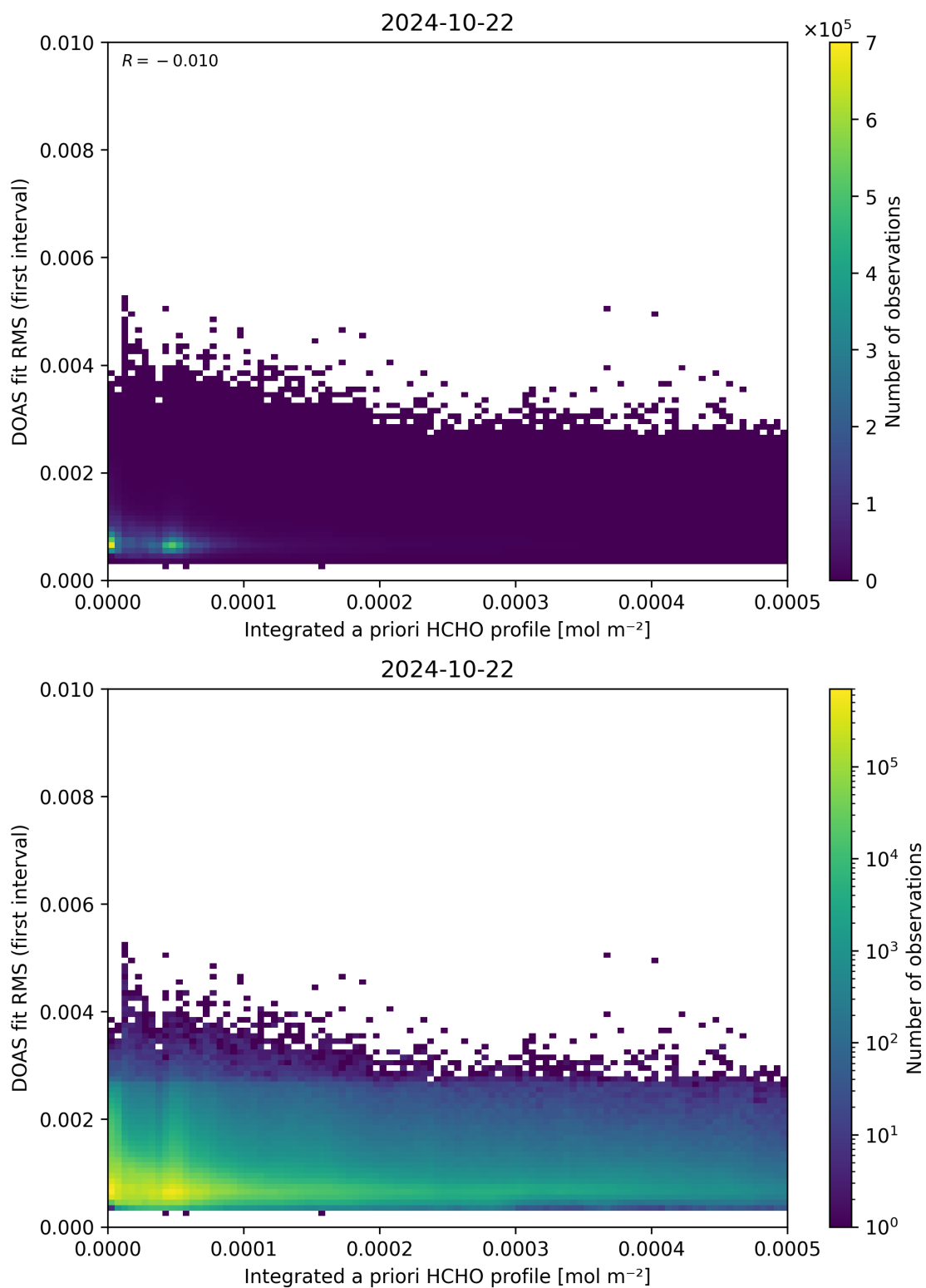
Figure 148: Scatter density plot of “Integrated a priori HCHO profile” against “DOAS fit RMS (first interval)” for 2024-10-21 to 2024-10-23.
