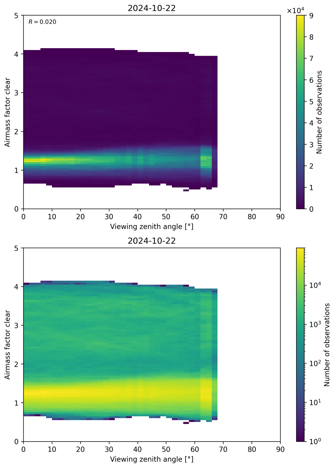
Figure 185: Scatter density plot of “Viewing zenith angle” against “Airmass factor clear” for 2024-10-21 to 2024-10-23.
