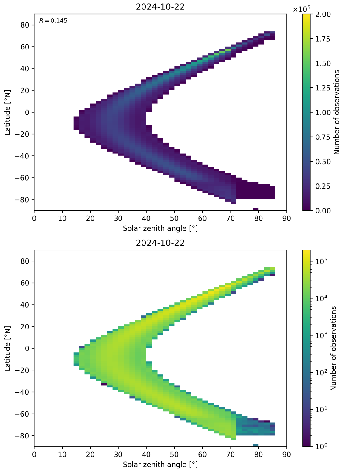
Figure 181: Scatter density plot of “Solar zenith angle” against “Latitude” for 2024-10-21 to 2024-10-23.
