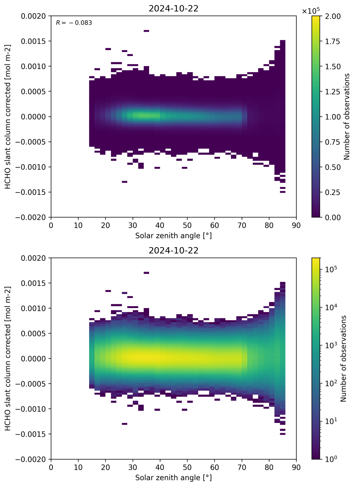
Figure 171: Scatter density plot of “Solar zenith angle” against “HCHO slant column corrected” for 2024-10-21 to 2024-10-23.
