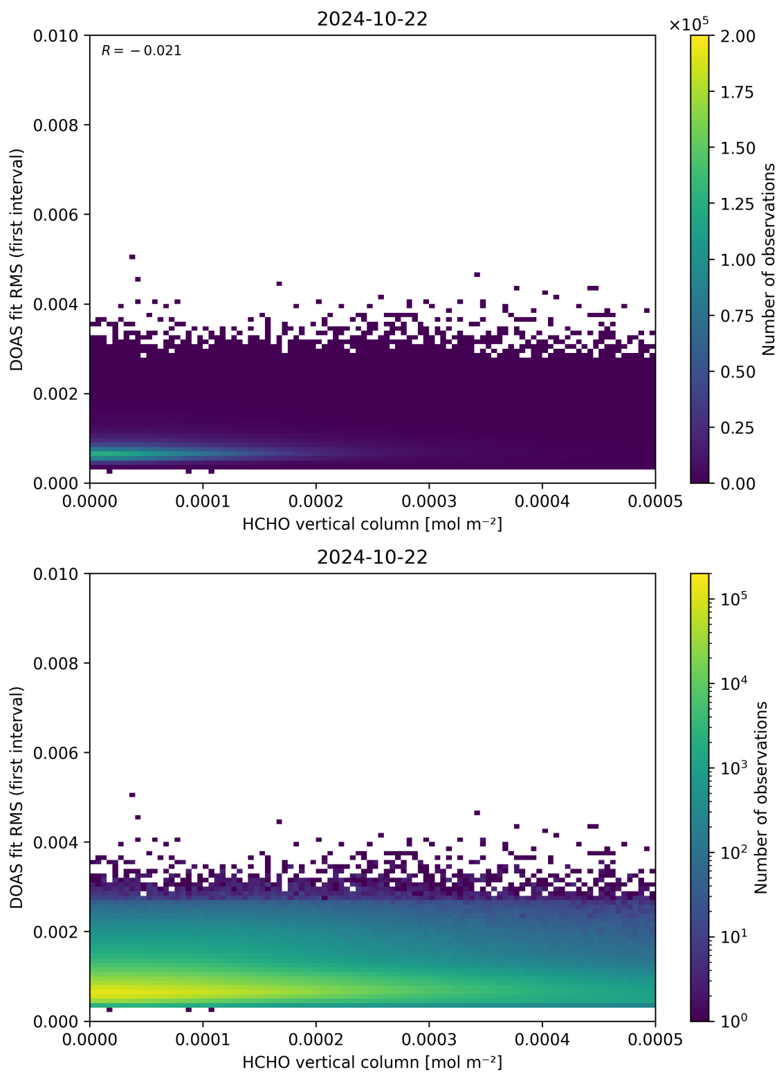
Figure 123: Scatter density plot of “HCHO vertical column” against “DOAS fit RMS (first interval)” for 2024-10-21 to 2024-10-23.
