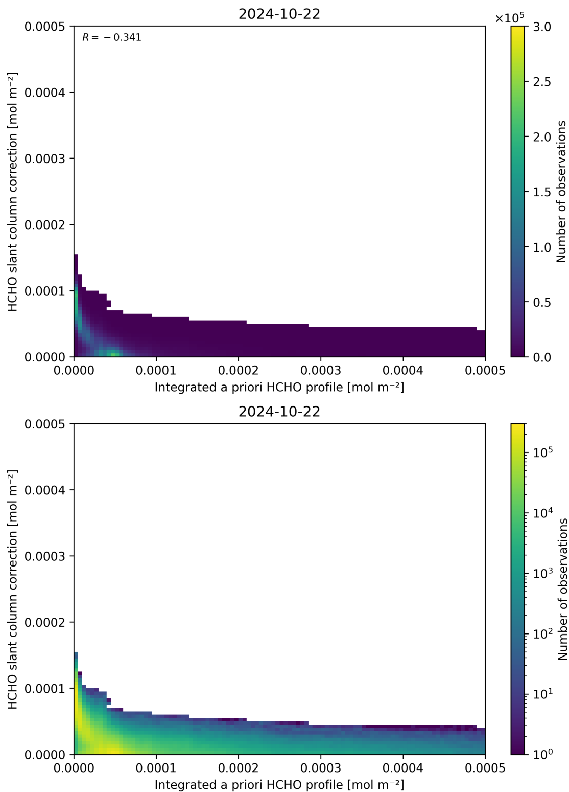
Figure 152: Scatter density plot of “Integrated a priori HCHO profile” against “HCHO slant column correction” for 2024-10-21 to 2024-10-23.
