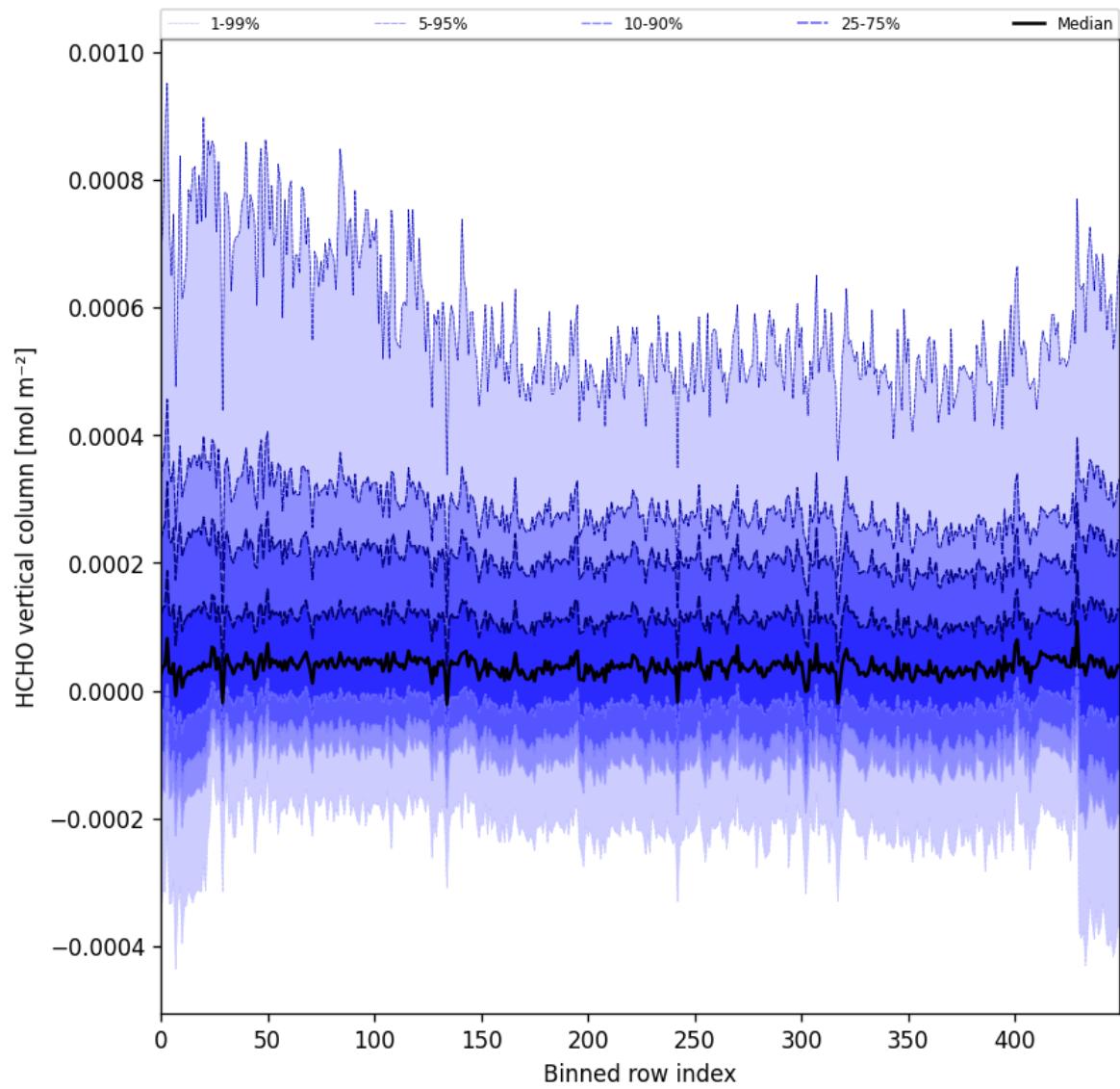
Figure 49: Along track statistics of “HCHO vertical column” for 2024-10-21 to 2024-10-23
