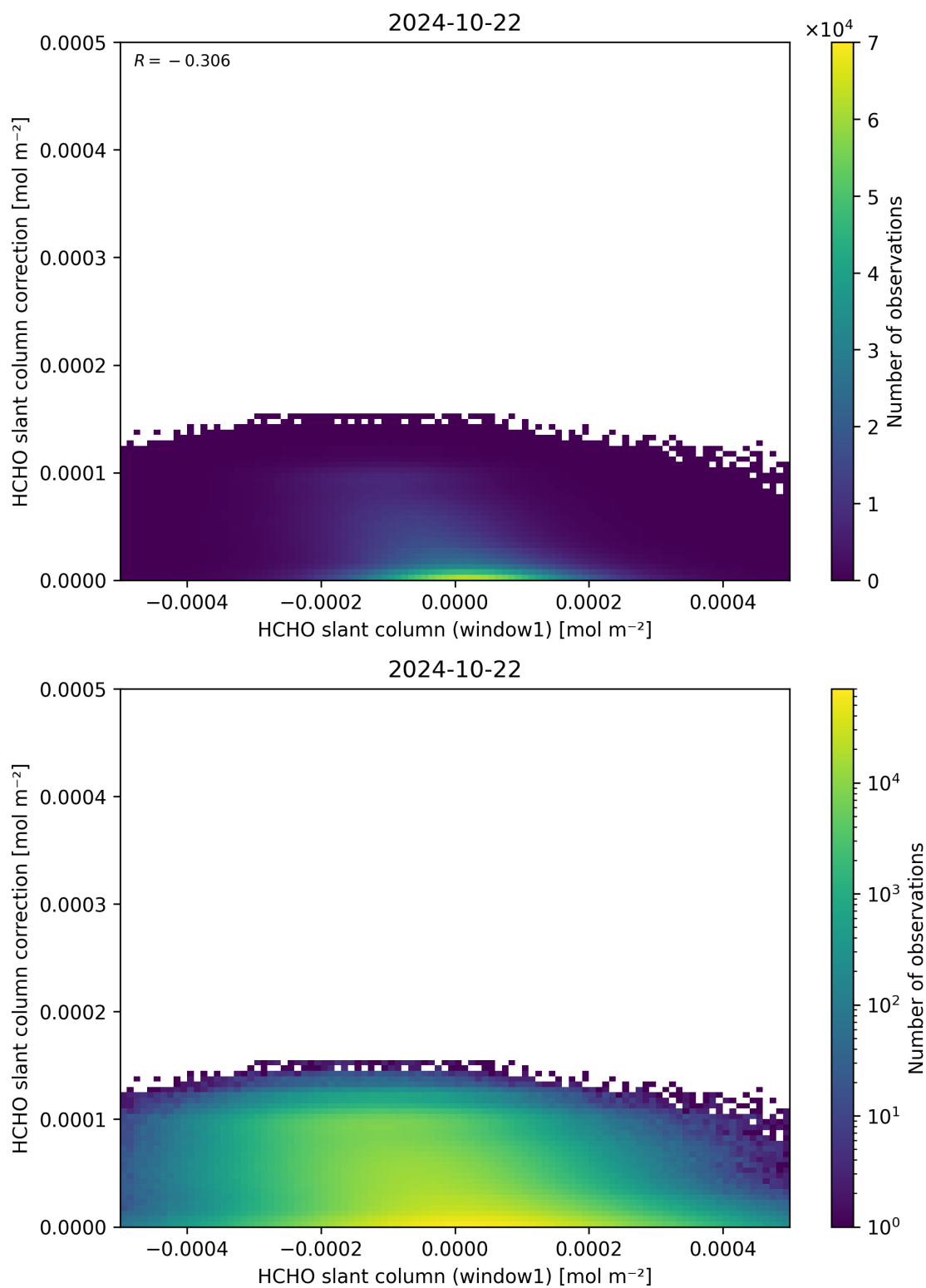
Figure 83: Scatter density plot of “HCHO slant column (window1)” against “HCHO slant column correction” for 2024-10-21 to 2024-10-23.
