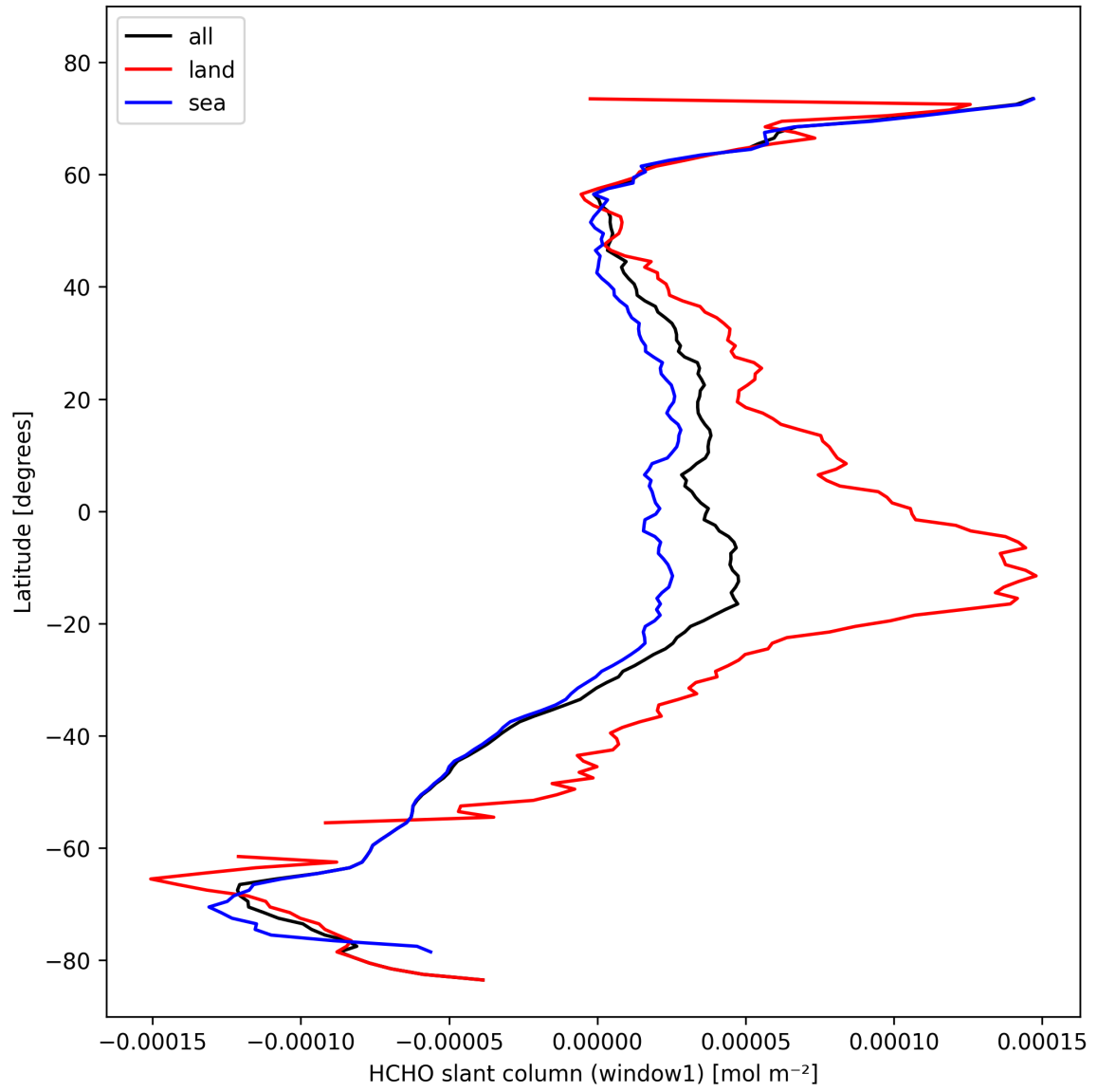
Figure 24: Zonal average of “HCHO slant column (window1)” for 2024-10-21 to 2024-10-23.
