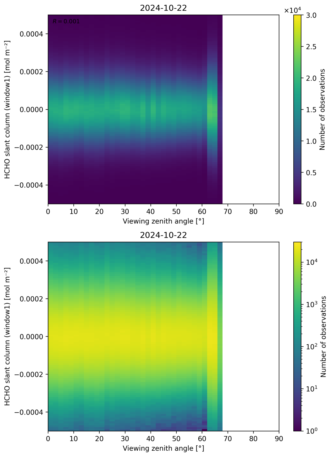
Figure 188: Scatter density plot of “Viewing zenith angle” against “HCHO slant column (window1)” for 2024-10-21 to 2024-10-23.
