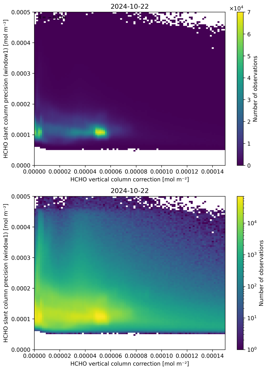
Figure 119: Scatter density plot of “HCHO vertical column correction” against “HCHO slant column precision (window1)” for 2024-10-21 to 2024-10-23.
