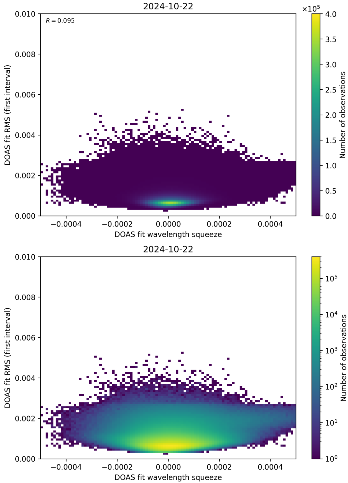
Figure 68: Scatter density plot of “DOAS fit wavelength squeeze” against “DOAS fit RMS (first interval)” for 2024-10-21 to 2024-10-23.
