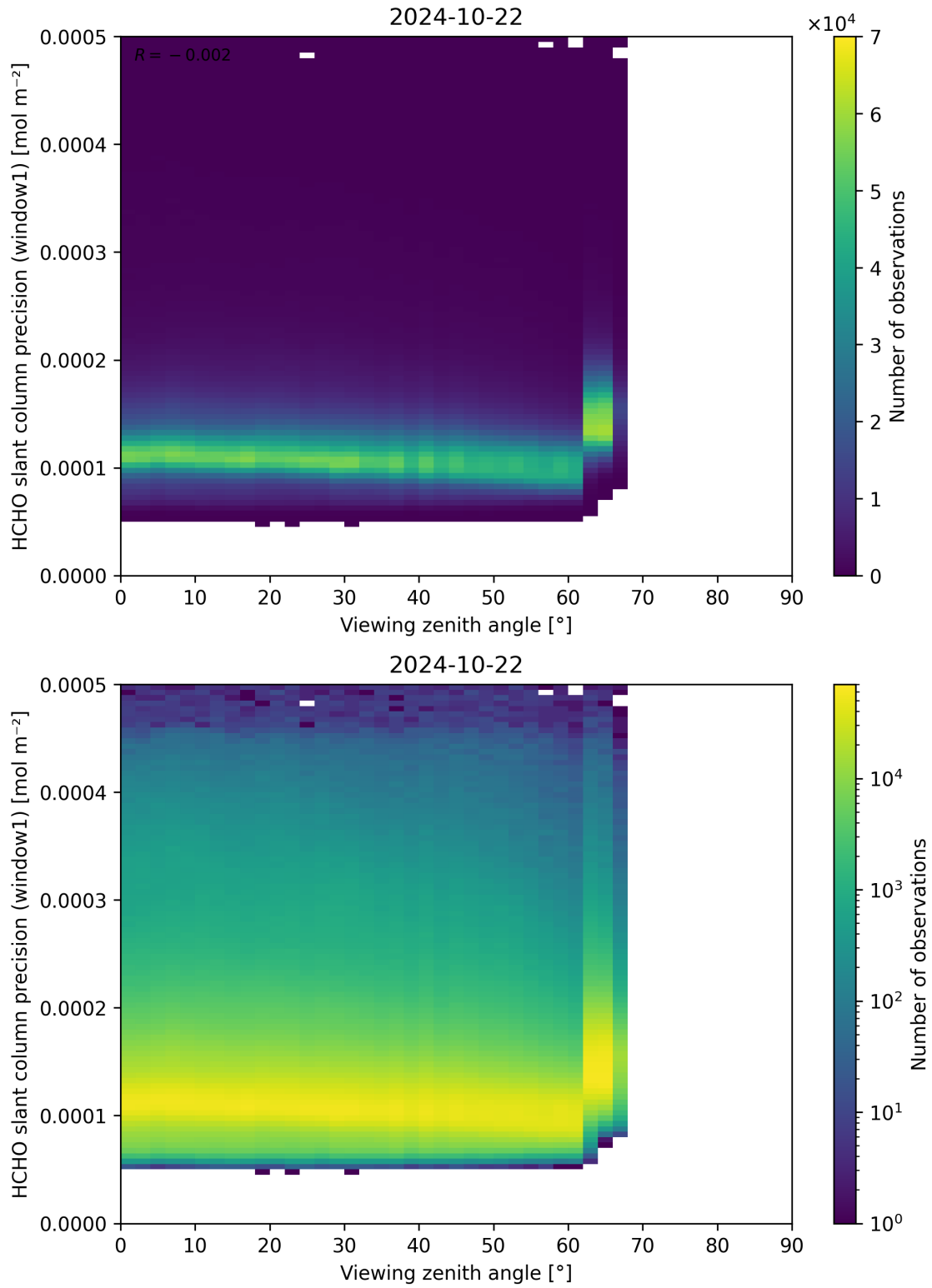
Figure 189: Scatter density plot of “Viewing zenith angle” against “HCHO slant column precision (window1)” for 2024-10-21 to 2024-10-23.
