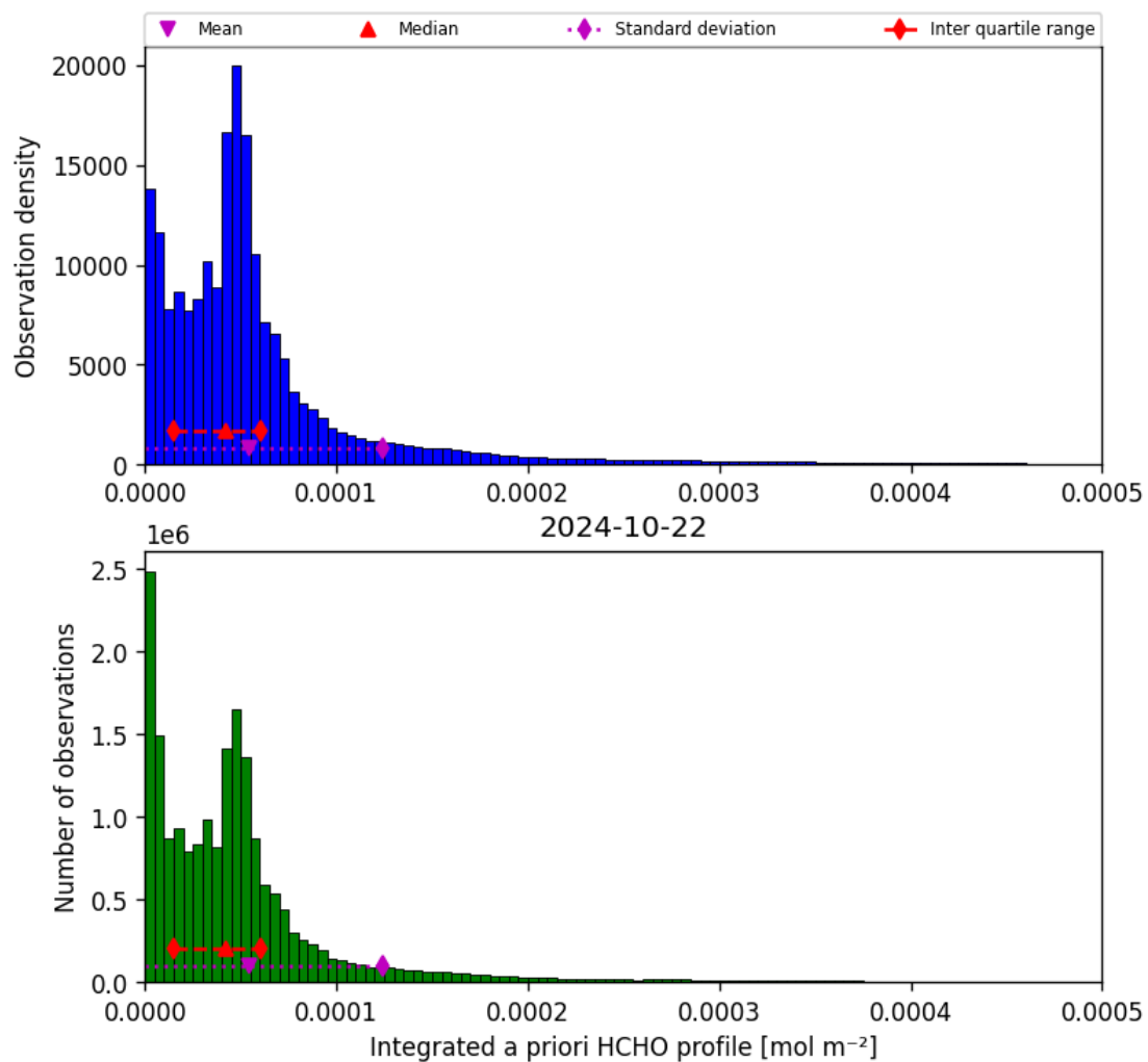
Figure 43: Histogram of “Integrated a priori HCHO profile” for 2024-10-21 to 2024-10-23
