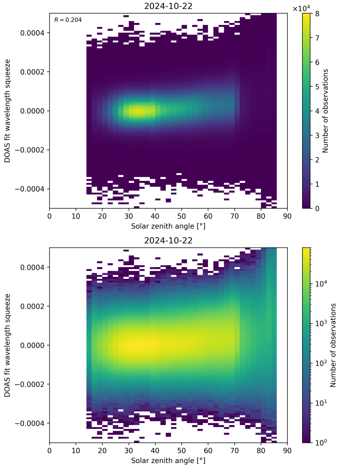
Figure 169: Scatter density plot of “Solar zenith angle” against “DOAS fit wavelength squeeze” for 2024-10-21 to 2024-10-23.
