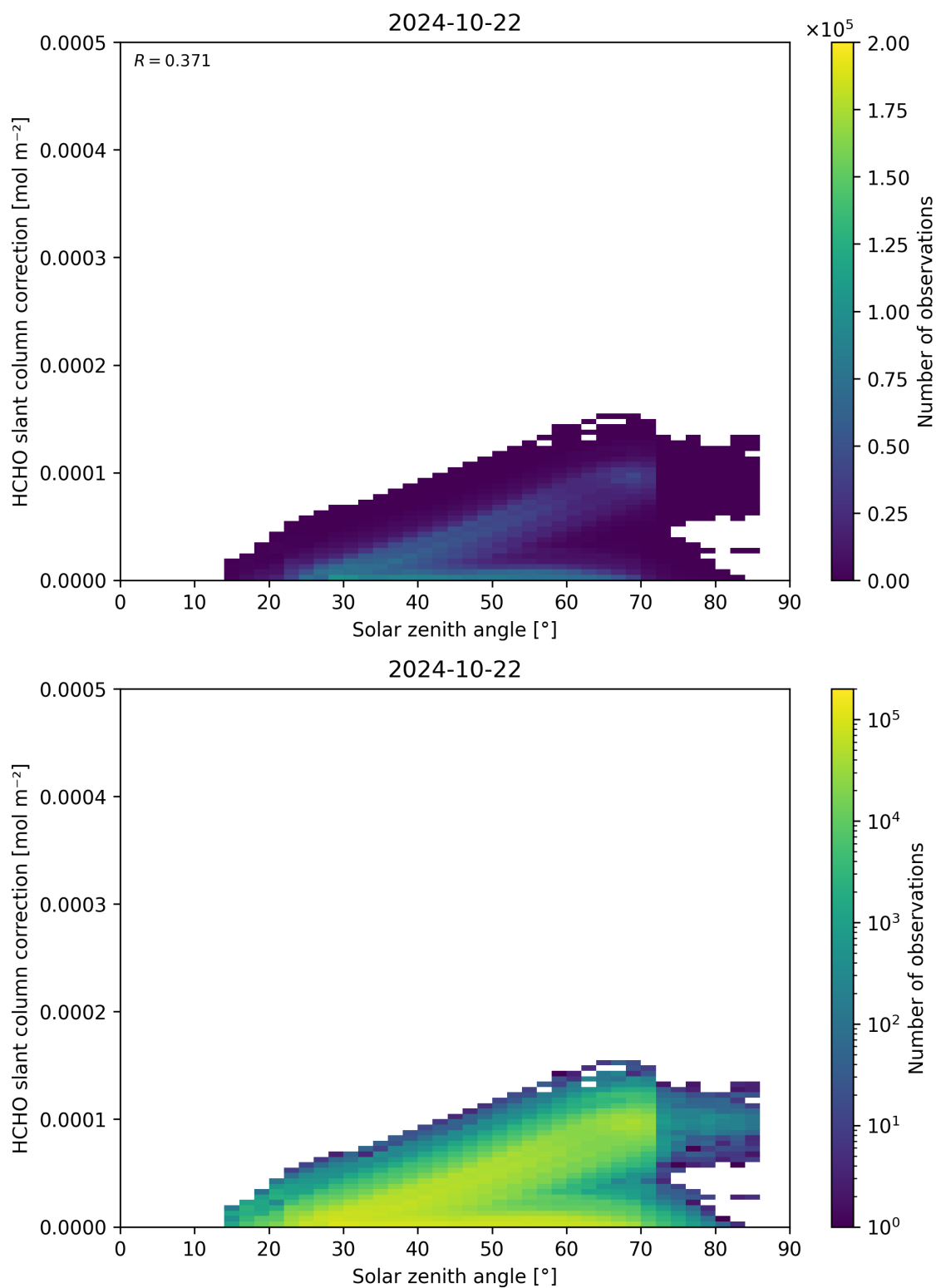
Figure 172: Scatter density plot of “Solar zenith angle” against “HCHO slant column correction” for 2024-10-21 to 2024-10-23.
