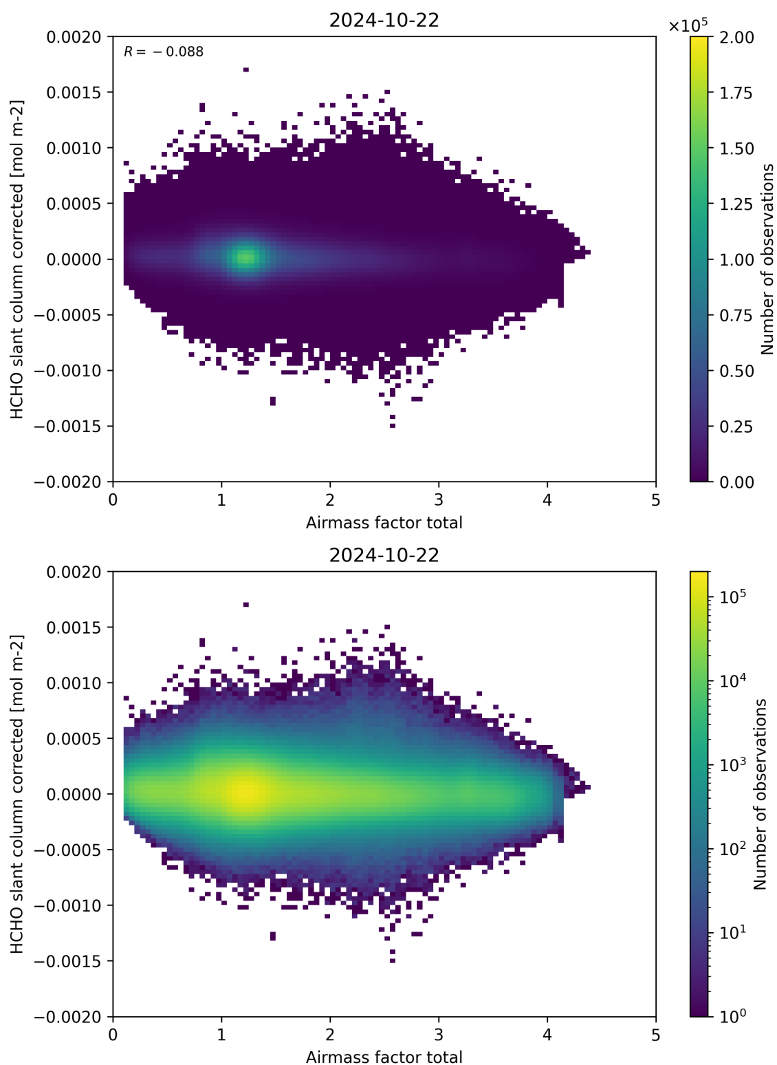
Figure 101: Scatter density plot of “Airmass factor total” against “HCHO slant column corrected” for 2024-10-21 to 2024-10-23.
