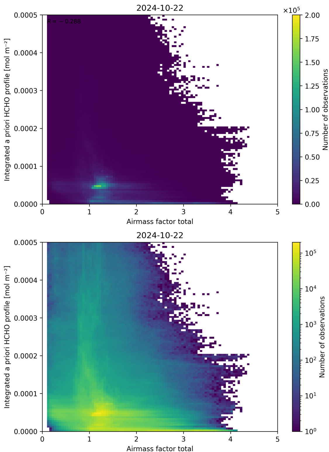
Figure 104: Scatter density plot of “Airmass factor total” against “Integrated a priori HCHO profile” for 2024-10-21 to 2024-10-23.
