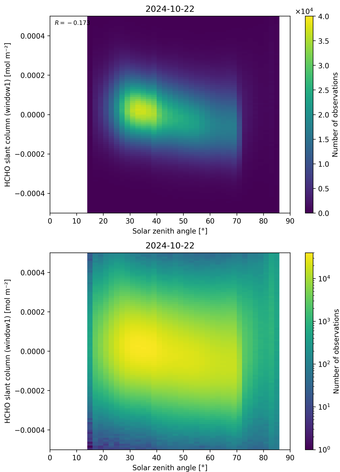
Figure 173: Scatter density plot of “Solar zenith angle” against “HCHO slant column (window1)” for 2024-10-21 to 2024-10-23.
