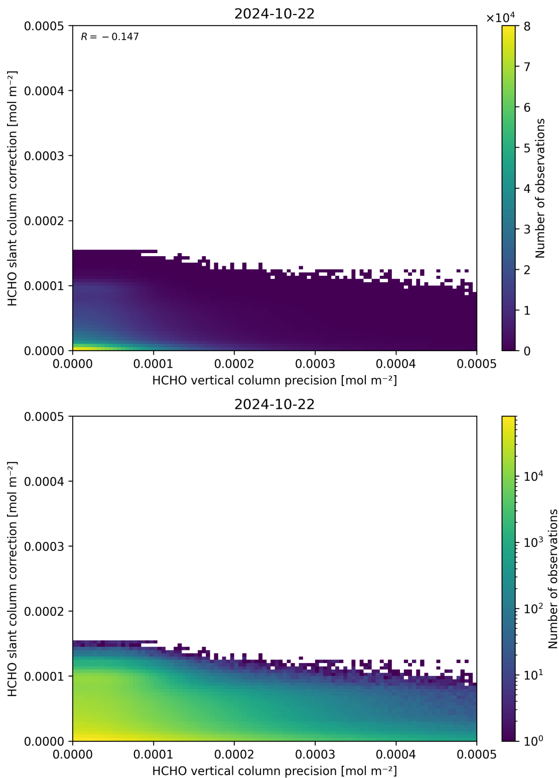
Figure 141: Scatter density plot of “HCHO vertical column precision” against “HCHO slant column correction” for 2024-10-21 to 2024-10-23.
