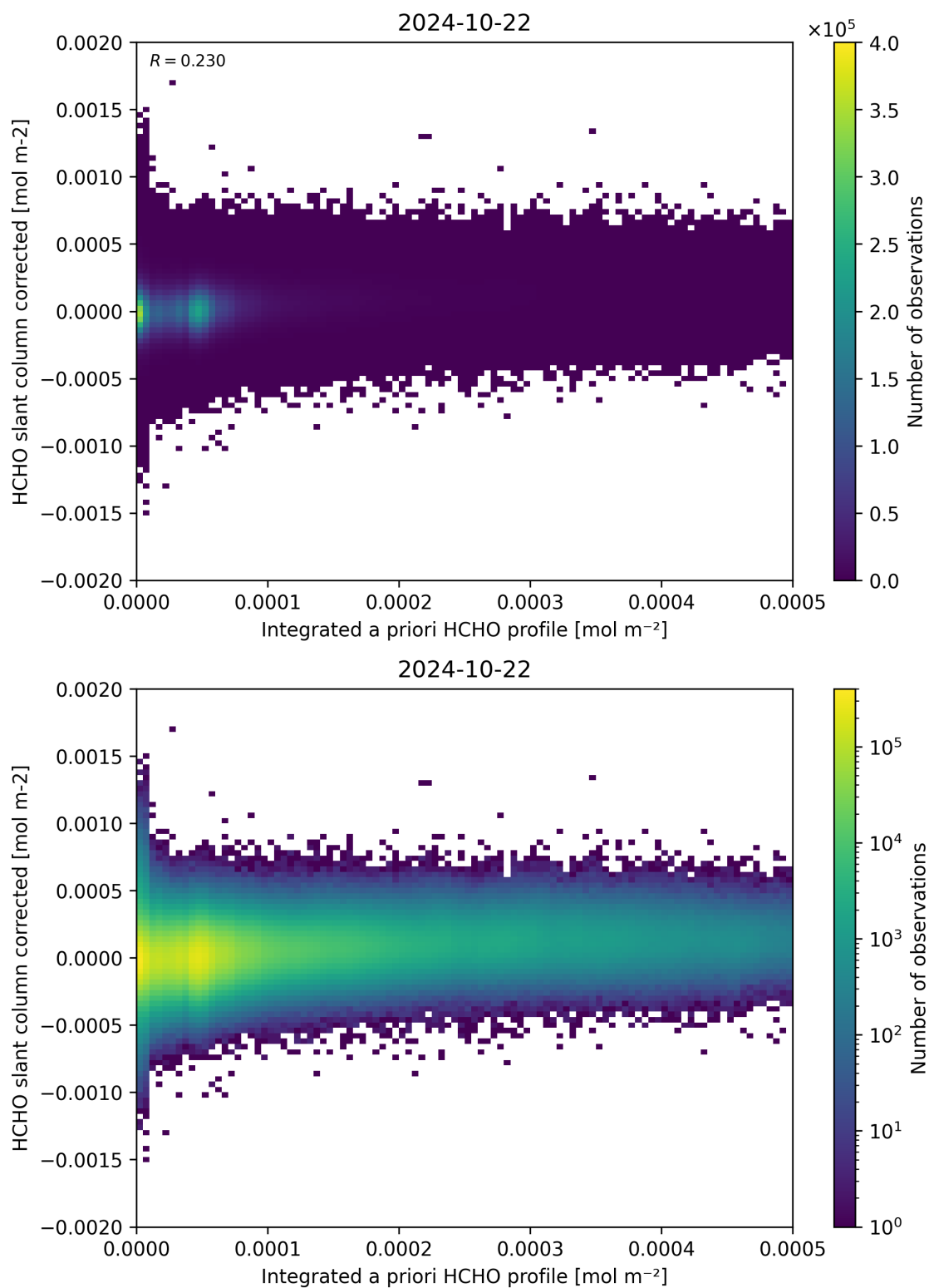
Figure 151: Scatter density plot of “Integrated a priori HCHO profile” against “HCHO slant column corrected” for 2024-10-21 to 2024-10-23.
