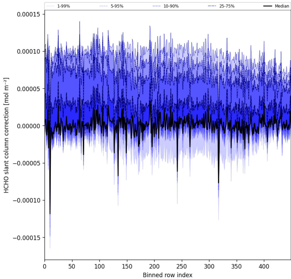
Figure 61: Along track statistics of “HCHO slant column correction” for 2024-10-21 to 2024-10-23
