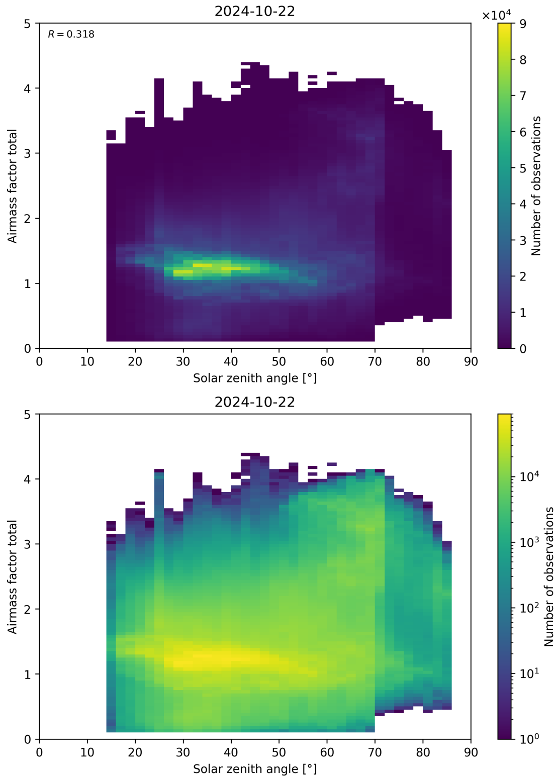
Figure 175: Scatter density plot of “Solar zenith angle” against “Airmass factor total” for 2024-10-21 to 2024-10-23.
