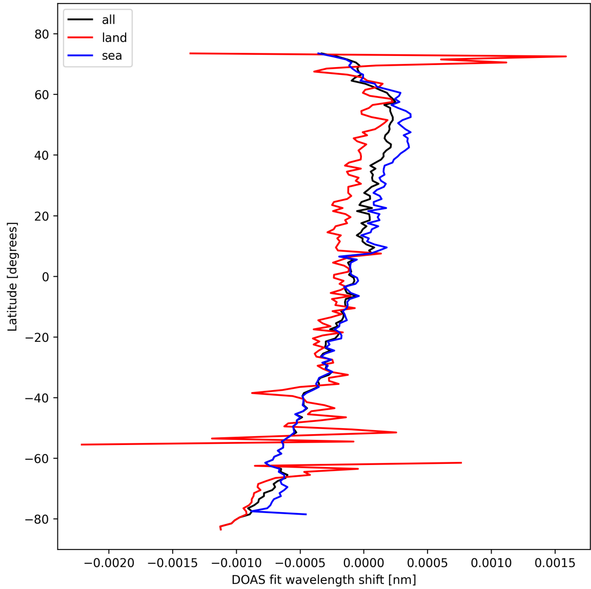
Figure 30: Zonal average of “DOAS fit wavelength shift” for 2024-10-21 to 2024-10-23.
