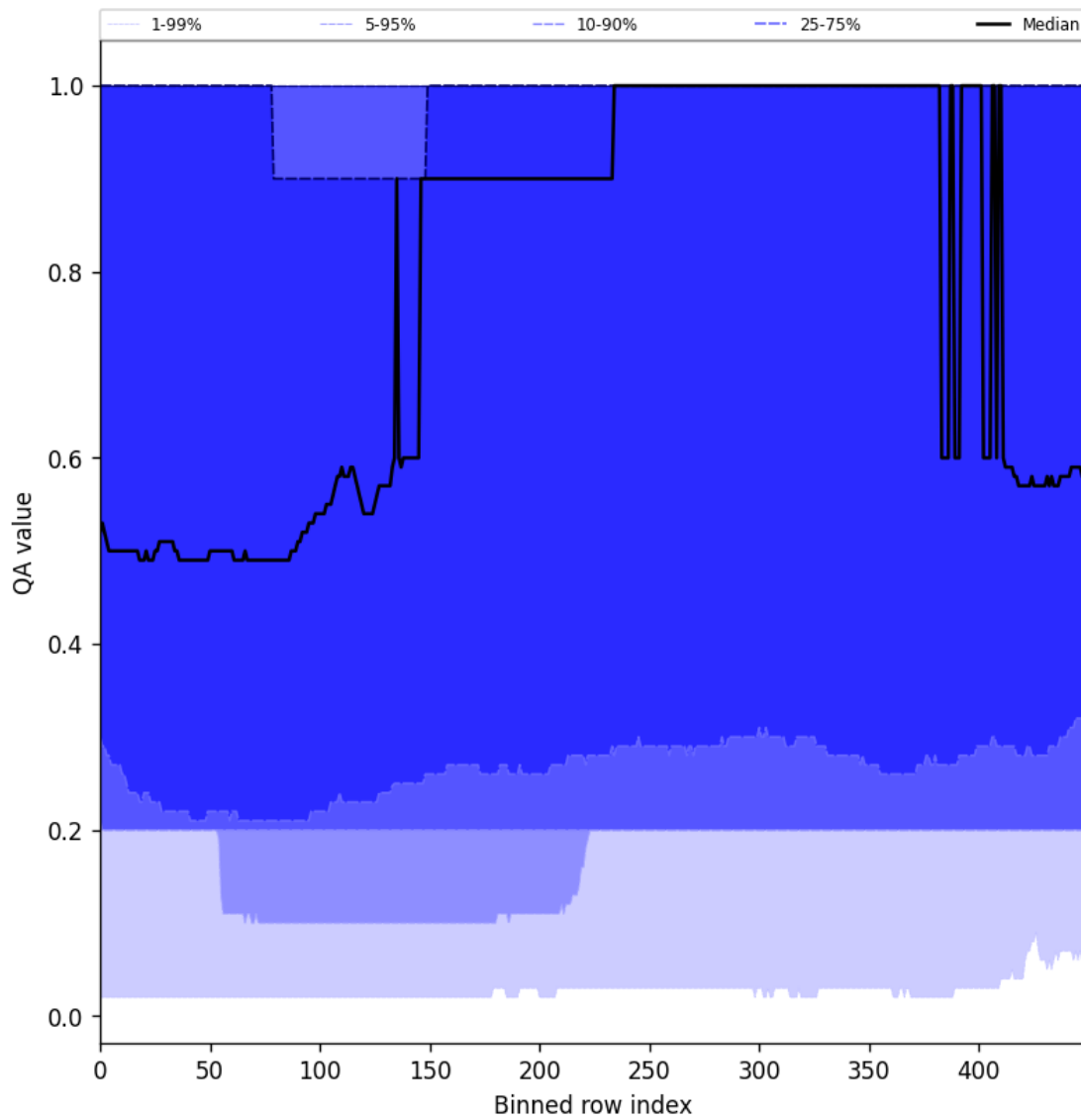
Figure 48: Along track statistics of “QA value” for 2024-10-21 to 2024-10-23
