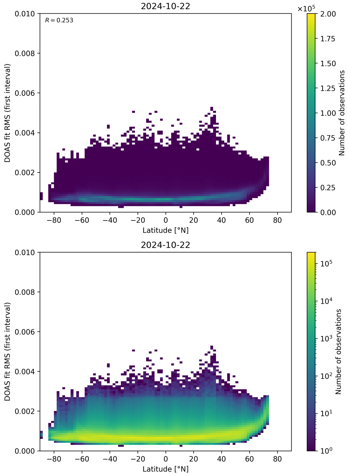
Figure 153: Scatter density plot of “Latitude” against “DOAS fit RMS (first interval)” for 2024-10-21 to 2024-10-23.
