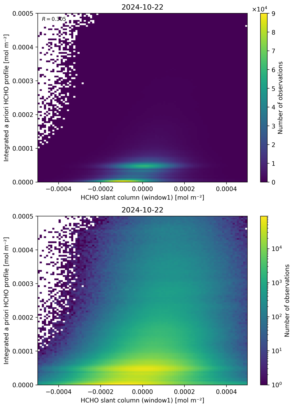
Figure 87: Scatter density plot of “HCHO slant column (window1)” against “Integrated a priori HCHO profile” for 2024-10-21 to 2024-10-23.
