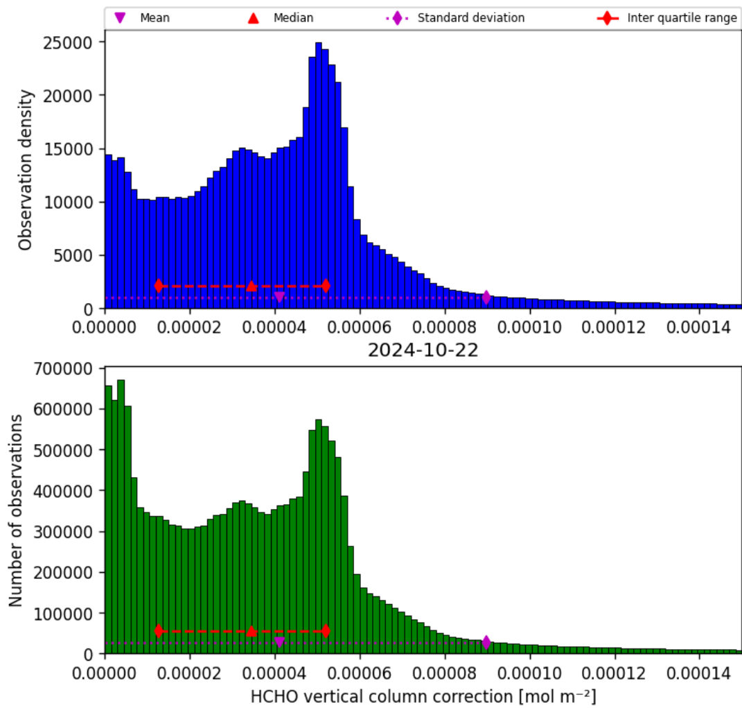
Figure 37: Histogram of “HCHO vertical column correction” for 2024-10-21 to 2024-10-23
