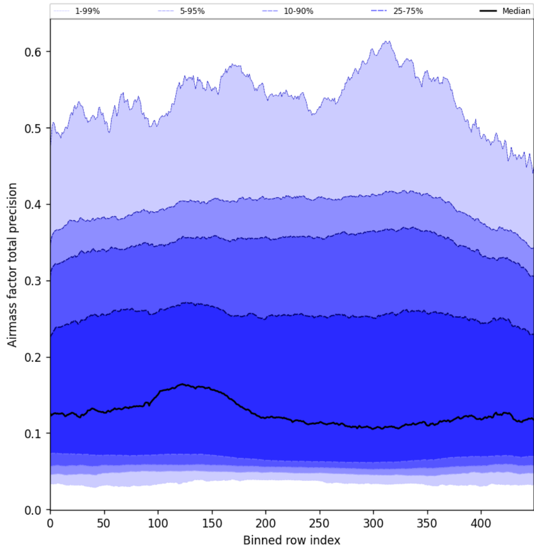
Figure 55: Along track statistics of “Airmass factor total precision” for 2024-10-21 to 2024-10-23
