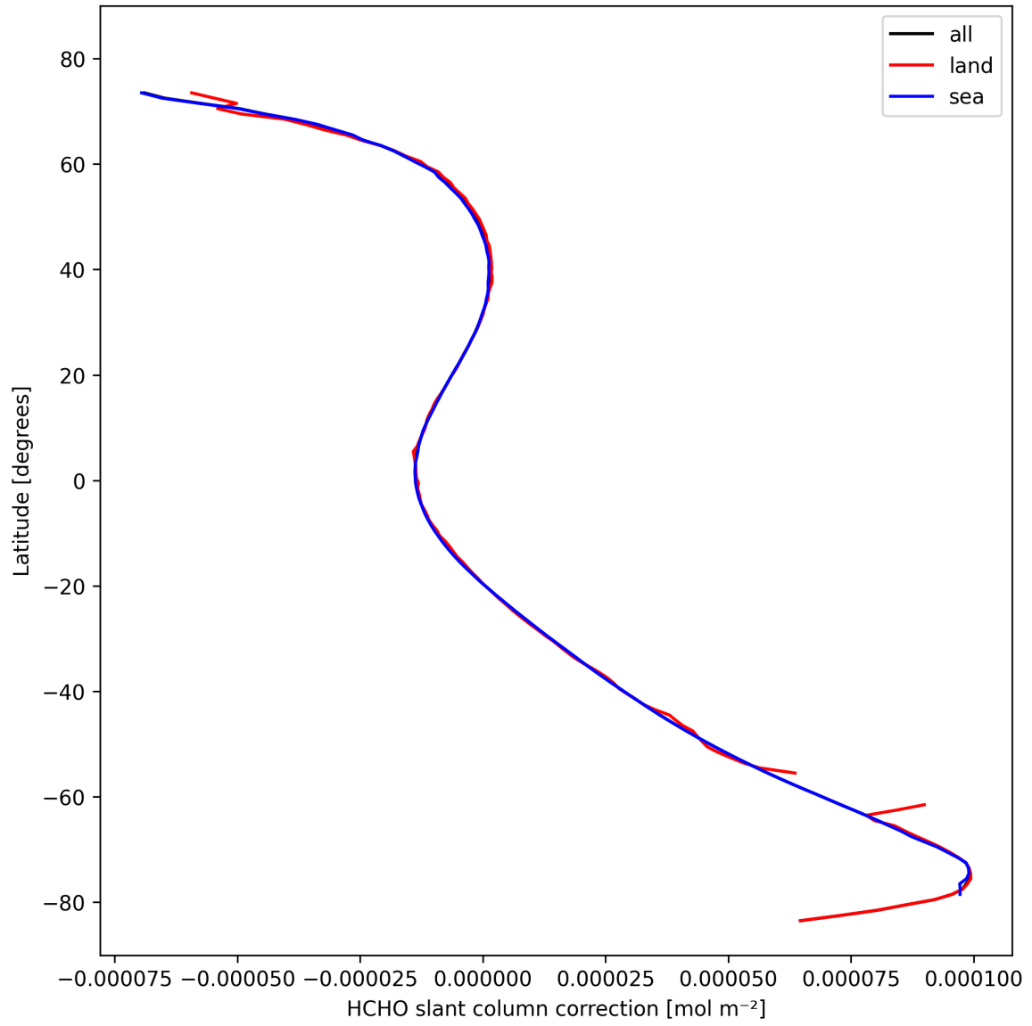
Figure 33: Zonal average of “HCHO slant column correction” for 2024-10-21 to 2024-10-23.
