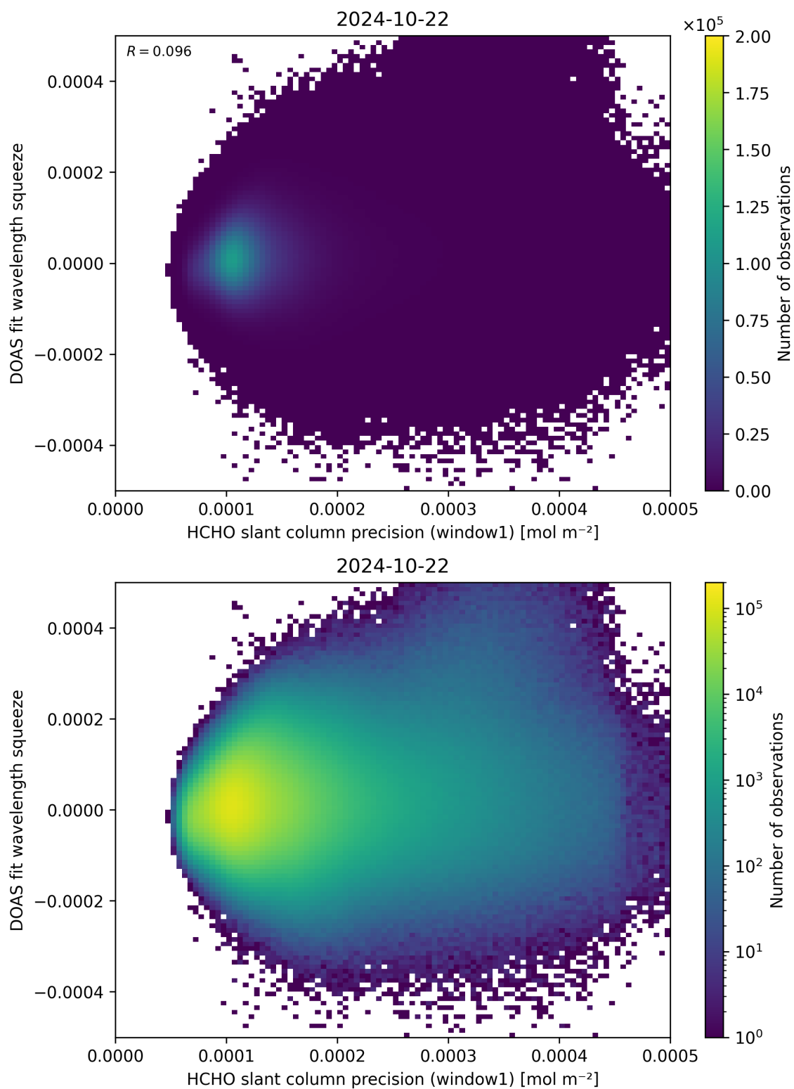
Figure 90: Scatter density plot of “HCHO slant column precision (window1)” against “DOAS fit wavelength squeeze” for 2024-10-21 to 2024-10-23.
