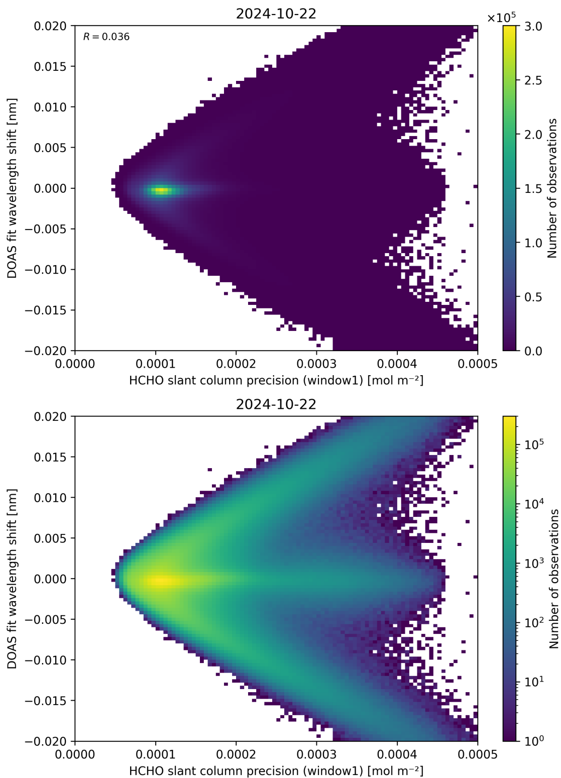
Figure 89: Scatter density plot of “HCHO slant column precision (window1)” against “DOAS fit wavelength shift” for 2024-10-21 to 2024-10-23.
