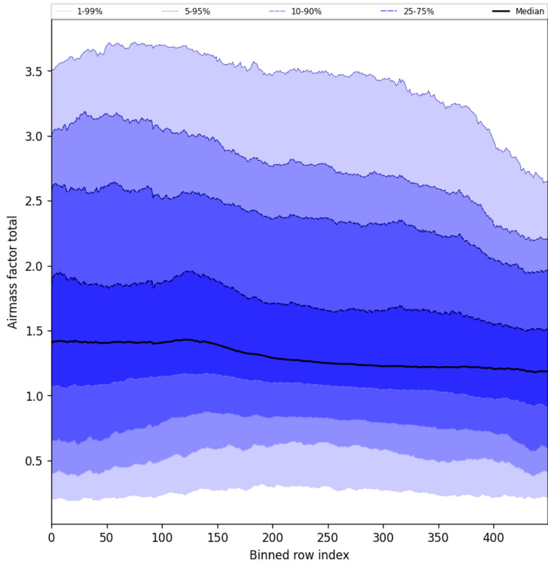
Figure 54: Along track statistics of “Airmass factor total” for 2024-10-21 to 2024-10-23
