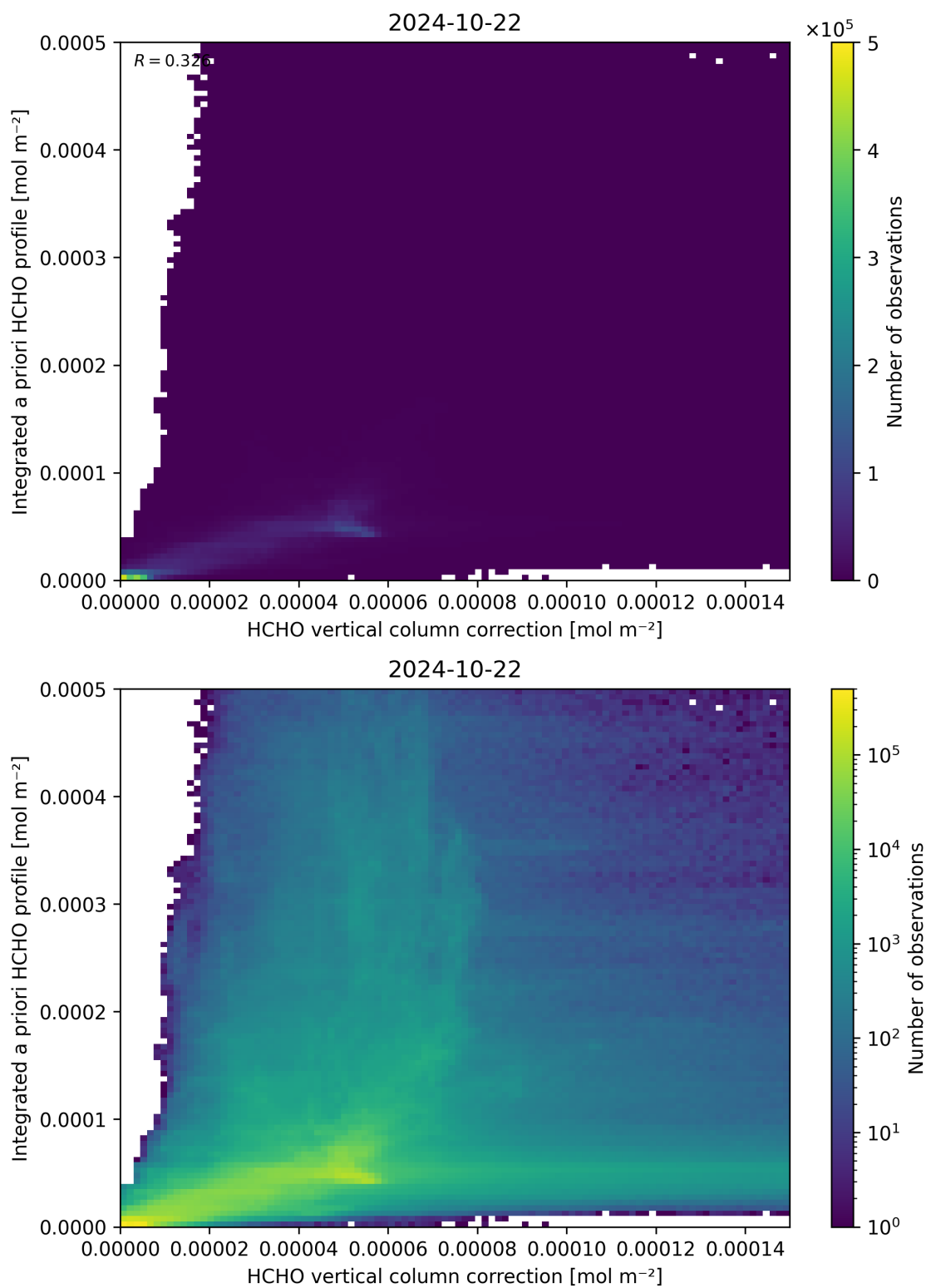
Figure 122: Scatter density plot of “HCHO vertical column correction” against “Integrated a priori HCHO profile” for 2024-10-21 to 2024-10-23.
