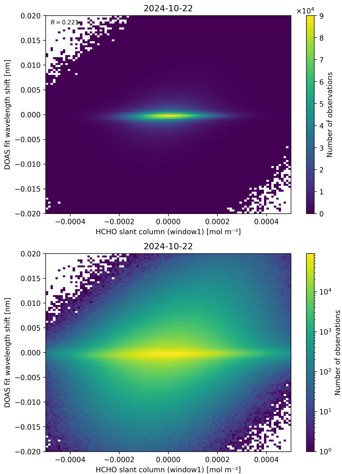
Figure 79: Scatter density plot of “HCHO slant column (window1)” against “DOAS fit wavelength shift” for 2024-10-21 to 2024-10-23.
