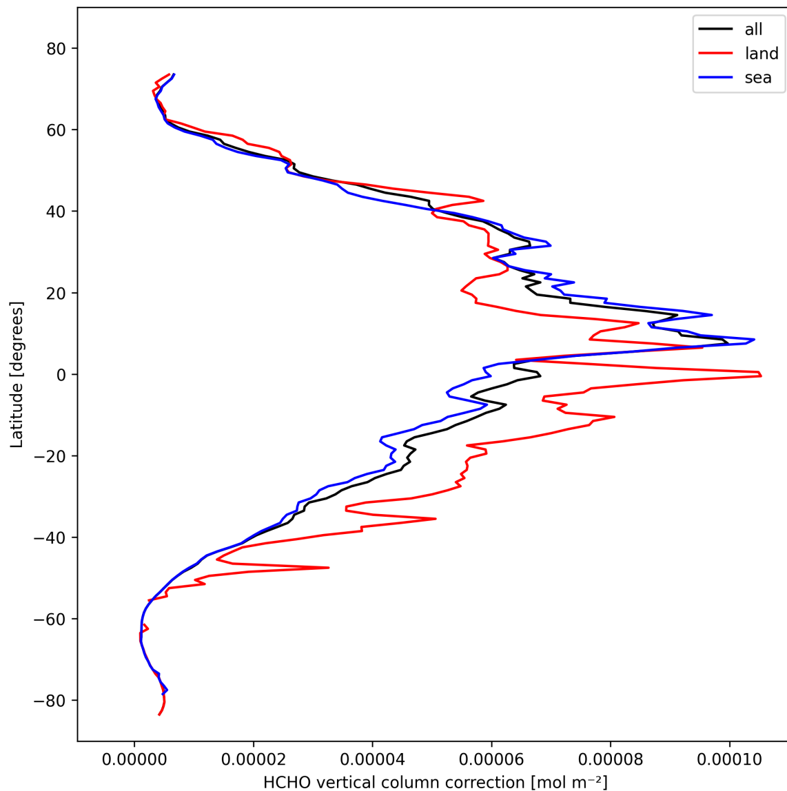
Figure 23: Zonal average of “HCHO vertical column correction” for 2024-10-21 to 2024-10-23.
