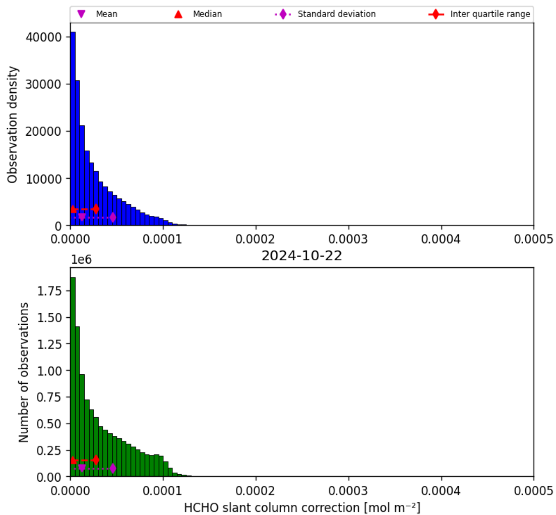
Figure 47: Histogram of “HCHO slant column correction” for 2024-10-21 to 2024-10-23
