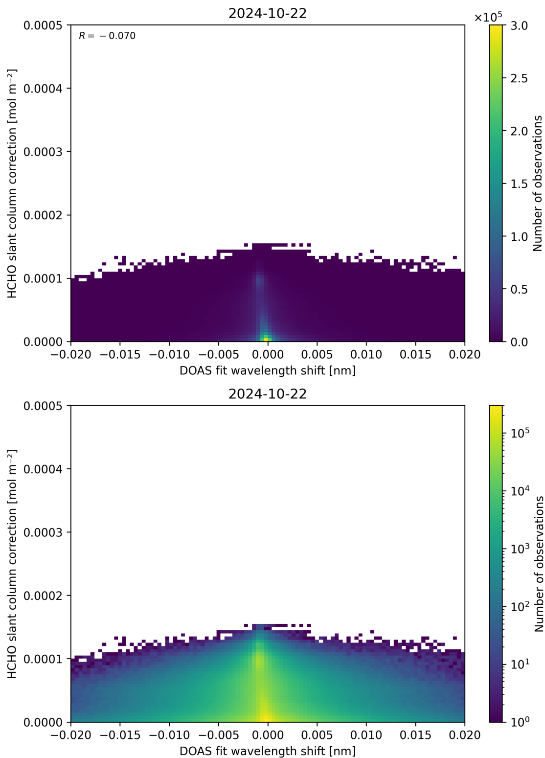
Figure 67: Scatter density plot of “DOAS fit wavelength shift” against “HCHO slant column correction” for 2024-10-21 to 2024-10-23.
