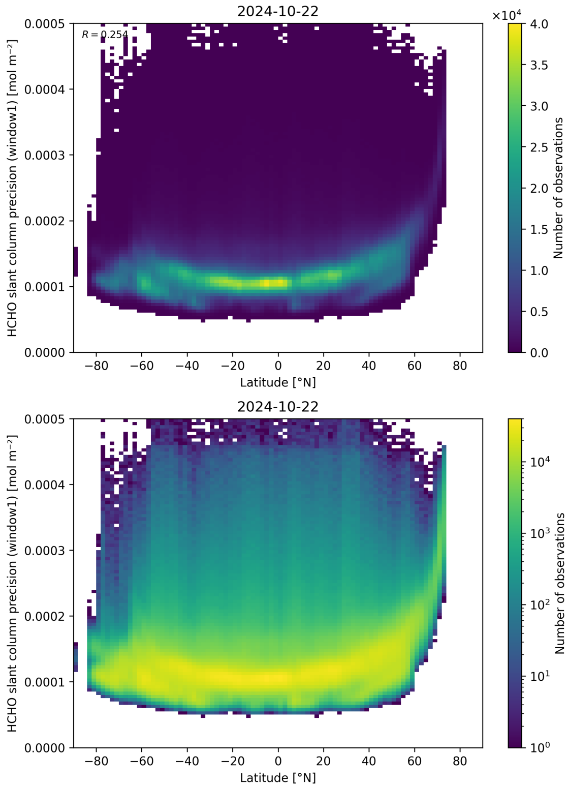
Figure 160: Scatter density plot of “Latitude” against “HCHO slant column precision (window1)” for 2024-10-21 to 2024-10-23.
