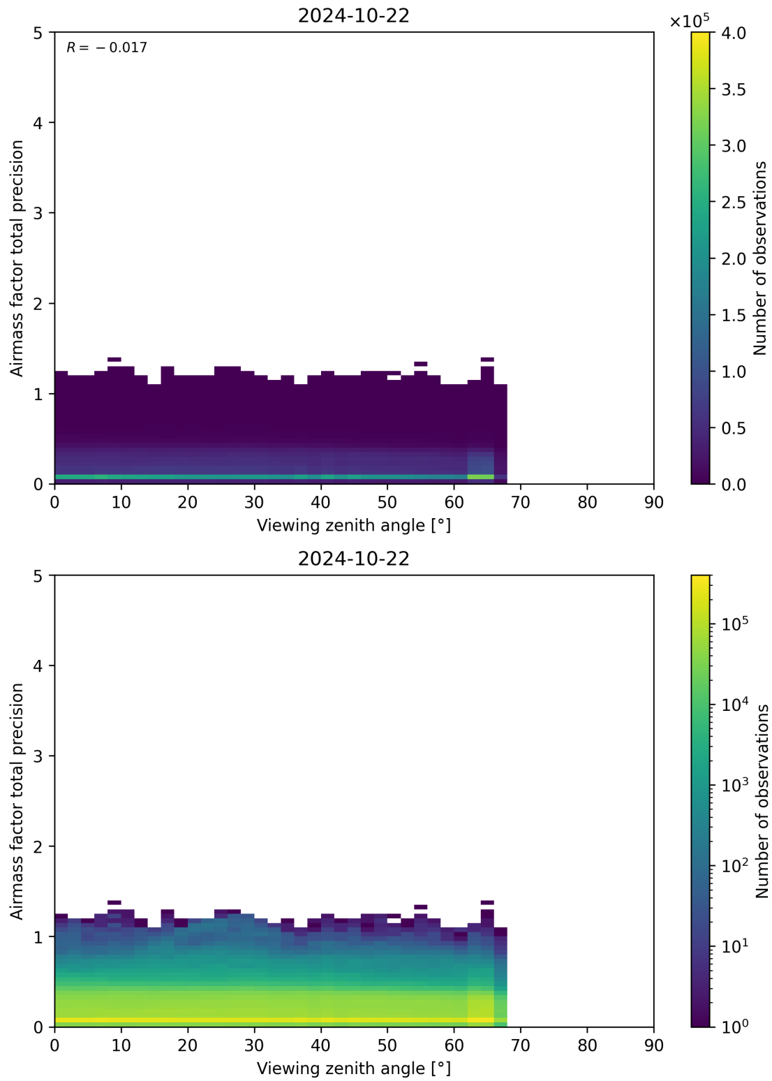
Figure 191: Scatter density plot of “Viewing zenith angle” against “Airmass factor total precision” for 2024-10-21 to 2024-10-23.
