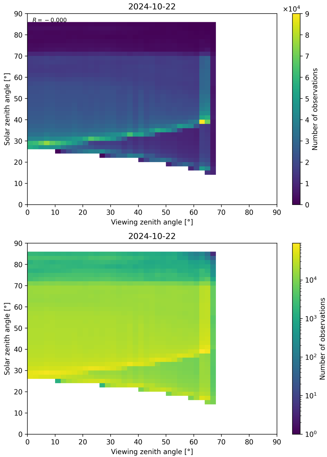
Figure 197: Scatter density plot of “Viewing zenith angle” against “Solar zenith angle” for 2024-10-21 to 2024-10-23.
