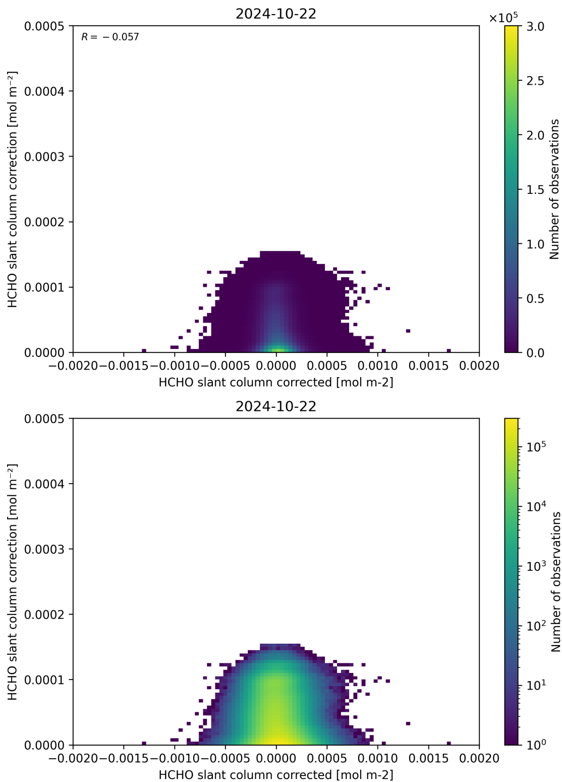
Figure 77: Scatter density plot of “HCHO slant column corrected” against “HCHO slant column correction” for 2024-10-21 to 2024-10-23.
