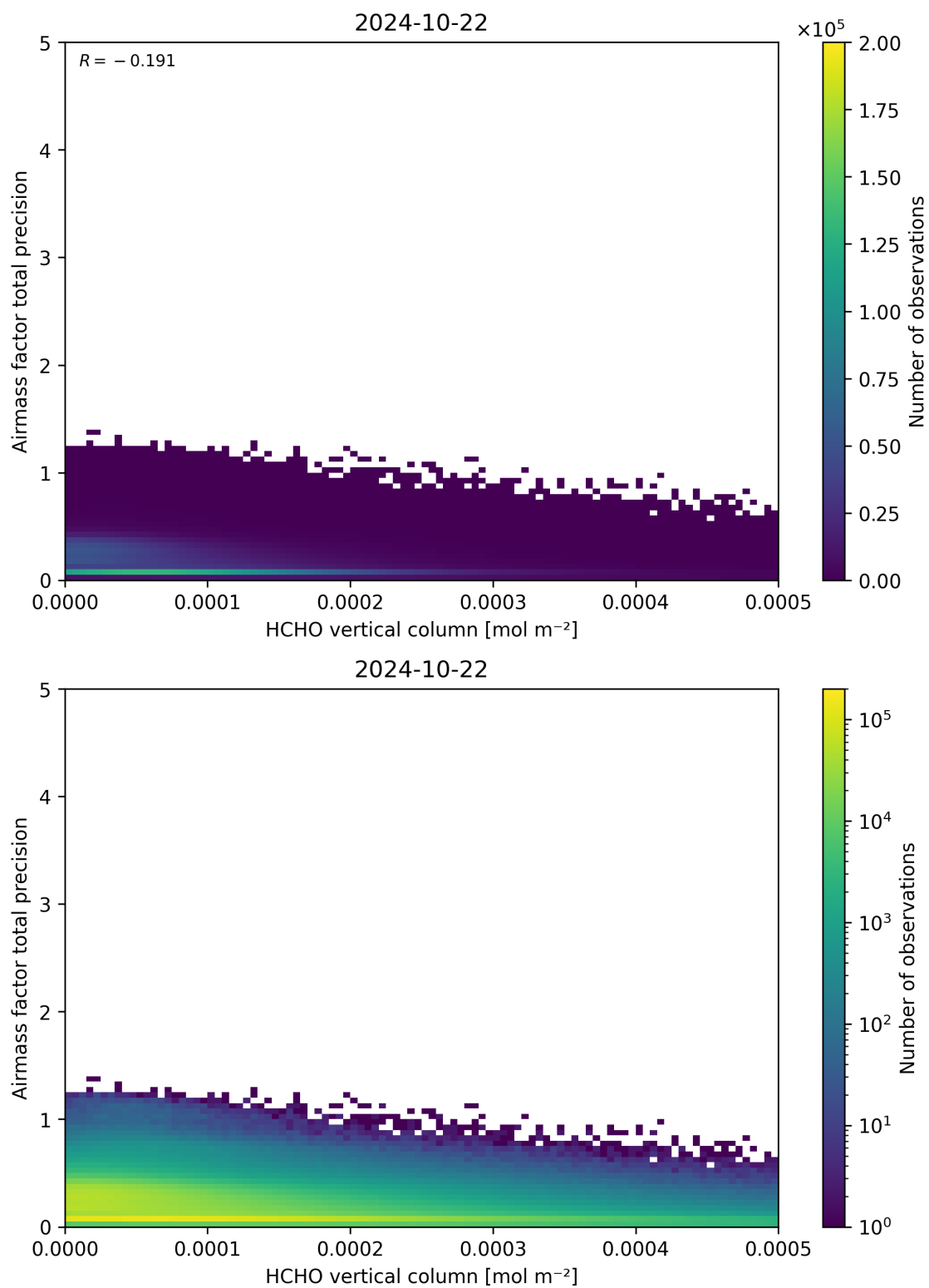
Figure 132: Scatter density plot of “HCHO vertical column” against “Airmass factor total precision” for 2024-10-21 to 2024-10-23.
