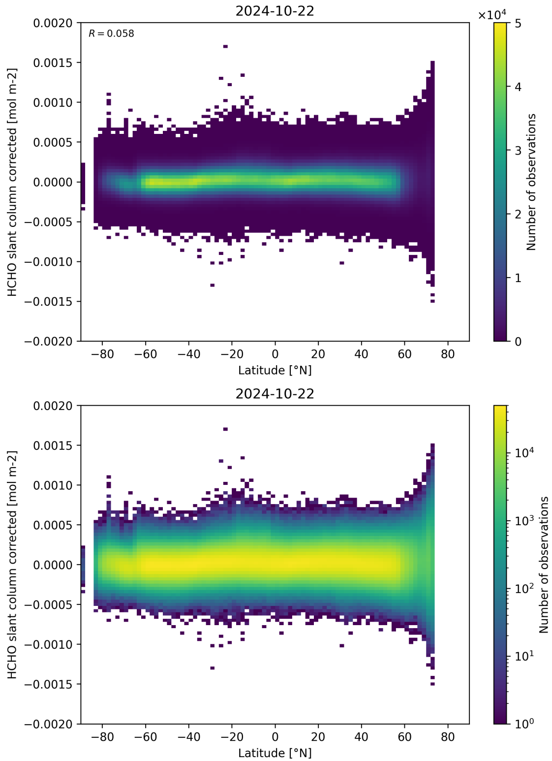
Figure 157: Scatter density plot of “Latitude” against “HCHO slant column corrected” for 2024-10-21 to 2024-10-23.
