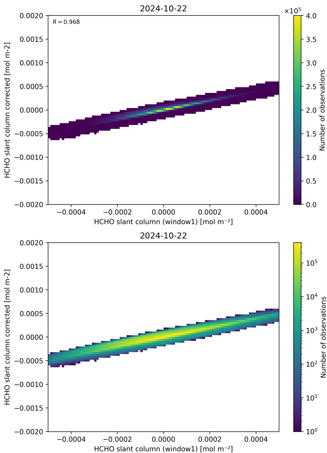
Figure 82: Scatter density plot of “HCHO slant column (window1)” against “HCHO slant column corrected” for 2024-10-21 to 2024-10-23.
