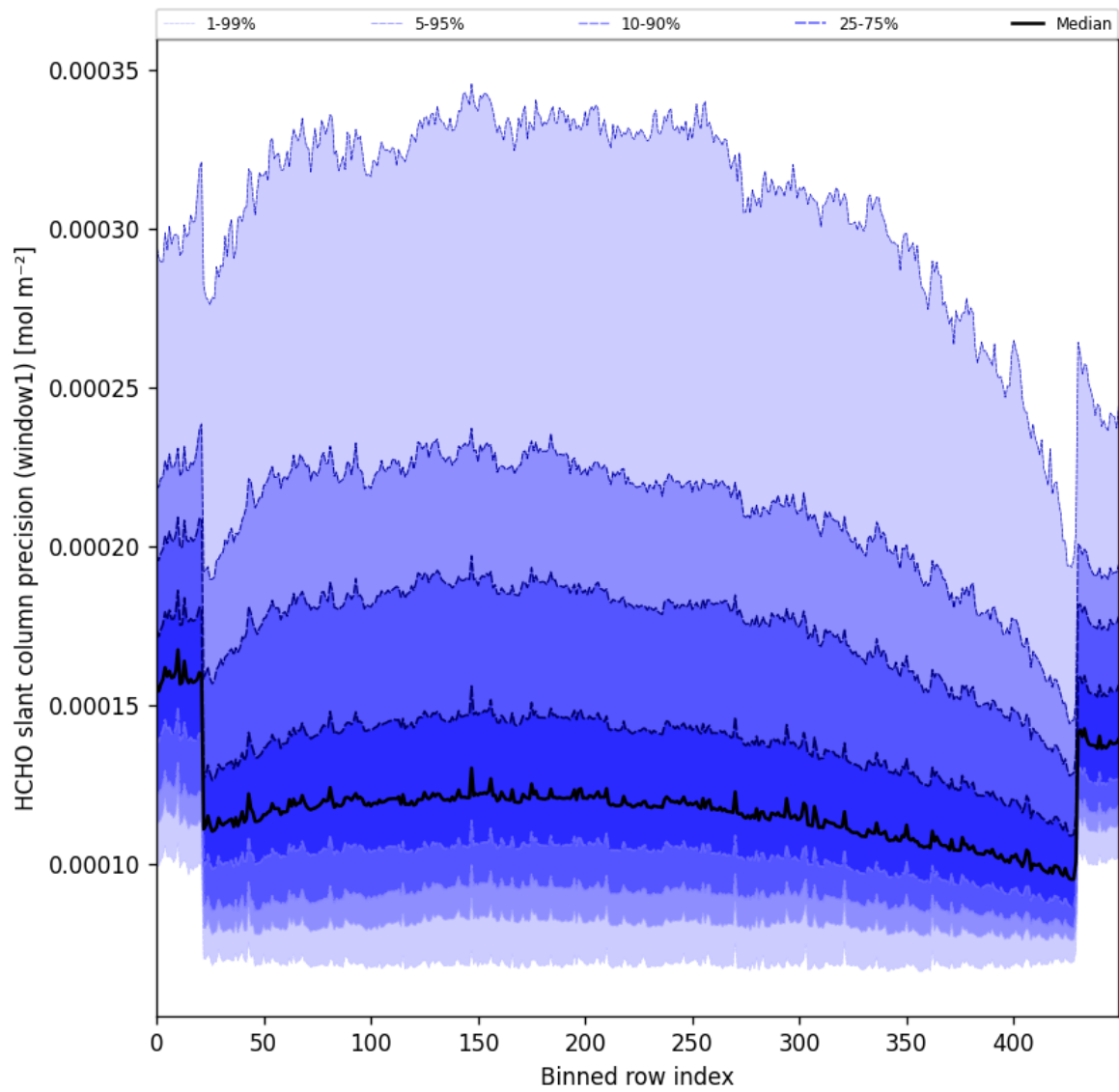
Figure 53: Along track statistics of “HCHO slant column precision (window1)” for 2024-10-21 to 2024-10-23
