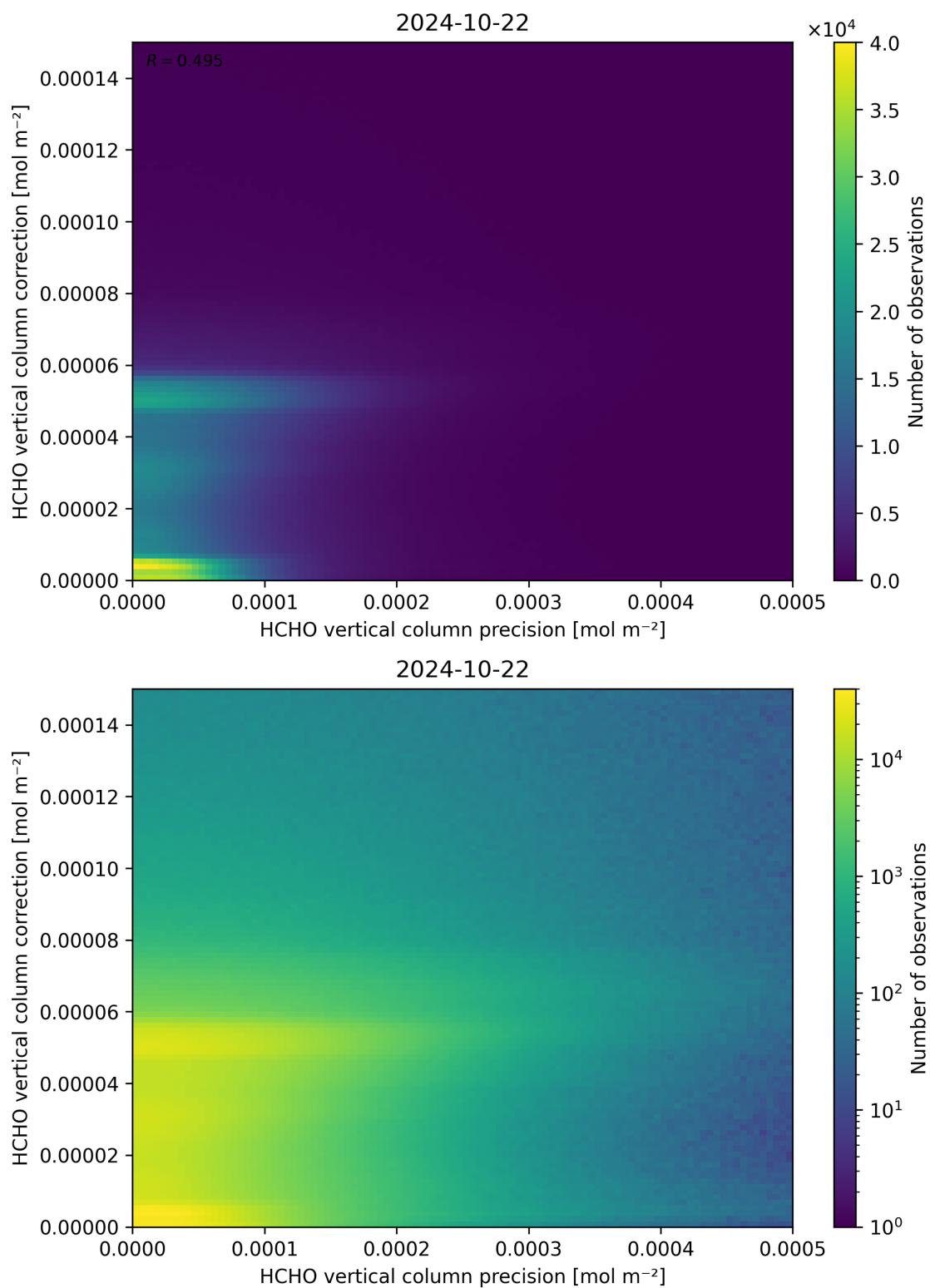
Figure 146: Scatter density plot of “HCHO vertical column precision” against “HCHO vertical column correction” for 2024-10-21 to 2024-10-23.
