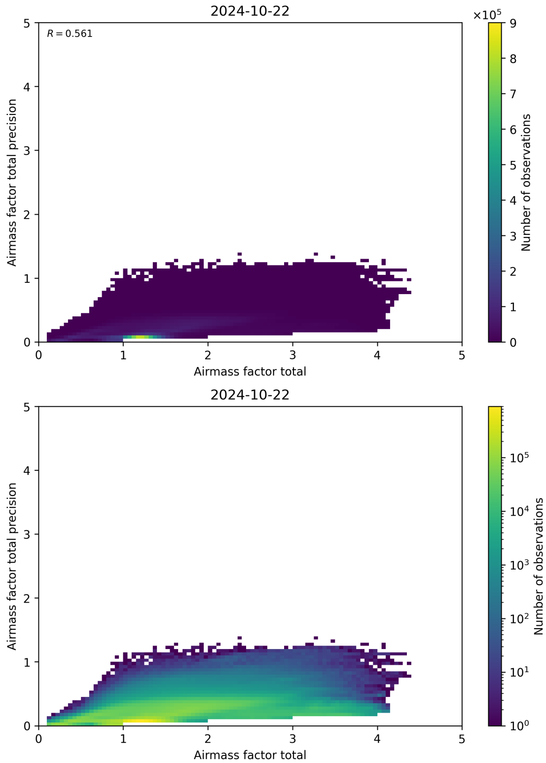
Figure 103: Scatter density plot of “Airmass factor total” against “Airmass factor total precision” for 2024-10-21 to 2024-10-23.
