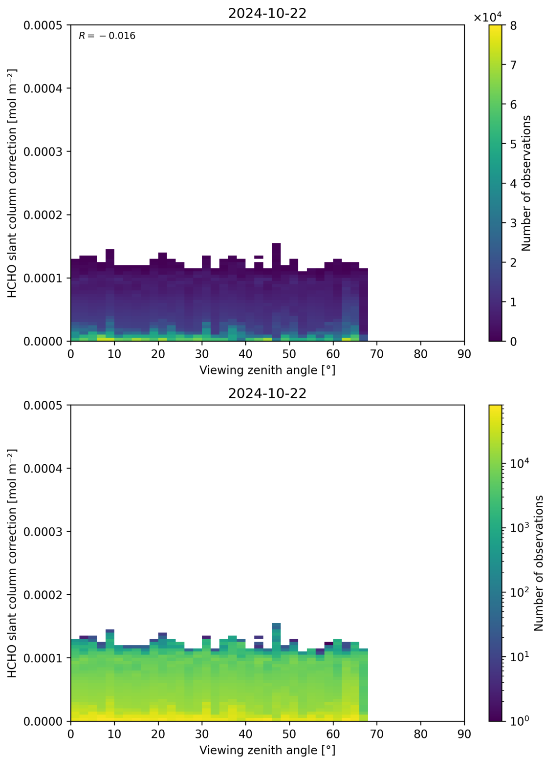
Figure 187: Scatter density plot of “Viewing zenith angle” against “HCHO slant column correction” for 2024-10-21 to 2024-10-23.
