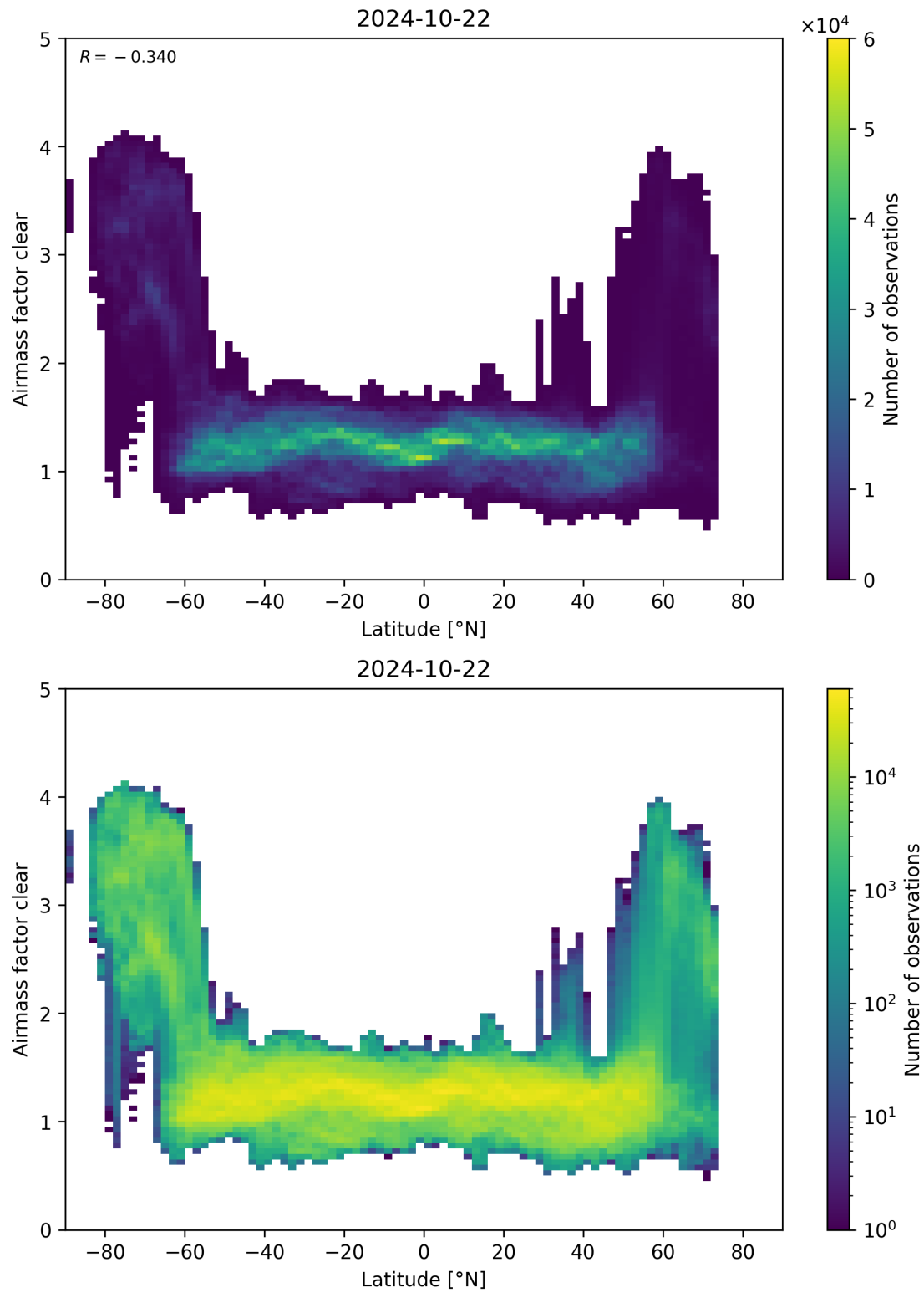
Figure 156: Scatter density plot of “Latitude” against “Airmass factor clear” for 2024-10-21 to 2024-10-23.
