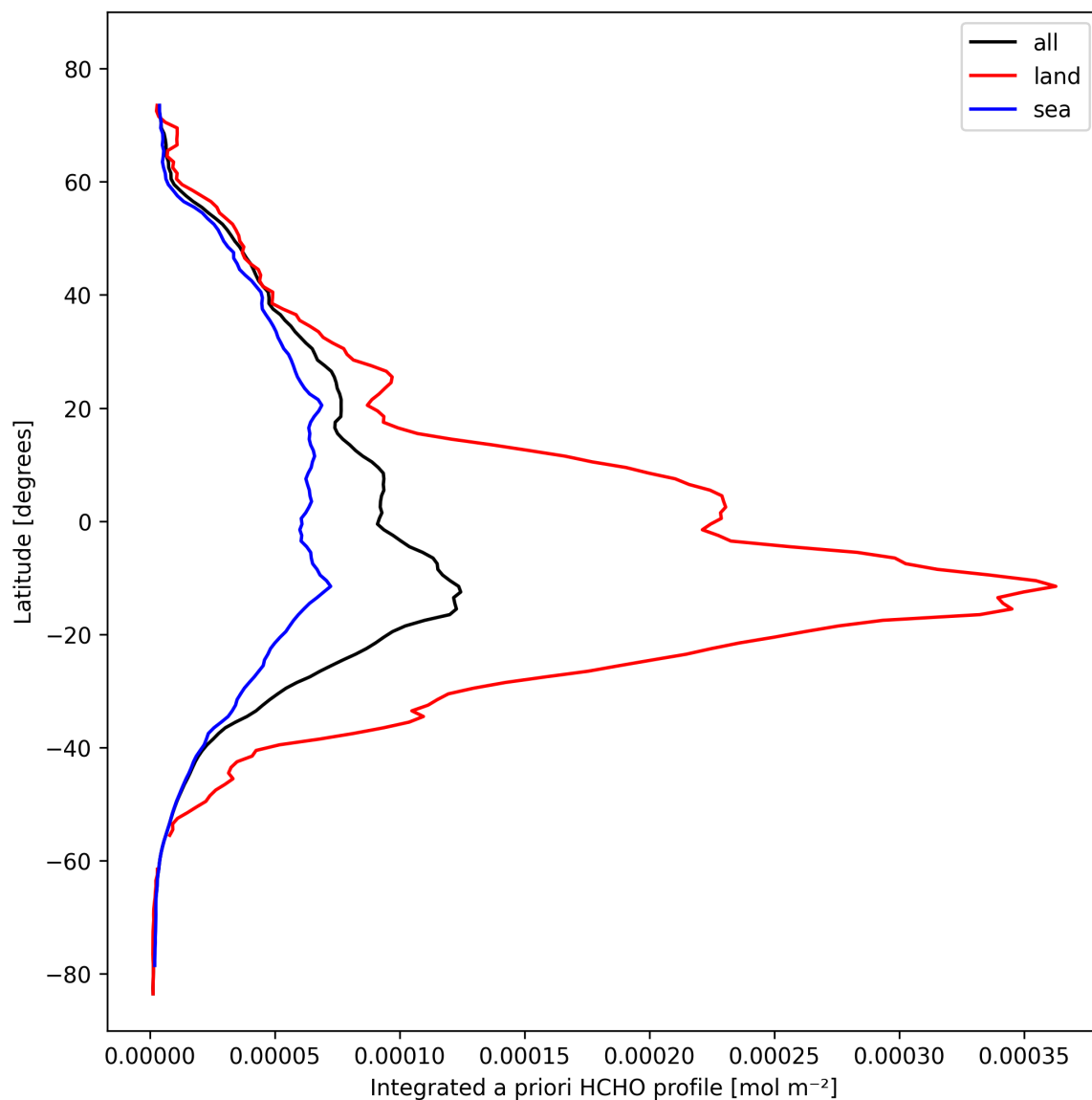
Figure 29: Zonal average of “Integrated a priori HCHO profile” for 2024-10-21 to 2024-10-23.
