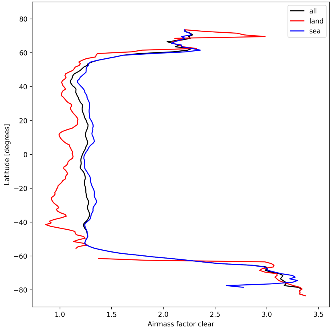
Figure 28: Zonal average of “Airmass factor clear” for 2024-10-21 to 2024-10-23.
