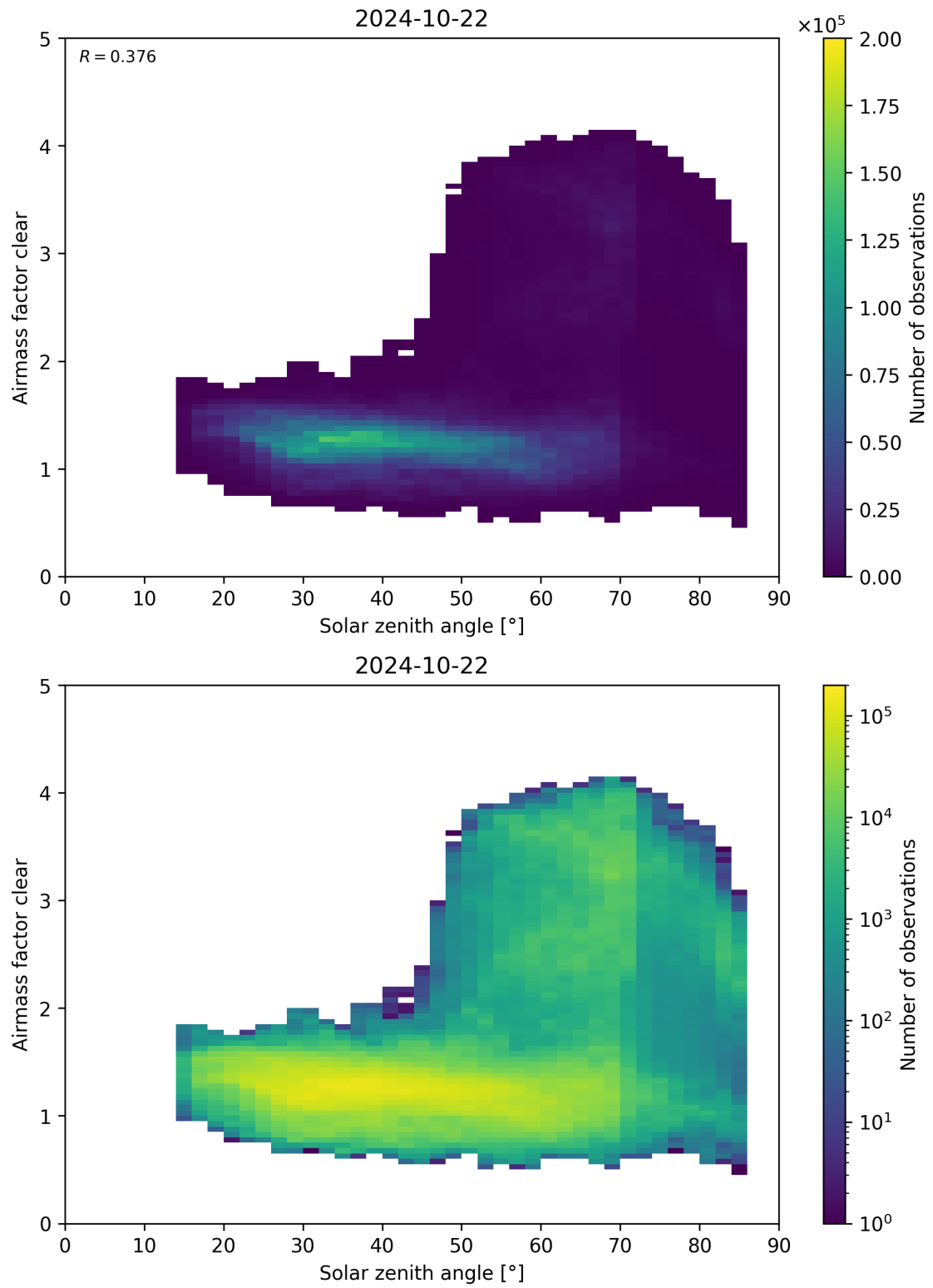
Figure 170: Scatter density plot of “Solar zenith angle” against “Airmass factor clear” for 2024-10-21 to 2024-10-23.
