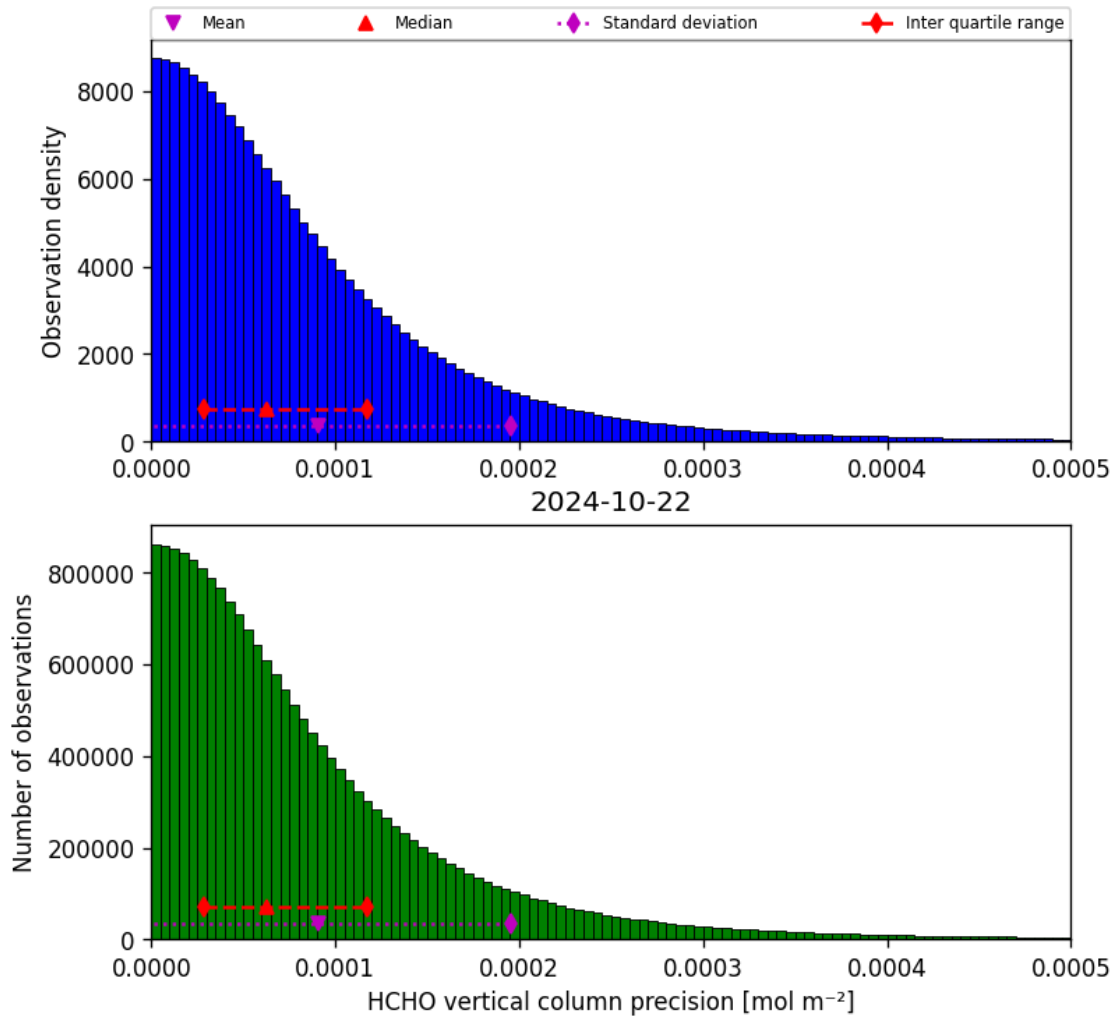
Figure 36: Histogram of “HCHO vertical column precision” for 2024-10-21 to 2024-10-23
