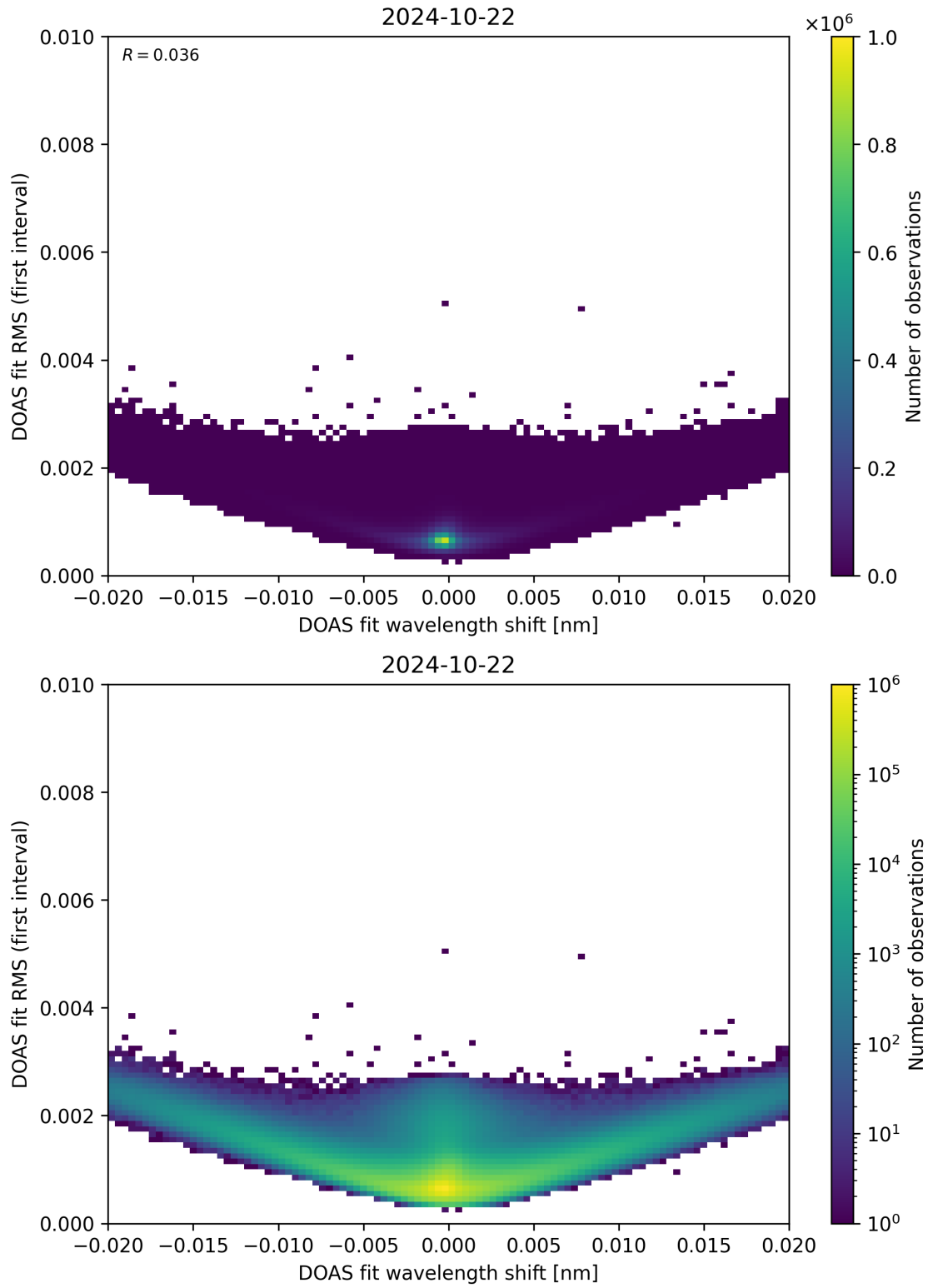
Figure 64: Scatter density plot of “DOAS fit wavelength shift” against “DOAS fit RMS (first interval)” for 2024-10-21 to 2024-10-23.
