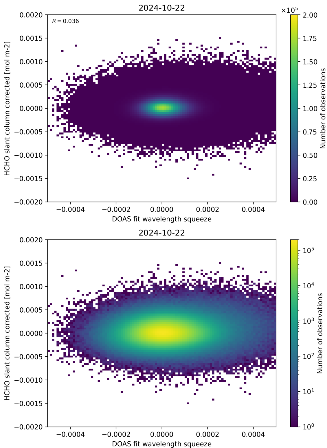
Figure 69: Scatter density plot of “DOAS fit wavelength squeeze” against “HCHO slant column corrected” for 2024-10-21 to 2024-10-23.
