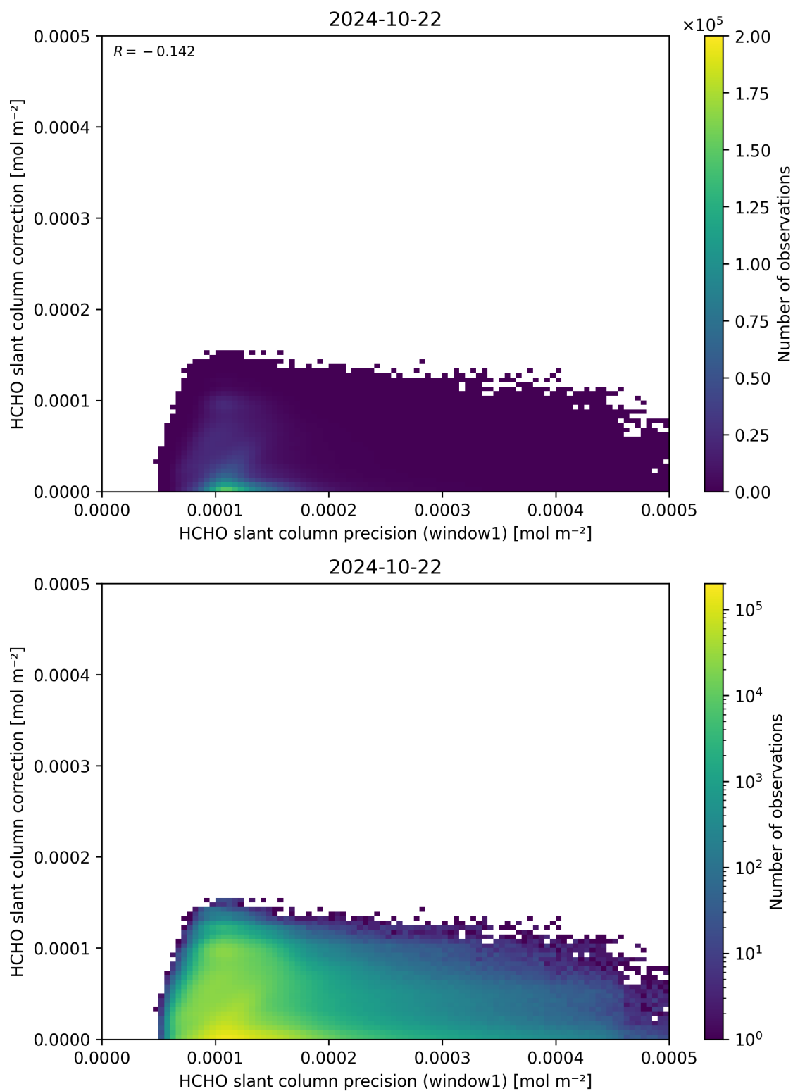
Figure 93: Scatter density plot of “HCHO slant column precision (window1)” against “HCHO slant column correction” for 2024-10-21 to 2024-10-23.
