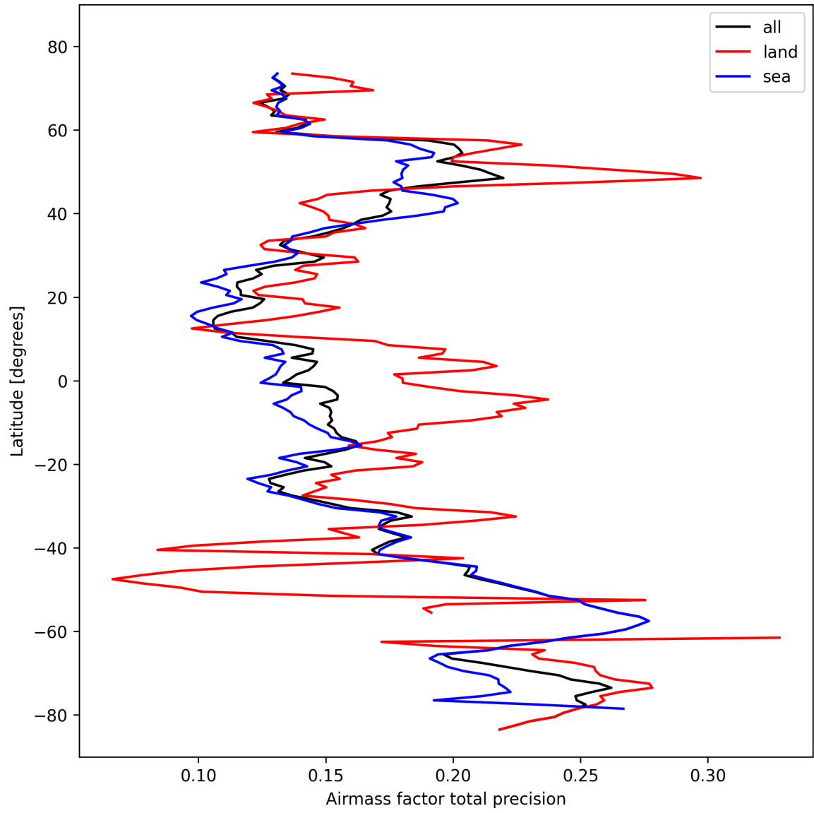
Figure 27: Zonal average of “Airmass factor total precision” for 2024-10-21 to 2024-10-23.
