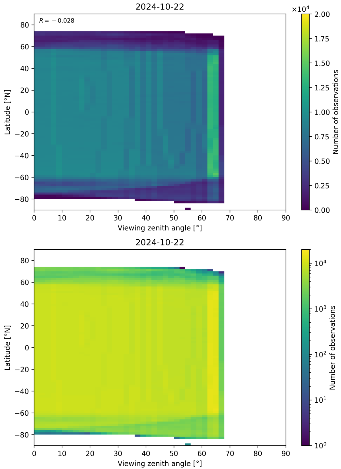
Figure 196: Scatter density plot of “Viewing zenith angle” against “Latitude” for 2024-10-21 to 2024-10-23.
