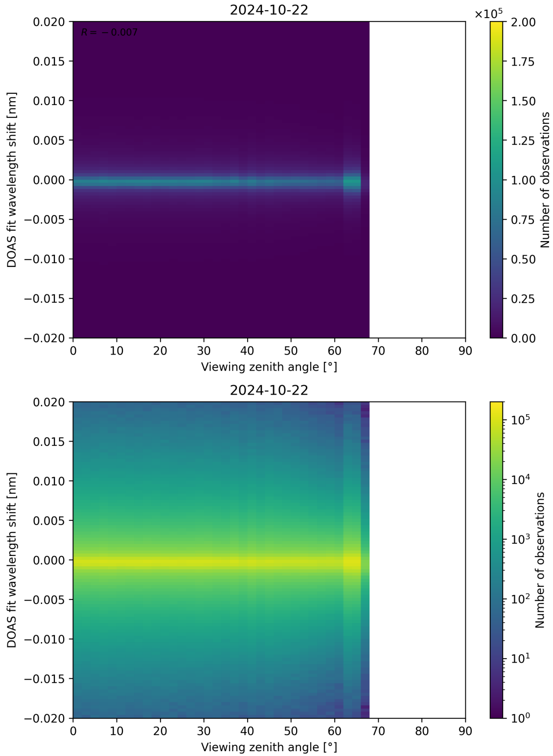
Figure 183: Scatter density plot of “Viewing zenith angle” against “DOAS fit wavelength shift” for 2024-10-21 to 2024-10-23.
