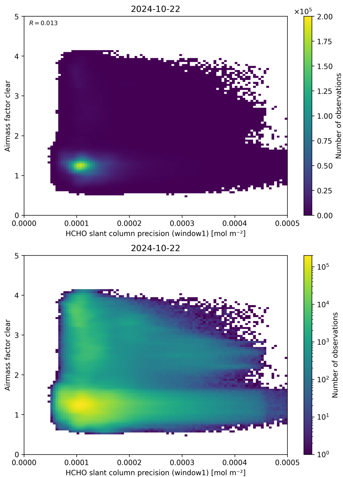
Figure 91: Scatter density plot of “HCHO slant column precision (window1)” against “Airmass factor clear” for 2024-10-21 to 2024-10-23.
