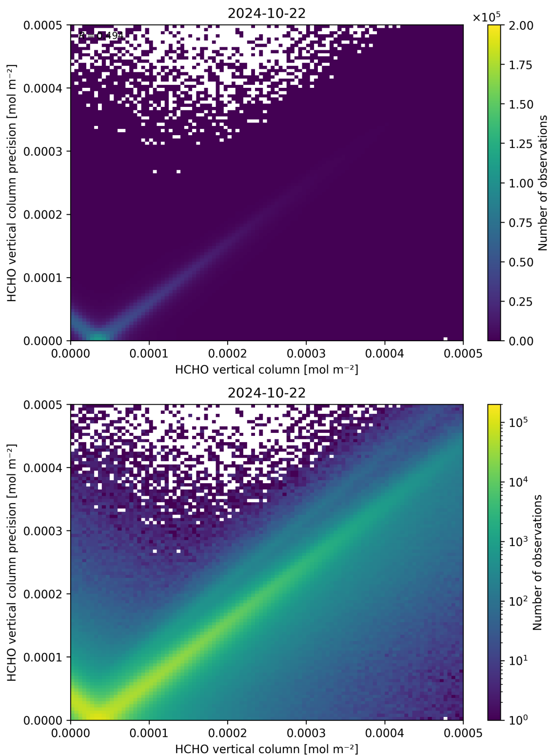
Figure 134: Scatter density plot of “HCHO vertical column” against “HCHO vertical column precision” for 2024-10-21 to 2024-10-23.
