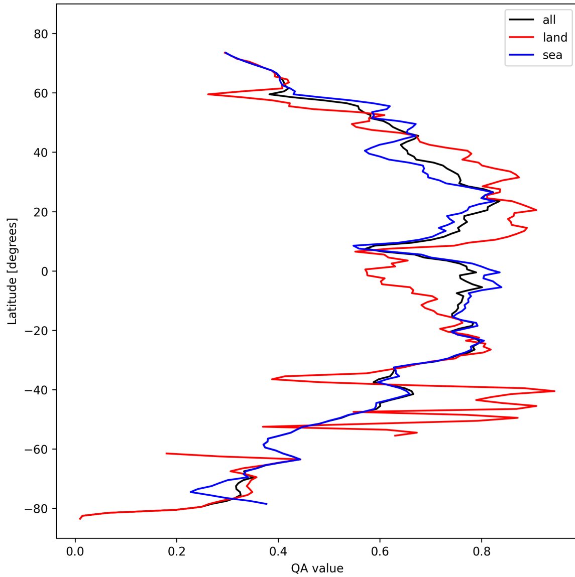
Figure 20: Zonal average of “QA value” for 2024-10-21 to 2024-10-23.
