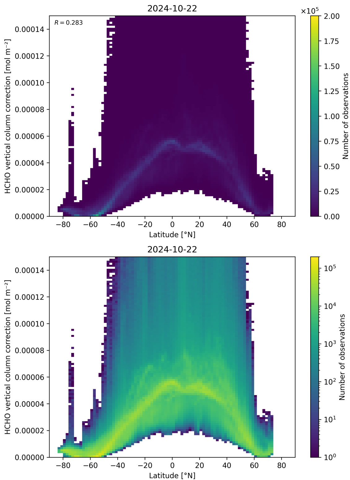
Figure 164: Scatter density plot of “Latitude” against “HCHO vertical column correction” for 2024-10-21 to 2024-10-23.
