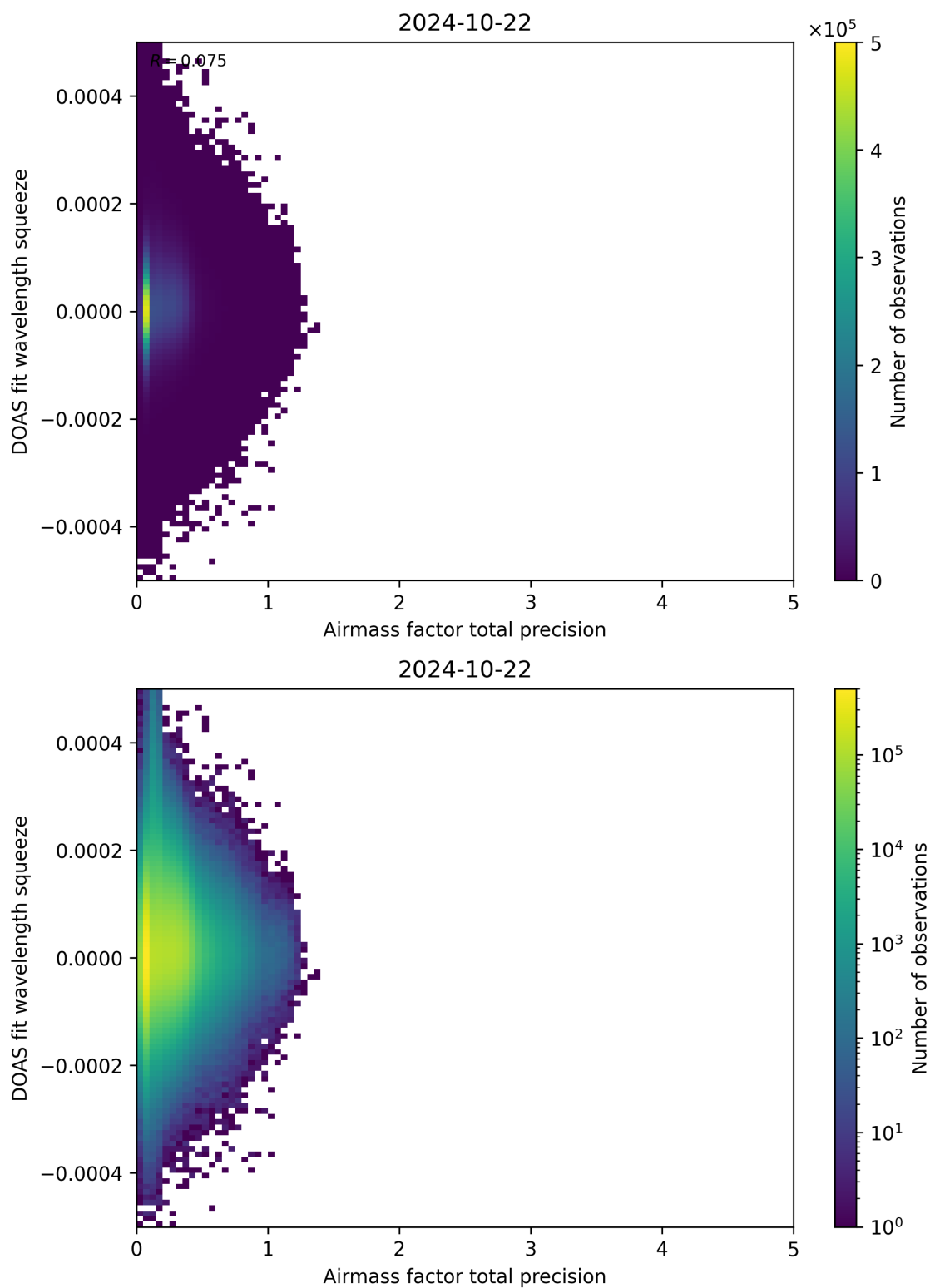
Figure 107: Scatter density plot of “Airmass factor total precision” against “DOAS fit wavelength squeeze” for 2024-10-21 to 2024-10-23.
