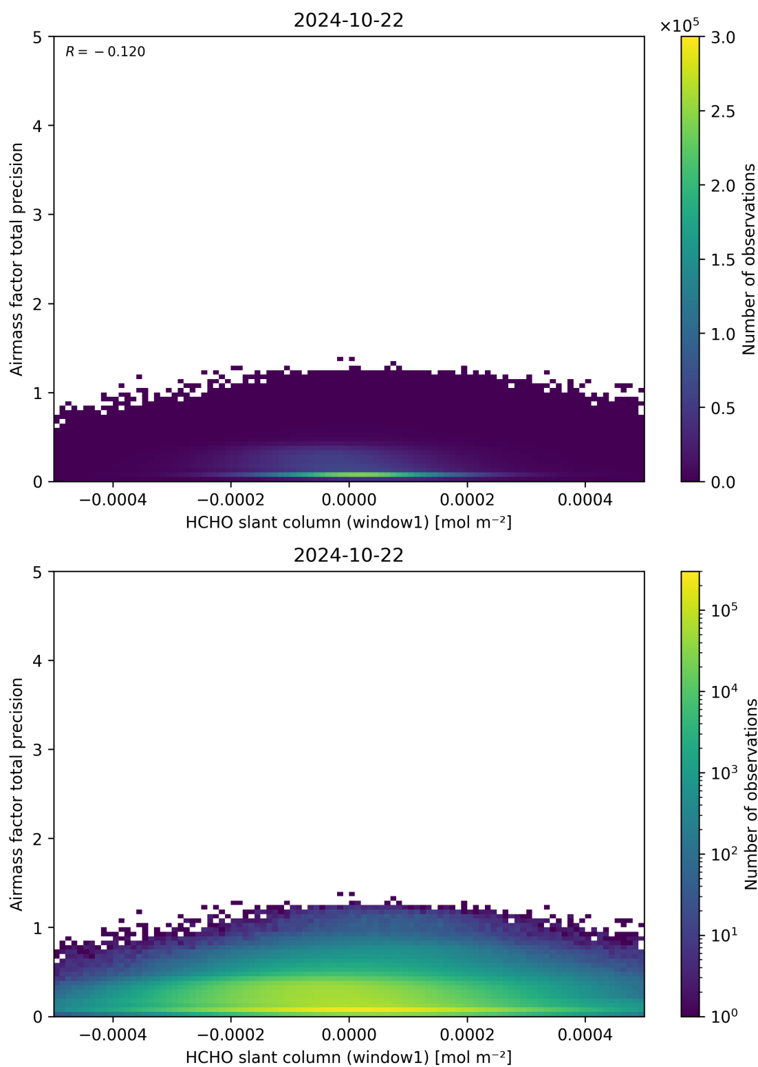
Figure 86: Scatter density plot of “HCHO slant column (window1)” against “Airmass factor total precision” for 2024-10-21 to 2024-10-23.
