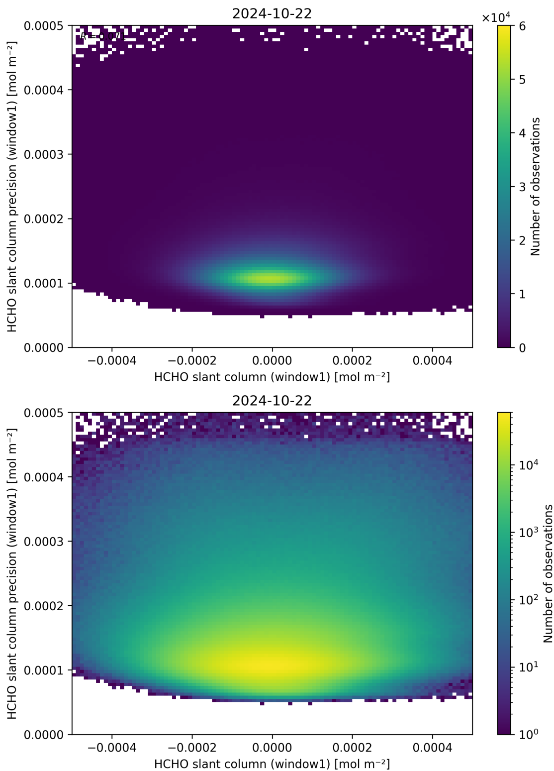
Figure 84: Scatter density plot of “HCHO slant column (window1)” against “HCHO slant column precision (window1)” for 2024-10-21 to 2024-10-23.
