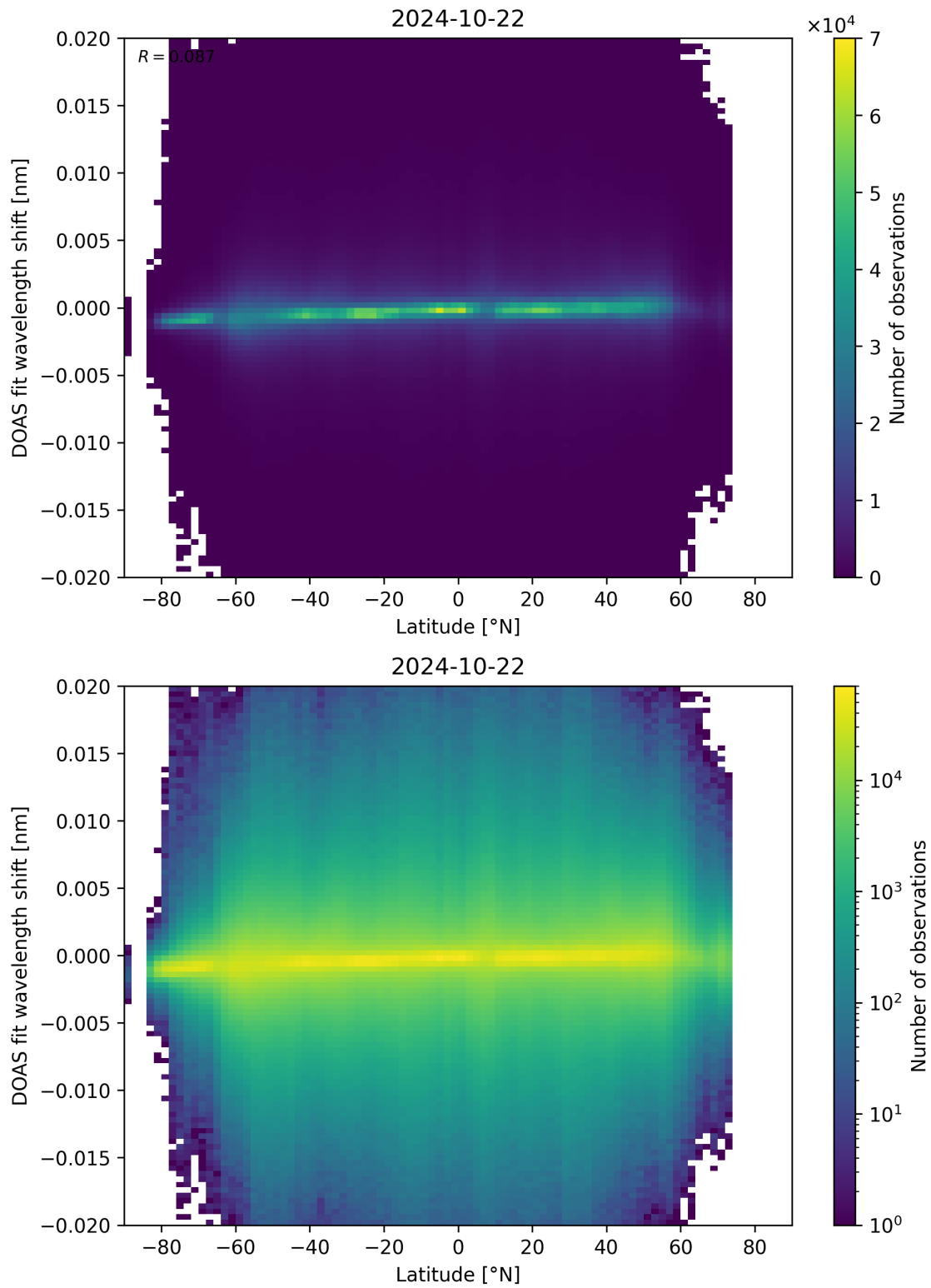
Figure 154: Scatter density plot of “Latitude” against “DOAS fit wavelength shift” for 2024-10-21 to 2024-10-23.
