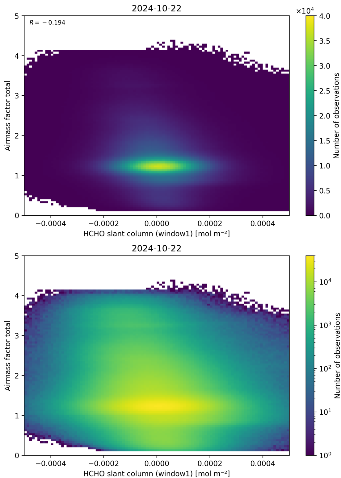
Figure 85: Scatter density plot of “HCHO slant column (window1)” against “Airmass factor total” for 2024-10-21 to 2024-10-23.
