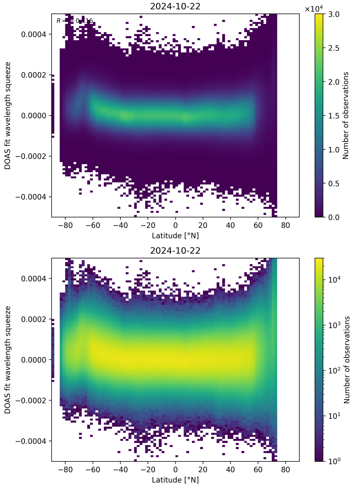
Figure 155: Scatter density plot of “Latitude” against “DOAS fit wavelength squeeze” for 2024-10-21 to 2024-10-23.
