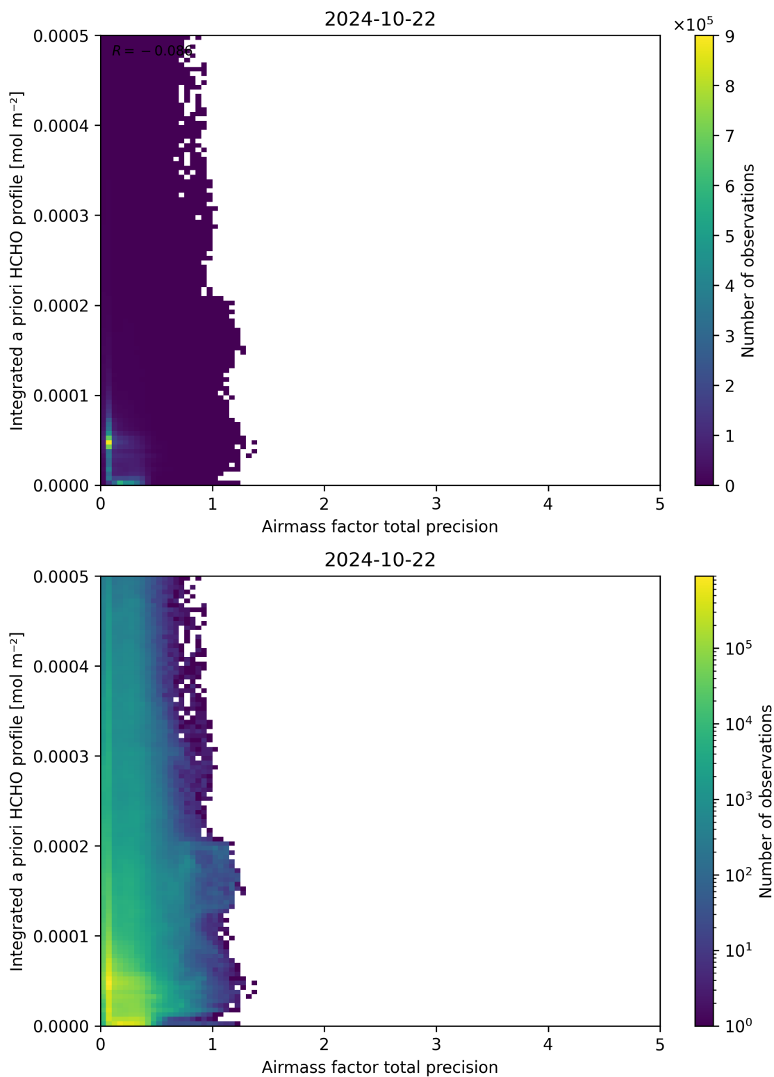
Figure 111: Scatter density plot of “Airmass factor total precision” against “Integrated a priori HCHO profile” for 2024-10-21 to 2024-10-23.
