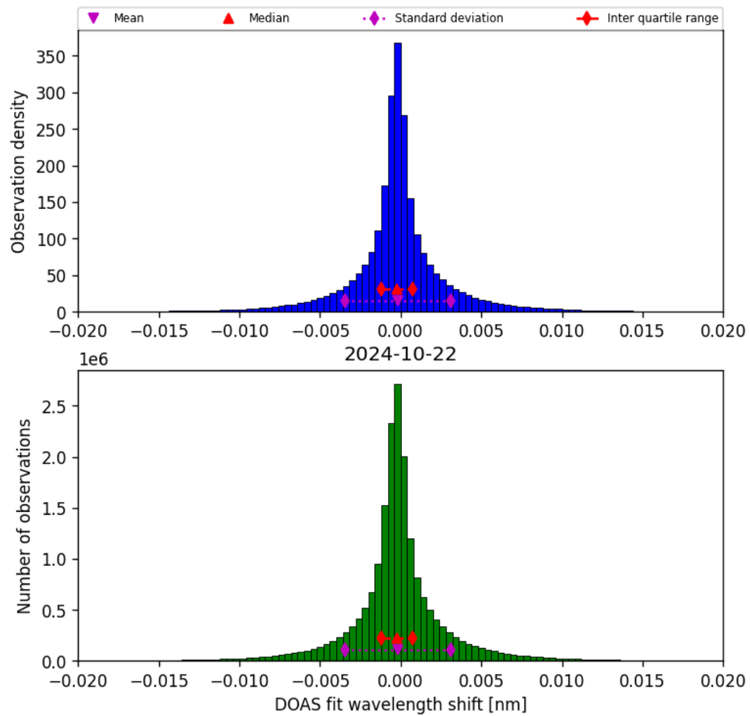
Figure 44: Histogram of “DOAS fit wavelength shift” for 2024-10-21 to 2024-10-23
