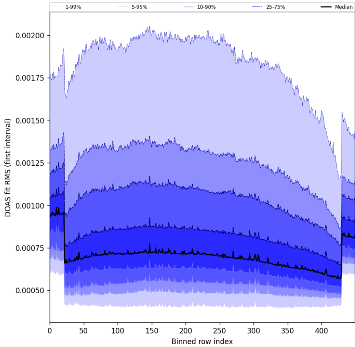
Figure 60: Along track statistics of “DOAS fit RMS (first interval)” for 2024-10-21 to 2024-10-23
