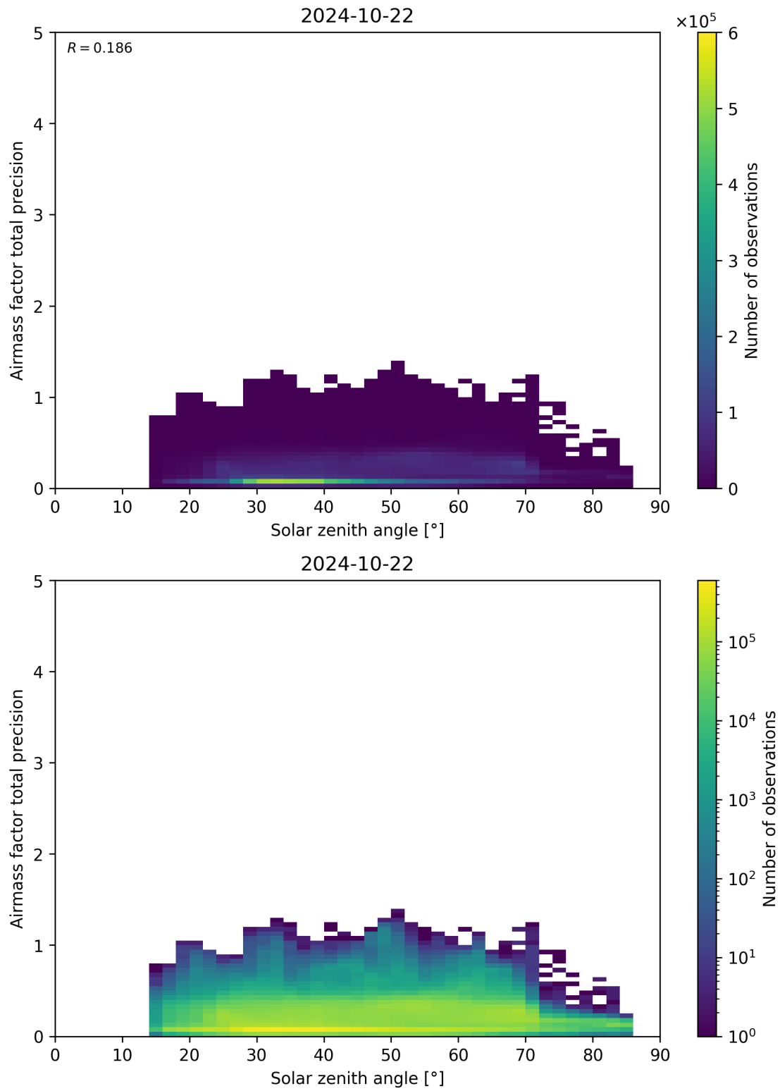
Figure 176: Scatter density plot of “Solar zenith angle” against “Airmass factor total precision” for 2024-10-21 to 2024-10-23.
