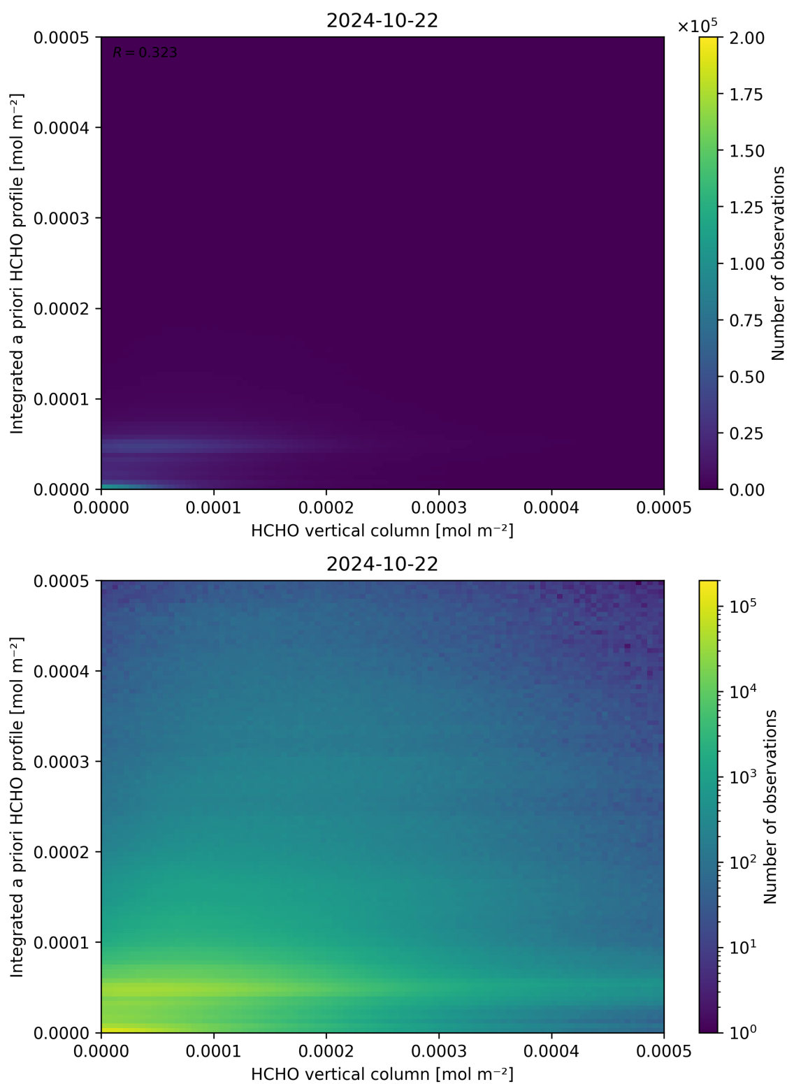
Figure 135: Scatter density plot of “HCHO vertical column” against “Integrated a priori HCHO profile” for 2024-10-21 to 2024-10-23.
