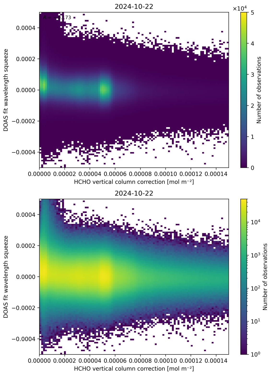
Figure 114: Scatter density plot of “HCHO vertical column correction” against “DOAS fit wavelength squeeze” for 2024-10-21 to 2024-10-23.
