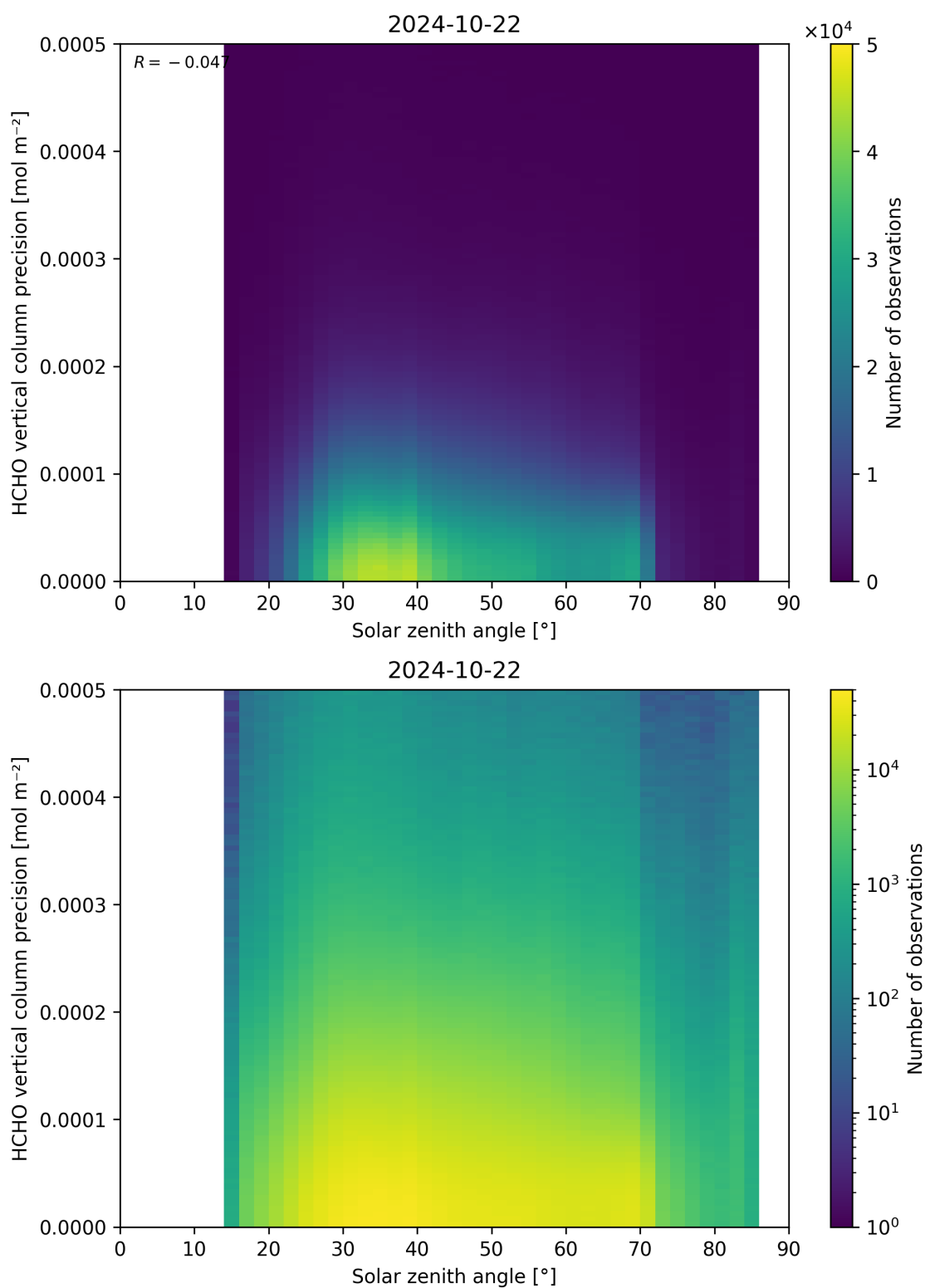
Figure 179: Scatter density plot of “Solar zenith angle” against “HCHO vertical column precision” for 2024-10-21 to 2024-10-23.
