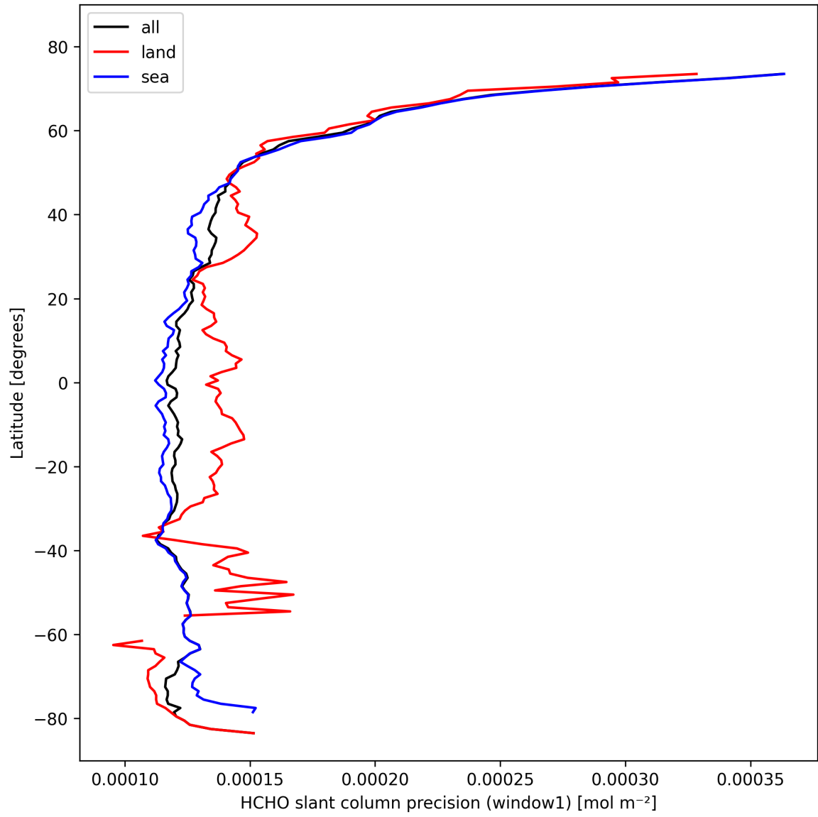
Figure 25: Zonal average of "HCHO slant column precision (window1)" for 2024-10-21 to 2024-10-23.
