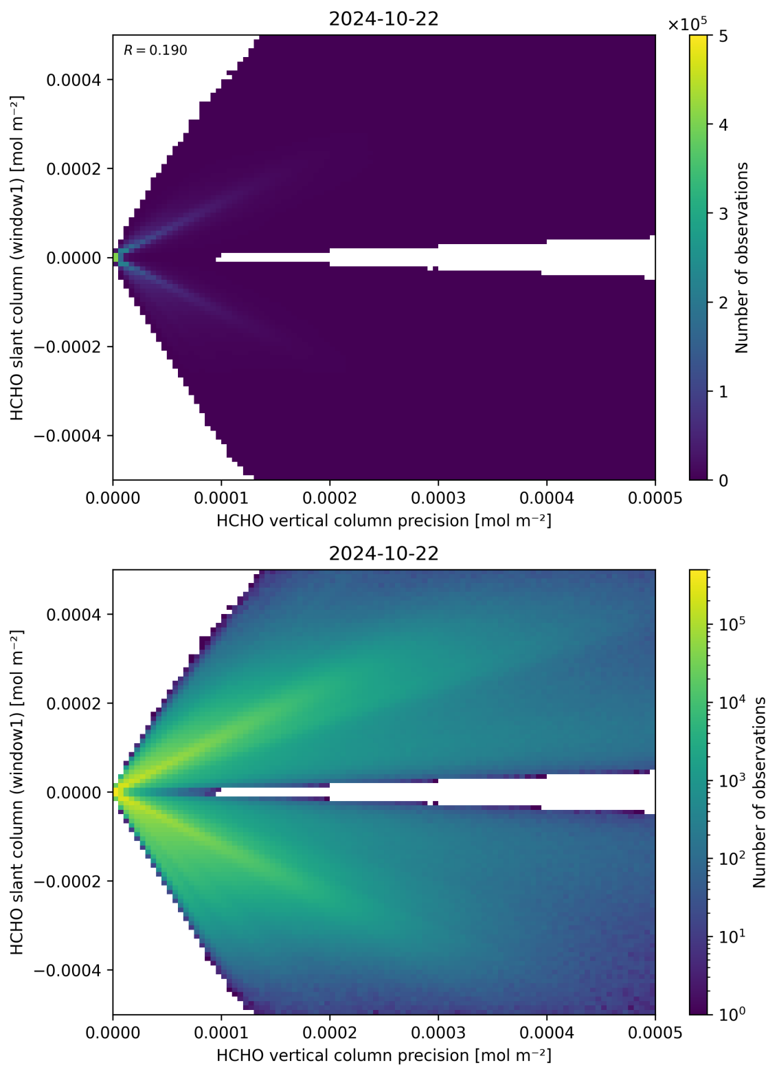
Figure 142: Scatter density plot of “HCHO vertical column precision” against “HCHO slant column (window1)” for 2024-10-21 to 2024-10-23.
