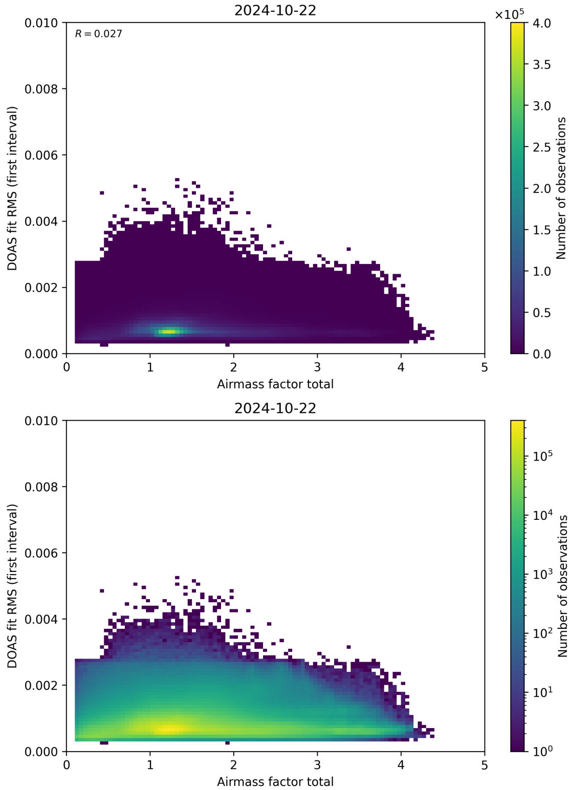
Figure 97: Scatter density plot of “Airmass factor total” against “DOAS fit RMS (first interval)” for 2024-10-21 to 2024-10-23.
