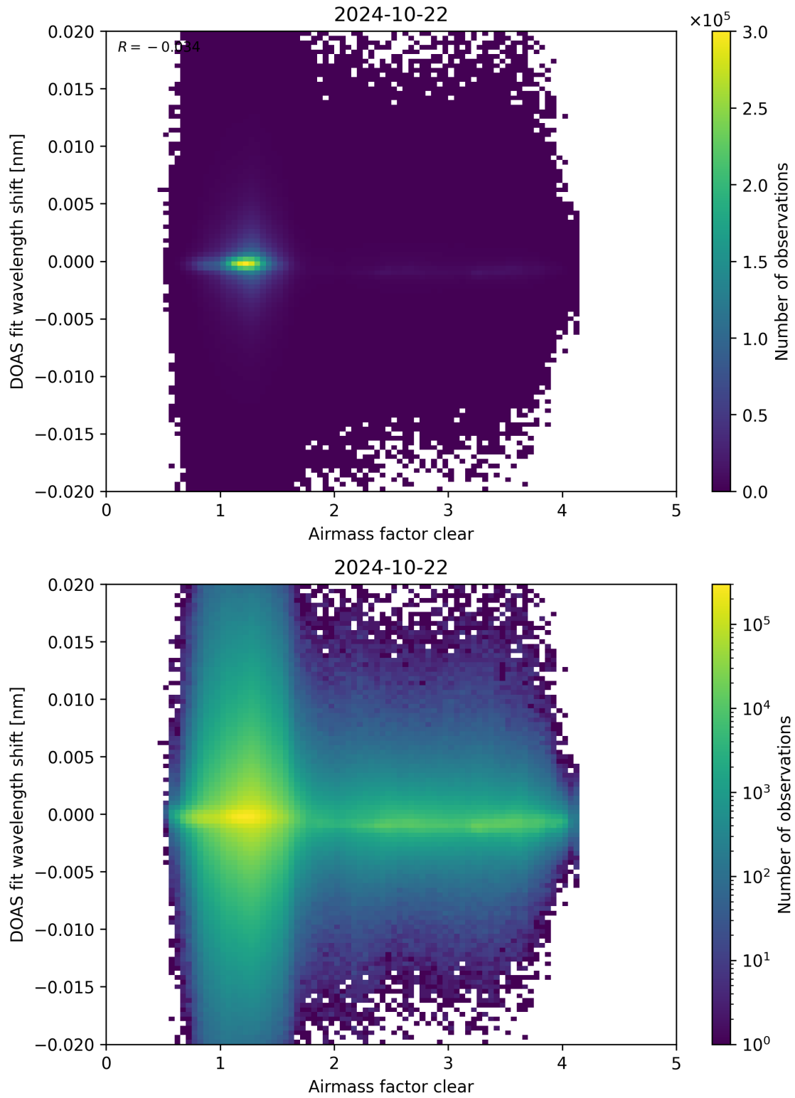
Figure 72: Scatter density plot of “Airmass factor clear” against “DOAS fit wavelength shift” for 2024-10-21 to 2024-10-23.
