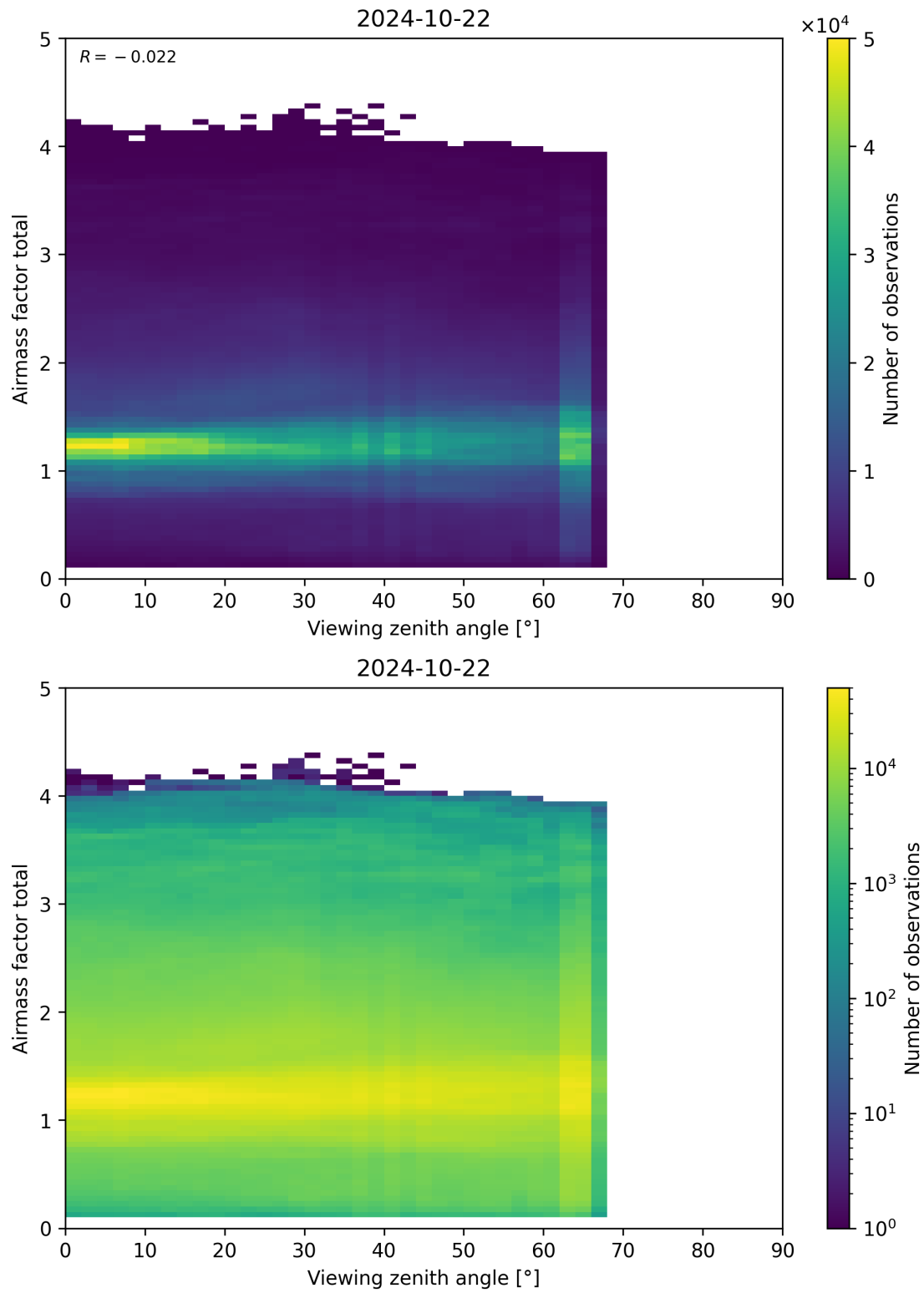
Figure 190: Scatter density plot of “Viewing zenith angle” against “Airmass factor total” for 2024-10-21 to 2024-10-23.
