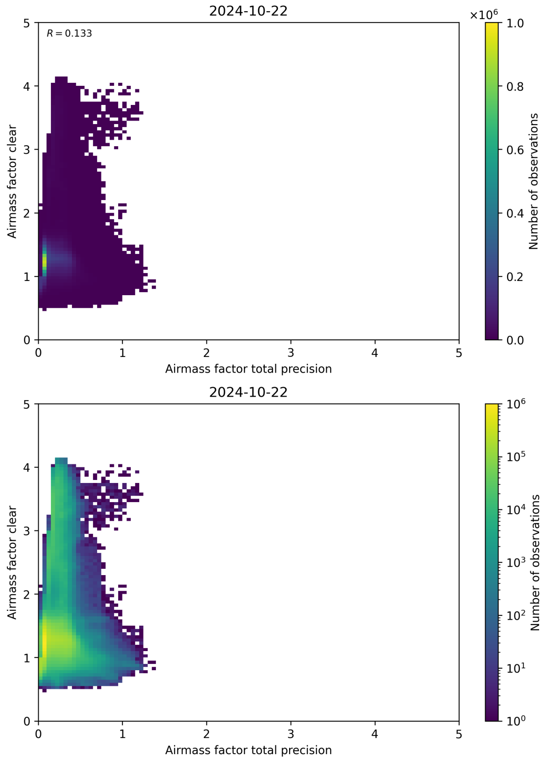
Figure 108: Scatter density plot of “Airmass factor total precision” against “Airmass factor clear” for 2024-10-21 to 2024-10-23.
