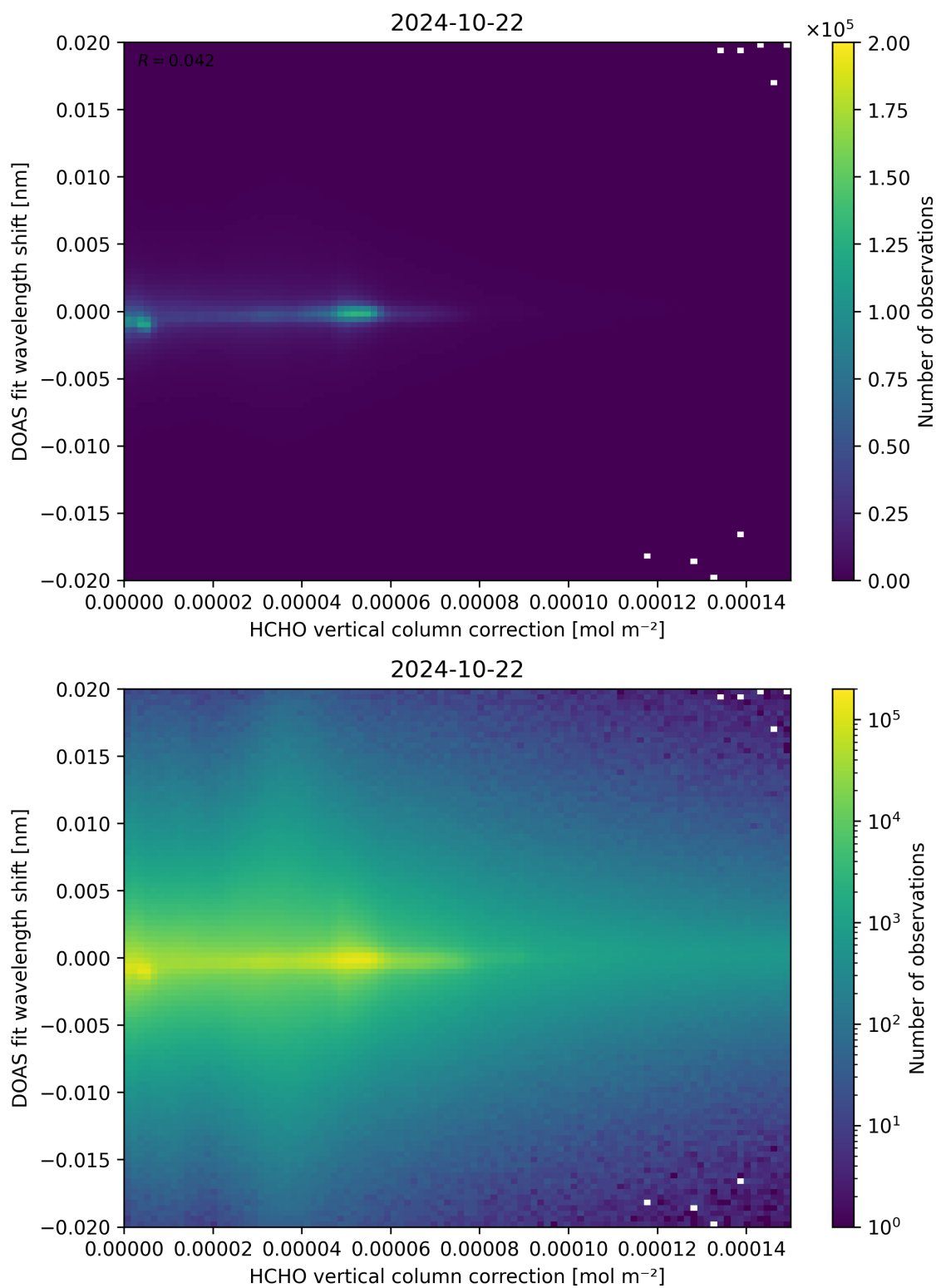
Figure 113: Scatter density plot of “HCHO vertical column correction” against “DOAS fit wavelength shift” for 2024-10-21 to 2024-10-23.
