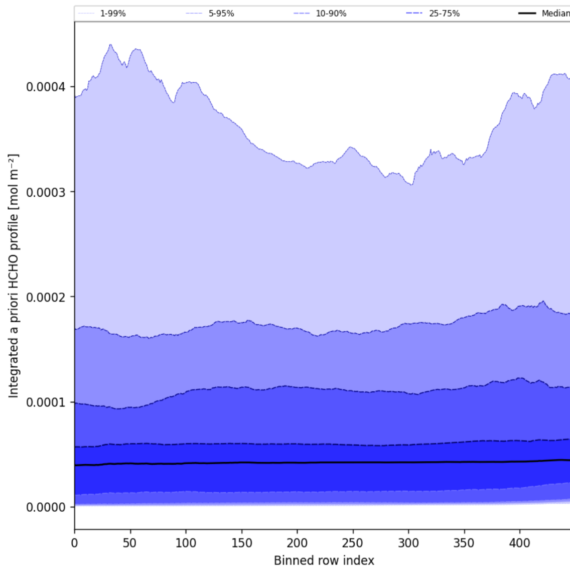
Figure 57: Along track statistics of "Integrated a priori HCHO profile" for 2024-10-21 to 2024-10-23
