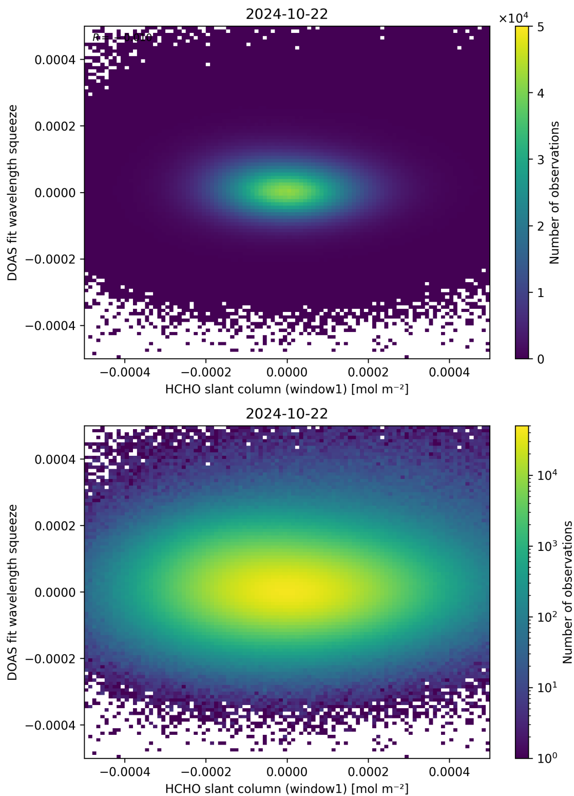
Figure 80: Scatter density plot of “HCHO slant column (window1)” against “DOAS fit wavelength squeeze” for 2024-10-21 to 2024-10-23.
