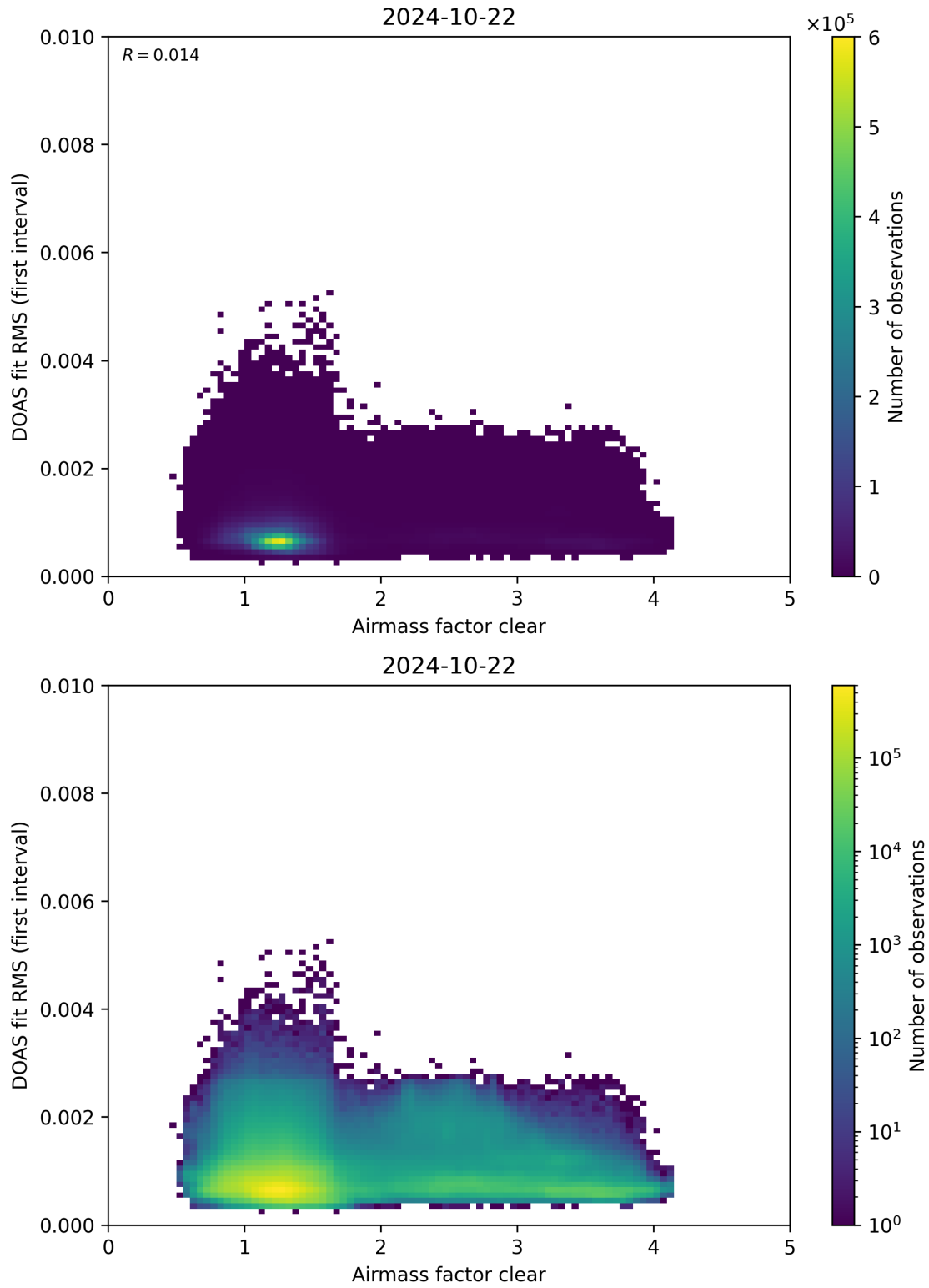
Figure 71: Scatter density plot of “Airmass factor clear” against “DOAS fit RMS (first interval)” for 2024-10-21 to 2024-10-23.
