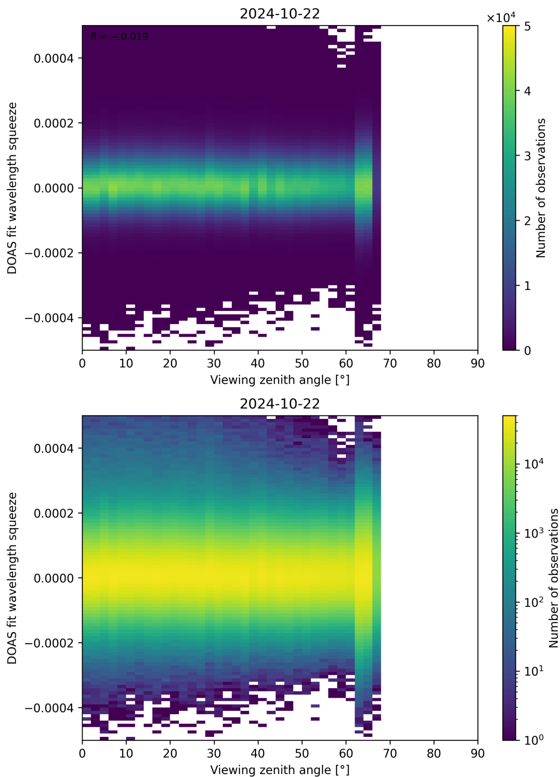
Figure 184: Scatter density plot of “Viewing zenith angle” against “DOAS fit wavelength squeeze” for 2024-10-21 to 2024-10-23.
