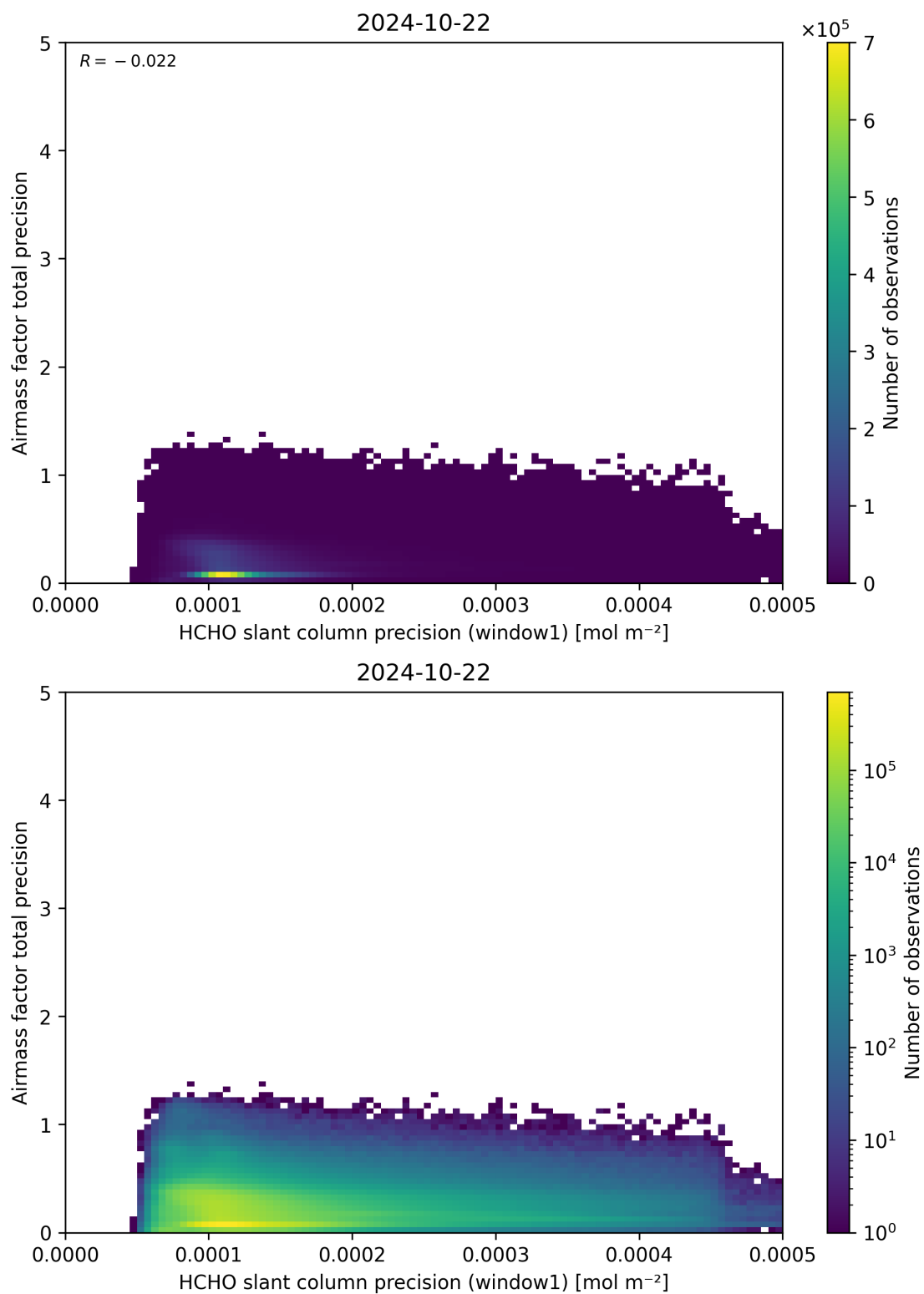
Figure 95: Scatter density plot of “HCHO slant column precision (window1)” against “Airmass factor total precision” for 2024-10-21 to 2024-10-23.
