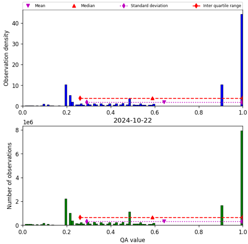
Figure 34: Histogram of “QA value” for 2024-10-21 to 2024-10-23
