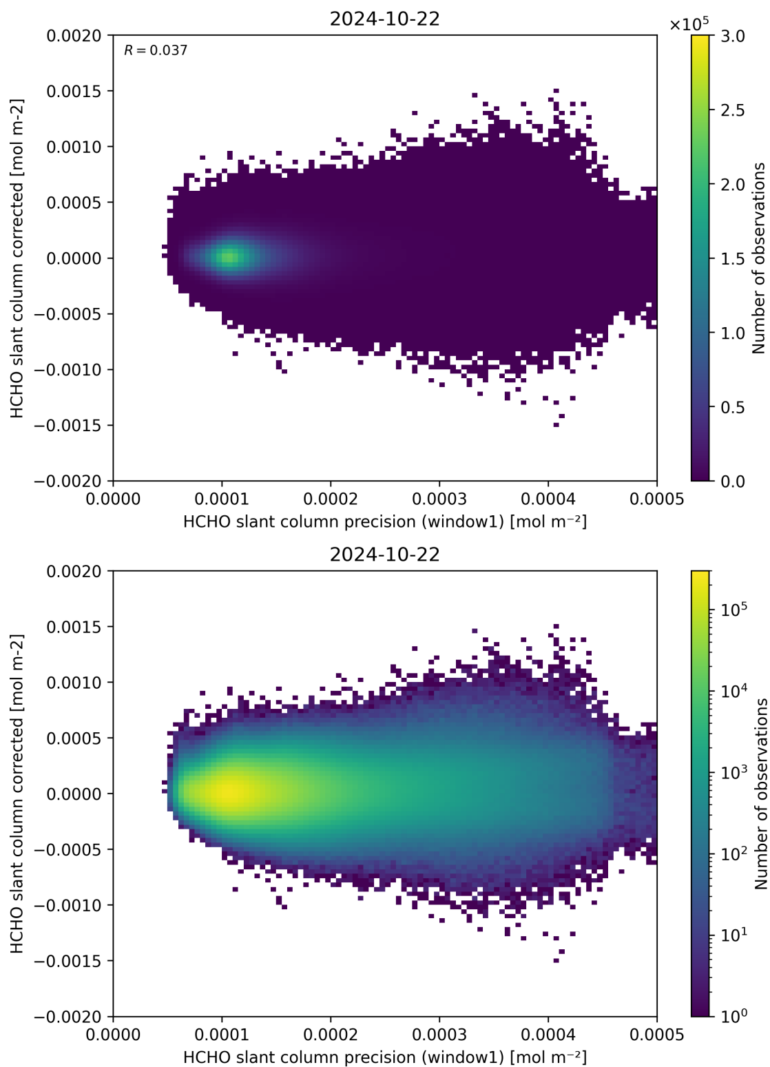
Figure 92: Scatter density plot of “HCHO slant column precision (window1)” against “HCHO slant column corrected” for 2024-10-21 to 2024-10-23.
