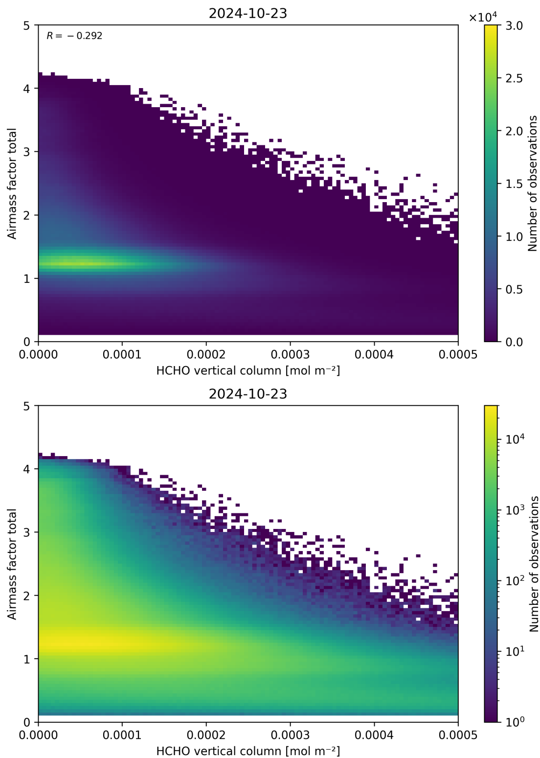
Figure 131: Scatter density plot of “HCHO vertical column” against “Airmass factor total” for 2024-10-22 to 2024-10-24.
