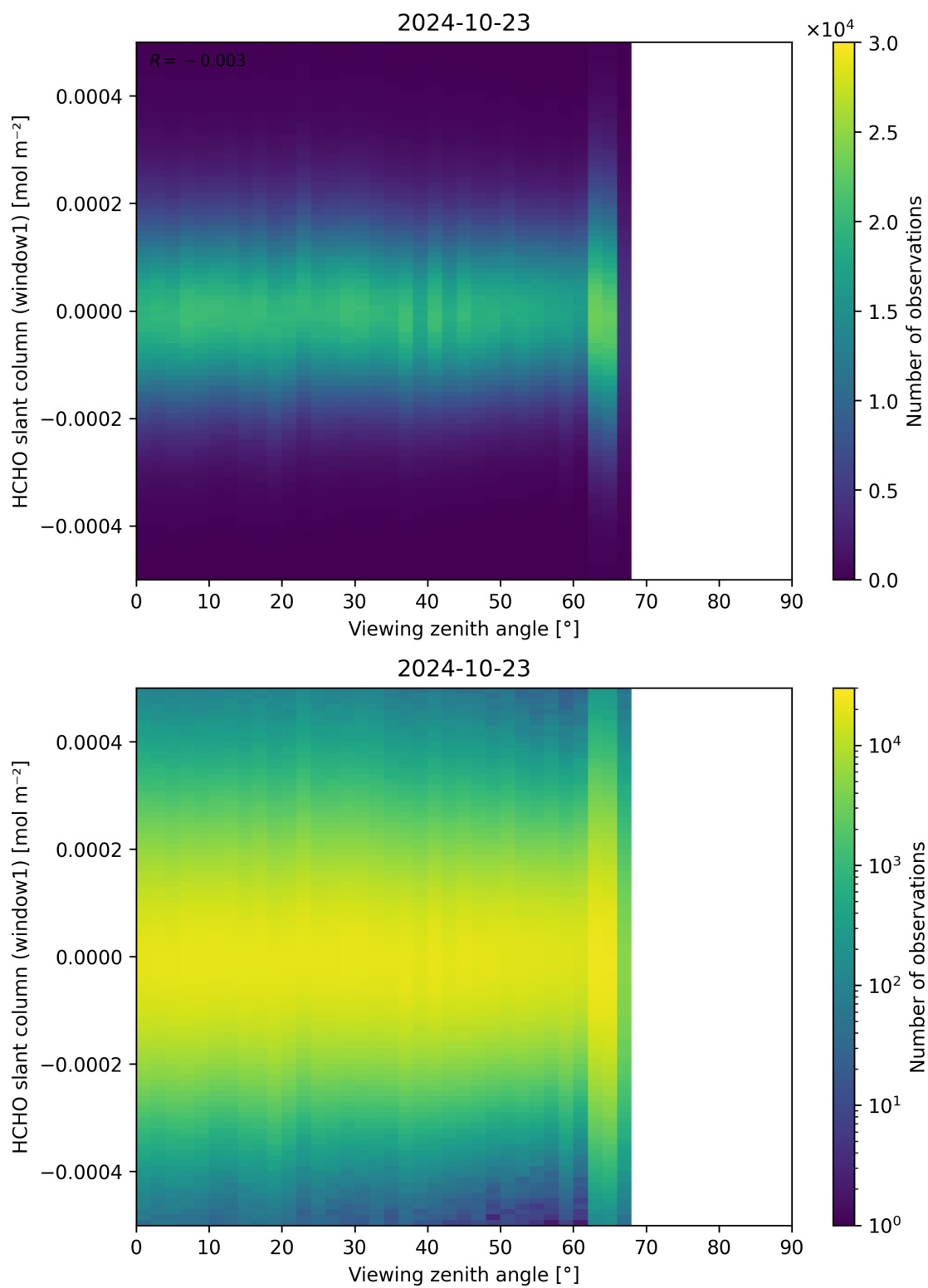
Figure 188: Scatter density plot of “Viewing zenith angle” against “HCHO slant column (window1)” for 2024-10-22 to 2024-10-24.
