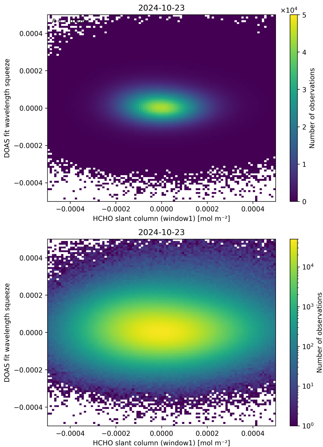
Figure 80: Scatter density plot of “HCHO slant column (window1)” against “DOAS fit wavelength squeeze” for 2024-10-22 to 2024-10-24.
