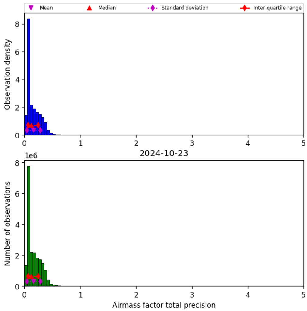
Figure 41: Histogram of “Airmass factor total precision” for 2024-10-22 to 2024-10-24
