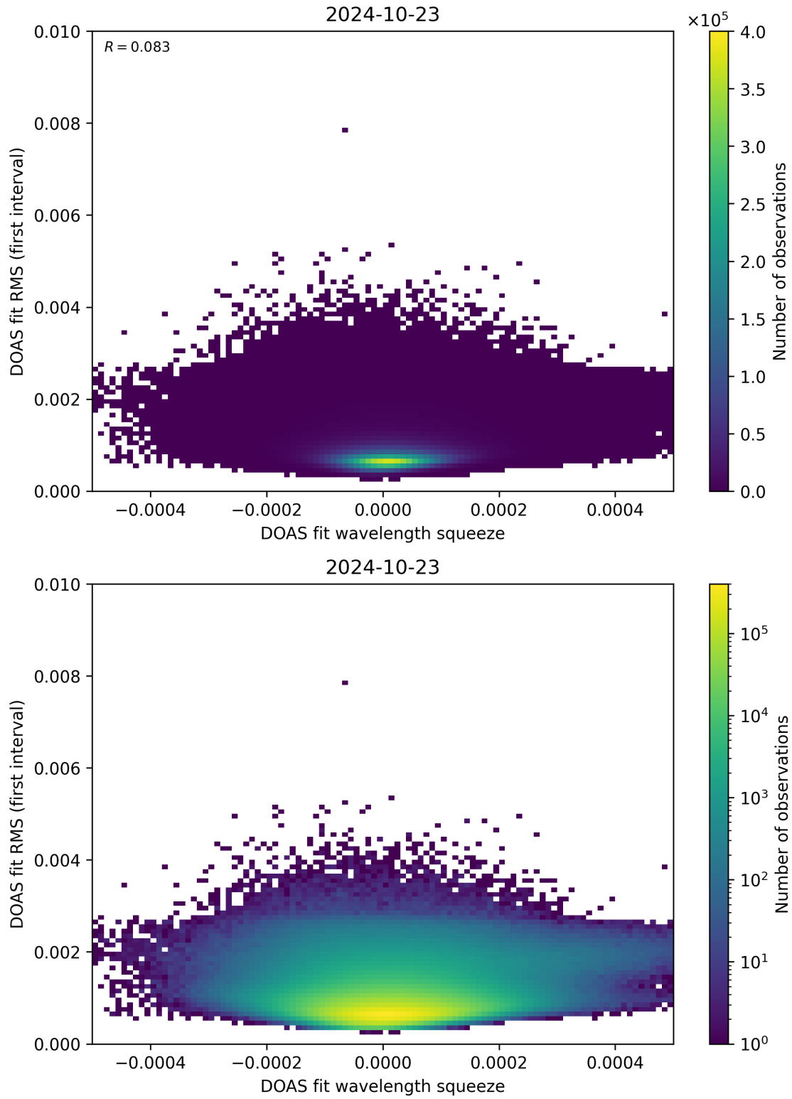
Figure 68: Scatter density plot of “DOAS fit wavelength squeeze” against “DOAS fit RMS (first interval)” for 2024-10-22 to 2024-10-24.
