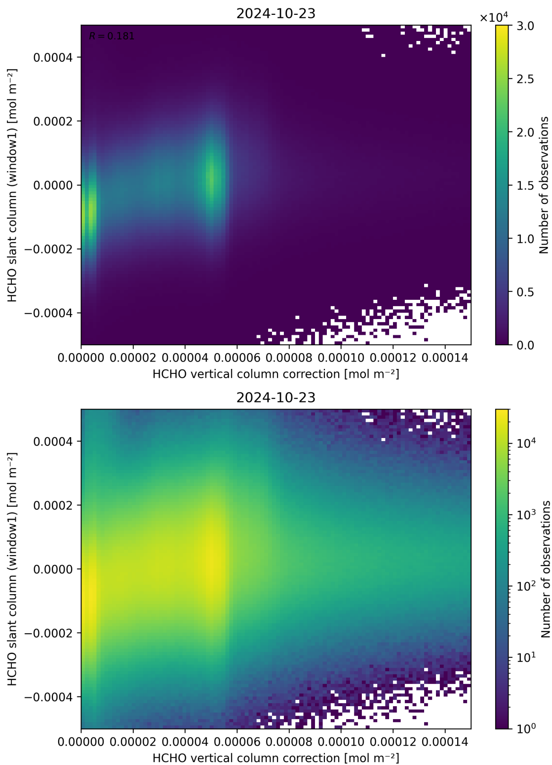
Figure 118: Scatter density plot of “HCHO vertical column correction” against “HCHO slant column (window1)” for 2024-10-22 to 2024-10-24.
