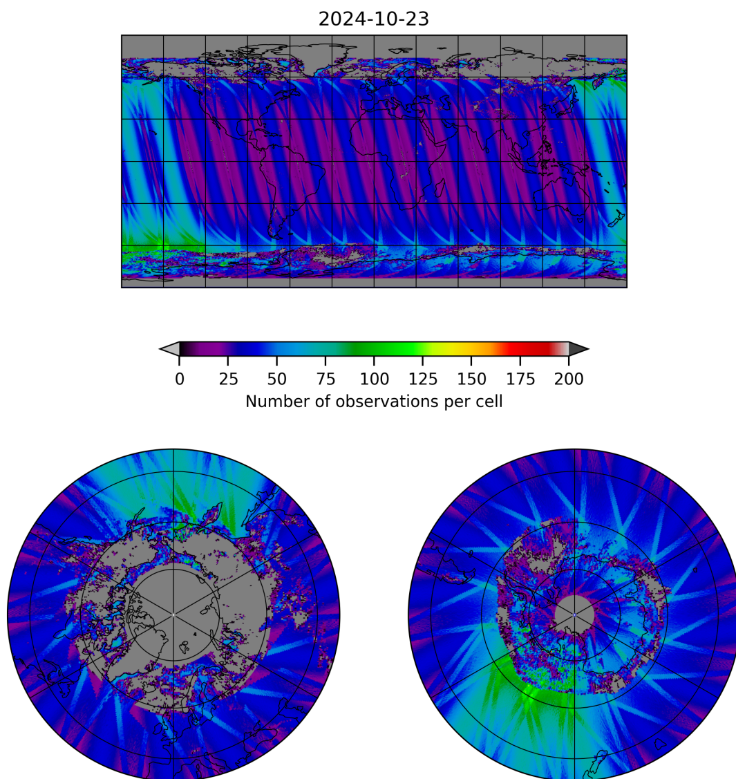
Figure 19: Map of the number of observations for 2024-10-22 to 2024-10-24
