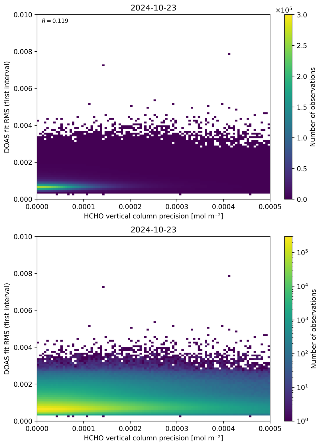
Figure 136: Scatter density plot of “HCHO vertical column precision” against “DOAS fit RMS (first interval)” for 2024-10-22 to 2024-10-24.
