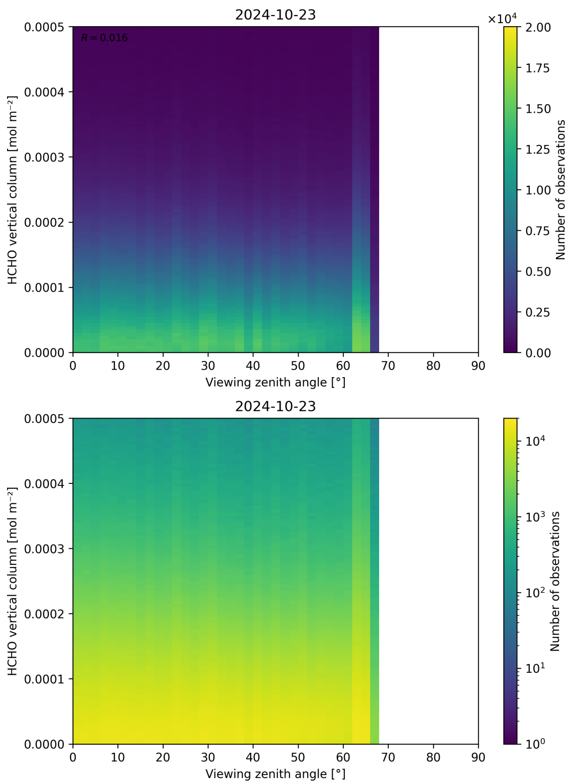
Figure 192: Scatter density plot of “Viewing zenith angle” against “HCHO vertical column” for 2024-10-22 to 2024-10-24.
