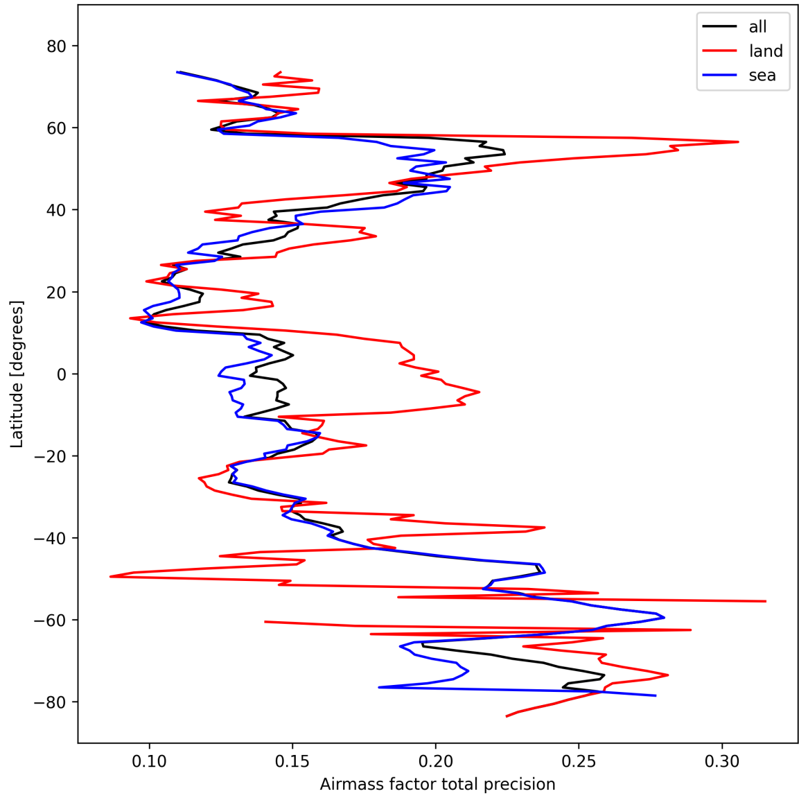
Figure 27: Zonal average of “Airmass factor total precision” for 2024-10-22 to 2024-10-24.
