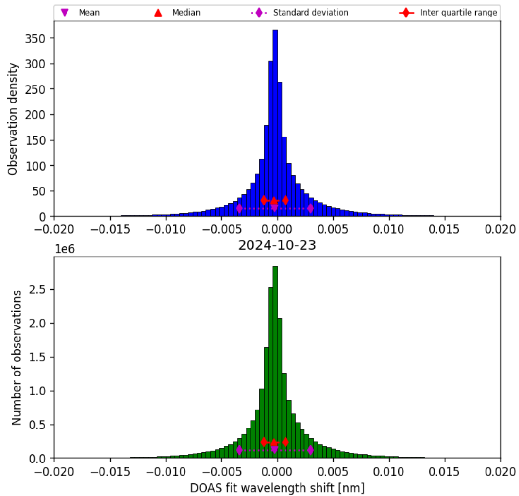
Figure 44: Histogram of “DOAS fit wavelength shift” for 2024-10-22 to 2024-10-24
