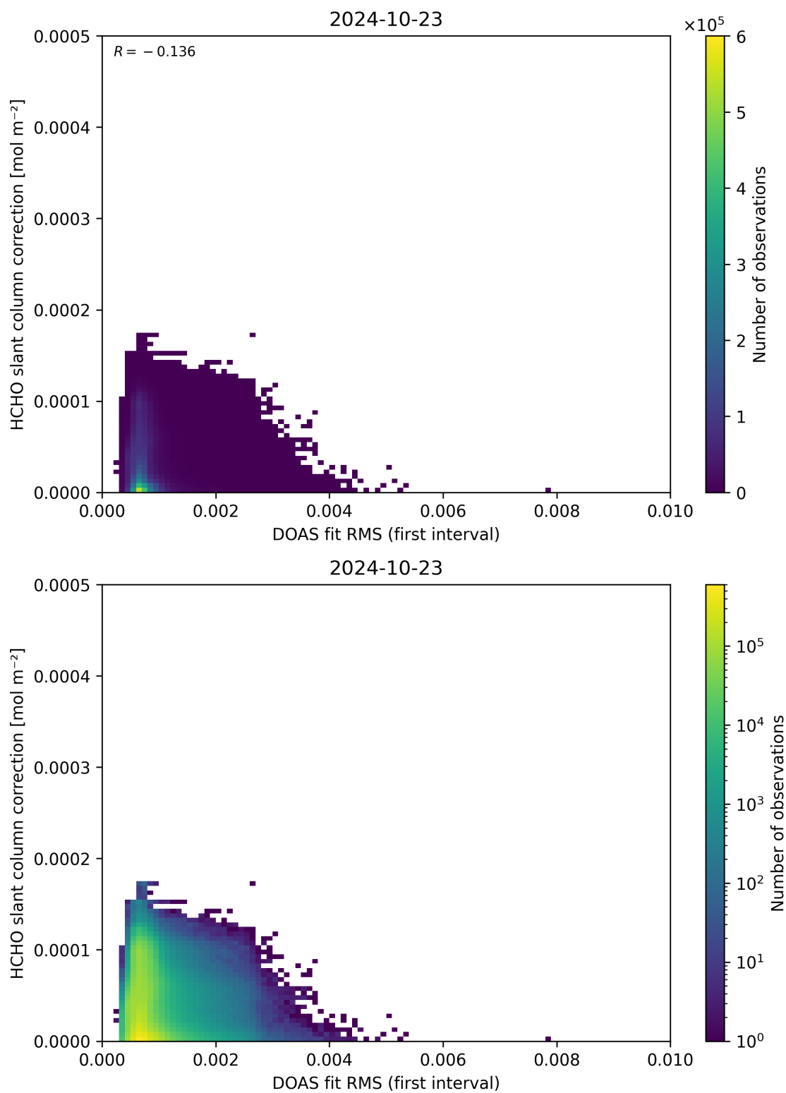
Figure 63: Scatter density plot of “DOAS fit RMS (first interval)” against “HCHO slant column correction” for 2024-10-22 to 2024-10-24.
