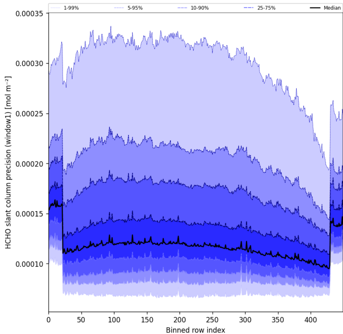
Figure 53: Along track statistics of “HCHO slant column precision (window1)” for 2024-10-22 to 2024-10-24
