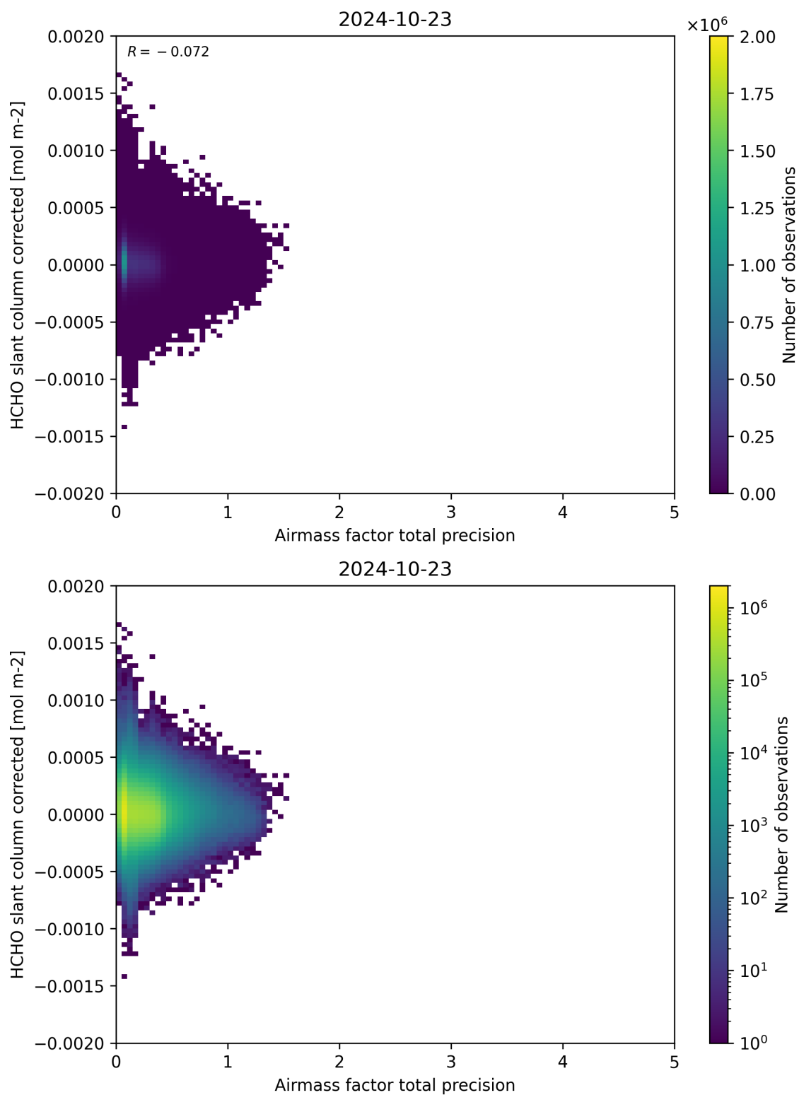
Figure 109: Scatter density plot of “Airmass factor total precision” against “HCHO slant column corrected” for 2024-10-22 to 2024-10-24.
