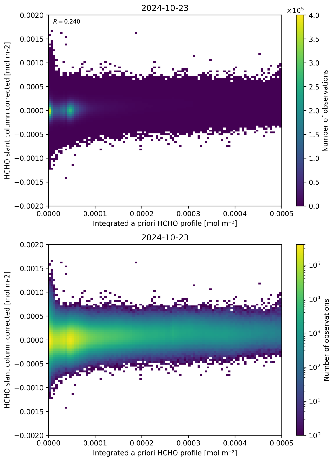
Figure 151: Scatter density plot of “Integrated a priori HCHO profile” against “HCHO slant column corrected” for 2024-10-22 to 2024-10-24.
