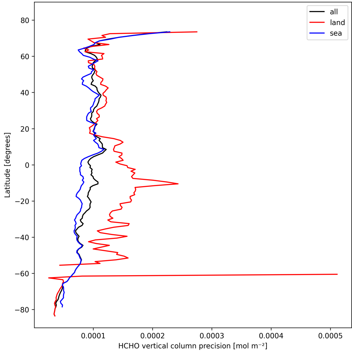
Figure 22: Zonal average of “HCHO vertical column precision” for 2024-10-22 to 2024-10-24.
