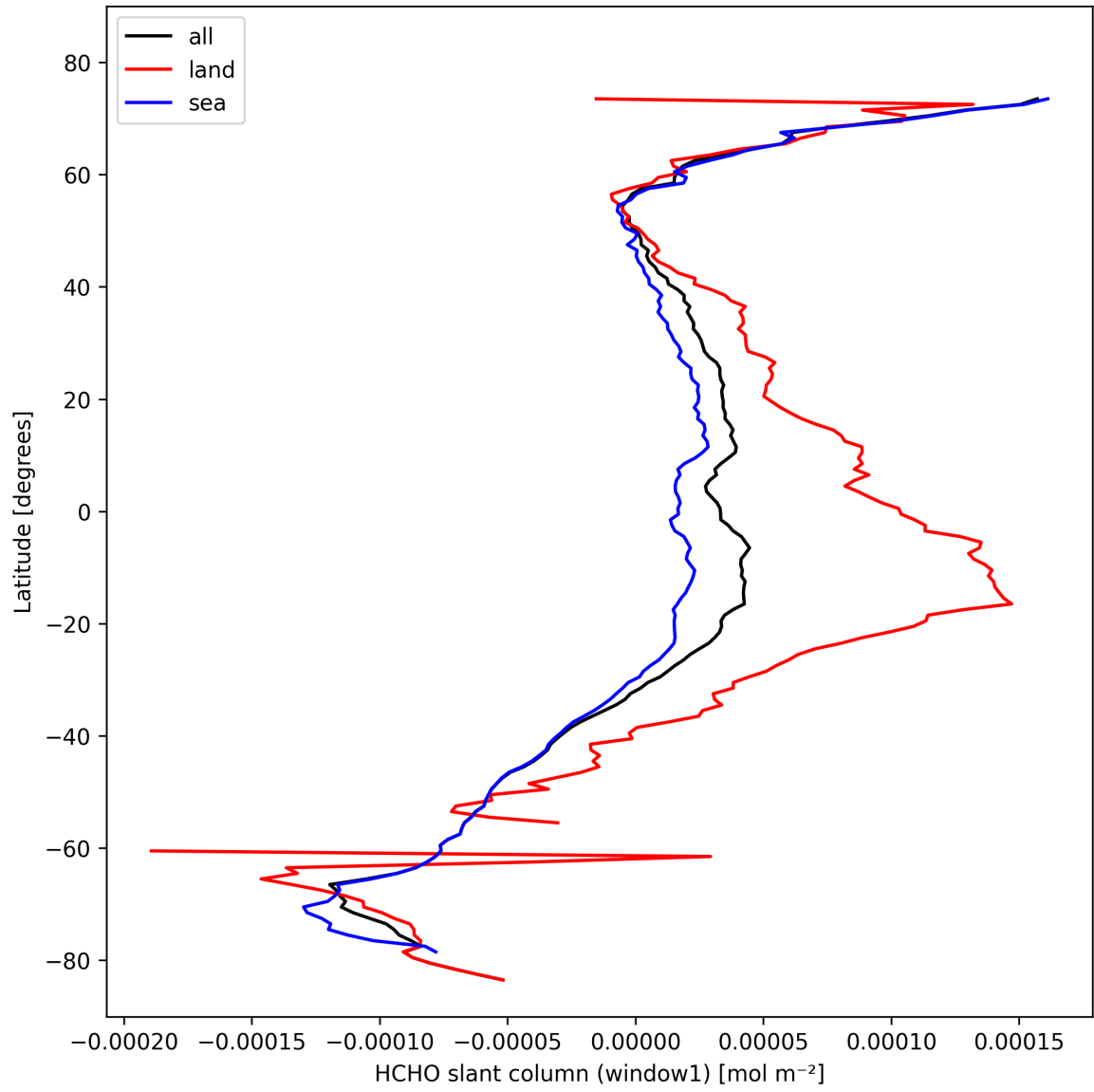
Figure 24: Zonal average of “HCHO slant column (window1)” for 2024-10-22 to 2024-10-24.
