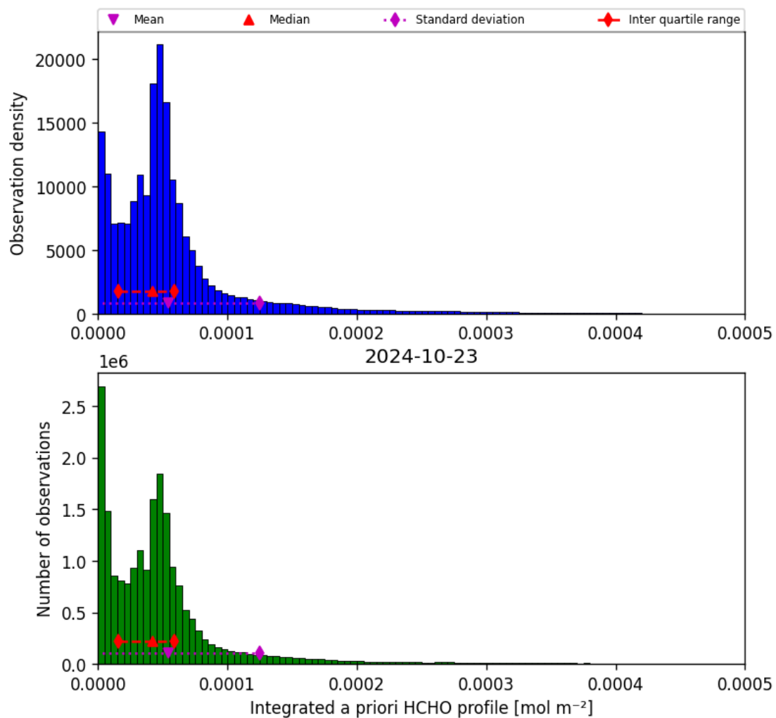
Figure 43: Histogram of “Integrated a priori HCHO profile” for 2024-10-22 to 2024-10-24
