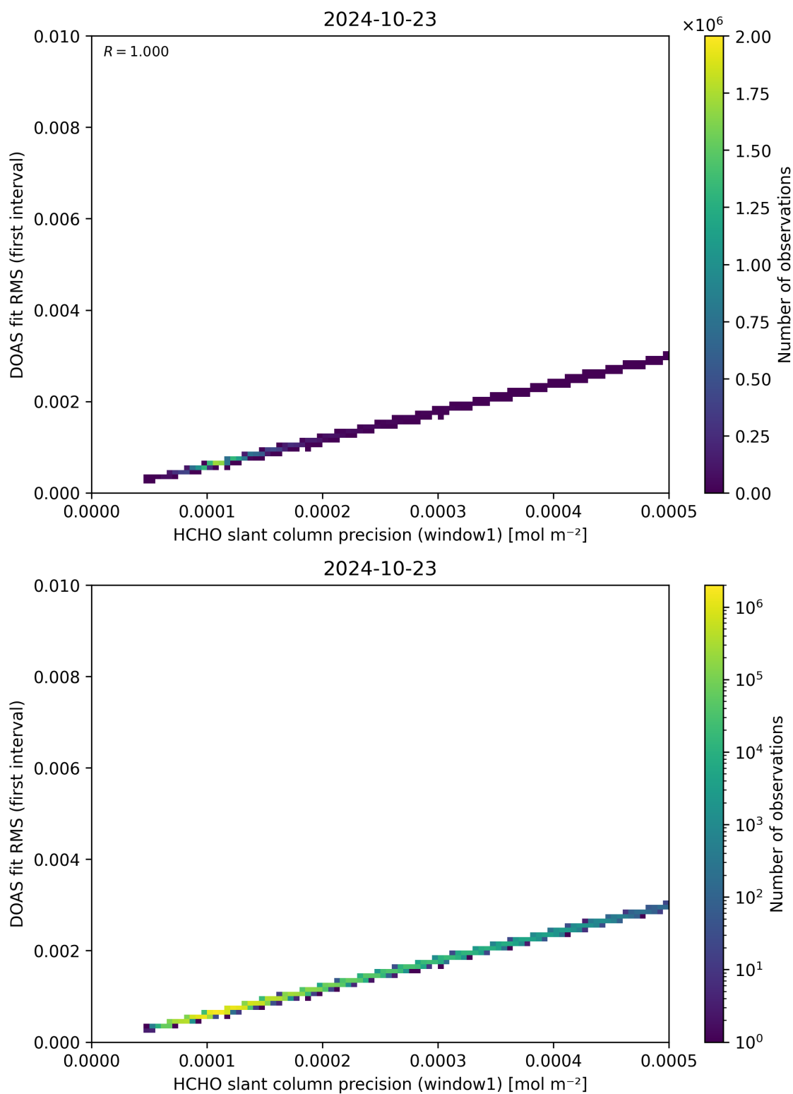
Figure 88: Scatter density plot of “HCHO slant column precision (window1)” against “DOAS fit RMS (first interval)” for 2024-10-22 to 2024-10-24.
