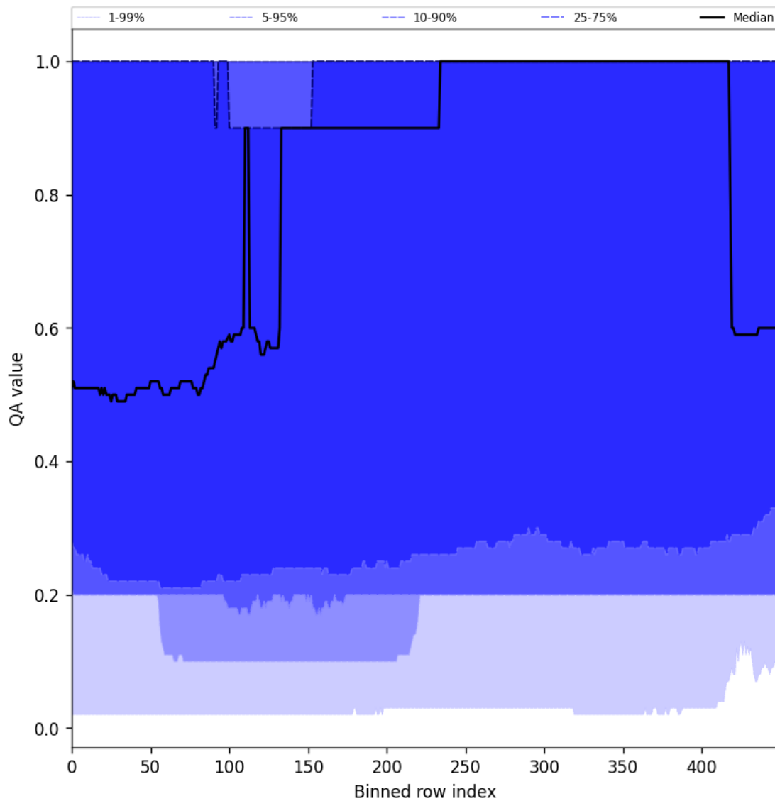
Figure 48: Along track statistics of “QA value” for 2024-10-22 to 2024-10-24
