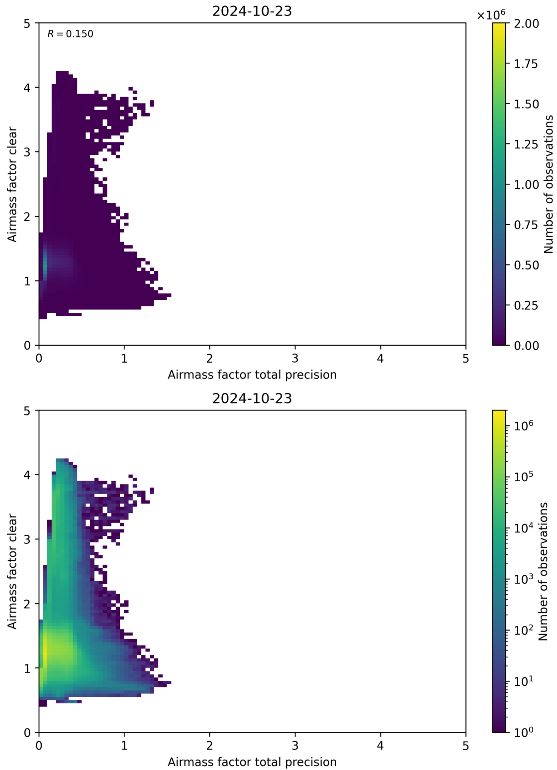
Figure 108: Scatter density plot of “Airmass factor total precision” against “Airmass factor clear” for 2024-10-22 to 2024-10-24.
