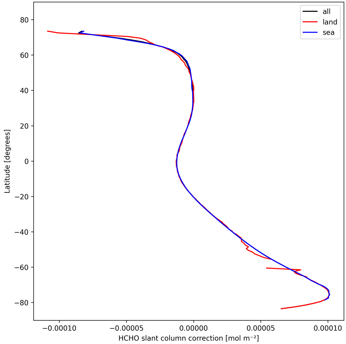
Figure 33: Zonal average of “HCHO slant column correction” for 2024-10-22 to 2024-10-24.
