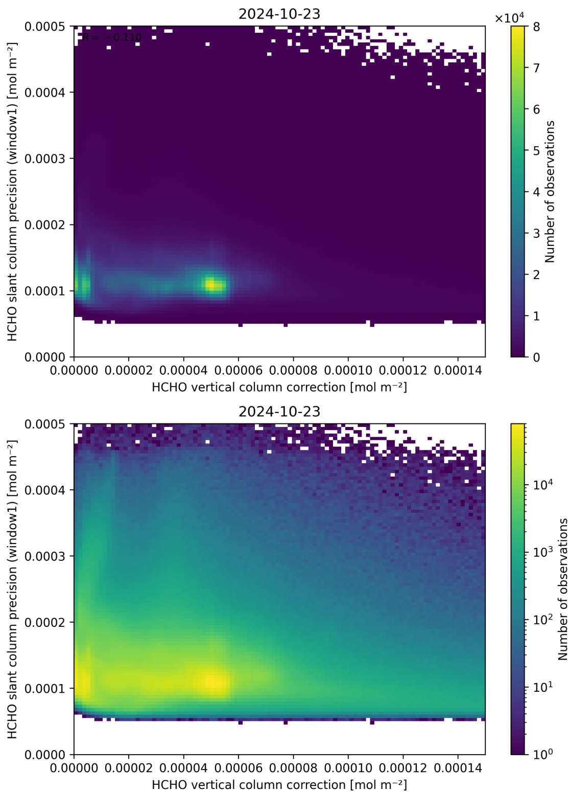
Figure 119: Scatter density plot of “HCHO vertical column correction” against “HCHO slant column precision (window1)” for 2024-10-22 to 2024-10-24.
