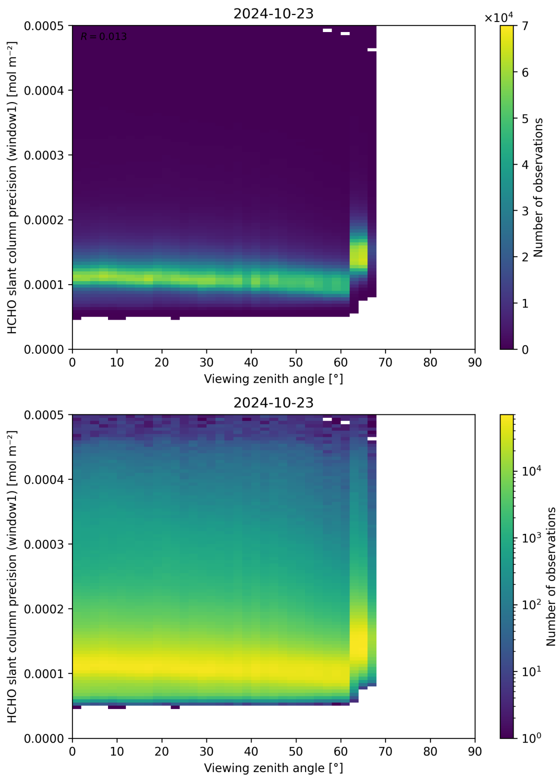
Figure 189: Scatter density plot of “Viewing zenith angle” against “HCHO slant column precision (window1)” for 2024-10-22 to 2024-10-24.
