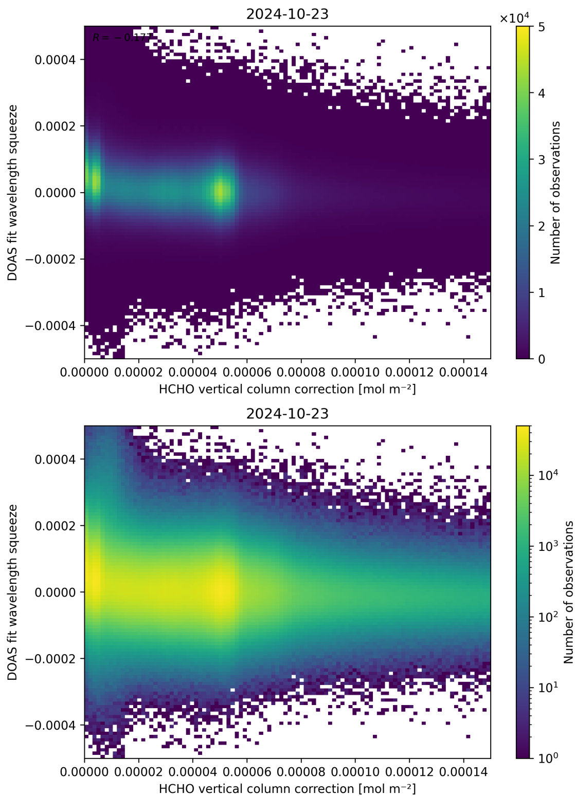
Figure 114: Scatter density plot of “HCHO vertical column correction” against “DOAS fit wavelength squeeze” for 2024-10-22 to 2024-10-24.
