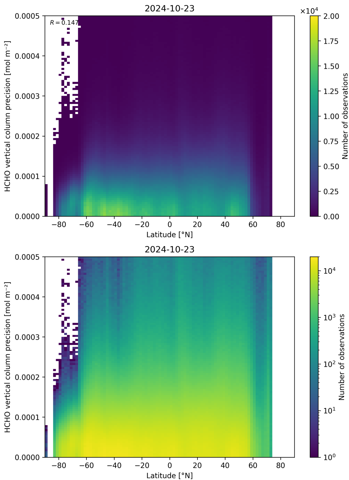
Figure 165: Scatter density plot of “Latitude” against “HCHO vertical column precision” for 2024-10-22 to 2024-10-24.
