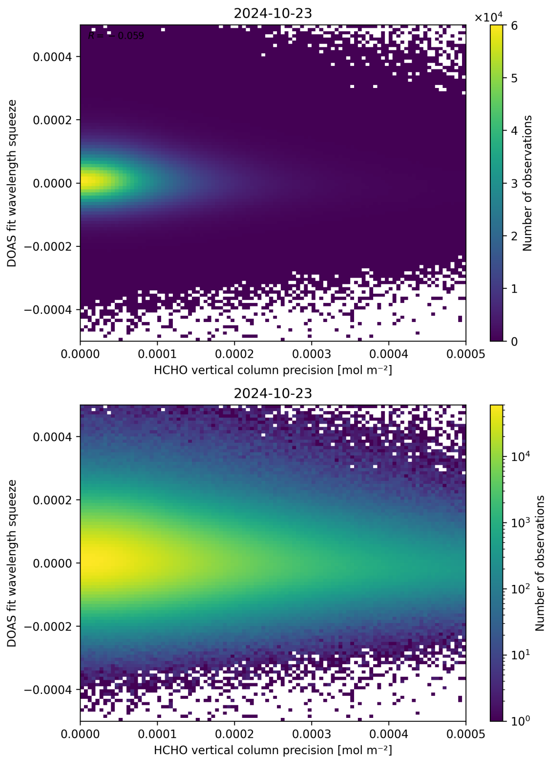
Figure 138: Scatter density plot of “HCHO vertical column precision” against “DOAS fit wavelength squeeze” for 2024-10-22 to 2024-10-24.
