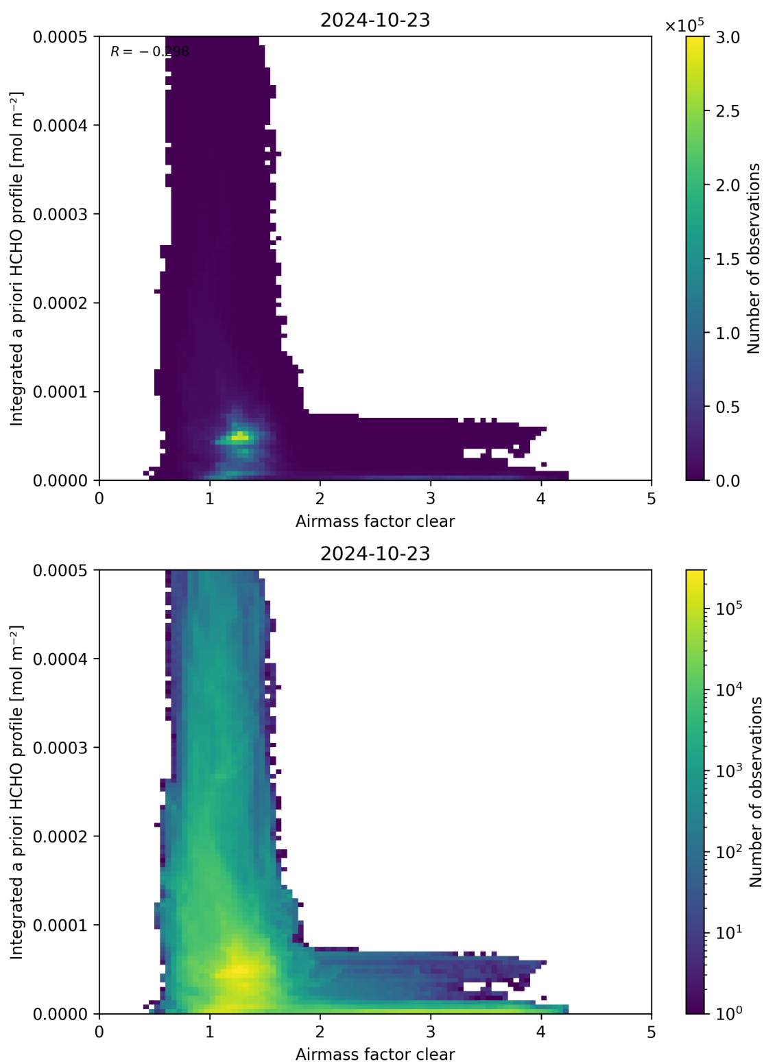
Figure 76: Scatter density plot of “Airmass factor clear” against “Integrated a priori HCHO profile” for 2024-10-22 to 2024-10-24.
