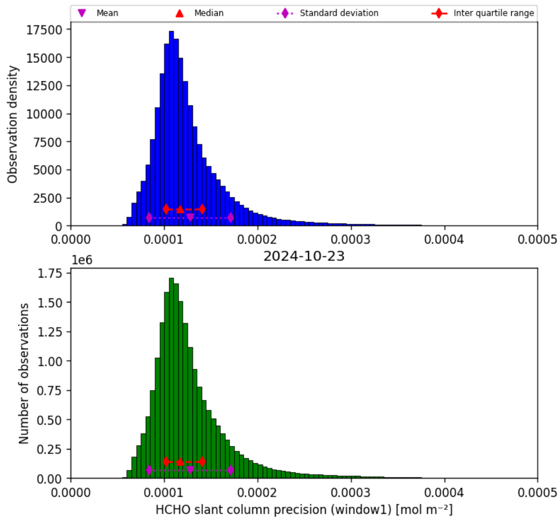
Figure 39: Histogram of “HCHO slant column precision (window1)” for 2024-10-22 to 2024-10-24
