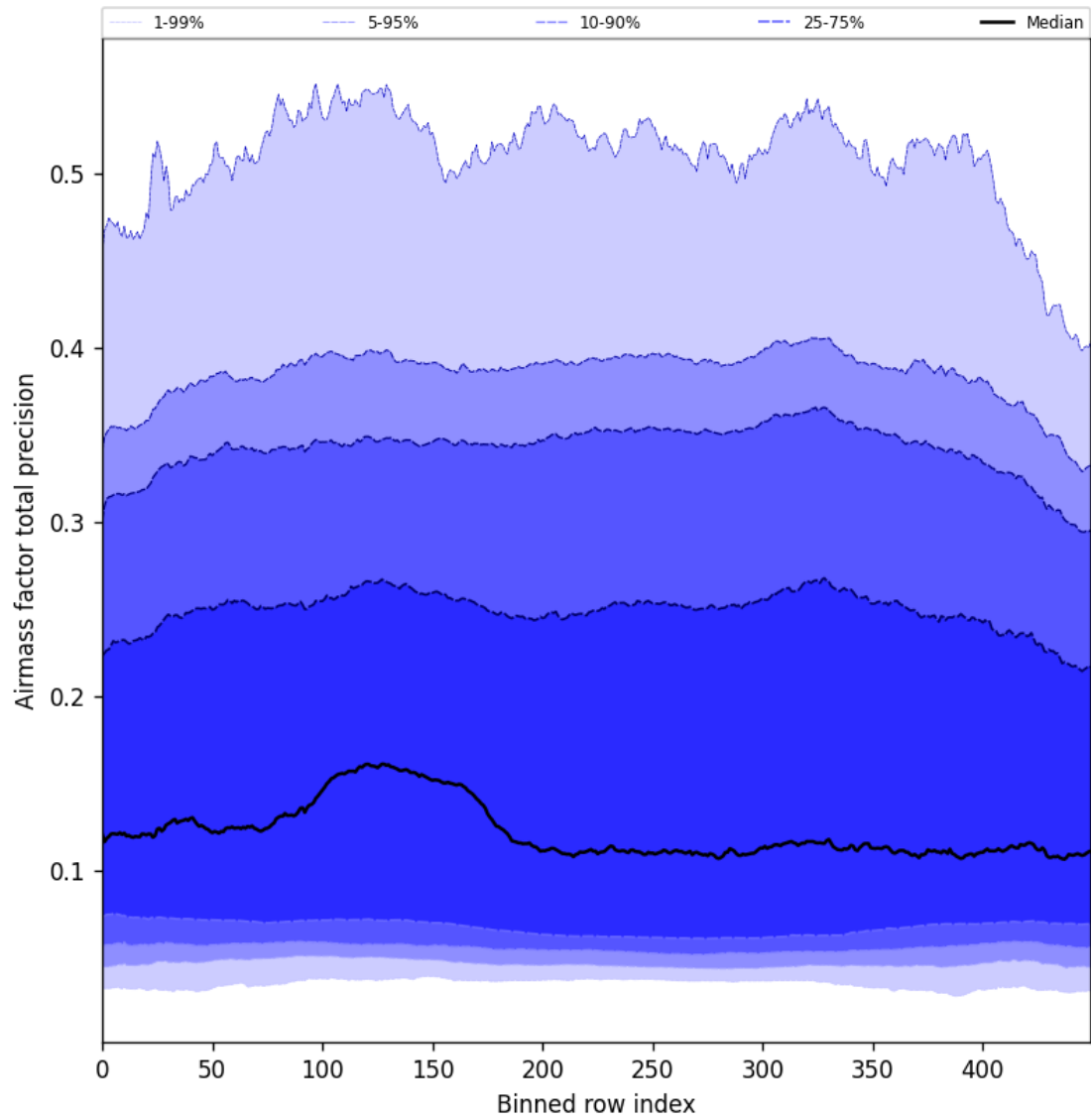
Figure 55: Along track statistics of “Airmass factor total precision” for 2024-10-22 to 2024-10-24
