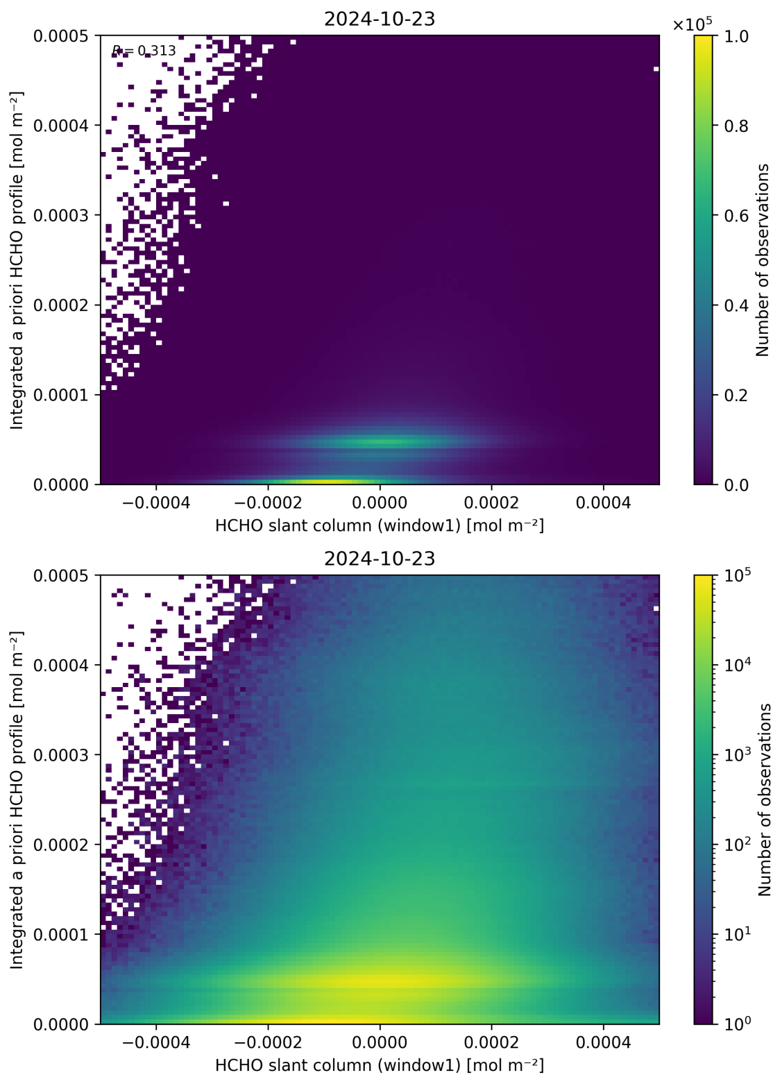
Figure 87: Scatter density plot of “HCHO slant column (window1)” against “Integrated a priori HCHO profile” for 2024-10-22 to 2024-10-24.
