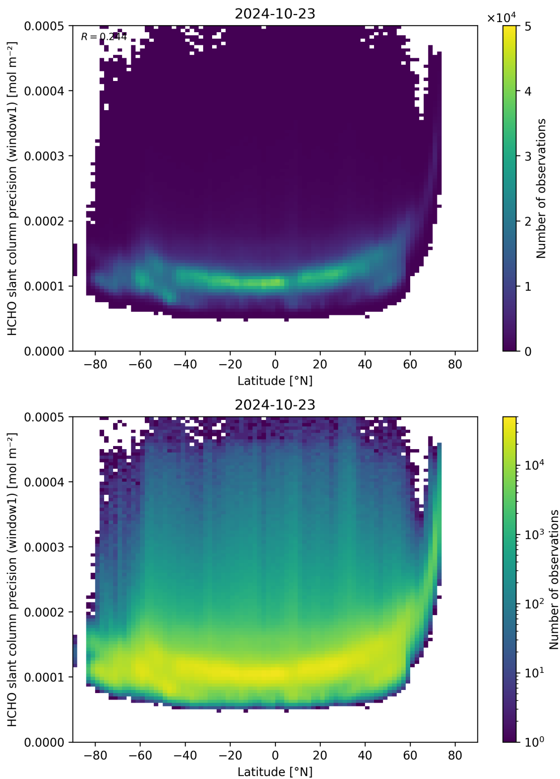
Figure 160: Scatter density plot of “Latitude” against “HCHO slant column precision (window1)” for 2024-10-22 to 2024-10-24.
