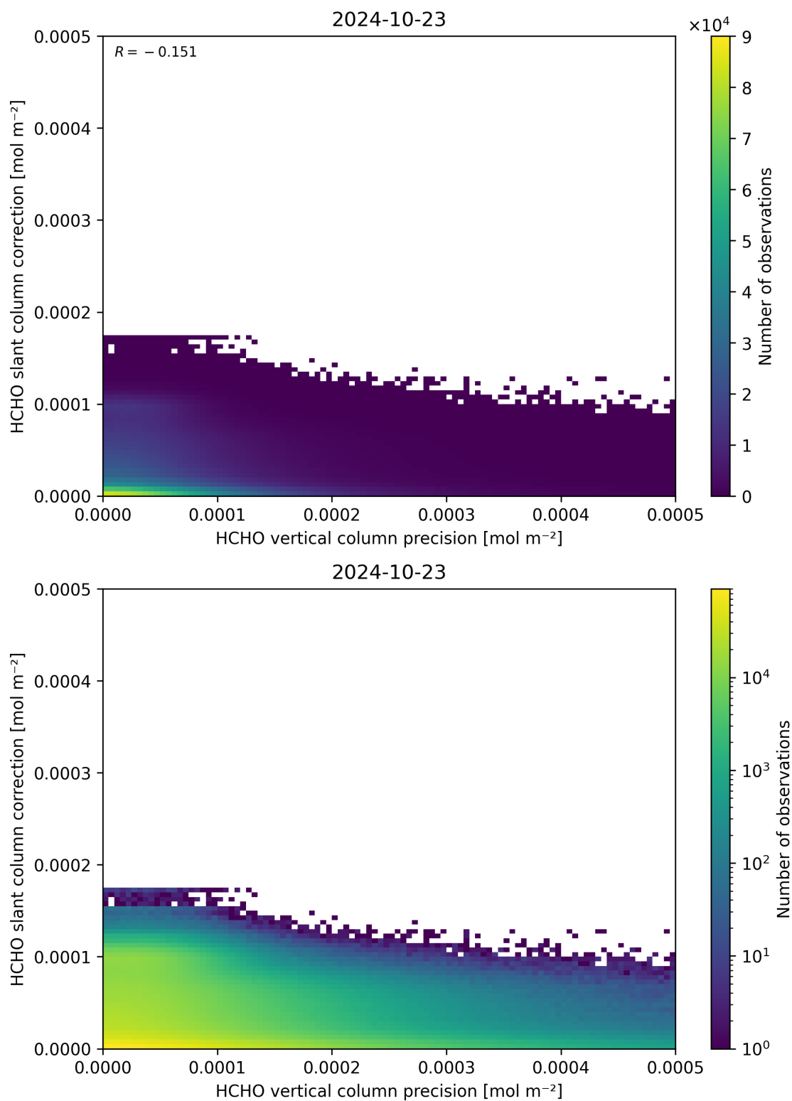
Figure 141: Scatter density plot of “HCHO vertical column precision” against “HCHO slant column correction” for 2024-10-22 to 2024-10-24.
