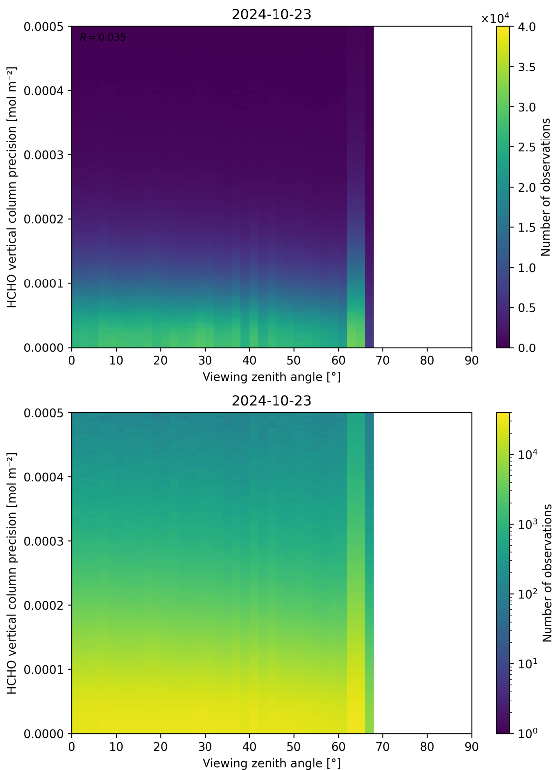
Figure 194: Scatter density plot of “Viewing zenith angle” against “HCHO vertical column precision” for 2024-10-22 to 2024-10-24.
