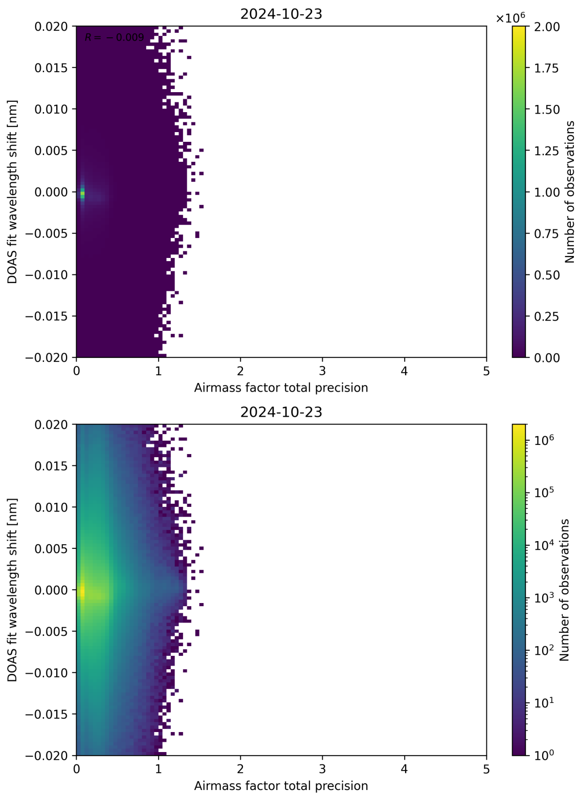
Figure 106: Scatter density plot of “Airmass factor total precision” against “DOAS fit wavelength shift” for 2024-10-22 to 2024-10-24.
