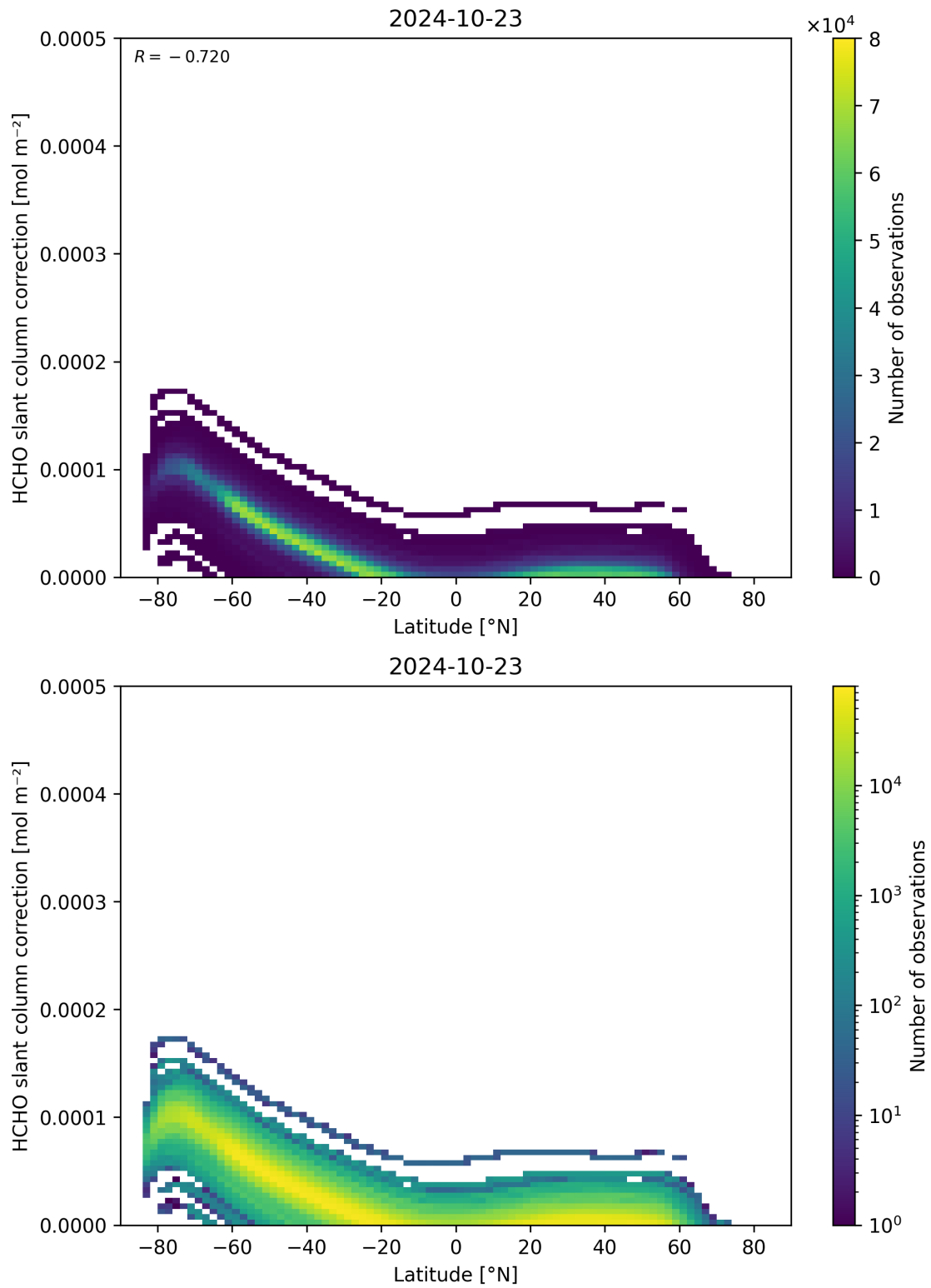
Figure 158: Scatter density plot of “Latitude” against “HCHO slant column correction” for 2024-10-22 to 2024-10-24.
