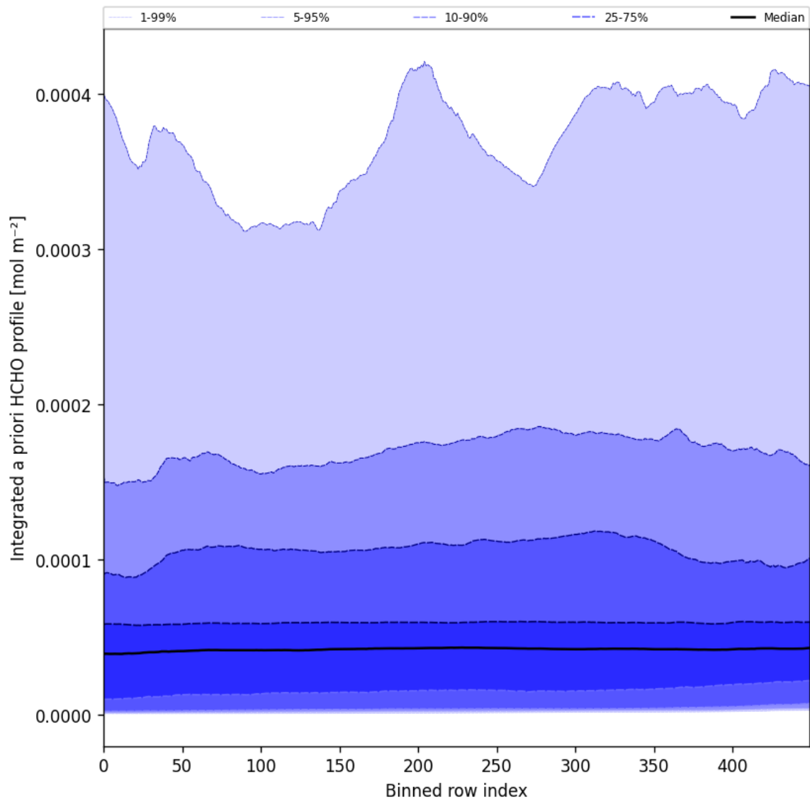
Figure 57: Along track statistics of “Integrated a priori HCHO profile” for 2024-10-22 to 2024-10-24
