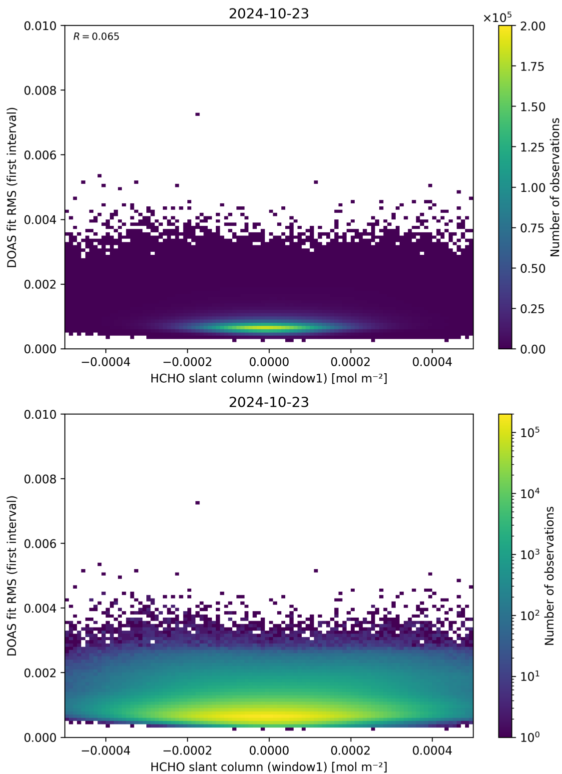
Figure 78: Scatter density plot of “HCHO slant column (window1)” against “DOAS fit RMS (first interval)” for 2024-10-22 to 2024-10-24.
