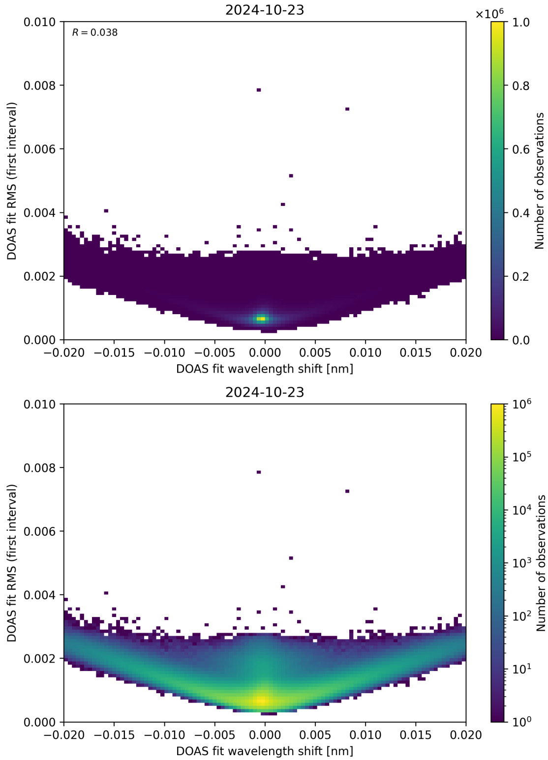
Figure 64: Scatter density plot of “DOAS fit wavelength shift” against “DOAS fit RMS (first interval)” for 2024-10-22 to 2024-10-24.
