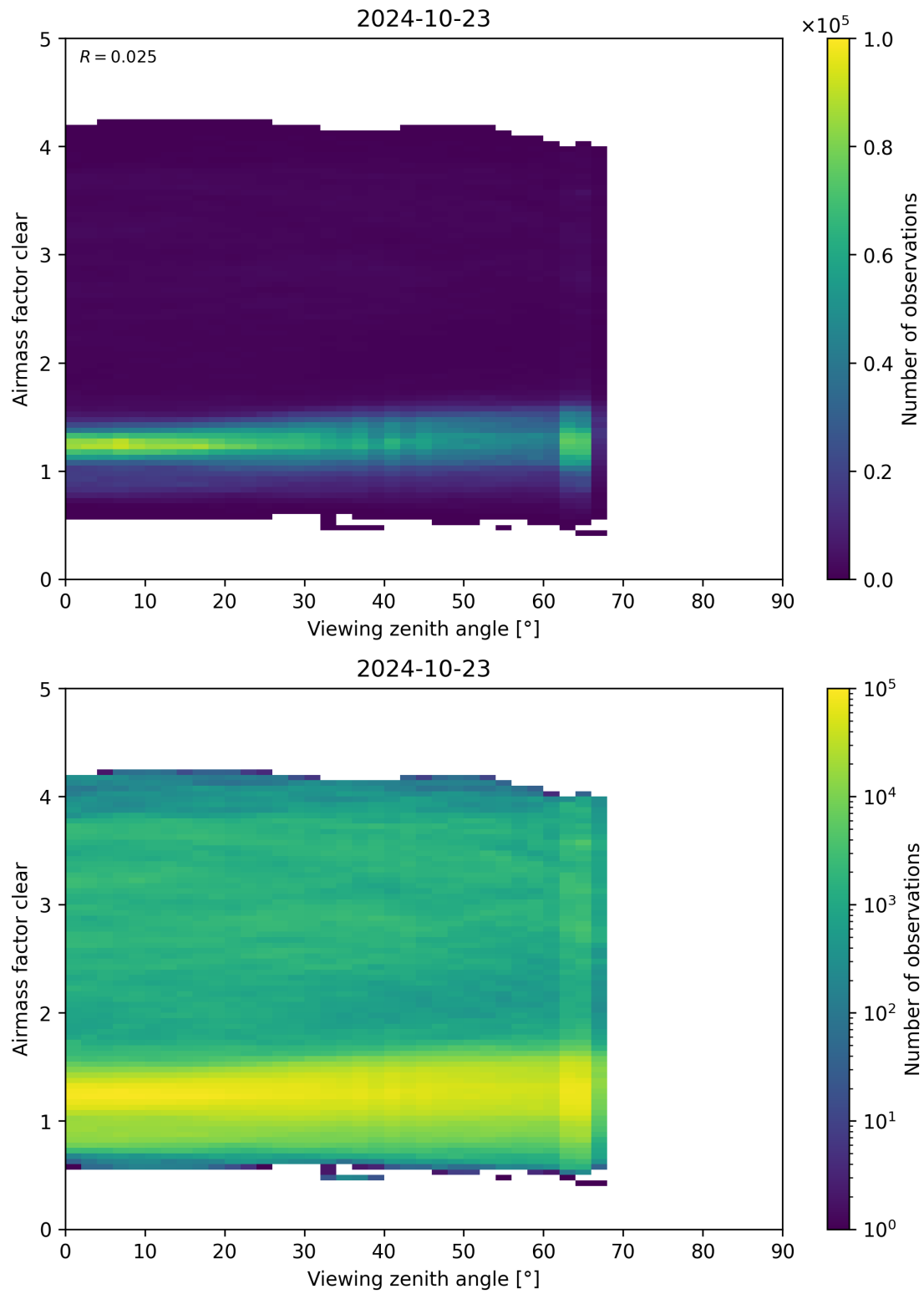
Figure 185: Scatter density plot of “Viewing zenith angle” against “Airmass factor clear” for 2024-10-22 to 2024-10-24.
