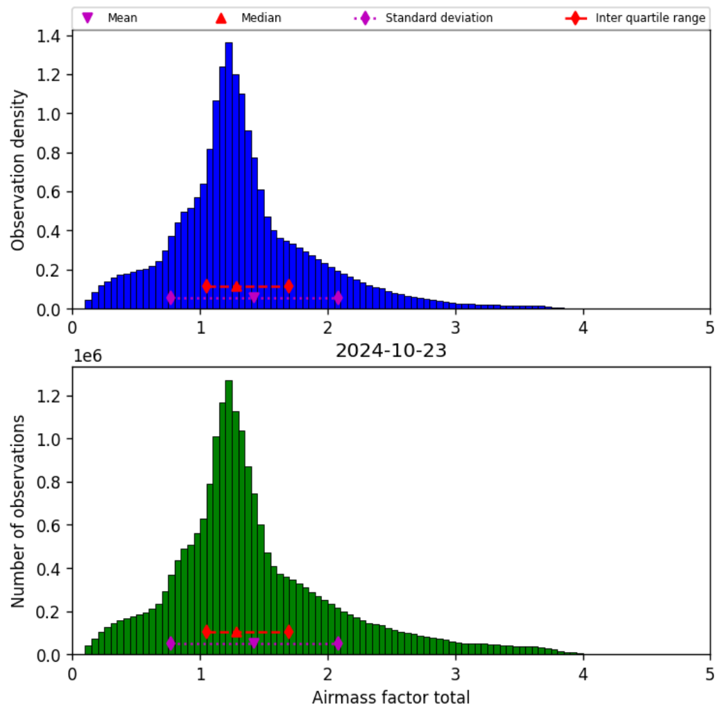
Figure 40: Histogram of “Airmass factor total” for 2024-10-22 to 2024-10-24
