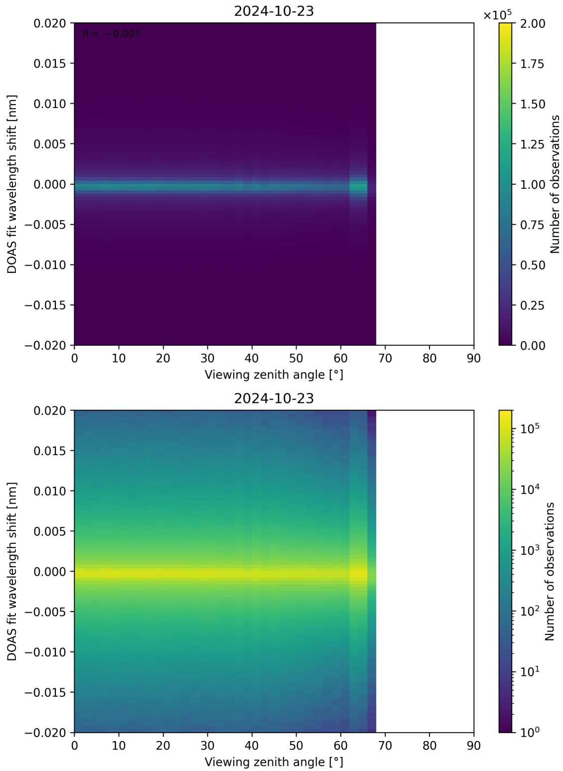
Figure 183: Scatter density plot of “Viewing zenith angle” against “DOAS fit wavelength shift” for 2024-10-22 to 2024-10-24.
