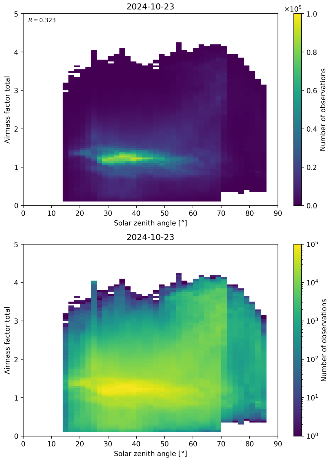
Figure 175: Scatter density plot of “Solar zenith angle” against “Airmass factor total” for 2024-10-22 to 2024-10-24.
