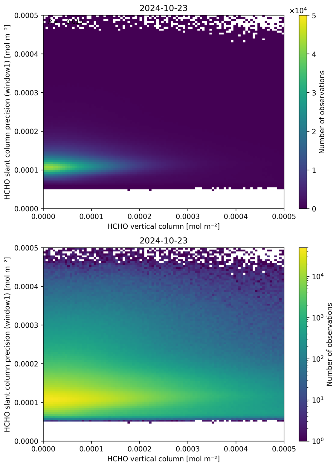
Figure 130: Scatter density plot of “HCHO vertical column” against “HCHO slant column precision (window1)” for 2024-10-22 to 2024-10-24.
