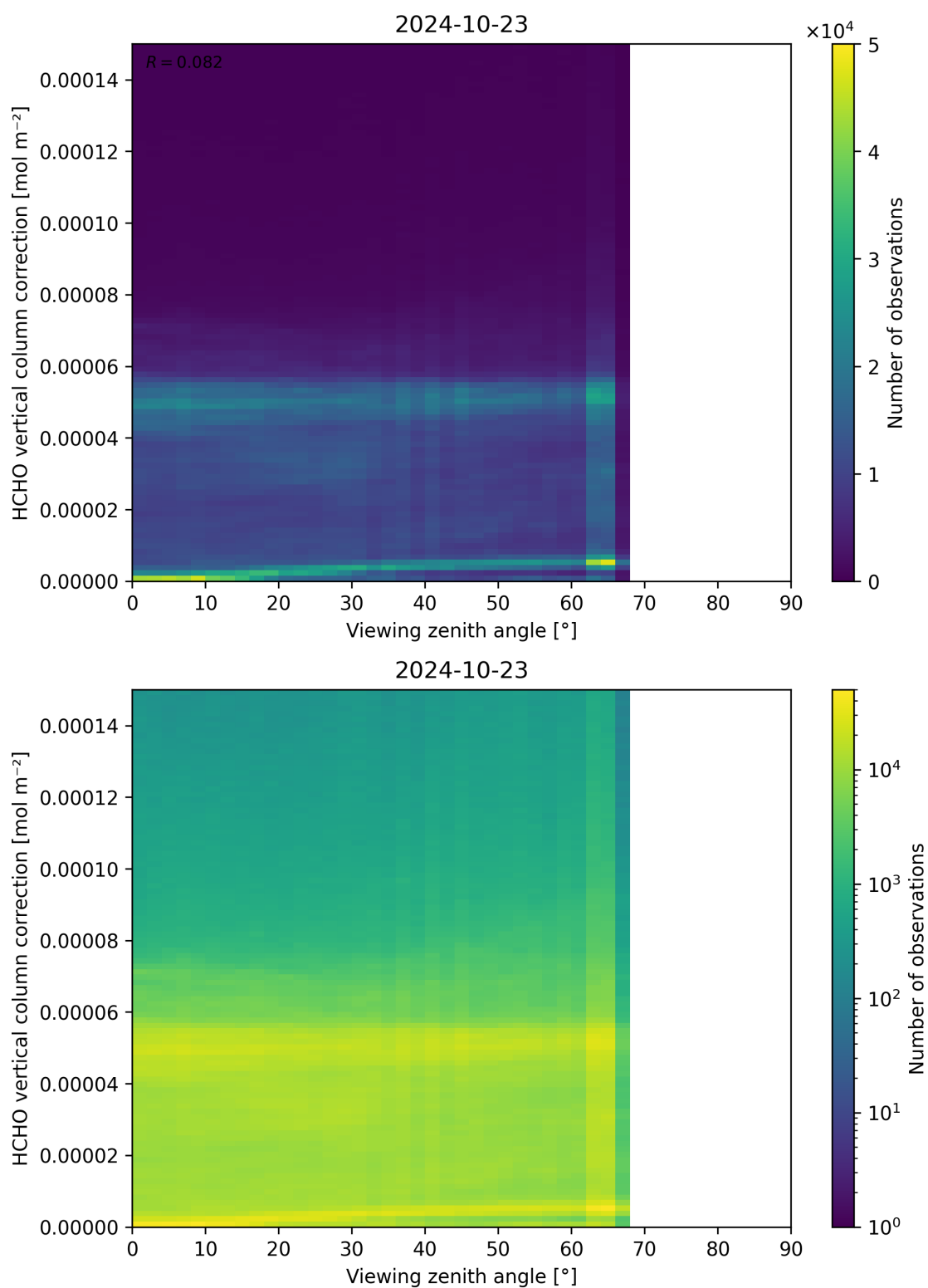
Figure 193: Scatter density plot of “Viewing zenith angle” against “HCHO vertical column correction” for 2024-10-22 to 2024-10-24.
