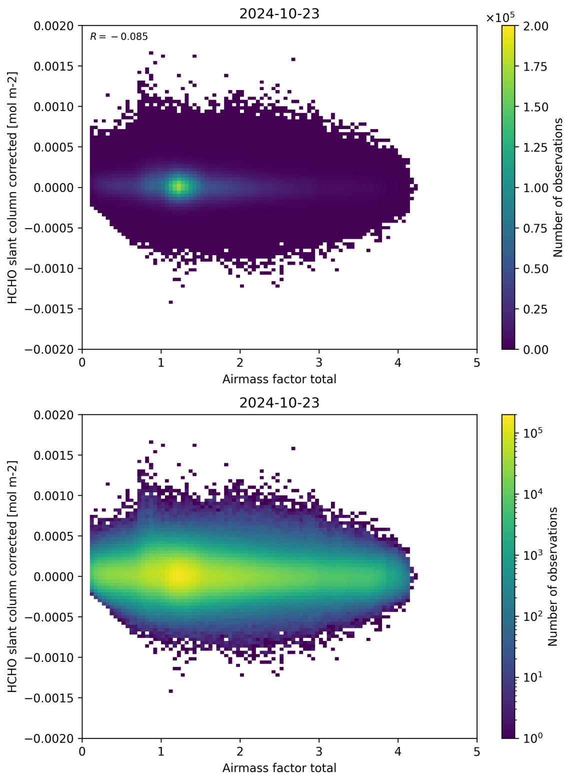
Figure 101: Scatter density plot of “Airmass factor total” against “HCHO slant column corrected” for 2024-10-22 to 2024-10-24.
