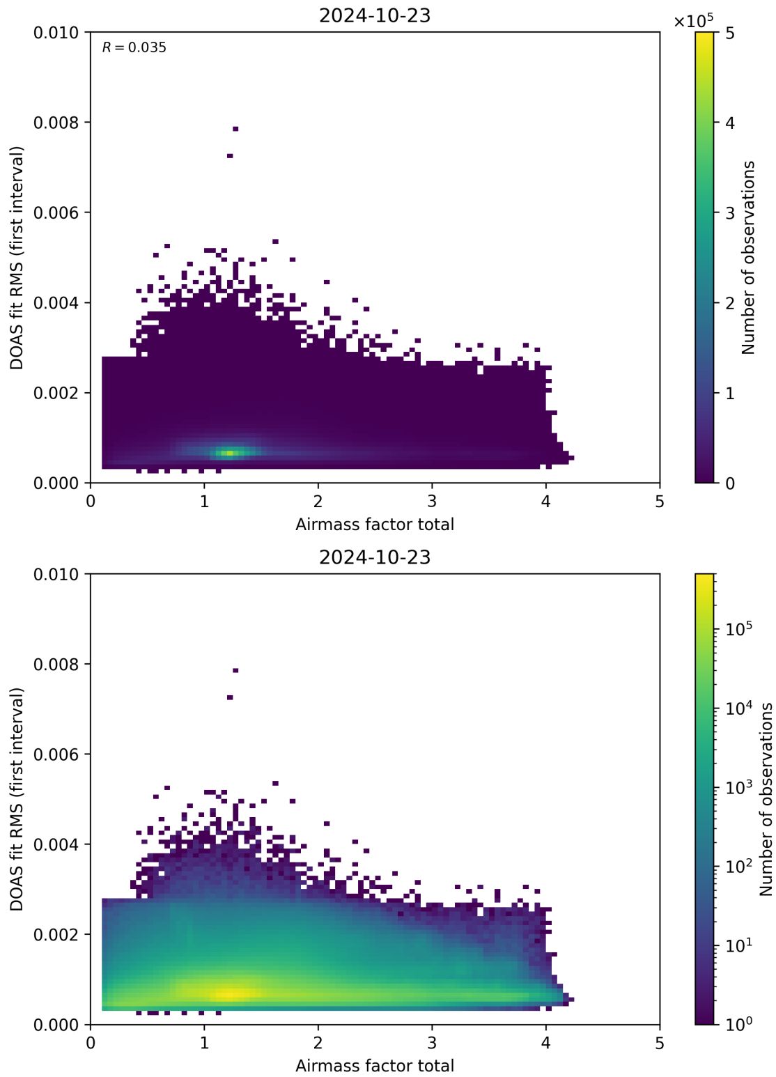
Figure 97: Scatter density plot of “Airmass factor total” against “DOAS fit RMS (first interval)” for 2024-10-22 to 2024-10-24.
