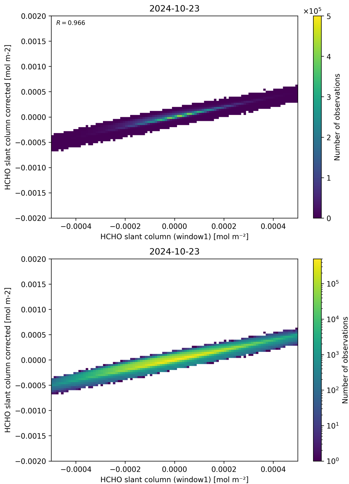
Figure 82: Scatter density plot of “HCHO slant column (window1)” against “HCHO slant column corrected” for 2024-10-22 to 2024-10-24.
