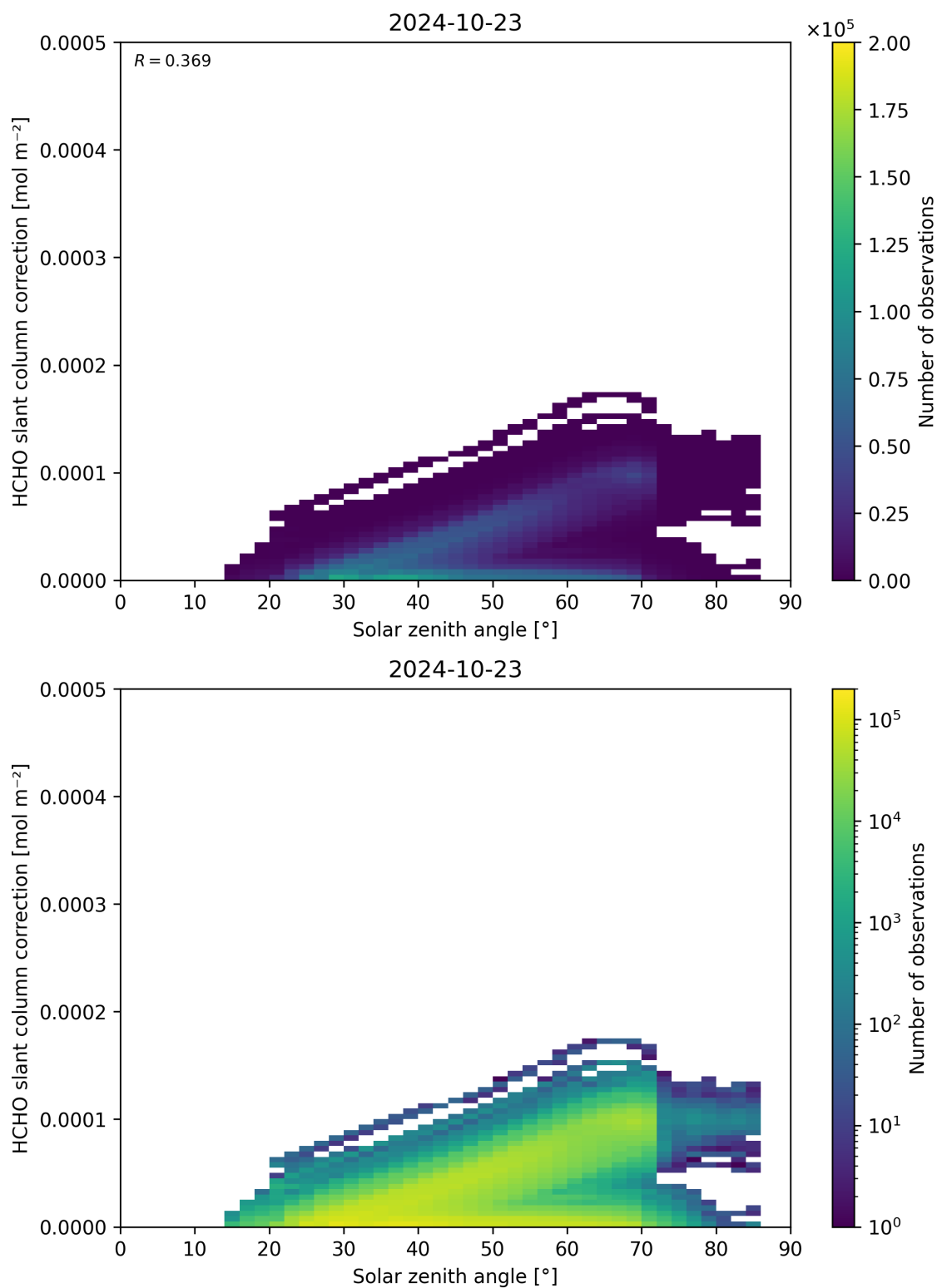
Figure 172: Scatter density plot of “Solar zenith angle” against “HCHO slant column correction” for 2024-10-22 to 2024-10-24.
