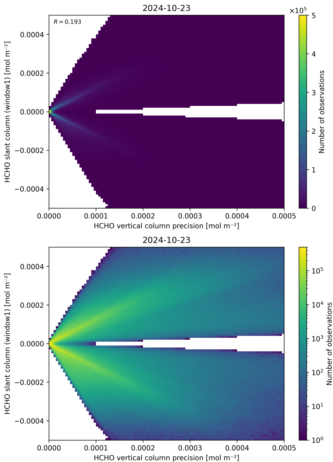
Figure 142: Scatter density plot of “HCHO vertical column precision” against “HCHO slant column (window1)” for 2024-10-22 to 2024-10-24.
