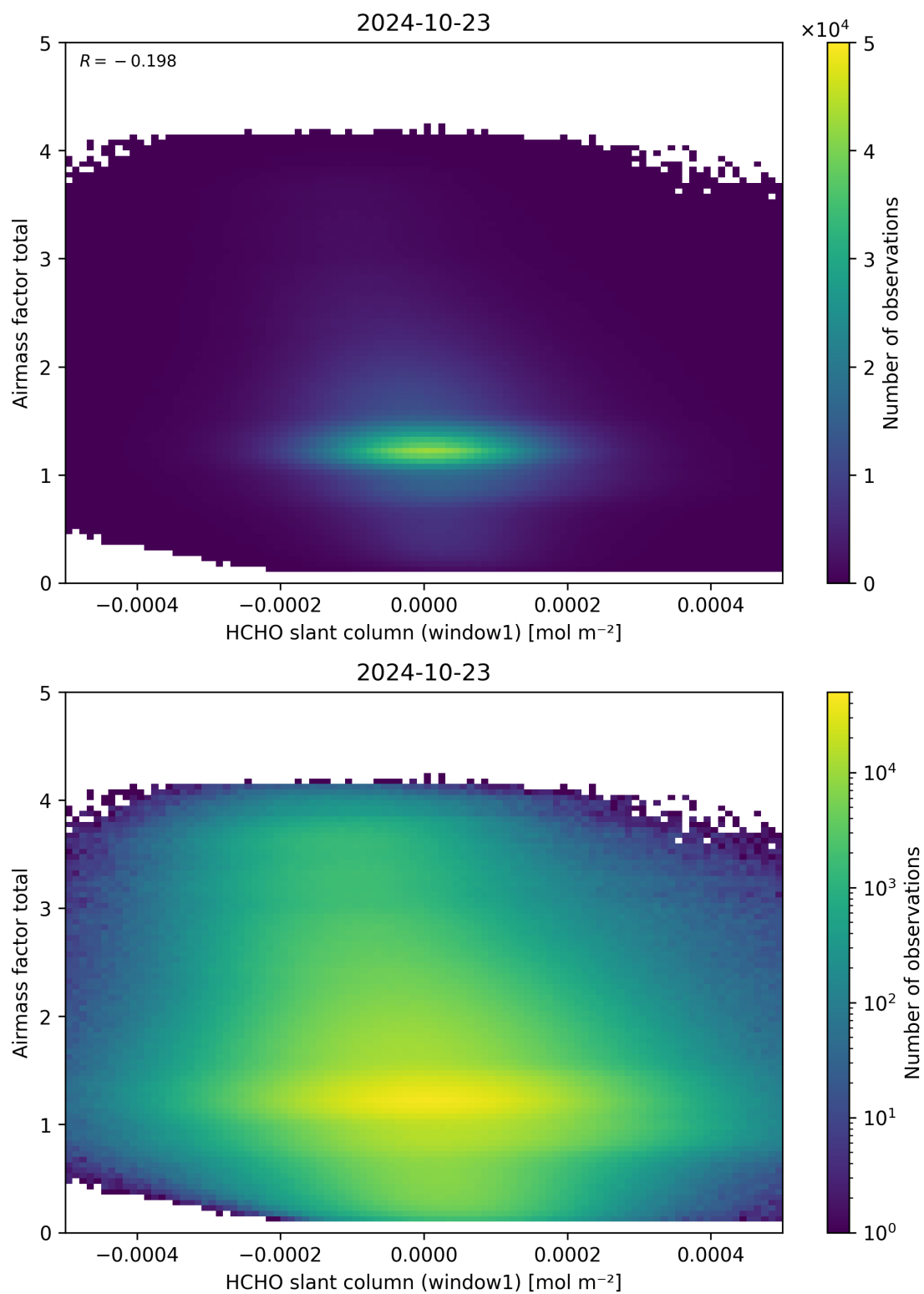
Figure 85: Scatter density plot of “HCHO slant column (window1)” against “Airmass factor total” for 2024-10-22 to 2024-10-24.
