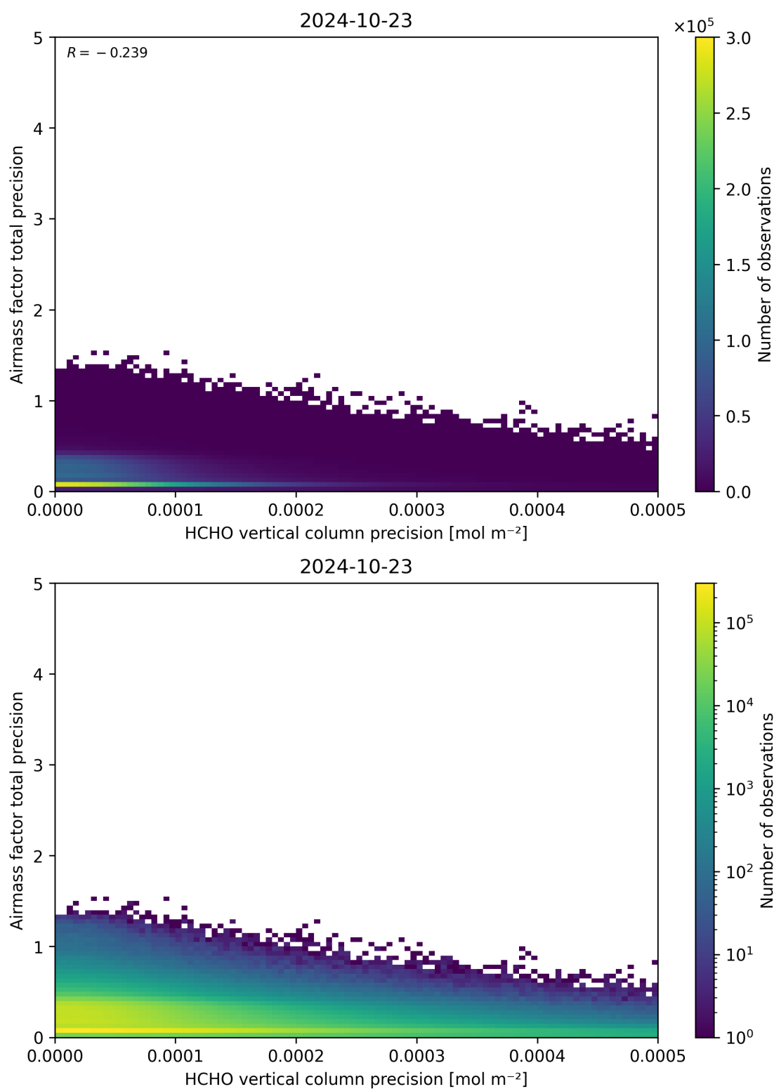
Figure 145: Scatter density plot of “HCHO vertical column precision” against “Airmass factor total precision” for 2024-10-22 to 2024-10-24.
