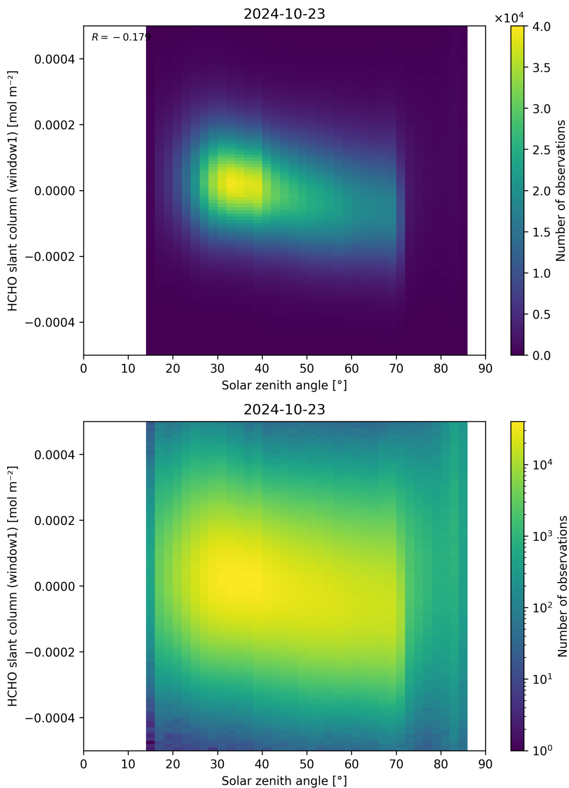
Figure 173: Scatter density plot of “Solar zenith angle” against “HCHO slant column (window1)” for 2024-10-22 to 2024-10-24.
