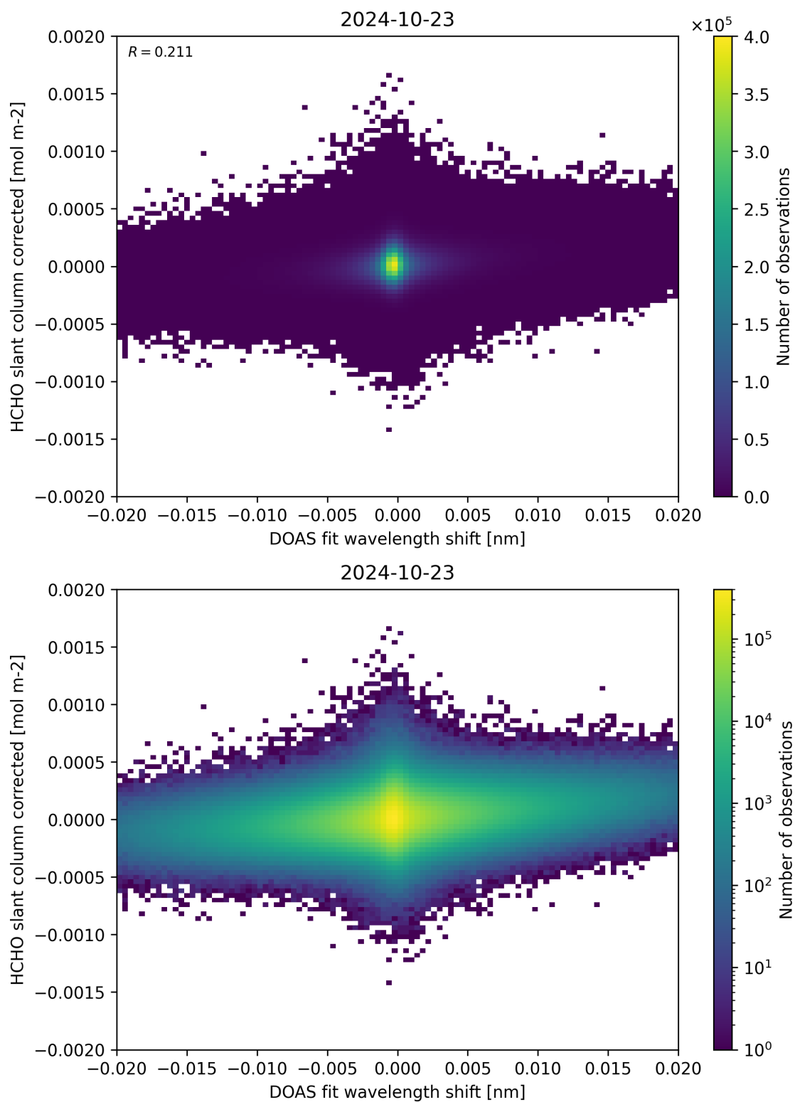
Figure 66: Scatter density plot of “DOAS fit wavelength shift” against “HCHO slant column corrected” for 2024-10-22 to 2024-10-24.
