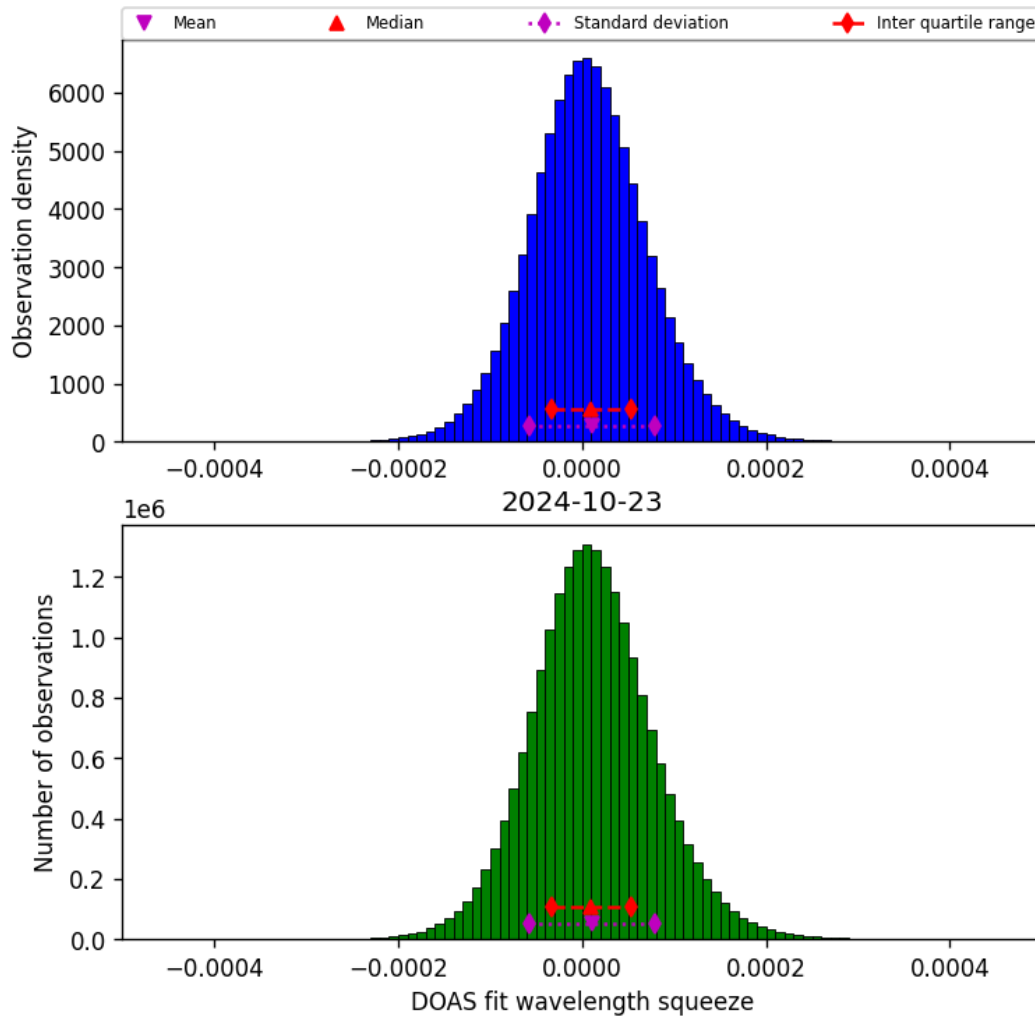
Figure 45: Histogram of “DOAS fit wavelength squeeze” for 2024-10-22 to 2024-10-24
