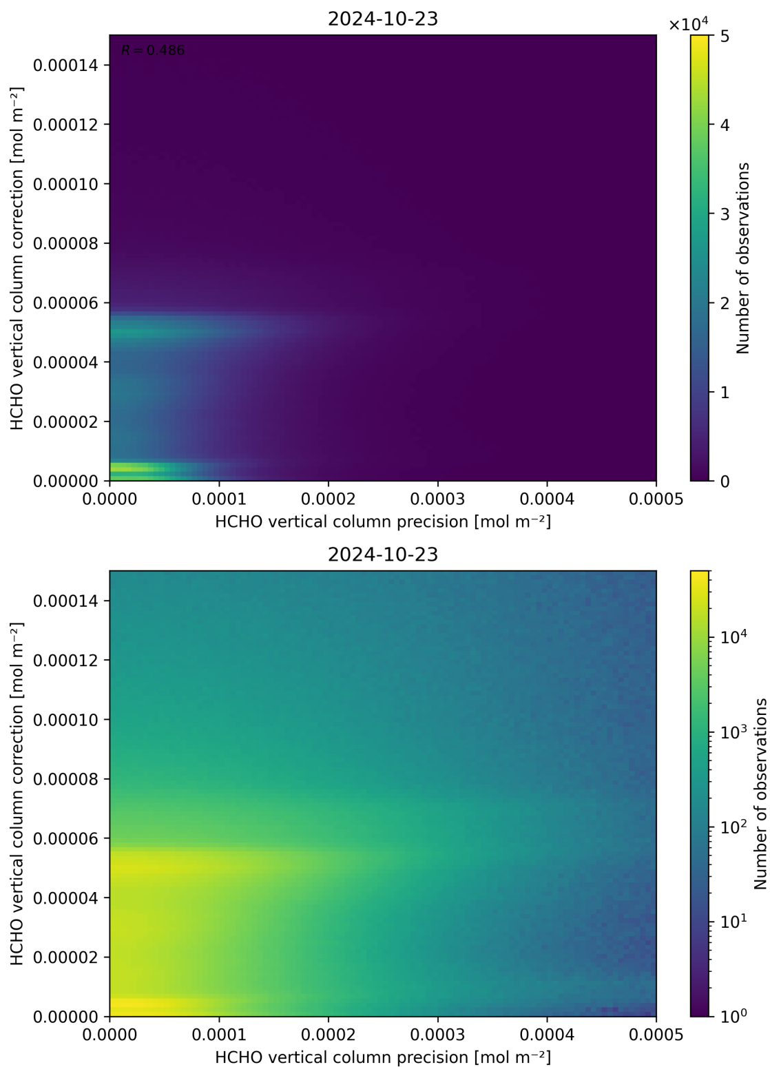
Figure 146: Scatter density plot of “HCHO vertical column precision” against “HCHO vertical column correction” for 2024-10-22 to 2024-10-24.
