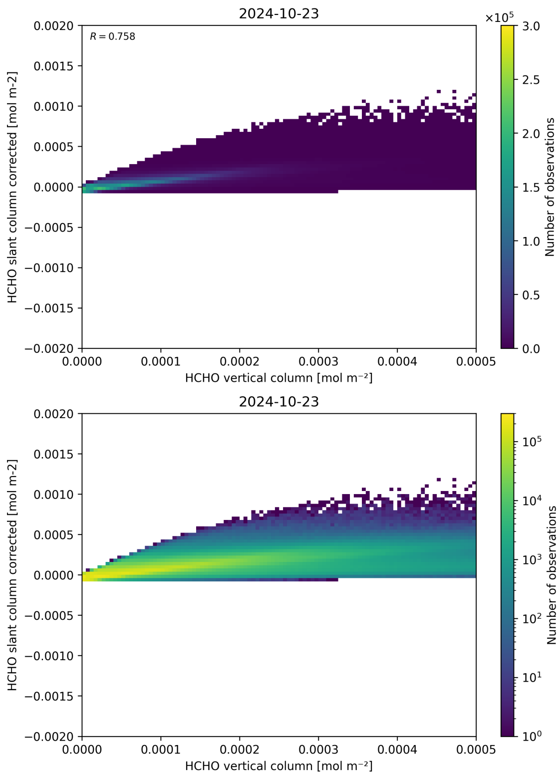
Figure 127: Scatter density plot of “HCHO vertical column” against “HCHO slant column corrected” for 2024-10-22 to 2024-10-24.
