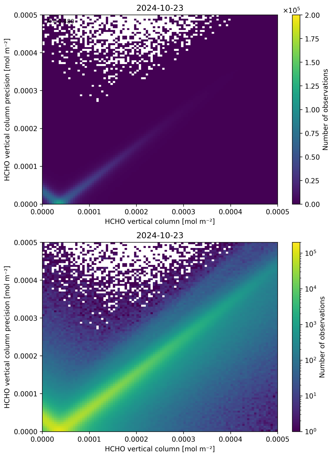
Figure 134: Scatter density plot of “HCHO vertical column” against “HCHO vertical column precision” for 2024-10-22 to 2024-10-24.
