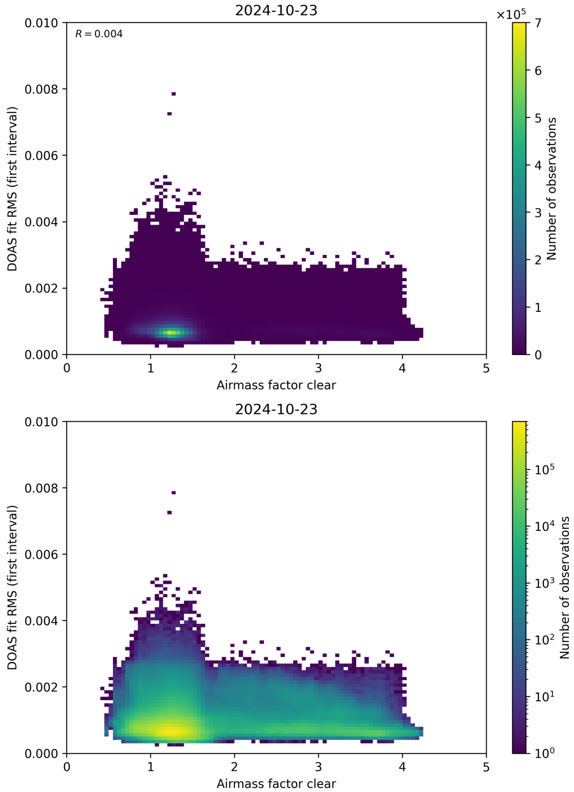
Figure 71: Scatter density plot of “Airmass factor clear” against “DOAS fit RMS (first interval)” for 2024-10-22 to 2024-10-24.
