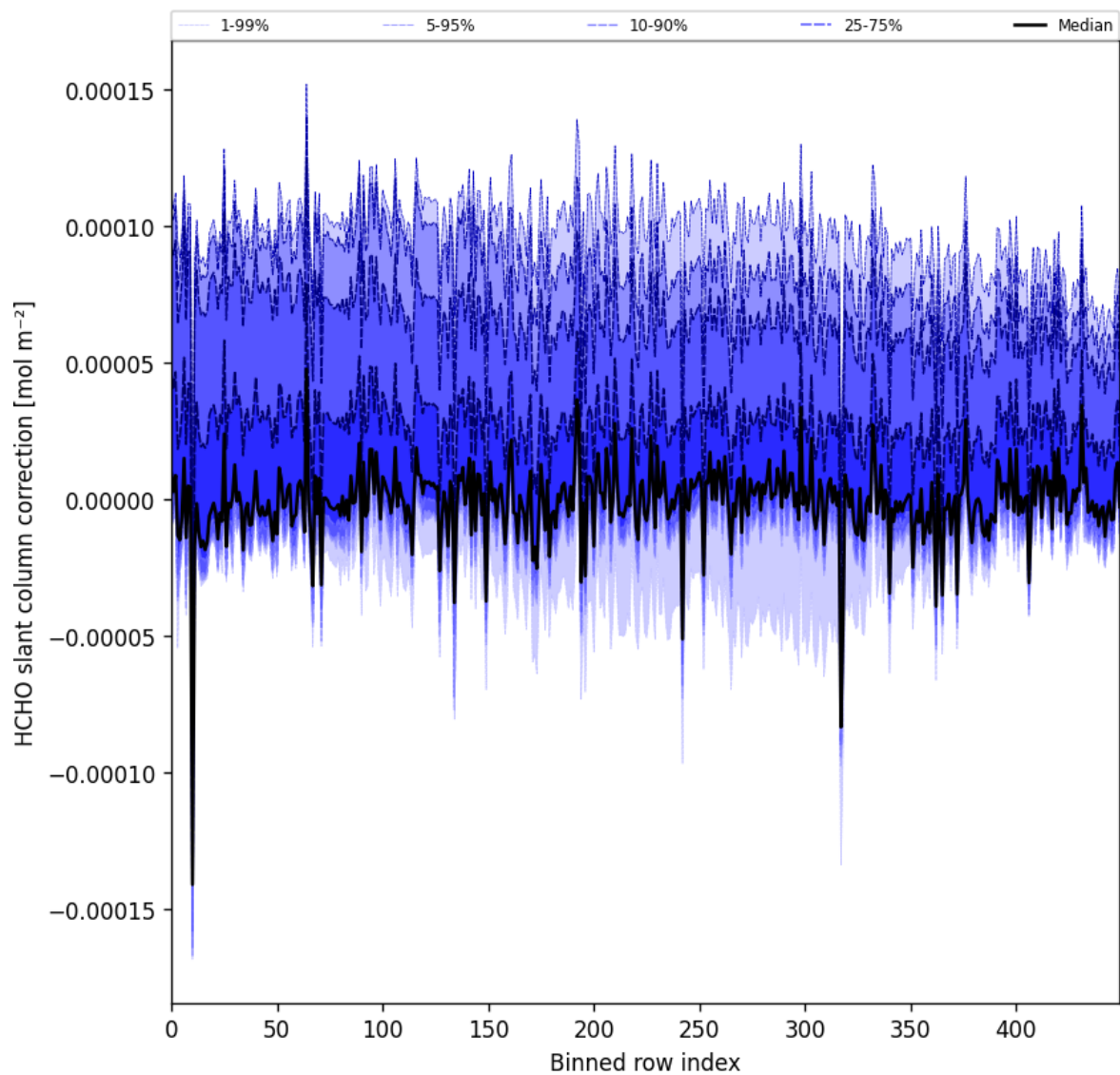
Figure 61: Along track statistics of “HCHO slant column correction” for 2024-10-22 to 2024-10-24
