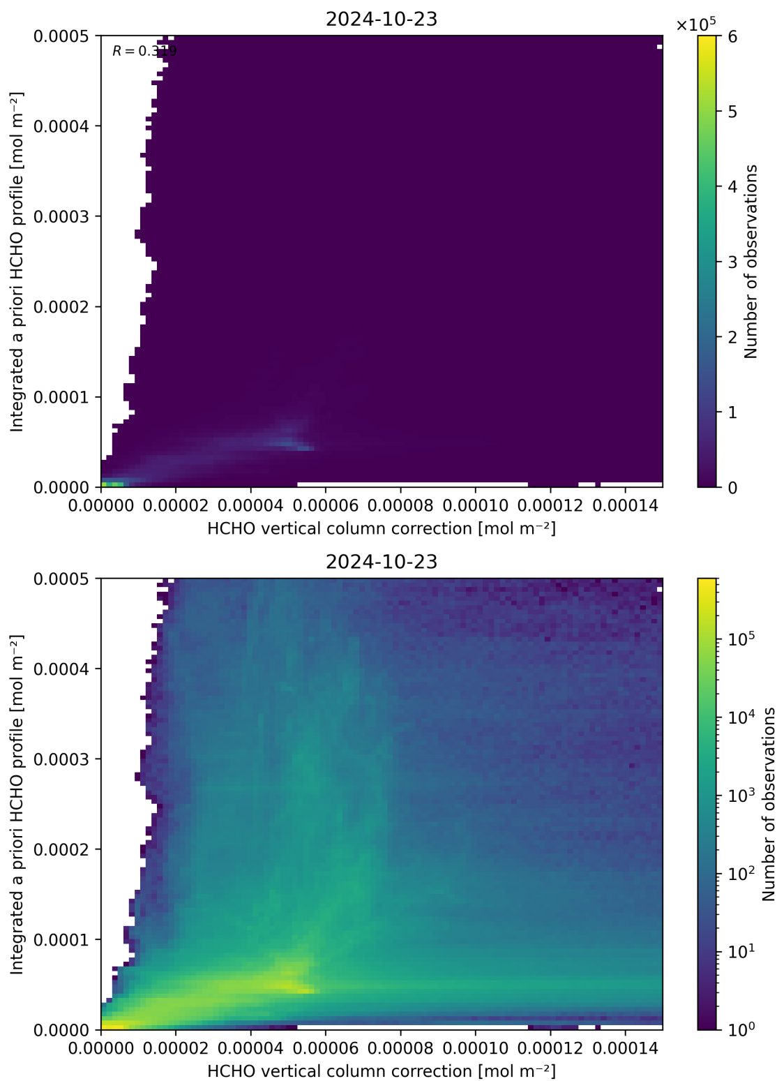
Figure 122: Scatter density plot of “HCHO vertical column correction” against “Integrated a priori HCHO profile” for 2024-10-22 to 2024-10-24.
