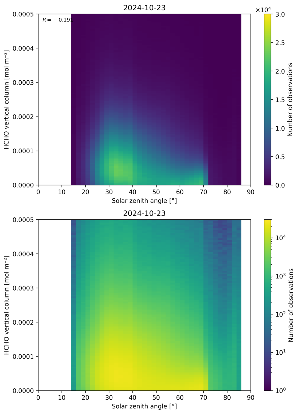
Figure 177: Scatter density plot of “Solar zenith angle” against “HCHO vertical column” for 2024-10-22 to 2024-10-24.
