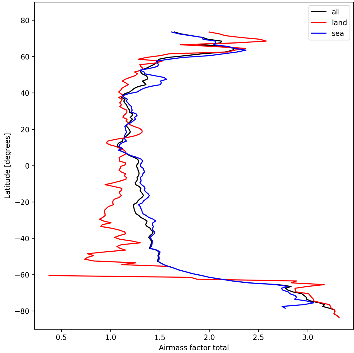
Figure 26: Zonal average of “Airmass factor total” for 2024-10-22 to 2024-10-24.
