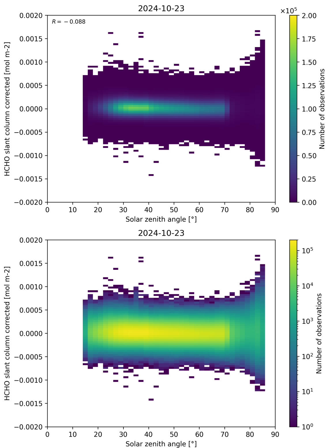
Figure 171: Scatter density plot of “Solar zenith angle” against “HCHO slant column corrected” for 2024-10-22 to 2024-10-24.
