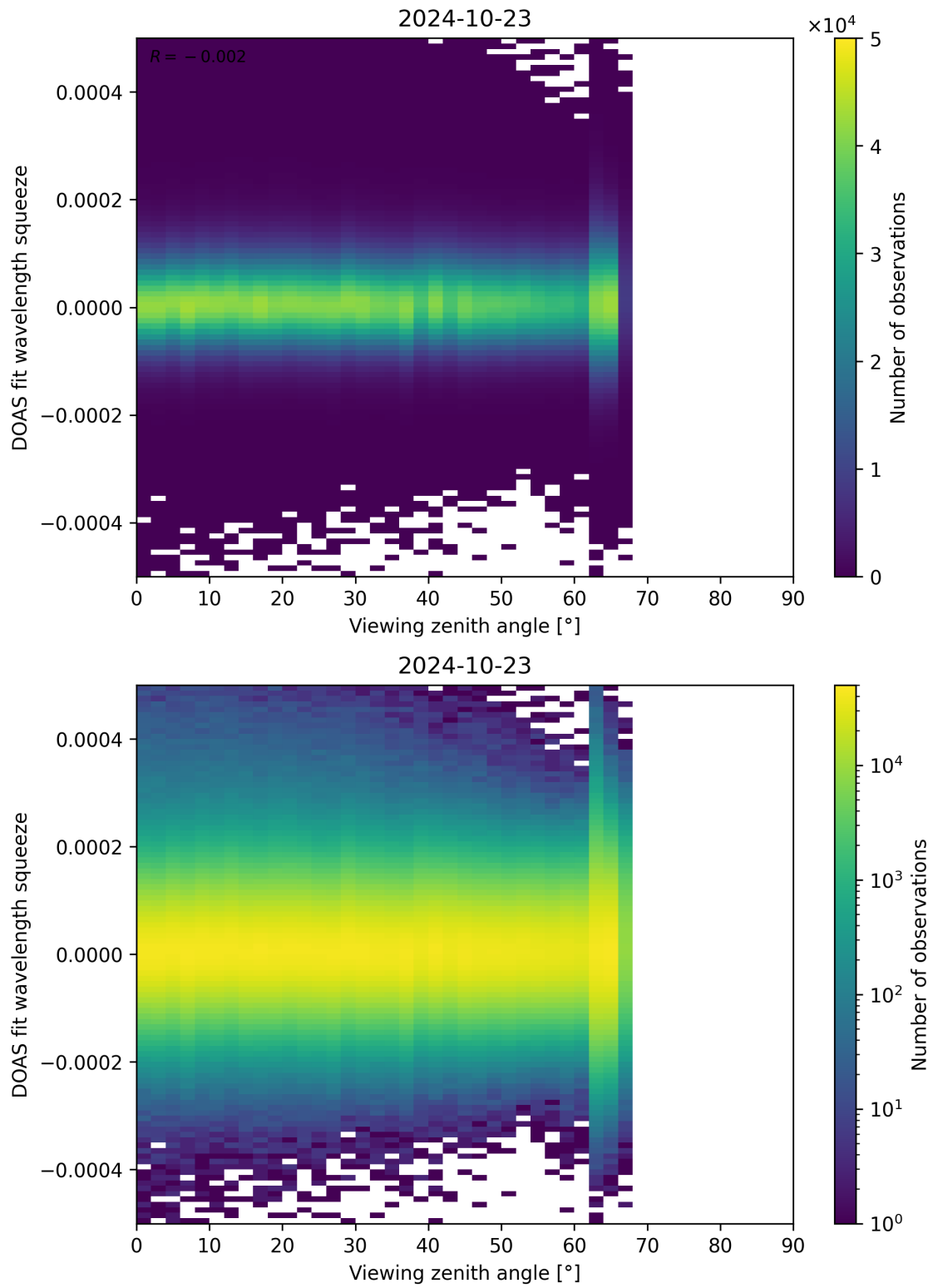
Figure 184: Scatter density plot of “Viewing zenith angle” against “DOAS fit wavelength squeeze” for 2024-10-22 to 2024-10-24.
