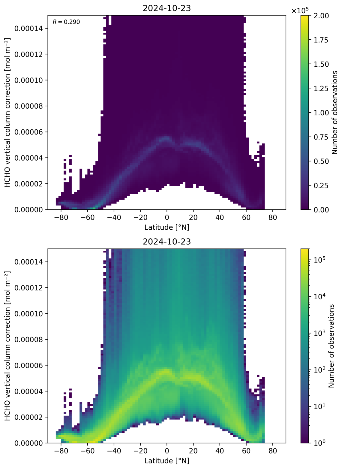
Figure 164: Scatter density plot of “Latitude” against “HCHO vertical column correction” for 2024-10-22 to 2024-10-24.
