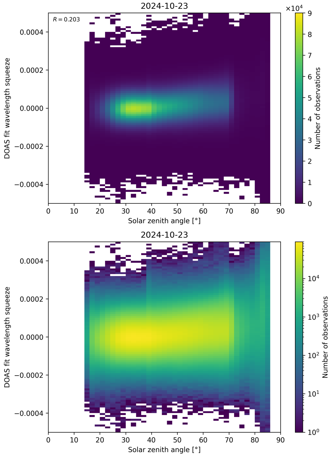
Figure 169: Scatter density plot of “Solar zenith angle” against “DOAS fit wavelength squeeze” for 2024-10-22 to 2024-10-24.
