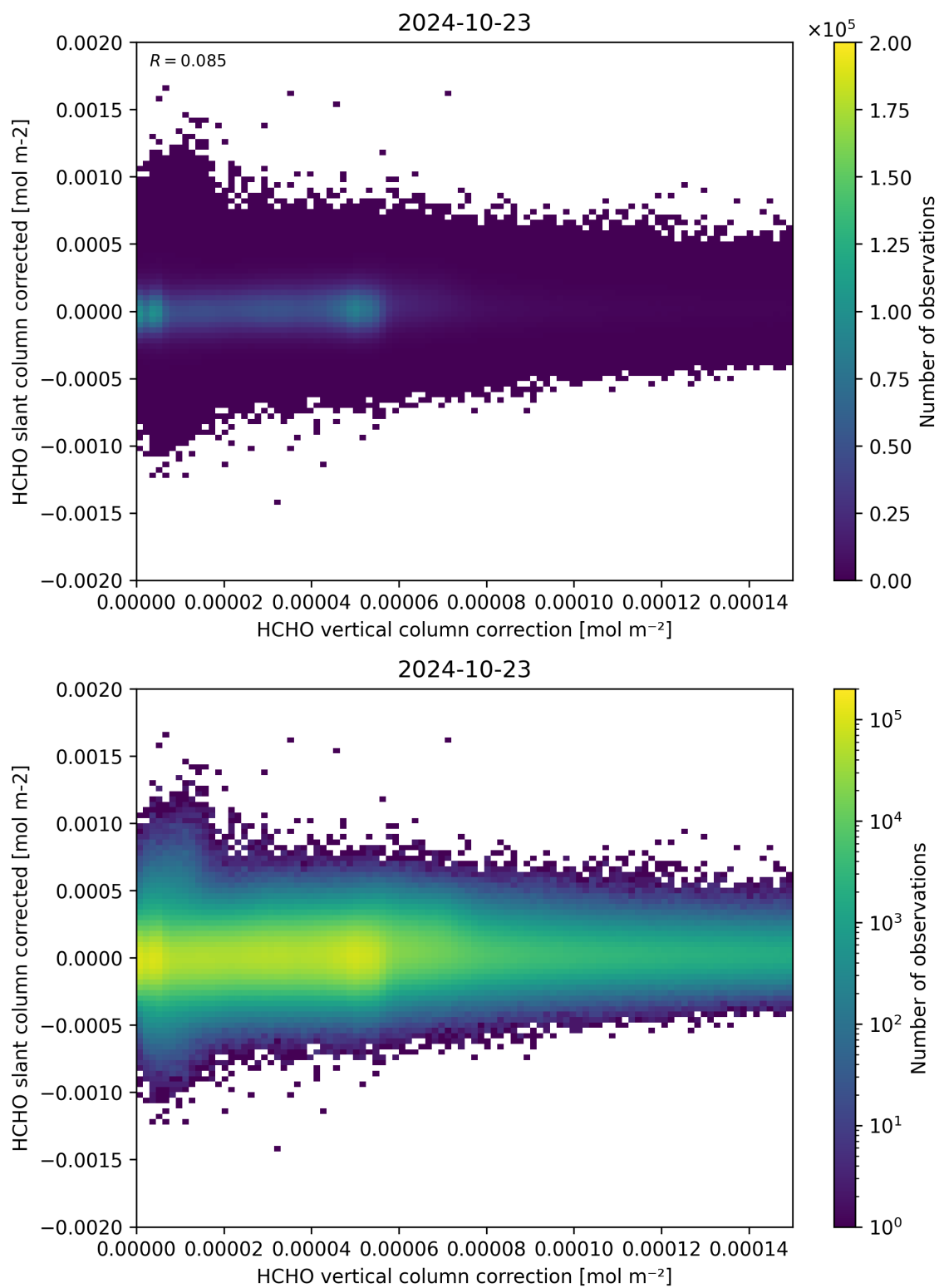
Figure 116: Scatter density plot of “HCHO vertical column correction” against “HCHO slant column corrected” for 2024-10-22 to 2024-10-24.
