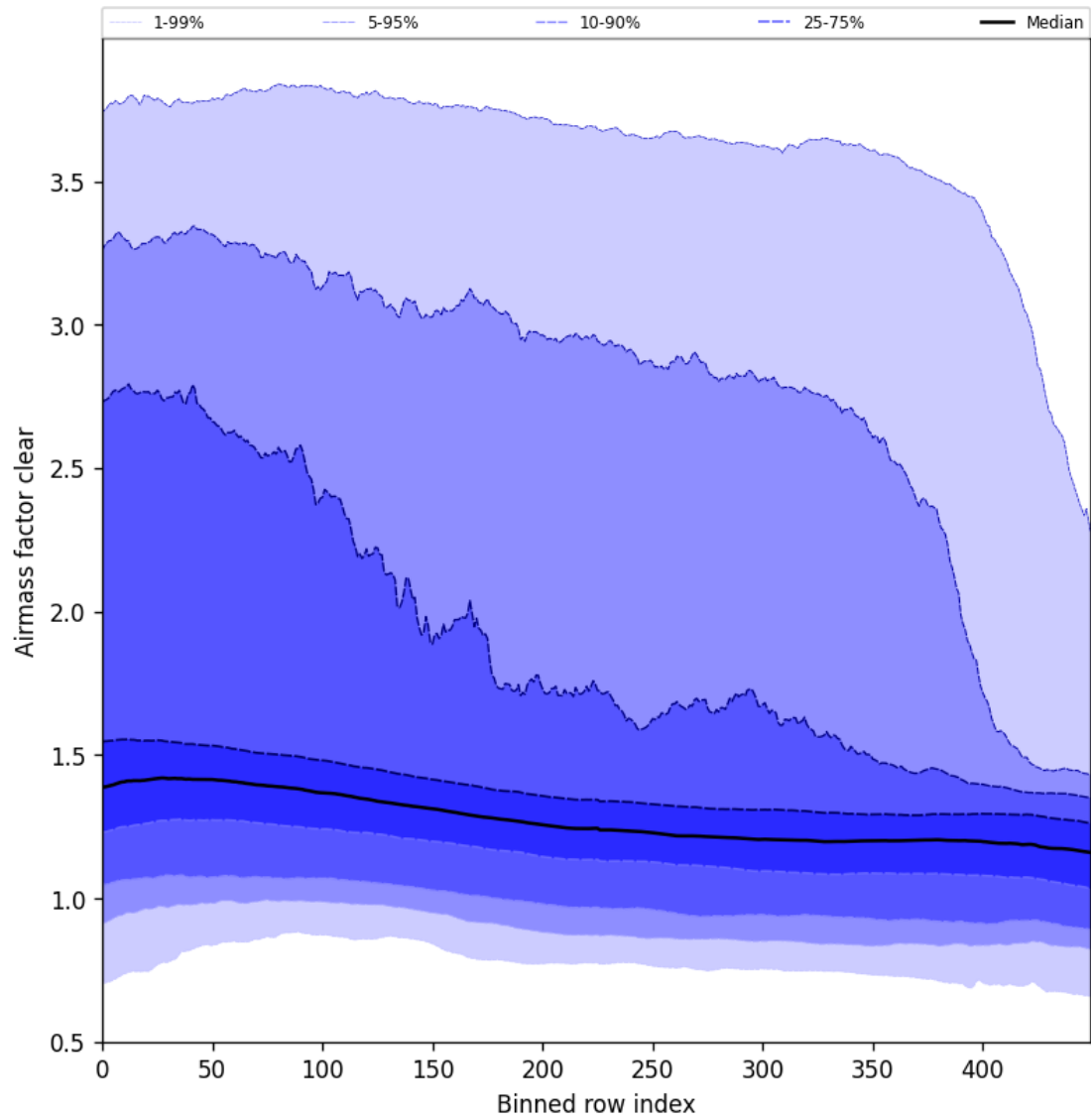
Figure 56: Along track statistics of “Airmass factor clear” for 2024-10-22 to 2024-10-24
