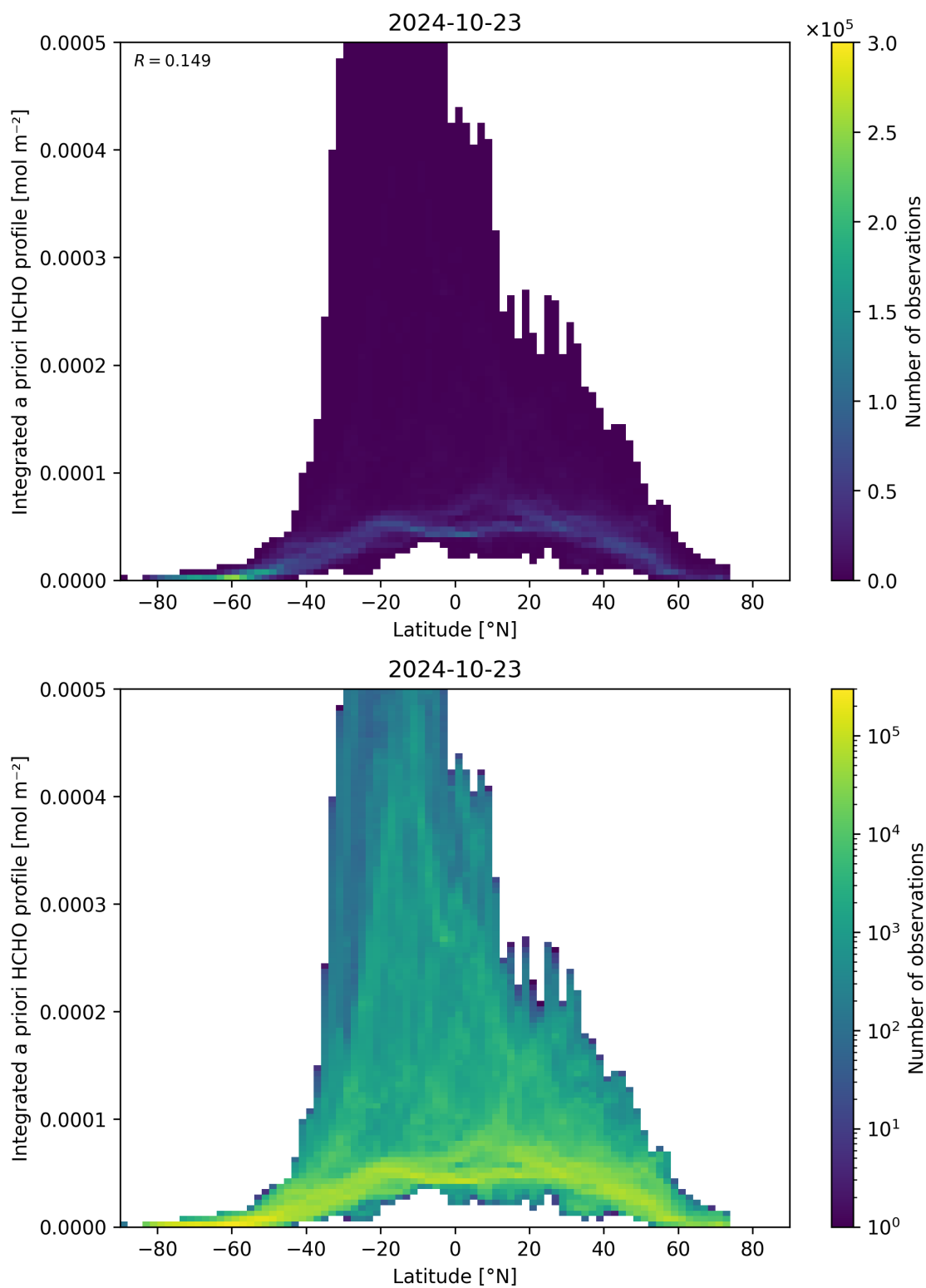
Figure 166: Scatter density plot of “Latitude” against “Integrated a priori HCHO profile” for 2024-10-22 to 2024-10-24.
