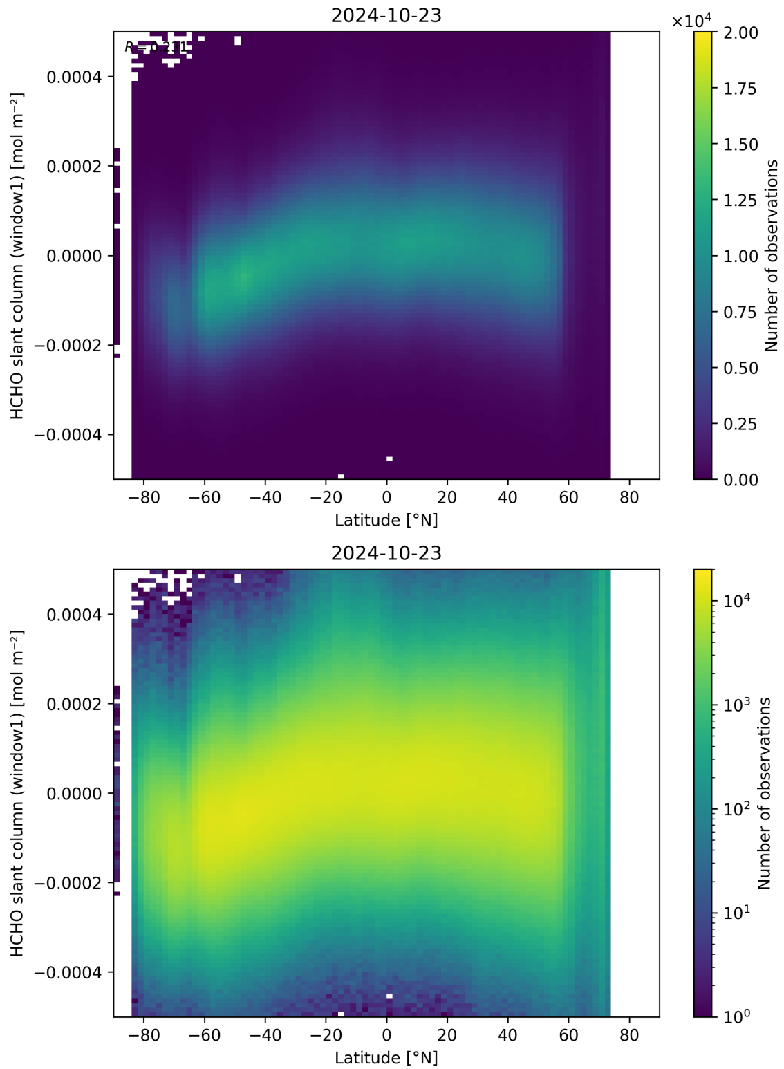
Figure 159: Scatter density plot of “Latitude” against “HCHO slant column (window1)” for 2024-10-22 to 2024-10-24.
