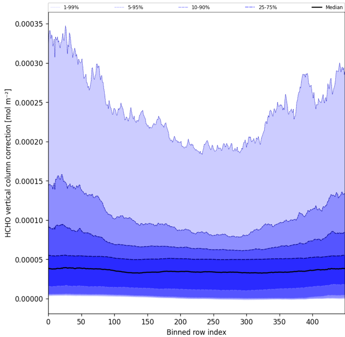
Figure 51: Along track statistics of “HCHO vertical column correction” for 2024-10-22 to 2024-10-24
