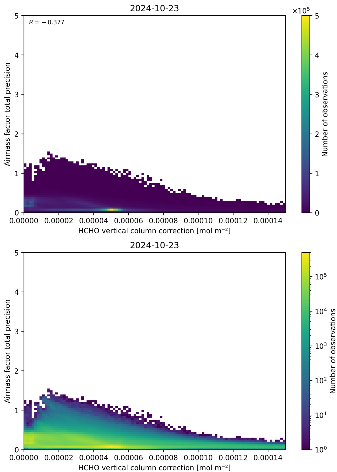
Figure 121: Scatter density plot of “HCHO vertical column correction” against “Airmass factor total precision” for 2024-10-22 to 2024-10-24.
