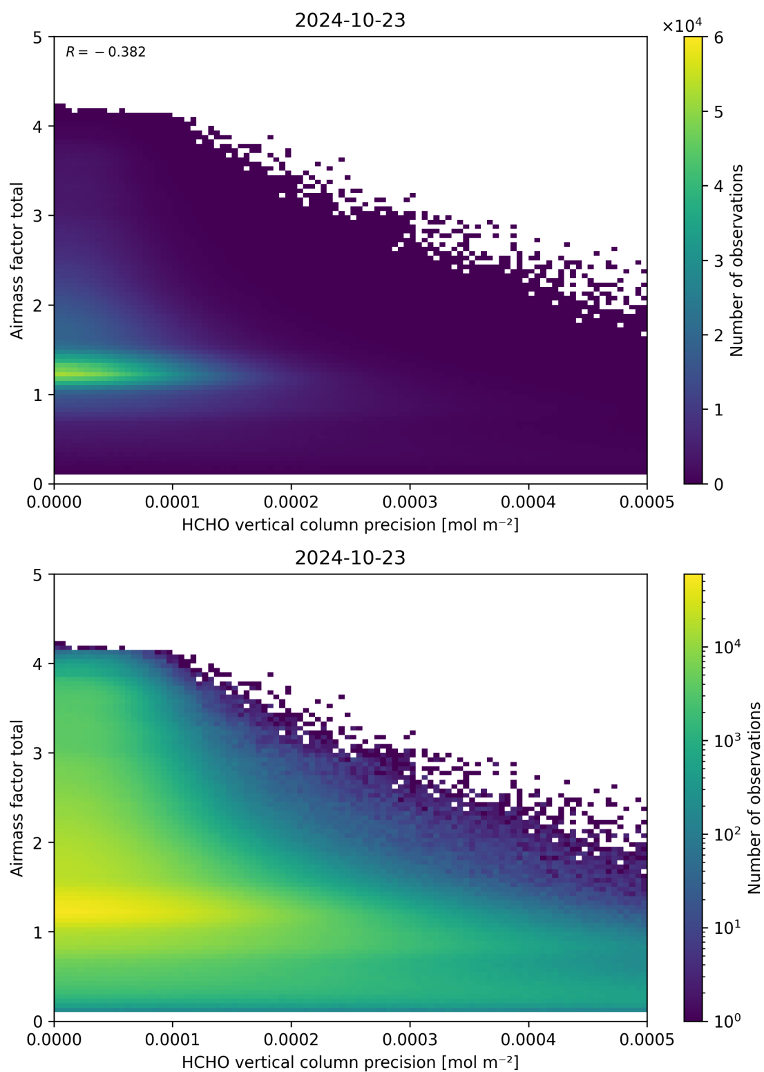
Figure 144: Scatter density plot of “HCHO vertical column precision” against “Airmass factor total” for 2024-10-22 to 2024-10-24.
