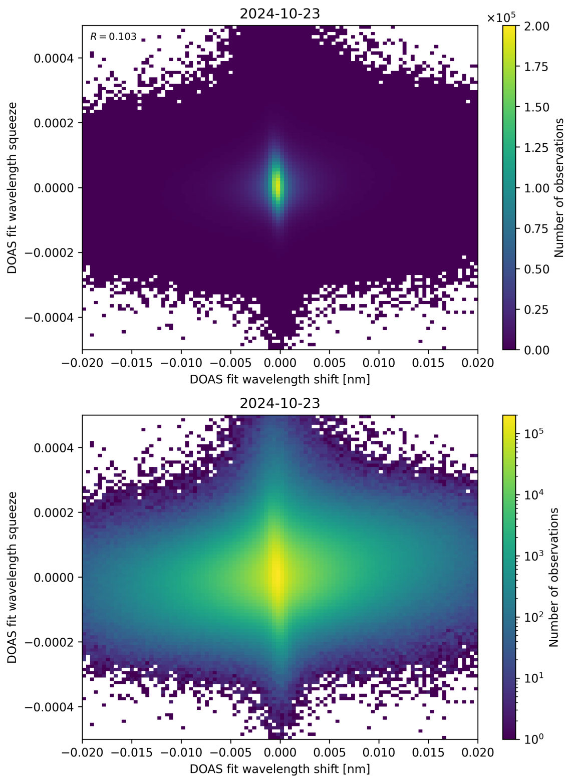
Figure 65: Scatter density plot of “DOAS fit wavelength shift” against “DOAS fit wavelength squeeze” for 2024-10-22 to 2024-10-24.
