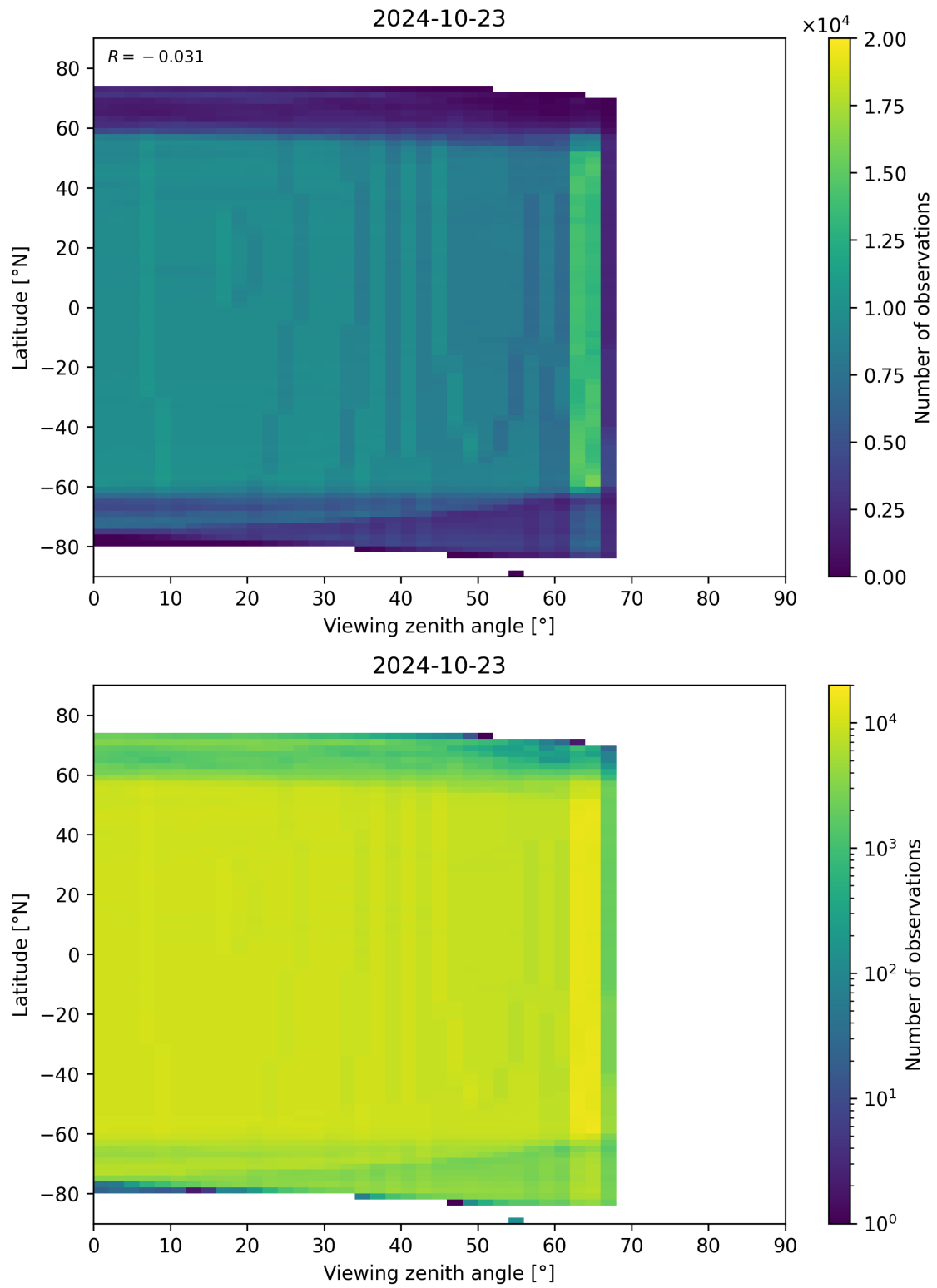
Figure 196: Scatter density plot of “Viewing zenith angle” against “Latitude” for 2024-10-22 to 2024-10-24.
