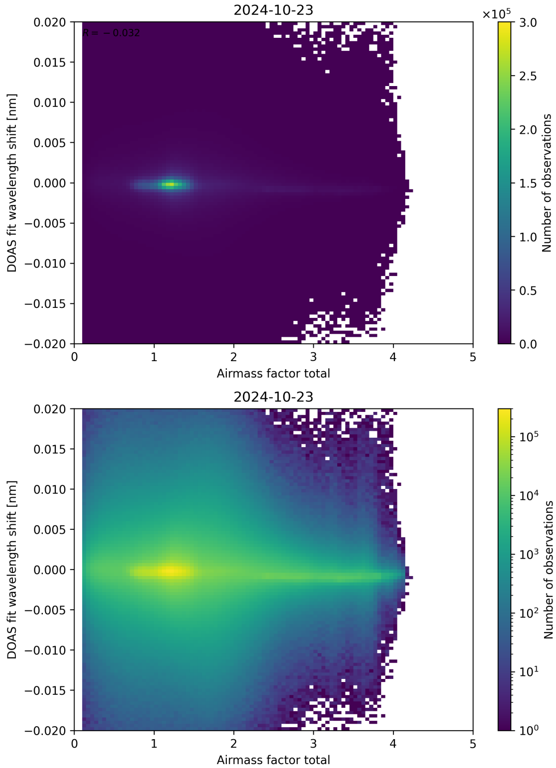
Figure 98: Scatter density plot of “Airmass factor total” against “DOAS fit wavelength shift” for 2024-10-22 to 2024-10-24.
