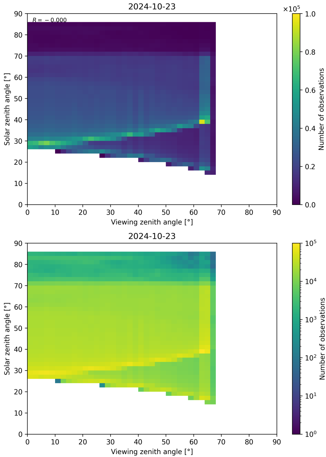
Figure 197: Scatter density plot of “Viewing zenith angle” against “Solar zenith angle” for 2024-10-22 to 2024-10-24.
