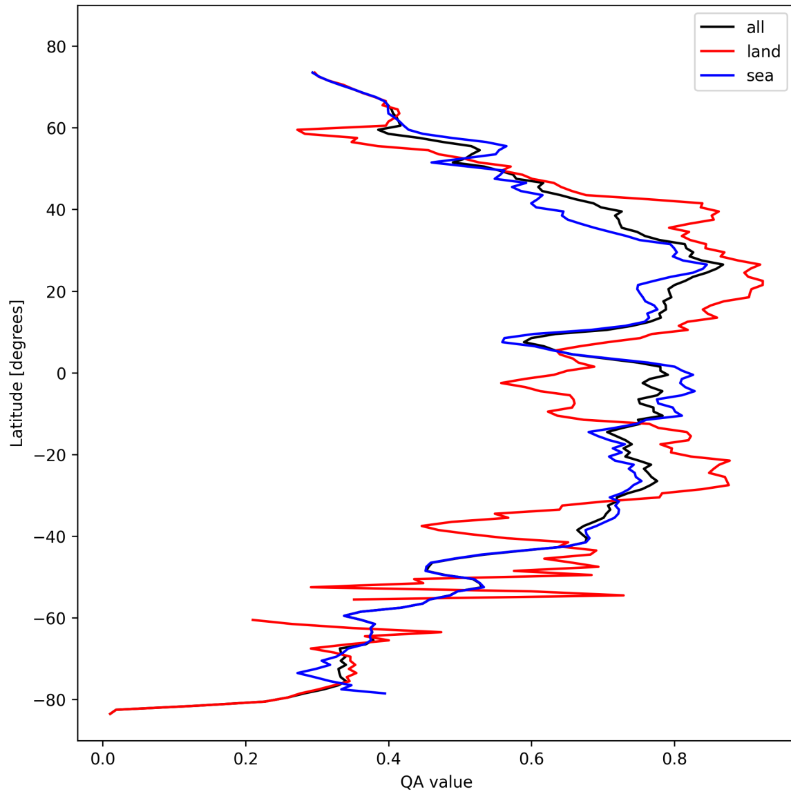
Figure 20: Zonal average of “QA value” for 2024-10-22 to 2024-10-24.
