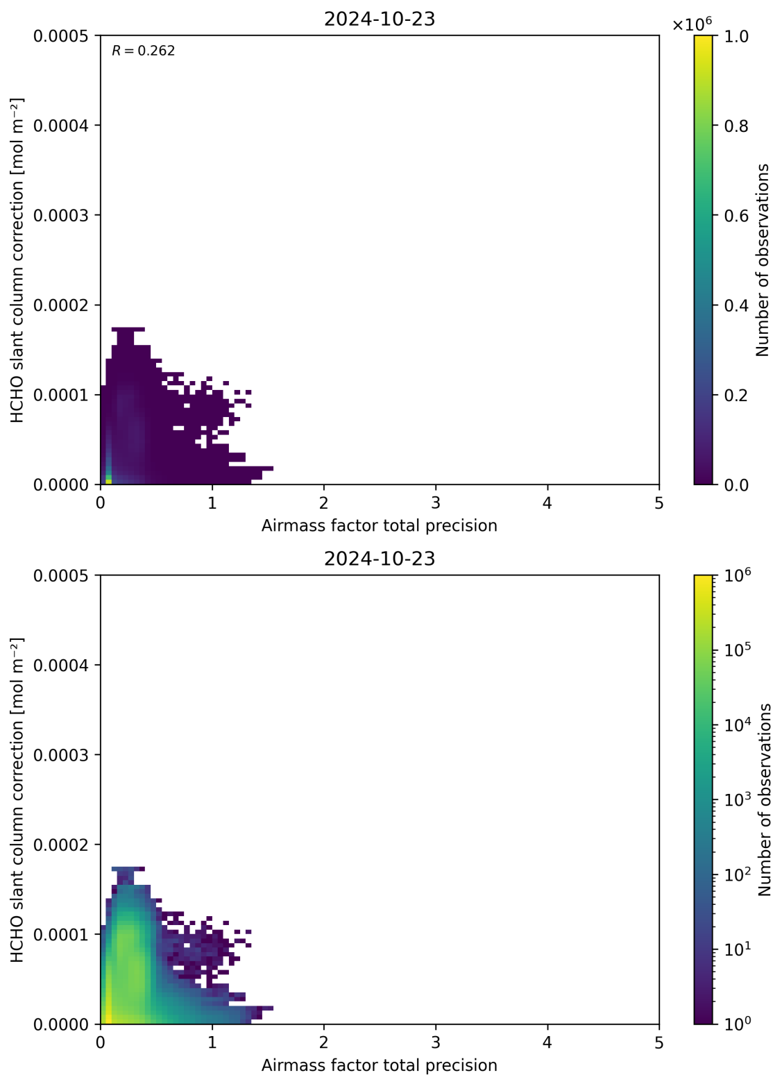
Figure 110: Scatter density plot of “Airmass factor total precision” against “HCHO slant column correction” for 2024-10-22 to 2024-10-24.
