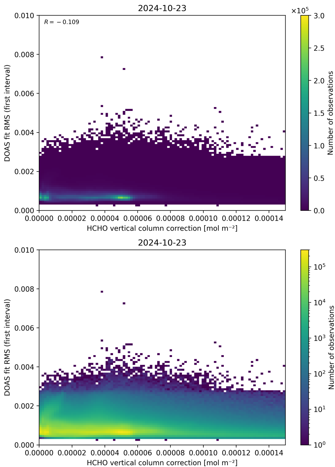
Figure 112: Scatter density plot of “HCHO vertical column correction” against “DOAS fit RMS (first interval)” for 2024-10-22 to 2024-10-24.
