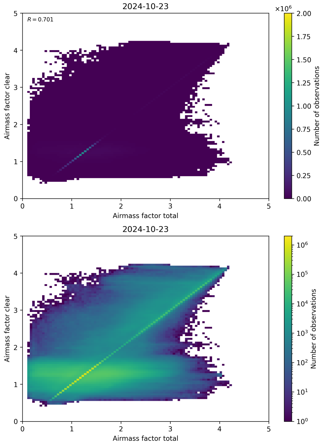
Figure 100: Scatter density plot of “Airmass factor total” against “Airmass factor clear” for 2024-10-22 to 2024-10-24.
