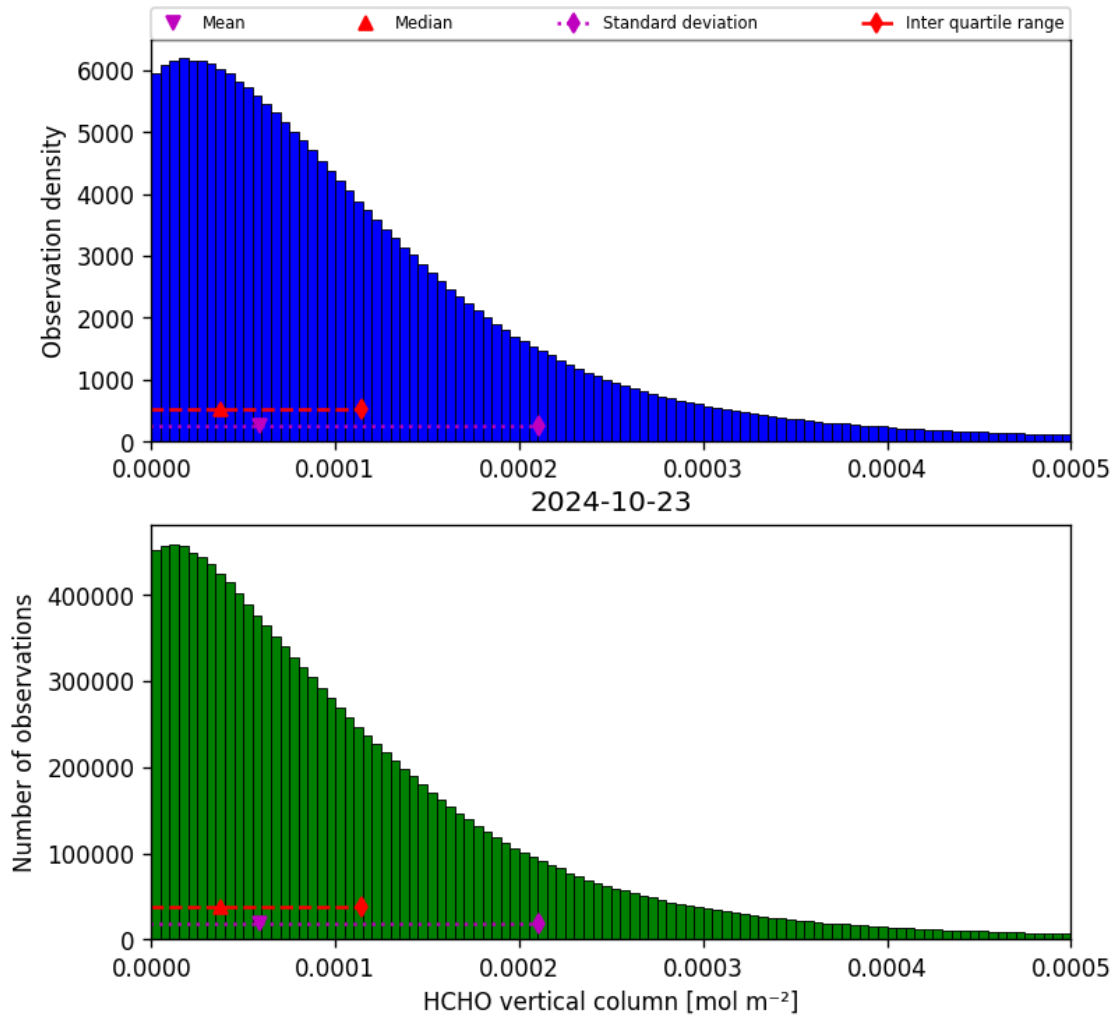
Figure 35: Histogram of “HCHO vertical column” for 2024-10-22 to 2024-10-24
