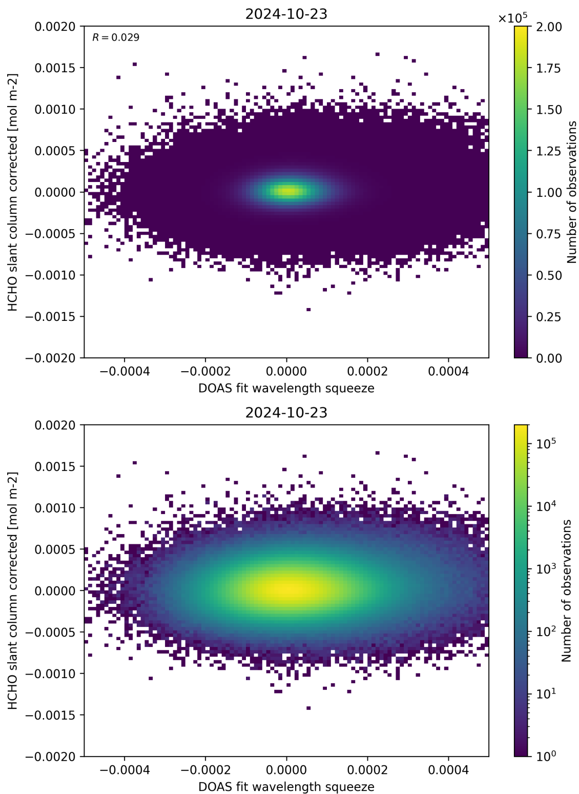
Figure 69: Scatter density plot of “DOAS fit wavelength squeeze” against “HCHO slant column corrected” for 2024-10-22 to 2024-10-24.
