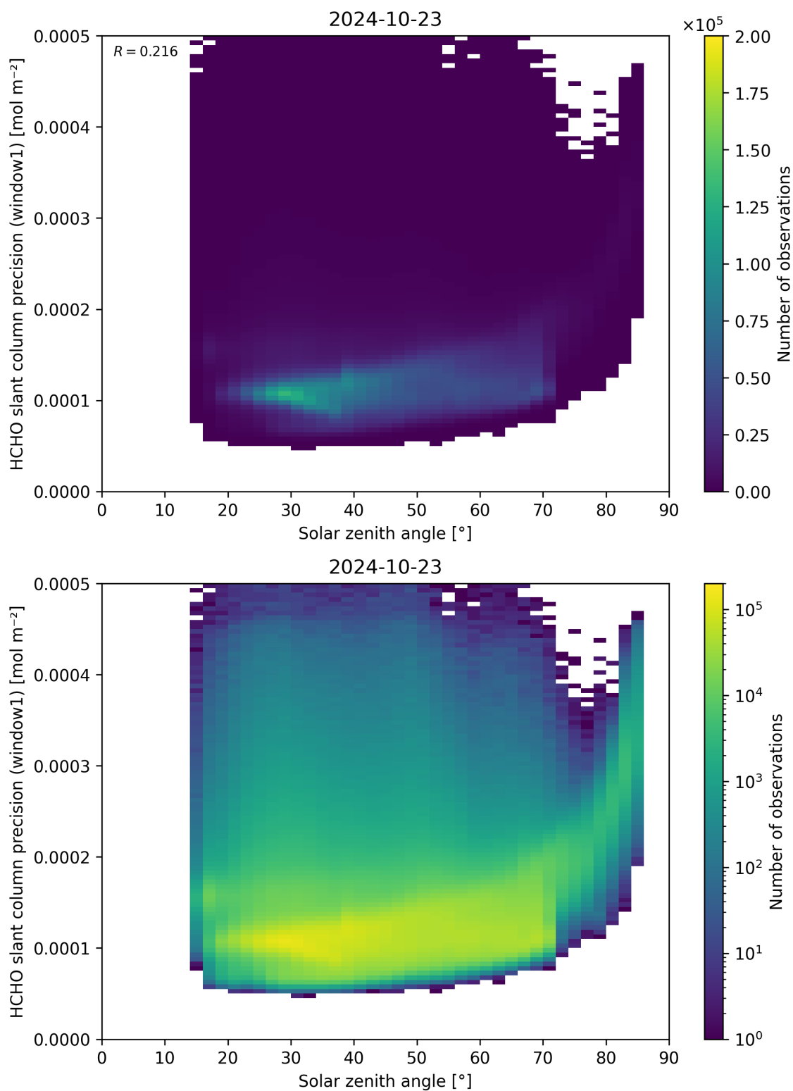
Figure 174: Scatter density plot of “Solar zenith angle” against “HCHO slant column precision (window1)” for 2024-10-22 to 2024-10-24.
