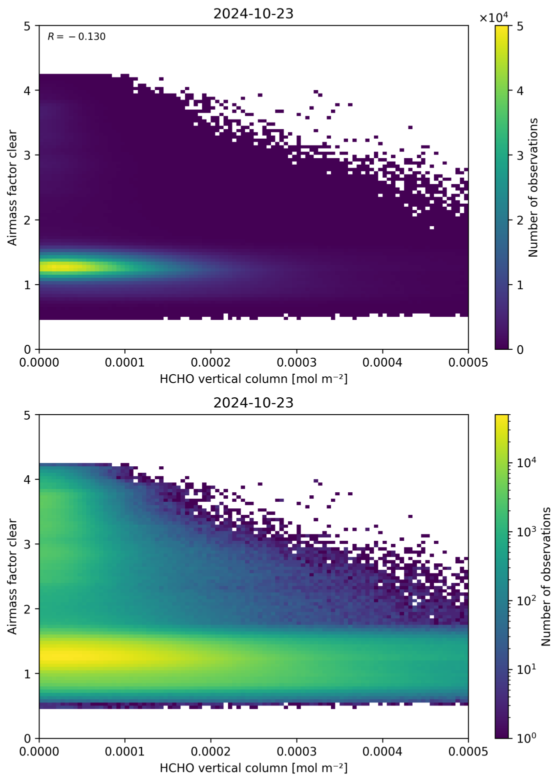
Figure 126: Scatter density plot of “HCHO vertical column” against “Airmass factor clear” for 2024-10-22 to 2024-10-24.
