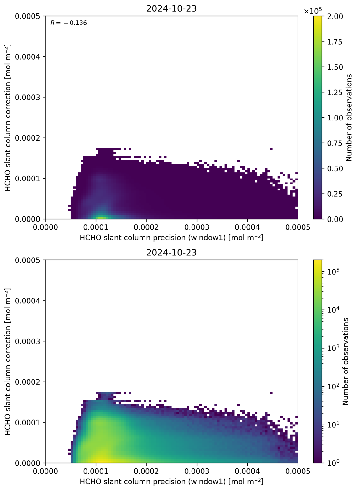
Figure 93: Scatter density plot of “HCHO slant column precision (window1)” against “HCHO slant column correction” for 2024-10-22 to 2024-10-24.
