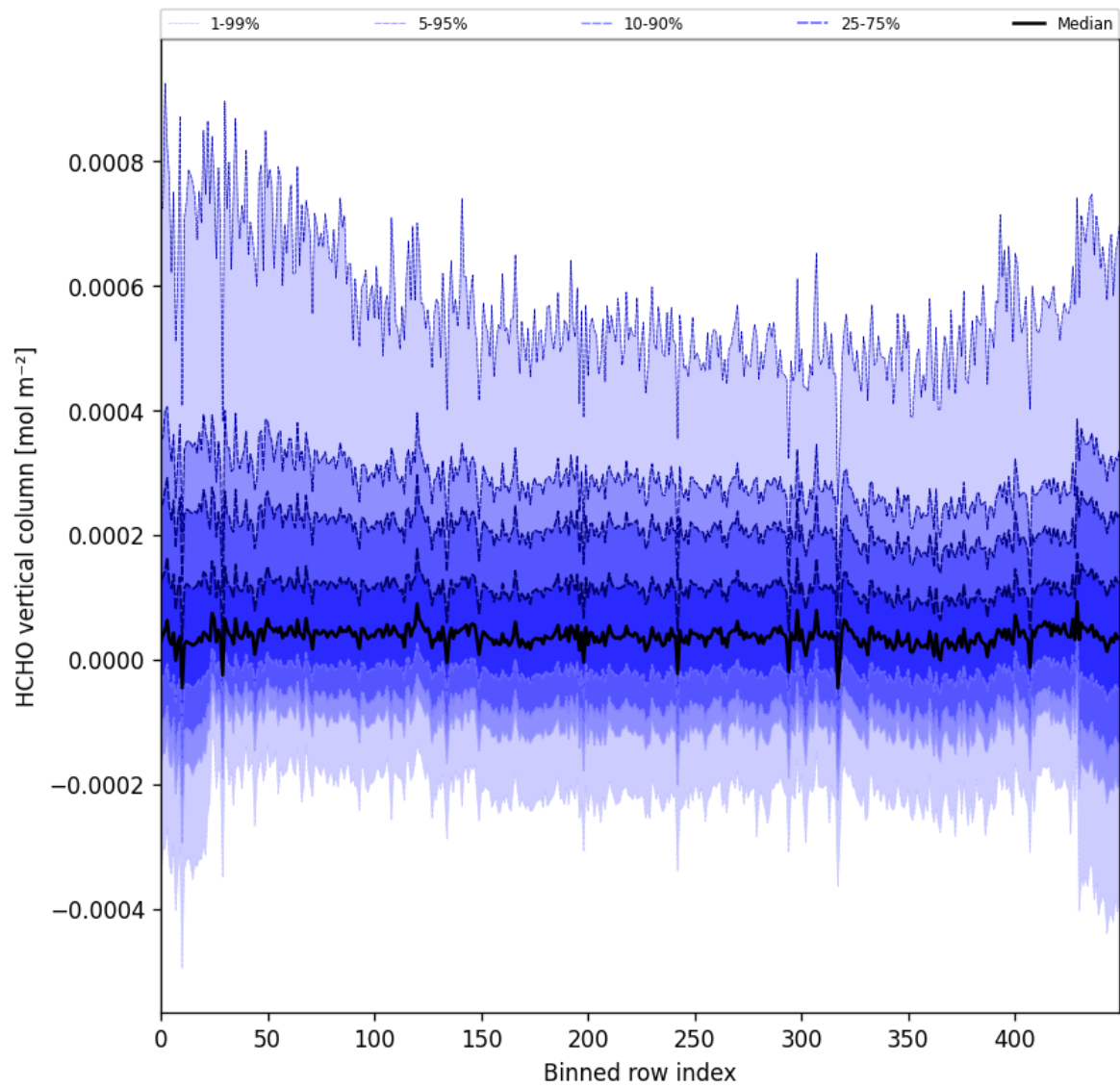
Figure 49: Along track statistics of “HCHO vertical column” for 2024-10-22 to 2024-10-24
