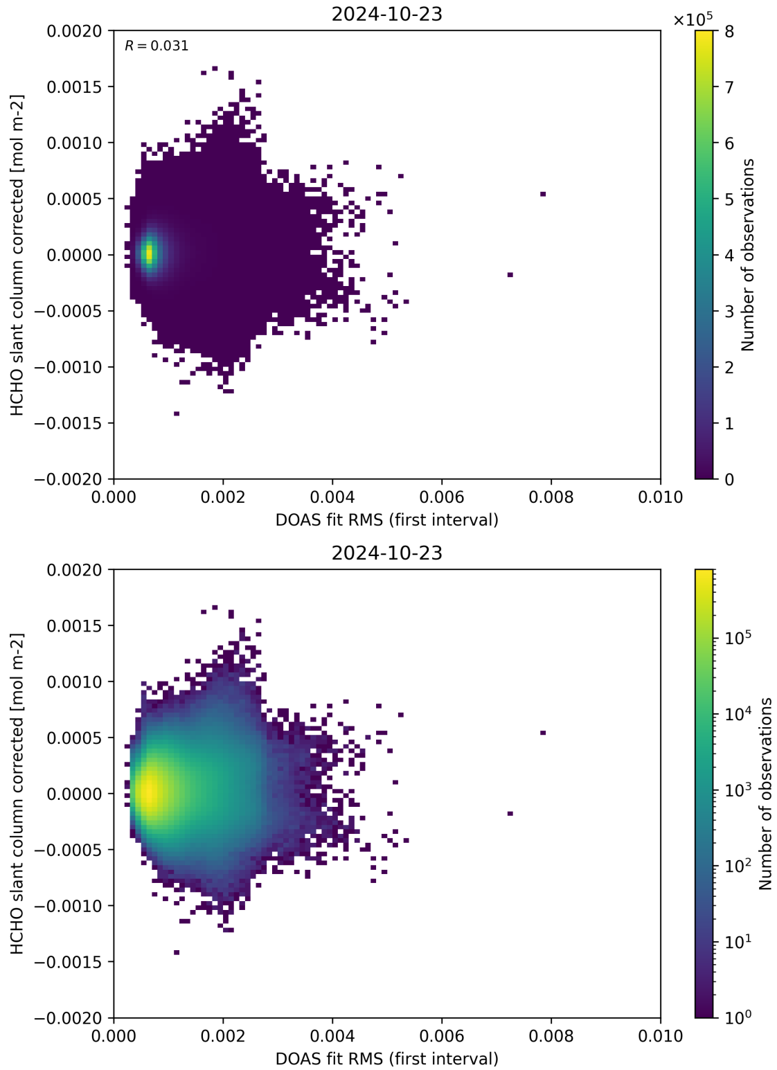
Figure 62: Scatter density plot of “DOAS fit RMS (first interval)” against “HCHO slant column corrected” for 2024-10-22 to 2024-10-24.
