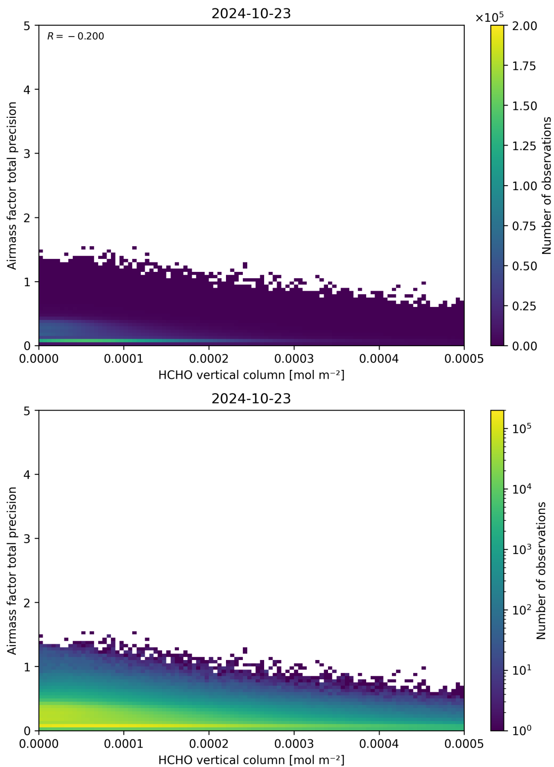
Figure 132: Scatter density plot of “HCHO vertical column” against “Airmass factor total precision” for 2024-10-22 to 2024-10-24.
