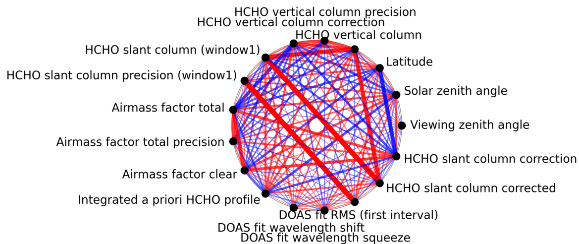
Figure 1: Map of correlation graph for 2024-10-22 to 2024-10-24.
