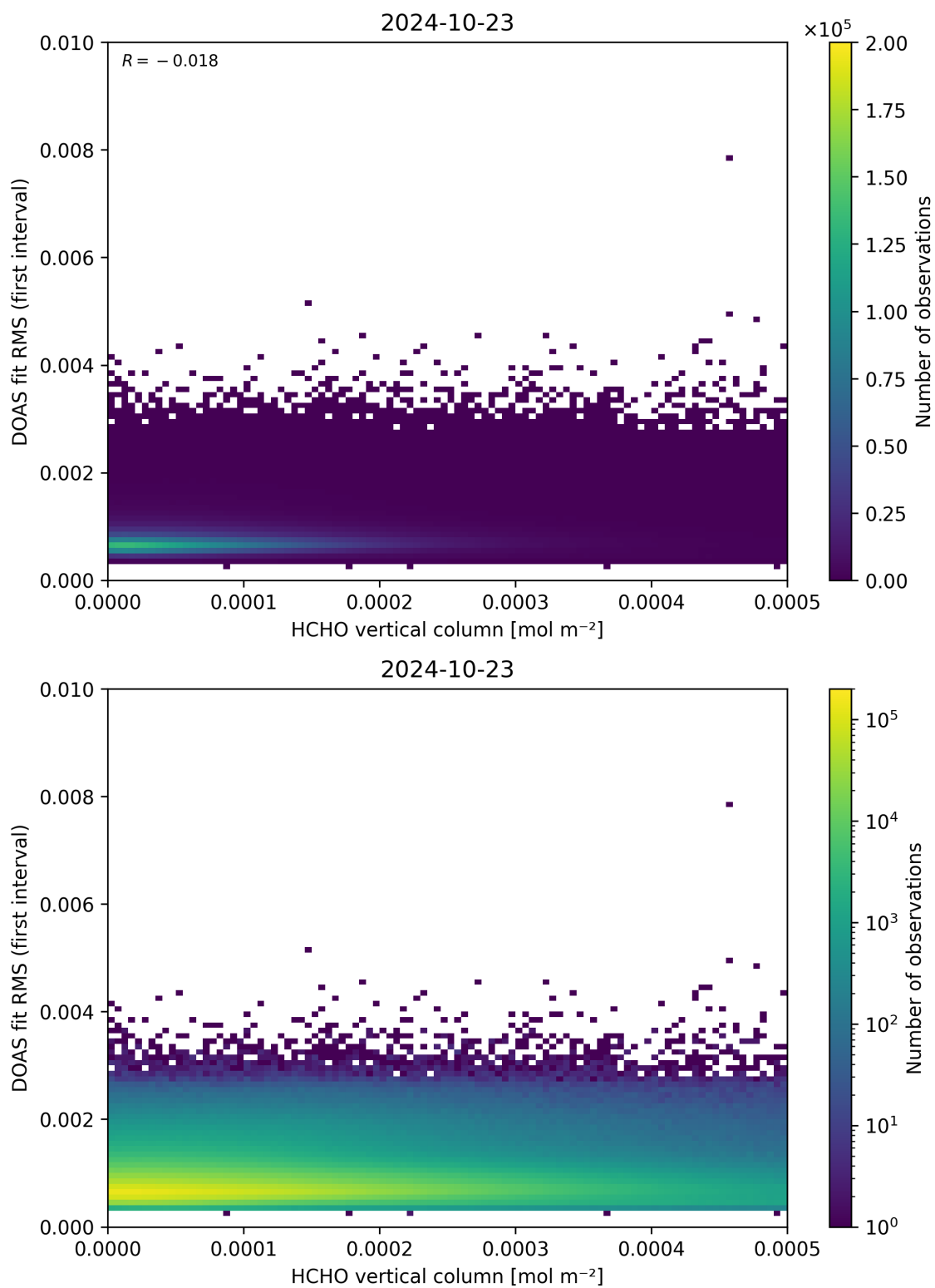
Figure 123: Scatter density plot of “HCHO vertical column” against “DOAS fit RMS (first interval)” for 2024-10-22 to 2024-10-24.
