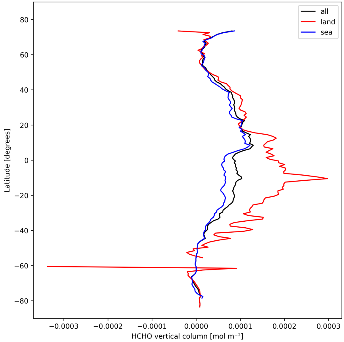
Figure 21: Zonal average of “HCHO vertical column” for 2024-10-22 to 2024-10-24.
