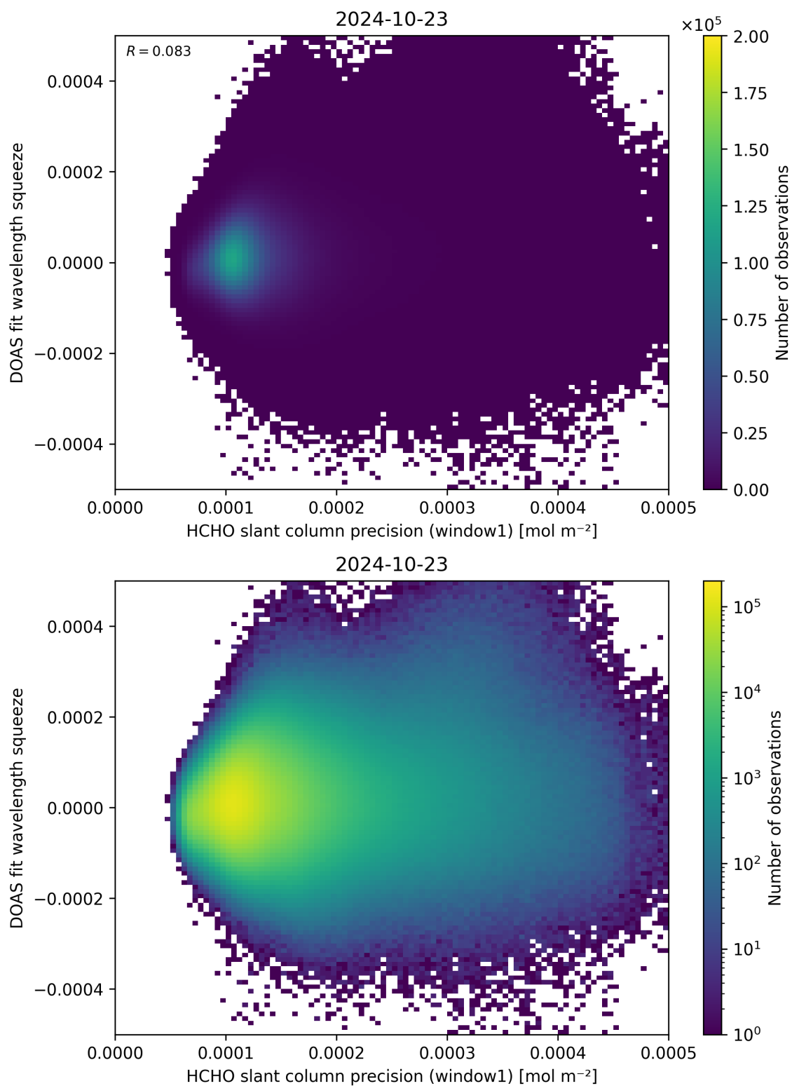
Figure 90: Scatter density plot of “HCHO slant column precision (window1)” against “DOAS fit wavelength squeeze” for 2024-10-22 to 2024-10-24.
