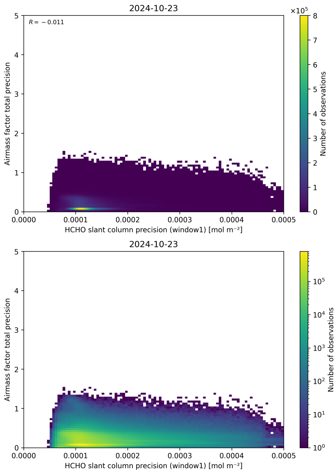
Figure 95: Scatter density plot of “HCHO slant column precision (window1)” against “Airmass factor total precision” for 2024-10-22 to 2024-10-24.
