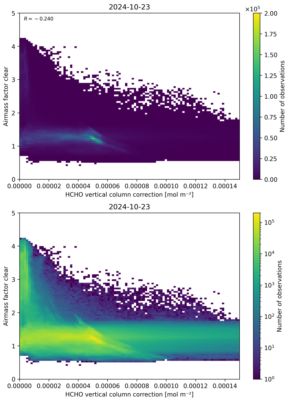
Figure 115: Scatter density plot of “HCHO vertical column correction” against “Airmass factor clear” for 2024-10-22 to 2024-10-24.
