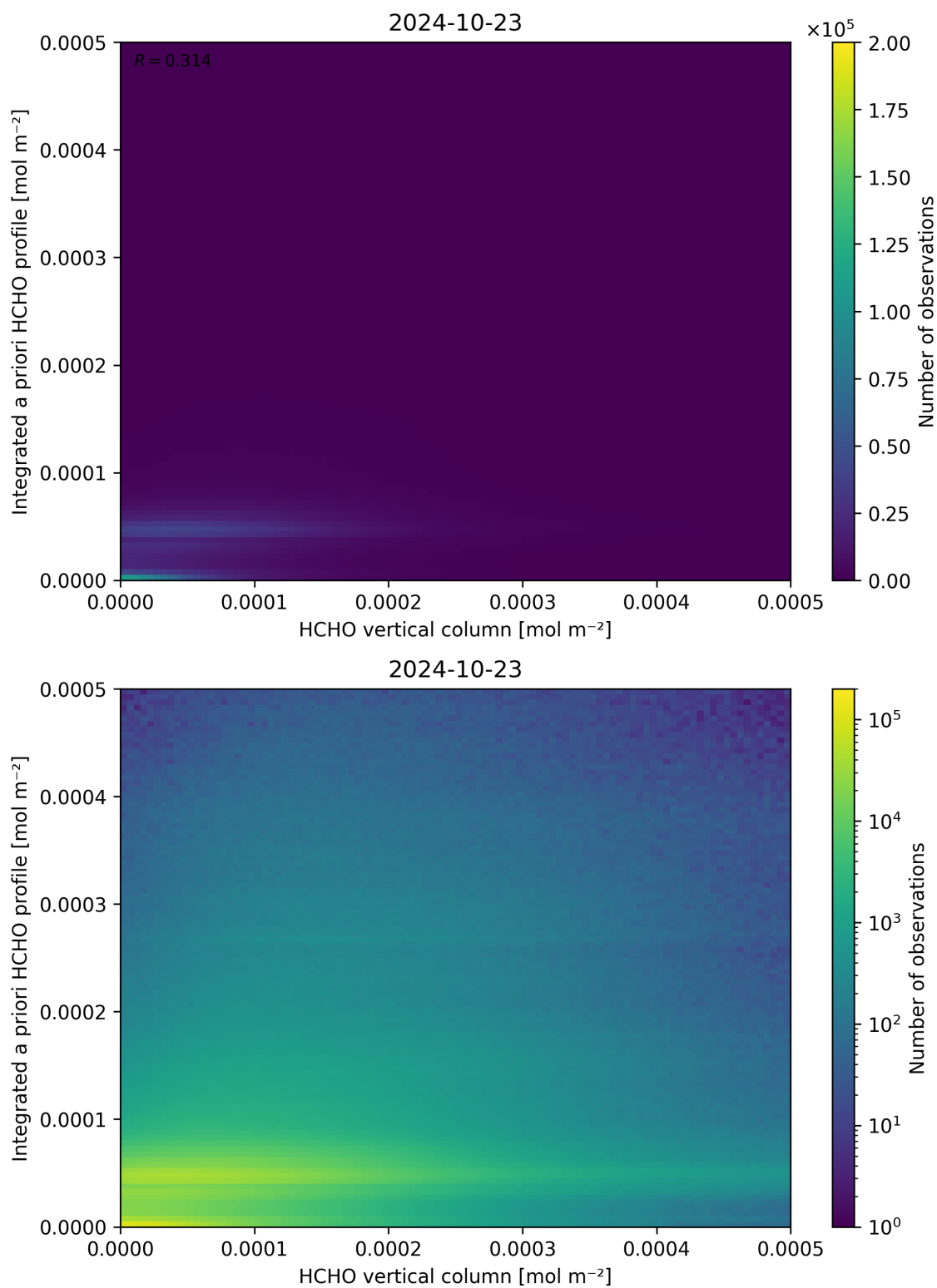
Figure 135: Scatter density plot of “HCHO vertical column” against “Integrated a priori HCHO profile” for 2024-10-22 to 2024-10-24.
