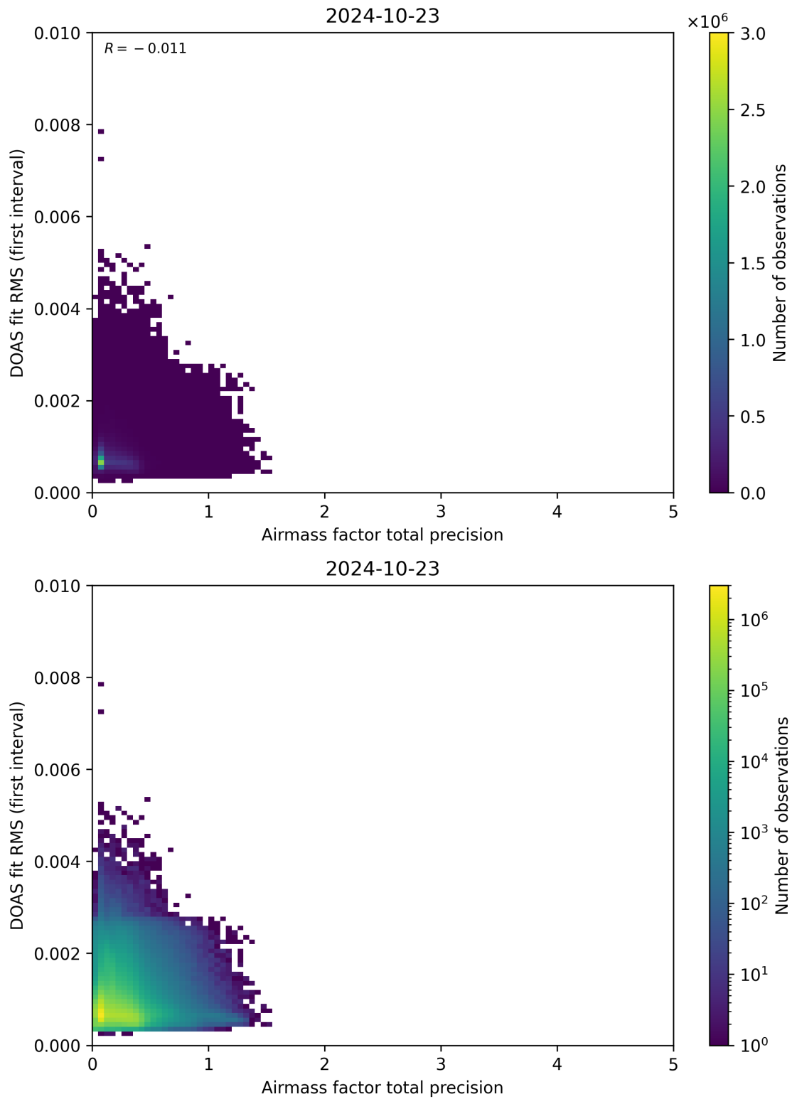
Figure 105: Scatter density plot of “Airmass factor total precision” against “DOAS fit RMS (first interval)” for 2024-10-22 to 2024-10-24.
