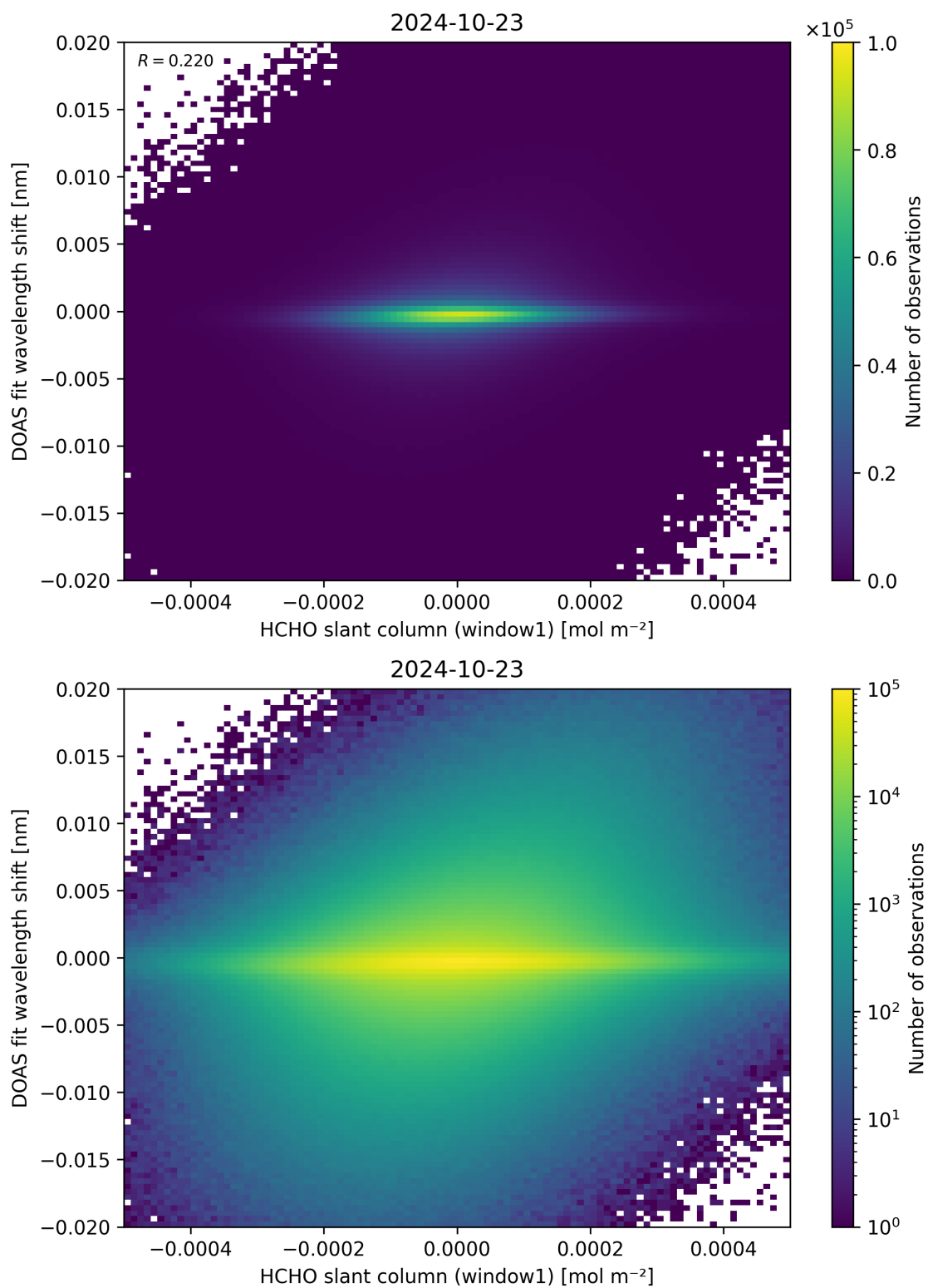
Figure 79: Scatter density plot of “HCHO slant column (window1)” against “DOAS fit wavelength shift” for 2024-10-22 to 2024-10-24.
