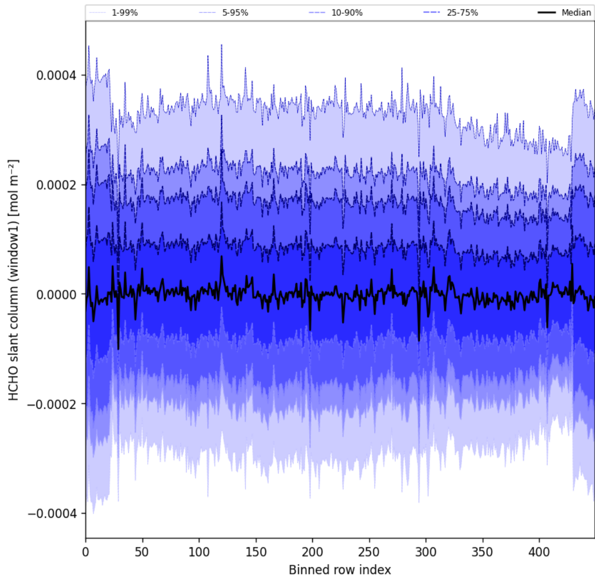
Figure 52: Along track statistics of “HCHO slant column (window1)” for 2024-10-22 to 2024-10-24
