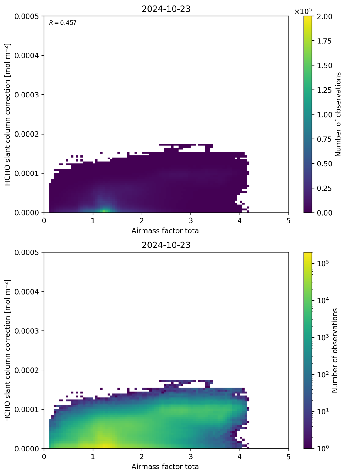
Figure 102: Scatter density plot of “Airmass factor total” against “HCHO slant column correction” for 2024-10-22 to 2024-10-24.
