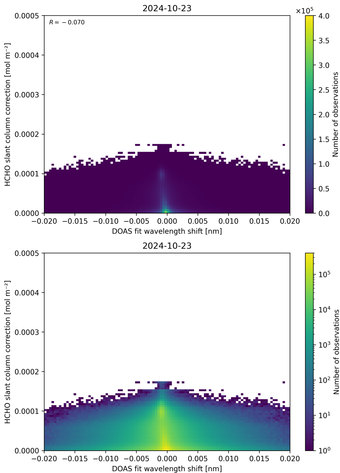
Figure 67: Scatter density plot of “DOAS fit wavelength shift” against “HCHO slant column correction” for 2024-10-22 to 2024-10-24.
