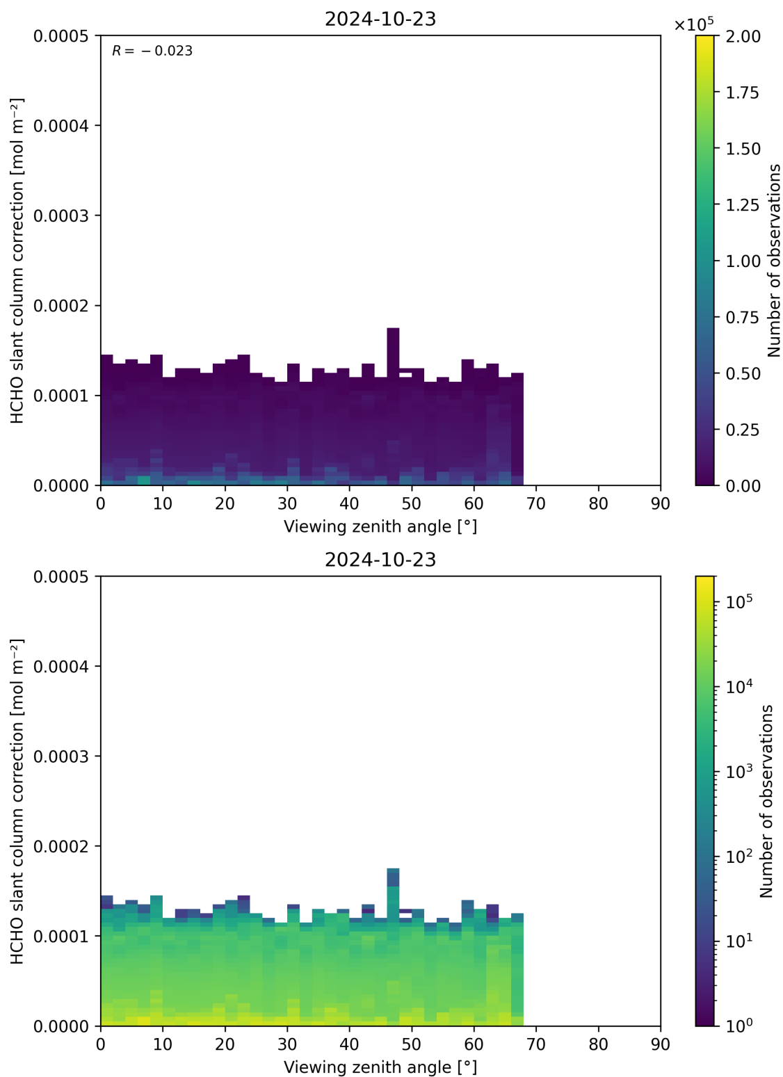
Figure 187: Scatter density plot of “Viewing zenith angle” against “HCHO slant column correction” for 2024-10-22 to 2024-10-24.
