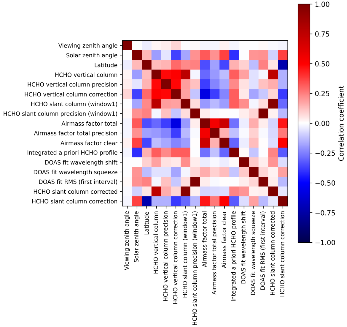
Figure 2: Map of correlation matrix for 2024-10-22 to 2024-10-24.
