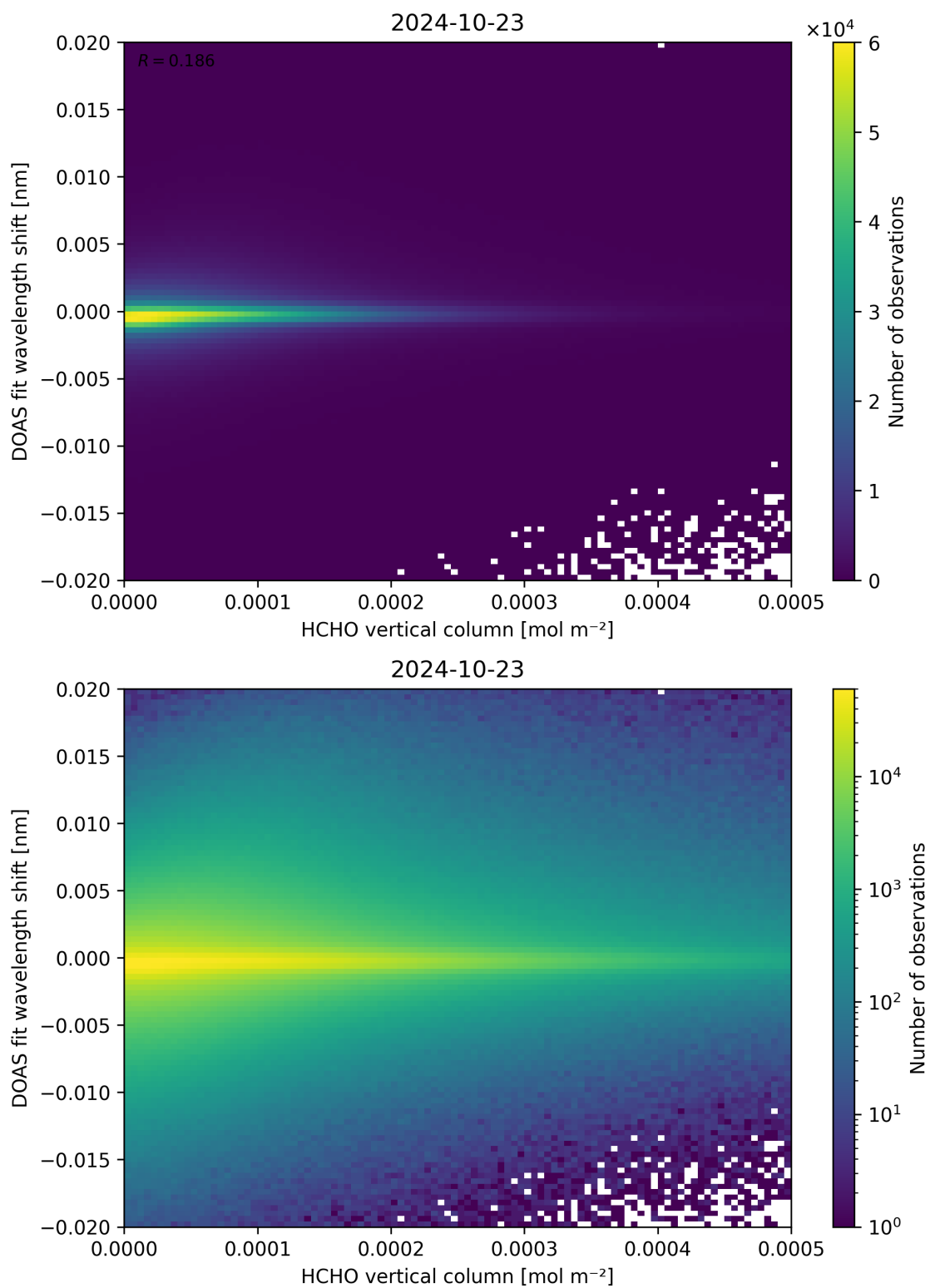
Figure 124: Scatter density plot of “HCHO vertical column” against “DOAS fit wavelength shift” for 2024-10-22 to 2024-10-24.
