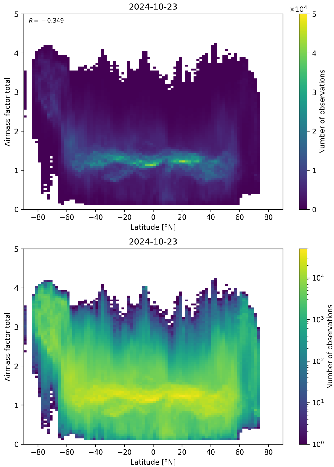
Figure 161: Scatter density plot of “Latitude” against “Airmass factor total” for 2024-10-22 to 2024-10-24.
