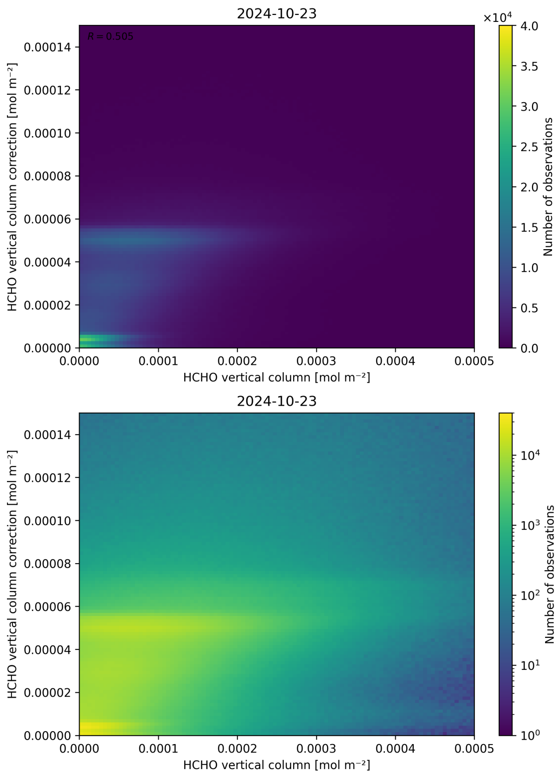
Figure 133: Scatter density plot of “HCHO vertical column” against “HCHO vertical column correction” for 2024-10-22 to 2024-10-24.
