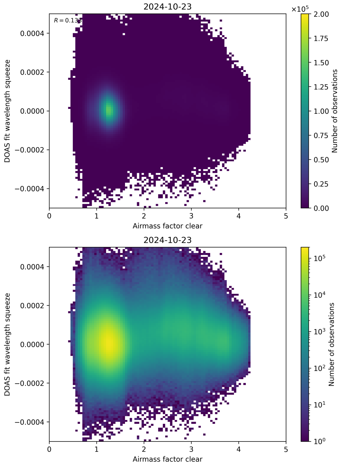
Figure 73: Scatter density plot of “Airmass factor clear” against “DOAS fit wavelength squeeze” for 2024-10-22 to 2024-10-24.
