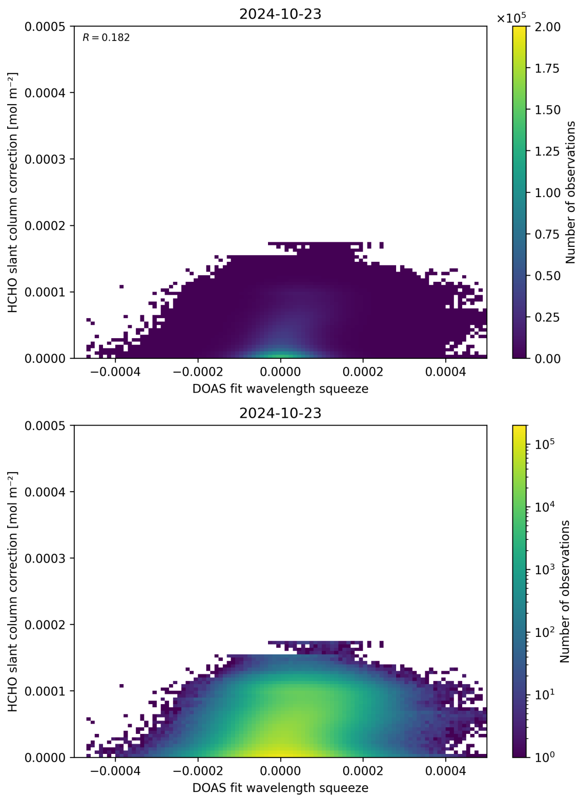
Figure 70: Scatter density plot of “DOAS fit wavelength squeeze” against “HCHO slant column correction” for 2024-10-22 to 2024-10-24.
