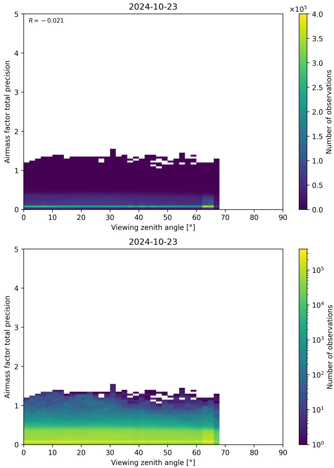
Figure 191: Scatter density plot of “Viewing zenith angle” against “Airmass factor total precision” for 2024-10-22 to 2024-10-24.
