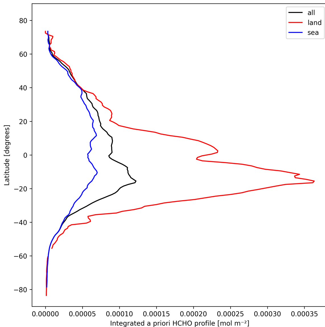
Figure 29: Zonal average of “Integrated a priori HCHO profile” for 2024-10-22 to 2024-10-24.
