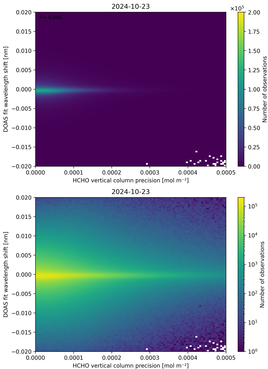
Figure 137: Scatter density plot of “HCHO vertical column precision” against “DOAS fit wavelength shift” for 2024-10-22 to 2024-10-24.
