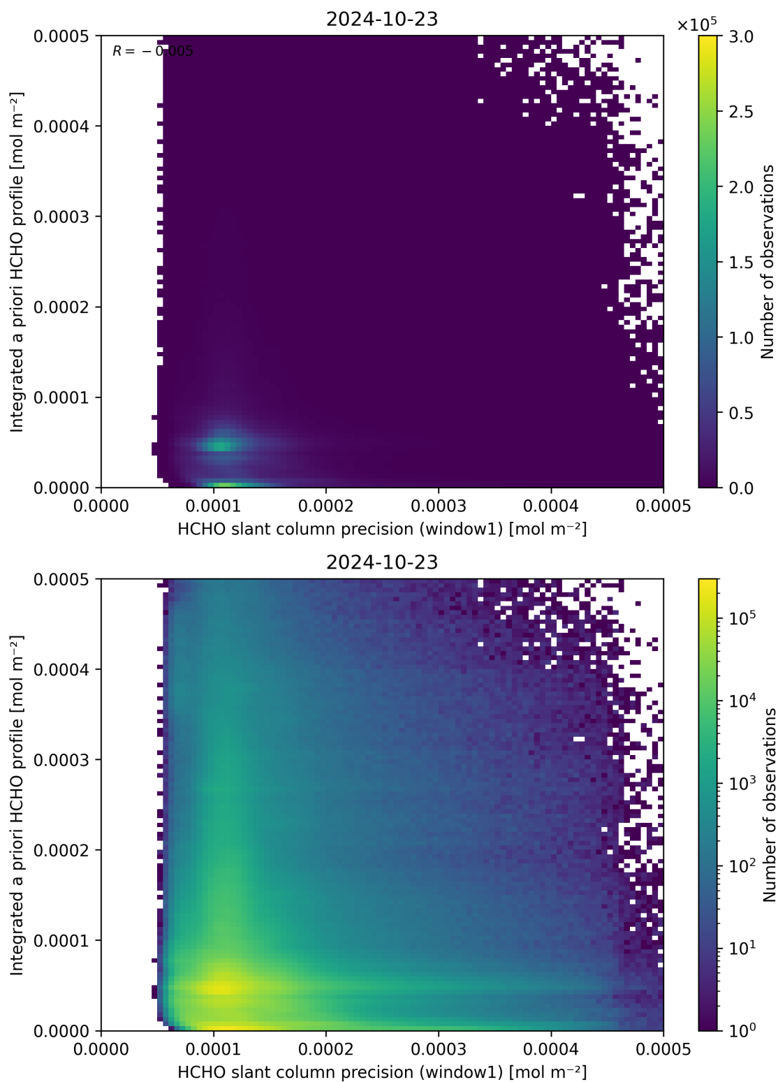
Figure 96: Scatter density plot of “HCHO slant column precision (window1)” against “Integrated a priori HCHO profile” for 2024-10-22 to 2024-10-24.
