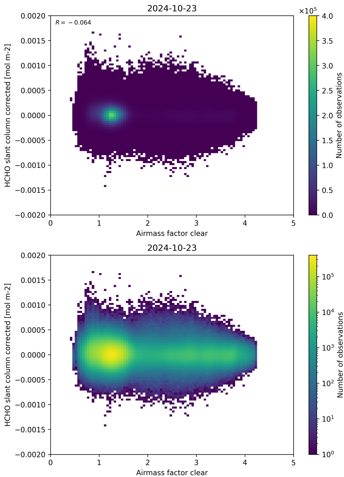
Figure 74: Scatter density plot of “Airmass factor clear” against “HCHO slant column corrected” for 2024-10-22 to 2024-10-24.
