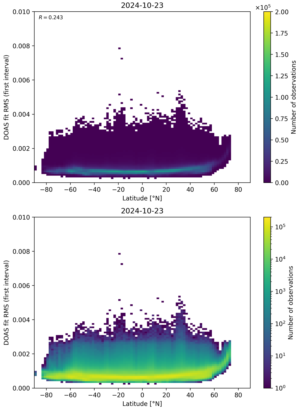
Figure 153: Scatter density plot of “Latitude” against “DOAS fit RMS (first interval)” for 2024-10-22 to 2024-10-24.
