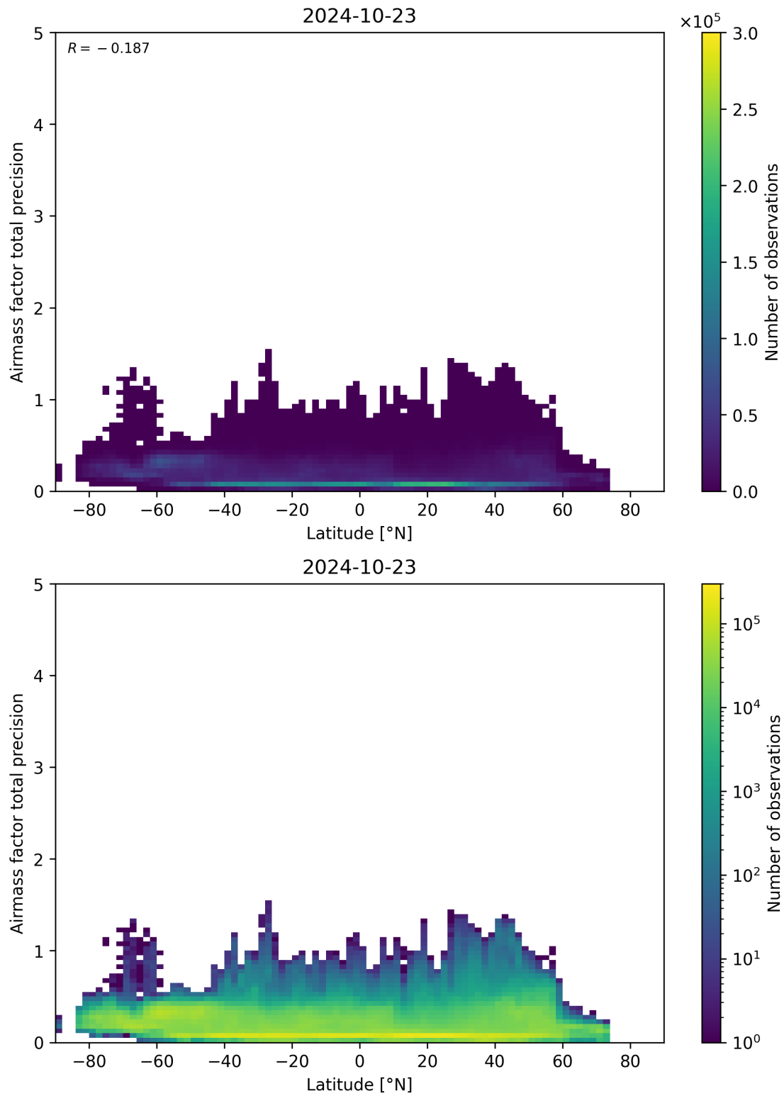
Figure 162: Scatter density plot of “Latitude” against “Airmass factor total precision” for 2024-10-22 to 2024-10-24.
