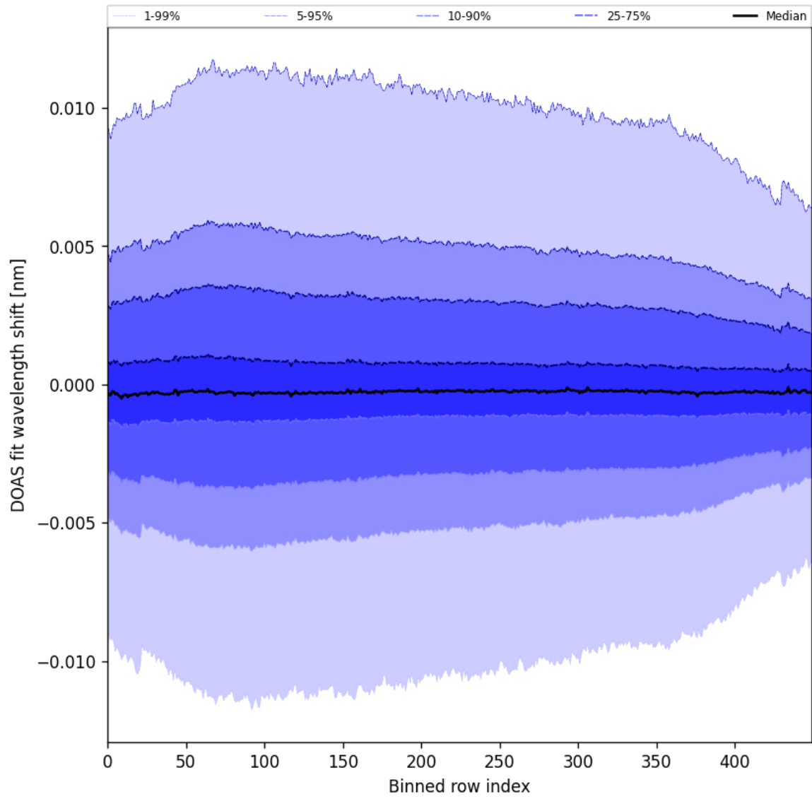
Figure 58: Along track statistics of “DOAS fit wavelength shift” for 2024-10-22 to 2024-10-24
