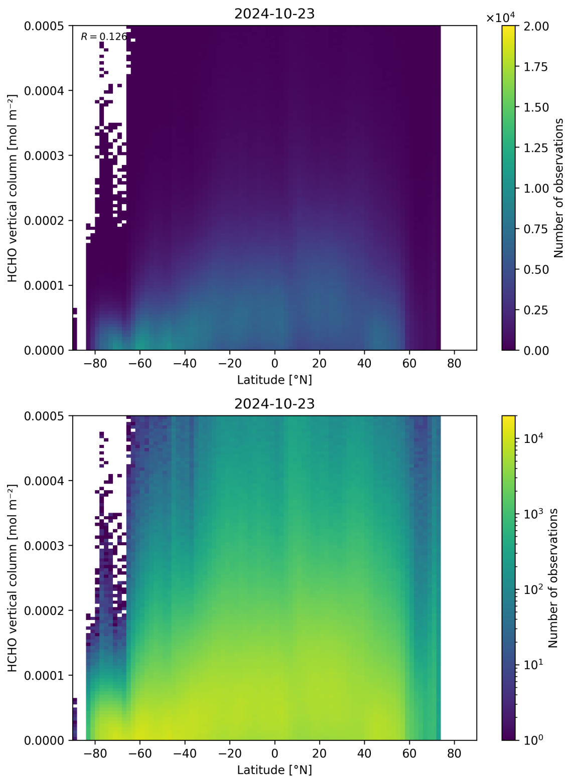
Figure 163: Scatter density plot of “Latitude” against “HCHO vertical column” for 2024-10-22 to 2024-10-24.
