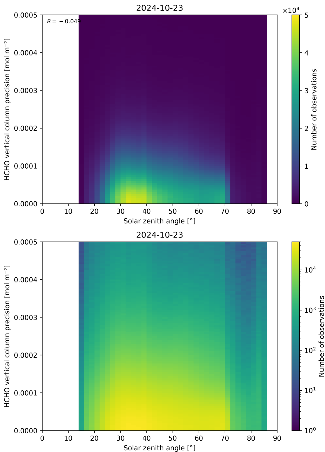
Figure 179: Scatter density plot of “Solar zenith angle” against “HCHO vertical column precision” for 2024-10-22 to 2024-10-24.
