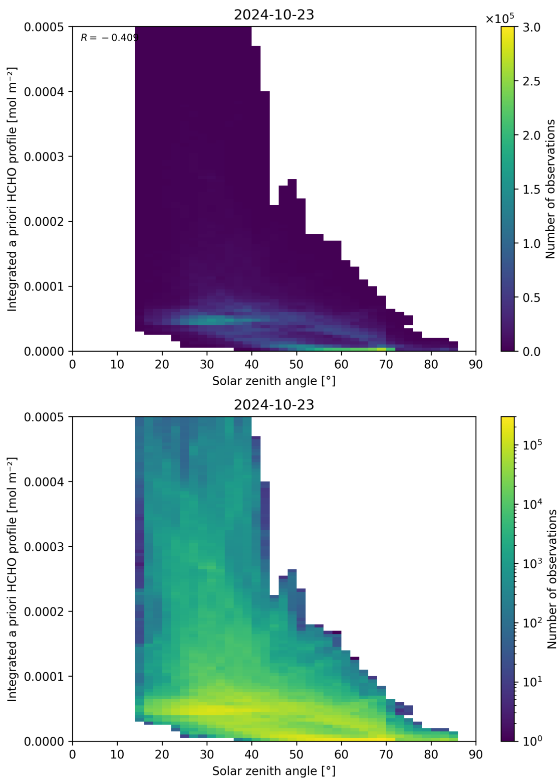
Figure 180: Scatter density plot of “Solar zenith angle” against “Integrated a priori HCHO profile” for 2024-10-22 to 2024-10-24.
