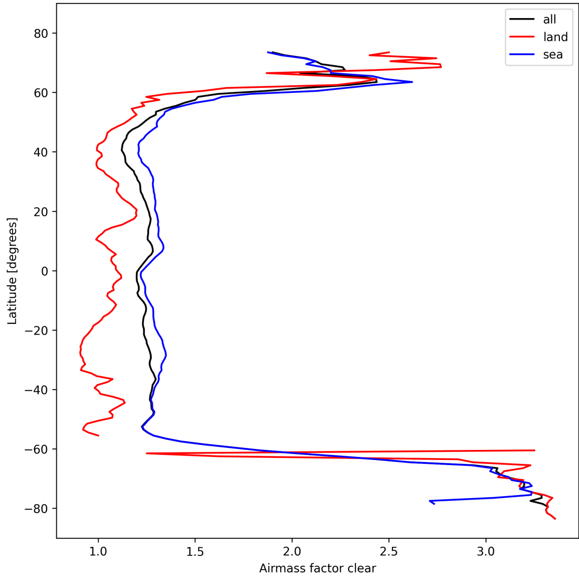
Figure 28: Zonal average of “Airmass factor clear” for 2024-10-22 to 2024-10-24.
