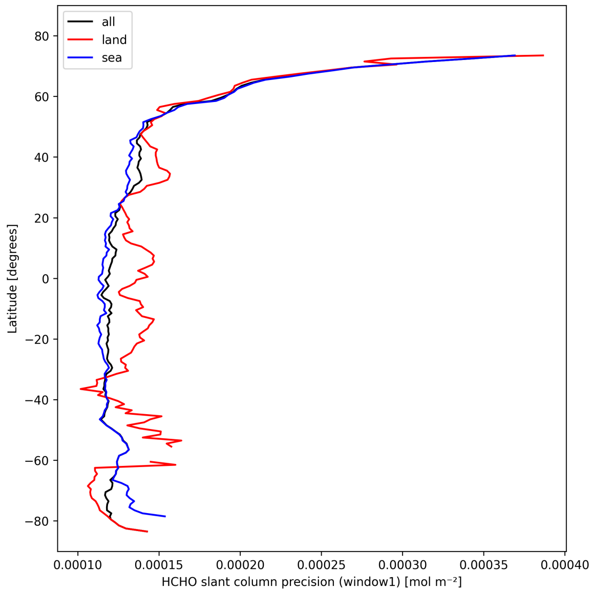
Figure 25: Zonal average of “HCHO slant column precision (window1)” for 2024-10-22 to 2024-10-24.
