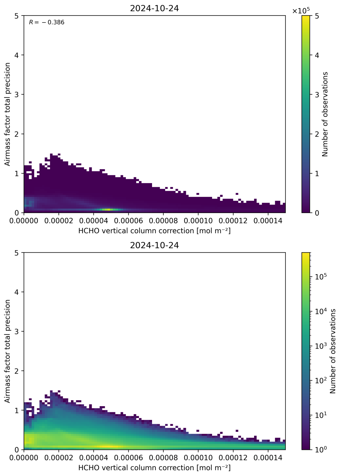
Figure 121: Scatter density plot of “HCHO vertical column correction” against “Airmass factor total precision” for 2024-10-24 to 2024-10-25.
