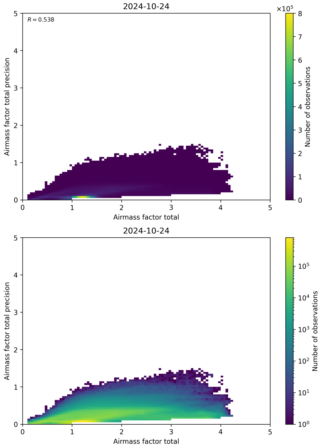
Figure 103: Scatter density plot of “Airmass factor total” against “Airmass factor total precision” for 2024-10-24 to 2024-10-25.
