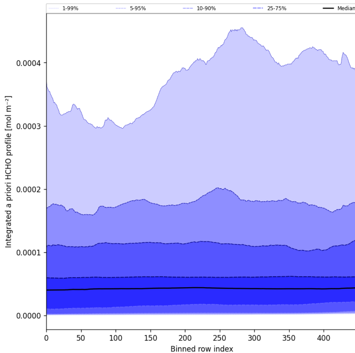
Figure 57: Along track statistics of “Integrated a priori HCHO profile” for 2024-10-24 to 2024-10-25
