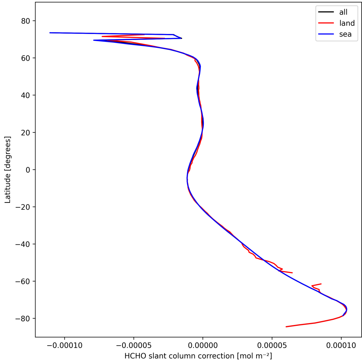
Figure 33: Zonal average of "HCHO slant column correction" for 2024-10-24 to 2024-10-25.
