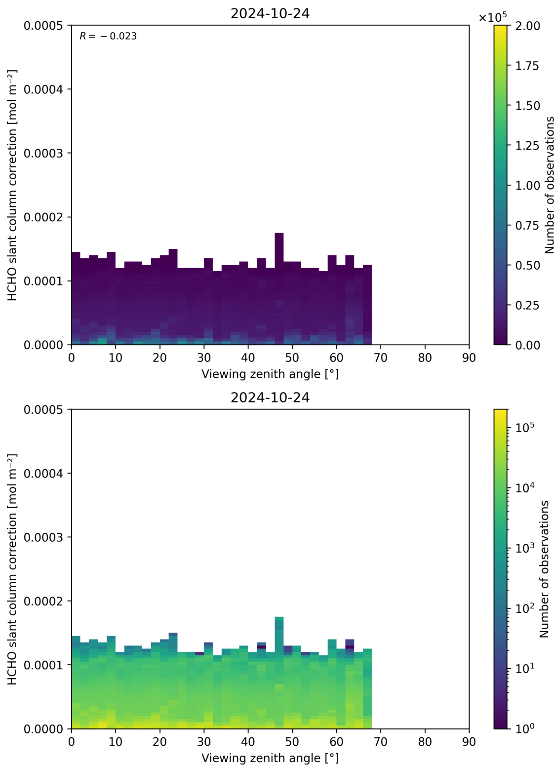
Figure 187: Scatter density plot of “Viewing zenith angle” against “HCHO slant column correction” for 2024-10-24 to 2024-10-25.
