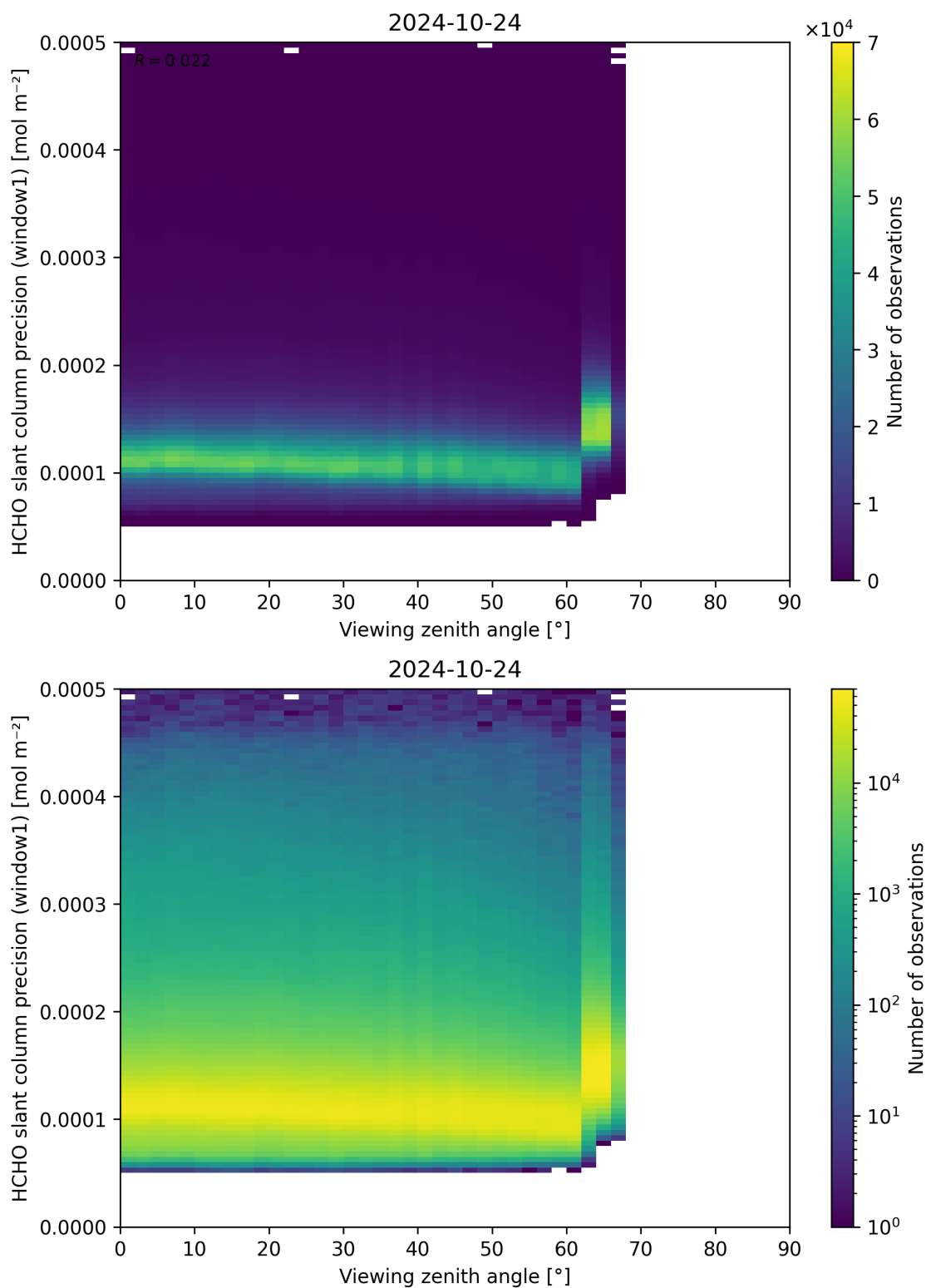
Figure 189: Scatter density plot of “Viewing zenith angle” against “HCHO slant column precision (window1)” for 2024-10-24 to 2024-10-25.
