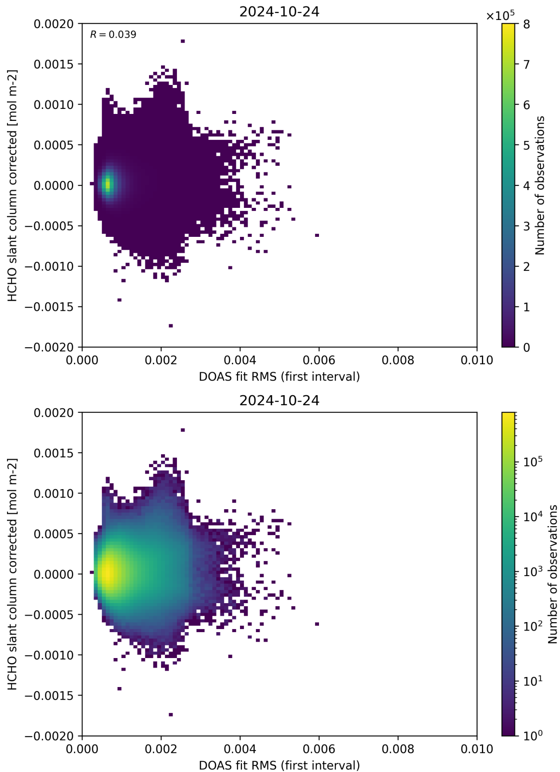
Figure 62: Scatter density plot of “DOAS fit RMS (first interval)” against “HCHO slant column corrected” for 2024-10-24 to 2024-10-25.
