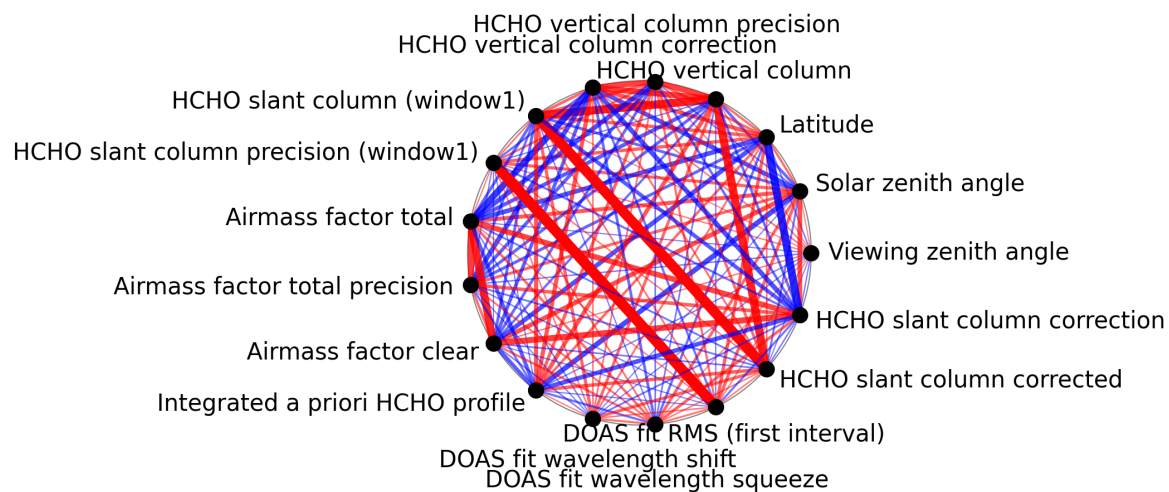
Figure 1: Map of correlation graph for 2024-10-24 to 2024-10-25.
