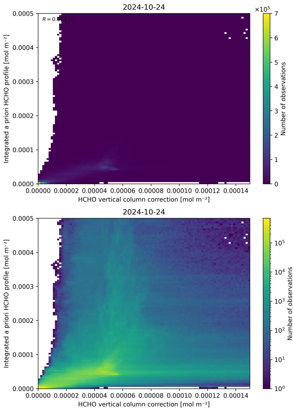
Figure 122: Scatter density plot of “HCHO vertical column correction” against “Integrated a priori HCHO profile” for 2024-10-24 to 2024-10-25.
