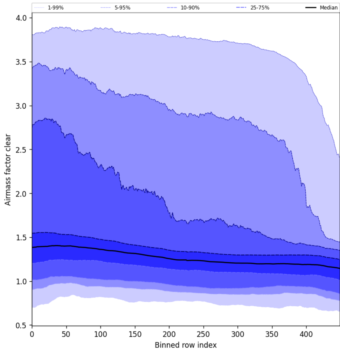
Figure 56: Along track statistics of “Airmass factor clear” for 2024-10-24 to 2024-10-25
