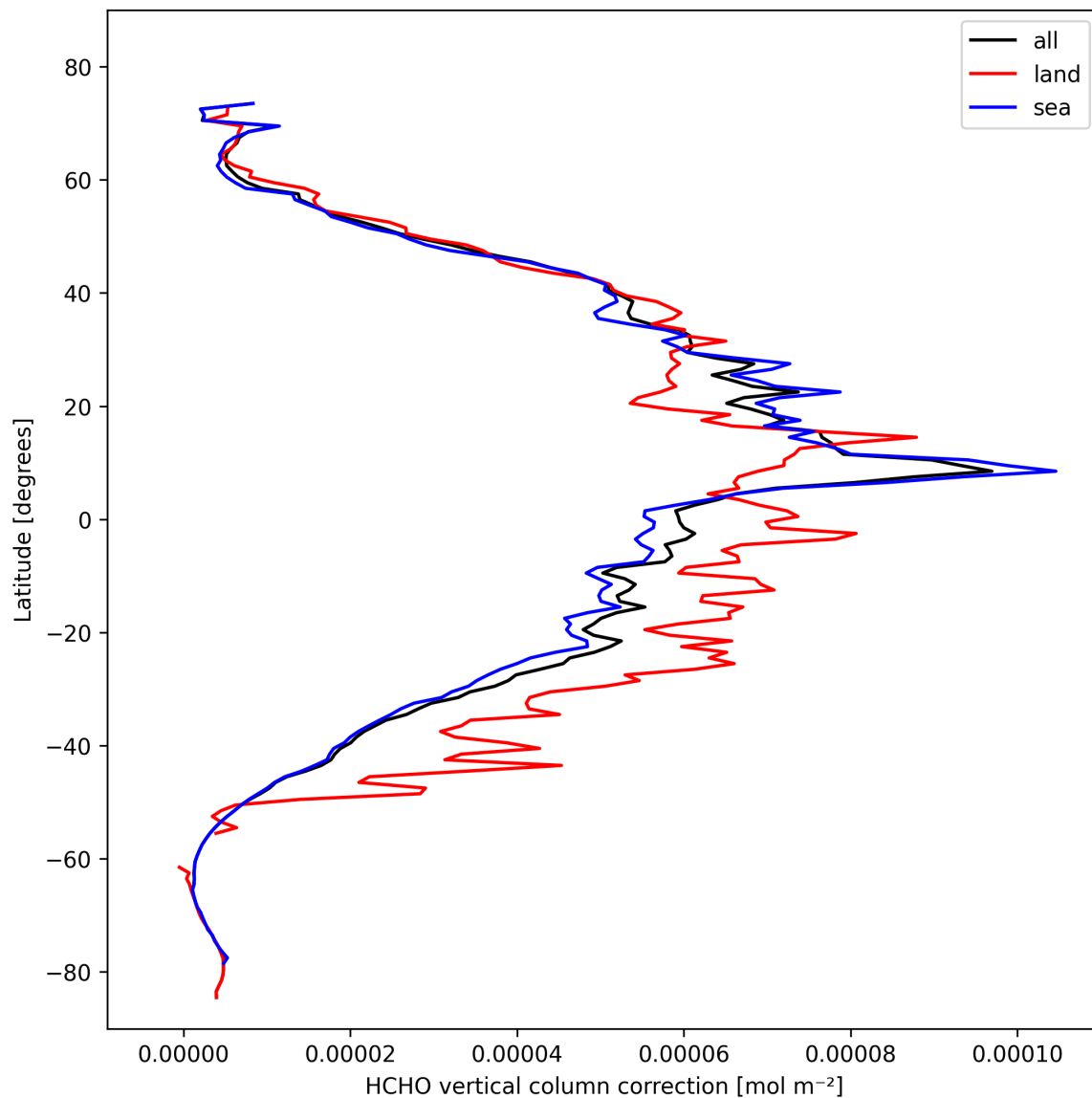
Figure 23: Zonal average of “HCHO vertical column correction” for 2024-10-24 to 2024-10-25.
