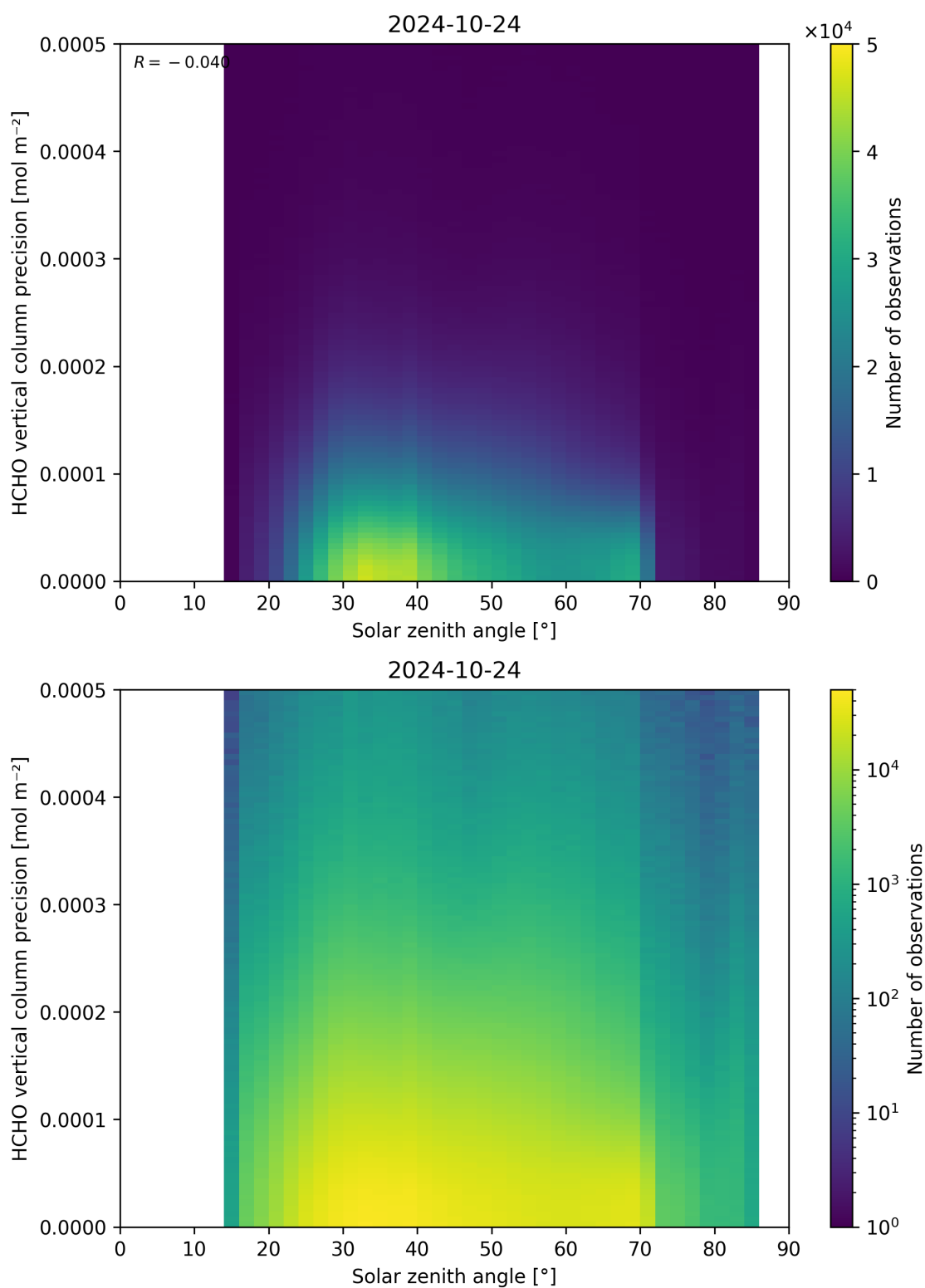
Figure 179: Scatter density plot of “Solar zenith angle” against “HCHO vertical column precision” for 2024-10-24 to 2024-10-25.
