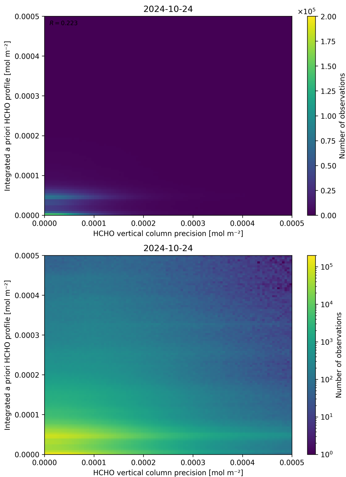
Figure 147: Scatter density plot of “HCHO vertical column precision” against “Integrated a priori HCHO profile” for 2024-10-24 to 2024-10-25.
