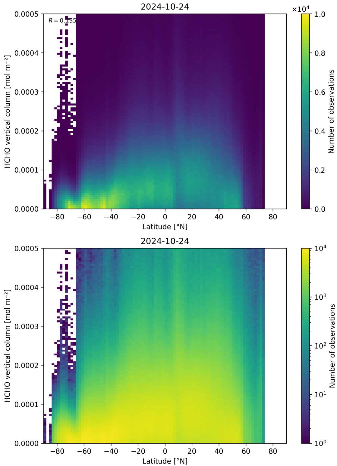
Figure 163: Scatter density plot of “Latitude” against “HCHO vertical column” for 2024-10-24 to 2024-10-25.
