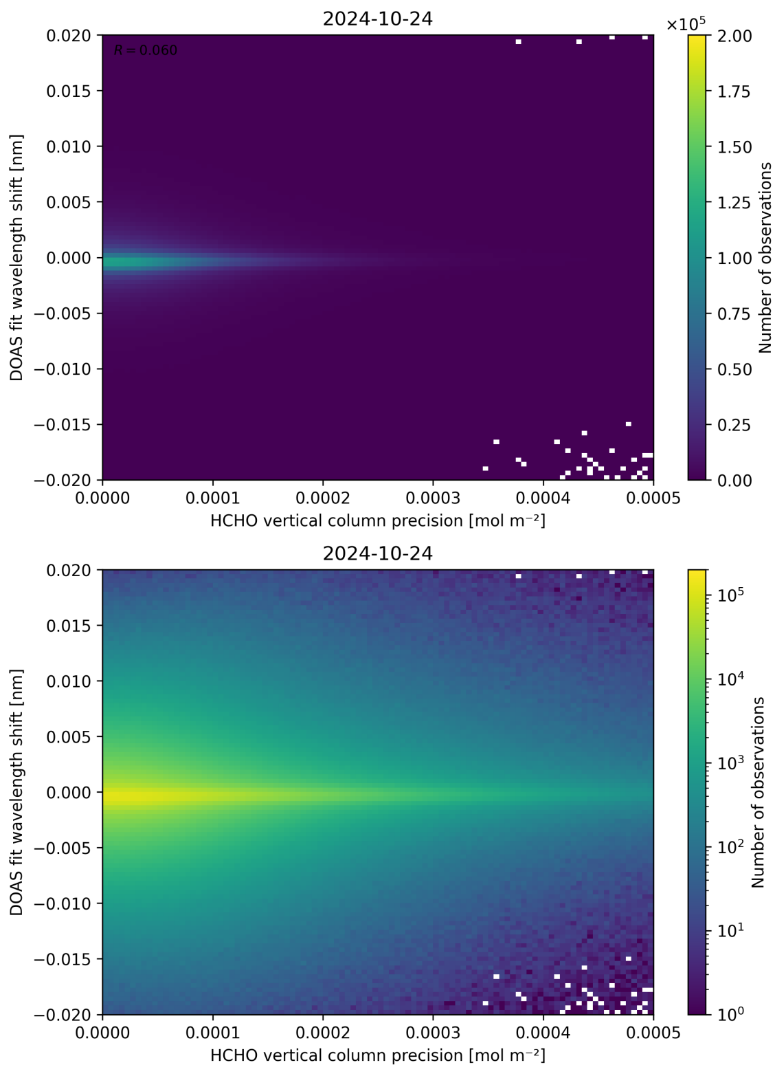
Figure 137: Scatter density plot of “HCHO vertical column precision” against “DOAS fit wavelength shift” for 2024-10-24 to 2024-10-25.
