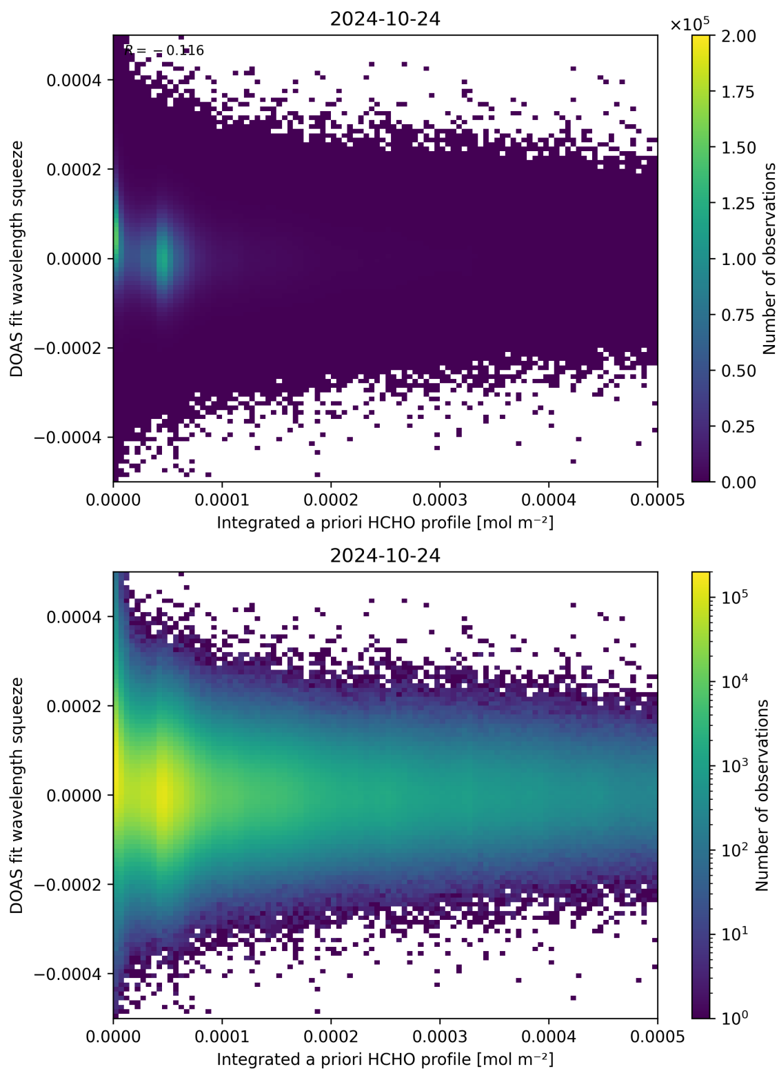
Figure 150: Scatter density plot of “Integrated a priori HCHO profile” against “DOAS fit wavelength squeeze” for 2024-10-24 to 2024-10-25.
