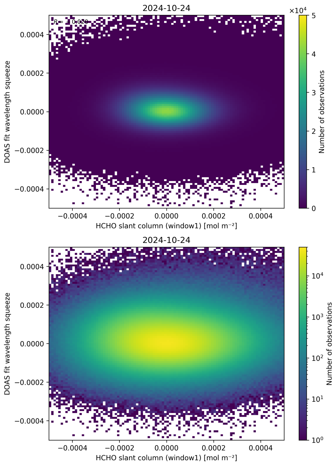
Figure 80: Scatter density plot of “HCHO slant column (window1)” against “DOAS fit wavelength squeeze” for 2024-10-24 to 2024-10-25.
