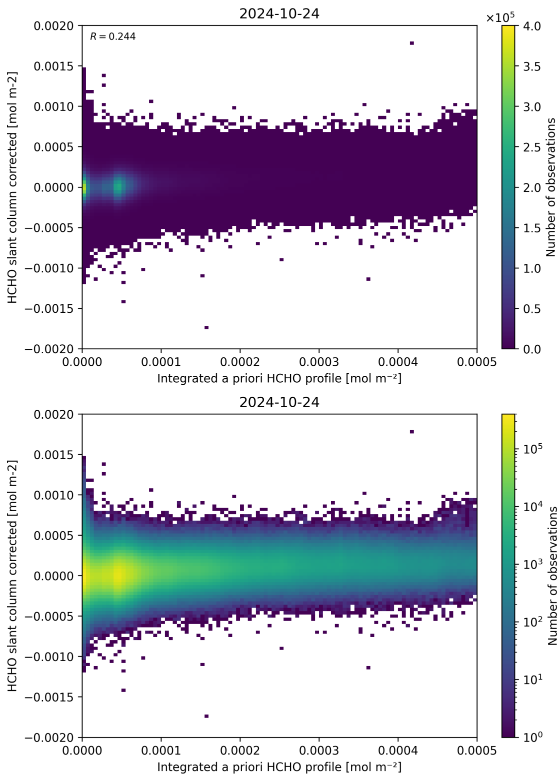
Figure 151: Scatter density plot of “Integrated a priori HCHO profile” against “HCHO slant column corrected” for 2024-10-24 to 2024-10-25.
