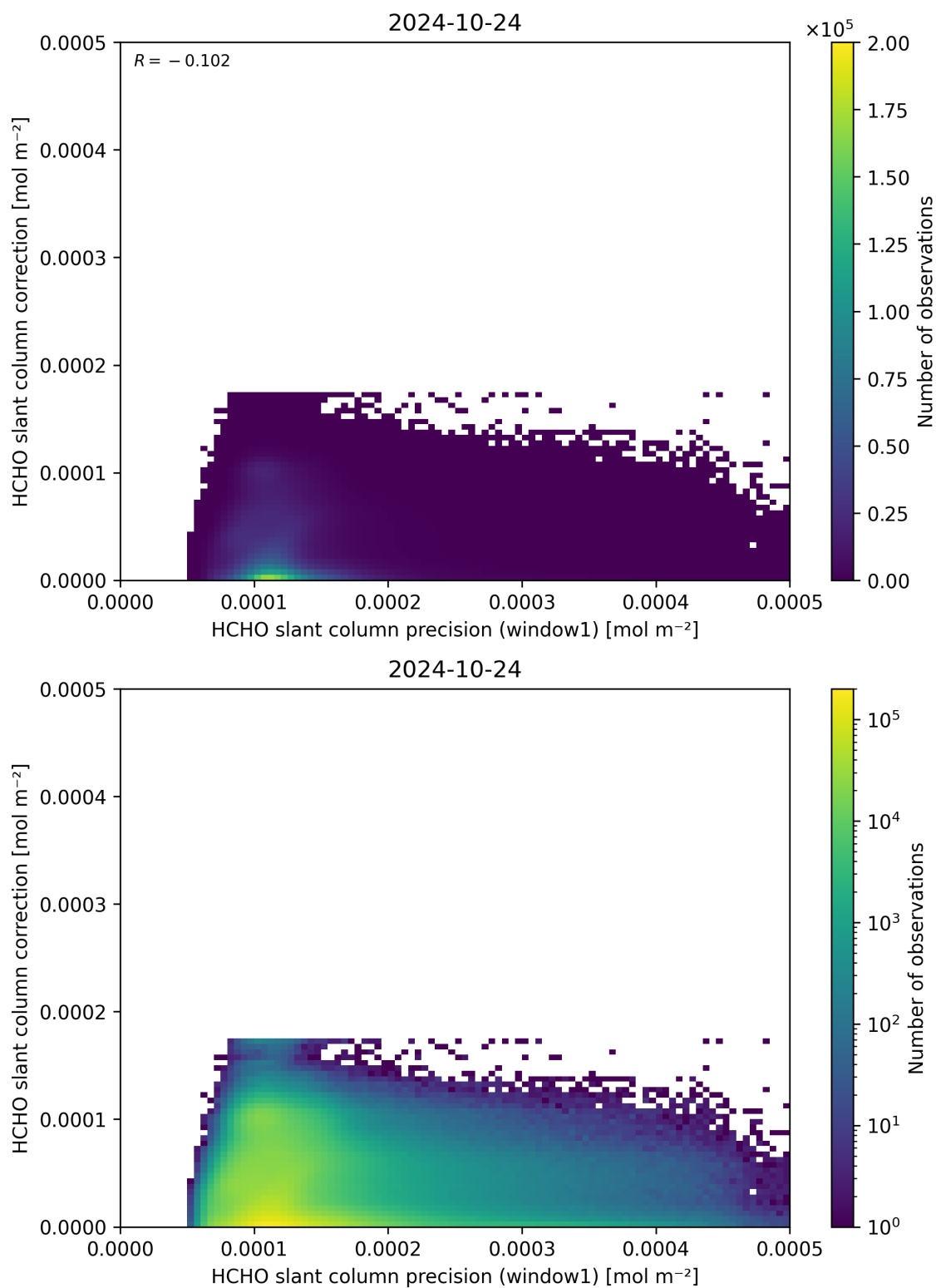
Figure 93: Scatter density plot of “HCHO slant column precision (window1)” against “HCHO slant column correction” for 2024-10-24 to 2024-10-25.
