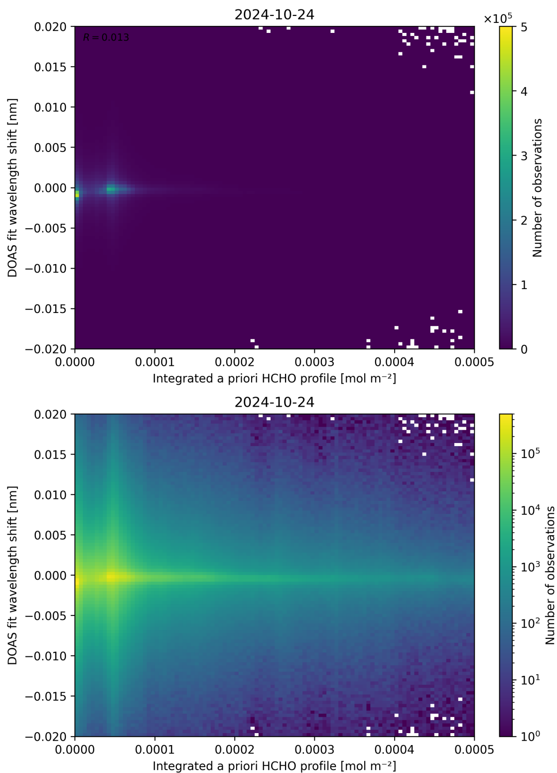
Figure 149: Scatter density plot of “Integrated a priori HCHO profile” against “DOAS fit wavelength shift” for 2024-10-24 to 2024-10-25.
