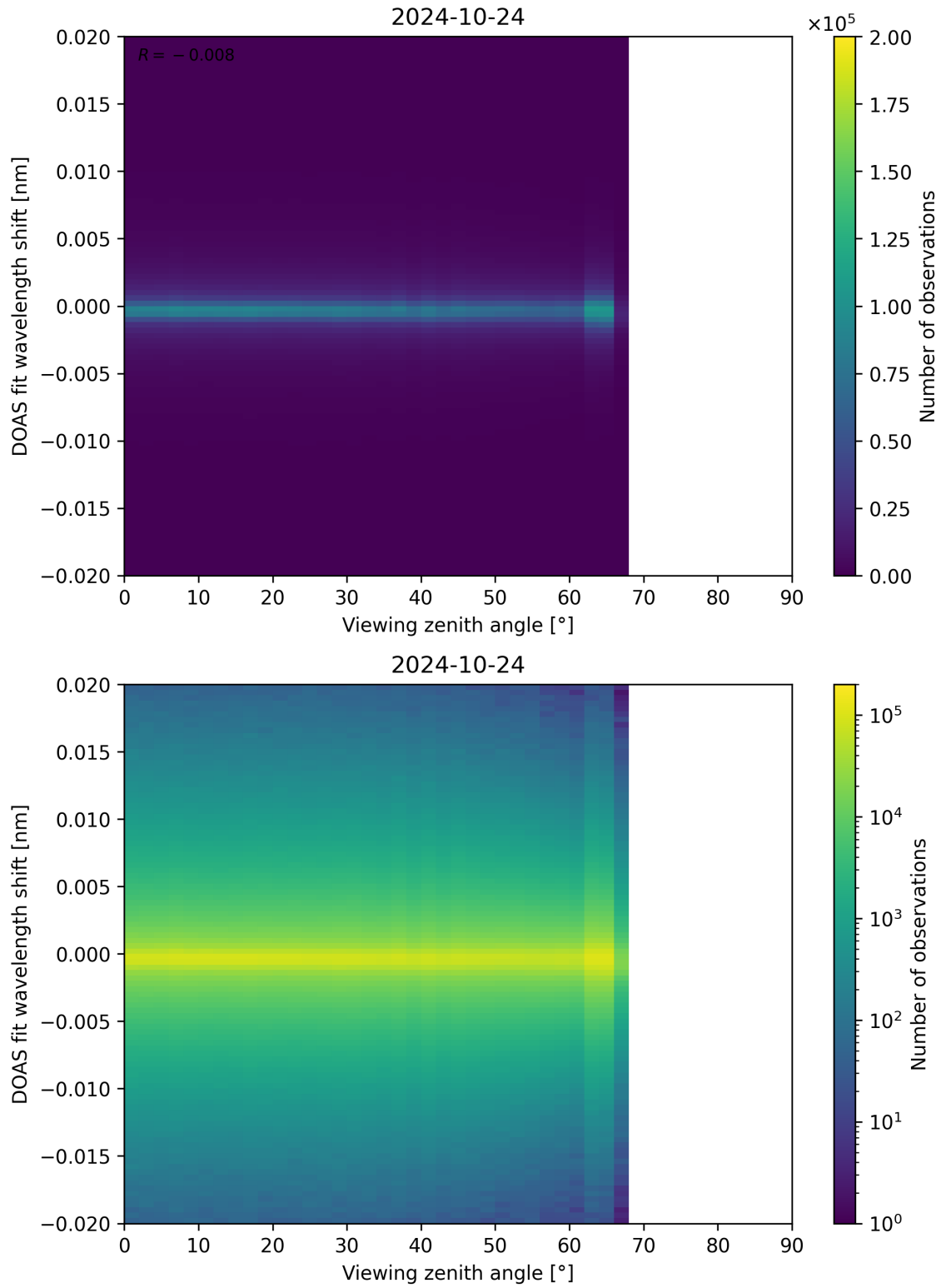
Figure 183: Scatter density plot of “Viewing zenith angle” against “DOAS fit wavelength shift” for 2024-10-24 to 2024-10-25.
