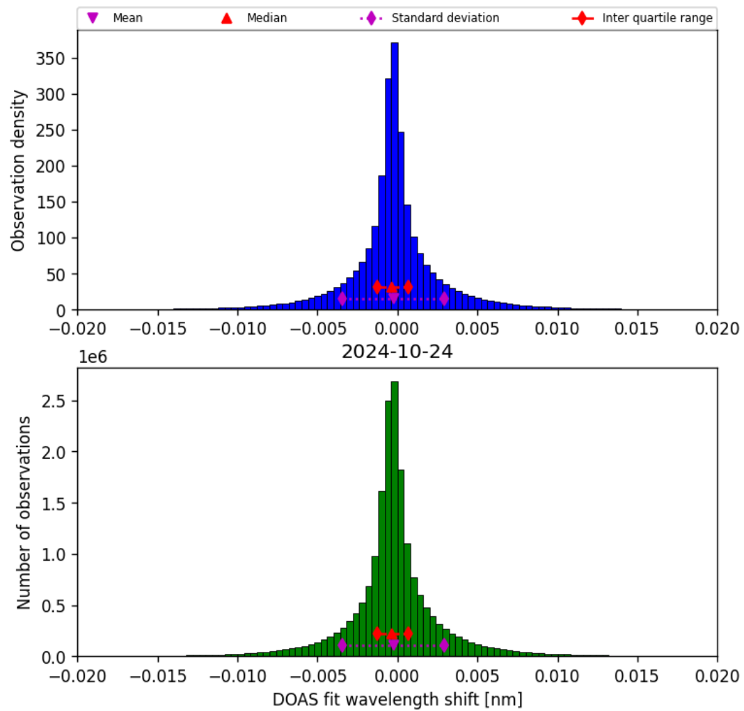
Figure 44: Histogram of “DOAS fit wavelength shift” for 2024-10-24 to 2024-10-25
