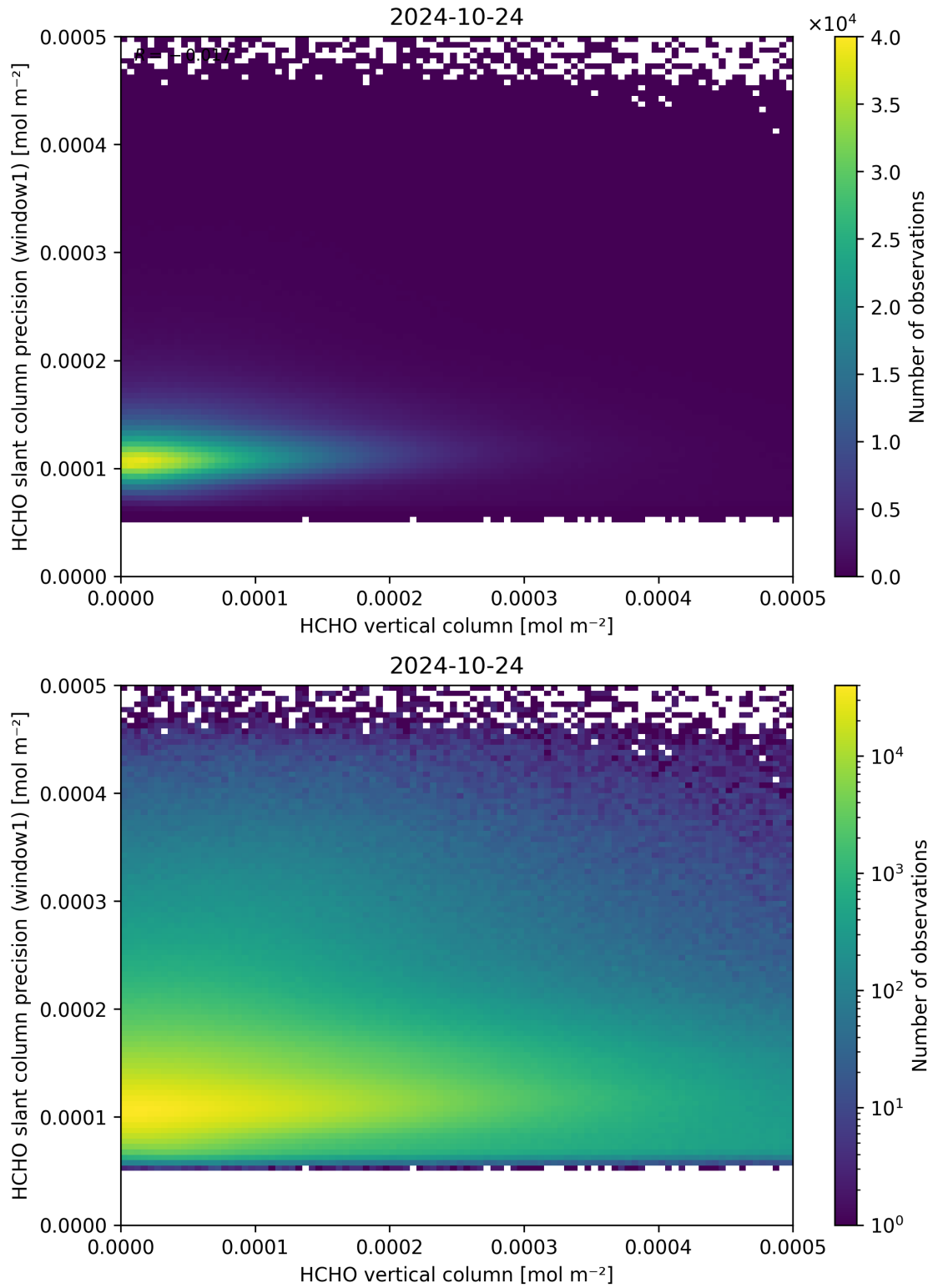
Figure 130: Scatter density plot of “HCHO vertical column” against “HCHO slant column precision (window1)” for 2024-10-24 to 2024-10-25.
