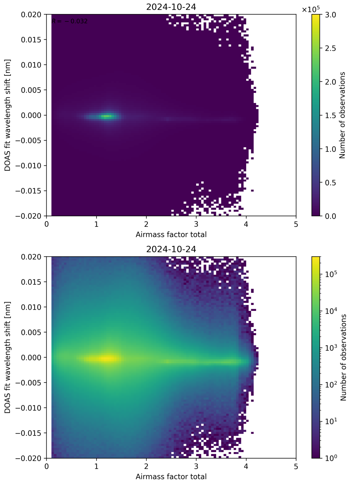
Figure 98: Scatter density plot of “Airmass factor total” against “DOAS fit wavelength shift” for 2024-10-24 to 2024-10-25.
