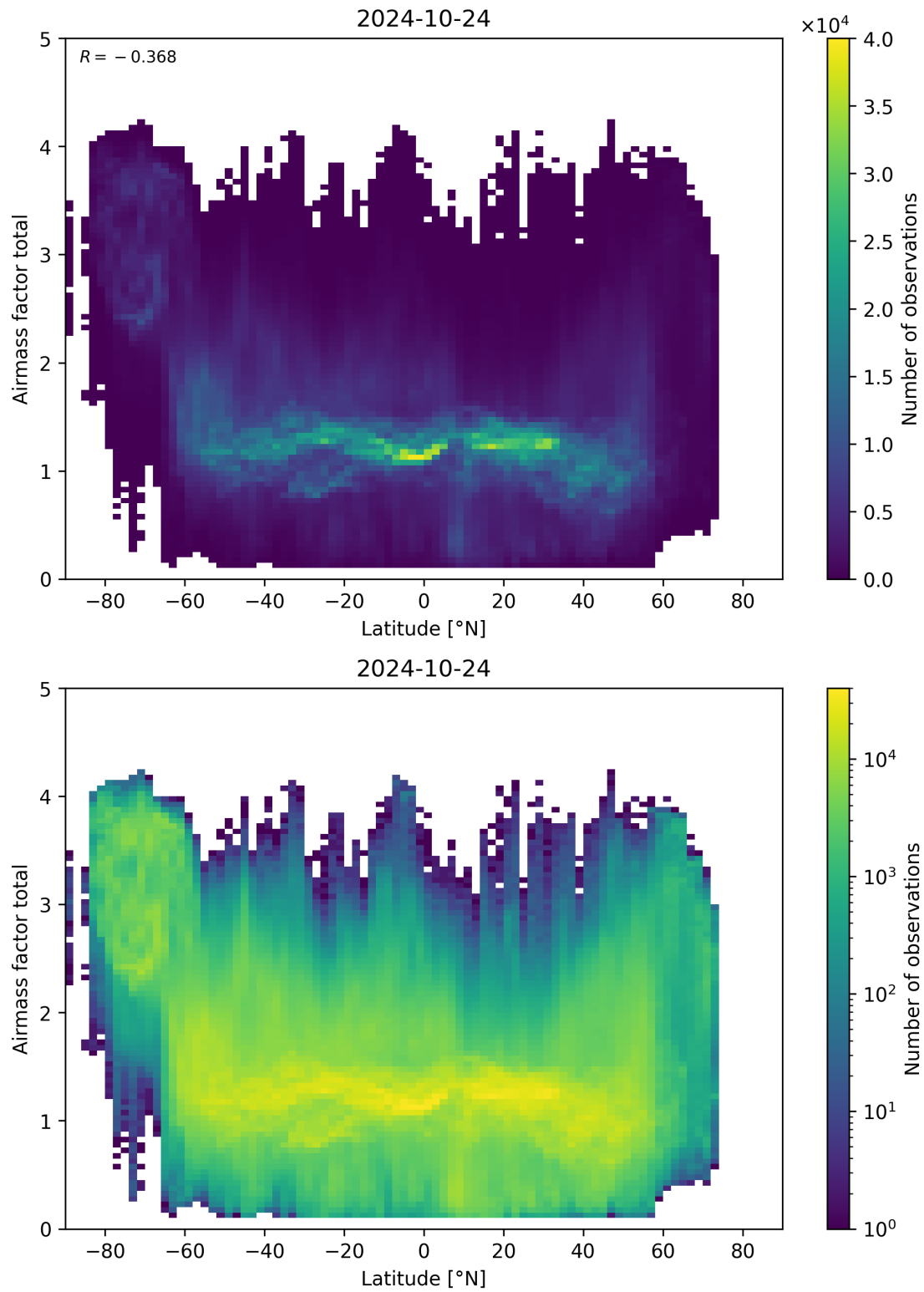
Figure 161: Scatter density plot of “Latitude” against “Airmass factor total” for 2024-10-24 to 2024-10-25.
