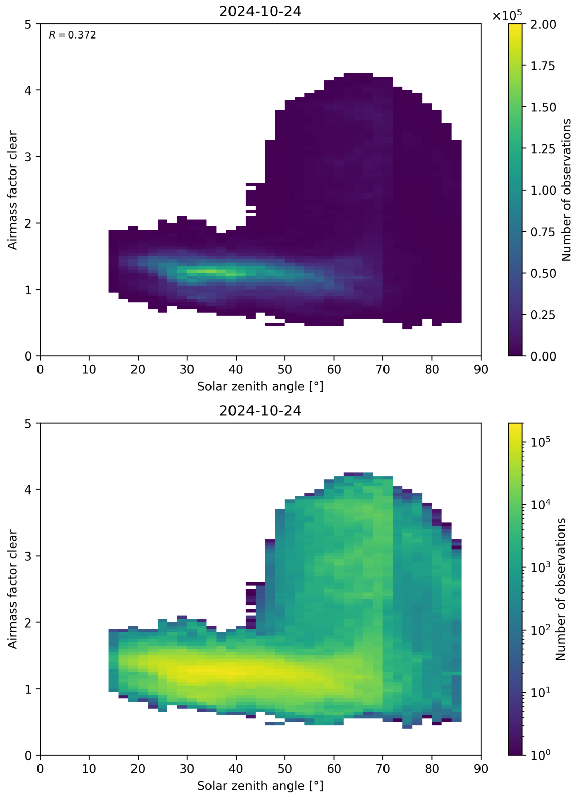
Figure 170: Scatter density plot of “Solar zenith angle” against “Airmass factor clear” for 2024-10-24 to 2024-10-25.
