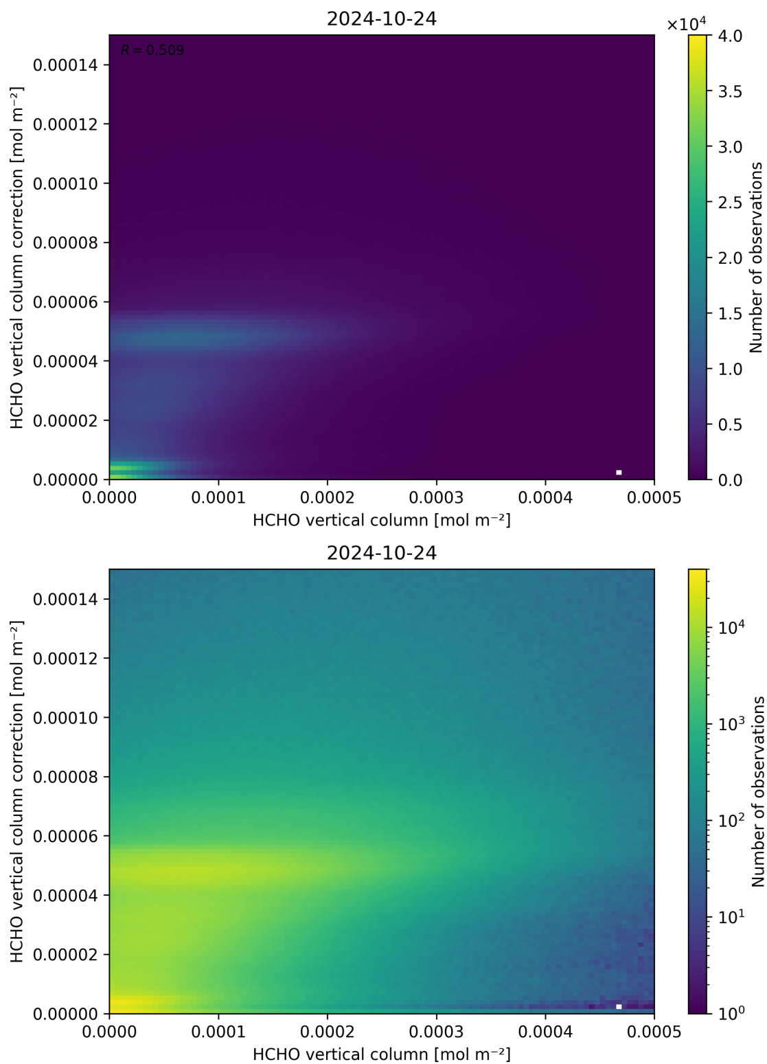
Figure 133: Scatter density plot of “HCHO vertical column” against “HCHO vertical column correction” for 2024-10-24 to 2024-10-25.
