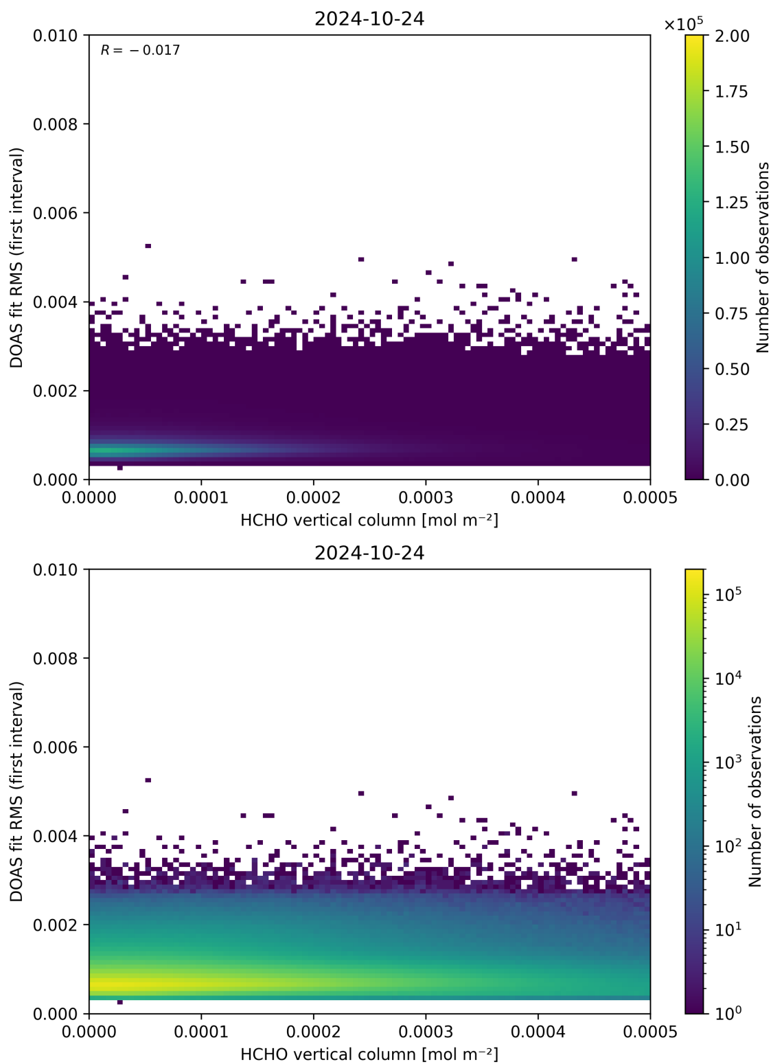
Figure 123: Scatter density plot of “HCHO vertical column” against “DOAS fit RMS (first interval)” for 2024-10-24 to 2024-10-25.
