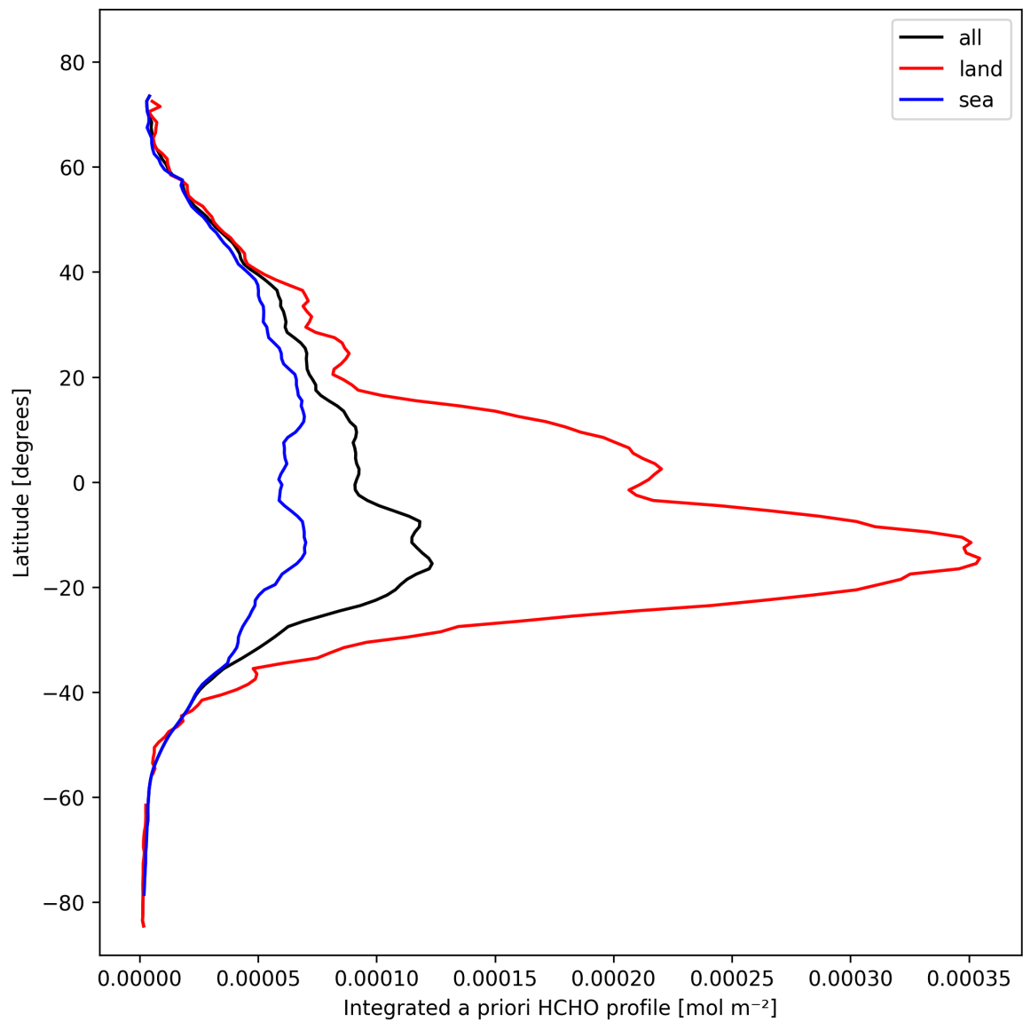
Figure 29: Zonal average of “Integrated a priori HCHO profile” for 2024-10-24 to 2024-10-25.
