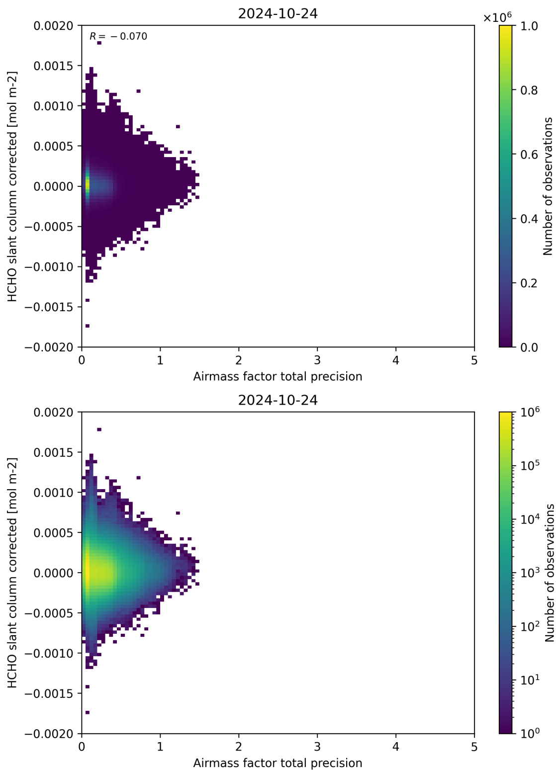
Figure 109: Scatter density plot of “Airmass factor total precision” against “HCHO slant column corrected” for 2024-10-24 to 2024-10-25.
