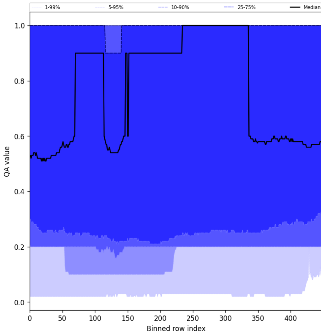
Figure 48: Along track statistics of “QA value” for 2024-10-24 to 2024-10-25
