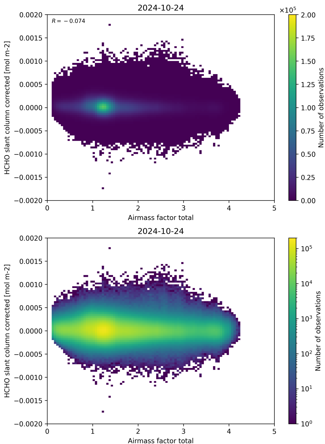
Figure 101: Scatter density plot of “Airmass factor total” against “HCHO slant column corrected” for 2024-10-24 to 2024-10-25.
