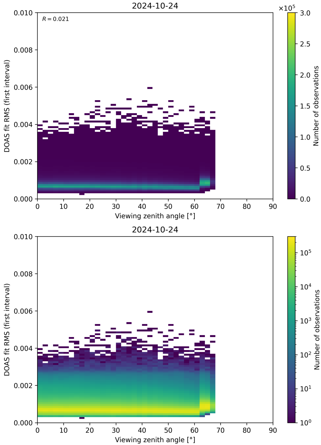
Figure 182: Scatter density plot of “Viewing zenith angle” against “DOAS fit RMS (first interval)” for 2024-10-24 to 2024-10-25.
