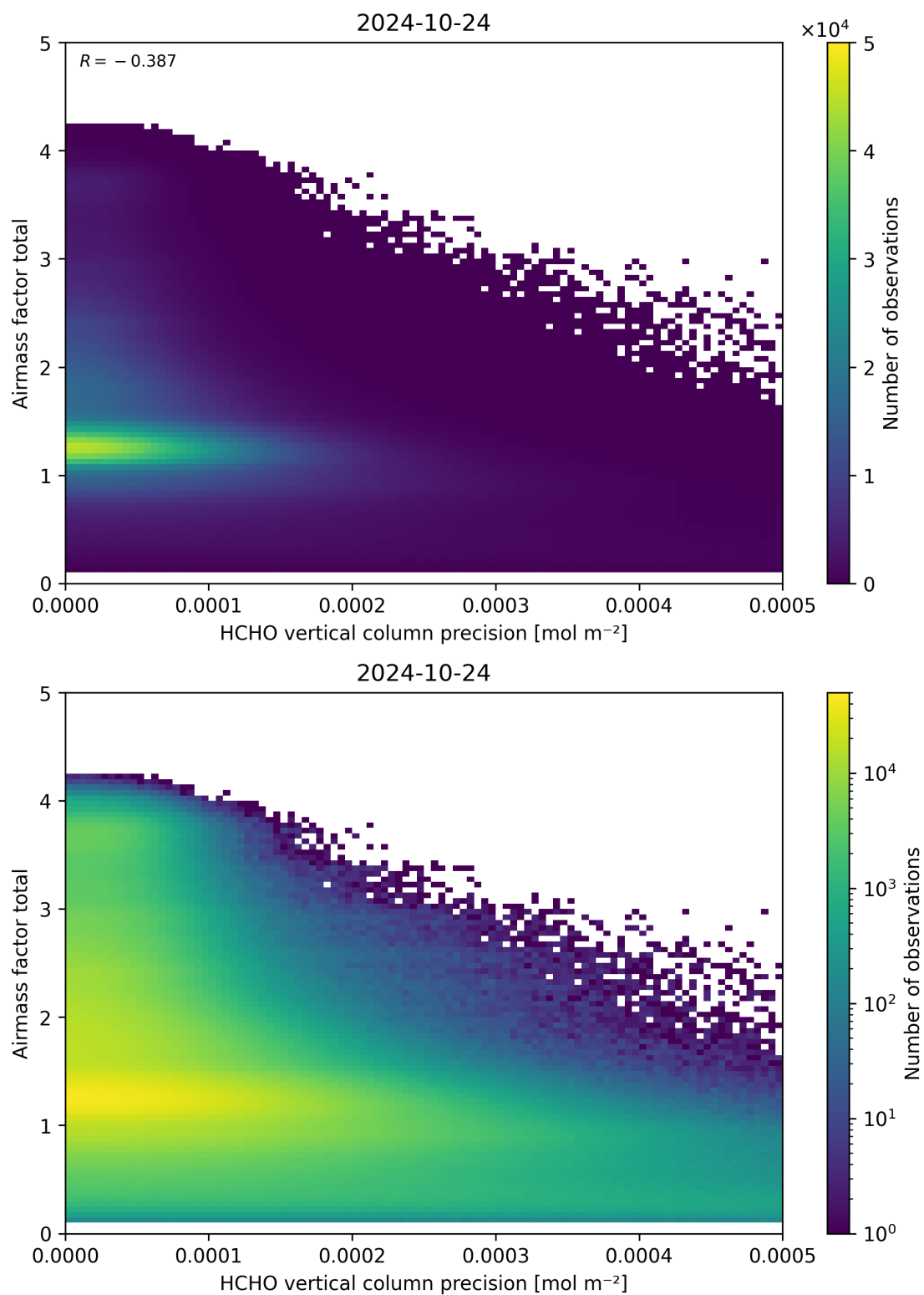
Figure 144: Scatter density plot of “HCHO vertical column precision” against “Airmass factor total” for 2024-10-24 to 2024-10-25.
