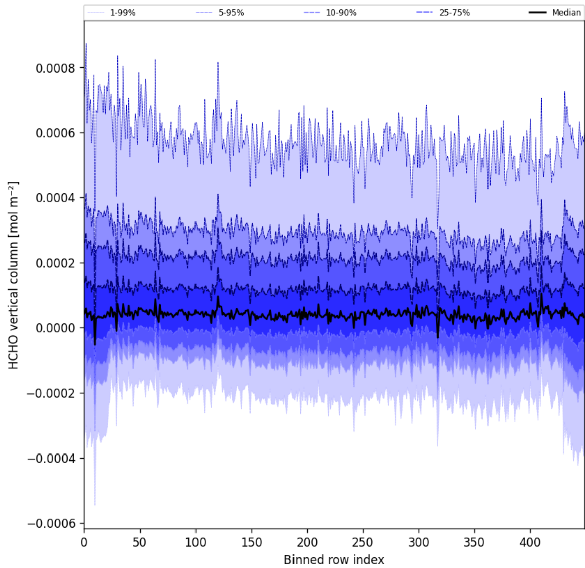
Figure 49: Along track statistics of “HCHO vertical column” for 2024-10-24 to 2024-10-25
