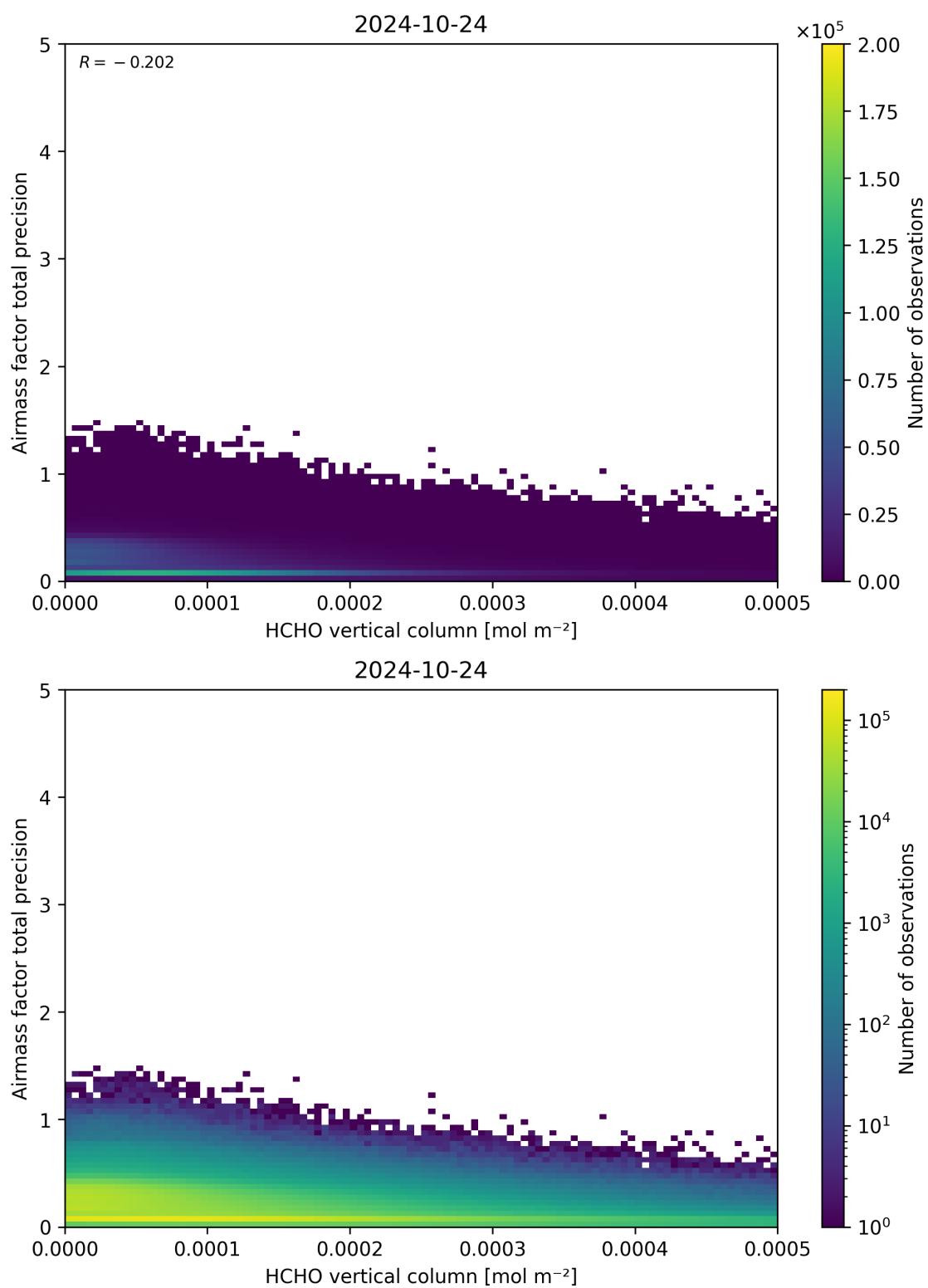
Figure 132: Scatter density plot of “HCHO vertical column” against “Airmass factor total precision” for 2024-10-24 to 2024-10-25.
