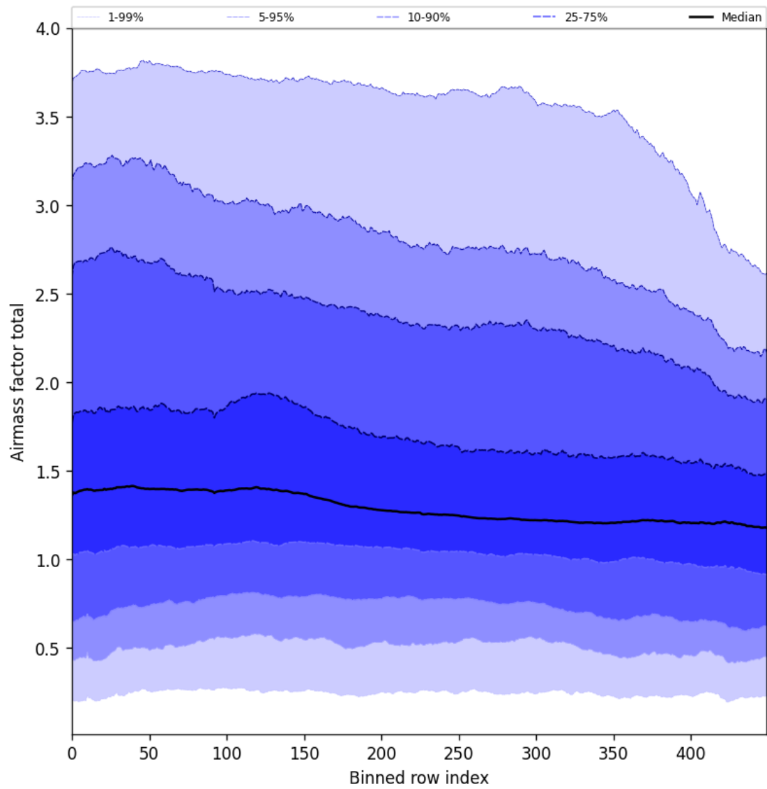
Figure 54: Along track statistics of “Airmass factor total” for 2024-10-24 to 2024-10-25
