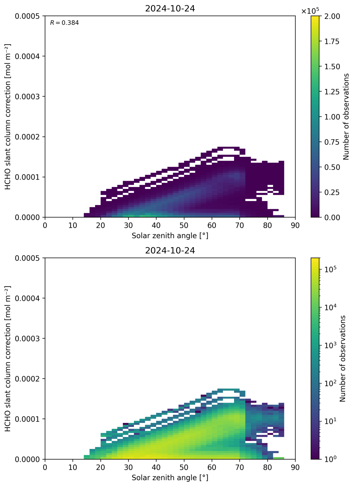
Figure 172: Scatter density plot of “Solar zenith angle” against “HCHO slant column correction” for 2024-10-24 to 2024-10-25.
