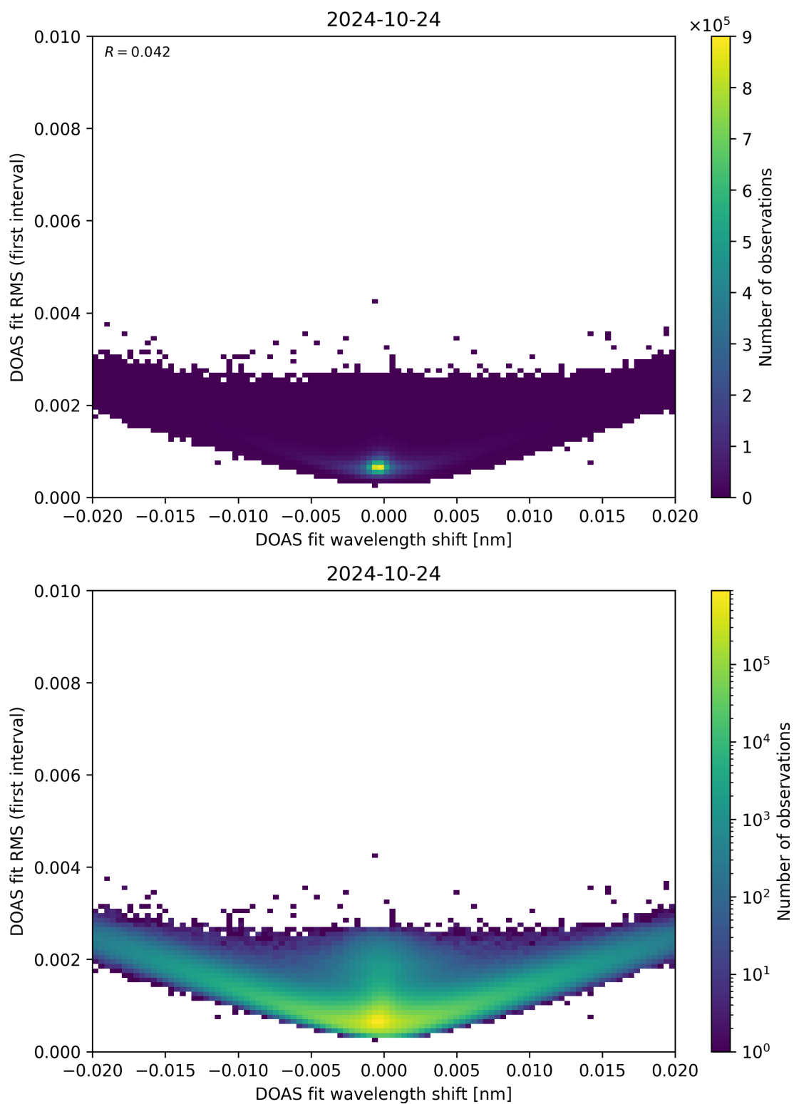
Figure 64: Scatter density plot of “DOAS fit wavelength shift” against “DOAS fit RMS (first interval)” for 2024-10-24 to 2024-10-25.
