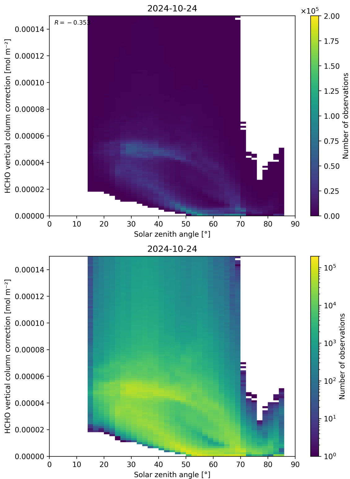
Figure 178: Scatter density plot of “Solar zenith angle” against “HCHO vertical column correction” for 2024-10-24 to 2024-10-25.
