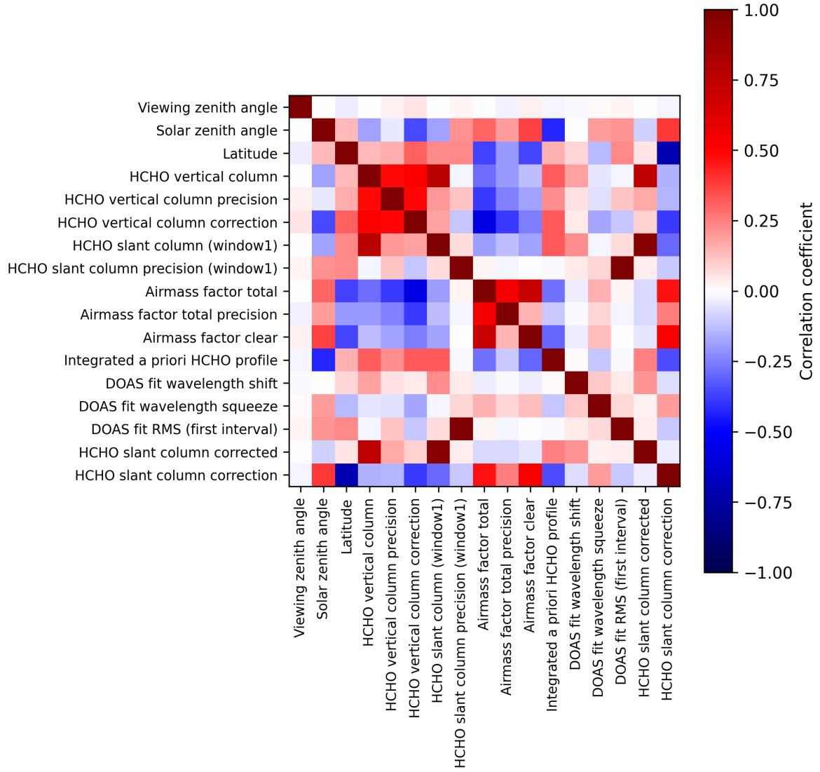
Figure 2: Map of correlation matrix for 2024-10-24 to 2024-10-25.
