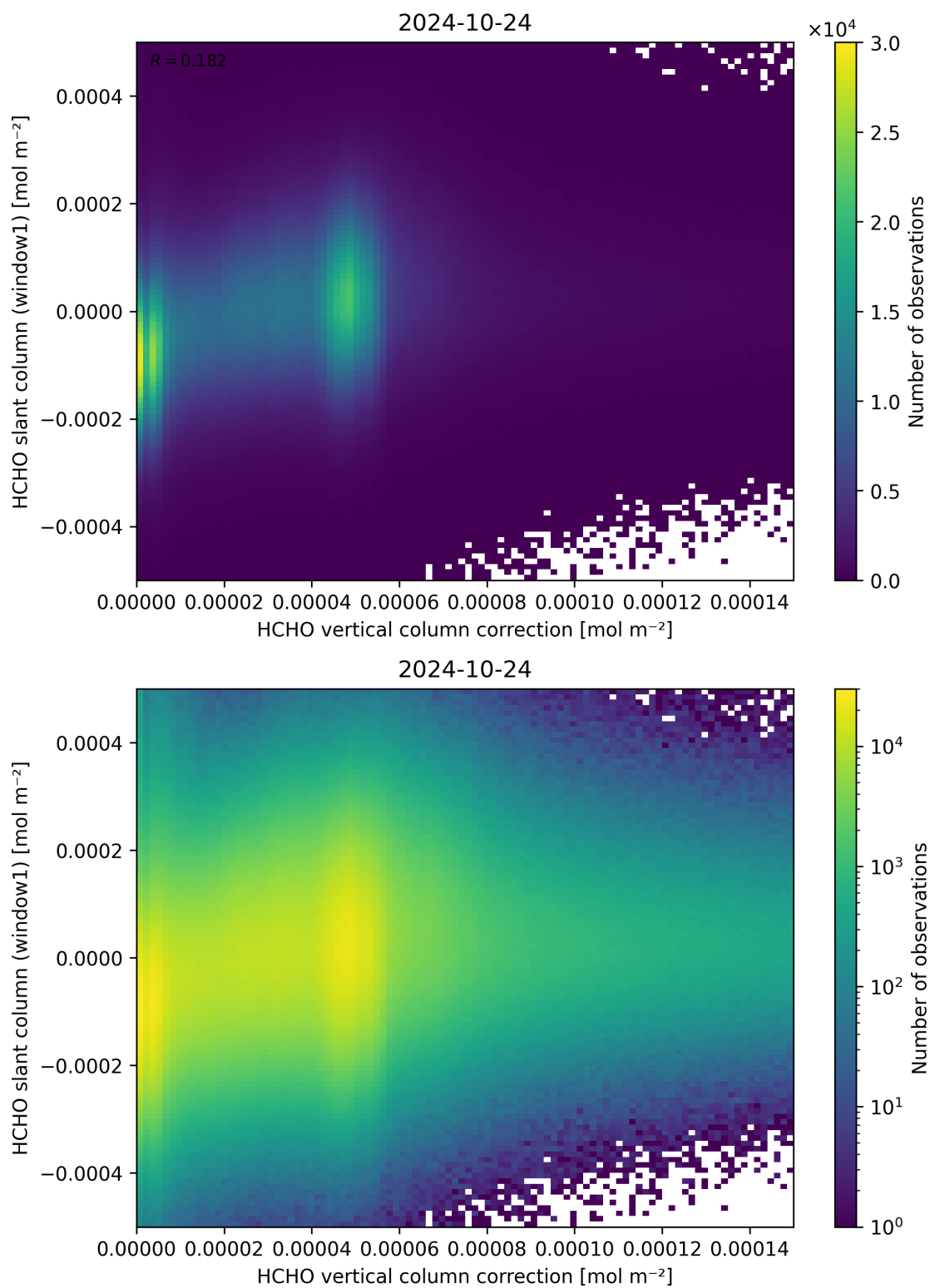
Figure 118: Scatter density plot of “HCHO vertical column correction” against “HCHO slant column (window1)” for 2024-10-24 to 2024-10-25.
