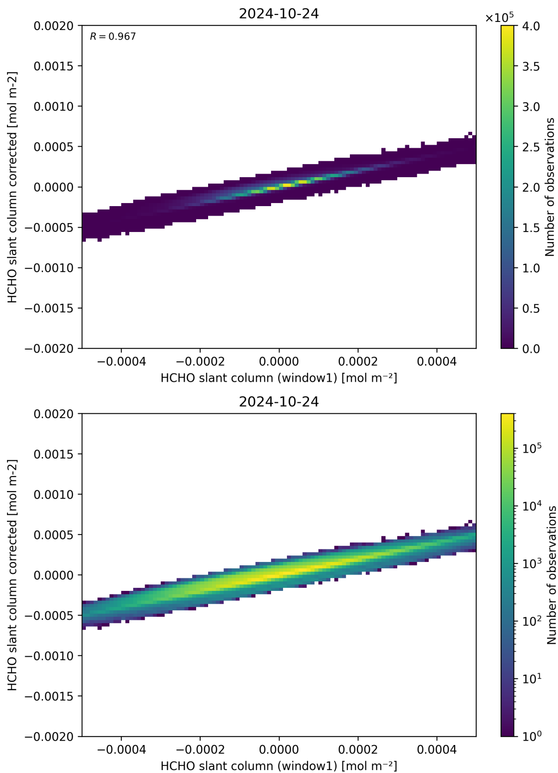
Figure 82: Scatter density plot of “HCHO slant column (window1)” against “HCHO slant column corrected” for 2024-10-24 to 2024-10-25.
