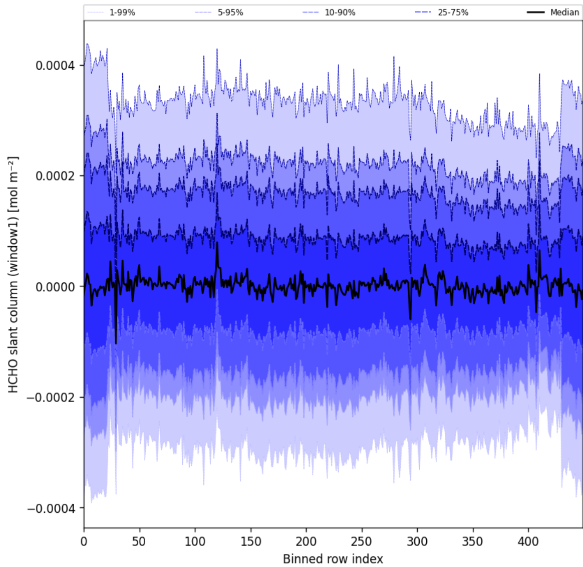
Figure 52: Along track statistics of “HCHO slant column (window1)” for 2024-10-24 to 2024-10-25
