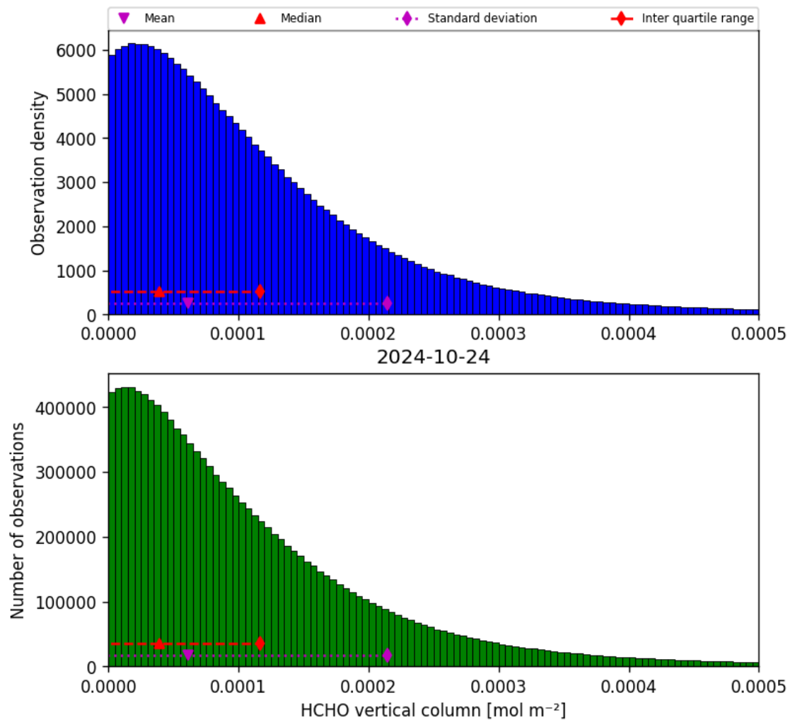
Figure 35: Histogram of “HCHO vertical column” for 2024-10-24 to 2024-10-25
