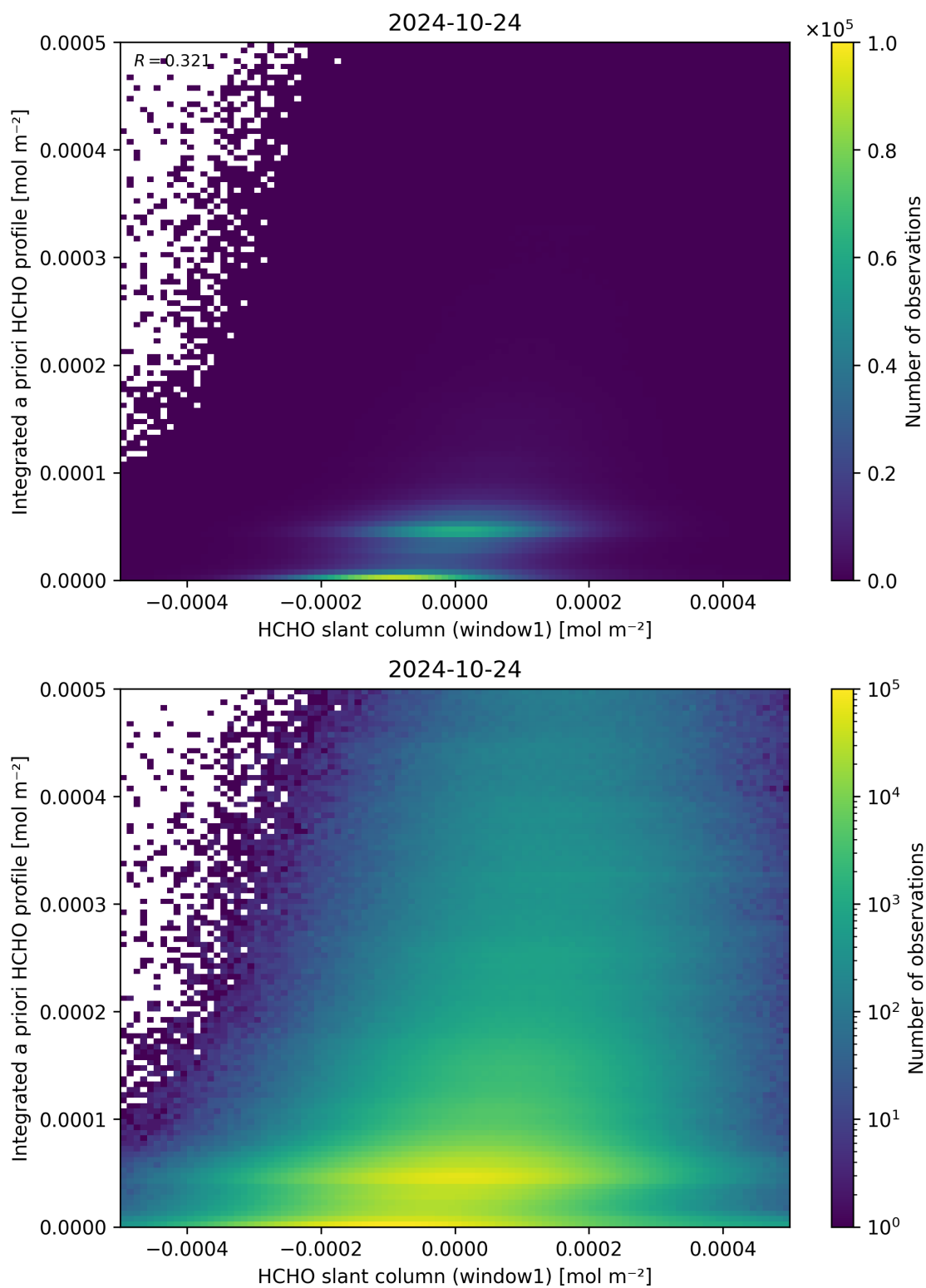
Figure 87: Scatter density plot of “HCHO slant column (window1)” against “Integrated a priori HCHO profile” for 2024-10-24 to 2024-10-25.
