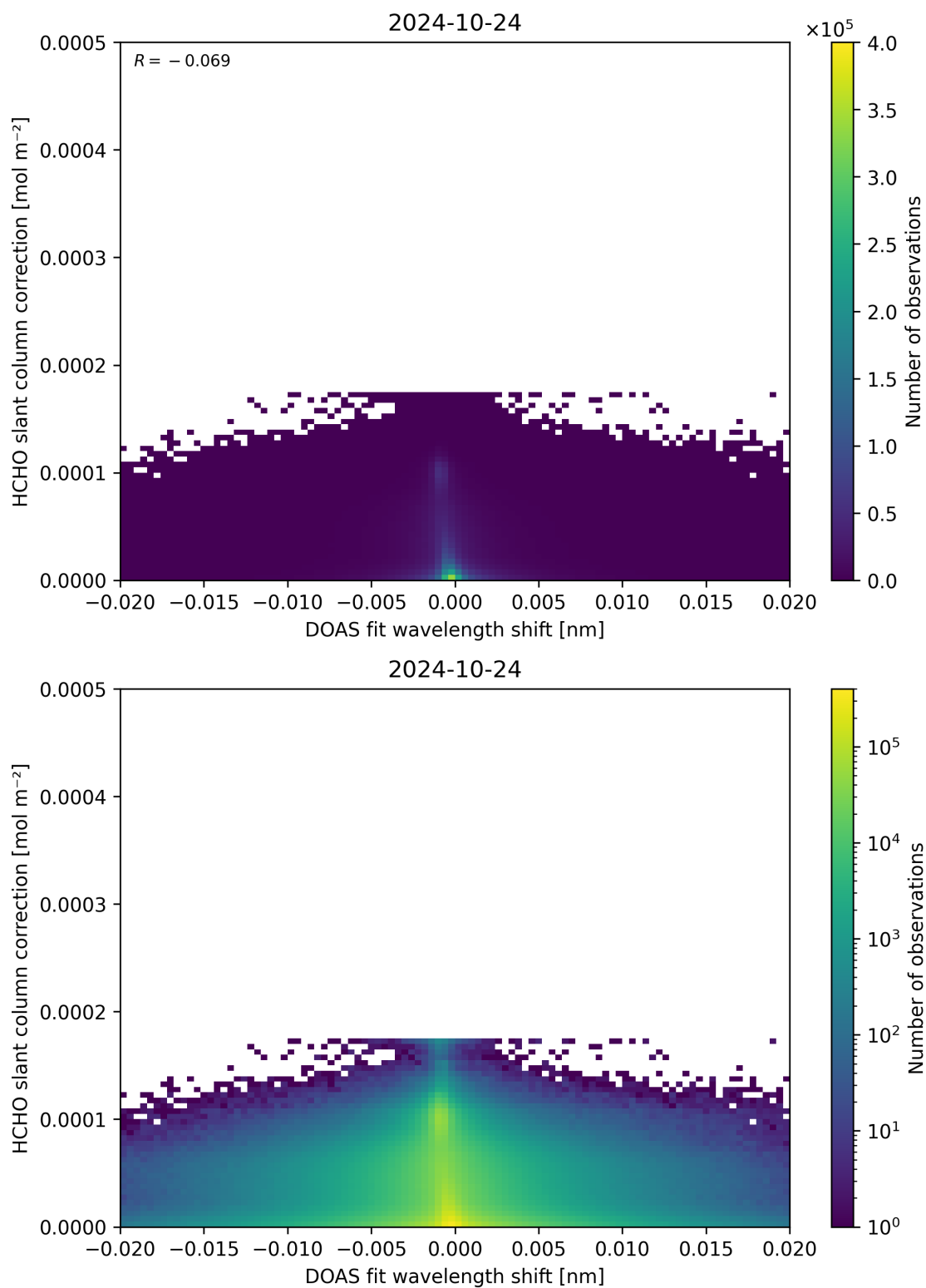
Figure 67: Scatter density plot of “DOAS fit wavelength shift” against “HCHO slant column correction” for 2024-10-24 to 2024-10-25.
