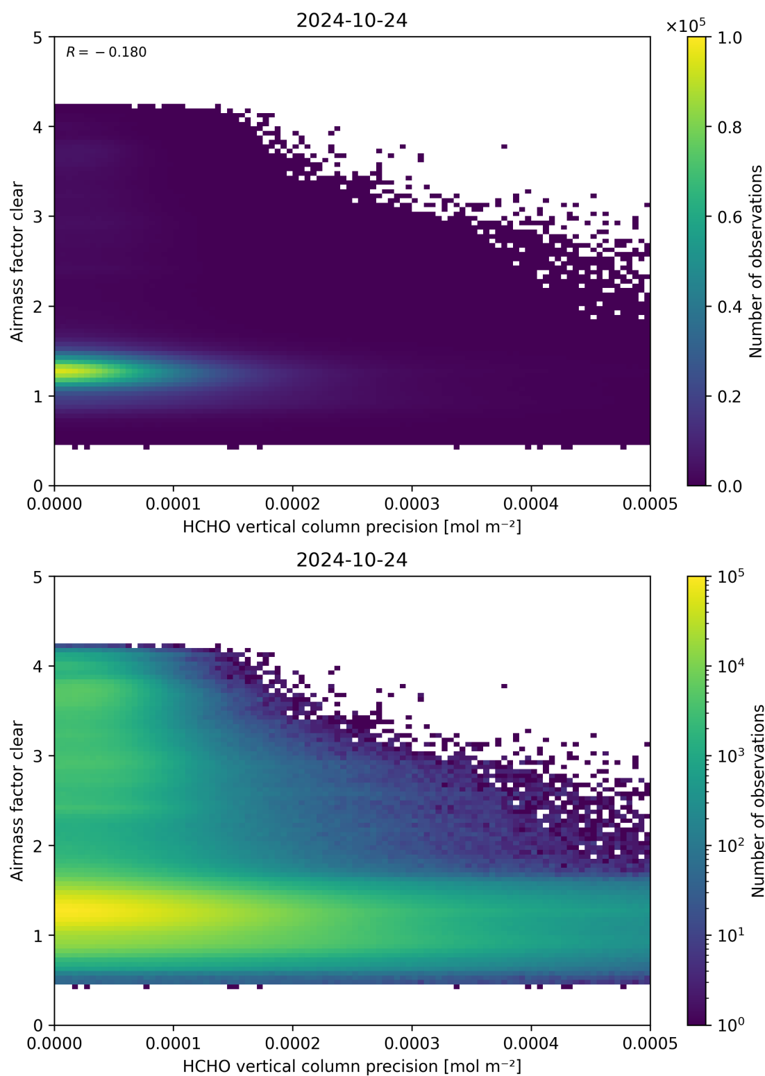
Figure 139: Scatter density plot of “HCHO vertical column precision” against “Airmass factor clear” for 2024-10-24 to 2024-10-25.
