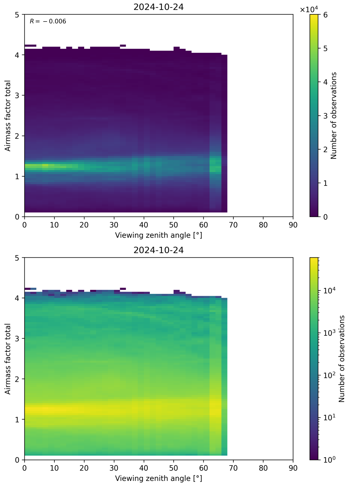
Figure 190: Scatter density plot of “Viewing zenith angle” against “Airmass factor total” for 2024-10-24 to 2024-10-25.
