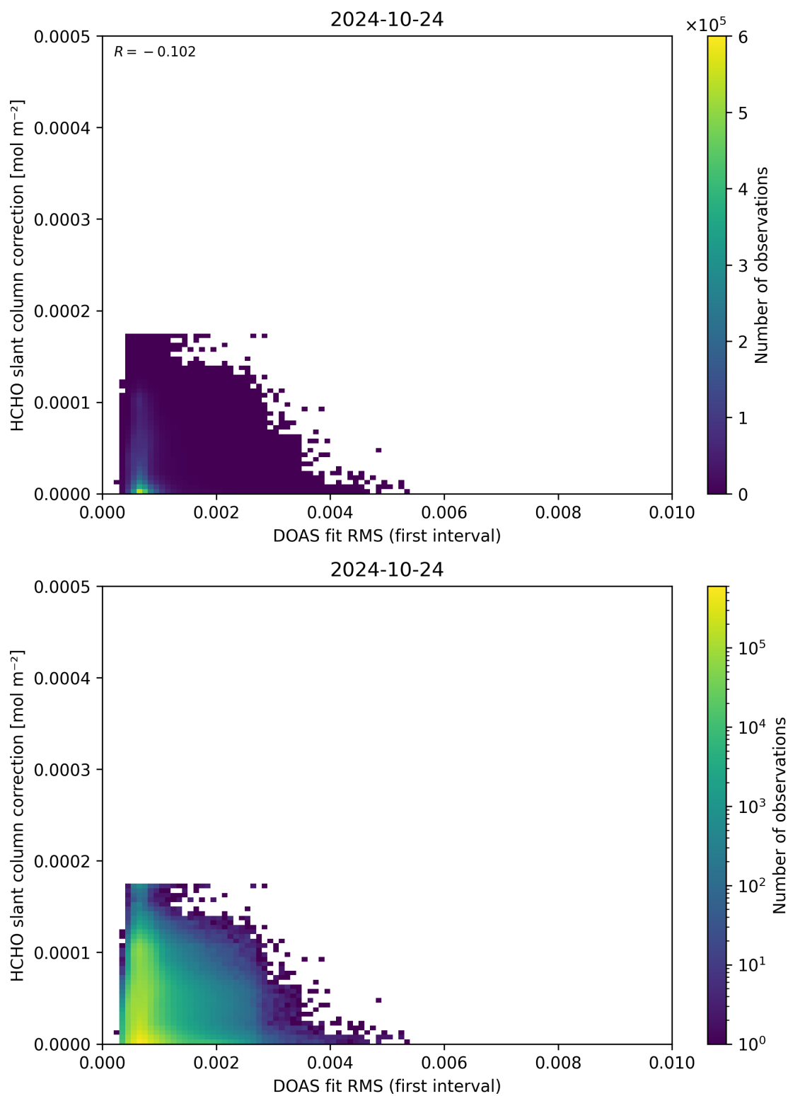
Figure 63: Scatter density plot of “DOAS fit RMS (first interval)” against “HCHO slant column correction” for 2024-10-24 to 2024-10-25.
