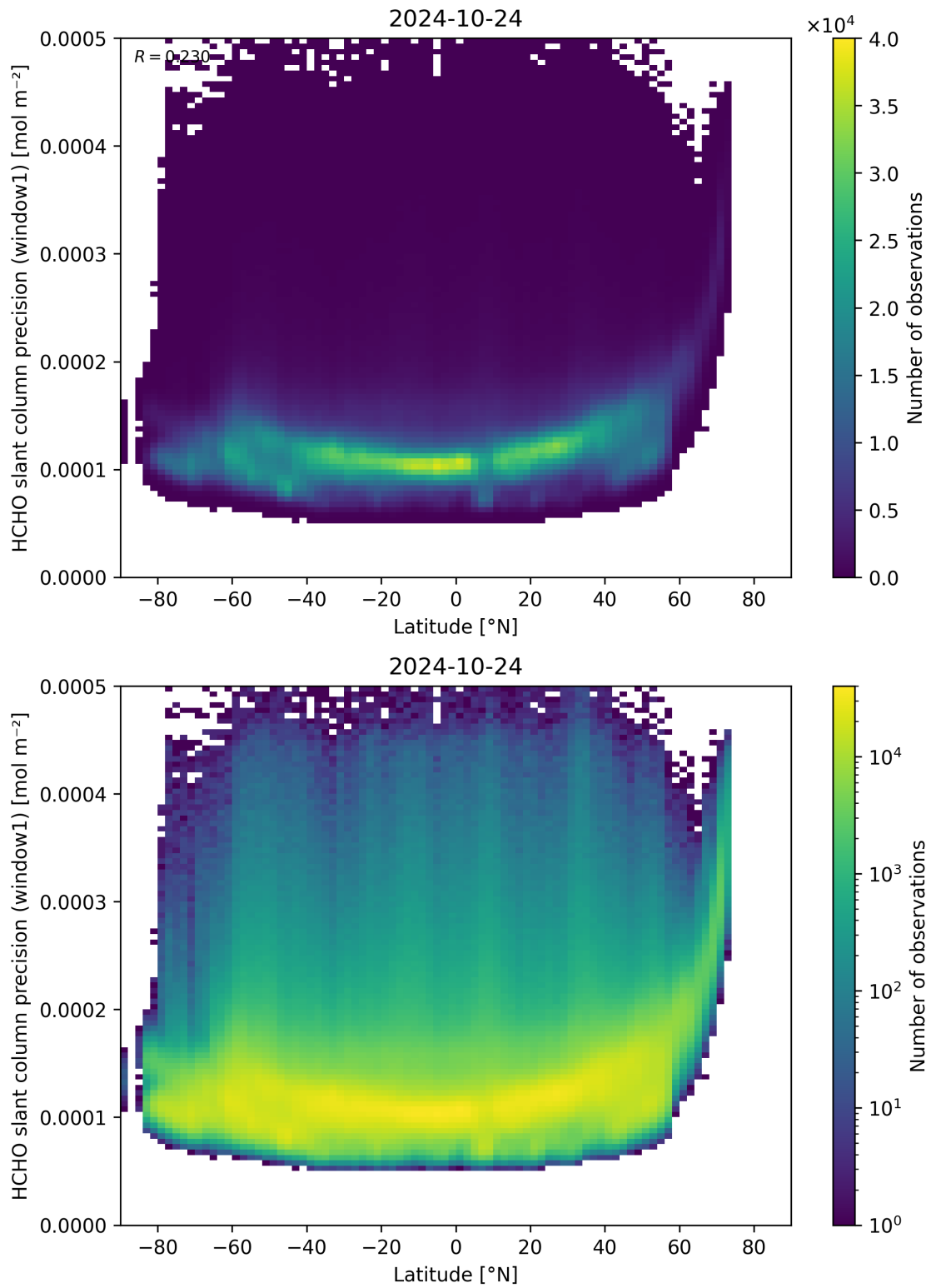
Figure 160: Scatter density plot of “Latitude” against “HCHO slant column precision (window1)” for 2024-10-24 to 2024-10-25.
