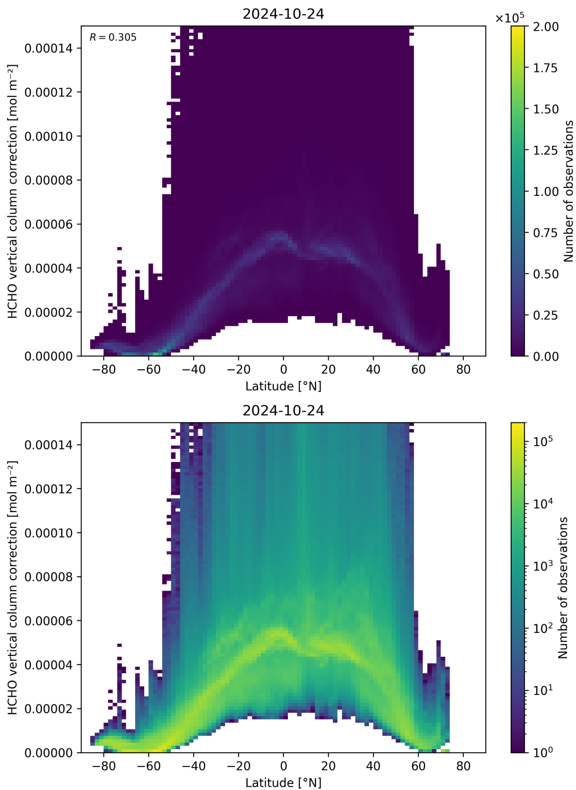
Figure 164: Scatter density plot of “Latitude” against “HCHO vertical column correction” for 2024-10-24 to 2024-10-25.
