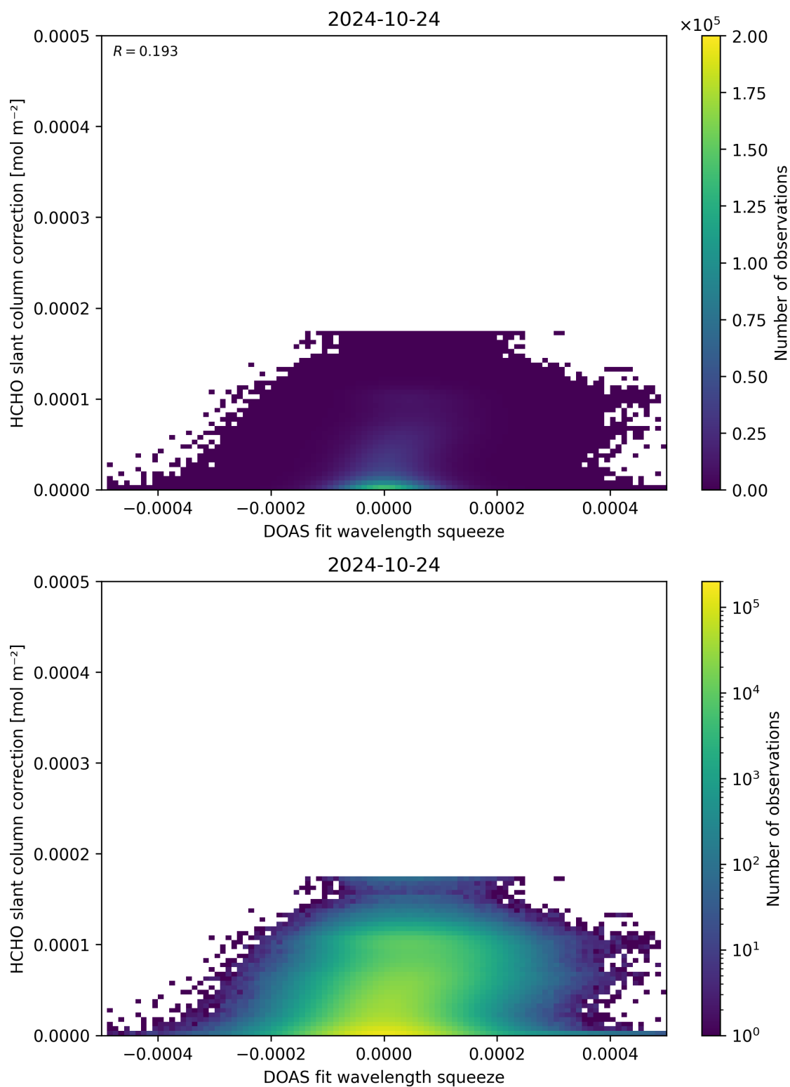
Figure 70: Scatter density plot of “DOAS fit wavelength squeeze” against “HCHO slant column correction” for 2024-10-24 to 2024-10-25.
