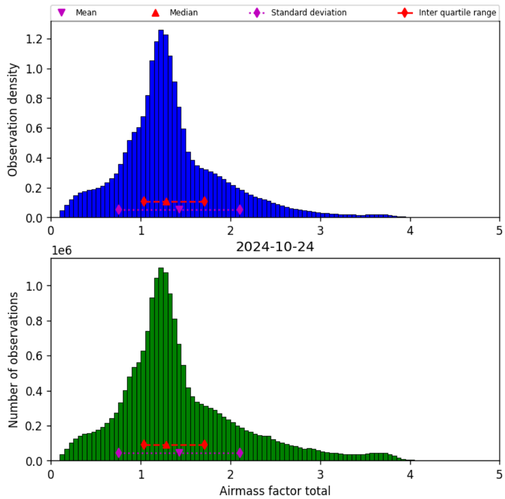
Figure 40: Histogram of “Airmass factor total” for 2024-10-24 to 2024-10-25
