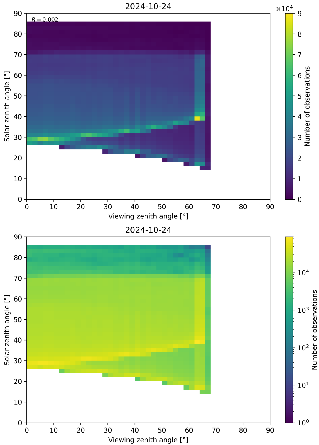
Figure 197: Scatter density plot of “Viewing zenith angle” against “Solar zenith angle” for 2024-10-24 to 2024-10-25.
