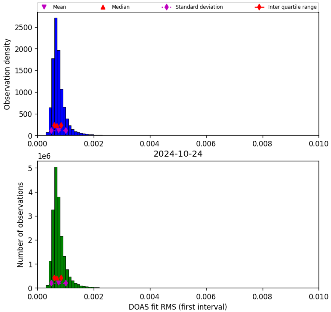
Figure 46: Histogram of “DOAS fit RMS (first interval)” for 2024-10-24 to 2024-10-25
