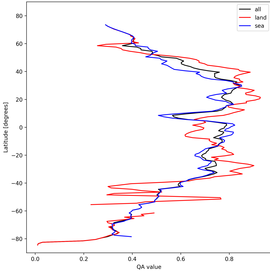
Figure 20: Zonal average of “QA value” for 2024-10-24 to 2024-10-25.
