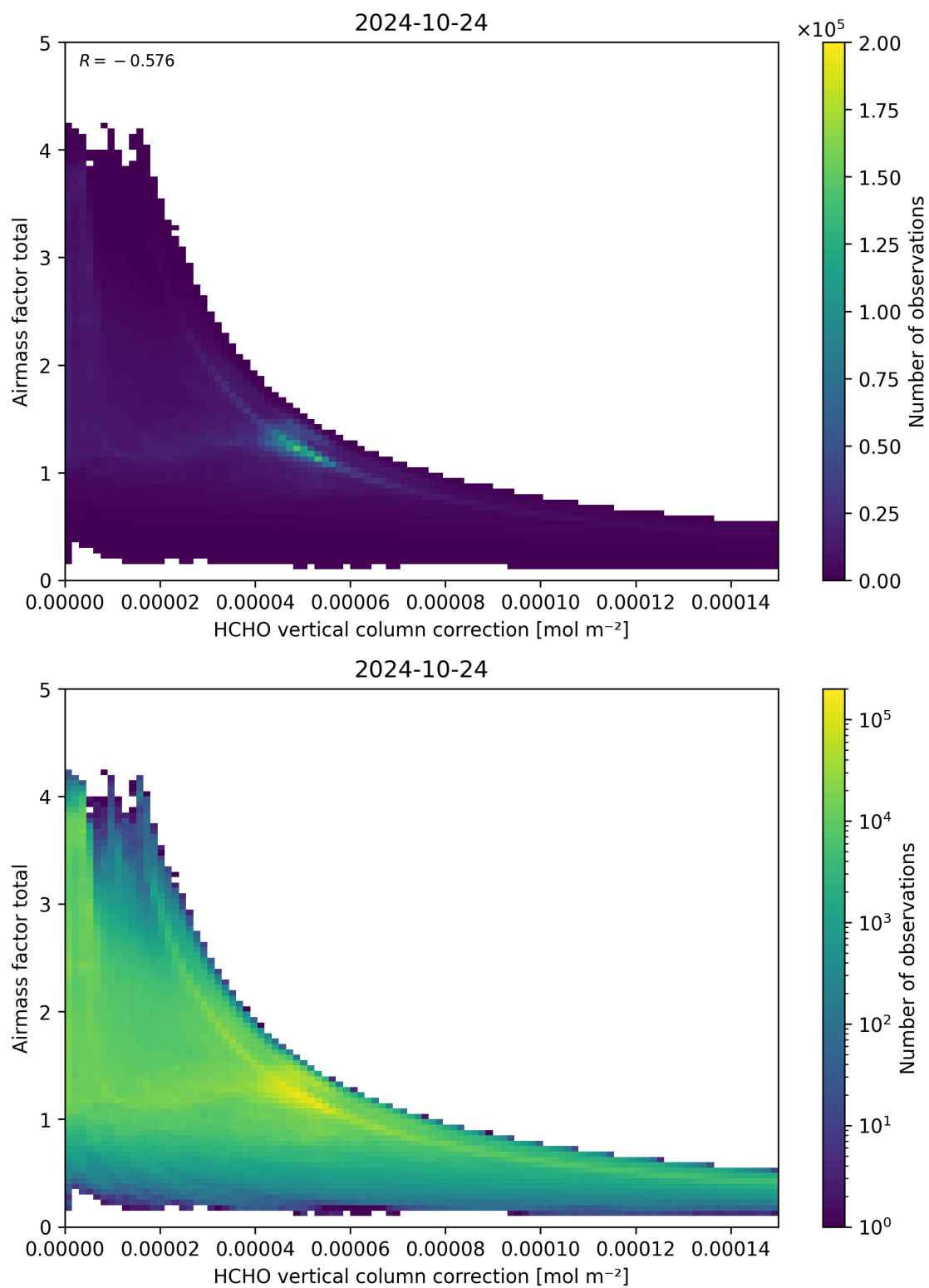
Figure 120: Scatter density plot of “HCHO vertical column correction” against “Airmass factor total” for 2024-10-24 to 2024-10-25.
