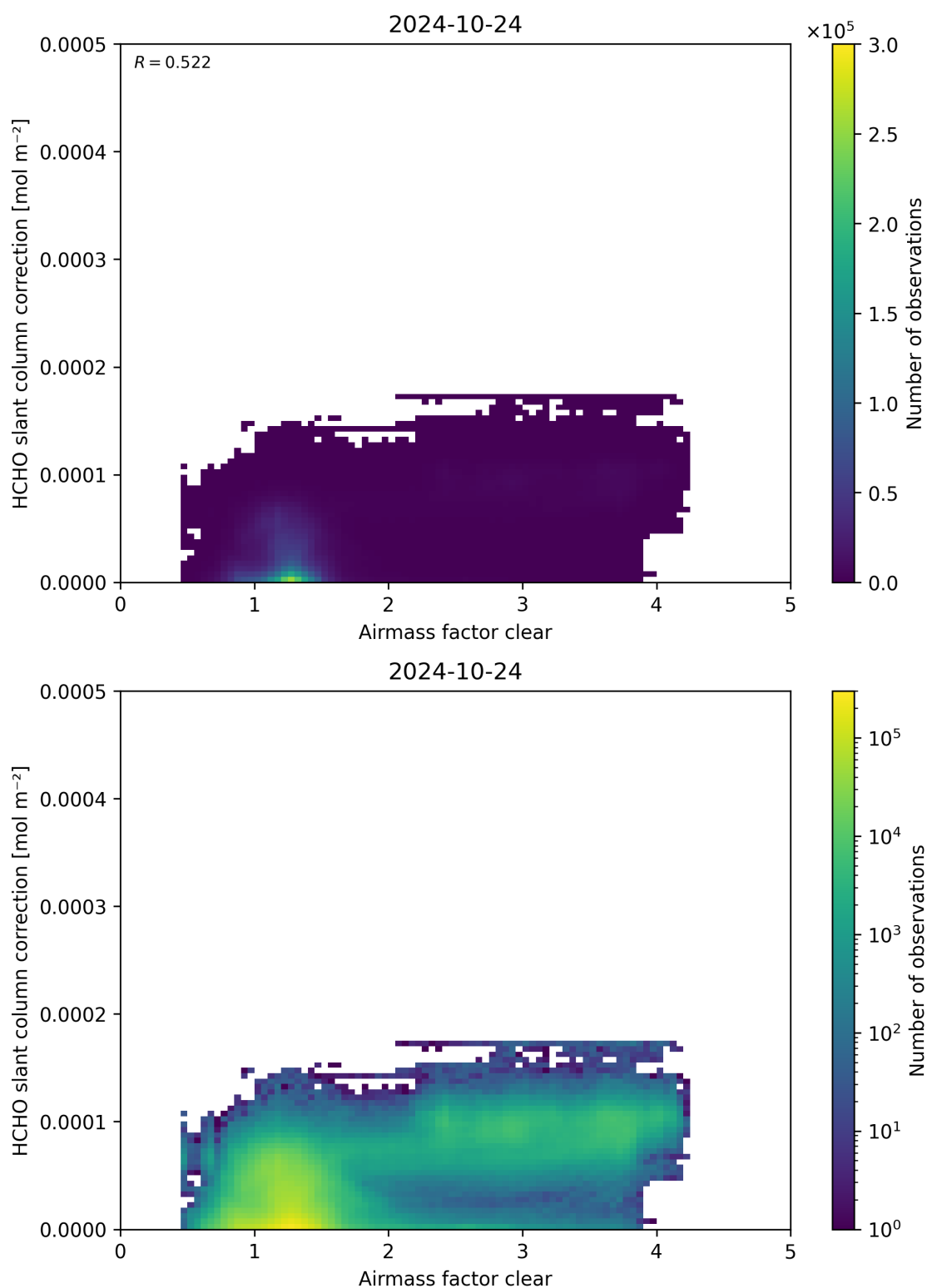
Figure 75: Scatter density plot of “Airmass factor clear” against “HCHO slant column correction” for 2024-10-24 to 2024-10-25.
