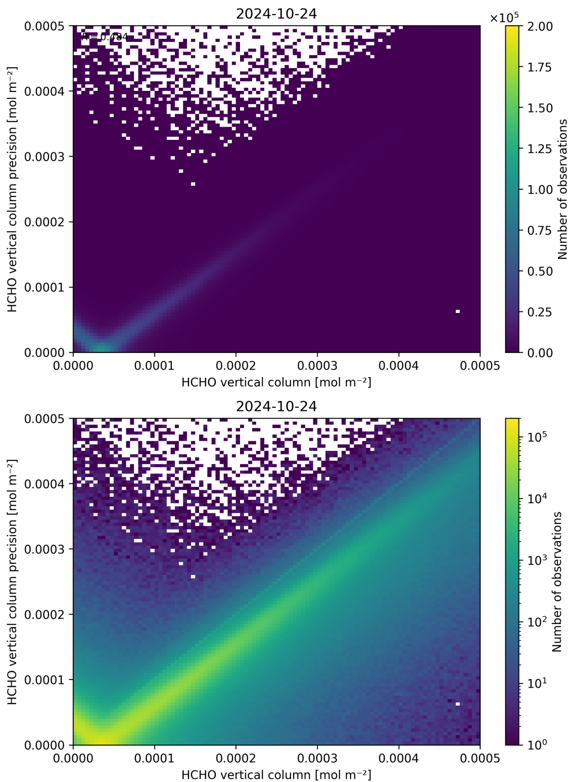
Figure 134: Scatter density plot of “HCHO vertical column” against “HCHO vertical column precision” for 2024-10-24 to 2024-10-25.
