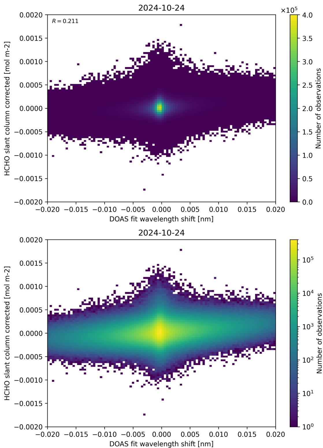
Figure 66: Scatter density plot of “DOAS fit wavelength shift” against “HCHO slant column corrected” for 2024-10-24 to 2024-10-25.
