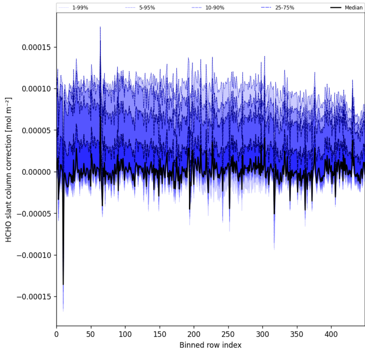
Figure 61: Along track statistics of “HCHO slant column correction” for 2024-10-24 to 2024-10-25
