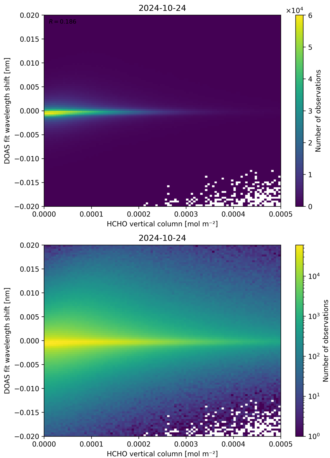
Figure 124: Scatter density plot of “HCHO vertical column” against “DOAS fit wavelength shift” for 2024-10-24 to 2024-10-25.
