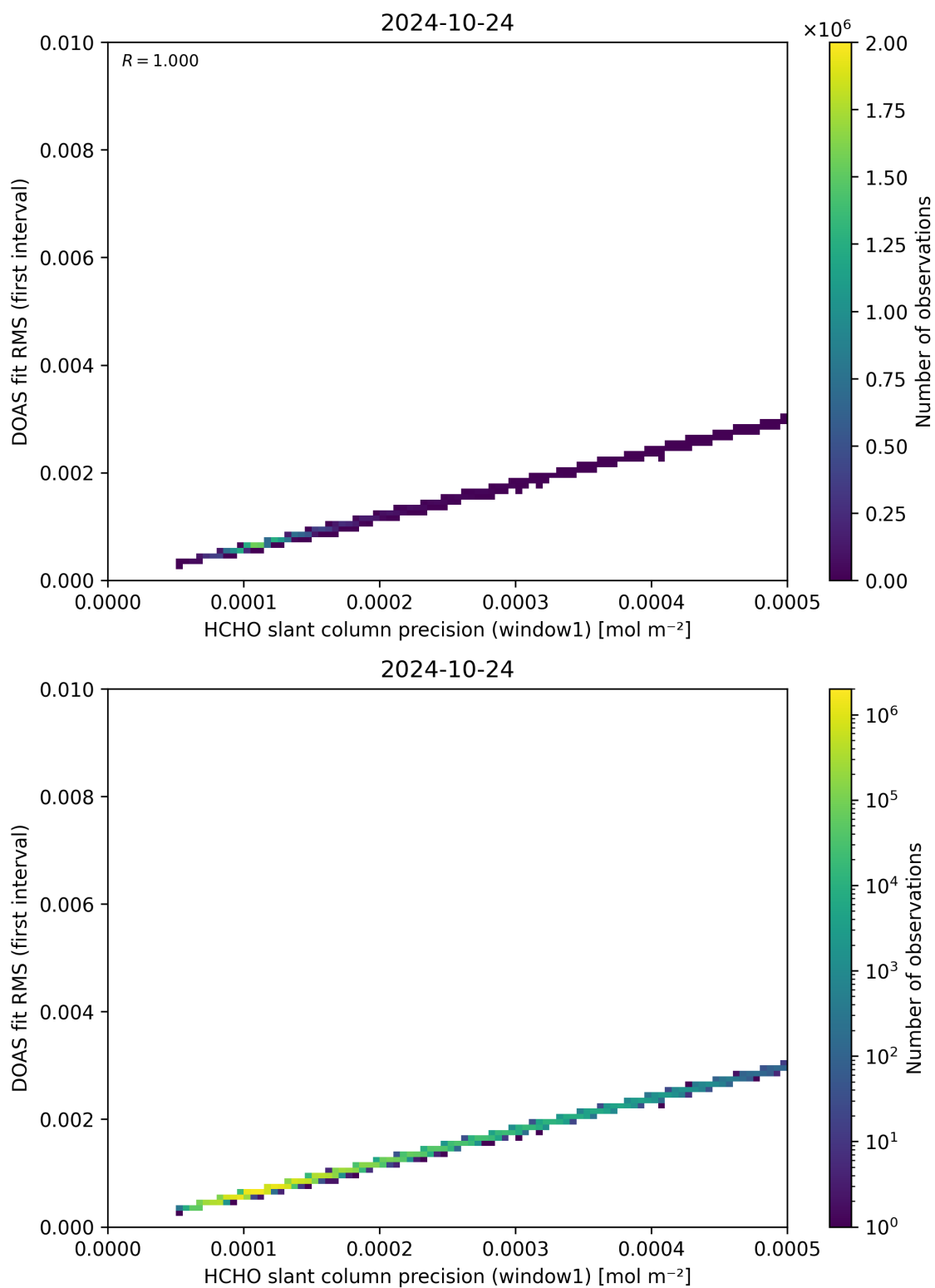
Figure 88: Scatter density plot of “HCHO slant column precision (window1)” against “DOAS fit RMS (first interval)” for 2024-10-24 to 2024-10-25.
