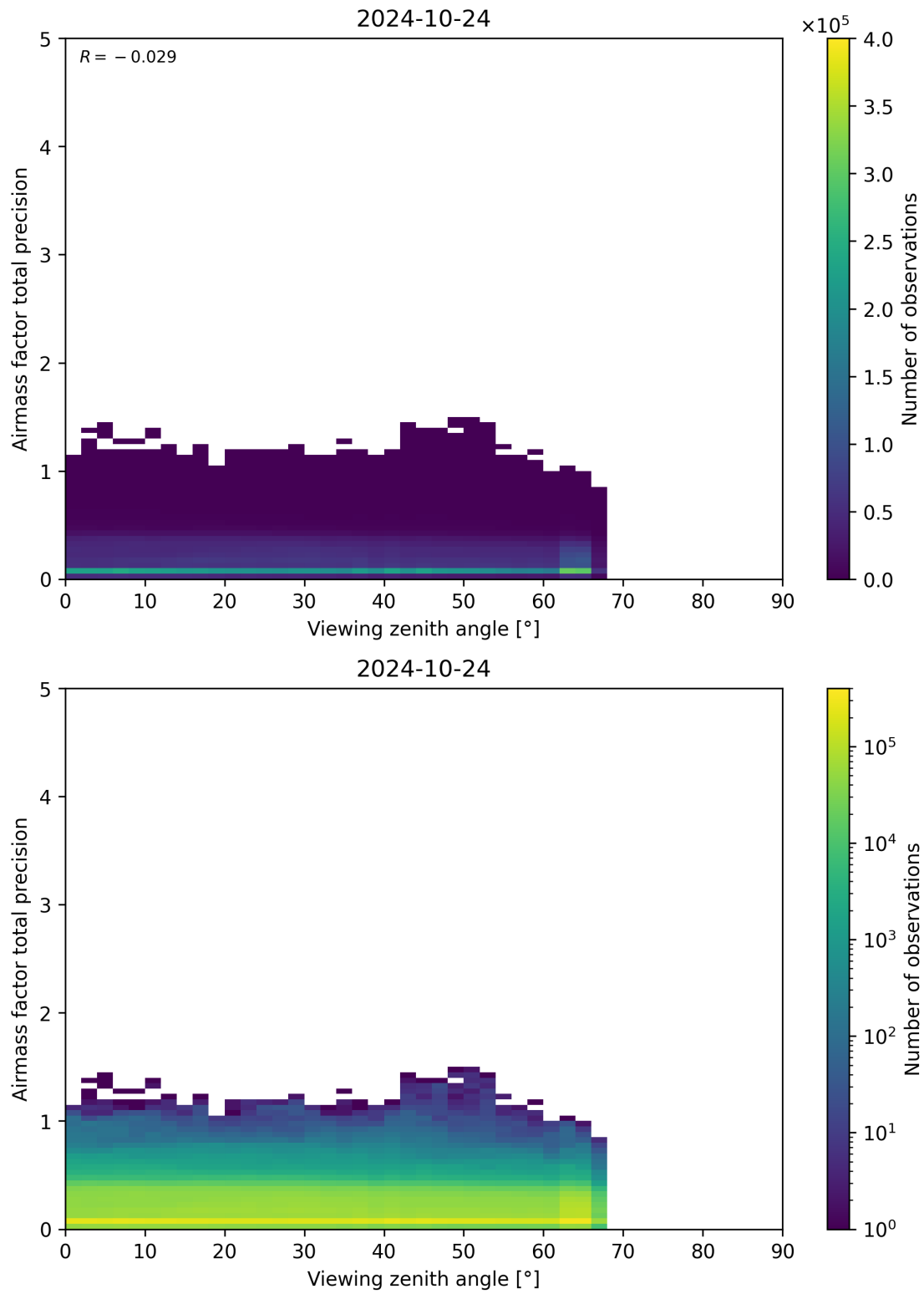
Figure 191: Scatter density plot of “Viewing zenith angle” against “Airmass factor total precision” for 2024-10-24 to 2024-10-25.
