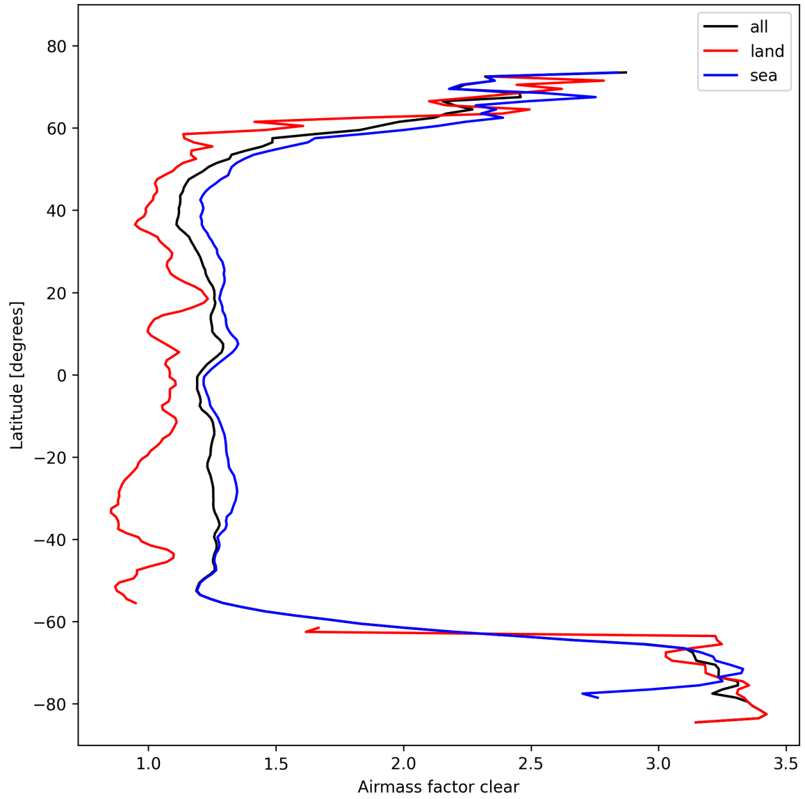
Figure 28: Zonal average of “Airmass factor clear” for 2024-10-24 to 2024-10-25.
