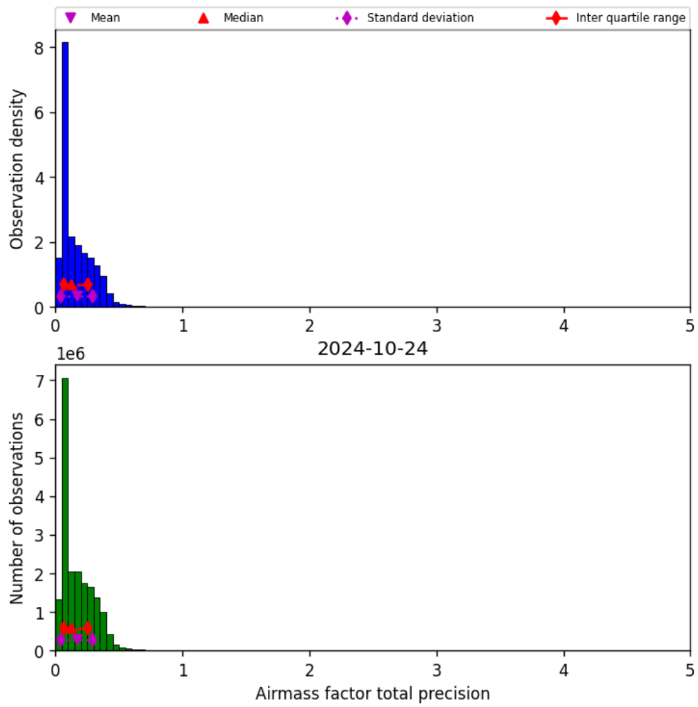
Figure 41: Histogram of “Airmass factor total precision” for 2024-10-24 to 2024-10-25
