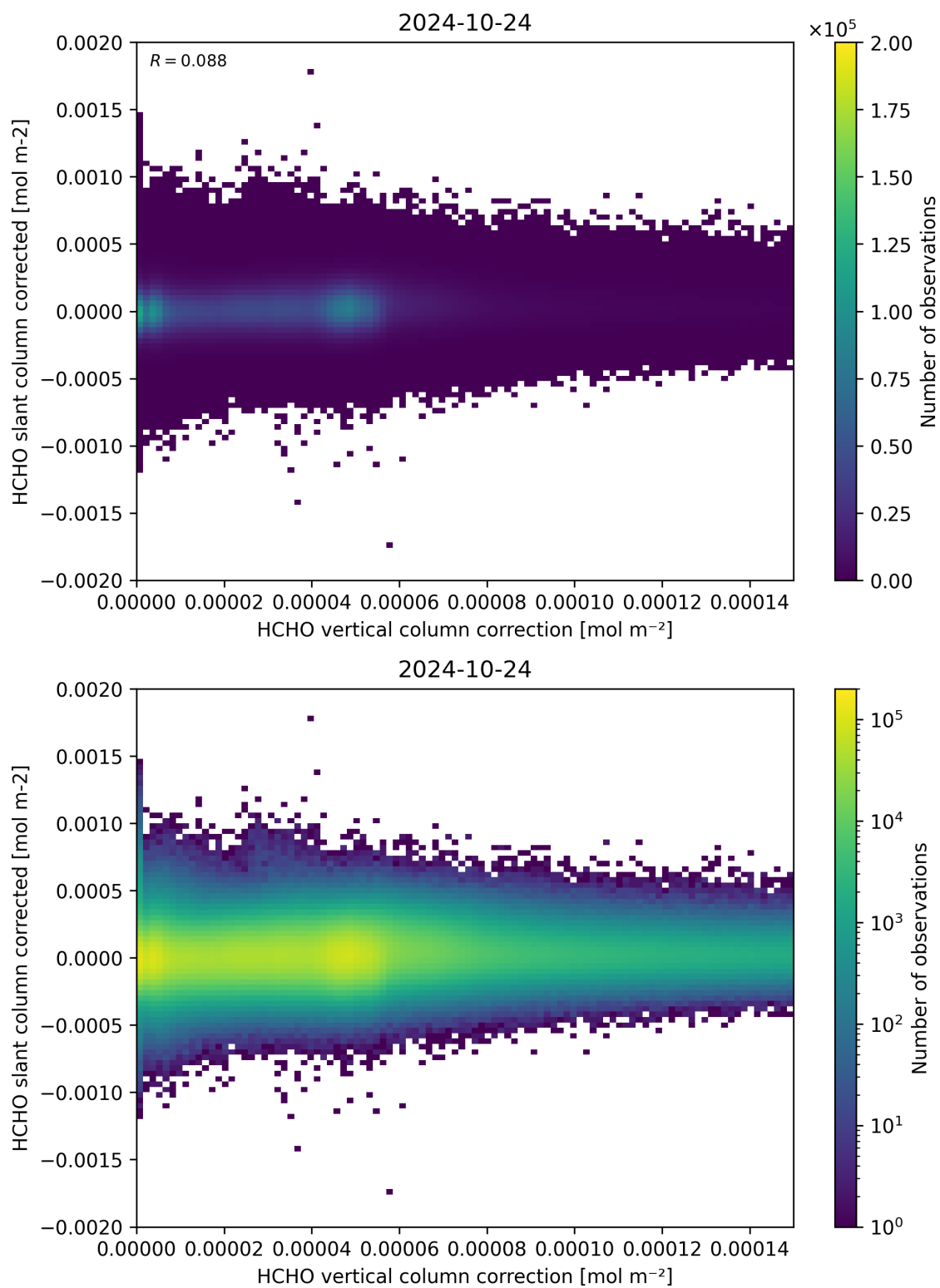
Figure 116: Scatter density plot of “HCHO vertical column correction” against “HCHO slant column corrected” for 2024-10-24 to 2024-10-25.
