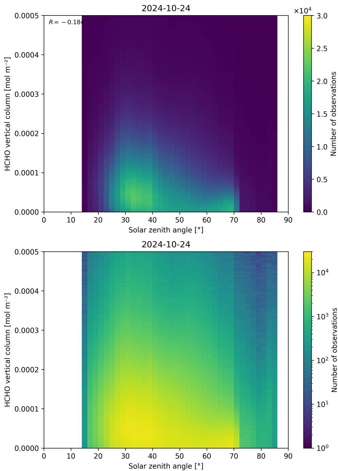
Figure 177: Scatter density plot of “Solar zenith angle” against “HCHO vertical column” for 2024-10-24 to 2024-10-25.
