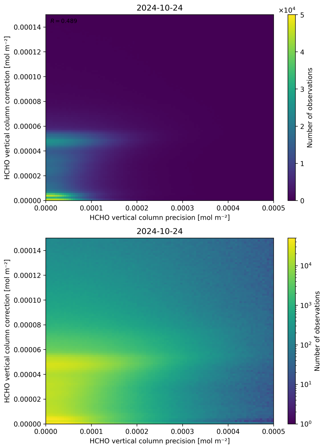
Figure 146: Scatter density plot of “HCHO vertical column precision” against “HCHO vertical column correction” for 2024-10-24 to 2024-10-25.
