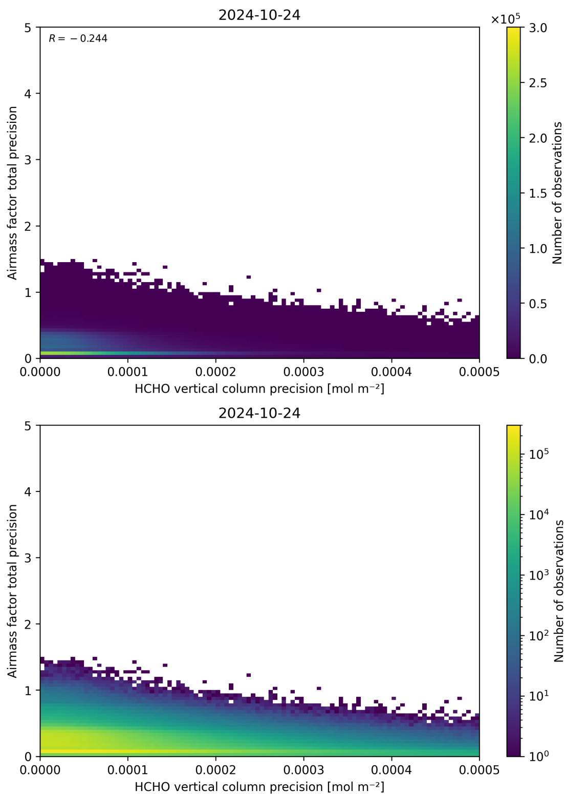
Figure 145: Scatter density plot of “HCHO vertical column precision” against “Airmass factor total precision” for 2024-10-24 to 2024-10-25.
