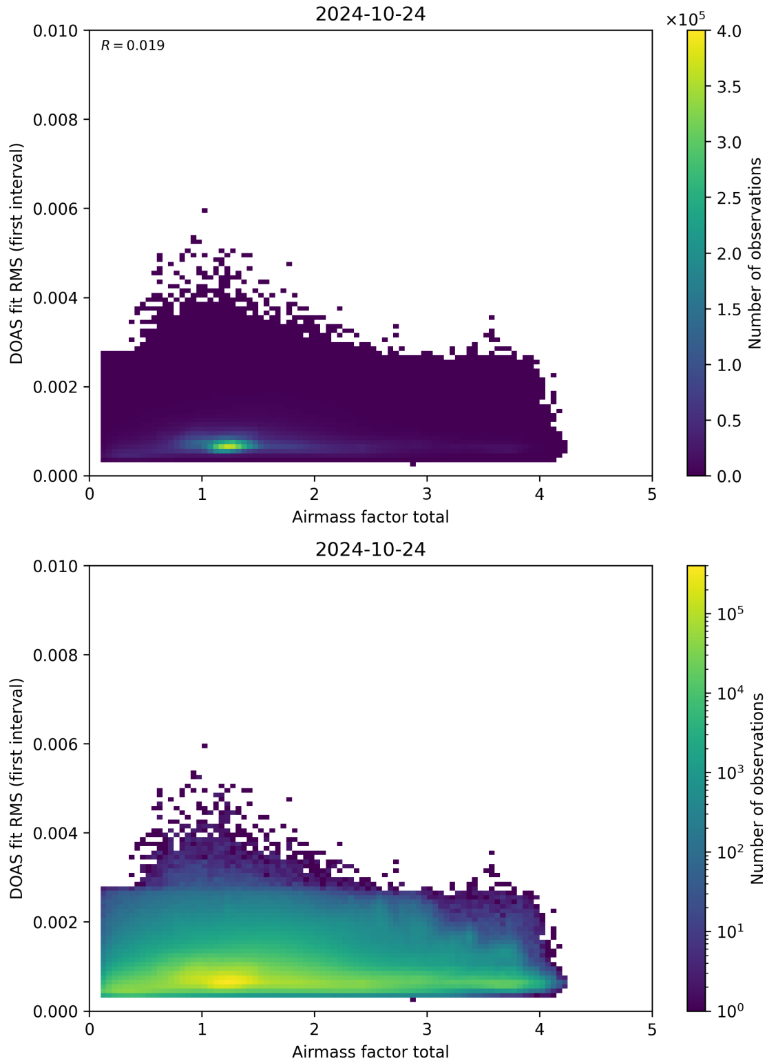
Figure 97: Scatter density plot of “Airmass factor total” against “DOAS fit RMS (first interval)” for 2024-10-24 to 2024-10-25.
