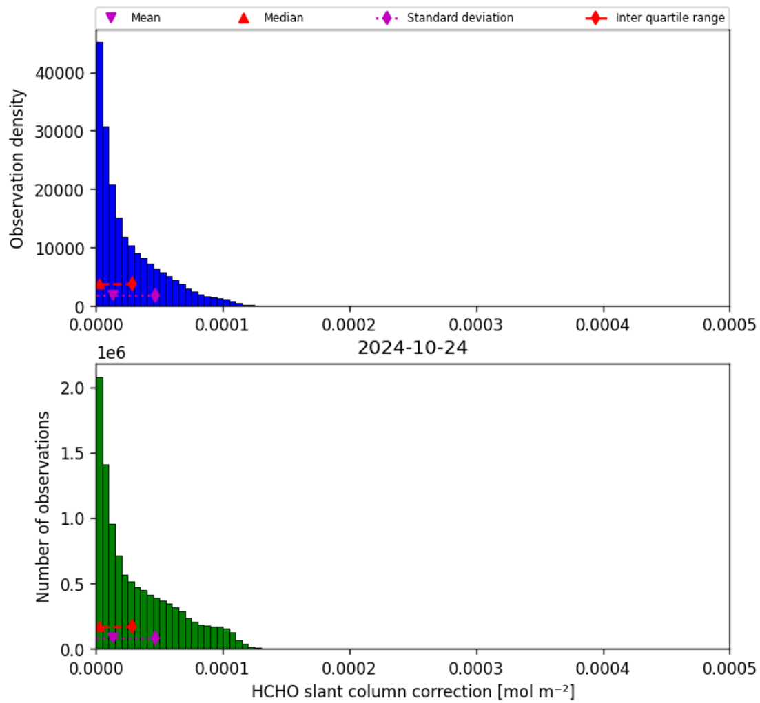
Figure 47: Histogram of “HCHO slant column correction” for 2024-10-24 to 2024-10-25
