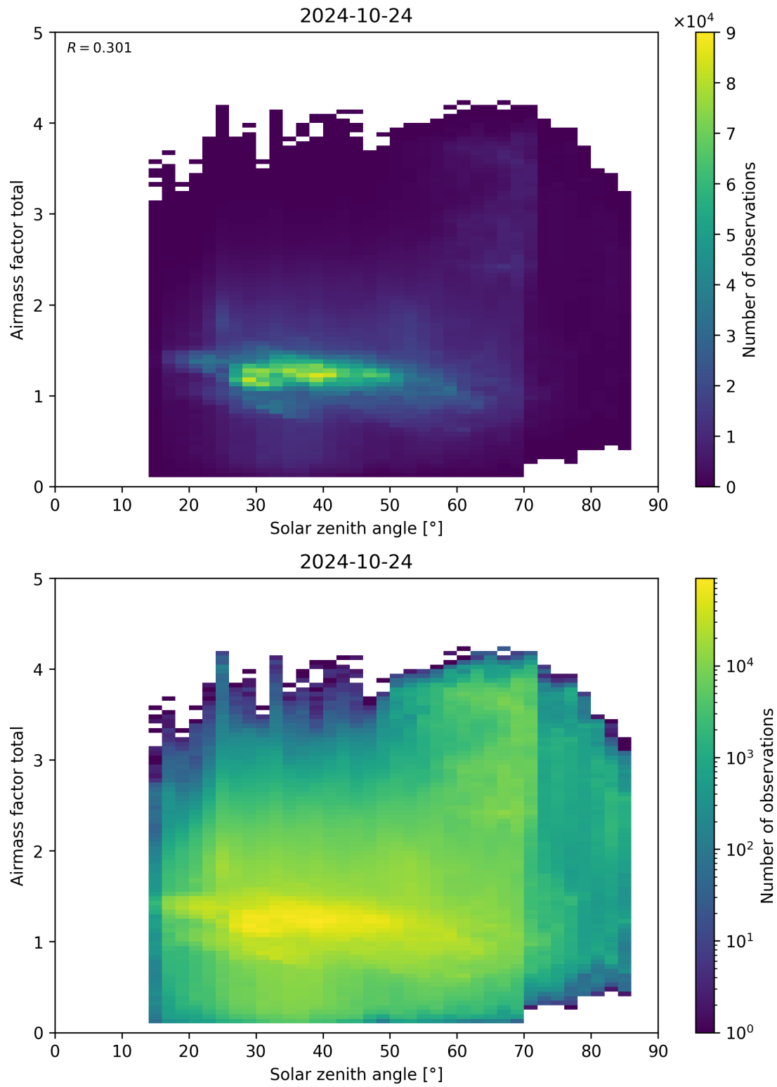
Figure 175: Scatter density plot of “Solar zenith angle” against “Airmass factor total” for 2024-10-24 to 2024-10-25.
