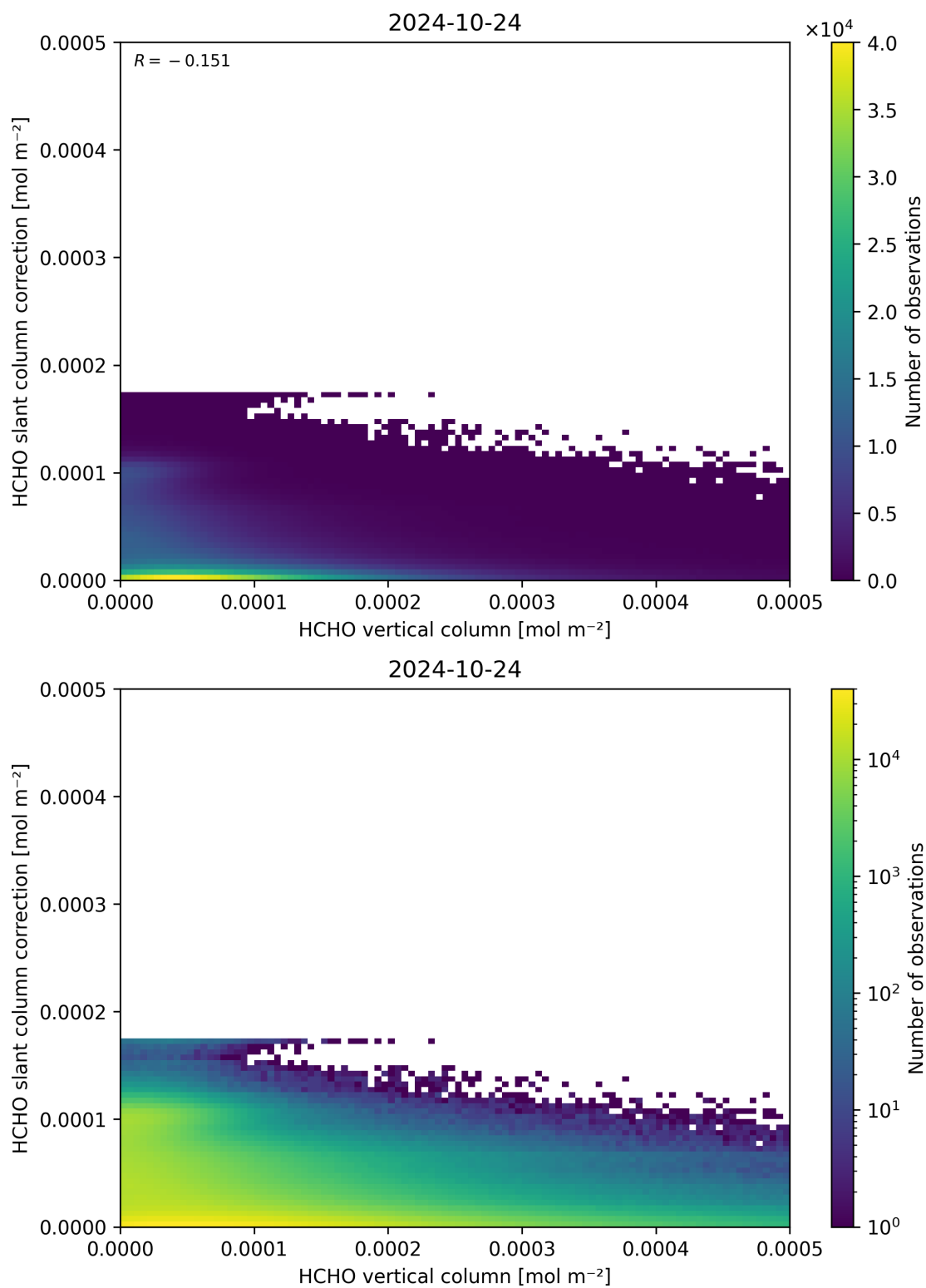
Figure 128: Scatter density plot of “HCHO vertical column” against “HCHO slant column correction” for 2024-10-24 to 2024-10-25.
