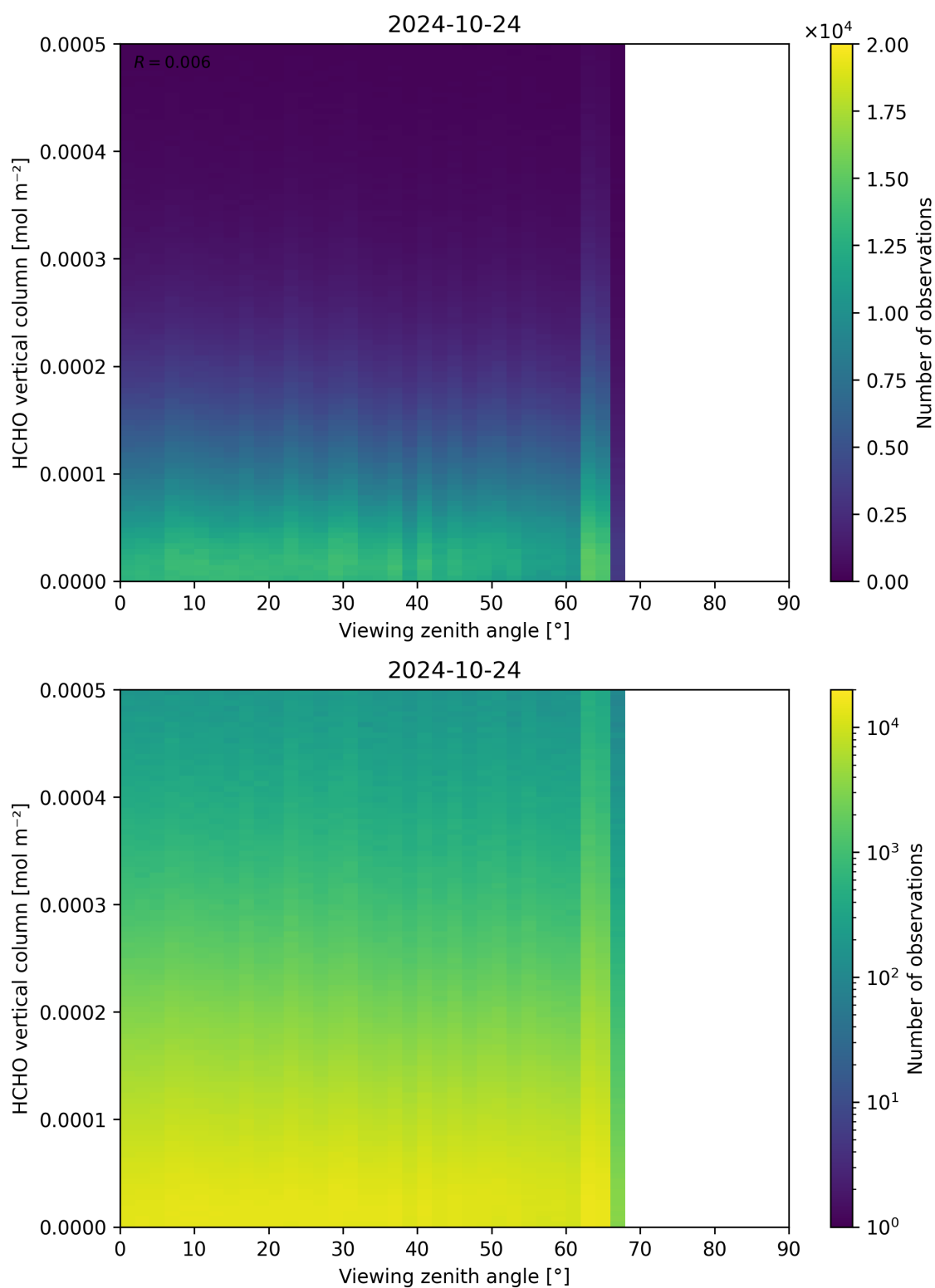
Figure 192: Scatter density plot of “Viewing zenith angle” against “HCHO vertical column” for 2024-10-24 to 2024-10-25.
