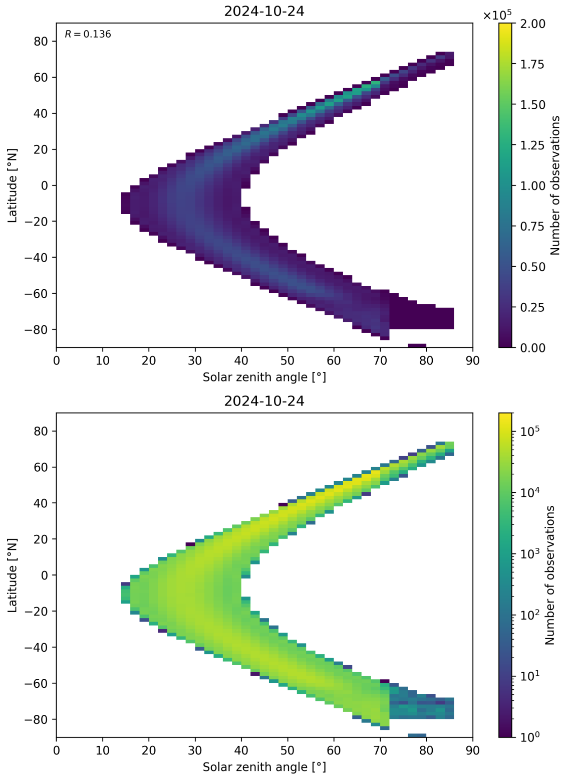
Figure 181: Scatter density plot of “Solar zenith angle” against “Latitude” for 2024-10-24 to 2024-10-25.
