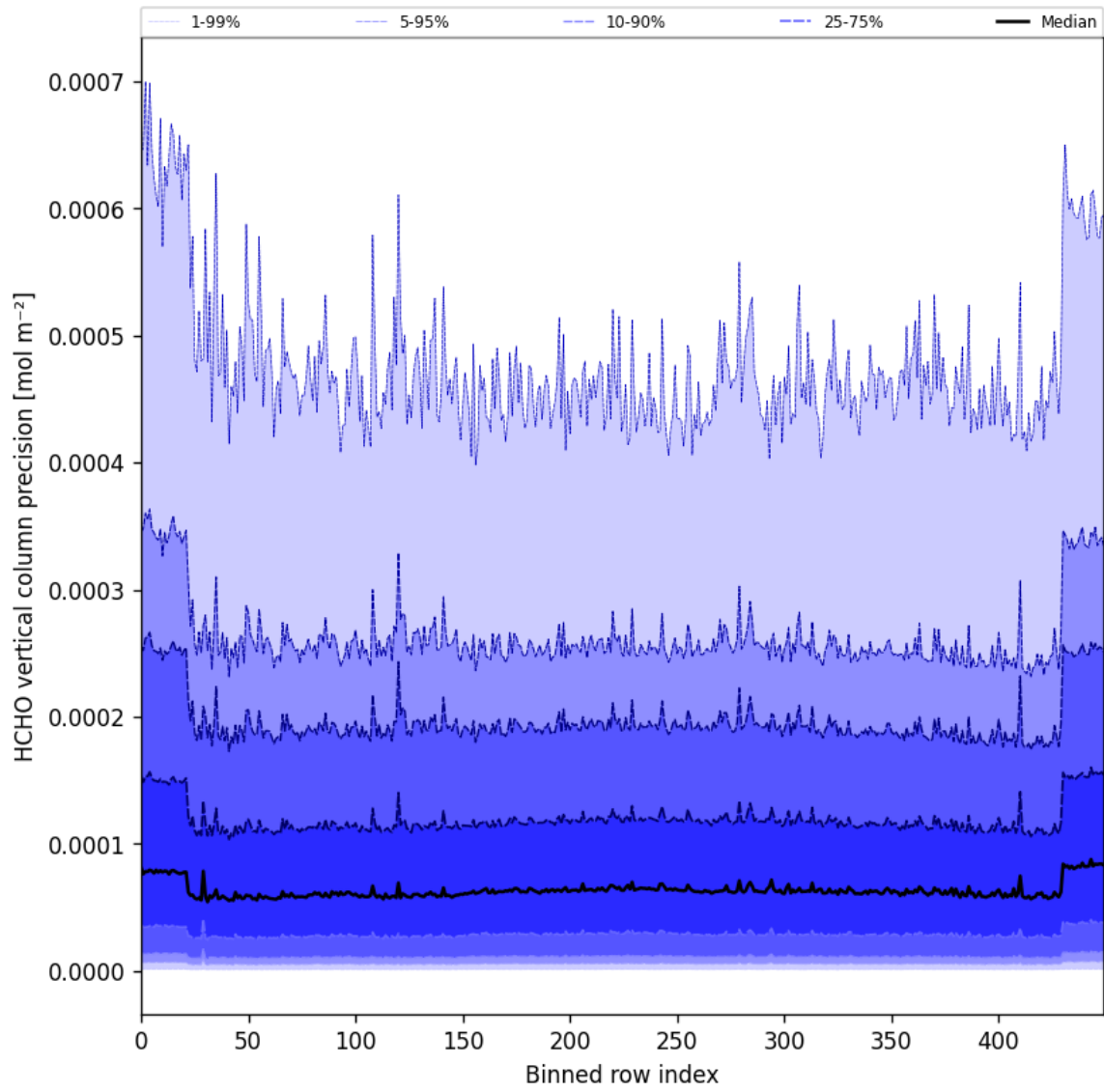
Figure 50: Along track statistics of “HCHO vertical column precision” for 2024-10-24 to 2024-10-25
