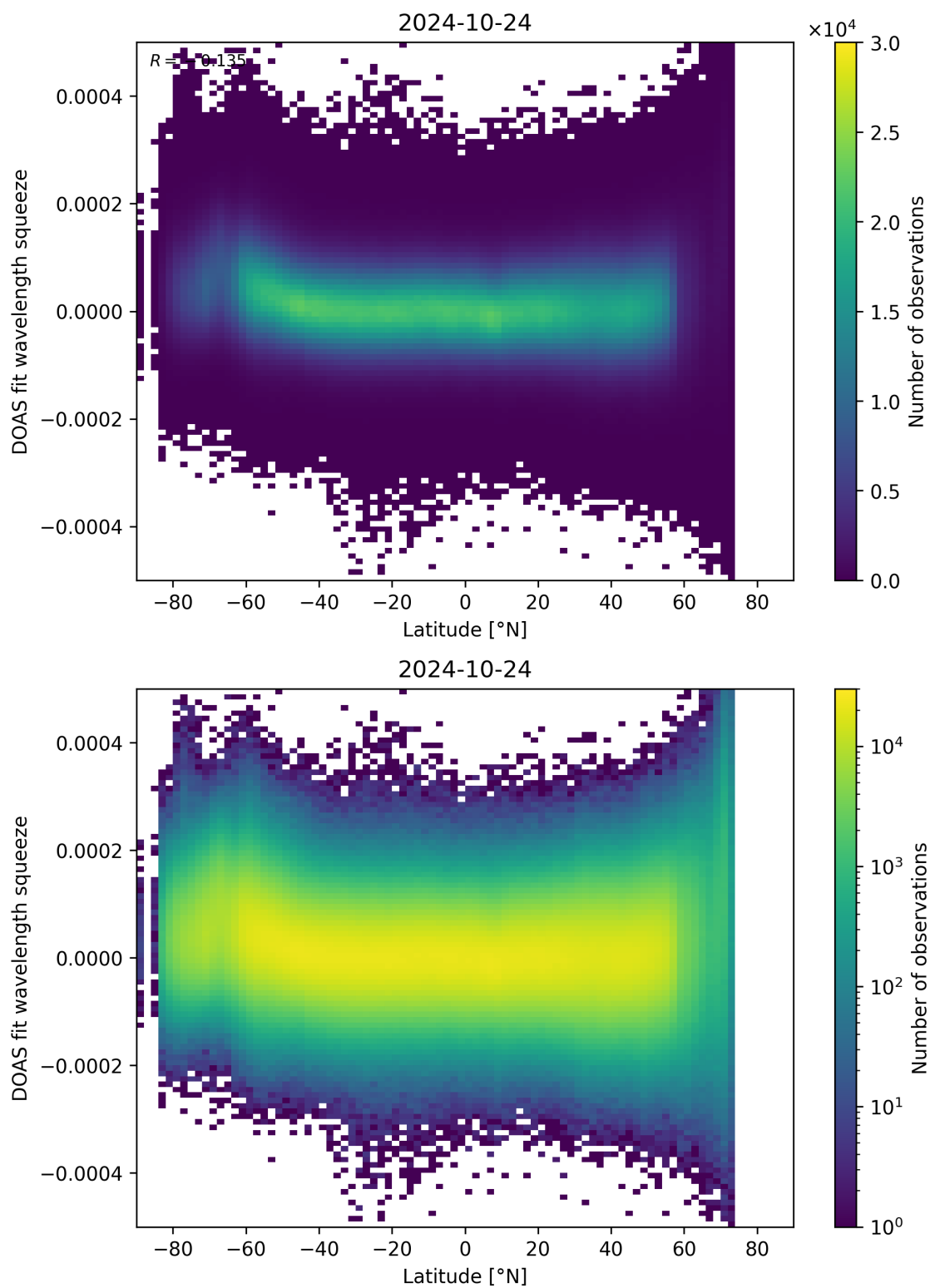
Figure 155: Scatter density plot of “Latitude” against “DOAS fit wavelength squeeze” for 2024-10-24 to 2024-10-25.
