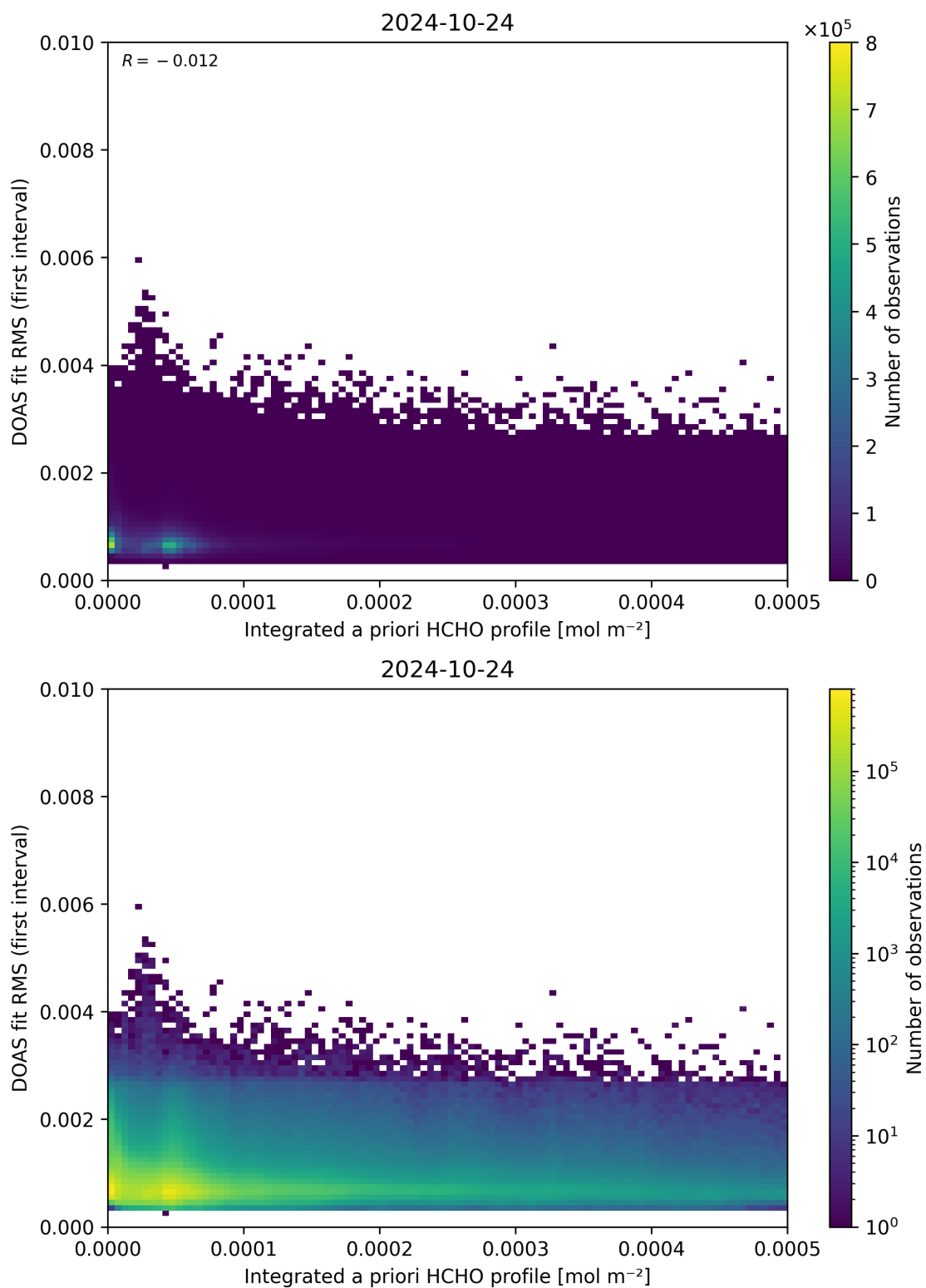
Figure 148: Scatter density plot of “Integrated a priori HCHO profile” against “DOAS fit RMS (first interval)” for 2024-10-24 to 2024-10-25.
