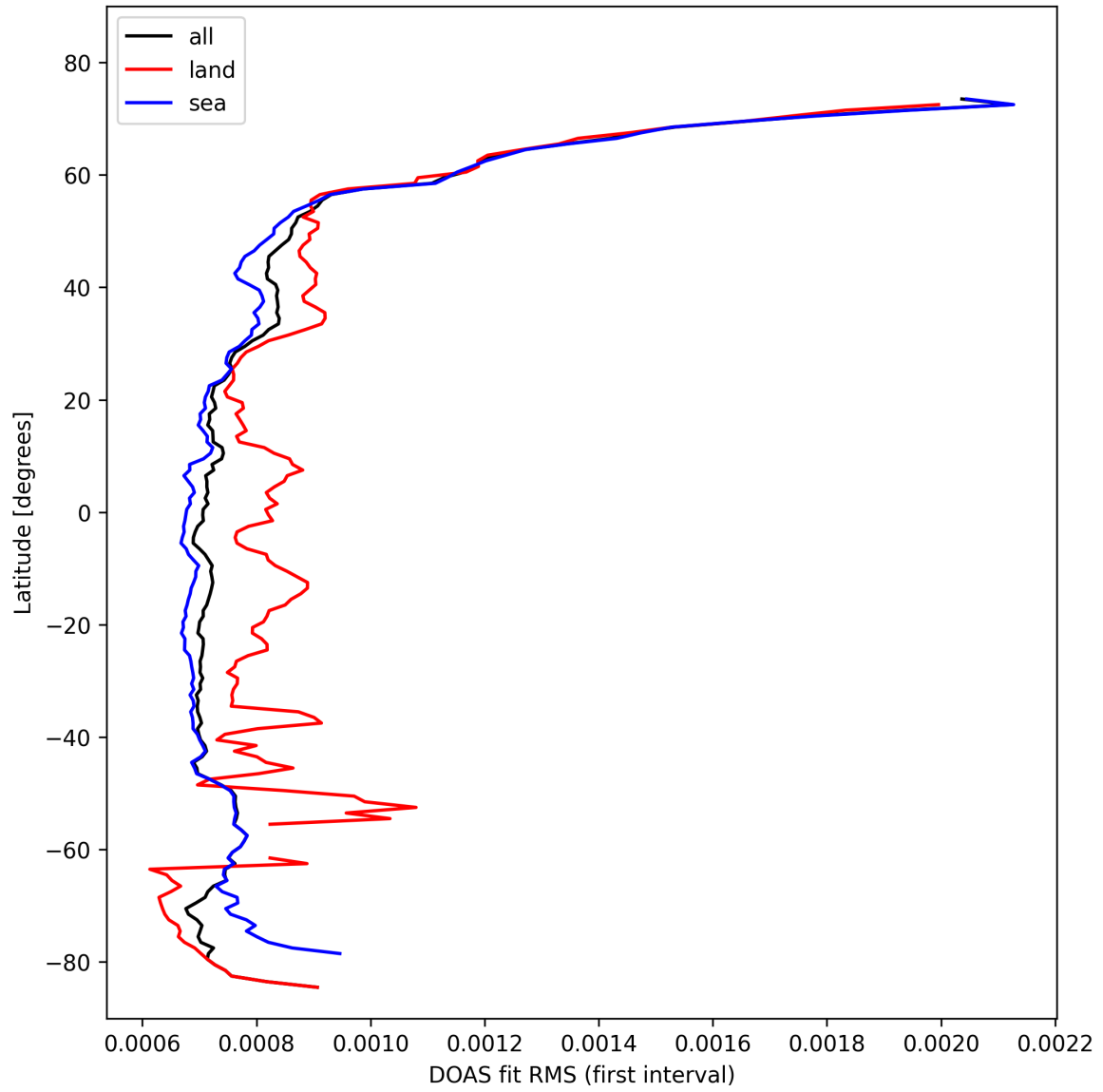
Figure 32: Zonal average of “DOAS fit RMS (first interval)” for 2024-10-24 to 2024-10-25.
