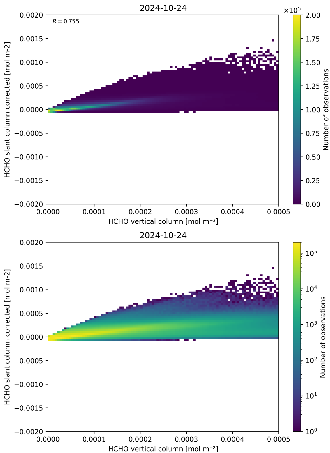
Figure 127: Scatter density plot of “HCHO vertical column” against “HCHO slant column corrected” for 2024-10-24 to 2024-10-25.
