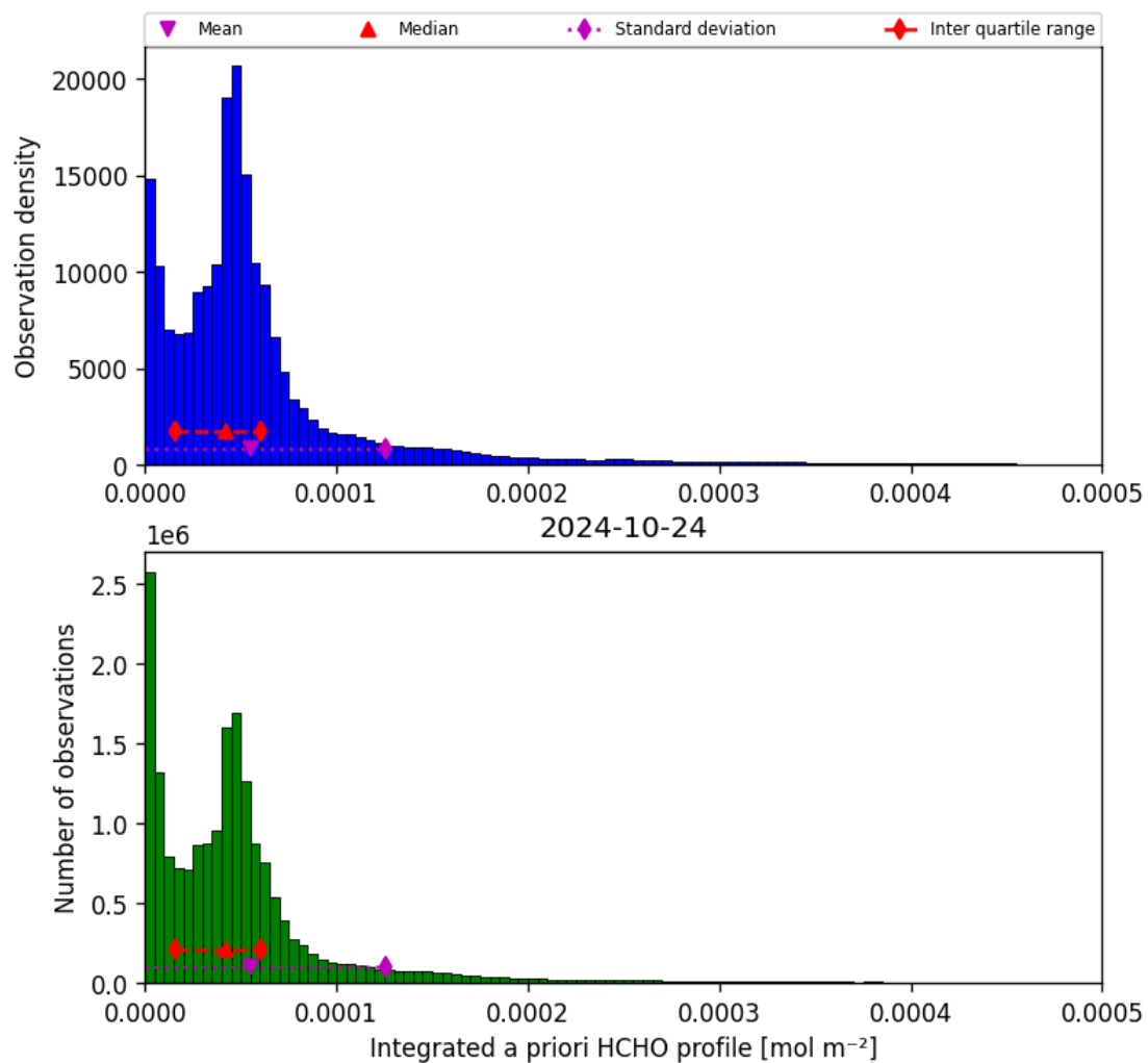
Figure 43: Histogram of “Integrated a priori HCHO profile” for 2024-10-24 to 2024-10-25
