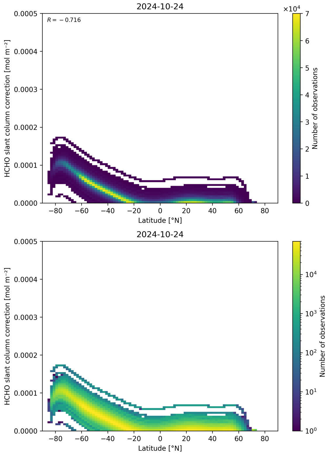
Figure 158: Scatter density plot of “Latitude” against “HCHO slant column correction” for 2024-10-24 to 2024-10-25.
