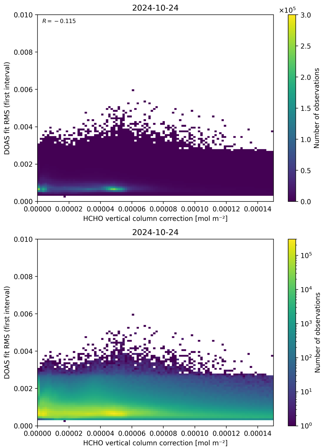
Figure 112: Scatter density plot of “HCHO vertical column correction” against “DOAS fit RMS (first interval)” for 2024-10-24 to 2024-10-25.
