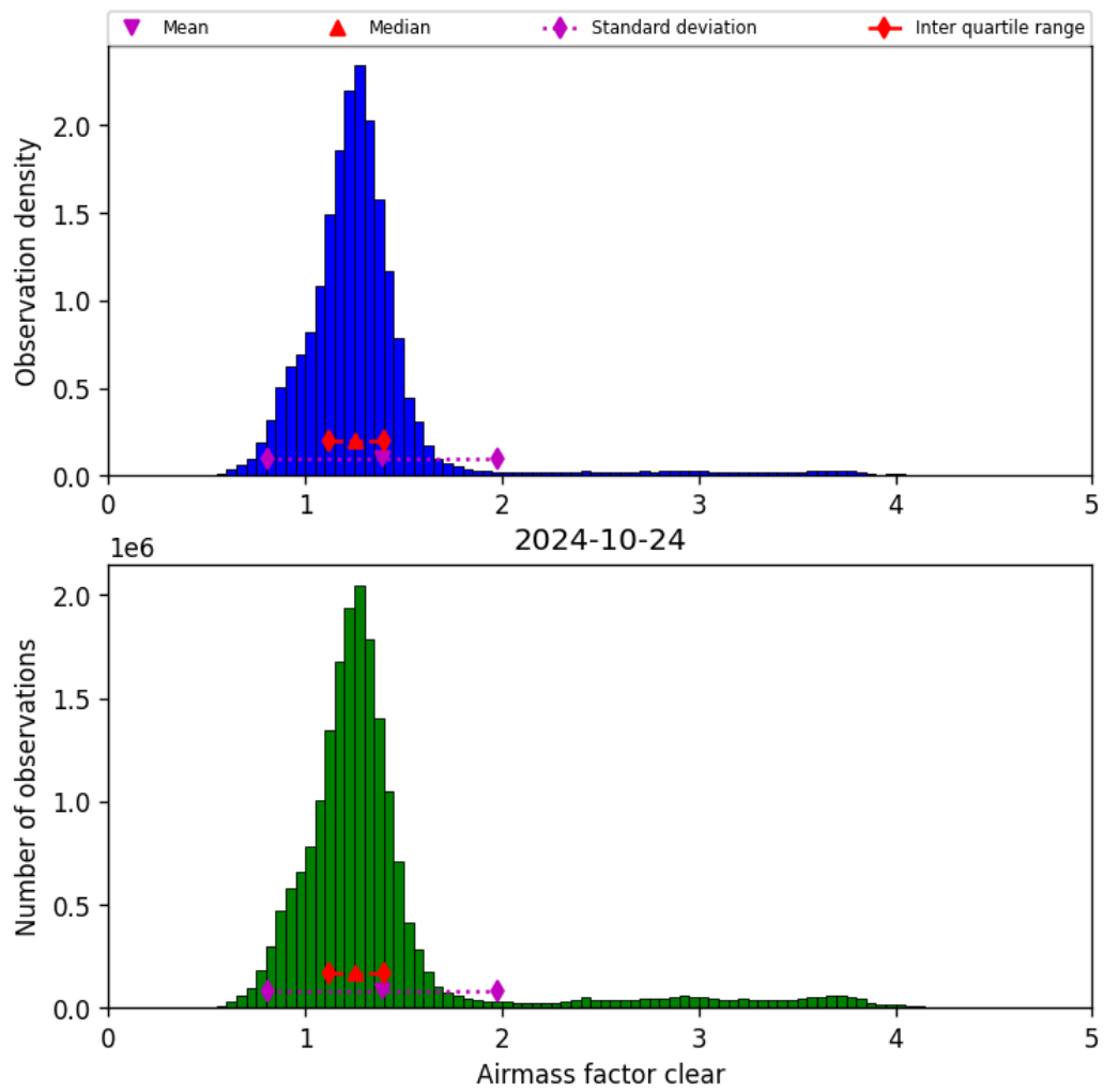
Figure 42: Histogram of “Airmass factor clear” for 2024-10-24 to 2024-10-25
