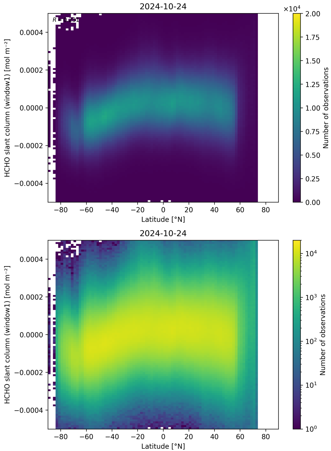
Figure 159: Scatter density plot of “Latitude” against “HCHO slant column (window1)” for 2024-10-24 to 2024-10-25.
