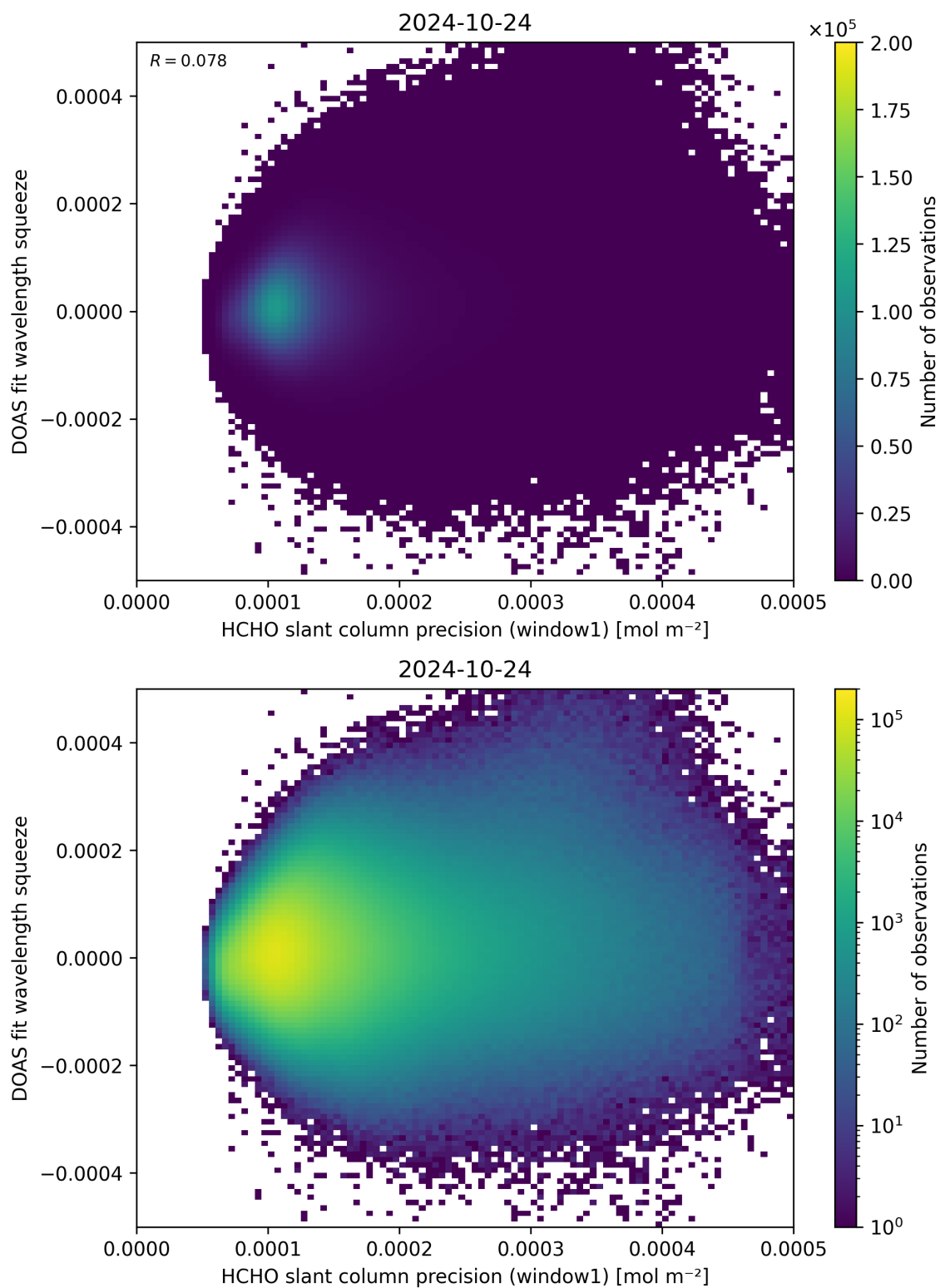
Figure 90: Scatter density plot of “HCHO slant column precision (window1)” against “DOAS fit wavelength squeeze” for 2024-10-24 to 2024-10-25.
