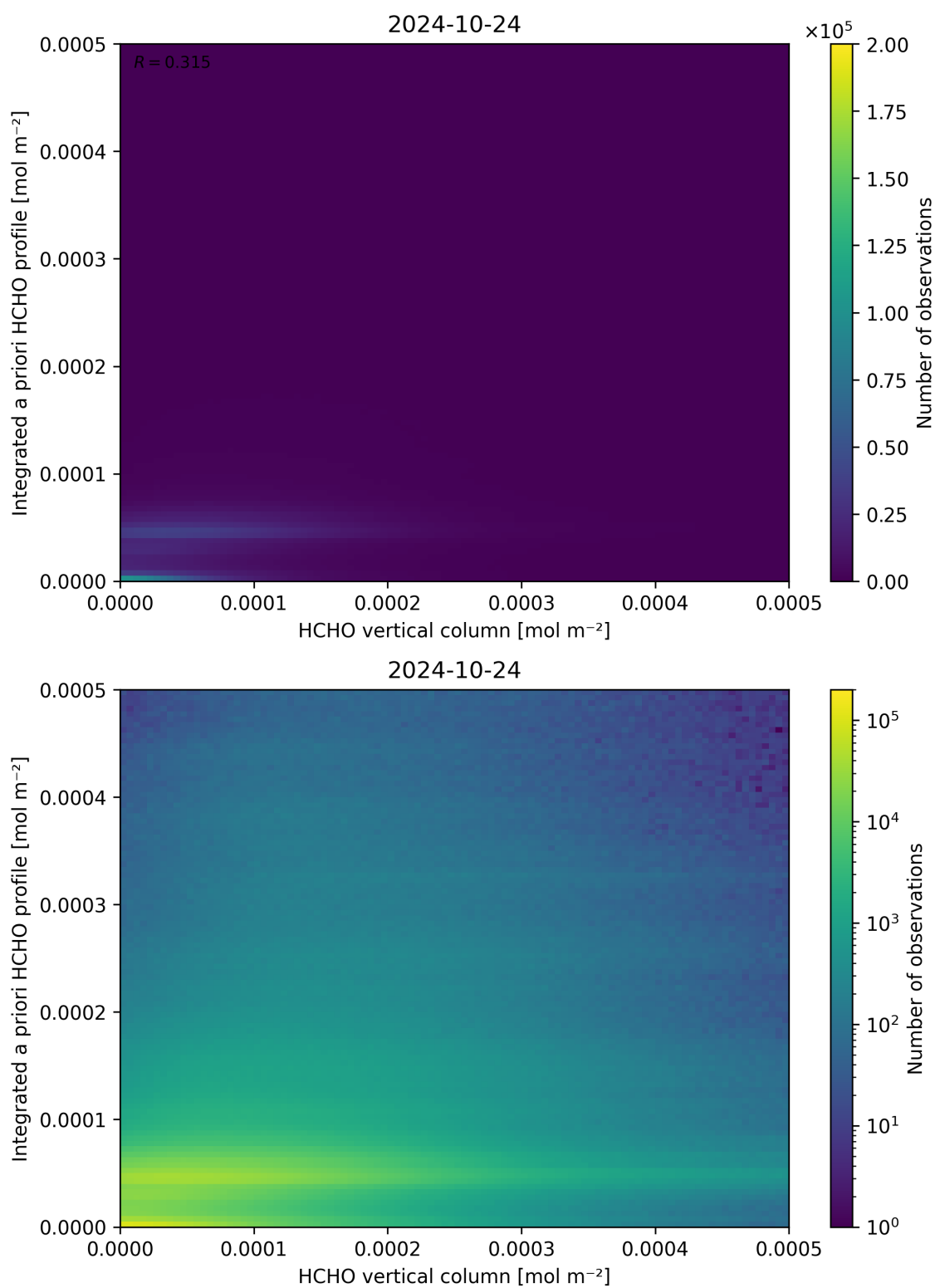
Figure 135: Scatter density plot of “HCHO vertical column” against “Integrated a priori HCHO profile” for 2024-10-24 to 2024-10-25.
