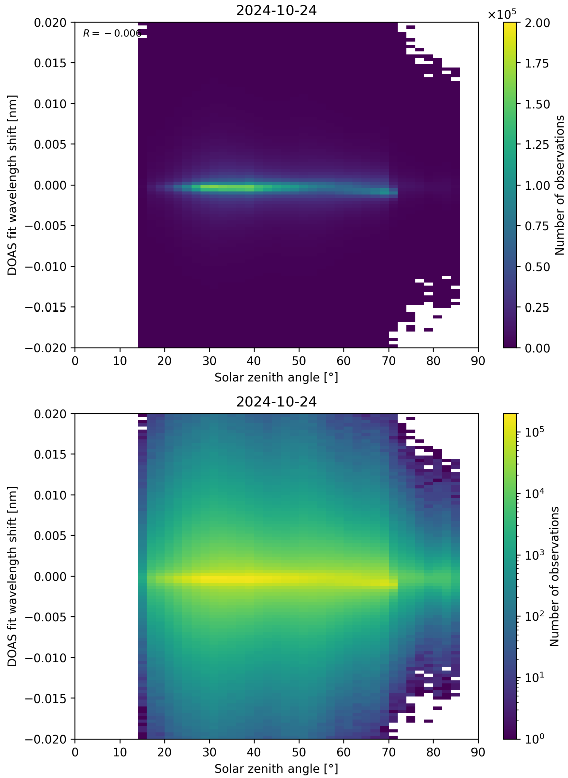
Figure 168: Scatter density plot of “Solar zenith angle” against “DOAS fit wavelength shift” for 2024-10-24 to 2024-10-25.
