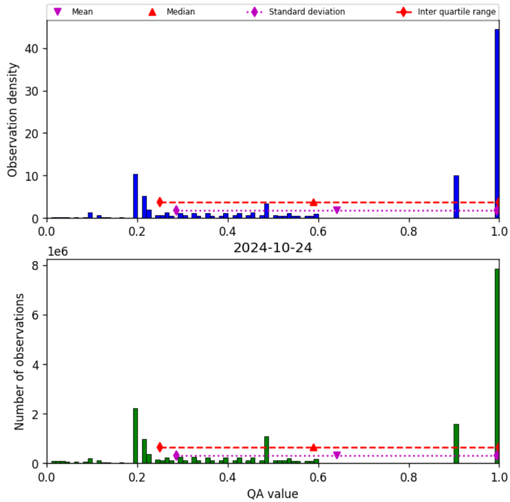
Figure 34: Histogram of “QA value” for 2024-10-24 to 2024-10-25
