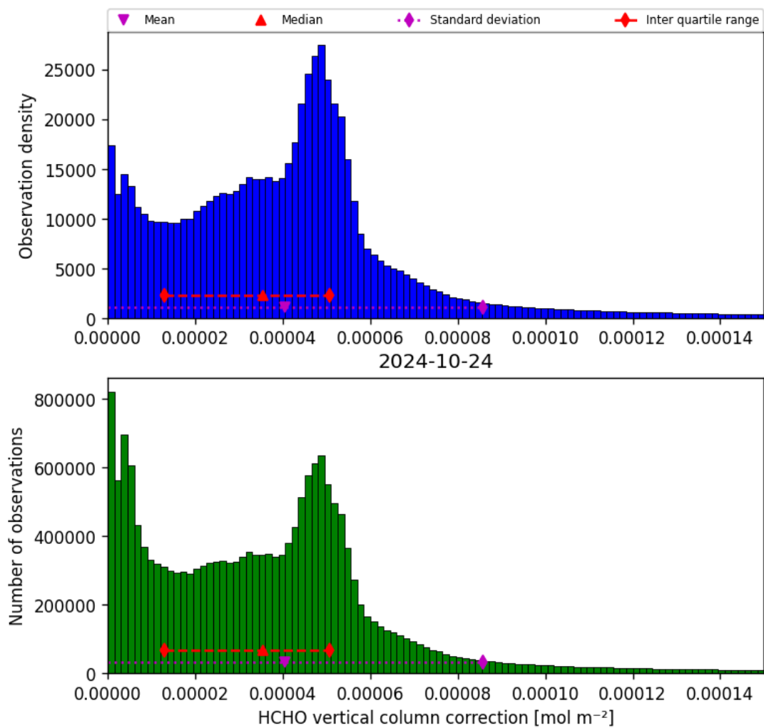
Figure 37: Histogram of “HCHO vertical column correction” for 2024-10-24 to 2024-10-25
