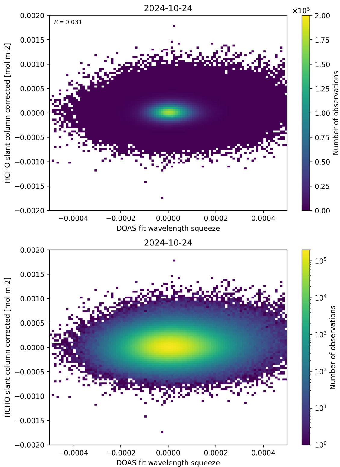
Figure 69: Scatter density plot of “DOAS fit wavelength squeeze” against “HCHO slant column corrected” for 2024-10-24 to 2024-10-25.
