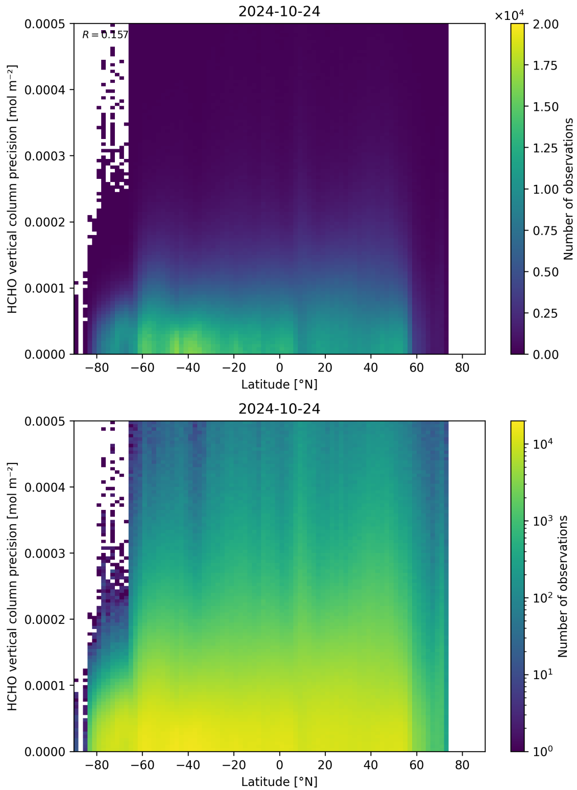
Figure 165: Scatter density plot of “Latitude” against “HCHO vertical column precision” for 2024-10-24 to 2024-10-25.
