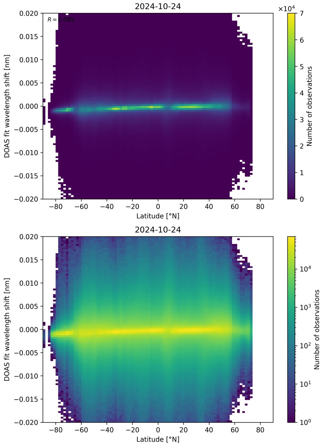
Figure 154: Scatter density plot of “Latitude” against “DOAS fit wavelength shift” for 2024-10-24 to 2024-10-25.
