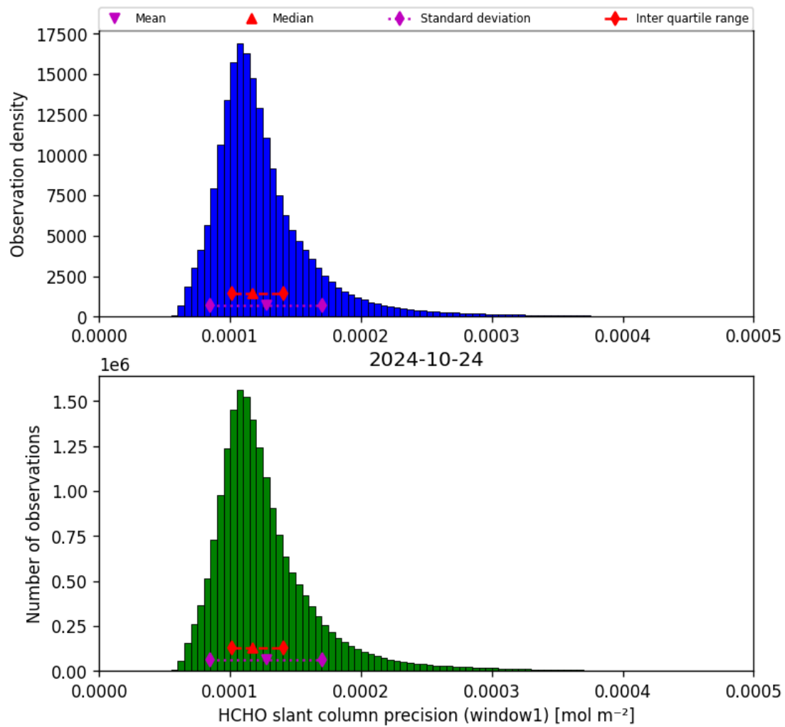
Figure 39: Histogram of “HCHO slant column precision (window1)” for 2024-10-24 to 2024-10-25
