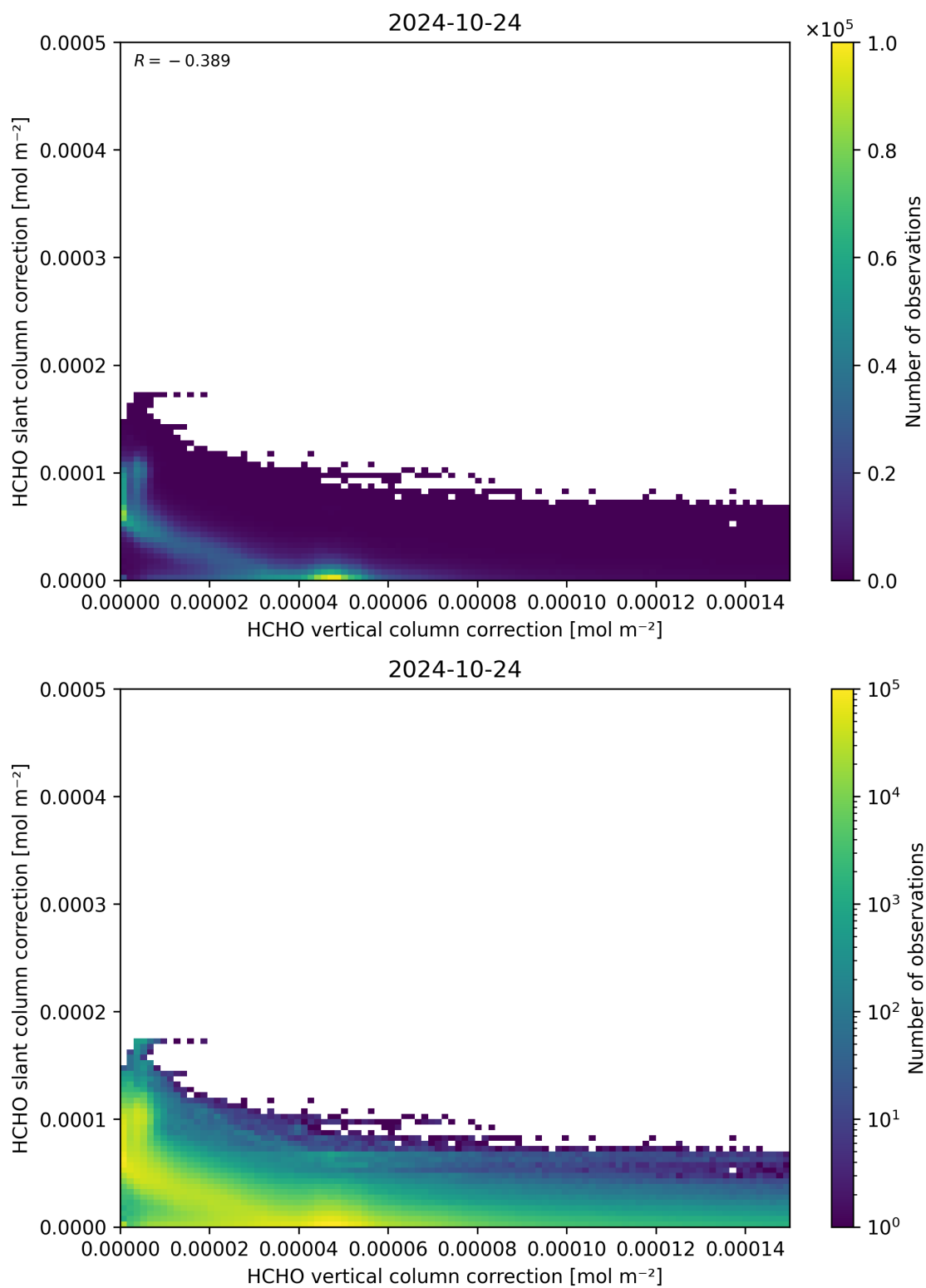
Figure 117: Scatter density plot of “HCHO vertical column correction” against “HCHO slant column correction” for 2024-10-24 to 2024-10-25.
