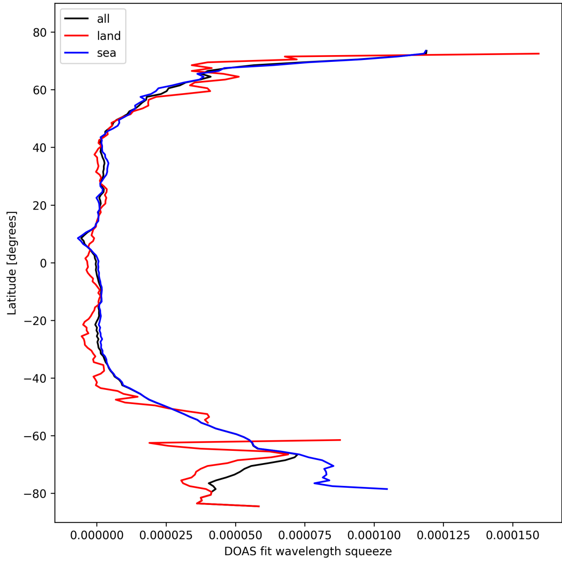
Figure 31: Zonal average of “DOAS fit wavelength squeeze” for 2024-10-24 to 2024-10-25.
