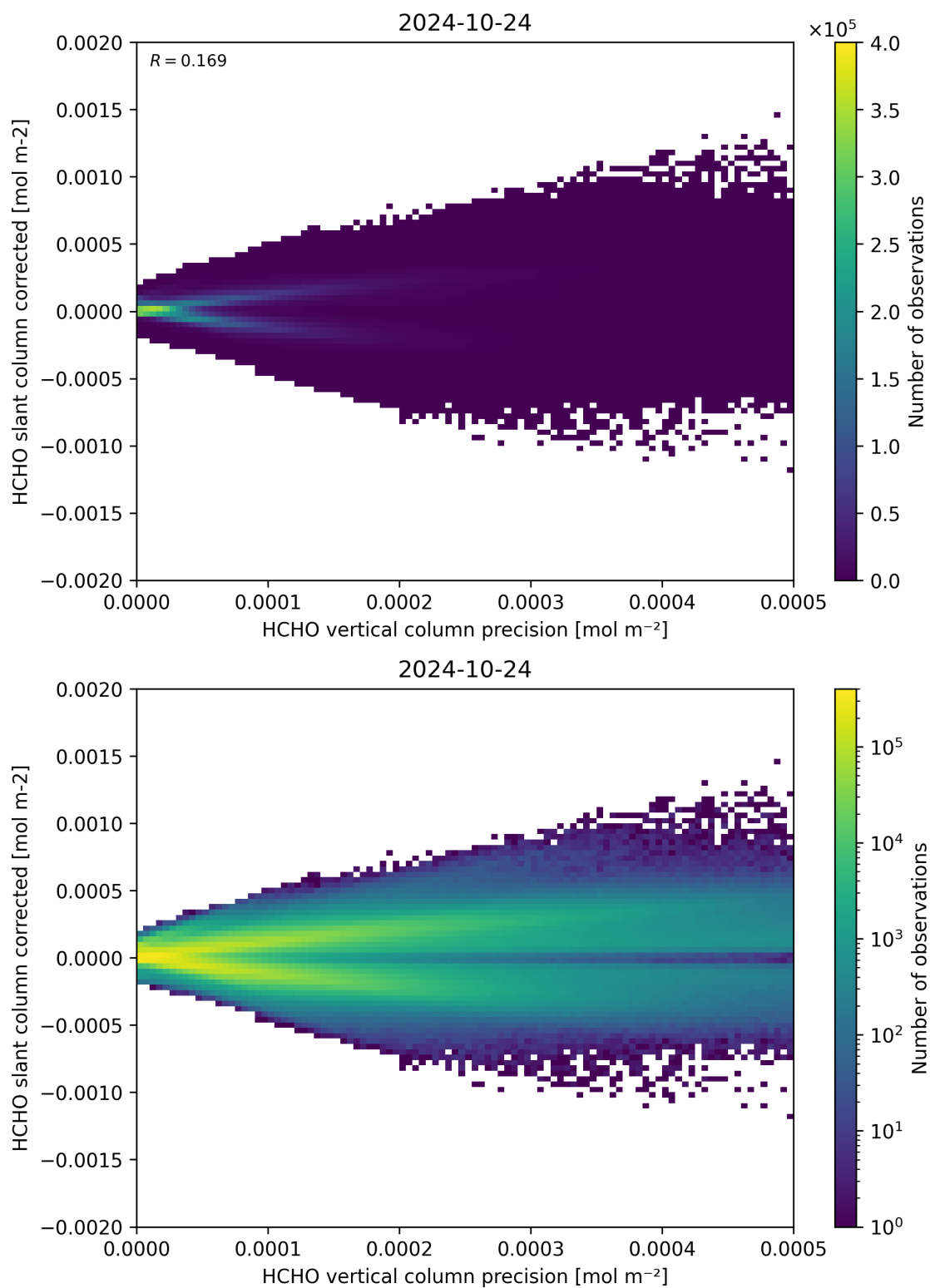
Figure 140: Scatter density plot of “HCHO vertical column precision” against “HCHO slant column corrected” for 2024-10-24 to 2024-10-25.
