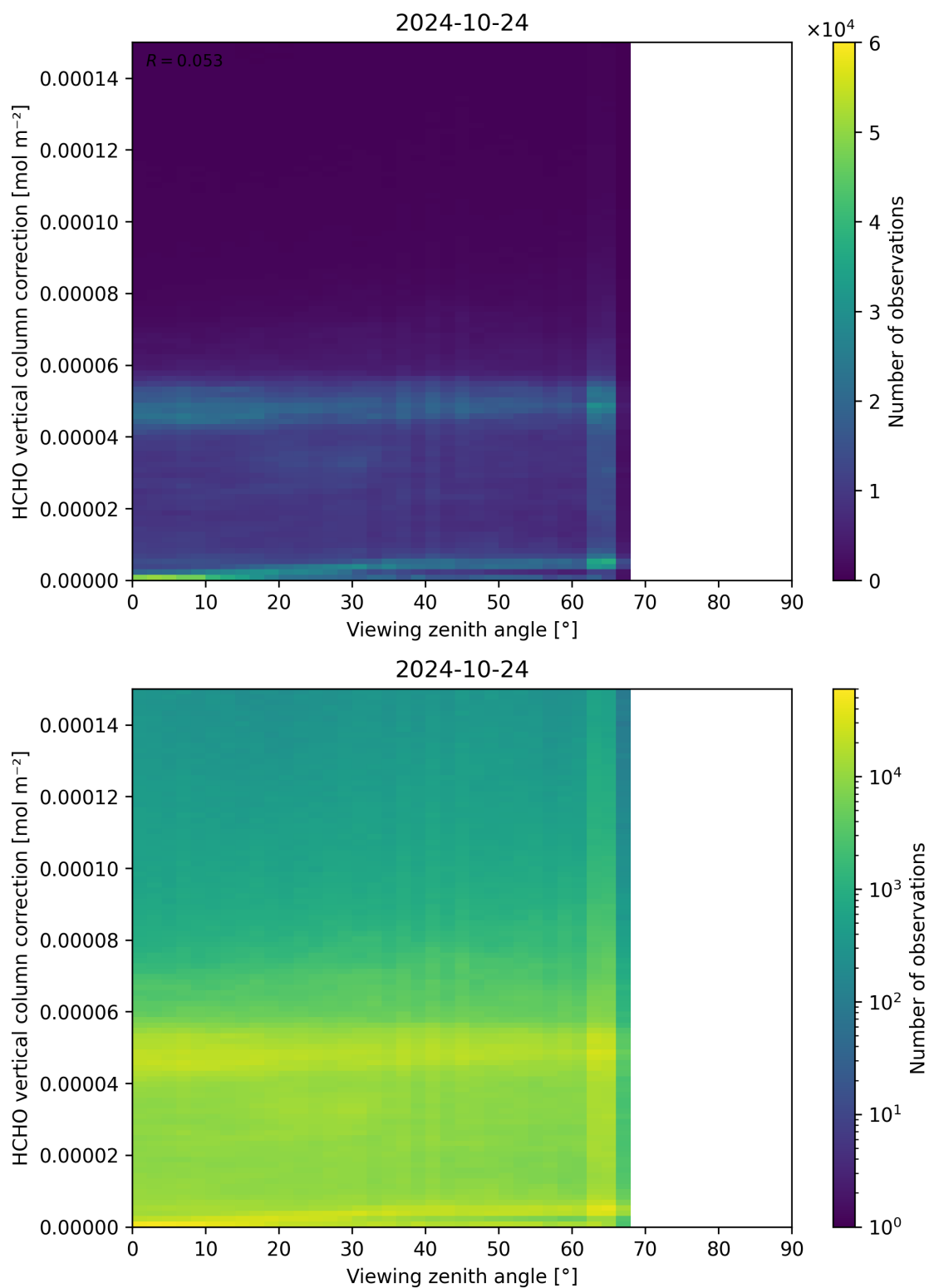
Figure 193: Scatter density plot of “Viewing zenith angle” against “HCHO vertical column correction” for 2024-10-24 to 2024-10-25.
