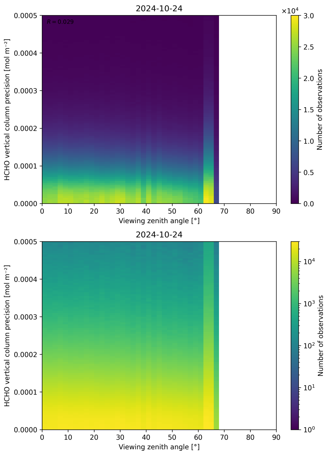
Figure 194: Scatter density plot of “Viewing zenith angle” against “HCHO vertical column precision” for 2024-10-24 to 2024-10-25.
