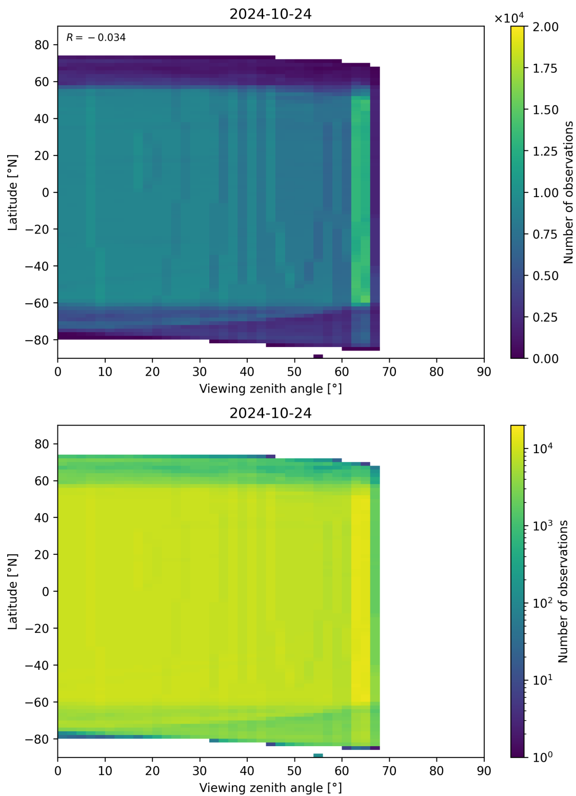
Figure 196: Scatter density plot of “Viewing zenith angle” against “Latitude” for 2024-10-24 to 2024-10-25.
