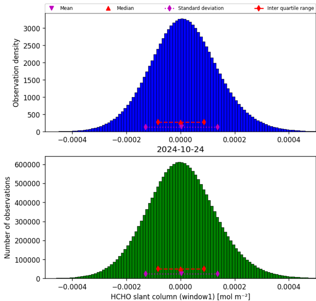
Figure 38: Histogram of “HCHO slant column (window1)” for 2024-10-24 to 2024-10-25
