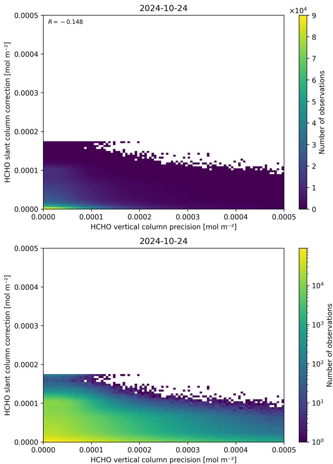
Figure 141: Scatter density plot of “HCHO vertical column precision” against “HCHO slant column correction” for 2024-10-24 to 2024-10-25.
