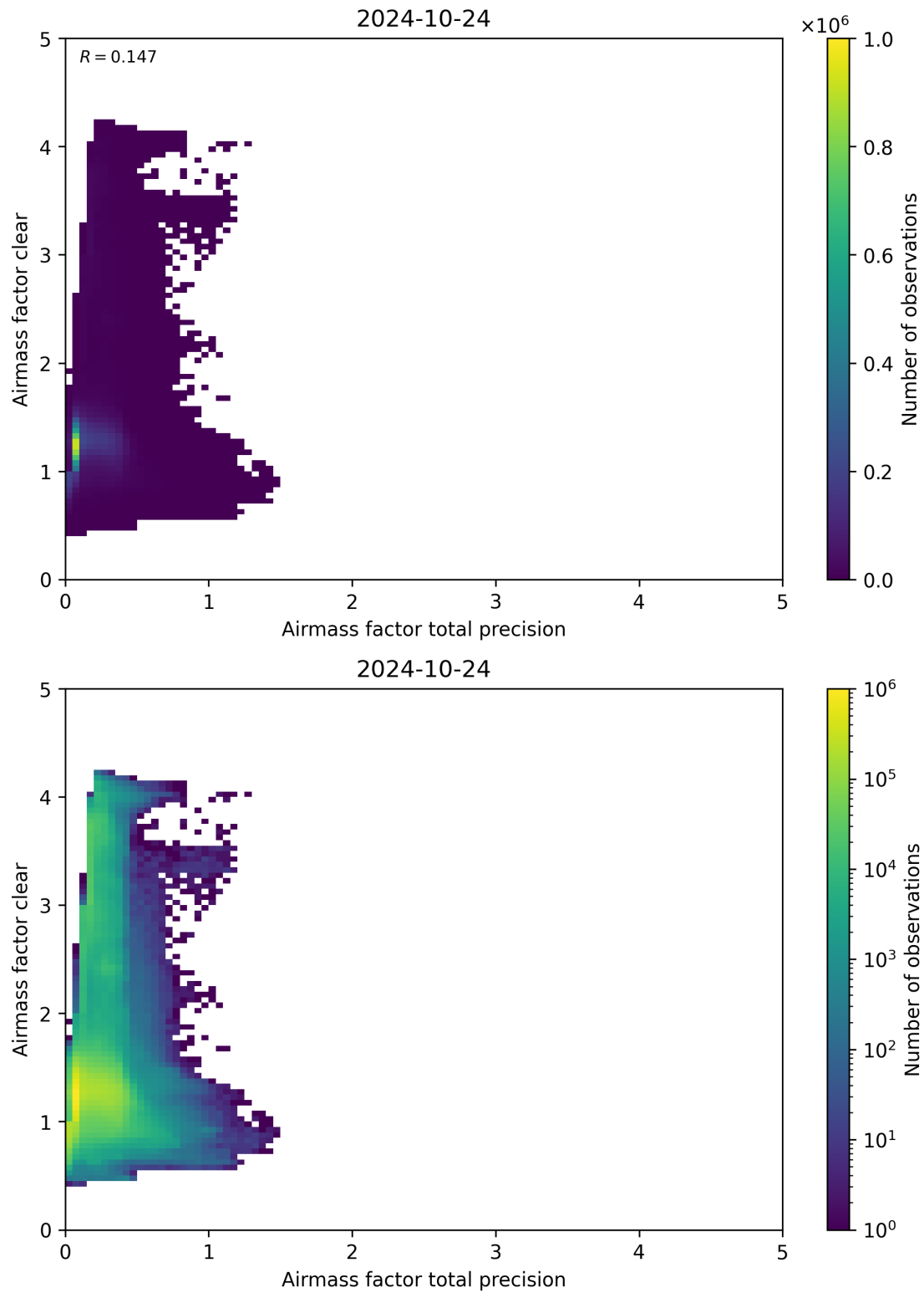
Figure 108: Scatter density plot of “Airmass factor total precision” against “Airmass factor clear” for 2024-10-24 to 2024-10-25.
