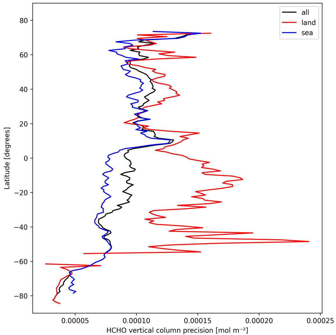
Figure 22: Zonal average of “HCHO vertical column precision” for 2024-10-24 to 2024-10-25.
