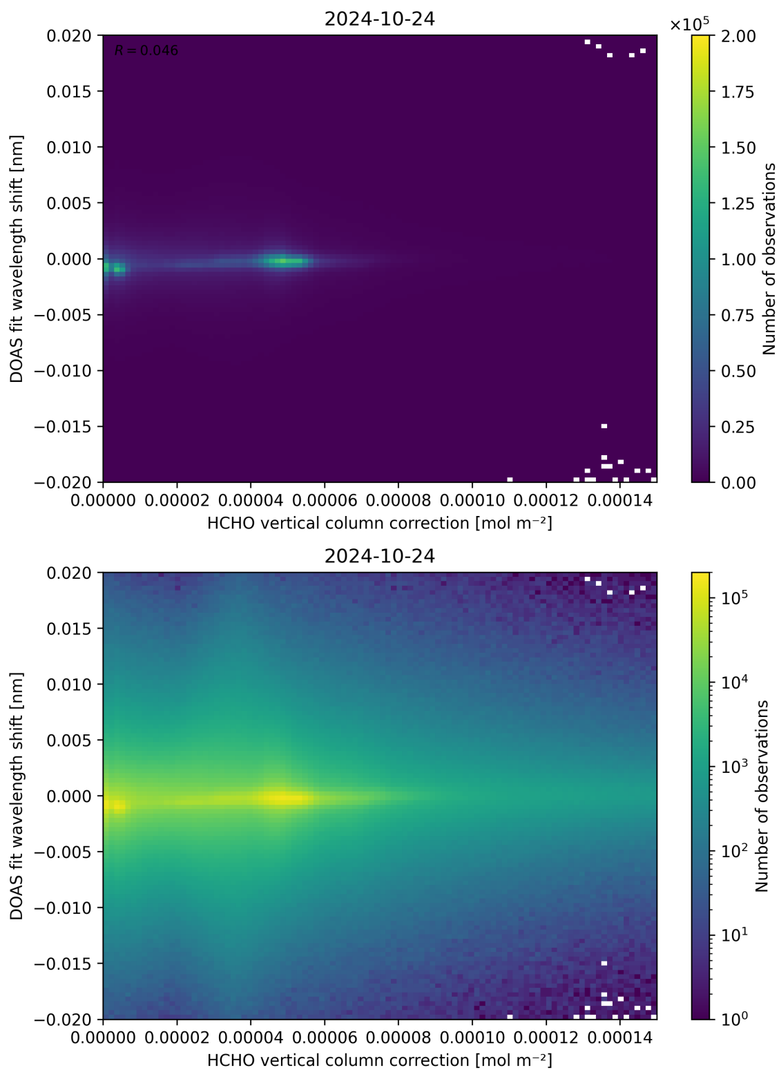
Figure 113: Scatter density plot of “HCHO vertical column correction” against “DOAS fit wavelength shift” for 2024-10-24 to 2024-10-25.
