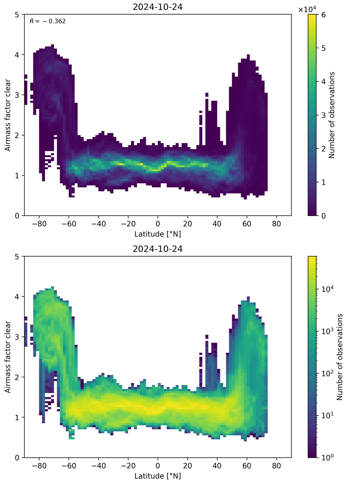
Figure 156: Scatter density plot of “Latitude” against “Airmass factor clear” for 2024-10-24 to 2024-10-25.
