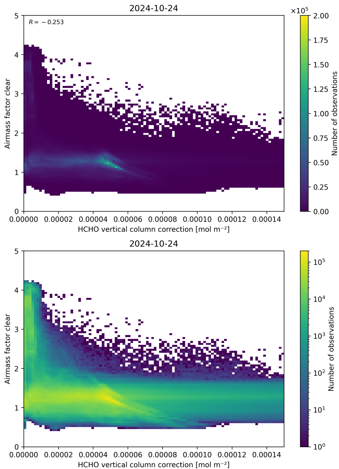
Figure 115: Scatter density plot of “HCHO vertical column correction” against “Airmass factor clear” for 2024-10-24 to 2024-10-25.
