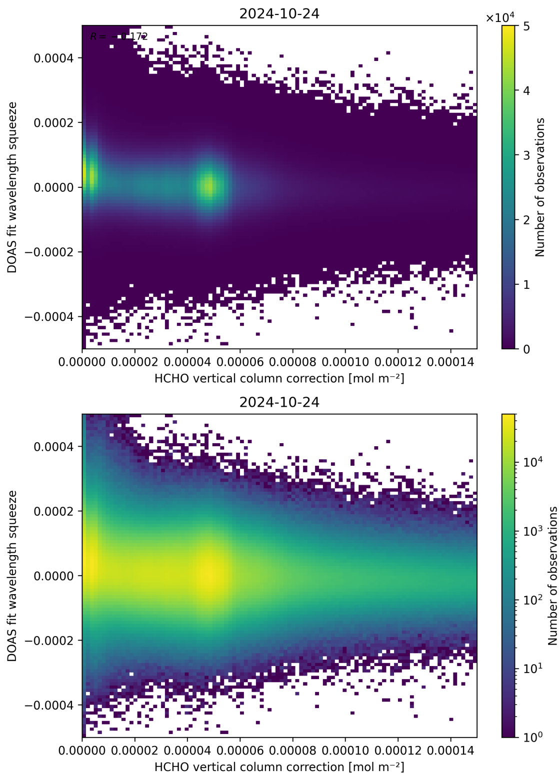
Figure 114: Scatter density plot of “HCHO vertical column correction” against “DOAS fit wavelength squeeze” for 2024-10-24 to 2024-10-25.
