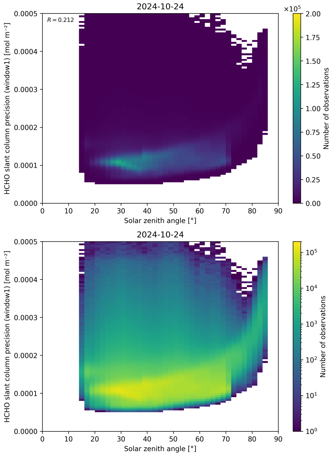
Figure 174: Scatter density plot of “Solar zenith angle” against “HCHO slant column precision (window1)” for 2024-10-24 to 2024-10-25.
