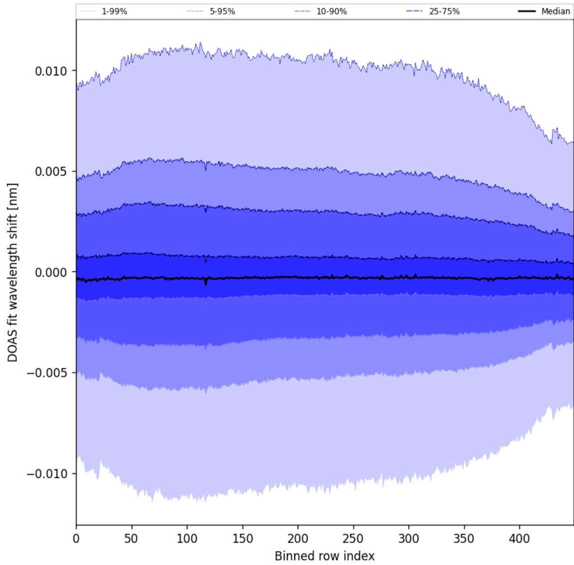
Figure 58: Along track statistics of “DOAS fit wavelength shift” for 2024-10-24 to 2024-10-25
