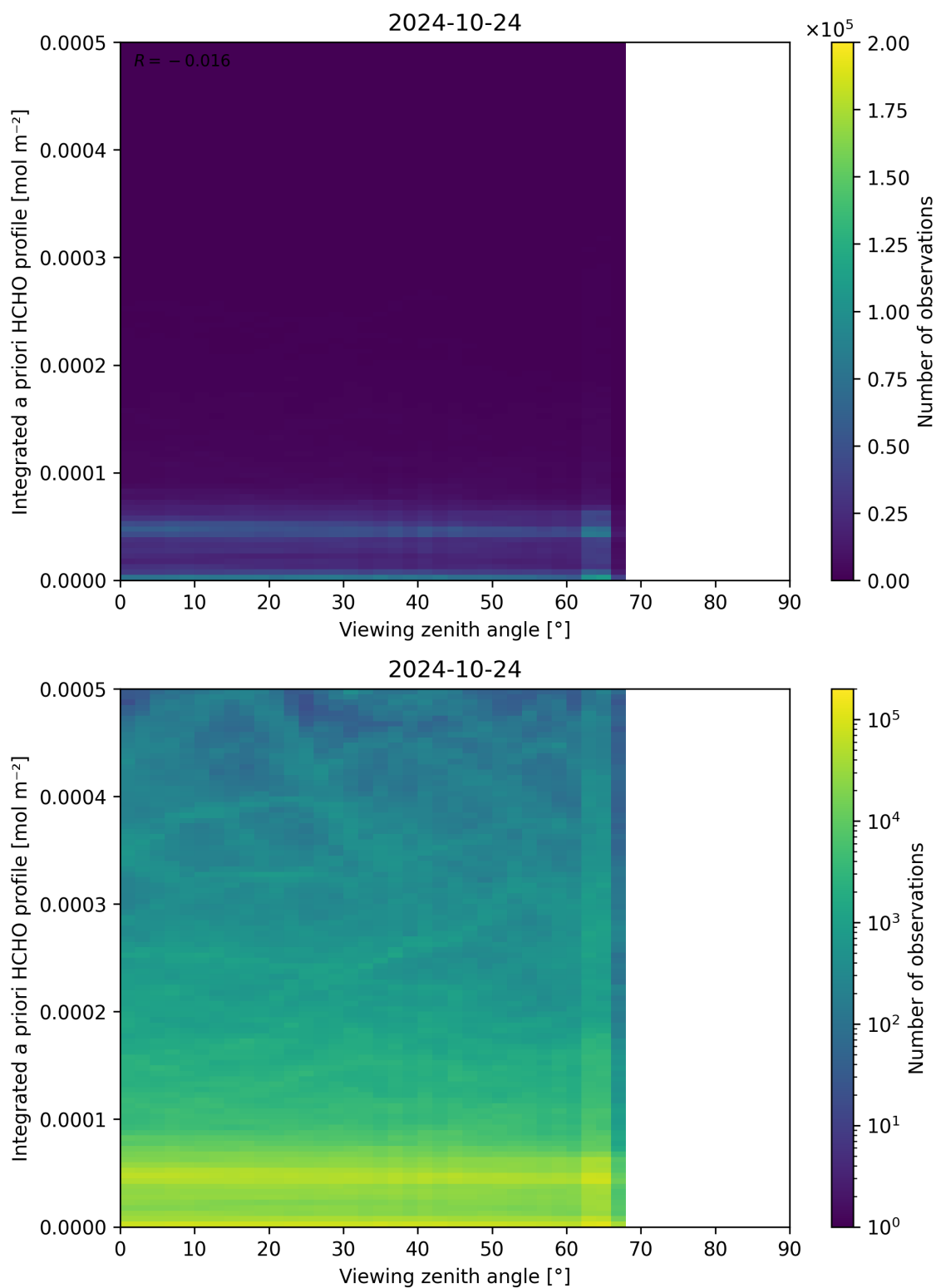
Figure 195: Scatter density plot of “Viewing zenith angle” against “Integrated a priori HCHO profile” for 2024-10-24 to 2024-10-25.
