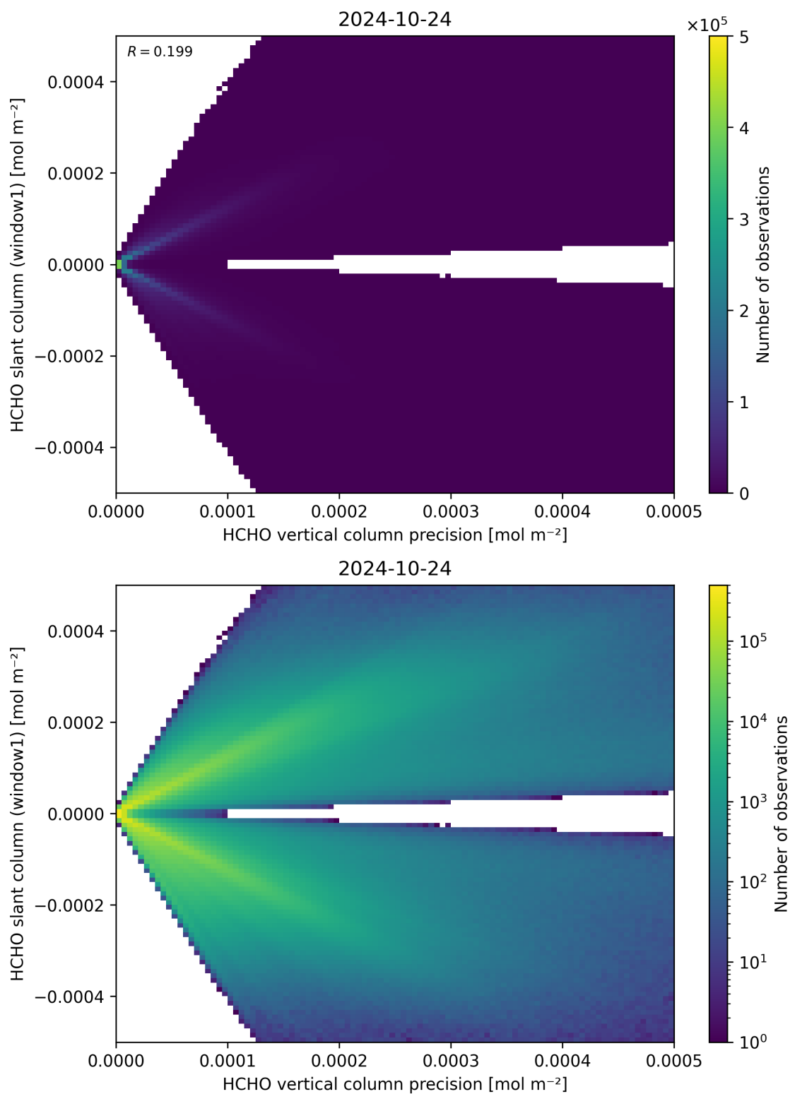
Figure 142: Scatter density plot of “HCHO vertical column precision” against “HCHO slant column (window1)” for 2024-10-24 to 2024-10-25.
