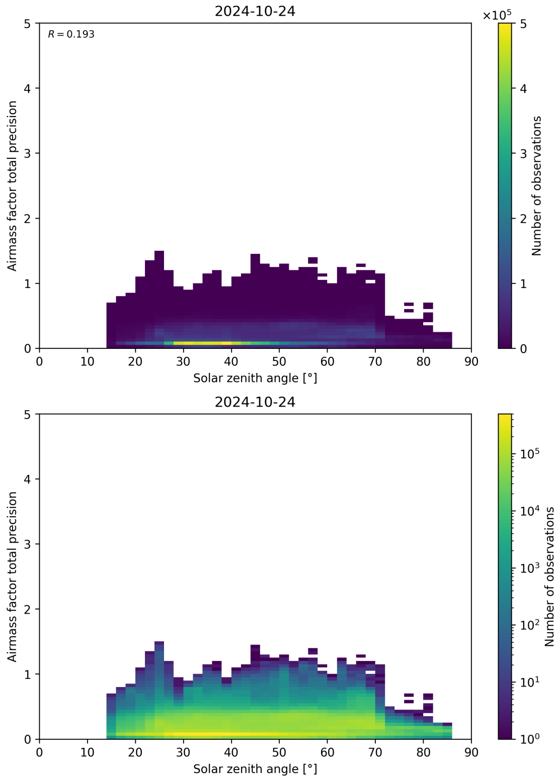
Figure 176: Scatter density plot of “Solar zenith angle” against “Airmass factor total precision” for 2024-10-24 to 2024-10-25.
