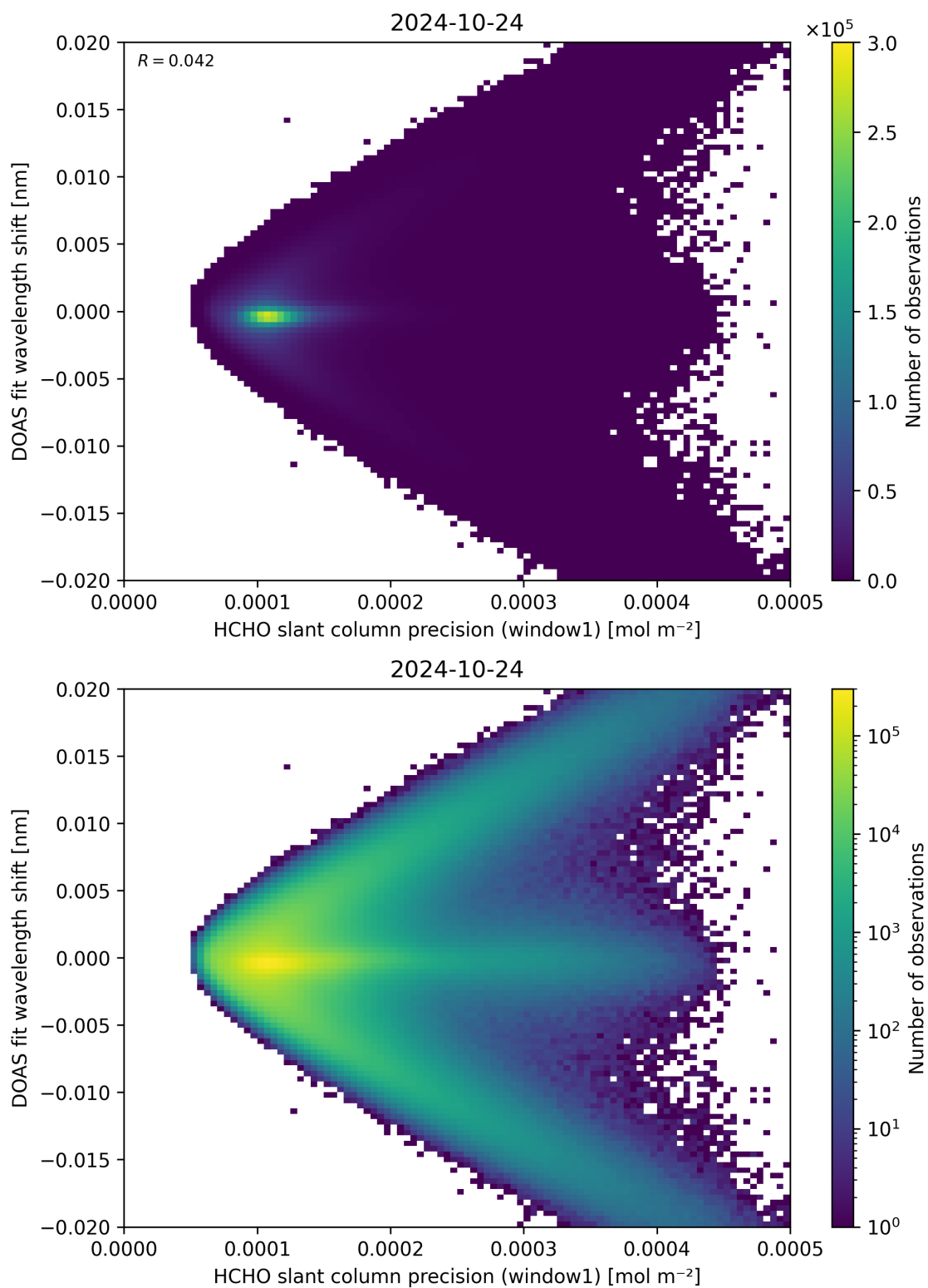
Figure 89: Scatter density plot of “HCHO slant column precision (window1)” against “DOAS fit wavelength shift” for 2024-10-24 to 2024-10-25.
