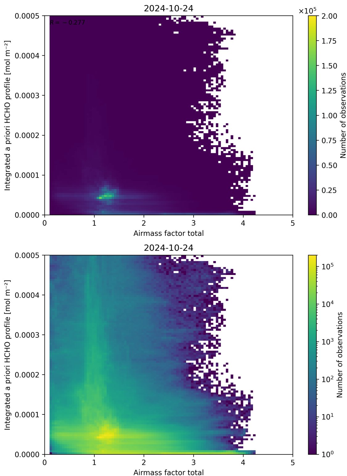
Figure 104: Scatter density plot of “Airmass factor total” against “Integrated a priori HCHO profile” for 2024-10-24 to 2024-10-25.
