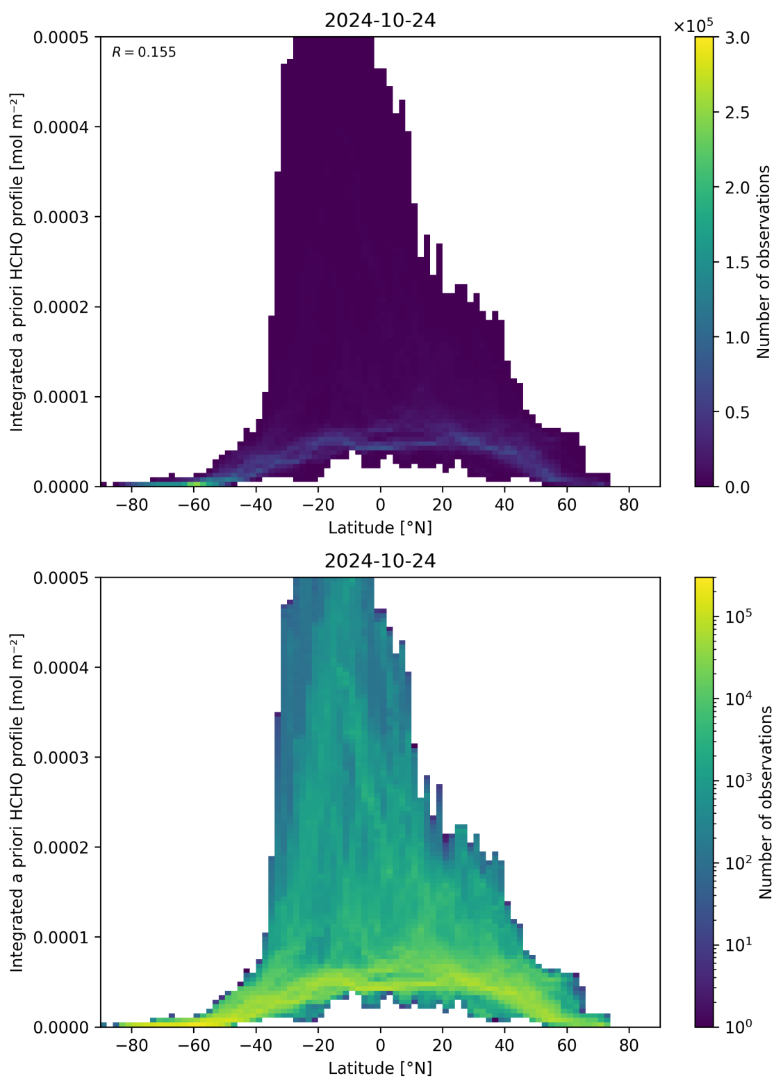
Figure 166: Scatter density plot of “Latitude” against “Integrated a priori HCHO profile” for 2024-10-24 to 2024-10-25.
