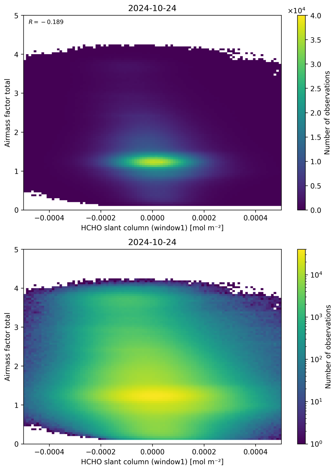
Figure 85: Scatter density plot of “HCHO slant column (window1)” against “Airmass factor total” for 2024-10-24 to 2024-10-25.
