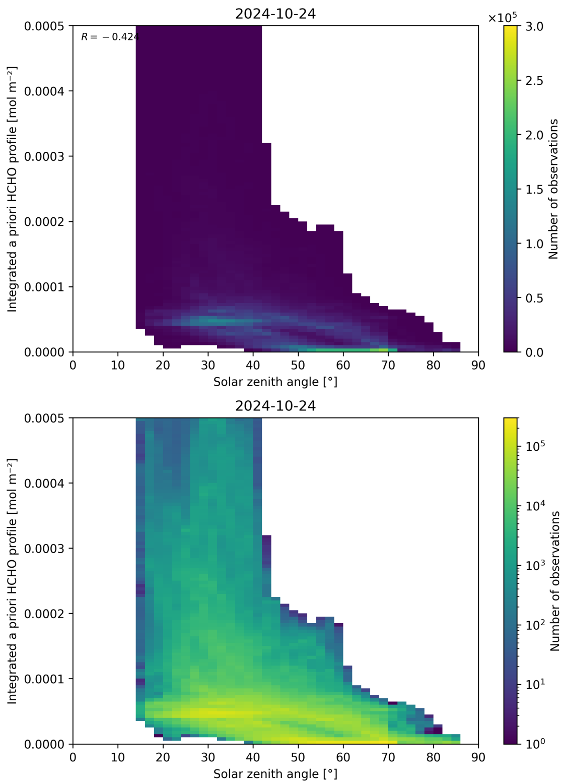
Figure 180: Scatter density plot of “Solar zenith angle” against “Integrated a priori HCHO profile” for 2024-10-24 to 2024-10-25.
