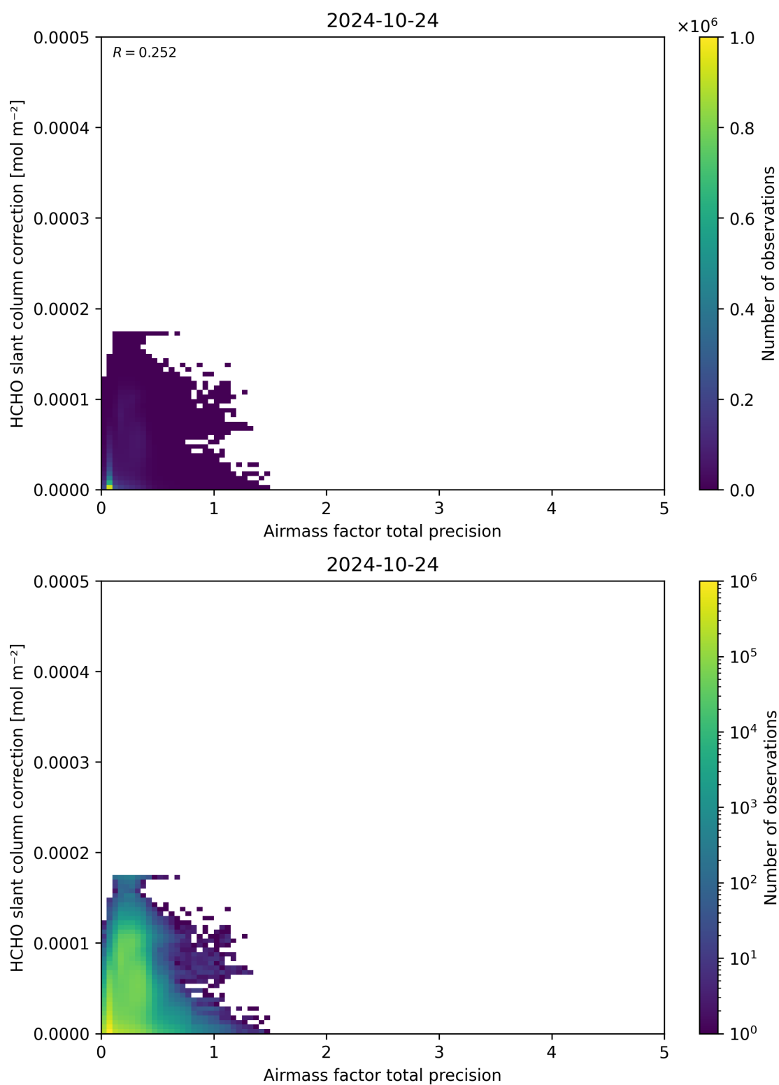
Figure 110: Scatter density plot of “Airmass factor total precision” against “HCHO slant column correction” for 2024-10-24 to 2024-10-25.
