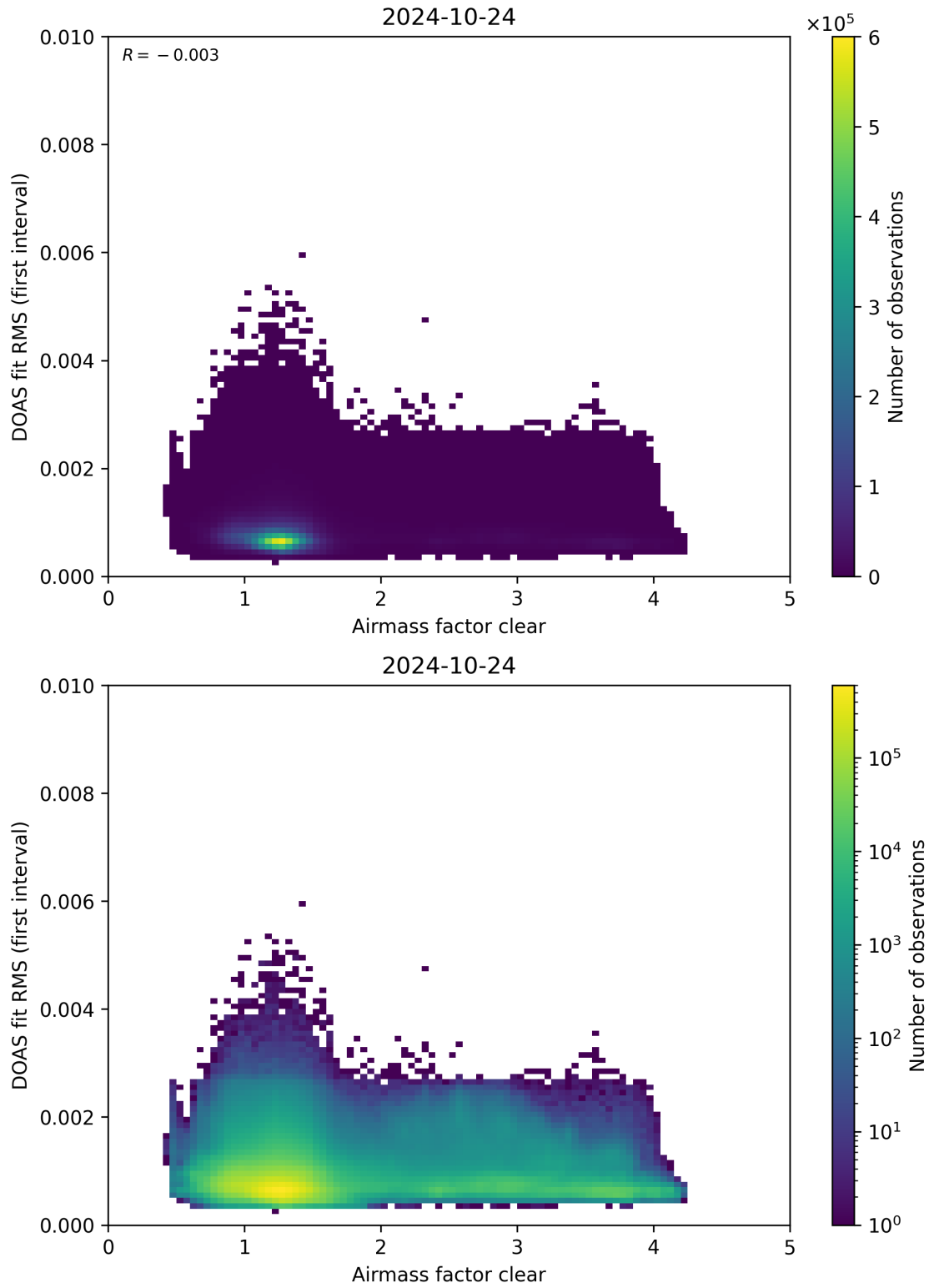
Figure 71: Scatter density plot of “Airmass factor clear” against “DOAS fit RMS (first interval)” for 2024-10-24 to 2024-10-25.
