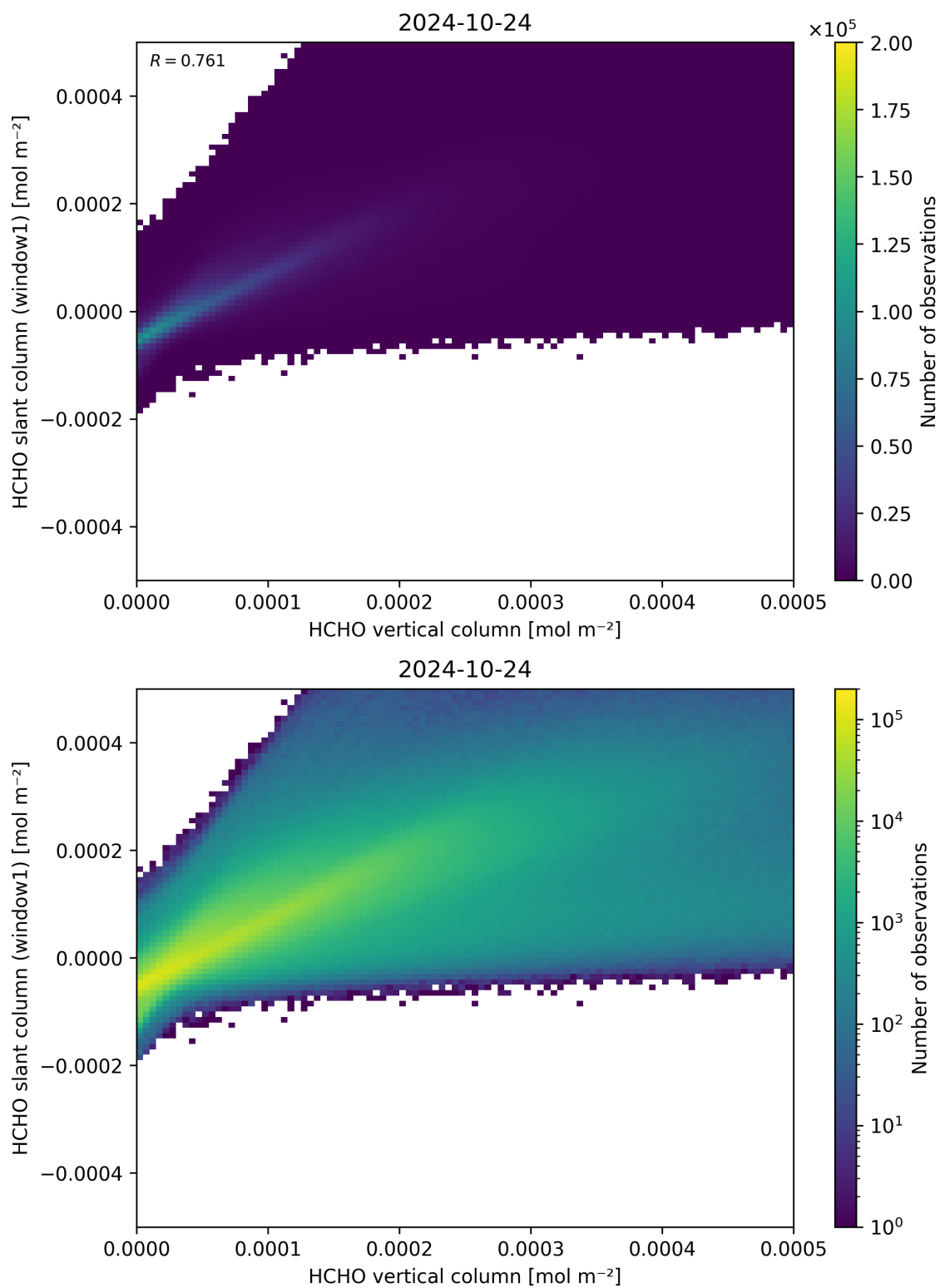
Figure 129: Scatter density plot of “HCHO vertical column” against “HCHO slant column (window1)” for 2024-10-24 to 2024-10-25.
