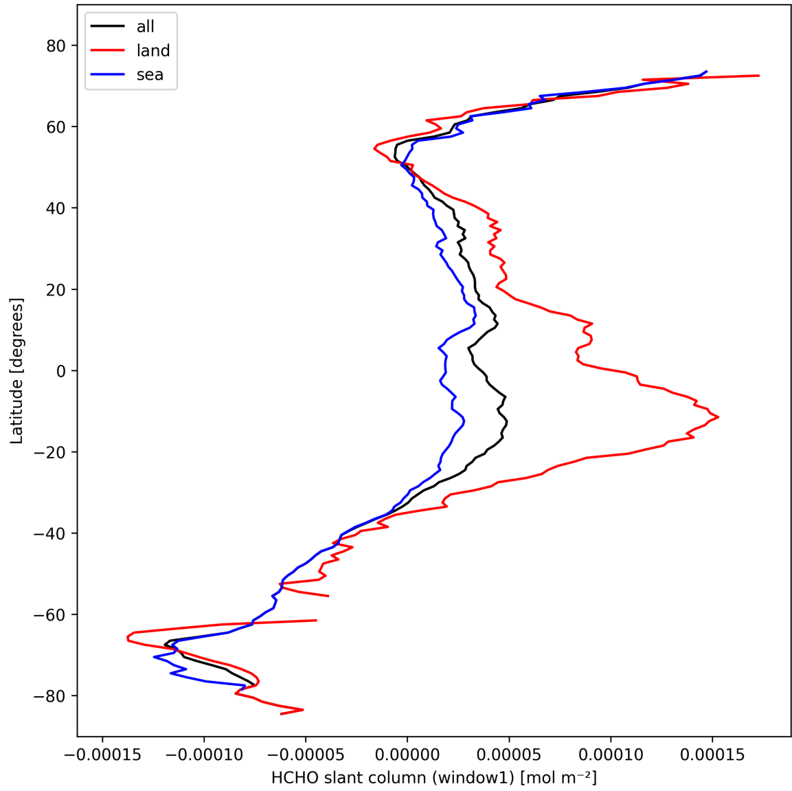
Figure 24: Zonal average of “HCHO slant column (window1)” for 2024-10-24 to 2024-10-25.
