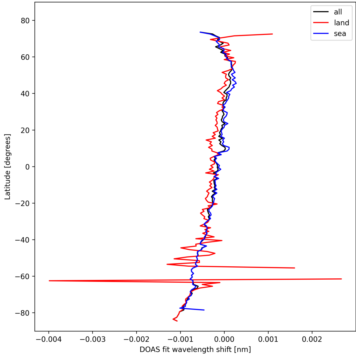
Figure 30: Zonal average of "DOAS fit wavelength shift" for 2024-10-24 to 2024-10-25.
