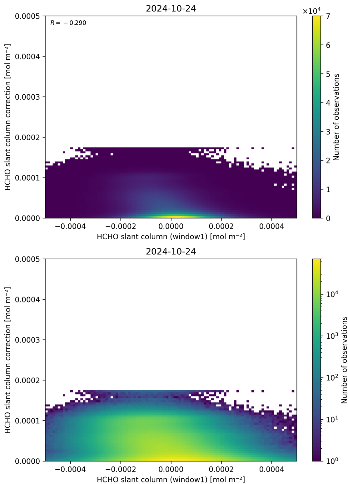
Figure 83: Scatter density plot of “HCHO slant column (window1)” against “HCHO slant column correction” for 2024-10-24 to 2024-10-25.
