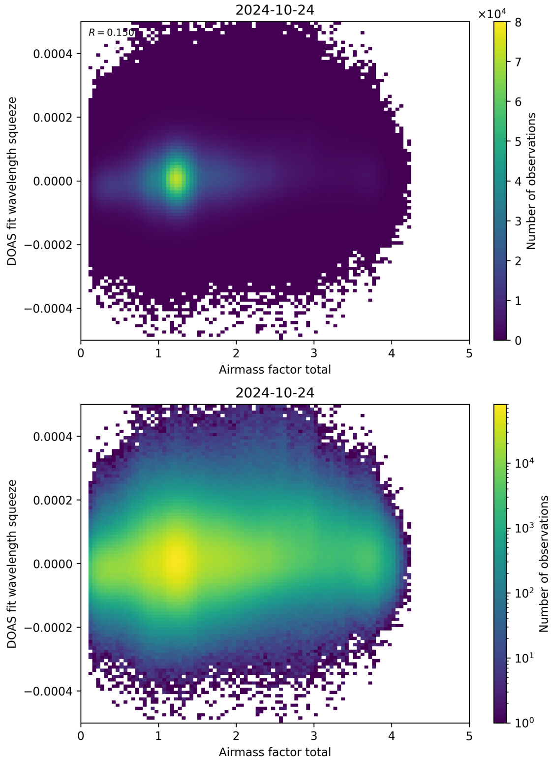
Figure 99: Scatter density plot of “Airmass factor total” against “DOAS fit wavelength squeeze” for 2024-10-24 to 2024-10-25.
