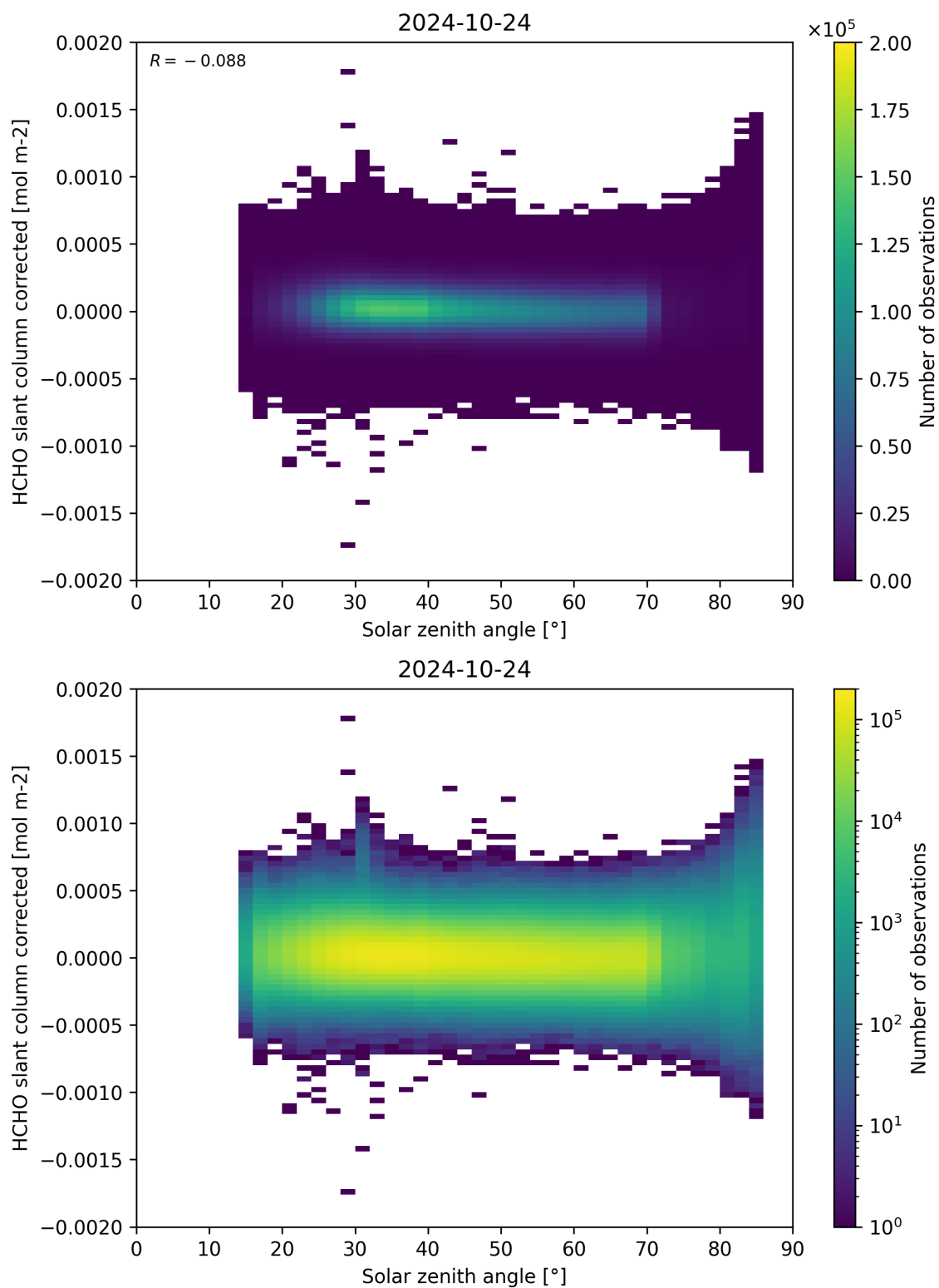
Figure 171: Scatter density plot of “Solar zenith angle” against “HCHO slant column corrected” for 2024-10-24 to 2024-10-25.
