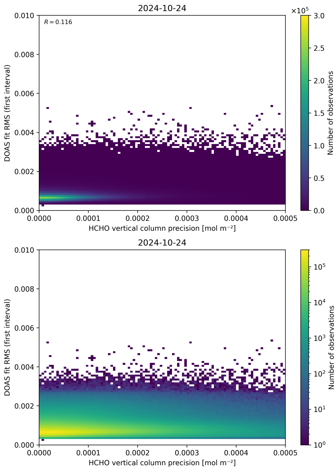
Figure 136: Scatter density plot of “HCHO vertical column precision” against “DOAS fit RMS (first interval)” for 2024-10-24 to 2024-10-25.
