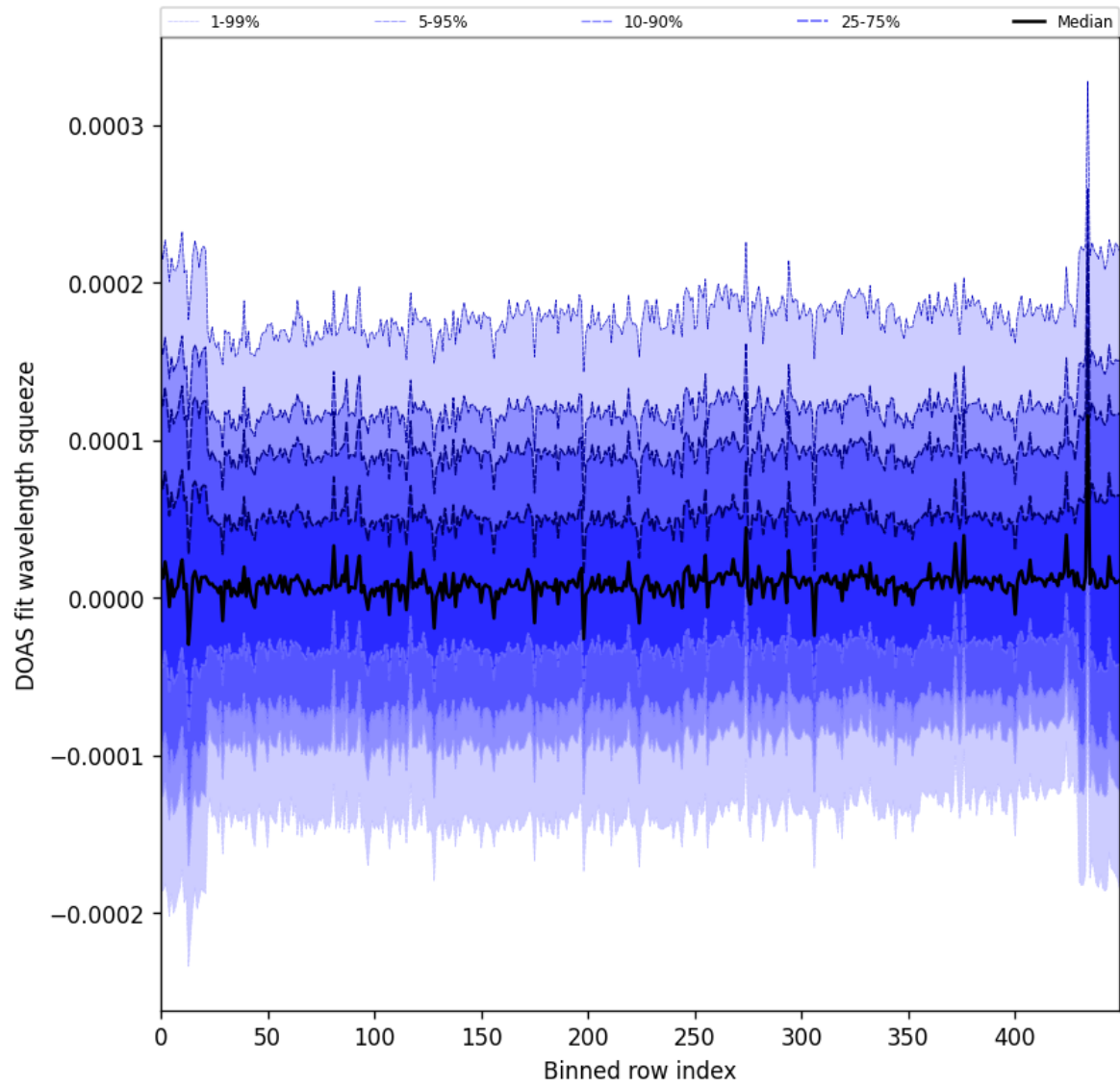
Figure 59: Along track statistics of “DOAS fit wavelength squeeze” for 2024-10-24 to 2024-10-25
