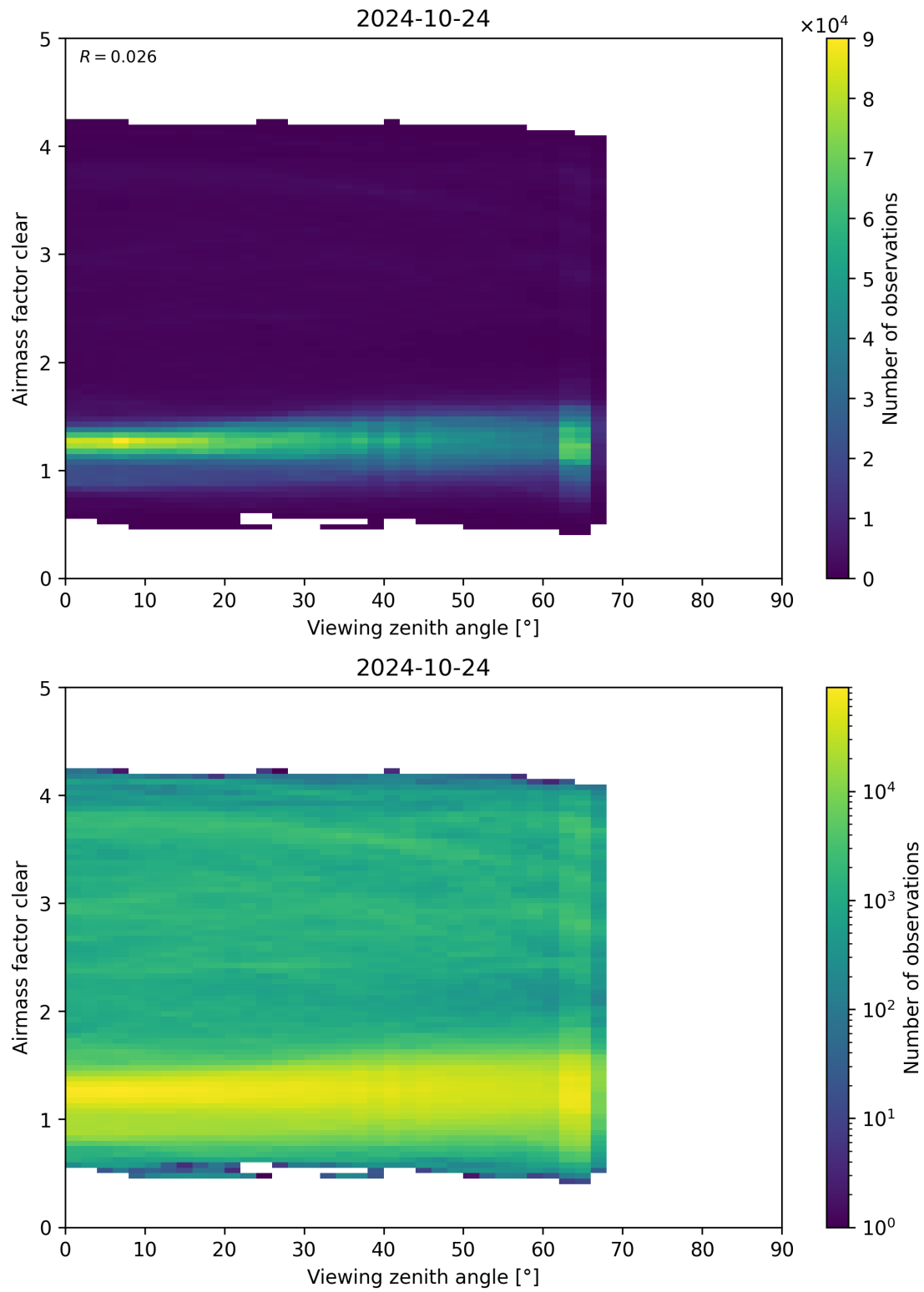
Figure 185: Scatter density plot of “Viewing zenith angle” against “Airmass factor clear” for 2024-10-24 to 2024-10-25.
