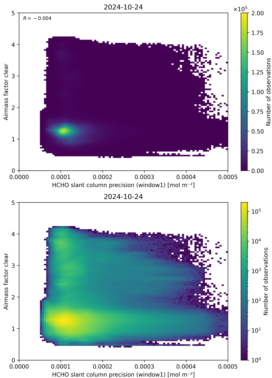
Figure 91: Scatter density plot of “HCHO slant column precision (window1)” against “Airmass factor clear” for 2024-10-24 to 2024-10-25.
