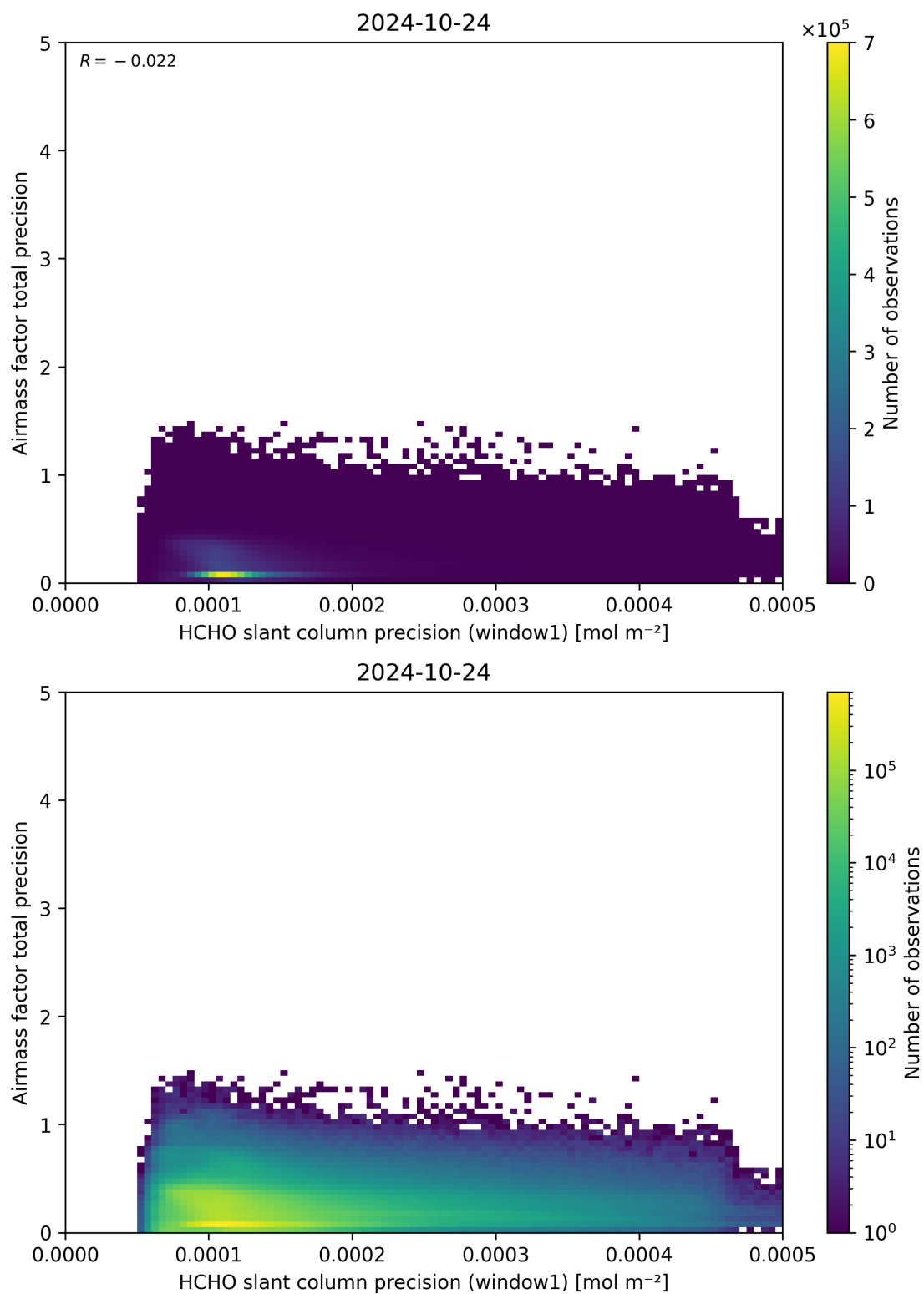
Figure 95: Scatter density plot of “HCHO slant column precision (window1)” against “Airmass factor total precision” for 2024-10-24 to 2024-10-25.
