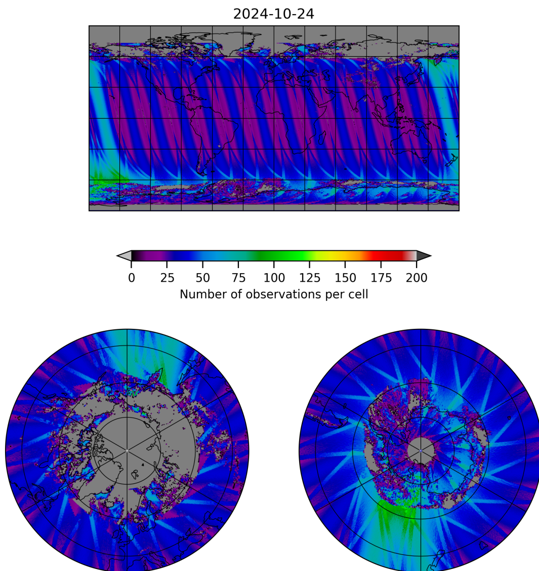
Figure 19: Map of the number of observations for 2024-10-24 to 2024-10-25
