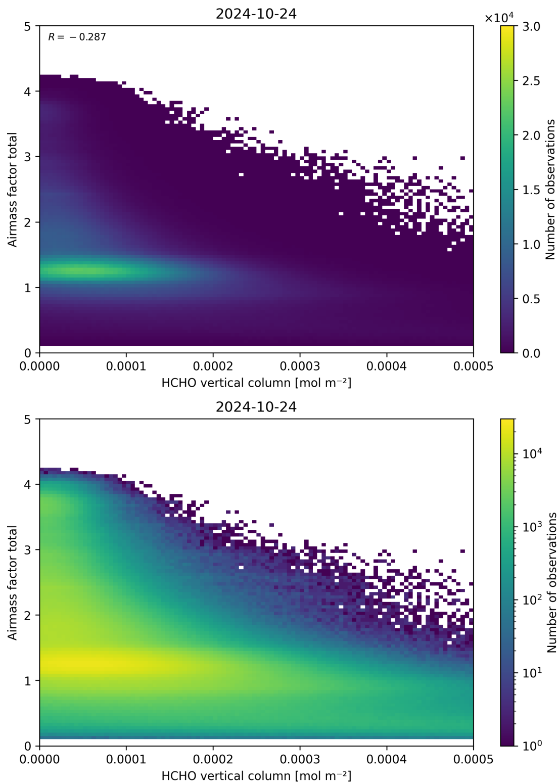
Figure 131: Scatter density plot of “HCHO vertical column” against “Airmass factor total” for 2024-10-24 to 2024-10-25.
