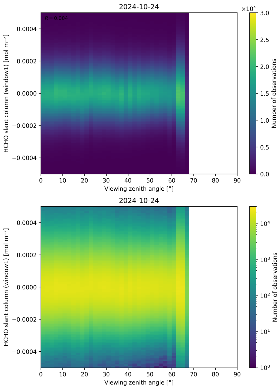
Figure 188: Scatter density plot of “Viewing zenith angle” against “HCHO slant column (window1)” for 2024-10-24 to 2024-10-25.
