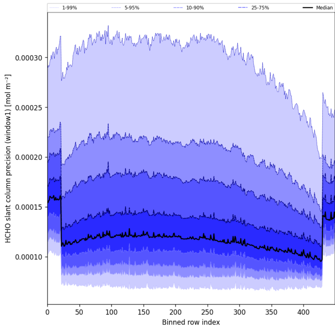
Figure 53: Along track statistics of “HCHO slant column precision (window1)” for 2024-10-24 to 2024-10-25
