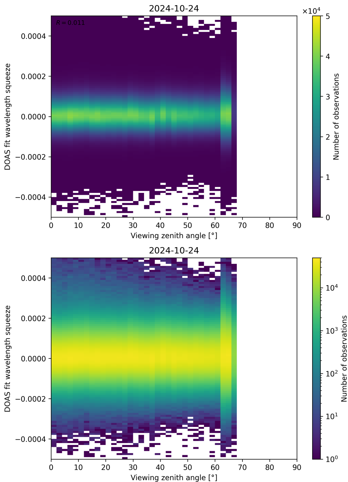
Figure 184: Scatter density plot of “Viewing zenith angle” against “DOAS fit wavelength squeeze” for 2024-10-24 to 2024-10-25.
