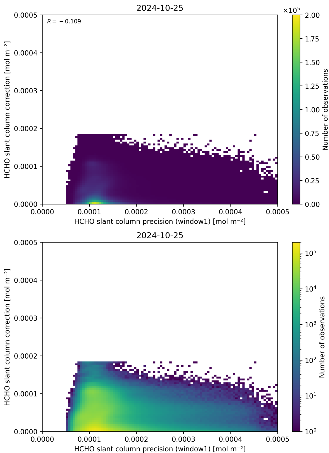
Figure 93: Scatter density plot of “HCHO slant column precision (window1)” against “HCHO slant column correction” for 2024-10-24 to 2024-10-26.
