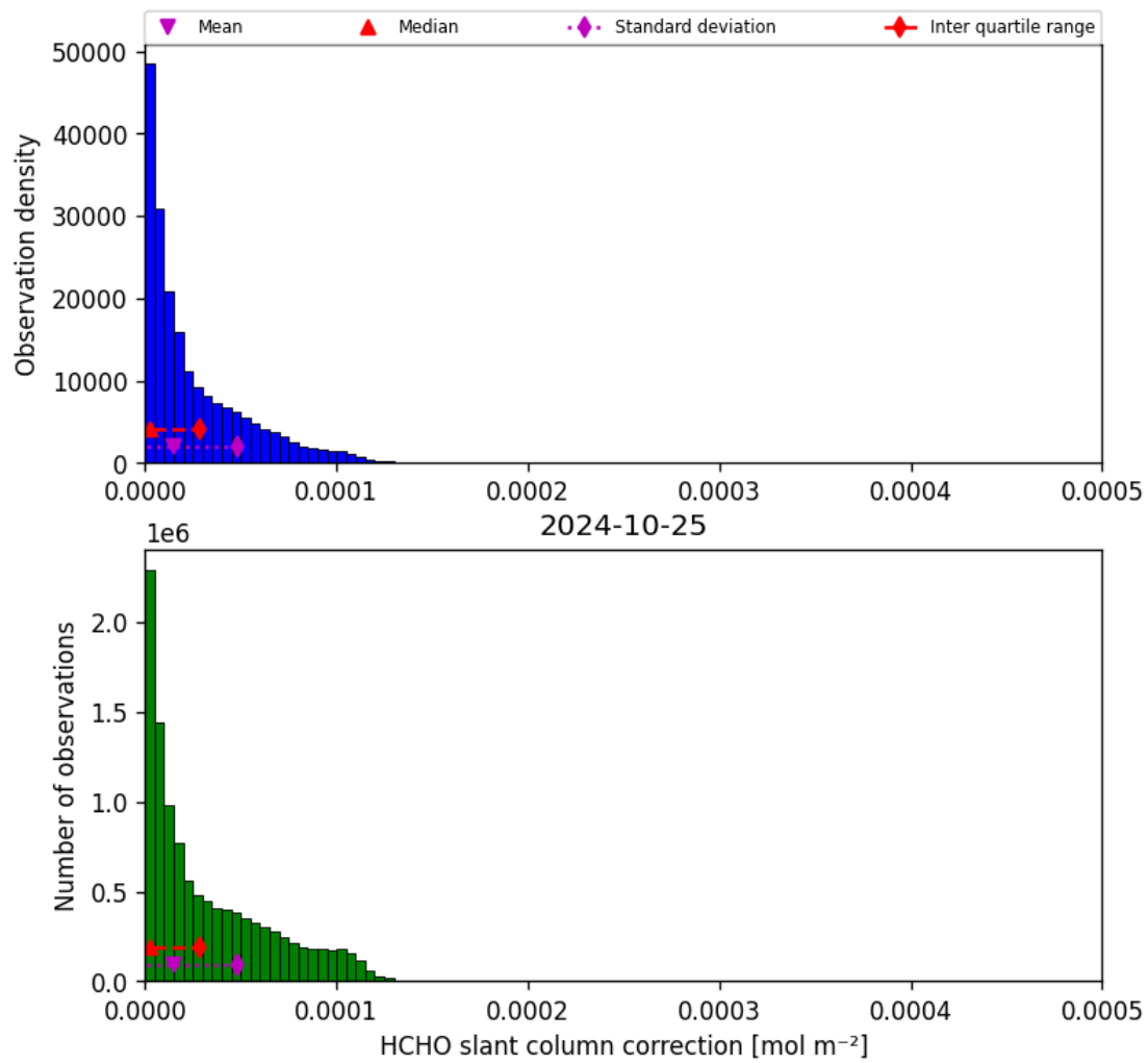
Figure 47: Histogram of “HCHO slant column correction” for 2024-10-24 to 2024-10-26
