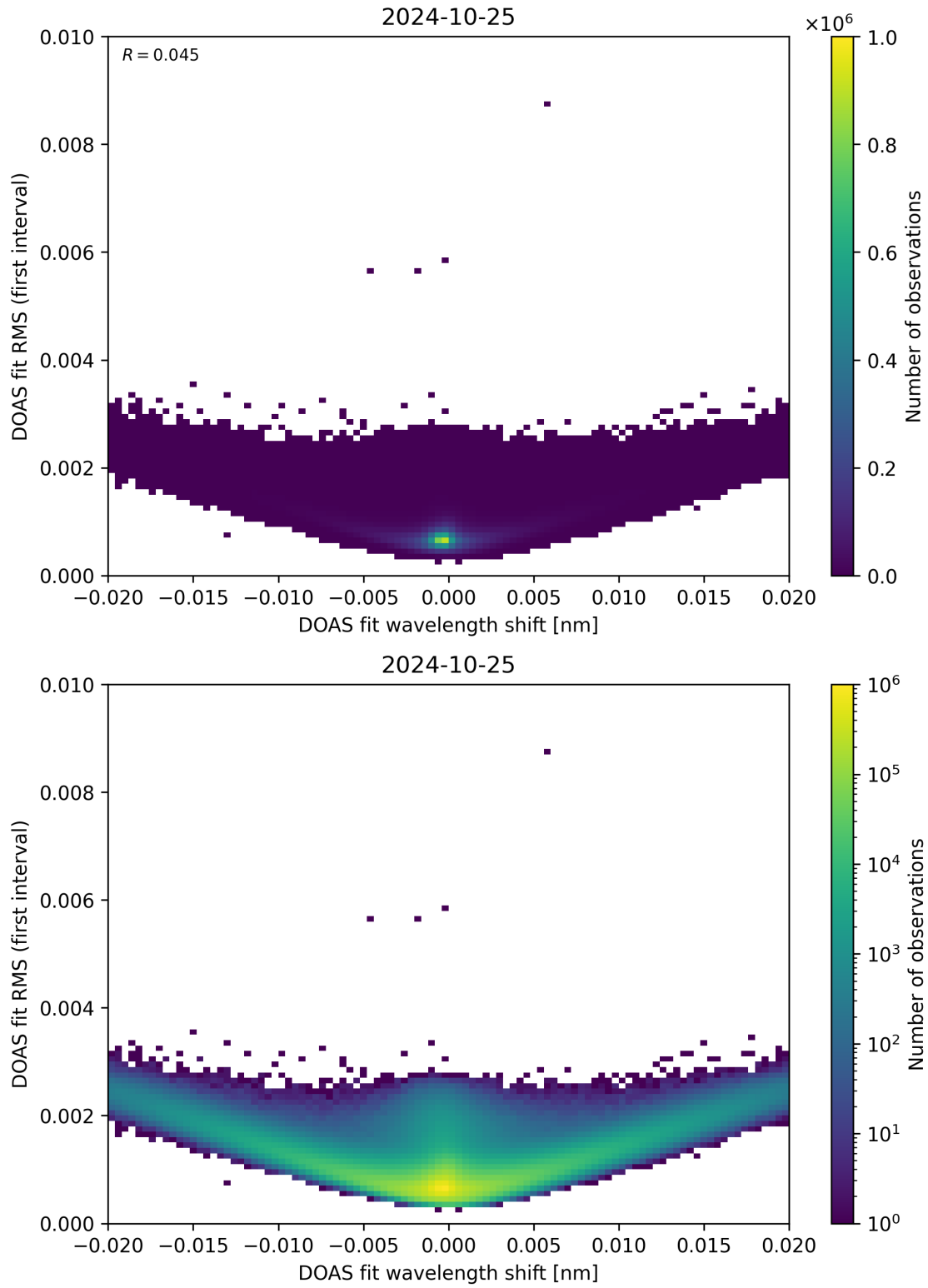
Figure 64: Scatter density plot of “DOAS fit wavelength shift” against “DOAS fit RMS (first interval)” for 2024-10-24 to 2024-10-26.
