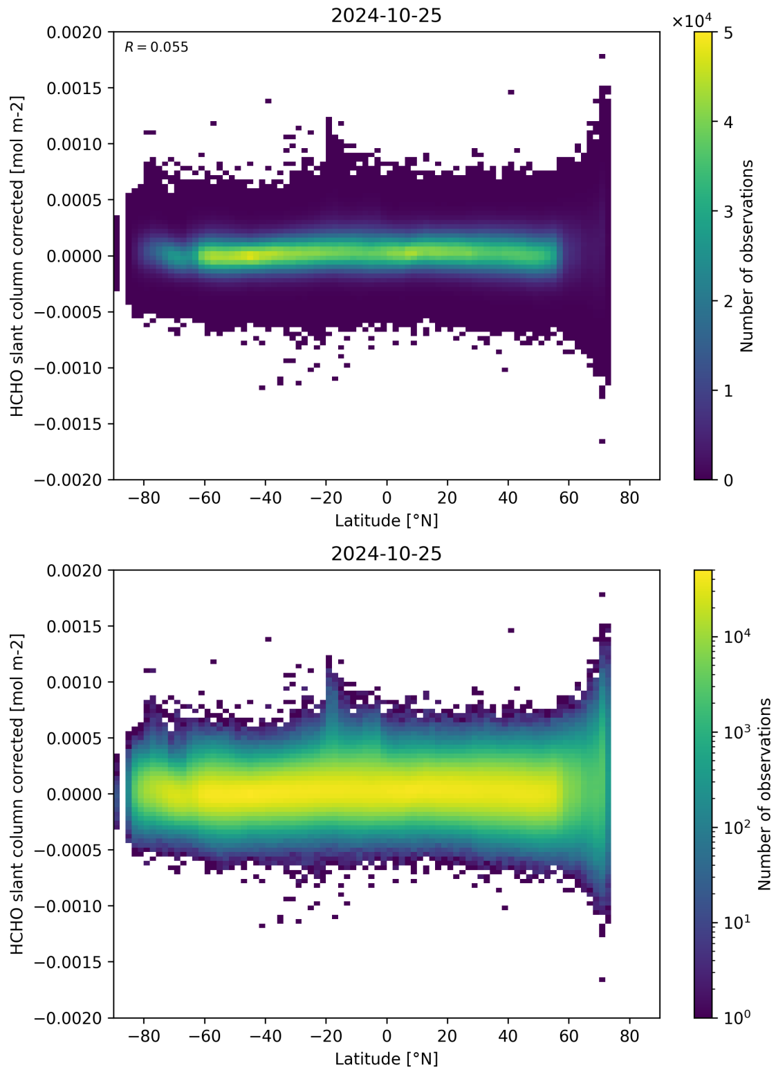
Figure 157: Scatter density plot of “Latitude” against “HCHO slant column corrected” for 2024-10-24 to 2024-10-26.
