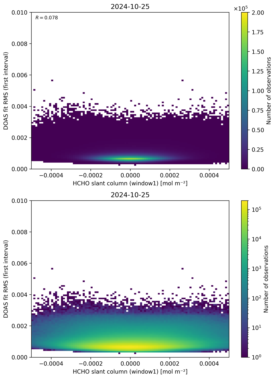
Figure 78: Scatter density plot of “HCHO slant column (window1)” against “DOAS fit RMS (first interval)” for 2024-10-24 to 2024-10-26.
