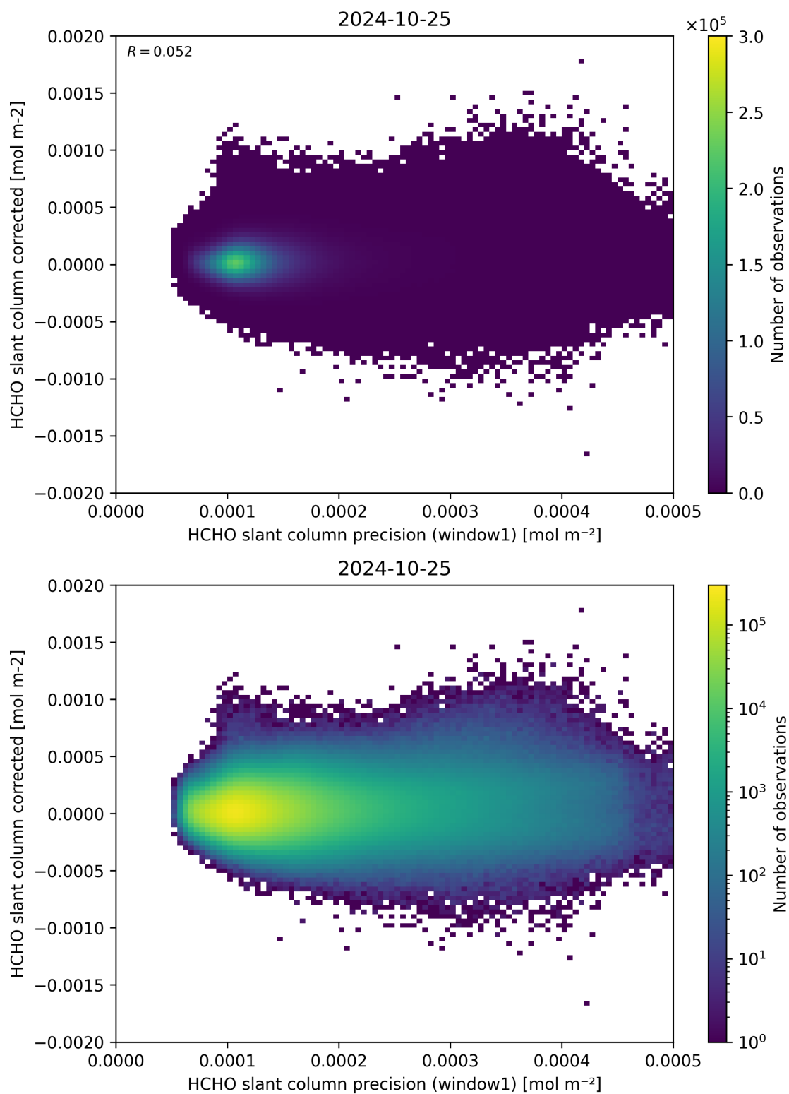
Figure 92: Scatter density plot of “HCHO slant column precision (window1)” against “HCHO slant column corrected” for 2024-10-24 to 2024-10-26.
