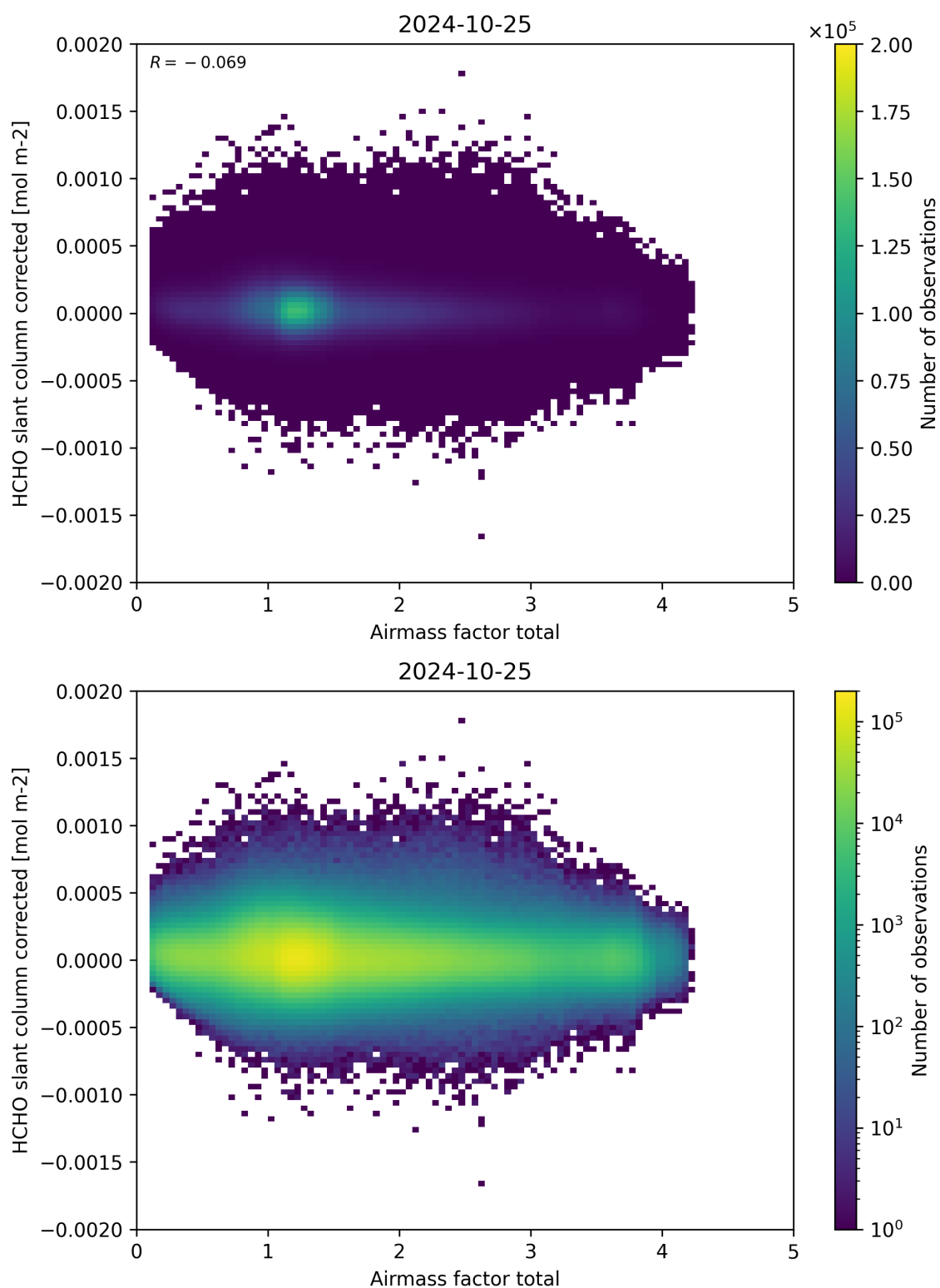
Figure 101: Scatter density plot of “Airmass factor total” against “HCHO slant column corrected” for 2024-10-24 to 2024-10-26.
