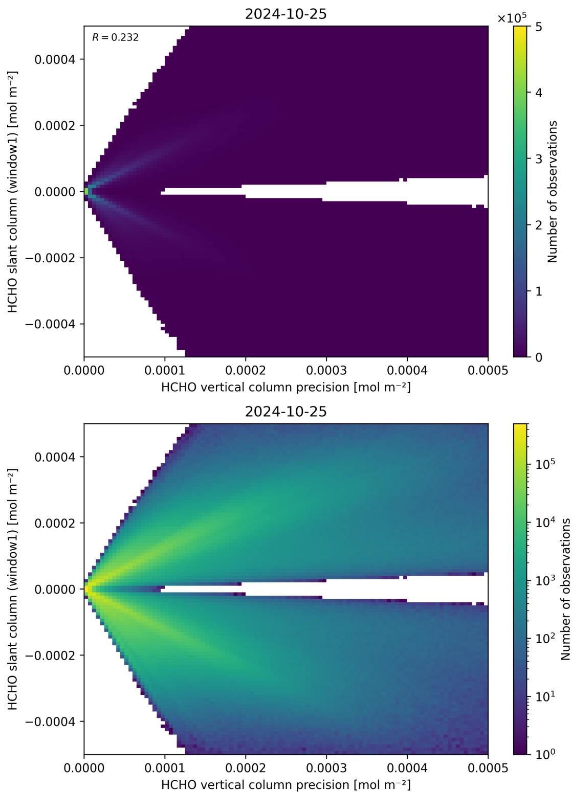
Figure 142: Scatter density plot of “HCHO vertical column precision” against “HCHO slant column (window1)” for 2024-10-24 to 2024-10-26.
