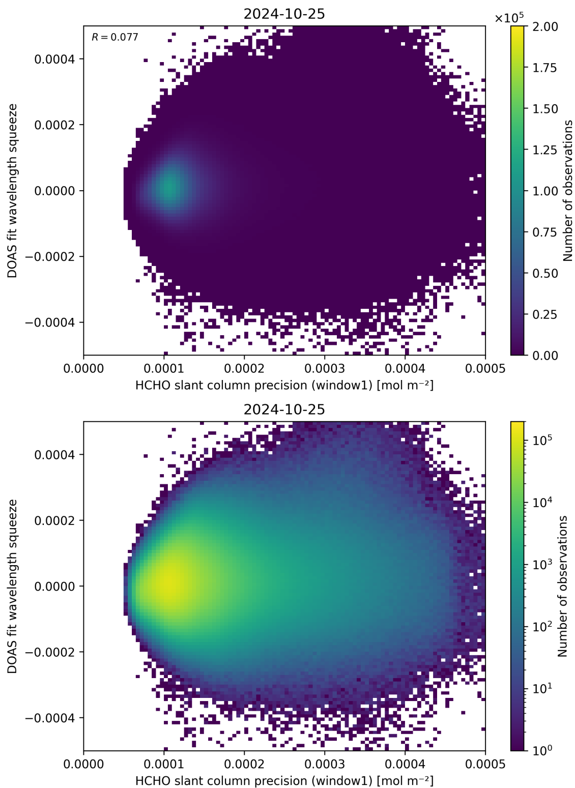
Figure 90: Scatter density plot of “HCHO slant column precision (window1)” against “DOAS fit wavelength squeeze” for 2024-10-24 to 2024-10-26.
