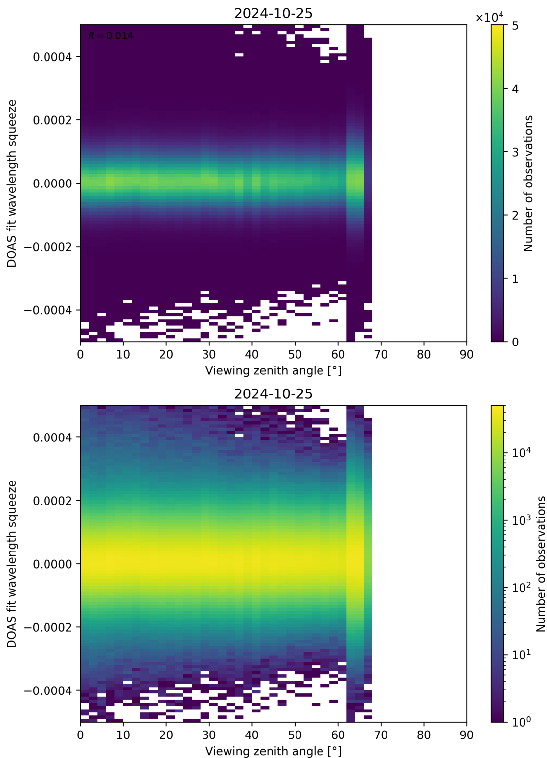
Figure 184: Scatter density plot of “Viewing zenith angle” against “DOAS fit wavelength squeeze” for 2024-10-24 to 2024-10-26.
