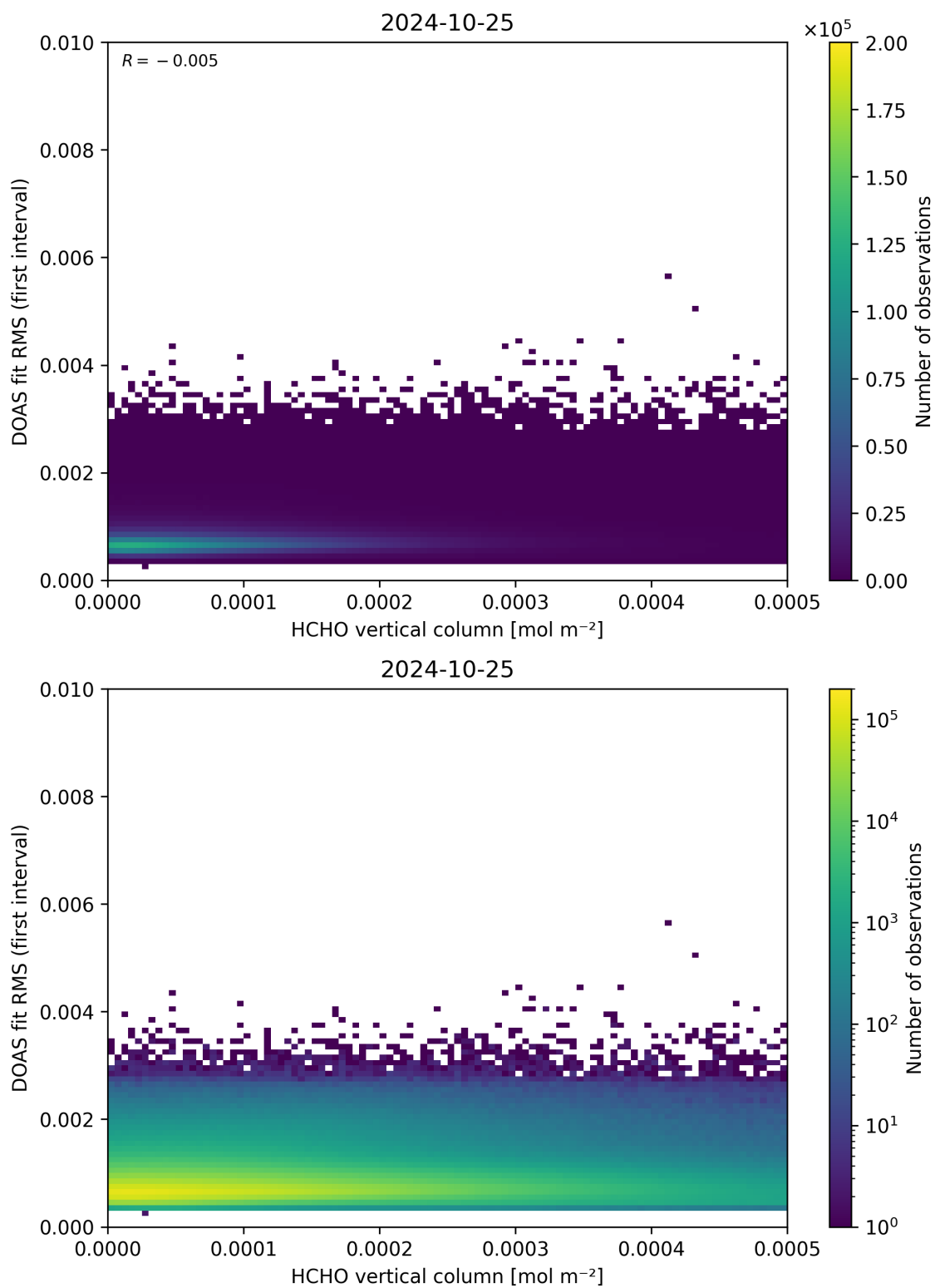
Figure 123: Scatter density plot of “HCHO vertical column” against “DOAS fit RMS (first interval)” for 2024-10-24 to 2024-10-26.
