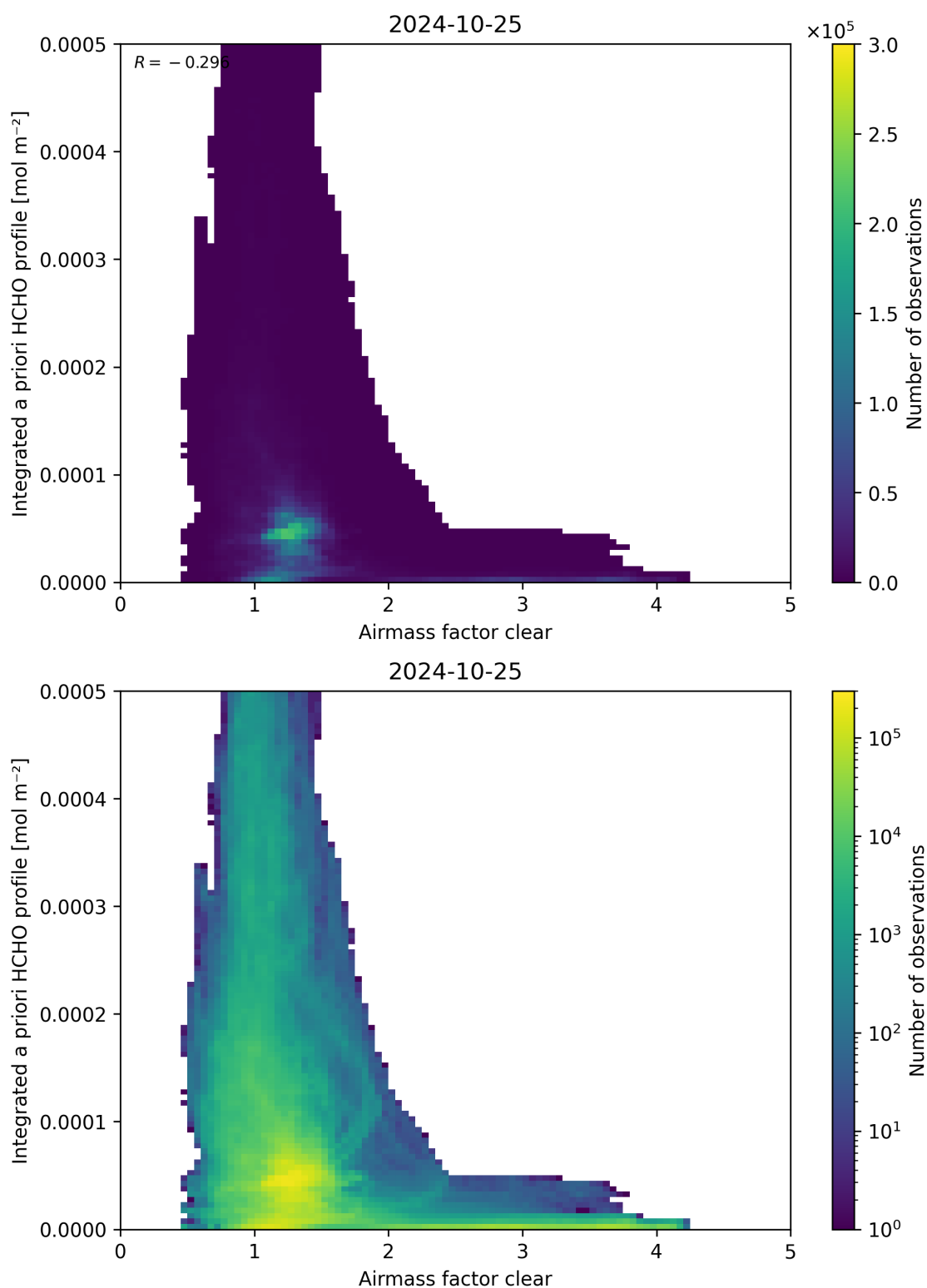
Figure 76: Scatter density plot of “Airmass factor clear” against “Integrated a priori HCHO profile” for 2024-10-24 to 2024-10-26.
