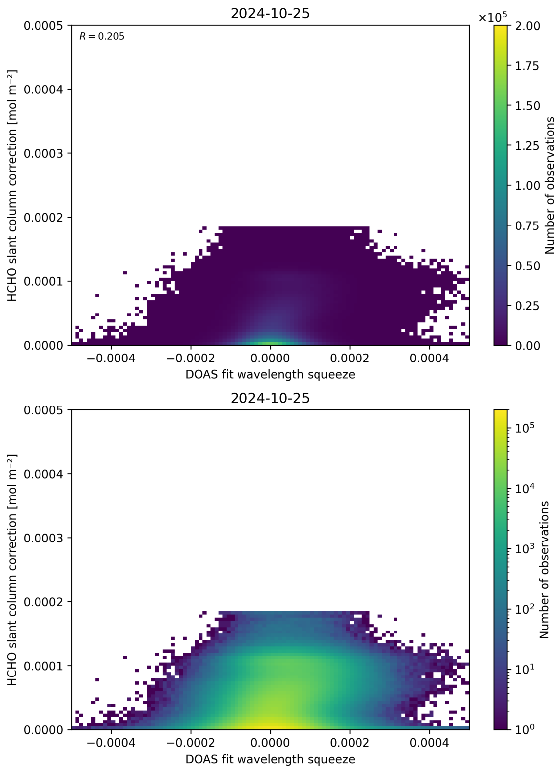
Figure 70: Scatter density plot of “DOAS fit wavelength squeeze” against “HCHO slant column correction” for 2024-10-24 to 2024-10-26.
