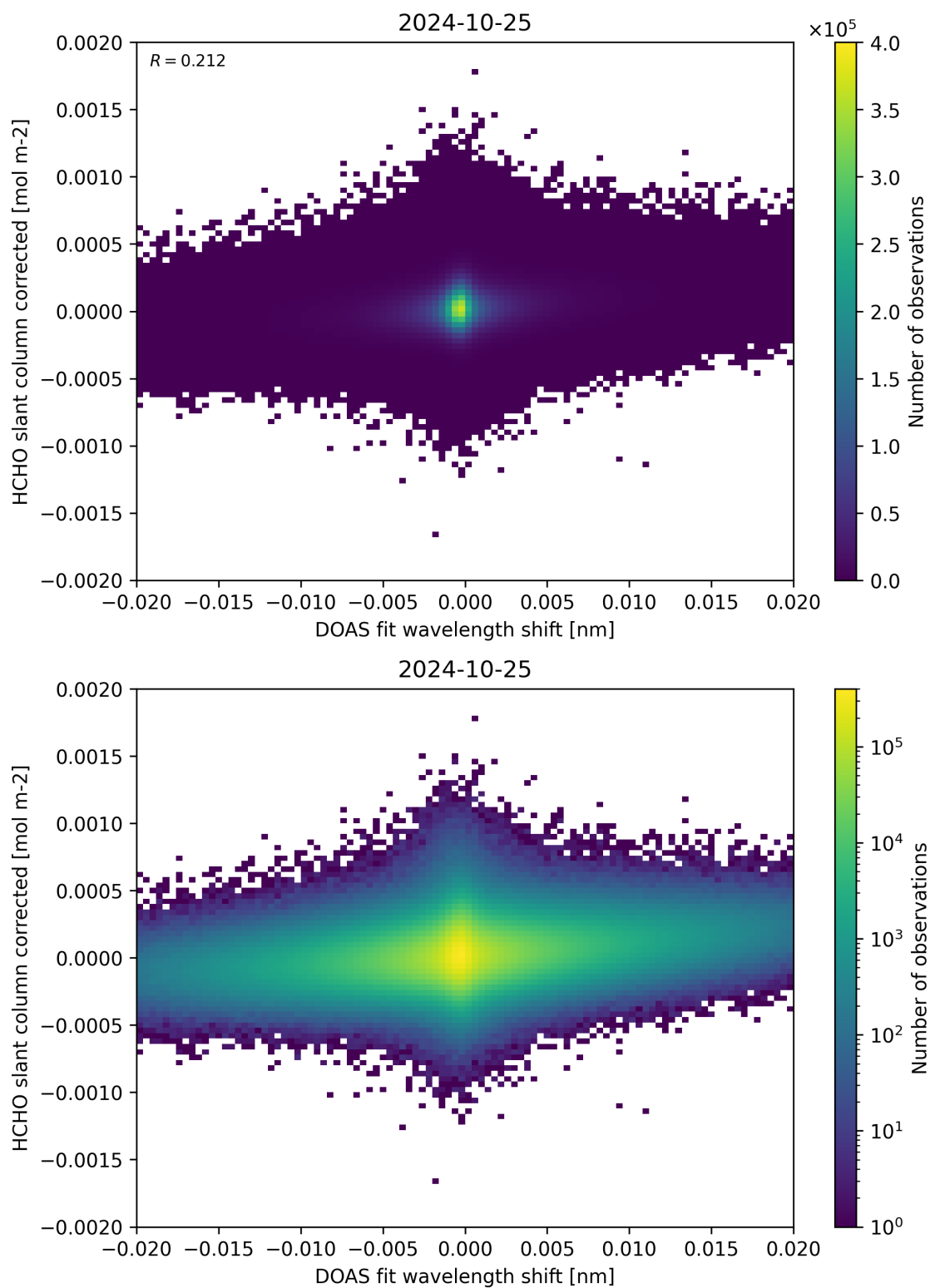
Figure 66: Scatter density plot of “DOAS fit wavelength shift” against “HCHO slant column corrected” for 2024-10-24 to 2024-10-26.
