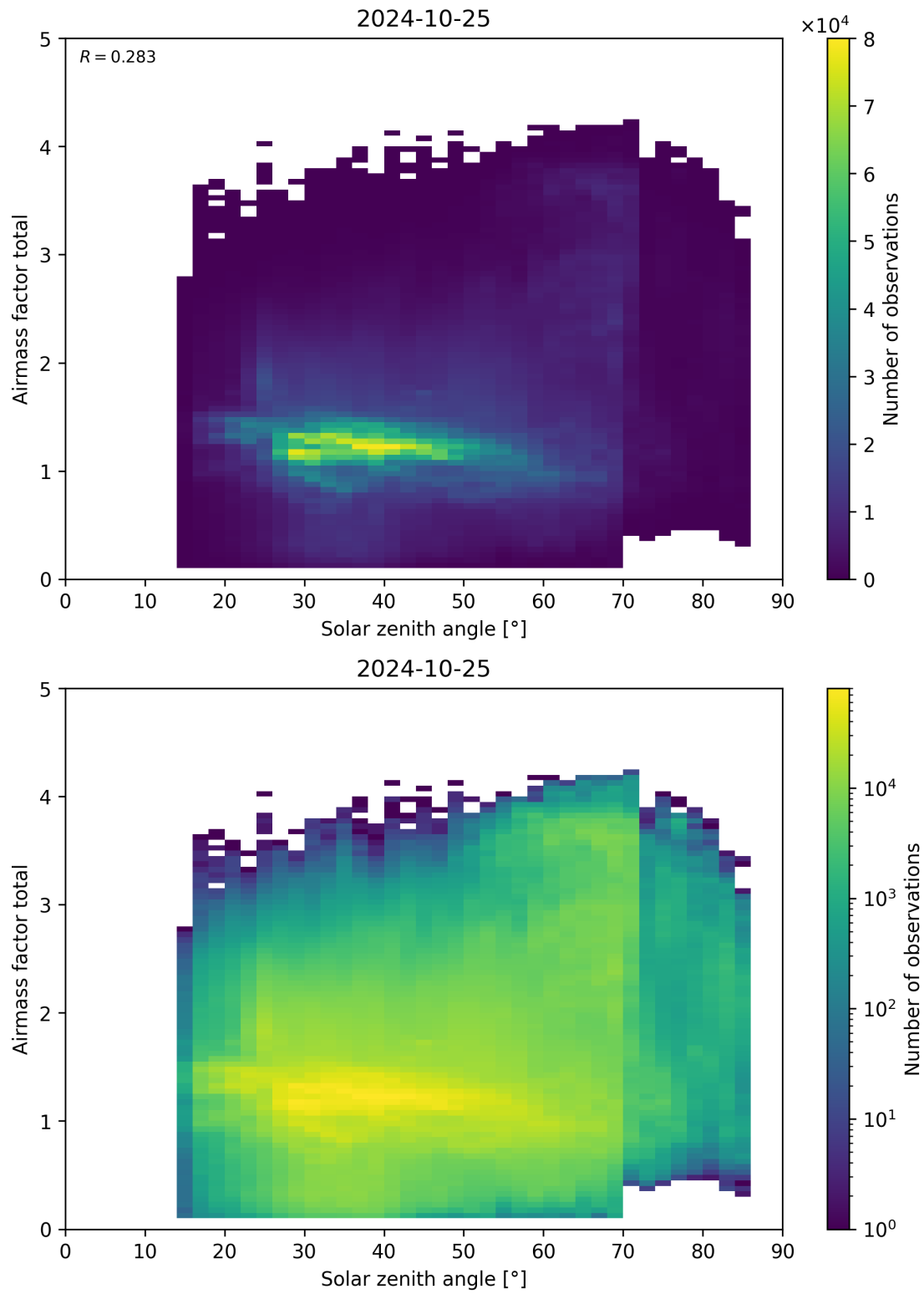
Figure 175: Scatter density plot of “Solar zenith angle” against “Airmass factor total” for 2024-10-24 to 2024-10-26.
