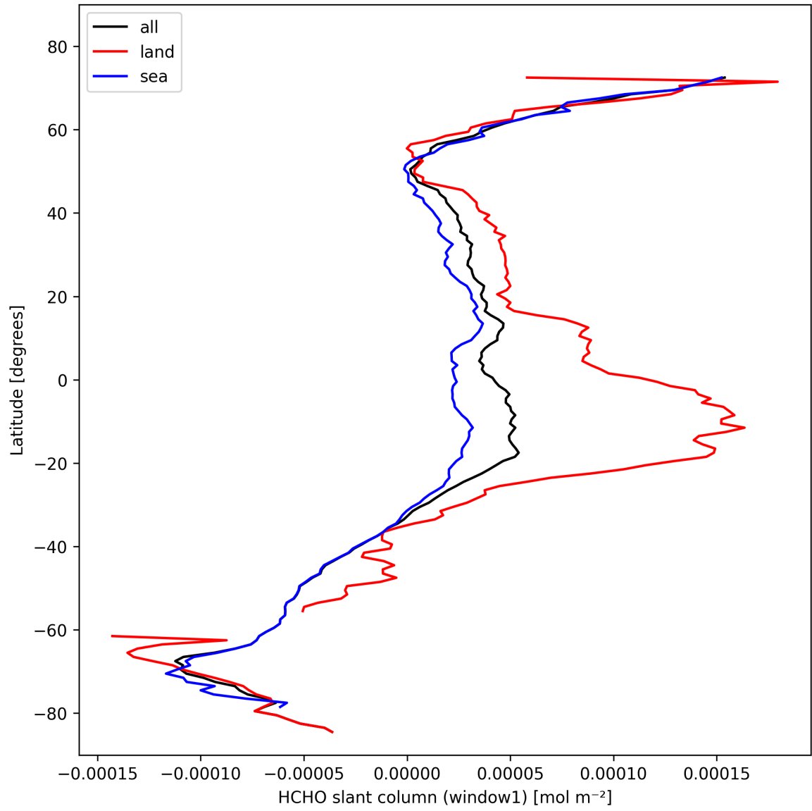
Figure 24: Zonal average of “HCHO slant column (window1)” for 2024-10-24 to 2024-10-26.
