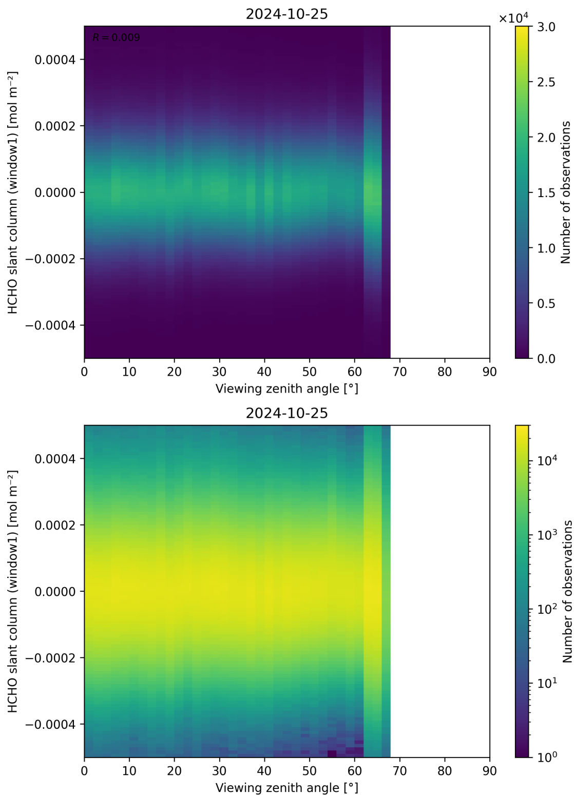
Figure 188: Scatter density plot of “Viewing zenith angle” against “HCHO slant column (window1)” for 2024-10-24 to 2024-10-26.
