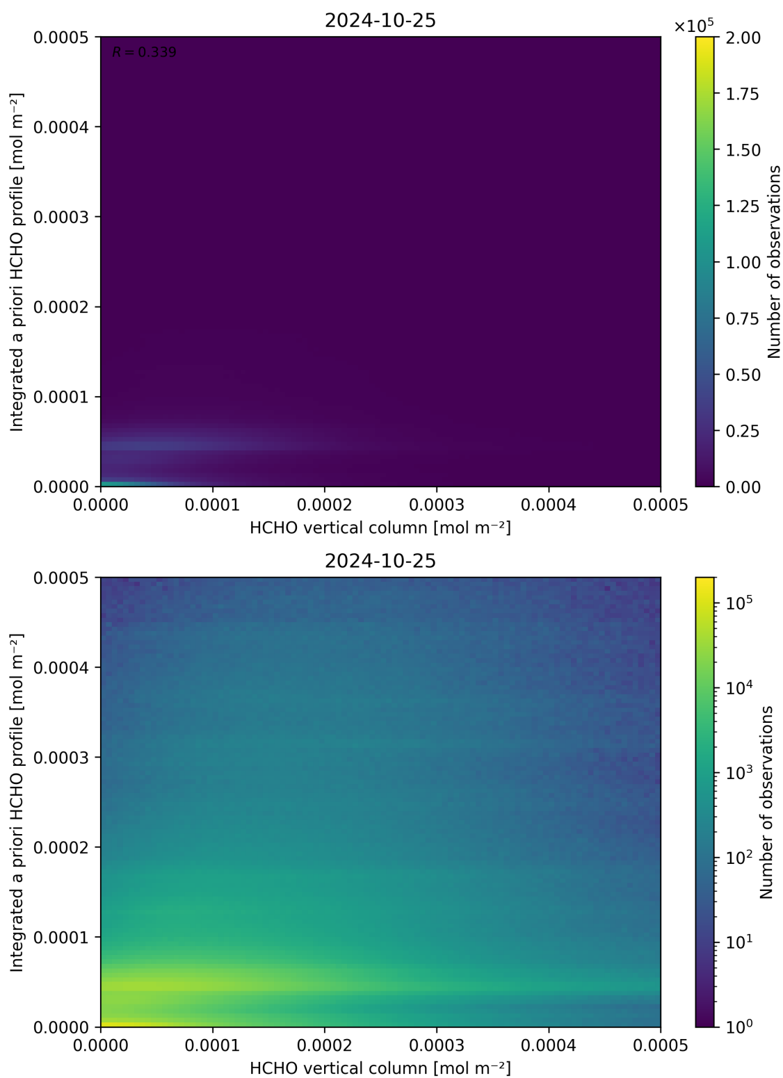
Figure 135: Scatter density plot of “HCHO vertical column” against “Integrated a priori HCHO profile” for 2024-10-24 to 2024-10-26.
