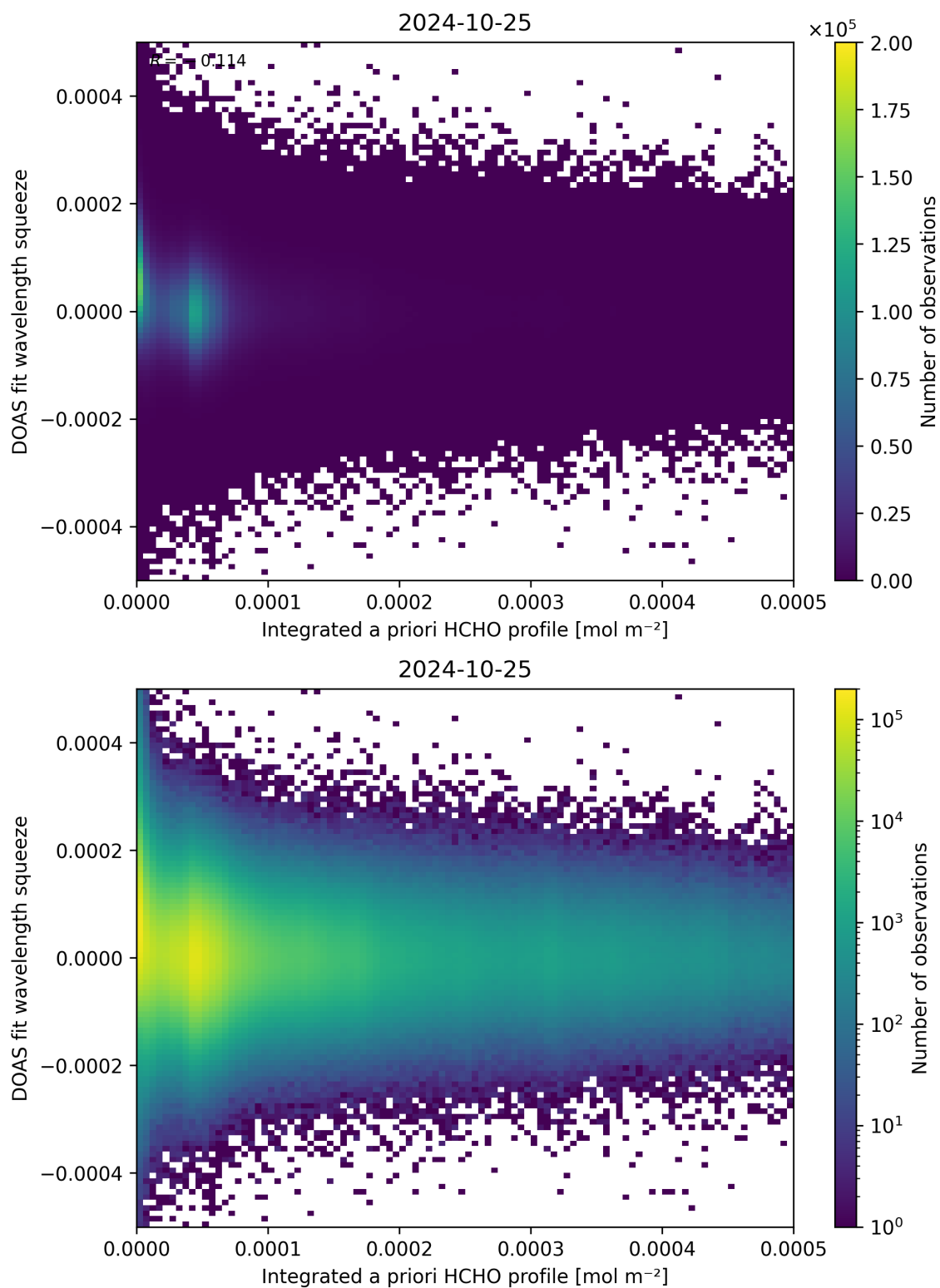
Figure 150: Scatter density plot of “Integrated a priori HCHO profile” against “DOAS fit wavelength squeeze” for 2024-10-24 to 2024-10-26.
