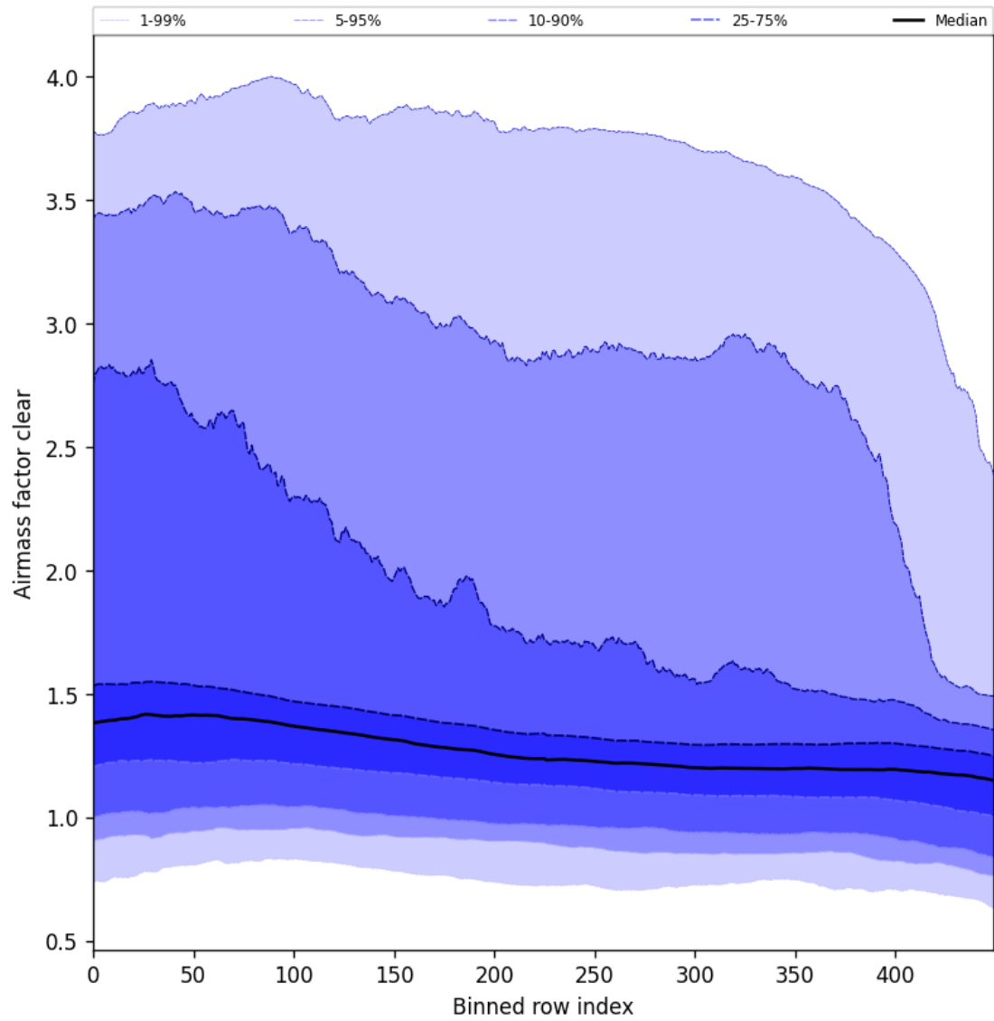
Figure 56: Along track statistics of “Airmass factor clear” for 2024-10-24 to 2024-10-26
