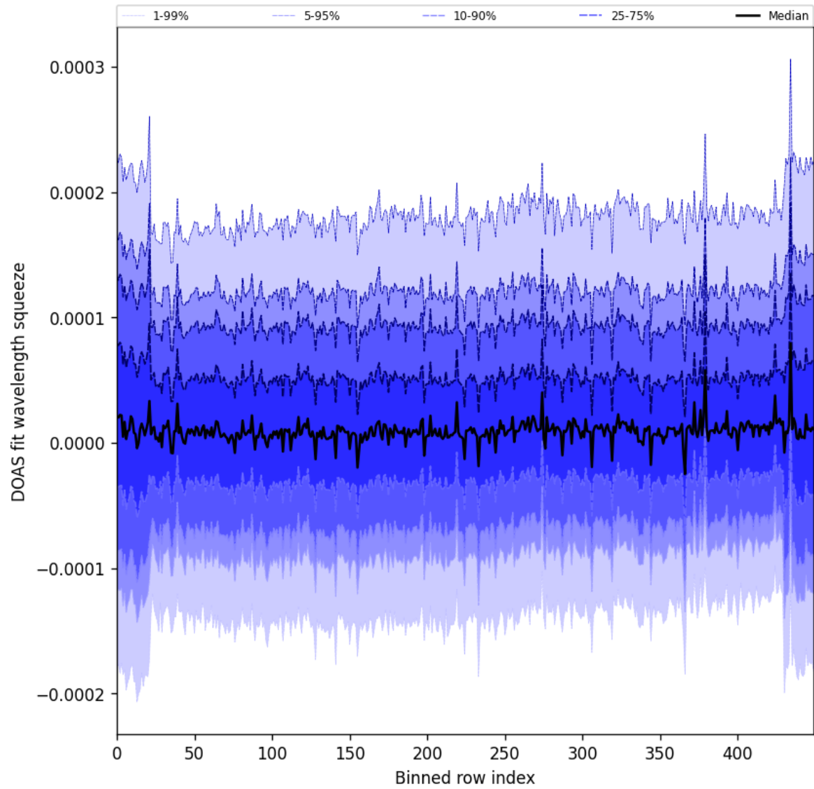
Figure 59: Along track statistics of “DOAS fit wavelength squeeze” for 2024-10-24 to 2024-10-26
