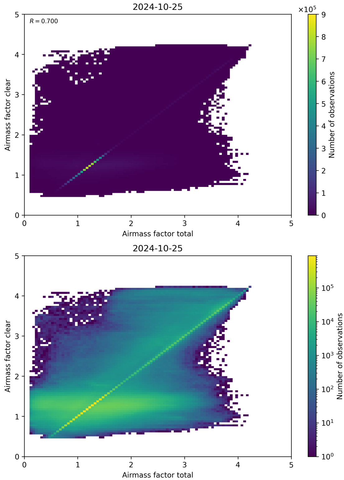
Figure 100: Scatter density plot of “Airmass factor total” against “Airmass factor clear” for 2024-10-24 to 2024-10-26.
