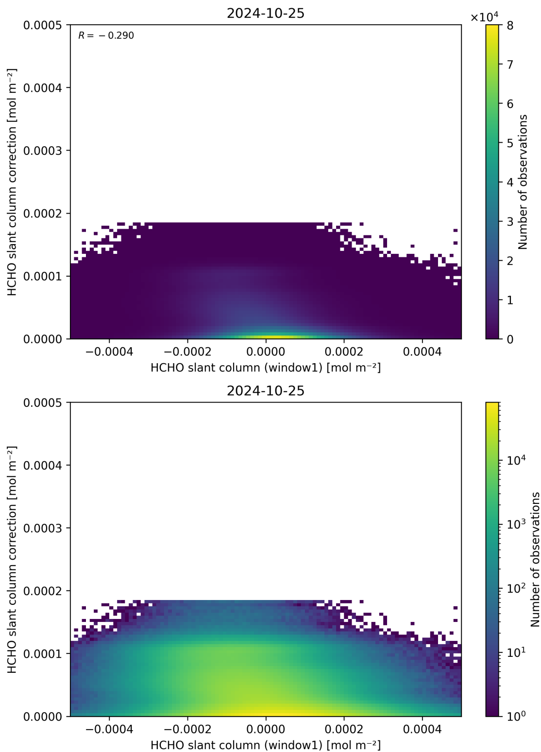
Figure 83: Scatter density plot of “HCHO slant column (window1)” against “HCHO slant column correction” for 2024-10-24 to 2024-10-26.
