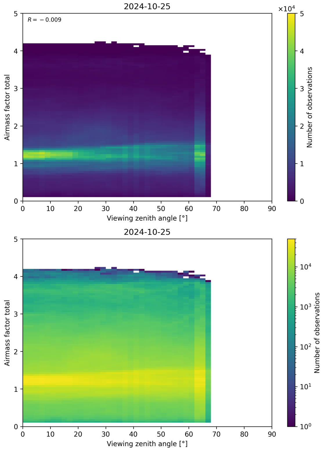
Figure 190: Scatter density plot of “Viewing zenith angle” against “Airmass factor total” for 2024-10-24 to 2024-10-26.
