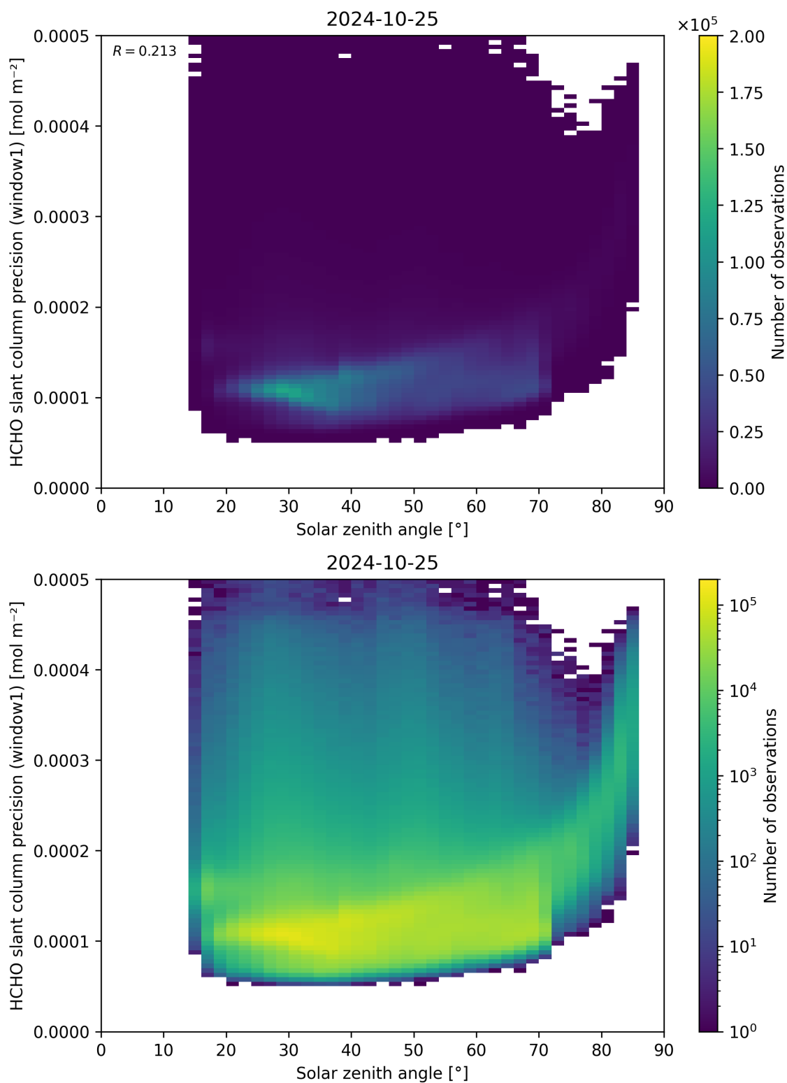
Figure 174: Scatter density plot of “Solar zenith angle” against “HCHO slant column precision (window1)” for 2024-10-24 to 2024-10-26.
