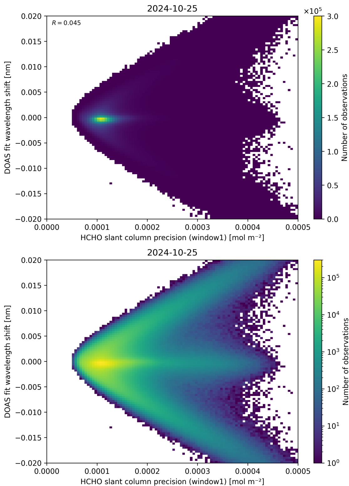
Figure 89: Scatter density plot of “HCHO slant column precision (window1)” against “DOAS fit wavelength shift” for 2024-10-24 to 2024-10-26.
