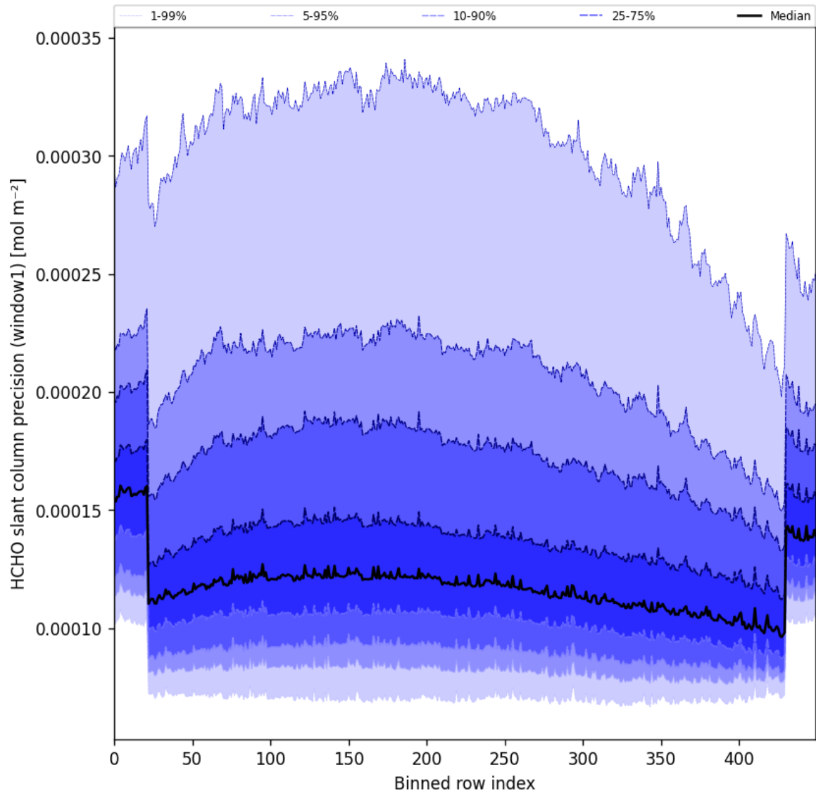
Figure 53: Along track statistics of “HCHO slant column precision (window1)” for 2024-10-24 to 2024-10-26
