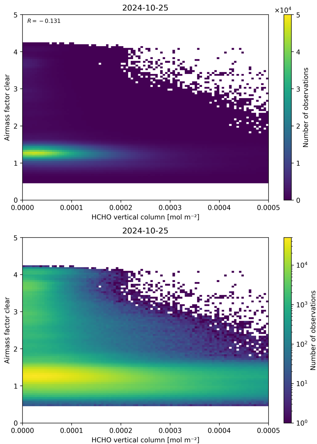
Figure 126: Scatter density plot of “HCHO vertical column” against “Airmass factor clear” for 2024-10-24 to 2024-10-26.
