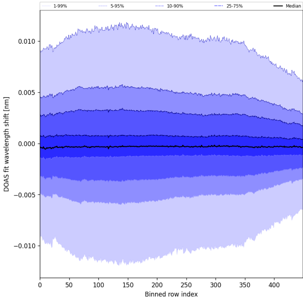
Figure 58: Along track statistics of “DOAS fit wavelength shift” for 2024-10-24 to 2024-10-26
