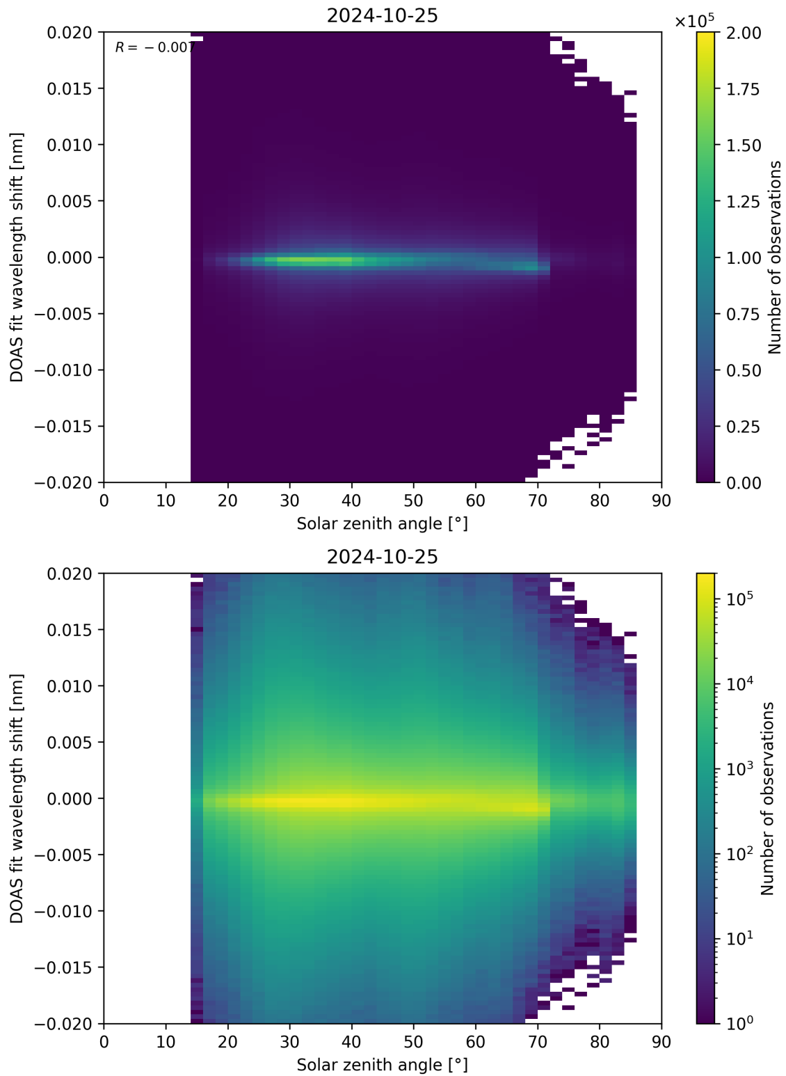
Figure 168: Scatter density plot of “Solar zenith angle” against “DOAS fit wavelength shift” for 2024-10-24 to 2024-10-26.
