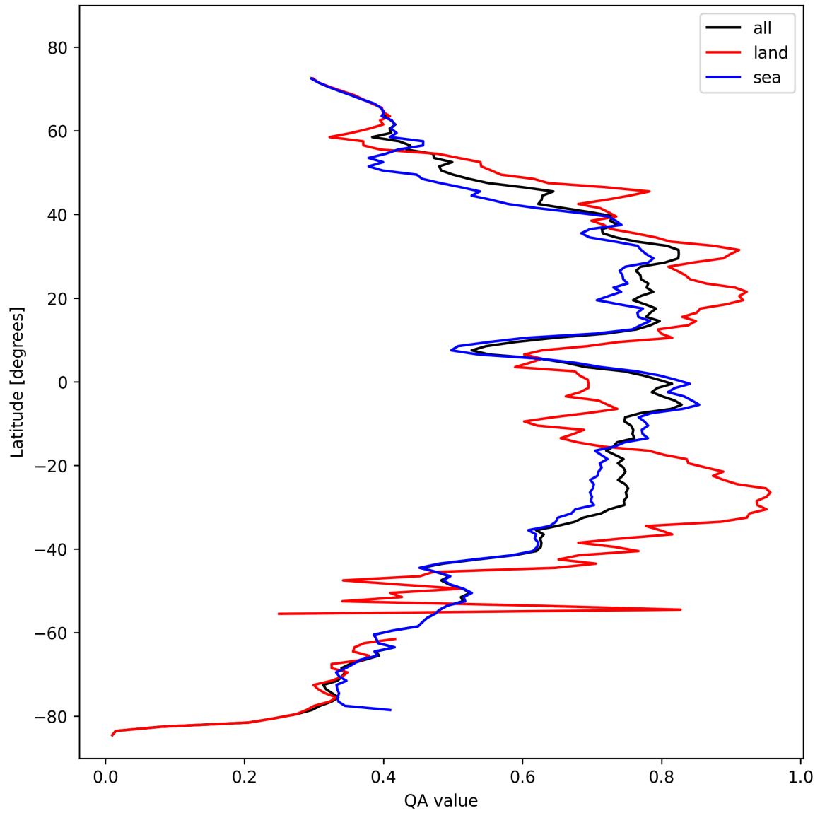
Figure 20: Zonal average of “QA value” for 2024-10-24 to 2024-10-26.
