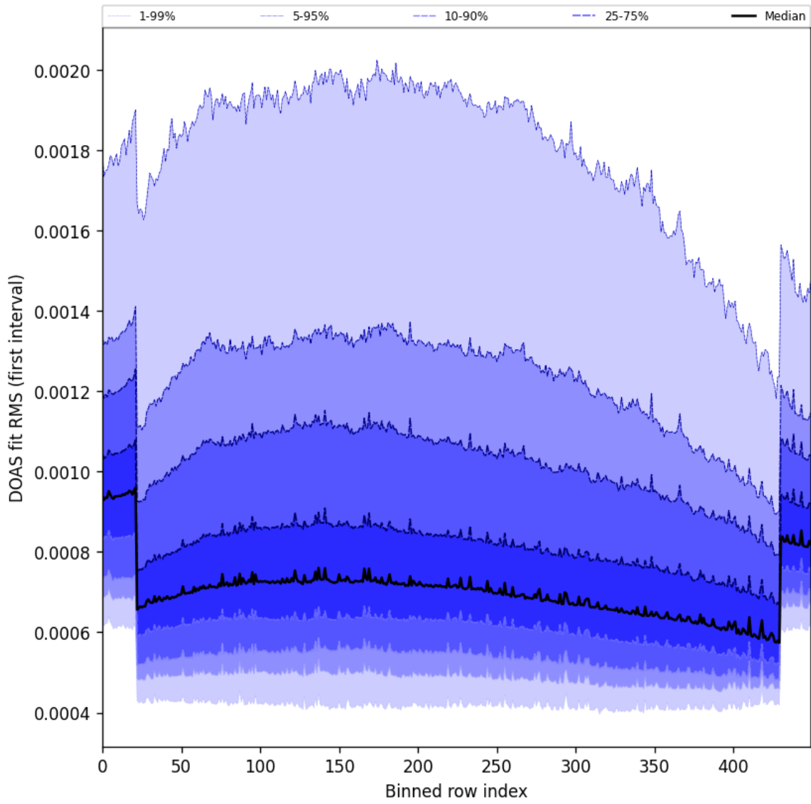
Figure 60: Along track statistics of “DOAS fit RMS (first interval)” for 2024-10-24 to 2024-10-26
