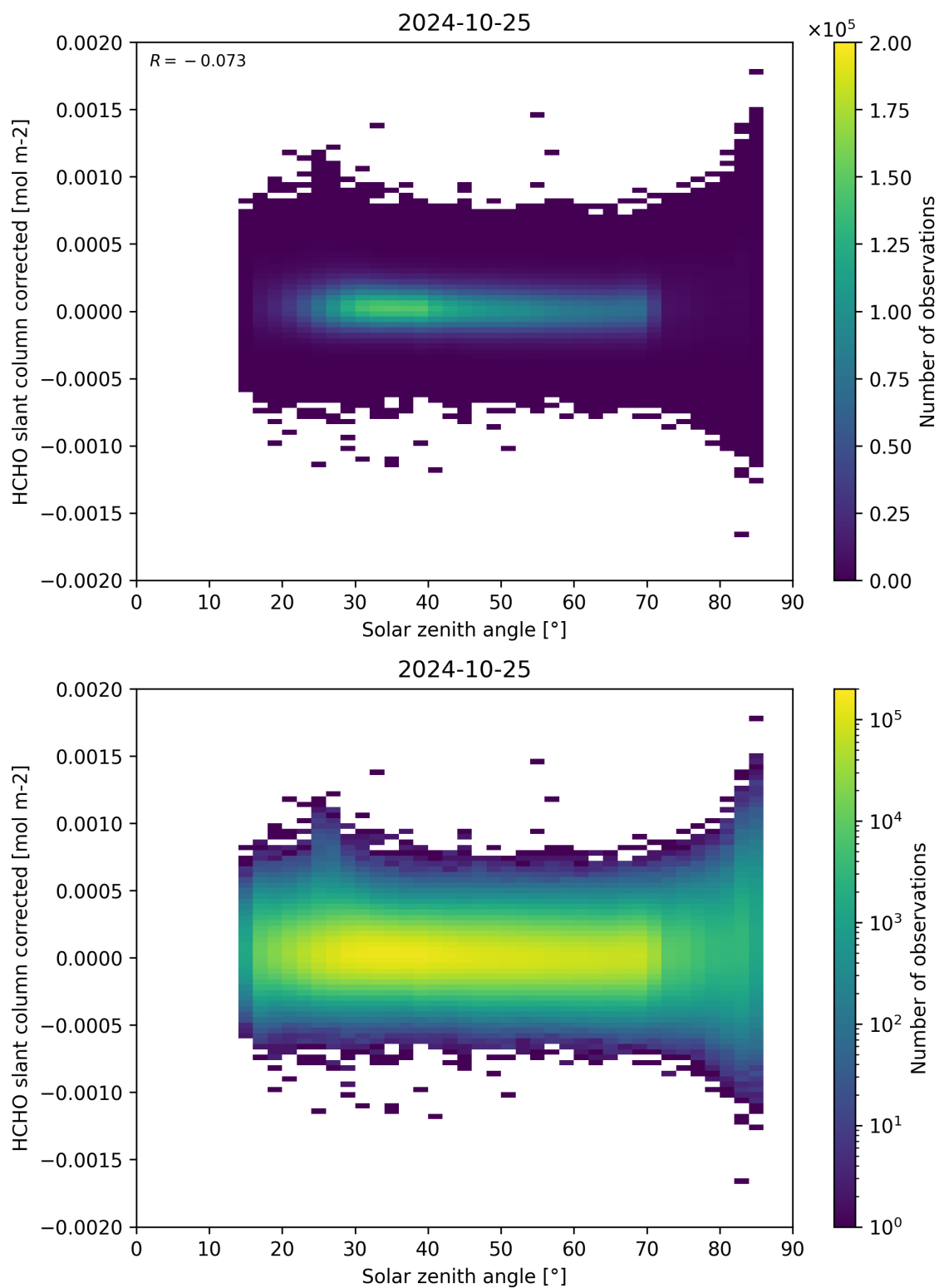
Figure 171: Scatter density plot of “Solar zenith angle” against “HCHO slant column corrected” for 2024-10-24 to 2024-10-26.
