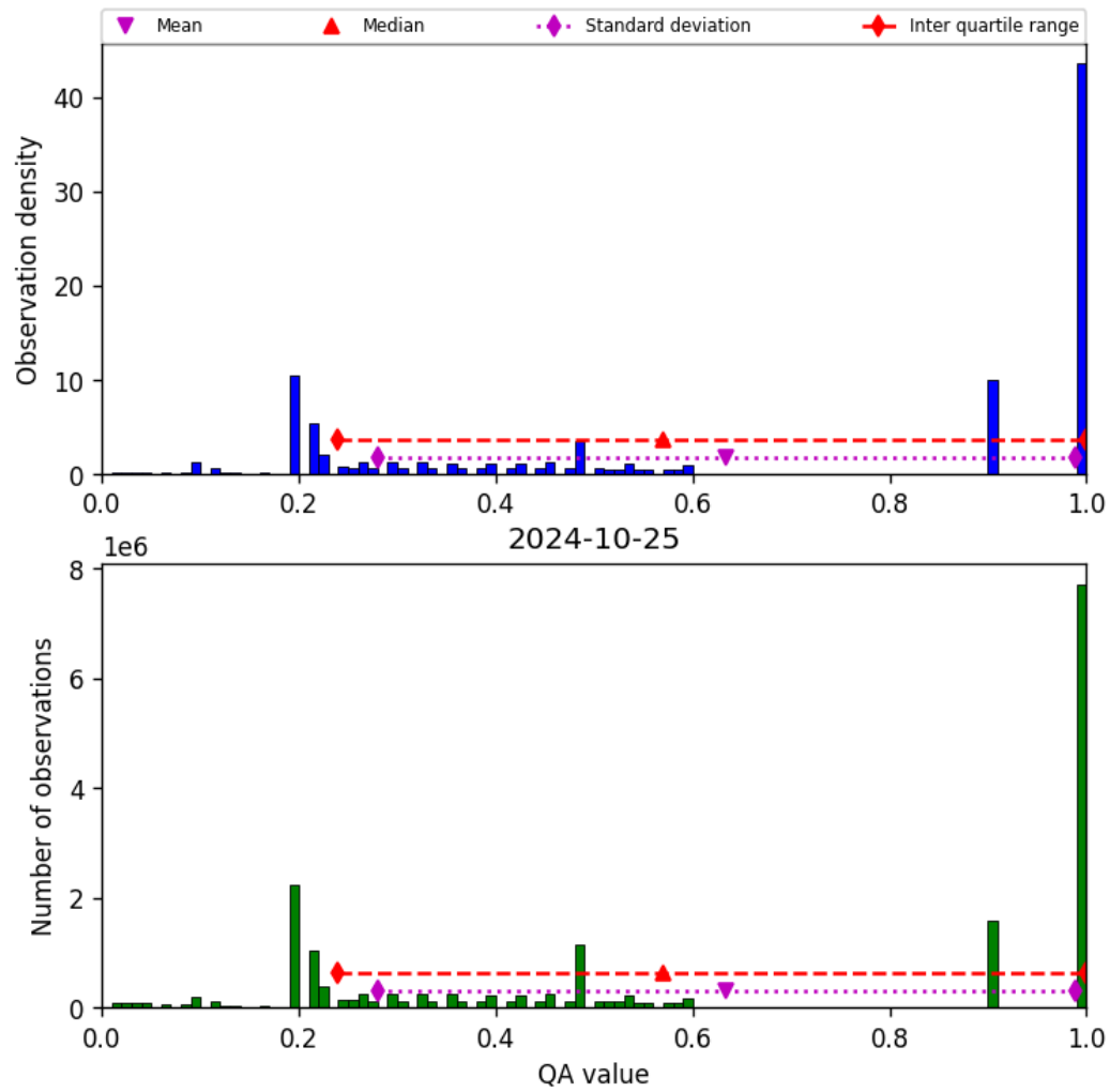
Figure 34: Histogram of “QA value” for 2024-10-24 to 2024-10-26
