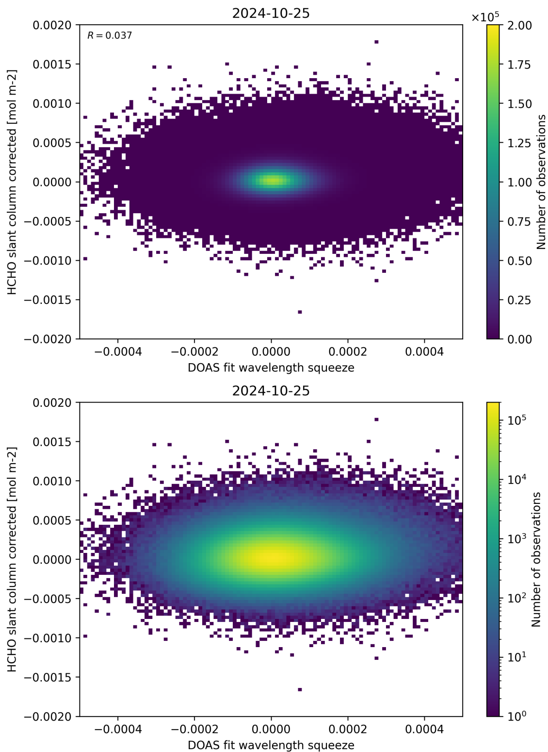
Figure 69: Scatter density plot of “DOAS fit wavelength squeeze” against “HCHO slant column corrected” for 2024-10-24 to 2024-10-26.
