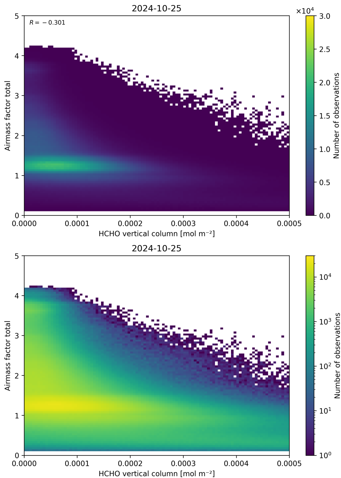
Figure 131: Scatter density plot of “HCHO vertical column” against “Airmass factor total” for 2024-10-24 to 2024-10-26.
