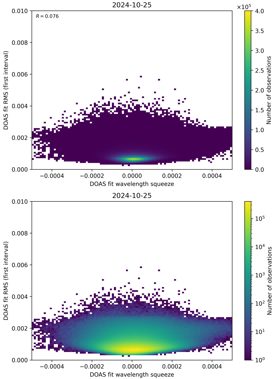
Figure 68: Scatter density plot of “DOAS fit wavelength squeeze” against “DOAS fit RMS (first interval)” for 2024-10-24 to 2024-10-26.
