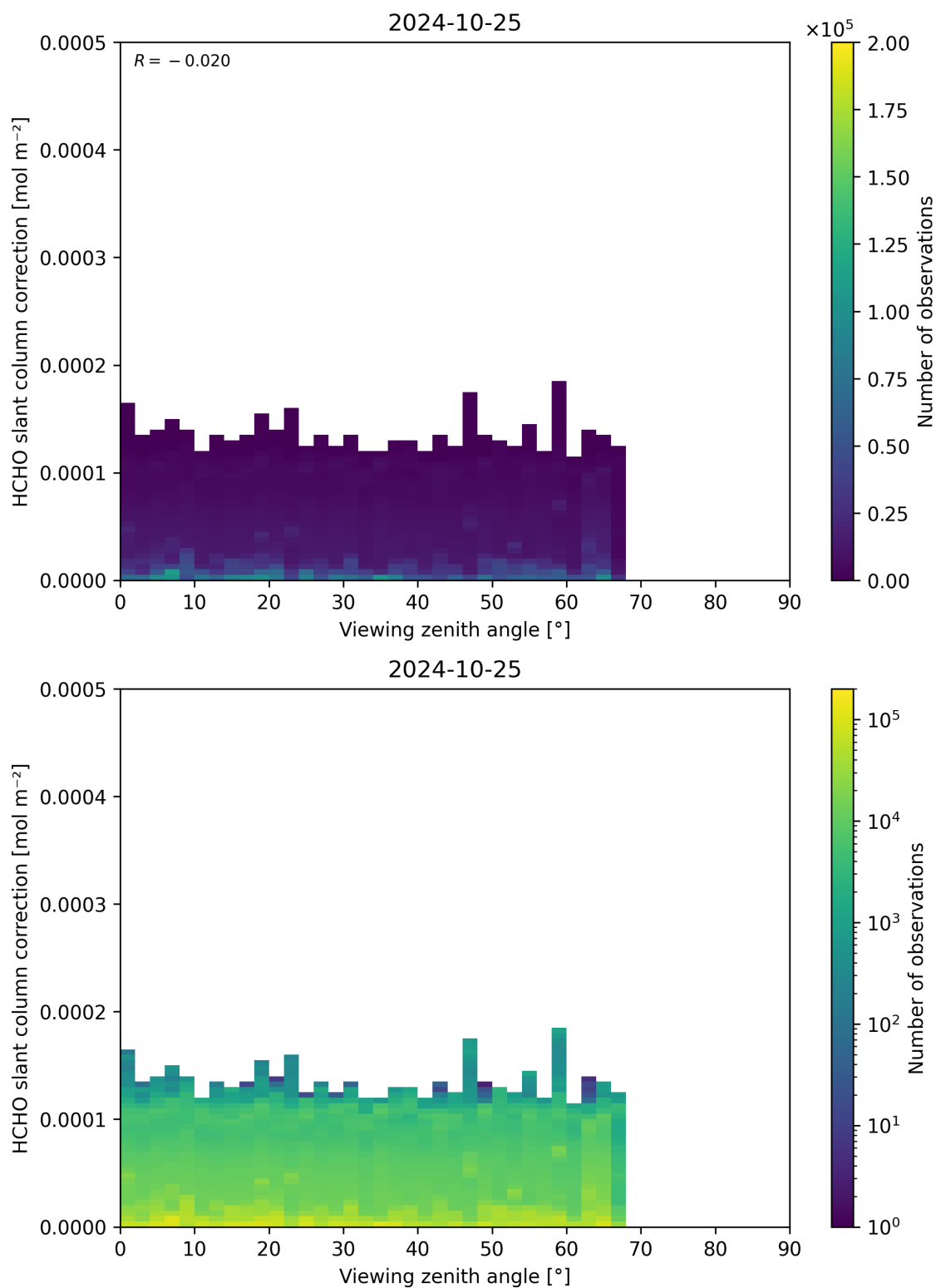
Figure 187: Scatter density plot of “Viewing zenith angle” against “HCHO slant column correction” for 2024-10-24 to 2024-10-26.
