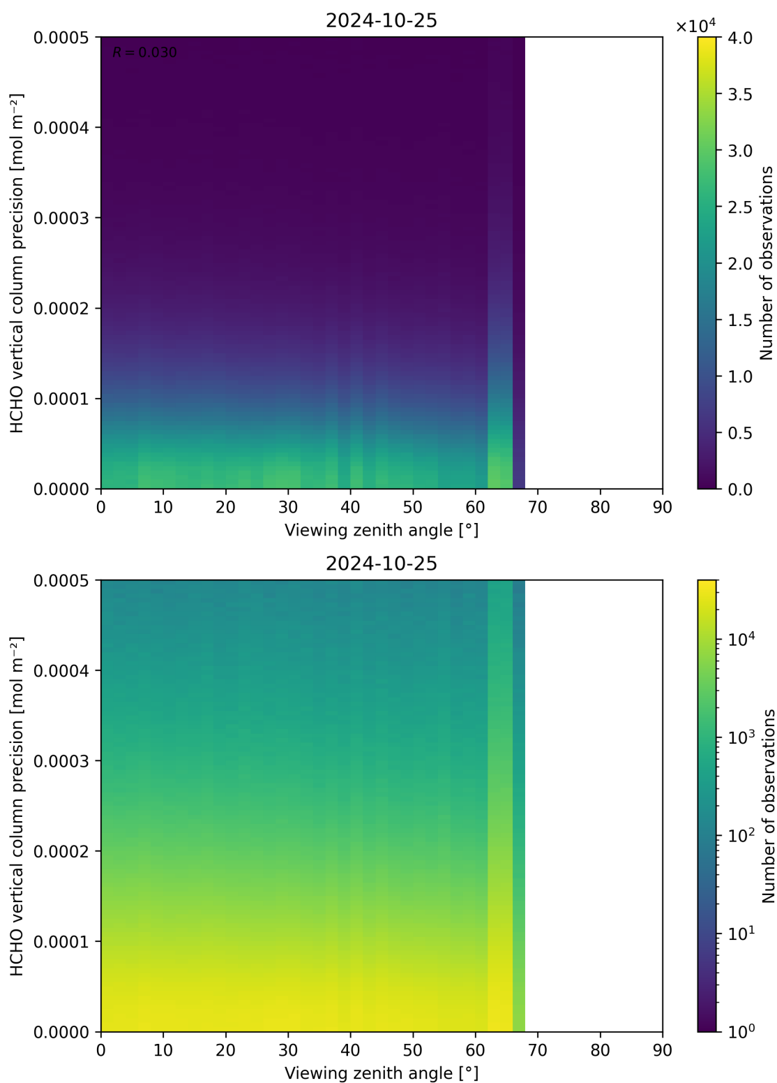
Figure 194: Scatter density plot of “Viewing zenith angle” against “HCHO vertical column precision” for 2024-10-24 to 2024-10-26.
