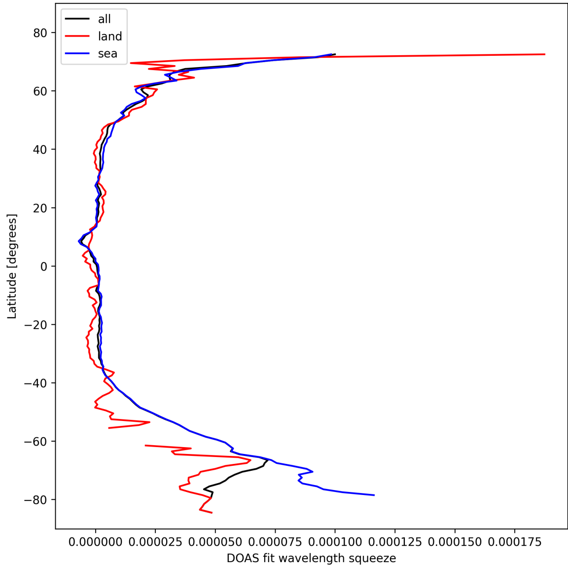
Figure 31: Zonal average of “DOAS fit wavelength squeeze” for 2024-10-24 to 2024-10-26.
