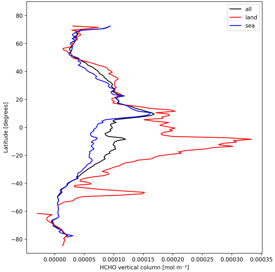
Figure 21: Zonal average of “HCHO vertical column” for 2024-10-24 to 2024-10-26.
