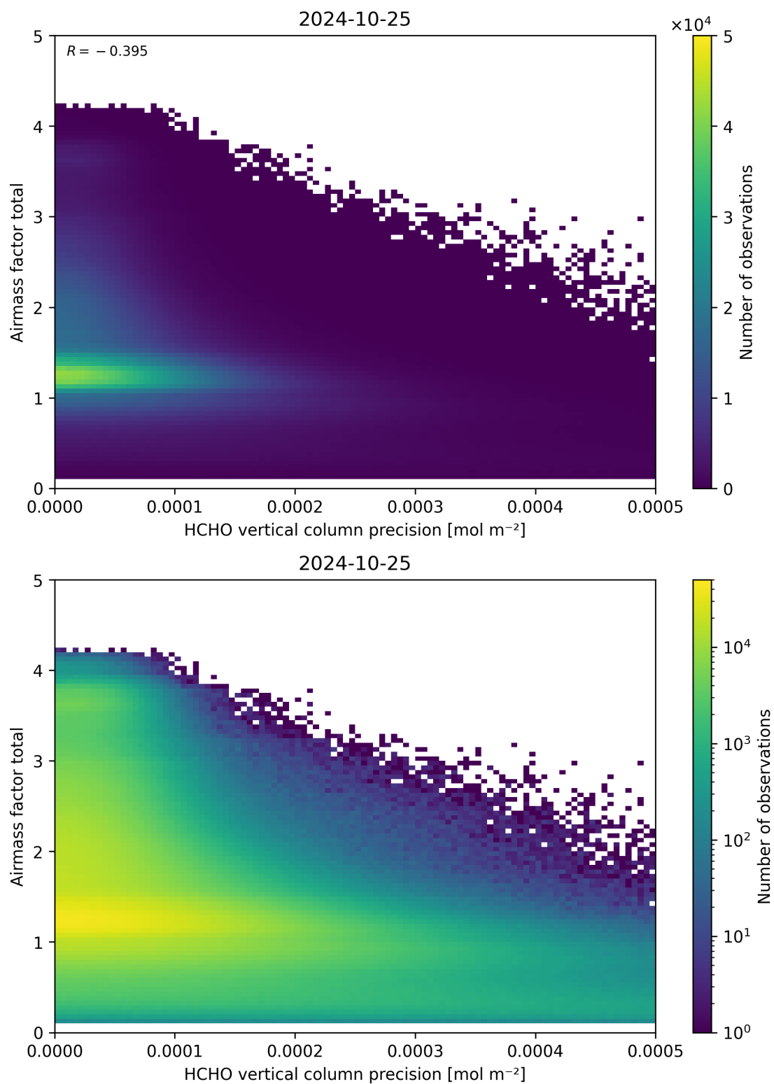
Figure 144: Scatter density plot of “HCHO vertical column precision” against “Airmass factor total” for 2024-10-24 to 2024-10-26.
