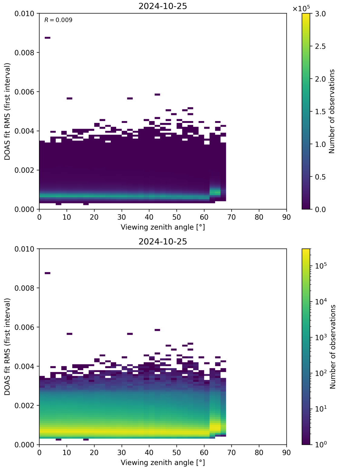
Figure 182: Scatter density plot of “Viewing zenith angle” against “DOAS fit RMS (first interval)” for 2024-10-24 to 2024-10-26.
