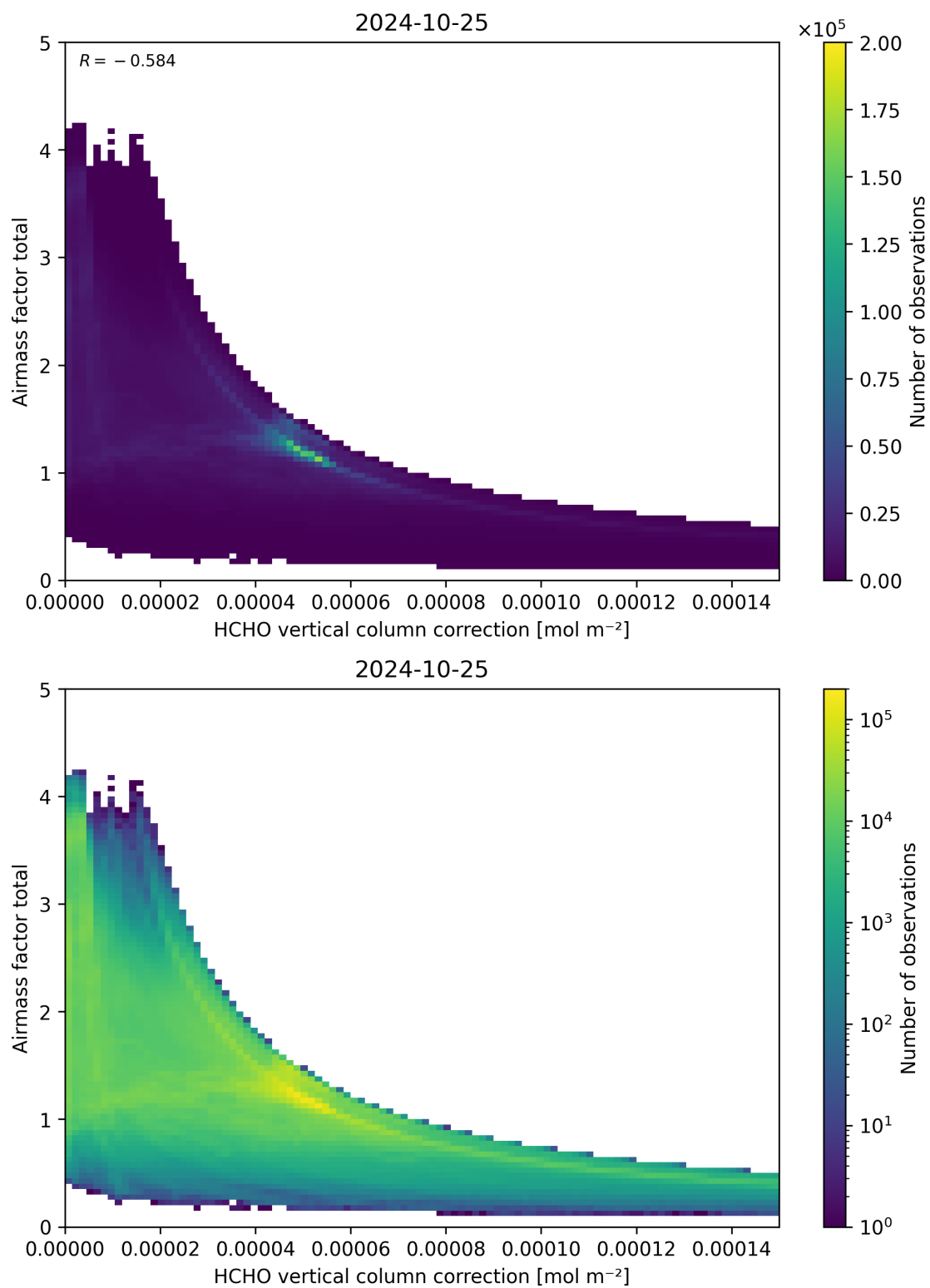
Figure 120: Scatter density plot of “HCHO vertical column correction” against “Airmass factor total” for 2024-10-24 to 2024-10-26.
