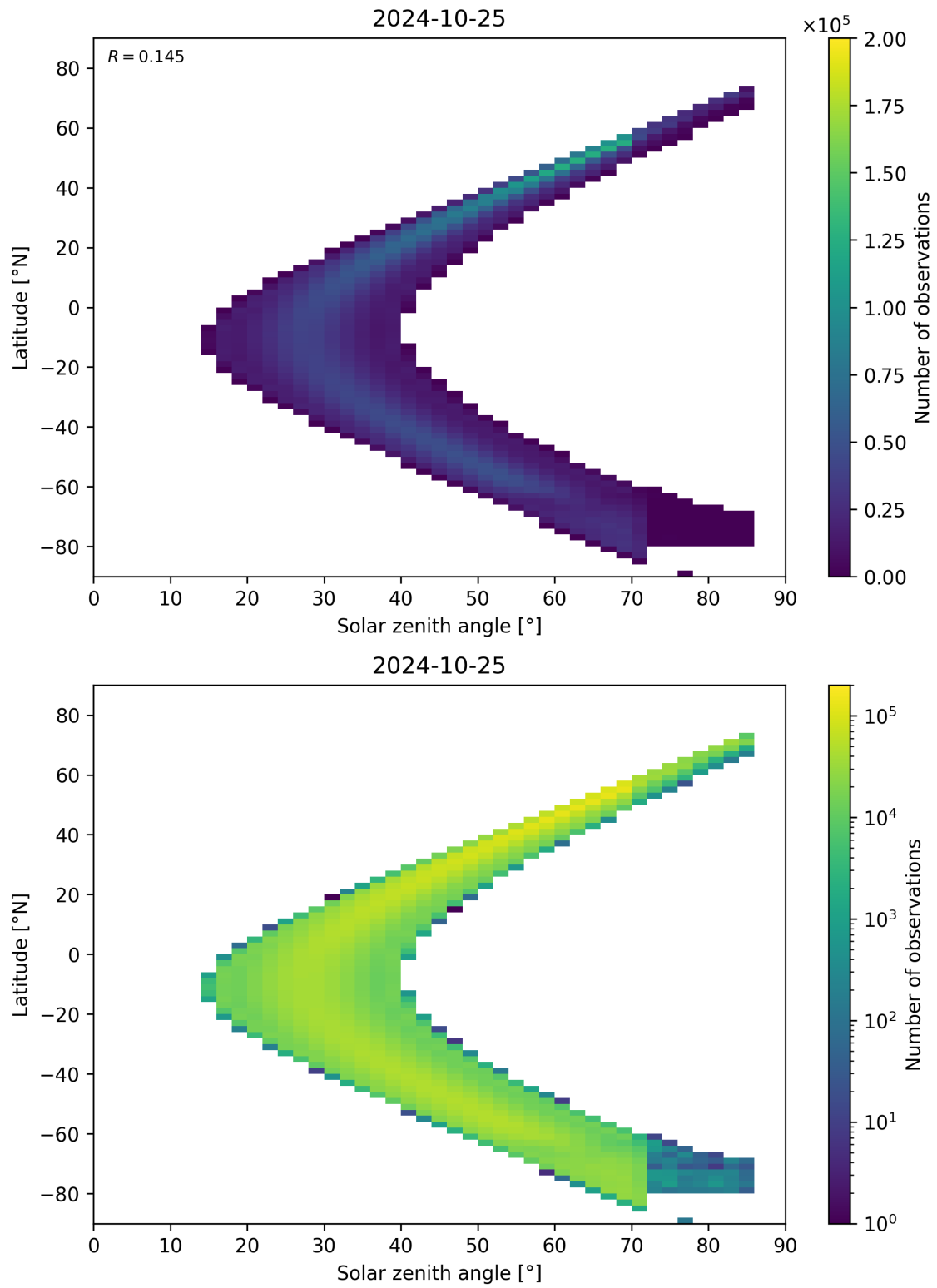
Figure 181: Scatter density plot of “Solar zenith angle” against “Latitude” for 2024-10-24 to 2024-10-26.
