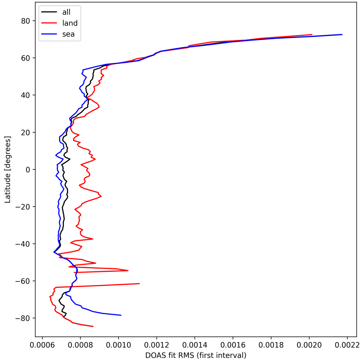
Figure 32: Zonal average of “DOAS fit RMS (first interval)” for 2024-10-24 to 2024-10-26.
