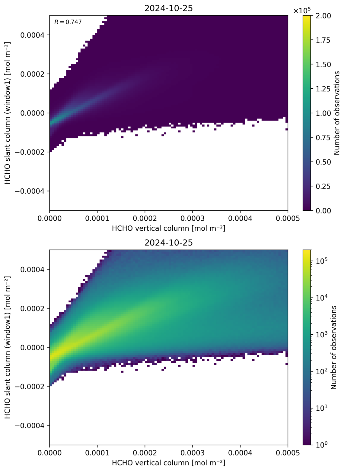
Figure 129: Scatter density plot of “HCHO vertical column” against “HCHO slant column (window1)” for 2024-10-24 to 2024-10-26.
