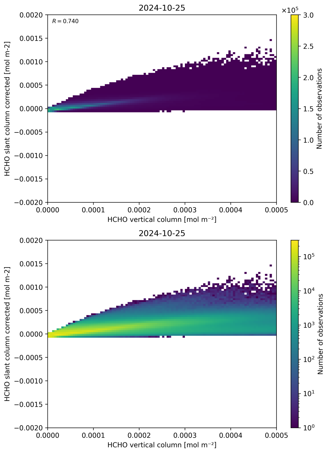
Figure 127: Scatter density plot of “HCHO vertical column” against “HCHO slant column corrected” for 2024-10-24 to 2024-10-26.
