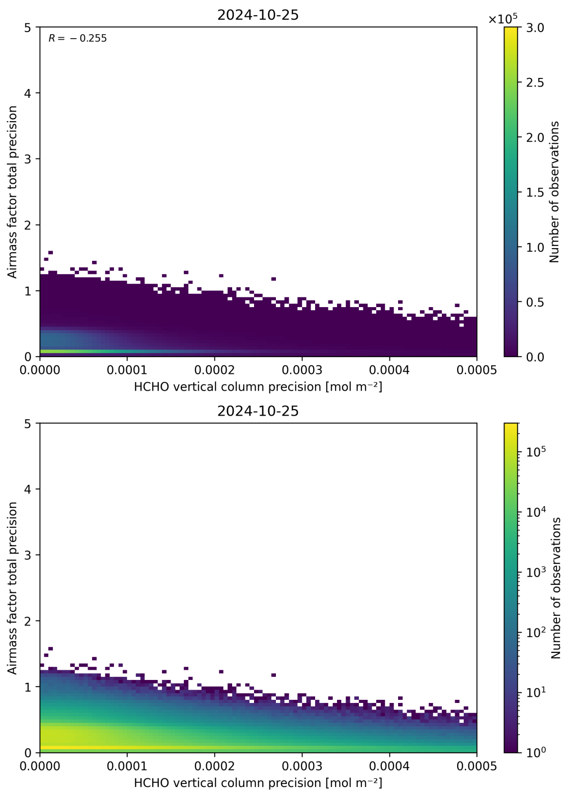
Figure 145: Scatter density plot of “HCHO vertical column precision” against “Airmass factor total precision” for 2024-10-24 to 2024-10-26.
