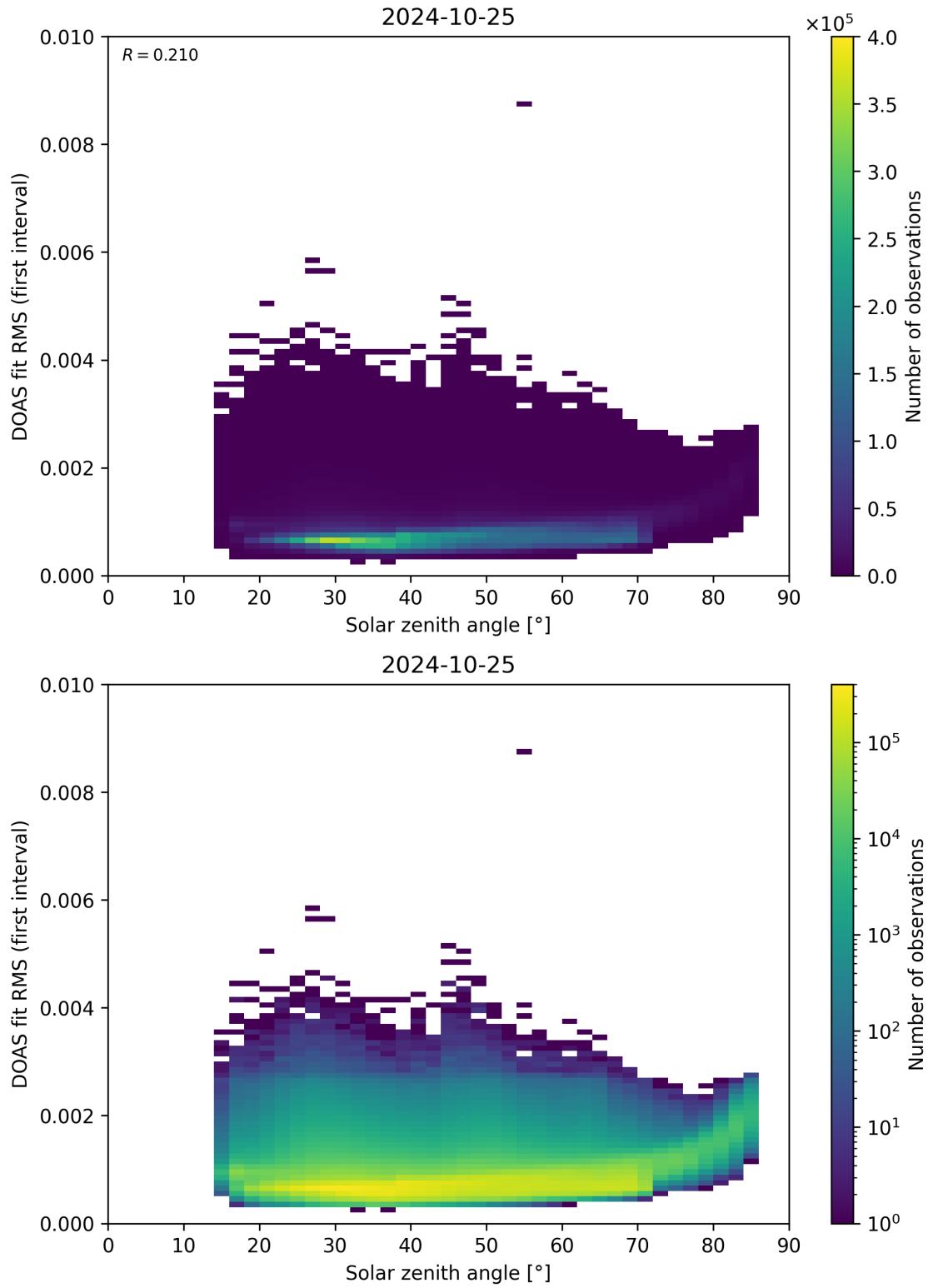
Figure 167: Scatter density plot of “Solar zenith angle” against “DOAS fit RMS (first interval)” for 2024-10-24 to 2024-10-26.
