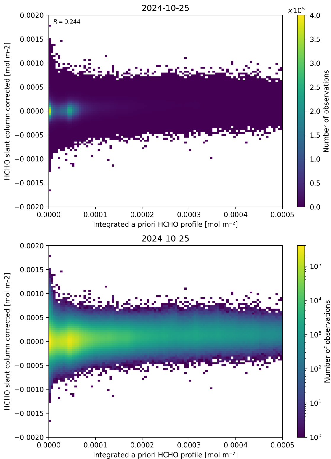
Figure 151: Scatter density plot of “Integrated a priori HCHO profile” against “HCHO slant column corrected” for 2024-10-24 to 2024-10-26.
