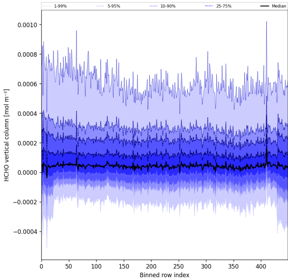
Figure 49: Along track statistics of “HCHO vertical column” for 2024-10-24 to 2024-10-26
