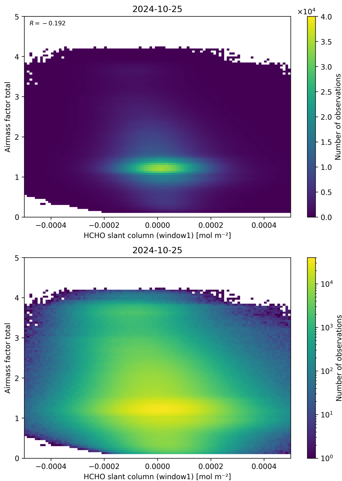
Figure 85: Scatter density plot of “HCHO slant column (window1)” against “Airmass factor total” for 2024-10-24 to 2024-10-26.
