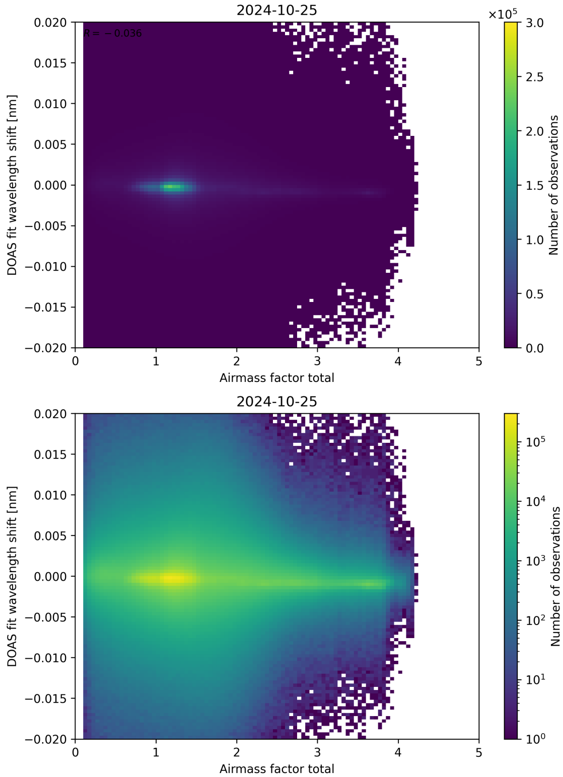
Figure 98: Scatter density plot of “Airmass factor total” against “DOAS fit wavelength shift” for 2024-10-24 to 2024-10-26.
