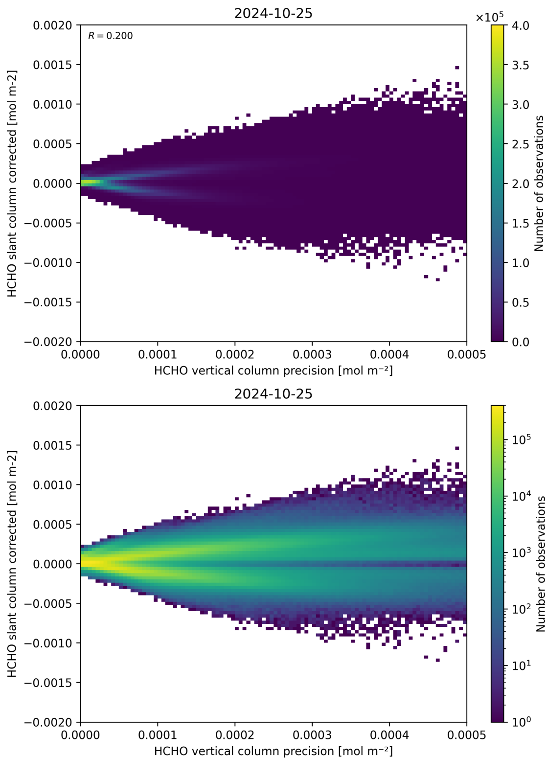
Figure 140: Scatter density plot of “HCHO vertical column precision” against “HCHO slant column corrected” for 2024-10-24 to 2024-10-26.
