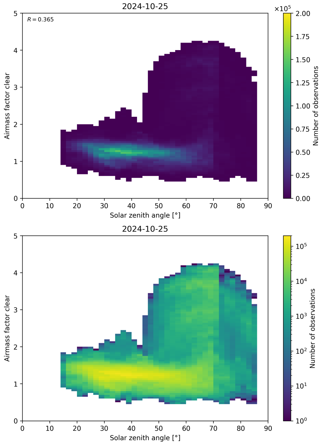
Figure 170: Scatter density plot of “Solar zenith angle” against “Airmass factor clear” for 2024-10-24 to 2024-10-26.
