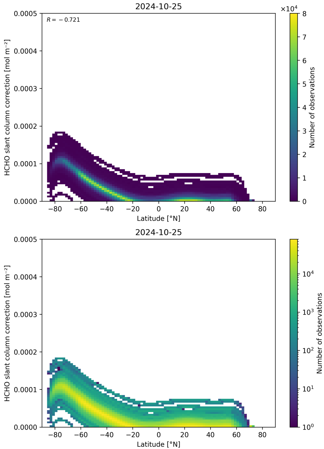
Figure 158: Scatter density plot of “Latitude” against “HCHO slant column correction” for 2024-10-24 to 2024-10-26.
