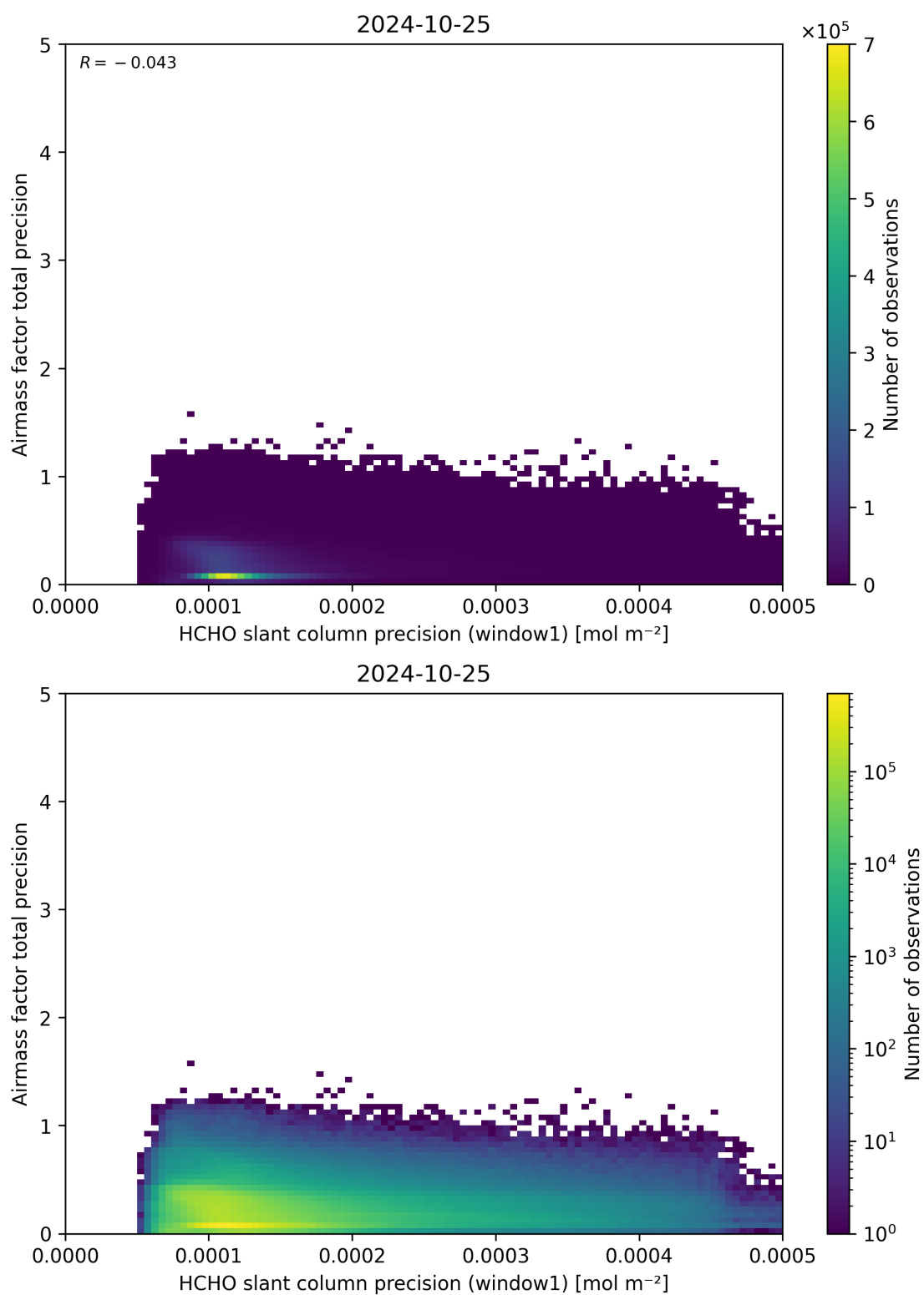
Figure 95: Scatter density plot of “HCHO slant column precision (window1)” against “Airmass factor total precision” for 2024-10-24 to 2024-10-26.
