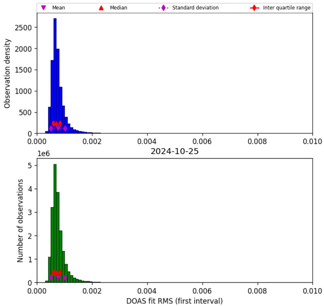
Figure 46: Histogram of “DOAS fit RMS (first interval)” for 2024-10-24 to 2024-10-26
