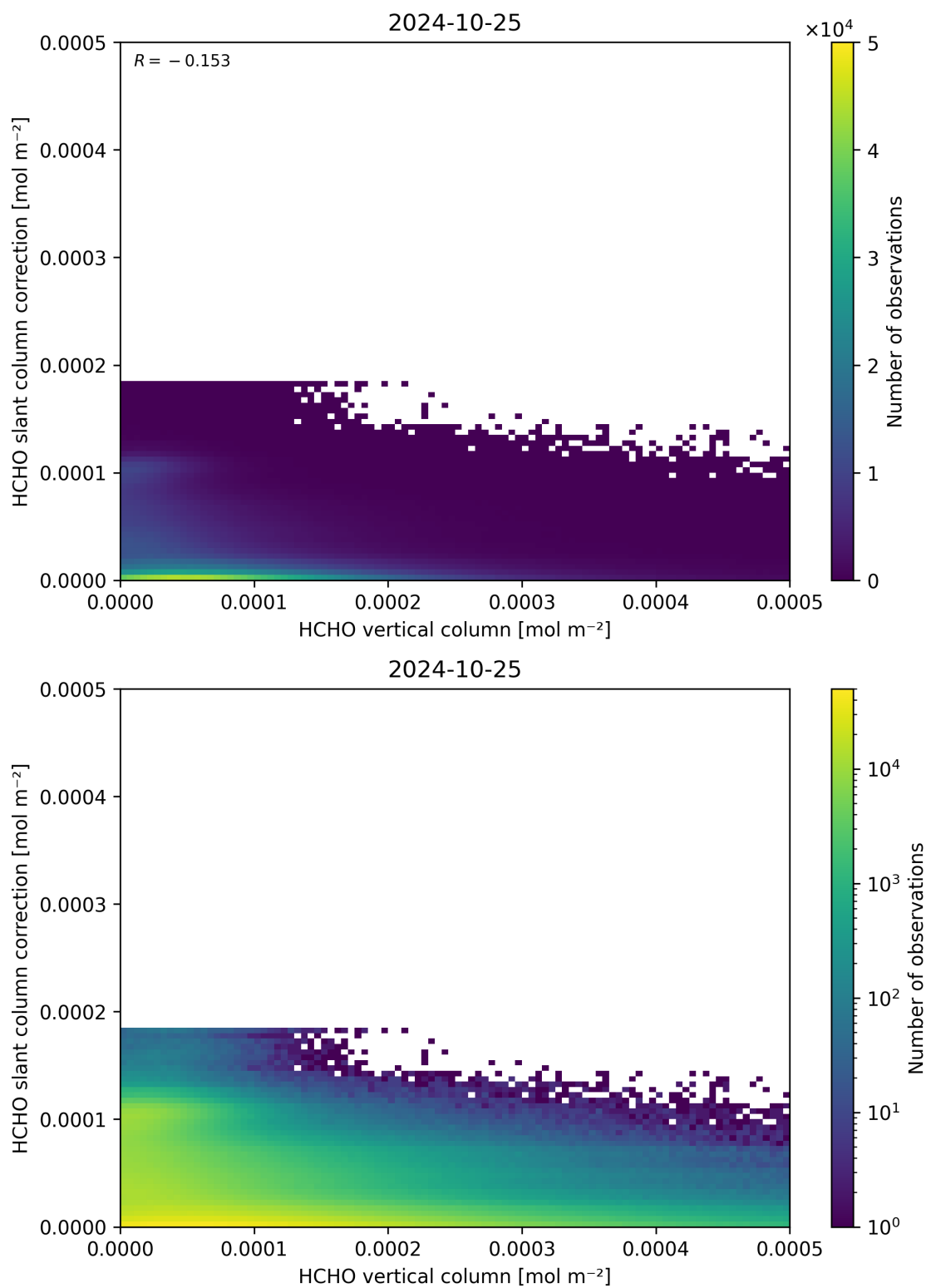
Figure 128: Scatter density plot of “HCHO vertical column” against “HCHO slant column correction” for 2024-10-24 to 2024-10-26.
