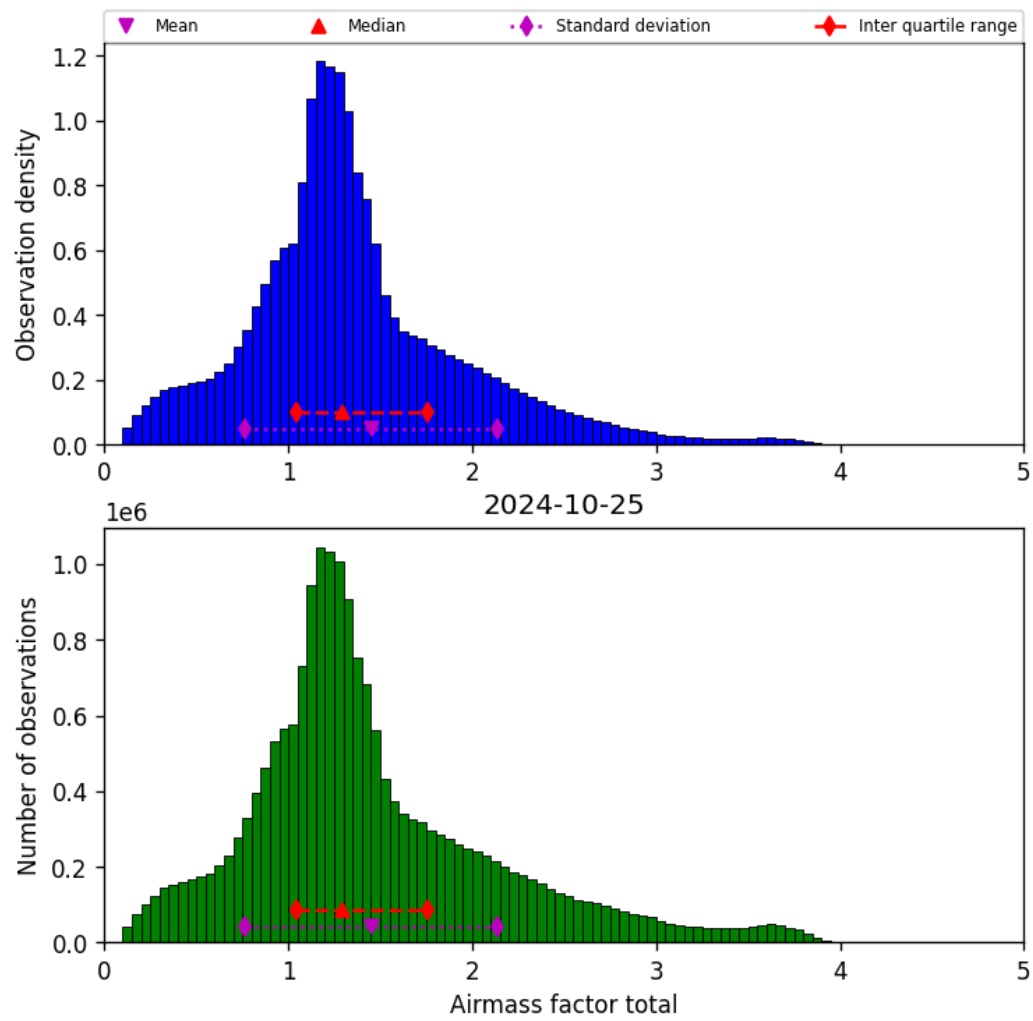
Figure 40: Histogram of “Airmass factor total” for 2024-10-24 to 2024-10-26
