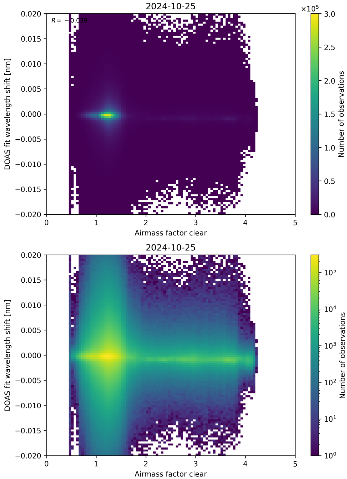
Figure 72: Scatter density plot of “Airmass factor clear” against “DOAS fit wavelength shift” for 2024-10-24 to 2024-10-26.
