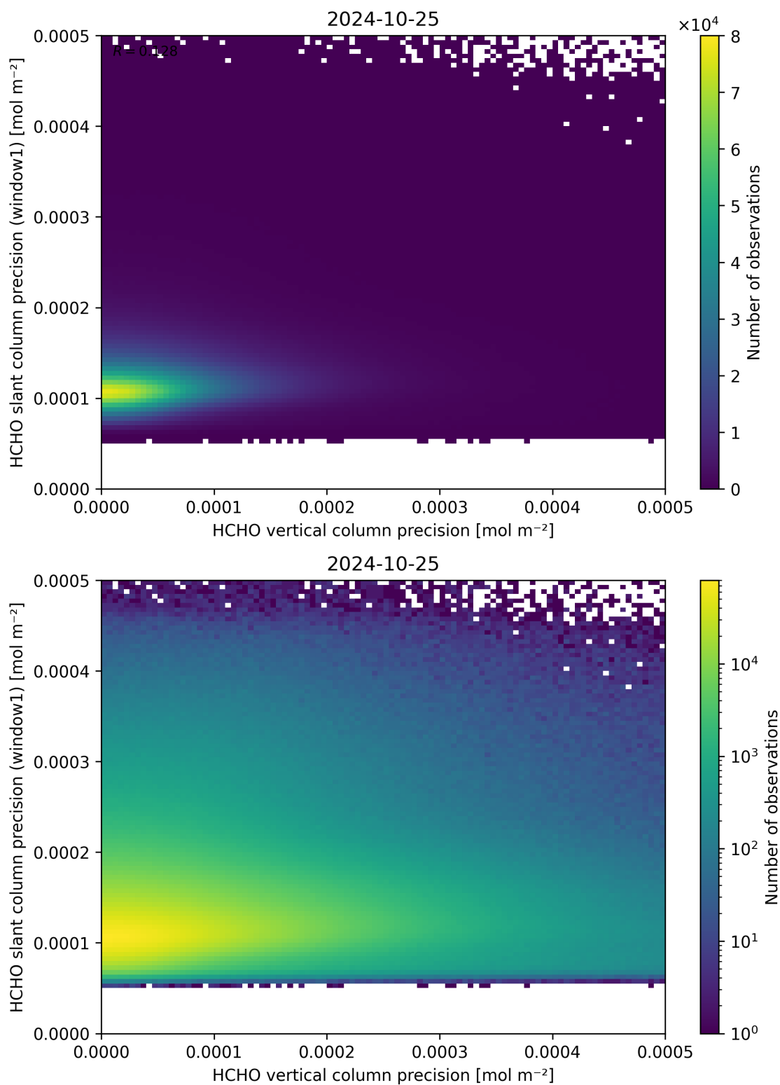
Figure 143: Scatter density plot of “HCHO vertical column precision” against “HCHO slant column precision (window1)” for 2024-10-24 to 2024-10-26.
