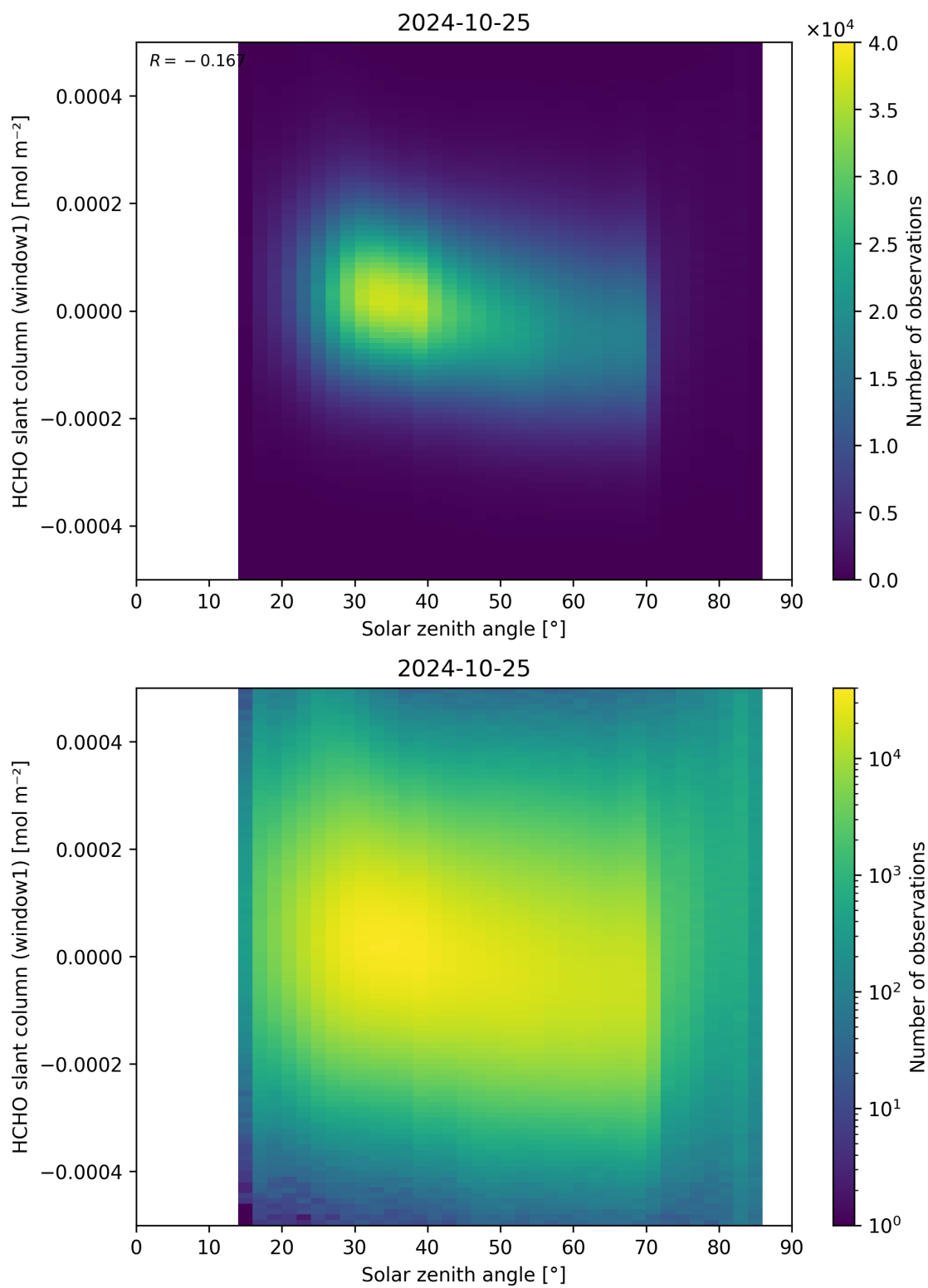
Figure 173: Scatter density plot of “Solar zenith angle” against “HCHO slant column (window1)” for 2024-10-24 to 2024-10-26.
