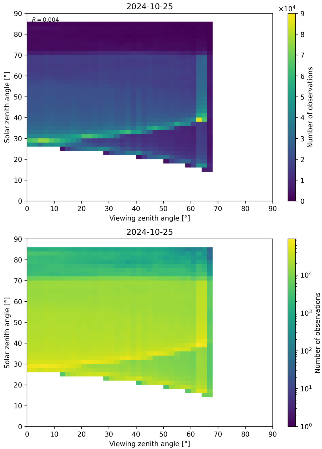
Figure 197: Scatter density plot of “Viewing zenith angle” against “Solar zenith angle” for 2024-10-24 to 2024-10-26.
