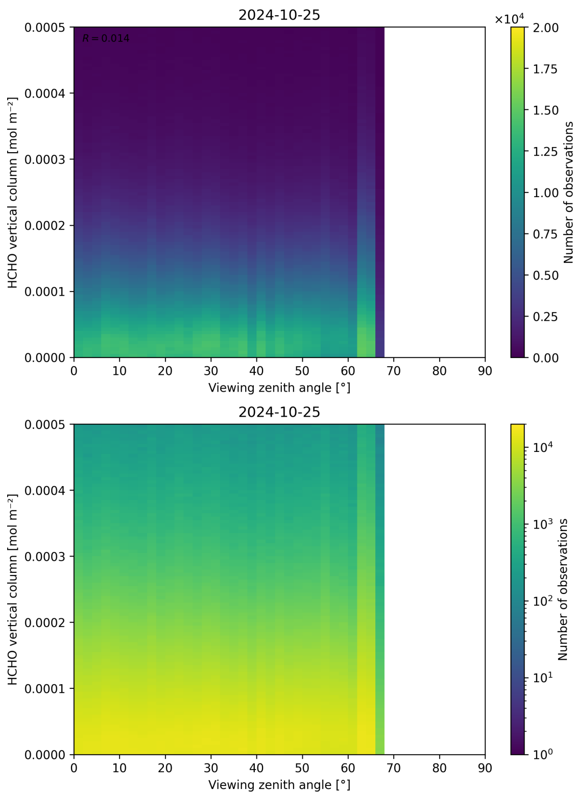
Figure 192: Scatter density plot of “Viewing zenith angle” against “HCHO vertical column” for 2024-10-24 to 2024-10-26.
