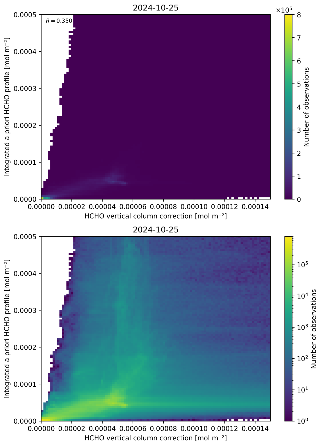
Figure 122: Scatter density plot of “HCHO vertical column correction” against “Integrated a priori HCHO profile” for 2024-10-24 to 2024-10-26.
