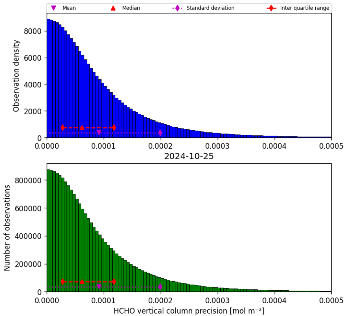
Figure 36: Histogram of “HCHO vertical column precision” for 2024-10-24 to 2024-10-26
