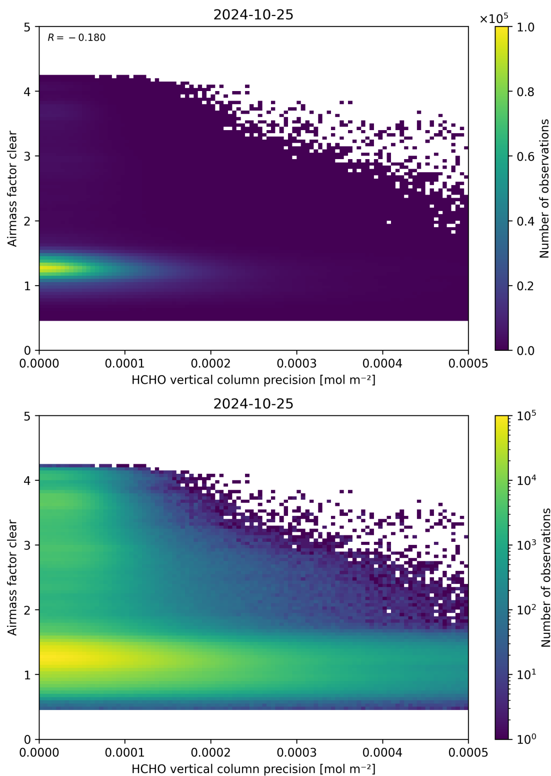
Figure 139: Scatter density plot of “HCHO vertical column precision” against “Airmass factor clear” for 2024-10-24 to 2024-10-26.
