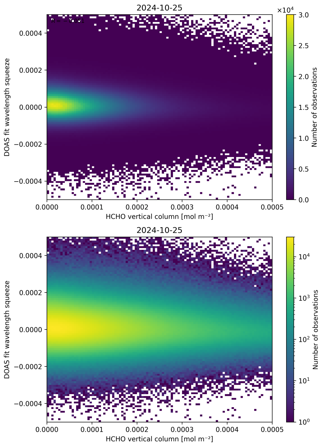
Figure 125: Scatter density plot of “HCHO vertical column” against “DOAS fit wavelength squeeze” for 2024-10-24 to 2024-10-26.
