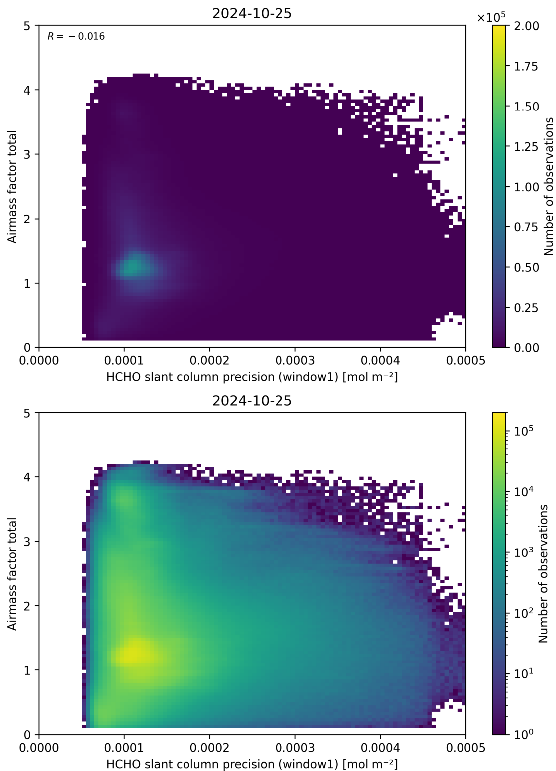
Figure 94: Scatter density plot of “HCHO slant column precision (window1)” against “Airmass factor total” for 2024-10-24 to 2024-10-26.
