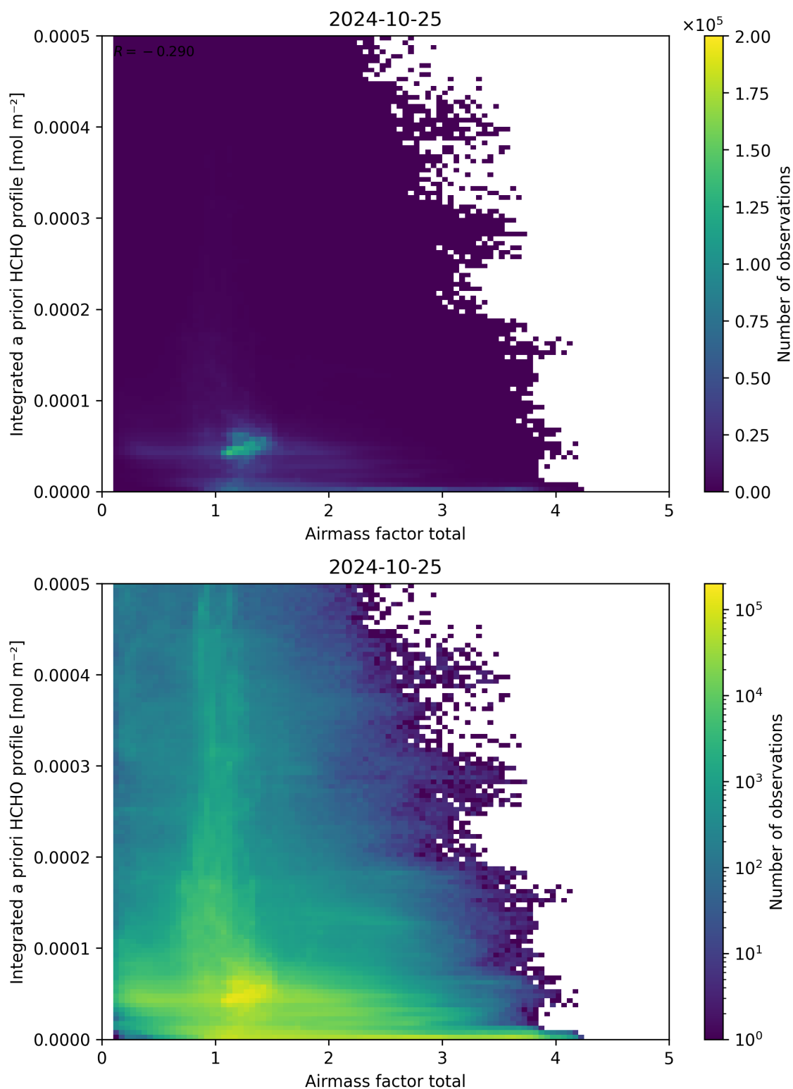
Figure 104: Scatter density plot of “Airmass factor total” against “Integrated a priori HCHO profile” for 2024-10-24 to 2024-10-26.
