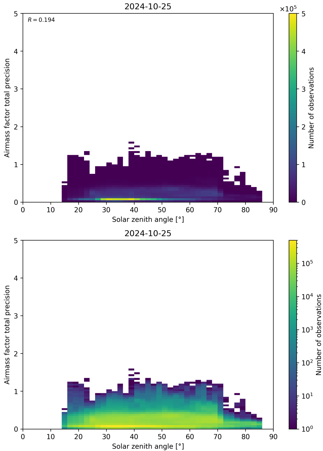
Figure 176: Scatter density plot of “Solar zenith angle” against “Airmass factor total precision” for 2024-10-24 to 2024-10-26.
