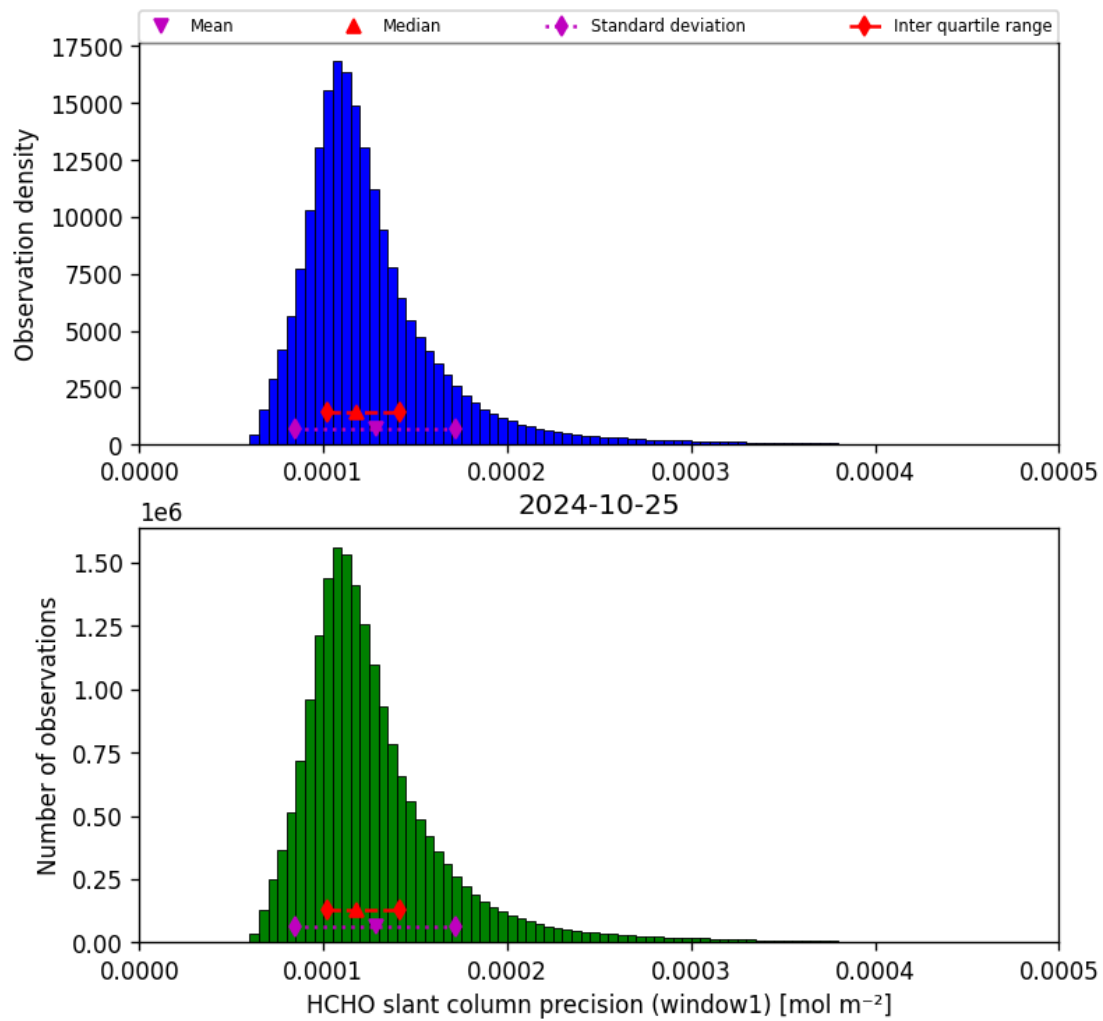
Figure 39: Histogram of “HCHO slant column precision (window1)” for 2024-10-24 to 2024-10-26
