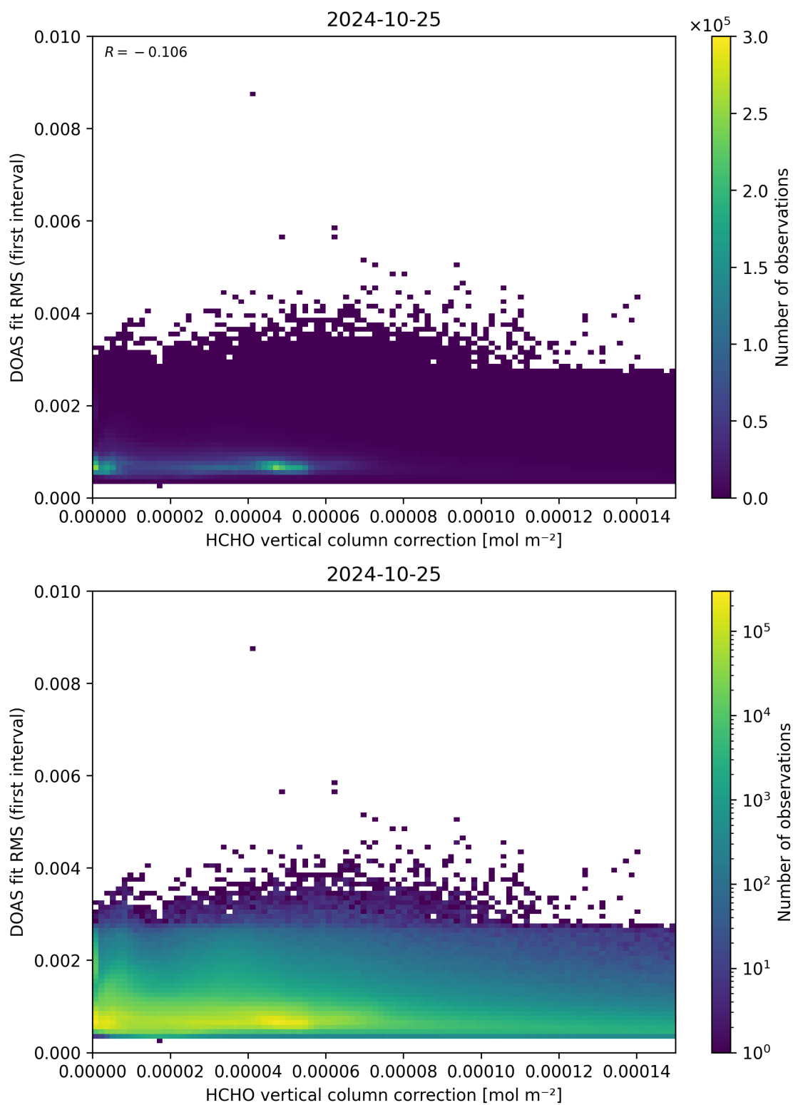
Figure 112: Scatter density plot of “HCHO vertical column correction” against “DOAS fit RMS (first interval)” for 2024-10-24 to 2024-10-26.
