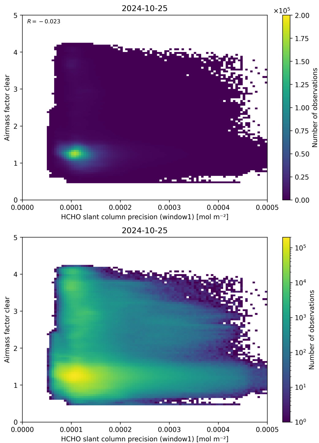
Figure 91: Scatter density plot of “HCHO slant column precision (window1)” against “Airmass factor clear” for 2024-10-24 to 2024-10-26.
