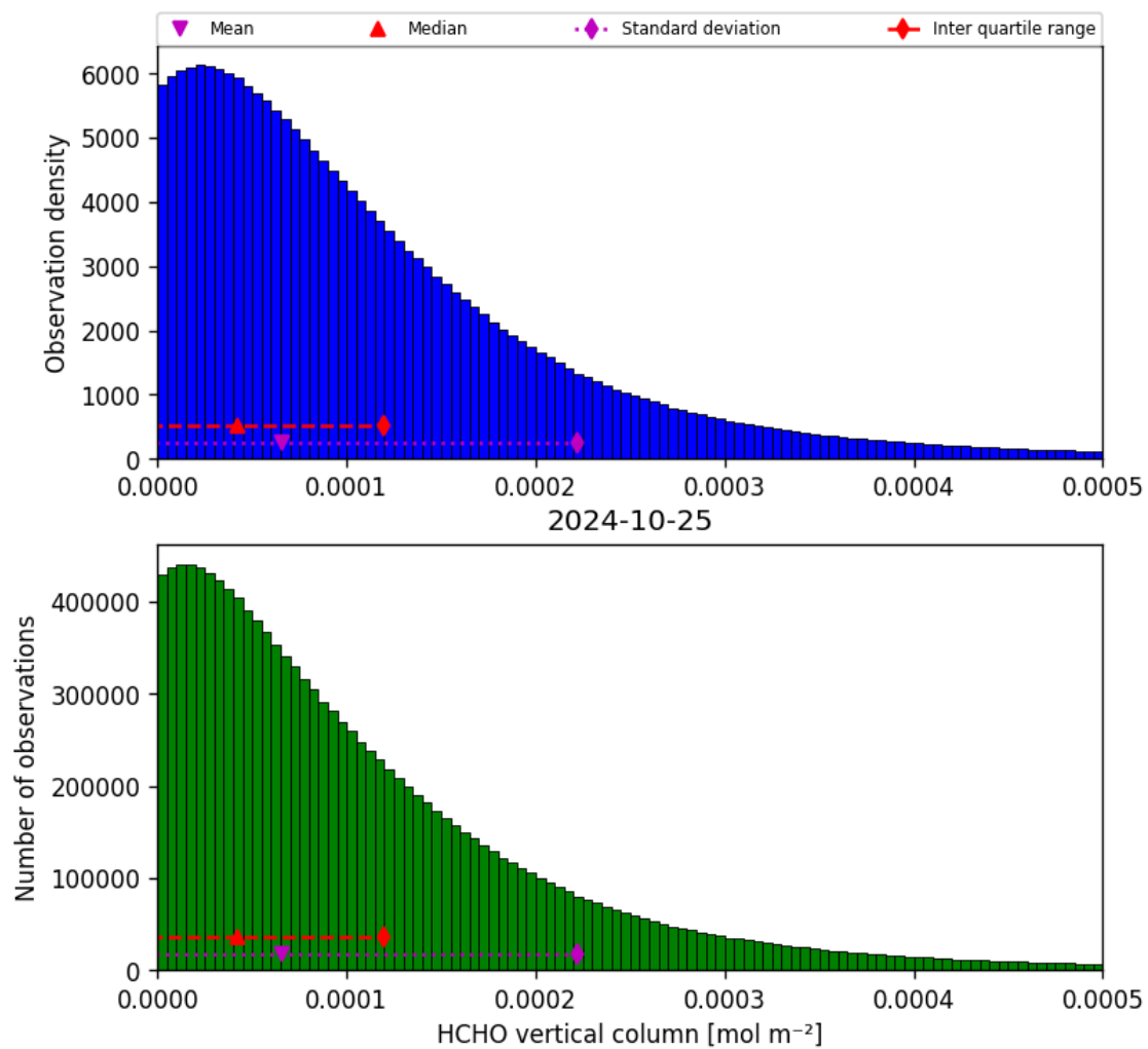
Figure 35: Histogram of “HCHO vertical column” for 2024-10-24 to 2024-10-26
