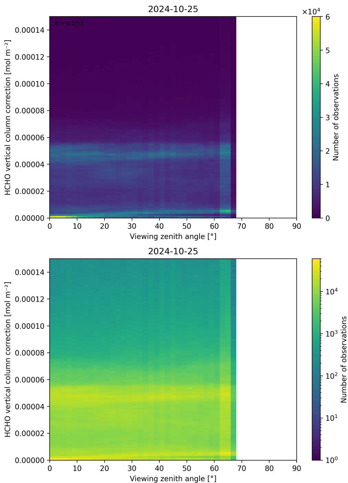
Figure 193: Scatter density plot of “Viewing zenith angle” against “HCHO vertical column correction” for 2024-10-24 to 2024-10-26.
