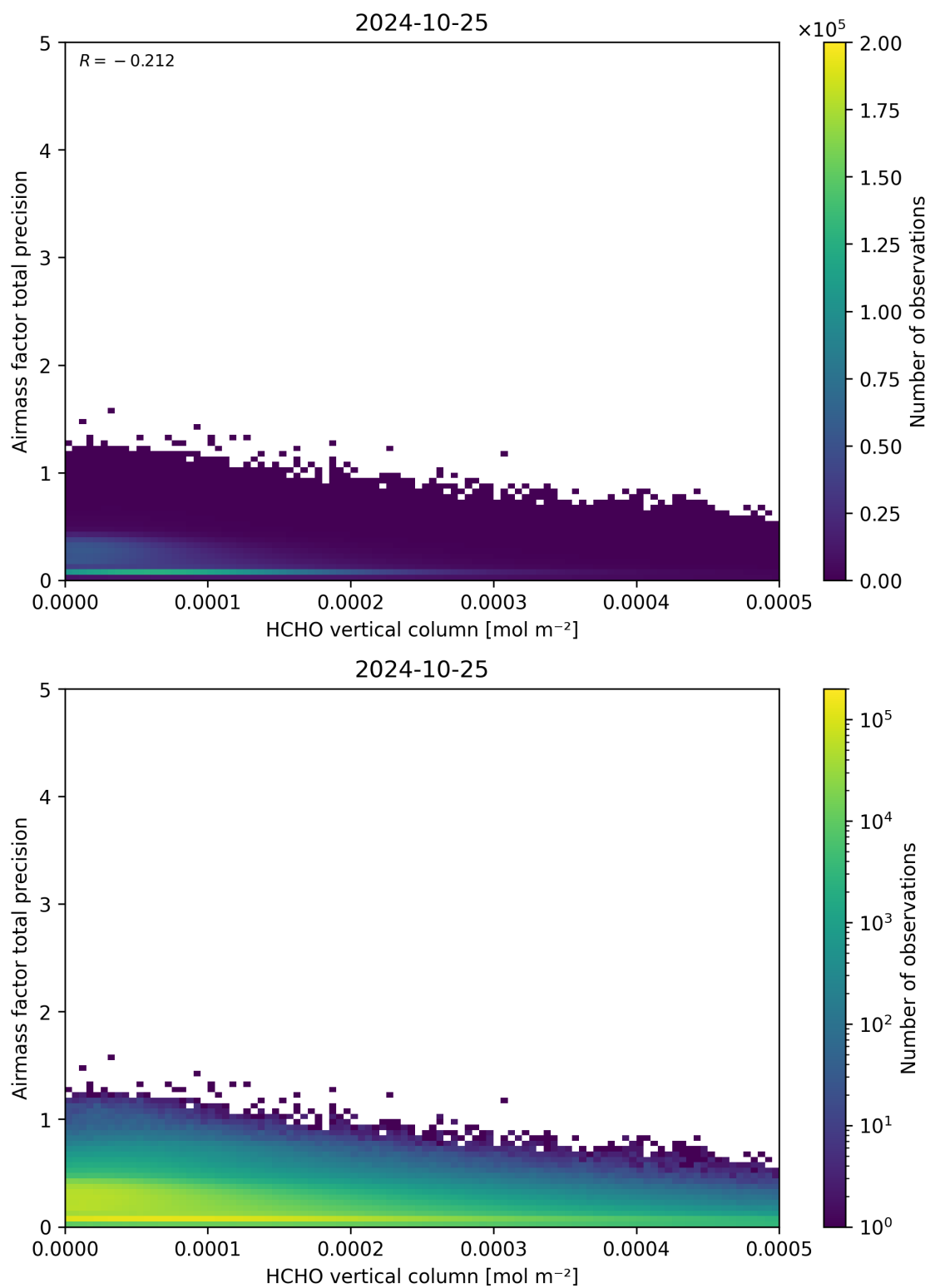
Figure 132: Scatter density plot of “HCHO vertical column” against “Airmass factor total precision” for 2024-10-24 to 2024-10-26.
