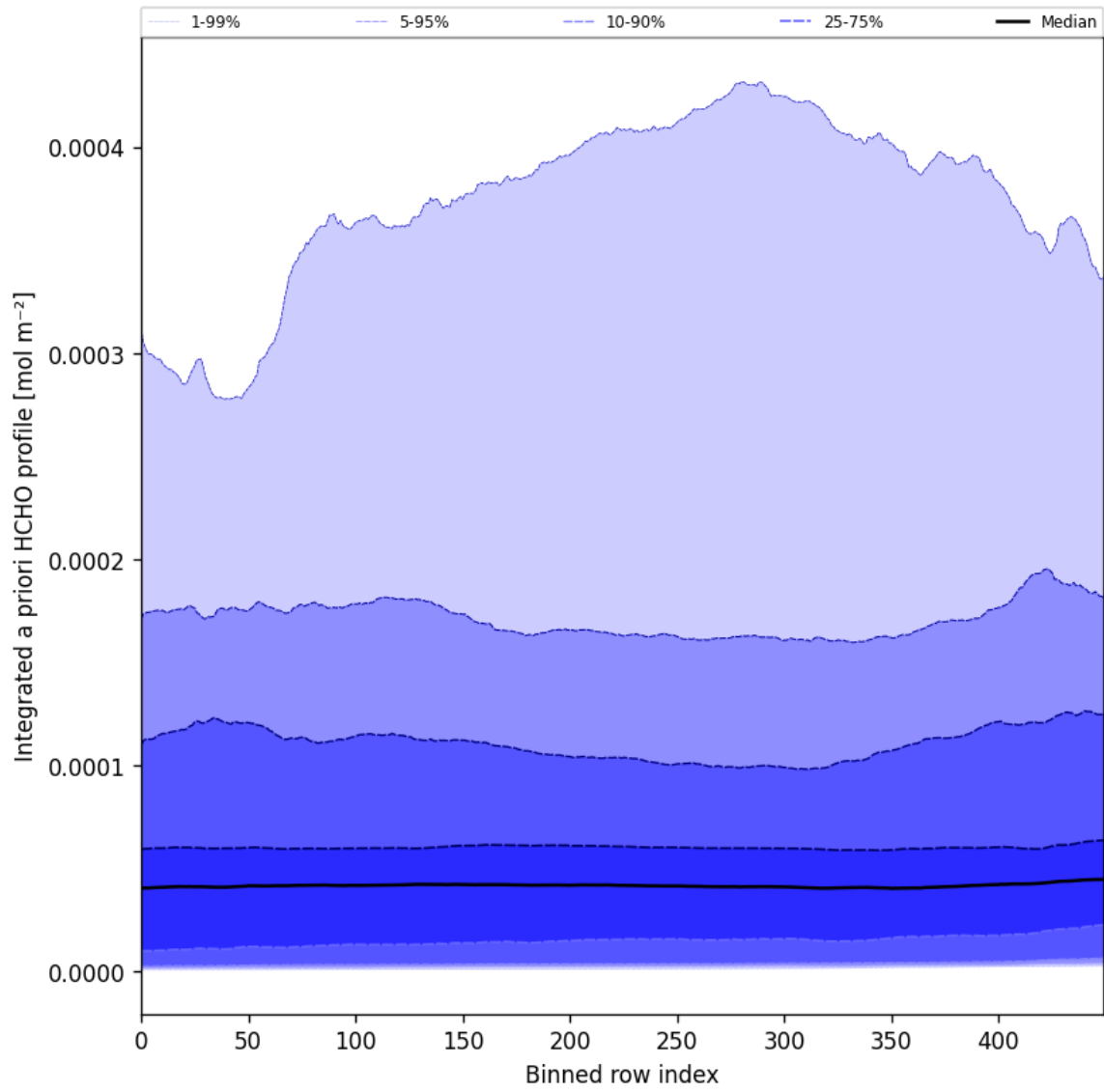
Figure 57: Along track statistics of “Integrated a priori HCHO profile” for 2024-10-24 to 2024-10-26
