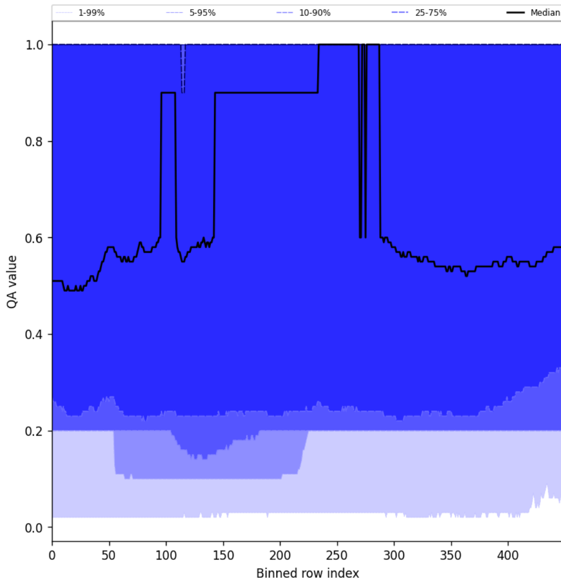
Figure 48: Along track statistics of “QA value” for 2024-10-24 to 2024-10-26
