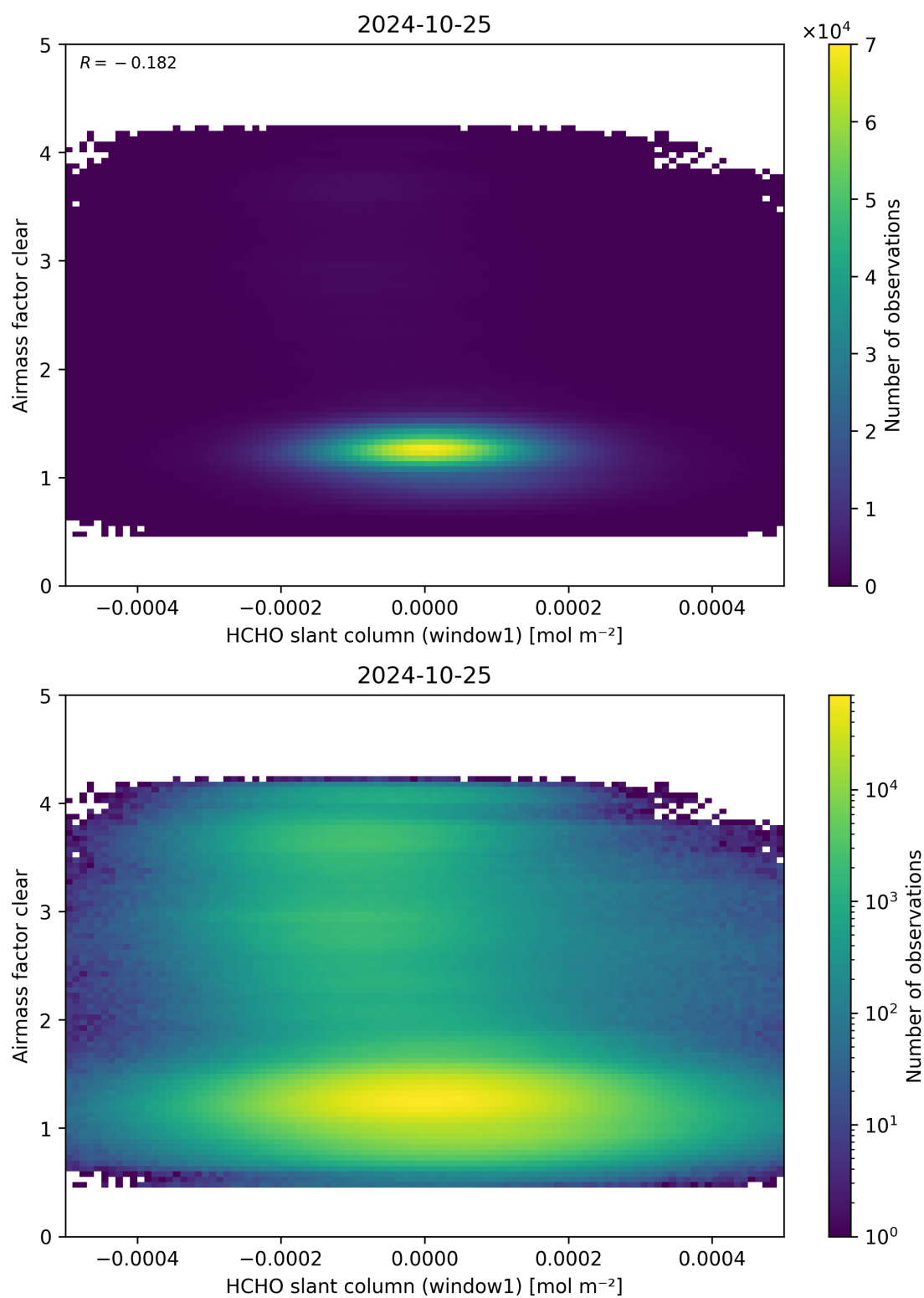
Figure 81: Scatter density plot of “HCHO slant column (window1)” against “Airmass factor clear” for 2024-10-24 to 2024-10-26.
