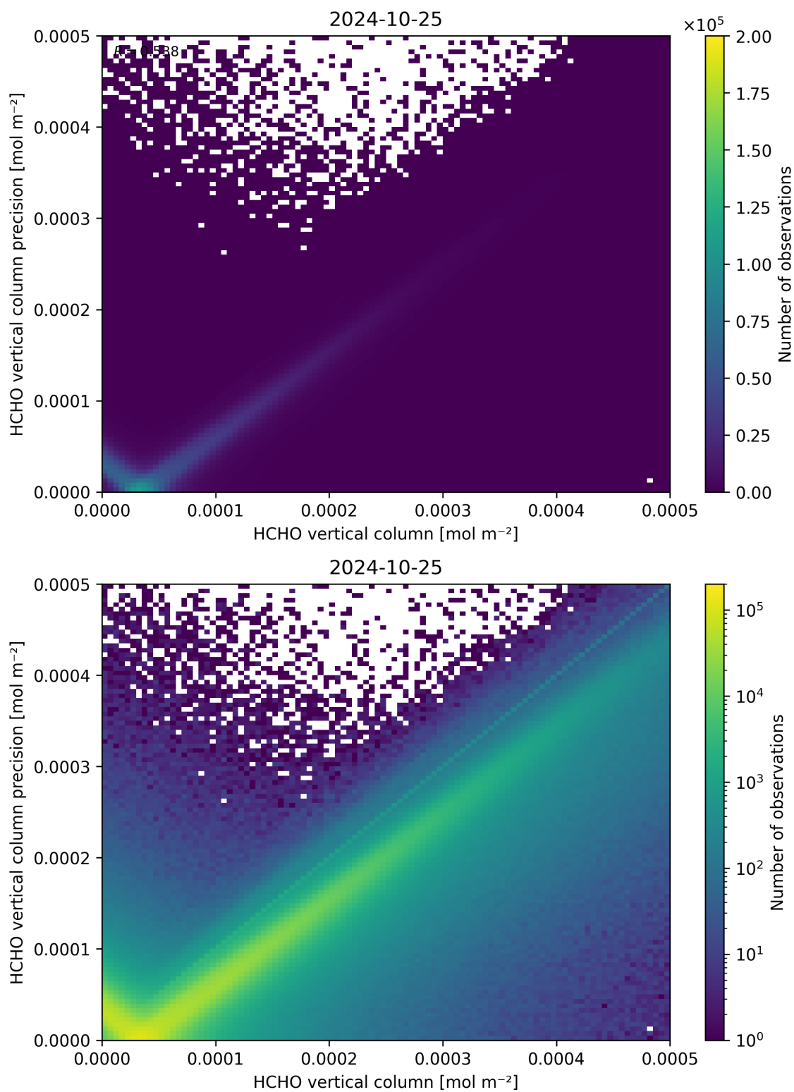
Figure 134: Scatter density plot of “HCHO vertical column” against “HCHO vertical column precision” for 2024-10-24 to 2024-10-26.
