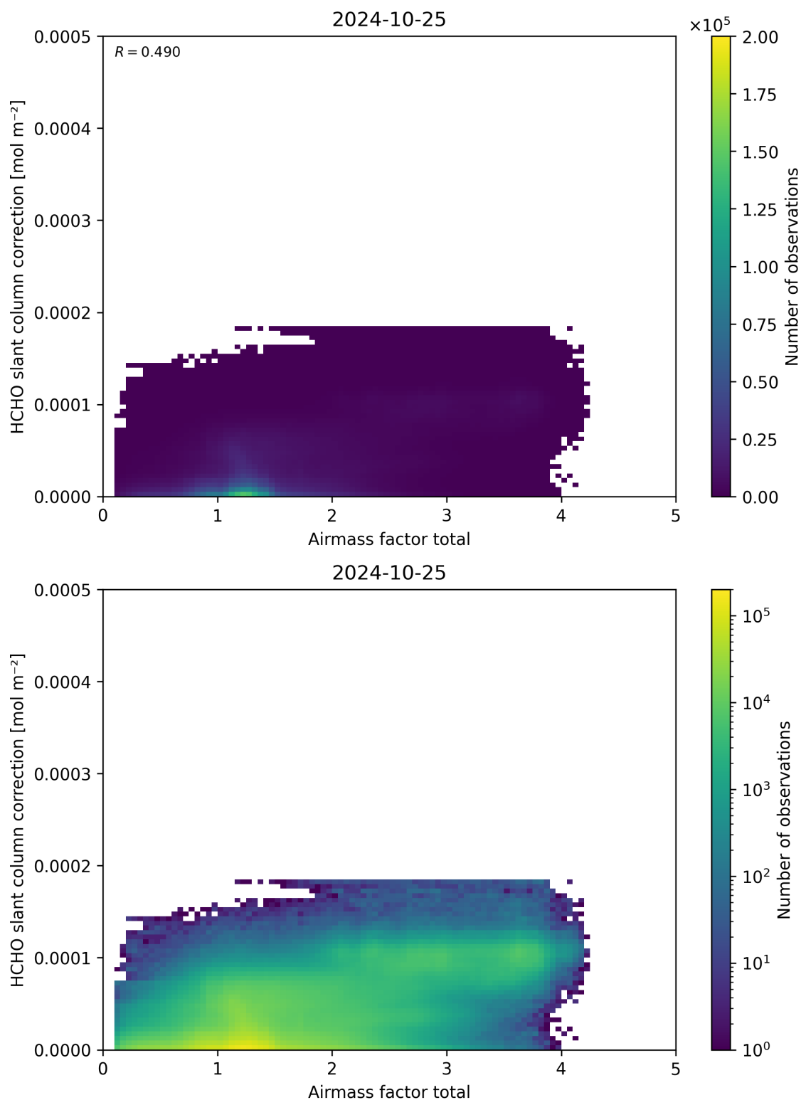
Figure 102: Scatter density plot of “Airmass factor total” against “HCHO slant column correction” for 2024-10-24 to 2024-10-26.
