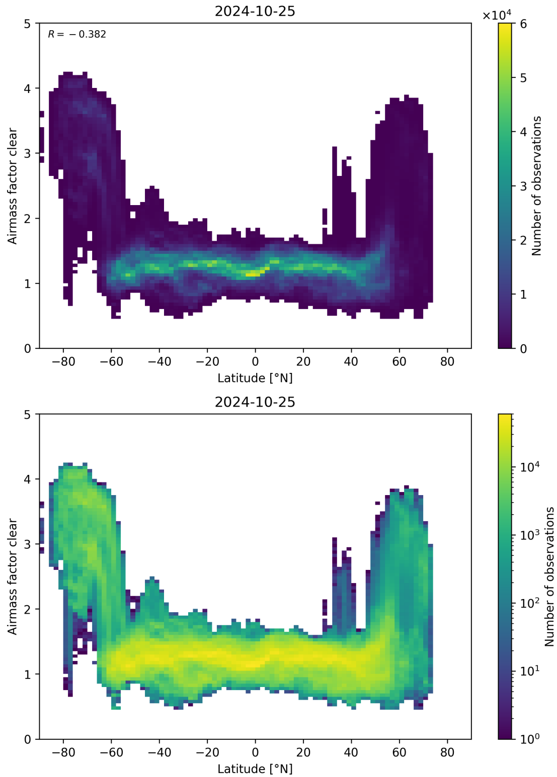
Figure 156: Scatter density plot of “Latitude” against “Airmass factor clear” for 2024-10-24 to 2024-10-26.
