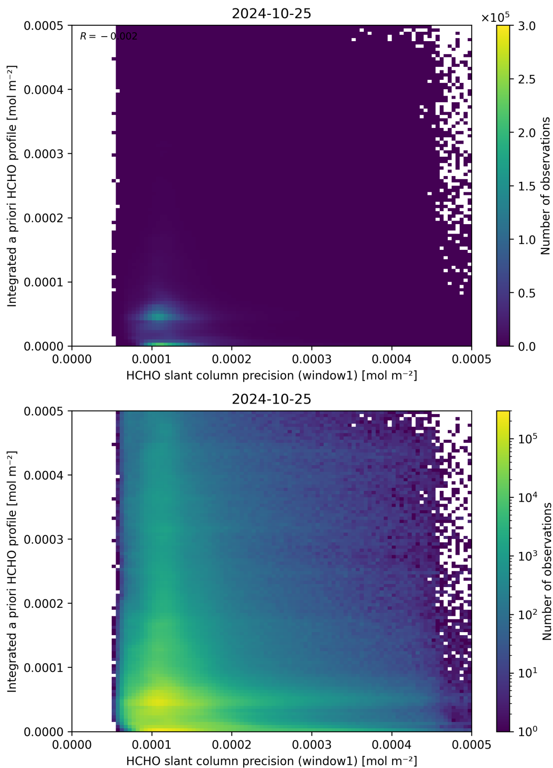
Figure 96: Scatter density plot of “HCHO slant column precision (window1)” against “Integrated a priori HCHO profile” for 2024-10-24 to 2024-10-26.
