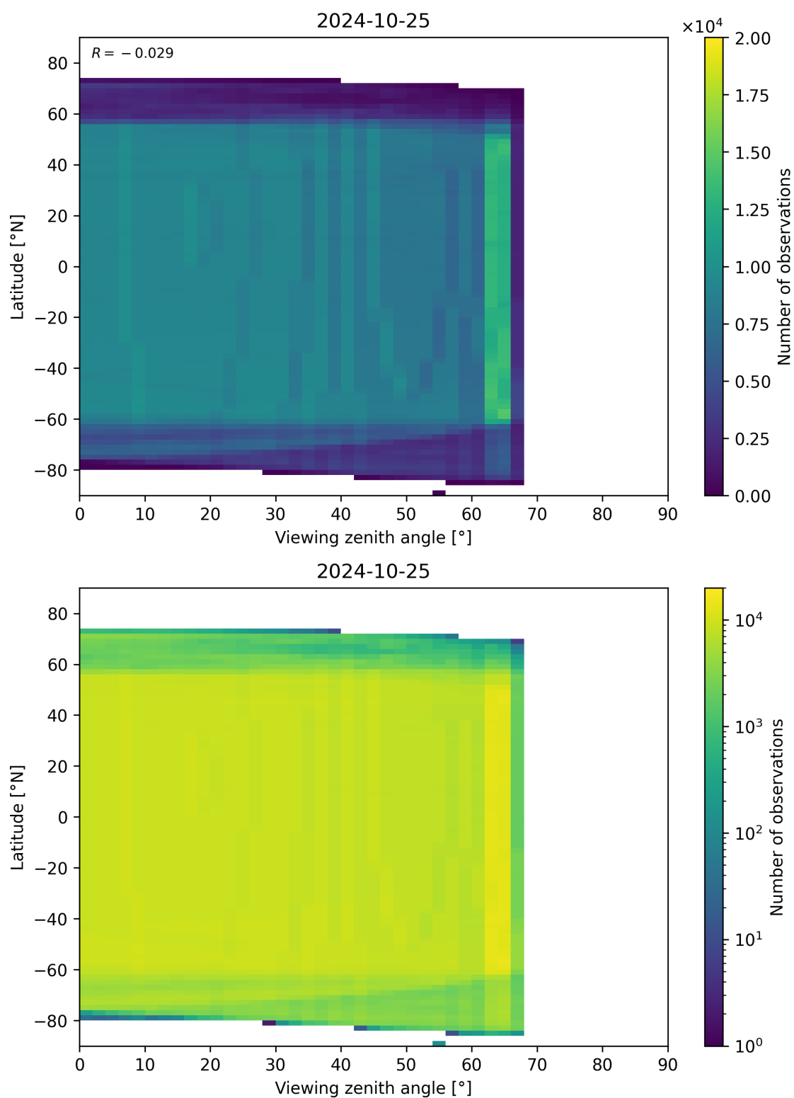
Figure 196: Scatter density plot of “Viewing zenith angle” against “Latitude” for 2024-10-24 to 2024-10-26.
