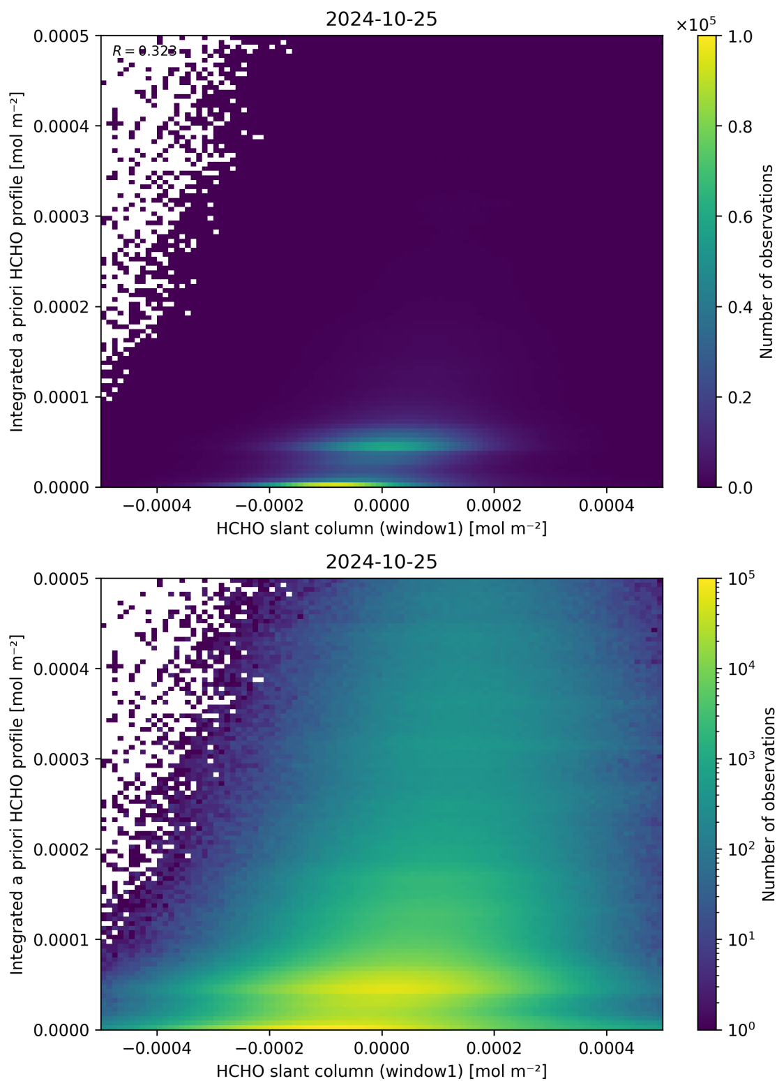
Figure 87: Scatter density plot of “HCHO slant column (window1)” against “Integrated a priori HCHO profile” for 2024-10-24 to 2024-10-26.
