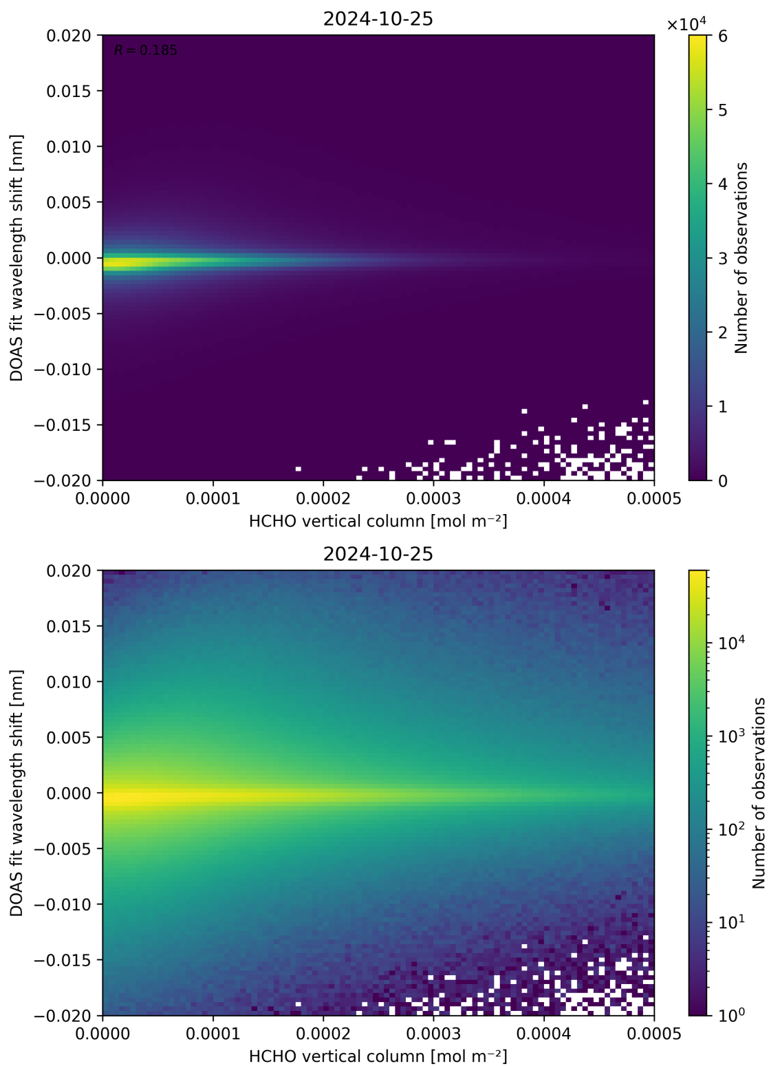
Figure 124: Scatter density plot of “HCHO vertical column” against “DOAS fit wavelength shift” for 2024-10-24 to 2024-10-26.
