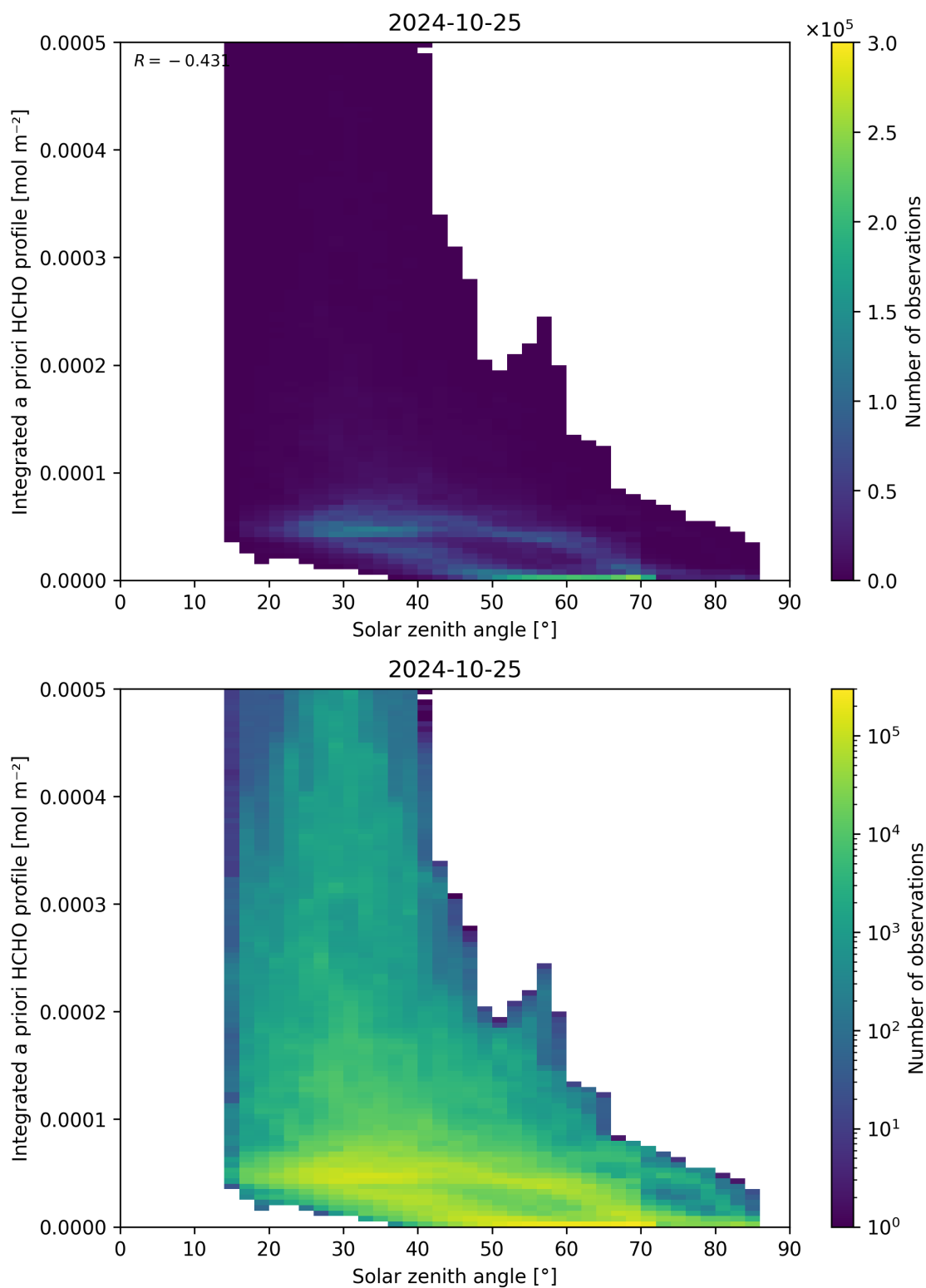
Figure 180: Scatter density plot of “Solar zenith angle” against “Integrated a priori HCHO profile” for 2024-10-24 to 2024-10-26.
