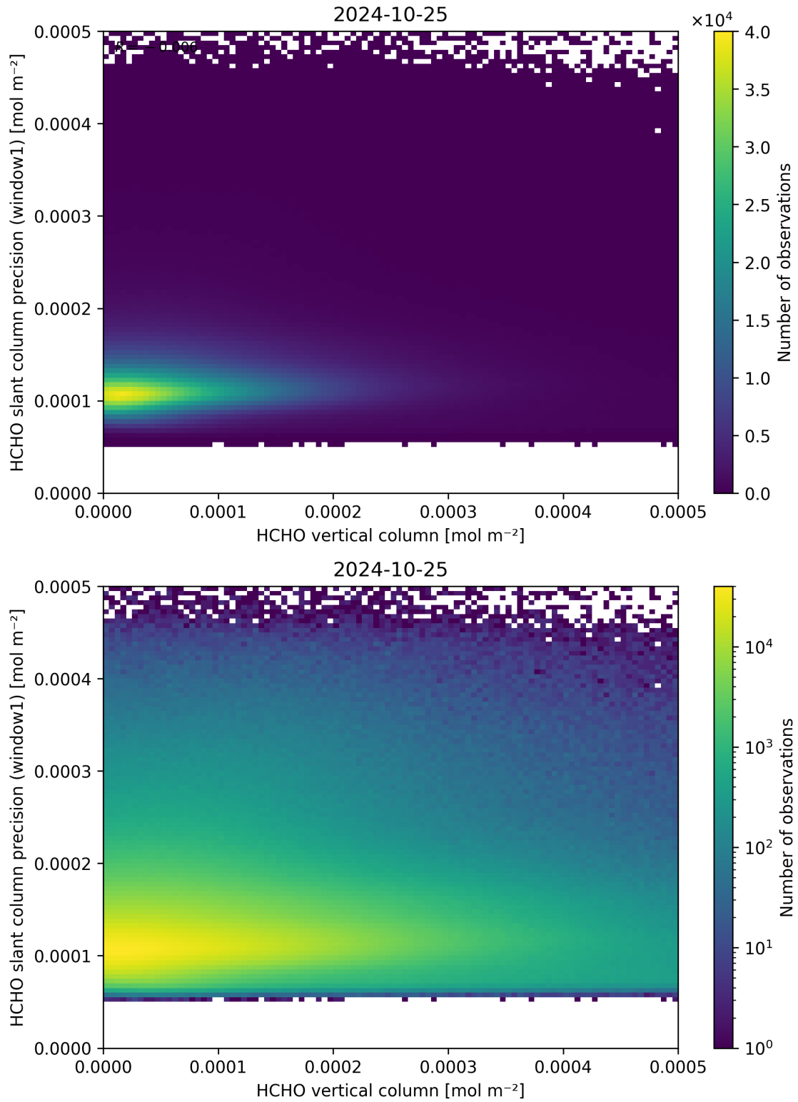
Figure 130: Scatter density plot of “HCHO vertical column” against “HCHO slant column precision (window1)” for 2024-10-24 to 2024-10-26.
