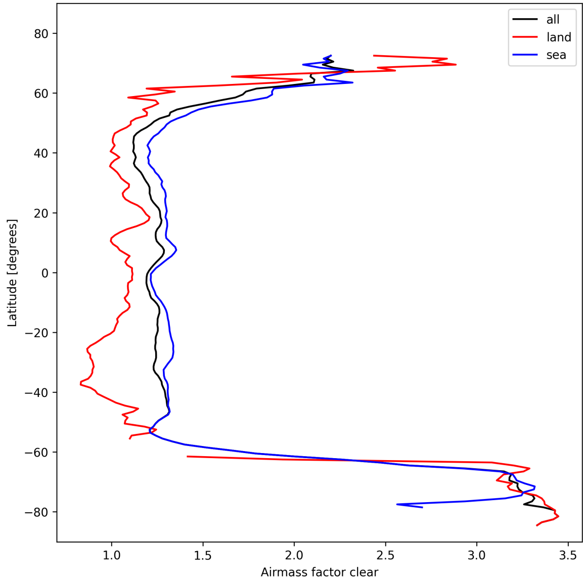
Figure 28: Zonal average of “Airmass factor clear” for 2024-10-24 to 2024-10-26.
