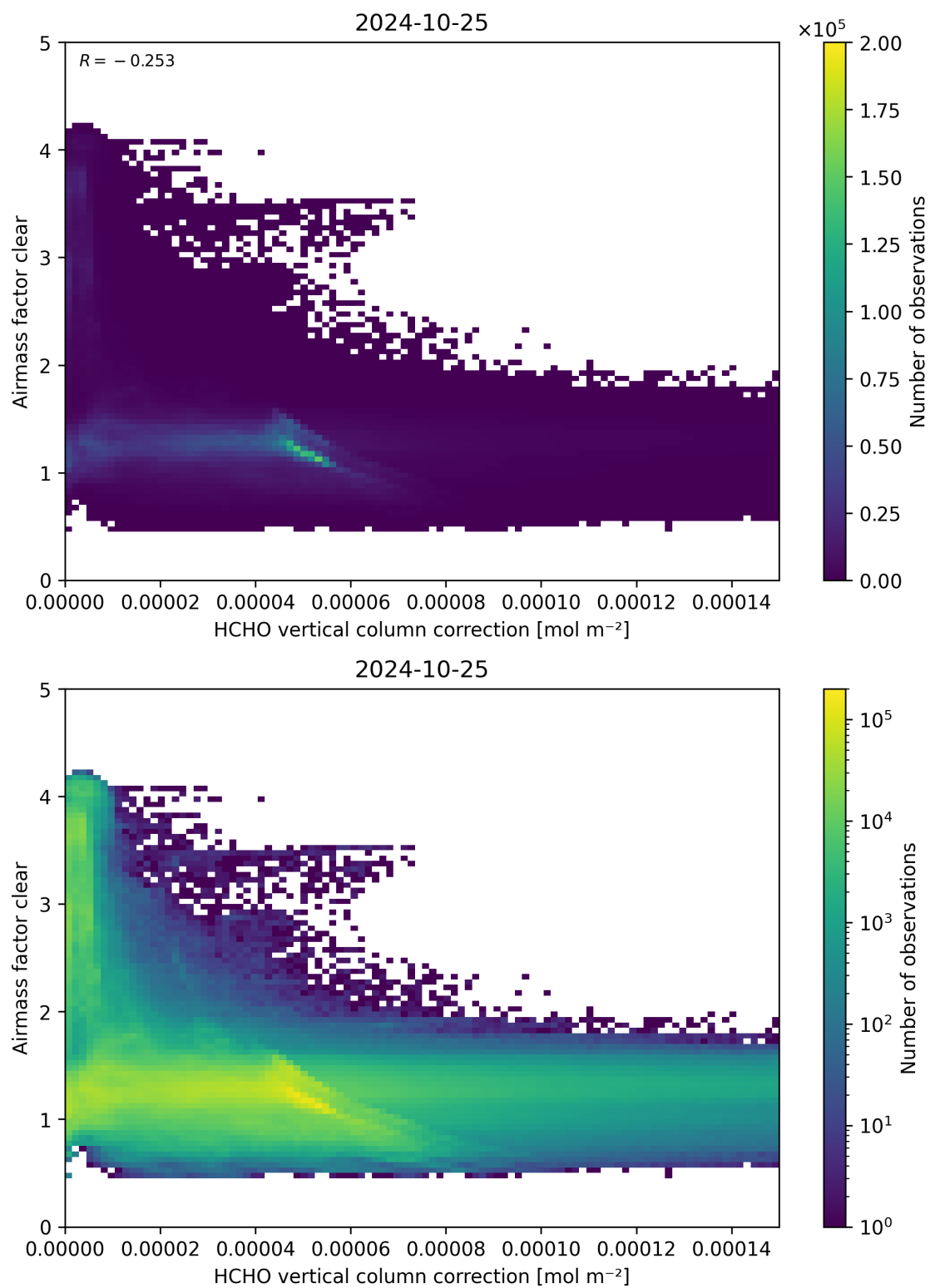
Figure 115: Scatter density plot of “HCHO vertical column correction” against “Airmass factor clear” for 2024-10-24 to 2024-10-26.
