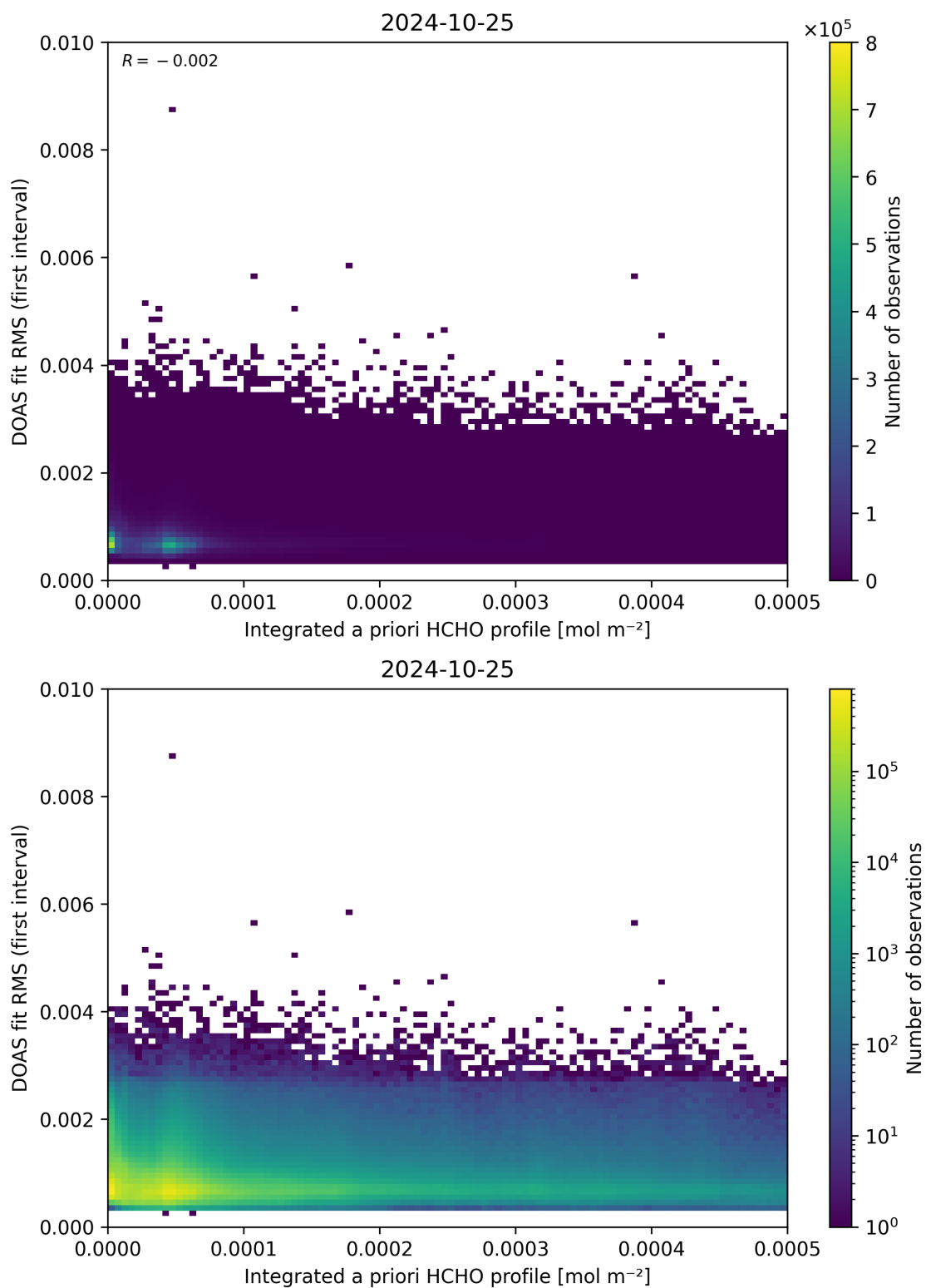
Figure 148: Scatter density plot of “Integrated a priori HCHO profile” against “DOAS fit RMS (first interval)” for 2024-10-24 to 2024-10-26.
