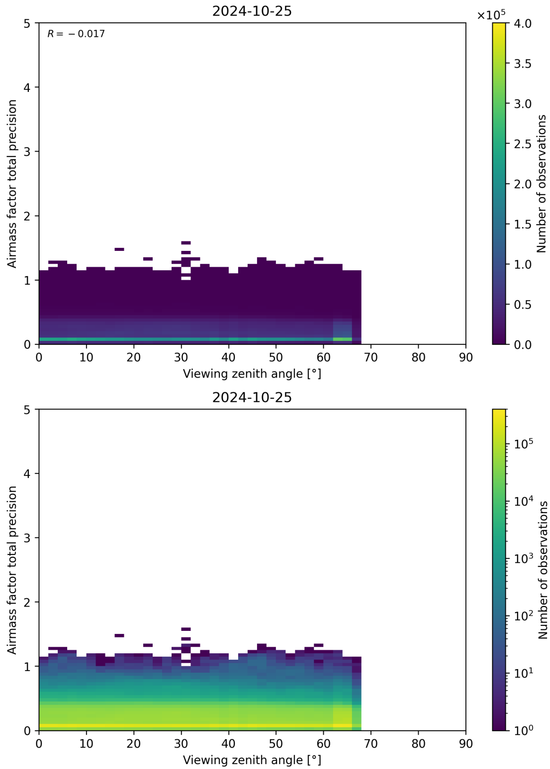
Figure 191: Scatter density plot of “Viewing zenith angle” against “Airmass factor total precision” for 2024-10-24 to 2024-10-26.
