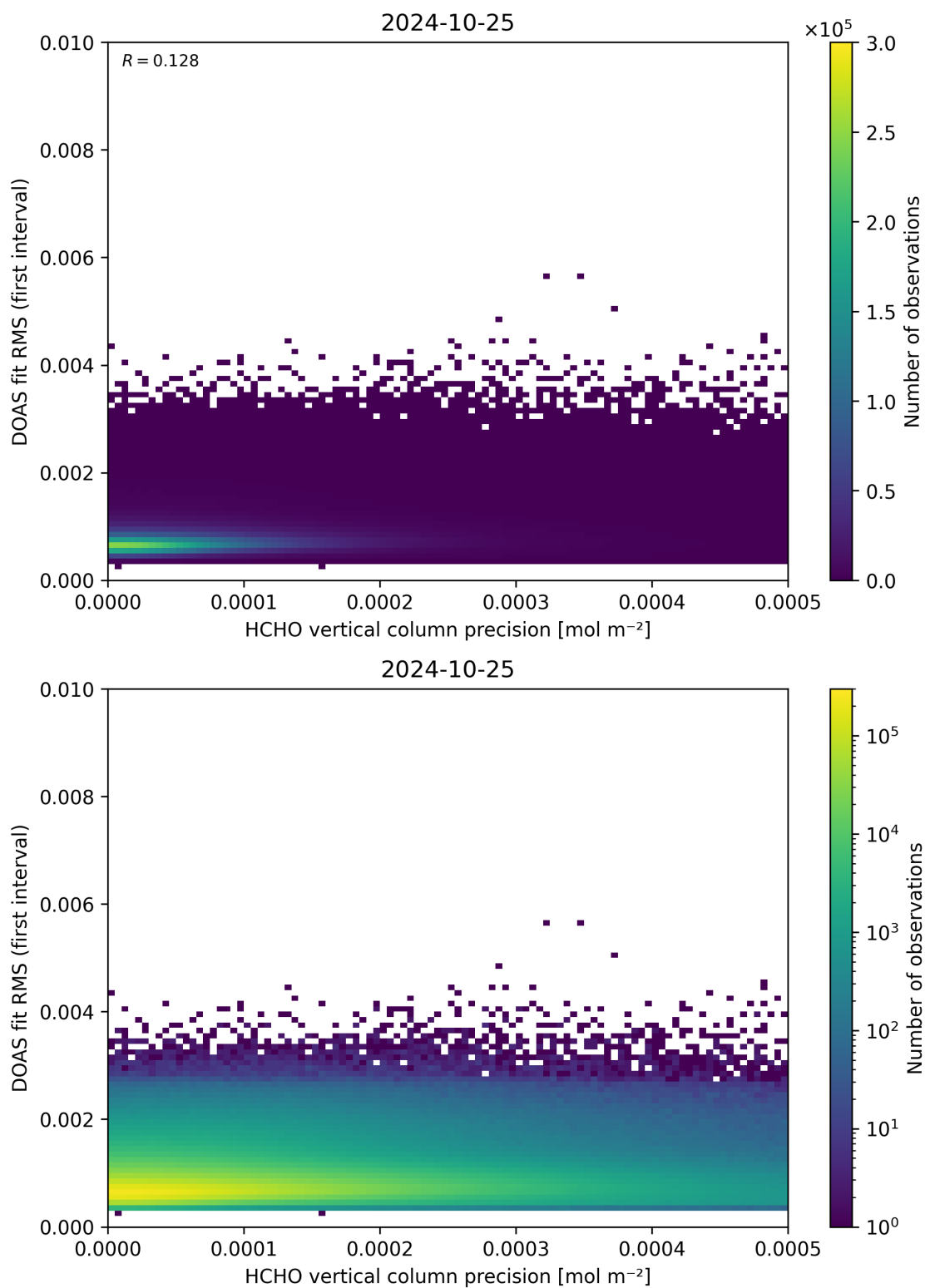
Figure 136: Scatter density plot of “HCHO vertical column precision” against “DOAS fit RMS (first interval)” for 2024-10-24 to 2024-10-26.
