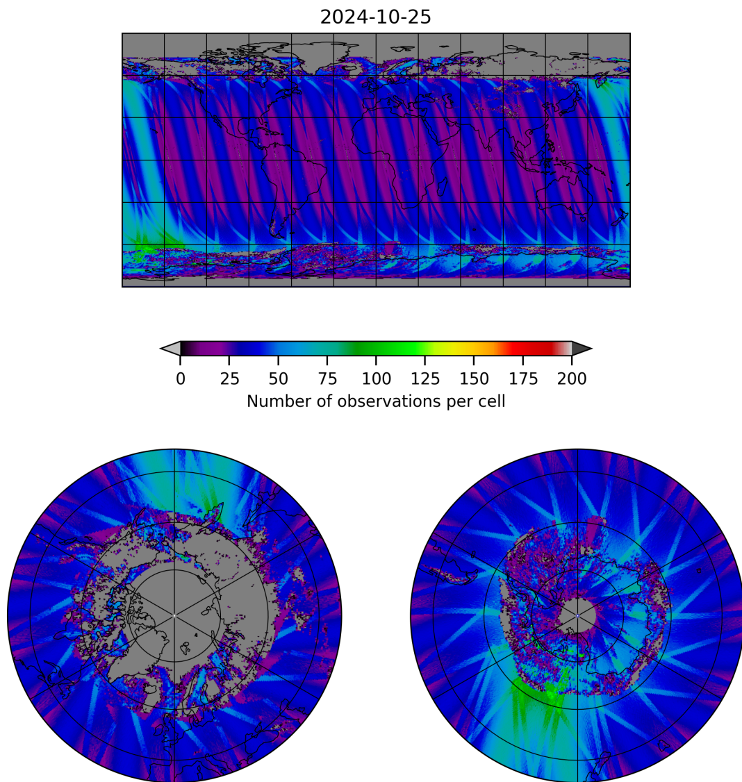
Figure 19: Map of the number of observations for 2024-10-24 to 2024-10-26
