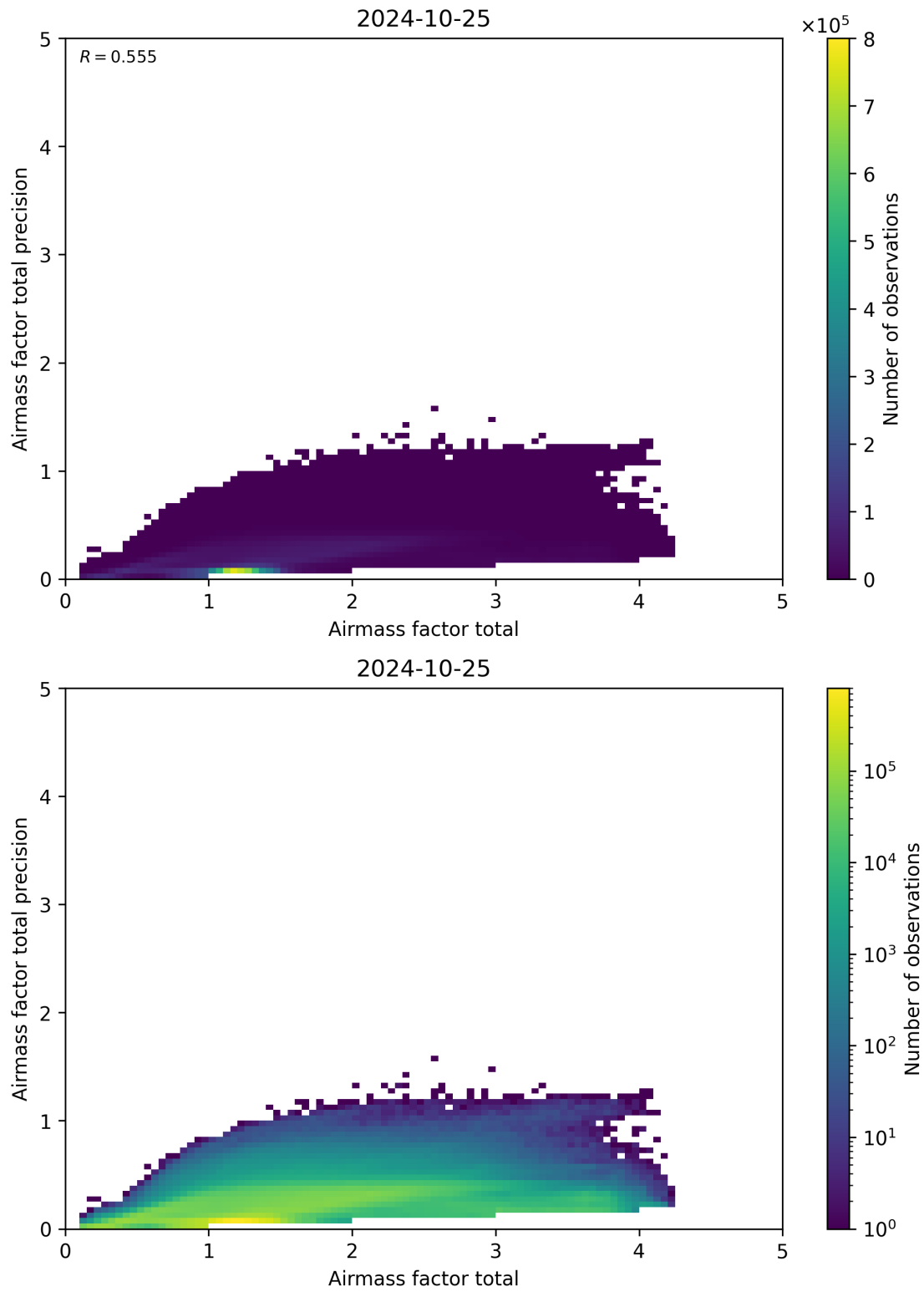
Figure 103: Scatter density plot of “Airmass factor total” against “Airmass factor total precision” for 2024-10-24 to 2024-10-26.
