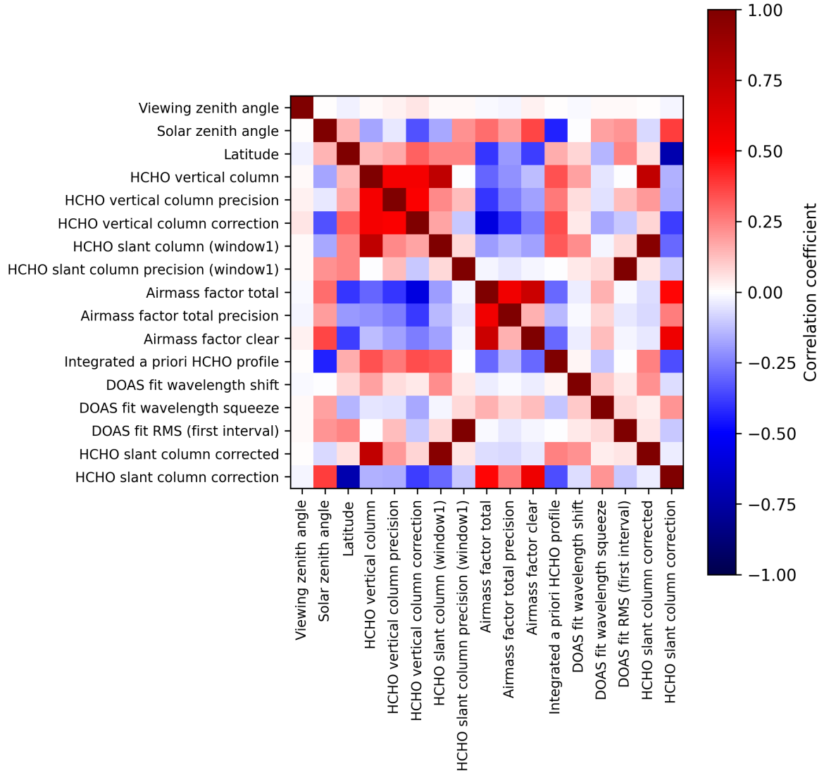
Figure 2: Map of correlation matrix for 2024-10-24 to 2024-10-26.
