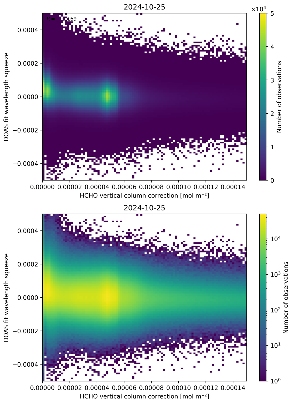
Figure 114: Scatter density plot of “HCHO vertical column correction” against “DOAS fit wavelength squeeze” for 2024-10-24 to 2024-10-26.
