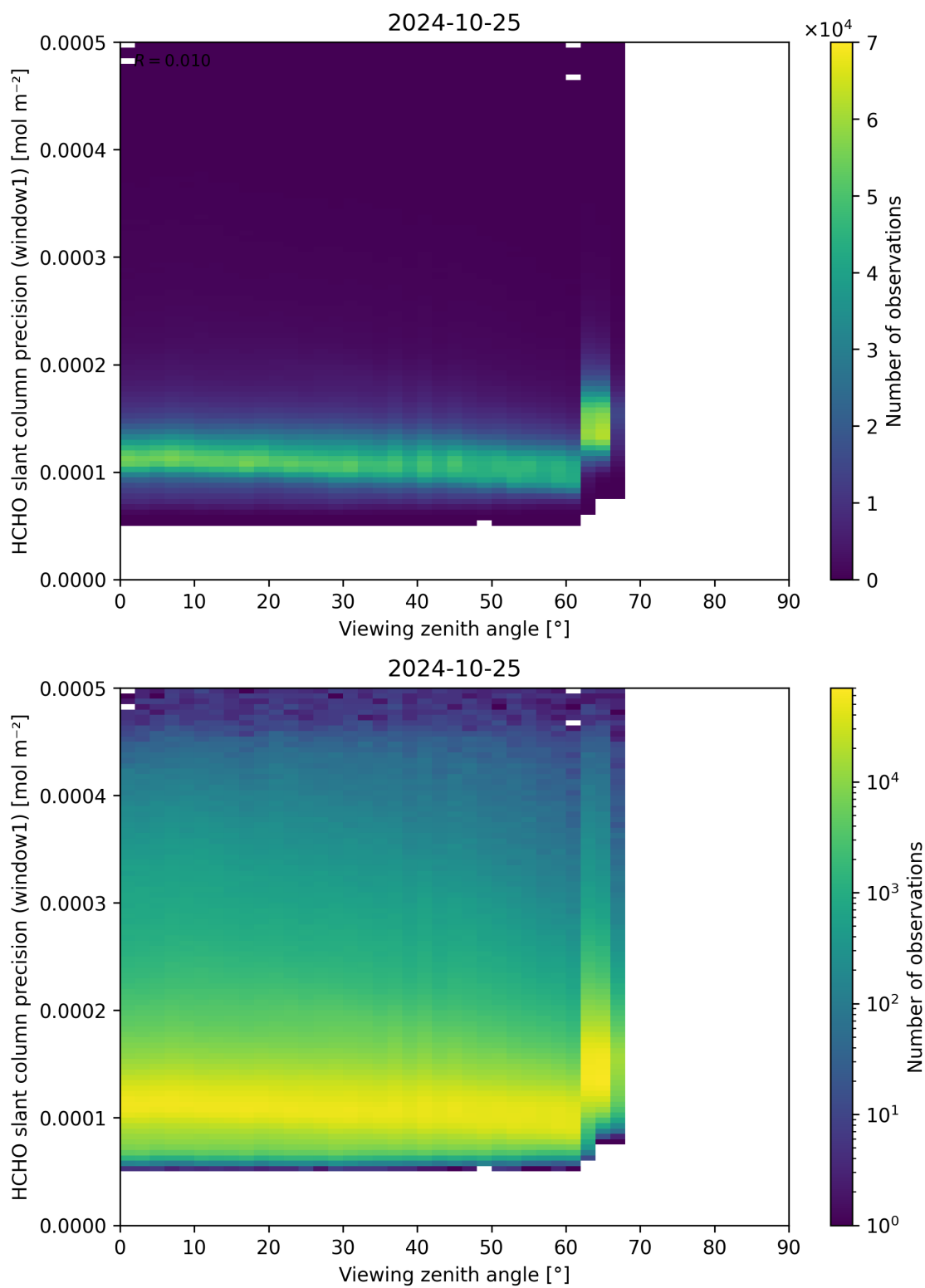
Figure 189: Scatter density plot of “Viewing zenith angle” against “HCHO slant column precision (window1)” for 2024-10-24 to 2024-10-26.
