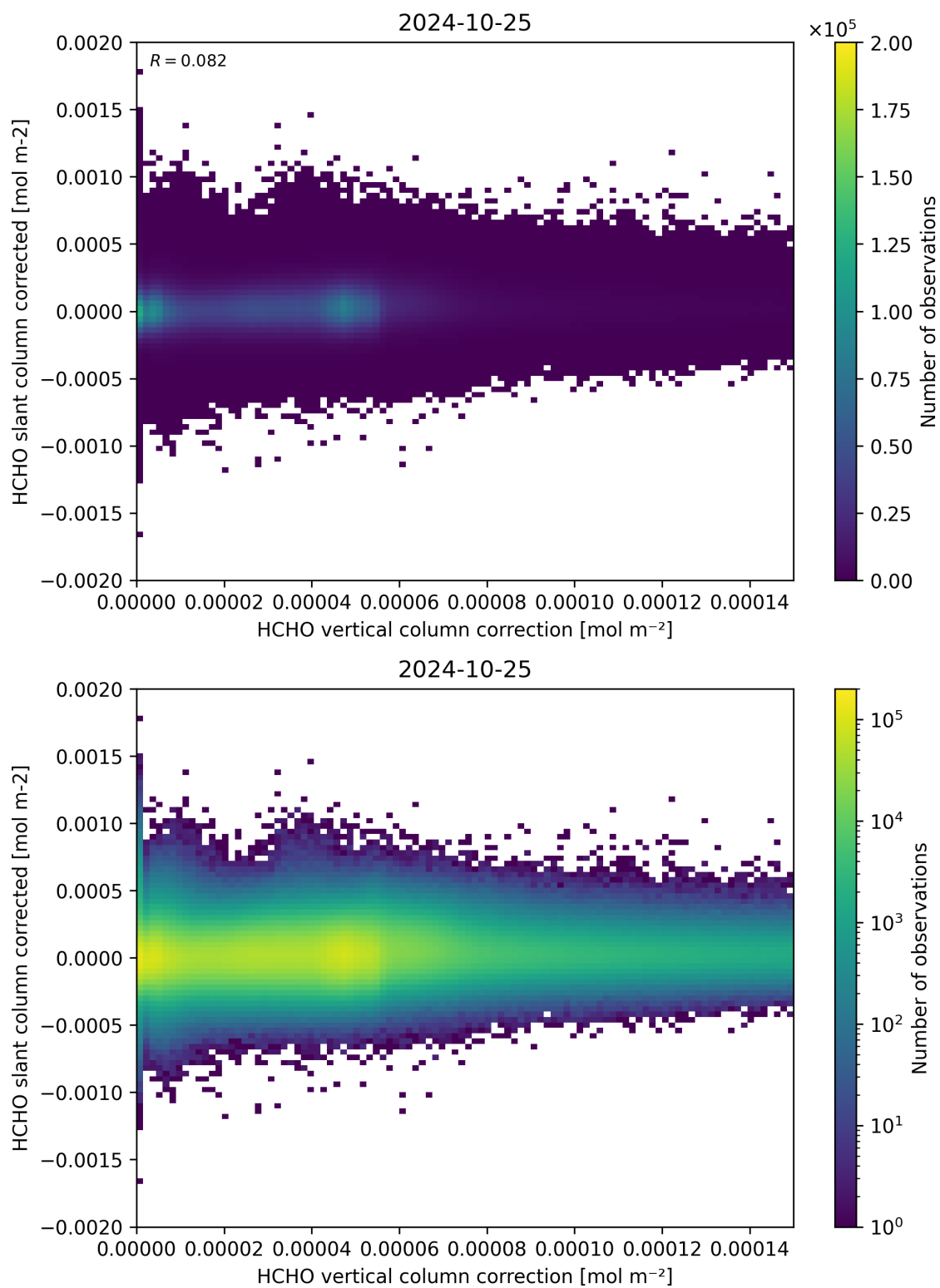
Figure 116: Scatter density plot of “HCHO vertical column correction” against “HCHO slant column corrected” for 2024-10-24 to 2024-10-26.
