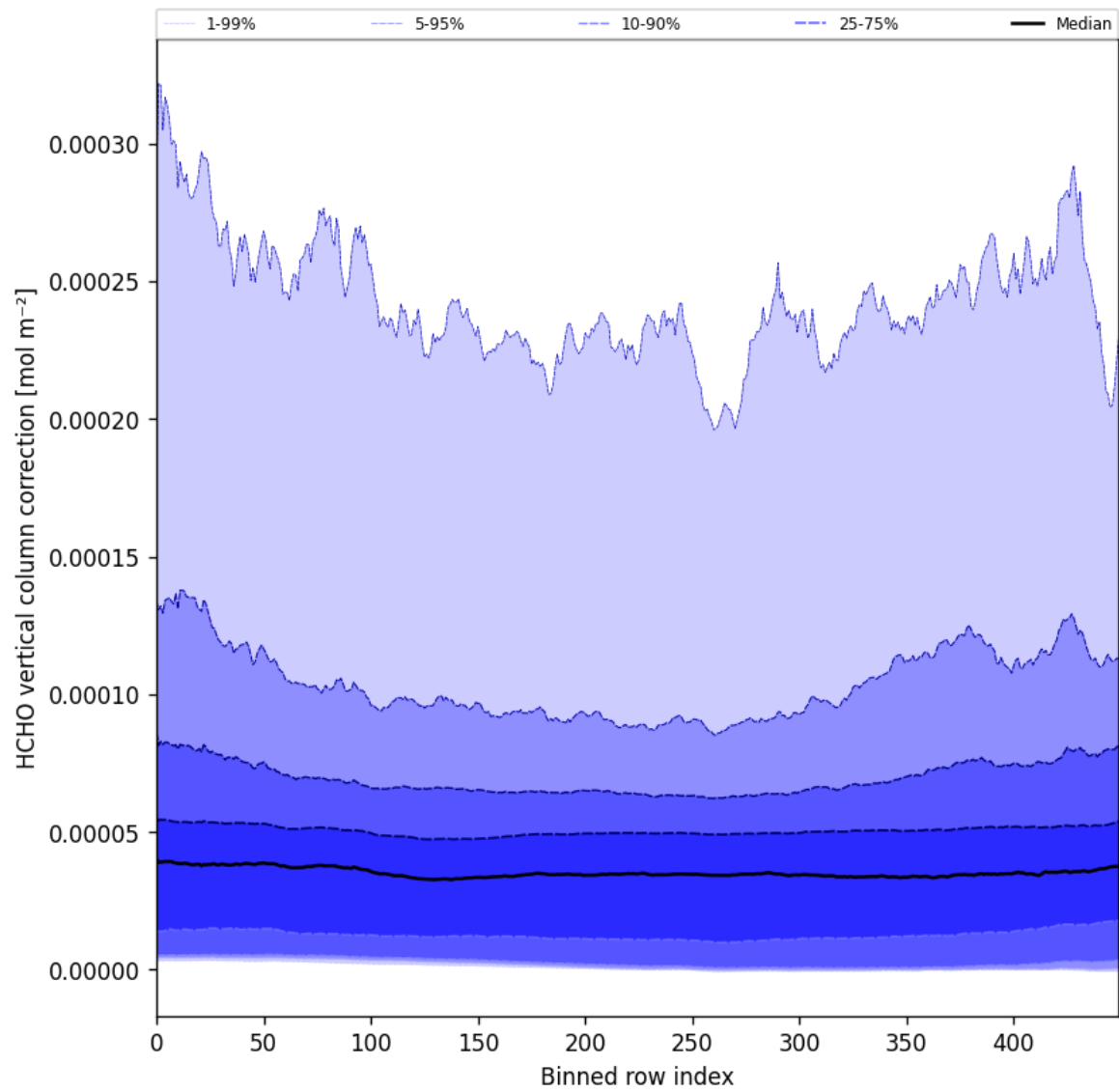
Figure 51: Along track statistics of “HCHO vertical column correction” for 2024-10-24 to 2024-10-26
