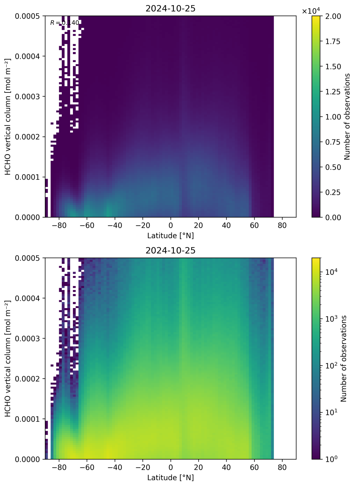
Figure 163: Scatter density plot of “Latitude” against “HCHO vertical column” for 2024-10-24 to 2024-10-26.
