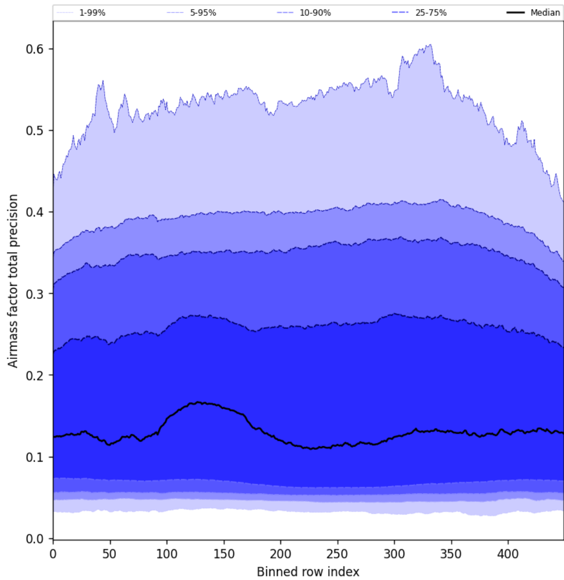
Figure 55: Along track statistics of “Airmass factor total precision” for 2024-10-24 to 2024-10-26
