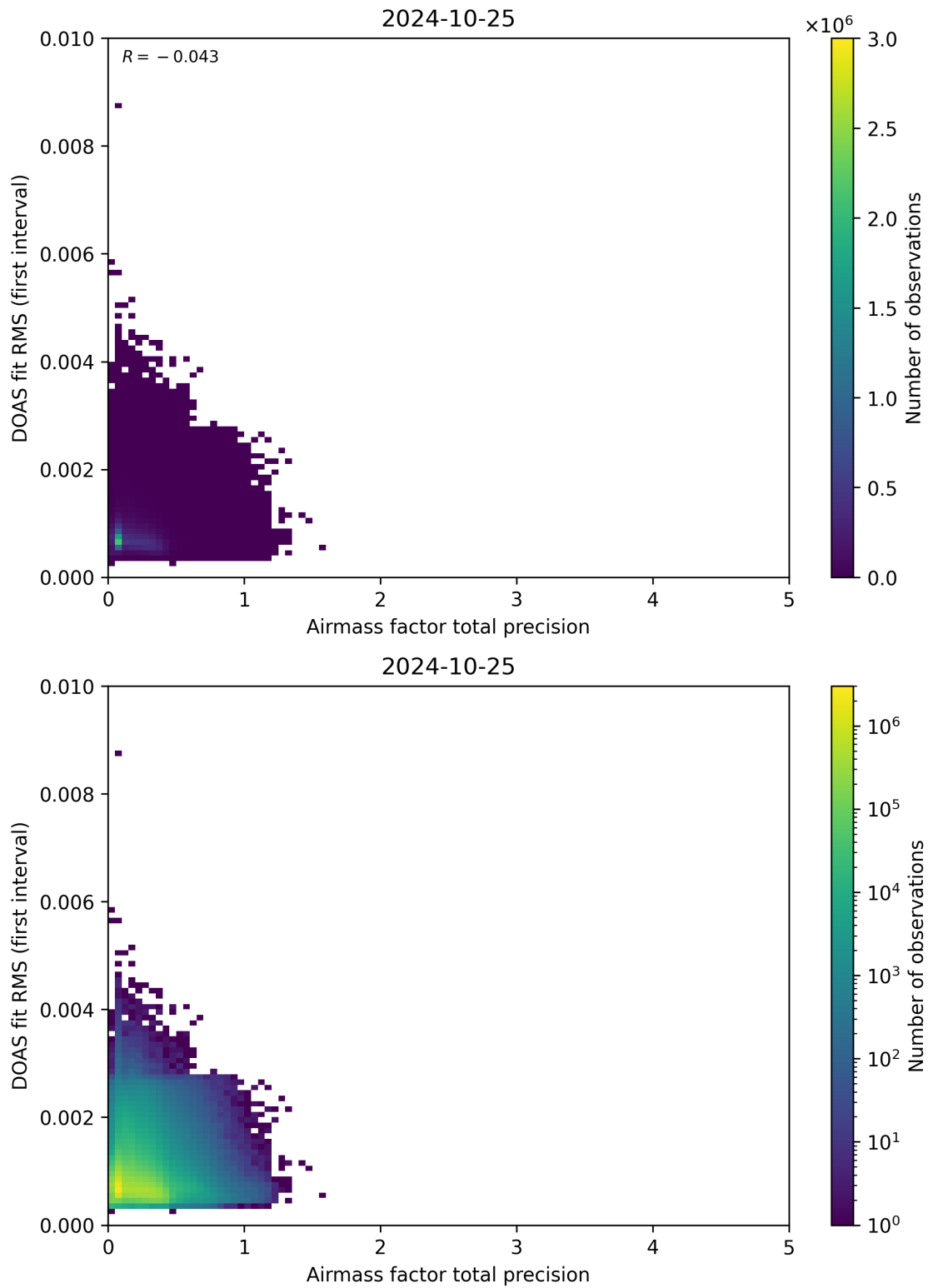
Figure 105: Scatter density plot of “Airmass factor total precision” against “DOAS fit RMS (first interval)” for 2024-10-24 to 2024-10-26.
