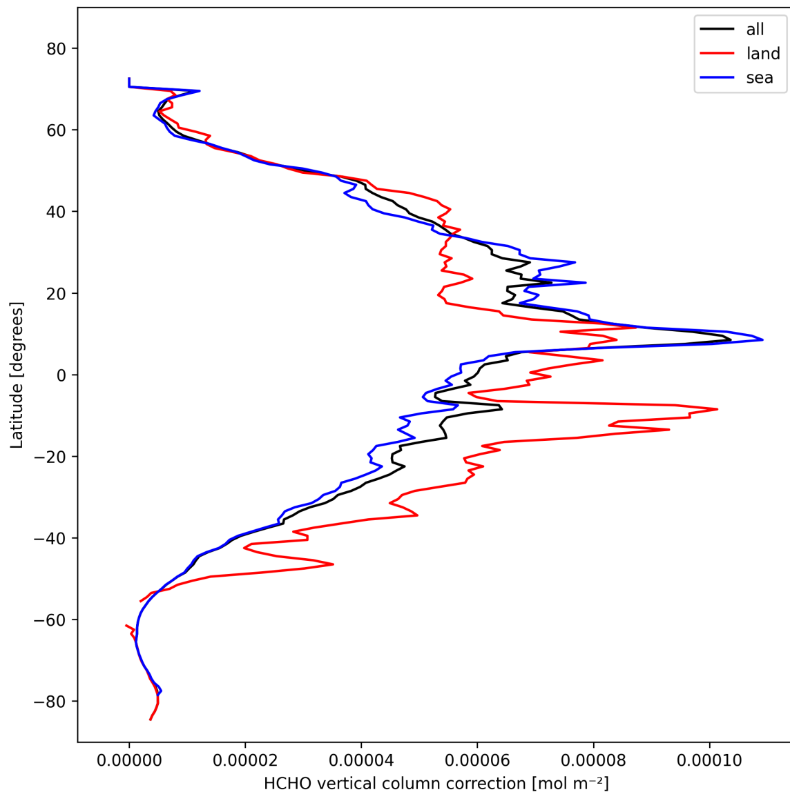
Figure 23: Zonal average of “HCHO vertical column correction” for 2024-10-24 to 2024-10-26.
