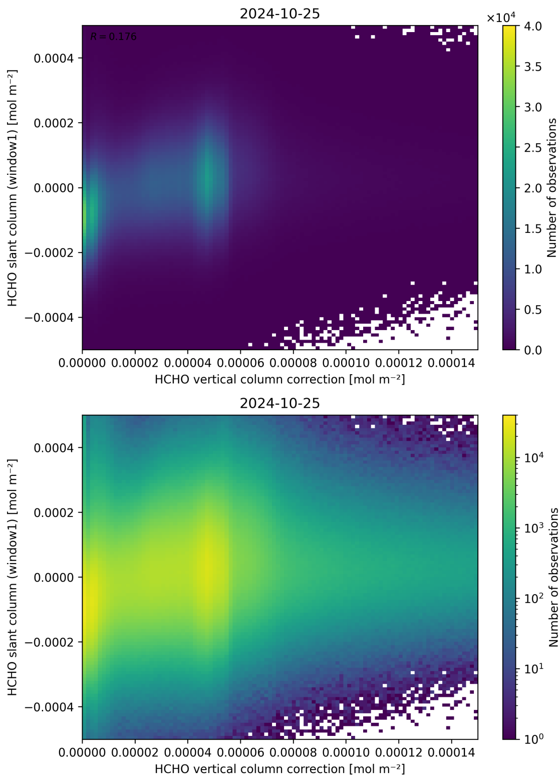
Figure 118: Scatter density plot of “HCHO vertical column correction” against “HCHO slant column (window1)” for 2024-10-24 to 2024-10-26.
