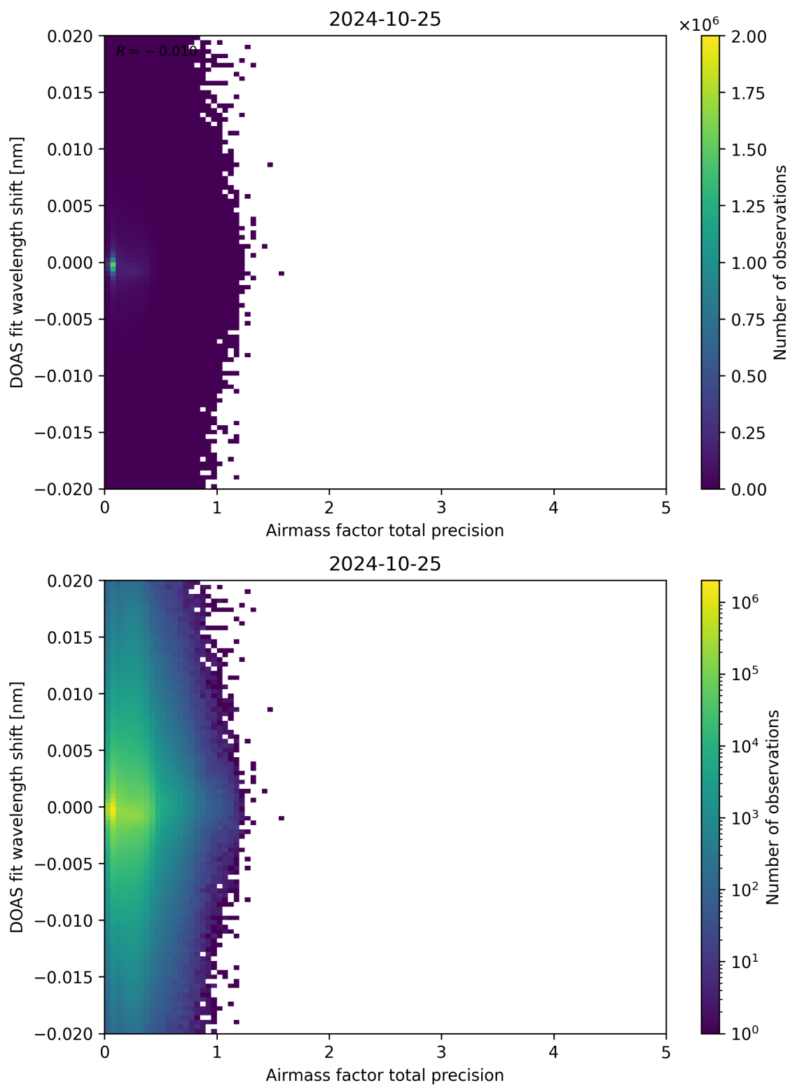
Figure 106: Scatter density plot of “Airmass factor total precision” against “DOAS fit wavelength shift” for 2024-10-24 to 2024-10-26.
