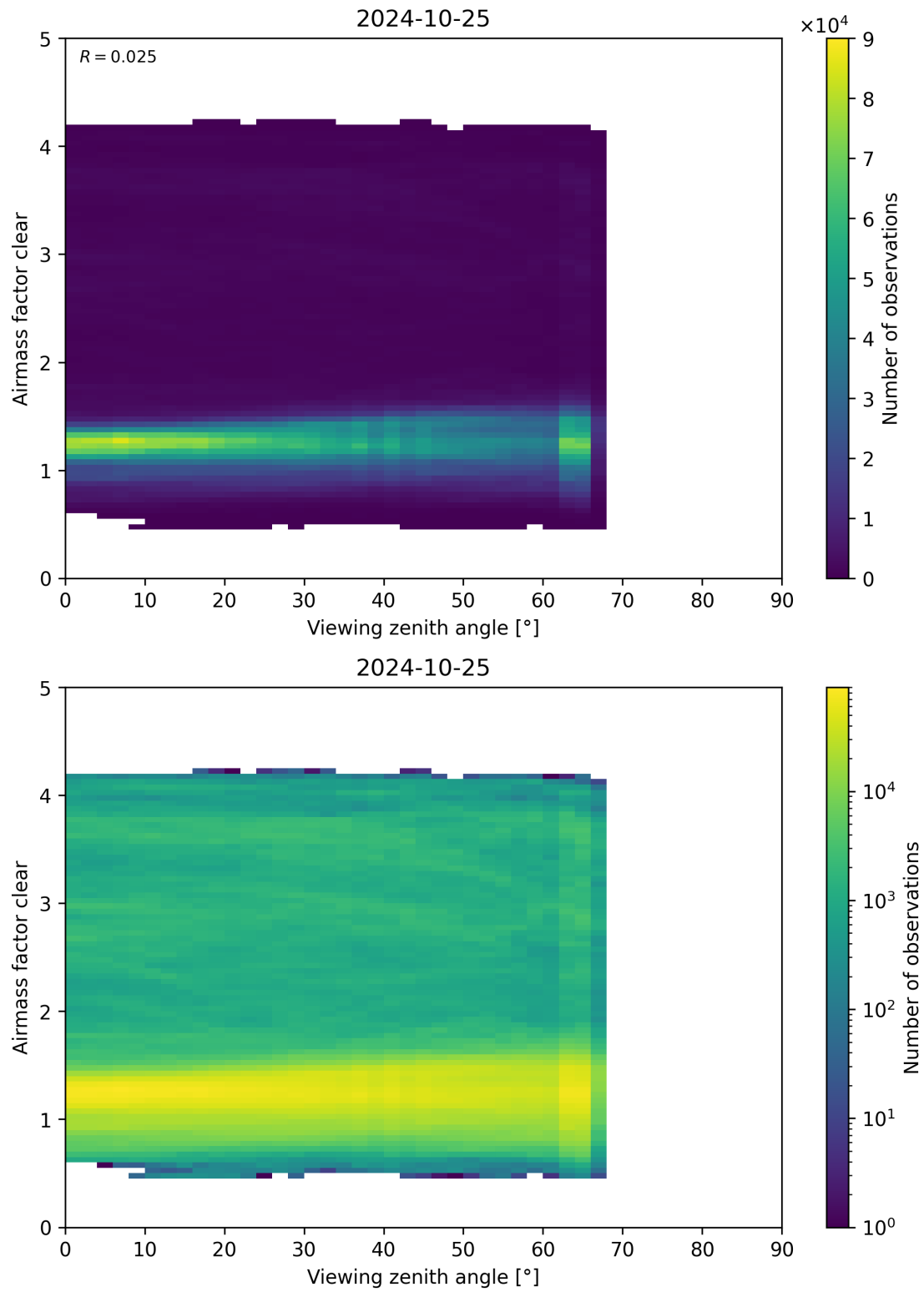
Figure 185: Scatter density plot of “Viewing zenith angle” against “Airmass factor clear” for 2024-10-24 to 2024-10-26.
