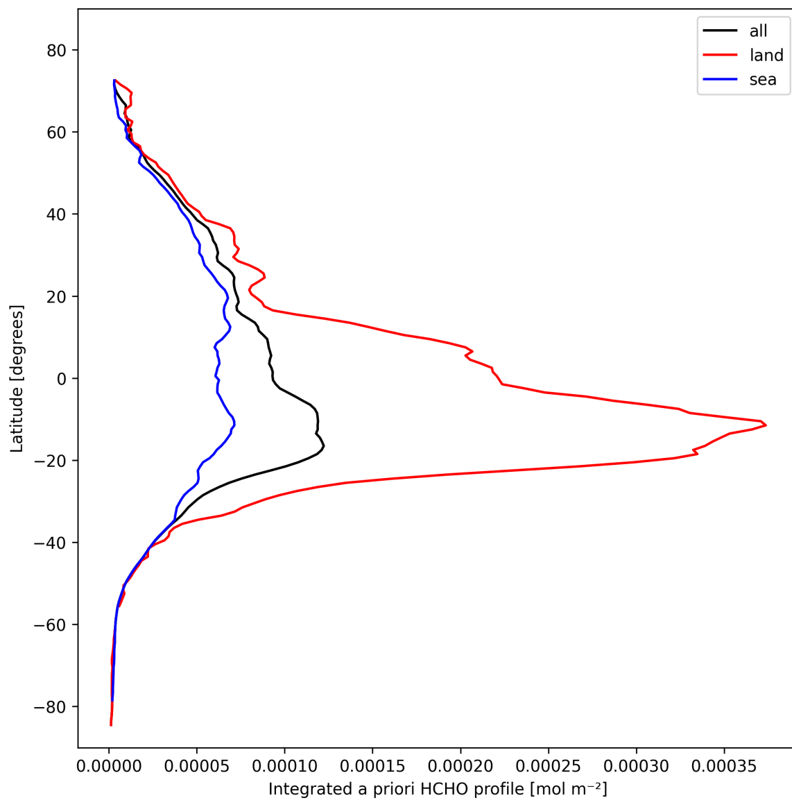
Figure 29: Zonal average of “Integrated a priori HCHO profile” for 2024-10-24 to 2024-10-26.
