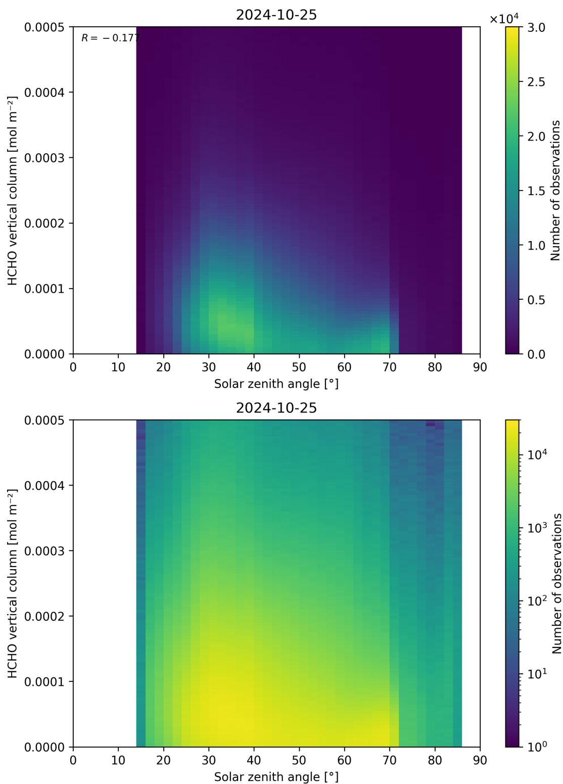
Figure 177: Scatter density plot of “Solar zenith angle” against “HCHO vertical column” for 2024-10-24 to 2024-10-26.
