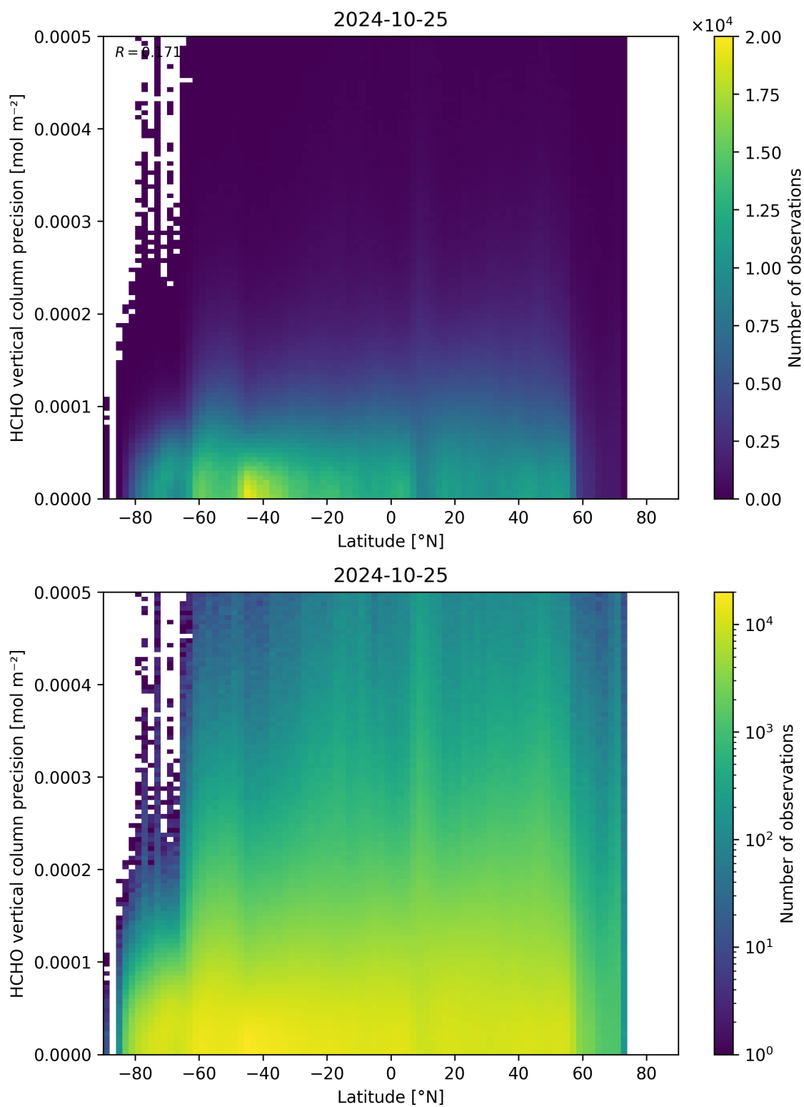
Figure 165: Scatter density plot of “Latitude” against “HCHO vertical column precision” for 2024-10-24 to 2024-10-26.
