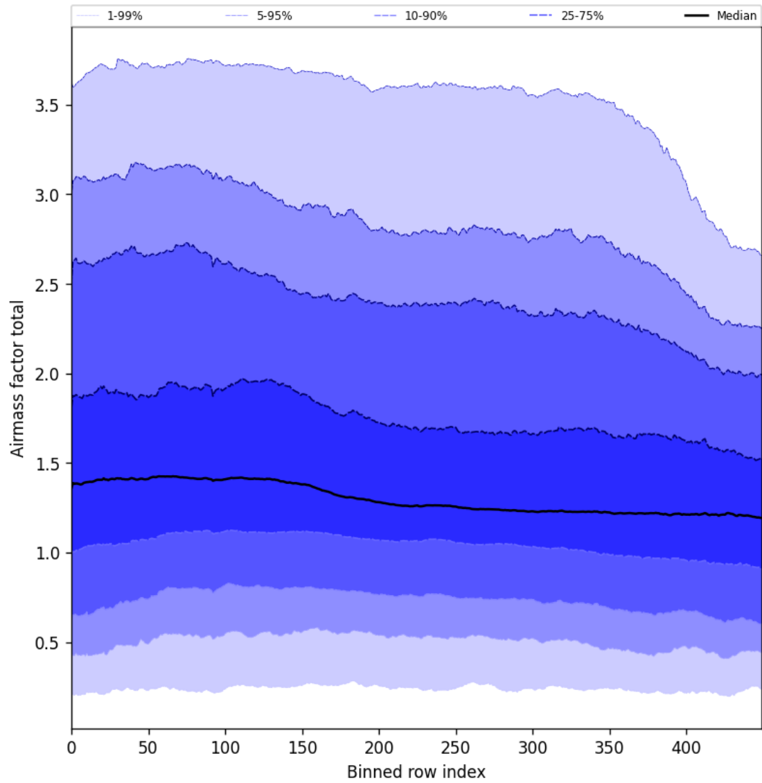
Figure 54: Along track statistics of “Airmass factor total” for 2024-10-24 to 2024-10-26
