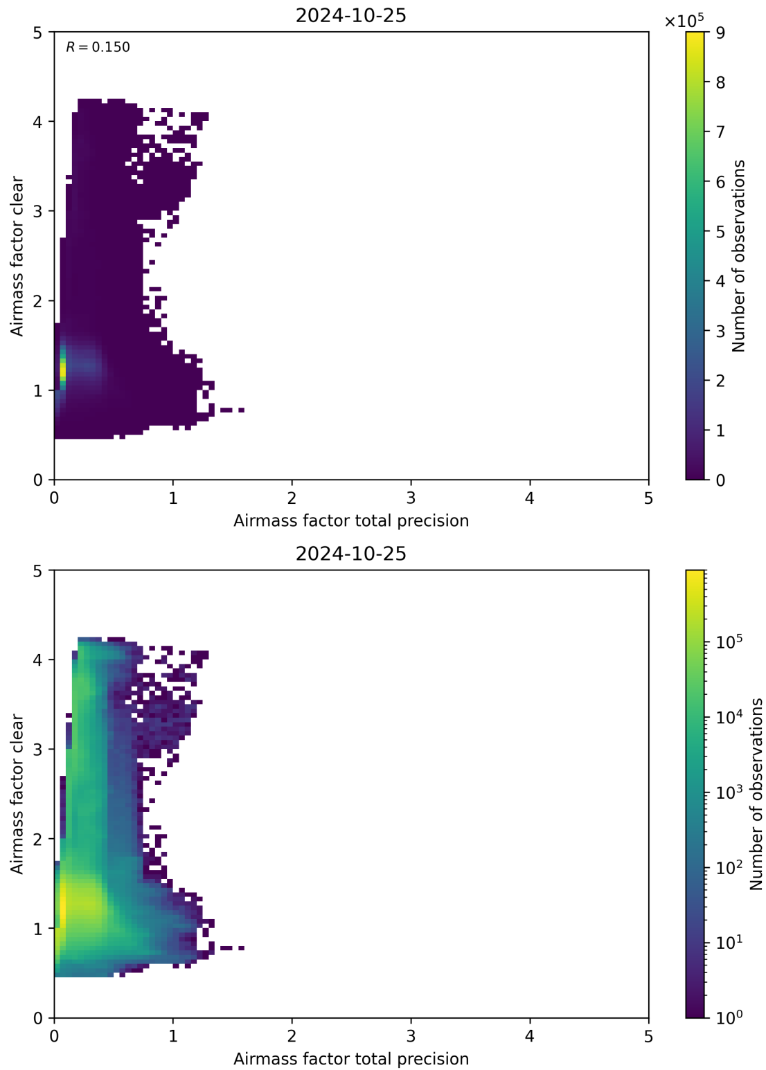
Figure 108: Scatter density plot of “Airmass factor total precision” against “Airmass factor clear” for 2024-10-24 to 2024-10-26.
