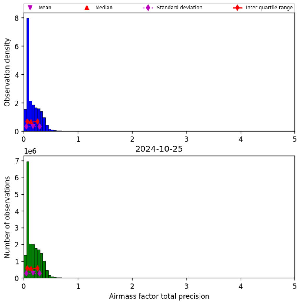
Figure 41: Histogram of “Airmass factor total precision” for 2024-10-24 to 2024-10-26
