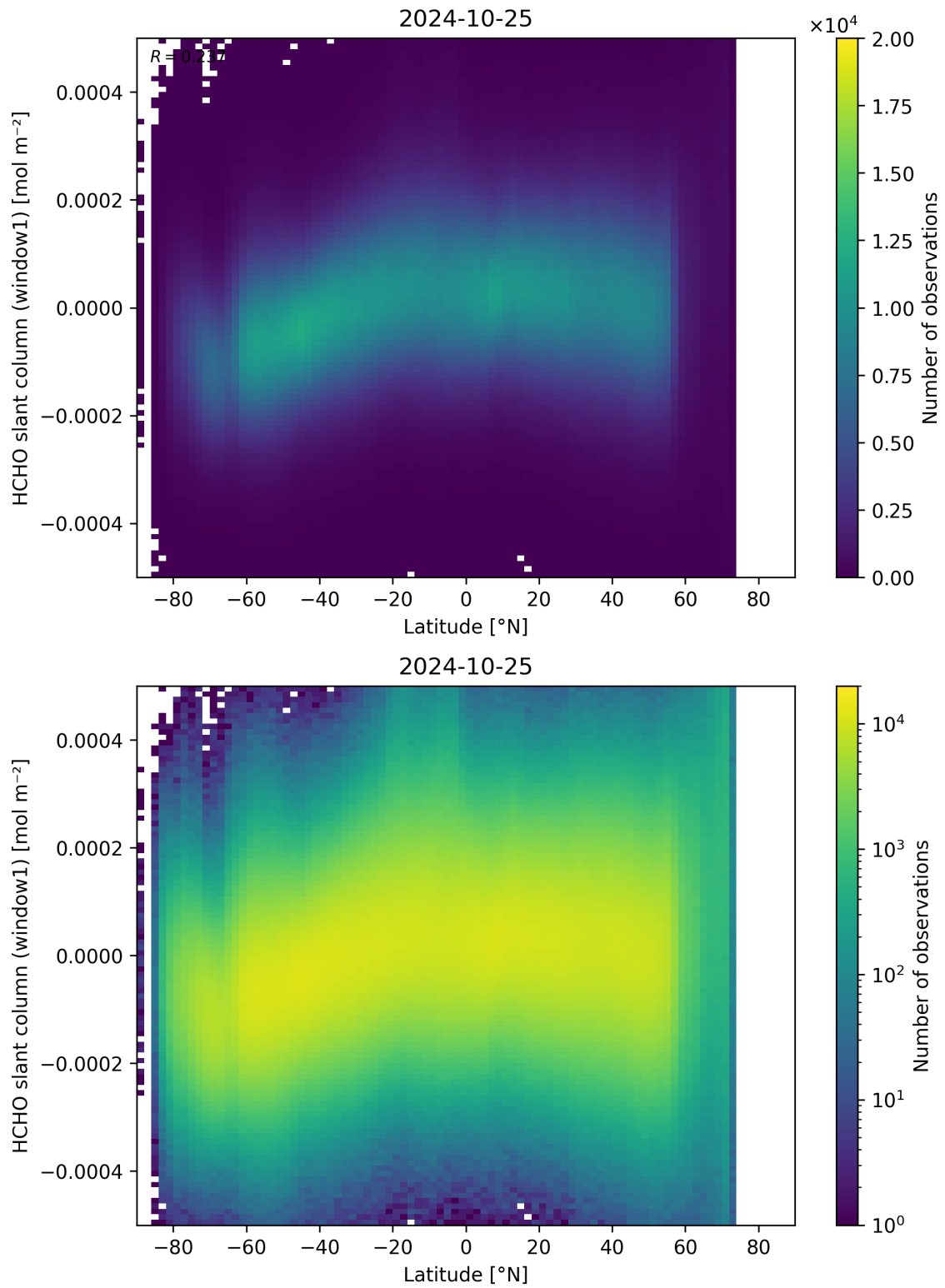
Figure 159: Scatter density plot of “Latitude” against “HCHO slant column (window1)” for 2024-10-24 to 2024-10-26.
