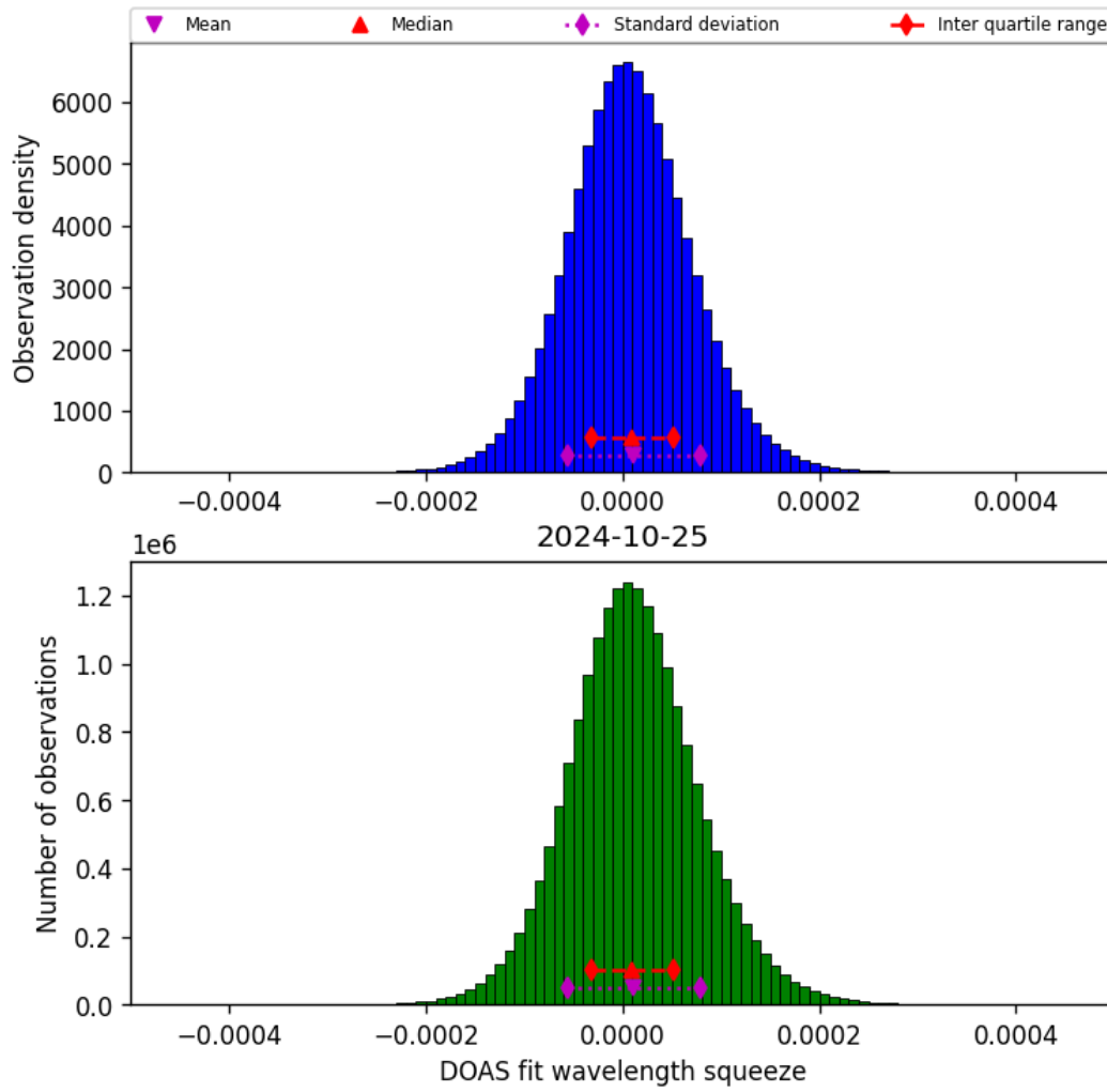
Figure 45: Histogram of “DOAS fit wavelength squeeze” for 2024-10-24 to 2024-10-26
