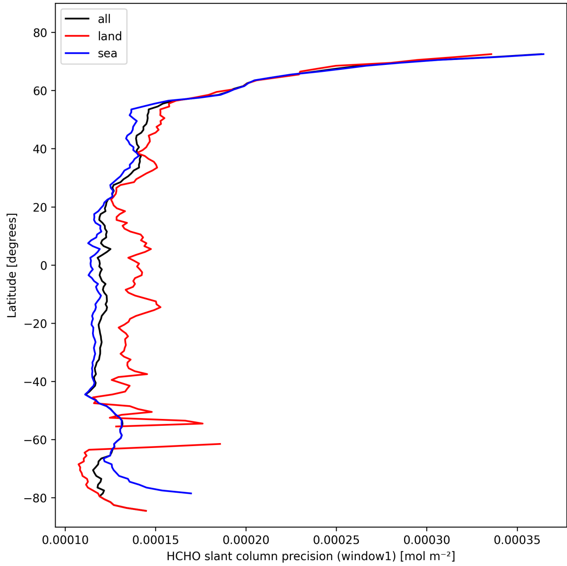
Figure 25: Zonal average of “HCHO slant column precision (window1)” for 2024-10-24 to 2024-10-26.
