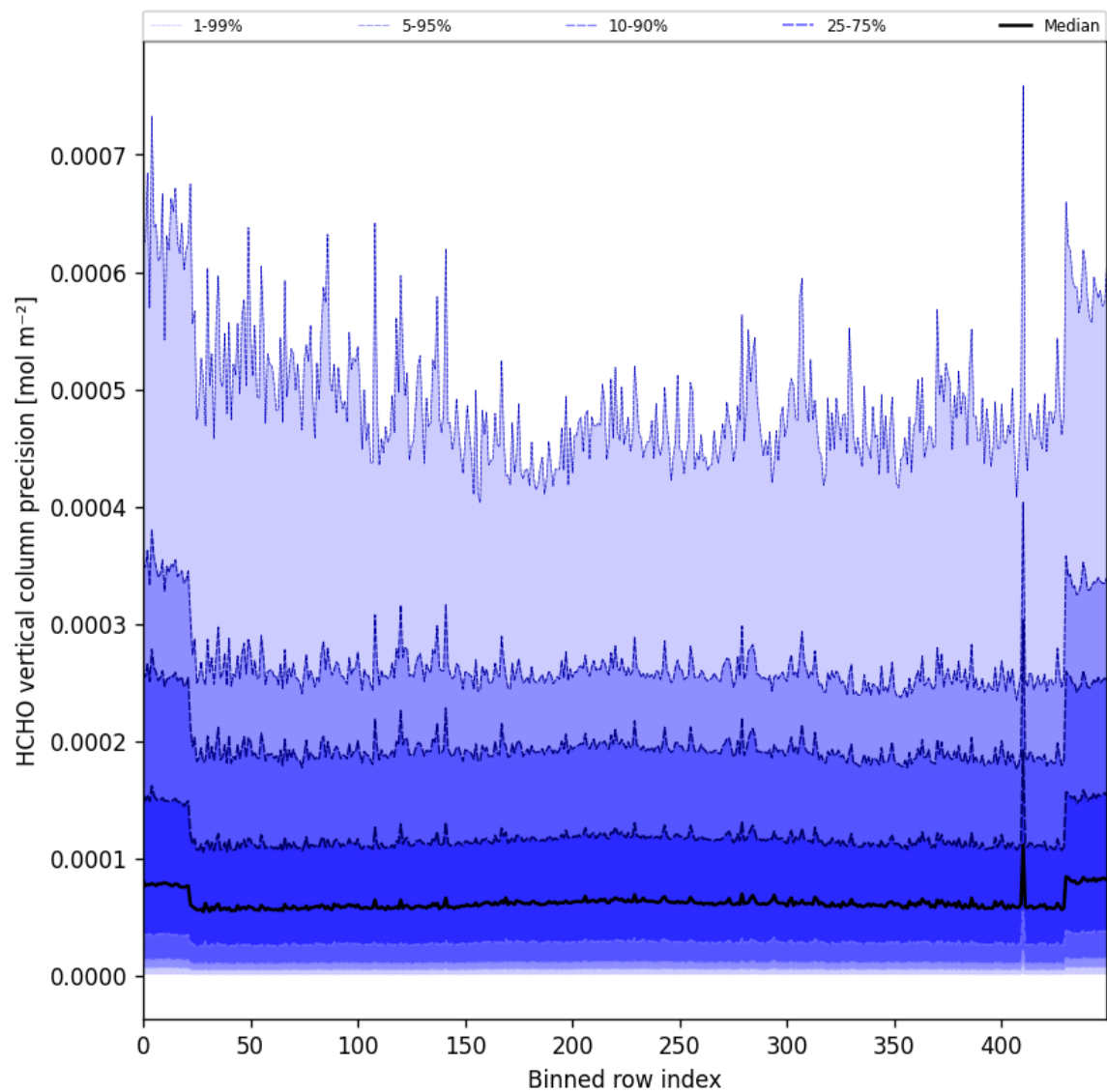
Figure 50: Along track statistics of "HCHO vertical column precision" for 2024-10-24 to 2024-10-26
