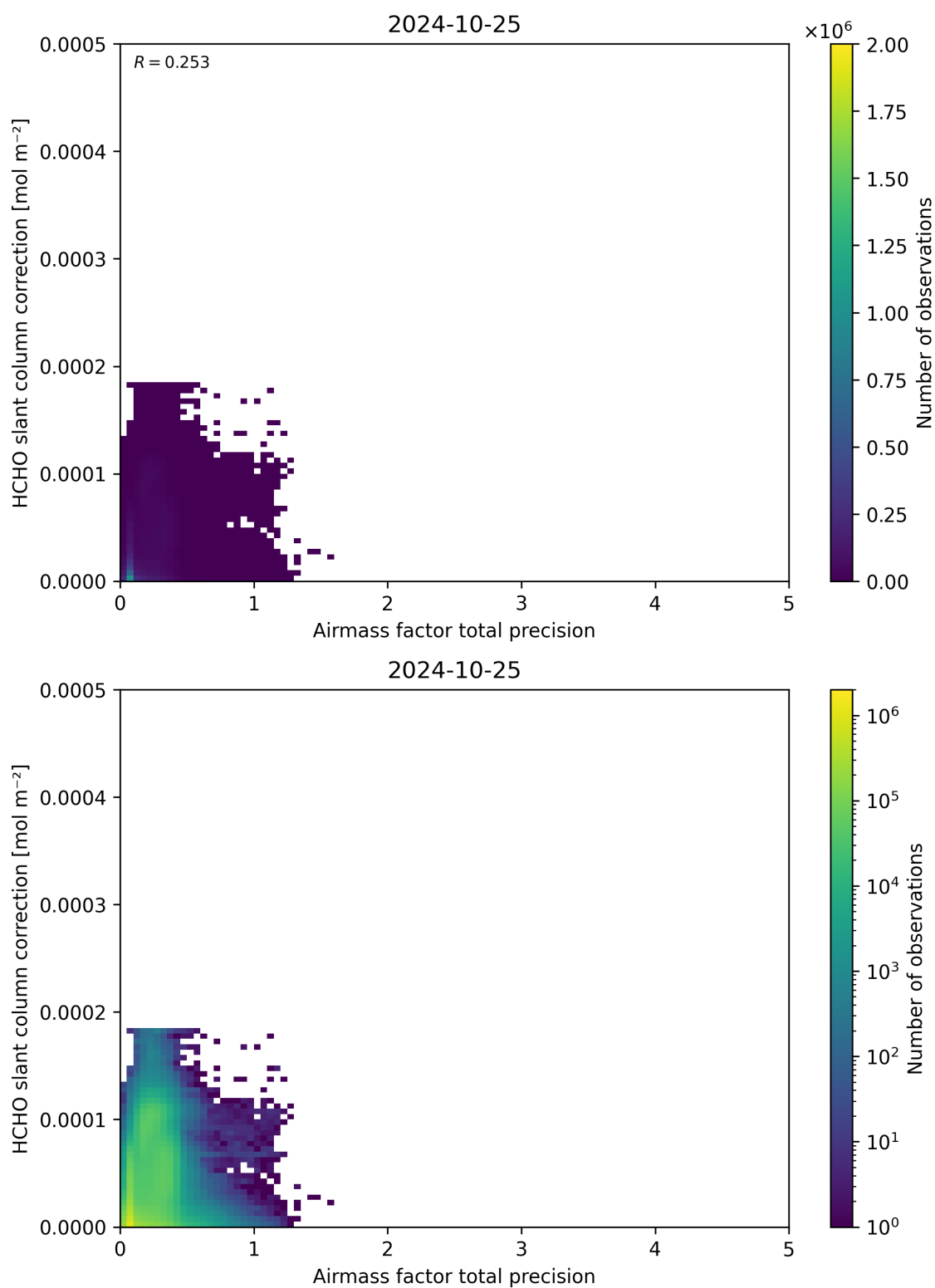
Figure 110: Scatter density plot of “Airmass factor total precision” against “HCHO slant column correction” for 2024-10-24 to 2024-10-26.
