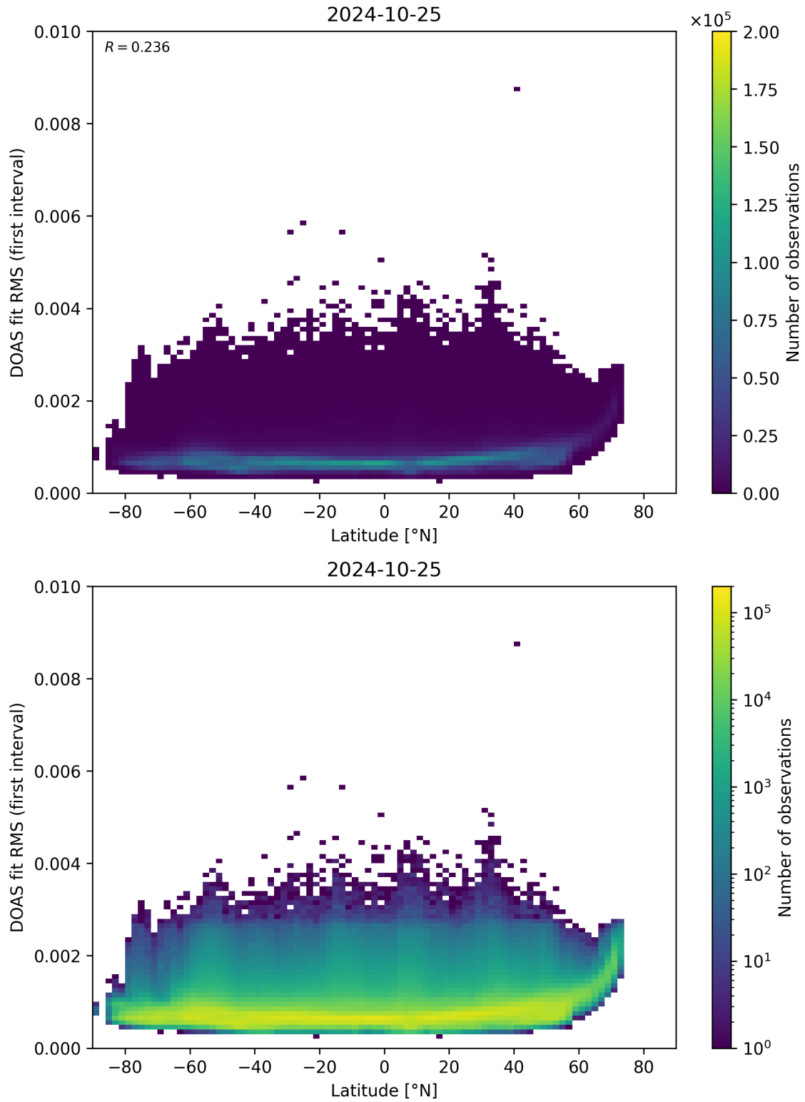
Figure 153: Scatter density plot of “Latitude” against “DOAS fit RMS (first interval)” for 2024-10-24 to 2024-10-26.
