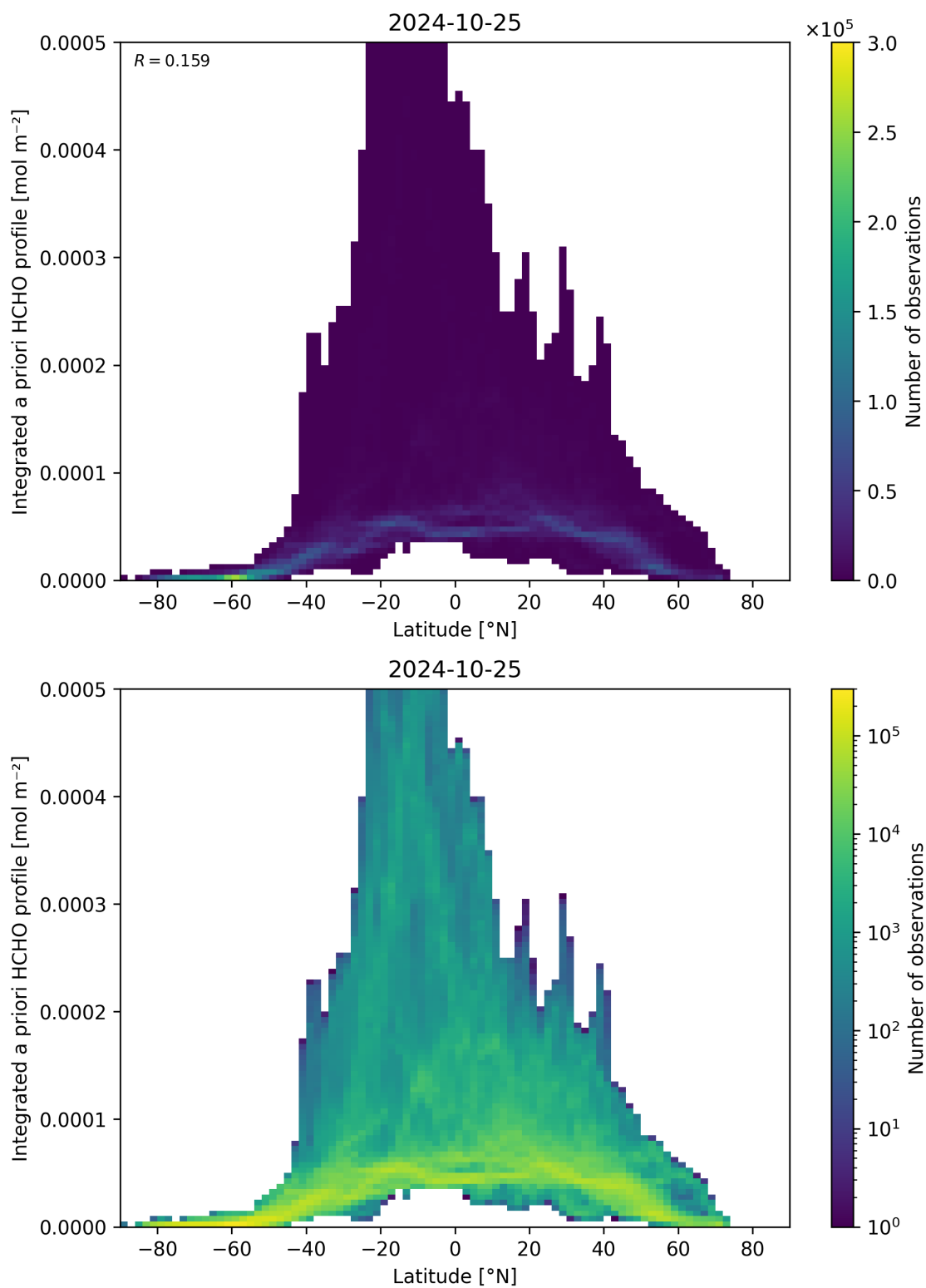
Figure 166: Scatter density plot of “Latitude” against “Integrated a priori HCHO profile” for 2024-10-24 to 2024-10-26.
