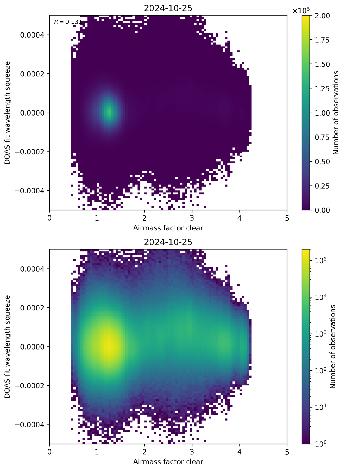
Figure 73: Scatter density plot of “Airmass factor clear” against “DOAS fit wavelength squeeze” for 2024-10-24 to 2024-10-26.
