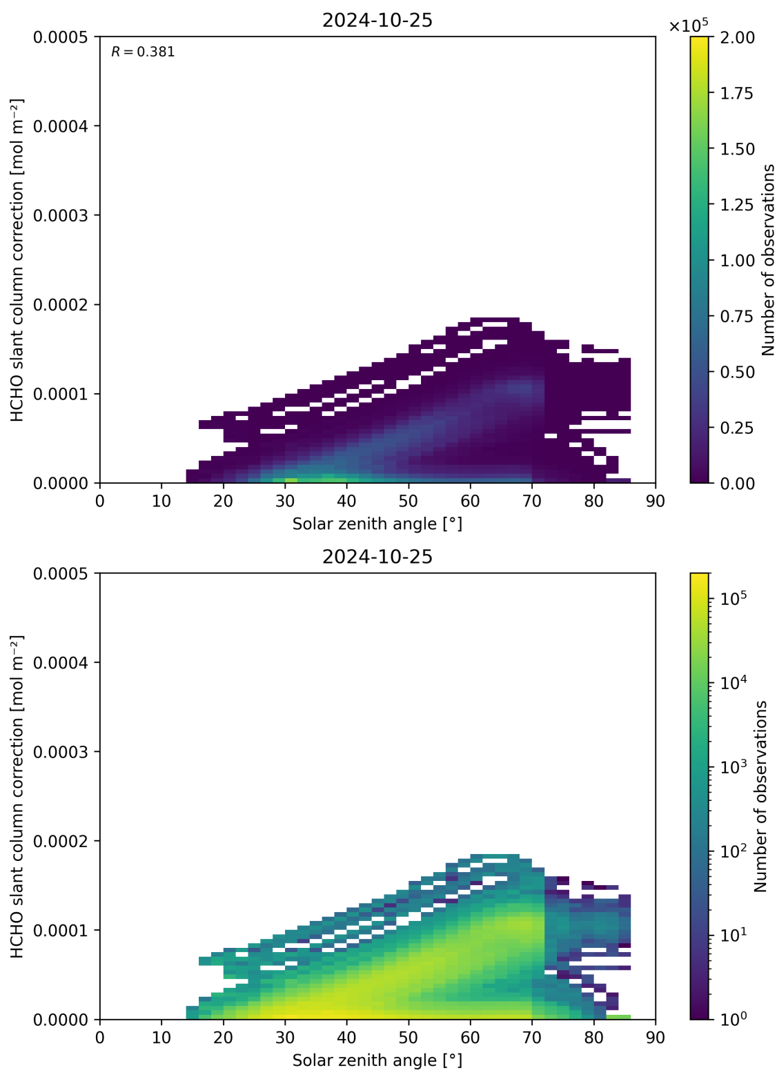
Figure 172: Scatter density plot of “Solar zenith angle” against “HCHO slant column correction” for 2024-10-24 to 2024-10-26.
