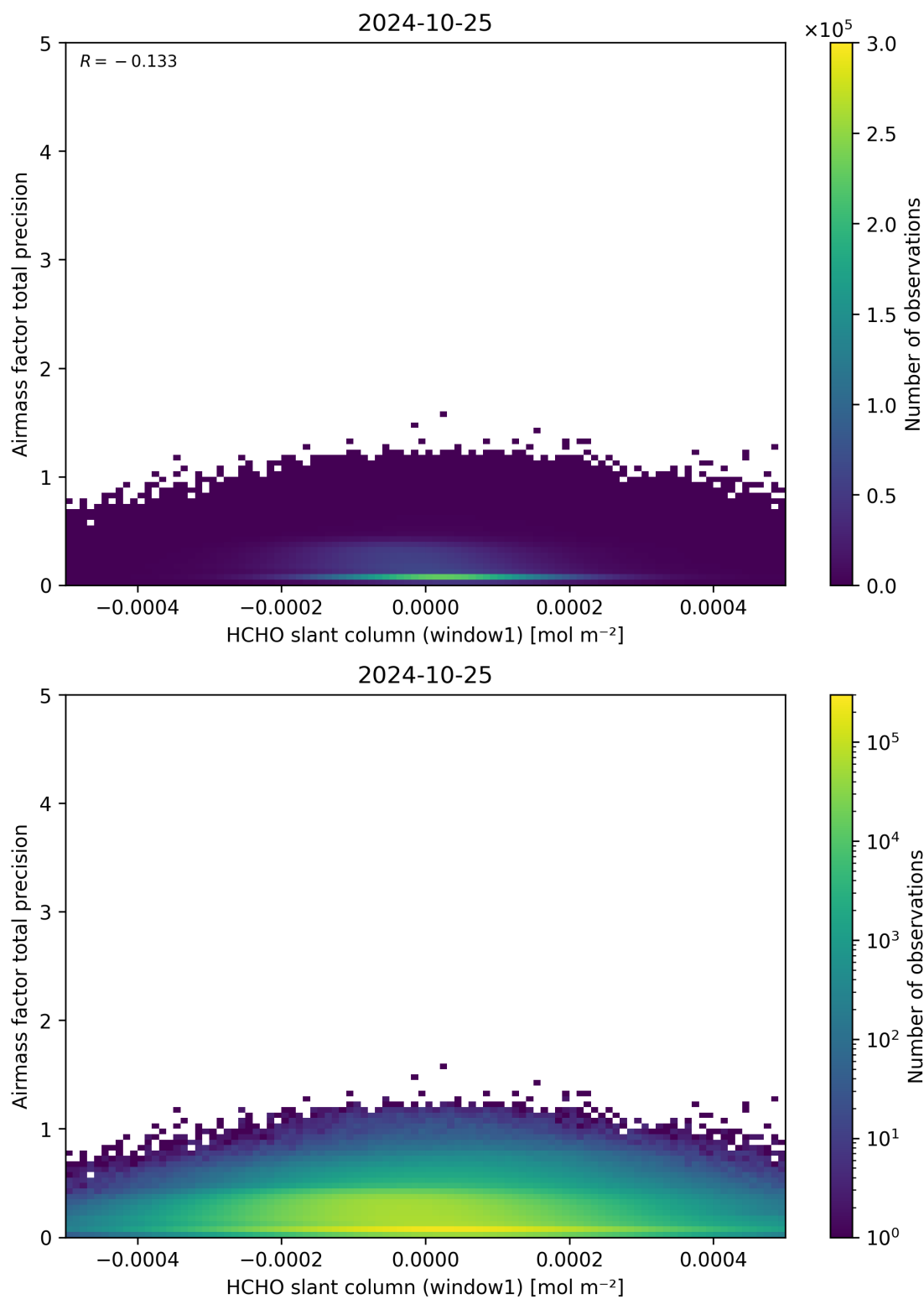
Figure 86: Scatter density plot of “HCHO slant column (window1)” against “Airmass factor total precision” for 2024-10-24 to 2024-10-26.
