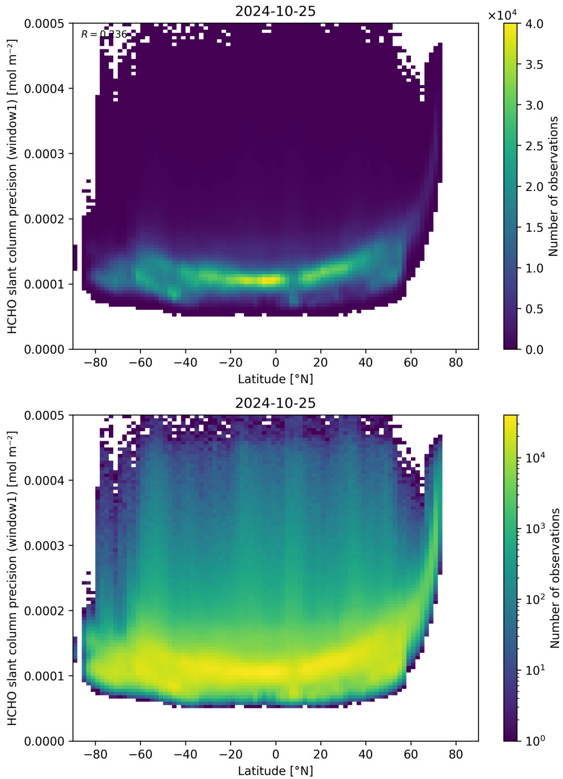
Figure 160: Scatter density plot of “Latitude” against “HCHO slant column precision (window1)” for 2024-10-24 to 2024-10-26.
