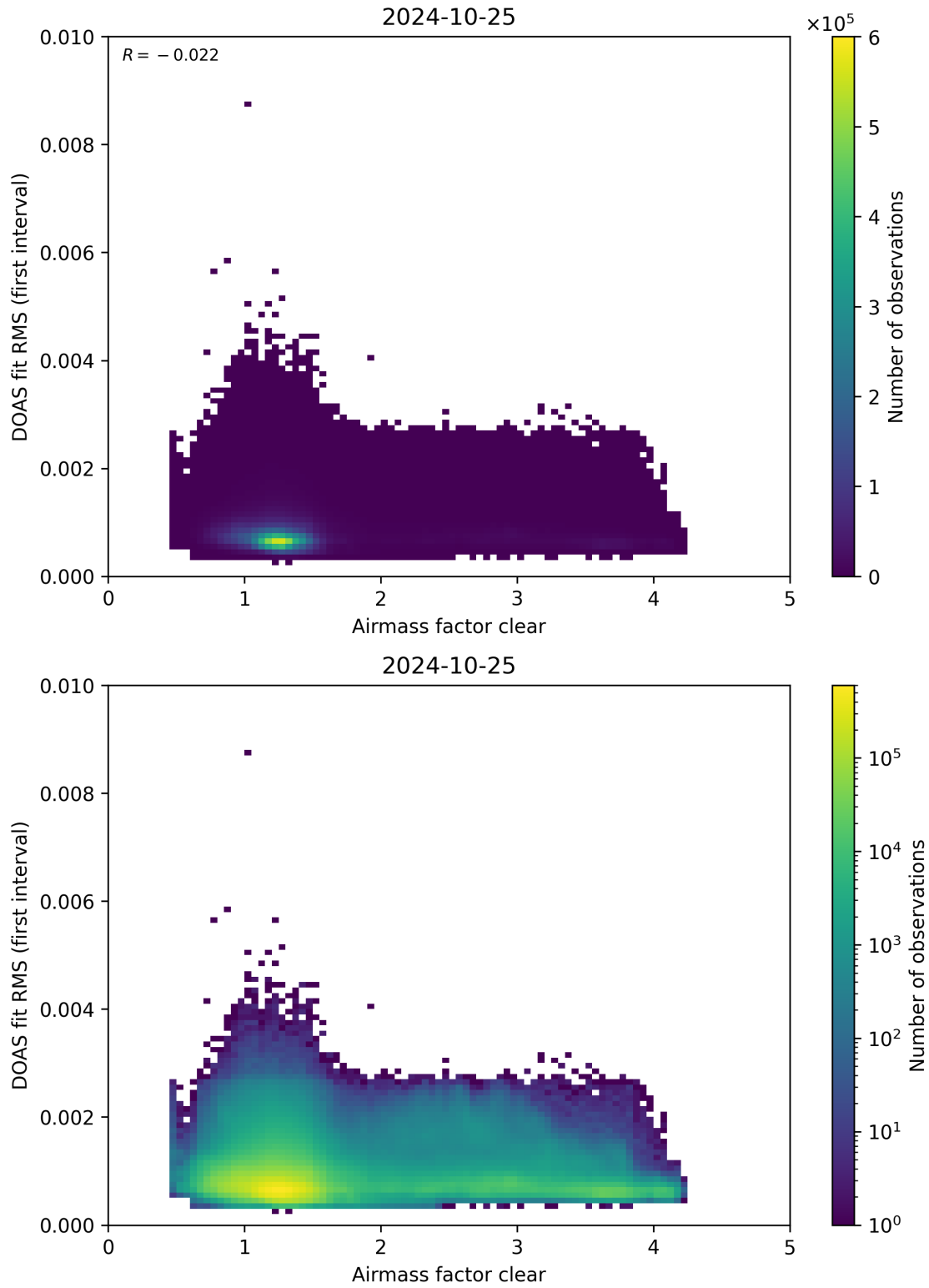
Figure 71: Scatter density plot of “Airmass factor clear” against “DOAS fit RMS (first interval)” for 2024-10-24 to 2024-10-26.
