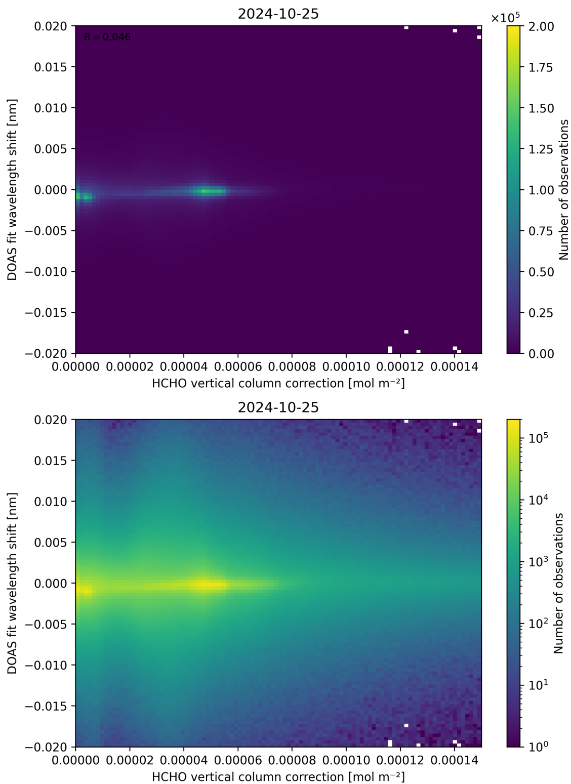
Figure 113: Scatter density plot of “HCHO vertical column correction” against “DOAS fit wavelength shift” for 2024-10-24 to 2024-10-26.
