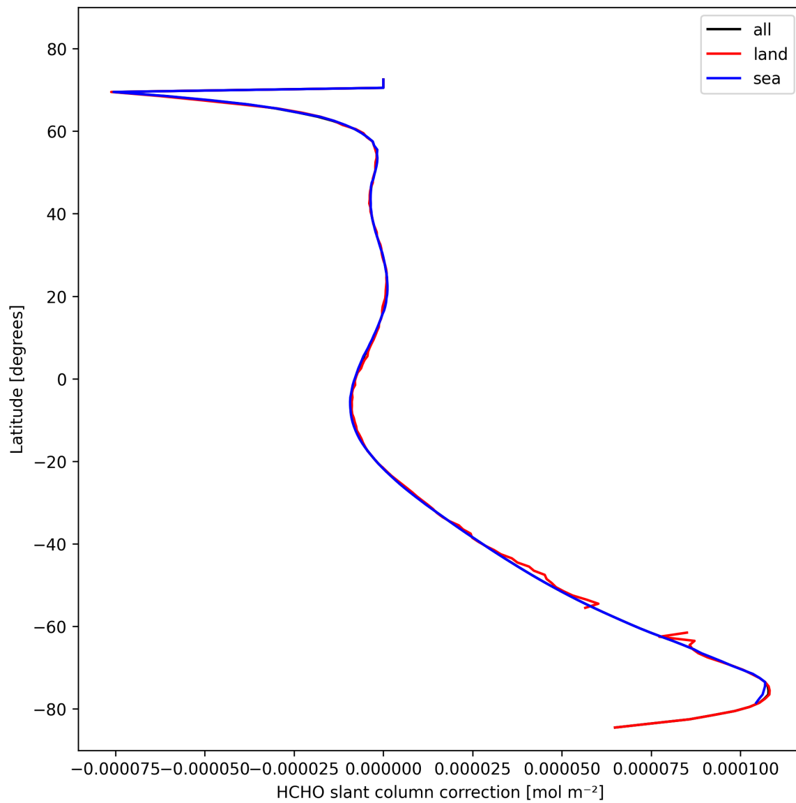
Figure 33: Zonal average of “HCHO slant column correction” for 2024-10-24 to 2024-10-26.
