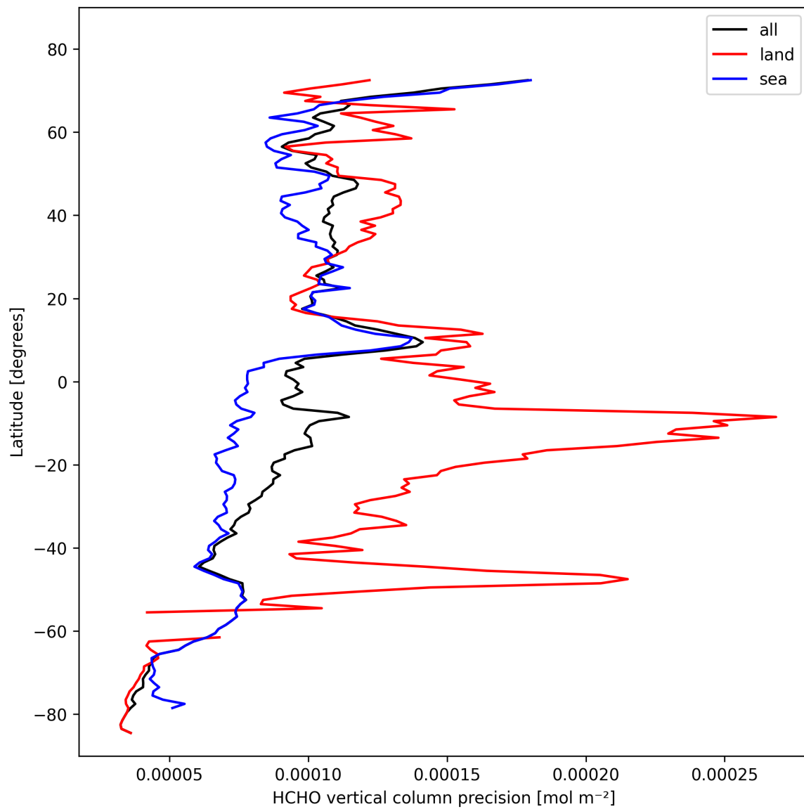
Figure 22: Zonal average of “HCHO vertical column precision” for 2024-10-24 to 2024-10-26.
