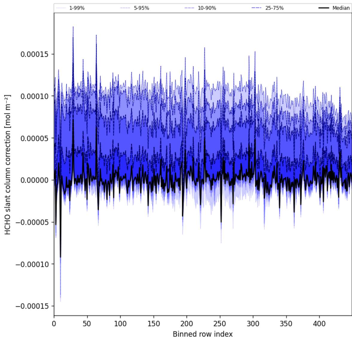
Figure 61: Along track statistics of "HCHO slant column correction" for 2024-10-24 to 2024-10-26
