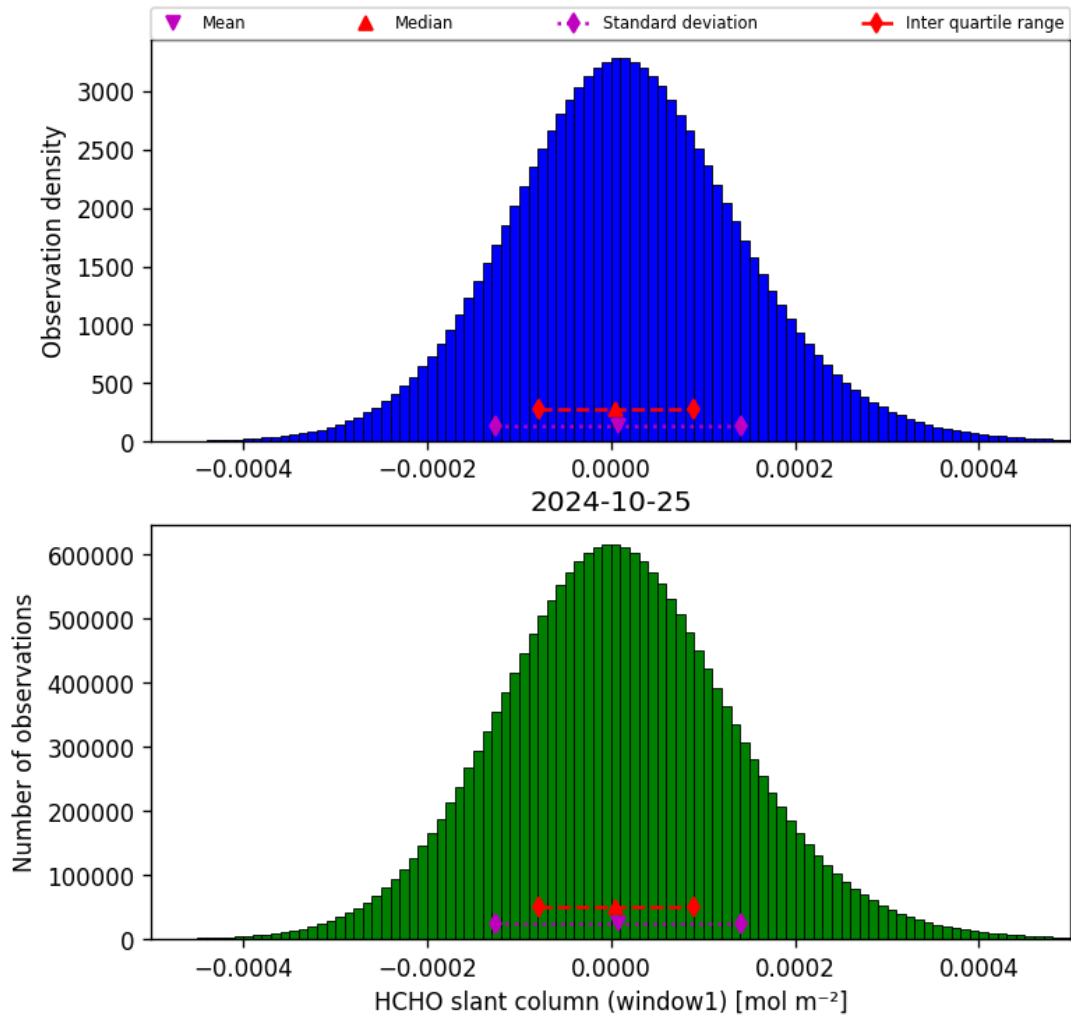
Figure 38: Histogram of “HCHO slant column (window1)” for 2024-10-24 to 2024-10-26
