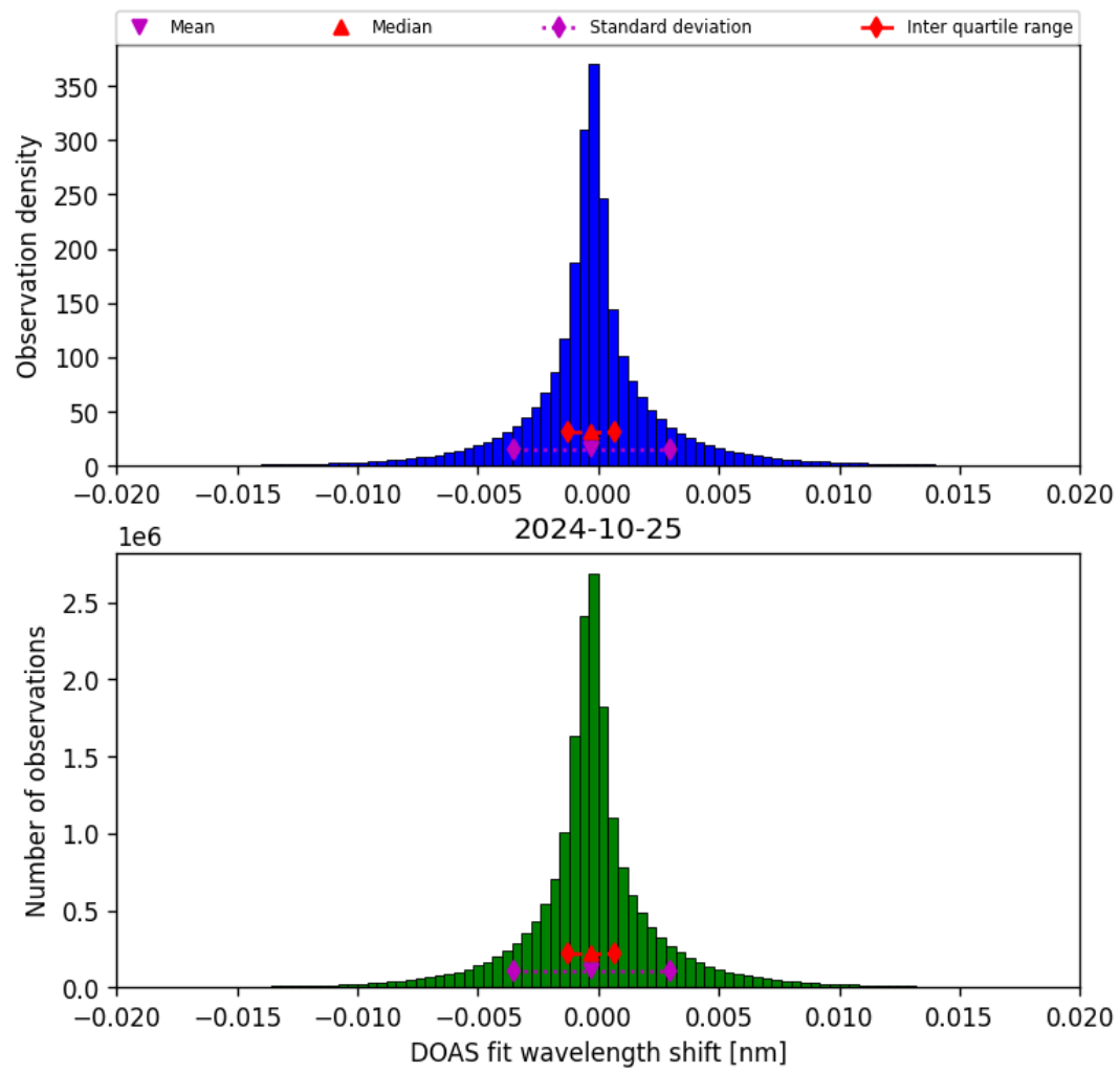
Figure 44: Histogram of “DOAS fit wavelength shift” for 2024-10-24 to 2024-10-26
