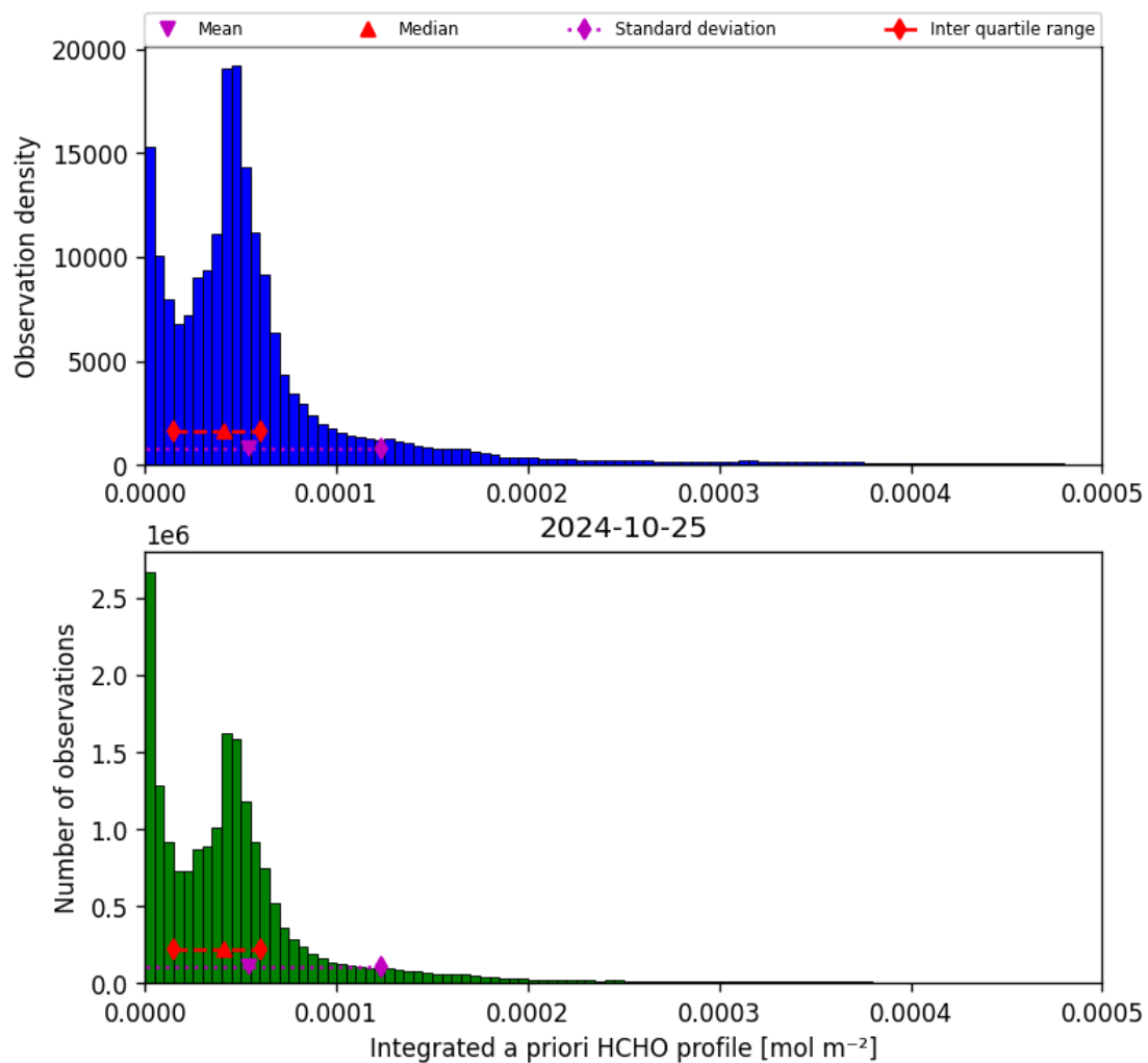
Figure 43: Histogram of “Integrated a priori HCHO profile” for 2024-10-24 to 2024-10-26
