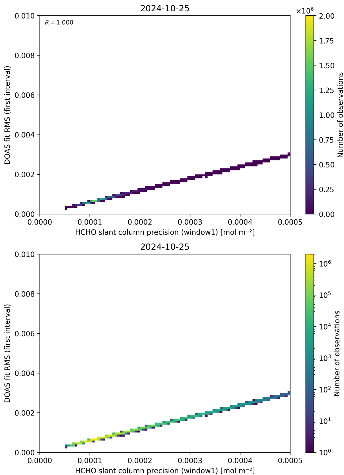
Figure 88: Scatter density plot of “HCHO slant column precision (window1)” against “DOAS fit RMS (first interval)” for 2024-10-24 to 2024-10-26.
