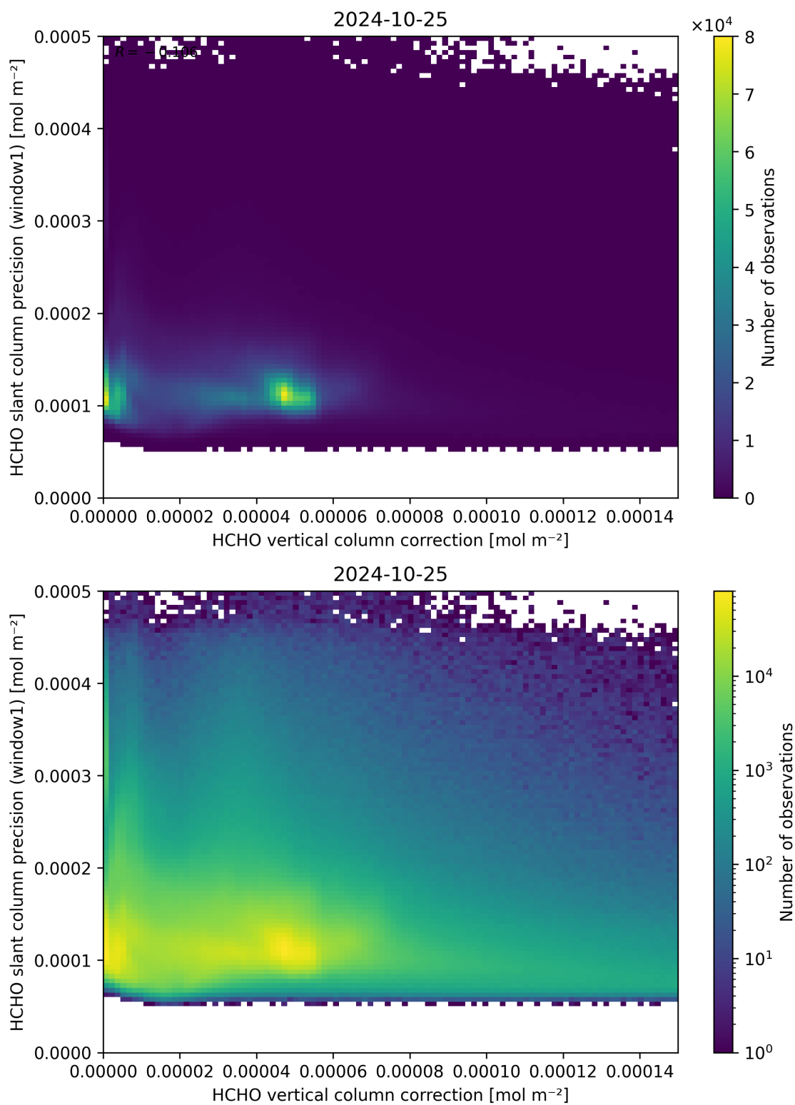
Figure 119: Scatter density plot of “HCHO vertical column correction” against “HCHO slant column precision (window1)” for 2024-10-24 to 2024-10-26.
