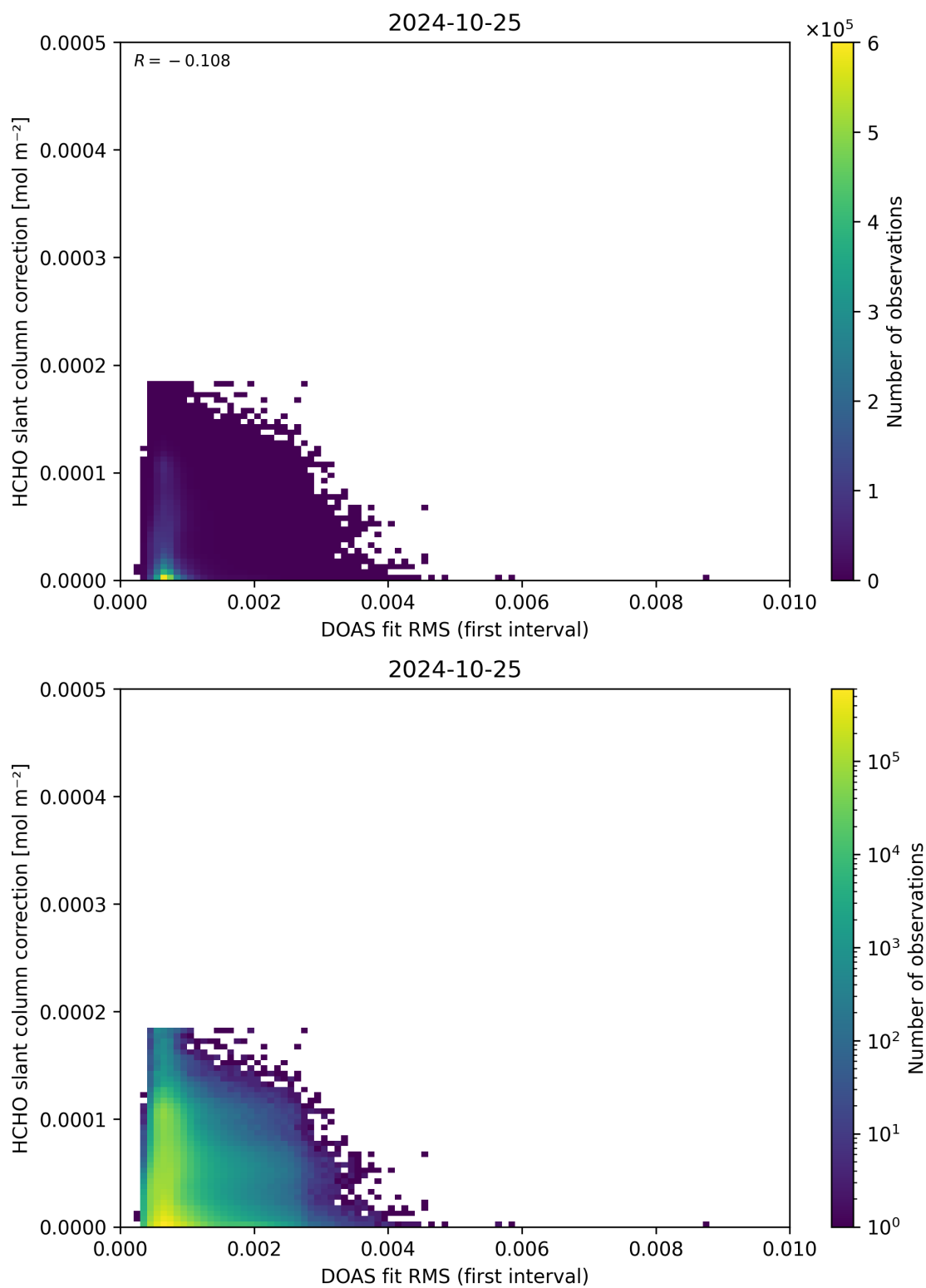
Figure 63: Scatter density plot of “DOAS fit RMS (first interval)” against “HCHO slant column correction” for 2024-10-24 to 2024-10-26.
