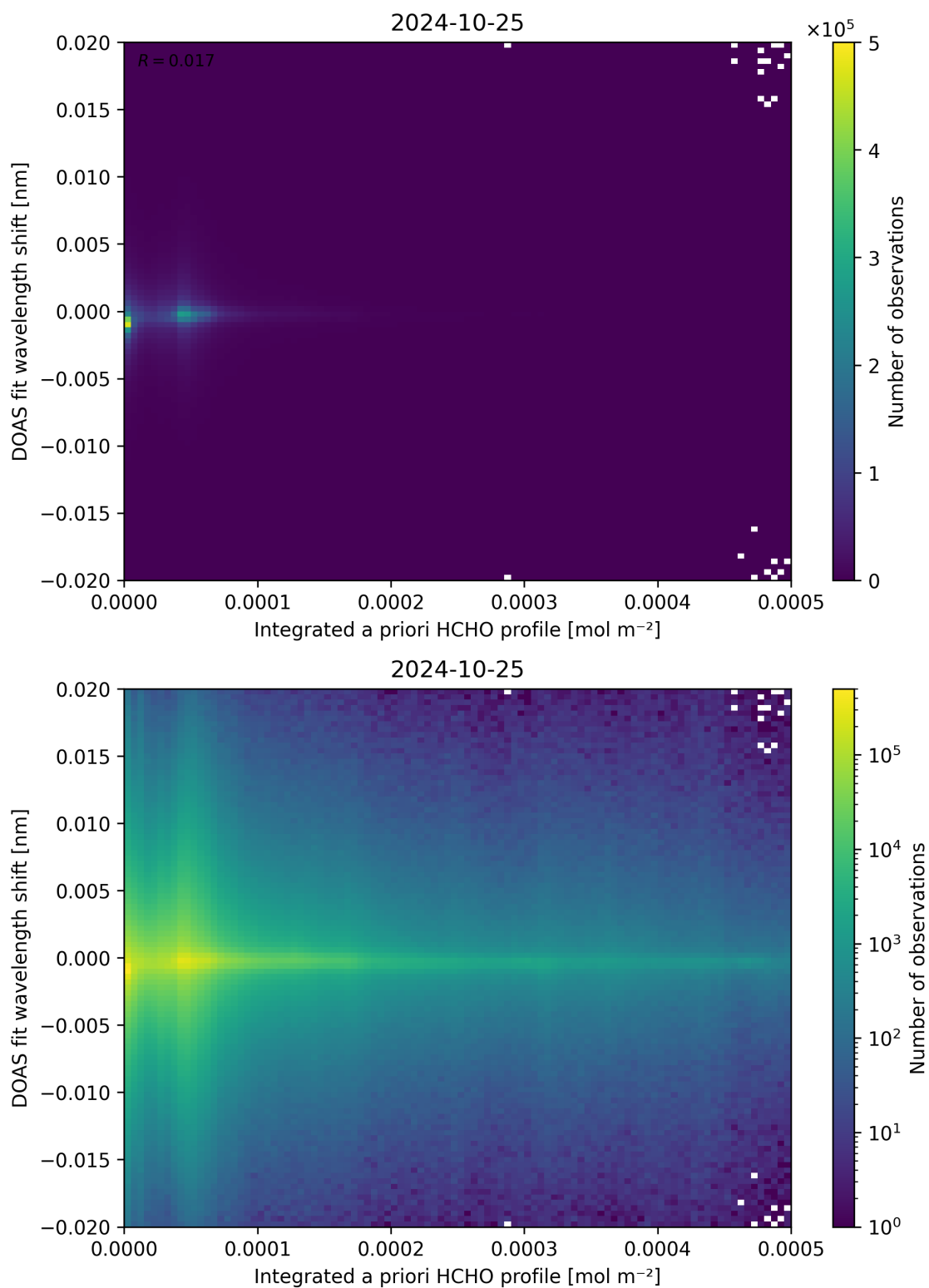
Figure 149: Scatter density plot of “Integrated a priori HCHO profile” against “DOAS fit wavelength shift” for 2024-10-24 to 2024-10-26.
