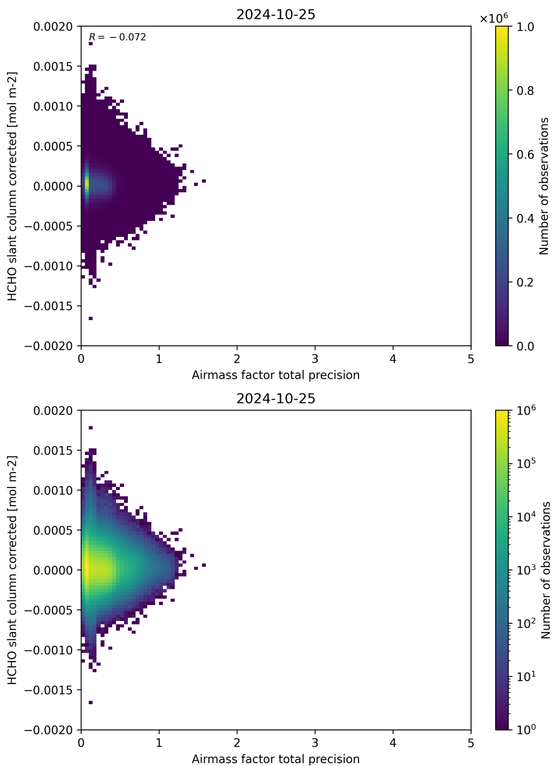
Figure 109: Scatter density plot of “Airmass factor total precision” against “HCHO slant column corrected” for 2024-10-24 to 2024-10-26.
