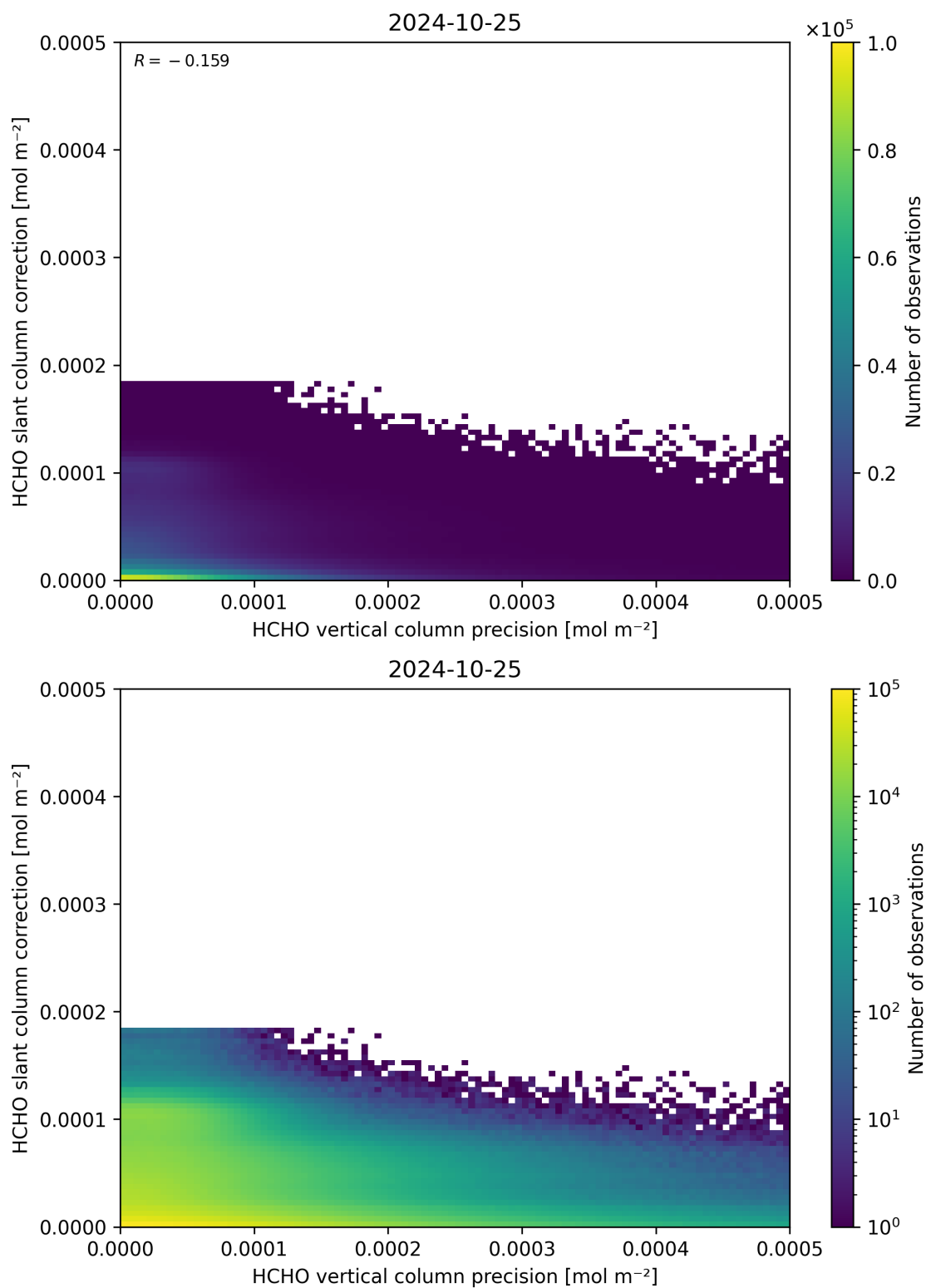
Figure 141: Scatter density plot of “HCHO vertical column precision” against “HCHO slant column correction” for 2024-10-24 to 2024-10-26.
