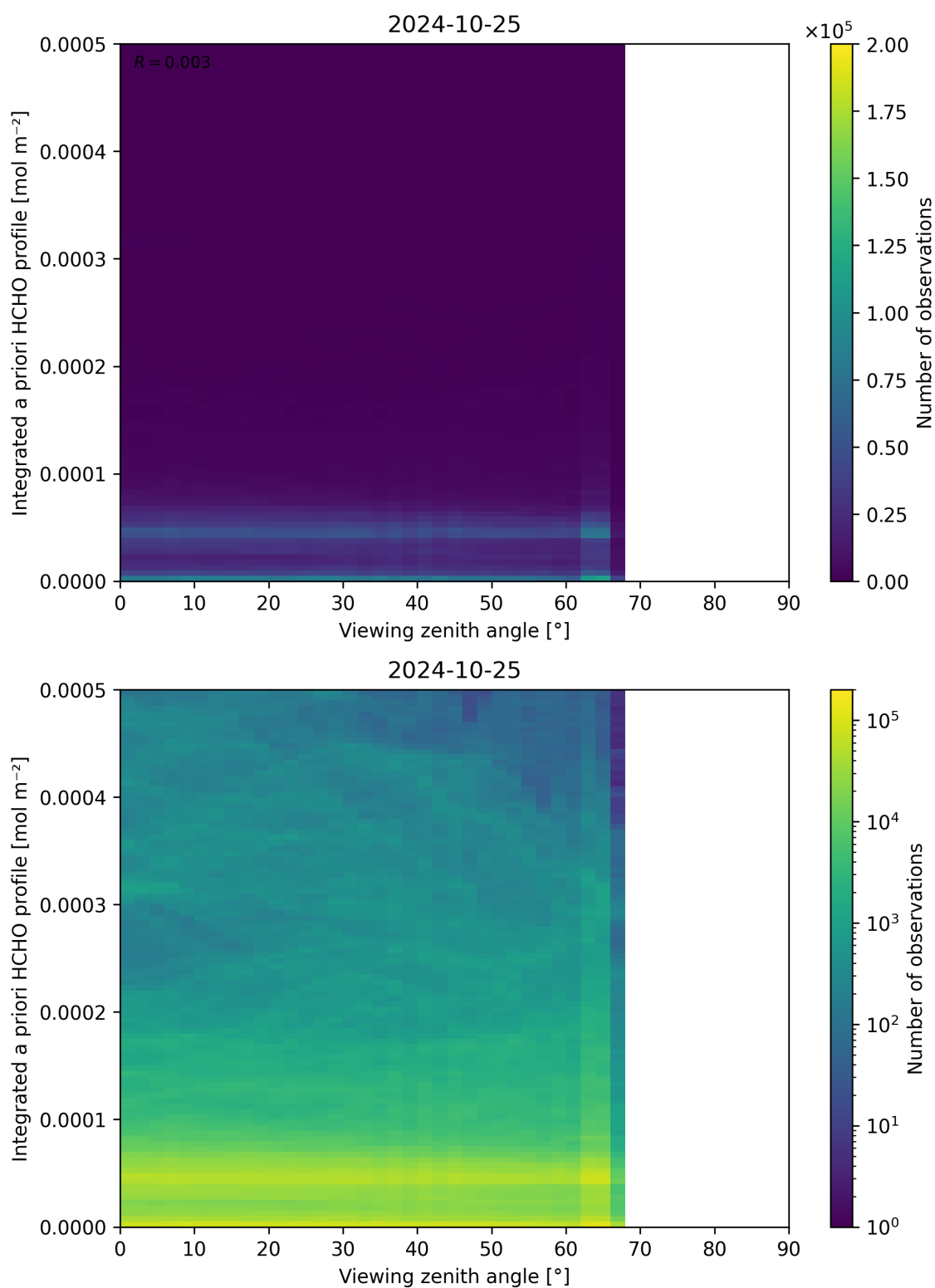
Figure 195: Scatter density plot of “Viewing zenith angle” against “Integrated a priori HCHO profile” for 2024-10-24 to 2024-10-26.
