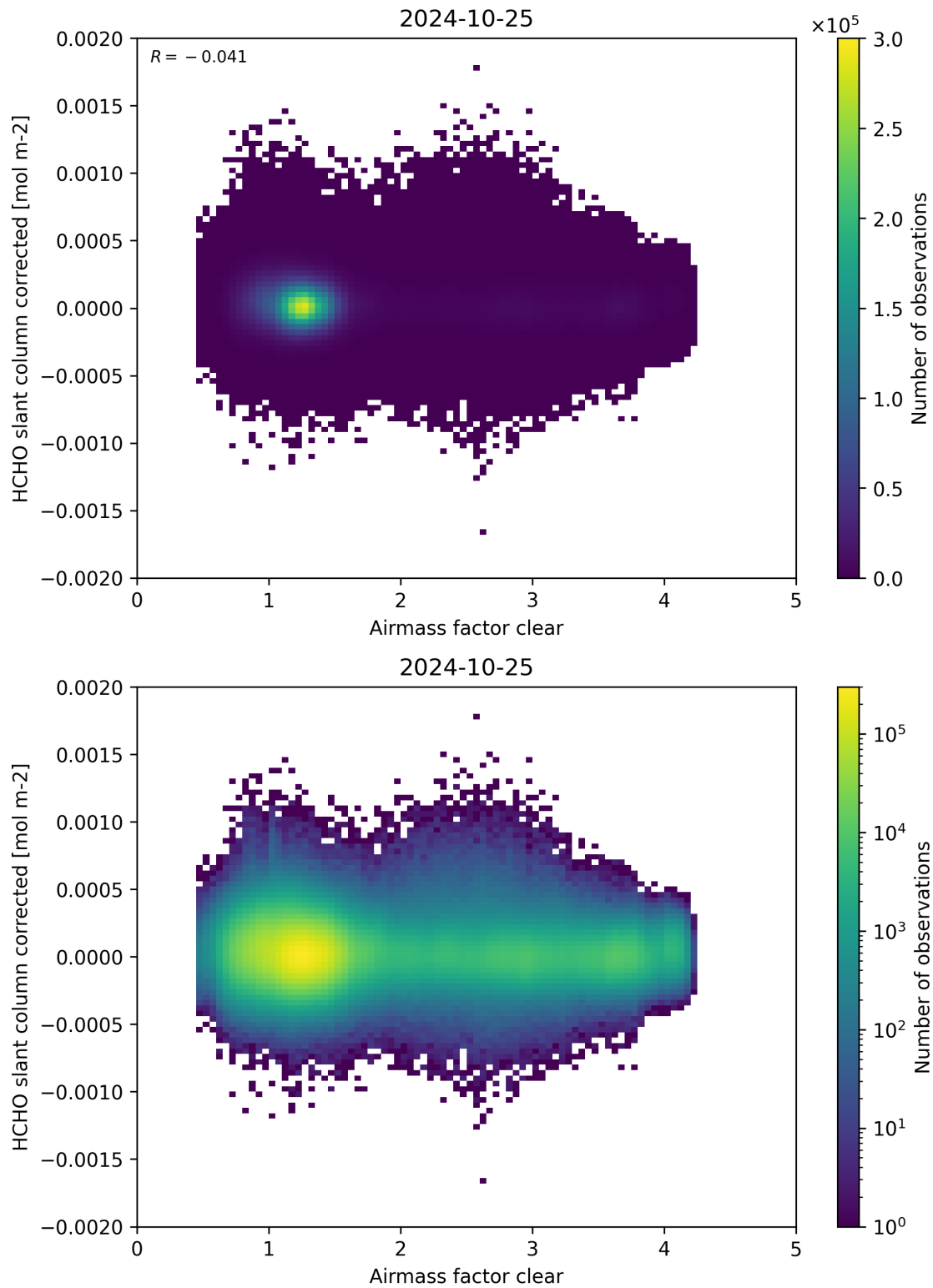
Figure 74: Scatter density plot of “Airmass factor clear” against “HCHO slant column corrected” for 2024-10-24 to 2024-10-26.
