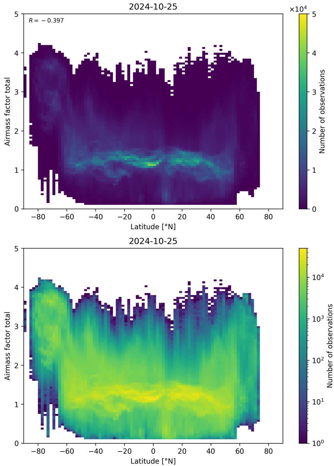
Figure 161: Scatter density plot of “Latitude” against “Airmass factor total” for 2024-10-24 to 2024-10-26.
