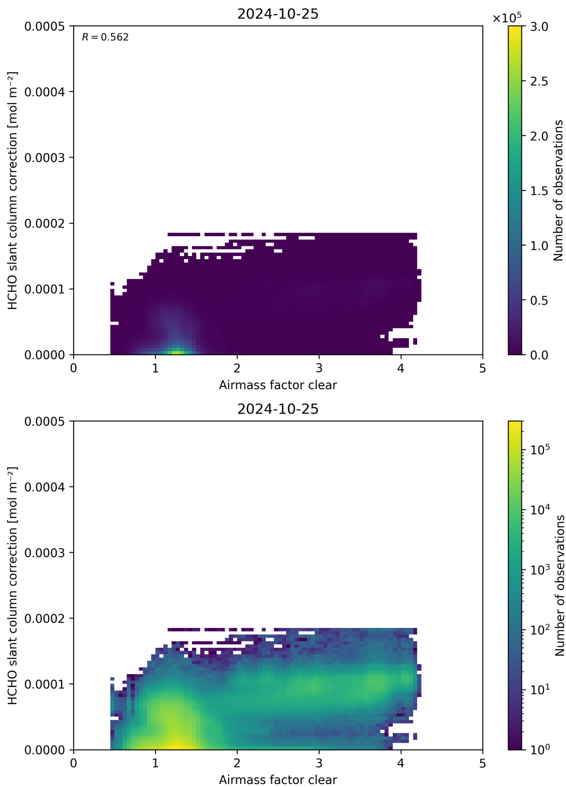
Figure 75: Scatter density plot of “Airmass factor clear” against “HCHO slant column correction” for 2024-10-24 to 2024-10-26.
