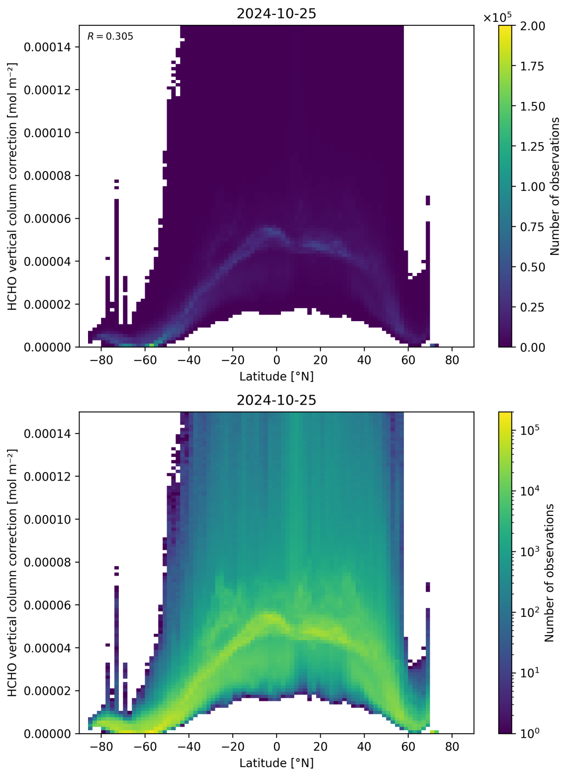
Figure 164: Scatter density plot of “Latitude” against “HCHO vertical column correction” for 2024-10-24 to 2024-10-26.
