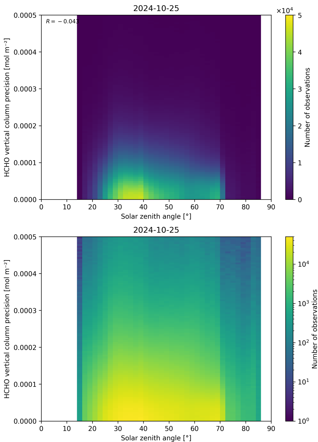
Figure 179: Scatter density plot of “Solar zenith angle” against “HCHO vertical column precision” for 2024-10-24 to 2024-10-26.
