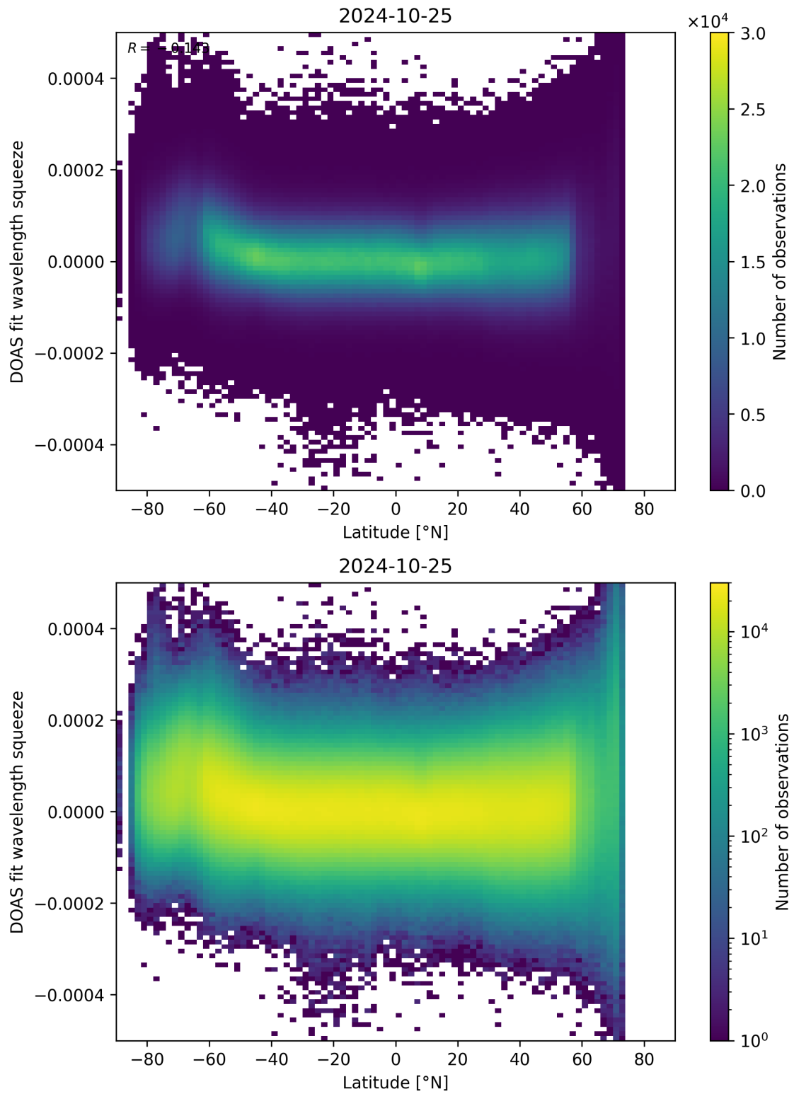
Figure 155: Scatter density plot of “Latitude” against “DOAS fit wavelength squeeze” for 2024-10-24 to 2024-10-26.
