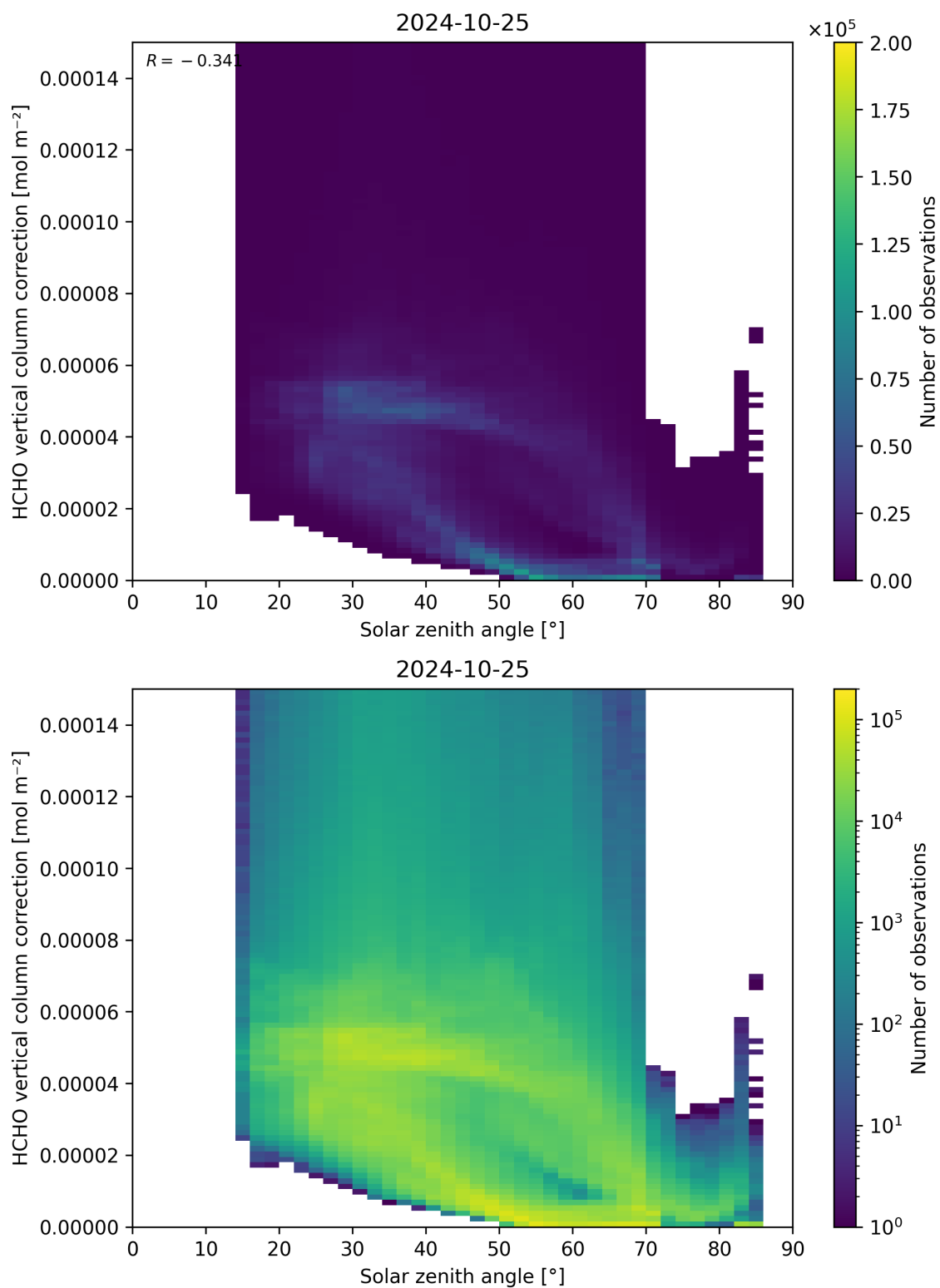
Figure 178: Scatter density plot of “Solar zenith angle” against “HCHO vertical column correction” for 2024-10-24 to 2024-10-26.
