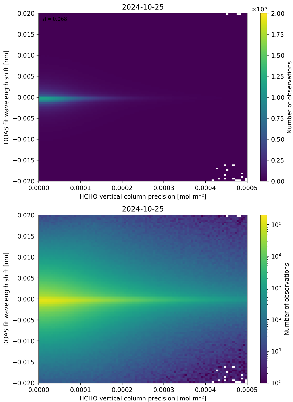
Figure 137: Scatter density plot of “HCHO vertical column precision” against “DOAS fit wavelength shift” for 2024-10-24 to 2024-10-26.
