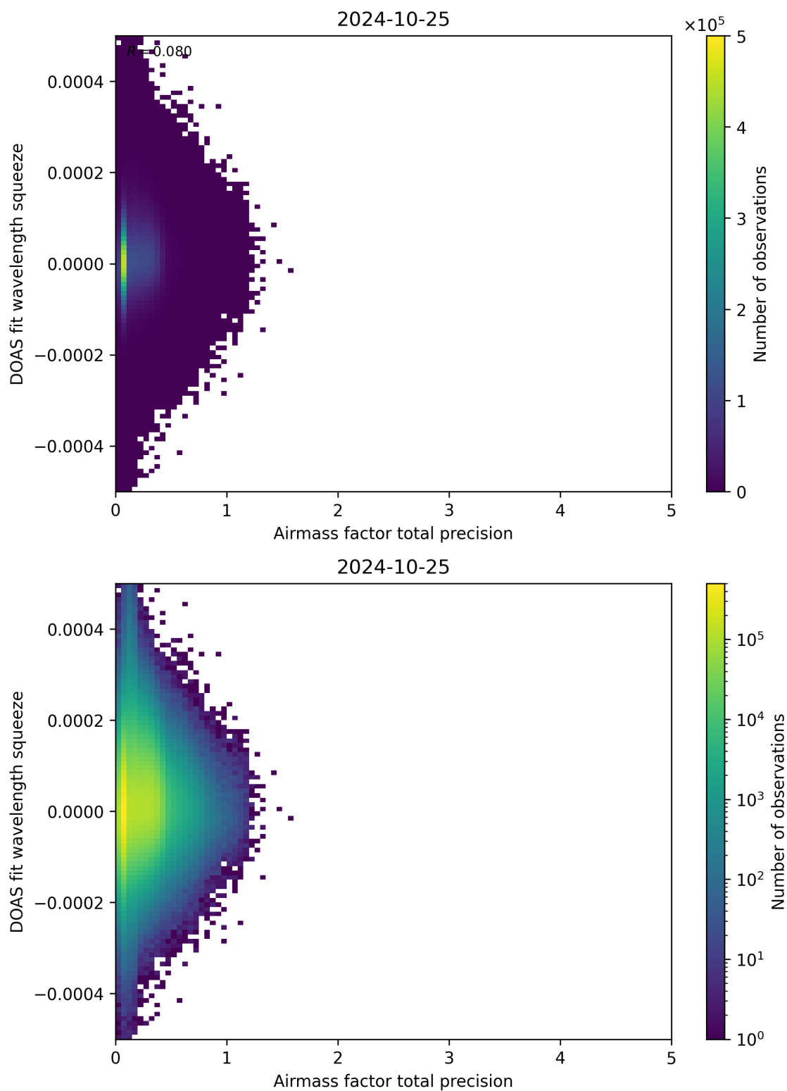
Figure 107: Scatter density plot of “Airmass factor total precision” against “DOAS fit wavelength squeeze” for 2024-10-24 to 2024-10-26.
