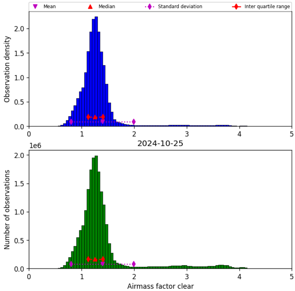
Figure 42: Histogram of “Airmass factor clear” for 2024-10-24 to 2024-10-26
