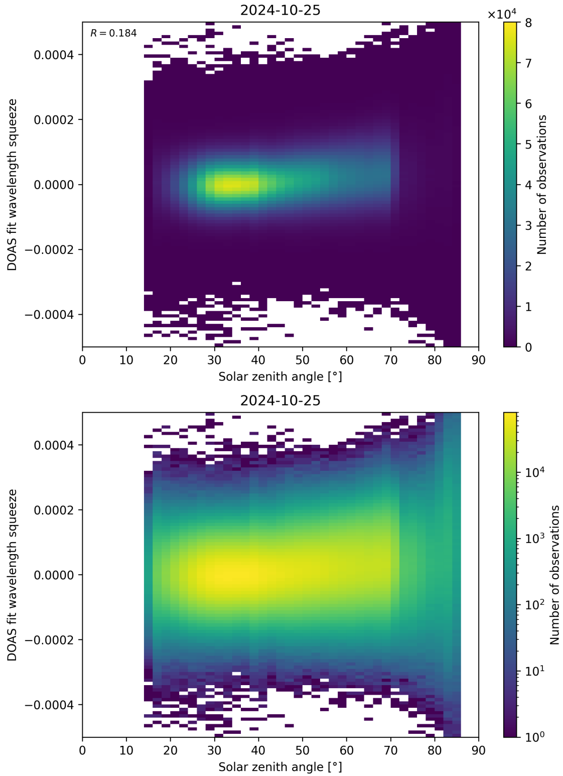
Figure 169: Scatter density plot of “Solar zenith angle” against “DOAS fit wavelength squeeze” for 2024-10-24 to 2024-10-26.
