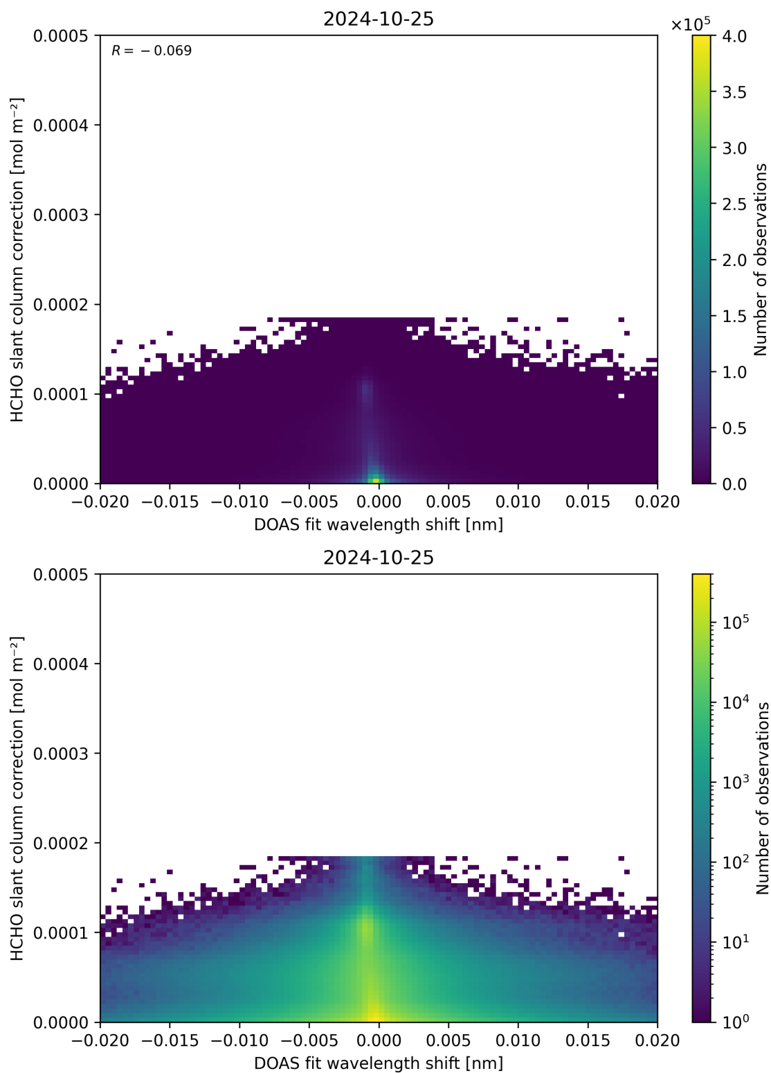
Figure 67: Scatter density plot of “DOAS fit wavelength shift” against “HCHO slant column correction” for 2024-10-24 to 2024-10-26.
