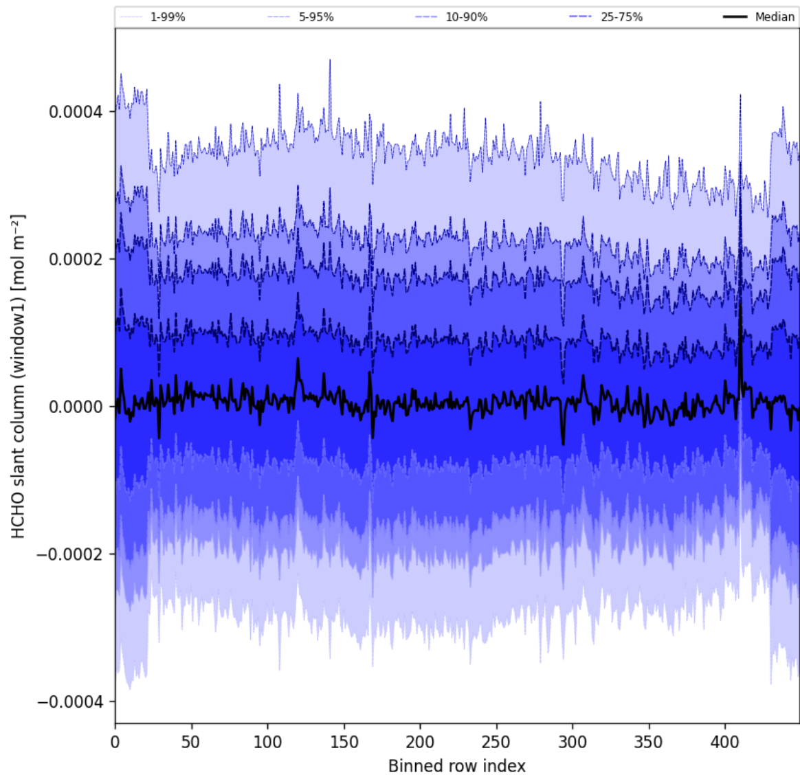
Figure 52: Along track statistics of “HCHO slant column (window1)” for 2024-10-24 to 2024-10-26
