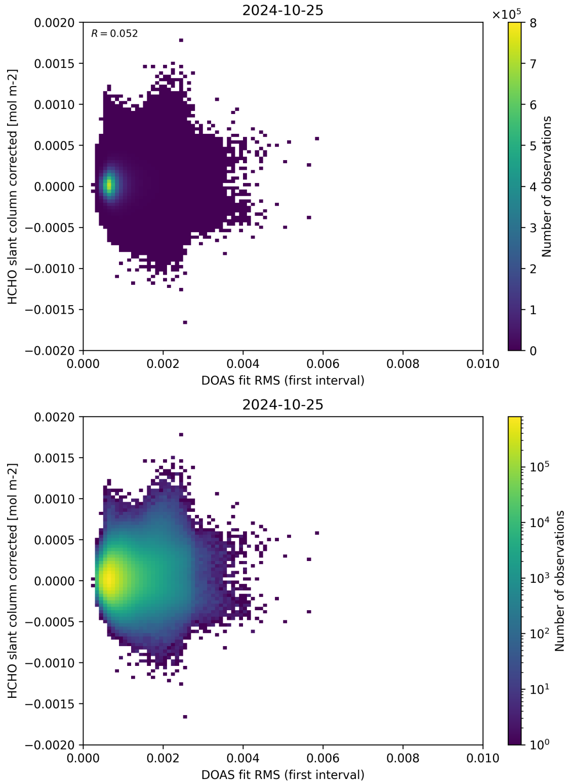
Figure 62: Scatter density plot of “DOAS fit RMS (first interval)” against “HCHO slant column corrected” for 2024-10-24 to 2024-10-26.
