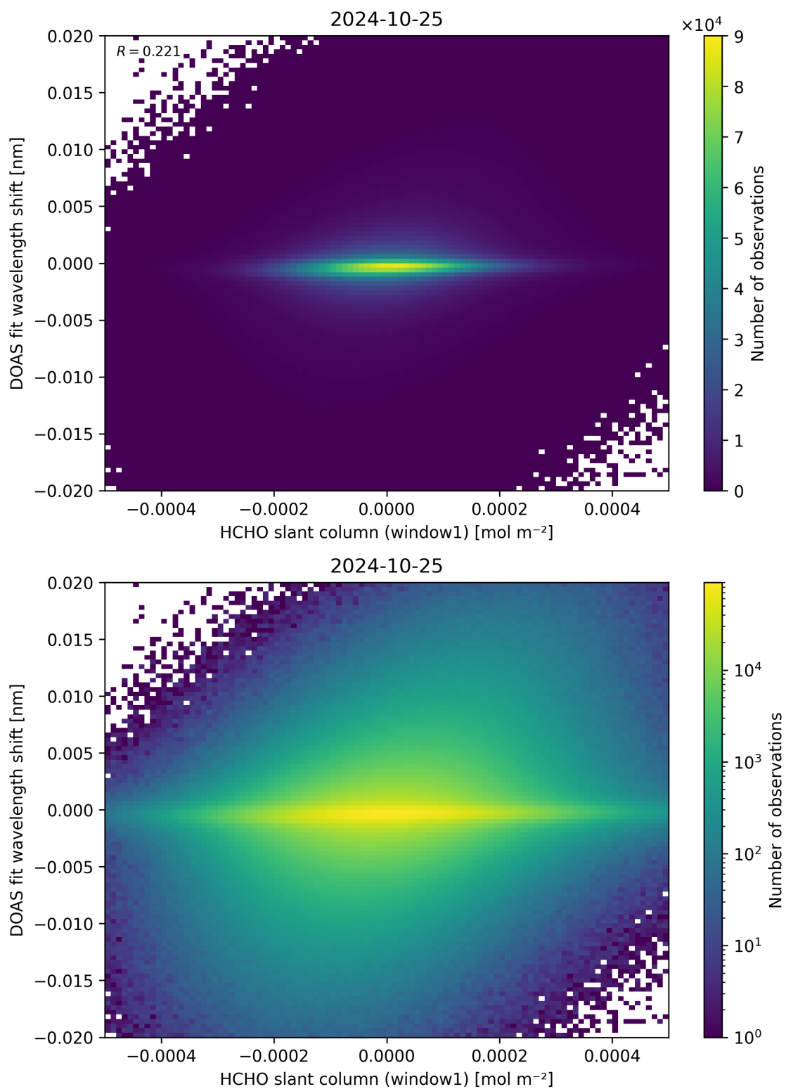
Figure 79: Scatter density plot of “HCHO slant column (window1)” against “DOAS fit wavelength shift” for 2024-10-24 to 2024-10-26.
