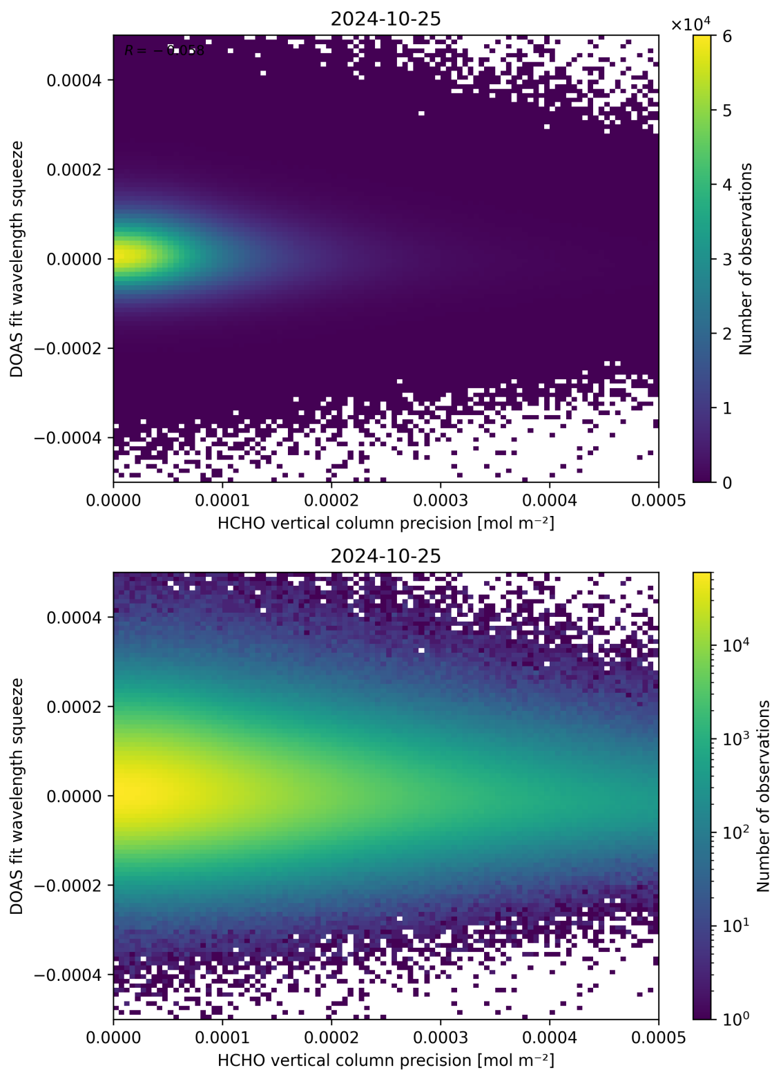
Figure 138: Scatter density plot of “HCHO vertical column precision” against “DOAS fit wavelength squeeze” for 2024-10-24 to 2024-10-26.
