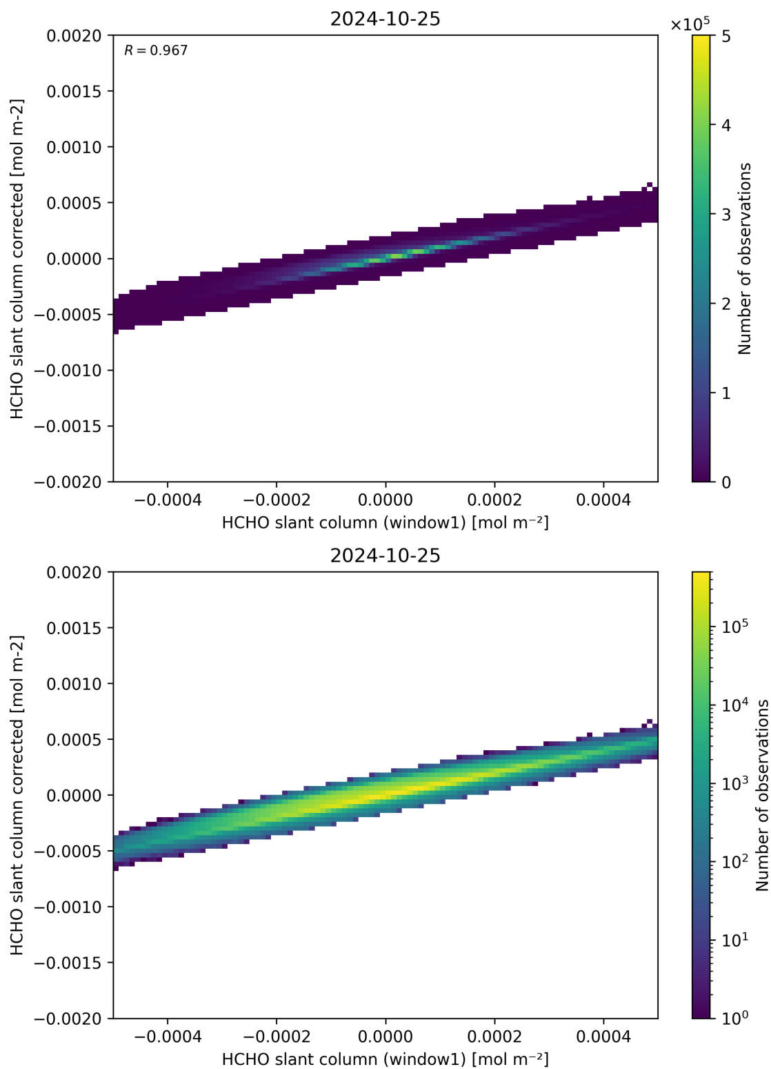
Figure 82: Scatter density plot of “HCHO slant column (window1)” against “HCHO slant column corrected” for 2024-10-24 to 2024-10-26.
