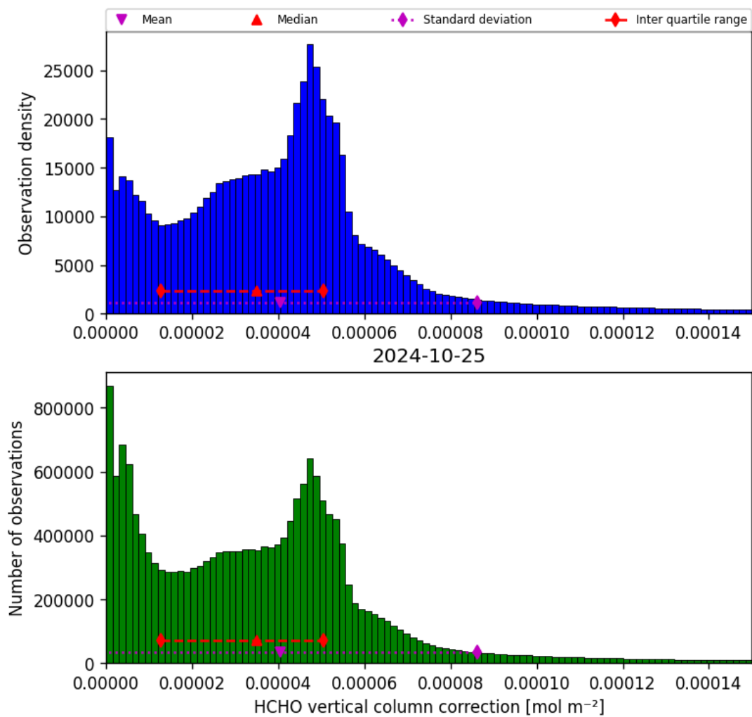
Figure 37: Histogram of “HCHO vertical column correction” for 2024-10-24 to 2024-10-26
