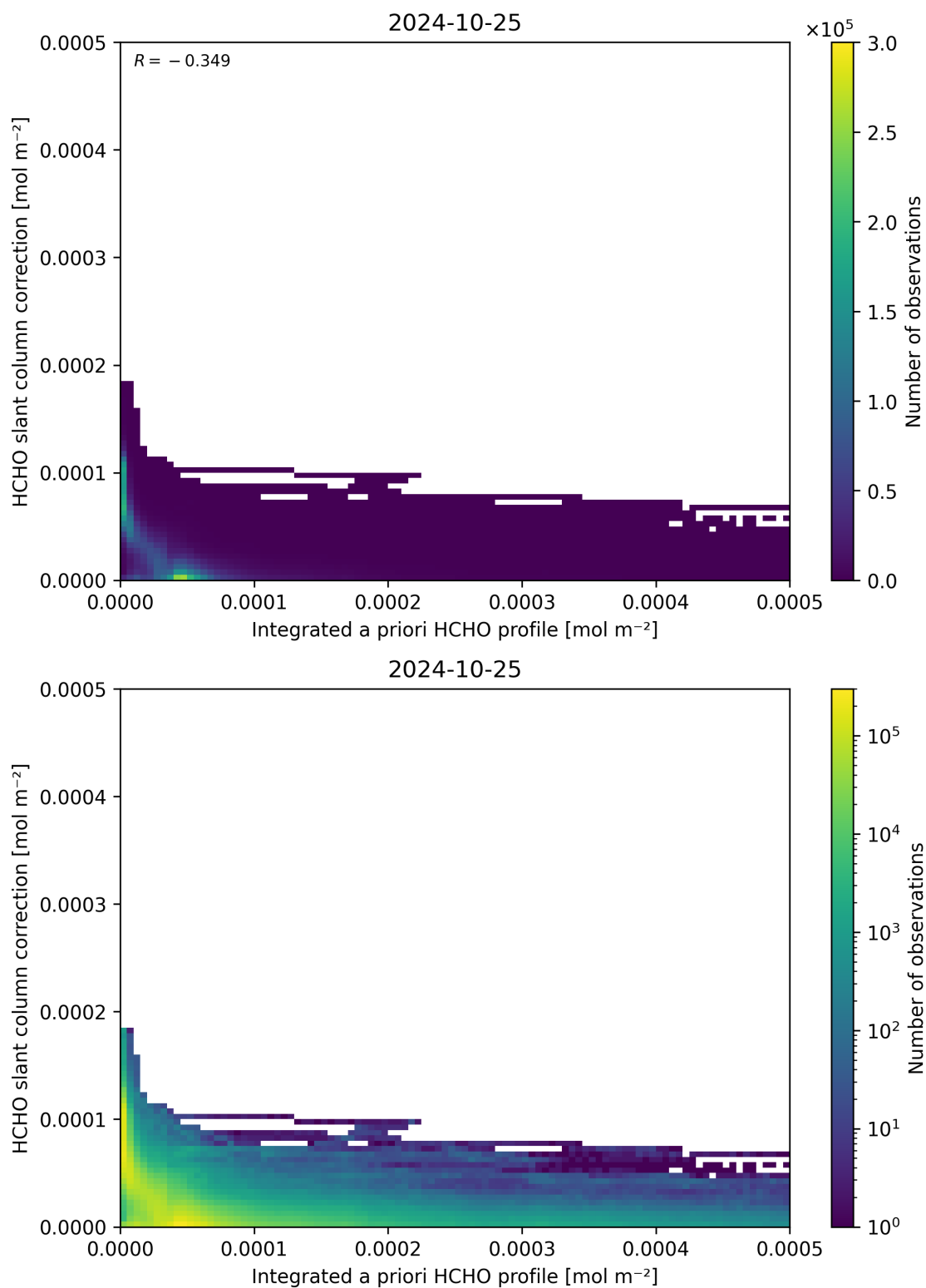
Figure 152: Scatter density plot of “Integrated a priori HCHO profile” against “HCHO slant column correction” for 2024-10-24 to 2024-10-26.
