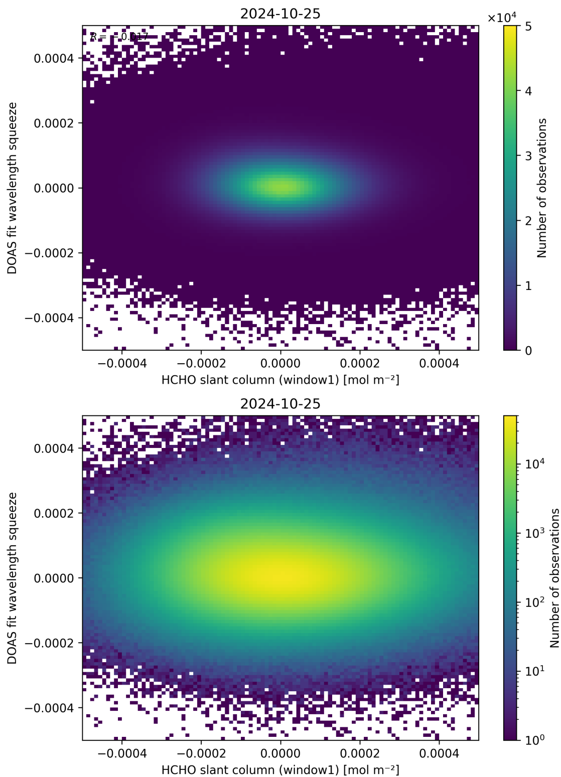
Figure 80: Scatter density plot of “HCHO slant column (window1)” against “DOAS fit wavelength squeeze” for 2024-10-24 to 2024-10-26.
