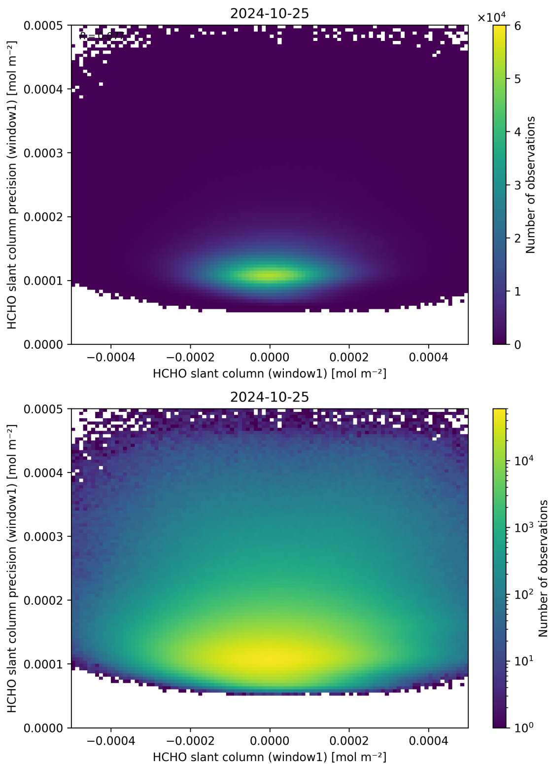
Figure 84: Scatter density plot of “HCHO slant column (window1)” against “HCHO slant column precision (window1)” for 2024-10-24 to 2024-10-26.
