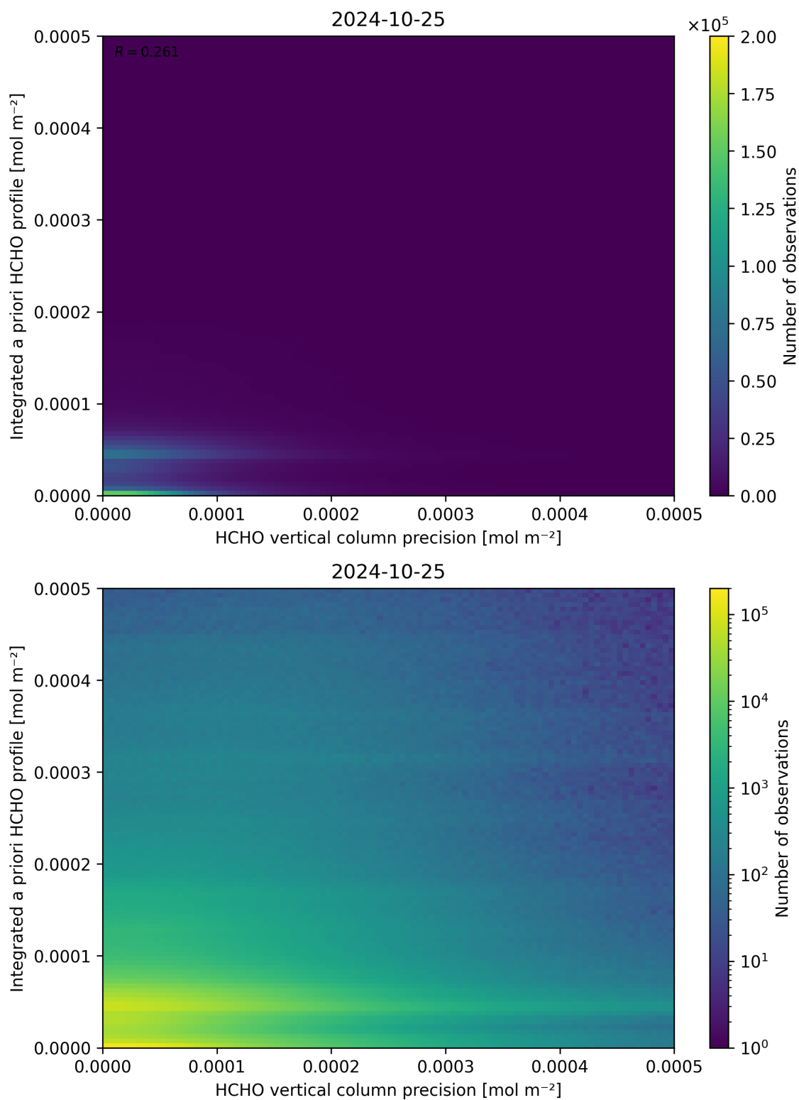
Figure 147: Scatter density plot of “HCHO vertical column precision” against “Integrated a priori HCHO profile” for 2024-10-24 to 2024-10-26.
