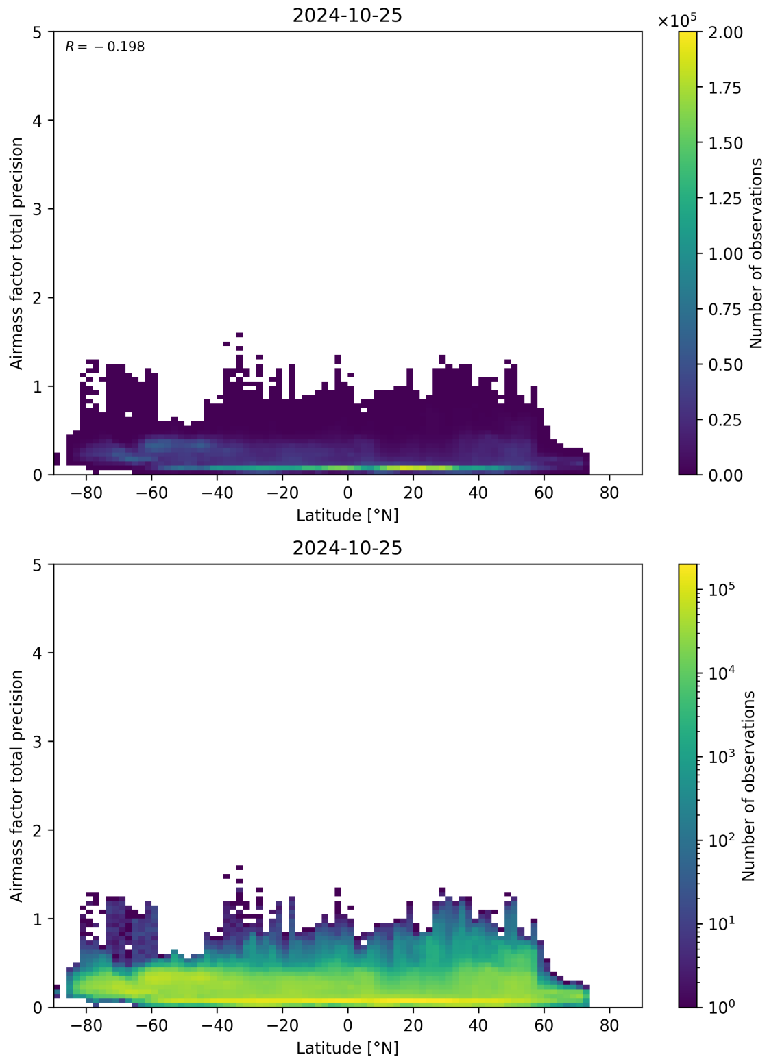
Figure 162: Scatter density plot of “Latitude” against “Airmass factor total precision” for 2024-10-24 to 2024-10-26.
