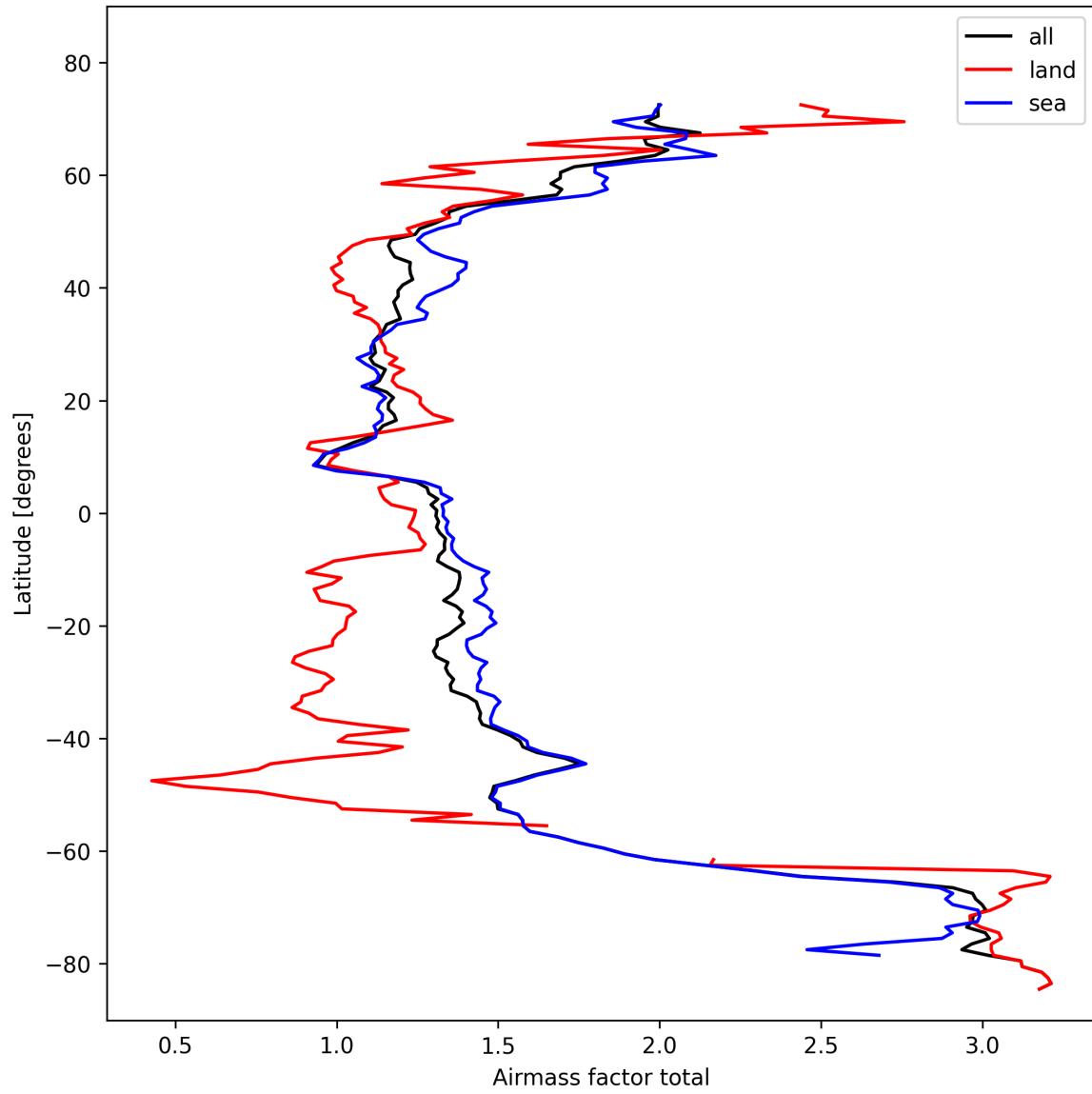
Figure 26: Zonal average of “Airmass factor total” for 2024-10-24 to 2024-10-26.
