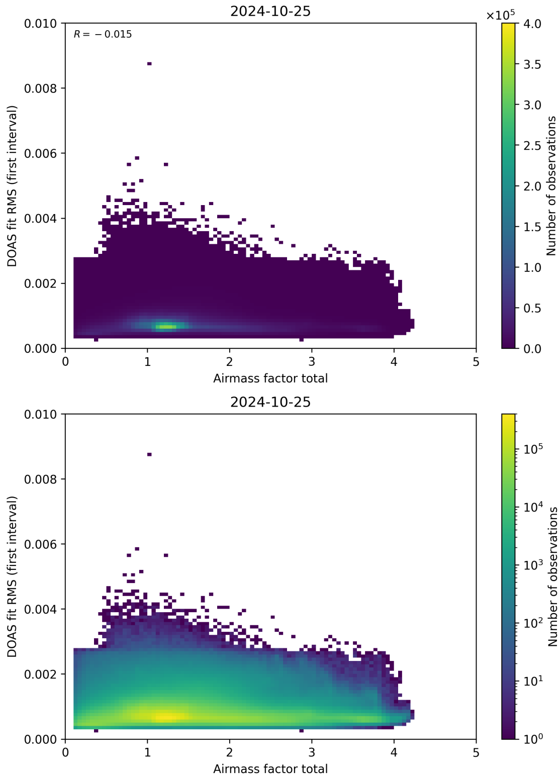
Figure 97: Scatter density plot of “Airmass factor total” against “DOAS fit RMS (first interval)” for 2024-10-24 to 2024-10-26.
