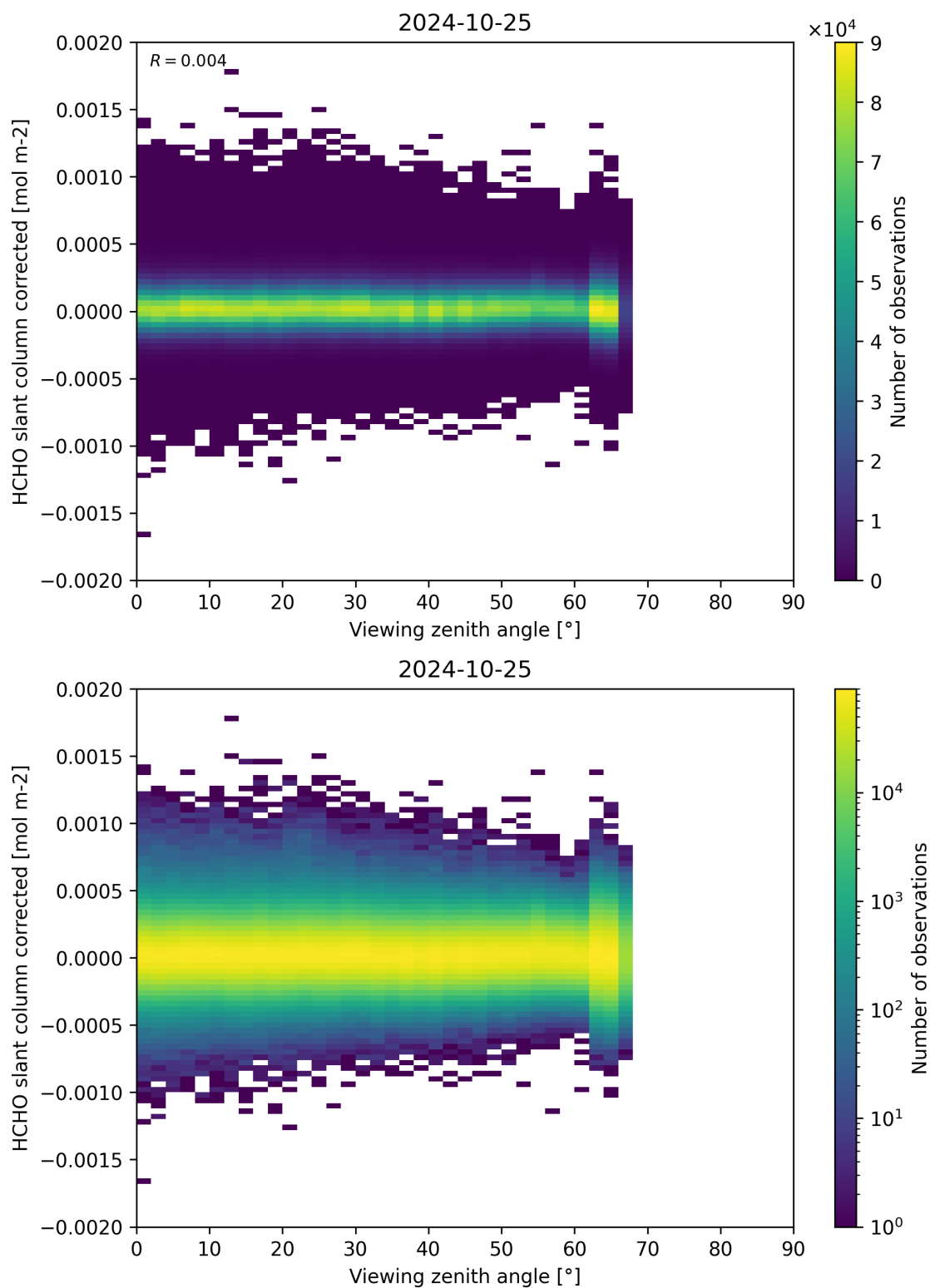
Figure 186: Scatter density plot of “Viewing zenith angle” against “HCHO slant column corrected” for 2024-10-24 to 2024-10-26.
