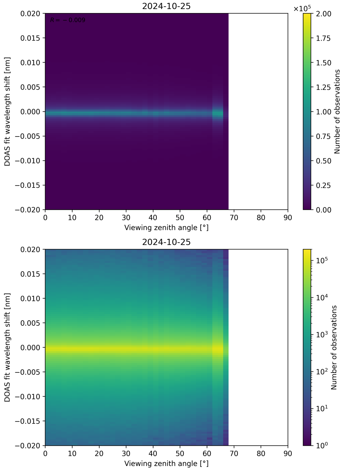
Figure 183: Scatter density plot of “Viewing zenith angle” against “DOAS fit wavelength shift” for 2024-10-24 to 2024-10-26.
