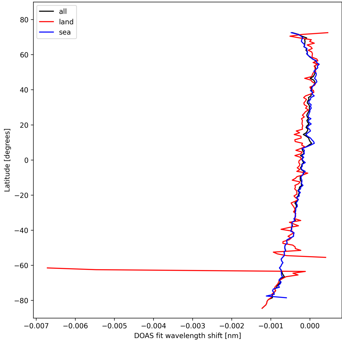
Figure 30: Zonal average of “DOAS fit wavelength shift” for 2024-10-24 to 2024-10-26.
