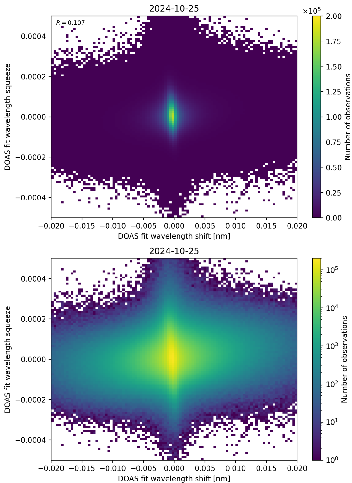
Figure 65: Scatter density plot of “DOAS fit wavelength shift” against “DOAS fit wavelength squeeze” for 2024-10-24 to 2024-10-26.
