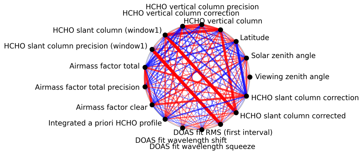
Figure 1: Map of correlation graph for 2024-10-24 to 2024-10-26.
