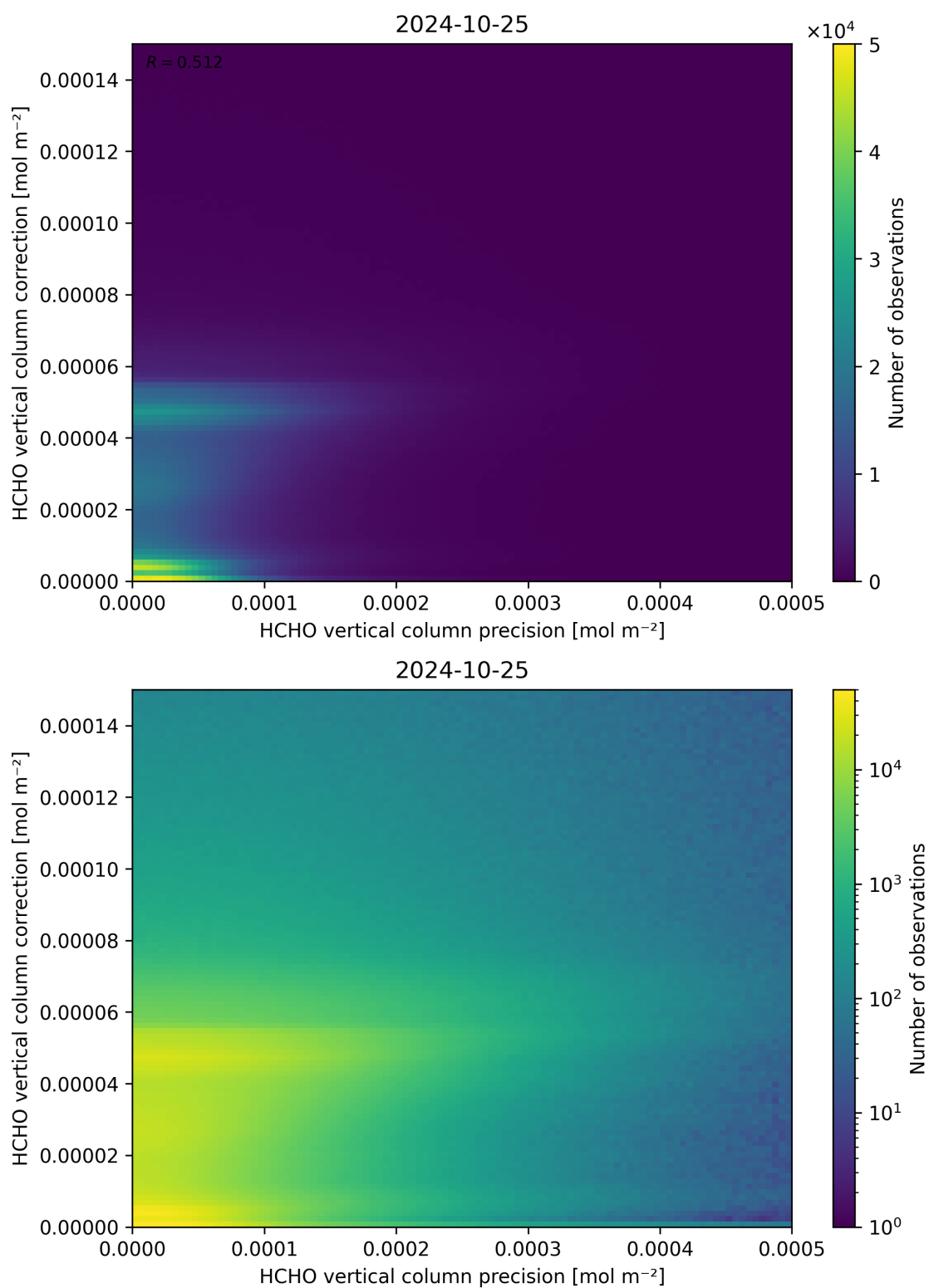
Figure 146: Scatter density plot of “HCHO vertical column precision” against “HCHO vertical column correction” for 2024-10-24 to 2024-10-26.
