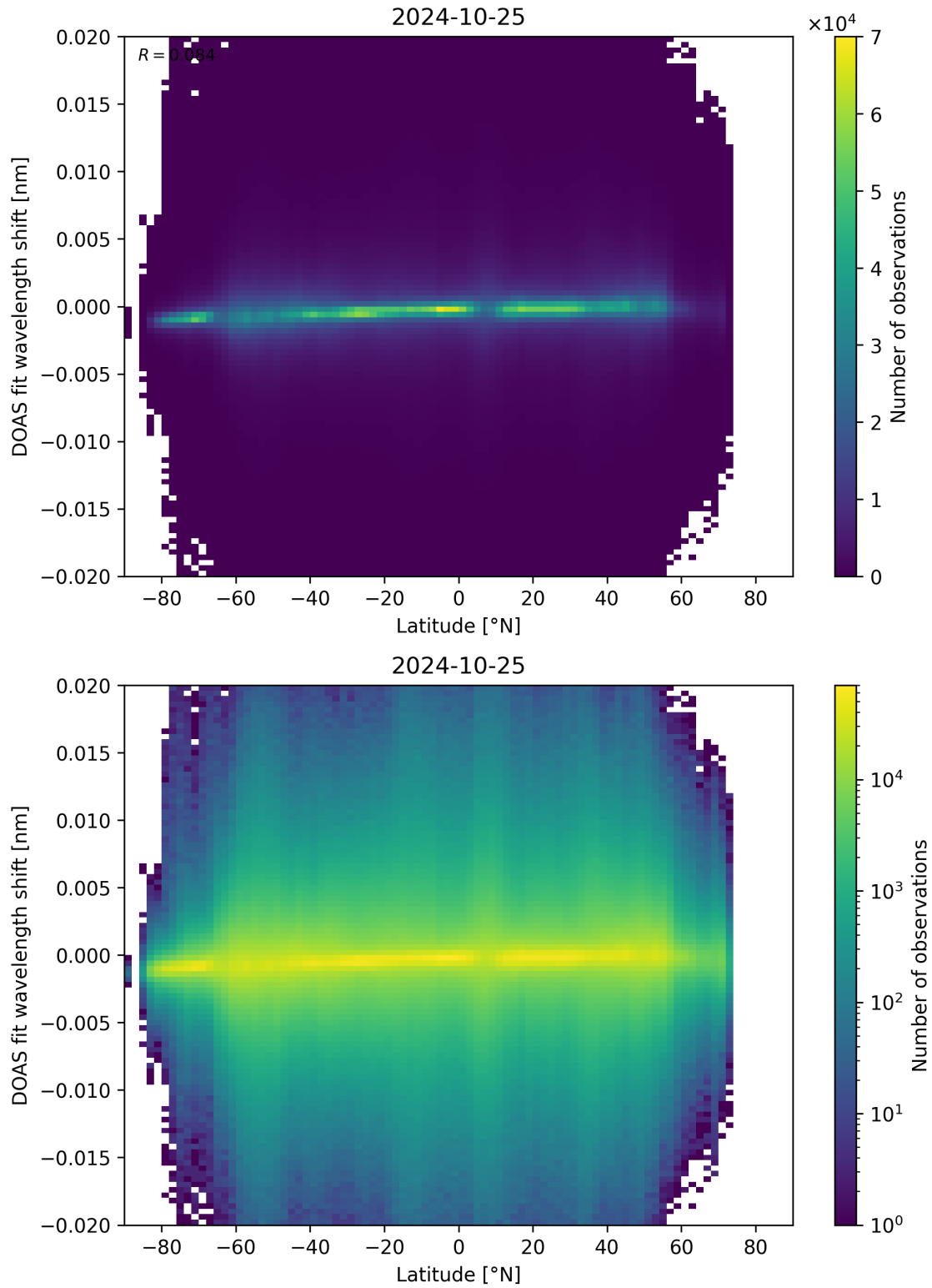
Figure 154: Scatter density plot of “Latitude” against “DOAS fit wavelength shift” for 2024-10-24 to 2024-10-26.
