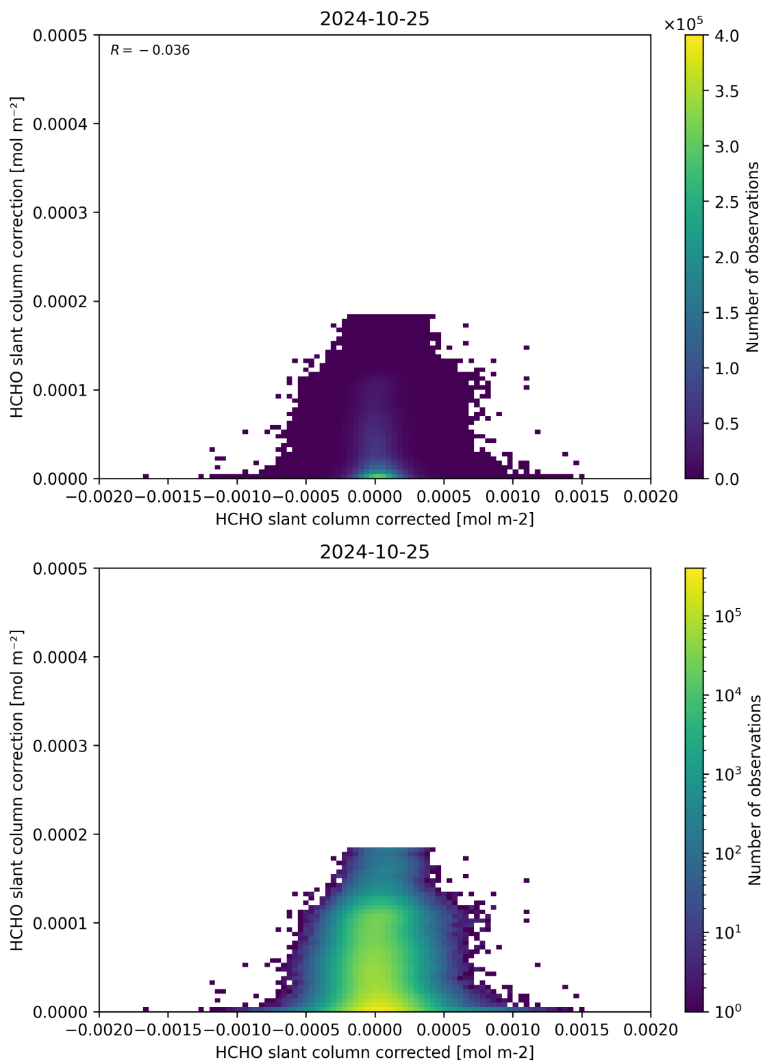
Figure 77: Scatter density plot of “HCHO slant column corrected” against “HCHO slant column correction” for 2024-10-24 to 2024-10-26.
