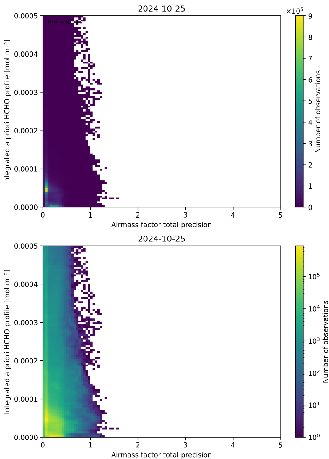
Figure 111: Scatter density plot of “Airmass factor total precision” against “Integrated a priori HCHO profile” for 2024-10-24 to 2024-10-26.
