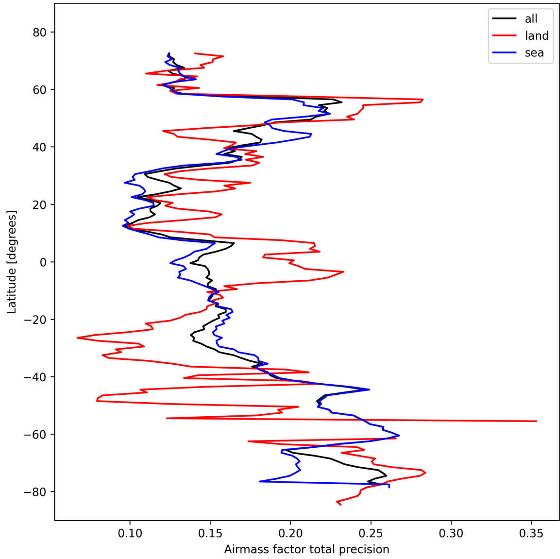
Figure 27: Zonal average of “Airmass factor total precision” for 2024-10-24 to 2024-10-26.
