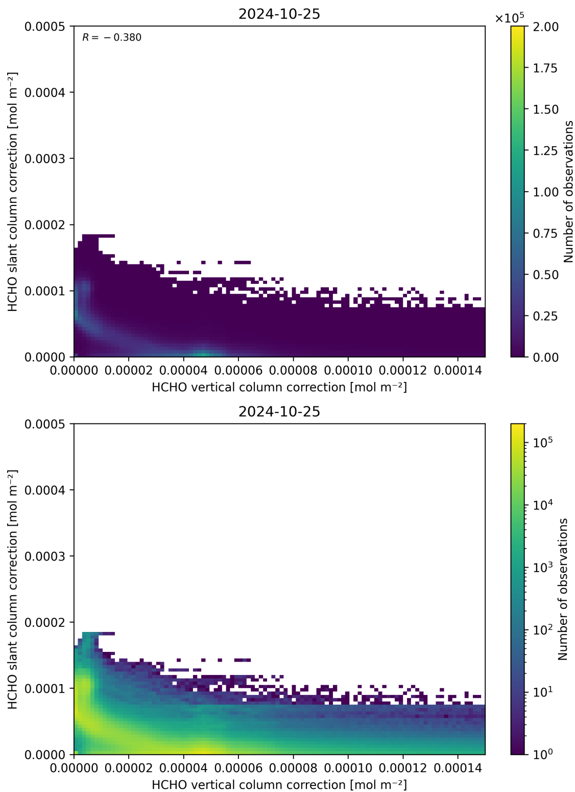
Figure 117: Scatter density plot of “HCHO vertical column correction” against “HCHO slant column correction” for 2024-10-24 to 2024-10-26.
