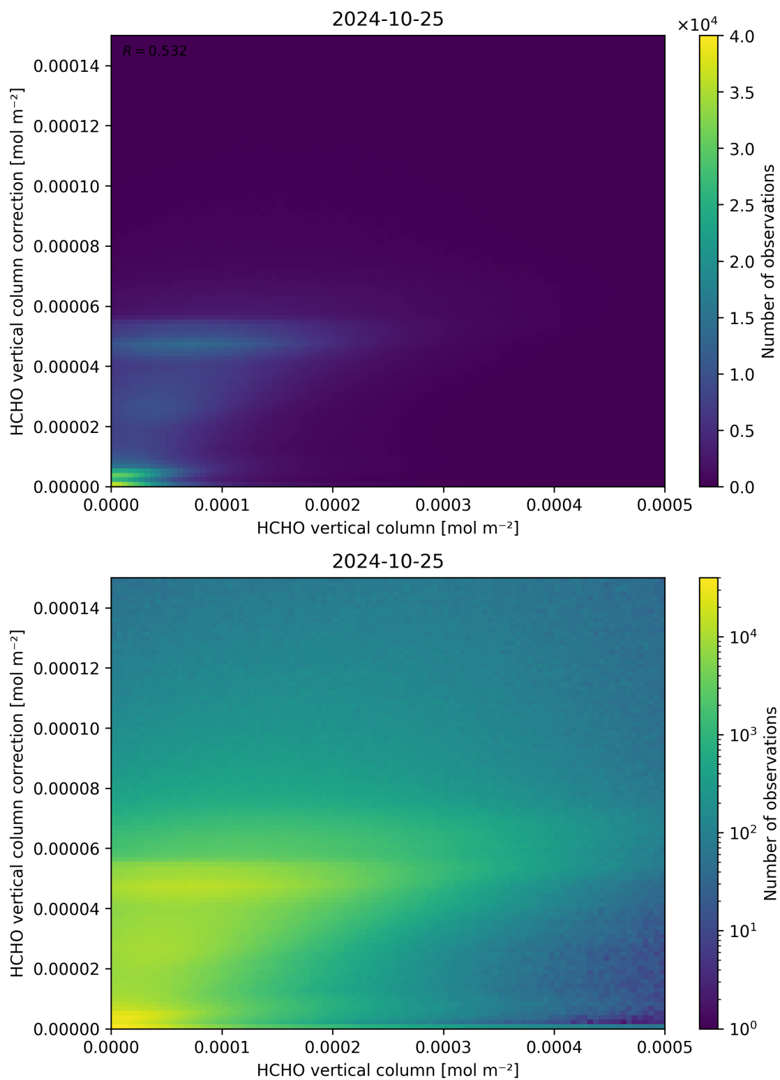
Figure 133: Scatter density plot of “HCHO vertical column” against “HCHO vertical column correction” for 2024-10-24 to 2024-10-26.
