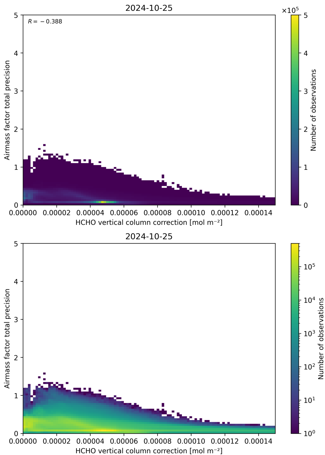
Figure 121: Scatter density plot of “HCHO vertical column correction” against “Airmass factor total precision” for 2024-10-24 to 2024-10-26.
