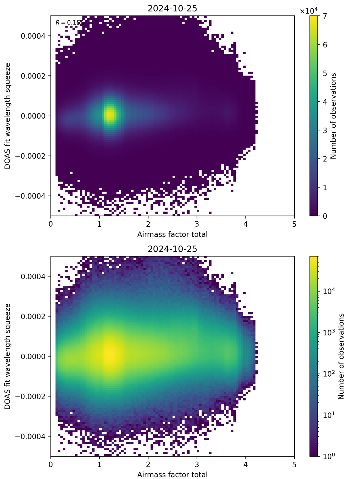
Figure 99: Scatter density plot of “Airmass factor total” against “DOAS fit wavelength squeeze” for 2024-10-24 to 2024-10-26.
