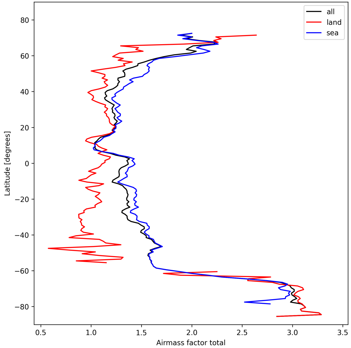
Figure 26: Zonal average of “Airmass factor total” for 2024-10-26 to 2024-10-28.
