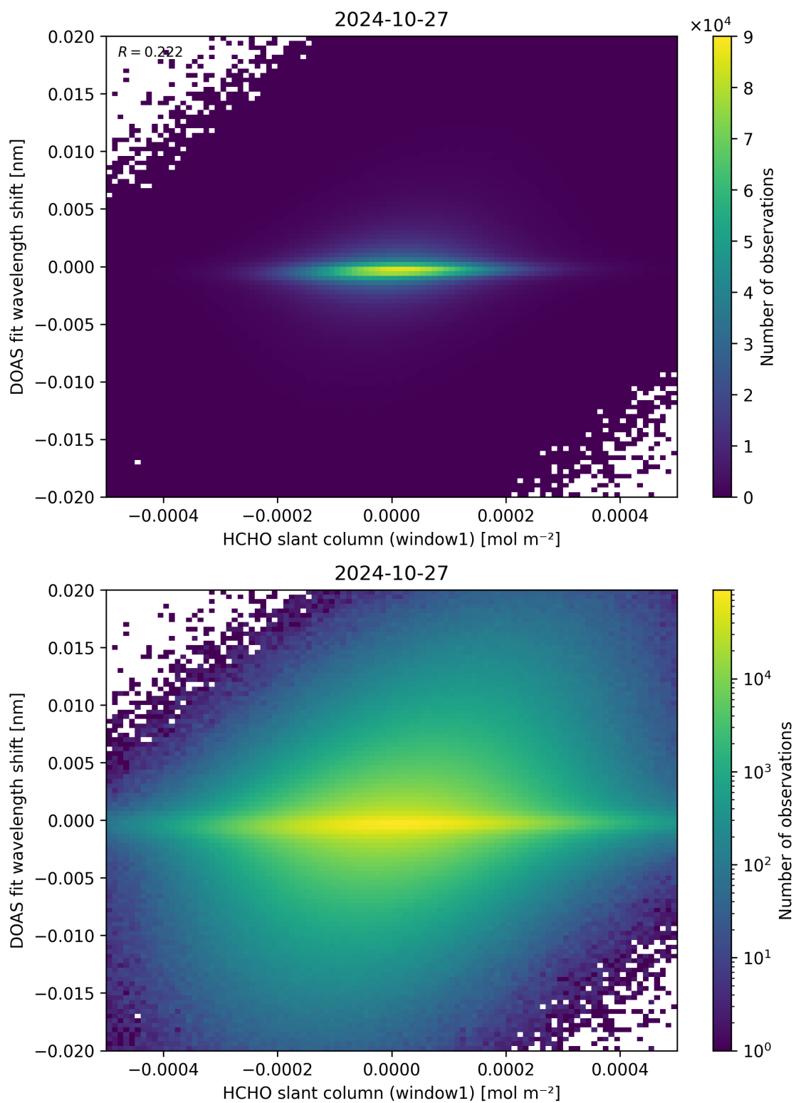
Figure 79: Scatter density plot of “HCHO slant column (window1)” against “DOAS fit wavelength shift” for 2024-10-26 to 2024-10-28.
