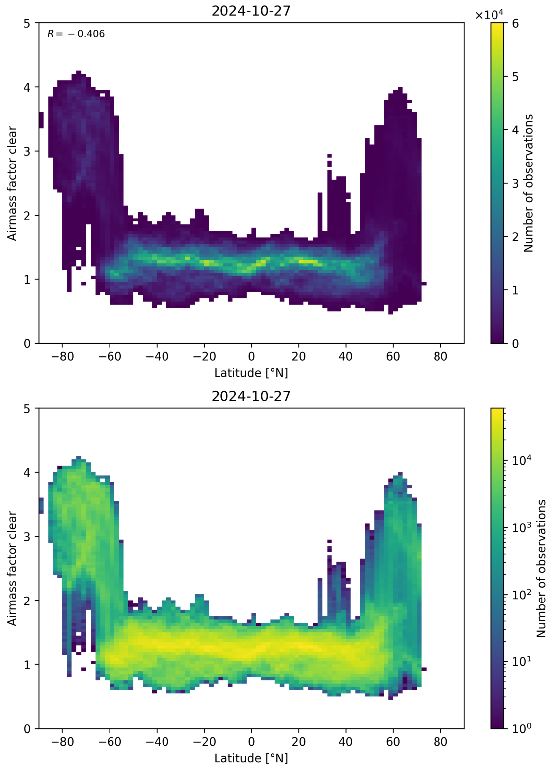
Figure 156: Scatter density plot of “Latitude” against “Airmass factor clear” for 2024-10-26 to 2024-10-28.
