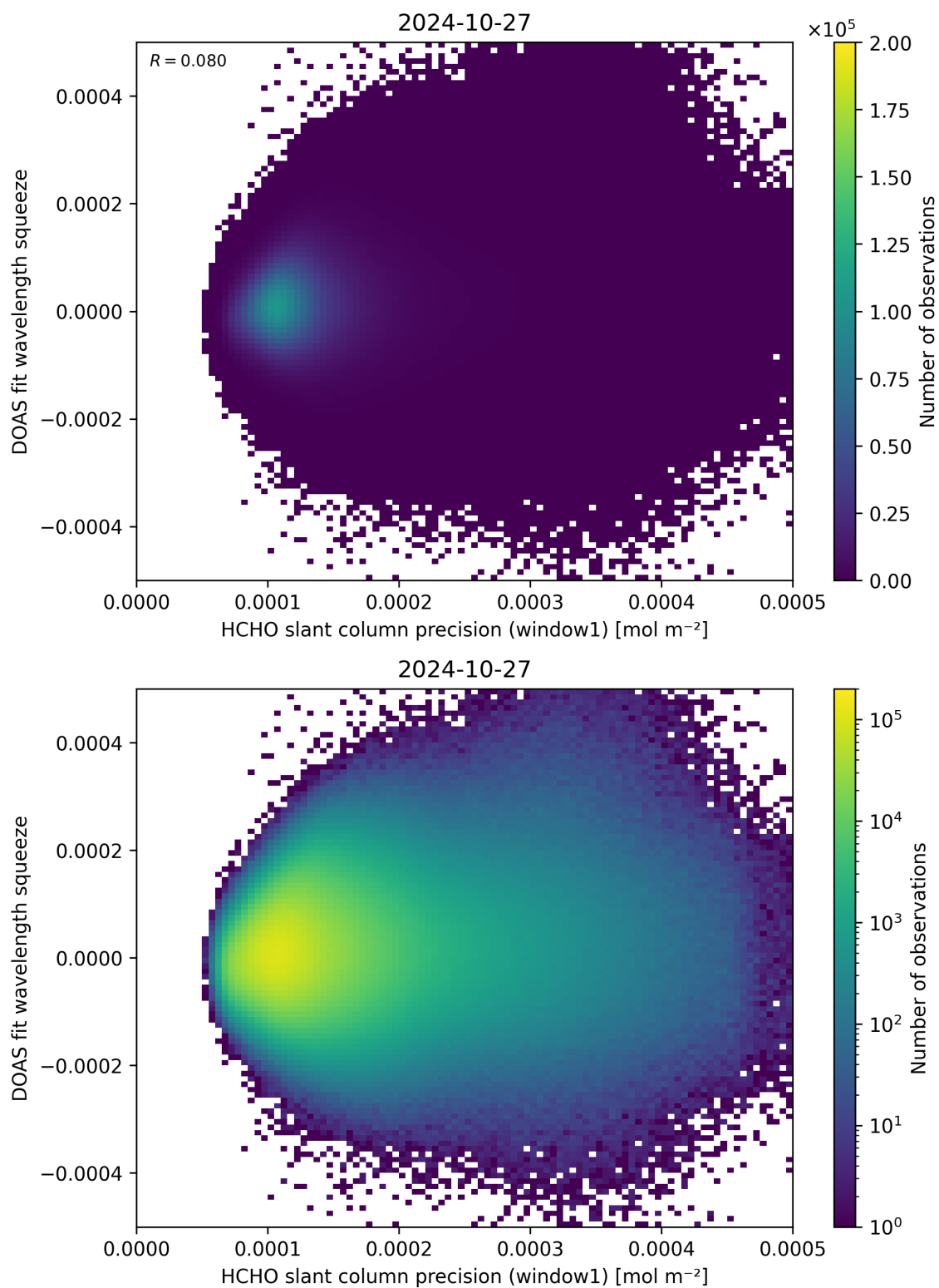
Figure 90: Scatter density plot of “HCHO slant column precision (window1)” against “DOAS fit wavelength squeeze” for 2024-10-26 to 2024-10-28.
