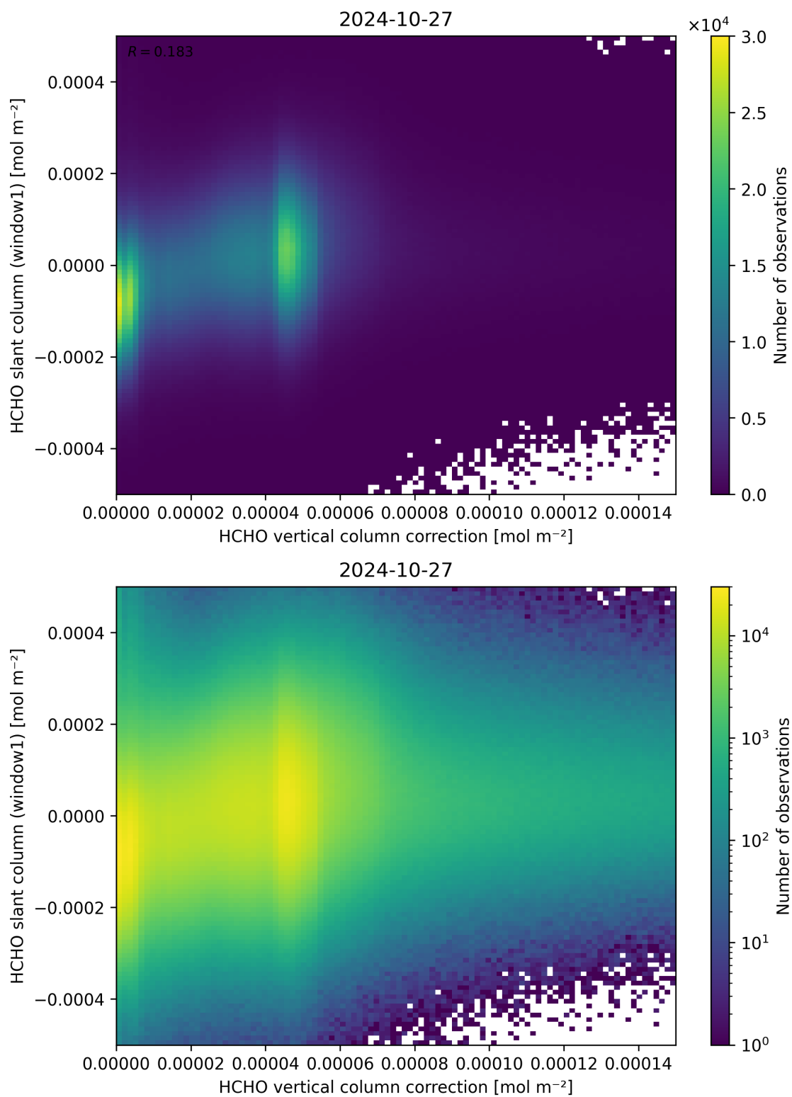
Figure 118: Scatter density plot of “HCHO vertical column correction” against “HCHO slant column (window1)” for 2024-10-26 to 2024-10-28.
