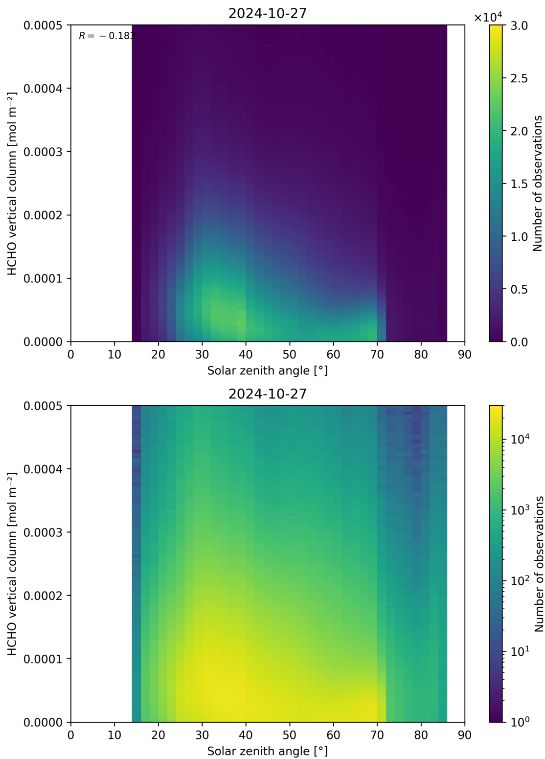
Figure 177: Scatter density plot of “Solar zenith angle” against “HCHO vertical column” for 2024-10-26 to 2024-10-28.
