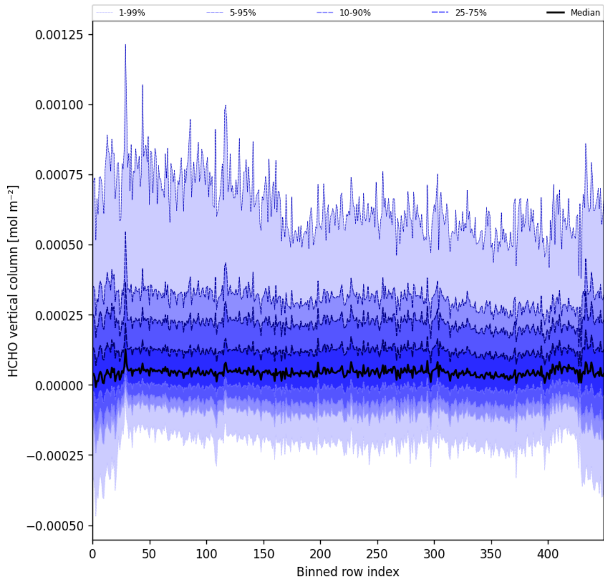
Figure 49: Along track statistics of “HCHO vertical column” for 2024-10-26 to 2024-10-28
