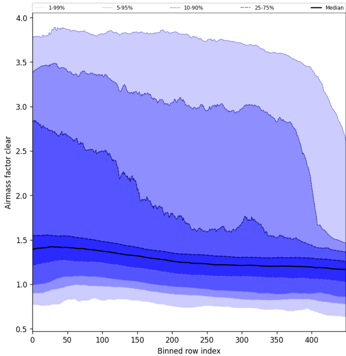
Figure 56: Along track statistics of “Airmass factor clear” for 2024-10-26 to 2024-10-28
