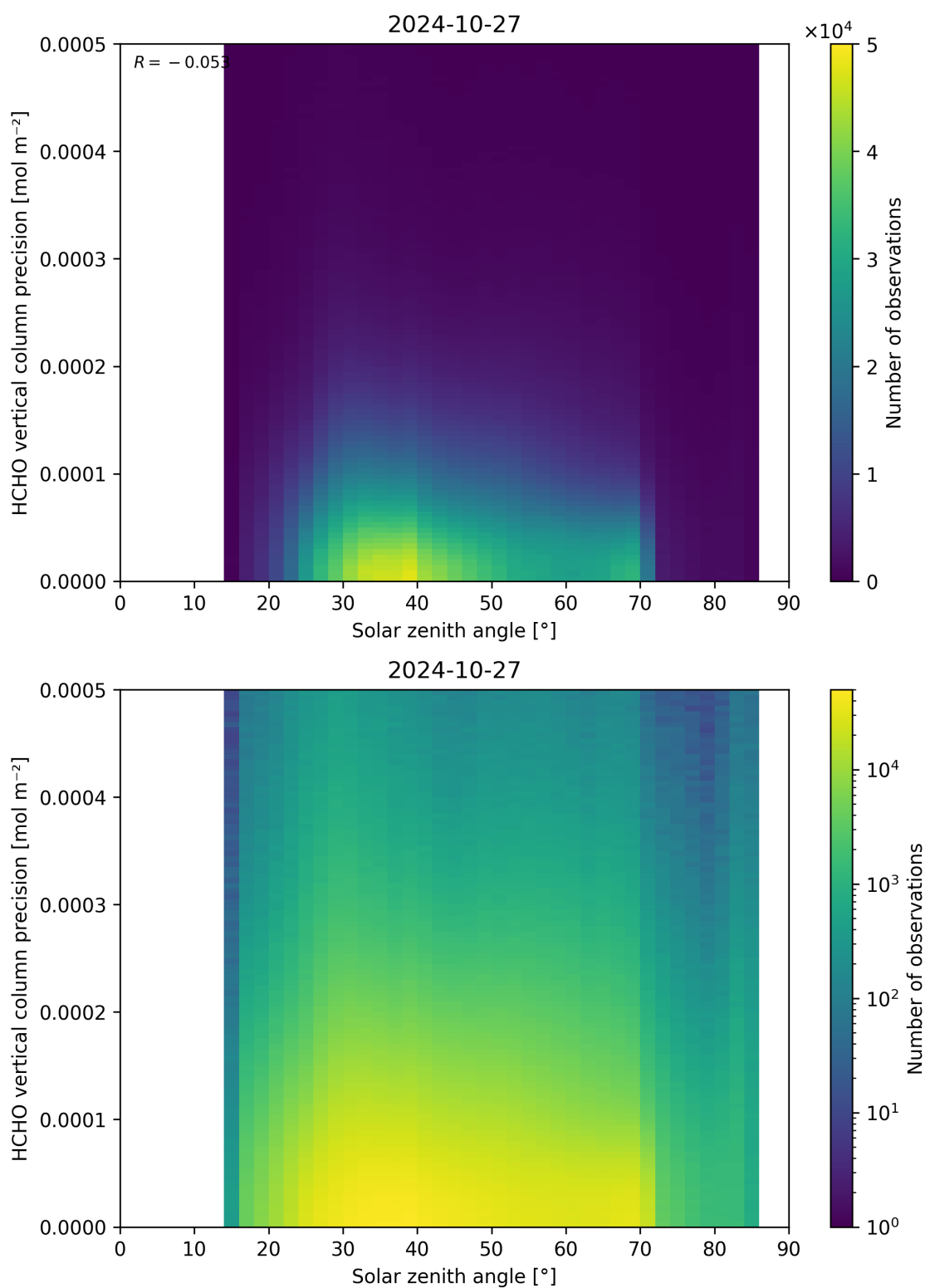
Figure 179: Scatter density plot of “Solar zenith angle” against “HCHO vertical column precision” for 2024-10-26 to 2024-10-28.
