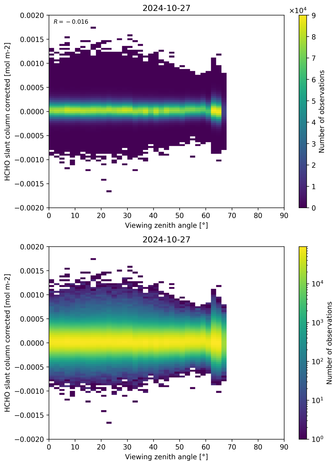
Figure 186: Scatter density plot of “Viewing zenith angle” against “HCHO slant column corrected” for 2024-10-26 to 2024-10-28.
