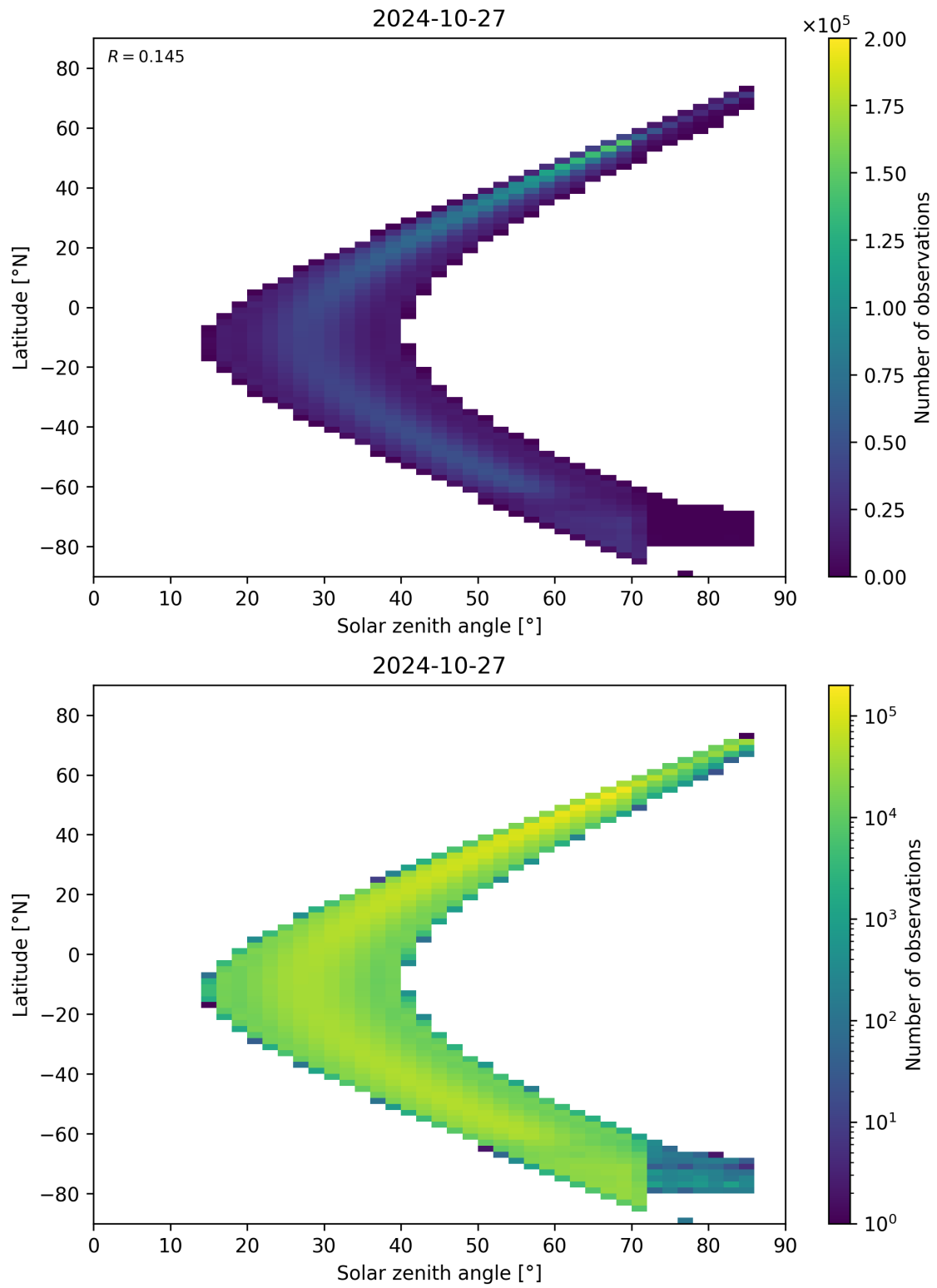
Figure 181: Scatter density plot of “Solar zenith angle” against “Latitude” for 2024-10-26 to 2024-10-28.
