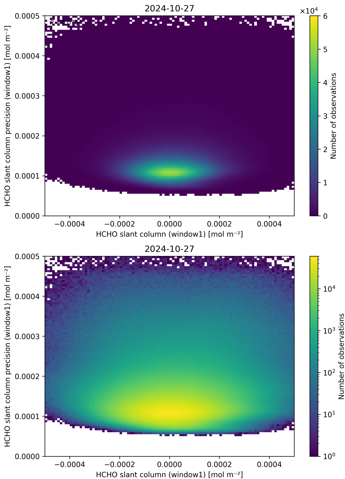
Figure 84: Scatter density plot of “HCHO slant column (window1)” against “HCHO slant column precision (window1)” for 2024-10-26 to 2024-10-28.
