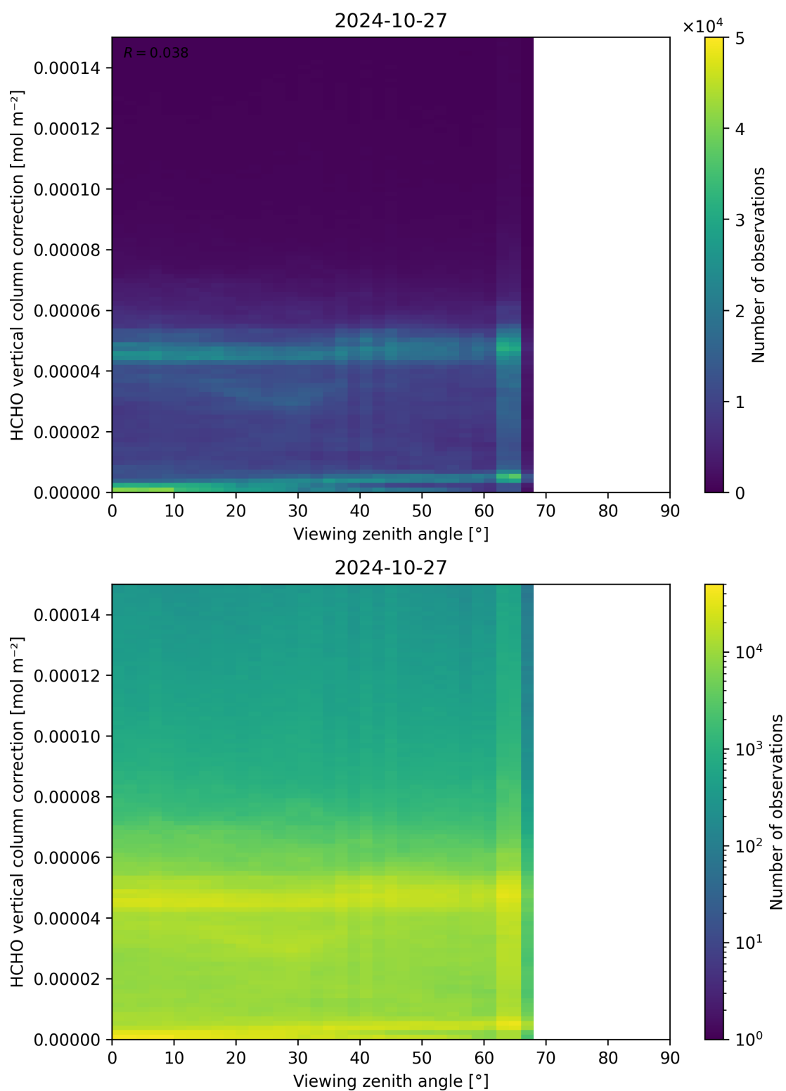
Figure 193: Scatter density plot of “Viewing zenith angle” against “HCHO vertical column correction” for 2024-10-26 to 2024-10-28.
