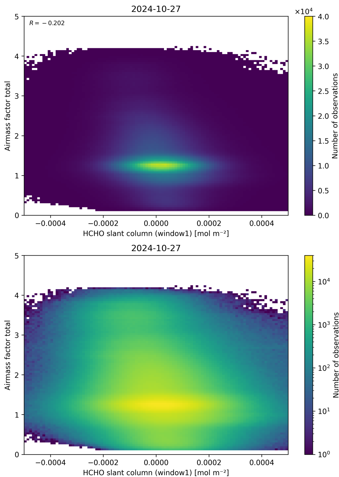
Figure 85: Scatter density plot of “HCHO slant column (window1)” against “Airmass factor total” for 2024-10-26 to 2024-10-28.
