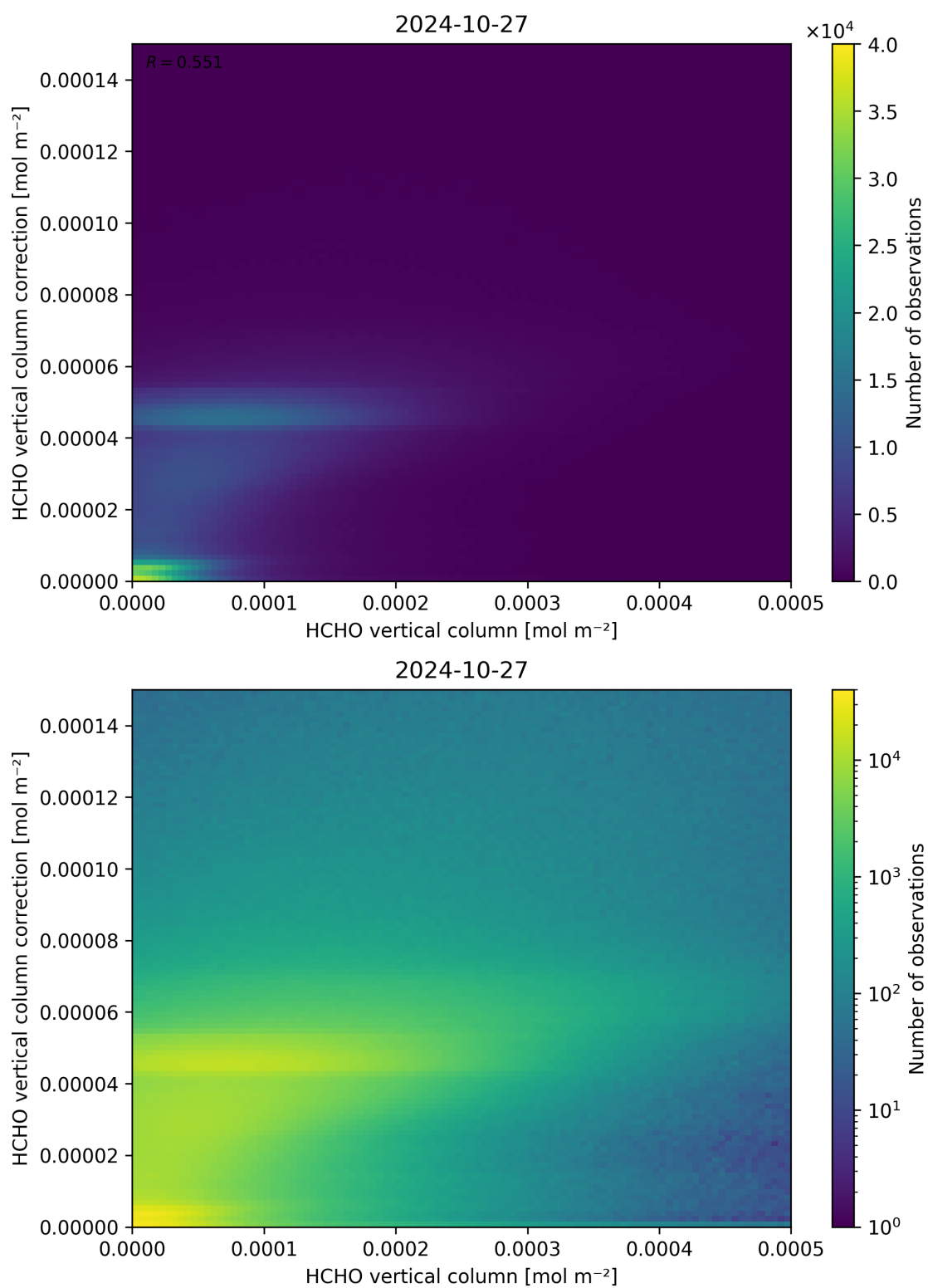
Figure 133: Scatter density plot of “HCHO vertical column” against “HCHO vertical column correction” for 2024-10-26 to 2024-10-28.
