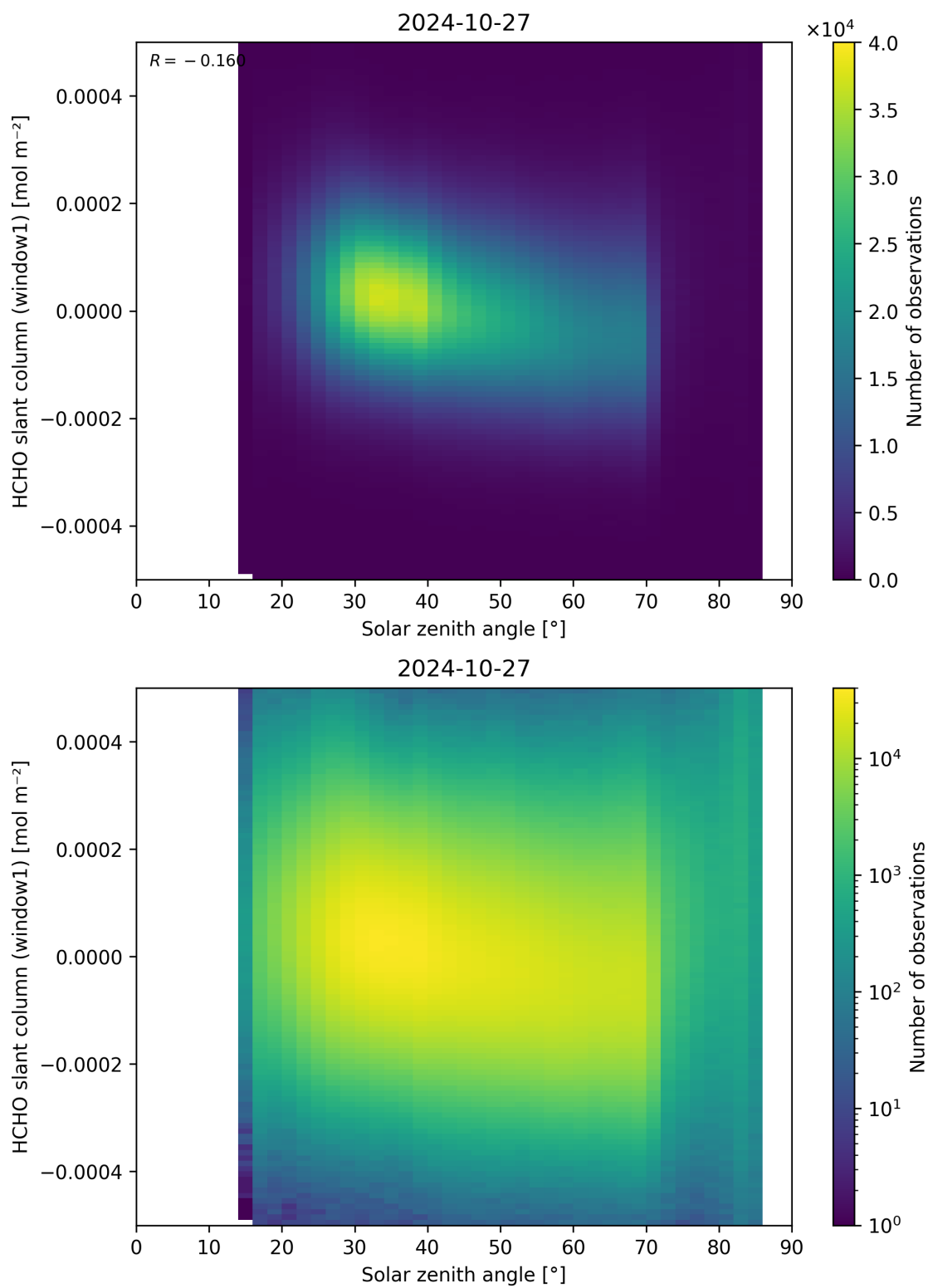
Figure 173: Scatter density plot of “Solar zenith angle” against “HCHO slant column (window1)” for 2024-10-26 to 2024-10-28.
