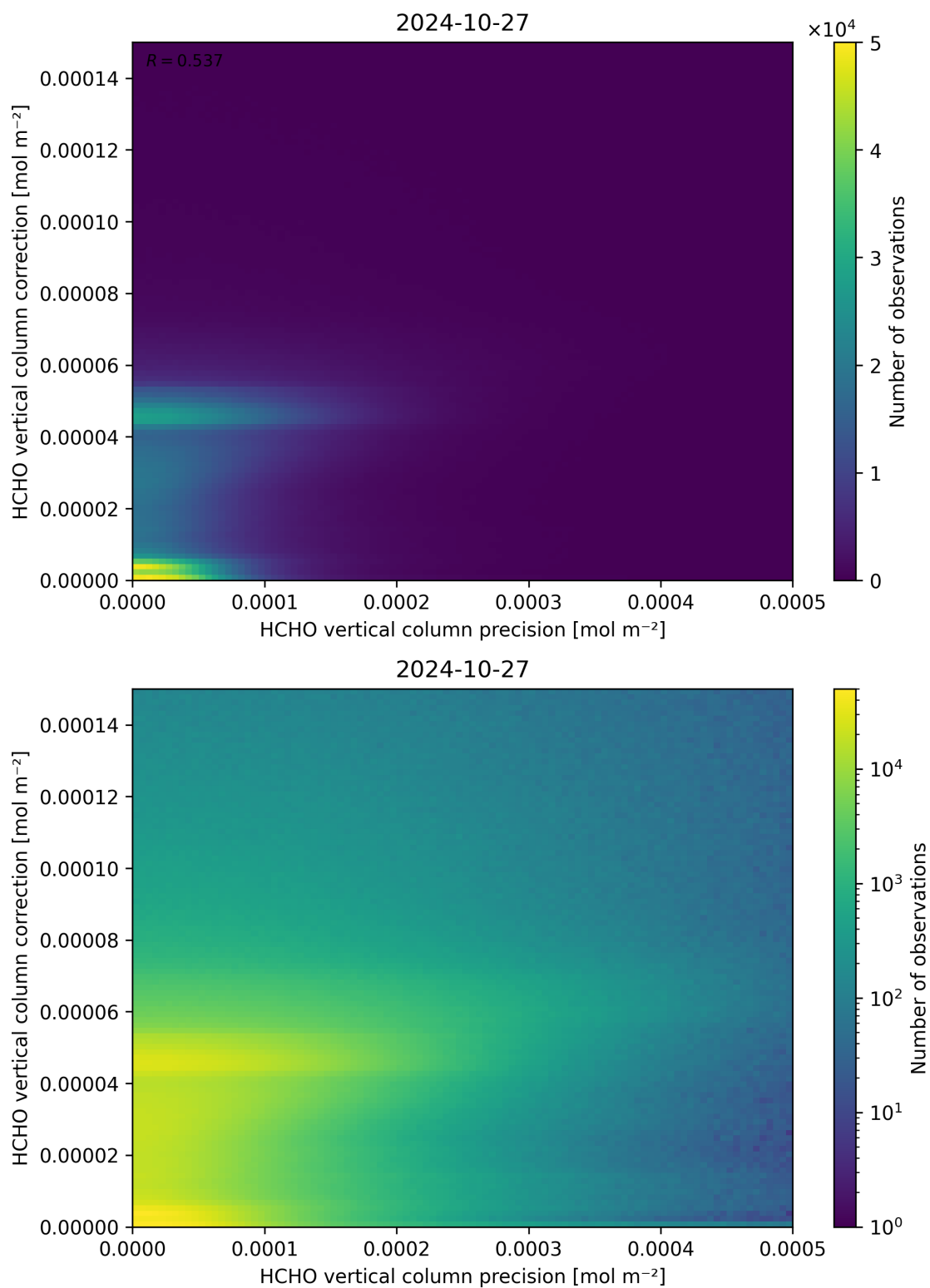
Figure 146: Scatter density plot of “HCHO vertical column precision” against “HCHO vertical column correction” for 2024-10-26 to 2024-10-28.
