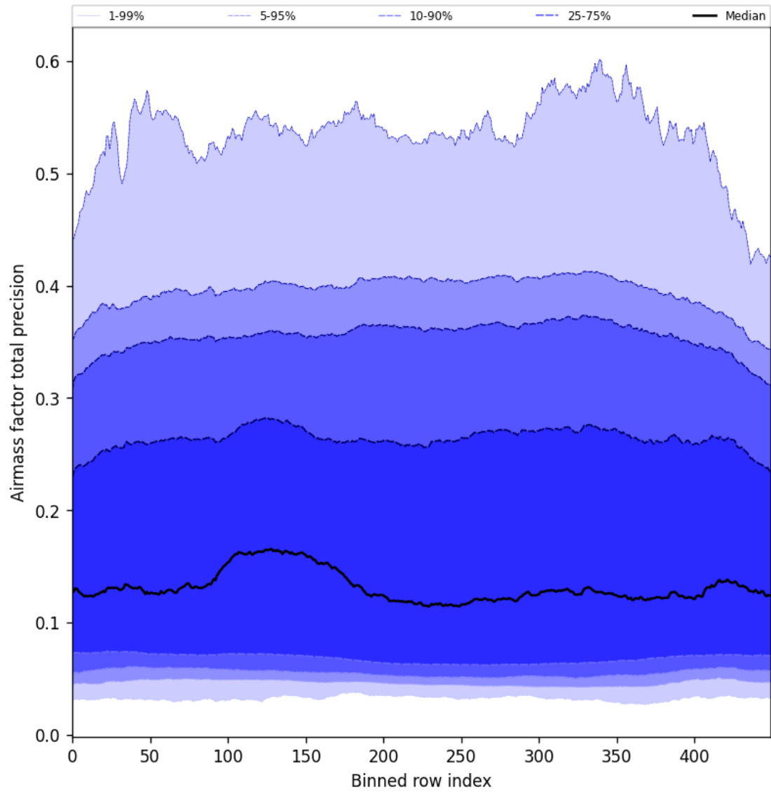
Figure 55: Along track statistics of “Airmass factor total precision” for 2024-10-26 to 2024-10-28
