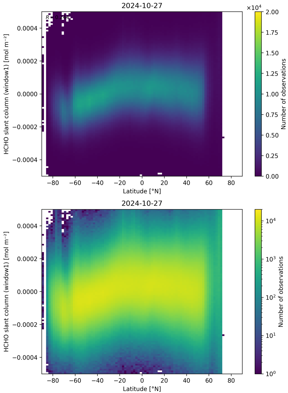
Figure 159: Scatter density plot of “Latitude” against “HCHO slant column (window1)” for 2024-10-26 to 2024-10-28.
