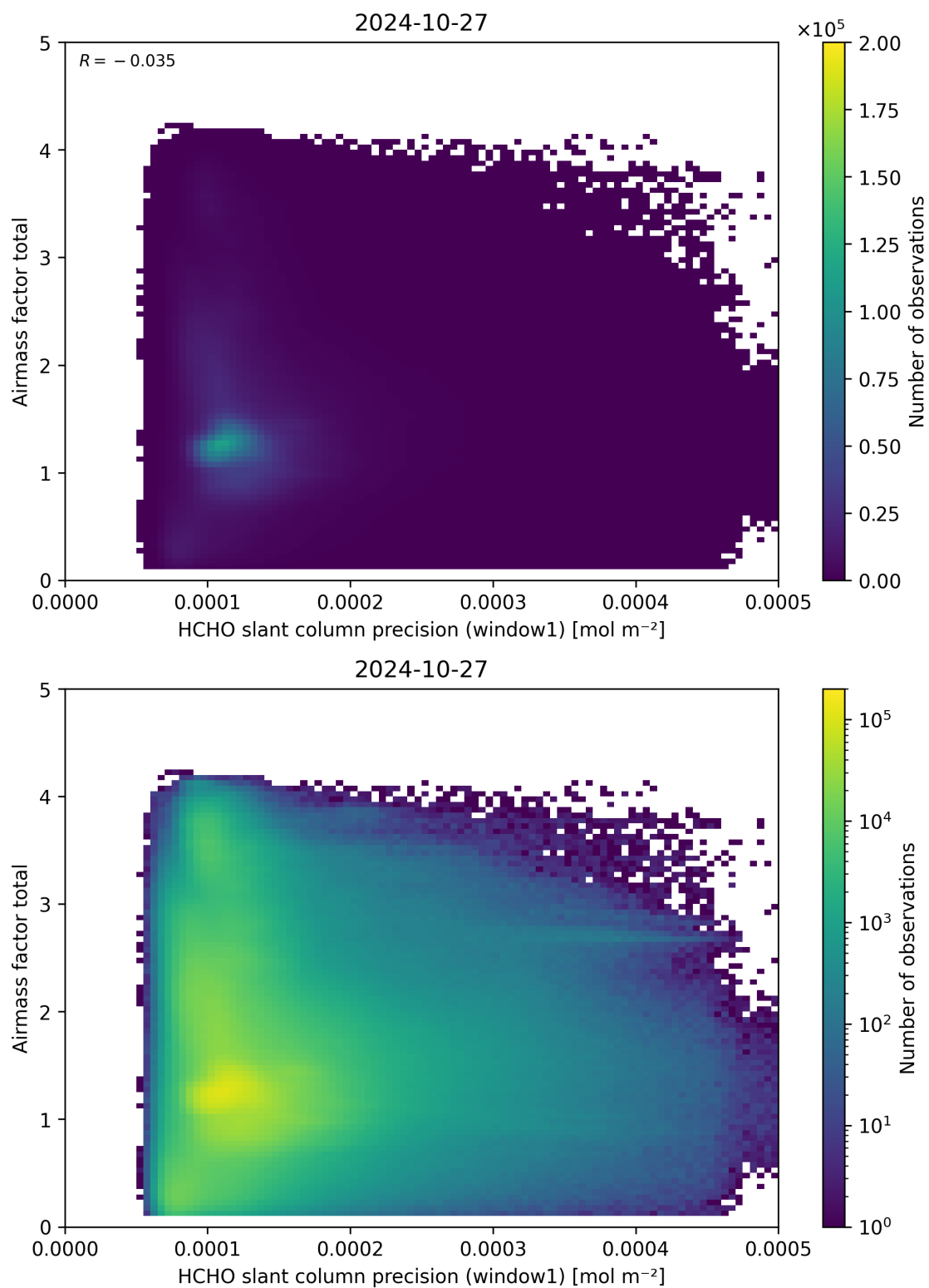
Figure 94: Scatter density plot of “HCHO slant column precision (window1)” against “Airmass factor total” for 2024-10-26 to 2024-10-28.
