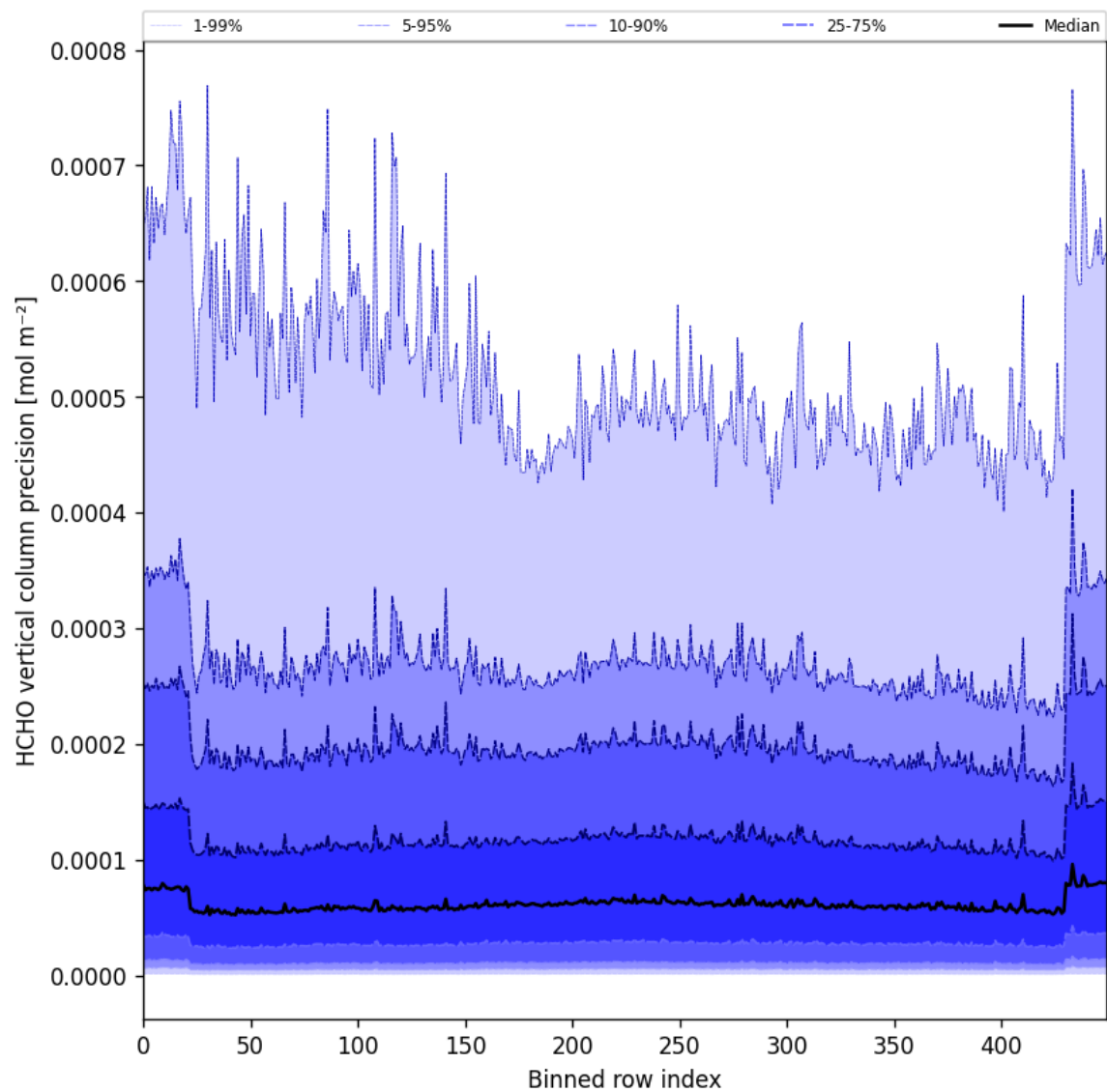
Figure 50: Along track statistics of “HCHO vertical column precision” for 2024-10-26 to 2024-10-28
