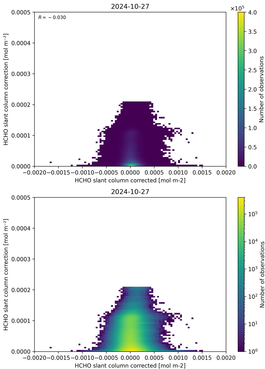
Figure 77: Scatter density plot of “HCHO slant column corrected” against “HCHO slant column correction” for 2024-10-26 to 2024-10-28.
