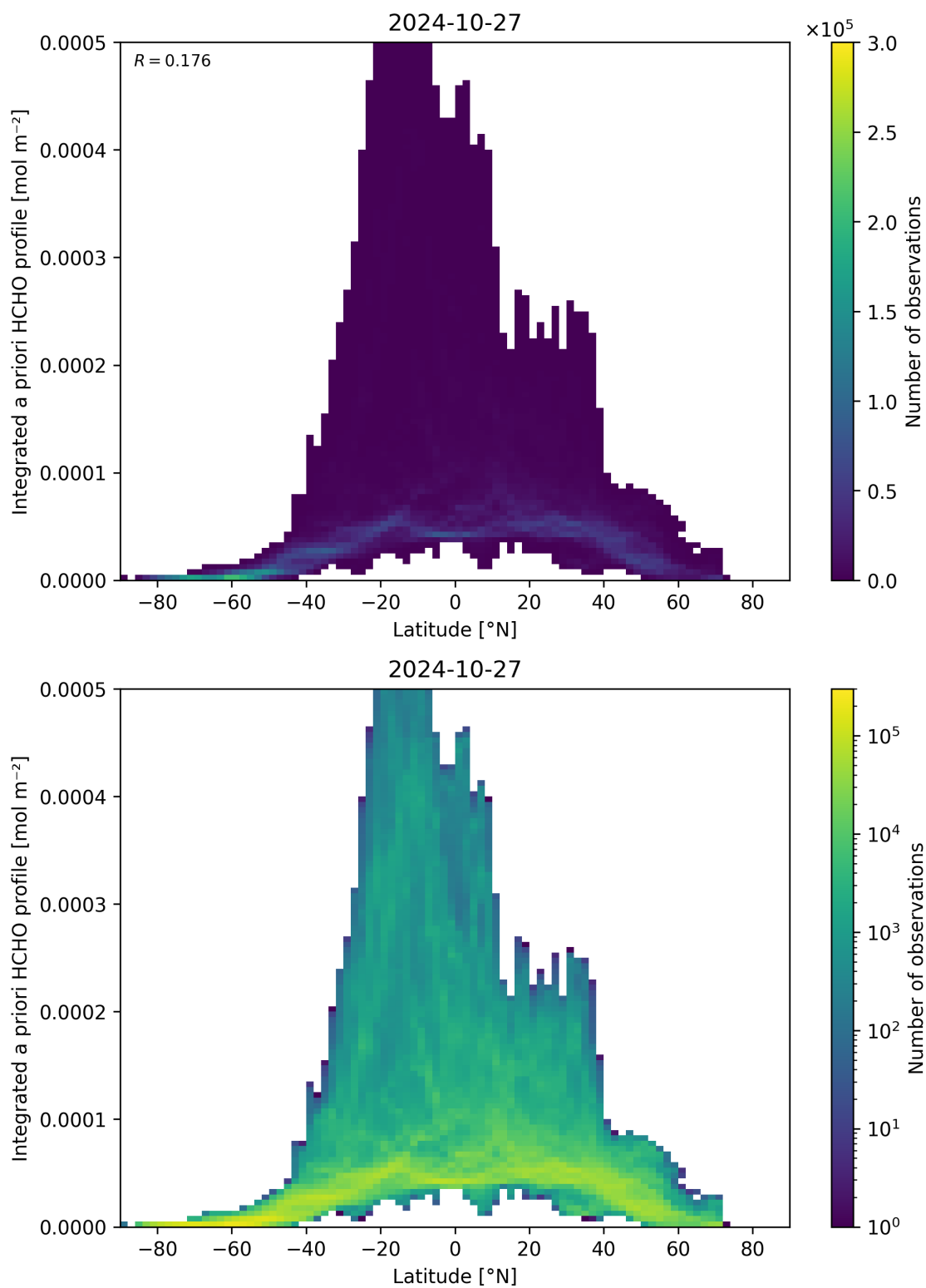
Figure 166: Scatter density plot of “Latitude” against “Integrated a priori HCHO profile” for 2024-10-26 to 2024-10-28.
