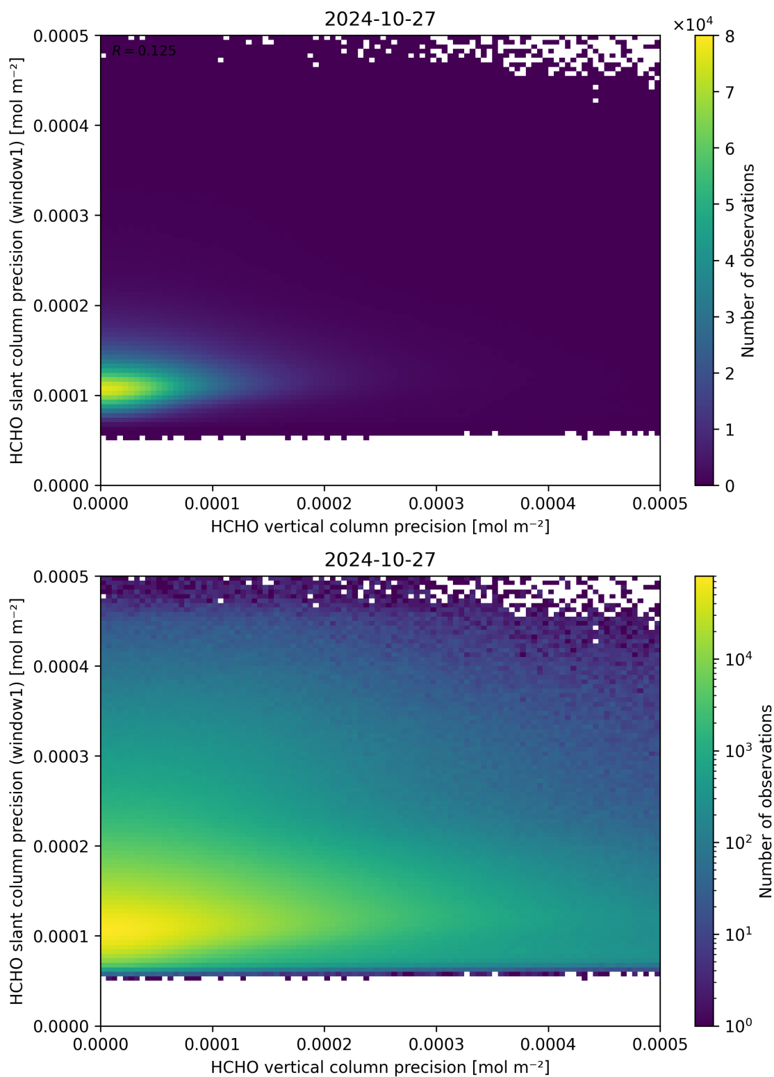
Figure 143: Scatter density plot of “HCHO vertical column precision” against “HCHO slant column precision (window1)” for 2024-10-26 to 2024-10-28.
