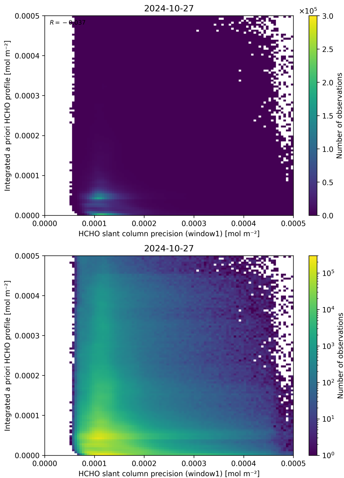
Figure 96: Scatter density plot of “HCHO slant column precision (window1)” against “Integrated a priori HCHO profile” for 2024-10-26 to 2024-10-28.
