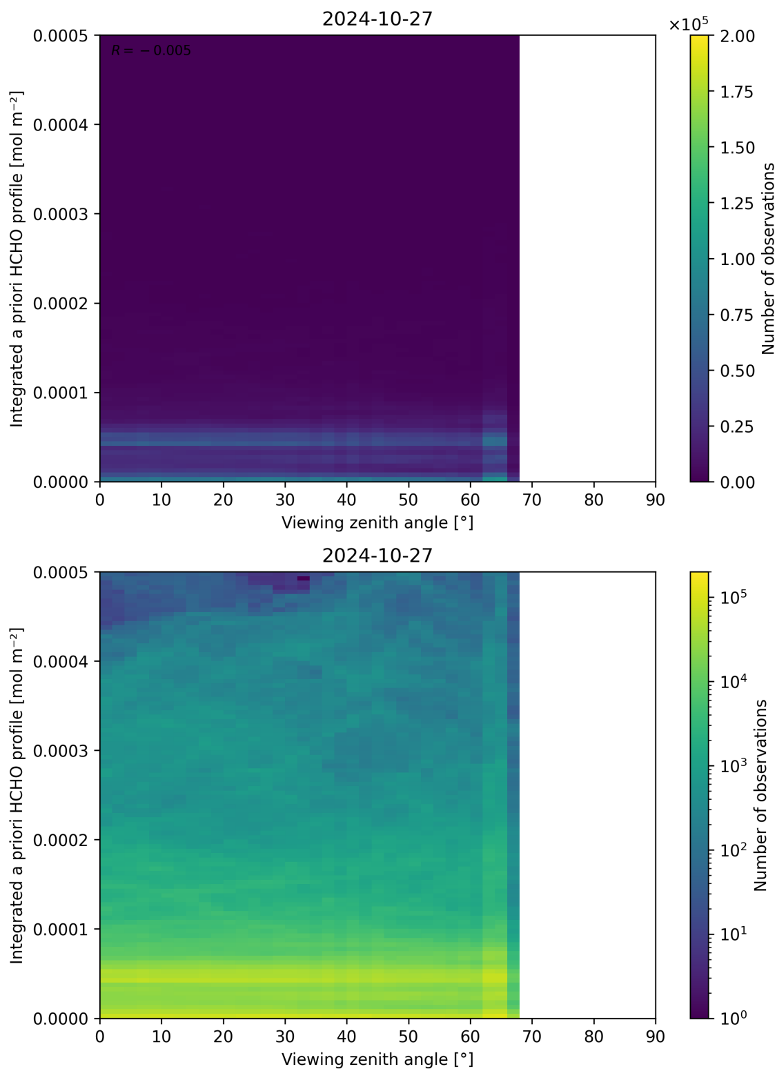
Figure 195: Scatter density plot of “Viewing zenith angle” against “Integrated a priori HCHO profile” for 2024-10-26 to 2024-10-28.
