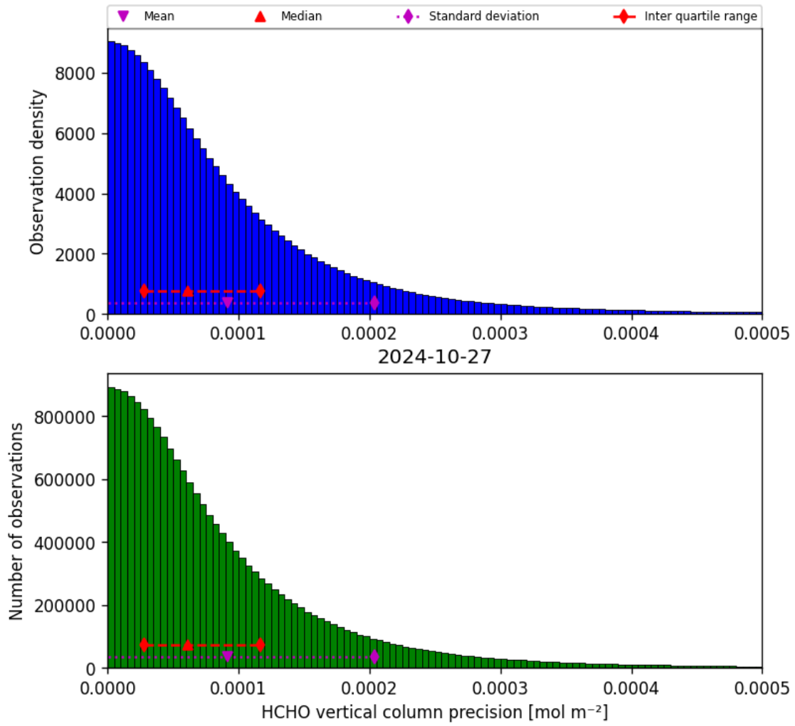
Figure 36: Histogram of “HCHO vertical column precision” for 2024-10-26 to 2024-10-28
