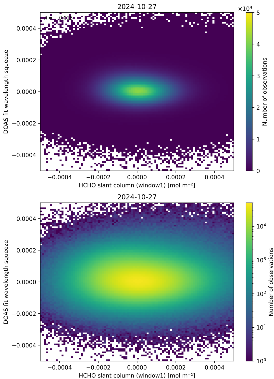
Figure 80: Scatter density plot of “HCHO slant column (window1)” against “DOAS fit wavelength squeeze” for 2024-10-26 to 2024-10-28.
