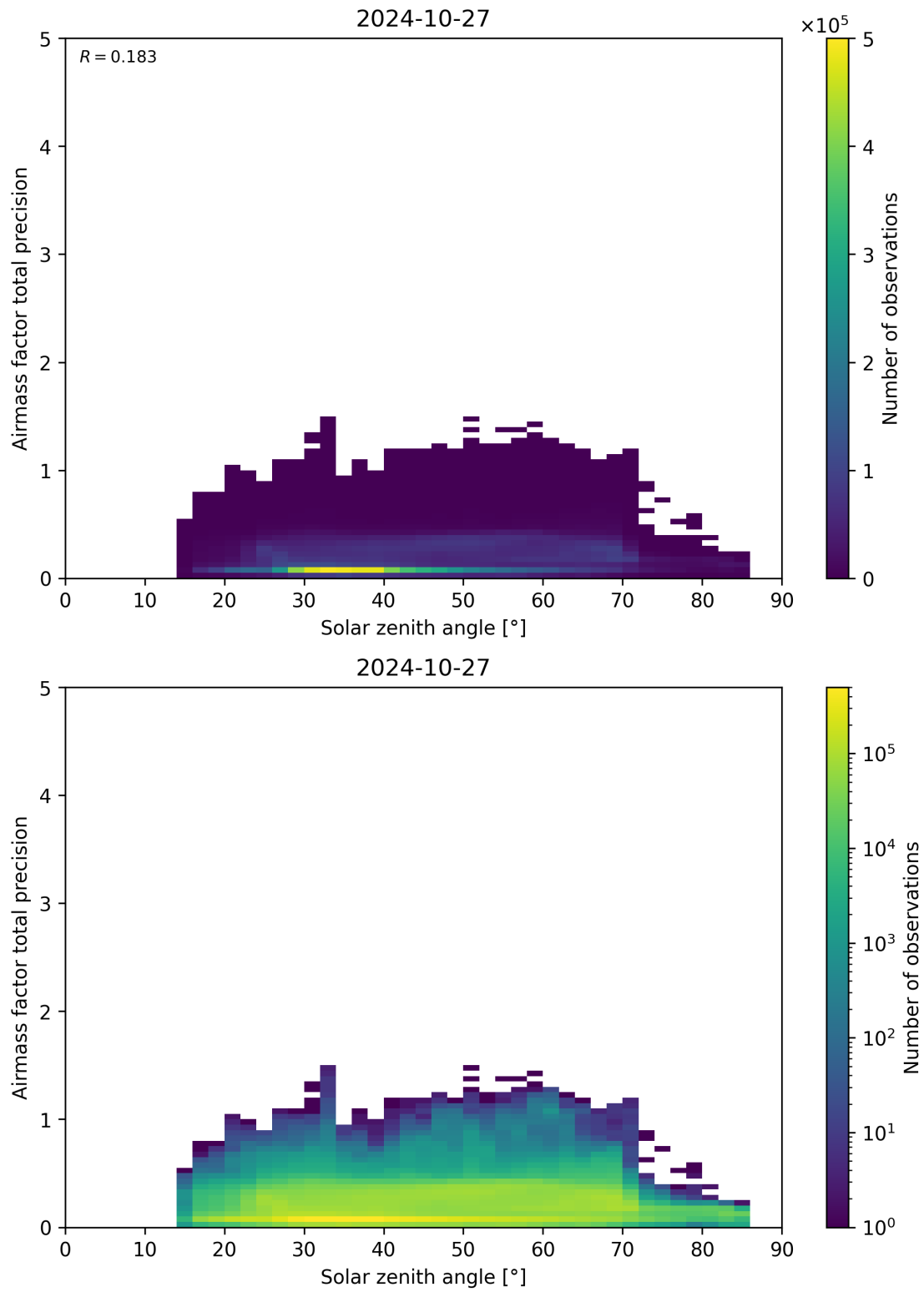
Figure 176: Scatter density plot of “Solar zenith angle” against “Airmass factor total precision” for 2024-10-26 to 2024-10-28.
