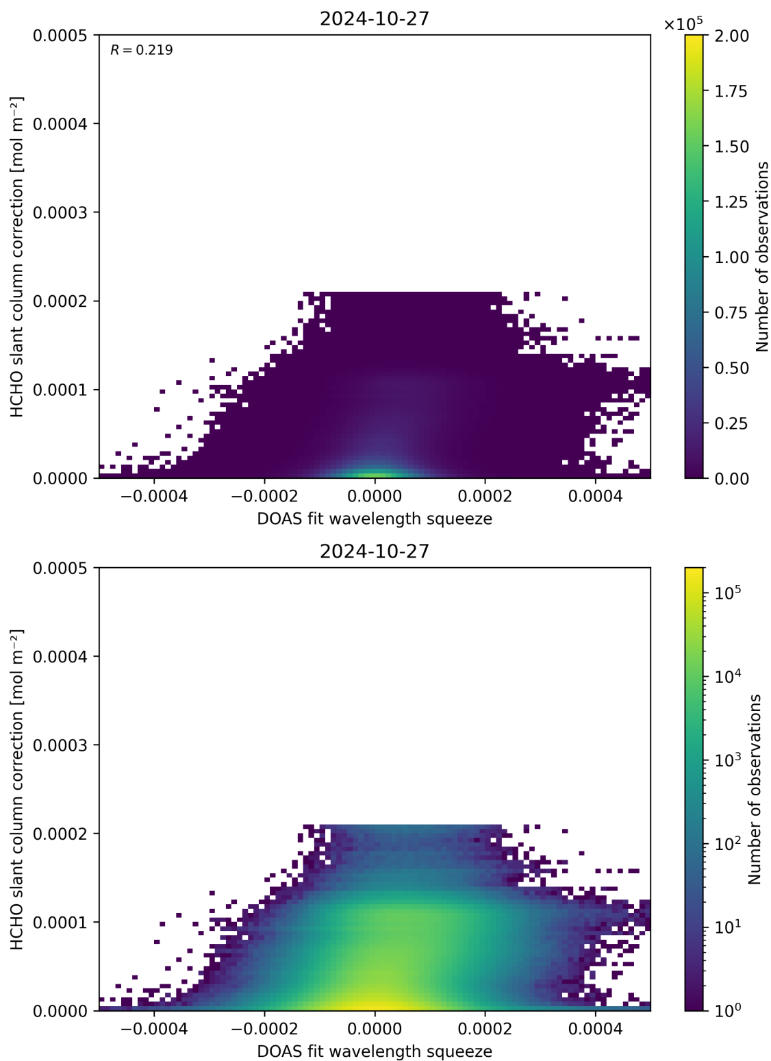
Figure 70: Scatter density plot of “DOAS fit wavelength squeeze” against “HCHO slant column correction” for 2024-10-26 to 2024-10-28.
