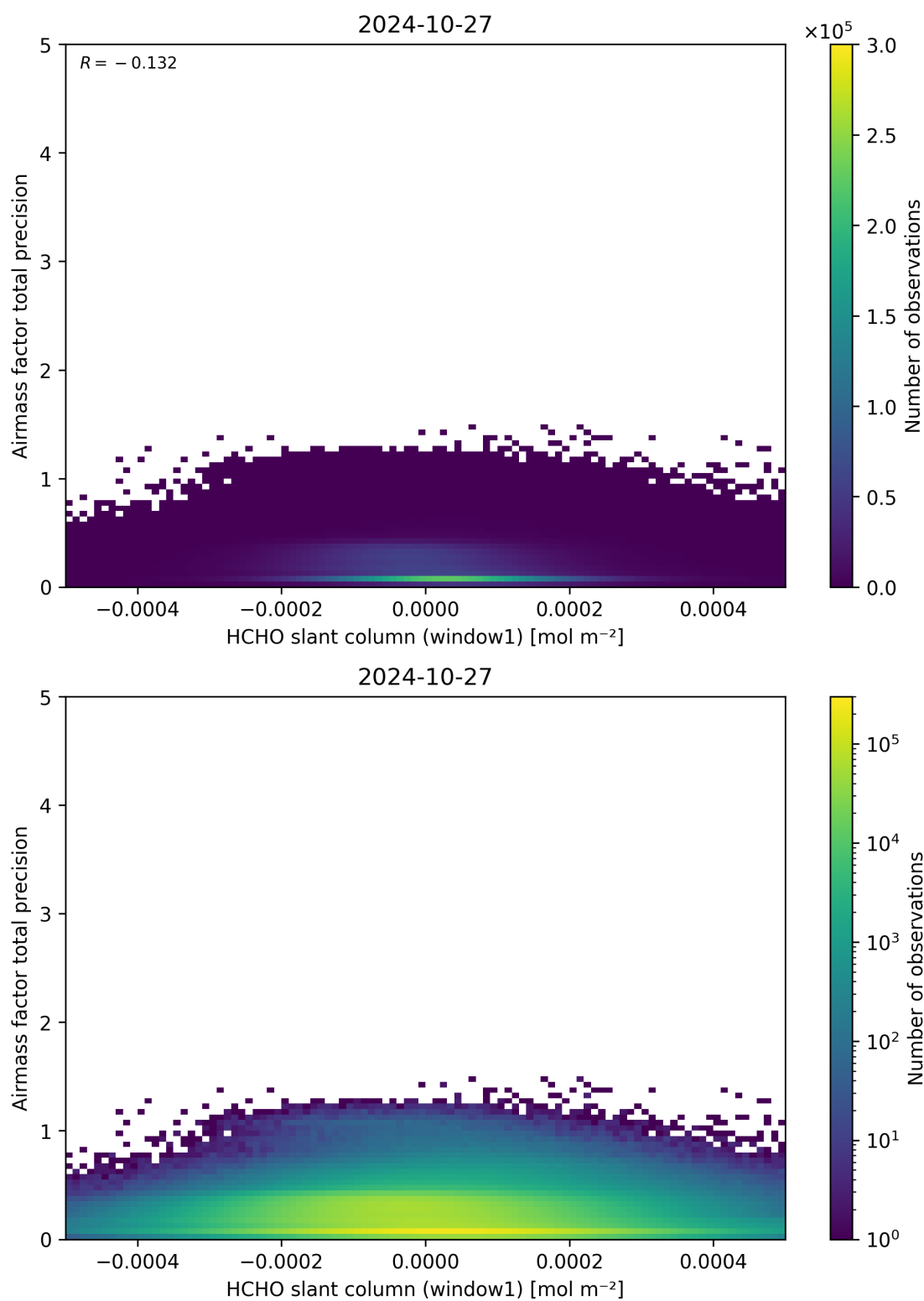
Figure 86: Scatter density plot of “HCHO slant column (window1)” against “Airmass factor total precision” for 2024-10-26 to 2024-10-28.
