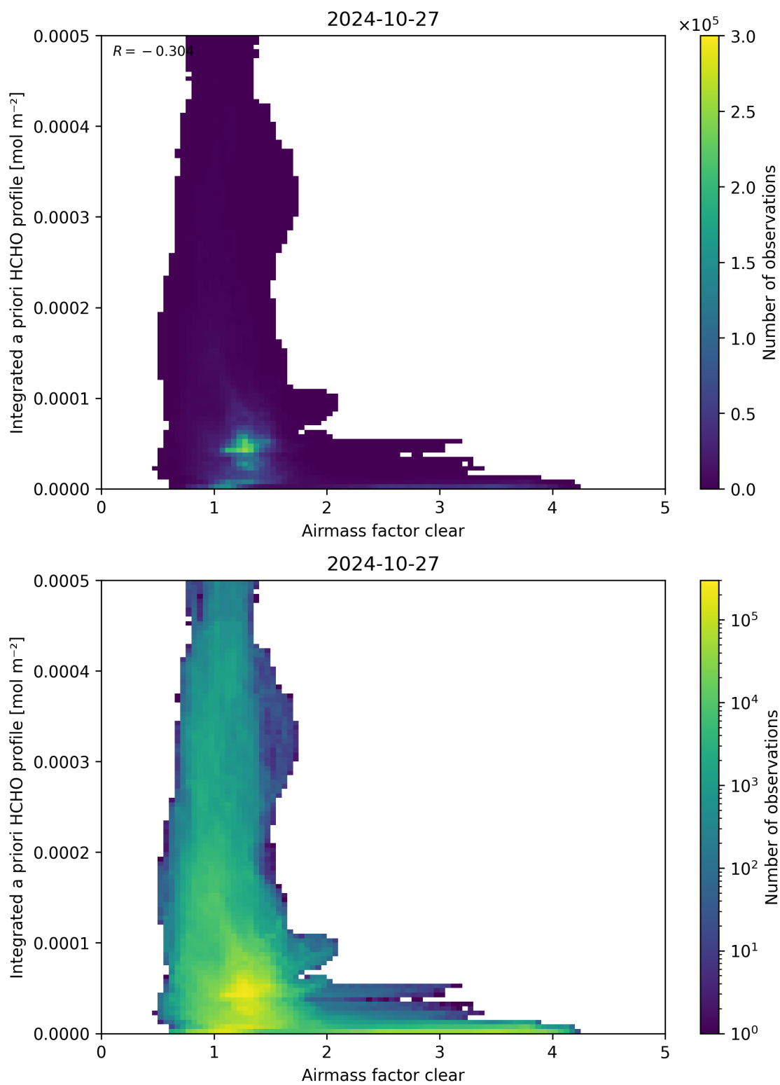
Figure 76: Scatter density plot of “Airmass factor clear” against “Integrated a priori HCHO profile” for 2024-10-26 to 2024-10-28.
