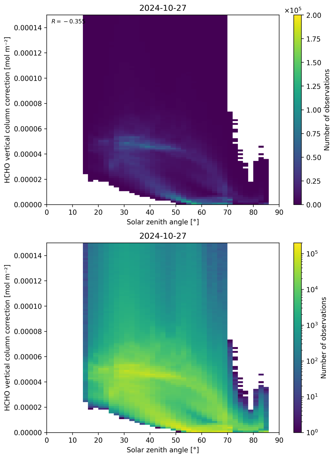
Figure 178: Scatter density plot of “Solar zenith angle” against “HCHO vertical column correction” for 2024-10-26 to 2024-10-28.
