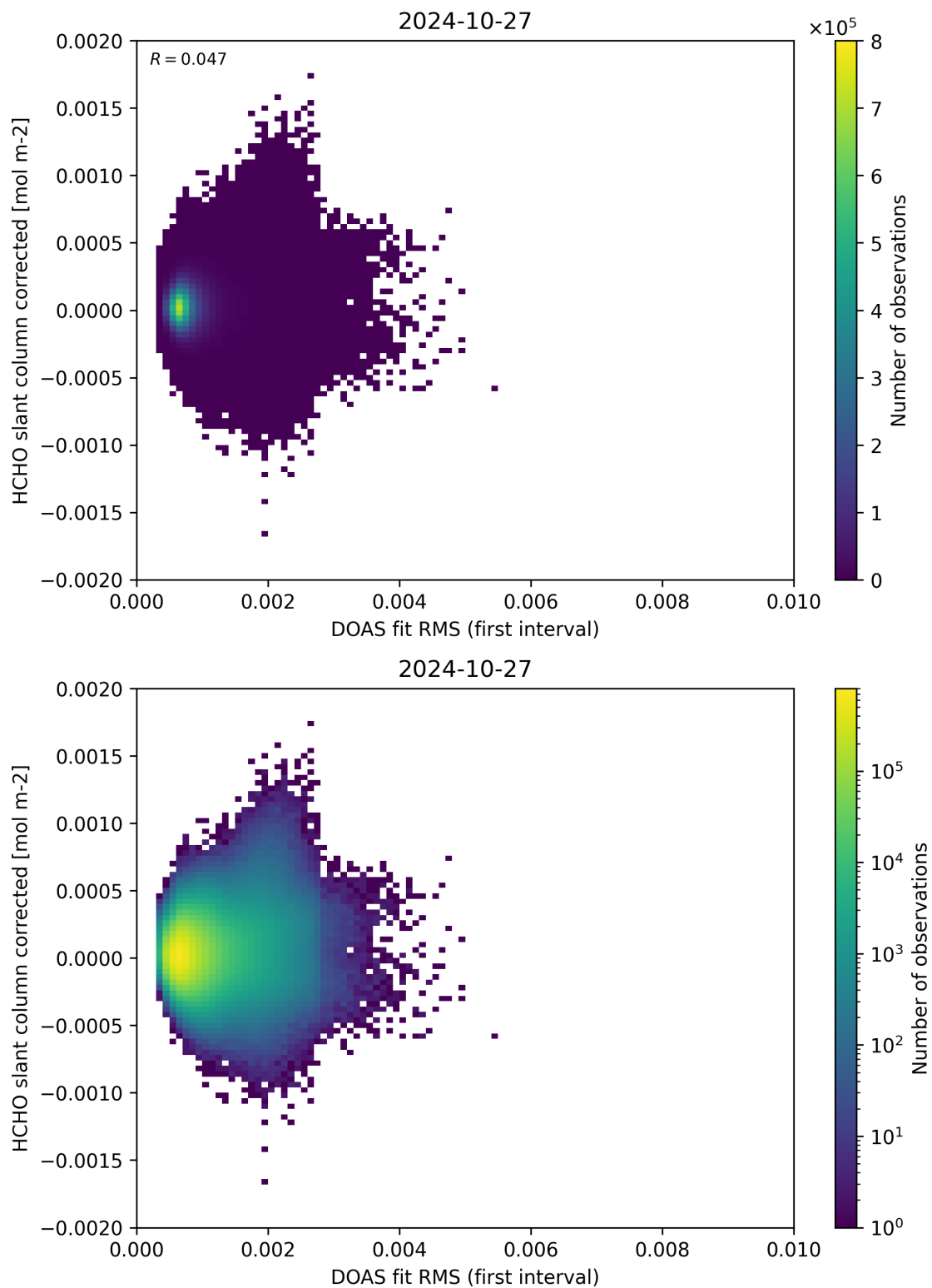
Figure 62: Scatter density plot of “DOAS fit RMS (first interval)” against “HCHO slant column corrected” for 2024-10-26 to 2024-10-28.
