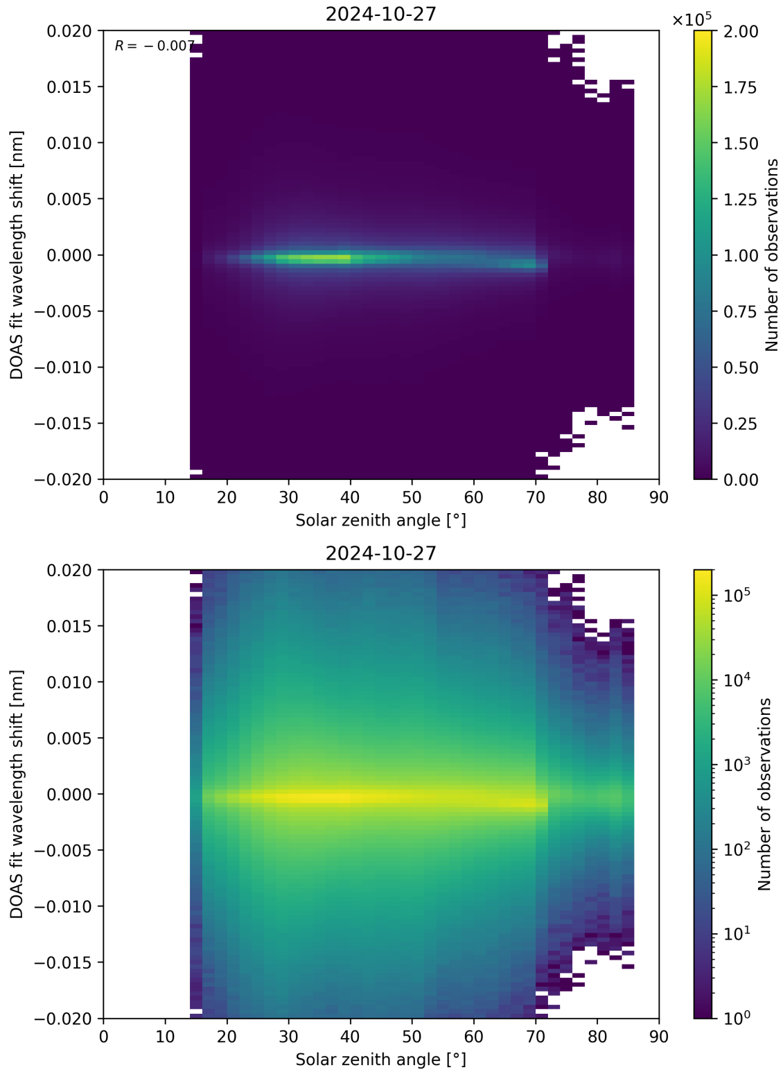
Figure 168: Scatter density plot of “Solar zenith angle” against “DOAS fit wavelength shift” for 2024-10-26 to 2024-10-28.
