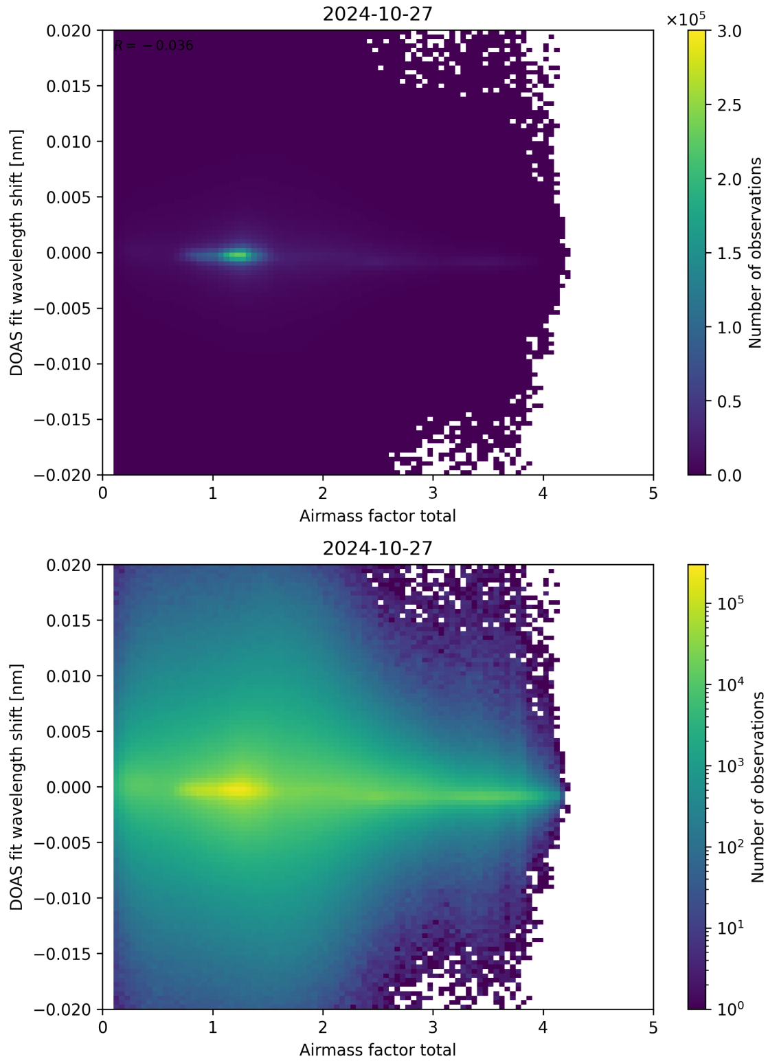
Figure 98: Scatter density plot of “Airmass factor total” against “DOAS fit wavelength shift” for 2024-10-26 to 2024-10-28.
