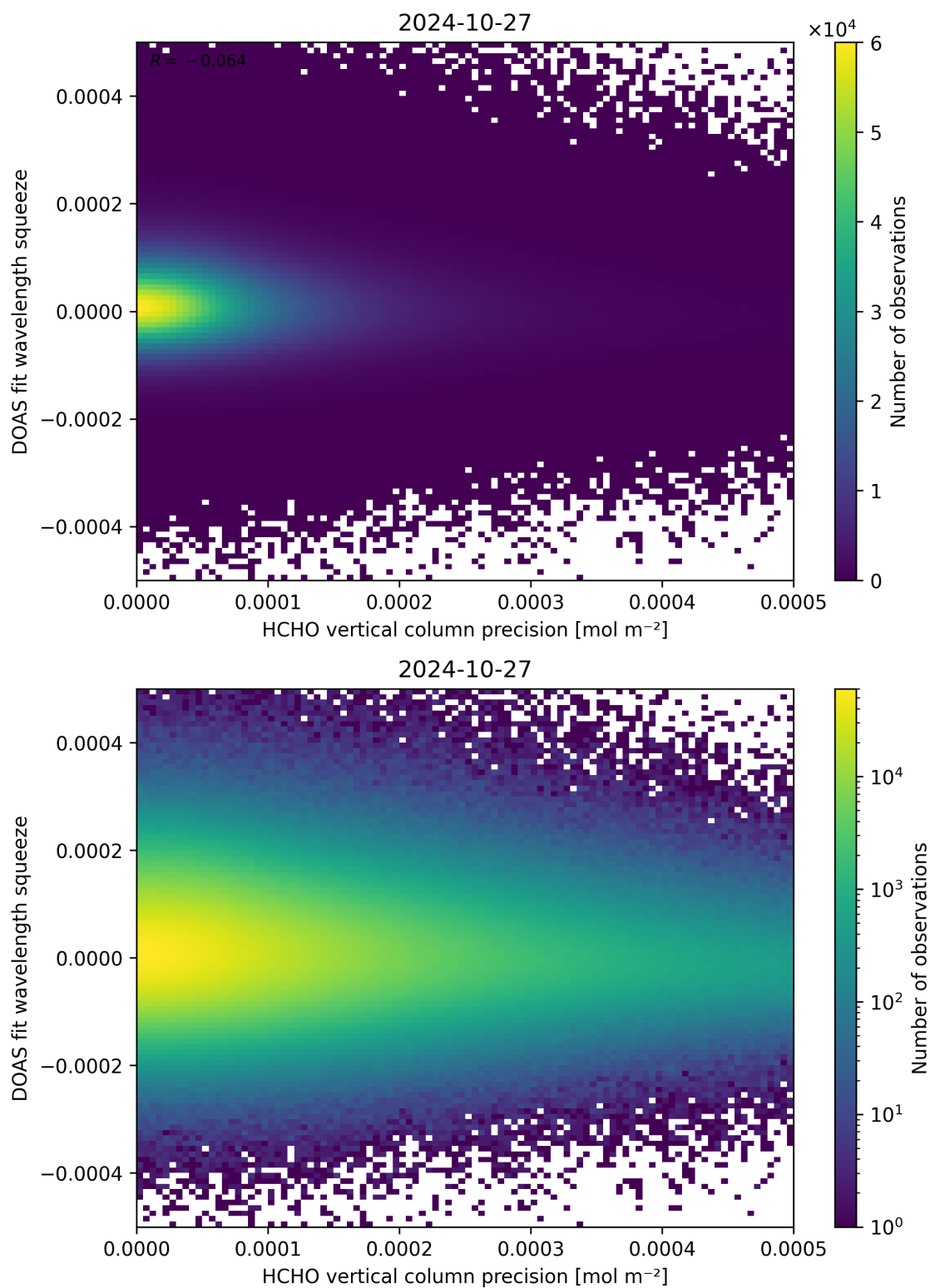
Figure 138: Scatter density plot of “HCHO vertical column precision” against “DOAS fit wavelength squeeze” for 2024-10-26 to 2024-10-28.
