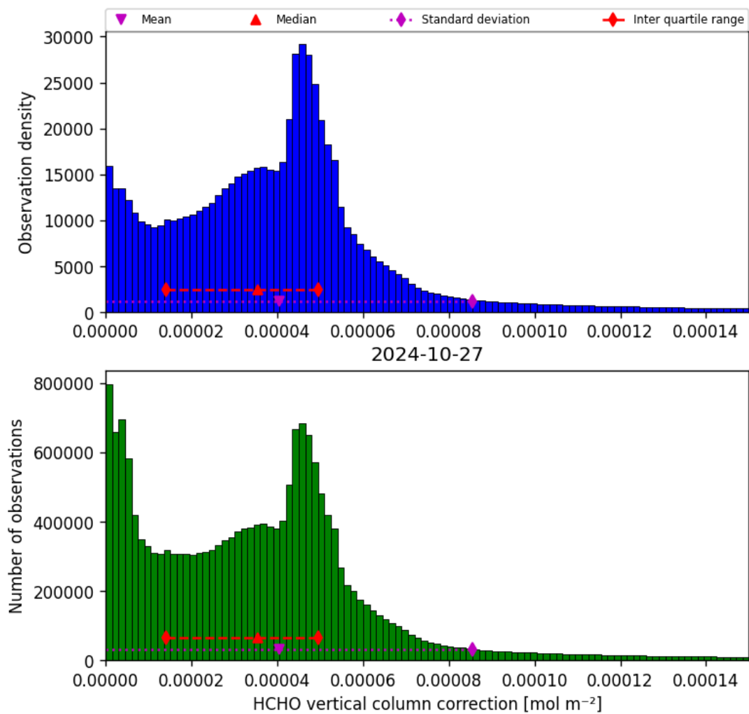
Figure 37: Histogram of “HCHO vertical column correction” for 2024-10-26 to 2024-10-28
