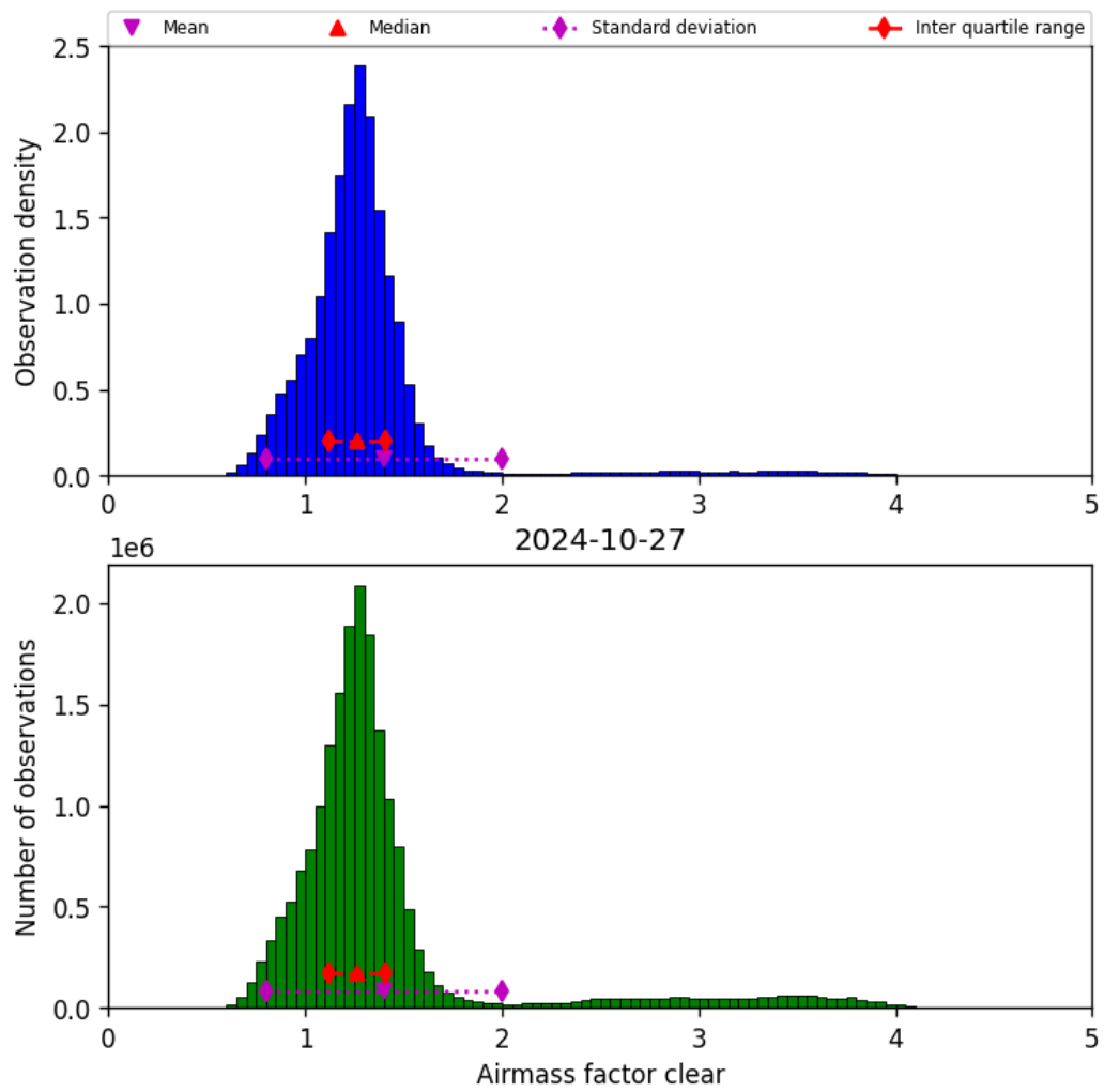
Figure 42: Histogram of “Airmass factor clear” for 2024-10-26 to 2024-10-28
