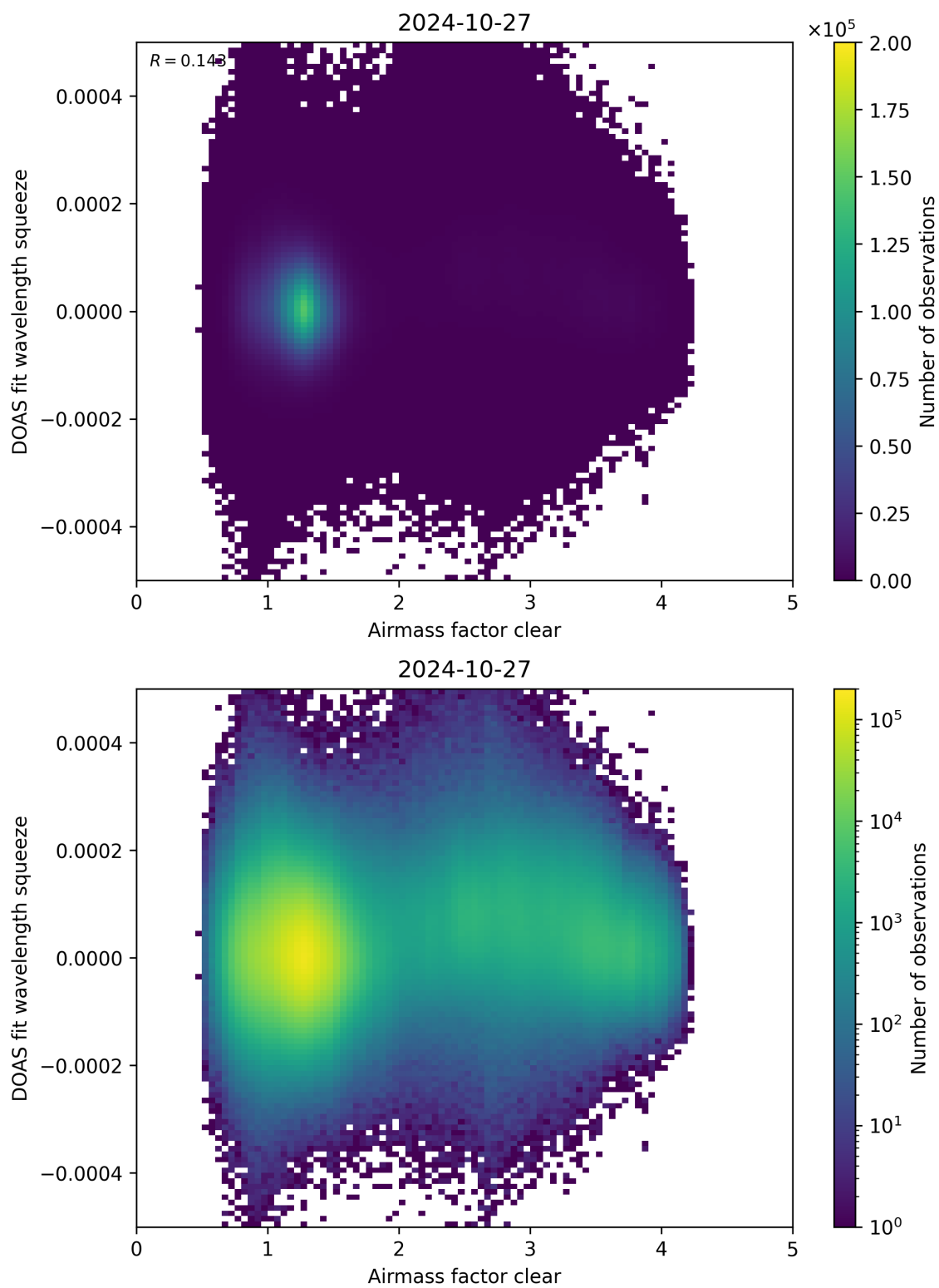
Figure 73: Scatter density plot of “Airmass factor clear” against “DOAS fit wavelength squeeze” for 2024-10-26 to 2024-10-28.
