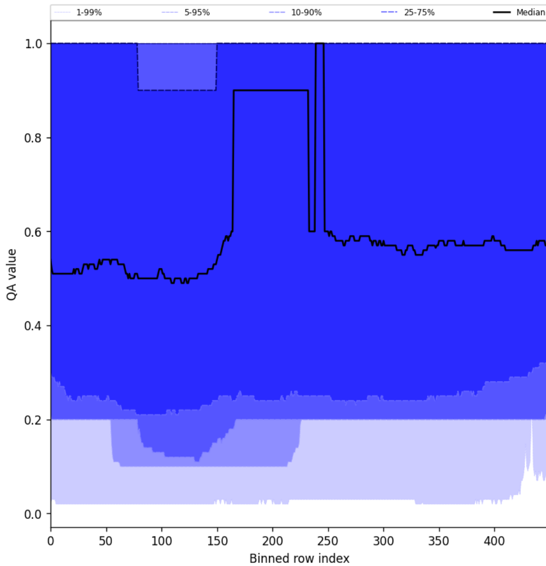
Figure 48: Along track statistics of “QA value” for 2024-10-26 to 2024-10-28
