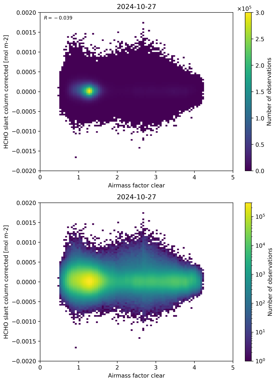
Figure 74: Scatter density plot of “Airmass factor clear” against “HCHO slant column corrected” for 2024-10-26 to 2024-10-28.
