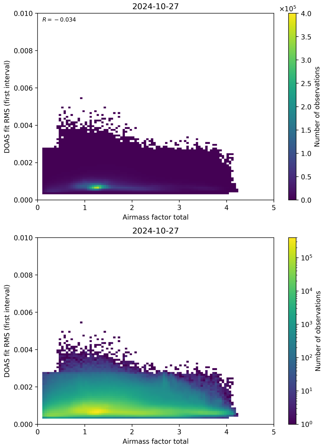
Figure 97: Scatter density plot of “Airmass factor total” against “DOAS fit RMS (first interval)” for 2024-10-26 to 2024-10-28.
