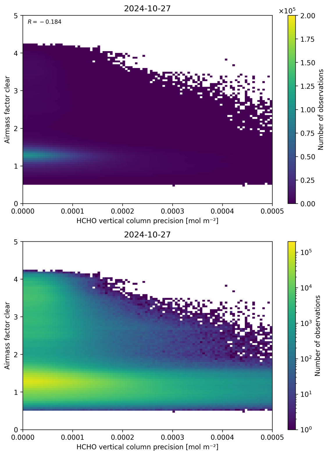
Figure 139: Scatter density plot of “HCHO vertical column precision” against “Airmass factor clear” for 2024-10-26 to 2024-10-28.
