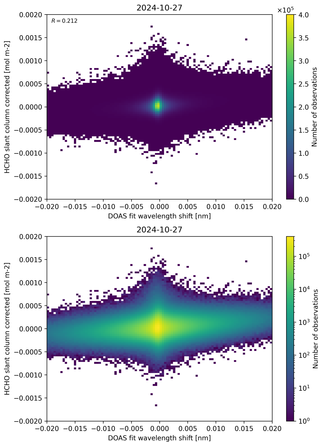
Figure 66: Scatter density plot of “DOAS fit wavelength shift” against “HCHO slant column corrected” for 2024-10-26 to 2024-10-28.
