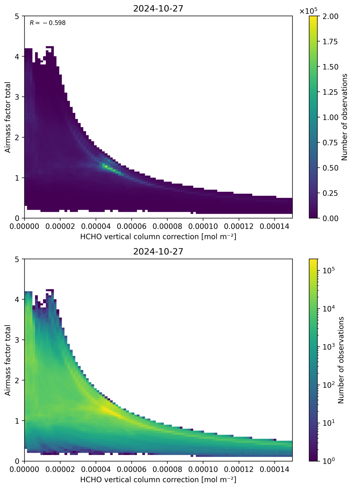
Figure 120: Scatter density plot of “HCHO vertical column correction” against “Airmass factor total” for 2024-10-26 to 2024-10-28.
