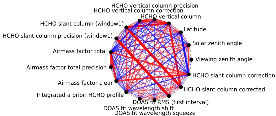
Figure 1: Map of correlation graph for 2024-10-26 to 2024-10-28.
