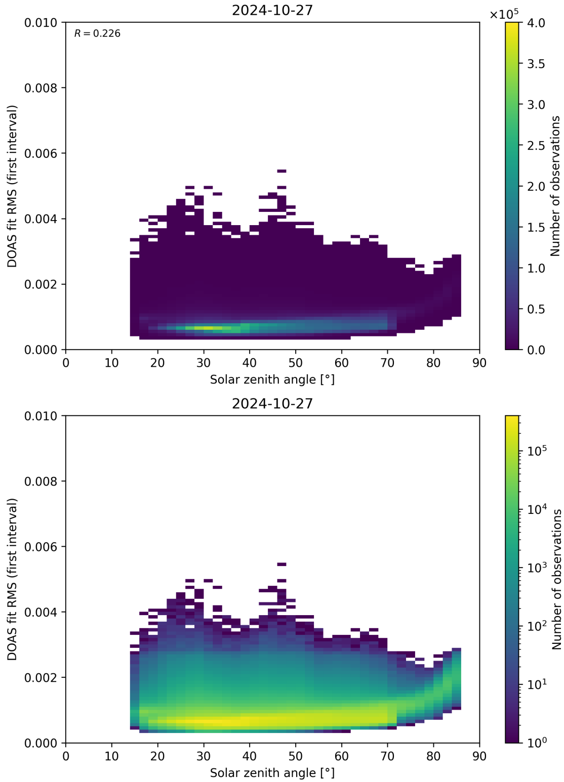
Figure 167: Scatter density plot of “Solar zenith angle” against “DOAS fit RMS (first interval)” for 2024-10-26 to 2024-10-28.
