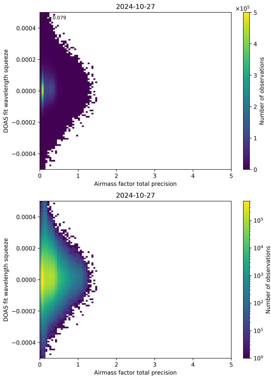
Figure 107: Scatter density plot of “Airmass factor total precision” against “DOAS fit wavelength squeeze” for 2024-10-26 to 2024-10-28.
