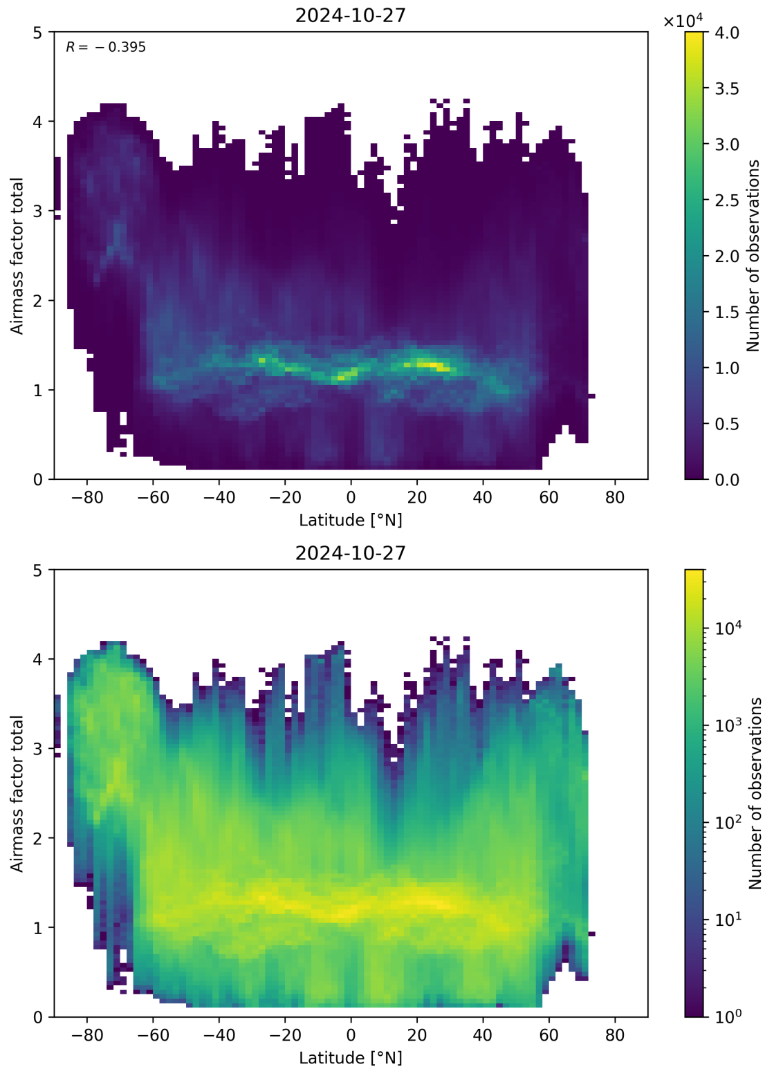
Figure 161: Scatter density plot of “Latitude” against “Airmass factor total” for 2024-10-26 to 2024-10-28.
