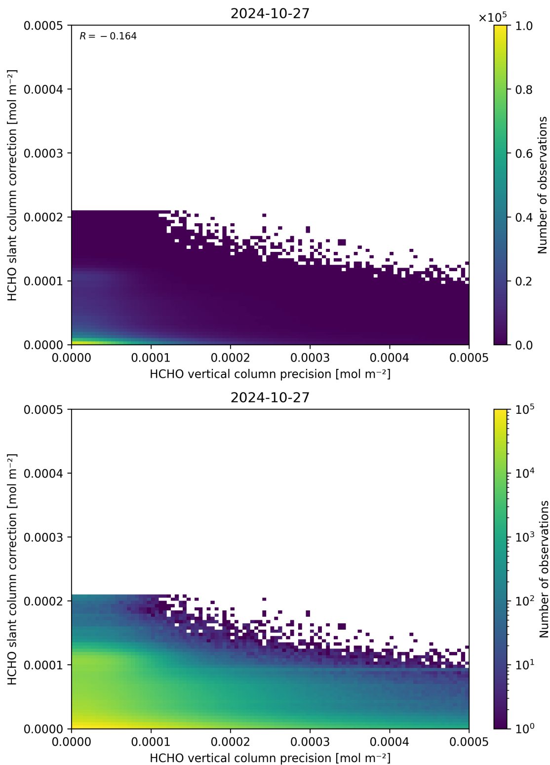
Figure 141: Scatter density plot of “HCHO vertical column precision” against “HCHO slant column correction” for 2024-10-26 to 2024-10-28.
