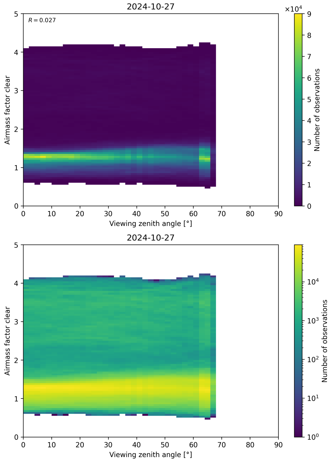
Figure 185: Scatter density plot of “Viewing zenith angle” against “Airmass factor clear” for 2024-10-26 to 2024-10-28.
