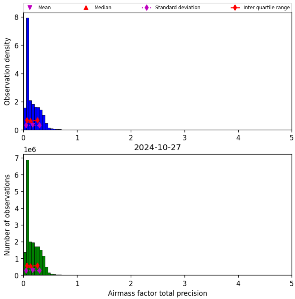
Figure 41: Histogram of “Airmass factor total precision” for 2024-10-26 to 2024-10-28
