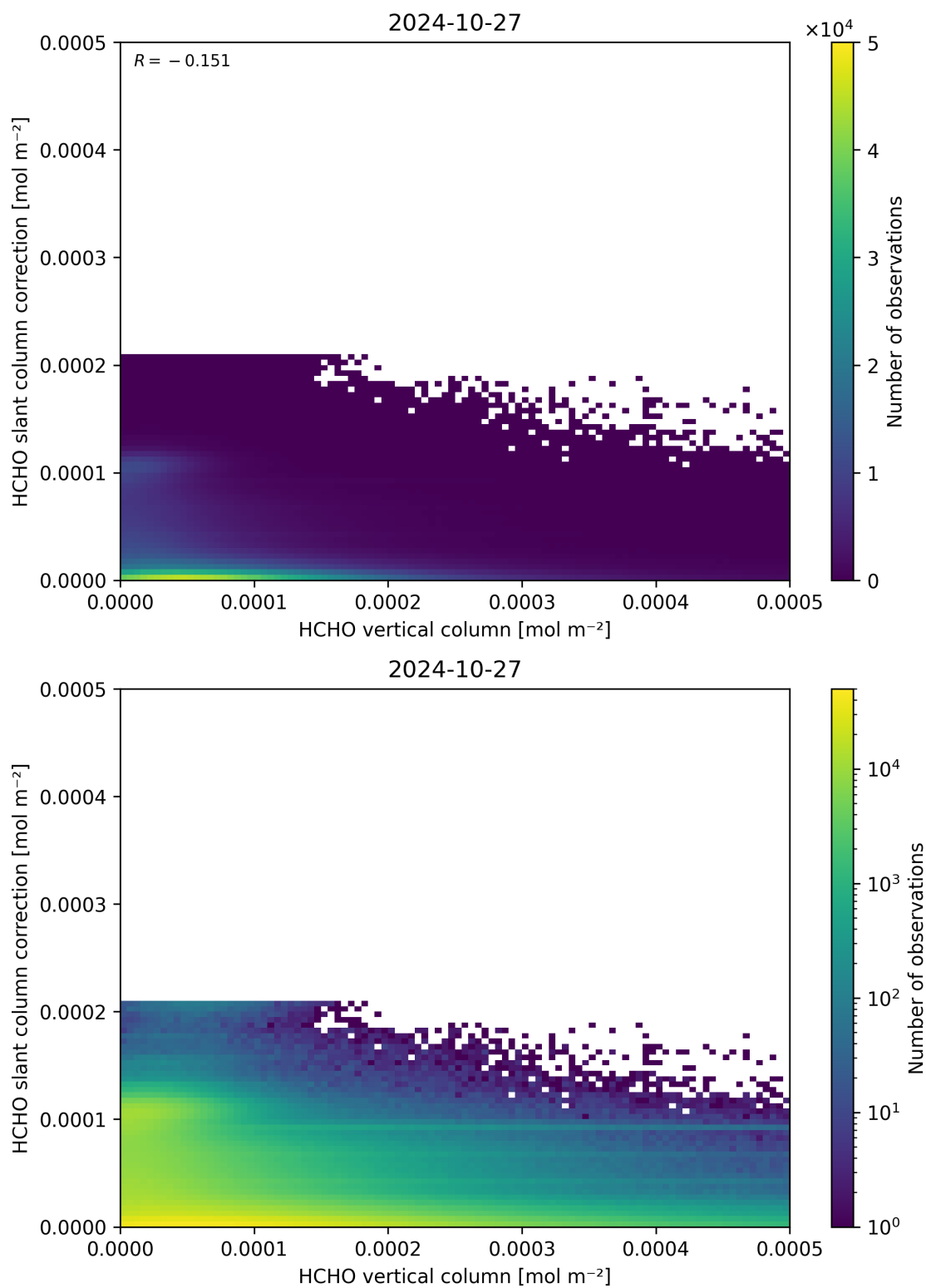
Figure 128: Scatter density plot of “HCHO vertical column” against “HCHO slant column correction” for 2024-10-26 to 2024-10-28.
