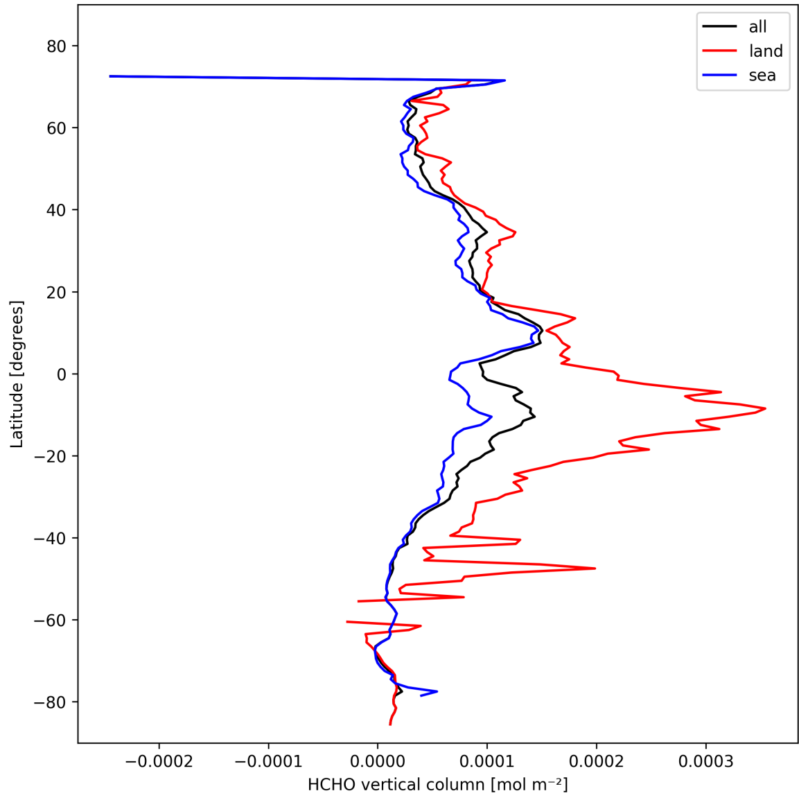
Figure 21: Zonal average of “HCHO vertical column” for 2024-10-26 to 2024-10-28.
