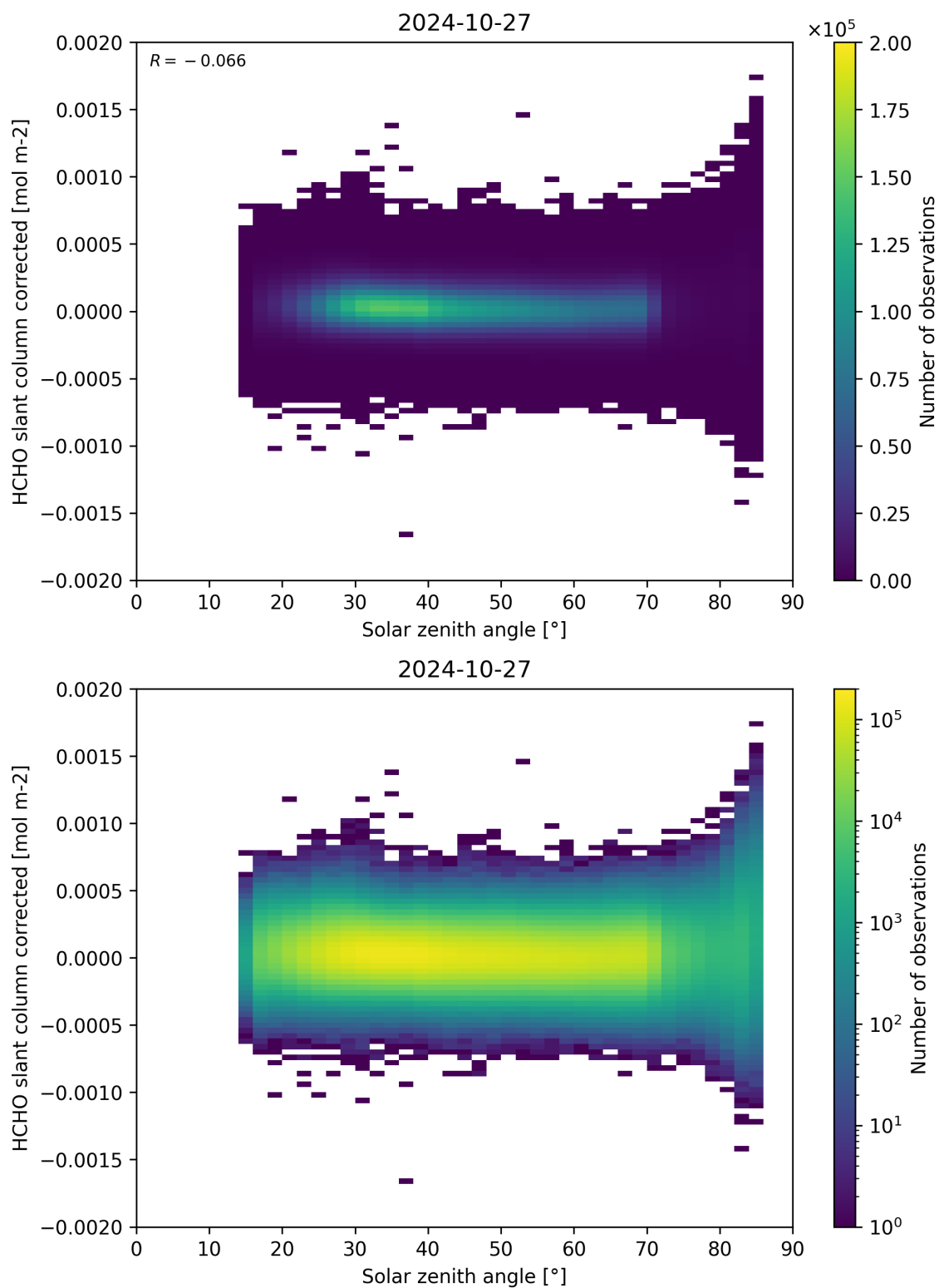
Figure 171: Scatter density plot of “Solar zenith angle” against “HCHO slant column corrected” for 2024-10-26 to 2024-10-28.
