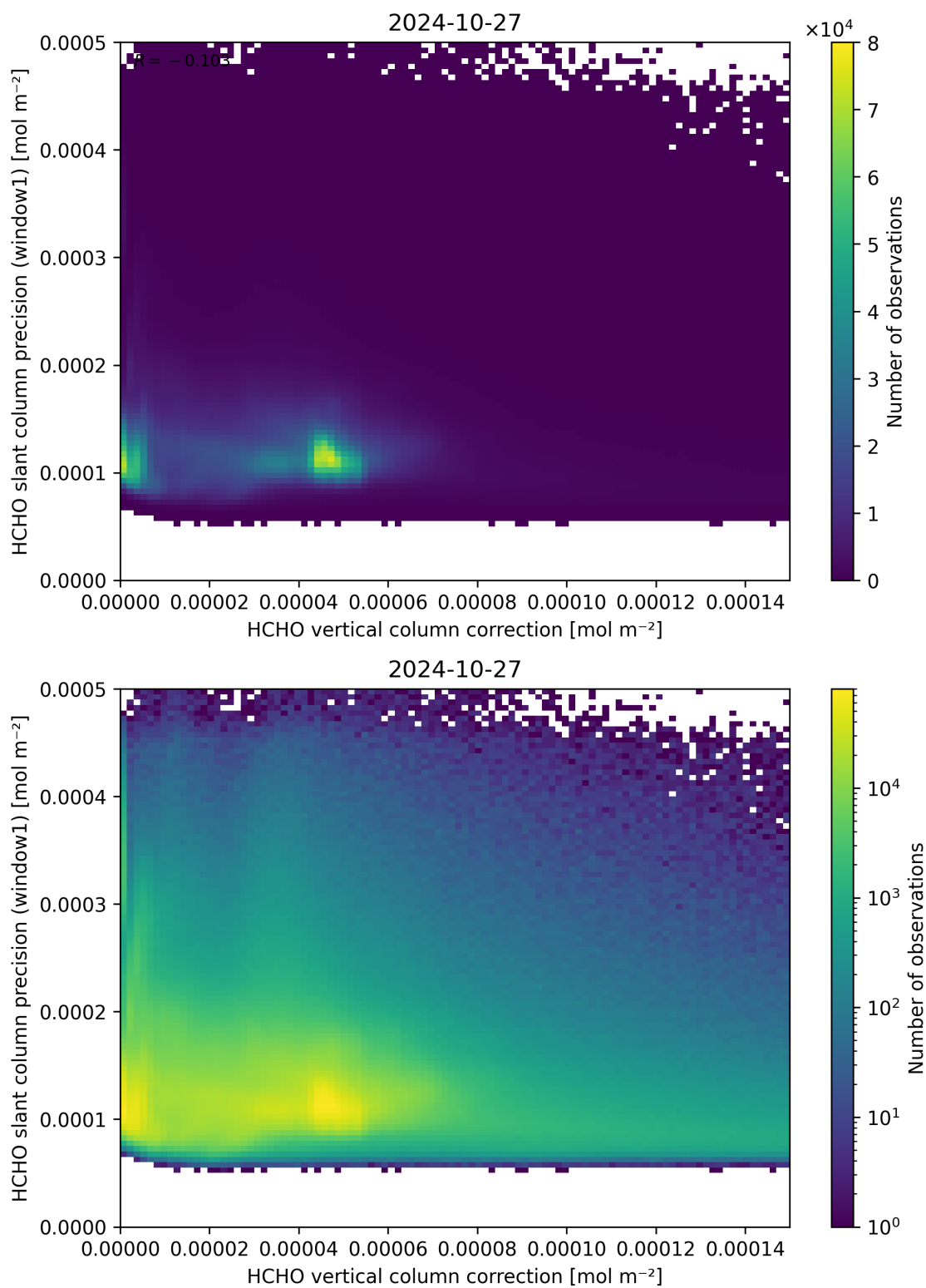
Figure 119: Scatter density plot of “HCHO vertical column correction” against “HCHO slant column precision (window1)” for 2024-10-26 to 2024-10-28.
