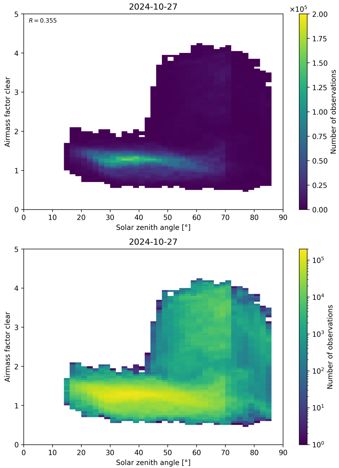
Figure 170: Scatter density plot of “Solar zenith angle” against “Airmass factor clear” for 2024-10-26 to 2024-10-28.
