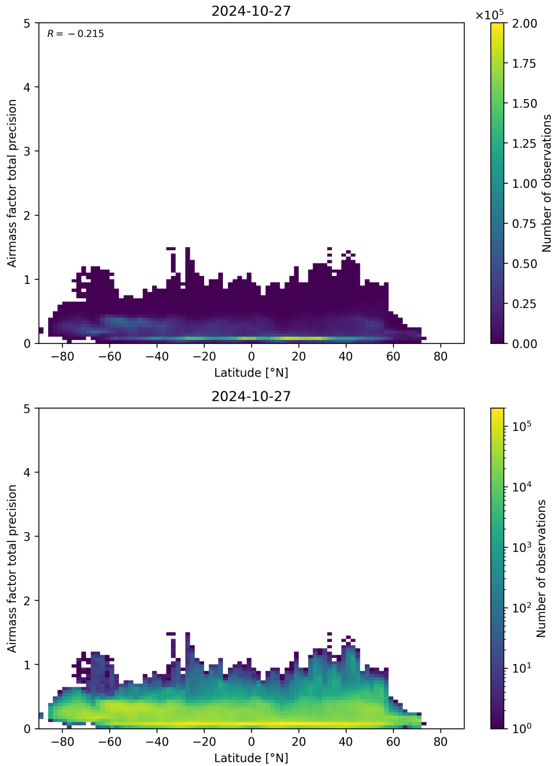
Figure 162: Scatter density plot of “Latitude” against “Airmass factor total precision” for 2024-10-26 to 2024-10-28.
