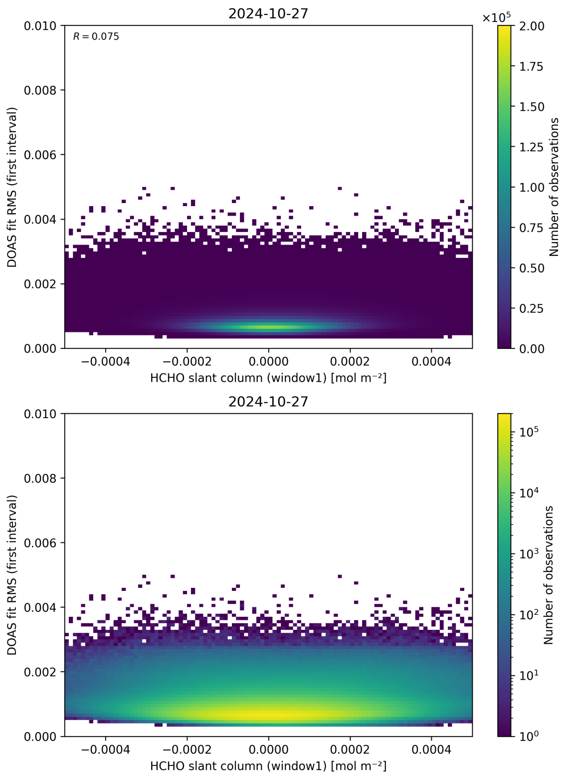
Figure 78: Scatter density plot of “HCHO slant column (window1)” against “DOAS fit RMS (first interval)” for 2024-10-26 to 2024-10-28.
