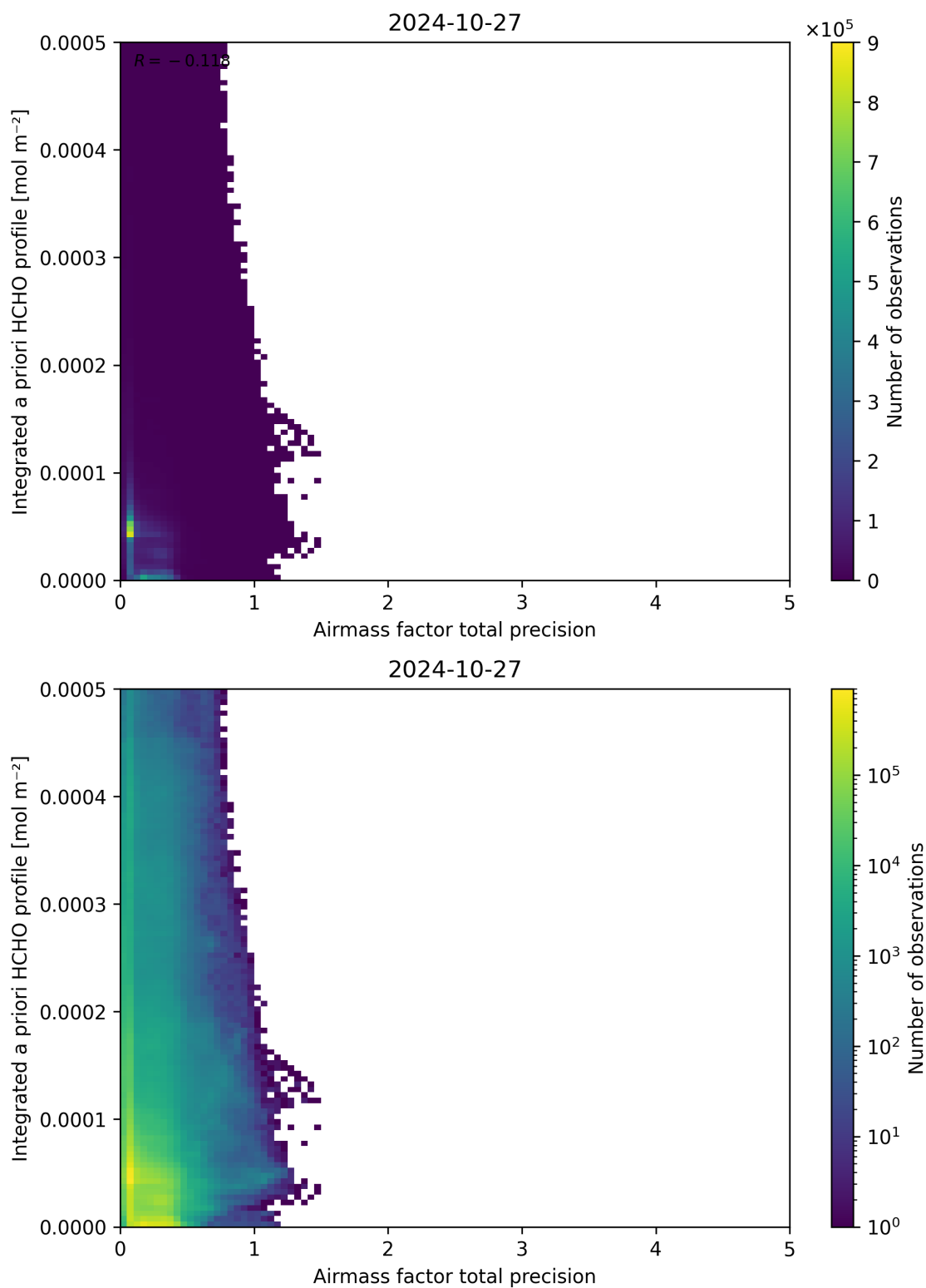
Figure 111: Scatter density plot of “Airmass factor total precision” against “Integrated a priori HCHO profile” for 2024-10-26 to 2024-10-28.
