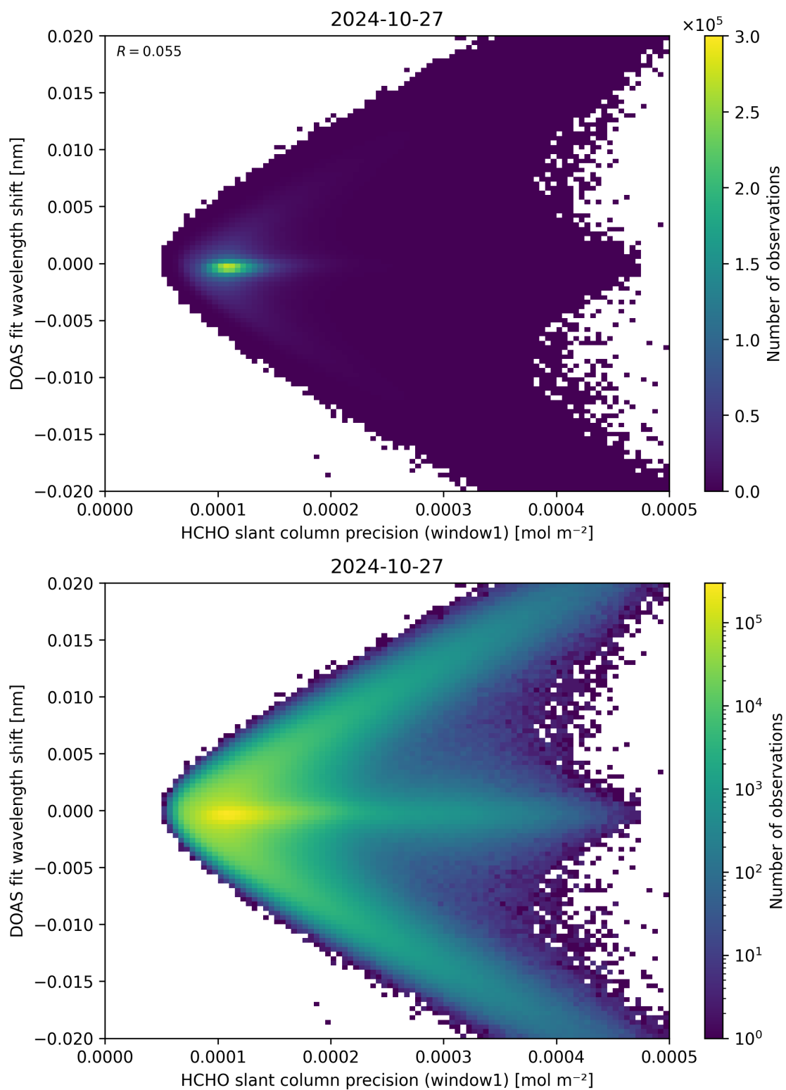
Figure 89: Scatter density plot of “HCHO slant column precision (window1)” against “DOAS fit wavelength shift” for 2024-10-26 to 2024-10-28.
