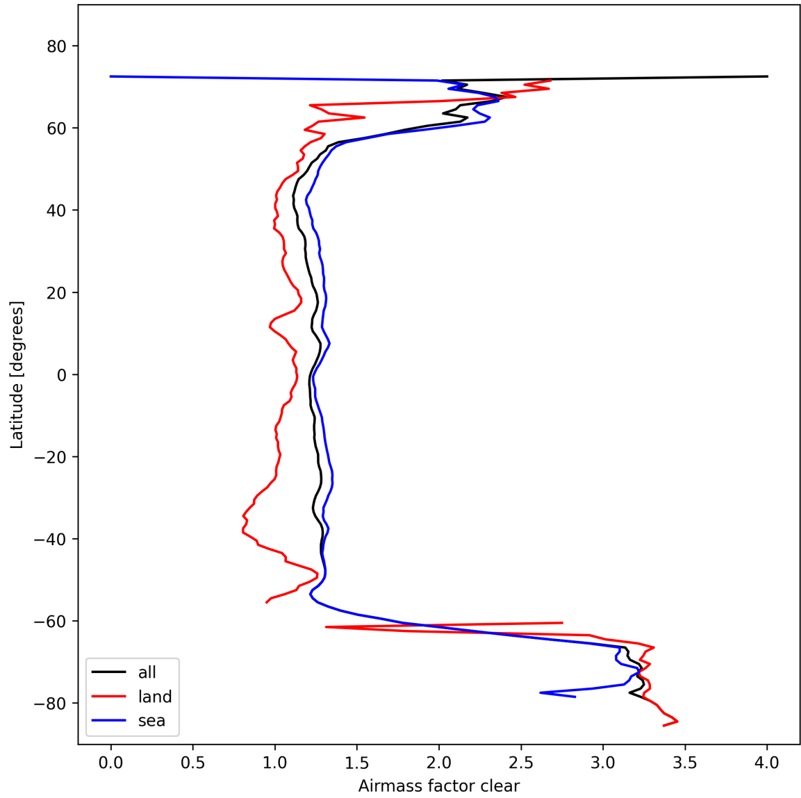
Figure 28: Zonal average of “Airmass factor clear” for 2024-10-26 to 2024-10-28.
