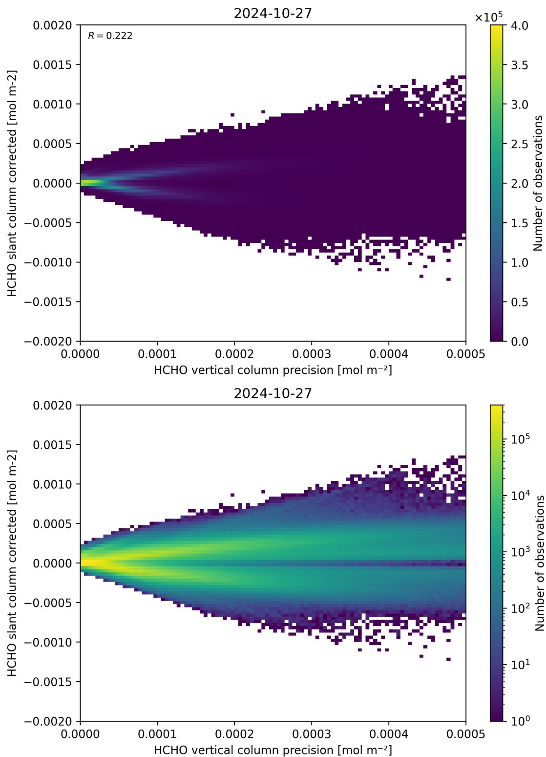
Figure 140: Scatter density plot of “HCHO vertical column precision” against “HCHO slant column corrected” for 2024-10-26 to 2024-10-28.
