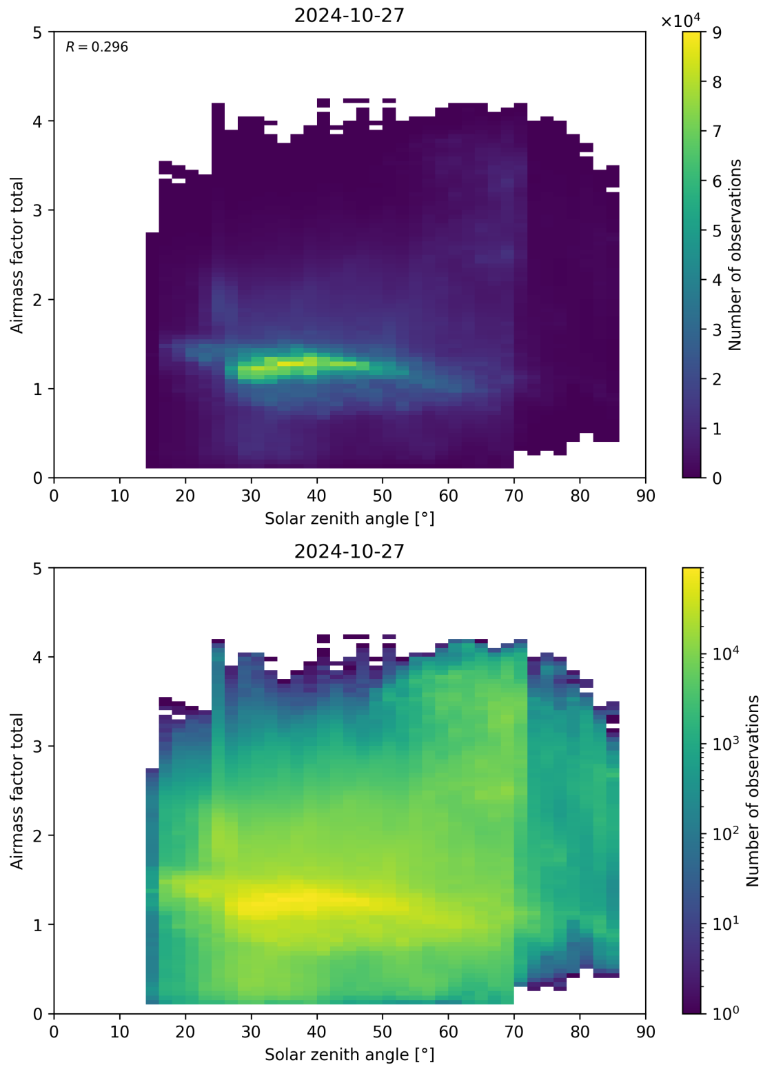
Figure 175: Scatter density plot of “Solar zenith angle” against “Airmass factor total” for 2024-10-26 to 2024-10-28.
