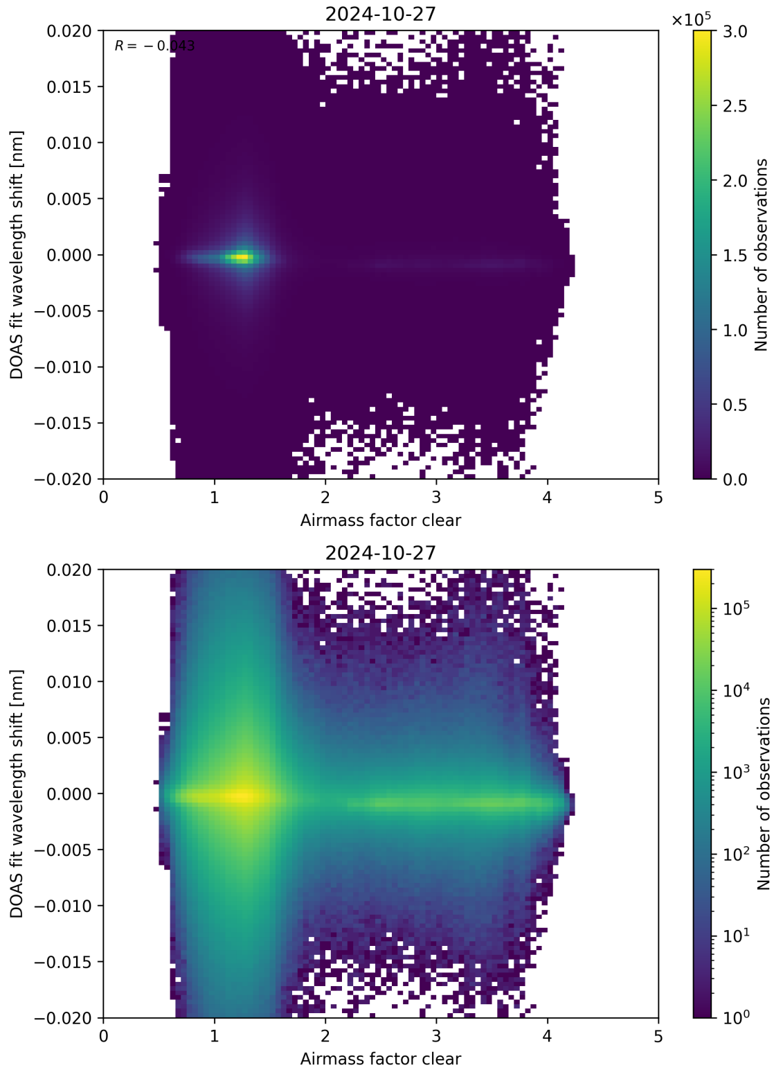
Figure 72: Scatter density plot of “Airmass factor clear” against “DOAS fit wavelength shift” for 2024-10-26 to 2024-10-28.
