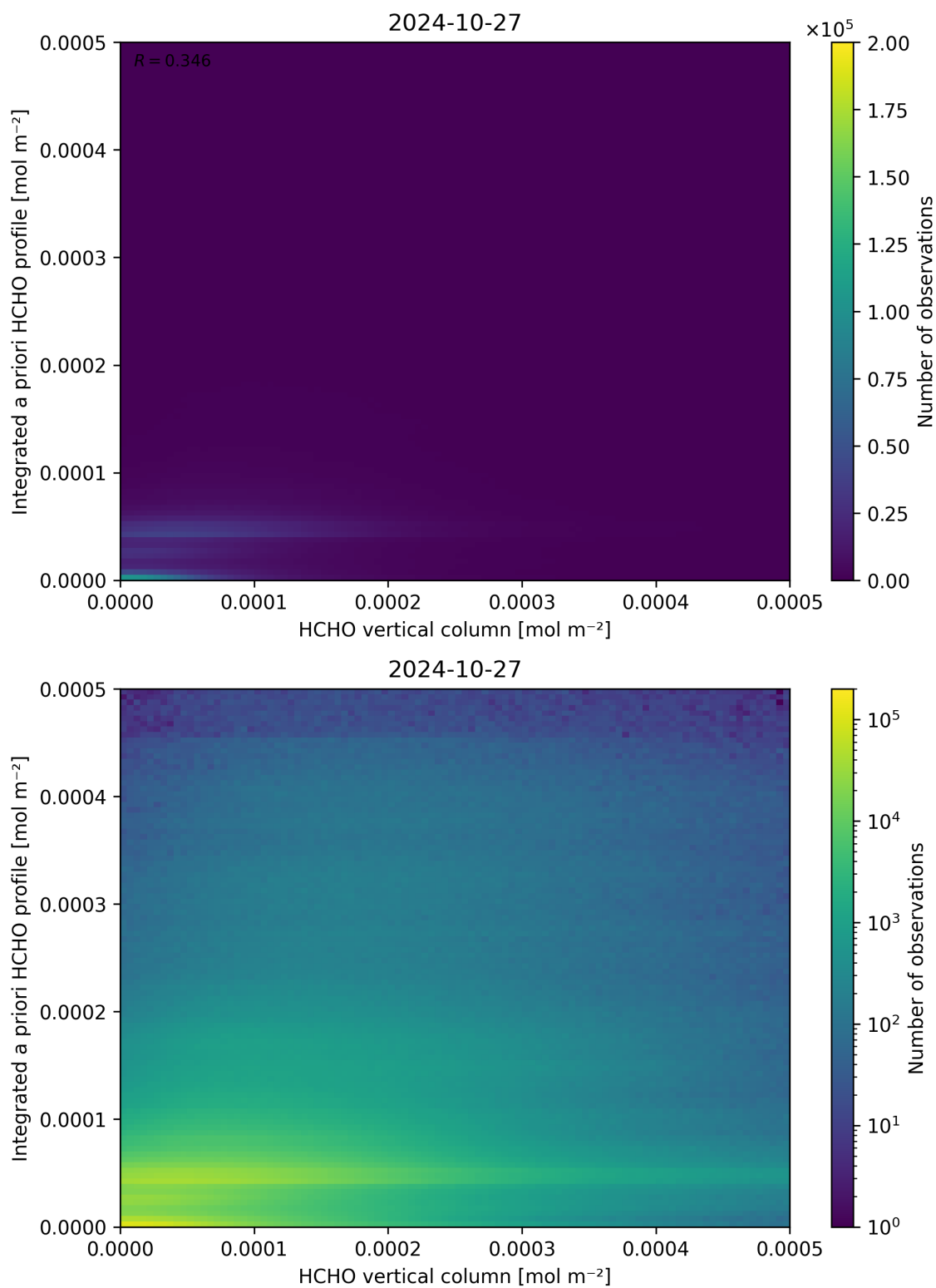
Figure 135: Scatter density plot of “HCHO vertical column” against “Integrated a priori HCHO profile” for 2024-10-26 to 2024-10-28.
