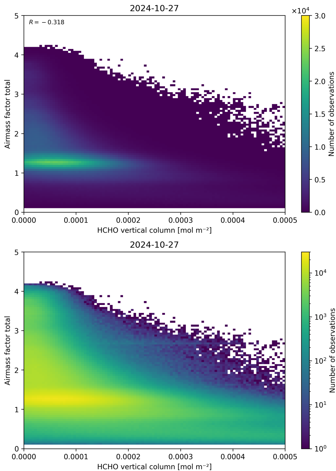
Figure 131: Scatter density plot of “HCHO vertical column” against “Airmass factor total” for 2024-10-26 to 2024-10-28.
