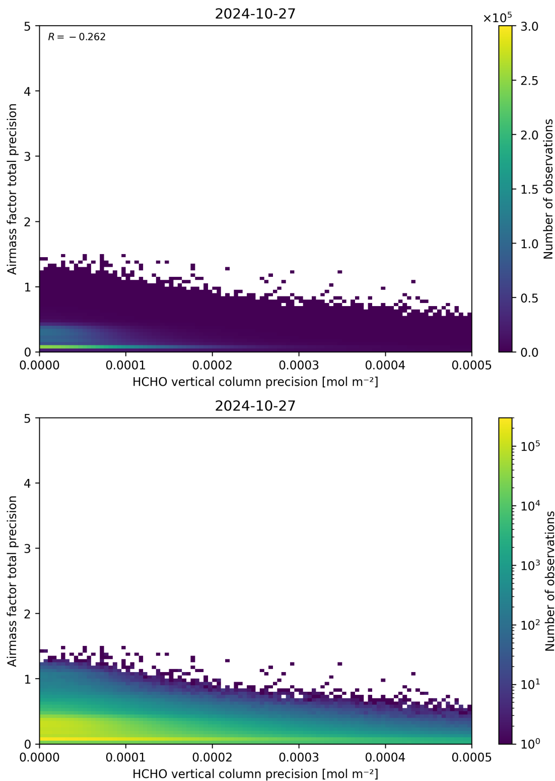
Figure 145: Scatter density plot of “HCHO vertical column precision” against “Airmass factor total precision” for 2024-10-26 to 2024-10-28.
