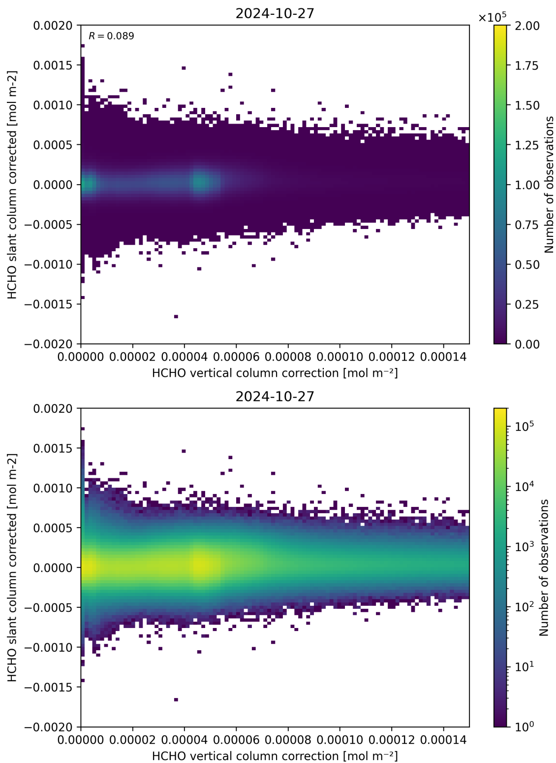
Figure 116: Scatter density plot of “HCHO vertical column correction” against “HCHO slant column corrected” for 2024-10-26 to 2024-10-28.
