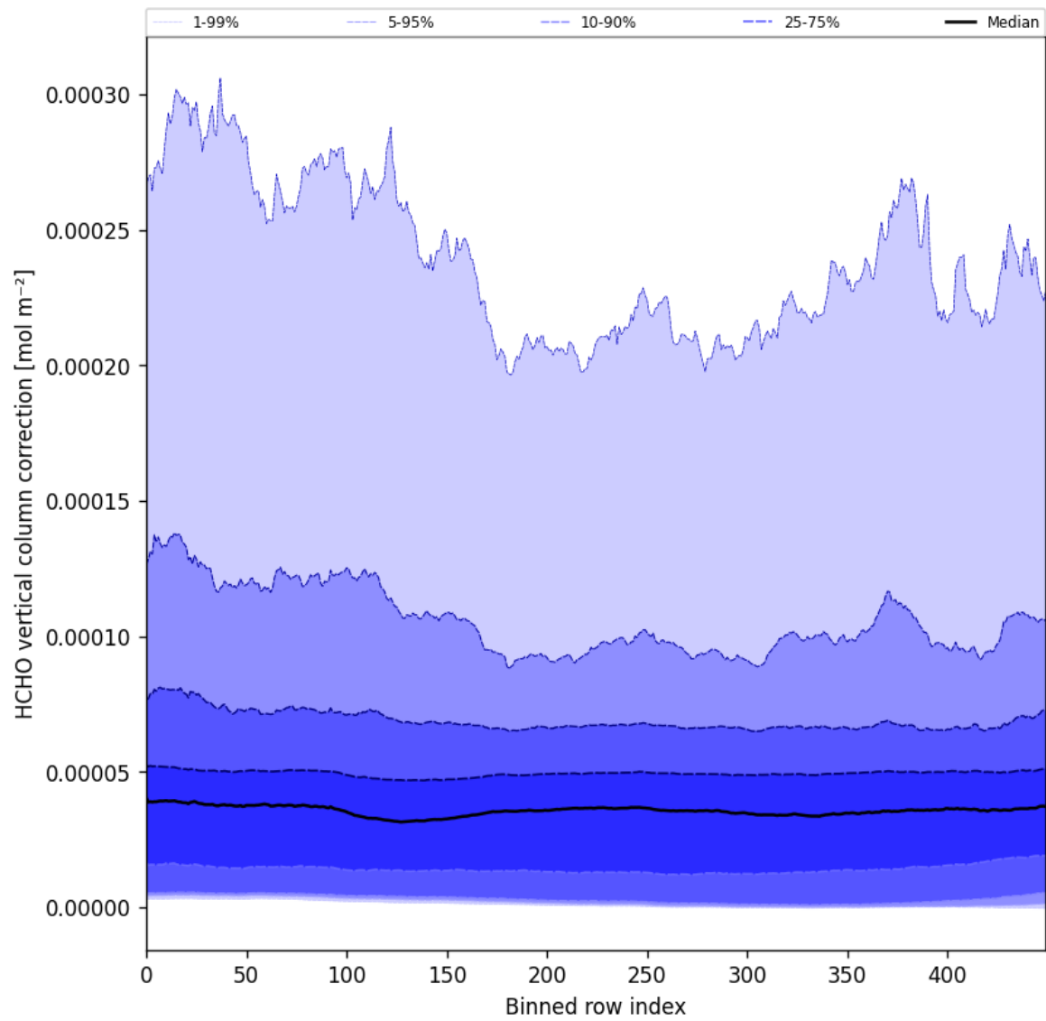
Figure 51: Along track statistics of “HCHO vertical column correction” for 2024-10-26 to 2024-10-28
