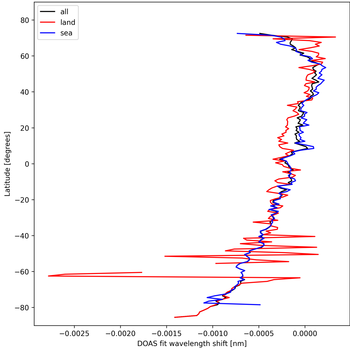
Figure 30: Zonal average of “DOAS fit wavelength shift” for 2024-10-26 to 2024-10-28.
