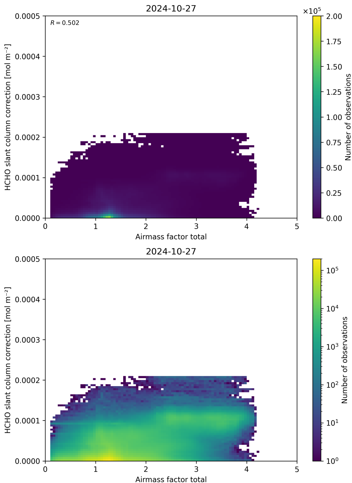
Figure 102: Scatter density plot of “Airmass factor total” against “HCHO slant column correction” for 2024-10-26 to 2024-10-28.
