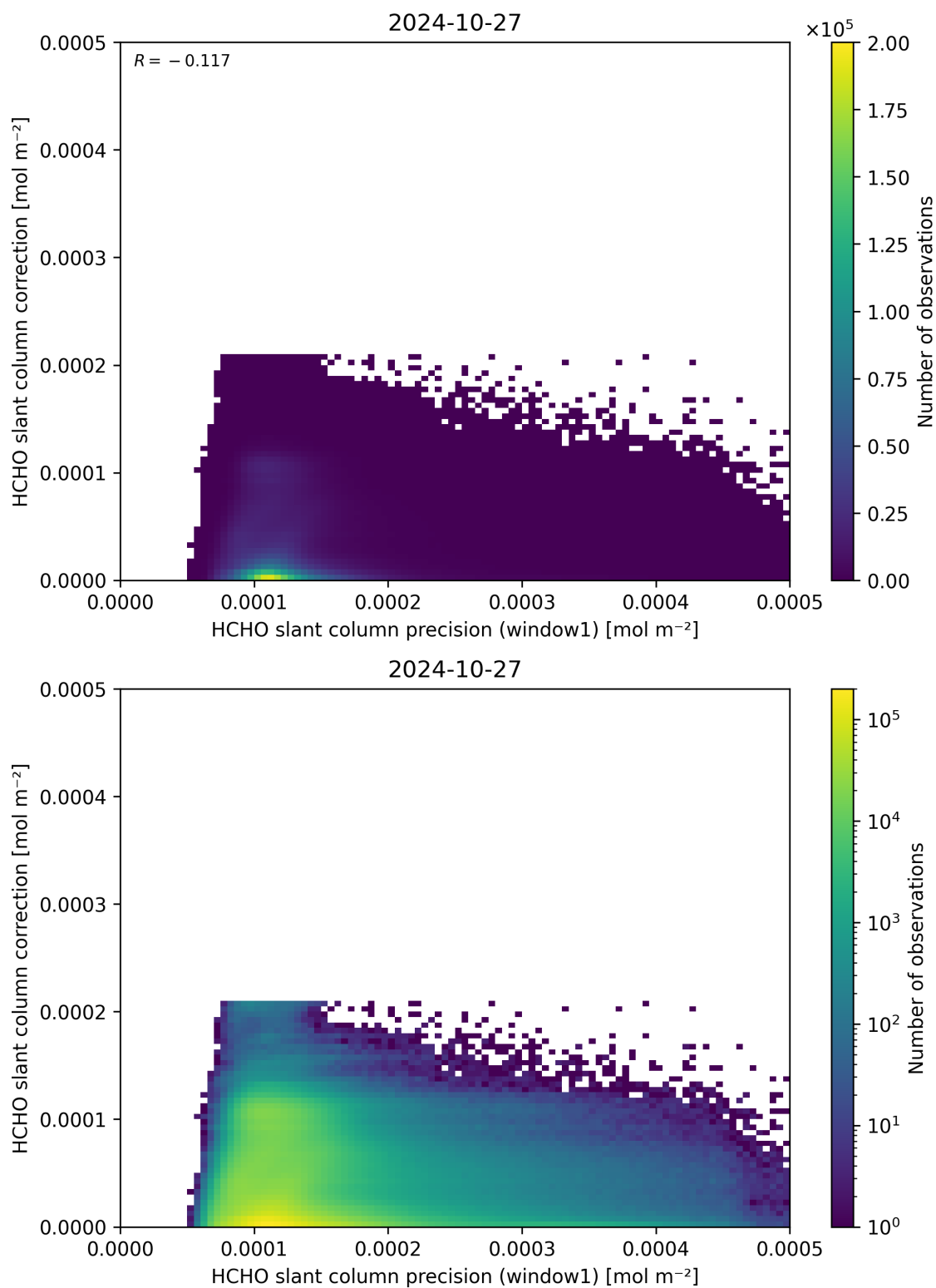
Figure 93: Scatter density plot of “HCHO slant column precision (window1)” against “HCHO slant column correction” for 2024-10-26 to 2024-10-28.
