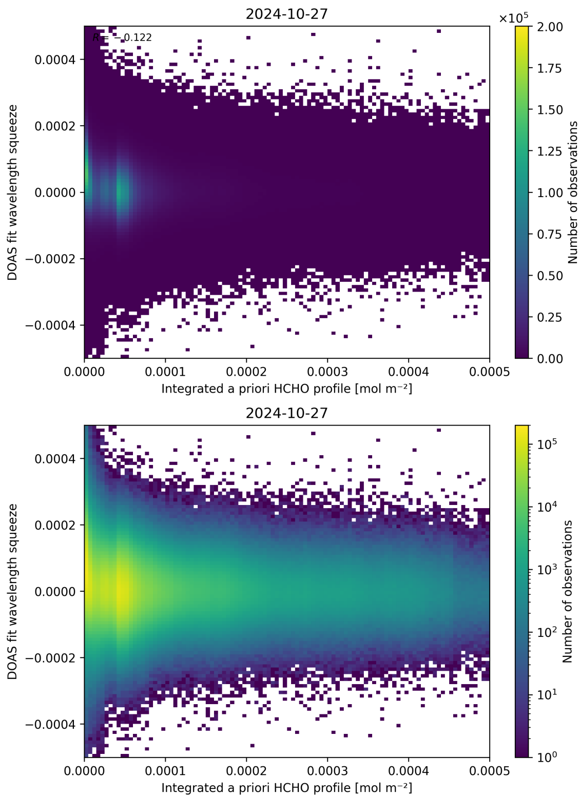
Figure 150: Scatter density plot of “Integrated a priori HCHO profile” against “DOAS fit wavelength squeeze” for 2024-10-26 to 2024-10-28.
