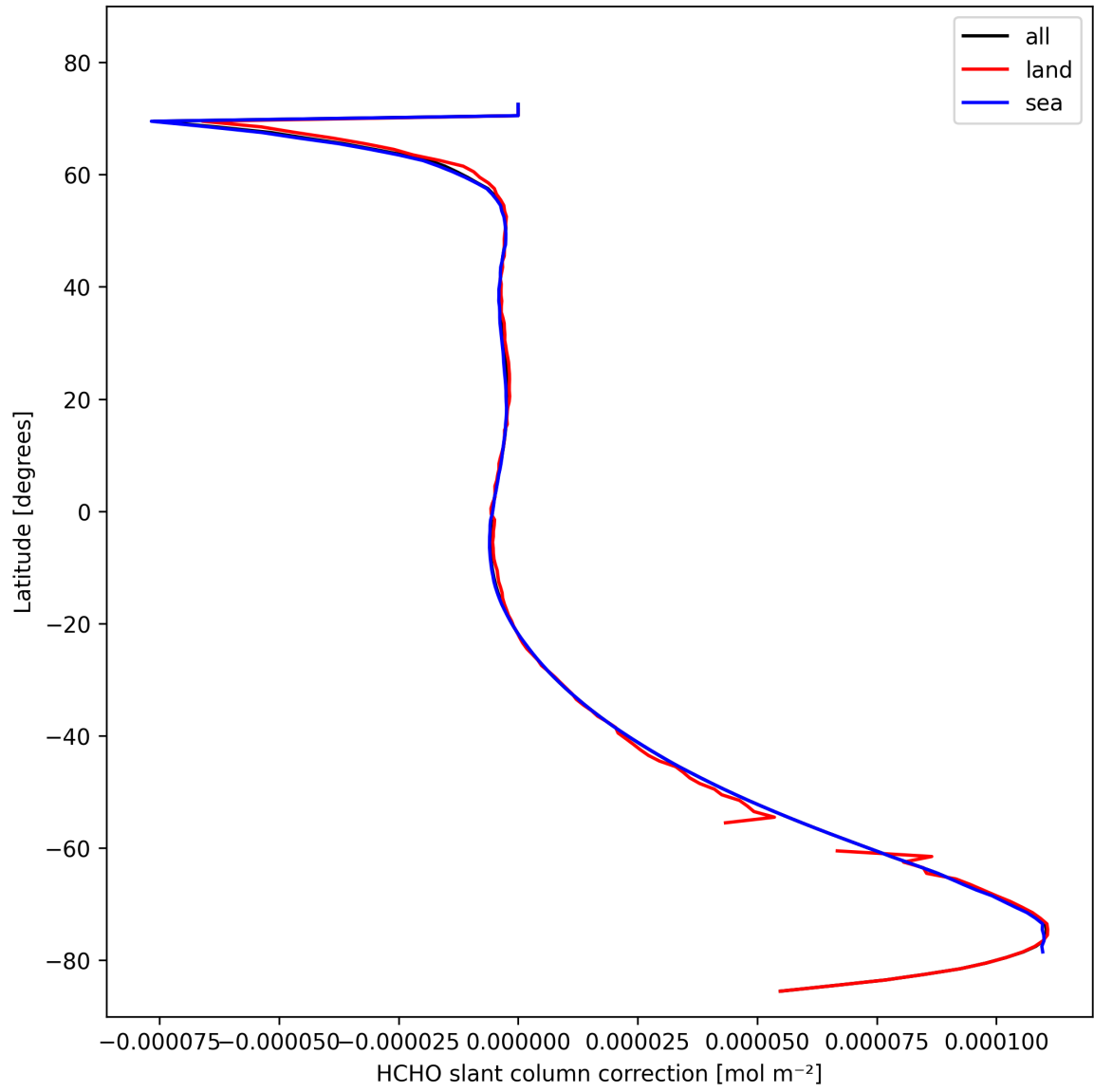
Figure 33: Zonal average of “HCHO slant column correction” for 2024-10-26 to 2024-10-28.
