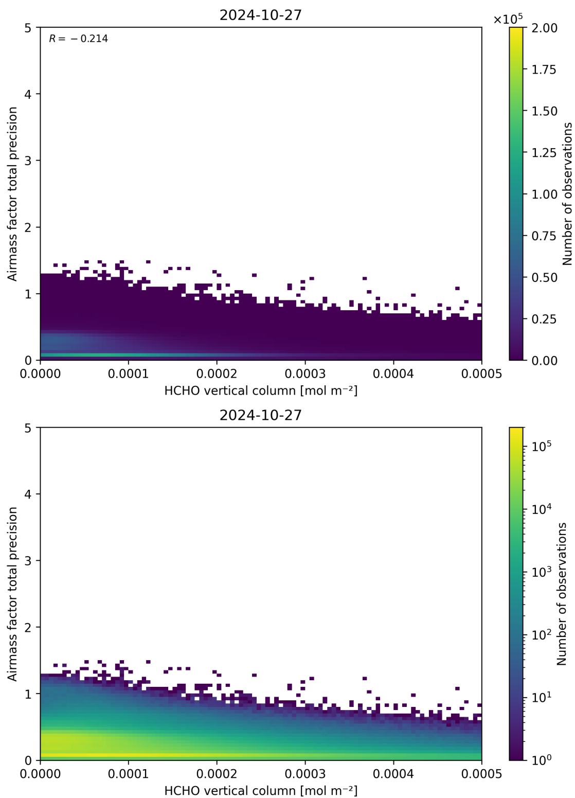
Figure 132: Scatter density plot of “HCHO vertical column” against “Airmass factor total precision” for 2024-10-26 to 2024-10-28.
