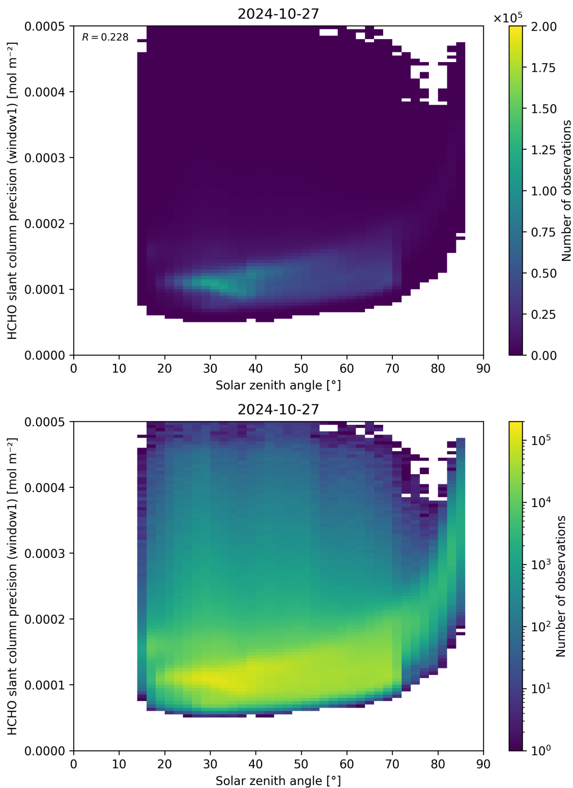
Figure 174: Scatter density plot of “Solar zenith angle” against “HCHO slant column precision (window1)” for 2024-10-26 to 2024-10-28.
