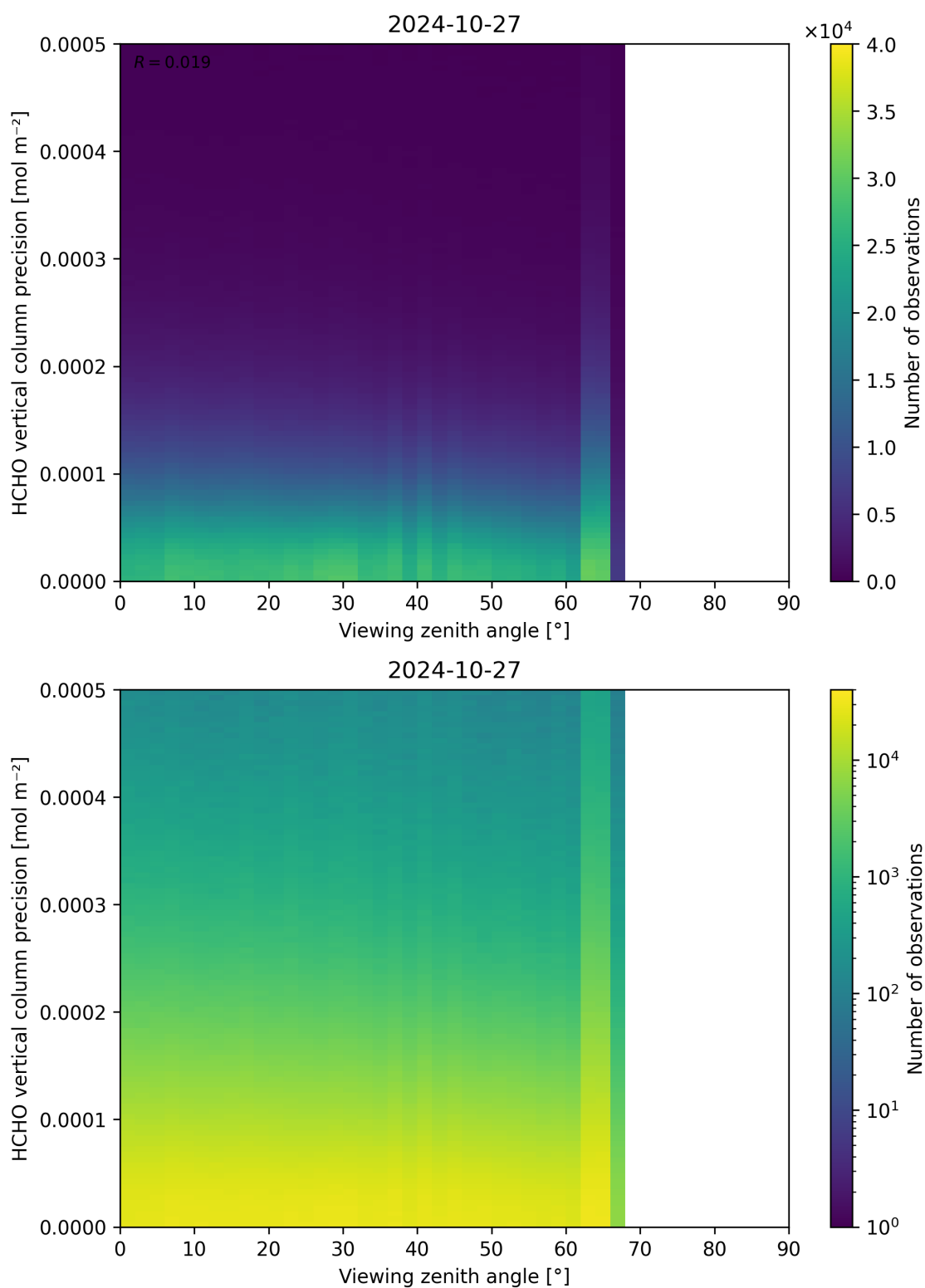
Figure 194: Scatter density plot of “Viewing zenith angle” against “HCHO vertical column precision” for 2024-10-26 to 2024-10-28.
