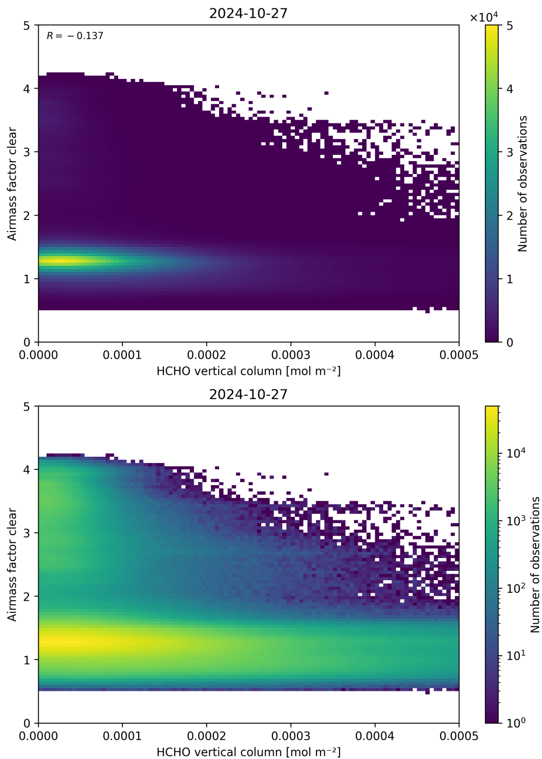
Figure 126: Scatter density plot of “HCHO vertical column” against “Airmass factor clear” for 2024-10-26 to 2024-10-28.
