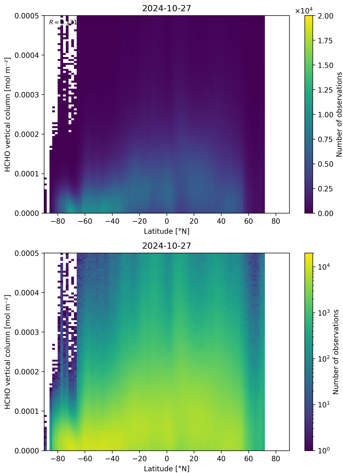
Figure 163: Scatter density plot of “Latitude” against “HCHO vertical column” for 2024-10-26 to 2024-10-28.
