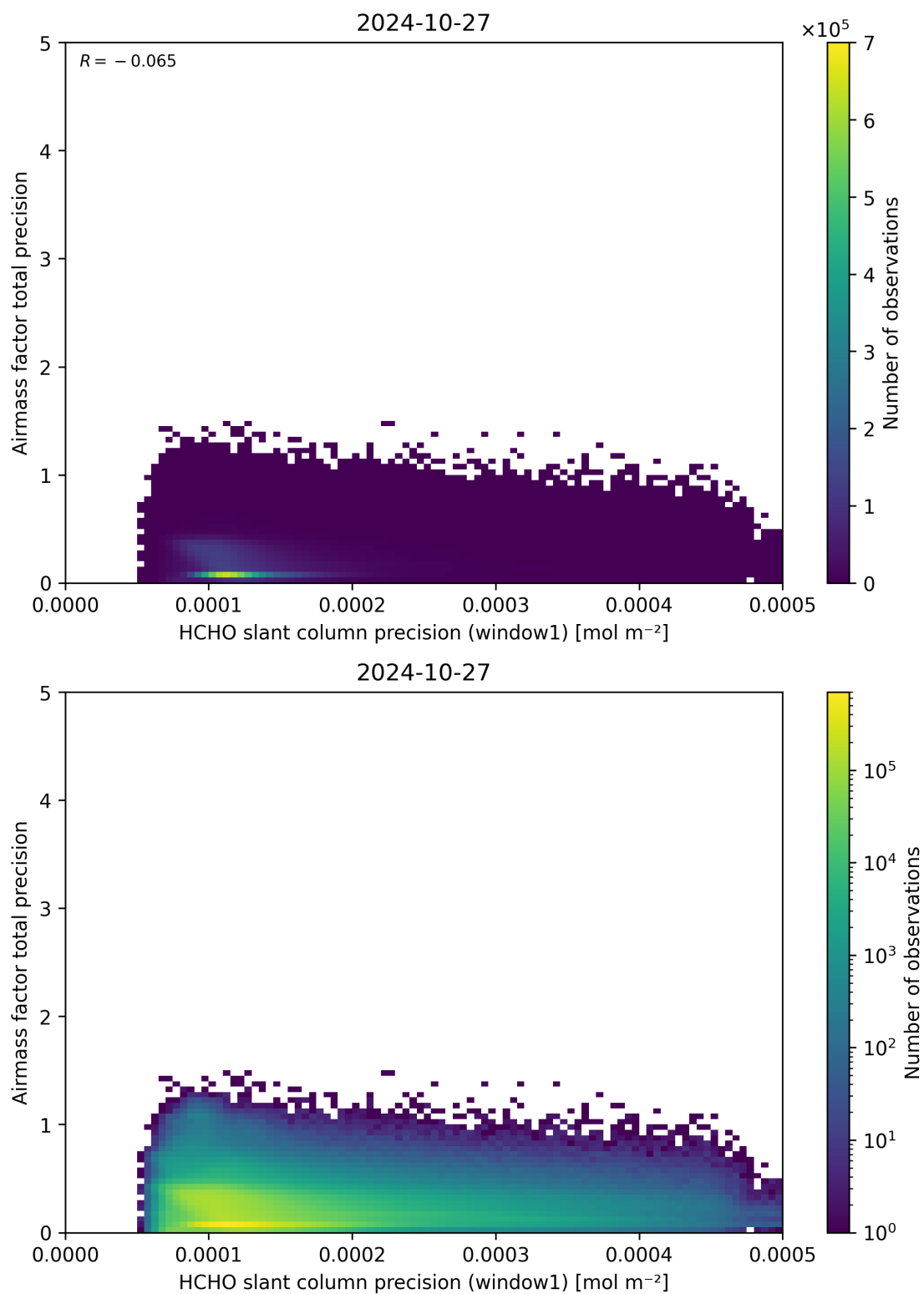
Figure 95: Scatter density plot of “HCHO slant column precision (window1)” against “Airmass factor total precision” for 2024-10-26 to 2024-10-28.
