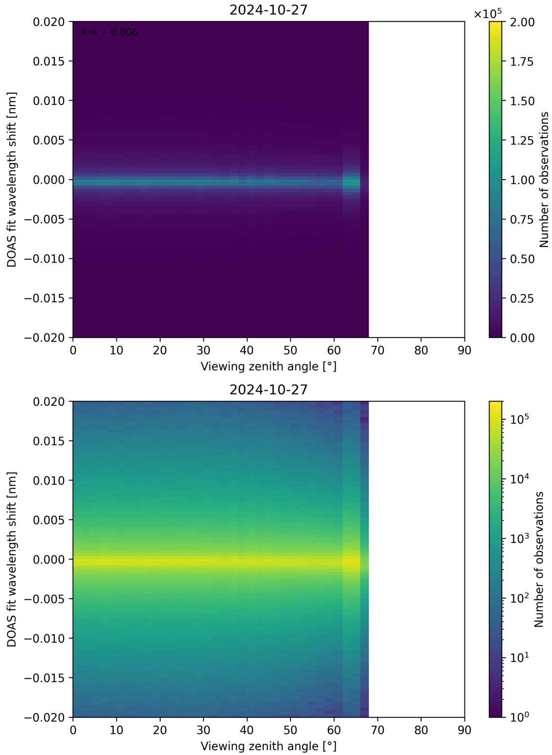
Figure 183: Scatter density plot of “Viewing zenith angle” against “DOAS fit wavelength shift” for 2024-10-26 to 2024-10-28.
