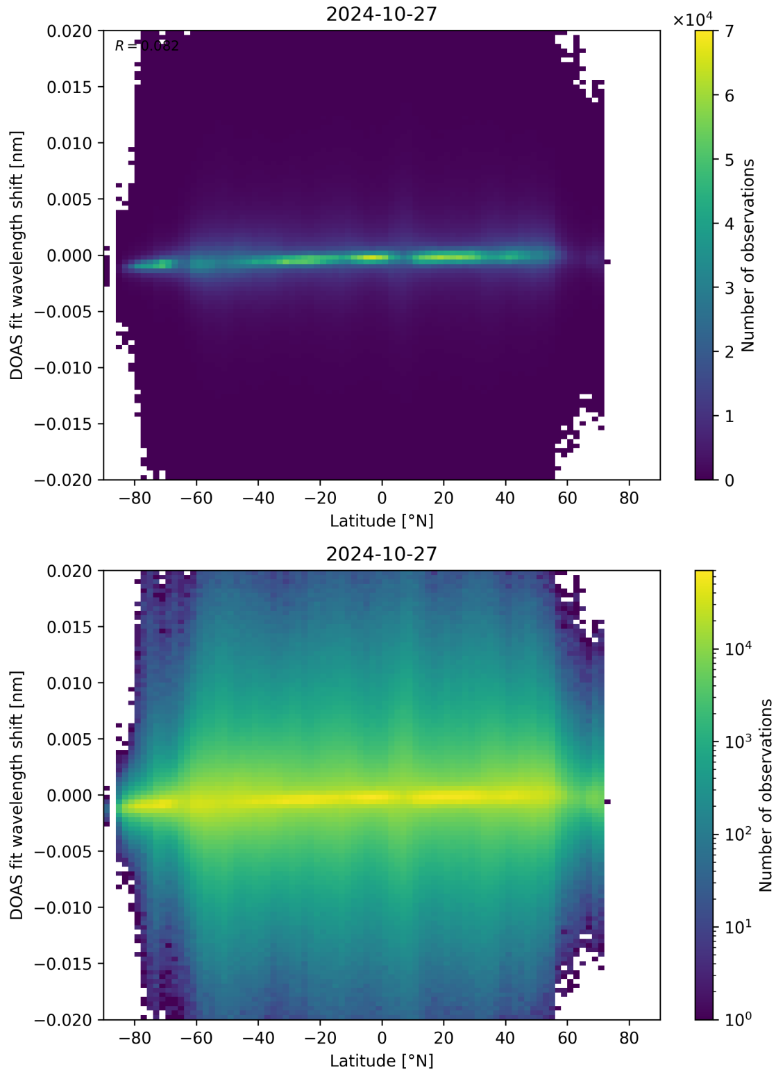
Figure 154: Scatter density plot of “Latitude” against “DOAS fit wavelength shift” for 2024-10-26 to 2024-10-28.
