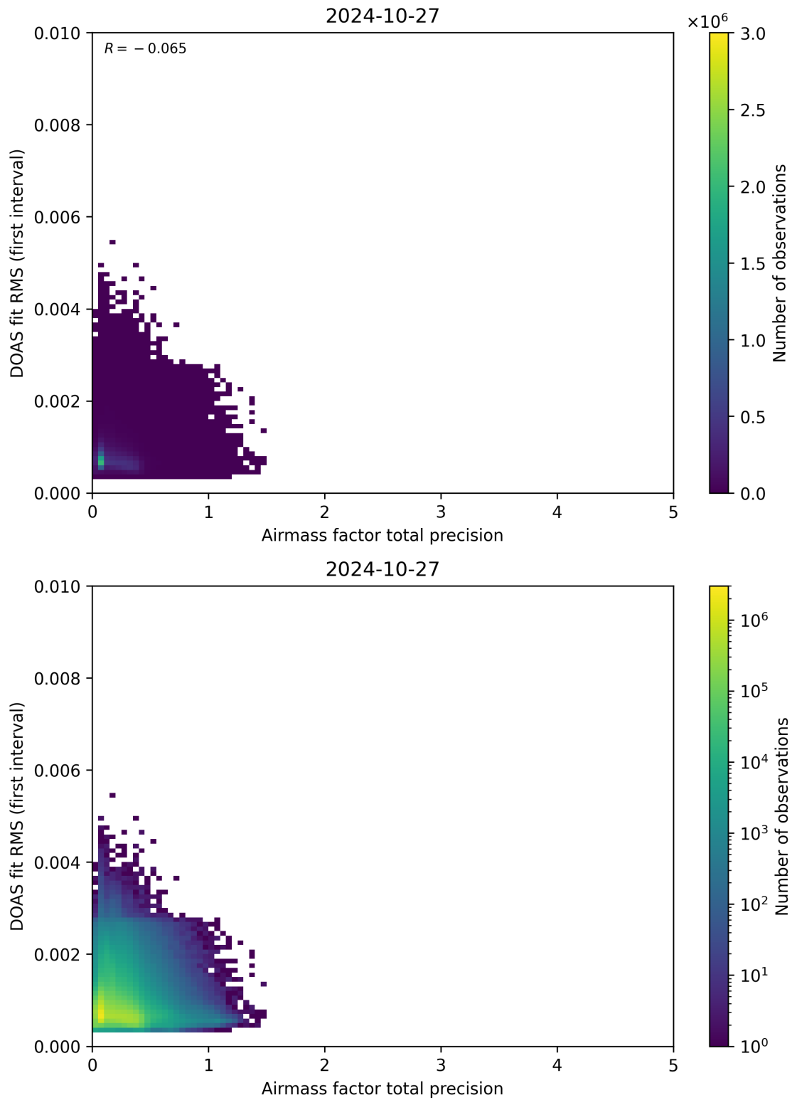
Figure 105: Scatter density plot of “Airmass factor total precision” against “DOAS fit RMS (first interval)” for 2024-10-26 to 2024-10-28.
