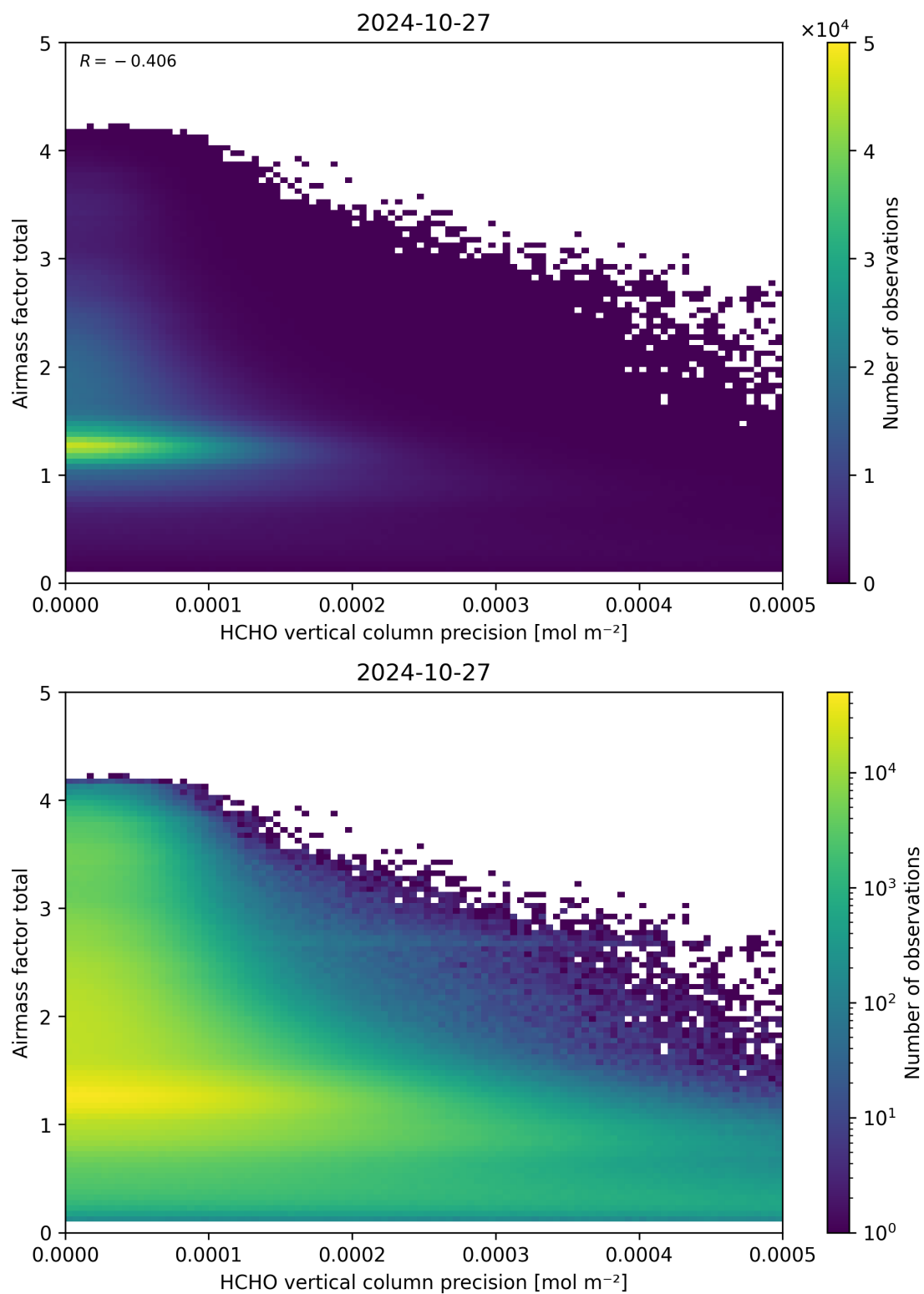
Figure 144: Scatter density plot of “HCHO vertical column precision” against “Airmass factor total” for 2024-10-26 to 2024-10-28.
