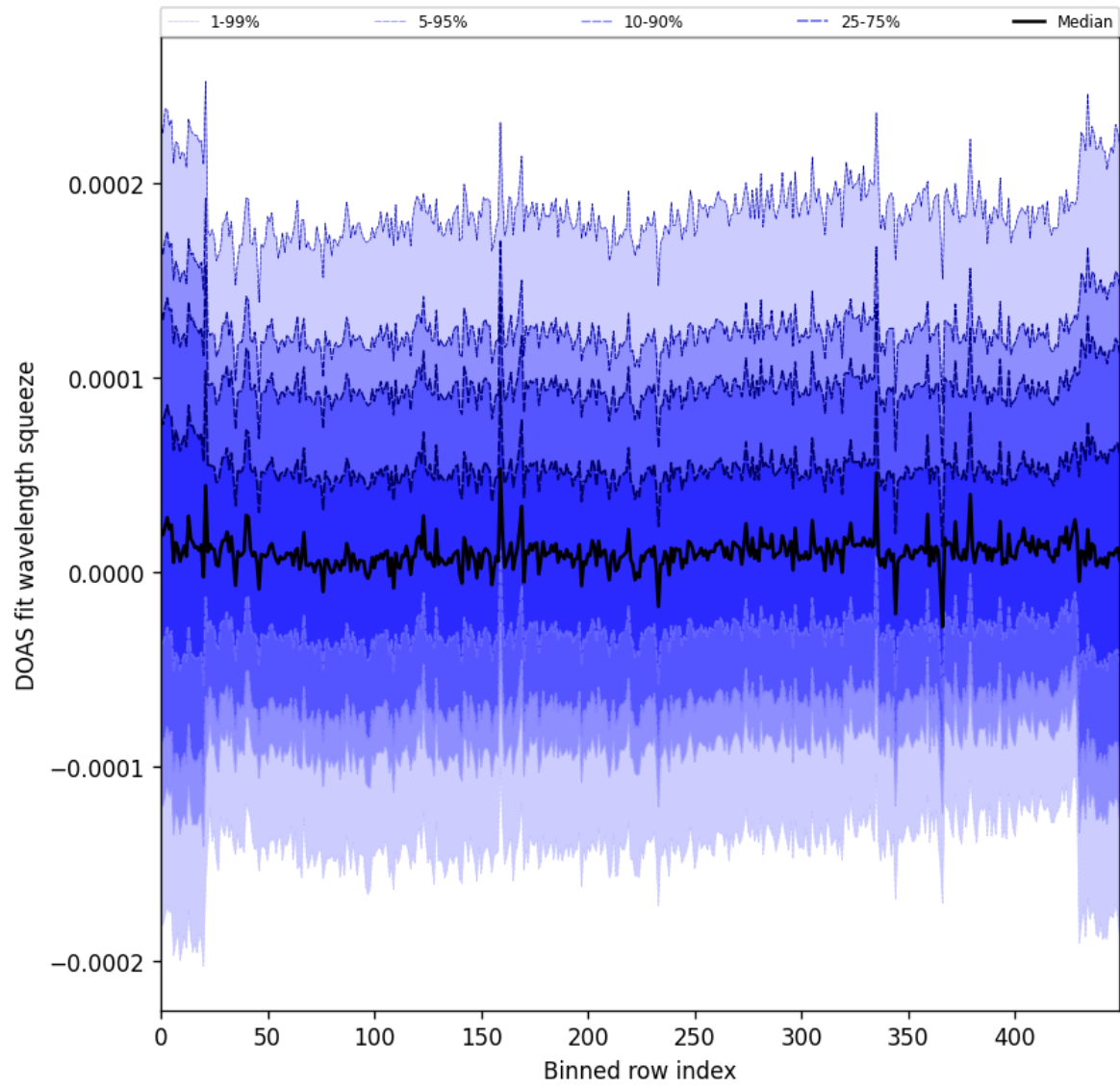
Figure 59: Along track statistics of “DOAS fit wavelength squeeze” for 2024-10-26 to 2024-10-28
