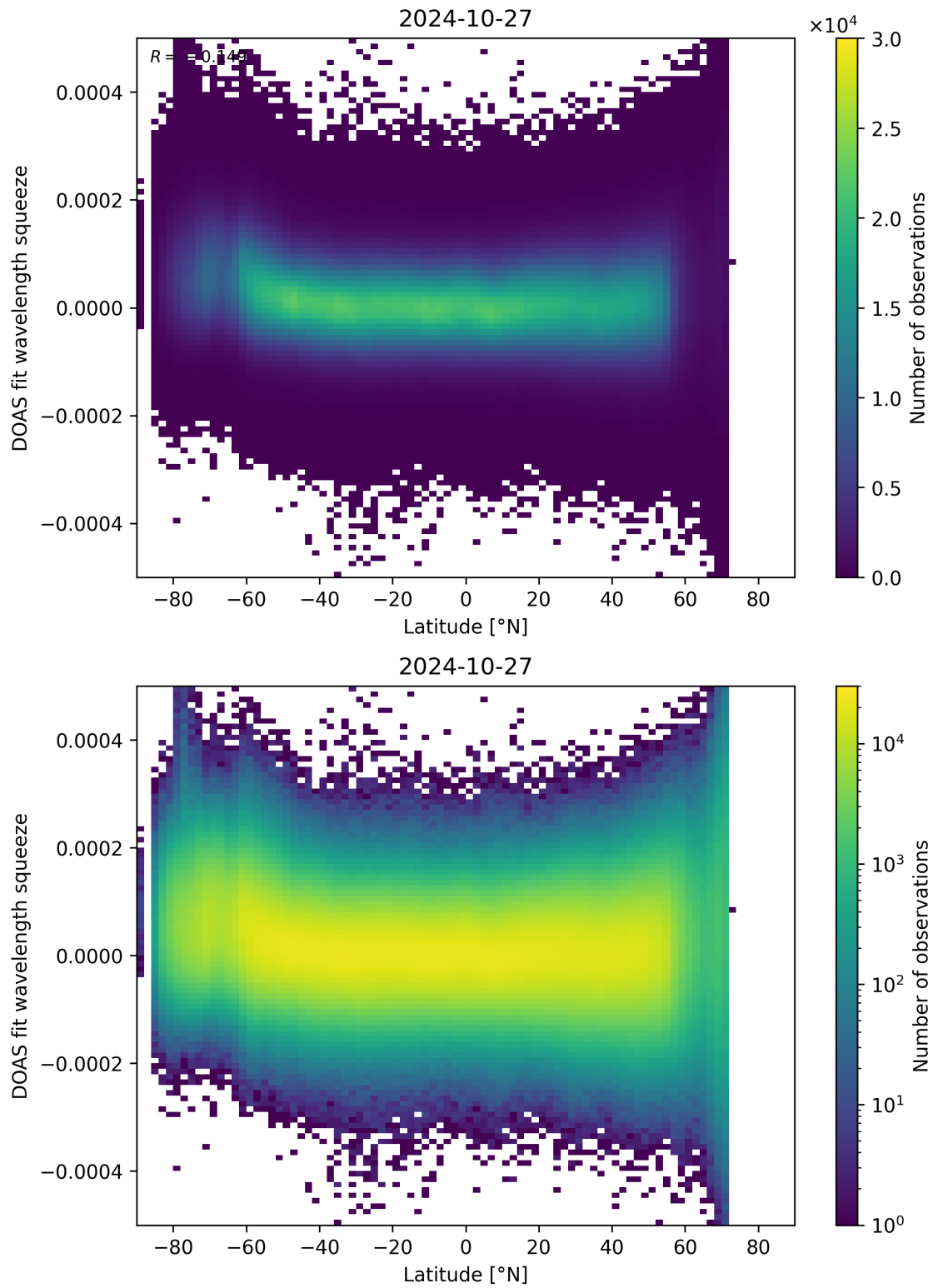
Figure 155: Scatter density plot of “Latitude” against “DOAS fit wavelength squeeze” for 2024-10-26 to 2024-10-28.
