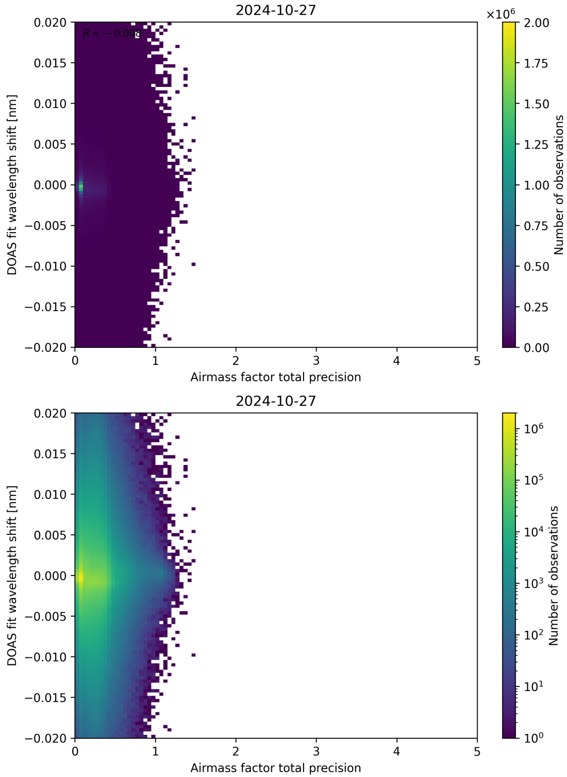
Figure 106: Scatter density plot of “Airmass factor total precision” against “DOAS fit wavelength shift” for 2024-10-26 to 2024-10-28.
