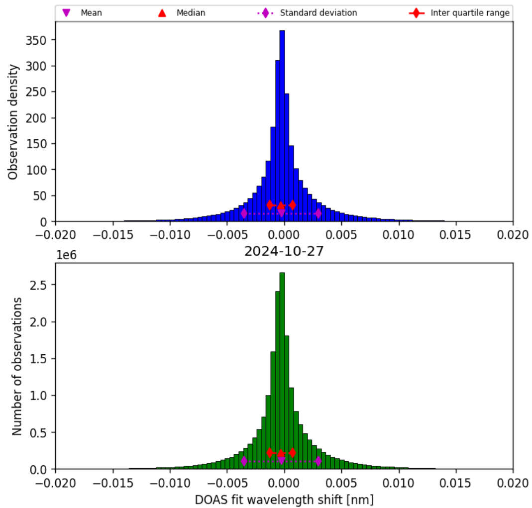
Figure 44: Histogram of “DOAS fit wavelength shift” for 2024-10-26 to 2024-10-28
