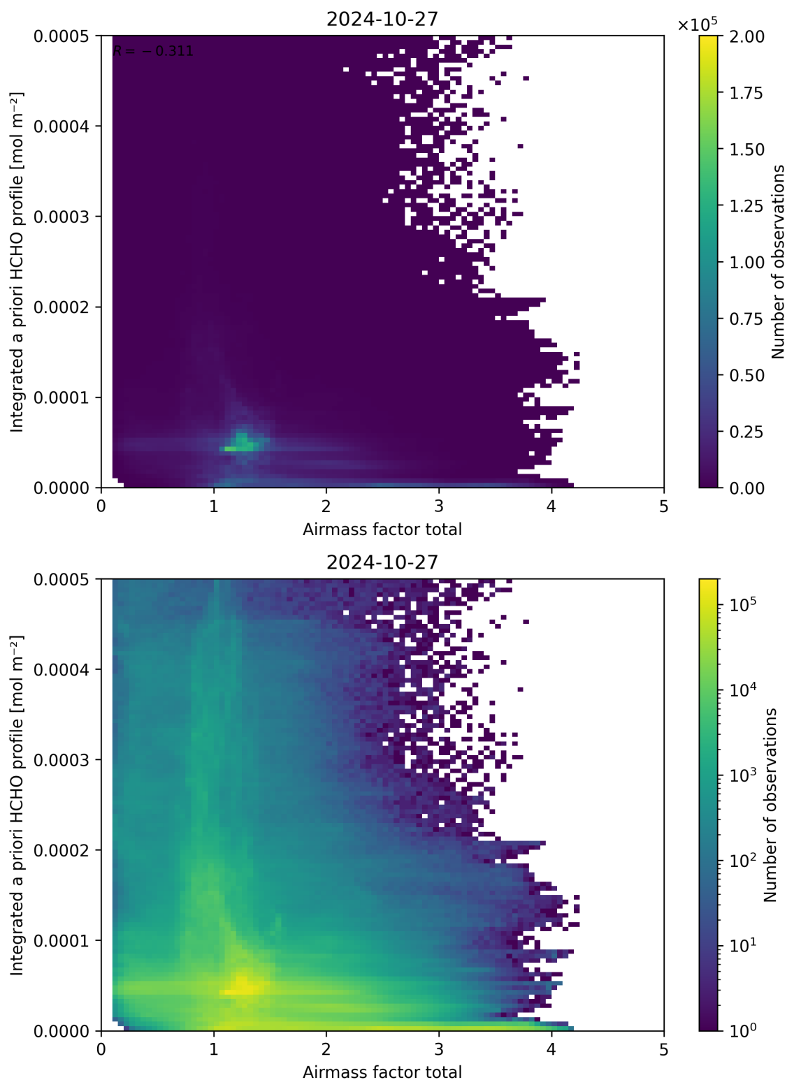
Figure 104: Scatter density plot of “Airmass factor total” against “Integrated a priori HCHO profile” for 2024-10-26 to 2024-10-28.
