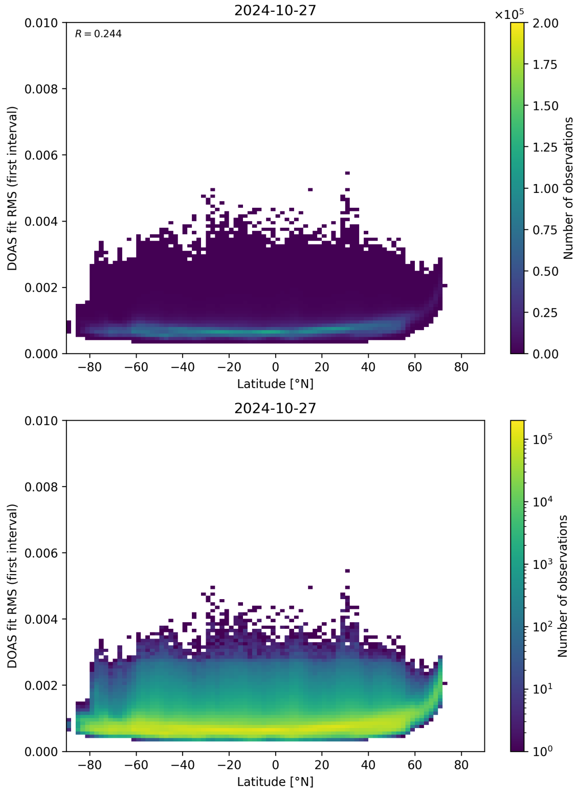
Figure 153: Scatter density plot of “Latitude” against “DOAS fit RMS (first interval)” for 2024-10-26 to 2024-10-28.
