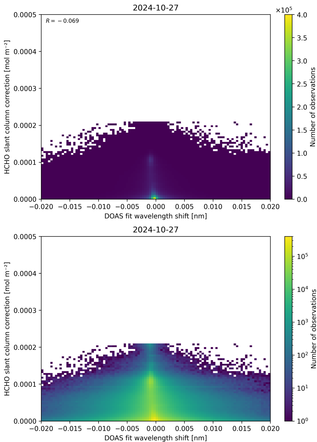
Figure 67: Scatter density plot of “DOAS fit wavelength shift” against “HCHO slant column correction” for 2024-10-26 to 2024-10-28.
