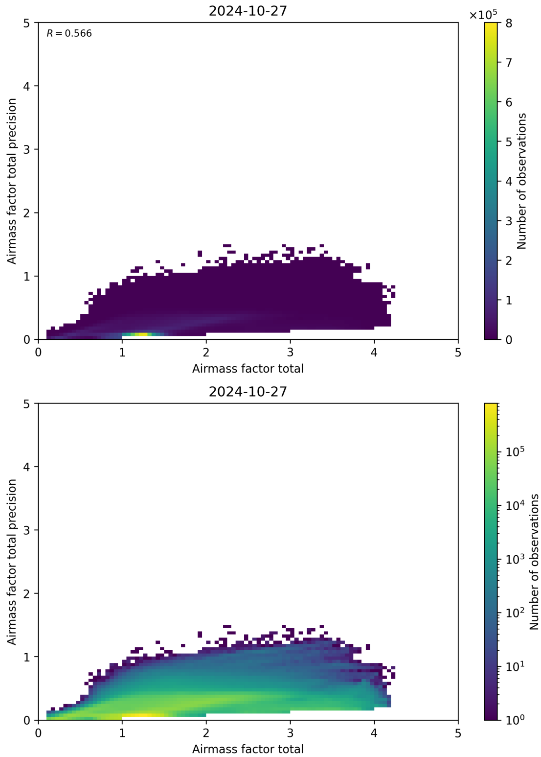
Figure 103: Scatter density plot of “Airmass factor total” against “Airmass factor total precision” for 2024-10-26 to 2024-10-28.
