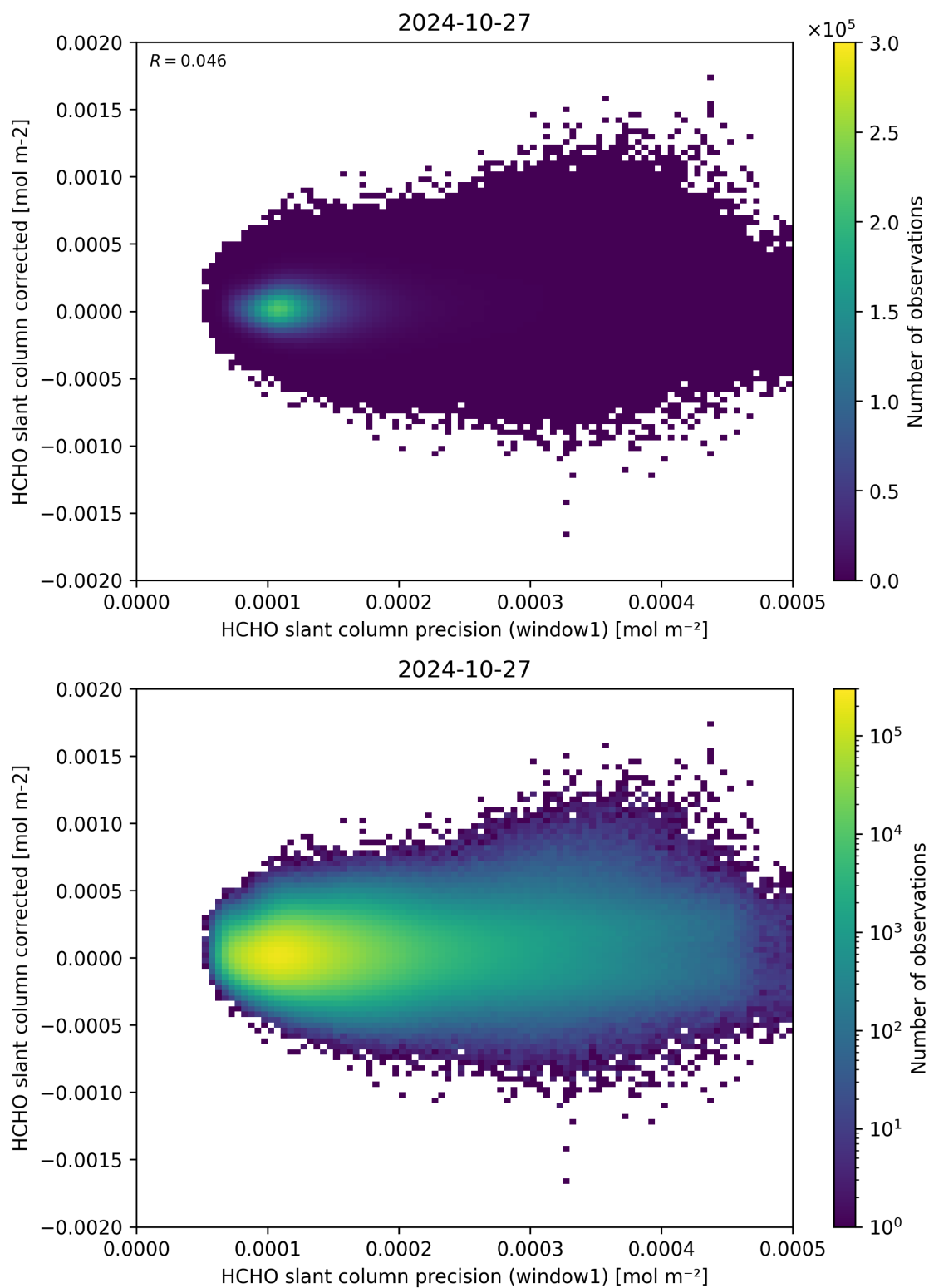
Figure 92: Scatter density plot of “HCHO slant column precision (window1)” against “HCHO slant column corrected” for 2024-10-26 to 2024-10-28.
