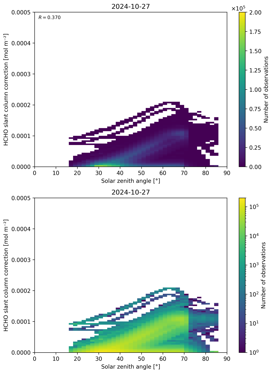
Figure 172: Scatter density plot of “Solar zenith angle” against “HCHO slant column correction” for 2024-10-26 to 2024-10-28.
