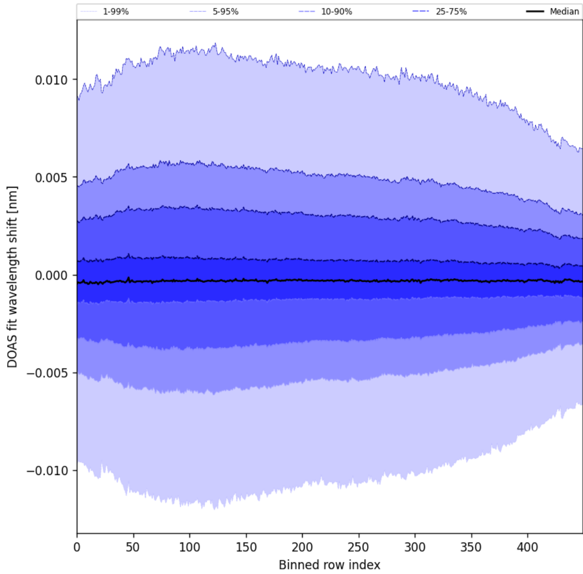
Figure 58: Along track statistics of “DOAS fit wavelength shift” for 2024-10-26 to 2024-10-28
