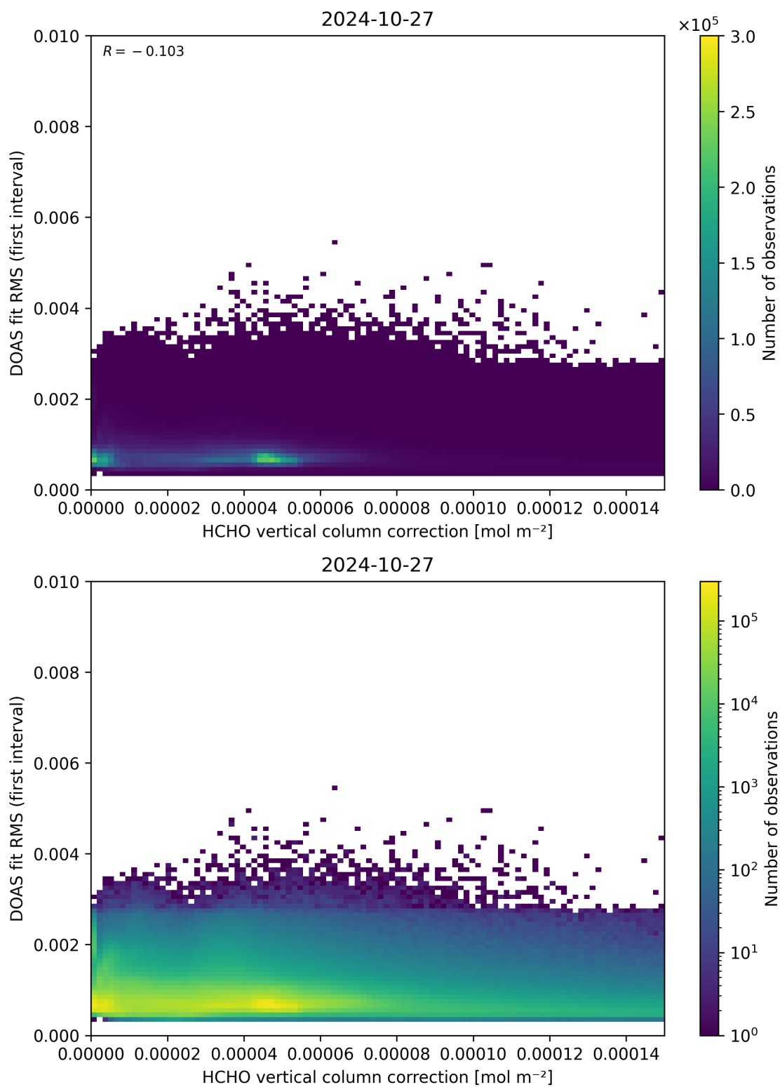
Figure 112: Scatter density plot of “HCHO vertical column correction” against “DOAS fit RMS (first interval)” for 2024-10-26 to 2024-10-28.
