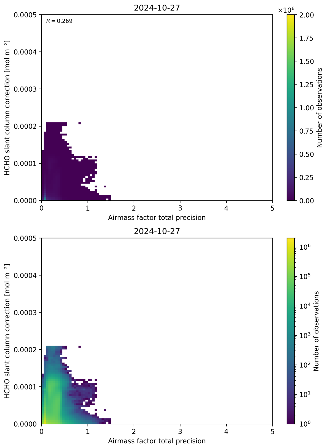
Figure 110: Scatter density plot of “Airmass factor total precision” against “HCHO slant column correction” for 2024-10-26 to 2024-10-28.
