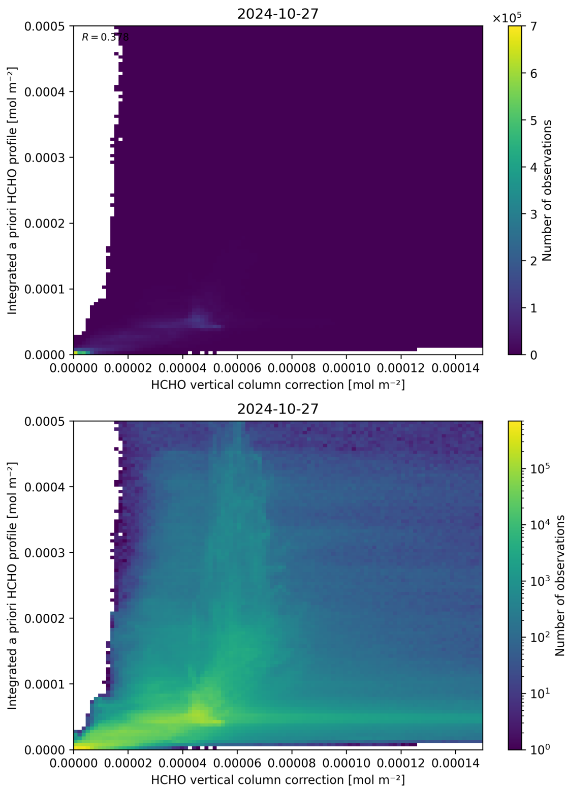
Figure 122: Scatter density plot of “HCHO vertical column correction” against “Integrated a priori HCHO profile” for 2024-10-26 to 2024-10-28.
