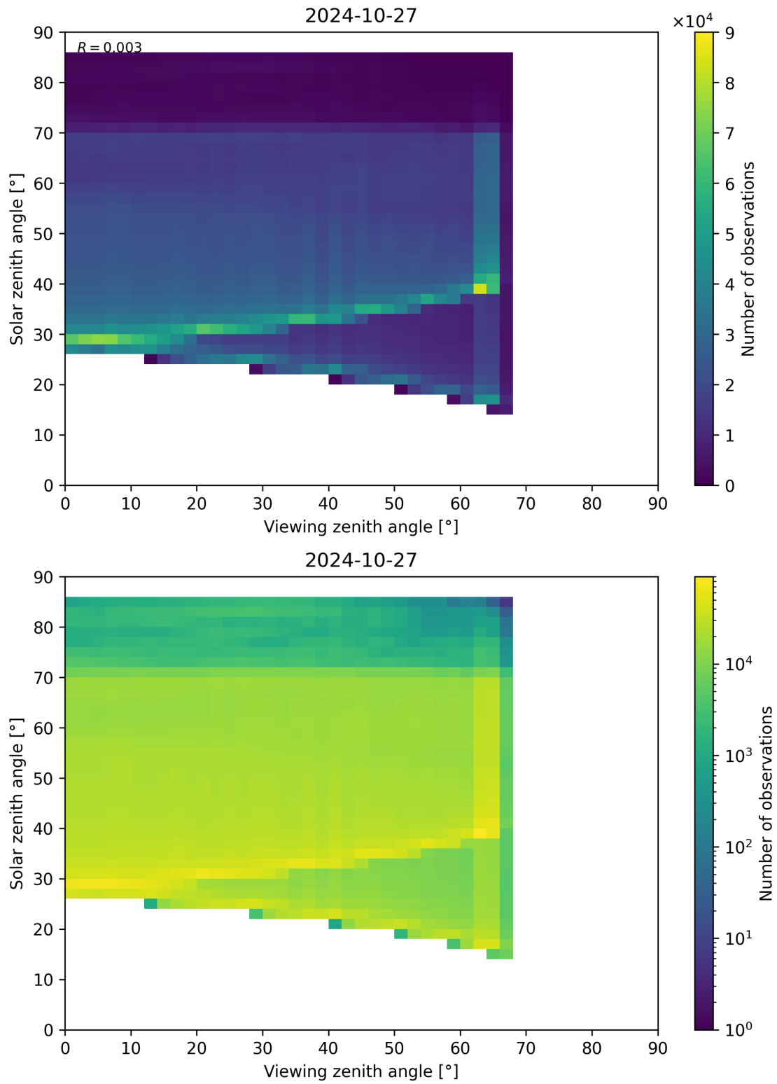
Figure 197: Scatter density plot of “Viewing zenith angle” against “Solar zenith angle” for 2024-10-26 to 2024-10-28.
