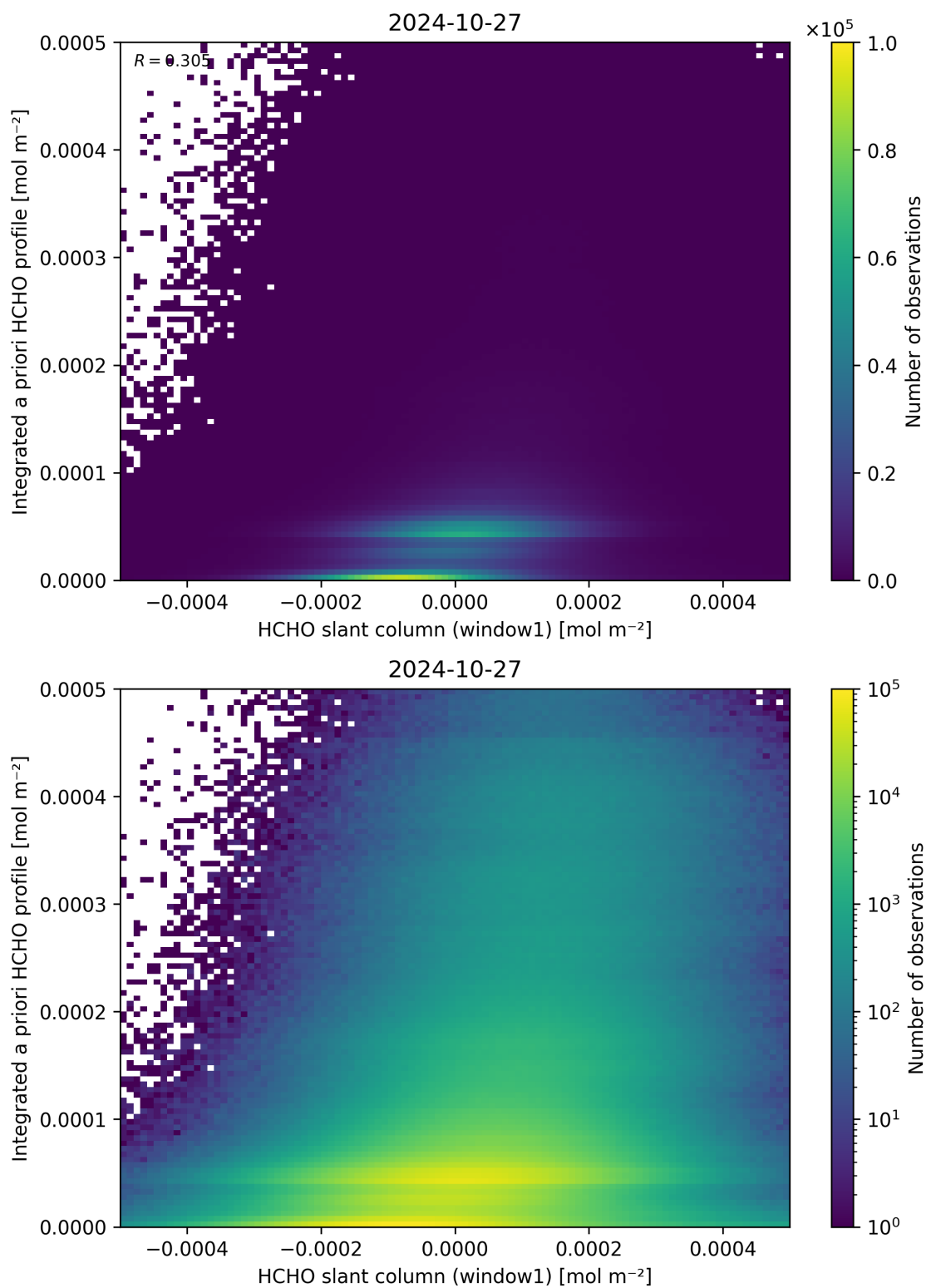
Figure 87: Scatter density plot of “HCHO slant column (window1)” against “Integrated a priori HCHO profile” for 2024-10-26 to 2024-10-28.
