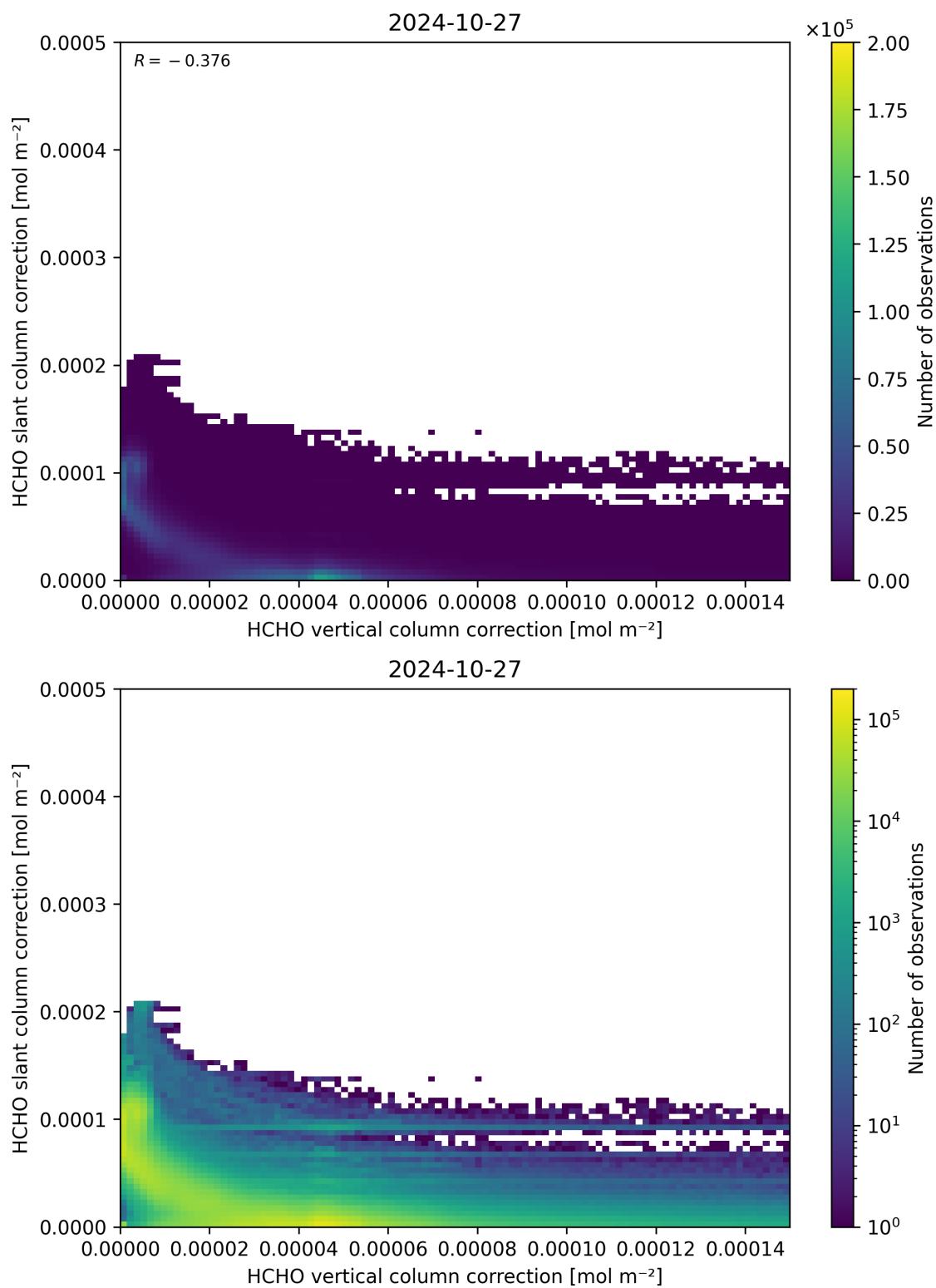
Figure 117: Scatter density plot of “HCHO vertical column correction” against “HCHO slant column correction” for 2024-10-26 to 2024-10-28.
