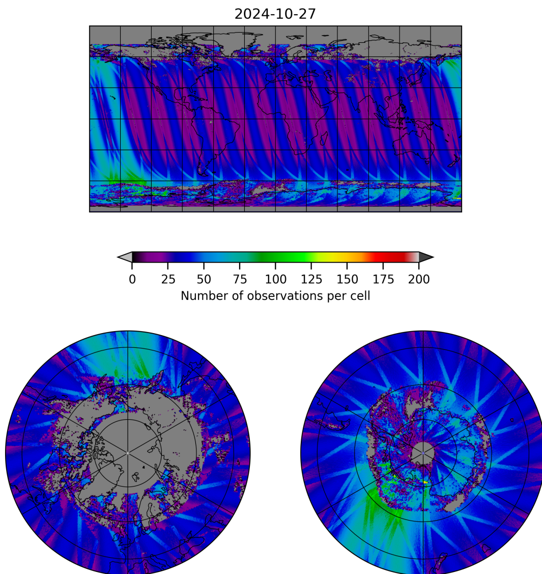
Figure 19: Map of the number of observations for 2024-10-26 to 2024-10-28
