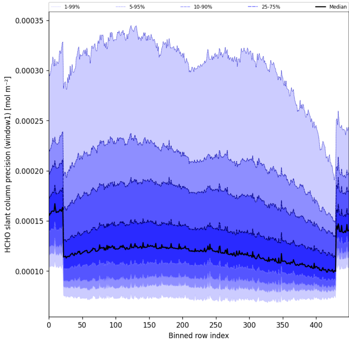
Figure 53: Along track statistics of “HCHO slant column precision (window1)” for 2024-10-26 to 2024-10-28
