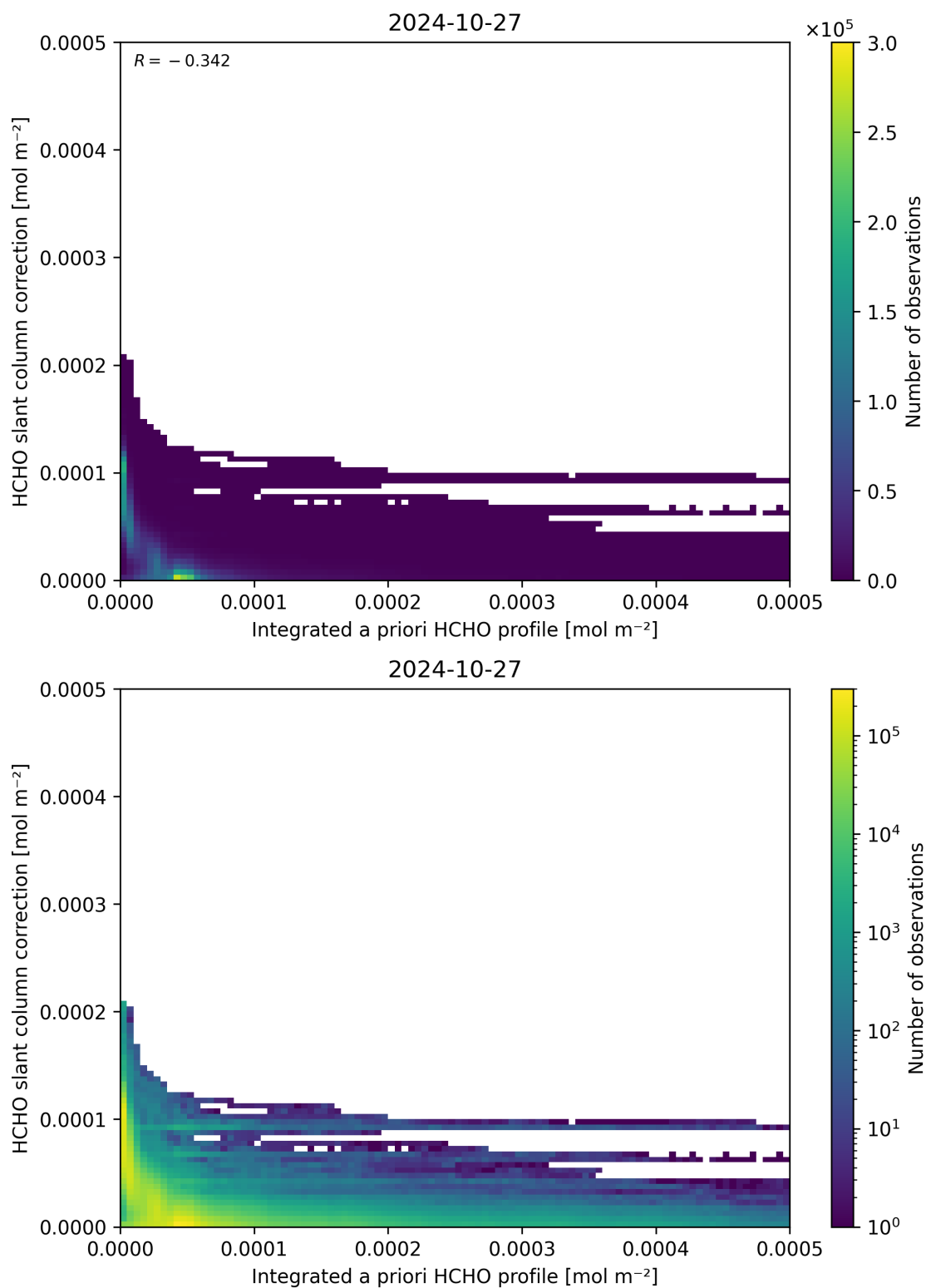
Figure 152: Scatter density plot of “Integrated a priori HCHO profile” against “HCHO slant column correction” for 2024-10-26 to 2024-10-28.
