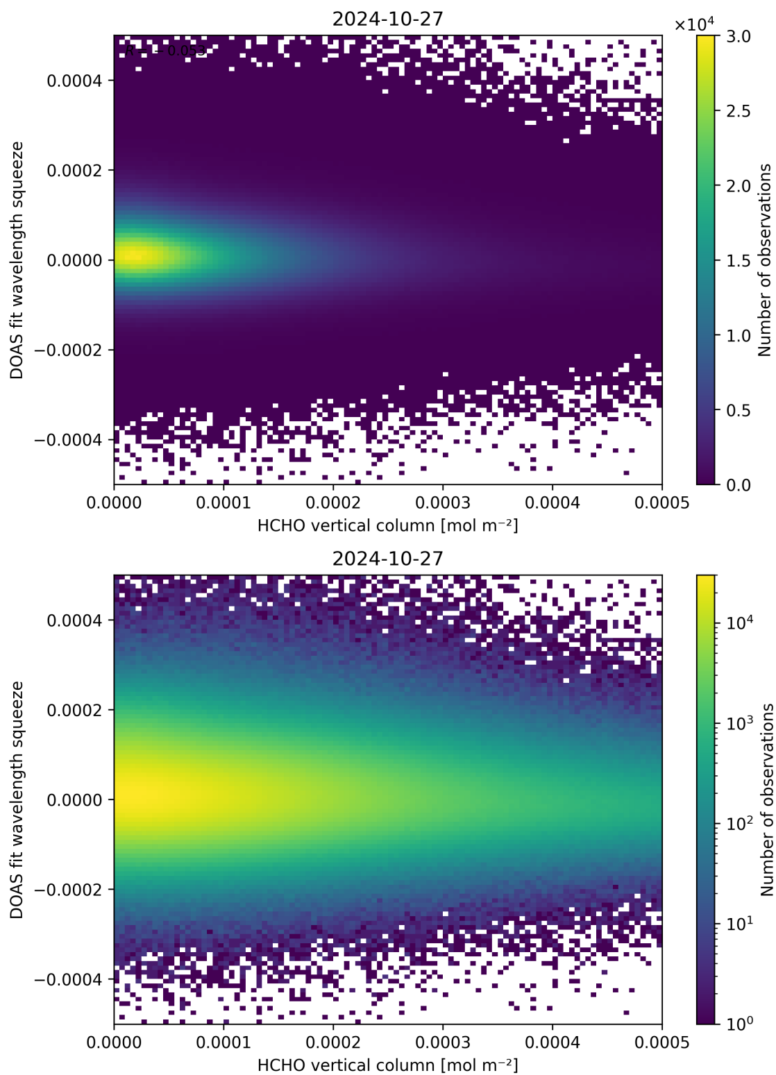
Figure 125: Scatter density plot of “HCHO vertical column” against “DOAS fit wavelength squeeze” for 2024-10-26 to 2024-10-28.
