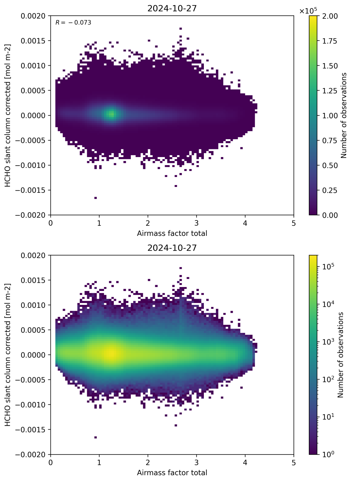
Figure 101: Scatter density plot of “Airmass factor total” against “HCHO slant column corrected” for 2024-10-26 to 2024-10-28.
