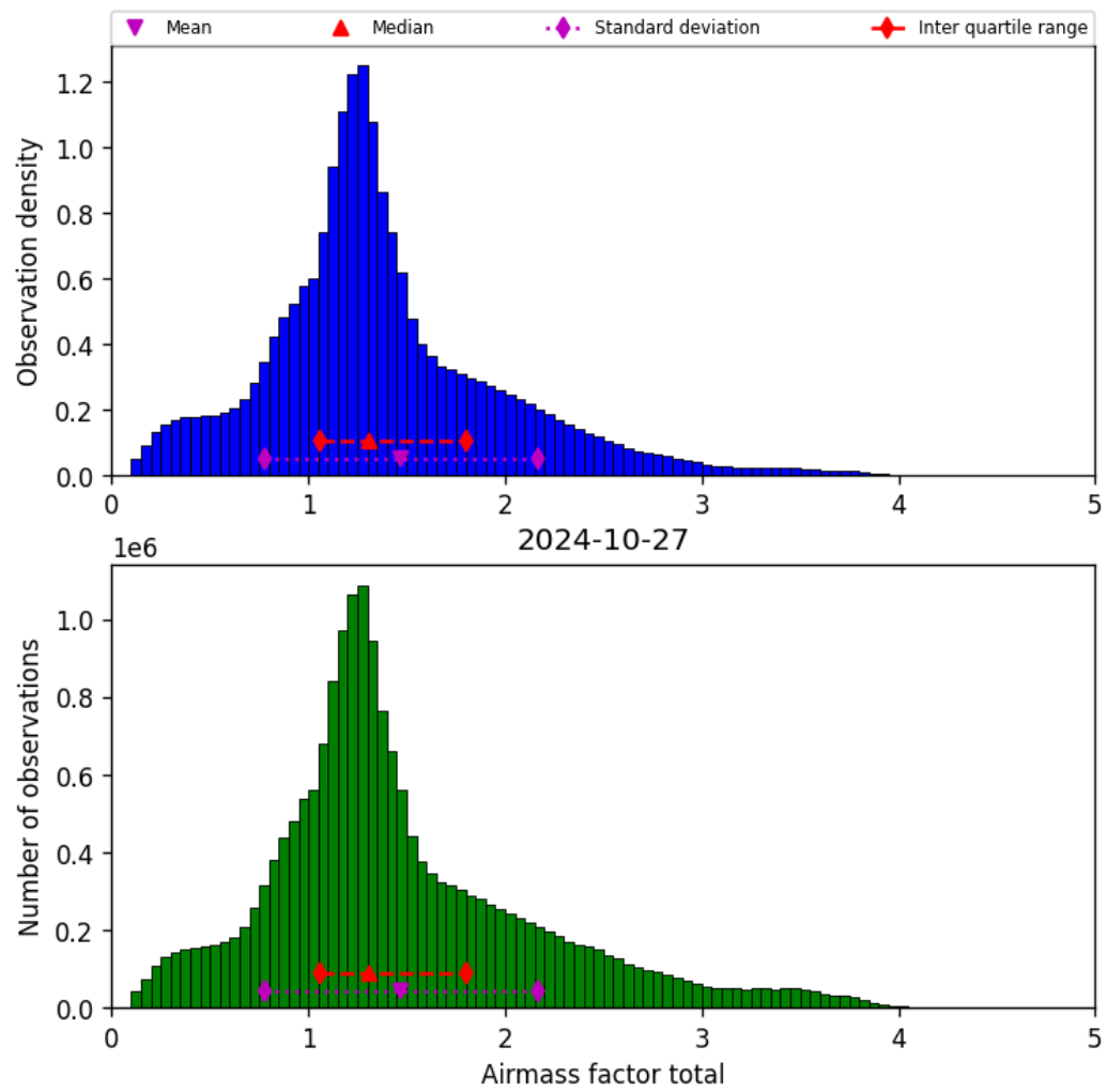
Figure 40: Histogram of “Airmass factor total” for 2024-10-26 to 2024-10-28
