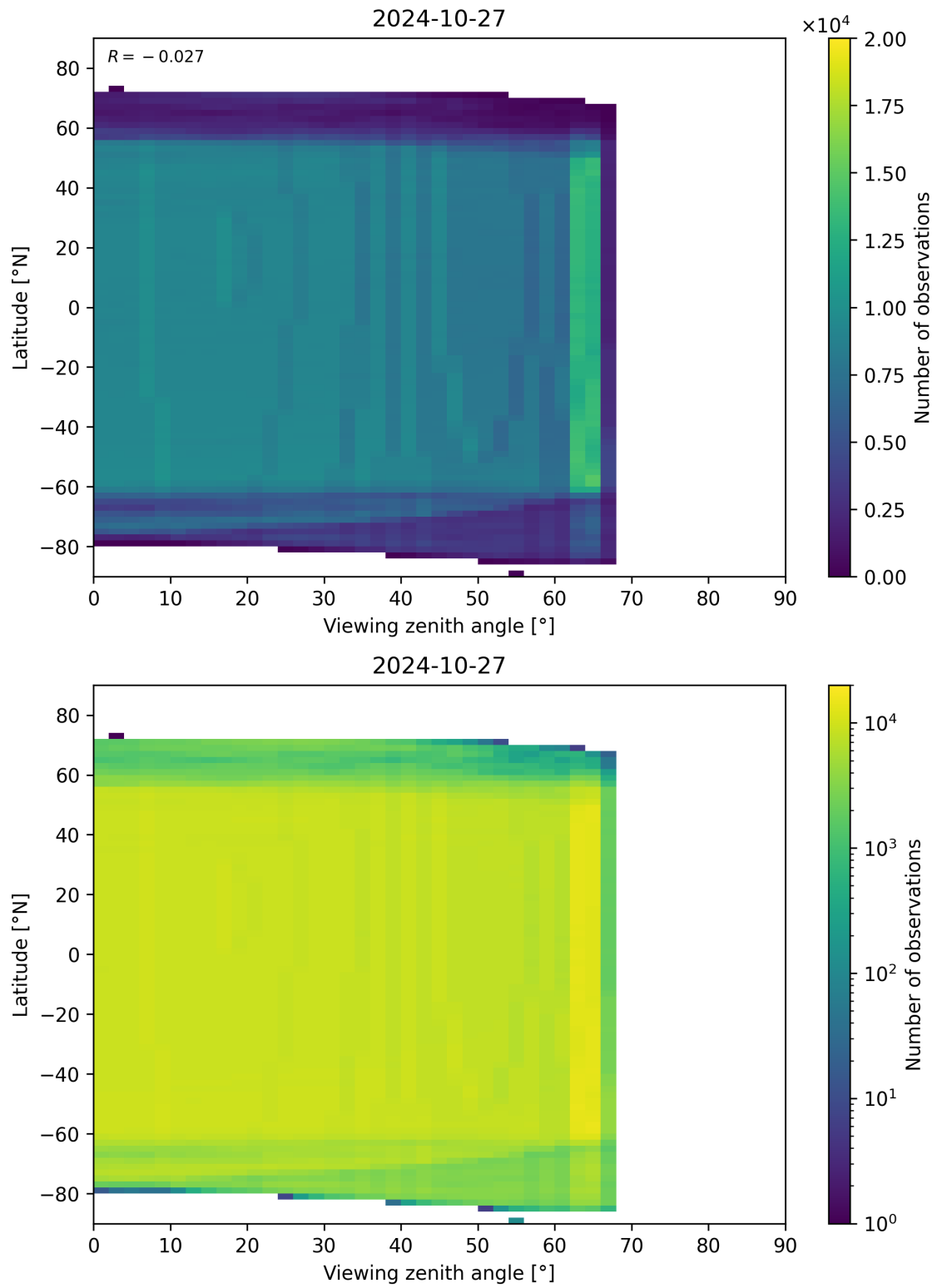
Figure 196: Scatter density plot of “Viewing zenith angle” against “Latitude” for 2024-10-26 to 2024-10-28.
