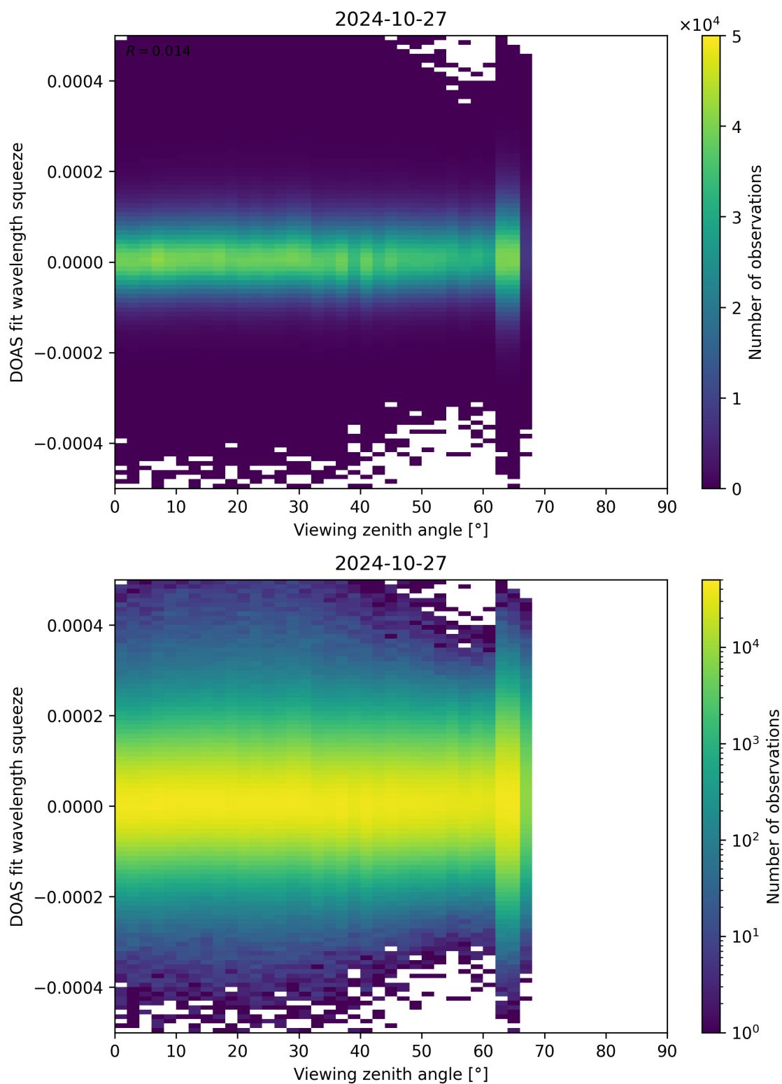
Figure 184: Scatter density plot of “Viewing zenith angle” against “DOAS fit wavelength squeeze” for 2024-10-26 to 2024-10-28.
