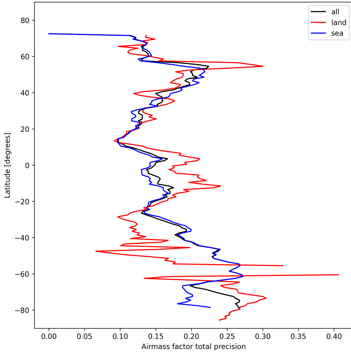
Figure 27: Zonal average of “Airmass factor total precision” for 2024-10-26 to 2024-10-28.
