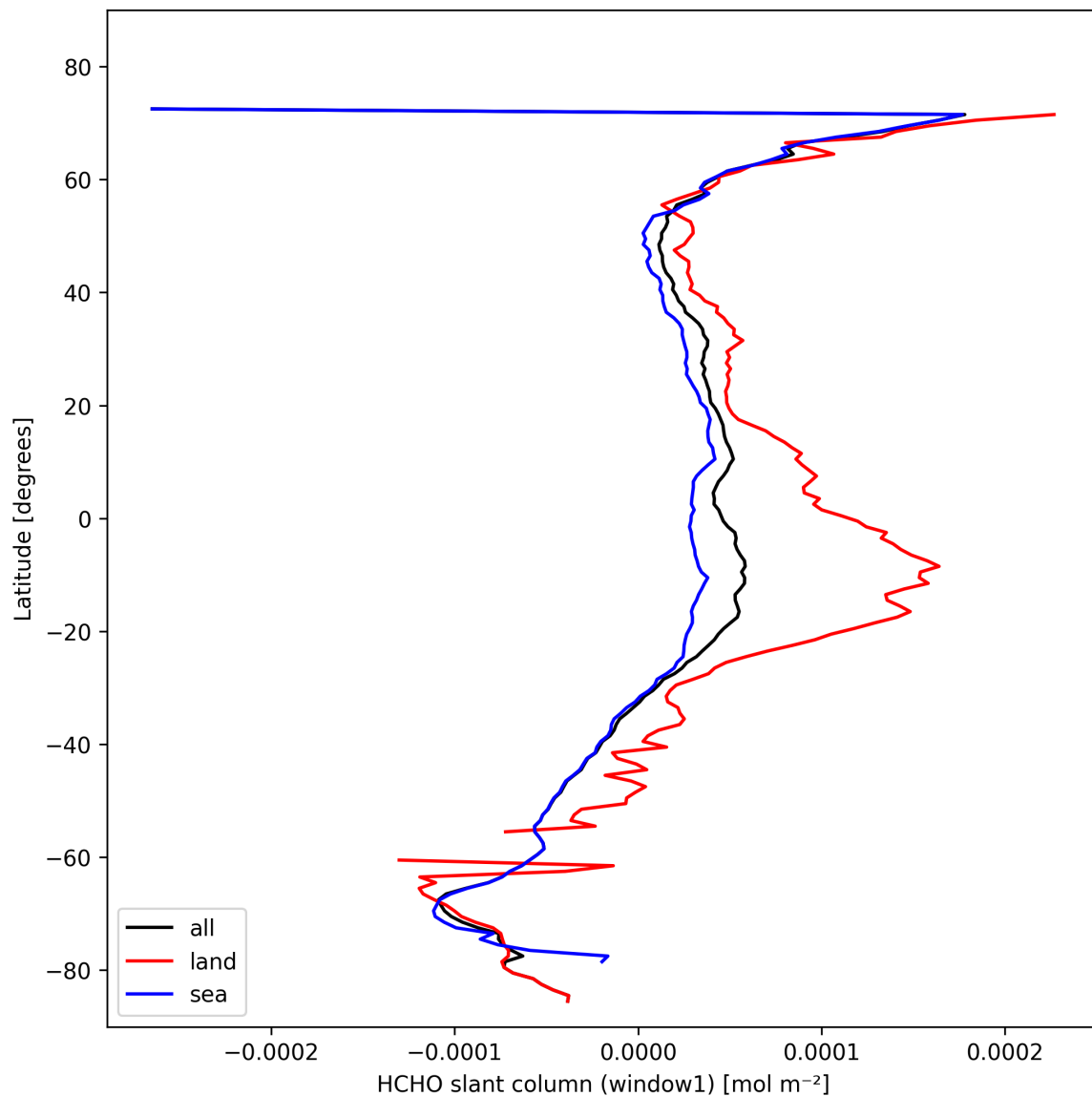
Figure 24: Zonal average of “HCHO slant column (window1)” for 2024-10-26 to 2024-10-28.
