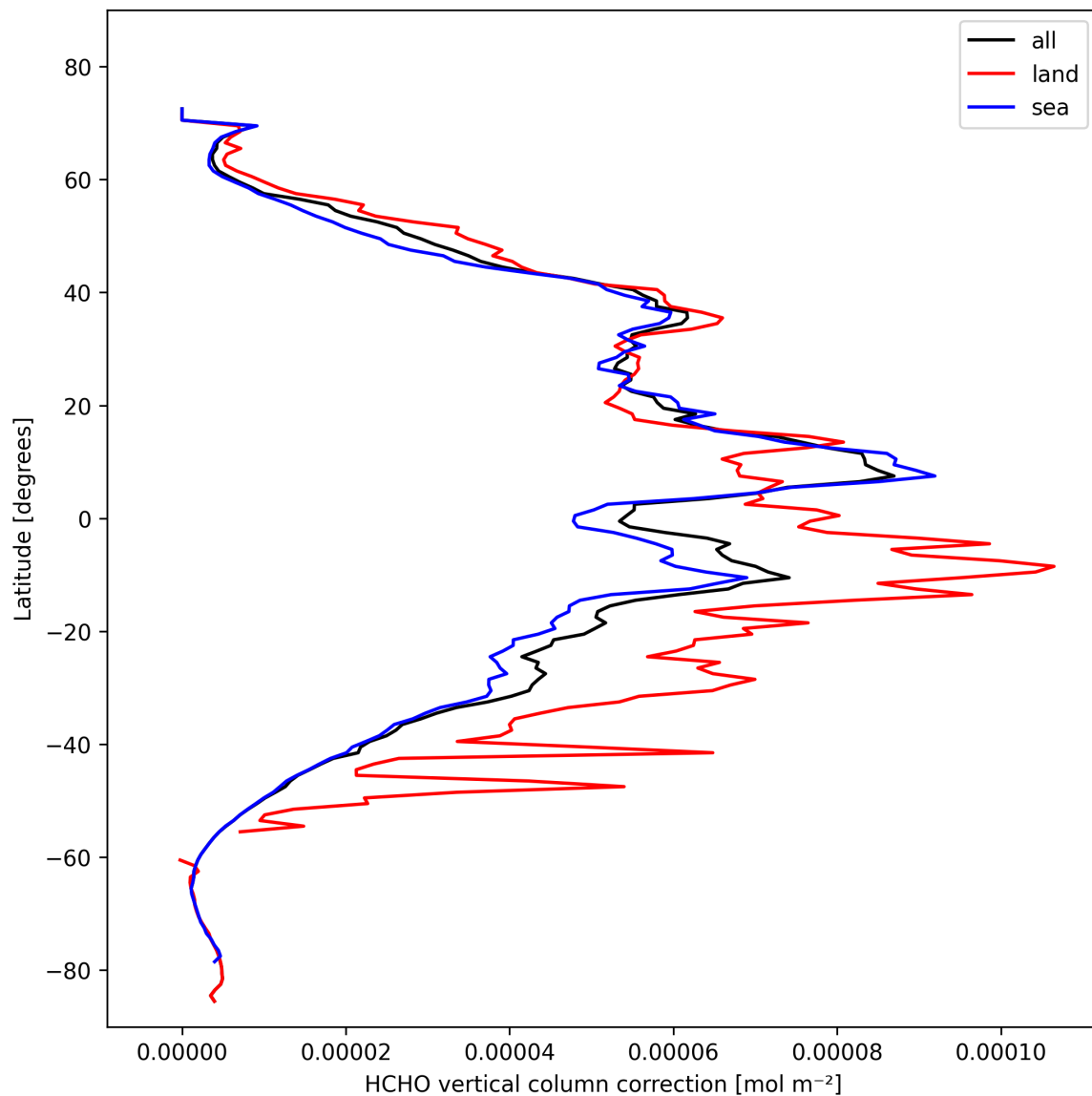
Figure 23: Zonal average of “HCHO vertical column correction” for 2024-10-26 to 2024-10-28.
