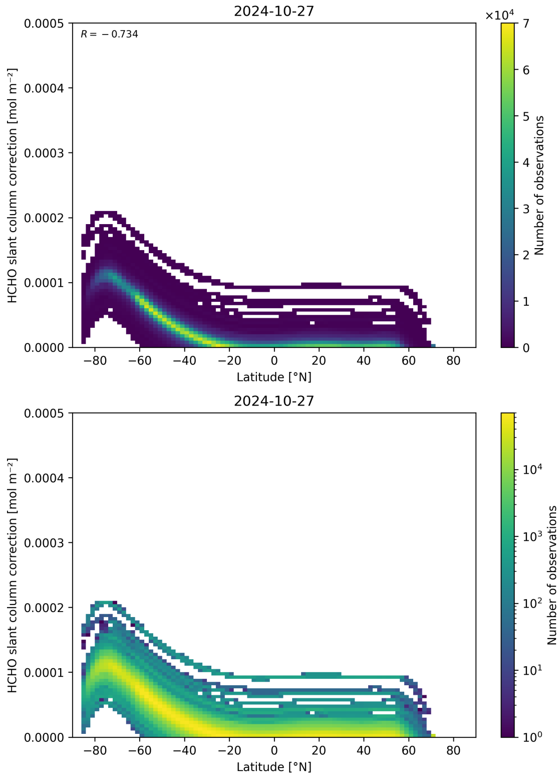
Figure 158: Scatter density plot of “Latitude” against “HCHO slant column correction” for 2024-10-26 to 2024-10-28.
