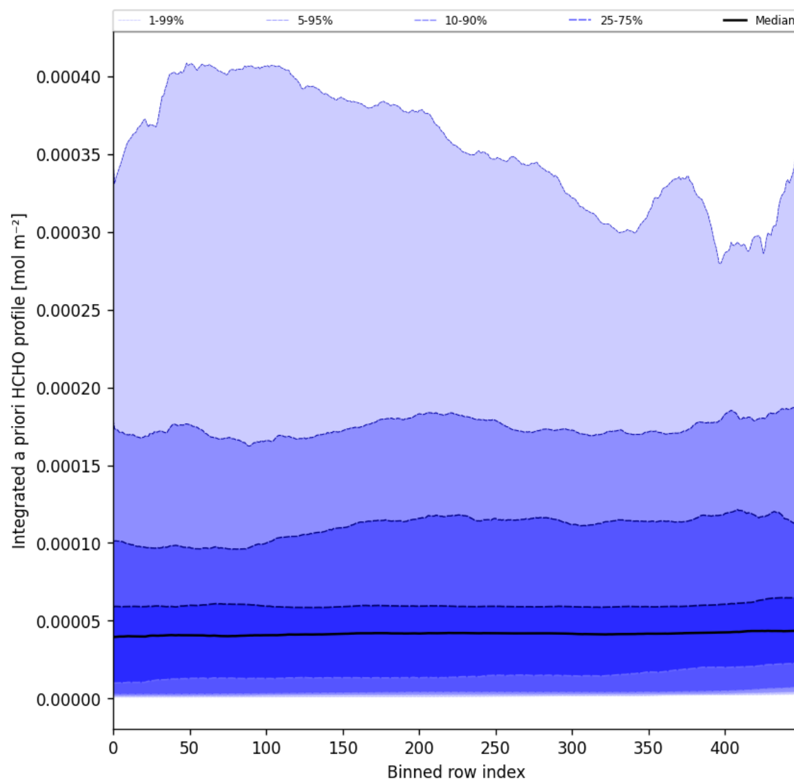
Figure 57: Along track statistics of “Integrated a priori HCHO profile” for 2024-10-26 to 2024-10-28
