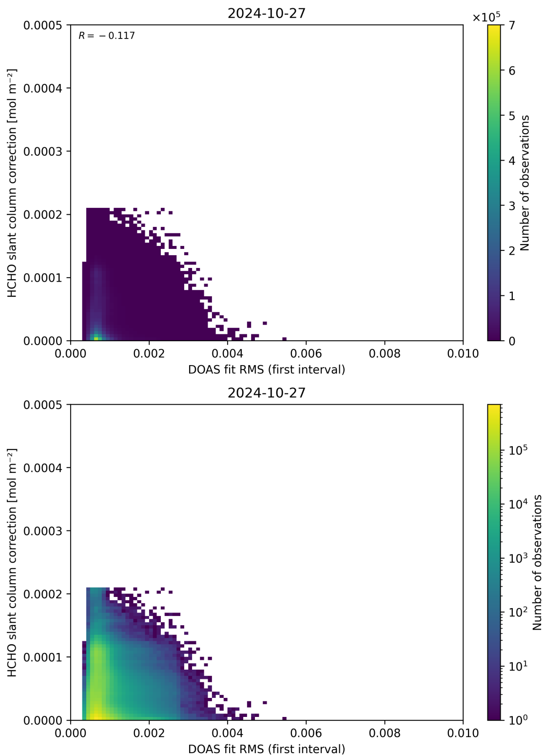
Figure 63: Scatter density plot of “DOAS fit RMS (first interval)” against “HCHO slant column correction” for 2024-10-26 to 2024-10-28.
