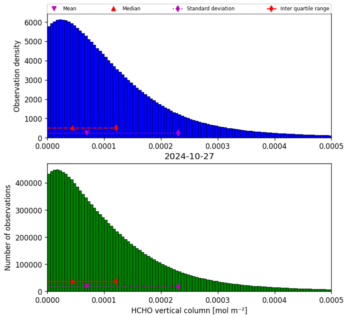
Figure 35: Histogram of “HCHO vertical column” for 2024-10-26 to 2024-10-28
