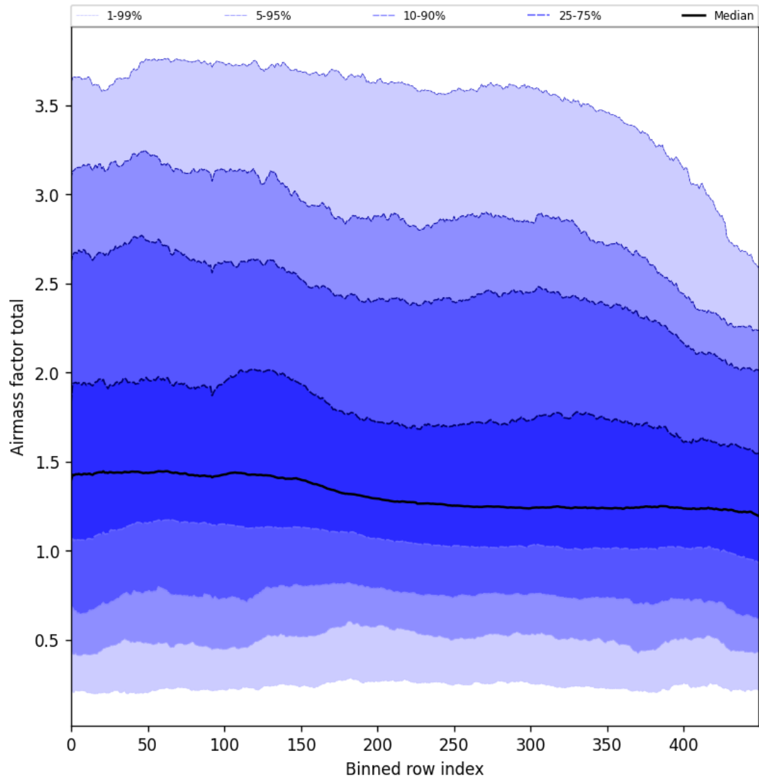
Figure 54: Along track statistics of “Airmass factor total” for 2024-10-26 to 2024-10-28
