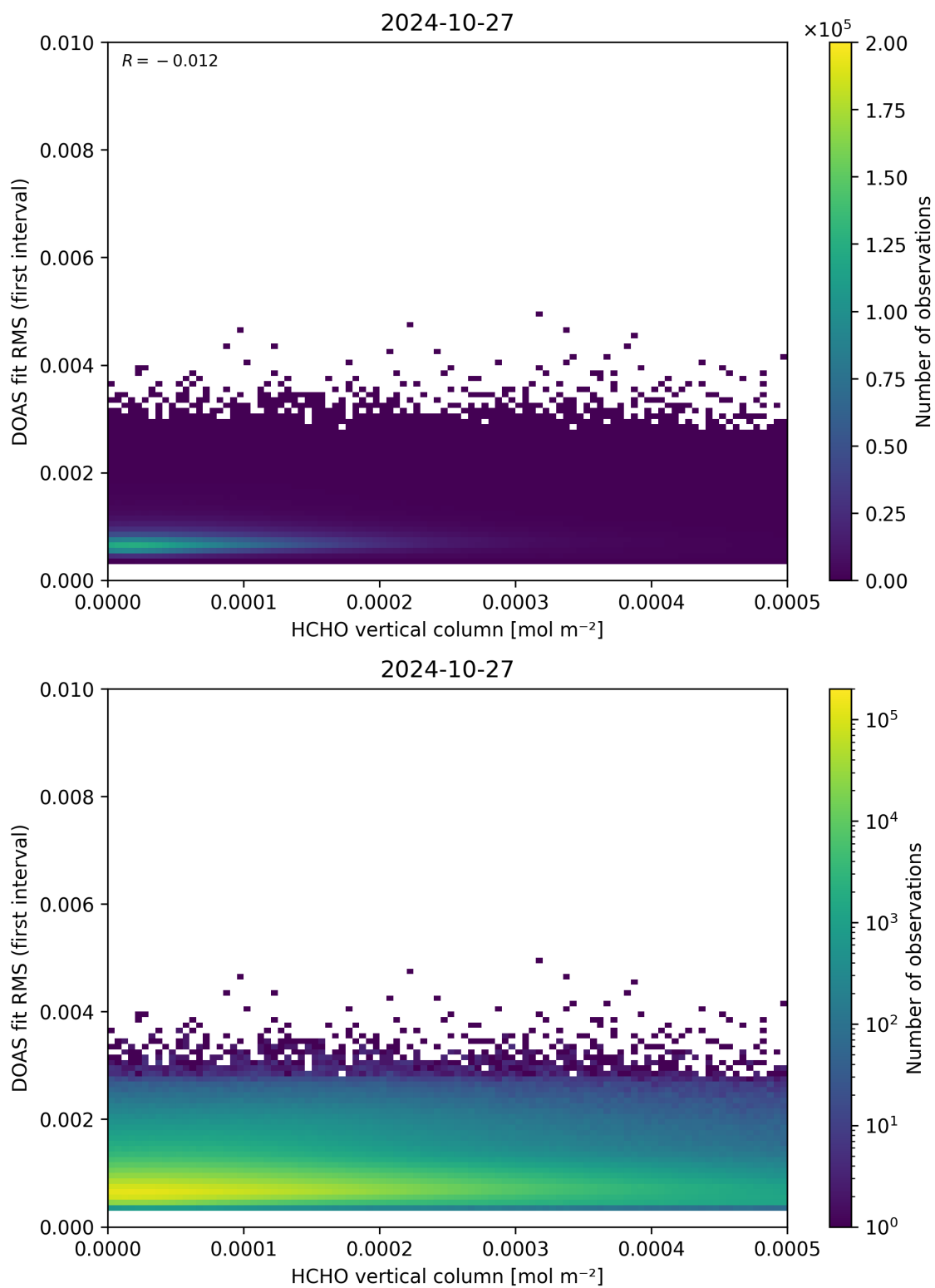
Figure 123: Scatter density plot of “HCHO vertical column” against “DOAS fit RMS (first interval)” for 2024-10-26 to 2024-10-28.
