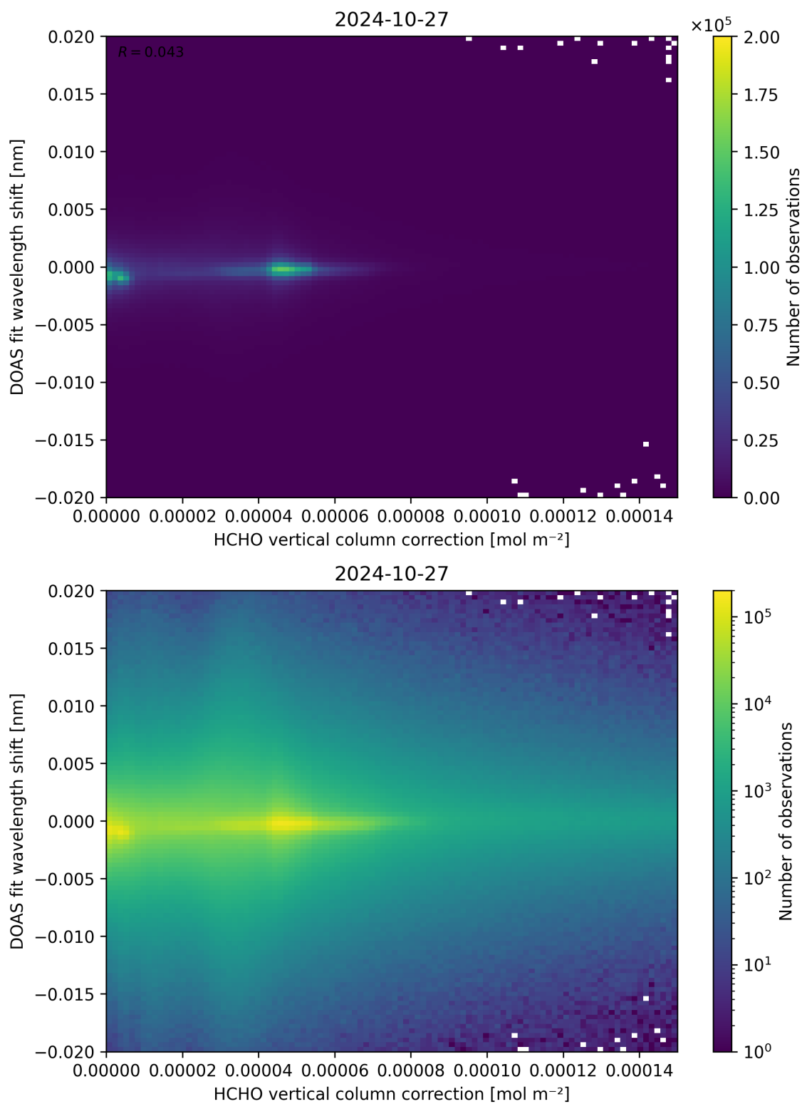
Figure 113: Scatter density plot of “HCHO vertical column correction” against “DOAS fit wavelength shift” for 2024-10-26 to 2024-10-28.
