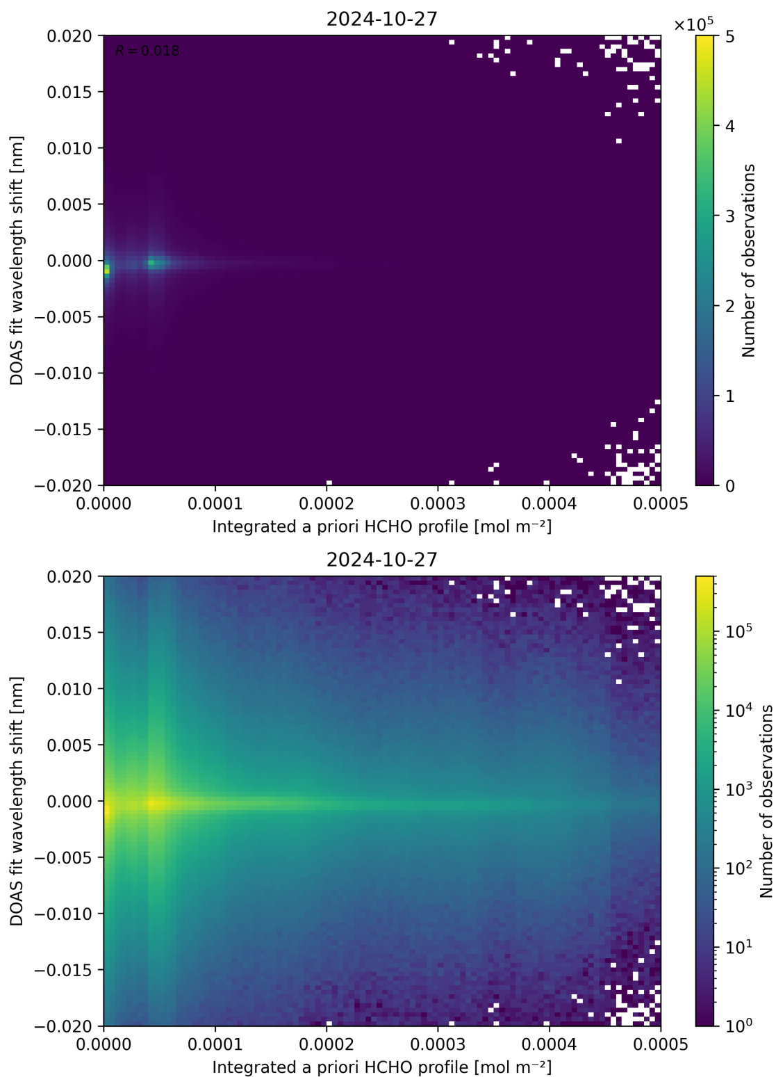
Figure 149: Scatter density plot of “Integrated a priori HCHO profile” against “DOAS fit wavelength shift” for 2024-10-26 to 2024-10-28.
