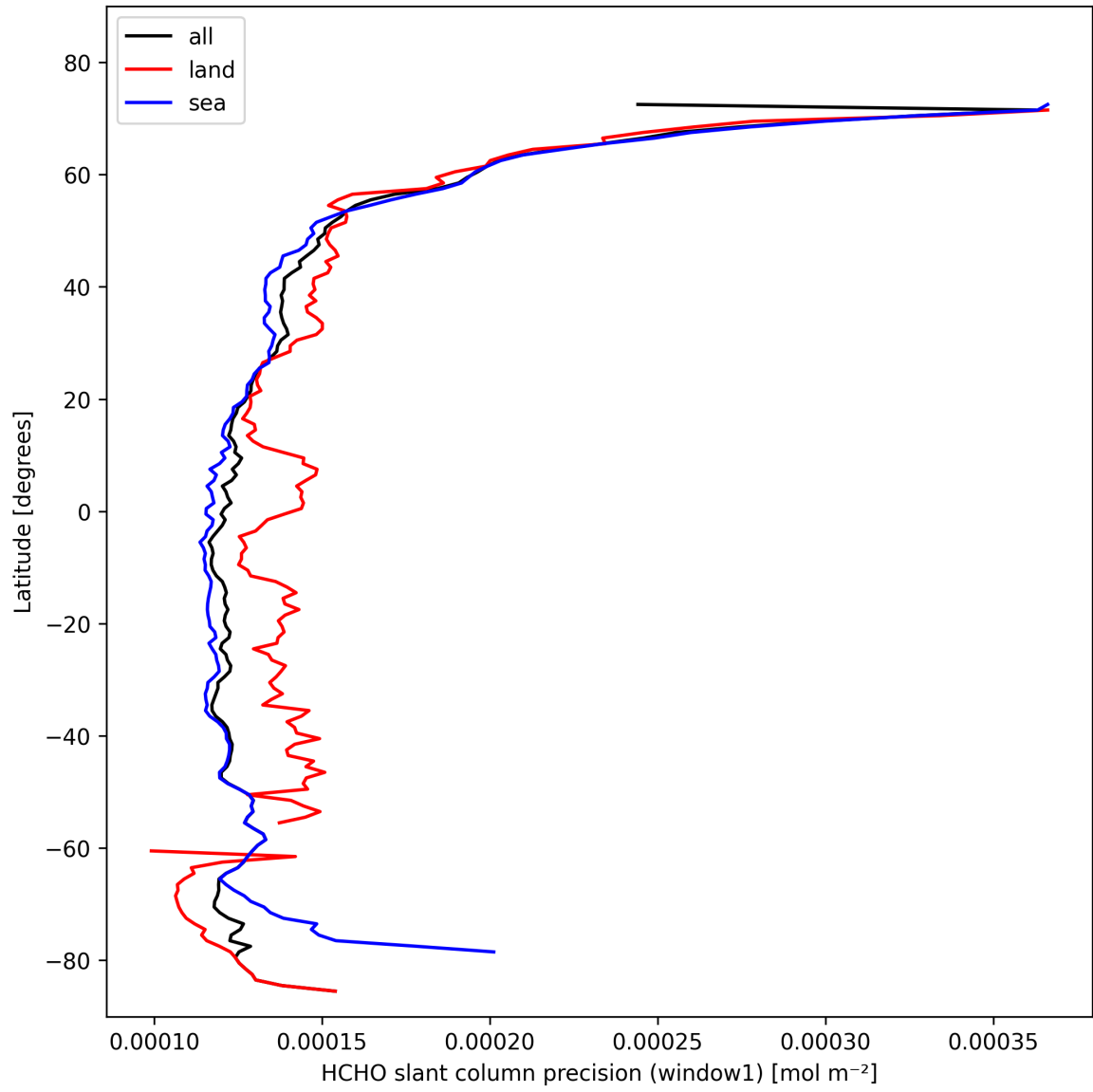
Figure 25: Zonal average of “HCHO slant column precision (window1)” for 2024-10-26 to 2024-10-28.
