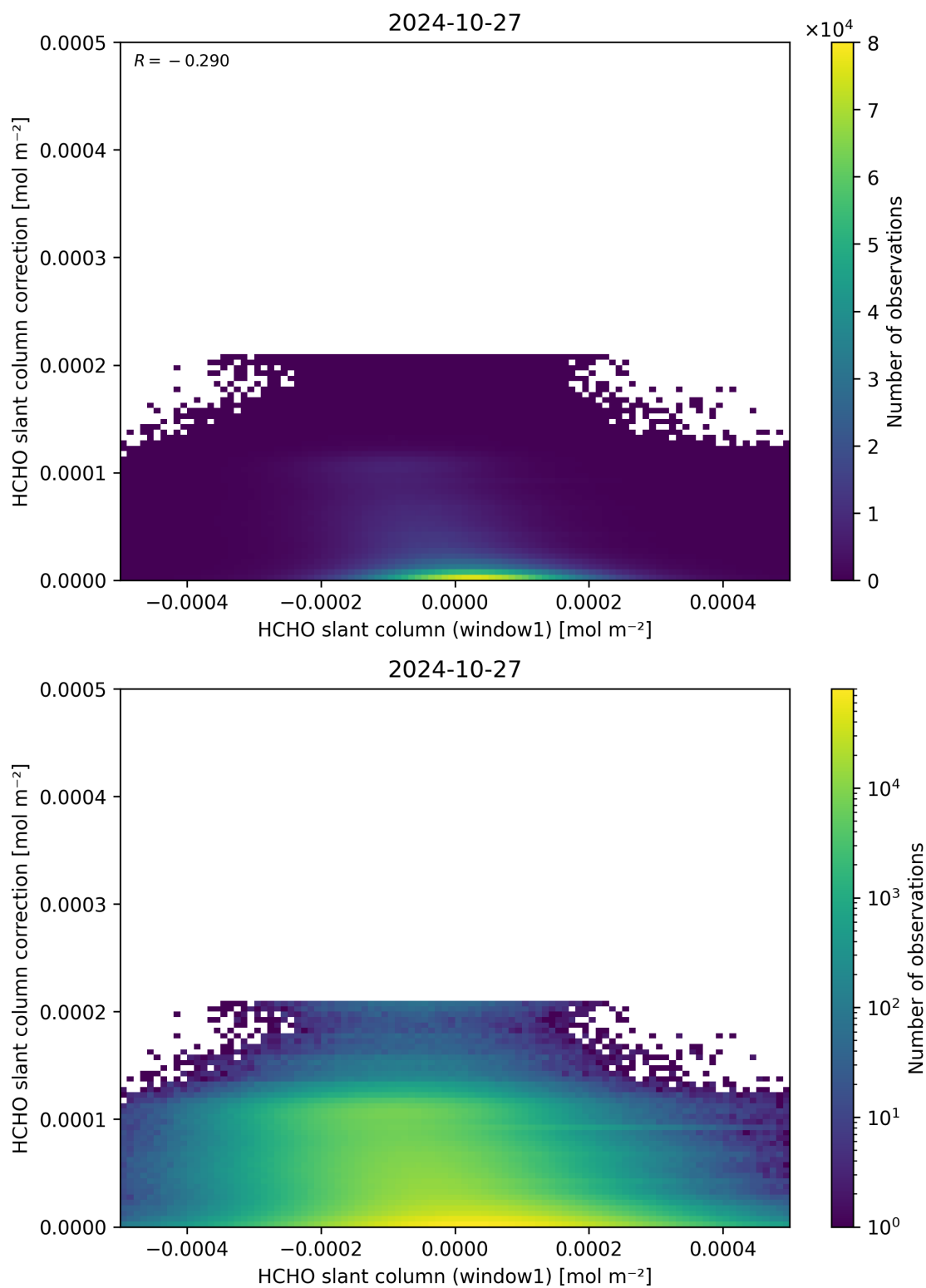
Figure 83: Scatter density plot of “HCHO slant column (window1)” against “HCHO slant column correction” for 2024-10-26 to 2024-10-28.
