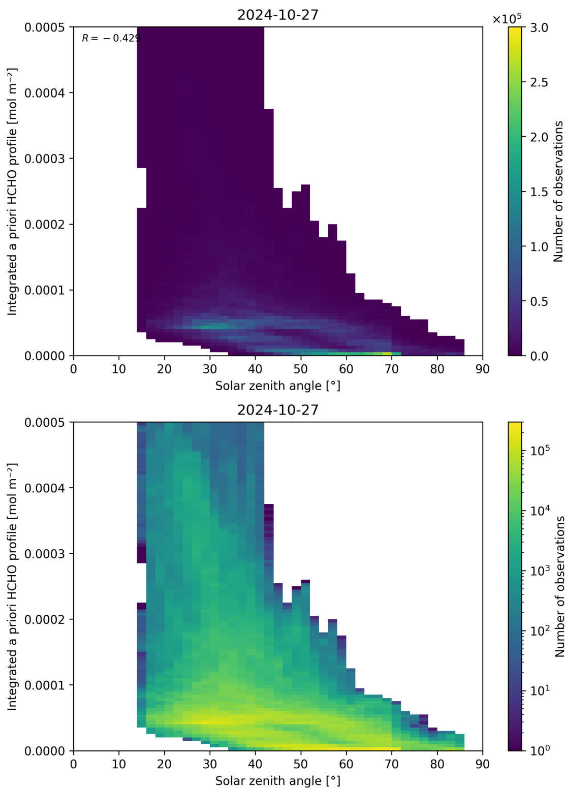
Figure 180: Scatter density plot of “Solar zenith angle” against “Integrated a priori HCHO profile” for 2024-10-26 to 2024-10-28.
