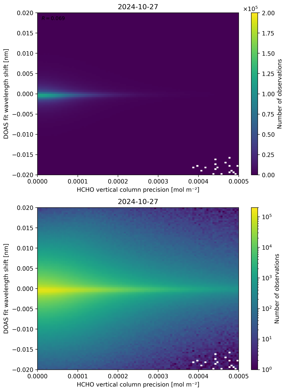
Figure 137: Scatter density plot of “HCHO vertical column precision” against “DOAS fit wavelength shift” for 2024-10-26 to 2024-10-28.
