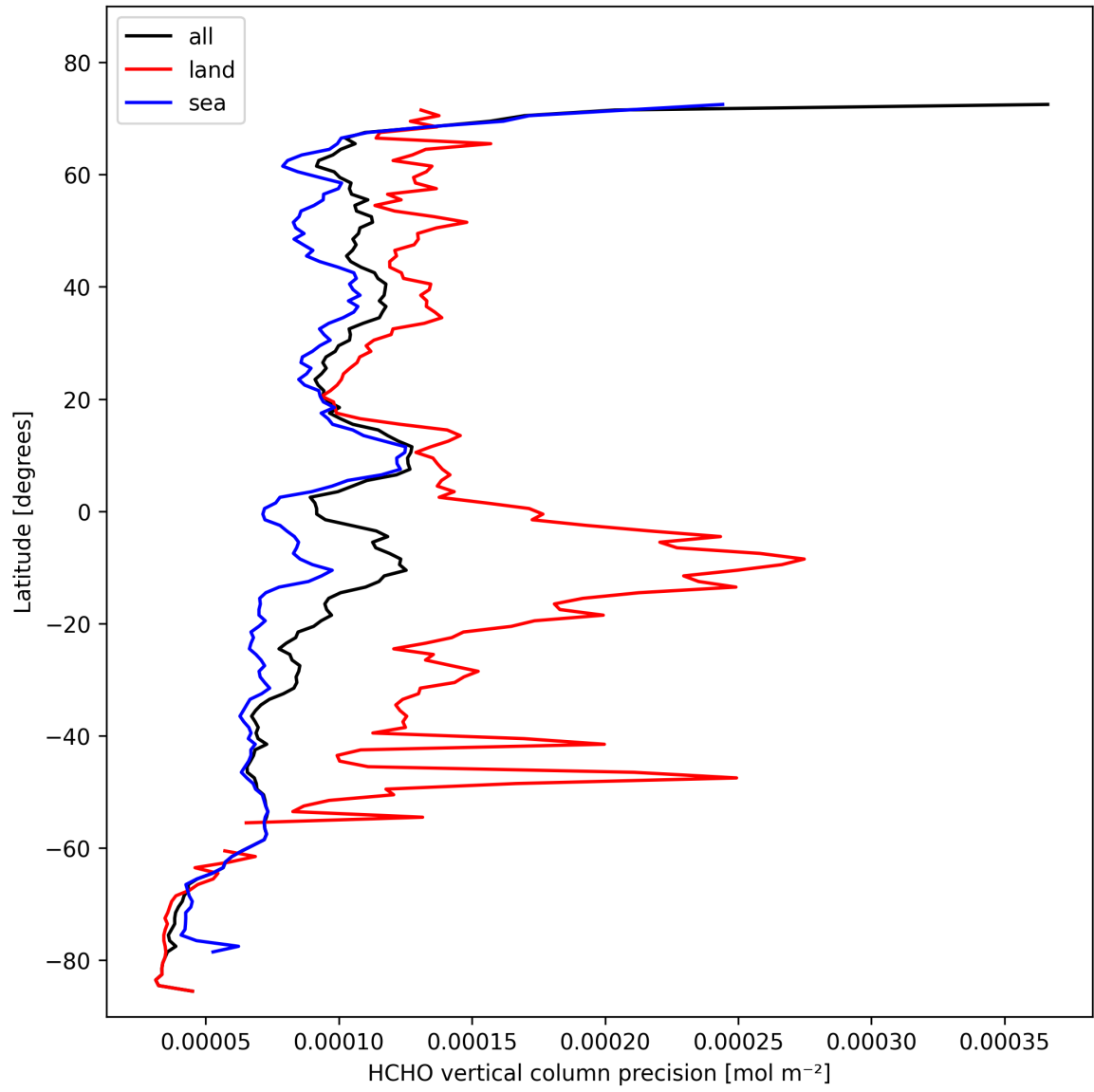
Figure 22: Zonal average of “HCHO vertical column precision” for 2024-10-26 to 2024-10-28.
