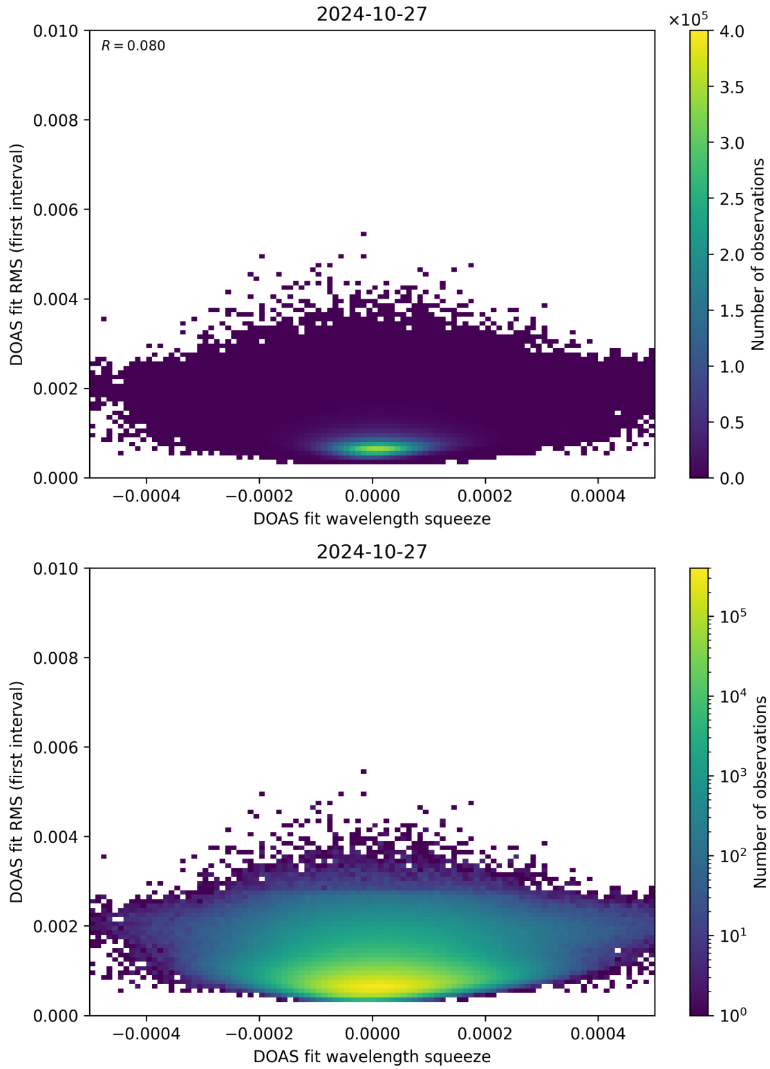
Figure 68: Scatter density plot of “DOAS fit wavelength squeeze” against “DOAS fit RMS (first interval)” for 2024-10-26 to 2024-10-28.
