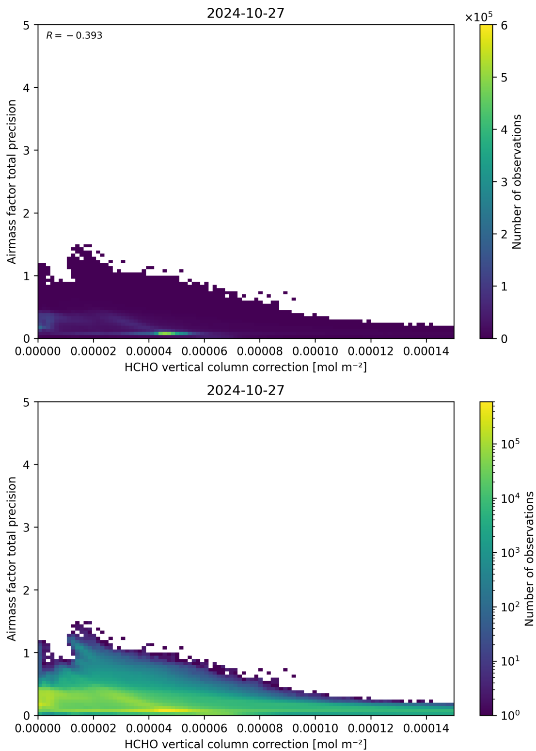
Figure 121: Scatter density plot of “HCHO vertical column correction” against “Airmass factor total precision” for 2024-10-26 to 2024-10-28.
