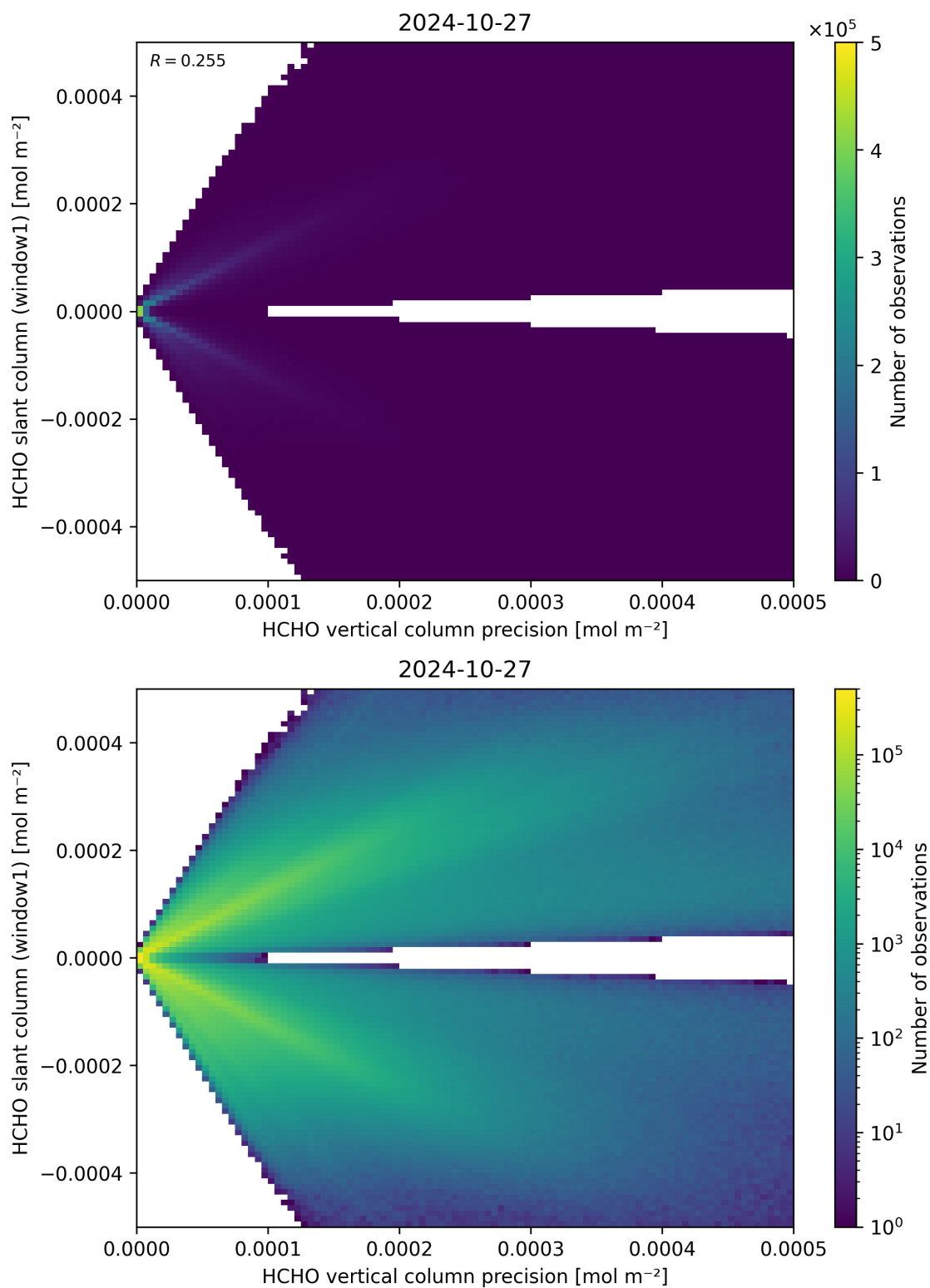
Figure 142: Scatter density plot of “HCHO vertical column precision” against “HCHO slant column (window1)” for 2024-10-26 to 2024-10-28.
