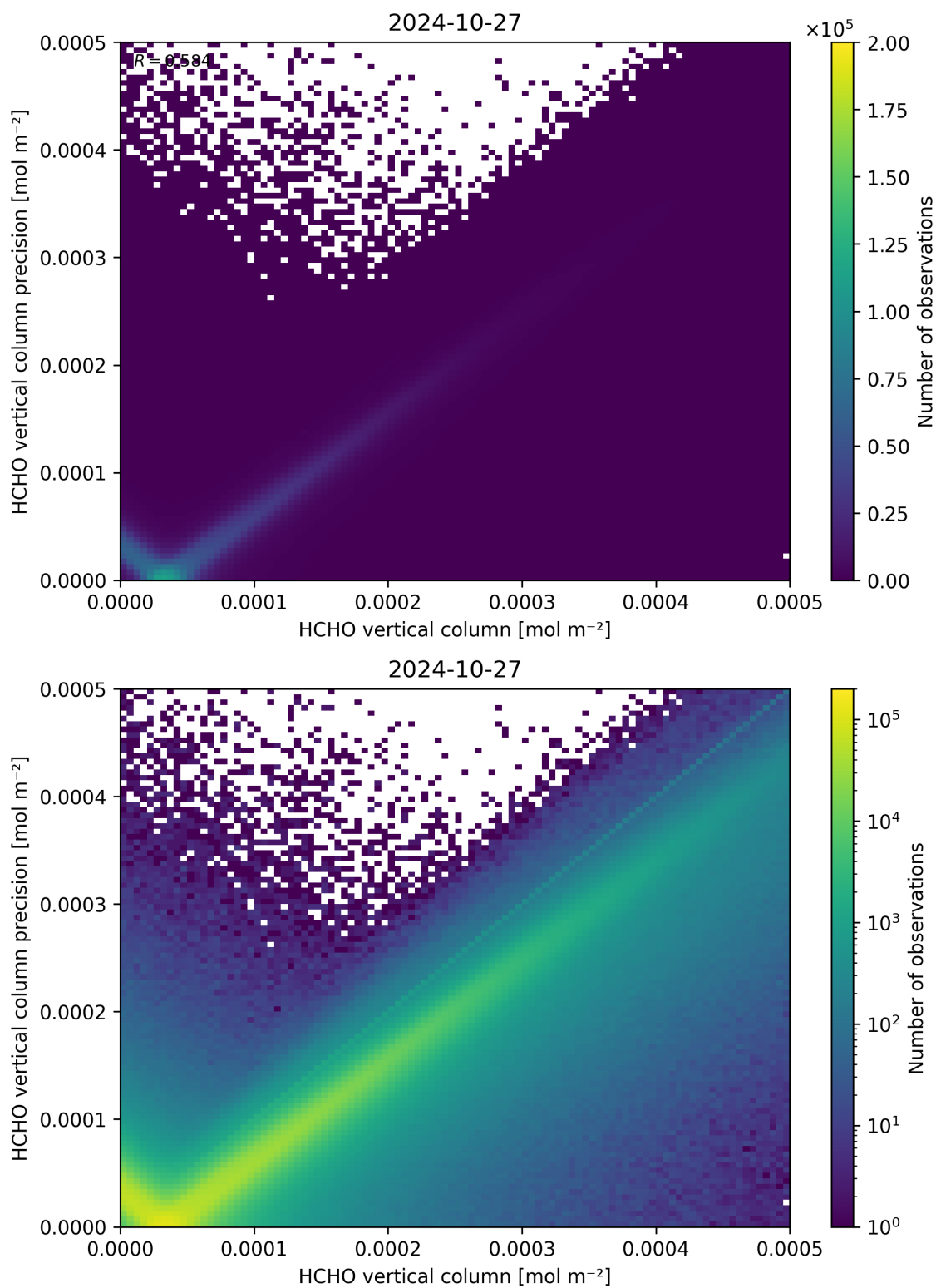
Figure 134: Scatter density plot of “HCHO vertical column” against “HCHO vertical column precision” for 2024-10-26 to 2024-10-28.
