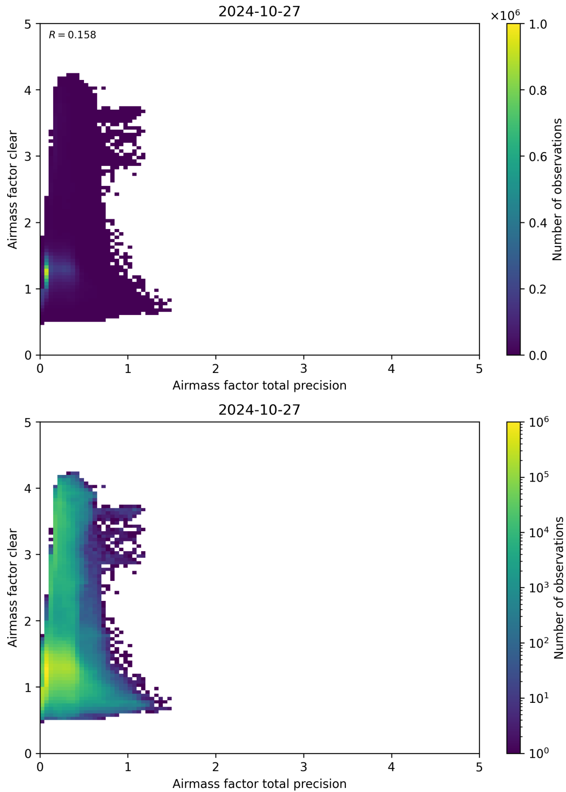
Figure 108: Scatter density plot of “Airmass factor total precision” against “Airmass factor clear” for 2024-10-26 to 2024-10-28.
