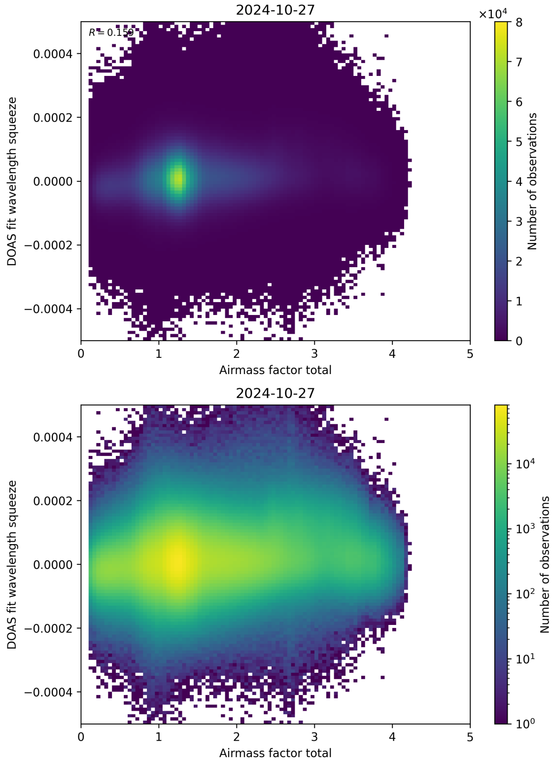
Figure 99: Scatter density plot of “Airmass factor total” against “DOAS fit wavelength squeeze” for 2024-10-26 to 2024-10-28.
