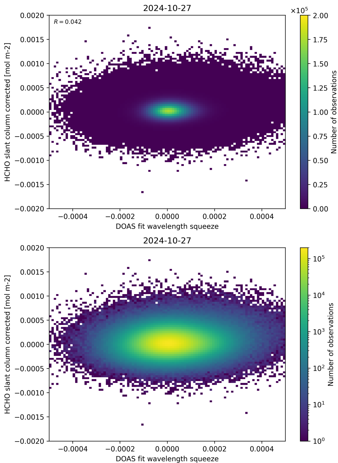
Figure 69: Scatter density plot of “DOAS fit wavelength squeeze” against “HCHO slant column corrected” for 2024-10-26 to 2024-10-28.
