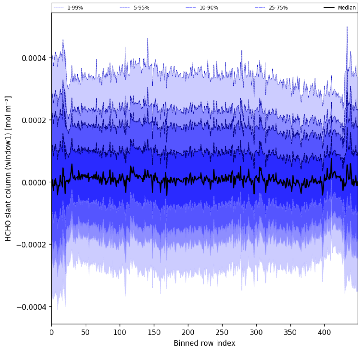
Figure 52: Along track statistics of “HCHO slant column (window1)” for 2024-10-26 to 2024-10-28
