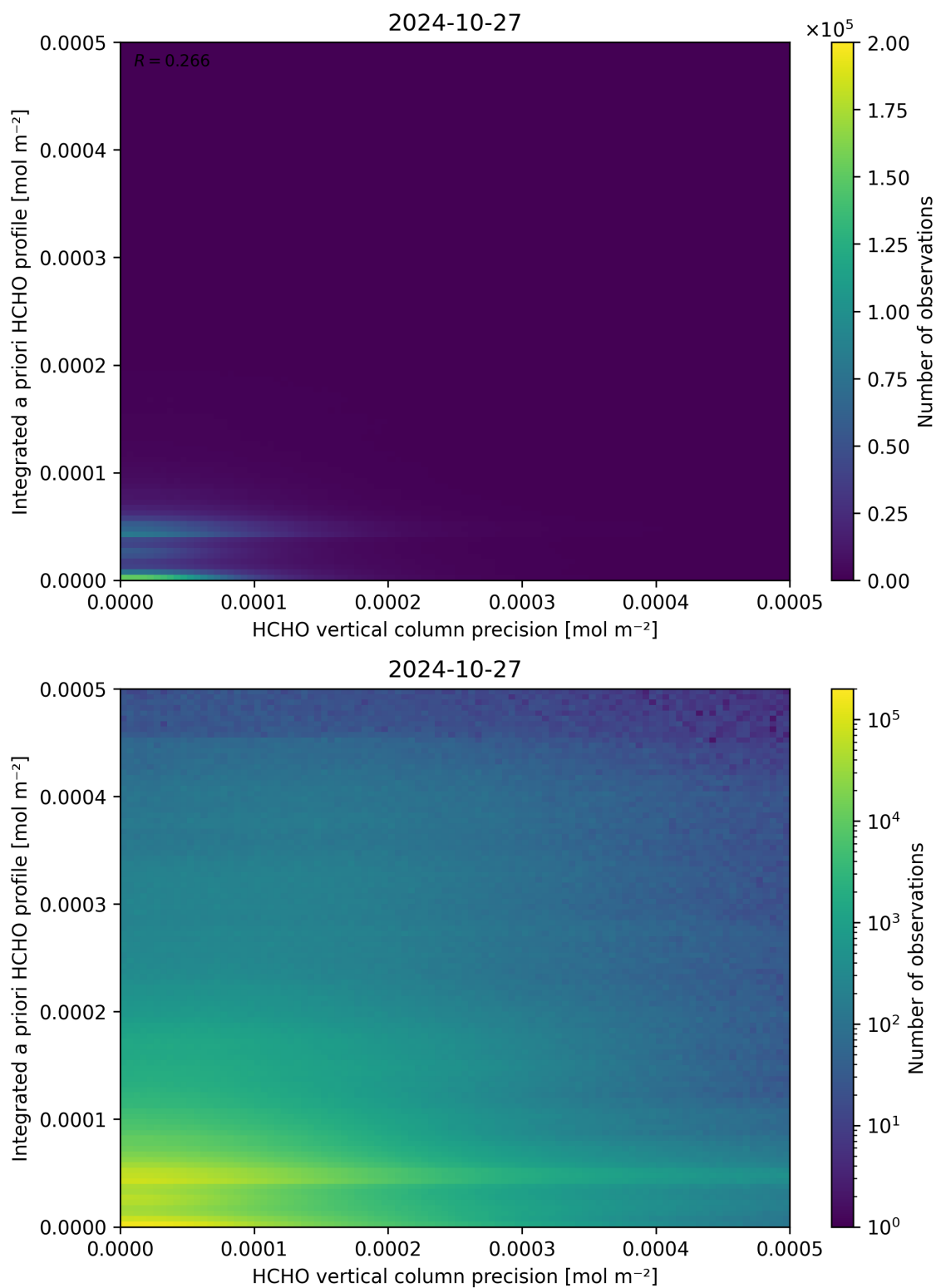
Figure 147: Scatter density plot of “HCHO vertical column precision” against “Integrated a priori HCHO profile” for 2024-10-26 to 2024-10-28.
