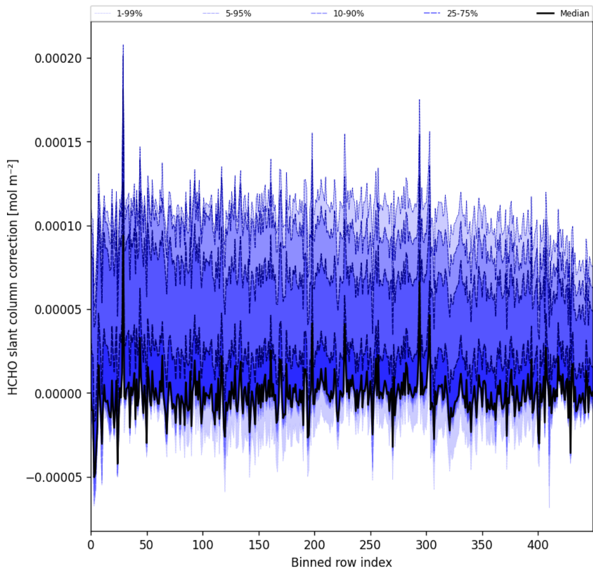
Figure 61: Along track statistics of “HCHO slant column correction” for 2024-10-26 to 2024-10-28
