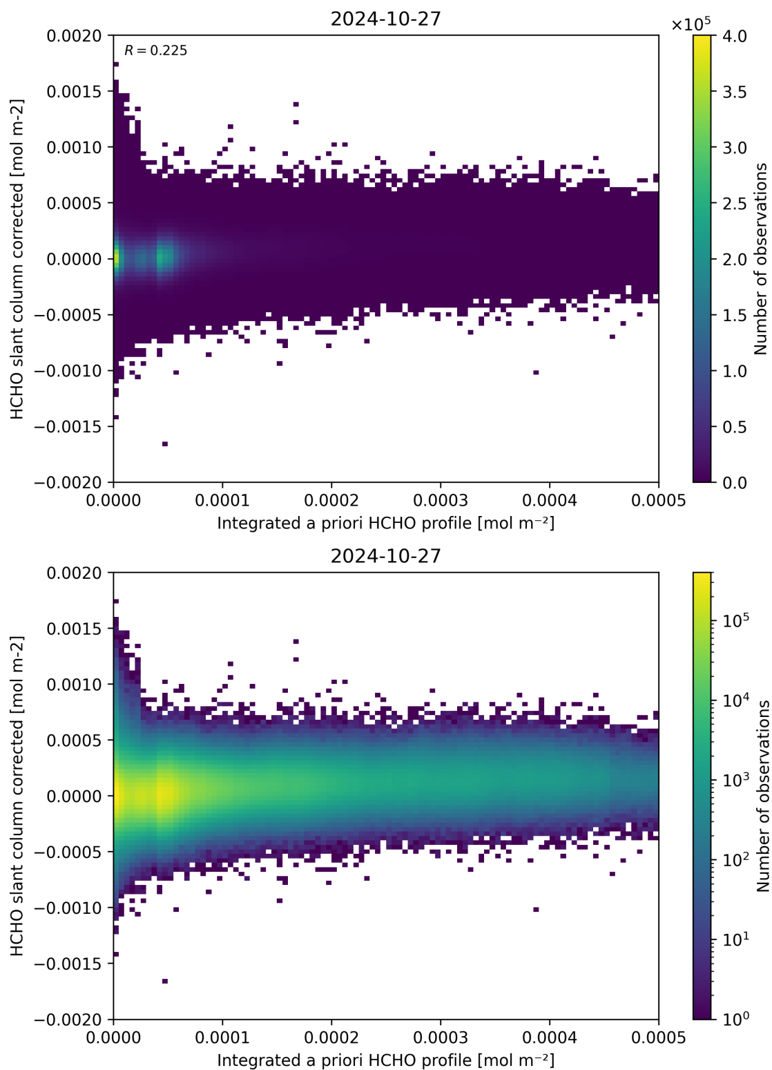
Figure 151: Scatter density plot of “Integrated a priori HCHO profile” against “HCHO slant column corrected” for 2024-10-26 to 2024-10-28.
