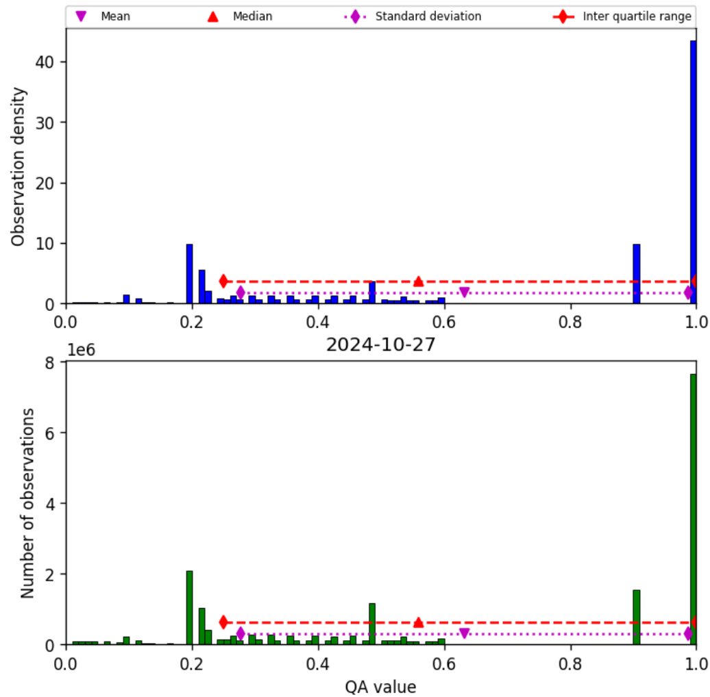
Figure 34: Histogram of “QA value” for 2024-10-26 to 2024-10-28
