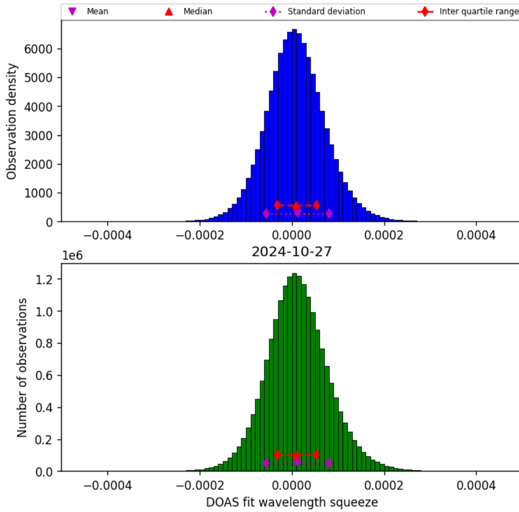
Figure 45: Histogram of “DOAS fit wavelength squeeze” for 2024-10-26 to 2024-10-28
