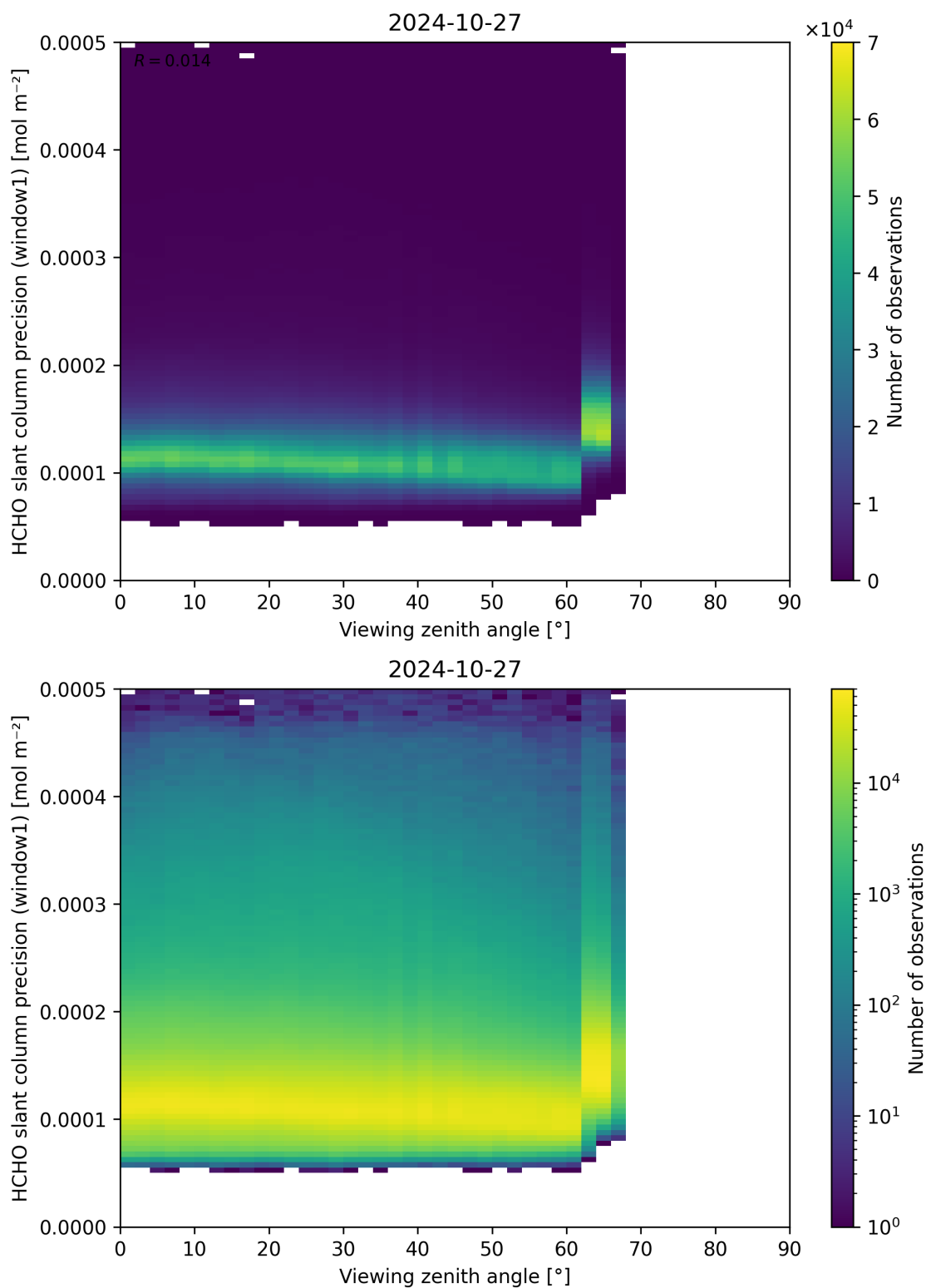
Figure 189: Scatter density plot of “Viewing zenith angle” against “HCHO slant column precision (window1)” for 2024-10-26 to 2024-10-28.
