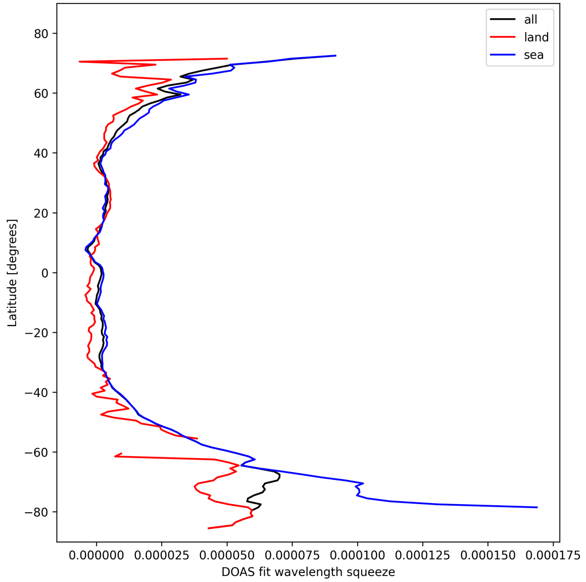
Figure 31: Zonal average of “DOAS fit wavelength squeeze” for 2024-10-26 to 2024-10-28.
