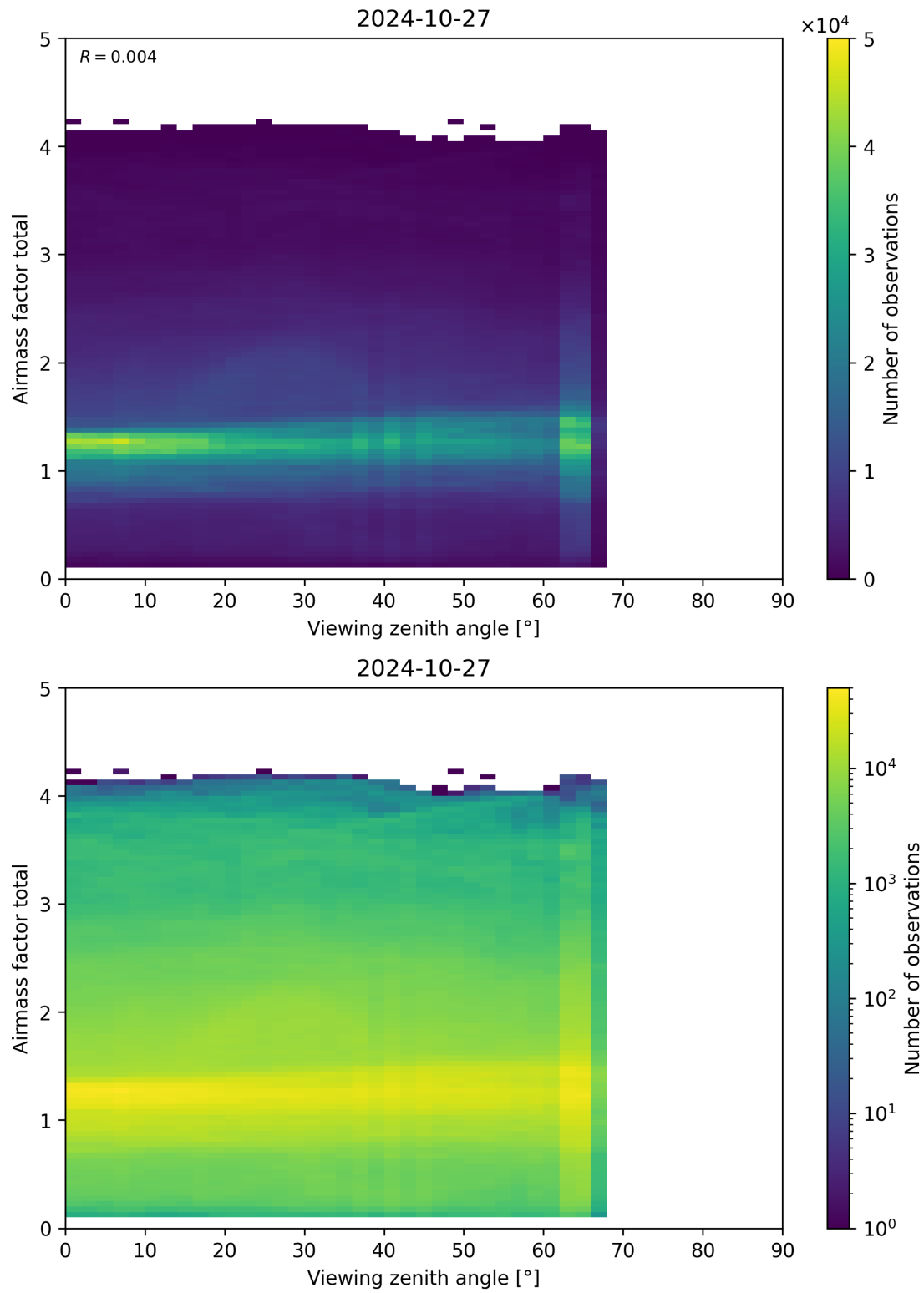
Figure 190: Scatter density plot of “Viewing zenith angle” against “Airmass factor total” for 2024-10-26 to 2024-10-28.
