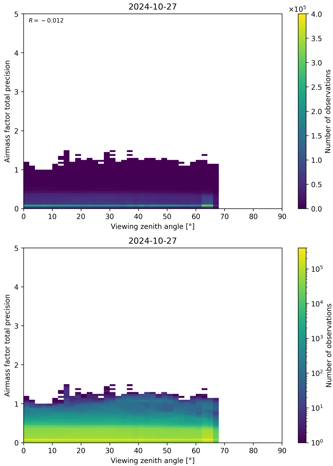
Figure 191: Scatter density plot of “Viewing zenith angle” against “Airmass factor total precision” for 2024-10-26 to 2024-10-28.
