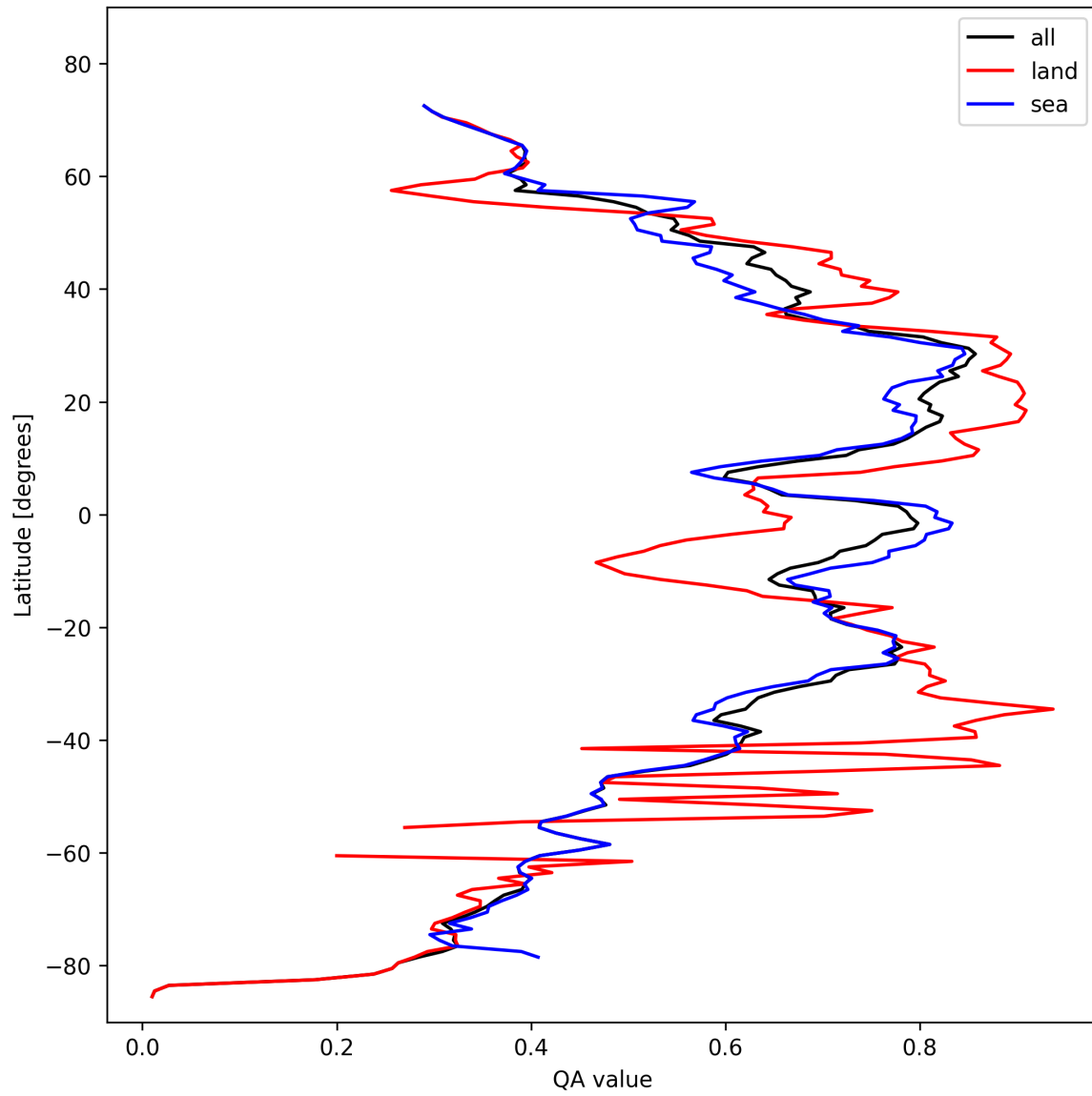
Figure 20: Zonal average of “QA value” for 2024-10-26 to 2024-10-28.
