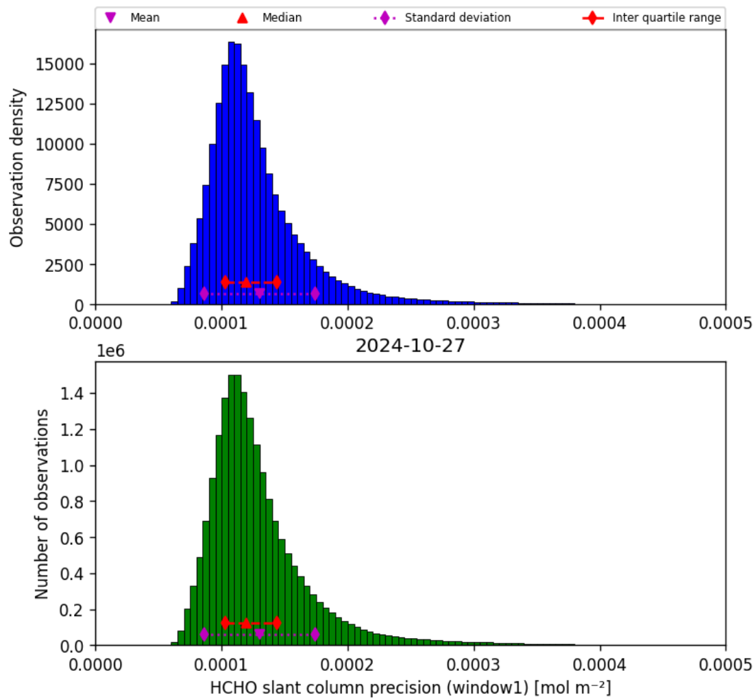
Figure 39: Histogram of “HCHO slant column precision (window1)” for 2024-10-26 to 2024-10-28
