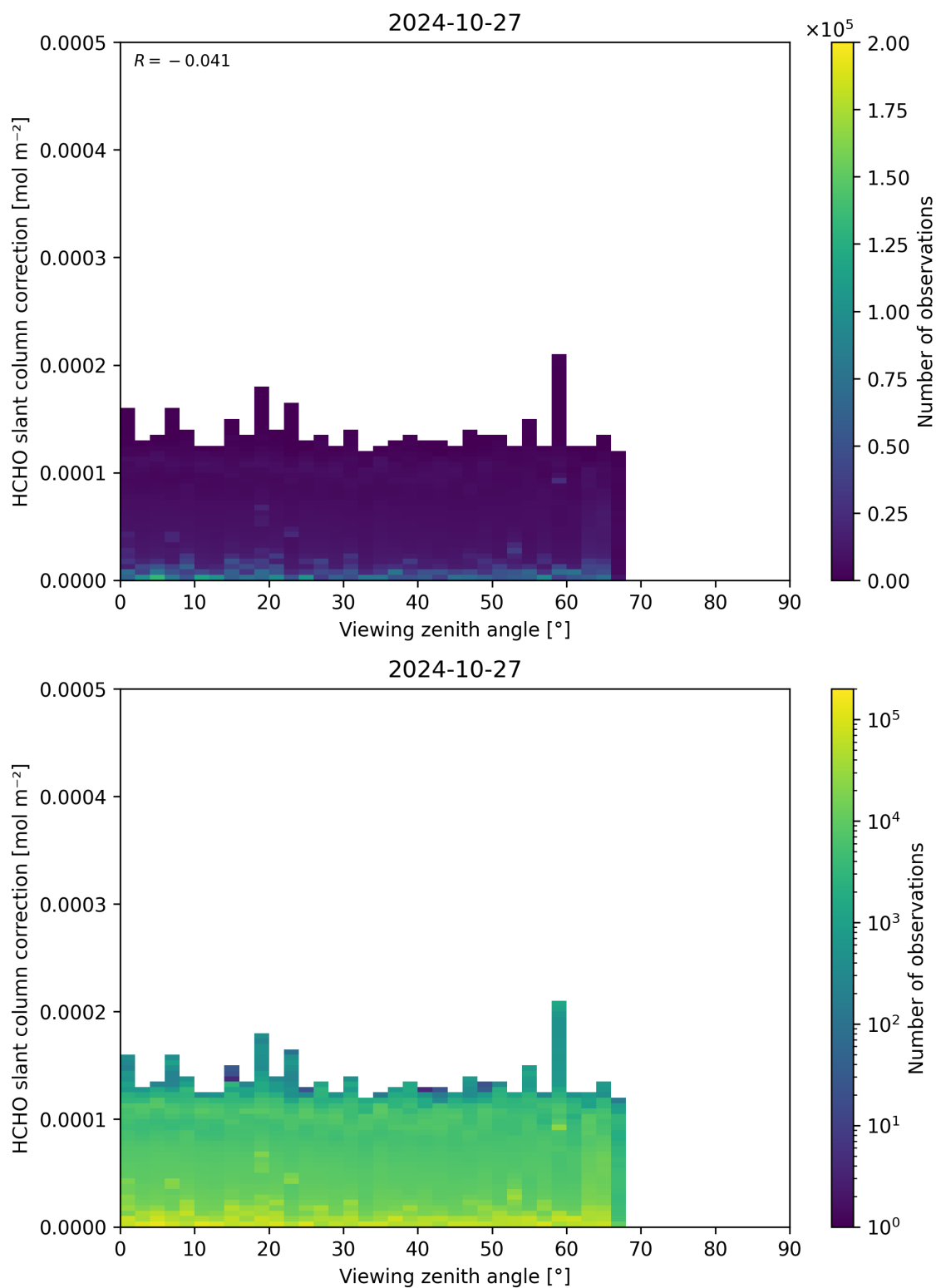
Figure 187: Scatter density plot of “Viewing zenith angle” against “HCHO slant column correction” for 2024-10-26 to 2024-10-28.
