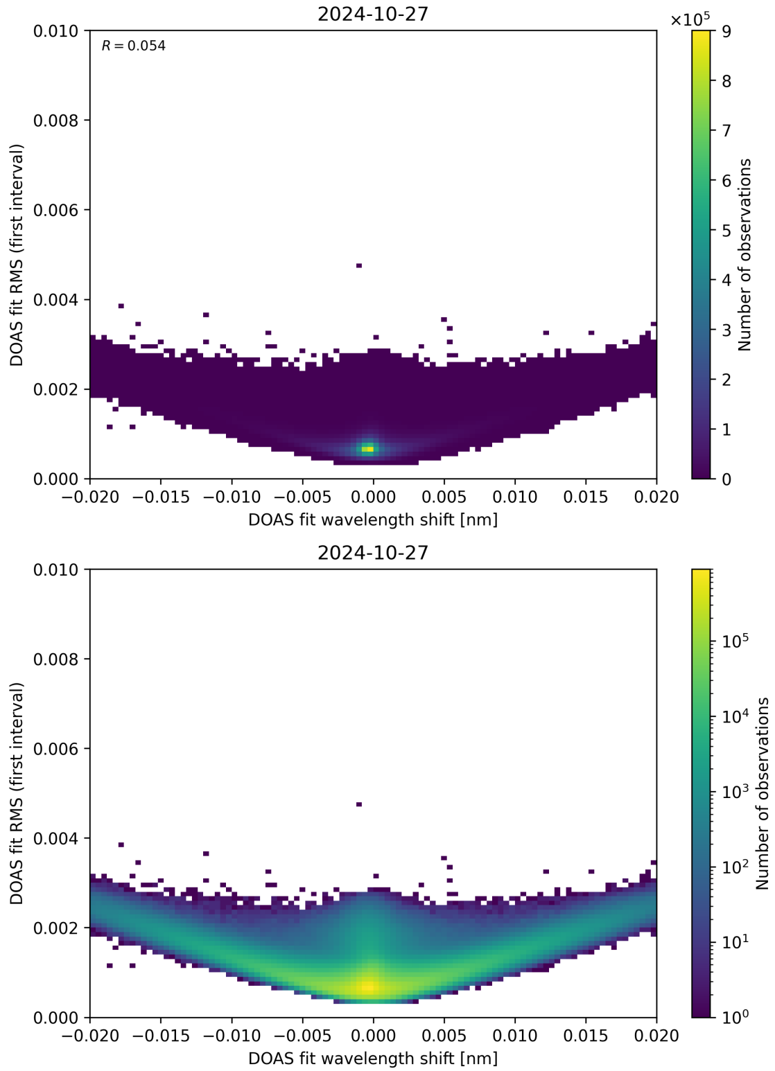
Figure 64: Scatter density plot of “DOAS fit wavelength shift” against “DOAS fit RMS (first interval)” for 2024-10-26 to 2024-10-28.
