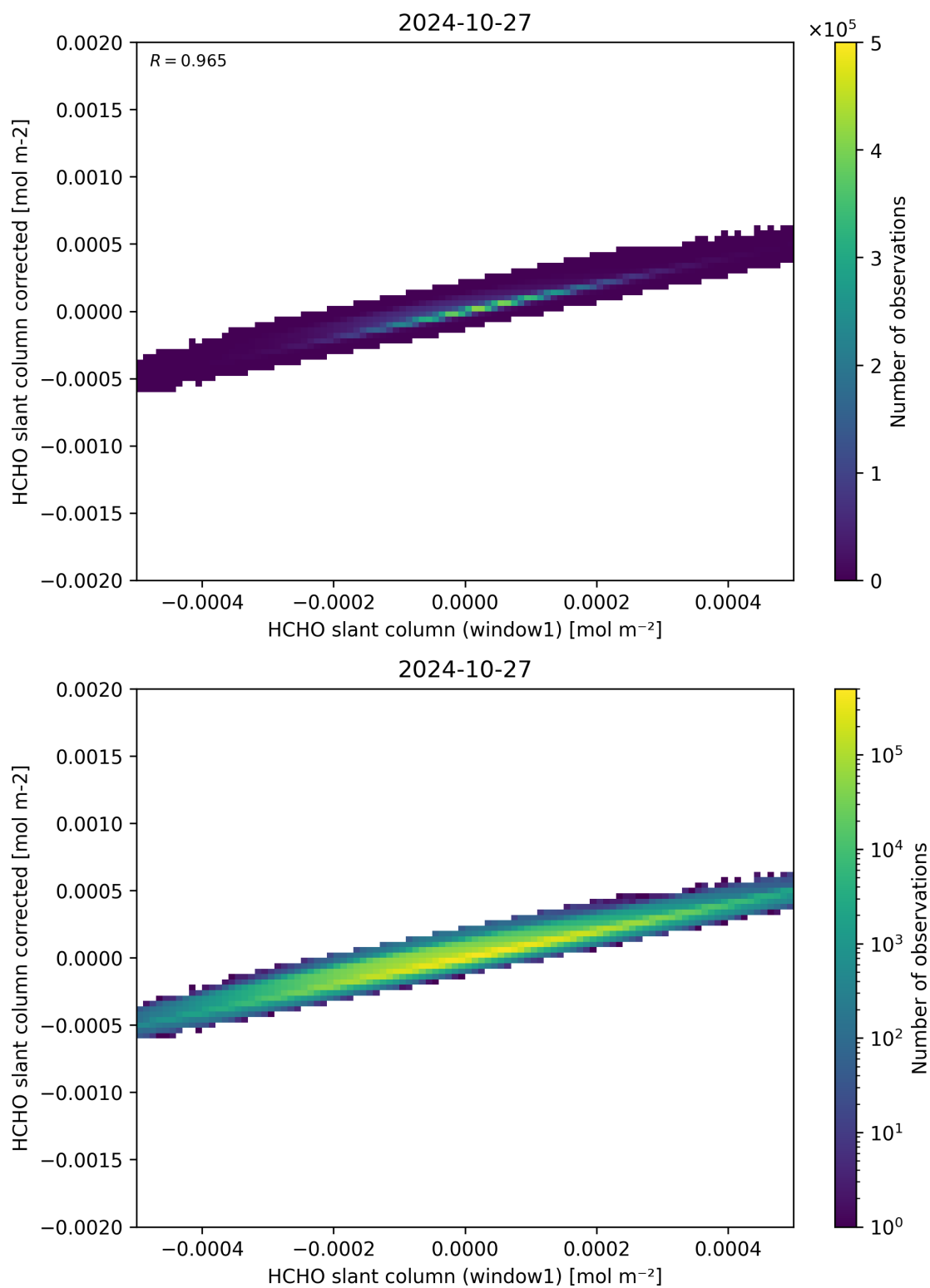
Figure 82: Scatter density plot of “HCHO slant column (window1)” against “HCHO slant column corrected” for 2024-10-26 to 2024-10-28.
