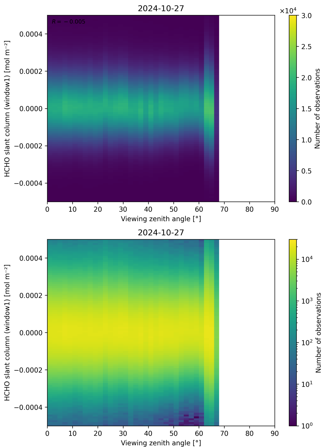
Figure 188: Scatter density plot of “Viewing zenith angle” against “HCHO slant column (window1)” for 2024-10-26 to 2024-10-28.
