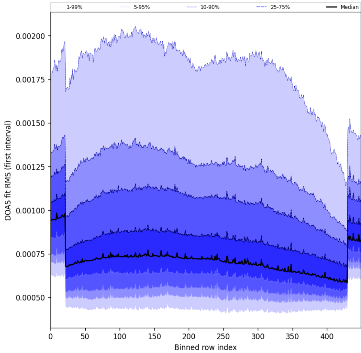
Figure 60: Along track statistics of “DOAS fit RMS (first interval)” for 2024-10-26 to 2024-10-28
