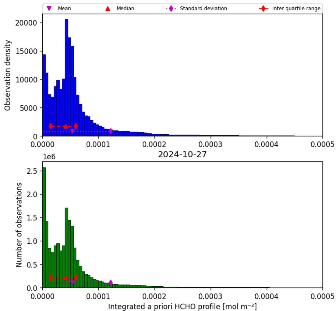
Figure 43: Histogram of “Integrated a priori HCHO profile” for 2024-10-26 to 2024-10-28
