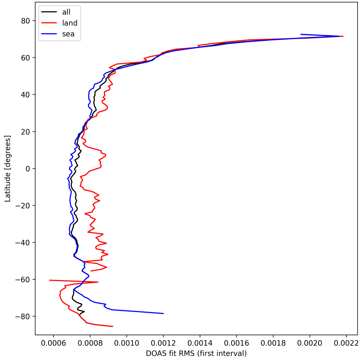
Figure 32: Zonal average of “DOAS fit RMS (first interval)” for 2024-10-26 to 2024-10-28.
