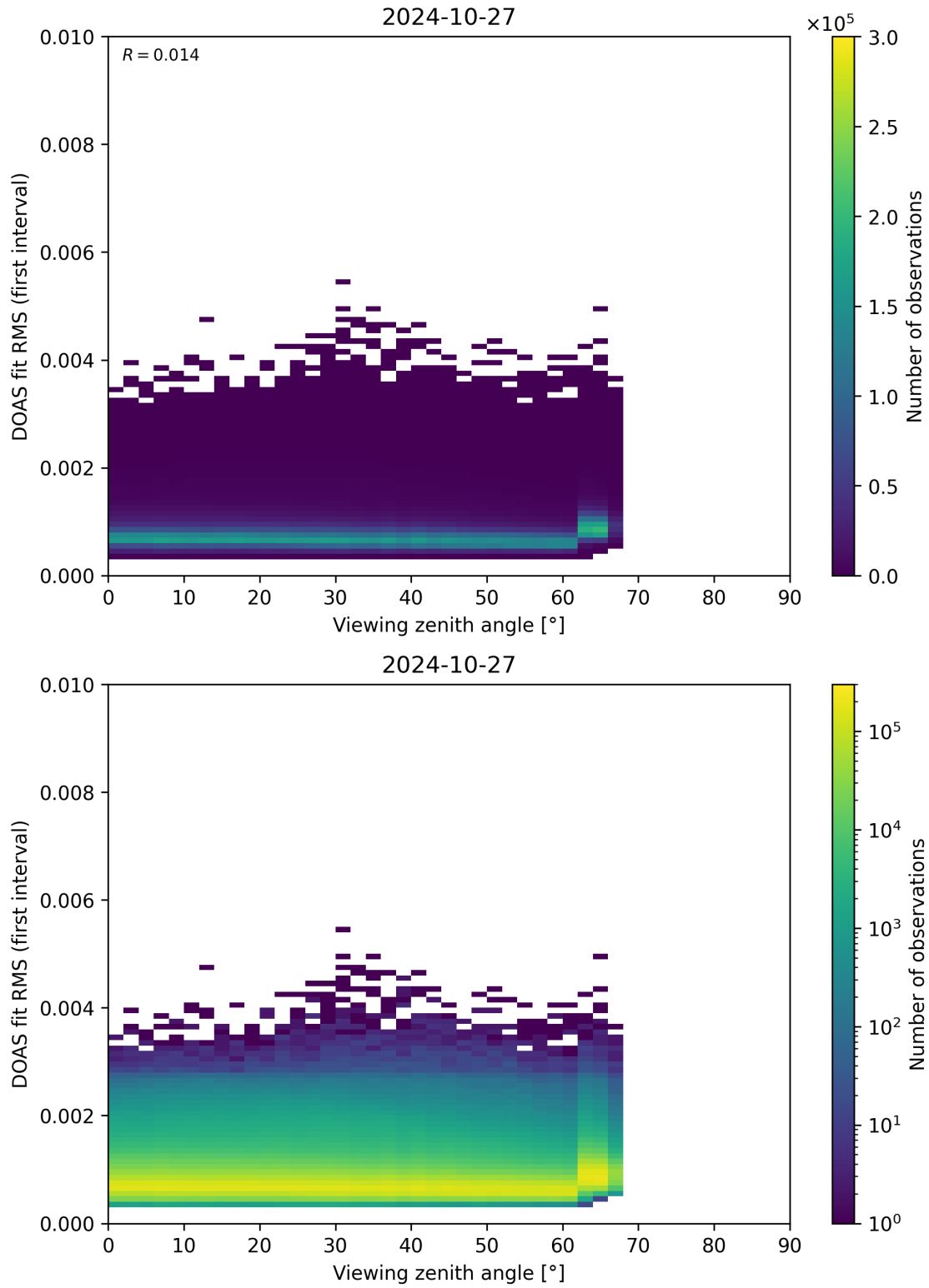
Figure 182: Scatter density plot of “Viewing zenith angle” against “DOAS fit RMS (first interval)” for 2024-10-26 to 2024-10-28.
