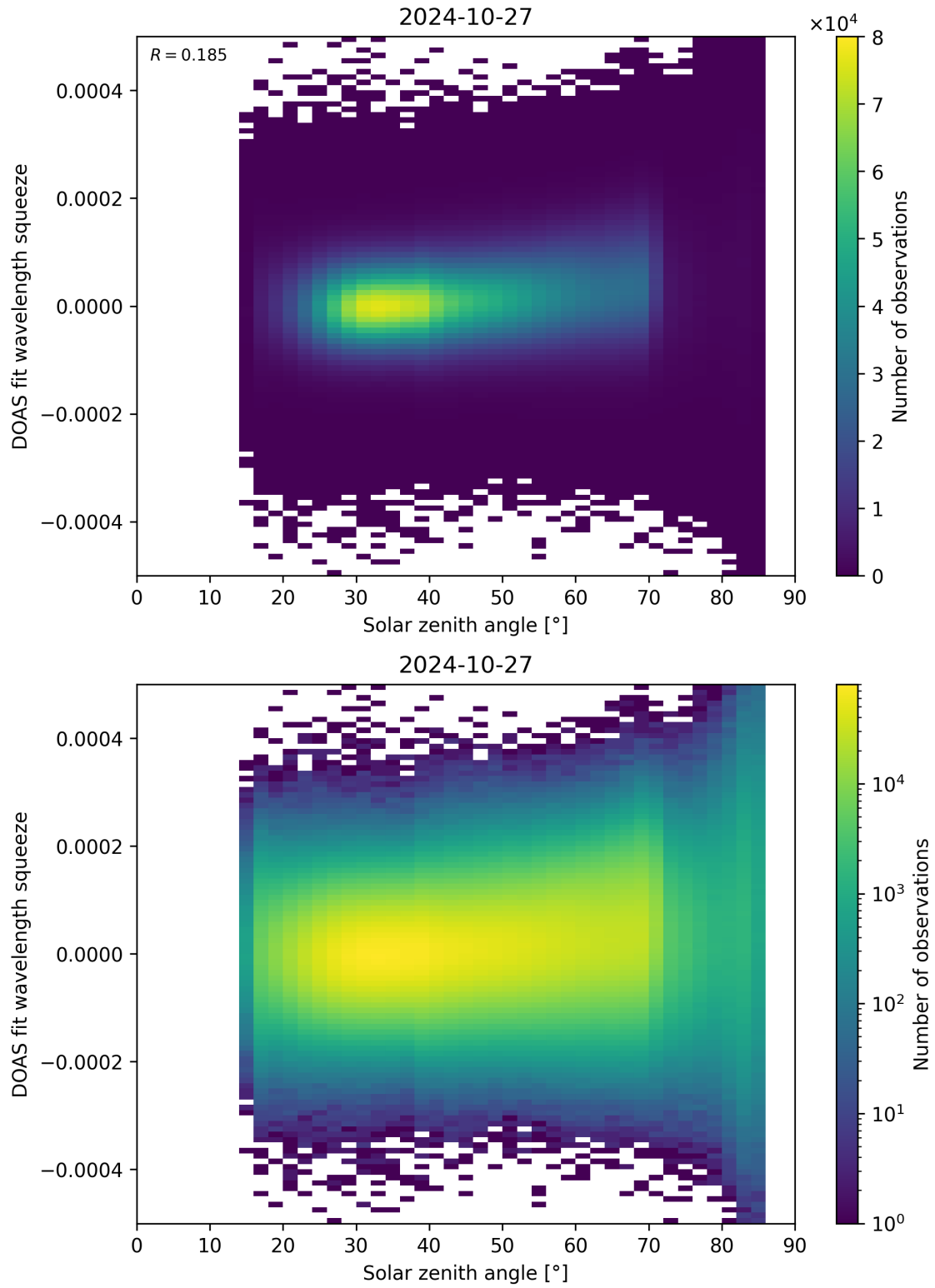
Figure 169: Scatter density plot of “Solar zenith angle” against “DOAS fit wavelength squeeze” for 2024-10-26 to 2024-10-28.
