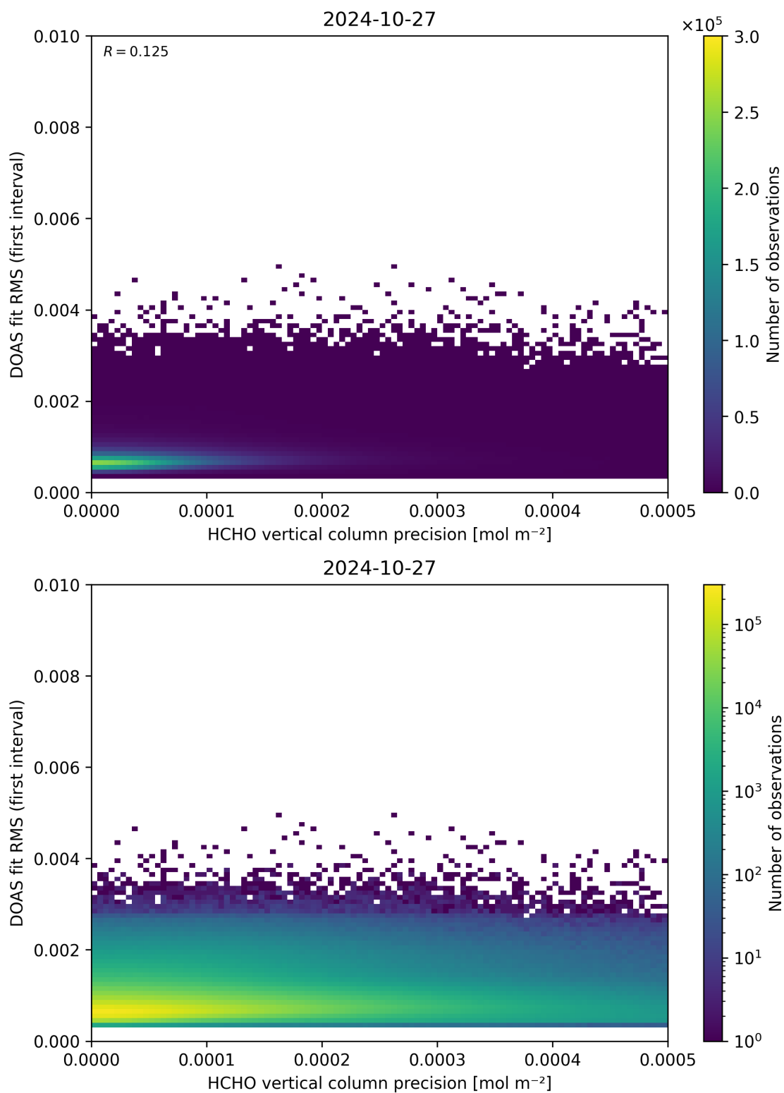
Figure 136: Scatter density plot of “HCHO vertical column precision” against “DOAS fit RMS (first interval)” for 2024-10-26 to 2024-10-28.
