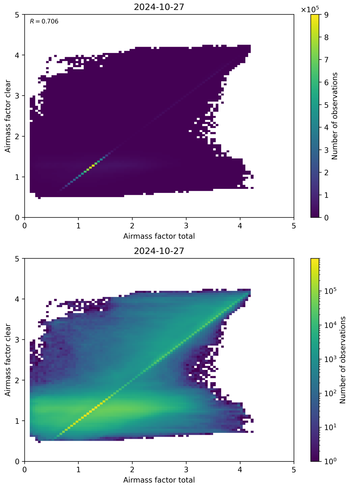
Figure 100: Scatter density plot of “Airmass factor total” against “Airmass factor clear” for 2024-10-26 to 2024-10-28.
