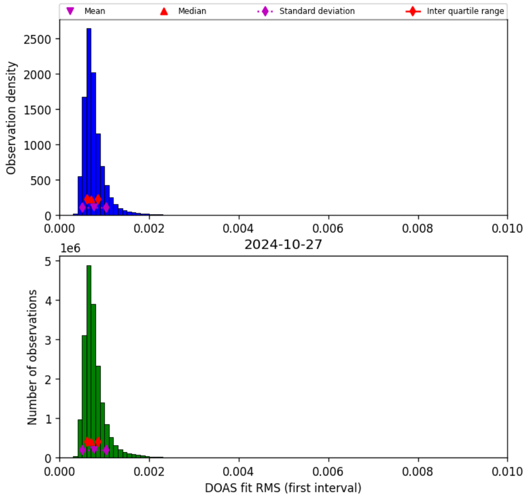
Figure 46: Histogram of “DOAS fit RMS (first interval)” for 2024-10-26 to 2024-10-28
