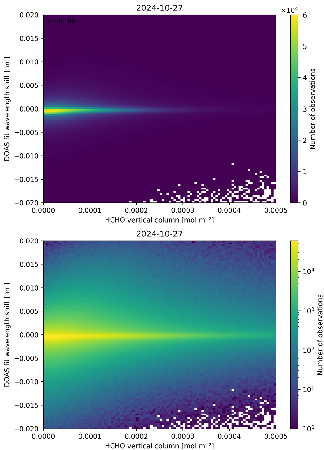
Figure 124: Scatter density plot of “HCHO vertical column” against “DOAS fit wavelength shift” for 2024-10-26 to 2024-10-28.
