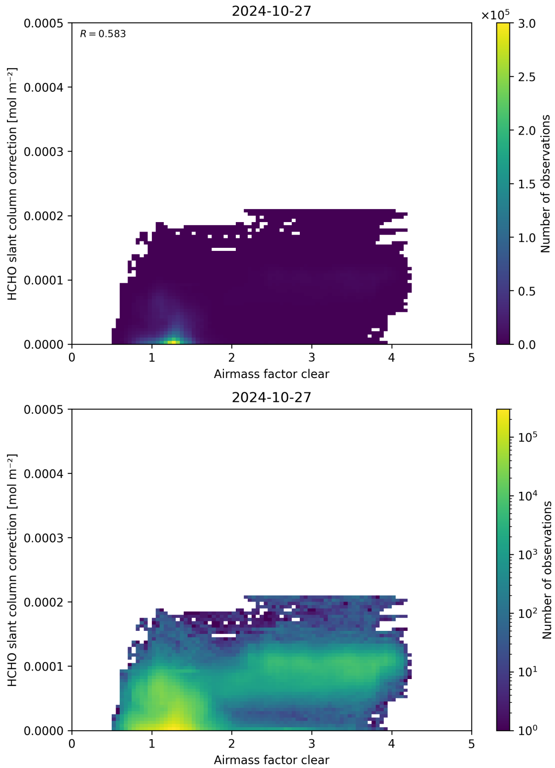
Figure 75: Scatter density plot of “Airmass factor clear” against “HCHO slant column correction” for 2024-10-26 to 2024-10-28.
