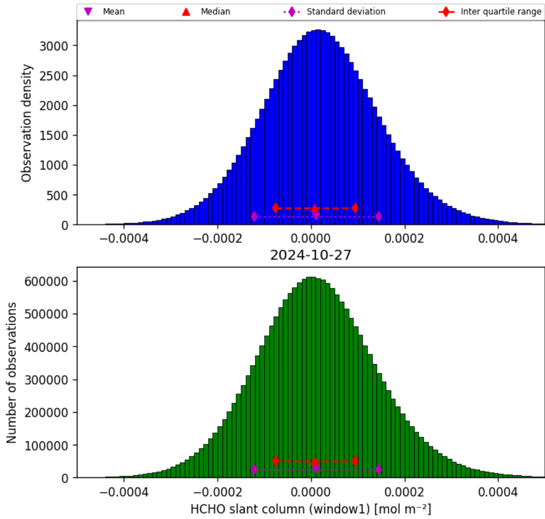
Figure 38: Histogram of “HCHO slant column (window1)” for 2024-10-26 to 2024-10-28
