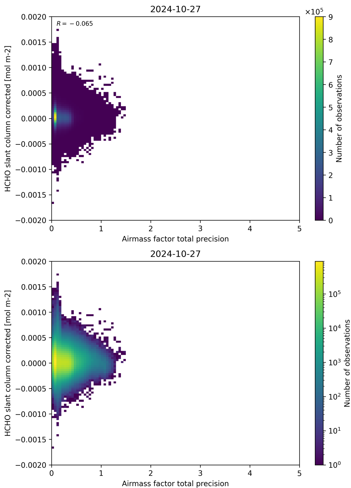
Figure 109: Scatter density plot of “Airmass factor total precision” against “HCHO slant column corrected” for 2024-10-26 to 2024-10-28.
