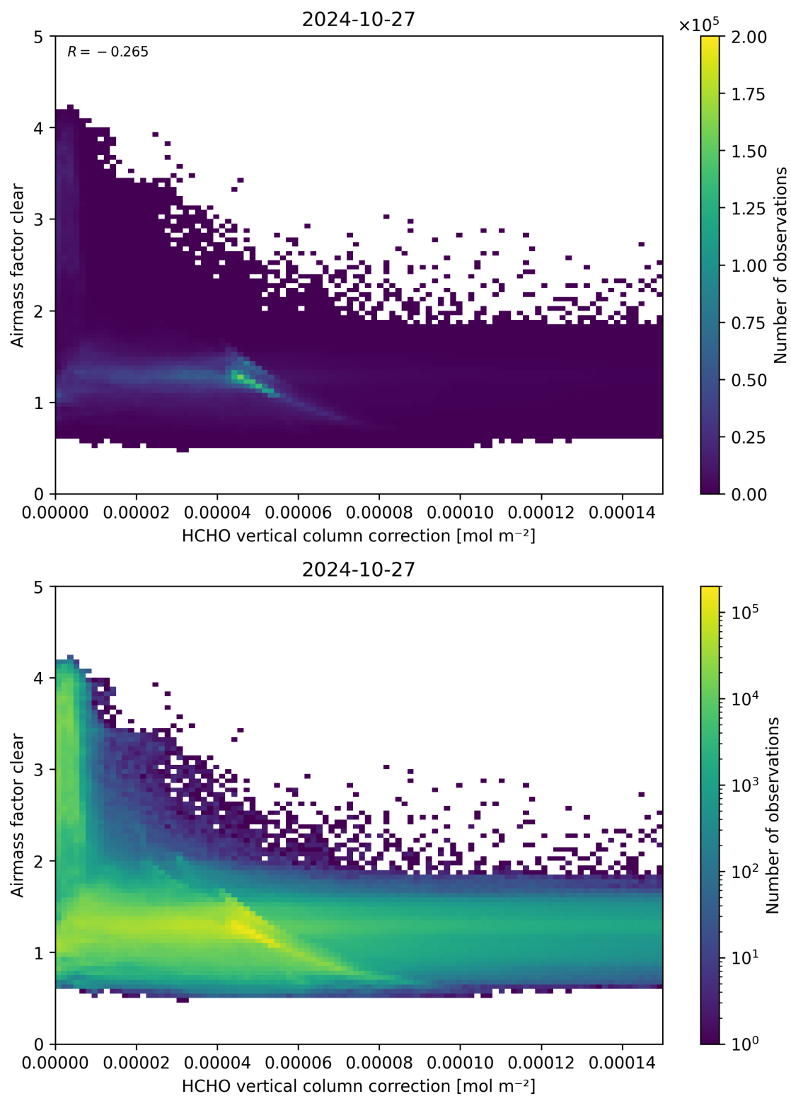
Figure 115: Scatter density plot of “HCHO vertical column correction” against “Airmass factor clear” for 2024-10-26 to 2024-10-28.
