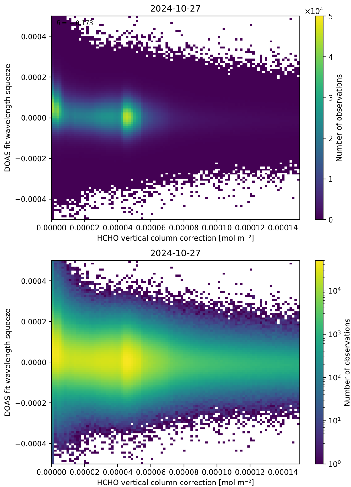
Figure 114: Scatter density plot of “HCHO vertical column correction” against “DOAS fit wavelength squeeze” for 2024-10-26 to 2024-10-28.
