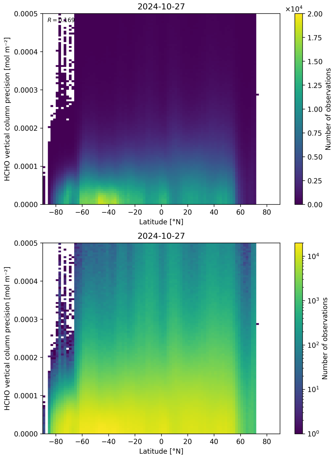
Figure 165: Scatter density plot of “Latitude” against “HCHO vertical column precision” for 2024-10-26 to 2024-10-28.
