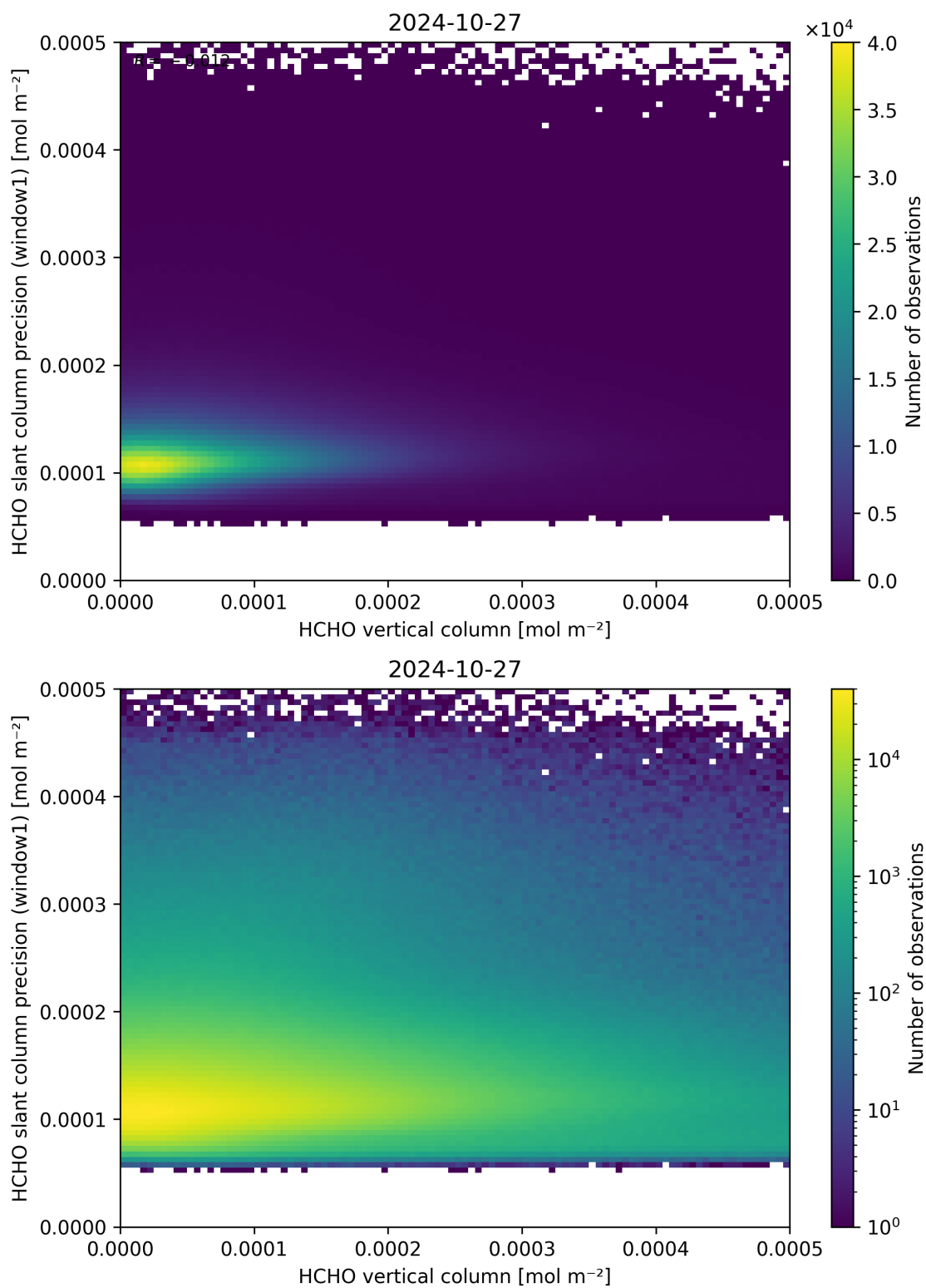
Figure 130: Scatter density plot of “HCHO vertical column” against “HCHO slant column precision (window1)” for 2024-10-26 to 2024-10-28.
