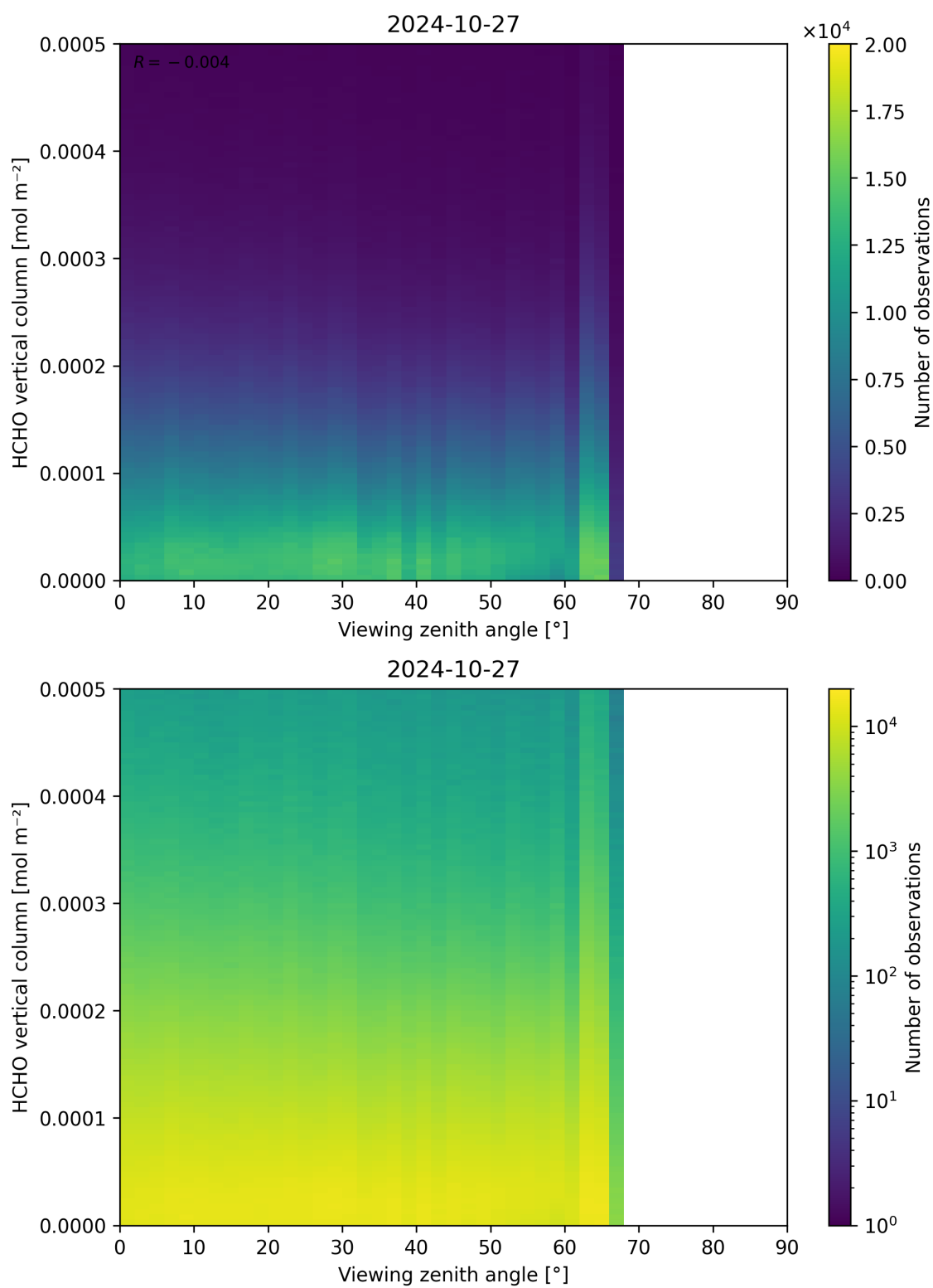
Figure 192: Scatter density plot of “Viewing zenith angle” against “HCHO vertical column” for 2024-10-26 to 2024-10-28.
