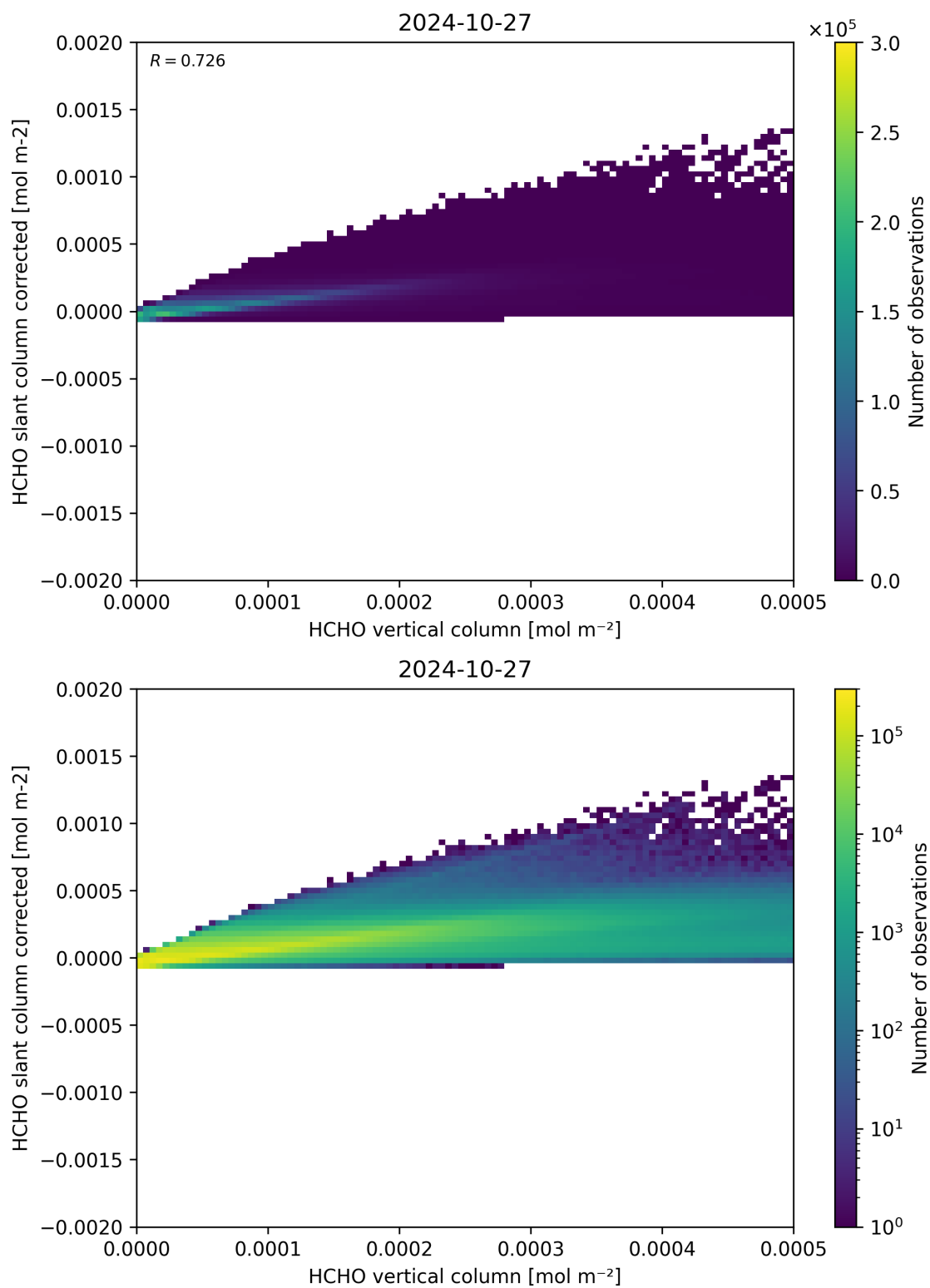
Figure 127: Scatter density plot of “HCHO vertical column” against “HCHO slant column corrected” for 2024-10-26 to 2024-10-28.
