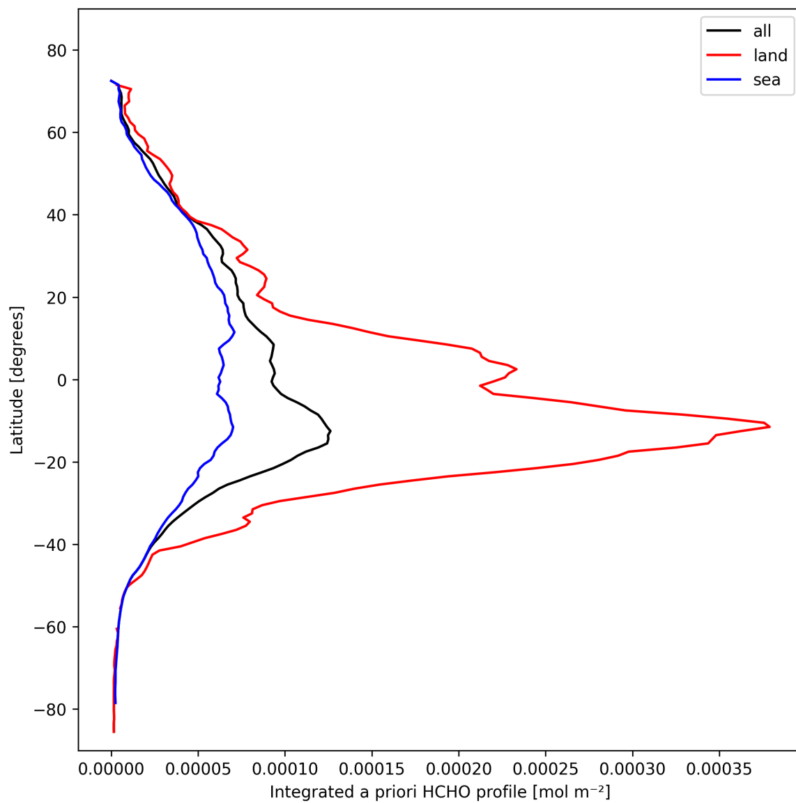
Figure 29: Zonal average of “Integrated a priori HCHO profile” for 2024-10-26 to 2024-10-28.
