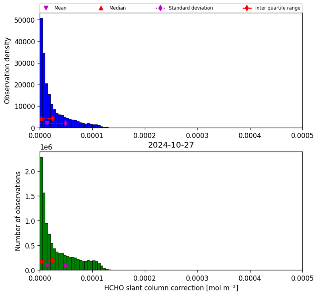
Figure 47: Histogram of “HCHO slant column correction” for 2024-10-26 to 2024-10-28
