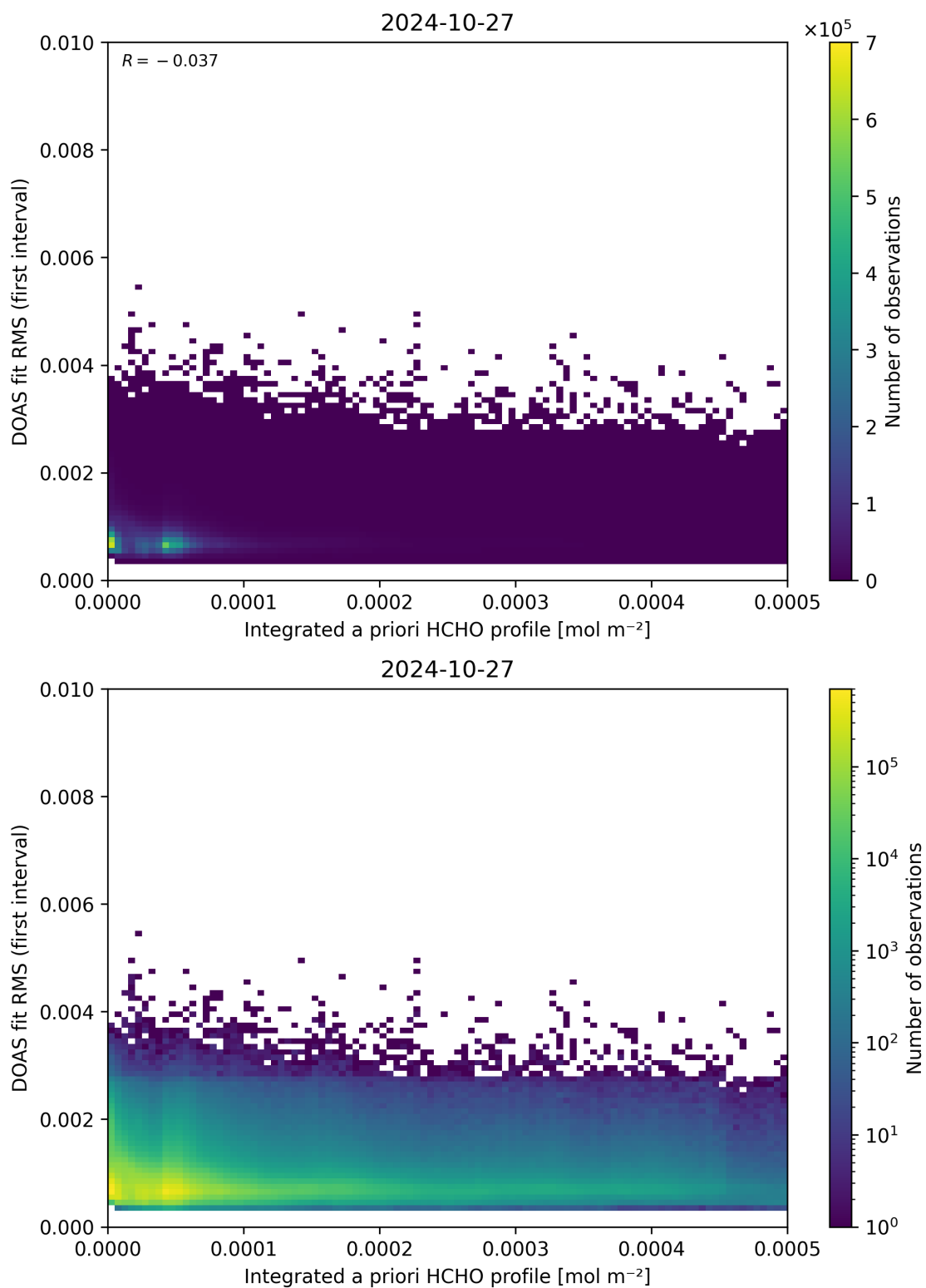
Figure 148: Scatter density plot of “Integrated a priori HCHO profile” against “DOAS fit RMS (first interval)” for 2024-10-26 to 2024-10-28.
