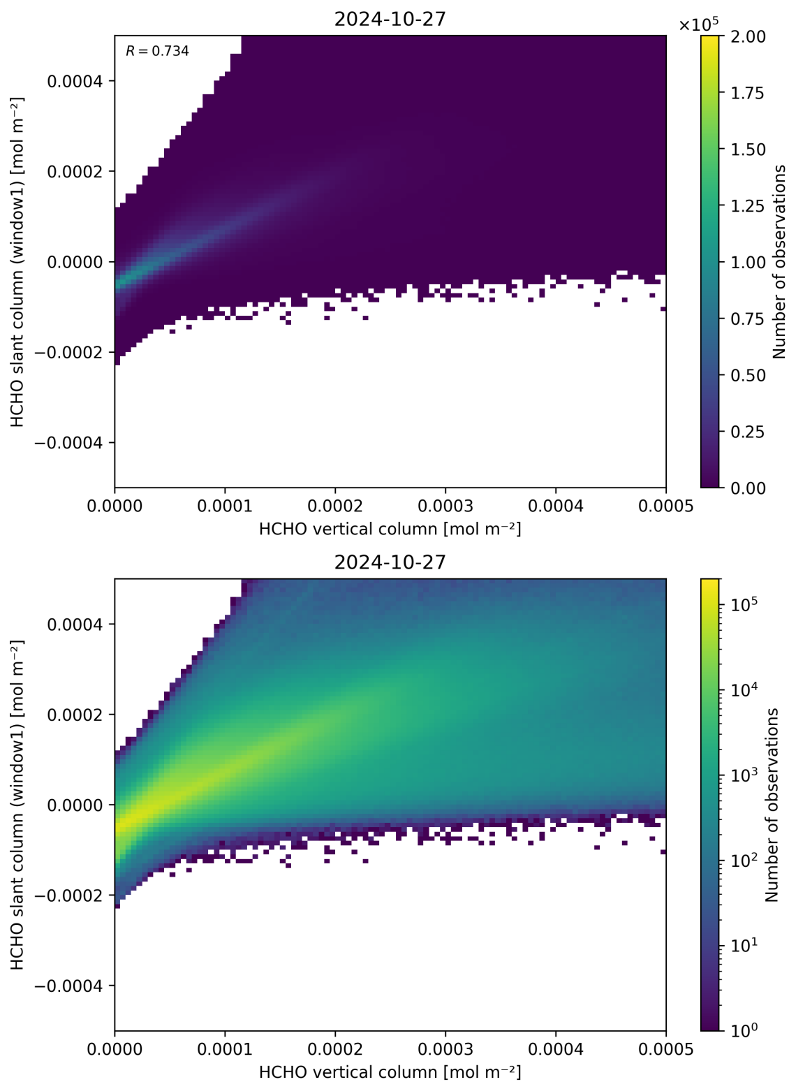
Figure 129: Scatter density plot of “HCHO vertical column” against “HCHO slant column (window1)” for 2024-10-26 to 2024-10-28.
