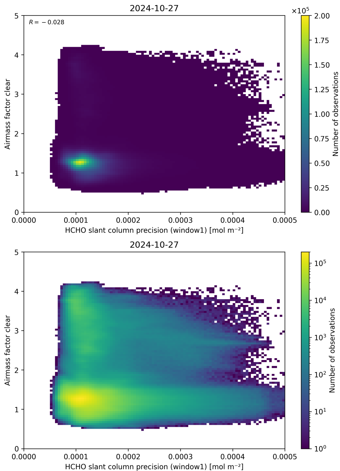
Figure 91: Scatter density plot of “HCHO slant column precision (window1)” against “Airmass factor clear” for 2024-10-26 to 2024-10-28.
