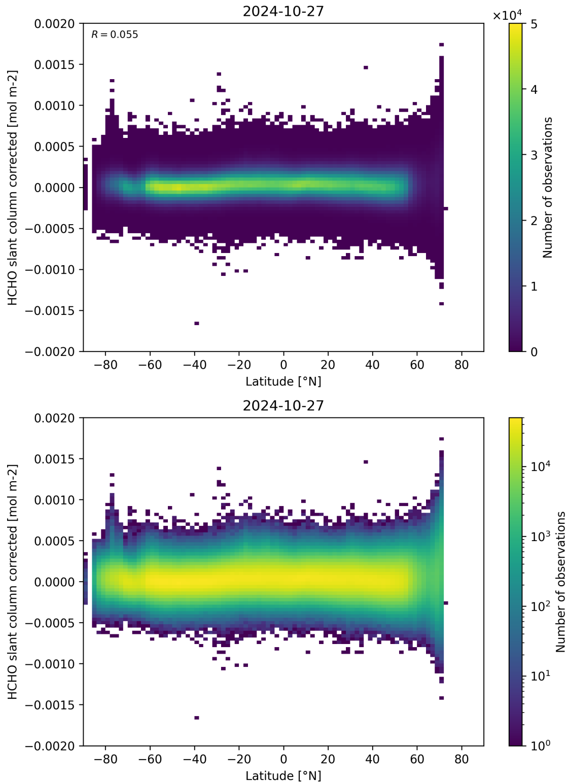
Figure 157: Scatter density plot of “Latitude” against “HCHO slant column corrected” for 2024-10-26 to 2024-10-28.
