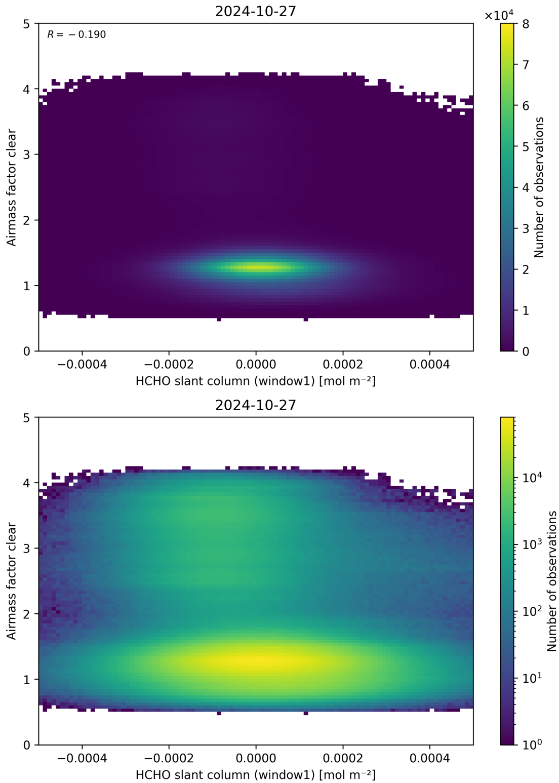
Figure 81: Scatter density plot of “HCHO slant column (window1)” against “Airmass factor clear” for 2024-10-26 to 2024-10-28.
