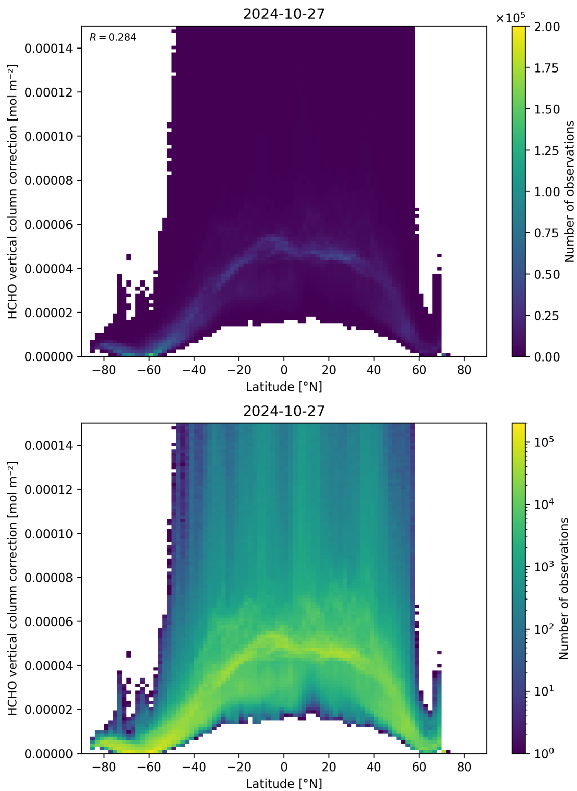
Figure 164: Scatter density plot of “Latitude” against “HCHO vertical column correction” for 2024-10-26 to 2024-10-28.
