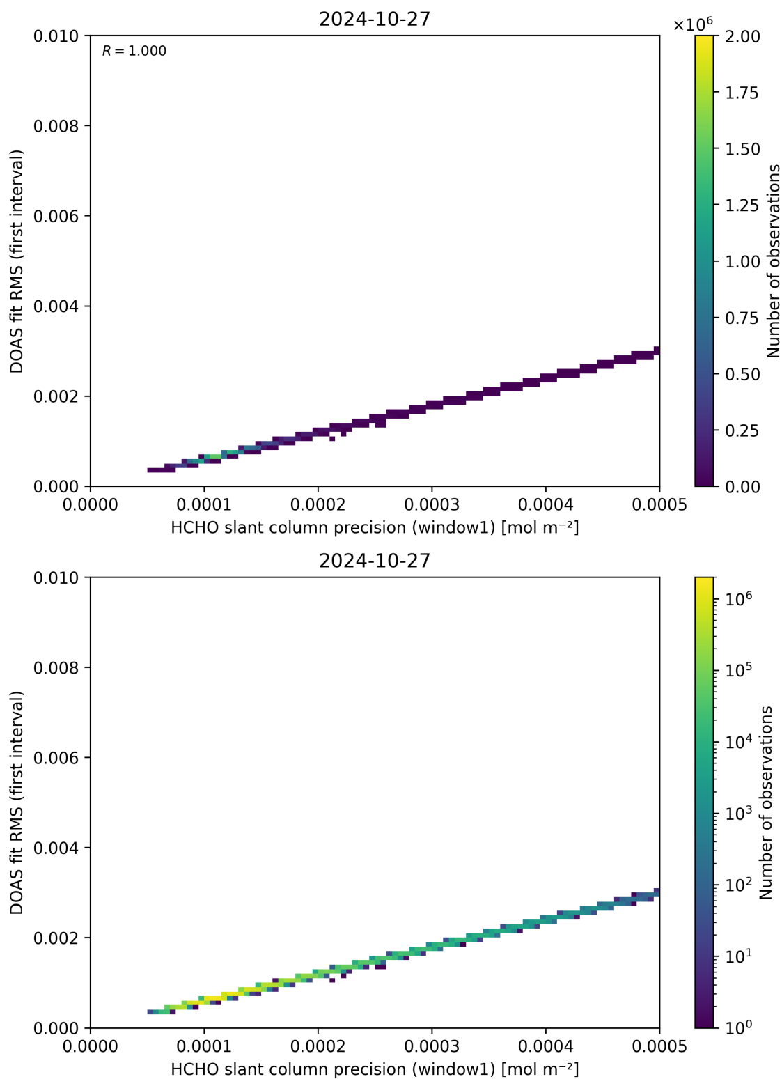
Figure 88: Scatter density plot of “HCHO slant column precision (window1)” against “DOAS fit RMS (first interval)” for 2024-10-26 to 2024-10-28.
