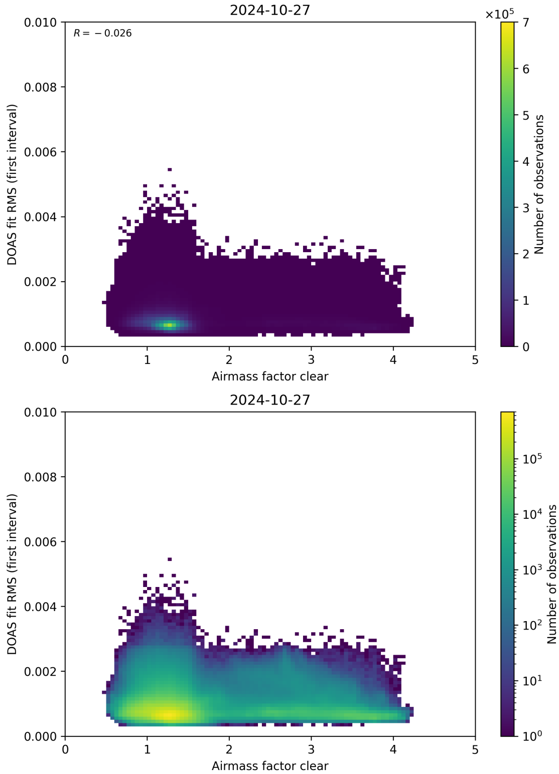
Figure 71: Scatter density plot of “Airmass factor clear” against “DOAS fit RMS (first interval)” for 2024-10-26 to 2024-10-28.
