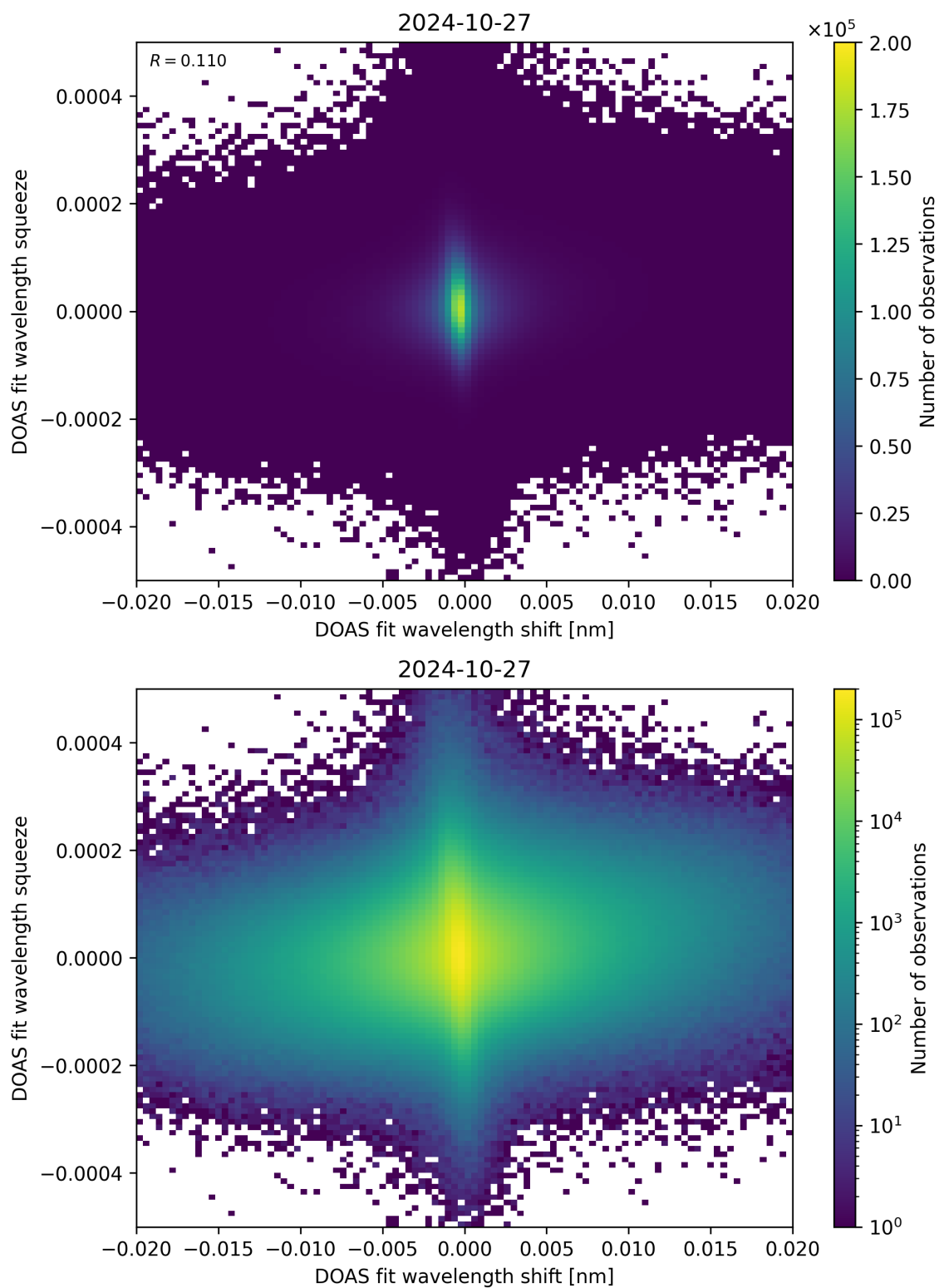
Figure 65: Scatter density plot of “DOAS fit wavelength shift” against “DOAS fit wavelength squeeze” for 2024-10-26 to 2024-10-28.
