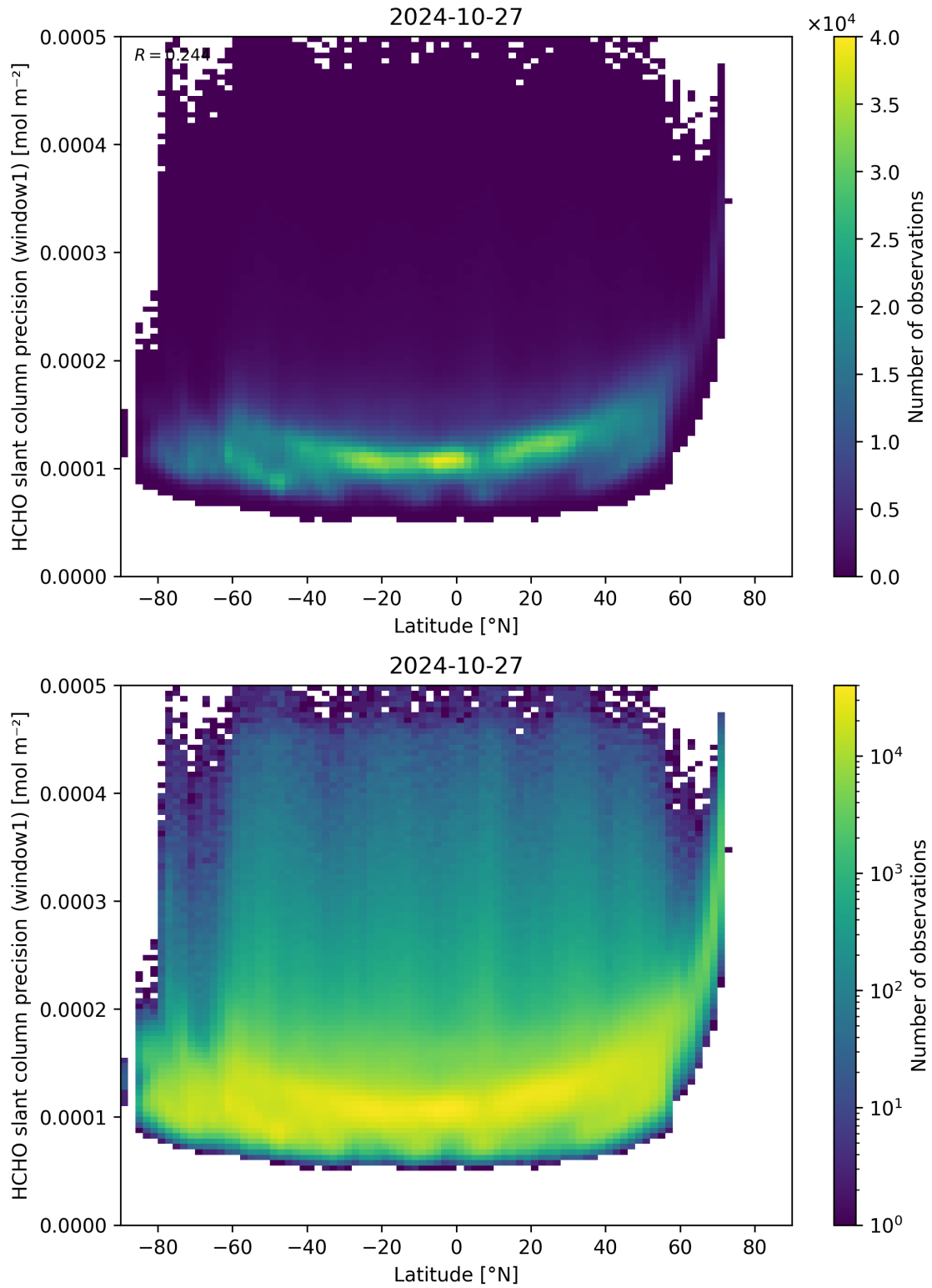
Figure 160: Scatter density plot of “Latitude” against “HCHO slant column precision (window1)” for 2024-10-26 to 2024-10-28.
