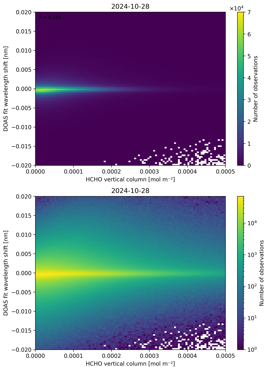
Figure 124: Scatter density plot of “HCHO vertical column” against “DOAS fit wavelength shift” for 2024-10-27 to 2024-10-29.
