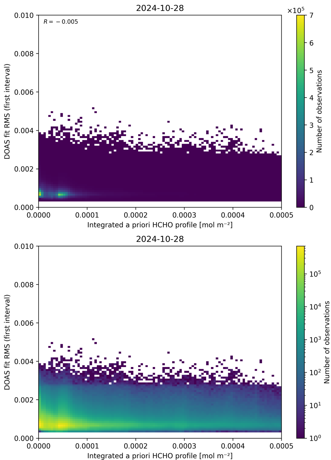
Figure 148: Scatter density plot of “Integrated a priori HCHO profile” against “DOAS fit RMS (first interval)” for 2024-10-27 to 2024-10-29.
