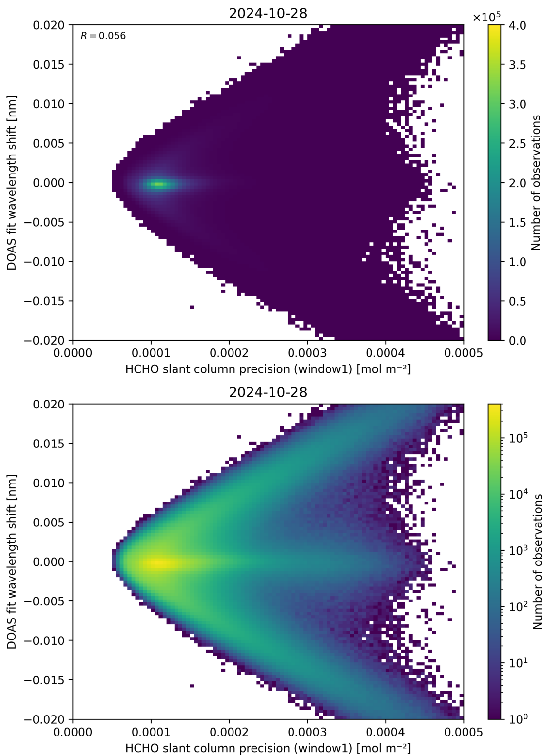
Figure 89: Scatter density plot of “HCHO slant column precision (window1)” against “DOAS fit wavelength shift” for 2024-10-27 to 2024-10-29.
