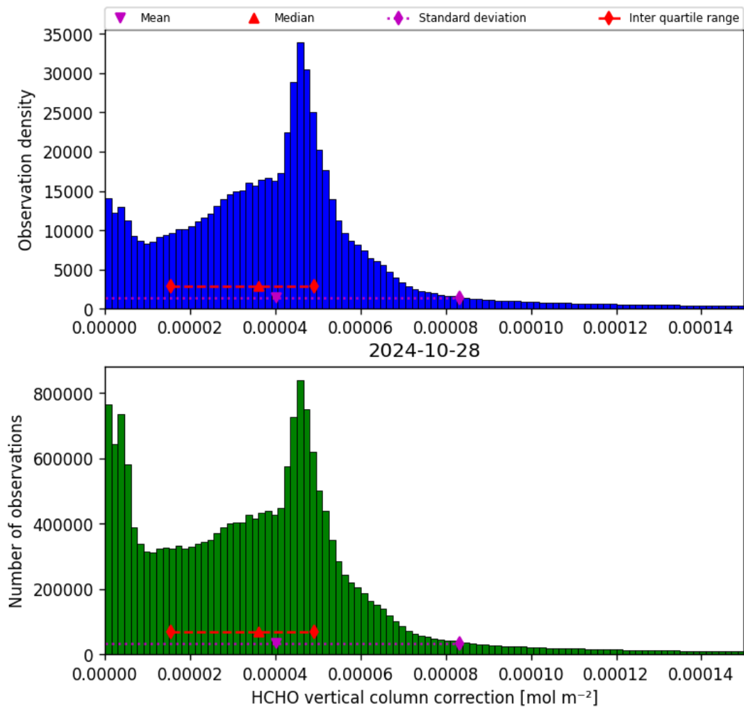
Figure 37: Histogram of “HCHO vertical column correction” for 2024-10-27 to 2024-10-29
