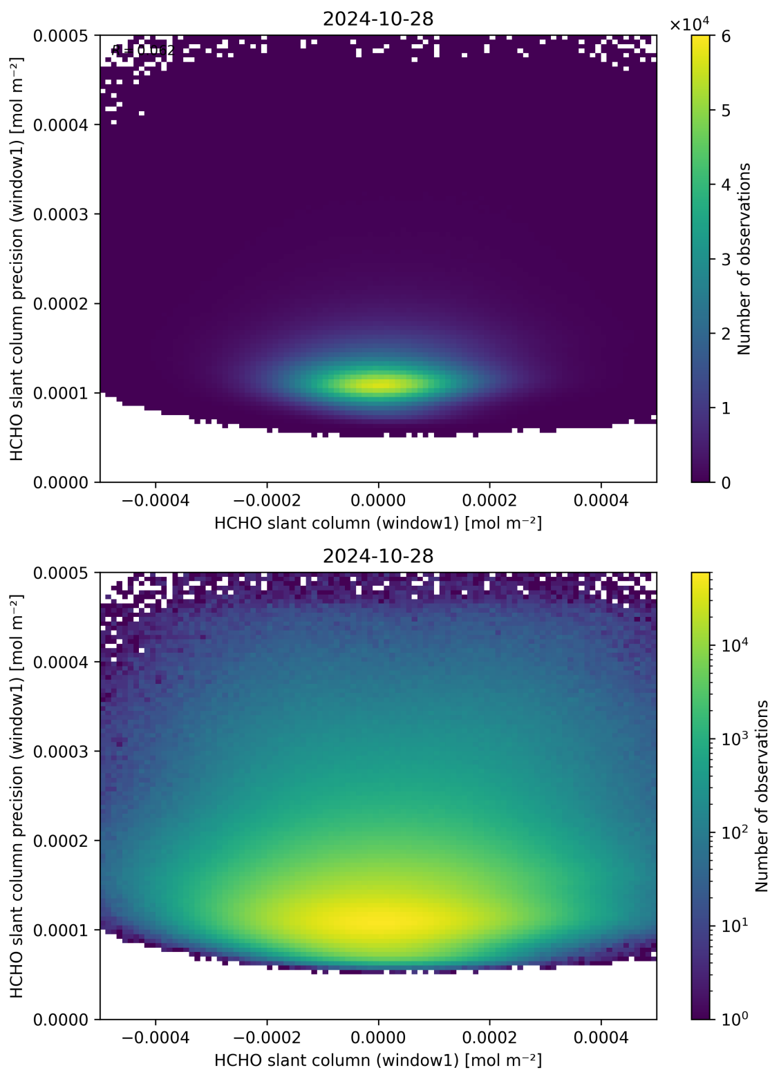
Figure 84: Scatter density plot of “HCHO slant column (window1)” against “HCHO slant column precision (window1)” for 2024-10-27 to 2024-10-29.
