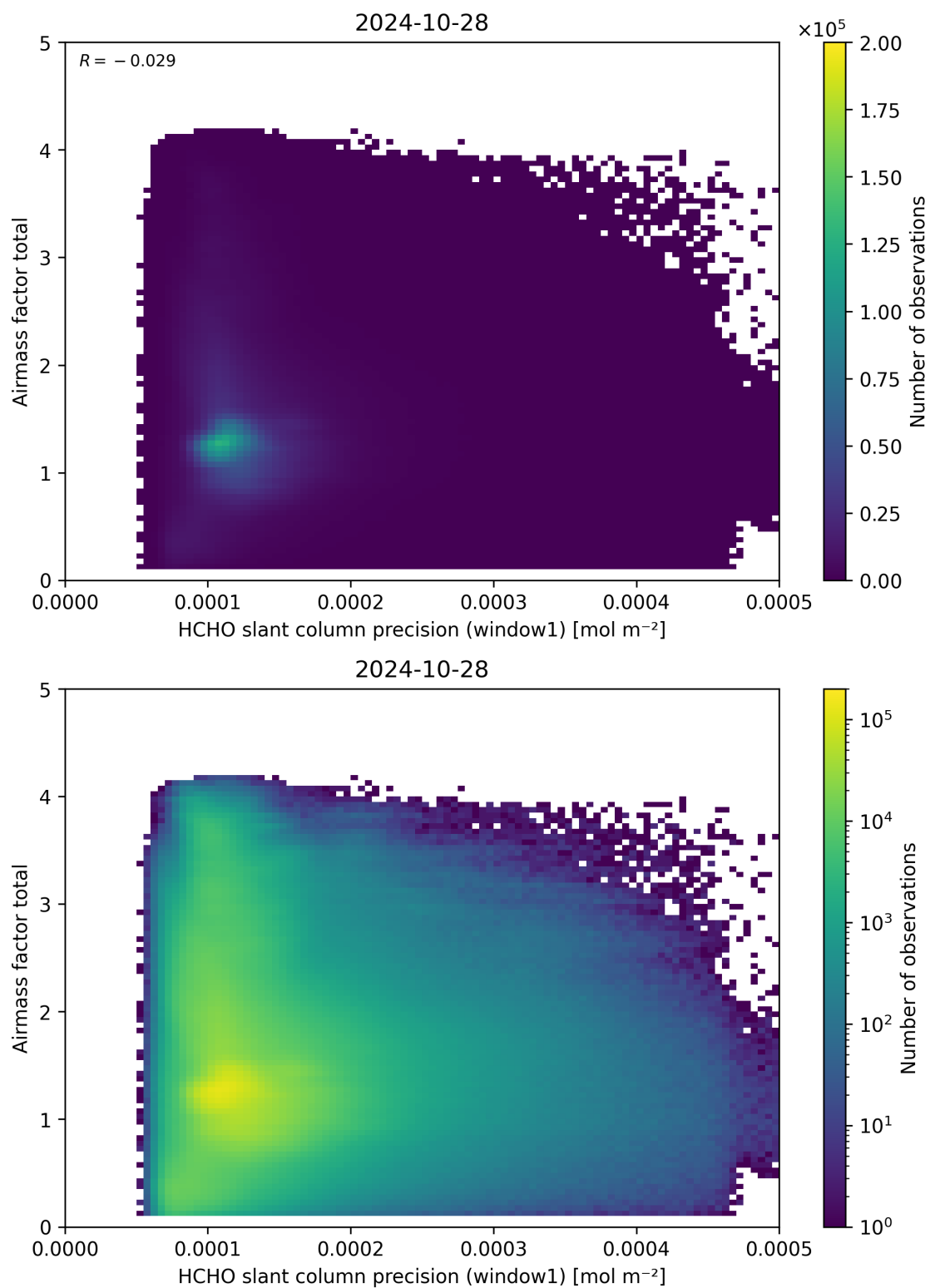
Figure 94: Scatter density plot of “HCHO slant column precision (window1)” against “Airmass factor total” for 2024-10-27 to 2024-10-29.
