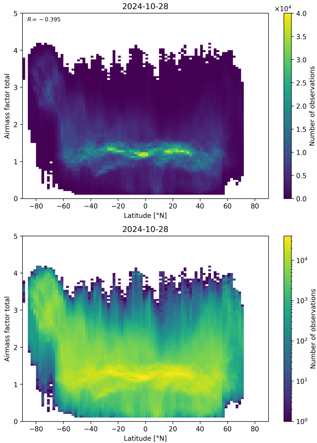
Figure 161: Scatter density plot of “Latitude” against “Airmass factor total” for 2024-10-27 to 2024-10-29.
