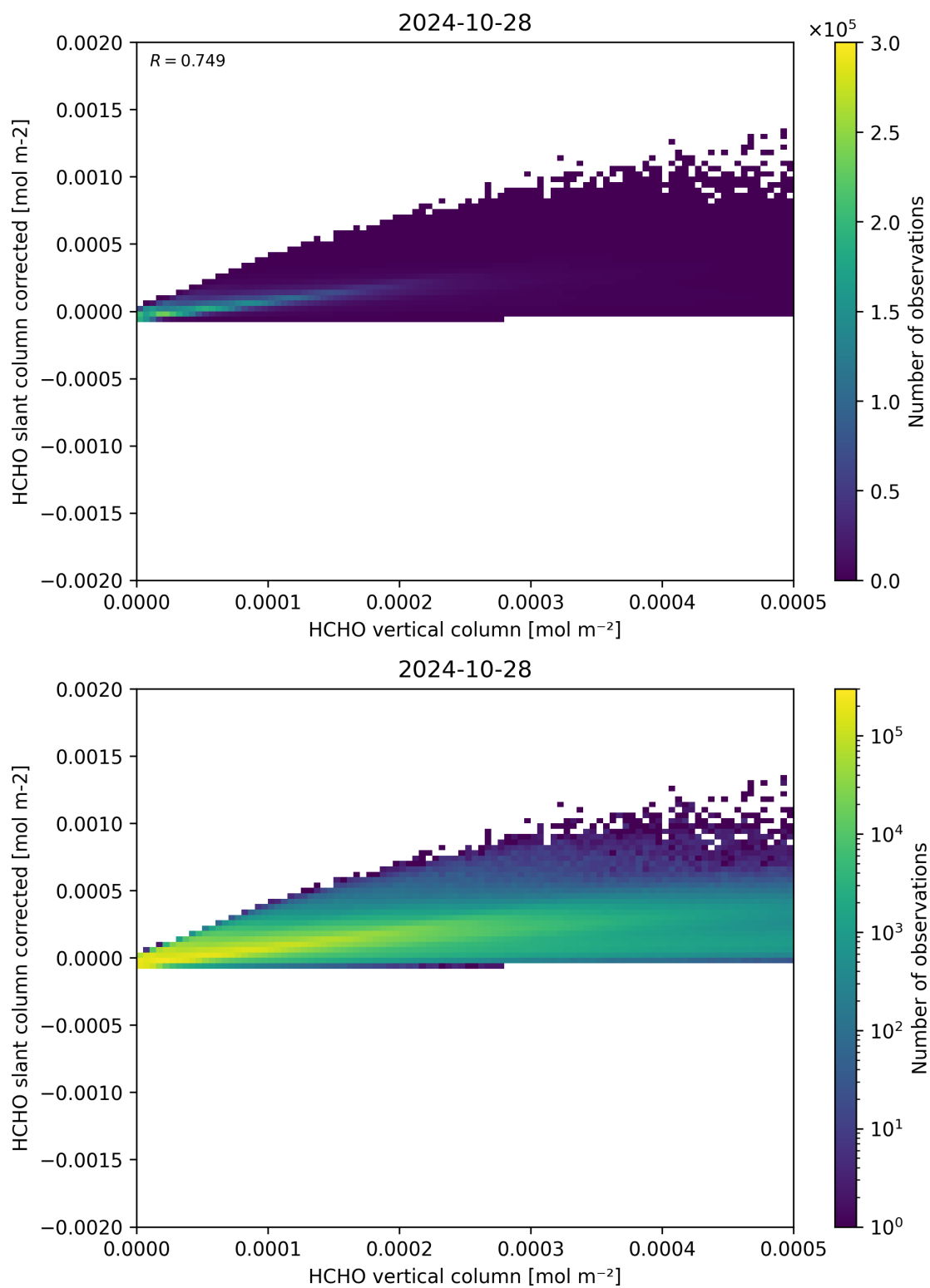
Figure 127: Scatter density plot of “HCHO vertical column” against “HCHO slant column corrected” for 2024-10-27 to 2024-10-29.
