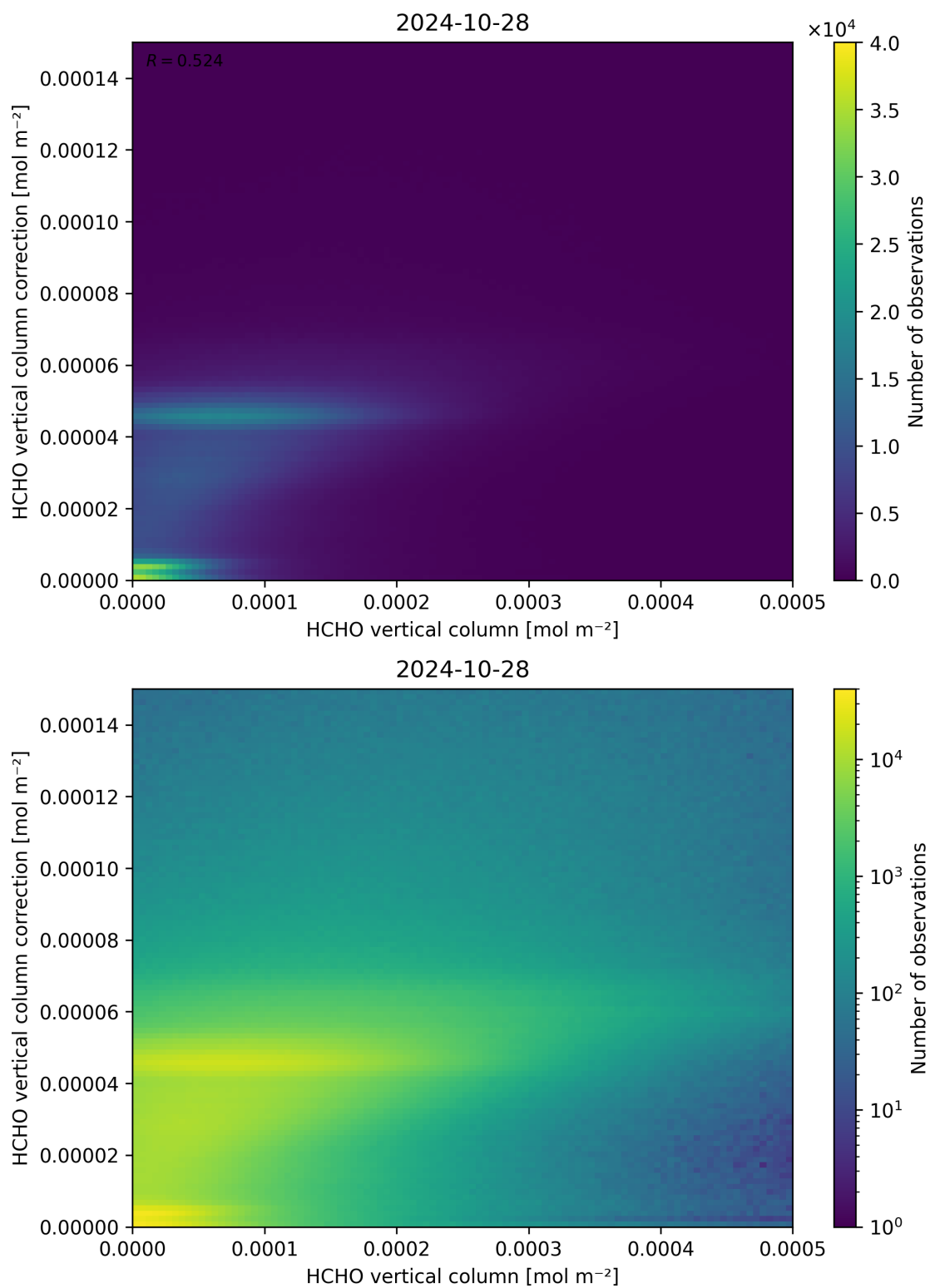
Figure 133: Scatter density plot of “HCHO vertical column” against “HCHO vertical column correction” for 2024-10-27 to 2024-10-29.
