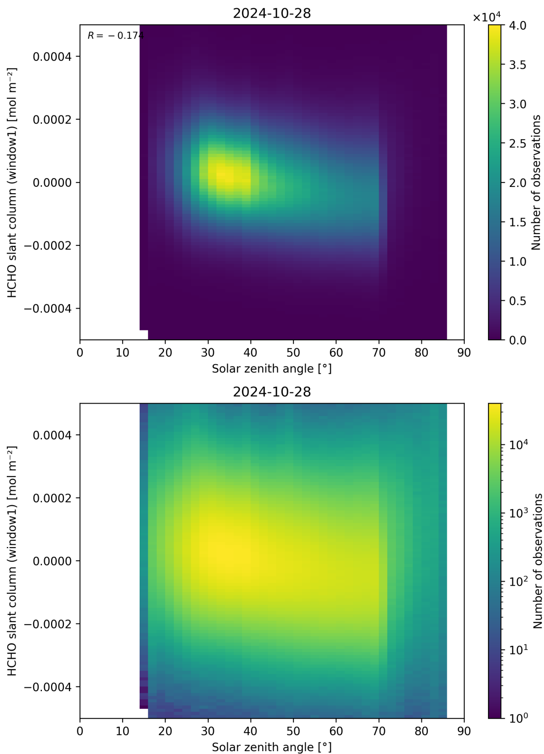
Figure 173: Scatter density plot of “Solar zenith angle” against “HCHO slant column (window1)” for 2024-10-27 to 2024-10-29.
