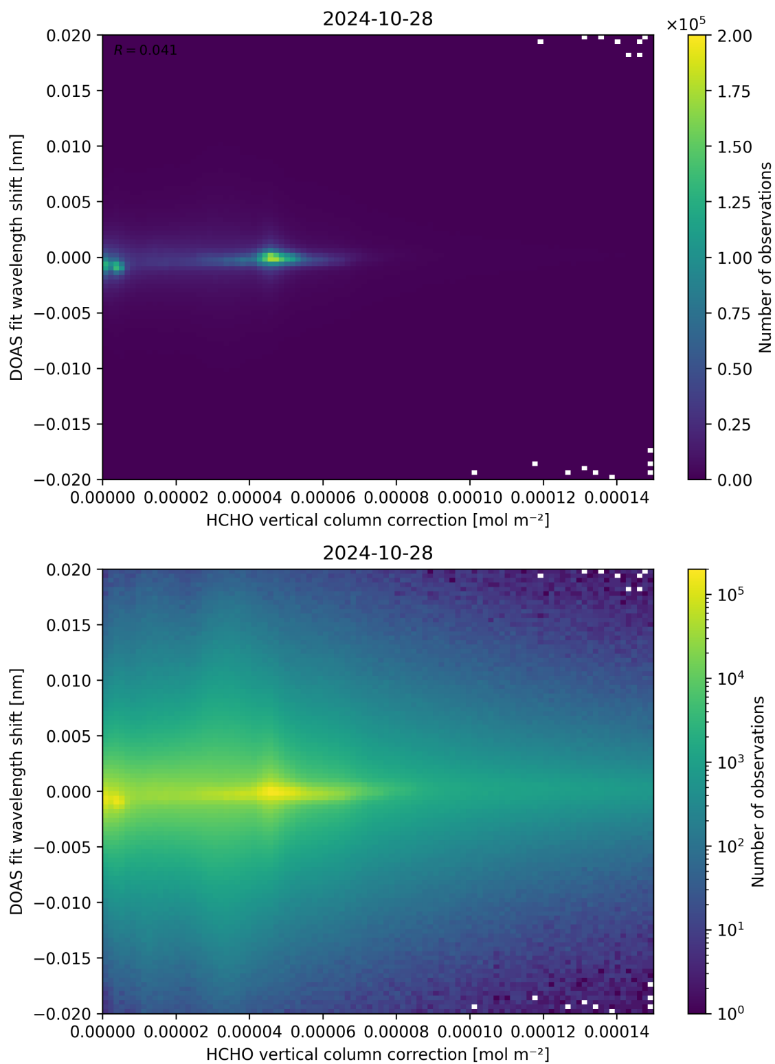
Figure 113: Scatter density plot of “HCHO vertical column correction” against “DOAS fit wavelength shift” for 2024-10-27 to 2024-10-29.
