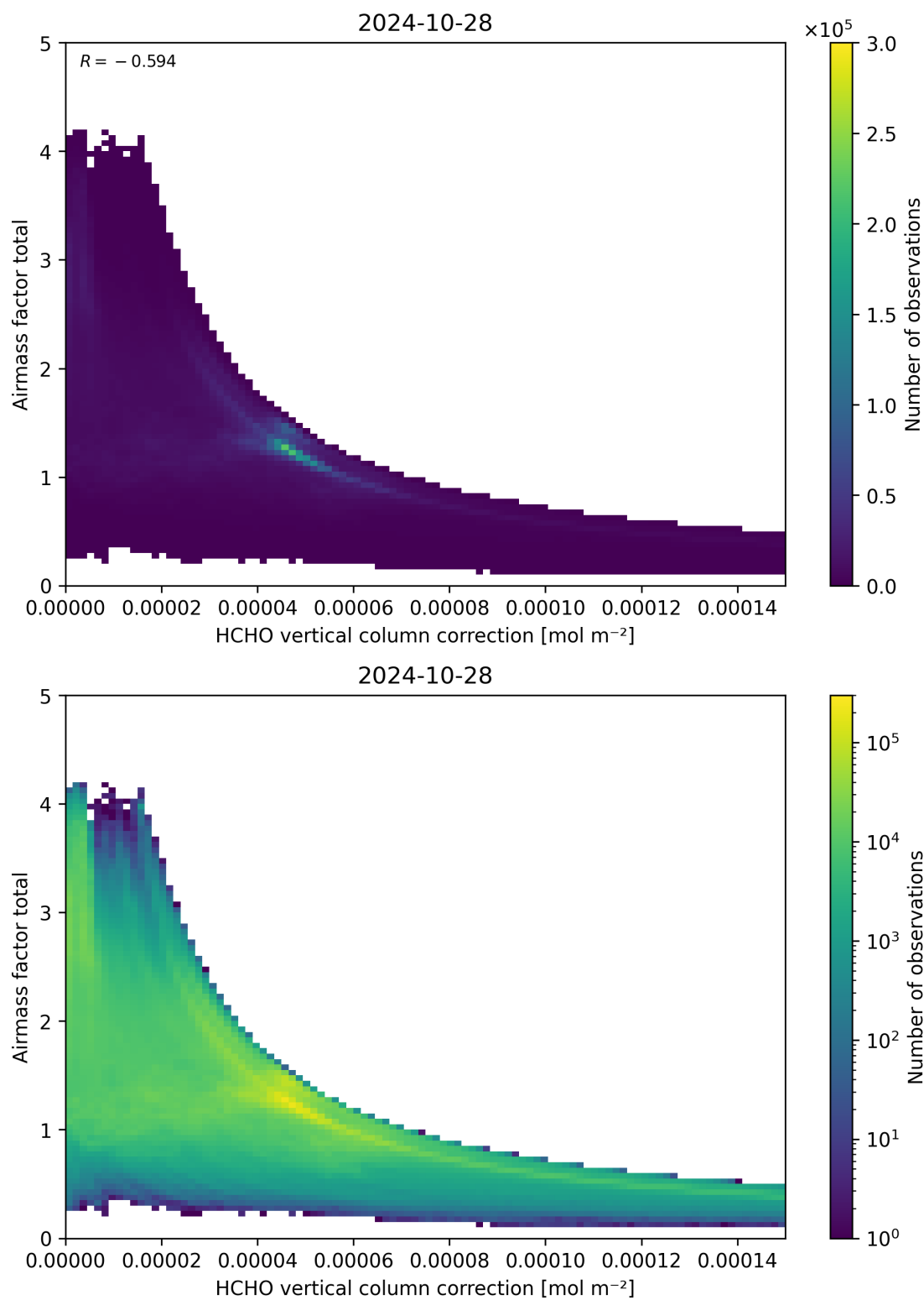
Figure 120: Scatter density plot of “HCHO vertical column correction” against “Airmass factor total” for 2024-10-27 to 2024-10-29.
