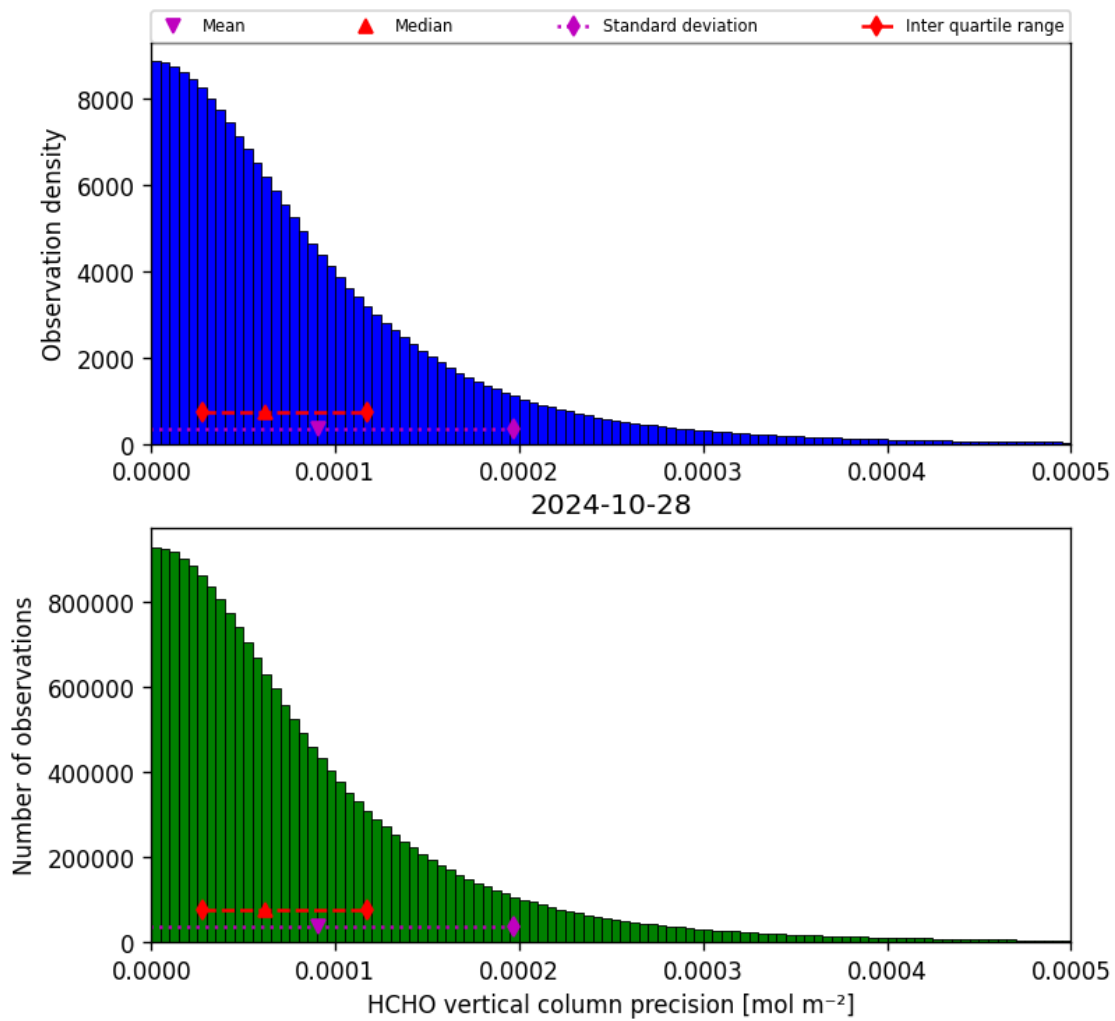
Figure 36: Histogram of “HCHO vertical column precision” for 2024-10-27 to 2024-10-29
