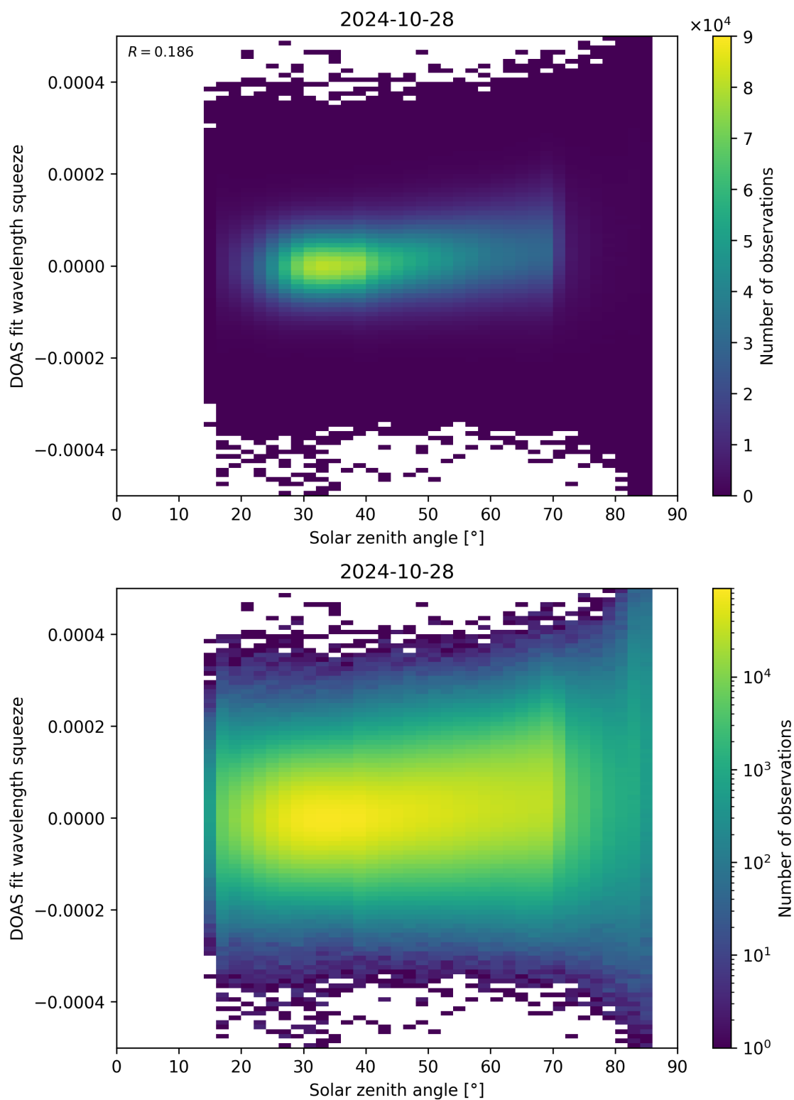
Figure 169: Scatter density plot of “Solar zenith angle” against “DOAS fit wavelength squeeze” for 2024-10-27 to 2024-10-29.
