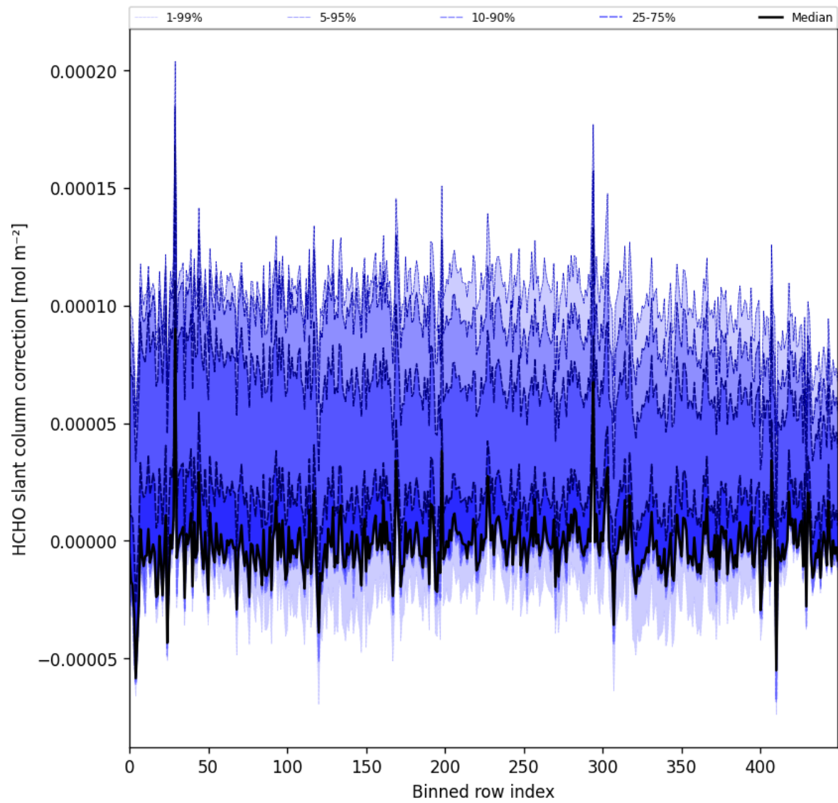
Figure 61: Along track statistics of “HCHO slant column correction” for 2024-10-27 to 2024-10-29
