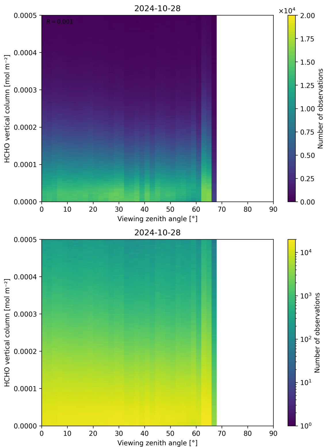
Figure 192: Scatter density plot of “Viewing zenith angle” against “HCHO vertical column” for 2024-10-27 to 2024-10-29.
