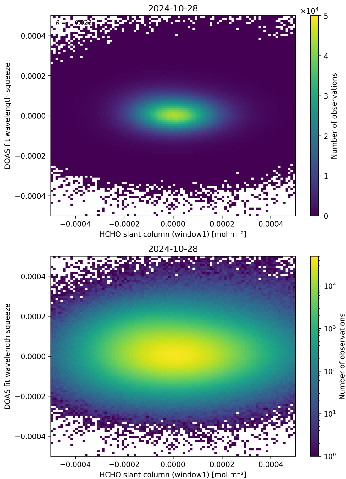
Figure 80: Scatter density plot of “HCHO slant column (window1)” against “DOAS fit wavelength squeeze” for 2024-10-27 to 2024-10-29.
