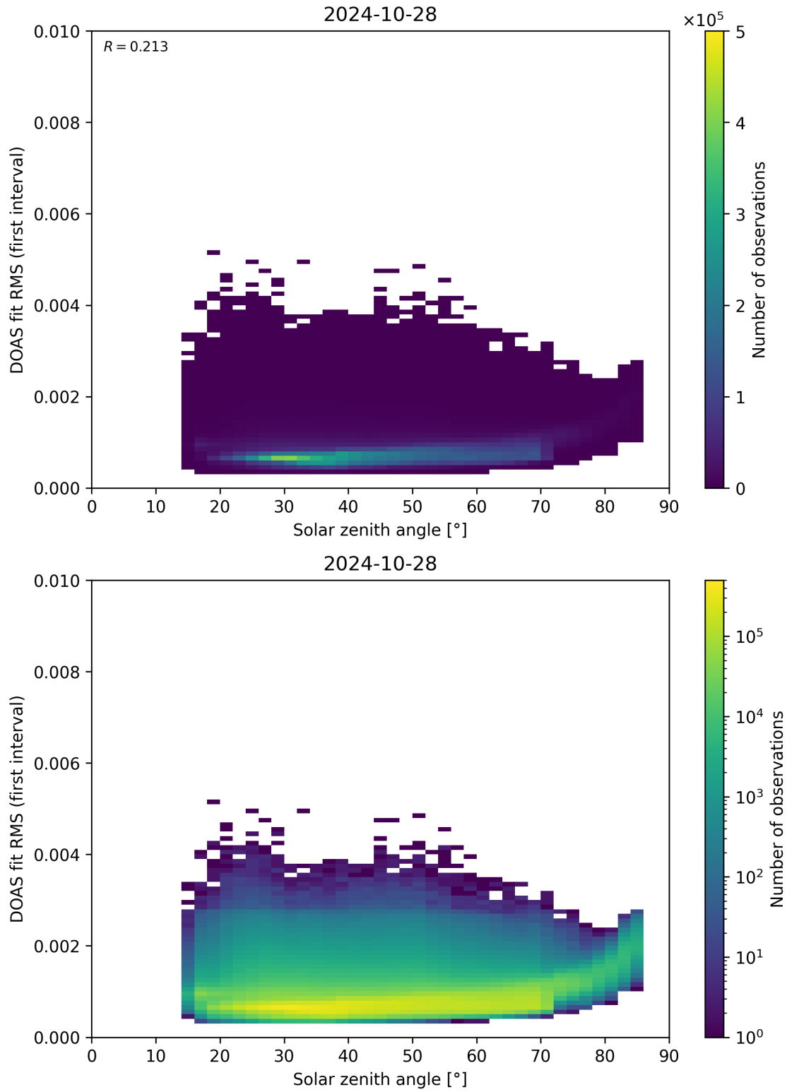
Figure 167: Scatter density plot of “Solar zenith angle” against “DOAS fit RMS (first interval)” for 2024-10-27 to 2024-10-29.
