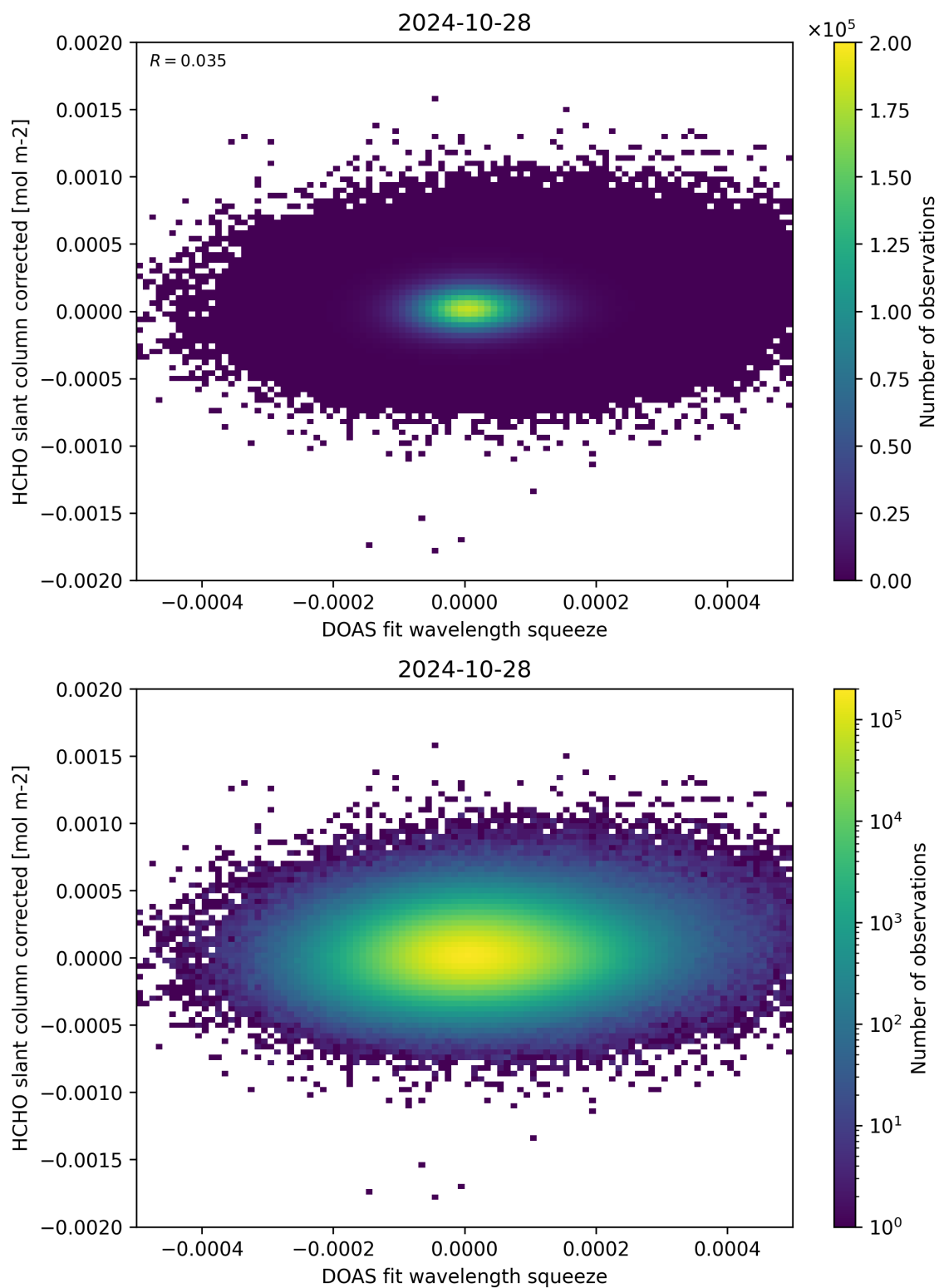
Figure 69: Scatter density plot of “DOAS fit wavelength squeeze” against “HCHO slant column corrected” for 2024-10-27 to 2024-10-29.
