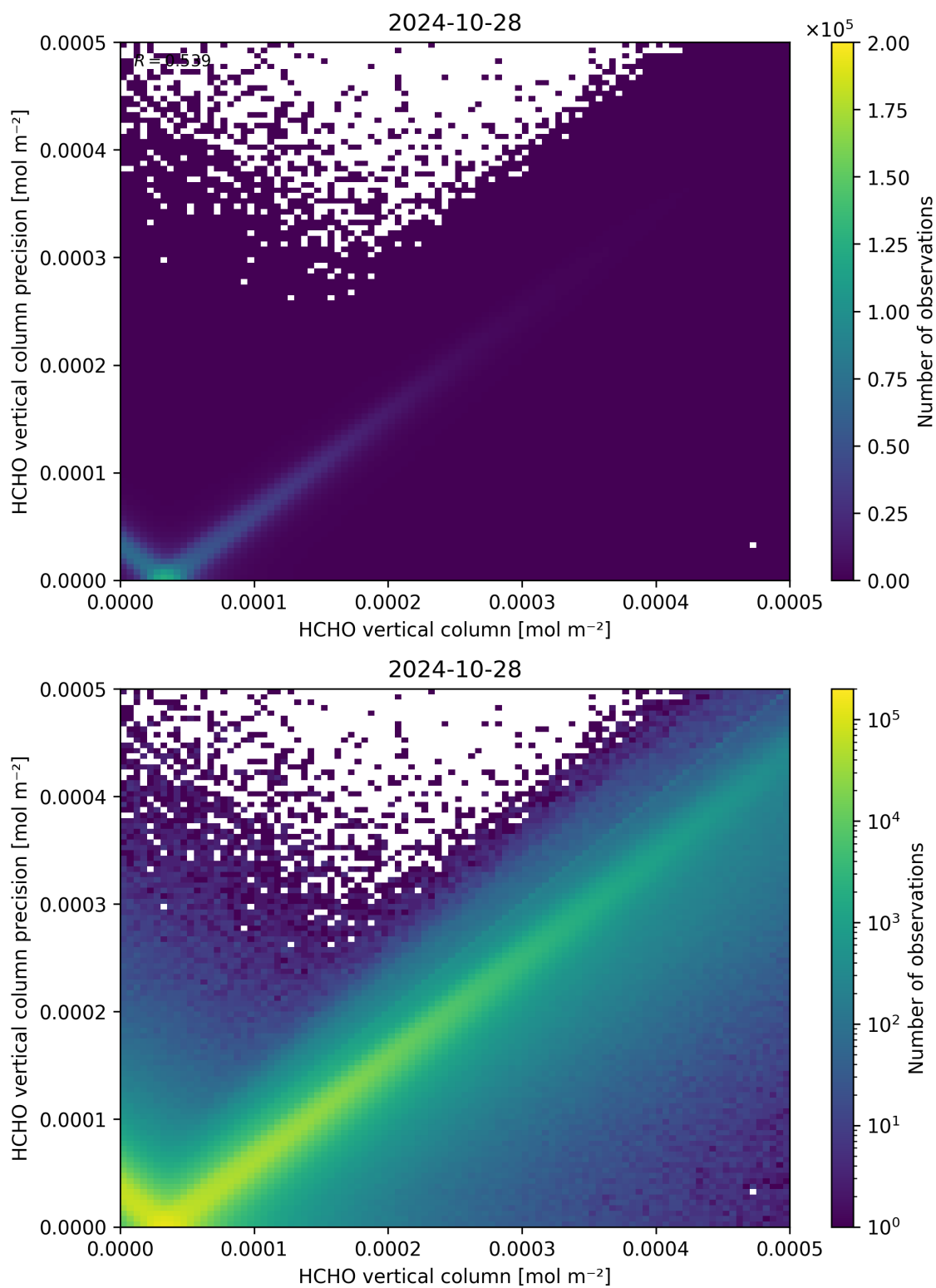
Figure 134: Scatter density plot of “HCHO vertical column” against “HCHO vertical column precision” for 2024-10-27 to 2024-10-29.
