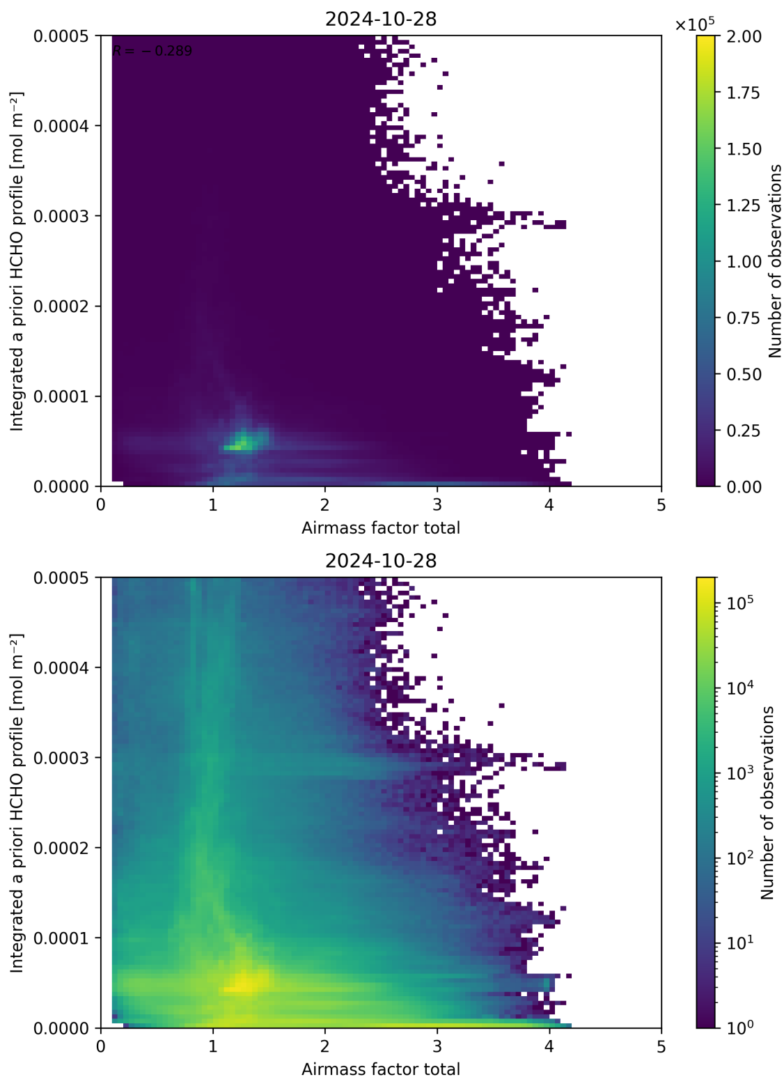
Figure 104: Scatter density plot of “Airmass factor total” against “Integrated a priori HCHO profile” for 2024-10-27 to 2024-10-29.
