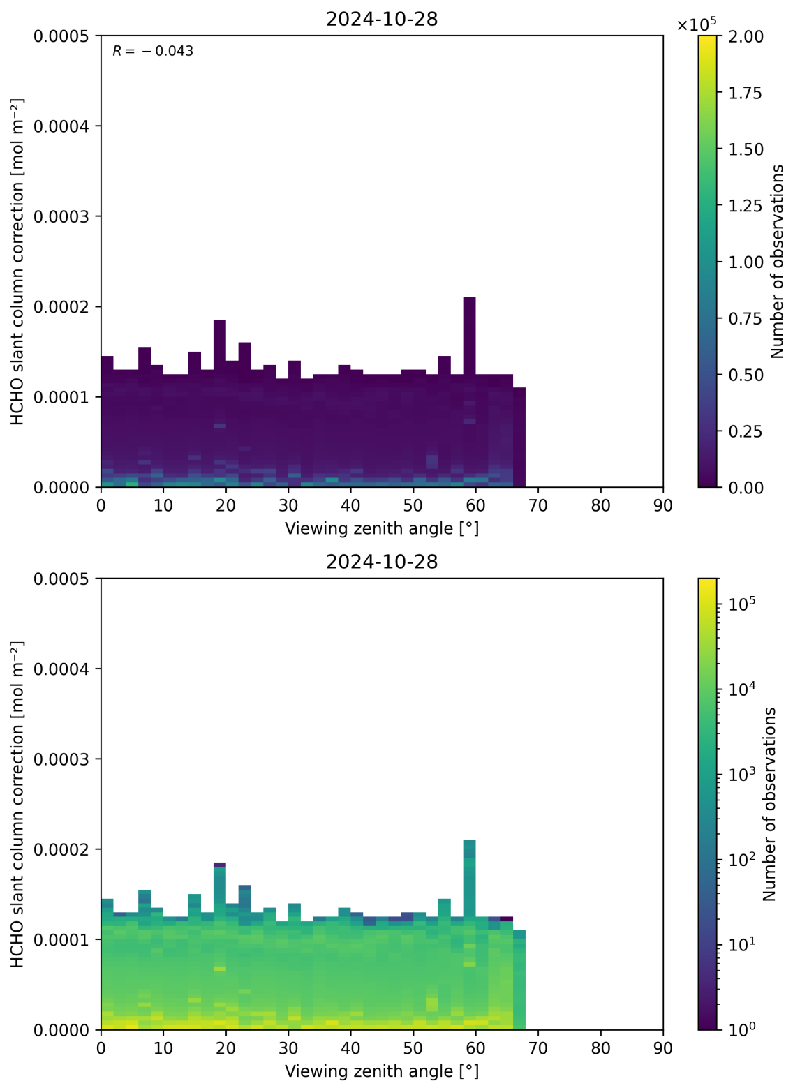
Figure 187: Scatter density plot of “Viewing zenith angle” against “HCHO slant column correction” for 2024-10-27 to 2024-10-29.
