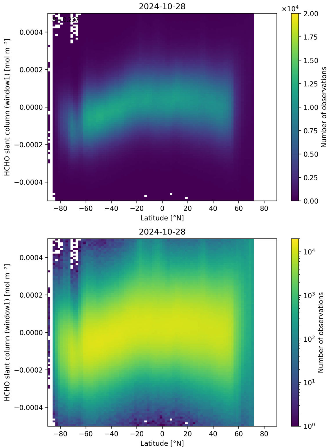
Figure 159: Scatter density plot of “Latitude” against “HCHO slant column (window1)” for 2024-10-27 to 2024-10-29.
