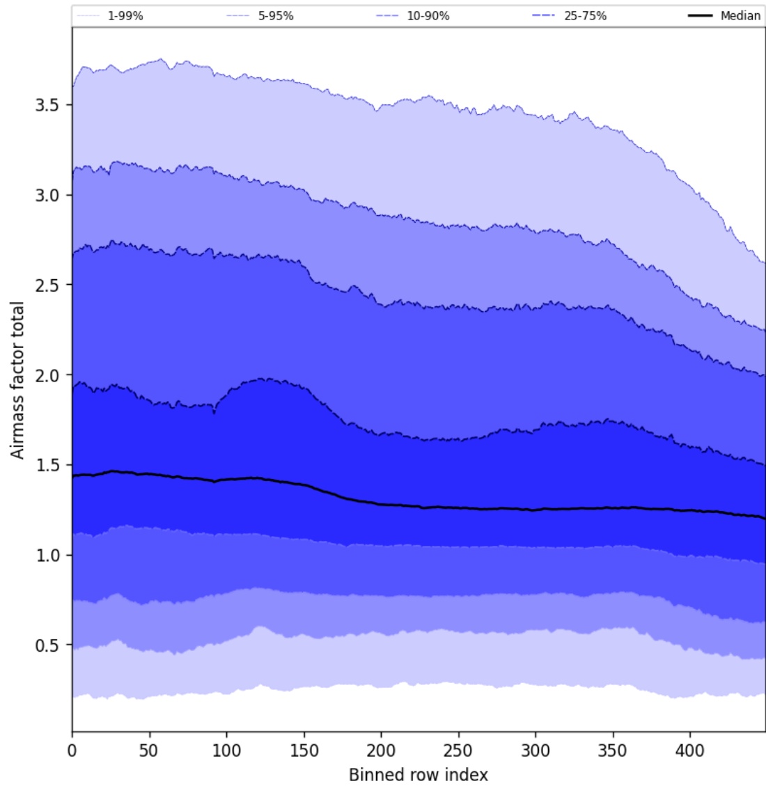
Figure 54: Along track statistics of “Airmass factor total” for 2024-10-27 to 2024-10-29
