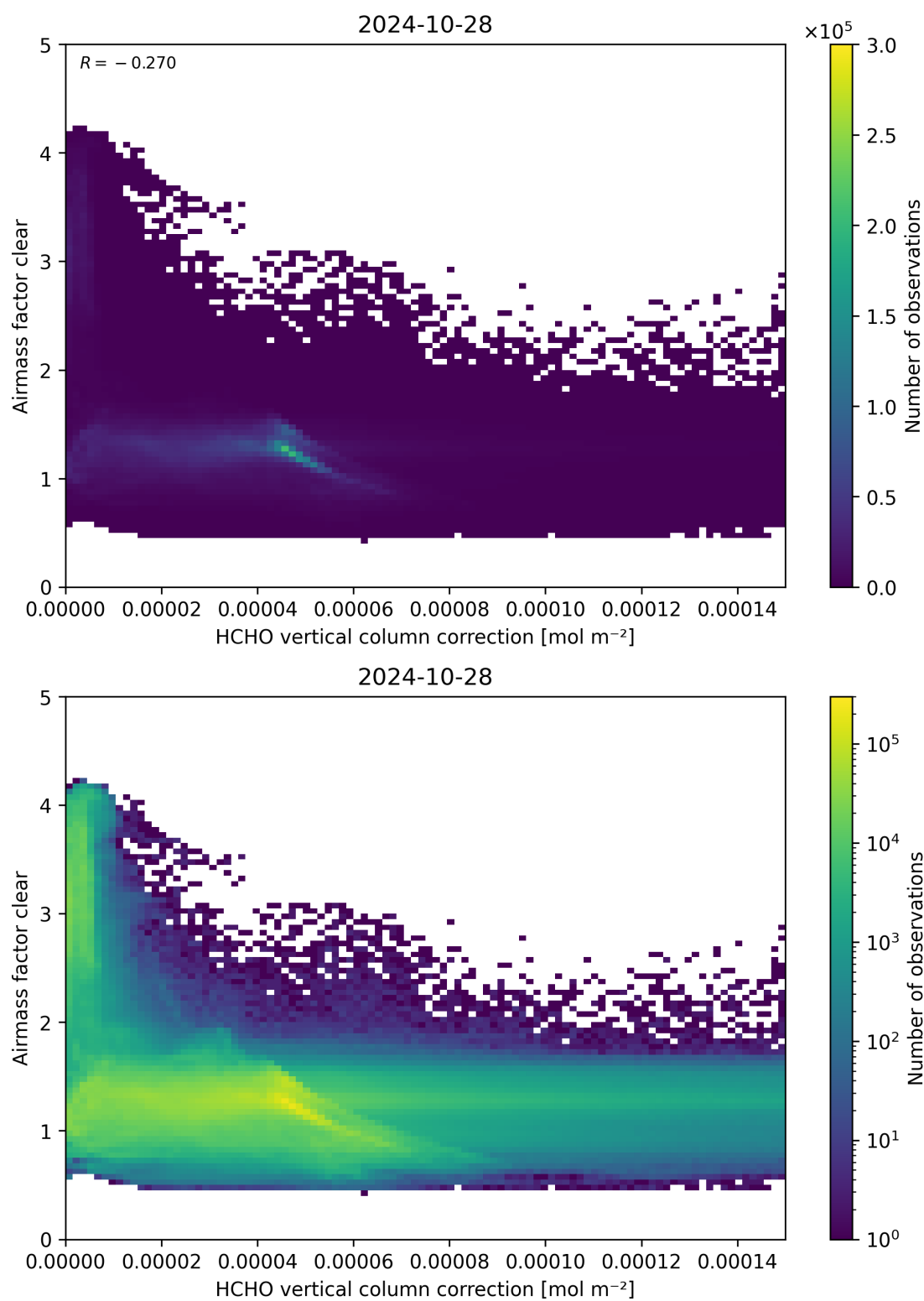
Figure 115: Scatter density plot of “HCHO vertical column correction” against “Airmass factor clear” for 2024-10-27 to 2024-10-29.
