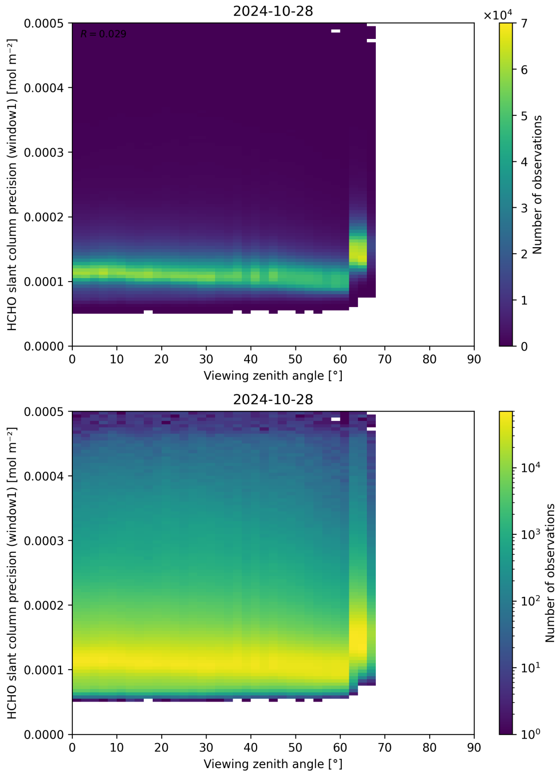
Figure 189: Scatter density plot of “Viewing zenith angle” against “HCHO slant column precision (window1)” for 2024-10-27 to 2024-10-29.
