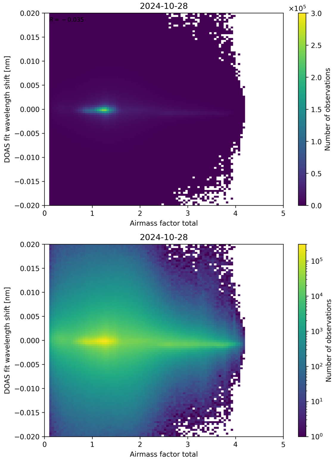
Figure 98: Scatter density plot of “Airmass factor total” against “DOAS fit wavelength shift” for 2024-10-27 to 2024-10-29.
