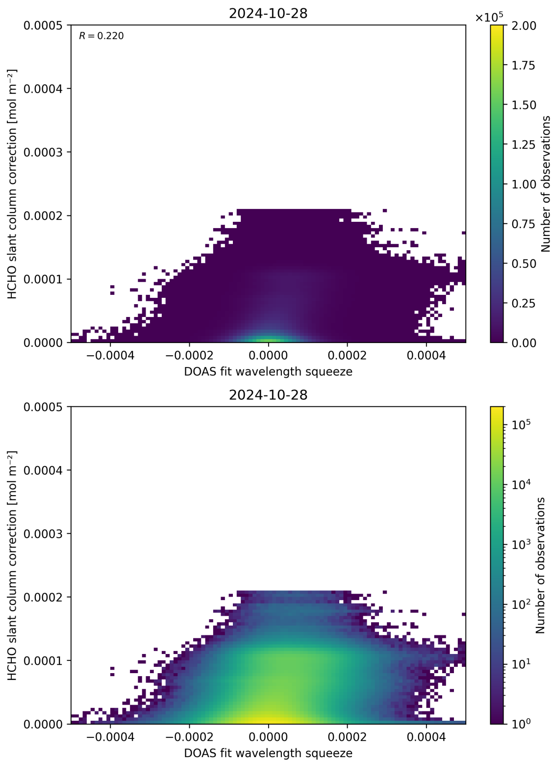
Figure 70: Scatter density plot of “DOAS fit wavelength squeeze” against “HCHO slant column correction” for 2024-10-27 to 2024-10-29.
