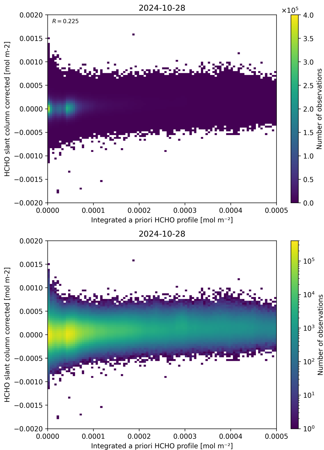
Figure 151: Scatter density plot of “Integrated a priori HCHO profile” against “HCHO slant column corrected” for 2024-10-27 to 2024-10-29.
