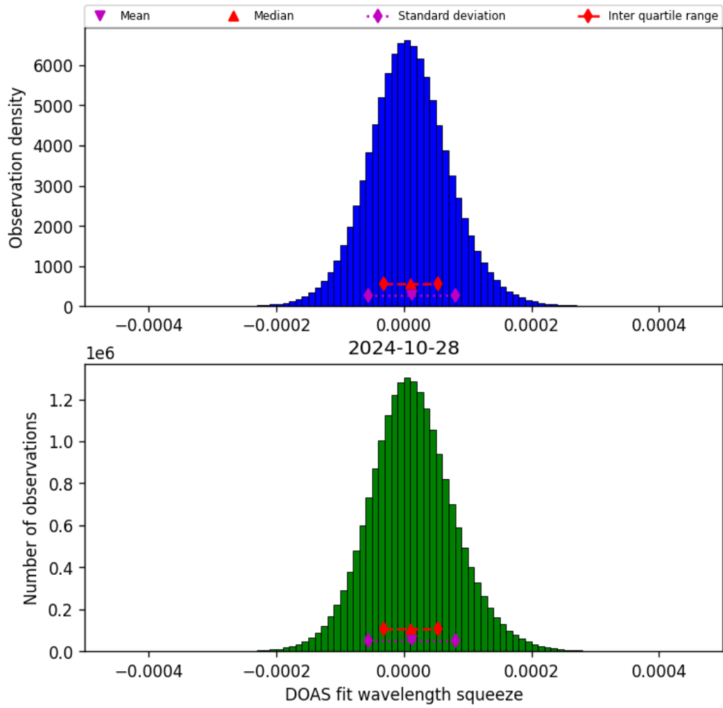
Figure 45: Histogram of “DOAS fit wavelength squeeze” for 2024-10-27 to 2024-10-29
