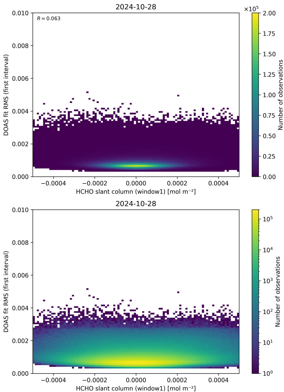
Figure 78: Scatter density plot of “HCHO slant column (window1)” against “DOAS fit RMS (first interval)” for 2024-10-27 to 2024-10-29.
