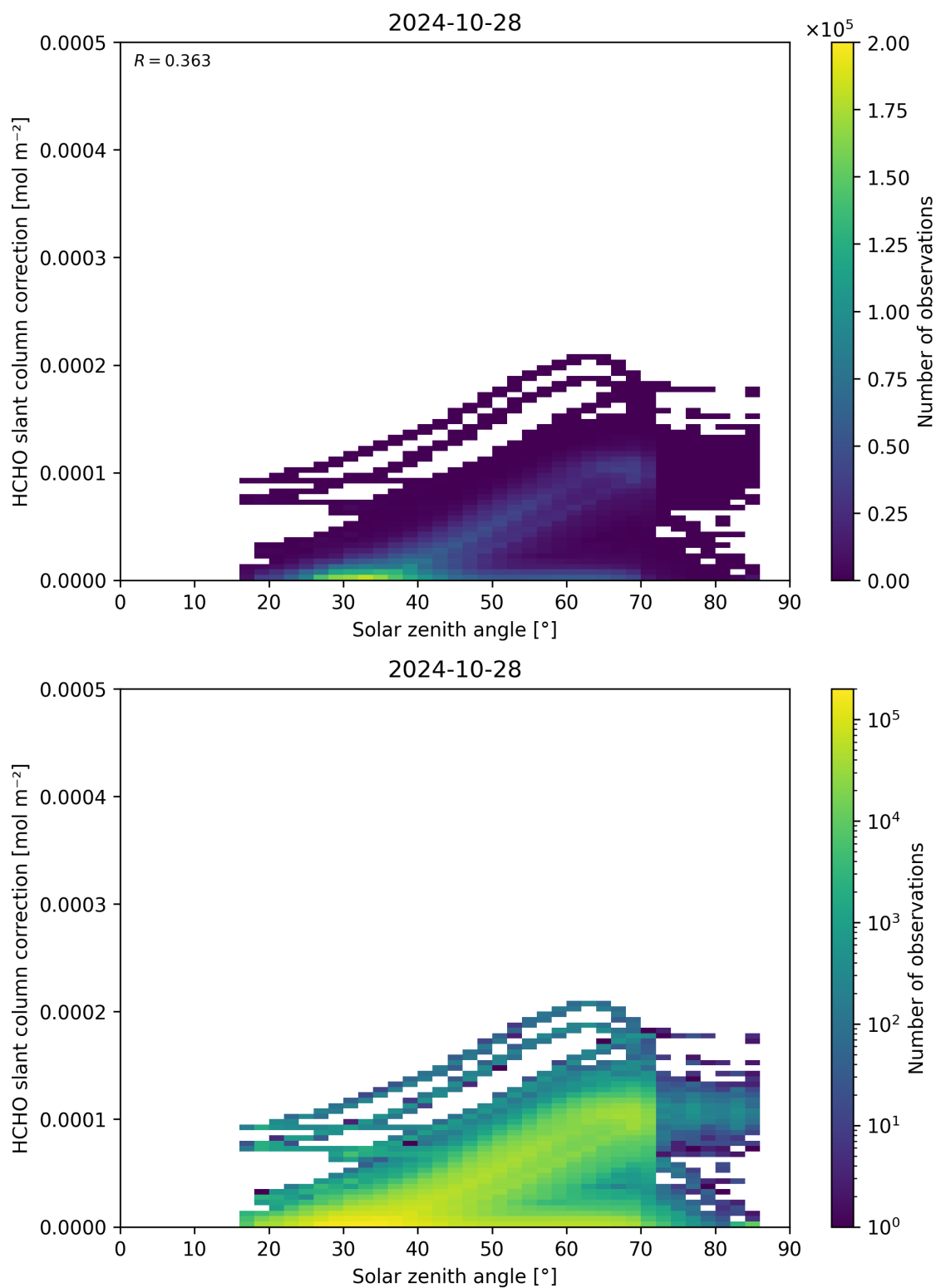
Figure 172: Scatter density plot of “Solar zenith angle” against “HCHO slant column correction” for 2024-10-27 to 2024-10-29.
