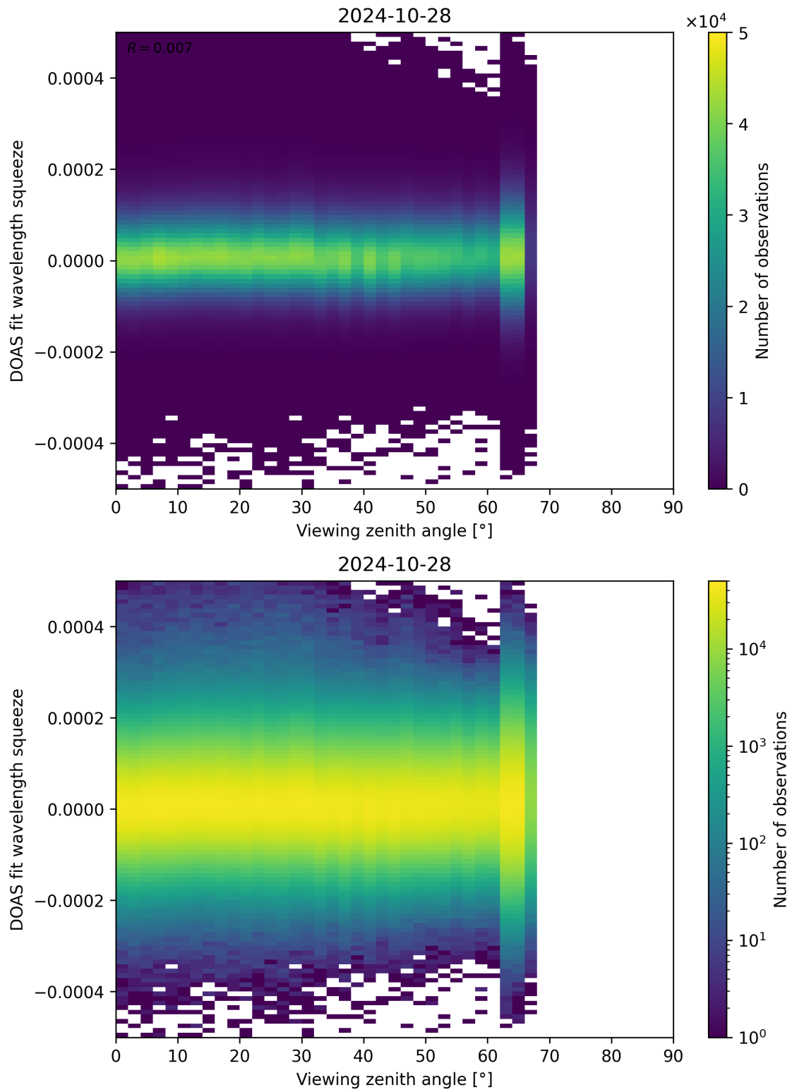
Figure 184: Scatter density plot of “Viewing zenith angle” against “DOAS fit wavelength squeeze” for 2024-10-27 to 2024-10-29.
