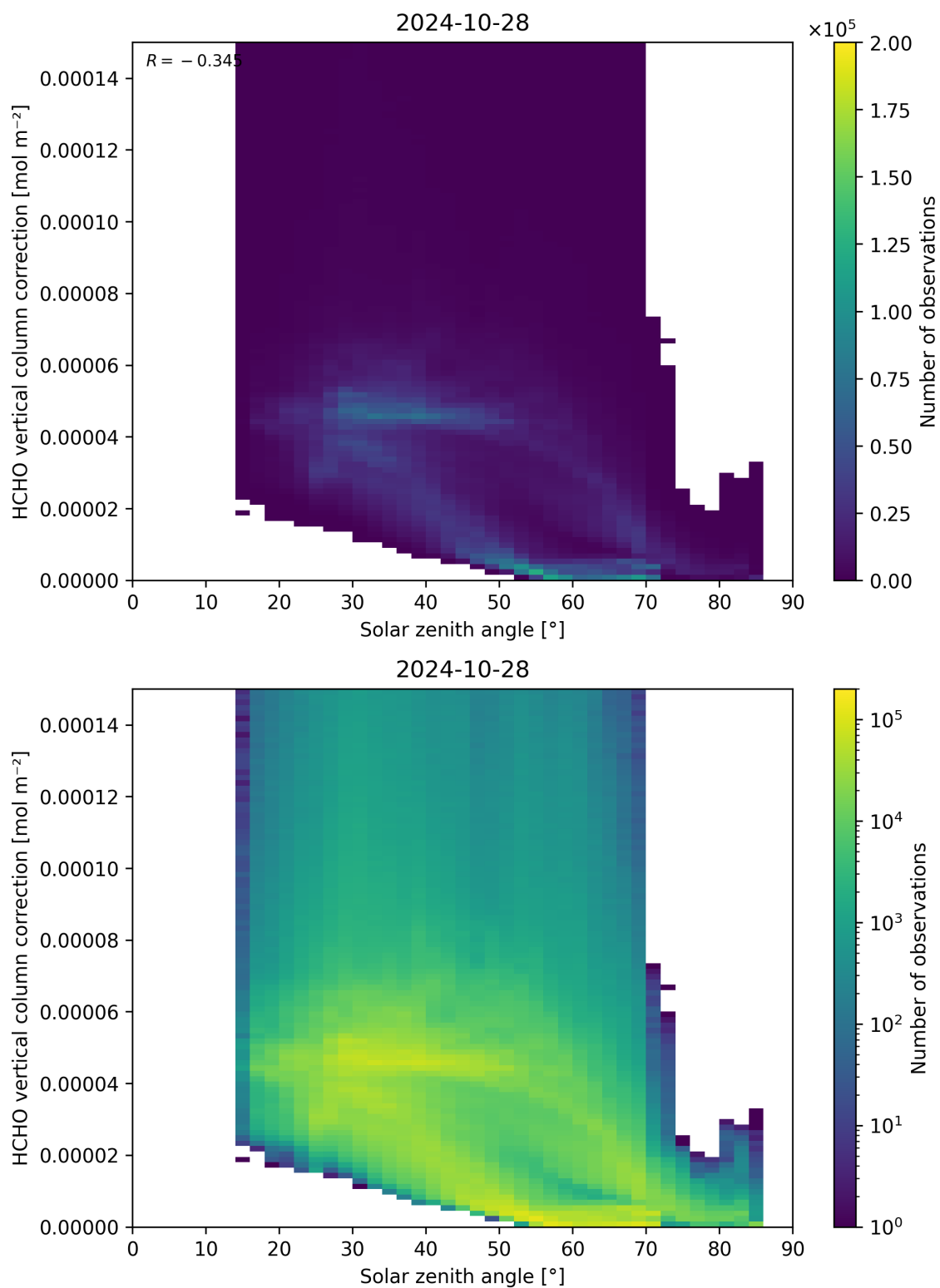
Figure 178: Scatter density plot of “Solar zenith angle” against “HCHO vertical column correction” for 2024-10-27 to 2024-10-29.
