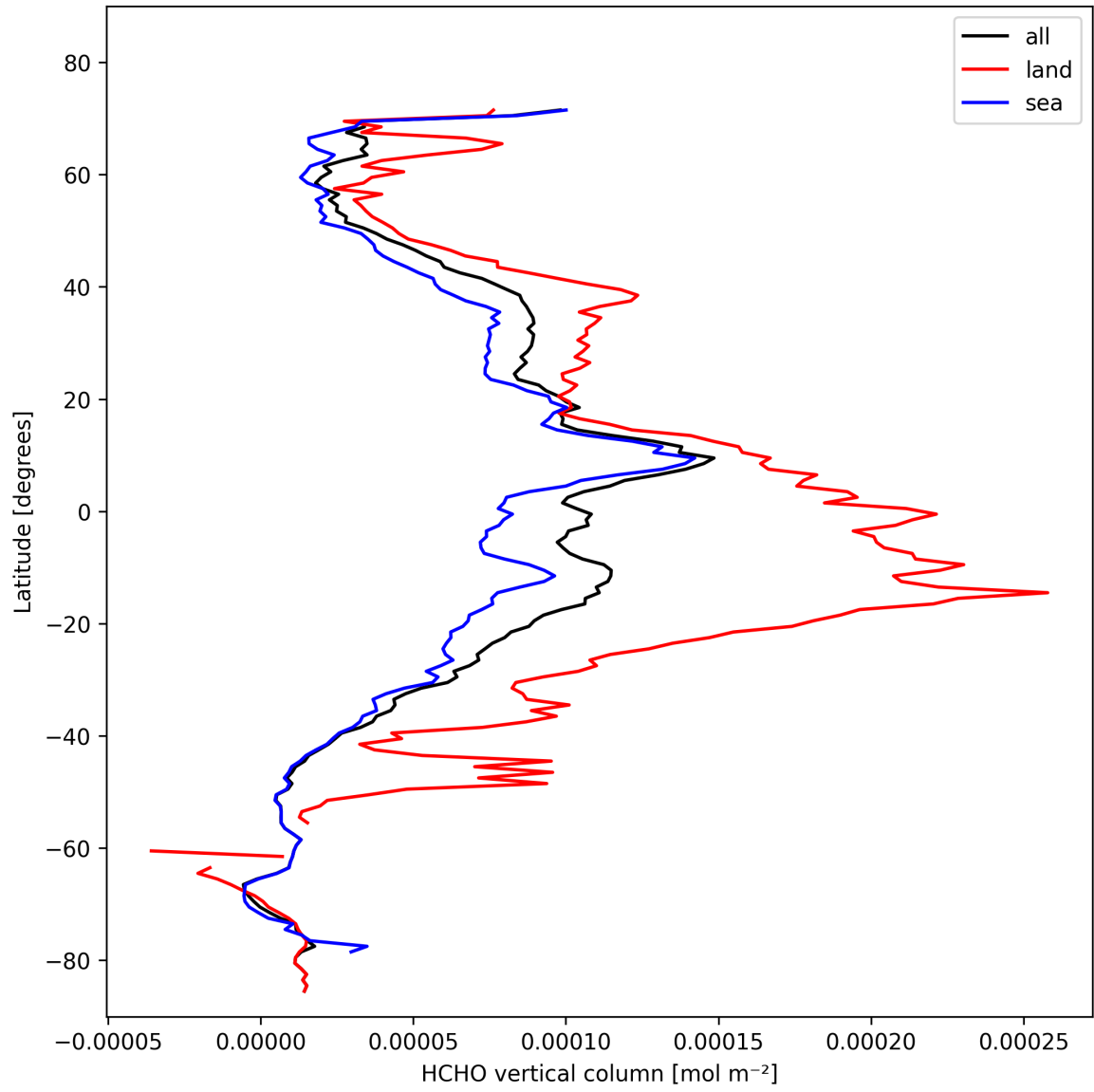
Figure 21: Zonal average of “HCHO vertical column” for 2024-10-27 to 2024-10-29.
