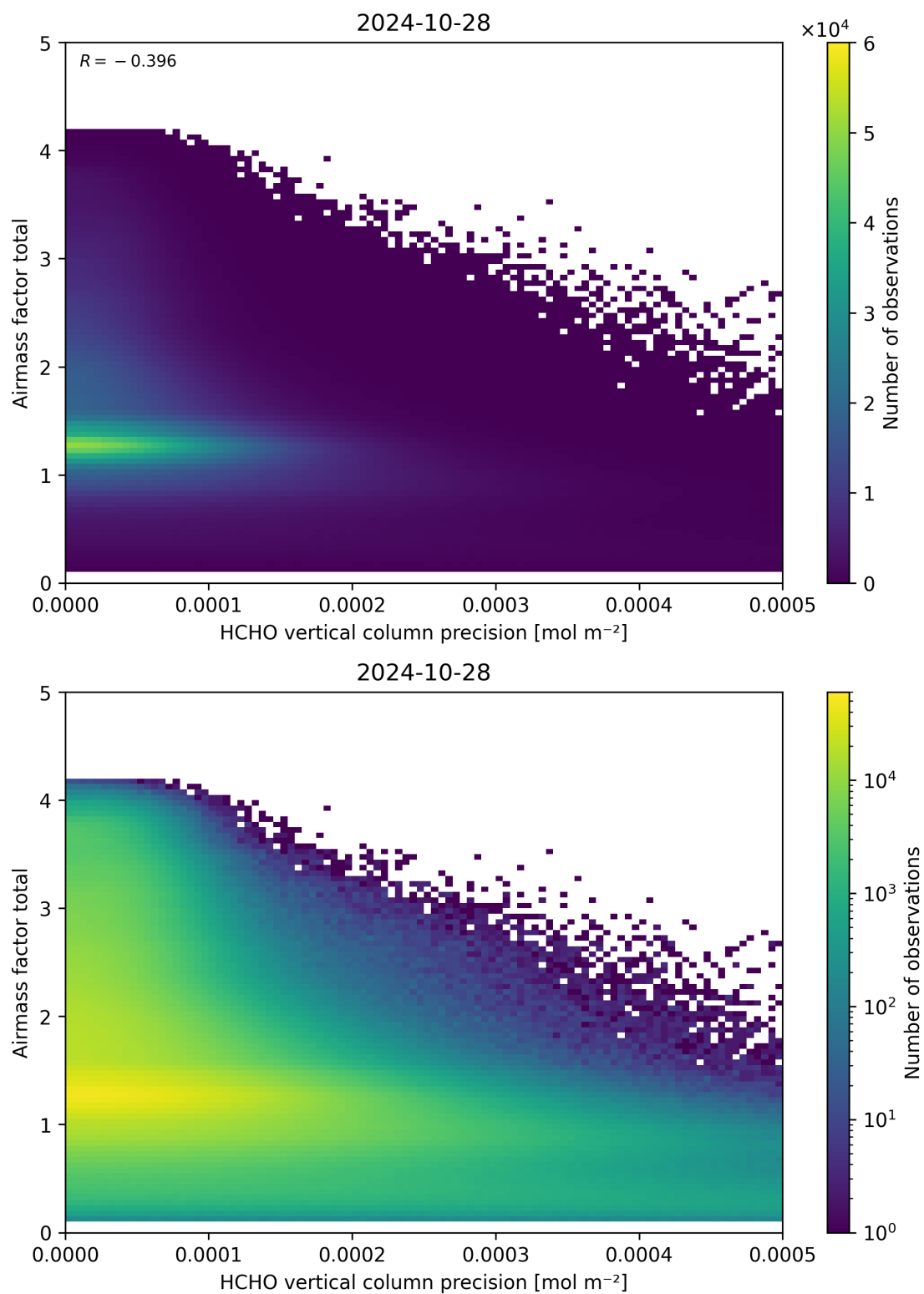
Figure 144: Scatter density plot of “HCHO vertical column precision” against “Airmass factor total” for 2024-10-27 to 2024-10-29.
