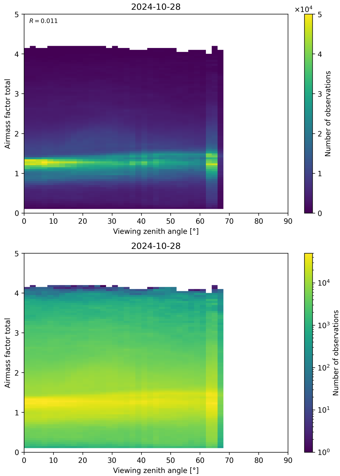
Figure 190: Scatter density plot of “Viewing zenith angle” against “Airmass factor total” for 2024-10-27 to 2024-10-29.
