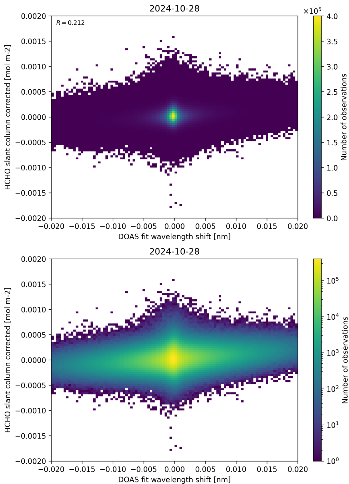
Figure 66: Scatter density plot of “DOAS fit wavelength shift” against “HCHO slant column corrected” for 2024-10-27 to 2024-10-29.
