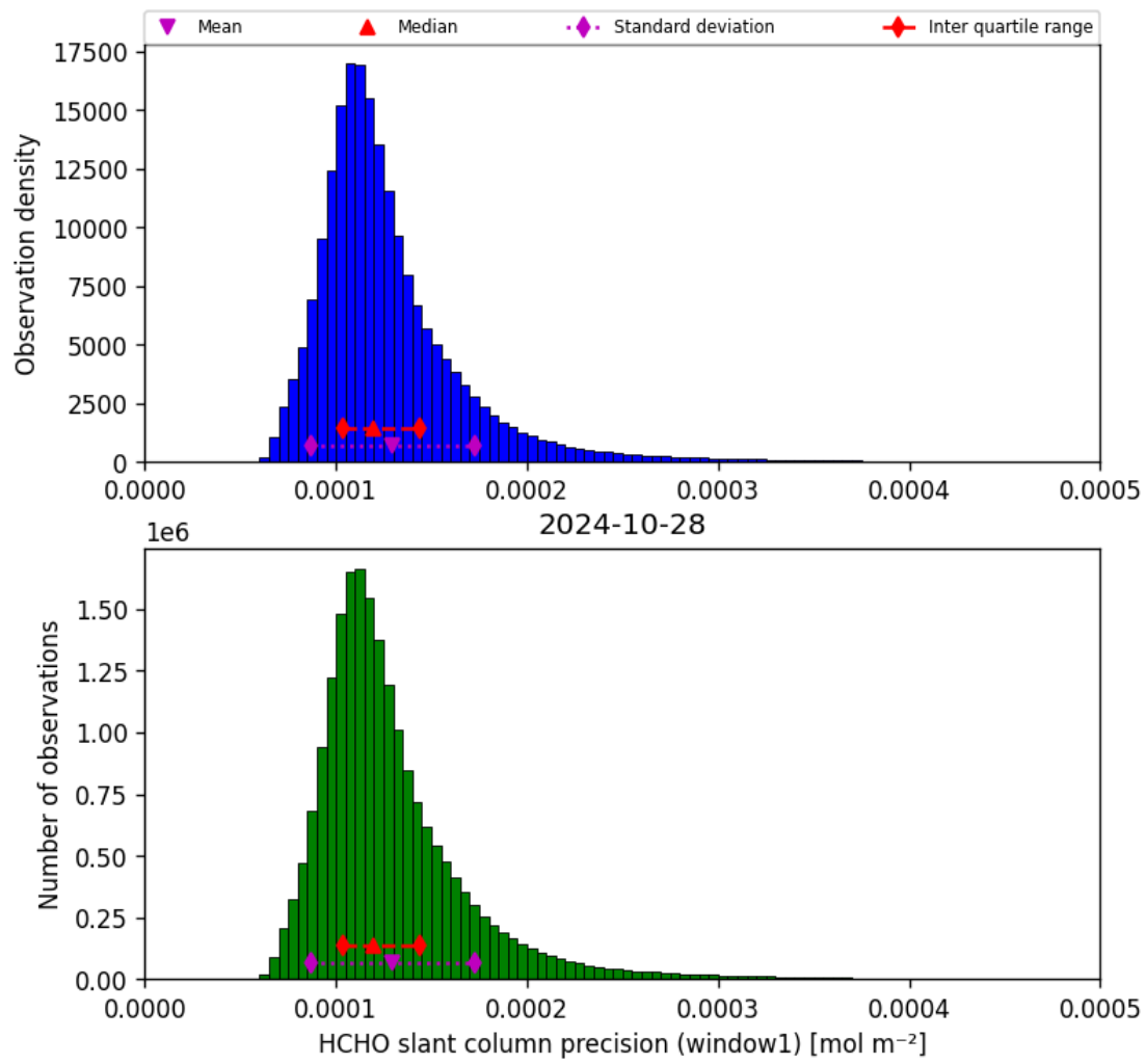
Figure 39: Histogram of “HCHO slant column precision (window1)” for 2024-10-27 to 2024-10-29
