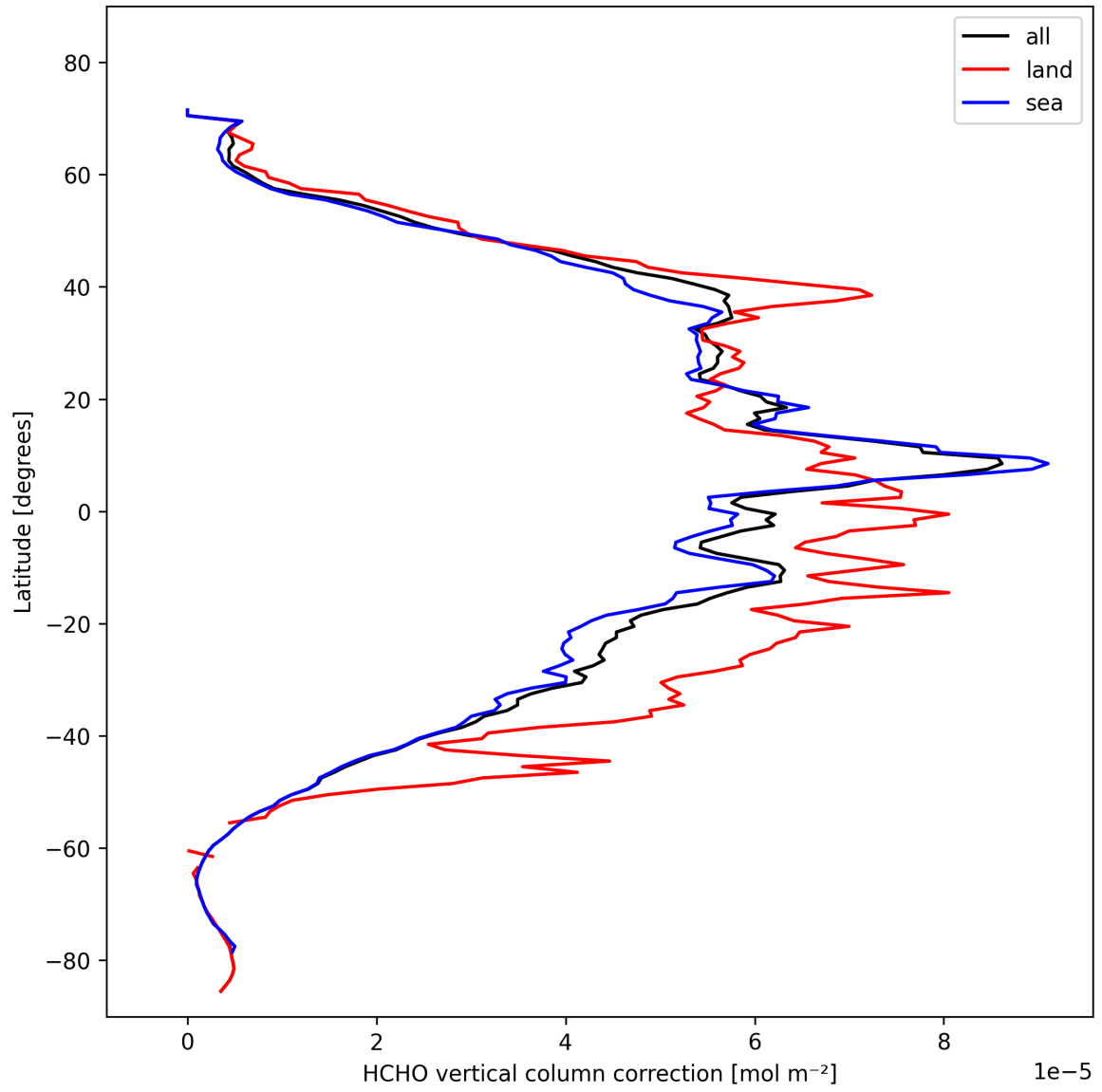
Figure 23: Zonal average of “HCHO vertical column correction” for 2024-10-27 to 2024-10-29.
