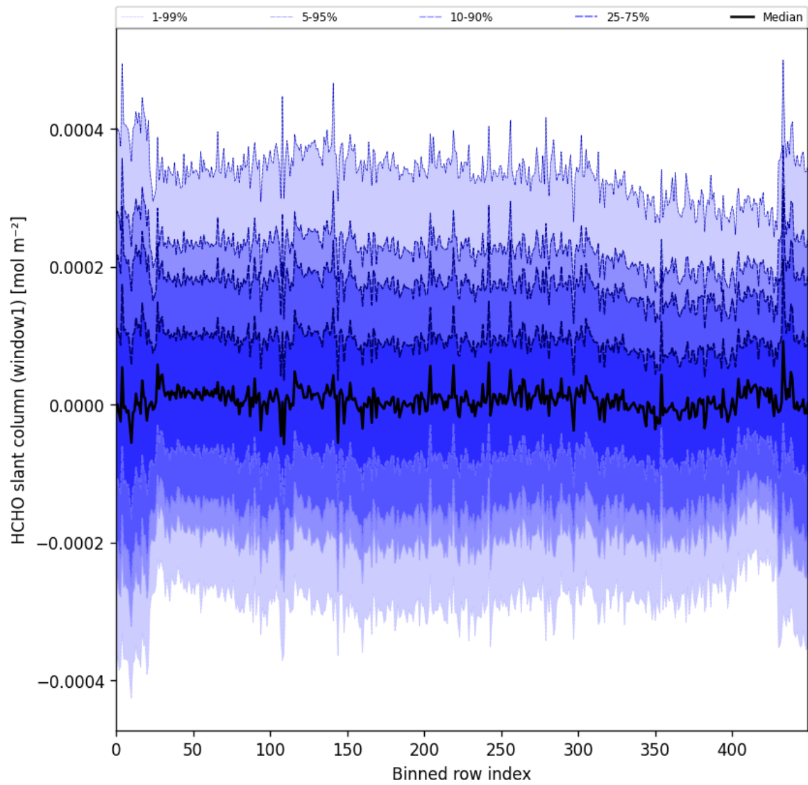
Figure 52: Along track statistics of “HCHO slant column (window1)” for 2024-10-27 to 2024-10-29
