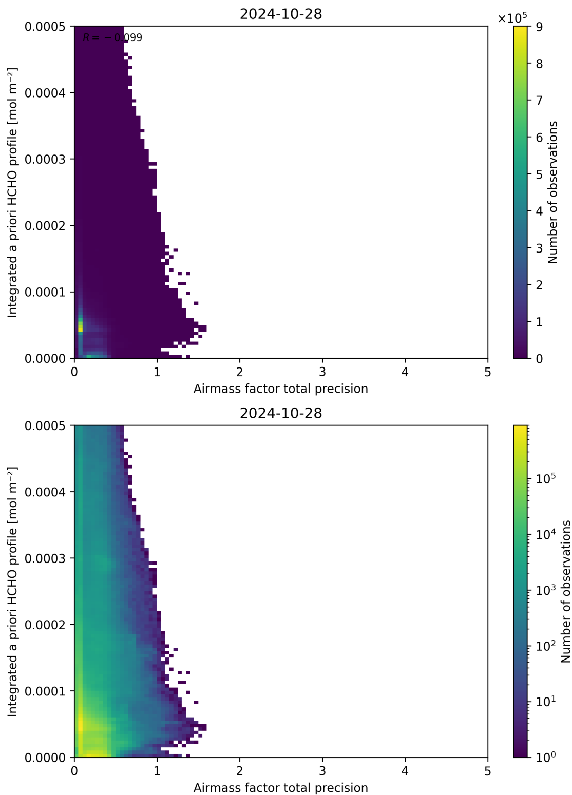
Figure 111: Scatter density plot of “Airmass factor total precision” against “Integrated a priori HCHO profile” for 2024-10-27 to 2024-10-29.
