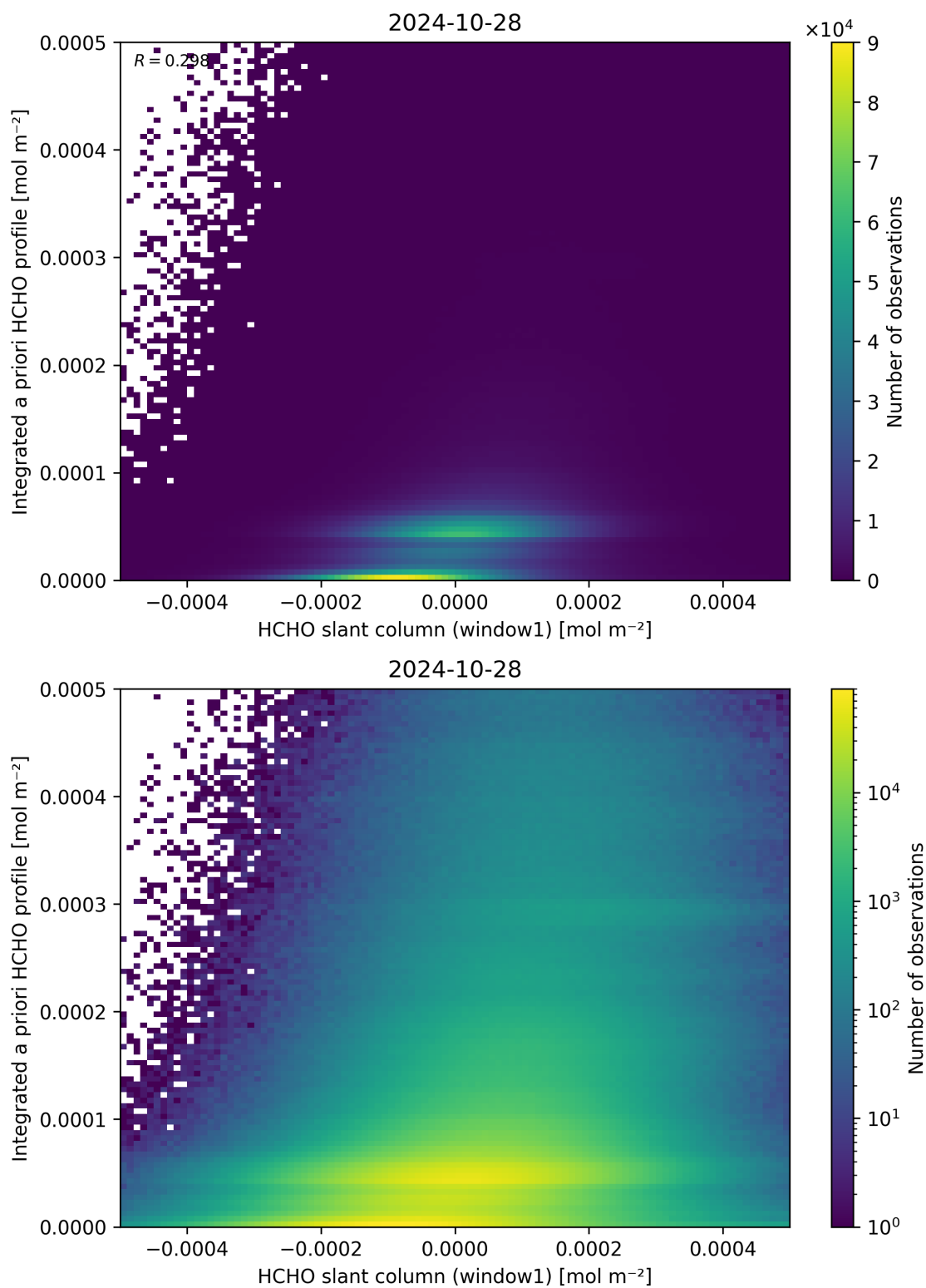
Figure 87: Scatter density plot of “HCHO slant column (window1)” against “Integrated a priori HCHO profile” for 2024-10-27 to 2024-10-29.
