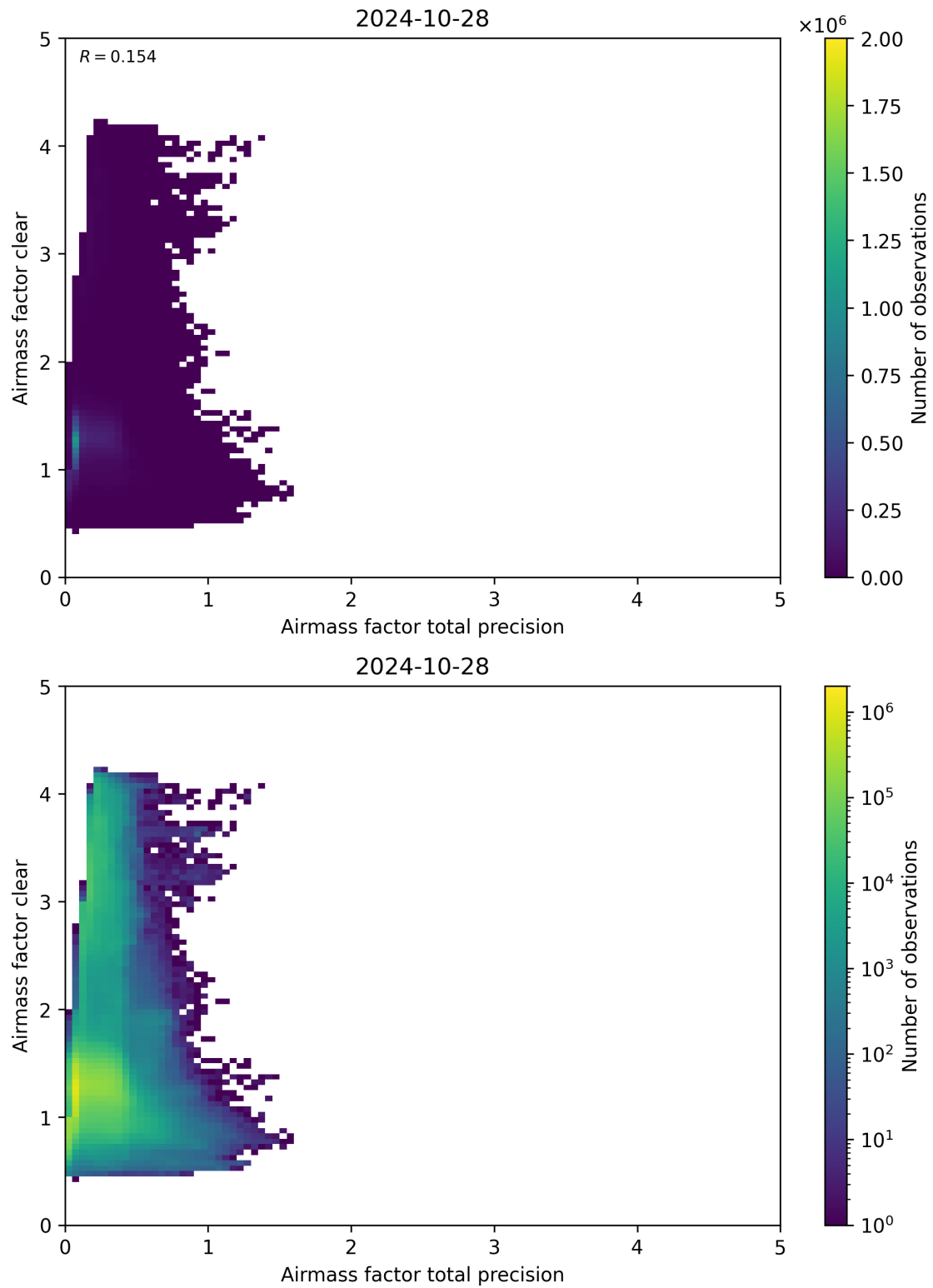
Figure 108: Scatter density plot of “Airmass factor total precision” against “Airmass factor clear” for 2024-10-27 to 2024-10-29.
