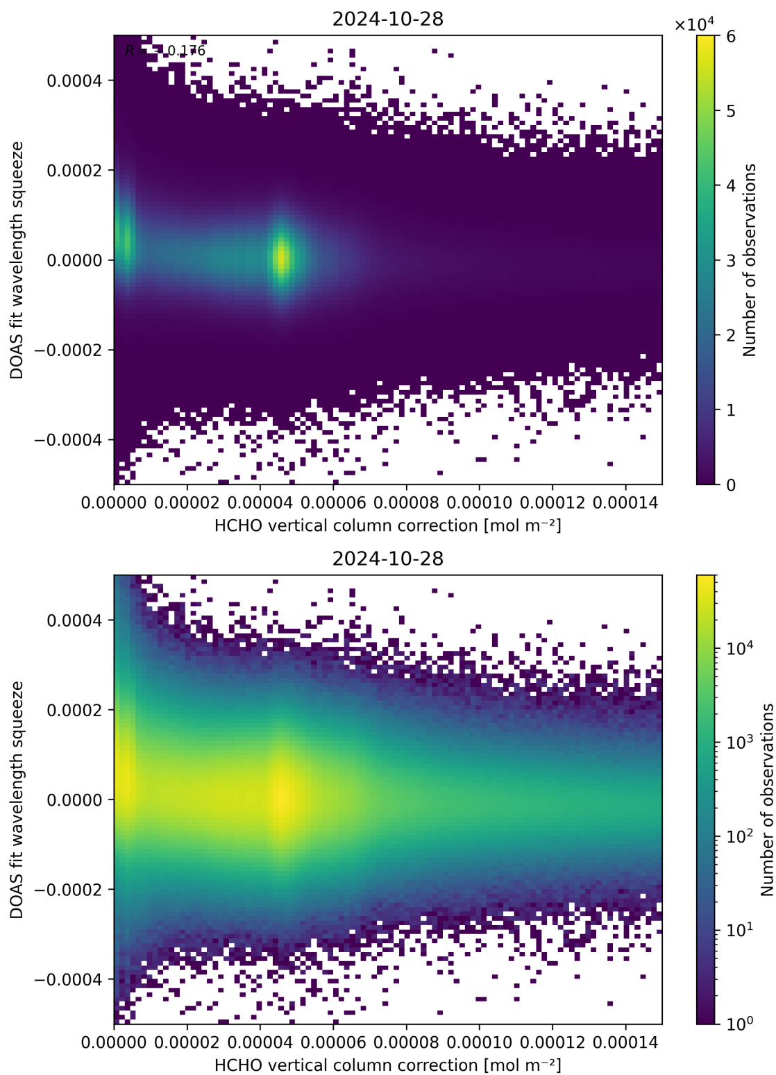
Figure 114: Scatter density plot of “HCHO vertical column correction” against “DOAS fit wavelength squeeze” for 2024-10-27 to 2024-10-29.
