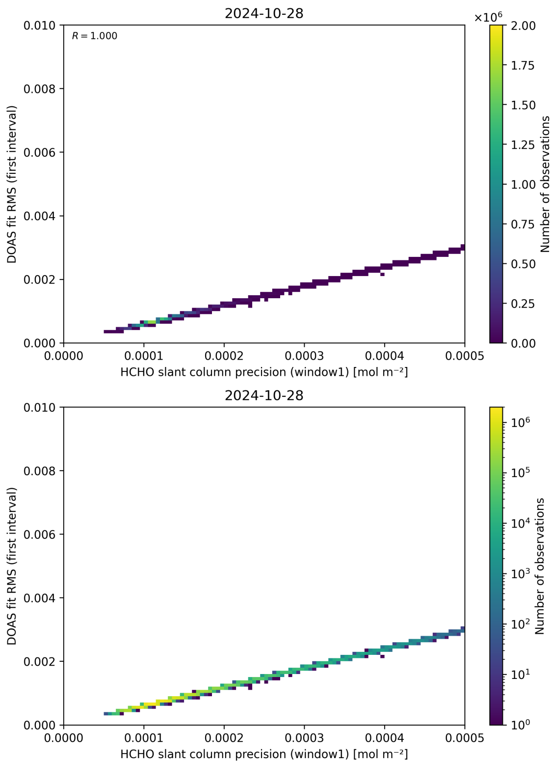
Figure 88: Scatter density plot of “HCHO slant column precision (window1)” against “DOAS fit RMS (first interval)” for 2024-10-27 to 2024-10-29.
