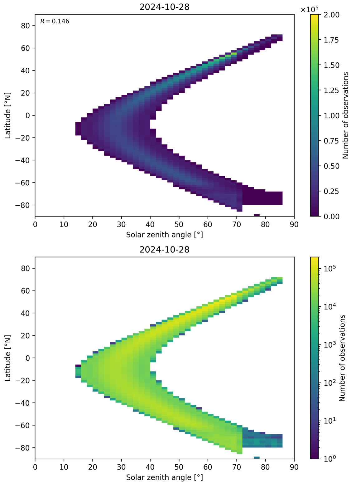
Figure 181: Scatter density plot of “Solar zenith angle” against “Latitude” for 2024-10-27 to 2024-10-29.
