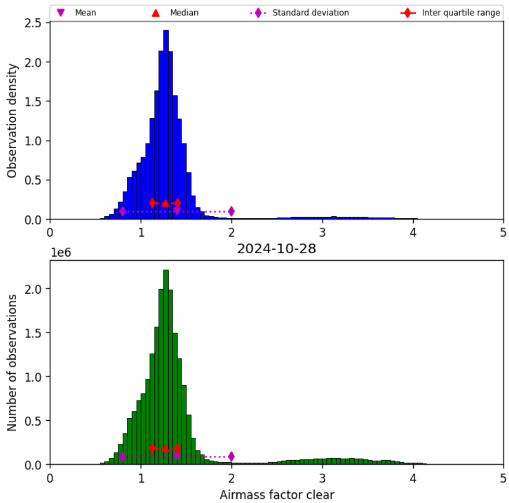
Figure 42: Histogram of “Airmass factor clear” for 2024-10-27 to 2024-10-29
