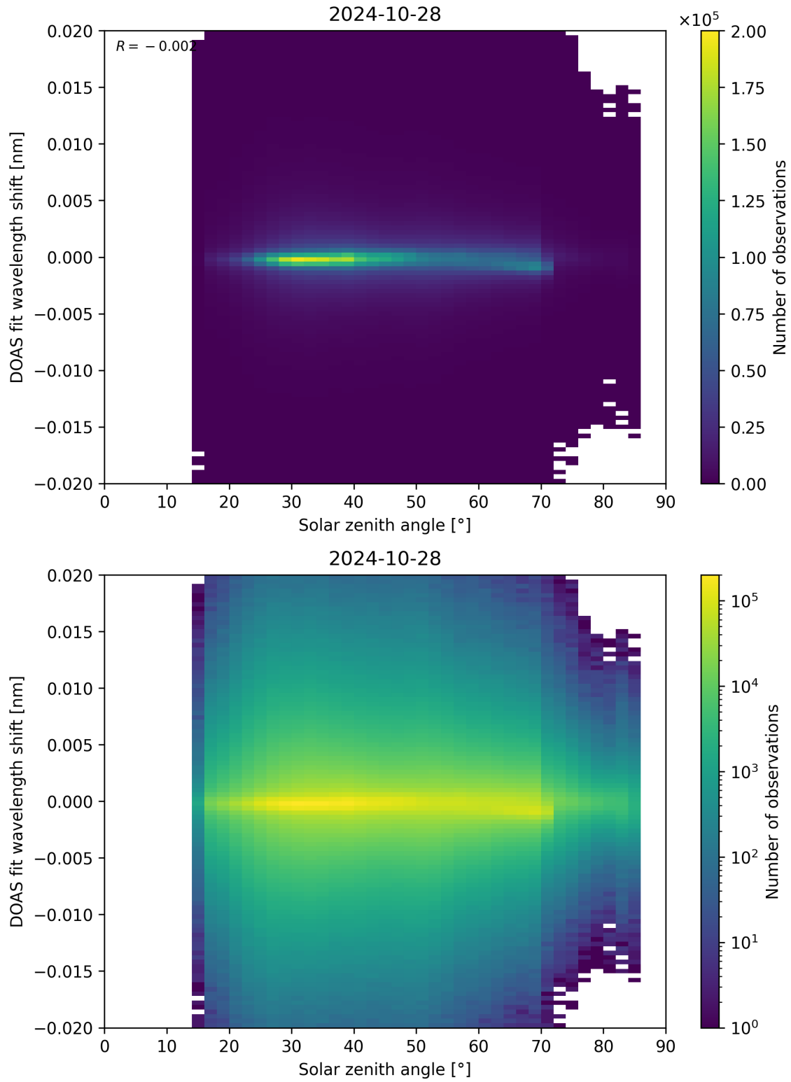
Figure 168: Scatter density plot of “Solar zenith angle” against “DOAS fit wavelength shift” for 2024-10-27 to 2024-10-29.
