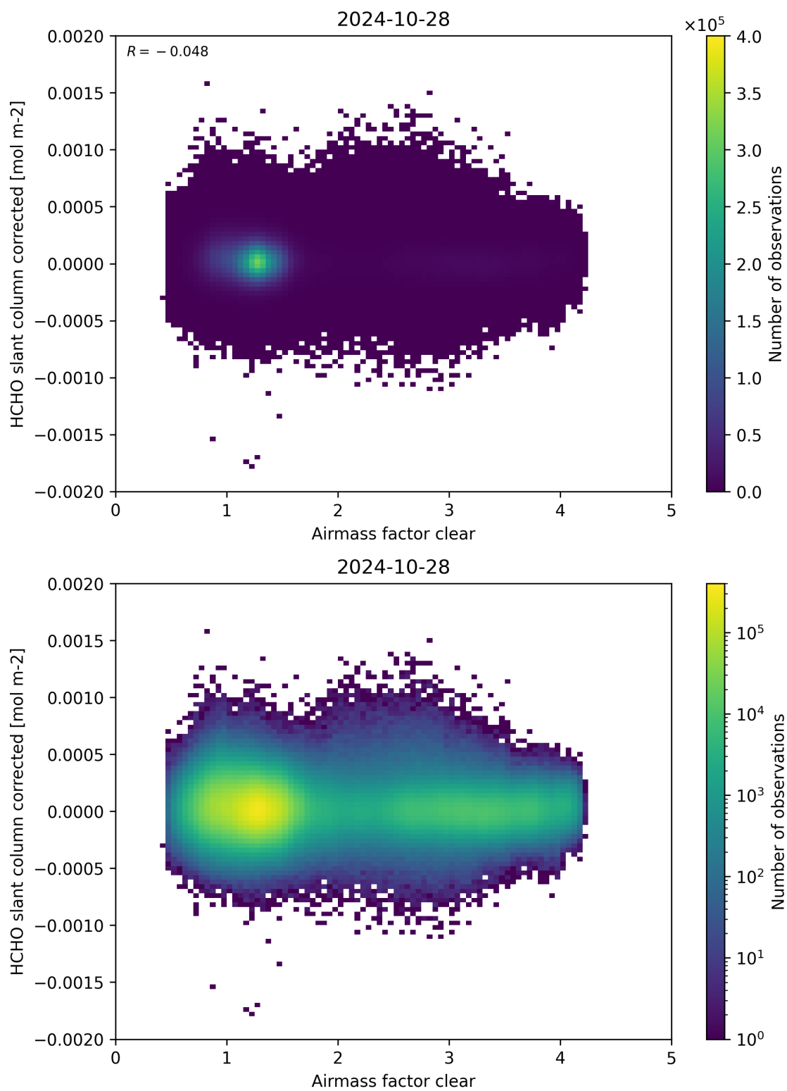
Figure 74: Scatter density plot of “Airmass factor clear” against “HCHO slant column corrected” for 2024-10-27 to 2024-10-29.
