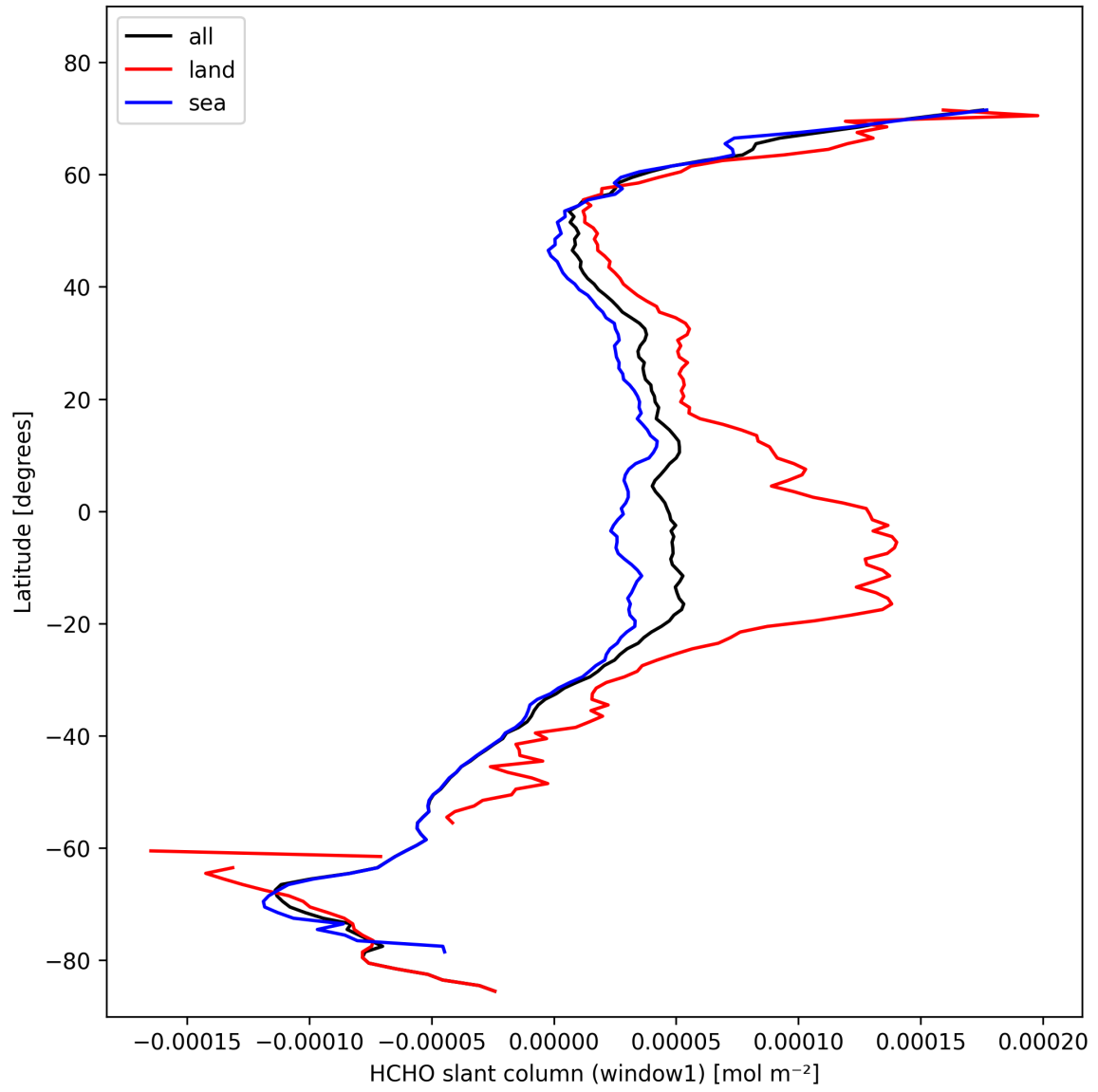
Figure 24: Zonal average of “HCHO slant column (window1)” for 2024-10-27 to 2024-10-29.
