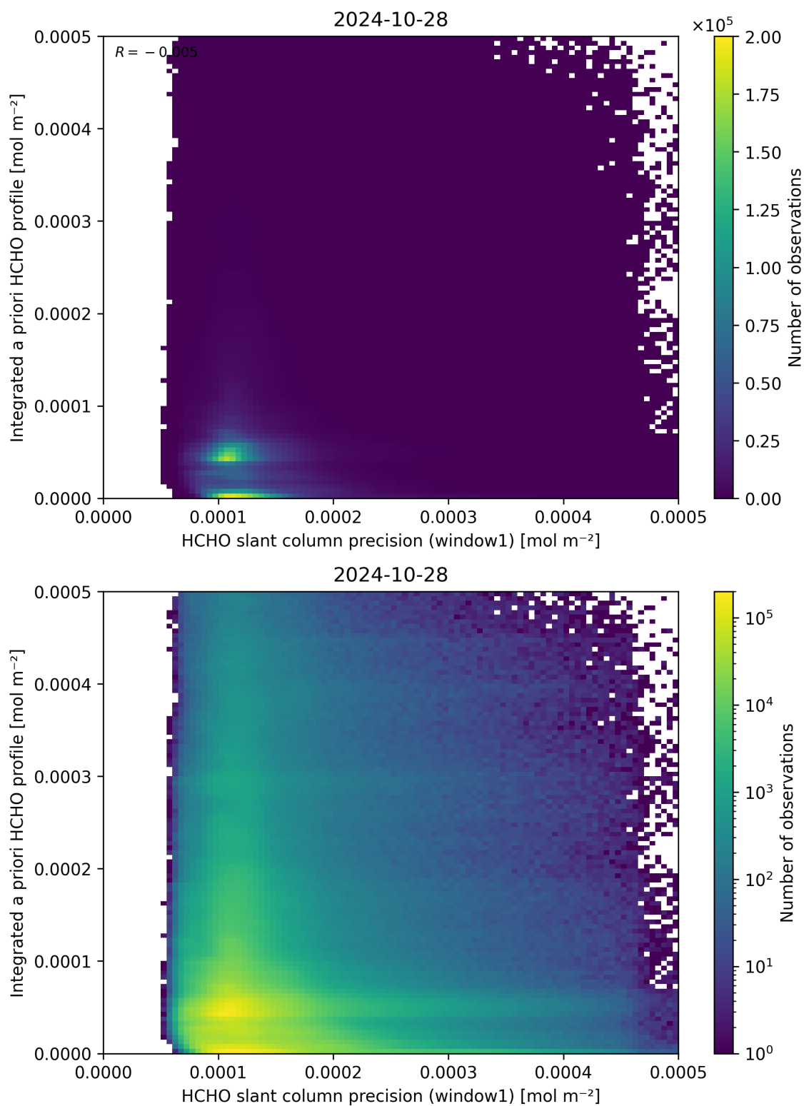
Figure 96: Scatter density plot of “HCHO slant column precision (window1)” against “Integrated a priori HCHO profile” for 2024-10-27 to 2024-10-29.
