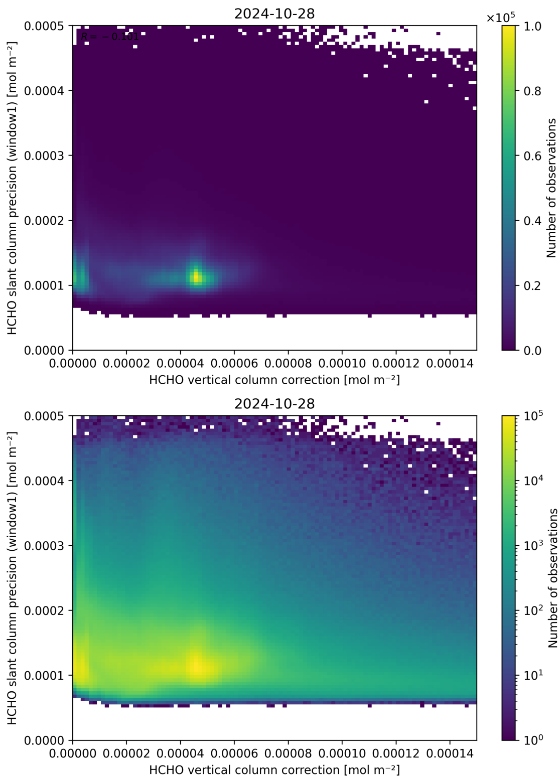
Figure 119: Scatter density plot of “HCHO vertical column correction” against “HCHO slant column precision (window1)” for 2024-10-27 to 2024-10-29.
