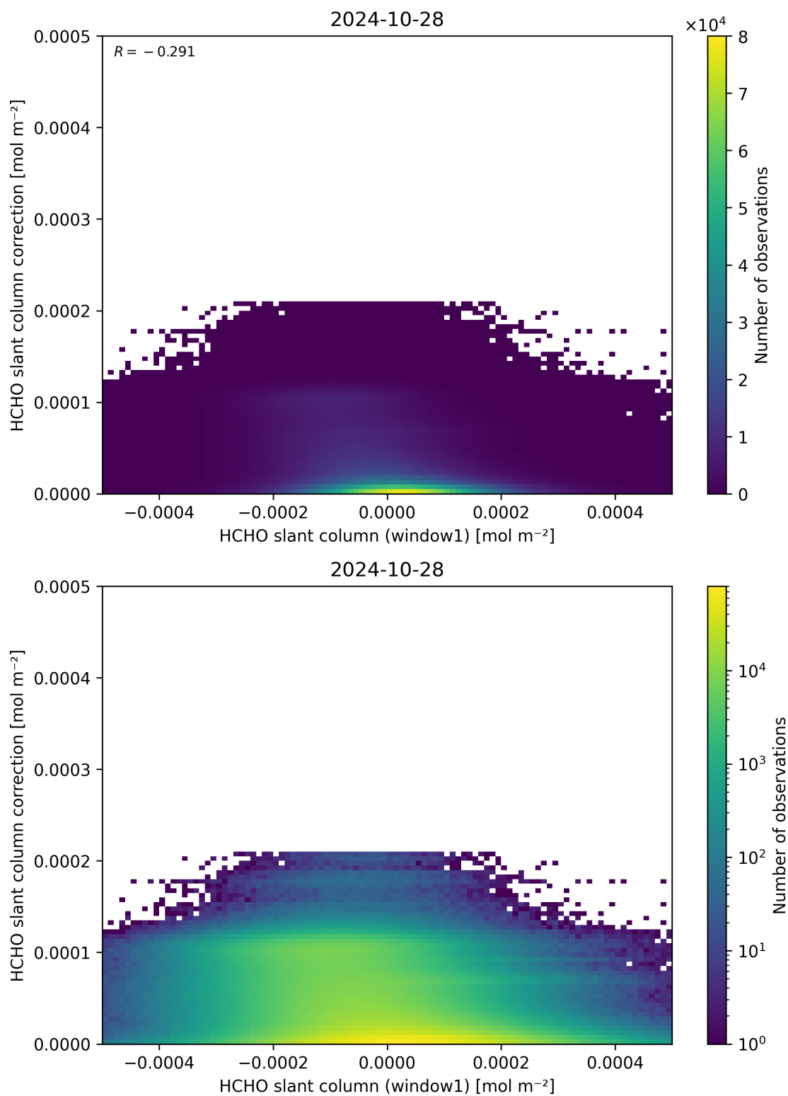
Figure 83: Scatter density plot of “HCHO slant column (window1)” against “HCHO slant column correction” for 2024-10-27 to 2024-10-29.
