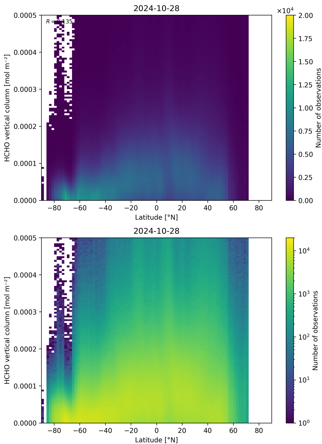
Figure 163: Scatter density plot of “Latitude” against “HCHO vertical column” for 2024-10-27 to 2024-10-29.
