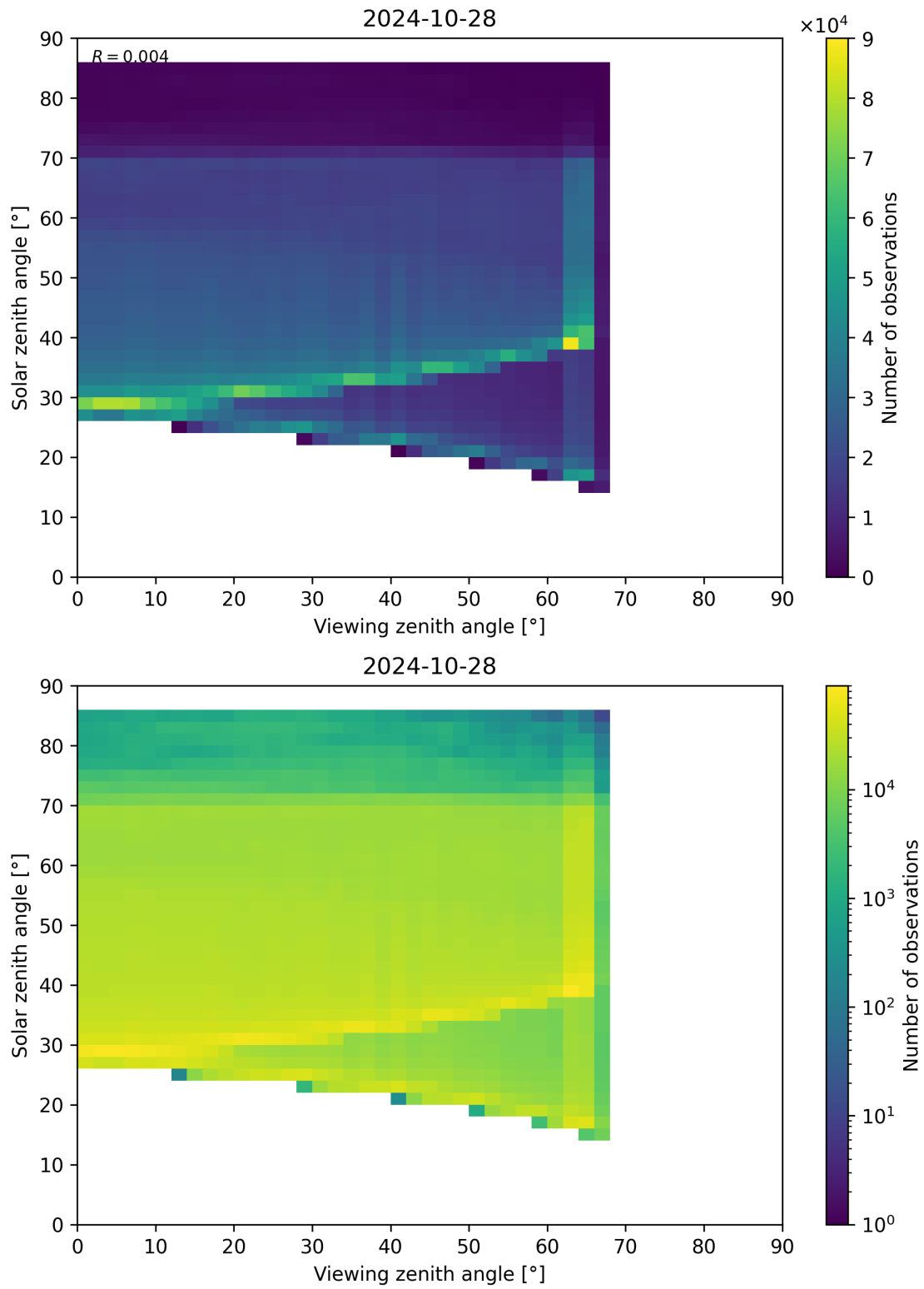
Figure 197: Scatter density plot of “Viewing zenith angle” against “Solar zenith angle” for 2024-10-27 to 2024-10-29.
