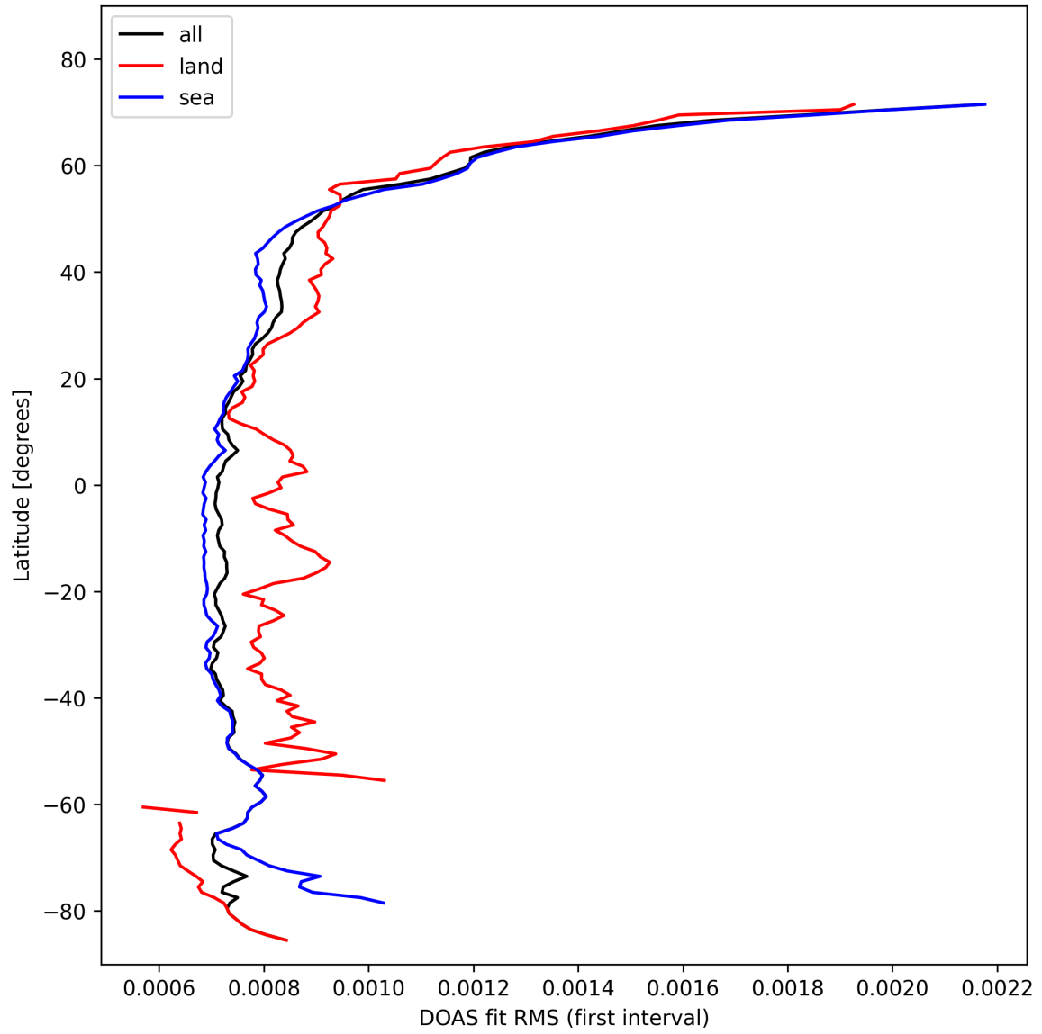
Figure 32: Zonal average of “DOAS fit RMS (first interval)” for 2024-10-27 to 2024-10-29.
