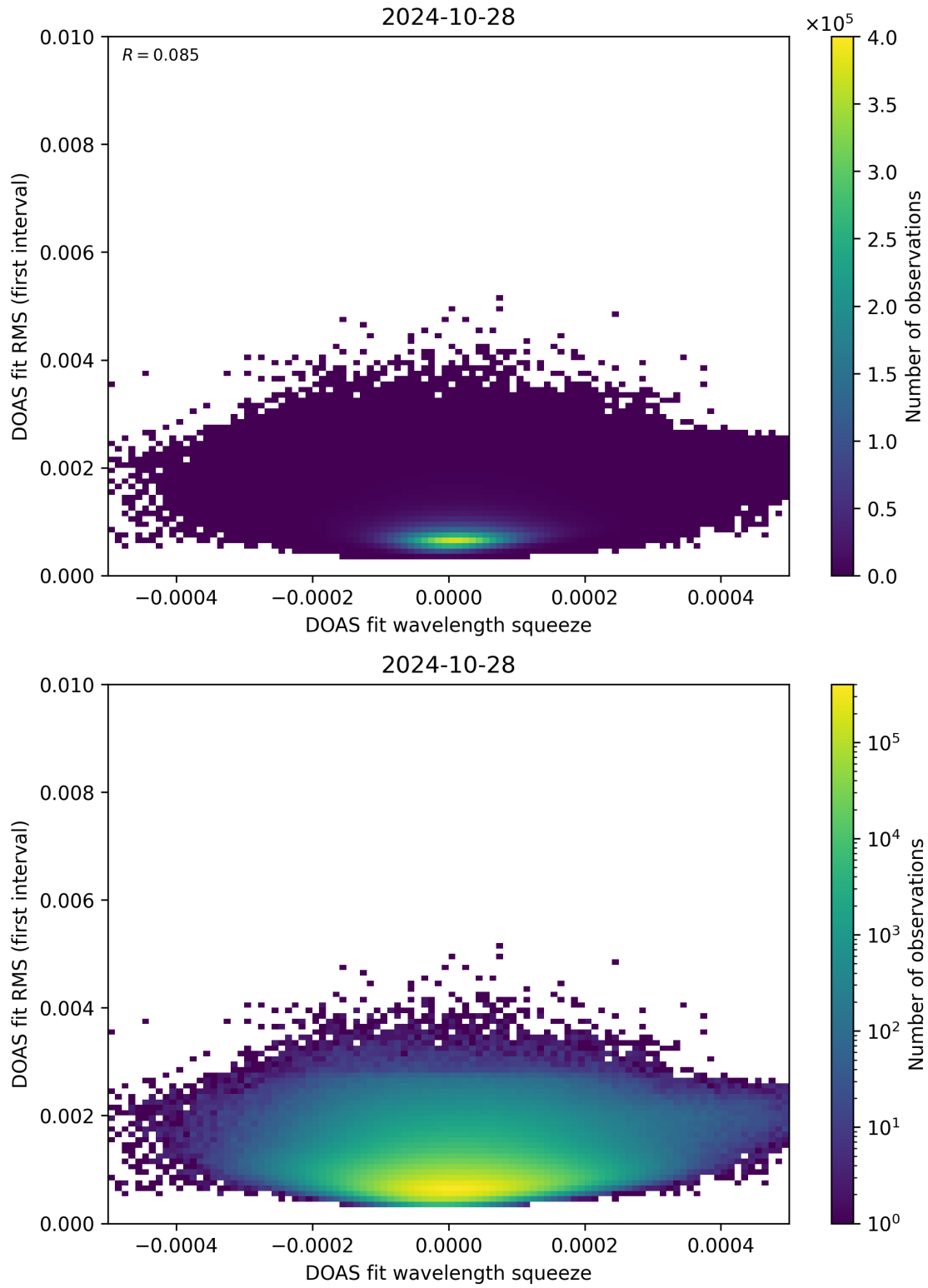
Figure 68: Scatter density plot of “DOAS fit wavelength squeeze” against “DOAS fit RMS (first interval)” for 2024-10-27 to 2024-10-29.
