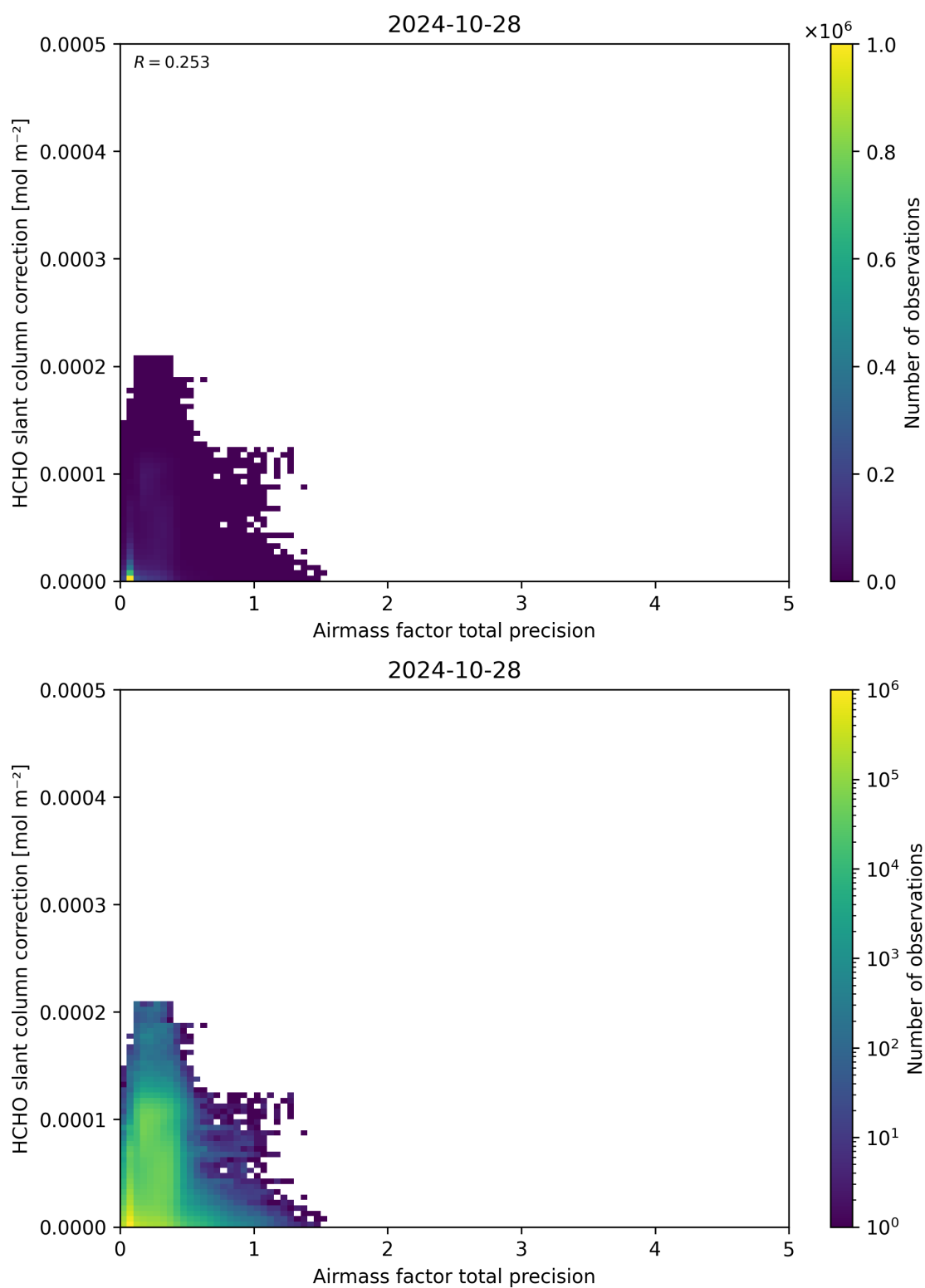
Figure 110: Scatter density plot of “Airmass factor total precision” against “HCHO slant column correction” for 2024-10-27 to 2024-10-29.
