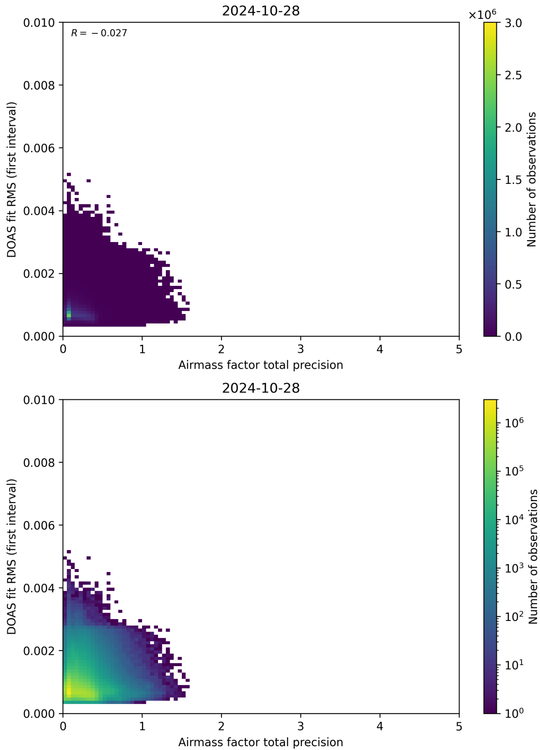
Figure 105: Scatter density plot of “Airmass factor total precision” against “DOAS fit RMS (first interval)” for 2024-10-27 to 2024-10-29.
