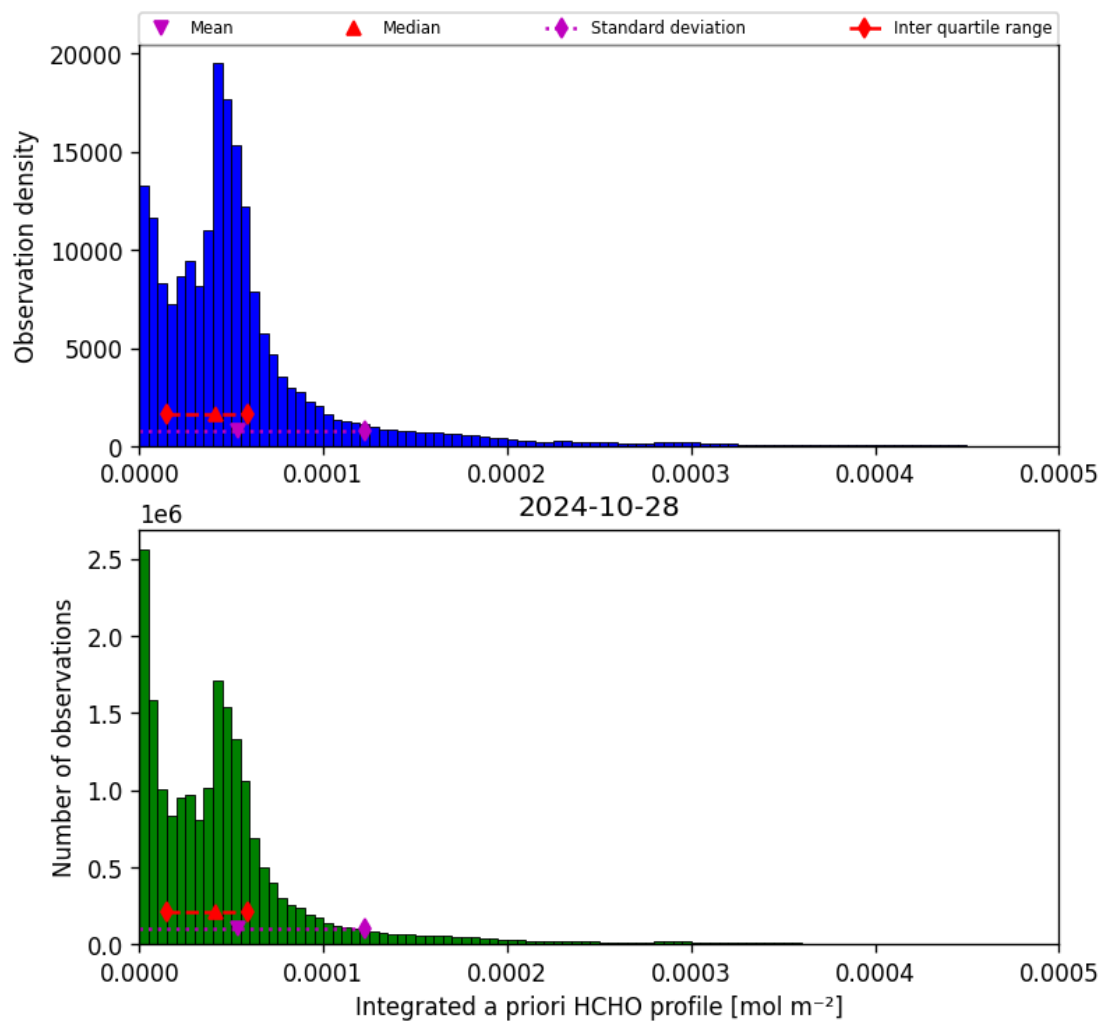
Figure 43: Histogram of “Integrated a priori HCHO profile” for 2024-10-27 to 2024-10-29
