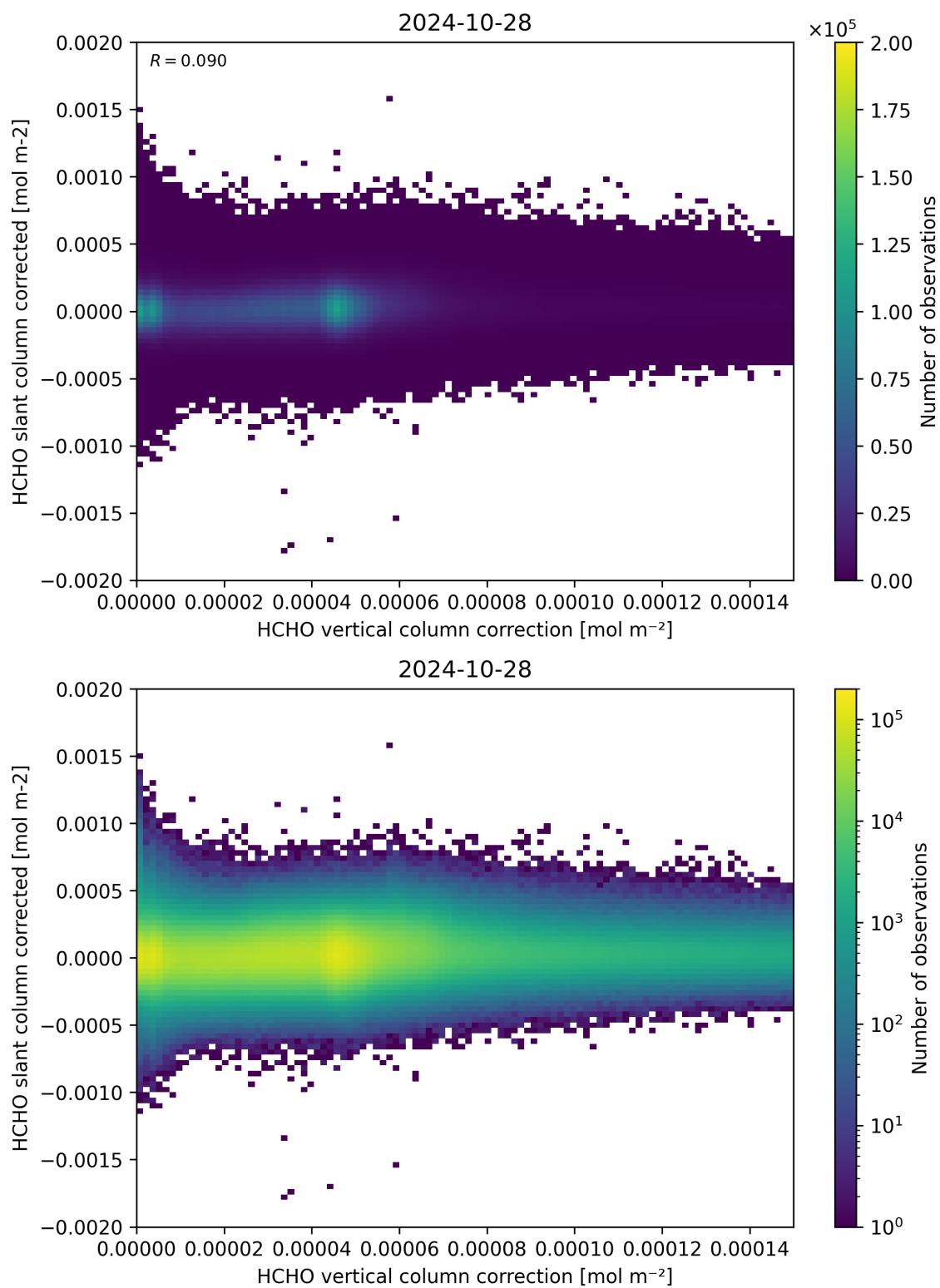
Figure 116: Scatter density plot of “HCHO vertical column correction” against “HCHO slant column corrected” for 2024-10-27 to 2024-10-29.
