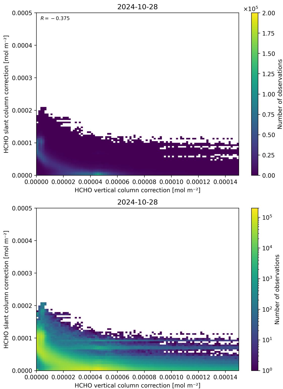
Figure 117: Scatter density plot of “HCHO vertical column correction” against “HCHO slant column correction” for 2024-10-27 to 2024-10-29.
