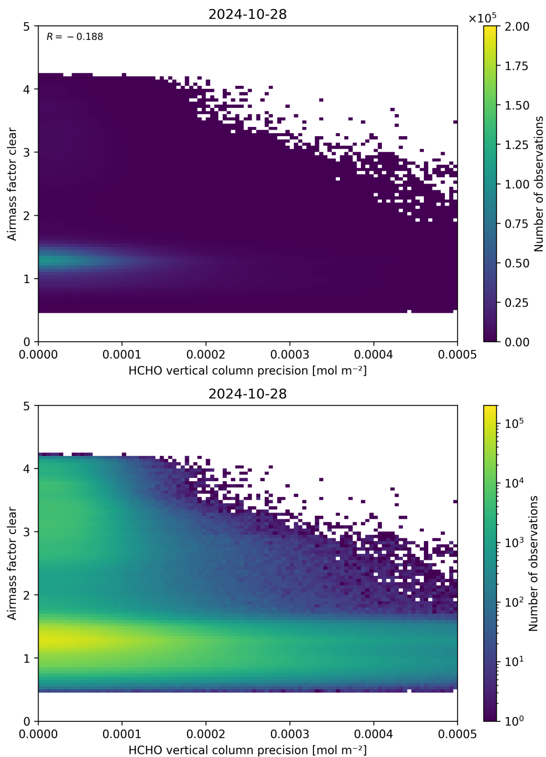
Figure 139: Scatter density plot of “HCHO vertical column precision” against “Airmass factor clear” for 2024-10-27 to 2024-10-29.
