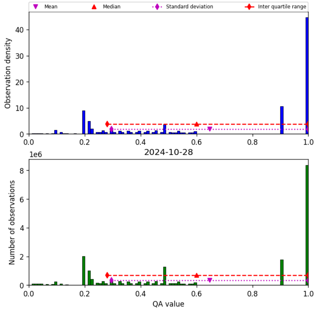
Figure 34: Histogram of “QA value” for 2024-10-27 to 2024-10-29
