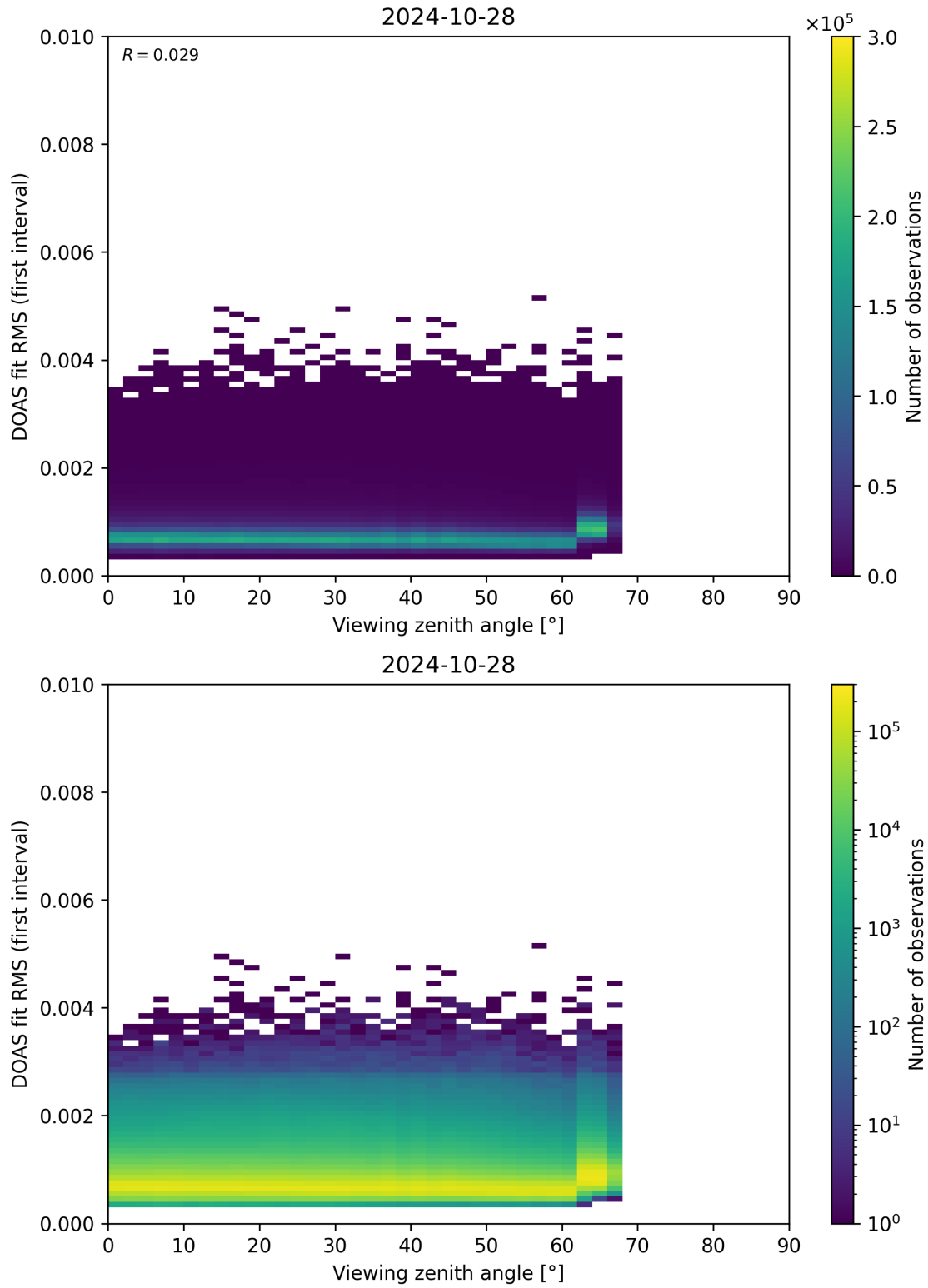
Figure 182: Scatter density plot of “Viewing zenith angle” against “DOAS fit RMS (first interval)” for 2024-10-27 to 2024-10-29.
