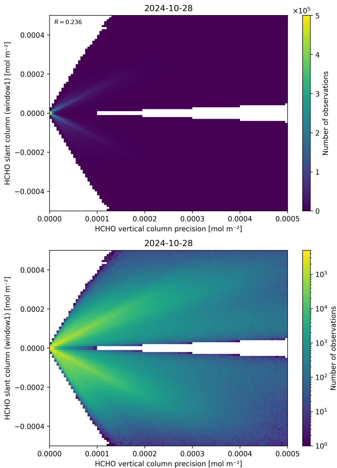
Figure 142: Scatter density plot of “HCHO vertical column precision” against “HCHO slant column (window1)” for 2024-10-27 to 2024-10-29.
