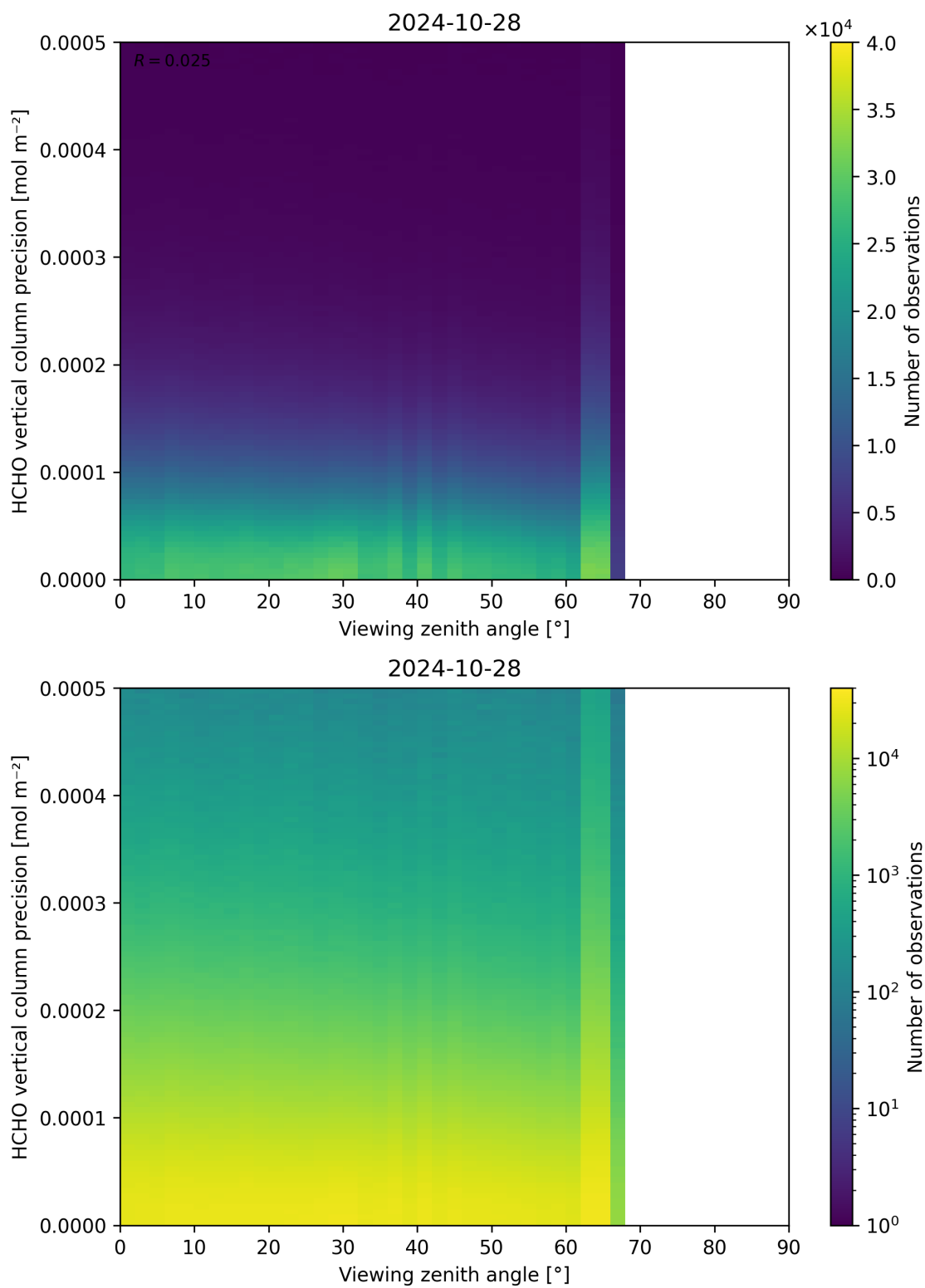
Figure 194: Scatter density plot of “Viewing zenith angle” against “HCHO vertical column precision” for 2024-10-27 to 2024-10-29.
