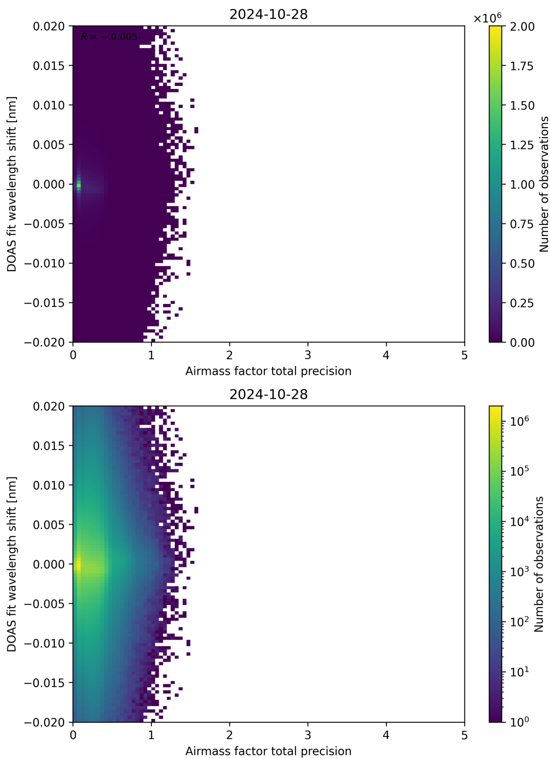
Figure 106: Scatter density plot of “Airmass factor total precision” against “DOAS fit wavelength shift” for 2024-10-27 to 2024-10-29.
