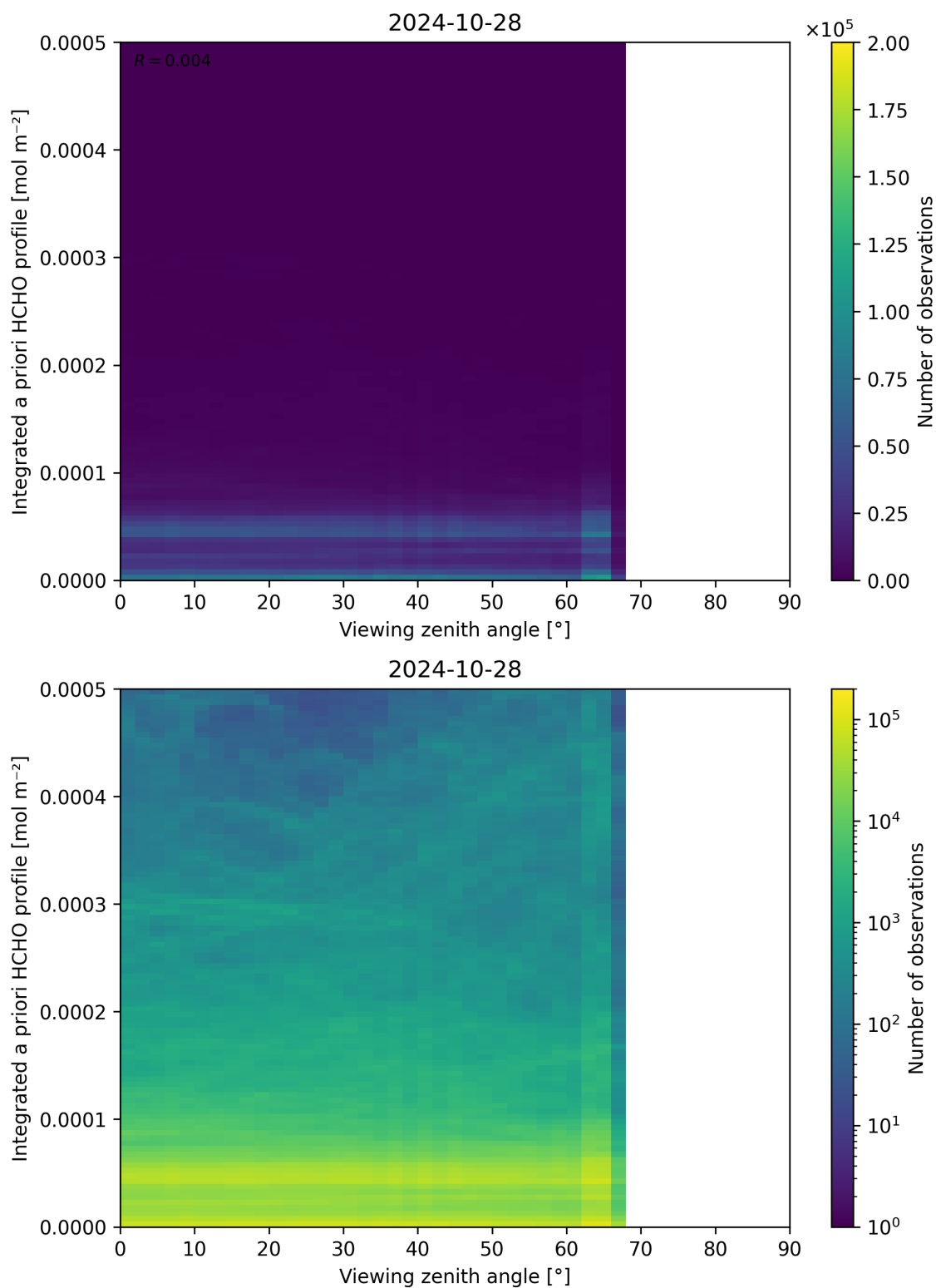
Figure 195: Scatter density plot of “Viewing zenith angle” against “Integrated a priori HCHO profile” for 2024-10-27 to 2024-10-29.
