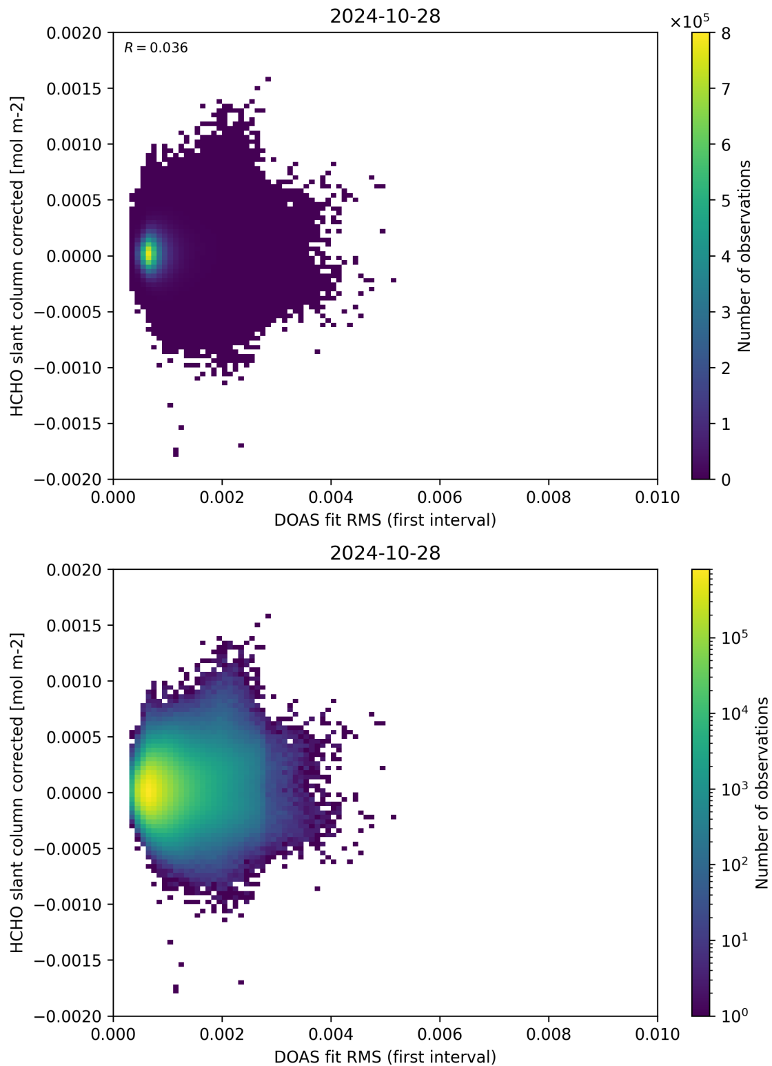
Figure 62: Scatter density plot of “DOAS fit RMS (first interval)” against “HCHO slant column corrected” for 2024-10-27 to 2024-10-29.
