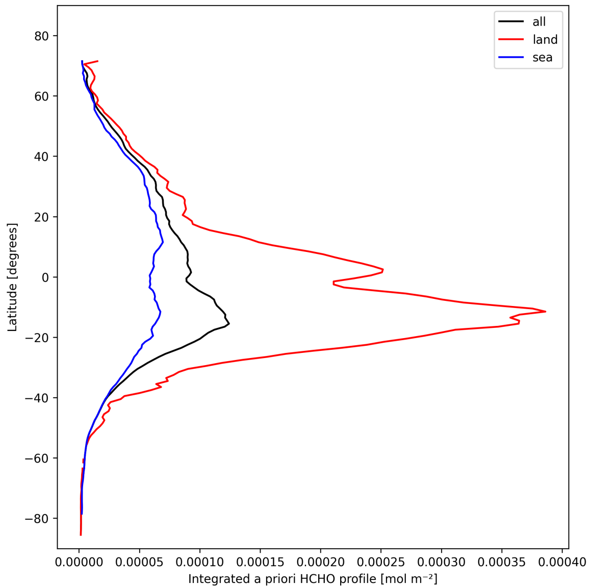
Figure 29: Zonal average of “Integrated a priori HCHO profile” for 2024-10-27 to 2024-10-29.
