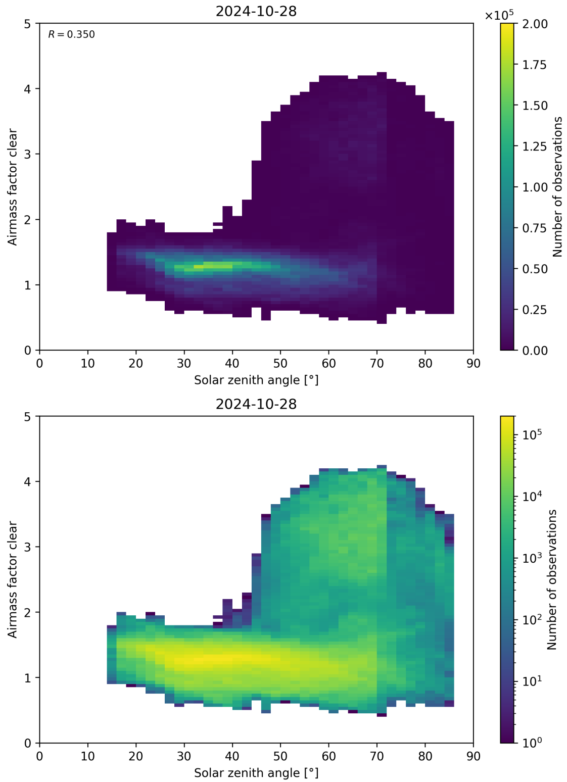
Figure 170: Scatter density plot of “Solar zenith angle” against “Airmass factor clear” for 2024-10-27 to 2024-10-29.
