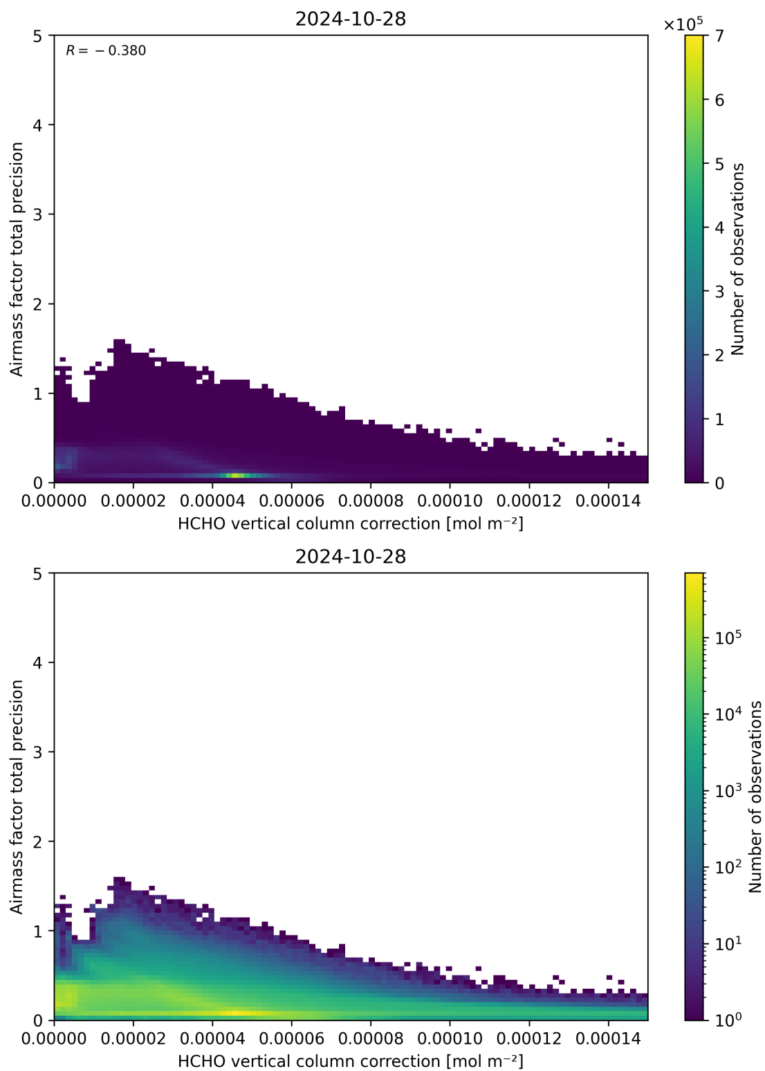
Figure 121: Scatter density plot of “HCHO vertical column correction” against “Airmass factor total precision” for 2024-10-27 to 2024-10-29.
