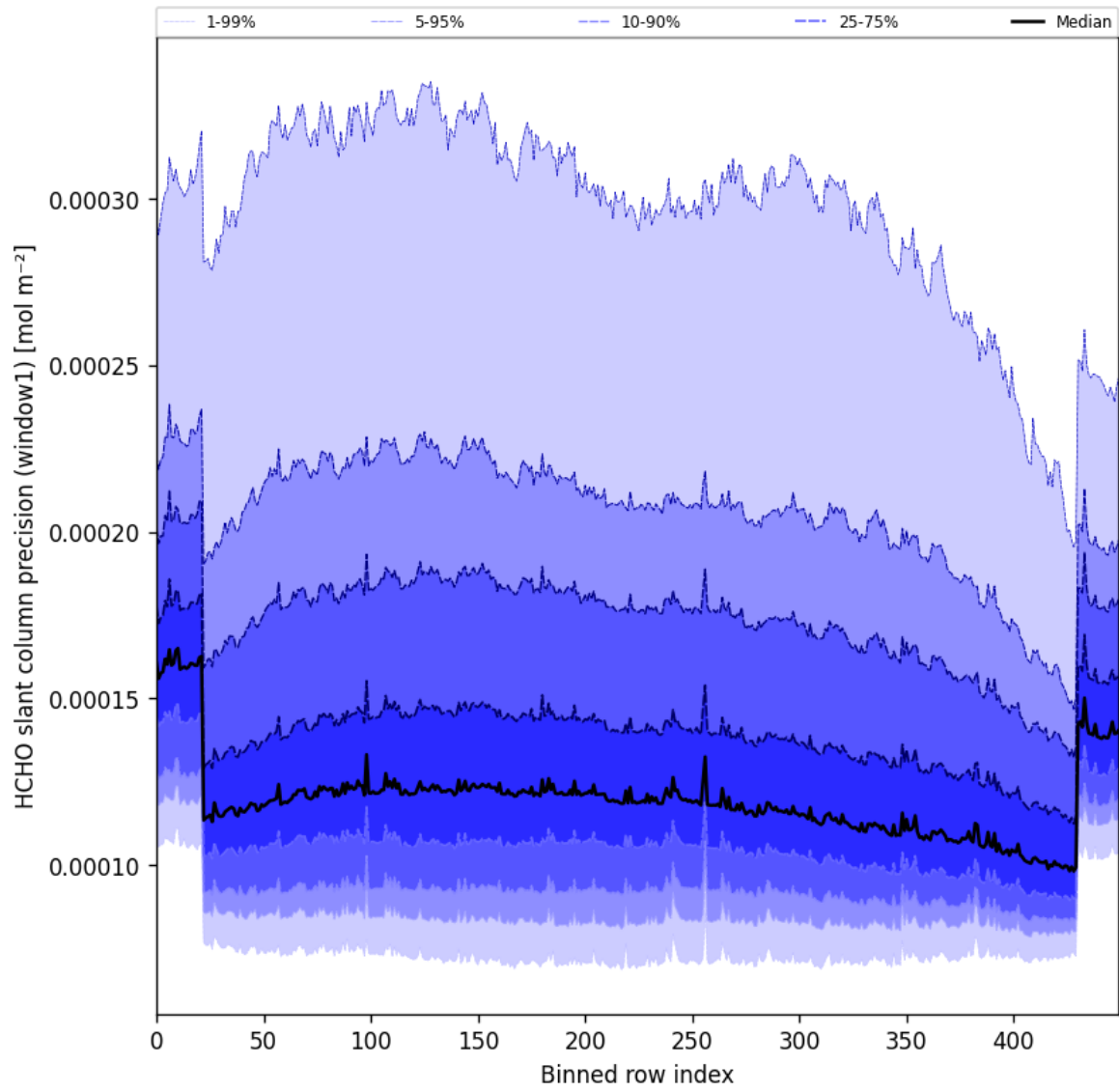
Figure 53: Along track statistics of “HCHO slant column precision (window1)” for 2024-10-27 to 2024-10-29
