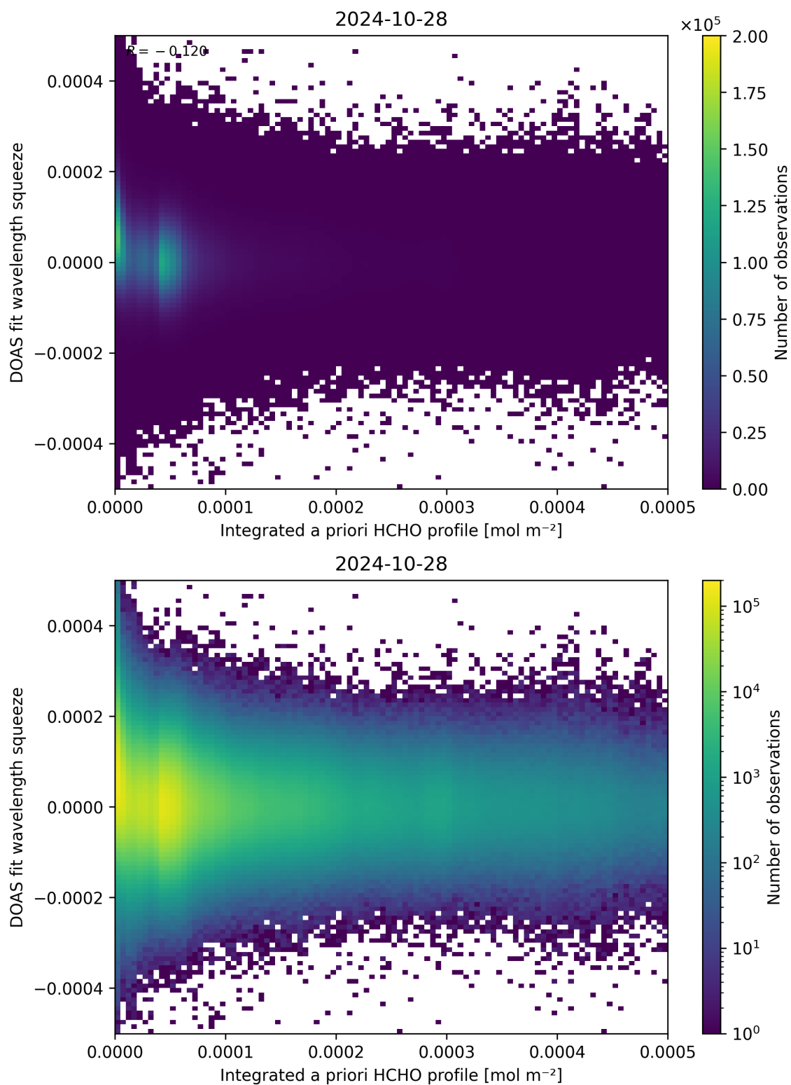
Figure 150: Scatter density plot of “Integrated a priori HCHO profile” against “DOAS fit wavelength squeeze” for 2024-10-27 to 2024-10-29.
