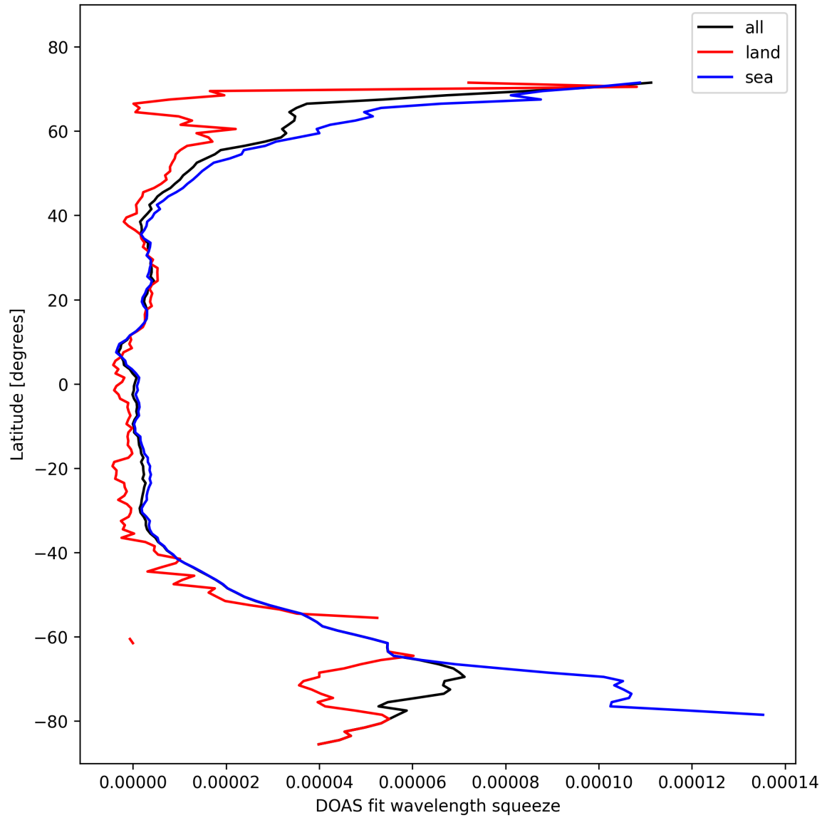
Figure 31: Zonal average of “DOAS fit wavelength squeeze” for 2024-10-27 to 2024-10-29.
