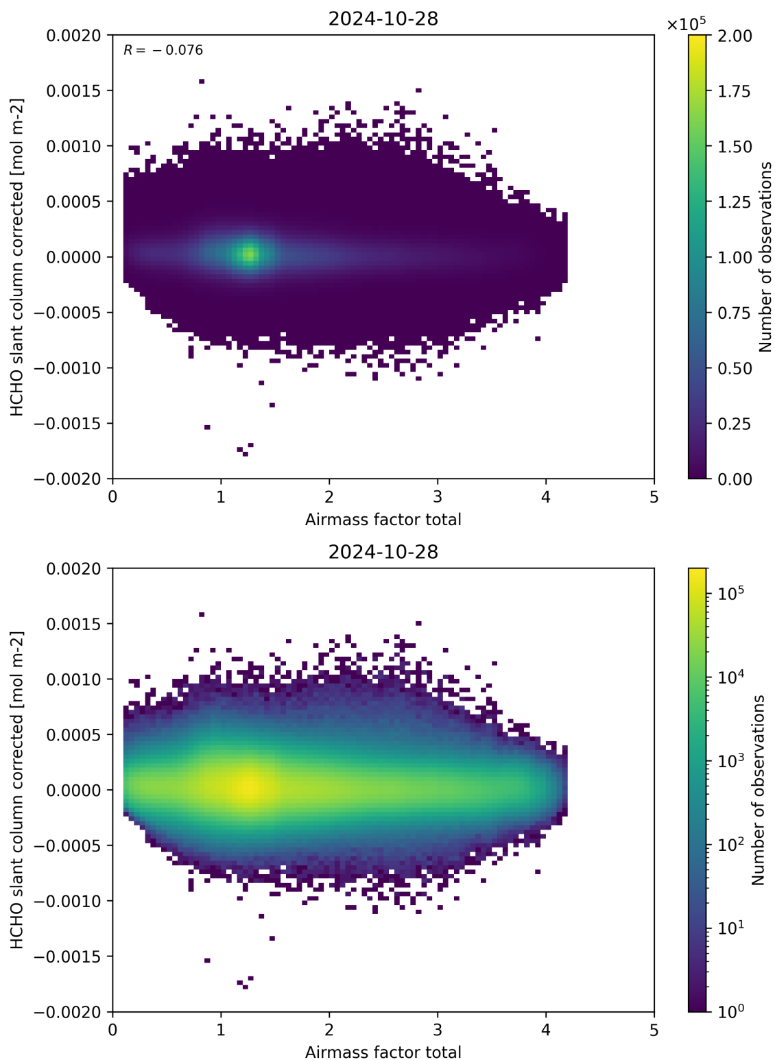
Figure 101: Scatter density plot of “Airmass factor total” against “HCHO slant column corrected” for 2024-10-27 to 2024-10-29.
