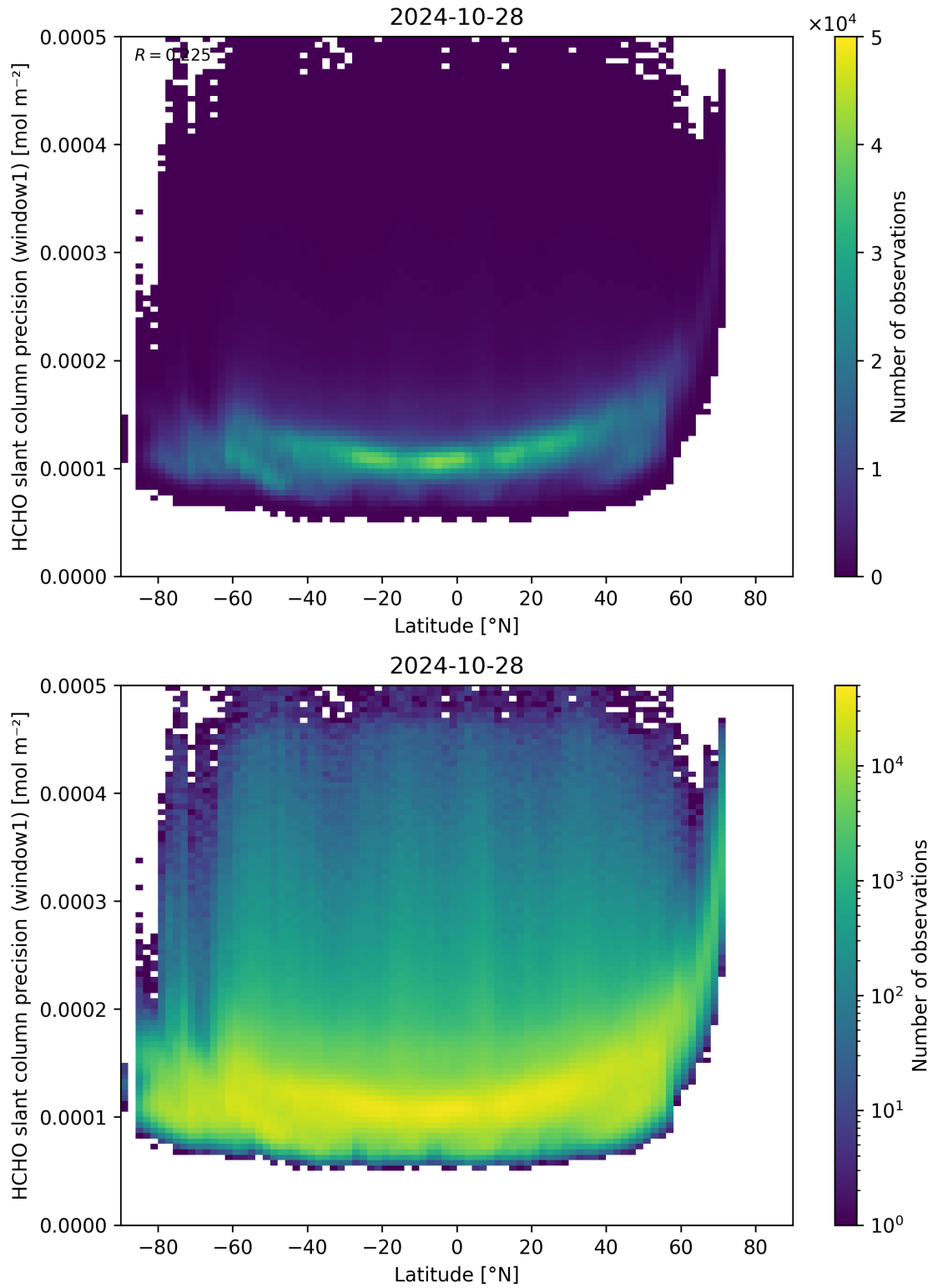
Figure 160: Scatter density plot of “Latitude” against “HCHO slant column precision (window1)” for 2024-10-27 to 2024-10-29.
