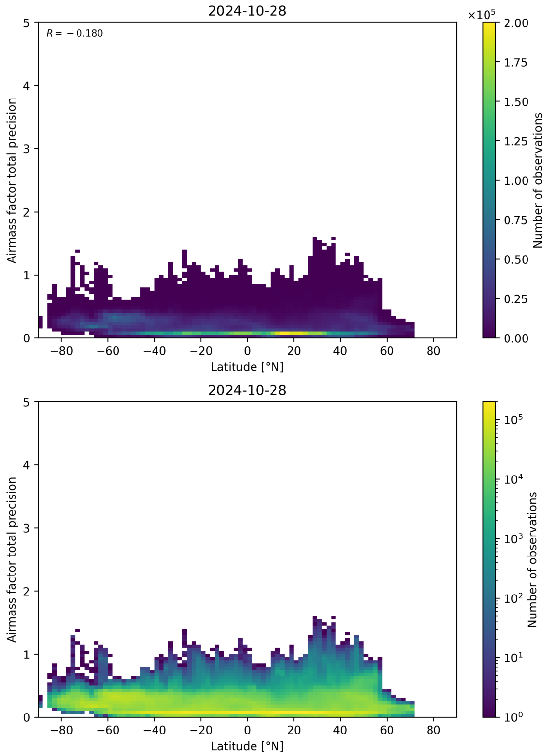
Figure 162: Scatter density plot of “Latitude” against “Airmass factor total precision” for 2024-10-27 to 2024-10-29.
