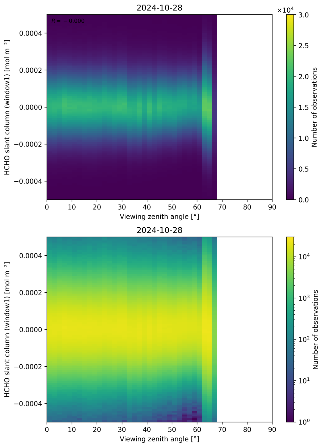
Figure 188: Scatter density plot of “Viewing zenith angle” against “HCHO slant column (window1)” for 2024-10-27 to 2024-10-29.
