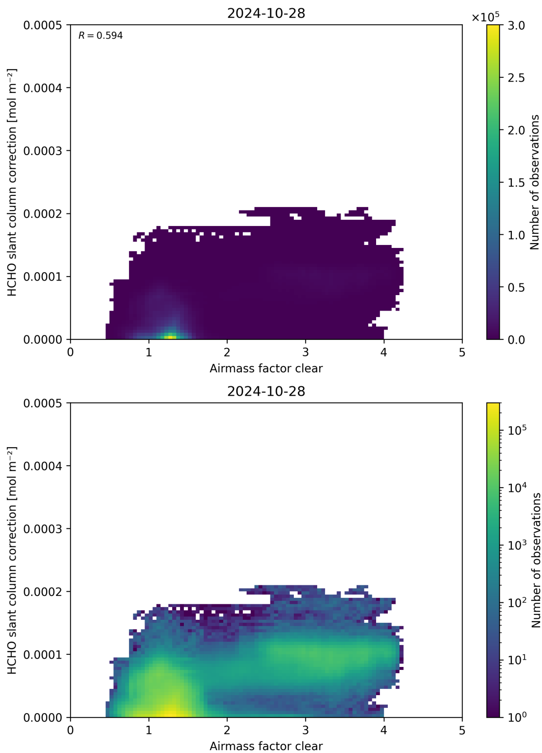
Figure 75: Scatter density plot of “Airmass factor clear” against “HCHO slant column correction” for 2024-10-27 to 2024-10-29.
