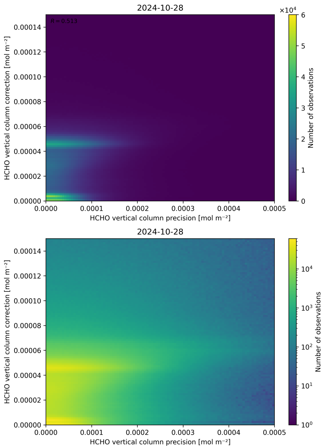
Figure 146: Scatter density plot of “HCHO vertical column precision” against “HCHO vertical column correction” for 2024-10-27 to 2024-10-29.
