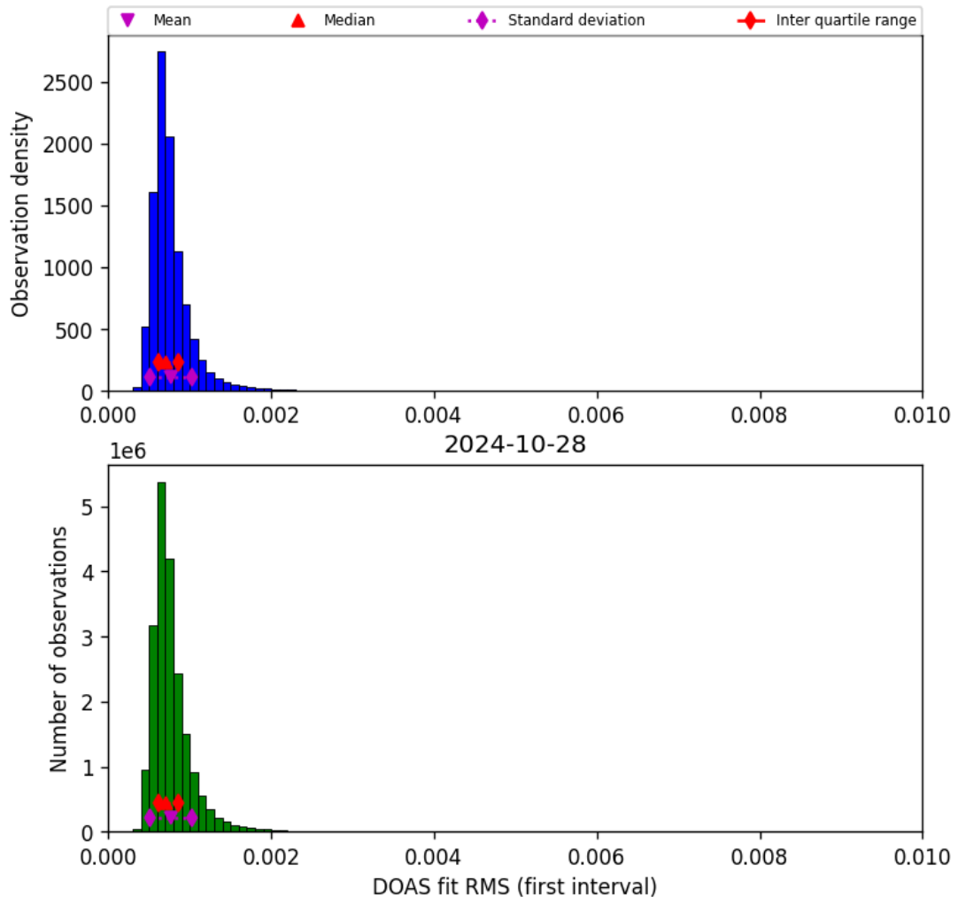
Figure 46: Histogram of “DOAS fit RMS (first interval)” for 2024-10-27 to 2024-10-29
