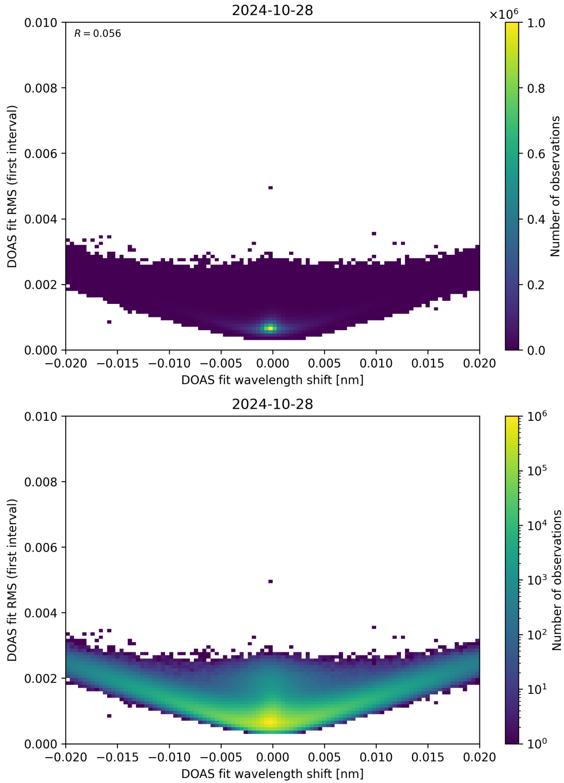
Figure 64: Scatter density plot of “DOAS fit wavelength shift” against “DOAS fit RMS (first interval)” for 2024-10-27 to 2024-10-29.
