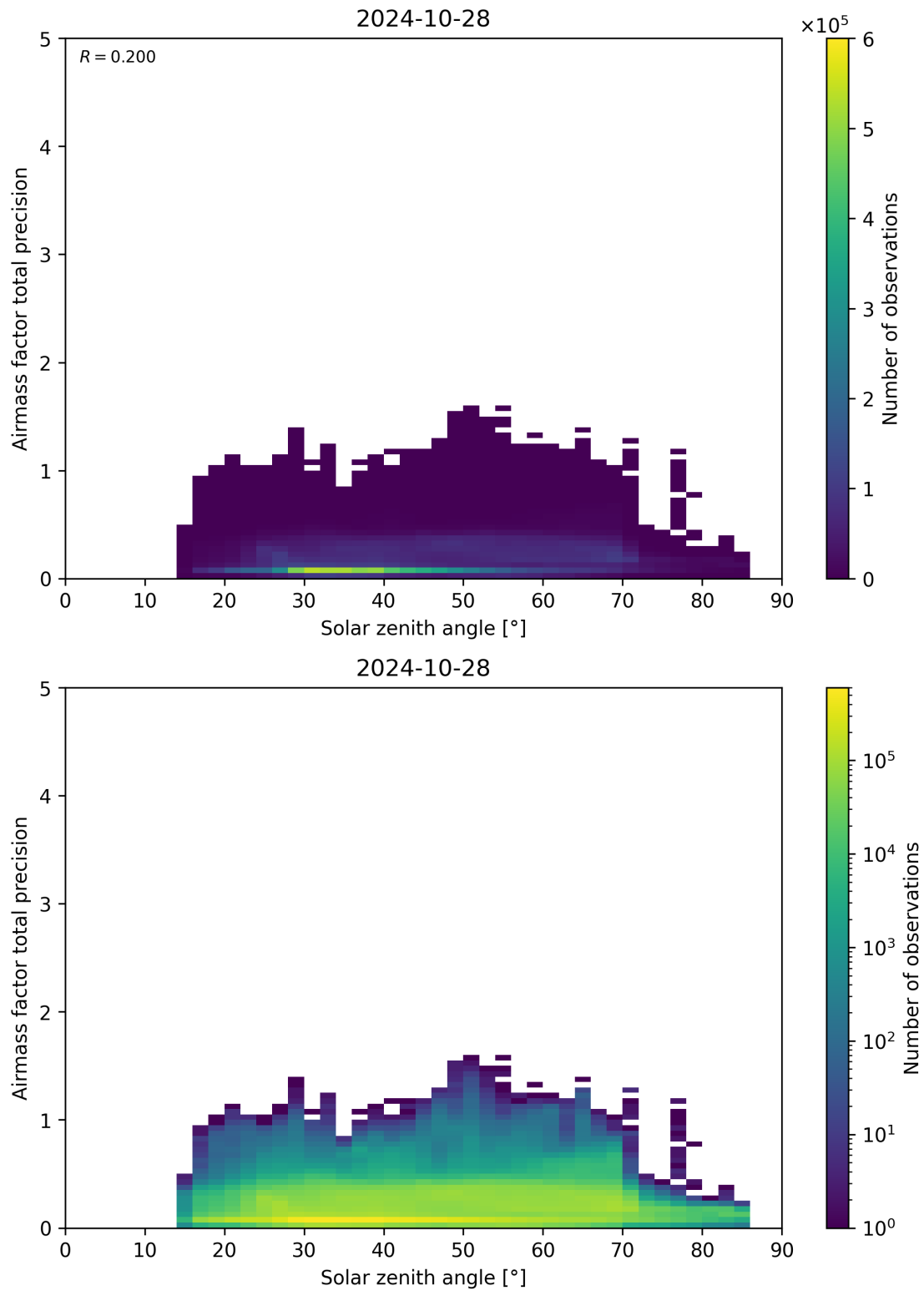
Figure 176: Scatter density plot of “Solar zenith angle” against “Airmass factor total precision” for 2024-10-27 to 2024-10-29.
