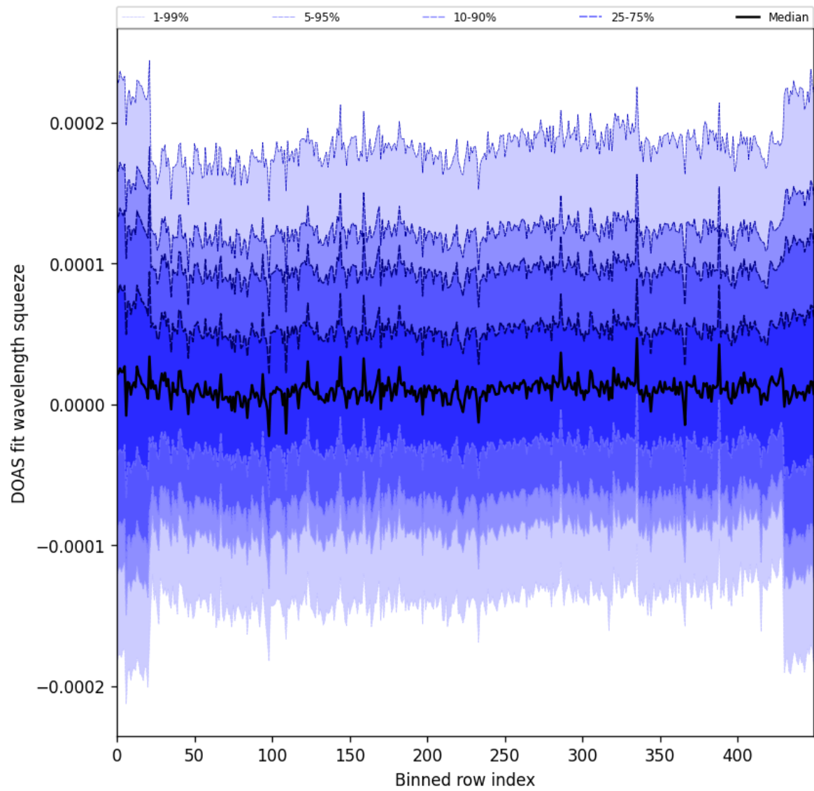
Figure 59: Along track statistics of “DOAS fit wavelength squeeze” for 2024-10-27 to 2024-10-29
