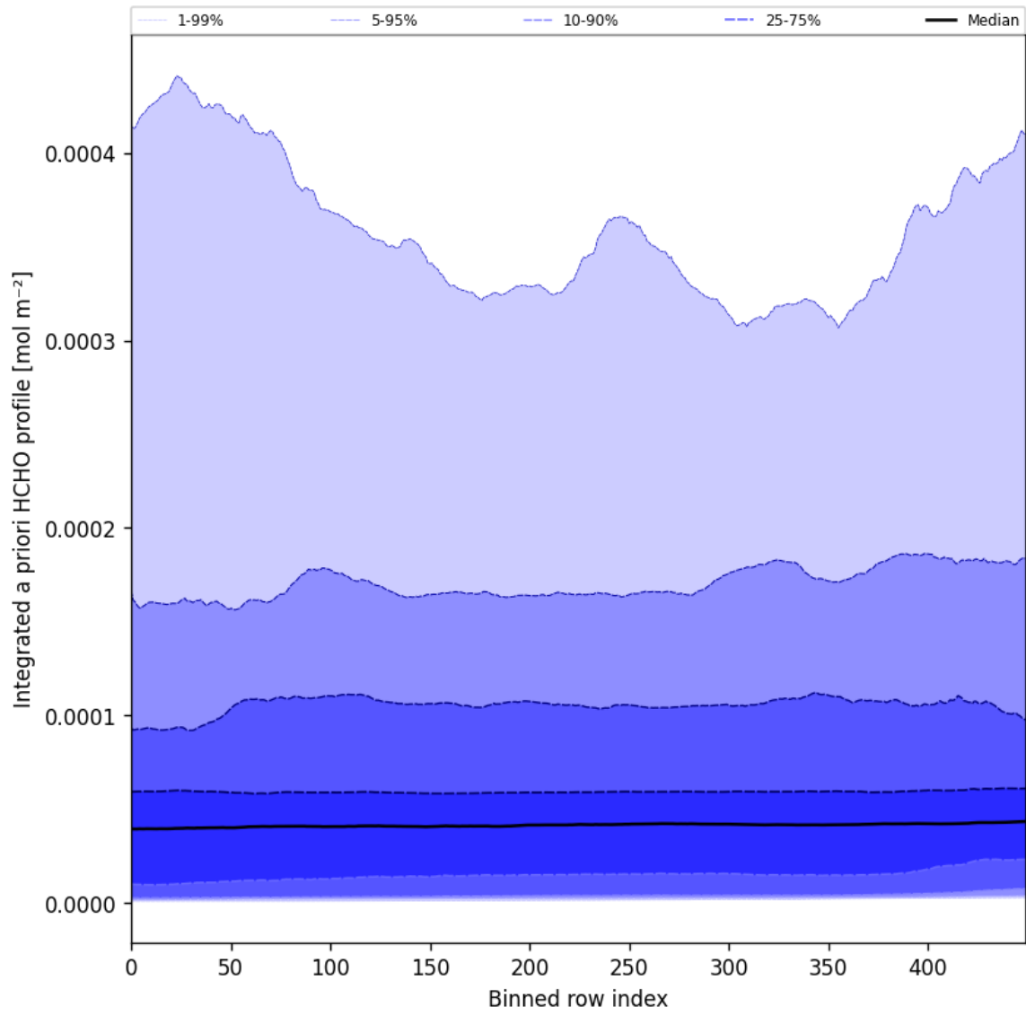
Figure 57: Along track statistics of “Integrated a priori HCHO profile” for 2024-10-27 to 2024-10-29
