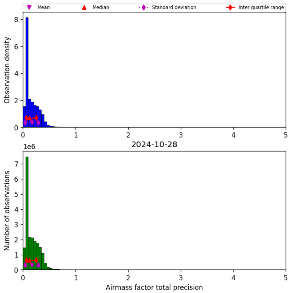
Figure 41: Histogram of “Airmass factor total precision” for 2024-10-27 to 2024-10-29
