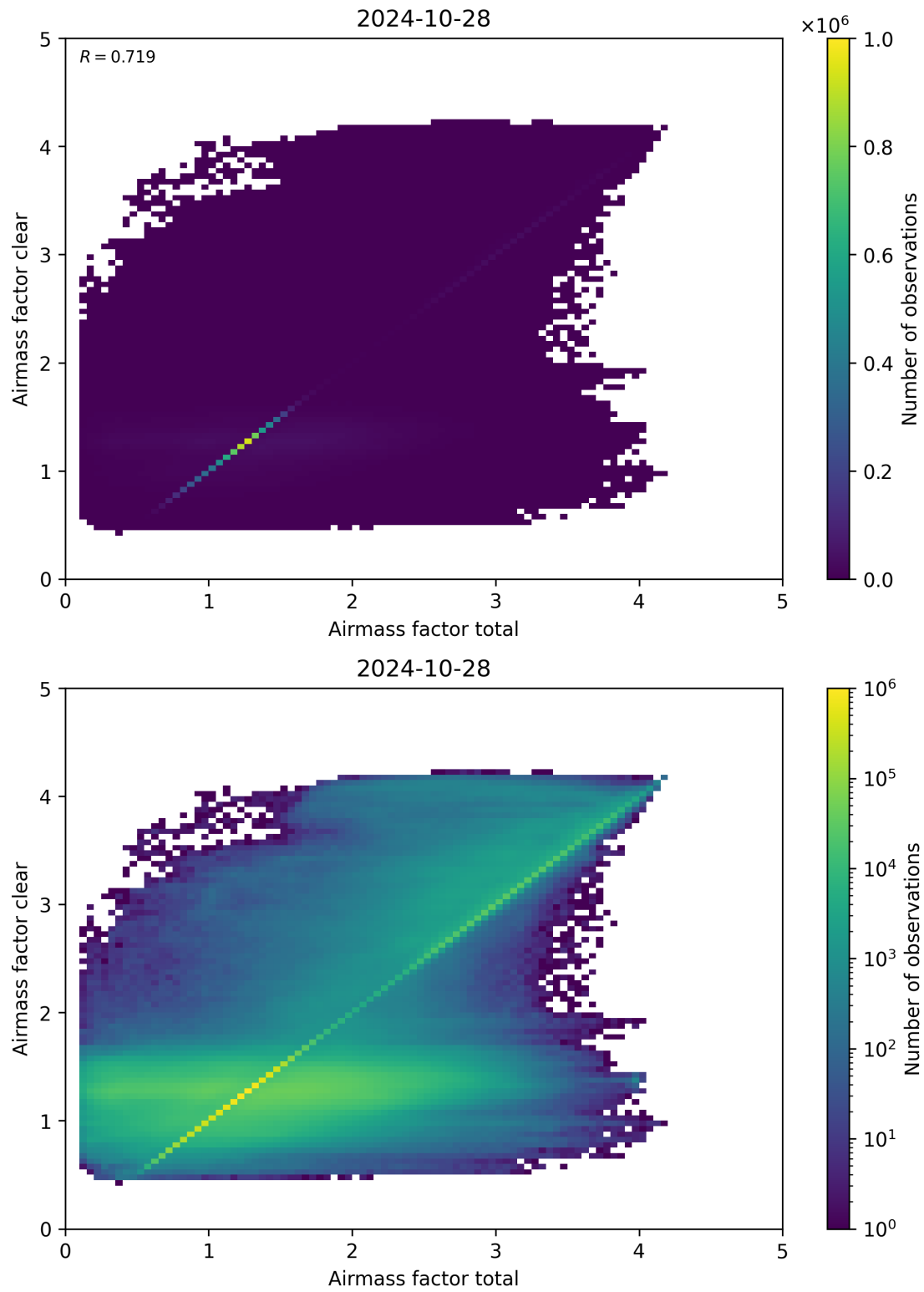
Figure 100: Scatter density plot of “Airmass factor total” against “Airmass factor clear” for 2024-10-27 to 2024-10-29.
