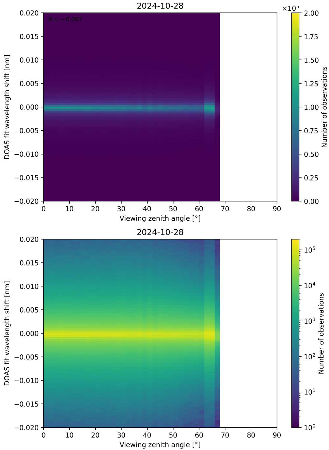
Figure 183: Scatter density plot of “Viewing zenith angle” against “DOAS fit wavelength shift” for 2024-10-27 to 2024-10-29.
