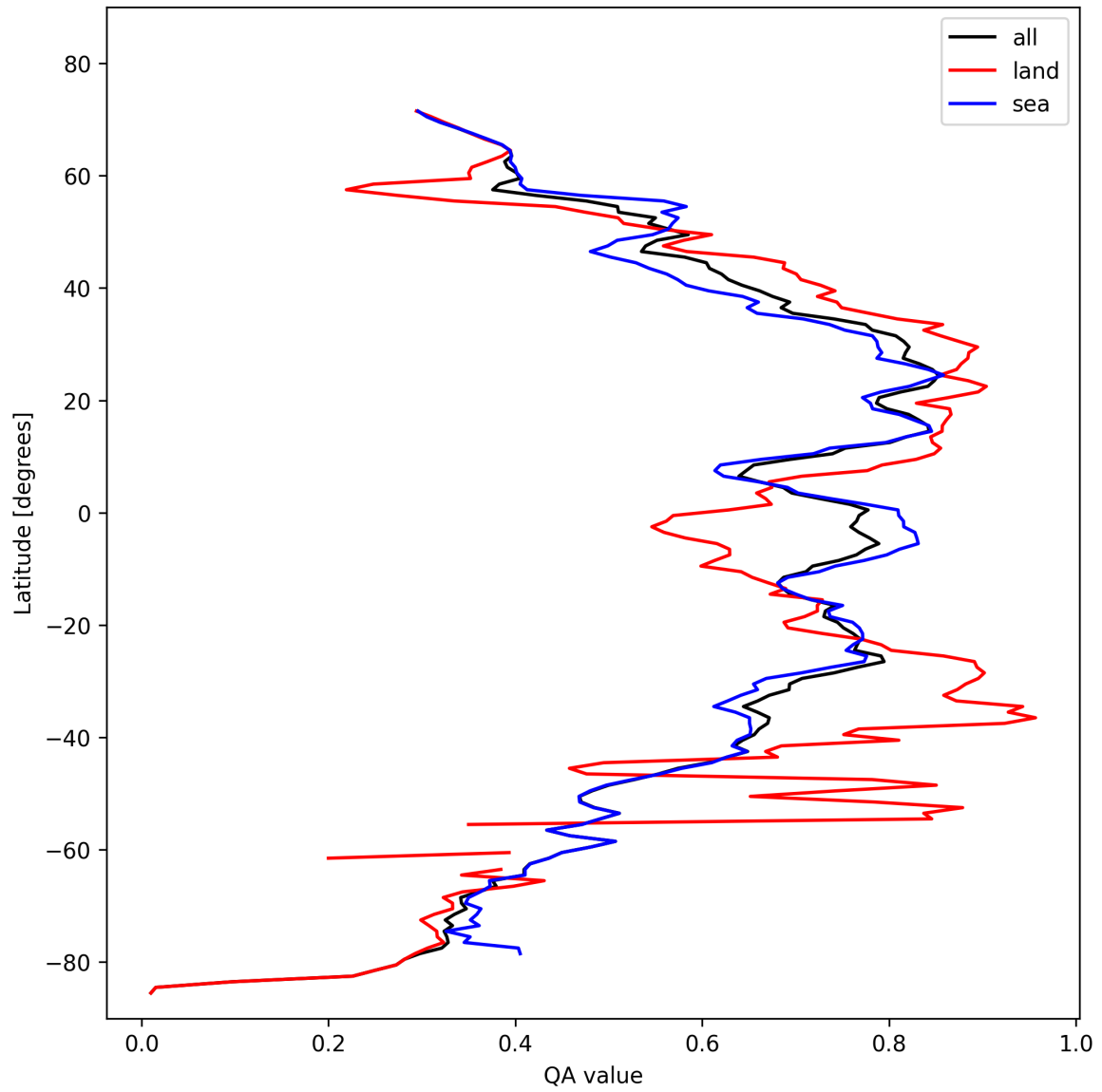
Figure 20: Zonal average of “QA value” for 2024-10-27 to 2024-10-29.
