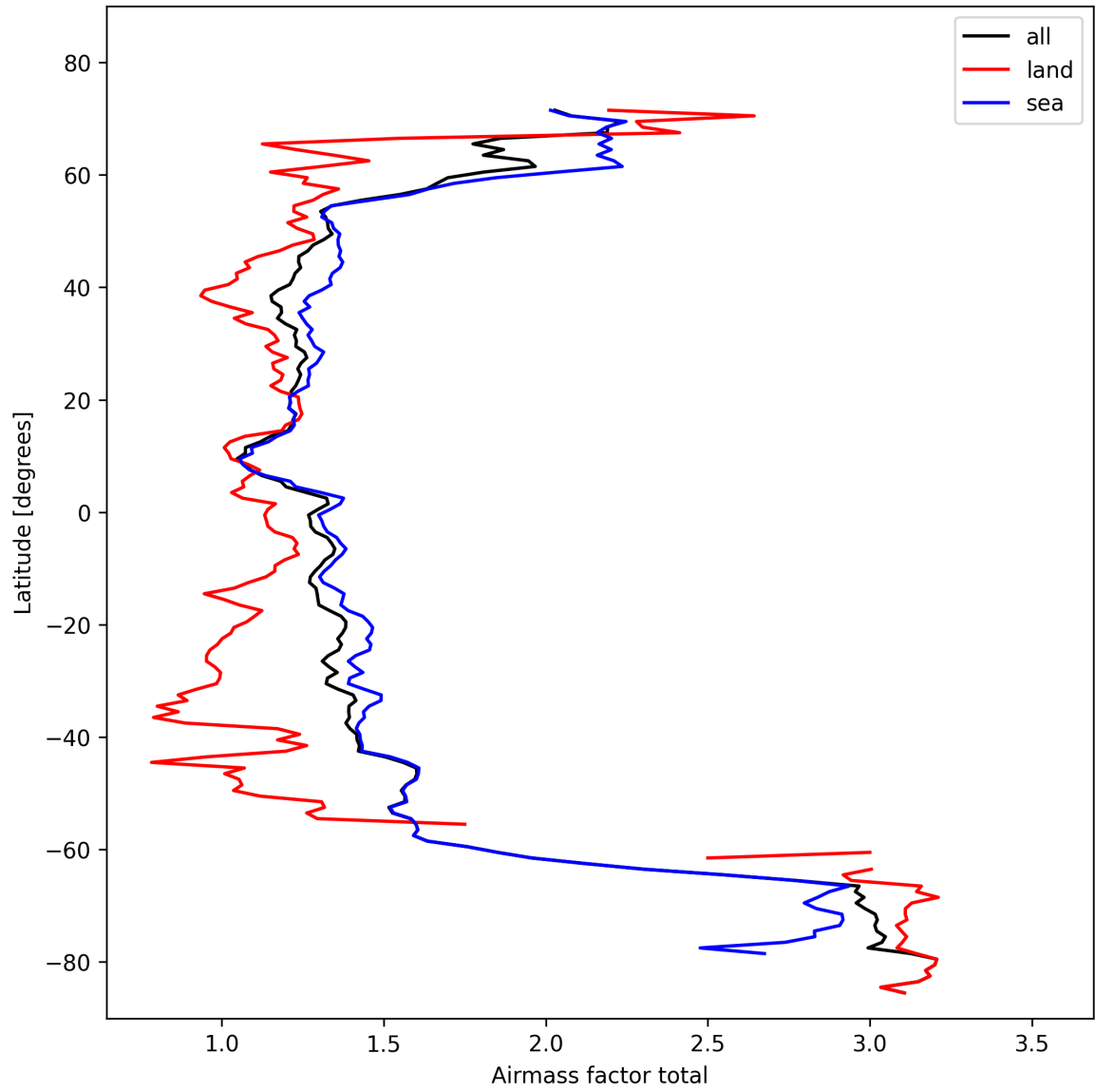
Figure 26: Zonal average of “Airmass factor total” for 2024-10-27 to 2024-10-29.
