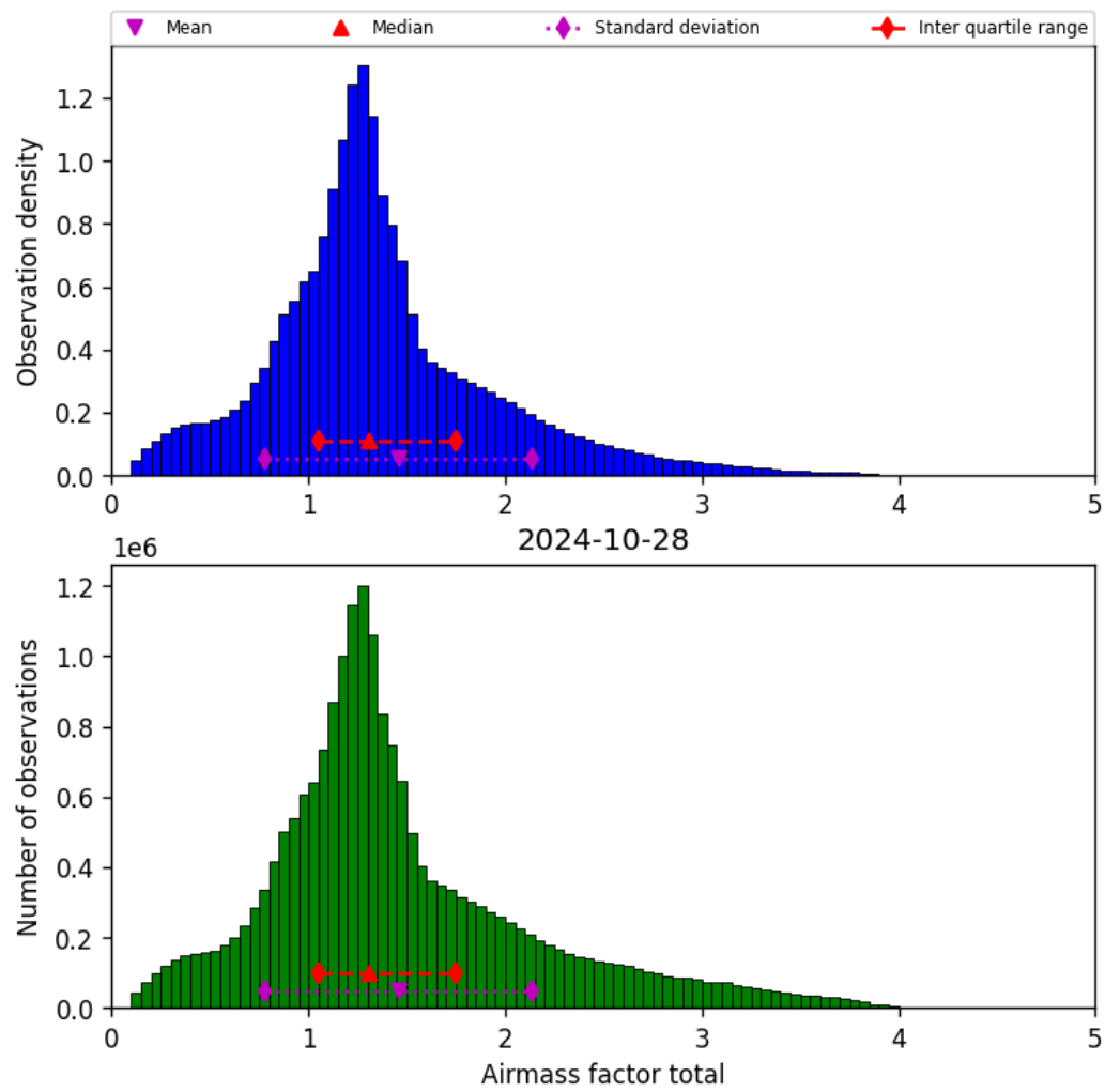
Figure 40: Histogram of “Airmass factor total” for 2024-10-27 to 2024-10-29
