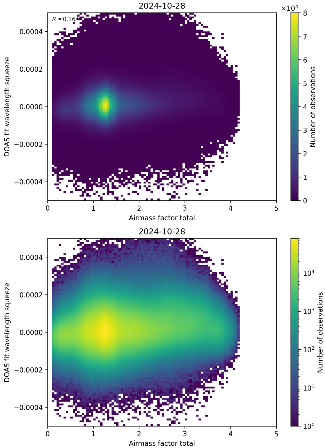
Figure 99: Scatter density plot of “Airmass factor total” against “DOAS fit wavelength squeeze” for 2024-10-27 to 2024-10-29.
