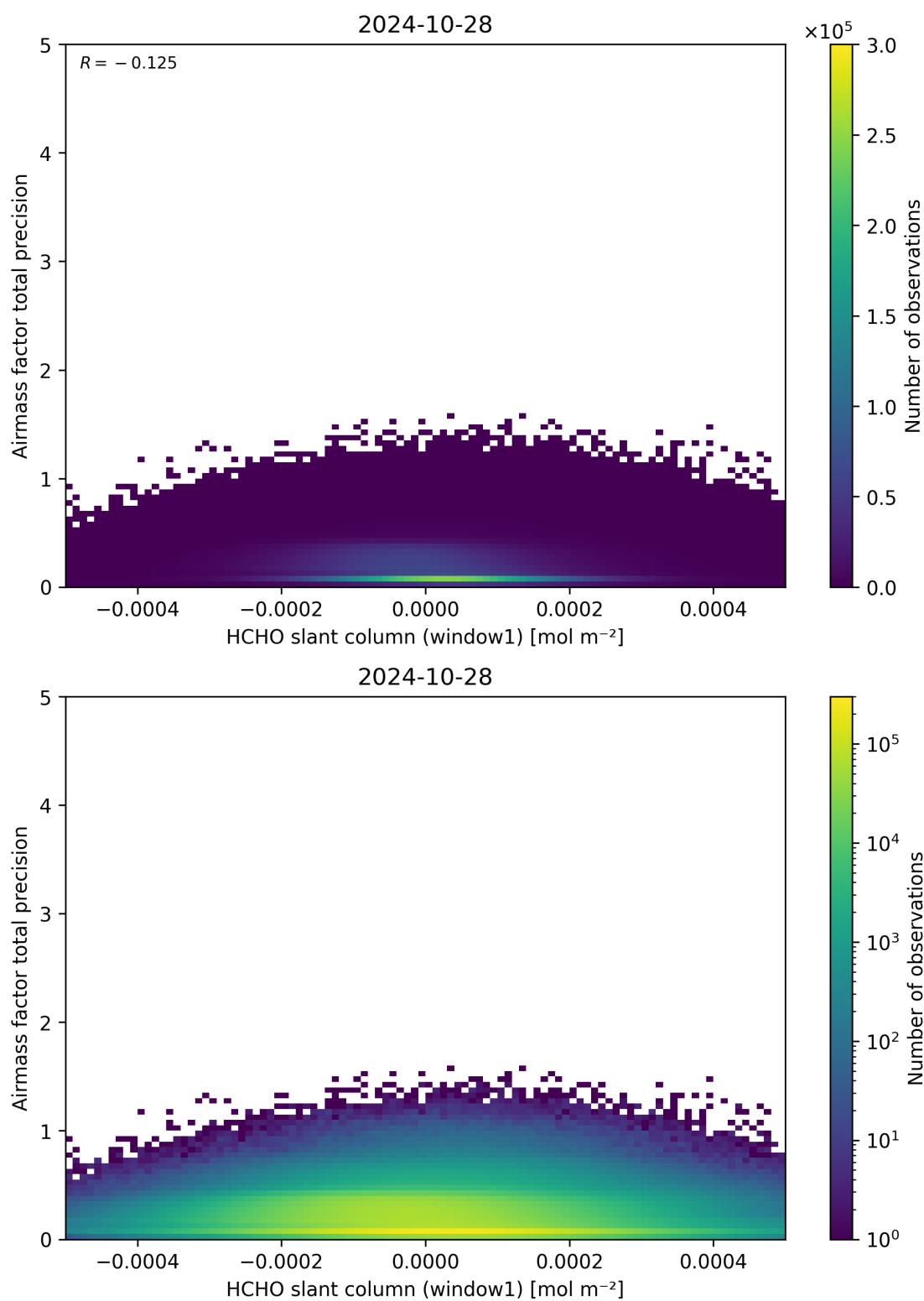
Figure 86: Scatter density plot of “HCHO slant column (window1)” against “Airmass factor total precision” for 2024-10-27 to 2024-10-29.
