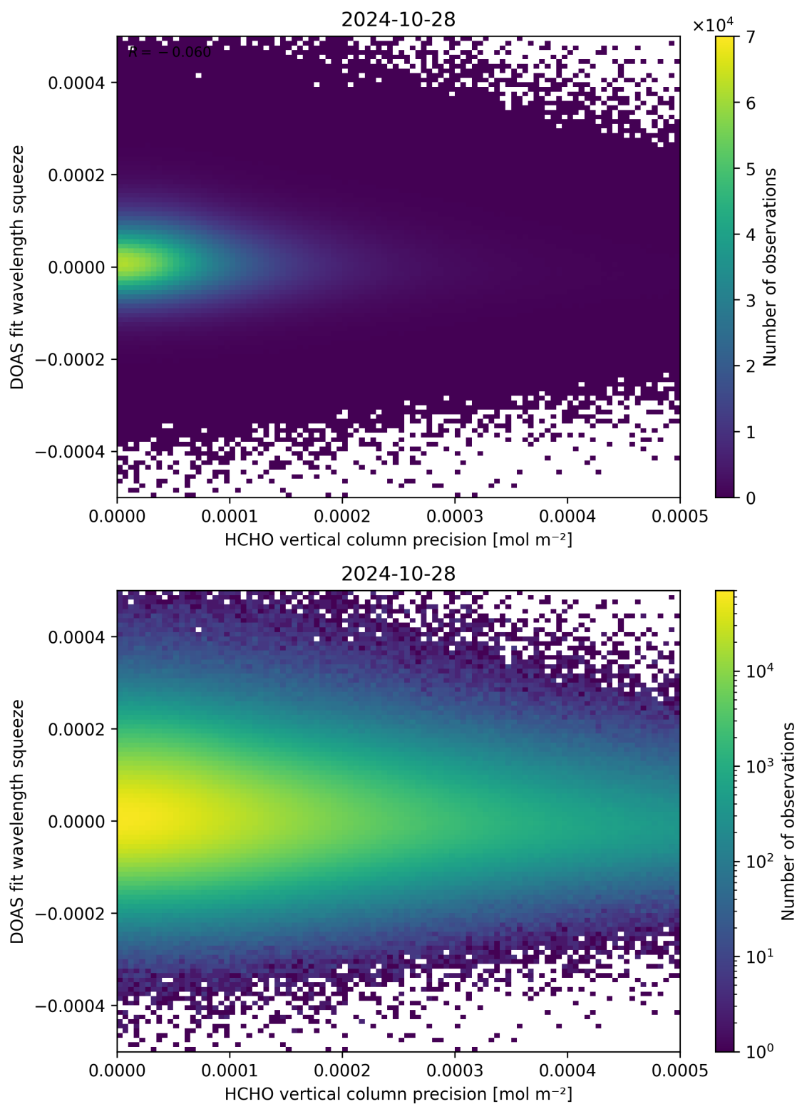
Figure 138: Scatter density plot of “HCHO vertical column precision” against “DOAS fit wavelength squeeze” for 2024-10-27 to 2024-10-29.
