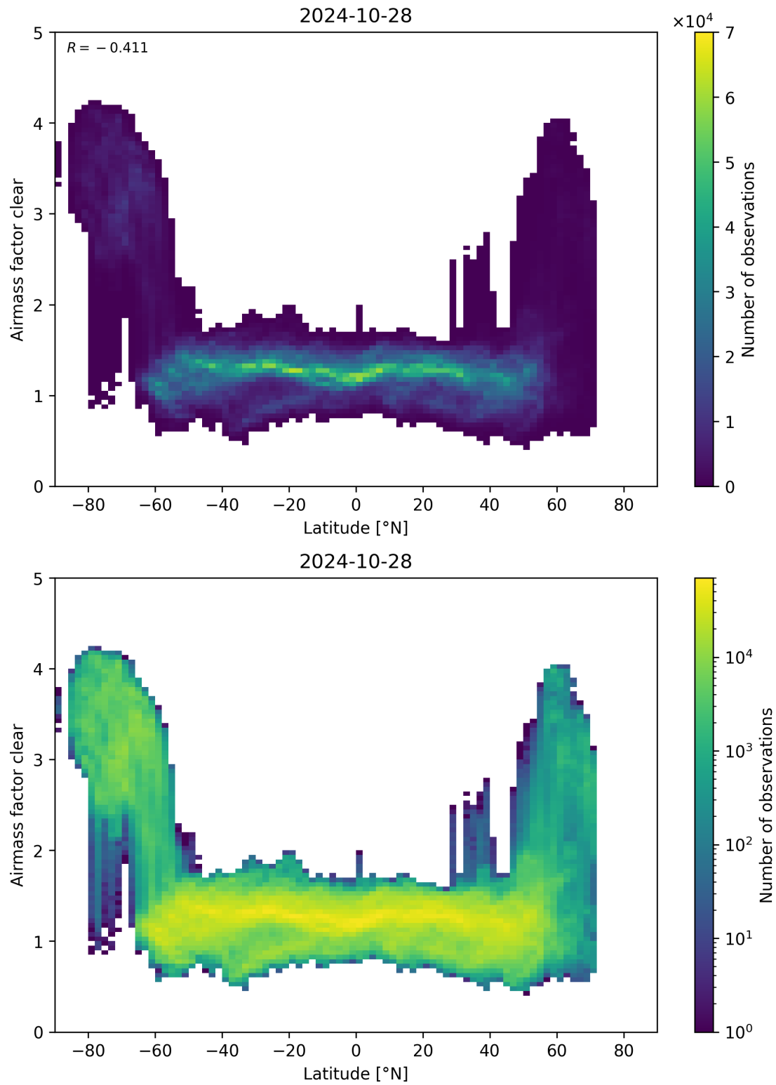
Figure 156: Scatter density plot of “Latitude” against “Airmass factor clear” for 2024-10-27 to 2024-10-29.
