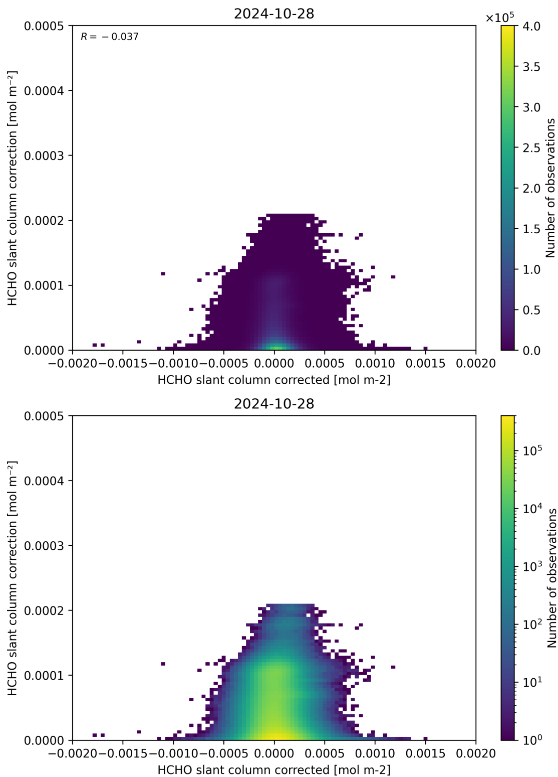
Figure 77: Scatter density plot of “HCHO slant column corrected” against “HCHO slant column correction” for 2024-10-27 to 2024-10-29.
