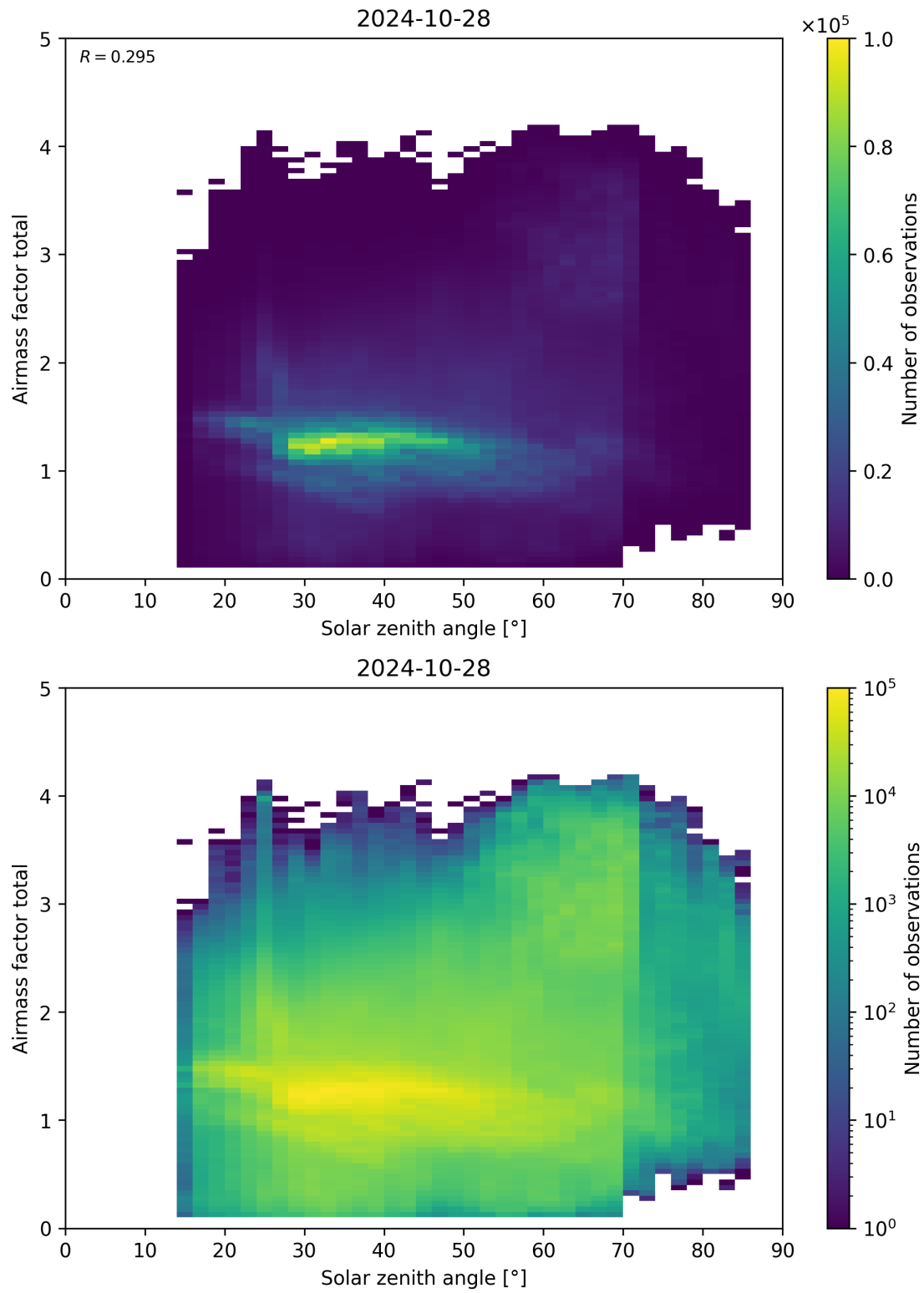
Figure 175: Scatter density plot of “Solar zenith angle” against “Airmass factor total” for 2024-10-27 to 2024-10-29.
