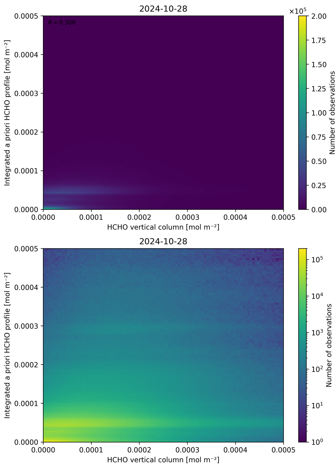
Figure 135: Scatter density plot of “HCHO vertical column” against “Integrated a priori HCHO profile” for 2024-10-27 to 2024-10-29.
