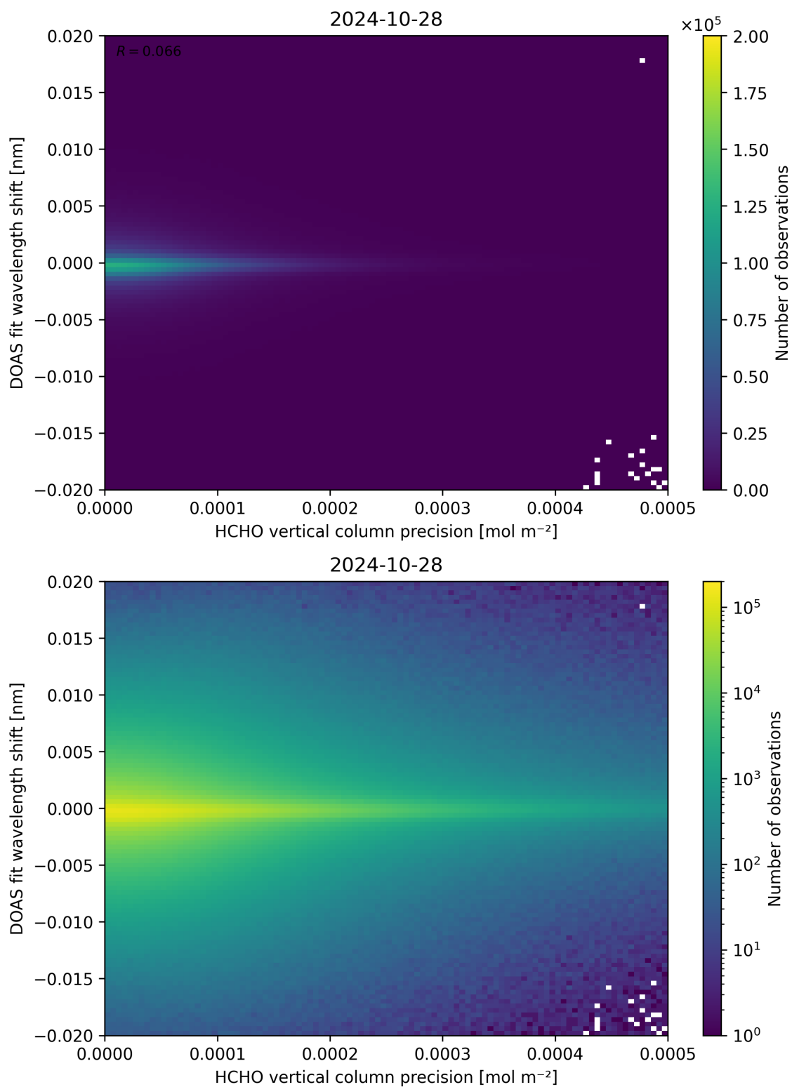
Figure 137: Scatter density plot of “HCHO vertical column precision” against “DOAS fit wavelength shift” for 2024-10-27 to 2024-10-29.
