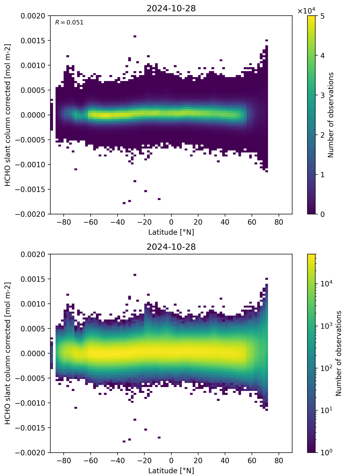
Figure 157: Scatter density plot of “Latitude” against “HCHO slant column corrected” for 2024-10-27 to 2024-10-29.
