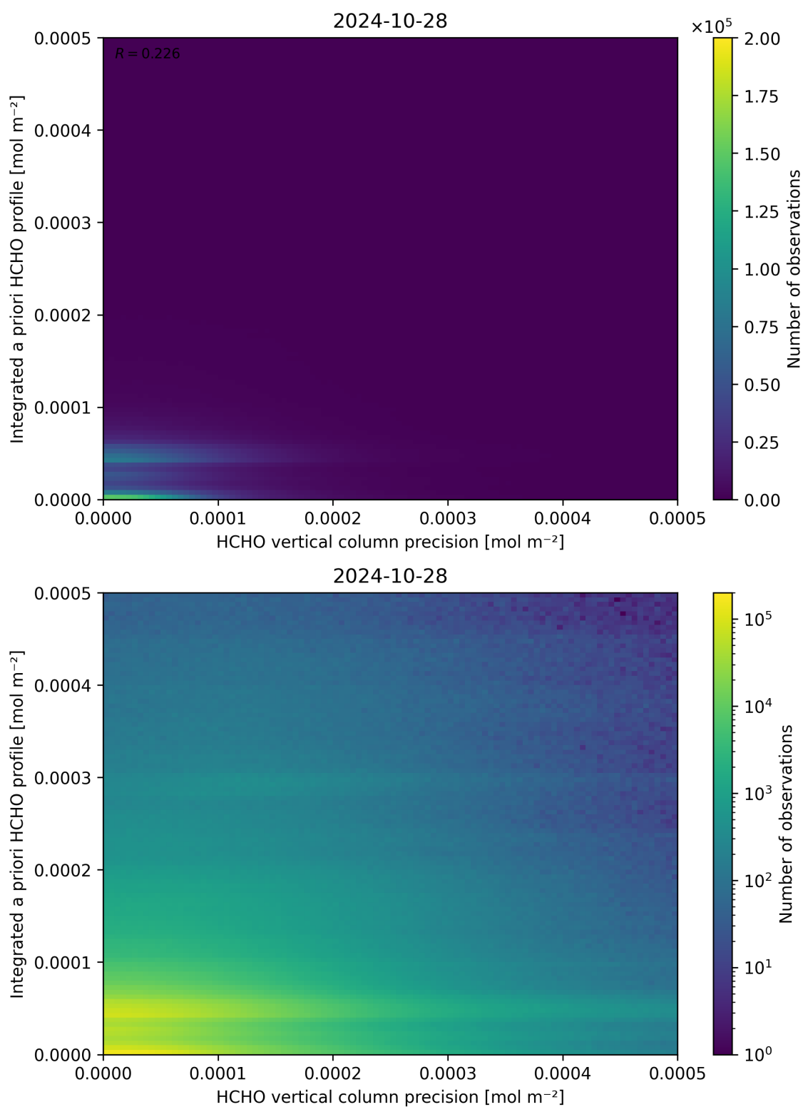
Figure 147: Scatter density plot of “HCHO vertical column precision” against “Integrated a priori HCHO profile” for 2024-10-27 to 2024-10-29.
