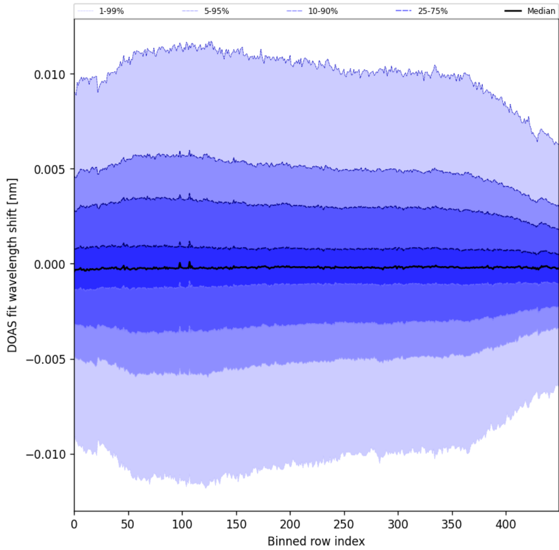
Figure 58: Along track statistics of “DOAS fit wavelength shift” for 2024-10-27 to 2024-10-29
