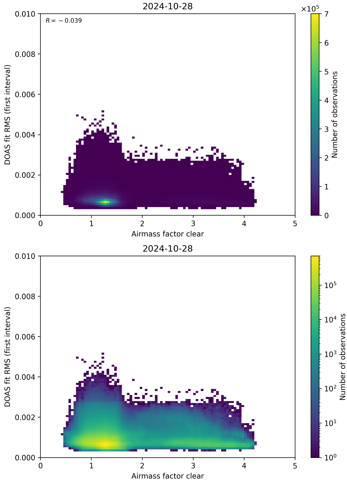
Figure 71: Scatter density plot of “Airmass factor clear” against “DOAS fit RMS (first interval)” for 2024-10-27 to 2024-10-29.
