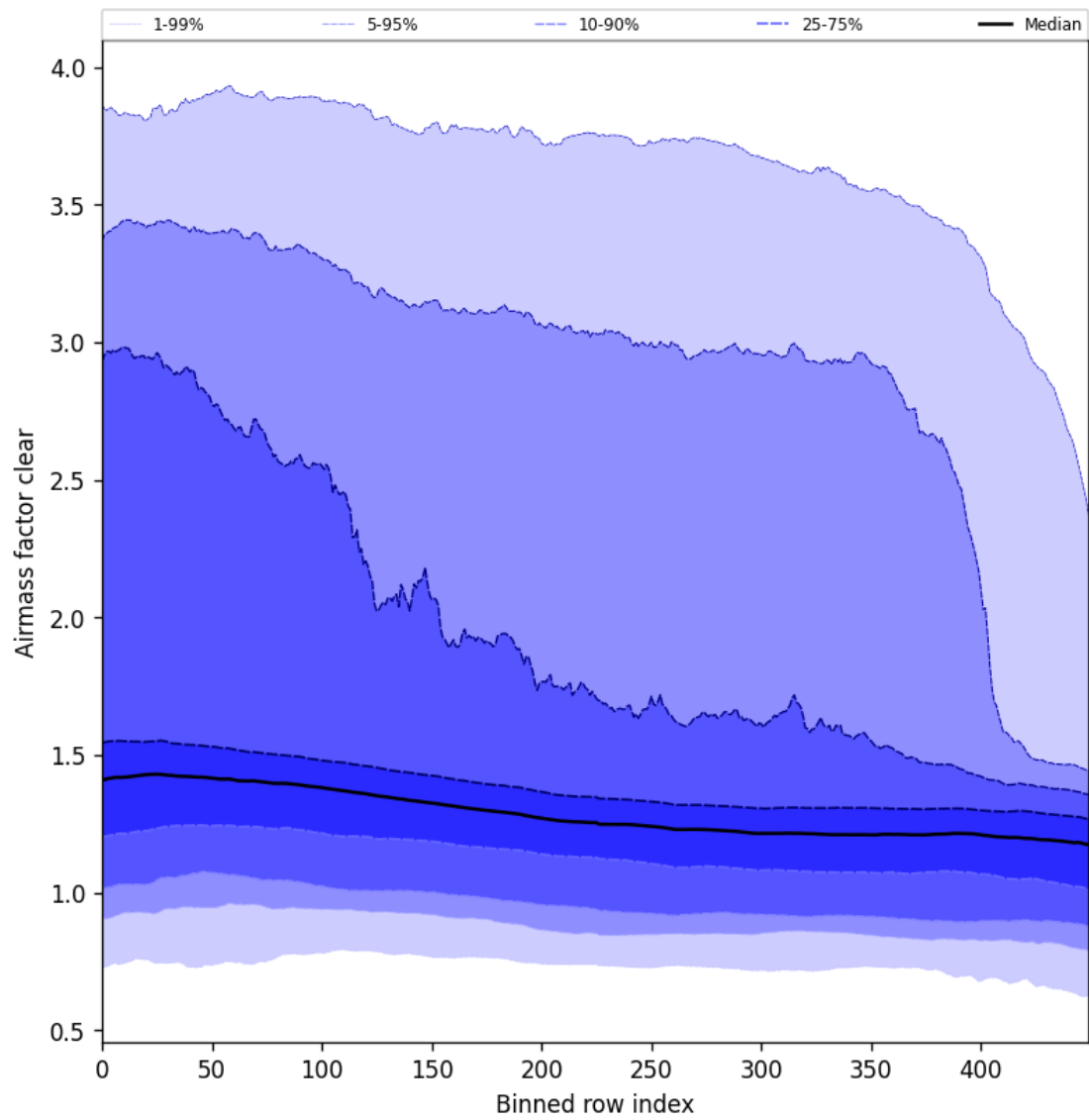
Figure 56: Along track statistics of “Airmass factor clear” for 2024-10-27 to 2024-10-29
