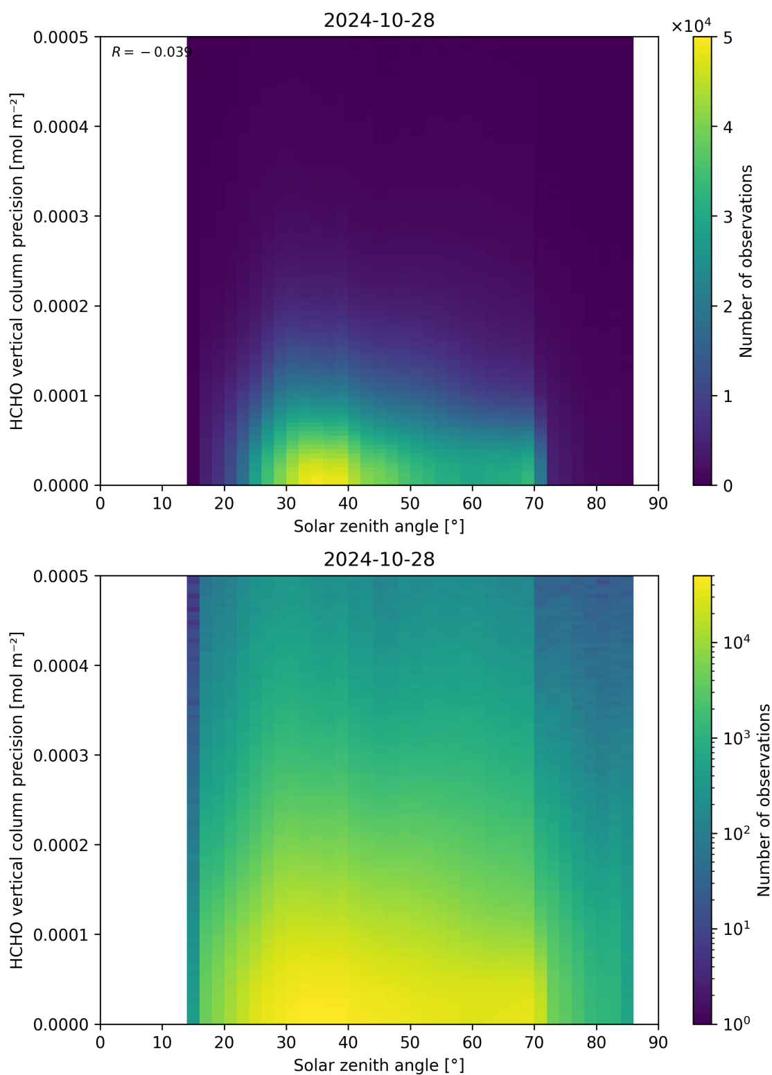
Figure 179: Scatter density plot of “Solar zenith angle” against “HCHO vertical column precision” for 2024-10-27 to 2024-10-29.
