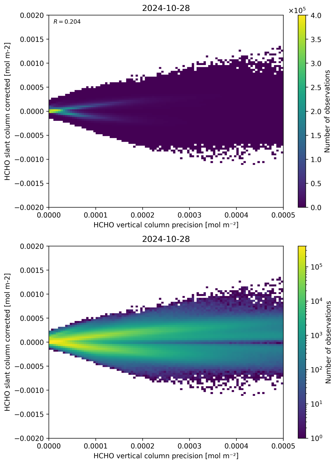
Figure 140: Scatter density plot of “HCHO vertical column precision” against “HCHO slant column corrected” for 2024-10-27 to 2024-10-29.
