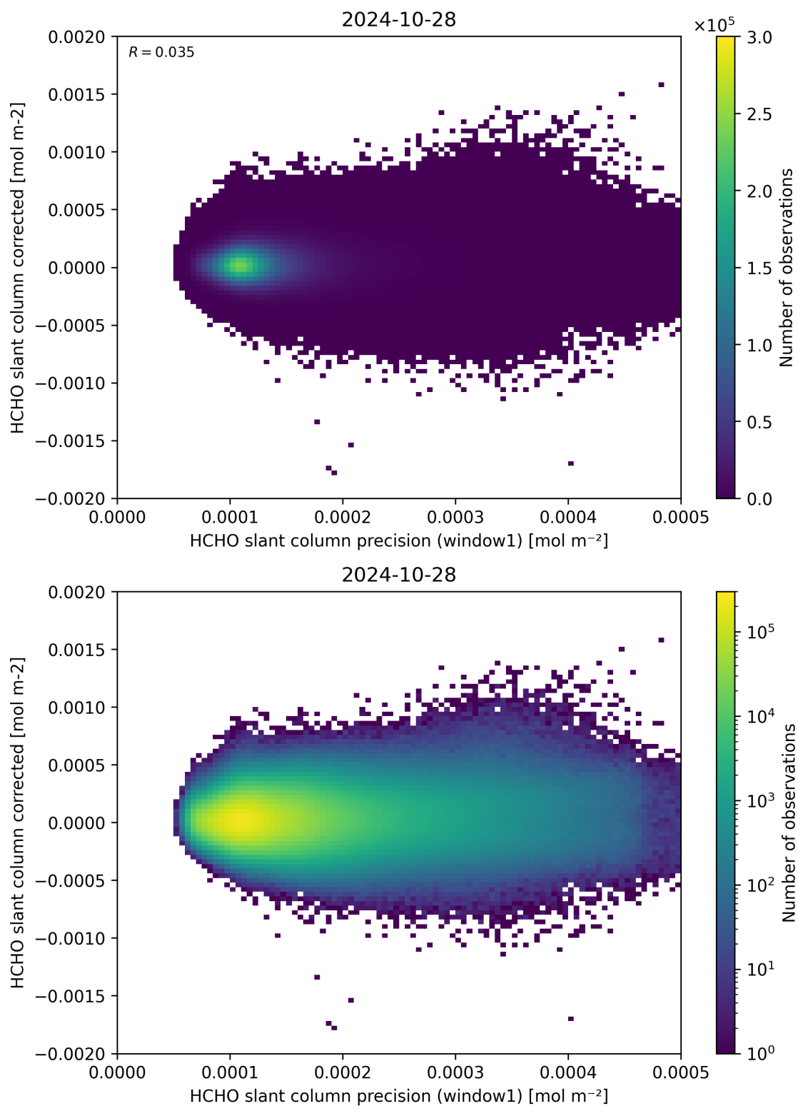
Figure 92: Scatter density plot of “HCHO slant column precision (window1)” against “HCHO slant column corrected” for 2024-10-27 to 2024-10-29.
