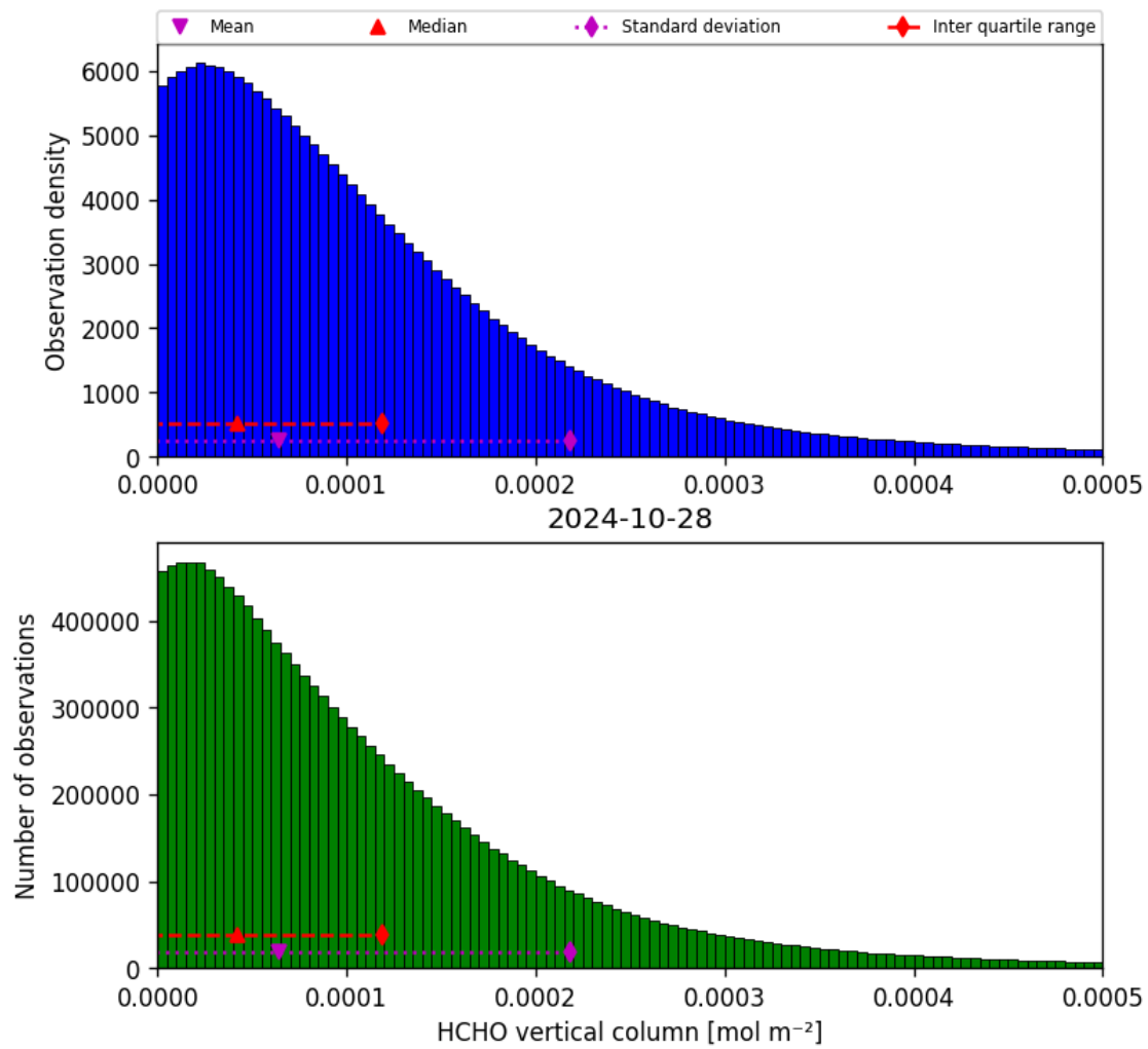
Figure 35: Histogram of “HCHO vertical column” for 2024-10-27 to 2024-10-29
