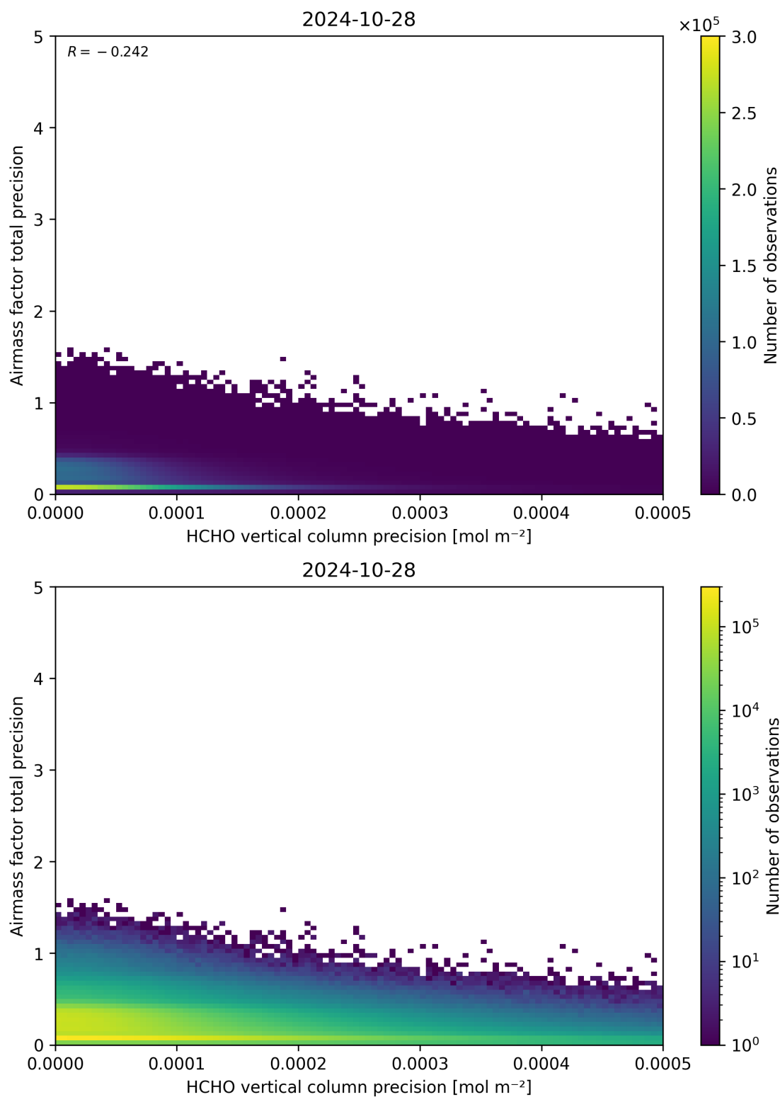
Figure 145: Scatter density plot of “HCHO vertical column precision” against “Airmass factor total precision” for 2024-10-27 to 2024-10-29.
