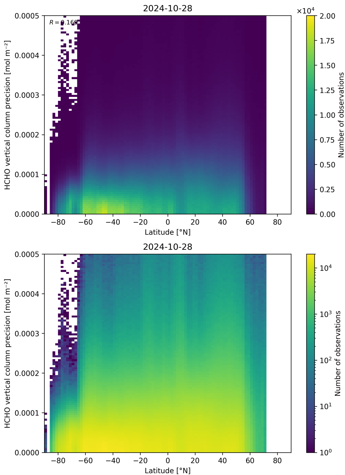
Figure 165: Scatter density plot of “Latitude” against “HCHO vertical column precision” for 2024-10-27 to 2024-10-29.
