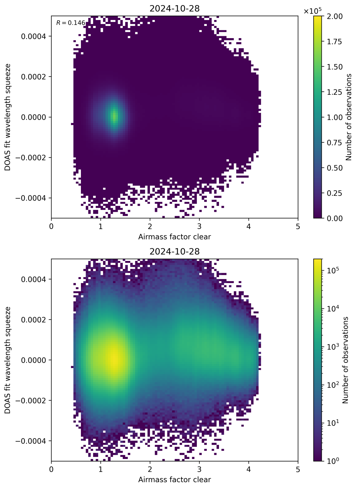
Figure 73: Scatter density plot of “Airmass factor clear” against “DOAS fit wavelength squeeze” for 2024-10-27 to 2024-10-29.
