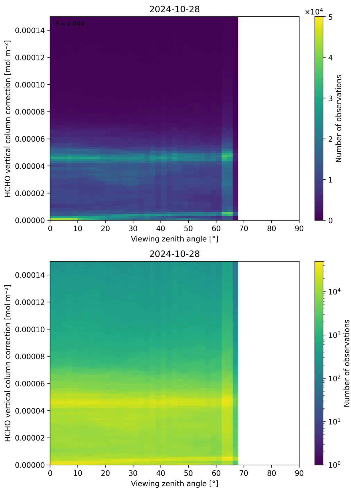
Figure 193: Scatter density plot of “Viewing zenith angle” against “HCHO vertical column correction” for 2024-10-27 to 2024-10-29.
