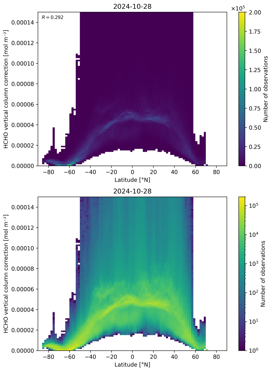
Figure 164: Scatter density plot of “Latitude” against “HCHO vertical column correction” for 2024-10-27 to 2024-10-29.
