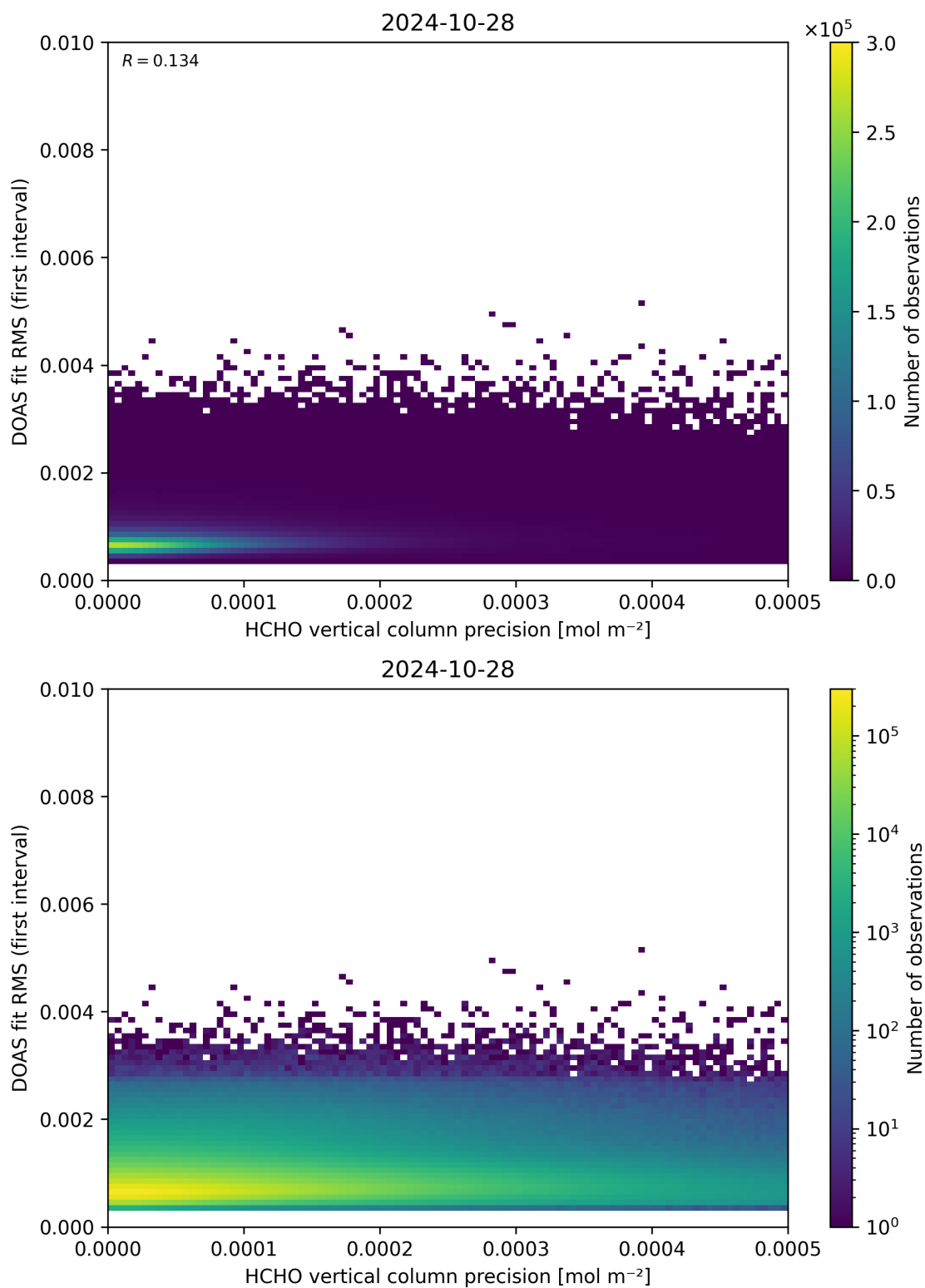
Figure 136: Scatter density plot of “HCHO vertical column precision” against “DOAS fit RMS (first interval)” for 2024-10-27 to 2024-10-29.
