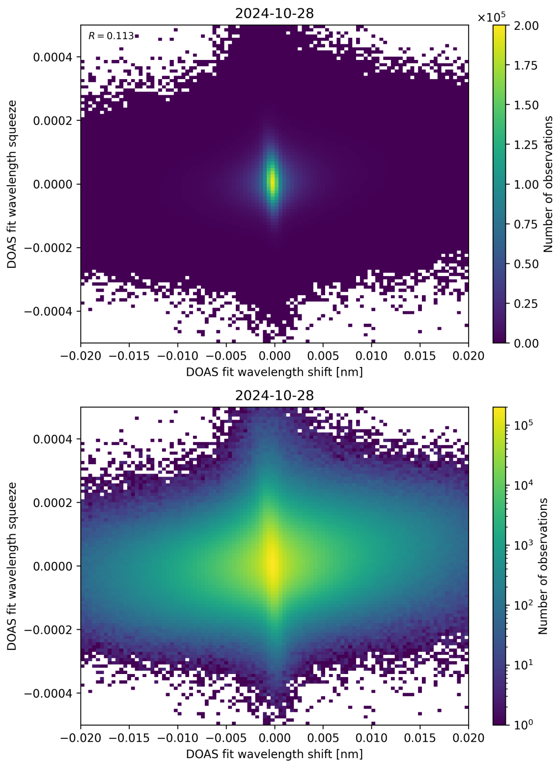
Figure 65: Scatter density plot of “DOAS fit wavelength shift” against “DOAS fit wavelength squeeze” for 2024-10-27 to 2024-10-29.
