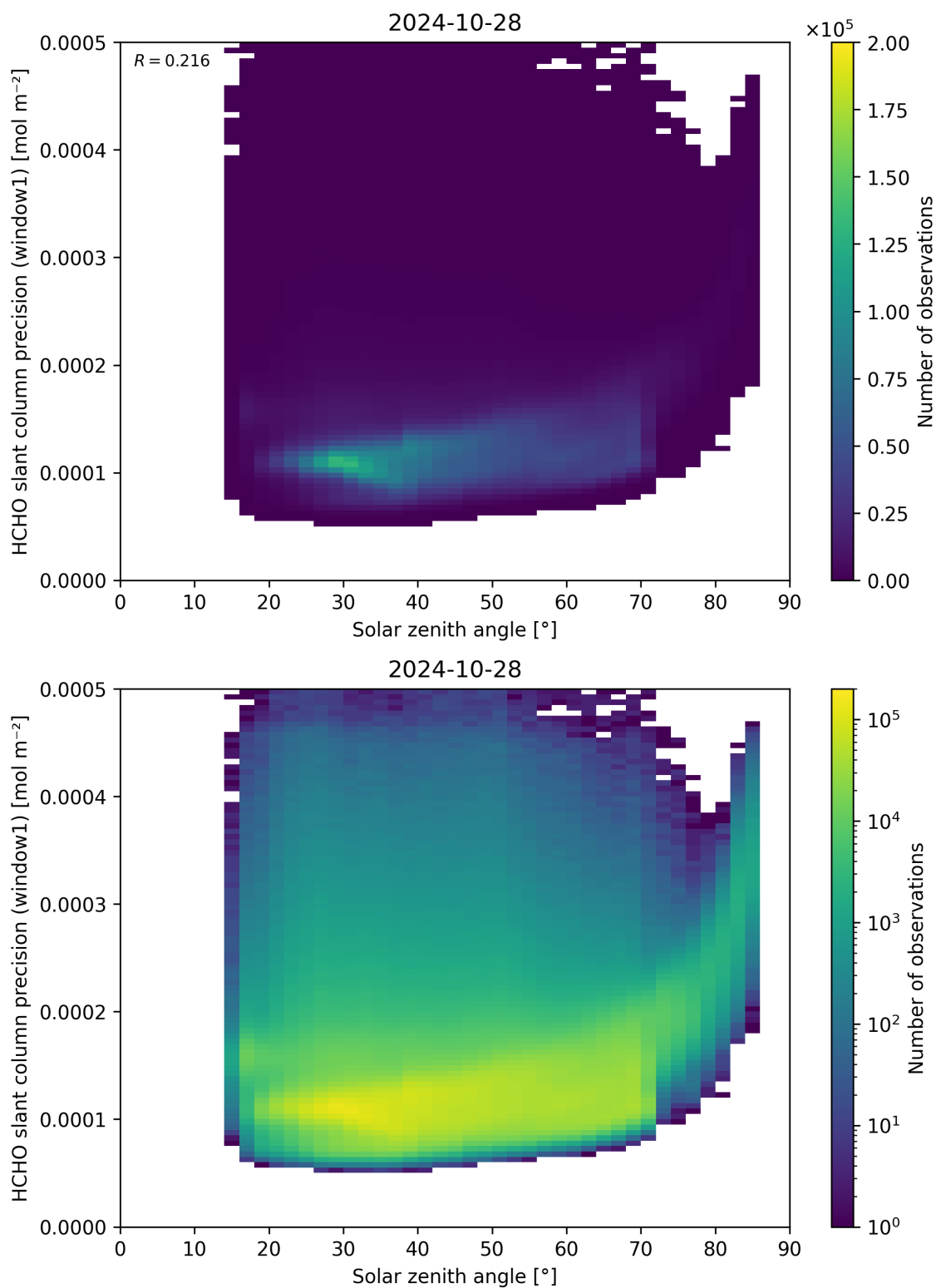
Figure 174: Scatter density plot of “Solar zenith angle” against “HCHO slant column precision (window1)” for 2024-10-27 to 2024-10-29.
