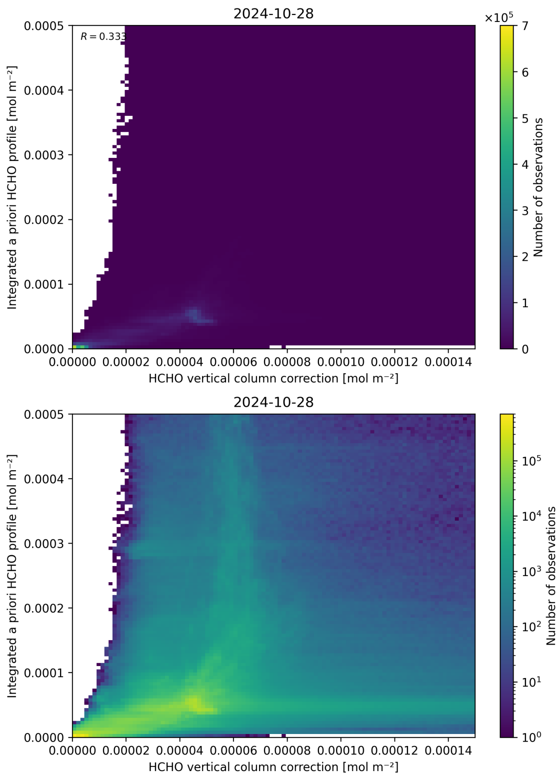
Figure 122: Scatter density plot of “HCHO vertical column correction” against “Integrated a priori HCHO profile” for 2024-10-27 to 2024-10-29.
