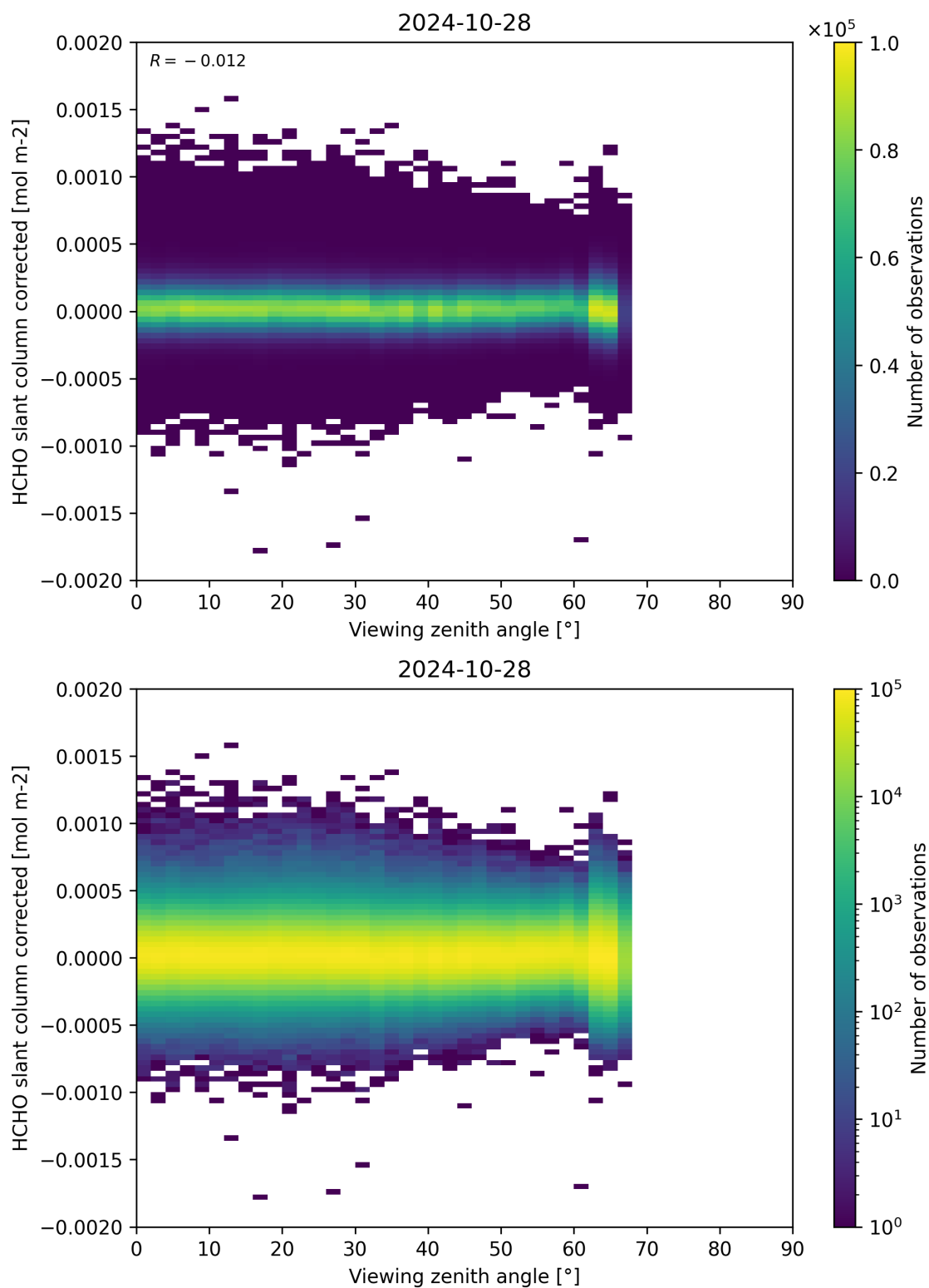
Figure 186: Scatter density plot of “Viewing zenith angle” against “HCHO slant column corrected” for 2024-10-27 to 2024-10-29.
