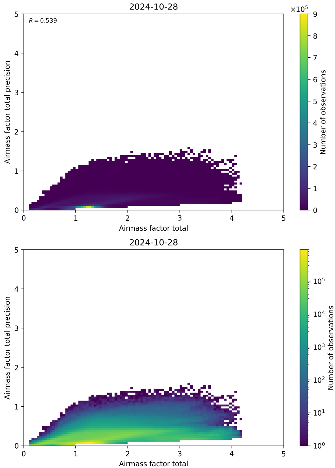
Figure 103: Scatter density plot of “Airmass factor total” against “Airmass factor total precision” for 2024-10-27 to 2024-10-29.
