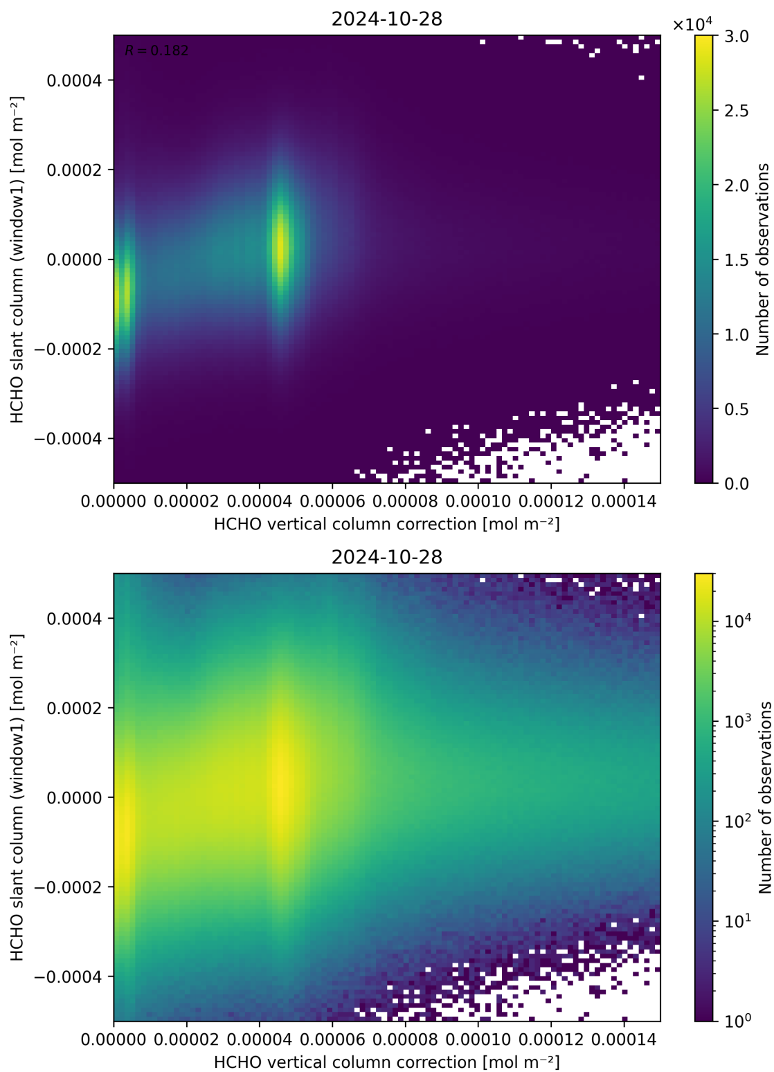
Figure 118: Scatter density plot of “HCHO vertical column correction” against “HCHO slant column (window1)” for 2024-10-27 to 2024-10-29.
