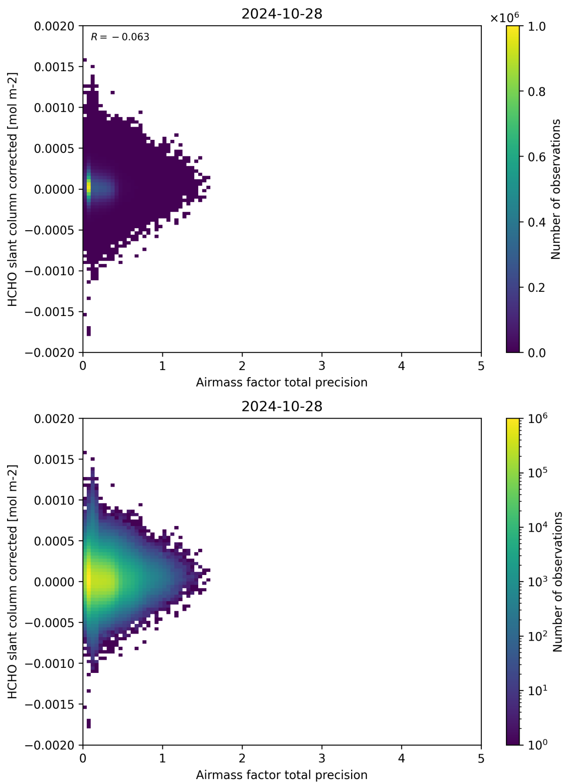
Figure 109: Scatter density plot of “Airmass factor total precision” against “HCHO slant column corrected” for 2024-10-27 to 2024-10-29.
