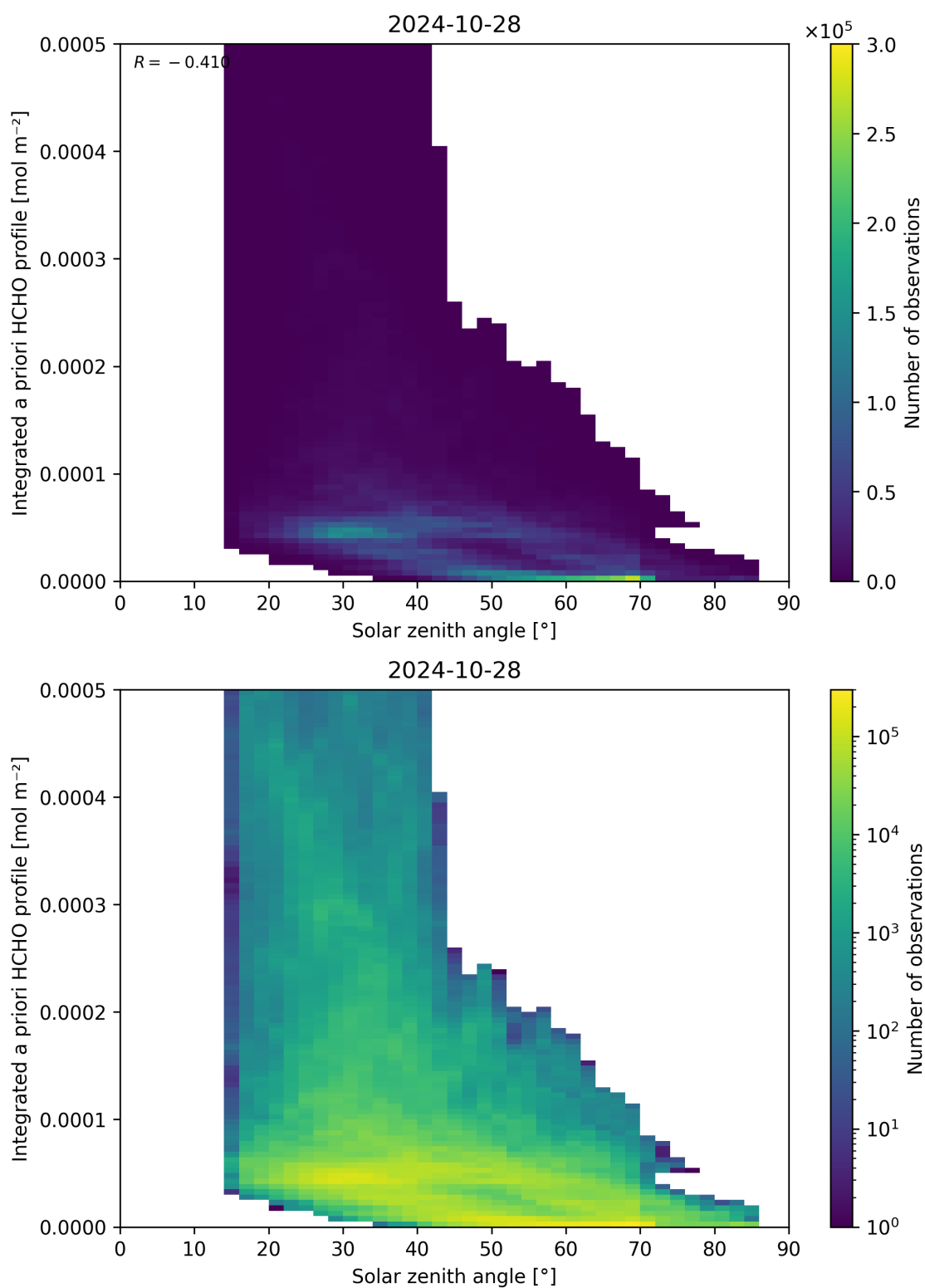
Figure 180: Scatter density plot of “Solar zenith angle” against “Integrated a priori HCHO profile” for 2024-10-27 to 2024-10-29.
