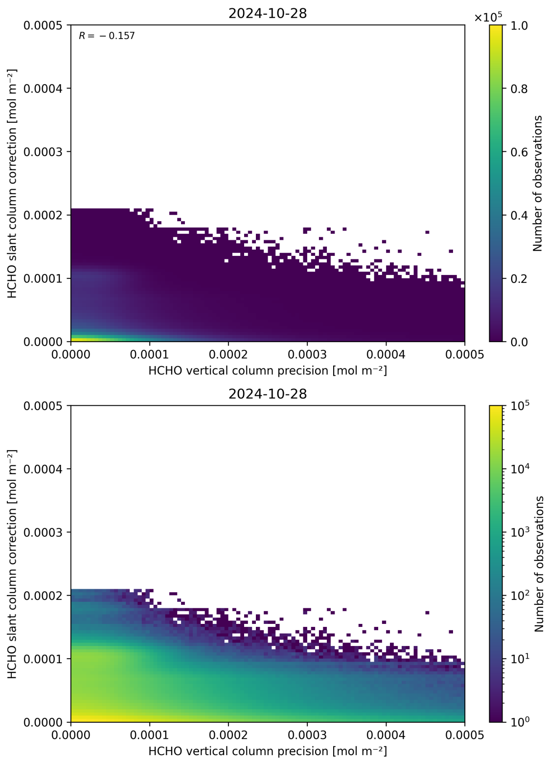
Figure 141: Scatter density plot of “HCHO vertical column precision” against “HCHO slant column correction” for 2024-10-27 to 2024-10-29.
