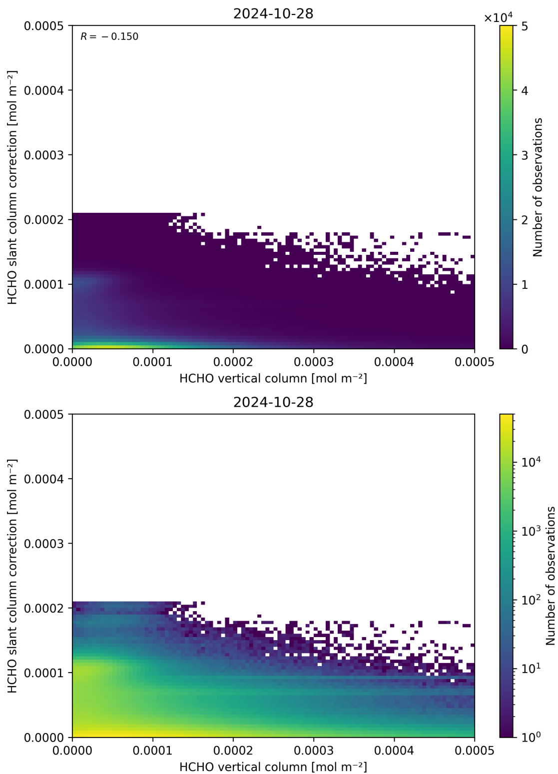
Figure 128: Scatter density plot of “HCHO vertical column” against “HCHO slant column correction” for 2024-10-27 to 2024-10-29.
