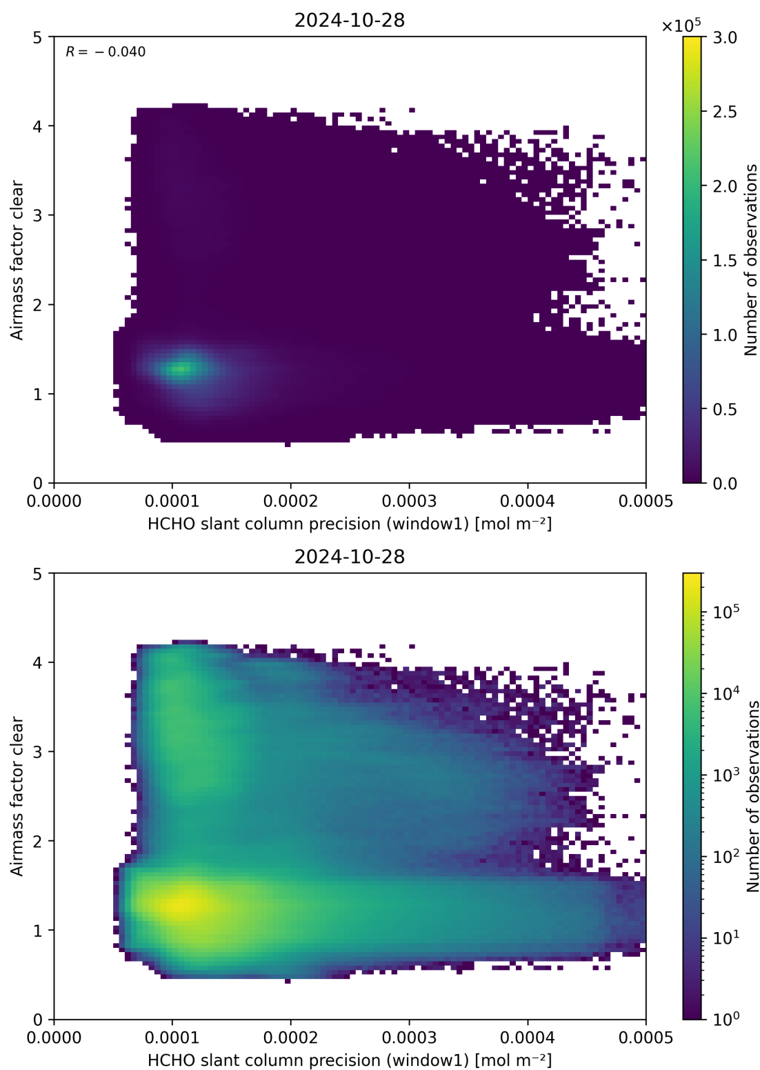
Figure 91: Scatter density plot of “HCHO slant column precision (window1)” against “Airmass factor clear” for 2024-10-27 to 2024-10-29.
