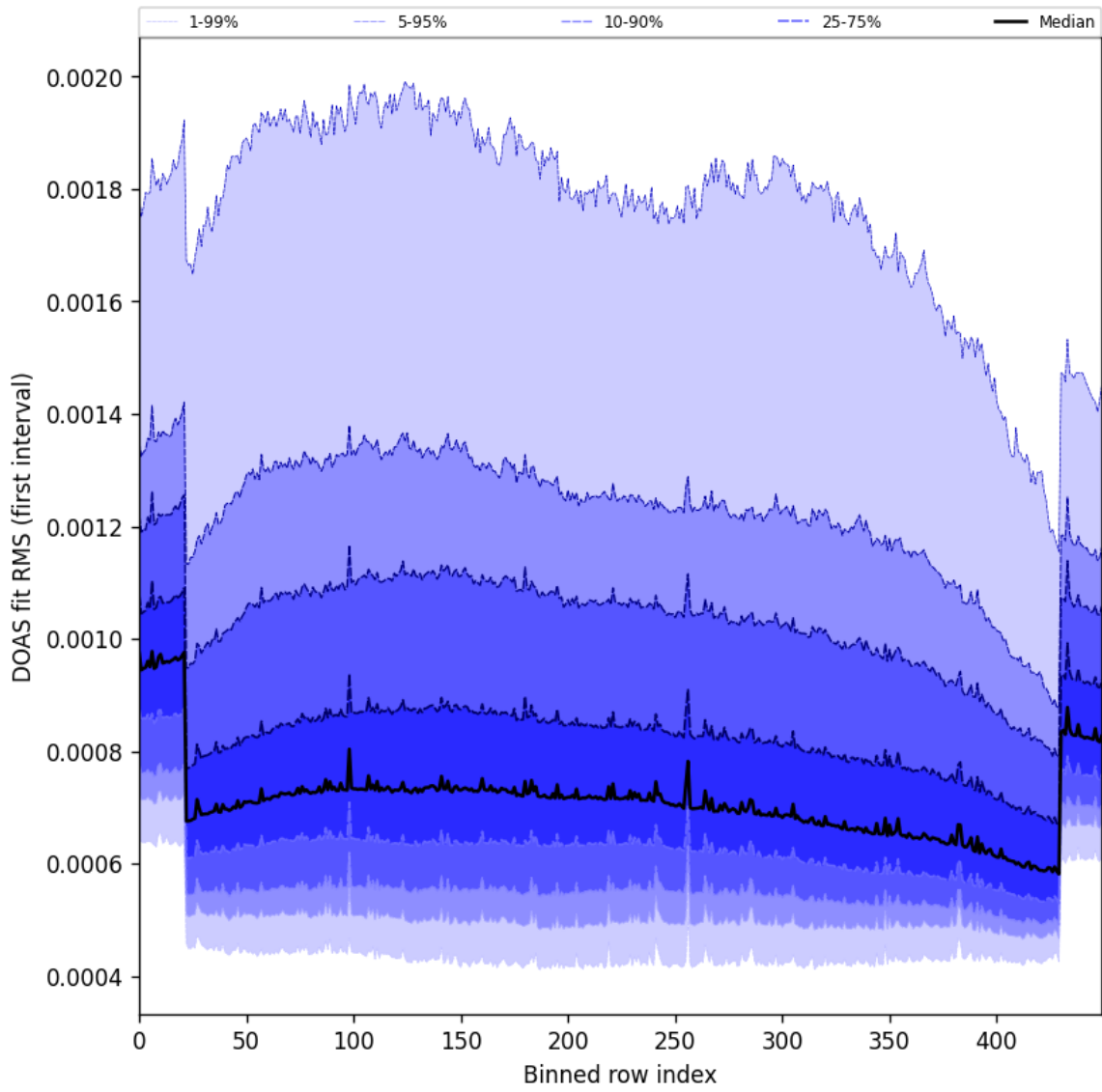
Figure 60: Along track statistics of “DOAS fit RMS (first interval)” for 2024-10-27 to 2024-10-29
