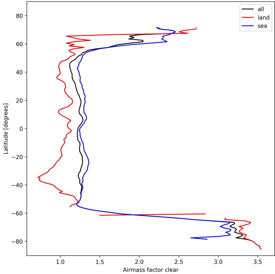
Figure 28: Zonal average of “Airmass factor clear” for 2024-10-27 to 2024-10-29.
