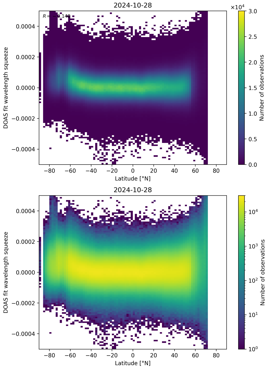
Figure 155: Scatter density plot of “Latitude” against “DOAS fit wavelength squeeze” for 2024-10-27 to 2024-10-29.
