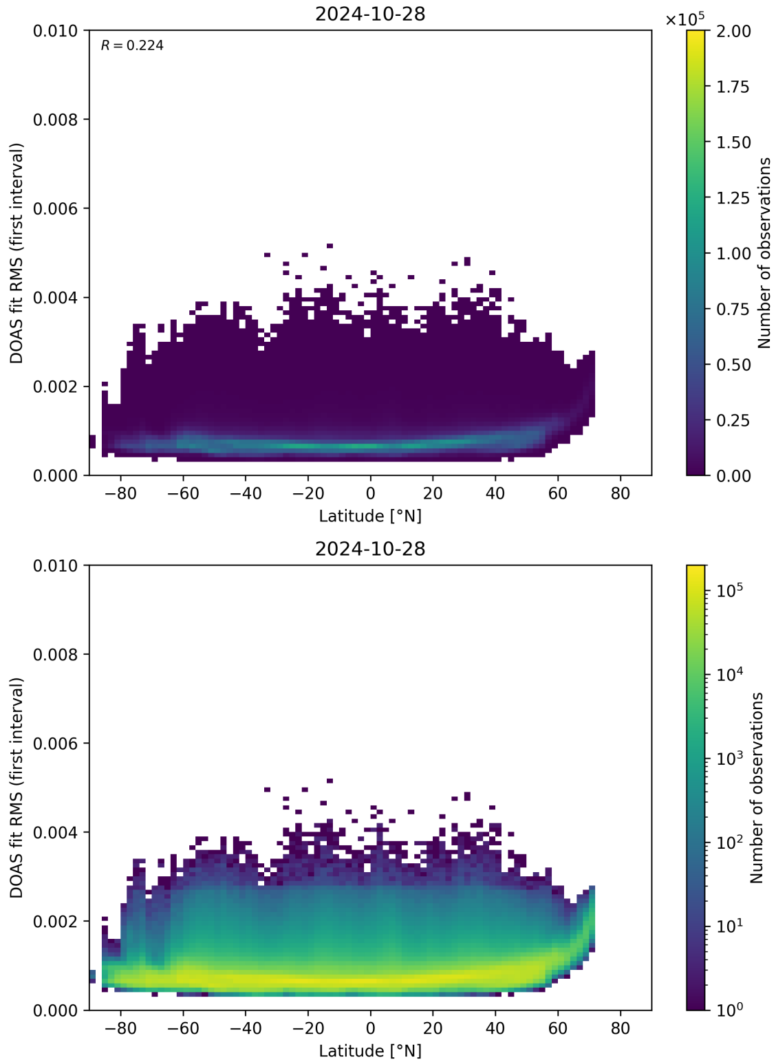
Figure 153: Scatter density plot of “Latitude” against “DOAS fit RMS (first interval)” for 2024-10-27 to 2024-10-29.
