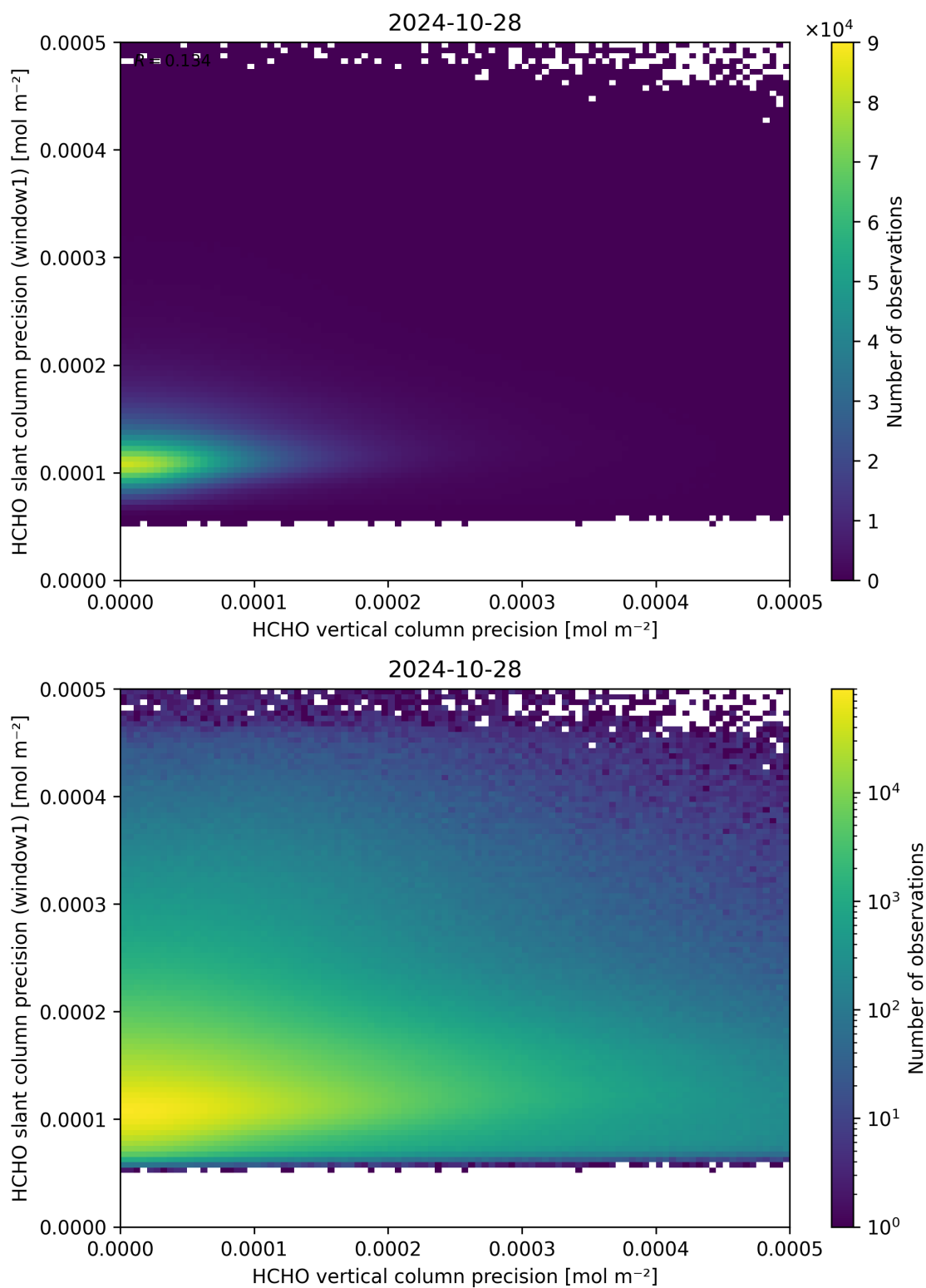
Figure 143: Scatter density plot of “HCHO vertical column precision” against “HCHO slant column precision (window1)” for 2024-10-27 to 2024-10-29.
