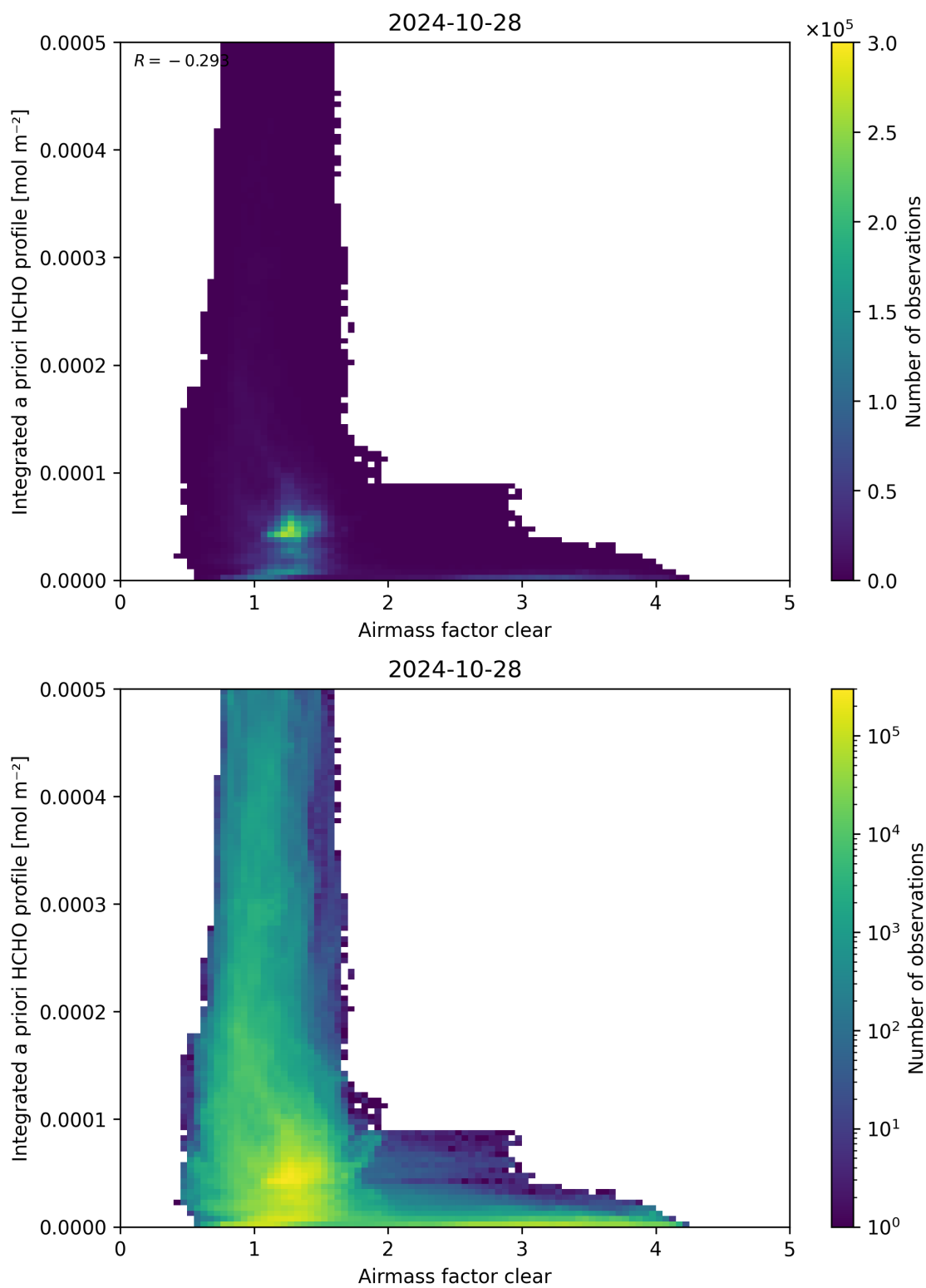
Figure 76: Scatter density plot of “Airmass factor clear” against “Integrated a priori HCHO profile” for 2024-10-27 to 2024-10-29.
