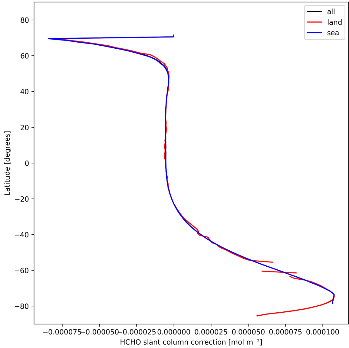
Figure 33: Zonal average of “HCHO slant column correction” for 2024-10-27 to 2024-10-29.
