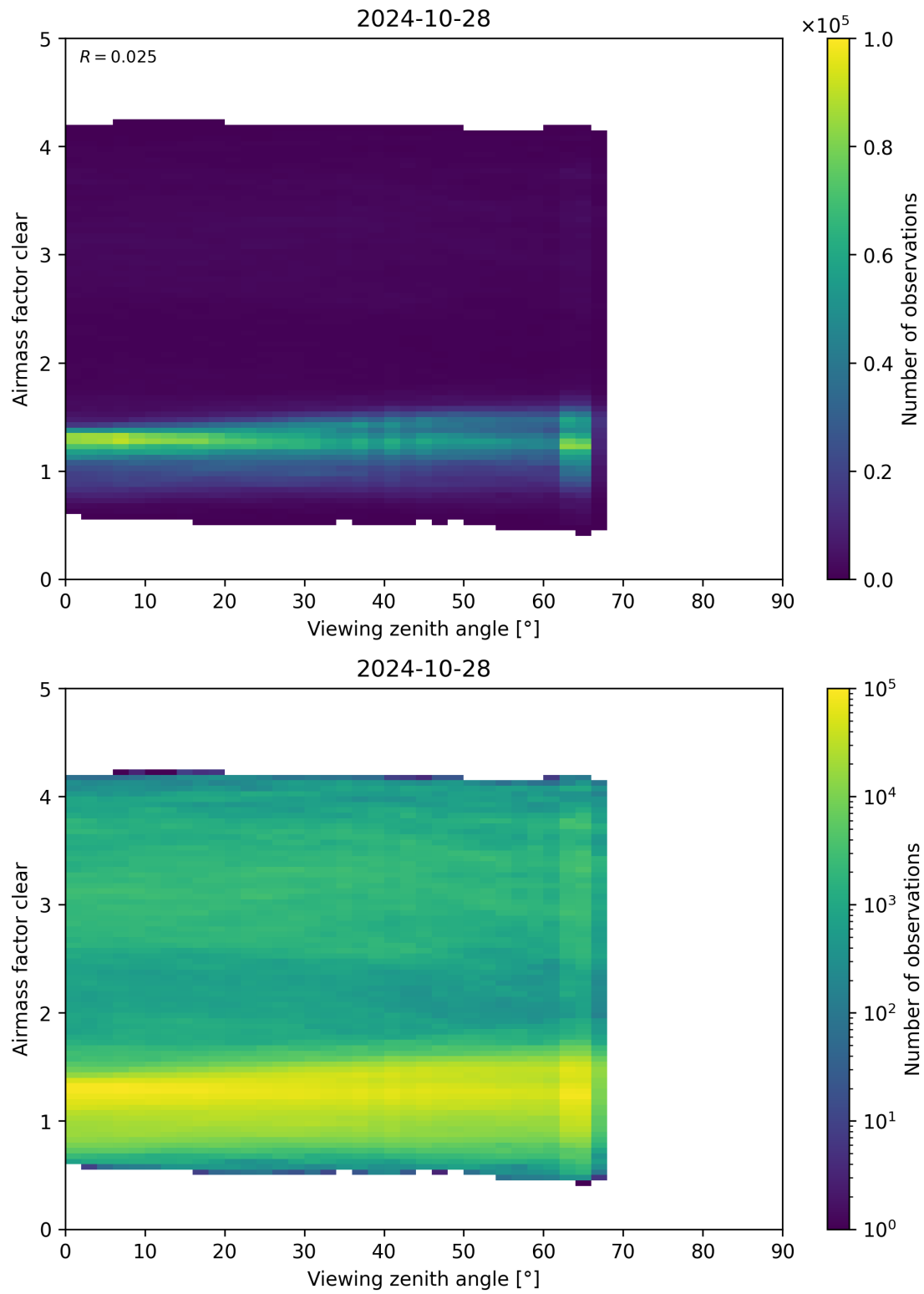
Figure 185: Scatter density plot of “Viewing zenith angle” against “Airmass factor clear” for 2024-10-27 to 2024-10-29.
