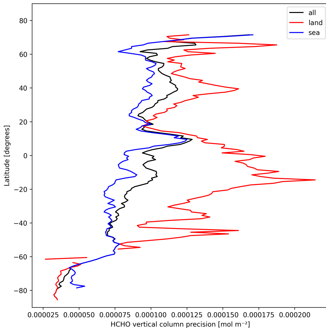
Figure 22: Zonal average of “HCHO vertical column precision” for 2024-10-27 to 2024-10-29.
