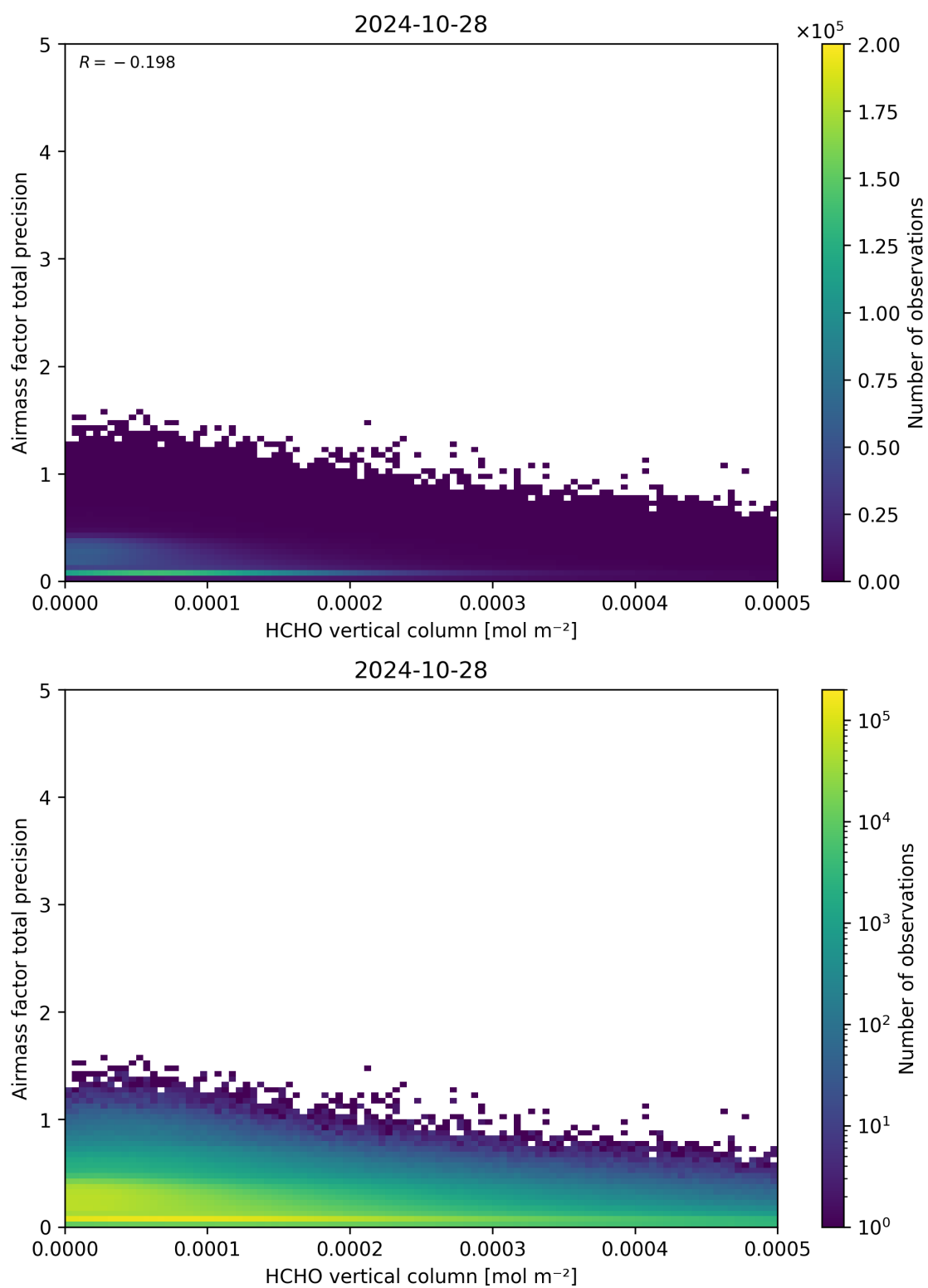
Figure 132: Scatter density plot of “HCHO vertical column” against “Airmass factor total precision” for 2024-10-27 to 2024-10-29.
