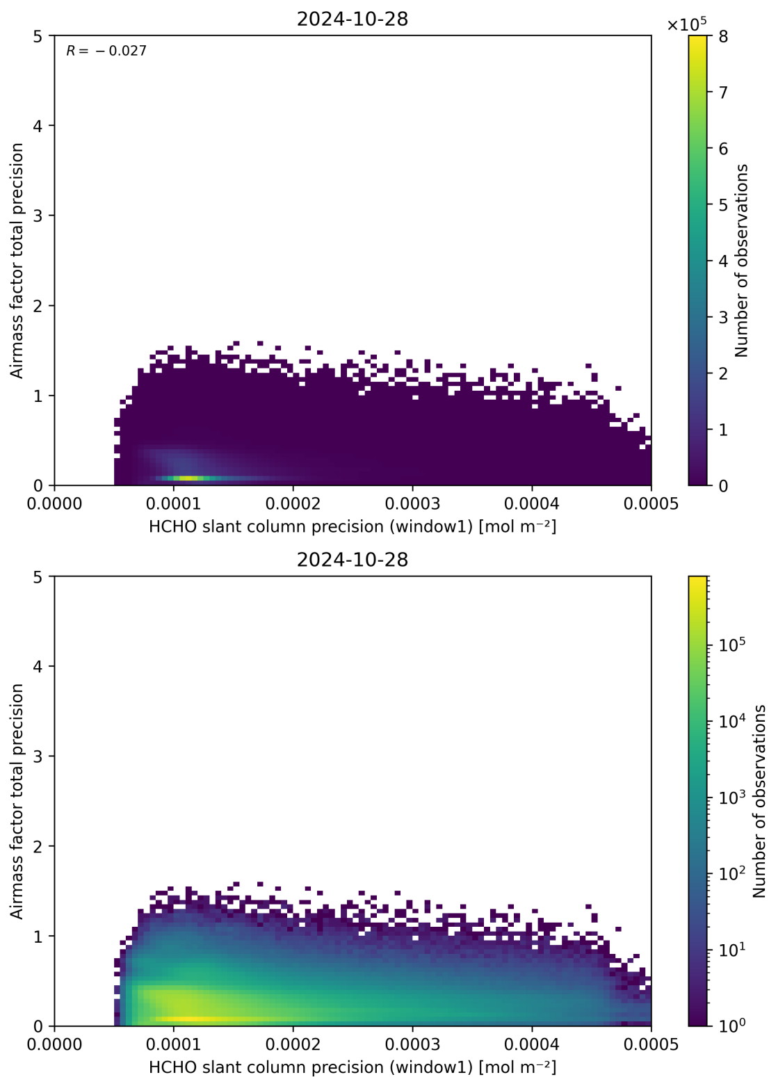
Figure 95: Scatter density plot of “HCHO slant column precision (window1)” against “Airmass factor total precision” for 2024-10-27 to 2024-10-29.
