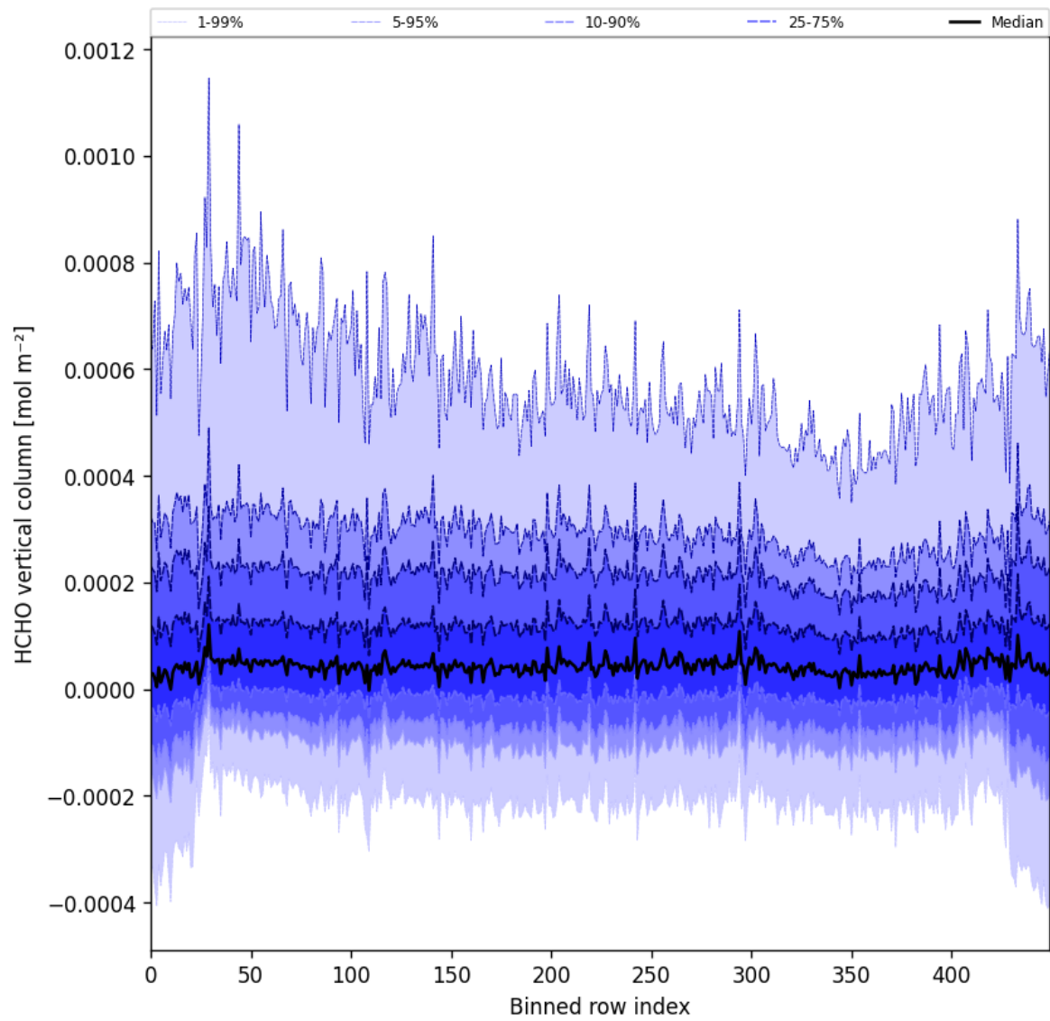
Figure 49: Along track statistics of “HCHO vertical column” for 2024-10-27 to 2024-10-29
