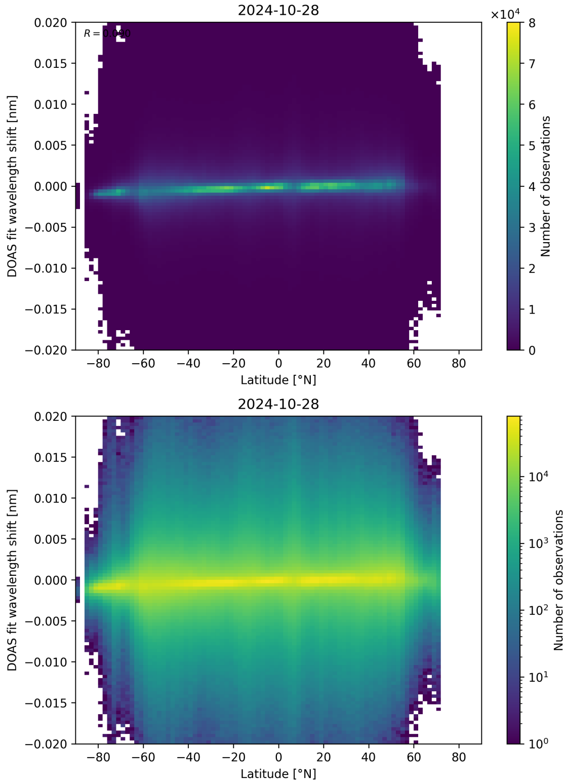
Figure 154: Scatter density plot of “Latitude” against “DOAS fit wavelength shift” for 2024-10-27 to 2024-10-29.
