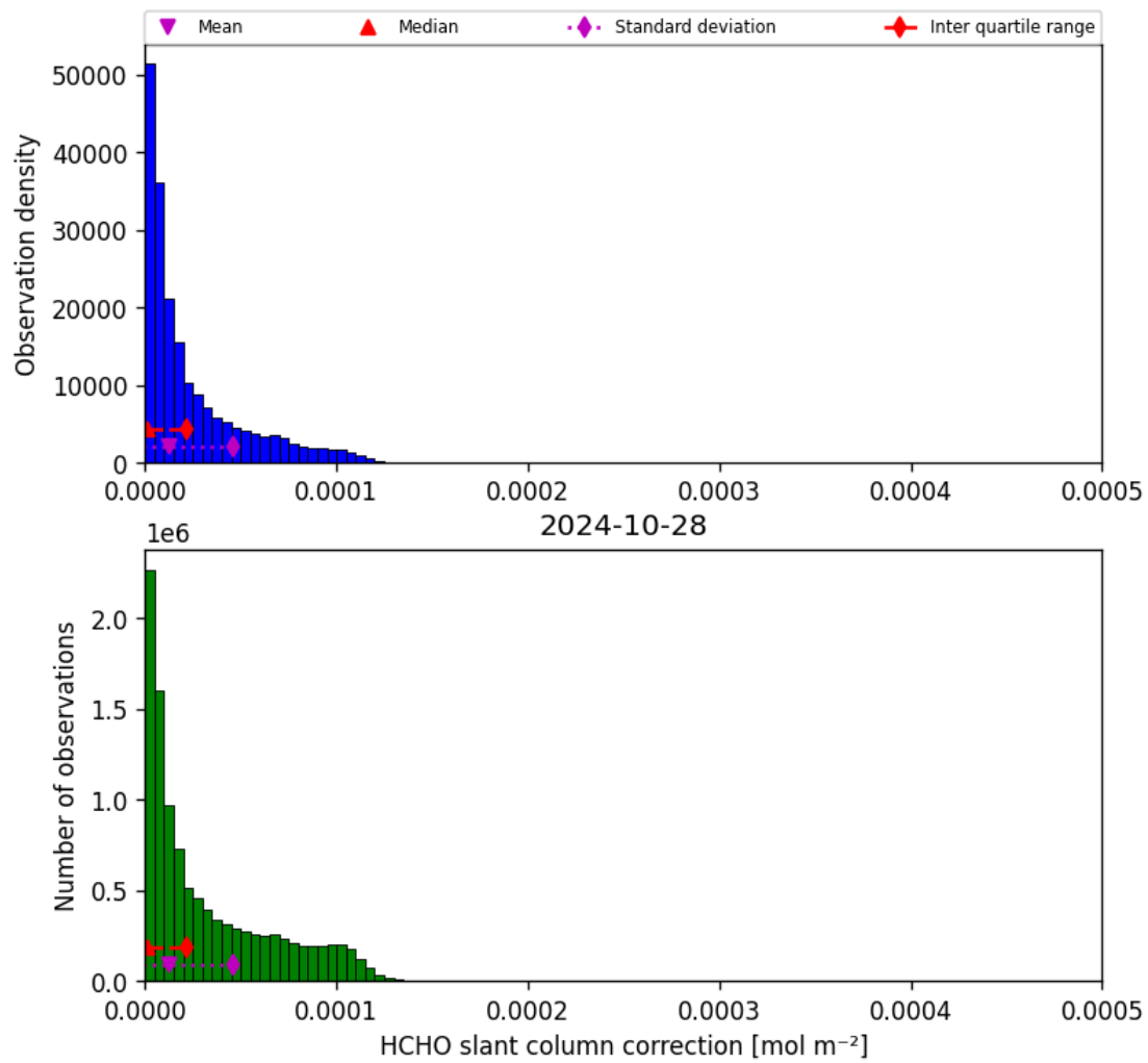
Figure 47: Histogram of “HCHO slant column correction” for 2024-10-27 to 2024-10-29
