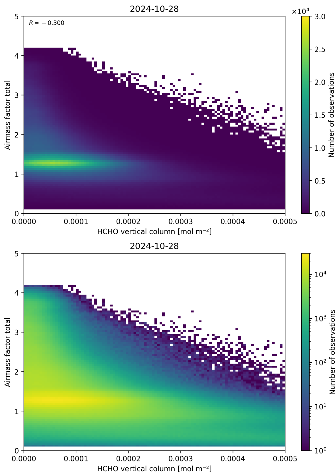
Figure 131: Scatter density plot of “HCHO vertical column” against “Airmass factor total” for 2024-10-27 to 2024-10-29.
