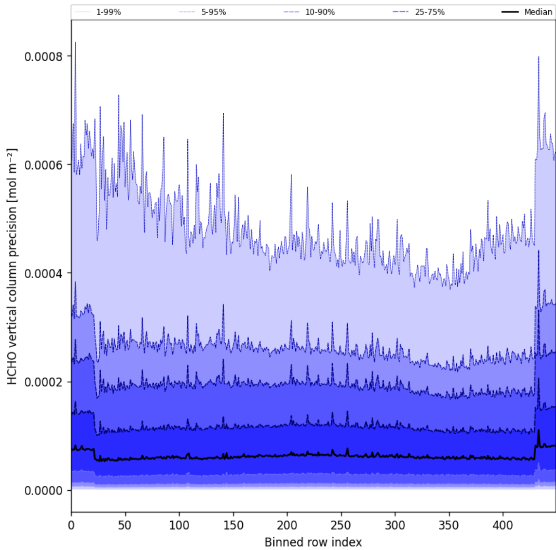
Figure 50: Along track statistics of “HCHO vertical column precision” for 2024-10-27 to 2024-10-29
