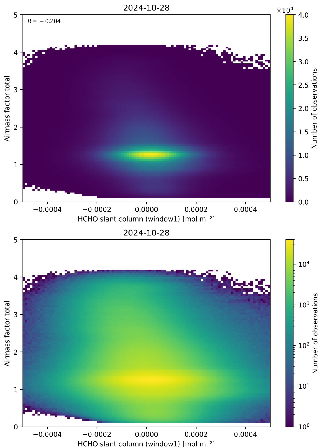
Figure 85: Scatter density plot of “HCHO slant column (window1)” against “Airmass factor total” for 2024-10-27 to 2024-10-29.
