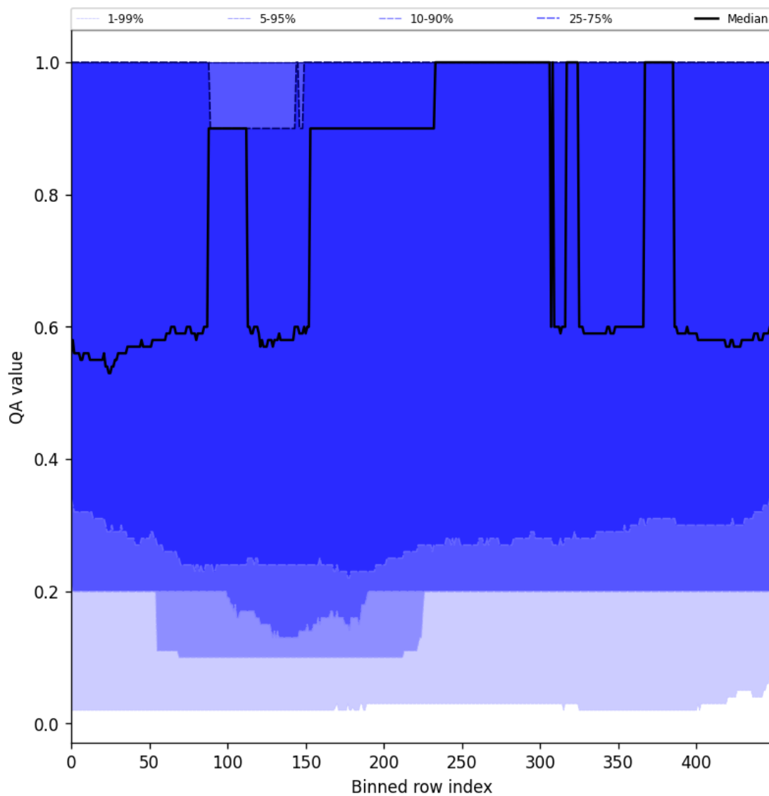
Figure 48: Along track statistics of “QA value” for 2024-10-27 to 2024-10-29
