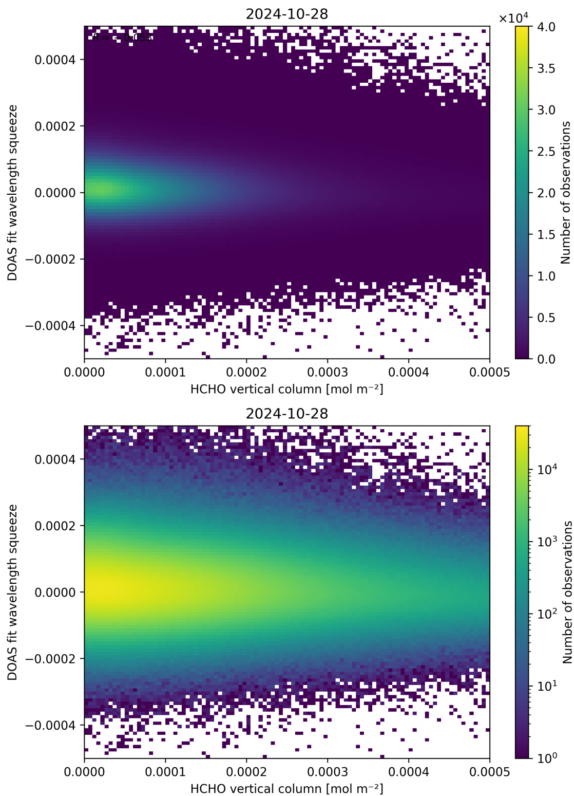
Figure 125: Scatter density plot of “HCHO vertical column” against “DOAS fit wavelength squeeze” for 2024-10-27 to 2024-10-29.
