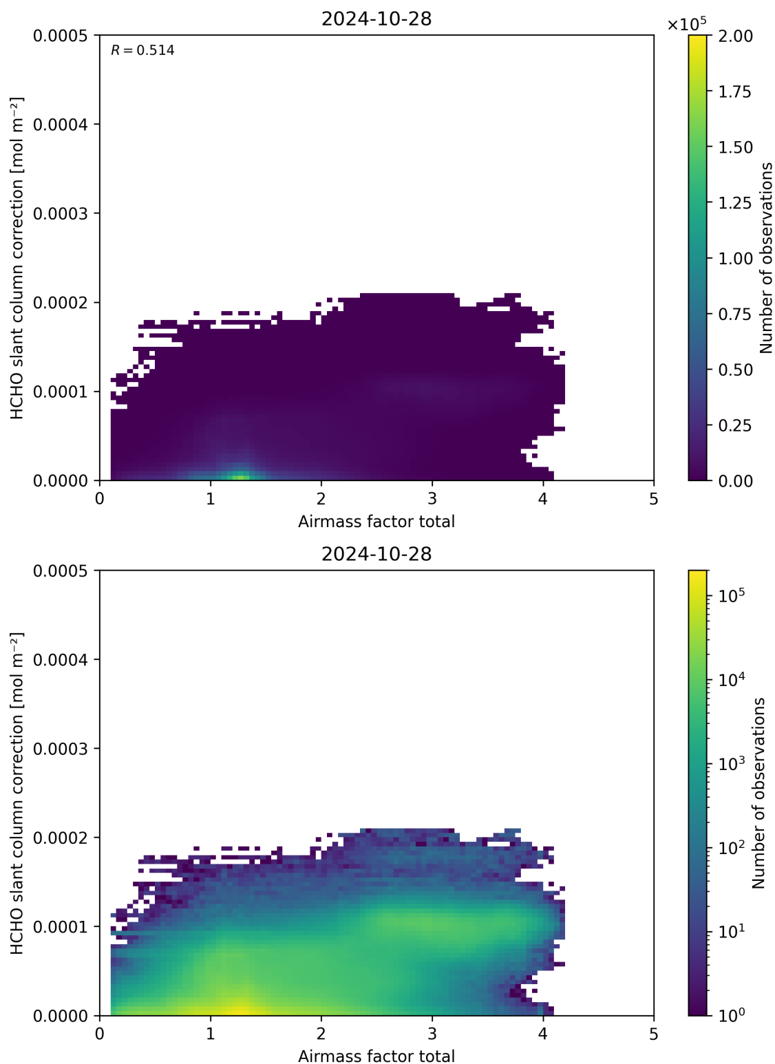
Figure 102: Scatter density plot of “Airmass factor total” against “HCHO slant column correction” for 2024-10-27 to 2024-10-29.
