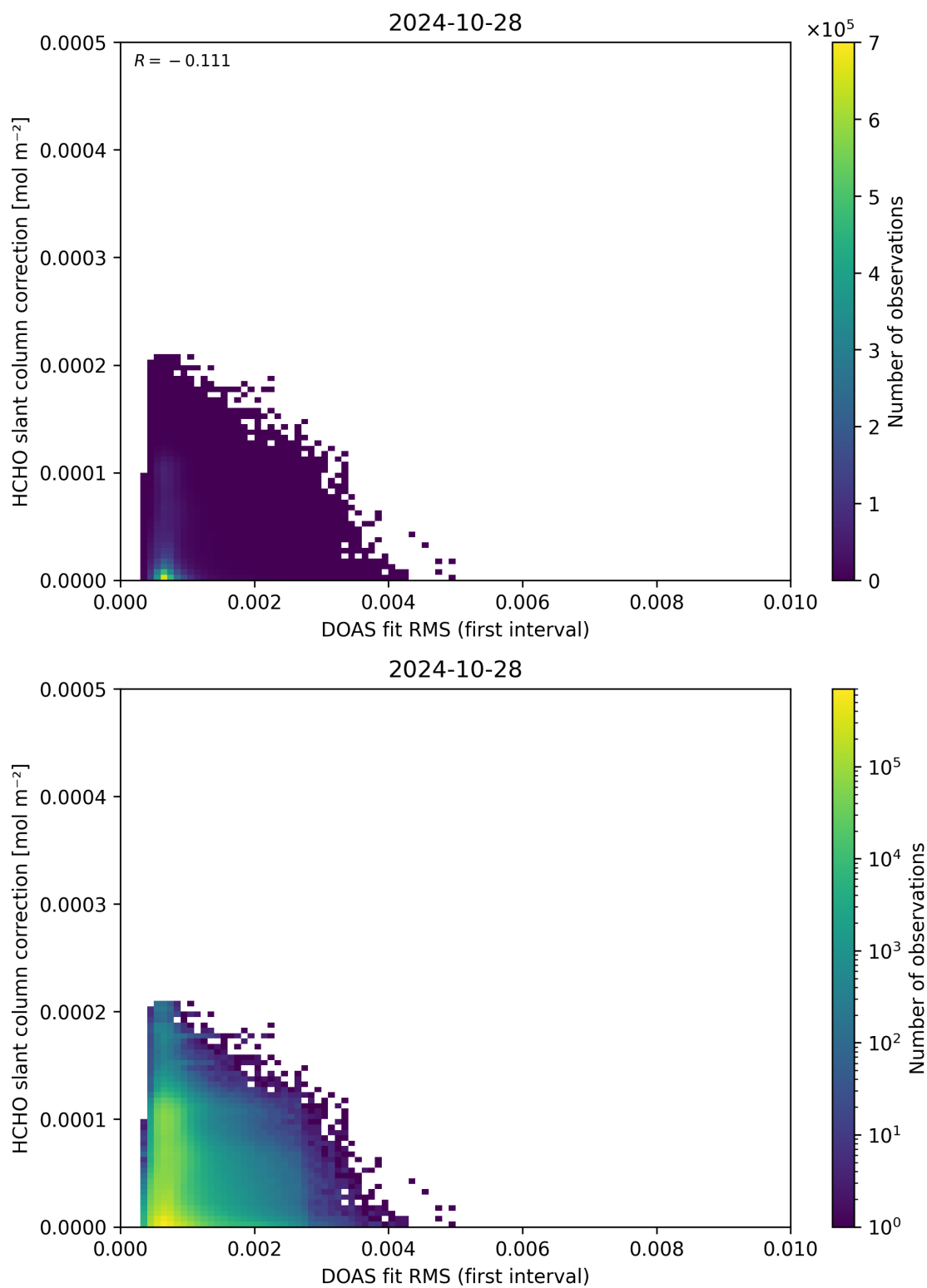
Figure 63: Scatter density plot of “DOAS fit RMS (first interval)” against “HCHO slant column correction” for 2024-10-27 to 2024-10-29.
