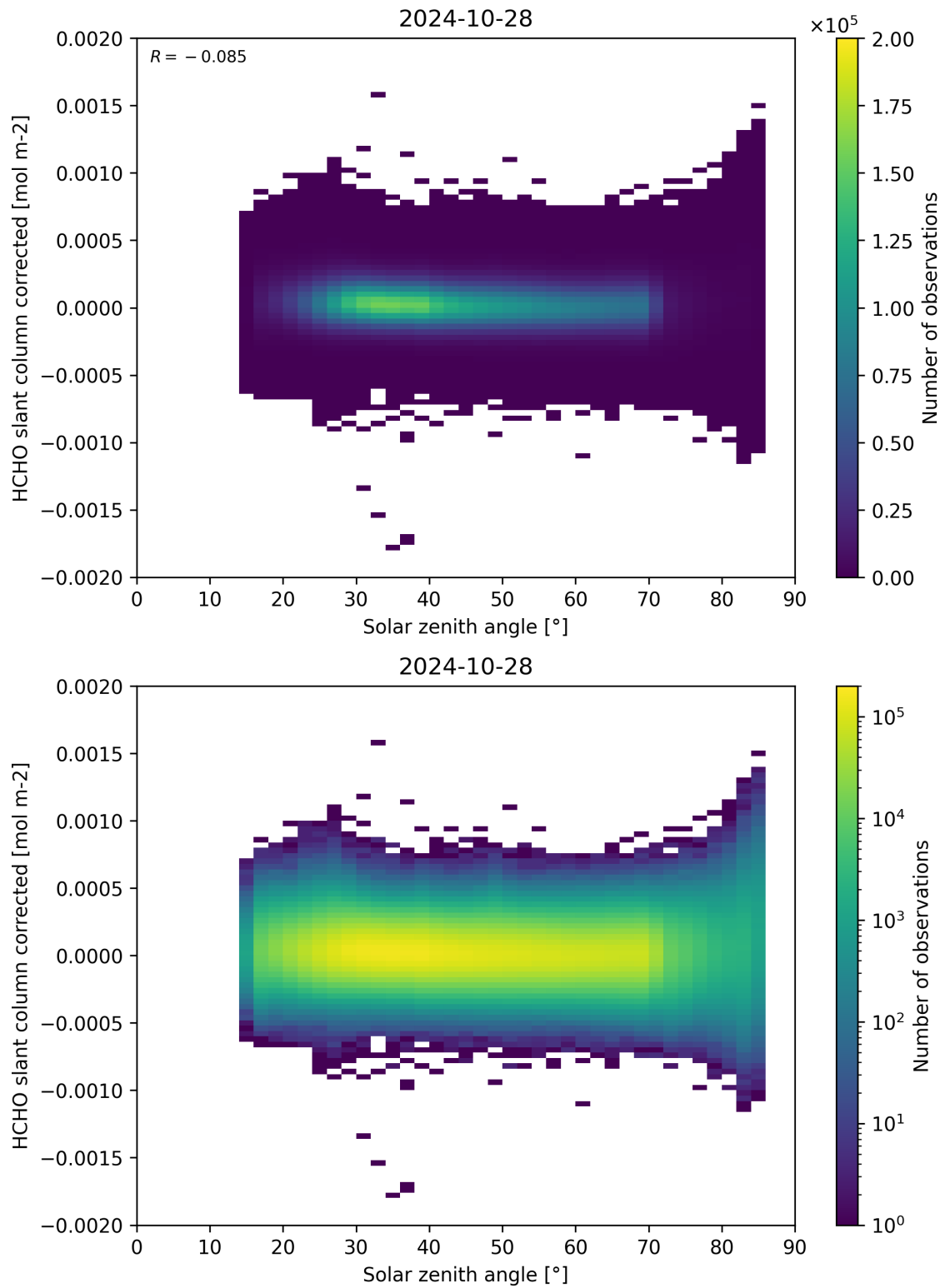
Figure 171: Scatter density plot of “Solar zenith angle” against “HCHO slant column corrected” for 2024-10-27 to 2024-10-29.
