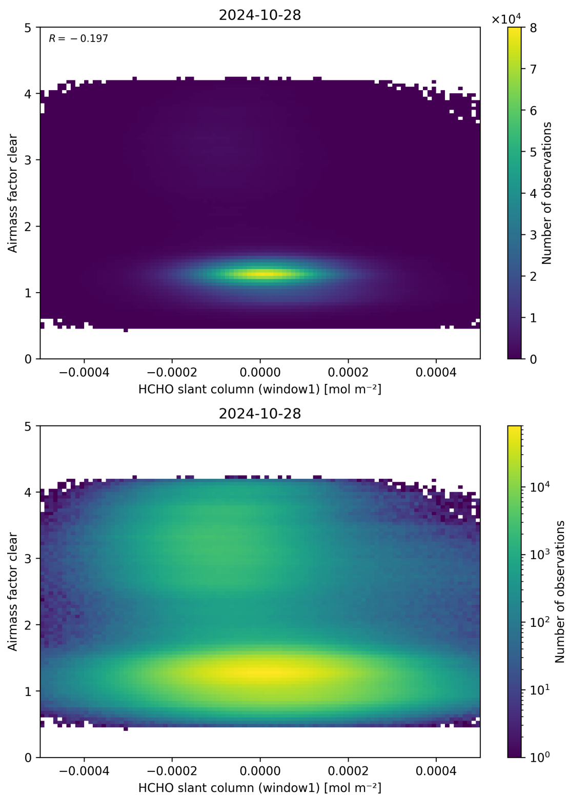
Figure 81: Scatter density plot of “HCHO slant column (window1)” against “Airmass factor clear” for 2024-10-27 to 2024-10-29.
