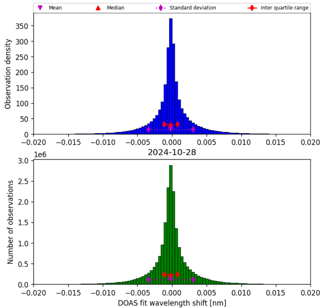
Figure 44: Histogram of “DOAS fit wavelength shift” for 2024-10-27 to 2024-10-29
