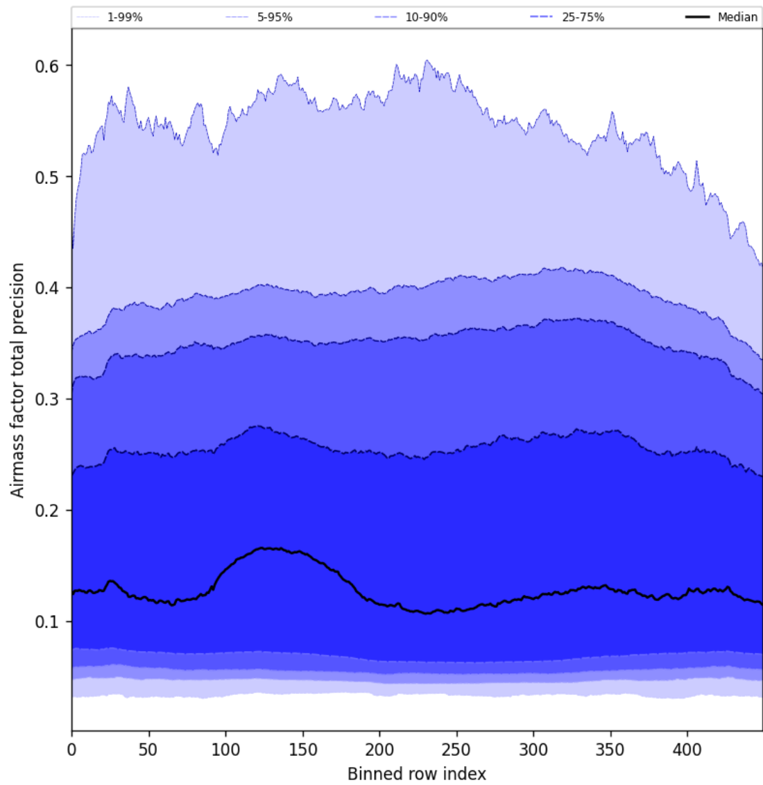
Figure 55: Along track statistics of “Airmass factor total precision” for 2024-10-27 to 2024-10-29
