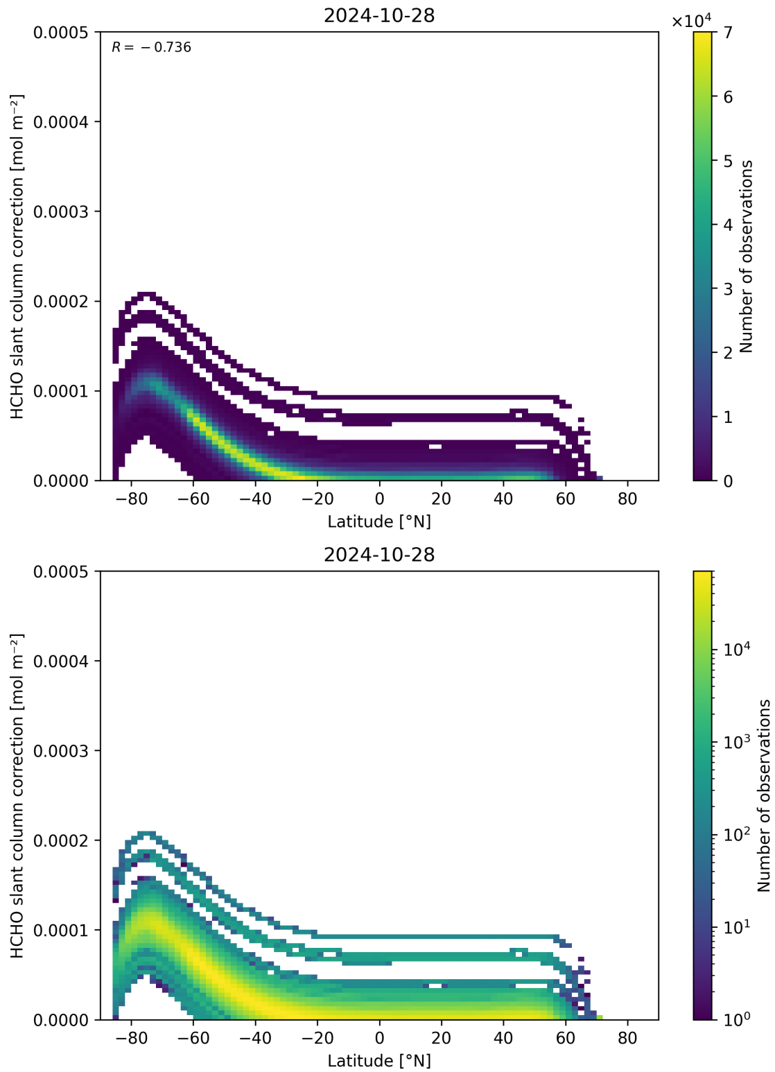
Figure 158: Scatter density plot of “Latitude” against “HCHO slant column correction” for 2024-10-27 to 2024-10-29.
