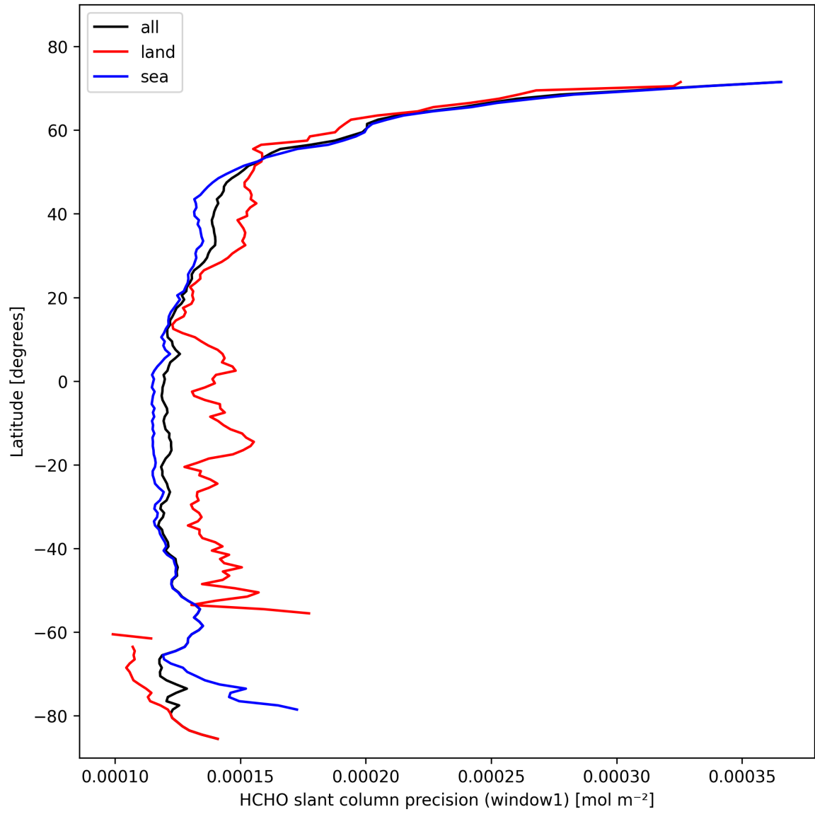
Figure 25: Zonal average of “HCHO slant column precision (window1)” for 2024-10-27 to 2024-10-29.
