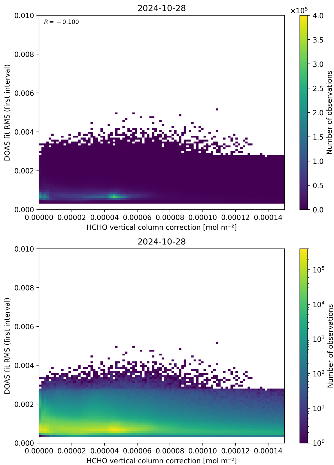
Figure 112: Scatter density plot of “HCHO vertical column correction” against “DOAS fit RMS (first interval)” for 2024-10-27 to 2024-10-29.
