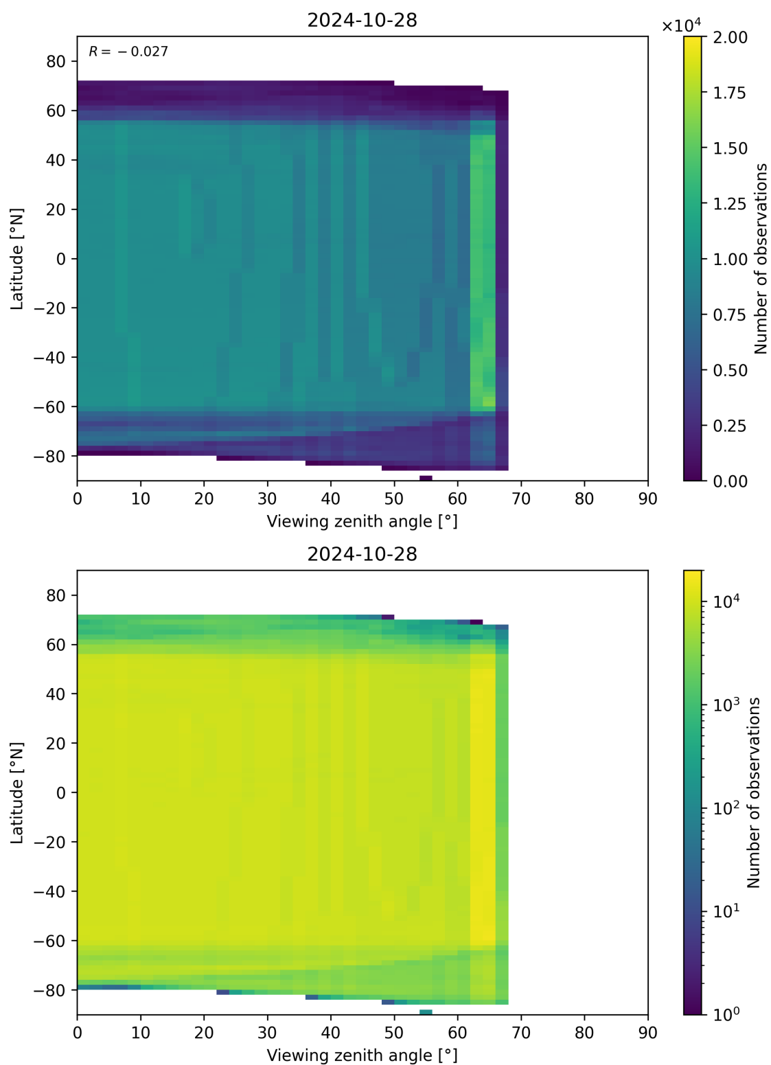
Figure 196: Scatter density plot of “Viewing zenith angle” against “Latitude” for 2024-10-27 to 2024-10-29.
