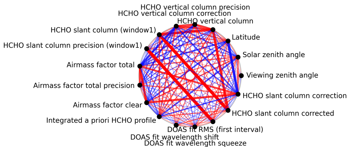
Figure 1: Map of correlation graph for 2024-10-27 to 2024-10-29.
