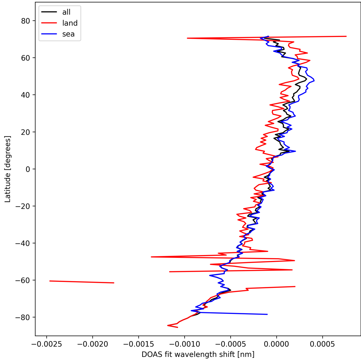
Figure 30: Zonal average of "DOAS fit wavelength shift" for 2024-10-27 to 2024-10-29.
