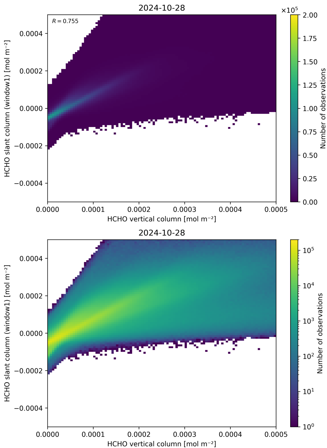
Figure 129: Scatter density plot of “HCHO vertical column” against “HCHO slant column (window1)” for 2024-10-27 to 2024-10-29.
