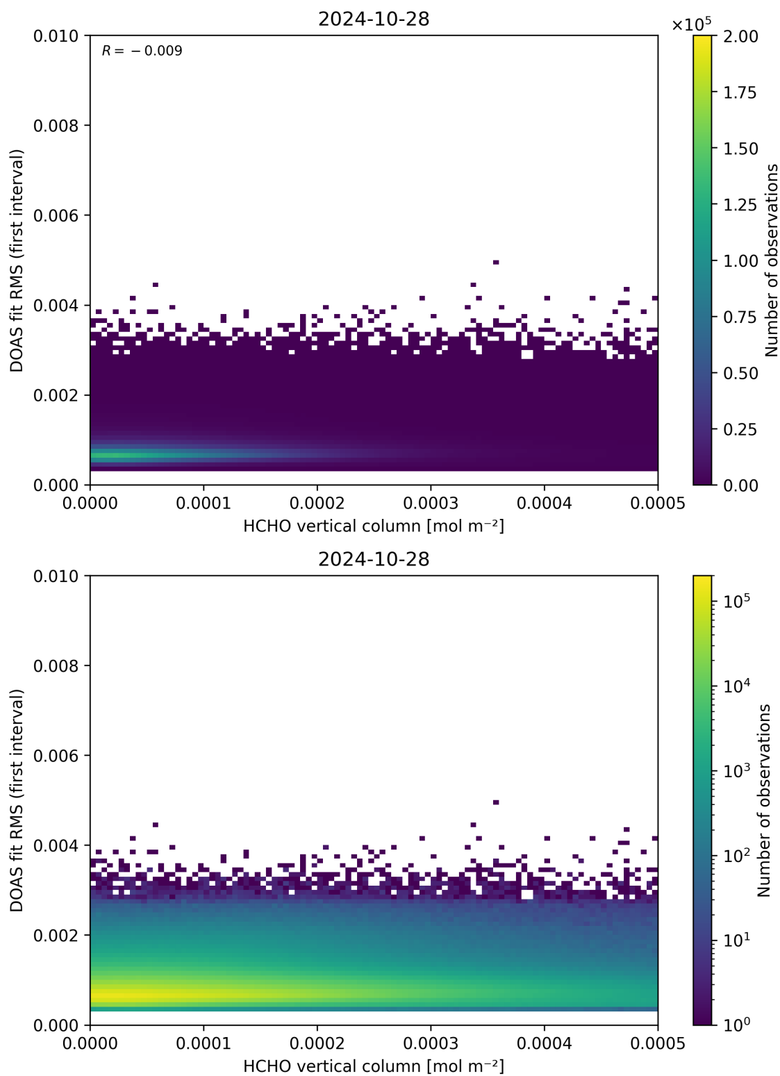
Figure 123: Scatter density plot of “HCHO vertical column” against “DOAS fit RMS (first interval)” for 2024-10-27 to 2024-10-29.
