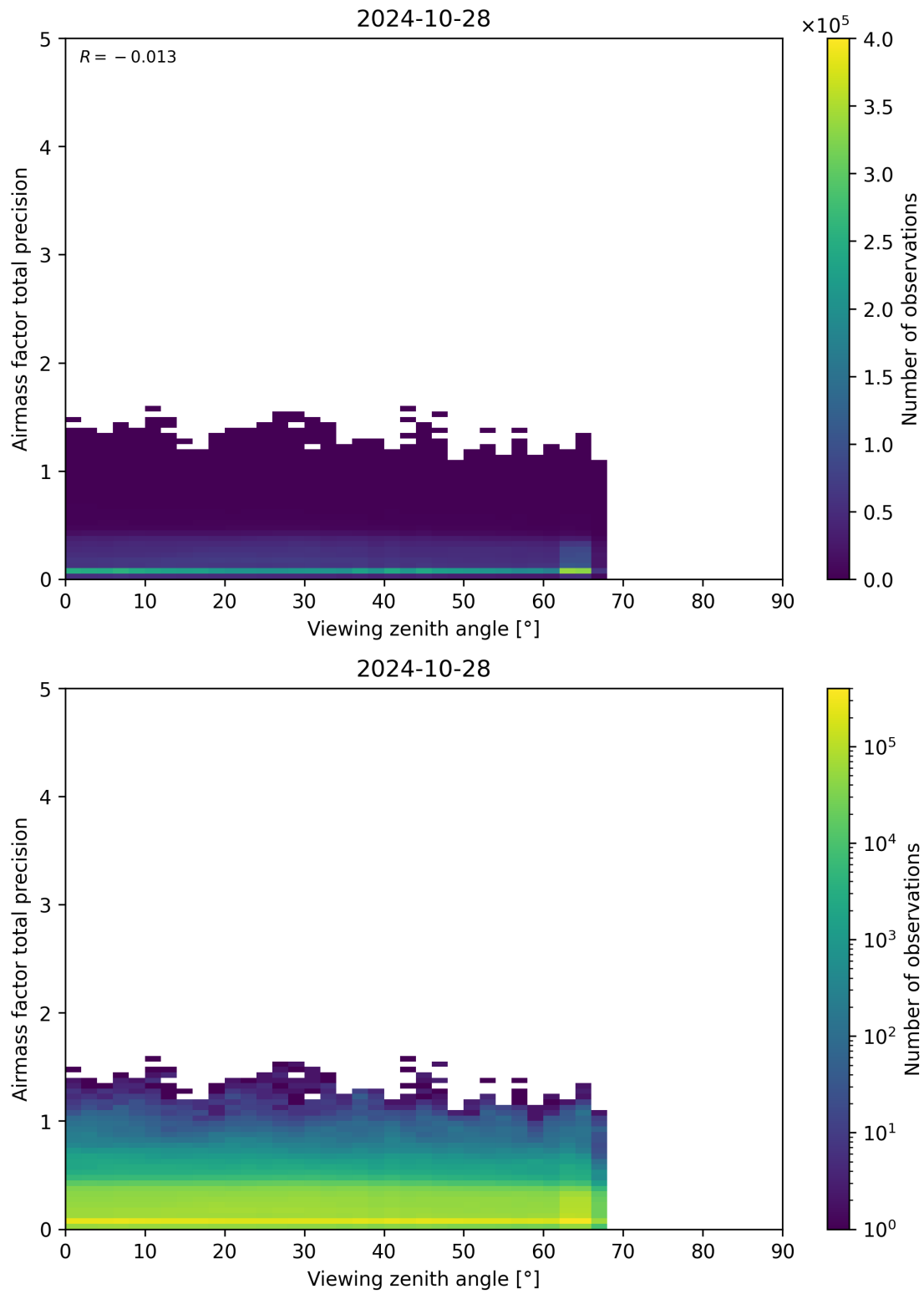
Figure 191: Scatter density plot of “Viewing zenith angle” against “Airmass factor total precision” for 2024-10-27 to 2024-10-29.
