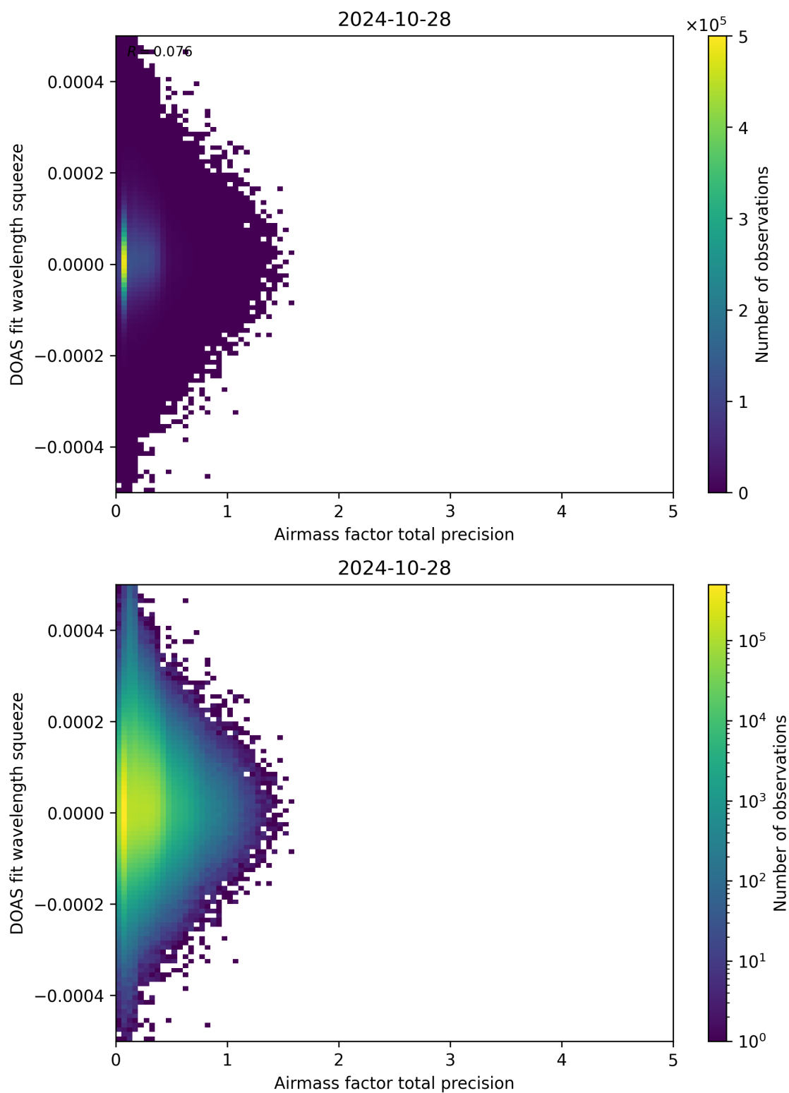
Figure 107: Scatter density plot of “Airmass factor total precision” against “DOAS fit wavelength squeeze” for 2024-10-27 to 2024-10-29.
