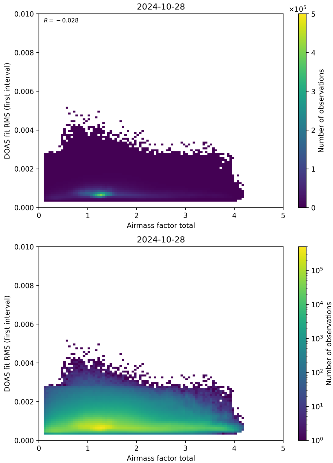
Figure 97: Scatter density plot of “Airmass factor total” against “DOAS fit RMS (first interval)” for 2024-10-27 to 2024-10-29.
