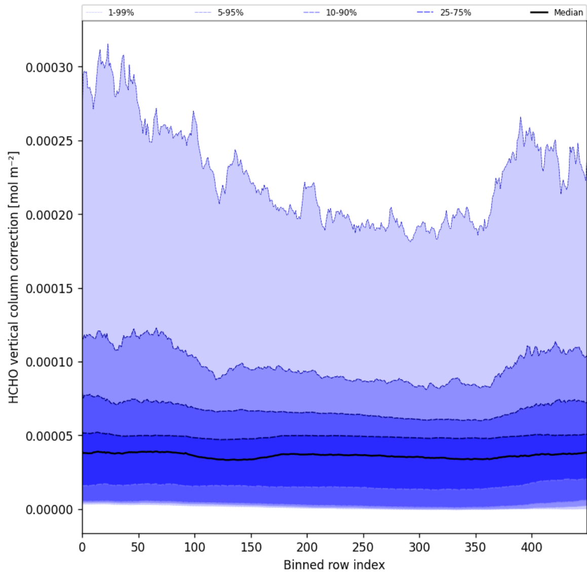
Figure 51: Along track statistics of “HCHO vertical column correction” for 2024-10-27 to 2024-10-29
