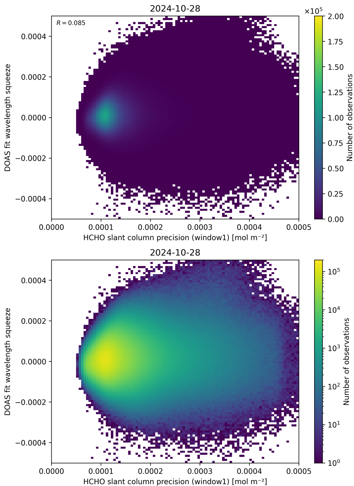
Figure 90: Scatter density plot of “HCHO slant column precision (window1)” against “DOAS fit wavelength squeeze” for 2024-10-27 to 2024-10-29.
