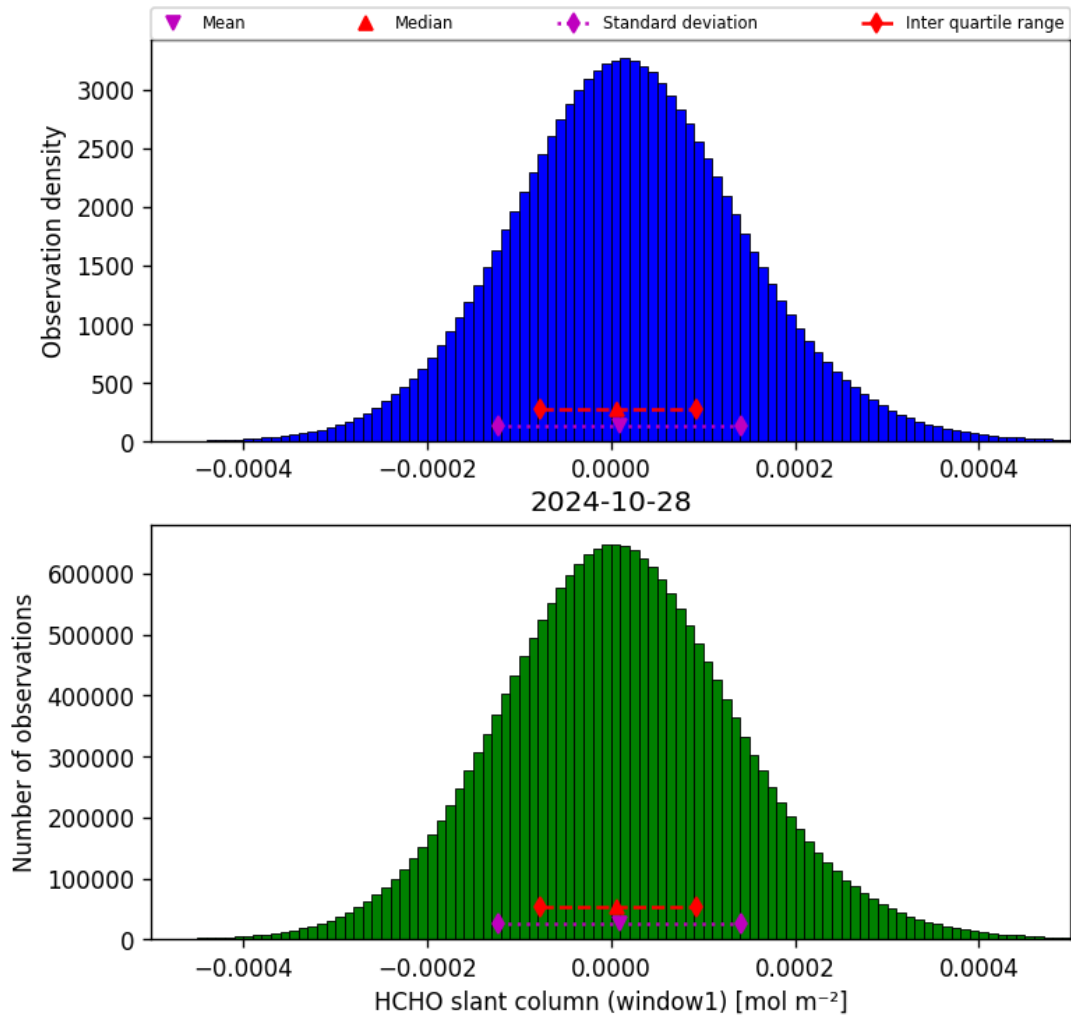
Figure 38: Histogram of “HCHO slant column (window1)” for 2024-10-27 to 2024-10-29
