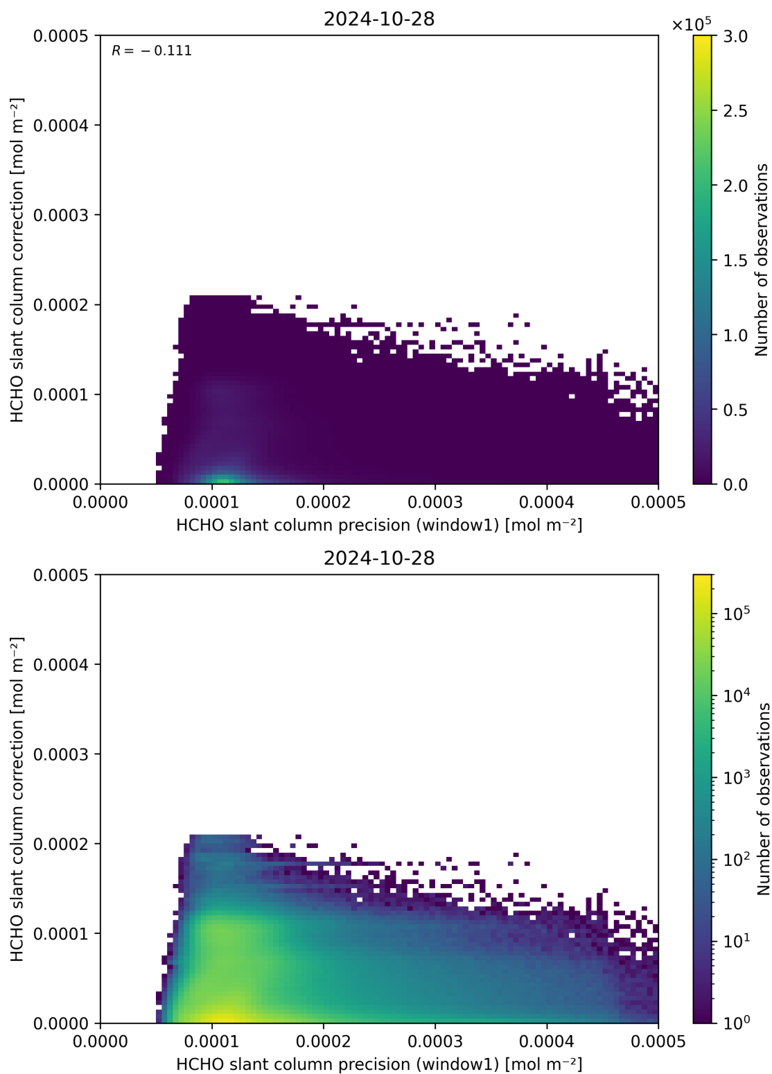
Figure 93: Scatter density plot of “HCHO slant column precision (window1)” against “HCHO slant column correction” for 2024-10-27 to 2024-10-29.
