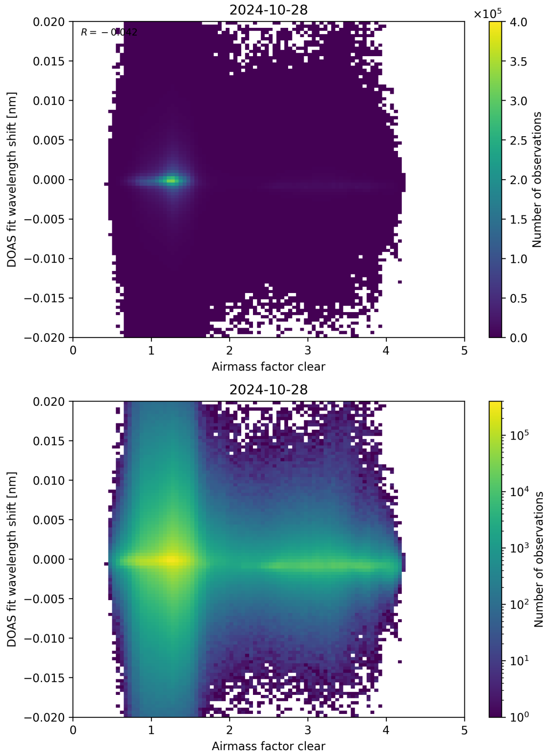
Figure 72: Scatter density plot of “Airmass factor clear” against “DOAS fit wavelength shift” for 2024-10-27 to 2024-10-29.
