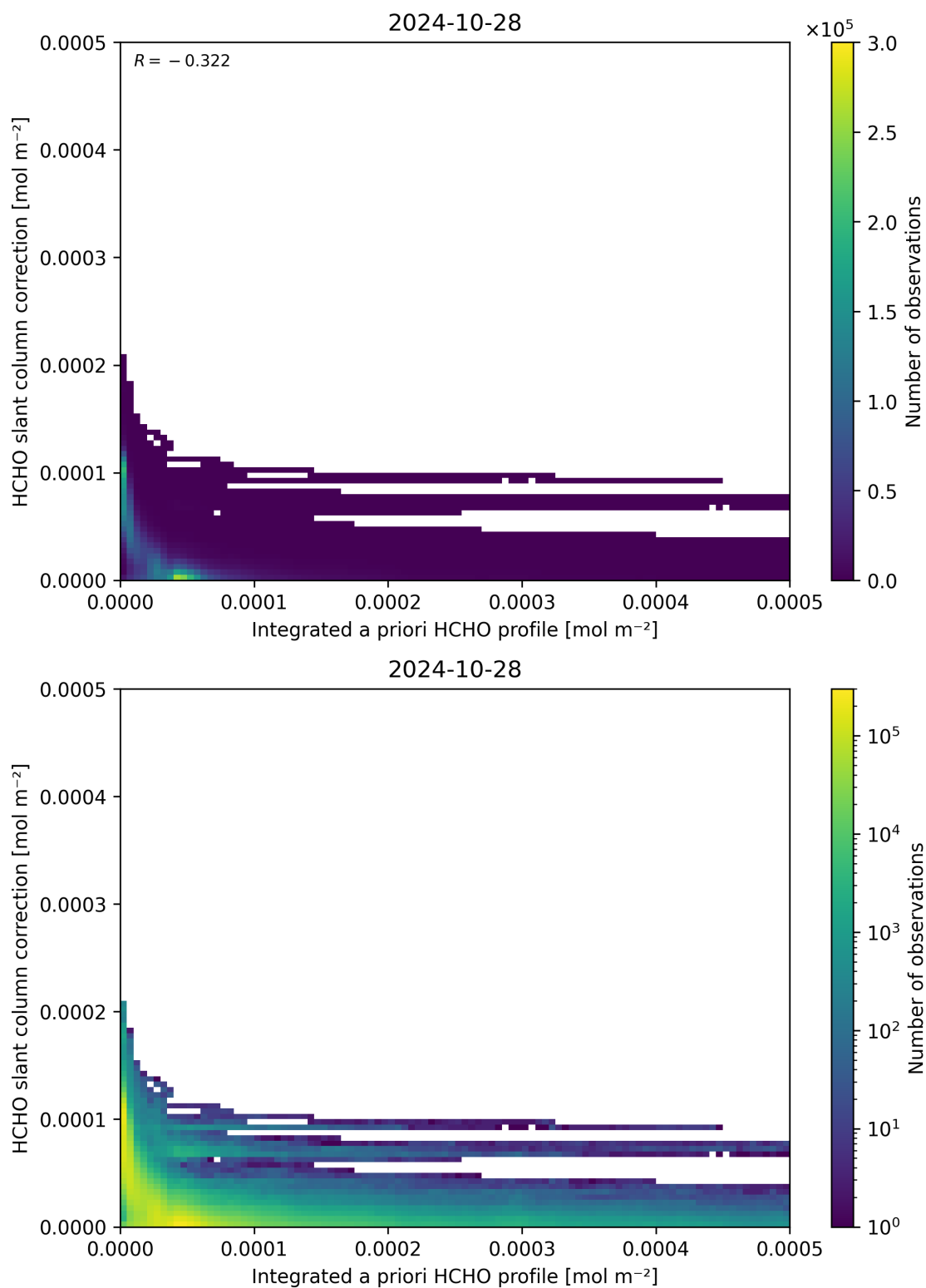
Figure 152: Scatter density plot of “Integrated a priori HCHO profile” against “HCHO slant column correction” for 2024-10-27 to 2024-10-29.
