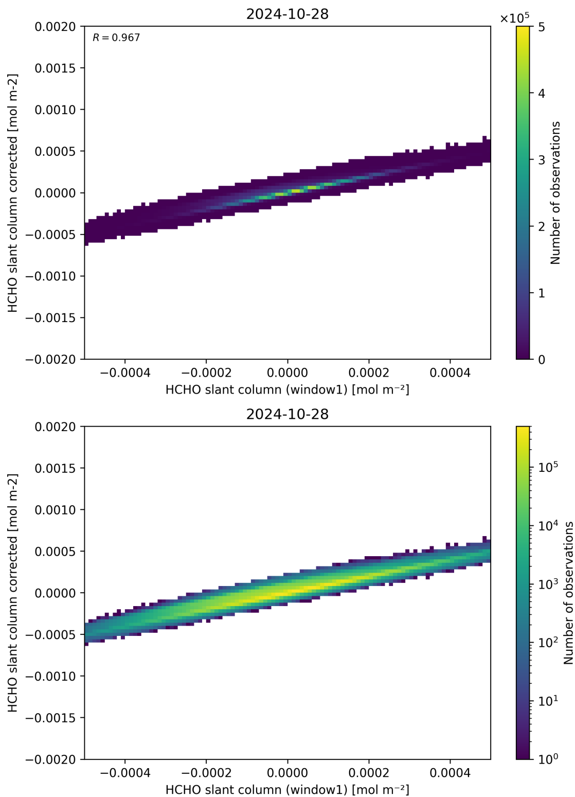
Figure 82: Scatter density plot of “HCHO slant column (window1)” against “HCHO slant column corrected” for 2024-10-27 to 2024-10-29.
