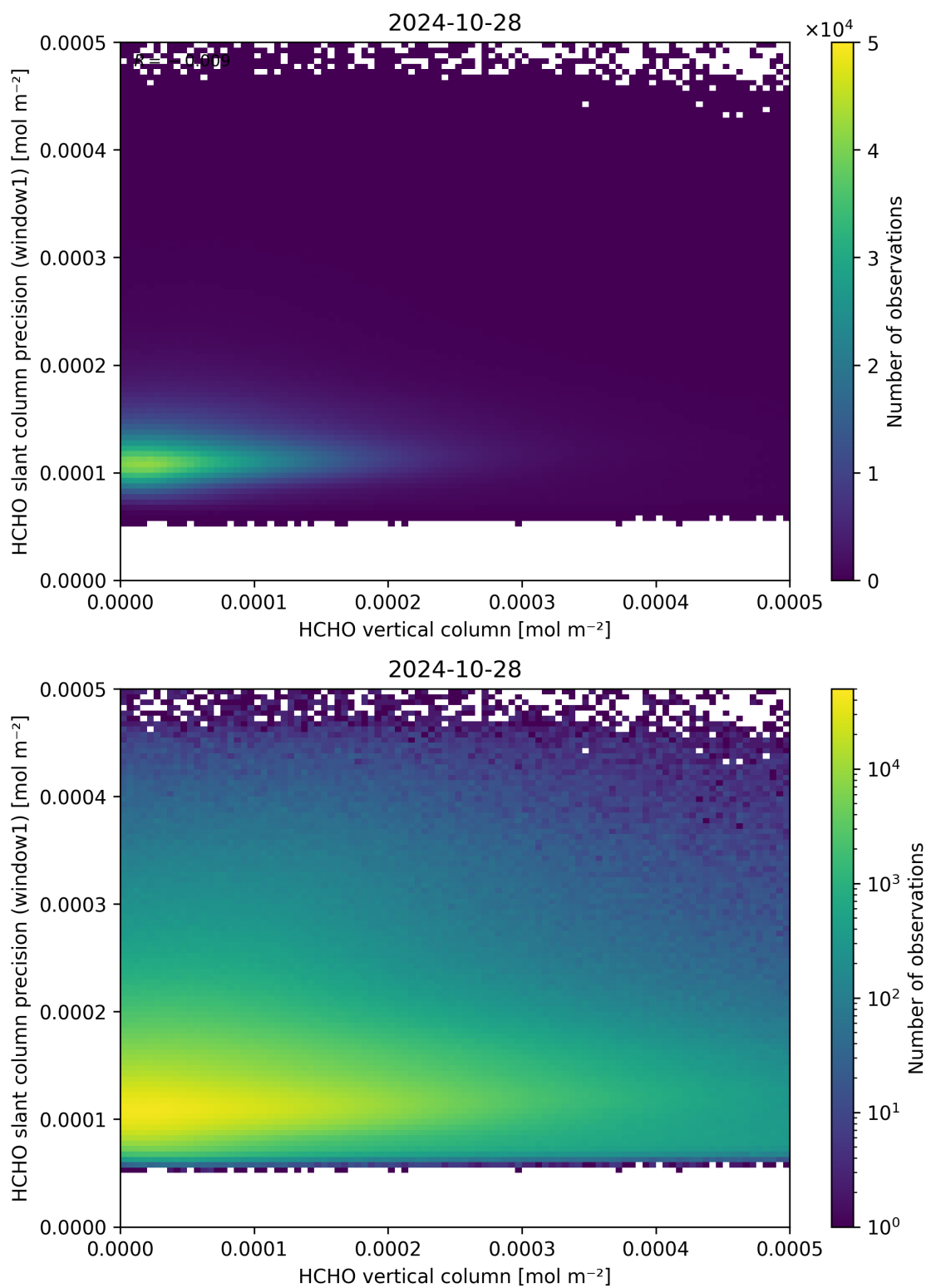
Figure 130: Scatter density plot of “HCHO vertical column” against “HCHO slant column precision (window1)” for 2024-10-27 to 2024-10-29.
