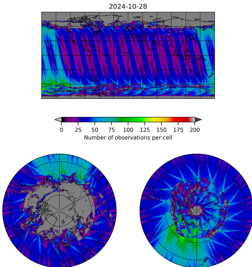
Figure 19: Map of the number of observations for 2024-10-27 to 2024-10-29
