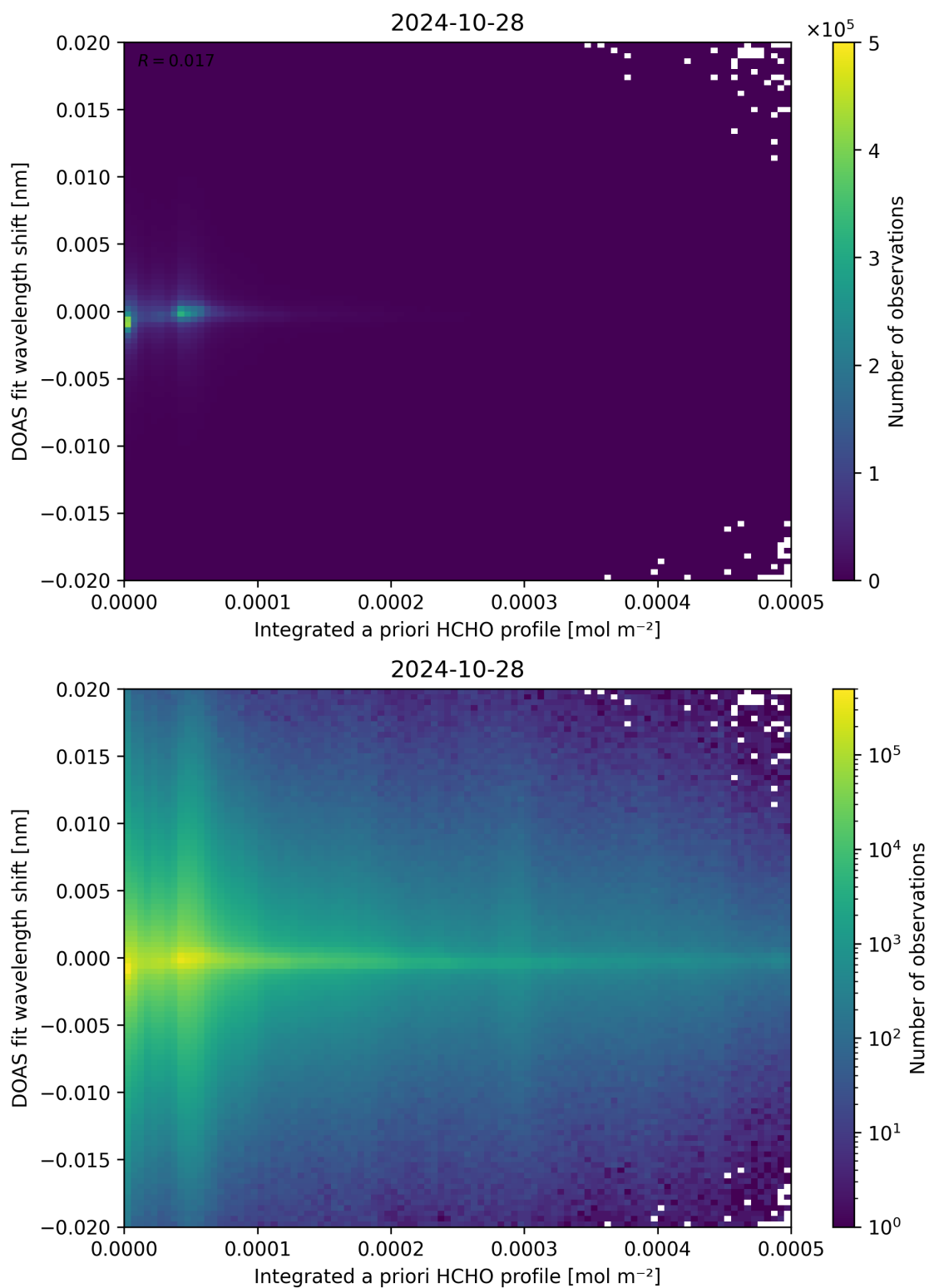
Figure 149: Scatter density plot of “Integrated a priori HCHO profile” against “DOAS fit wavelength shift” for 2024-10-27 to 2024-10-29.
