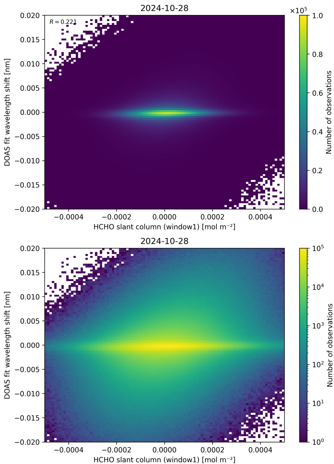
Figure 79: Scatter density plot of “HCHO slant column (window1)” against “DOAS fit wavelength shift” for 2024-10-27 to 2024-10-29.
