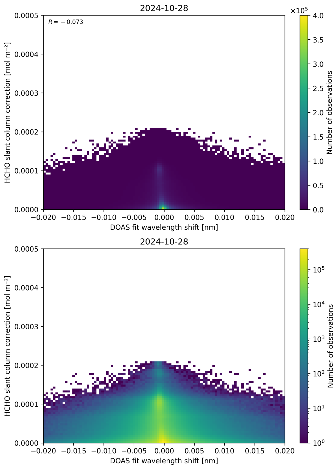
Figure 67: Scatter density plot of “DOAS fit wavelength shift” against “HCHO slant column correction” for 2024-10-27 to 2024-10-29.
