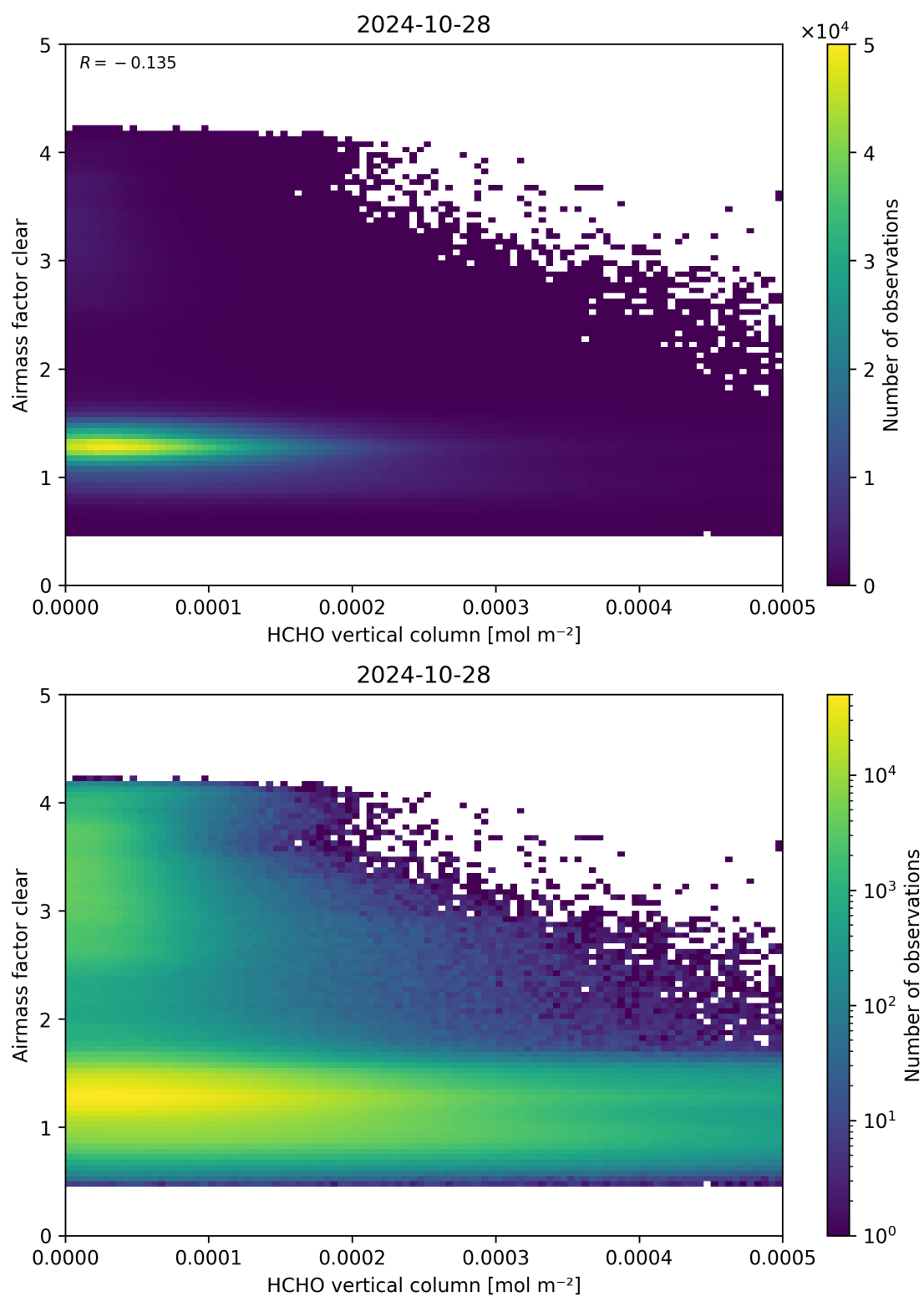
Figure 126: Scatter density plot of “HCHO vertical column” against “Airmass factor clear” for 2024-10-27 to 2024-10-29.
