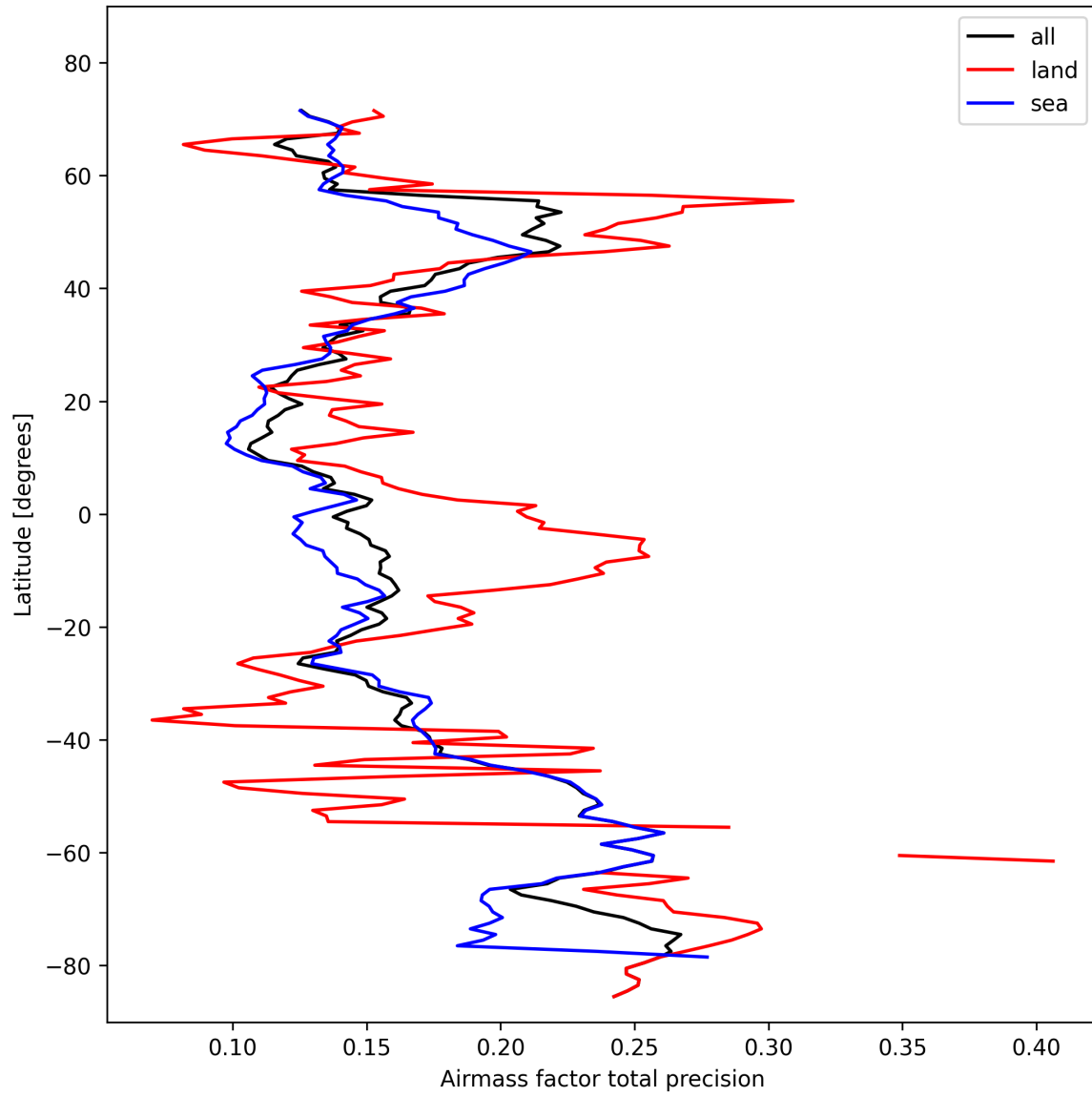
Figure 27: Zonal average of “Airmass factor total precision” for 2024-10-27 to 2024-10-29.
