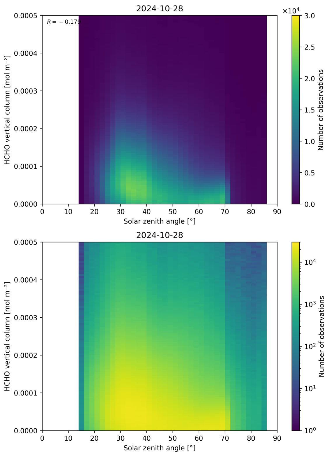
Figure 177: Scatter density plot of “Solar zenith angle” against “HCHO vertical column” for 2024-10-27 to 2024-10-29.
