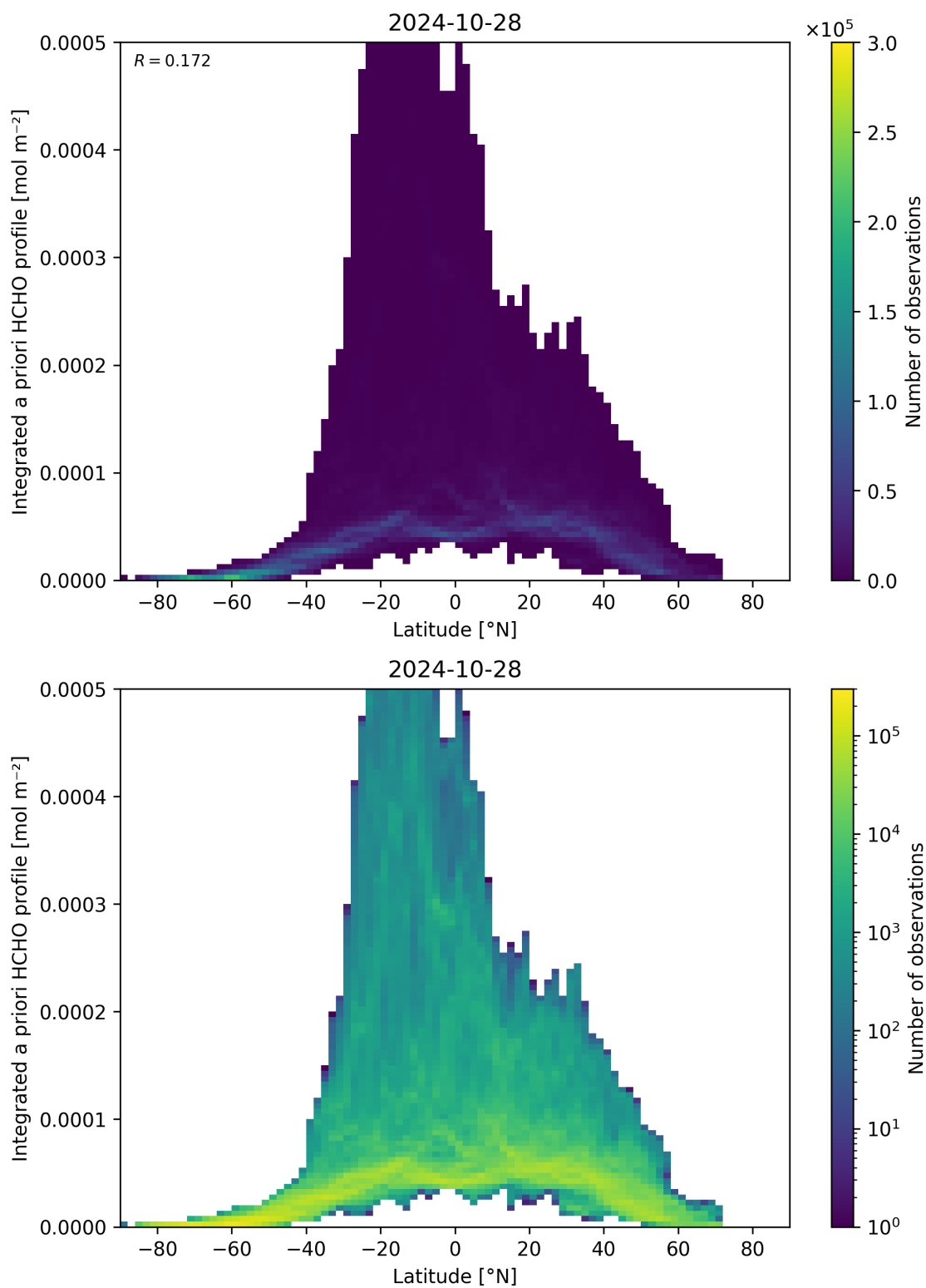
Figure 166: Scatter density plot of “Latitude” against “Integrated a priori HCHO profile” for 2024-10-27 to 2024-10-29.
