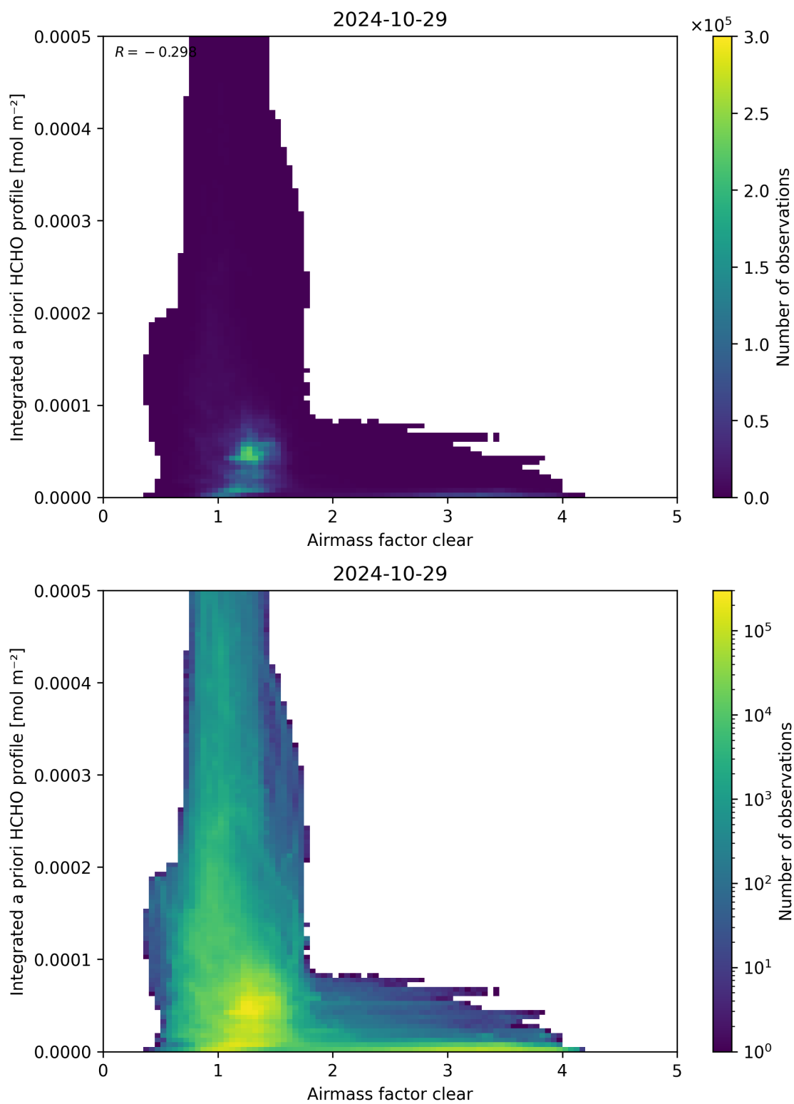
Figure 76: Scatter density plot of “Airmass factor clear” against “Integrated a priori HCHO profile” for 2024-10-29 to 2024-10-30.
