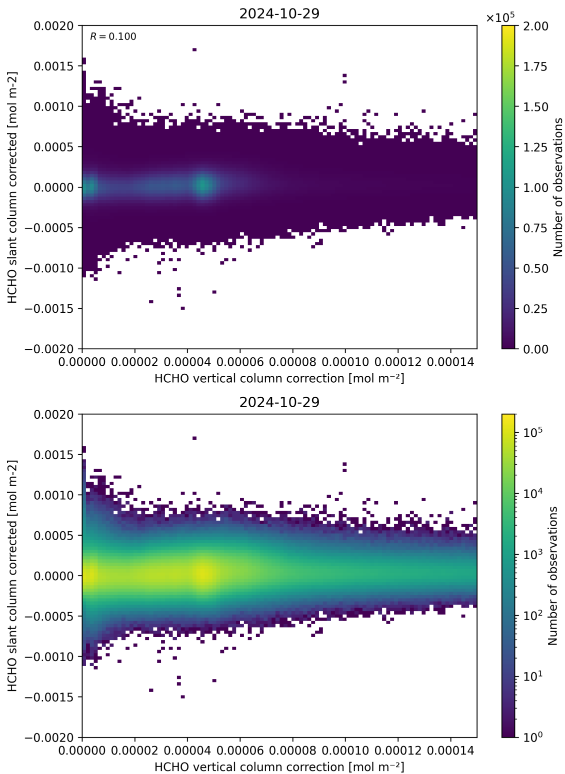
Figure 116: Scatter density plot of “HCHO vertical column correction” against “HCHO slant column corrected” for 2024-10-29 to 2024-10-30.
