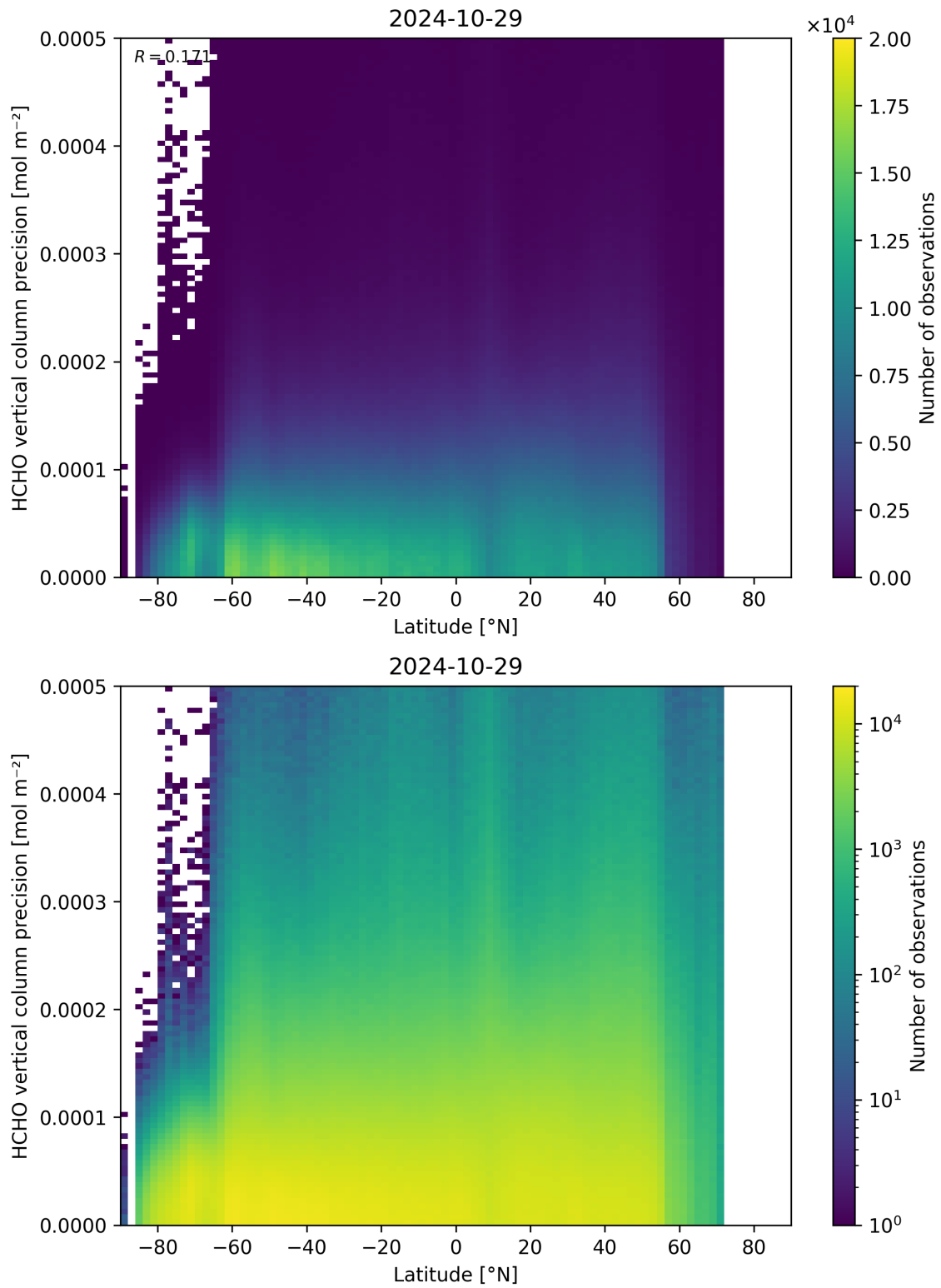
Figure 165: Scatter density plot of “Latitude” against “HCHO vertical column precision” for 2024-10-29 to 2024-10-30.
