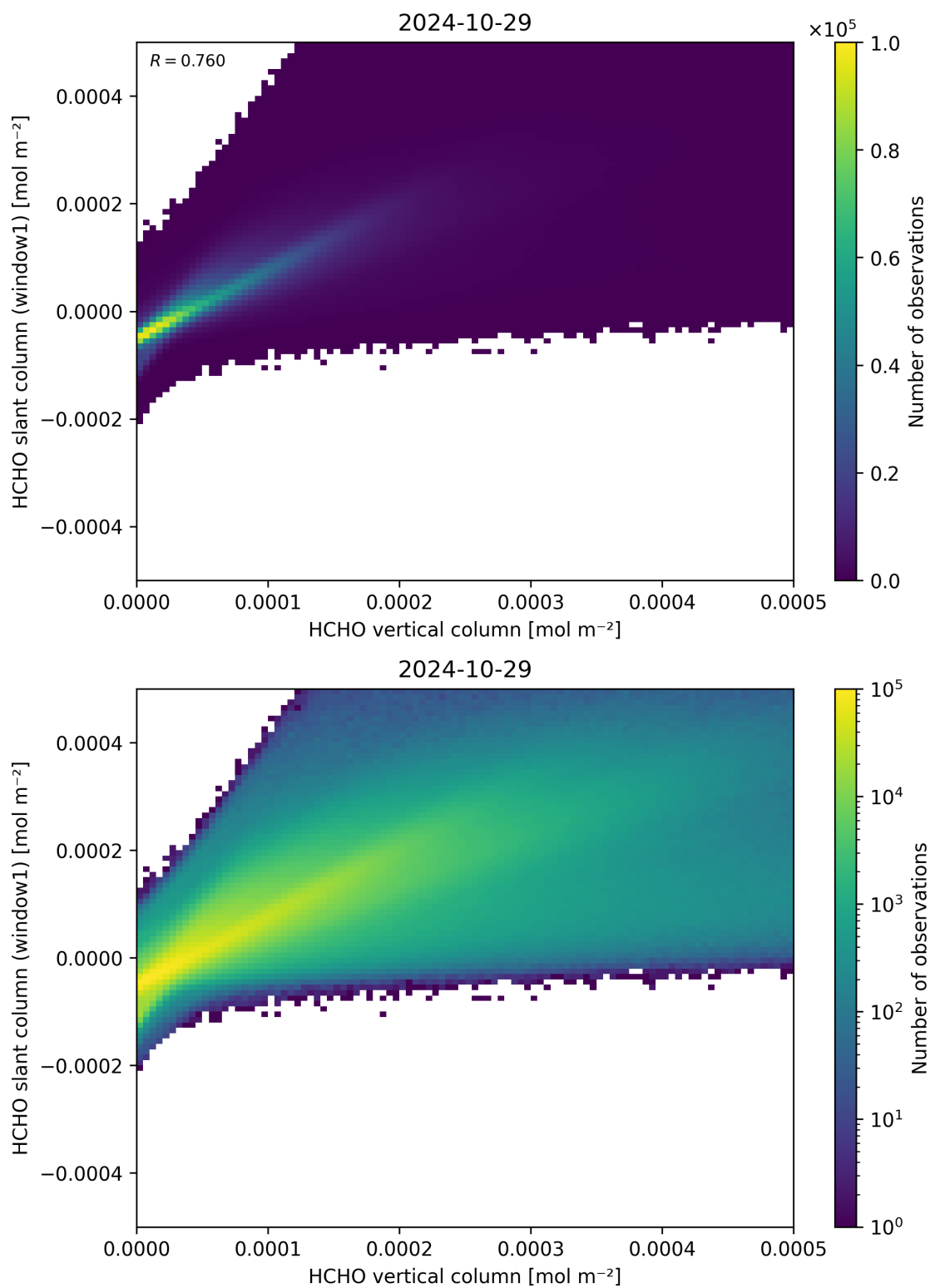
Figure 129: Scatter density plot of “HCHO vertical column” against “HCHO slant column (window1)” for 2024-10-29 to 2024-10-30.
