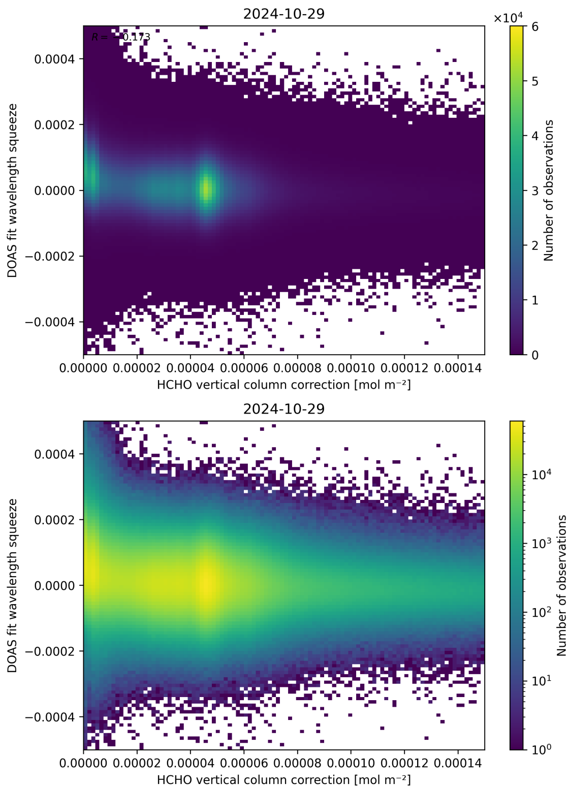
Figure 114: Scatter density plot of “HCHO vertical column correction” against “DOAS fit wavelength squeeze” for 2024-10-29 to 2024-10-30.
