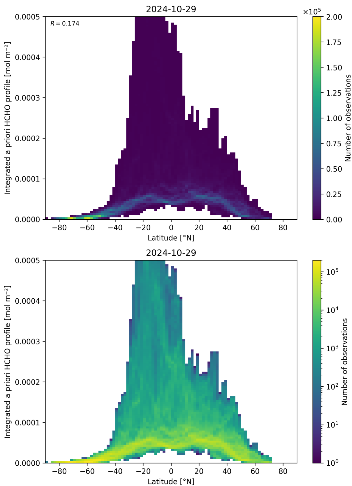
Figure 166: Scatter density plot of “Latitude” against “Integrated a priori HCHO profile” for 2024-10-29 to 2024-10-30.
