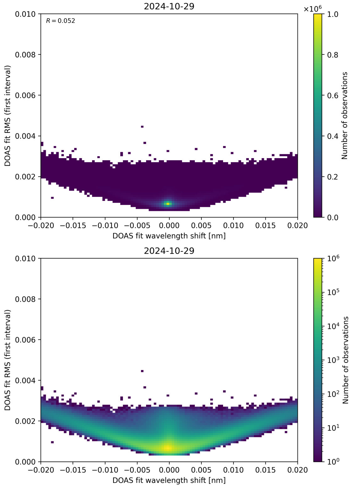
Figure 64: Scatter density plot of “DOAS fit wavelength shift” against “DOAS fit RMS (first interval)” for 2024-10-29 to 2024-10-30.
