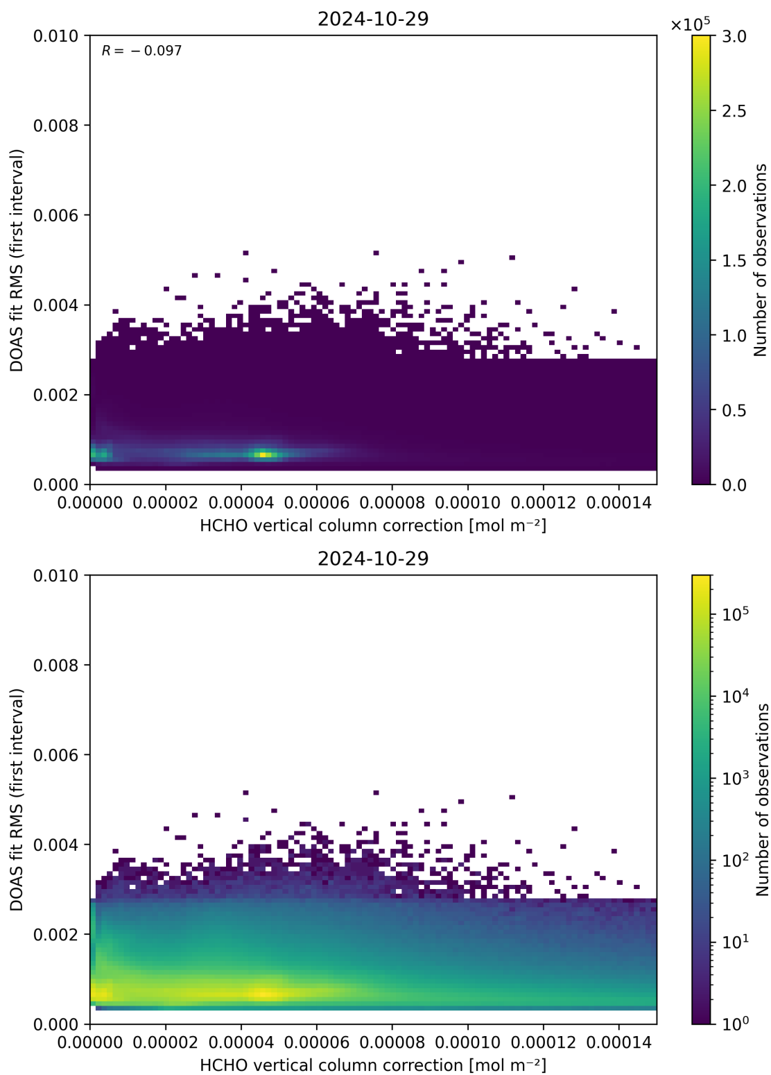
Figure 112: Scatter density plot of “HCHO vertical column correction” against “DOAS fit RMS (first interval)” for 2024-10-29 to 2024-10-30.
