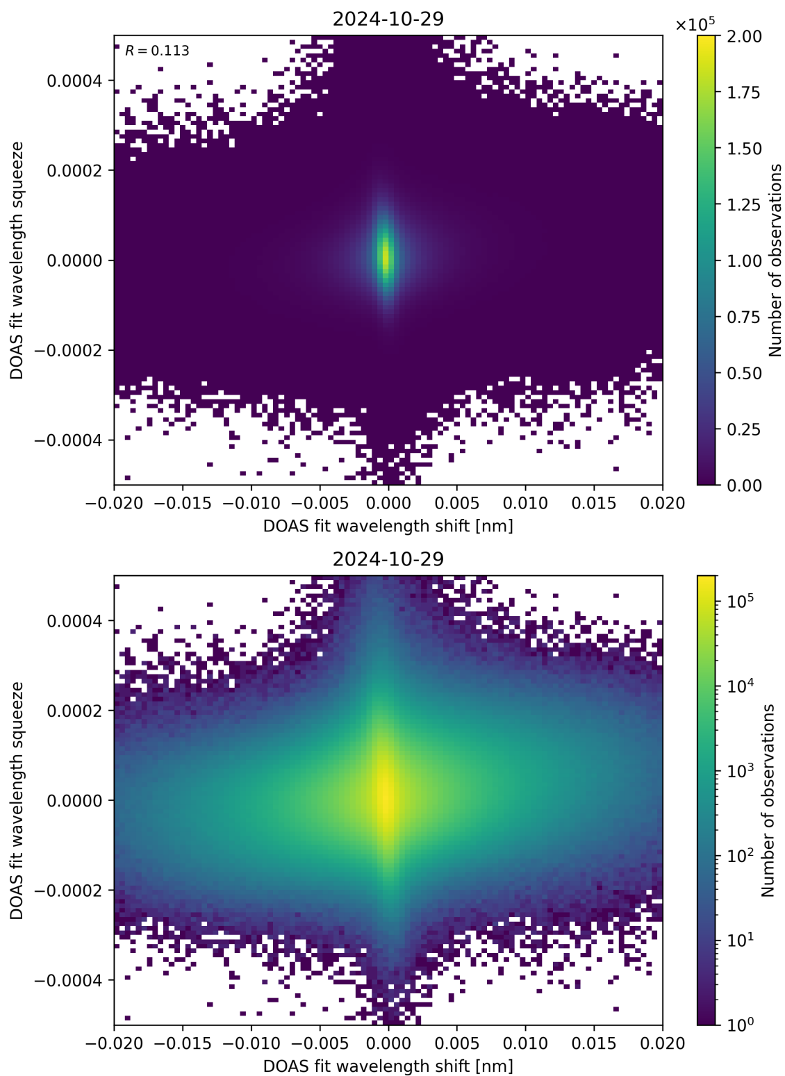
Figure 65: Scatter density plot of “DOAS fit wavelength shift” against “DOAS fit wavelength squeeze” for 2024-10-29 to 2024-10-30.
