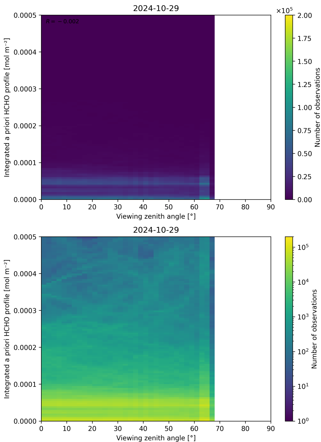
Figure 195: Scatter density plot of “Viewing zenith angle” against “Integrated a priori HCHO profile” for 2024-10-29 to 2024-10-30.
