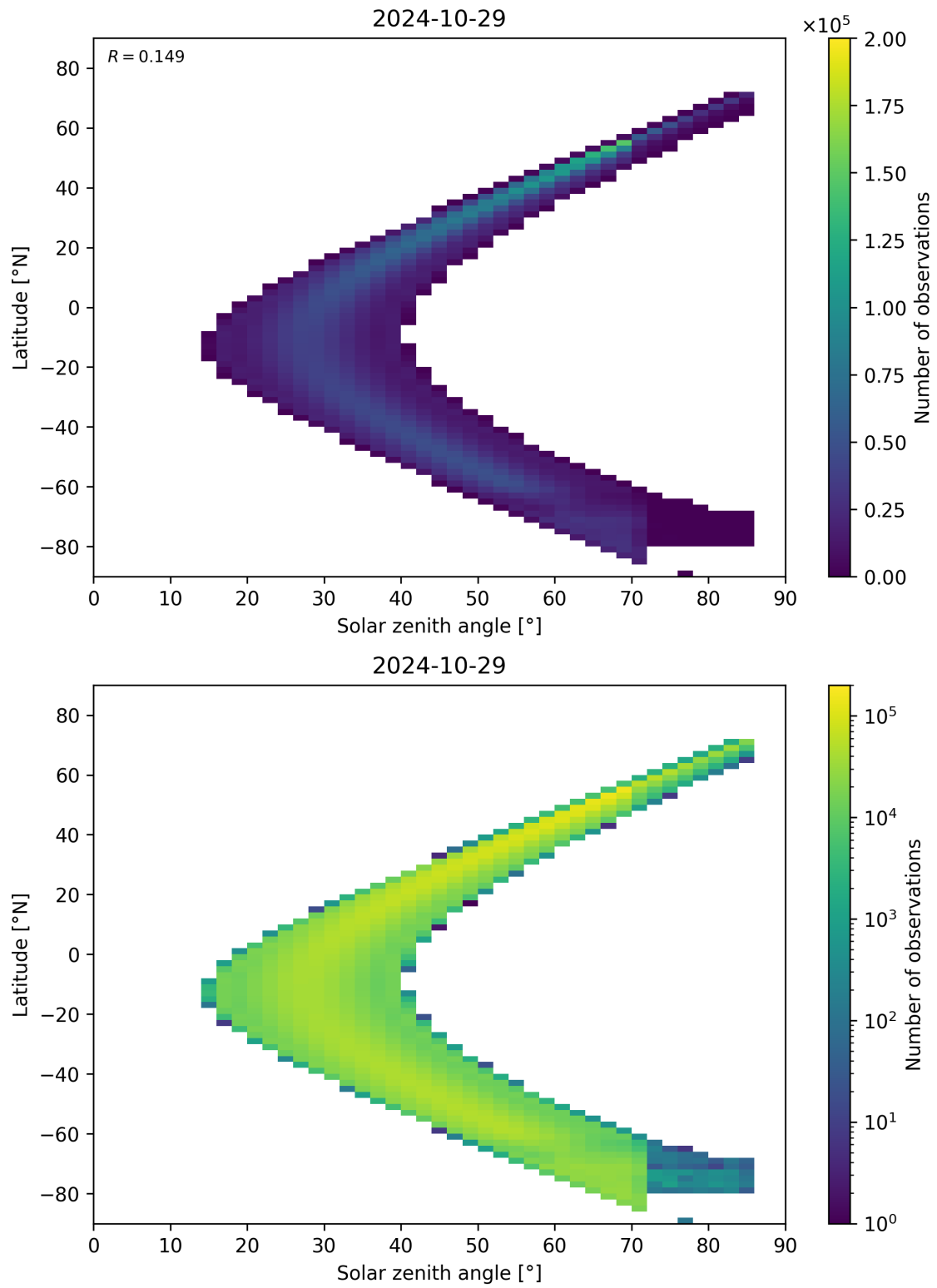
Figure 181: Scatter density plot of “Solar zenith angle” against “Latitude” for 2024-10-29 to 2024-10-30.
