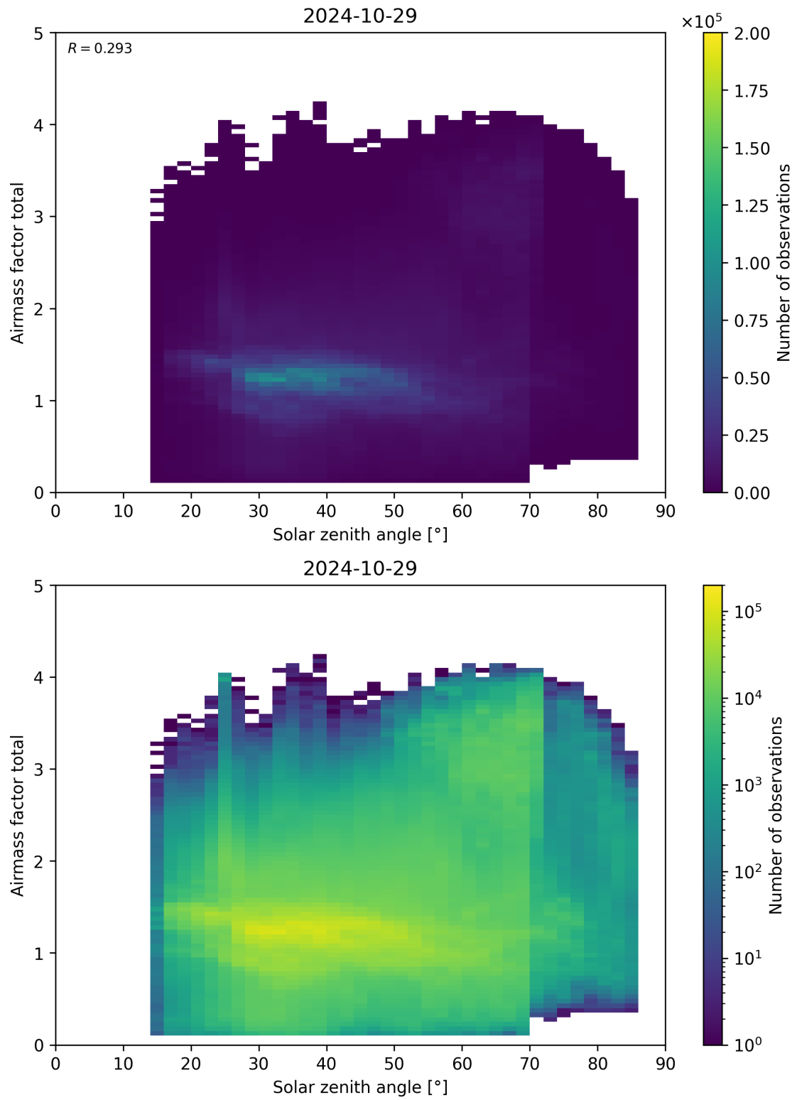
Figure 175: Scatter density plot of “Solar zenith angle” against “Airmass factor total” for 2024-10-29 to 2024-10-30.
