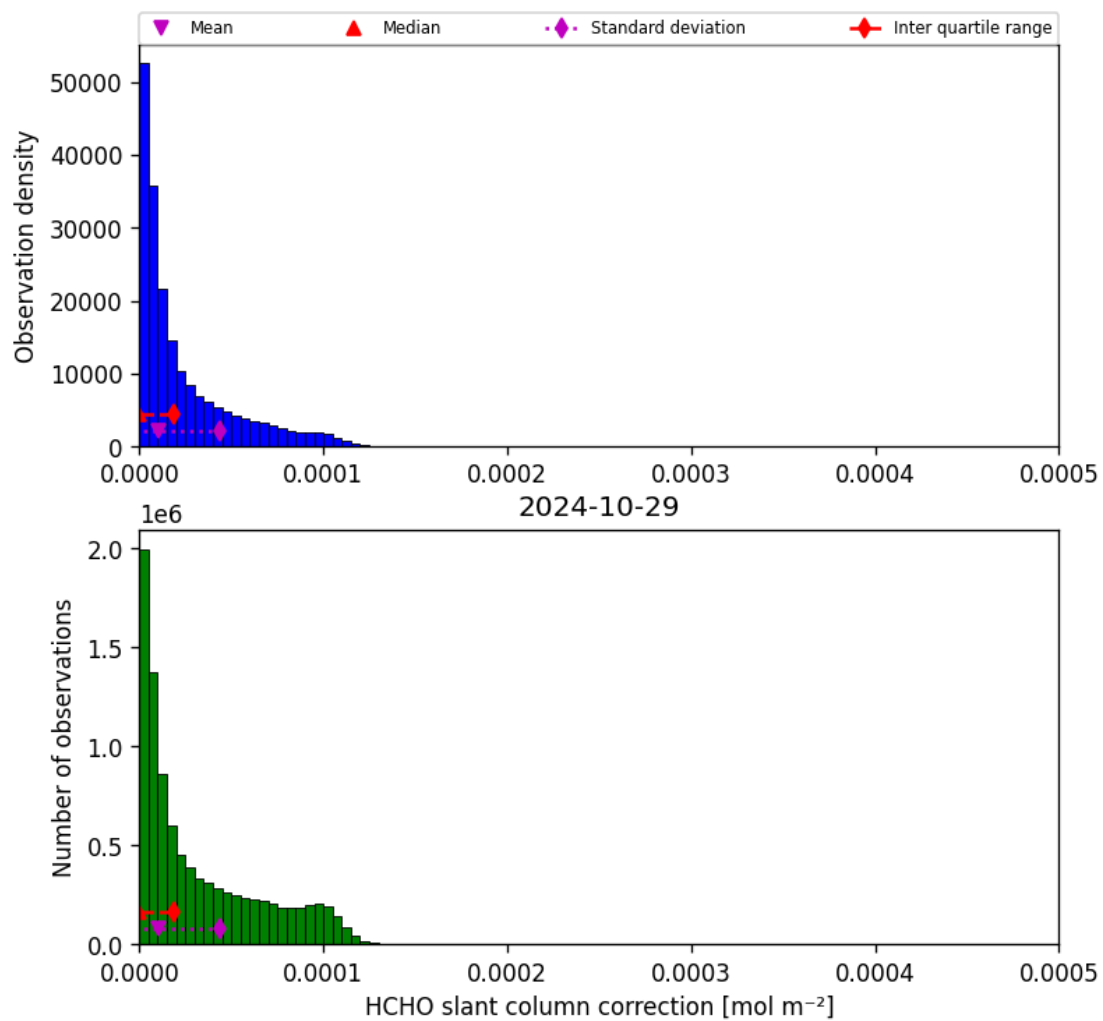
Figure 47: Histogram of “HCHO slant column correction” for 2024-10-29 to 2024-10-30
