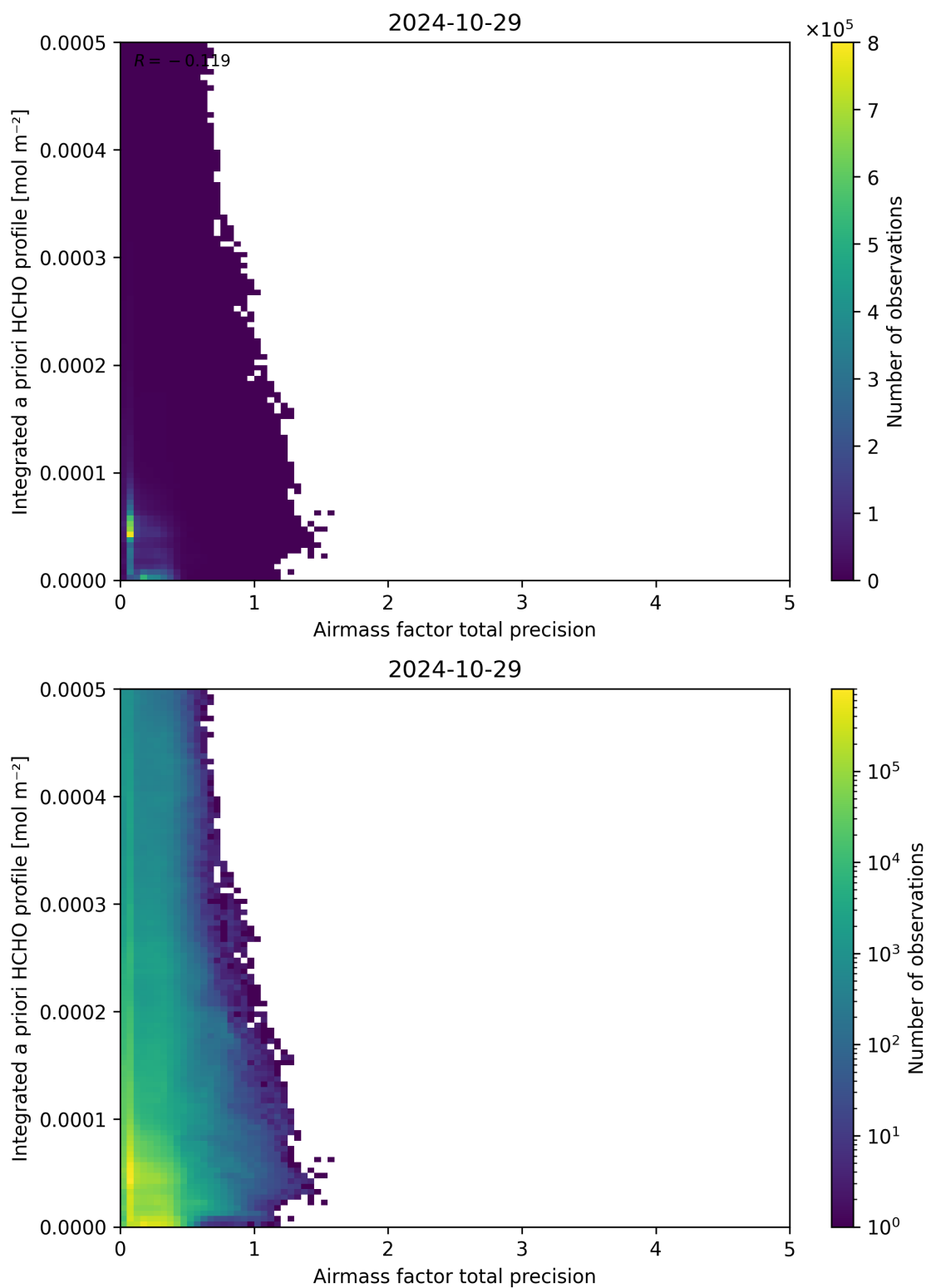
Figure 111: Scatter density plot of “Airmass factor total precision” against “Integrated a priori HCHO profile” for 2024-10-29 to 2024-10-30.
