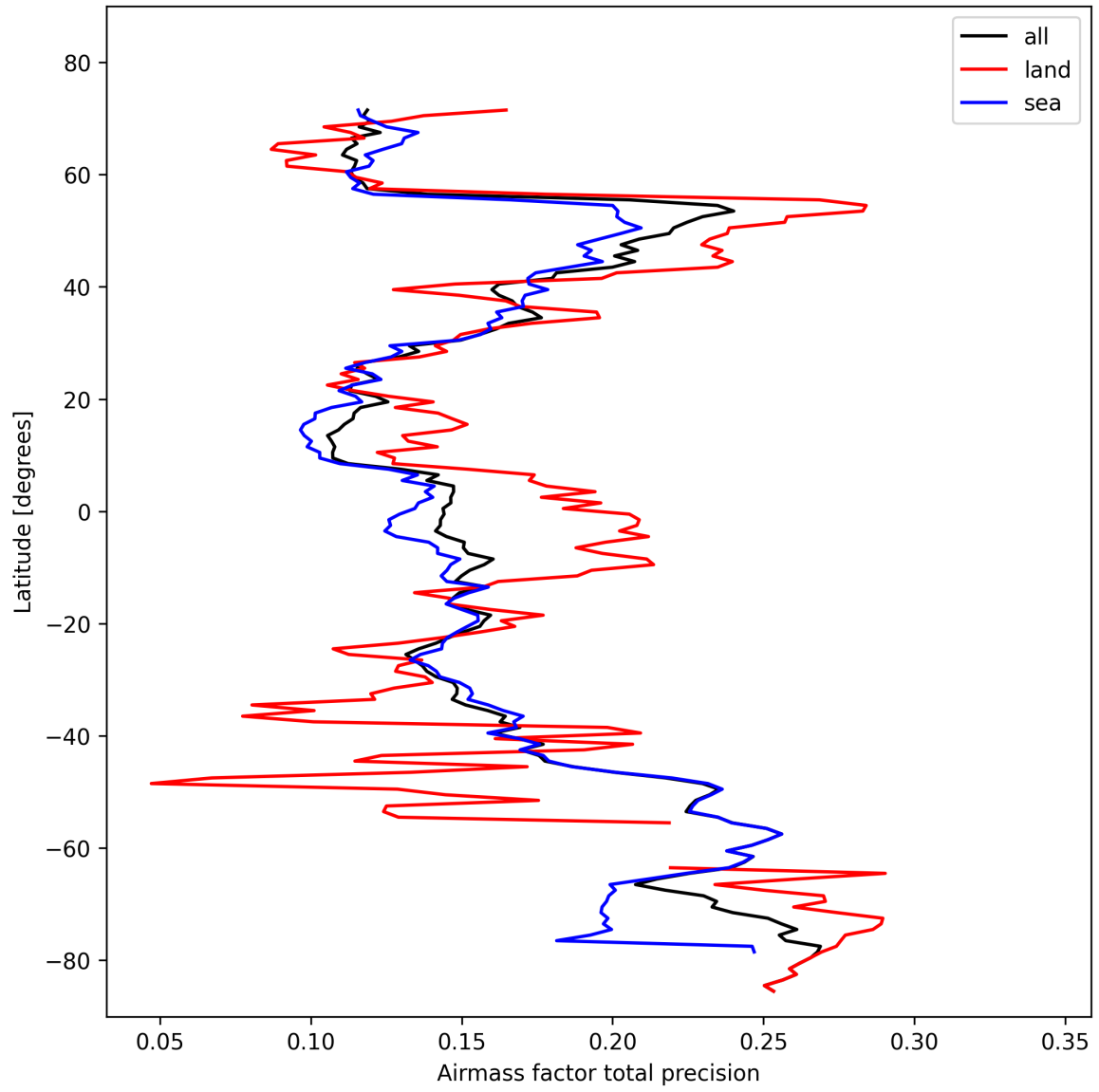
Figure 27: Zonal average of “Airmass factor total precision” for 2024-10-29 to 2024-10-30.
