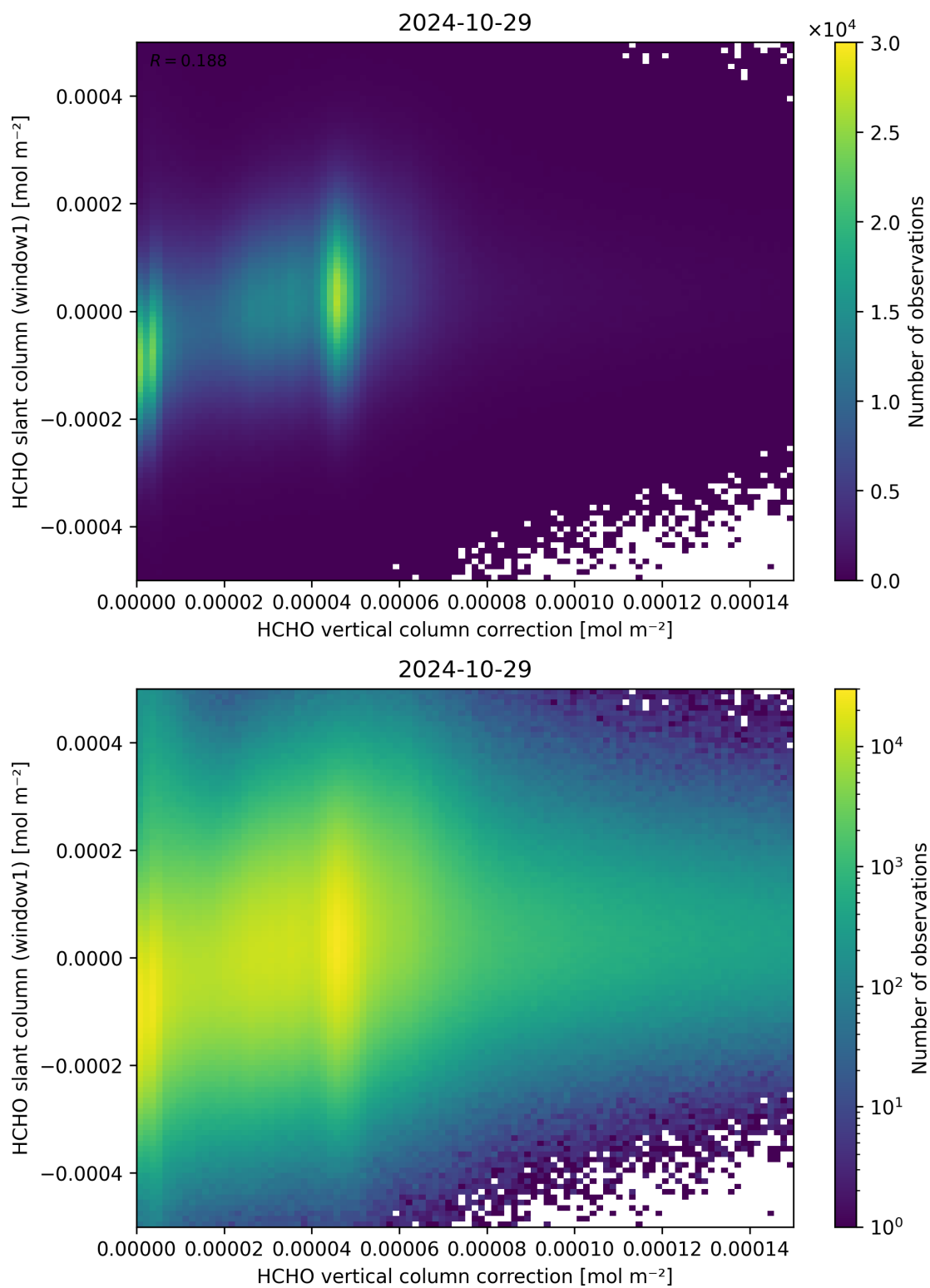
Figure 118: Scatter density plot of “HCHO vertical column correction” against “HCHO slant column (window1)” for 2024-10-29 to 2024-10-30.
