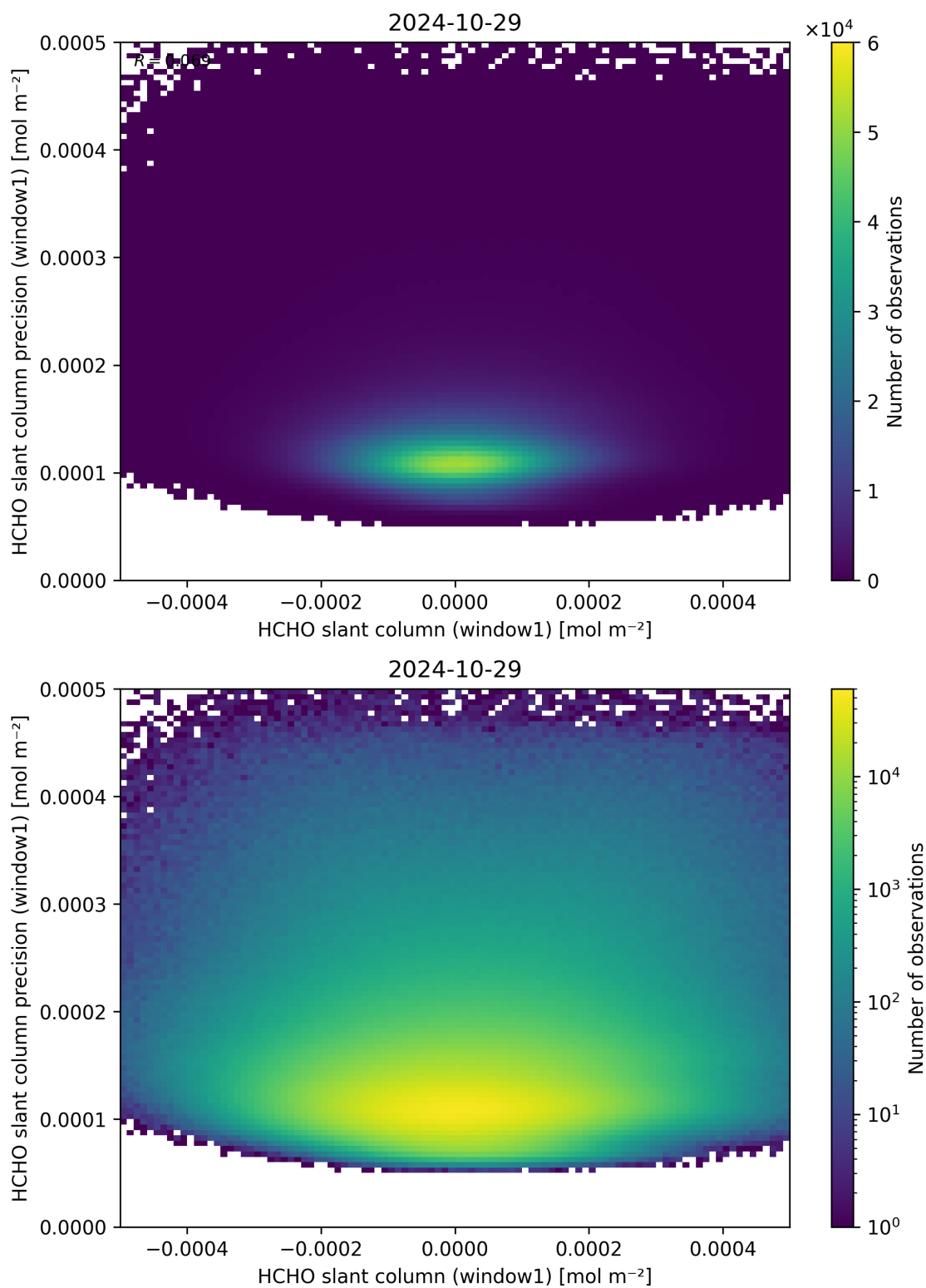
Figure 84: Scatter density plot of “HCHO slant column (window1)” against “HCHO slant column precision (window1)” for 2024-10-29 to 2024-10-30.
