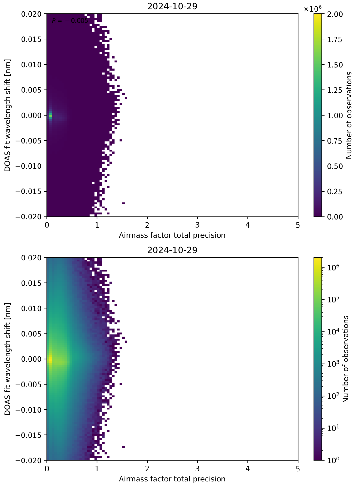
Figure 106: Scatter density plot of “Airmass factor total precision” against “DOAS fit wavelength shift” for 2024-10-29 to 2024-10-30.
