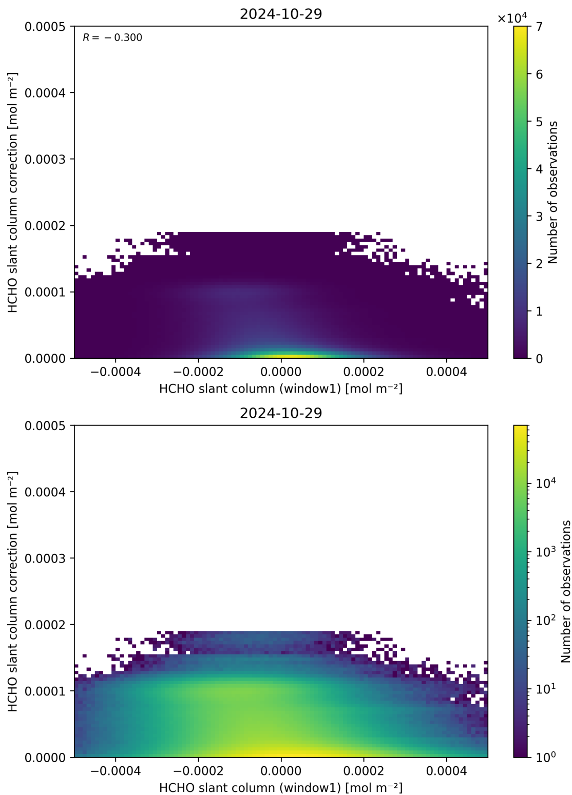
Figure 83: Scatter density plot of “HCHO slant column (window1)” against “HCHO slant column correction” for 2024-10-29 to 2024-10-30.
