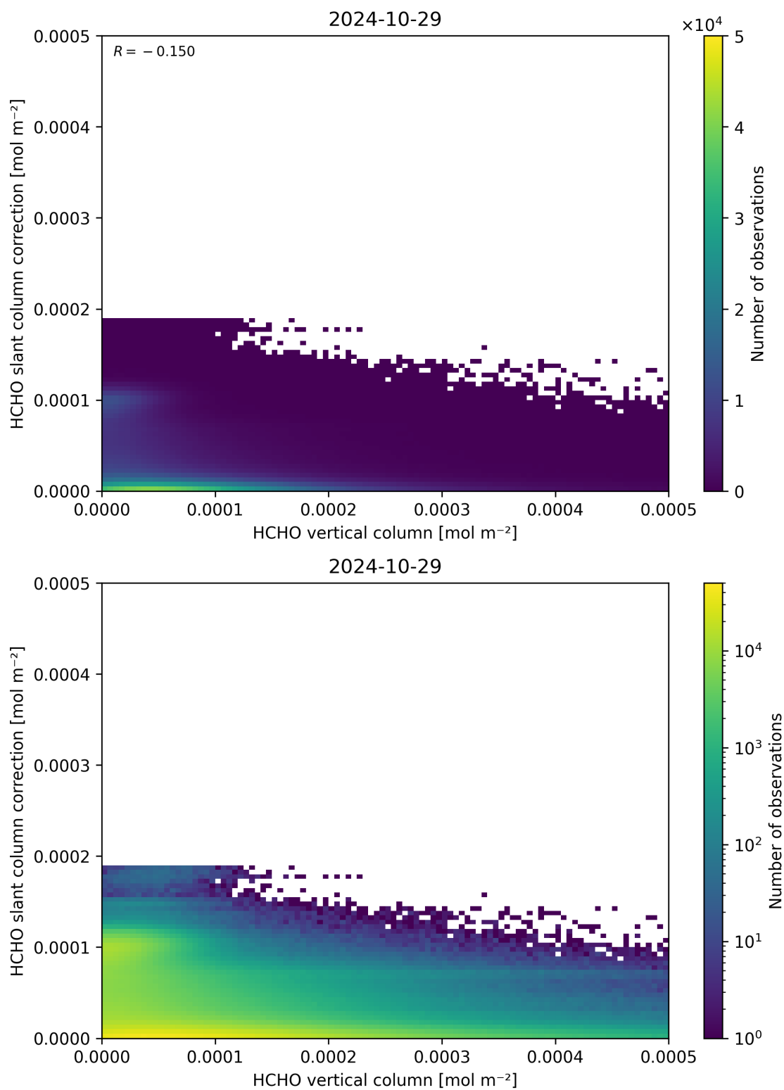
Figure 128: Scatter density plot of “HCHO vertical column” against “HCHO slant column correction” for 2024-10-29 to 2024-10-30.
