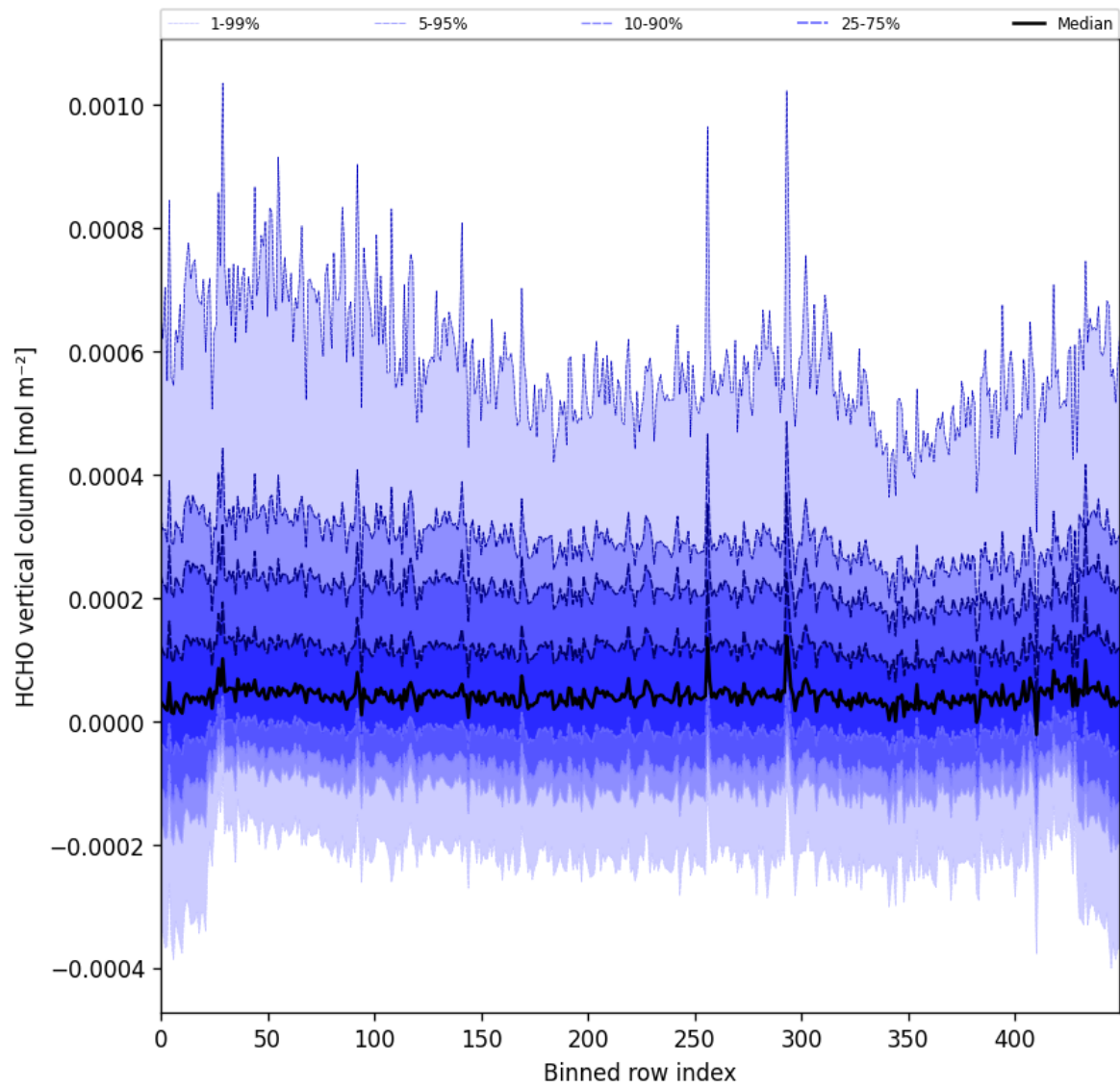
Figure 49: Along track statistics of “HCHO vertical column” for 2024-10-29 to 2024-10-30
