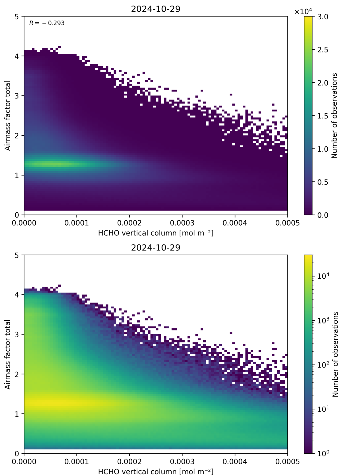
Figure 131: Scatter density plot of “HCHO vertical column” against “Airmass factor total” for 2024-10-29 to 2024-10-30.
