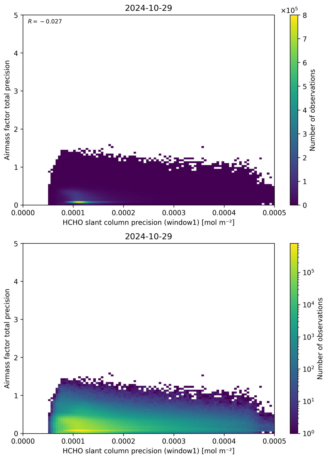
Figure 95: Scatter density plot of “HCHO slant column precision (window1)” against “Airmass factor total precision” for 2024-10-29 to 2024-10-30.
