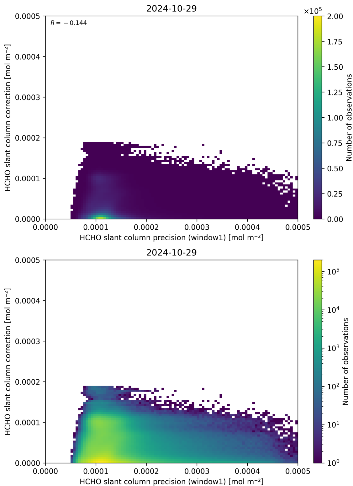
Figure 93: Scatter density plot of “HCHO slant column precision (window1)” against “HCHO slant column correction” for 2024-10-29 to 2024-10-30.
