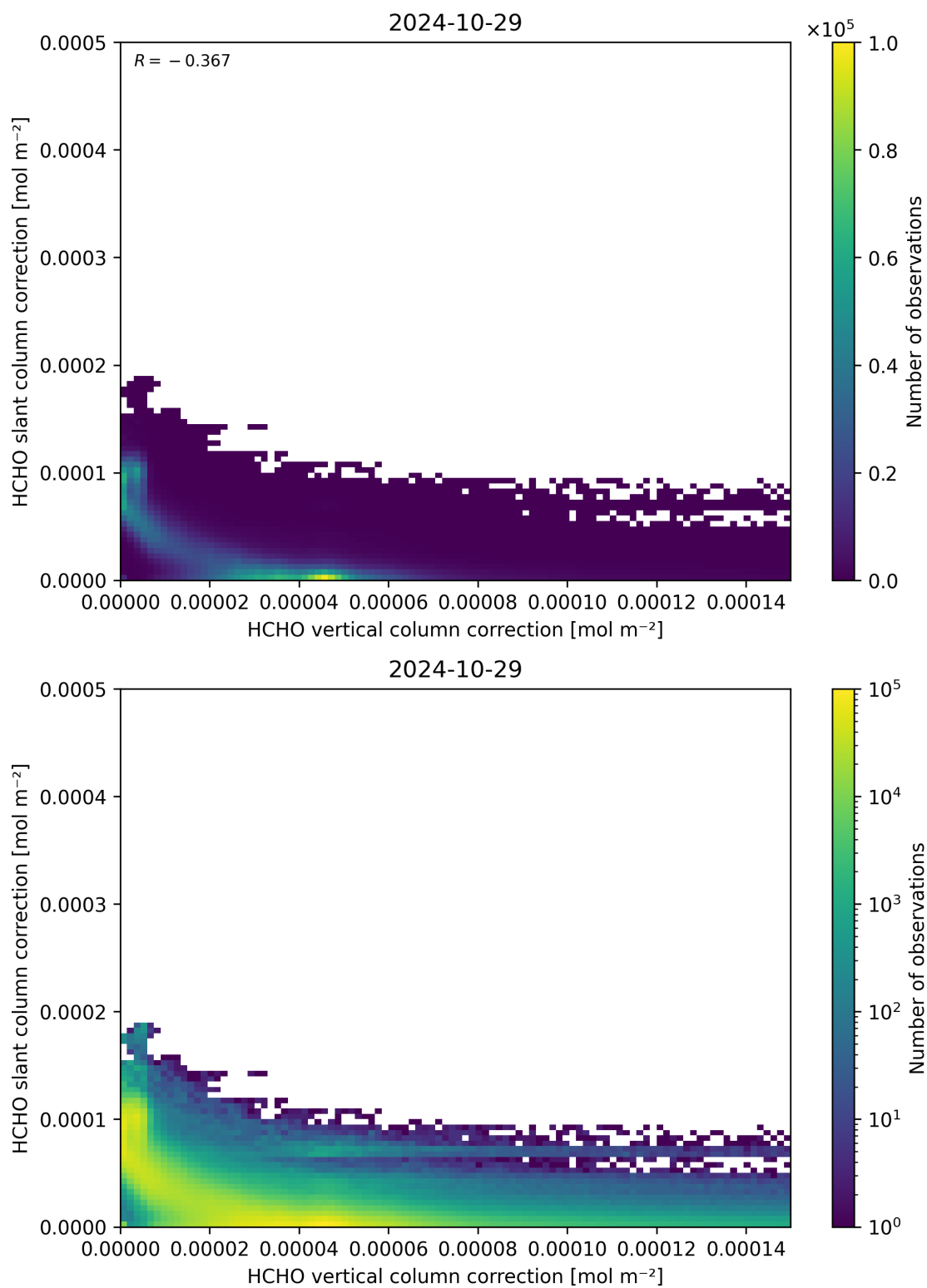
Figure 117: Scatter density plot of “HCHO vertical column correction” against “HCHO slant column correction” for 2024-10-29 to 2024-10-30.
