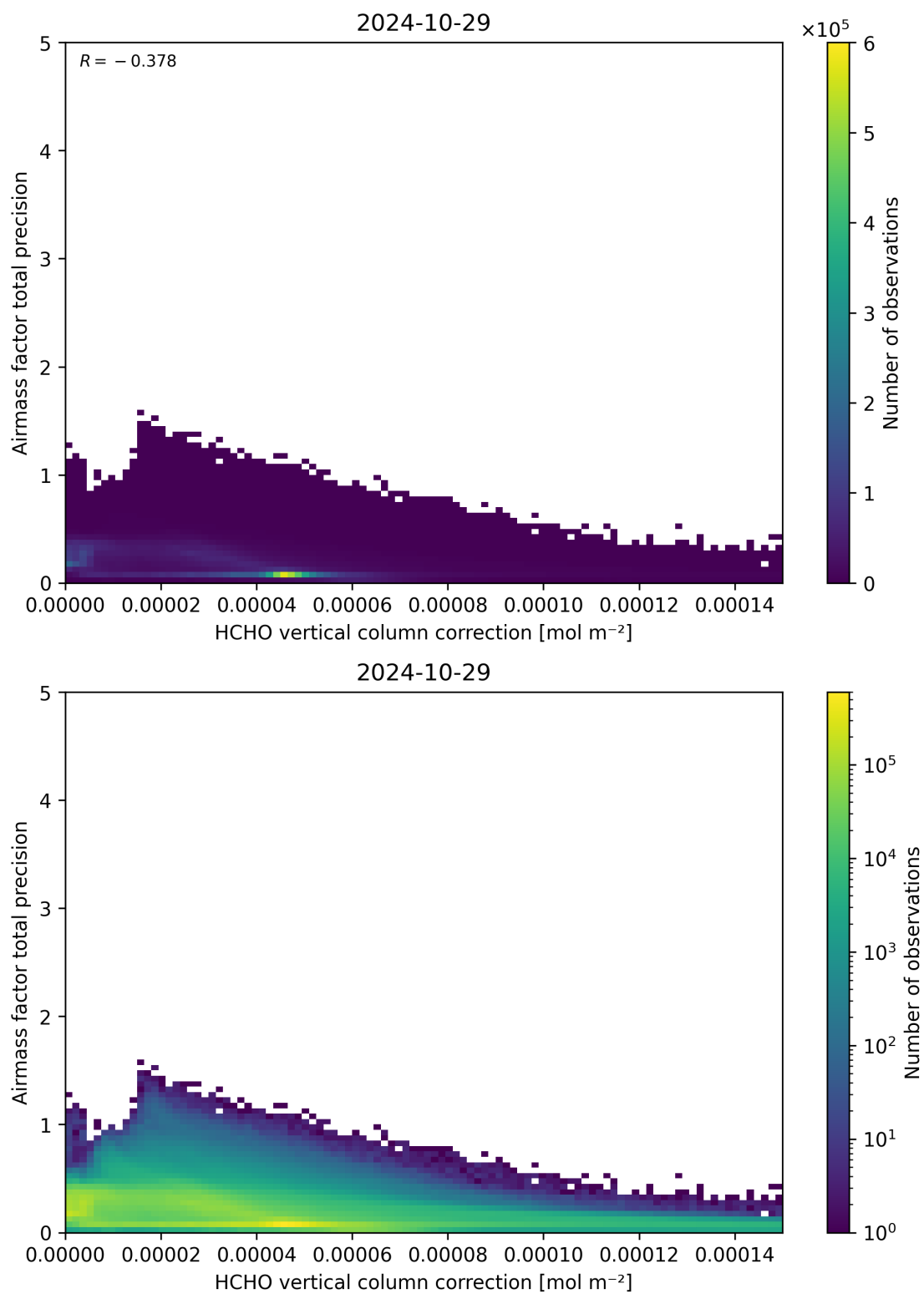
Figure 121: Scatter density plot of “HCHO vertical column correction” against “Airmass factor total precision” for 2024-10-29 to 2024-10-30.
