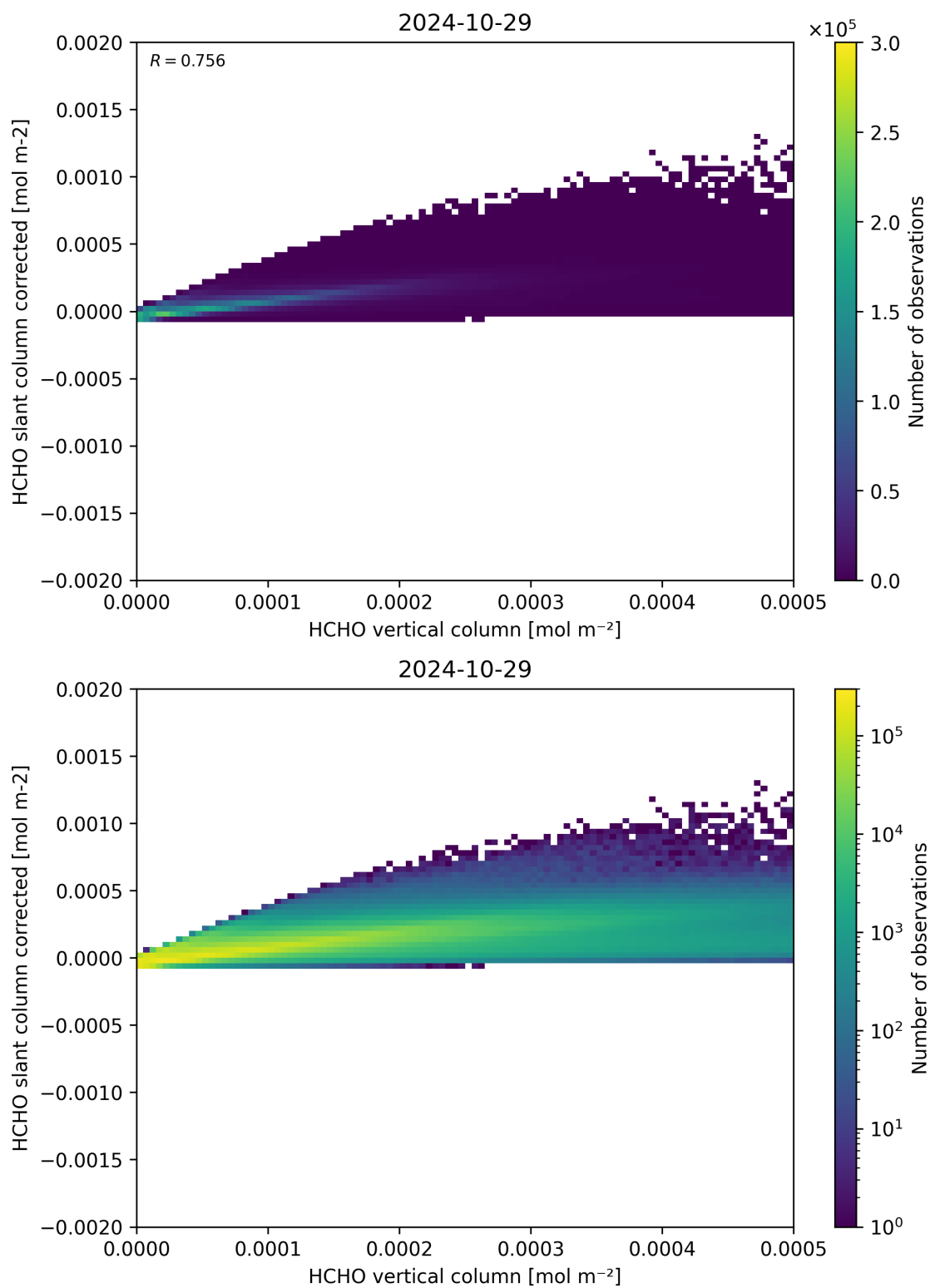
Figure 127: Scatter density plot of “HCHO vertical column” against “HCHO slant column corrected” for 2024-10-29 to 2024-10-30.
