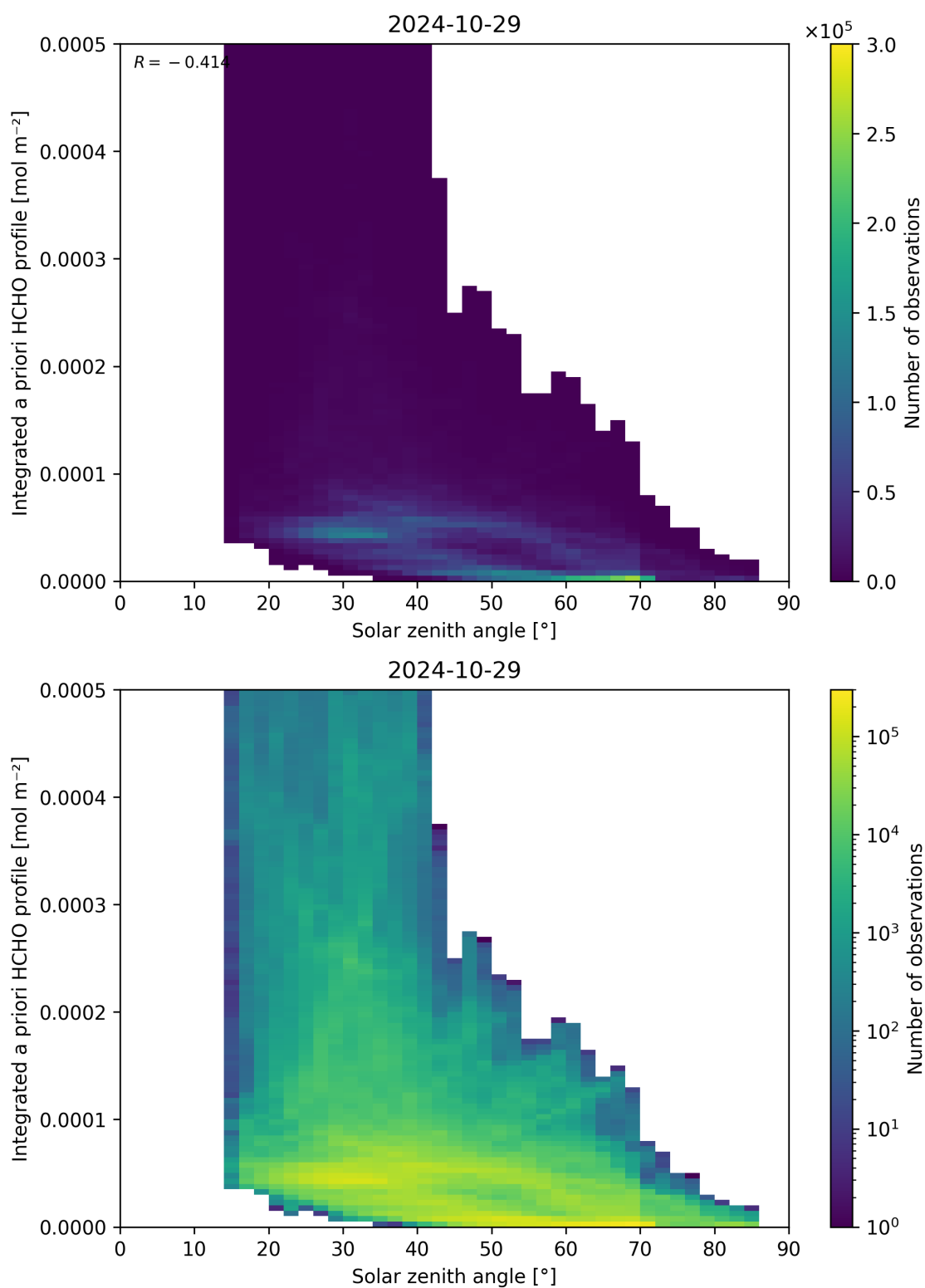
Figure 180: Scatter density plot of “Solar zenith angle” against “Integrated a priori HCHO profile” for 2024-10-29 to 2024-10-30.
