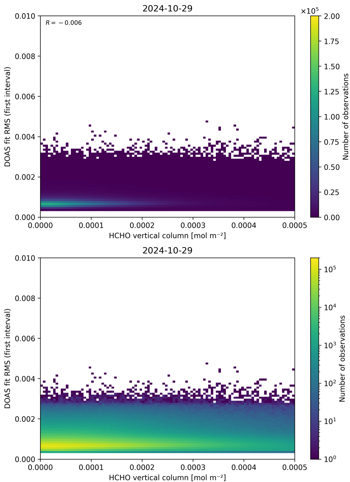
Figure 123: Scatter density plot of “HCHO vertical column” against “DOAS fit RMS (first interval)” for 2024-10-29 to 2024-10-30.
