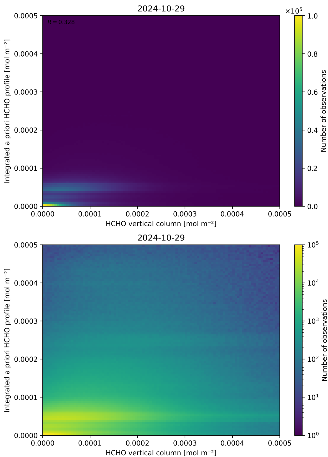
Figure 135: Scatter density plot of “HCHO vertical column” against “Integrated a priori HCHO profile” for 2024-10-29 to 2024-10-30.
