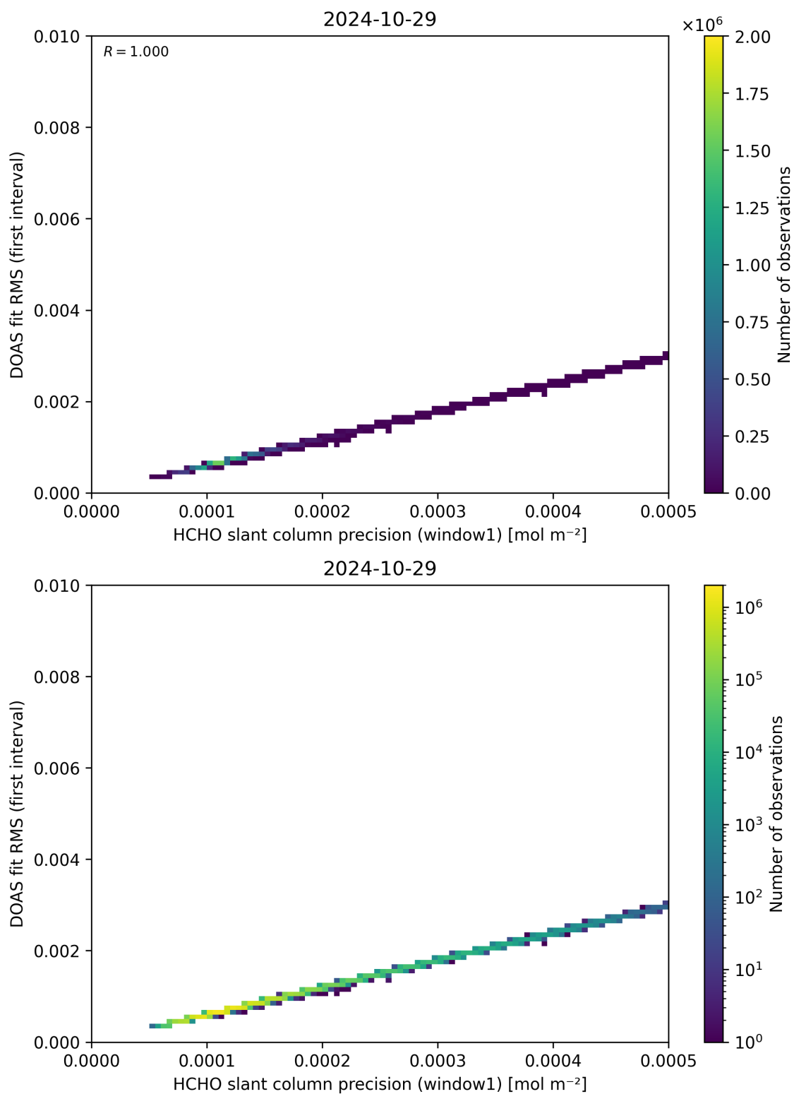
Figure 88: Scatter density plot of “HCHO slant column precision (window1)” against “DOAS fit RMS (first interval)” for 2024-10-29 to 2024-10-30.
