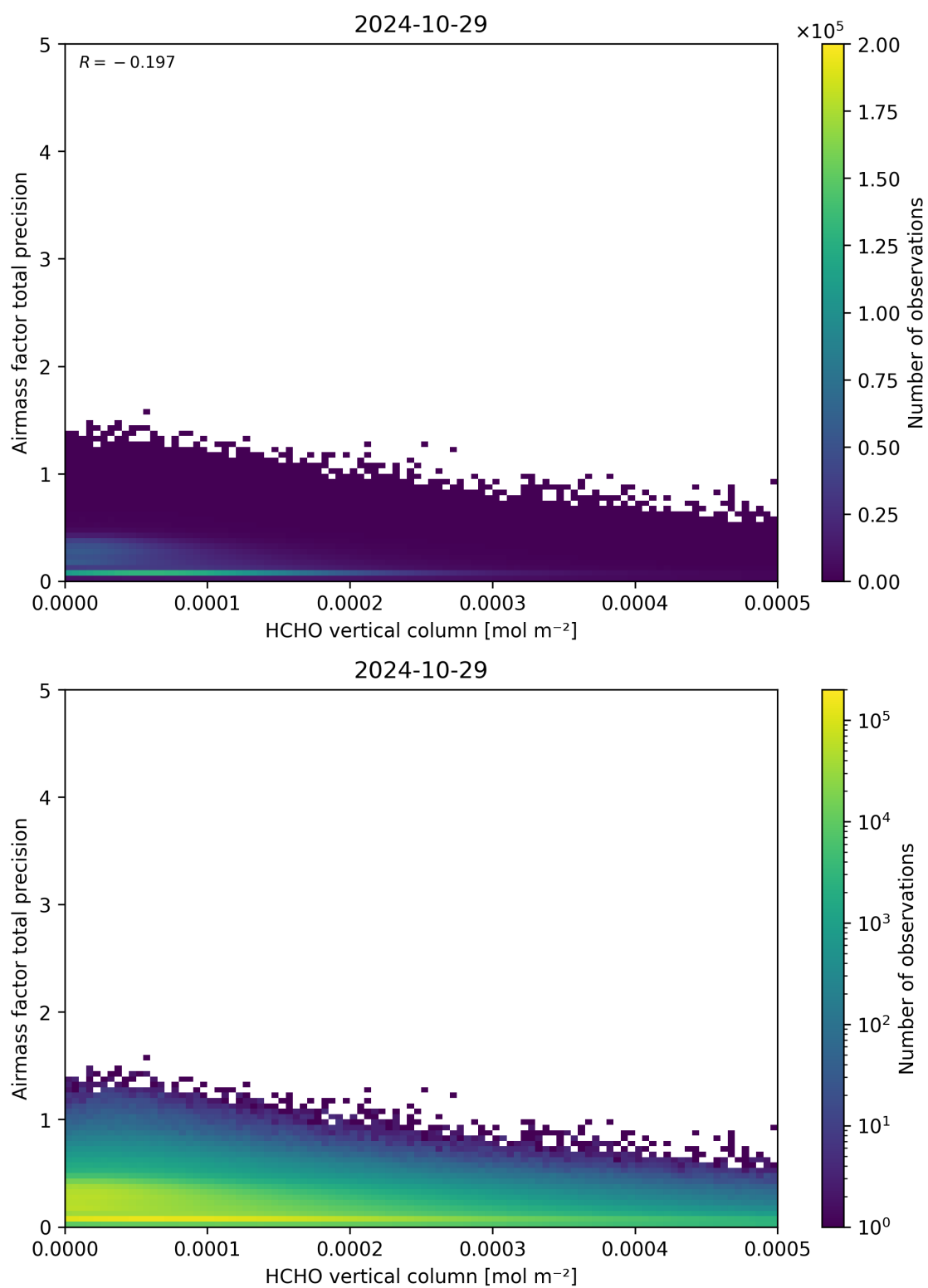
Figure 132: Scatter density plot of “HCHO vertical column” against “Airmass factor total precision” for 2024-10-29 to 2024-10-30.
