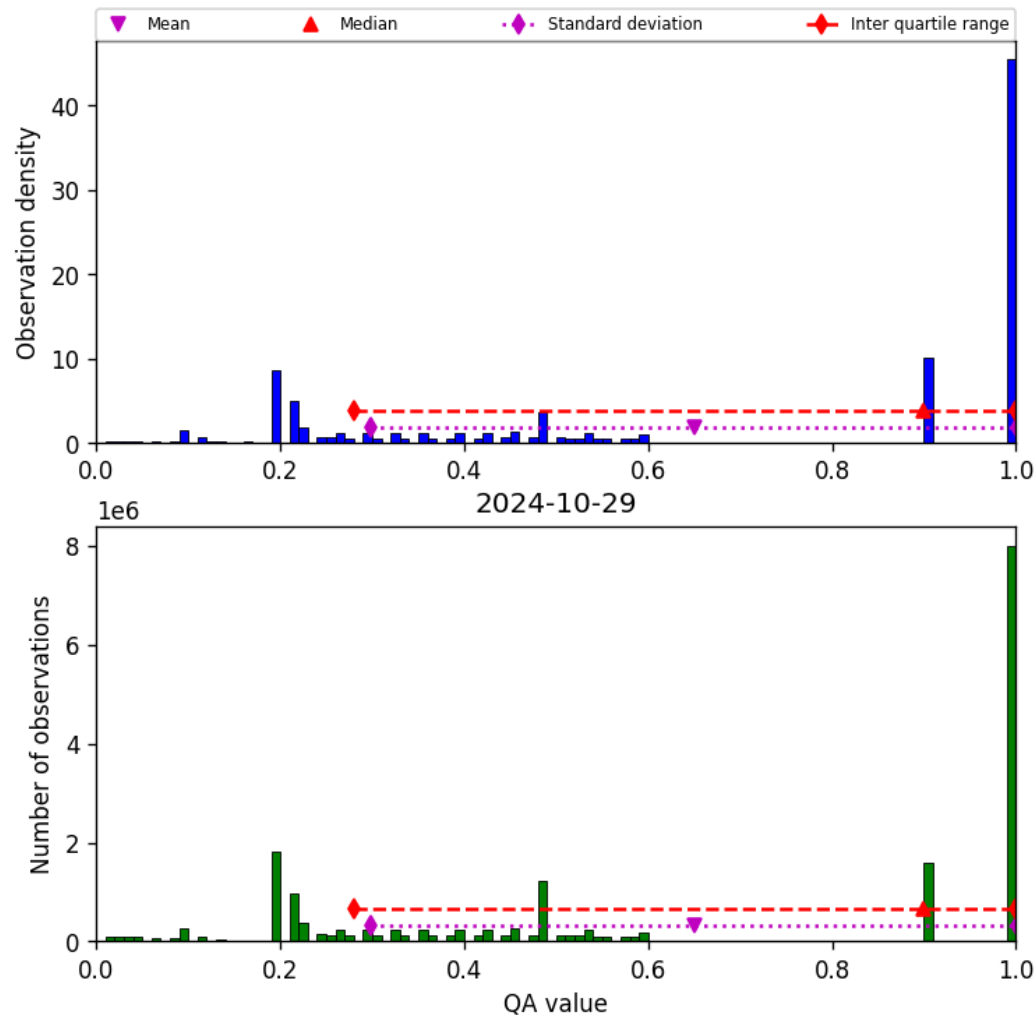
Figure 34: Histogram of “QA value” for 2024-10-29 to 2024-10-30
