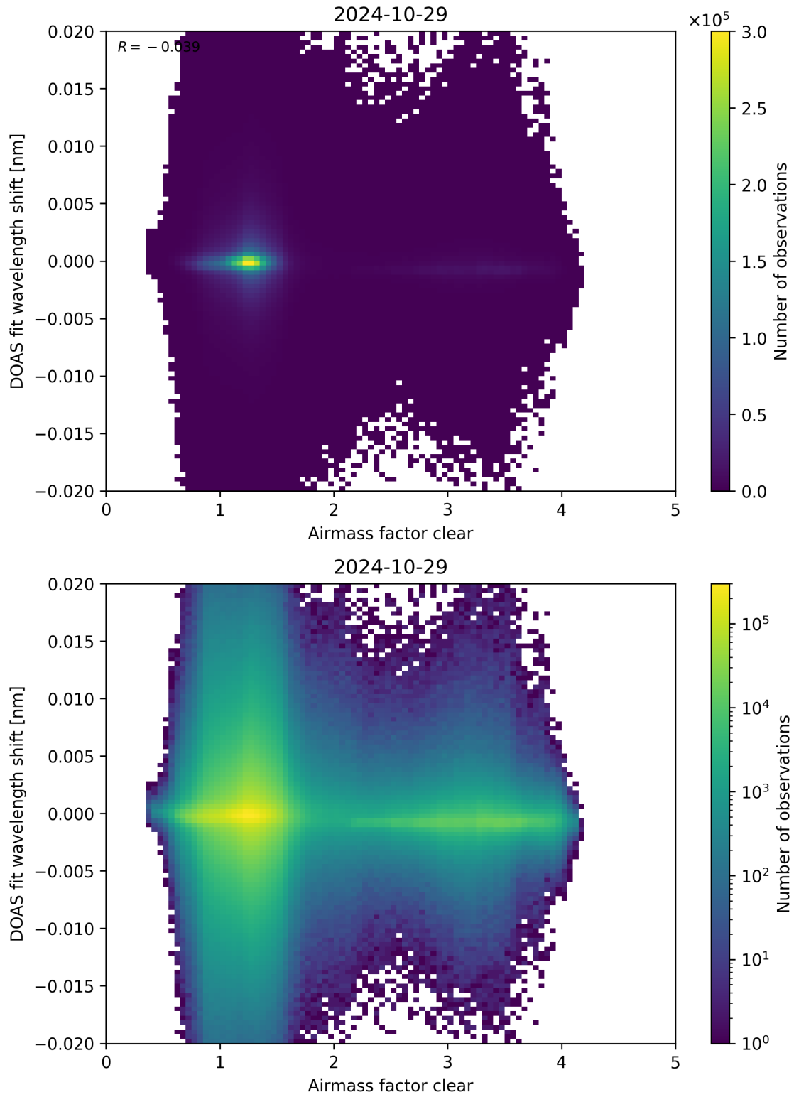
Figure 72: Scatter density plot of “Airmass factor clear” against “DOAS fit wavelength shift” for 2024-10-29 to 2024-10-30.
