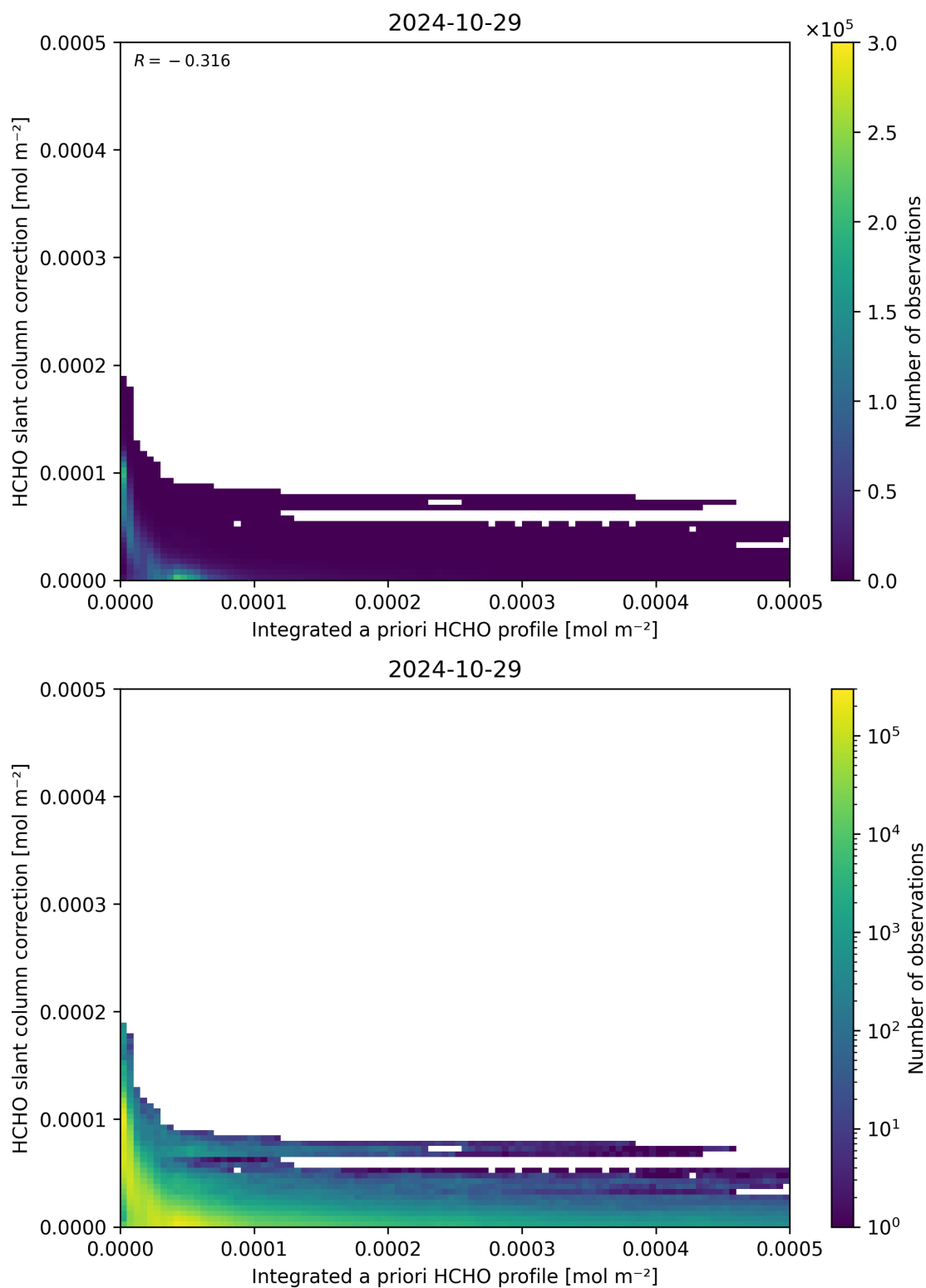
Figure 152: Scatter density plot of “Integrated a priori HCHO profile” against “HCHO slant column correction” for 2024-10-29 to 2024-10-30.
