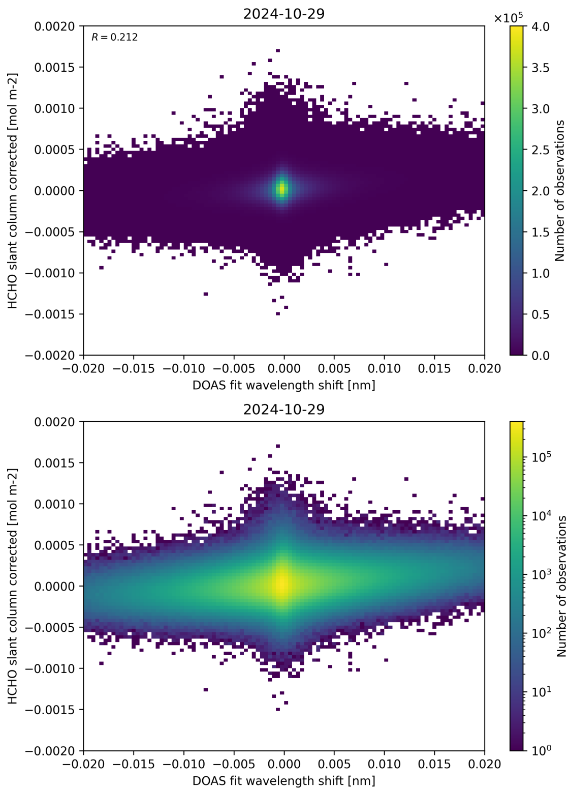
Figure 66: Scatter density plot of “DOAS fit wavelength shift” against “HCHO slant column corrected” for 2024-10-29 to 2024-10-30.
