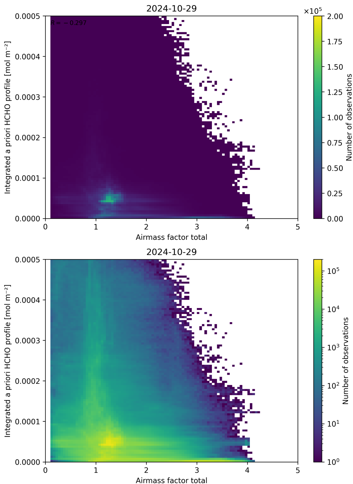
Figure 104: Scatter density plot of “Airmass factor total” against “Integrated a priori HCHO profile” for 2024-10-29 to 2024-10-30.
