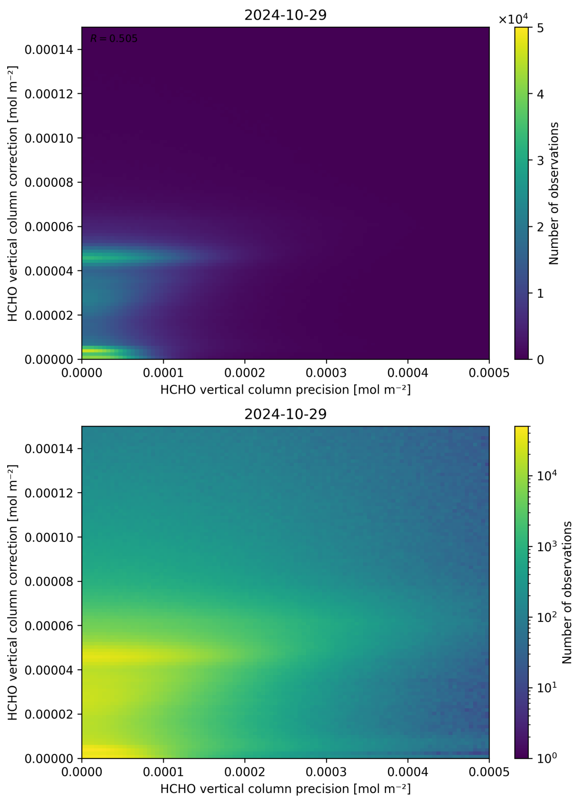
Figure 146: Scatter density plot of “HCHO vertical column precision” against “HCHO vertical column correction” for 2024-10-29 to 2024-10-30.
