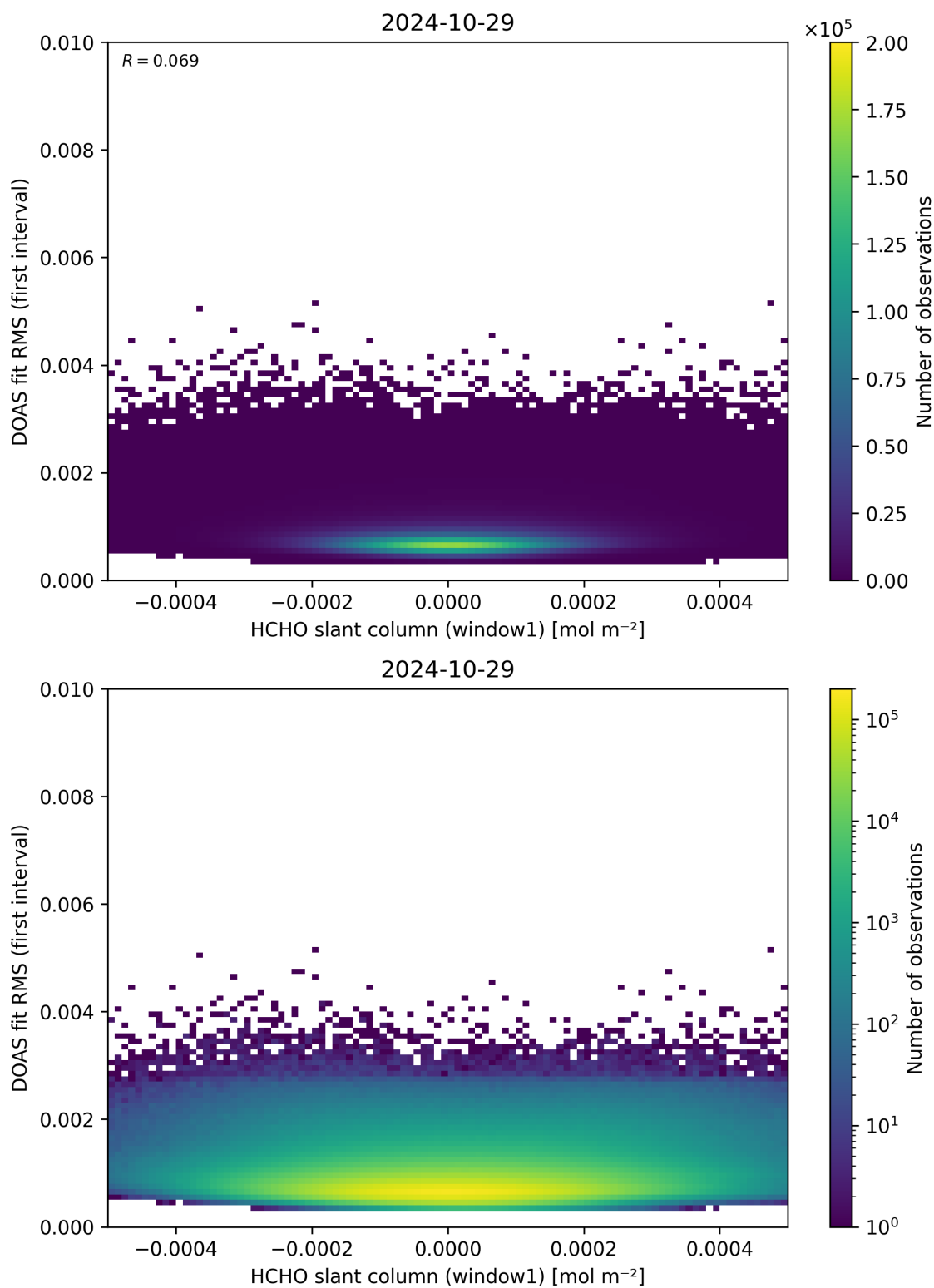
Figure 78: Scatter density plot of “HCHO slant column (window1)” against “DOAS fit RMS (first interval)” for 2024-10-29 to 2024-10-30.
