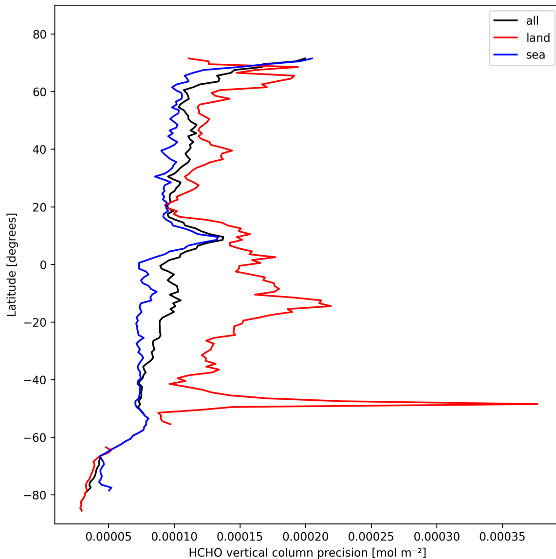
Figure 22: Zonal average of “HCHO vertical column precision” for 2024-10-29 to 2024-10-30.
