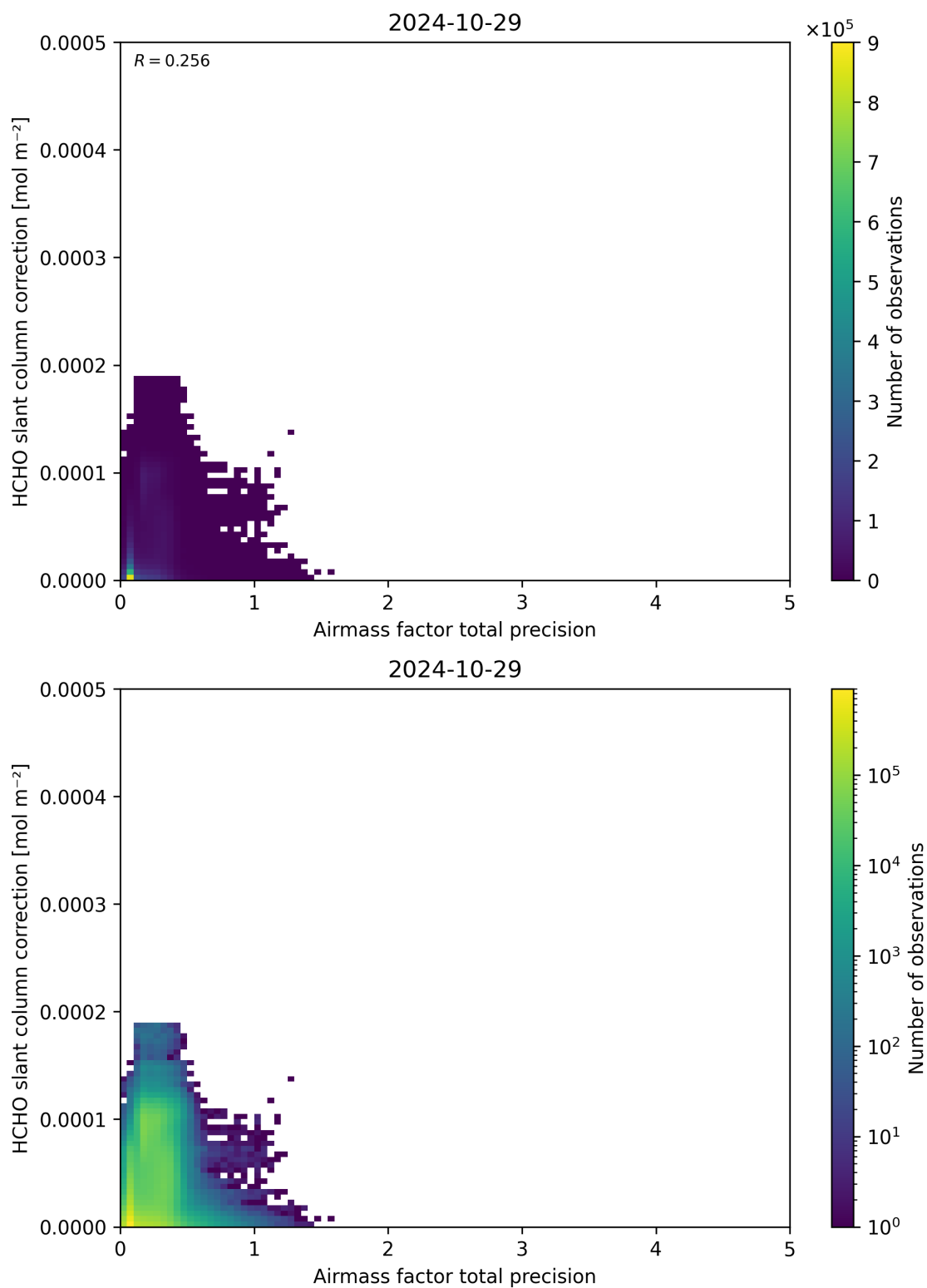
Figure 110: Scatter density plot of “Airmass factor total precision” against “HCHO slant column correction” for 2024-10-29 to 2024-10-30.
