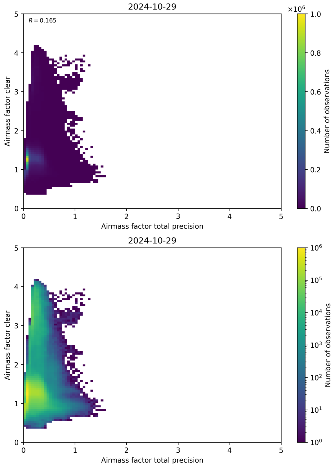
Figure 108: Scatter density plot of “Airmass factor total precision” against “Airmass factor clear” for 2024-10-29 to 2024-10-30.
