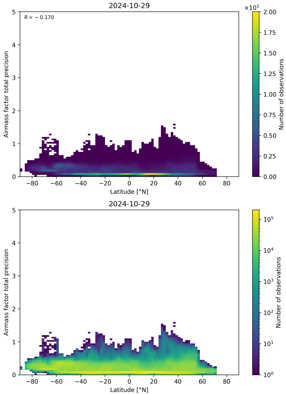
Figure 162: Scatter density plot of “Latitude” against “Airmass factor total precision” for 2024-10-29 to 2024-10-30.
