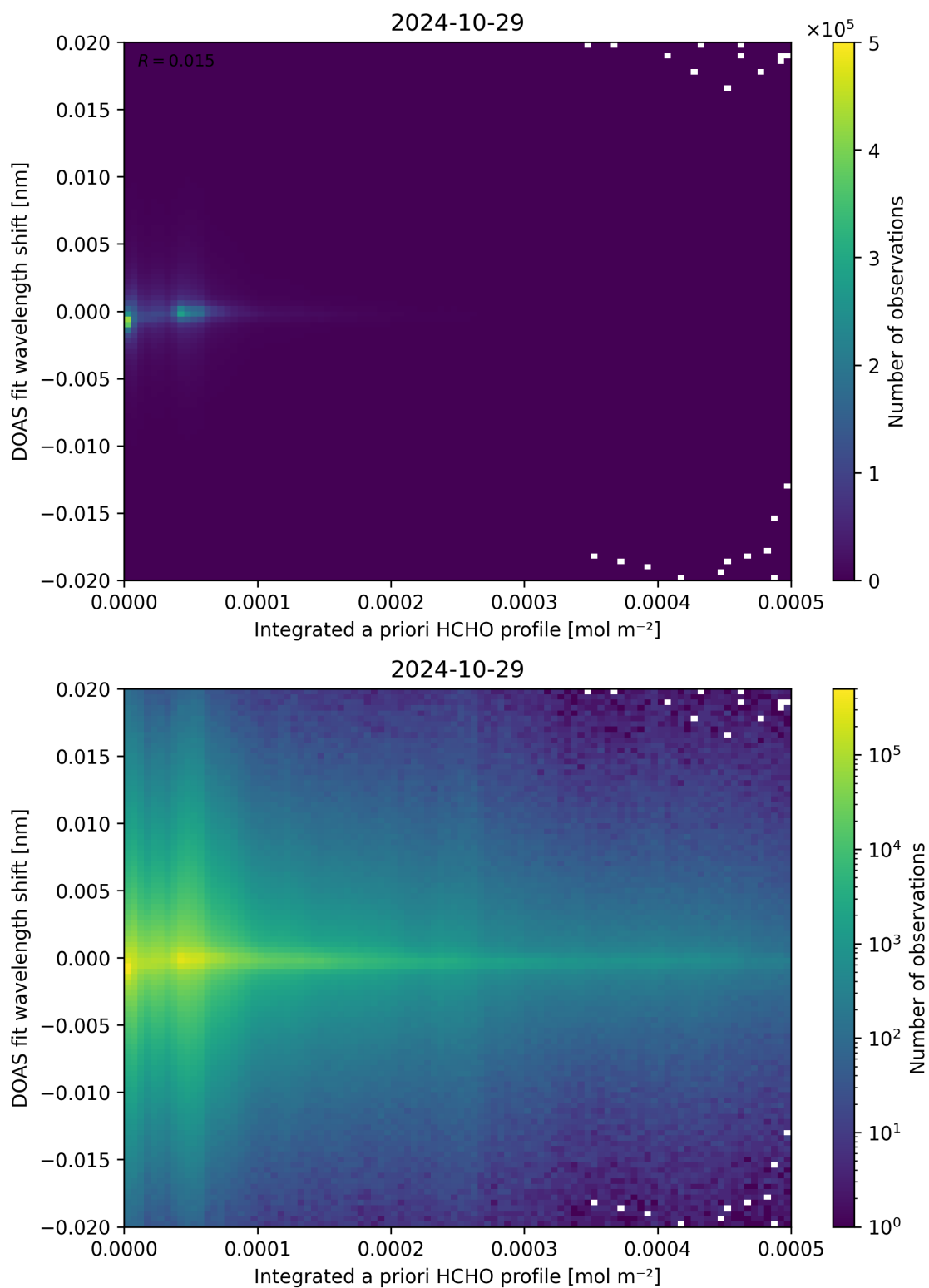
Figure 149: Scatter density plot of “Integrated a priori HCHO profile” against “DOAS fit wavelength shift” for 2024-10-29 to 2024-10-30.
