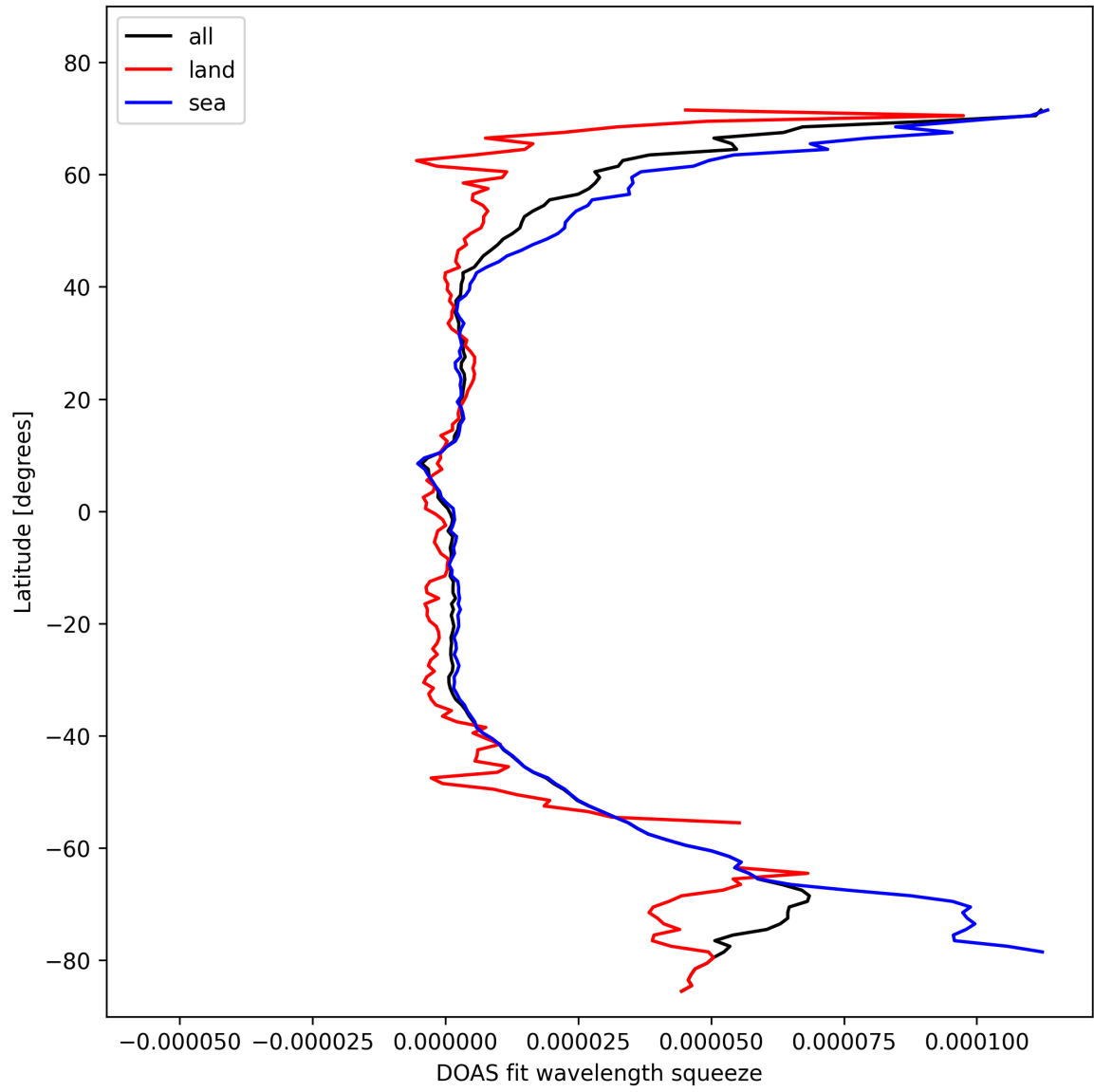
Figure 31: Zonal average of "DOAS fit wavelength squeeze" for 2024-10-29 to 2024-10-30.
