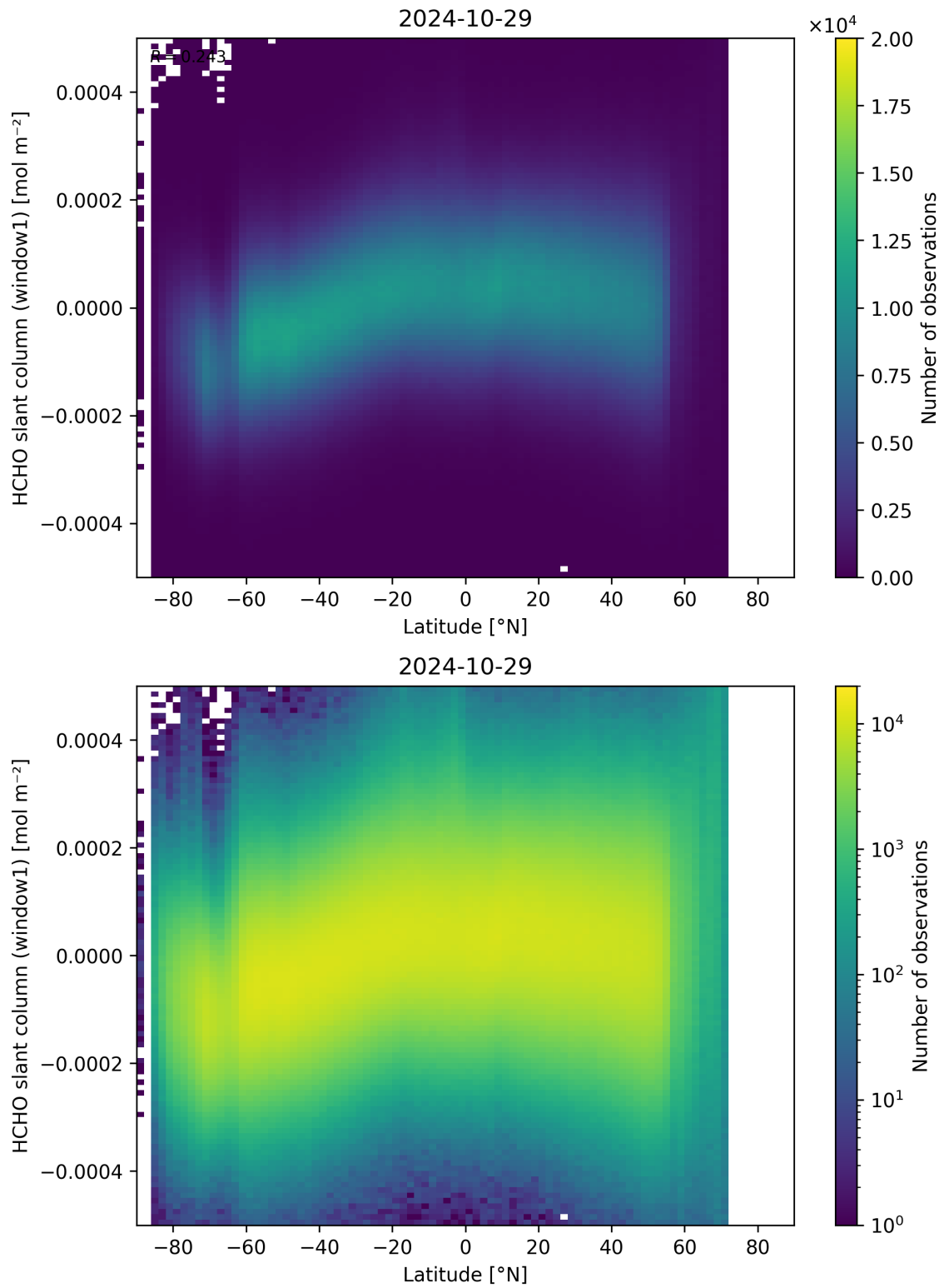
Figure 159: Scatter density plot of “Latitude” against “HCHO slant column (window1)” for 2024-10-29 to 2024-10-30.
