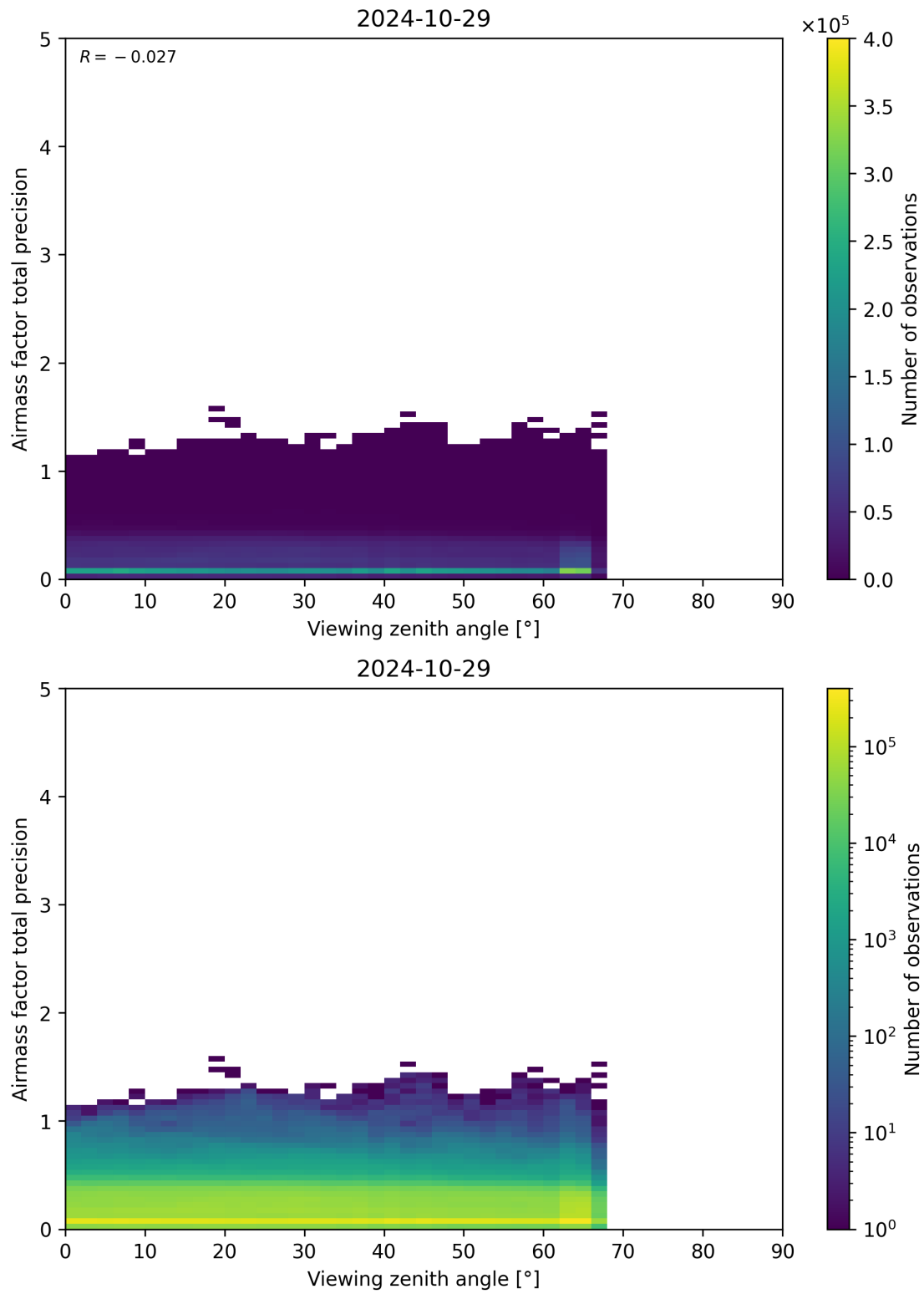
Figure 191: Scatter density plot of “Viewing zenith angle” against “Airmass factor total precision” for 2024-10-29 to 2024-10-30.
