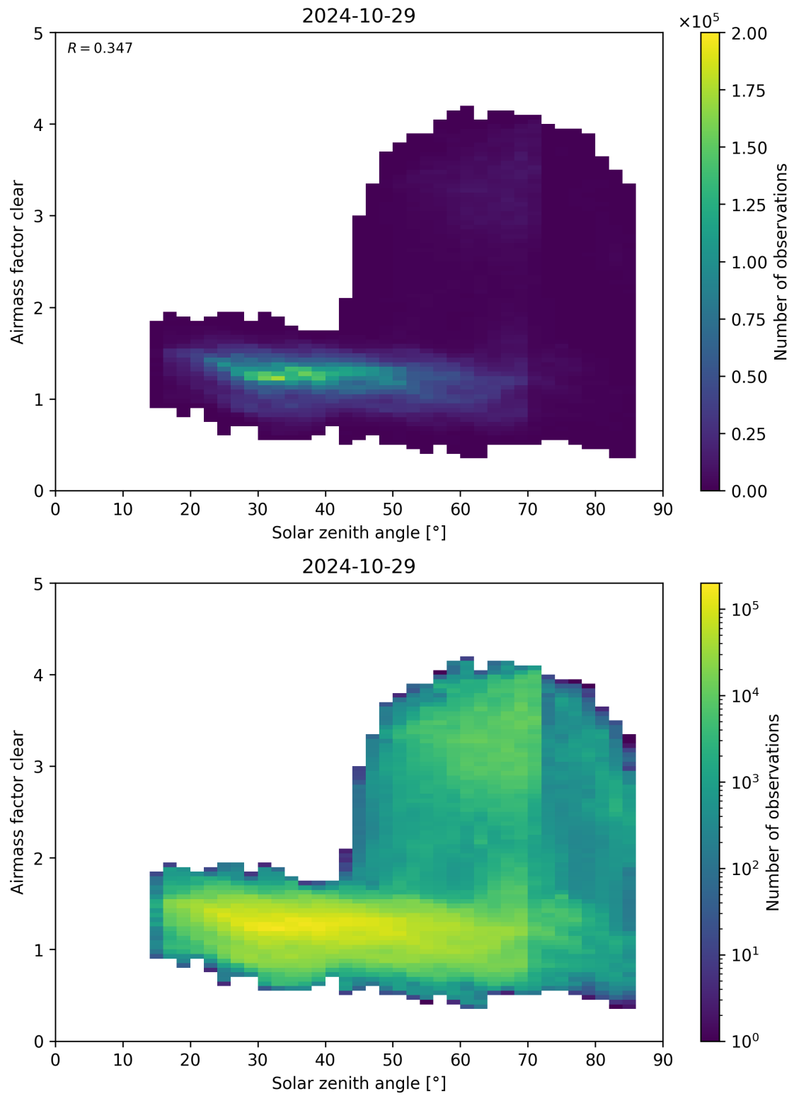
Figure 170: Scatter density plot of “Solar zenith angle” against “Airmass factor clear” for 2024-10-29 to 2024-10-30.
