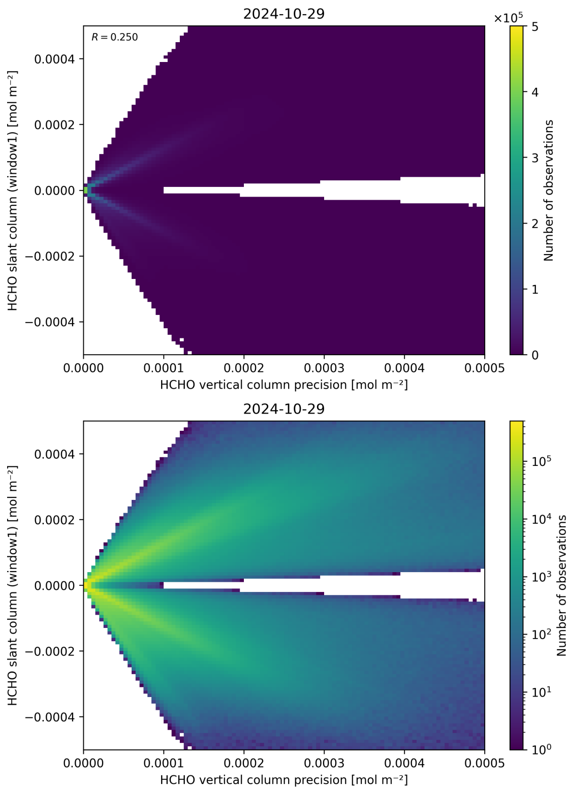
Figure 142: Scatter density plot of “HCHO vertical column precision” against “HCHO slant column (window1)” for 2024-10-29 to 2024-10-30.
