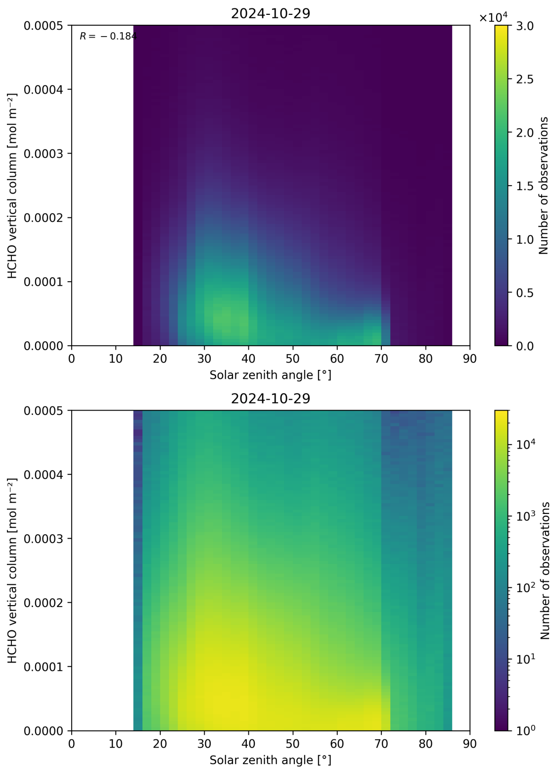
Figure 177: Scatter density plot of “Solar zenith angle” against “HCHO vertical column” for 2024-10-29 to 2024-10-30.
