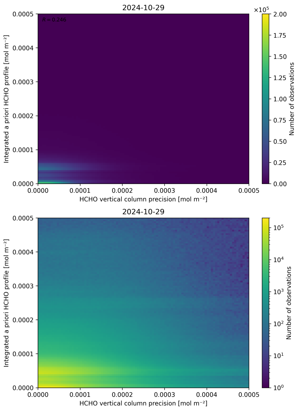
Figure 147: Scatter density plot of “HCHO vertical column precision” against “Integrated a priori HCHO profile” for 2024-10-29 to 2024-10-30.
