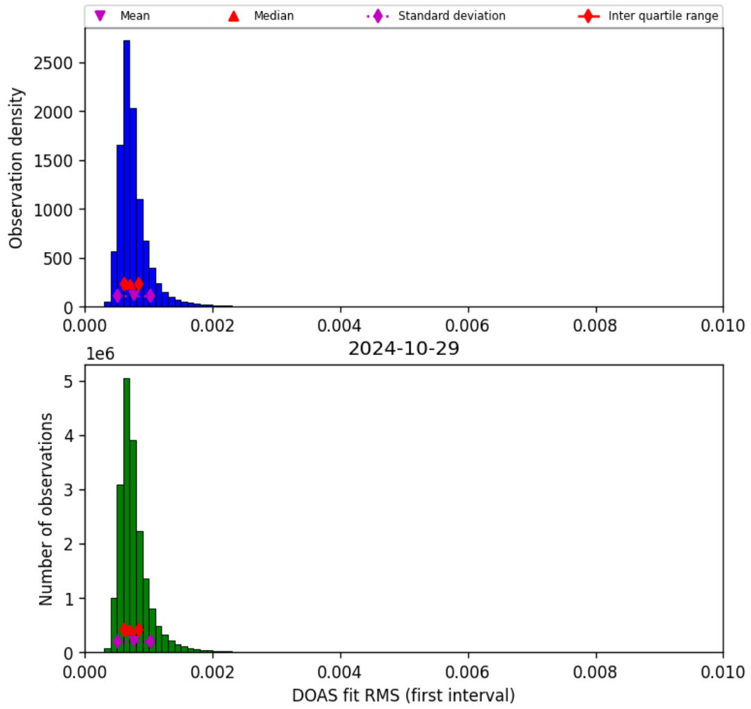
Figure 46: Histogram of “DOAS fit RMS (first interval)” for 2024-10-29 to 2024-10-30
