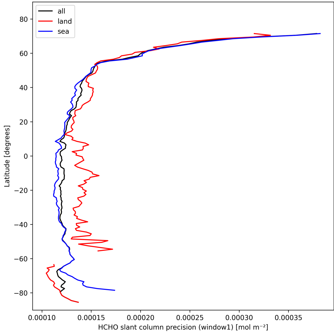
Figure 25: Zonal average of “HCHO slant column precision (window1)” for 2024-10-29 to 2024-10-30.
