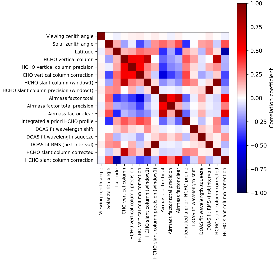
Figure 2: Map of correlation matrix for 2024-10-29 to 2024-10-30.
