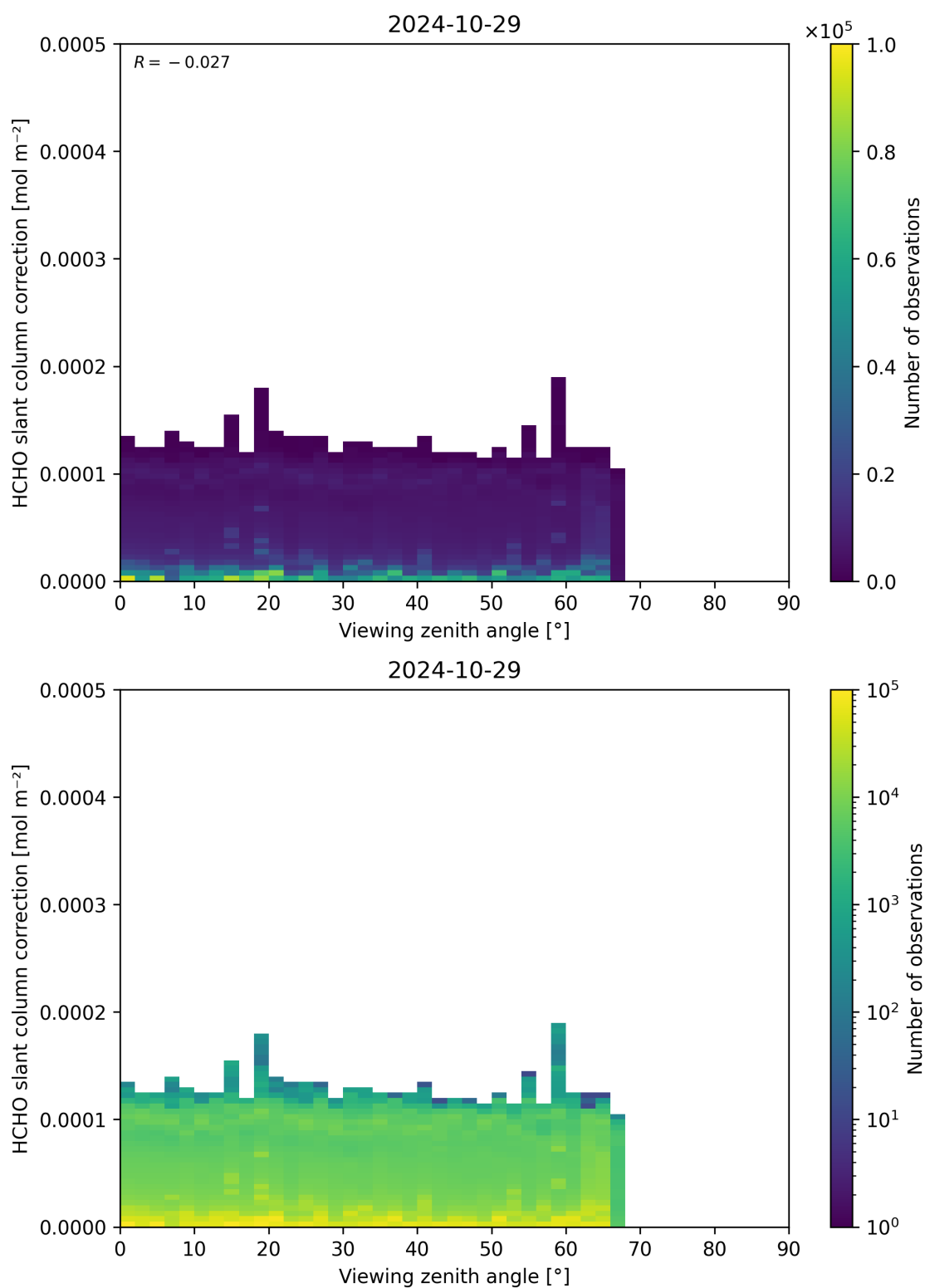
Figure 187: Scatter density plot of “Viewing zenith angle” against “HCHO slant column correction” for 2024-10-29 to 2024-10-30.
