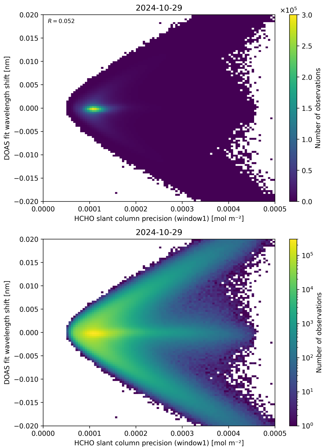
Figure 89: Scatter density plot of “HCHO slant column precision (window1)” against “DOAS fit wavelength shift” for 2024-10-29 to 2024-10-30.
