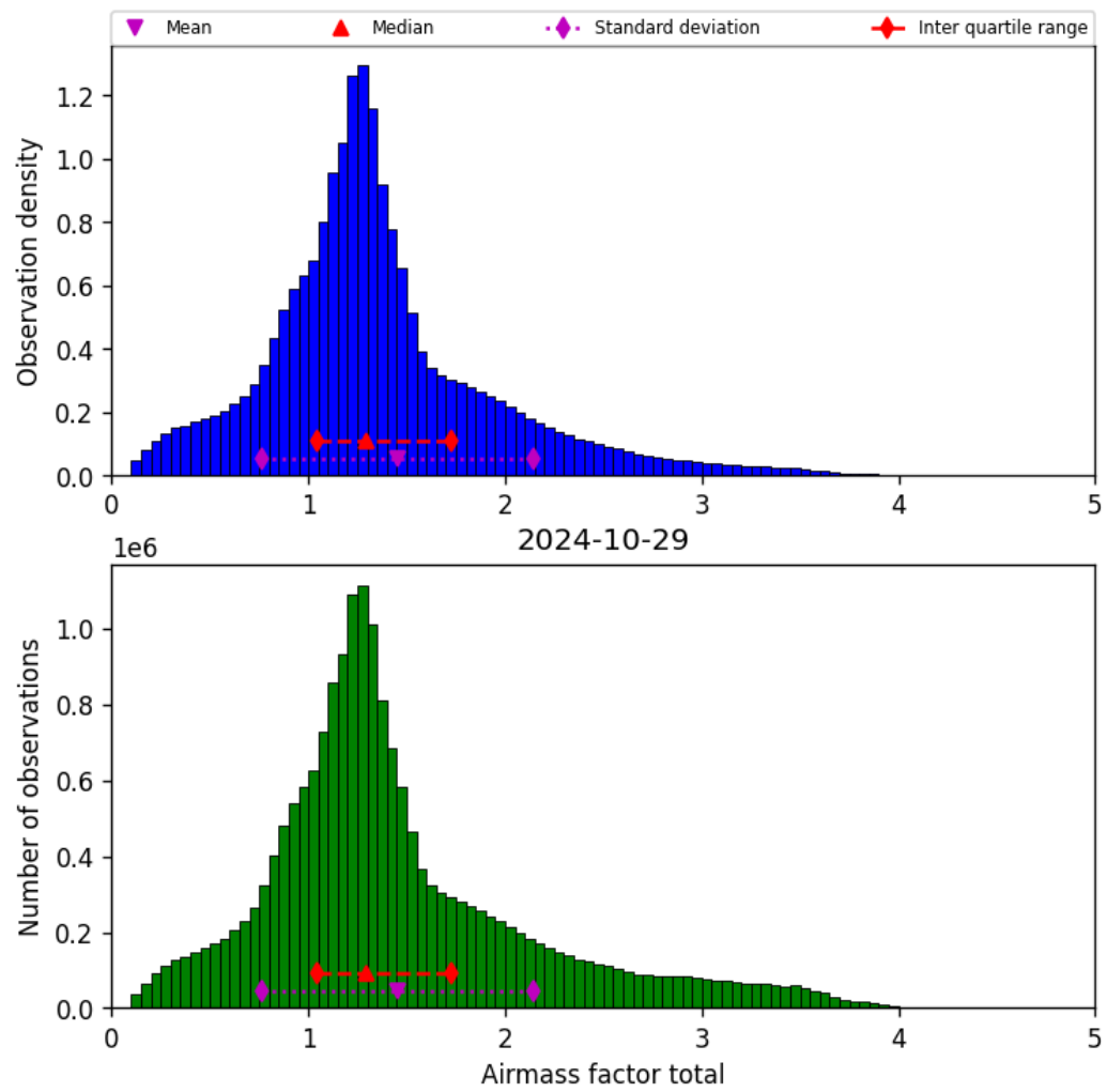
Figure 40: Histogram of “Airmass factor total” for 2024-10-29 to 2024-10-30
