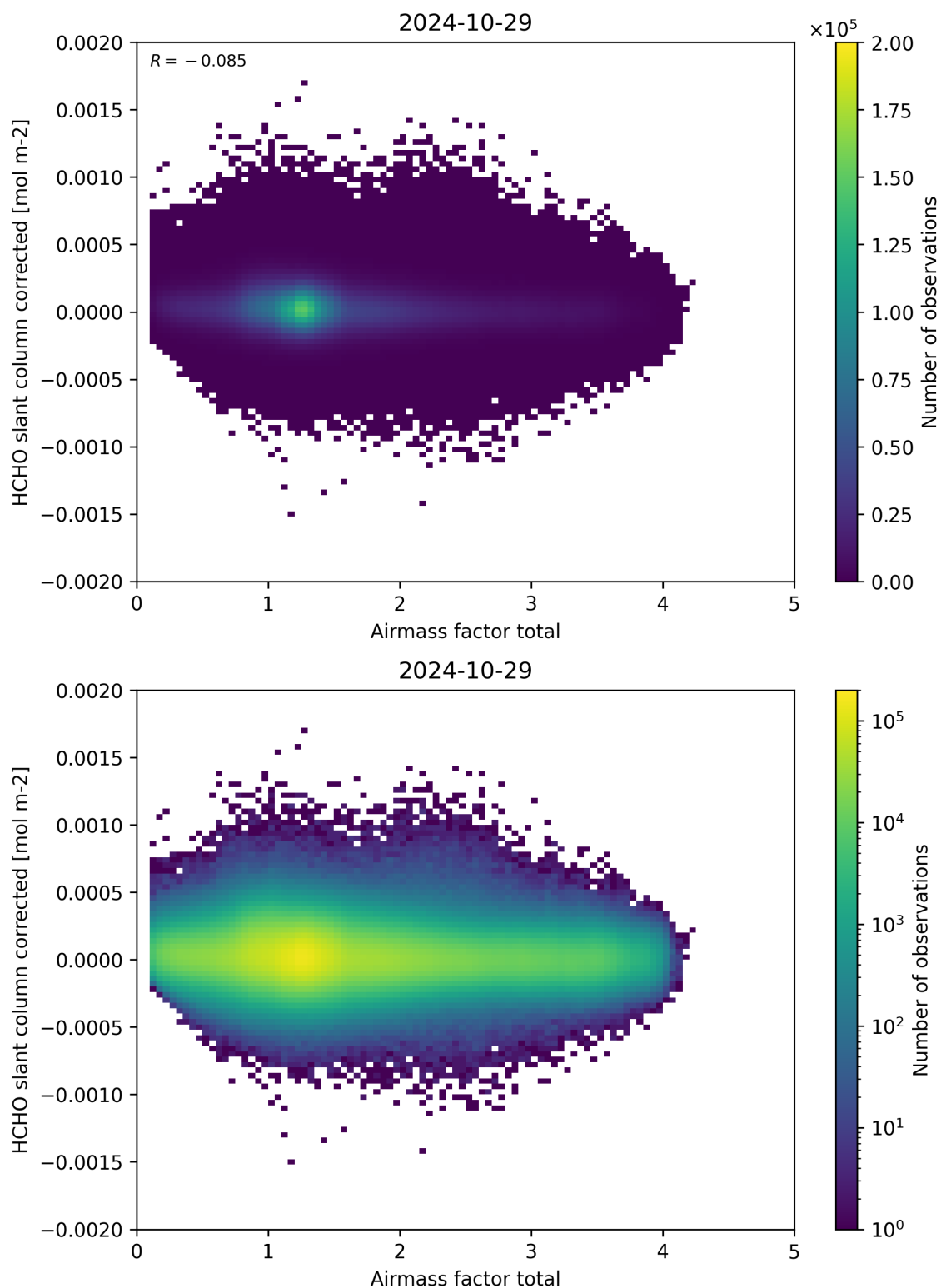
Figure 101: Scatter density plot of “Airmass factor total” against “HCHO slant column corrected” for 2024-10-29 to 2024-10-30.
