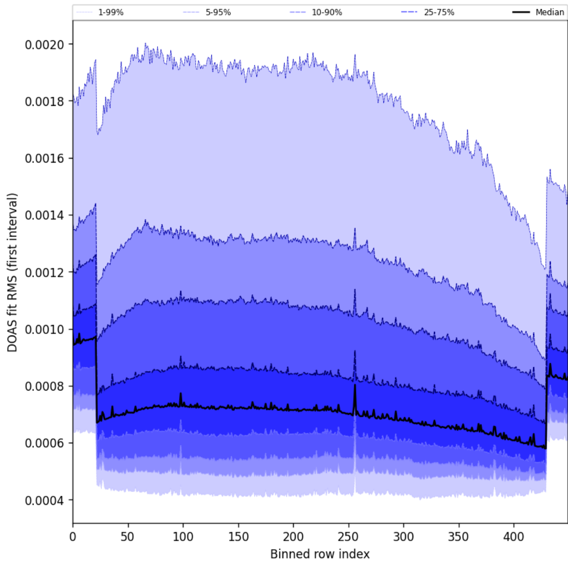
Figure 60: Along track statistics of “DOAS fit RMS (first interval)” for 2024-10-29 to 2024-10-30
