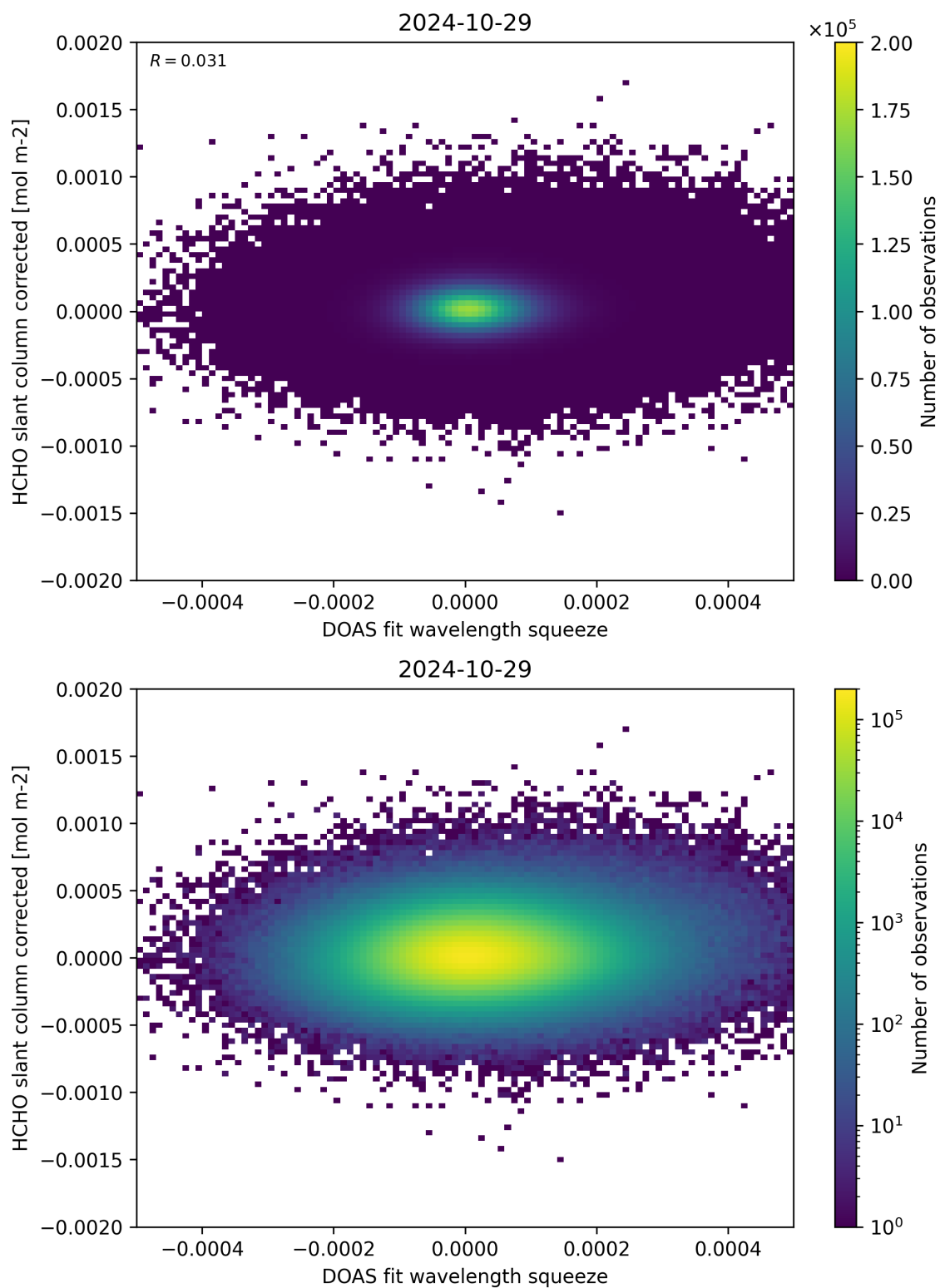
Figure 69: Scatter density plot of “DOAS fit wavelength squeeze” against “HCHO slant column corrected” for 2024-10-29 to 2024-10-30.
