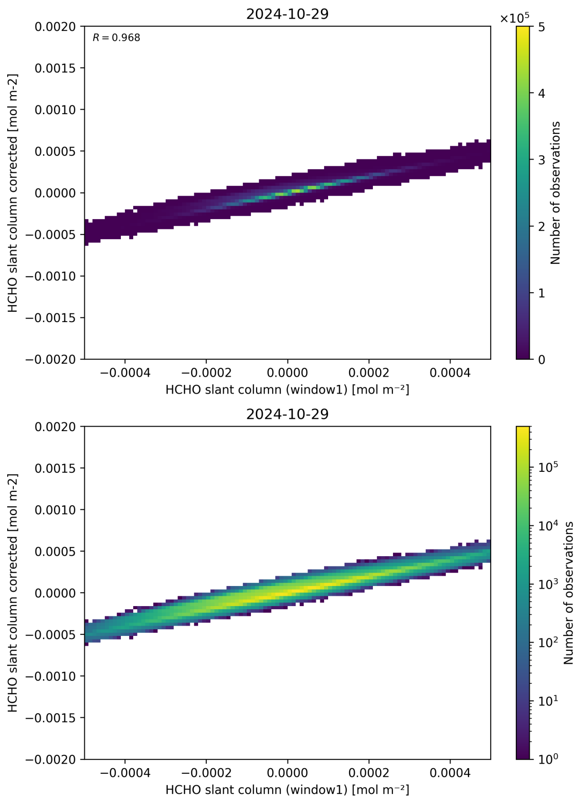
Figure 82: Scatter density plot of “HCHO slant column (window1)” against “HCHO slant column corrected” for 2024-10-29 to 2024-10-30.
