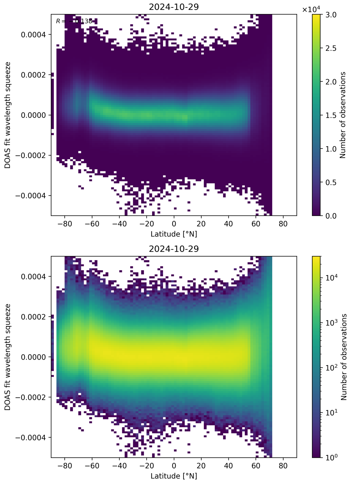
Figure 155: Scatter density plot of “Latitude” against “DOAS fit wavelength squeeze” for 2024-10-29 to 2024-10-30.
