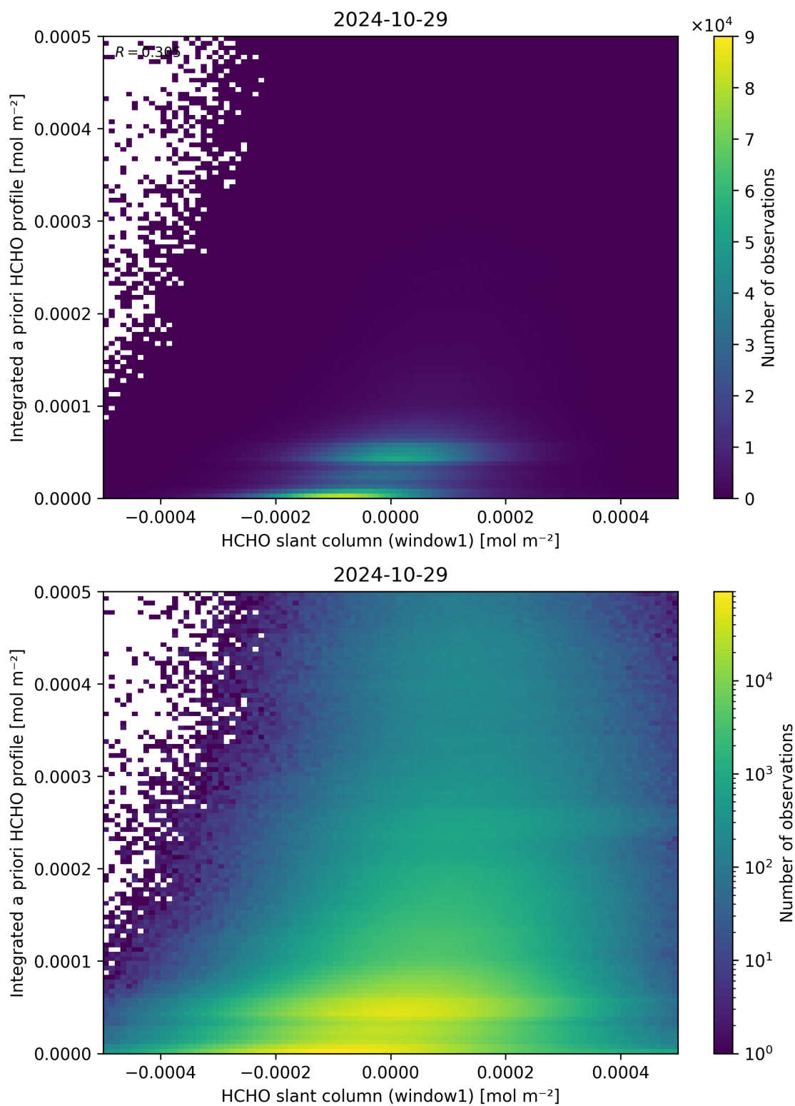
Figure 87: Scatter density plot of “HCHO slant column (window1)” against “Integrated a priori HCHO profile” for 2024-10-29 to 2024-10-30.
