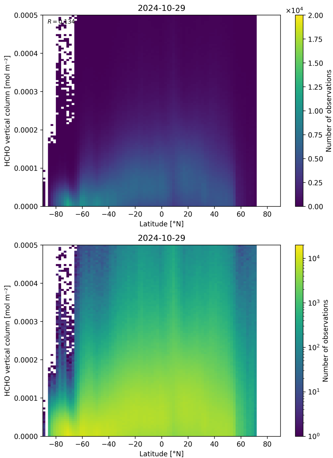
Figure 163: Scatter density plot of “Latitude” against “HCHO vertical column” for 2024-10-29 to 2024-10-30.
