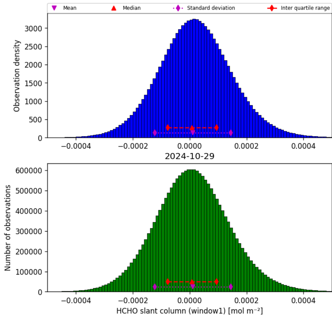
Figure 38: Histogram of “HCHO slant column (window1)” for 2024-10-29 to 2024-10-30
