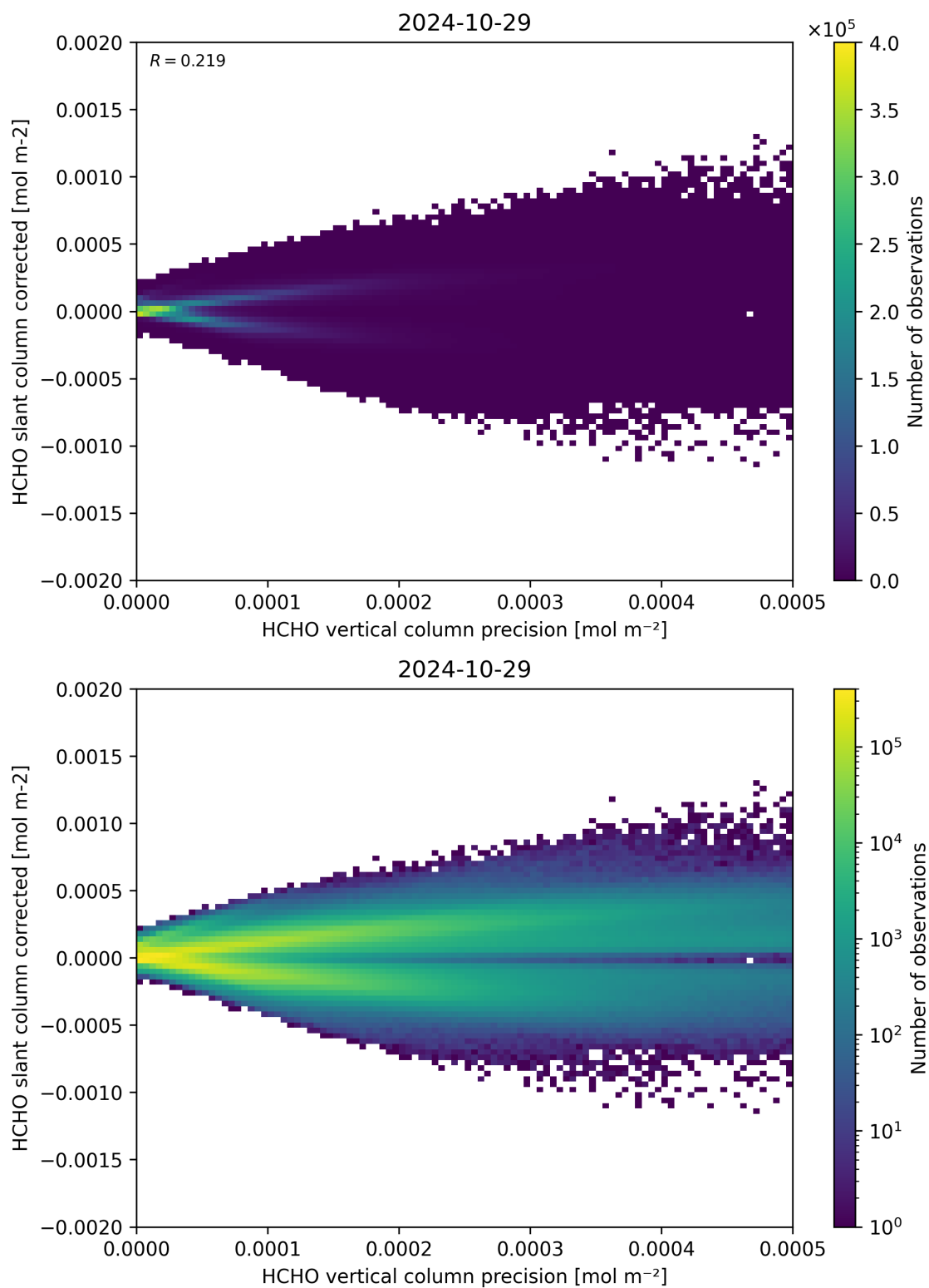
Figure 140: Scatter density plot of “HCHO vertical column precision” against “HCHO slant column corrected” for 2024-10-29 to 2024-10-30.
