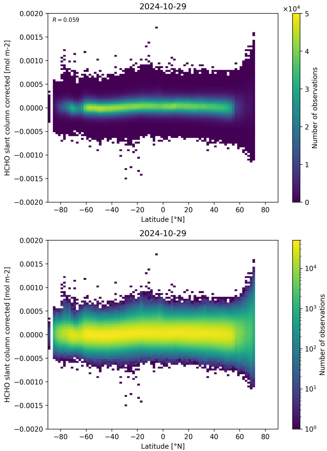
Figure 157: Scatter density plot of “Latitude” against “HCHO slant column corrected” for 2024-10-29 to 2024-10-30.
