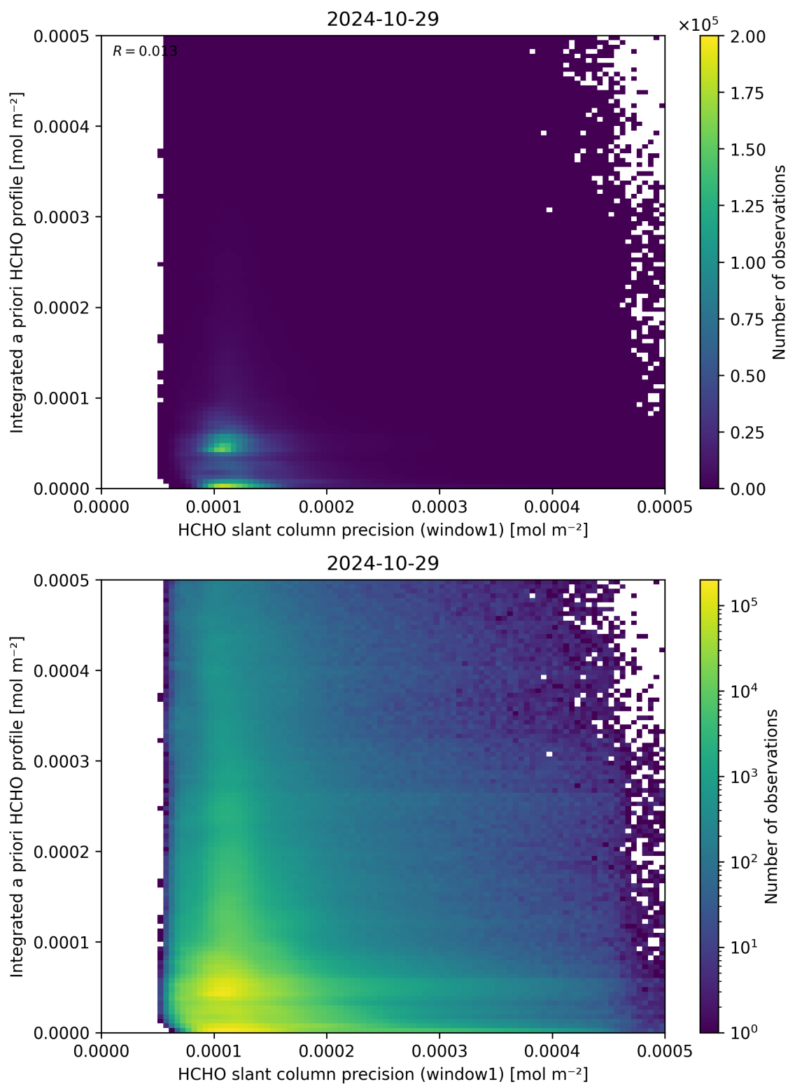
Figure 96: Scatter density plot of “HCHO slant column precision (window1)” against “Integrated a priori HCHO profile” for 2024-10-29 to 2024-10-30.
