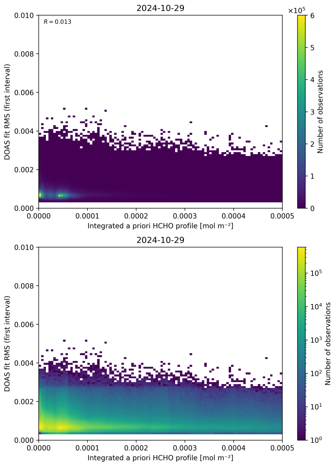
Figure 148: Scatter density plot of “Integrated a priori HCHO profile” against “DOAS fit RMS (first interval)” for 2024-10-29 to 2024-10-30.
