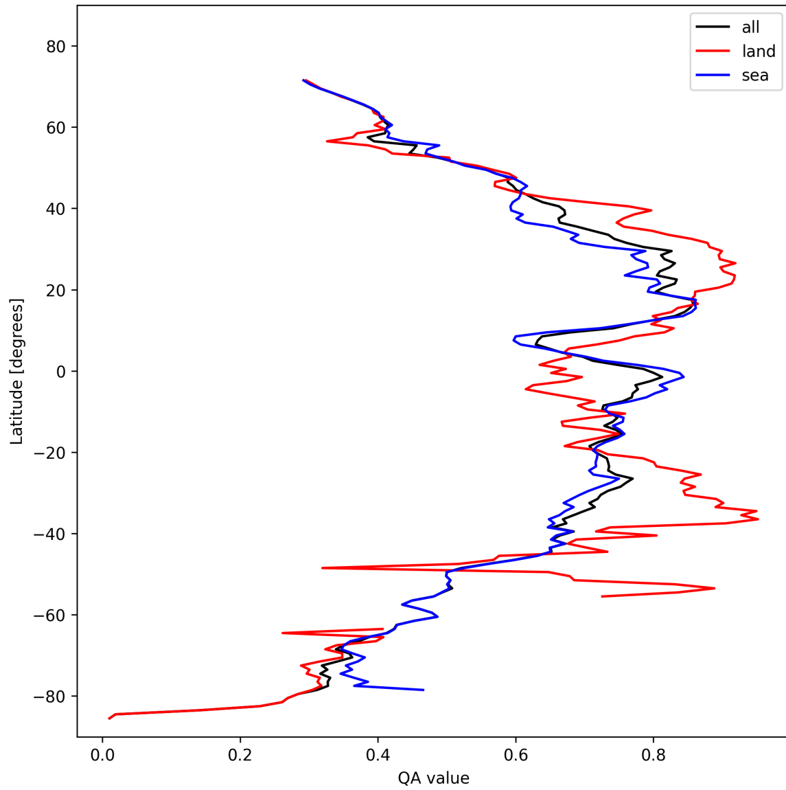
Figure 20: Zonal average of “QA value” for 2024-10-29 to 2024-10-30.
