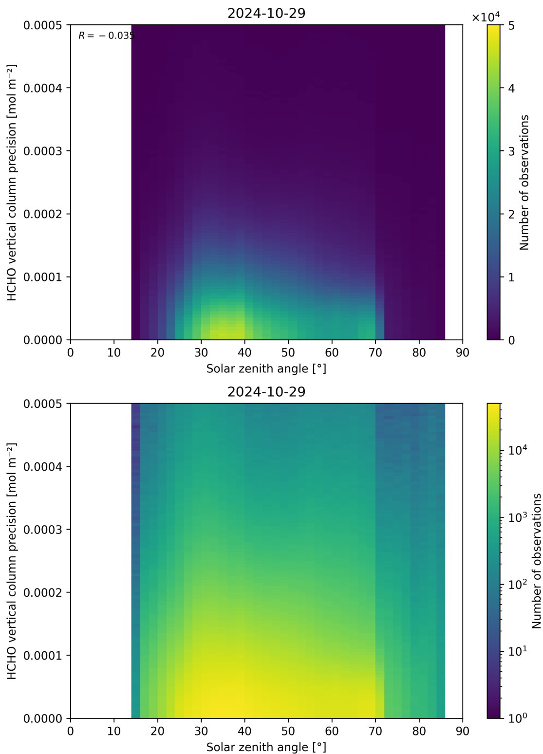
Figure 179: Scatter density plot of “Solar zenith angle” against “HCHO vertical column precision” for 2024-10-29 to 2024-10-30.
