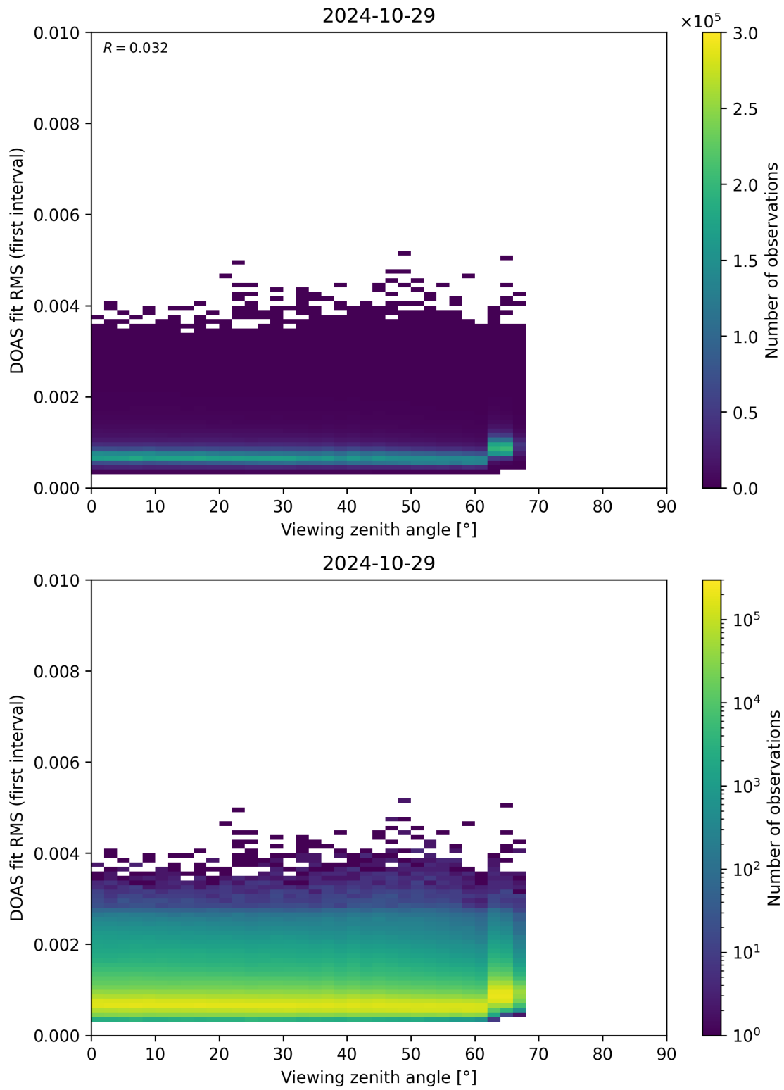
Figure 182: Scatter density plot of “Viewing zenith angle” against “DOAS fit RMS (first interval)” for 2024-10-29 to 2024-10-30.
