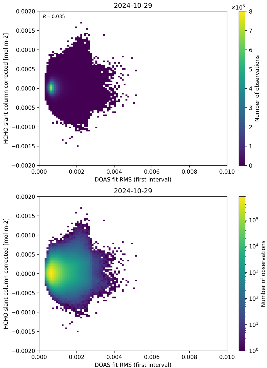
Figure 62: Scatter density plot of “DOAS fit RMS (first interval)” against “HCHO slant column corrected” for 2024-10-29 to 2024-10-30.
