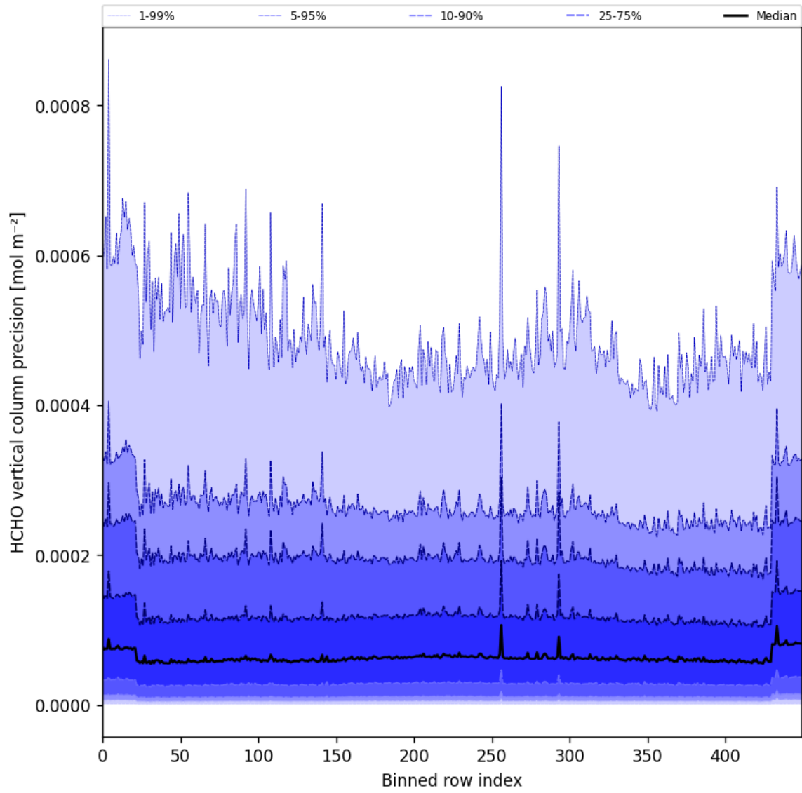
Figure 50: Along track statistics of “HCHO vertical column precision” for 2024-10-29 to 2024-10-30
