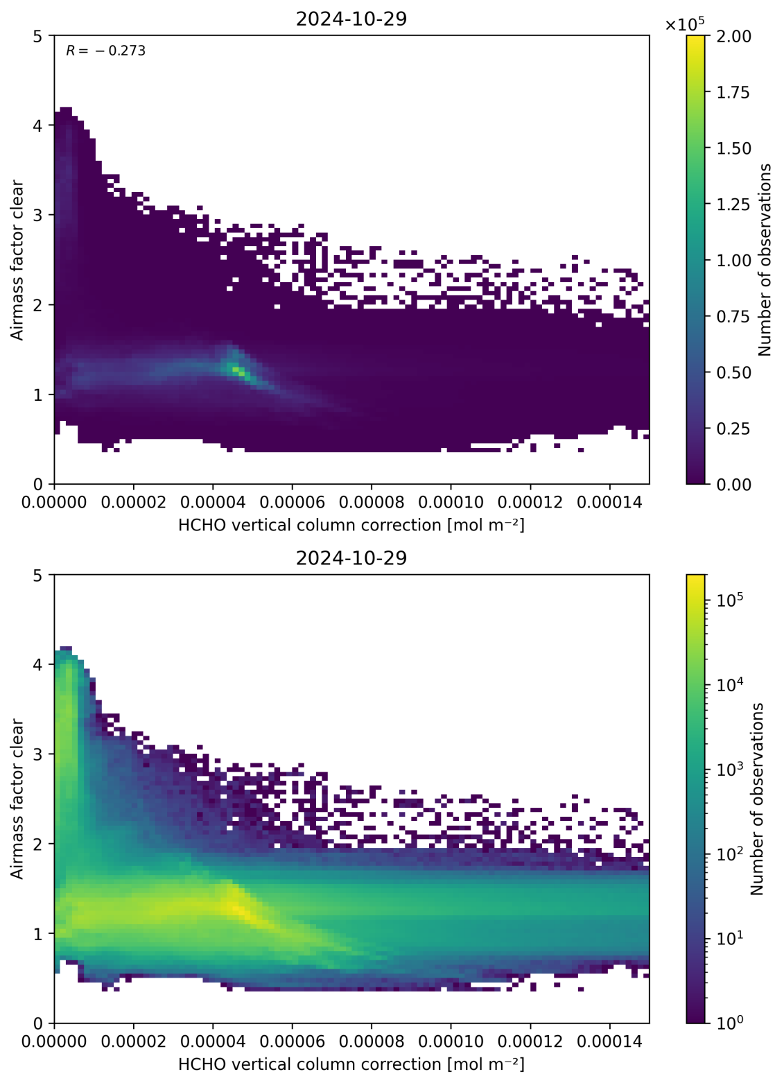
Figure 115: Scatter density plot of “HCHO vertical column correction” against “Airmass factor clear” for 2024-10-29 to 2024-10-30.
