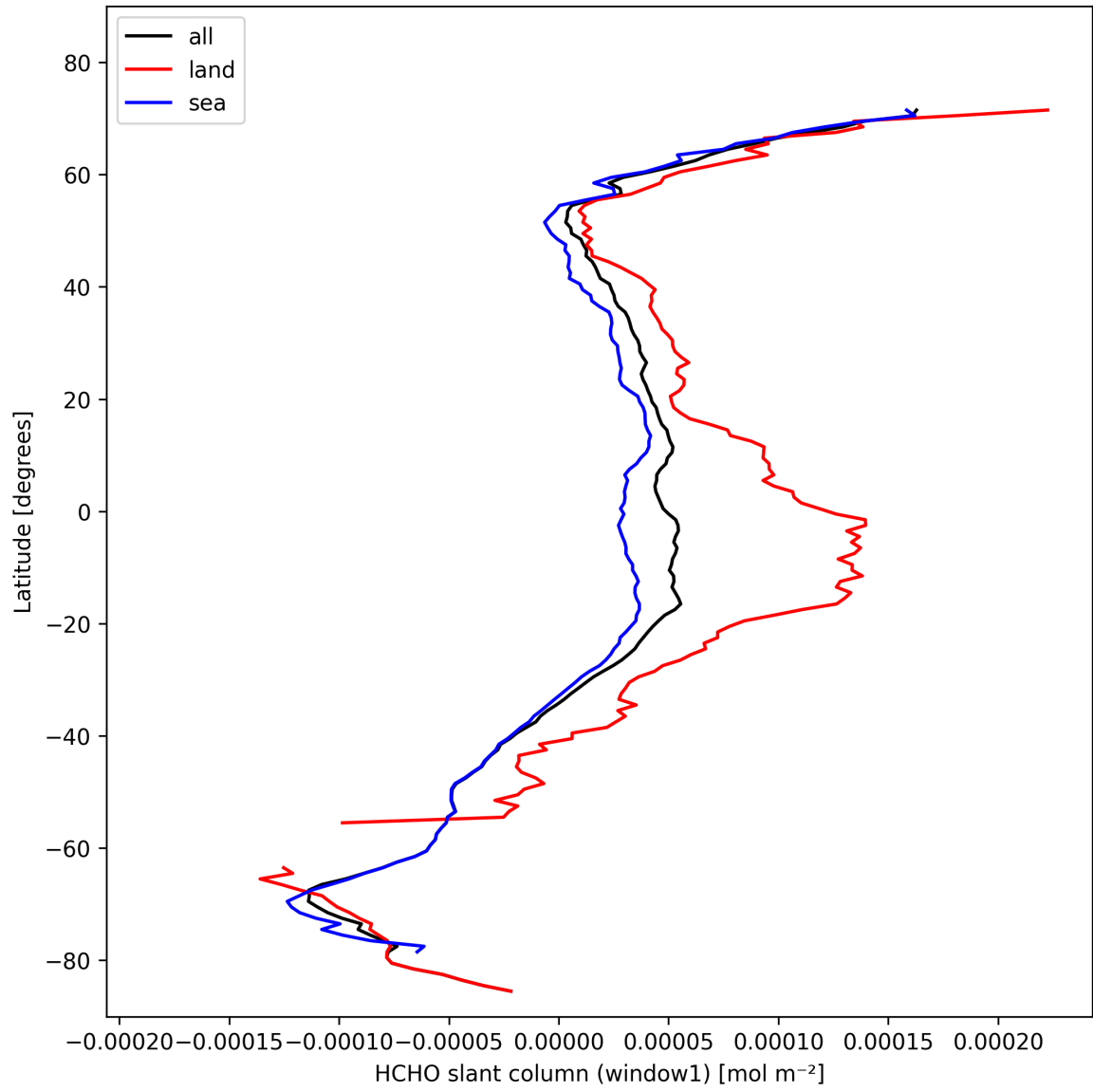
Figure 24: Zonal average of “HCHO slant column (window1)” for 2024-10-29 to 2024-10-30.
