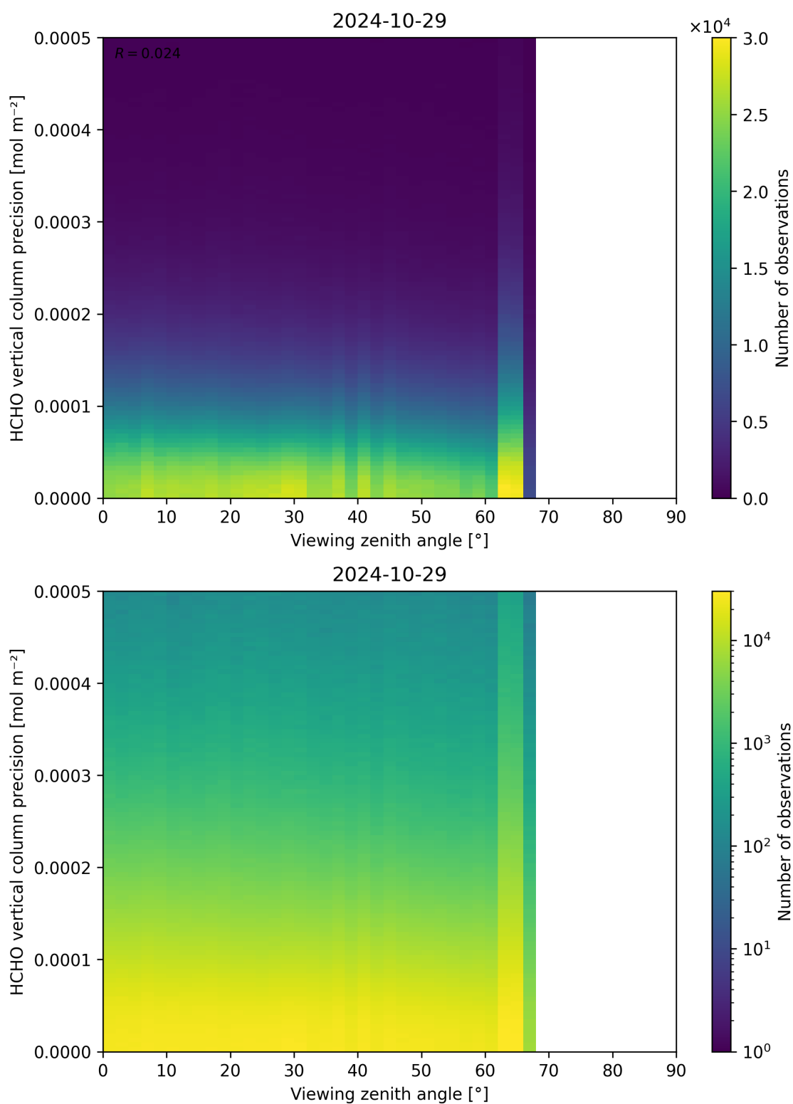
Figure 194: Scatter density plot of “Viewing zenith angle” against “HCHO vertical column precision” for 2024-10-29 to 2024-10-30.
