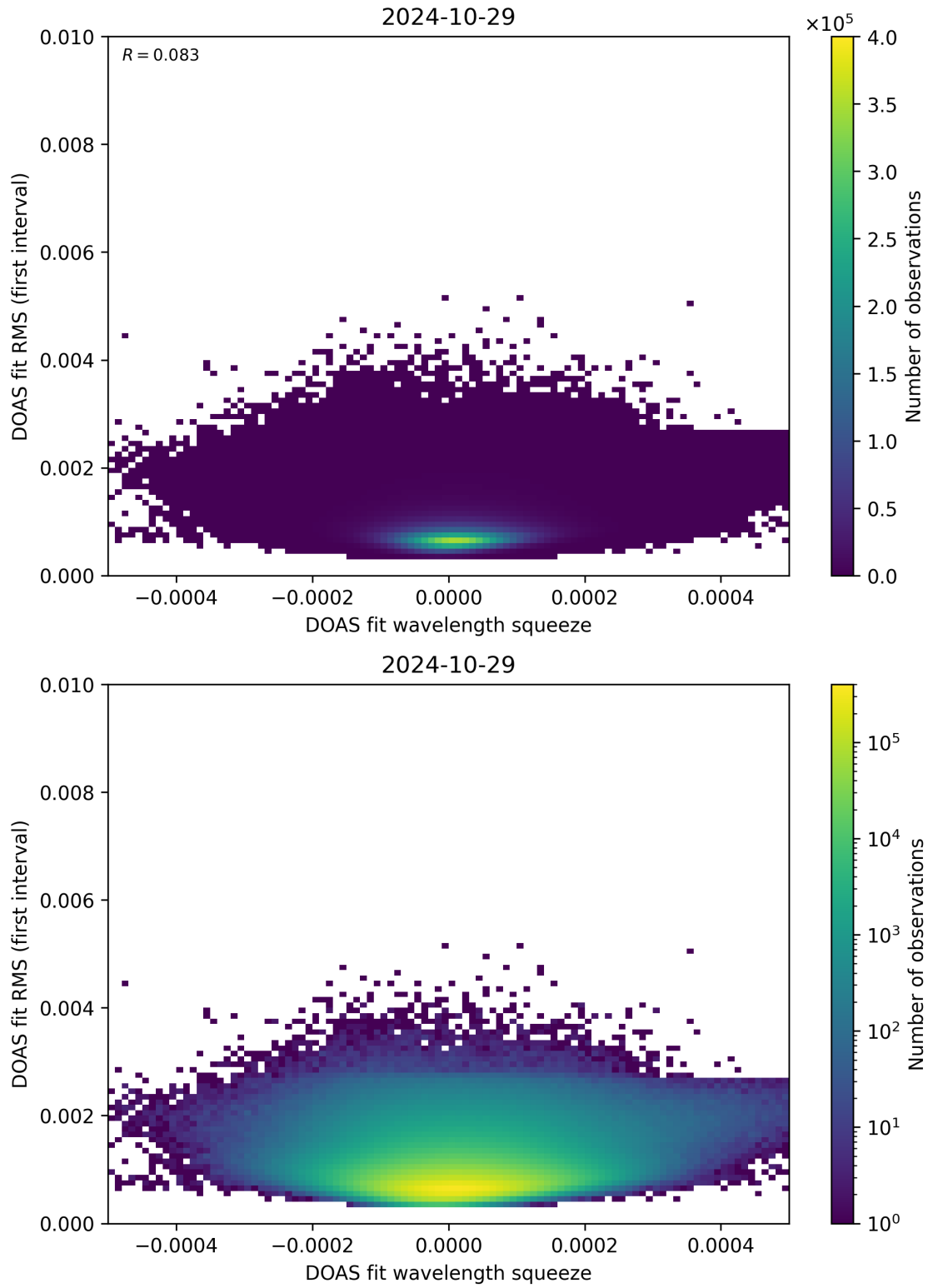
Figure 68: Scatter density plot of “DOAS fit wavelength squeeze” against “DOAS fit RMS (first interval)” for 2024-10-29 to 2024-10-30.
