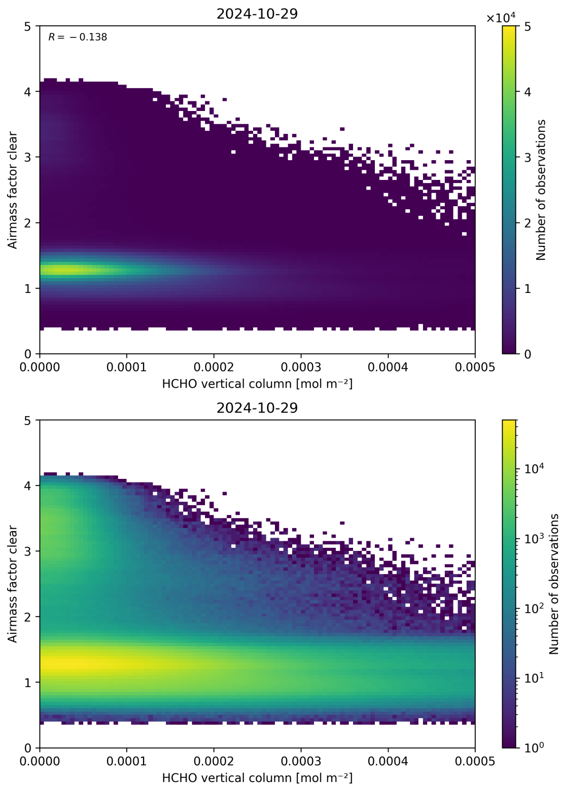
Figure 126: Scatter density plot of “HCHO vertical column” against “Airmass factor clear” for 2024-10-29 to 2024-10-30.
