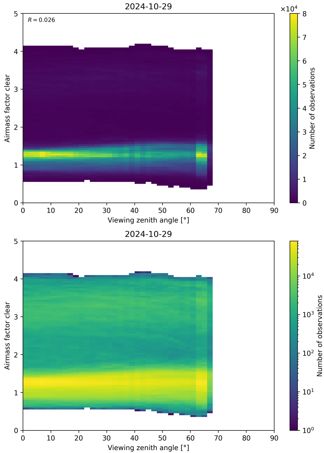
Figure 185: Scatter density plot of “Viewing zenith angle” against “Airmass factor clear” for 2024-10-29 to 2024-10-30.
