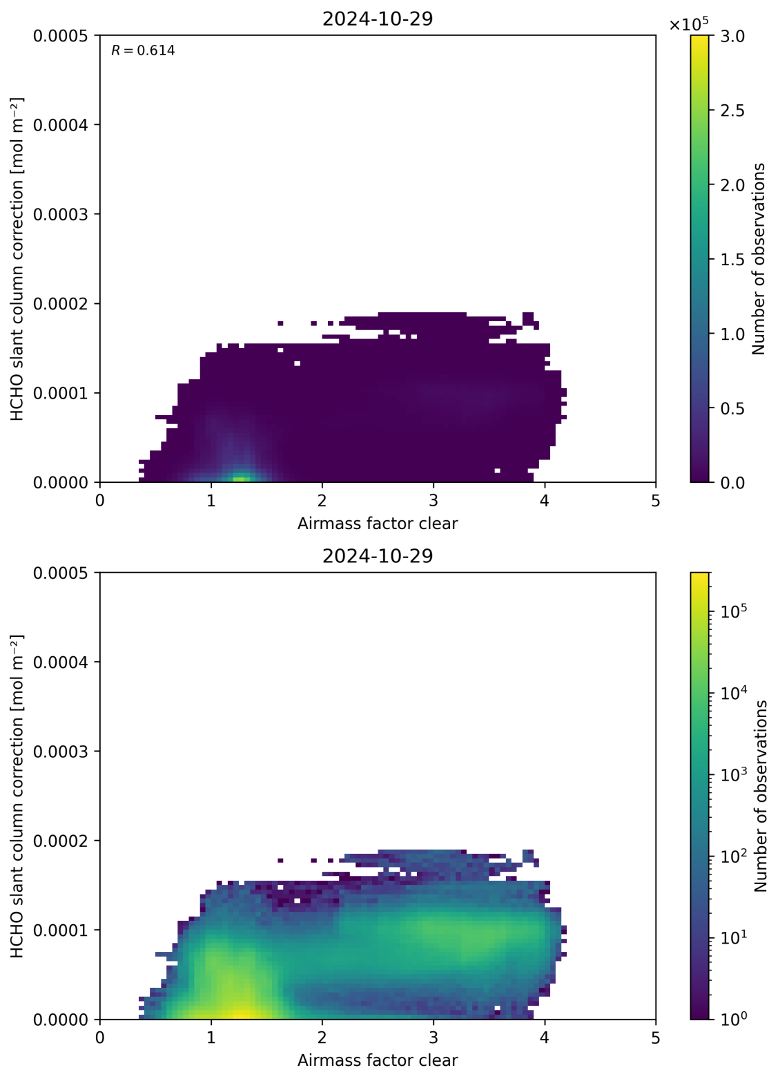
Figure 75: Scatter density plot of “Airmass factor clear” against “HCHO slant column correction” for 2024-10-29 to 2024-10-30.
