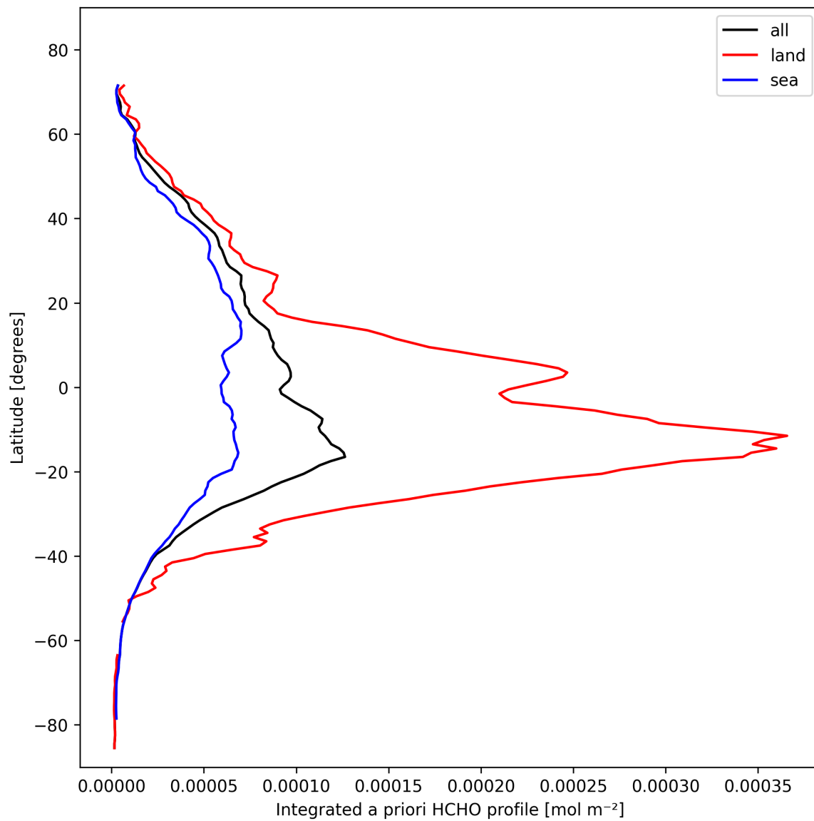
Figure 29: Zonal average of “Integrated a priori HCHO profile” for 2024-10-29 to 2024-10-30.
