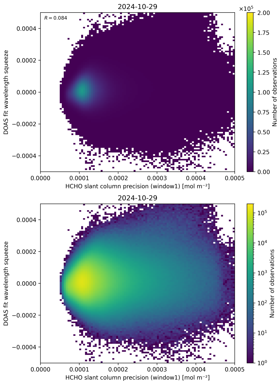
Figure 90: Scatter density plot of “HCHO slant column precision (window1)” against “DOAS fit wavelength squeeze” for 2024-10-29 to 2024-10-30.
