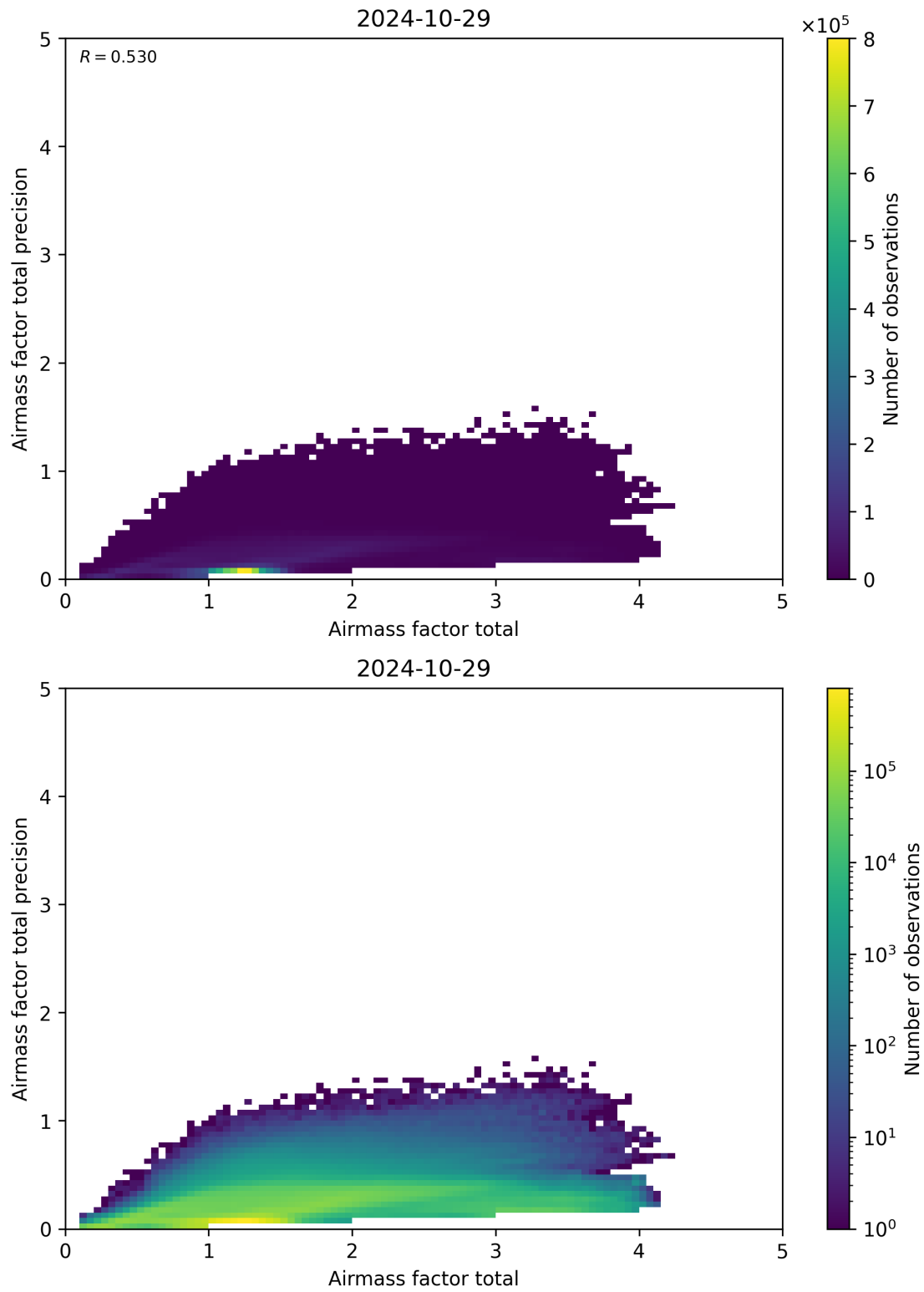
Figure 103: Scatter density plot of “Airmass factor total” against “Airmass factor total precision” for 2024-10-29 to 2024-10-30.
