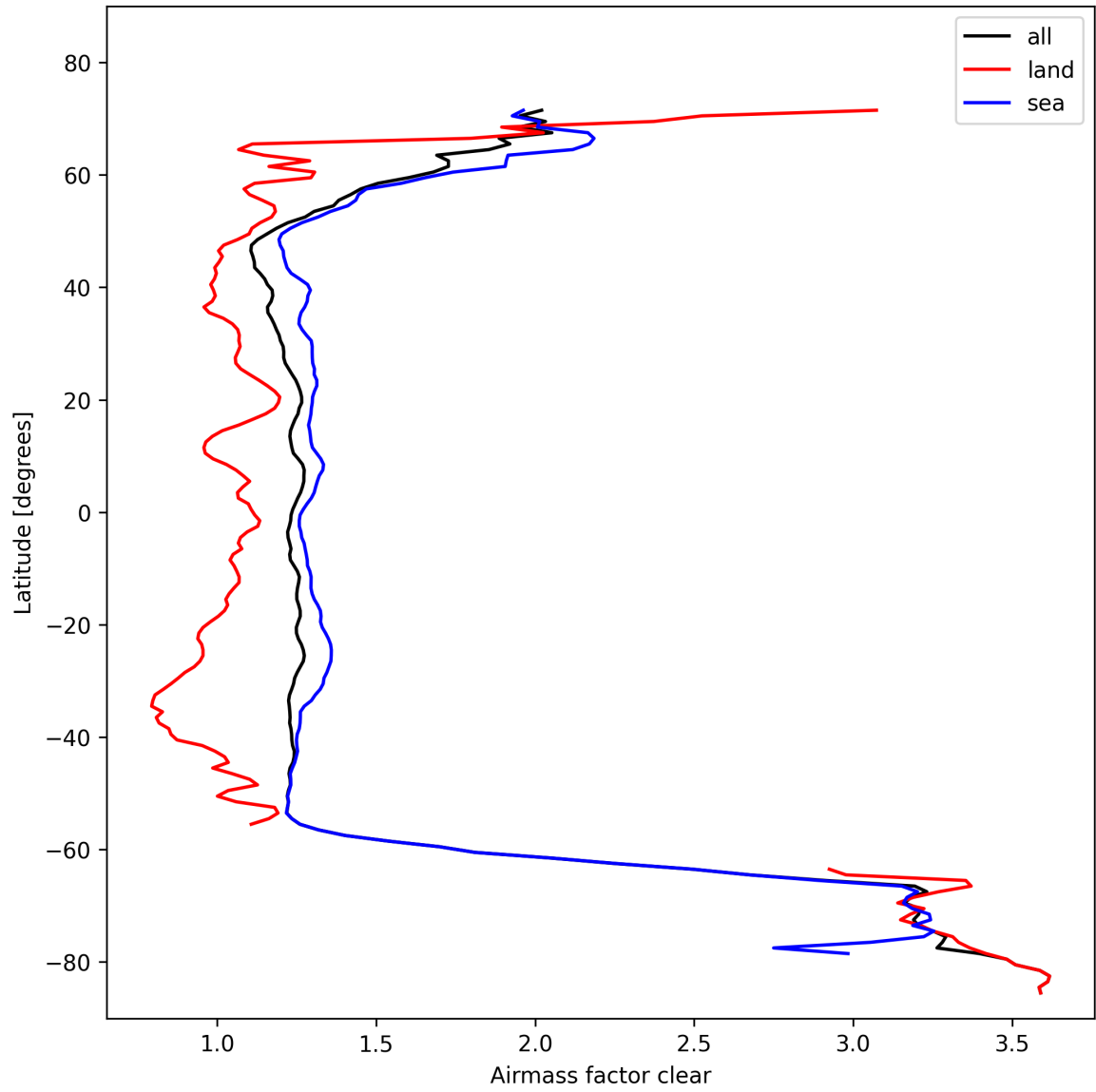
Figure 28: Zonal average of “Airmass factor clear” for 2024-10-29 to 2024-10-30.
