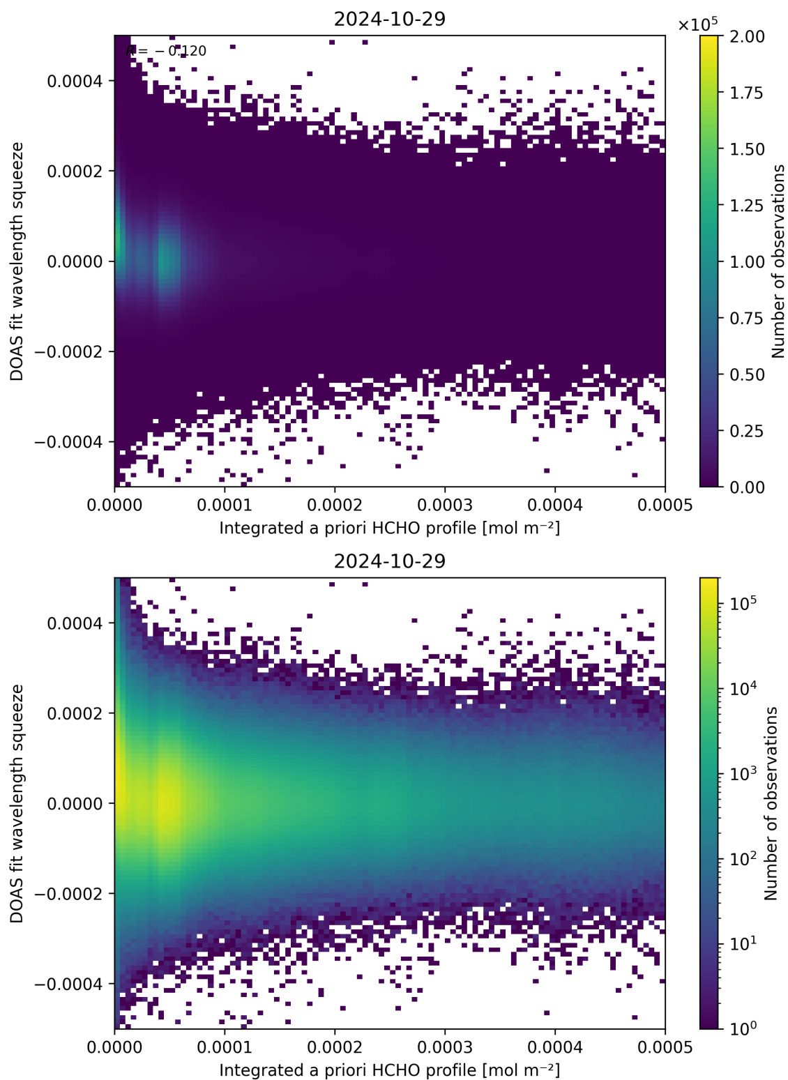
Figure 150: Scatter density plot of “Integrated a priori HCHO profile” against “DOAS fit wavelength squeeze” for 2024-10-29 to 2024-10-30.
