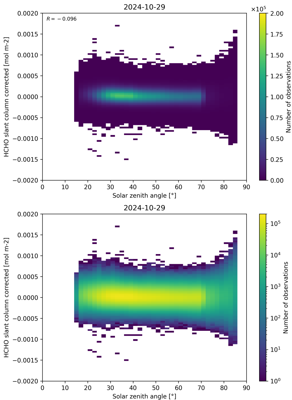
Figure 171: Scatter density plot of “Solar zenith angle” against “HCHO slant column corrected” for 2024-10-29 to 2024-10-30.
