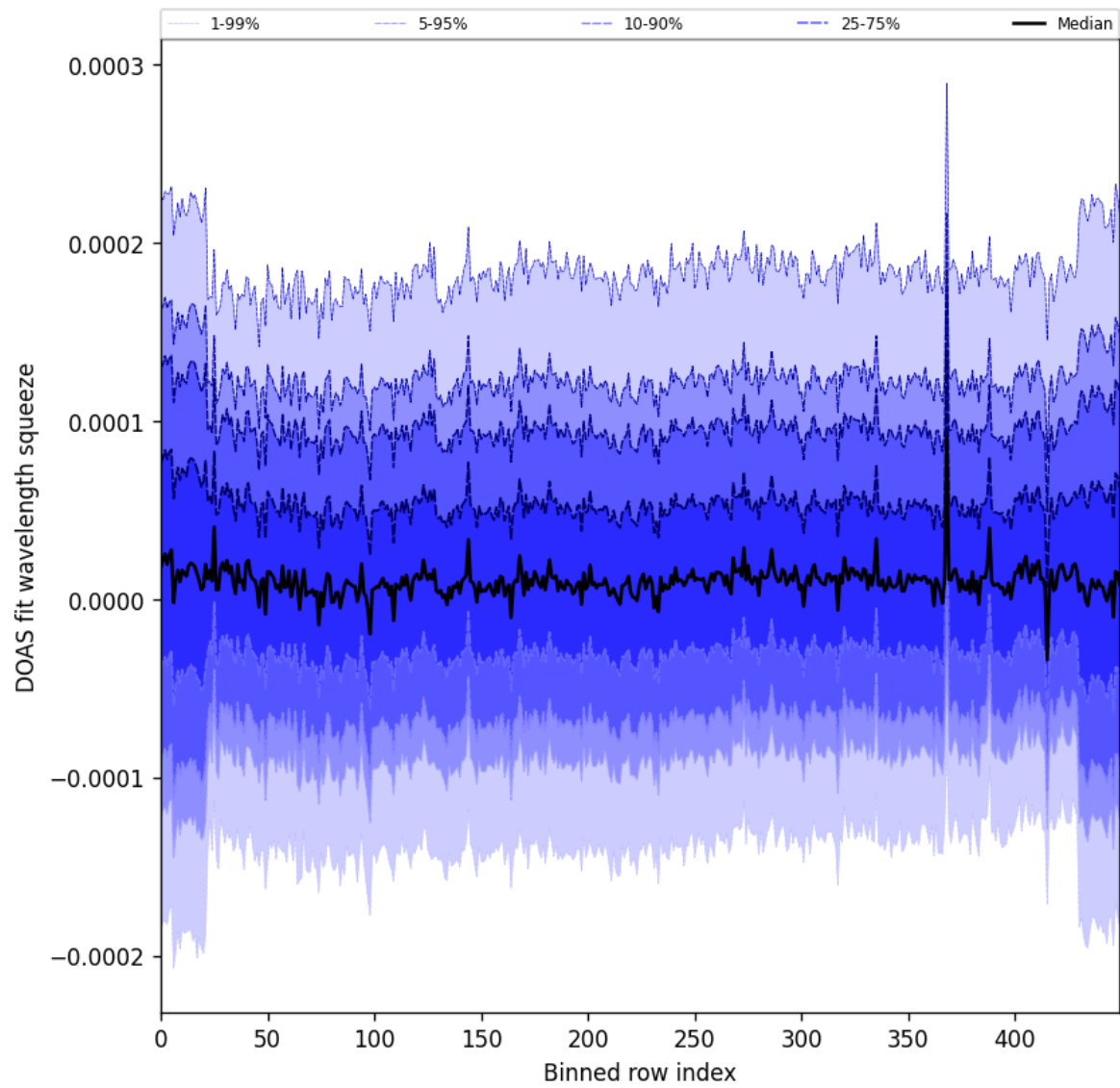
Figure 59: Along track statistics of “DOAS fit wavelength squeeze” for 2024-10-29 to 2024-10-30
