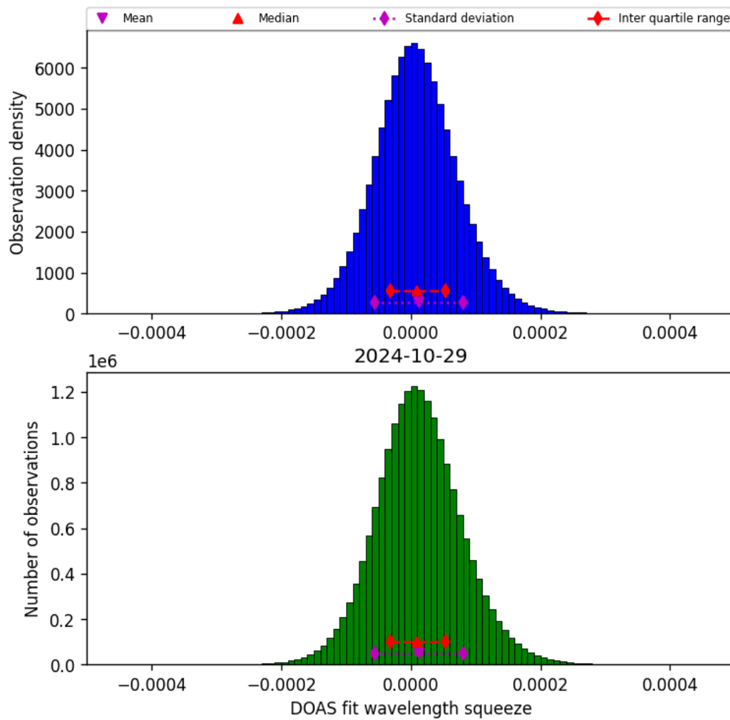
Figure 45: Histogram of “DOAS fit wavelength squeeze” for 2024-10-29 to 2024-10-30
