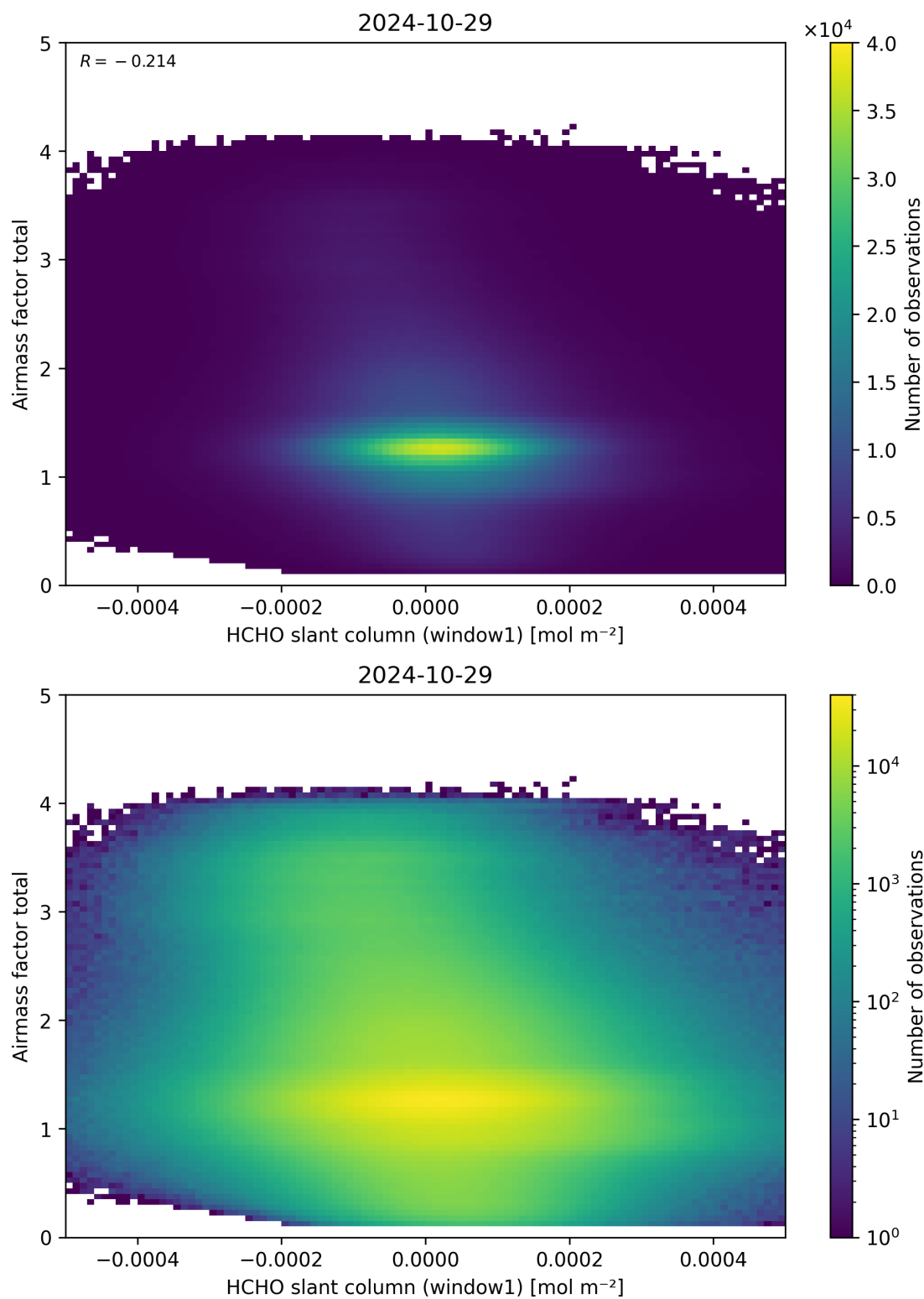
Figure 85: Scatter density plot of “HCHO slant column (window1)” against “Airmass factor total” for 2024-10-29 to 2024-10-30.
