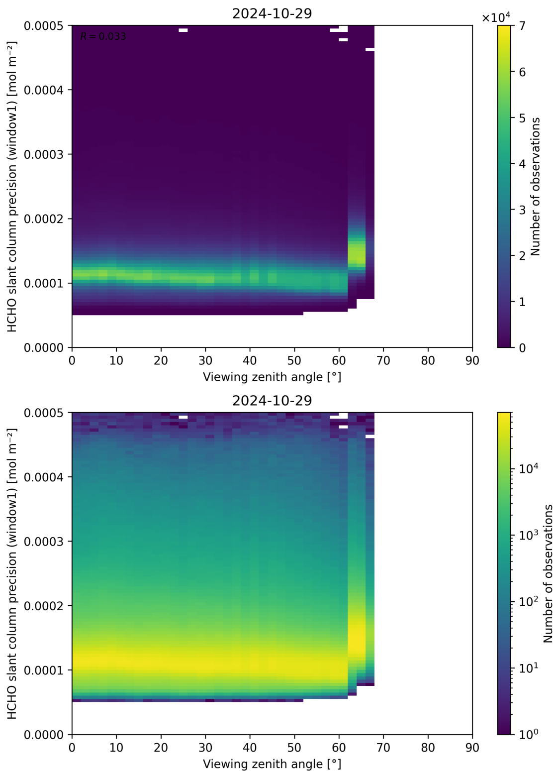
Figure 189: Scatter density plot of “Viewing zenith angle” against “HCHO slant column precision (window1)” for 2024-10-29 to 2024-10-30.
