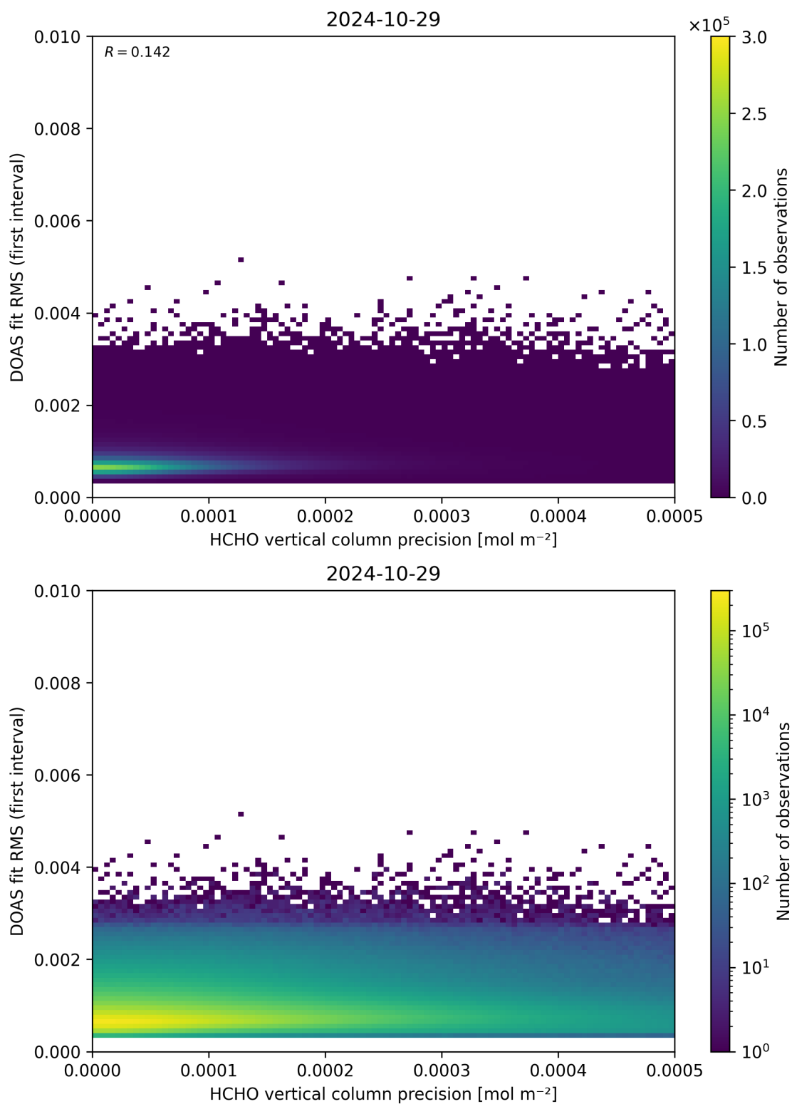
Figure 136: Scatter density plot of “HCHO vertical column precision” against “DOAS fit RMS (first interval)” for 2024-10-29 to 2024-10-30.
