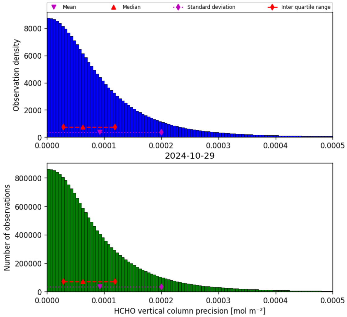
Figure 36: Histogram of “HCHO vertical column precision” for 2024-10-29 to 2024-10-30
