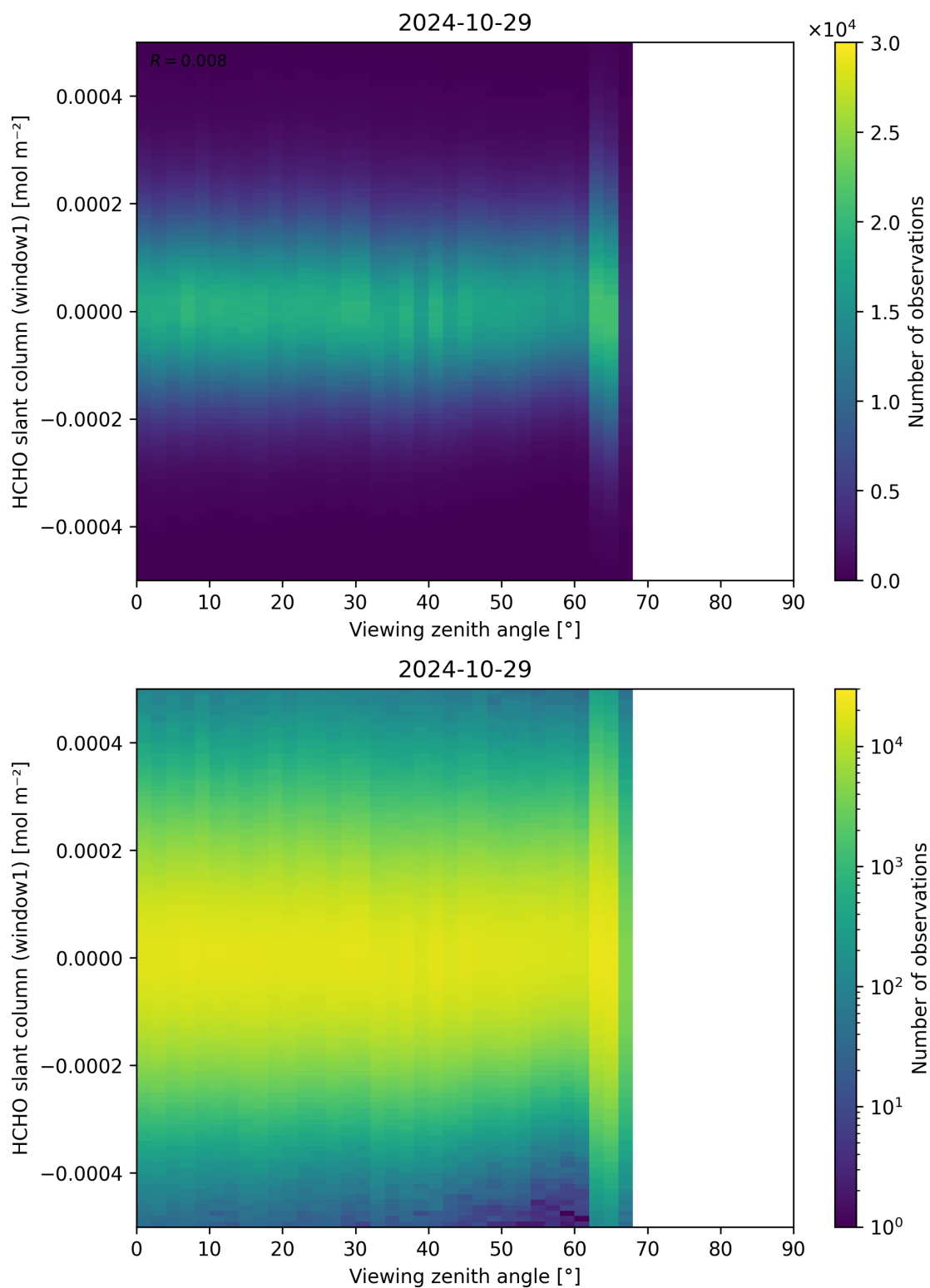
Figure 188: Scatter density plot of “Viewing zenith angle” against “HCHO slant column (window1)” for 2024-10-29 to 2024-10-30.
