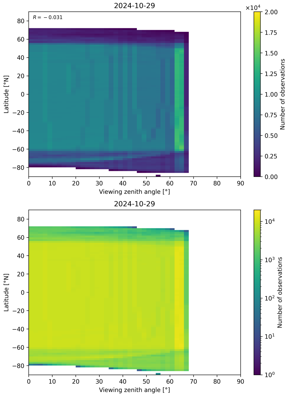
Figure 196: Scatter density plot of “Viewing zenith angle” against “Latitude” for 2024-10-29 to 2024-10-30.
