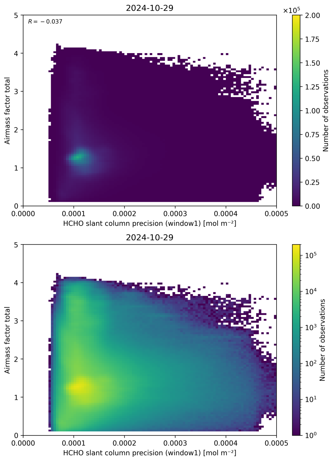
Figure 94: Scatter density plot of “HCHO slant column precision (window1)” against “Airmass factor total” for 2024-10-29 to 2024-10-30.
