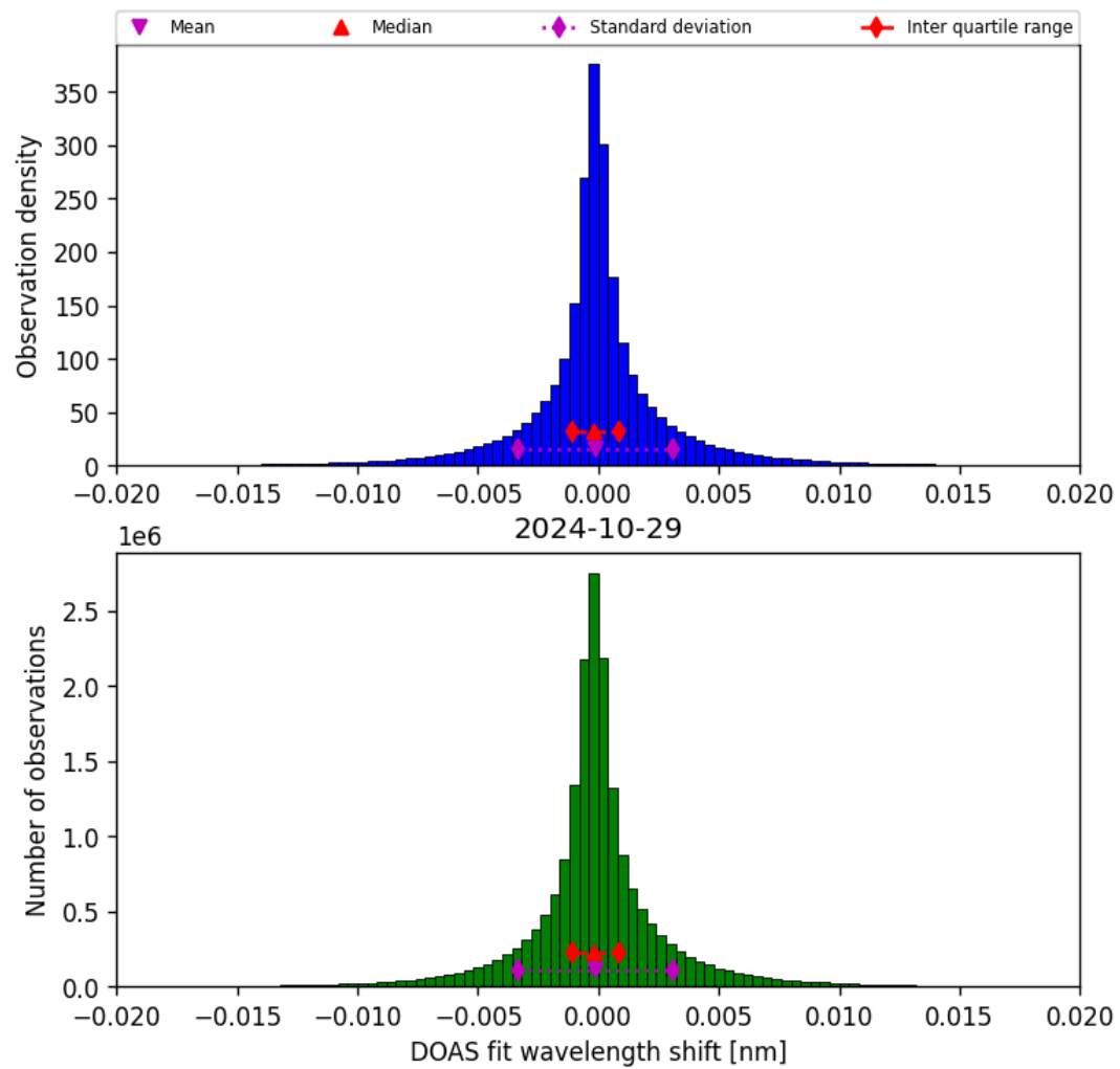
Figure 44: Histogram of “DOAS fit wavelength shift” for 2024-10-29 to 2024-10-30
