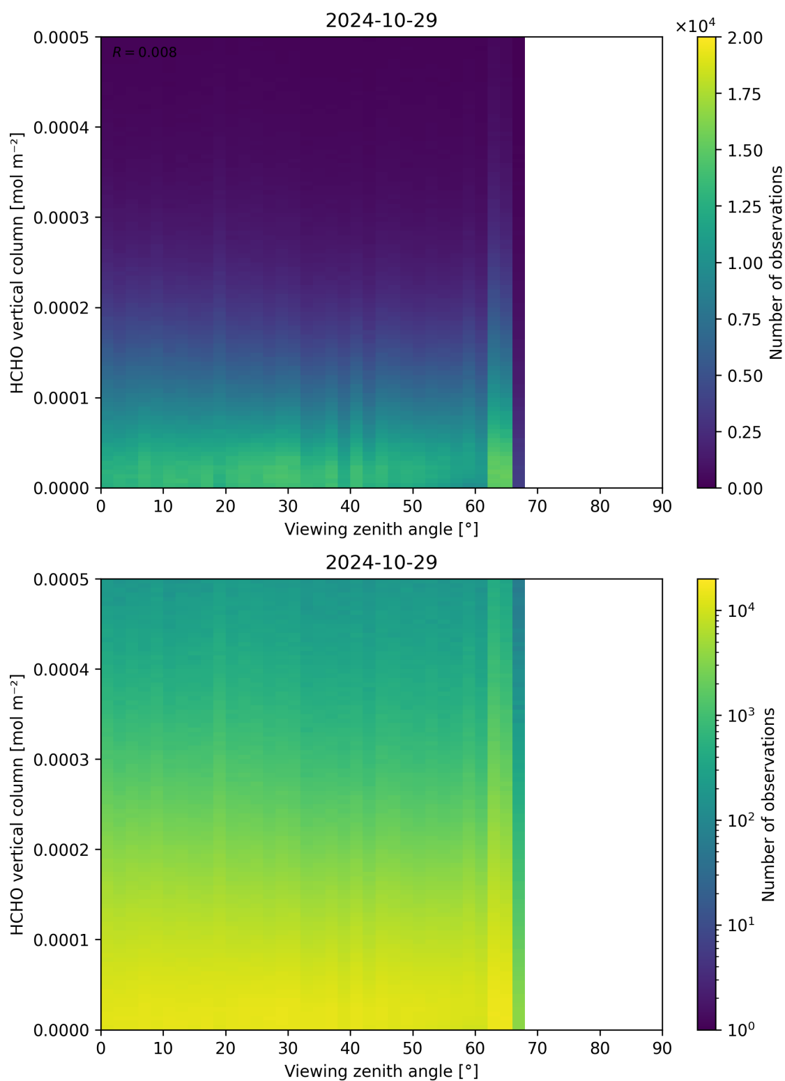
Figure 192: Scatter density plot of “Viewing zenith angle” against “HCHO vertical column” for 2024-10-29 to 2024-10-30.
