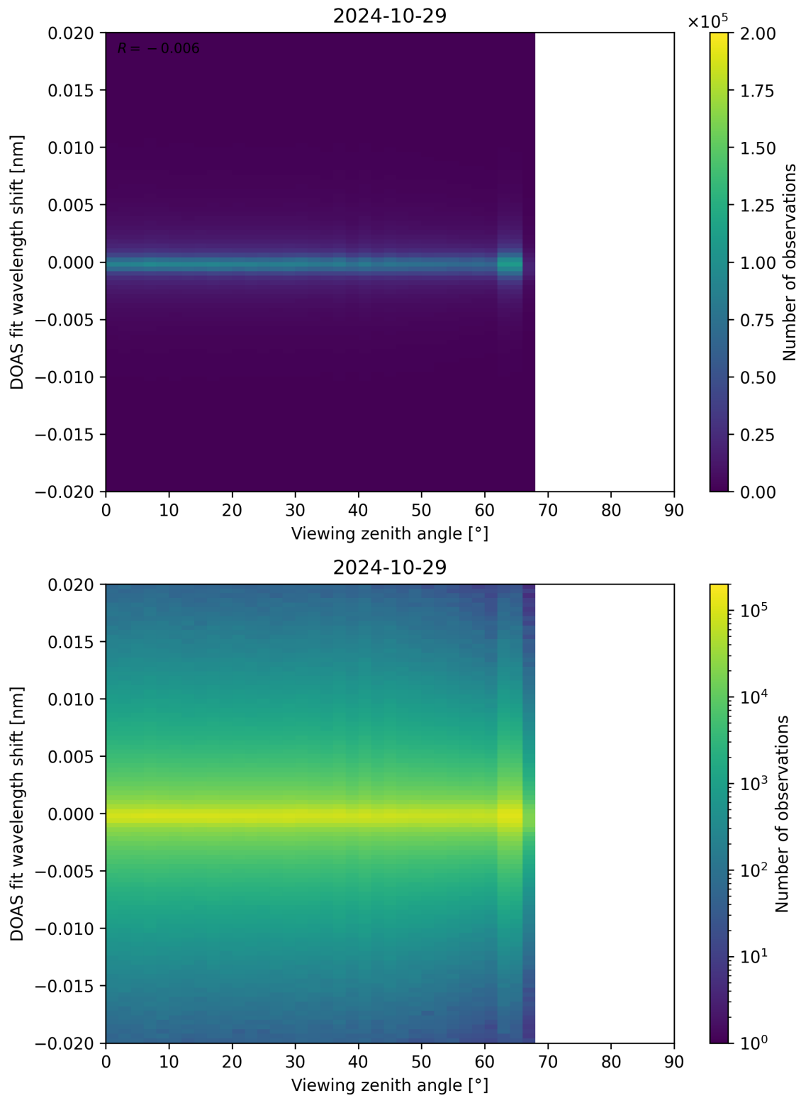
Figure 183: Scatter density plot of “Viewing zenith angle” against “DOAS fit wavelength shift” for 2024-10-29 to 2024-10-30.
