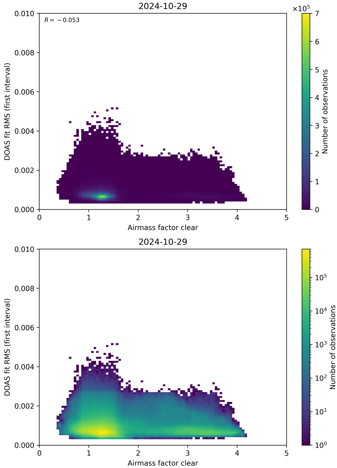
Figure 71: Scatter density plot of “Airmass factor clear” against “DOAS fit RMS (first interval)” for 2024-10-29 to 2024-10-30.
