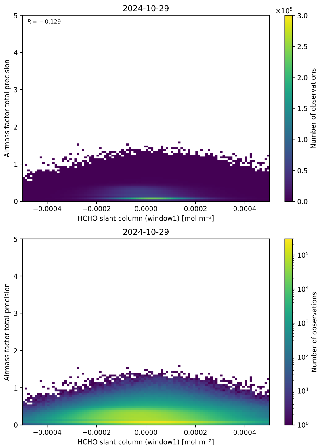
Figure 86: Scatter density plot of “HCHO slant column (window1)” against “Airmass factor total precision” for 2024-10-29 to 2024-10-30.
