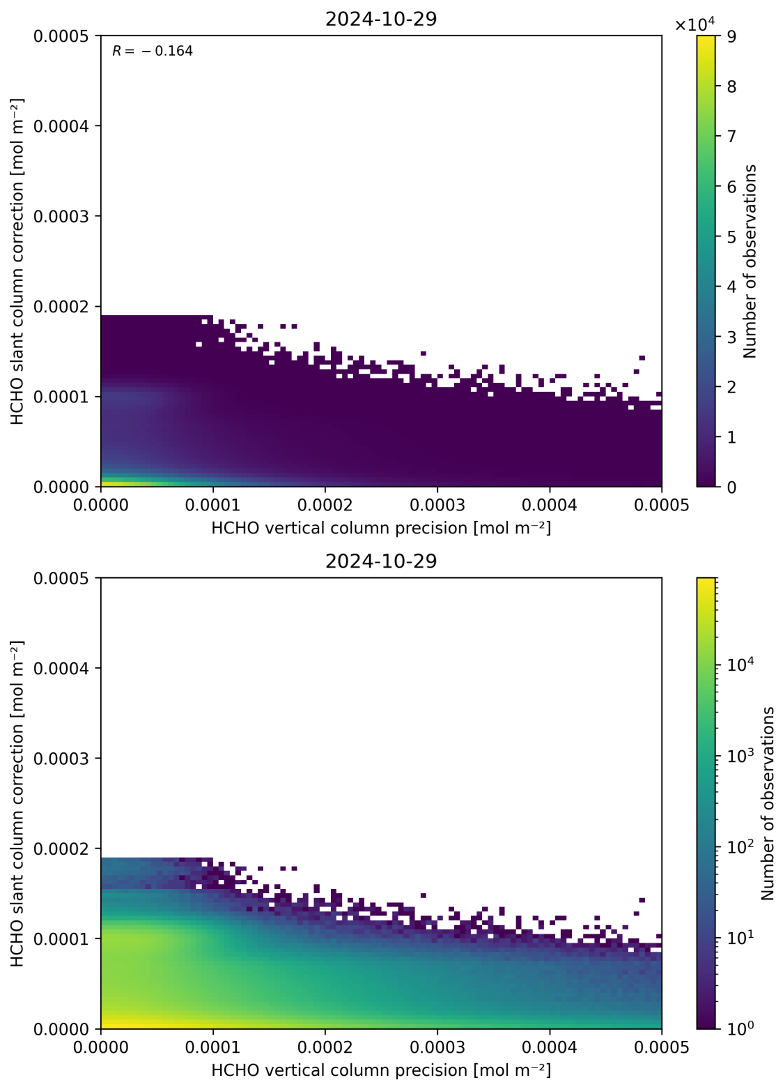
Figure 141: Scatter density plot of “HCHO vertical column precision” against “HCHO slant column correction” for 2024-10-29 to 2024-10-30.
