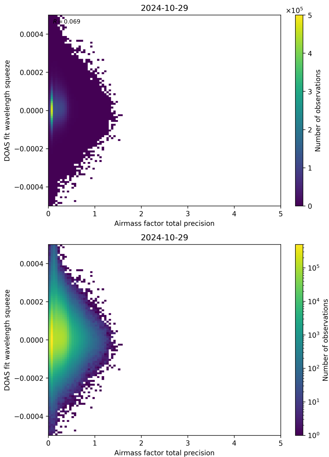
Figure 107: Scatter density plot of “Airmass factor total precision” against “DOAS fit wavelength squeeze” for 2024-10-29 to 2024-10-30.
