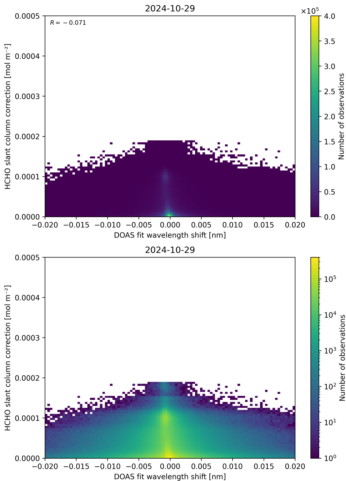
Figure 67: Scatter density plot of “DOAS fit wavelength shift” against “HCHO slant column correction” for 2024-10-29 to 2024-10-30.
