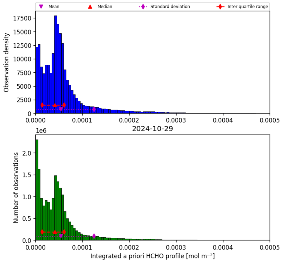
Figure 43: Histogram of “Integrated a priori HCHO profile” for 2024-10-29 to 2024-10-30
