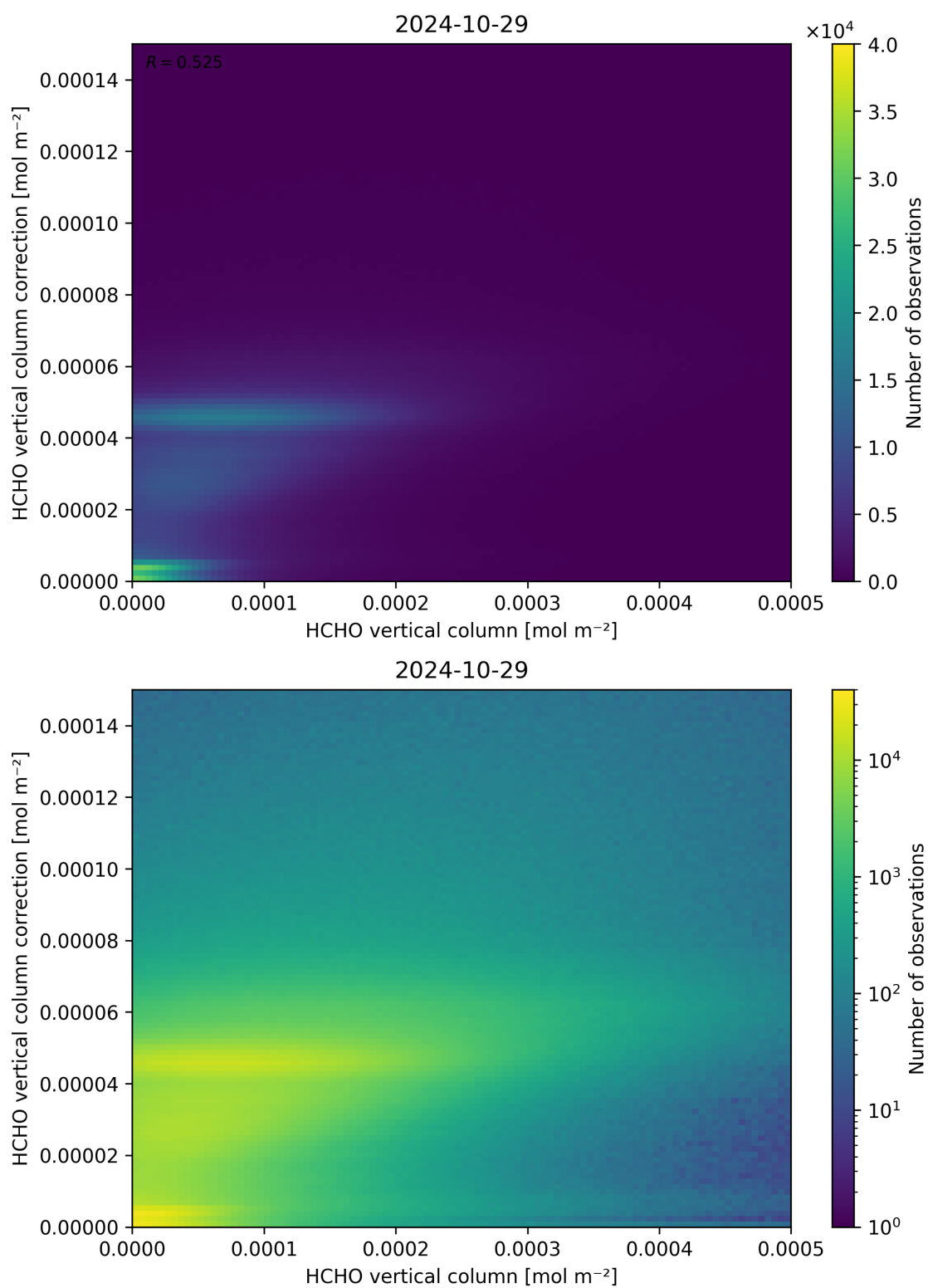
Figure 133: Scatter density plot of “HCHO vertical column” against “HCHO vertical column correction” for 2024-10-29 to 2024-10-30.
