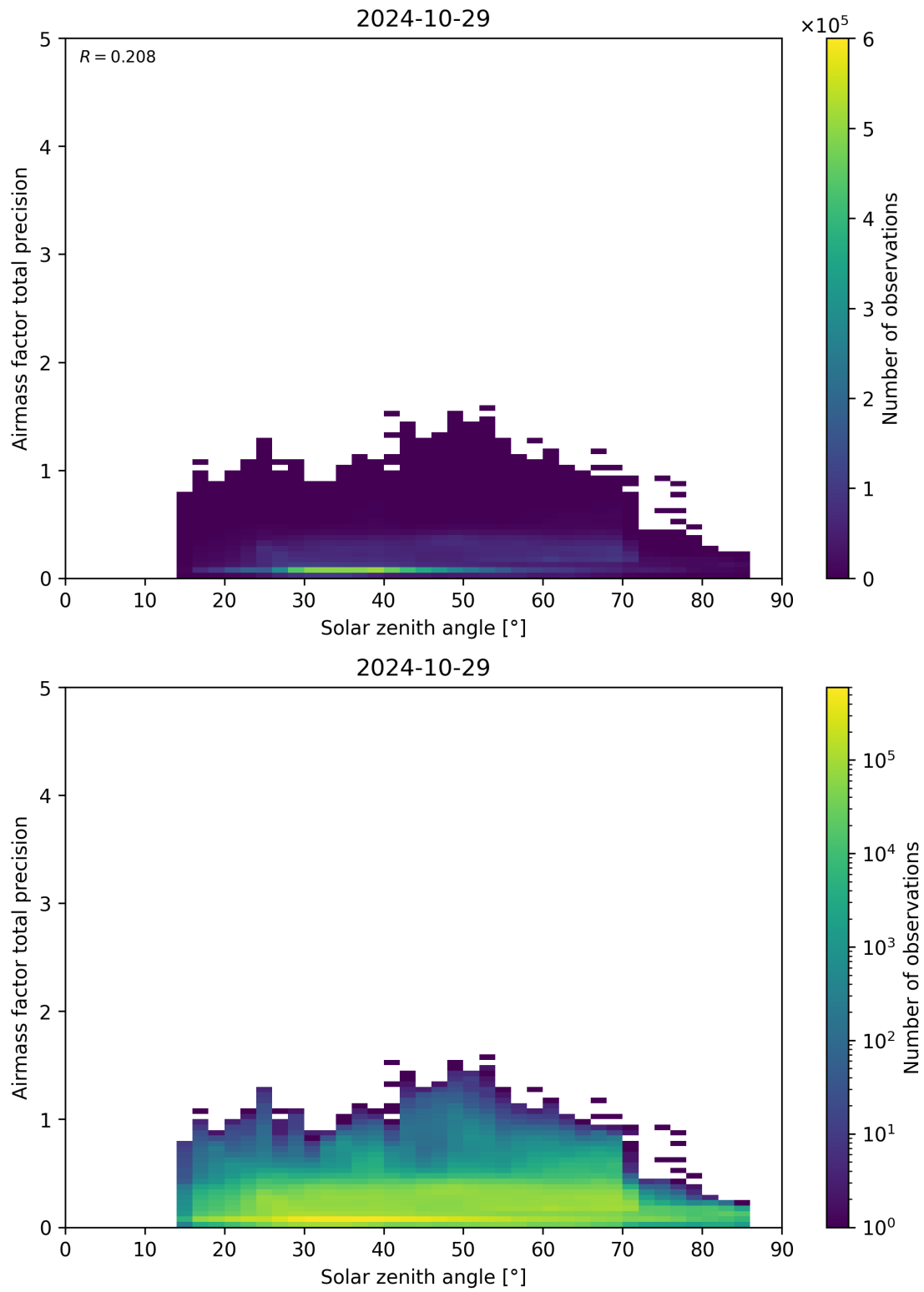
Figure 176: Scatter density plot of “Solar zenith angle” against “Airmass factor total precision” for 2024-10-29 to 2024-10-30.
