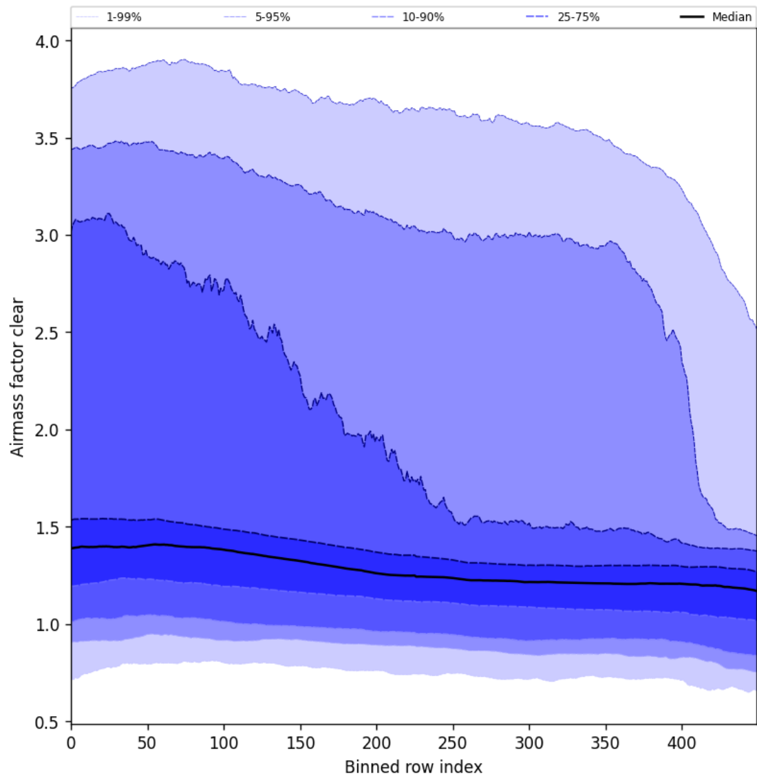
Figure 56: Along track statistics of “Airmass factor clear” for 2024-10-29 to 2024-10-30
