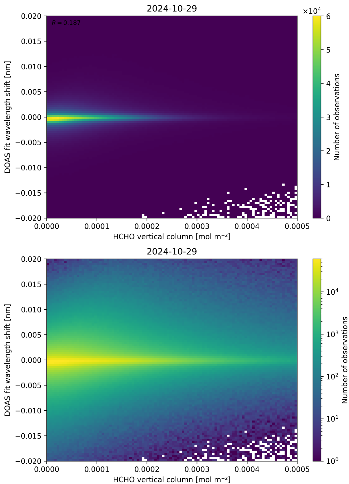
Figure 124: Scatter density plot of “HCHO vertical column” against “DOAS fit wavelength shift” for 2024-10-29 to 2024-10-30.
