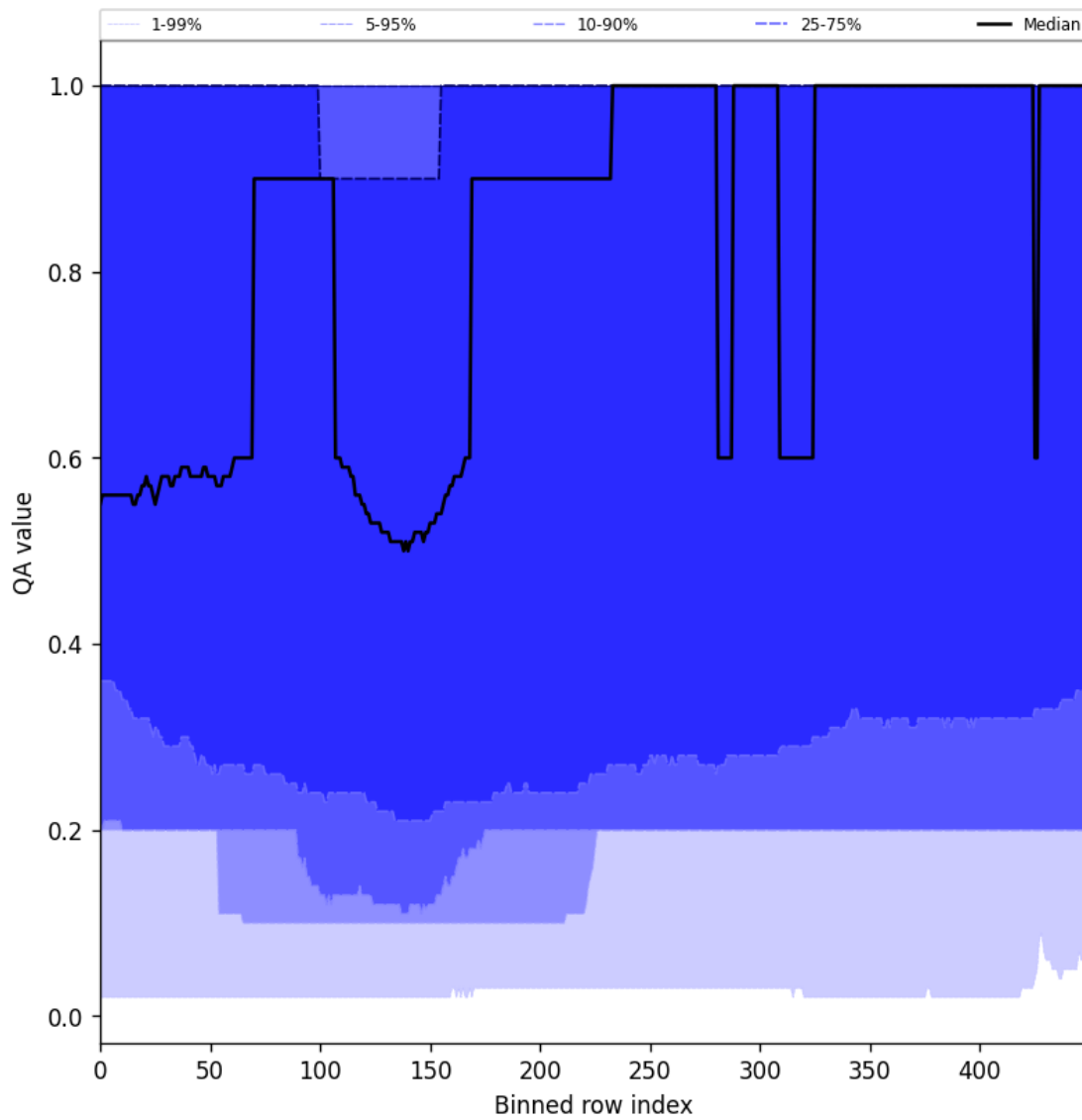
Figure 48: Along track statistics of “QA value” for 2024-10-29 to 2024-10-30
