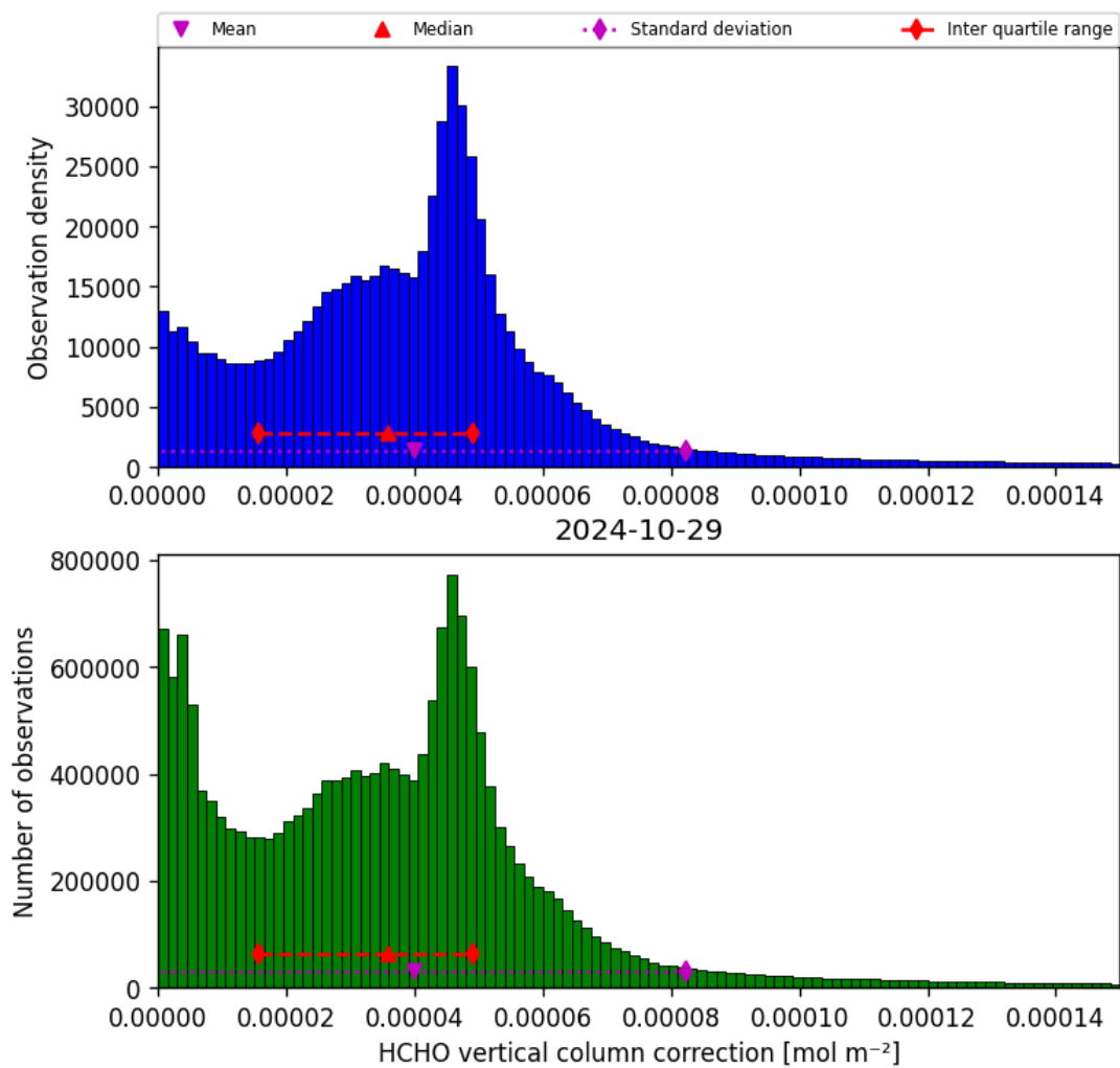
Figure 37: Histogram of “HCHO vertical column correction” for 2024-10-29 to 2024-10-30
