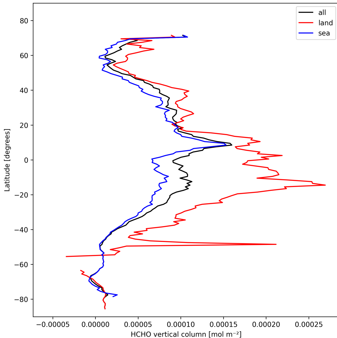
Figure 21: Zonal average of “HCHO vertical column” for 2024-10-29 to 2024-10-30.
