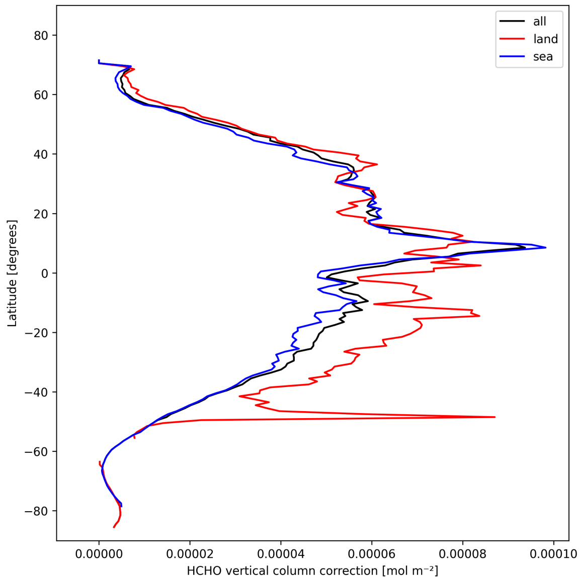
Figure 23: Zonal average of “HCHO vertical column correction” for 2024-10-29 to 2024-10-30.
