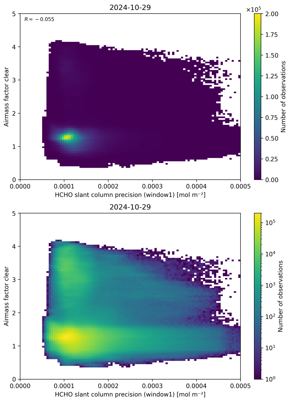
Figure 91: Scatter density plot of “HCHO slant column precision (window1)” against “Airmass factor clear” for 2024-10-29 to 2024-10-30.
