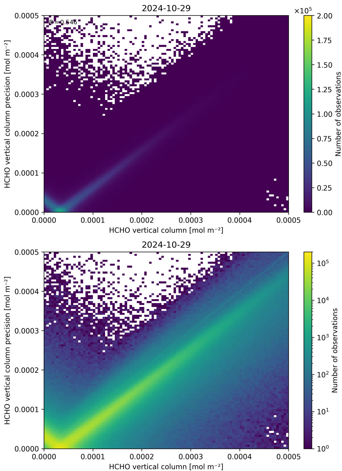
Figure 134: Scatter density plot of “HCHO vertical column” against “HCHO vertical column precision” for 2024-10-29 to 2024-10-30.
