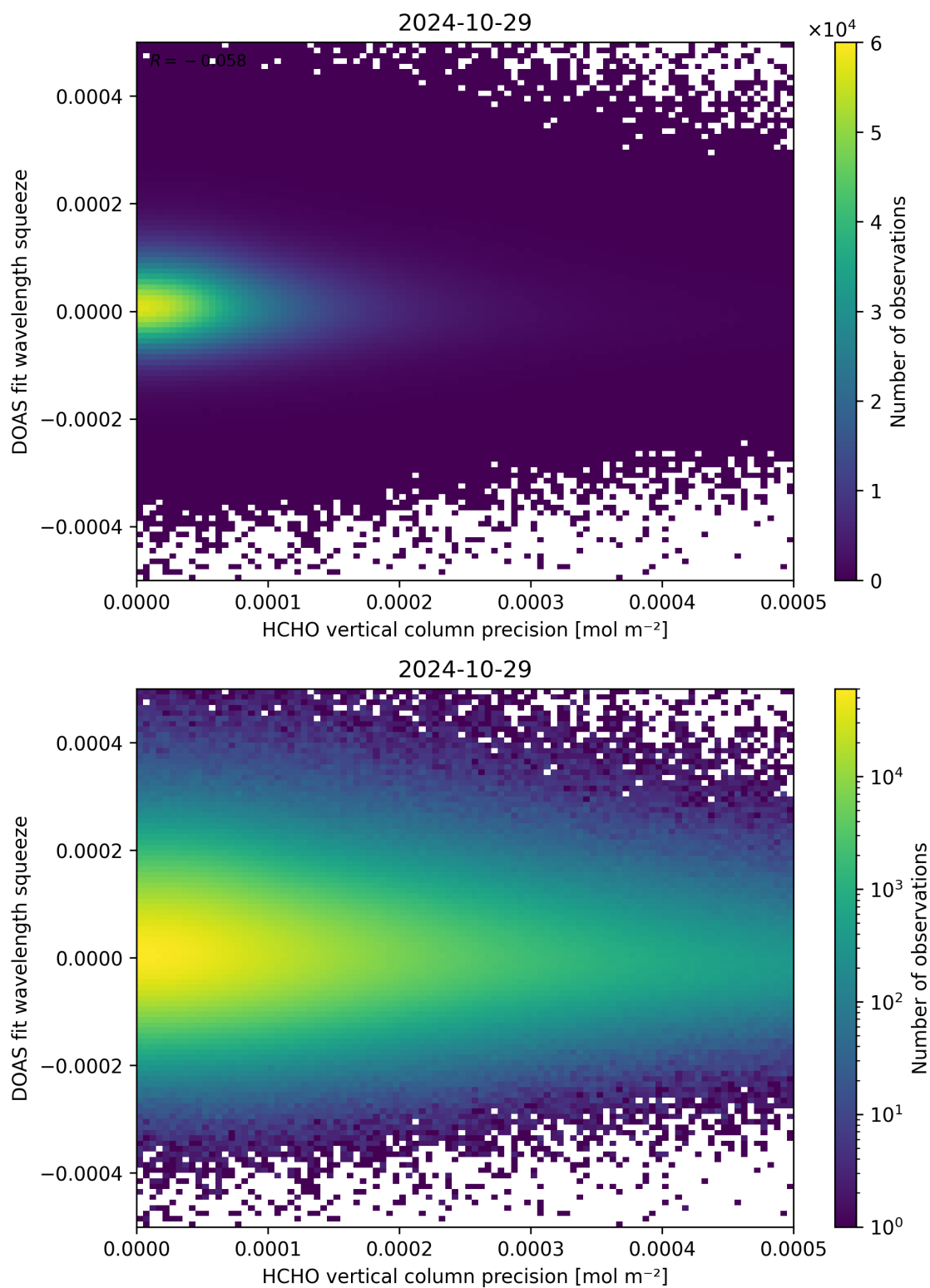
Figure 138: Scatter density plot of “HCHO vertical column precision” against “DOAS fit wavelength squeeze” for 2024-10-29 to 2024-10-30.
