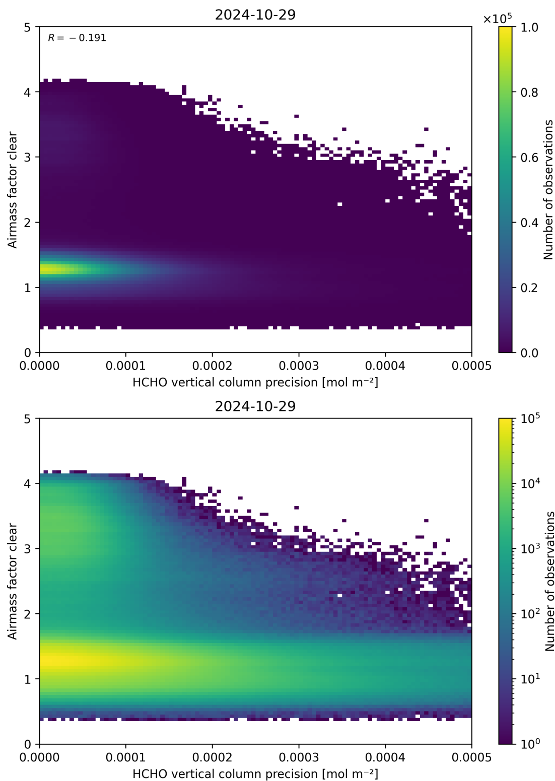
Figure 139: Scatter density plot of “HCHO vertical column precision” against “Airmass factor clear” for 2024-10-29 to 2024-10-30.
