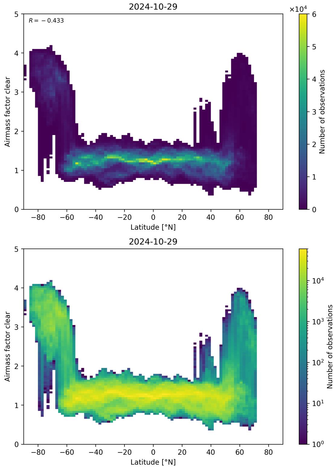
Figure 156: Scatter density plot of “Latitude” against “Airmass factor clear” for 2024-10-29 to 2024-10-30.
