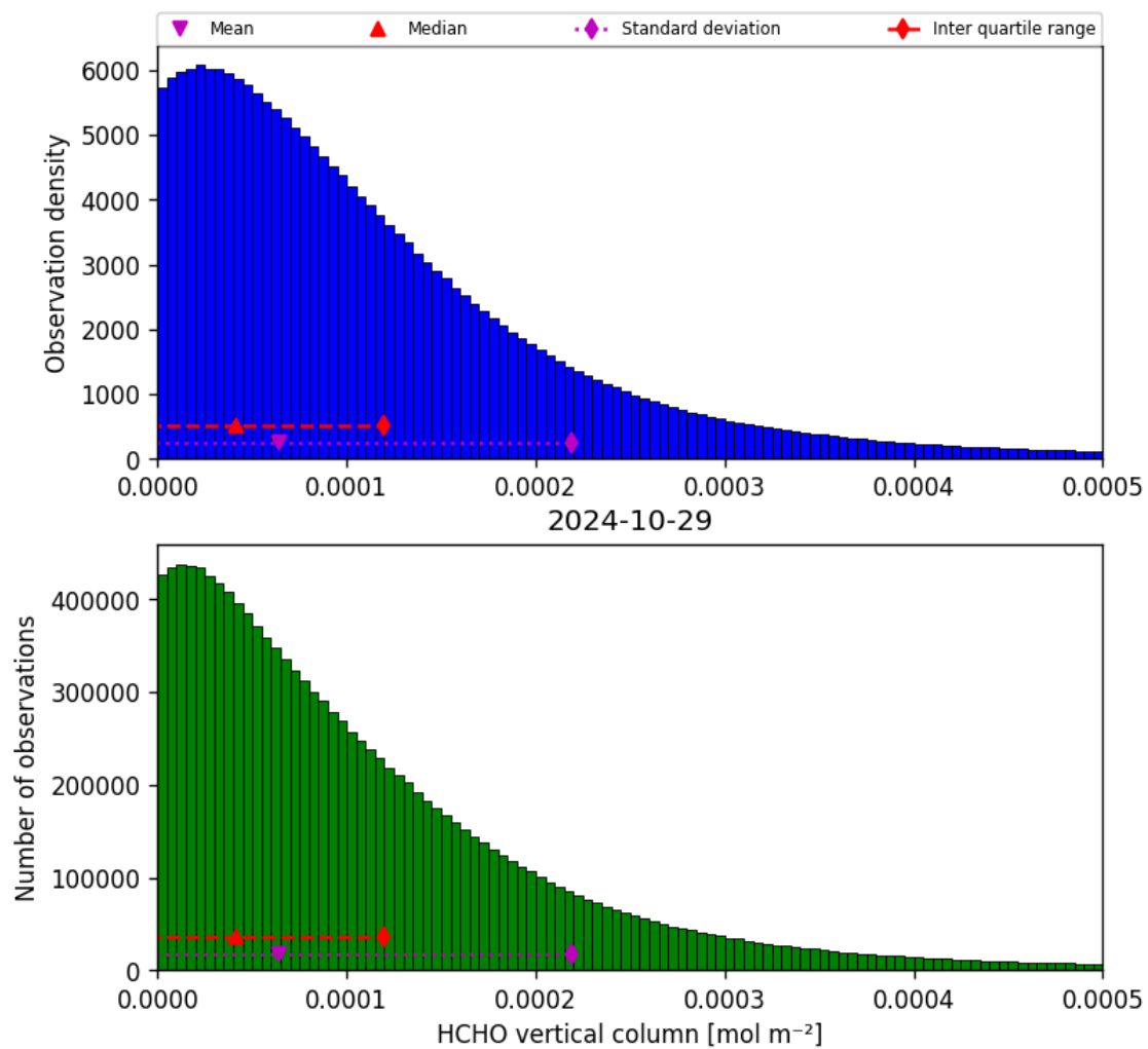
Figure 35: Histogram of “HCHO vertical column” for 2024-10-29 to 2024-10-30
