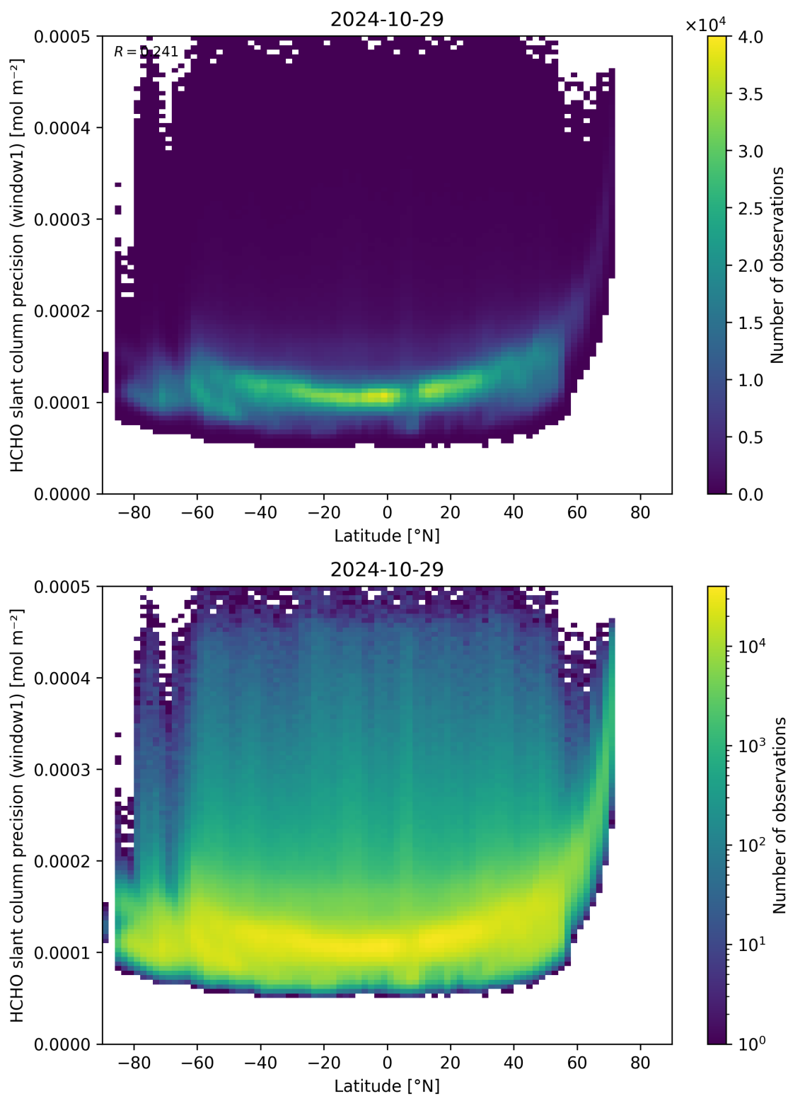
Figure 160: Scatter density plot of “Latitude” against “HCHO slant column precision (window1)” for 2024-10-29 to 2024-10-30.
