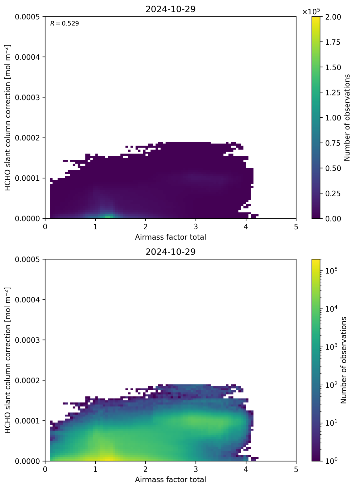
Figure 102: Scatter density plot of “Airmass factor total” against “HCHO slant column correction” for 2024-10-29 to 2024-10-30.
