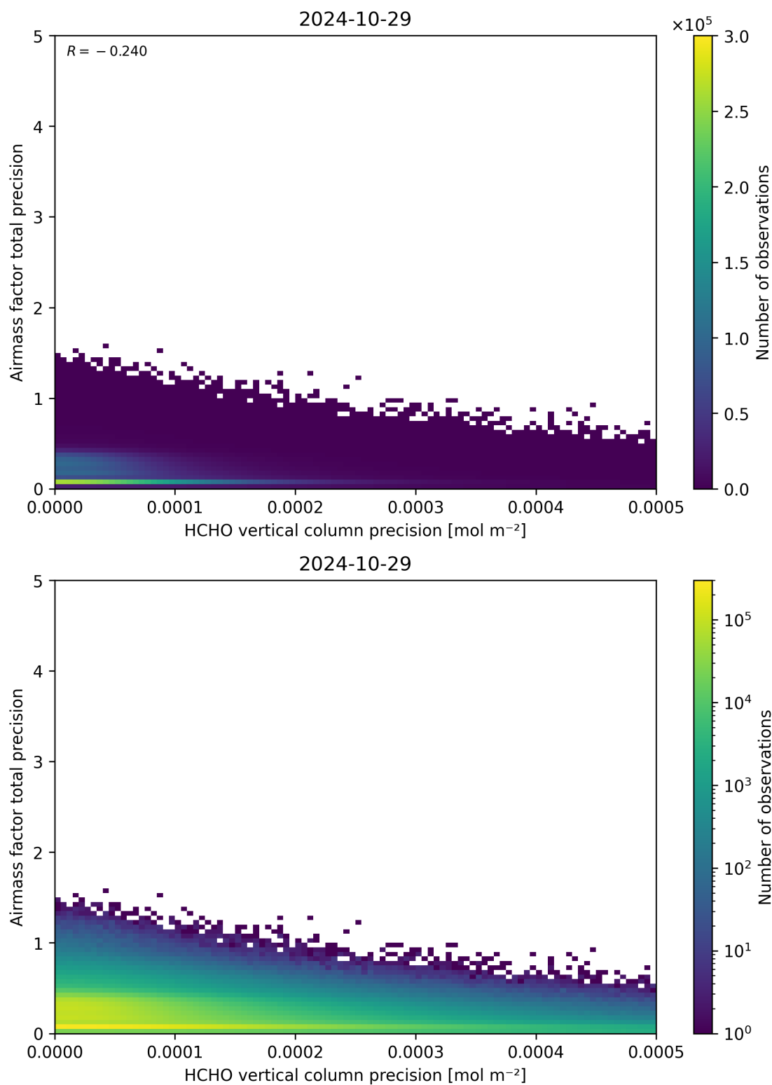
Figure 145: Scatter density plot of “HCHO vertical column precision” against “Airmass factor total precision” for 2024-10-29 to 2024-10-30.
