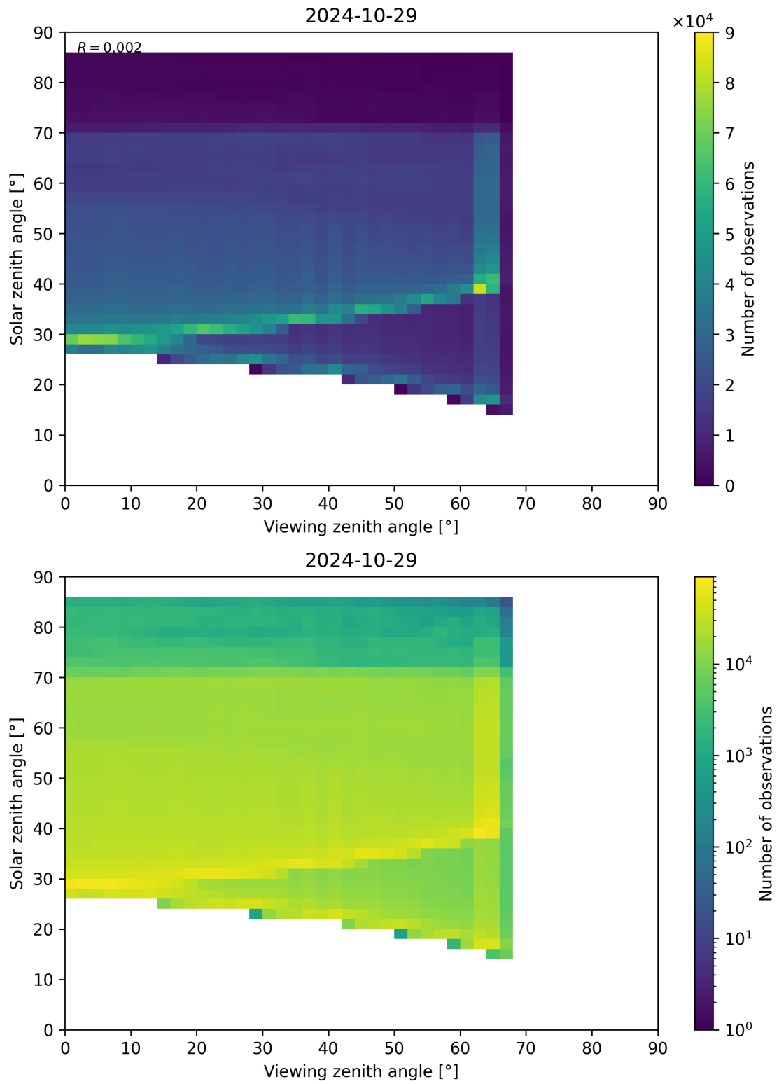
Figure 197: Scatter density plot of “Viewing zenith angle” against “Solar zenith angle” for 2024-10-29 to 2024-10-30.
