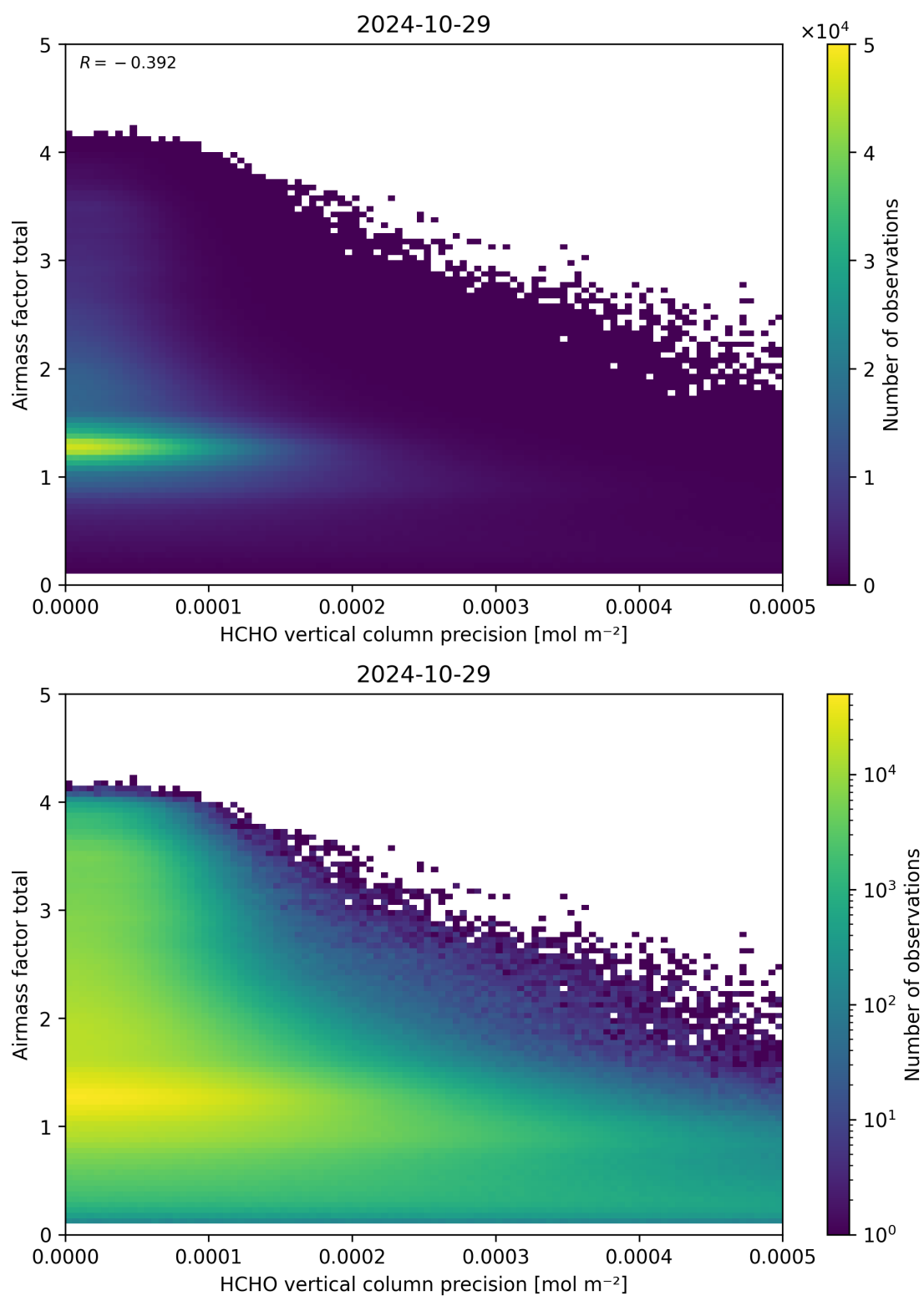
Figure 144: Scatter density plot of “HCHO vertical column precision” against “Airmass factor total” for 2024-10-29 to 2024-10-30.
