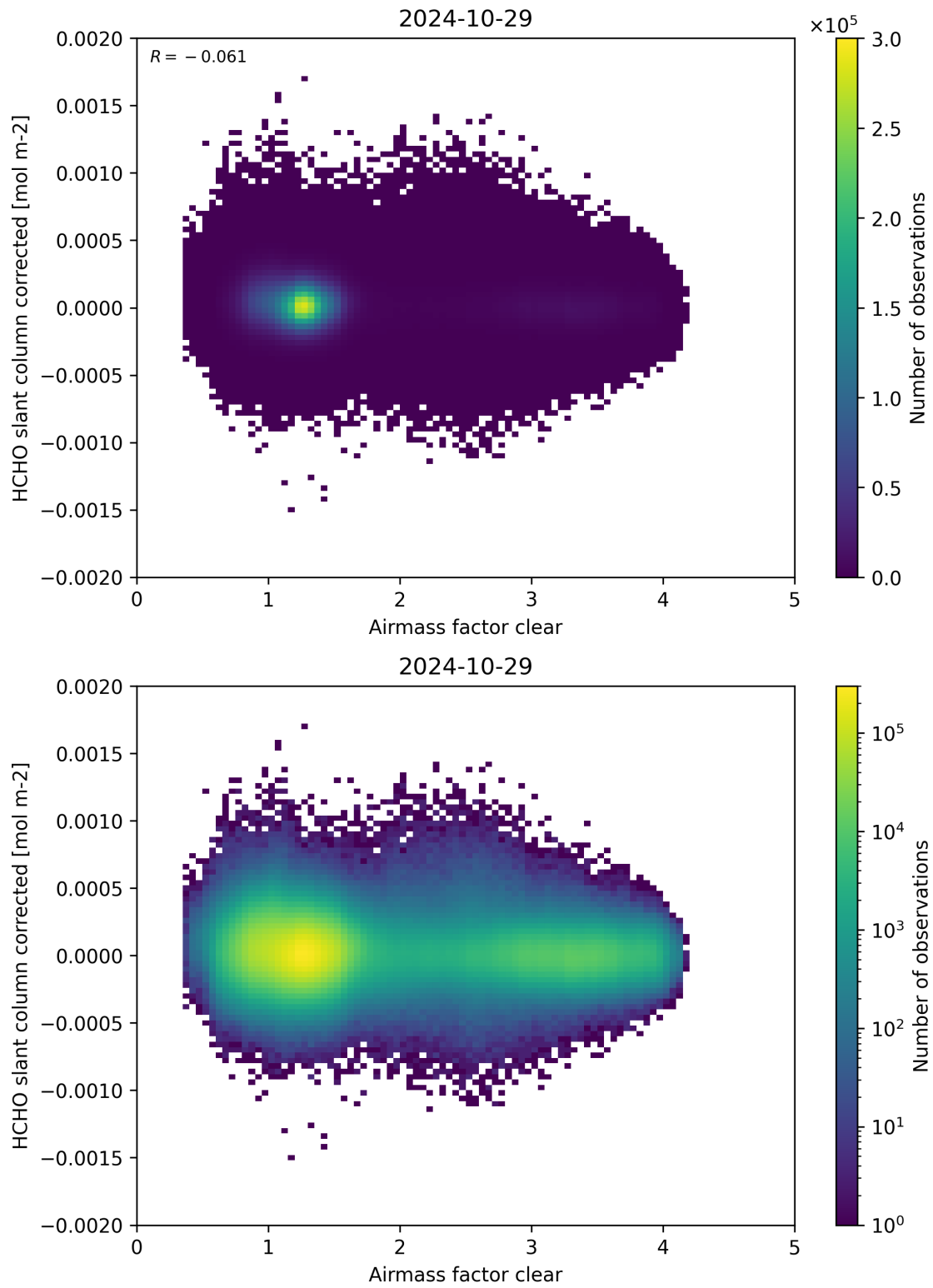
Figure 74: Scatter density plot of “Airmass factor clear” against “HCHO slant column corrected” for 2024-10-29 to 2024-10-30.
