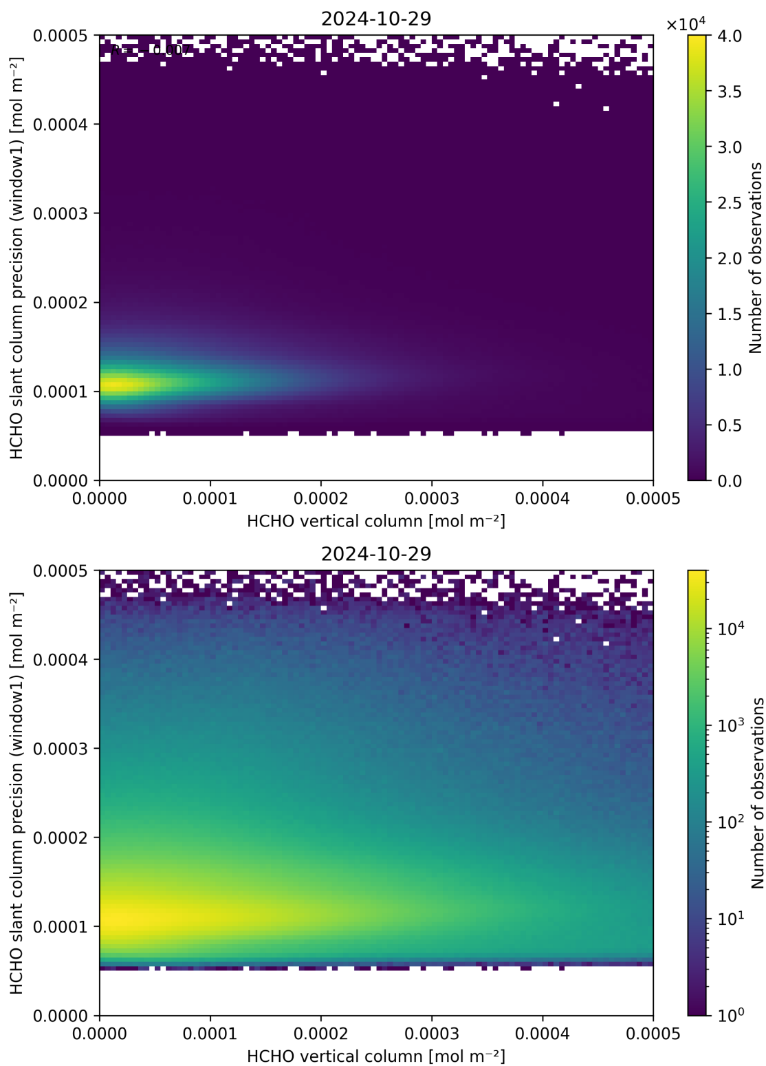
Figure 130: Scatter density plot of “HCHO vertical column” against “HCHO slant column precision (window1)” for 2024-10-29 to 2024-10-30.
