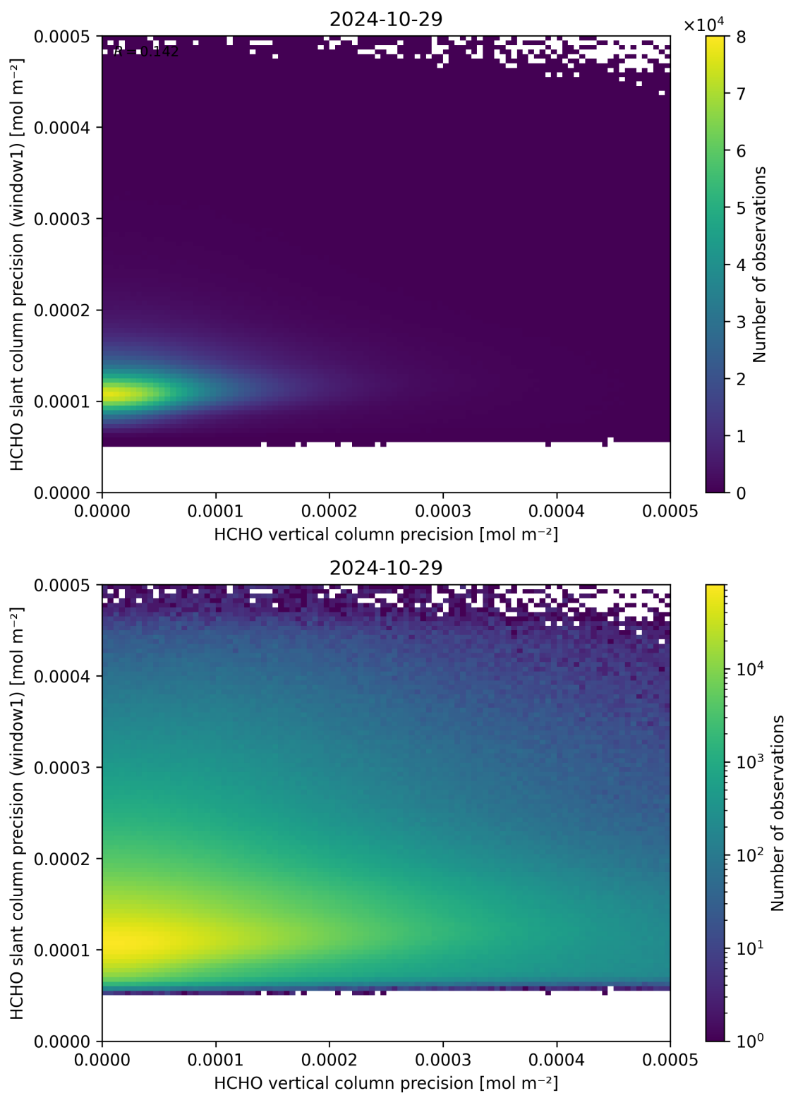
Figure 143: Scatter density plot of “HCHO vertical column precision” against “HCHO slant column precision (window1)” for 2024-10-29 to 2024-10-30.
