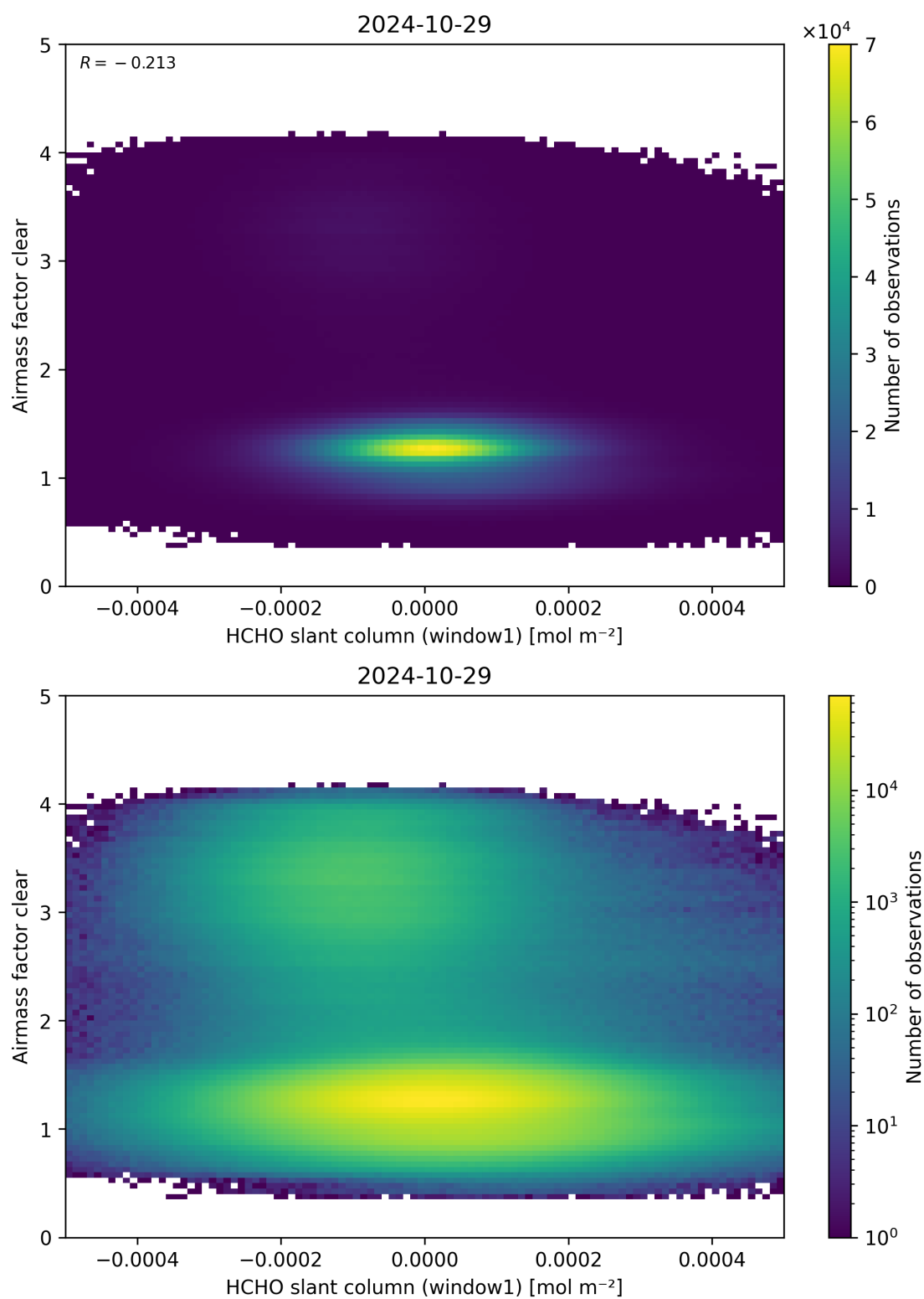
Figure 81: Scatter density plot of “HCHO slant column (window1)” against “Airmass factor clear” for 2024-10-29 to 2024-10-30.
