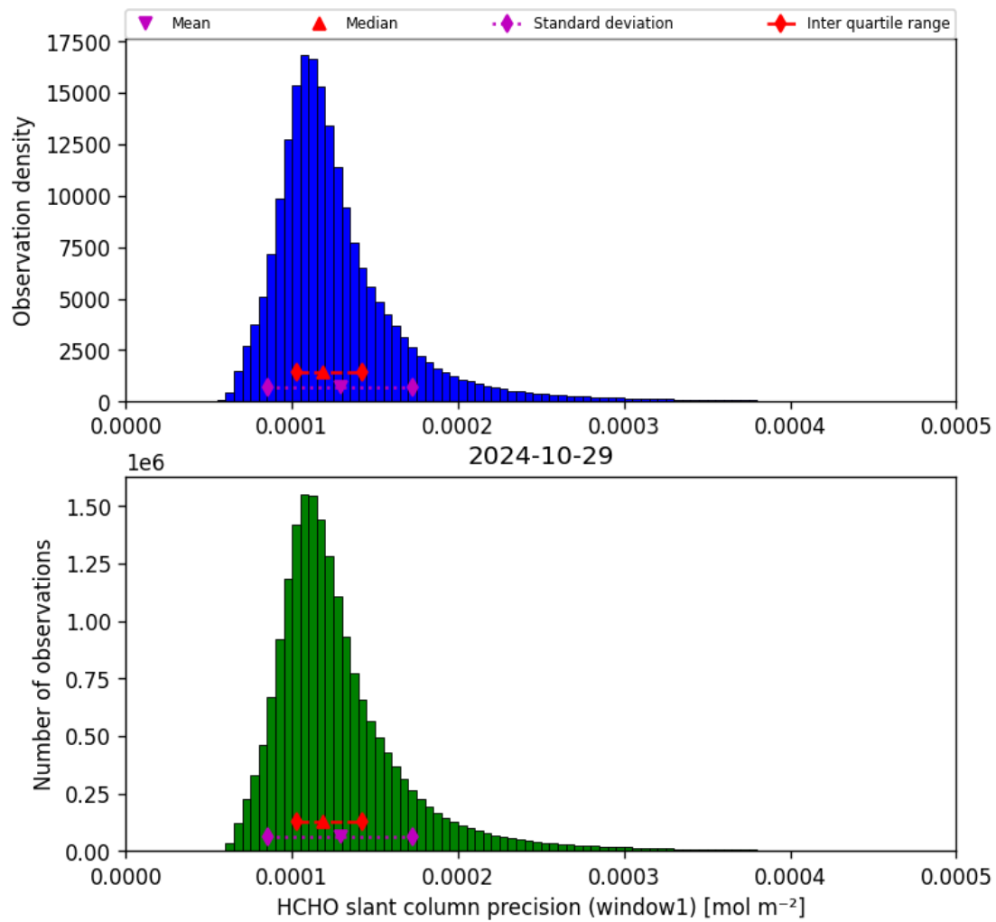
Figure 39: Histogram of “HCHO slant column precision (window1)” for 2024-10-29 to 2024-10-30
