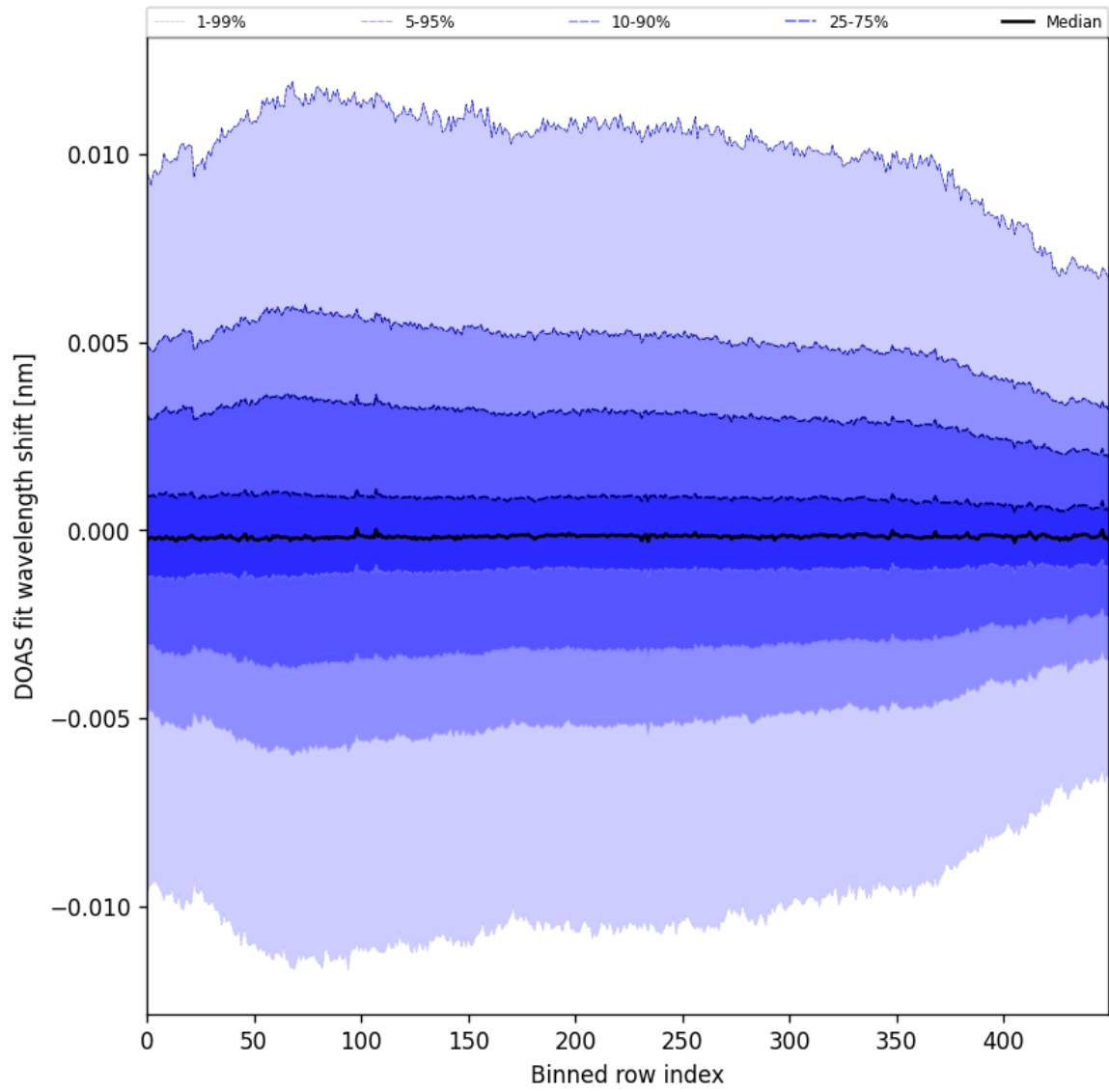
Figure 58: Along track statistics of “DOAS fit wavelength shift” for 2024-10-29 to 2024-10-30
