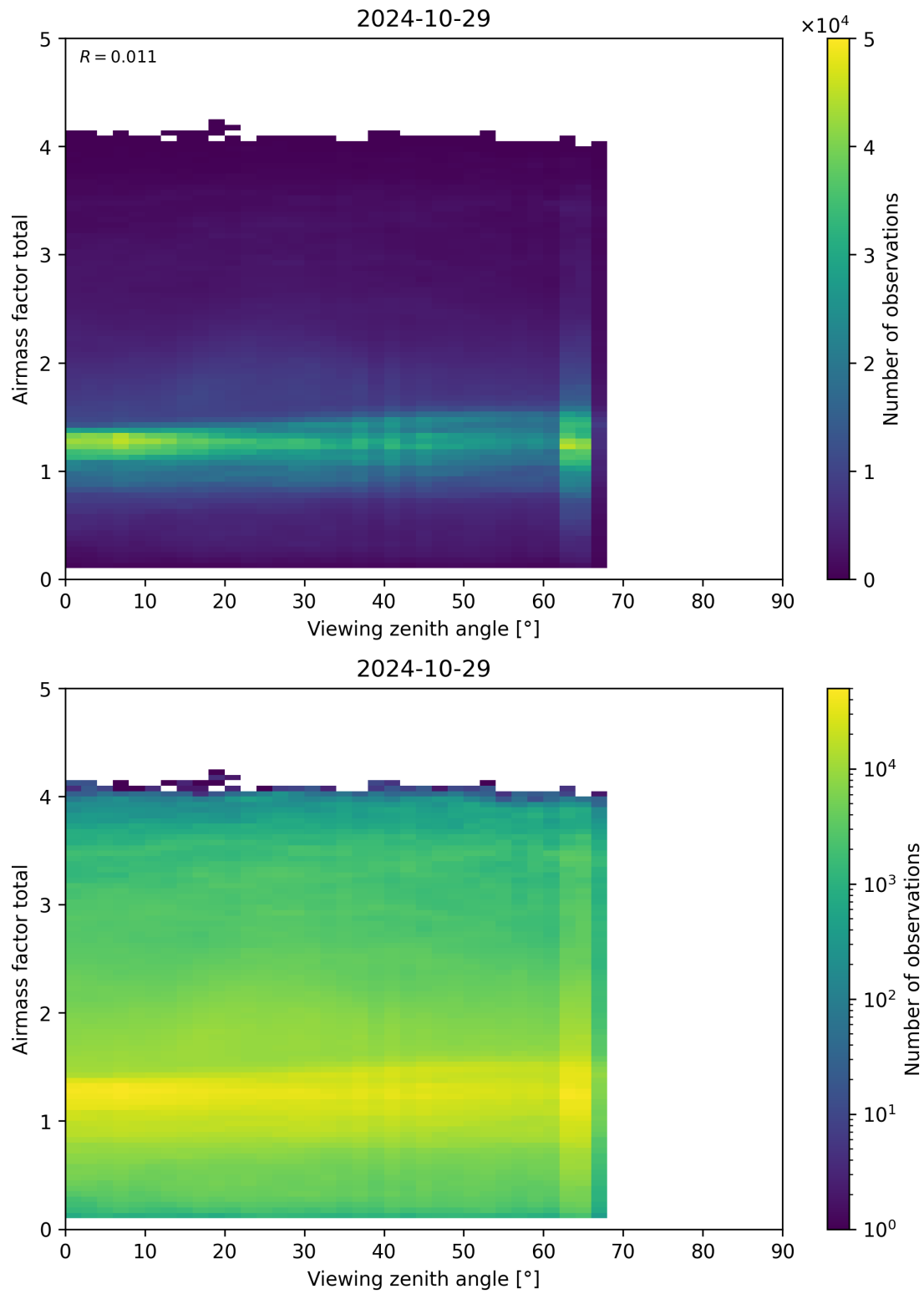
Figure 190: Scatter density plot of “Viewing zenith angle” against “Airmass factor total” for 2024-10-29 to 2024-10-30.
