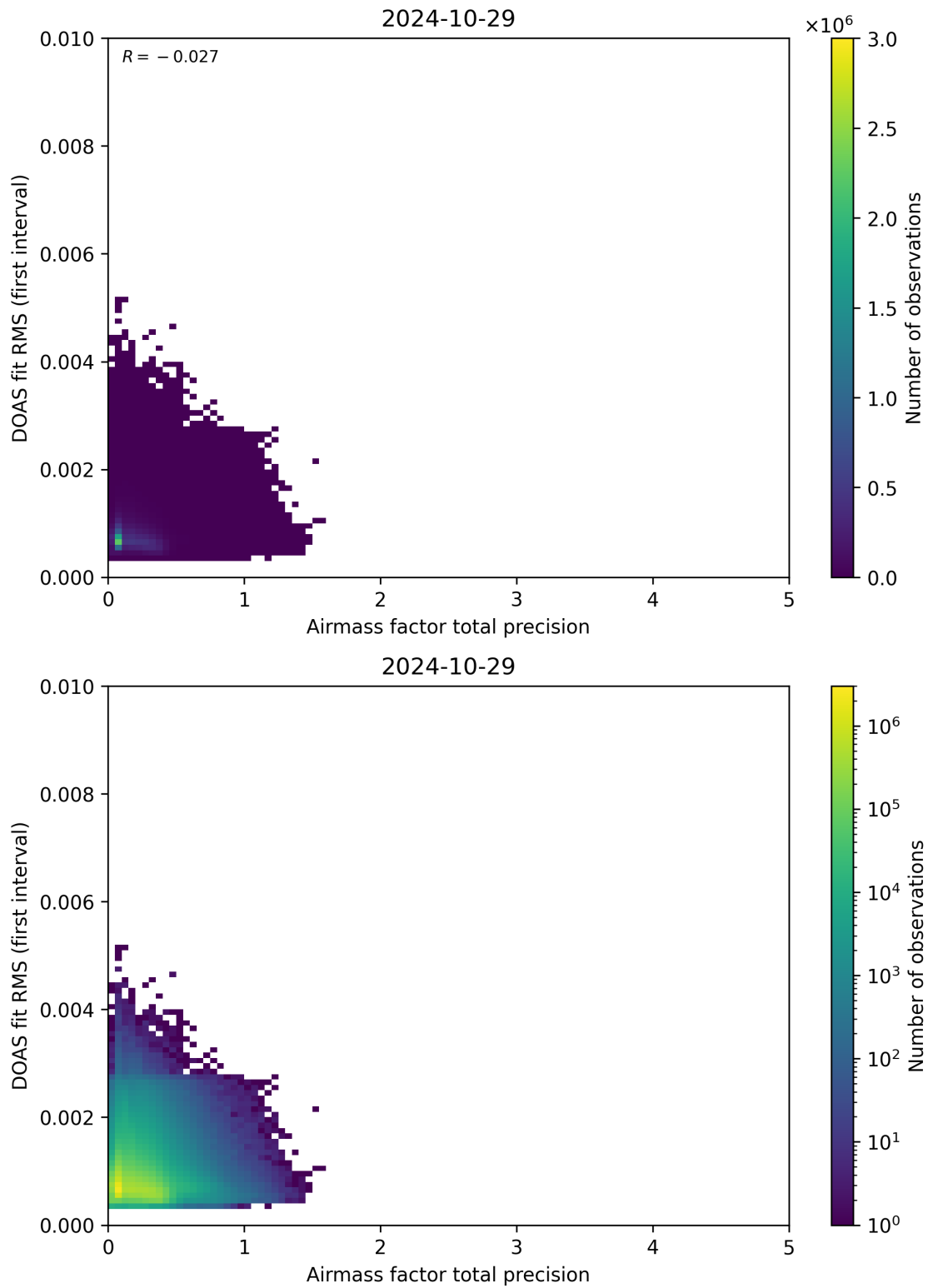
Figure 105: Scatter density plot of “Airmass factor total precision” against “DOAS fit RMS (first interval)” for 2024-10-29 to 2024-10-30.
