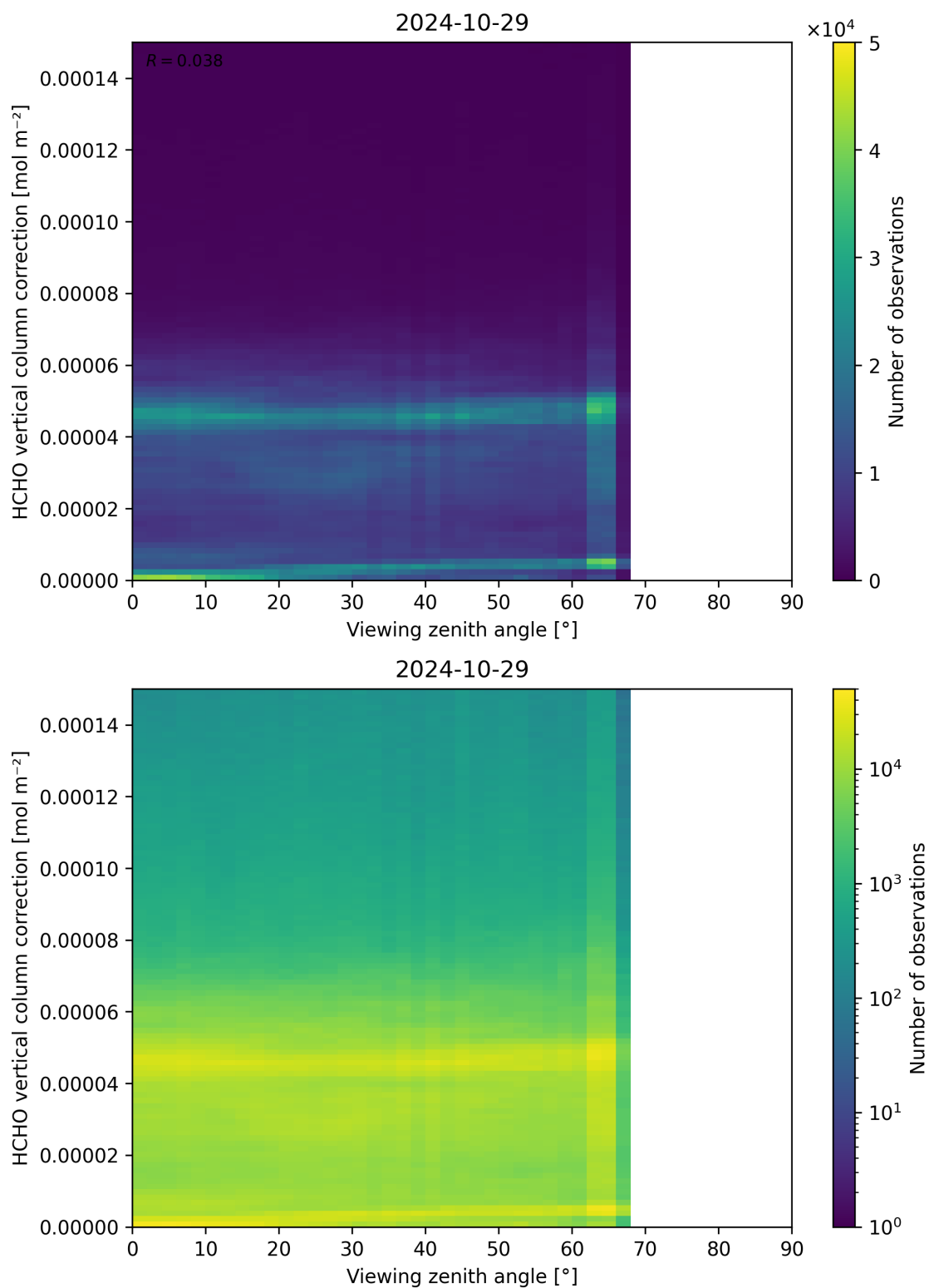
Figure 193: Scatter density plot of “Viewing zenith angle” against “HCHO vertical column correction” for 2024-10-29 to 2024-10-30.
