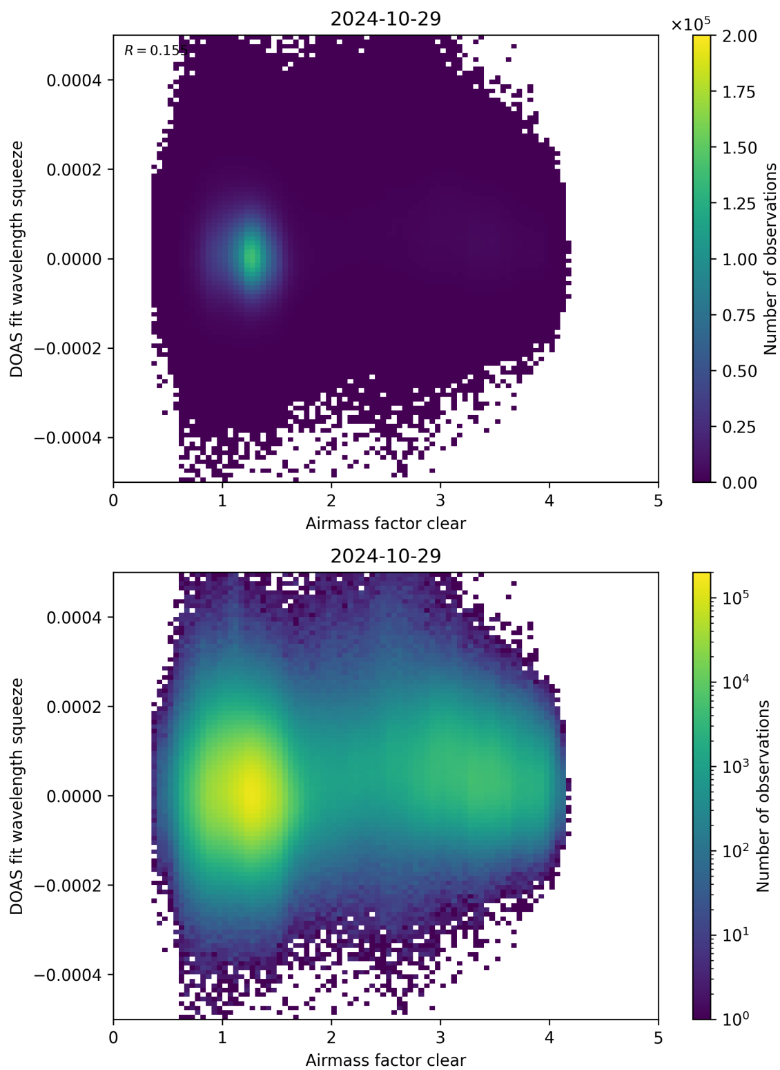
Figure 73: Scatter density plot of “Airmass factor clear” against “DOAS fit wavelength squeeze” for 2024-10-29 to 2024-10-30.
