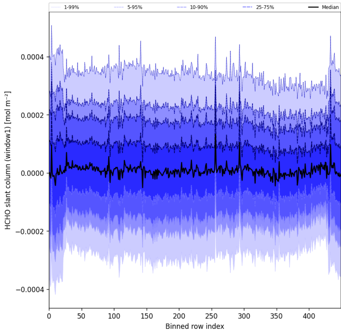
Figure 52: Along track statistics of “HCHO slant column (window1)” for 2024-10-29 to 2024-10-30
