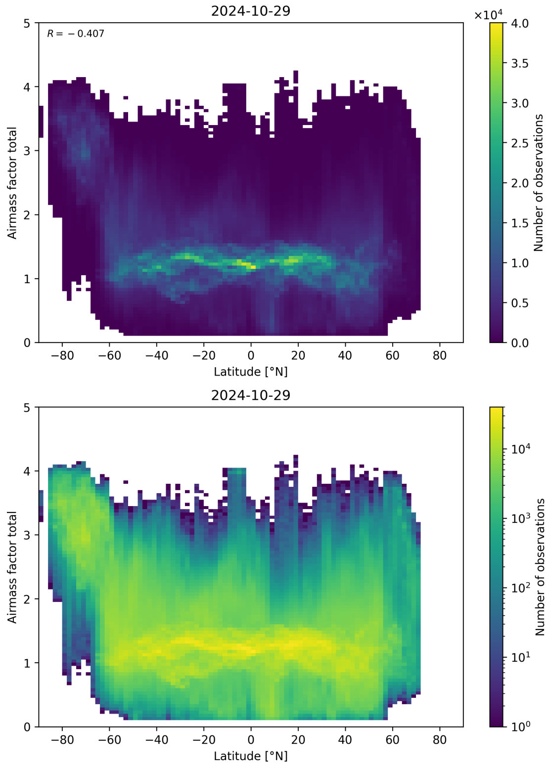
Figure 161: Scatter density plot of “Latitude” against “Airmass factor total” for 2024-10-29 to 2024-10-30.
