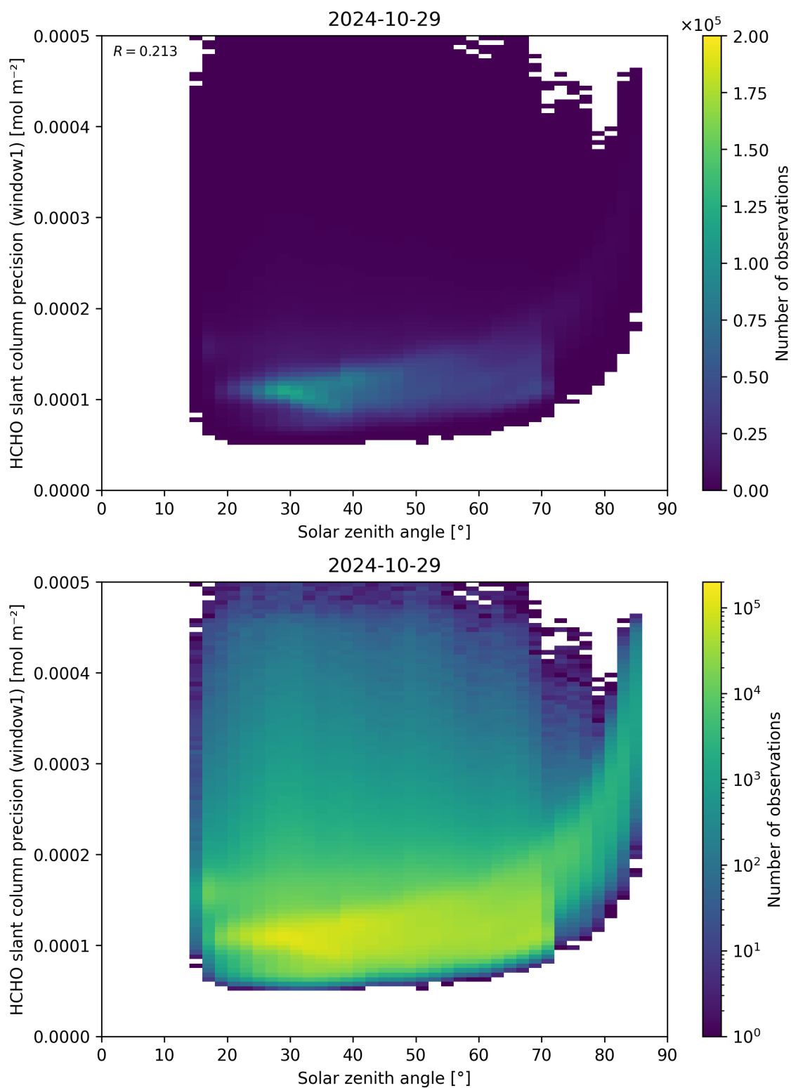
Figure 174: Scatter density plot of “Solar zenith angle” against “HCHO slant column precision (window1)” for 2024-10-29 to 2024-10-30.
