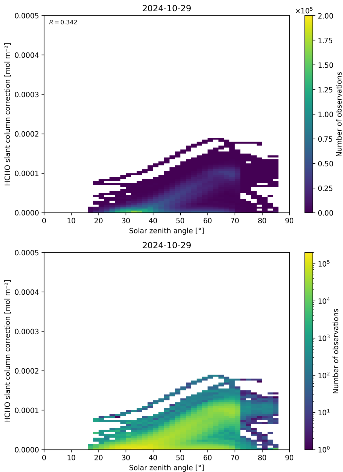
Figure 172: Scatter density plot of “Solar zenith angle” against “HCHO slant column correction” for 2024-10-29 to 2024-10-30.
