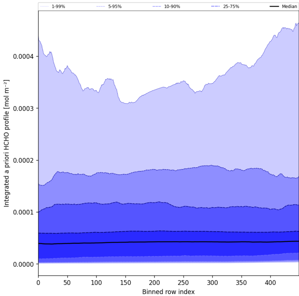
Figure 57: Along track statistics of "Integrated a priori HCHO profile" for 2024-10-29 to 2024-10-30
