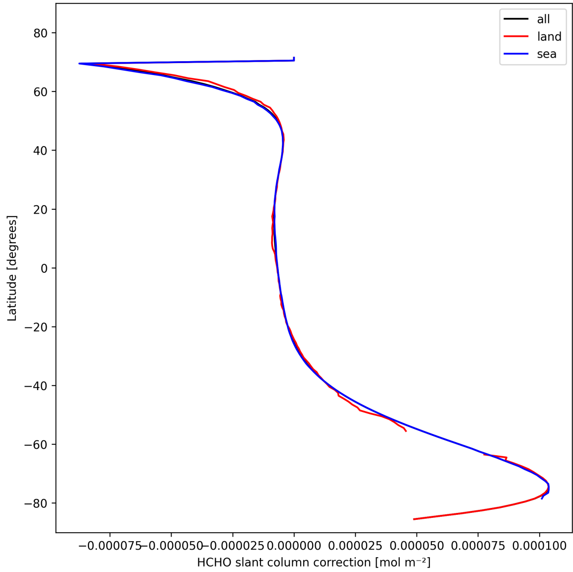
Figure 33: Zonal average of “HCHO slant column correction” for 2024-10-29 to 2024-10-30.
