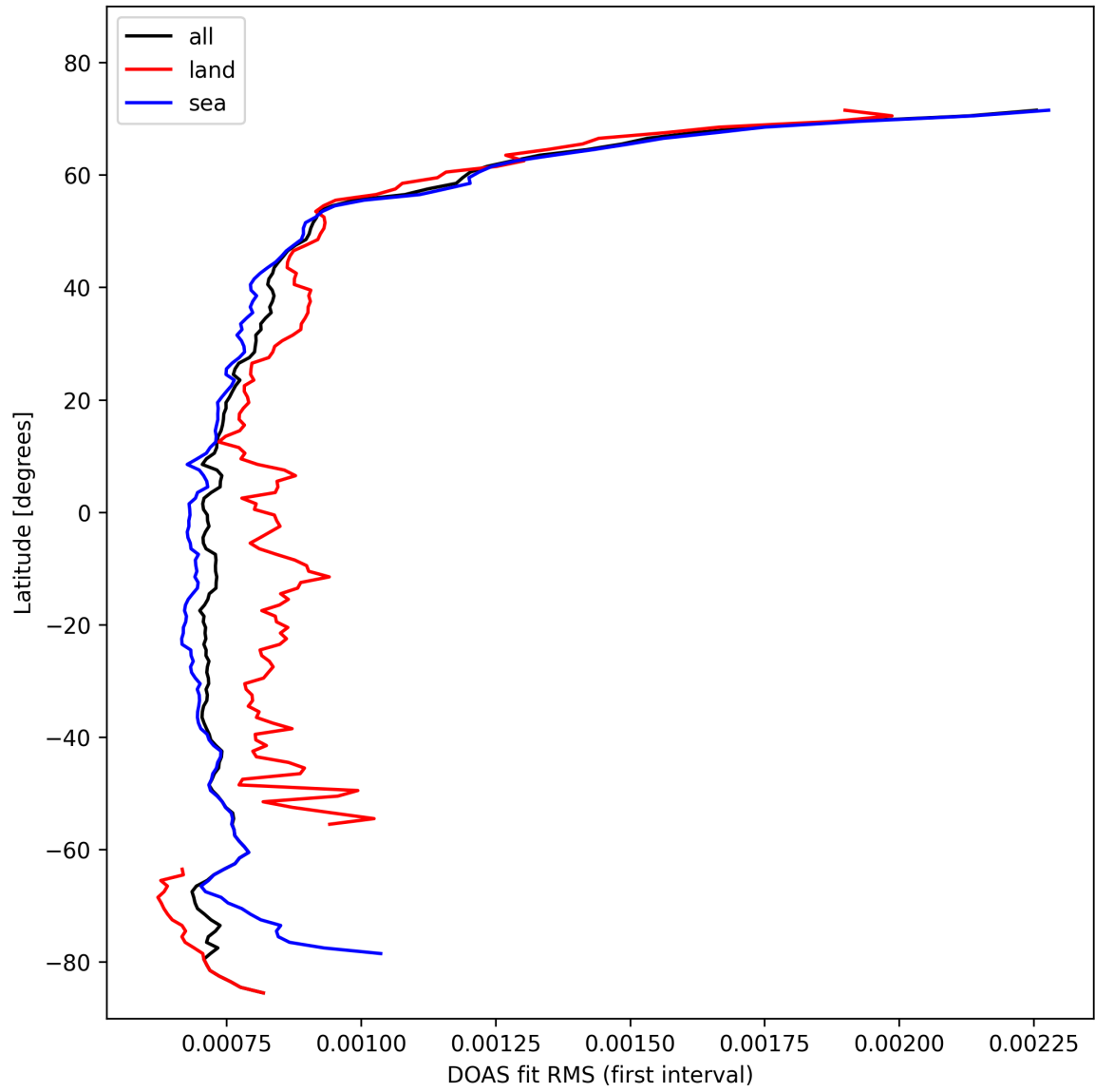
Figure 32: Zonal average of “DOAS fit RMS (first interval)” for 2024-10-29 to 2024-10-30.
