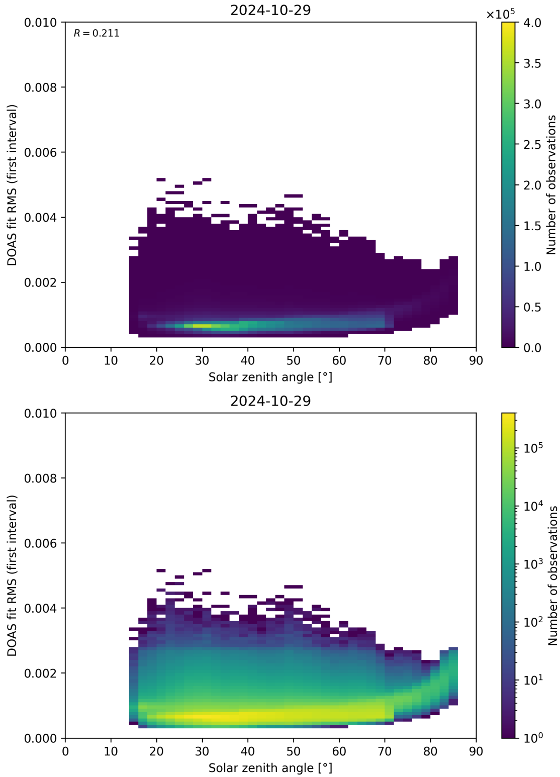
Figure 167: Scatter density plot of “Solar zenith angle” against “DOAS fit RMS (first interval)” for 2024-10-29 to 2024-10-30.
