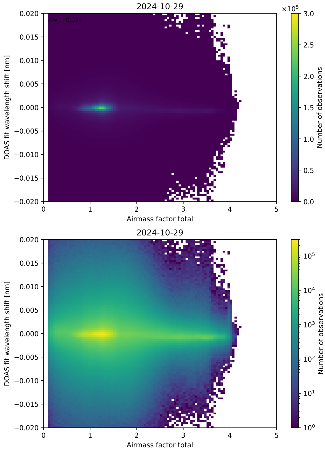
Figure 98: Scatter density plot of “Airmass factor total” against “DOAS fit wavelength shift” for 2024-10-29 to 2024-10-30.
