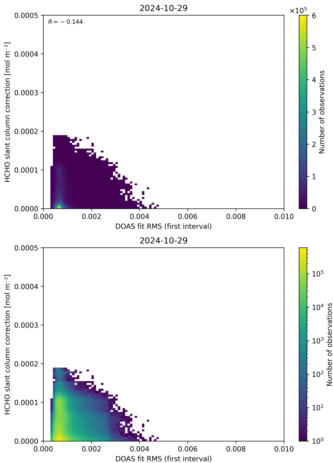
Figure 63: Scatter density plot of “DOAS fit RMS (first interval)” against “HCHO slant column correction” for 2024-10-29 to 2024-10-30.
