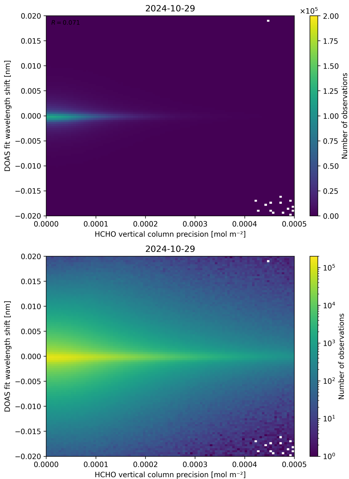
Figure 137: Scatter density plot of “HCHO vertical column precision” against “DOAS fit wavelength shift” for 2024-10-29 to 2024-10-30.
