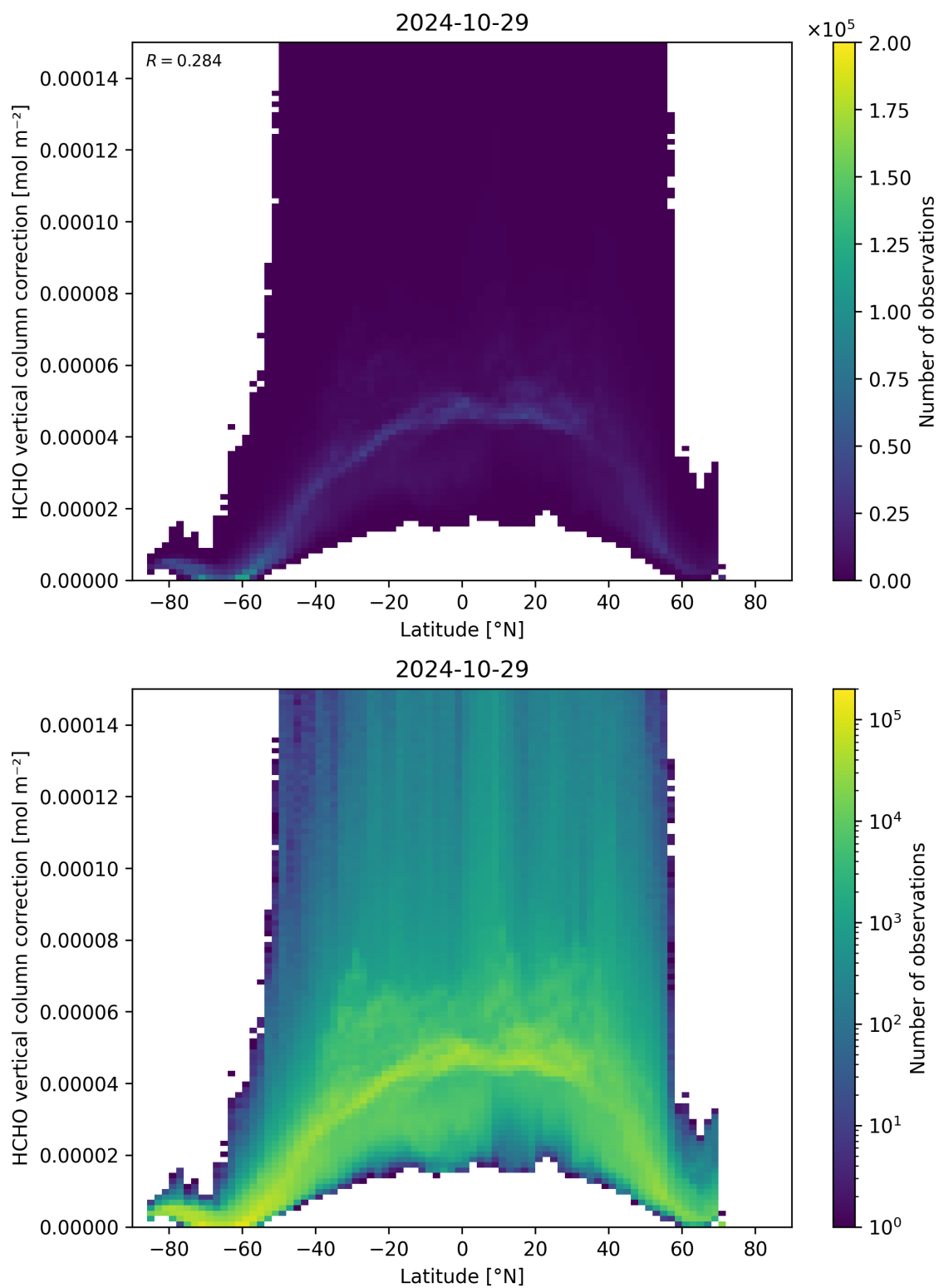
Figure 164: Scatter density plot of “Latitude” against “HCHO vertical column correction” for 2024-10-29 to 2024-10-30.
