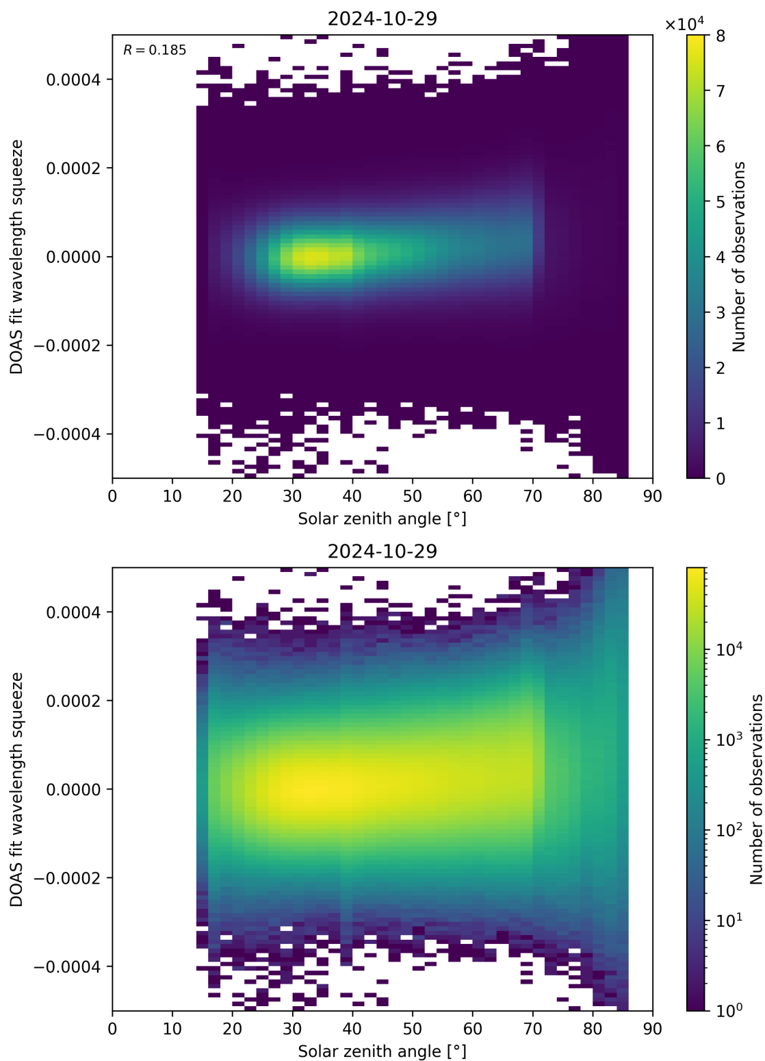
Figure 169: Scatter density plot of “Solar zenith angle” against “DOAS fit wavelength squeeze” for 2024-10-29 to 2024-10-30.
