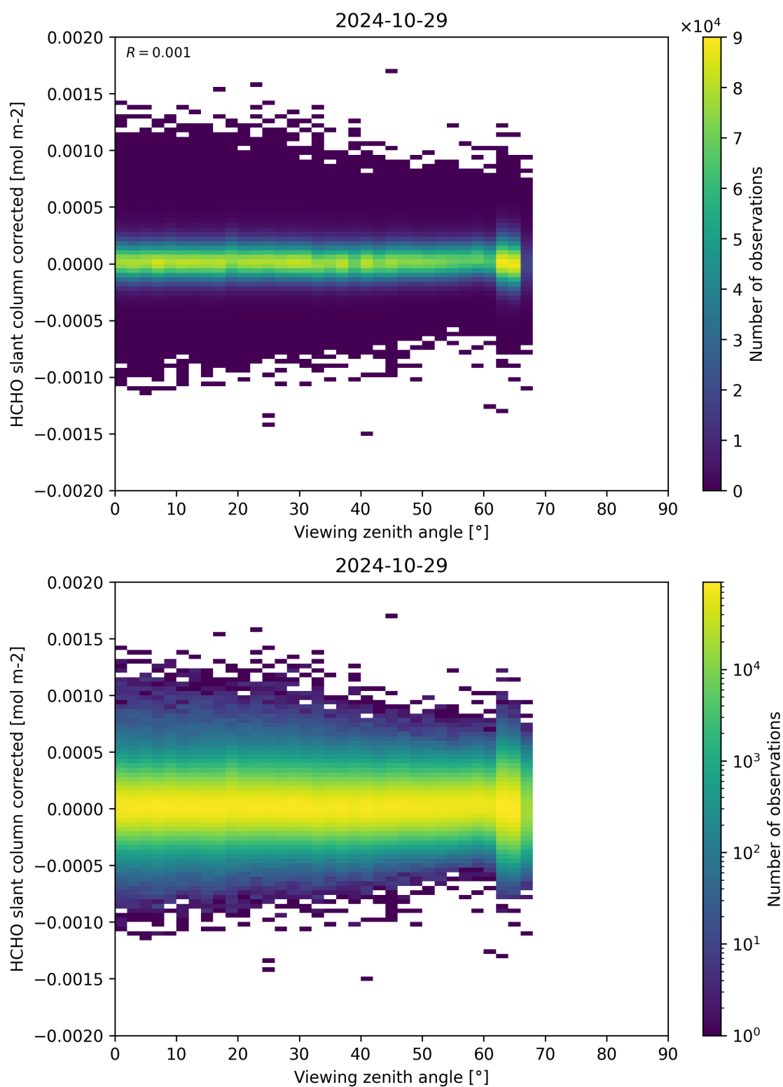
Figure 186: Scatter density plot of “Viewing zenith angle” against “HCHO slant column corrected” for 2024-10-29 to 2024-10-30.
