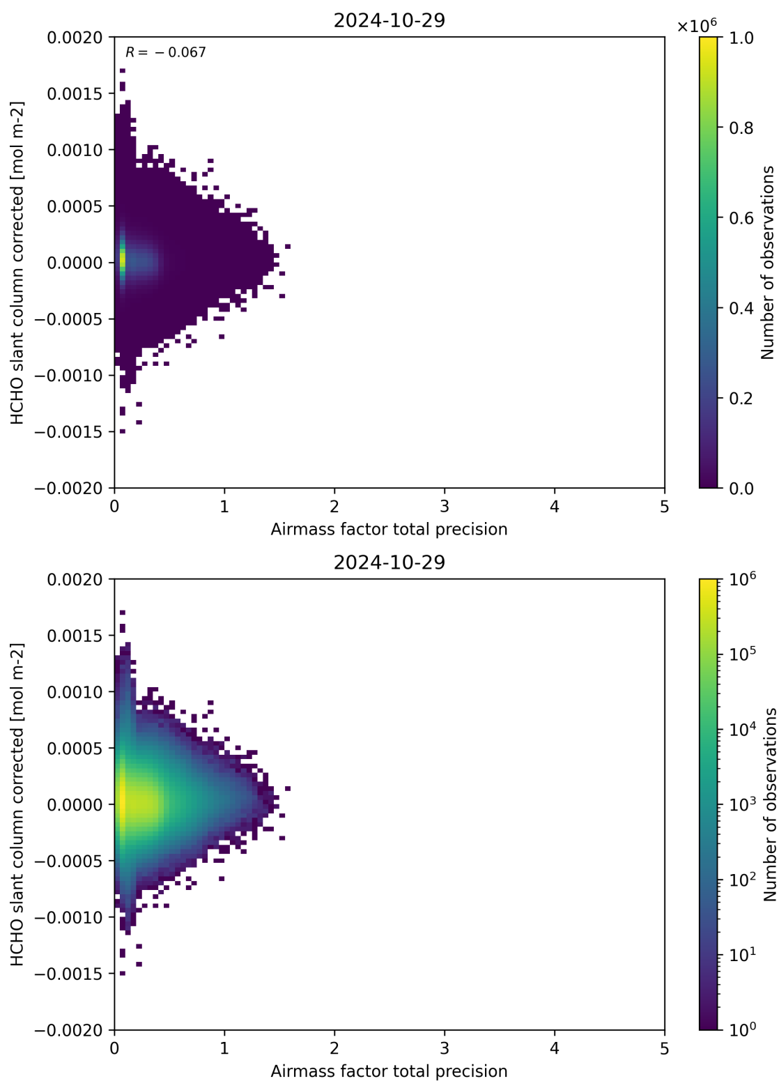
Figure 109: Scatter density plot of “Airmass factor total precision” against “HCHO slant column corrected” for 2024-10-29 to 2024-10-30.
