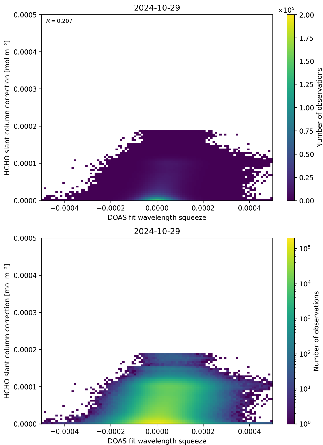
Figure 70: Scatter density plot of “DOAS fit wavelength squeeze” against “HCHO slant column correction” for 2024-10-29 to 2024-10-30.
