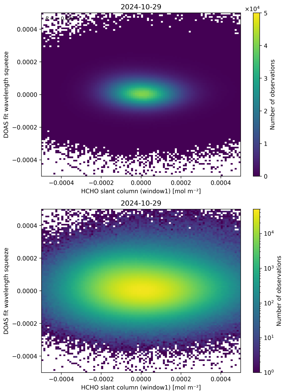
Figure 80: Scatter density plot of “HCHO slant column (window1)” against “DOAS fit wavelength squeeze” for 2024-10-29 to 2024-10-30.
