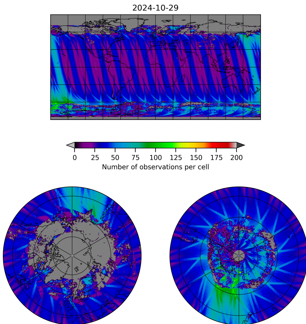
Figure 19: Map of the number of observations for 2024-10-29 to 2024-10-30
