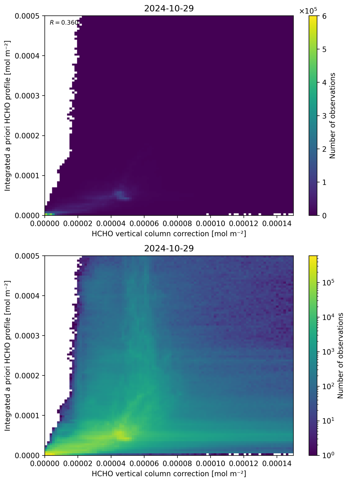
Figure 122: Scatter density plot of “HCHO vertical column correction” against “Integrated a priori HCHO profile” for 2024-10-29 to 2024-10-30.
