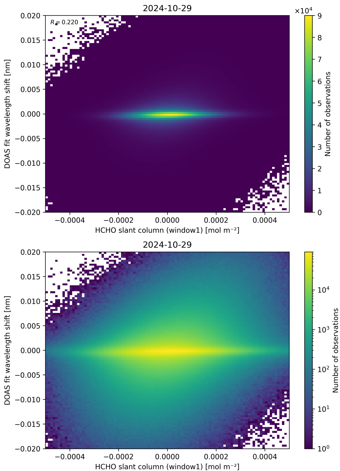
Figure 79: Scatter density plot of “HCHO slant column (window1)” against “DOAS fit wavelength shift” for 2024-10-29 to 2024-10-30.
