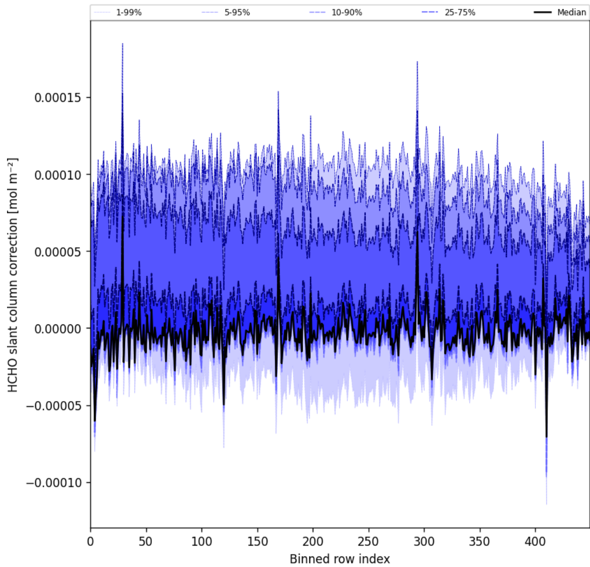
Figure 61: Along track statistics of “HCHO slant column correction” for 2024-10-29 to 2024-10-30
