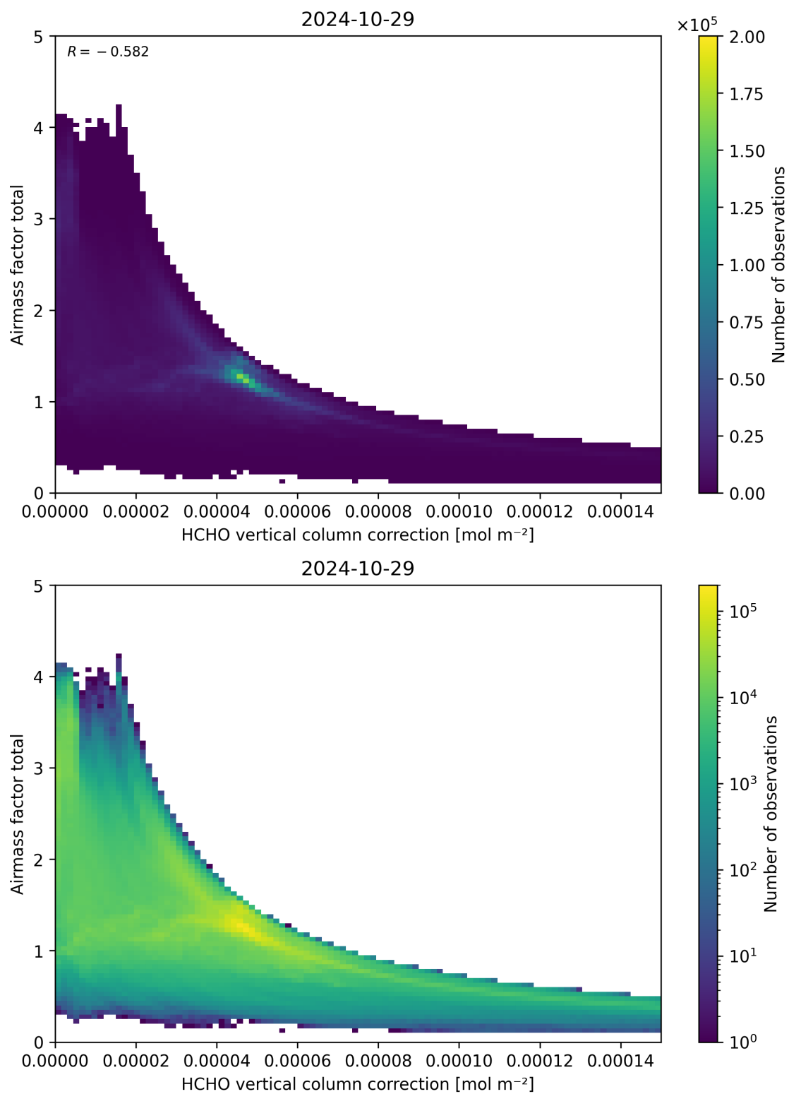
Figure 120: Scatter density plot of “HCHO vertical column correction” against “Airmass factor total” for 2024-10-29 to 2024-10-30.
