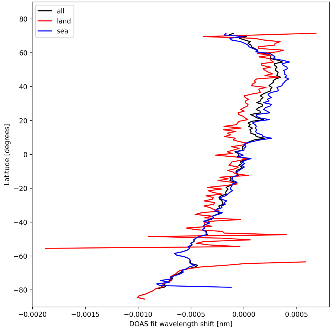
Figure 30: Zonal average of "DOAS fit wavelength shift" for 2024-10-29 to 2024-10-30.
