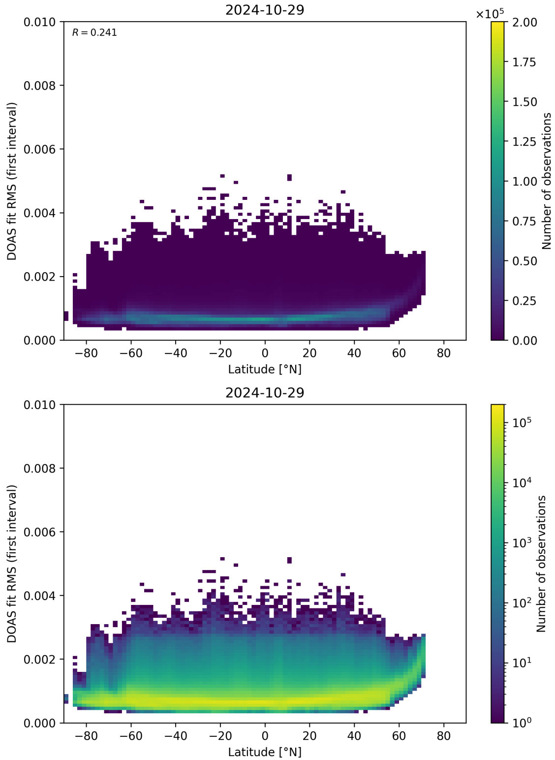
Figure 153: Scatter density plot of “Latitude” against “DOAS fit RMS (first interval)” for 2024-10-29 to 2024-10-30.
