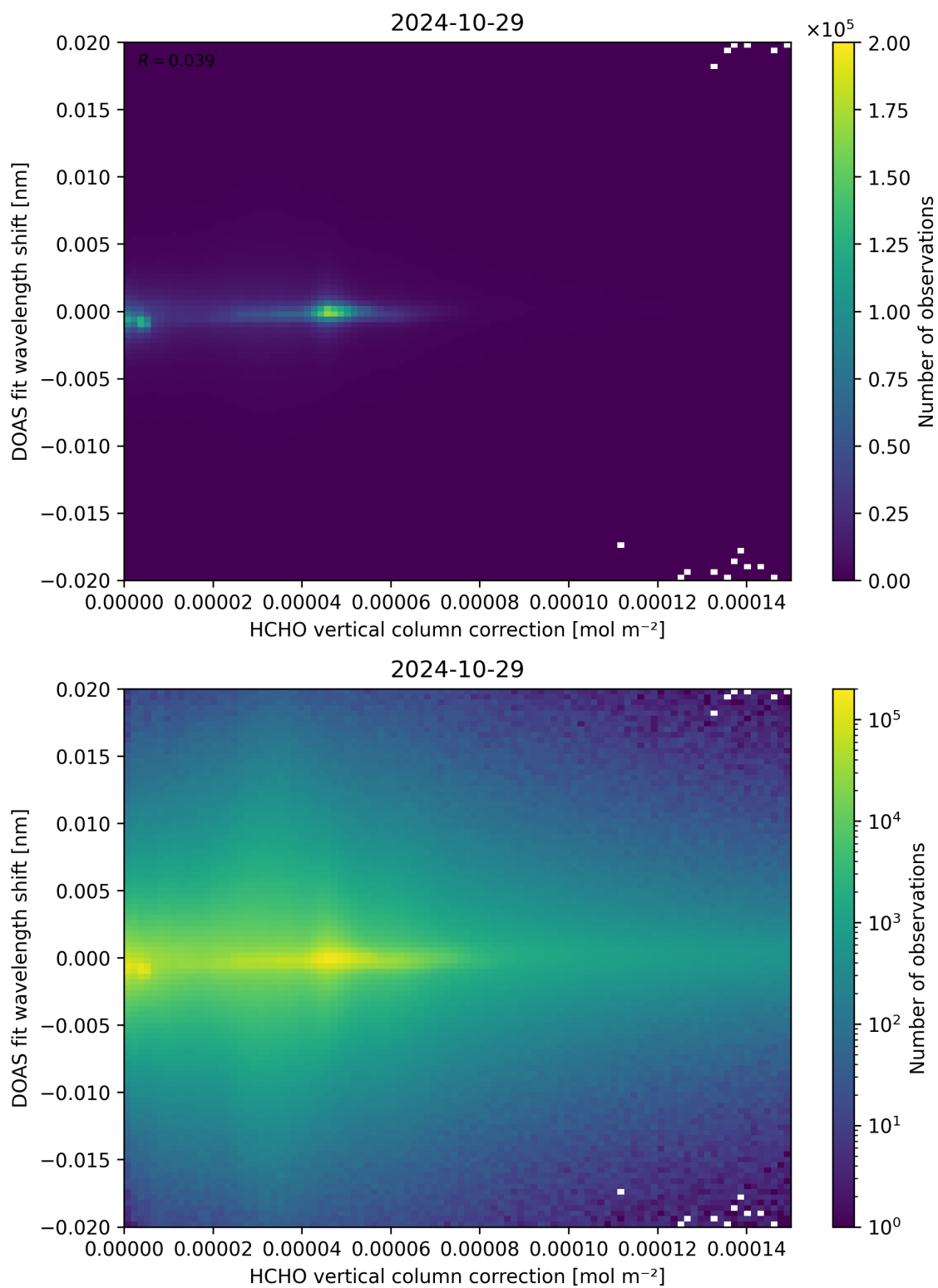
Figure 113: Scatter density plot of “HCHO vertical column correction” against “DOAS fit wavelength shift” for 2024-10-29 to 2024-10-30.
