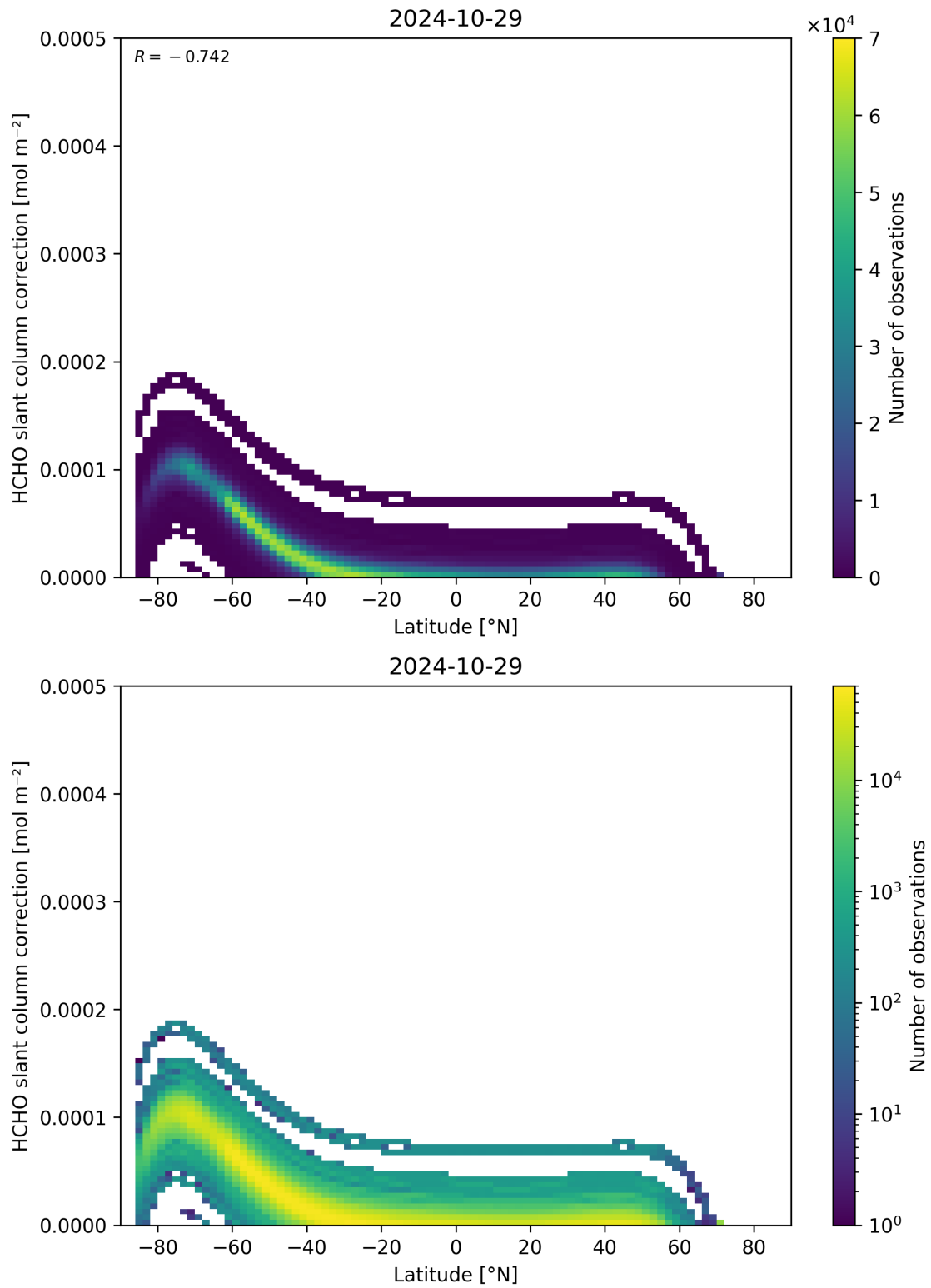
Figure 158: Scatter density plot of “Latitude” against “HCHO slant column correction” for 2024-10-29 to 2024-10-30.
