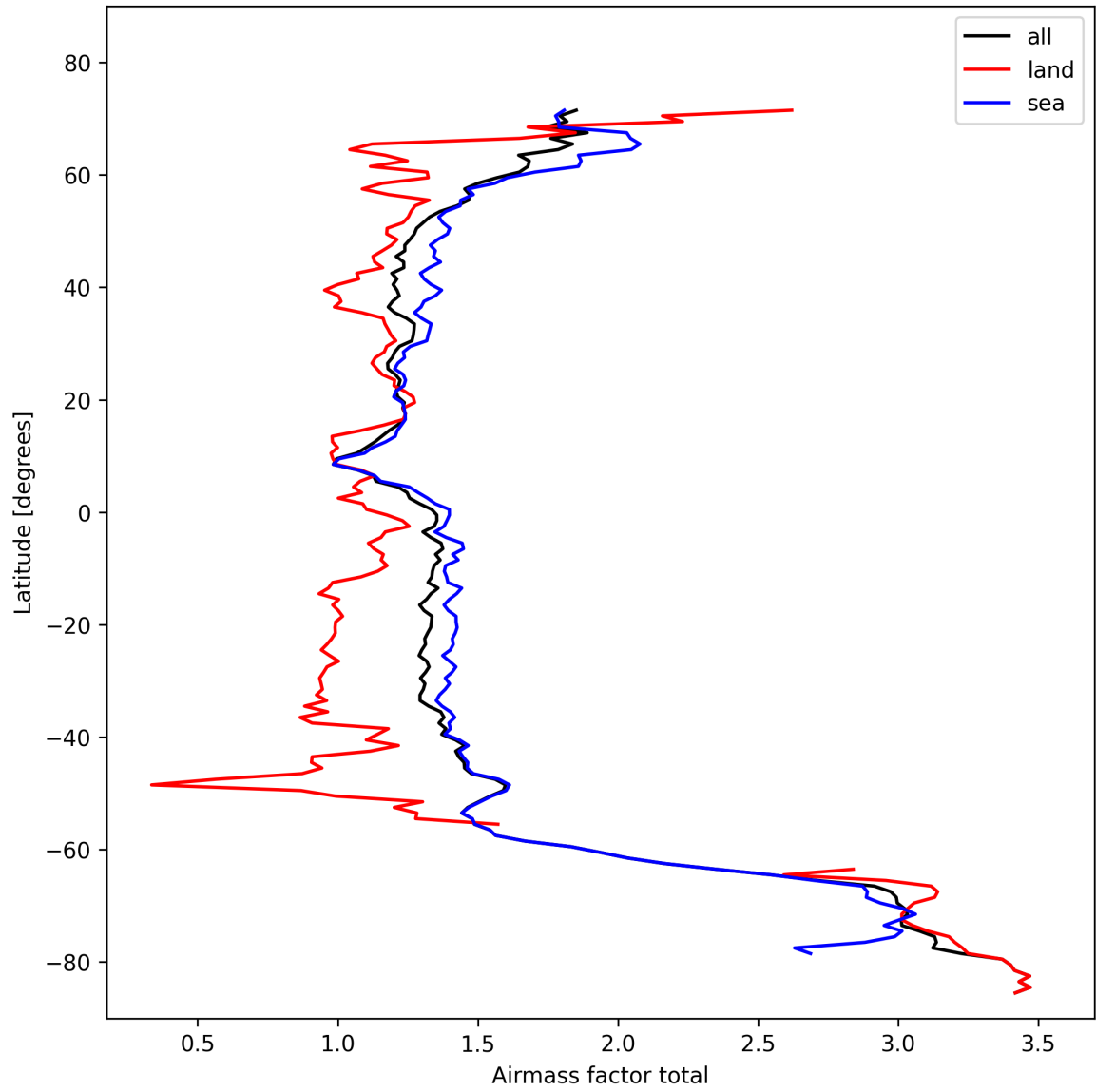
Figure 26: Zonal average of “Airmass factor total” for 2024-10-29 to 2024-10-30.
