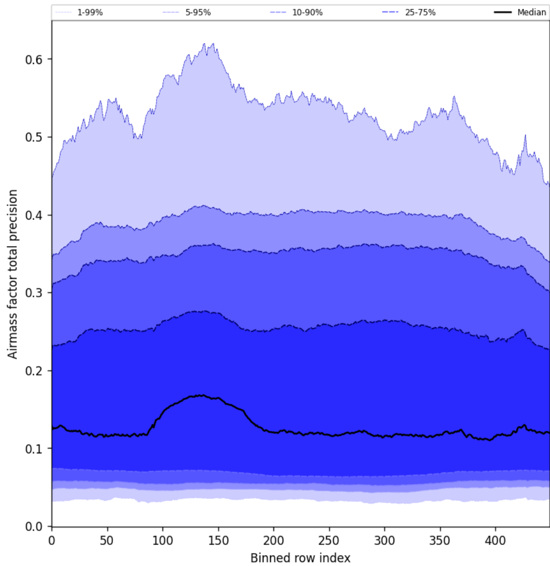
Figure 55: Along track statistics of “Airmass factor total precision” for 2024-10-29 to 2024-10-30
