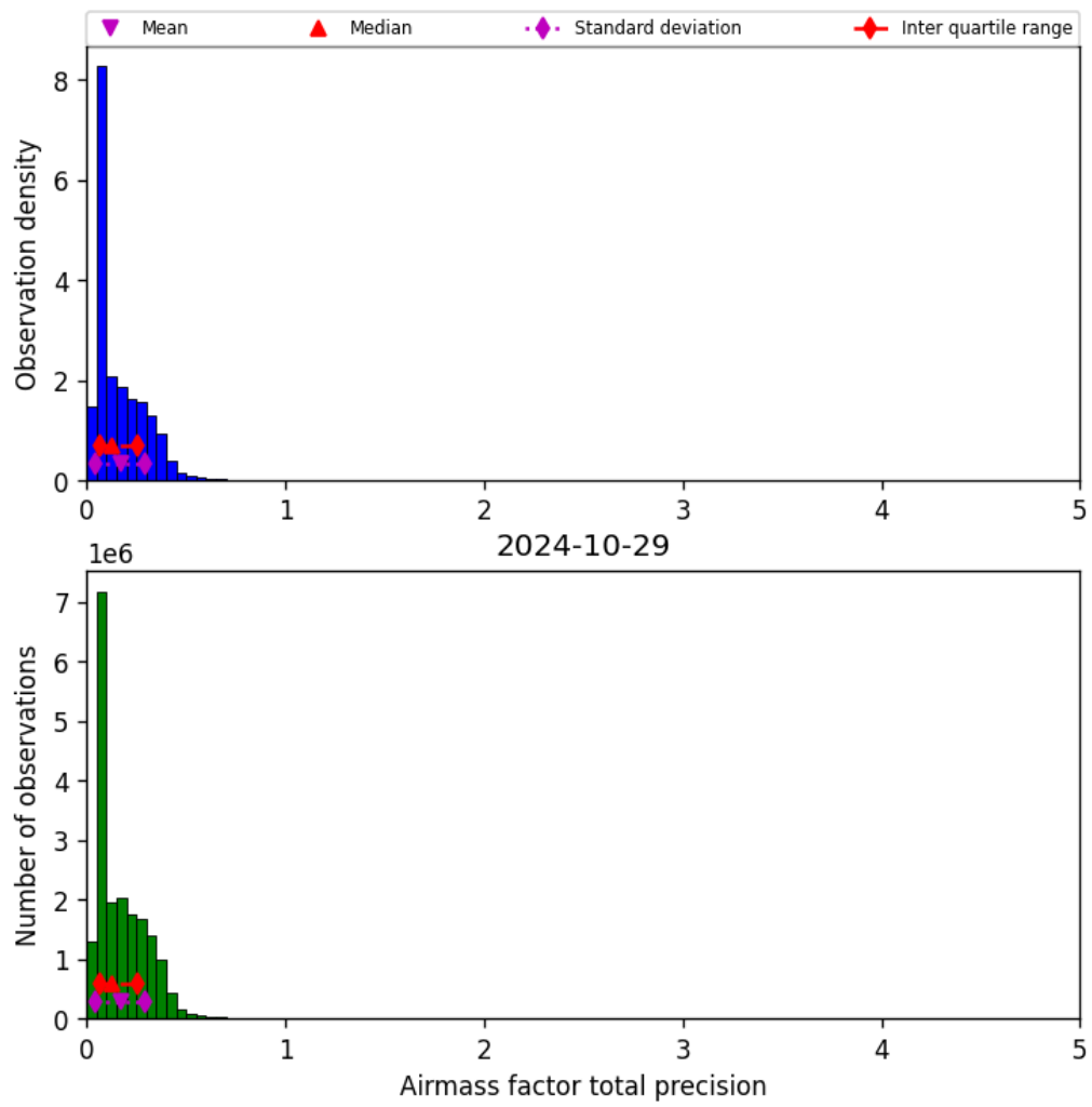
Figure 41: Histogram of “Airmass factor total precision” for 2024-10-29 to 2024-10-30
