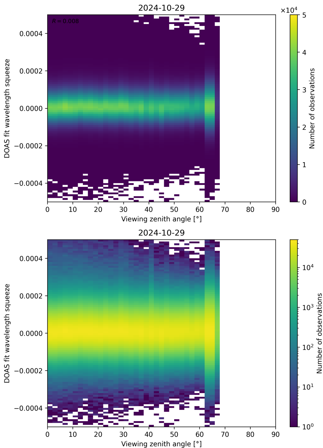
Figure 184: Scatter density plot of “Viewing zenith angle” against “DOAS fit wavelength squeeze” for 2024-10-29 to 2024-10-30.
