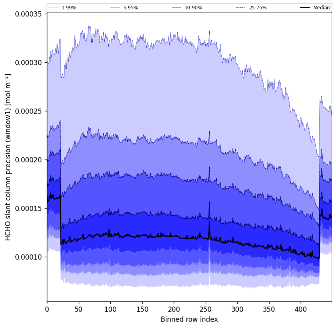
Figure 53: Along track statistics of “HCHO slant column precision (window1)” for 2024-10-29 to 2024-10-30
