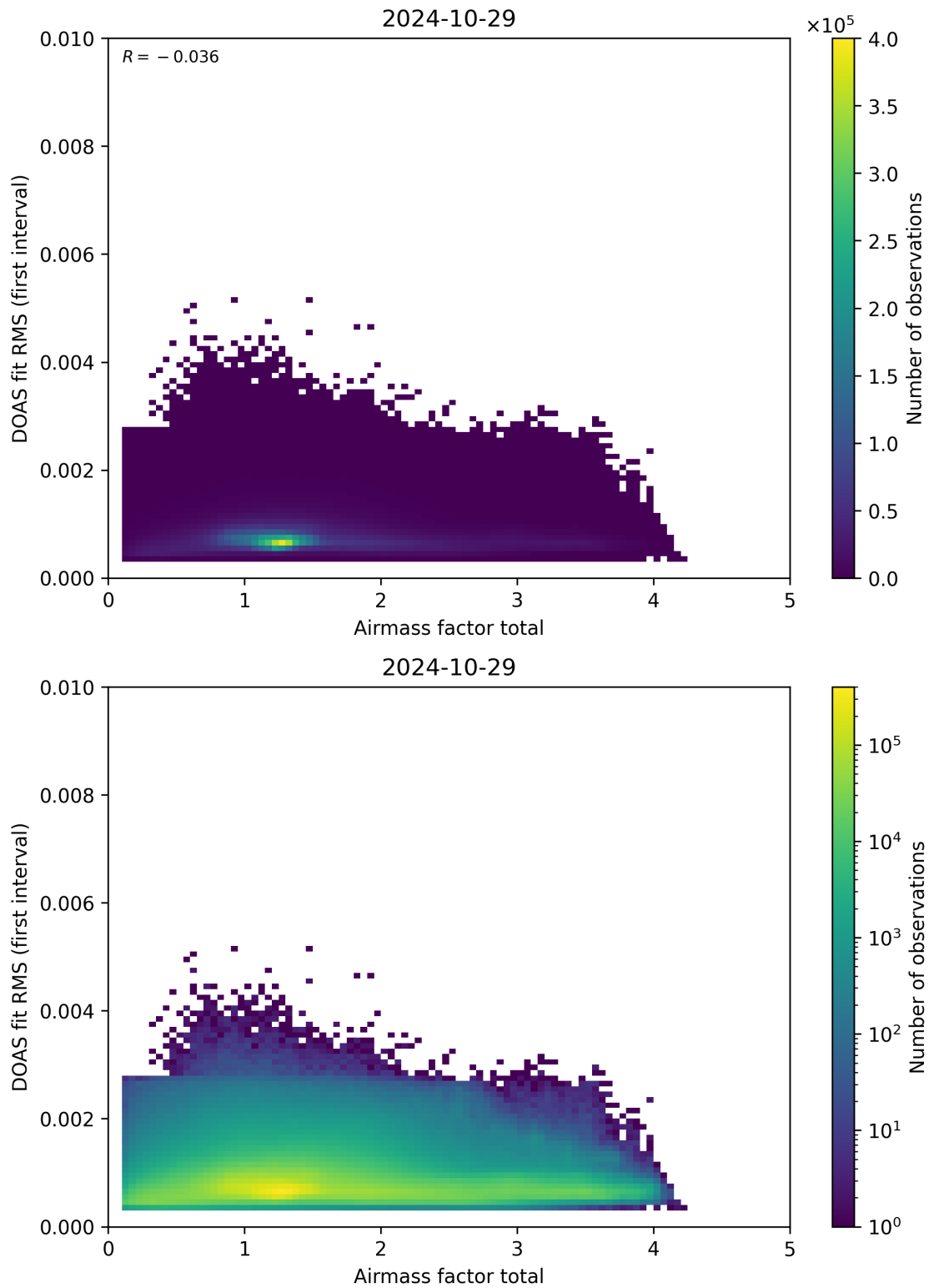
Figure 97: Scatter density plot of “Airmass factor total” against “DOAS fit RMS (first interval)” for 2024-10-29 to 2024-10-30.
