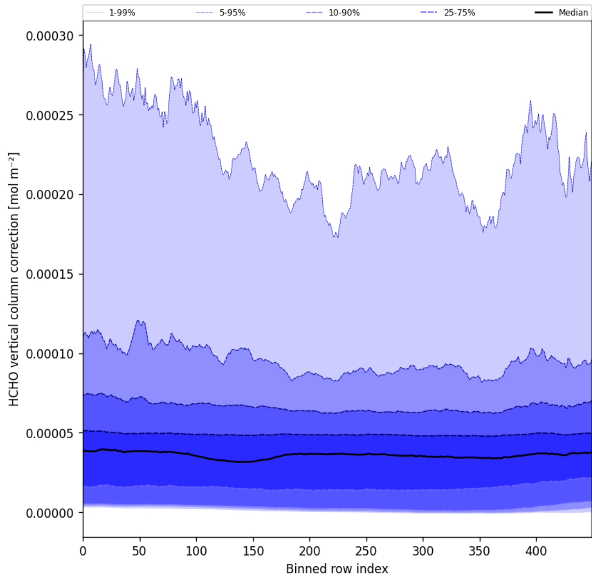
Figure 51: Along track statistics of “HCHO vertical column correction” for 2024-10-29 to 2024-10-30
