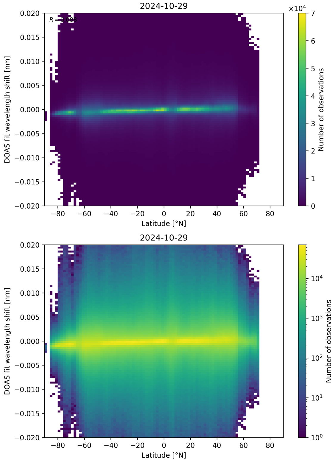
Figure 154: Scatter density plot of “Latitude” against “DOAS fit wavelength shift” for 2024-10-29 to 2024-10-30.
