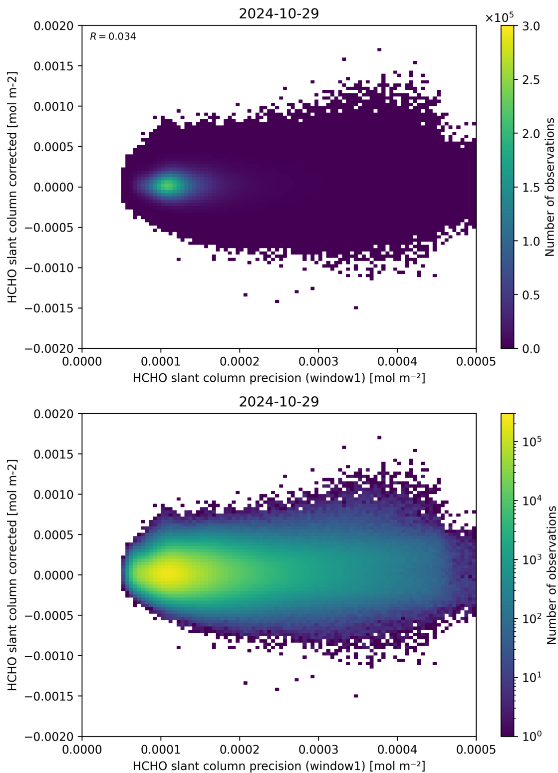
Figure 92: Scatter density plot of “HCHO slant column precision (window1)” against “HCHO slant column corrected” for 2024-10-29 to 2024-10-30.
