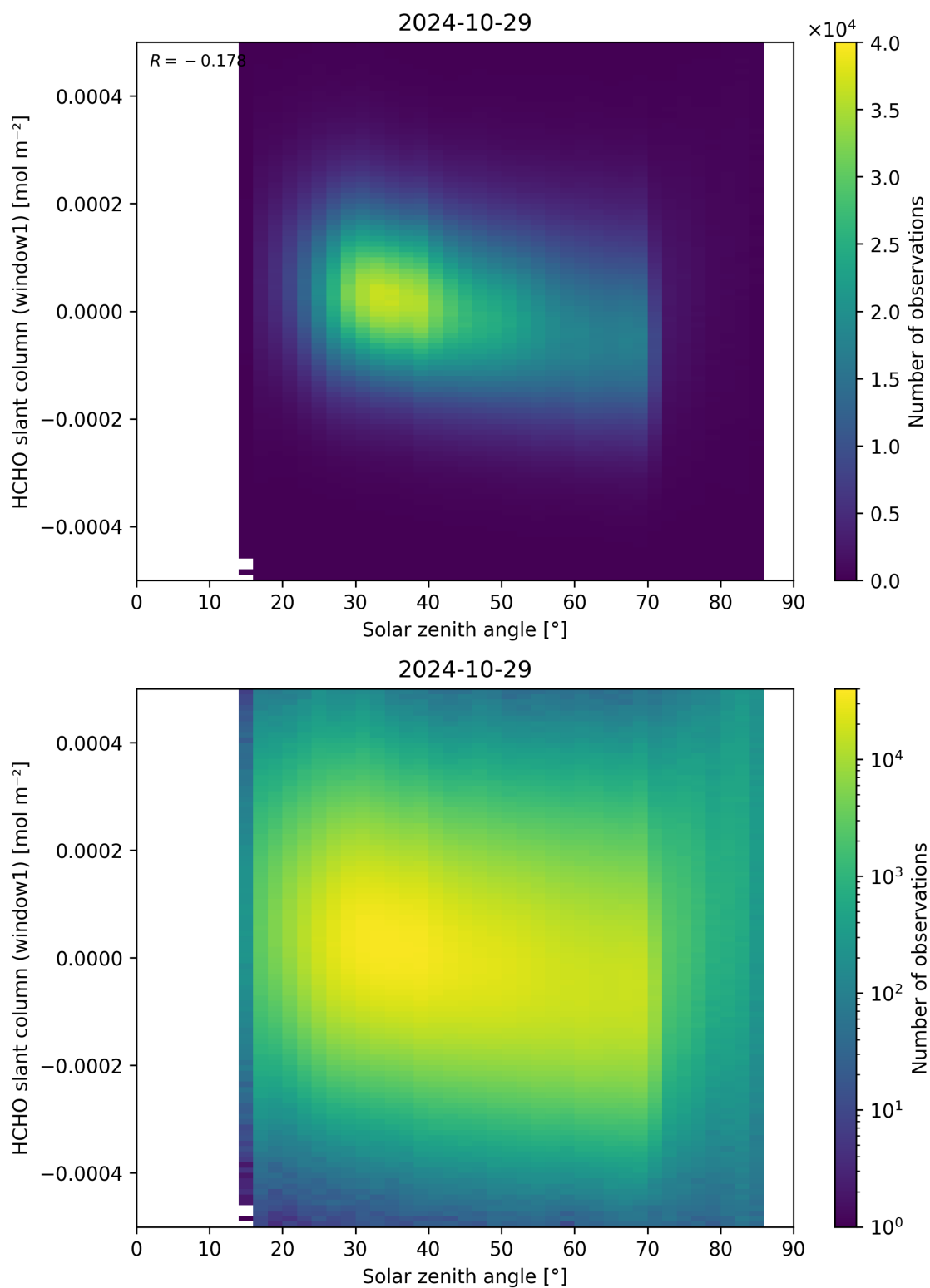
Figure 173: Scatter density plot of “Solar zenith angle” against “HCHO slant column (window1)” for 2024-10-29 to 2024-10-30.
