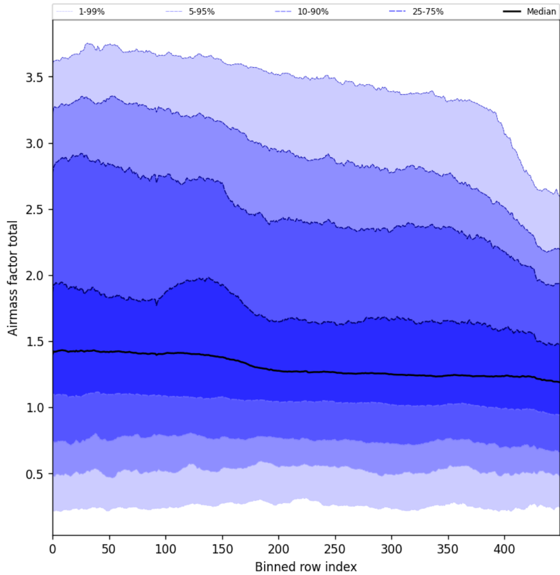
Figure 54: Along track statistics of “Airmass factor total” for 2024-10-29 to 2024-10-30
