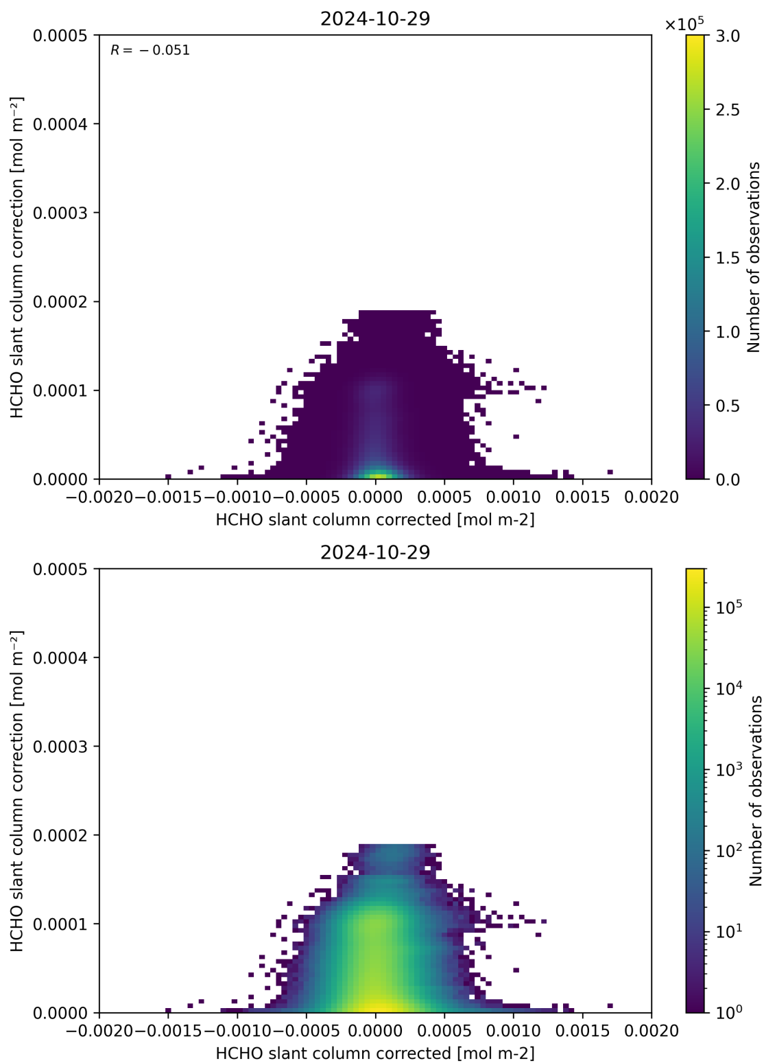
Figure 77: Scatter density plot of “HCHO slant column corrected” against “HCHO slant column correction” for 2024-10-29 to 2024-10-30.
