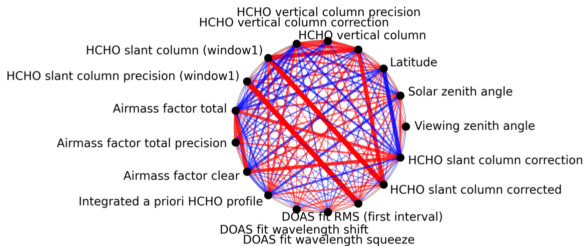
Figure 1: Map of correlation graph for 2024-10-29 to 2024-10-30.
