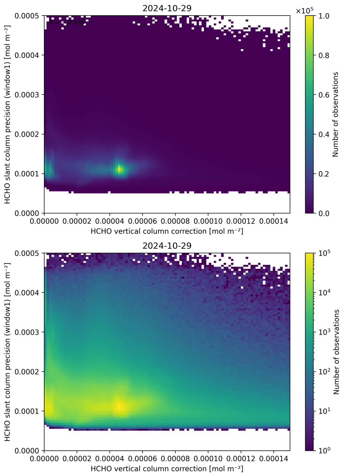
Figure 119: Scatter density plot of “HCHO vertical column correction” against “HCHO slant column precision (window1)” for 2024-10-29 to 2024-10-30.
