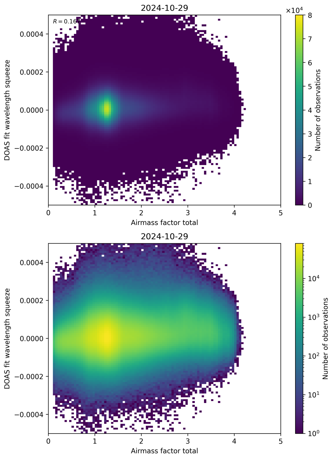
Figure 99: Scatter density plot of “Airmass factor total” against “DOAS fit wavelength squeeze” for 2024-10-29 to 2024-10-30.
