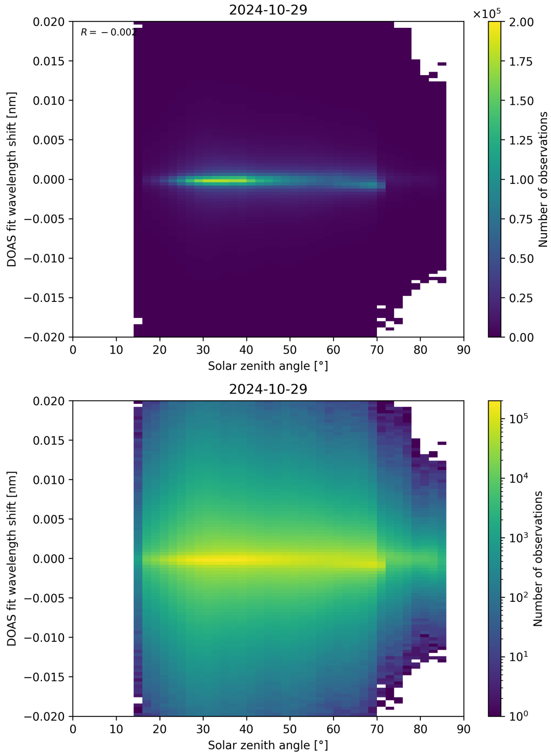
Figure 168: Scatter density plot of “Solar zenith angle” against “DOAS fit wavelength shift” for 2024-10-29 to 2024-10-30.
