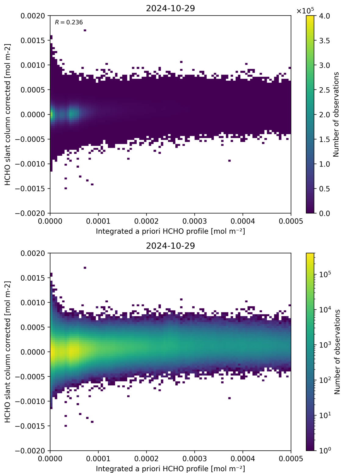
Figure 151: Scatter density plot of “Integrated a priori HCHO profile” against “HCHO slant column corrected” for 2024-10-29 to 2024-10-30.
