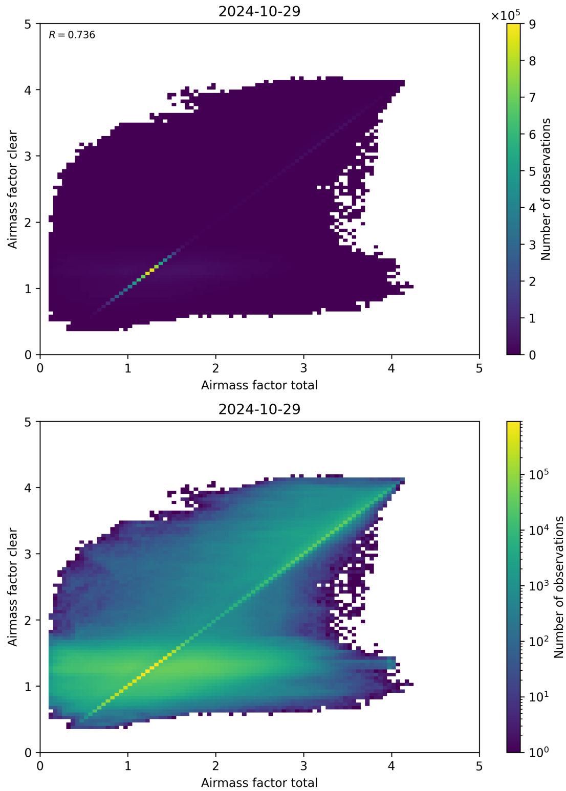
Figure 100: Scatter density plot of “Airmass factor total” against “Airmass factor clear” for 2024-10-29 to 2024-10-30.
