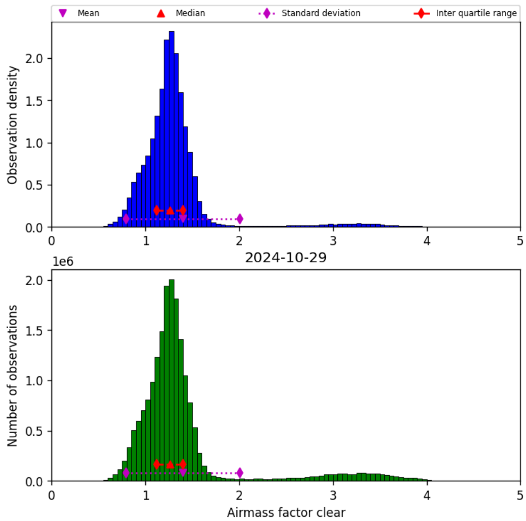
Figure 42: Histogram of “Airmass factor clear” for 2024-10-29 to 2024-10-30
