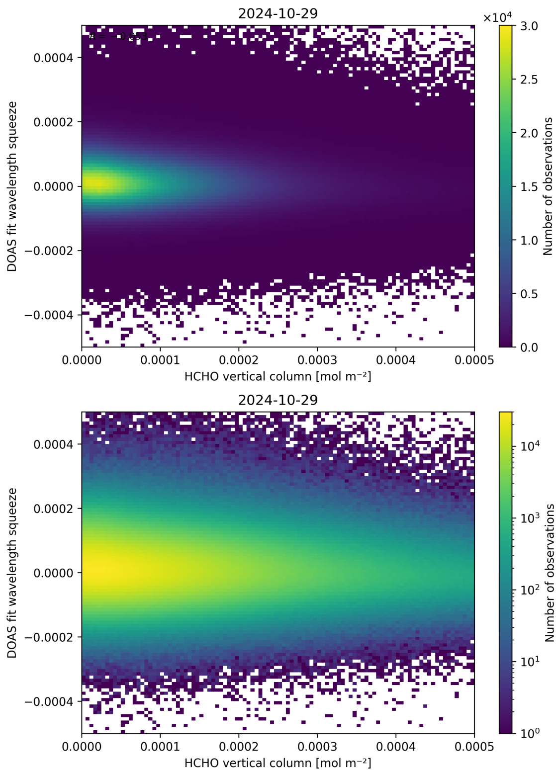
Figure 125: Scatter density plot of “HCHO vertical column” against “DOAS fit wavelength squeeze” for 2024-10-29 to 2024-10-30.
