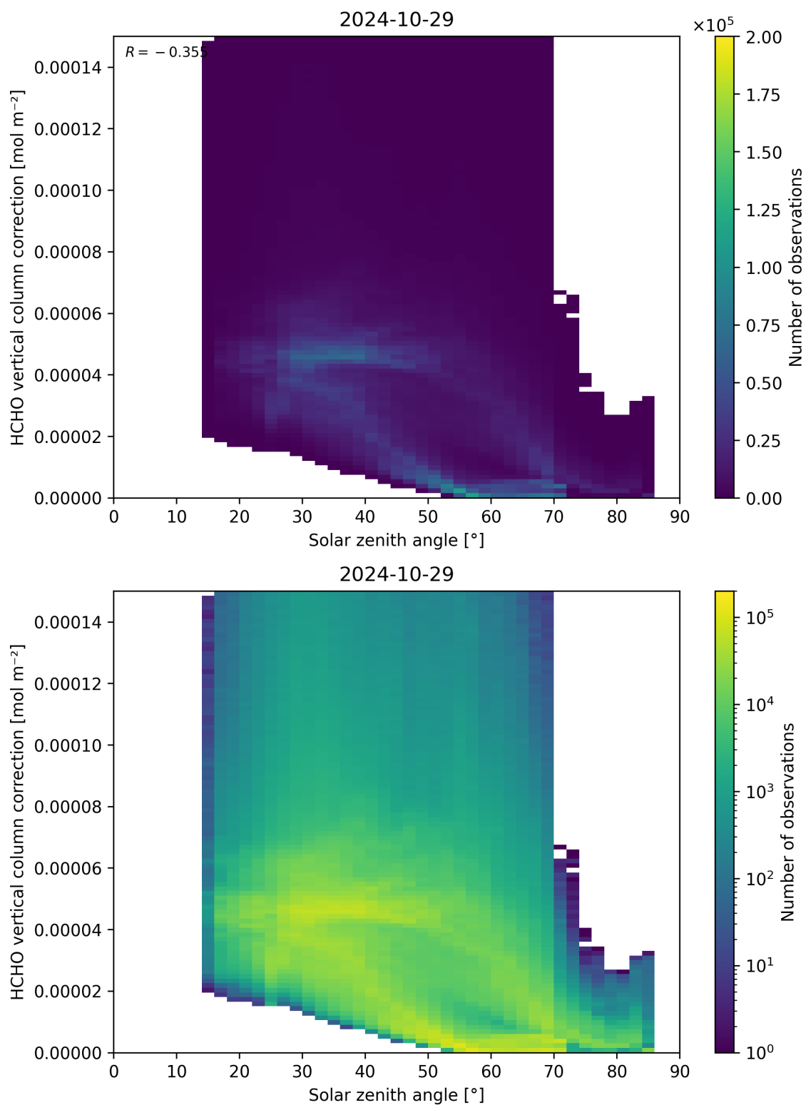
Figure 178: Scatter density plot of “Solar zenith angle” against “HCHO vertical column correction” for 2024-10-29 to 2024-10-30.
