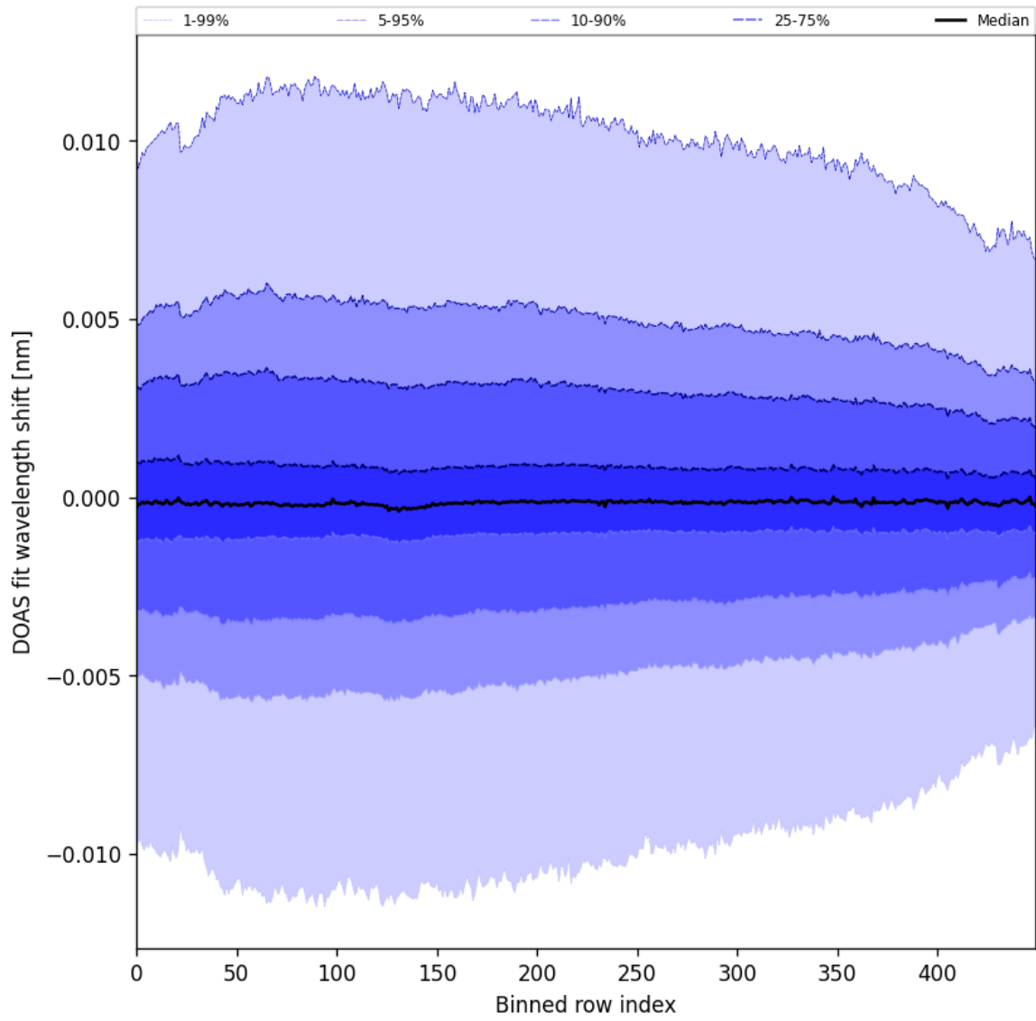
Figure 58: Along track statistics of “DOAS fit wavelength shift” for 2024-10-30 to 2024-10-31
