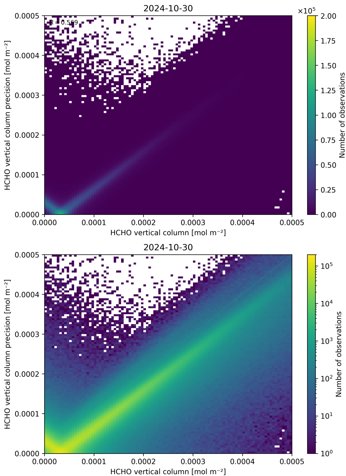
Figure 134: Scatter density plot of “HCHO vertical column” against “HCHO vertical column precision” for 2024-10-30 to 2024-10-31.
