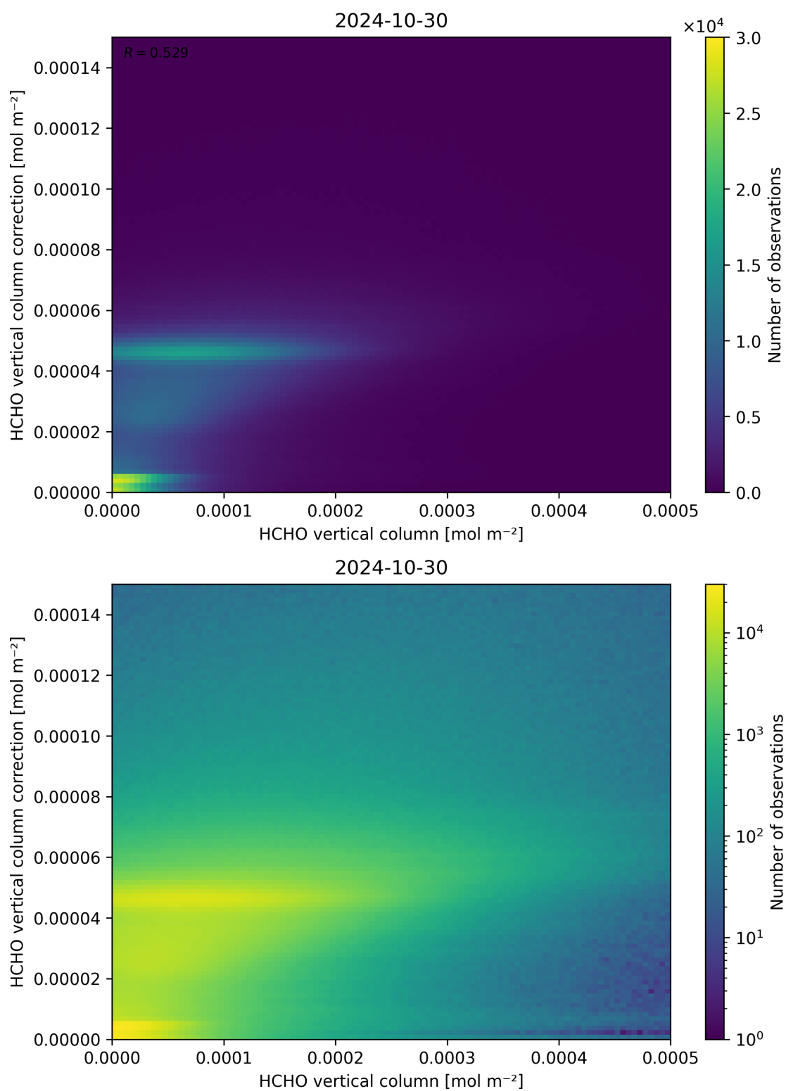
Figure 133: Scatter density plot of “HCHO vertical column” against “HCHO vertical column correction” for 2024-10-30 to 2024-10-31.
