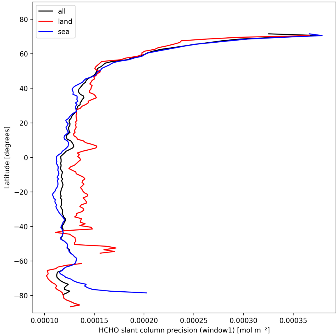
Figure 25: Zonal average of "HCHO slant column precision (window1)" for 2024-10-30 to 2024-10-31.
