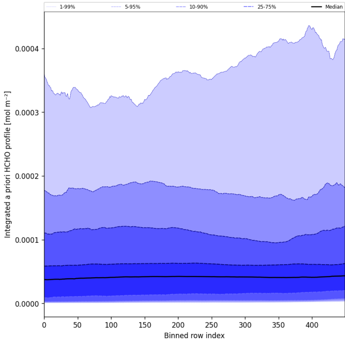
Figure 57: Along track statistics of "Integrated a priori HCHO profile" for 2024-10-30 to 2024-10-31
