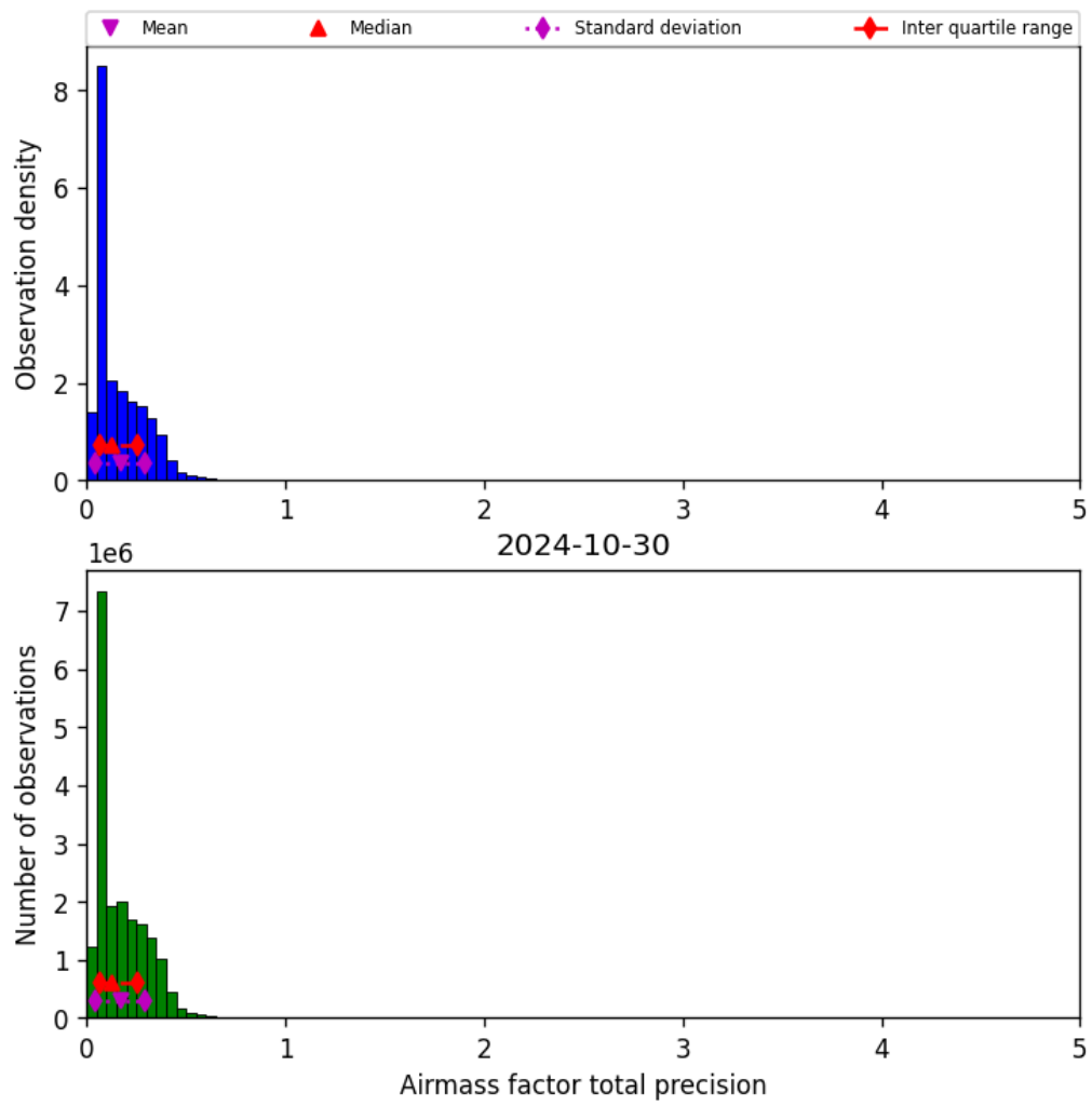
Figure 41: Histogram of “Airmass factor total precision” for 2024-10-30 to 2024-10-31
