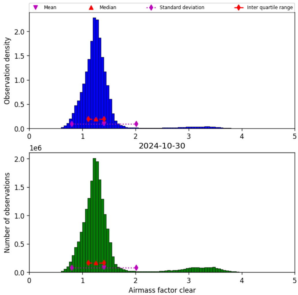
Figure 42: Histogram of “Airmass factor clear” for 2024-10-30 to 2024-10-31
