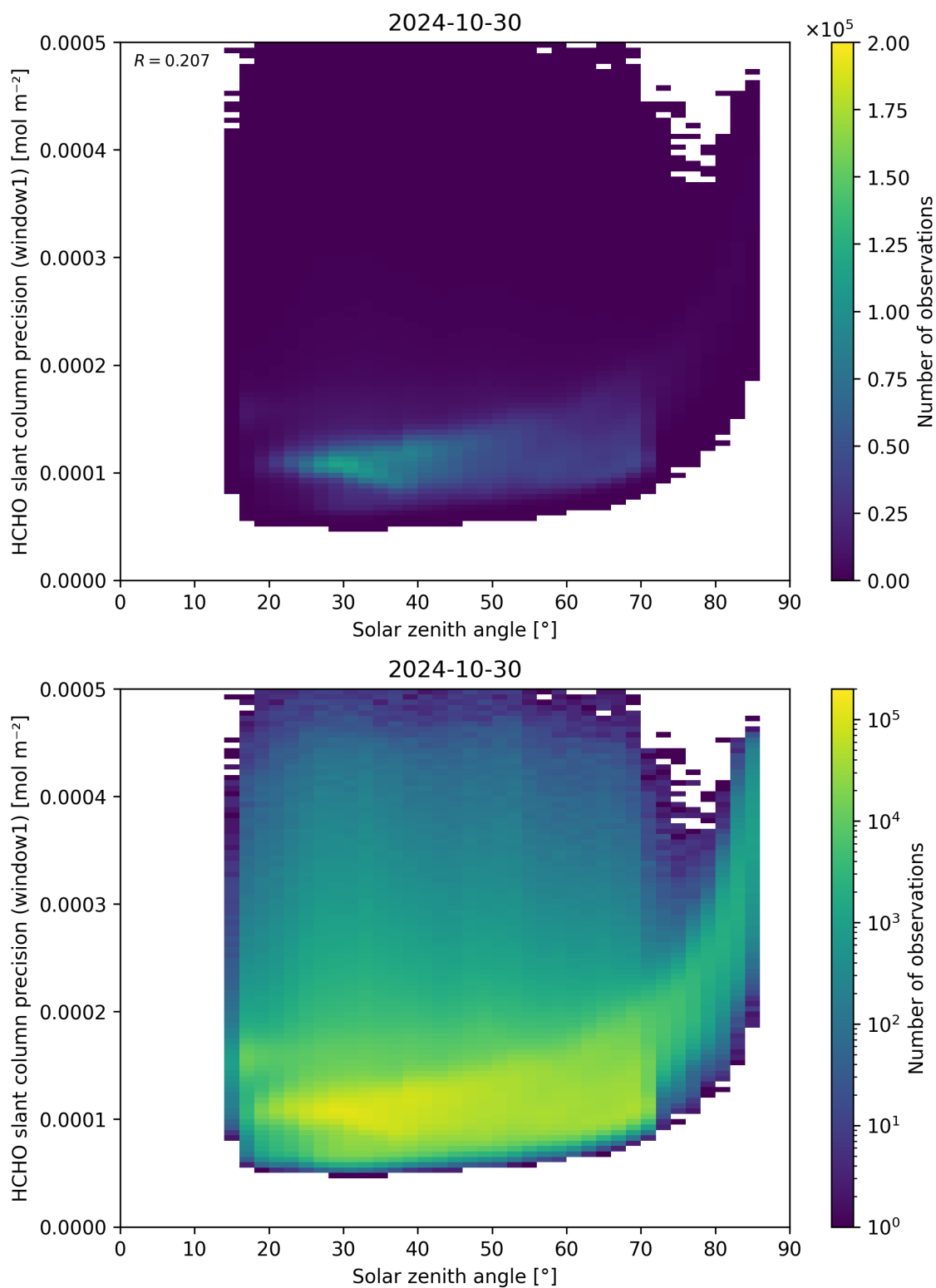
Figure 174: Scatter density plot of “Solar zenith angle” against “HCHO slant column precision (window1)” for 2024-10-30 to 2024-10-31.
