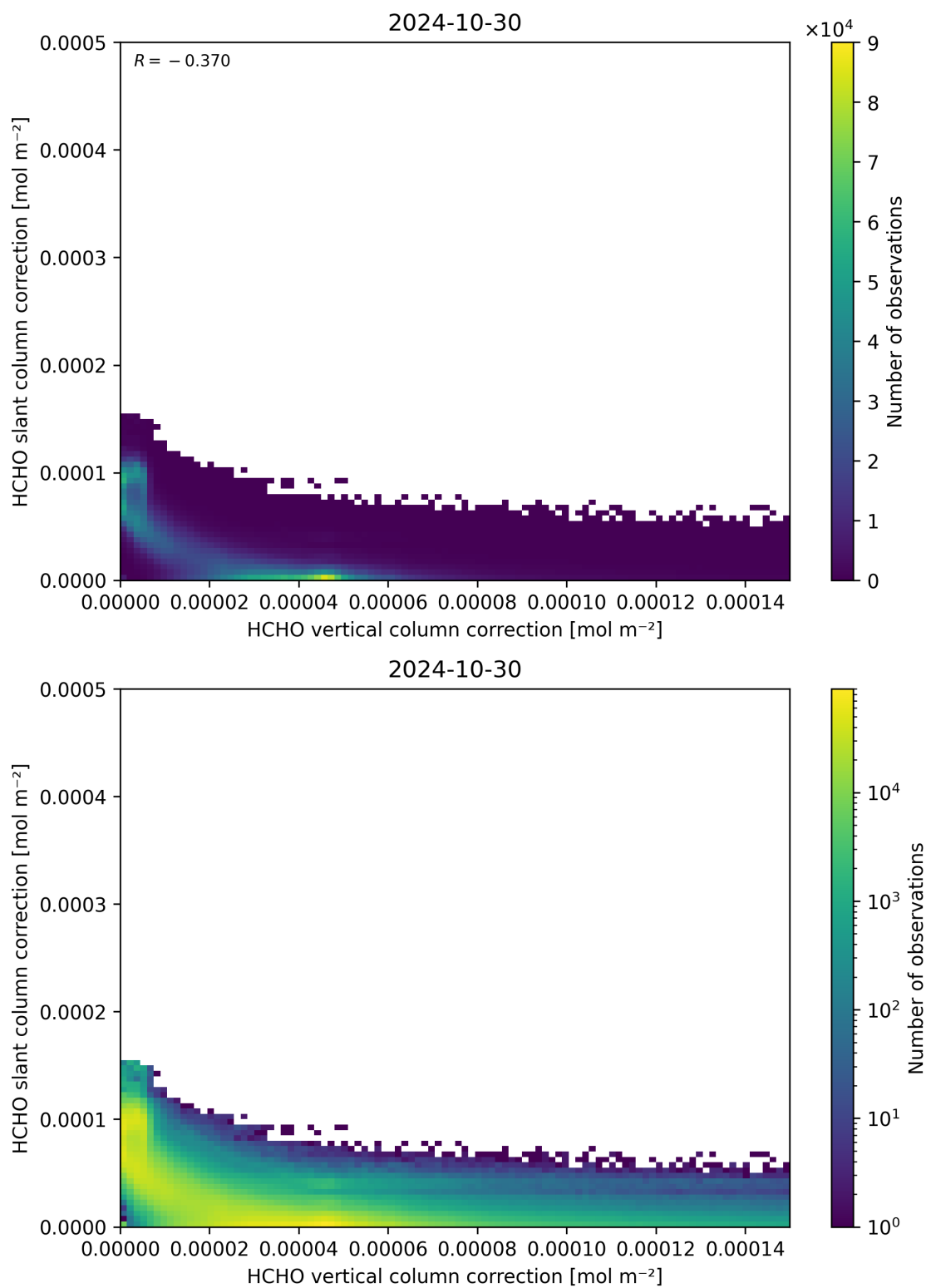
Figure 117: Scatter density plot of “HCHO vertical column correction” against “HCHO slant column correction” for 2024-10-30 to 2024-10-31.
