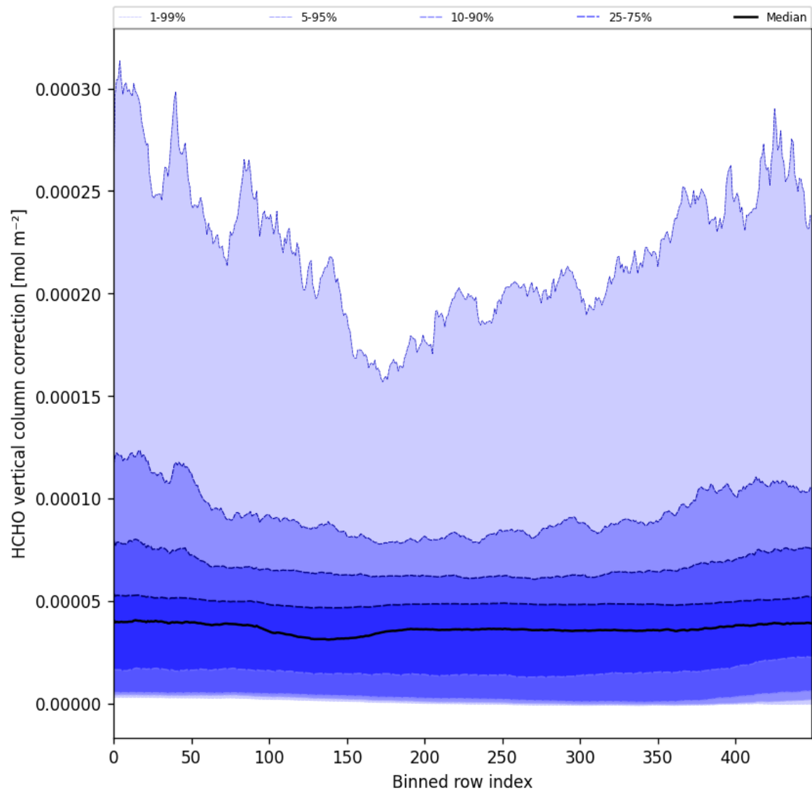
Figure 51: Along track statistics of “HCHO vertical column correction” for 2024-10-30 to 2024-10-31
