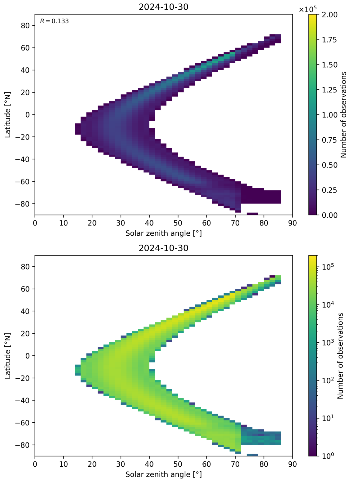
Figure 181: Scatter density plot of “Solar zenith angle” against “Latitude” for 2024-10-30 to 2024-10-31.
