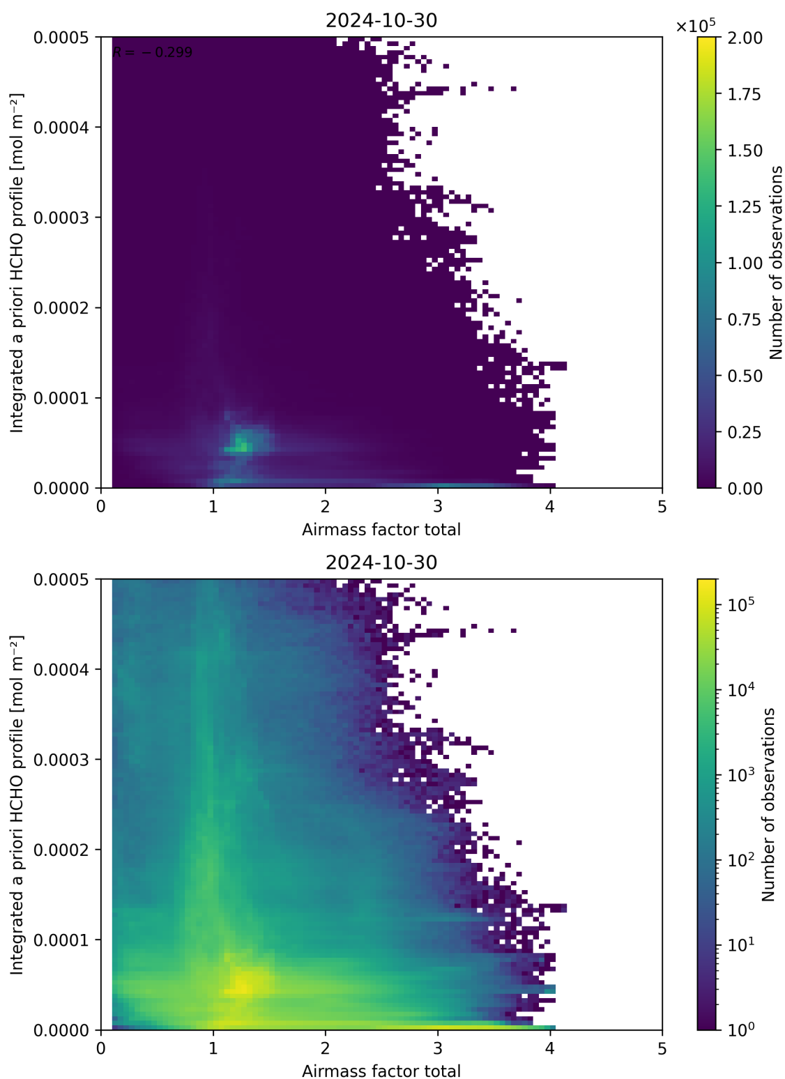
Figure 104: Scatter density plot of “Airmass factor total” against “Integrated a priori HCHO profile” for 2024-10-30 to 2024-10-31.
