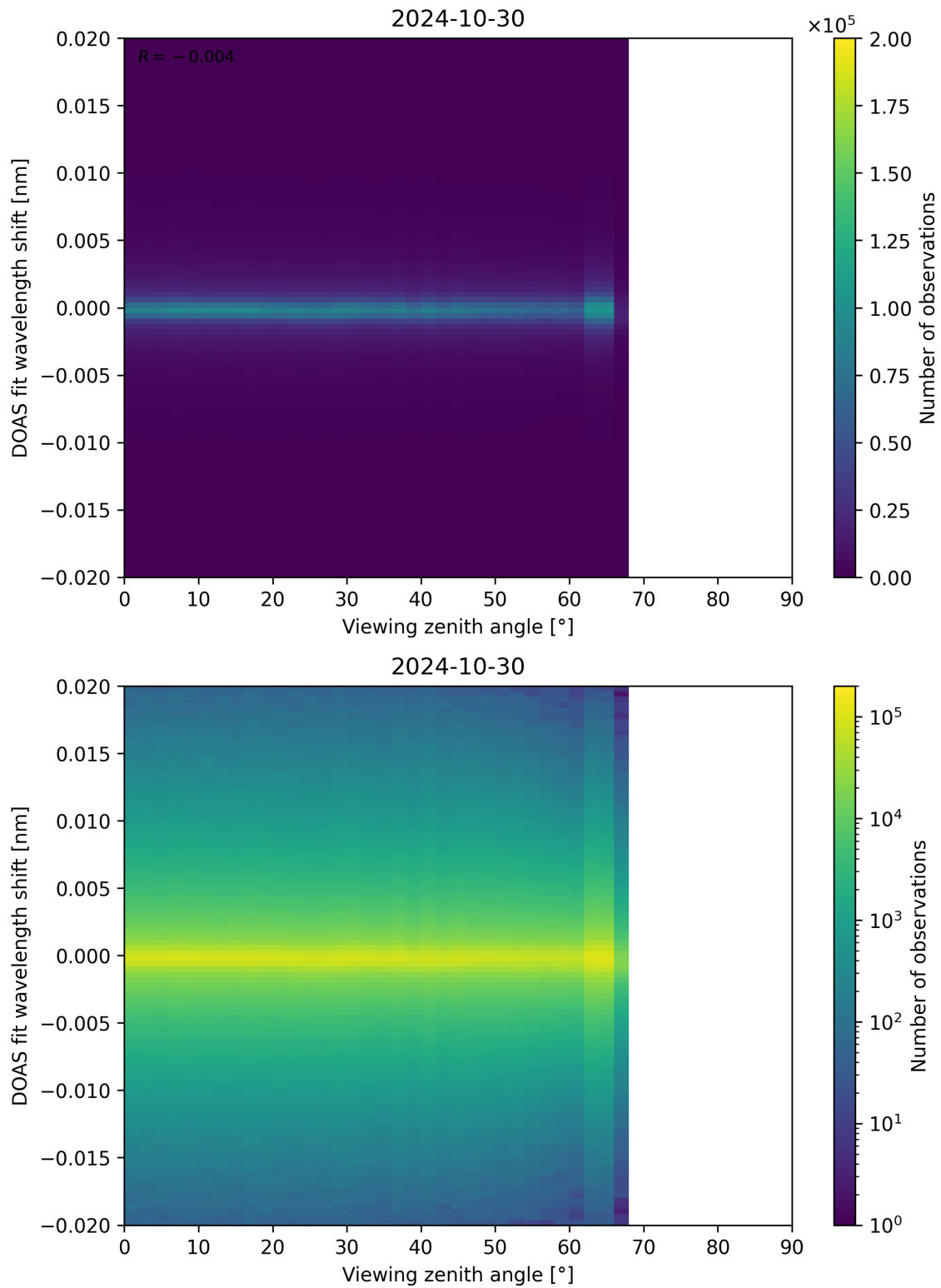
Figure 183: Scatter density plot of “Viewing zenith angle” against “DOAS fit wavelength shift” for 2024-10-30 to 2024-10-31.
