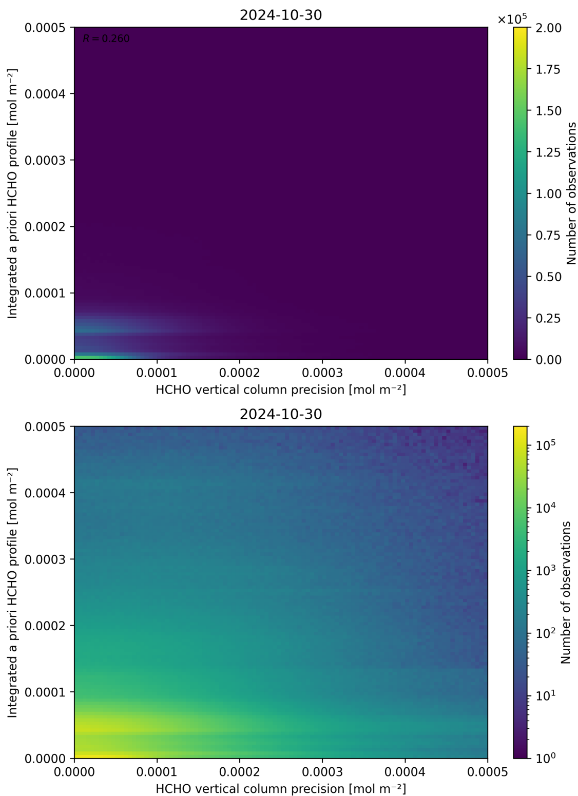
Figure 147: Scatter density plot of “HCHO vertical column precision” against “Integrated a priori HCHO profile” for 2024-10-30 to 2024-10-31.
