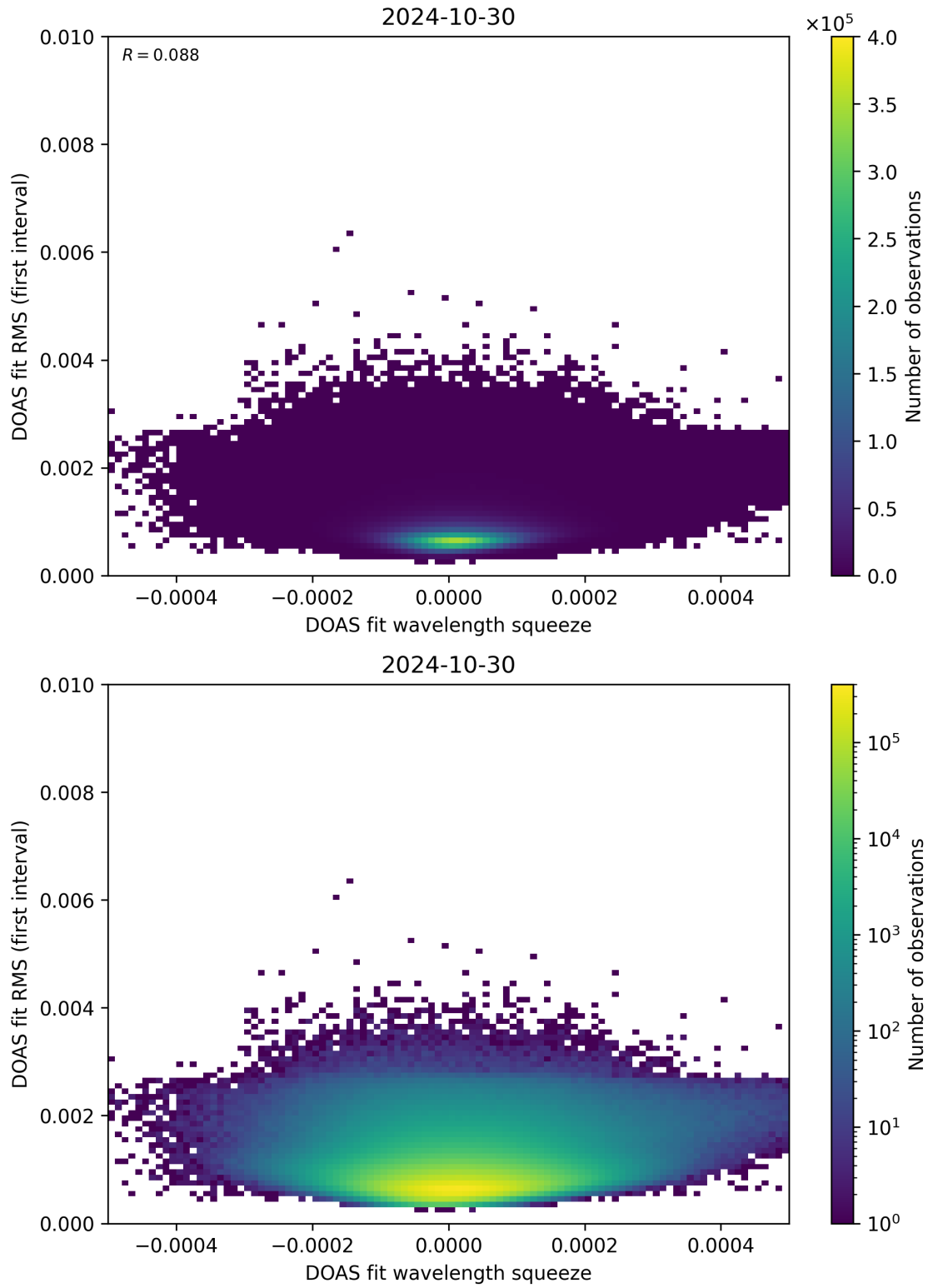
Figure 68: Scatter density plot of “DOAS fit wavelength squeeze” against “DOAS fit RMS (first interval)” for 2024-10-30 to 2024-10-31.
