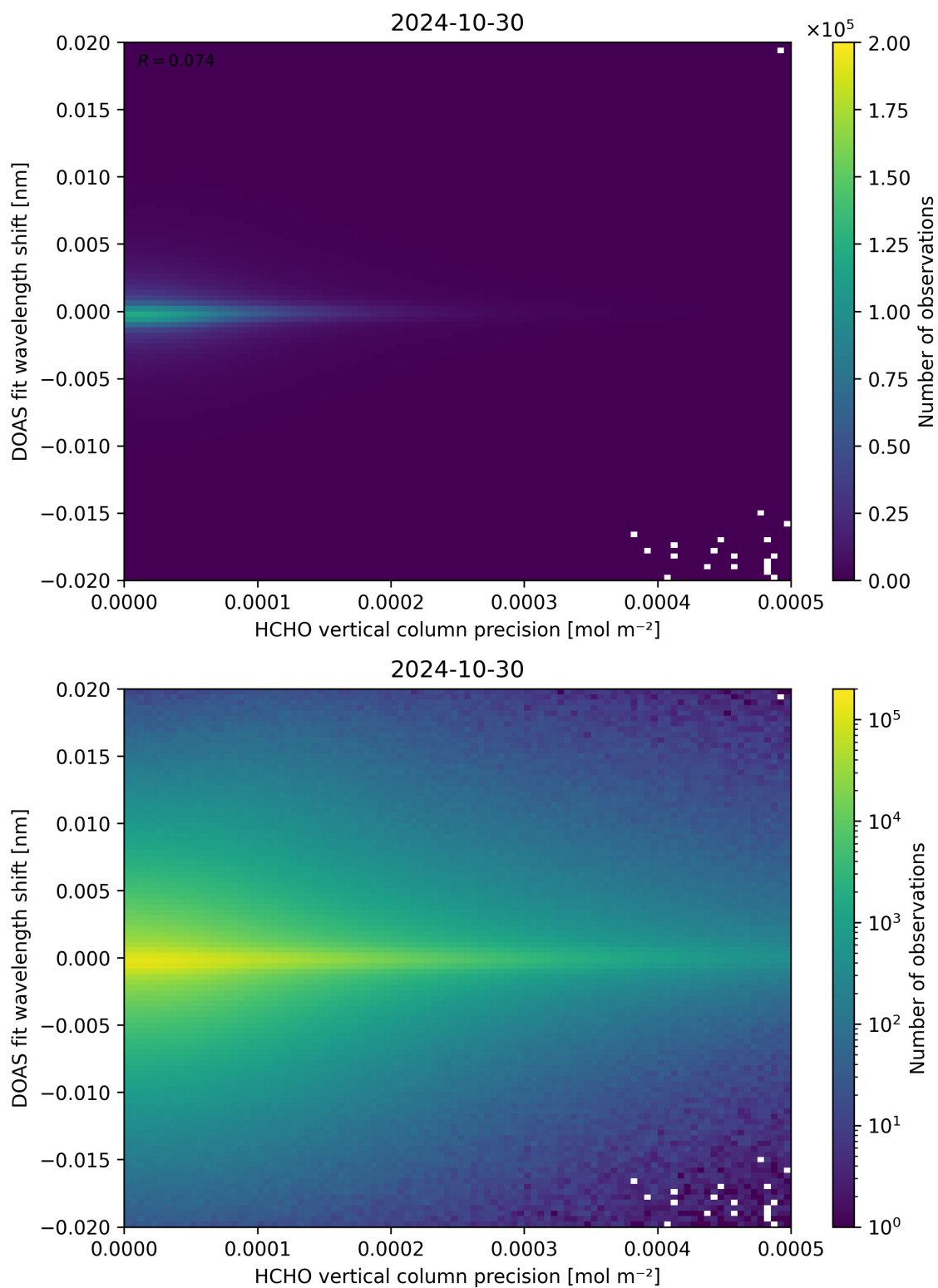
Figure 137: Scatter density plot of “HCHO vertical column precision” against “DOAS fit wavelength shift” for 2024-10-30 to 2024-10-31.
