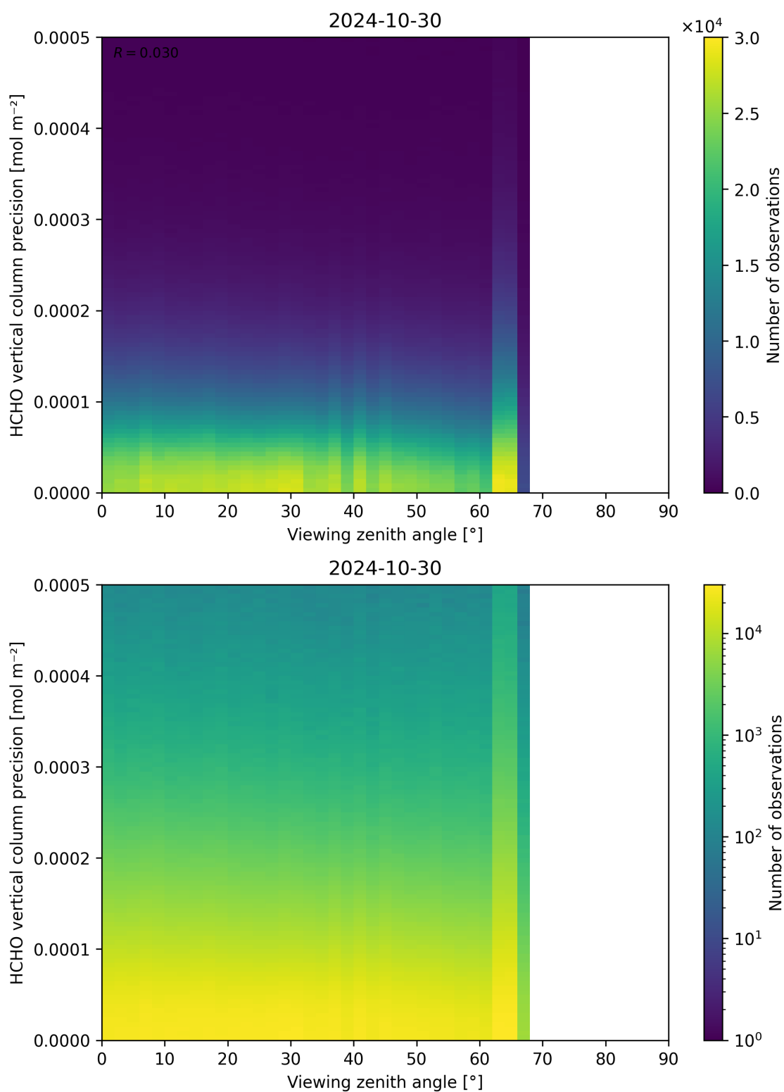
Figure 194: Scatter density plot of “Viewing zenith angle” against “HCHO vertical column precision” for 2024-10-30 to 2024-10-31.
