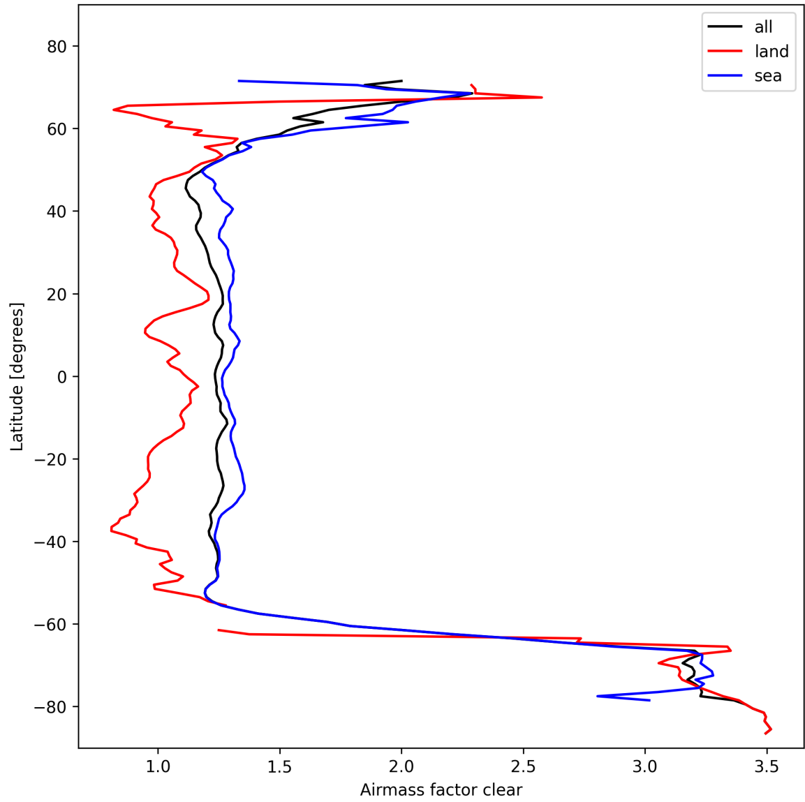
Figure 28: Zonal average of “Airmass factor clear” for 2024-10-30 to 2024-10-31.
