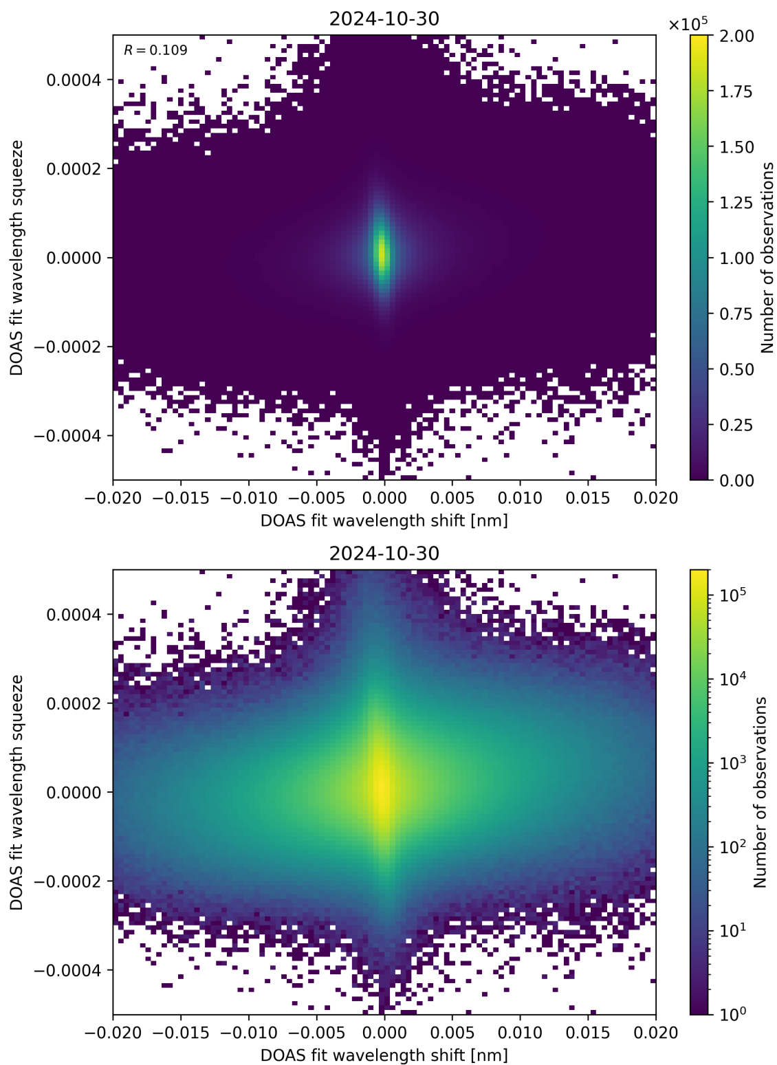
Figure 65: Scatter density plot of “DOAS fit wavelength shift” against “DOAS fit wavelength squeeze” for 2024-10-30 to 2024-10-31.
