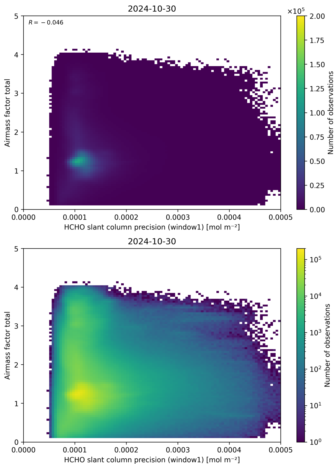
Figure 94: Scatter density plot of “HCHO slant column precision (window1)” against “Airmass factor total” for 2024-10-30 to 2024-10-31.
