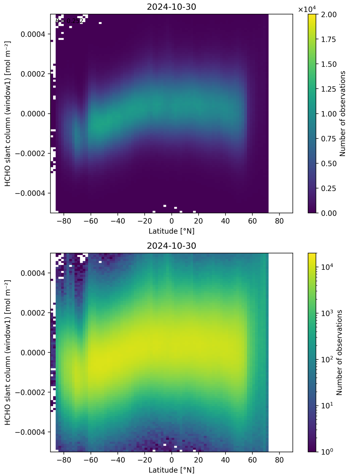
Figure 159: Scatter density plot of “Latitude” against “HCHO slant column (window1)” for 2024-10-30 to 2024-10-31.
