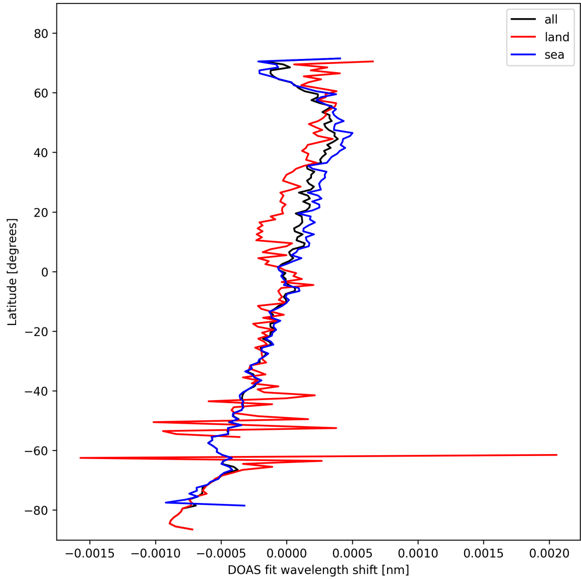
Figure 30: Zonal average of "DOAS fit wavelength shift" for 2024-10-30 to 2024-10-31.
