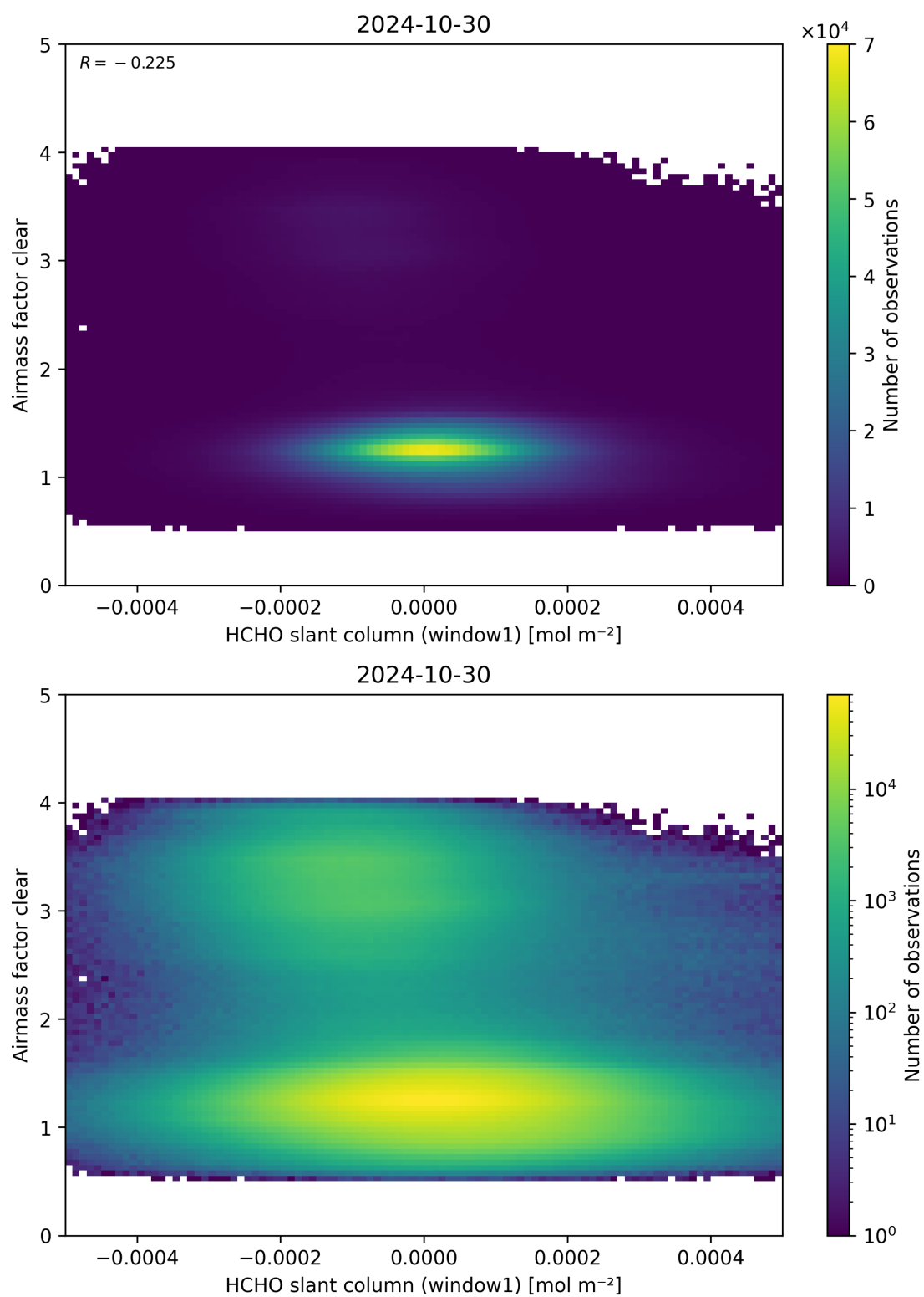
Figure 81: Scatter density plot of “HCHO slant column (window1)” against “Airmass factor clear” for 2024-10-30 to 2024-10-31.
