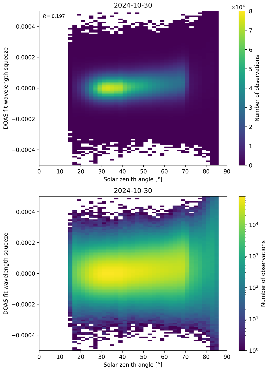
Figure 169: Scatter density plot of “Solar zenith angle” against “DOAS fit wavelength squeeze” for 2024-10-30 to 2024-10-31.
