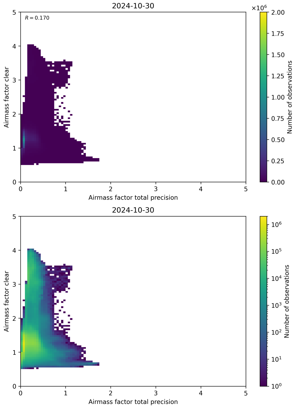
Figure 108: Scatter density plot of “Airmass factor total precision” against “Airmass factor clear” for 2024-10-30 to 2024-10-31.
