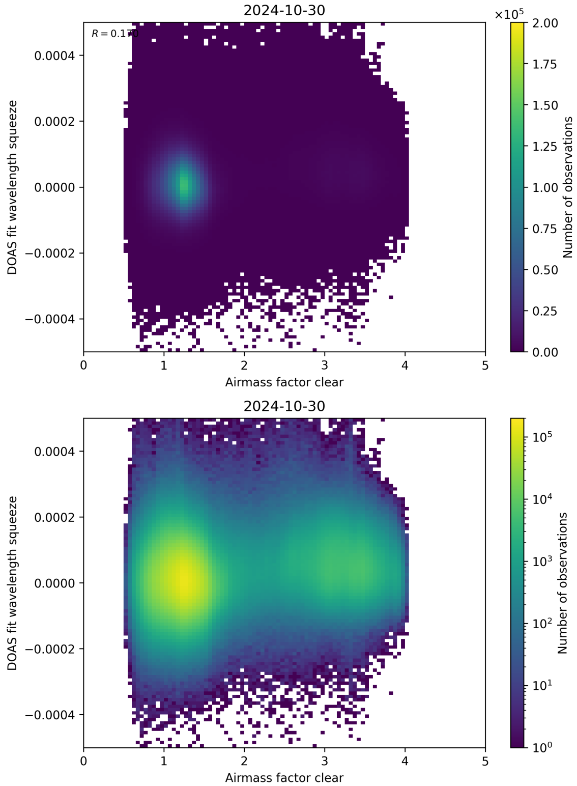
Figure 73: Scatter density plot of “Airmass factor clear” against “DOAS fit wavelength squeeze” for 2024-10-30 to 2024-10-31.
