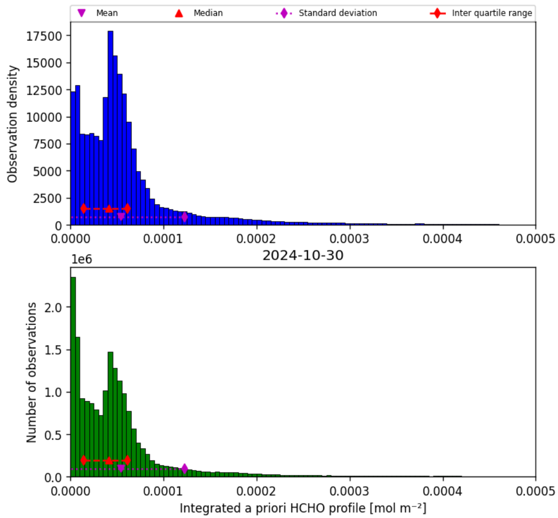
Figure 43: Histogram of “Integrated a priori HCHO profile” for 2024-10-30 to 2024-10-31
