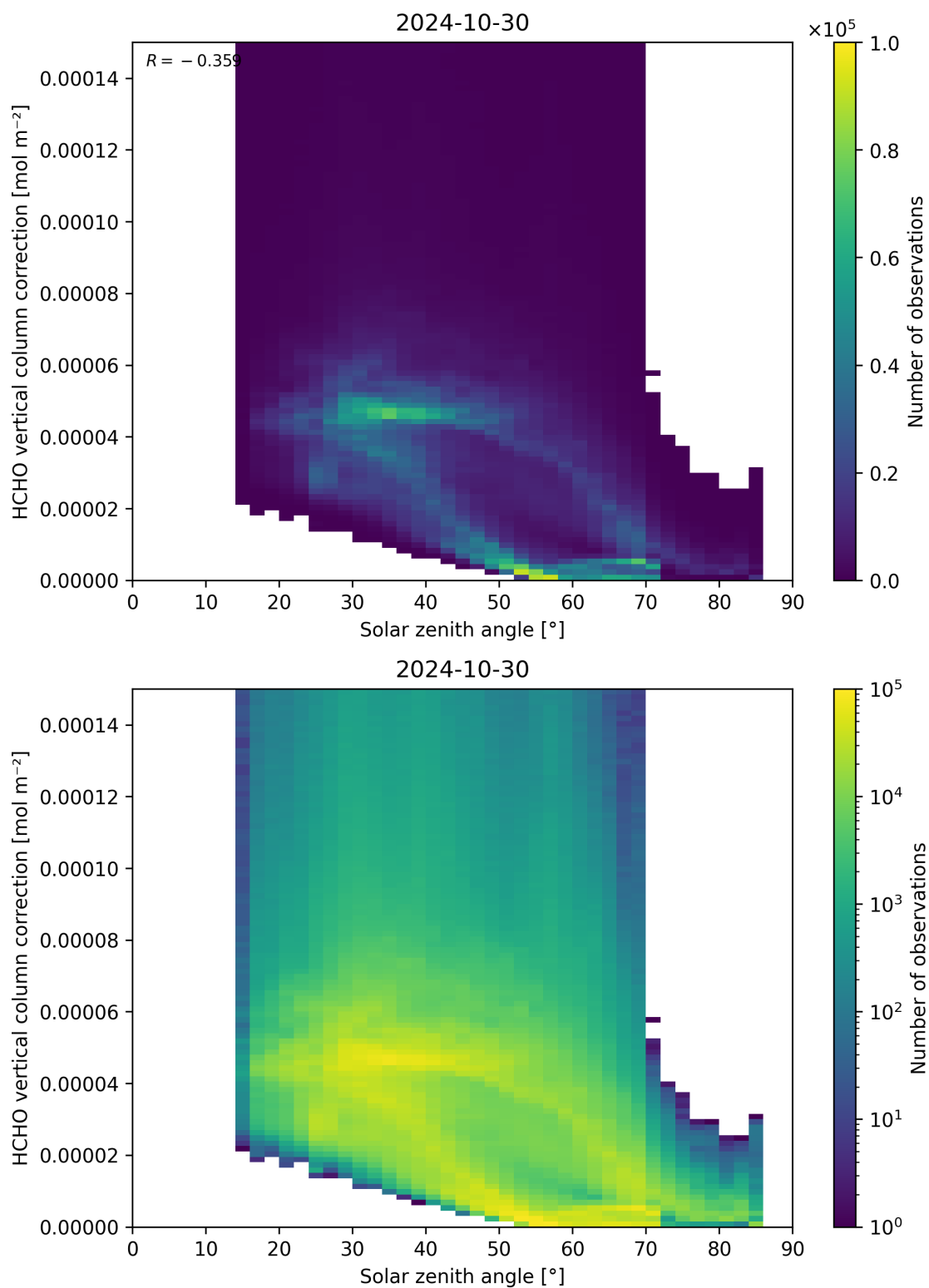
Figure 178: Scatter density plot of “Solar zenith angle” against “HCHO vertical column correction” for 2024-10-30 to 2024-10-31.
