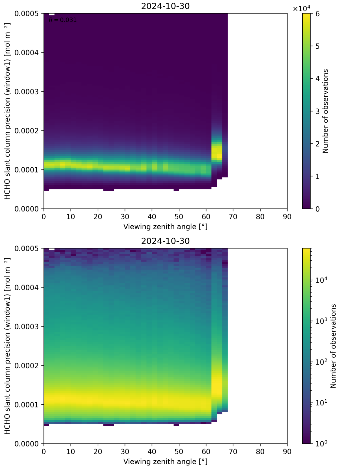
Figure 189: Scatter density plot of “Viewing zenith angle” against “HCHO slant column precision (window1)” for 2024-10-30 to 2024-10-31.
