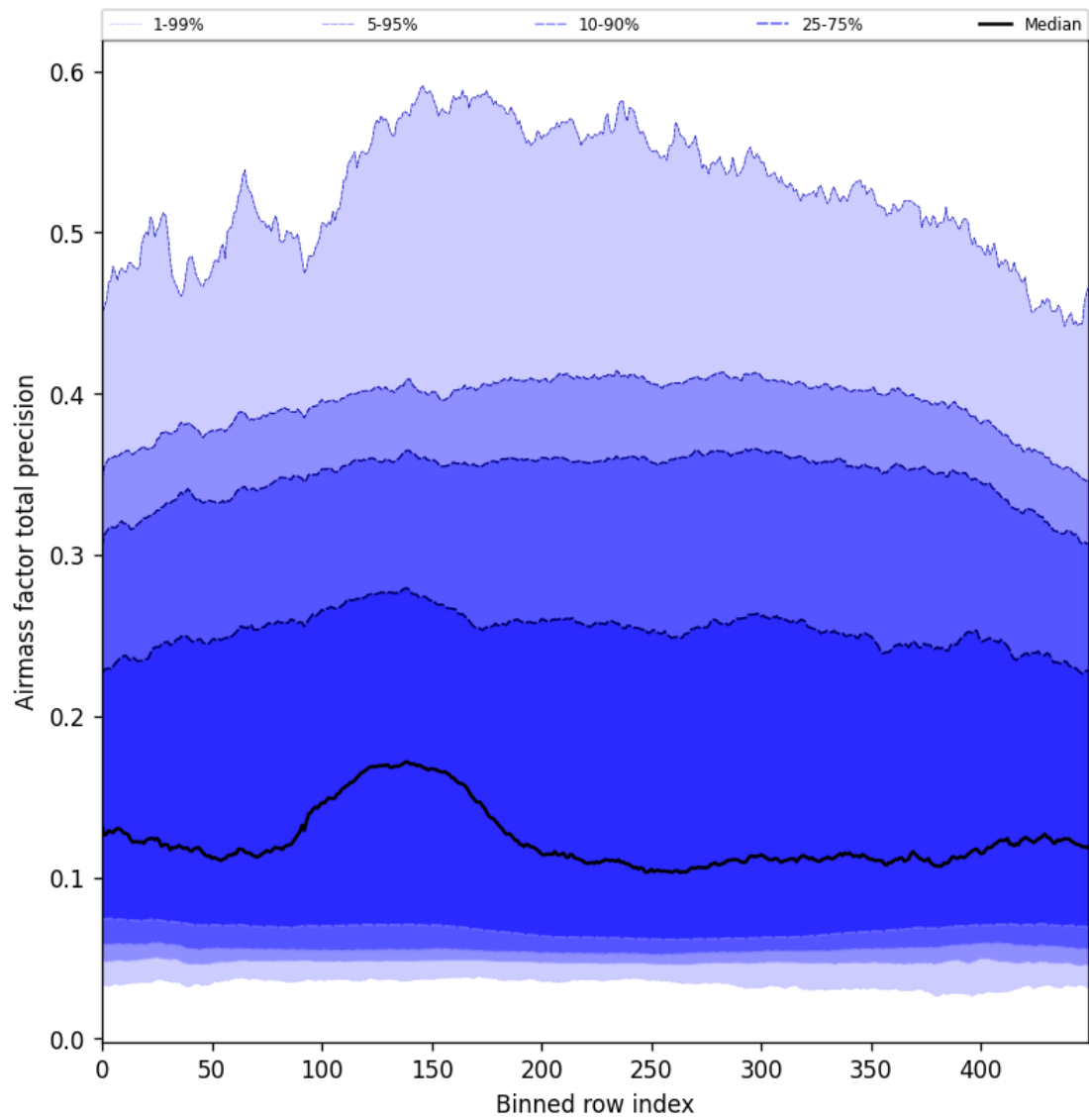
Figure 55: Along track statistics of “Airmass factor total precision” for 2024-10-30 to 2024-10-31
