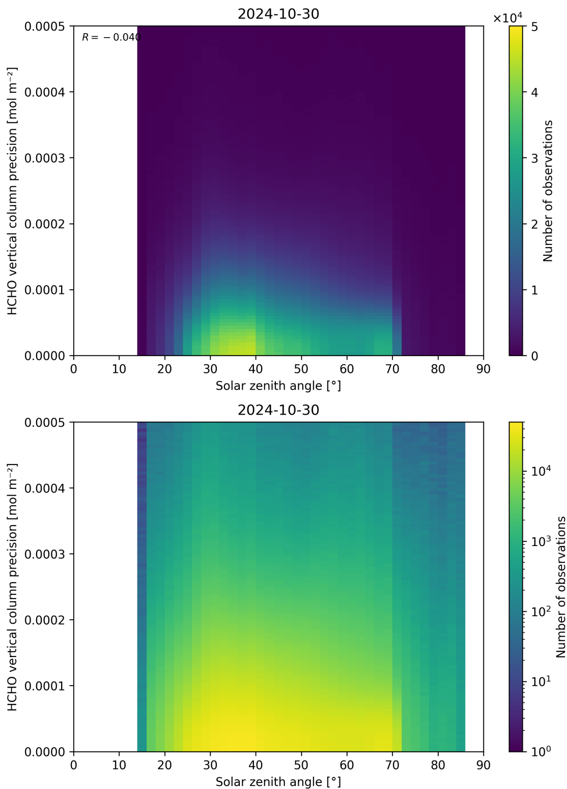
Figure 179: Scatter density plot of “Solar zenith angle” against “HCHO vertical column precision” for 2024-10-30 to 2024-10-31.
