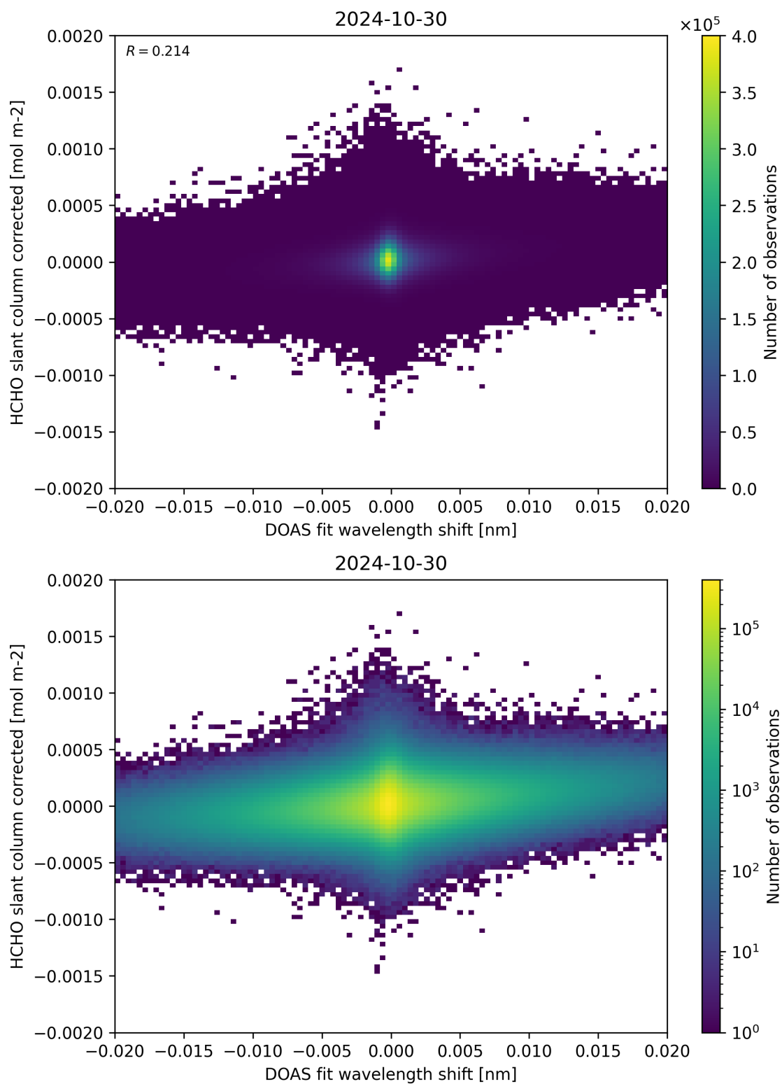
Figure 66: Scatter density plot of “DOAS fit wavelength shift” against “HCHO slant column corrected” for 2024-10-30 to 2024-10-31.
