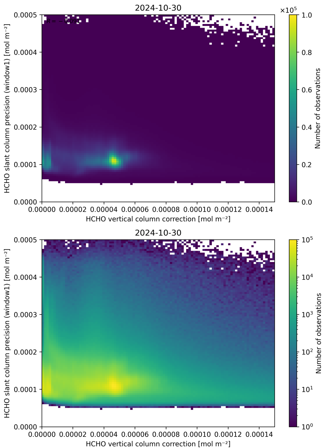
Figure 119: Scatter density plot of “HCHO vertical column correction” against “HCHO slant column precision (window1)” for 2024-10-30 to 2024-10-31.
