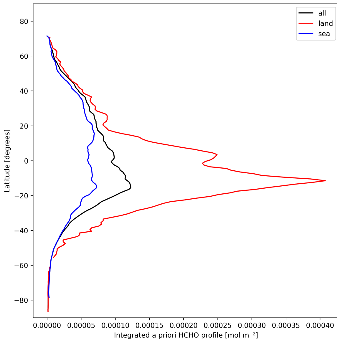
Figure 29: Zonal average of “Integrated a priori HCHO profile” for 2024-10-30 to 2024-10-31.
