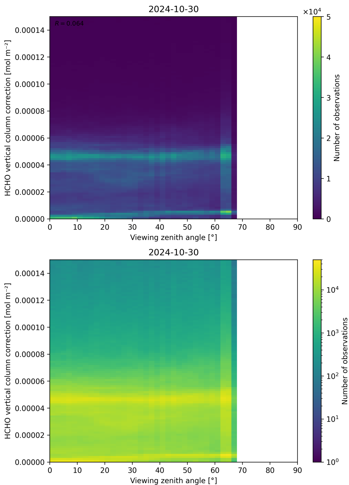
Figure 193: Scatter density plot of “Viewing zenith angle” against “HCHO vertical column correction” for 2024-10-30 to 2024-10-31.
