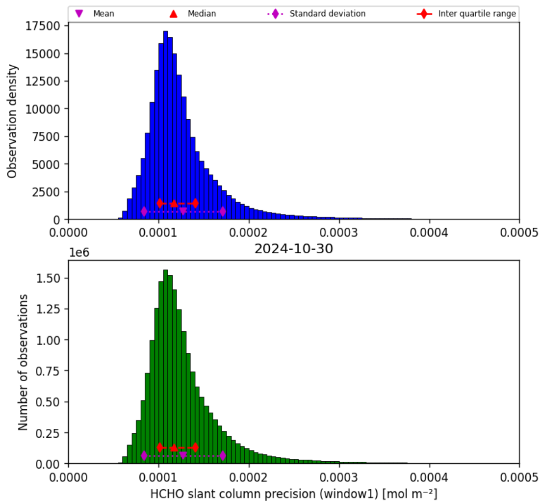
Figure 39: Histogram of “HCHO slant column precision (window1)” for 2024-10-30 to 2024-10-31
