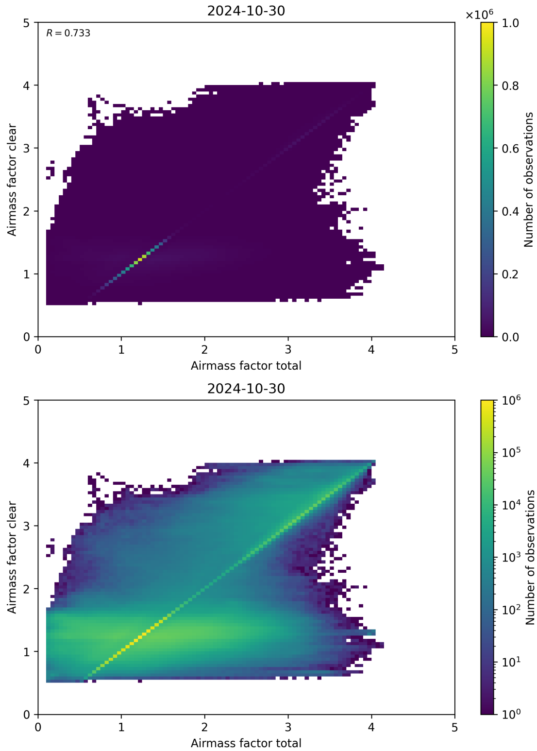
Figure 100: Scatter density plot of “Airmass factor total” against “Airmass factor clear” for 2024-10-30 to 2024-10-31.
