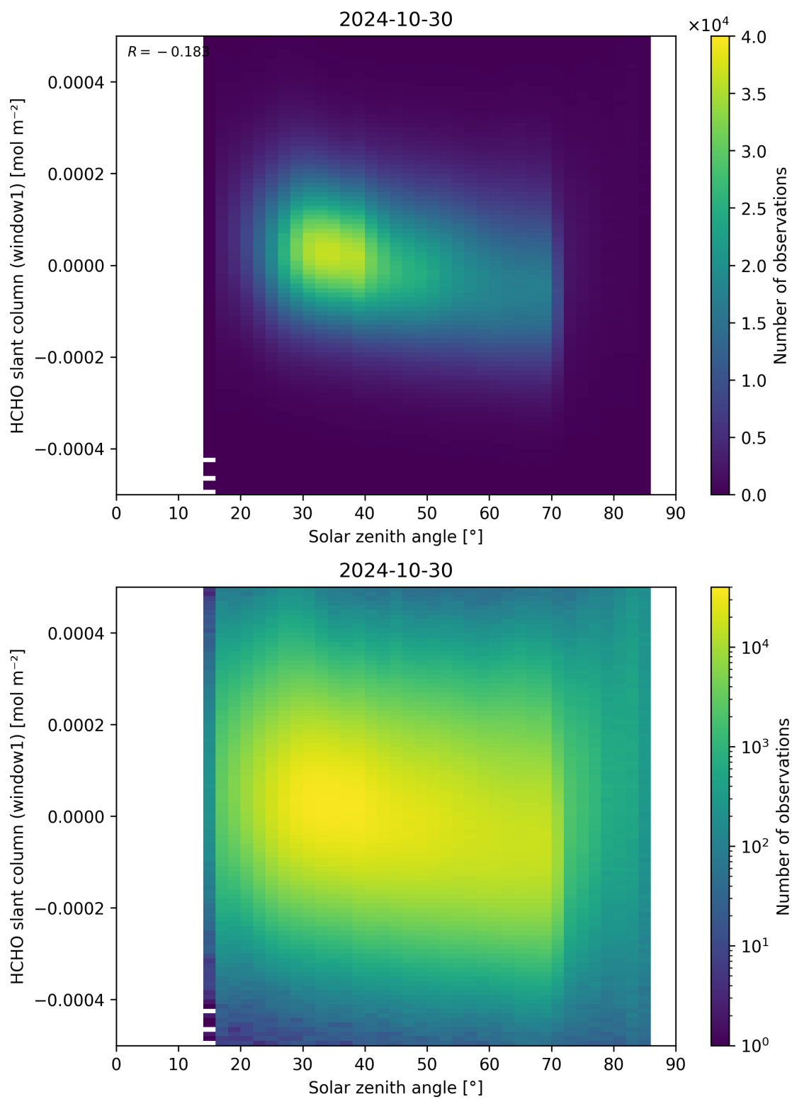
Figure 173: Scatter density plot of “Solar zenith angle” against “HCHO slant column (window1)” for 2024-10-30 to 2024-10-31.
