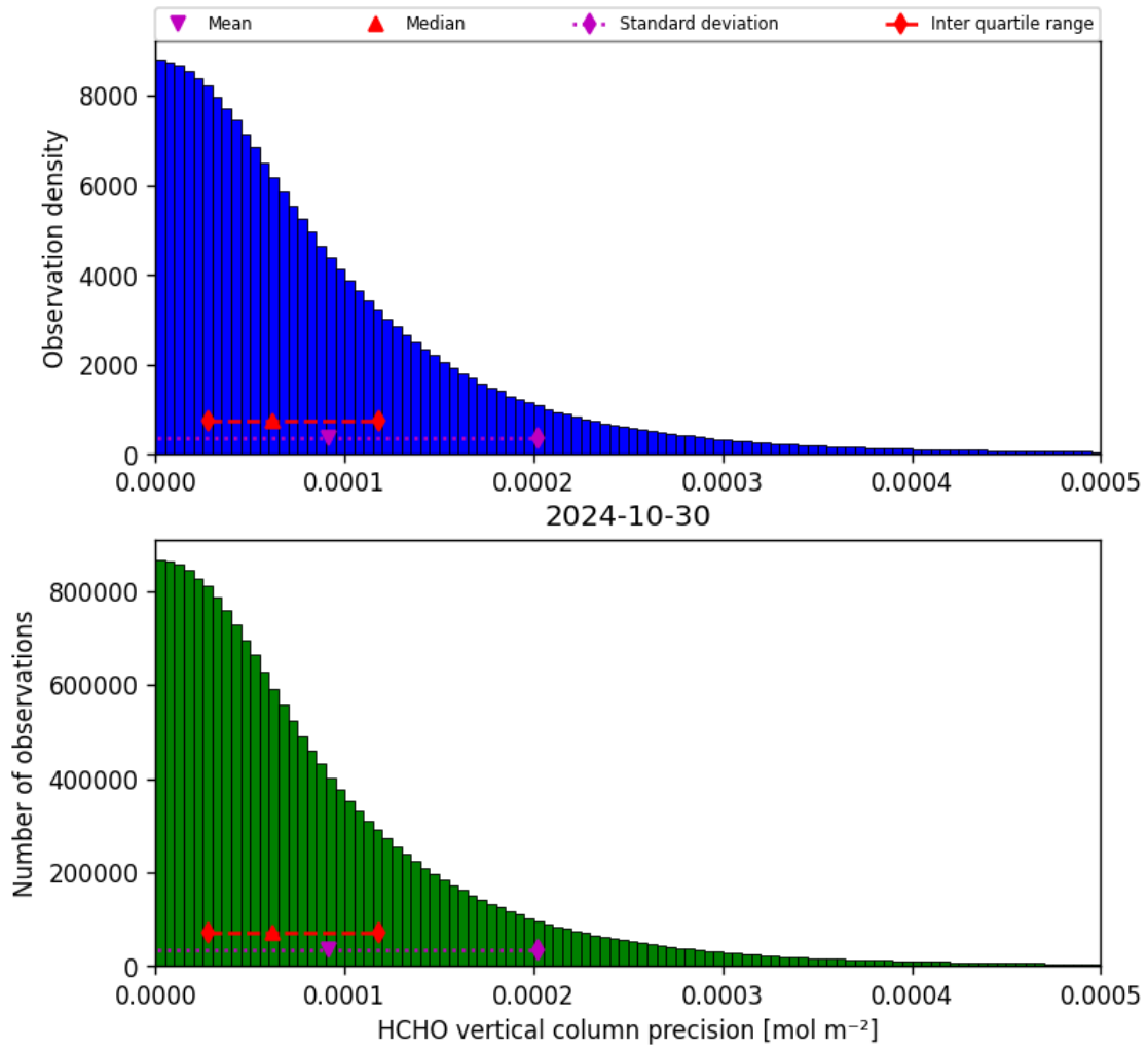
Figure 36: Histogram of “HCHO vertical column precision” for 2024-10-30 to 2024-10-31
