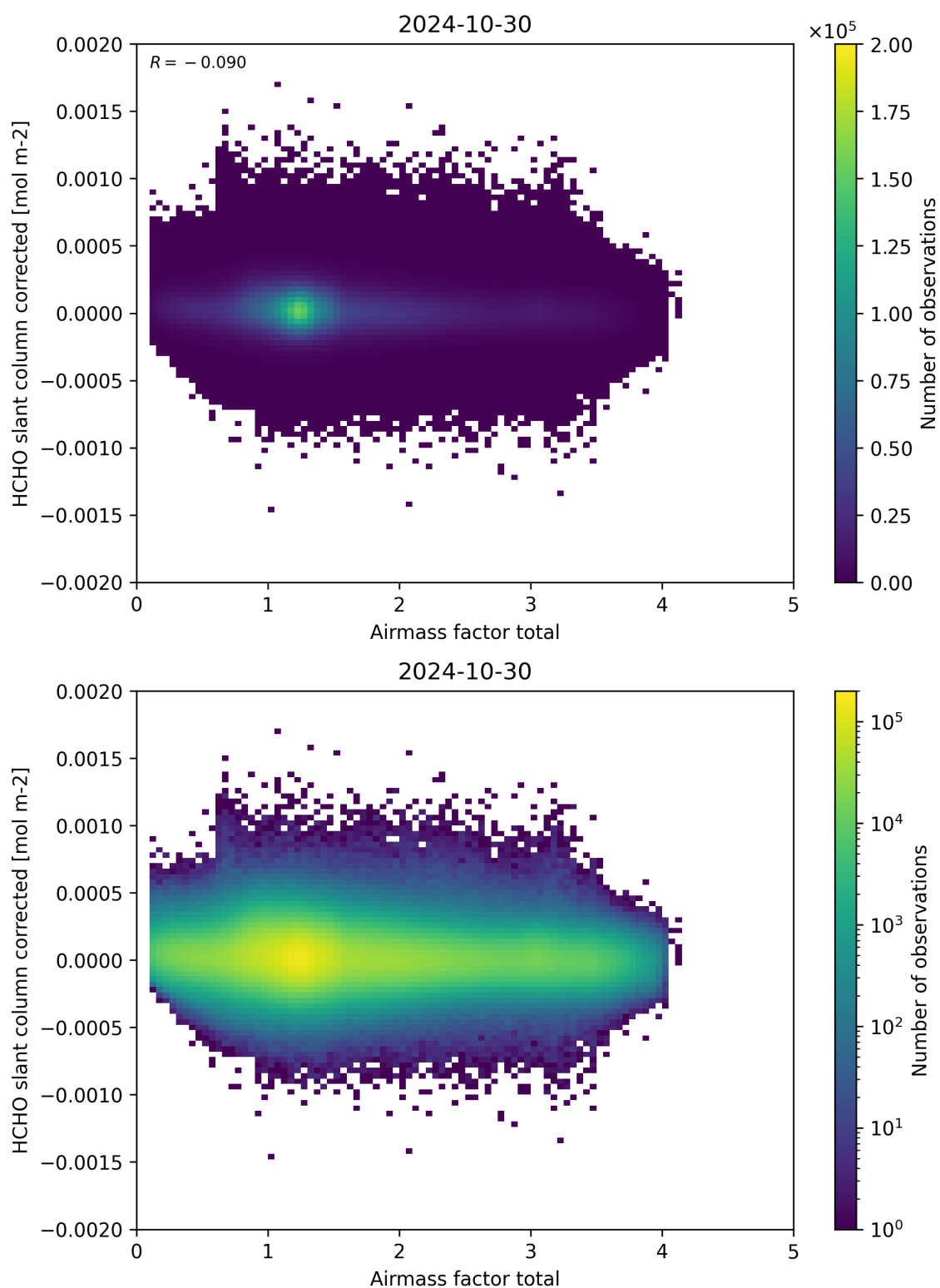
Figure 101: Scatter density plot of “Airmass factor total” against “HCHO slant column corrected” for 2024-10-30 to 2024-10-31.
