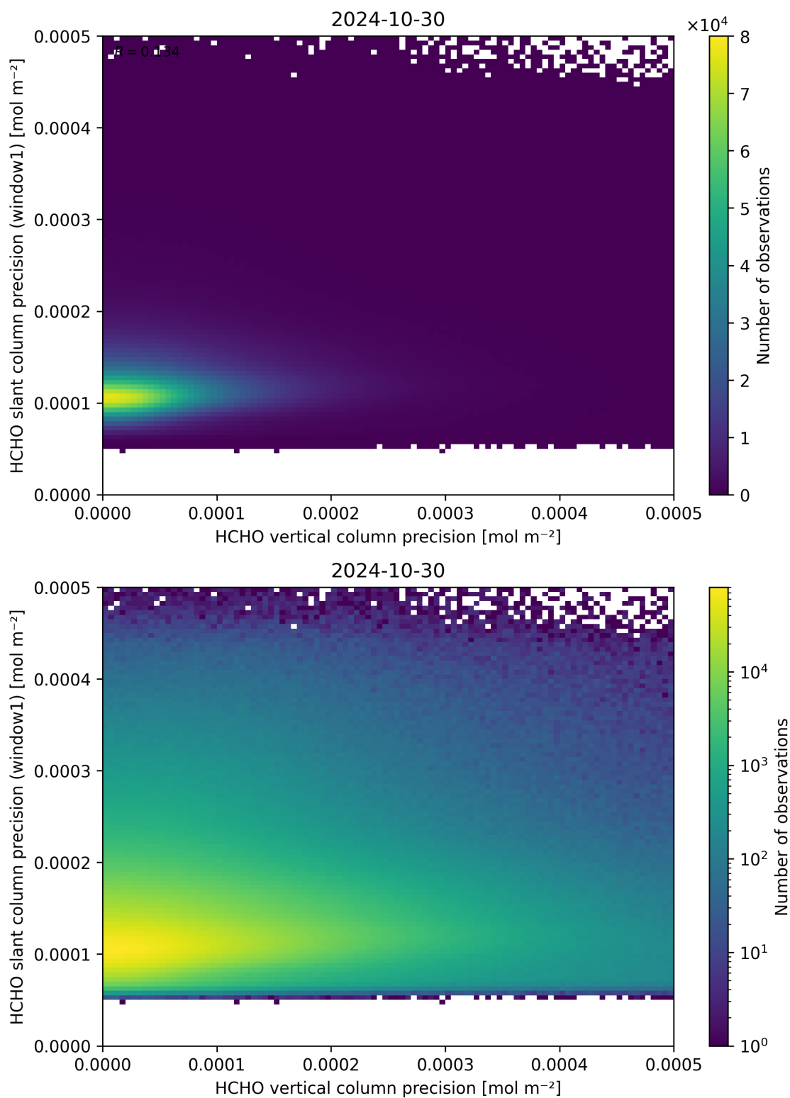
Figure 143: Scatter density plot of “HCHO vertical column precision” against “HCHO slant column precision (window1)” for 2024-10-30 to 2024-10-31.
