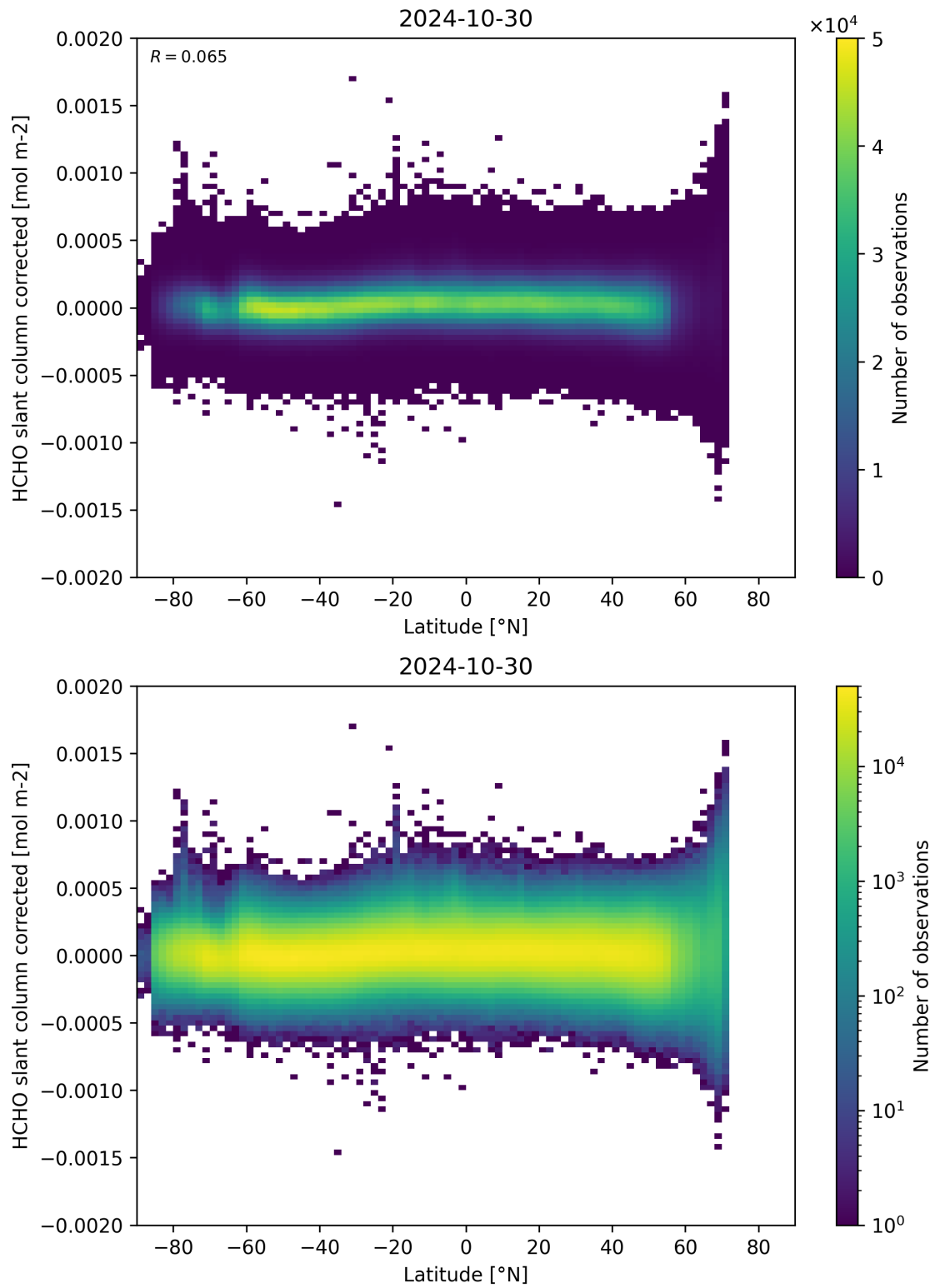
Figure 157: Scatter density plot of “Latitude” against “HCHO slant column corrected” for 2024-10-30 to 2024-10-31.
