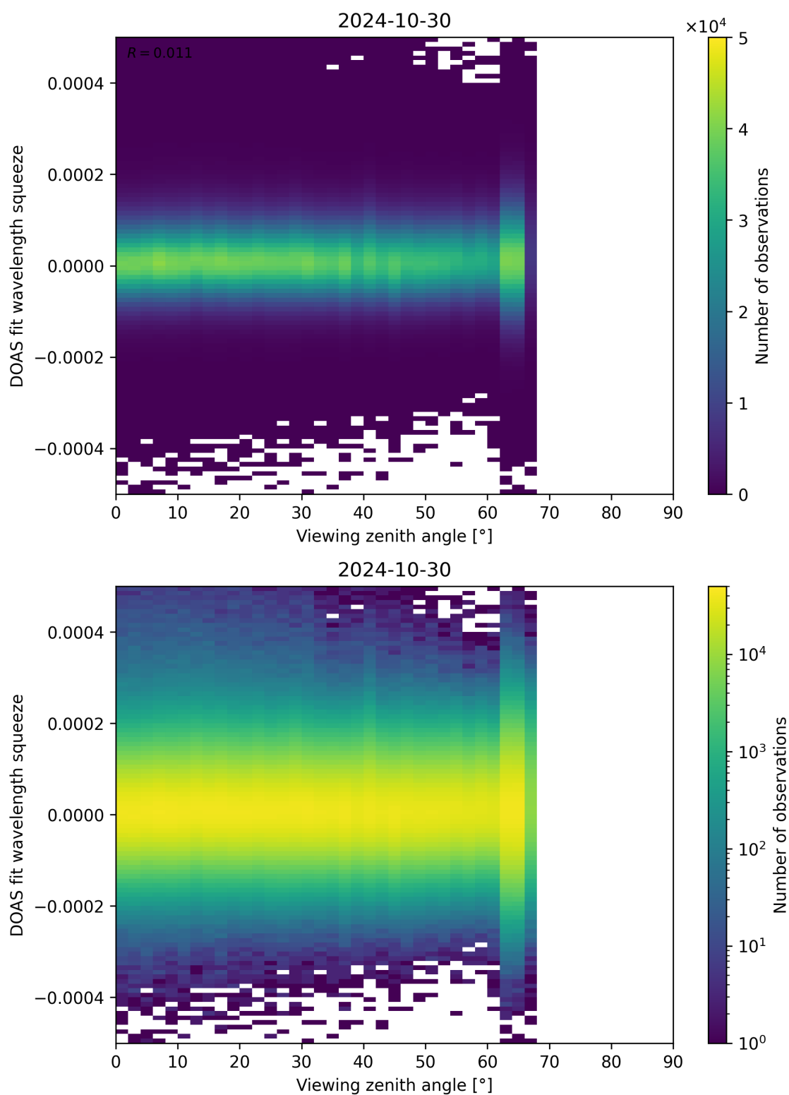
Figure 184: Scatter density plot of “Viewing zenith angle” against “DOAS fit wavelength squeeze” for 2024-10-30 to 2024-10-31.
