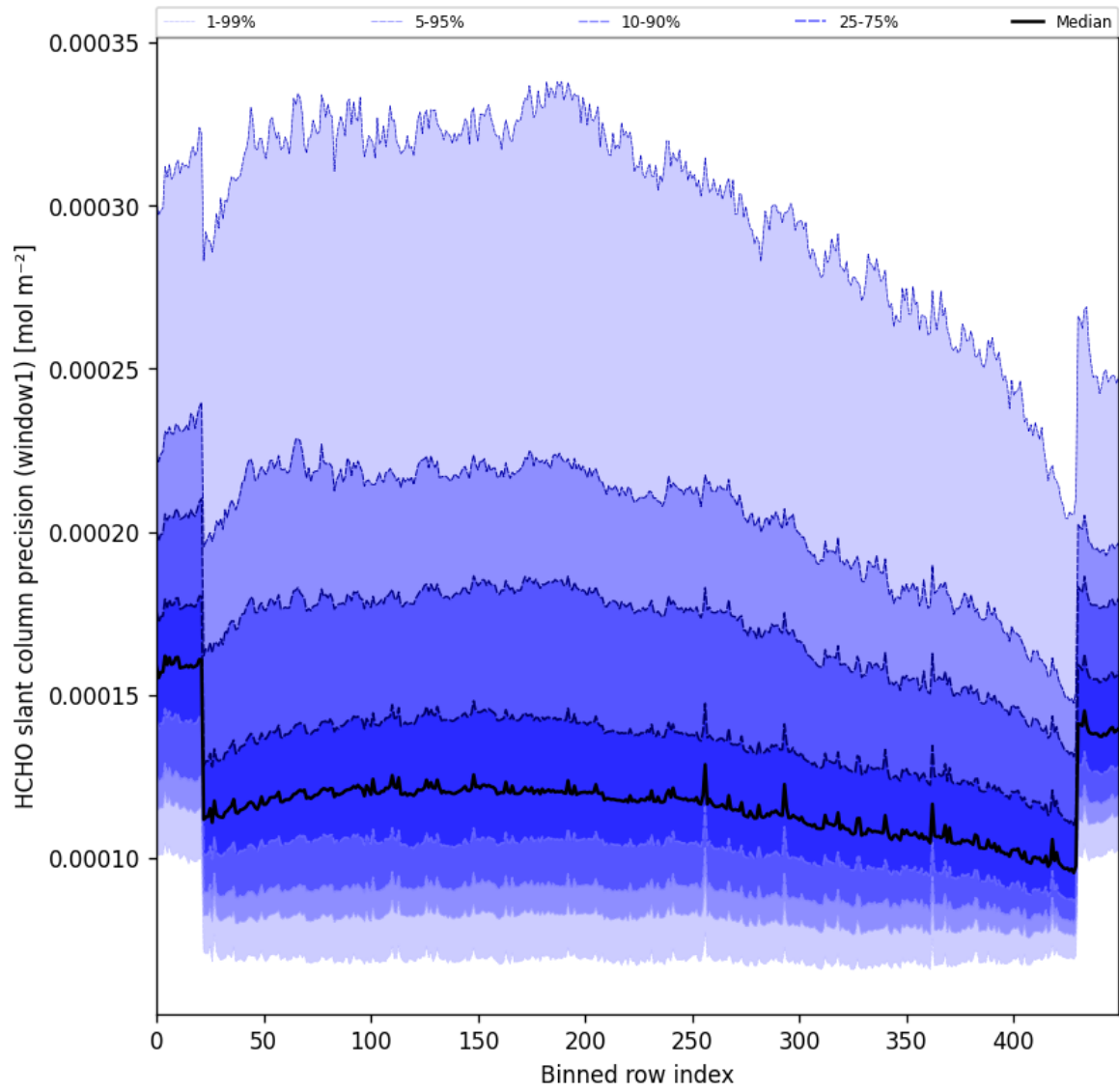
Figure 53: Along track statistics of “HCHO slant column precision (window1)” for 2024-10-30 to 2024-10-31
