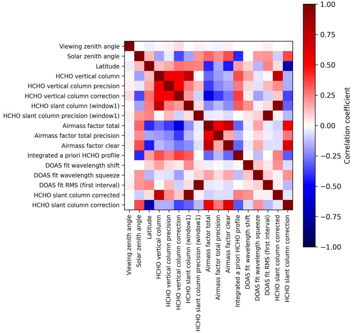
Figure 2: Map of correlation matrix for 2024-10-30 to 2024-10-31.
