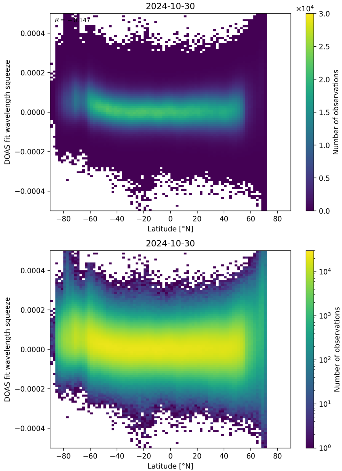
Figure 155: Scatter density plot of “Latitude” against “DOAS fit wavelength squeeze” for 2024-10-30 to 2024-10-31.
