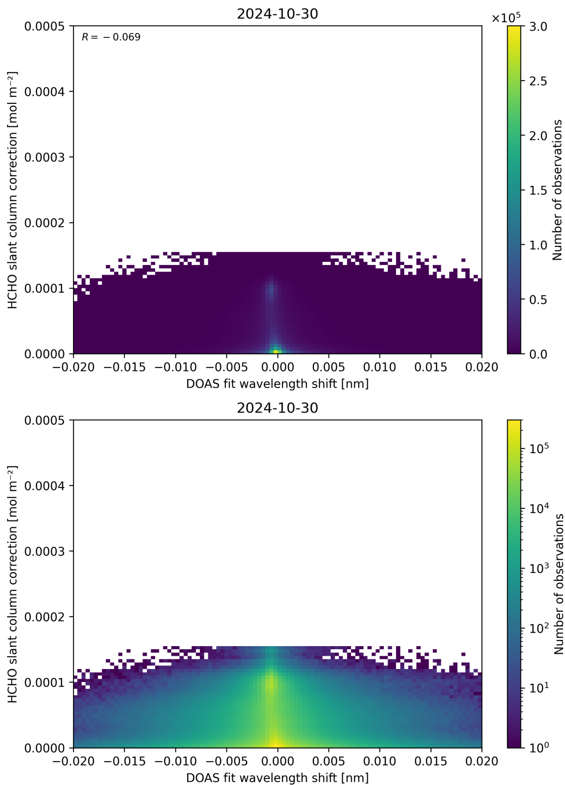
Figure 67: Scatter density plot of “DOAS fit wavelength shift” against “HCHO slant column correction” for 2024-10-30 to 2024-10-31.
