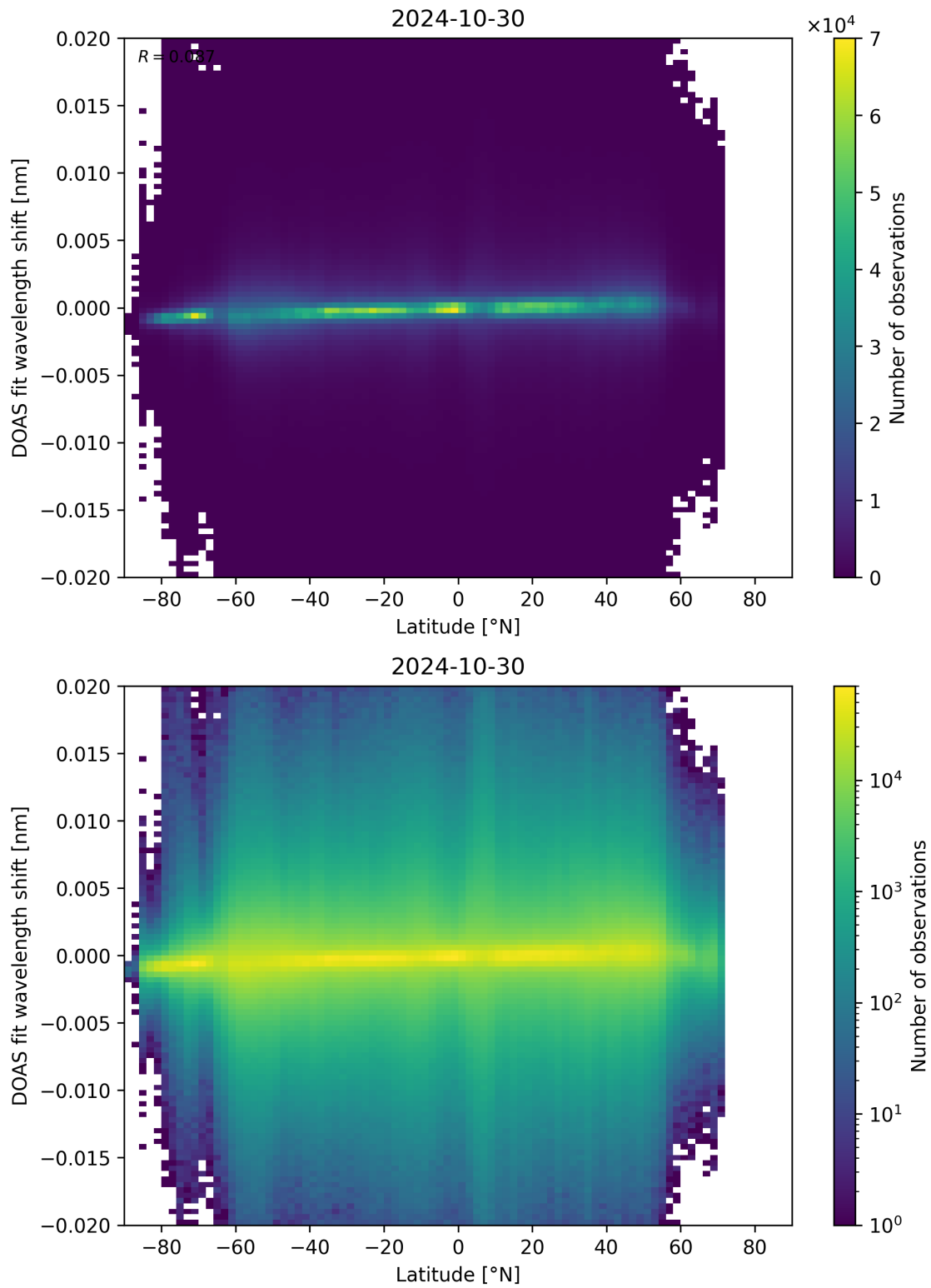
Figure 154: Scatter density plot of “Latitude” against “DOAS fit wavelength shift” for 2024-10-30 to 2024-10-31.
