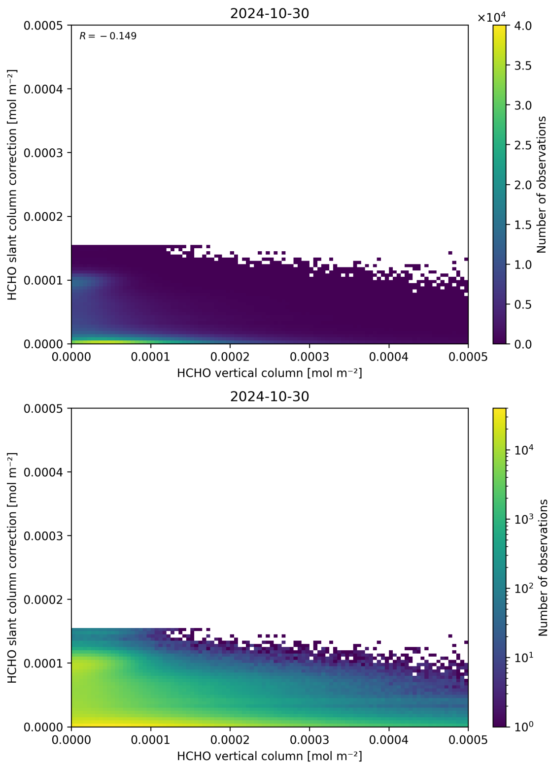
Figure 128: Scatter density plot of “HCHO vertical column” against “HCHO slant column correction” for 2024-10-30 to 2024-10-31.
