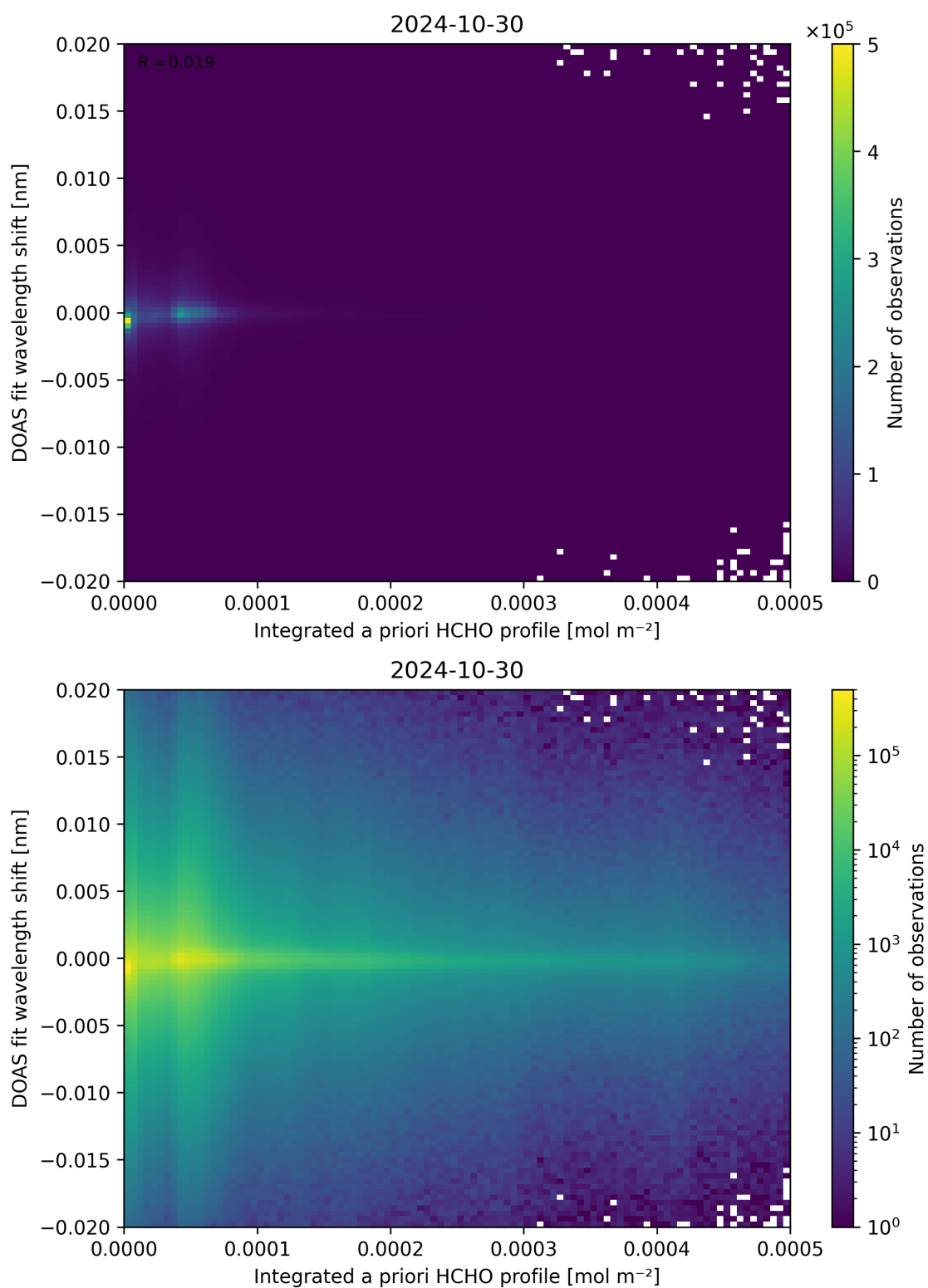
Figure 149: Scatter density plot of “Integrated a priori HCHO profile” against “DOAS fit wavelength shift” for 2024-10-30 to 2024-10-31.
