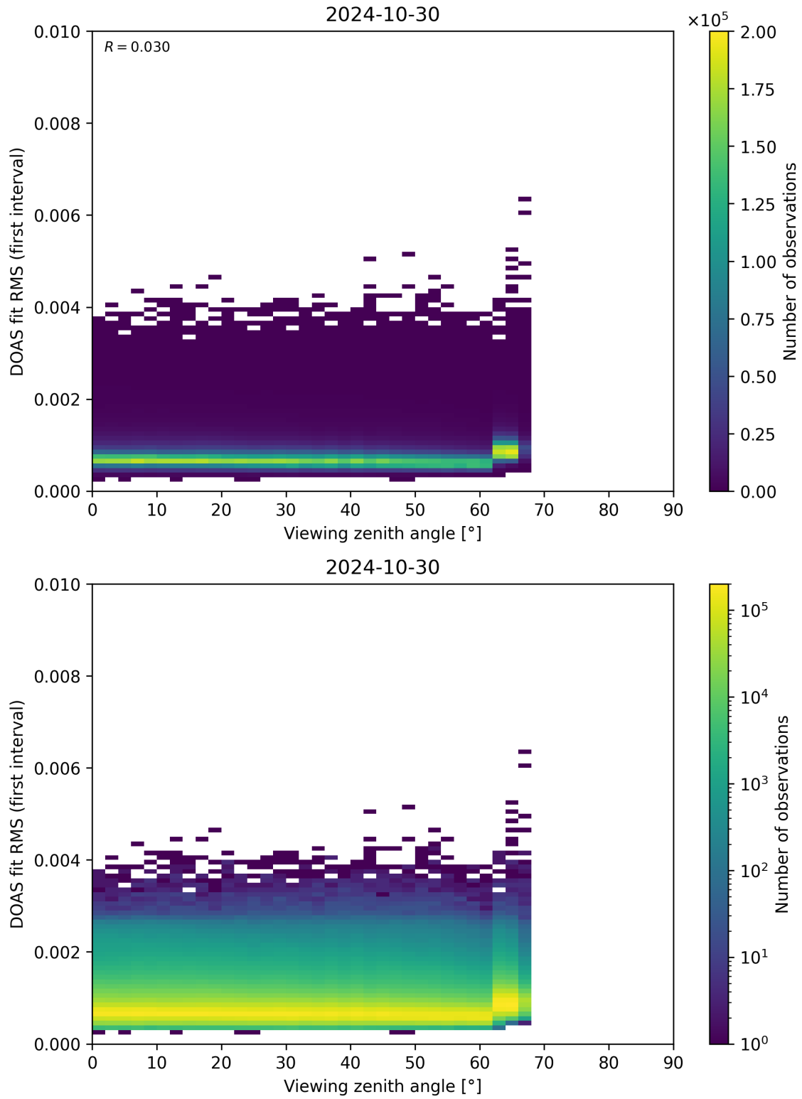
Figure 182: Scatter density plot of “Viewing zenith angle” against “DOAS fit RMS (first interval)” for 2024-10-30 to 2024-10-31.
