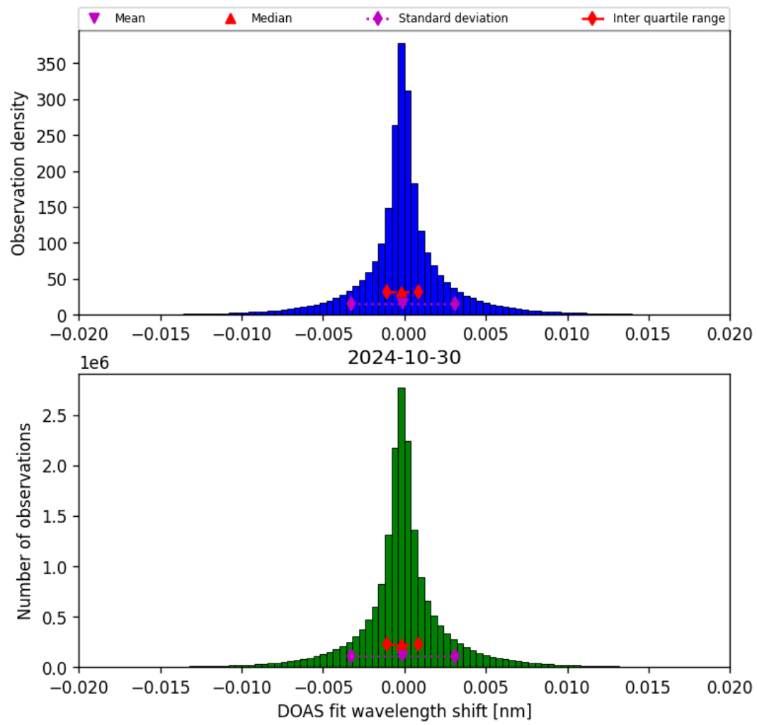
Figure 44: Histogram of “DOAS fit wavelength shift” for 2024-10-30 to 2024-10-31
