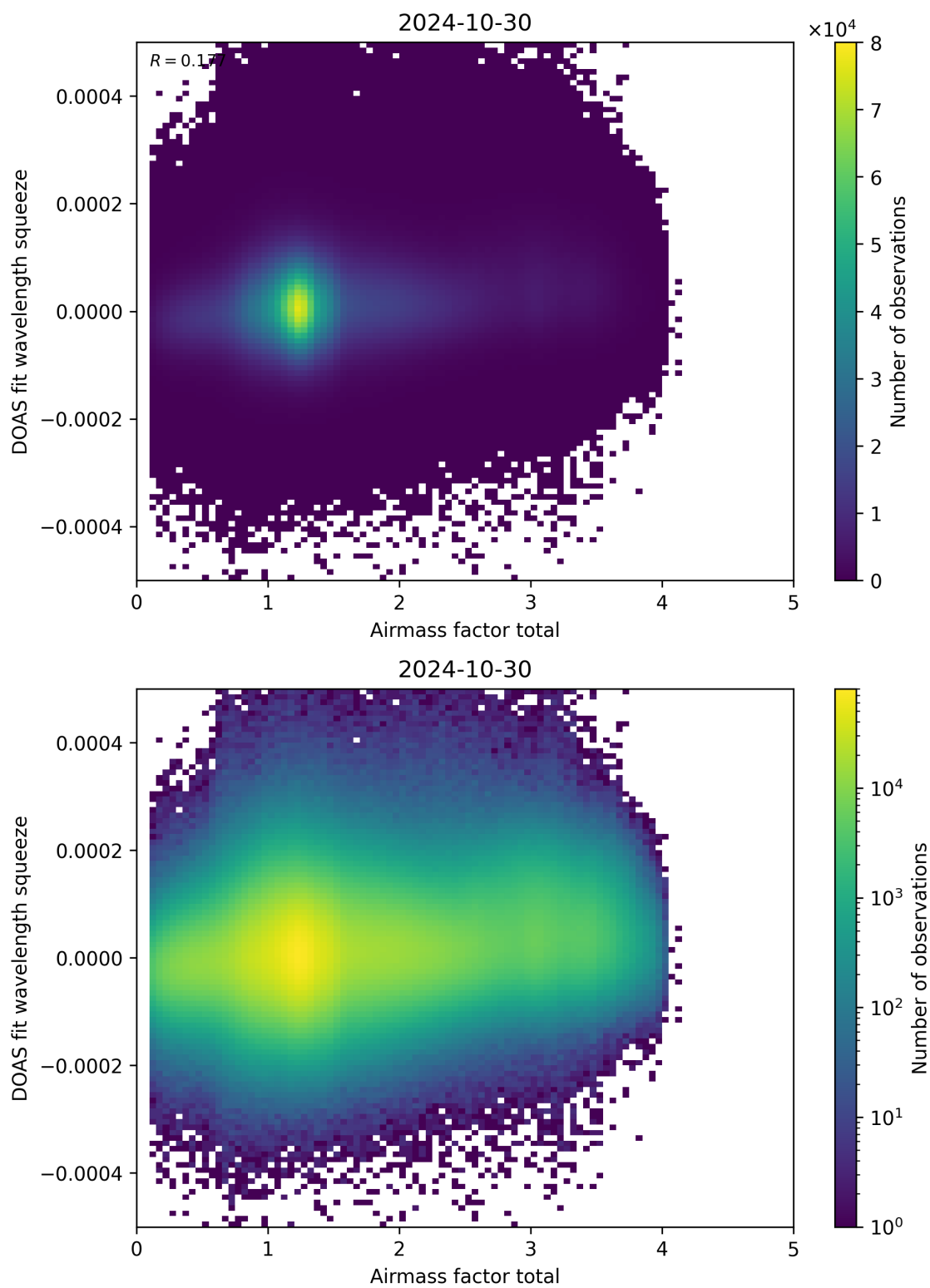
Figure 99: Scatter density plot of “Airmass factor total” against “DOAS fit wavelength squeeze” for 2024-10-30 to 2024-10-31.
