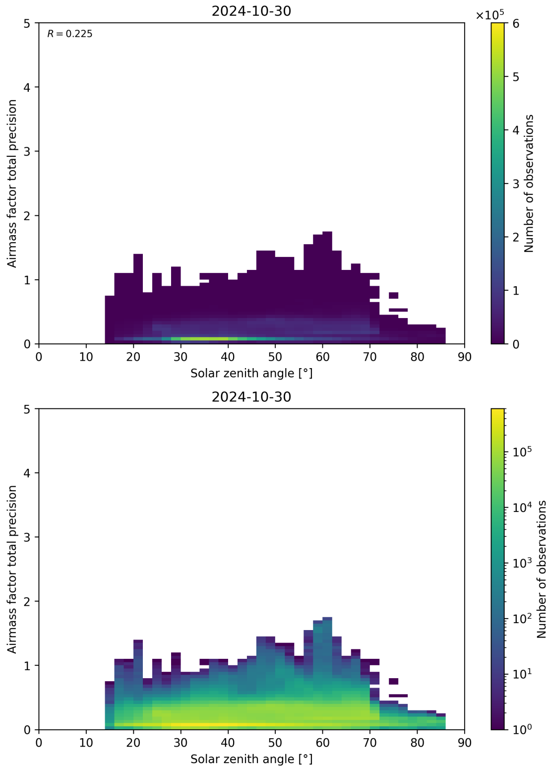
Figure 176: Scatter density plot of “Solar zenith angle” against “Airmass factor total precision” for 2024-10-30 to 2024-10-31.
