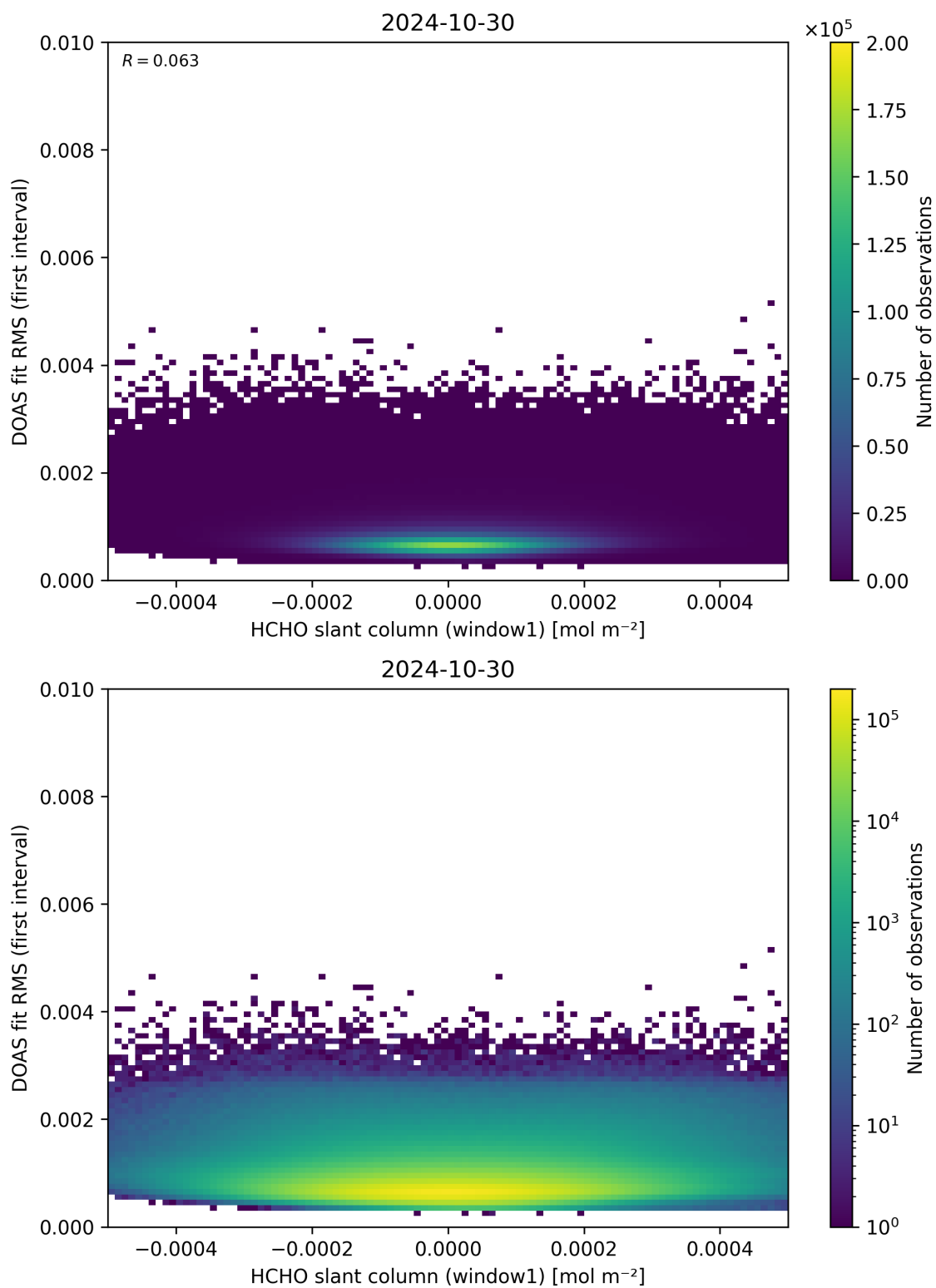
Figure 78: Scatter density plot of “HCHO slant column (window1)” against “DOAS fit RMS (first interval)” for 2024-10-30 to 2024-10-31.
