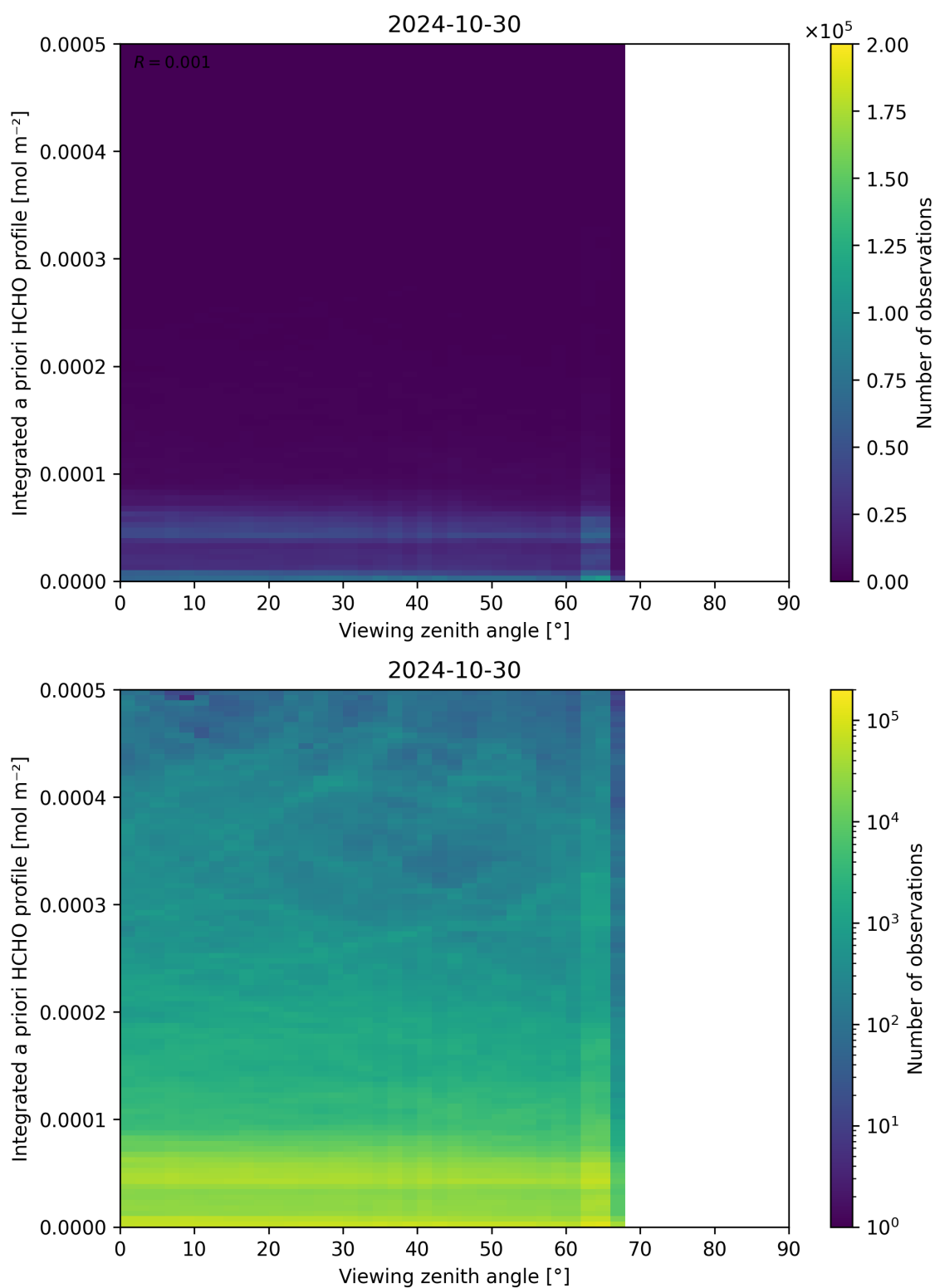
Figure 195: Scatter density plot of “Viewing zenith angle” against “Integrated a priori HCHO profile” for 2024-10-30 to 2024-10-31.
