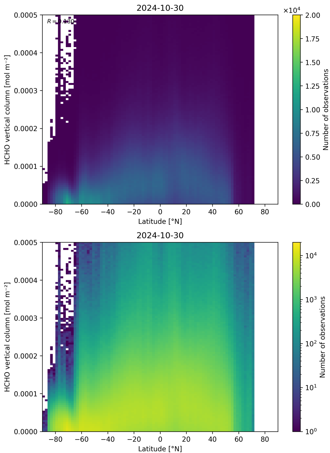
Figure 163: Scatter density plot of “Latitude” against “HCHO vertical column” for 2024-10-30 to 2024-10-31.
