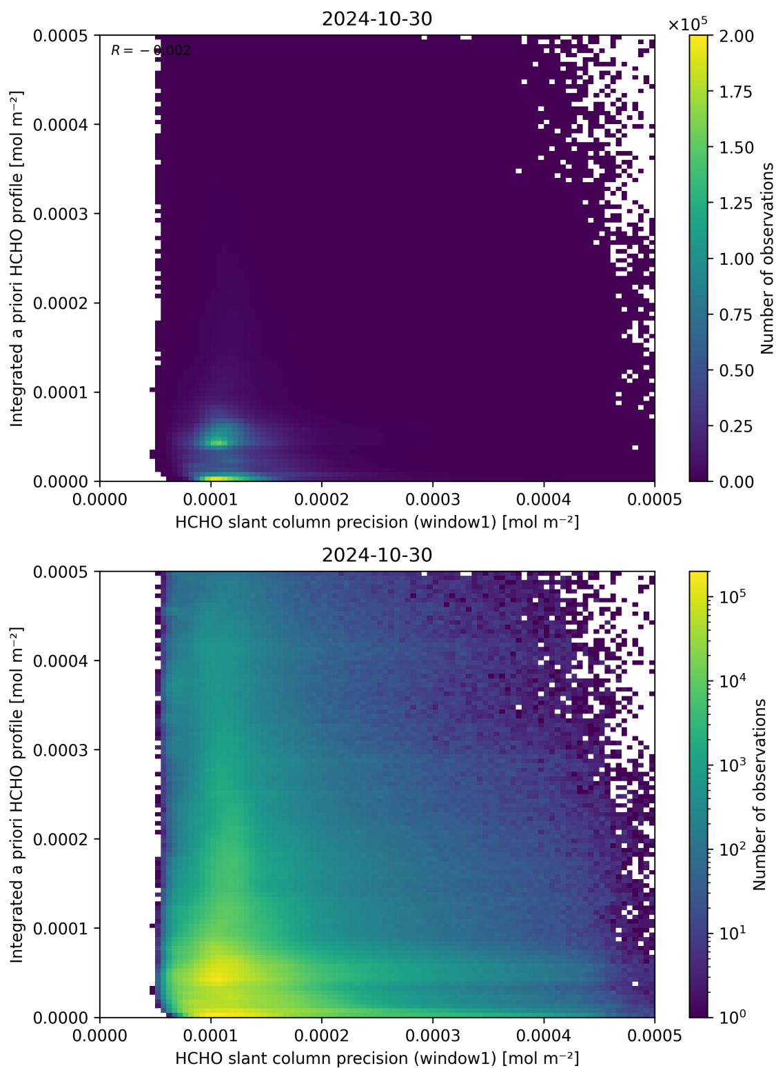
Figure 96: Scatter density plot of “HCHO slant column precision (window1)” against “Integrated a priori HCHO profile” for 2024-10-30 to 2024-10-31.
