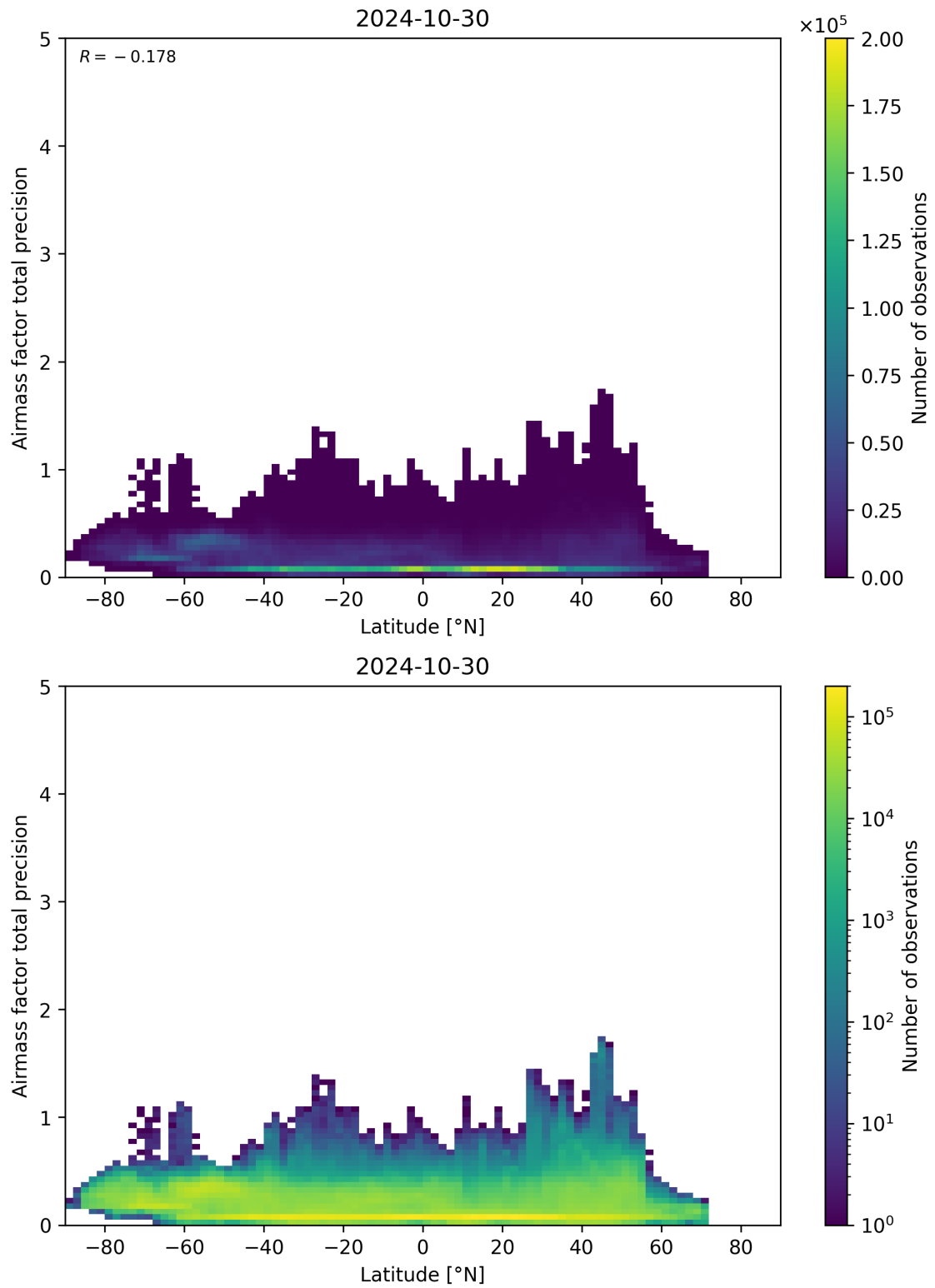
Figure 162: Scatter density plot of “Latitude” against “Airmass factor total precision” for 2024-10-30 to 2024-10-31.
