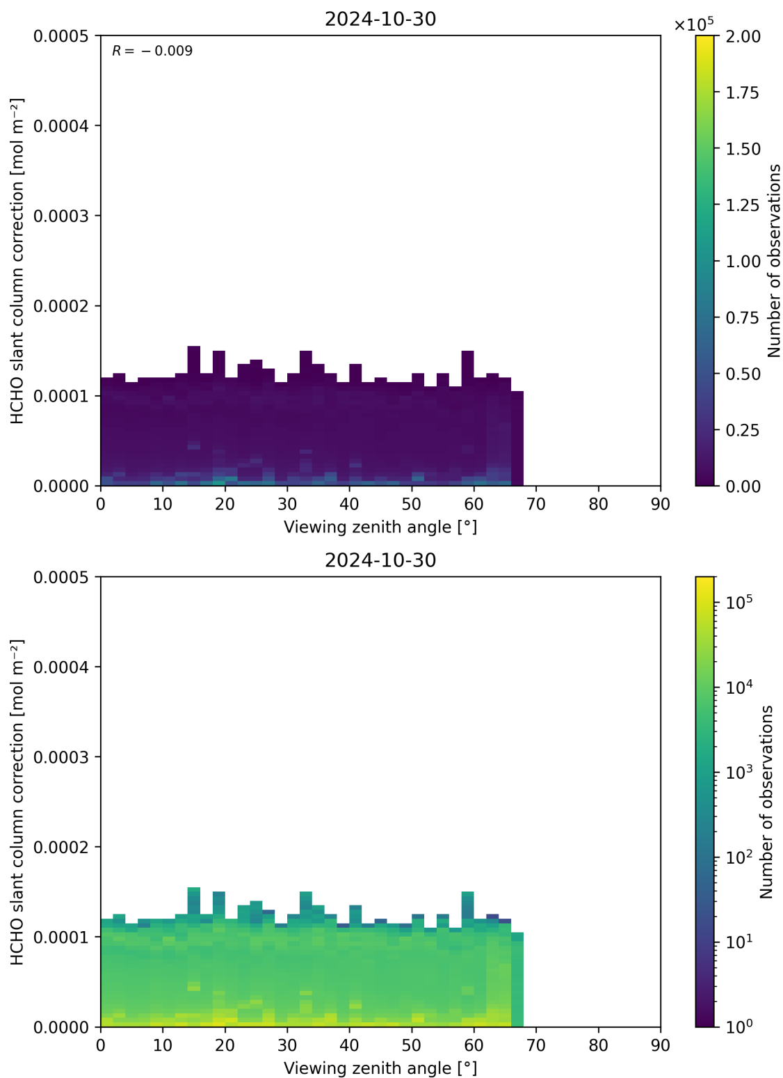
Figure 187: Scatter density plot of “Viewing zenith angle” against “HCHO slant column correction” for 2024-10-30 to 2024-10-31.
