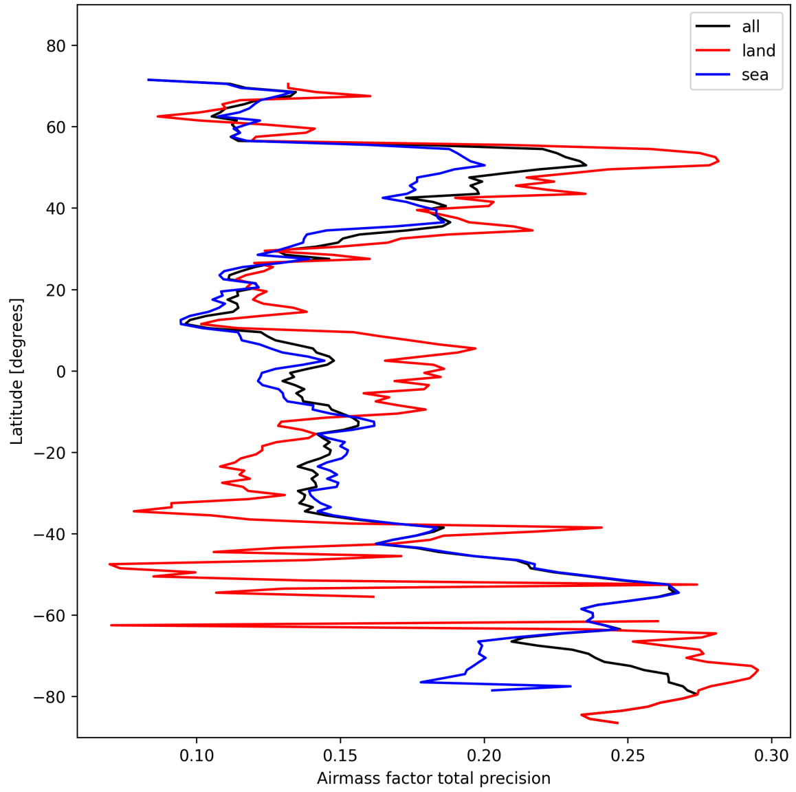
Figure 27: Zonal average of “Airmass factor total precision” for 2024-10-30 to 2024-10-31.
