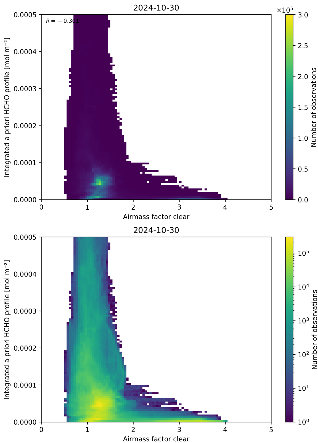
Figure 76: Scatter density plot of “Airmass factor clear” against “Integrated a priori HCHO profile” for 2024-10-30 to 2024-10-31.
