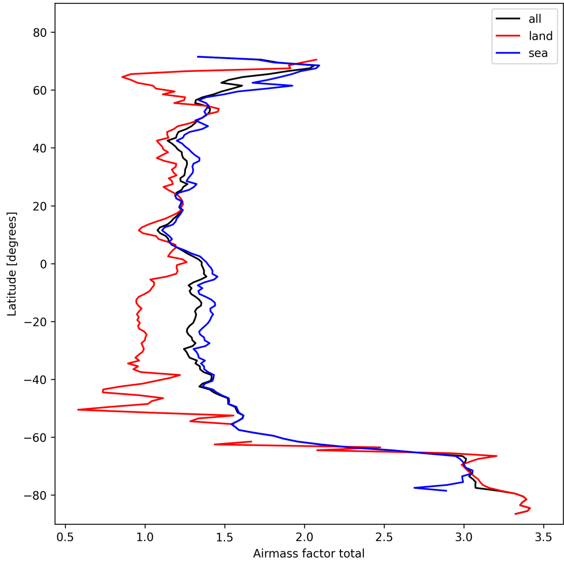
Figure 26: Zonal average of “Airmass factor total” for 2024-10-30 to 2024-10-31.
