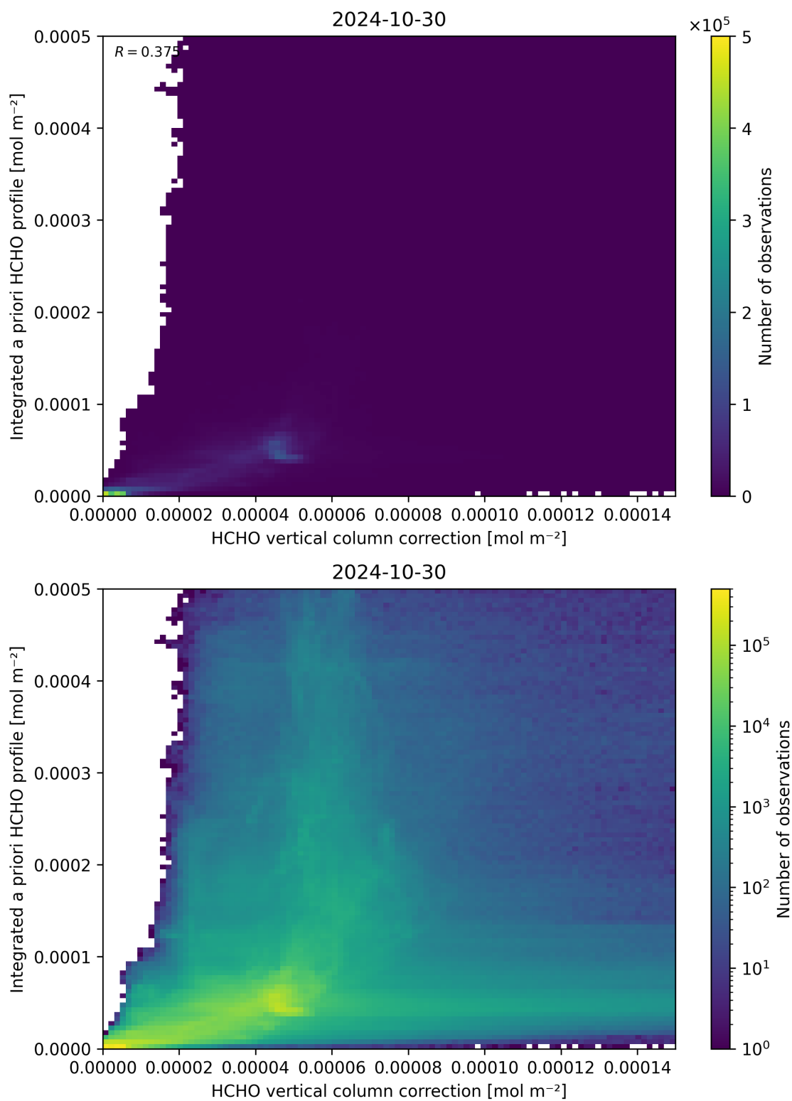
Figure 122: Scatter density plot of “HCHO vertical column correction” against “Integrated a priori HCHO profile” for 2024-10-30 to 2024-10-31.
