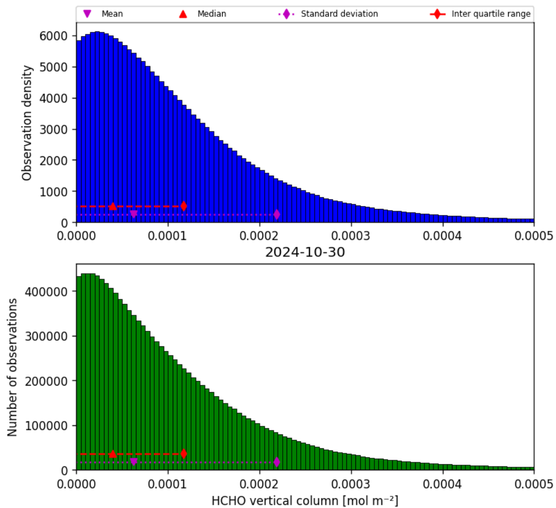
Figure 35: Histogram of “HCHO vertical column” for 2024-10-30 to 2024-10-31
