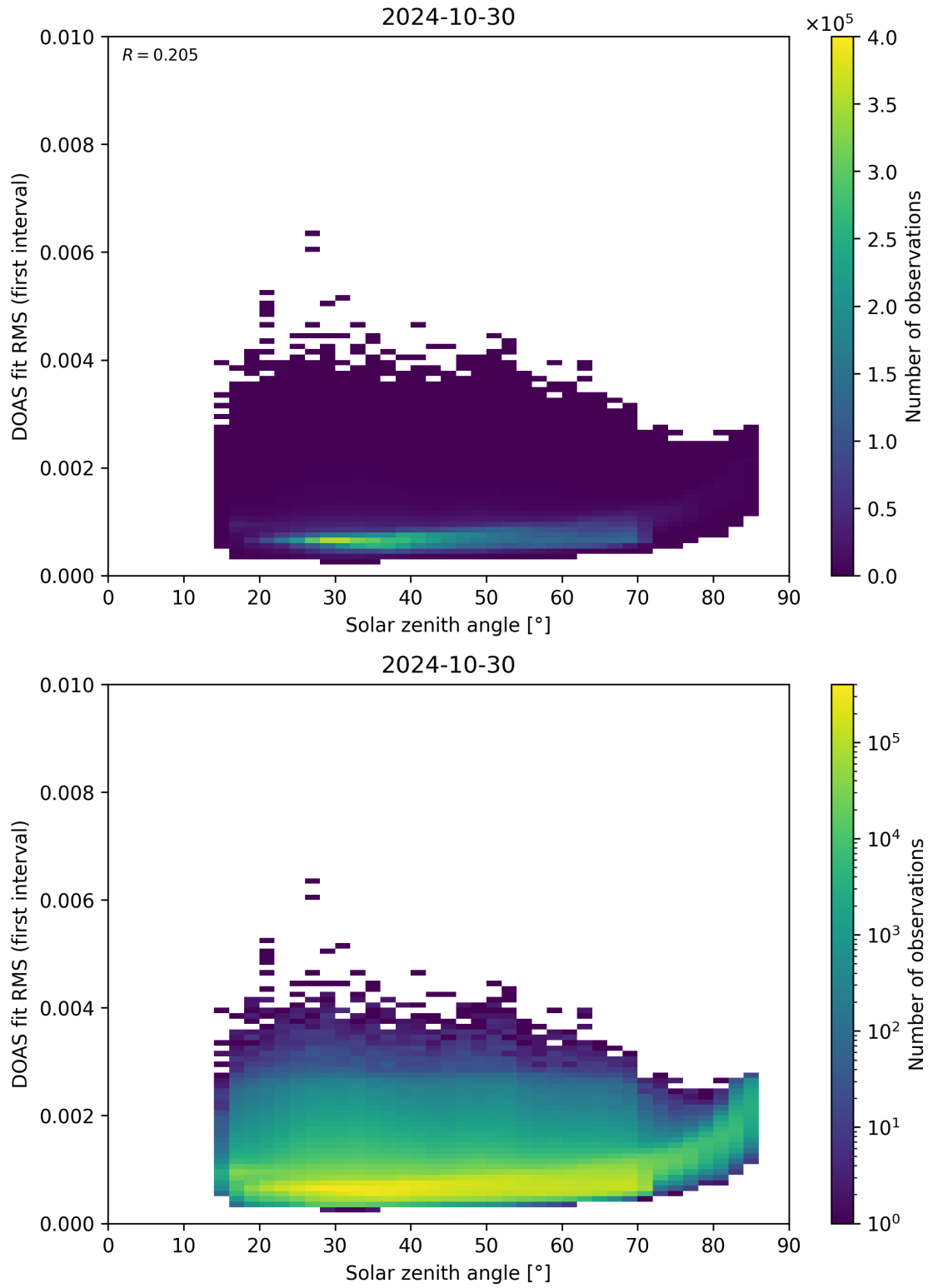
Figure 167: Scatter density plot of “Solar zenith angle” against “DOAS fit RMS (first interval)” for 2024-10-30 to 2024-10-31.
