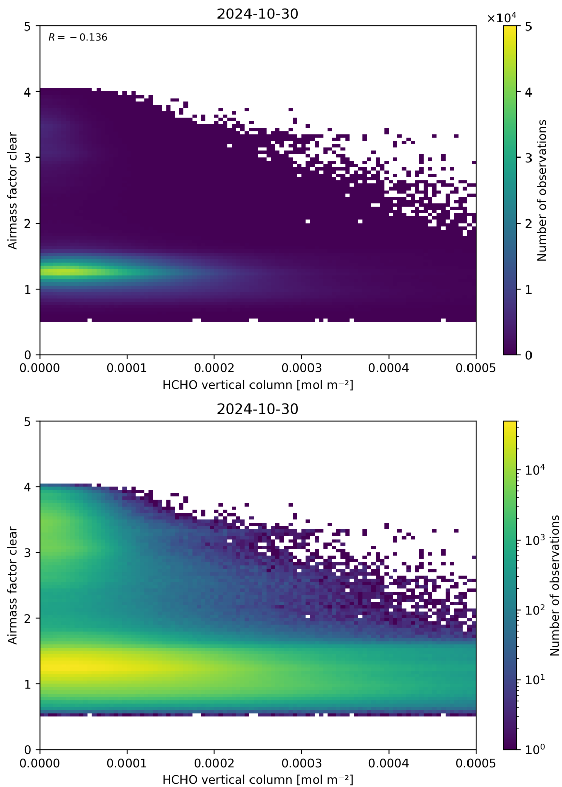
Figure 126: Scatter density plot of “HCHO vertical column” against “Airmass factor clear” for 2024-10-30 to 2024-10-31.
