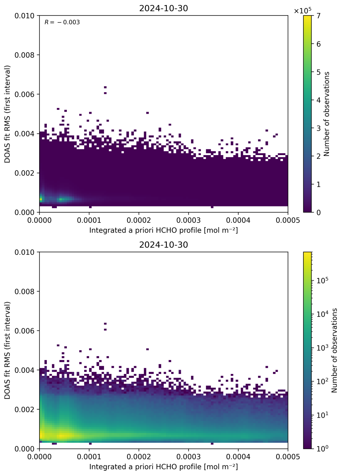
Figure 148: Scatter density plot of “Integrated a priori HCHO profile” against “DOAS fit RMS (first interval)” for 2024-10-30 to 2024-10-31.
