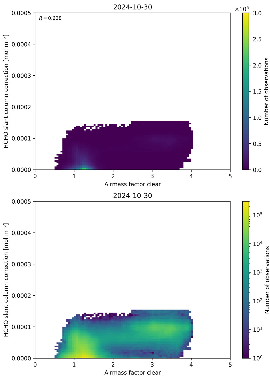
Figure 75: Scatter density plot of “Airmass factor clear” against “HCHO slant column correction” for 2024-10-30 to 2024-10-31.
