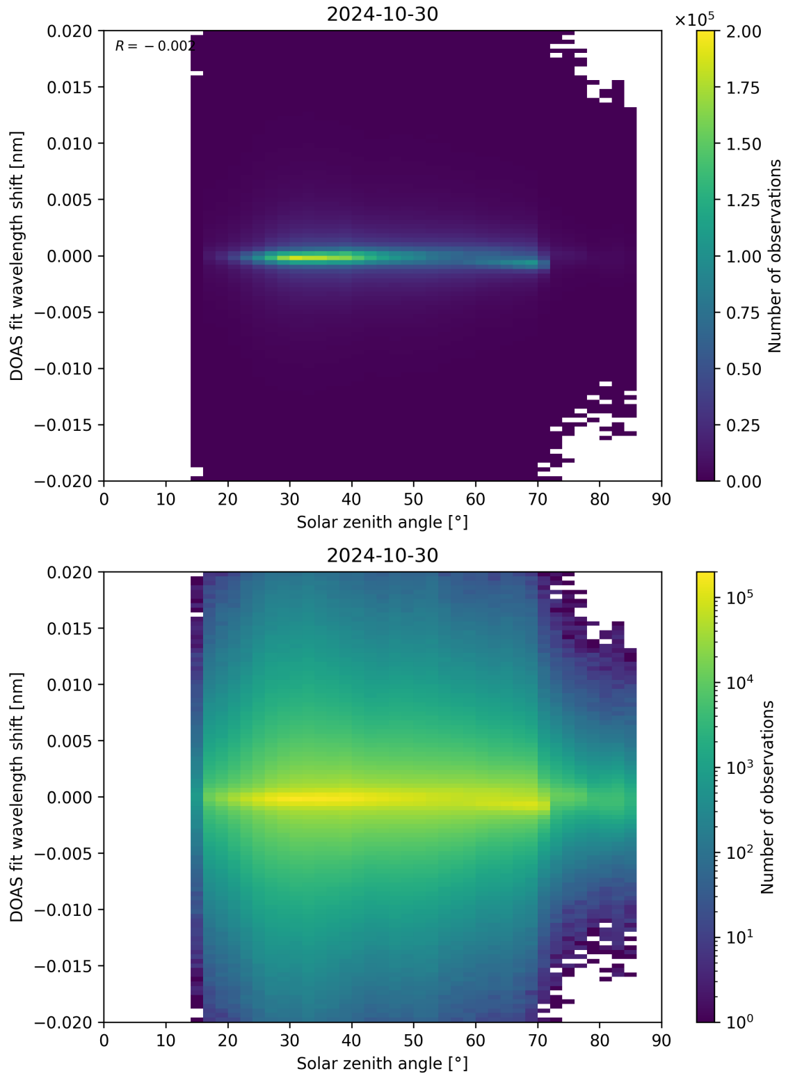
Figure 168: Scatter density plot of “Solar zenith angle” against “DOAS fit wavelength shift” for 2024-10-30 to 2024-10-31.
