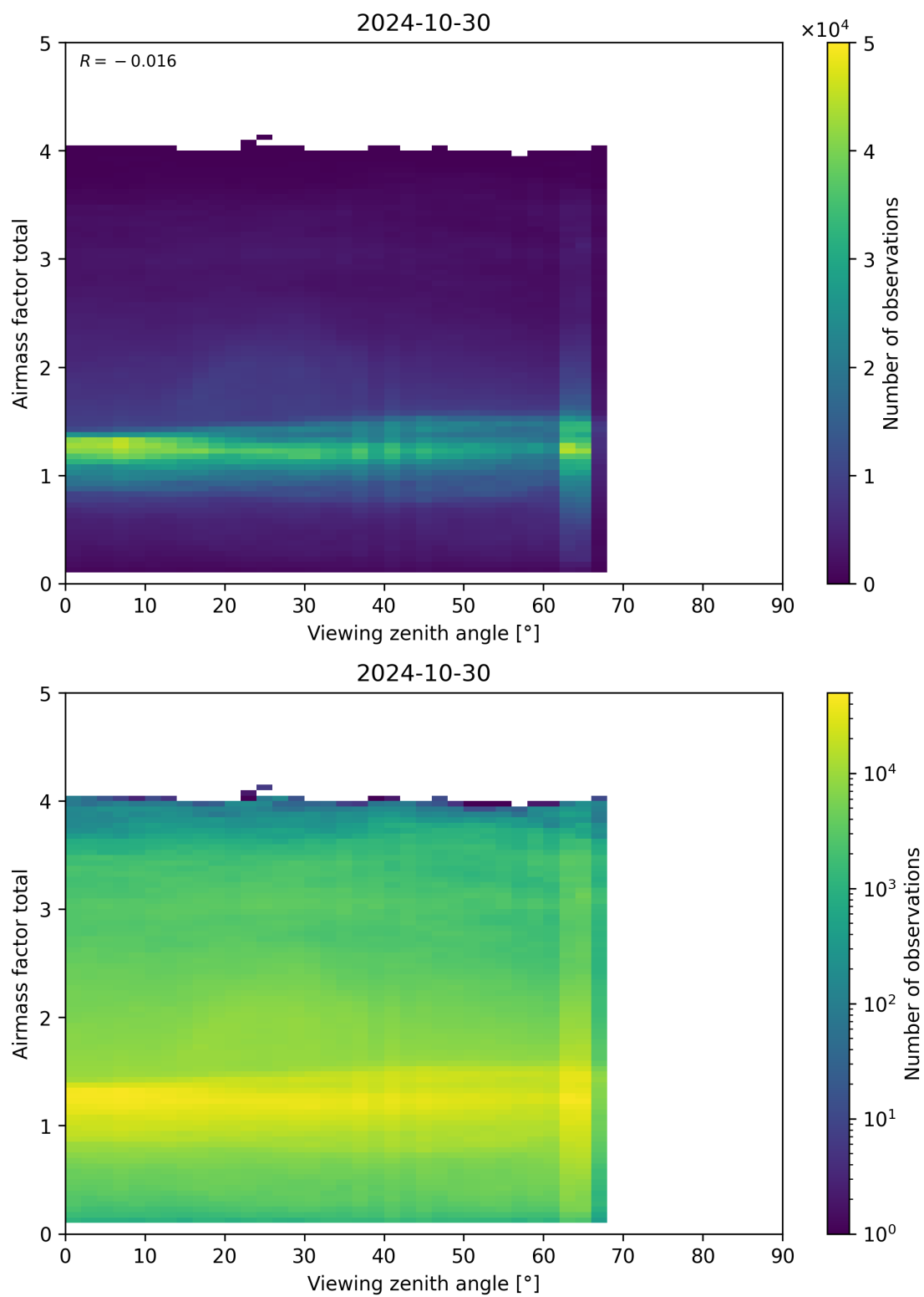
Figure 190: Scatter density plot of “Viewing zenith angle” against “Airmass factor total” for 2024-10-30 to 2024-10-31.
