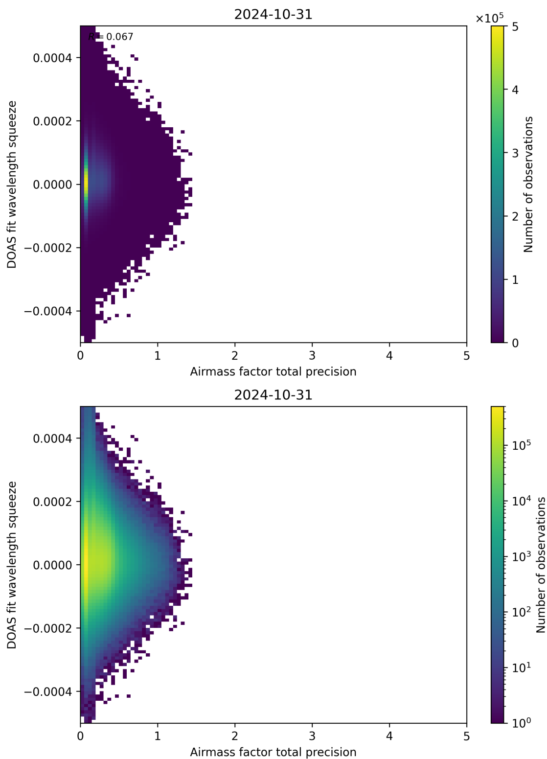
Figure 107: Scatter density plot of “Airmass factor total precision” against “DOAS fit wavelength squeeze” for 2024-10-30 to 2024-11-01.
