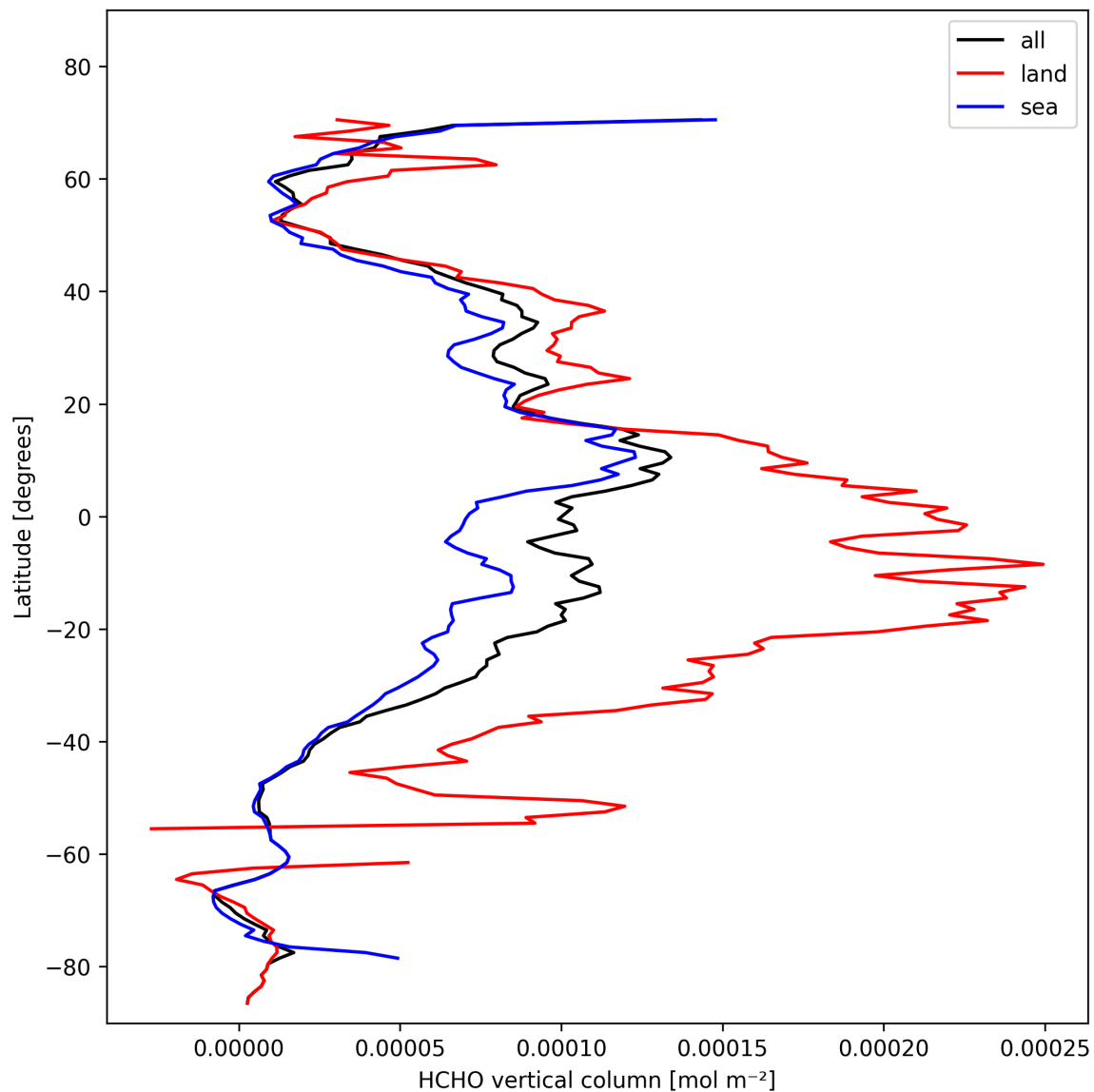
Figure 21: Zonal average of “HCHO vertical column” for 2024-10-30 to 2024-11-01.
