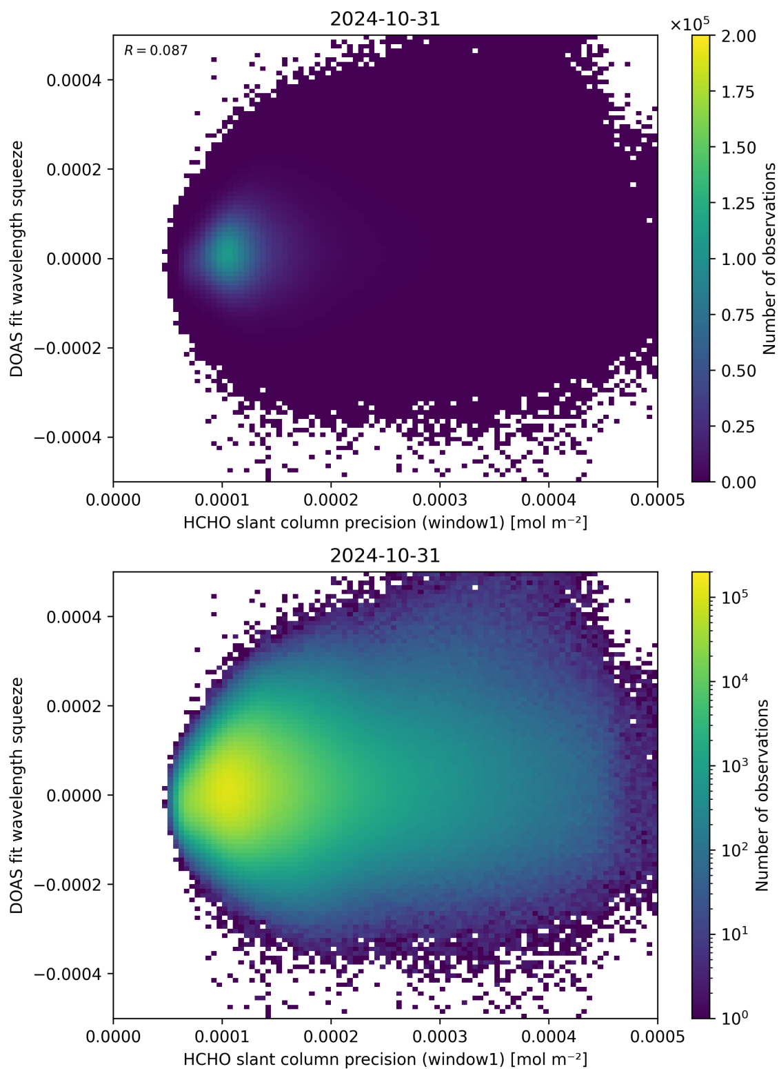
Figure 90: Scatter density plot of “HCHO slant column precision (window1)” against “DOAS fit wavelength squeeze” for 2024-10-30 to 2024-11-01.
