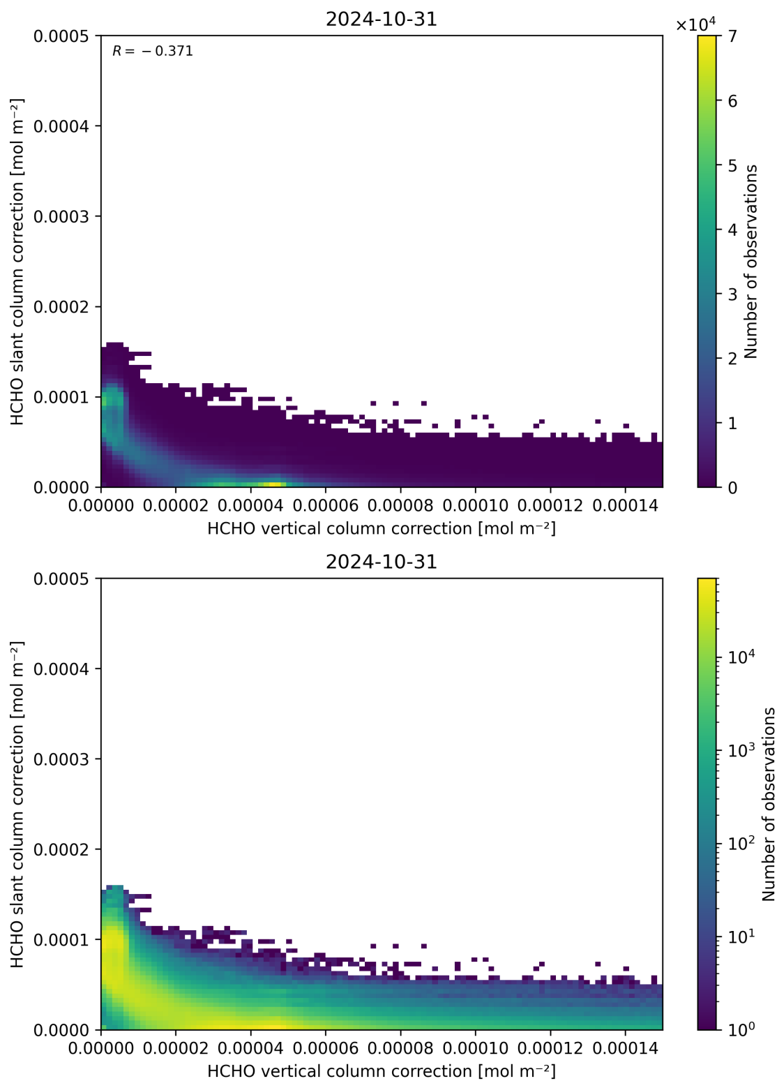
Figure 117: Scatter density plot of “HCHO vertical column correction” against “HCHO slant column correction” for 2024-10-30 to 2024-11-01.
