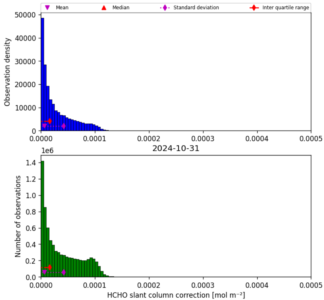
Figure 47: Histogram of “HCHO slant column correction” for 2024-10-30 to 2024-11-01
