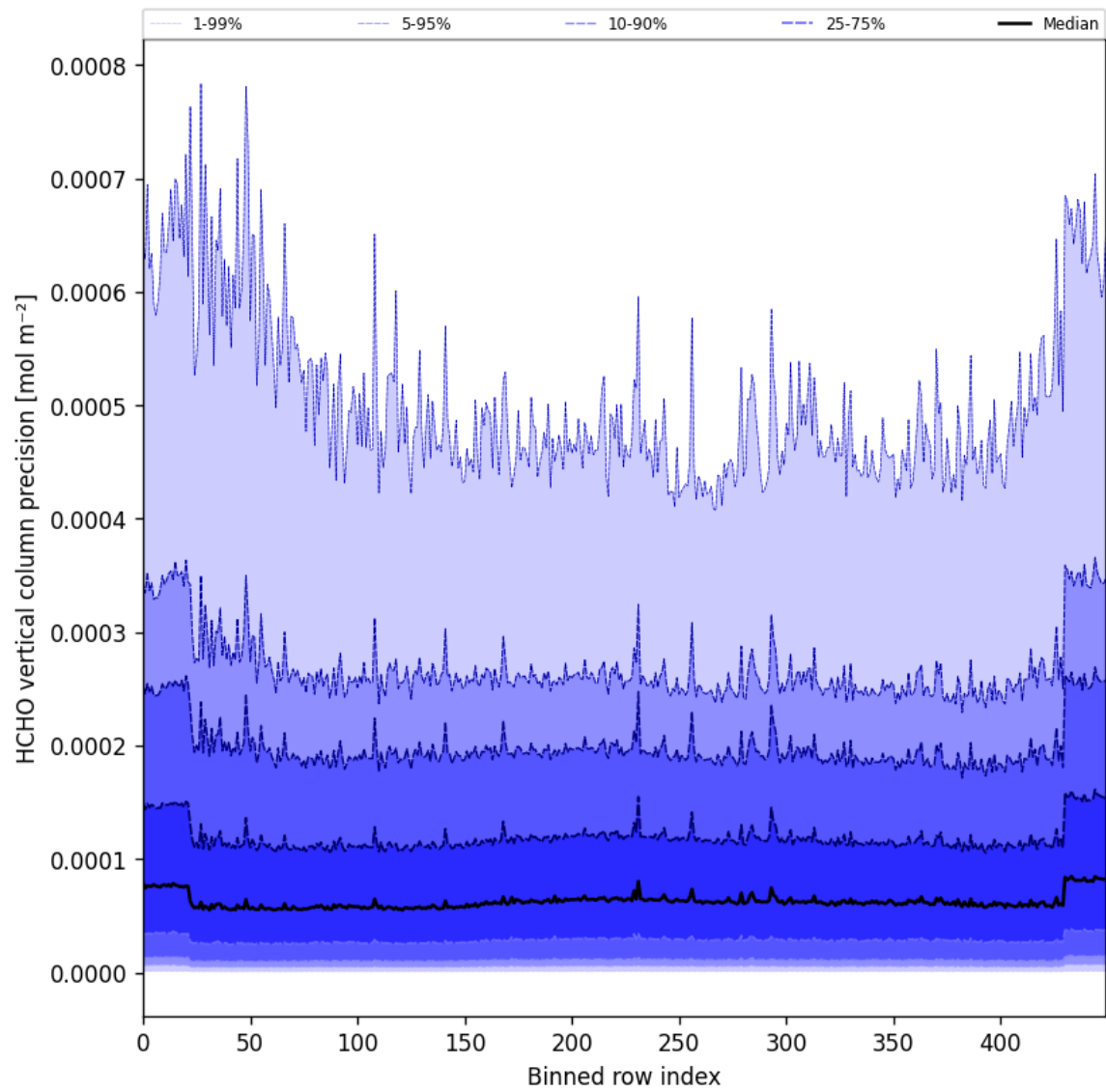
Figure 50: Along track statistics of “HCHO vertical column precision” for 2024-10-30 to 2024-11-01
