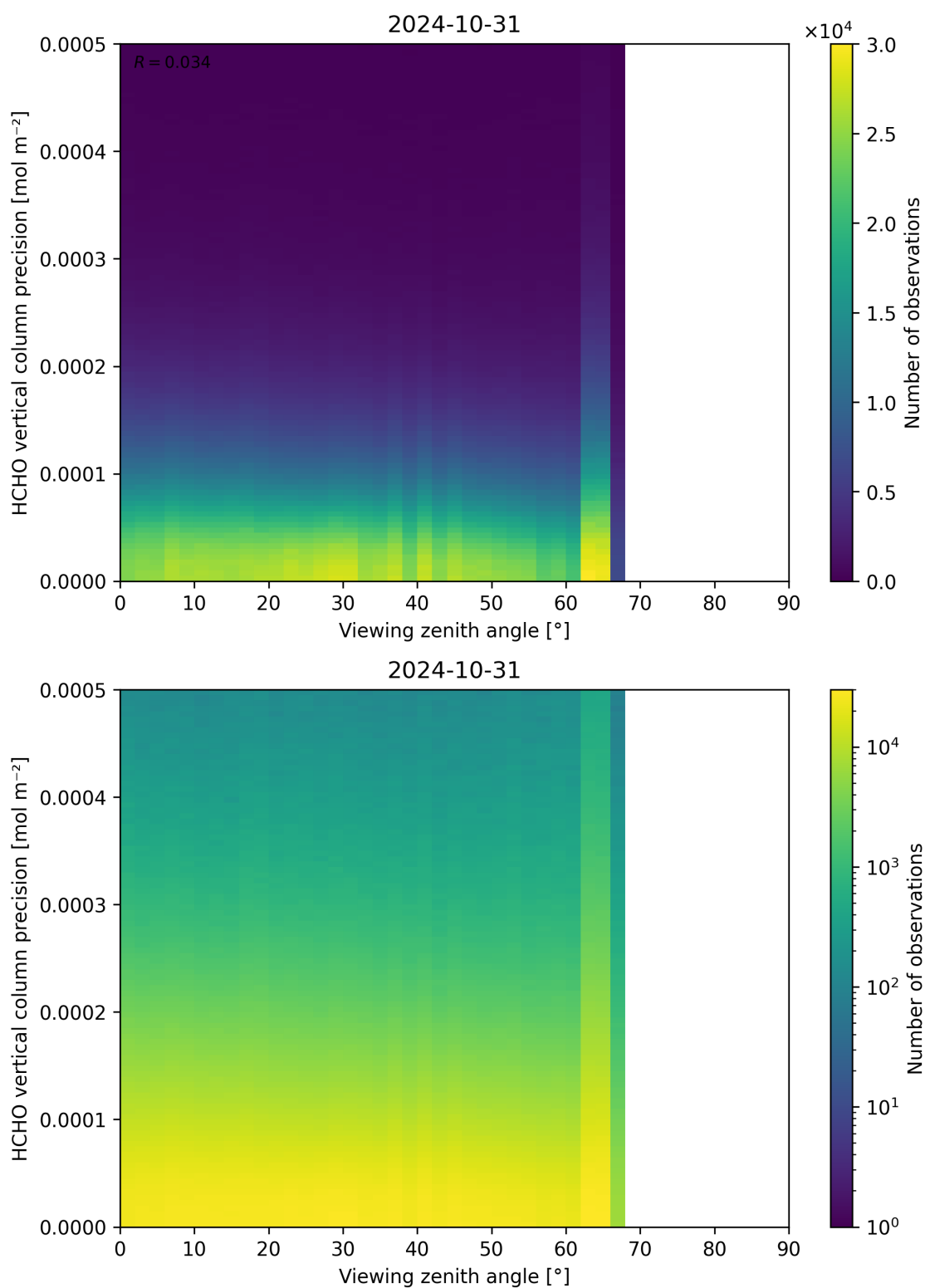
Figure 194: Scatter density plot of “Viewing zenith angle” against “HCHO vertical column precision” for 2024-10-30 to 2024-11-01.
