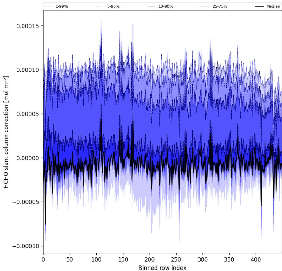
Figure 61: Along track statistics of “HCHO slant column correction” for 2024-10-30 to 2024-11-01
