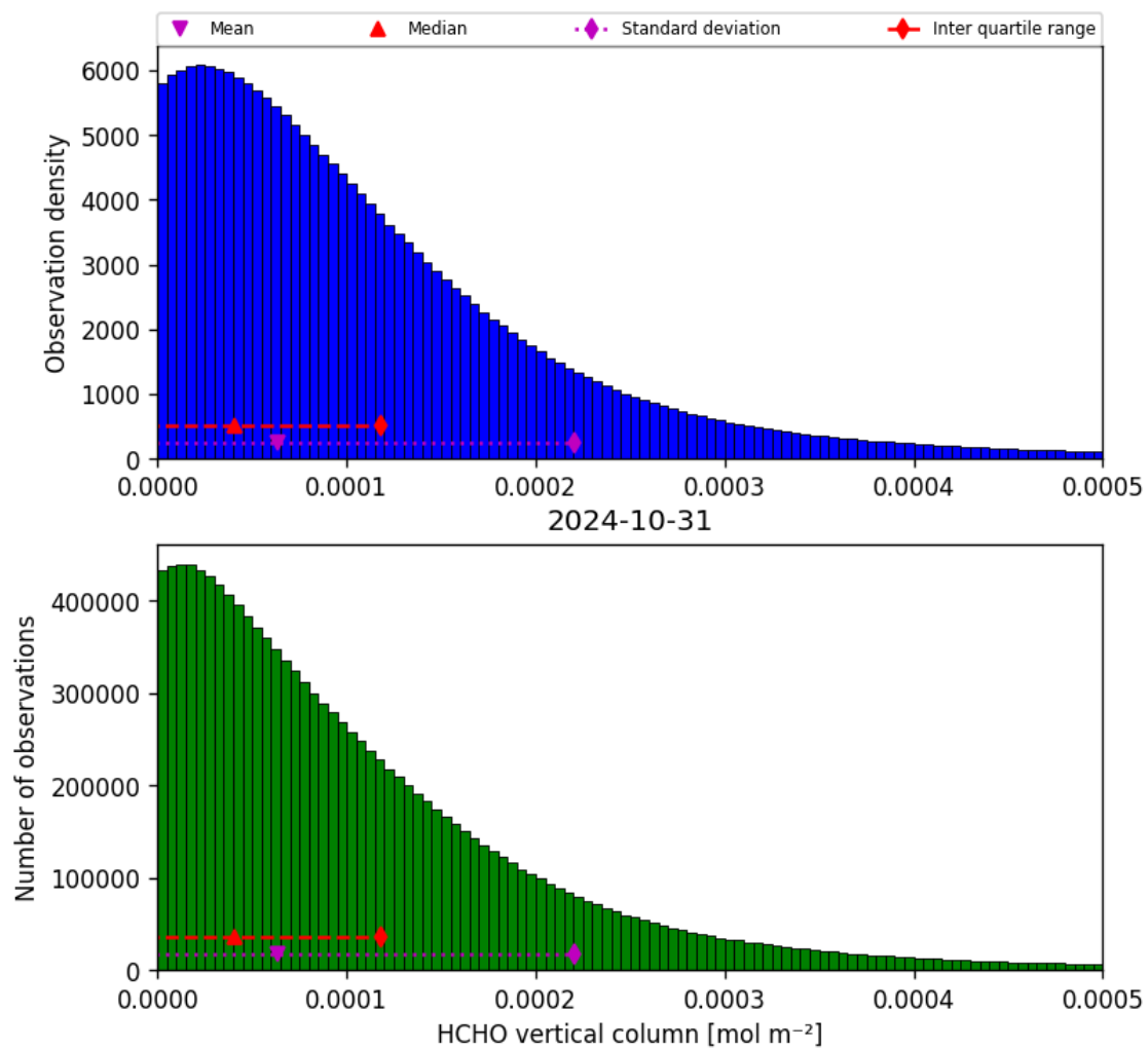
Figure 35: Histogram of “HCHO vertical column” for 2024-10-30 to 2024-11-01
