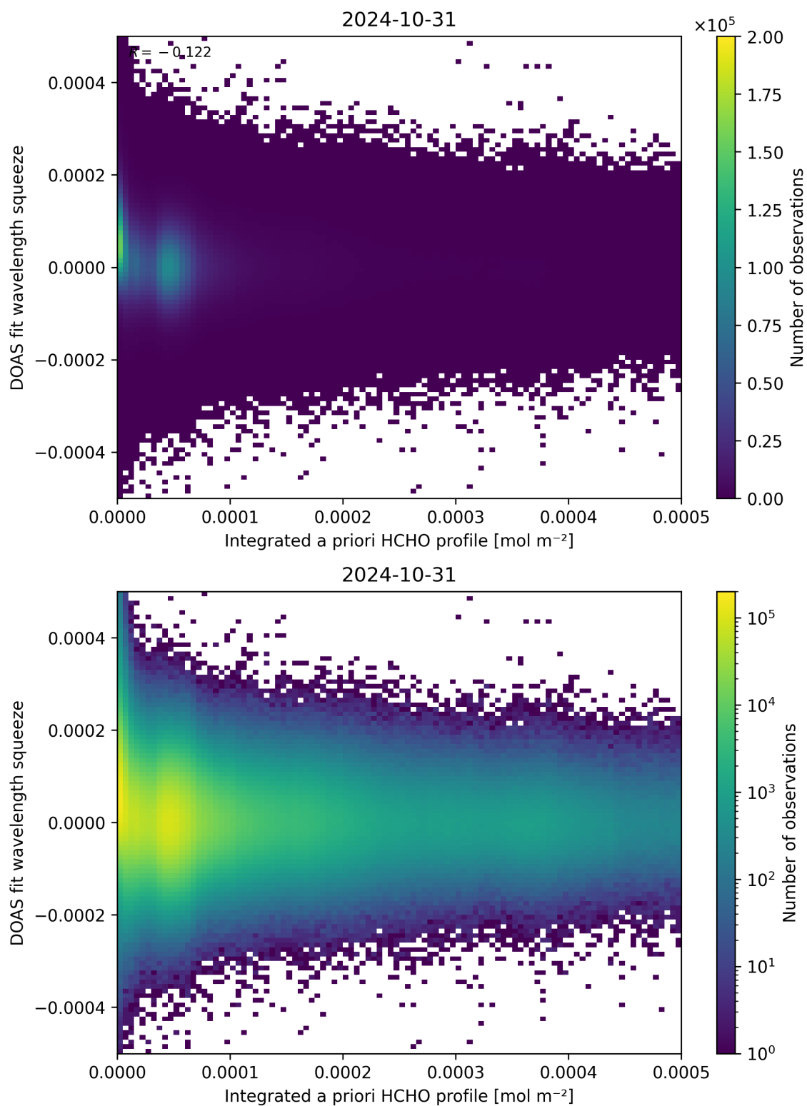
Figure 150: Scatter density plot of “Integrated a priori HCHO profile” against “DOAS fit wavelength squeeze” for 2024-10-30 to 2024-11-01.
