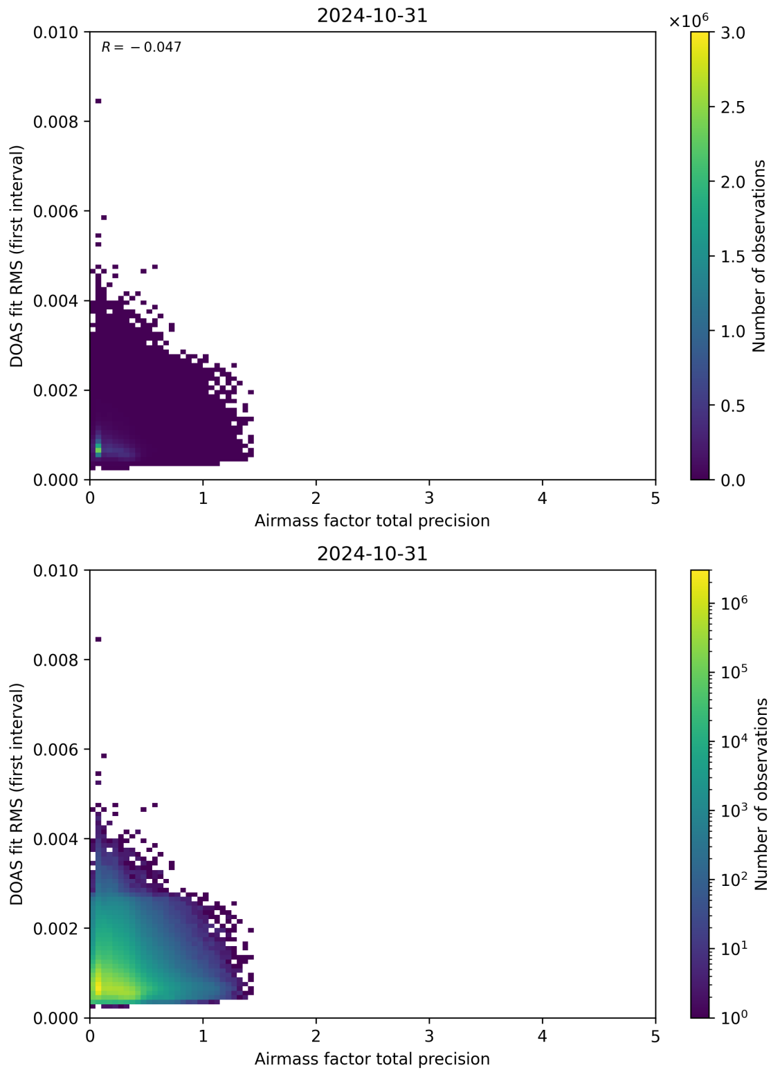
Figure 105: Scatter density plot of “Airmass factor total precision” against “DOAS fit RMS (first interval)” for 2024-10-30 to 2024-11-01.
