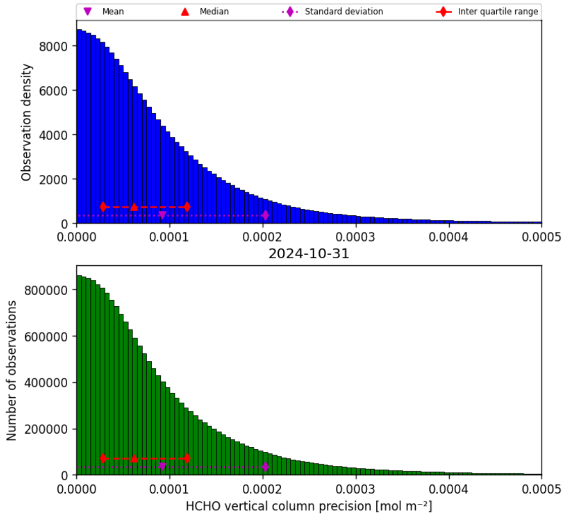
Figure 36: Histogram of “HCHO vertical column precision” for 2024-10-30 to 2024-11-01
