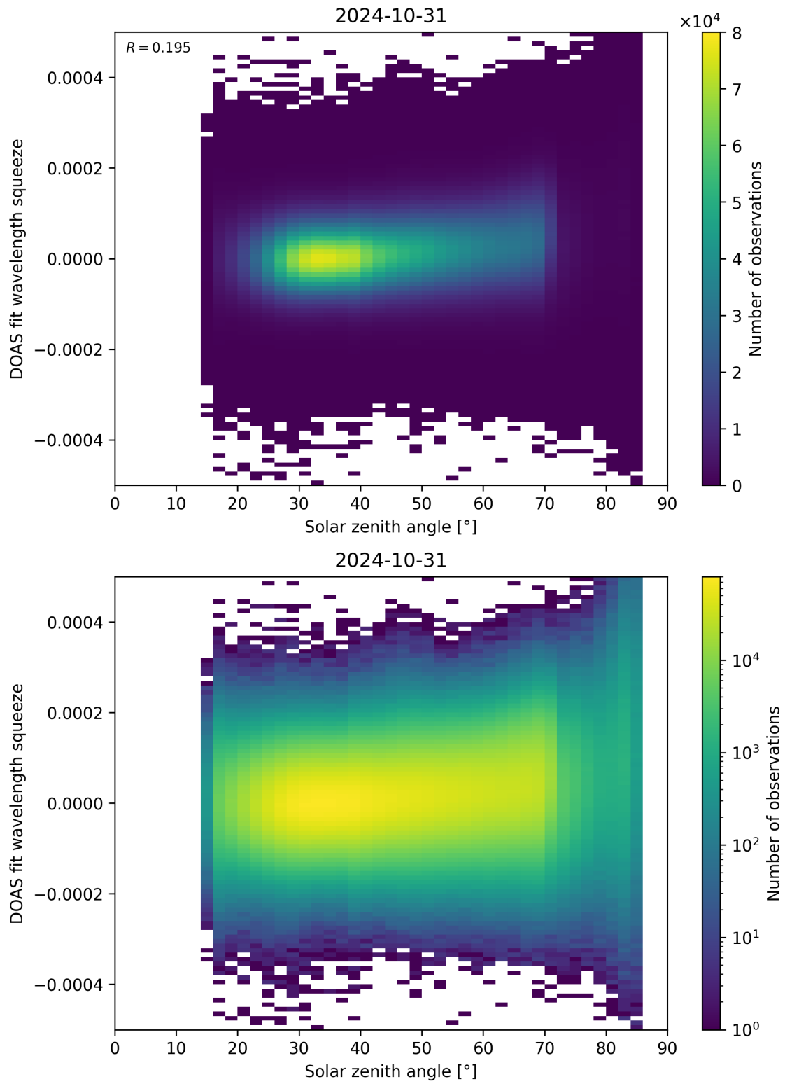
Figure 169: Scatter density plot of “Solar zenith angle” against “DOAS fit wavelength squeeze” for 2024-10-30 to 2024-11-01.
