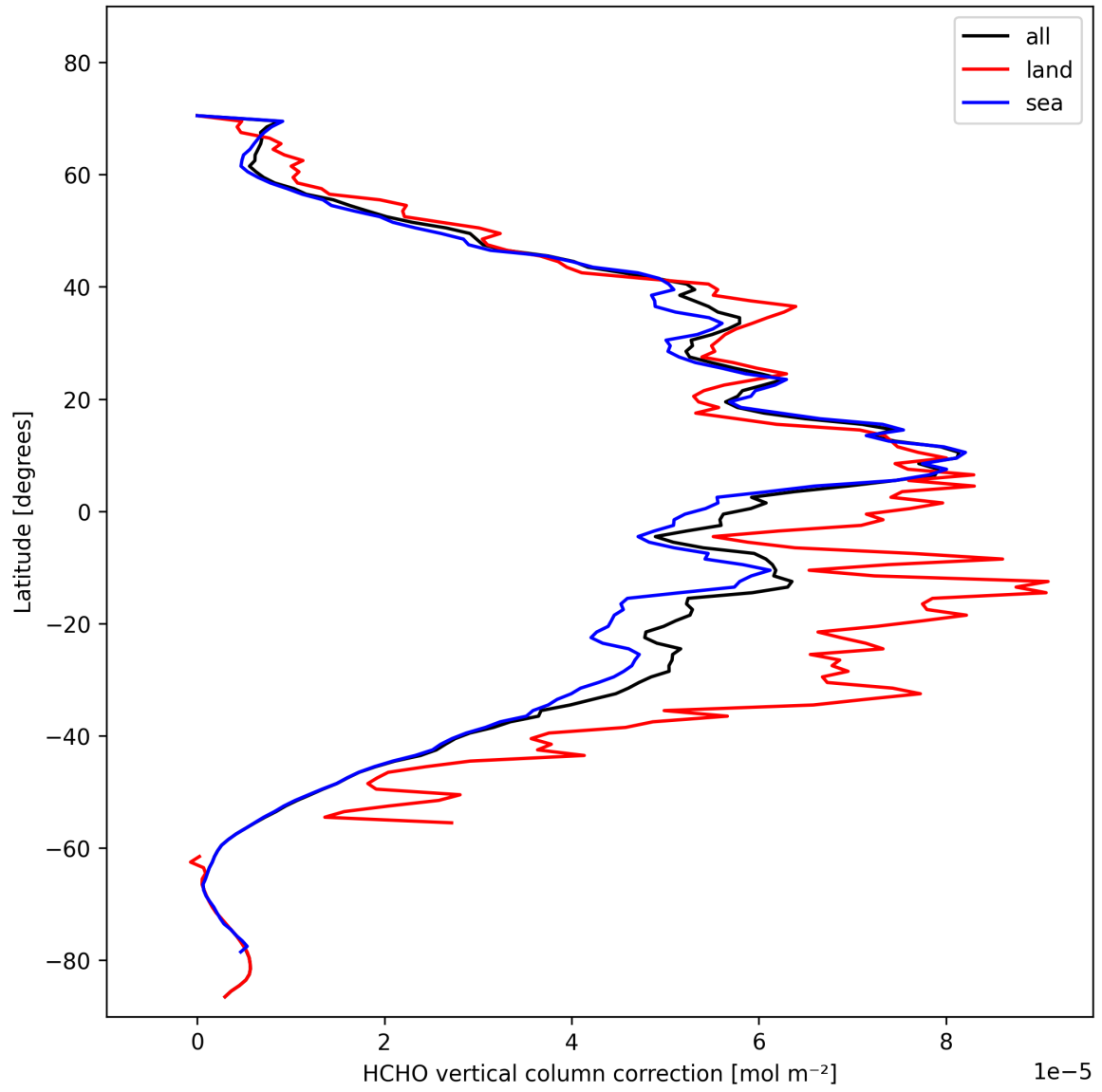
Figure 23: Zonal average of “HCHO vertical column correction” for 2024-10-30 to 2024-11-01.
