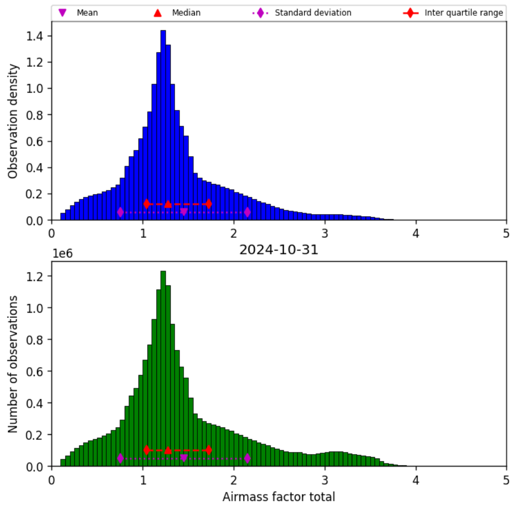
Figure 40: Histogram of “Airmass factor total” for 2024-10-30 to 2024-11-01
