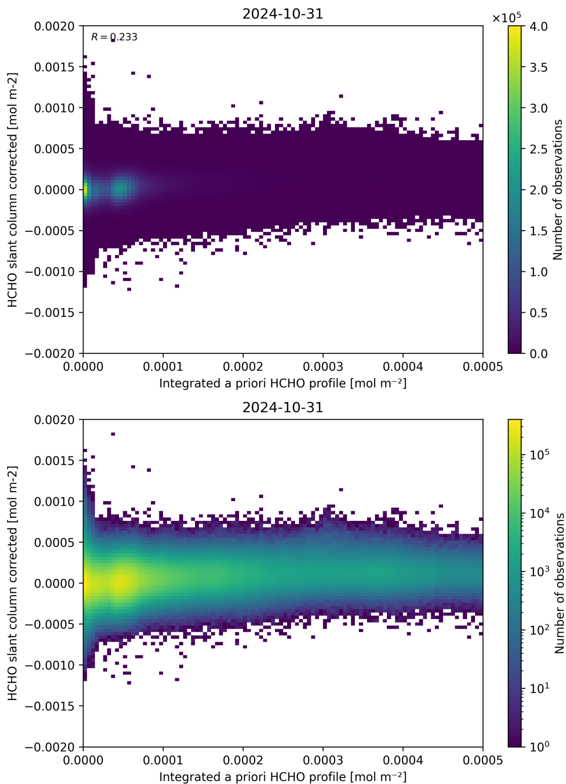
Figure 151: Scatter density plot of “Integrated a priori HCHO profile” against “HCHO slant column corrected” for 2024-10-30 to 2024-11-01.
