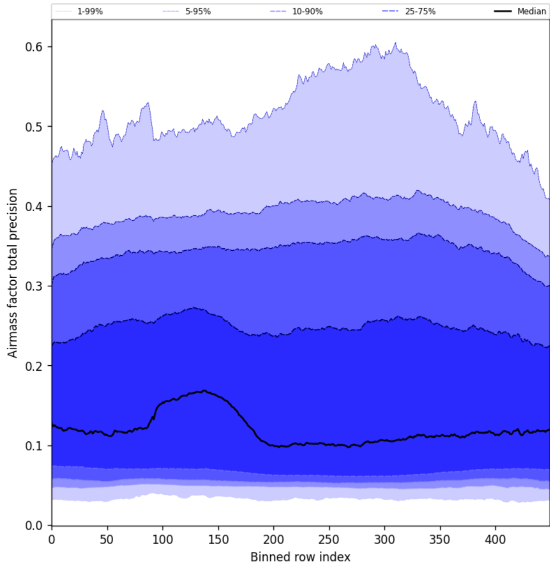
Figure 55: Along track statistics of “Airmass factor total precision” for 2024-10-30 to 2024-11-01
