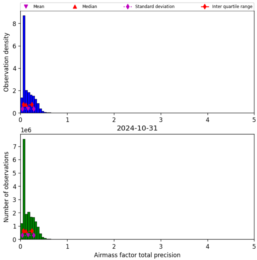
Figure 41: Histogram of “Airmass factor total precision” for 2024-10-30 to 2024-11-01
