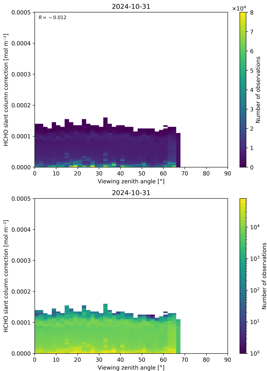
Figure 187: Scatter density plot of “Viewing zenith angle” against “HCHO slant column correction” for 2024-10-30 to 2024-11-01.
