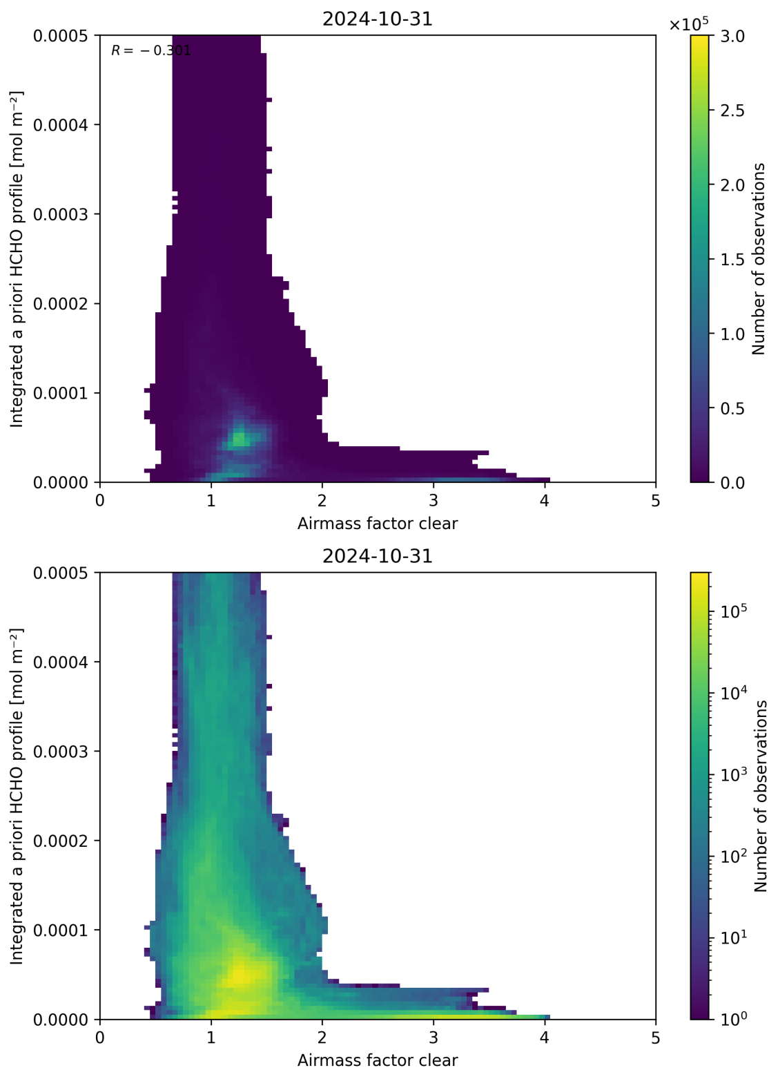
Figure 76: Scatter density plot of “Airmass factor clear” against “Integrated a priori HCHO profile” for 2024-10-30 to 2024-11-01.
