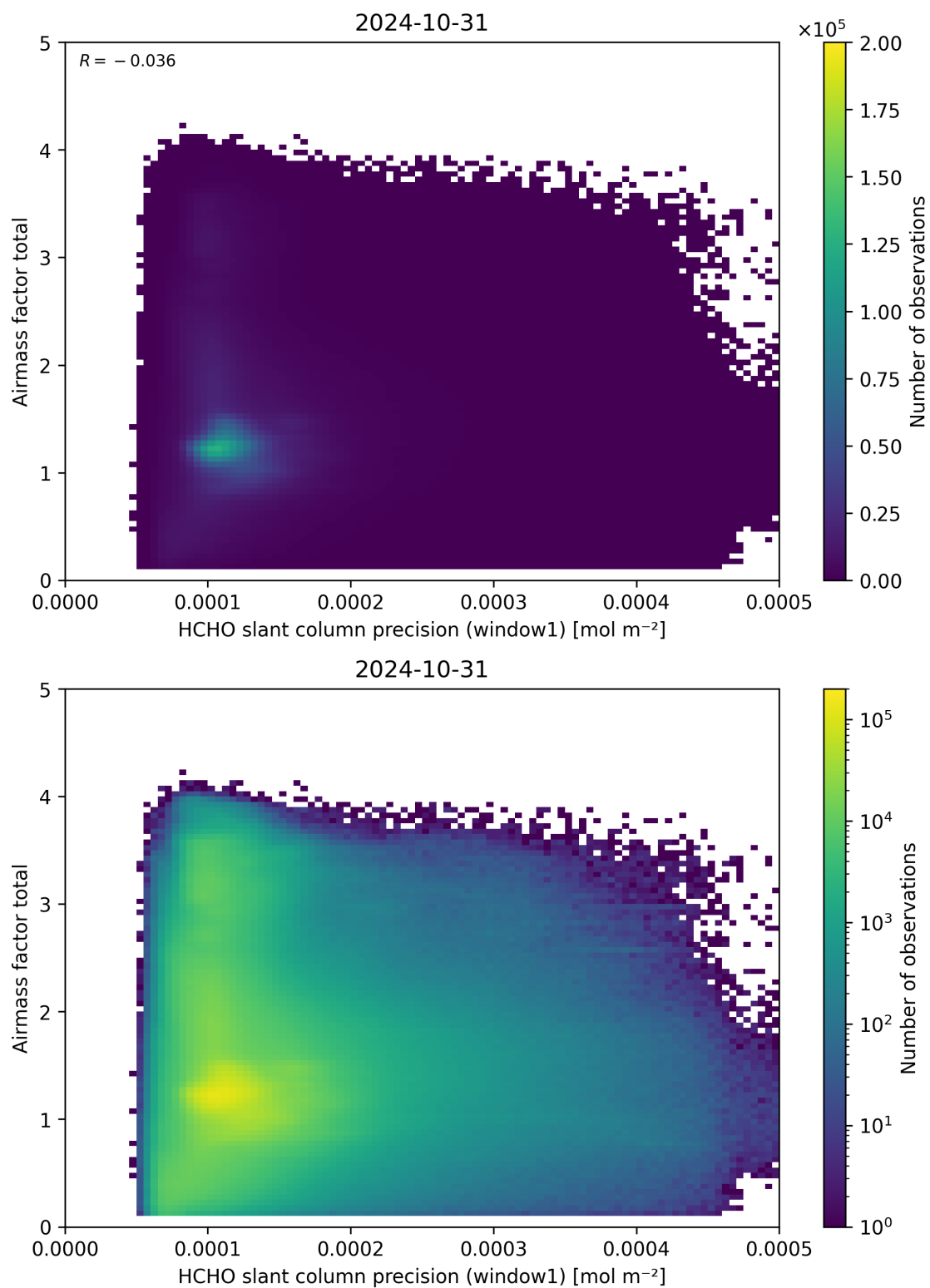
Figure 94: Scatter density plot of “HCHO slant column precision (window1)” against “Airmass factor total” for 2024-10-30 to 2024-11-01.
