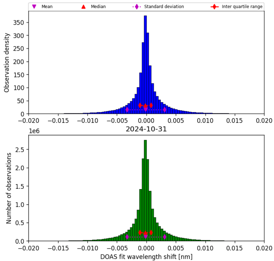
Figure 44: Histogram of “DOAS fit wavelength shift” for 2024-10-30 to 2024-11-01
