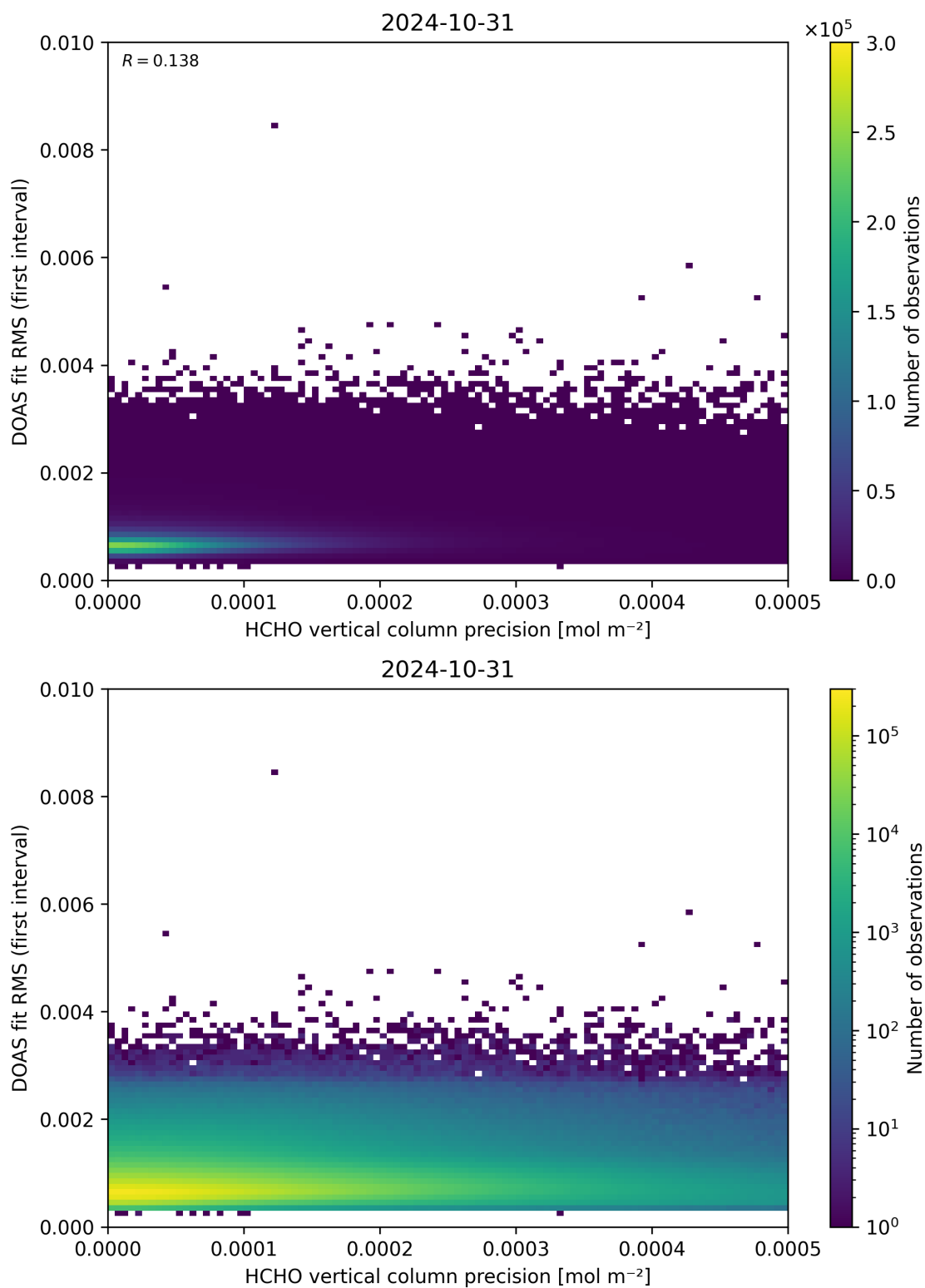
Figure 136: Scatter density plot of “HCHO vertical column precision” against “DOAS fit RMS (first interval)” for 2024-10-30 to 2024-11-01.
