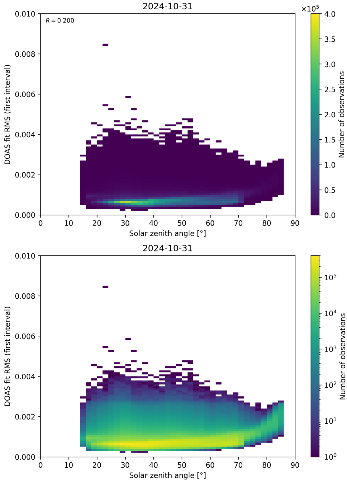
Figure 167: Scatter density plot of “Solar zenith angle” against “DOAS fit RMS (first interval)” for 2024-10-30 to 2024-11-01.
