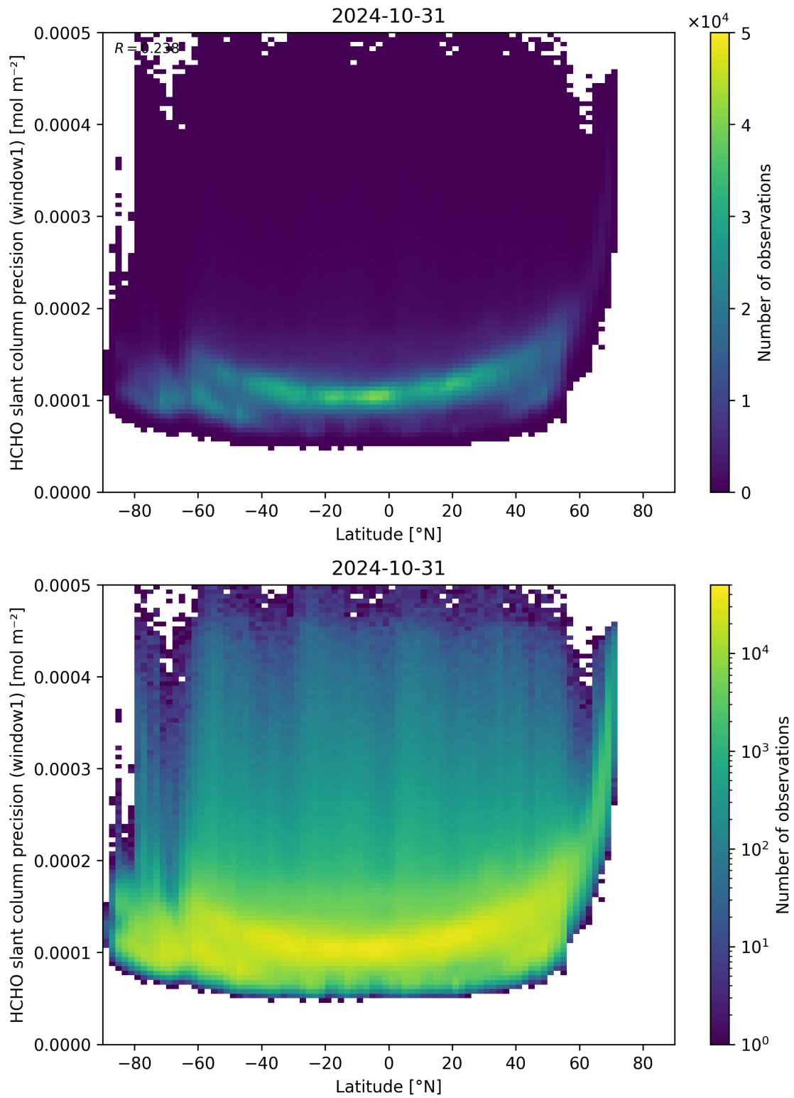
Figure 160: Scatter density plot of “Latitude” against “HCHO slant column precision (window1)” for 2024-10-30 to 2024-11-01.
