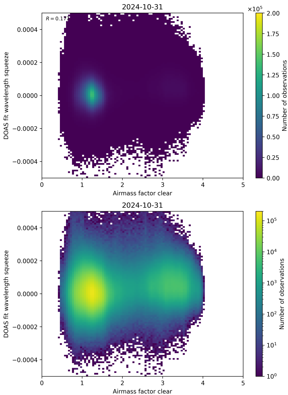
Figure 73: Scatter density plot of “Airmass factor clear” against “DOAS fit wavelength squeeze” for 2024-10-30 to 2024-11-01.
