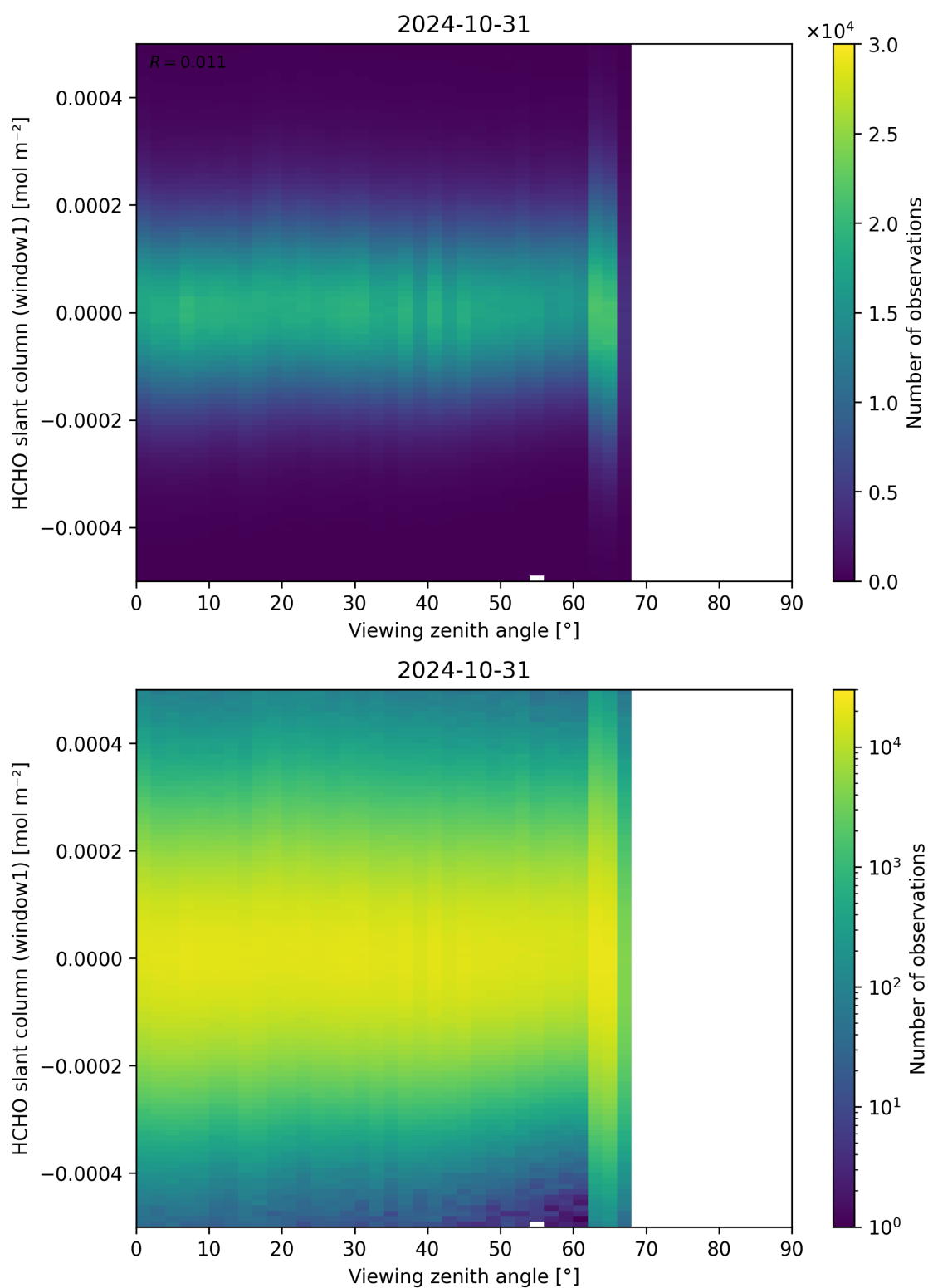
Figure 188: Scatter density plot of “Viewing zenith angle” against “HCHO slant column (window1)” for 2024-10-30 to 2024-11-01.
