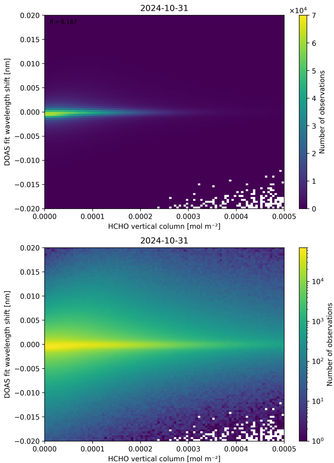
Figure 124: Scatter density plot of “HCHO vertical column” against “DOAS fit wavelength shift” for 2024-10-30 to 2024-11-01.
