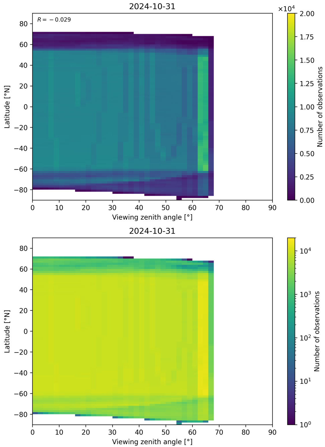
Figure 196: Scatter density plot of “Viewing zenith angle” against “Latitude” for 2024-10-30 to 2024-11-01.
