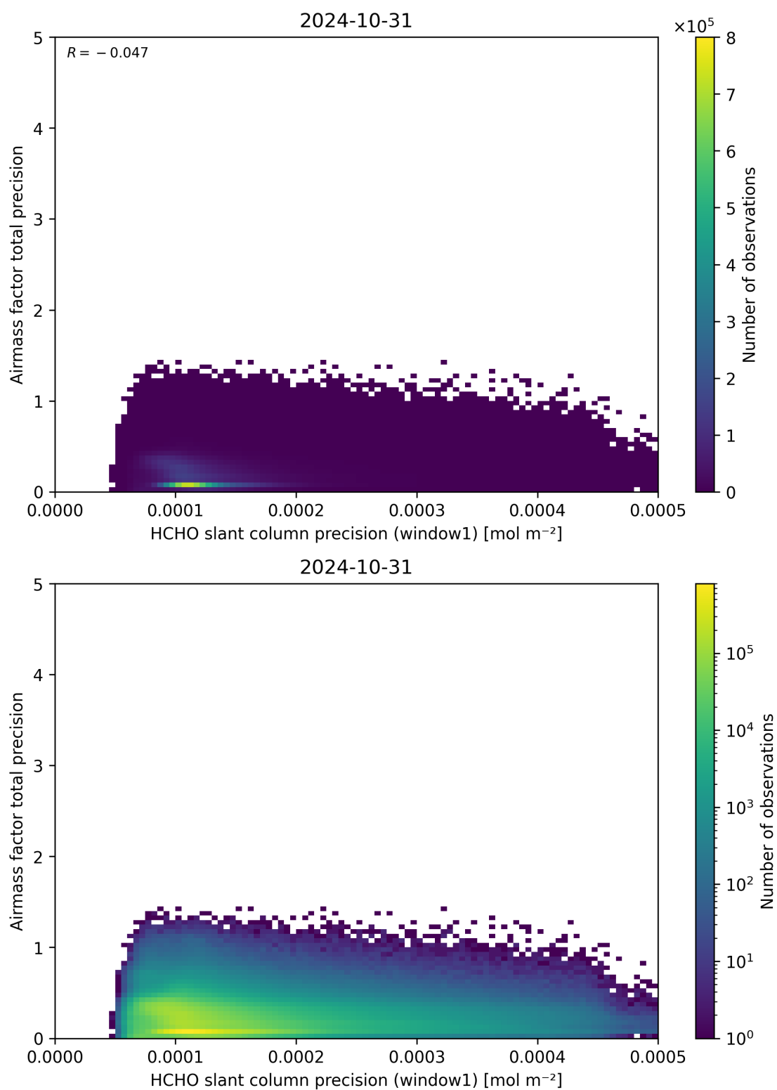
Figure 95: Scatter density plot of “HCHO slant column precision (window1)” against “Airmass factor total precision” for 2024-10-30 to 2024-11-01.
