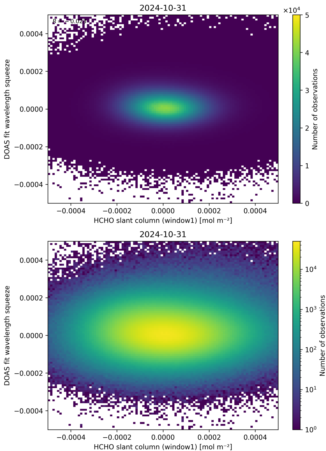
Figure 80: Scatter density plot of “HCHO slant column (window1)” against “DOAS fit wavelength squeeze” for 2024-10-30 to 2024-11-01.
