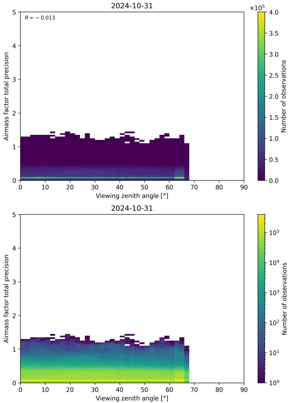
Figure 191: Scatter density plot of “Viewing zenith angle” against “Airmass factor total precision” for 2024-10-30 to 2024-11-01.
