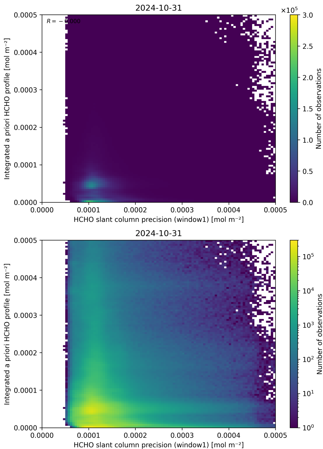
Figure 96: Scatter density plot of “HCHO slant column precision (window1)” against “Integrated a priori HCHO profile” for 2024-10-30 to 2024-11-01.
