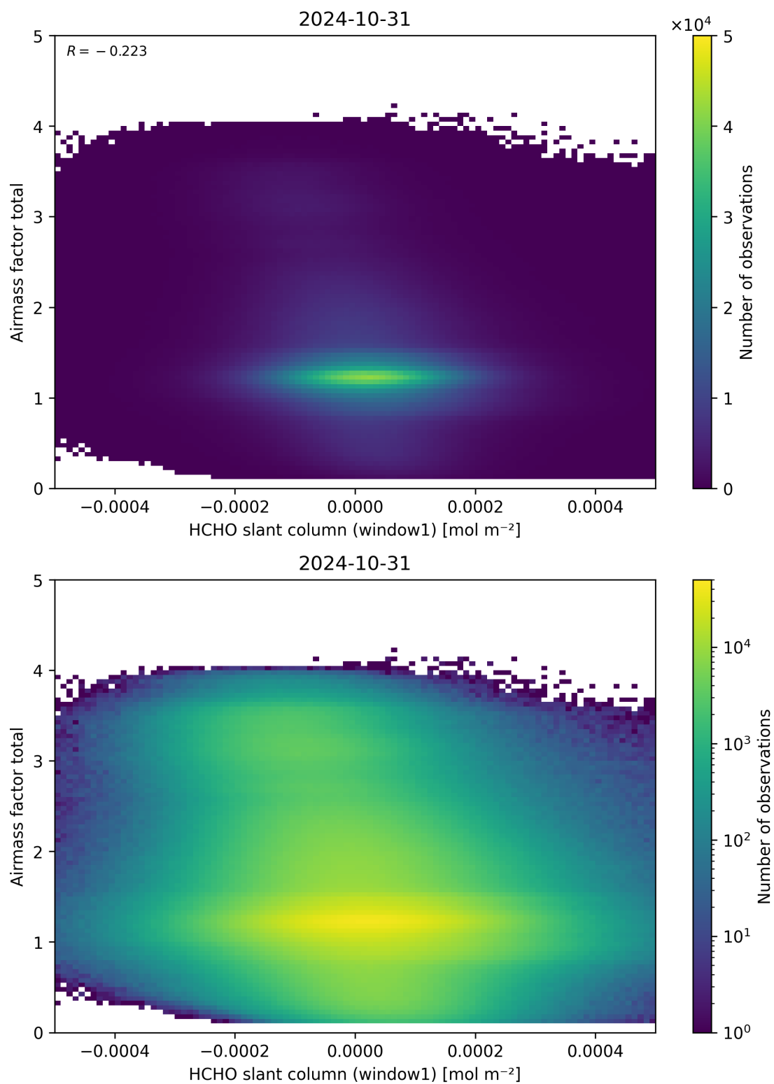
Figure 85: Scatter density plot of “HCHO slant column (window1)” against “Airmass factor total” for 2024-10-30 to 2024-11-01.
