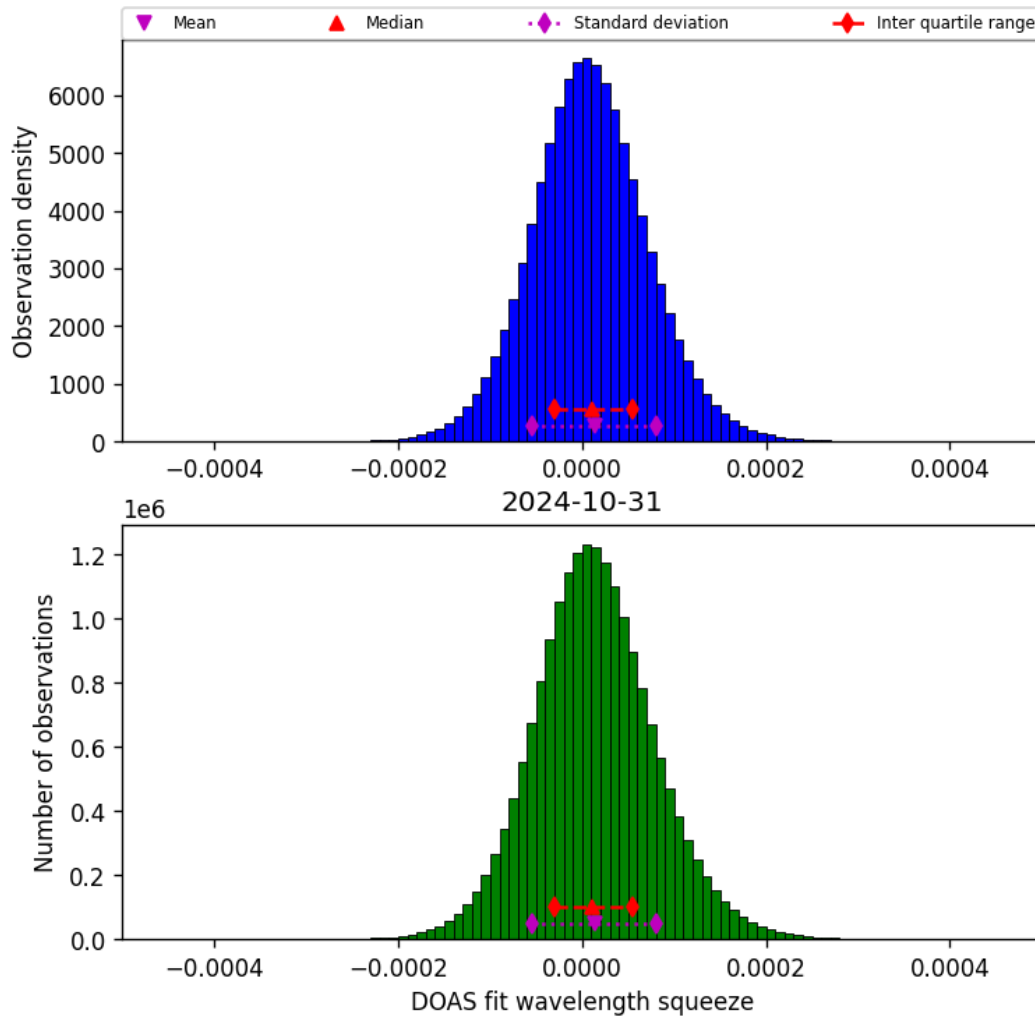
Figure 45: Histogram of “DOAS fit wavelength squeeze” for 2024-10-30 to 2024-11-01
