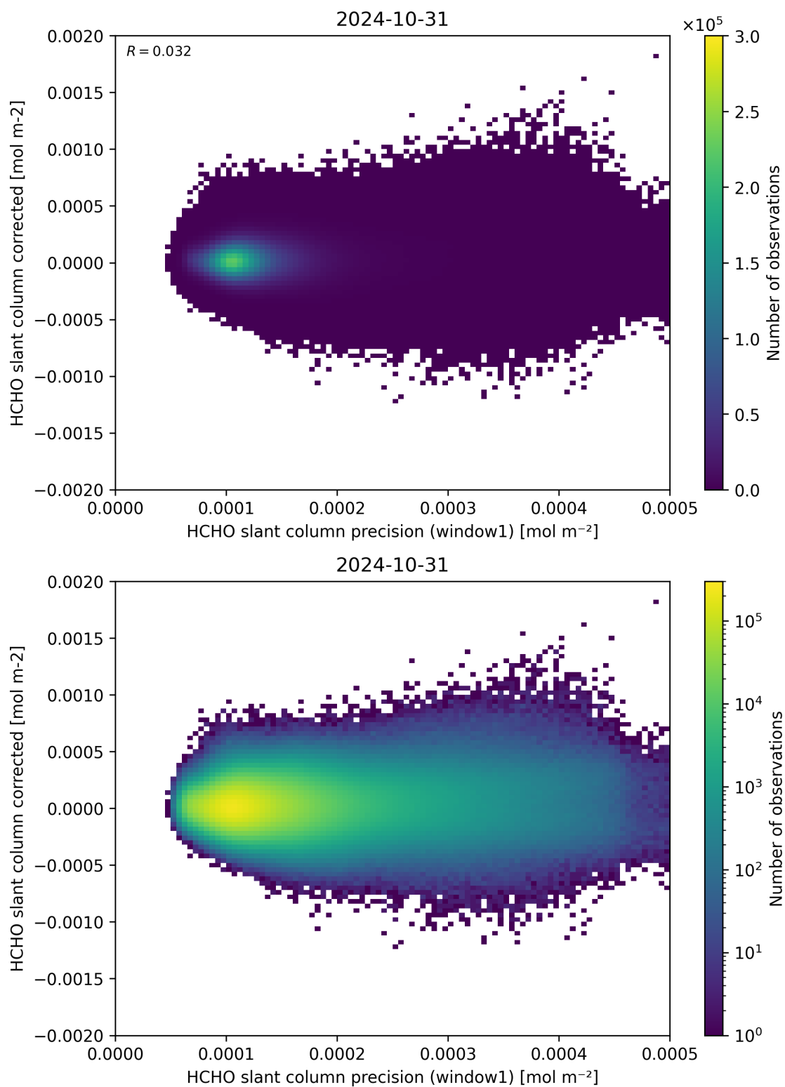
Figure 92: Scatter density plot of “HCHO slant column precision (window1)” against “HCHO slant column corrected” for 2024-10-30 to 2024-11-01.
