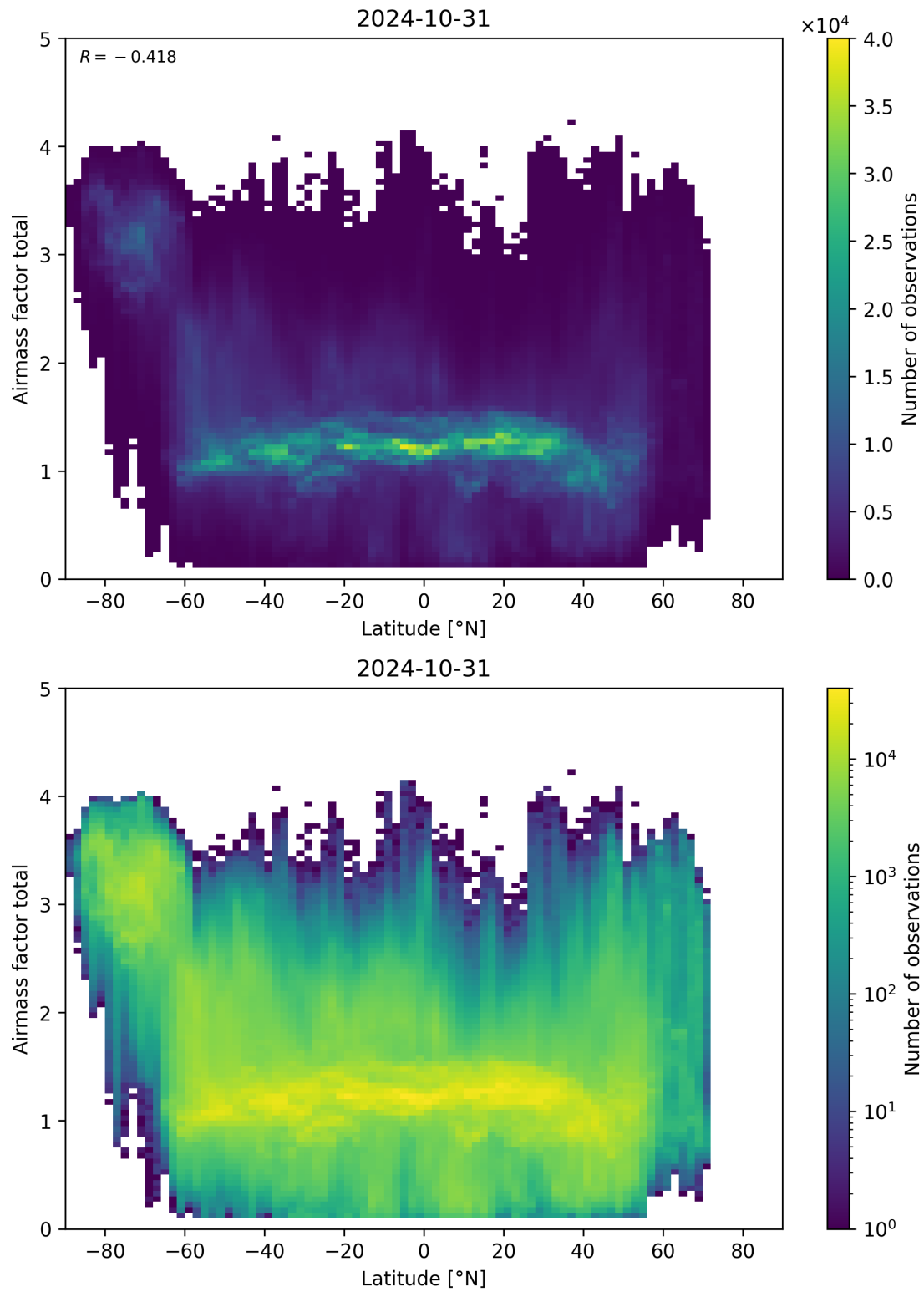
Figure 161: Scatter density plot of “Latitude” against “Airmass factor total” for 2024-10-30 to 2024-11-01.
