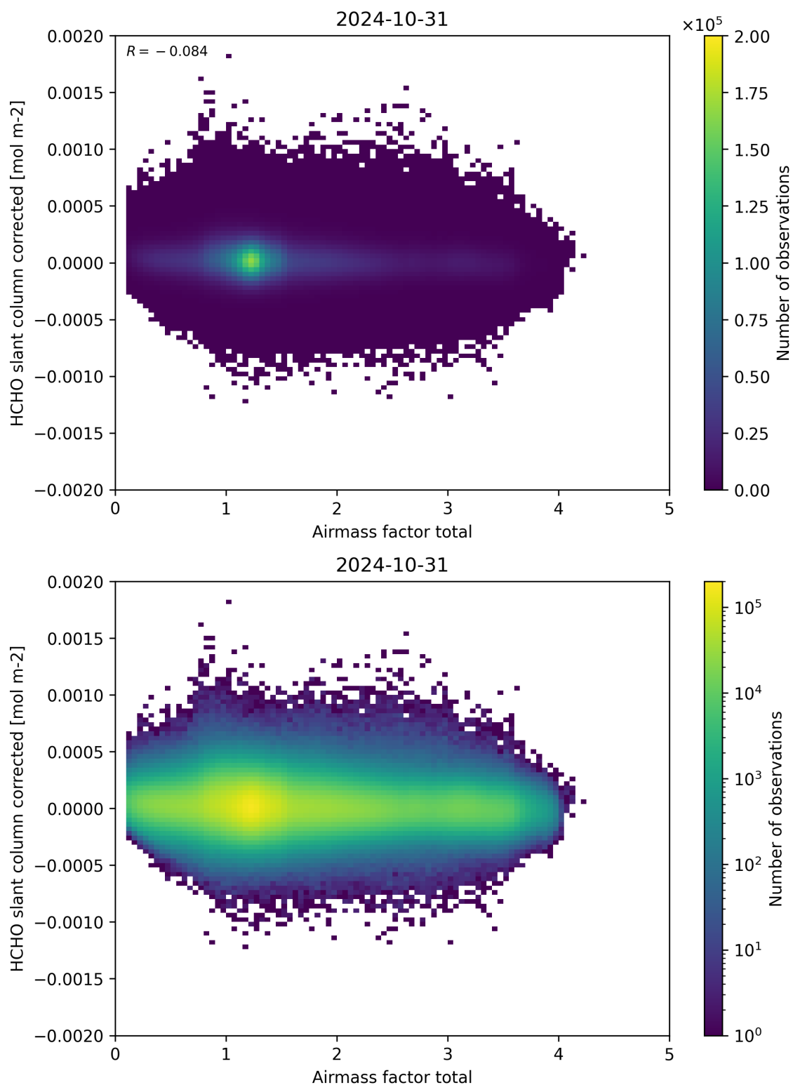
Figure 101: Scatter density plot of “Airmass factor total” against “HCHO slant column corrected” for 2024-10-30 to 2024-11-01.
