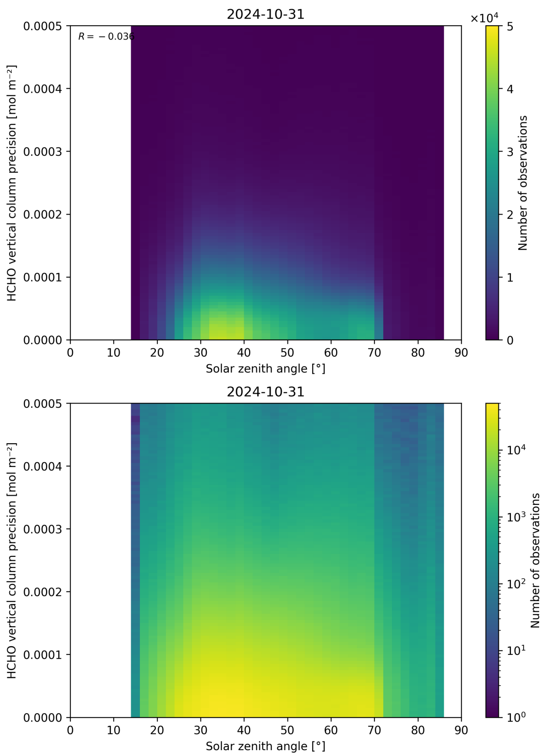
Figure 179: Scatter density plot of “Solar zenith angle” against “HCHO vertical column precision” for 2024-10-30 to 2024-11-01.
