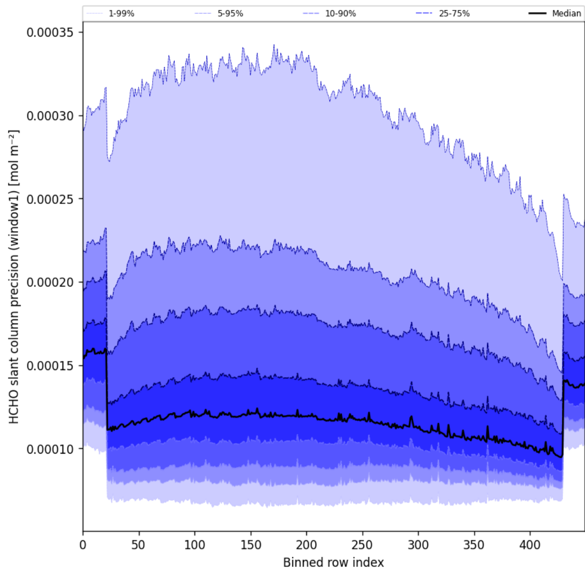
Figure 53: Along track statistics of “HCHO slant column precision (window1)” for 2024-10-30 to 2024-11-01
