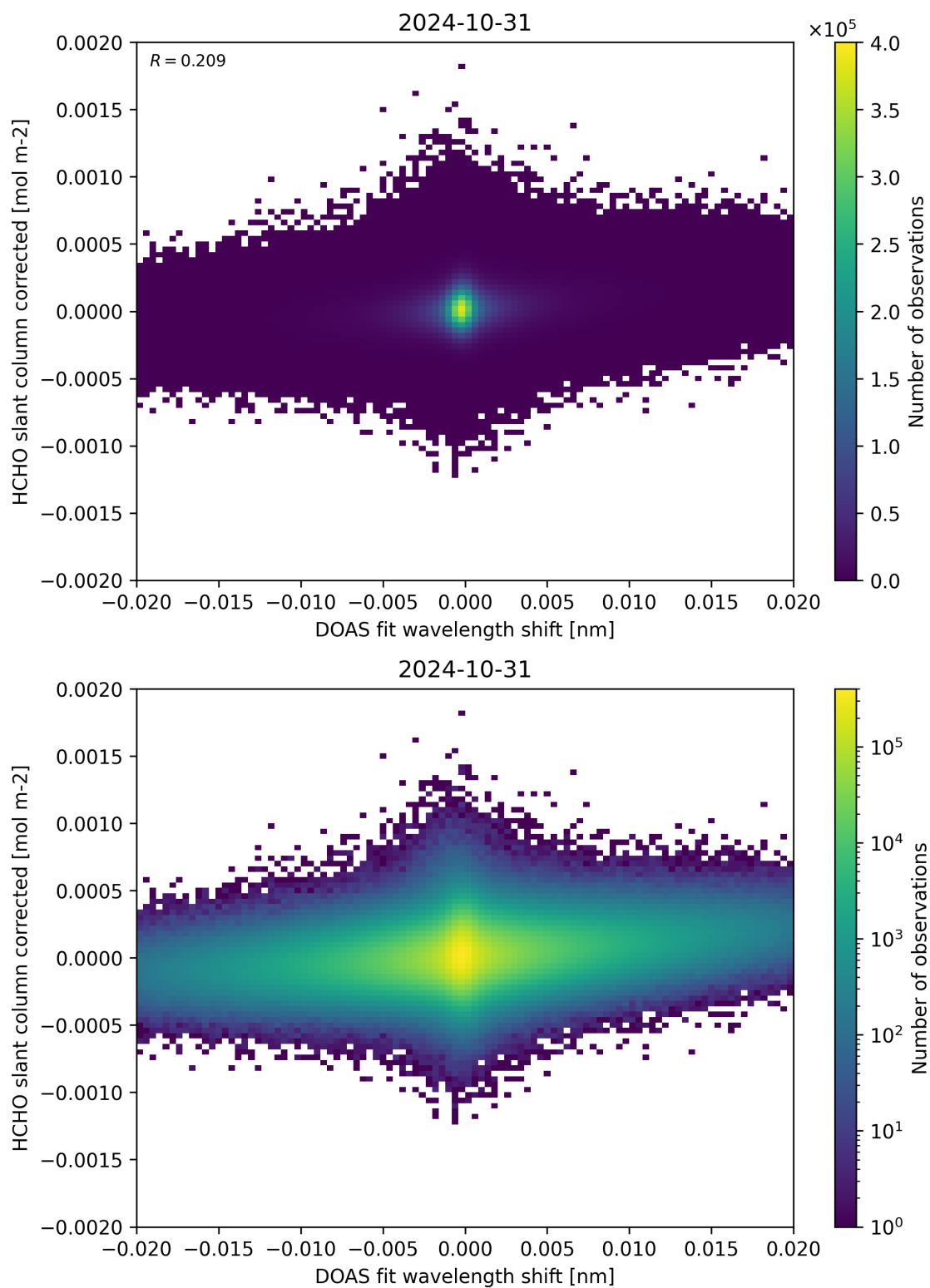
Figure 66: Scatter density plot of “DOAS fit wavelength shift” against “HCHO slant column corrected” for 2024-10-30 to 2024-11-01.
