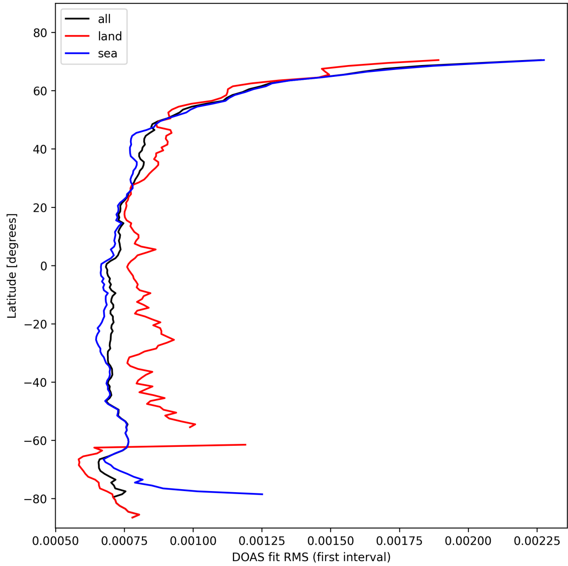
Figure 32: Zonal average of “DOAS fit RMS (first interval)” for 2024-10-30 to 2024-11-01.
