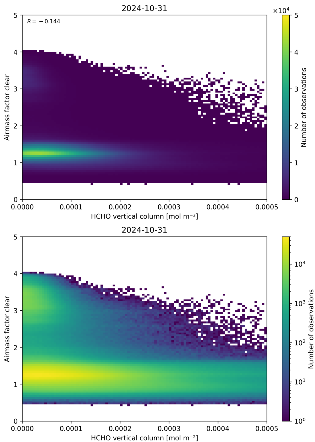
Figure 126: Scatter density plot of “HCHO vertical column” against “Airmass factor clear” for 2024-10-30 to 2024-11-01.
