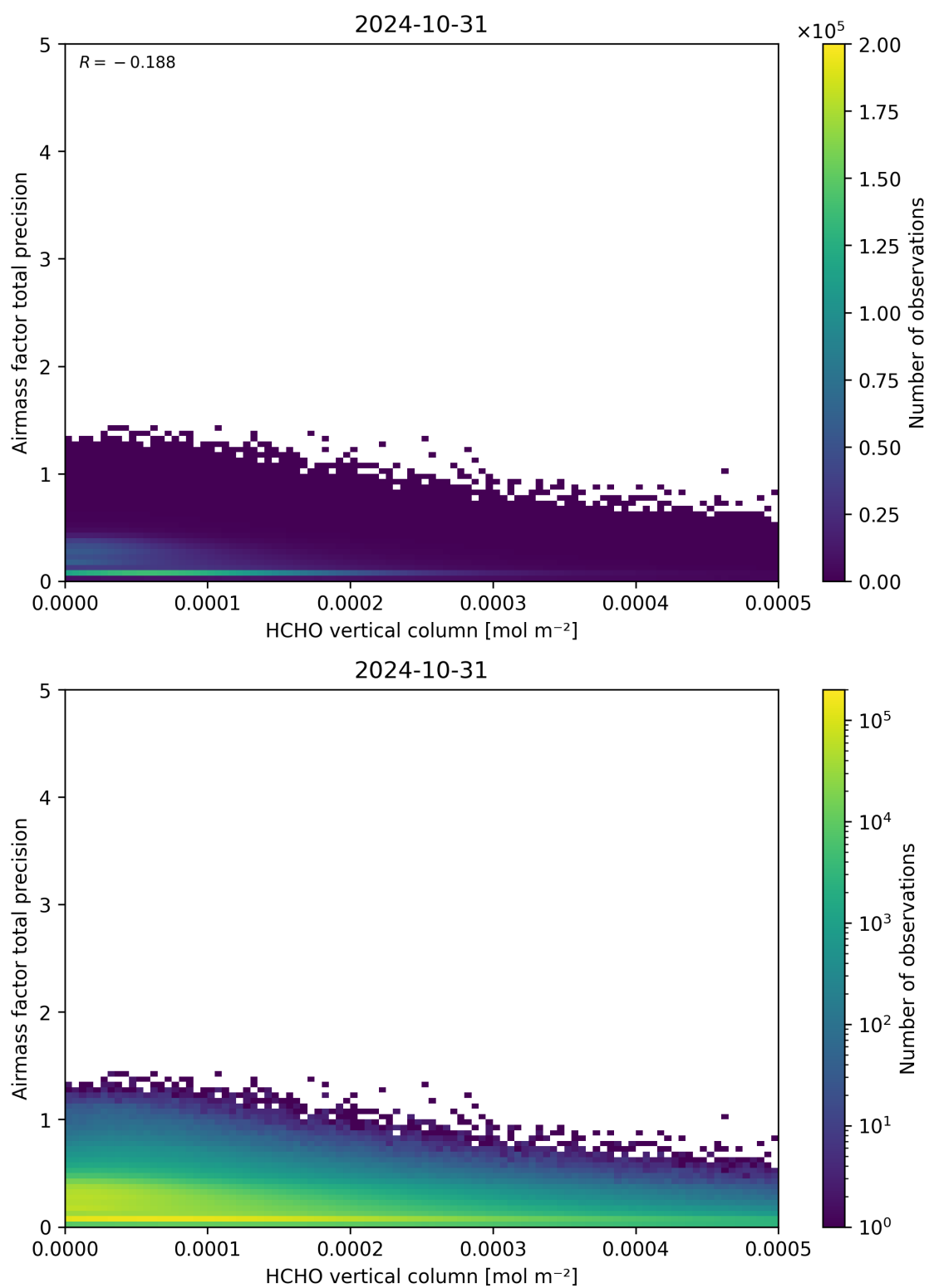
Figure 132: Scatter density plot of “HCHO vertical column” against “Airmass factor total precision” for 2024-10-30 to 2024-11-01.
