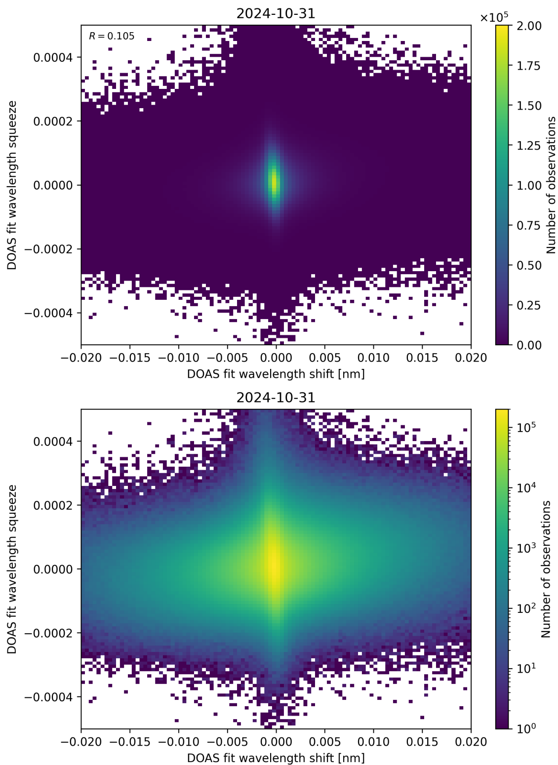
Figure 65: Scatter density plot of “DOAS fit wavelength shift” against “DOAS fit wavelength squeeze” for 2024-10-30 to 2024-11-01.
