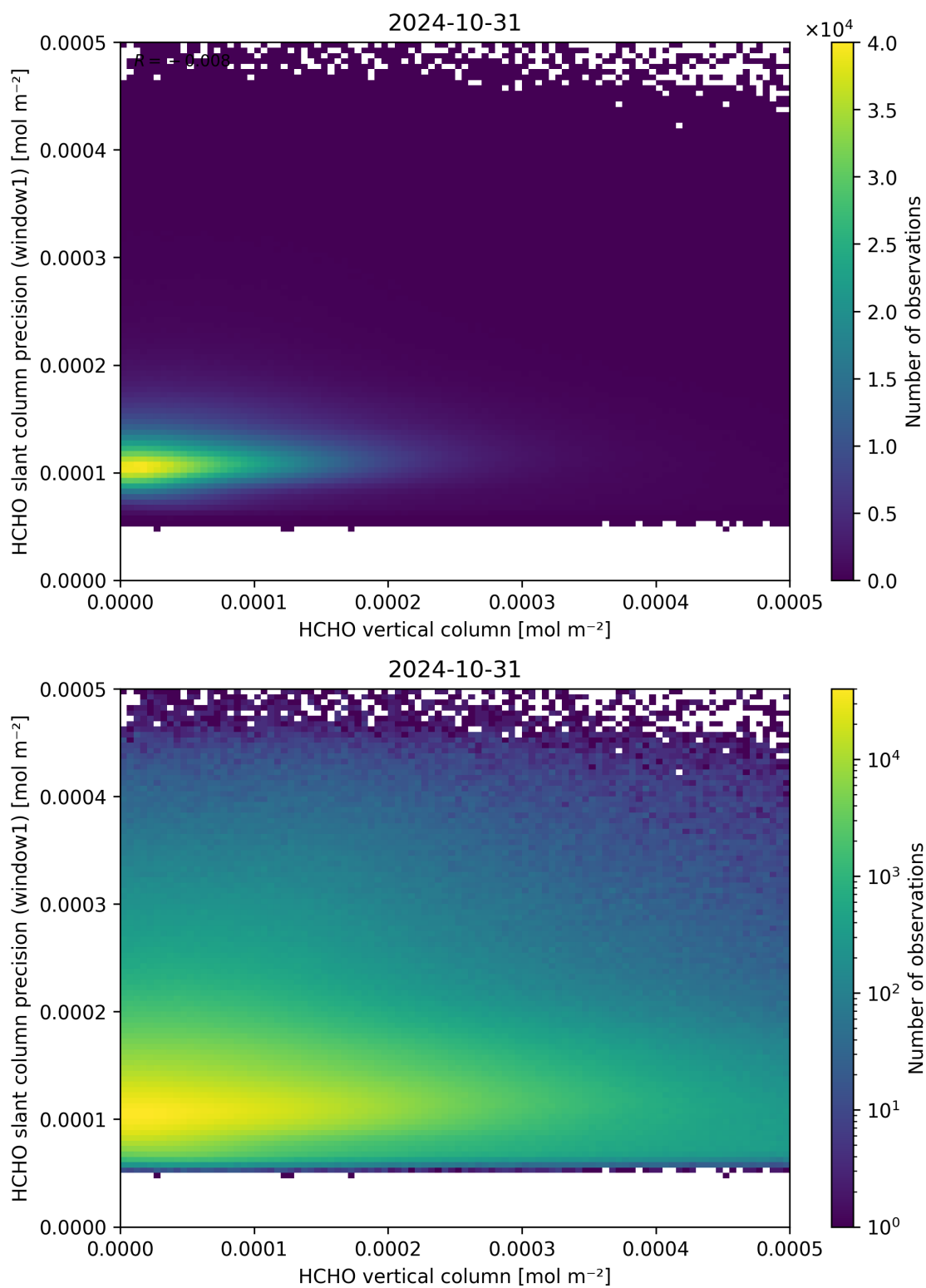
Figure 130: Scatter density plot of “HCHO vertical column” against “HCHO slant column precision (window1)” for 2024-10-30 to 2024-11-01.
