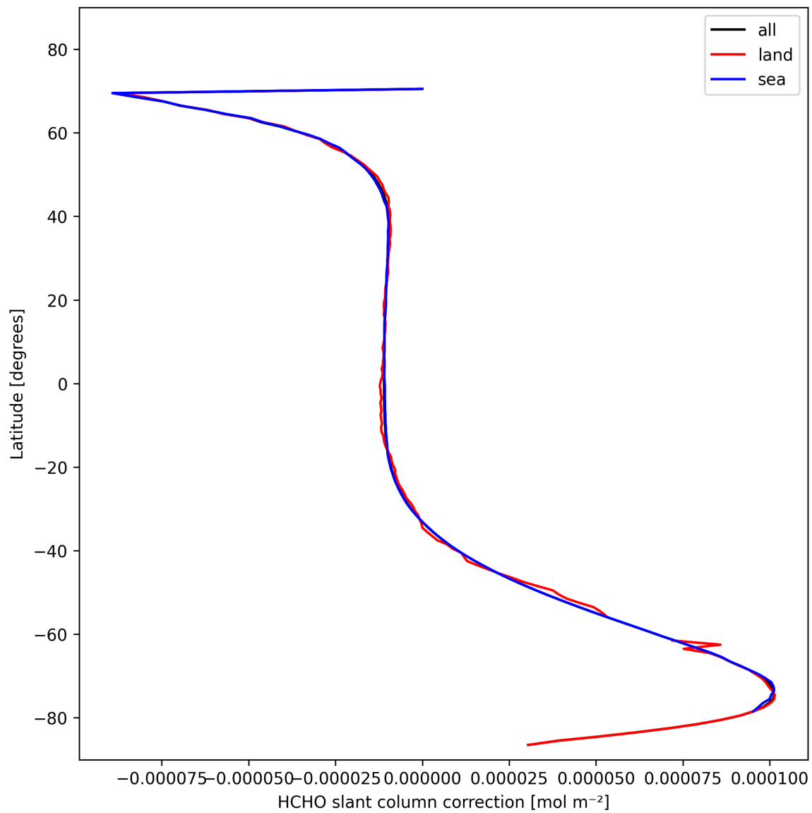
Figure 33: Zonal average of “HCHO slant column correction” for 2024-10-30 to 2024-11-01.
