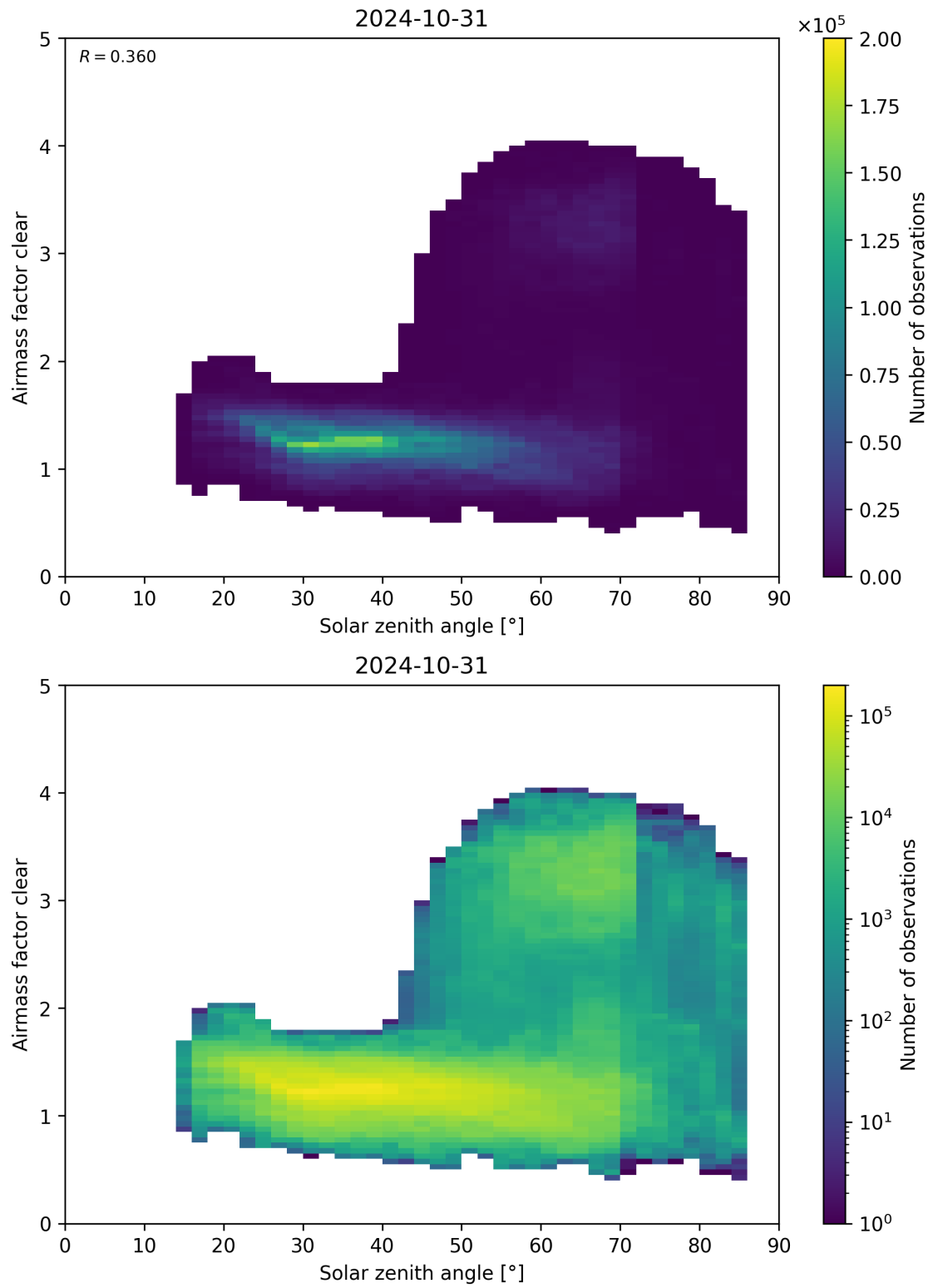
Figure 170: Scatter density plot of “Solar zenith angle” against “Airmass factor clear” for 2024-10-30 to 2024-11-01.
