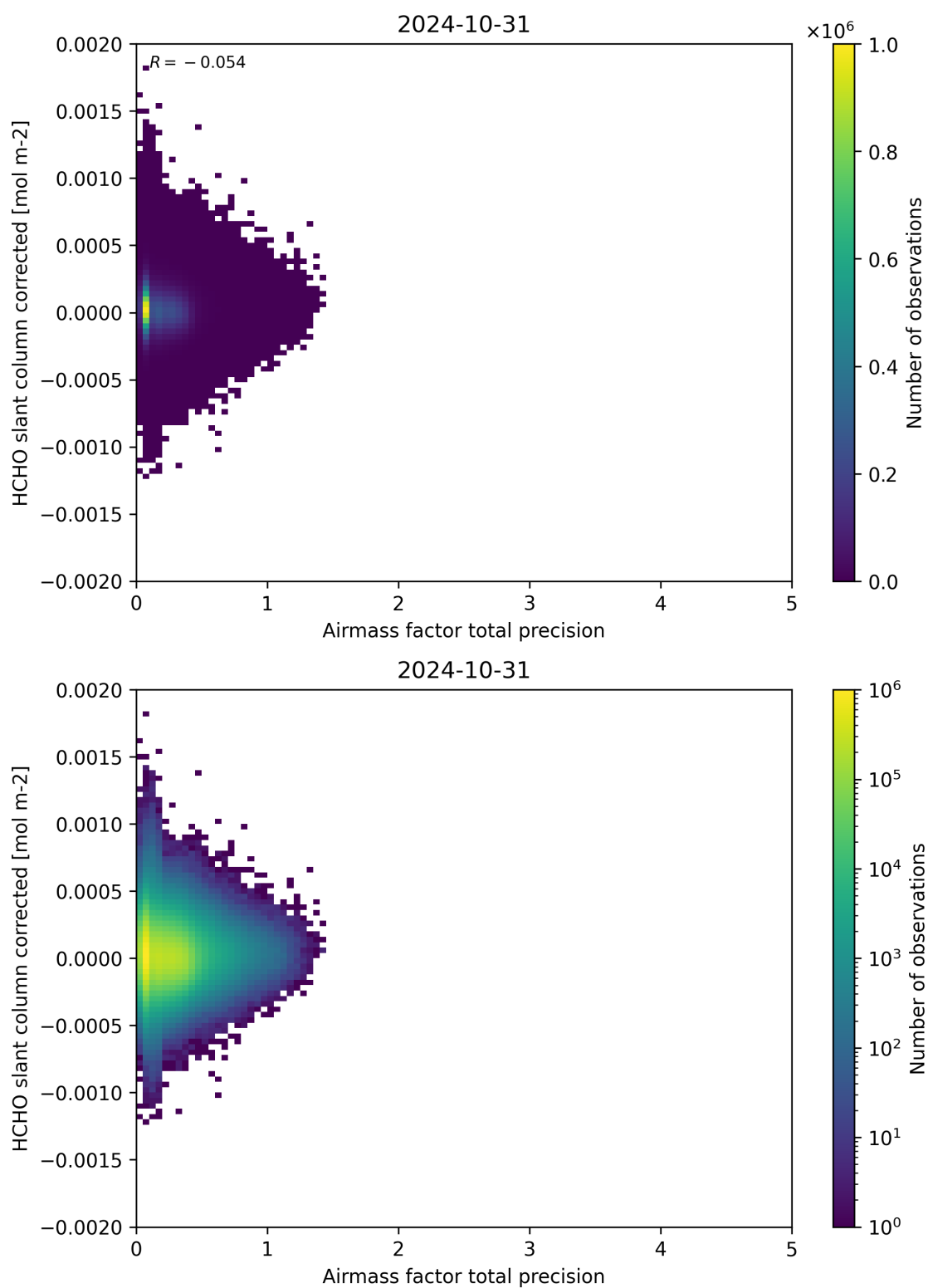
Figure 109: Scatter density plot of “Airmass factor total precision” against “HCHO slant column corrected” for 2024-10-30 to 2024-11-01.
