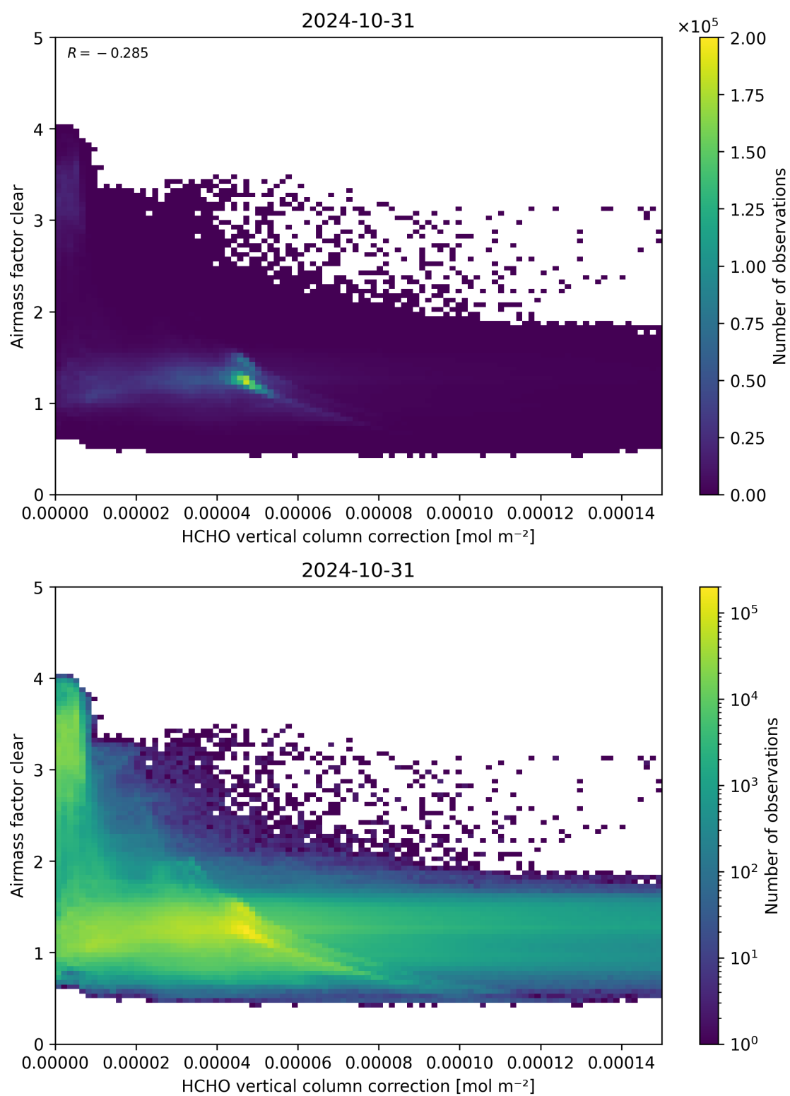
Figure 115: Scatter density plot of “HCHO vertical column correction” against “Airmass factor clear” for 2024-10-30 to 2024-11-01.
