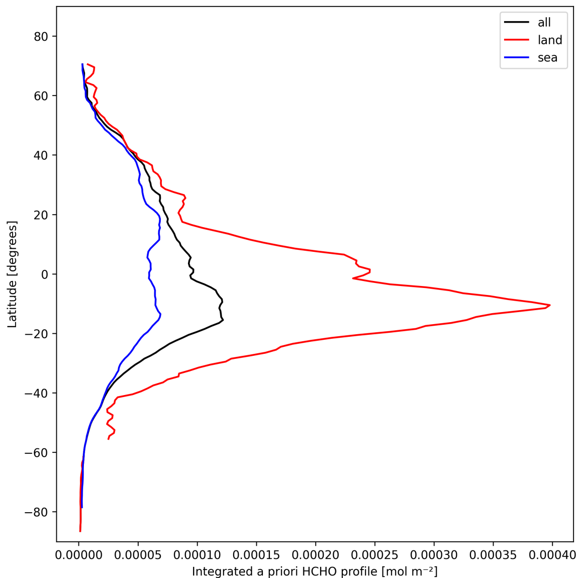
Figure 29: Zonal average of “Integrated a priori HCHO profile” for 2024-10-30 to 2024-11-01.
