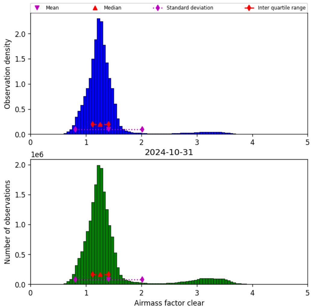
Figure 42: Histogram of “Airmass factor clear” for 2024-10-30 to 2024-11-01
