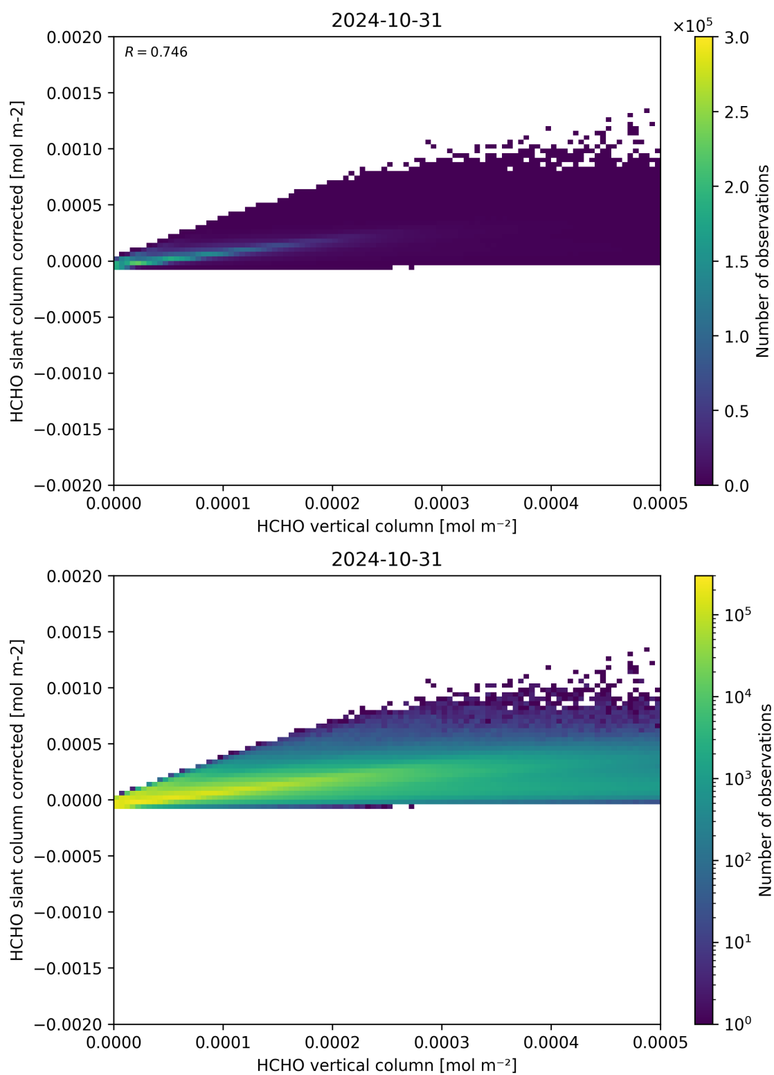
Figure 127: Scatter density plot of “HCHO vertical column” against “HCHO slant column corrected” for 2024-10-30 to 2024-11-01.
