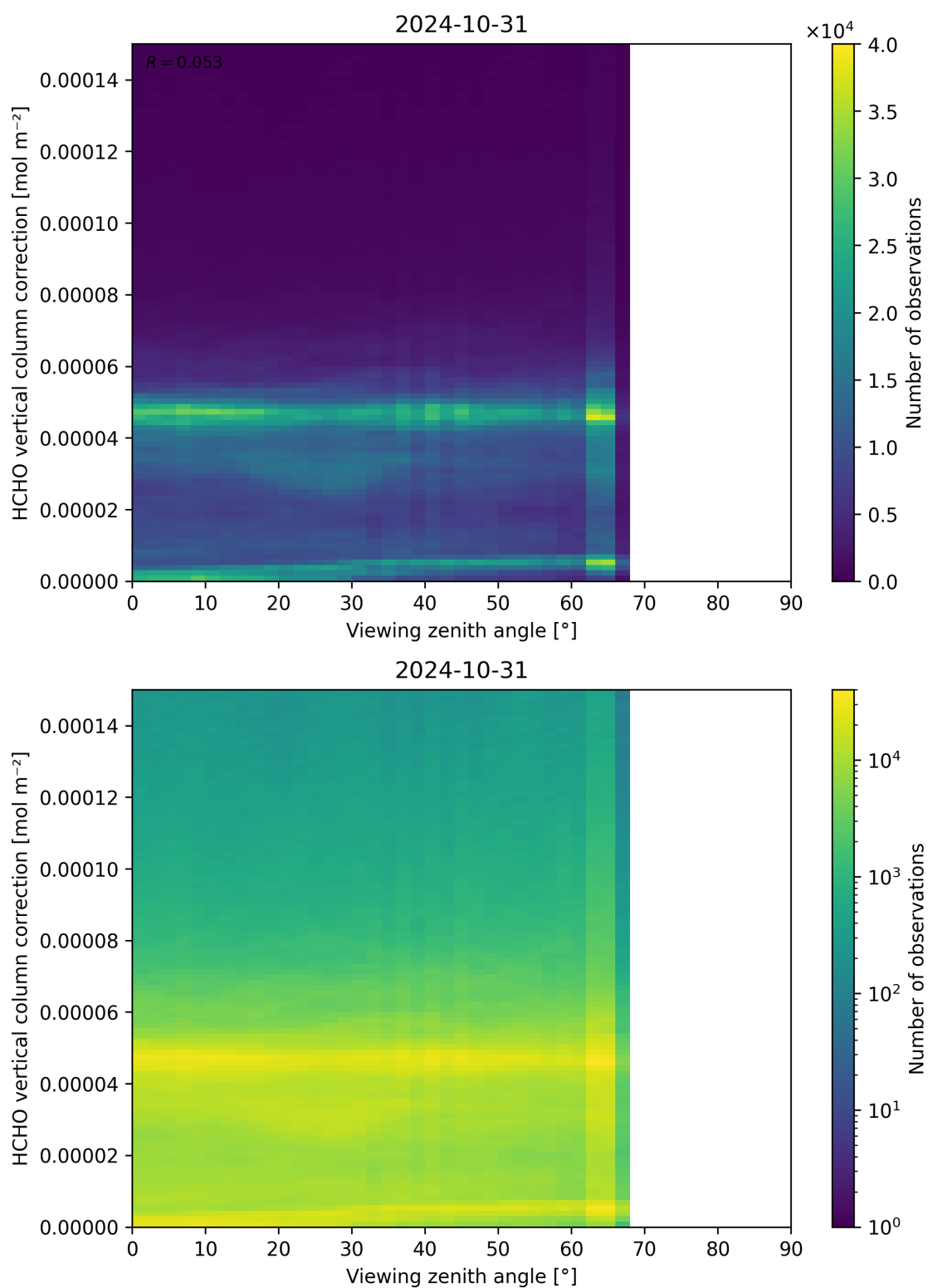
Figure 193: Scatter density plot of “Viewing zenith angle” against “HCHO vertical column correction” for 2024-10-30 to 2024-11-01.
