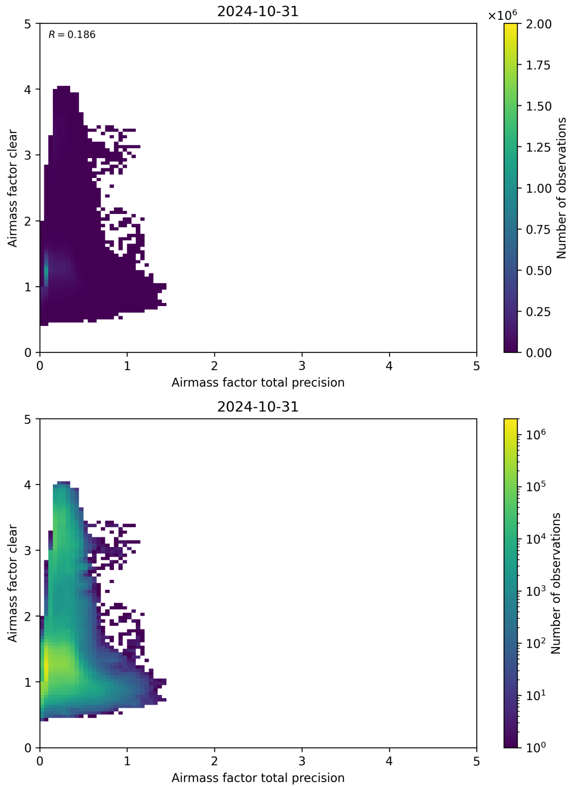
Figure 108: Scatter density plot of “Airmass factor total precision” against “Airmass factor clear” for 2024-10-30 to 2024-11-01.
