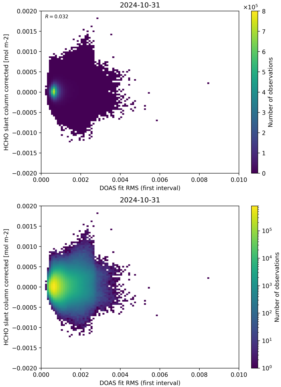
Figure 62: Scatter density plot of “DOAS fit RMS (first interval)” against “HCHO slant column corrected” for 2024-10-30 to 2024-11-01.
