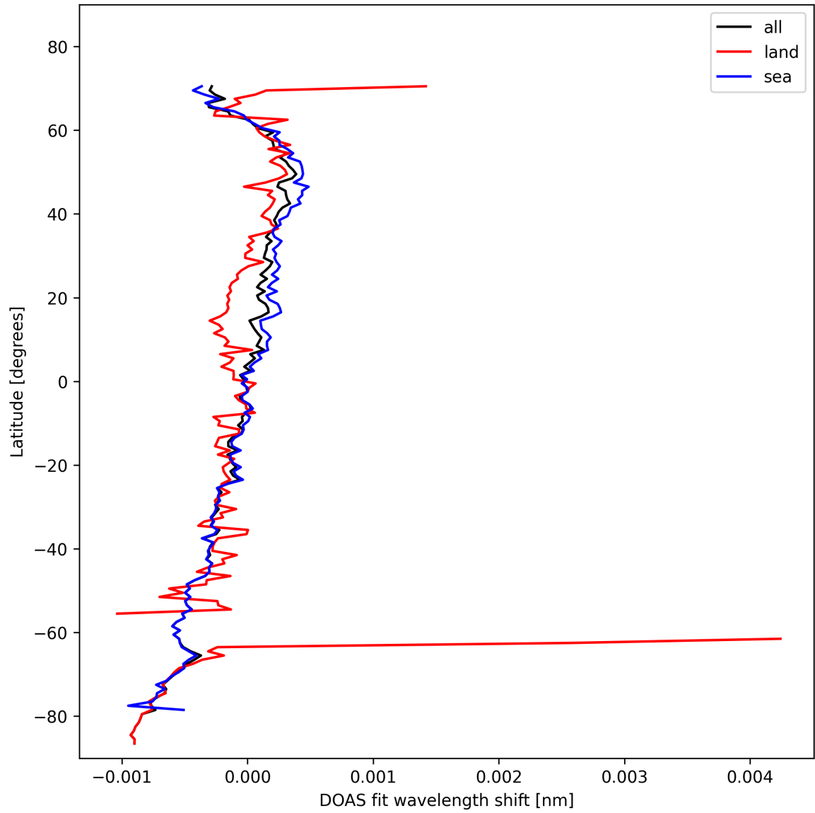
Figure 30: Zonal average of “DOAS fit wavelength shift” for 2024-10-30 to 2024-11-01.
