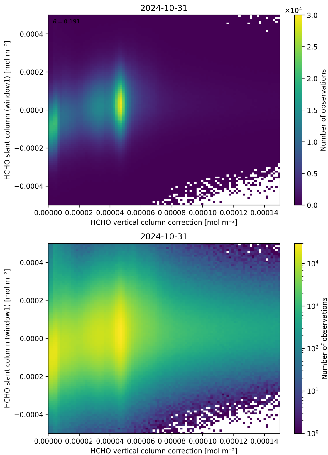
Figure 118: Scatter density plot of “HCHO vertical column correction” against “HCHO slant column (window1)” for 2024-10-30 to 2024-11-01.
