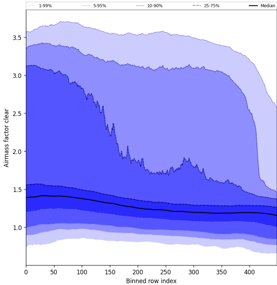
Figure 56: Along track statistics of “Airmass factor clear” for 2024-10-30 to 2024-11-01
