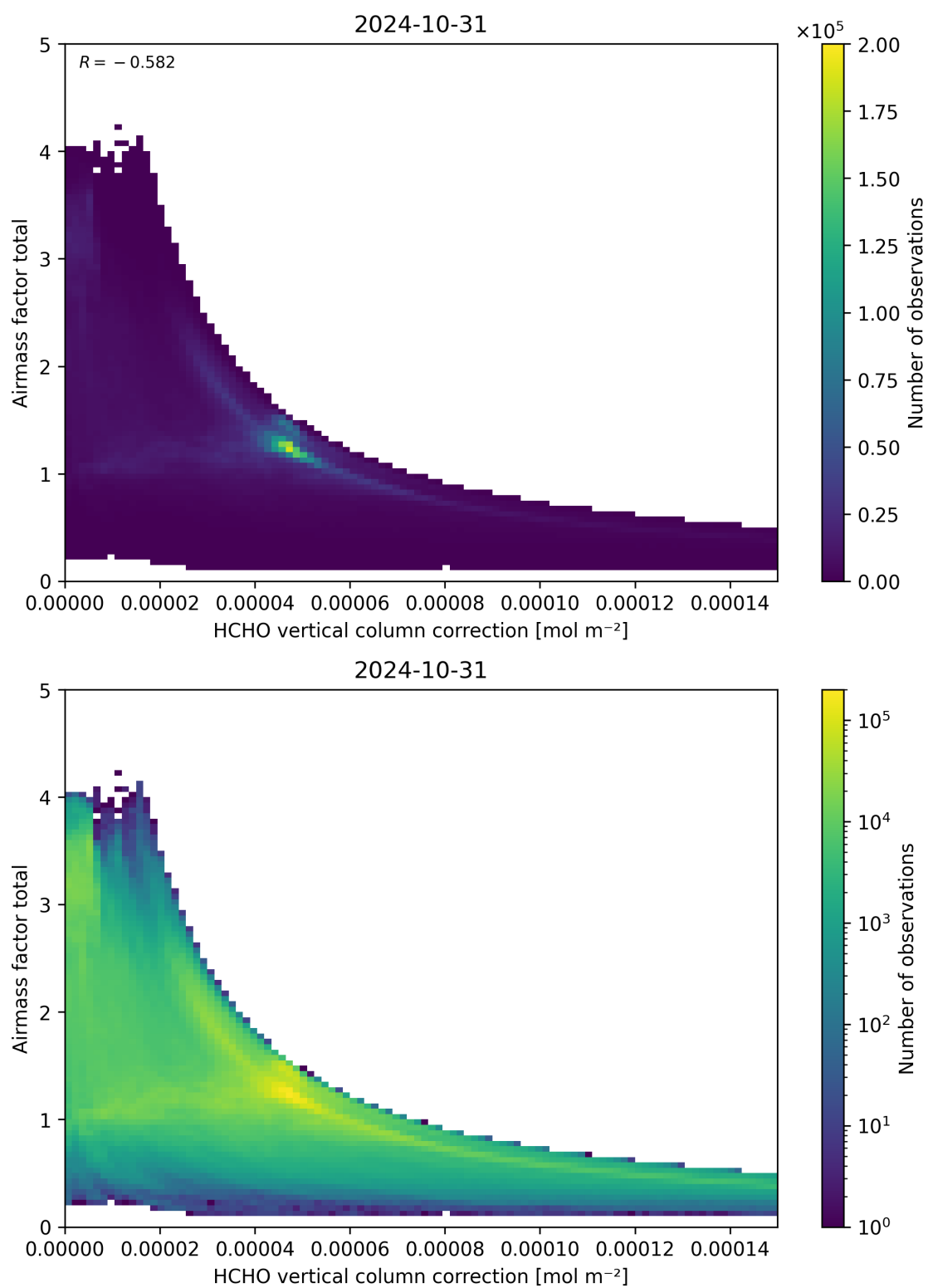
Figure 120: Scatter density plot of “HCHO vertical column correction” against “Airmass factor total” for 2024-10-30 to 2024-11-01.
