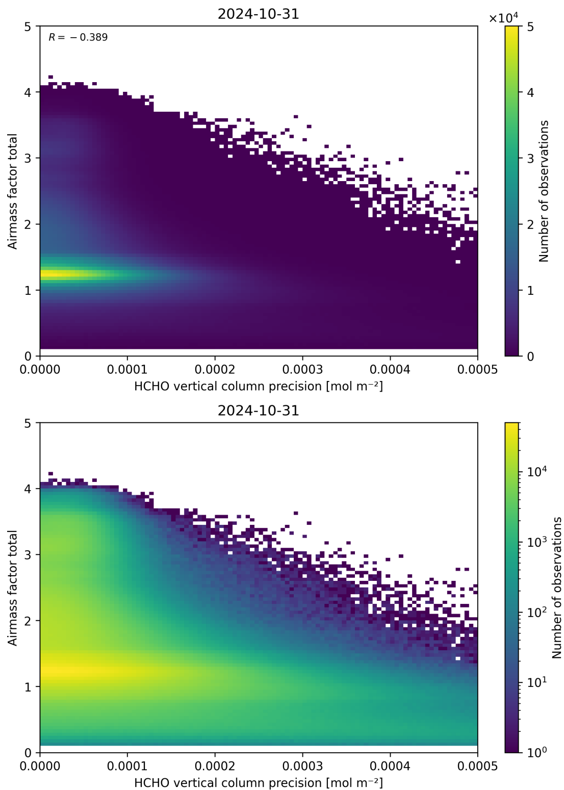
Figure 144: Scatter density plot of “HCHO vertical column precision” against “Airmass factor total” for 2024-10-30 to 2024-11-01.
