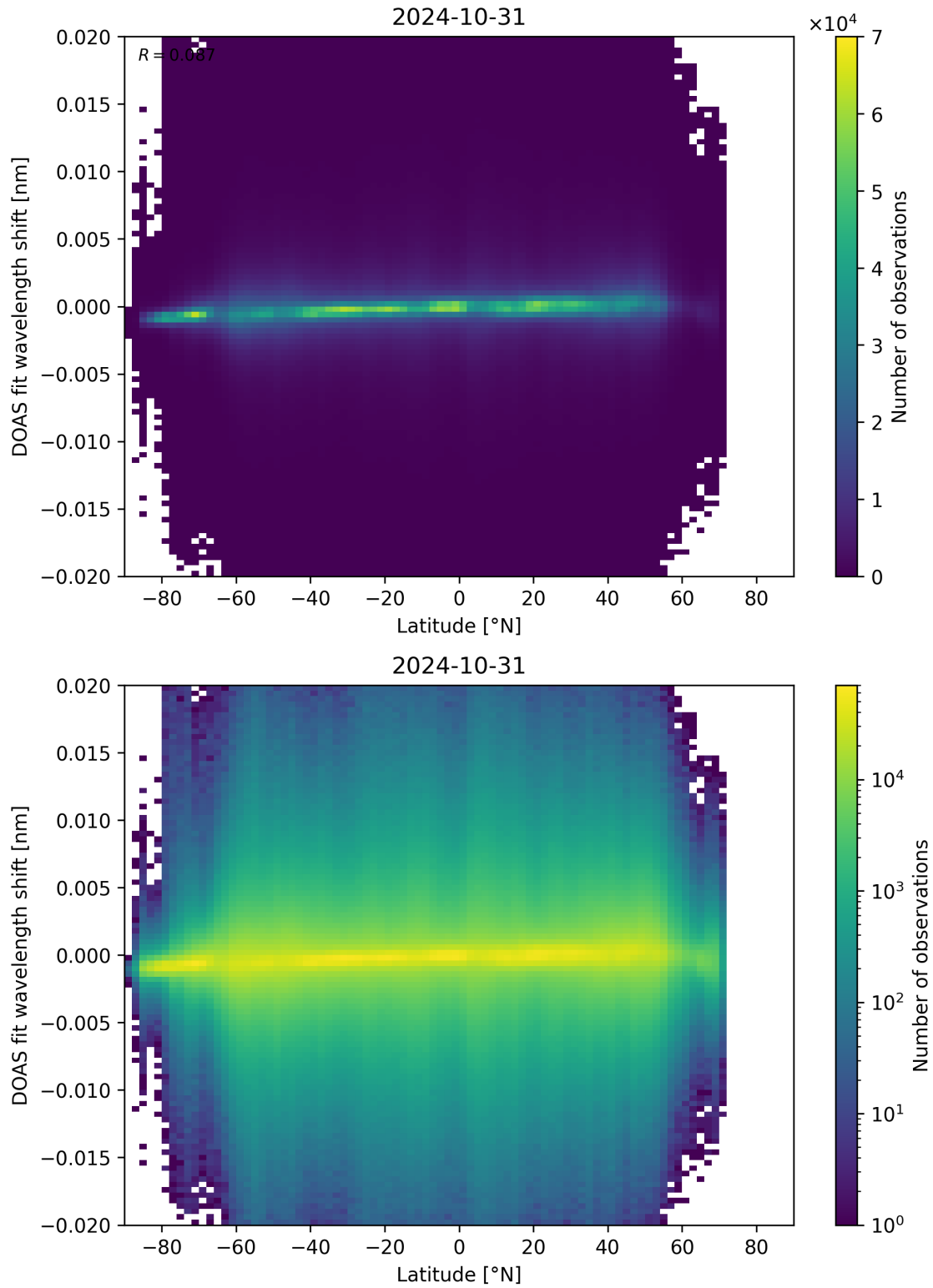
Figure 154: Scatter density plot of “Latitude” against “DOAS fit wavelength shift” for 2024-10-30 to 2024-11-01.
