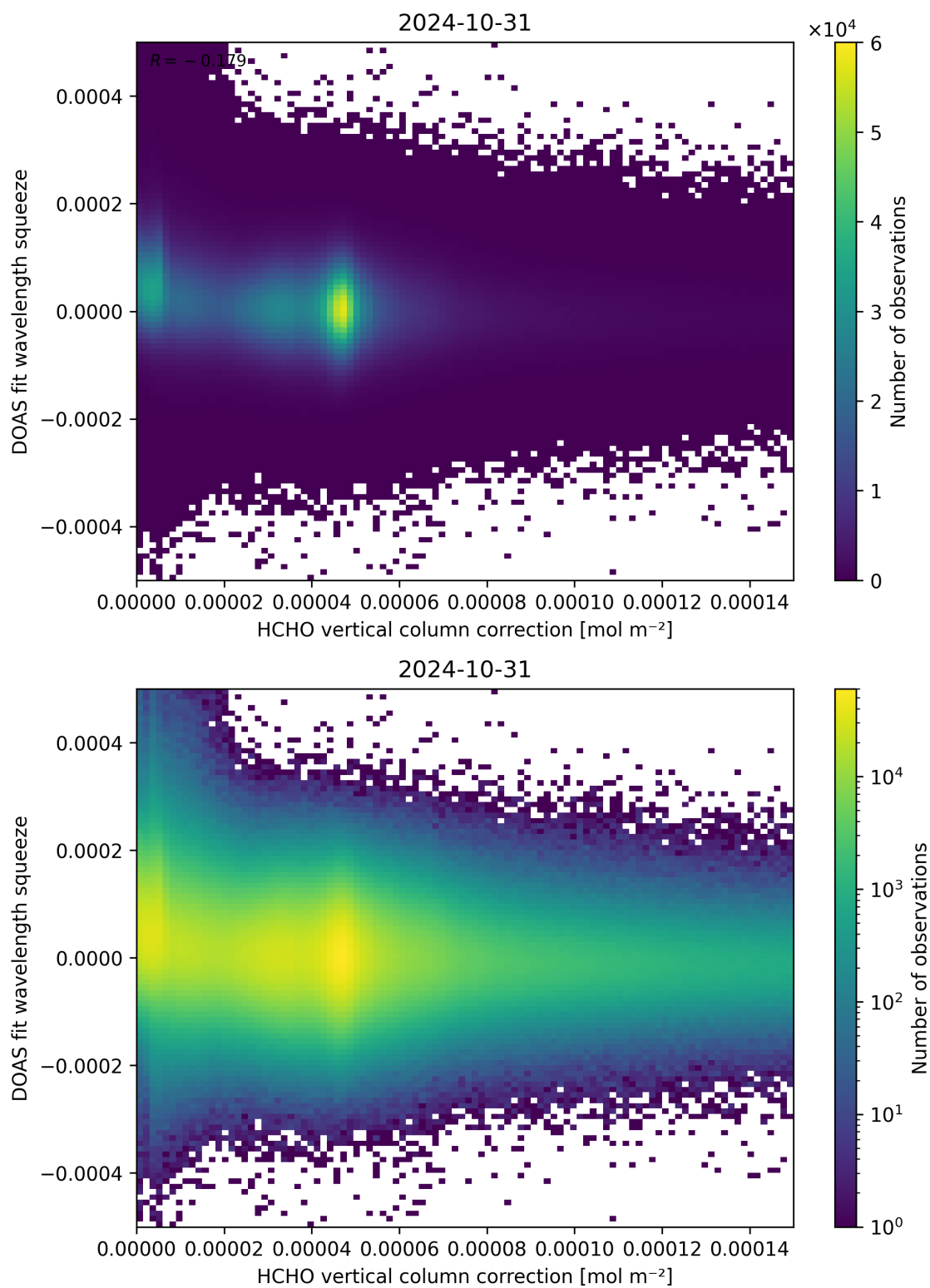
Figure 114: Scatter density plot of “HCHO vertical column correction” against “DOAS fit wavelength squeeze” for 2024-10-30 to 2024-11-01.
