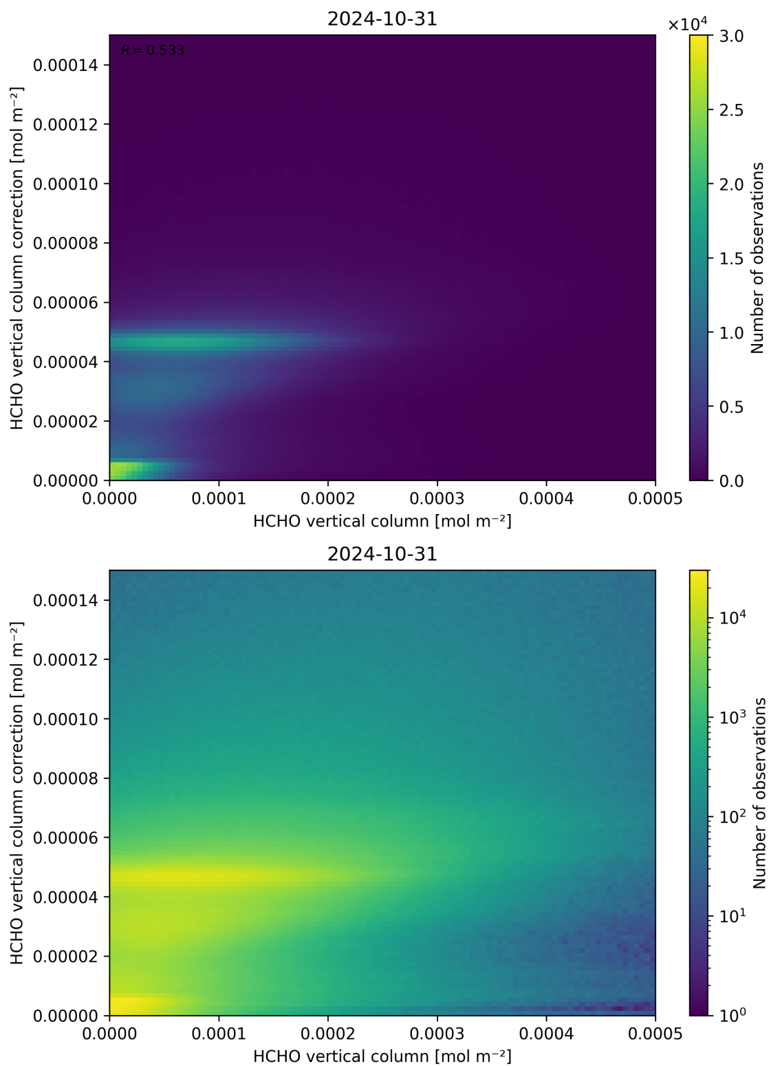
Figure 133: Scatter density plot of “HCHO vertical column” against “HCHO vertical column correction” for 2024-10-30 to 2024-11-01.
