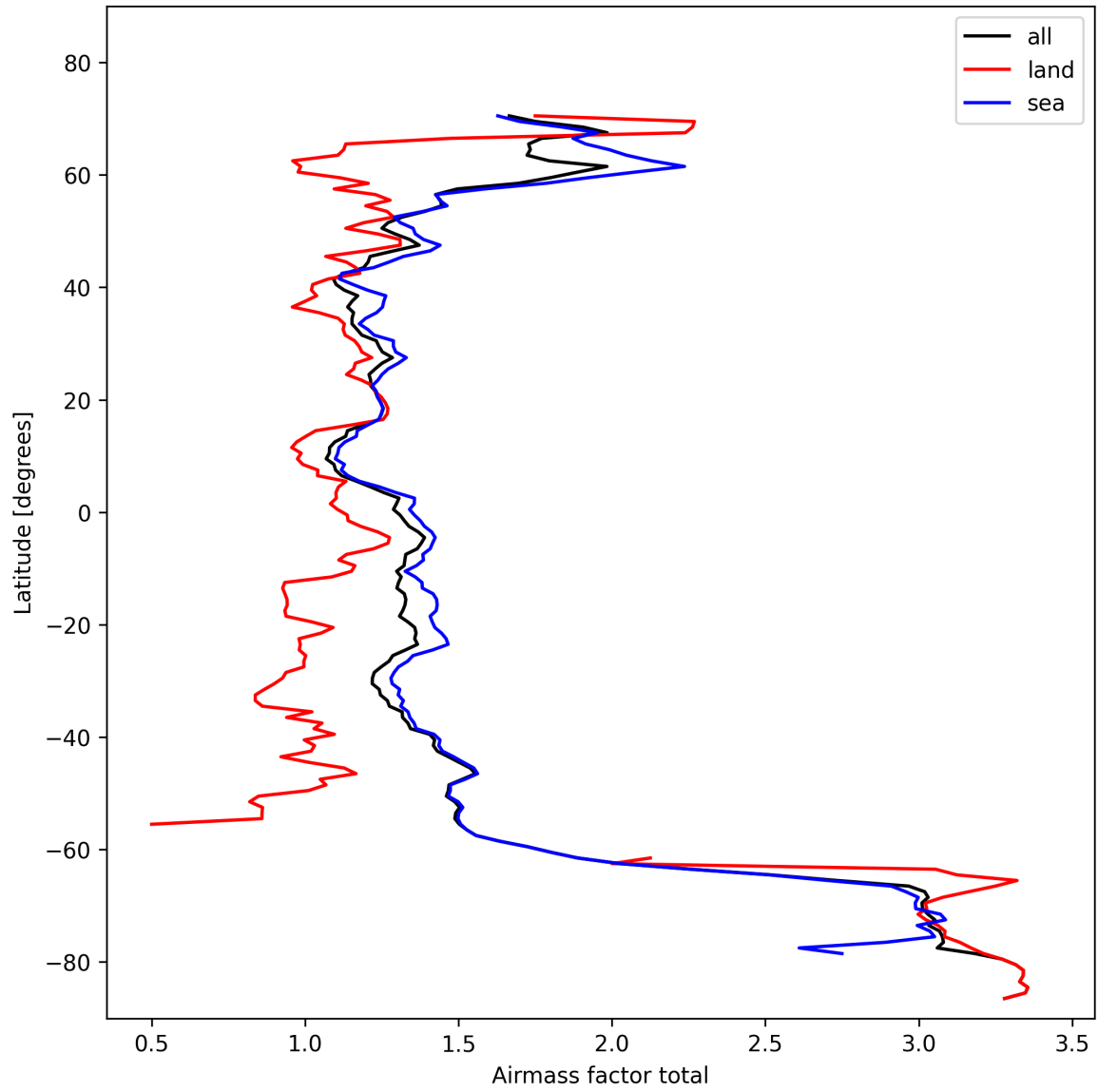
Figure 26: Zonal average of “Airmass factor total” for 2024-10-30 to 2024-11-01.
