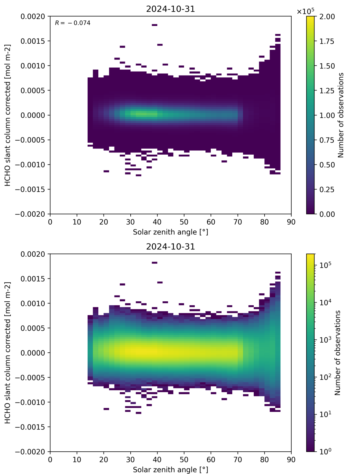
Figure 171: Scatter density plot of “Solar zenith angle” against “HCHO slant column corrected” for 2024-10-30 to 2024-11-01.
