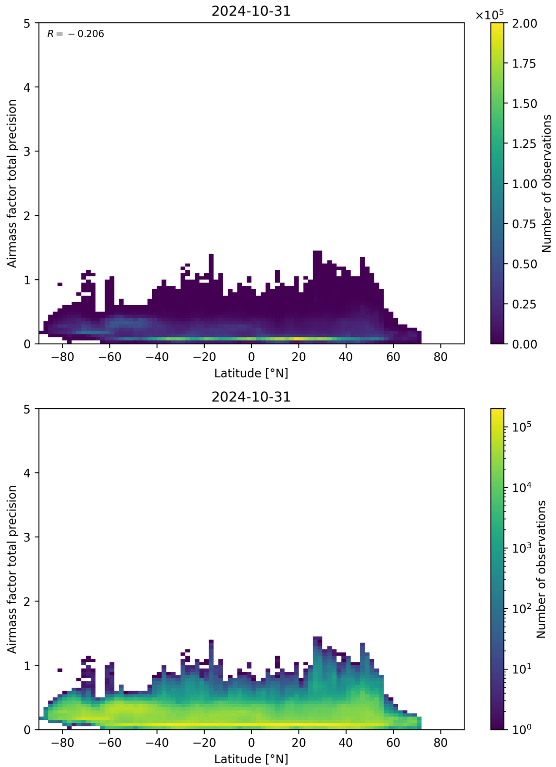
Figure 162: Scatter density plot of “Latitude” against “Airmass factor total precision” for 2024-10-30 to 2024-11-01.
