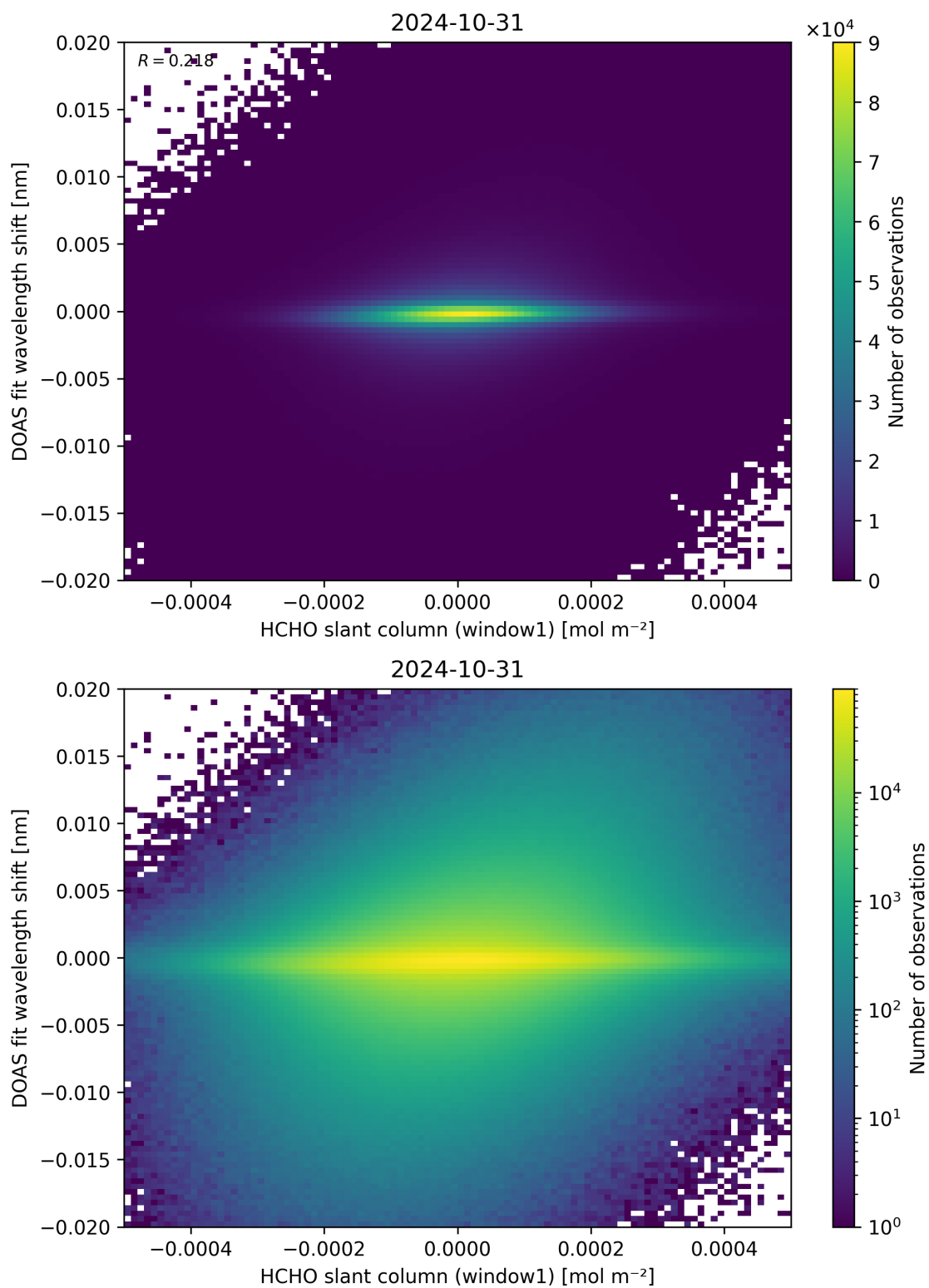
Figure 79: Scatter density plot of “HCHO slant column (window1)” against “DOAS fit wavelength shift” for 2024-10-30 to 2024-11-01.
