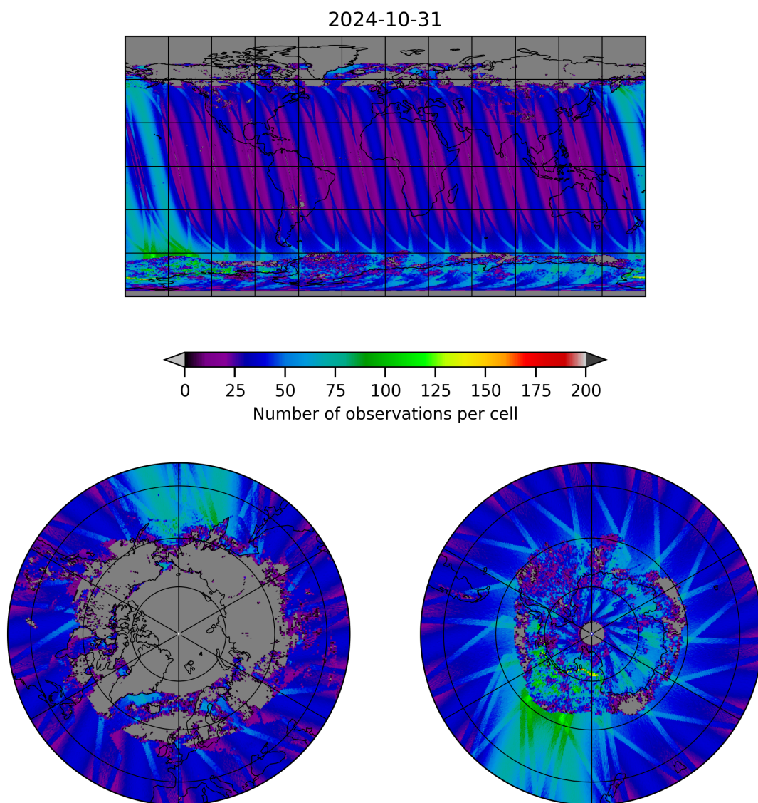
Figure 19: Map of the number of observations for 2024-10-30 to 2024-11-01
