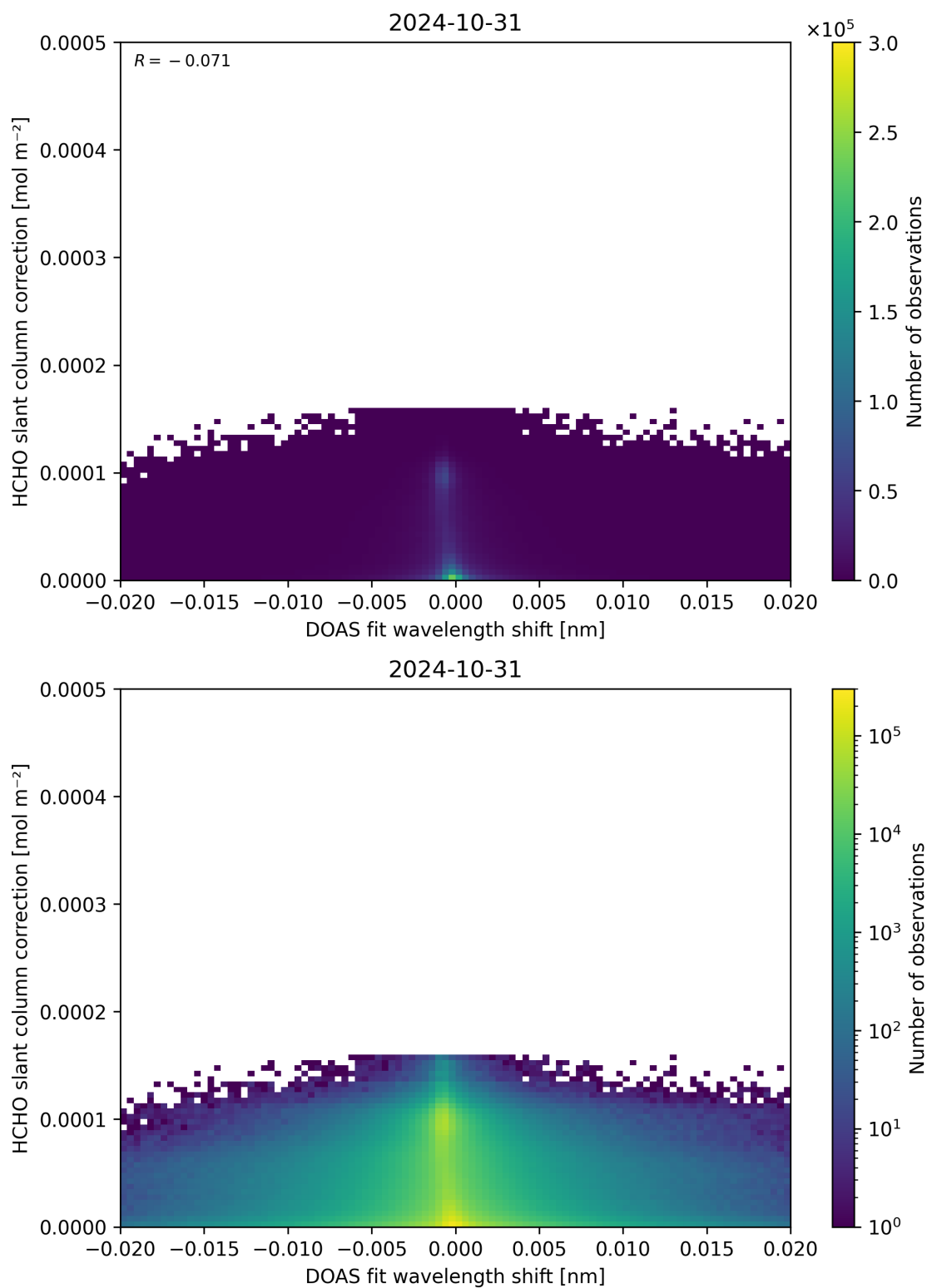
Figure 67: Scatter density plot of “DOAS fit wavelength shift” against “HCHO slant column correction” for 2024-10-30 to 2024-11-01.
