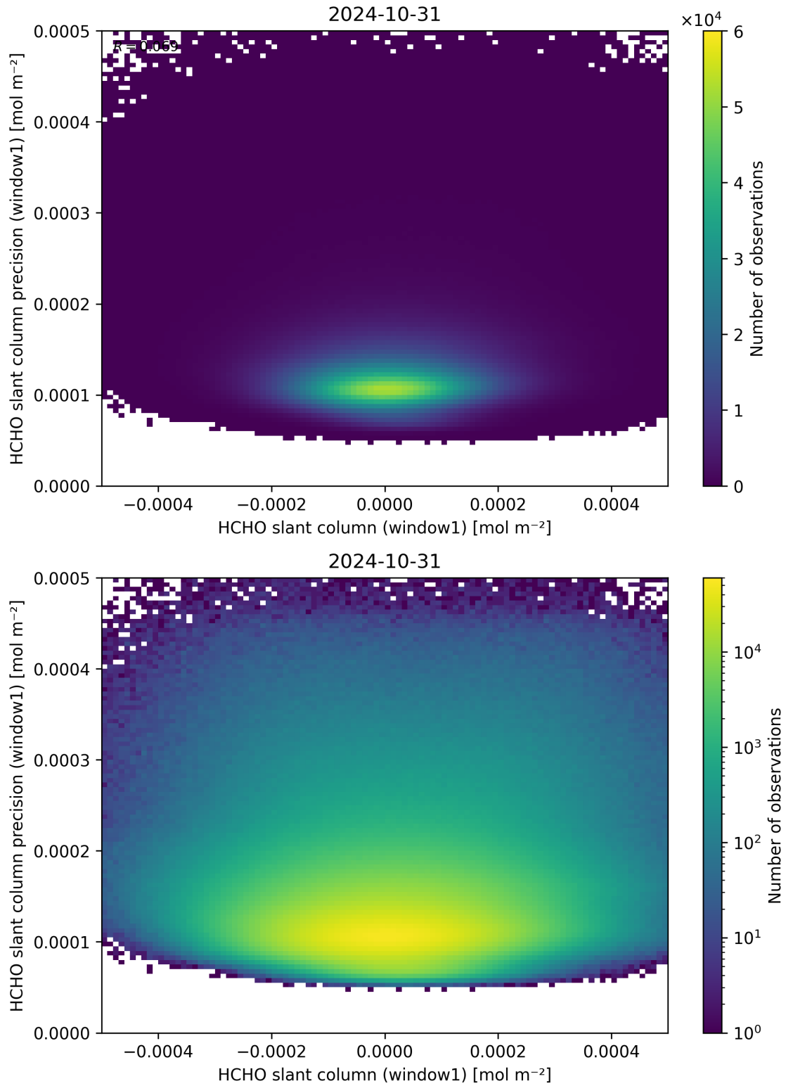
Figure 84: Scatter density plot of “HCHO slant column (window1)” against “HCHO slant column precision (window1)” for 2024-10-30 to 2024-11-01.
