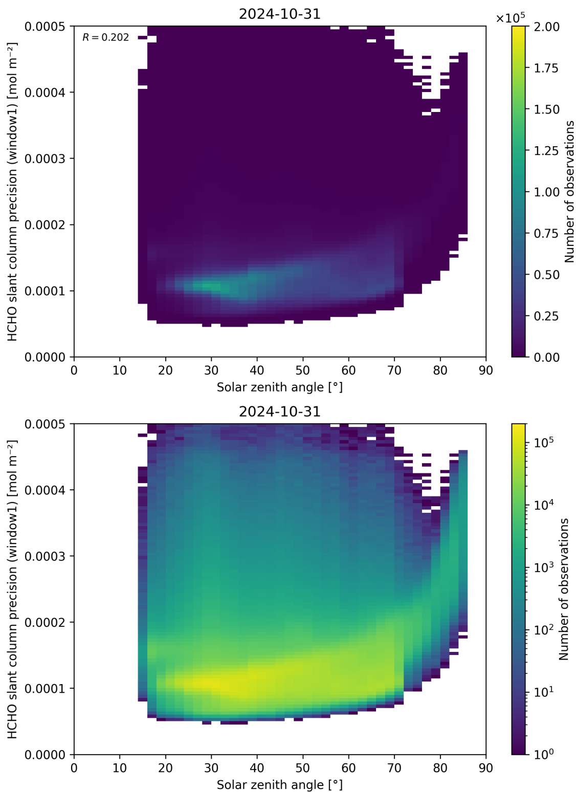
Figure 174: Scatter density plot of “Solar zenith angle” against “HCHO slant column precision (window1)” for 2024-10-30 to 2024-11-01.
