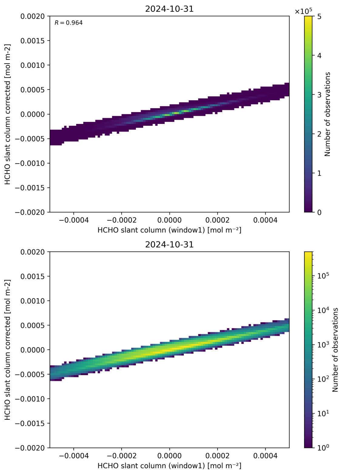
Figure 82: Scatter density plot of “HCHO slant column (window1)” against “HCHO slant column corrected” for 2024-10-30 to 2024-11-01.
