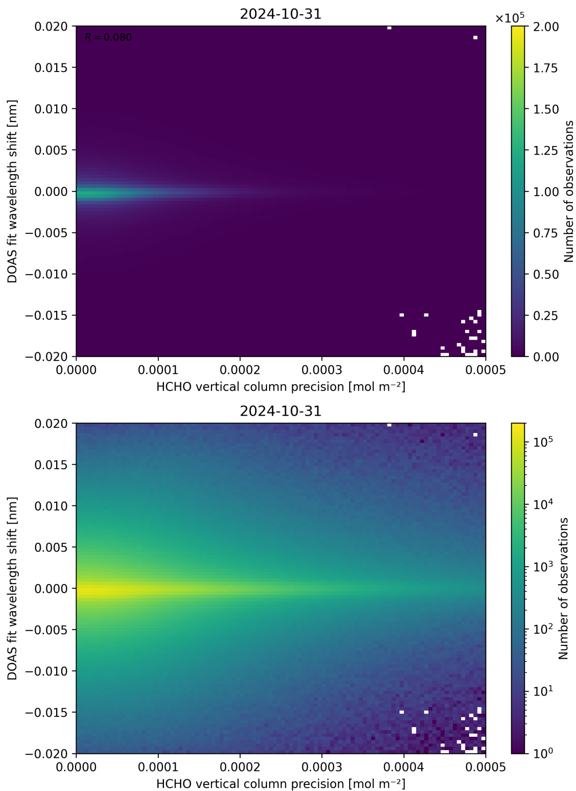
Figure 137: Scatter density plot of “HCHO vertical column precision” against “DOAS fit wavelength shift” for 2024-10-30 to 2024-11-01.
