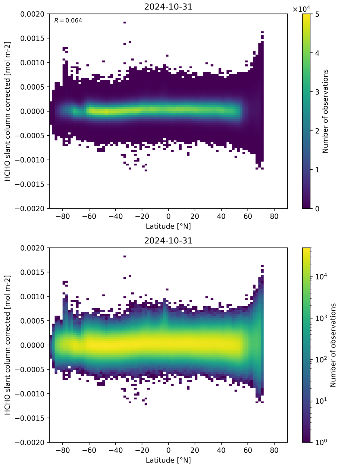
Figure 157: Scatter density plot of “Latitude” against “HCHO slant column corrected” for 2024-10-30 to 2024-11-01.
