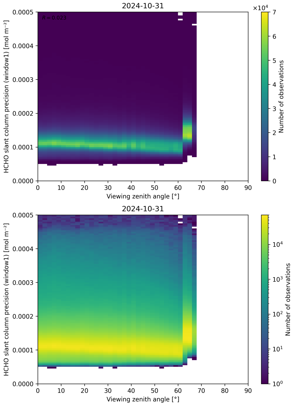
Figure 189: Scatter density plot of “Viewing zenith angle” against “HCHO slant column precision (window1)” for 2024-10-30 to 2024-11-01.
