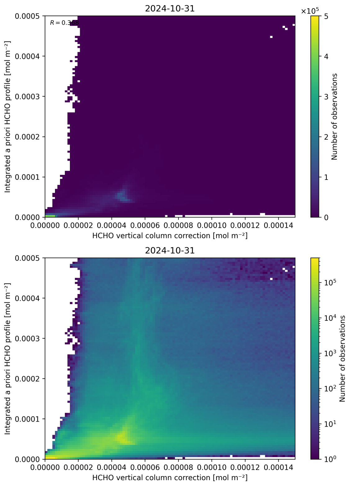
Figure 122: Scatter density plot of “HCHO vertical column correction” against “Integrated a priori HCHO profile” for 2024-10-30 to 2024-11-01.
