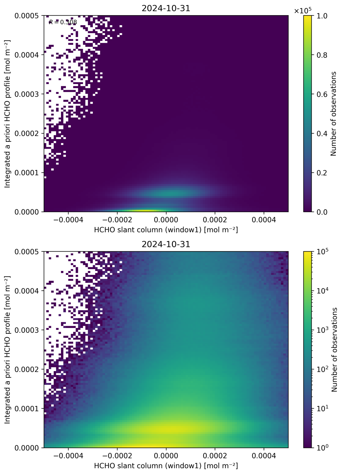
Figure 87: Scatter density plot of “HCHO slant column (window1)” against “Integrated a priori HCHO profile” for 2024-10-30 to 2024-11-01.
