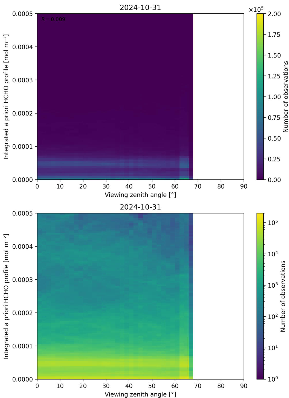
Figure 195: Scatter density plot of “Viewing zenith angle” against “Integrated a priori HCHO profile” for 2024-10-30 to 2024-11-01.
