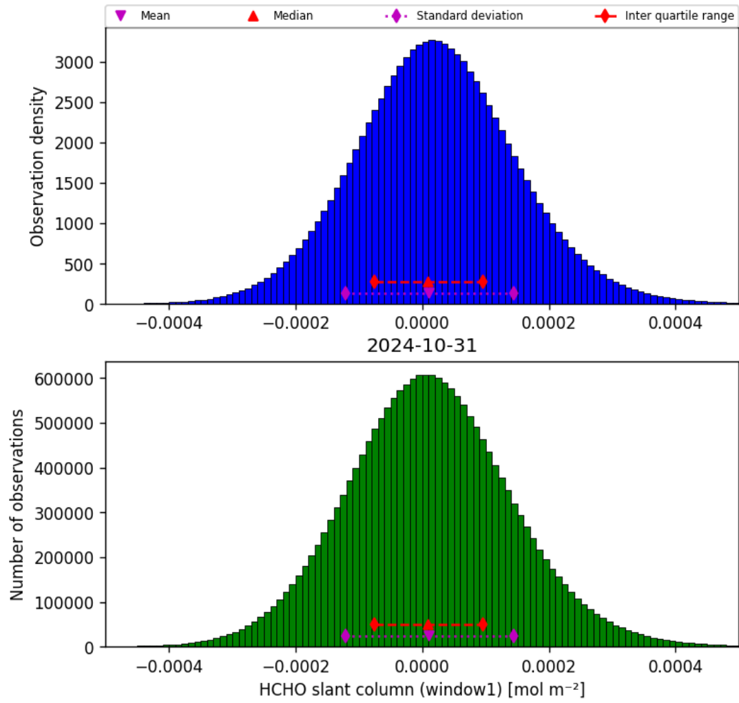
Figure 38: Histogram of “HCHO slant column (window1)” for 2024-10-30 to 2024-11-01
