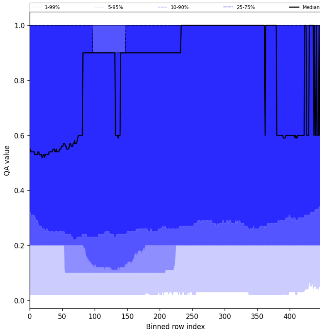
Figure 48: Along track statistics of “QA value” for 2024-10-30 to 2024-11-01
