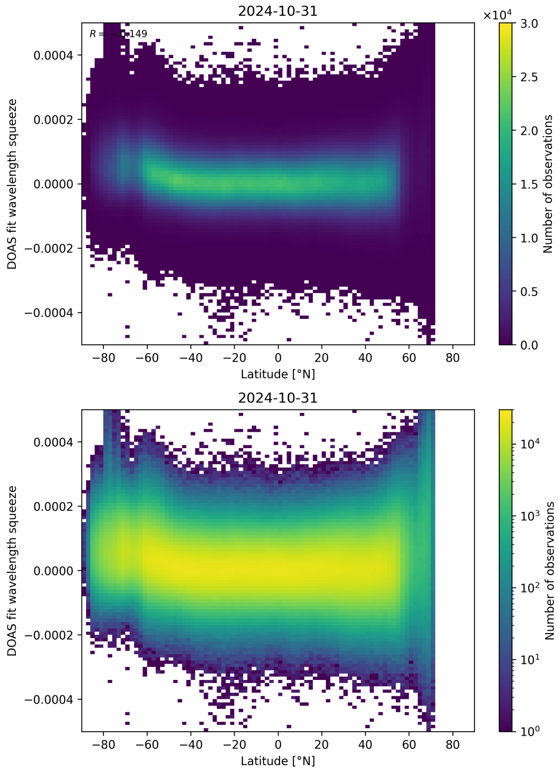
Figure 155: Scatter density plot of “Latitude” against “DOAS fit wavelength squeeze” for 2024-10-30 to 2024-11-01.
