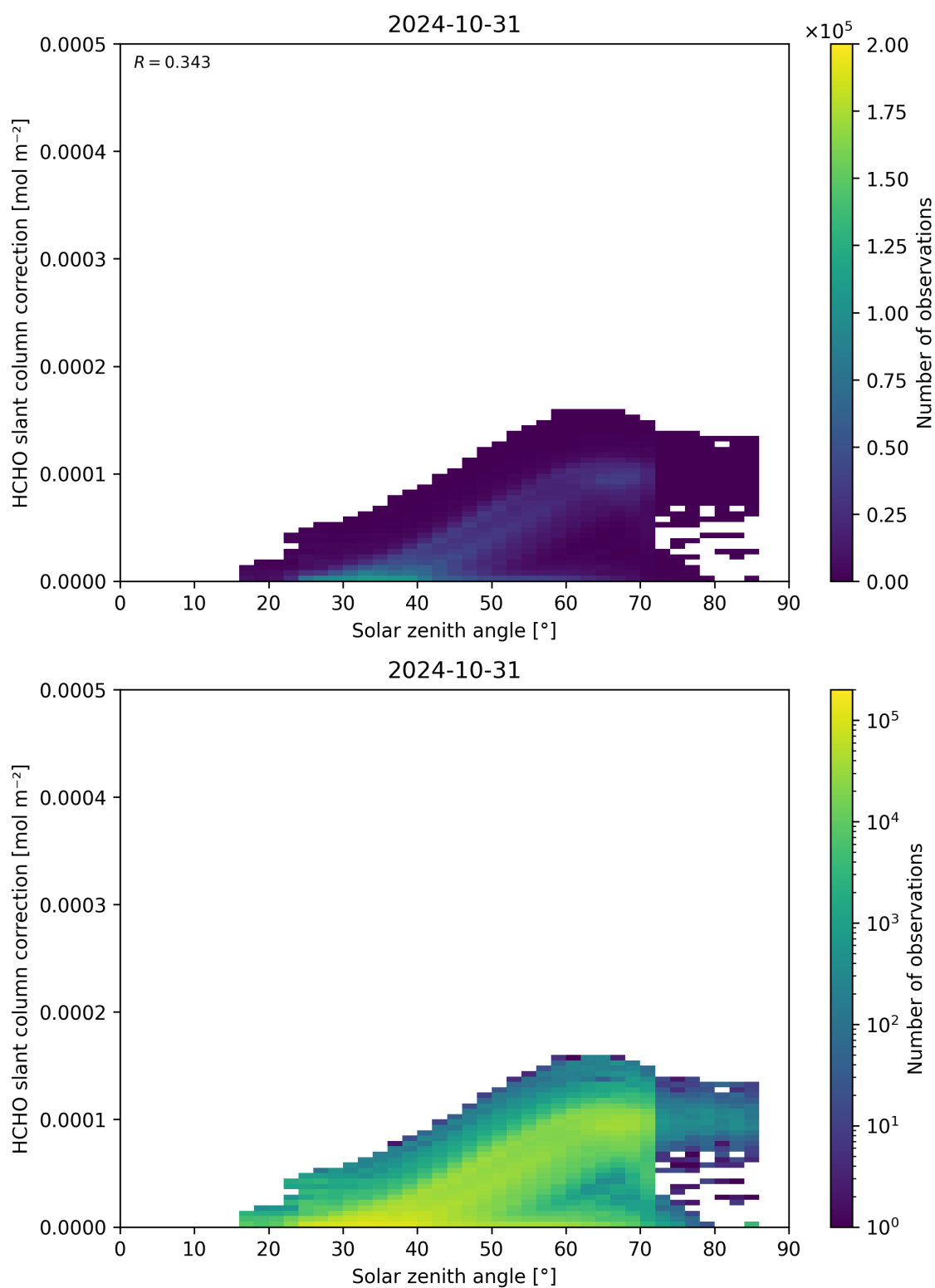
Figure 172: Scatter density plot of “Solar zenith angle” against “HCHO slant column correction” for 2024-10-30 to 2024-11-01.
