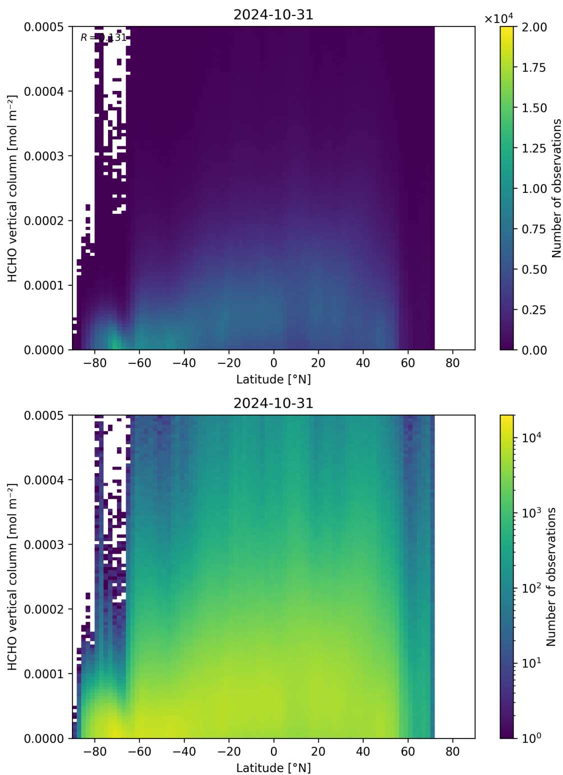
Figure 163: Scatter density plot of “Latitude” against “HCHO vertical column” for 2024-10-30 to 2024-11-01.
