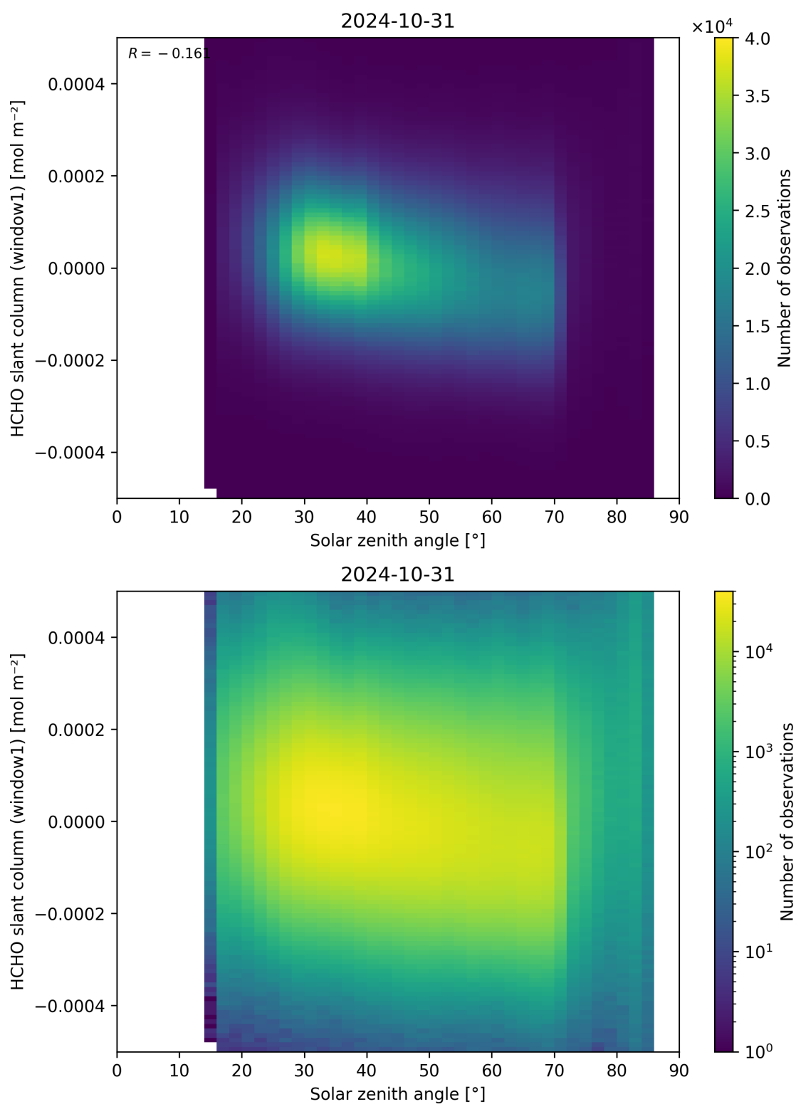
Figure 173: Scatter density plot of “Solar zenith angle” against “HCHO slant column (window1)” for 2024-10-30 to 2024-11-01.
