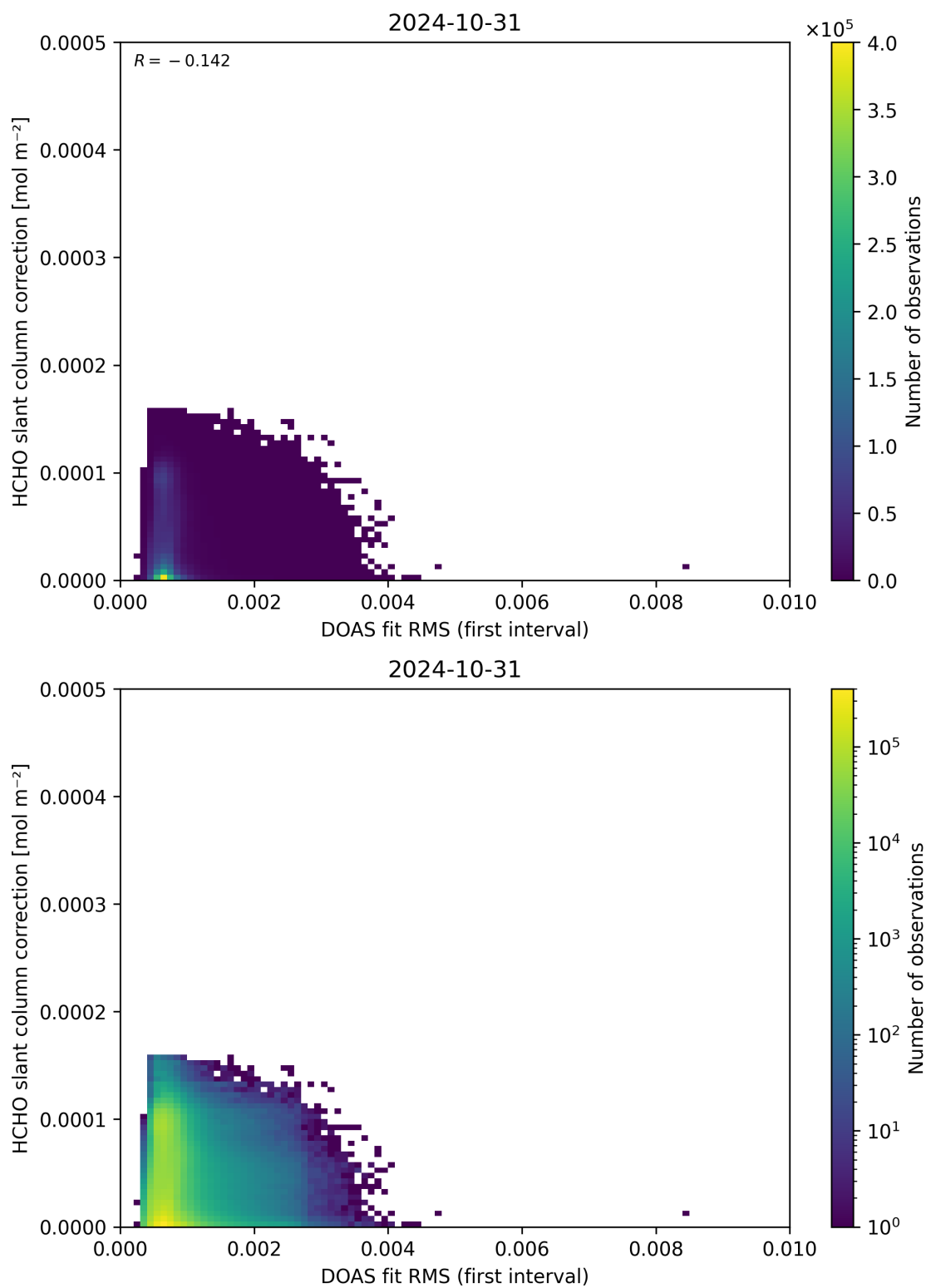
Figure 63: Scatter density plot of “DOAS fit RMS (first interval)” against “HCHO slant column correction” for 2024-10-30 to 2024-11-01.
