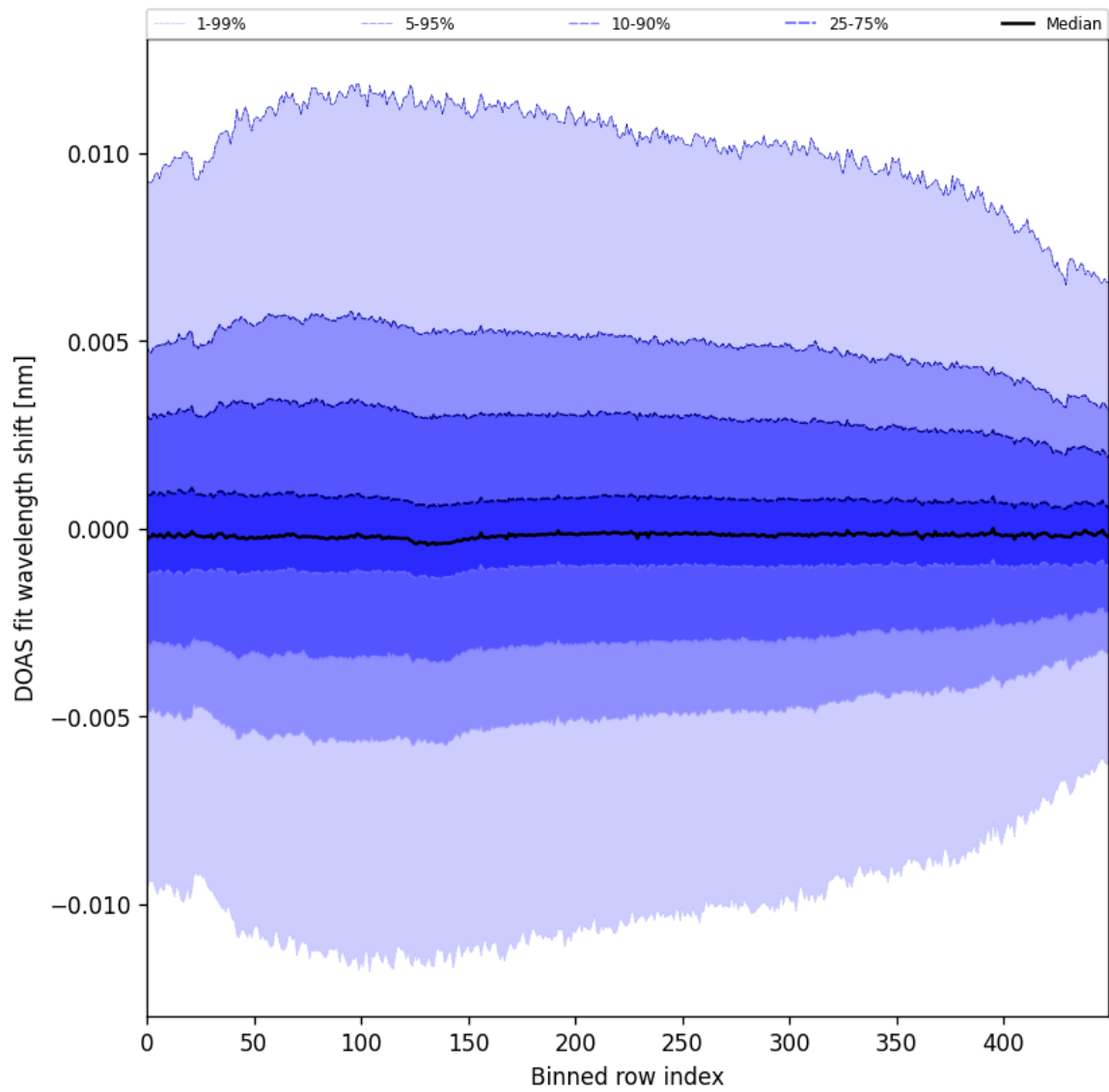
Figure 58: Along track statistics of “DOAS fit wavelength shift” for 2024-10-30 to 2024-11-01
