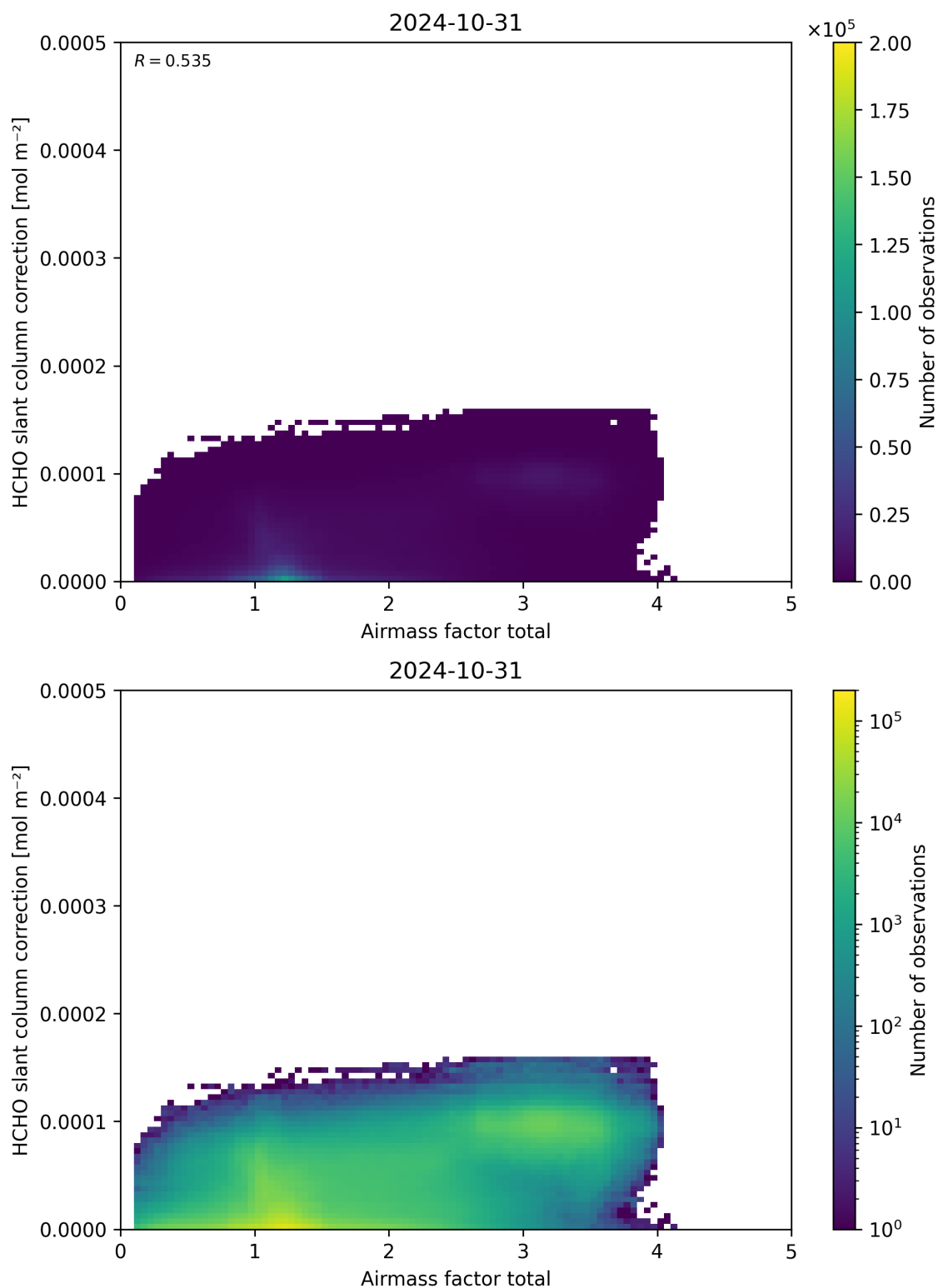
Figure 102: Scatter density plot of “Airmass factor total” against “HCHO slant column correction” for 2024-10-30 to 2024-11-01.
