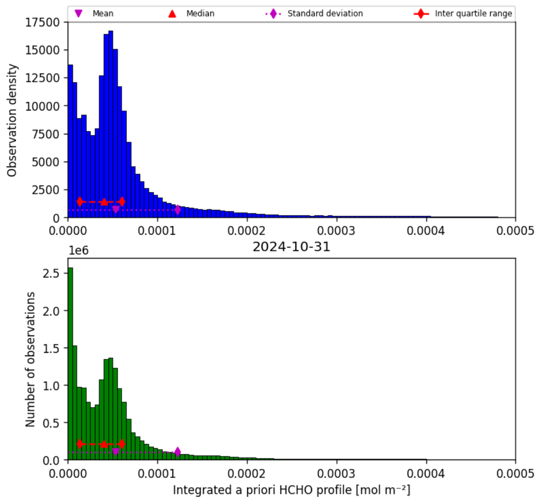
Figure 43: Histogram of “Integrated a priori HCHO profile” for 2024-10-30 to 2024-11-01
