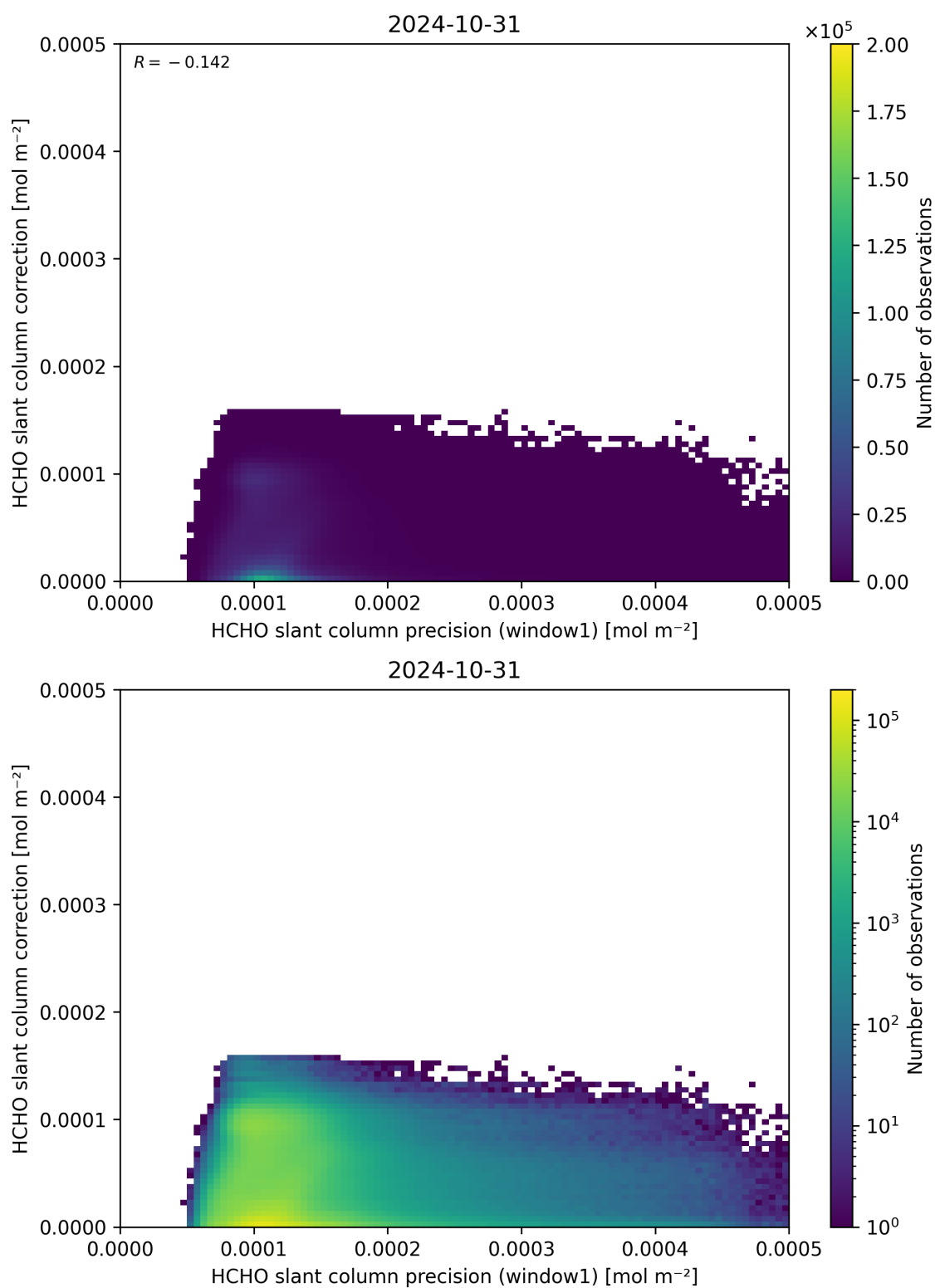
Figure 93: Scatter density plot of “HCHO slant column precision (window1)” against “HCHO slant column correction” for 2024-10-30 to 2024-11-01.
