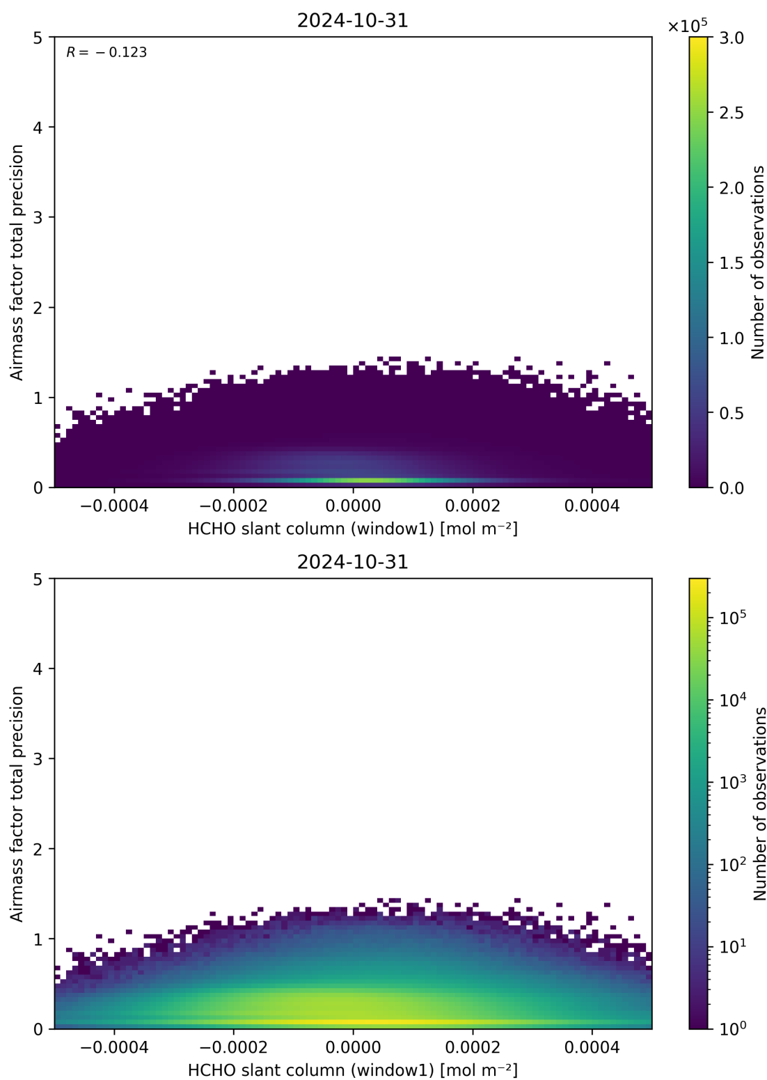
Figure 86: Scatter density plot of “HCHO slant column (window1)” against “Airmass factor total precision” for 2024-10-30 to 2024-11-01.
