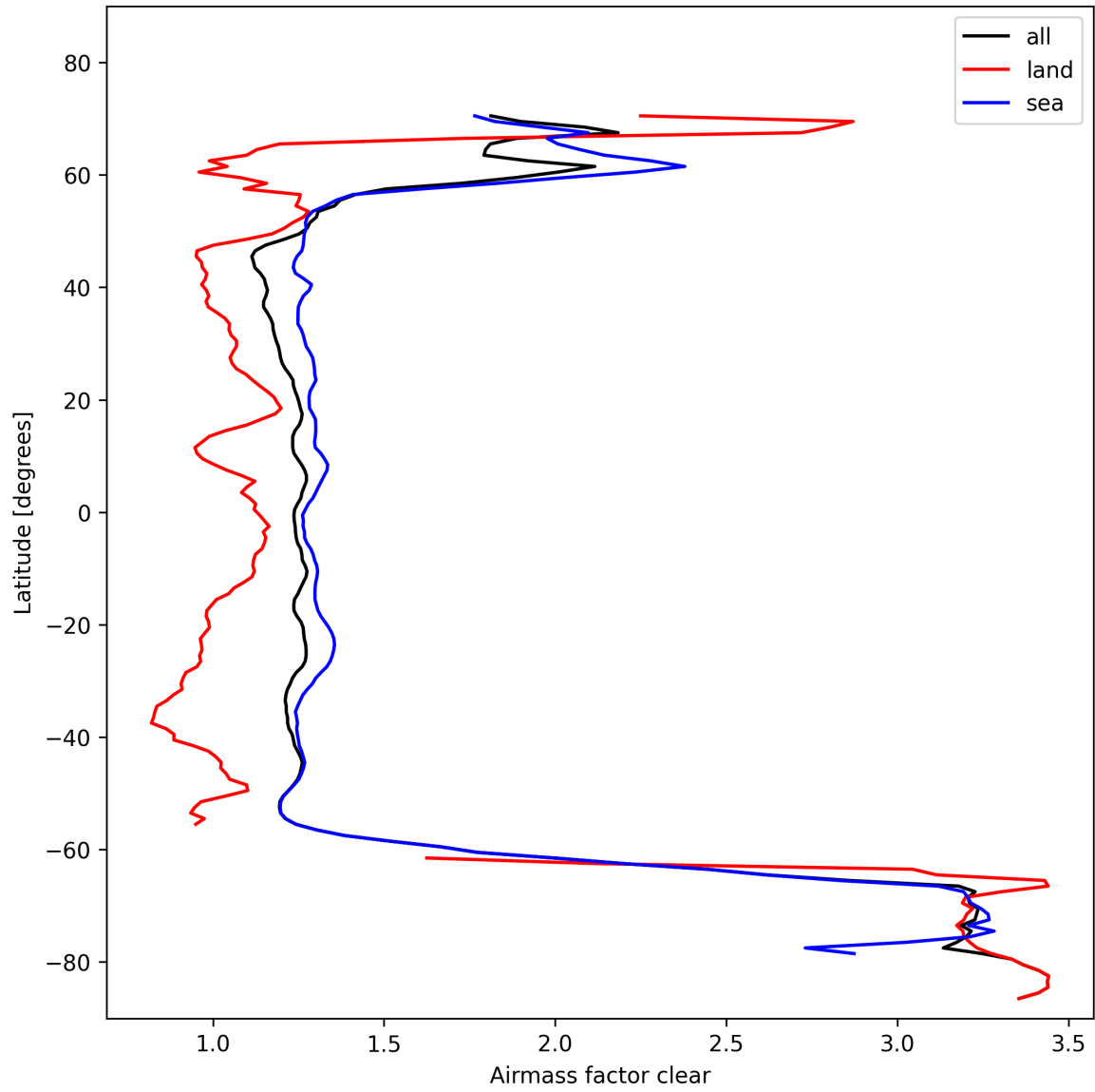
Figure 28: Zonal average of “Airmass factor clear” for 2024-10-30 to 2024-11-01.
