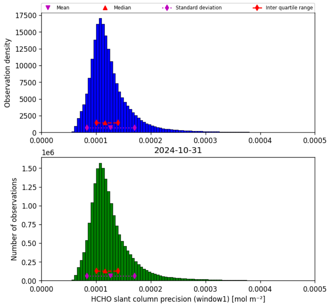
Figure 39: Histogram of “HCHO slant column precision (window1)” for 2024-10-30 to 2024-11-01
