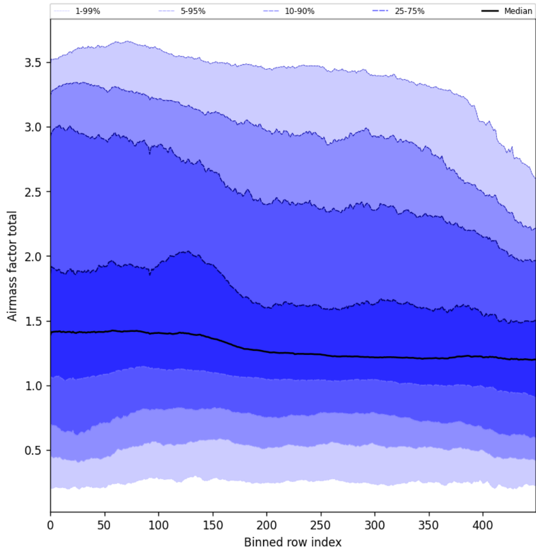
Figure 54: Along track statistics of “Airmass factor total” for 2024-10-30 to 2024-11-01
