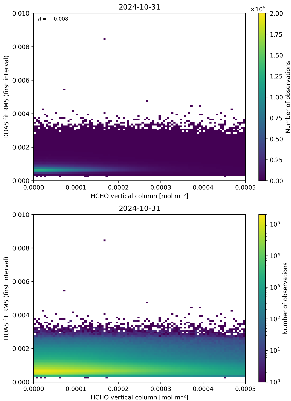
Figure 123: Scatter density plot of “HCHO vertical column” against “DOAS fit RMS (first interval)” for 2024-10-30 to 2024-11-01.
