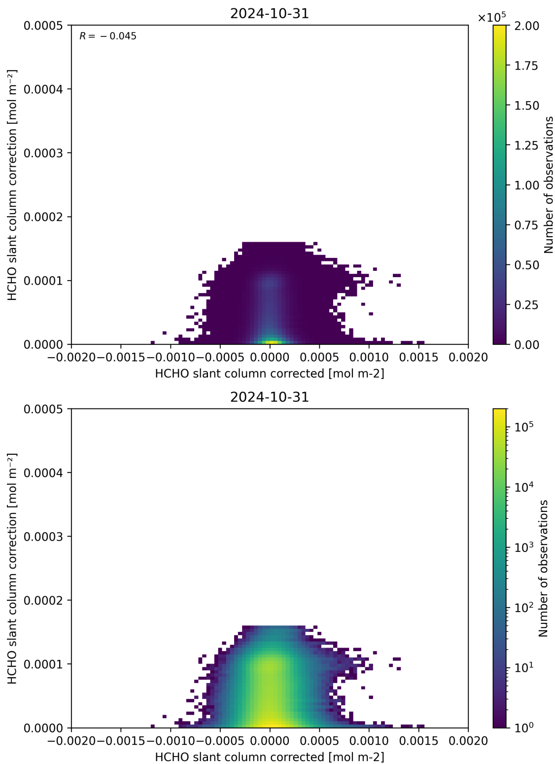
Figure 77: Scatter density plot of “HCHO slant column corrected” against “HCHO slant column correction” for 2024-10-30 to 2024-11-01.
