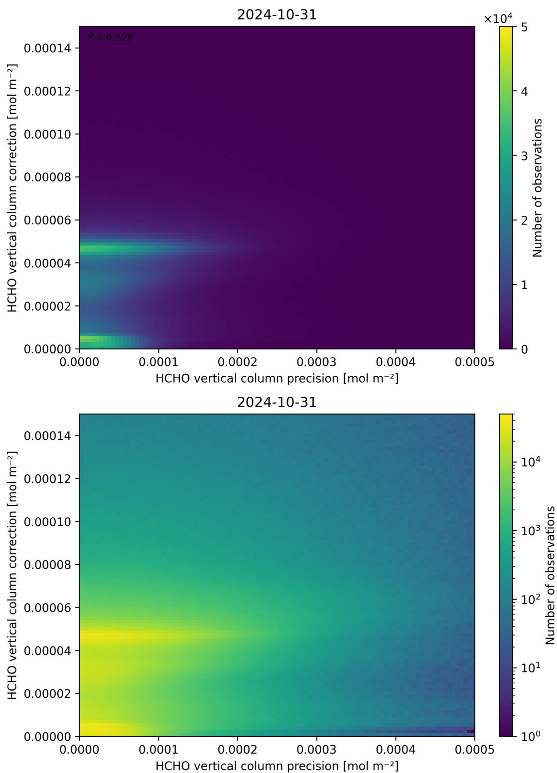
Figure 146: Scatter density plot of “HCHO vertical column precision” against “HCHO vertical column correction” for 2024-10-30 to 2024-11-01.
