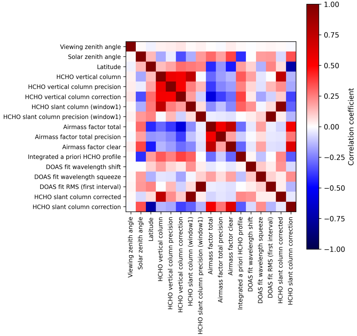
Figure 2: Map of correlation matrix for 2024-10-30 to 2024-11-01.
