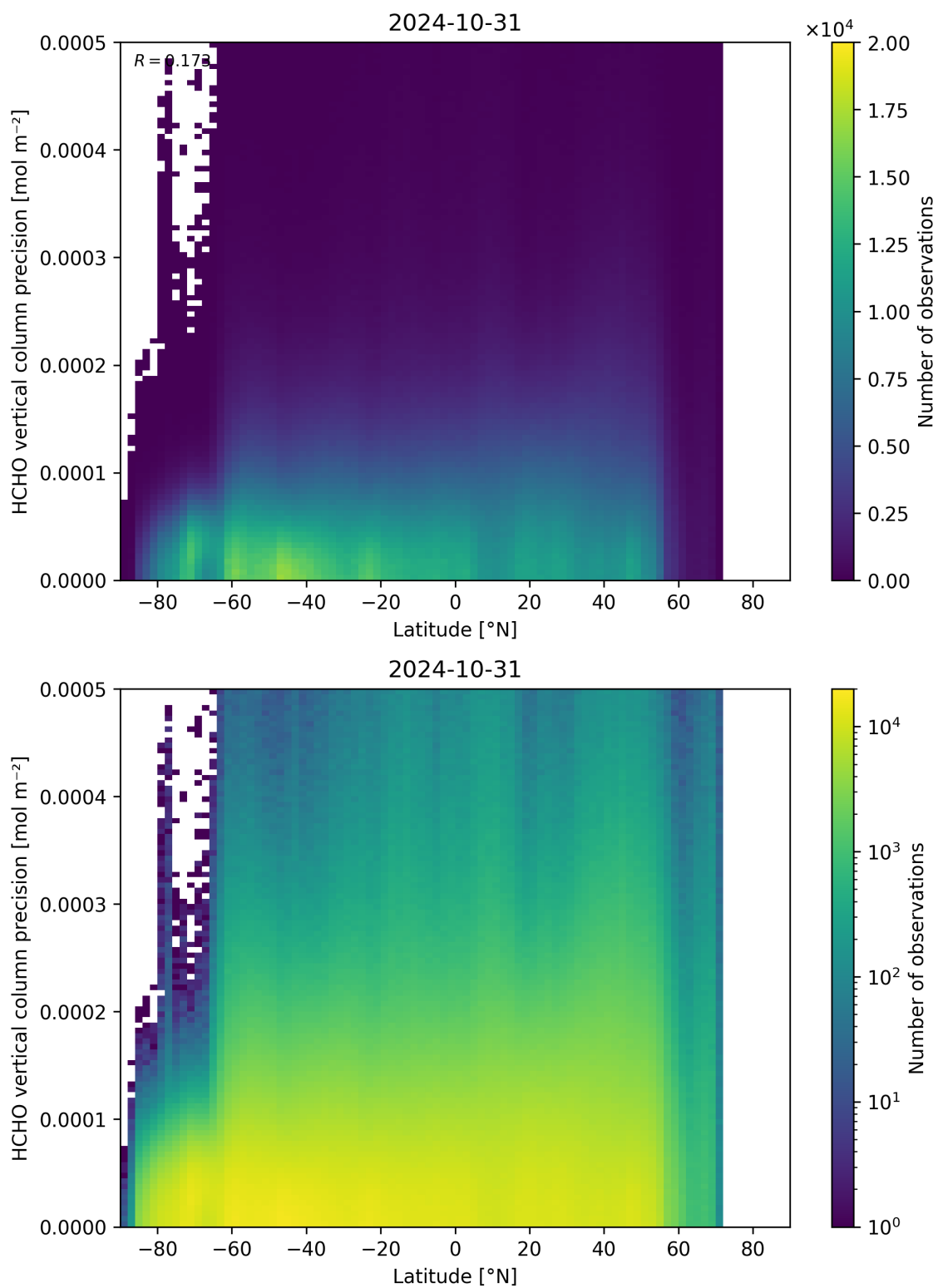
Figure 165: Scatter density plot of “Latitude” against “HCHO vertical column precision” for 2024-10-30 to 2024-11-01.
