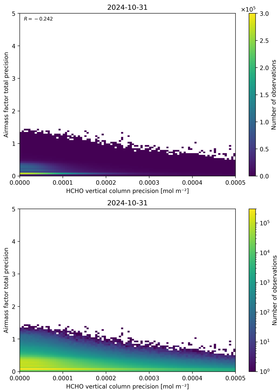
Figure 145: Scatter density plot of “HCHO vertical column precision” against “Airmass factor total precision” for 2024-10-30 to 2024-11-01.
