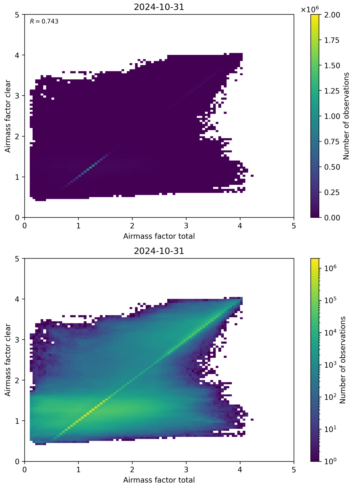
Figure 100: Scatter density plot of “Airmass factor total” against “Airmass factor clear” for 2024-10-30 to 2024-11-01.
