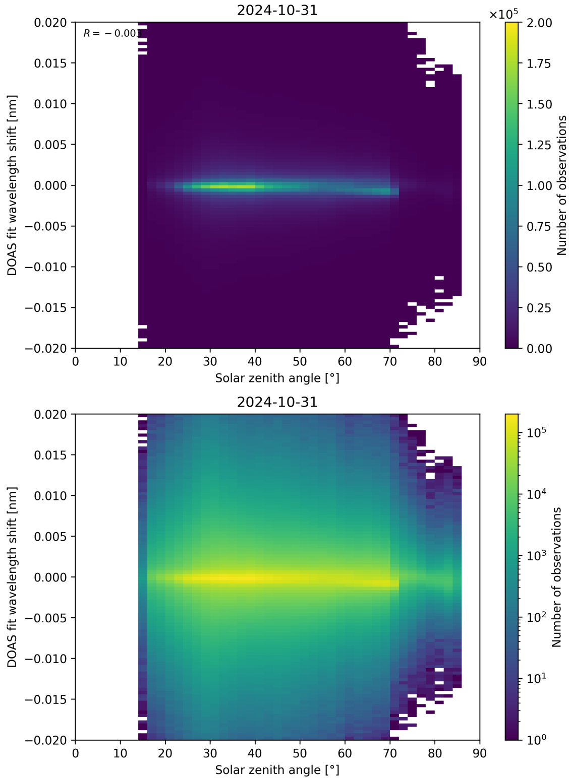
Figure 168: Scatter density plot of “Solar zenith angle” against “DOAS fit wavelength shift” for 2024-10-30 to 2024-11-01.
