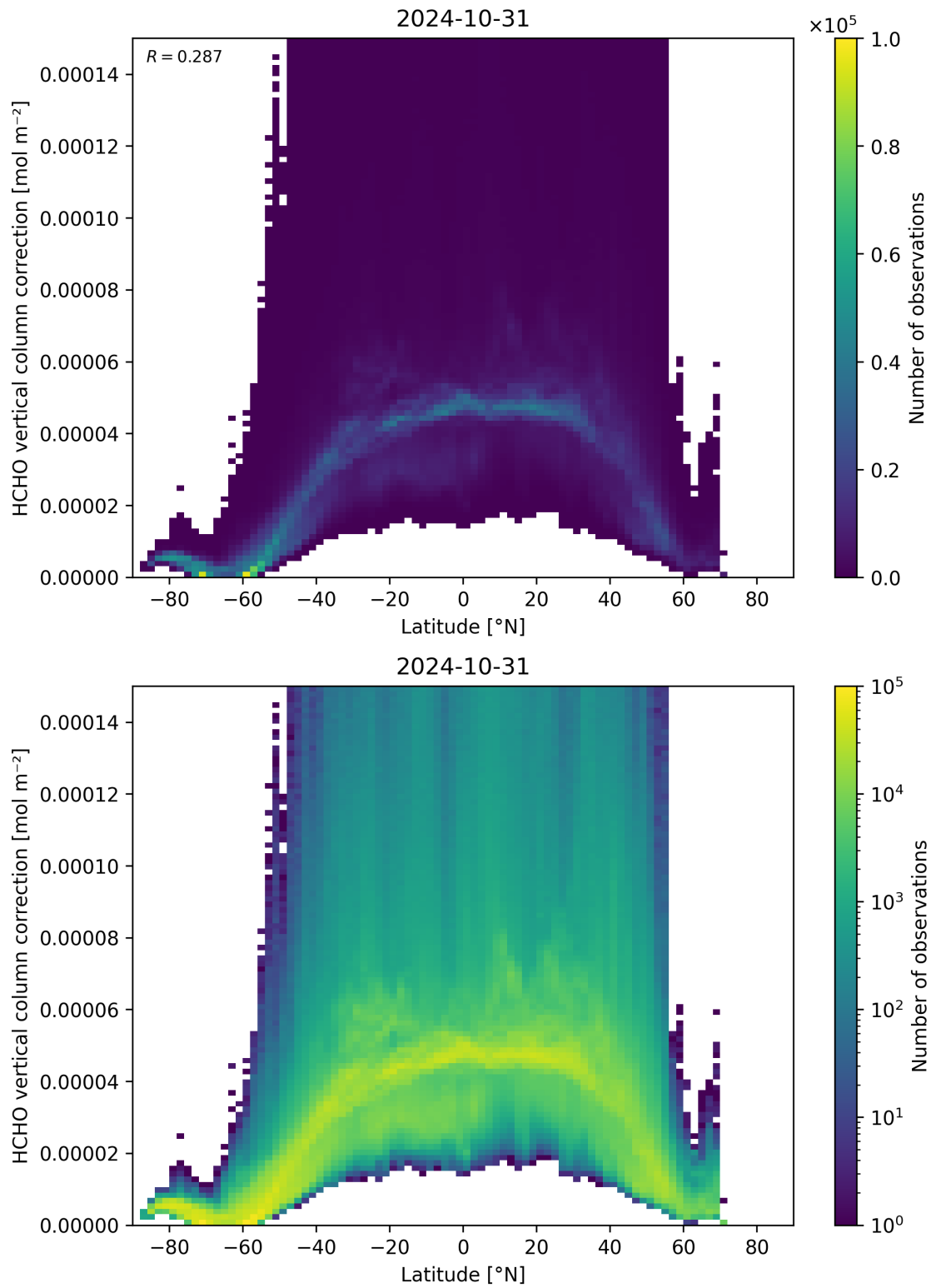
Figure 164: Scatter density plot of “Latitude” against “HCHO vertical column correction” for 2024-10-30 to 2024-11-01.
