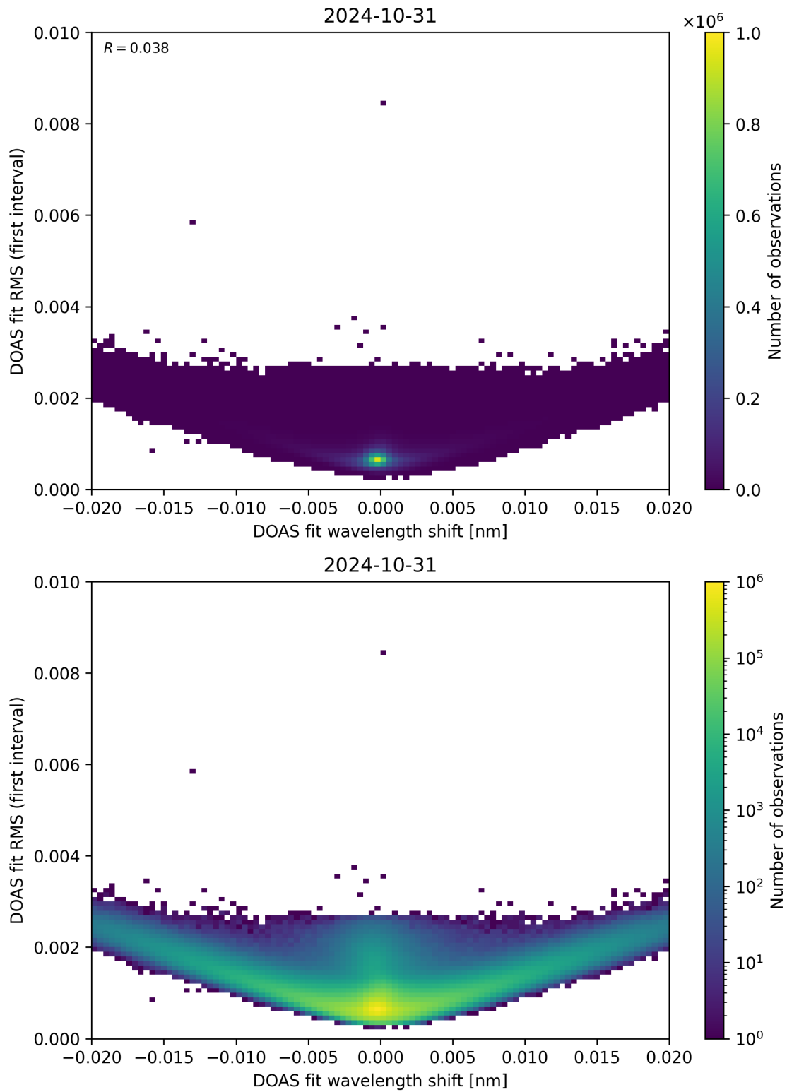
Figure 64: Scatter density plot of “DOAS fit wavelength shift” against “DOAS fit RMS (first interval)” for 2024-10-30 to 2024-11-01.
