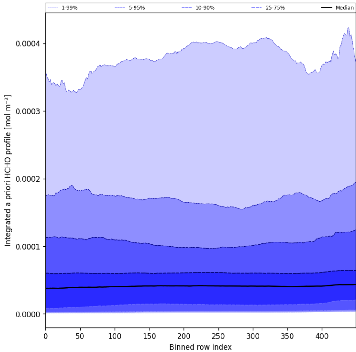
Figure 57: Along track statistics of "Integrated a priori HCHO profile" for 2024-10-30 to 2024-11-01
