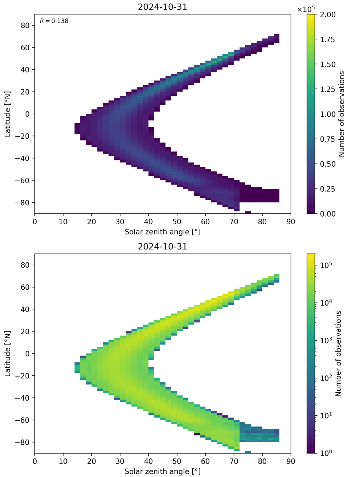
Figure 181: Scatter density plot of “Solar zenith angle” against “Latitude” for 2024-10-30 to 2024-11-01.
