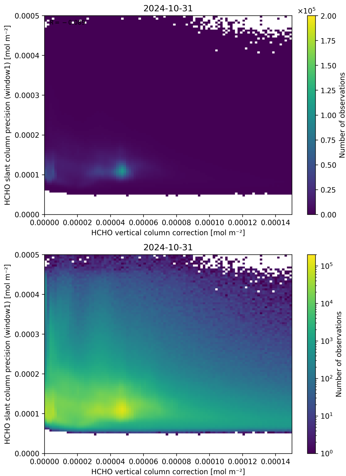
Figure 119: Scatter density plot of “HCHO vertical column correction” against “HCHO slant column precision (window1)” for 2024-10-30 to 2024-11-01.
