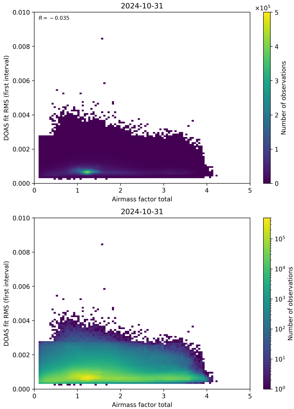
Figure 97: Scatter density plot of “Airmass factor total” against “DOAS fit RMS (first interval)” for 2024-10-30 to 2024-11-01.
