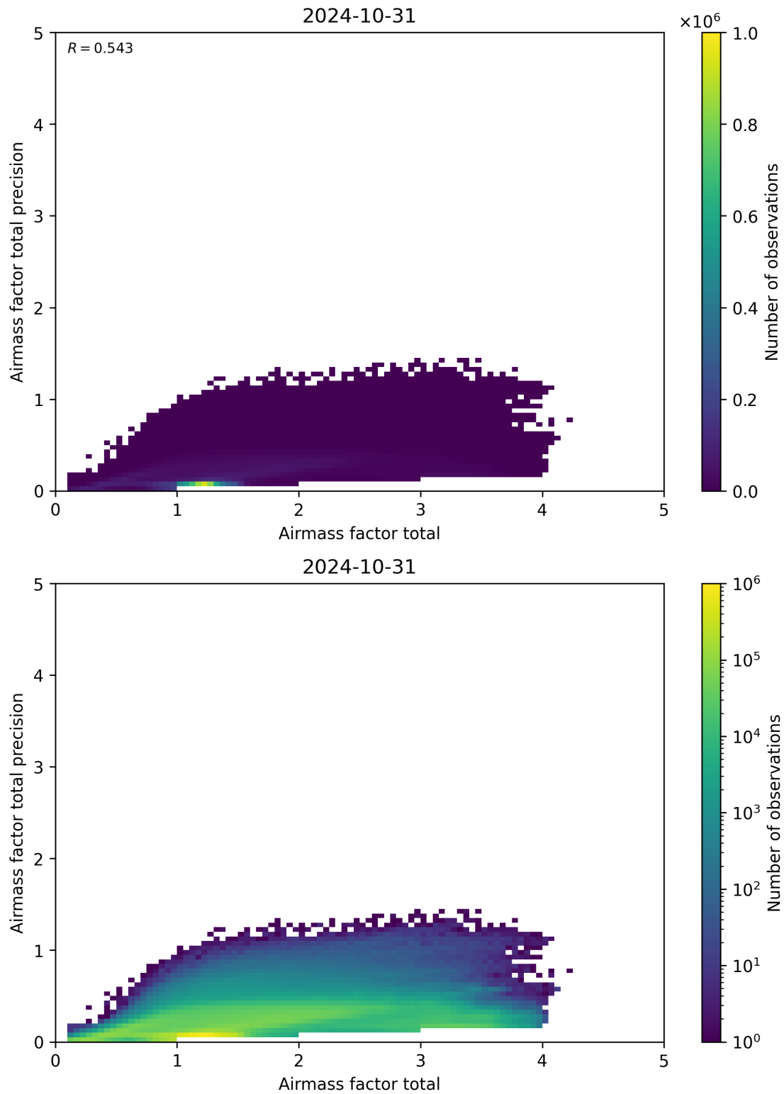
Figure 103: Scatter density plot of “Airmass factor total” against “Airmass factor total precision” for 2024-10-30 to 2024-11-01.
