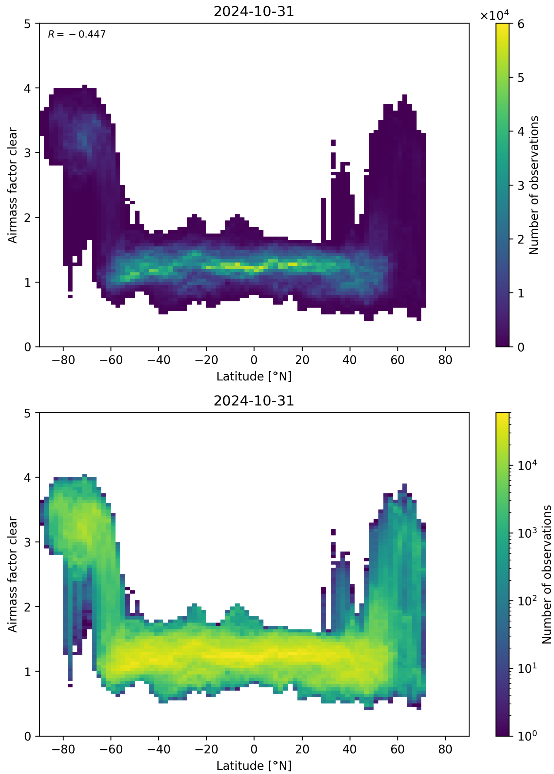
Figure 156: Scatter density plot of “Latitude” against “Airmass factor clear” for 2024-10-30 to 2024-11-01.
