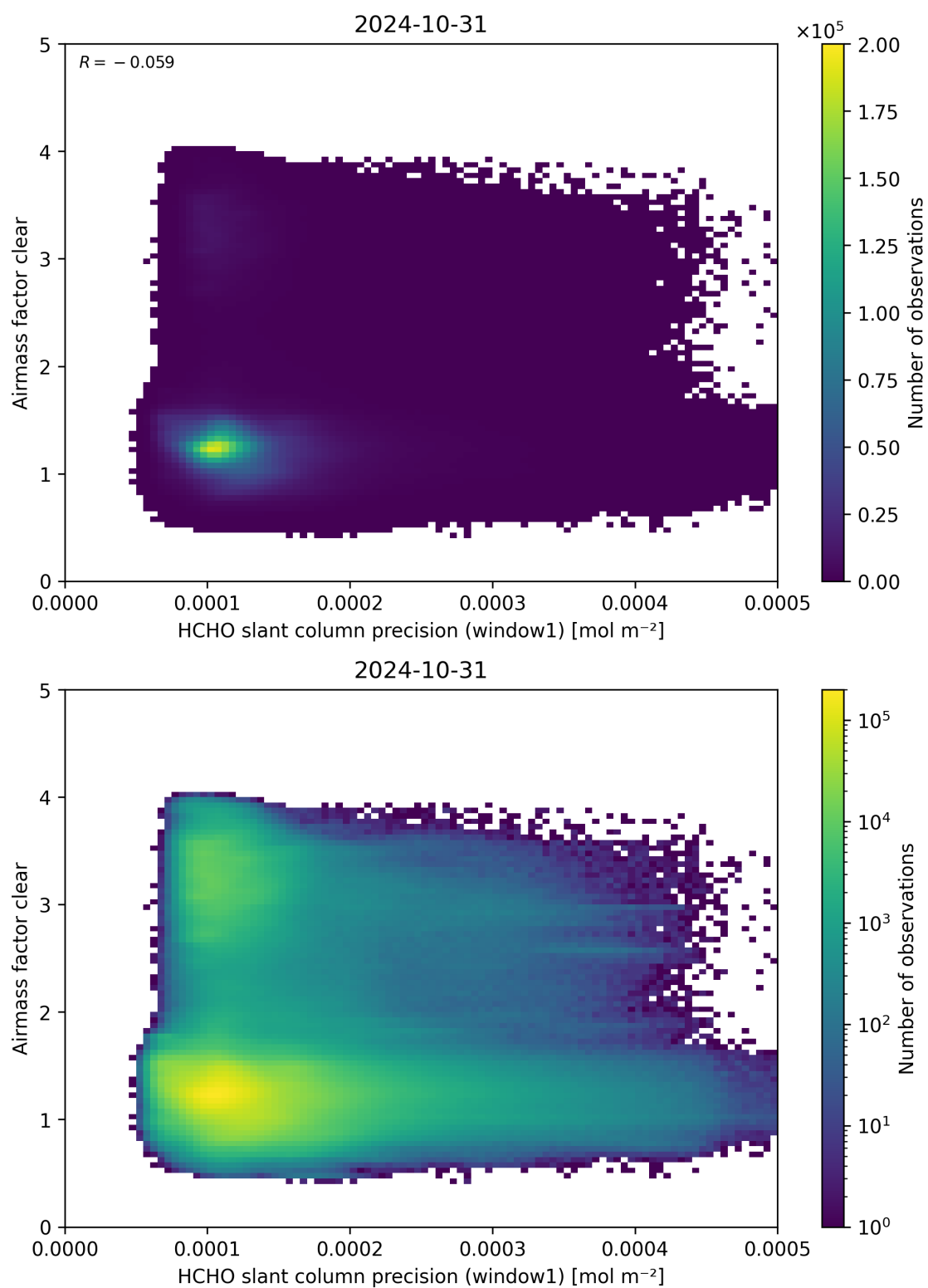
Figure 91: Scatter density plot of “HCHO slant column precision (window1)” against “Airmass factor clear” for 2024-10-30 to 2024-11-01.
