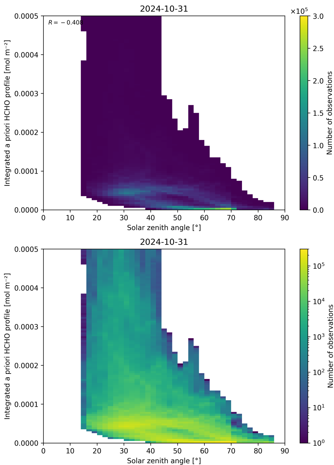
Figure 180: Scatter density plot of “Solar zenith angle” against “Integrated a priori HCHO profile” for 2024-10-30 to 2024-11-01.
