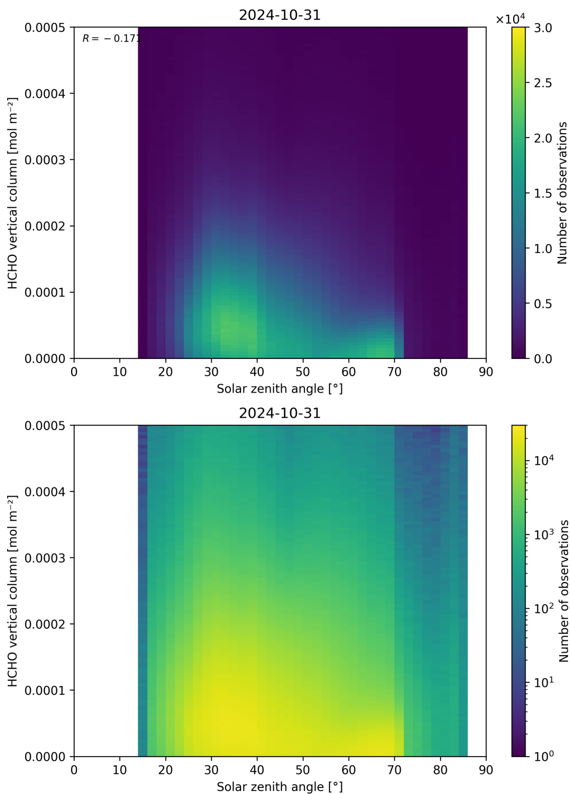
Figure 177: Scatter density plot of “Solar zenith angle” against “HCHO vertical column” for 2024-10-30 to 2024-11-01.
