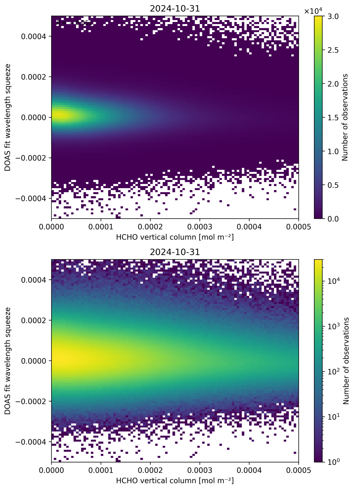
Figure 125: Scatter density plot of “HCHO vertical column” against “DOAS fit wavelength squeeze” for 2024-10-30 to 2024-11-01.
