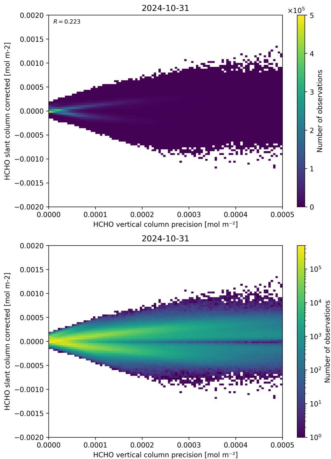
Figure 140: Scatter density plot of “HCHO vertical column precision” against “HCHO slant column corrected” for 2024-10-30 to 2024-11-01.
