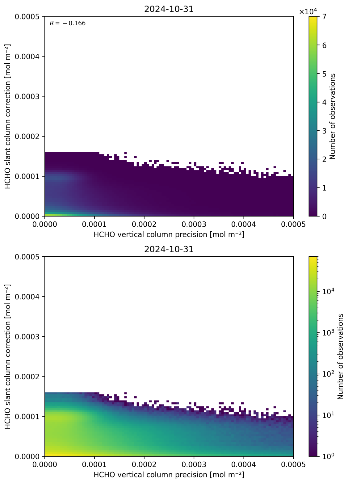
Figure 141: Scatter density plot of “HCHO vertical column precision” against “HCHO slant column correction” for 2024-10-30 to 2024-11-01.
