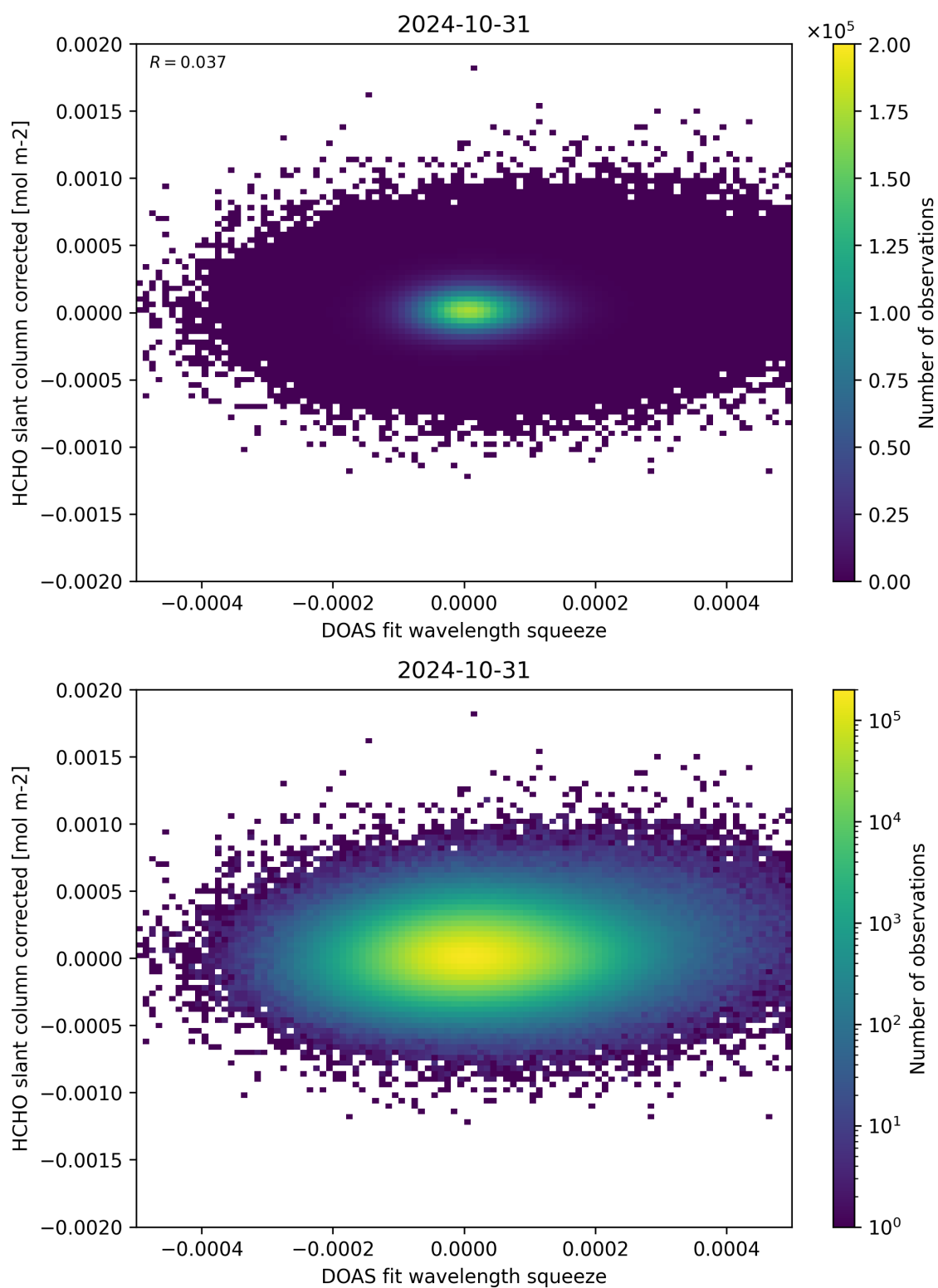
Figure 69: Scatter density plot of “DOAS fit wavelength squeeze” against “HCHO slant column corrected” for 2024-10-30 to 2024-11-01.
