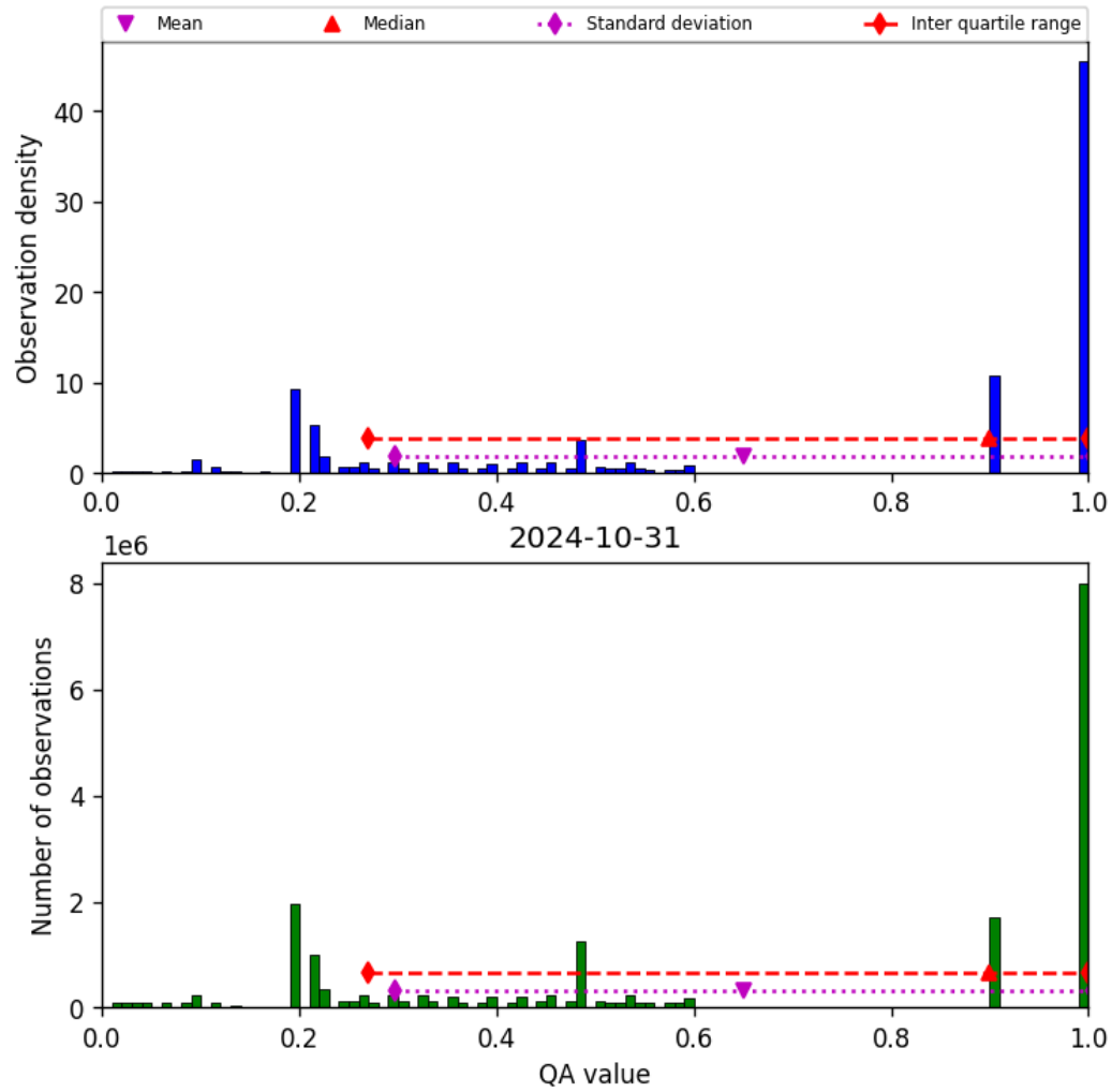
Figure 34: Histogram of “QA value” for 2024-10-30 to 2024-11-01
