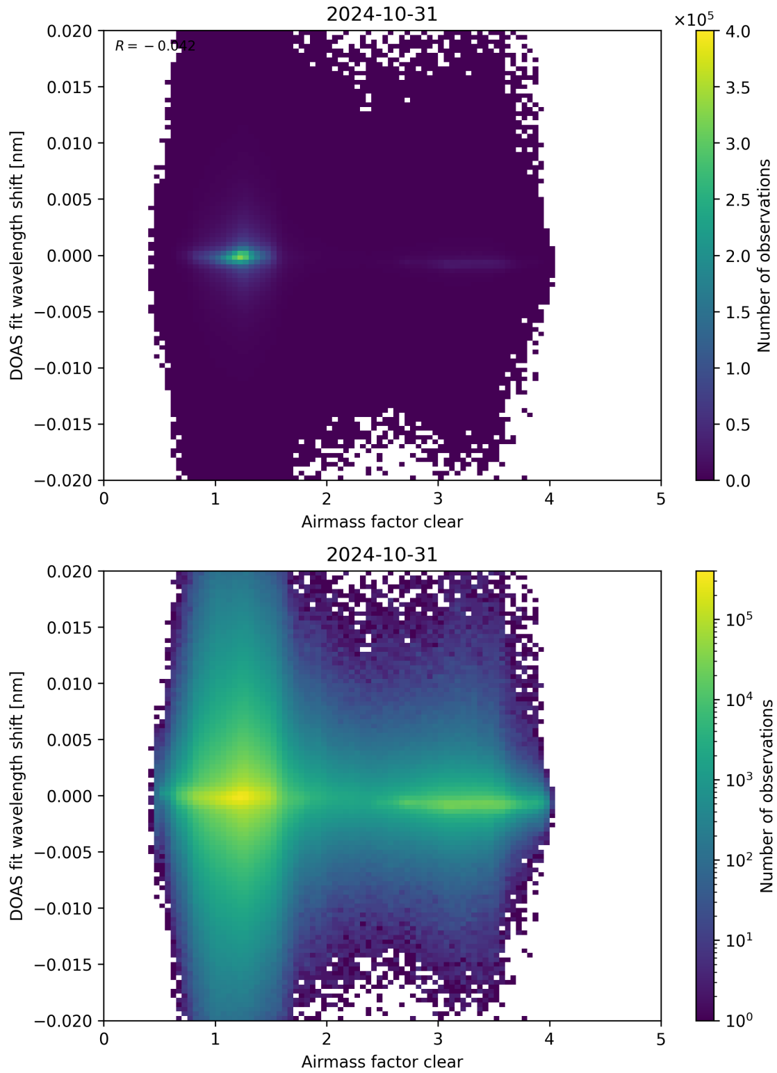
Figure 72: Scatter density plot of “Airmass factor clear” against “DOAS fit wavelength shift” for 2024-10-30 to 2024-11-01.
