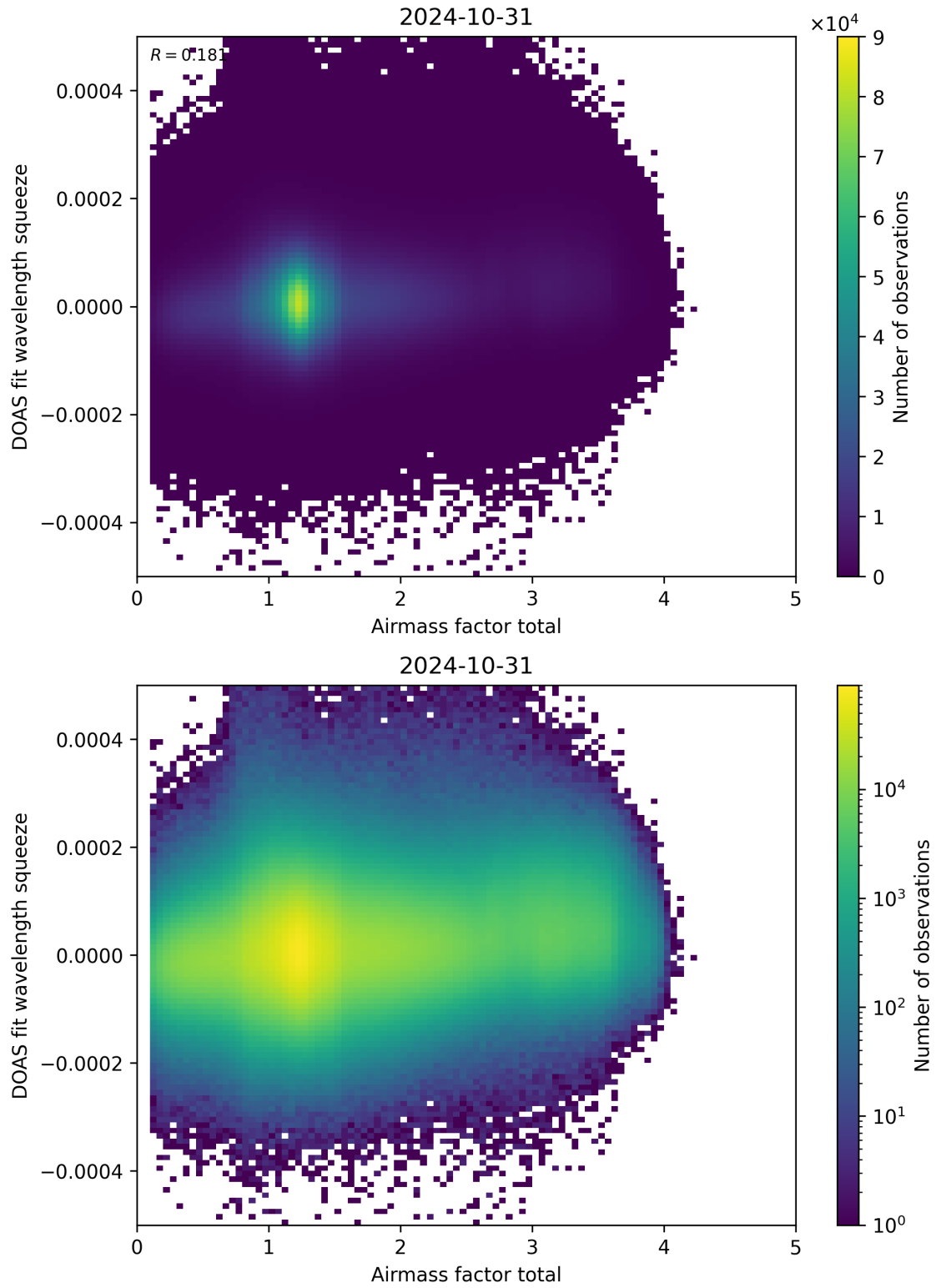
Figure 99: Scatter density plot of “Airmass factor total” against “DOAS fit wavelength squeeze” for 2024-10-30 to 2024-11-01.
