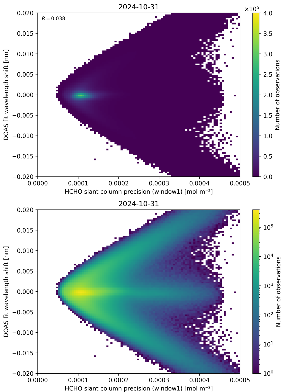
Figure 89: Scatter density plot of “HCHO slant column precision (window1)” against “DOAS fit wavelength shift” for 2024-10-30 to 2024-11-01.
