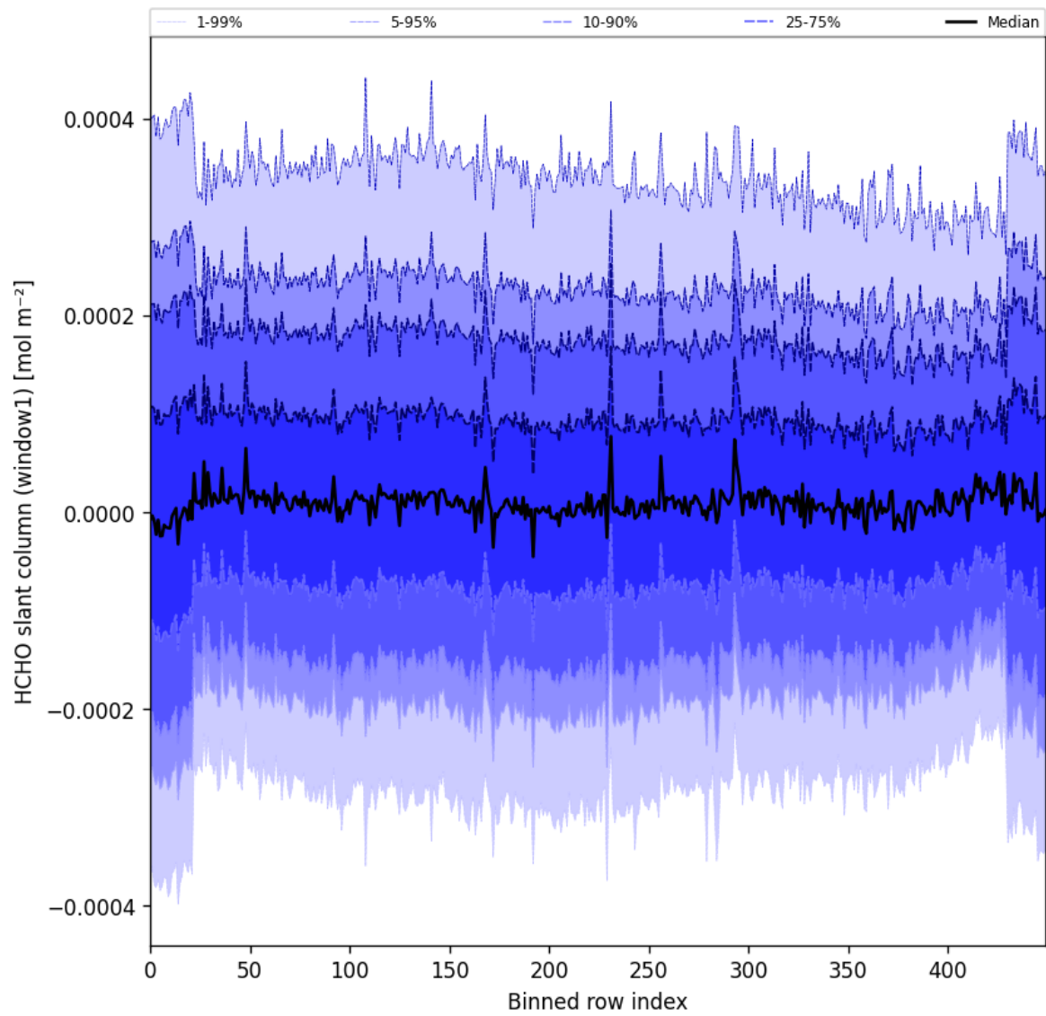
Figure 52: Along track statistics of “HCHO slant column (window1)” for 2024-10-30 to 2024-11-01
