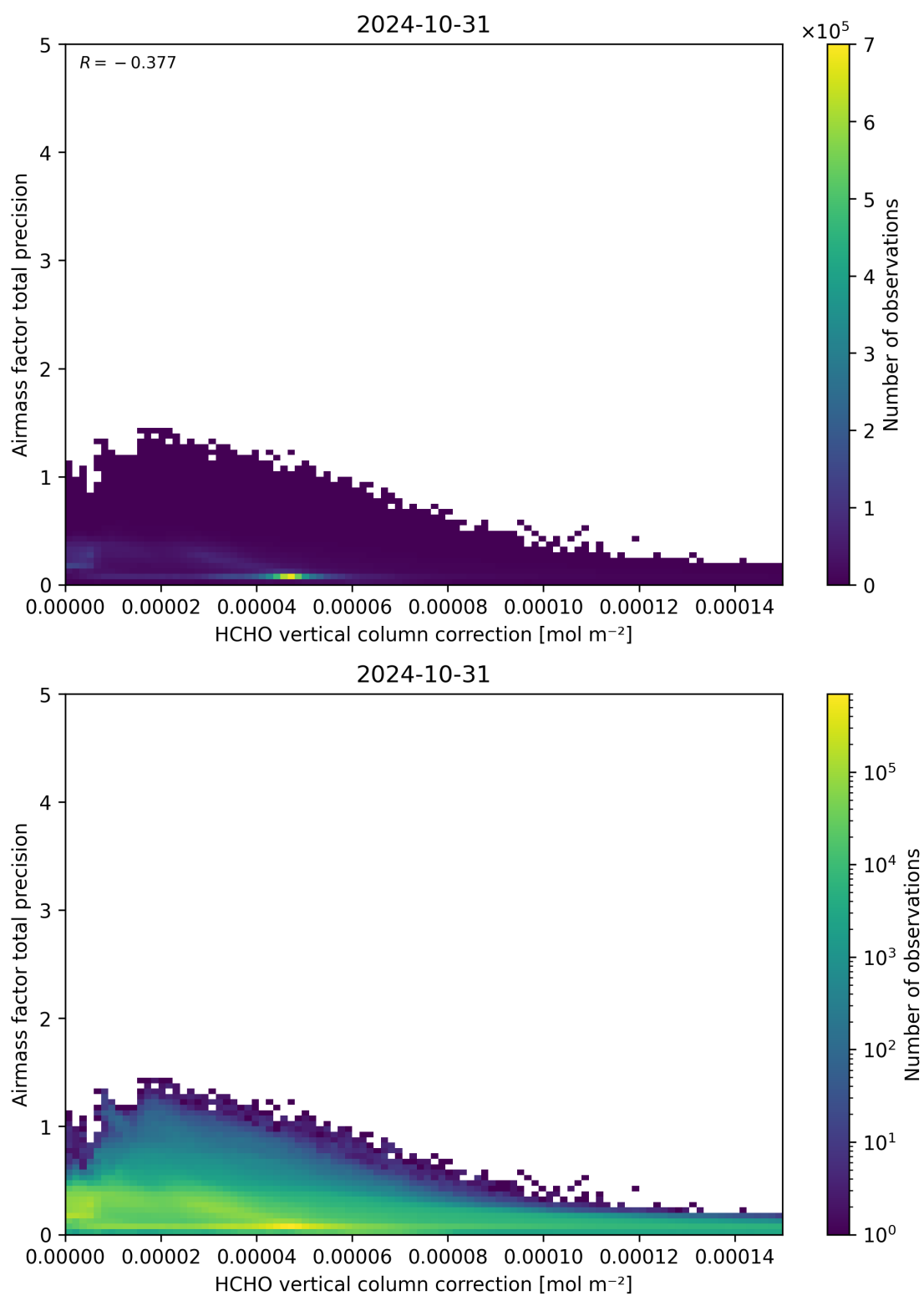
Figure 121: Scatter density plot of “HCHO vertical column correction” against “Airmass factor total precision” for 2024-10-30 to 2024-11-01.
