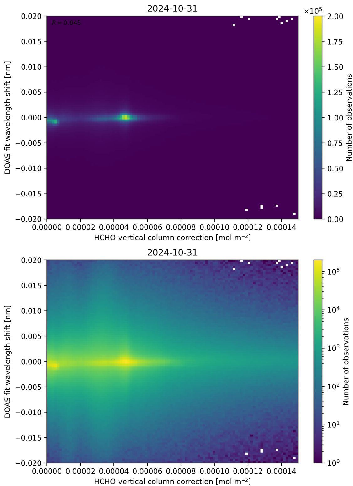
Figure 113: Scatter density plot of “HCHO vertical column correction” against “DOAS fit wavelength shift” for 2024-10-30 to 2024-11-01.
