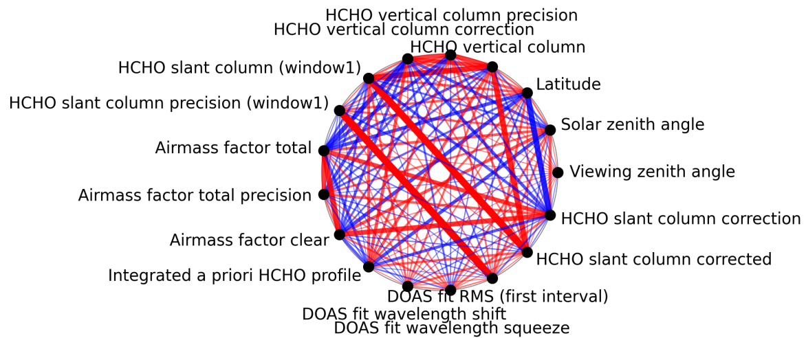
Figure 1: Map of correlation graph for 2024-10-30 to 2024-11-01.
