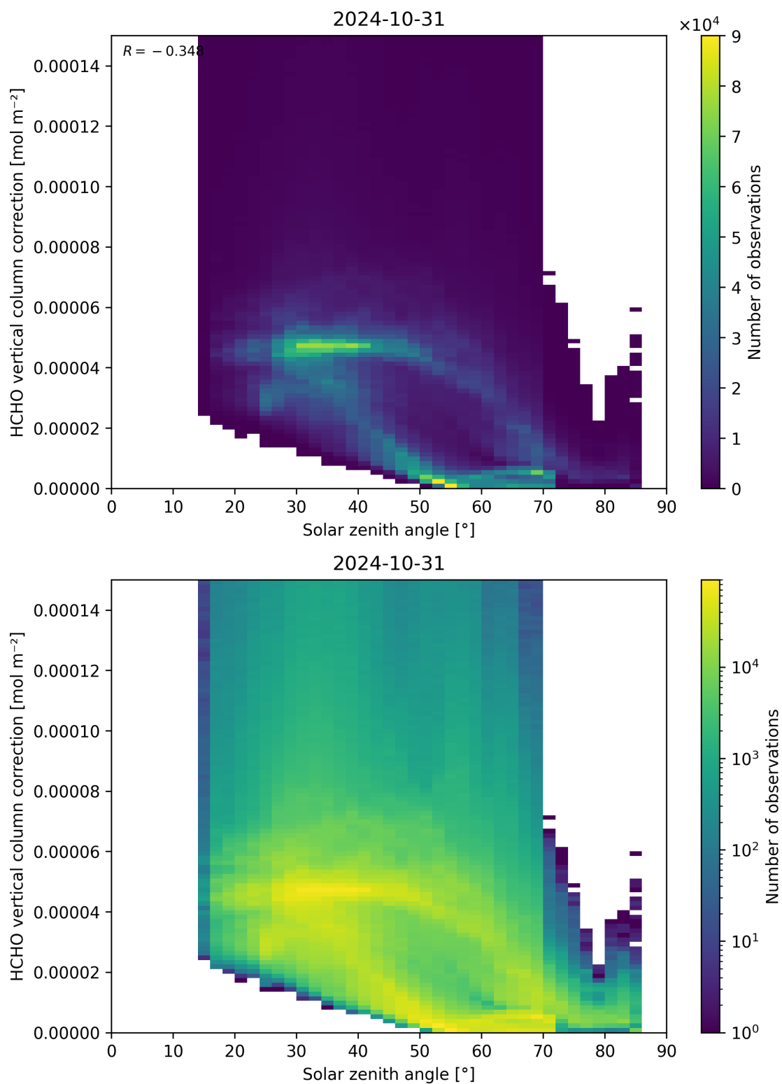
Figure 178: Scatter density plot of “Solar zenith angle” against “HCHO vertical column correction” for 2024-10-30 to 2024-11-01.
