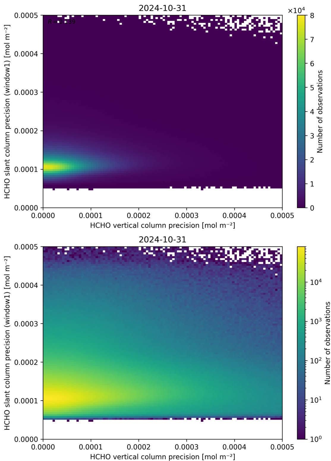
Figure 143: Scatter density plot of “HCHO vertical column precision” against “HCHO slant column precision (window1)” for 2024-10-30 to 2024-11-01.
