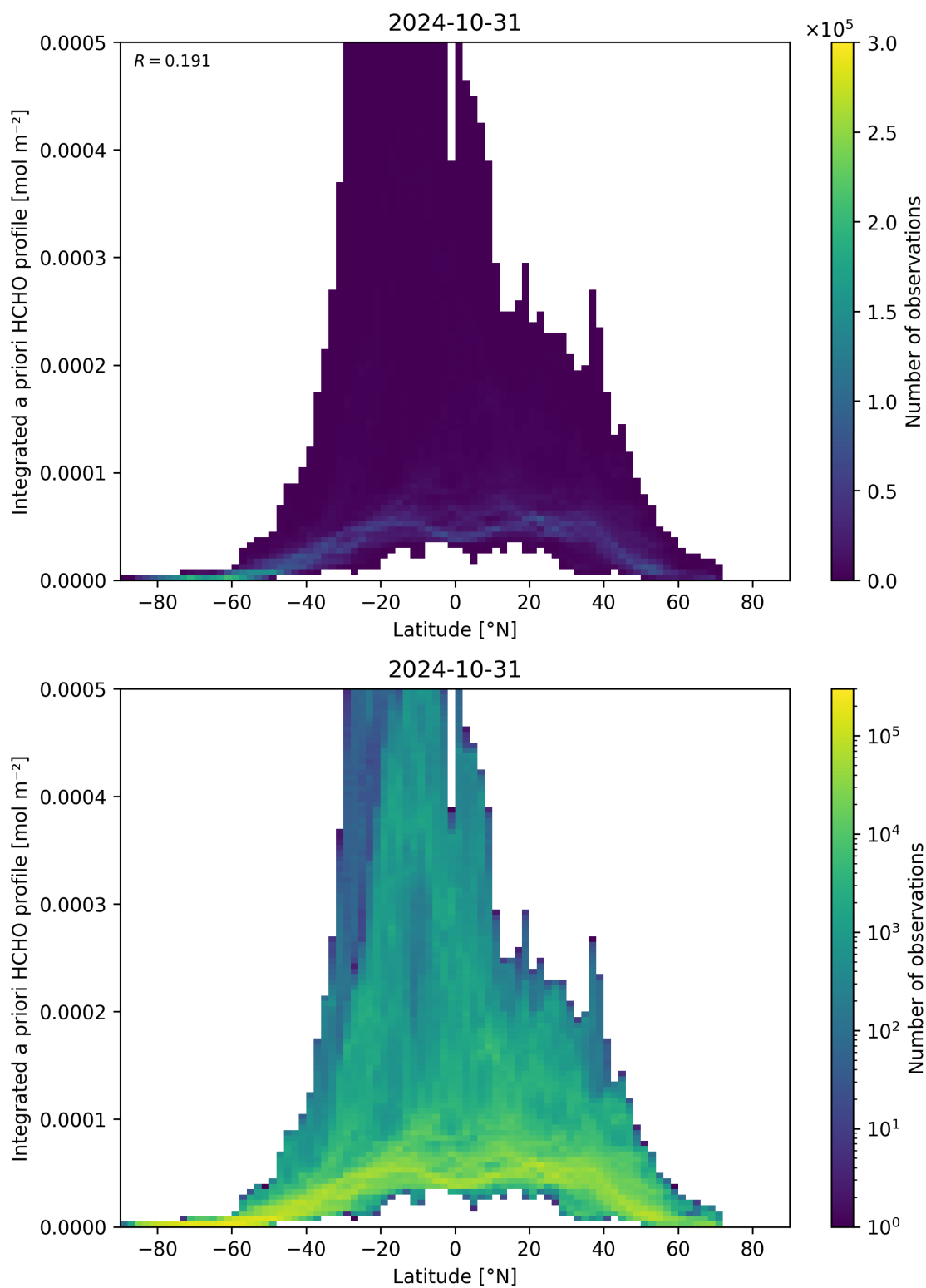
Figure 166: Scatter density plot of “Latitude” against “Integrated a priori HCHO profile” for 2024-10-30 to 2024-11-01.
