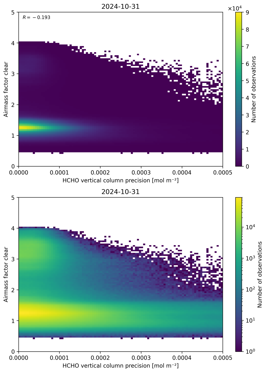
Figure 139: Scatter density plot of “HCHO vertical column precision” against “Airmass factor clear” for 2024-10-30 to 2024-11-01.
