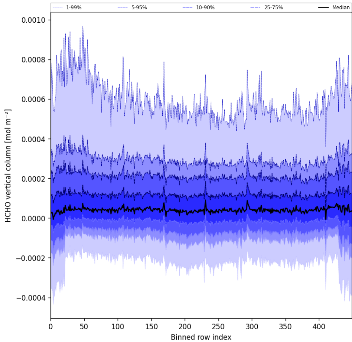
Figure 49: Along track statistics of “HCHO vertical column” for 2024-10-30 to 2024-11-01
