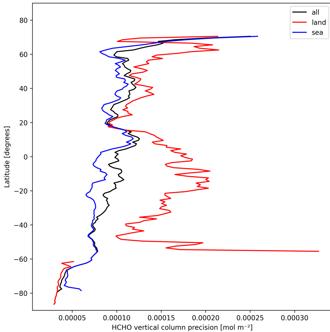
Figure 22: Zonal average of “HCHO vertical column precision” for 2024-10-30 to 2024-11-01.
