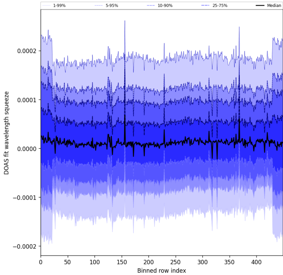
Figure 59: Along track statistics of “DOAS fit wavelength squeeze” for 2024-10-30 to 2024-11-01
