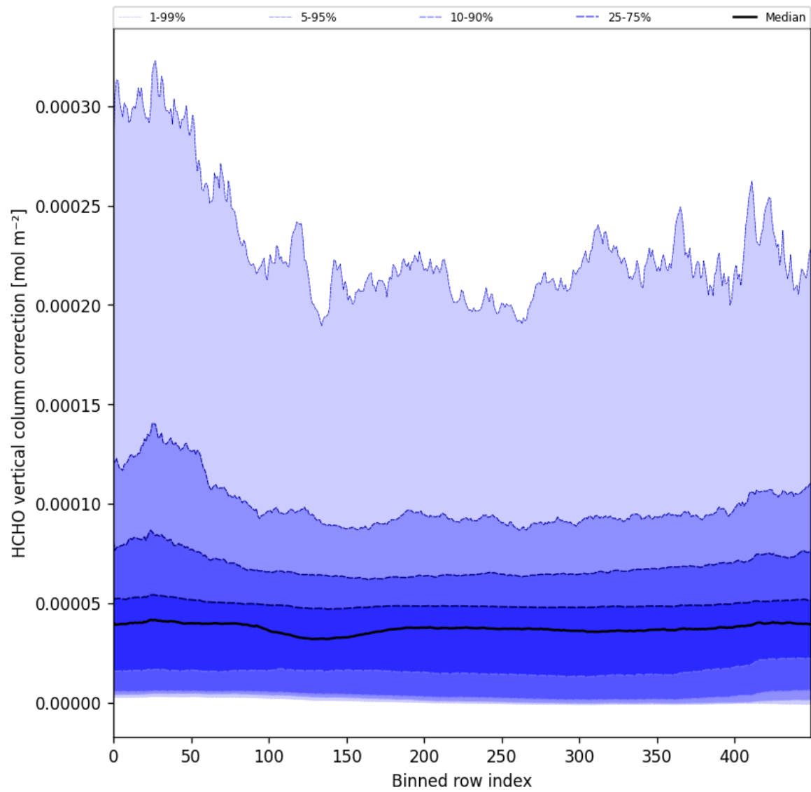
Figure 51: Along track statistics of “HCHO vertical column correction” for 2024-10-30 to 2024-11-01
