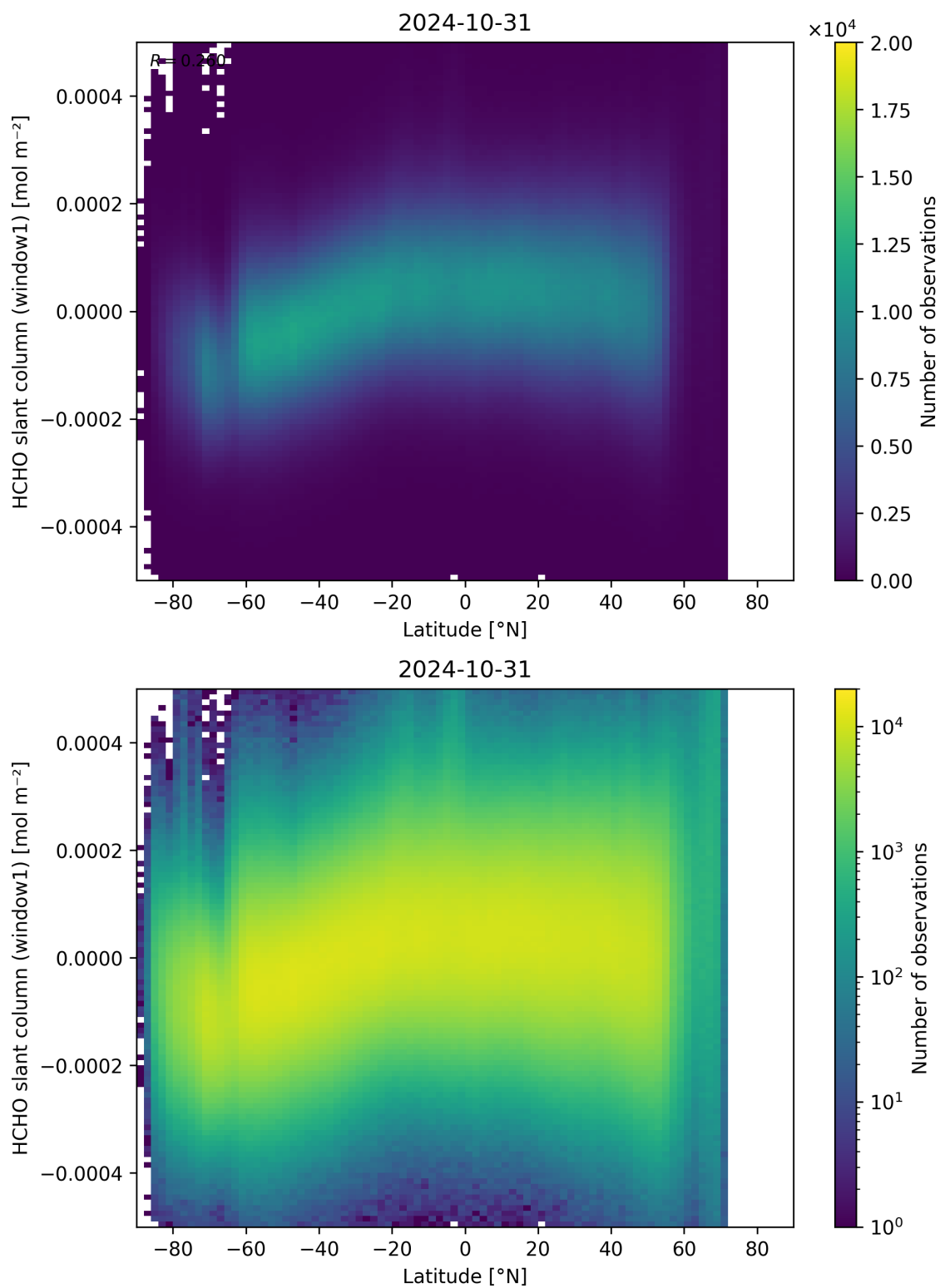
Figure 159: Scatter density plot of “Latitude” against “HCHO slant column (window1)” for 2024-10-30 to 2024-11-01.
