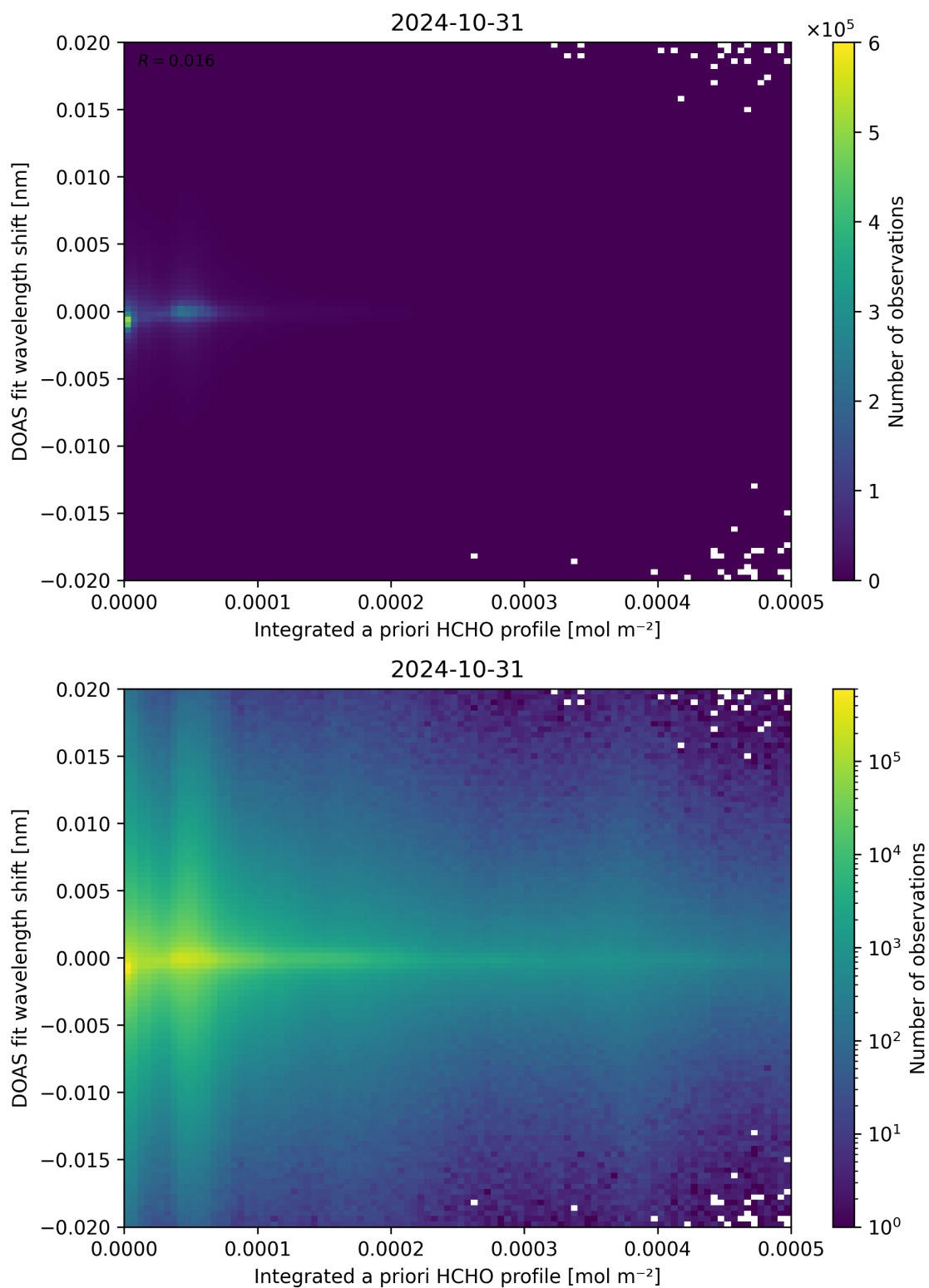
Figure 149: Scatter density plot of “Integrated a priori HCHO profile” against “DOAS fit wavelength shift” for 2024-10-30 to 2024-11-01.
