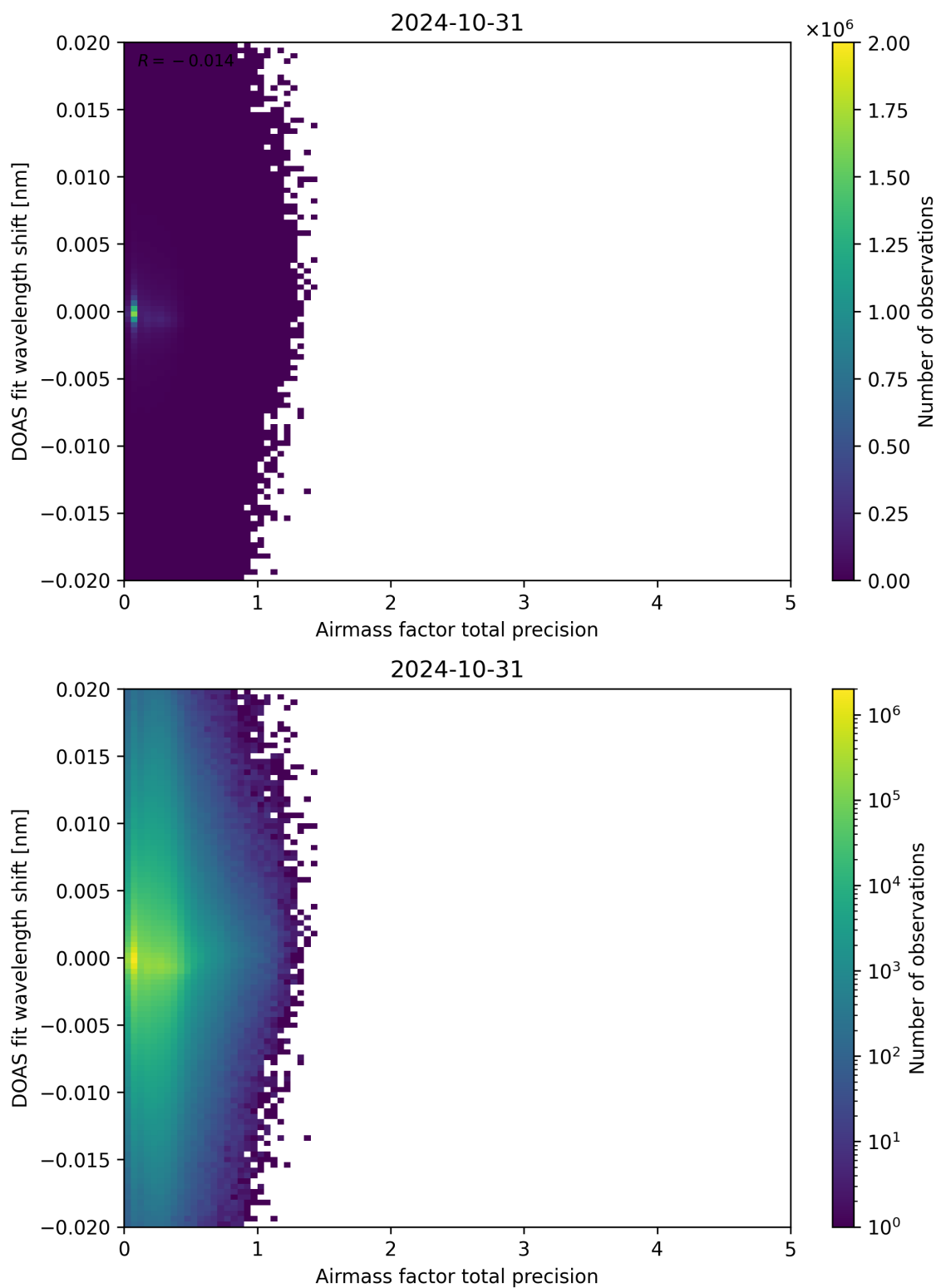
Figure 106: Scatter density plot of “Airmass factor total precision” against “DOAS fit wavelength shift” for 2024-10-30 to 2024-11-01.
