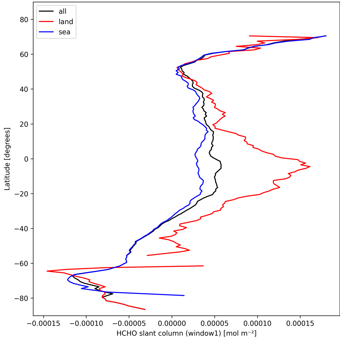
Figure 24: Zonal average of “HCHO slant column (window1)” for 2024-10-30 to 2024-11-01.
