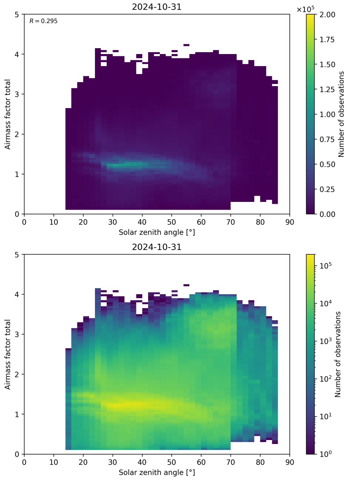
Figure 175: Scatter density plot of “Solar zenith angle” against “Airmass factor total” for 2024-10-30 to 2024-11-01.
