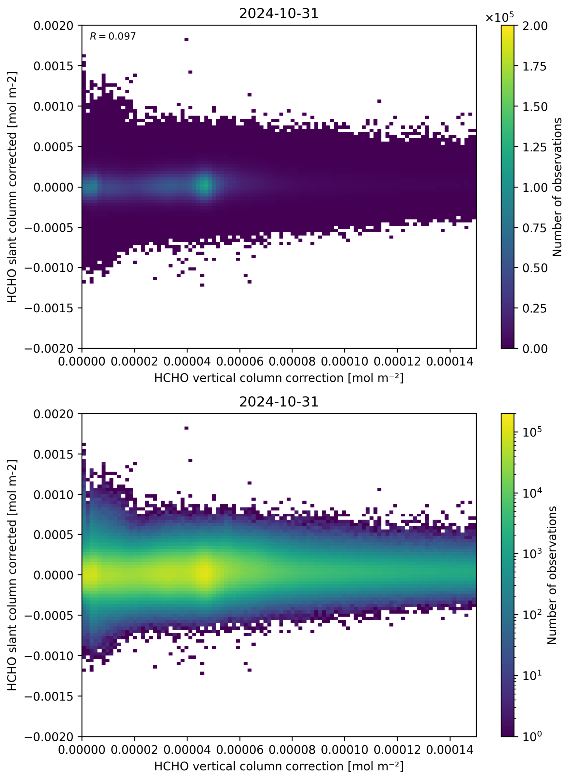
Figure 116: Scatter density plot of “HCHO vertical column correction” against “HCHO slant column corrected” for 2024-10-30 to 2024-11-01.
