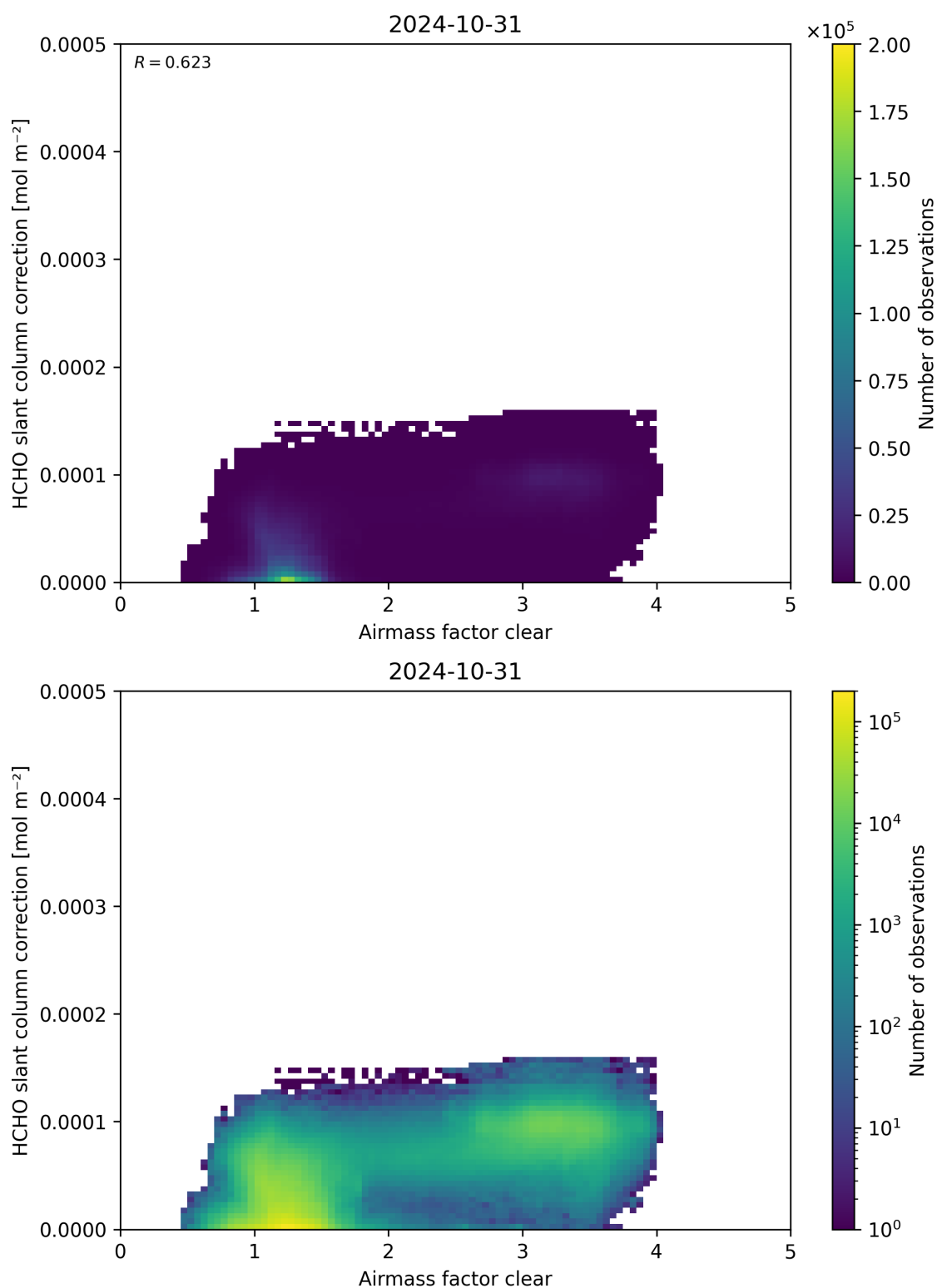
Figure 75: Scatter density plot of “Airmass factor clear” against “HCHO slant column correction” for 2024-10-30 to 2024-11-01.
