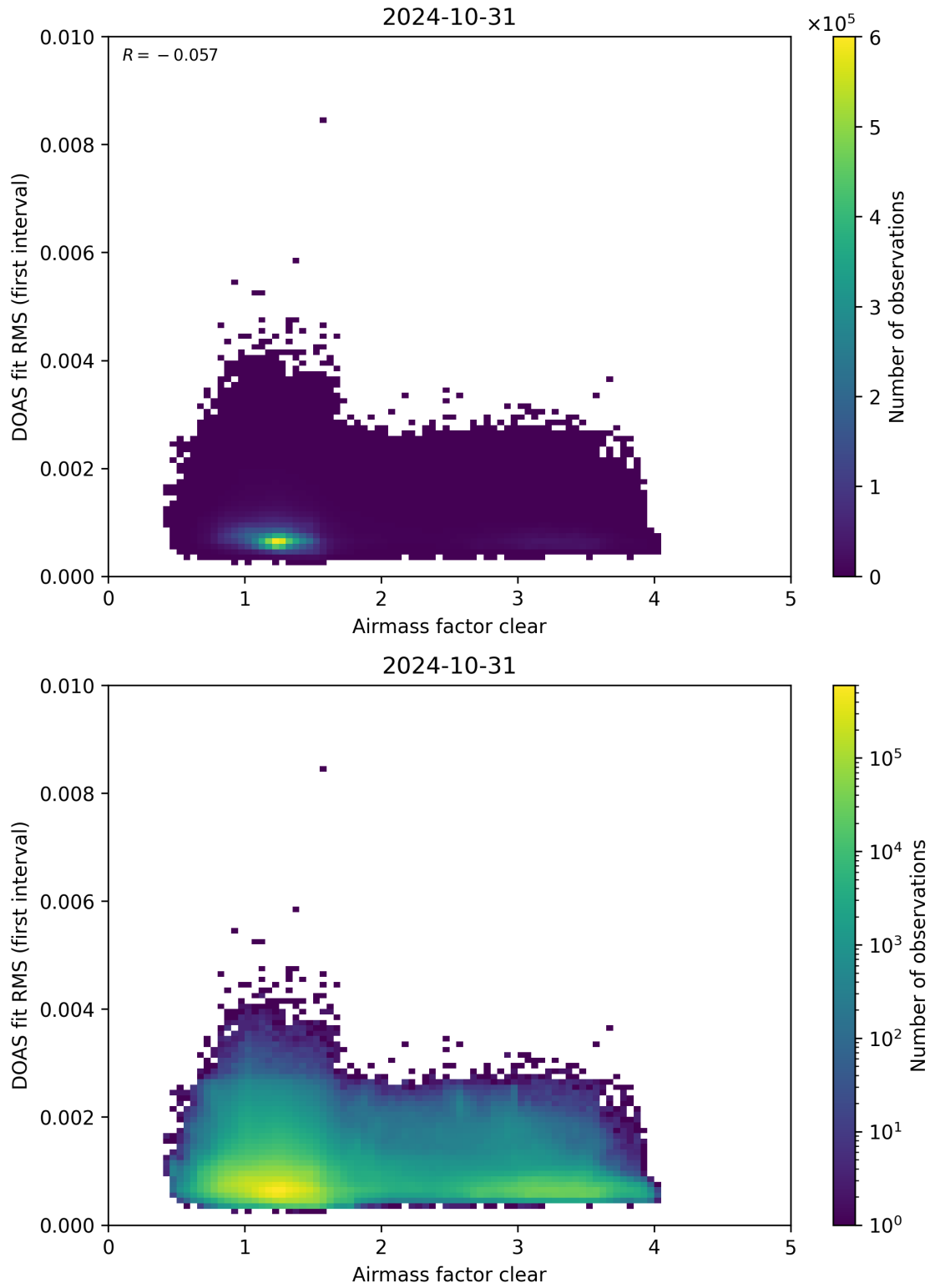
Figure 71: Scatter density plot of “Airmass factor clear” against “DOAS fit RMS (first interval)” for 2024-10-30 to 2024-11-01.
