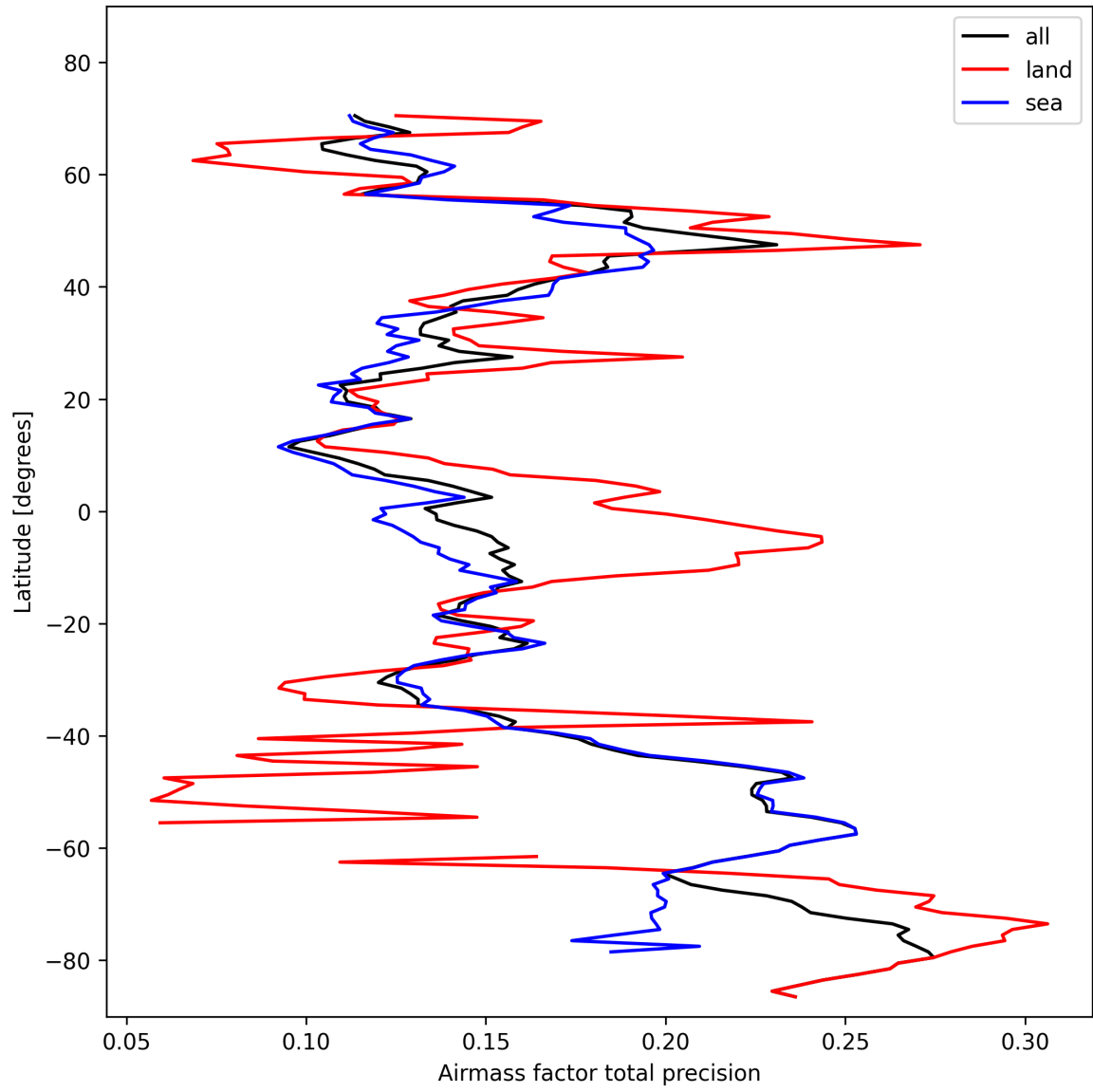
Figure 27: Zonal average of “Airmass factor total precision” for 2024-10-30 to 2024-11-01.
