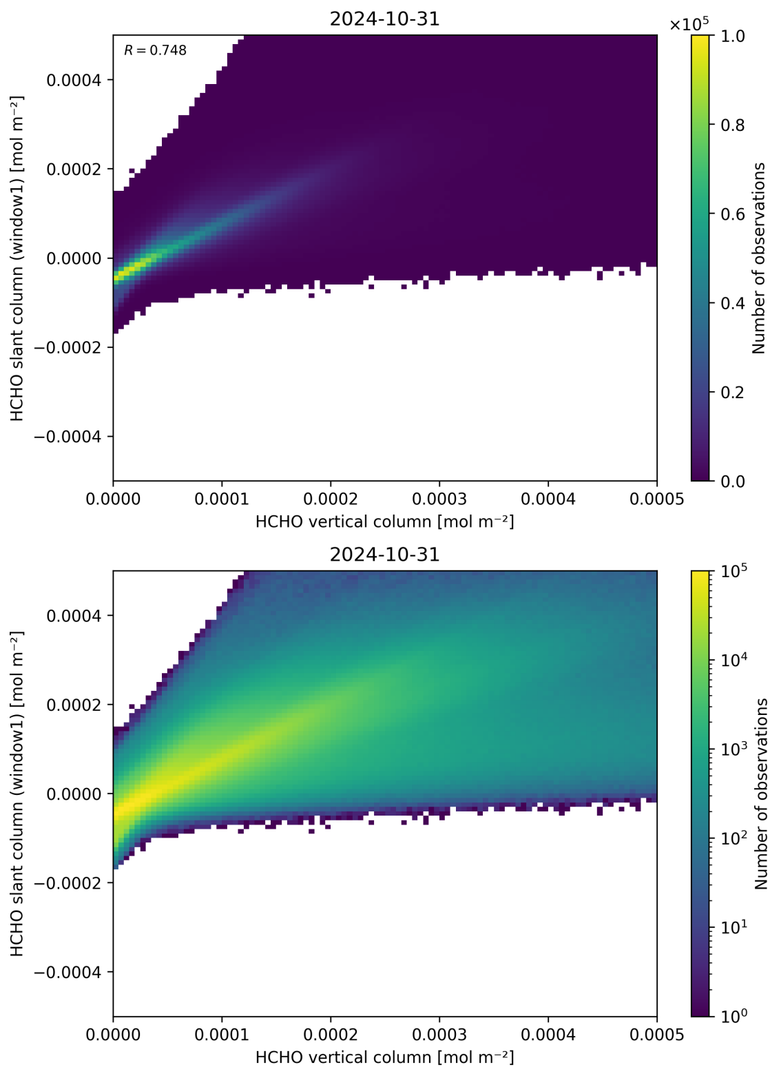
Figure 129: Scatter density plot of “HCHO vertical column” against “HCHO slant column (window1)” for 2024-10-30 to 2024-11-01.
