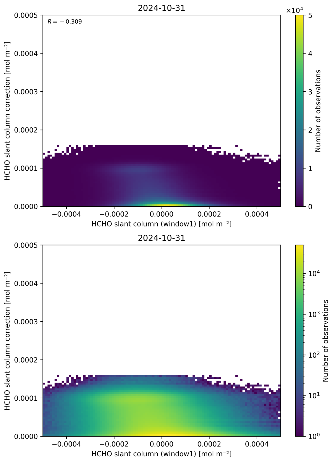
Figure 83: Scatter density plot of “HCHO slant column (window1)” against “HCHO slant column correction” for 2024-10-30 to 2024-11-01.
