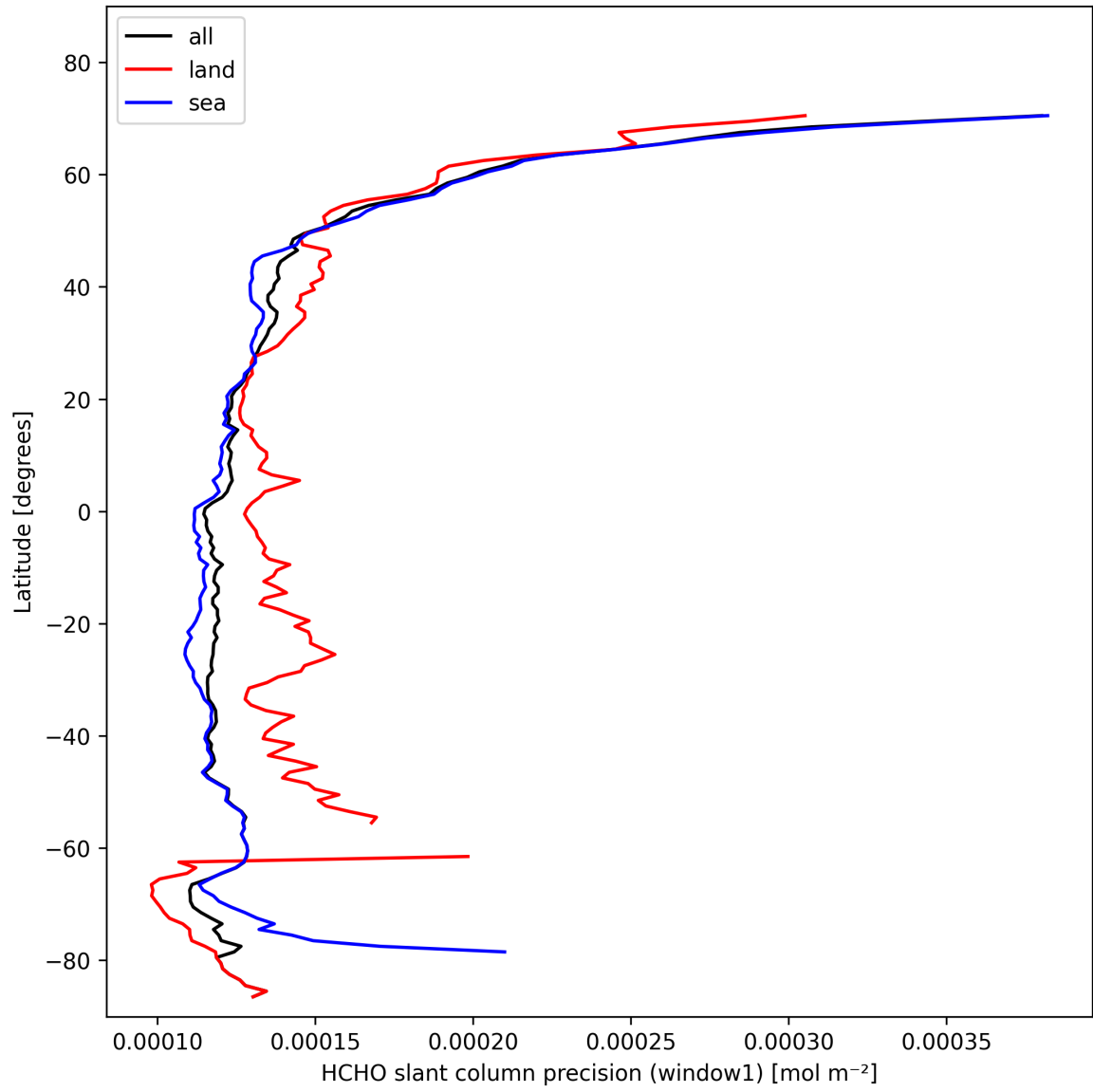
Figure 25: Zonal average of “HCHO slant column precision (window1)” for 2024-10-30 to 2024-11-01.
