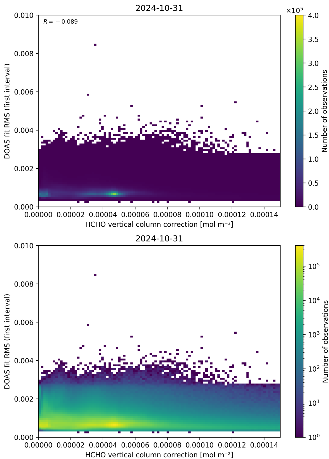
Figure 112: Scatter density plot of “HCHO vertical column correction” against “DOAS fit RMS (first interval)” for 2024-10-30 to 2024-11-01.
