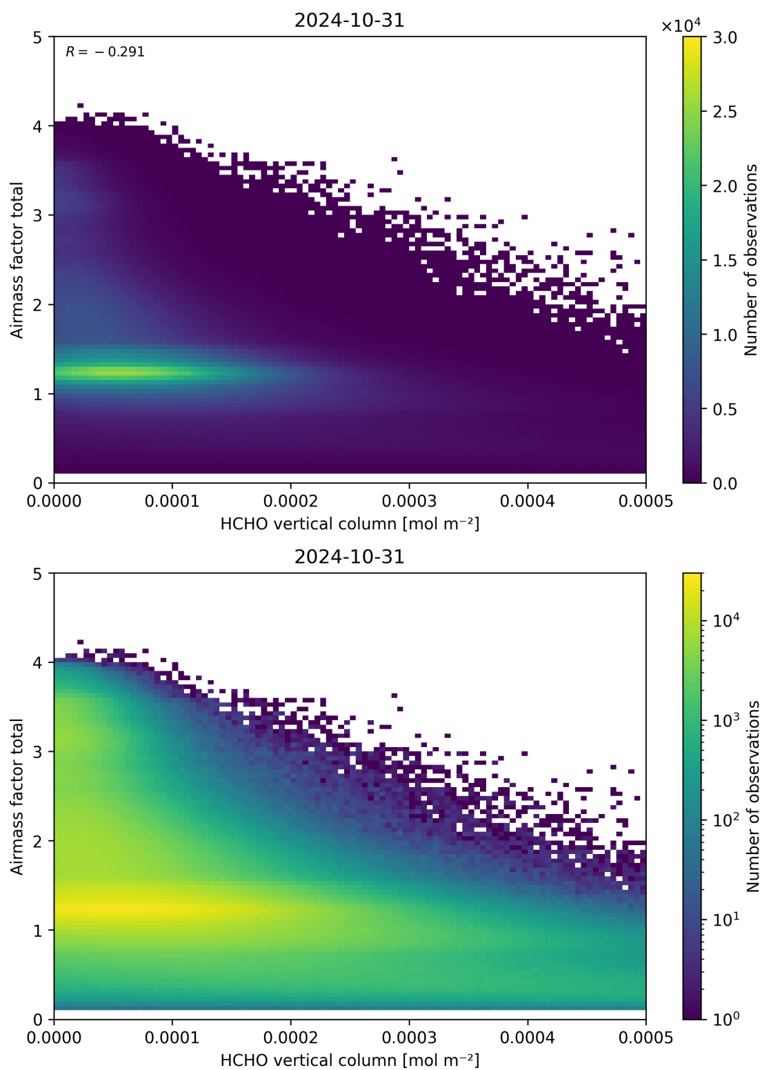
Figure 131: Scatter density plot of “HCHO vertical column” against “Airmass factor total” for 2024-10-30 to 2024-11-01.
