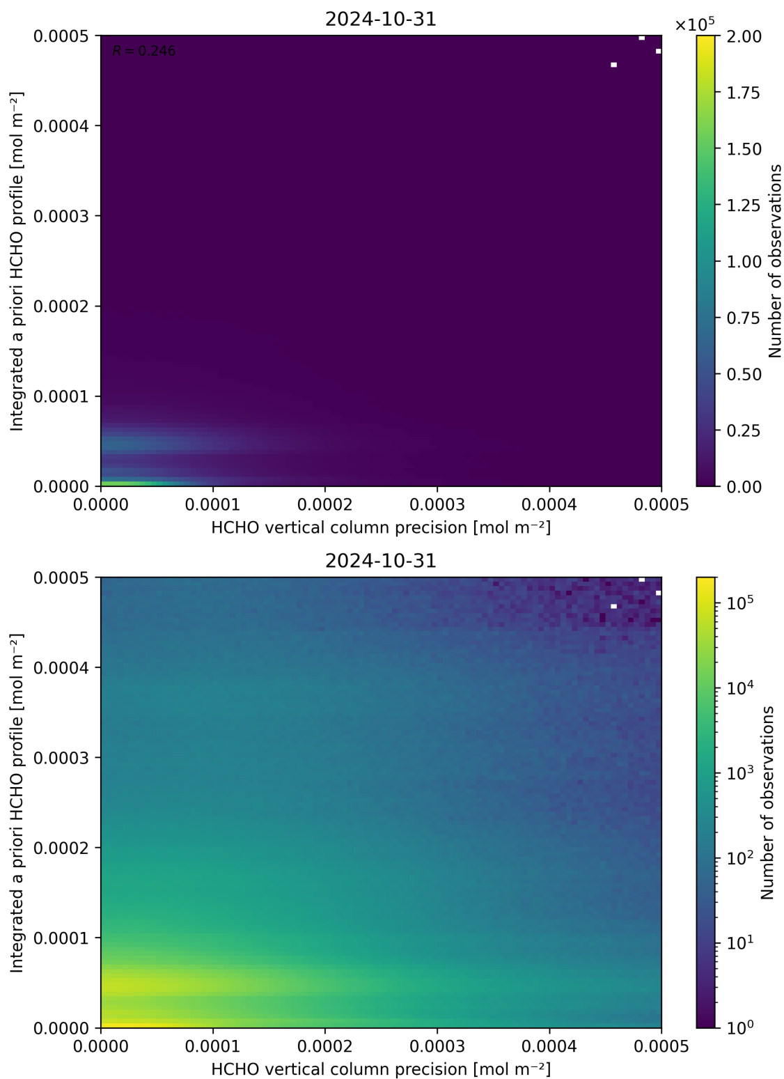
Figure 147: Scatter density plot of “HCHO vertical column precision” against “Integrated a priori HCHO profile” for 2024-10-30 to 2024-11-01.
