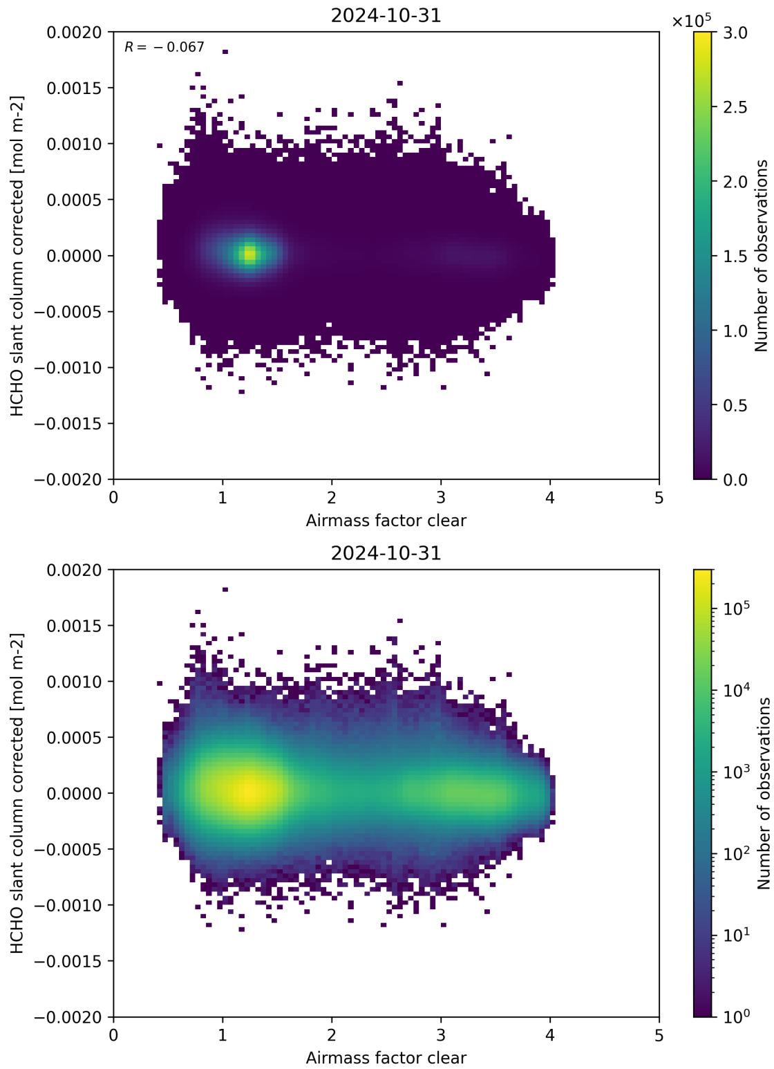
Figure 74: Scatter density plot of “Airmass factor clear” against “HCHO slant column corrected” for 2024-10-30 to 2024-11-01.
