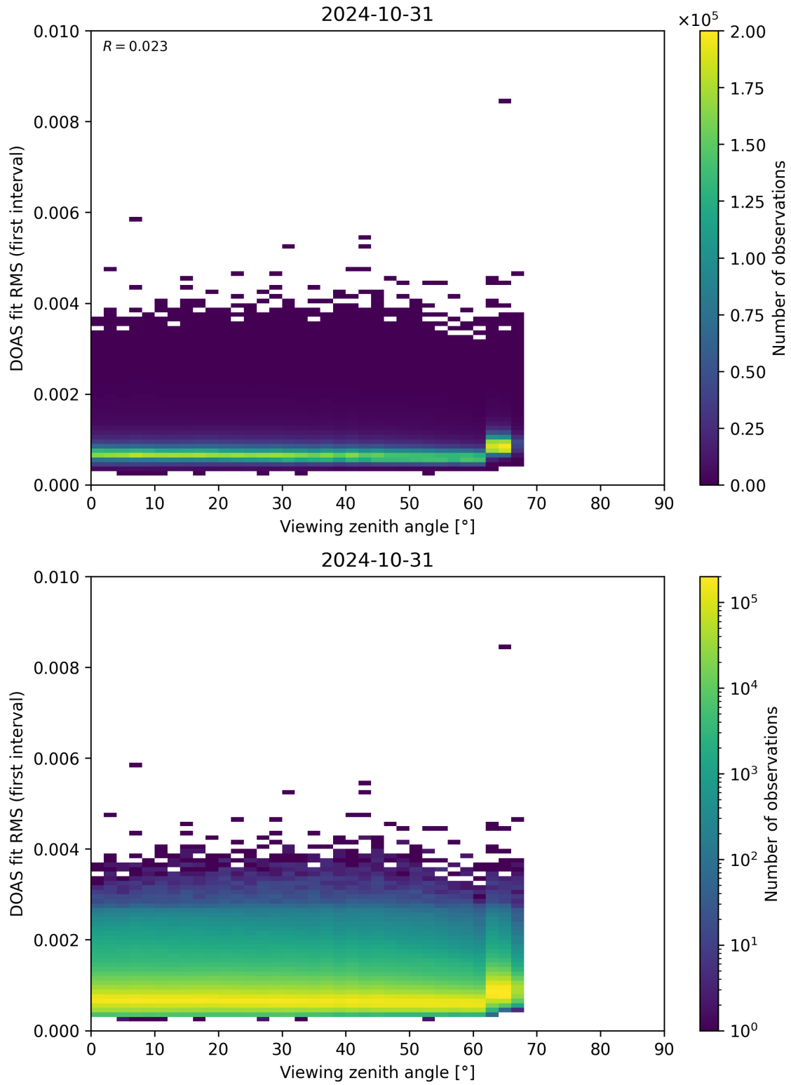
Figure 182: Scatter density plot of “Viewing zenith angle” against “DOAS fit RMS (first interval)” for 2024-10-30 to 2024-11-01.
