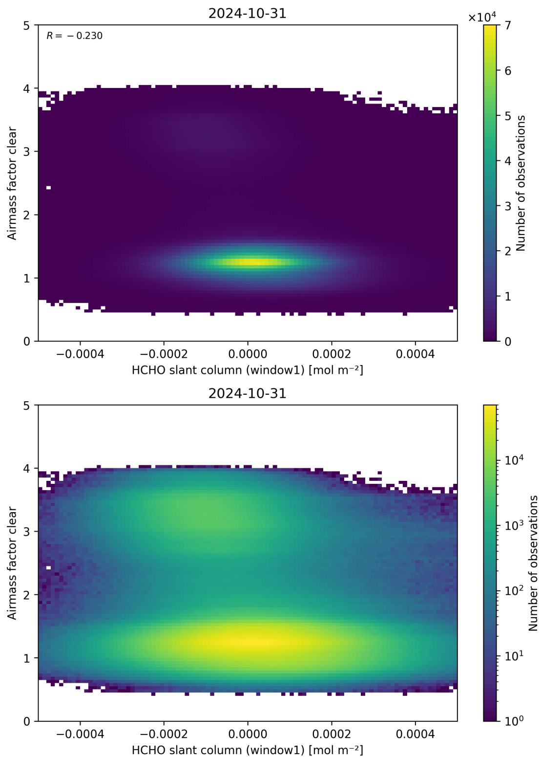
Figure 81: Scatter density plot of “HCHO slant column (window1)” against “Airmass factor clear” for 2024-10-30 to 2024-11-01.
