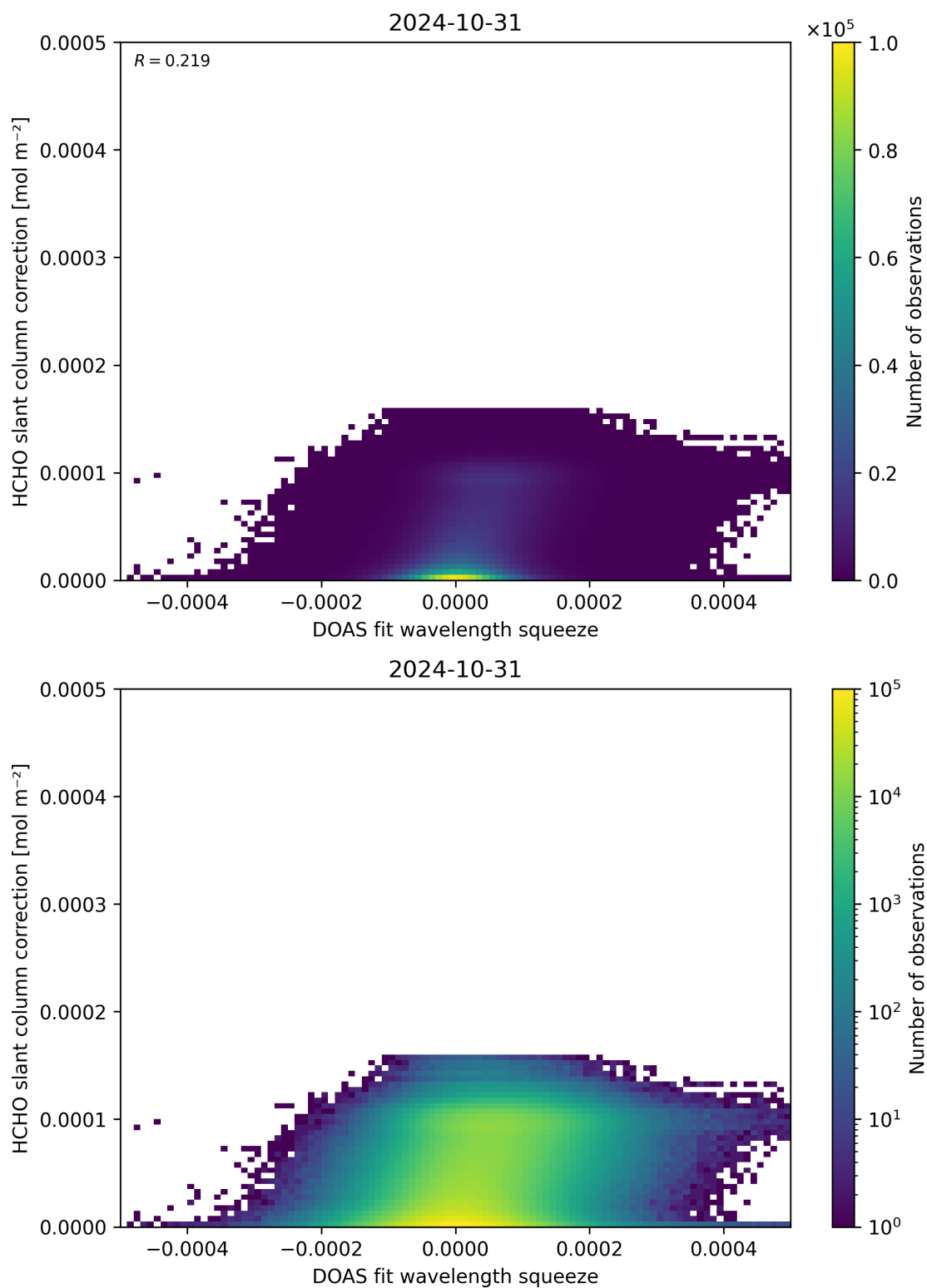
Figure 70: Scatter density plot of “DOAS fit wavelength squeeze” against “HCHO slant column correction” for 2024-10-30 to 2024-11-01.
