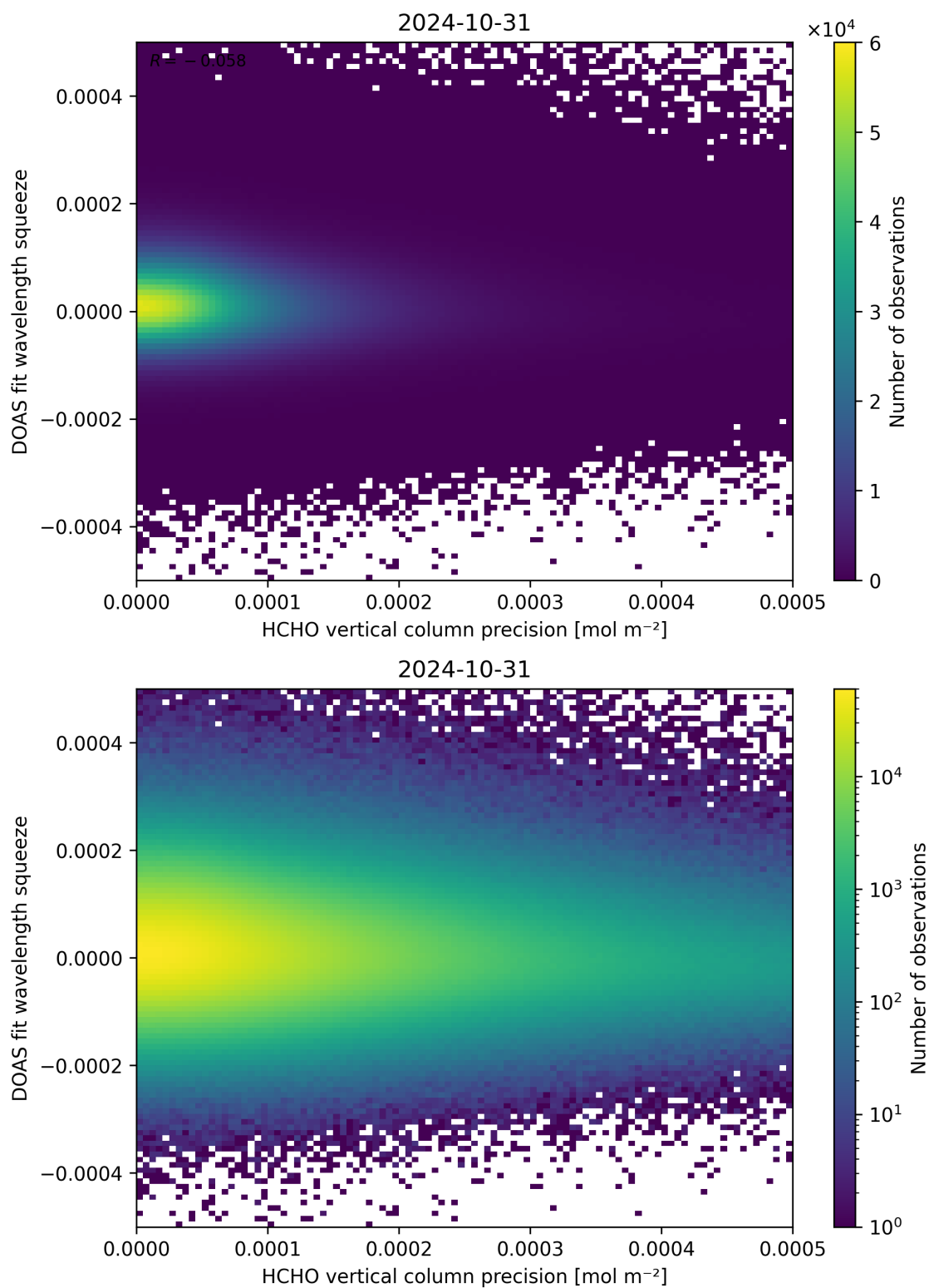
Figure 138: Scatter density plot of “HCHO vertical column precision” against “DOAS fit wavelength squeeze” for 2024-10-30 to 2024-11-01.
