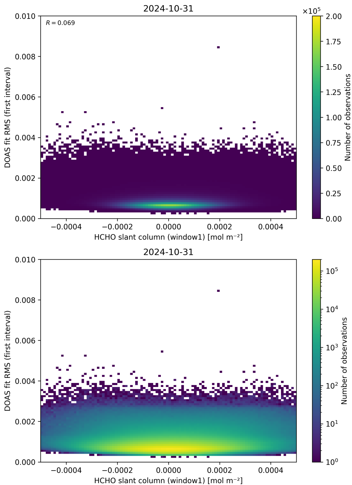
Figure 78: Scatter density plot of “HCHO slant column (window1)” against “DOAS fit RMS (first interval)” for 2024-10-30 to 2024-11-01.
