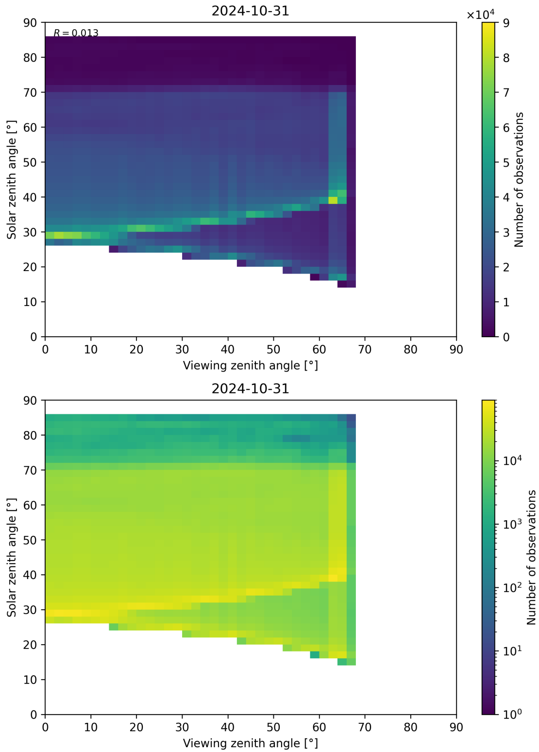
Figure 197: Scatter density plot of “Viewing zenith angle” against “Solar zenith angle” for 2024-10-30 to 2024-11-01.
