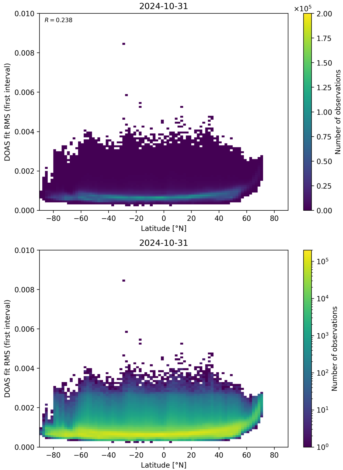
Figure 153: Scatter density plot of “Latitude” against “DOAS fit RMS (first interval)” for 2024-10-30 to 2024-11-01.
