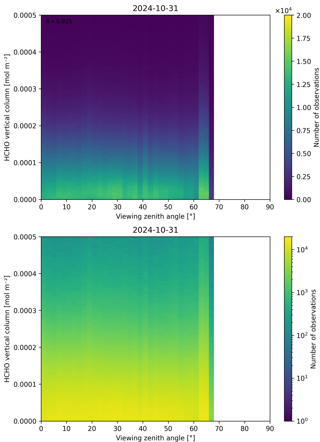
Figure 192: Scatter density plot of “Viewing zenith angle” against “HCHO vertical column” for 2024-10-30 to 2024-11-01.
