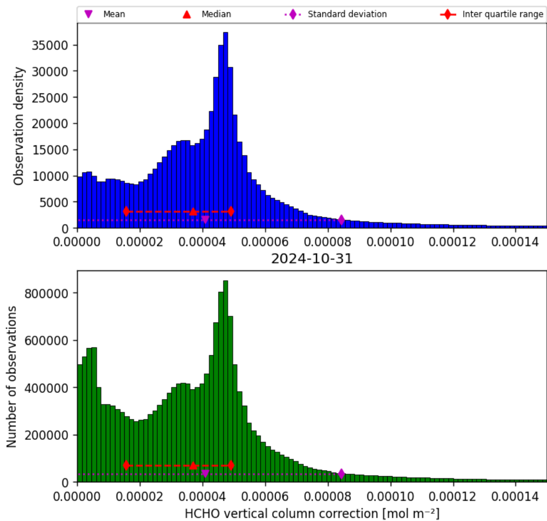
Figure 37: Histogram of “HCHO vertical column correction” for 2024-10-30 to 2024-11-01
