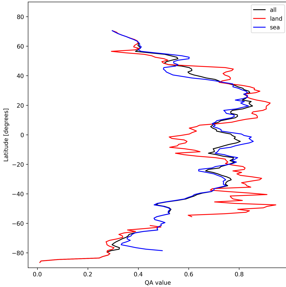
Figure 20: Zonal average of “QA value” for 2024-10-30 to 2024-11-01.
