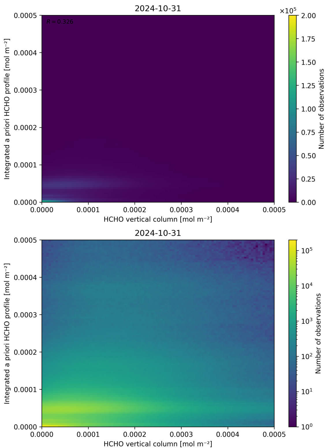
Figure 135: Scatter density plot of “HCHO vertical column” against “Integrated a priori HCHO profile” for 2024-10-30 to 2024-11-01.
