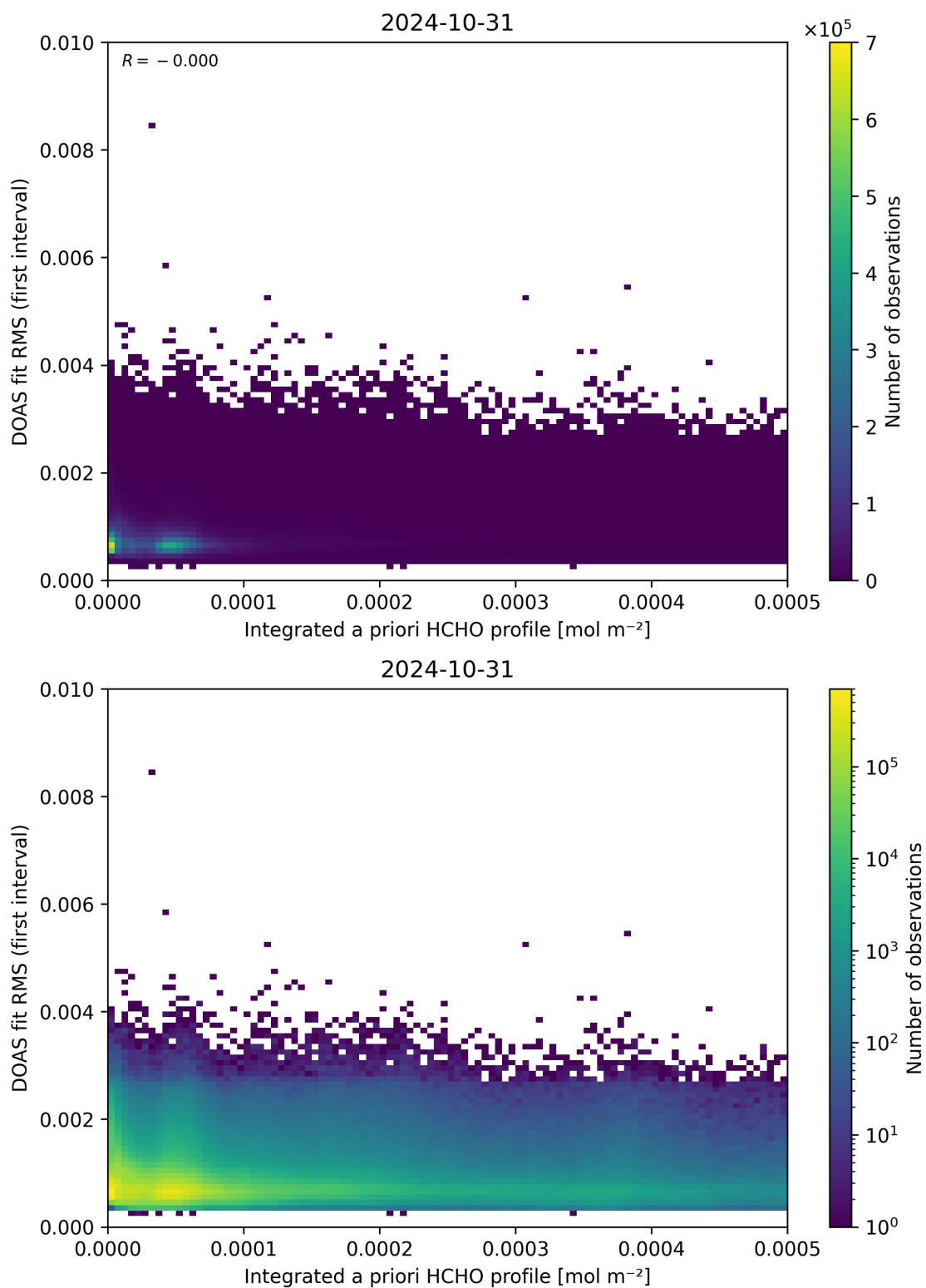
Figure 148: Scatter density plot of “Integrated a priori HCHO profile” against “DOAS fit RMS (first interval)” for 2024-10-30 to 2024-11-01.
