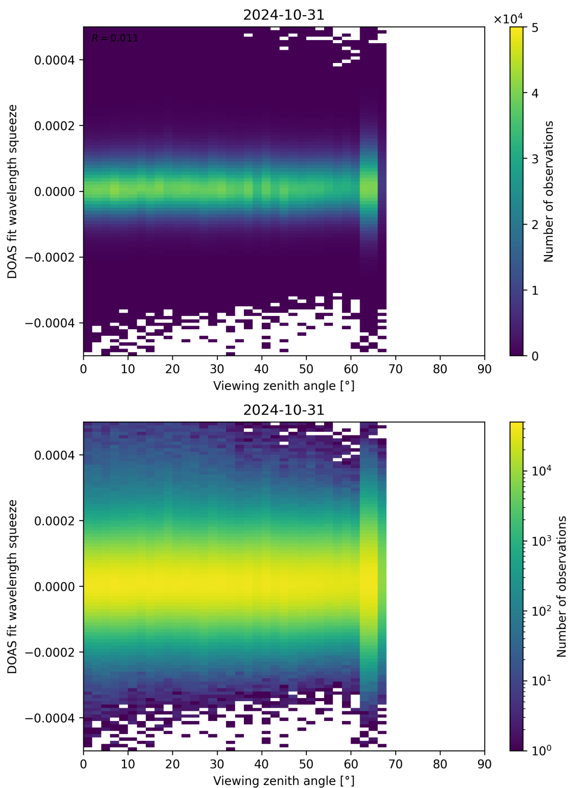
Figure 184: Scatter density plot of “Viewing zenith angle” against “DOAS fit wavelength squeeze” for 2024-10-30 to 2024-11-01.
