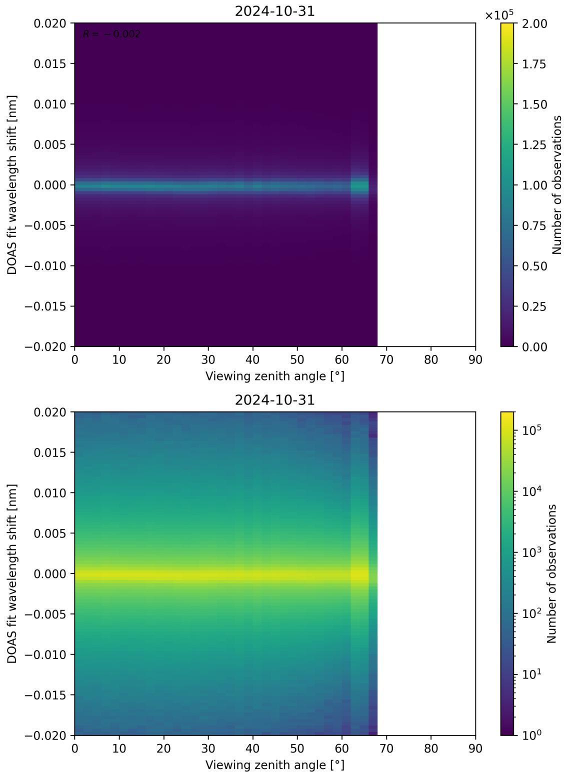
Figure 183: Scatter density plot of “Viewing zenith angle” against “DOAS fit wavelength shift” for 2024-10-30 to 2024-11-01.
