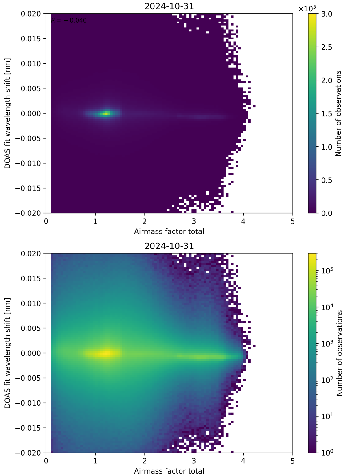
Figure 98: Scatter density plot of “Airmass factor total” against “DOAS fit wavelength shift” for 2024-10-30 to 2024-11-01.
