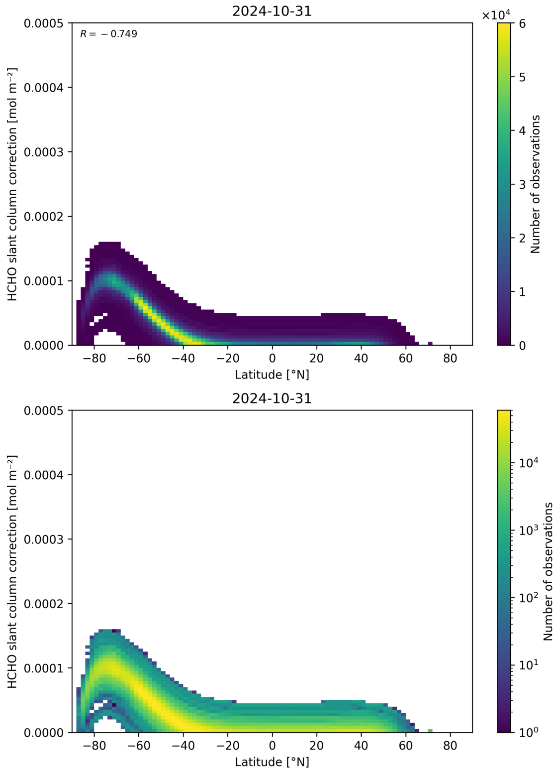
Figure 158: Scatter density plot of “Latitude” against “HCHO slant column correction” for 2024-10-30 to 2024-11-01.
