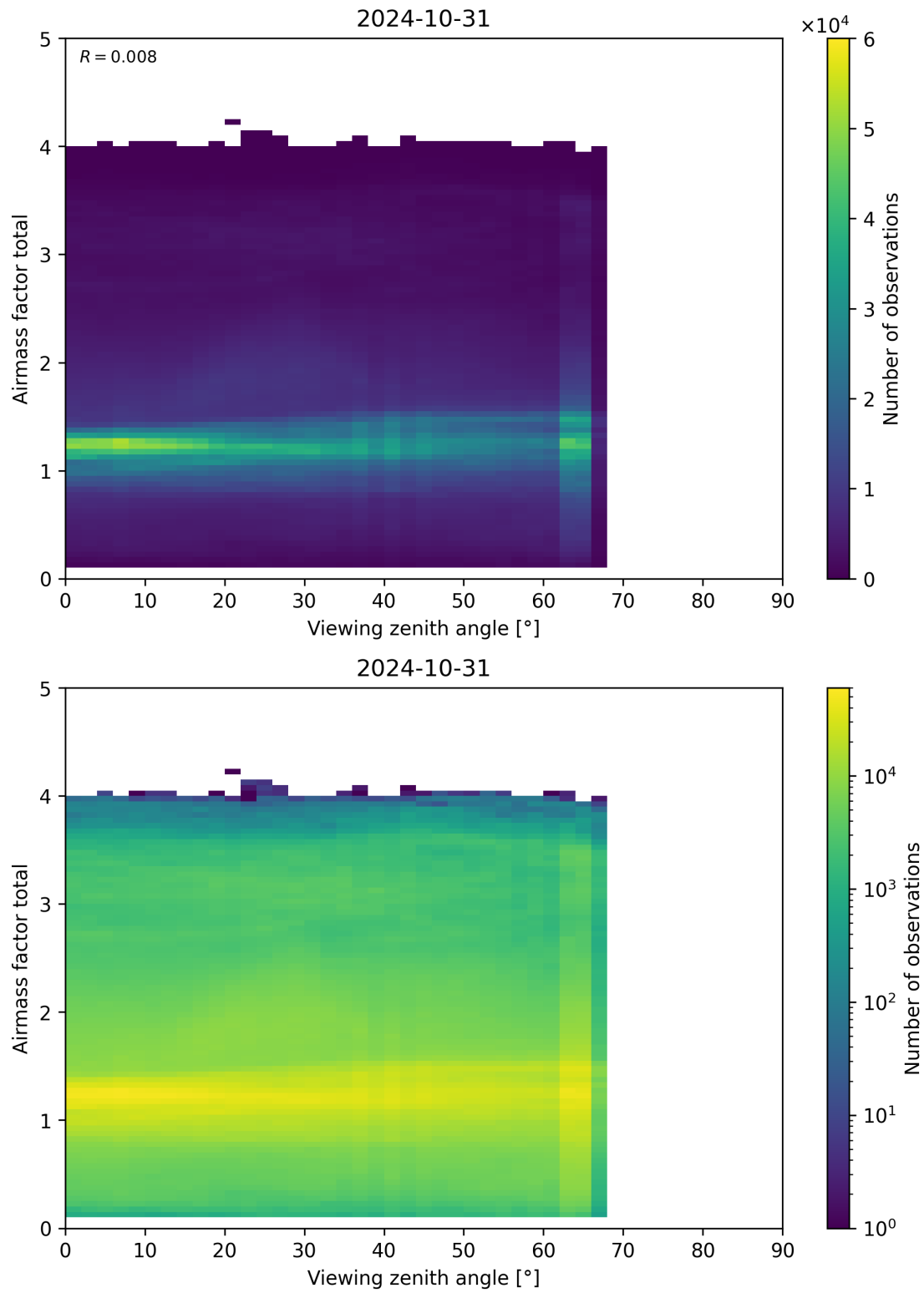
Figure 190: Scatter density plot of “Viewing zenith angle” against “Airmass factor total” for 2024-10-30 to 2024-11-01.
