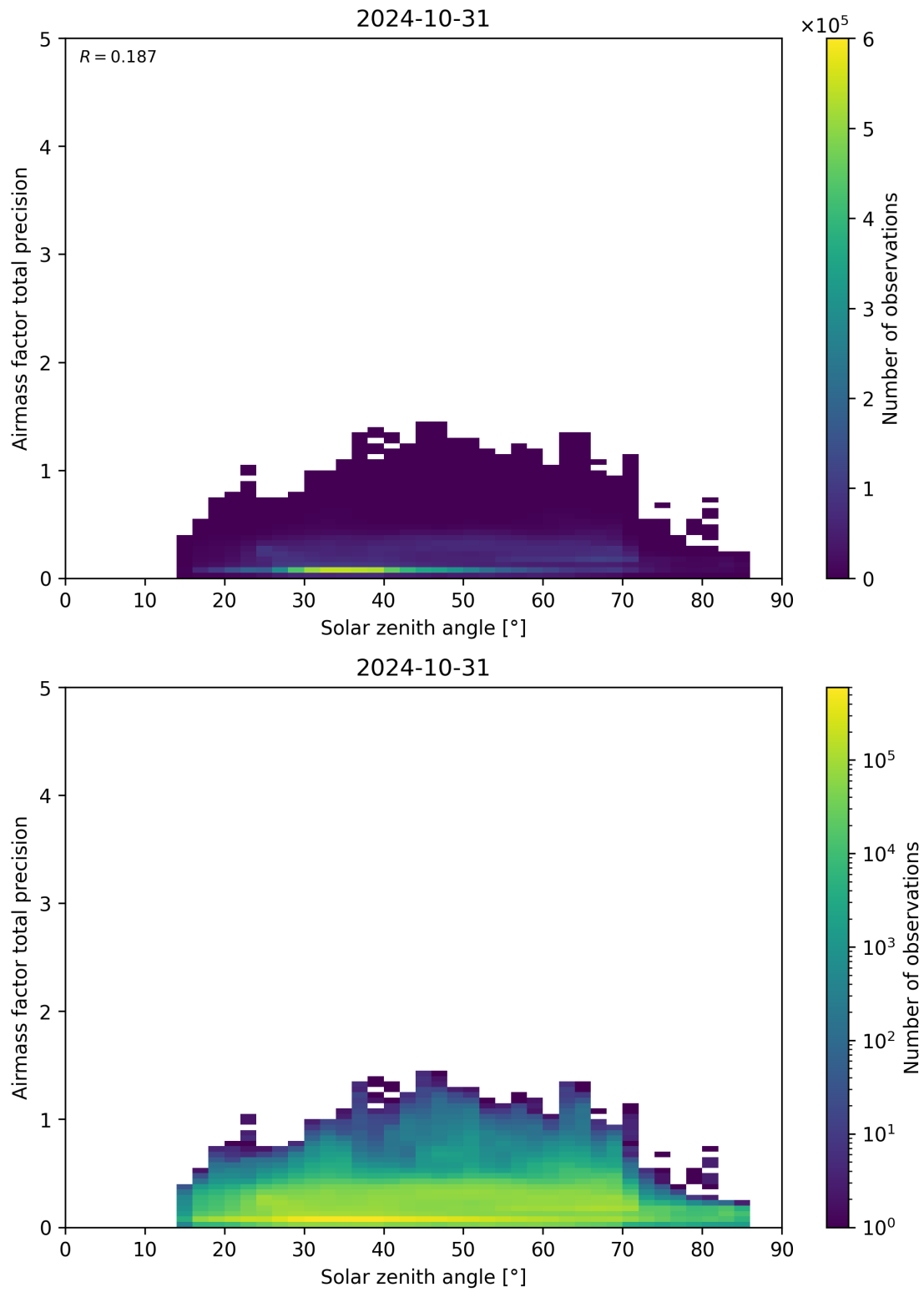
Figure 176: Scatter density plot of “Solar zenith angle” against “Airmass factor total precision” for 2024-10-30 to 2024-11-01.
