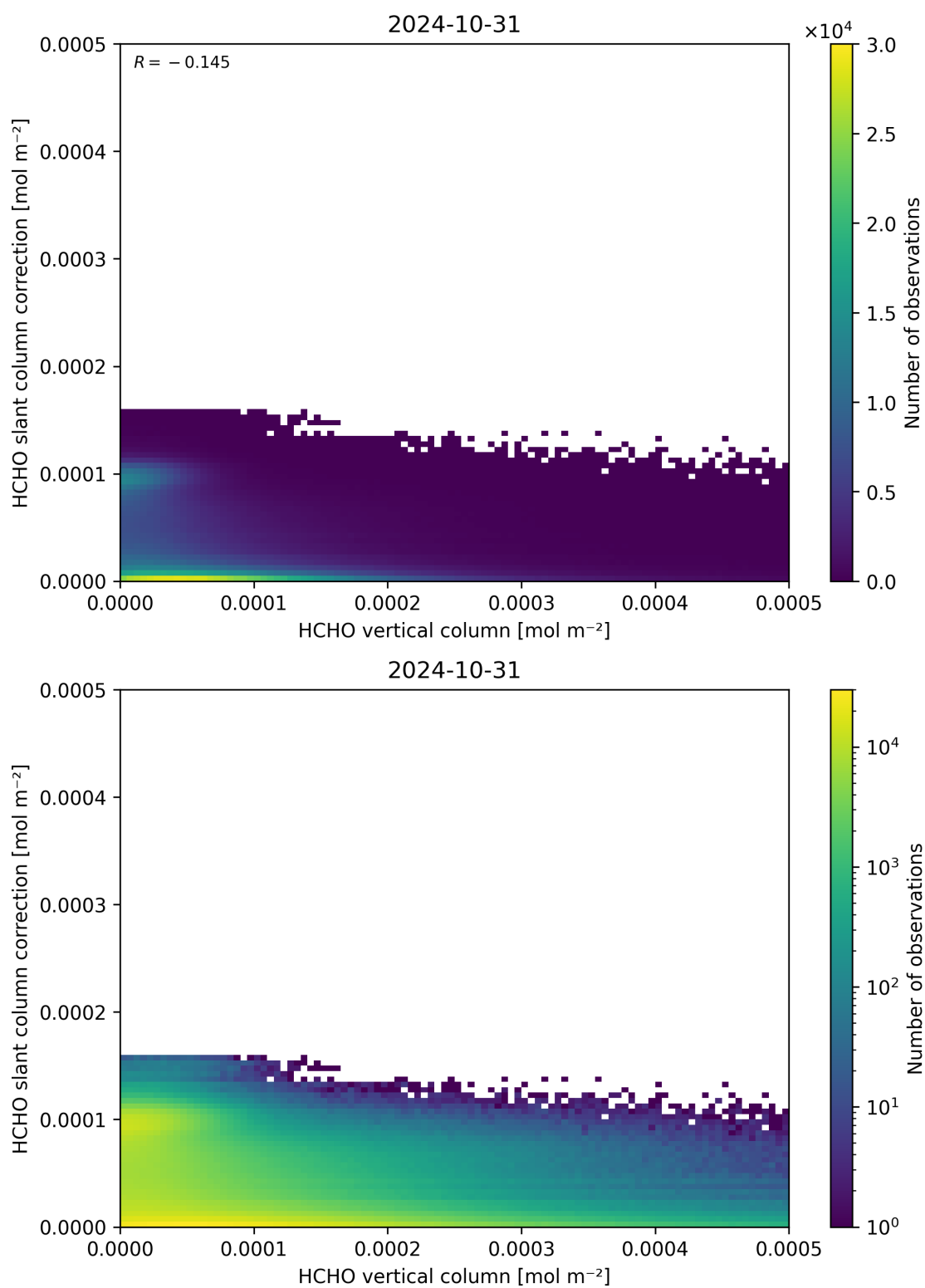
Figure 128: Scatter density plot of “HCHO vertical column” against “HCHO slant column correction” for 2024-10-30 to 2024-11-01.
