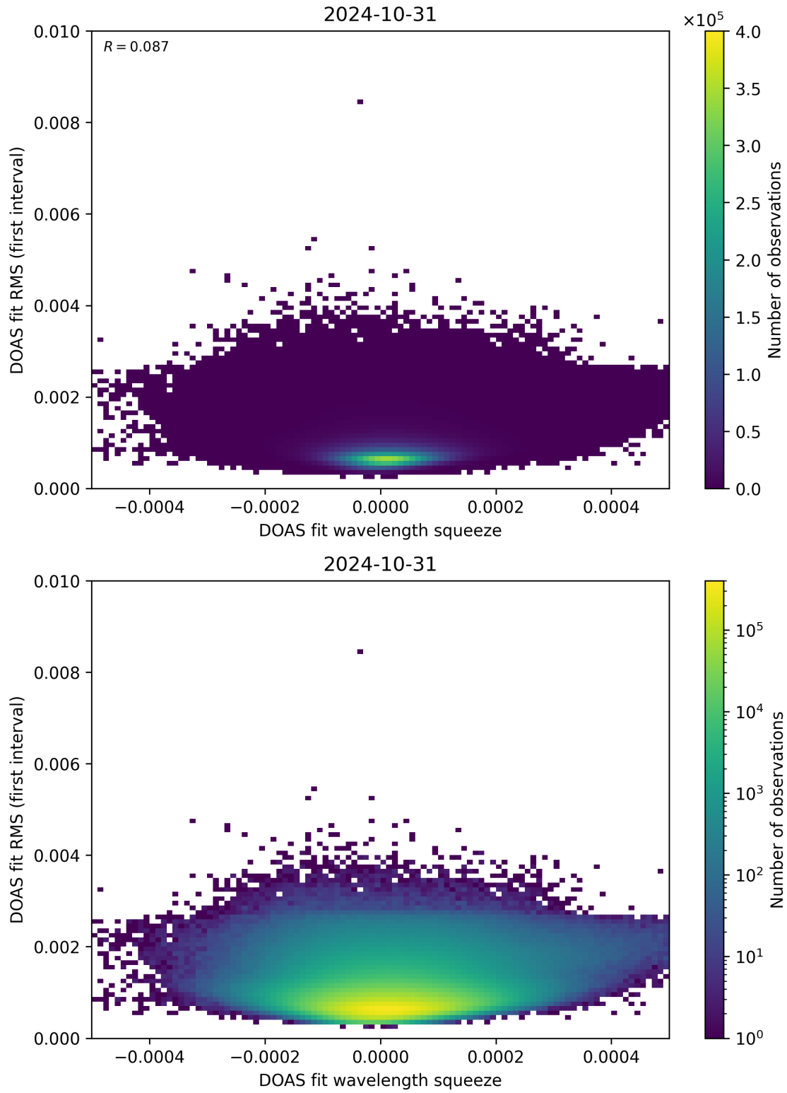
Figure 68: Scatter density plot of “DOAS fit wavelength squeeze” against “DOAS fit RMS (first interval)” for 2024-10-30 to 2024-11-01.
