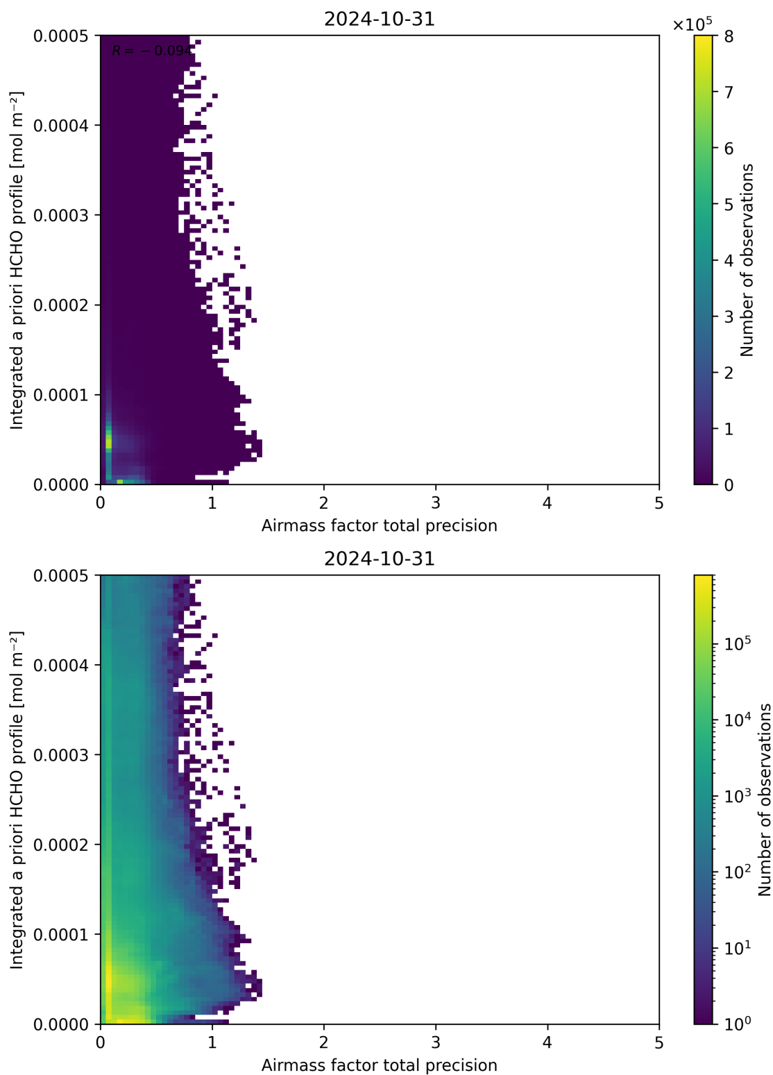
Figure 111: Scatter density plot of “Airmass factor total precision” against “Integrated a priori HCHO profile” for 2024-10-30 to 2024-11-01.
