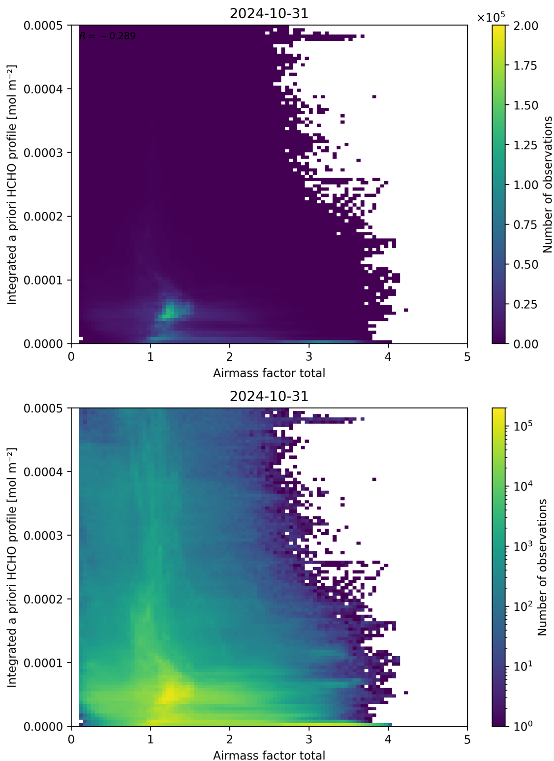
Figure 104: Scatter density plot of “Airmass factor total” against “Integrated a priori HCHO profile” for 2024-10-30 to 2024-11-01.
