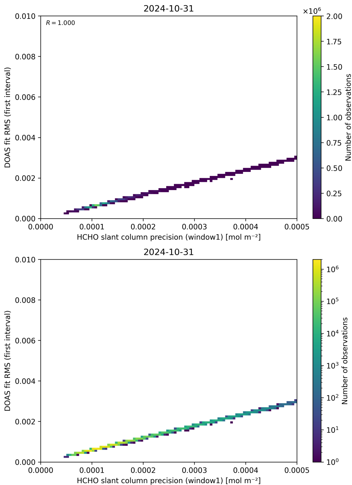
Figure 88: Scatter density plot of “HCHO slant column precision (window1)” against “DOAS fit RMS (first interval)” for 2024-10-30 to 2024-11-01.
