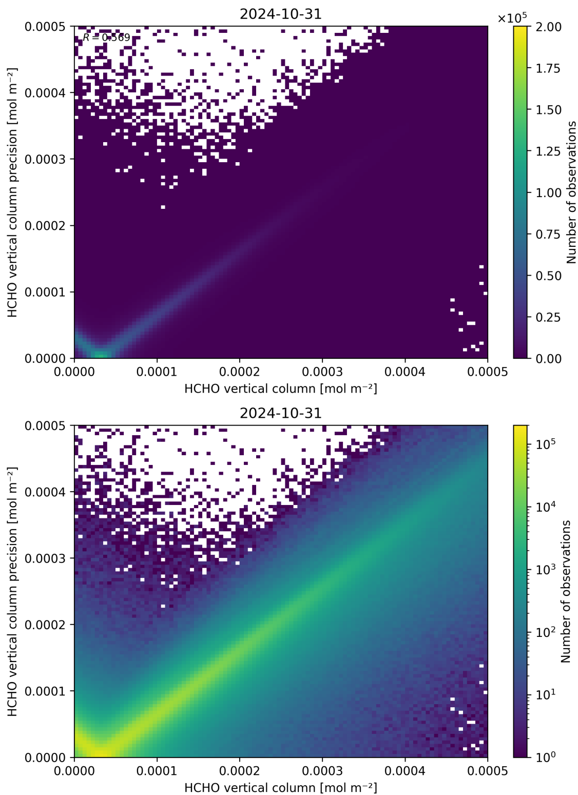
Figure 134: Scatter density plot of “HCHO vertical column” against “HCHO vertical column precision” for 2024-10-30 to 2024-11-01.
