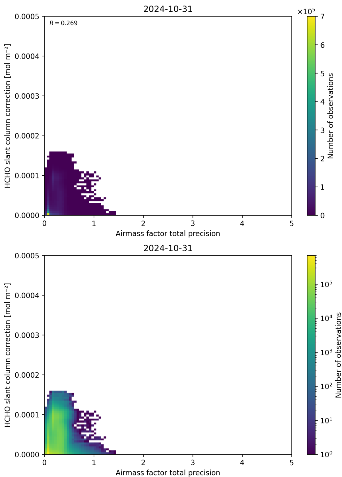
Figure 110: Scatter density plot of “Airmass factor total precision” against “HCHO slant column correction” for 2024-10-30 to 2024-11-01.
