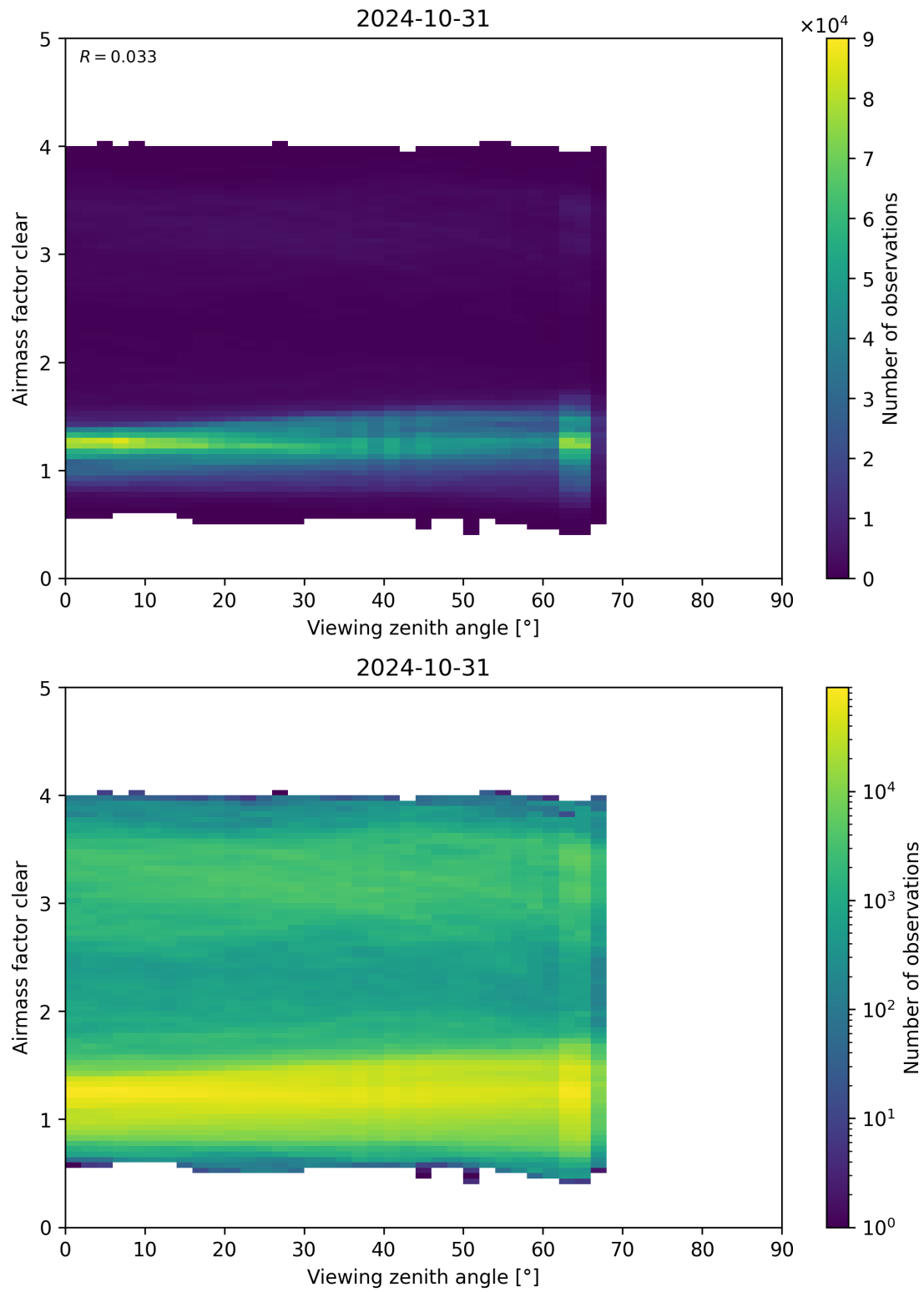
Figure 185: Scatter density plot of “Viewing zenith angle” against “Airmass factor clear” for 2024-10-30 to 2024-11-01.
