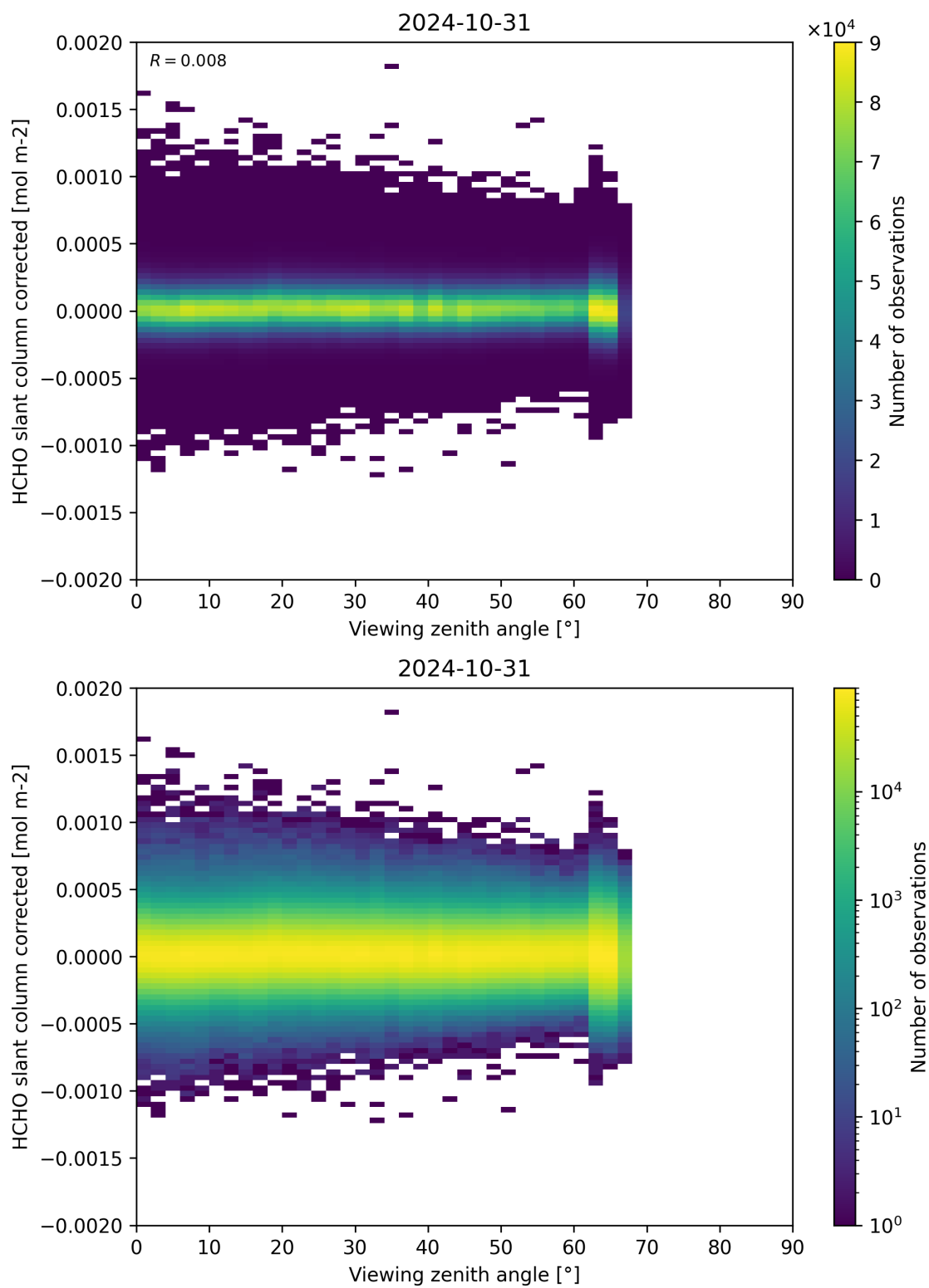
Figure 186: Scatter density plot of “Viewing zenith angle” against “HCHO slant column corrected” for 2024-10-30 to 2024-11-01.
