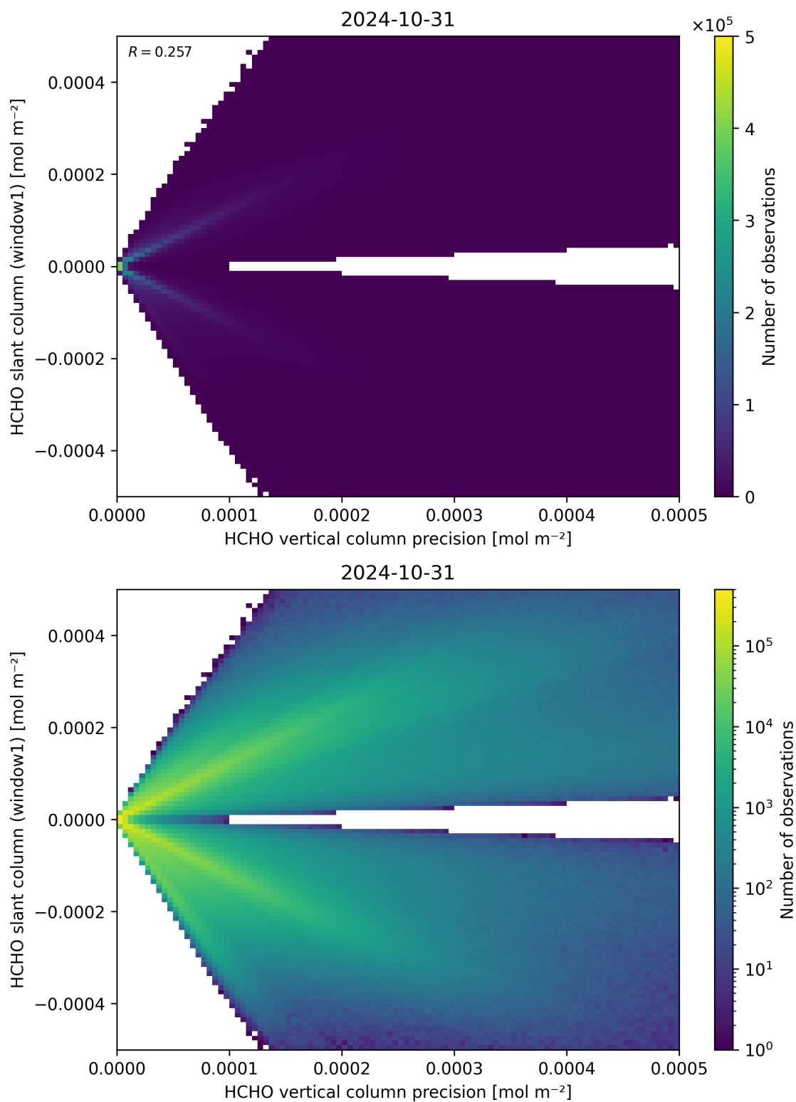
Figure 142: Scatter density plot of “HCHO vertical column precision” against “HCHO slant column (window1)” for 2024-10-30 to 2024-11-01.
