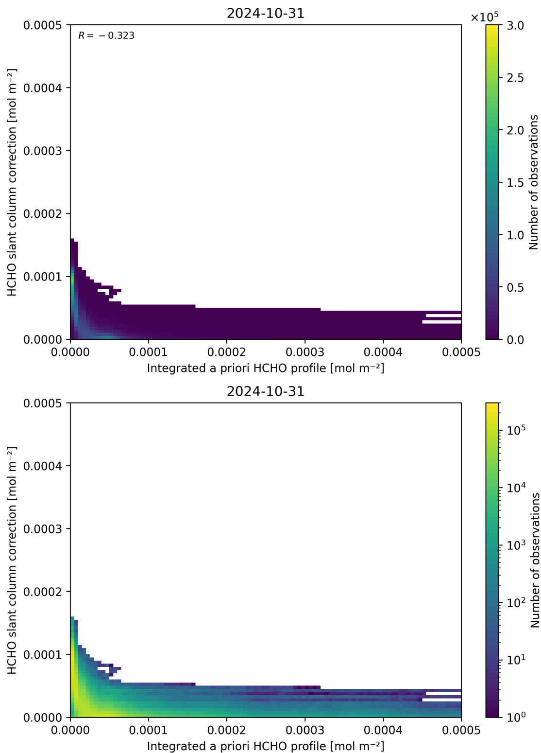
Figure 152: Scatter density plot of “Integrated a priori HCHO profile” against “HCHO slant column correction” for 2024-10-30 to 2024-11-01.
