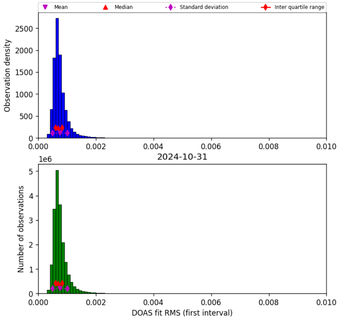
Figure 46: Histogram of “DOAS fit RMS (first interval)” for 2024-10-30 to 2024-11-01
