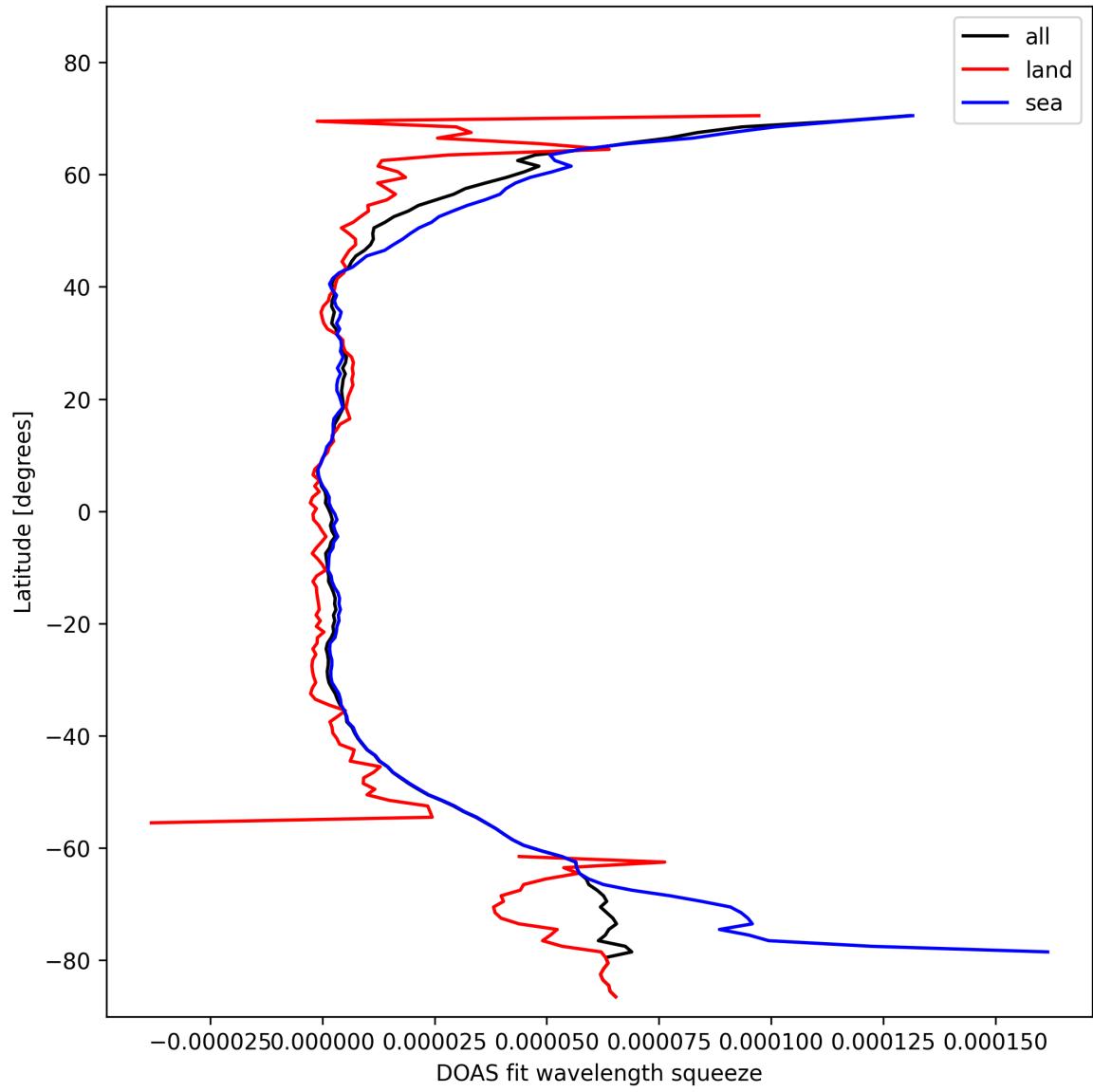
Figure 31: Zonal average of “DOAS fit wavelength squeeze” for 2024-10-30 to 2024-11-01.
