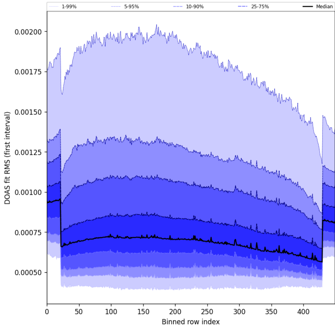
Figure 60: Along track statistics of “DOAS fit RMS (first interval)” for 2024-10-30 to 2024-11-01
