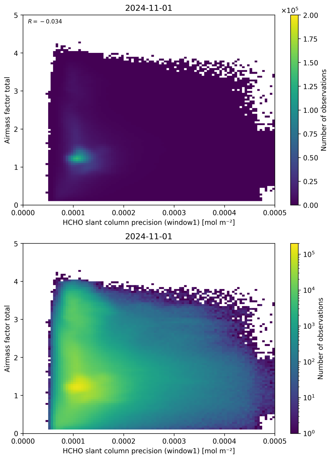
Figure 94: Scatter density plot of “HCHO slant column precision (window1)” against “Airmass factor total” for 2024-10-31 to 2024-11-02.
