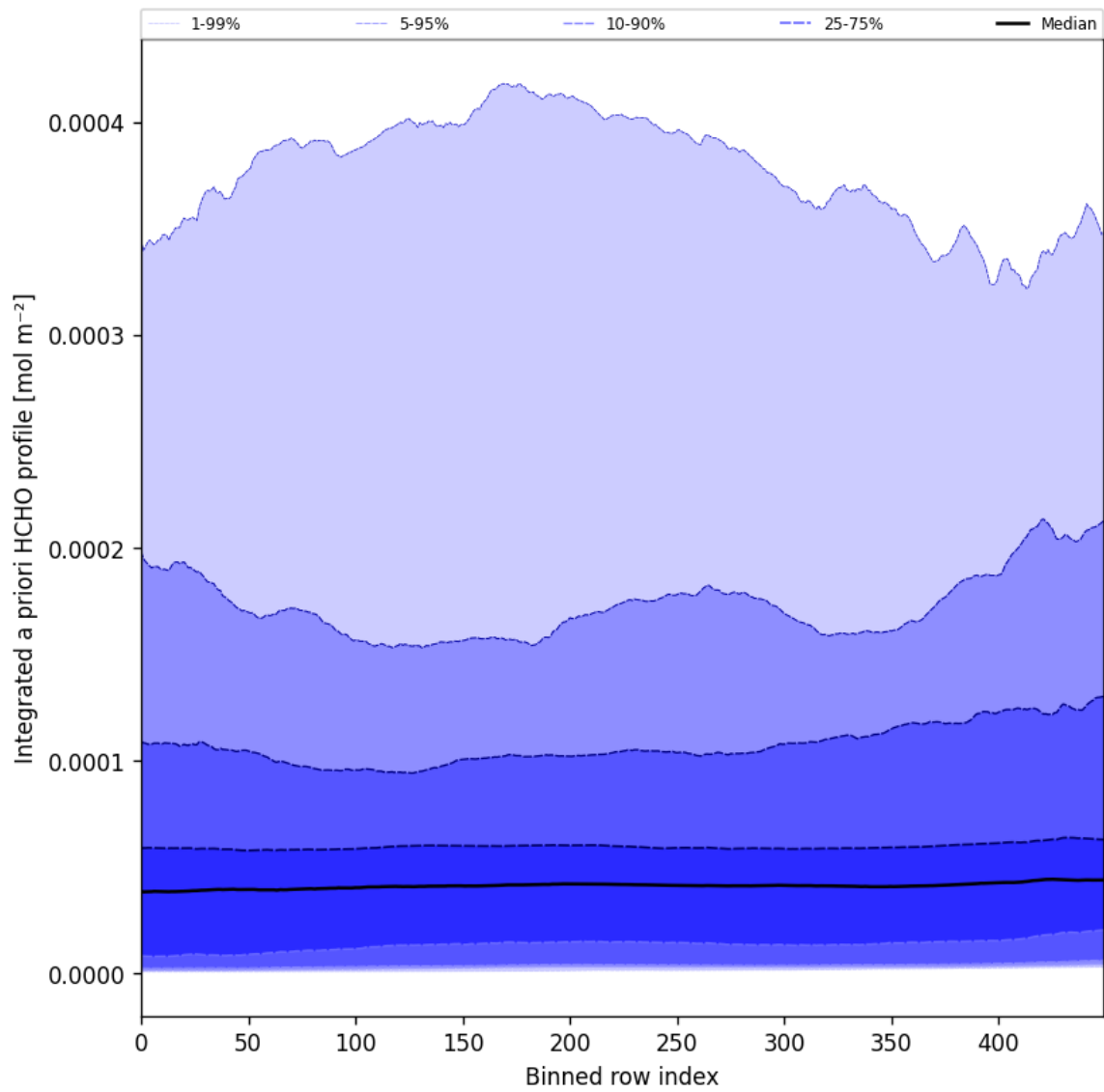
Figure 57: Along track statistics of “Integrated a priori HCHO profile” for 2024-10-31 to 2024-11-02
