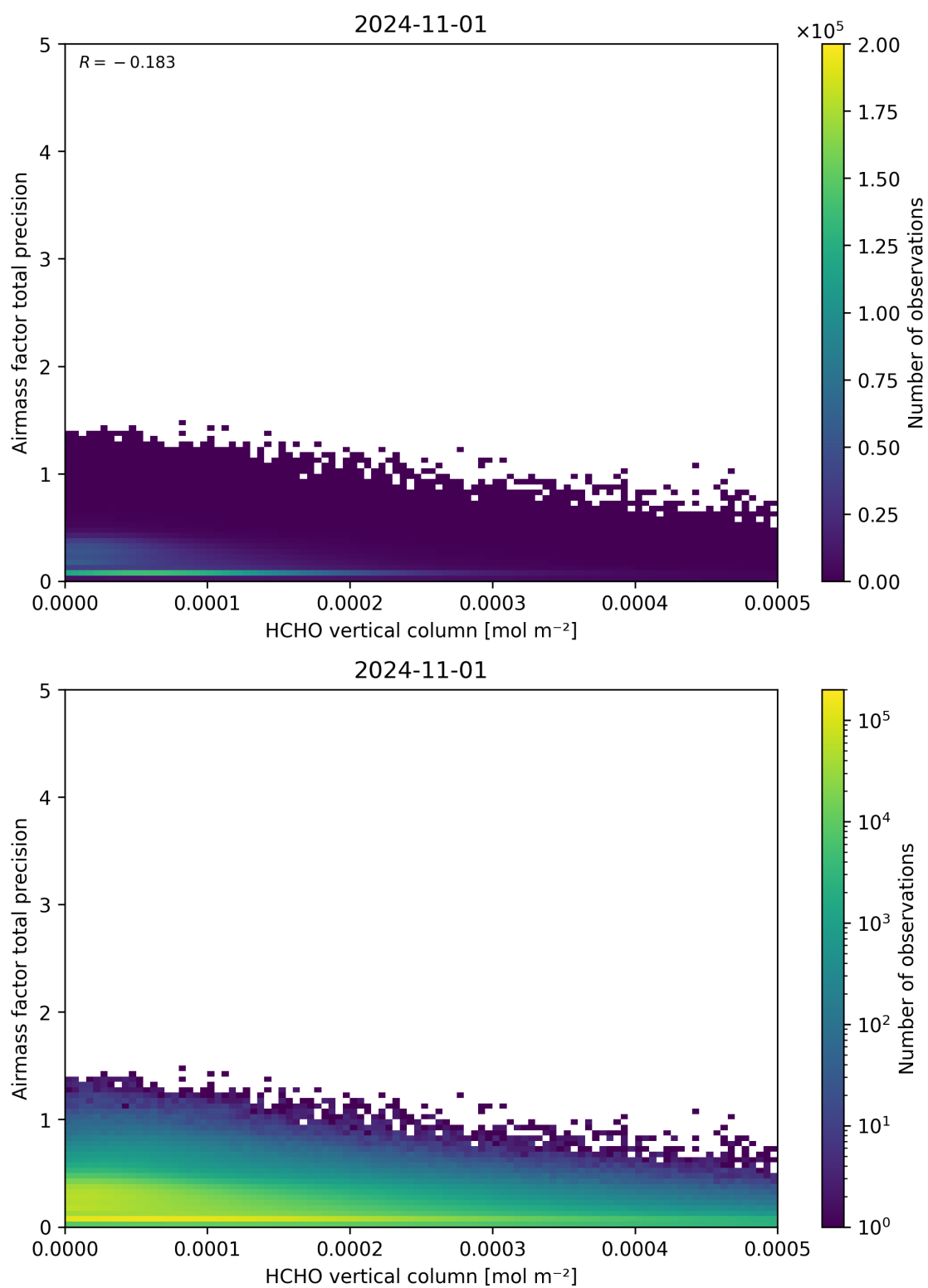
Figure 132: Scatter density plot of “HCHO vertical column” against “Airmass factor total precision” for 2024-10-31 to 2024-11-02.
