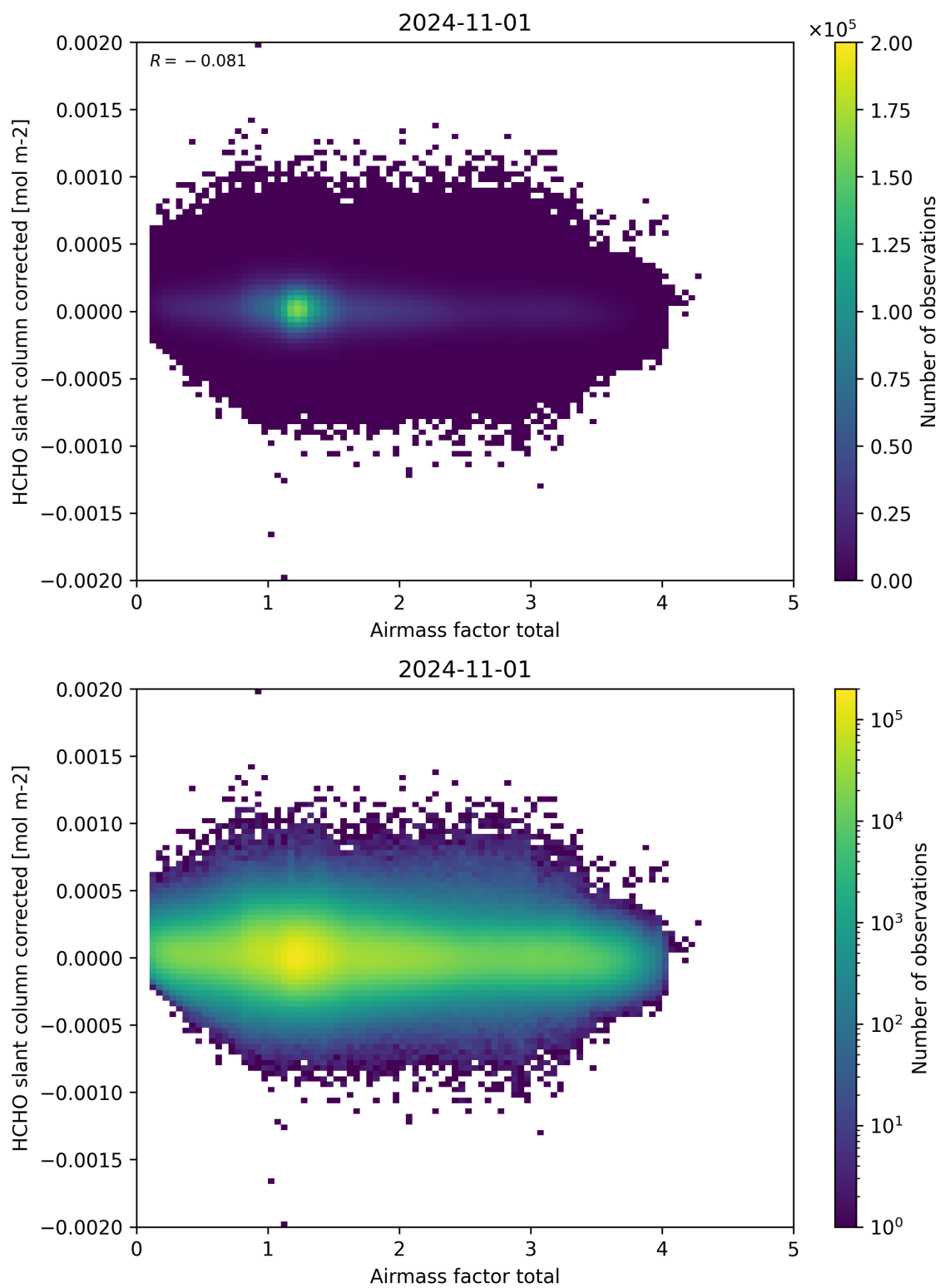
Figure 101: Scatter density plot of “Airmass factor total” against “HCHO slant column corrected” for 2024-10-31 to 2024-11-02.
