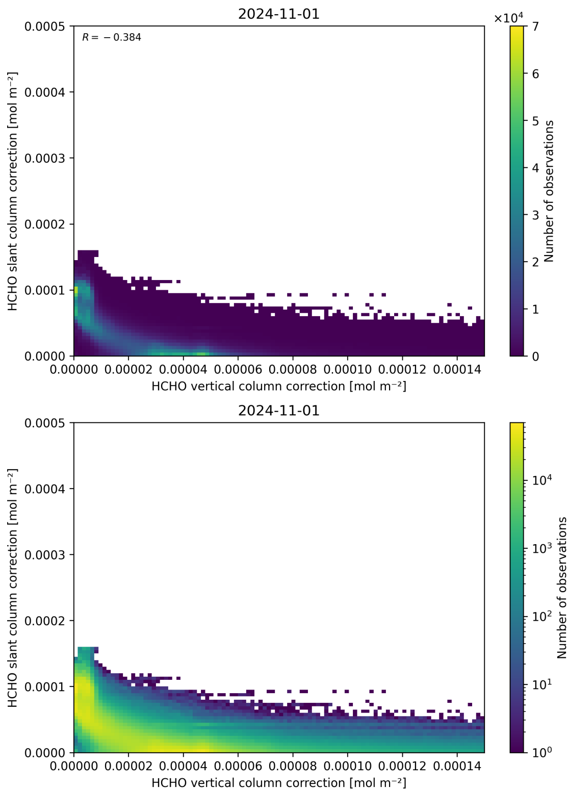
Figure 117: Scatter density plot of “HCHO vertical column correction” against “HCHO slant column correction” for 2024-10-31 to 2024-11-02.
