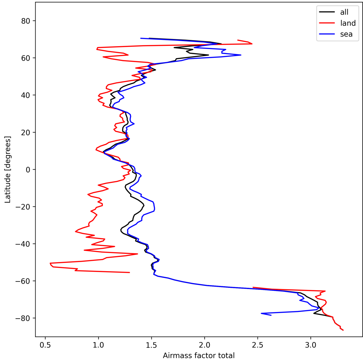
Figure 26: Zonal average of “Airmass factor total” for 2024-10-31 to 2024-11-02.
