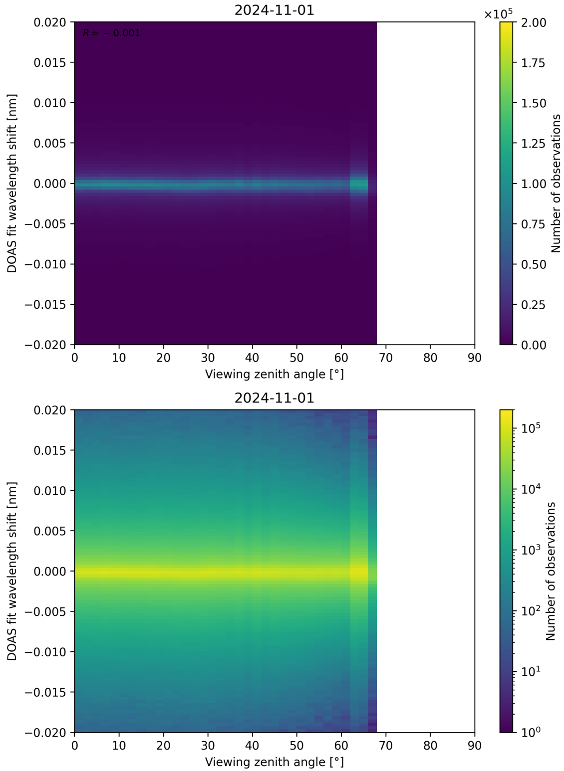
Figure 183: Scatter density plot of “Viewing zenith angle” against “DOAS fit wavelength shift” for 2024-10-31 to 2024-11-02.
