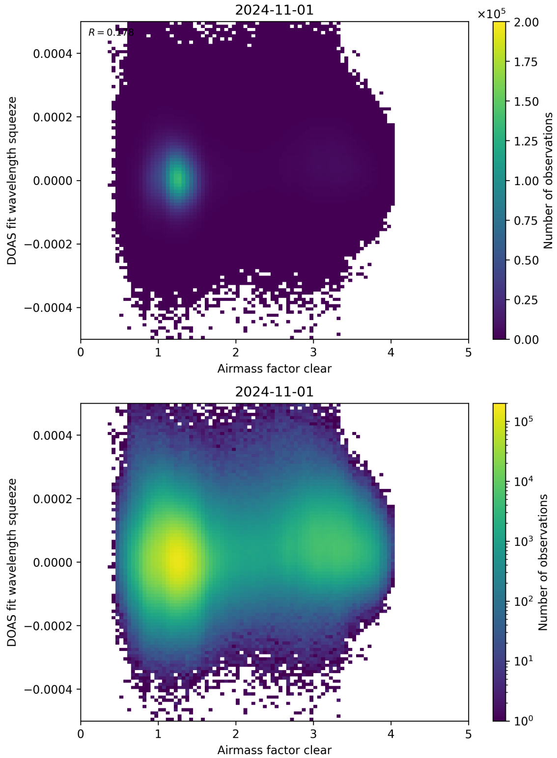
Figure 73: Scatter density plot of “Airmass factor clear” against “DOAS fit wavelength squeeze” for 2024-10-31 to 2024-11-02.
