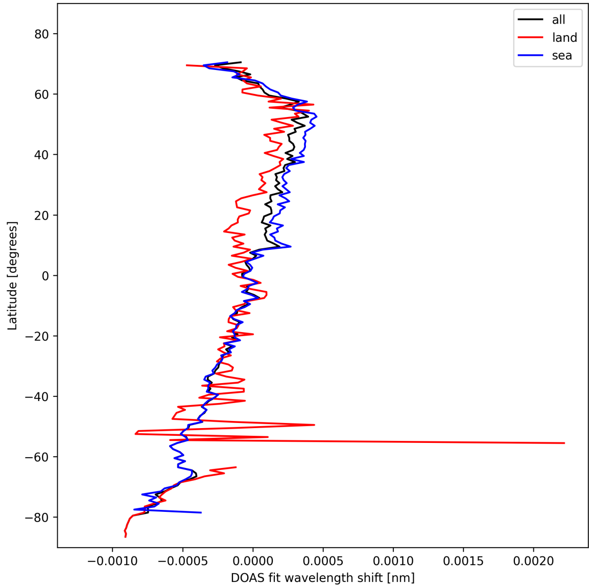
Figure 30: Zonal average of “DOAS fit wavelength shift” for 2024-10-31 to 2024-11-02.
