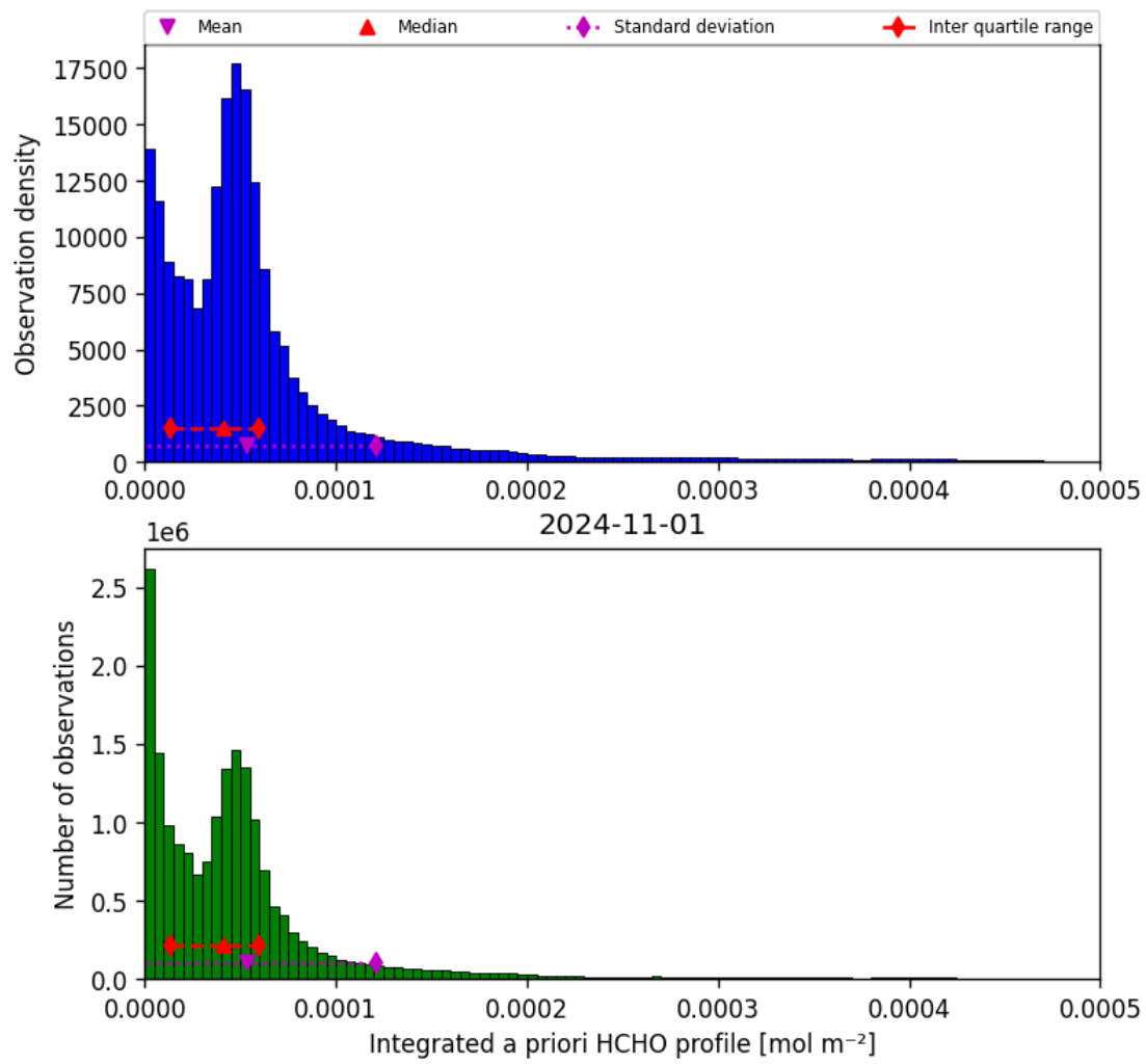
Figure 43: Histogram of “Integrated a priori HCHO profile” for 2024-10-31 to 2024-11-02
