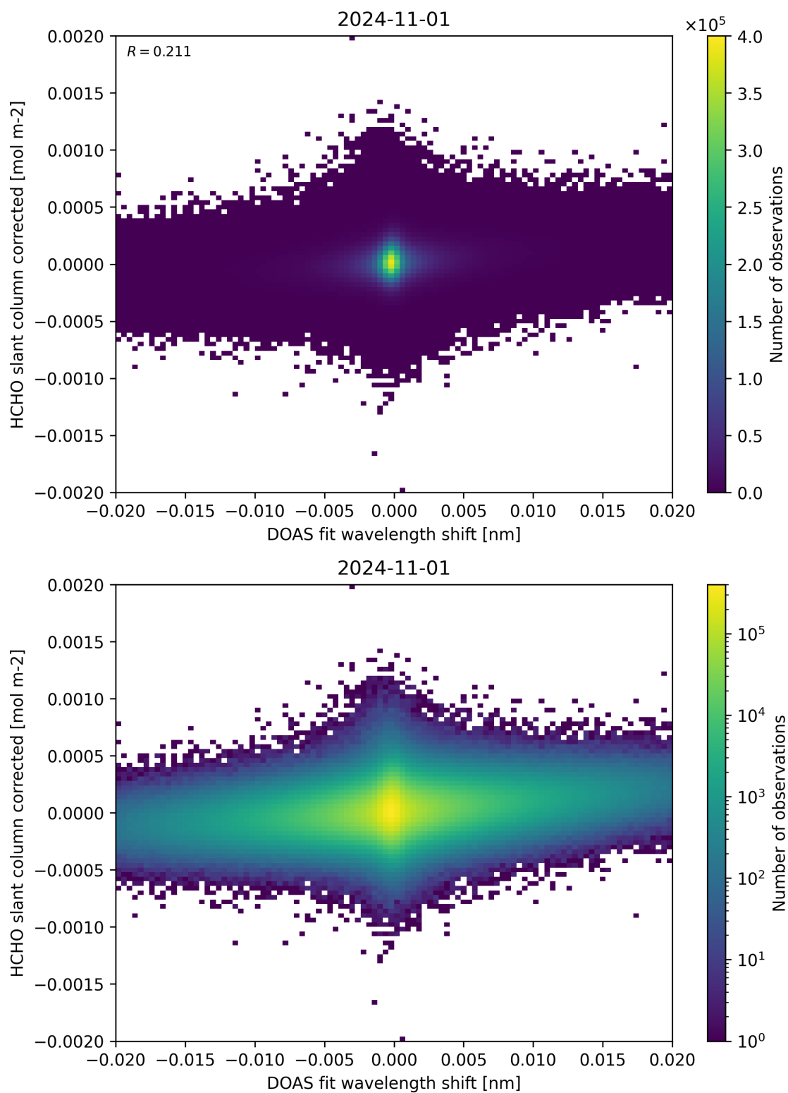
Figure 66: Scatter density plot of “DOAS fit wavelength shift” against “HCHO slant column corrected” for 2024-10-31 to 2024-11-02.
