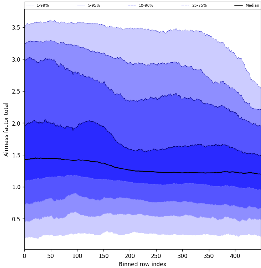
Figure 54: Along track statistics of “Airmass factor total” for 2024-10-31 to 2024-11-02
