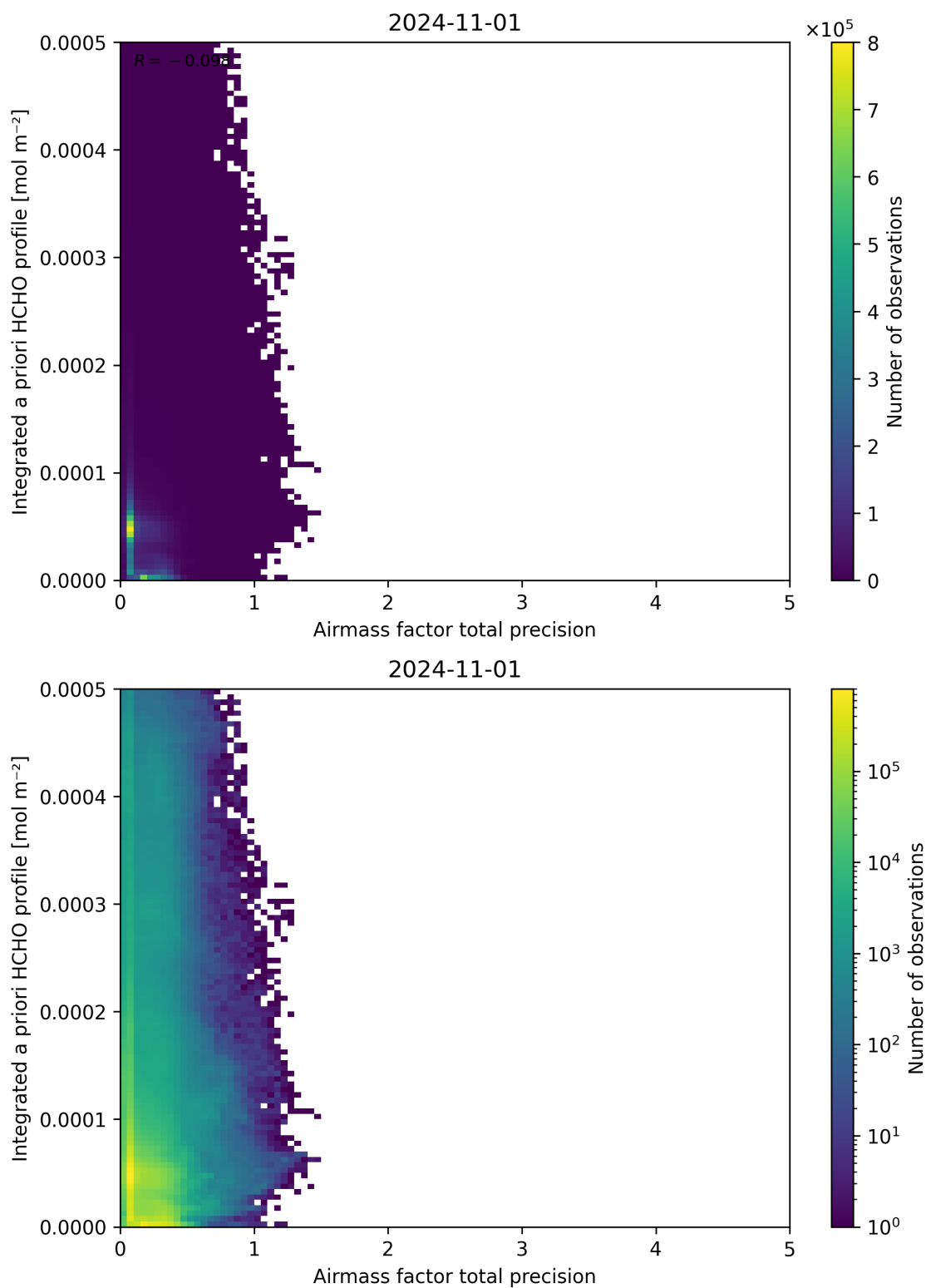
Figure 111: Scatter density plot of “Airmass factor total precision” against “Integrated a priori HCHO profile” for 2024-10-31 to 2024-11-02.
