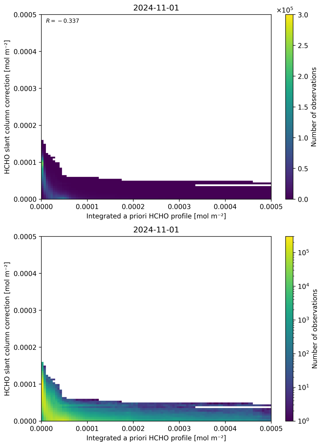
Figure 152: Scatter density plot of “Integrated a priori HCHO profile” against “HCHO slant column correction” for 2024-10-31 to 2024-11-02.
