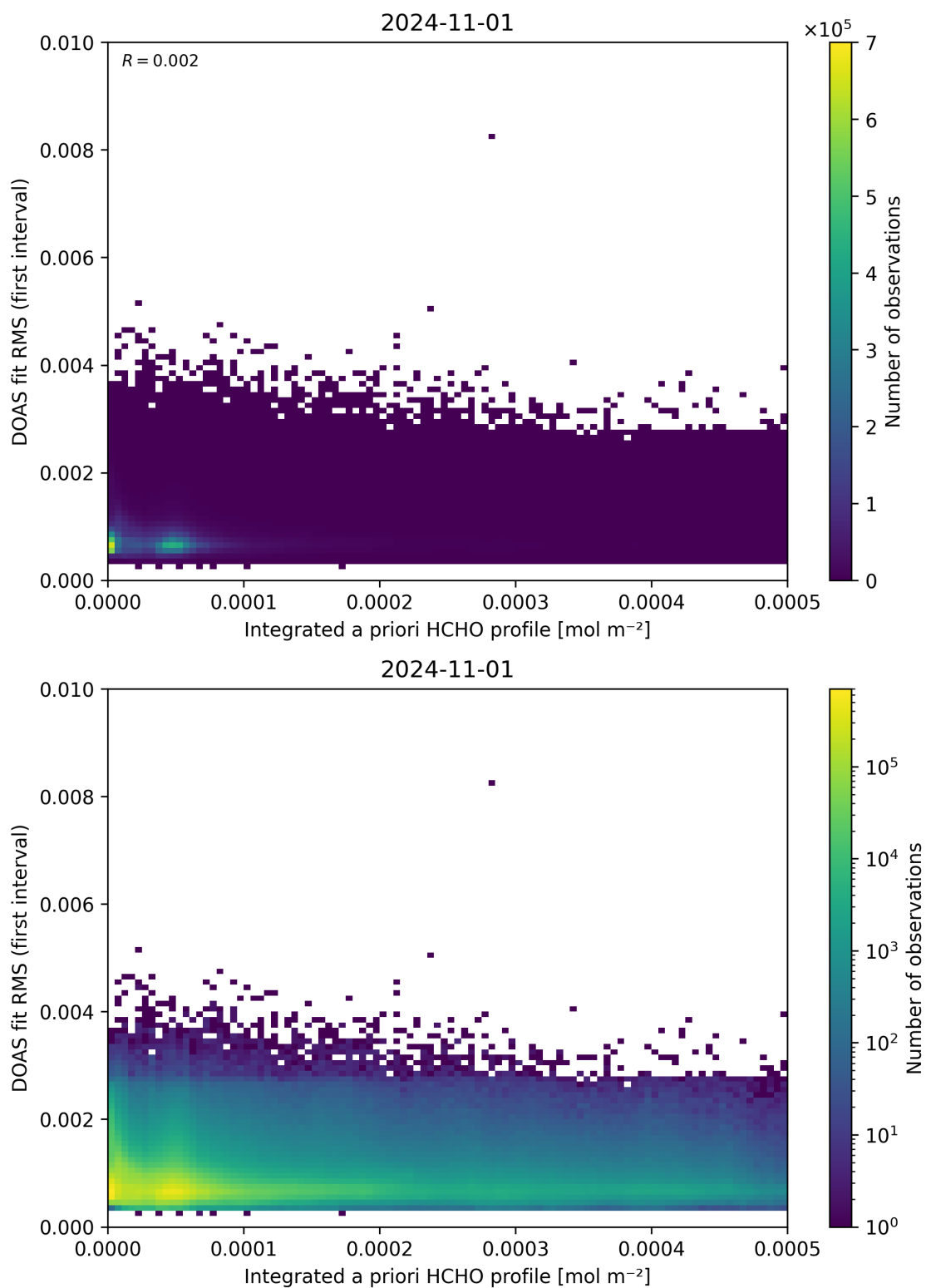
Figure 148: Scatter density plot of “Integrated a priori HCHO profile” against “DOAS fit RMS (first interval)” for 2024-10-31 to 2024-11-02.
