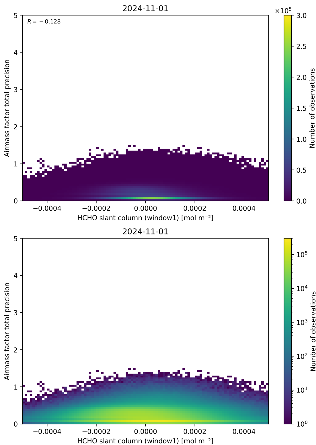
Figure 86: Scatter density plot of “HCHO slant column (window1)” against “Airmass factor total precision” for 2024-10-31 to 2024-11-02.
