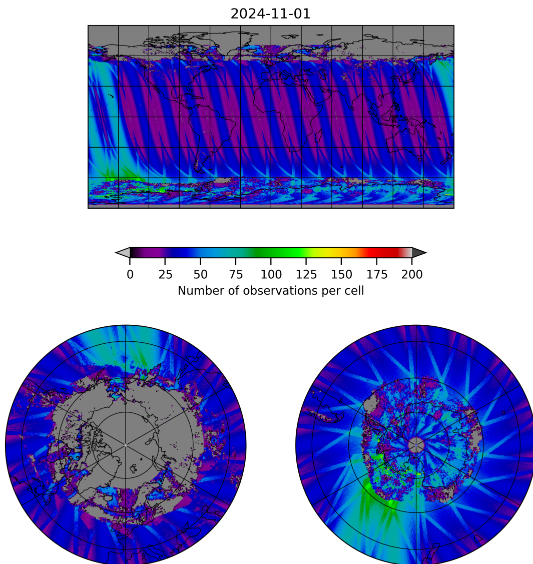
Figure 19: Map of the number of observations for 2024-10-31 to 2024-11-02
