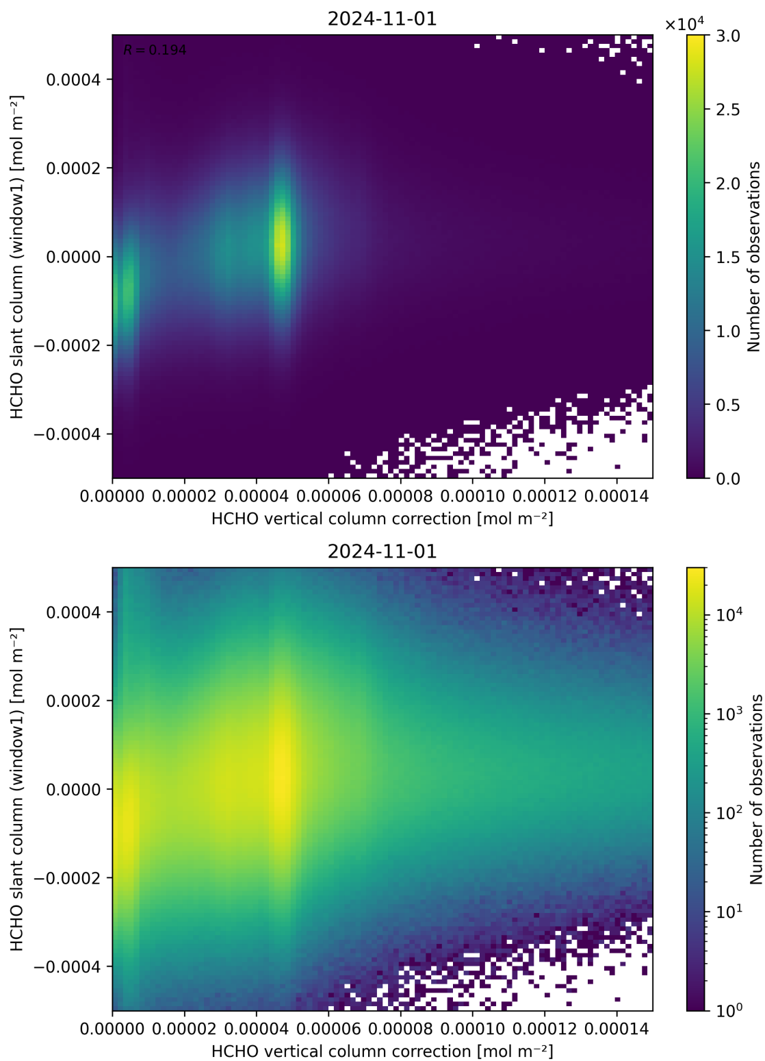
Figure 118: Scatter density plot of “HCHO vertical column correction” against “HCHO slant column (window1)” for 2024-10-31 to 2024-11-02.
