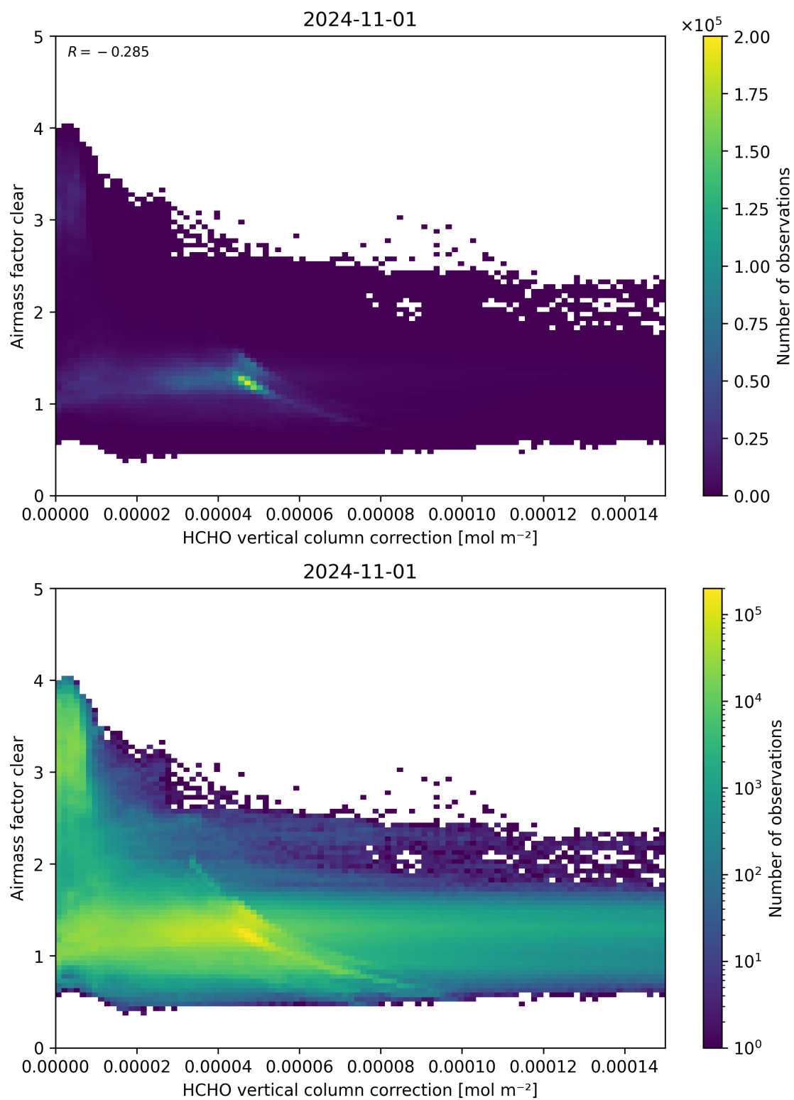
Figure 115: Scatter density plot of “HCHO vertical column correction” against “Airmass factor clear” for 2024-10-31 to 2024-11-02.
