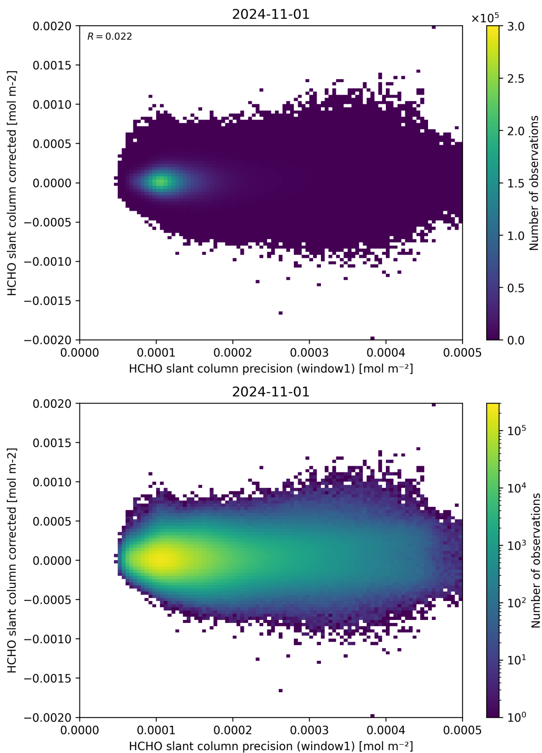
Figure 92: Scatter density plot of “HCHO slant column precision (window1)” against “HCHO slant column corrected” for 2024-10-31 to 2024-11-02.
