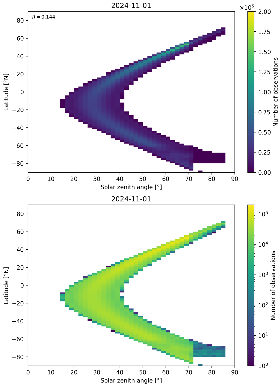
Figure 181: Scatter density plot of “Solar zenith angle” against “Latitude” for 2024-10-31 to 2024-11-02.
