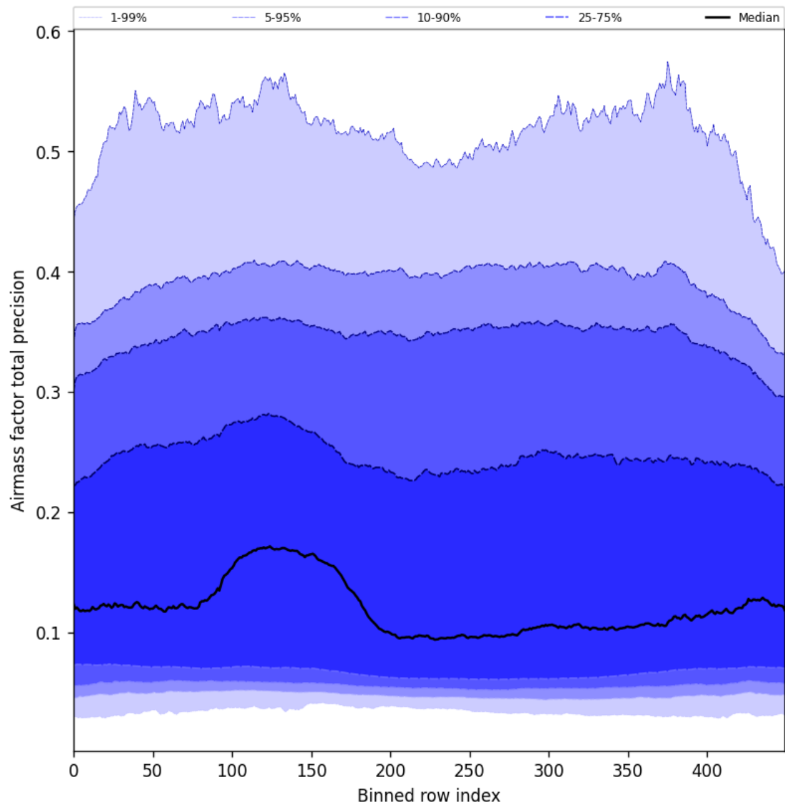
Figure 55: Along track statistics of “Airmass factor total precision” for 2024-10-31 to 2024-11-02
