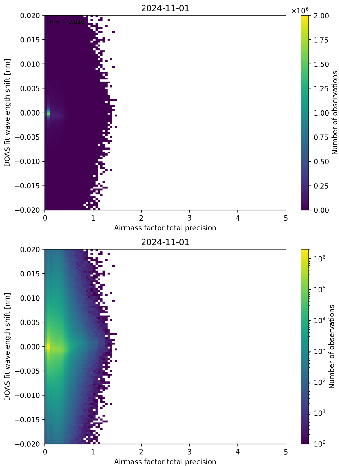
Figure 106: Scatter density plot of “Airmass factor total precision” against “DOAS fit wavelength shift” for 2024-10-31 to 2024-11-02.
