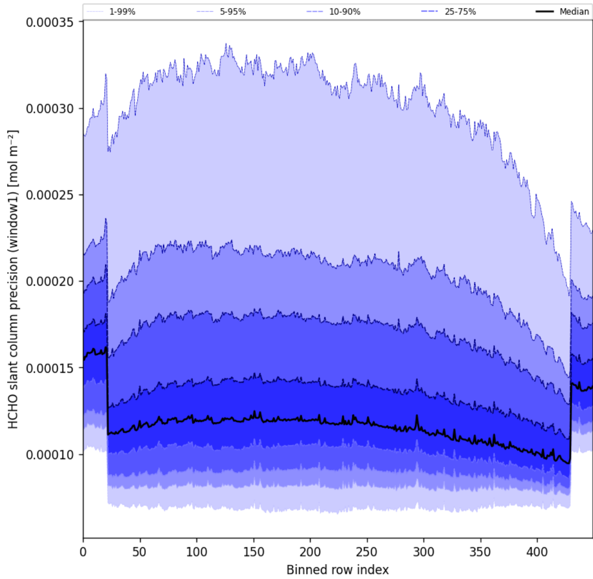
Figure 53: Along track statistics of “HCHO slant column precision (window1)” for 2024-10-31 to 2024-11-02
