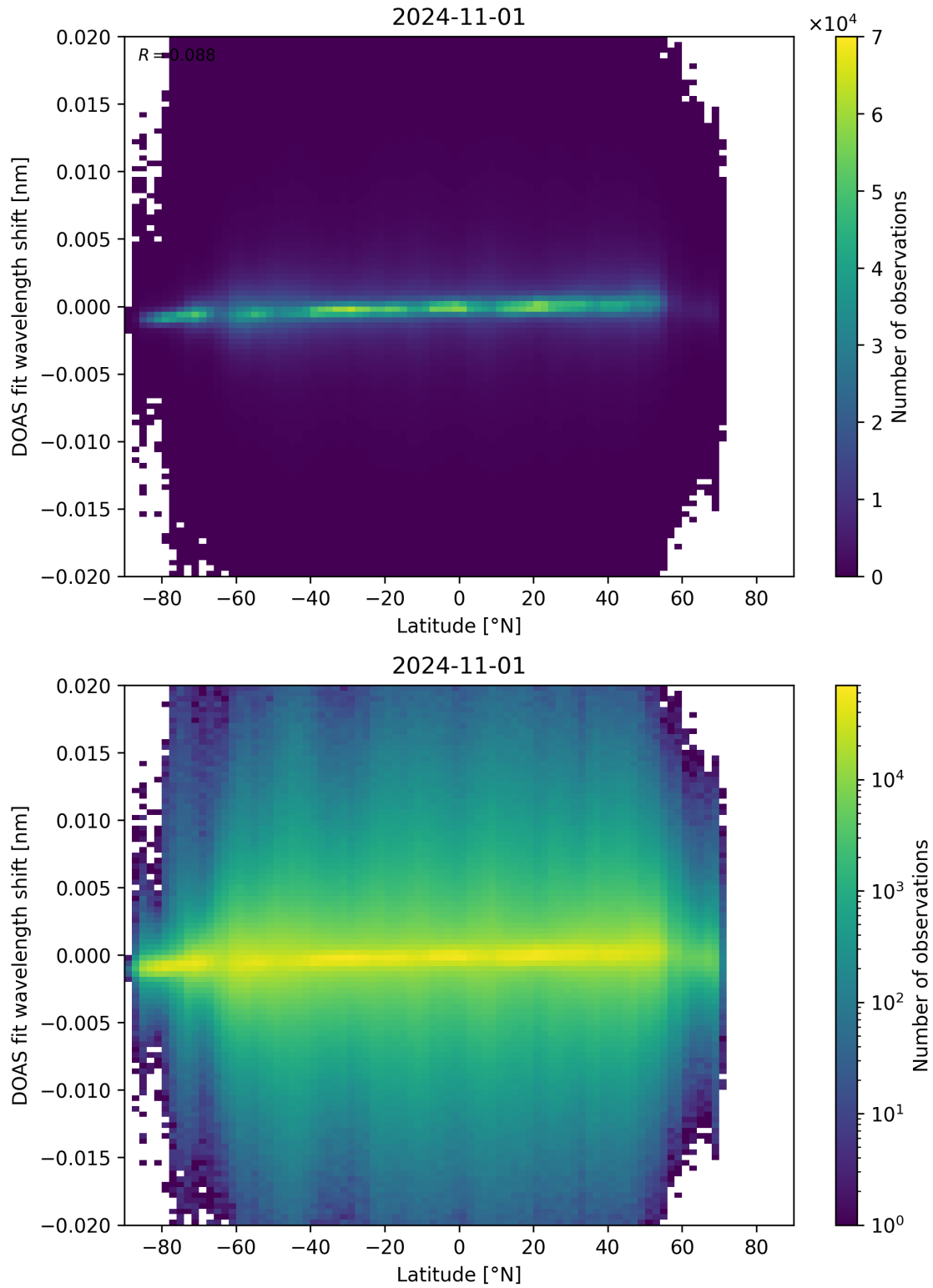
Figure 154: Scatter density plot of “Latitude” against “DOAS fit wavelength shift” for 2024-10-31 to 2024-11-02.
