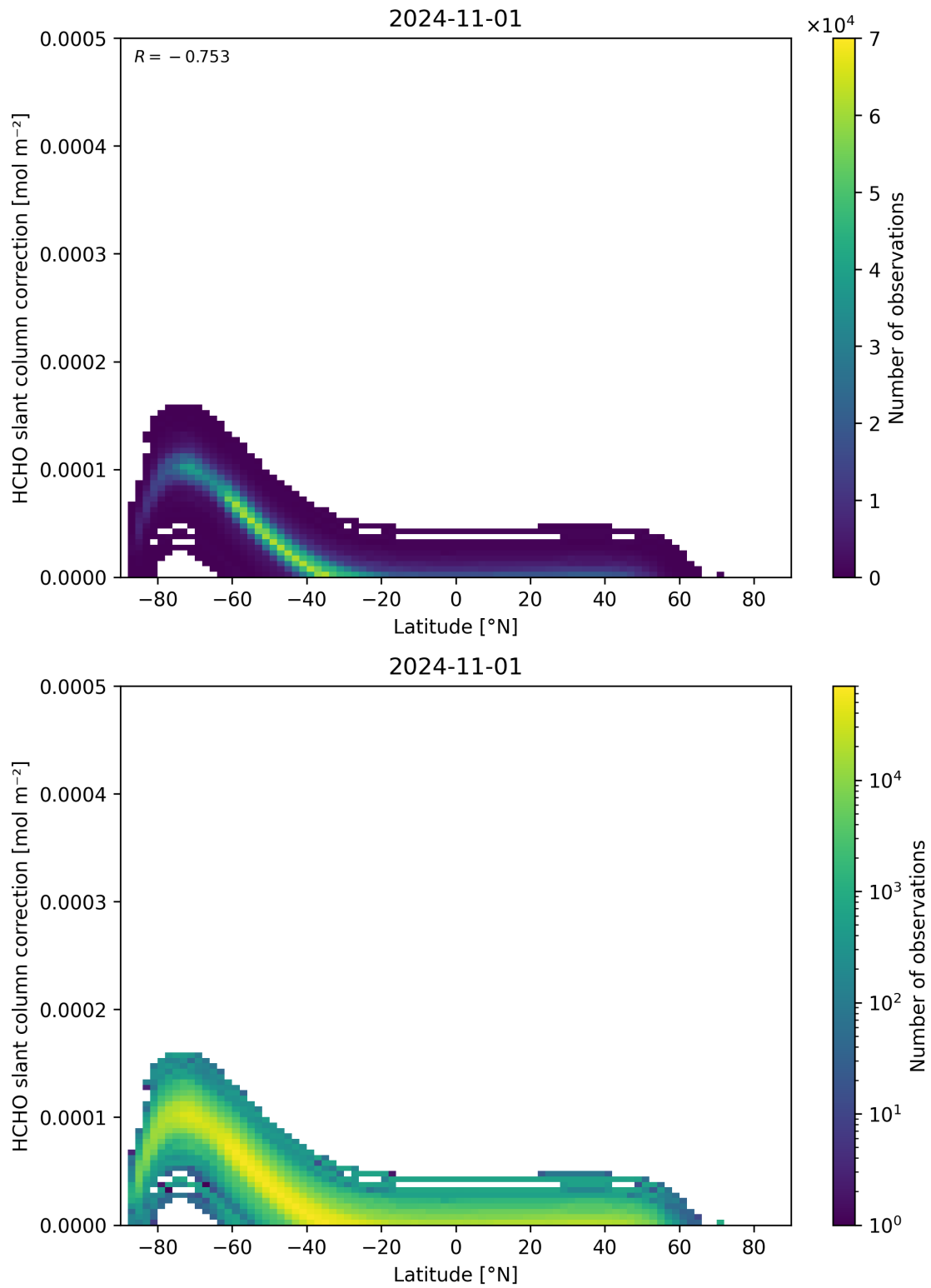
Figure 158: Scatter density plot of “Latitude” against “HCHO slant column correction” for 2024-10-31 to 2024-11-02.
