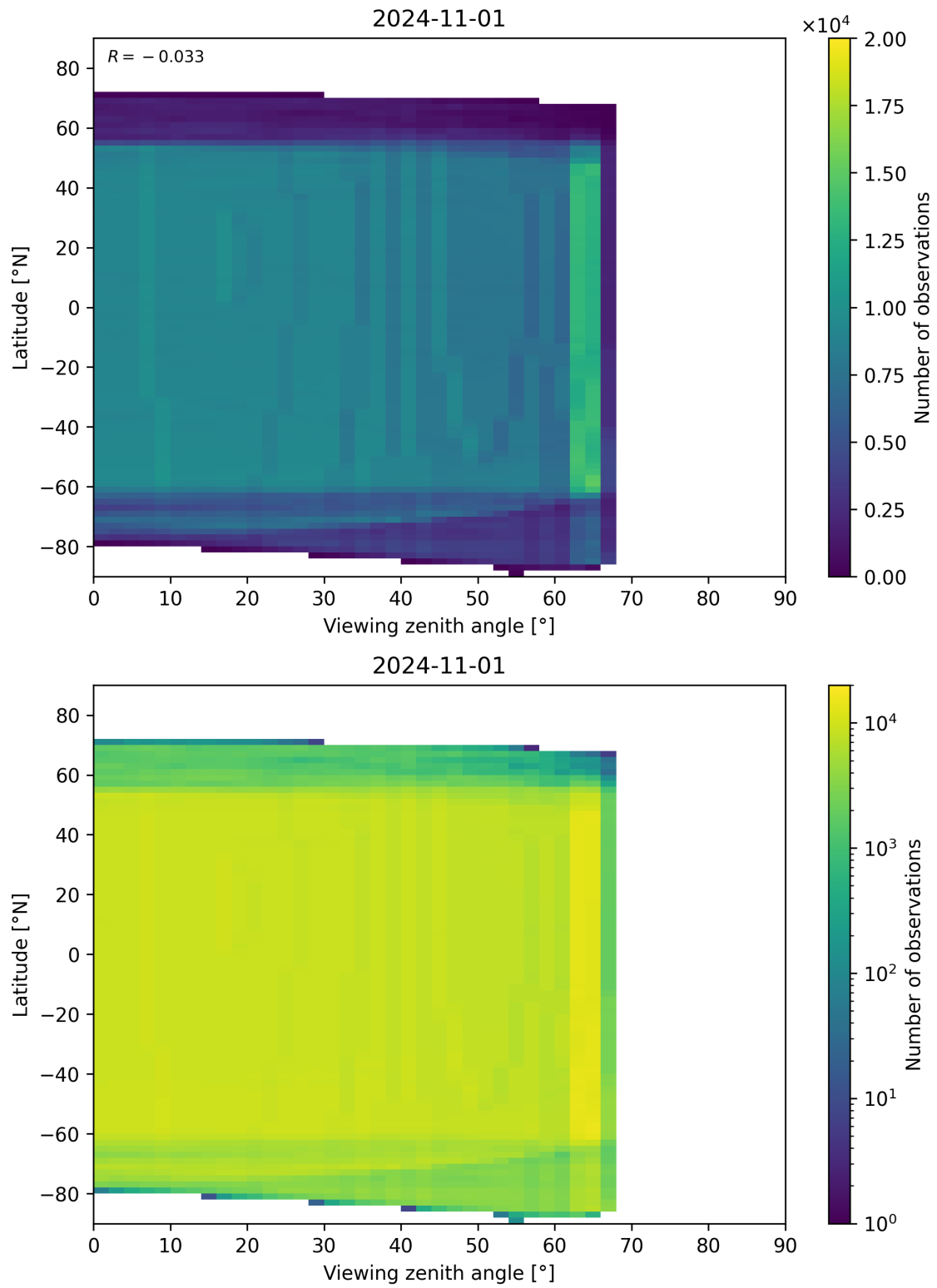
Figure 196: Scatter density plot of “Viewing zenith angle” against “Latitude” for 2024-10-31 to 2024-11-02.
