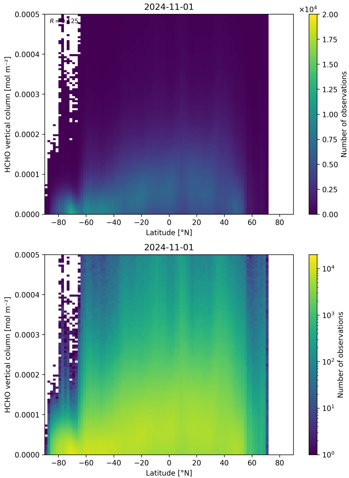
Figure 163: Scatter density plot of “Latitude” against “HCHO vertical column” for 2024-10-31 to 2024-11-02.
