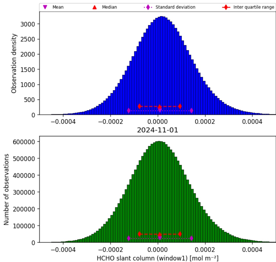
Figure 38: Histogram of “HCHO slant column (window1)” for 2024-10-31 to 2024-11-02
