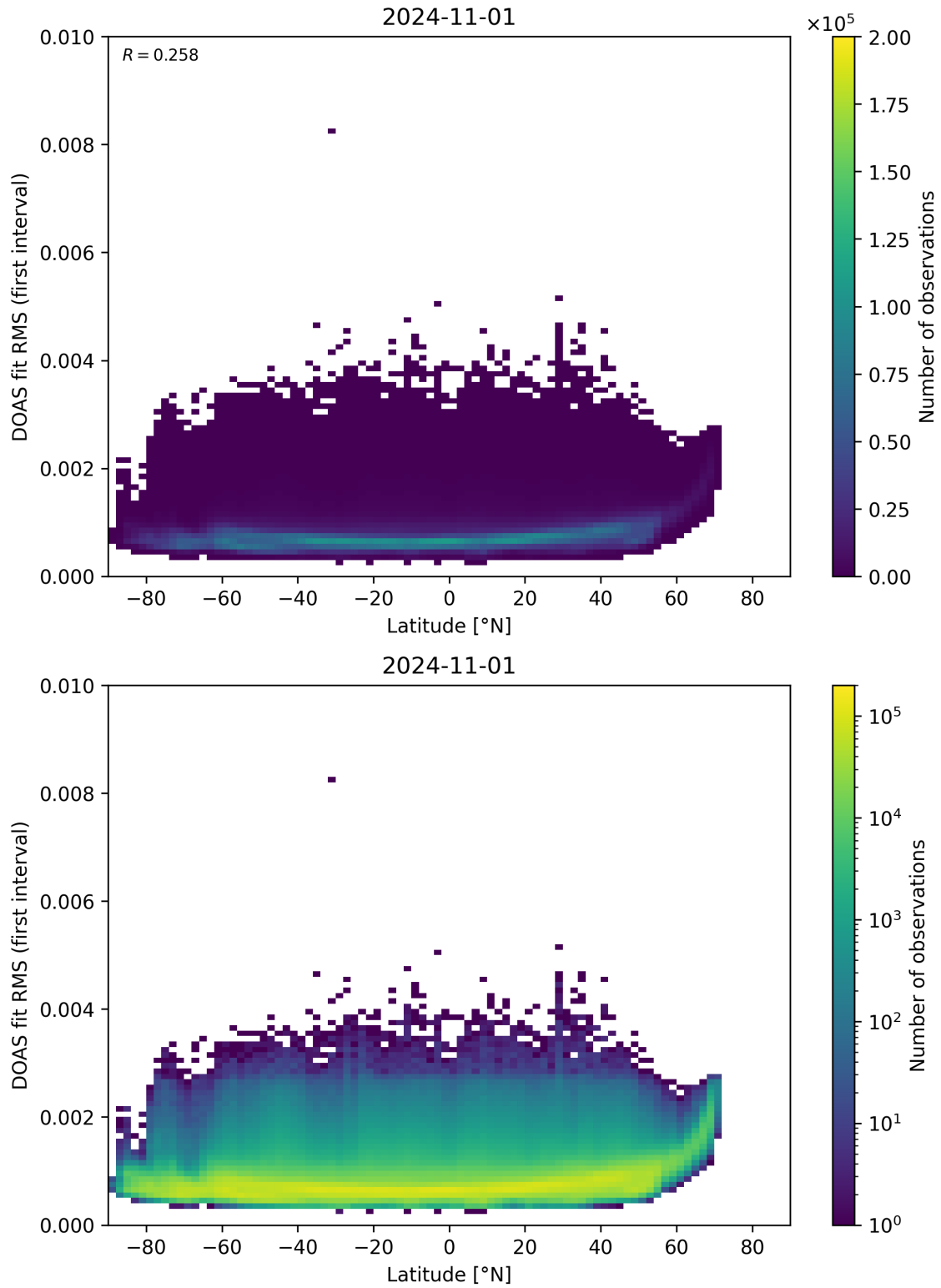
Figure 153: Scatter density plot of “Latitude” against “DOAS fit RMS (first interval)” for 2024-10-31 to 2024-11-02.
