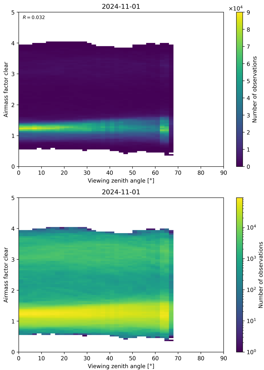
Figure 185: Scatter density plot of “Viewing zenith angle” against “Airmass factor clear” for 2024-10-31 to 2024-11-02.
