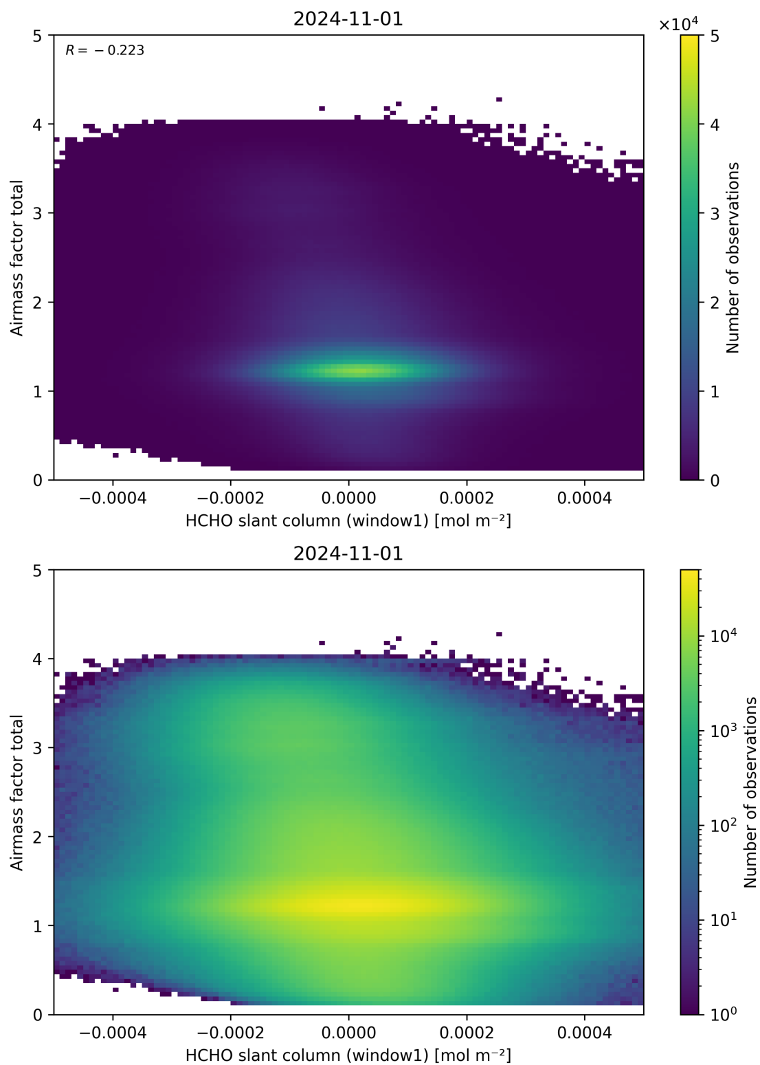
Figure 85: Scatter density plot of “HCHO slant column (window1)” against “Airmass factor total” for 2024-10-31 to 2024-11-02.
