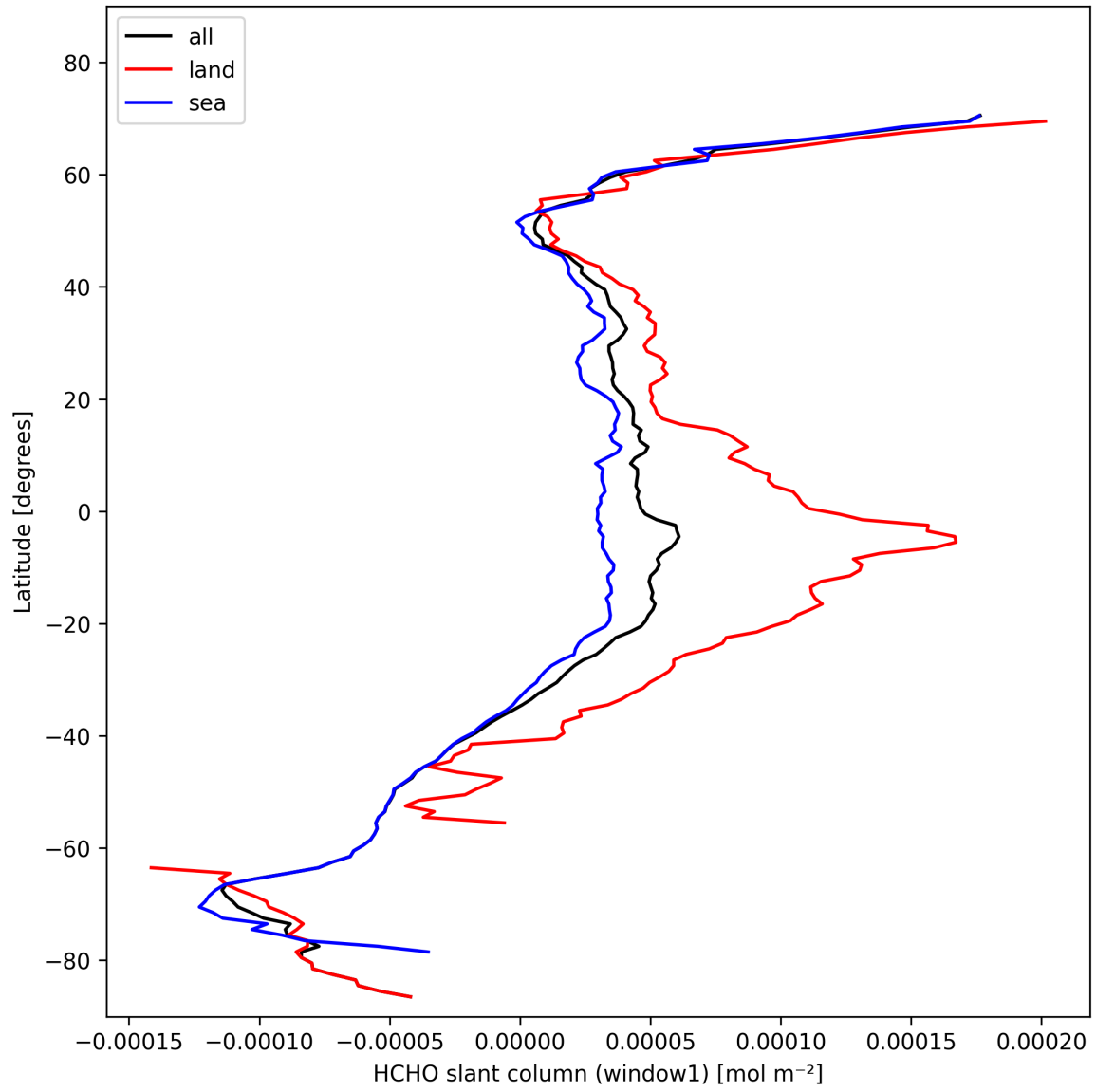
Figure 24: Zonal average of “HCHO slant column (window1)” for 2024-10-31 to 2024-11-02.
