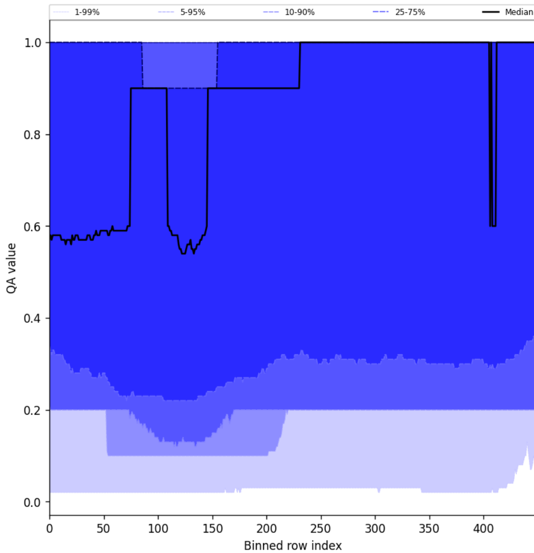
Figure 48: Along track statistics of “QA value” for 2024-10-31 to 2024-11-02
