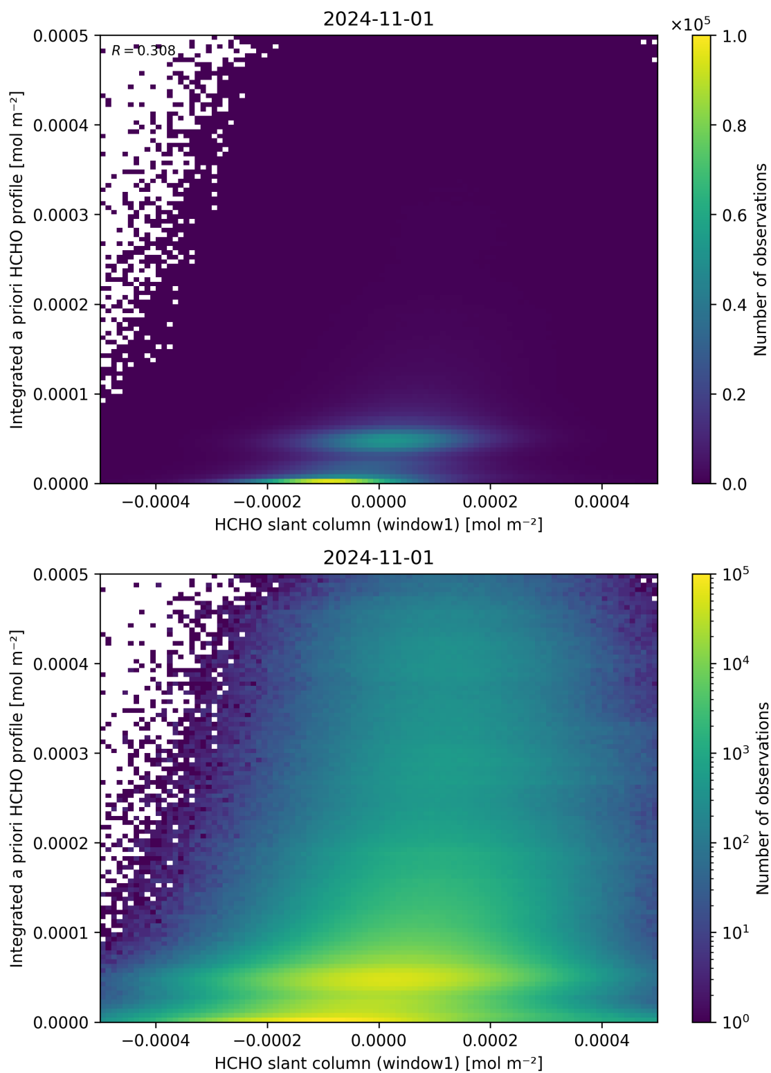
Figure 87: Scatter density plot of “HCHO slant column (window1)” against “Integrated a priori HCHO profile” for 2024-10-31 to 2024-11-02.
