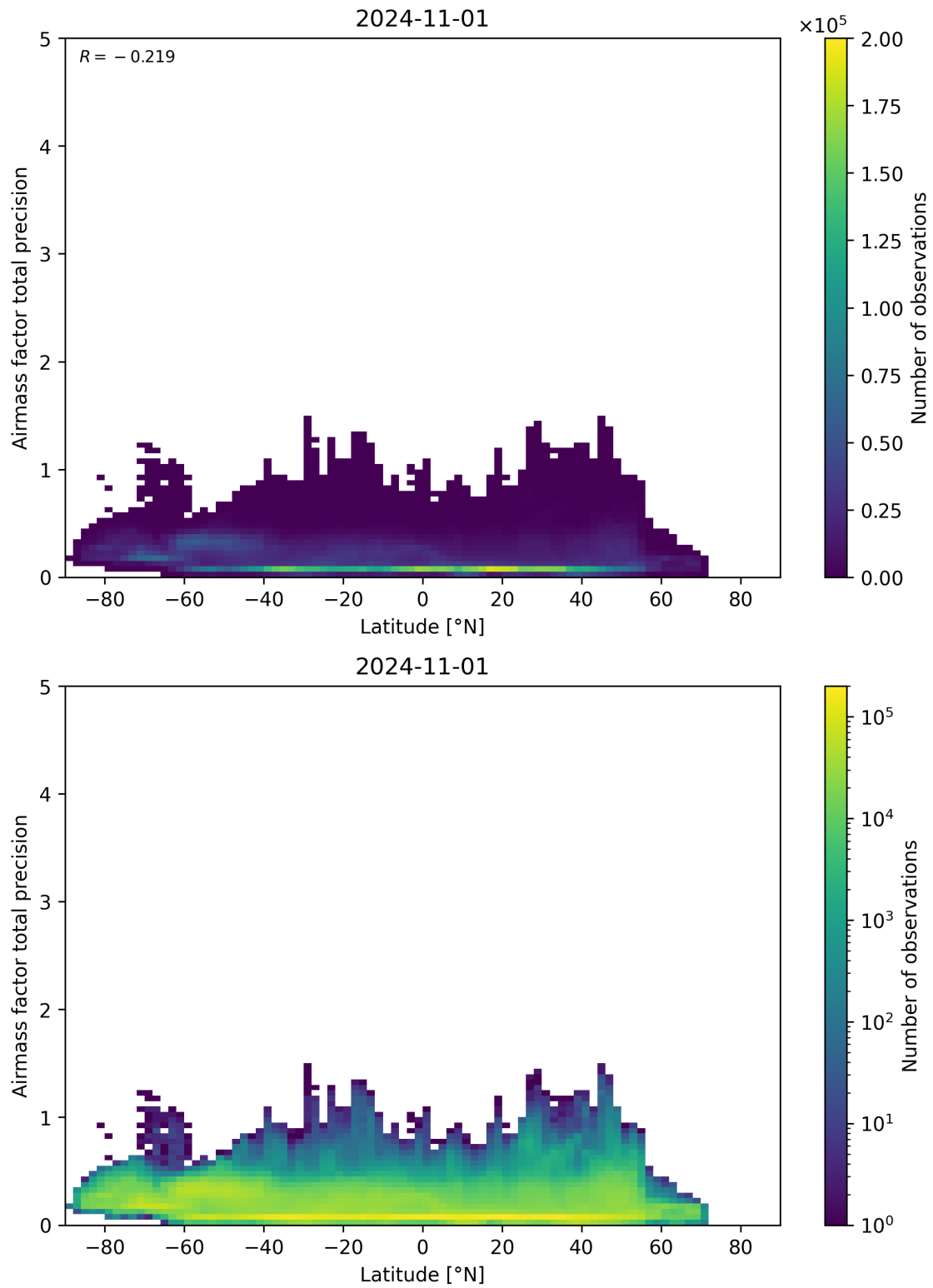
Figure 162: Scatter density plot of “Latitude” against “Airmass factor total precision” for 2024-10-31 to 2024-11-02.
