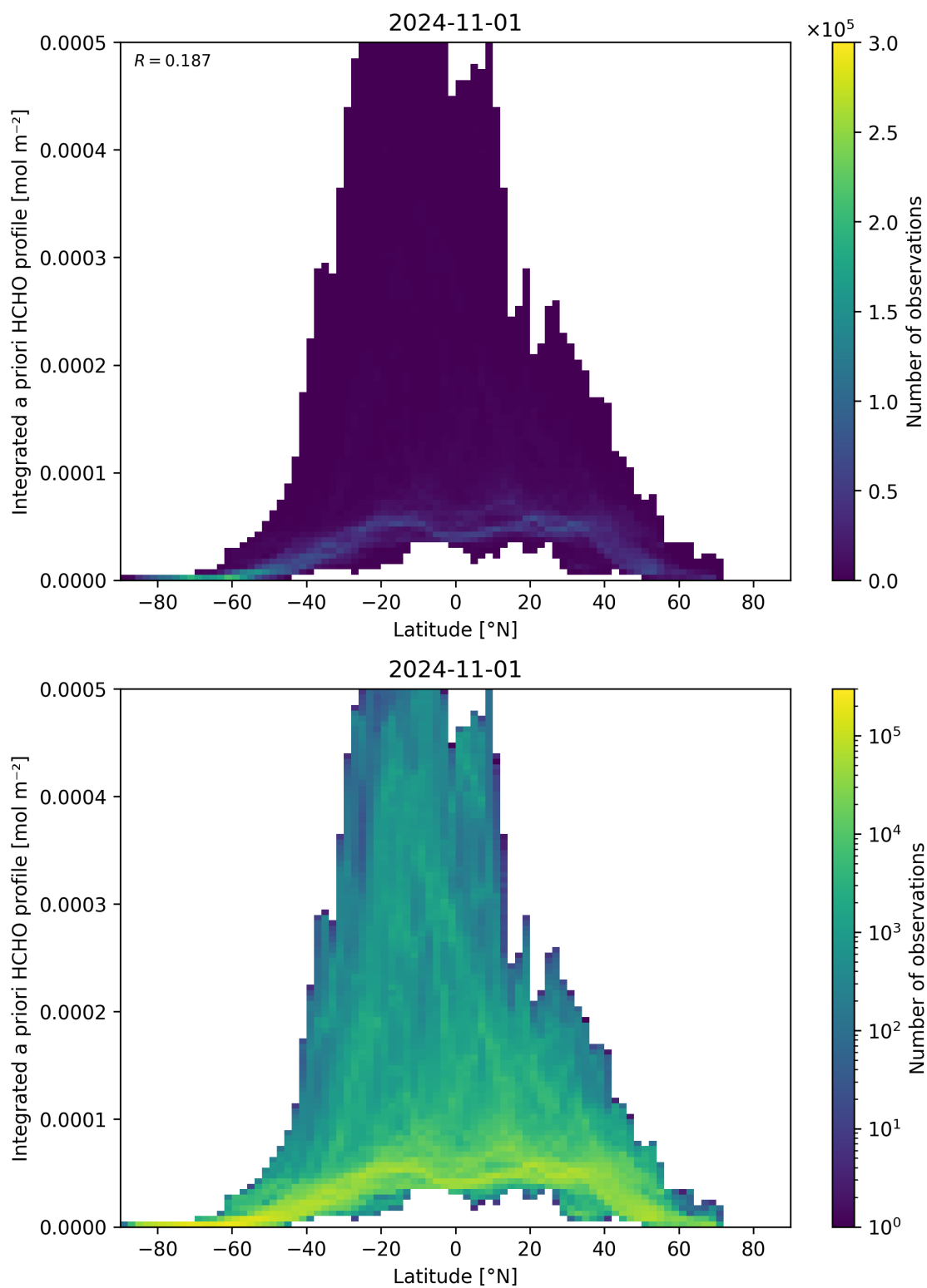
Figure 166: Scatter density plot of “Latitude” against “Integrated a priori HCHO profile” for 2024-10-31 to 2024-11-02.
