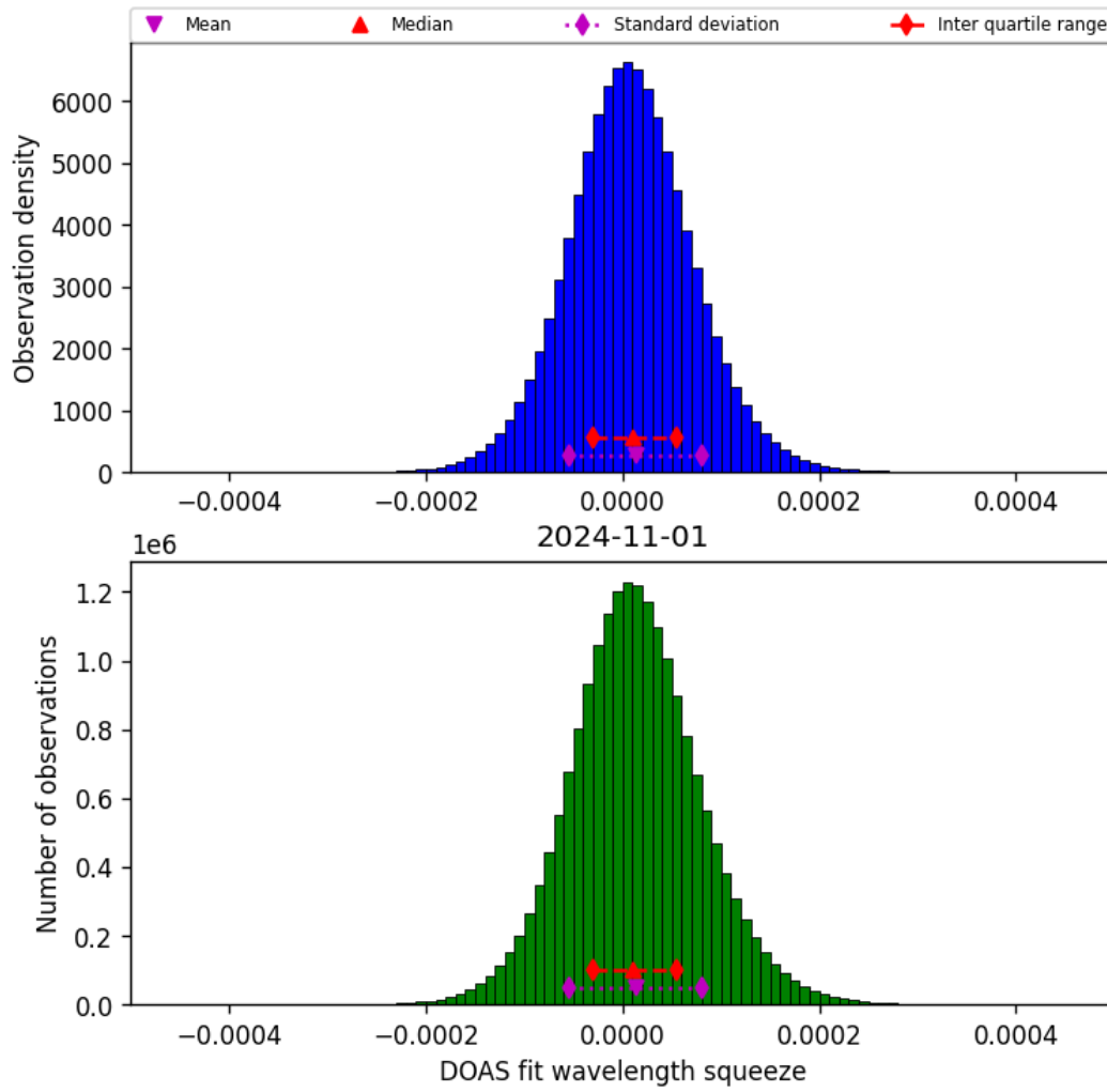
Figure 45: Histogram of “DOAS fit wavelength squeeze” for 2024-10-31 to 2024-11-02
