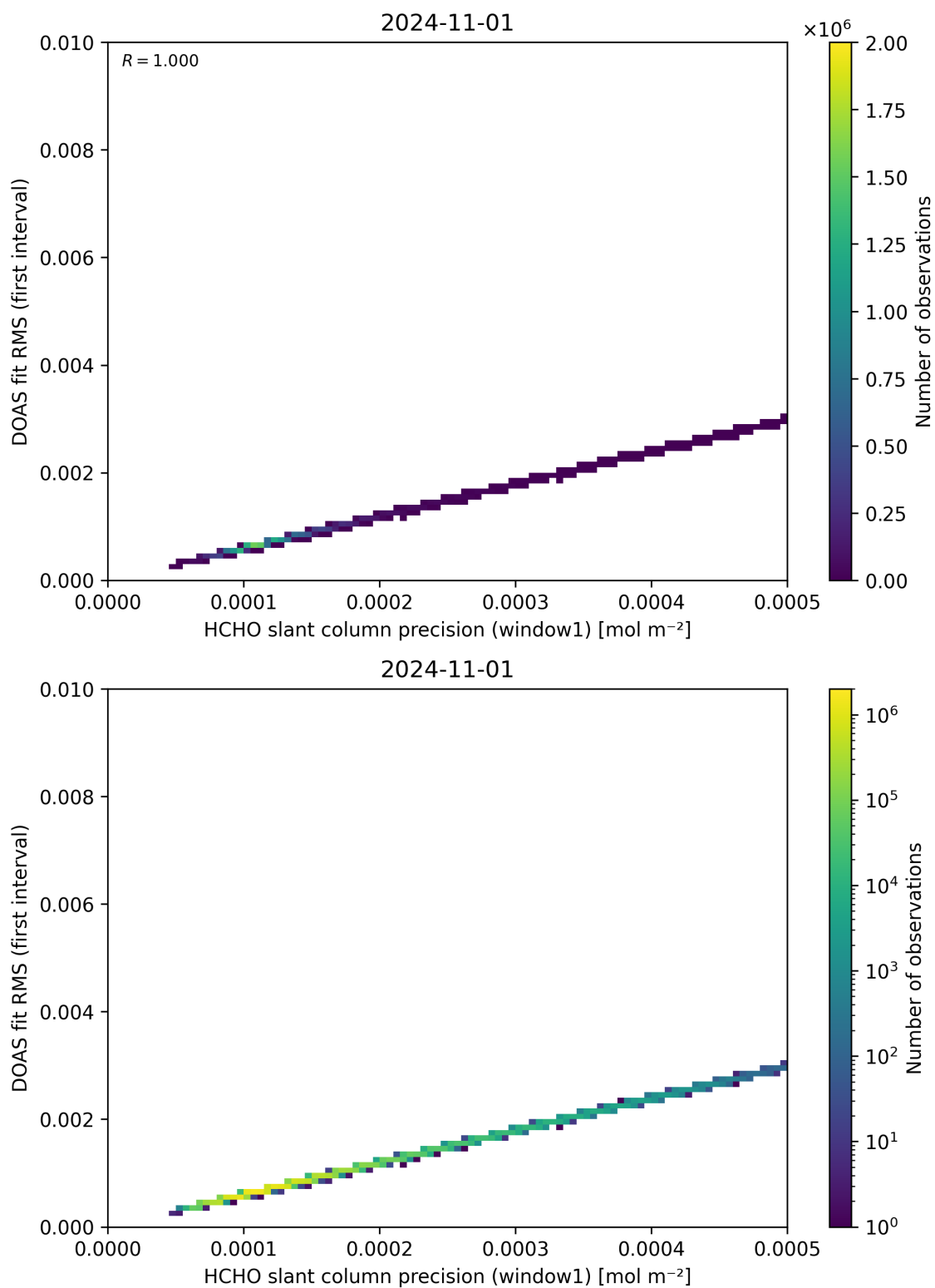
Figure 88: Scatter density plot of “HCHO slant column precision (window1)” against “DOAS fit RMS (first interval)” for 2024-10-31 to 2024-11-02.
