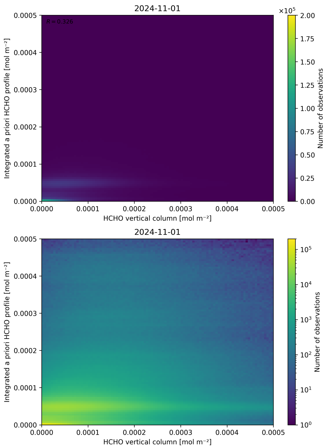
Figure 135: Scatter density plot of “HCHO vertical column” against “Integrated a priori HCHO profile” for 2024-10-31 to 2024-11-02.
