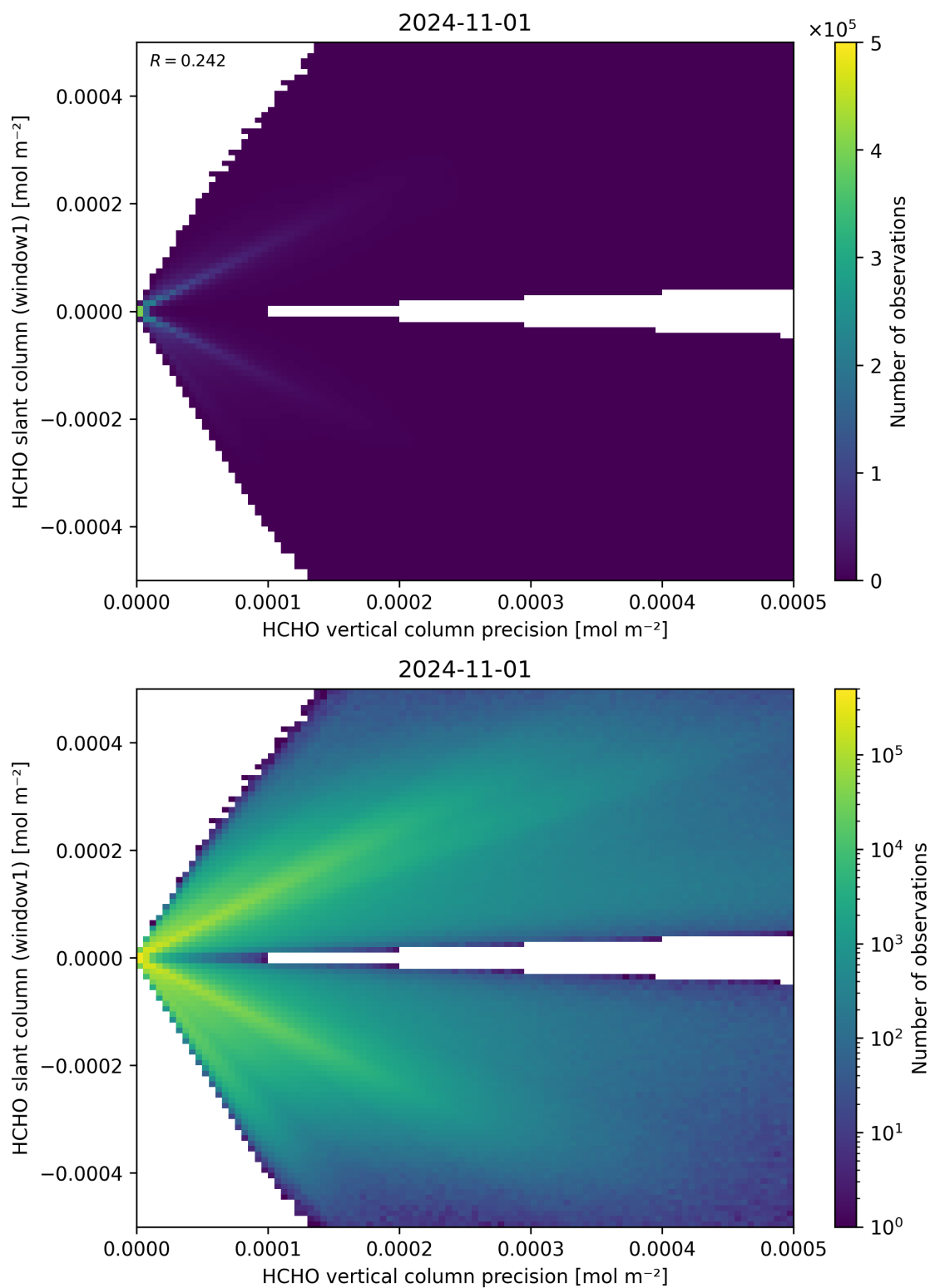
Figure 142: Scatter density plot of “HCHO vertical column precision” against “HCHO slant column (window1)” for 2024-10-31 to 2024-11-02.
