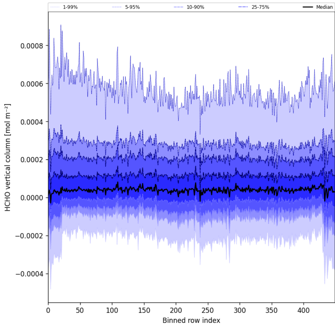
Figure 49: Along track statistics of “HCHO vertical column” for 2024-10-31 to 2024-11-02
