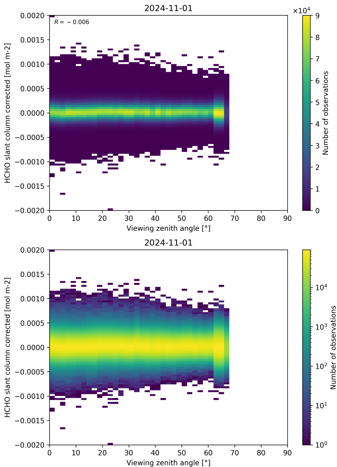
Figure 186: Scatter density plot of “Viewing zenith angle” against “HCHO slant column corrected” for 2024-10-31 to 2024-11-02.
