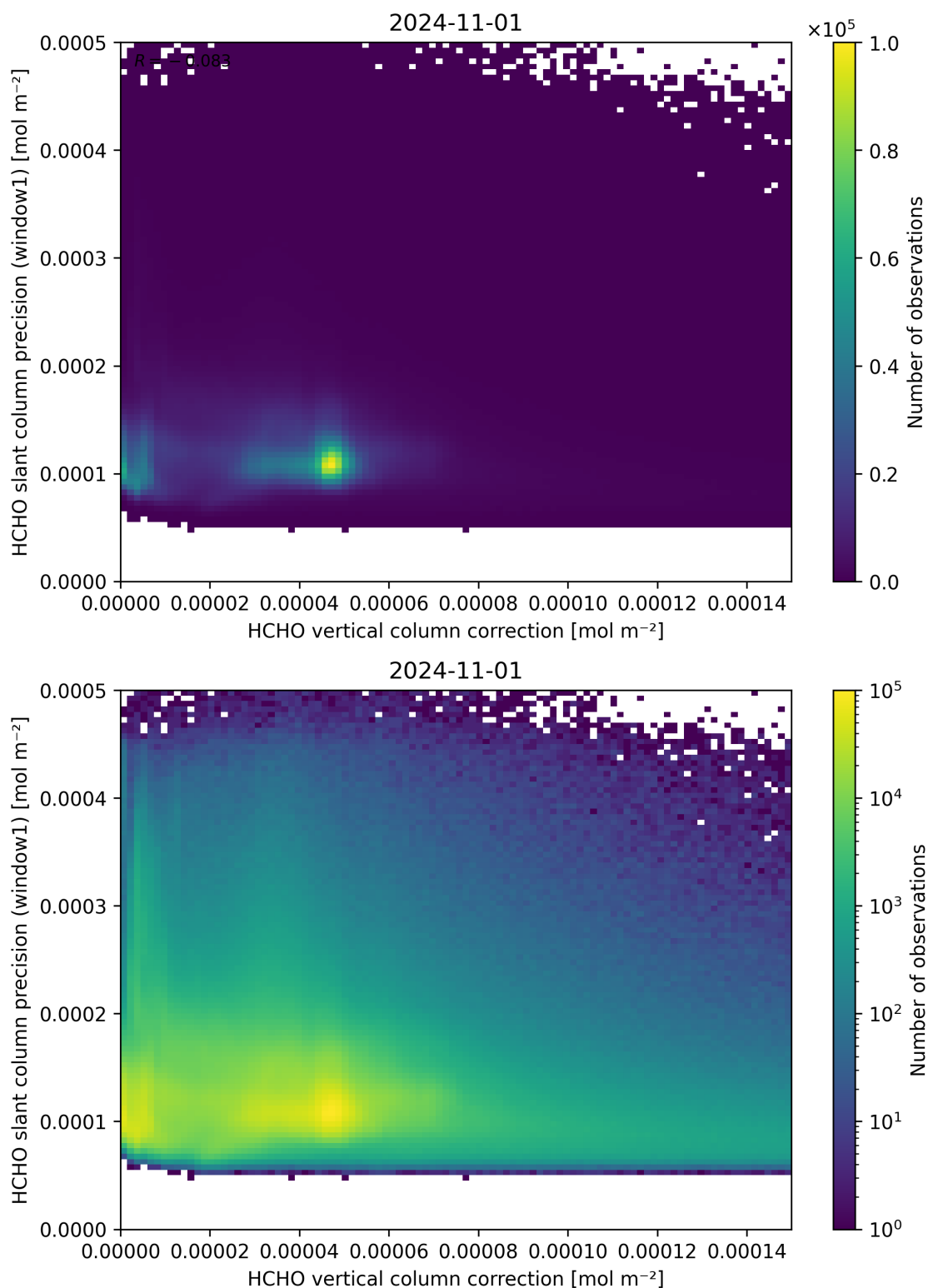
Figure 119: Scatter density plot of “HCHO vertical column correction” against “HCHO slant column precision (window1)” for 2024-10-31 to 2024-11-02.
