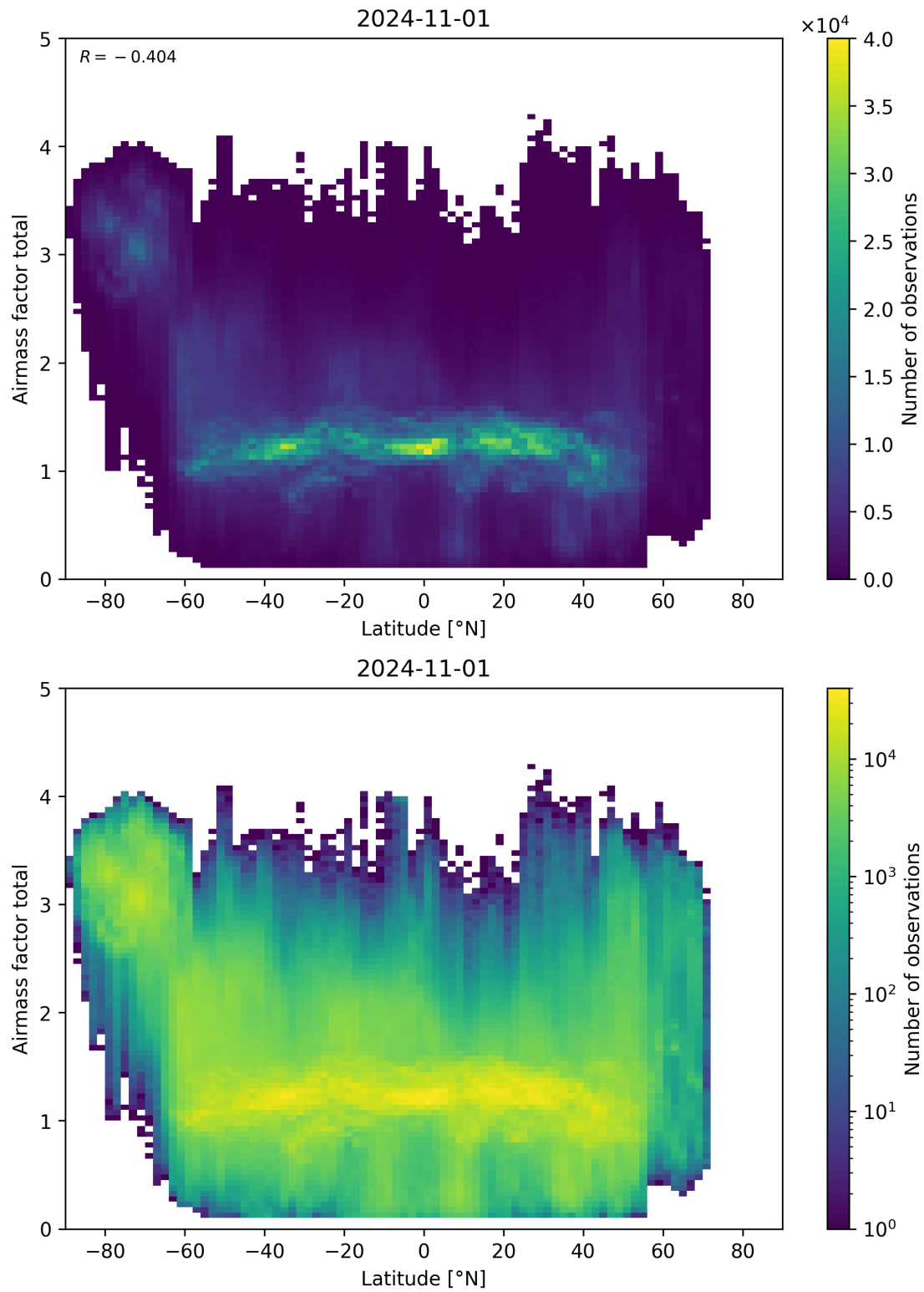
Figure 161: Scatter density plot of “Latitude” against “Airmass factor total” for 2024-10-31 to 2024-11-02.
