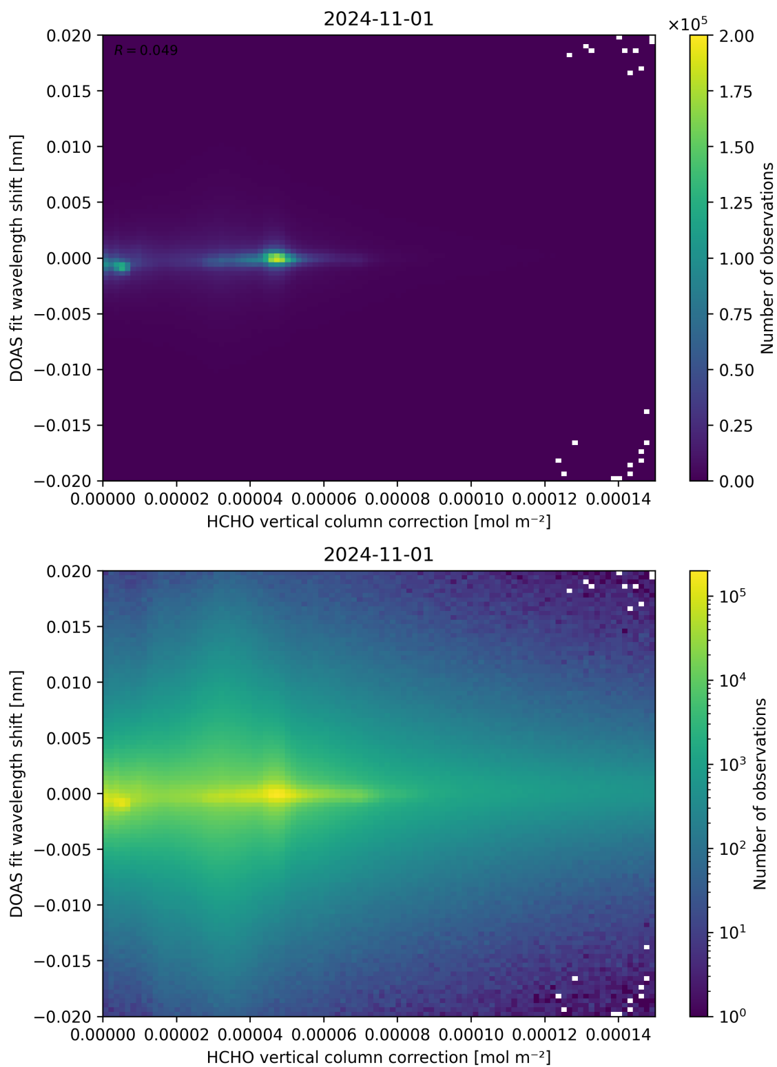
Figure 113: Scatter density plot of “HCHO vertical column correction” against “DOAS fit wavelength shift” for 2024-10-31 to 2024-11-02.
