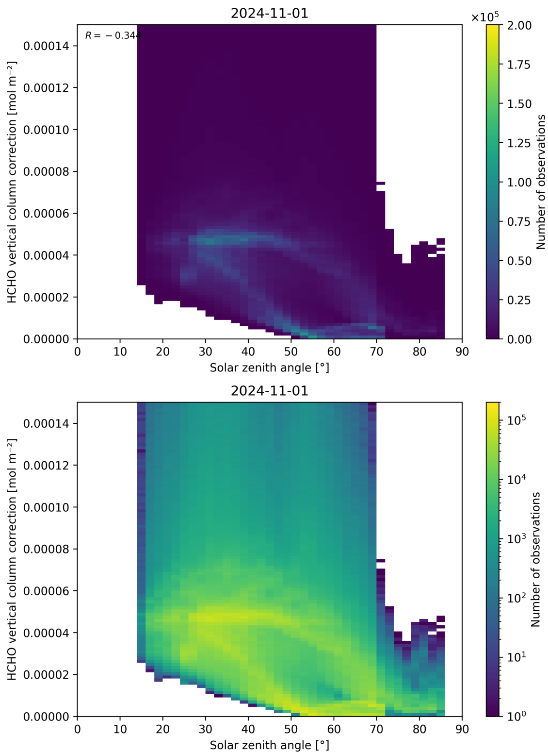
Figure 178: Scatter density plot of “Solar zenith angle” against “HCHO vertical column correction” for 2024-10-31 to 2024-11-02.
