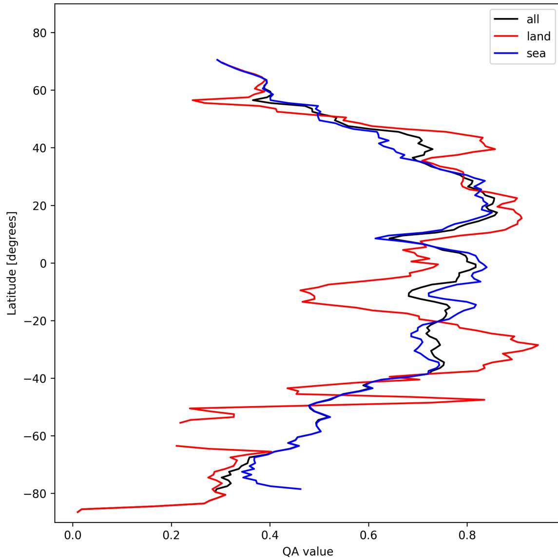
Figure 20: Zonal average of “QA value” for 2024-10-31 to 2024-11-02.
