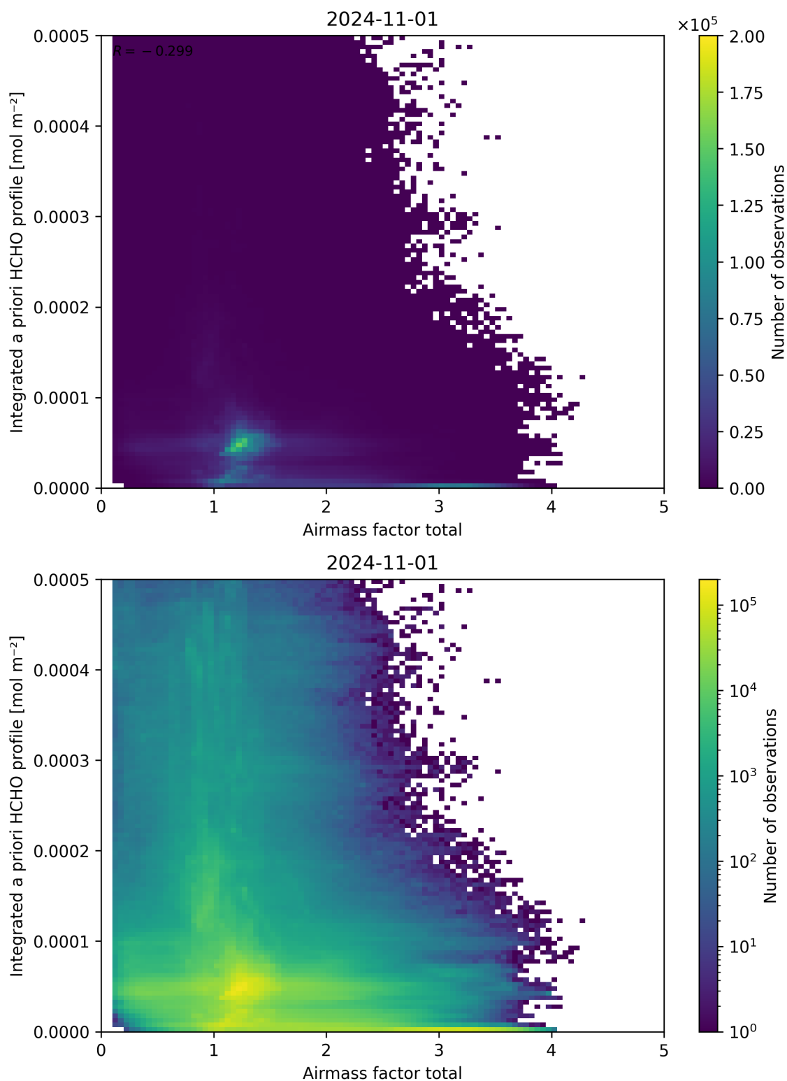
Figure 104: Scatter density plot of “Airmass factor total” against “Integrated a priori HCHO profile” for 2024-10-31 to 2024-11-02.
