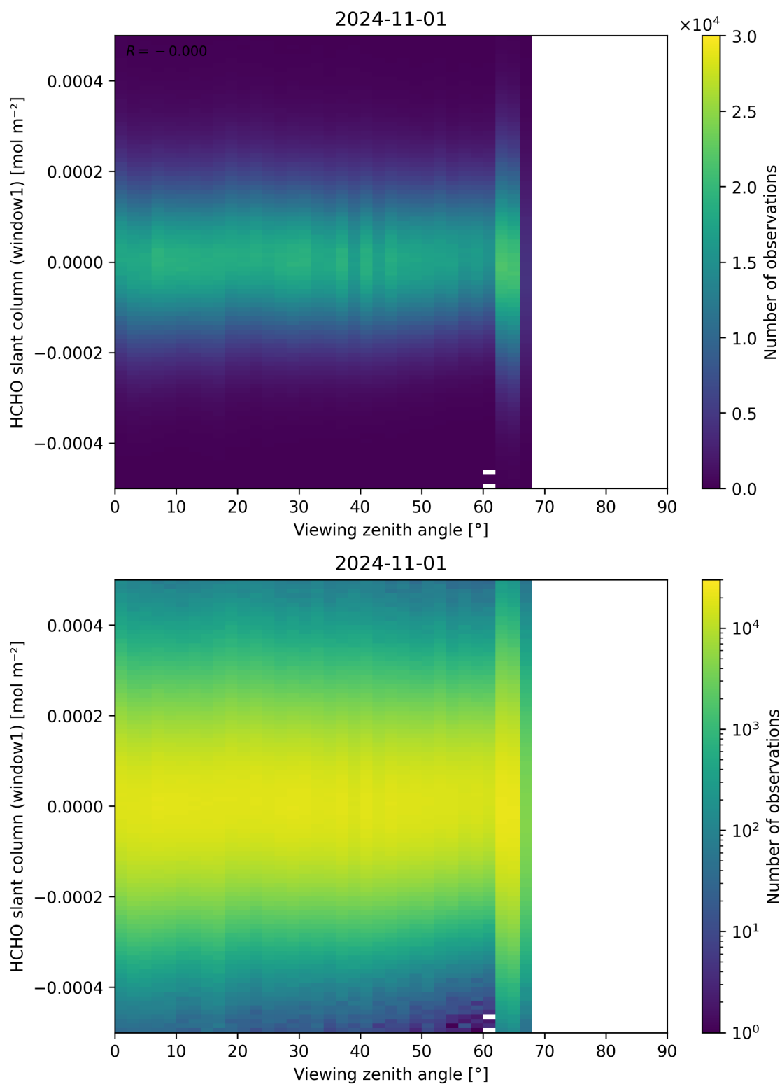
Figure 188: Scatter density plot of “Viewing zenith angle” against “HCHO slant column (window1)” for 2024-10-31 to 2024-11-02.
