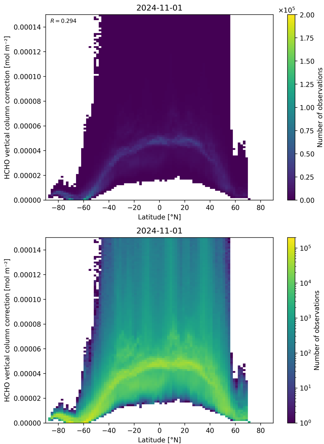
Figure 164: Scatter density plot of “Latitude” against “HCHO vertical column correction” for 2024-10-31 to 2024-11-02.
