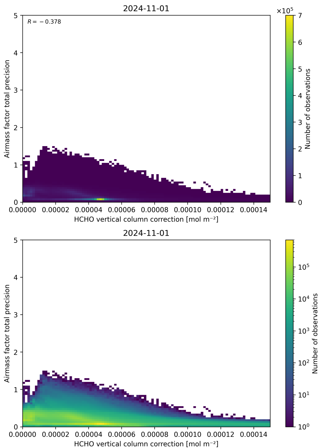
Figure 121: Scatter density plot of “HCHO vertical column correction” against “Airmass factor total precision” for 2024-10-31 to 2024-11-02.
