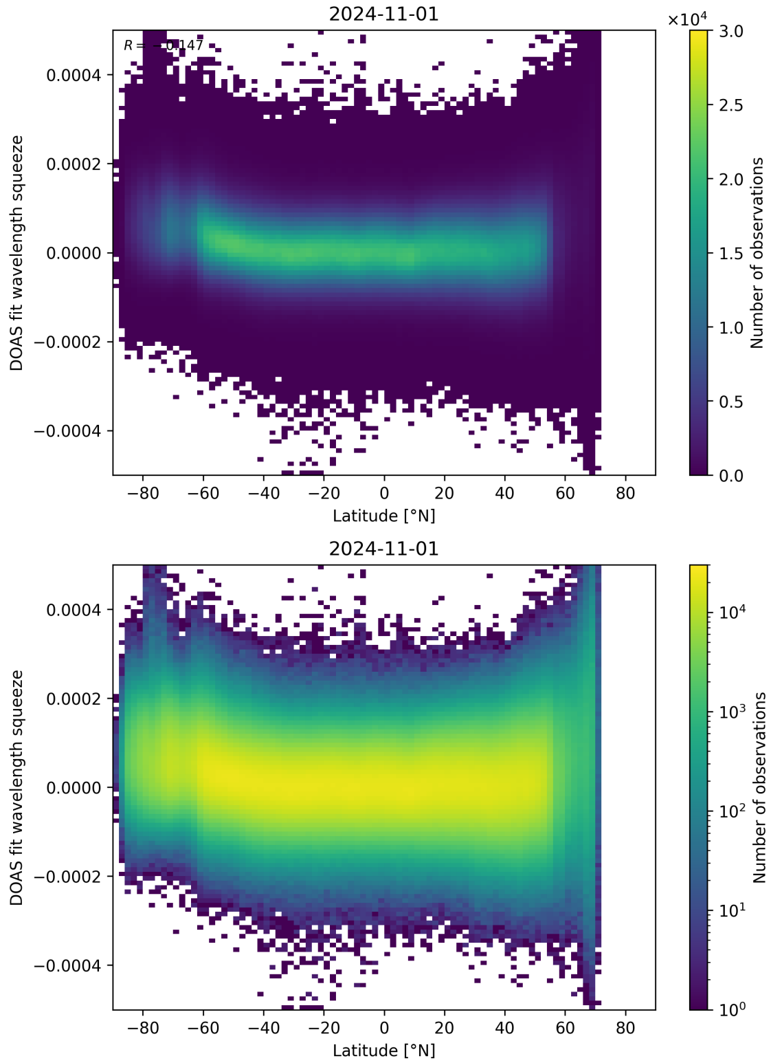
Figure 155: Scatter density plot of “Latitude” against “DOAS fit wavelength squeeze” for 2024-10-31 to 2024-11-02.
