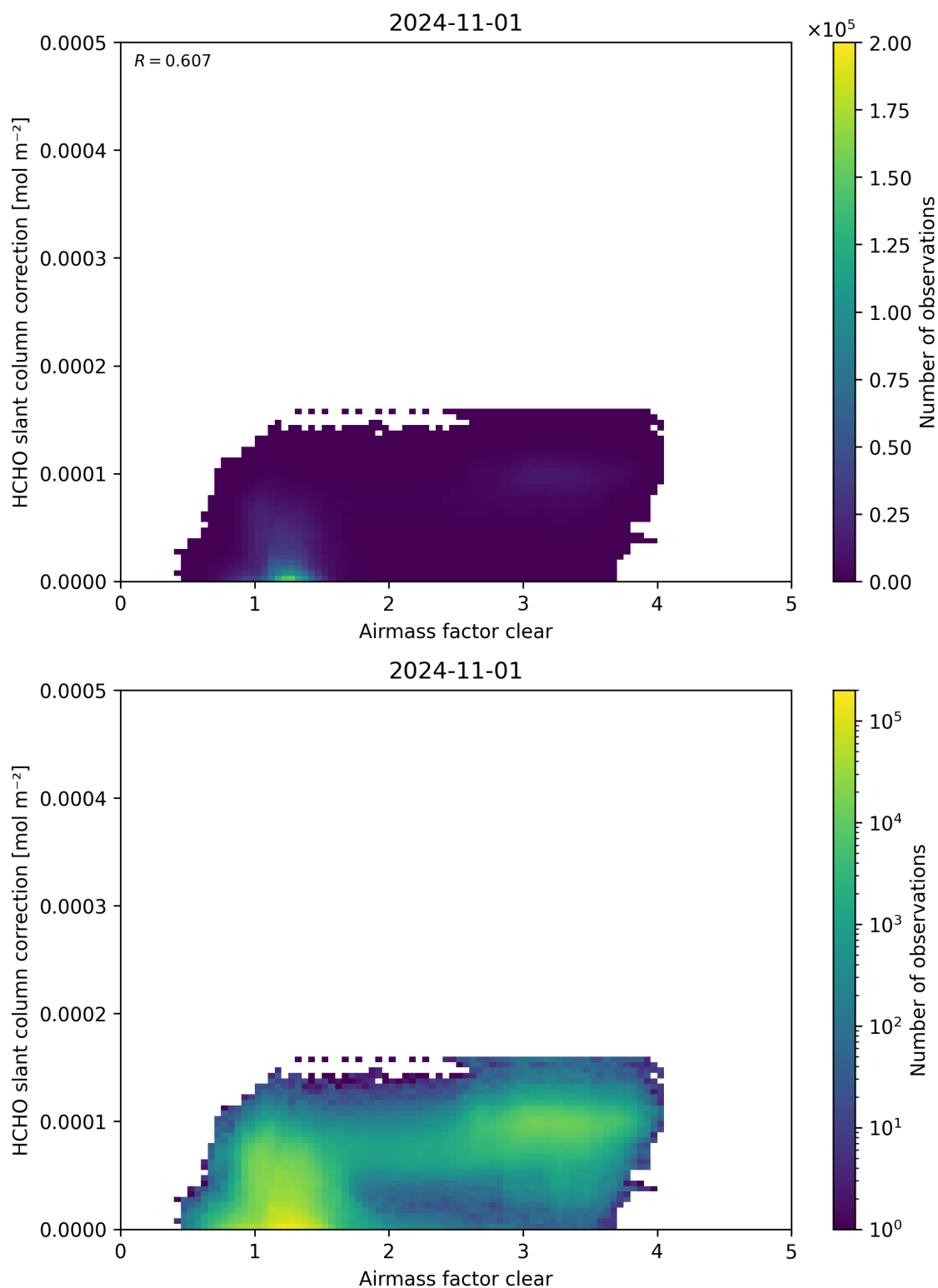
Figure 75: Scatter density plot of “Airmass factor clear” against “HCHO slant column correction” for 2024-10-31 to 2024-11-02.
