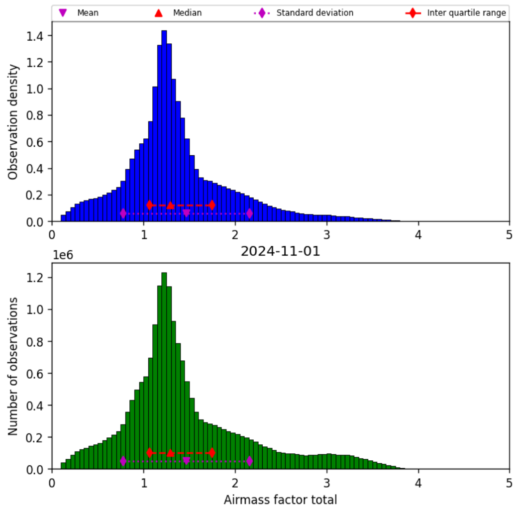
Figure 40: Histogram of “Airmass factor total” for 2024-10-31 to 2024-11-02
