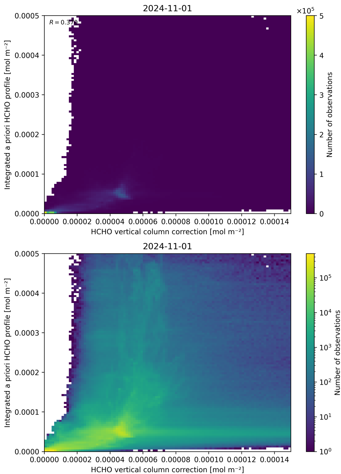
Figure 122: Scatter density plot of “HCHO vertical column correction” against “Integrated a priori HCHO profile” for 2024-10-31 to 2024-11-02.
