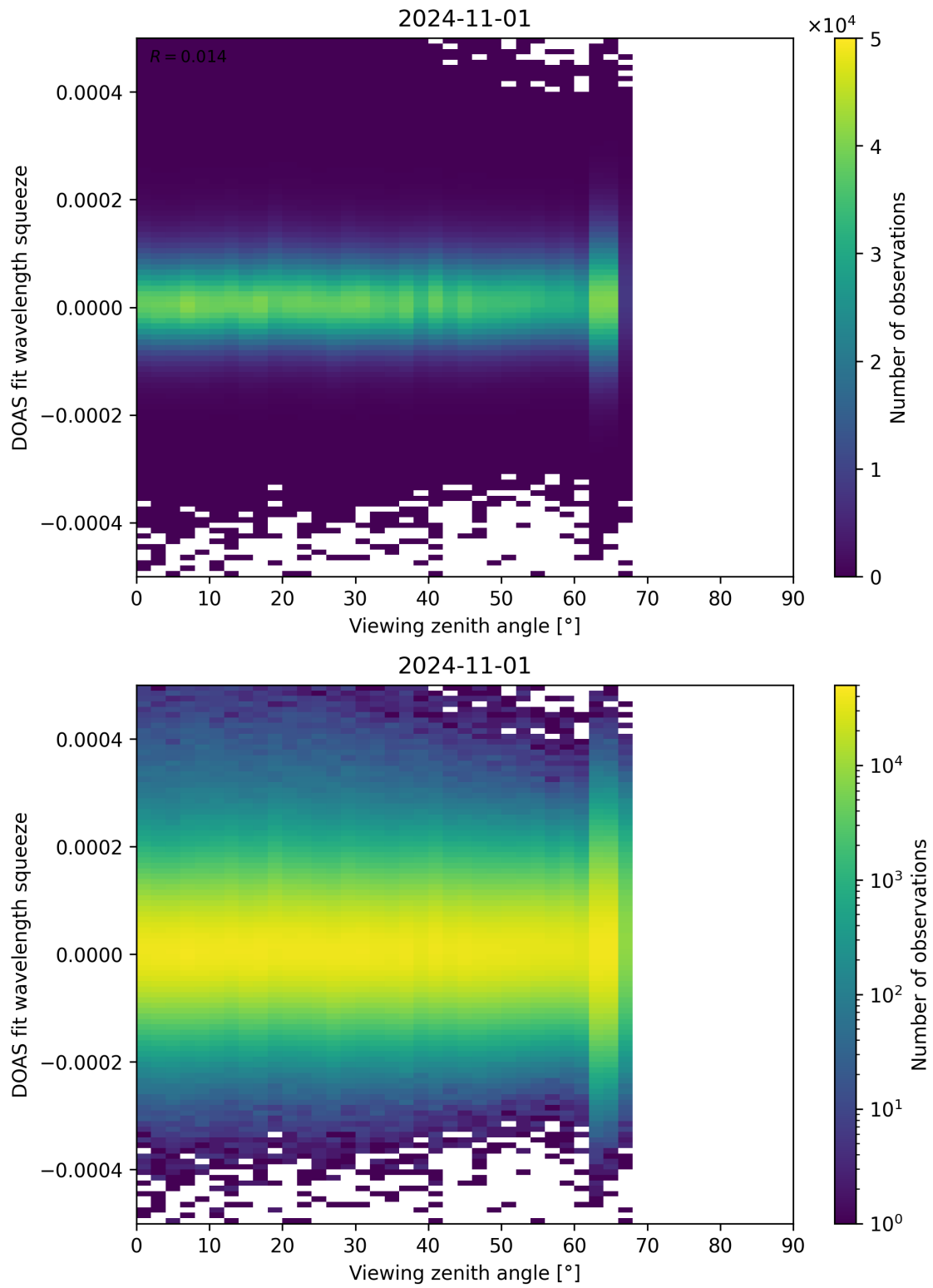
Figure 184: Scatter density plot of “Viewing zenith angle” against “DOAS fit wavelength squeeze” for 2024-10-31 to 2024-11-02.
