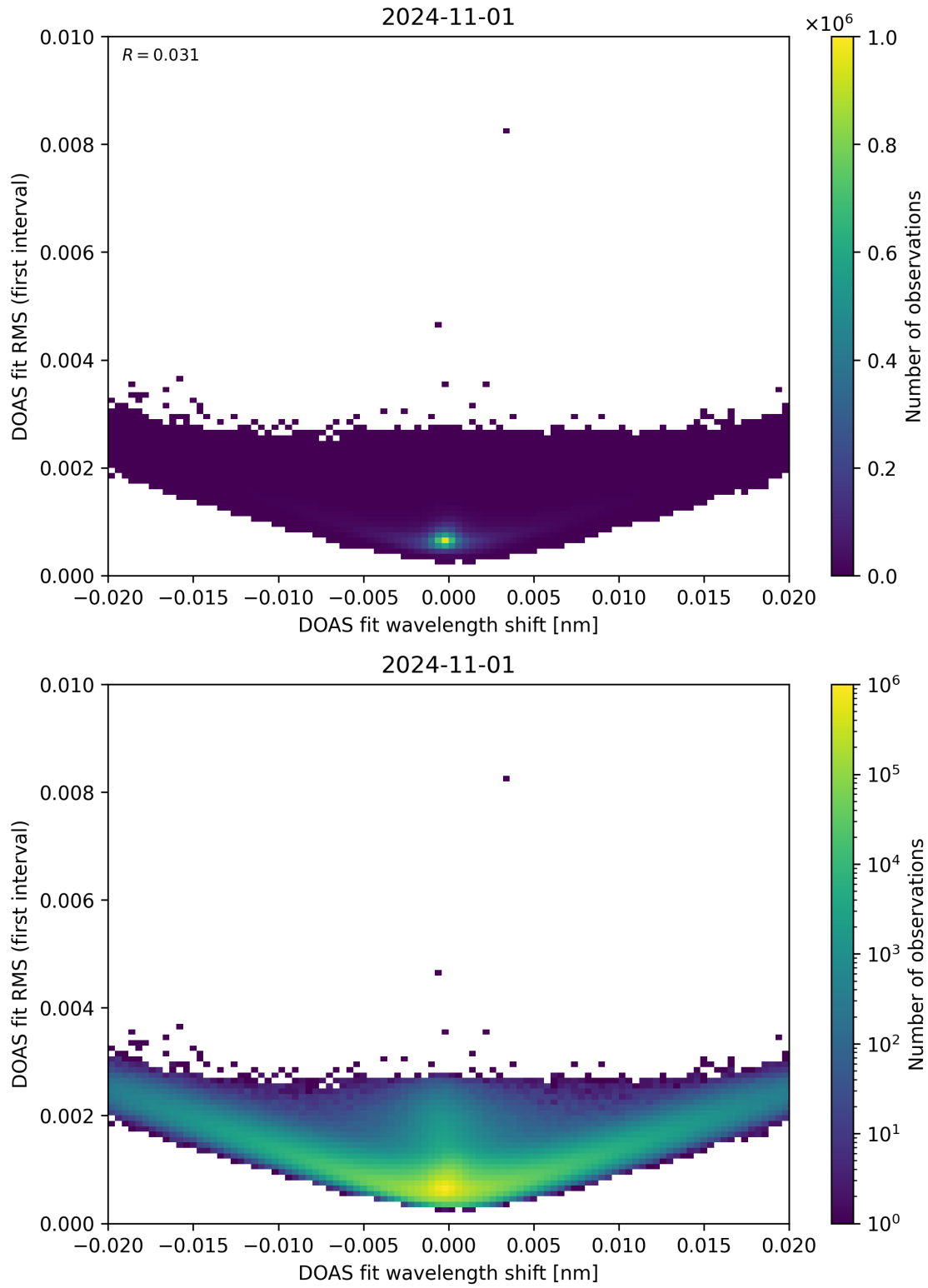
Figure 64: Scatter density plot of “DOAS fit wavelength shift” against “DOAS fit RMS (first interval)” for 2024-10-31 to 2024-11-02.
