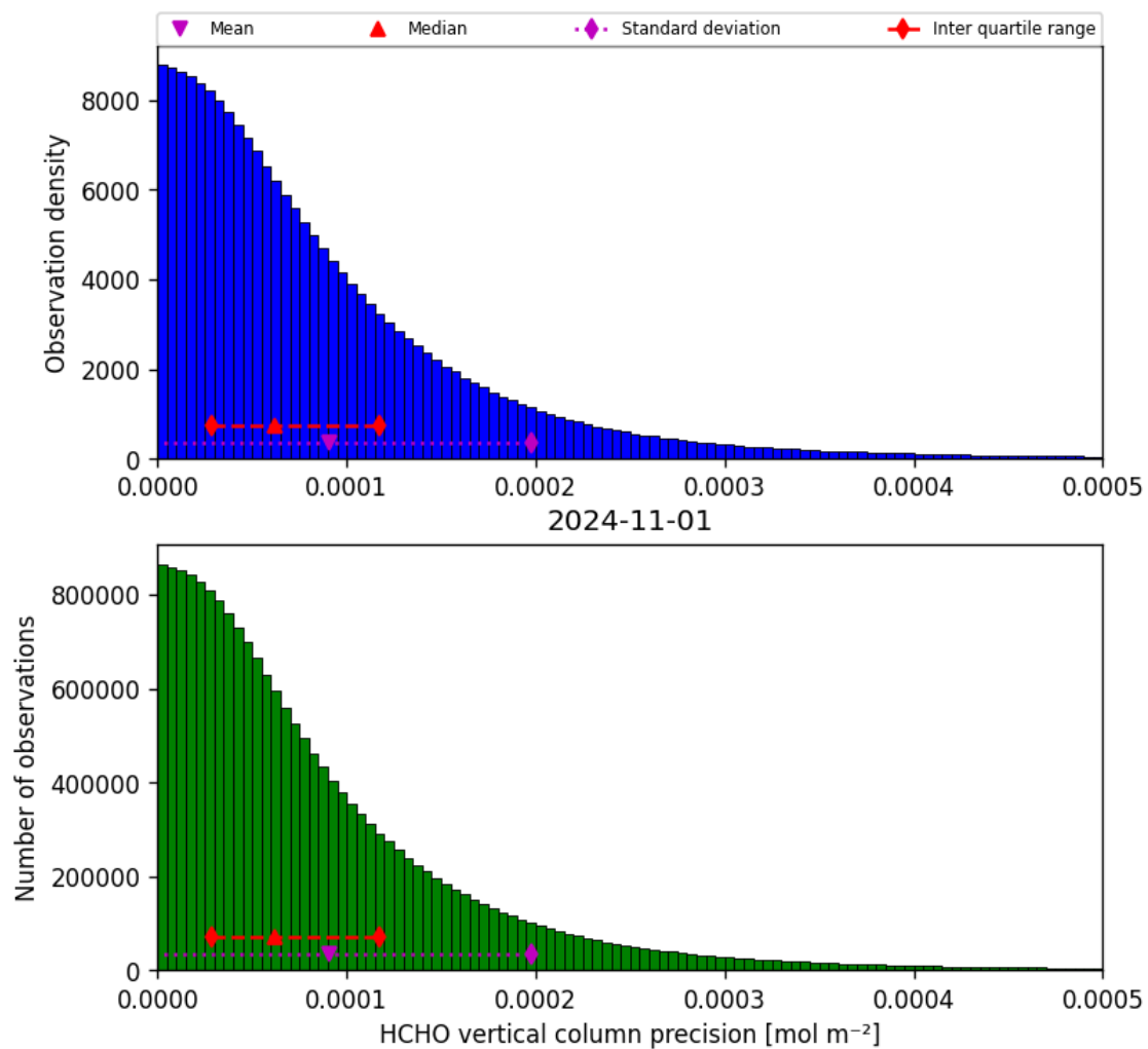
Figure 36: Histogram of “HCHO vertical column precision” for 2024-10-31 to 2024-11-02
