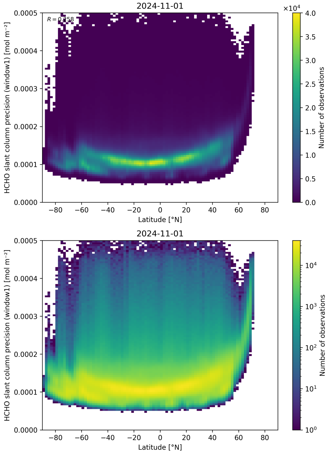
Figure 160: Scatter density plot of “Latitude” against “HCHO slant column precision (window1)” for 2024-10-31 to 2024-11-02.
