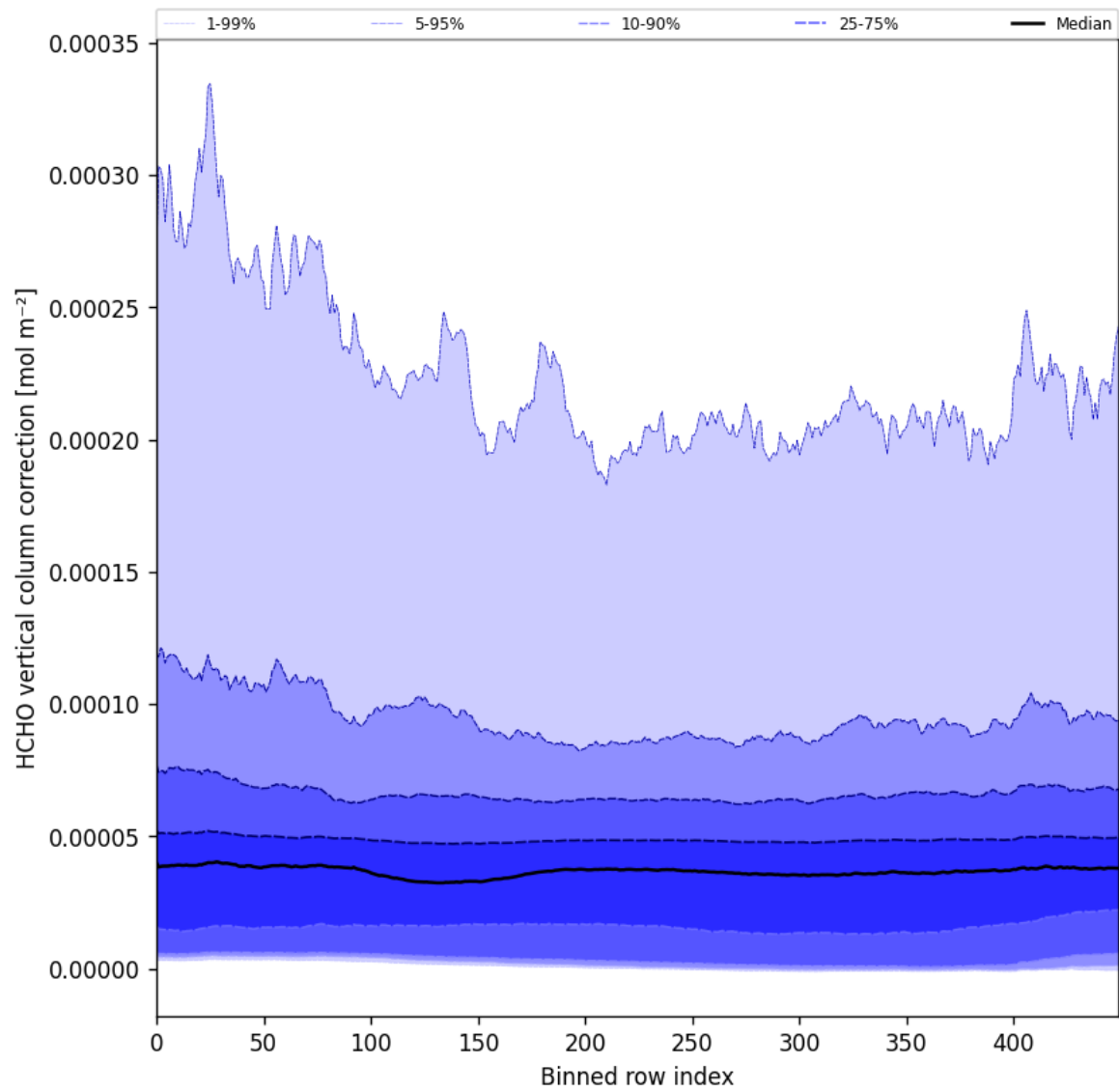
Figure 51: Along track statistics of “HCHO vertical column correction” for 2024-10-31 to 2024-11-02
