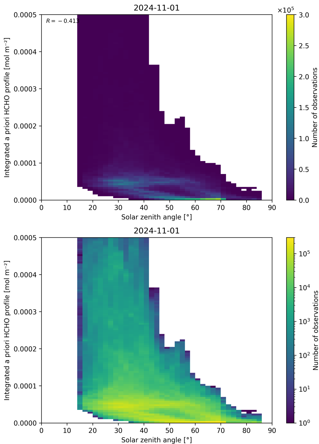
Figure 180: Scatter density plot of “Solar zenith angle” against “Integrated a priori HCHO profile” for 2024-10-31 to 2024-11-02.
