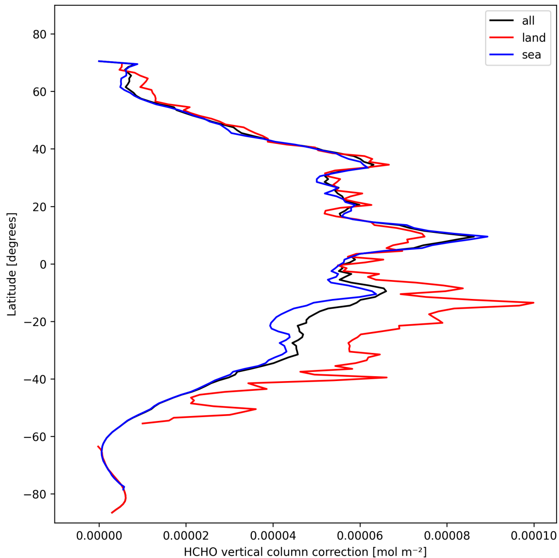
Figure 23: Zonal average of “HCHO vertical column correction” for 2024-10-31 to 2024-11-02.
