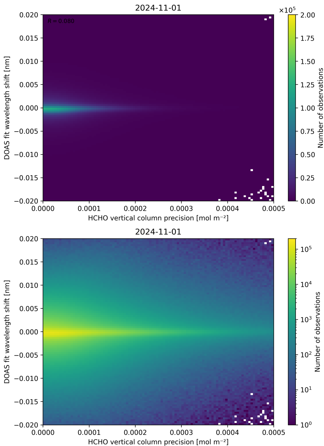
Figure 137: Scatter density plot of “HCHO vertical column precision” against “DOAS fit wavelength shift” for 2024-10-31 to 2024-11-02.
