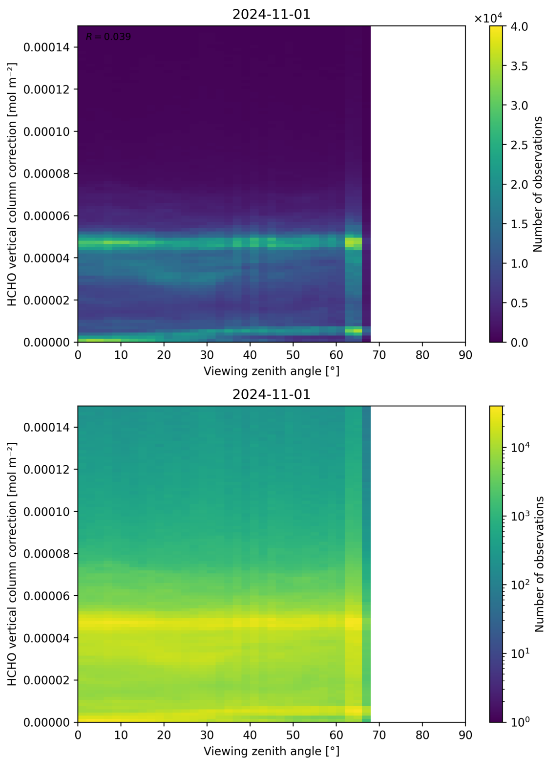
Figure 193: Scatter density plot of “Viewing zenith angle” against “HCHO vertical column correction” for 2024-10-31 to 2024-11-02.
