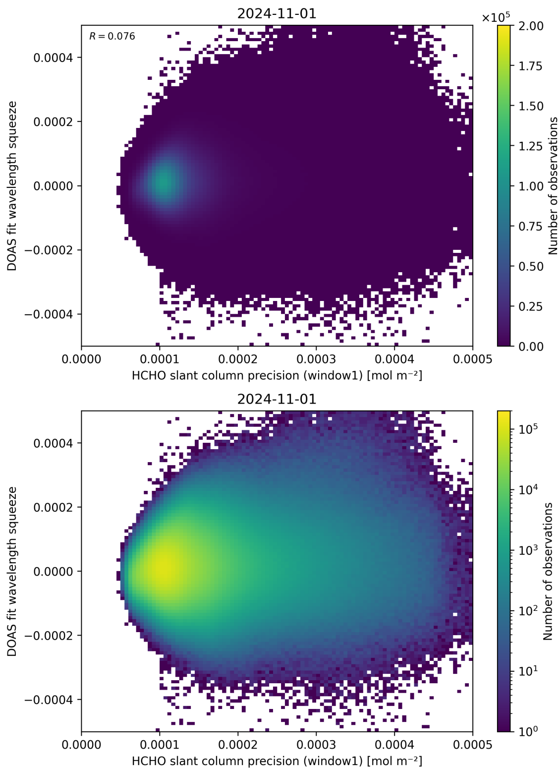
Figure 90: Scatter density plot of “HCHO slant column precision (window1)” against “DOAS fit wavelength squeeze” for 2024-10-31 to 2024-11-02.
