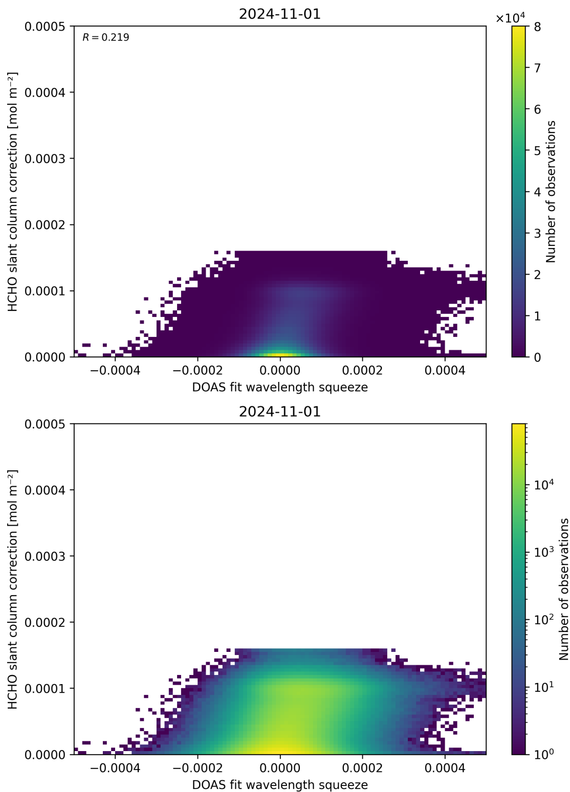
Figure 70: Scatter density plot of “DOAS fit wavelength squeeze” against “HCHO slant column correction” for 2024-10-31 to 2024-11-02.
