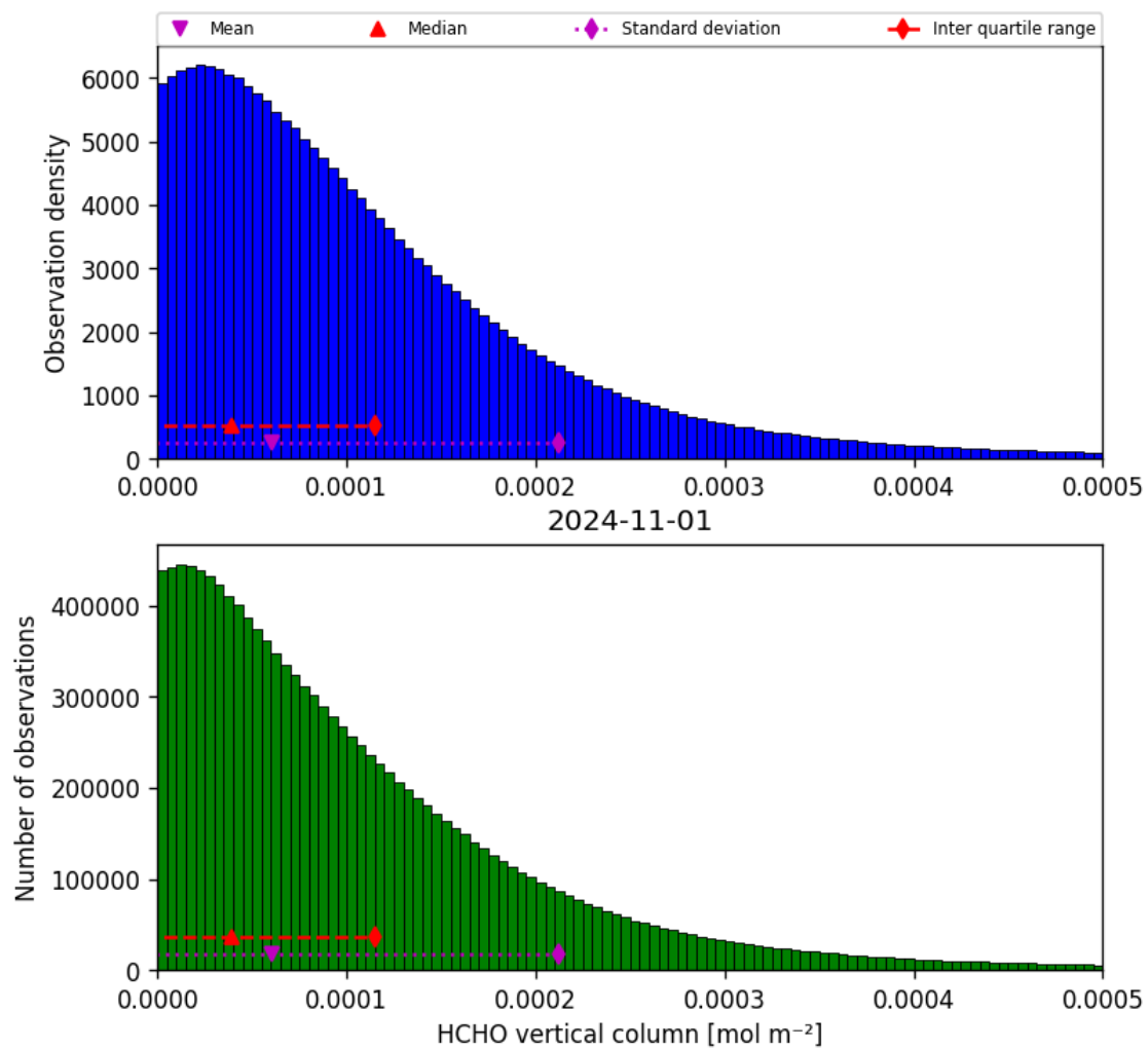
Figure 35: Histogram of “HCHO vertical column” for 2024-10-31 to 2024-11-02
