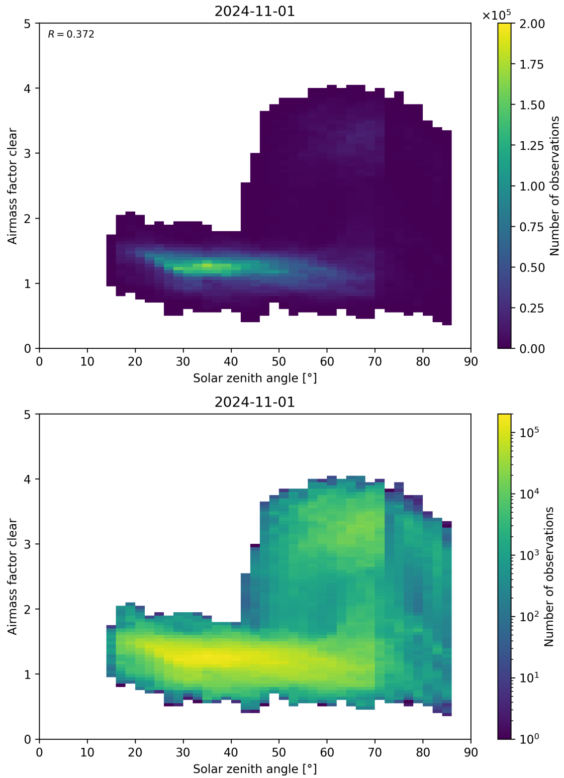
Figure 170: Scatter density plot of “Solar zenith angle” against “Airmass factor clear” for 2024-10-31 to 2024-11-02.
