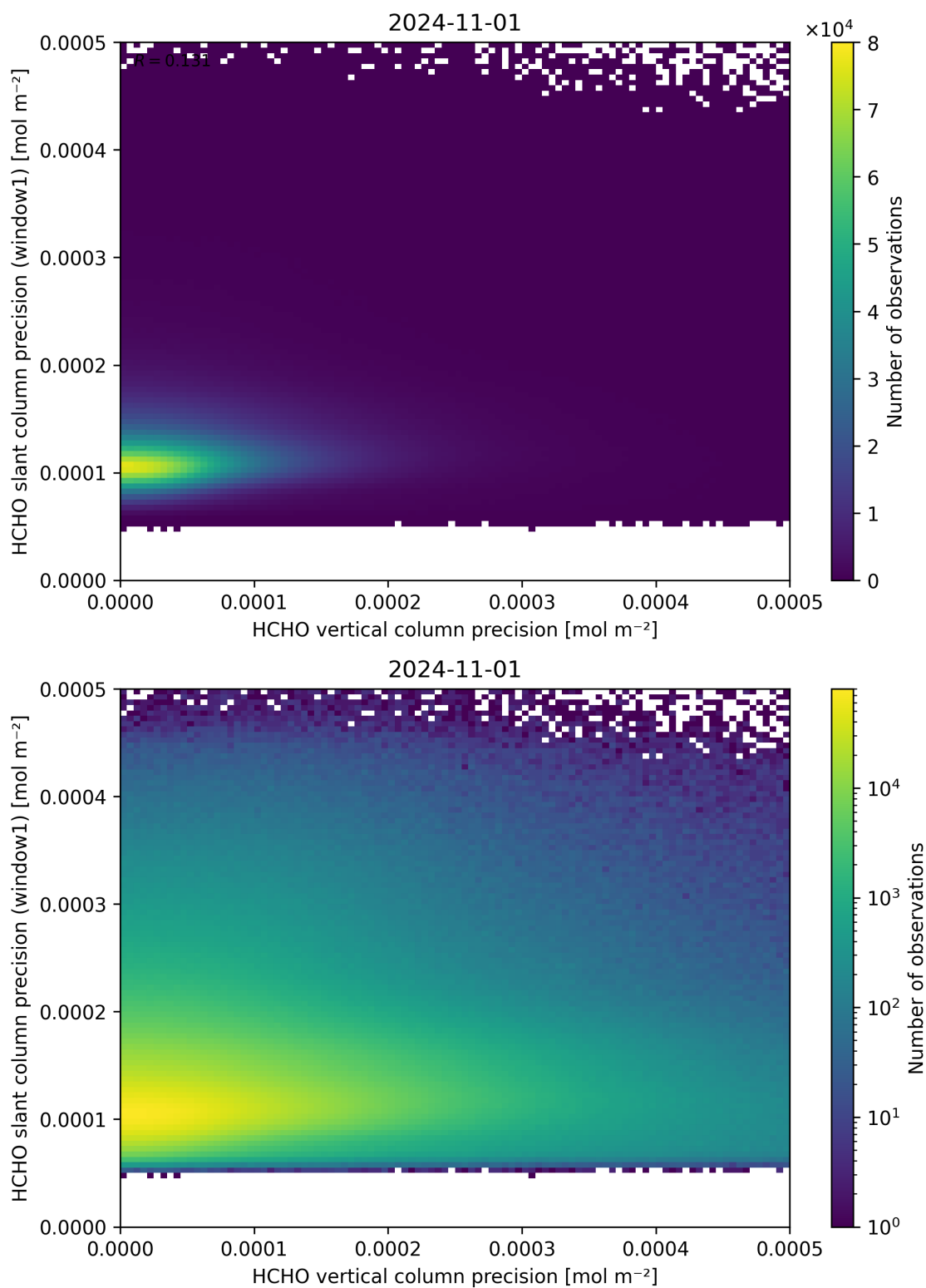
Figure 143: Scatter density plot of “HCHO vertical column precision” against “HCHO slant column precision (window1)” for 2024-10-31 to 2024-11-02.
