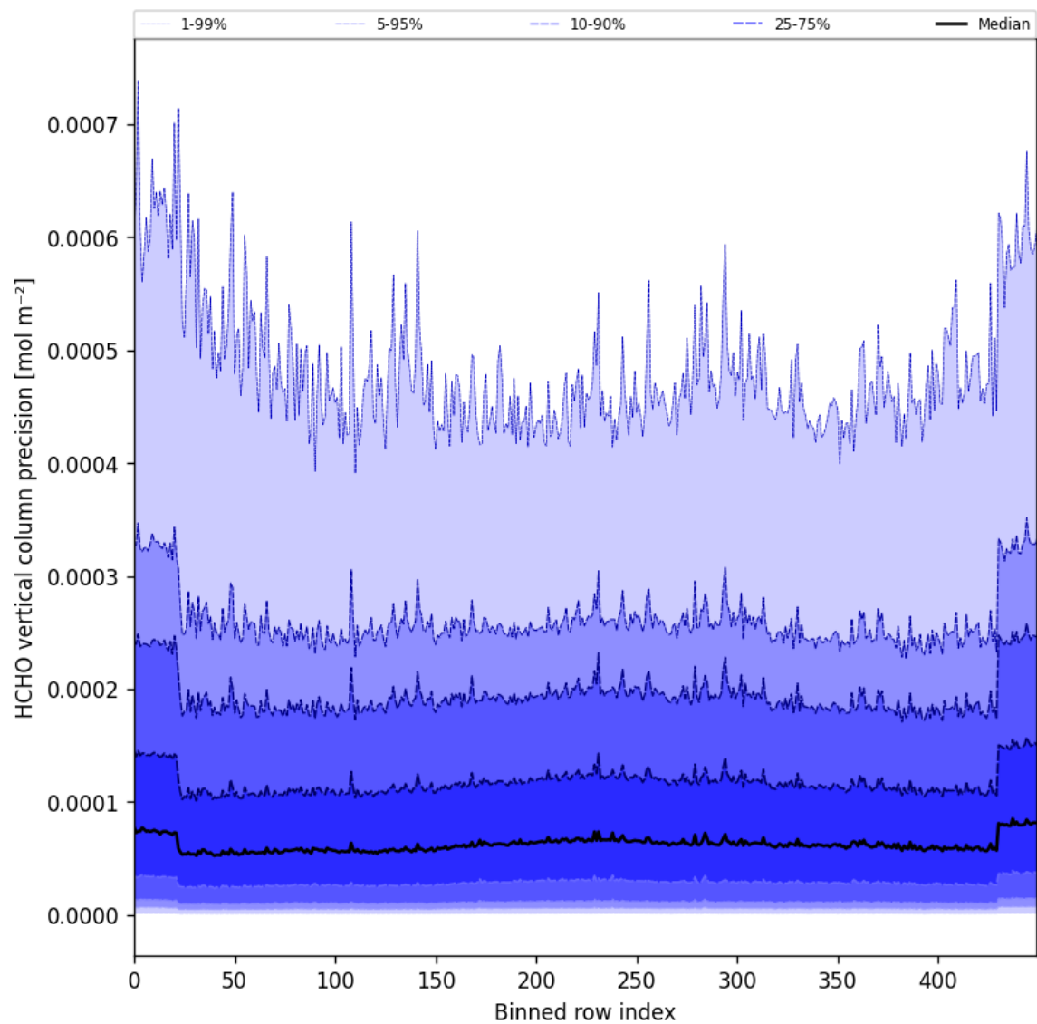
Figure 50: Along track statistics of “HCHO vertical column precision” for 2024-10-31 to 2024-11-02
