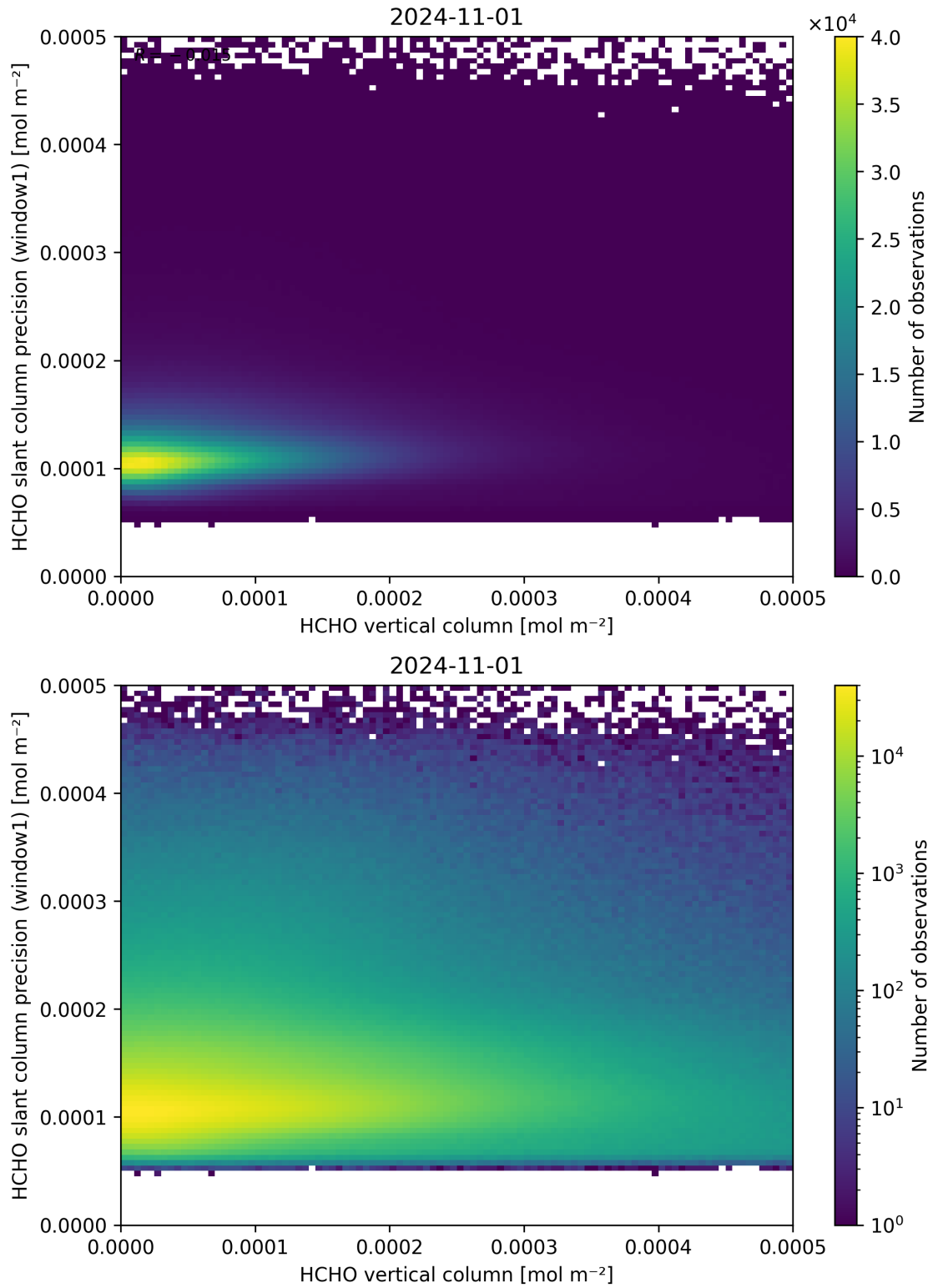
Figure 130: Scatter density plot of “HCHO vertical column” against “HCHO slant column precision (window1)” for 2024-10-31 to 2024-11-02.
