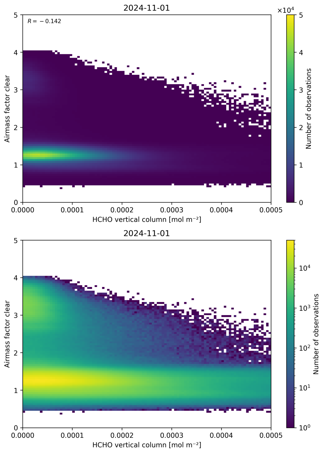
Figure 126: Scatter density plot of “HCHO vertical column” against “Airmass factor clear” for 2024-10-31 to 2024-11-02.
