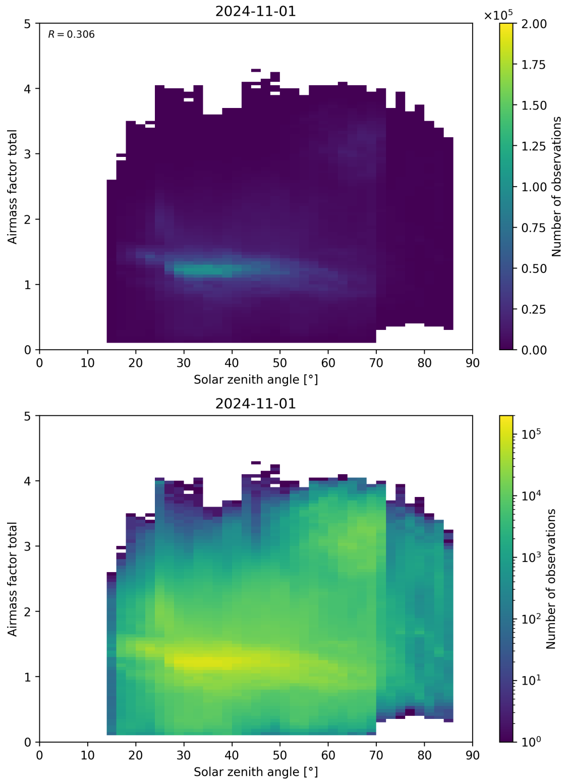
Figure 175: Scatter density plot of “Solar zenith angle” against “Airmass factor total” for 2024-10-31 to 2024-11-02.
