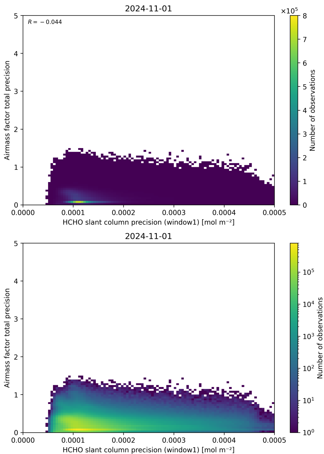
Figure 95: Scatter density plot of “HCHO slant column precision (window1)” against “Airmass factor total precision” for 2024-10-31 to 2024-11-02.
