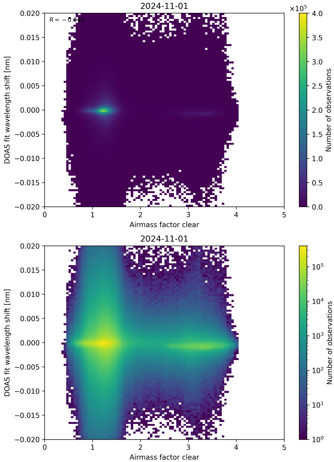
Figure 72: Scatter density plot of “Airmass factor clear” against “DOAS fit wavelength shift” for 2024-10-31 to 2024-11-02.
