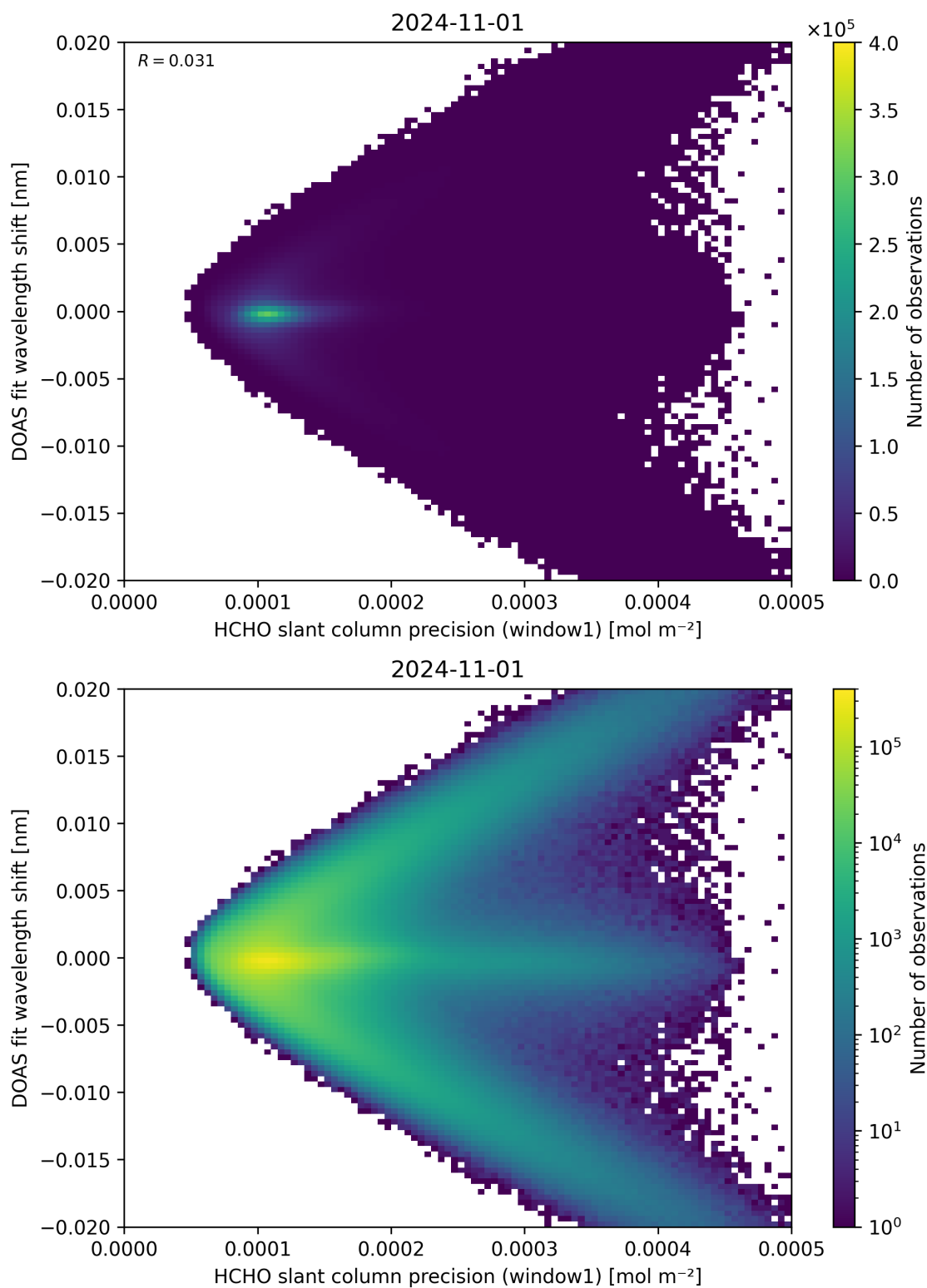
Figure 89: Scatter density plot of “HCHO slant column precision (window1)” against “DOAS fit wavelength shift” for 2024-10-31 to 2024-11-02.
