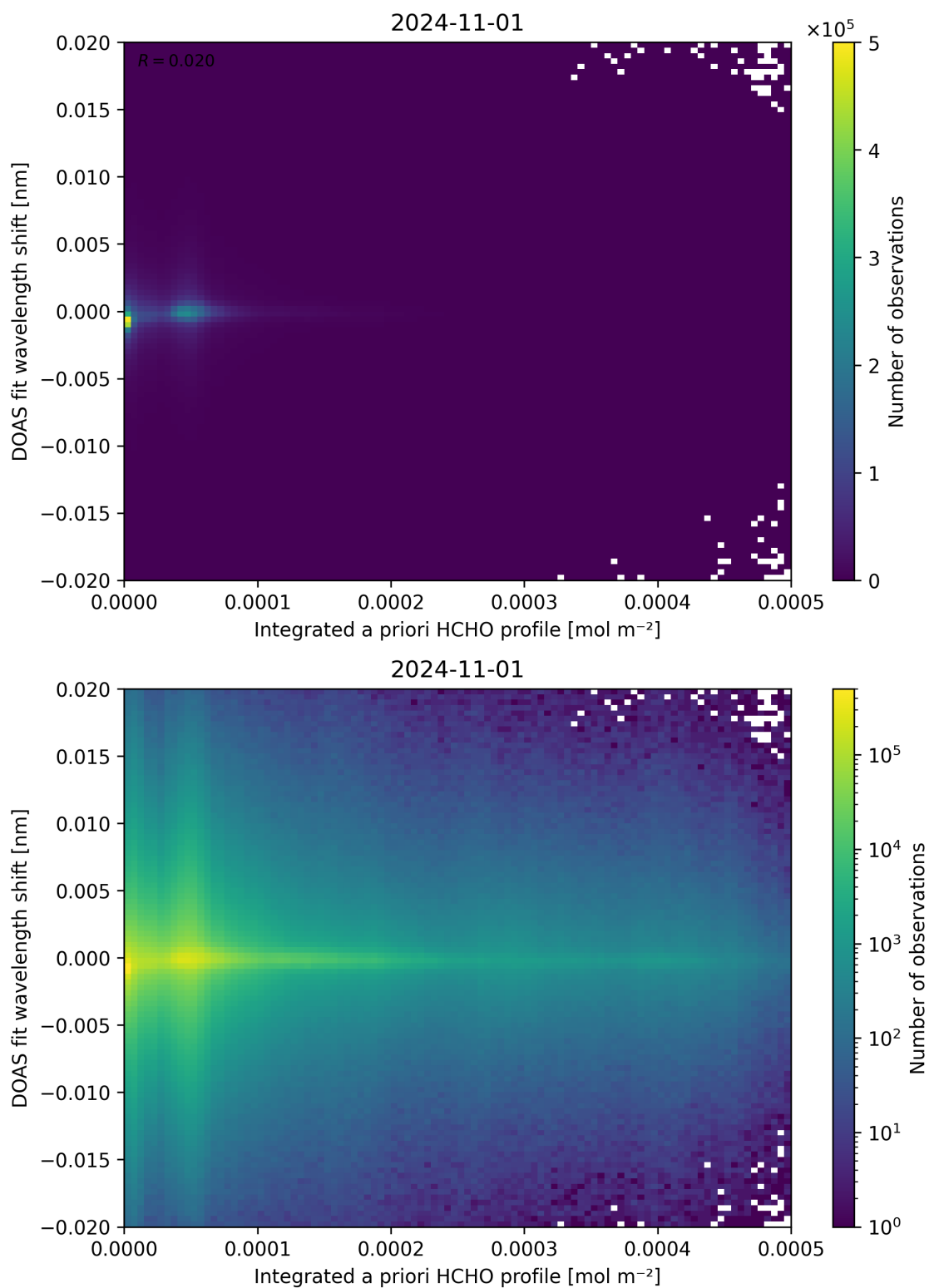
Figure 149: Scatter density plot of “Integrated a priori HCHO profile” against “DOAS fit wavelength shift” for 2024-10-31 to 2024-11-02.
