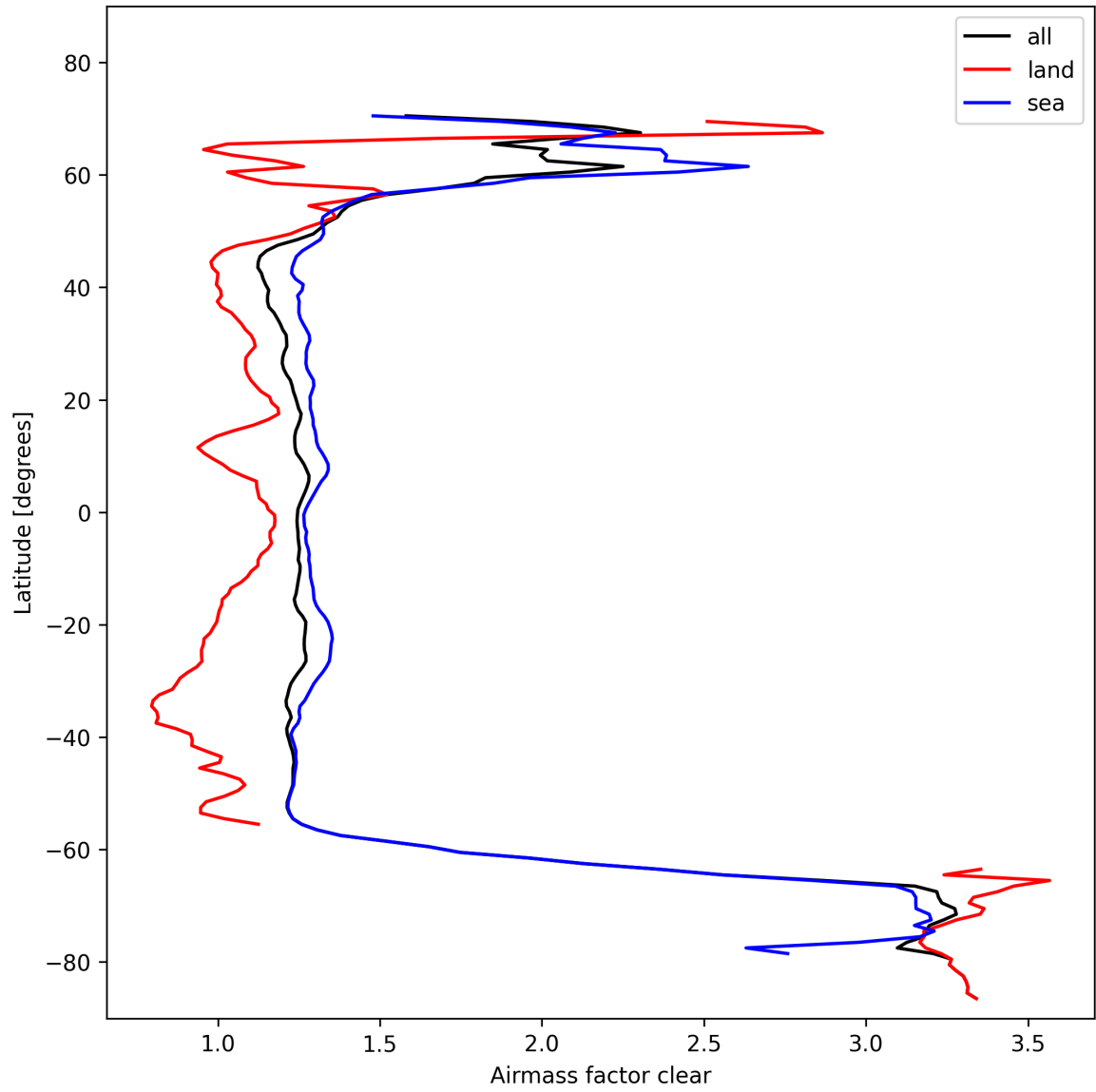
Figure 28: Zonal average of “Airmass factor clear” for 2024-10-31 to 2024-11-02.
