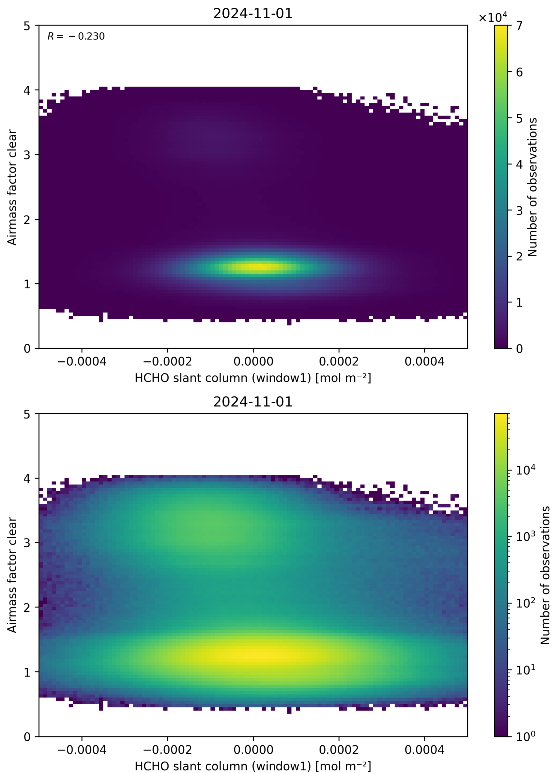
Figure 81: Scatter density plot of “HCHO slant column (window1)” against “Airmass factor clear” for 2024-10-31 to 2024-11-02.
