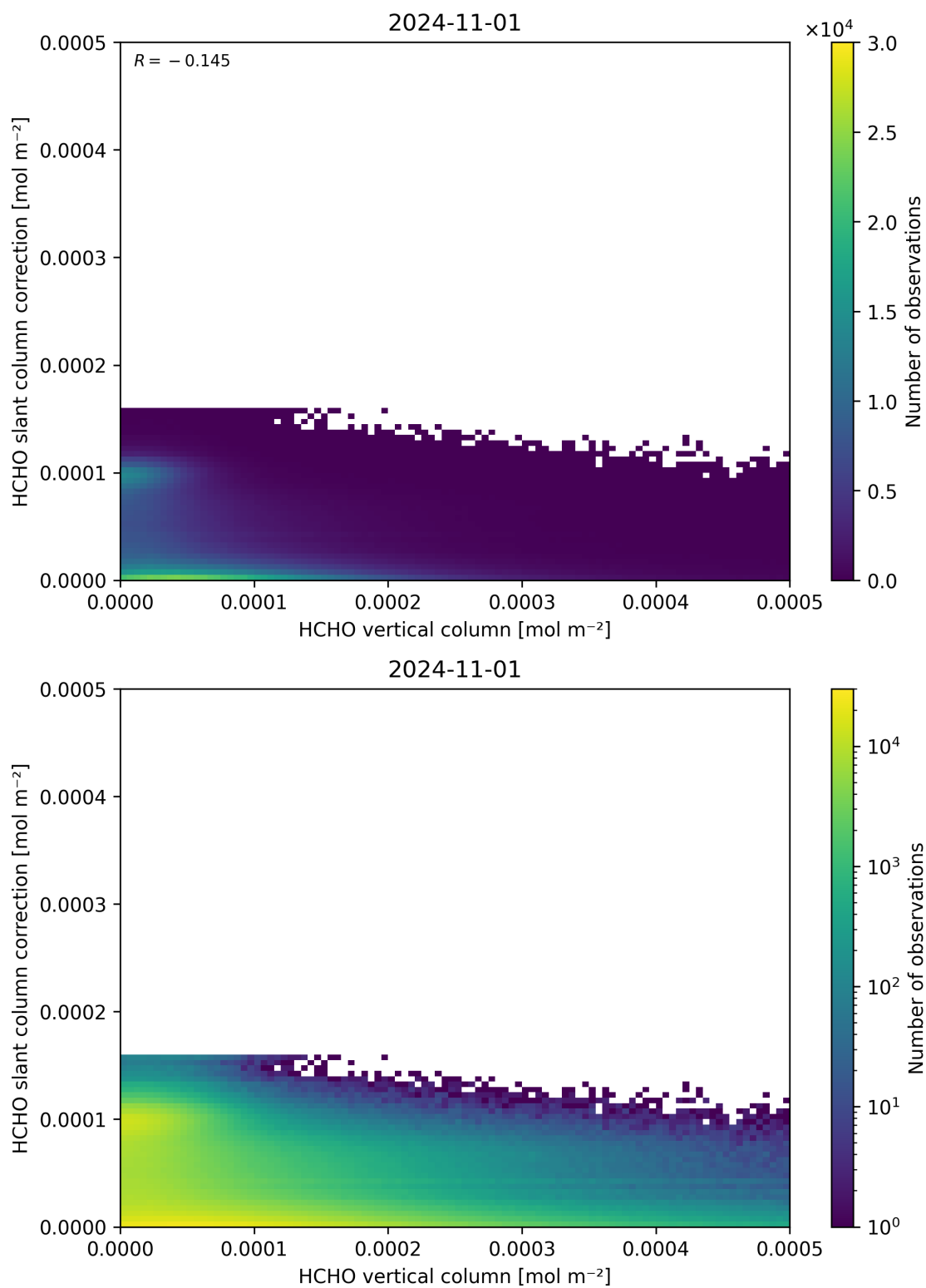
Figure 128: Scatter density plot of “HCHO vertical column” against “HCHO slant column correction” for 2024-10-31 to 2024-11-02.
