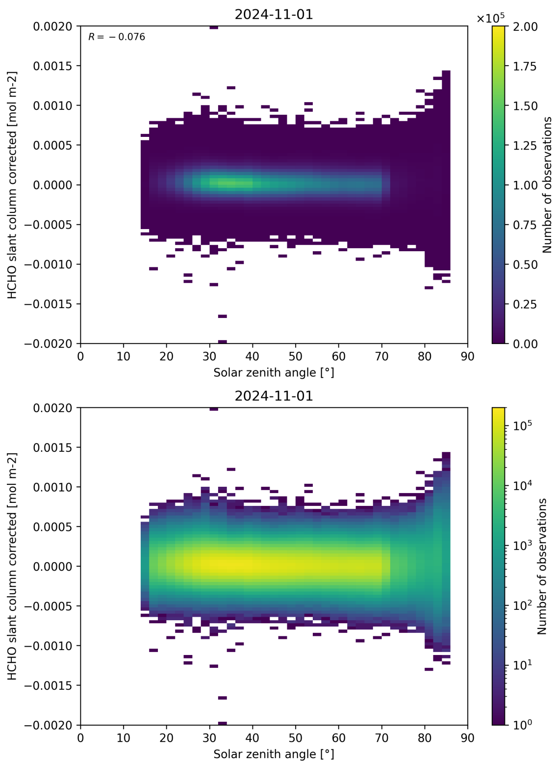
Figure 171: Scatter density plot of “Solar zenith angle” against “HCHO slant column corrected” for 2024-10-31 to 2024-11-02.
