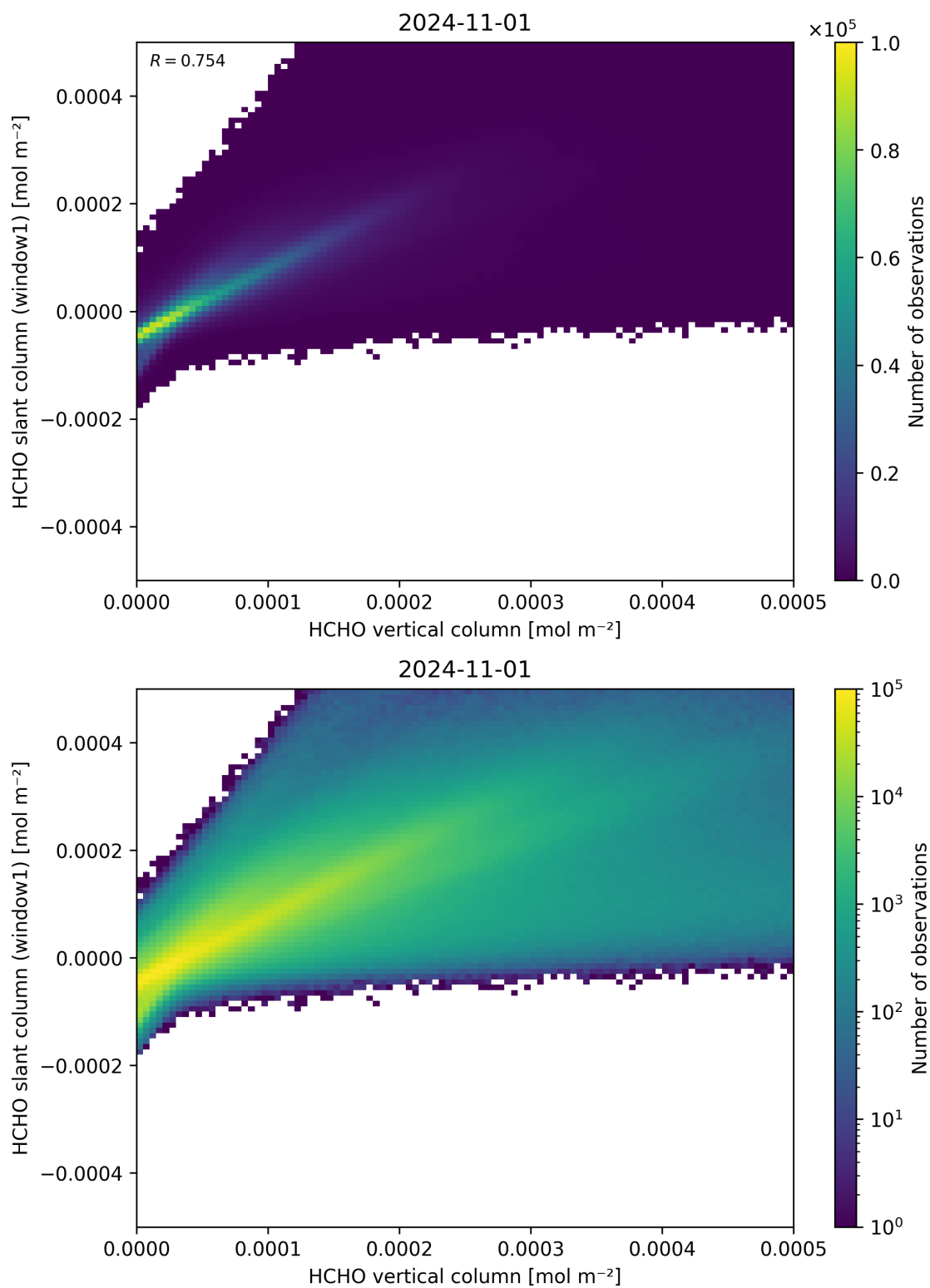
Figure 129: Scatter density plot of “HCHO vertical column” against “HCHO slant column (window1)” for 2024-10-31 to 2024-11-02.
