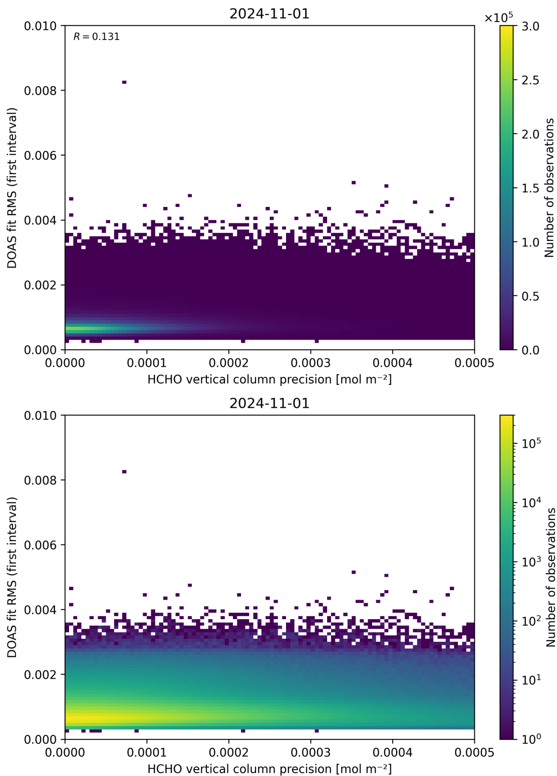
Figure 136: Scatter density plot of “HCHO vertical column precision” against “DOAS fit RMS (first interval)” for 2024-10-31 to 2024-11-02.
