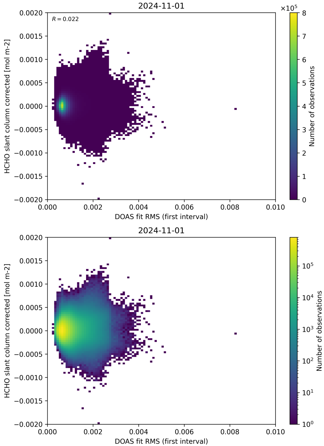
Figure 62: Scatter density plot of “DOAS fit RMS (first interval)” against “HCHO slant column corrected” for 2024-10-31 to 2024-11-02.
