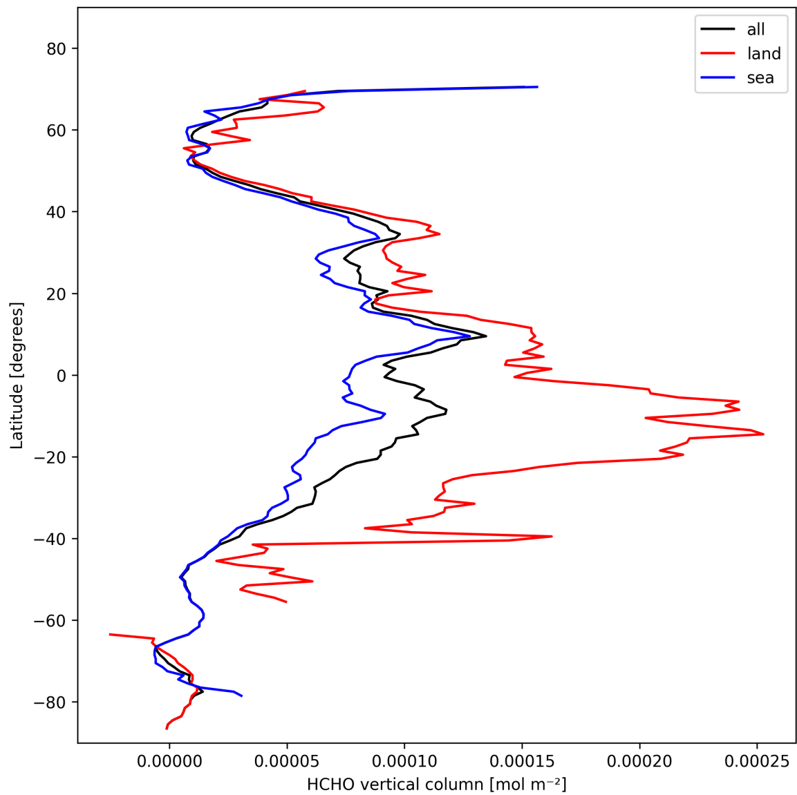
Figure 21: Zonal average of “HCHO vertical column” for 2024-10-31 to 2024-11-02.
