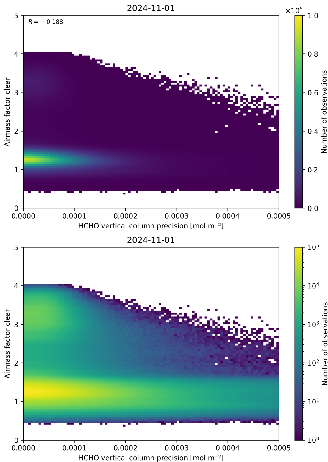
Figure 139: Scatter density plot of “HCHO vertical column precision” against “Airmass factor clear” for 2024-10-31 to 2024-11-02.
