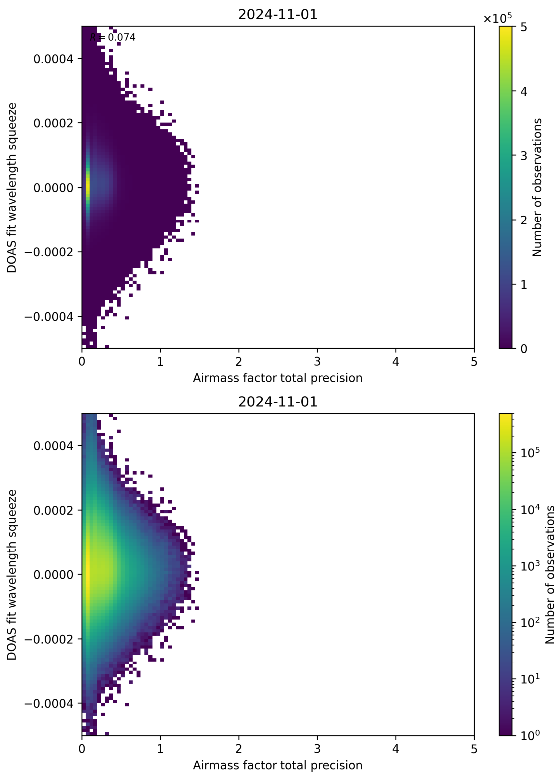
Figure 107: Scatter density plot of “Airmass factor total precision” against “DOAS fit wavelength squeeze” for 2024-10-31 to 2024-11-02.
