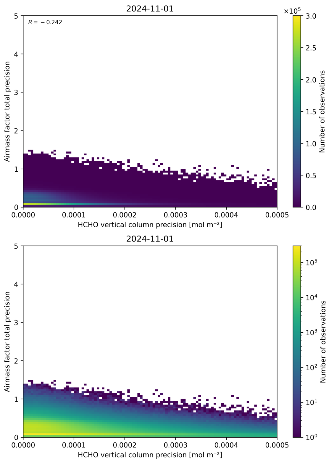
Figure 145: Scatter density plot of “HCHO vertical column precision” against “Airmass factor total precision” for 2024-10-31 to 2024-11-02.
