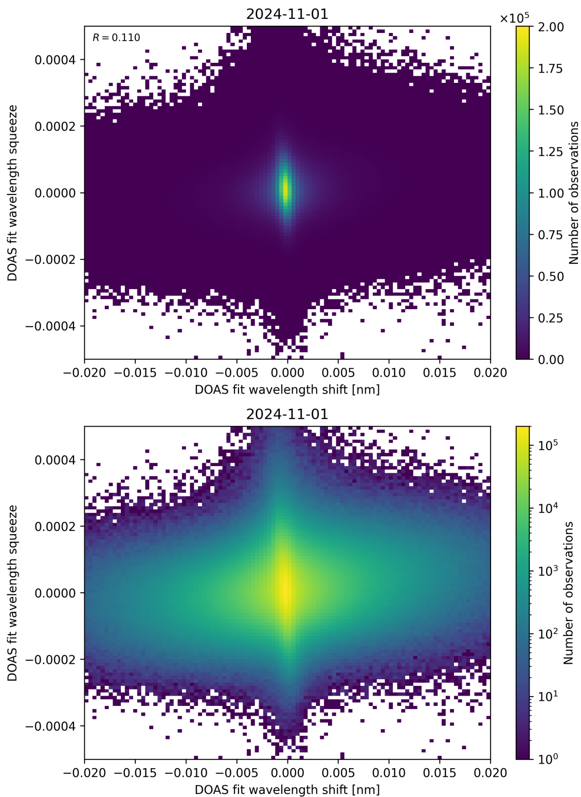
Figure 65: Scatter density plot of “DOAS fit wavelength shift” against “DOAS fit wavelength squeeze” for 2024-10-31 to 2024-11-02.
