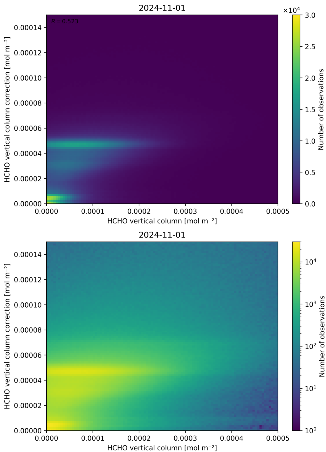
Figure 133: Scatter density plot of “HCHO vertical column” against “HCHO vertical column correction” for 2024-10-31 to 2024-11-02.
