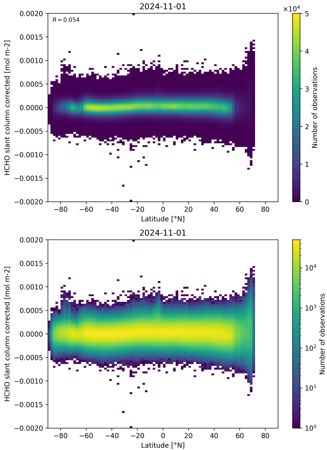
Figure 157: Scatter density plot of “Latitude” against “HCHO slant column corrected” for 2024-10-31 to 2024-11-02.
