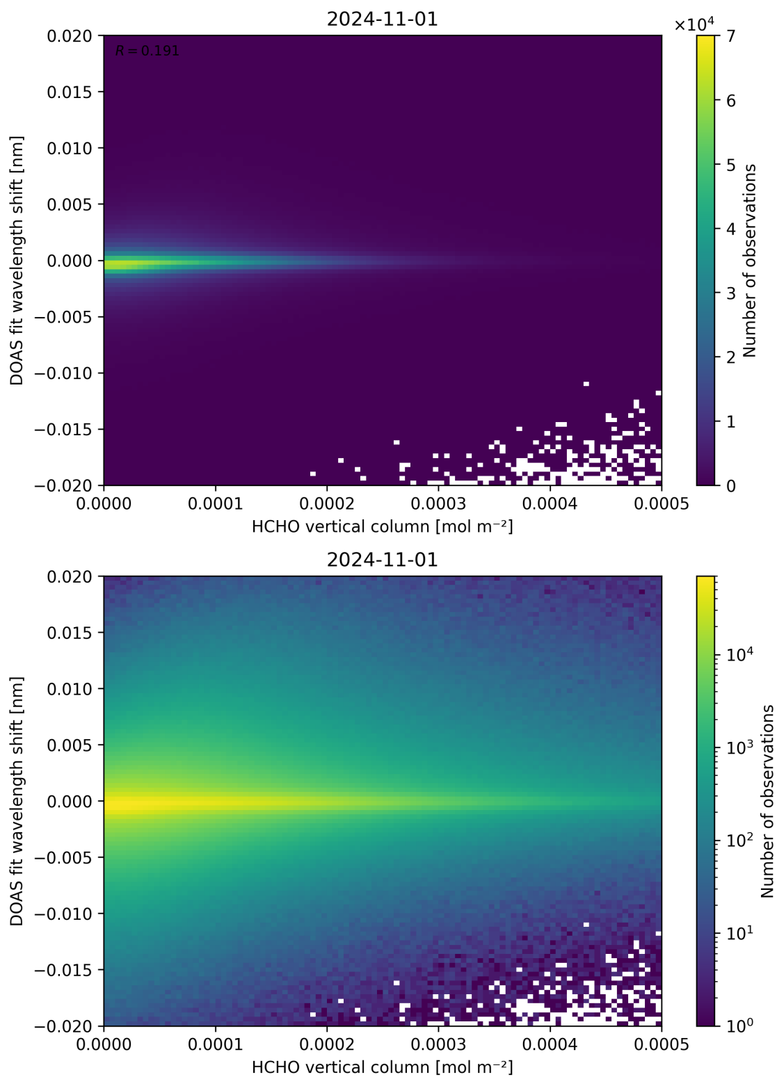
Figure 124: Scatter density plot of “HCHO vertical column” against “DOAS fit wavelength shift” for 2024-10-31 to 2024-11-02.
