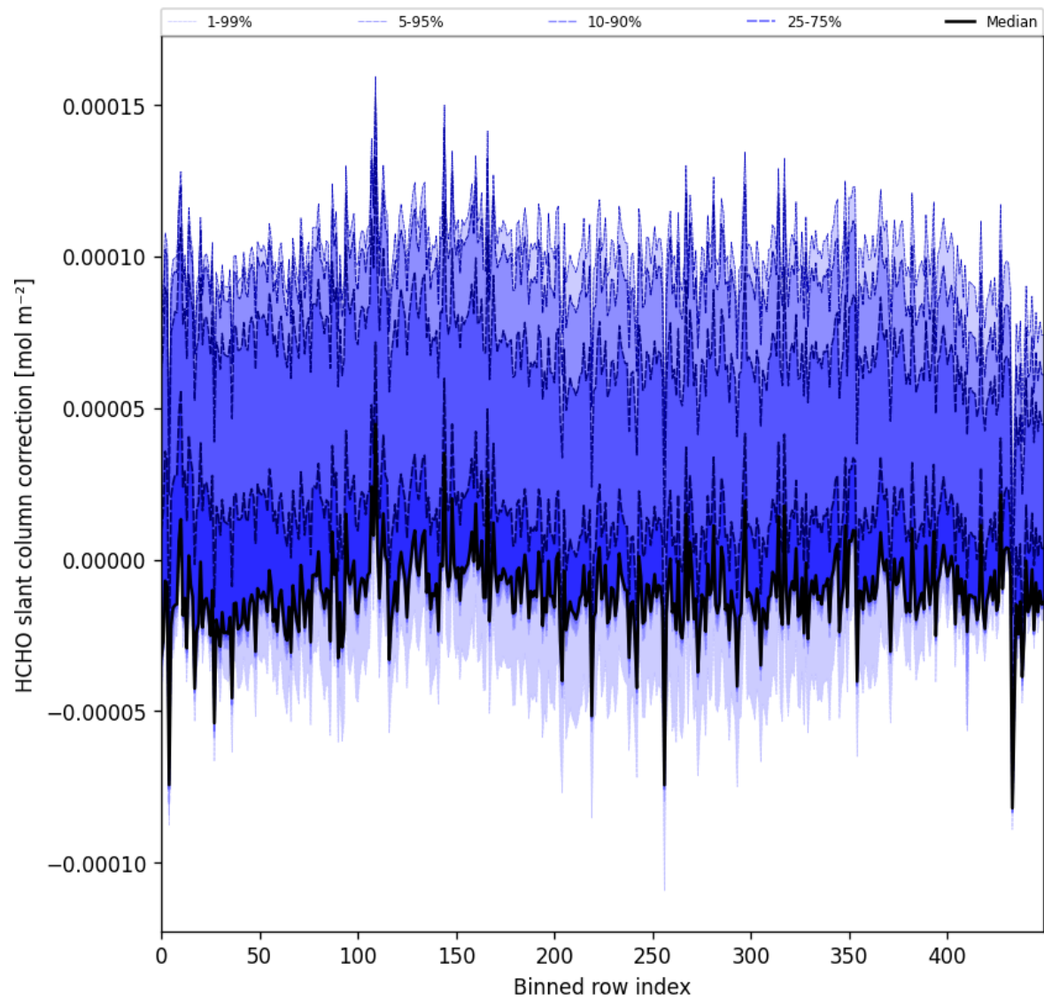
Figure 61: Along track statistics of “HCHO slant column correction” for 2024-10-31 to 2024-11-02
