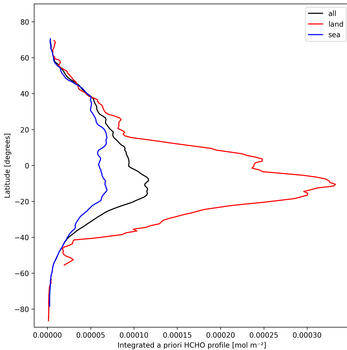
Figure 29: Zonal average of “Integrated a priori HCHO profile” for 2024-10-31 to 2024-11-02.
