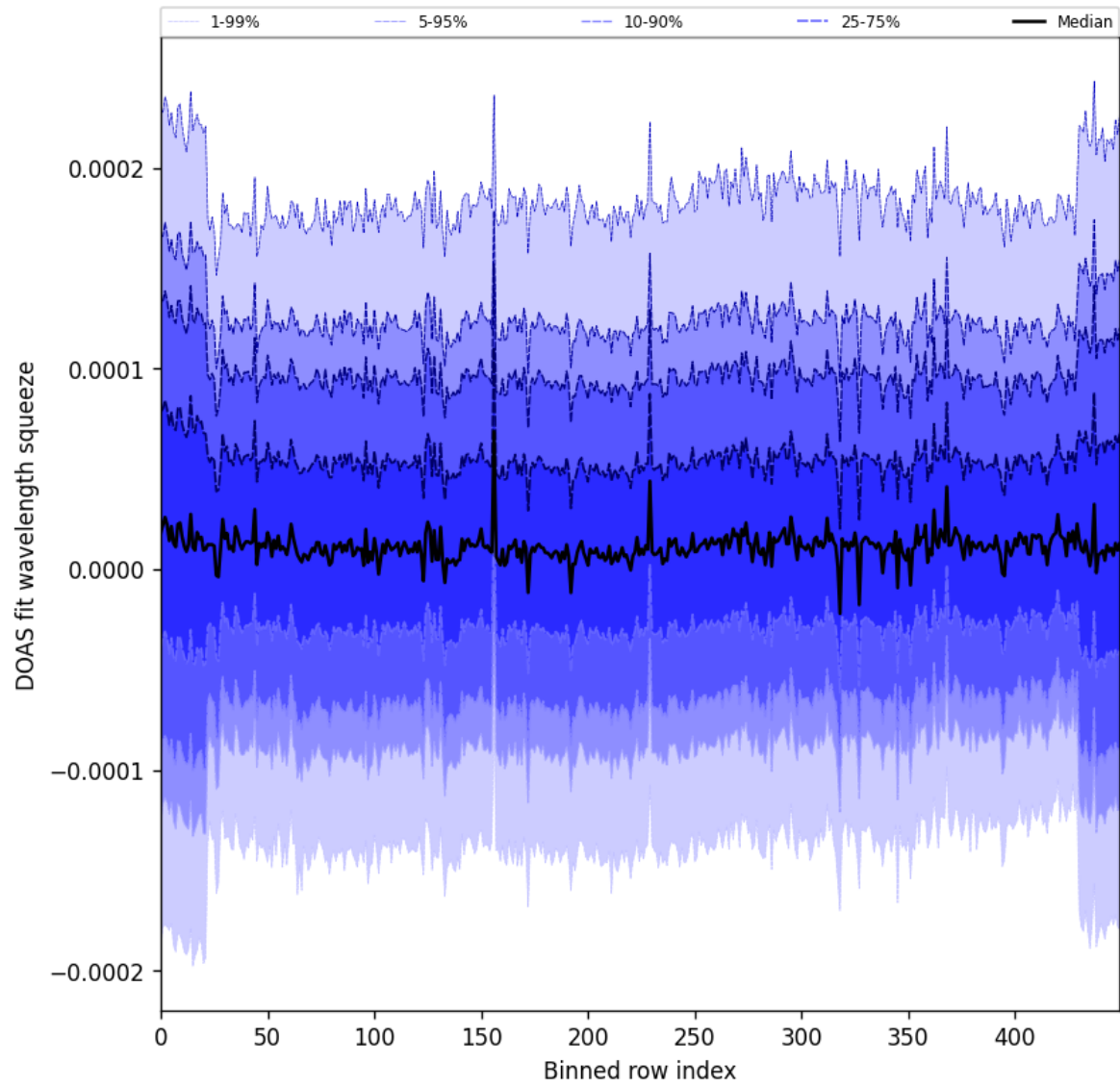
Figure 59: Along track statistics of “DOAS fit wavelength squeeze” for 2024-10-31 to 2024-11-02
