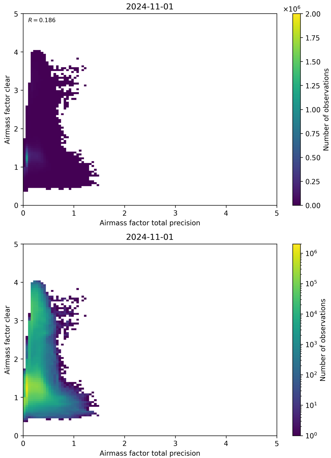
Figure 108: Scatter density plot of “Airmass factor total precision” against “Airmass factor clear” for 2024-10-31 to 2024-11-02.
