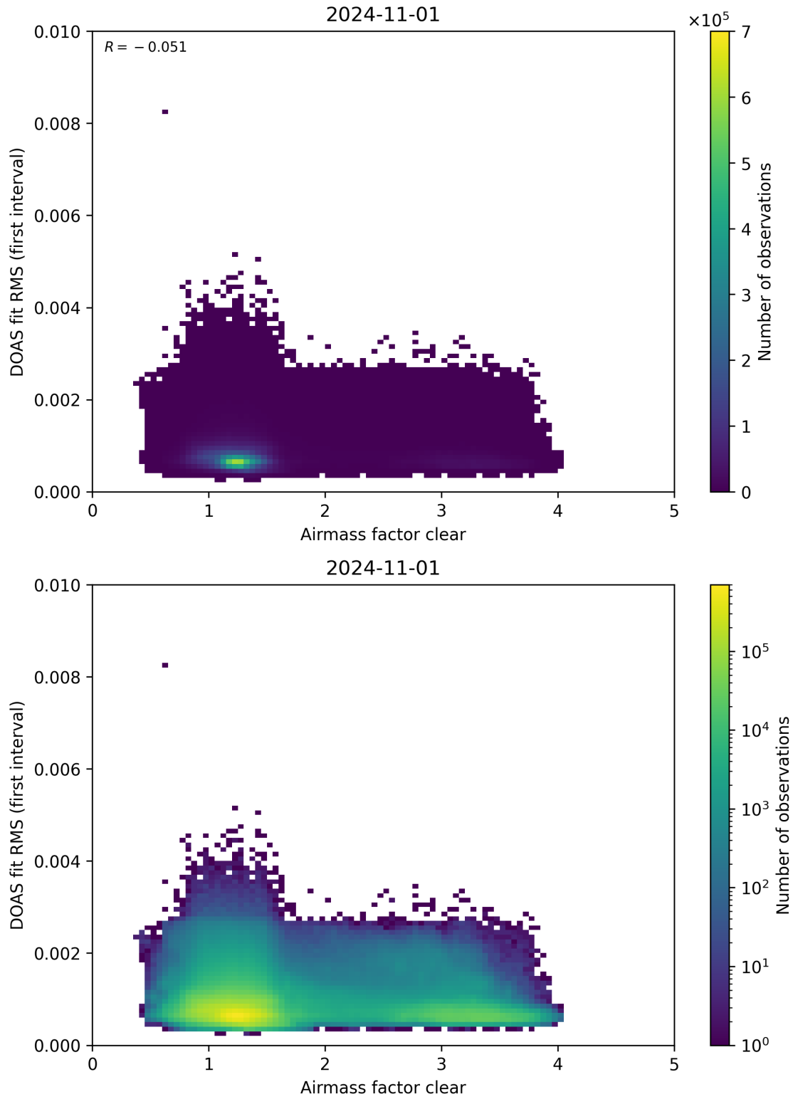
Figure 71: Scatter density plot of “Airmass factor clear” against “DOAS fit RMS (first interval)” for 2024-10-31 to 2024-11-02.
