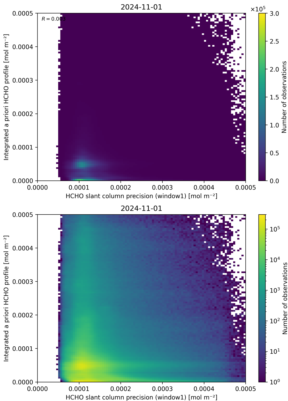
Figure 96: Scatter density plot of “HCHO slant column precision (window1)” against “Integrated a priori HCHO profile” for 2024-10-31 to 2024-11-02.
