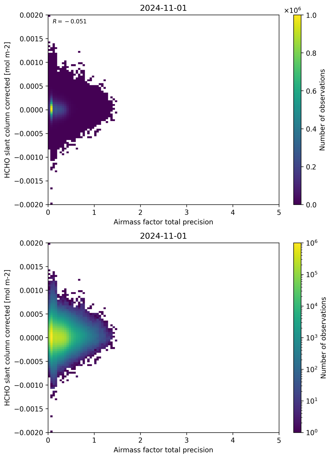
Figure 109: Scatter density plot of “Airmass factor total precision” against “HCHO slant column corrected” for 2024-10-31 to 2024-11-02.
