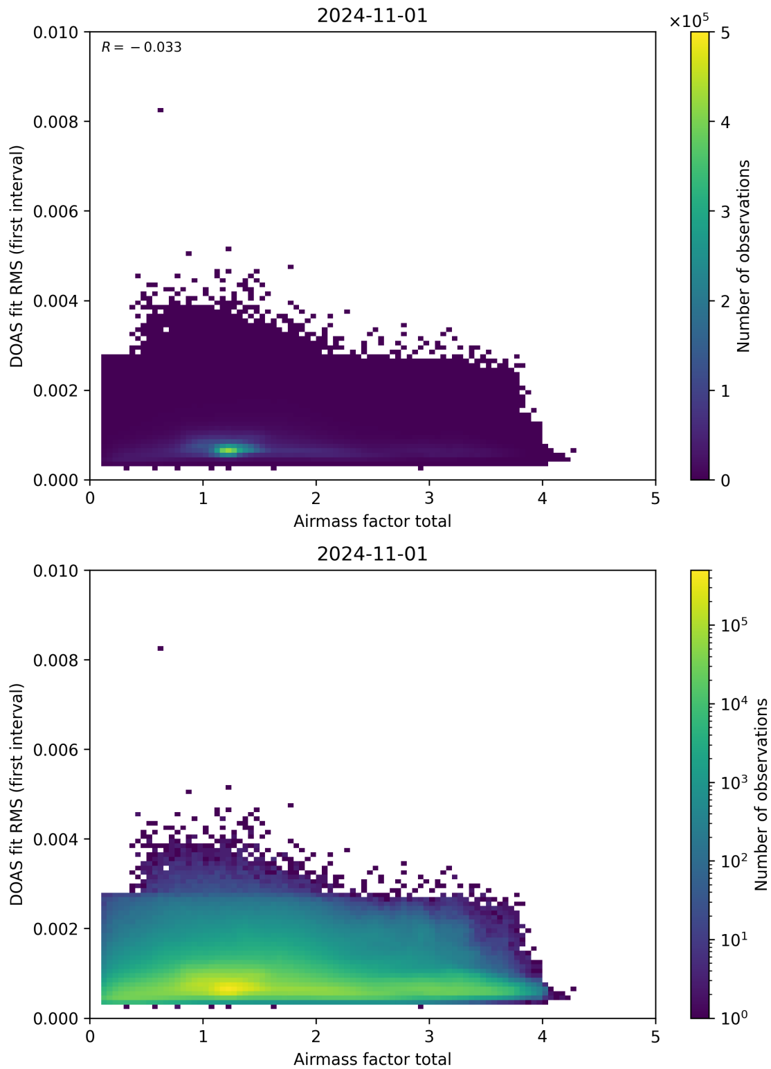
Figure 97: Scatter density plot of “Airmass factor total” against “DOAS fit RMS (first interval)” for 2024-10-31 to 2024-11-02.
