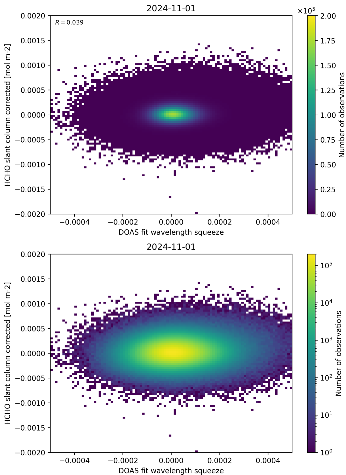
Figure 69: Scatter density plot of “DOAS fit wavelength squeeze” against “HCHO slant column corrected” for 2024-10-31 to 2024-11-02.
