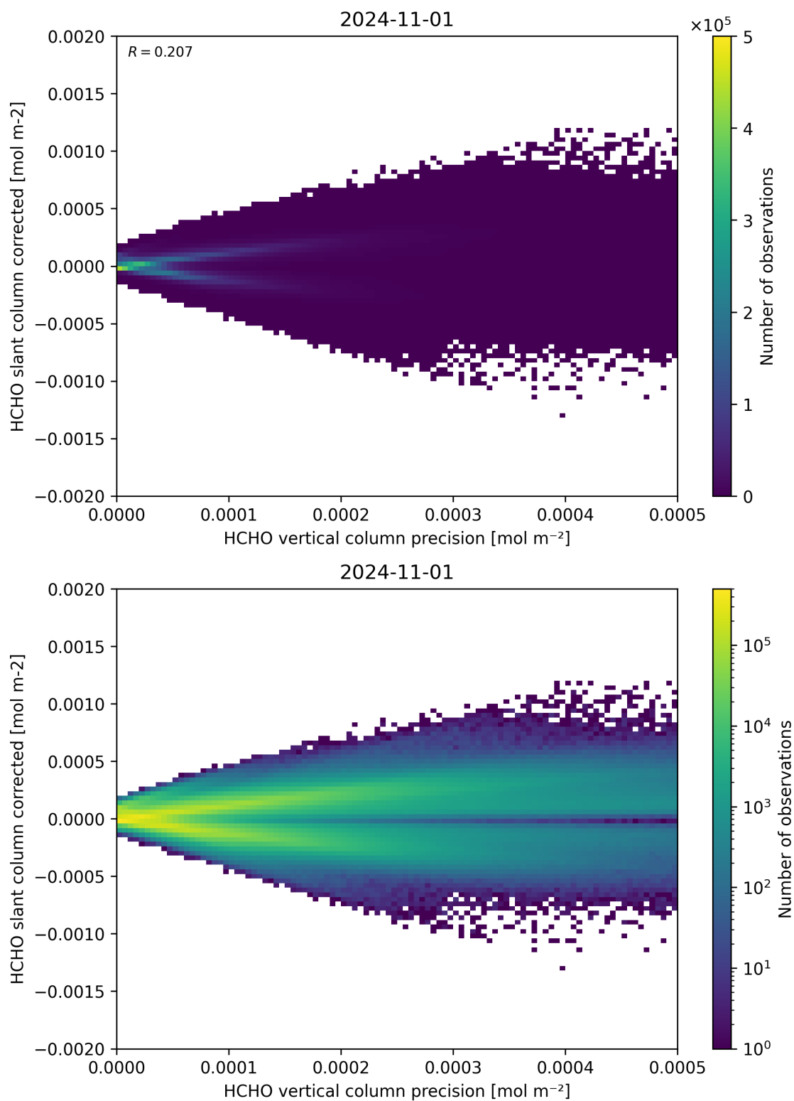
Figure 140: Scatter density plot of “HCHO vertical column precision” against “HCHO slant column corrected” for 2024-10-31 to 2024-11-02.
