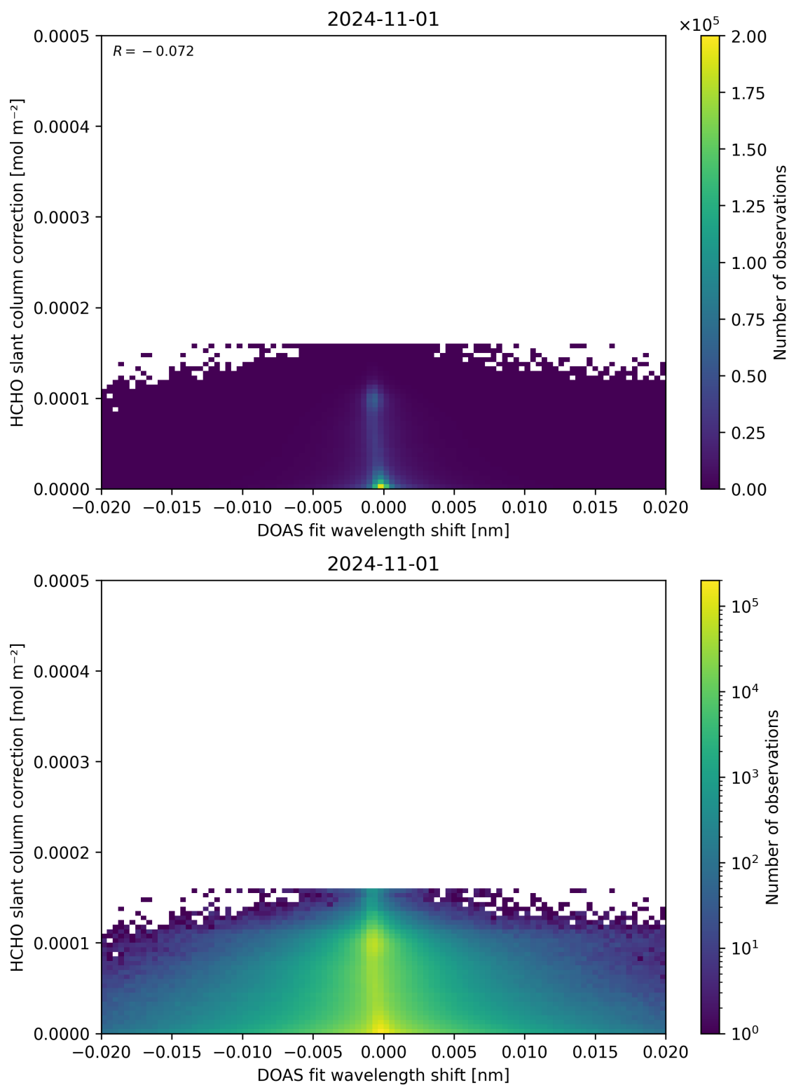
Figure 67: Scatter density plot of “DOAS fit wavelength shift” against “HCHO slant column correction” for 2024-10-31 to 2024-11-02.
