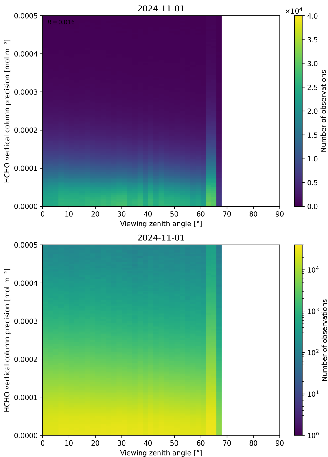
Figure 194: Scatter density plot of “Viewing zenith angle” against “HCHO vertical column precision” for 2024-10-31 to 2024-11-02.
