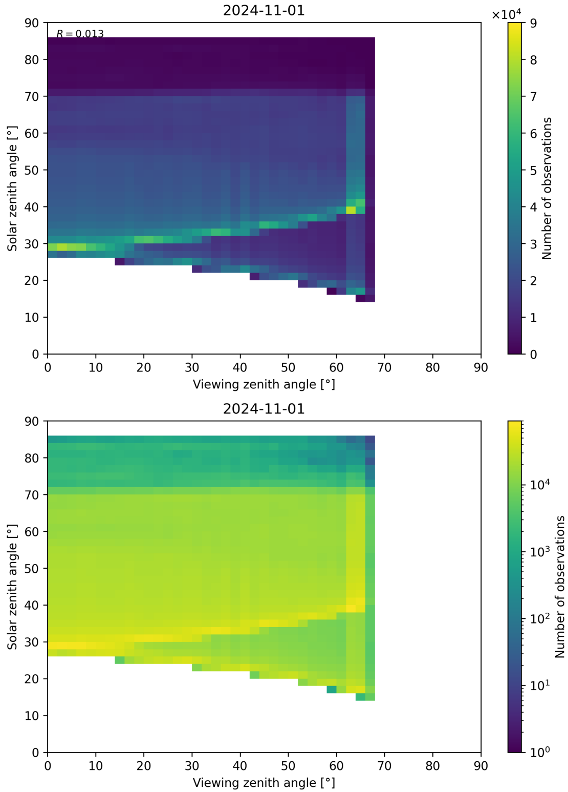
Figure 197: Scatter density plot of “Viewing zenith angle” against “Solar zenith angle” for 2024-10-31 to 2024-11-02.
