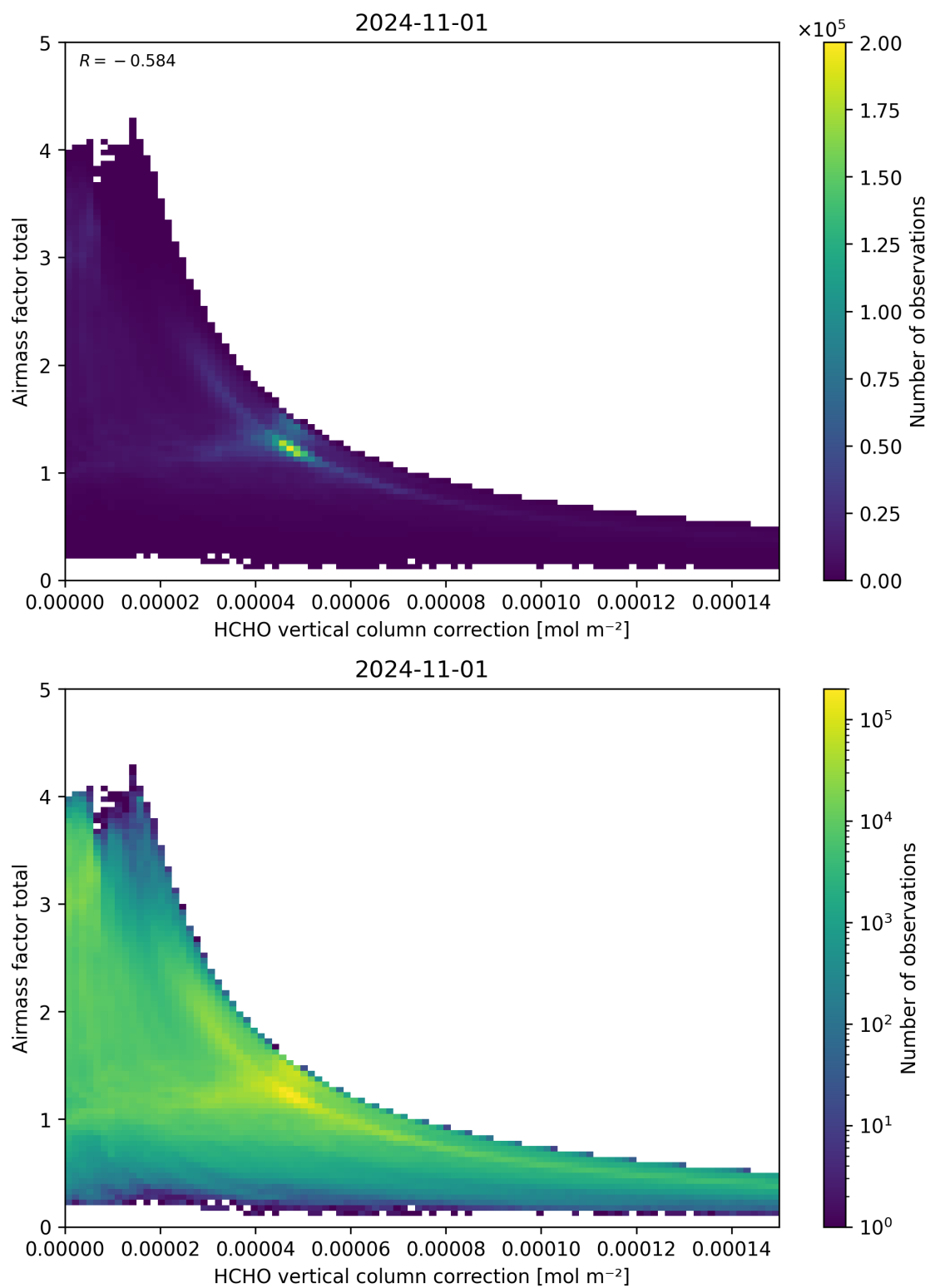
Figure 120: Scatter density plot of “HCHO vertical column correction” against “Airmass factor total” for 2024-10-31 to 2024-11-02.
