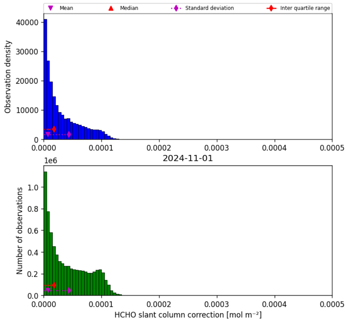
Figure 47: Histogram of “HCHO slant column correction” for 2024-10-31 to 2024-11-02
