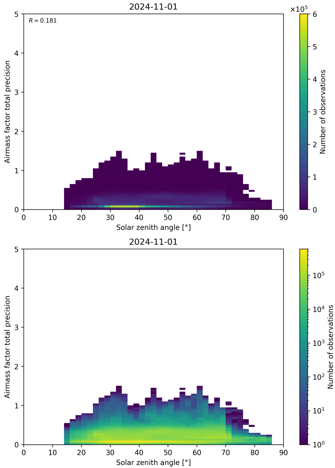
Figure 176: Scatter density plot of “Solar zenith angle” against “Airmass factor total precision” for 2024-10-31 to 2024-11-02.
