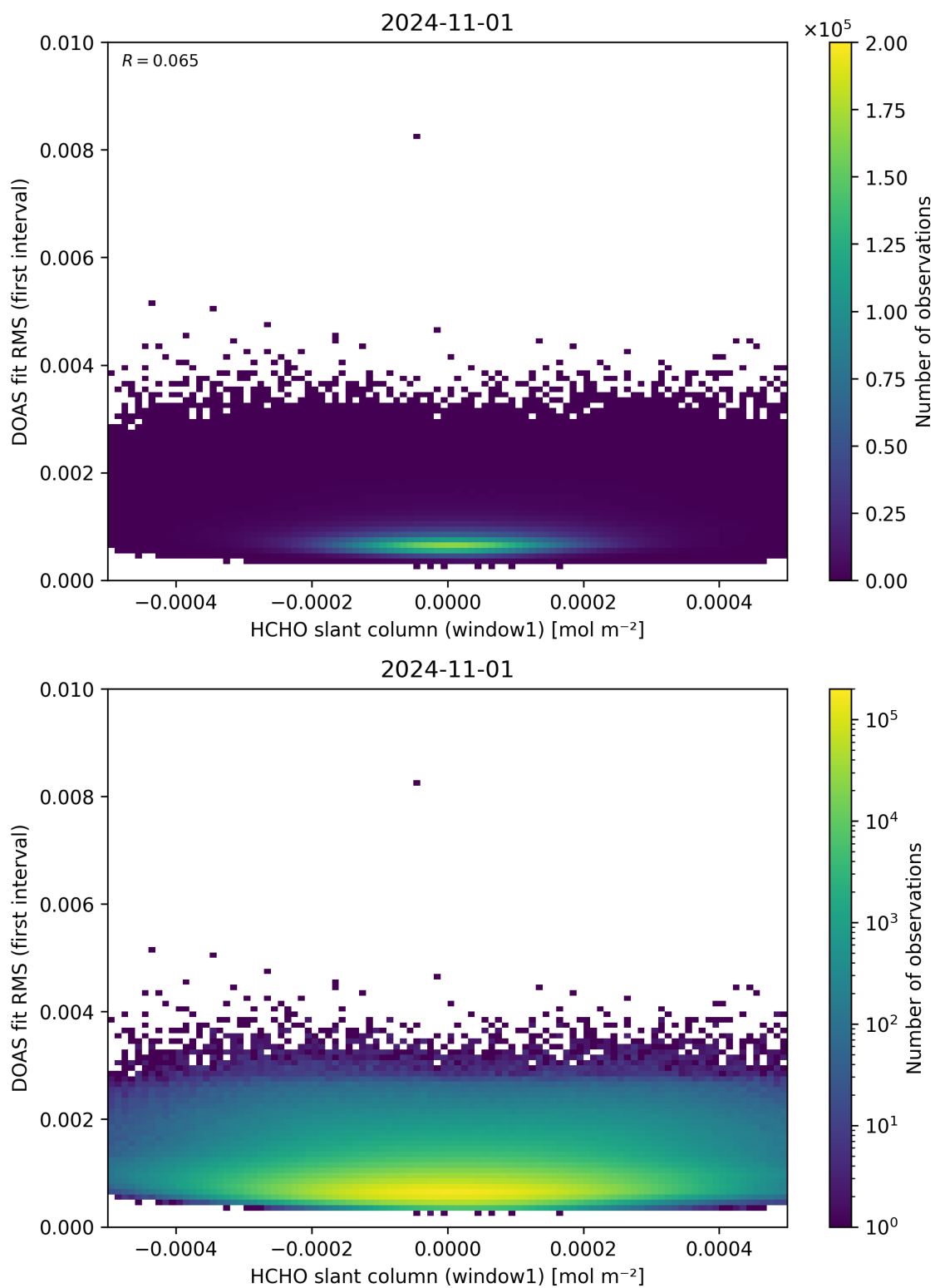
Figure 78: Scatter density plot of “HCHO slant column (window1)” against “DOAS fit RMS (first interval)” for 2024-10-31 to 2024-11-02.
