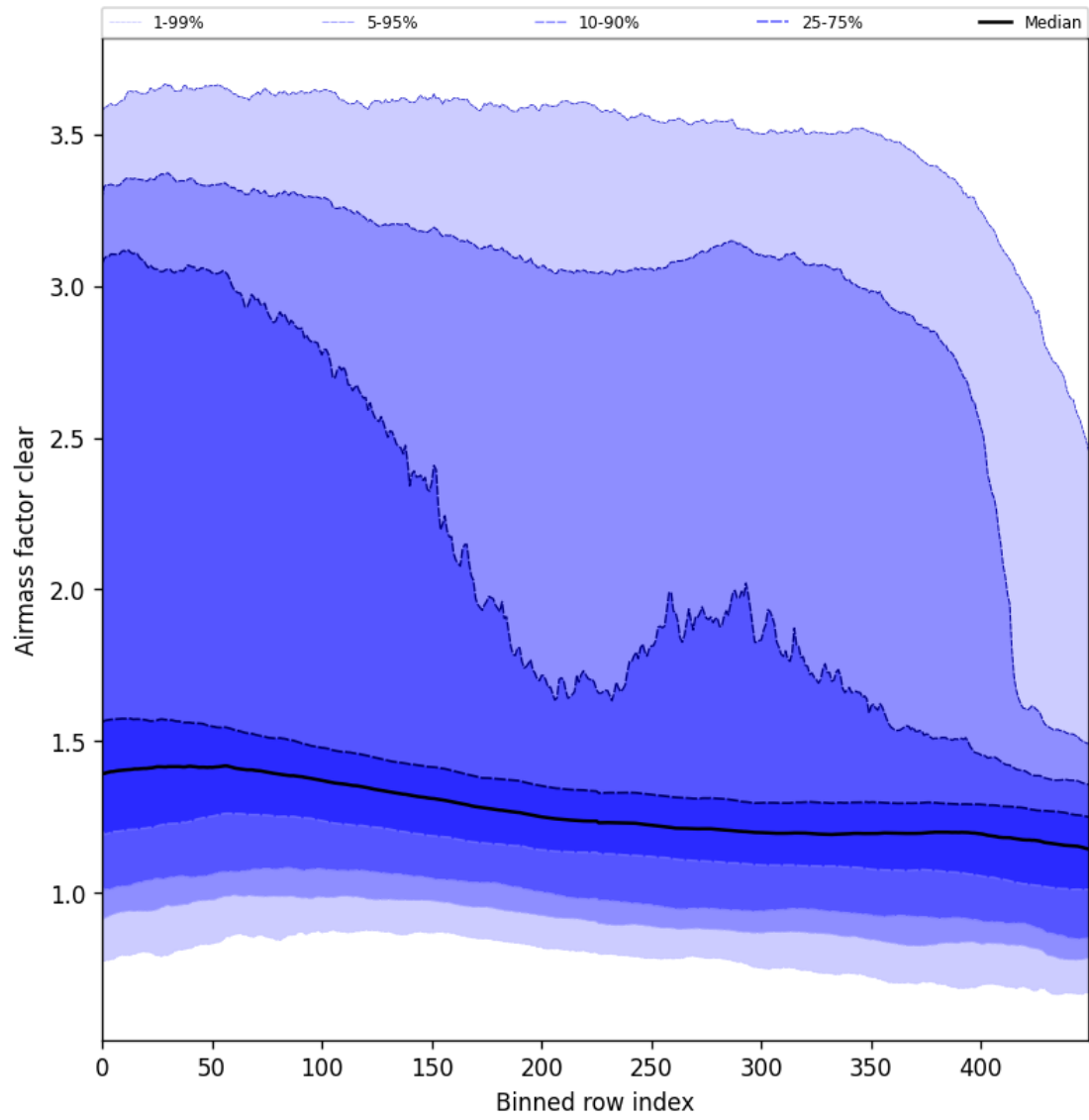
Figure 56: Along track statistics of “Airmass factor clear” for 2024-10-31 to 2024-11-02
