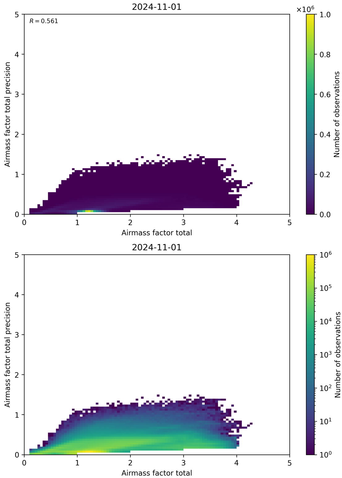
Figure 103: Scatter density plot of “Airmass factor total” against “Airmass factor total precision” for 2024-10-31 to 2024-11-02.
