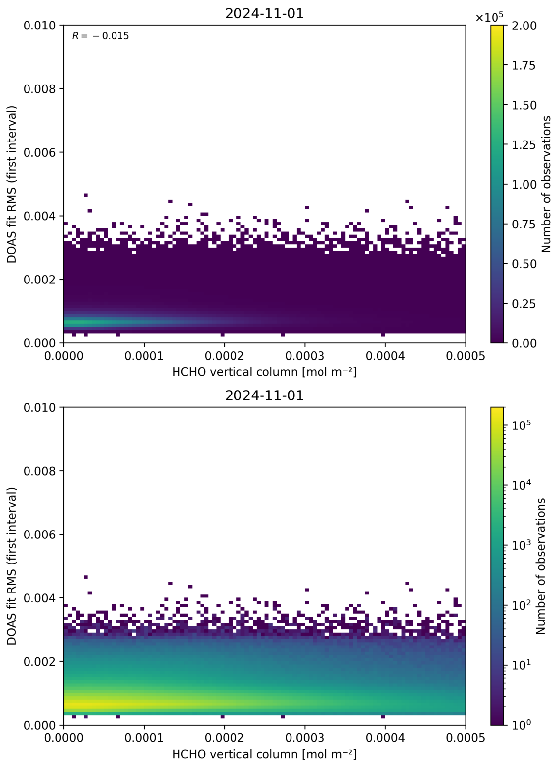
Figure 123: Scatter density plot of “HCHO vertical column” against “DOAS fit RMS (first interval)” for 2024-10-31 to 2024-11-02.
