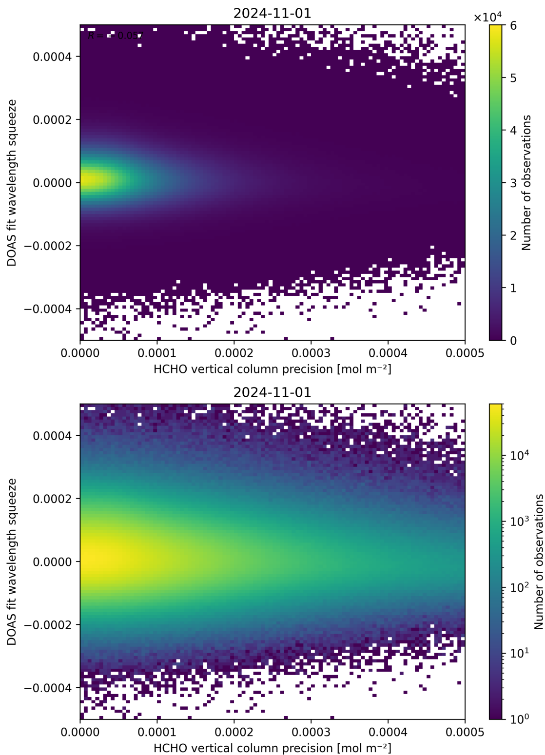
Figure 138: Scatter density plot of “HCHO vertical column precision” against “DOAS fit wavelength squeeze” for 2024-10-31 to 2024-11-02.
