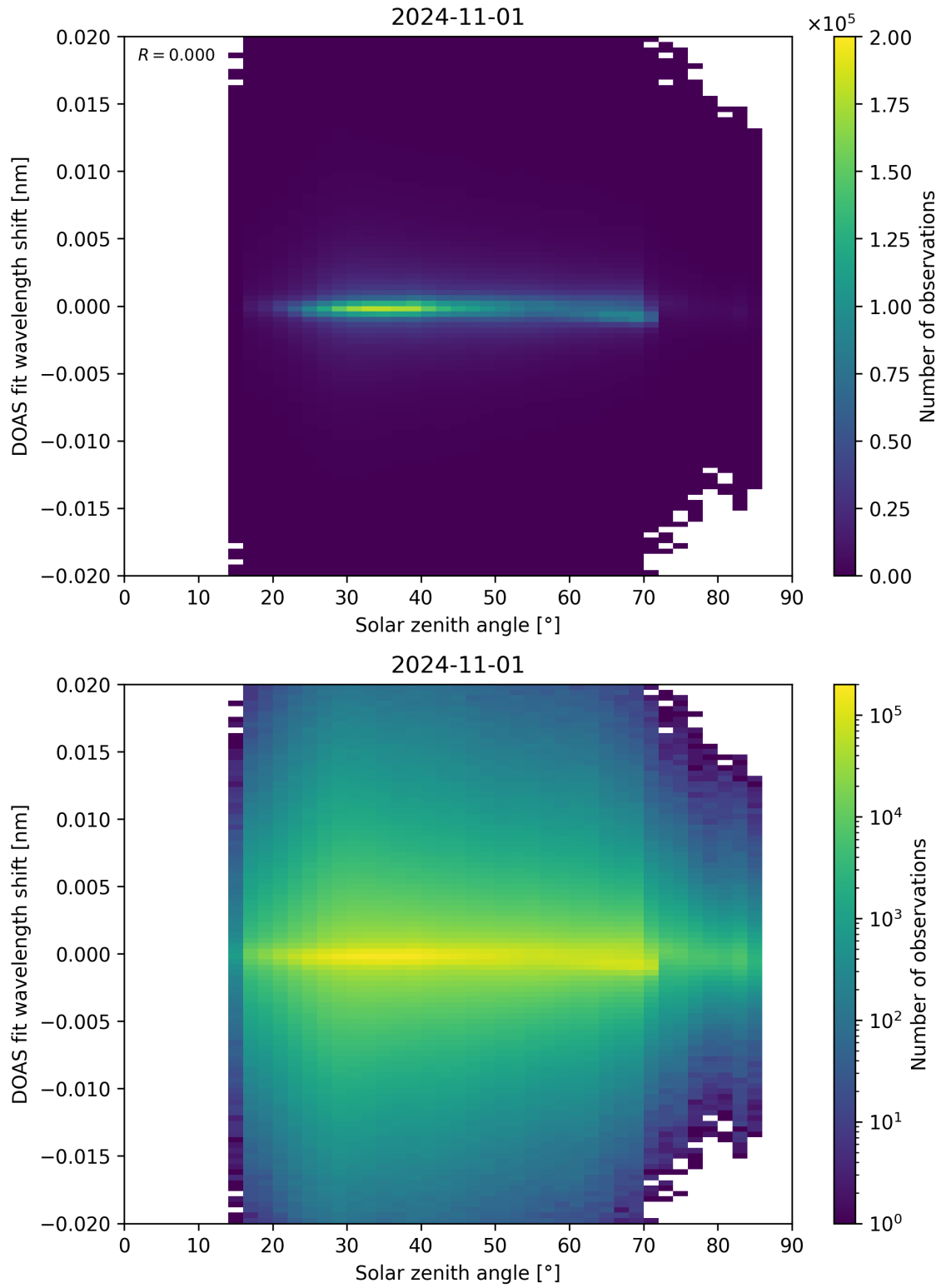
Figure 168: Scatter density plot of “Solar zenith angle” against “DOAS fit wavelength shift” for 2024-10-31 to 2024-11-02.
