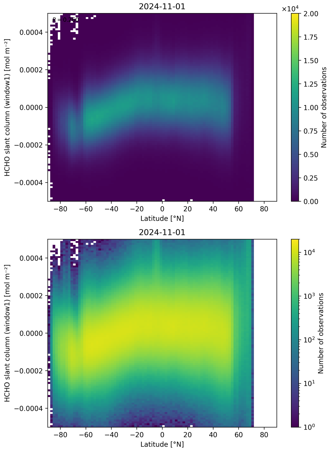
Figure 159: Scatter density plot of “Latitude” against “HCHO slant column (window1)” for 2024-10-31 to 2024-11-02.
