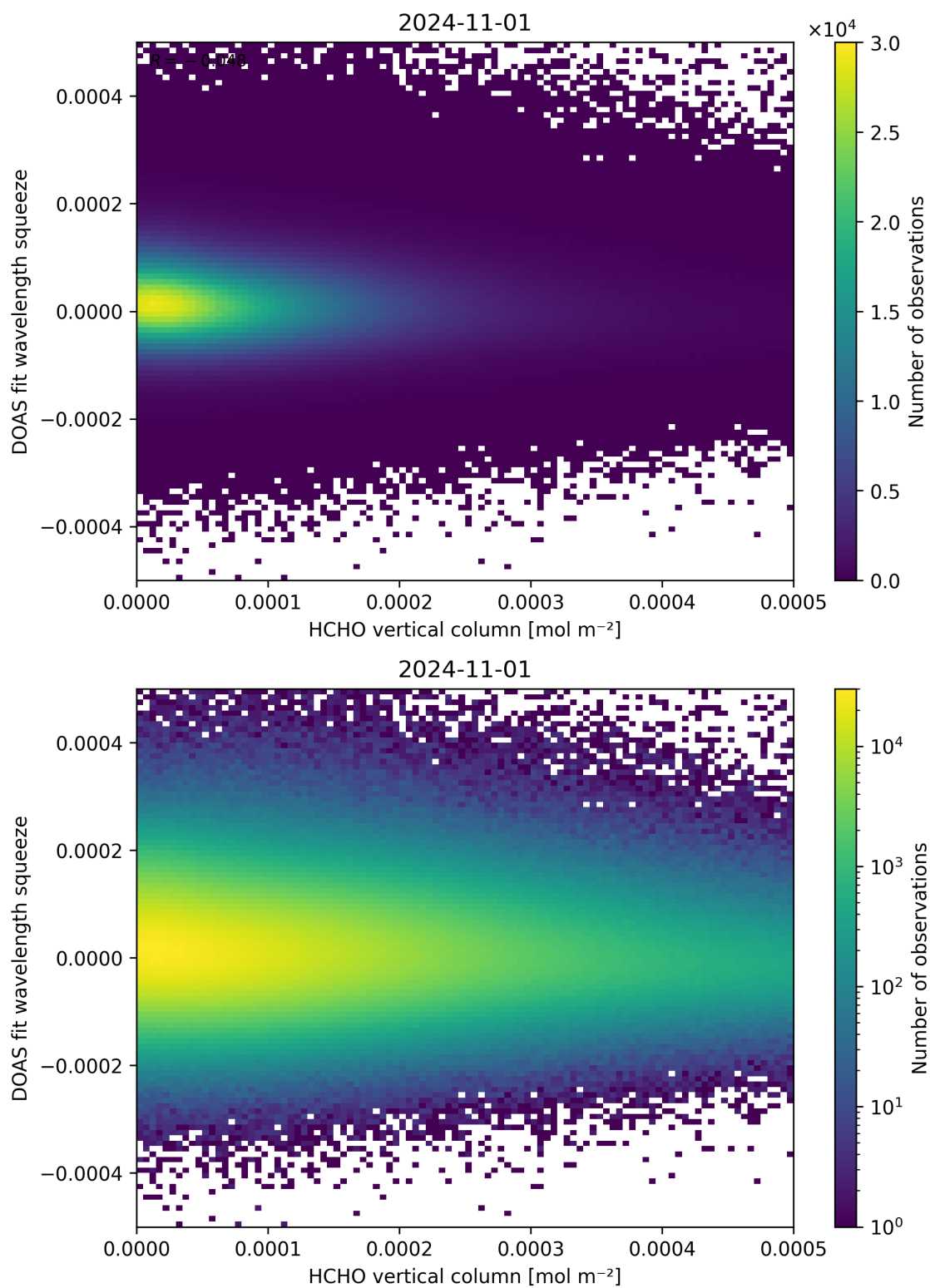
Figure 125: Scatter density plot of “HCHO vertical column” against “DOAS fit wavelength squeeze” for 2024-10-31 to 2024-11-02.
