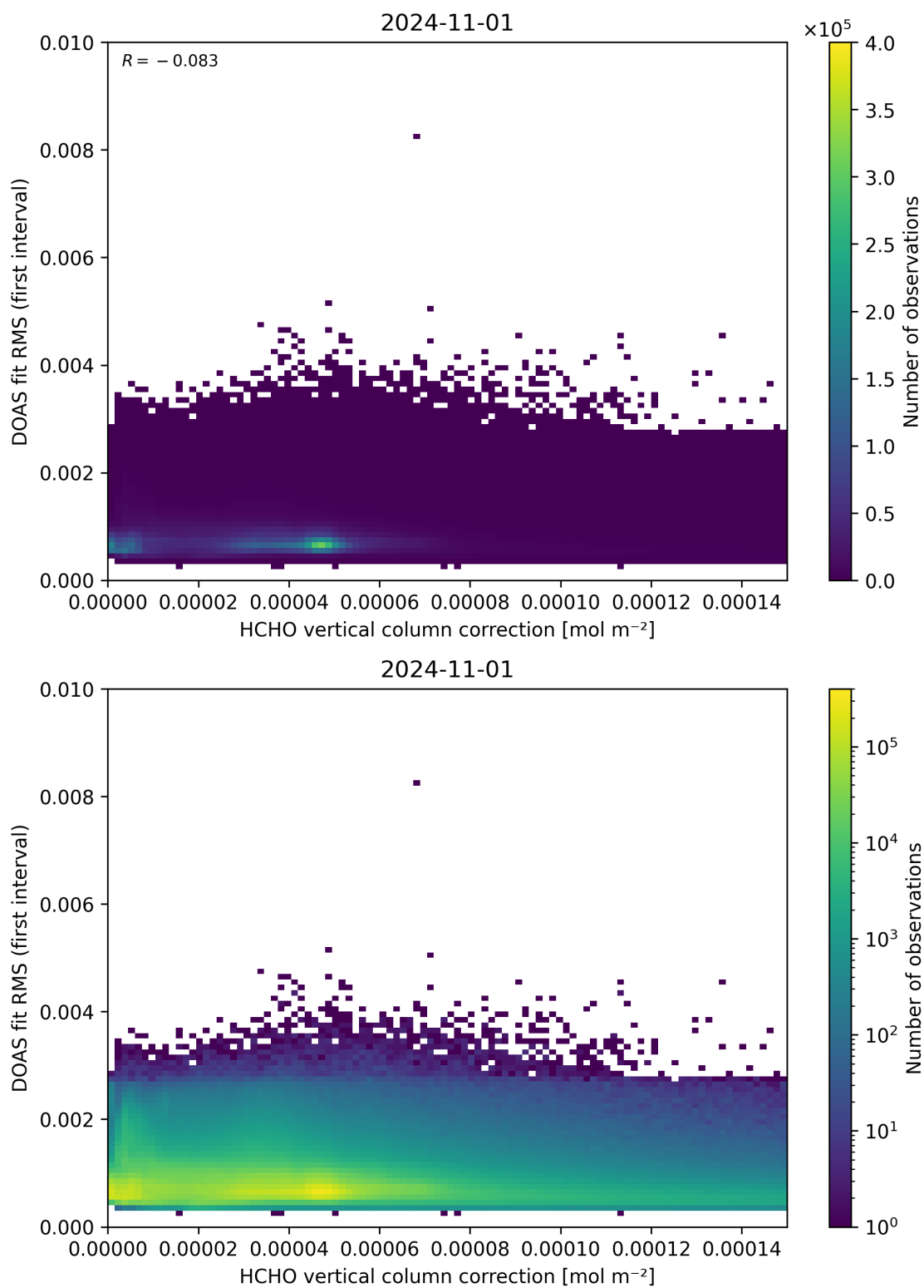
Figure 112: Scatter density plot of “HCHO vertical column correction” against “DOAS fit RMS (first interval)” for 2024-10-31 to 2024-11-02.
