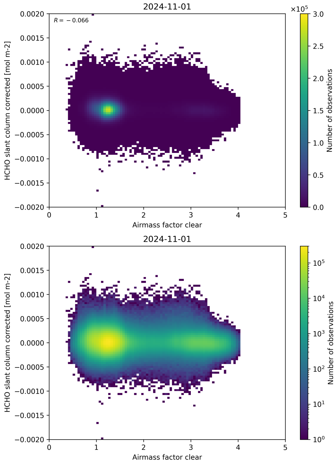
Figure 74: Scatter density plot of “Airmass factor clear” against “HCHO slant column corrected” for 2024-10-31 to 2024-11-02.
