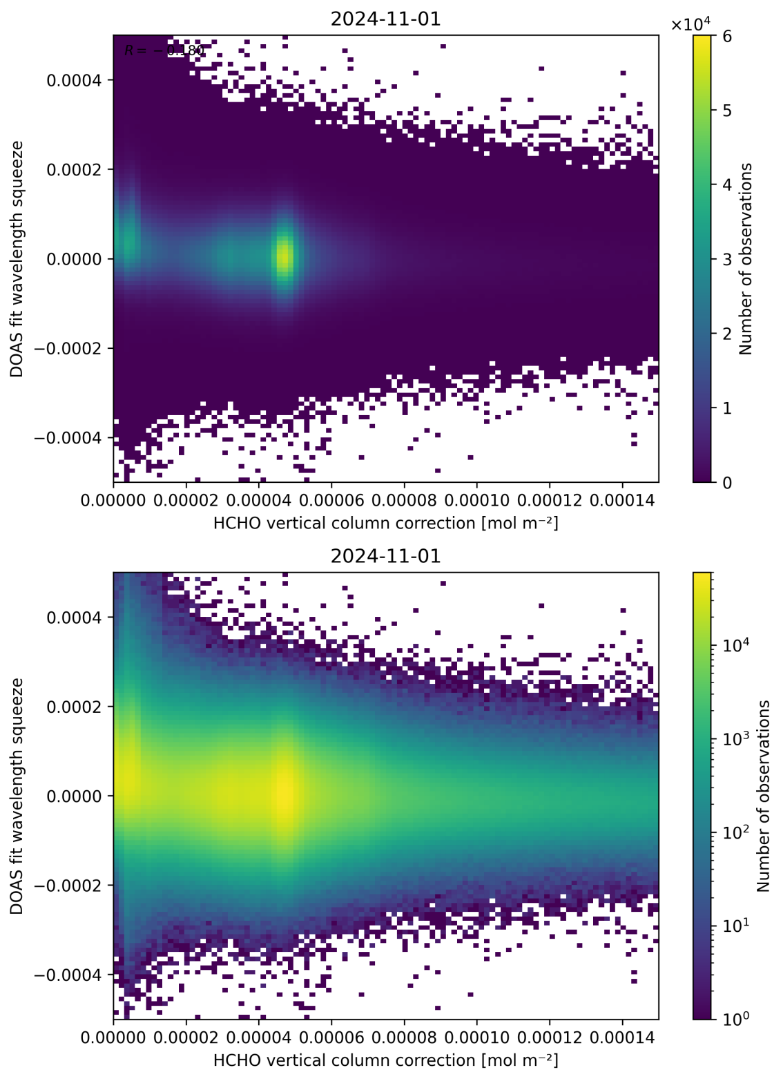
Figure 114: Scatter density plot of “HCHO vertical column correction” against “DOAS fit wavelength squeeze” for 2024-10-31 to 2024-11-02.
