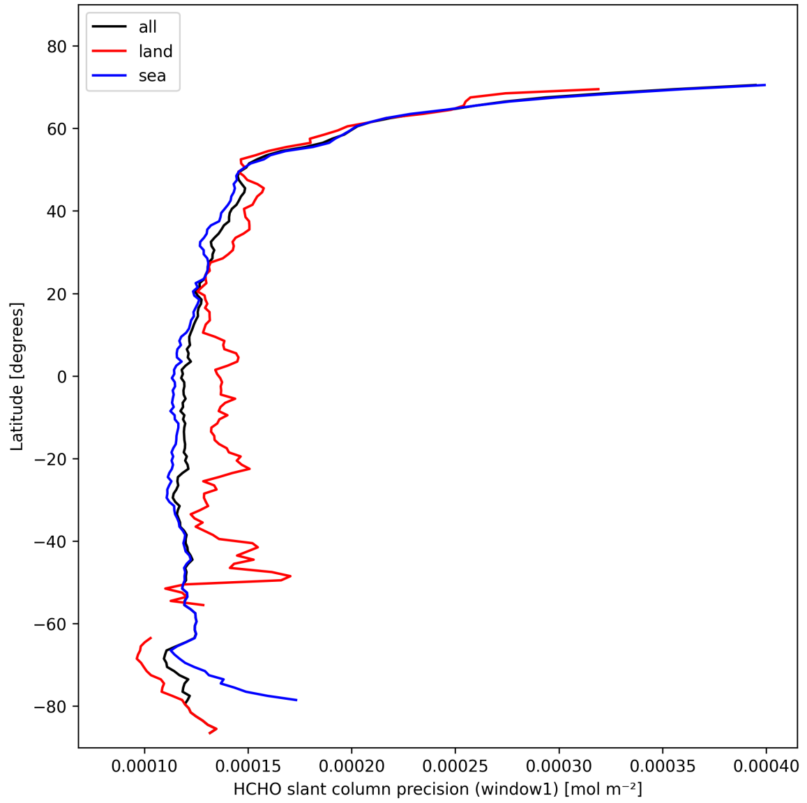
Figure 25: Zonal average of “HCHO slant column precision (window1)” for 2024-10-31 to 2024-11-02.
