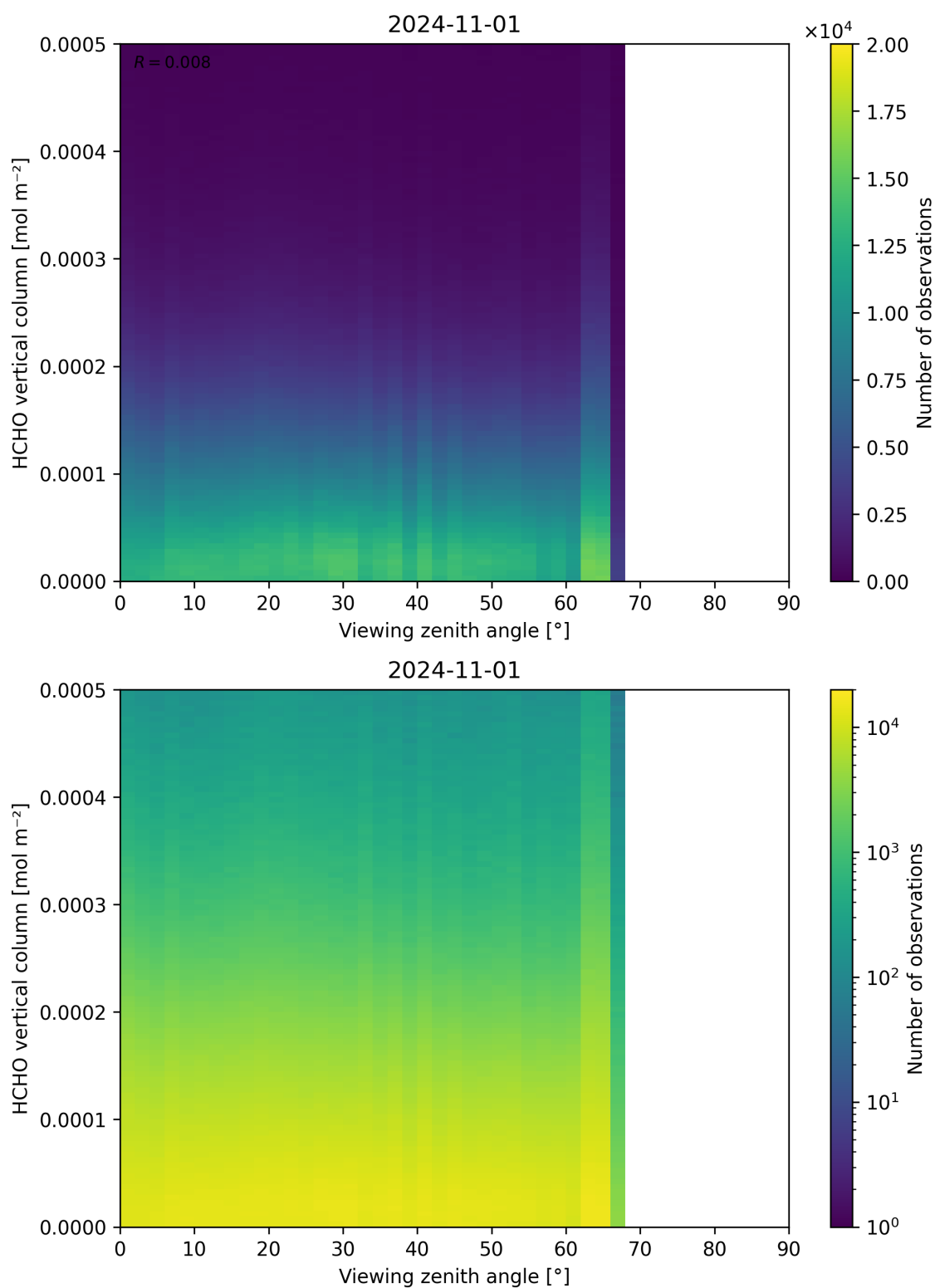
Figure 192: Scatter density plot of “Viewing zenith angle” against “HCHO vertical column” for 2024-10-31 to 2024-11-02.
