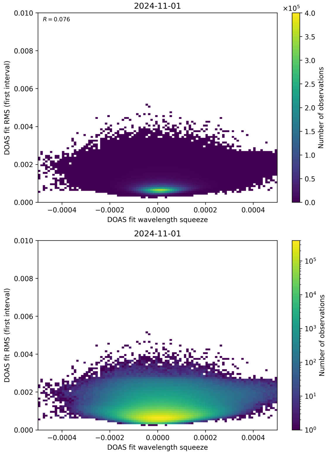
Figure 68: Scatter density plot of “DOAS fit wavelength squeeze” against “DOAS fit RMS (first interval)” for 2024-10-31 to 2024-11-02.
