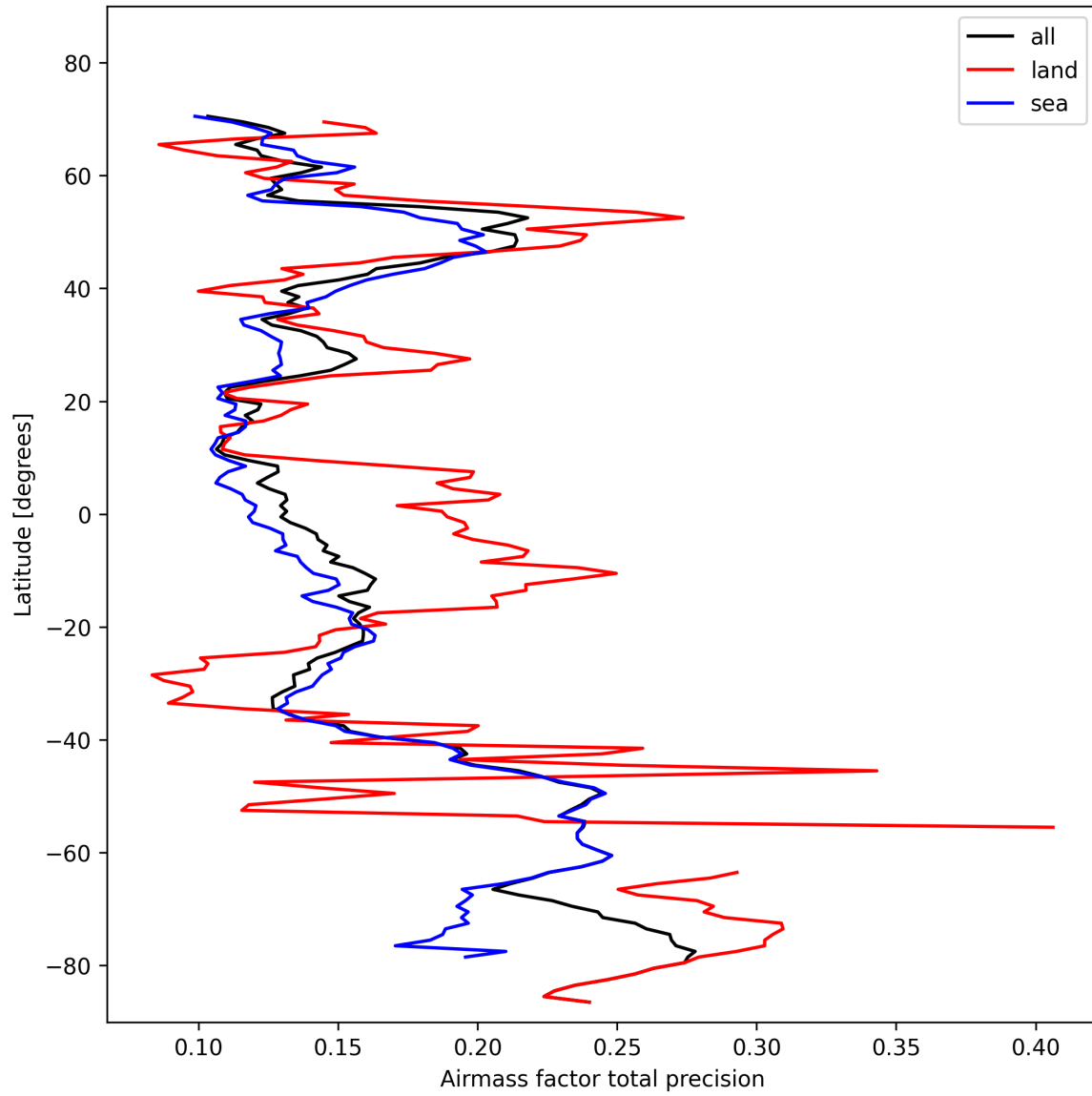
Figure 27: Zonal average of “Airmass factor total precision” for 2024-10-31 to 2024-11-02.
