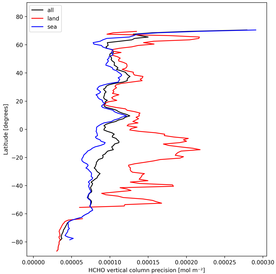
Figure 22: Zonal average of “HCHO vertical column precision” for 2024-10-31 to 2024-11-02.
