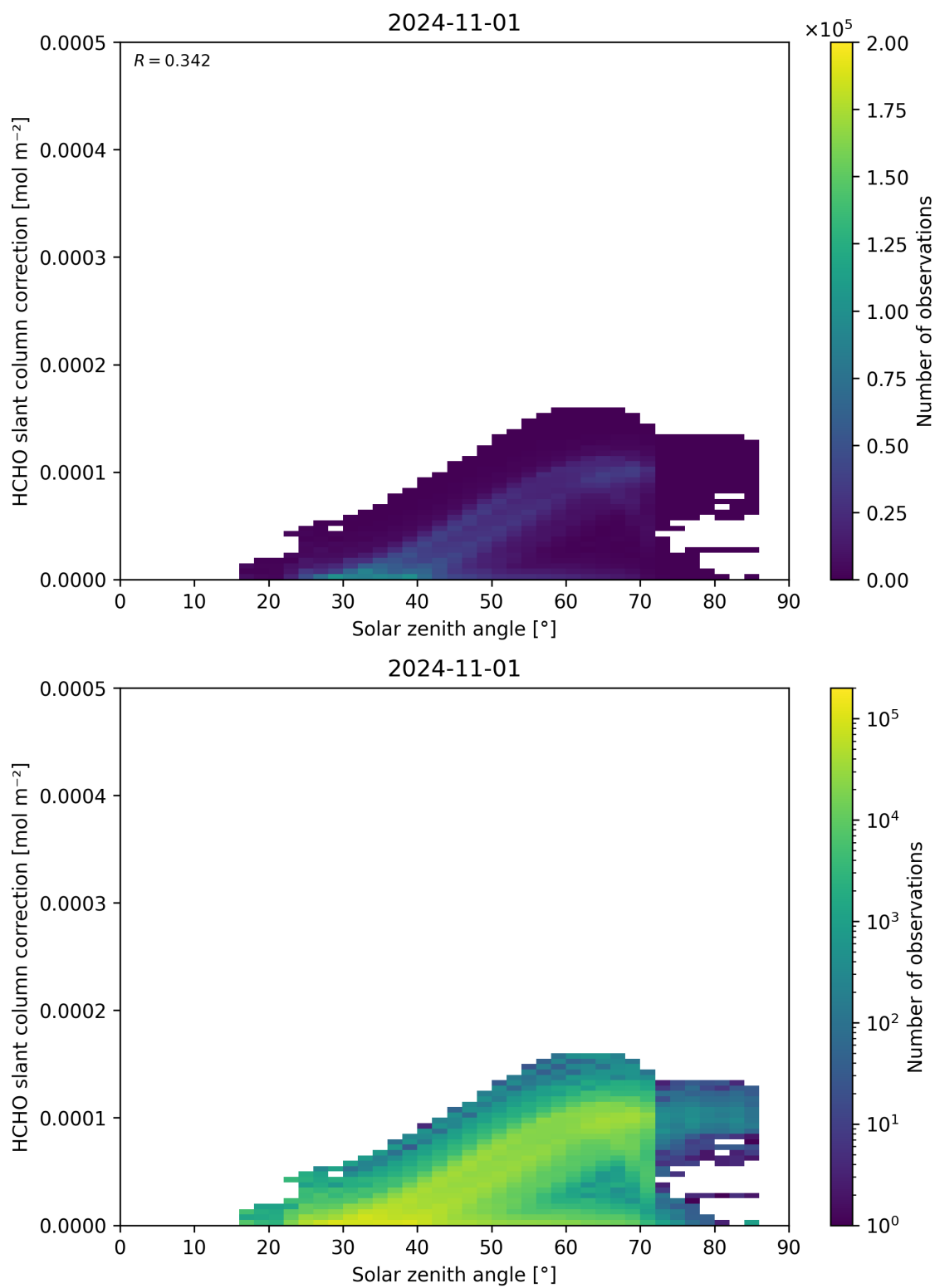
Figure 172: Scatter density plot of “Solar zenith angle” against “HCHO slant column correction” for 2024-10-31 to 2024-11-02.
