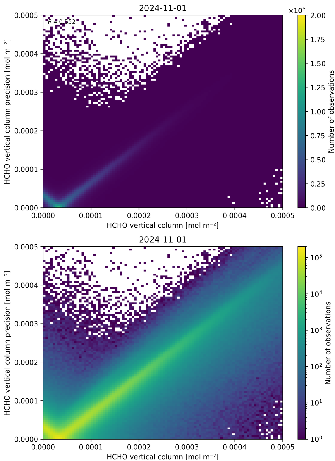
Figure 134: Scatter density plot of “HCHO vertical column” against “HCHO vertical column precision” for 2024-10-31 to 2024-11-02.
