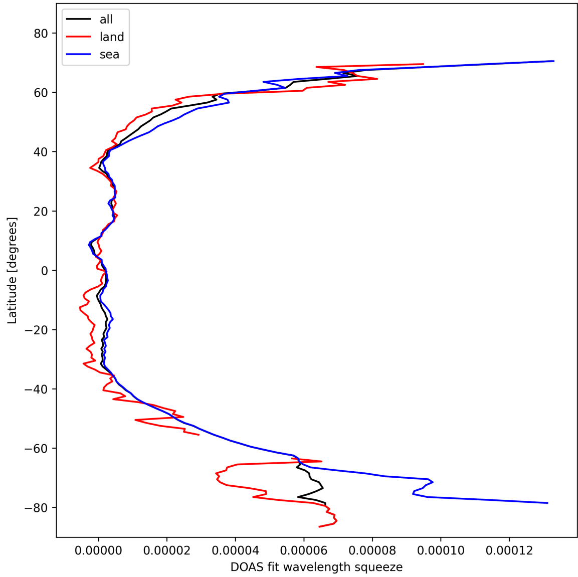
Figure 31: Zonal average of “DOAS fit wavelength squeeze” for 2024-10-31 to 2024-11-02.
