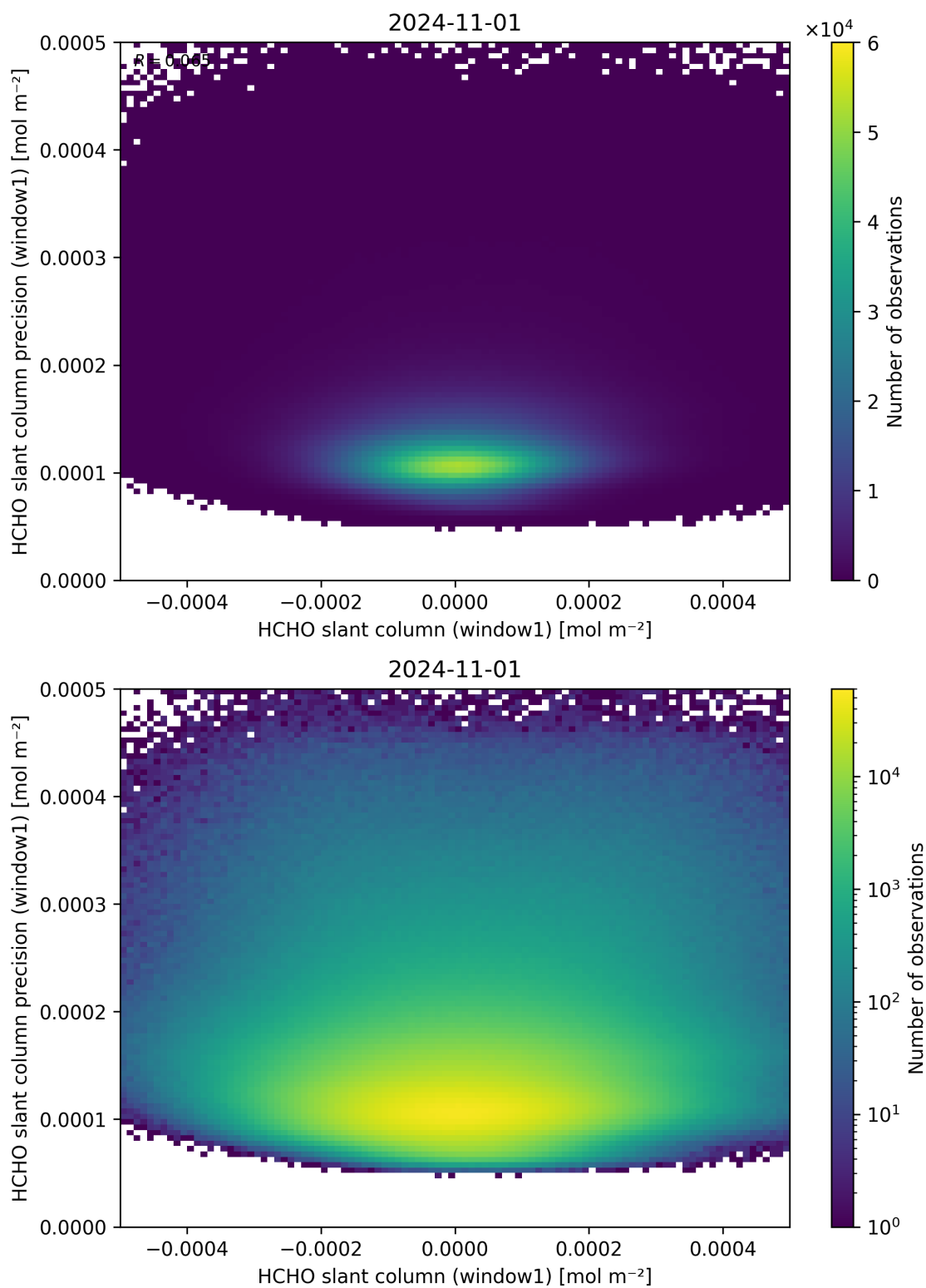
Figure 84: Scatter density plot of “HCHO slant column (window1)” against “HCHO slant column precision (window1)” for 2024-10-31 to 2024-11-02.
