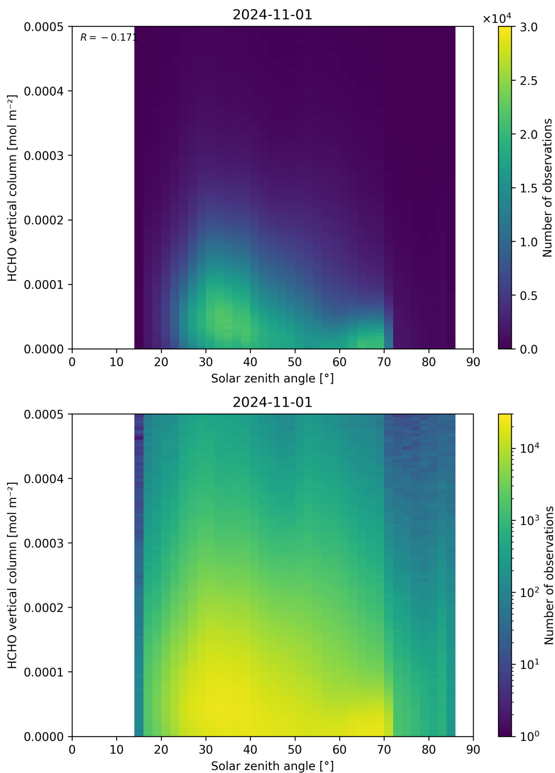
Figure 177: Scatter density plot of “Solar zenith angle” against “HCHO vertical column” for 2024-10-31 to 2024-11-02.
