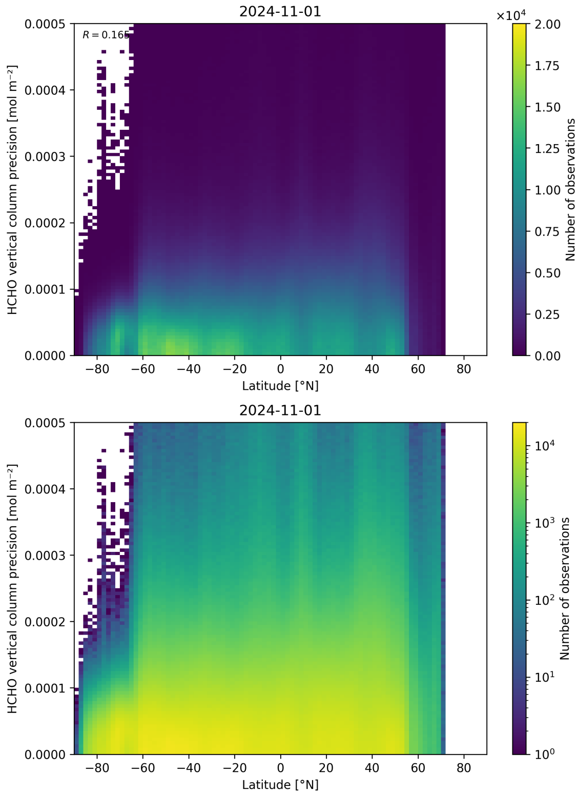
Figure 165: Scatter density plot of “Latitude” against “HCHO vertical column precision” for 2024-10-31 to 2024-11-02.
