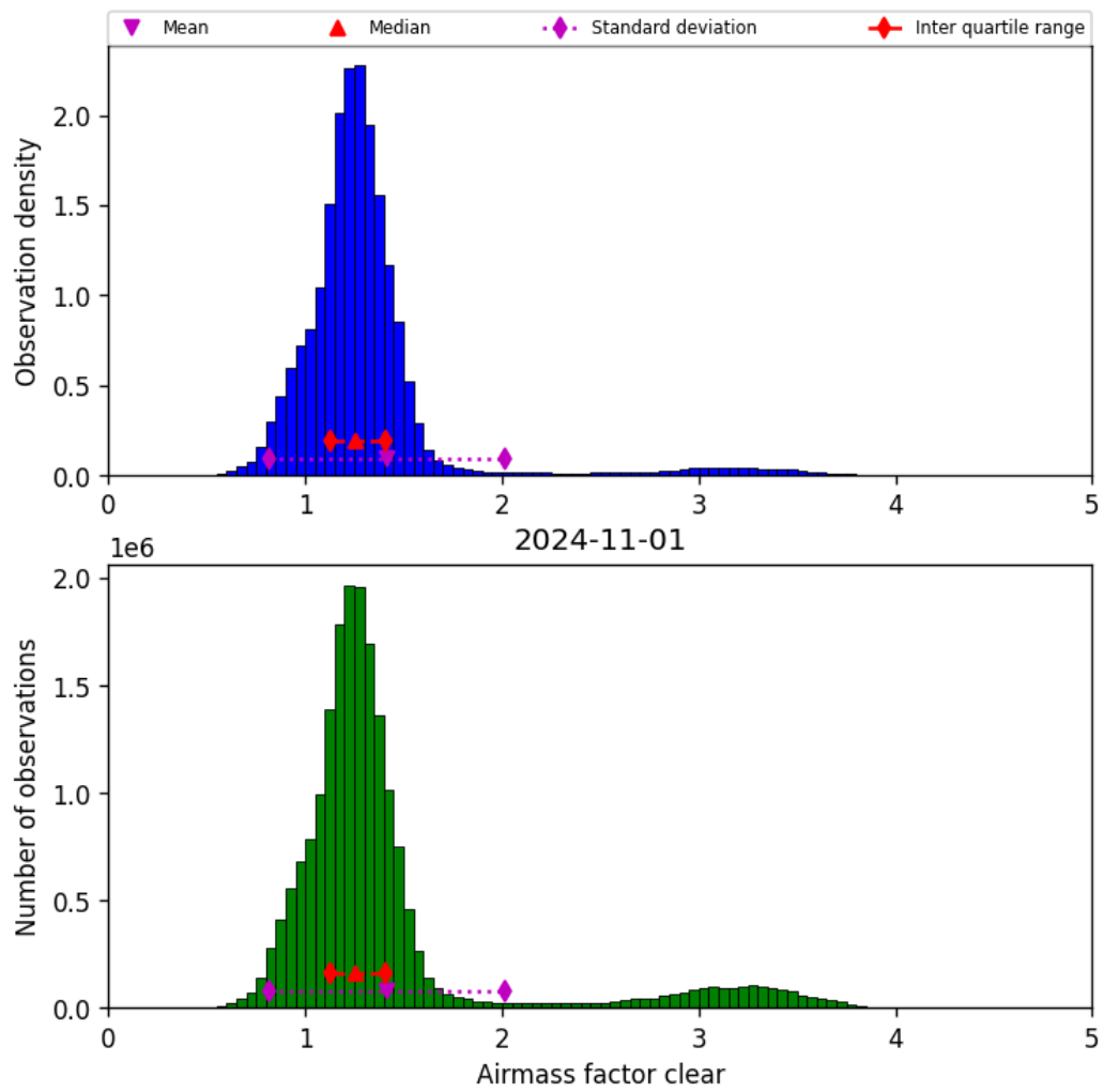
Figure 42: Histogram of “Airmass factor clear” for 2024-10-31 to 2024-11-02
