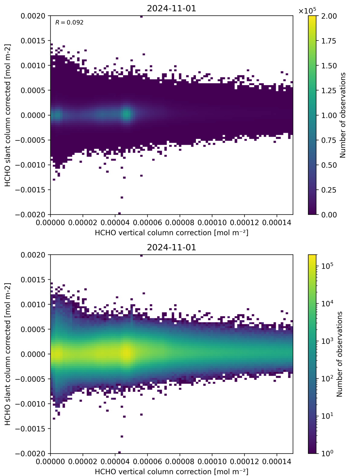
Figure 116: Scatter density plot of “HCHO vertical column correction” against “HCHO slant column corrected” for 2024-10-31 to 2024-11-02.
