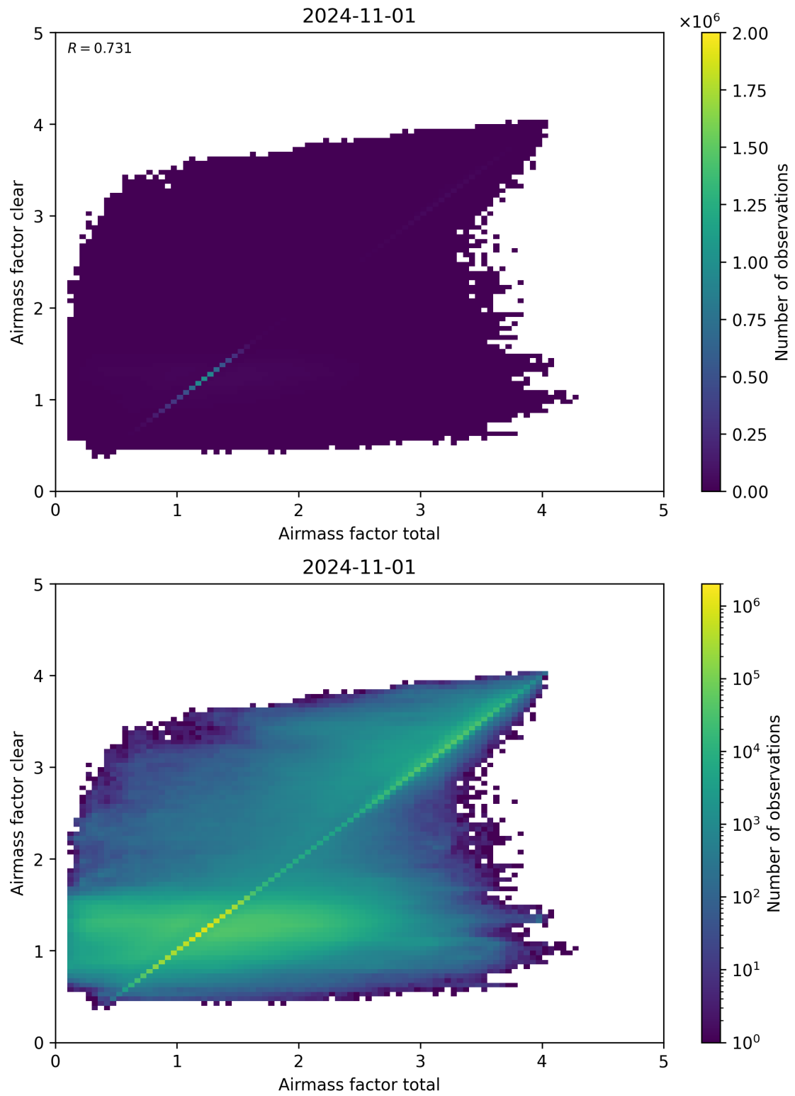
Figure 100: Scatter density plot of “Airmass factor total” against “Airmass factor clear” for 2024-10-31 to 2024-11-02.
