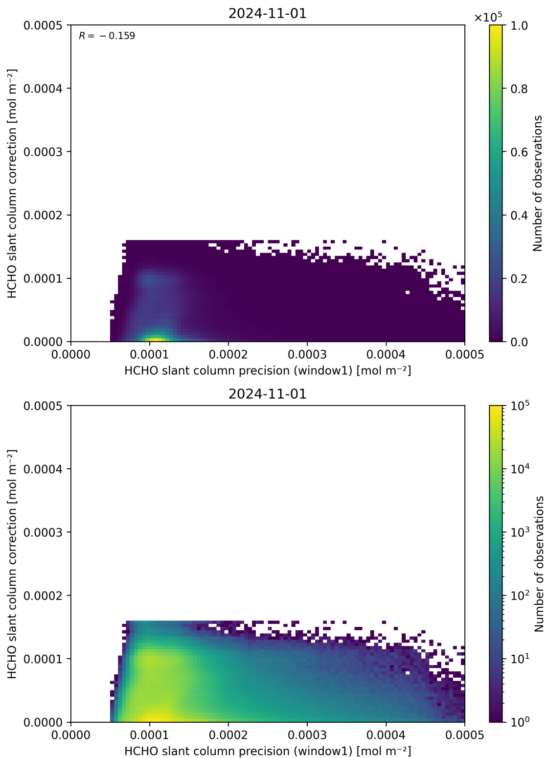
Figure 93: Scatter density plot of “HCHO slant column precision (window1)” against “HCHO slant column correction” for 2024-10-31 to 2024-11-02.
