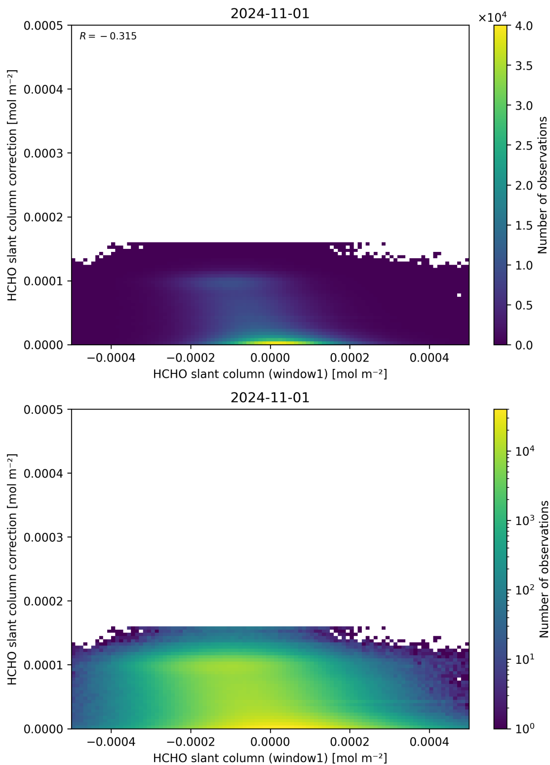
Figure 83: Scatter density plot of “HCHO slant column (window1)” against “HCHO slant column correction” for 2024-10-31 to 2024-11-02.
