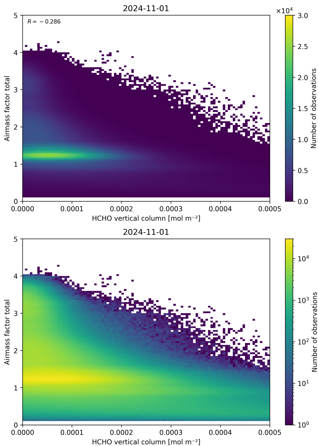
Figure 131: Scatter density plot of “HCHO vertical column” against “Airmass factor total” for 2024-10-31 to 2024-11-02.
