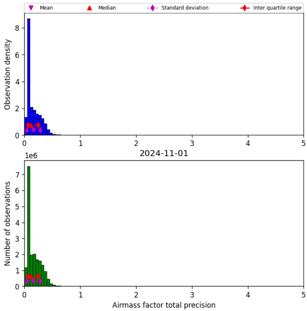
Figure 41: Histogram of “Airmass factor total precision” for 2024-10-31 to 2024-11-02
