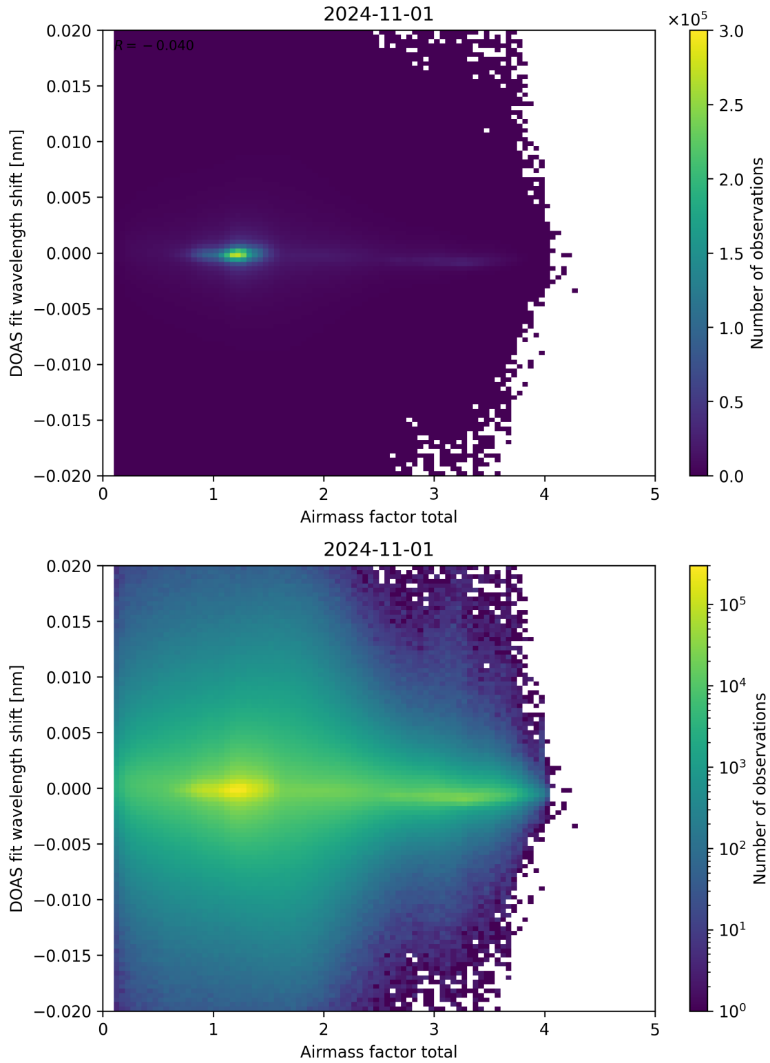
Figure 98: Scatter density plot of “Airmass factor total” against “DOAS fit wavelength shift” for 2024-10-31 to 2024-11-02.
