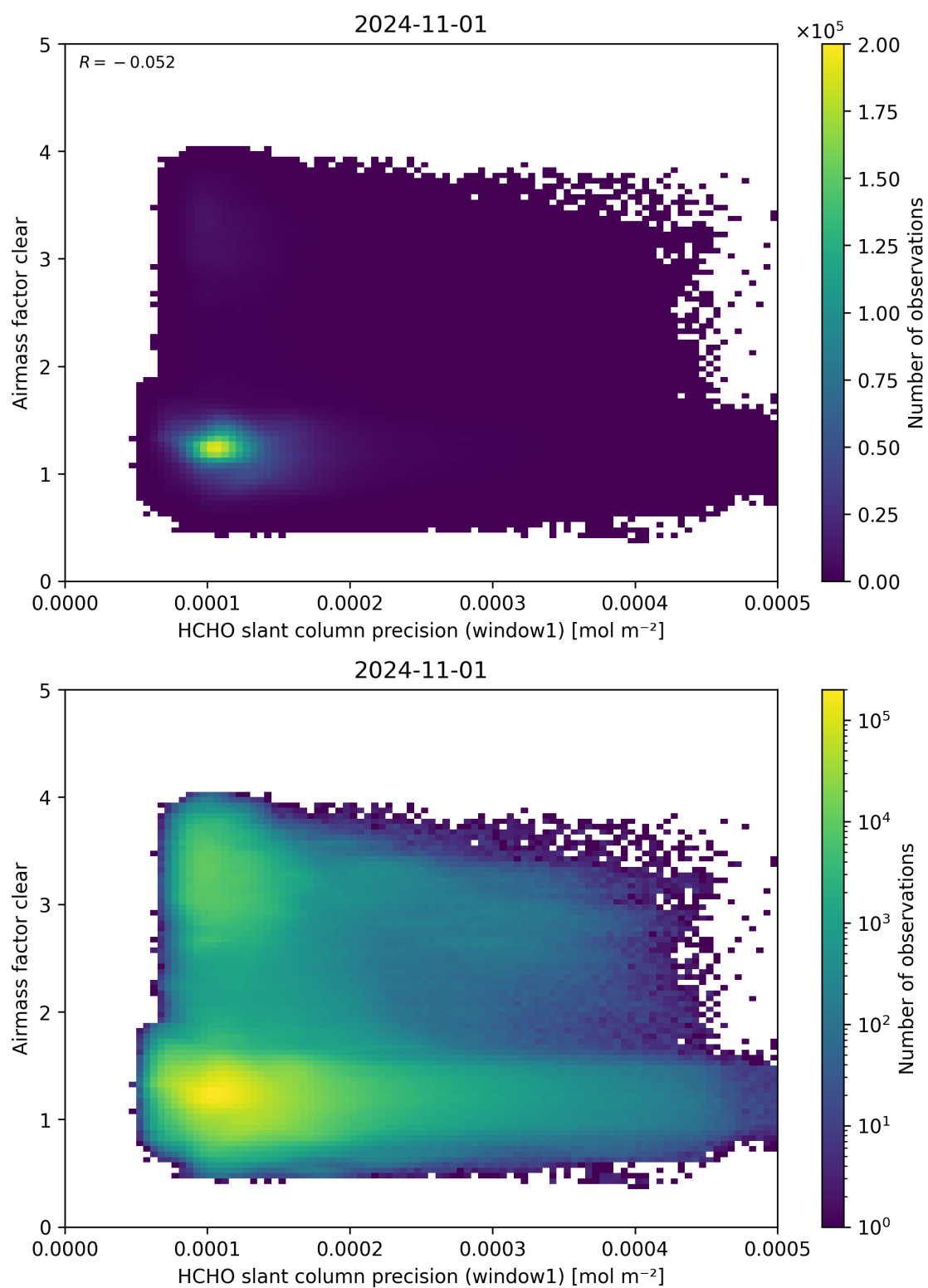
Figure 91: Scatter density plot of “HCHO slant column precision (window1)” against “Airmass factor clear” for 2024-10-31 to 2024-11-02.
