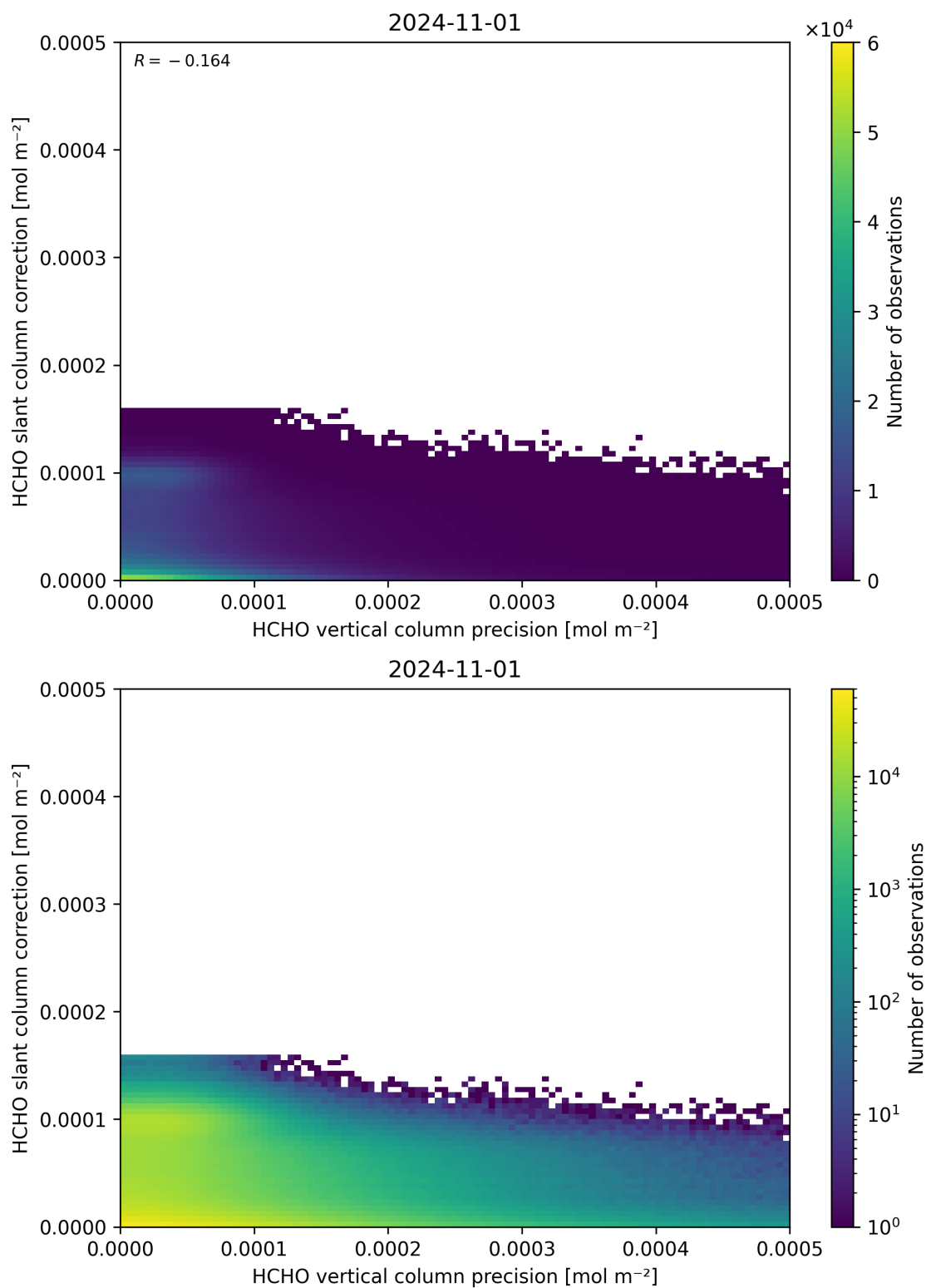
Figure 141: Scatter density plot of “HCHO vertical column precision” against “HCHO slant column correction” for 2024-10-31 to 2024-11-02.
