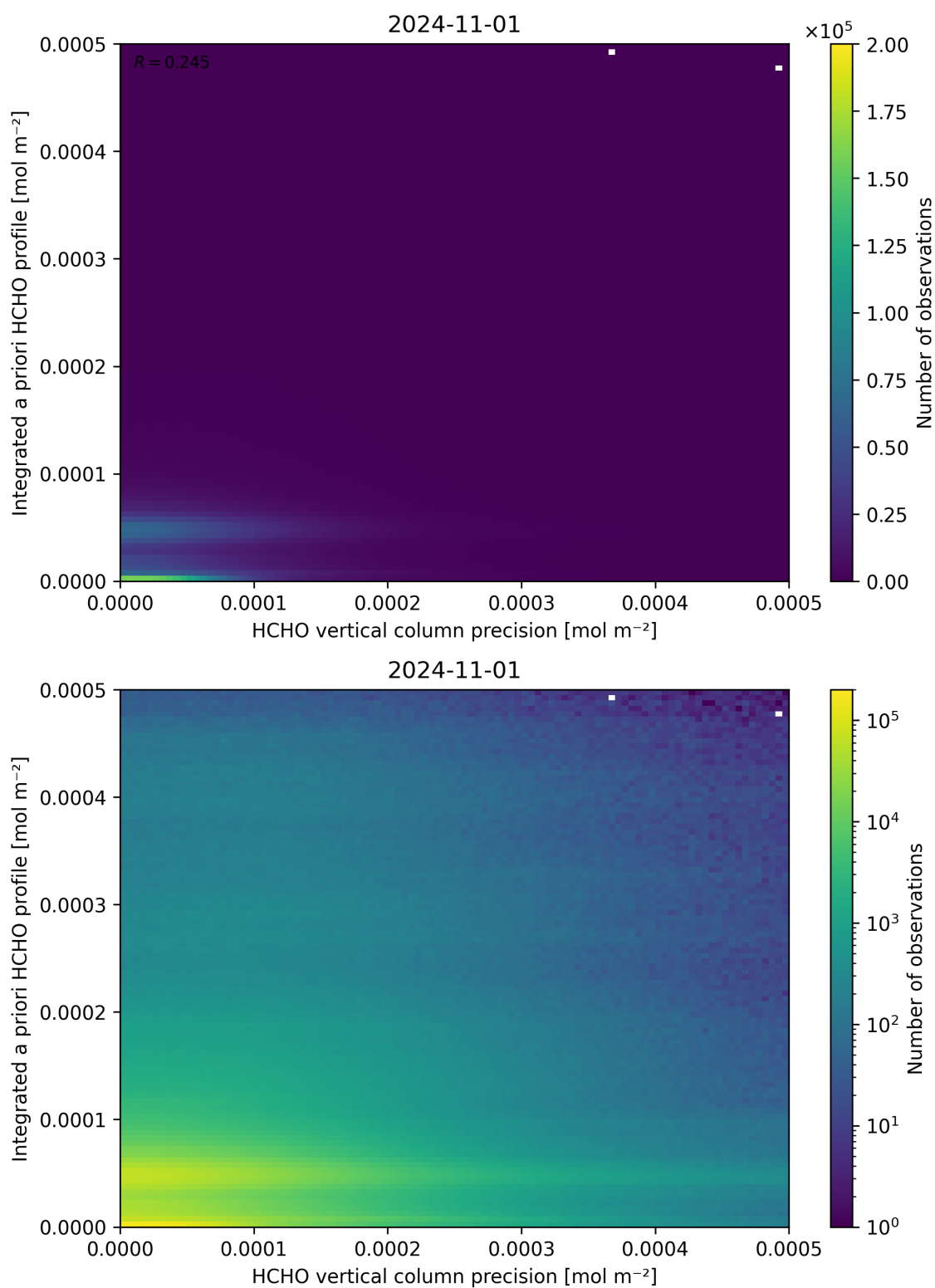
Figure 147: Scatter density plot of “HCHO vertical column precision” against “Integrated a priori HCHO profile” for 2024-10-31 to 2024-11-02.
