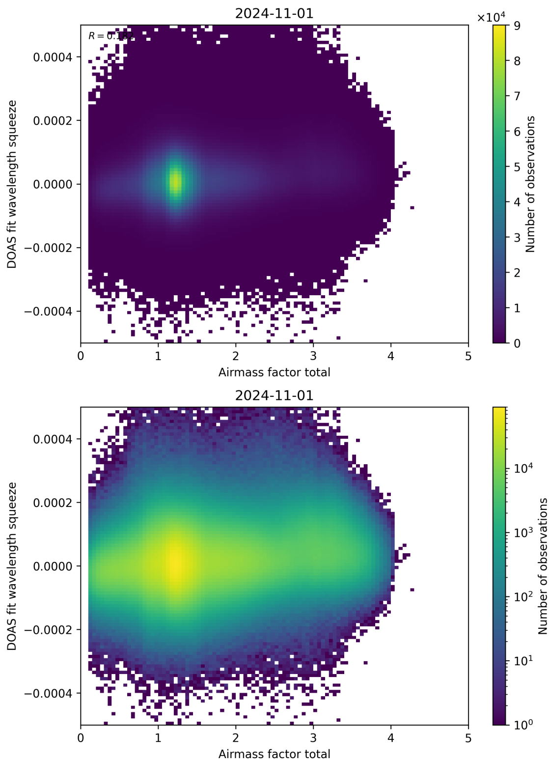
Figure 99: Scatter density plot of “Airmass factor total” against “DOAS fit wavelength squeeze” for 2024-10-31 to 2024-11-02.
