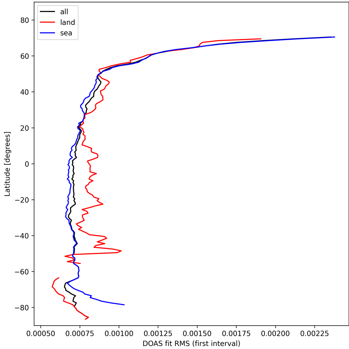
Figure 32: Zonal average of “DOAS fit RMS (first interval)” for 2024-10-31 to 2024-11-02.
