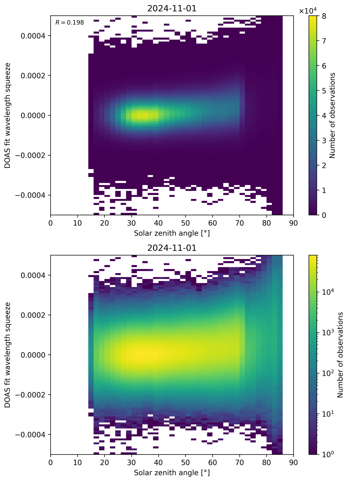
Figure 169: Scatter density plot of “Solar zenith angle” against “DOAS fit wavelength squeeze” for 2024-10-31 to 2024-11-02.
