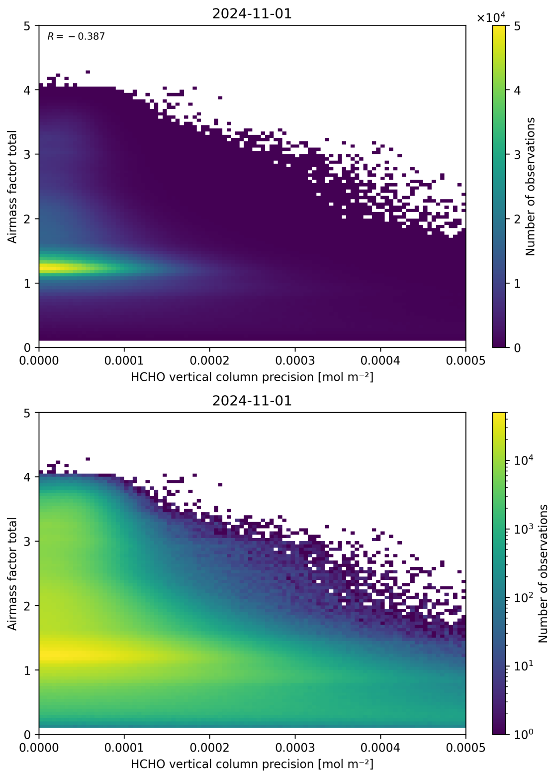
Figure 144: Scatter density plot of “HCHO vertical column precision” against “Airmass factor total” for 2024-10-31 to 2024-11-02.
