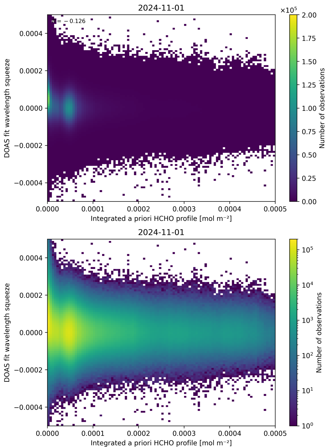
Figure 150: Scatter density plot of “Integrated a priori HCHO profile” against “DOAS fit wavelength squeeze” for 2024-10-31 to 2024-11-02.
