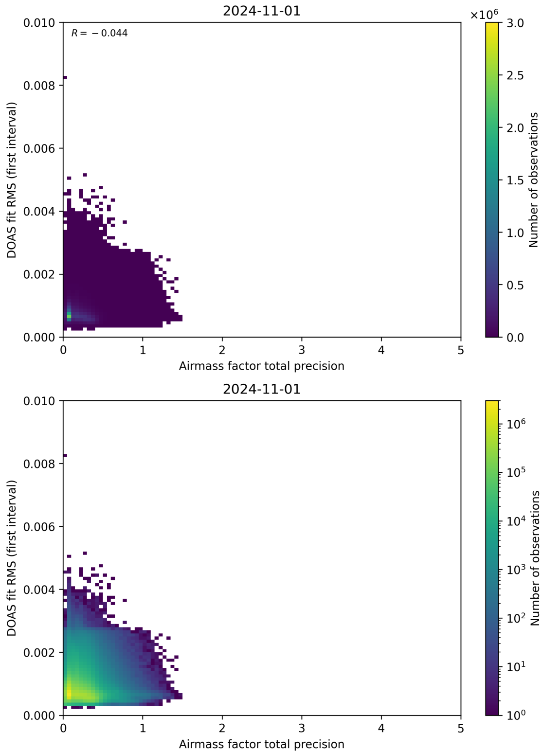
Figure 105: Scatter density plot of “Airmass factor total precision” against “DOAS fit RMS (first interval)” for 2024-10-31 to 2024-11-02.
