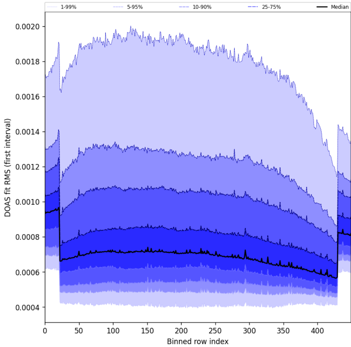
Figure 60: Along track statistics of “DOAS fit RMS (first interval)” for 2024-10-31 to 2024-11-02
