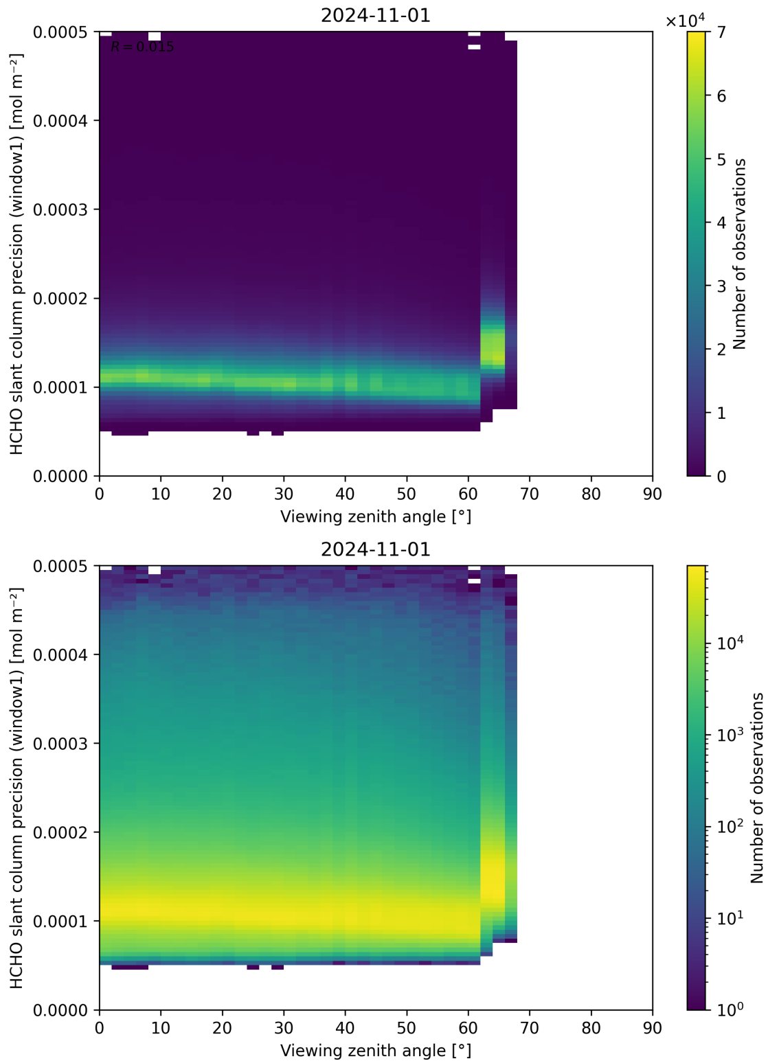
Figure 189: Scatter density plot of “Viewing zenith angle” against “HCHO slant column precision (window1)” for 2024-10-31 to 2024-11-02.
