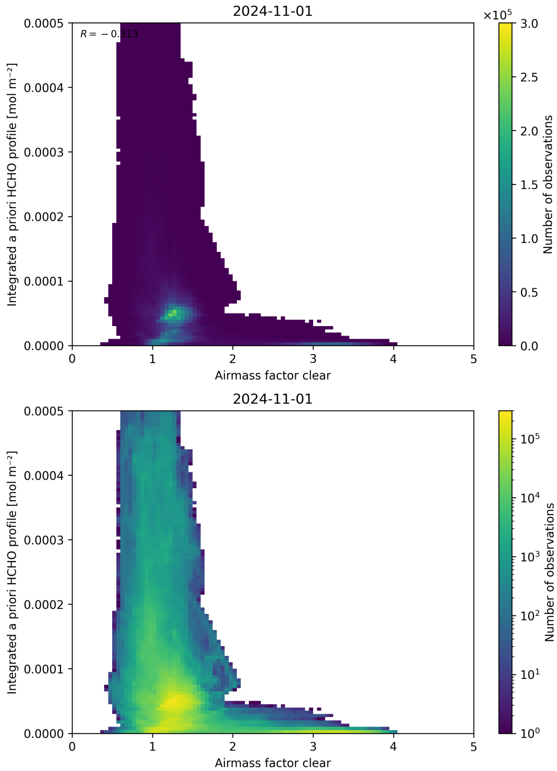
Figure 76: Scatter density plot of “Airmass factor clear” against “Integrated a priori HCHO profile” for 2024-10-31 to 2024-11-02.
