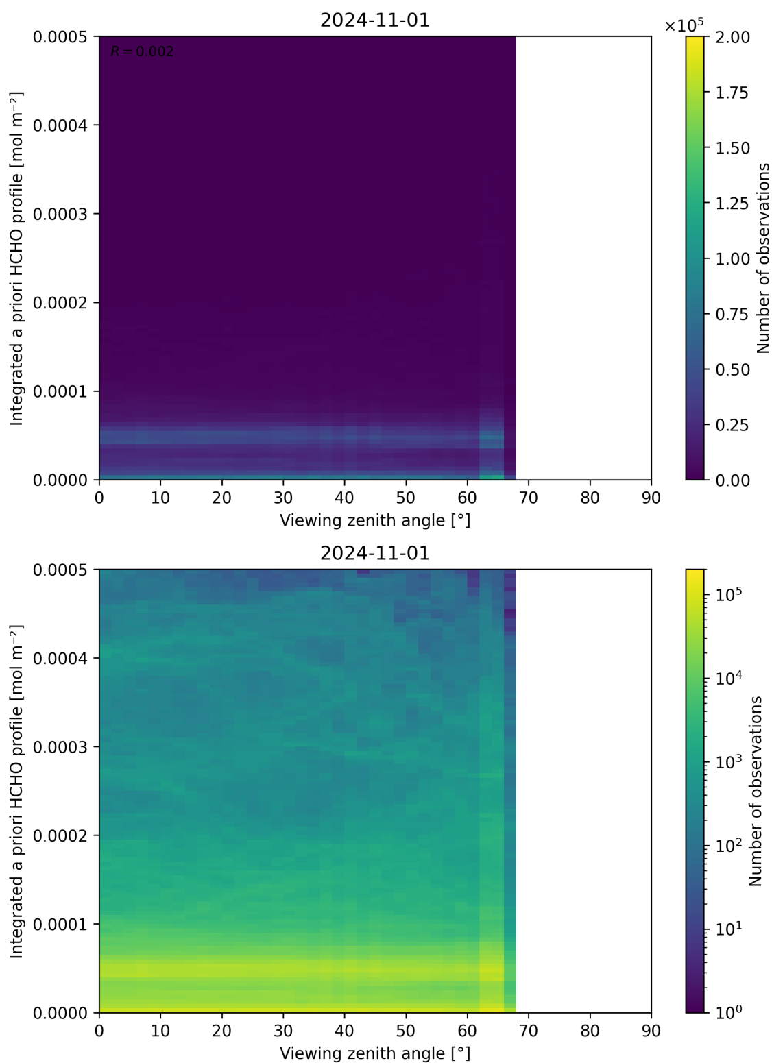
Figure 195: Scatter density plot of “Viewing zenith angle” against “Integrated a priori HCHO profile” for 2024-10-31 to 2024-11-02.
