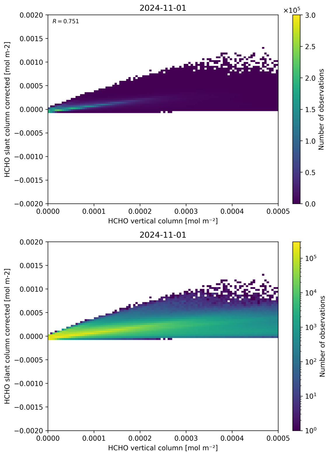
Figure 127: Scatter density plot of “HCHO vertical column” against “HCHO slant column corrected” for 2024-10-31 to 2024-11-02.
