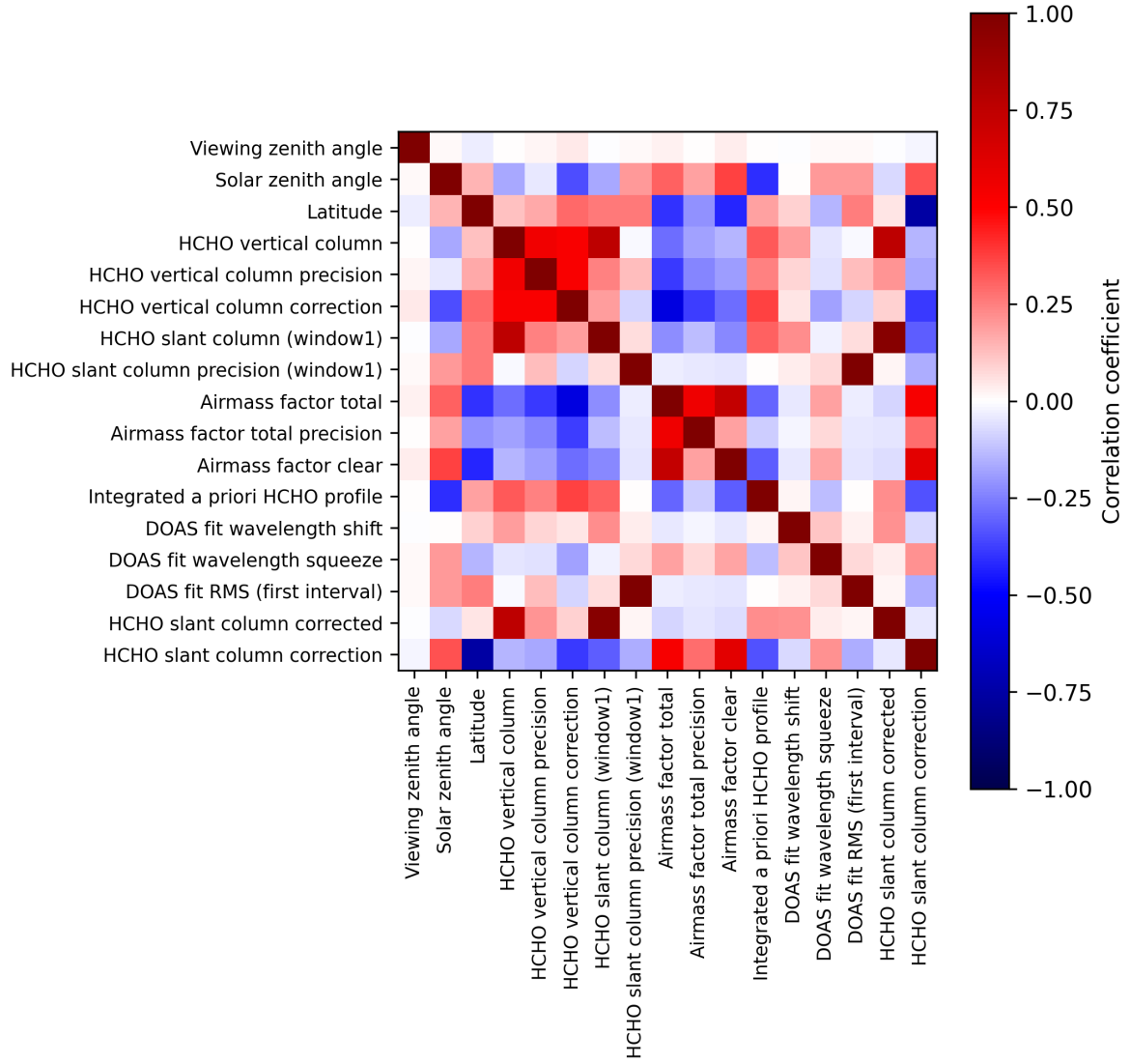
Figure 2: Map of correlation matrix for 2024-10-31 to 2024-11-02.
