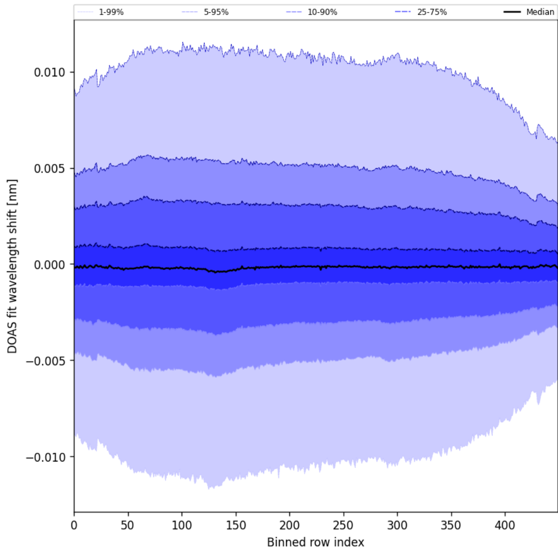
Figure 58: Along track statistics of “DOAS fit wavelength shift” for 2024-10-31 to 2024-11-02
