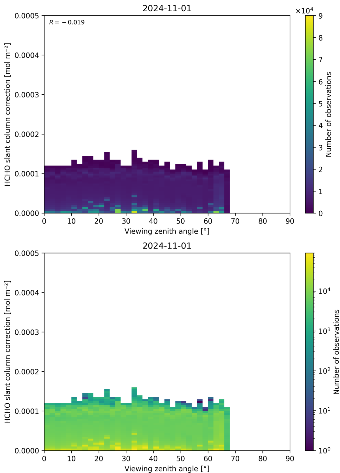
Figure 187: Scatter density plot of “Viewing zenith angle” against “HCHO slant column correction” for 2024-10-31 to 2024-11-02.
