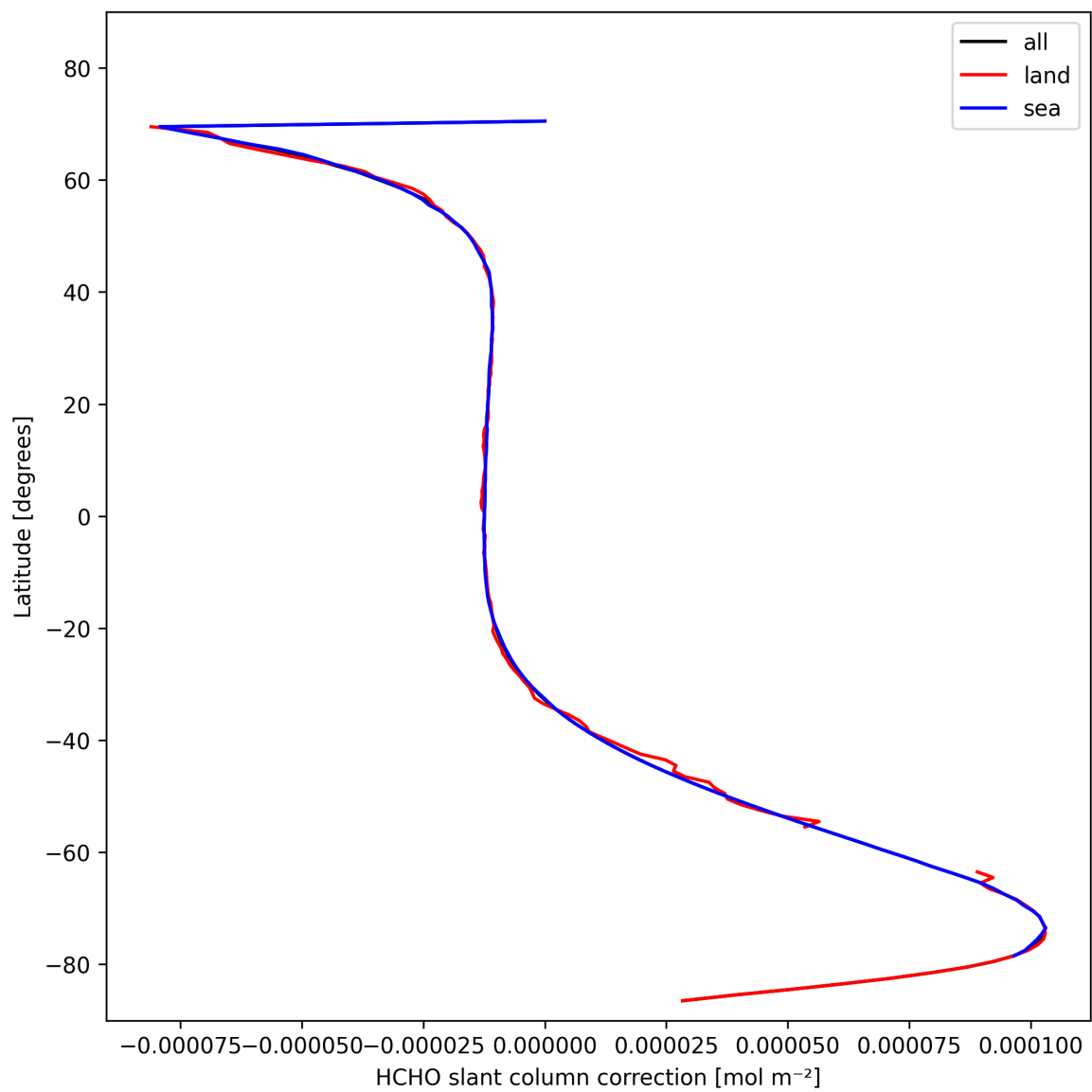
Figure 33: Zonal average of “HCHO slant column correction” for 2024-10-31 to 2024-11-02.
