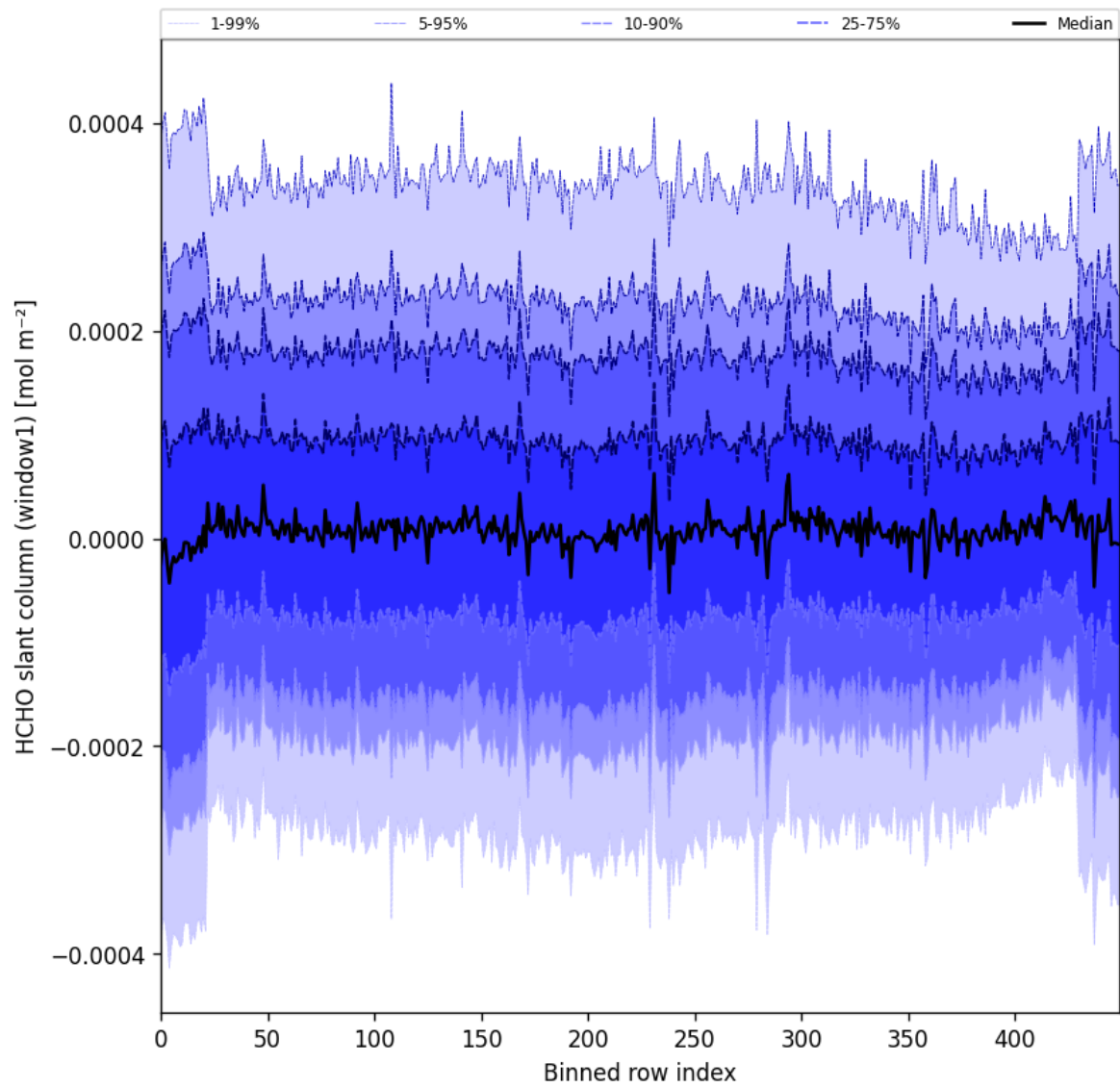
Figure 52: Along track statistics of “HCHO slant column (window1)” for 2024-10-31 to 2024-11-02
