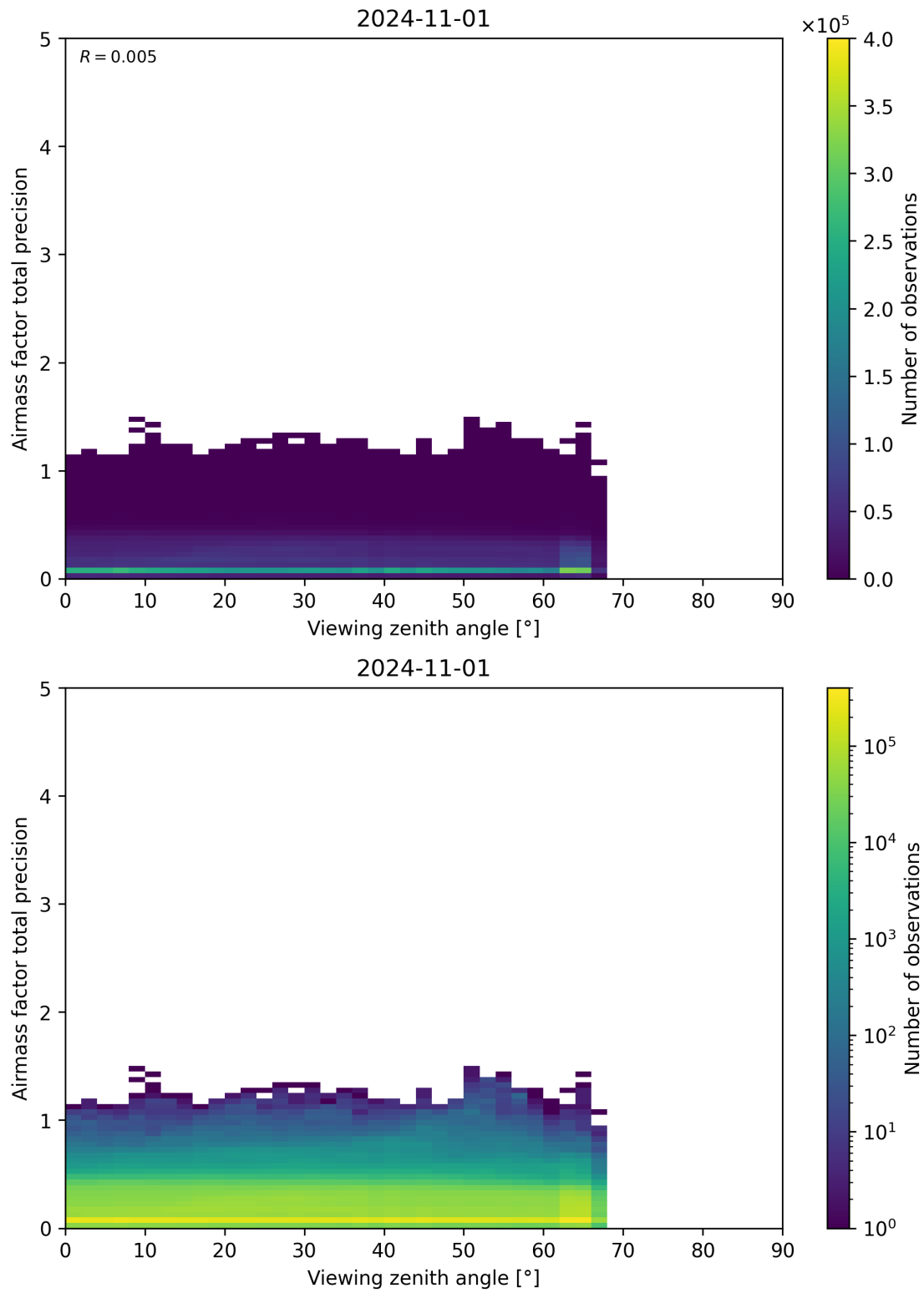
Figure 191: Scatter density plot of “Viewing zenith angle” against “Airmass factor total precision” for 2024-10-31 to 2024-11-02.
