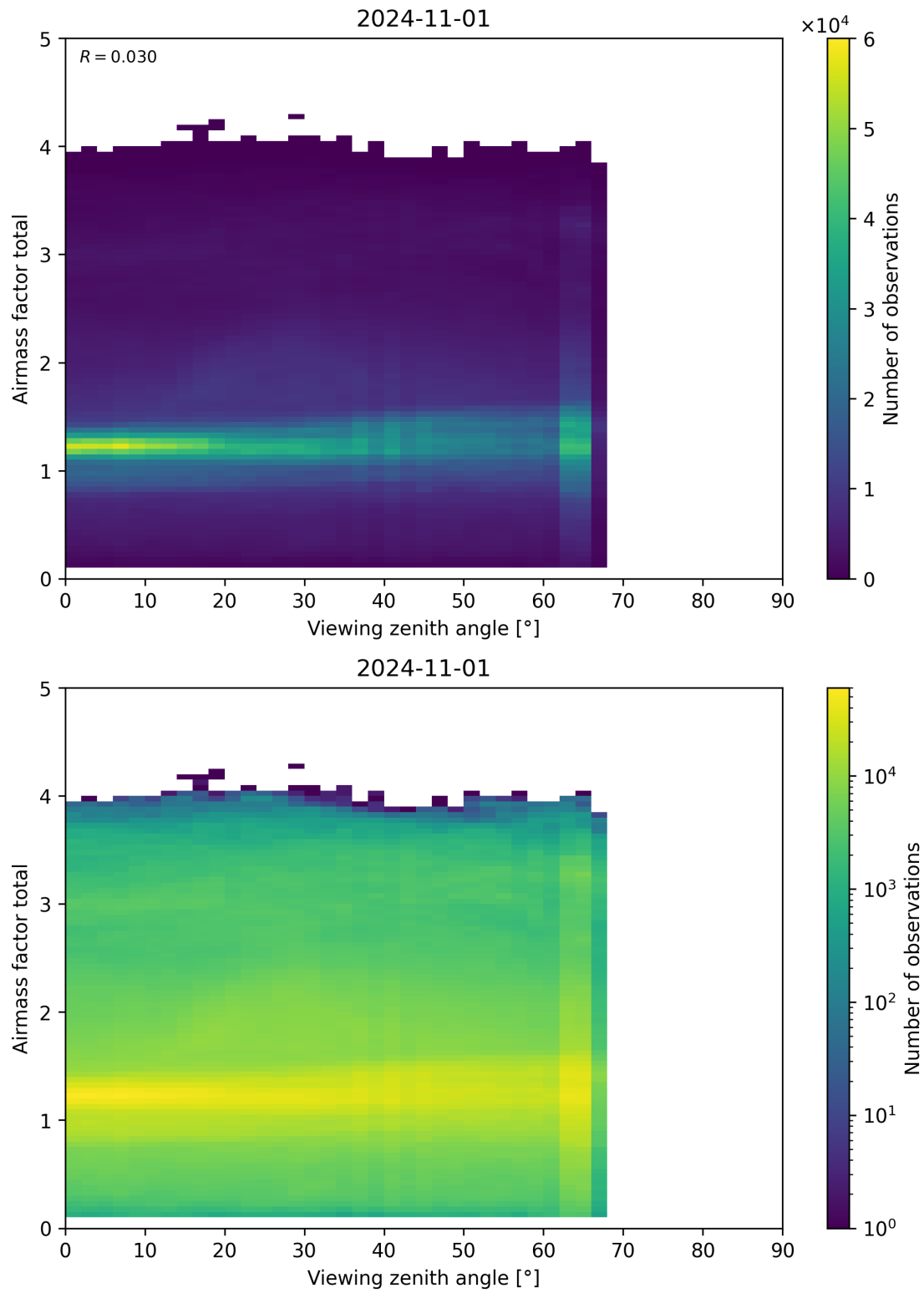
Figure 190: Scatter density plot of “Viewing zenith angle” against “Airmass factor total” for 2024-10-31 to 2024-11-02.
