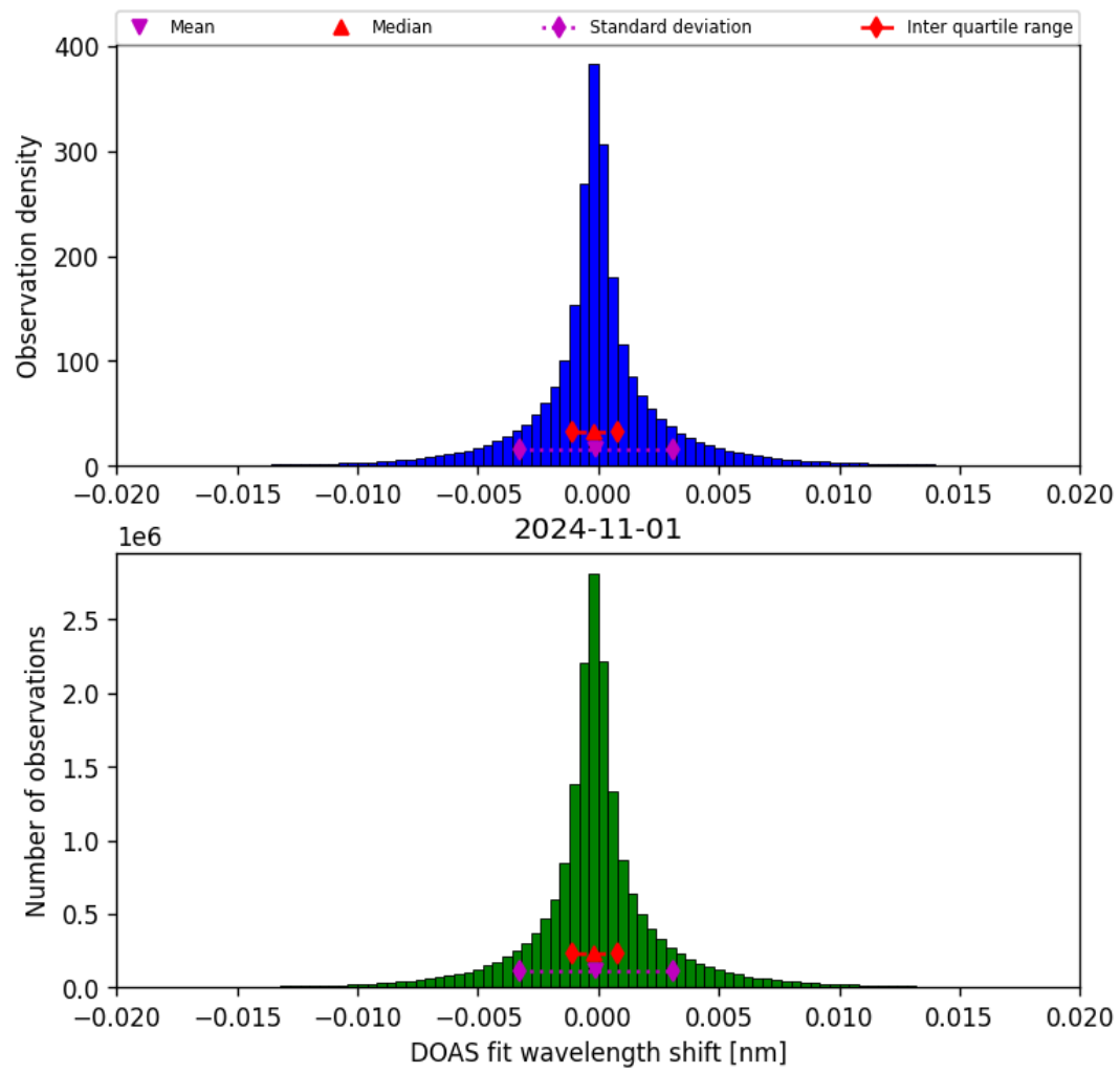
Figure 44: Histogram of “DOAS fit wavelength shift” for 2024-10-31 to 2024-11-02
