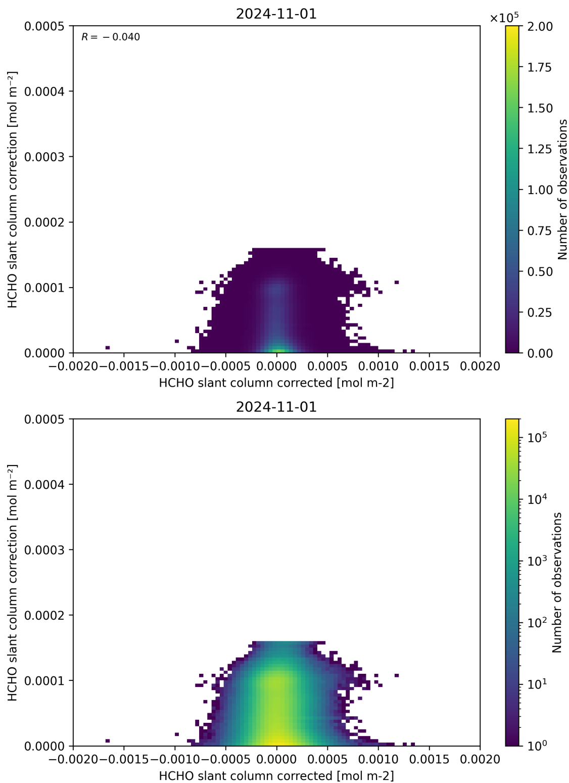
Figure 77: Scatter density plot of “HCHO slant column corrected” against “HCHO slant column correction” for 2024-10-31 to 2024-11-02.
