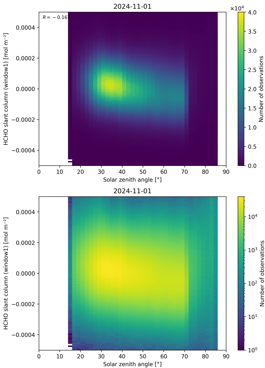
Figure 173: Scatter density plot of “Solar zenith angle” against “HCHO slant column (window1)” for 2024-10-31 to 2024-11-02.
