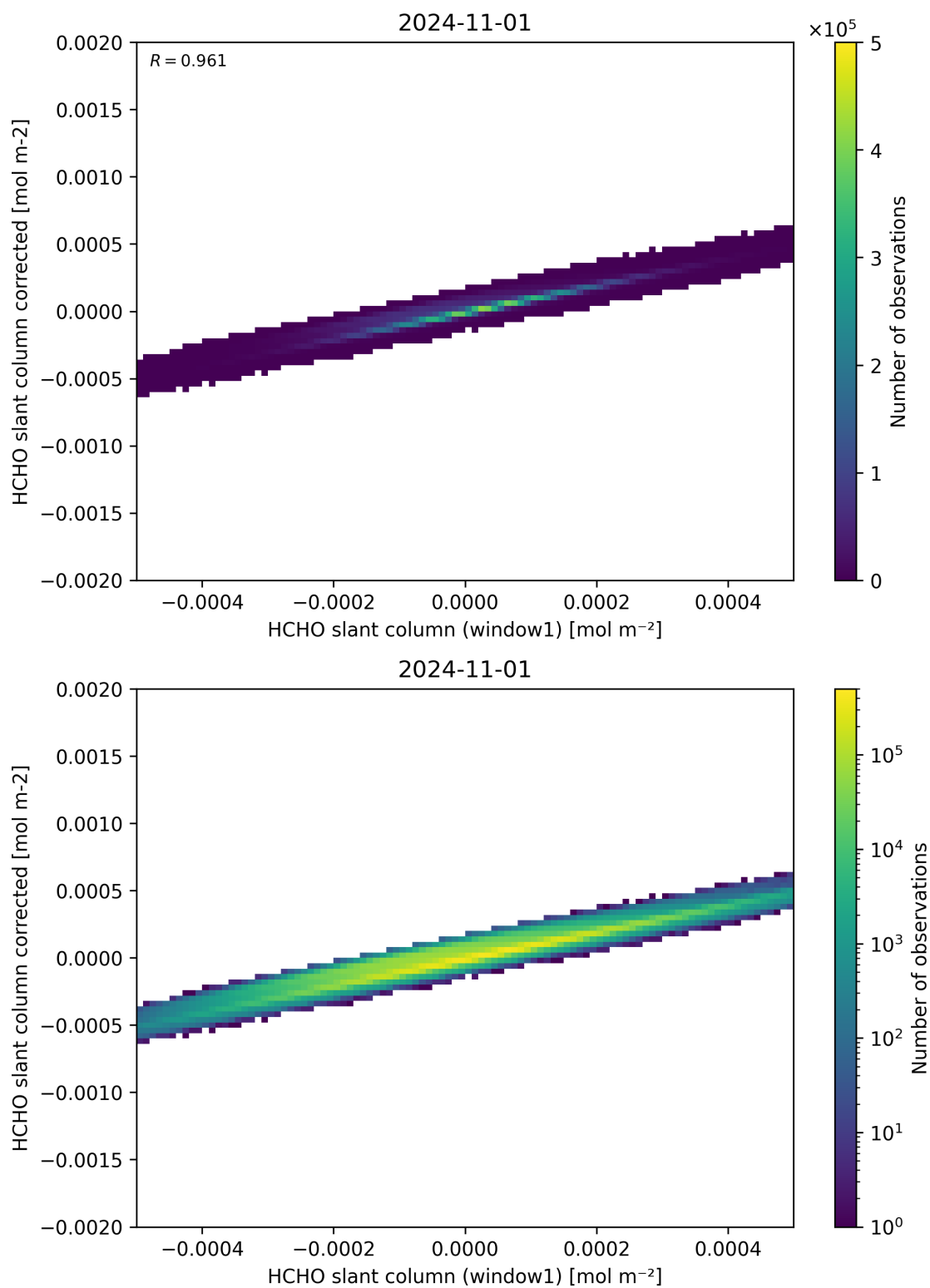
Figure 82: Scatter density plot of “HCHO slant column (window1)” against “HCHO slant column corrected” for 2024-10-31 to 2024-11-02.
