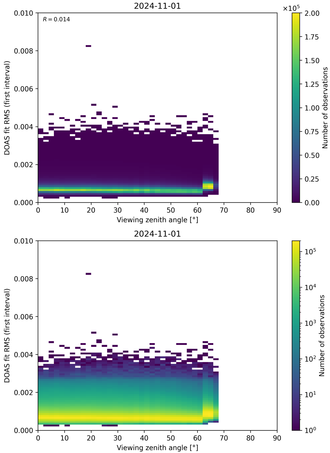
Figure 182: Scatter density plot of “Viewing zenith angle” against “DOAS fit RMS (first interval)” for 2024-10-31 to 2024-11-02.
