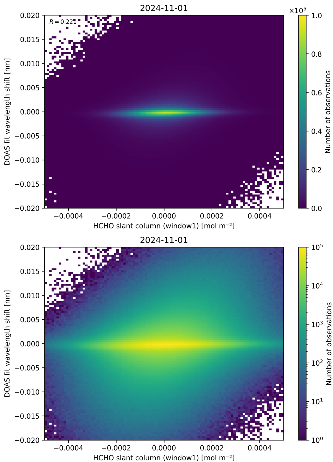
Figure 79: Scatter density plot of “HCHO slant column (window1)” against “DOAS fit wavelength shift” for 2024-10-31 to 2024-11-02.
