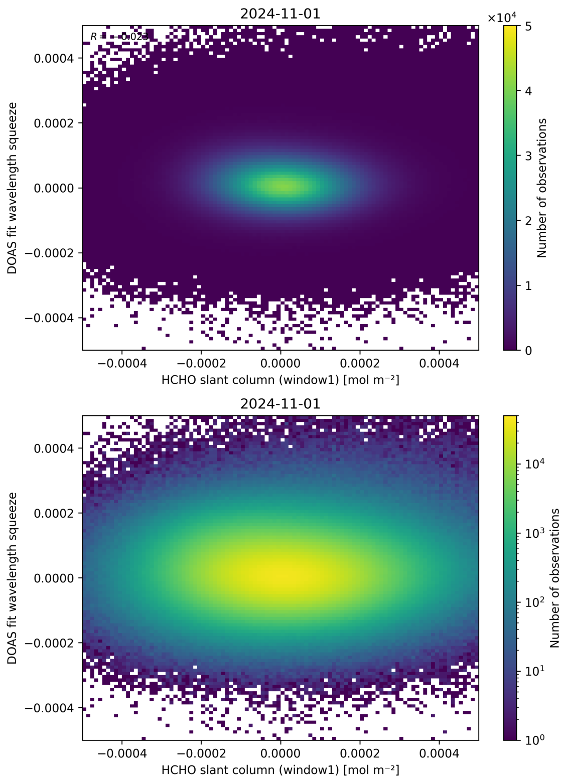
Figure 80: Scatter density plot of “HCHO slant column (window1)” against “DOAS fit wavelength squeeze” for 2024-10-31 to 2024-11-02.
