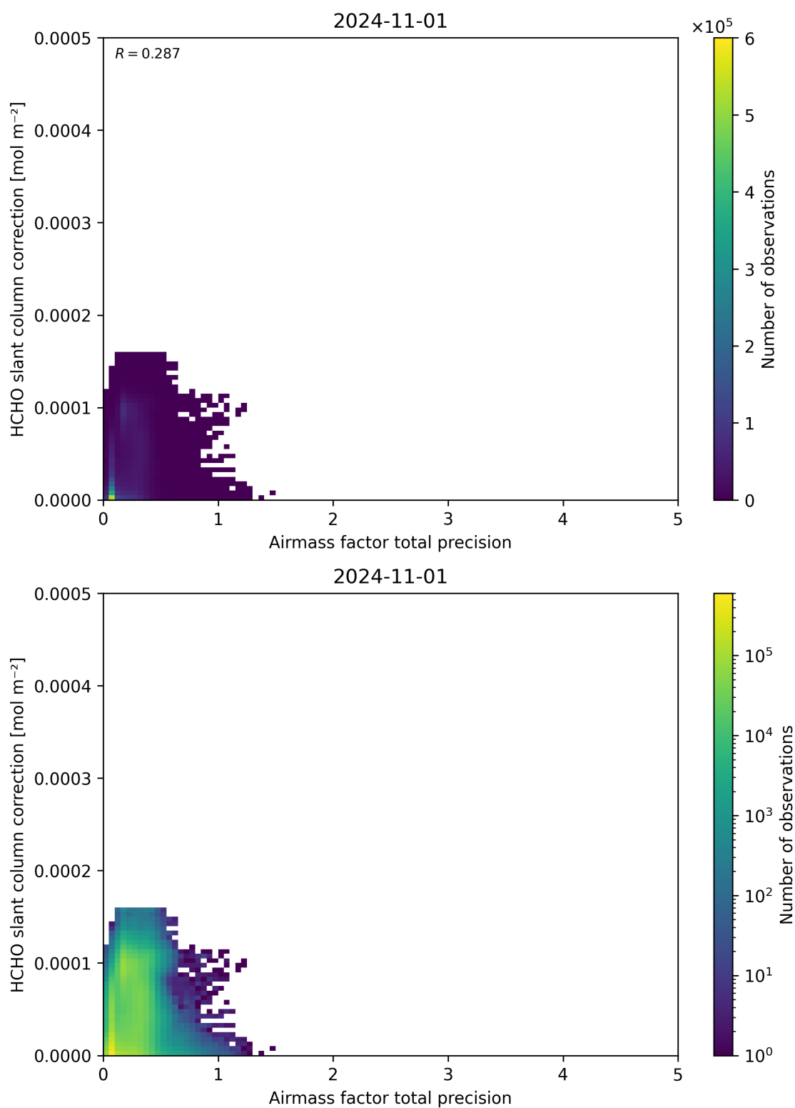
Figure 110: Scatter density plot of “Airmass factor total precision” against “HCHO slant column correction” for 2024-10-31 to 2024-11-02.
