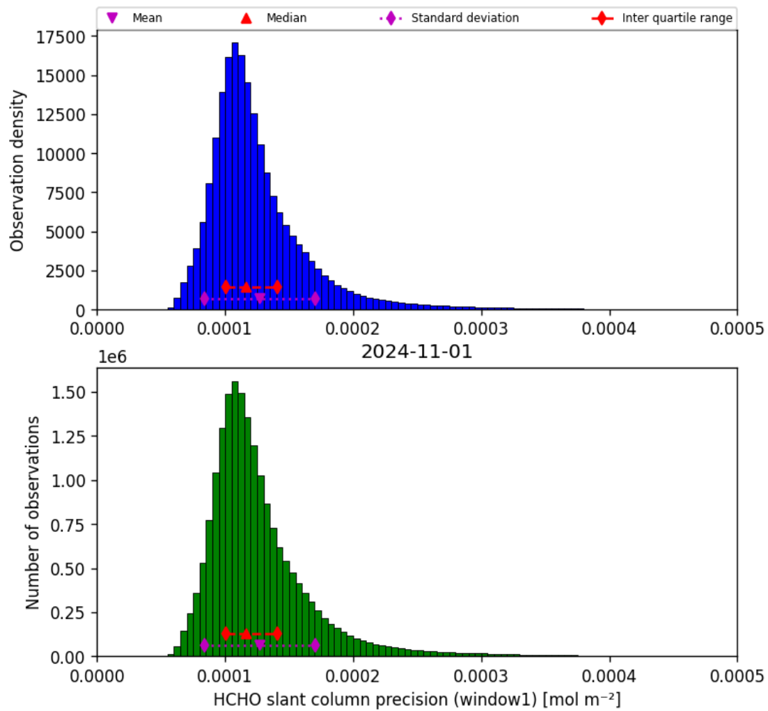
Figure 39: Histogram of “HCHO slant column precision (window1)” for 2024-10-31 to 2024-11-02
