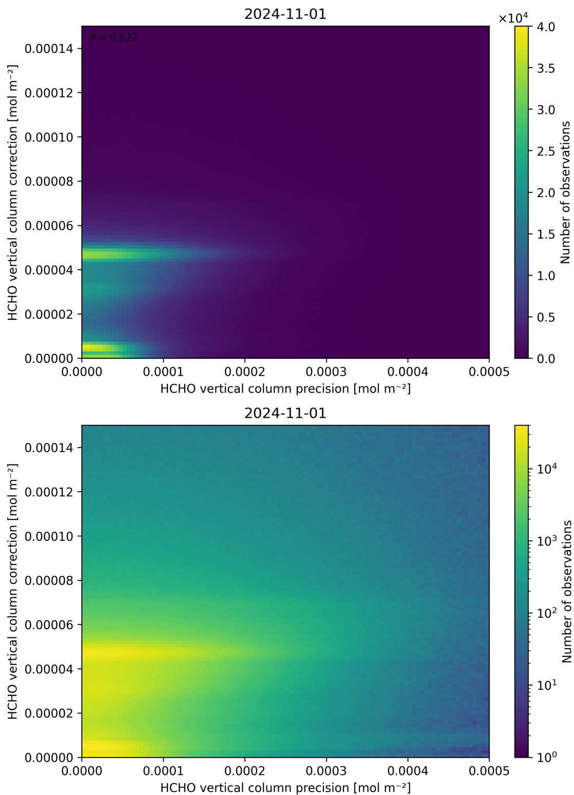
Figure 146: Scatter density plot of “HCHO vertical column precision” against “HCHO vertical column correction” for 2024-10-31 to 2024-11-02.
