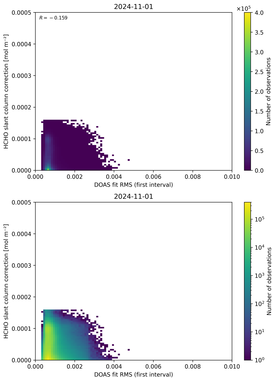
Figure 63: Scatter density plot of “DOAS fit RMS (first interval)” against “HCHO slant column correction” for 2024-10-31 to 2024-11-02.
