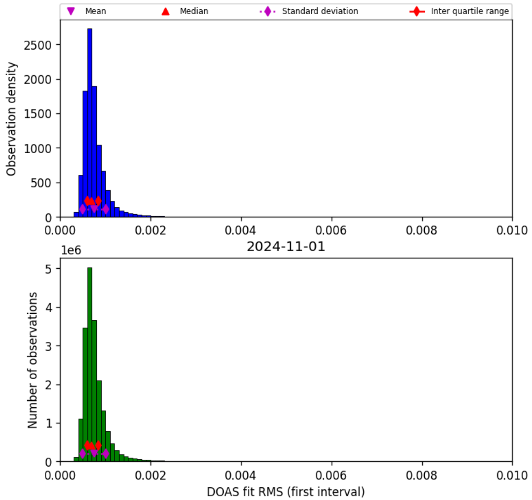
Figure 46: Histogram of “DOAS fit RMS (first interval)” for 2024-10-31 to 2024-11-02
