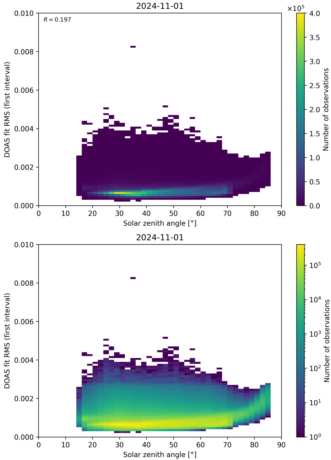
Figure 167: Scatter density plot of “Solar zenith angle” against “DOAS fit RMS (first interval)” for 2024-10-31 to 2024-11-02.
