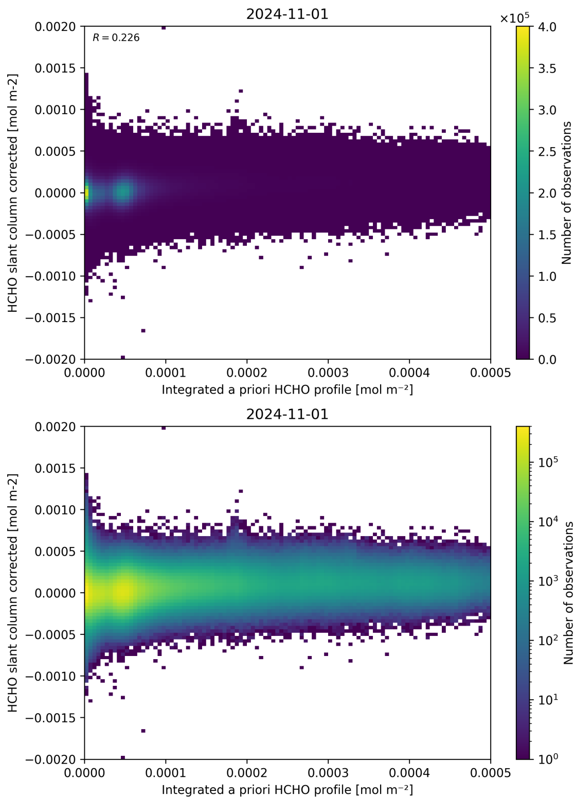
Figure 151: Scatter density plot of “Integrated a priori HCHO profile” against “HCHO slant column corrected” for 2024-10-31 to 2024-11-02.
