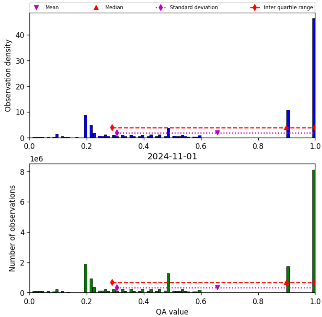
Figure 34: Histogram of “QA value” for 2024-10-31 to 2024-11-02
