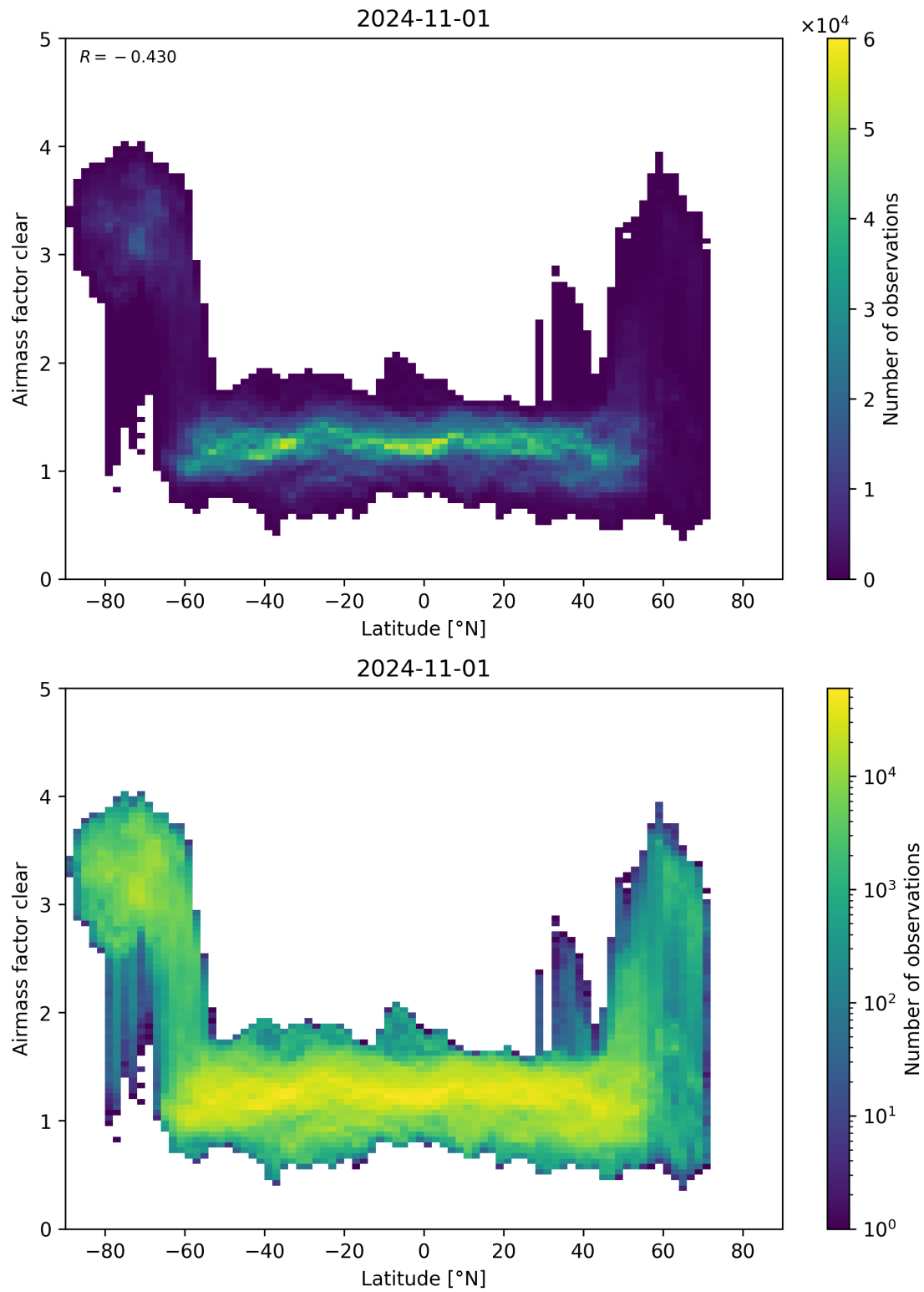
Figure 156: Scatter density plot of “Latitude” against “Airmass factor clear” for 2024-10-31 to 2024-11-02.
