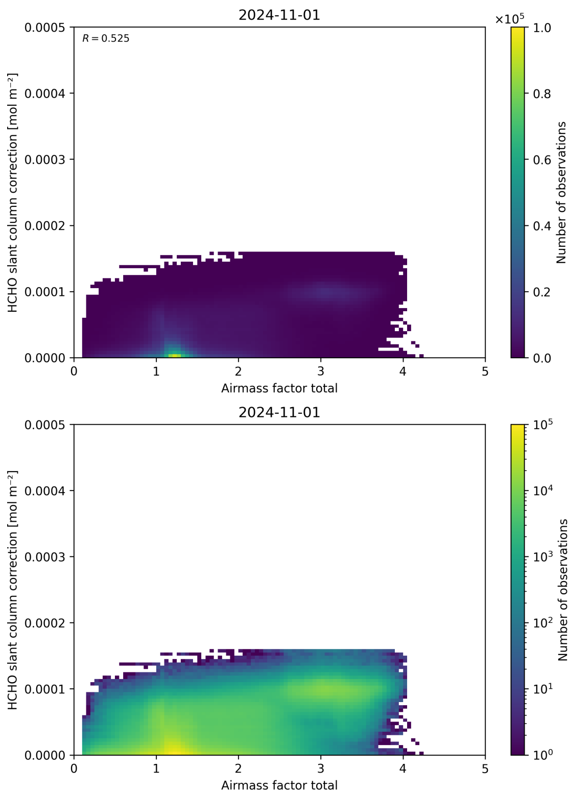
Figure 102: Scatter density plot of “Airmass factor total” against “HCHO slant column correction” for 2024-10-31 to 2024-11-02.
