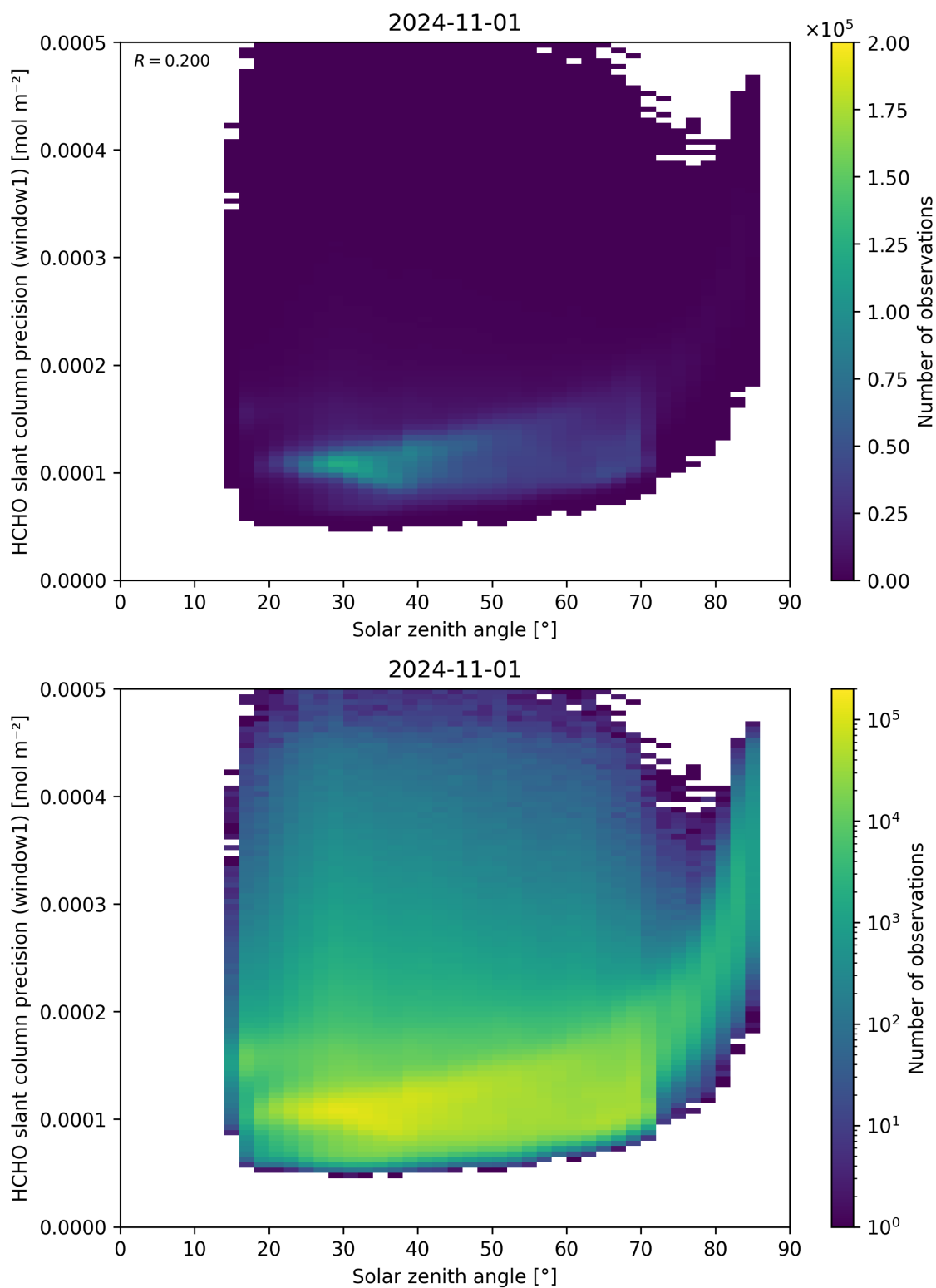
Figure 174: Scatter density plot of “Solar zenith angle” against “HCHO slant column precision (window1)” for 2024-10-31 to 2024-11-02.
