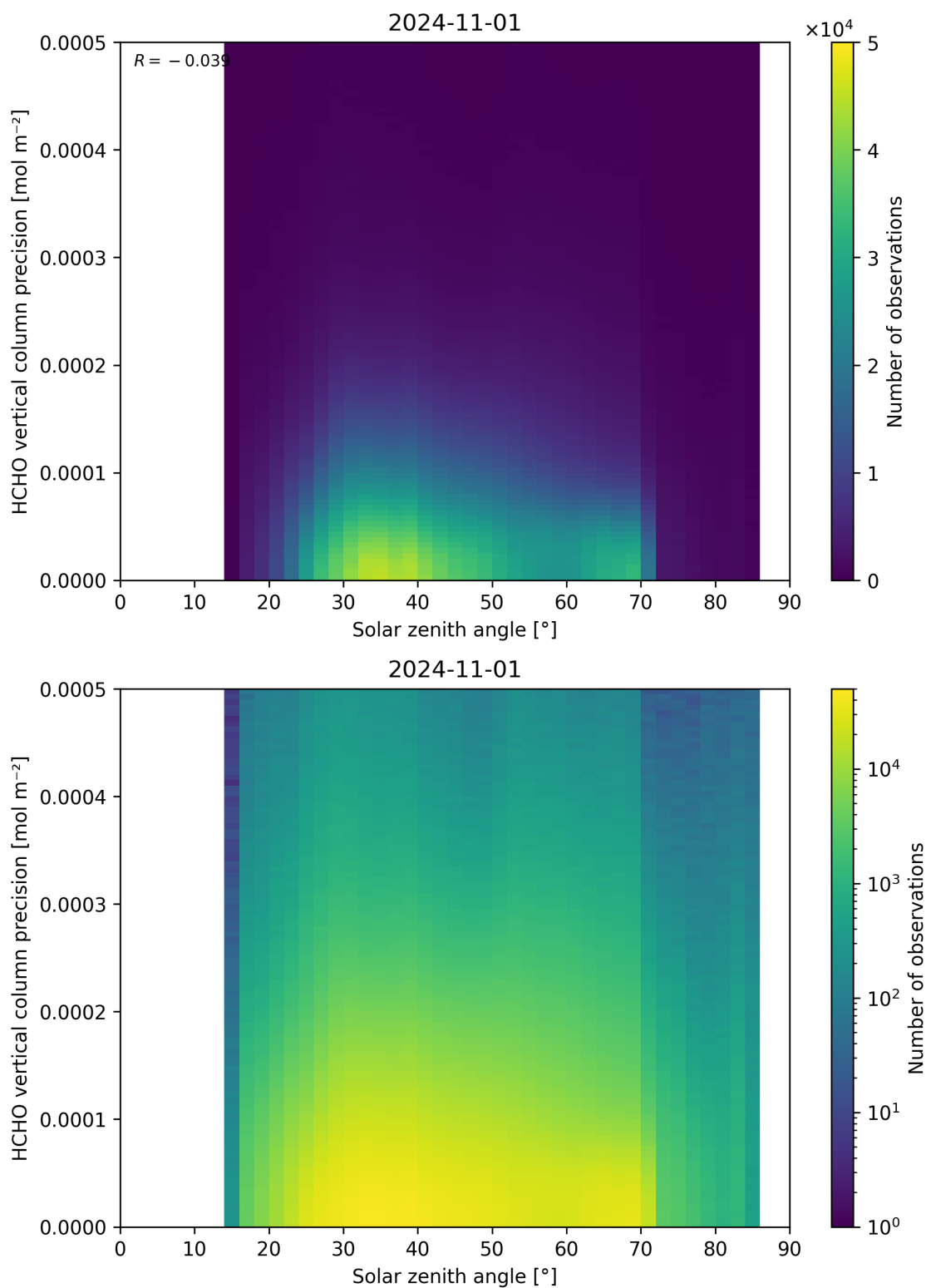
Figure 179: Scatter density plot of “Solar zenith angle” against “HCHO vertical column precision” for 2024-10-31 to 2024-11-02.
