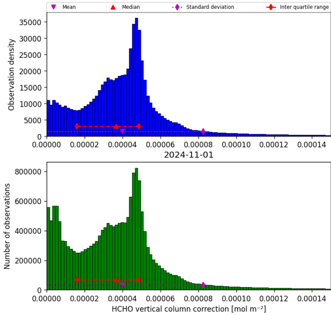
Figure 37: Histogram of “HCHO vertical column correction” for 2024-10-31 to 2024-11-02
