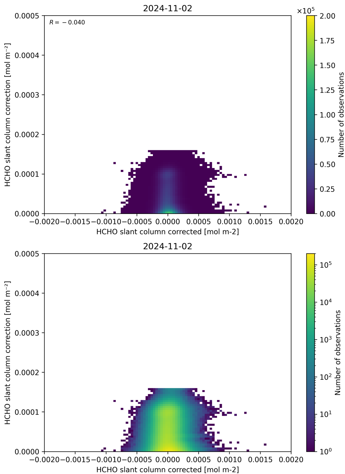
Figure 77: Scatter density plot of “HCHO slant column corrected” against “HCHO slant column correction” for 2024-11-01 to 2024-11-03.
