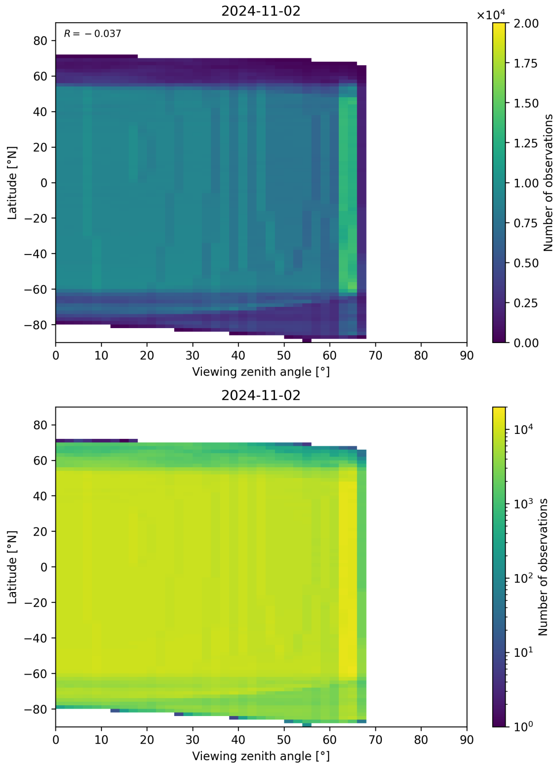
Figure 196: Scatter density plot of “Viewing zenith angle” against “Latitude” for 2024-11-01 to 2024-11-03.
