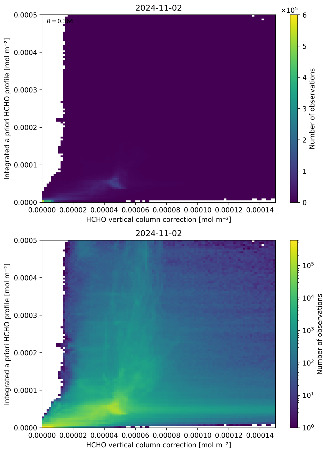
Figure 122: Scatter density plot of “HCHO vertical column correction” against “Integrated a priori HCHO profile” for 2024-11-01 to 2024-11-03.
