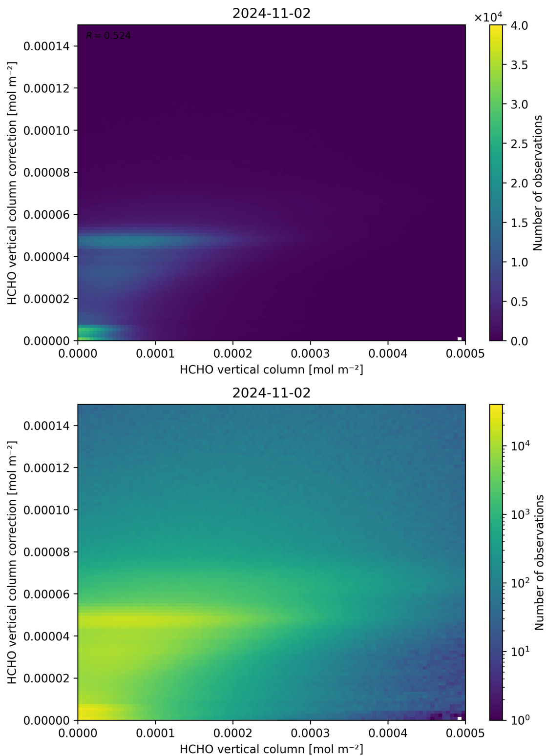
Figure 133: Scatter density plot of “HCHO vertical column” against “HCHO vertical column correction” for 2024-11-01 to 2024-11-03.
