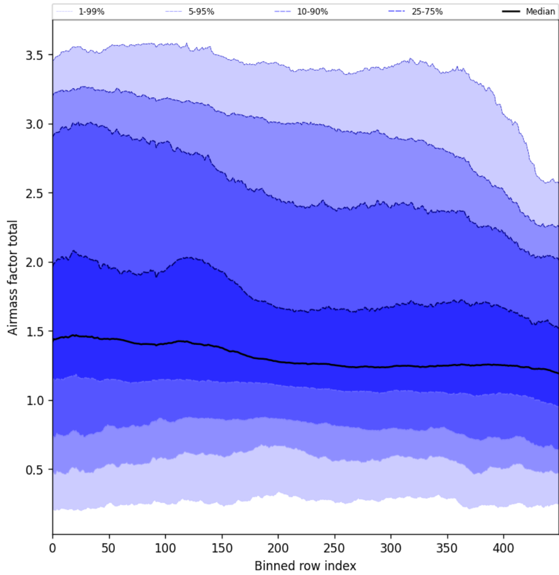
Figure 54: Along track statistics of “Airmass factor total” for 2024-11-01 to 2024-11-03
