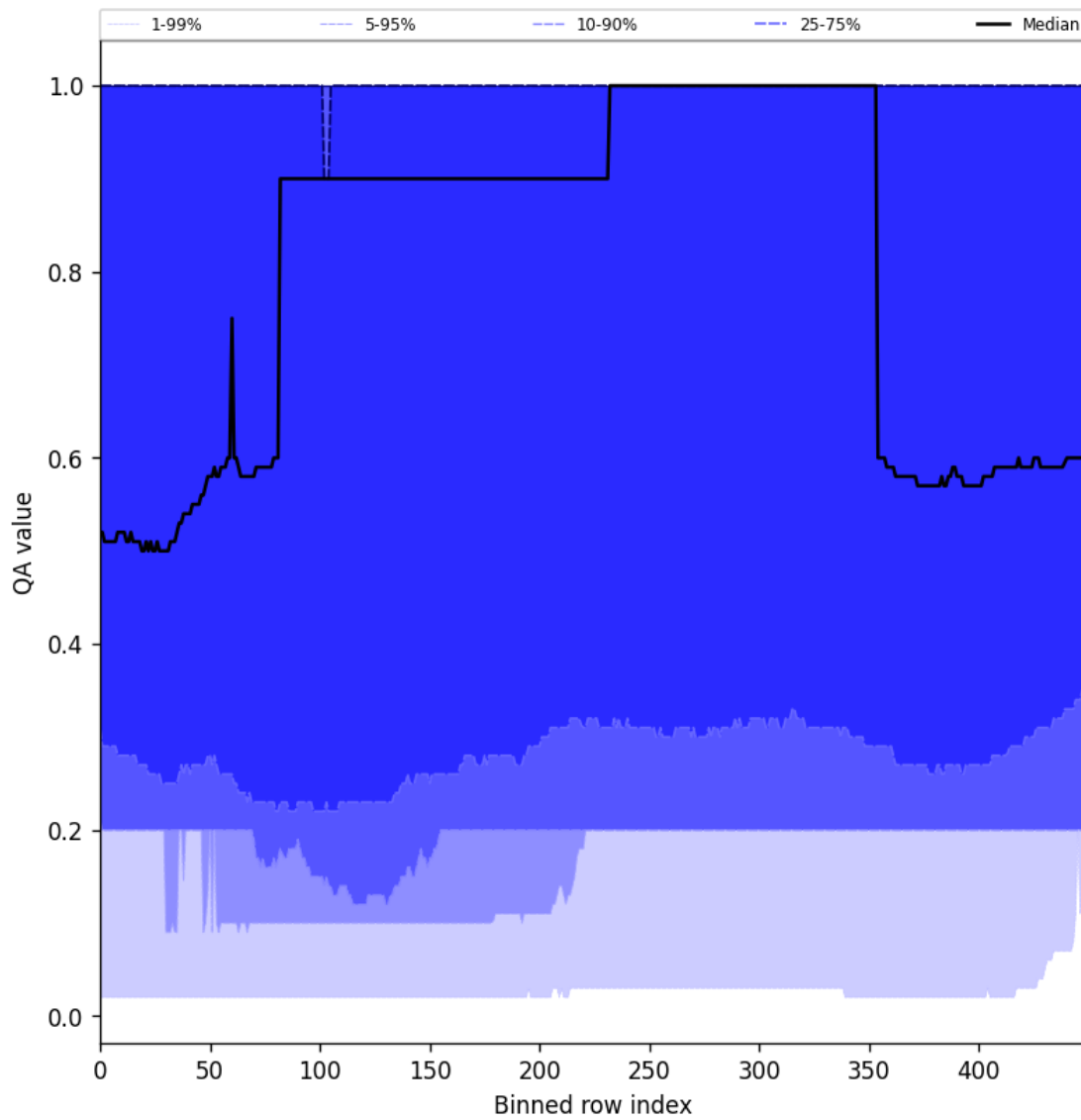
Figure 48: Along track statistics of “QA value” for 2024-11-01 to 2024-11-03
