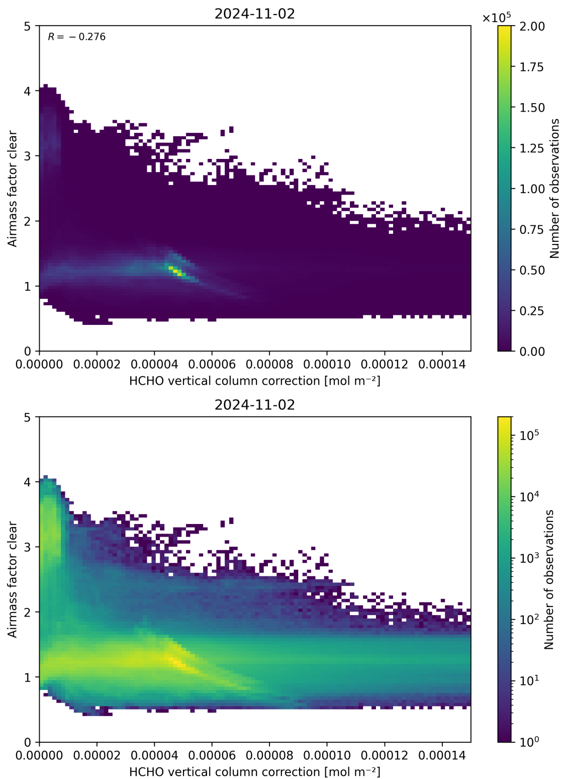
Figure 115: Scatter density plot of “HCHO vertical column correction” against “Airmass factor clear” for 2024-11-01 to 2024-11-03.
