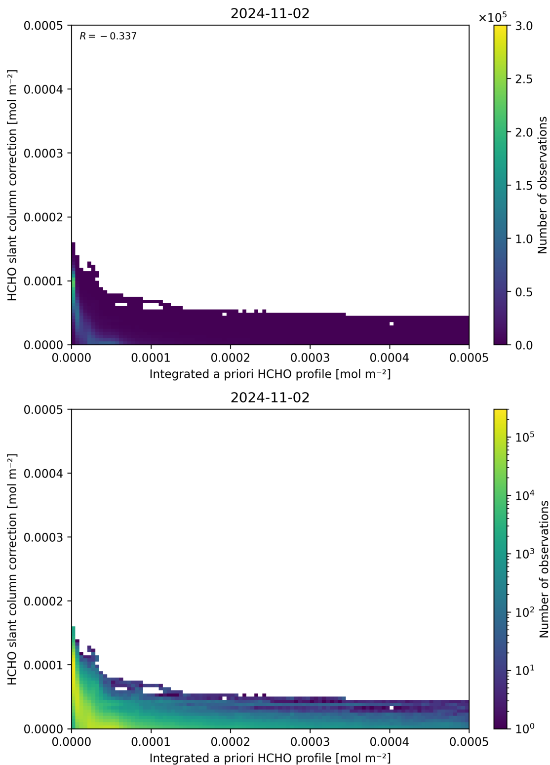
Figure 152: Scatter density plot of “Integrated a priori HCHO profile” against “HCHO slant column correction” for 2024-11-01 to 2024-11-03.
