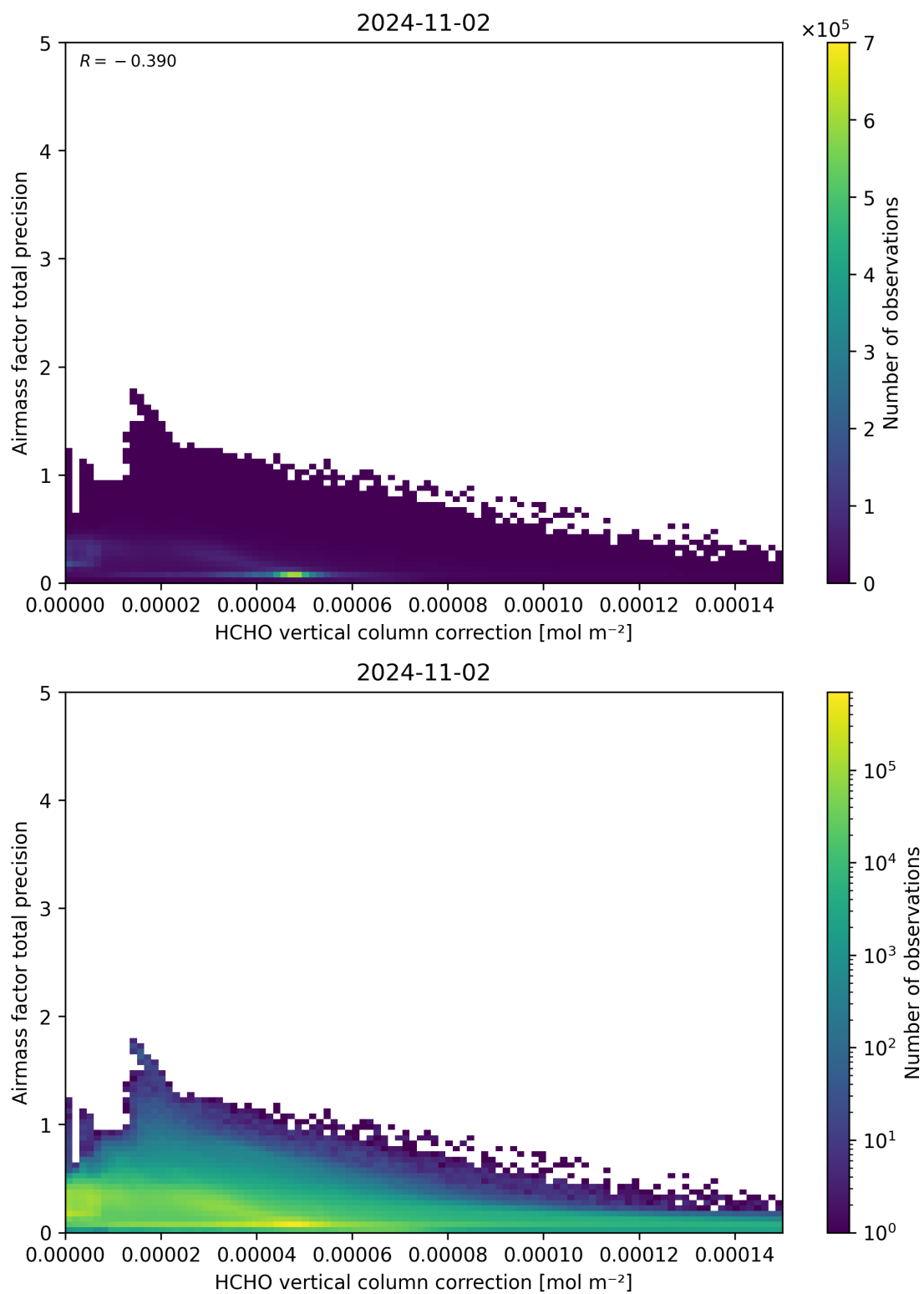
Figure 121: Scatter density plot of “HCHO vertical column correction” against “Airmass factor total precision” for 2024-11-01 to 2024-11-03.
