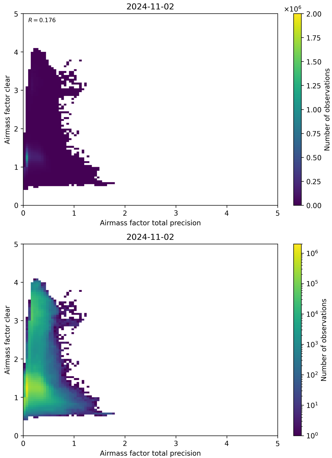
Figure 108: Scatter density plot of “Airmass factor total precision” against “Airmass factor clear” for 2024-11-01 to 2024-11-03.
