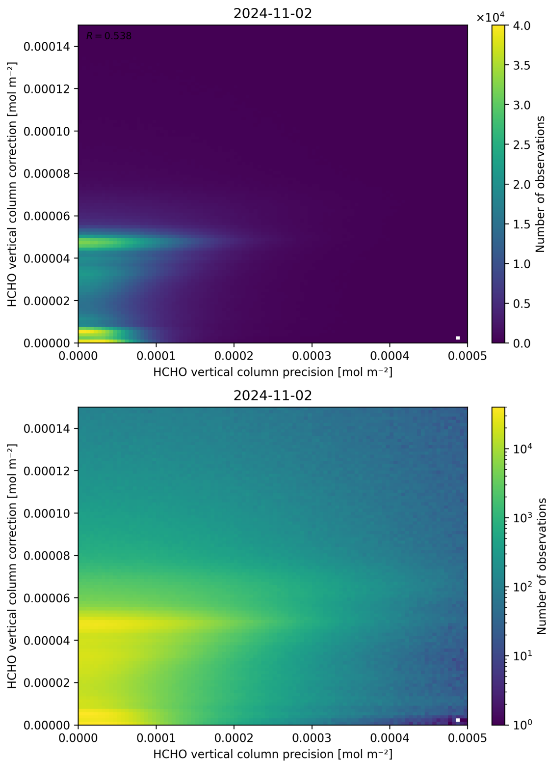
Figure 146: Scatter density plot of “HCHO vertical column precision” against “HCHO vertical column correction” for 2024-11-01 to 2024-11-03.
