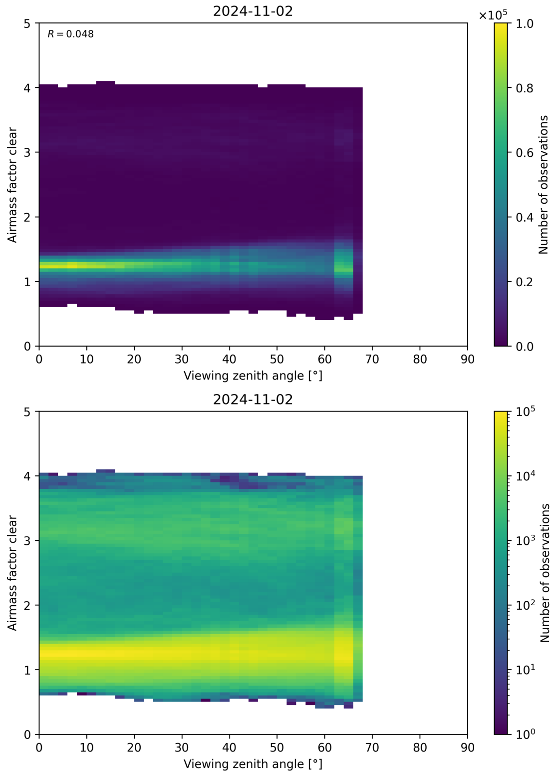
Figure 185: Scatter density plot of “Viewing zenith angle” against “Airmass factor clear” for 2024-11-01 to 2024-11-03.
