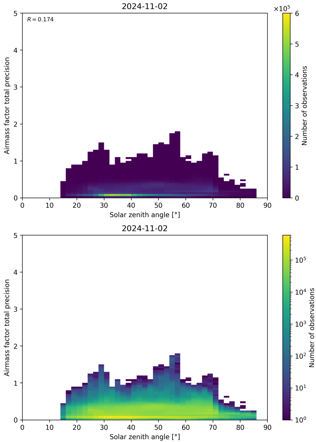
Figure 176: Scatter density plot of “Solar zenith angle” against “Airmass factor total precision” for 2024-11-01 to 2024-11-03.
