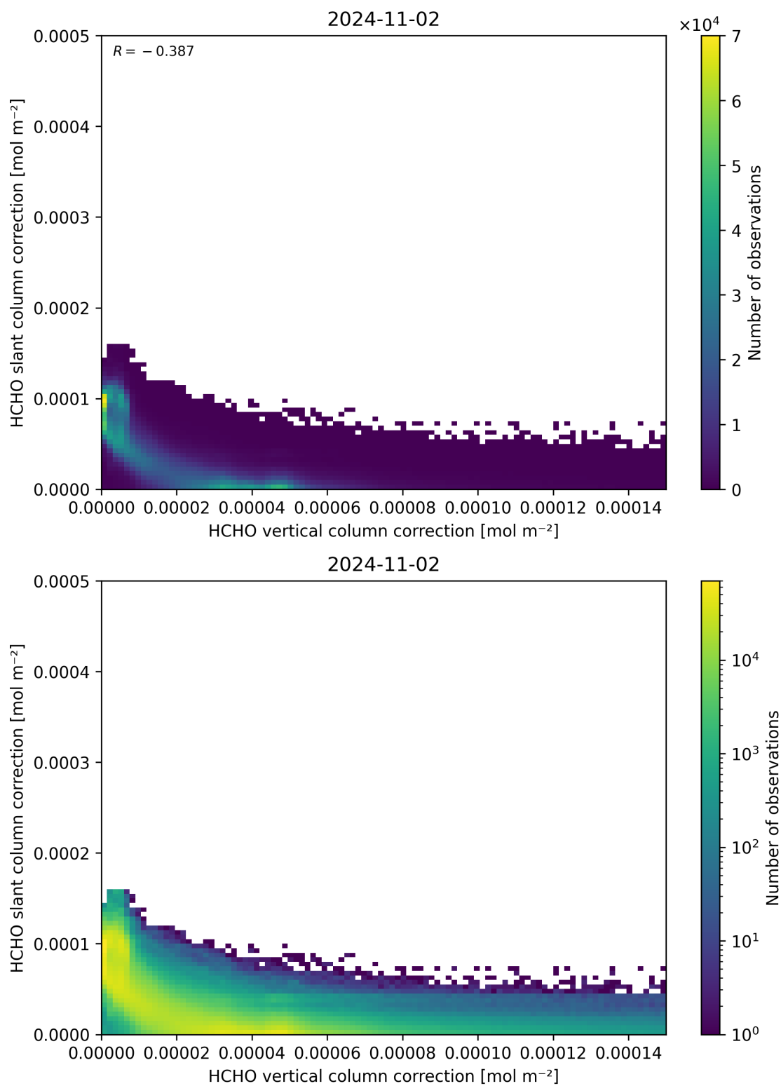
Figure 117: Scatter density plot of “HCHO vertical column correction” against “HCHO slant column correction” for 2024-11-01 to 2024-11-03.
