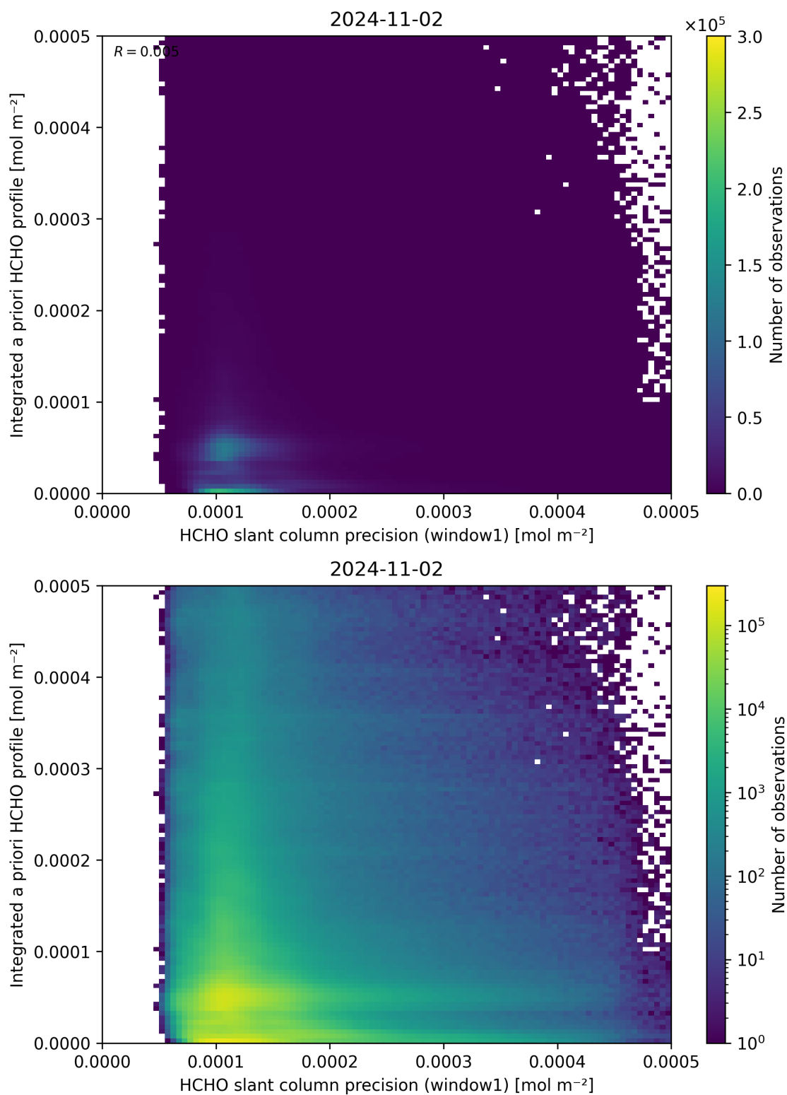
Figure 96: Scatter density plot of “HCHO slant column precision (window1)” against “Integrated a priori HCHO profile” for 2024-11-01 to 2024-11-03.
