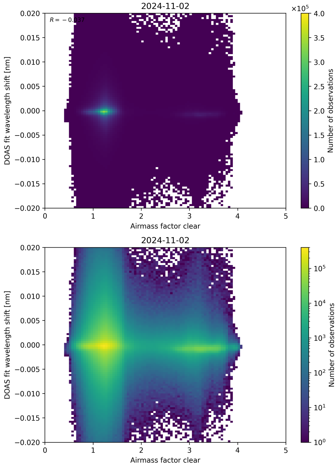
Figure 72: Scatter density plot of “Airmass factor clear” against “DOAS fit wavelength shift” for 2024-11-01 to 2024-11-03.
