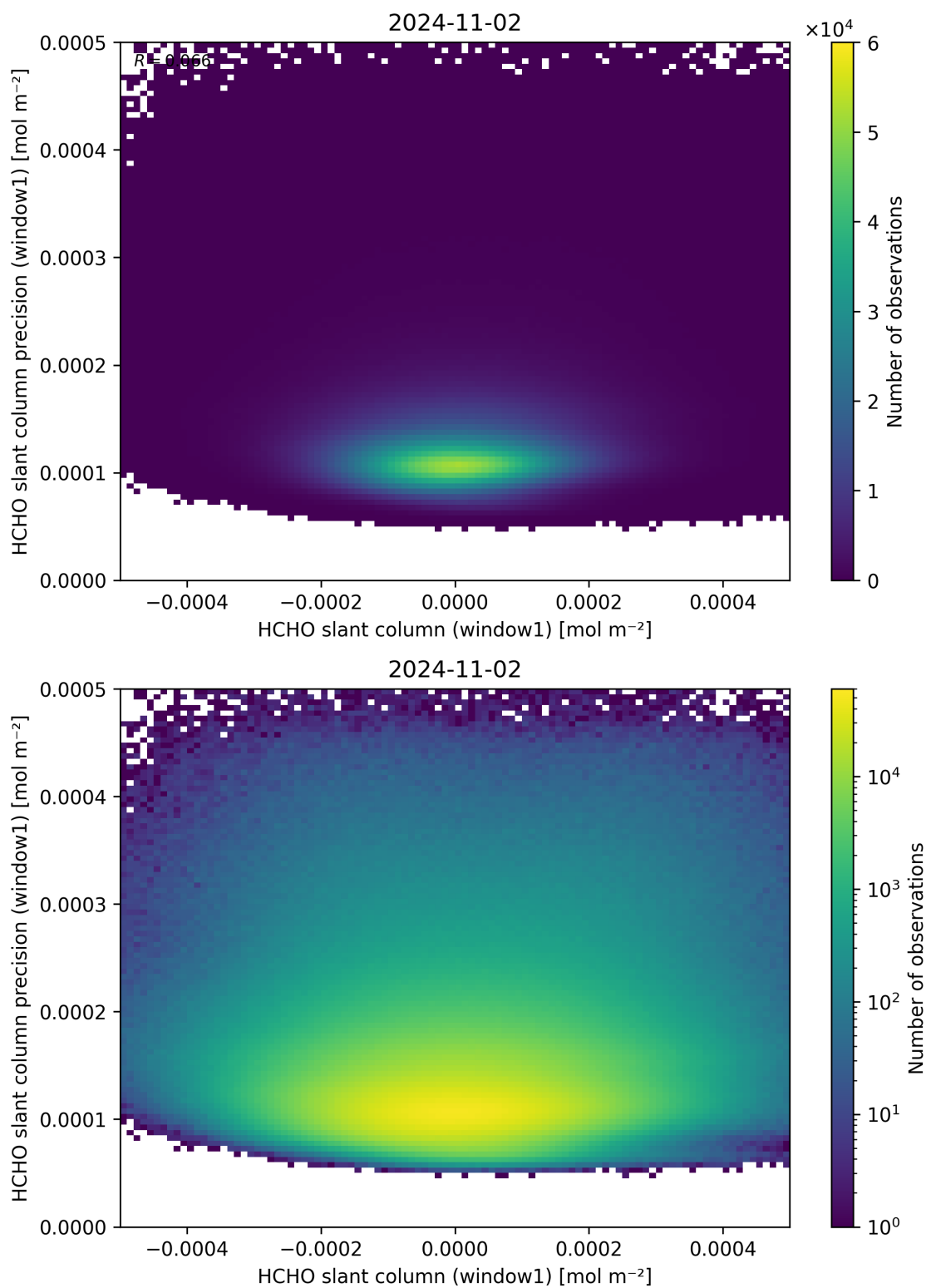
Figure 84: Scatter density plot of “HCHO slant column (window1)” against “HCHO slant column precision (window1)” for 2024-11-01 to 2024-11-03.
