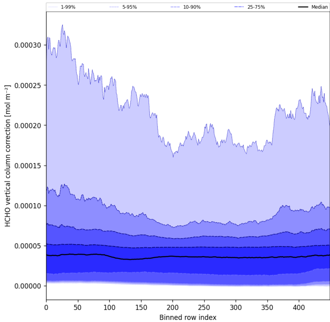
Figure 51: Along track statistics of “HCHO vertical column correction” for 2024-11-01 to 2024-11-03
