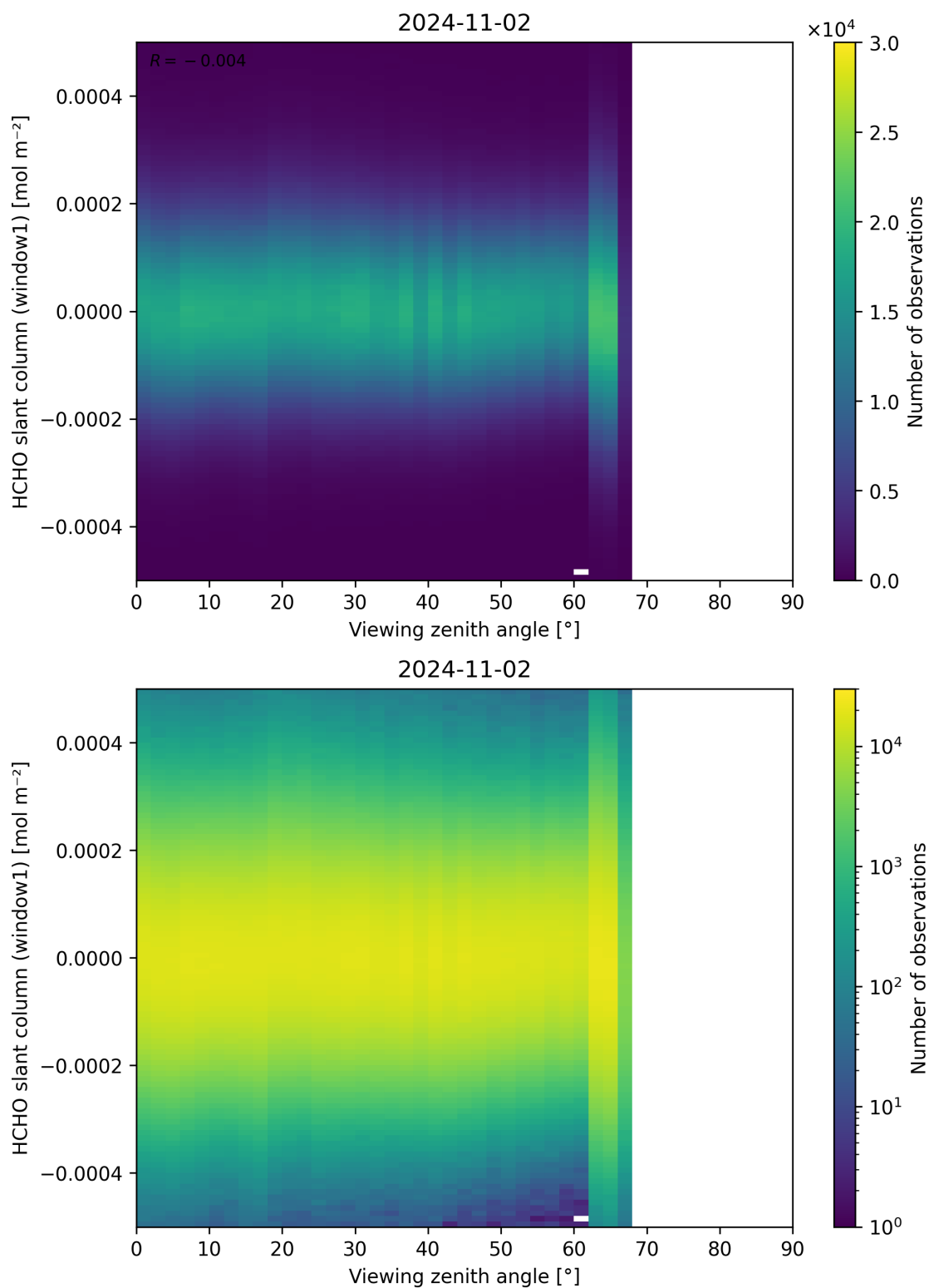
Figure 188: Scatter density plot of “Viewing zenith angle” against “HCHO slant column (window1)” for 2024-11-01 to 2024-11-03.
