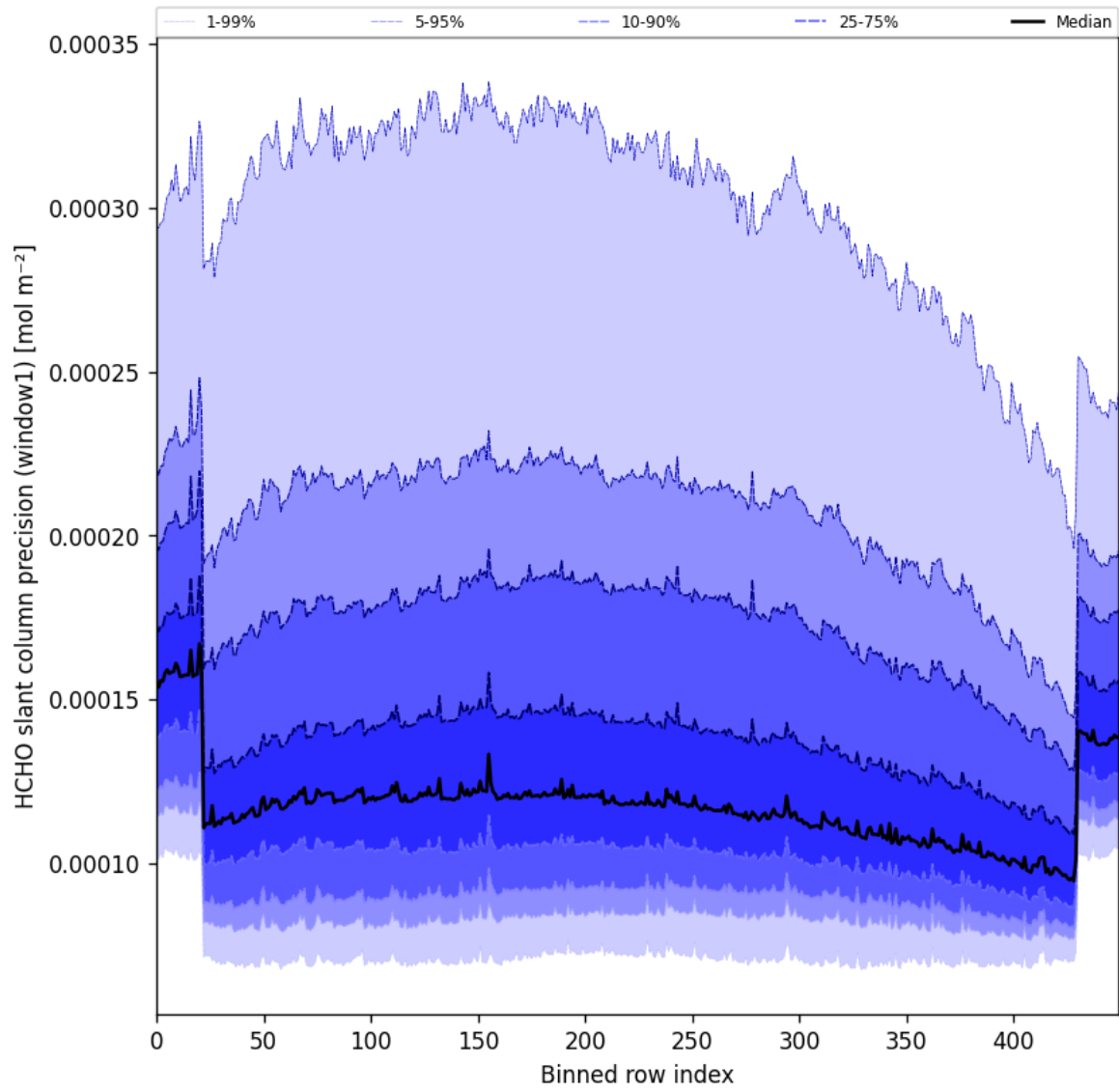
Figure 53: Along track statistics of “HCHO slant column precision (window1)” for 2024-11-01 to 2024-11-03
