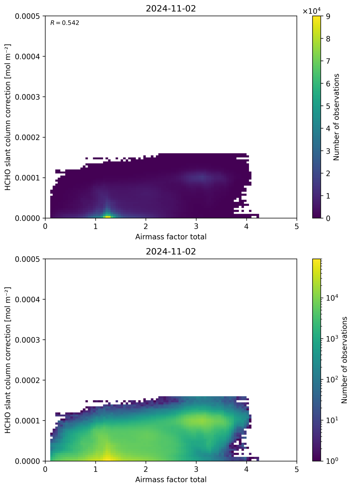
Figure 102: Scatter density plot of “Airmass factor total” against “HCHO slant column correction” for 2024-11-01 to 2024-11-03.
