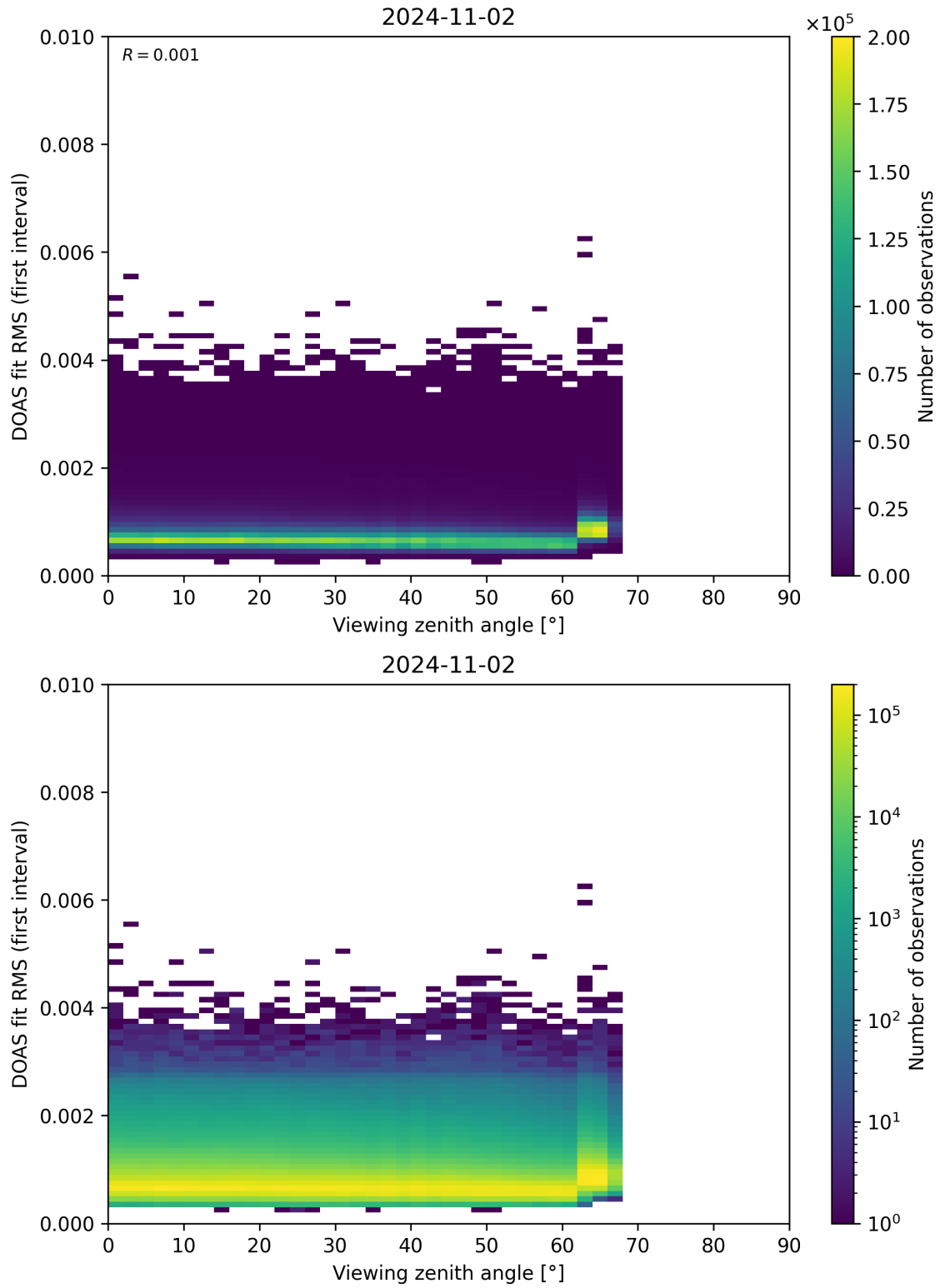
Figure 182: Scatter density plot of “Viewing zenith angle” against “DOAS fit RMS (first interval)” for 2024-11-01 to 2024-11-03.
