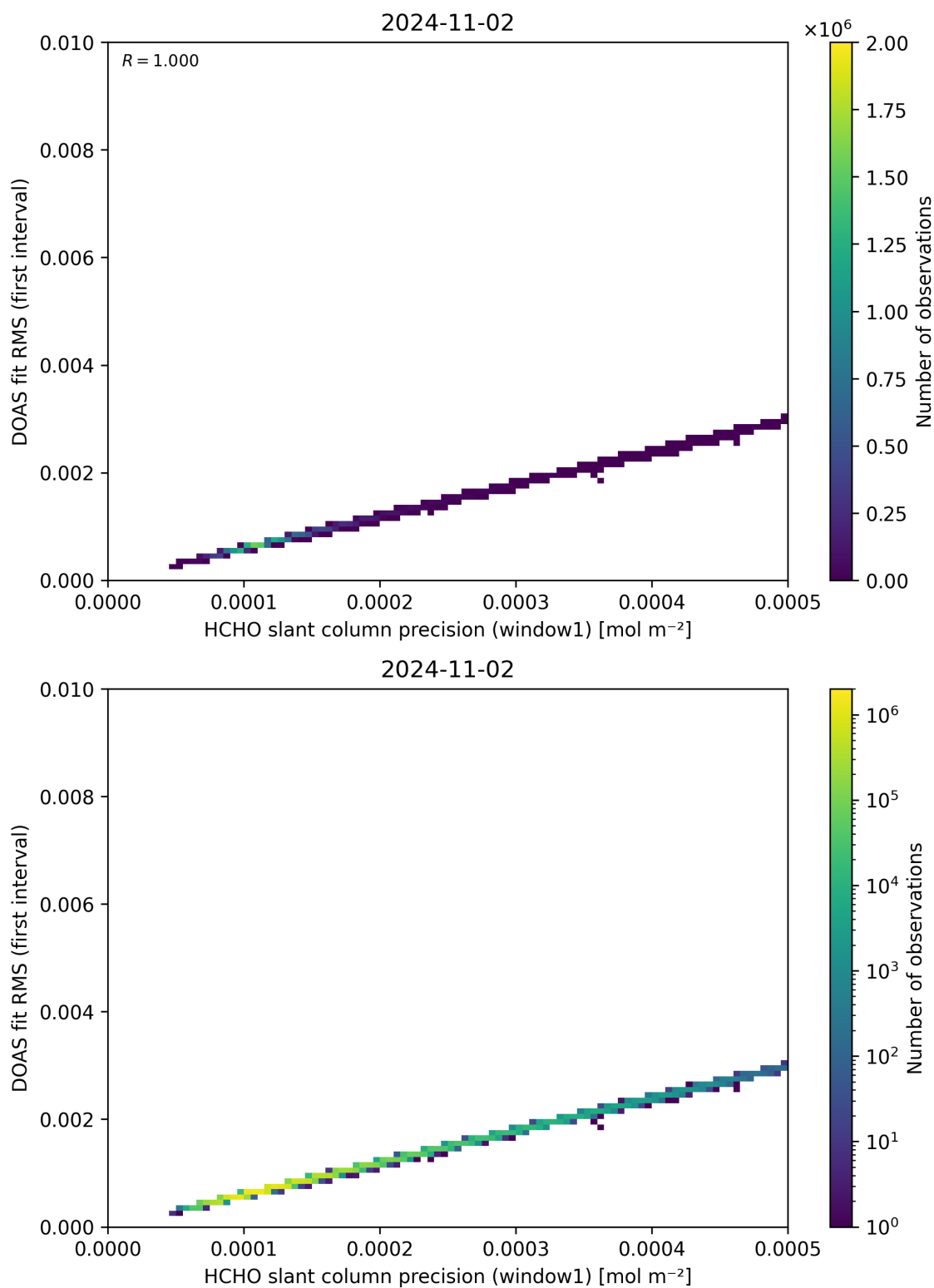
Figure 88: Scatter density plot of “HCHO slant column precision (window1)” against “DOAS fit RMS (first interval)” for 2024-11-01 to 2024-11-03.
