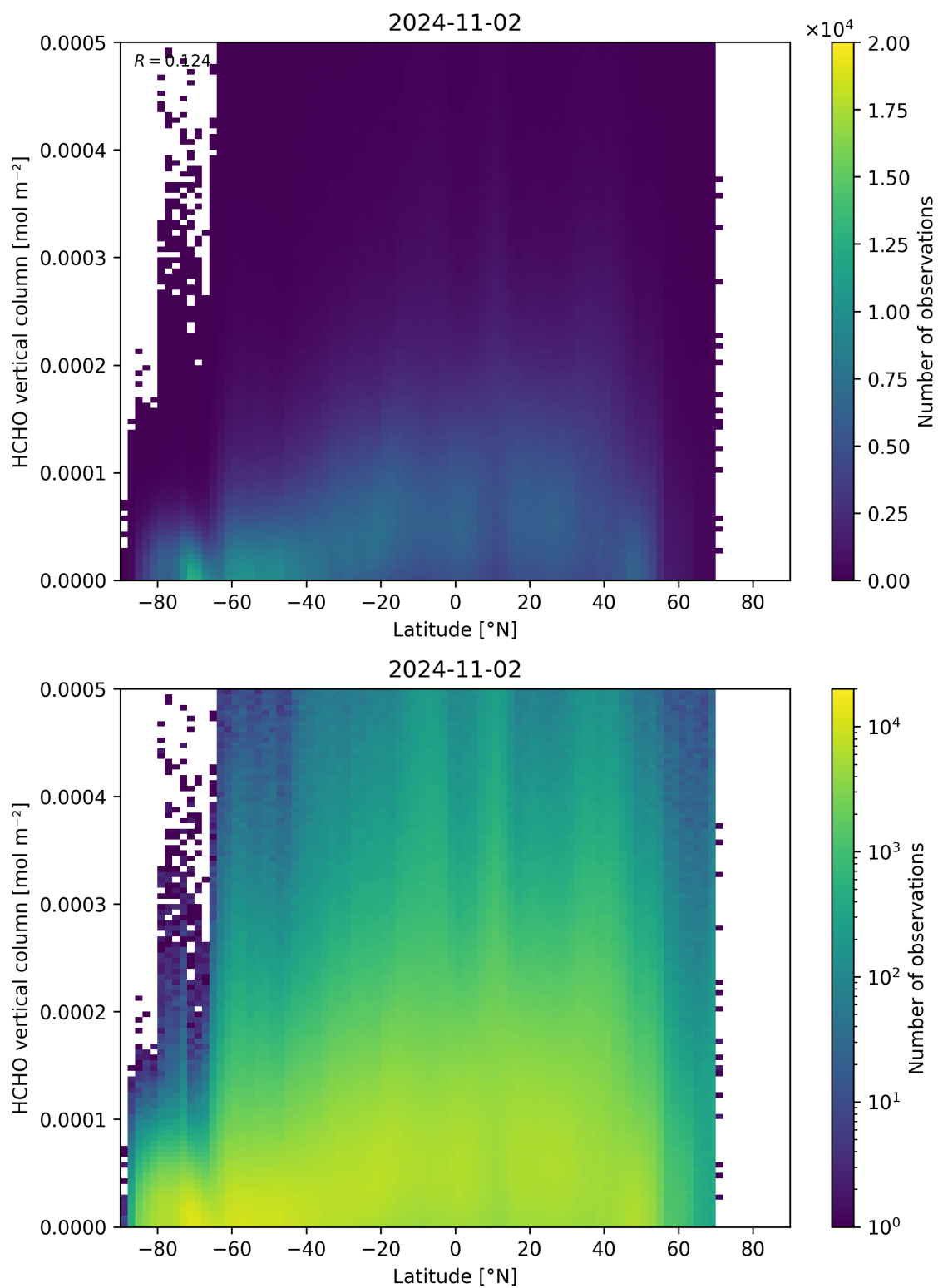
Figure 163: Scatter density plot of “Latitude” against “HCHO vertical column” for 2024-11-01 to 2024-11-03.
