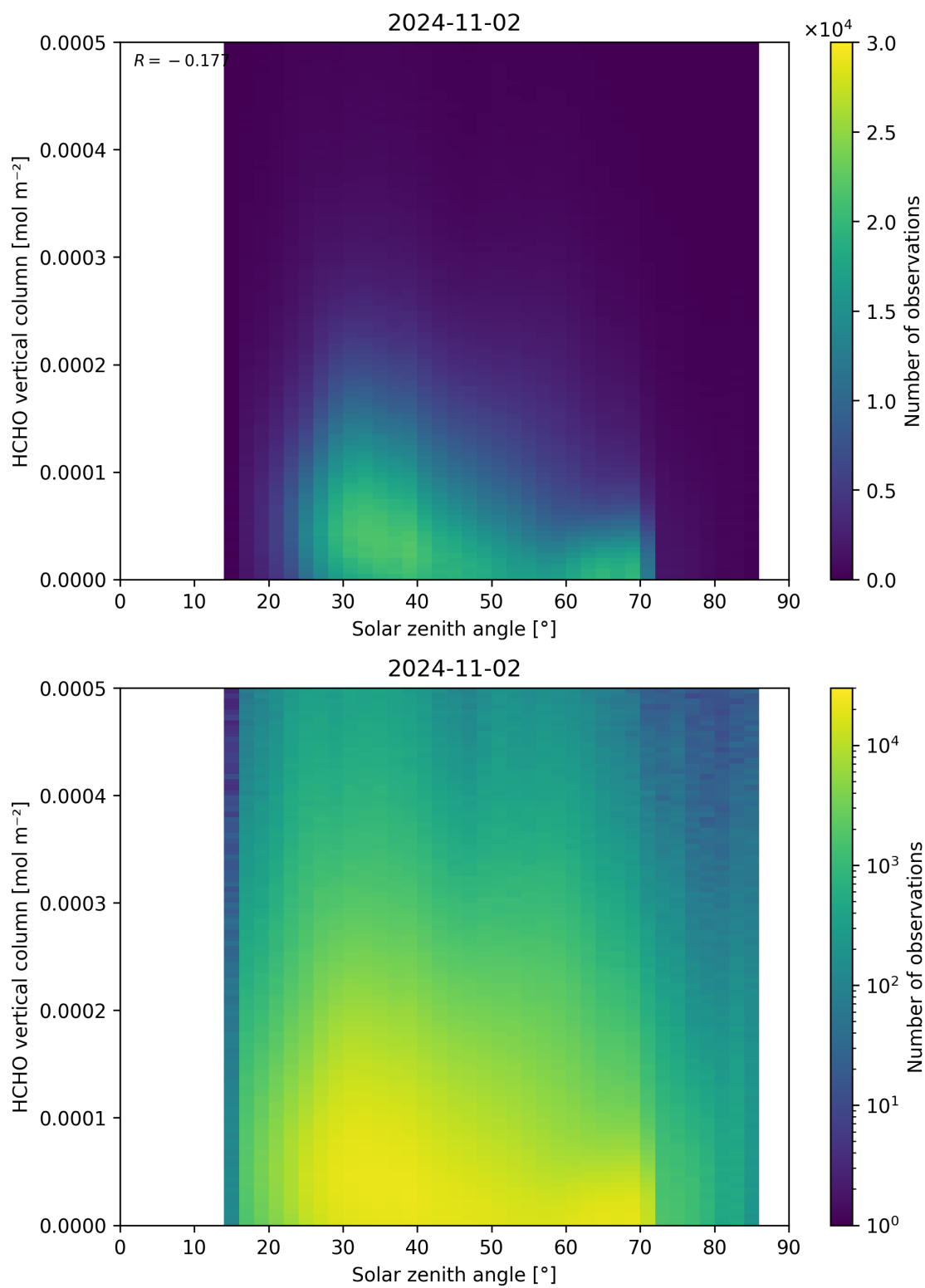
Figure 177: Scatter density plot of “Solar zenith angle” against “HCHO vertical column” for 2024-11-01 to 2024-11-03.
