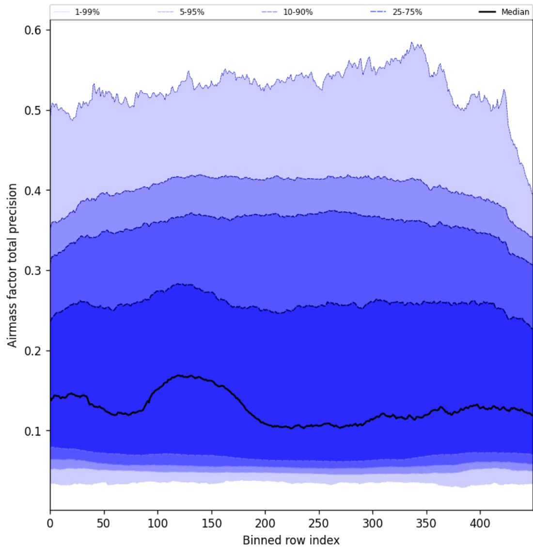
Figure 55: Along track statistics of “Airmass factor total precision” for 2024-11-01 to 2024-11-03
