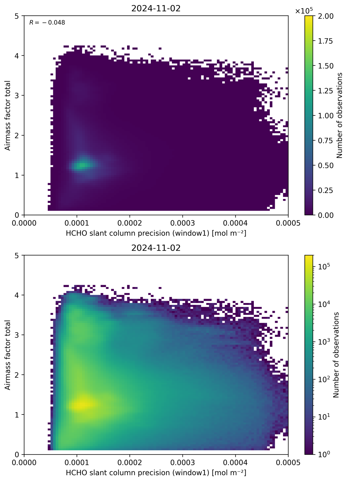
Figure 94: Scatter density plot of “HCHO slant column precision (window1)” against “Airmass factor total” for 2024-11-01 to 2024-11-03.
