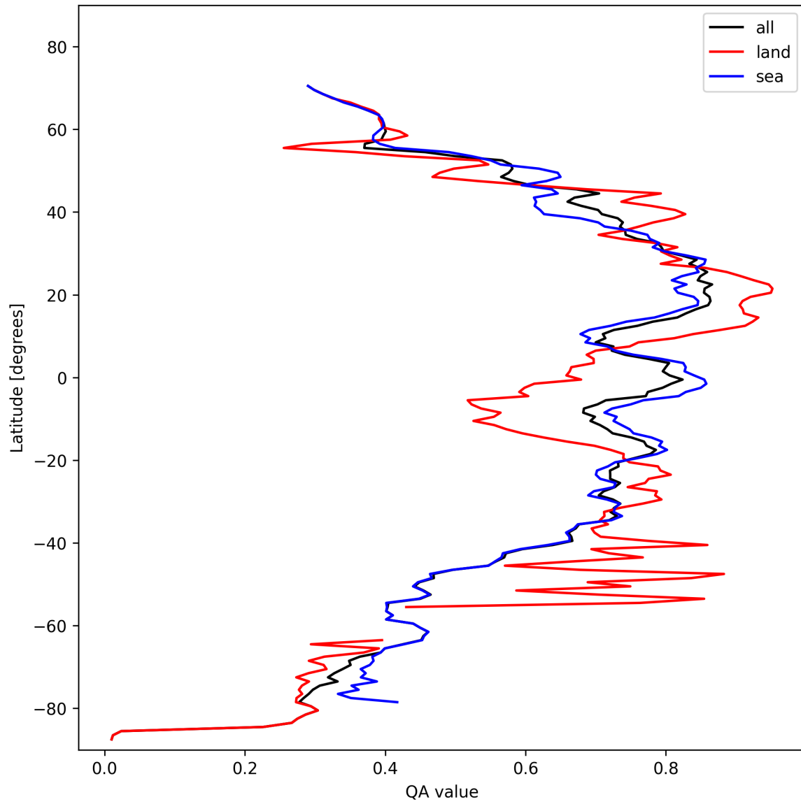
Figure 20: Zonal average of “QA value” for 2024-11-01 to 2024-11-03.
