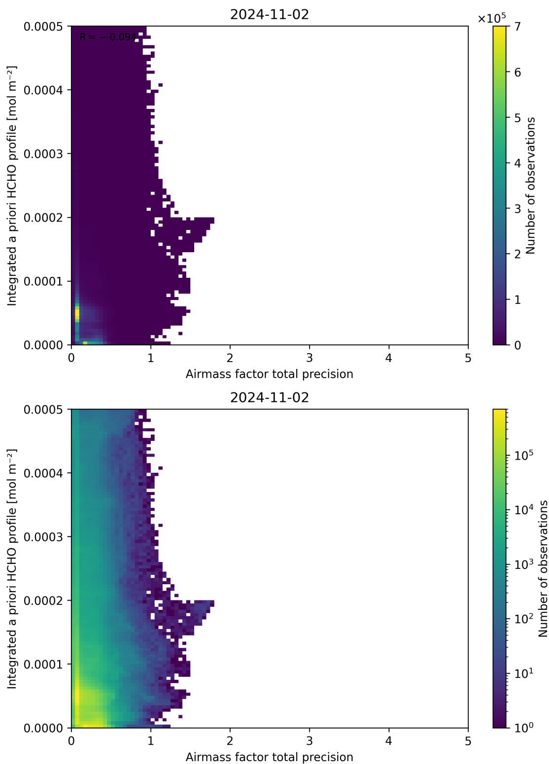
Figure 111: Scatter density plot of “Airmass factor total precision” against “Integrated a priori HCHO profile” for 2024-11-01 to 2024-11-03.
