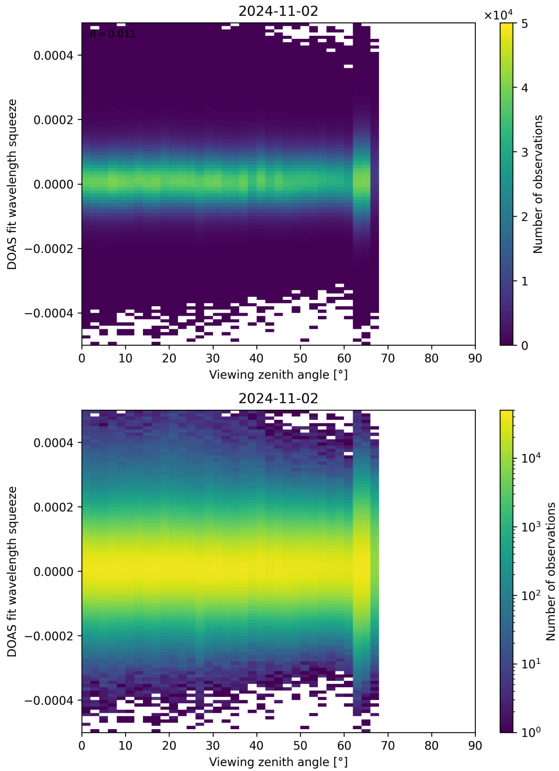
Figure 184: Scatter density plot of “Viewing zenith angle” against “DOAS fit wavelength squeeze” for 2024-11-01 to 2024-11-03.
