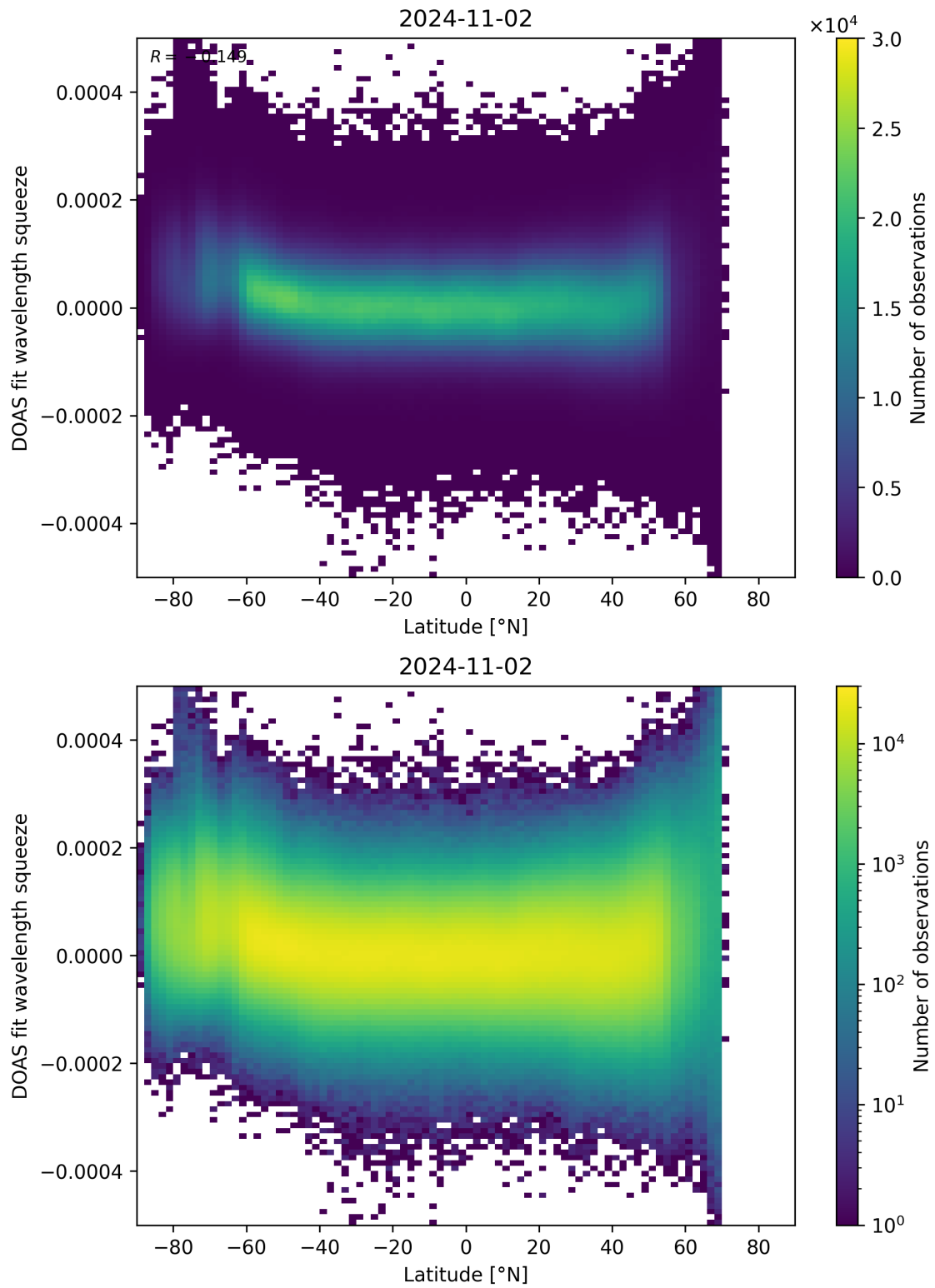
Figure 155: Scatter density plot of “Latitude” against “DOAS fit wavelength squeeze” for 2024-11-01 to 2024-11-03.
