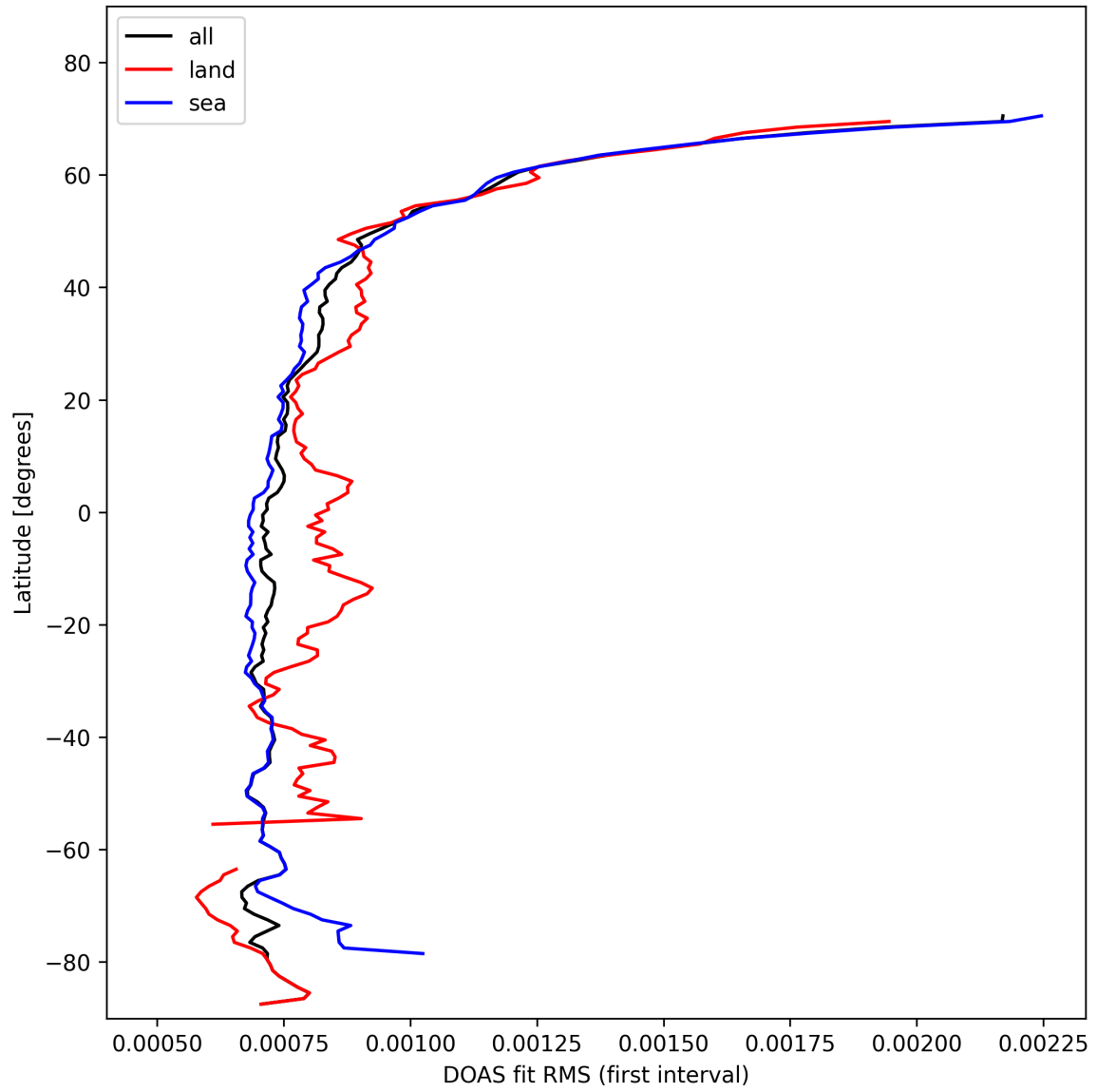
Figure 32: Zonal average of “DOAS fit RMS (first interval)” for 2024-11-01 to 2024-11-03.
