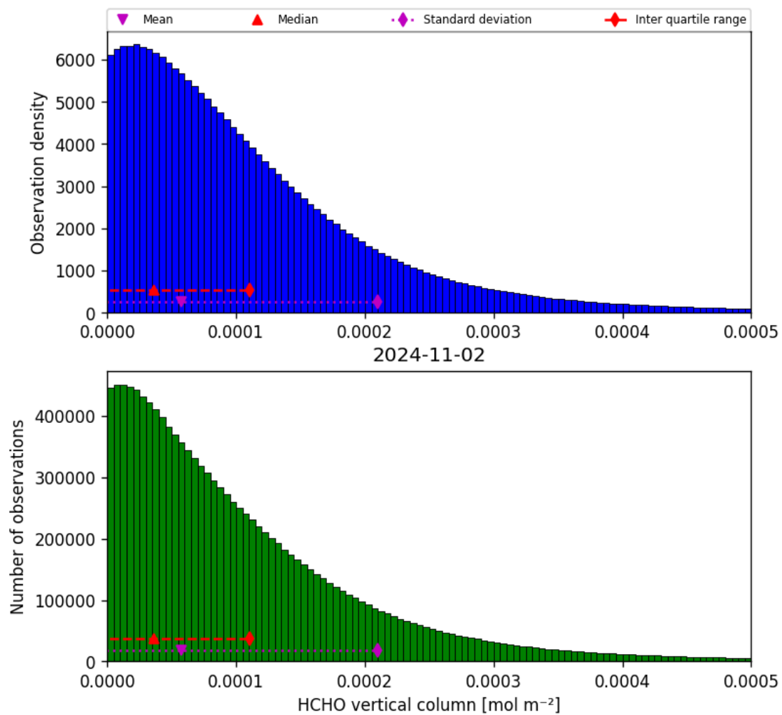
Figure 35: Histogram of “HCHO vertical column” for 2024-11-01 to 2024-11-03
