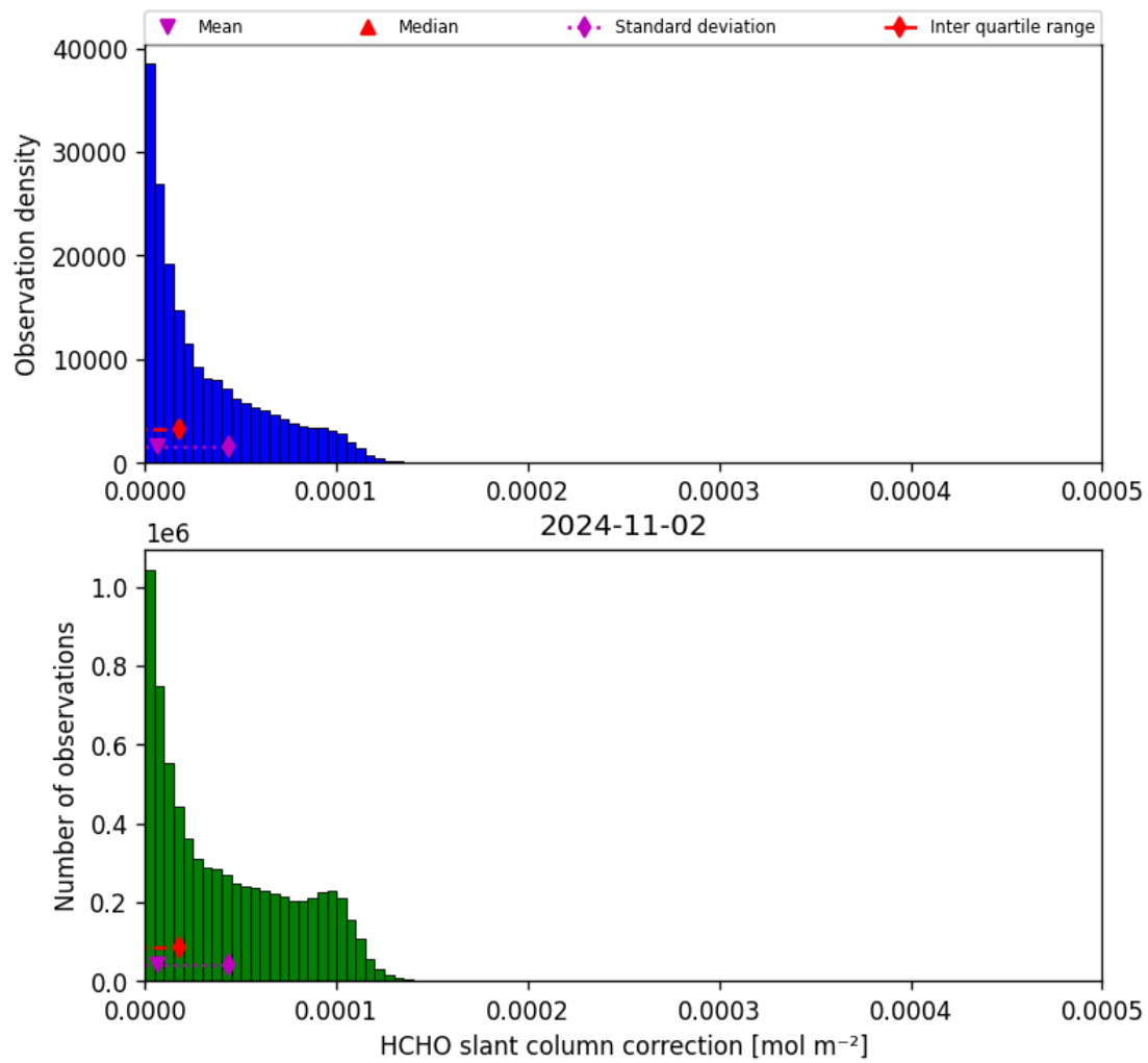
Figure 47: Histogram of “HCHO slant column correction” for 2024-11-01 to 2024-11-03
