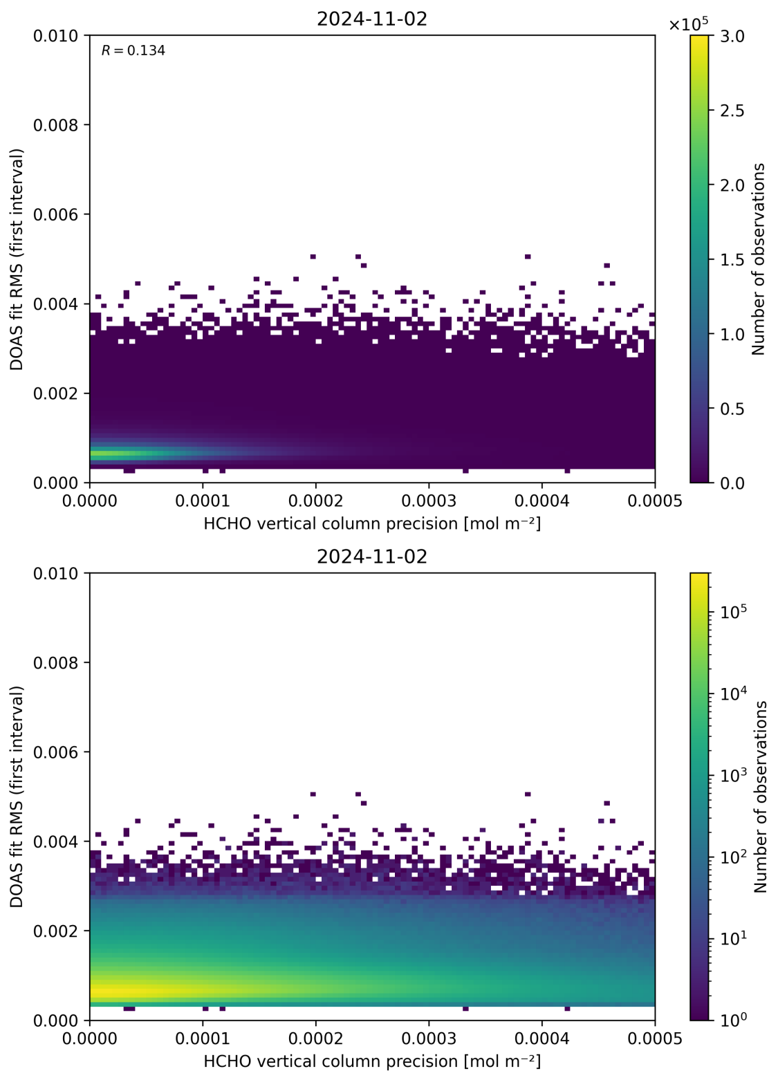
Figure 136: Scatter density plot of “HCHO vertical column precision” against “DOAS fit RMS (first interval)” for 2024-11-01 to 2024-11-03.
