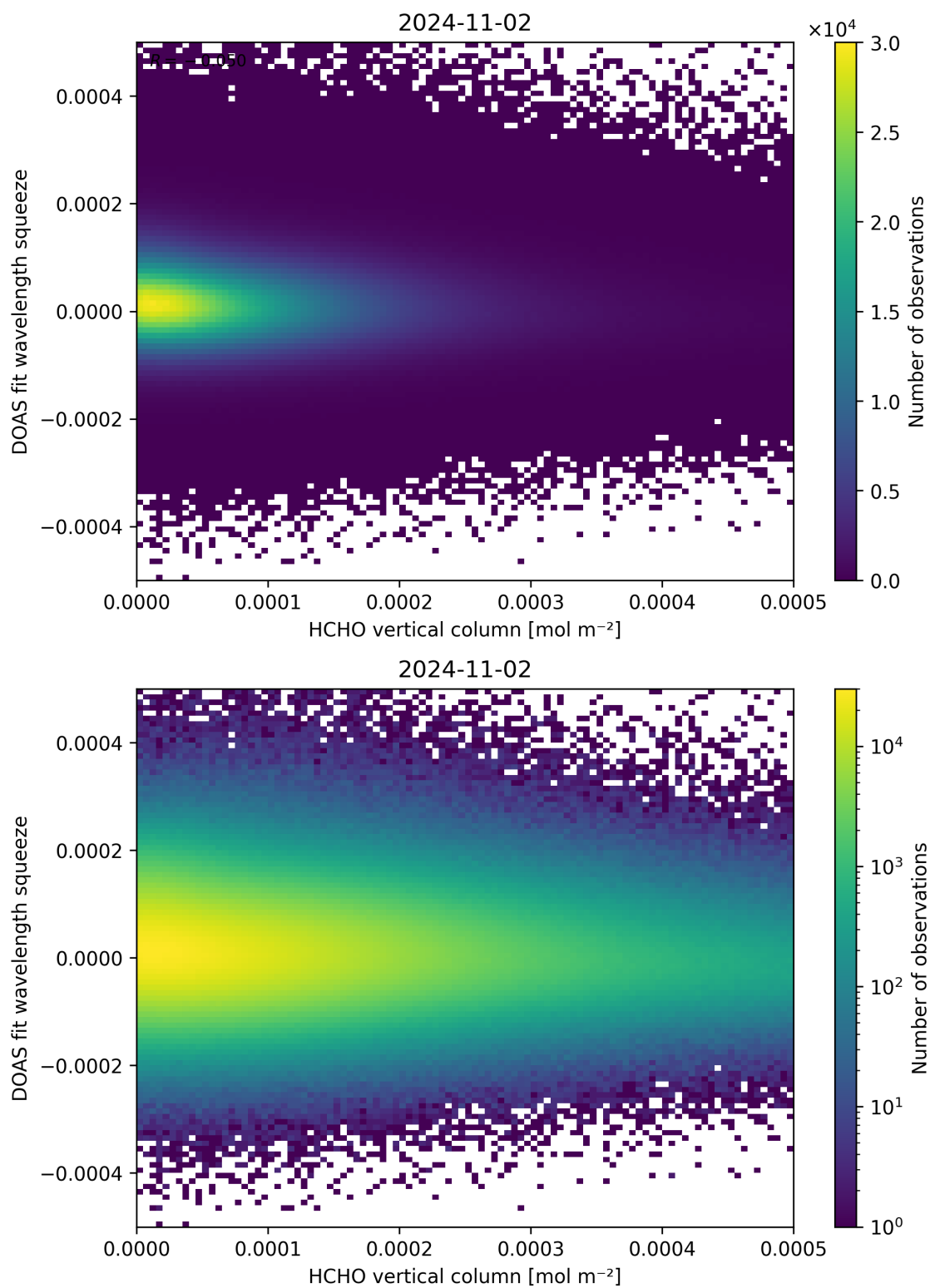
Figure 125: Scatter density plot of “HCHO vertical column” against “DOAS fit wavelength squeeze” for 2024-11-01 to 2024-11-03.
