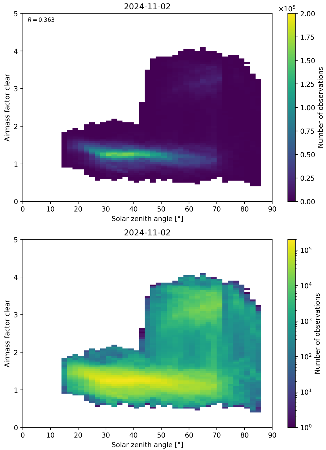
Figure 170: Scatter density plot of “Solar zenith angle” against “Airmass factor clear” for 2024-11-01 to 2024-11-03.
