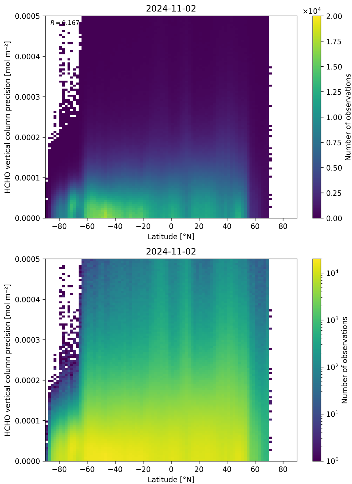
Figure 165: Scatter density plot of “Latitude” against “HCHO vertical column precision” for 2024-11-01 to 2024-11-03.
