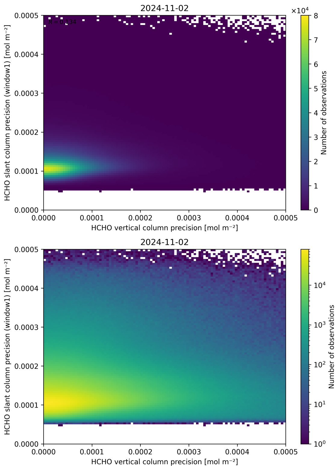
Figure 143: Scatter density plot of “HCHO vertical column precision” against “HCHO slant column precision (window1)” for 2024-11-01 to 2024-11-03.
