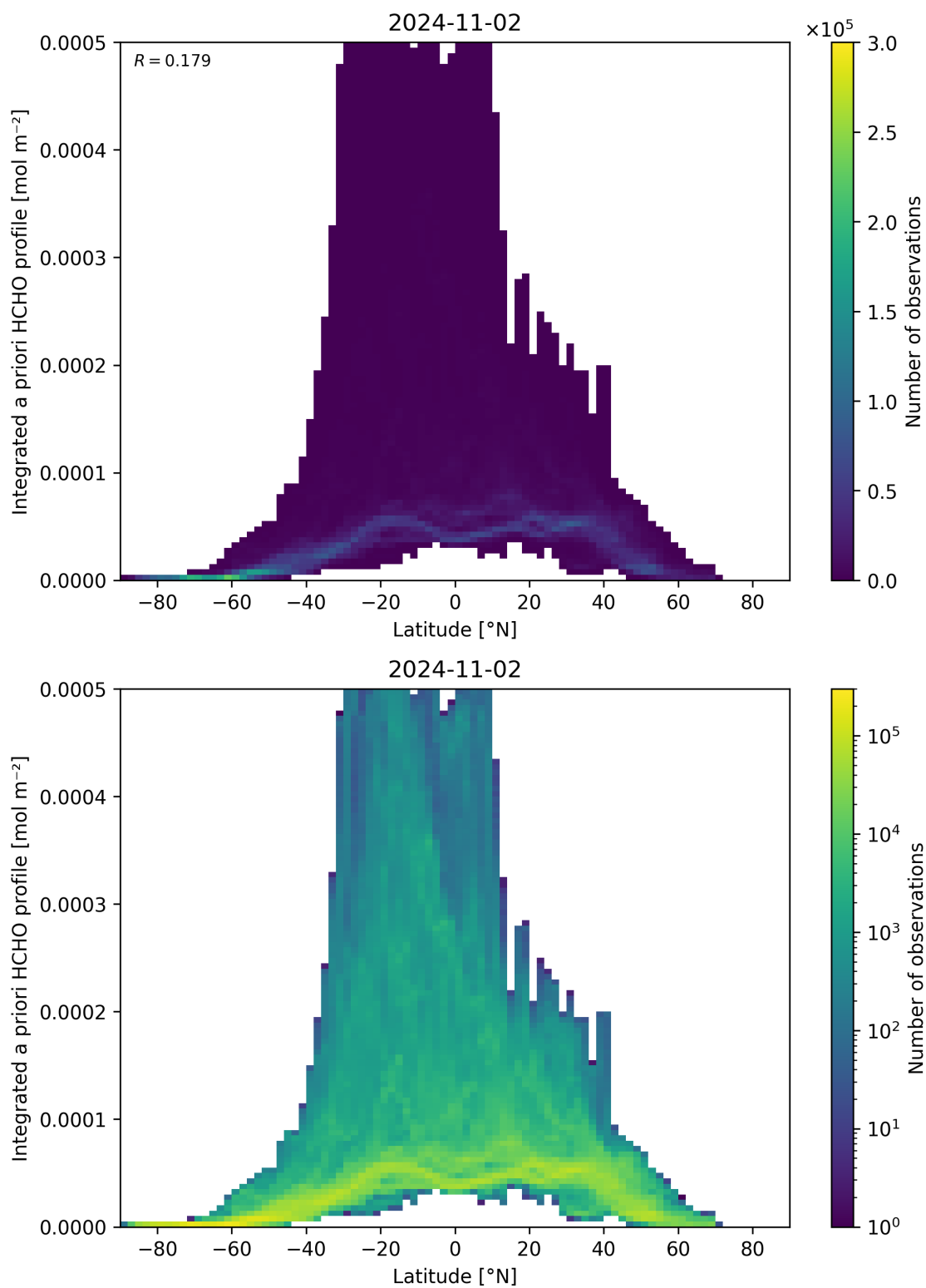
Figure 166: Scatter density plot of “Latitude” against “Integrated a priori HCHO profile” for 2024-11-01 to 2024-11-03.
