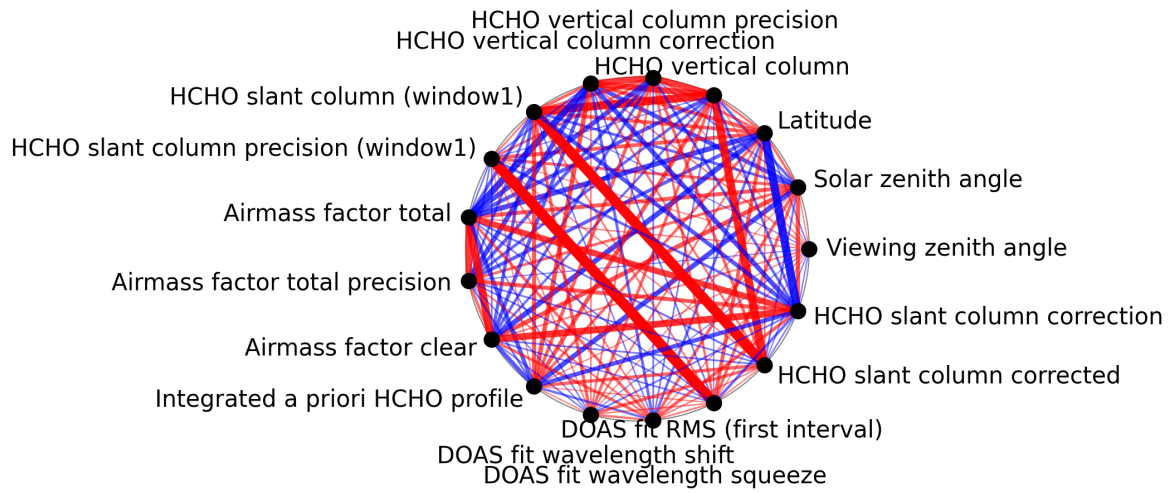
Figure 1: Map of correlation graph for 2024-11-01 to 2024-11-03.
