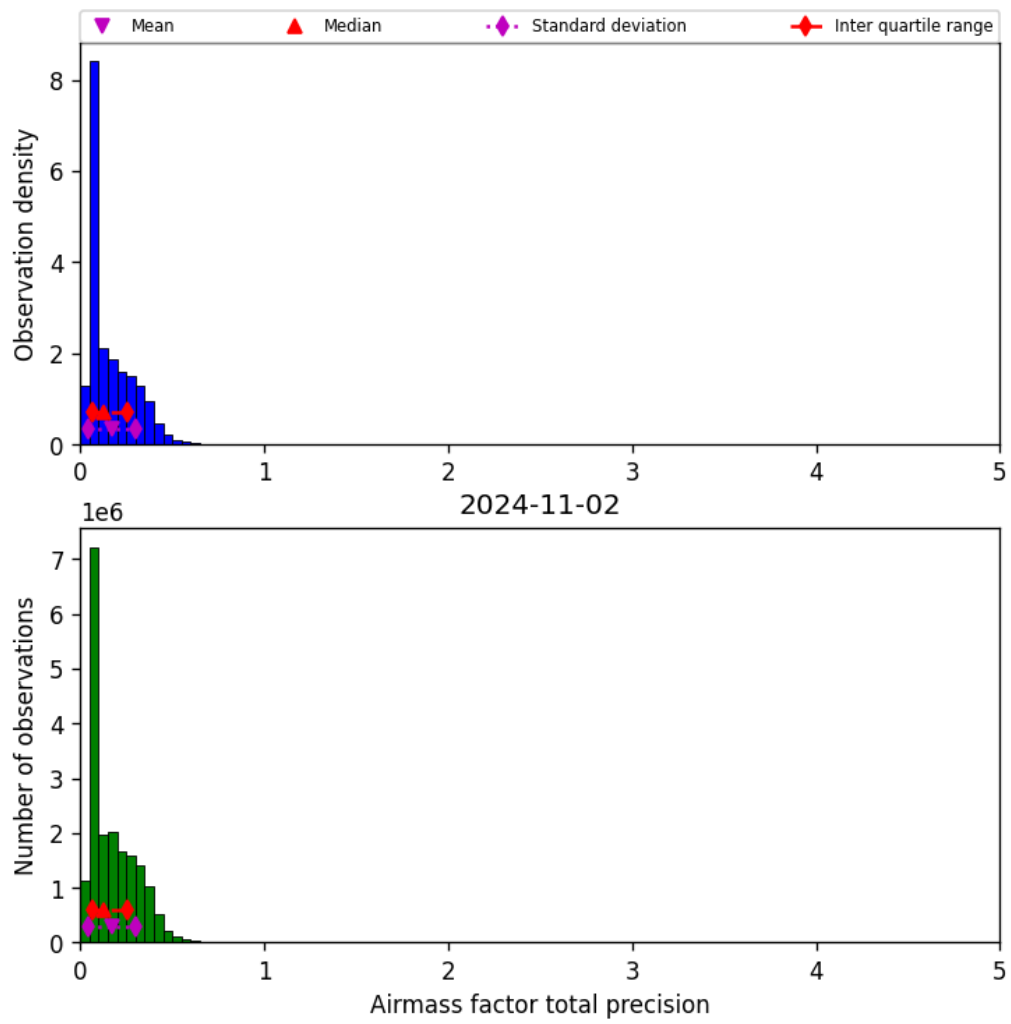
Figure 41: Histogram of “Airmass factor total precision” for 2024-11-01 to 2024-11-03
