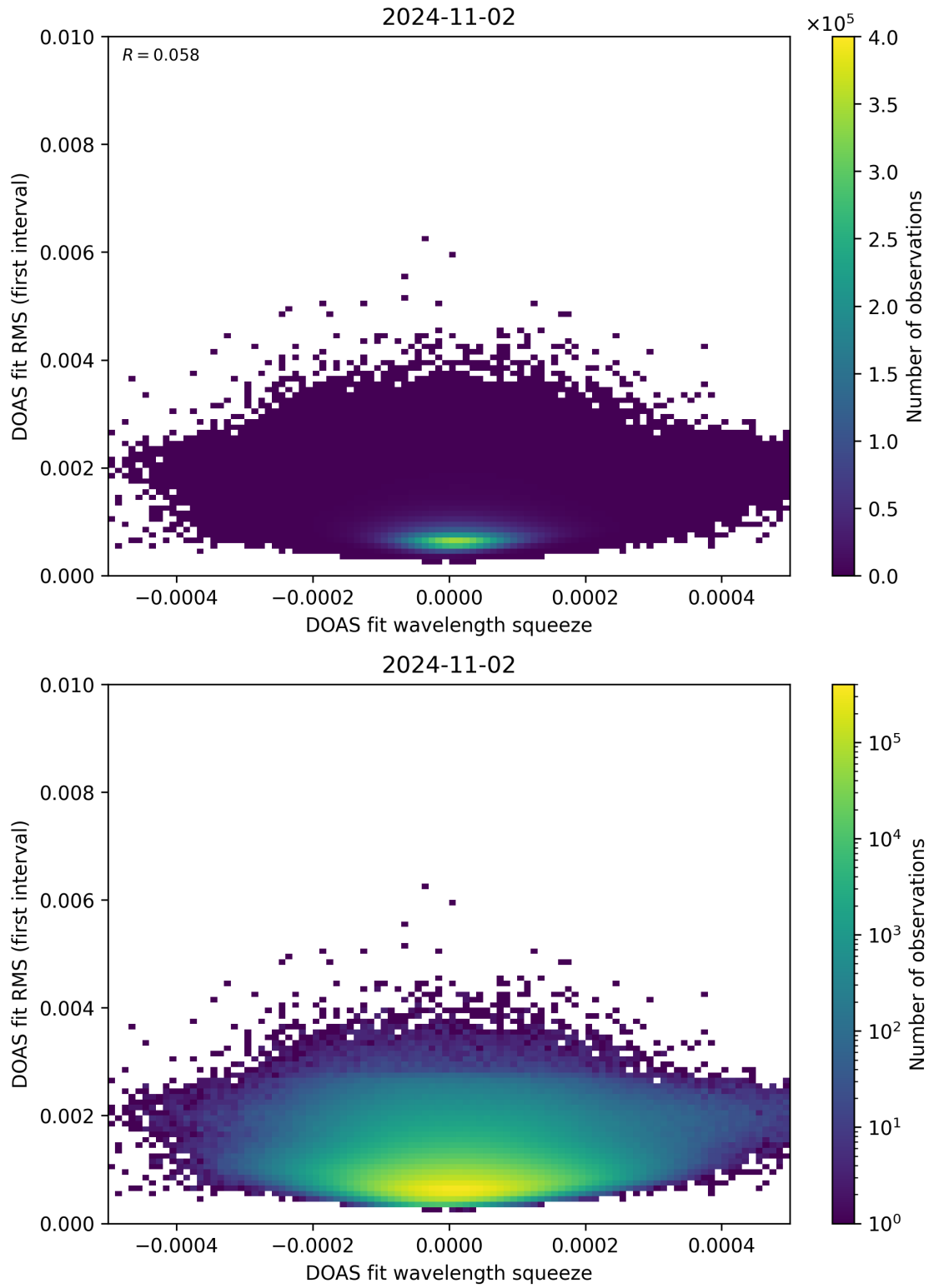
Figure 68: Scatter density plot of “DOAS fit wavelength squeeze” against “DOAS fit RMS (first interval)” for 2024-11-01 to 2024-11-03.
