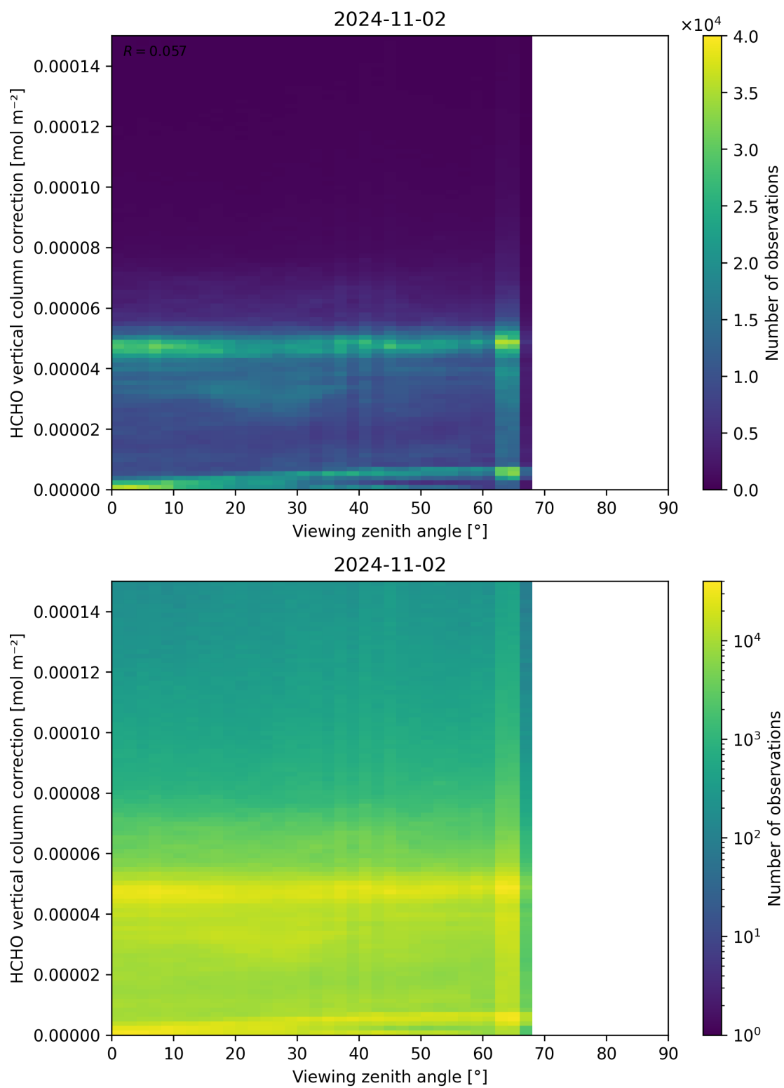
Figure 193: Scatter density plot of “Viewing zenith angle” against “HCHO vertical column correction” for 2024-11-01 to 2024-11-03.
