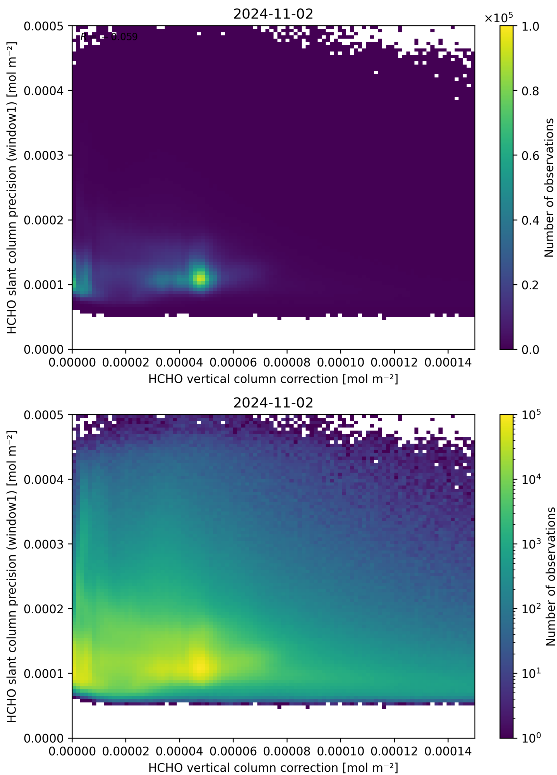
Figure 119: Scatter density plot of “HCHO vertical column correction” against “HCHO slant column precision (window1)” for 2024-11-01 to 2024-11-03.
