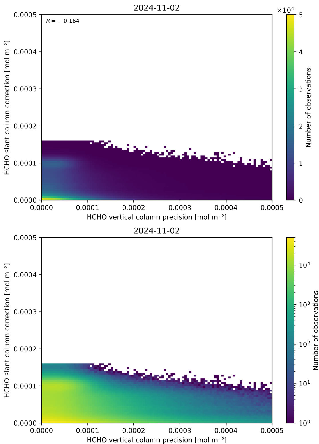
Figure 141: Scatter density plot of “HCHO vertical column precision” against “HCHO slant column correction” for 2024-11-01 to 2024-11-03.
