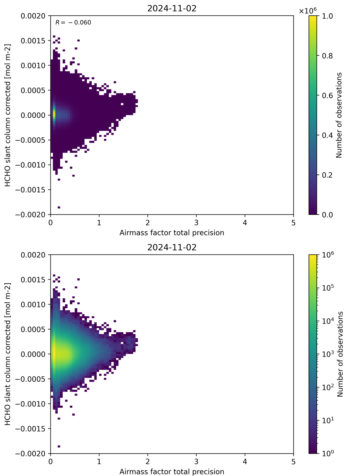
Figure 109: Scatter density plot of “Airmass factor total precision” against “HCHO slant column corrected” for 2024-11-01 to 2024-11-03.
