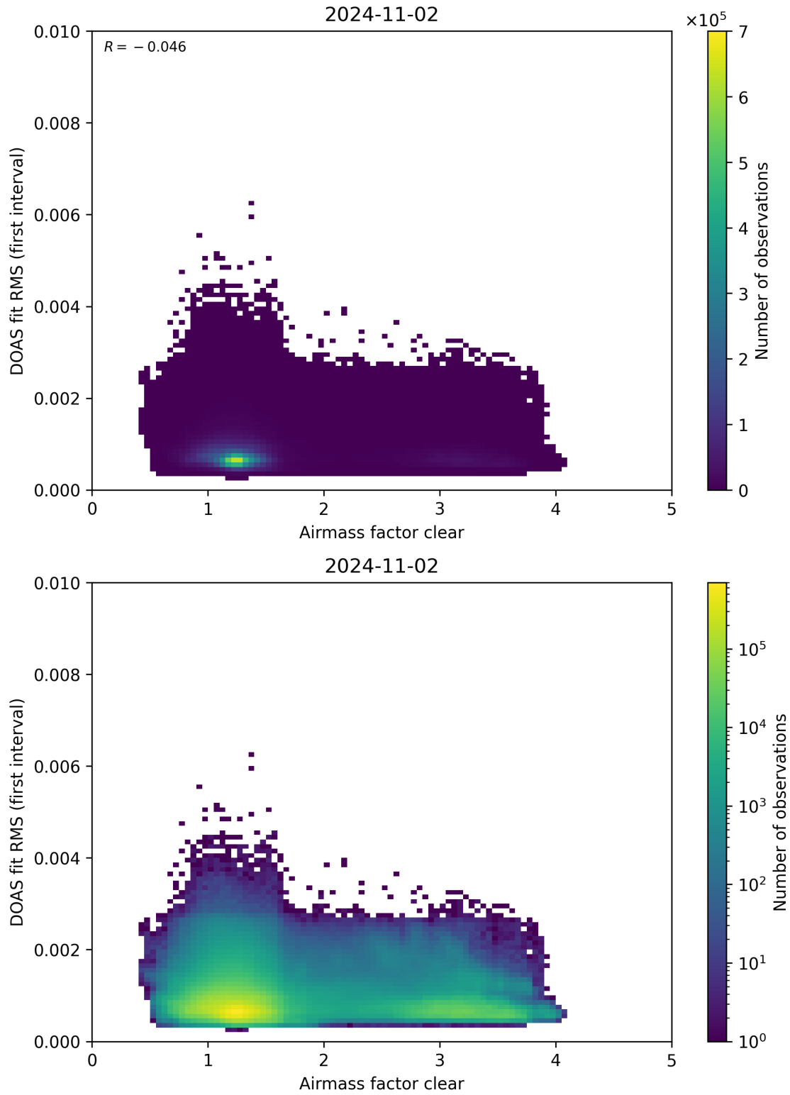
Figure 71: Scatter density plot of “Airmass factor clear” against “DOAS fit RMS (first interval)” for 2024-11-01 to 2024-11-03.
