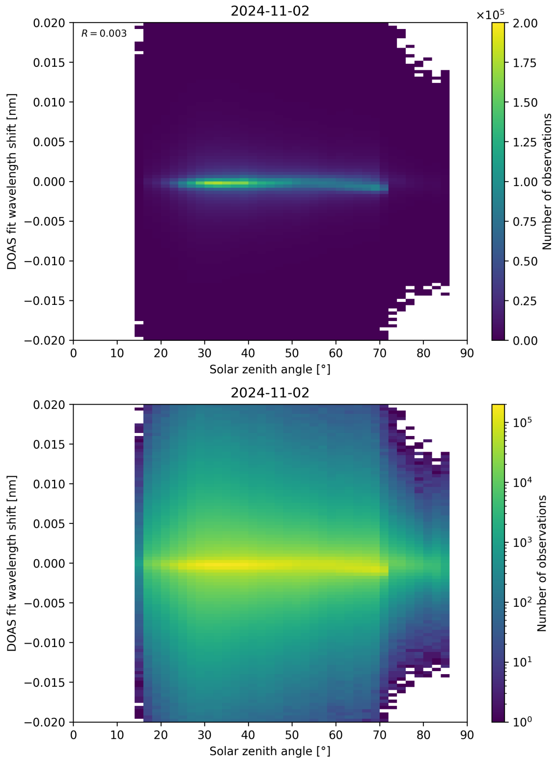
Figure 168: Scatter density plot of “Solar zenith angle” against “DOAS fit wavelength shift” for 2024-11-01 to 2024-11-03.
