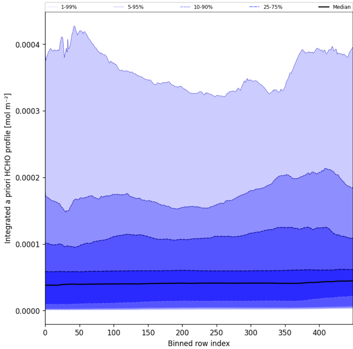
Figure 57: Along track statistics of "Integrated a priori HCHO profile" for 2024-11-01 to 2024-11-03
