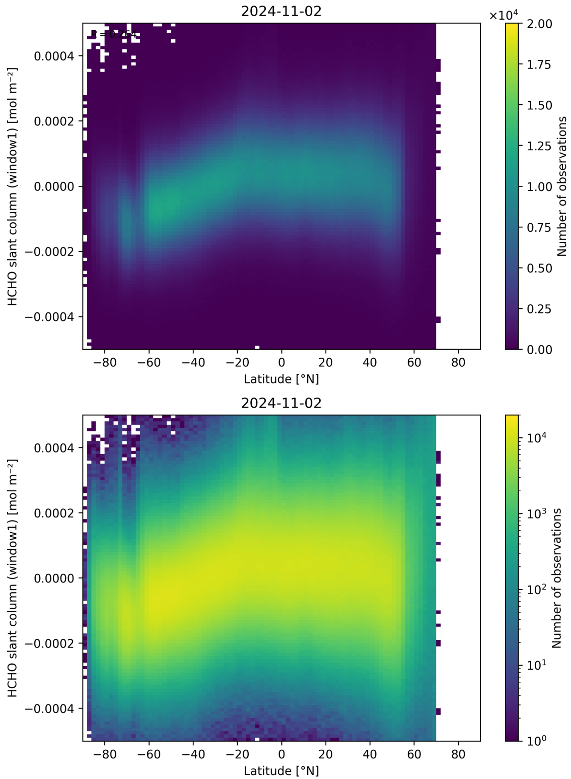
Figure 159: Scatter density plot of “Latitude” against “HCHO slant column (window1)” for 2024-11-01 to 2024-11-03.
