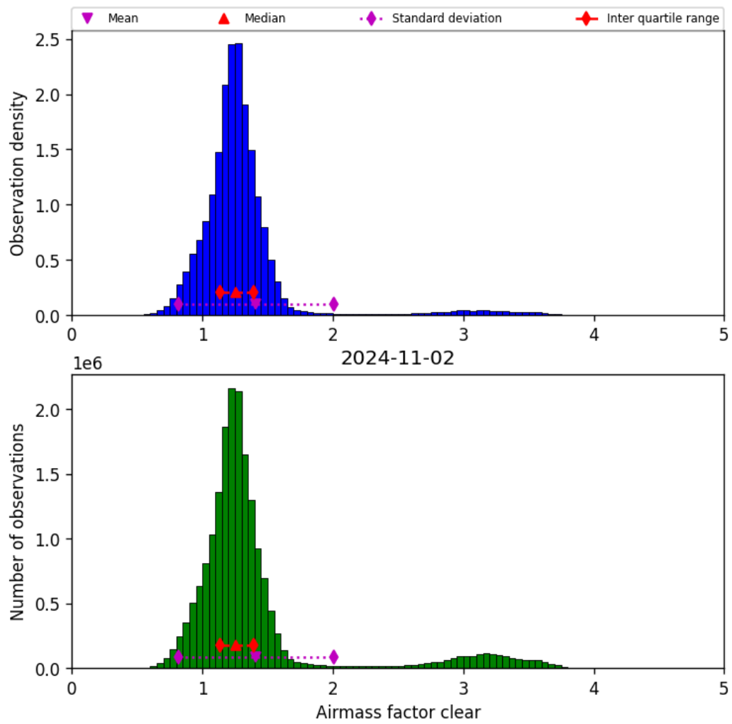
Figure 42: Histogram of “Airmass factor clear” for 2024-11-01 to 2024-11-03
