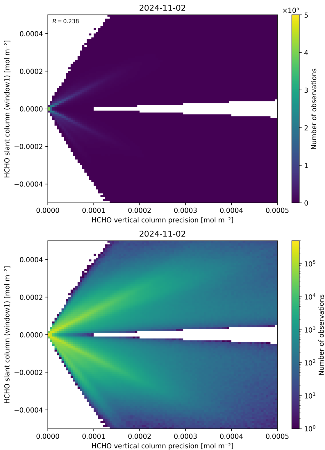
Figure 142: Scatter density plot of “HCHO vertical column precision” against “HCHO slant column (window1)” for 2024-11-01 to 2024-11-03.
