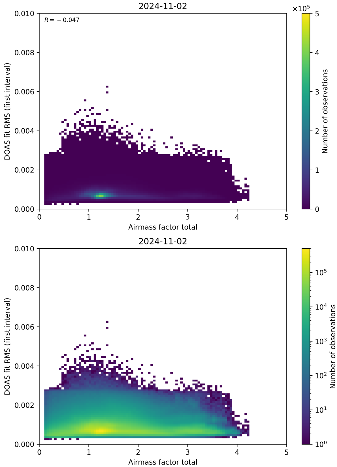
Figure 97: Scatter density plot of “Airmass factor total” against “DOAS fit RMS (first interval)” for 2024-11-01 to 2024-11-03.
