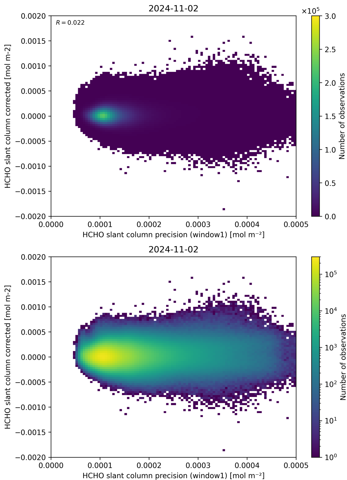
Figure 92: Scatter density plot of “HCHO slant column precision (window1)” against “HCHO slant column corrected” for 2024-11-01 to 2024-11-03.
