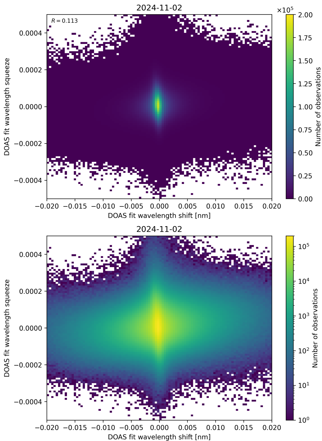
Figure 65: Scatter density plot of “DOAS fit wavelength shift” against “DOAS fit wavelength squeeze” for 2024-11-01 to 2024-11-03.
