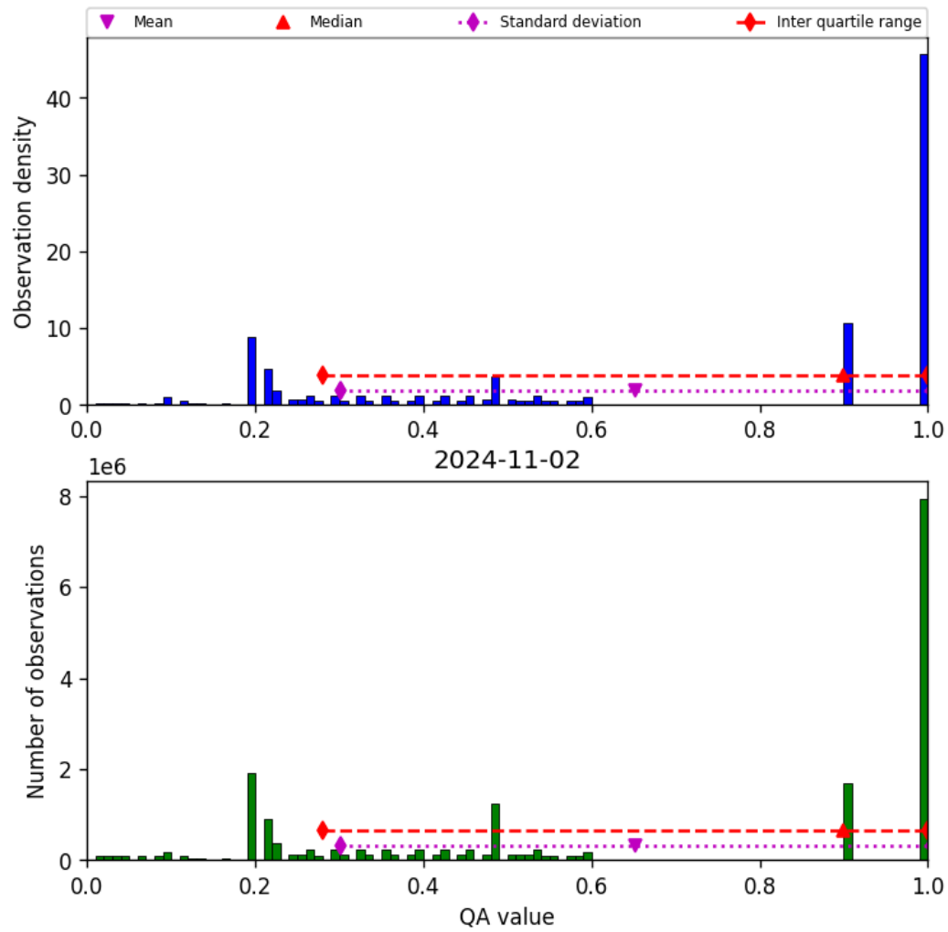
Figure 34: Histogram of “QA value” for 2024-11-01 to 2024-11-03
