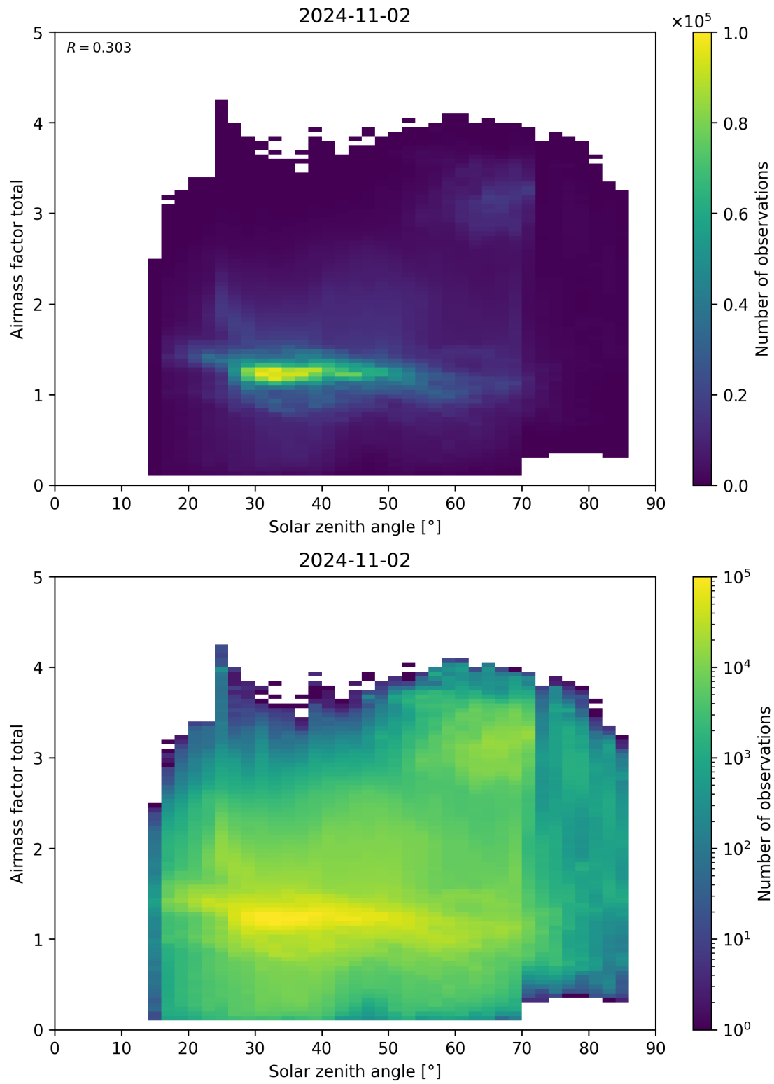
Figure 175: Scatter density plot of “Solar zenith angle” against “Airmass factor total” for 2024-11-01 to 2024-11-03.
