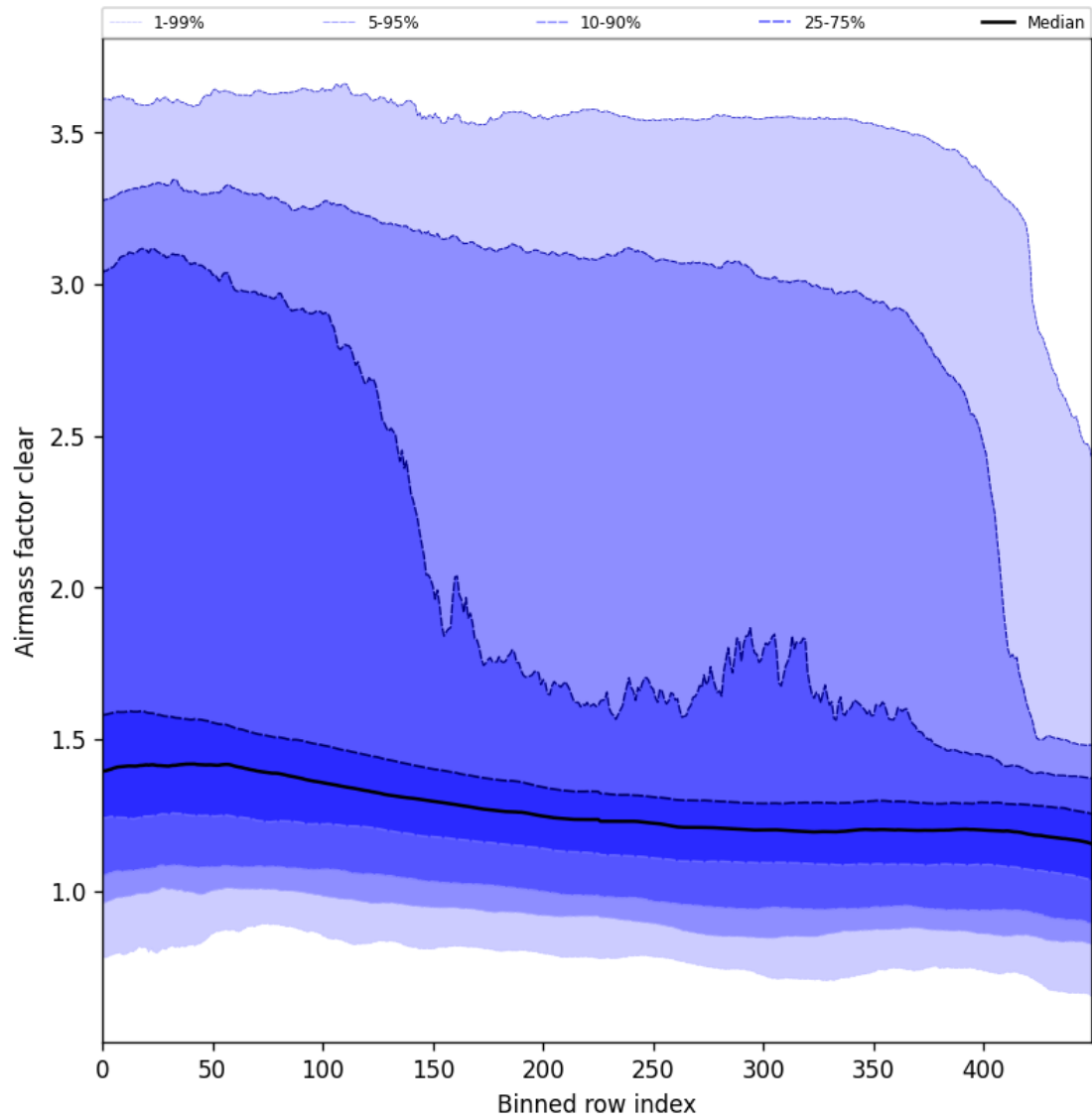
Figure 56: Along track statistics of “Airmass factor clear” for 2024-11-01 to 2024-11-03
