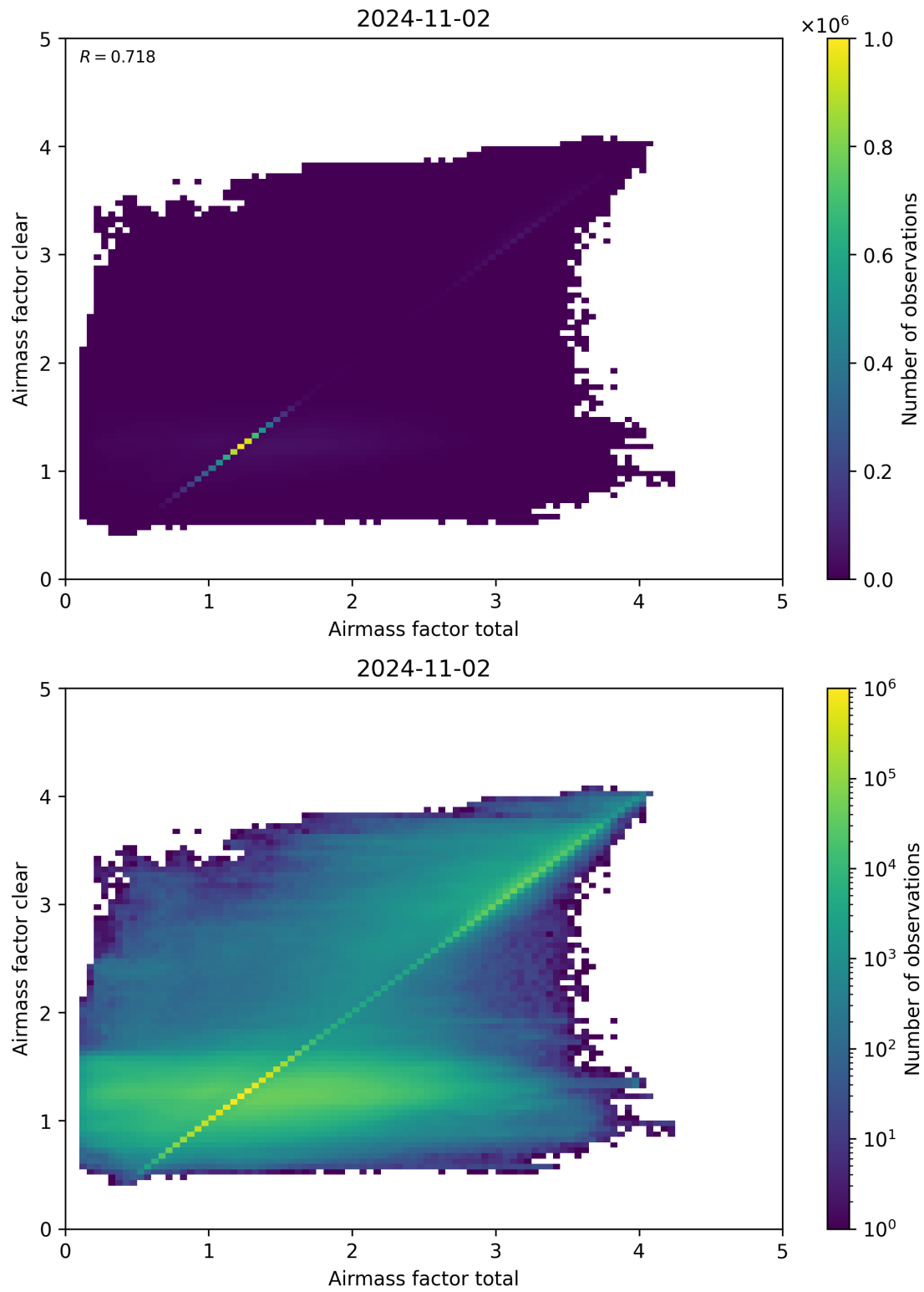
Figure 100: Scatter density plot of “Airmass factor total” against “Airmass factor clear” for 2024-11-01 to 2024-11-03.
