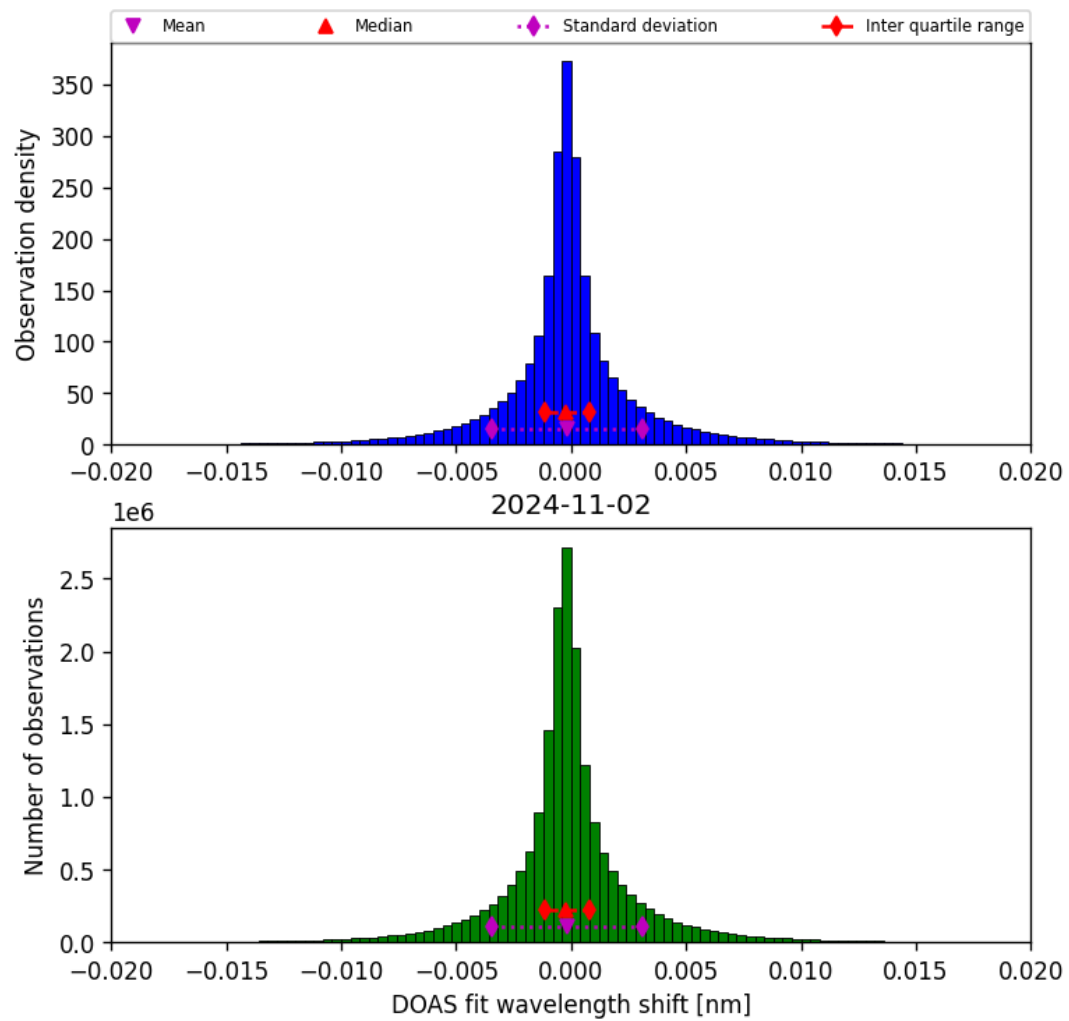
Figure 44: Histogram of “DOAS fit wavelength shift” for 2024-11-01 to 2024-11-03
