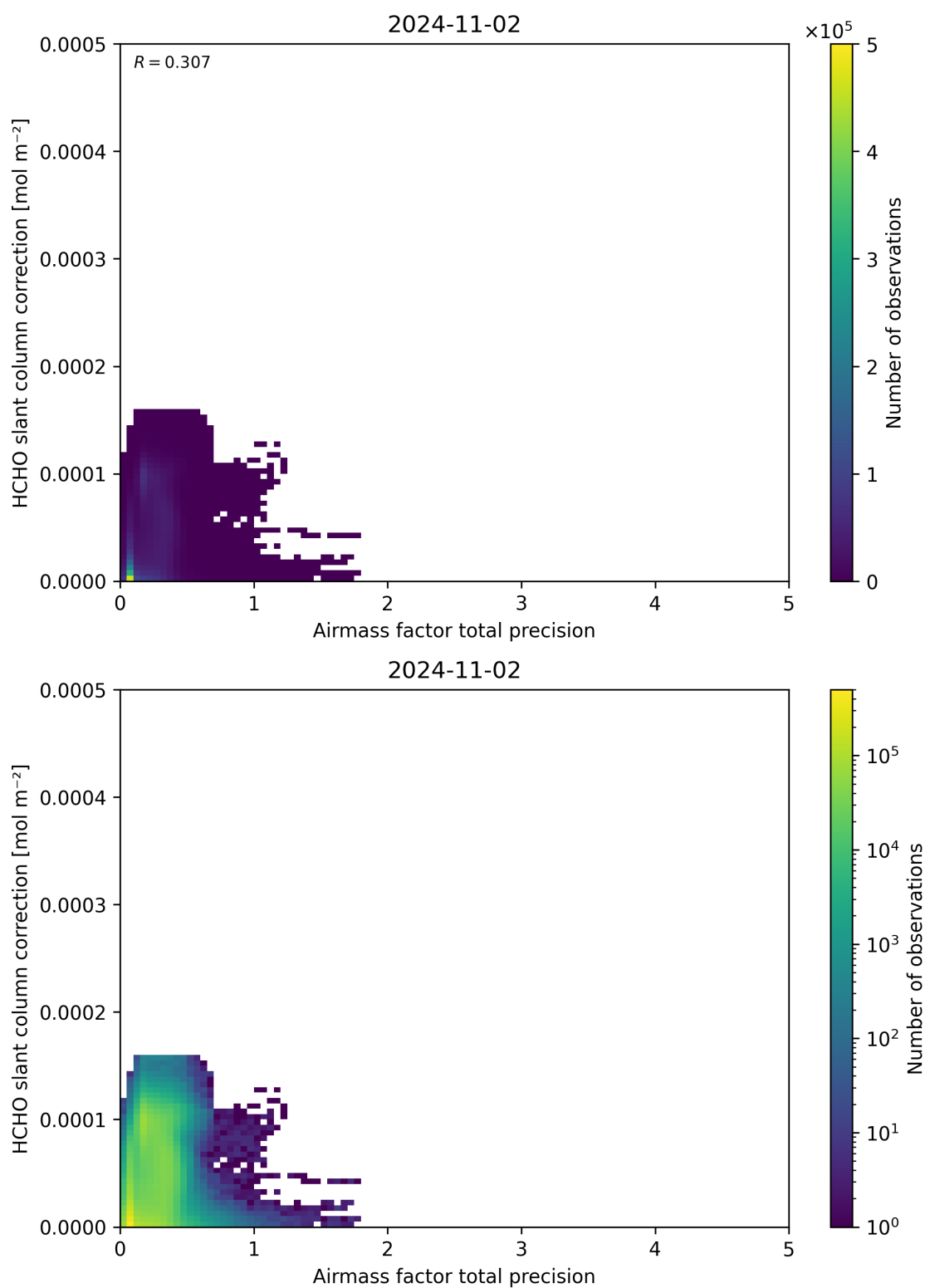
Figure 110: Scatter density plot of “Airmass factor total precision” against “HCHO slant column correction” for 2024-11-01 to 2024-11-03.
