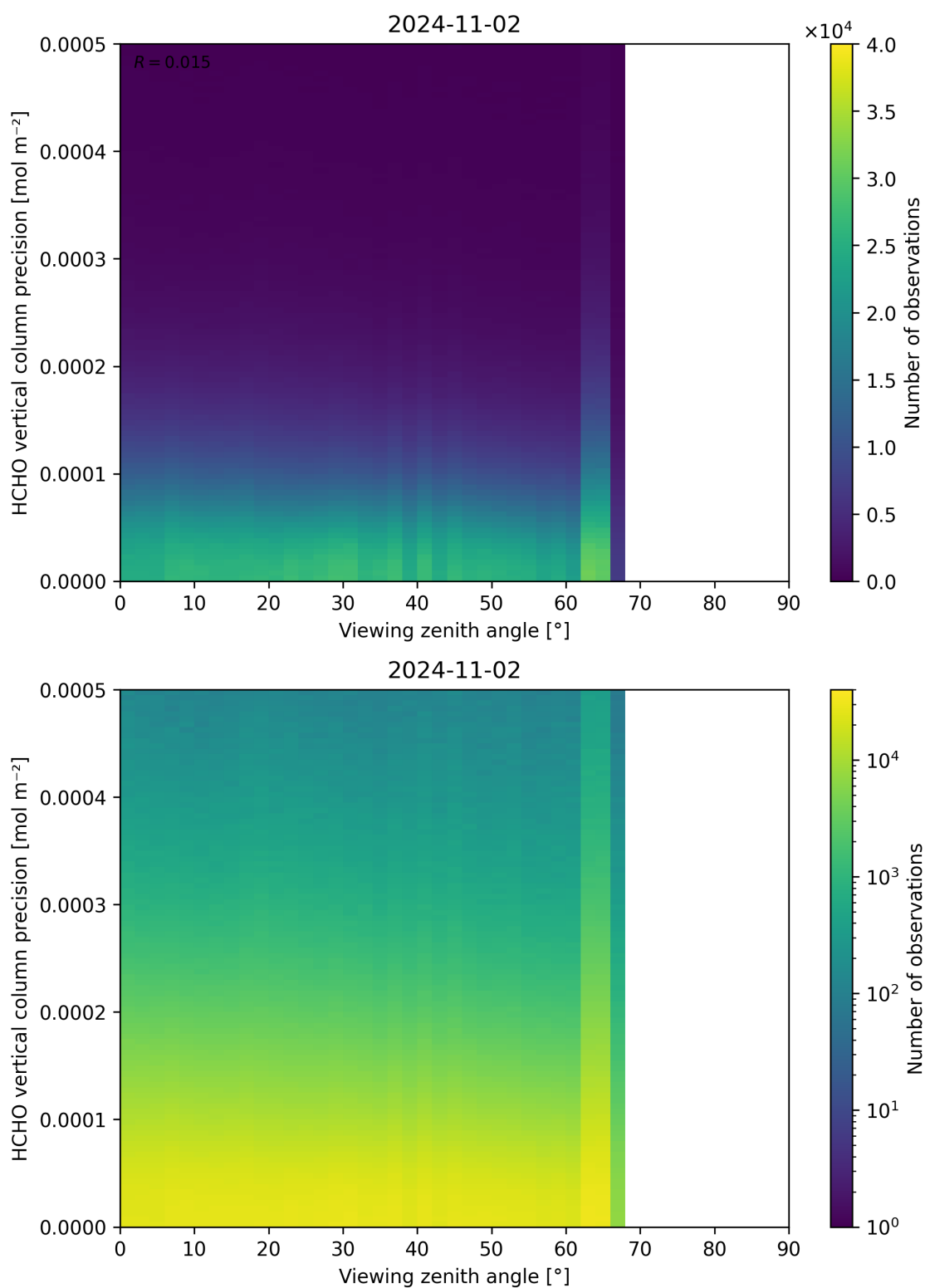
Figure 194: Scatter density plot of “Viewing zenith angle” against “HCHO vertical column precision” for 2024-11-01 to 2024-11-03.
