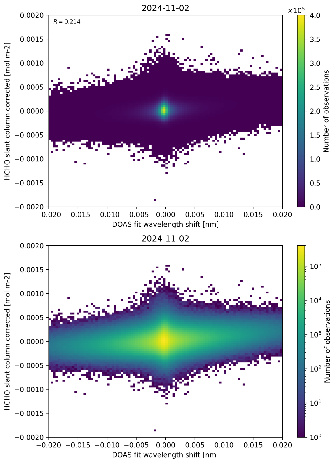
Figure 66: Scatter density plot of “DOAS fit wavelength shift” against “HCHO slant column corrected” for 2024-11-01 to 2024-11-03.
