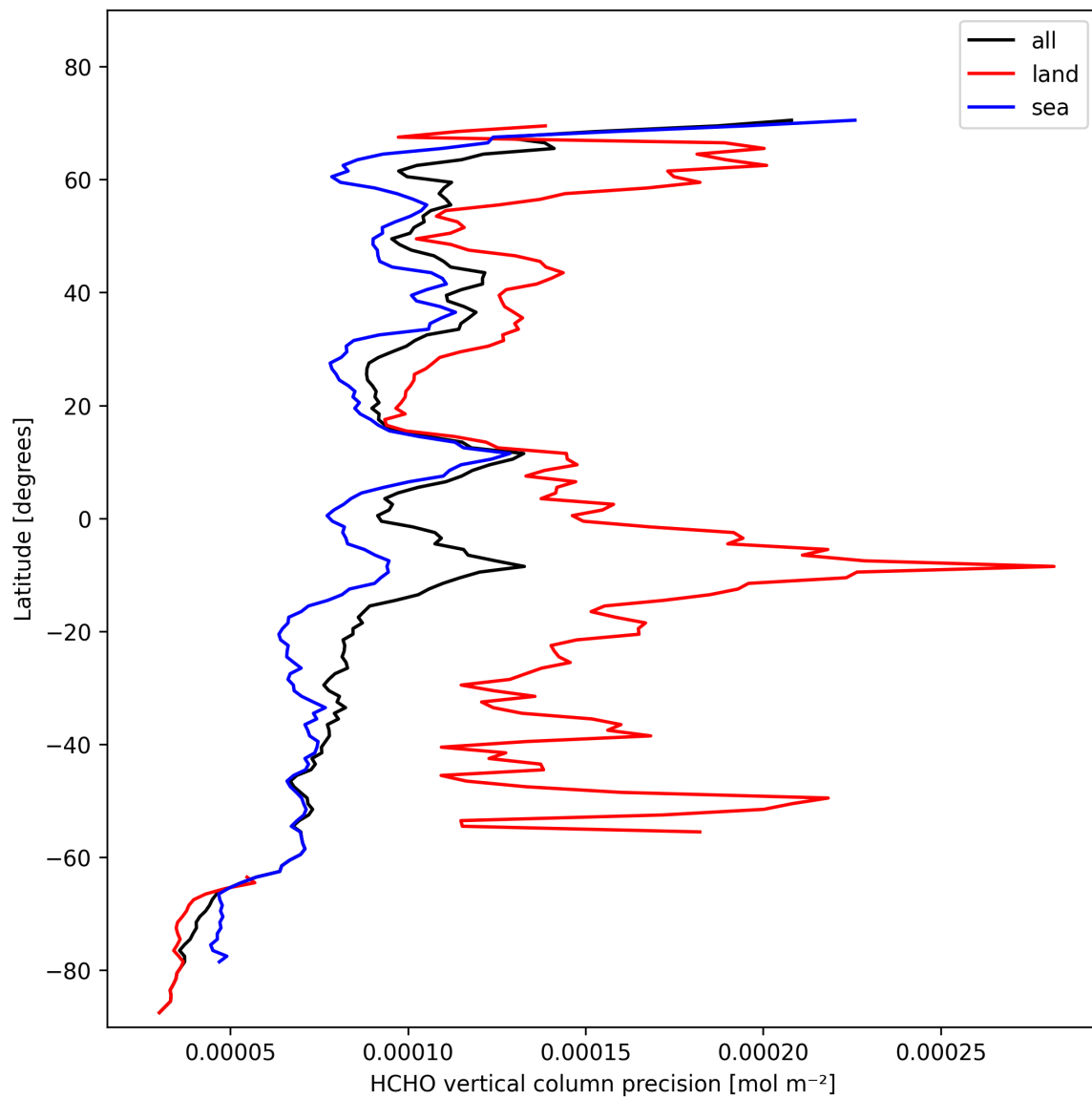
Figure 22: Zonal average of “HCHO vertical column precision” for 2024-11-01 to 2024-11-03.
