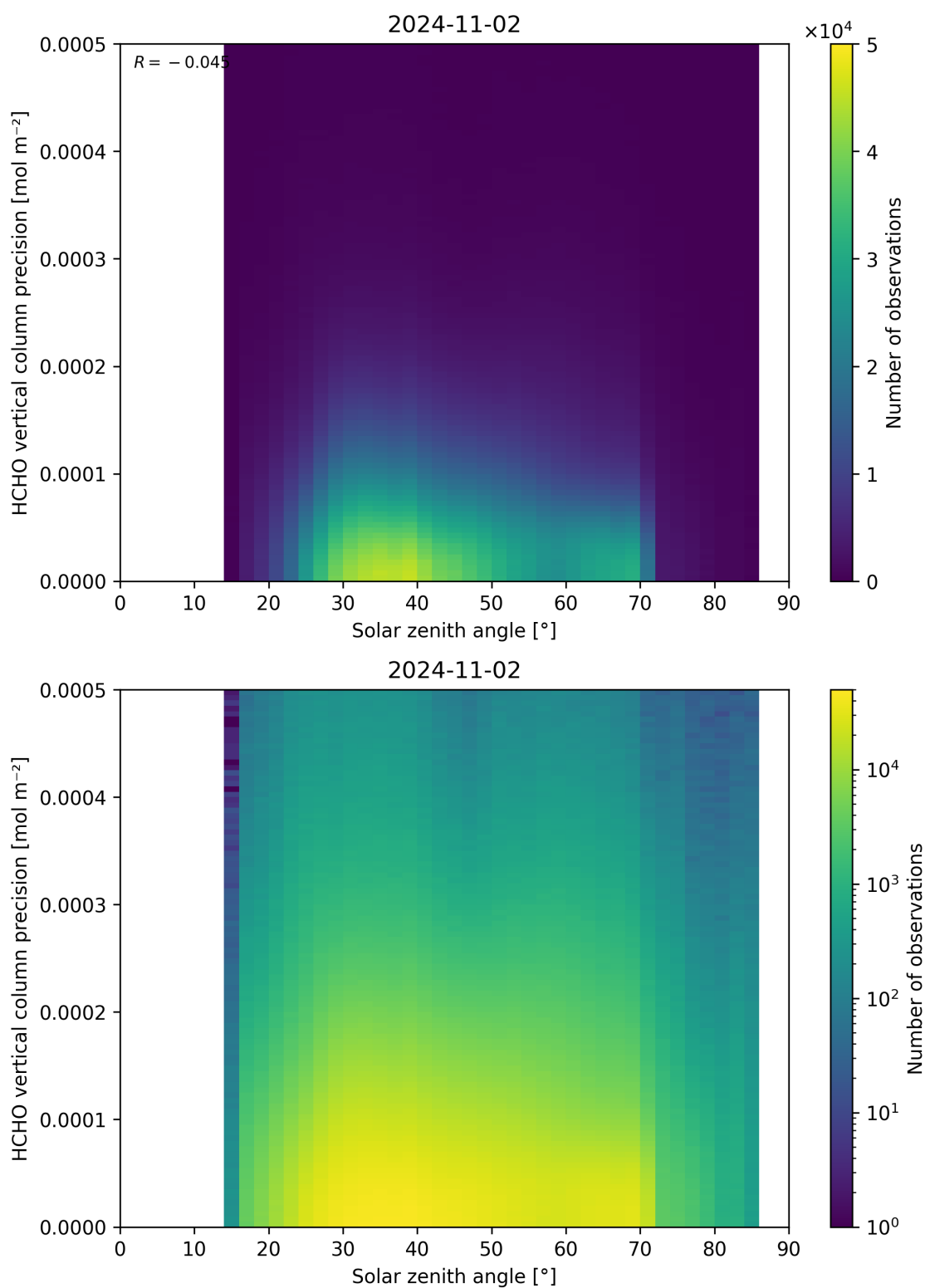
Figure 179: Scatter density plot of “Solar zenith angle” against “HCHO vertical column precision” for 2024-11-01 to 2024-11-03.
