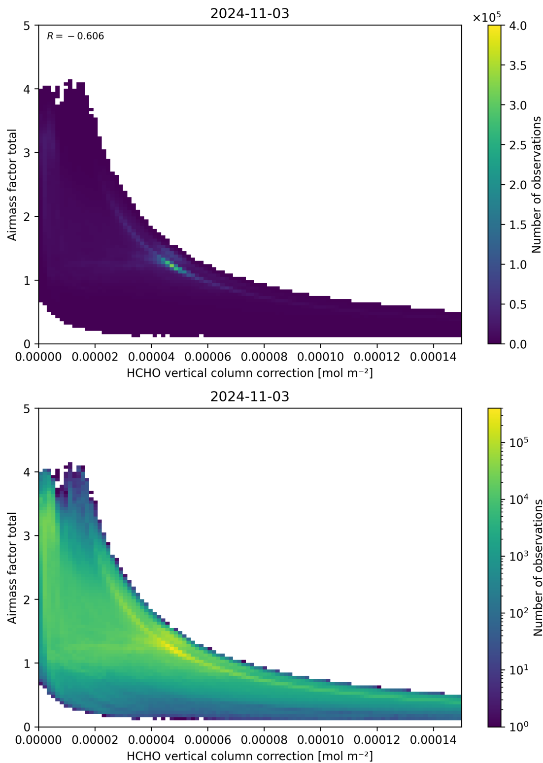
Figure 120: Scatter density plot of “HCHO vertical column correction” against “Airmass factor total” for 2024-11-02 to 2024-11-04.
