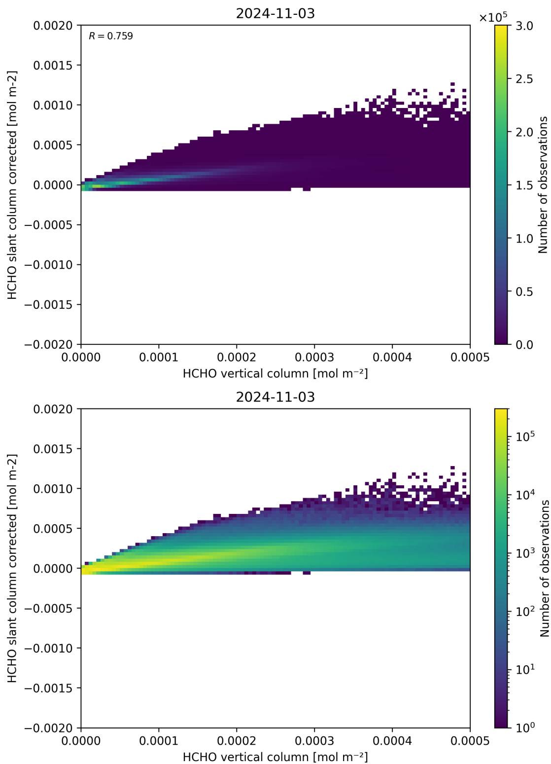
Figure 127: Scatter density plot of “HCHO vertical column” against “HCHO slant column corrected” for 2024-11-02 to 2024-11-04.
