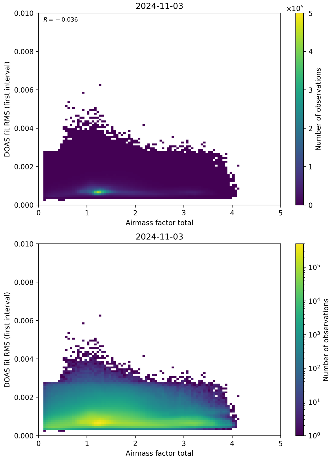
Figure 97: Scatter density plot of “Airmass factor total” against “DOAS fit RMS (first interval)” for 2024-11-02 to 2024-11-04.
