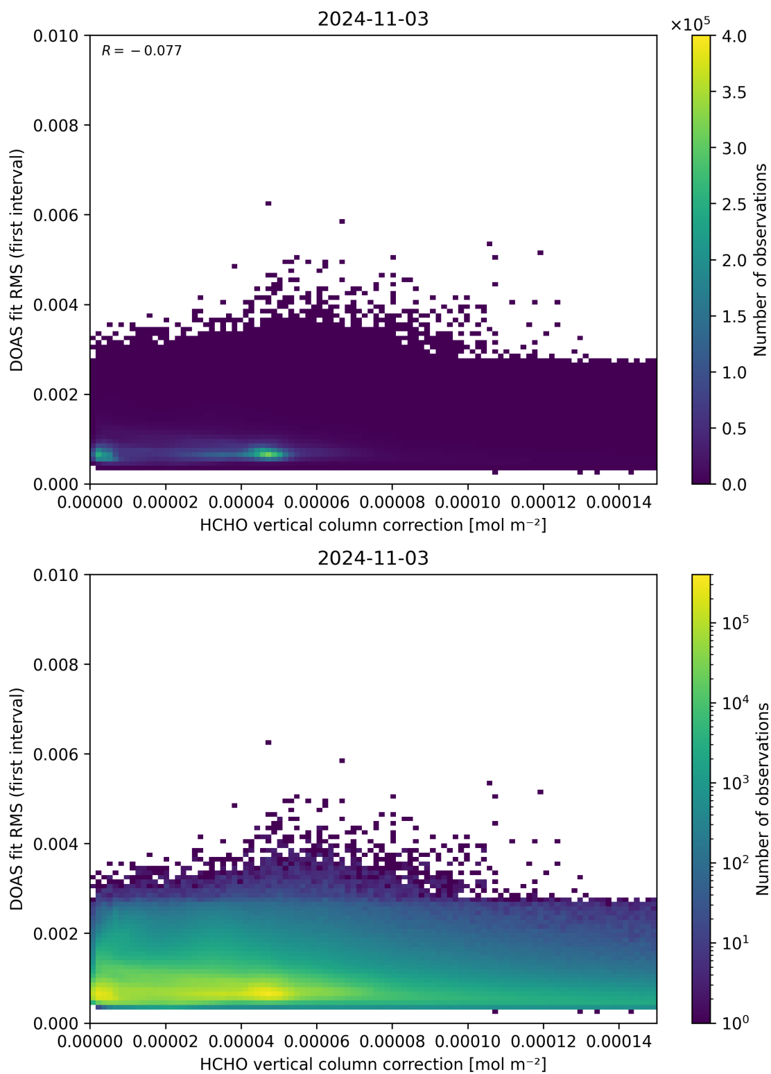
Figure 112: Scatter density plot of “HCHO vertical column correction” against “DOAS fit RMS (first interval)” for 2024-11-02 to 2024-11-04.
