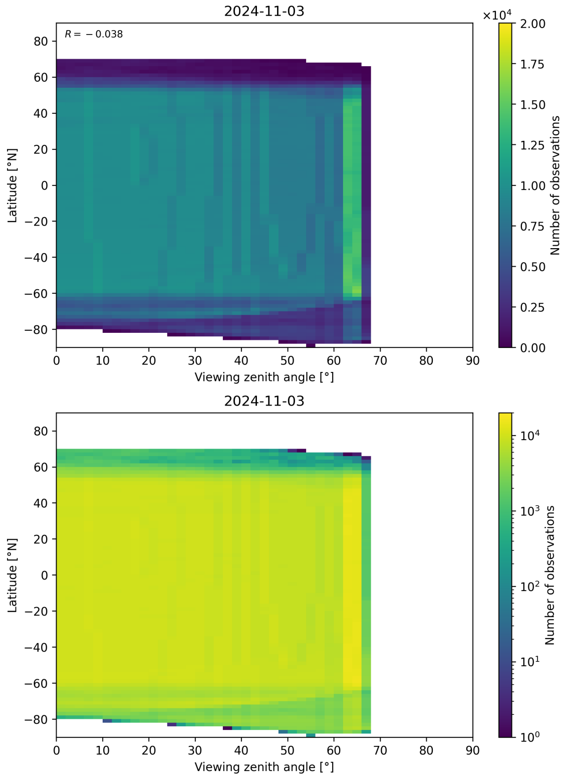
Figure 196: Scatter density plot of “Viewing zenith angle” against “Latitude” for 2024-11-02 to 2024-11-04.
