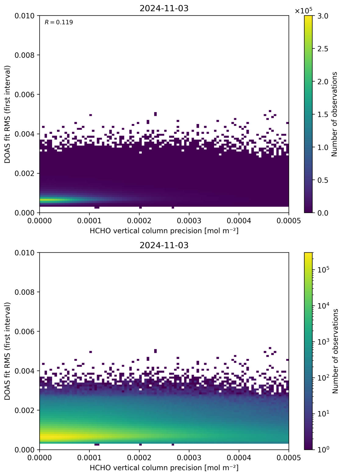
Figure 136: Scatter density plot of “HCHO vertical column precision” against “DOAS fit RMS (first interval)” for 2024-11-02 to 2024-11-04.
