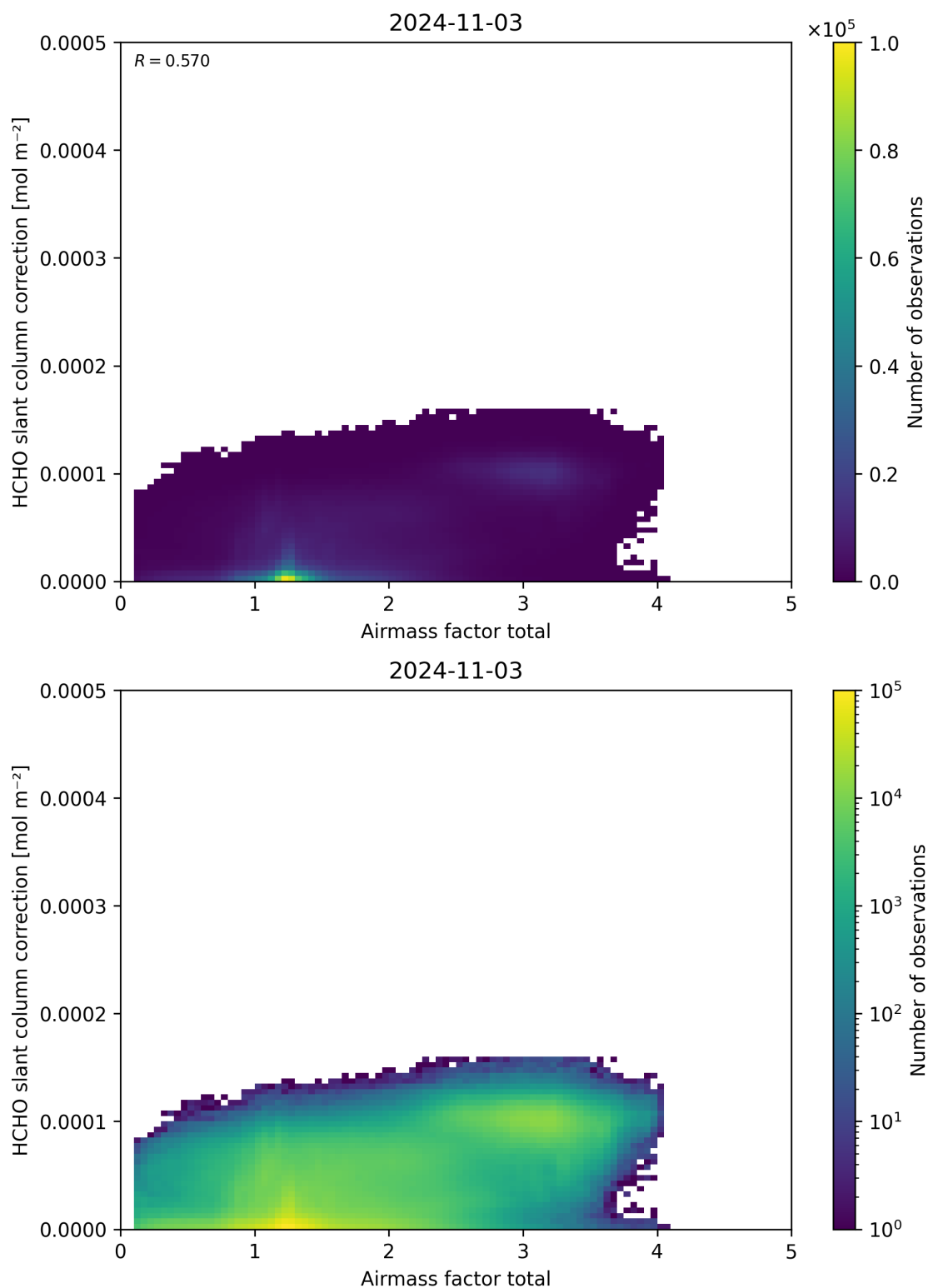
Figure 102: Scatter density plot of “Airmass factor total” against “HCHO slant column correction” for 2024-11-02 to 2024-11-04.
