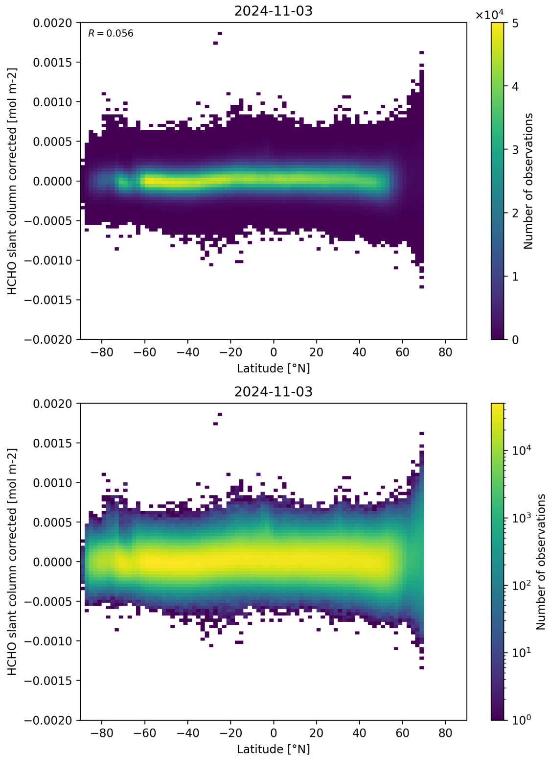
Figure 157: Scatter density plot of “Latitude” against “HCHO slant column corrected” for 2024-11-02 to 2024-11-04.
