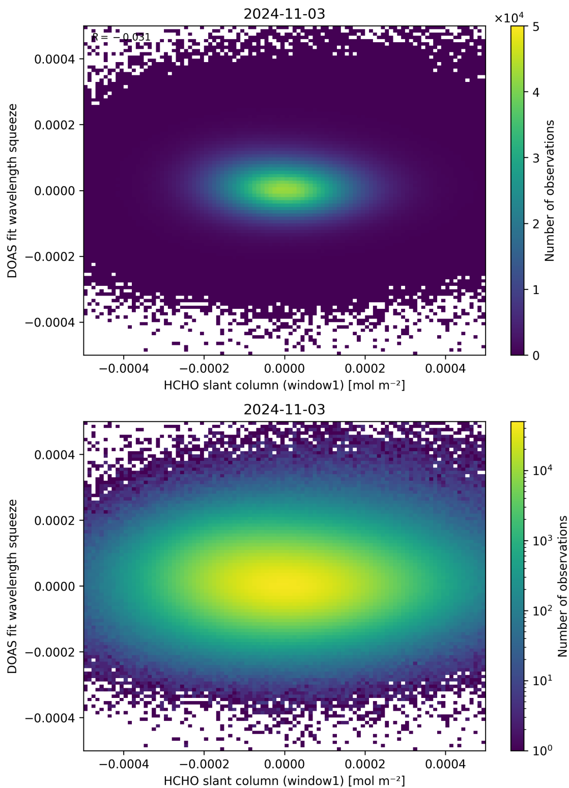
Figure 80: Scatter density plot of “HCHO slant column (window1)” against “DOAS fit wavelength squeeze” for 2024-11-02 to 2024-11-04.
