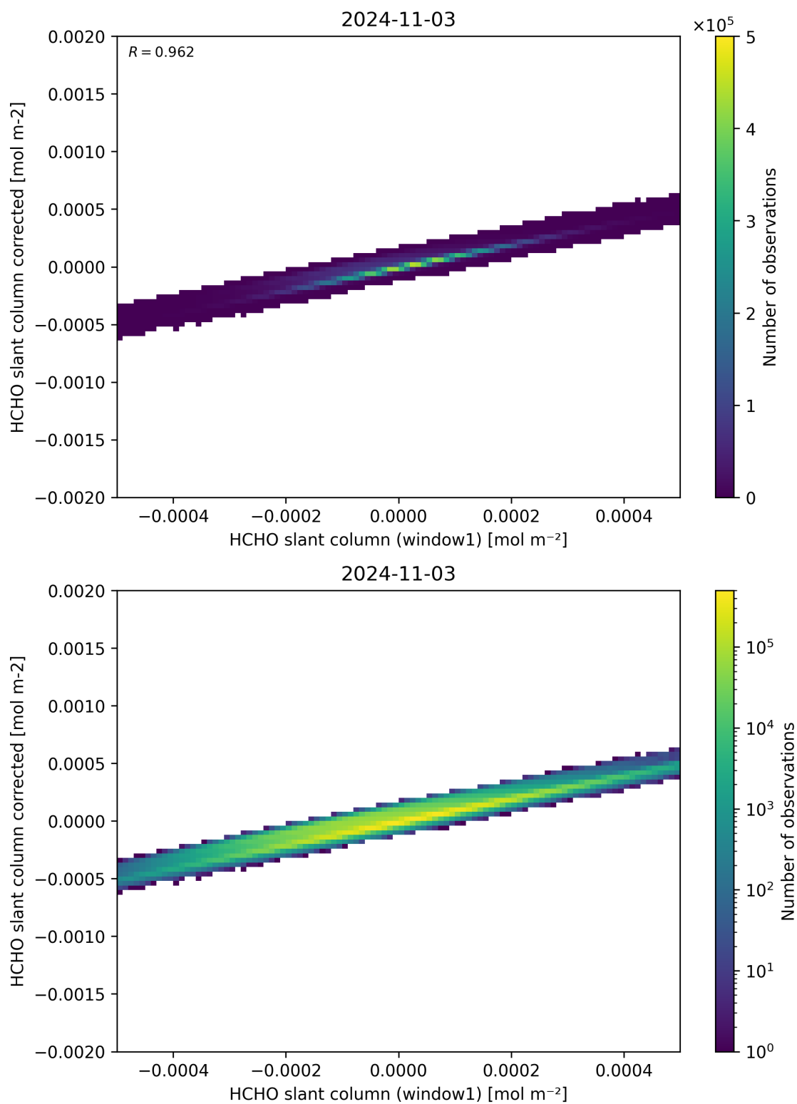
Figure 82: Scatter density plot of “HCHO slant column (window1)” against “HCHO slant column corrected” for 2024-11-02 to 2024-11-04.
