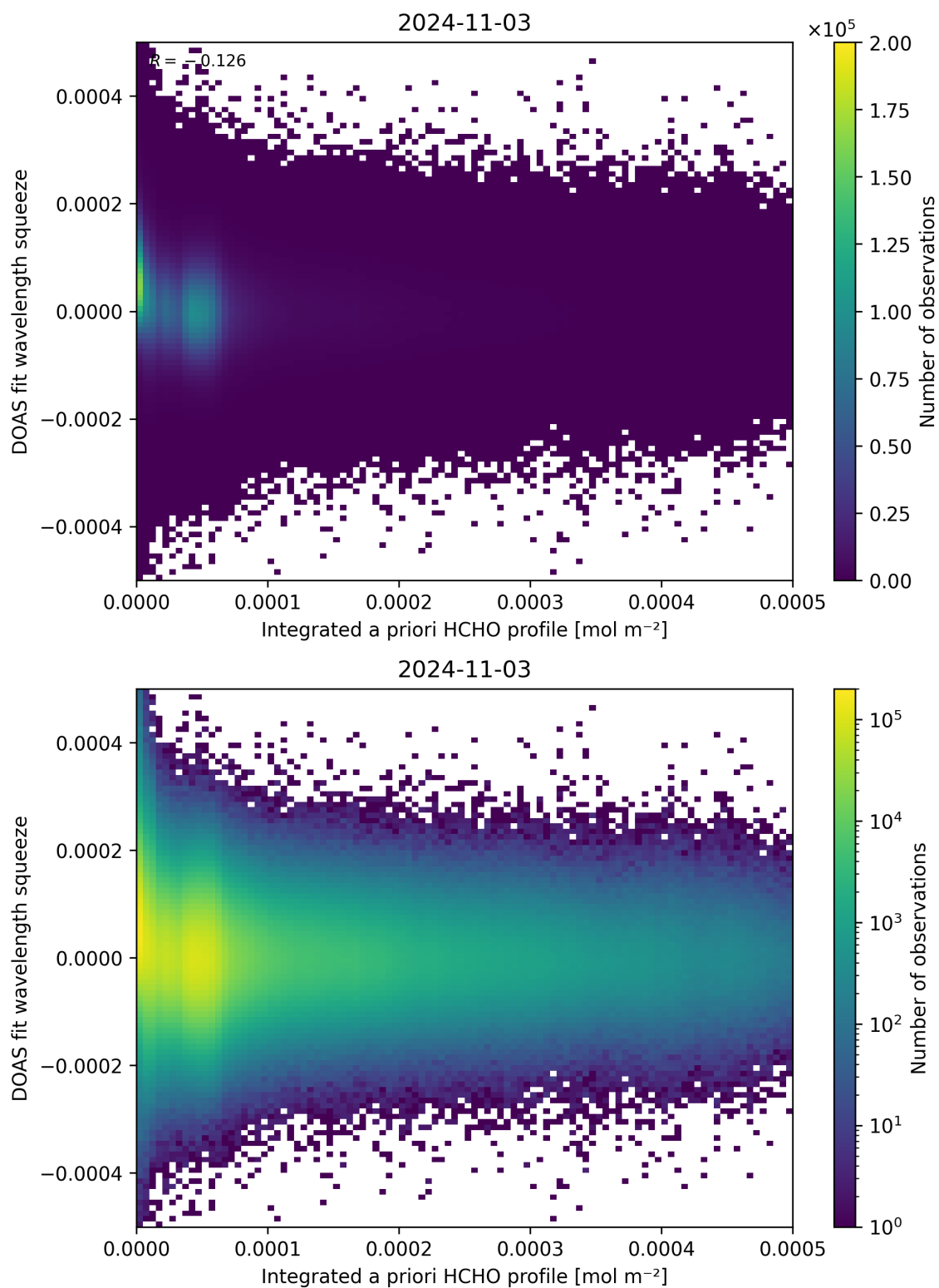
Figure 150: Scatter density plot of “Integrated a priori HCHO profile” against “DOAS fit wavelength squeeze” for 2024-11-02 to 2024-11-04.
