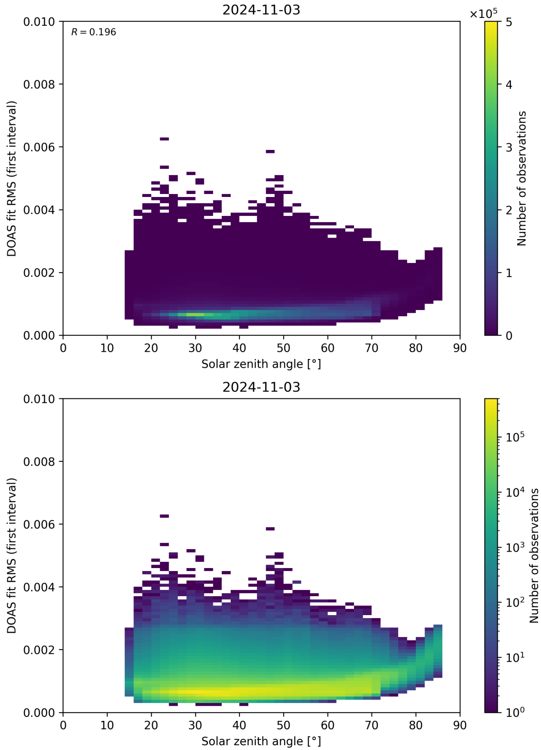
Figure 167: Scatter density plot of “Solar zenith angle” against “DOAS fit RMS (first interval)” for 2024-11-02 to 2024-11-04.
