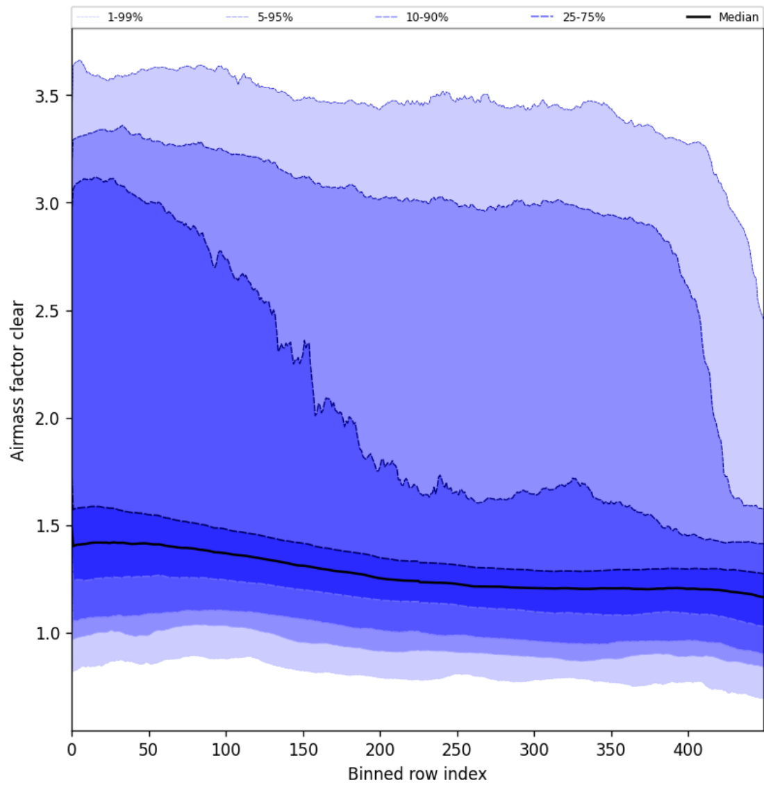
Figure 56: Along track statistics of “Airmass factor clear” for 2024-11-02 to 2024-11-04
