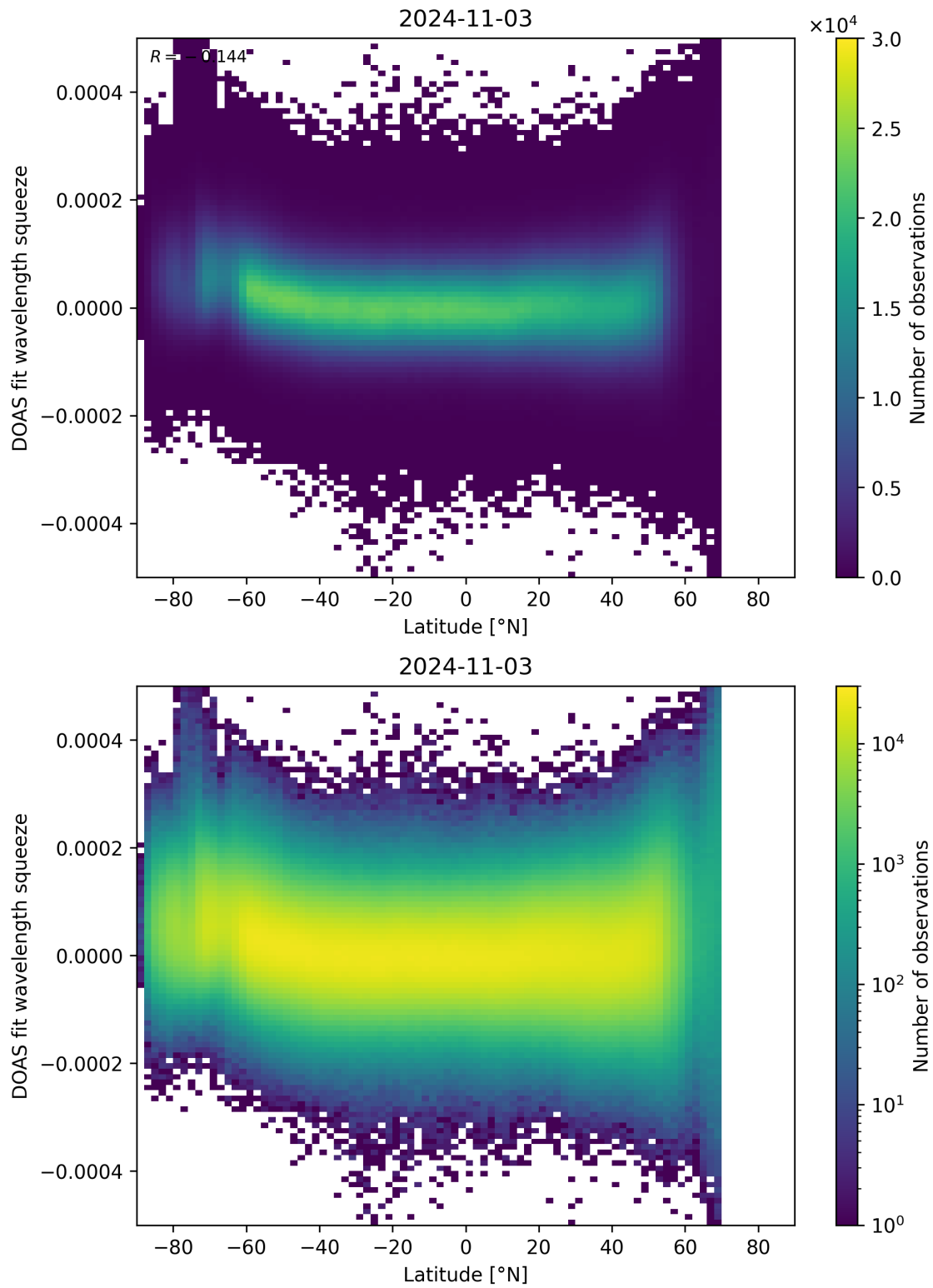
Figure 155: Scatter density plot of “Latitude” against “DOAS fit wavelength squeeze” for 2024-11-02 to 2024-11-04.
