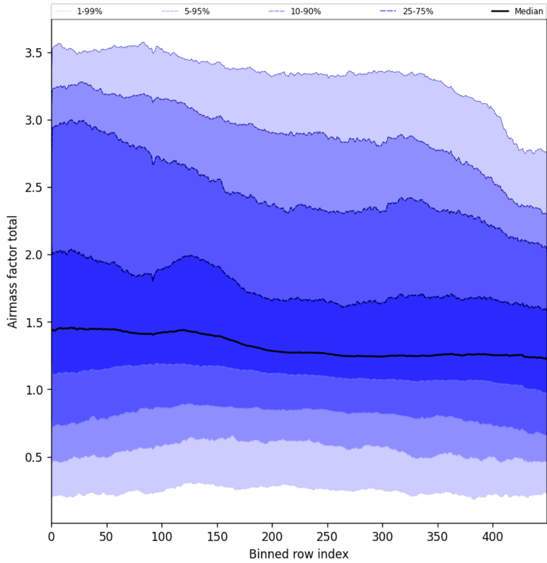
Figure 54: Along track statistics of “Airmass factor total” for 2024-11-02 to 2024-11-04
