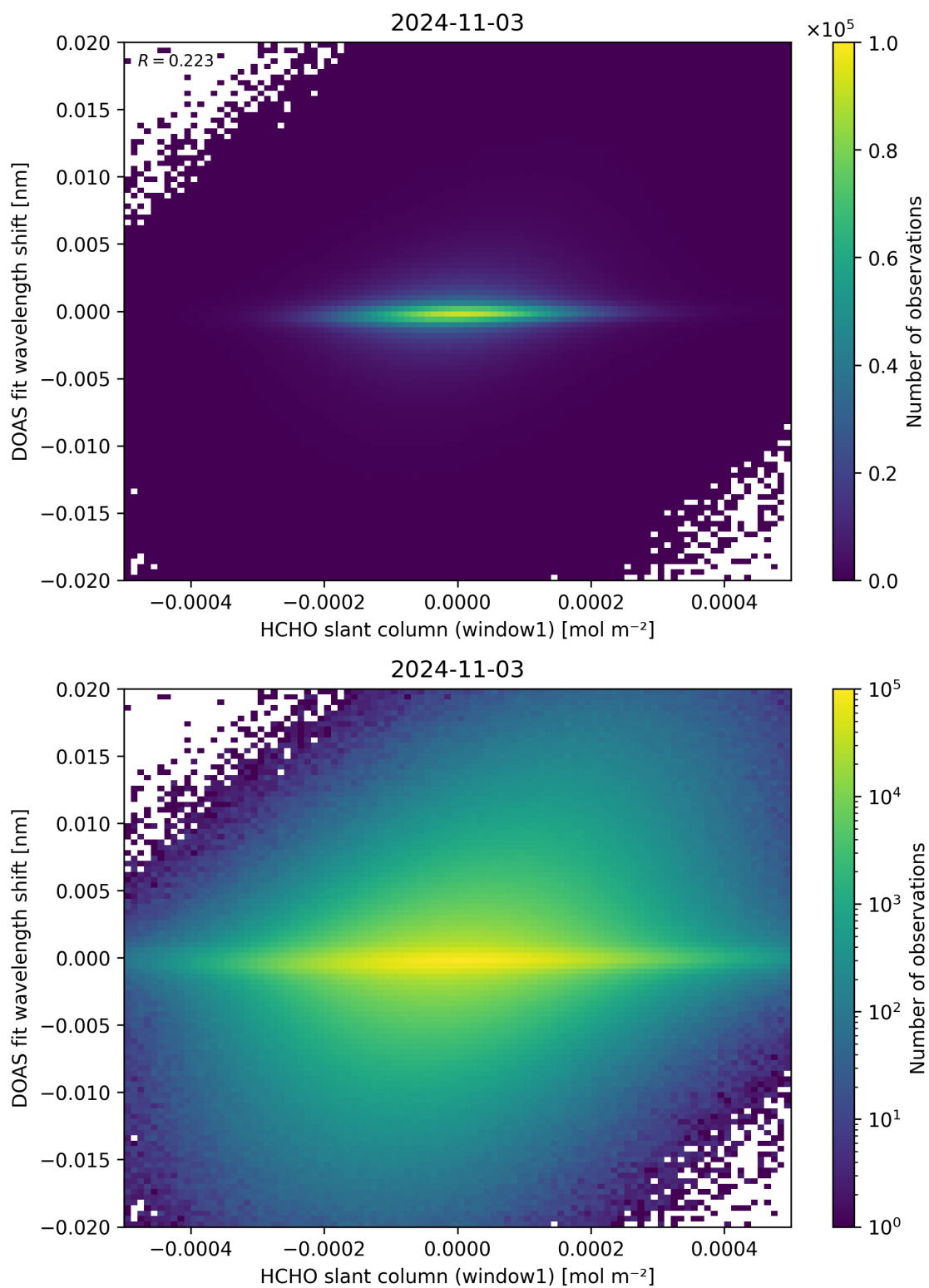
Figure 79: Scatter density plot of “HCHO slant column (window1)” against “DOAS fit wavelength shift” for 2024-11-02 to 2024-11-04.
