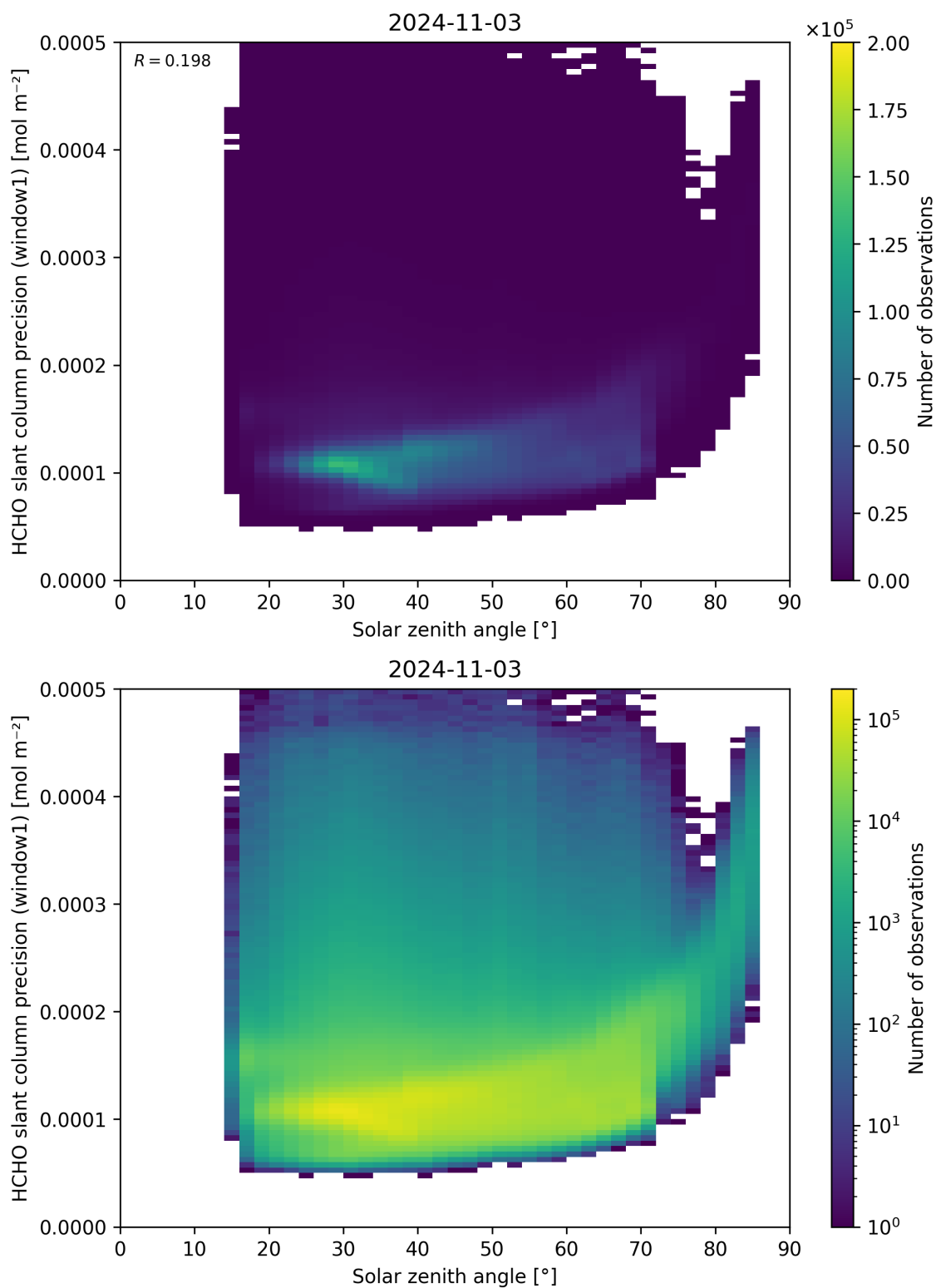
Figure 174: Scatter density plot of “Solar zenith angle” against “HCHO slant column precision (window1)” for 2024-11-02 to 2024-11-04.
