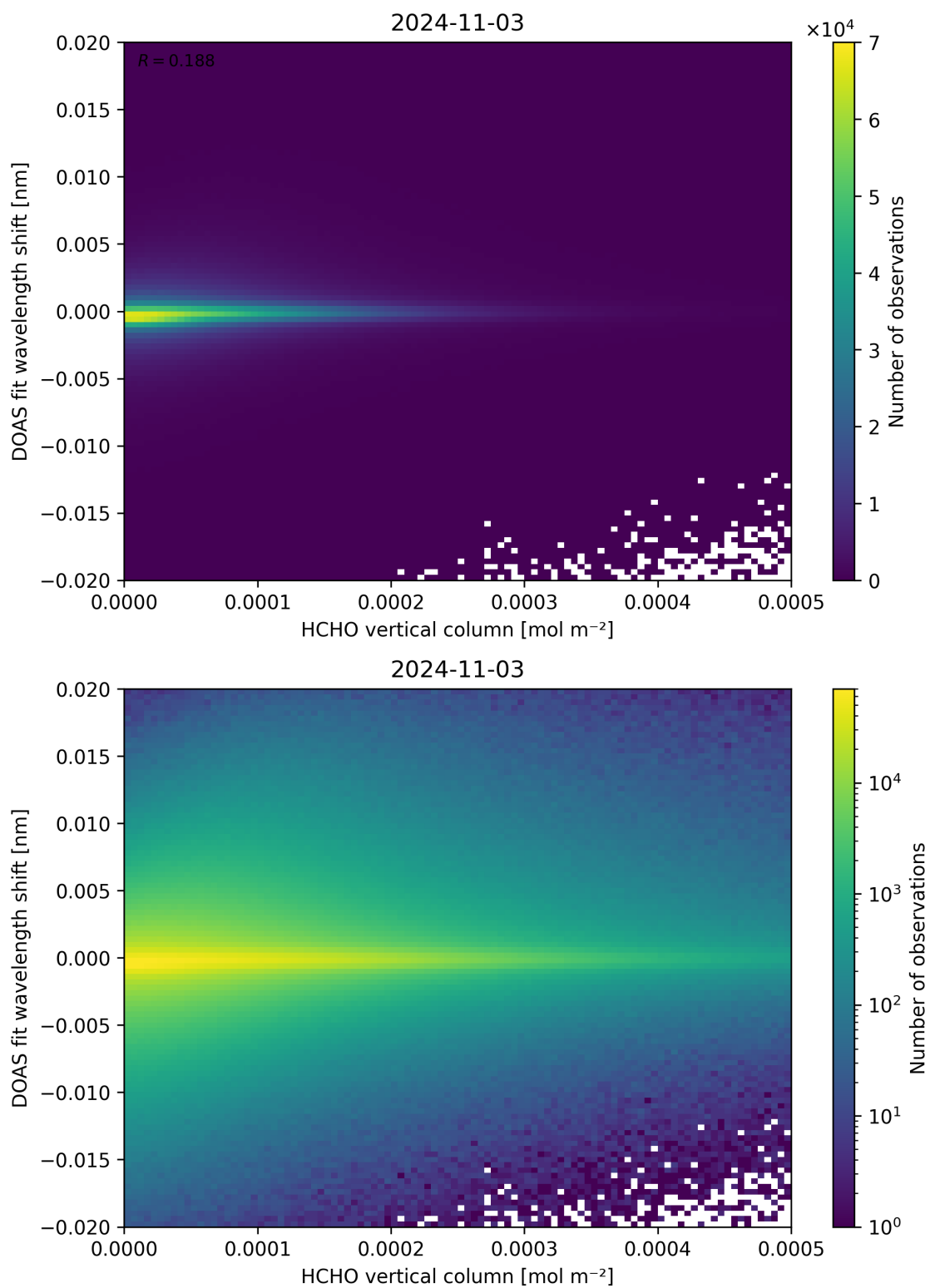
Figure 124: Scatter density plot of “HCHO vertical column” against “DOAS fit wavelength shift” for 2024-11-02 to 2024-11-04.
