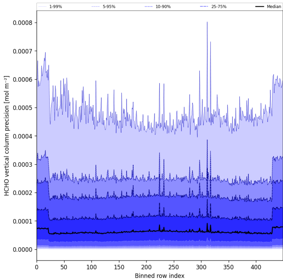
Figure 50: Along track statistics of “HCHO vertical column precision” for 2024-11-02 to 2024-11-04
