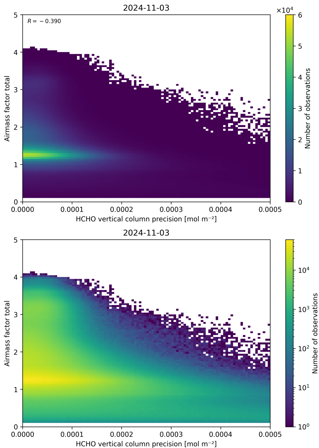
Figure 144: Scatter density plot of “HCHO vertical column precision” against “Airmass factor total” for 2024-11-02 to 2024-11-04.
