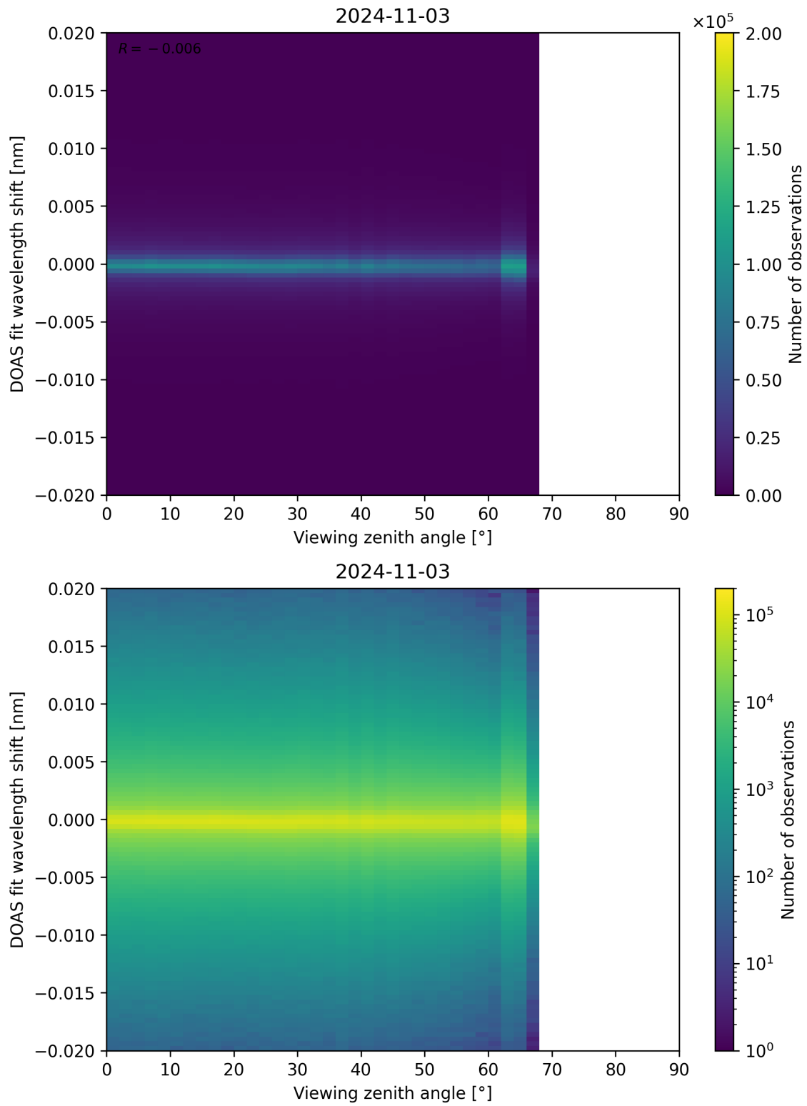
Figure 183: Scatter density plot of “Viewing zenith angle” against “DOAS fit wavelength shift” for 2024-11-02 to 2024-11-04.
