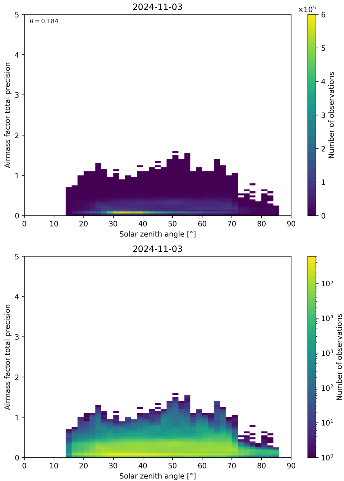
Figure 176: Scatter density plot of “Solar zenith angle” against “Airmass factor total precision” for 2024-11-02 to 2024-11-04.
