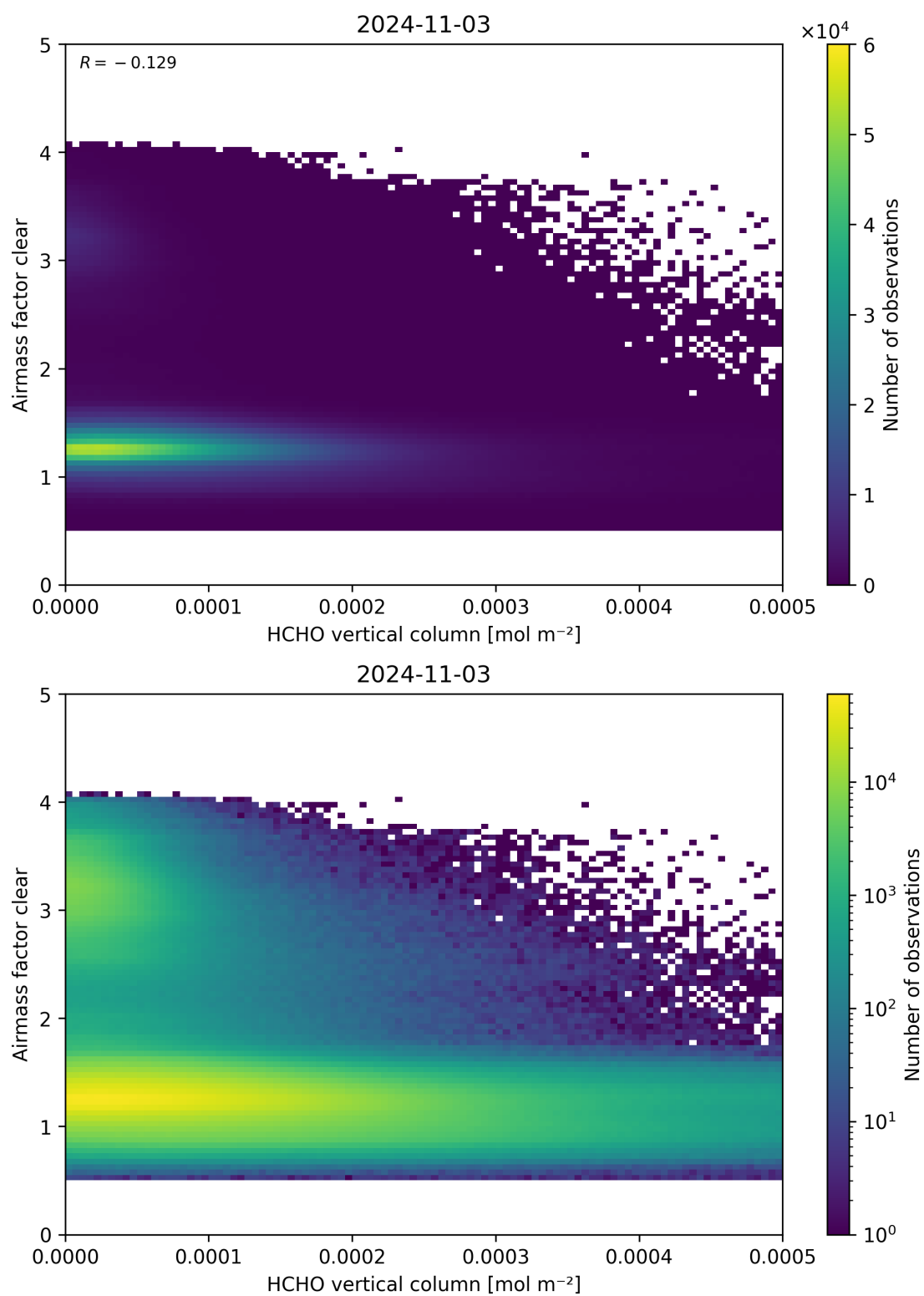
Figure 126: Scatter density plot of “HCHO vertical column” against “Airmass factor clear” for 2024-11-02 to 2024-11-04.
