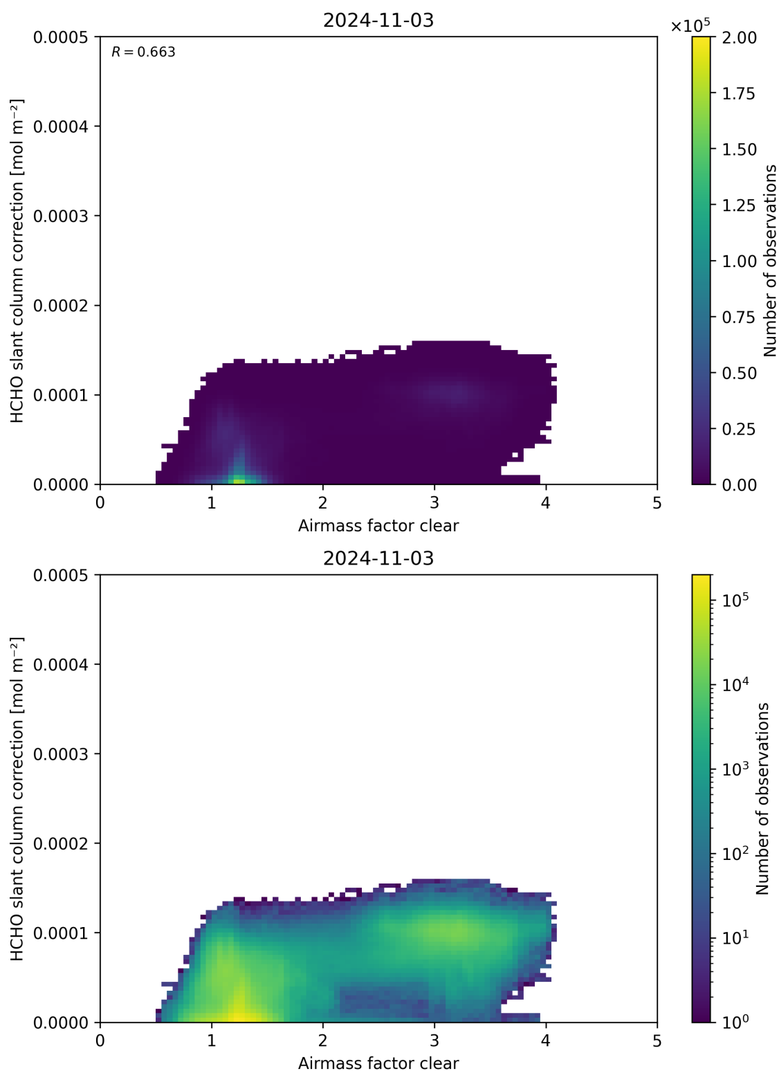
Figure 75: Scatter density plot of “Airmass factor clear” against “HCHO slant column correction” for 2024-11-02 to 2024-11-04.
