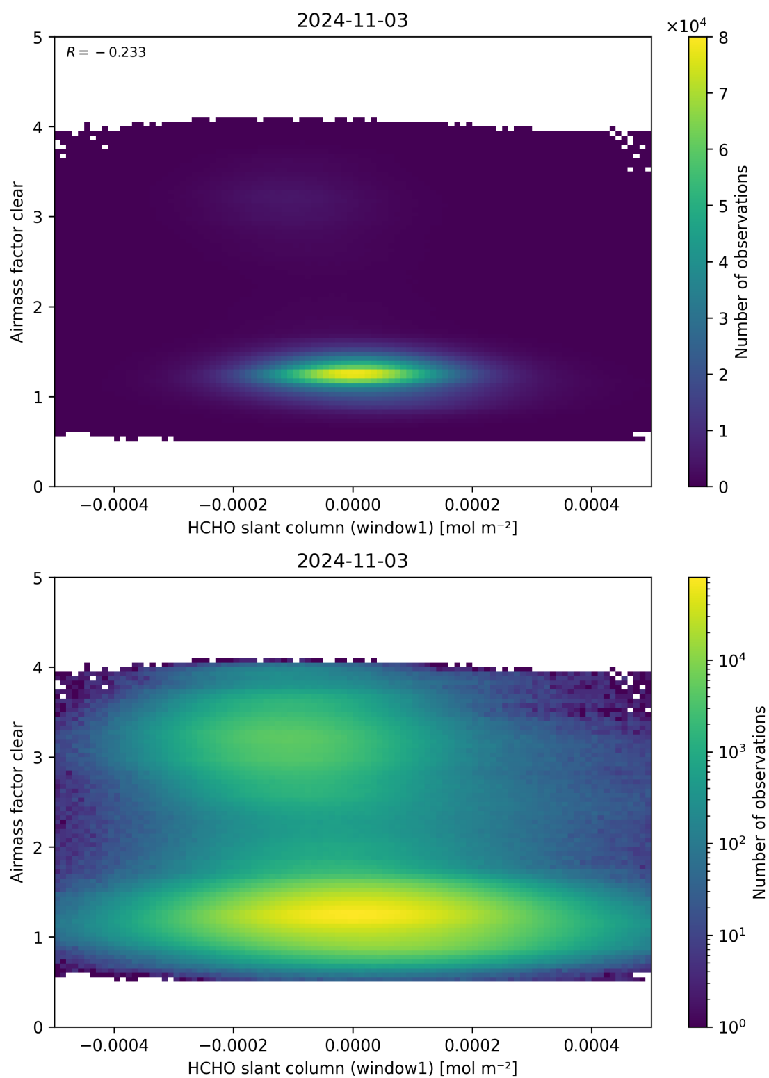
Figure 81: Scatter density plot of “HCHO slant column (window1)” against “Airmass factor clear” for 2024-11-02 to 2024-11-04.
