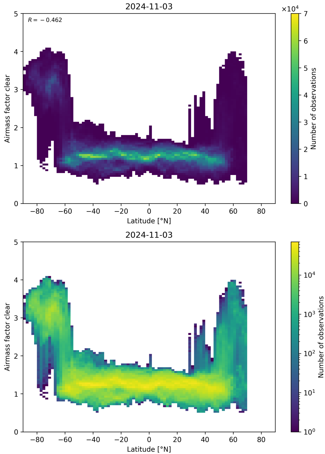
Figure 156: Scatter density plot of “Latitude” against “Airmass factor clear” for 2024-11-02 to 2024-11-04.
