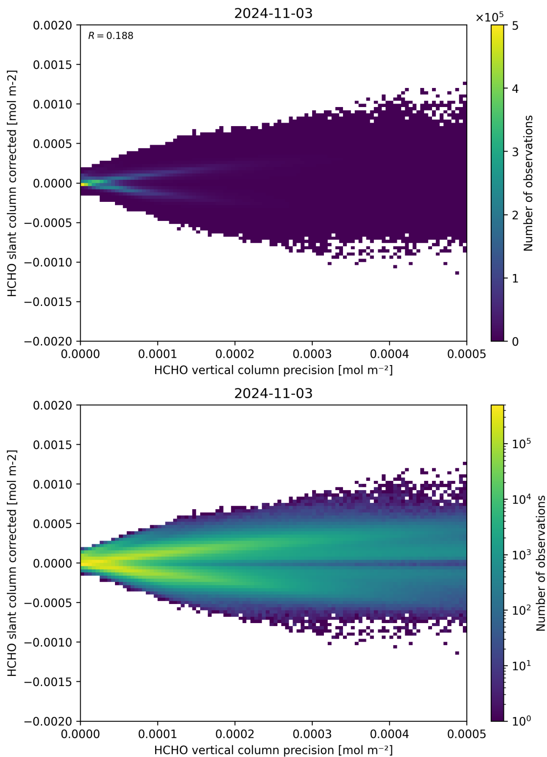
Figure 140: Scatter density plot of “HCHO vertical column precision” against “HCHO slant column corrected” for 2024-11-02 to 2024-11-04.
