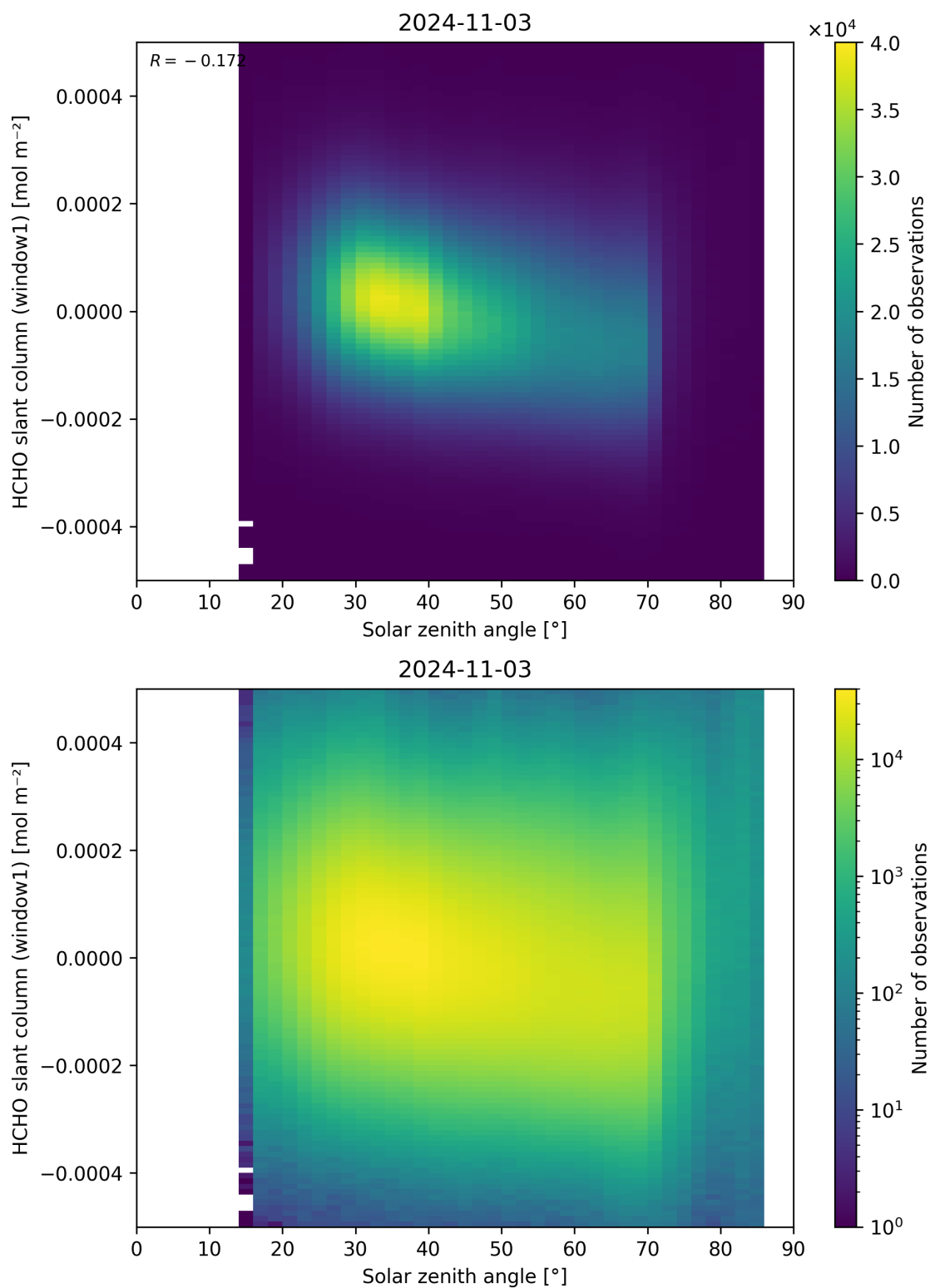
Figure 173: Scatter density plot of “Solar zenith angle” against “HCHO slant column (window1)” for 2024-11-02 to 2024-11-04.
