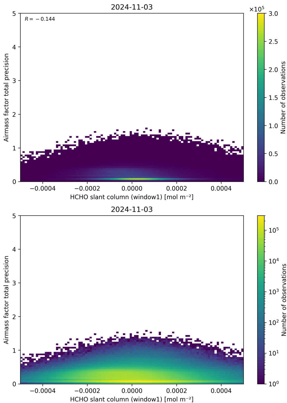
Figure 86: Scatter density plot of “HCHO slant column (window1)” against “Airmass factor total precision” for 2024-11-02 to 2024-11-04.
