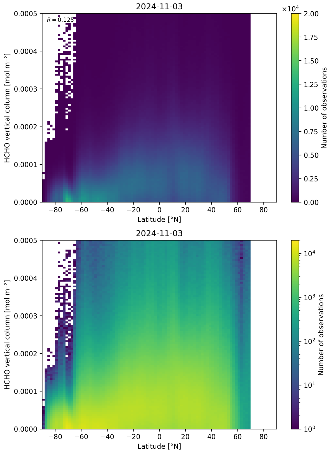
Figure 163: Scatter density plot of “Latitude” against “HCHO vertical column” for 2024-11-02 to 2024-11-04.
