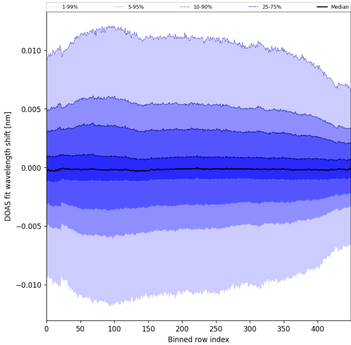
Figure 58: Along track statistics of “DOAS fit wavelength shift” for 2024-11-02 to 2024-11-04
