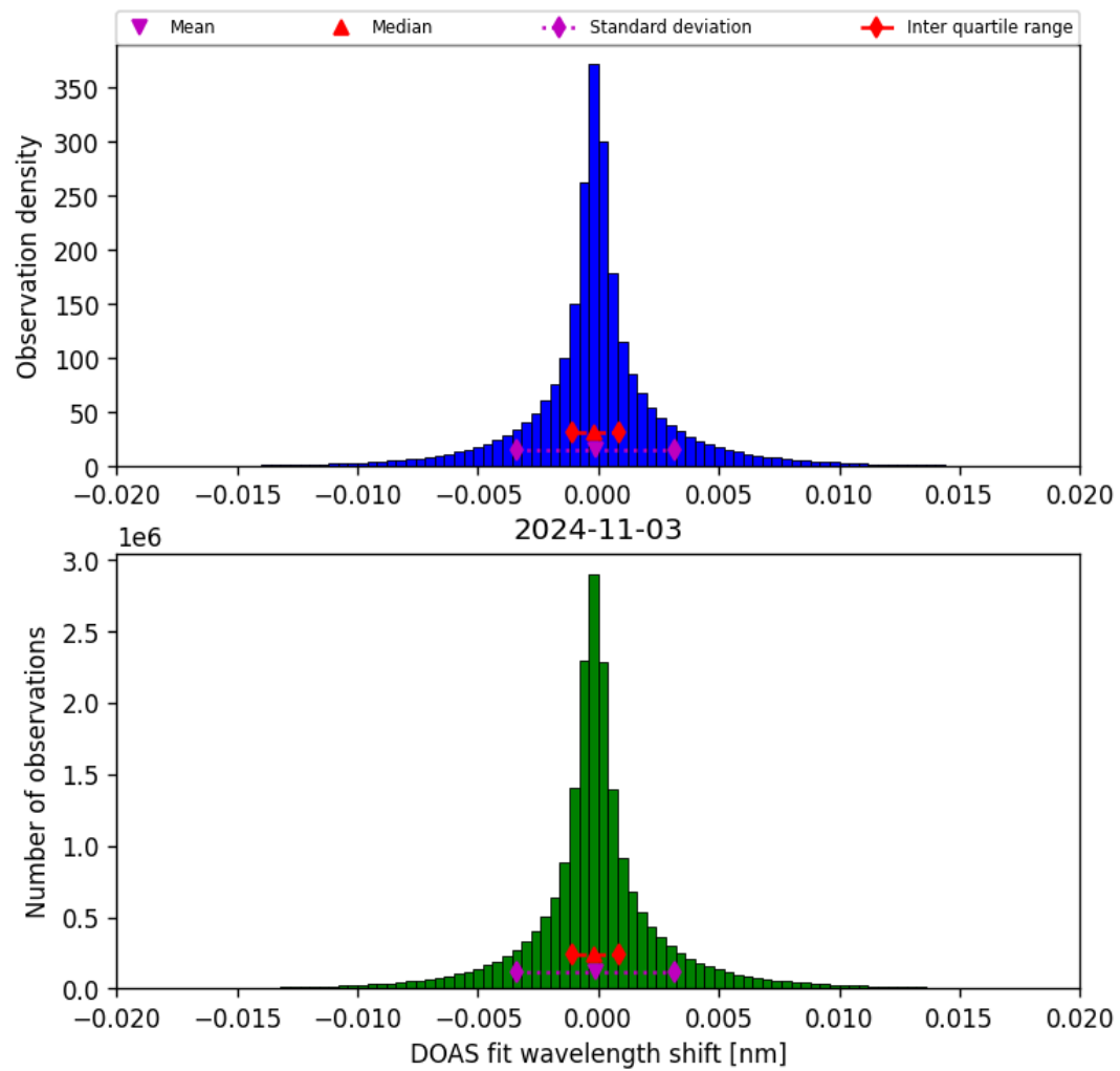
Figure 44: Histogram of “DOAS fit wavelength shift” for 2024-11-02 to 2024-11-04
