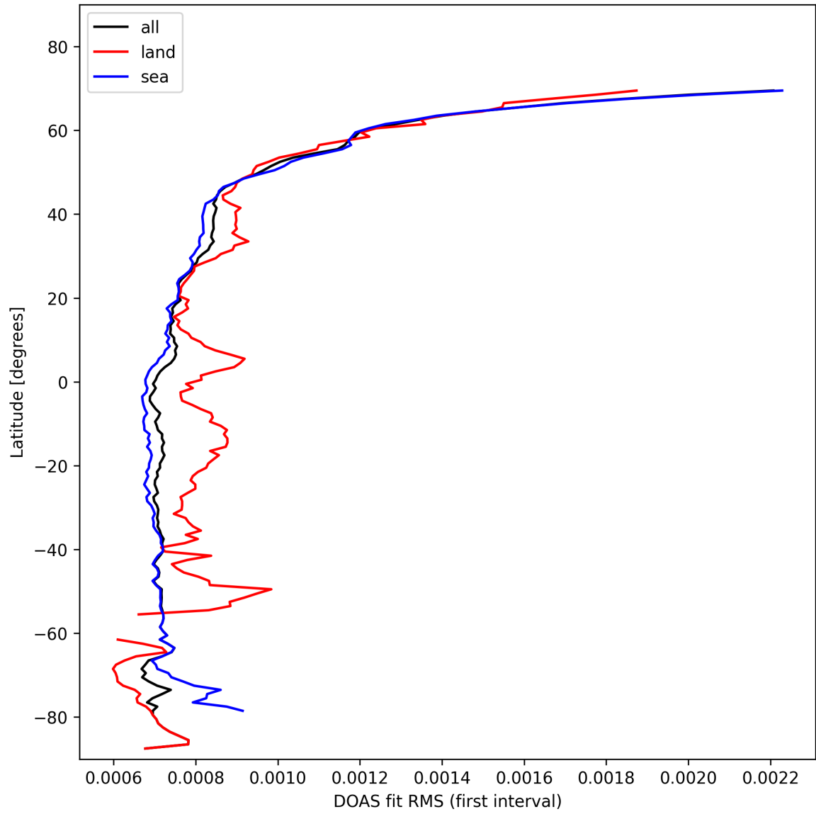
Figure 32: Zonal average of “DOAS fit RMS (first interval)” for 2024-11-02 to 2024-11-04.
