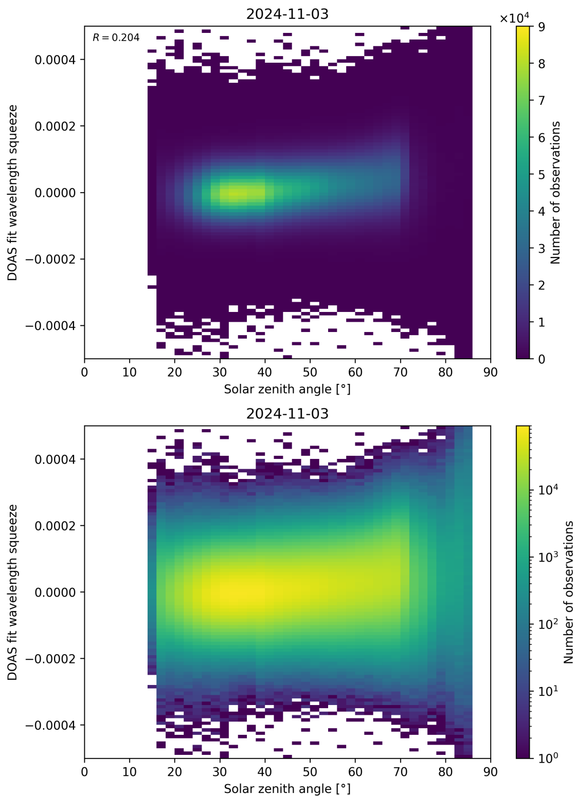
Figure 169: Scatter density plot of “Solar zenith angle” against “DOAS fit wavelength squeeze” for 2024-11-02 to 2024-11-04.
