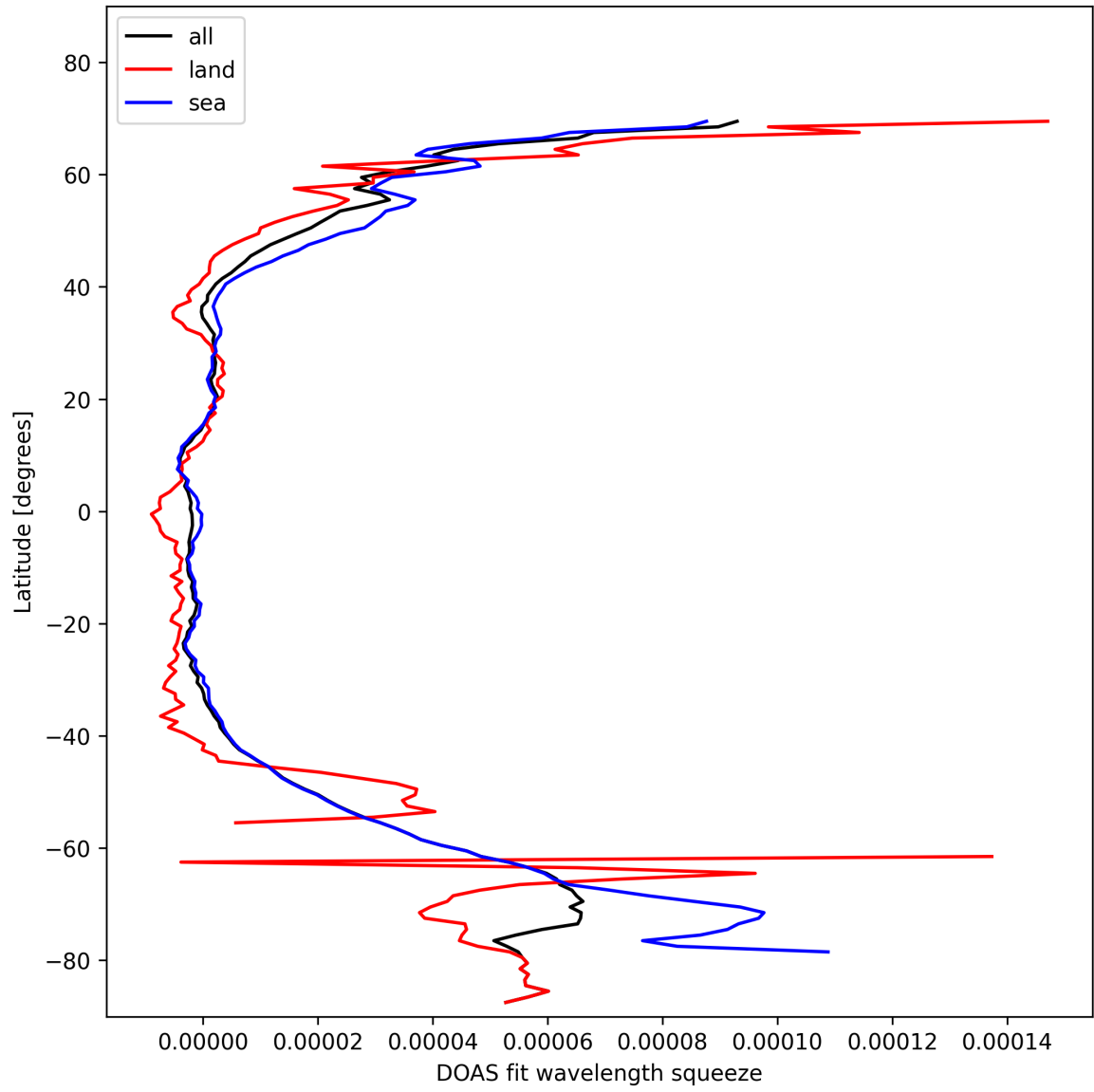
Figure 31: Zonal average of “DOAS fit wavelength squeeze” for 2024-11-02 to 2024-11-04.
