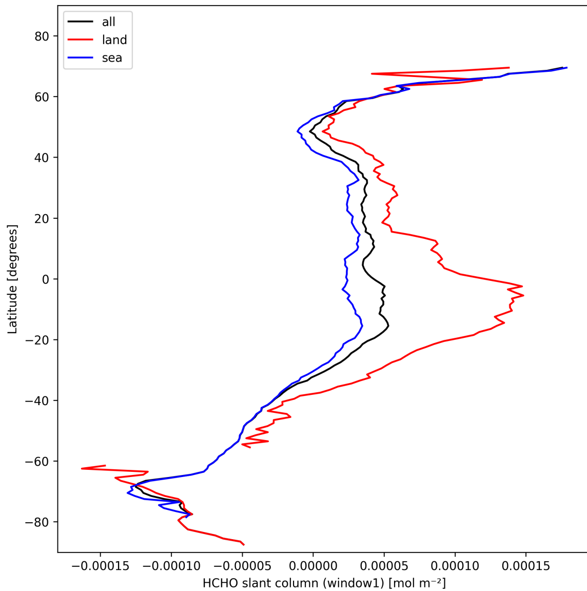
Figure 24: Zonal average of “HCHO slant column (window1)” for 2024-11-02 to 2024-11-04.
