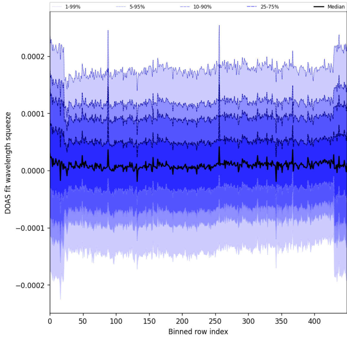
Figure 59: Along track statistics of “DOAS fit wavelength squeeze” for 2024-11-02 to 2024-11-04
