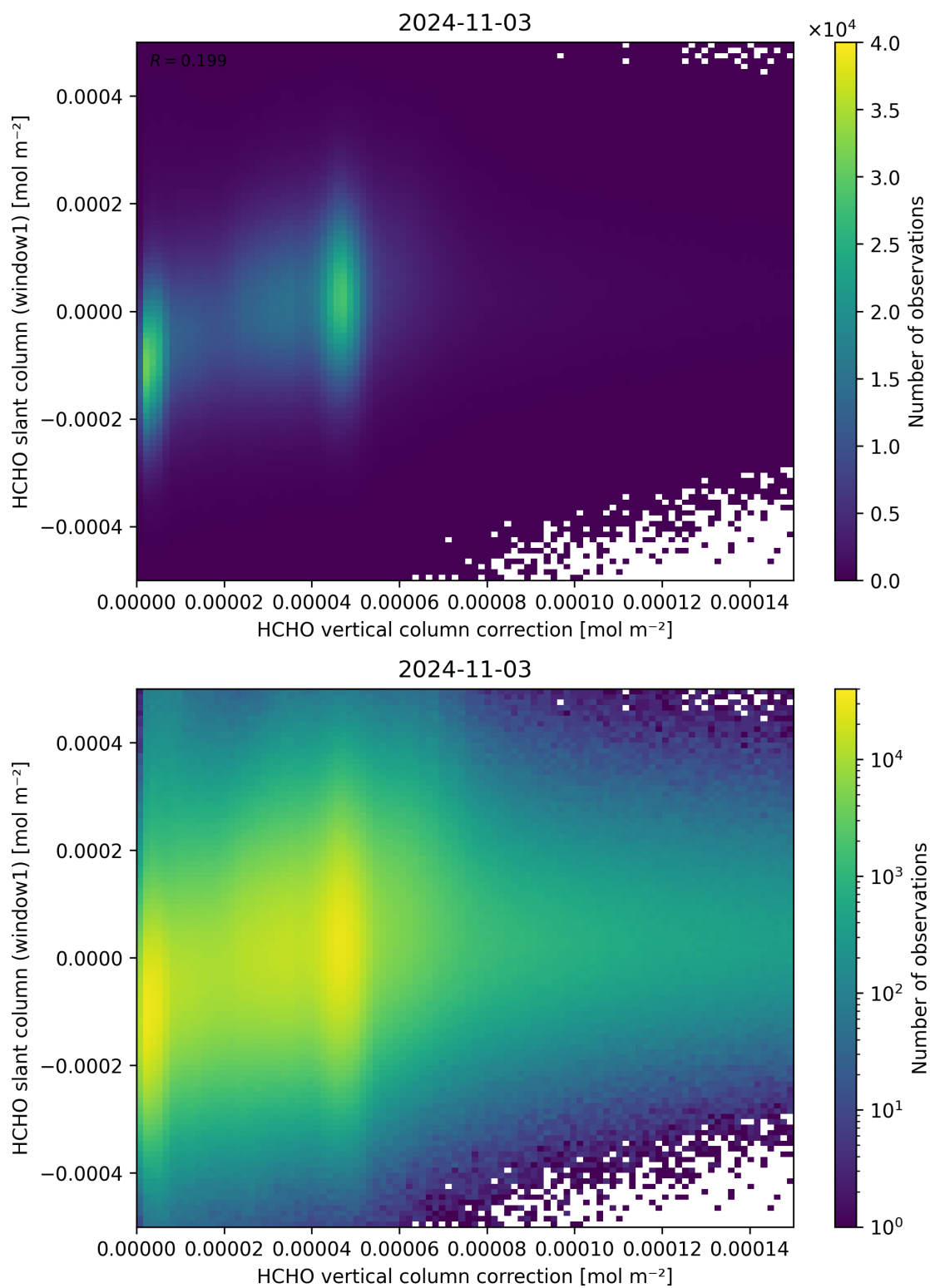
Figure 118: Scatter density plot of “HCHO vertical column correction” against “HCHO slant column (window1)” for 2024-11-02 to 2024-11-04.
