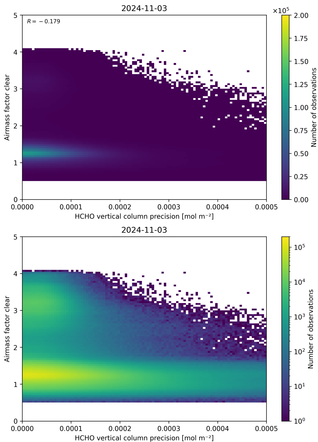
Figure 139: Scatter density plot of “HCHO vertical column precision” against “Airmass factor clear” for 2024-11-02 to 2024-11-04.
