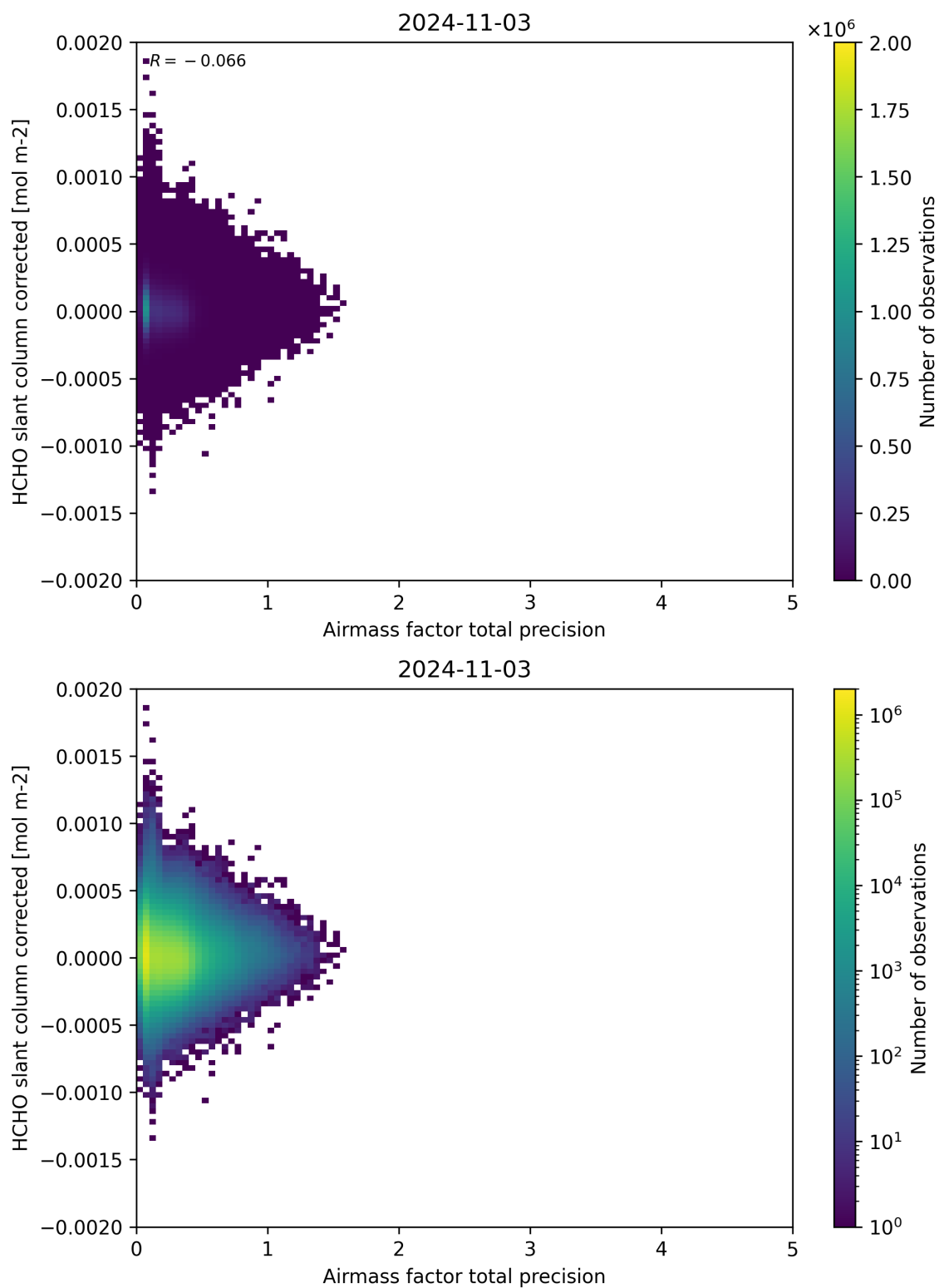
Figure 109: Scatter density plot of “Airmass factor total precision” against “HCHO slant column corrected” for 2024-11-02 to 2024-11-04.
