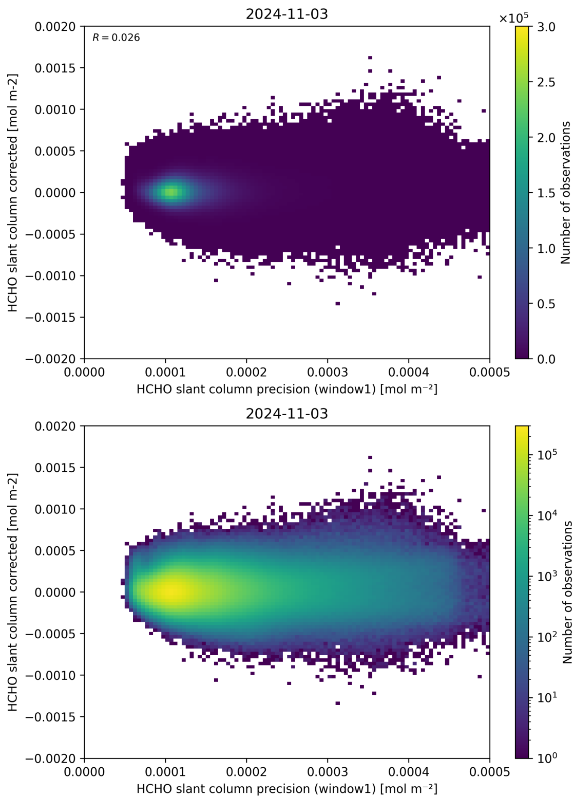
Figure 92: Scatter density plot of “HCHO slant column precision (window1)” against “HCHO slant column corrected” for 2024-11-02 to 2024-11-04.
