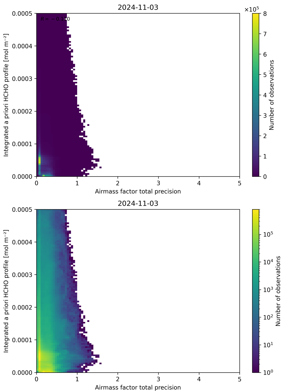
Figure 111: Scatter density plot of “Airmass factor total precision” against “Integrated a priori HCHO profile” for 2024-11-02 to 2024-11-04.
