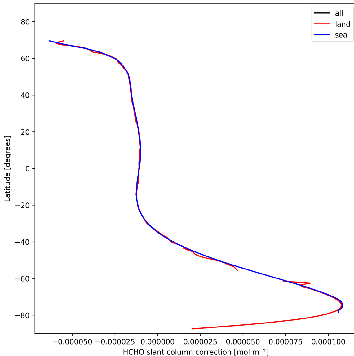
Figure 33: Zonal average of “HCHO slant column correction” for 2024-11-02 to 2024-11-04.
