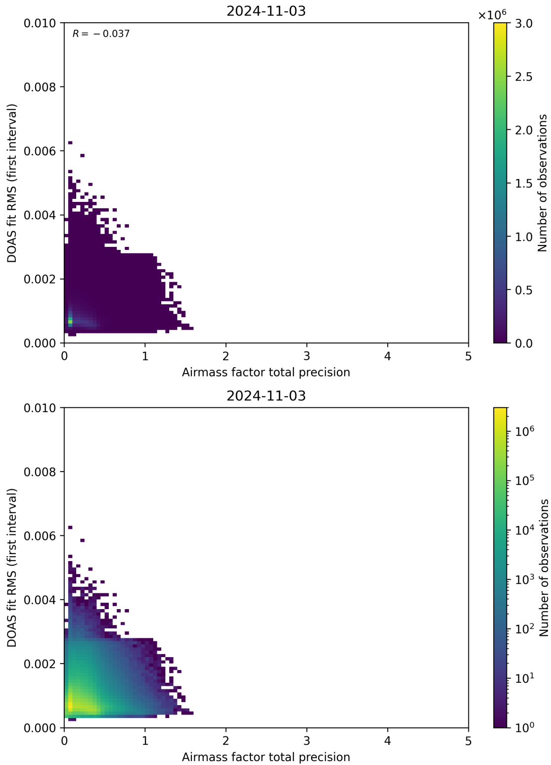
Figure 105: Scatter density plot of “Airmass factor total precision” against “DOAS fit RMS (first interval)” for 2024-11-02 to 2024-11-04.
