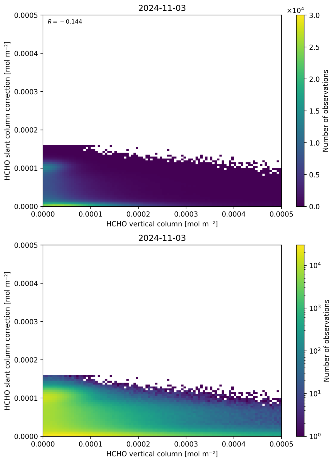
Figure 128: Scatter density plot of “HCHO vertical column” against “HCHO slant column correction” for 2024-11-02 to 2024-11-04.
