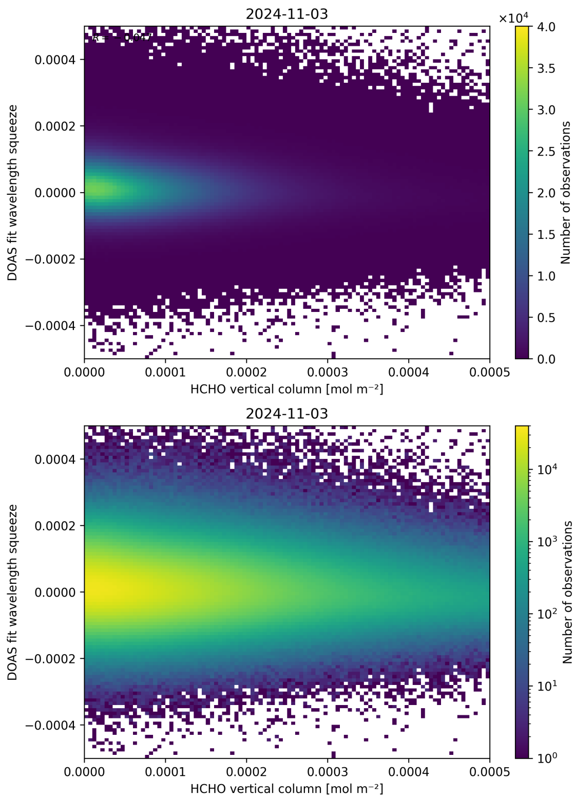
Figure 125: Scatter density plot of “HCHO vertical column” against “DOAS fit wavelength squeeze” for 2024-11-02 to 2024-11-04.
