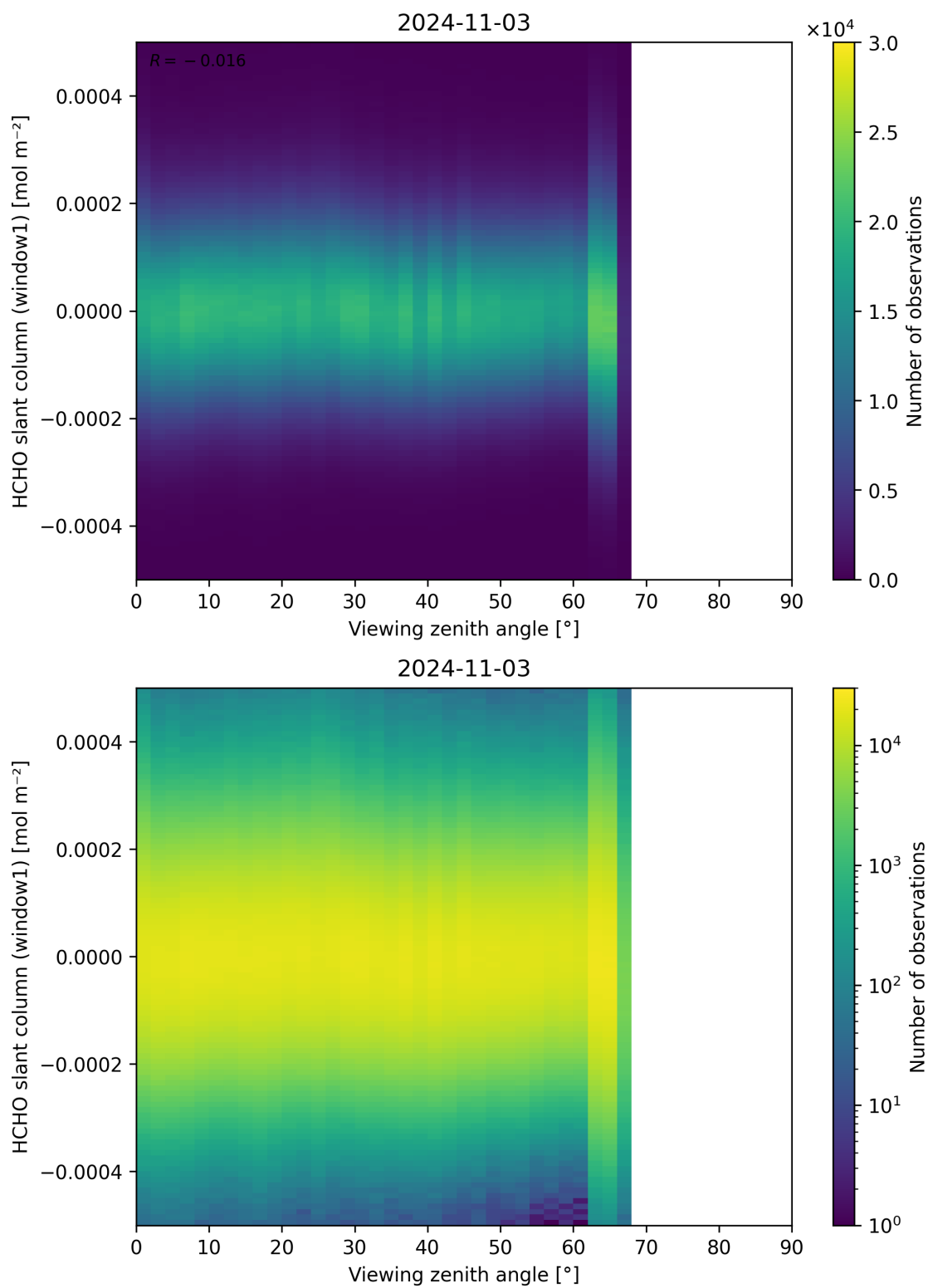
Figure 188: Scatter density plot of “Viewing zenith angle” against “HCHO slant column (window1)” for 2024-11-02 to 2024-11-04.
