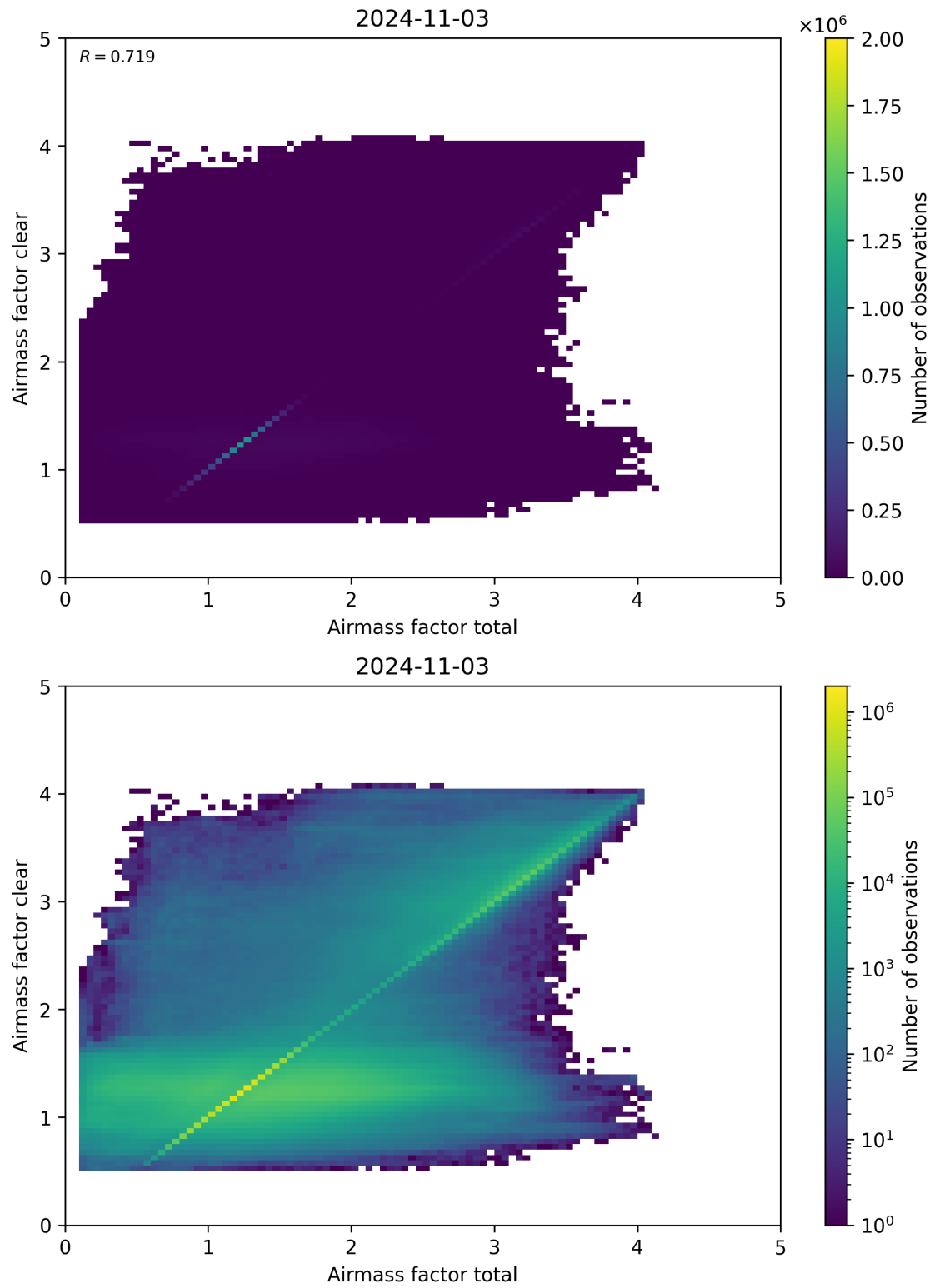
Figure 100: Scatter density plot of “Airmass factor total” against “Airmass factor clear” for 2024-11-02 to 2024-11-04.
