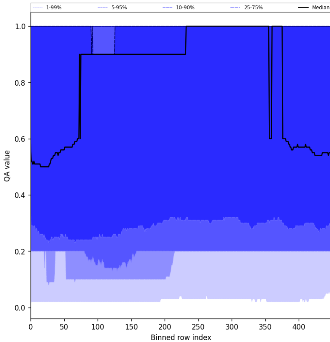
Figure 48: Along track statistics of “QA value” for 2024-11-02 to 2024-11-04
