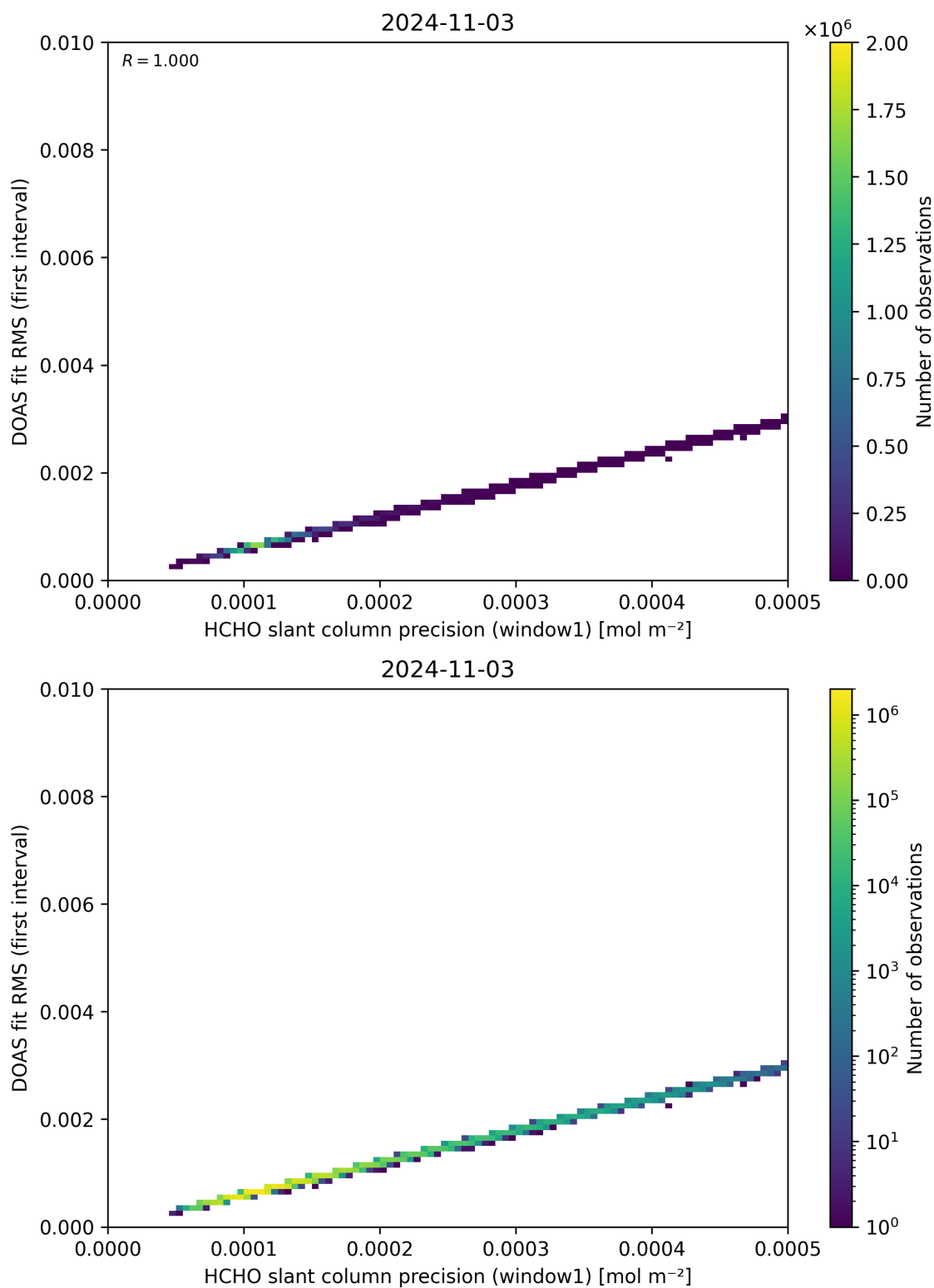
Figure 88: Scatter density plot of “HCHO slant column precision (window1)” against “DOAS fit RMS (first interval)” for 2024-11-02 to 2024-11-04.
