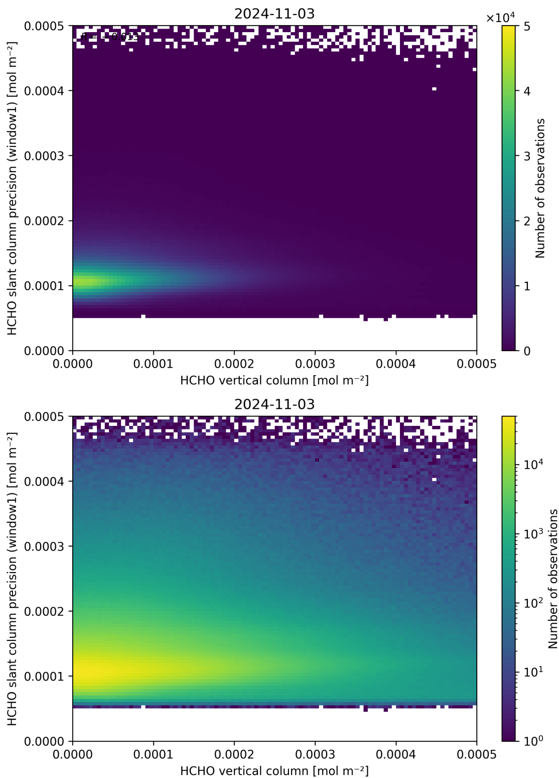
Figure 130: Scatter density plot of “HCHO vertical column” against “HCHO slant column precision (window1)” for 2024-11-02 to 2024-11-04.
