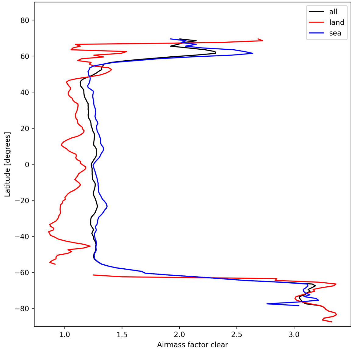
Figure 28: Zonal average of “Airmass factor clear” for 2024-11-02 to 2024-11-04.
