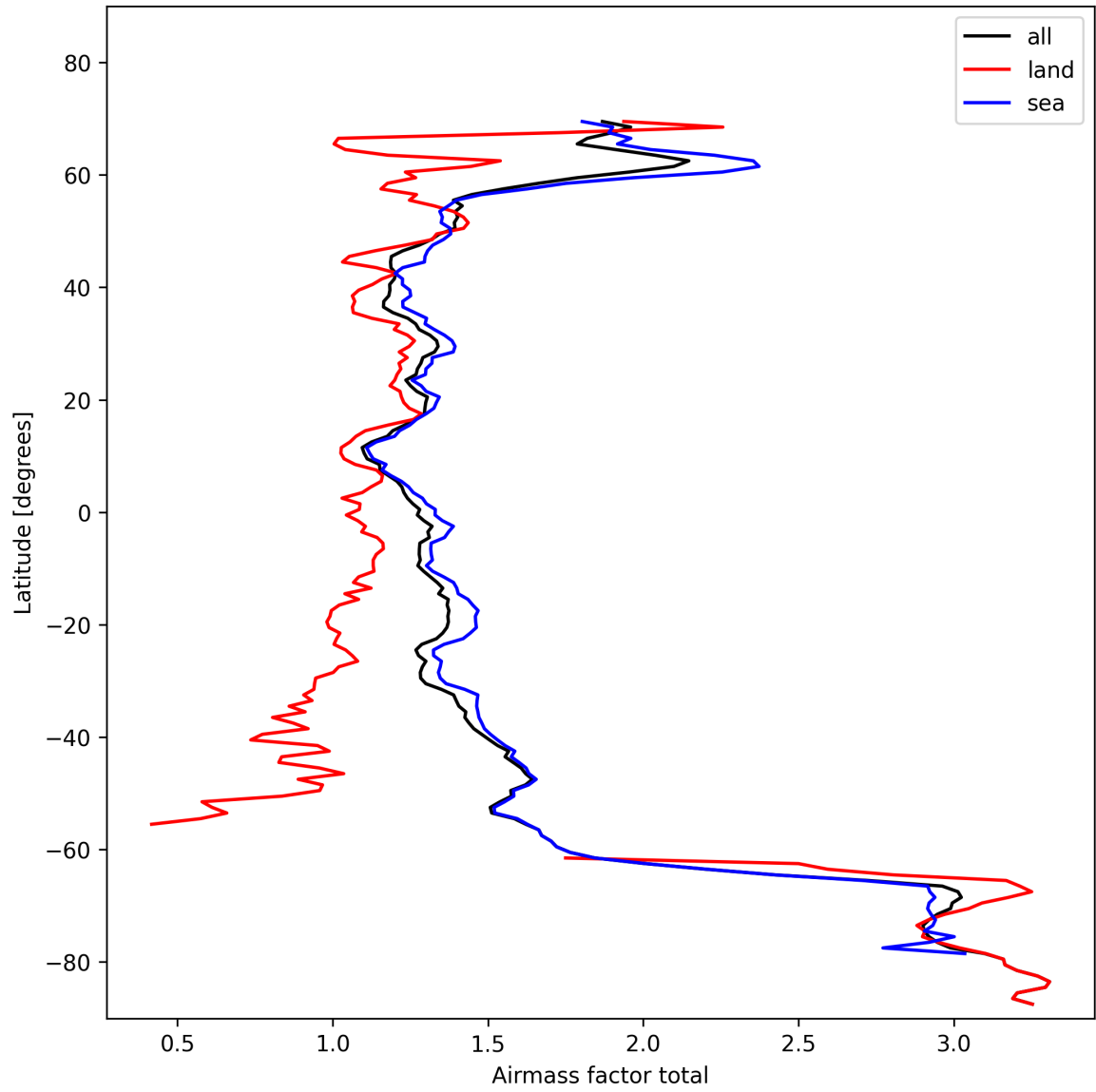
Figure 26: Zonal average of “Airmass factor total” for 2024-11-02 to 2024-11-04.
