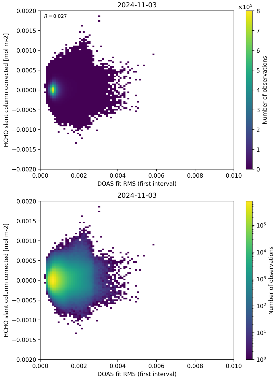
Figure 62: Scatter density plot of “DOAS fit RMS (first interval)” against “HCHO slant column corrected” for 2024-11-02 to 2024-11-04.
