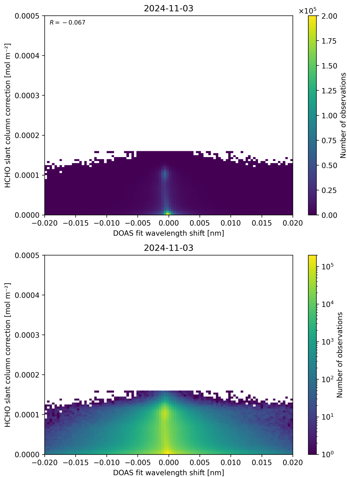
Figure 67: Scatter density plot of “DOAS fit wavelength shift” against “HCHO slant column correction” for 2024-11-02 to 2024-11-04.
