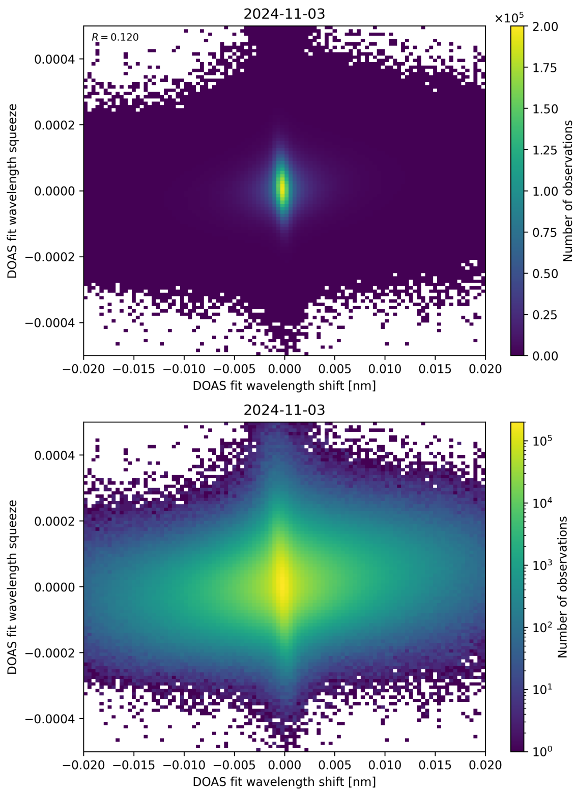
Figure 65: Scatter density plot of “DOAS fit wavelength shift” against “DOAS fit wavelength squeeze” for 2024-11-02 to 2024-11-04.
