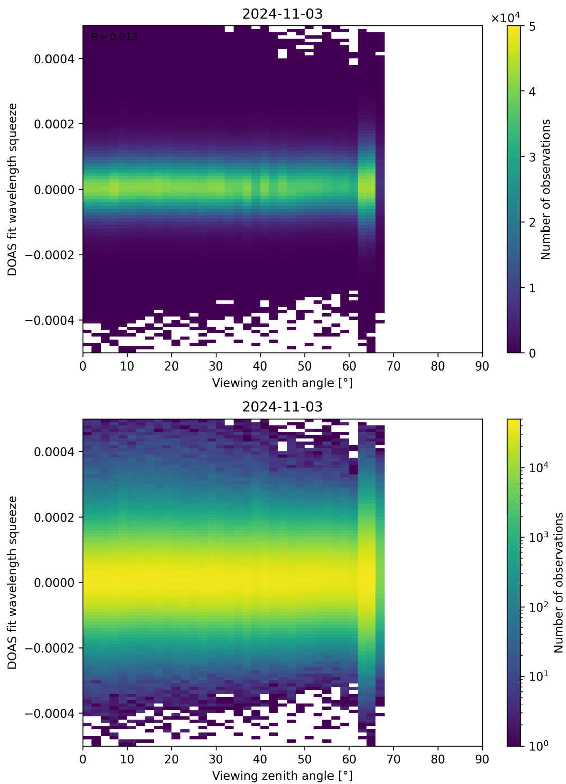
Figure 184: Scatter density plot of “Viewing zenith angle” against “DOAS fit wavelength squeeze” for 2024-11-02 to 2024-11-04.
