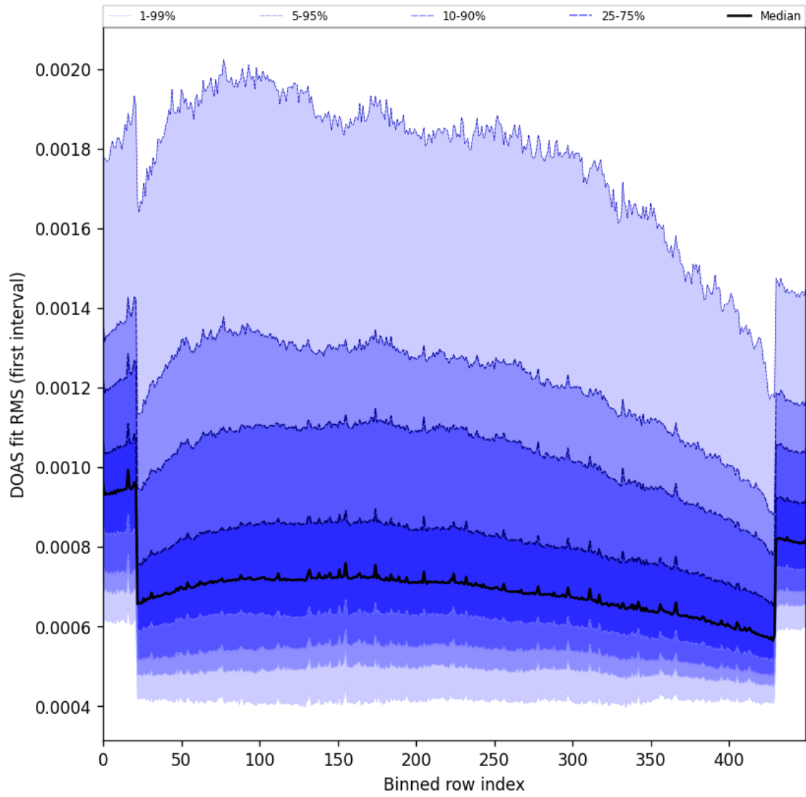
Figure 60: Along track statistics of “DOAS fit RMS (first interval)” for 2024-11-02 to 2024-11-04
