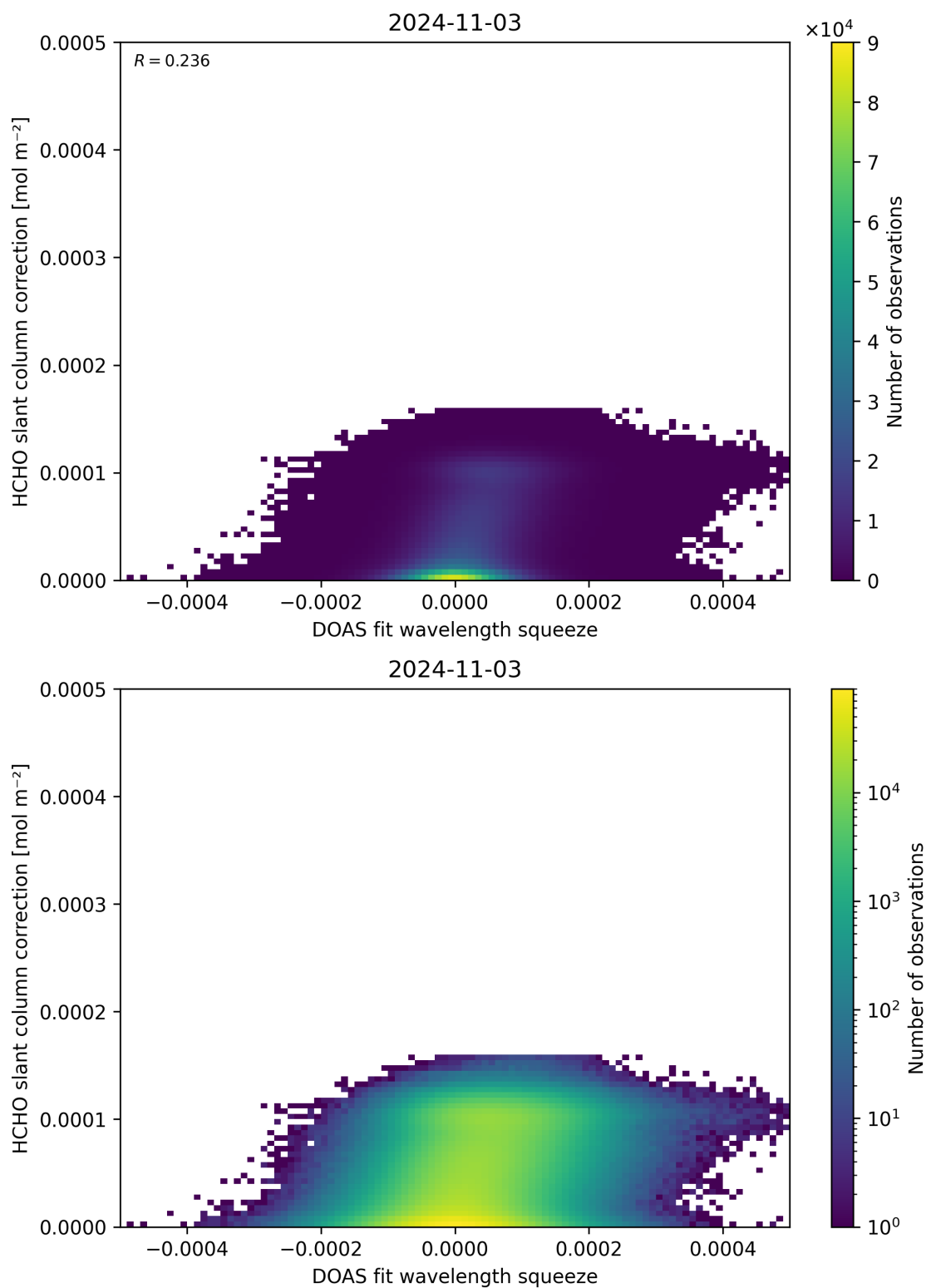
Figure 70: Scatter density plot of “DOAS fit wavelength squeeze” against “HCHO slant column correction” for 2024-11-02 to 2024-11-04.
