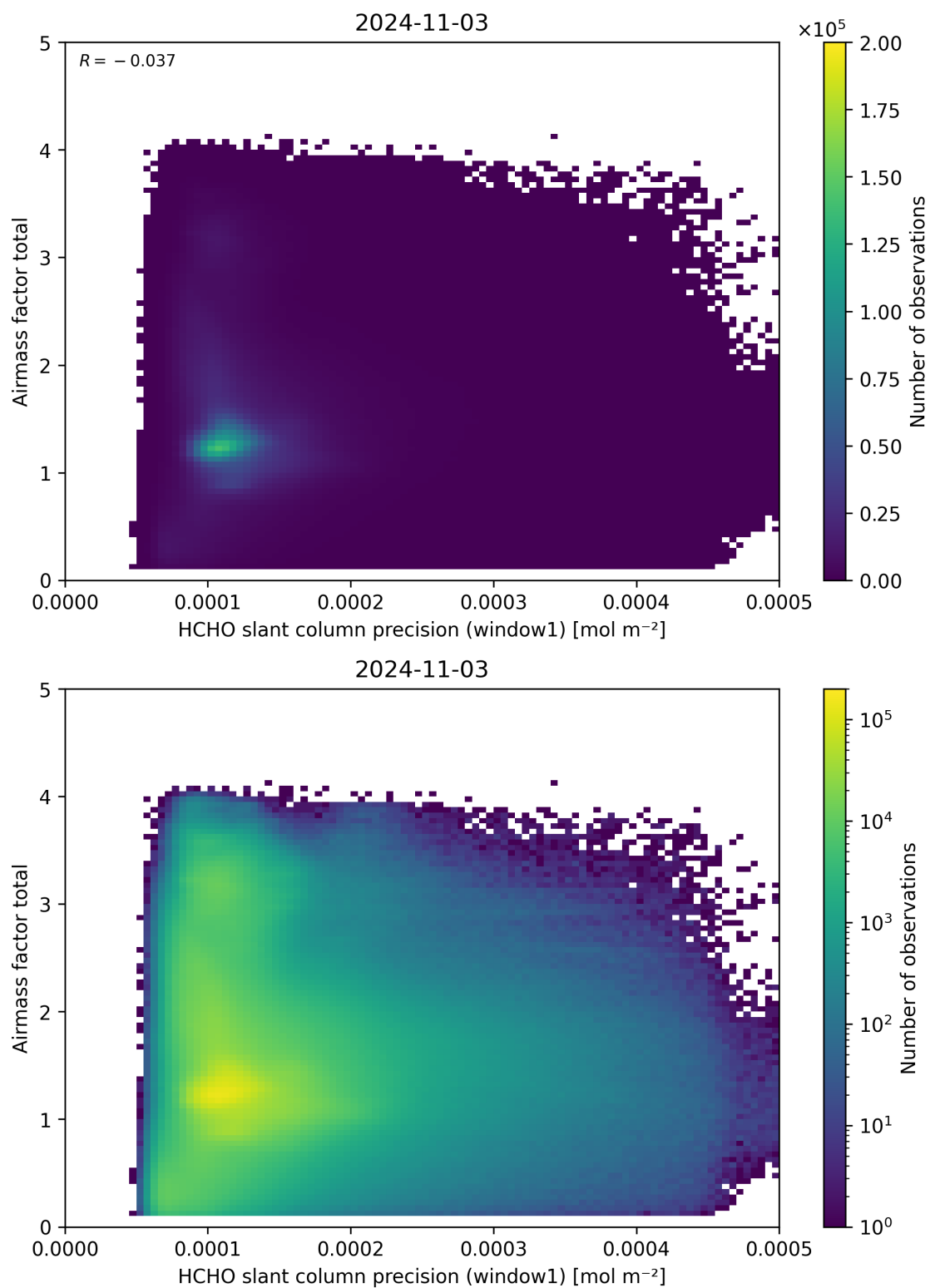
Figure 94: Scatter density plot of “HCHO slant column precision (window1)” against “Airmass factor total” for 2024-11-02 to 2024-11-04.
