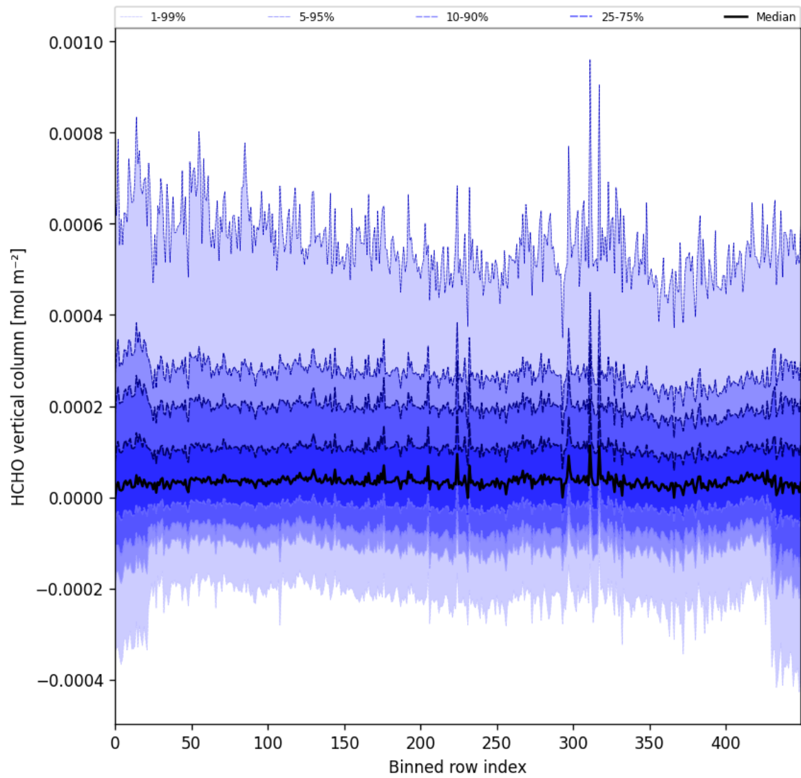
Figure 49: Along track statistics of “HCHO vertical column” for 2024-11-02 to 2024-11-04
