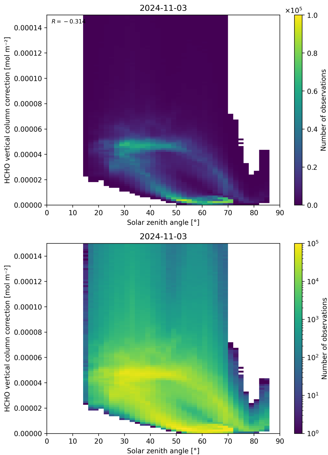
Figure 178: Scatter density plot of “Solar zenith angle” against “HCHO vertical column correction” for 2024-11-02 to 2024-11-04.
