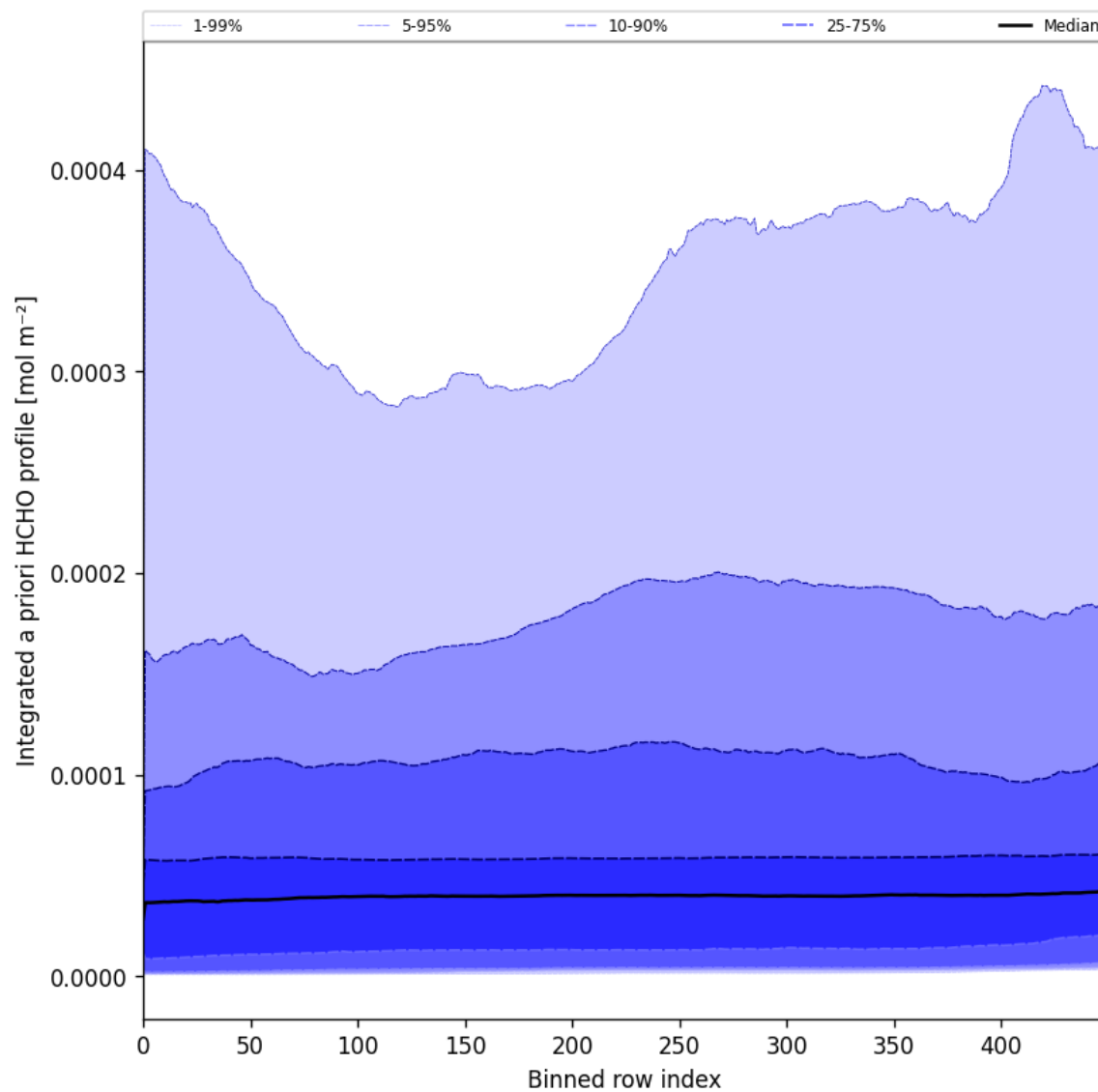
Figure 57: Along track statistics of “Integrated a priori HCHO profile” for 2024-11-02 to 2024-11-04
