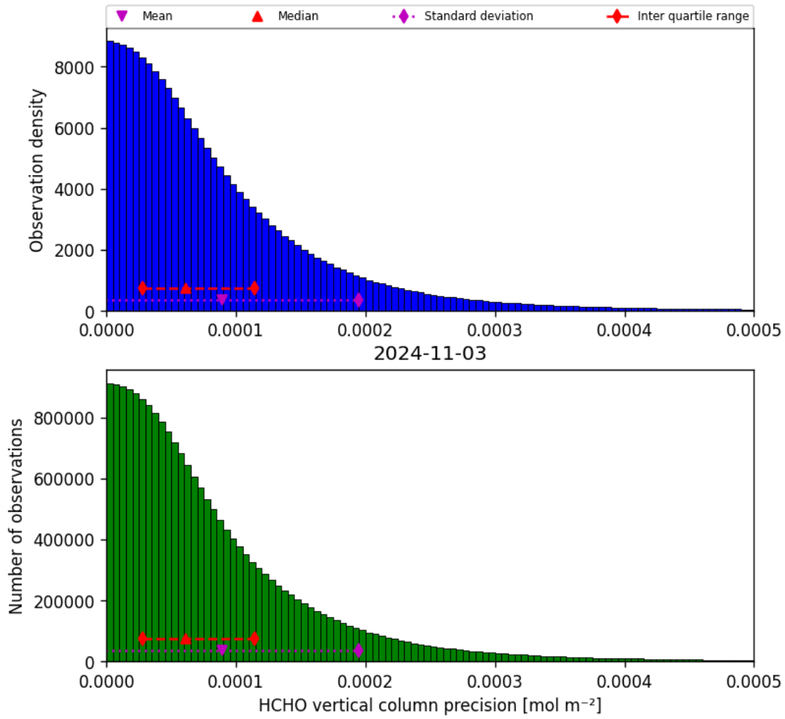
Figure 36: Histogram of “HCHO vertical column precision” for 2024-11-02 to 2024-11-04
