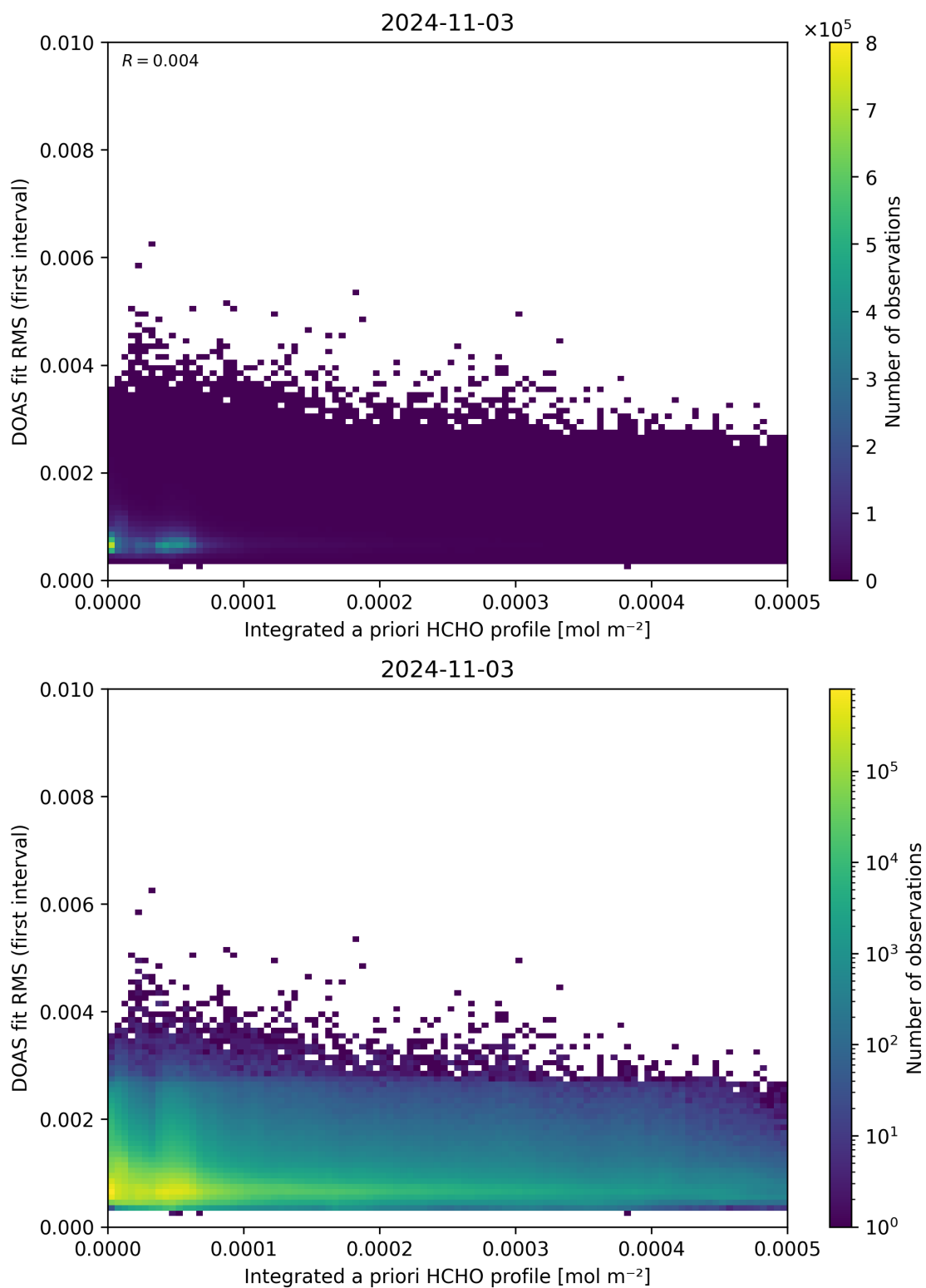
Figure 148: Scatter density plot of “Integrated a priori HCHO profile” against “DOAS fit RMS (first interval)” for 2024-11-02 to 2024-11-04.
