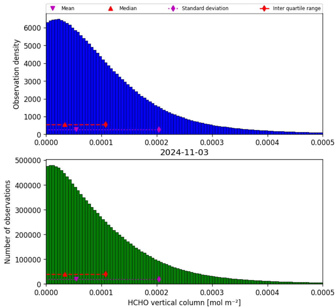
Figure 35: Histogram of “HCHO vertical column” for 2024-11-02 to 2024-11-04
