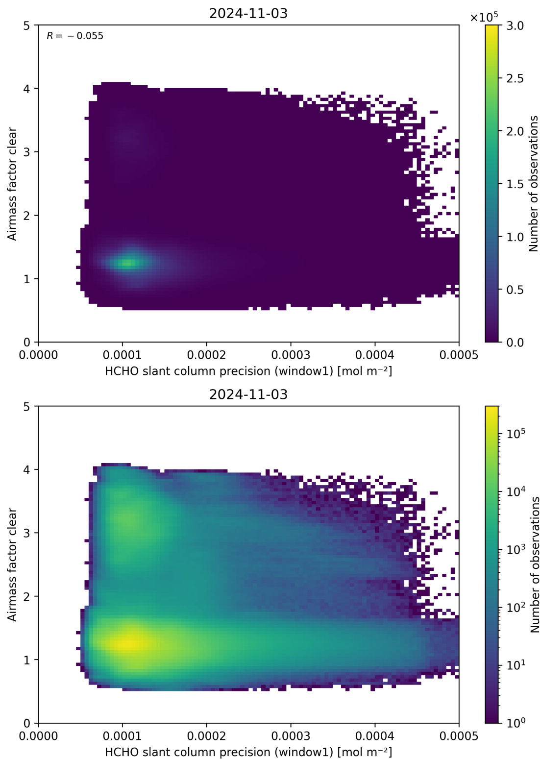
Figure 91: Scatter density plot of “HCHO slant column precision (window1)” against “Airmass factor clear” for 2024-11-02 to 2024-11-04.
