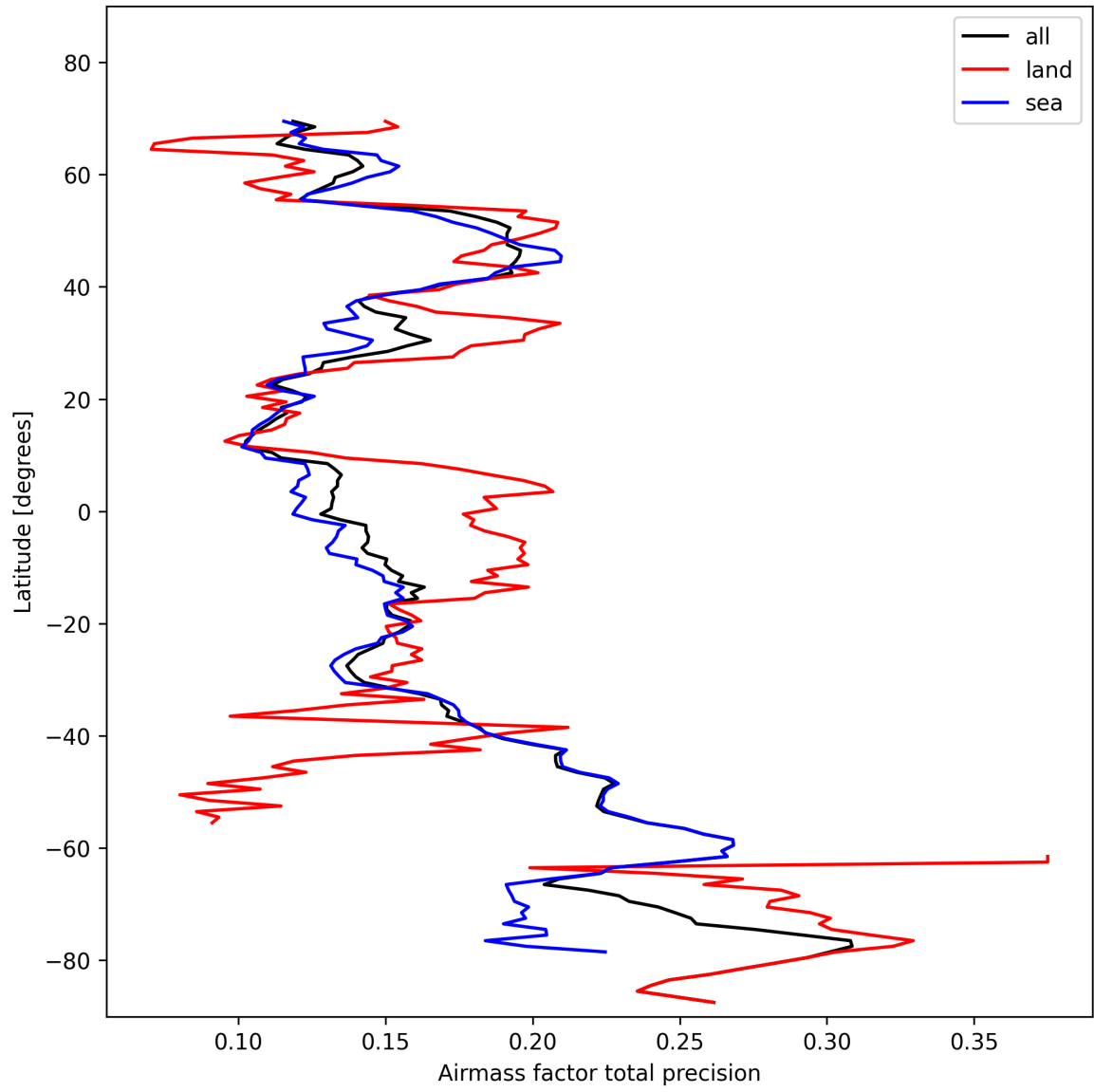
Figure 27: Zonal average of “Airmass factor total precision” for 2024-11-02 to 2024-11-04.
