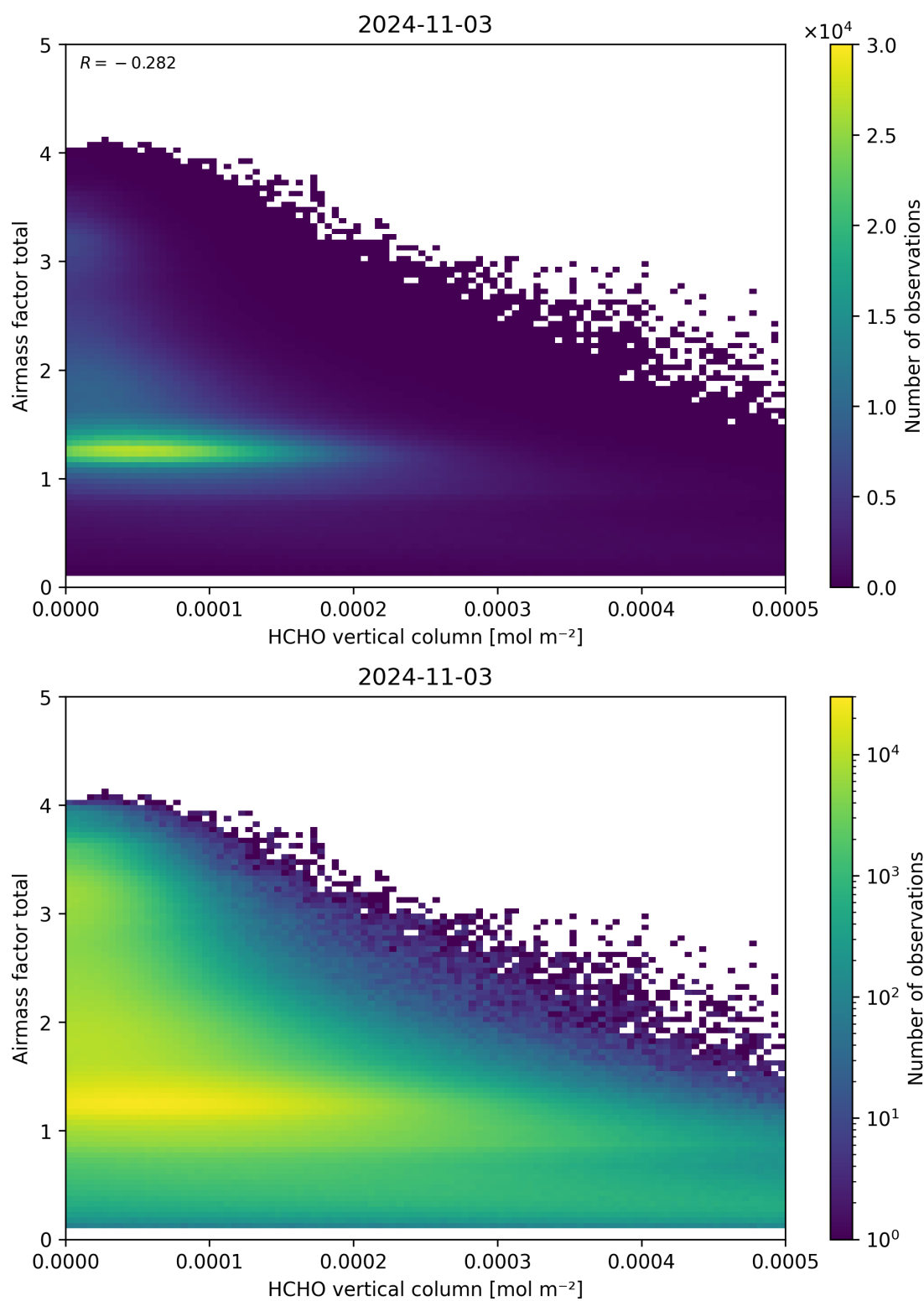
Figure 131: Scatter density plot of “HCHO vertical column” against “Airmass factor total” for 2024-11-02 to 2024-11-04.
