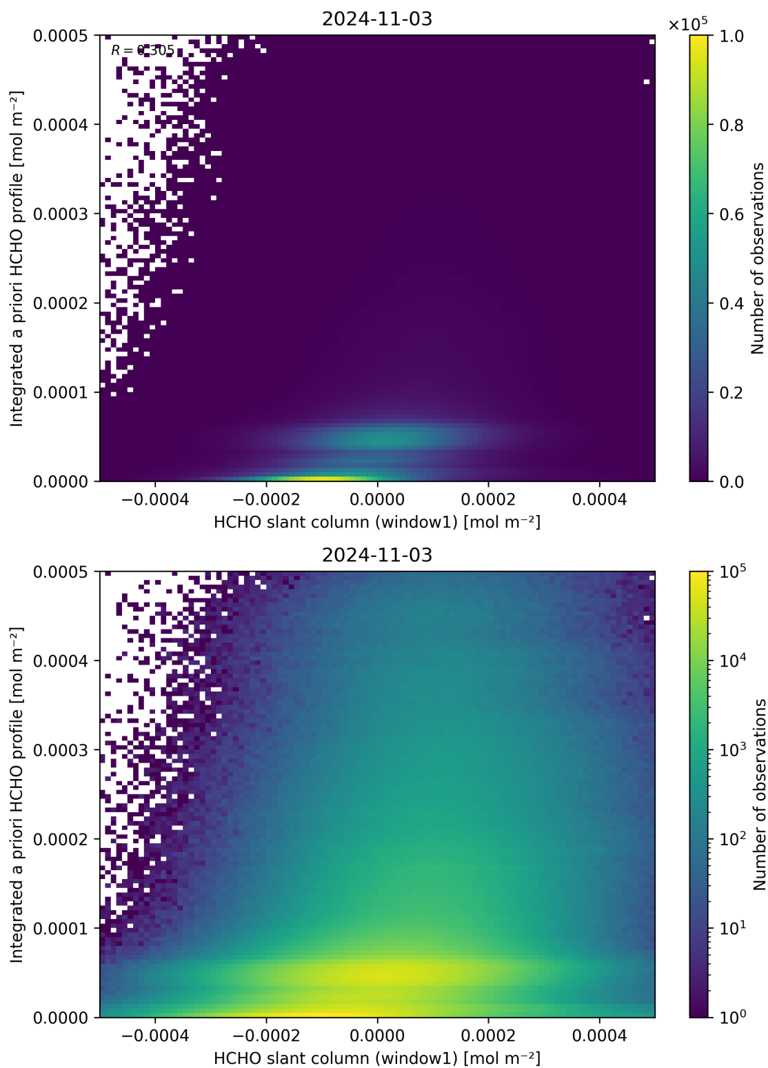
Figure 87: Scatter density plot of “HCHO slant column (window1)” against “Integrated a priori HCHO profile” for 2024-11-02 to 2024-11-04.
