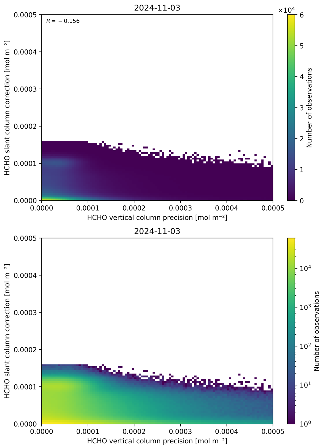
Figure 141: Scatter density plot of “HCHO vertical column precision” against “HCHO slant column correction” for 2024-11-02 to 2024-11-04.
