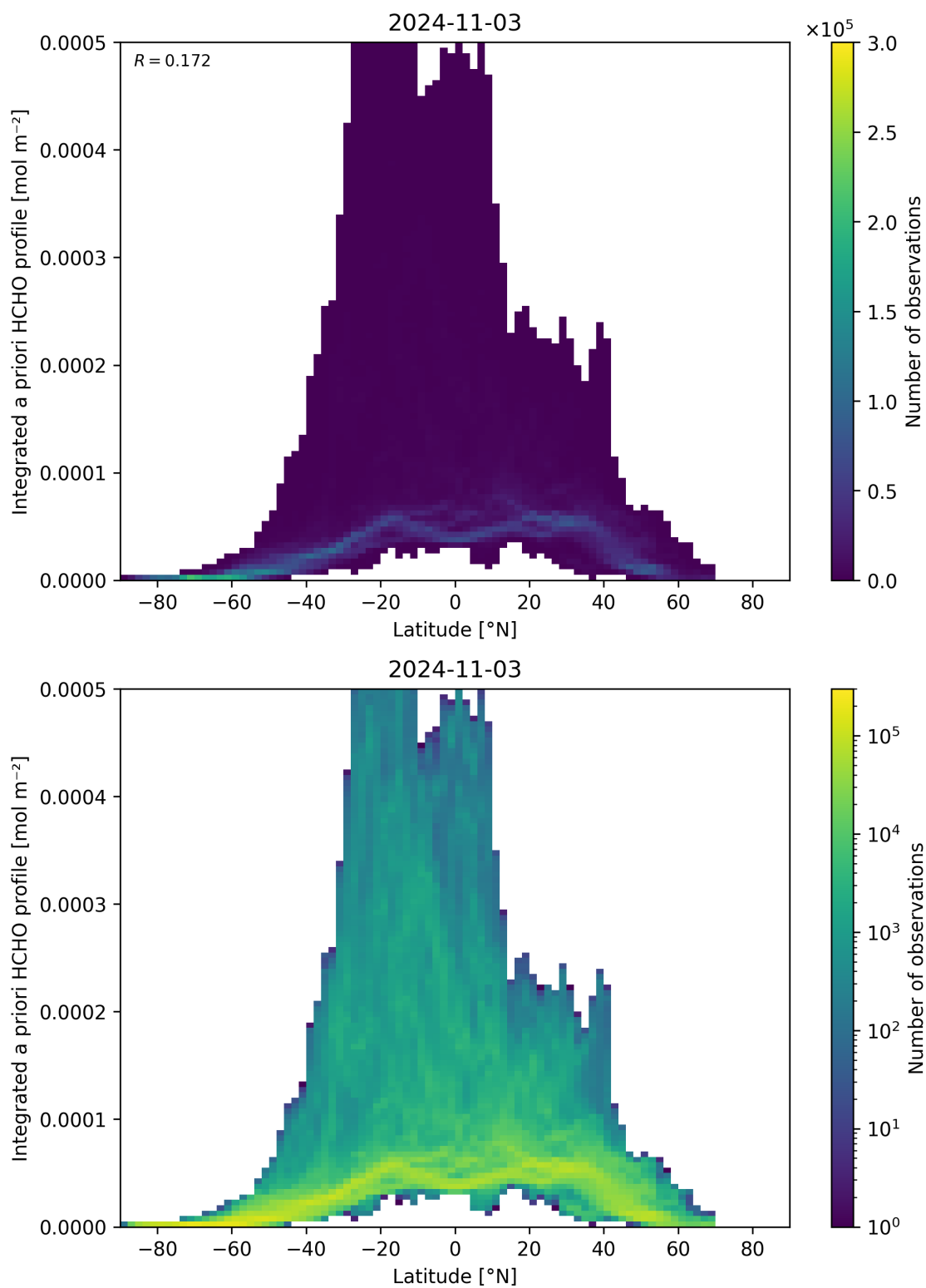
Figure 166: Scatter density plot of “Latitude” against “Integrated a priori HCHO profile” for 2024-11-02 to 2024-11-04.
