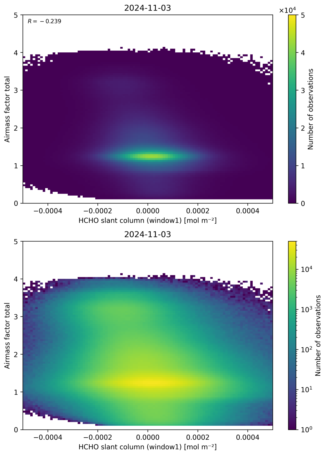
Figure 85: Scatter density plot of “HCHO slant column (window1)” against “Airmass factor total” for 2024-11-02 to 2024-11-04.
