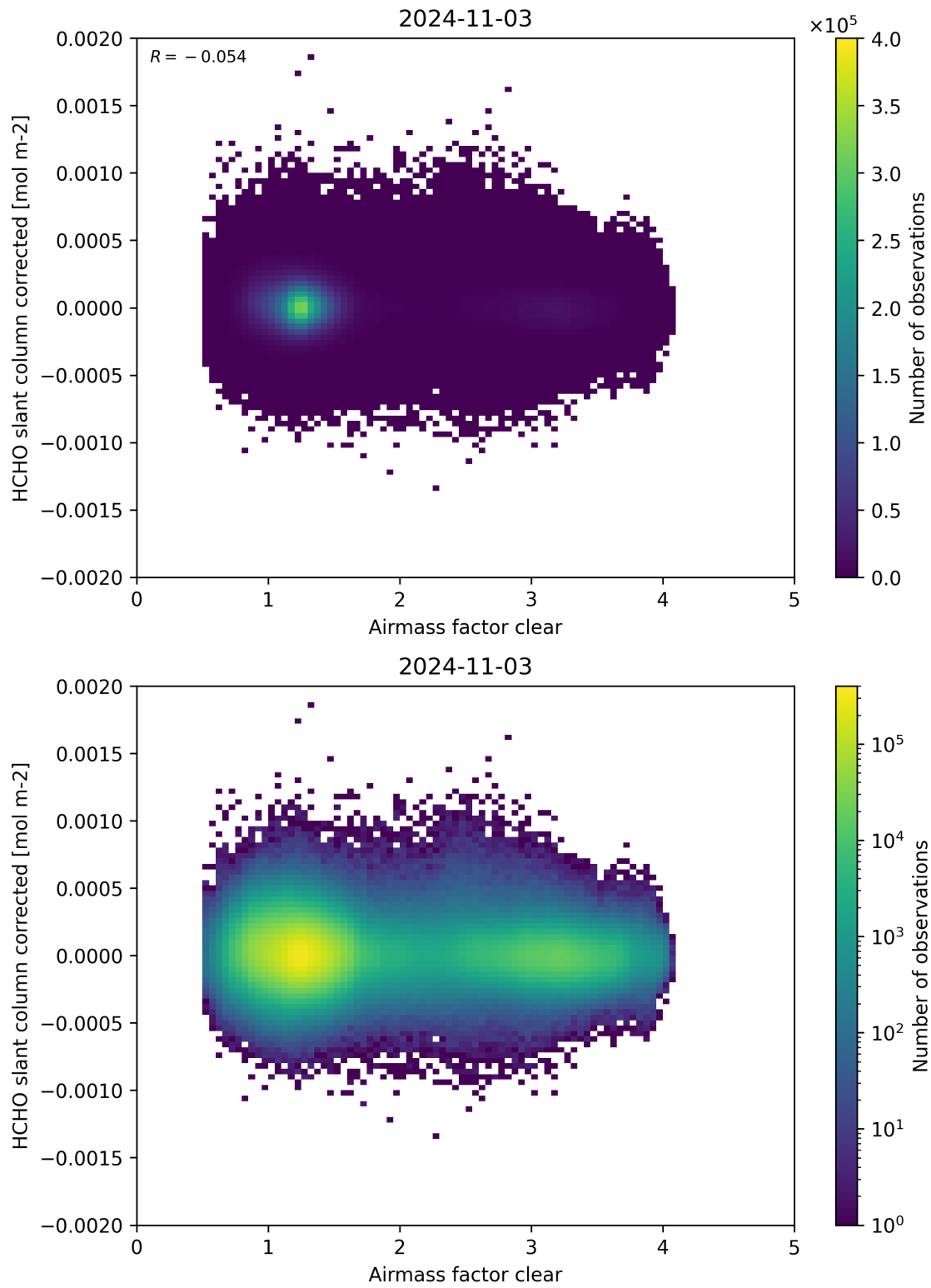
Figure 74: Scatter density plot of “Airmass factor clear” against “HCHO slant column corrected” for 2024-11-02 to 2024-11-04.
