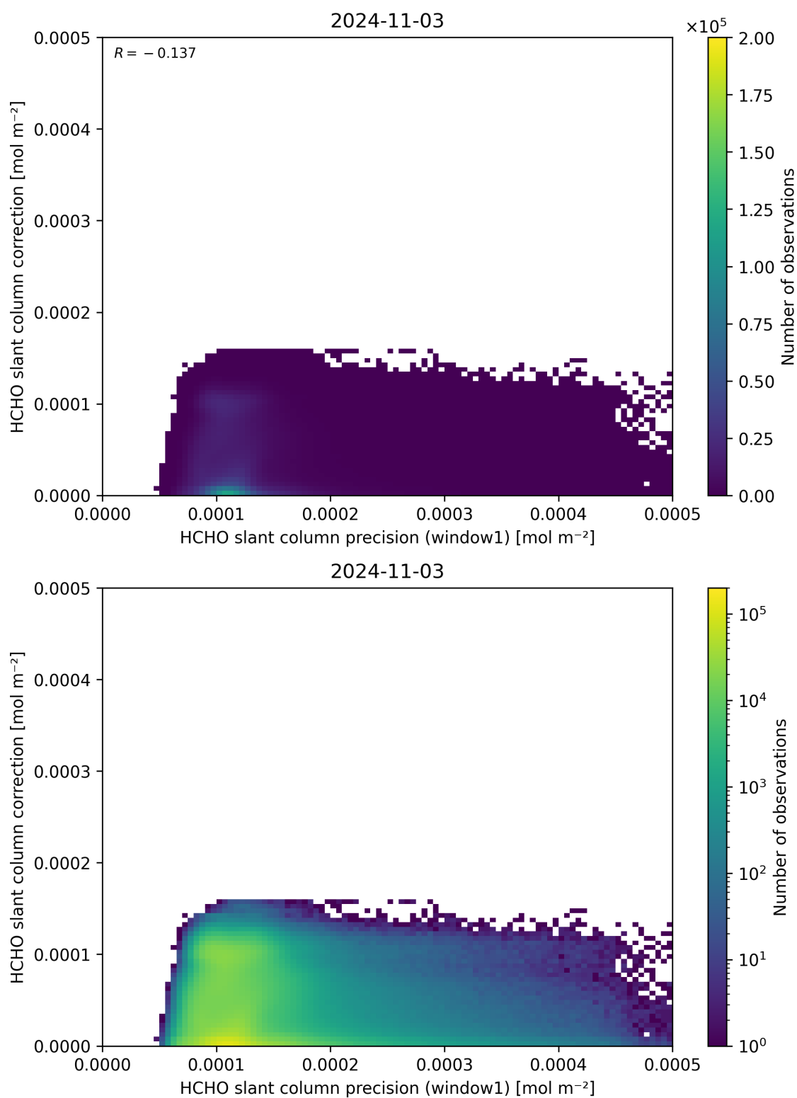
Figure 93: Scatter density plot of “HCHO slant column precision (window1)” against “HCHO slant column correction” for 2024-11-02 to 2024-11-04.
