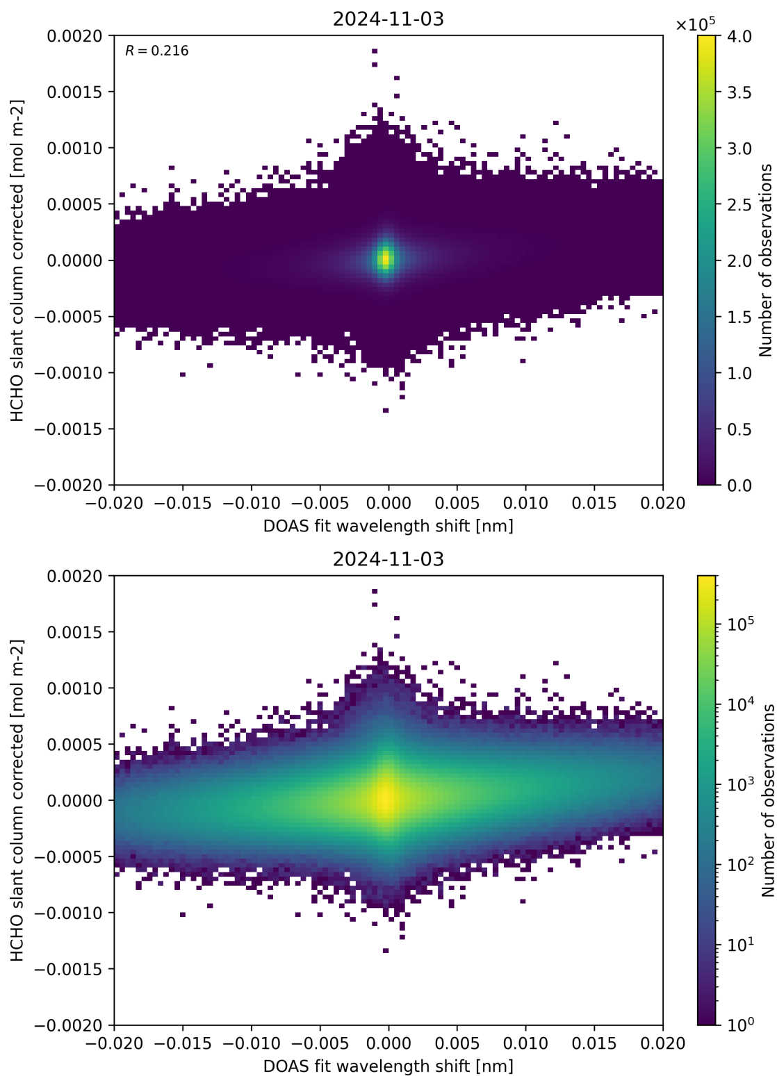
Figure 66: Scatter density plot of “DOAS fit wavelength shift” against “HCHO slant column corrected” for 2024-11-02 to 2024-11-04.
