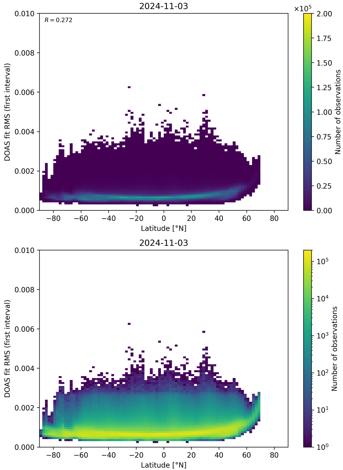
Figure 153: Scatter density plot of “Latitude” against “DOAS fit RMS (first interval)” for 2024-11-02 to 2024-11-04.
