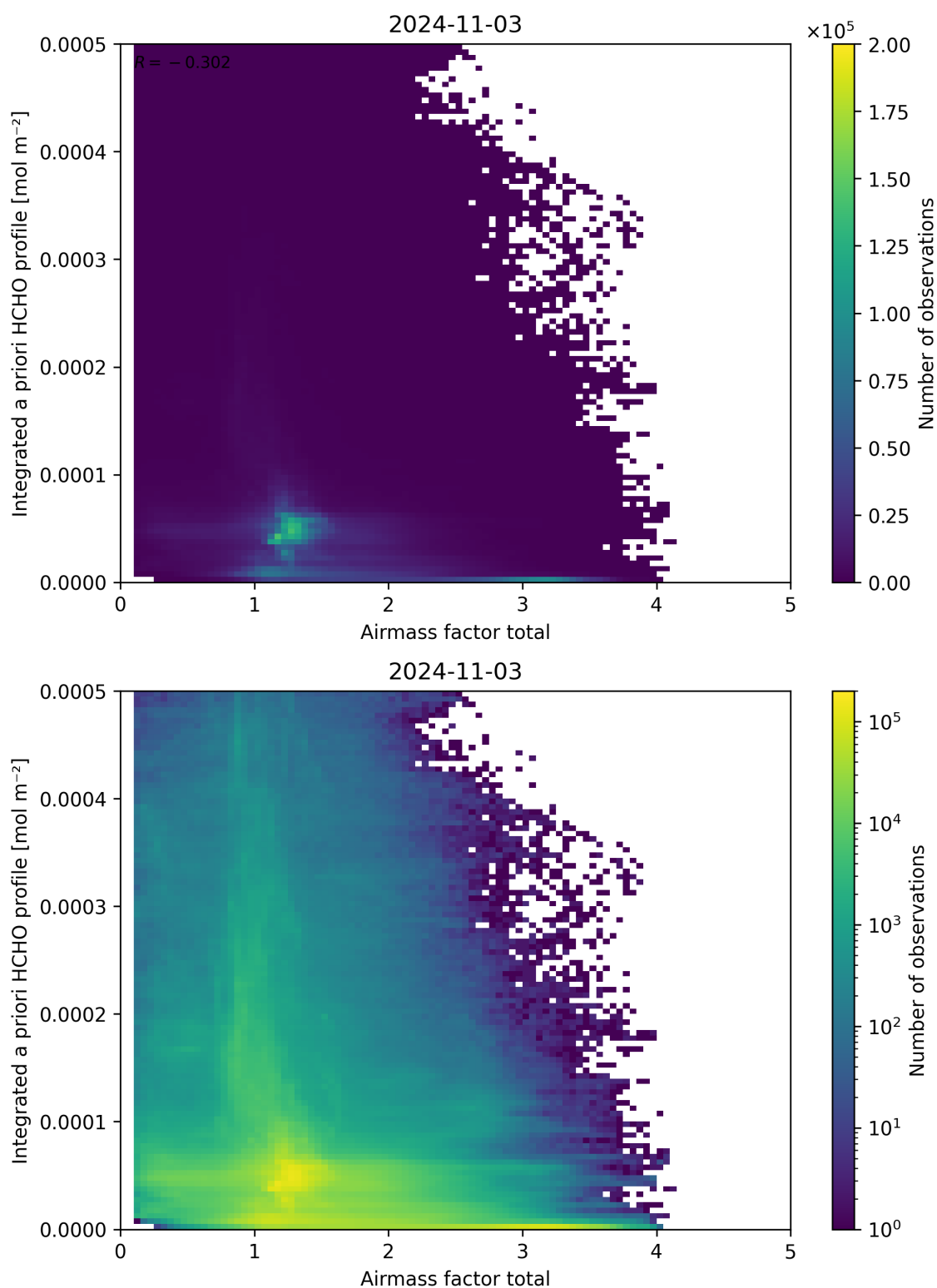
Figure 104: Scatter density plot of “Airmass factor total” against “Integrated a priori HCHO profile” for 2024-11-02 to 2024-11-04.
