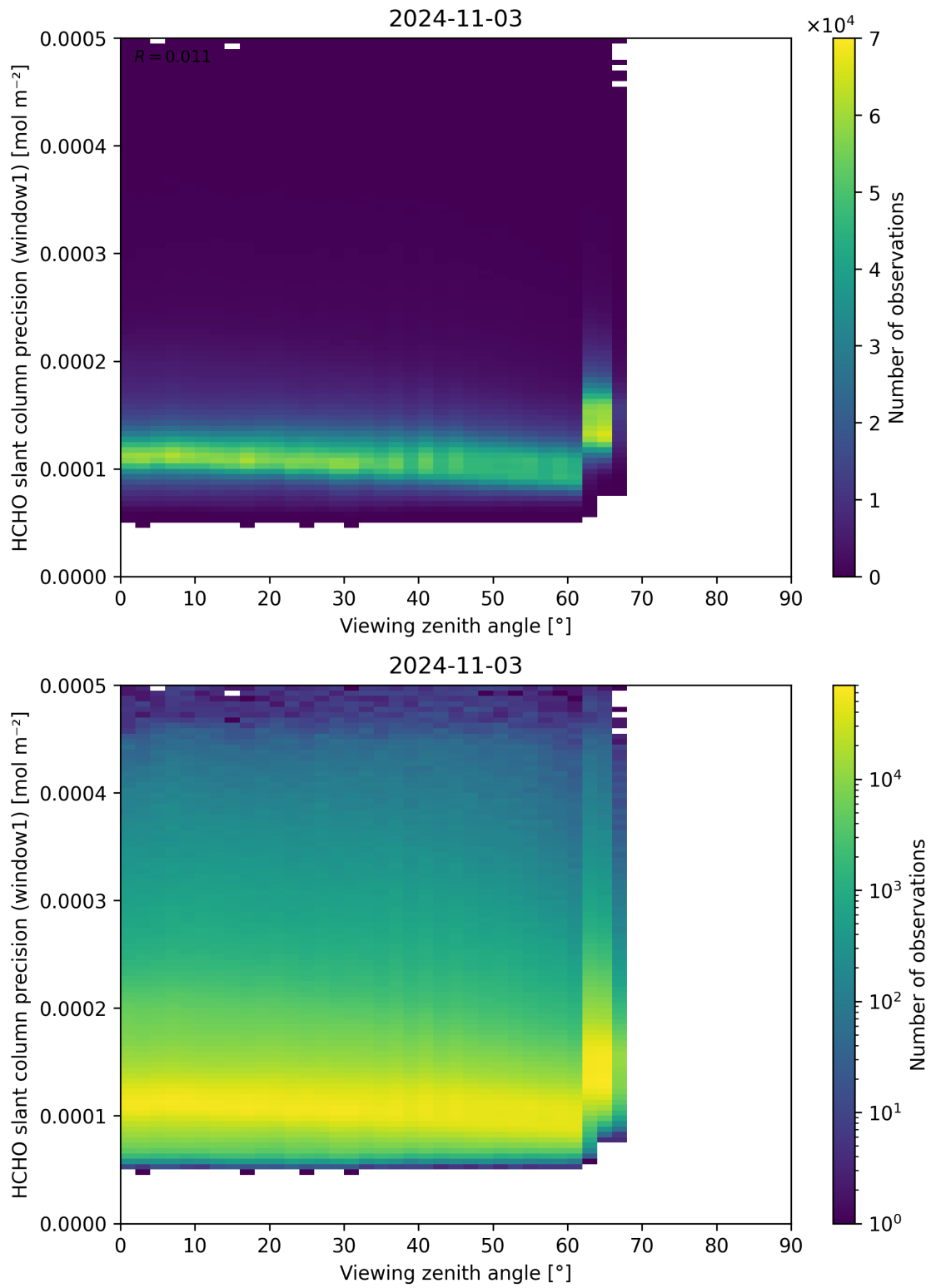
Figure 189: Scatter density plot of “Viewing zenith angle” against “HCHO slant column precision (window1)” for 2024-11-02 to 2024-11-04.
