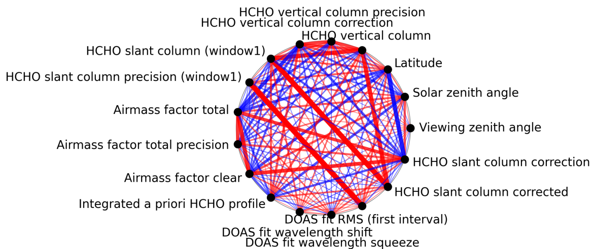
Figure 1: Map of correlation graph for 2024-11-02 to 2024-11-04.
