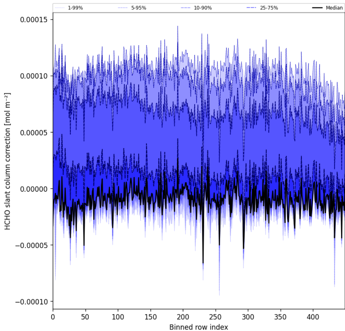
Figure 61: Along track statistics of “HCHO slant column correction” for 2024-11-02 to 2024-11-04
