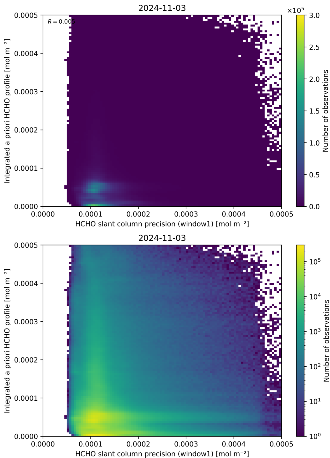
Figure 96: Scatter density plot of “HCHO slant column precision (window1)” against “Integrated a priori HCHO profile” for 2024-11-02 to 2024-11-04.
