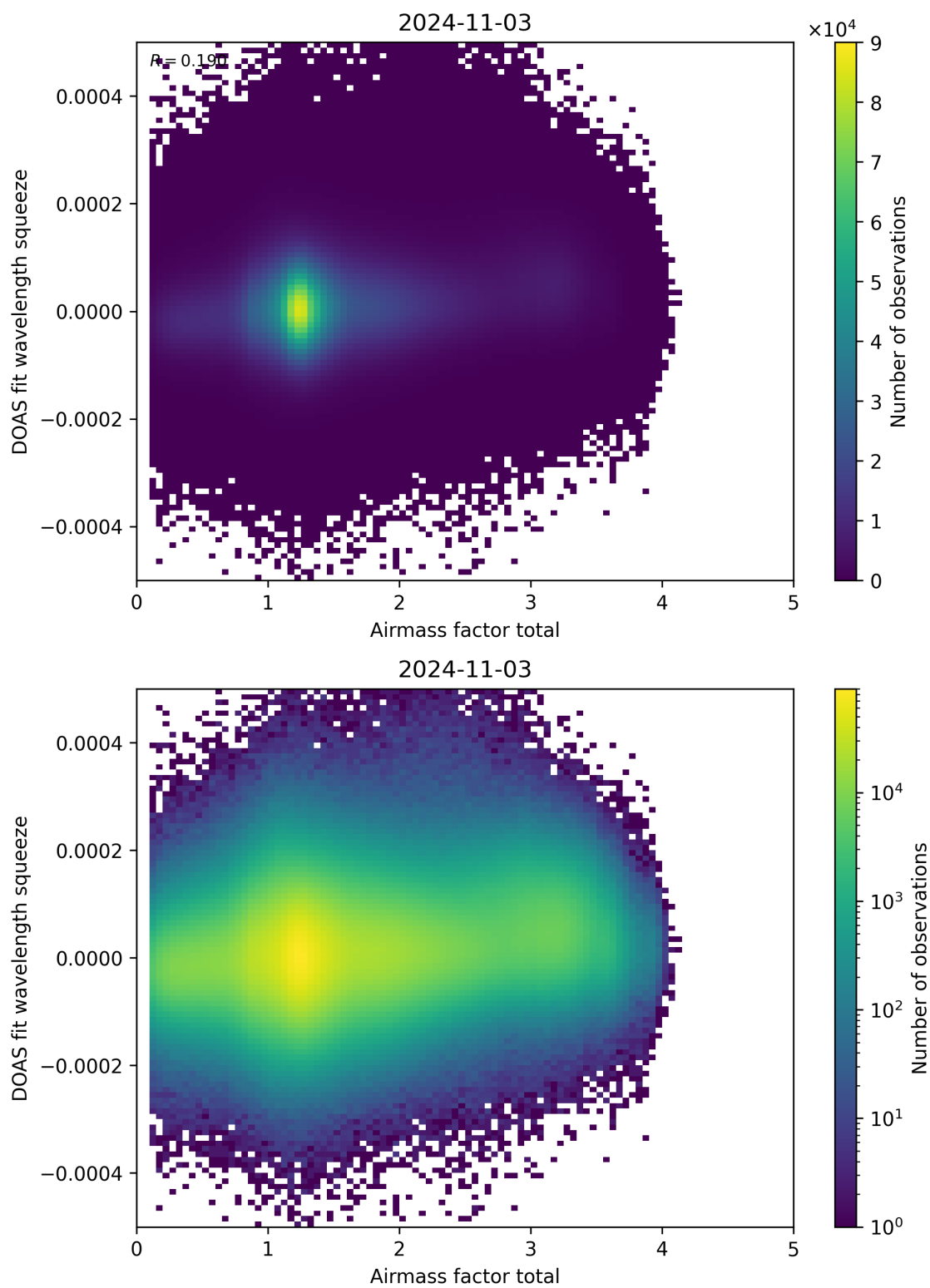
Figure 99: Scatter density plot of “Airmass factor total” against “DOAS fit wavelength squeeze” for 2024-11-02 to 2024-11-04.
