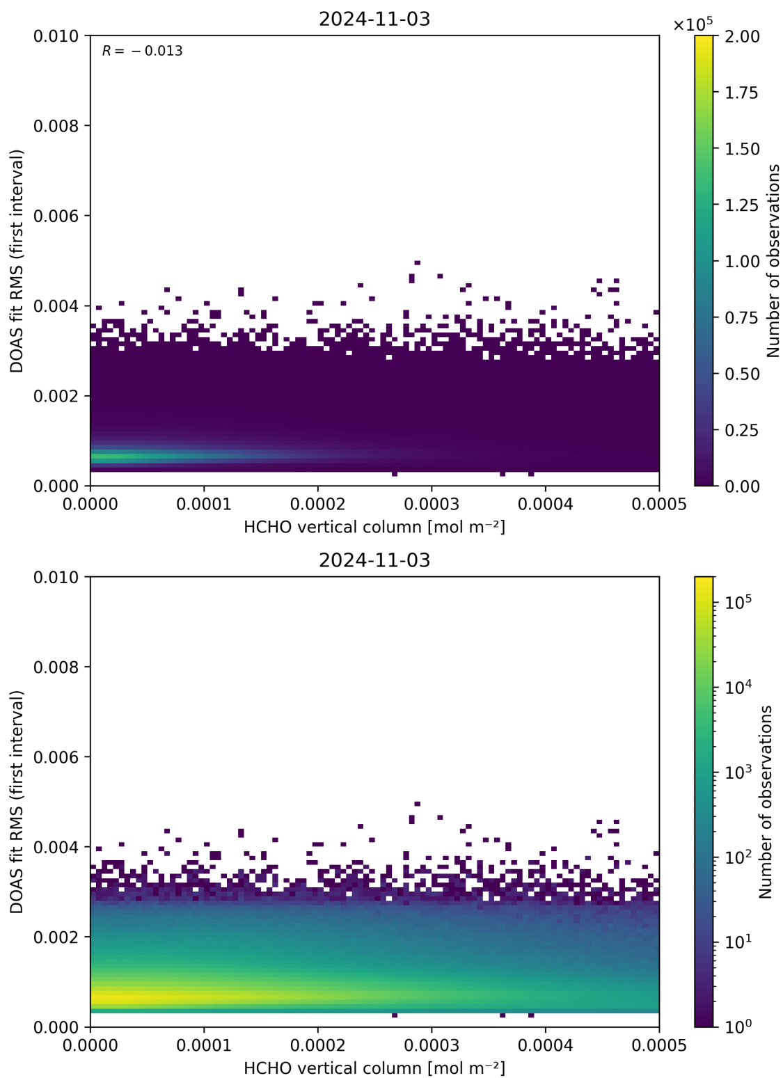
Figure 123: Scatter density plot of “HCHO vertical column” against “DOAS fit RMS (first interval)” for 2024-11-02 to 2024-11-04.
