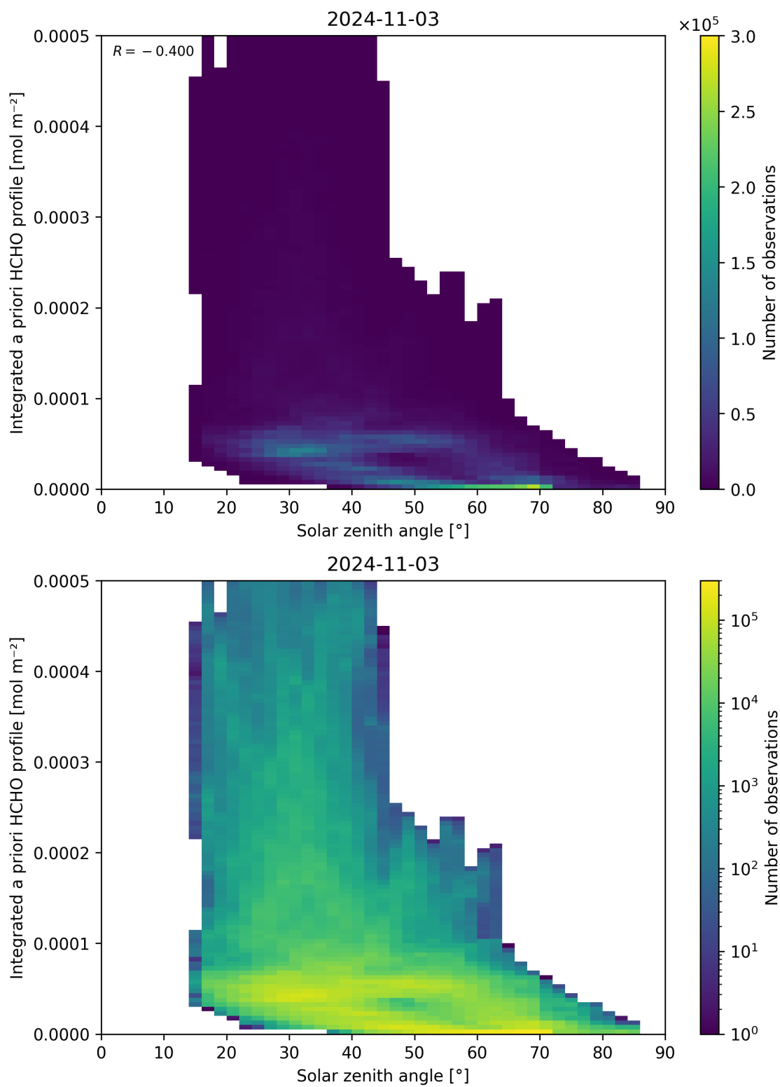
Figure 180: Scatter density plot of “Solar zenith angle” against “Integrated a priori HCHO profile” for 2024-11-02 to 2024-11-04.
