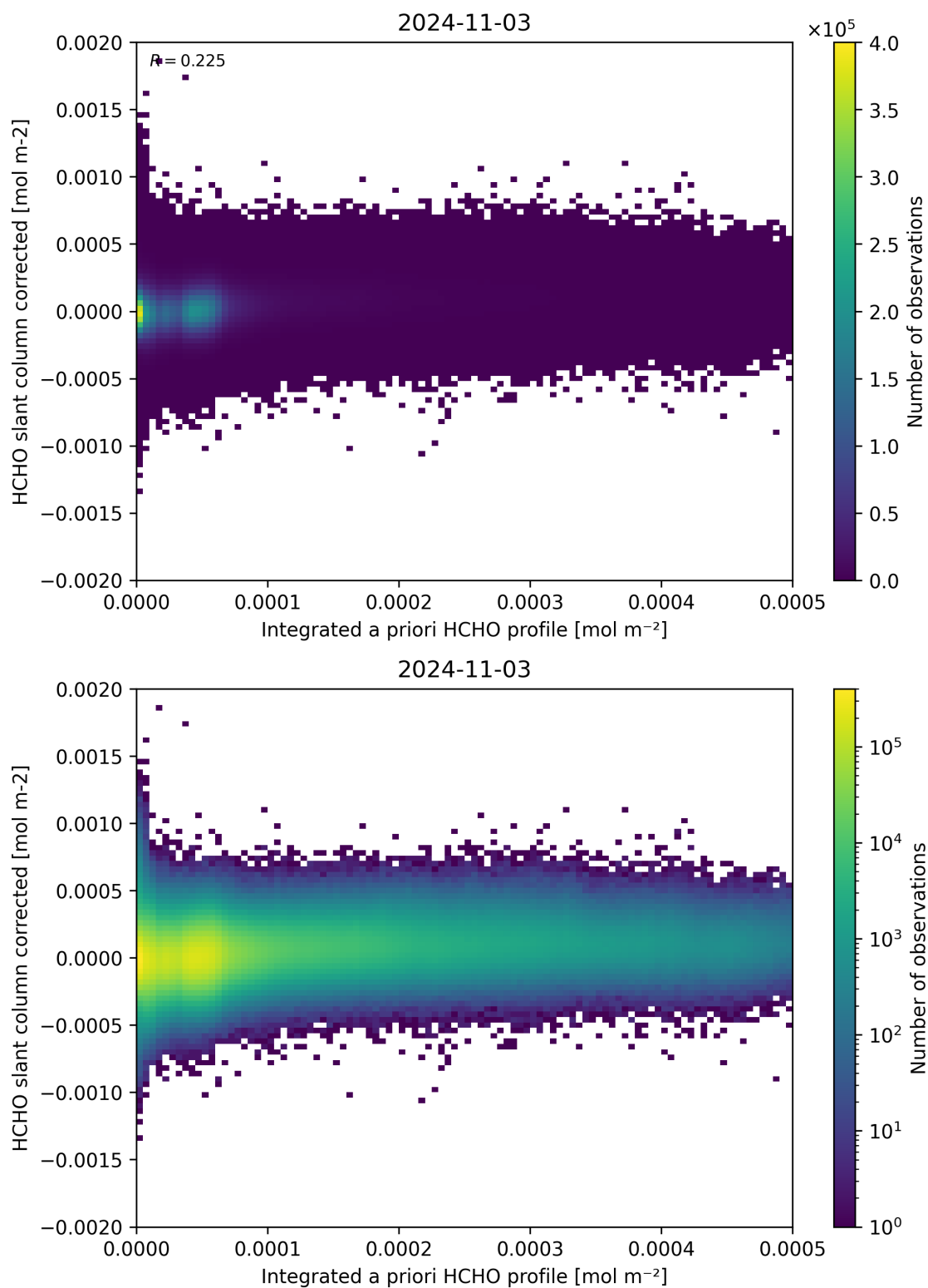
Figure 151: Scatter density plot of “Integrated a priori HCHO profile” against “HCHO slant column corrected” for 2024-11-02 to 2024-11-04.
