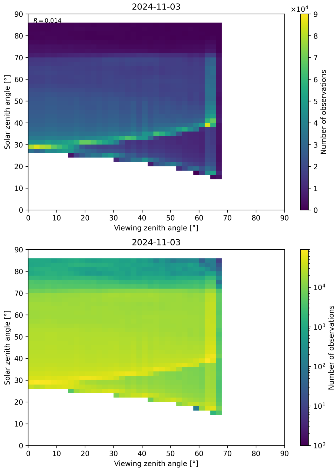
Figure 197: Scatter density plot of “Viewing zenith angle” against “Solar zenith angle” for 2024-11-02 to 2024-11-04.
