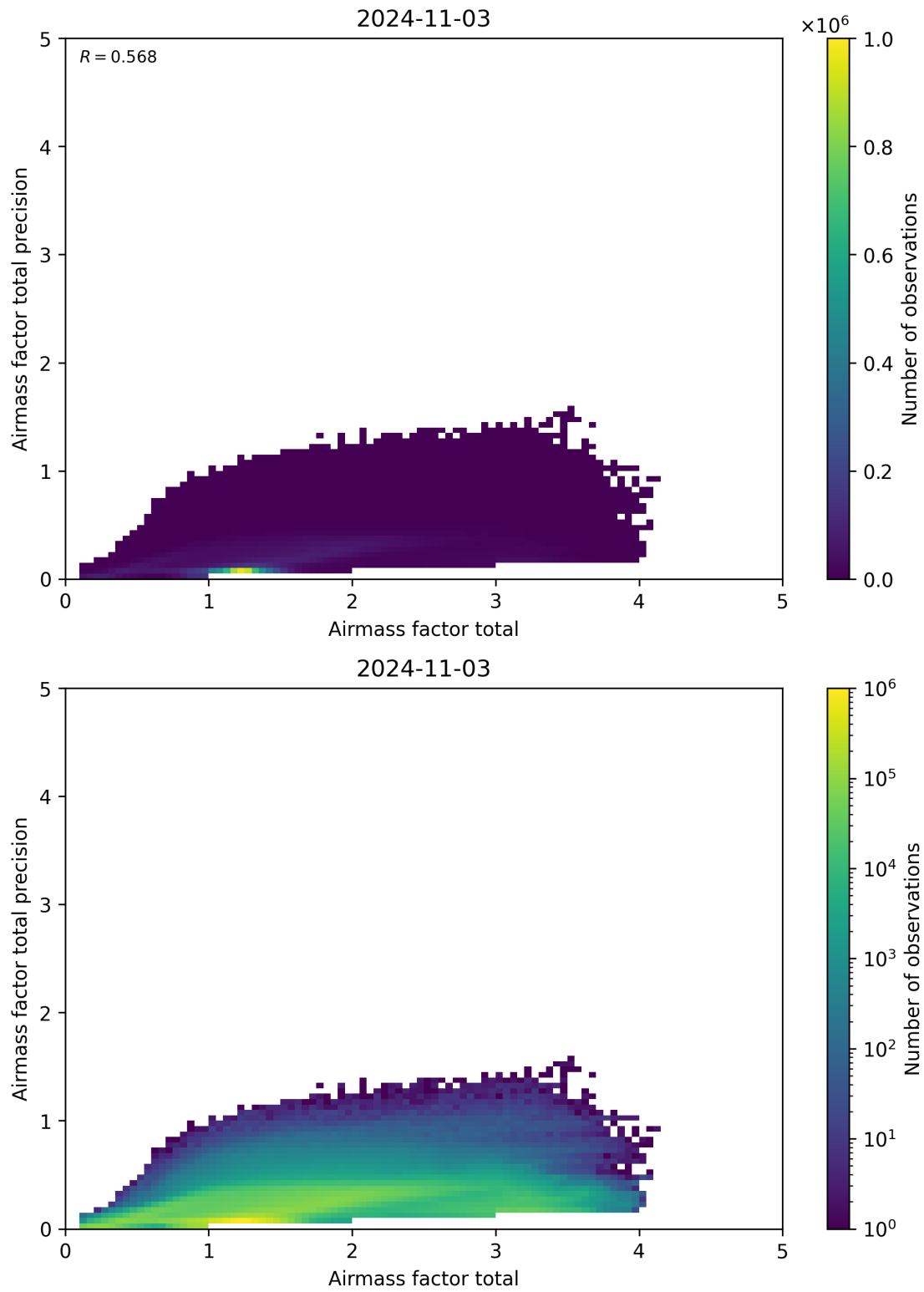
Figure 103: Scatter density plot of “Airmass factor total” against “Airmass factor total precision” for 2024-11-02 to 2024-11-04.
