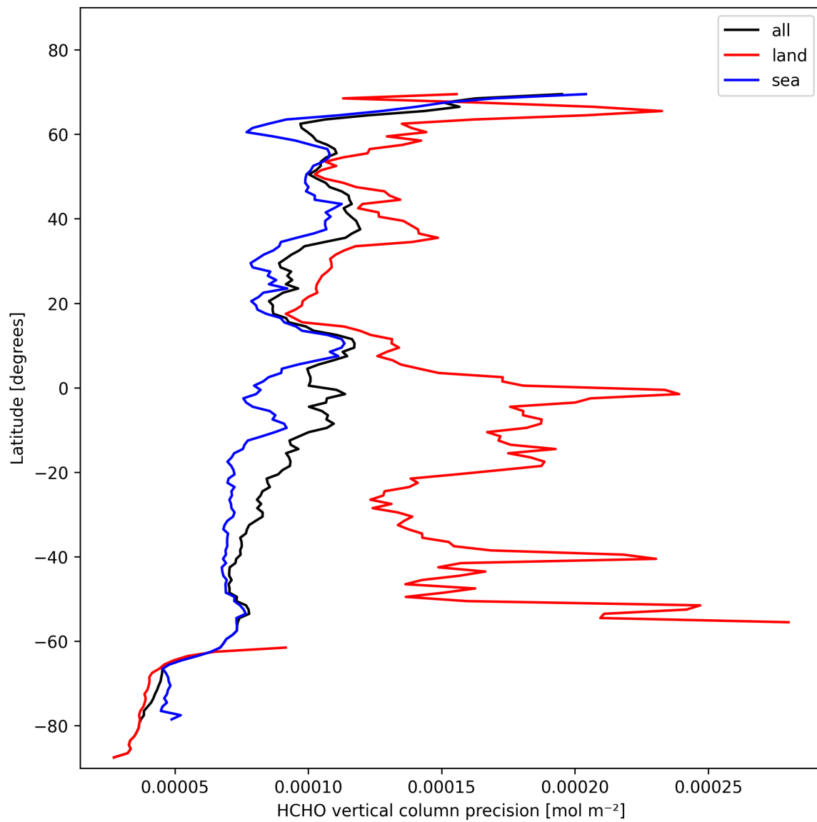
Figure 22: Zonal average of “HCHO vertical column precision” for 2024-11-02 to 2024-11-04.
