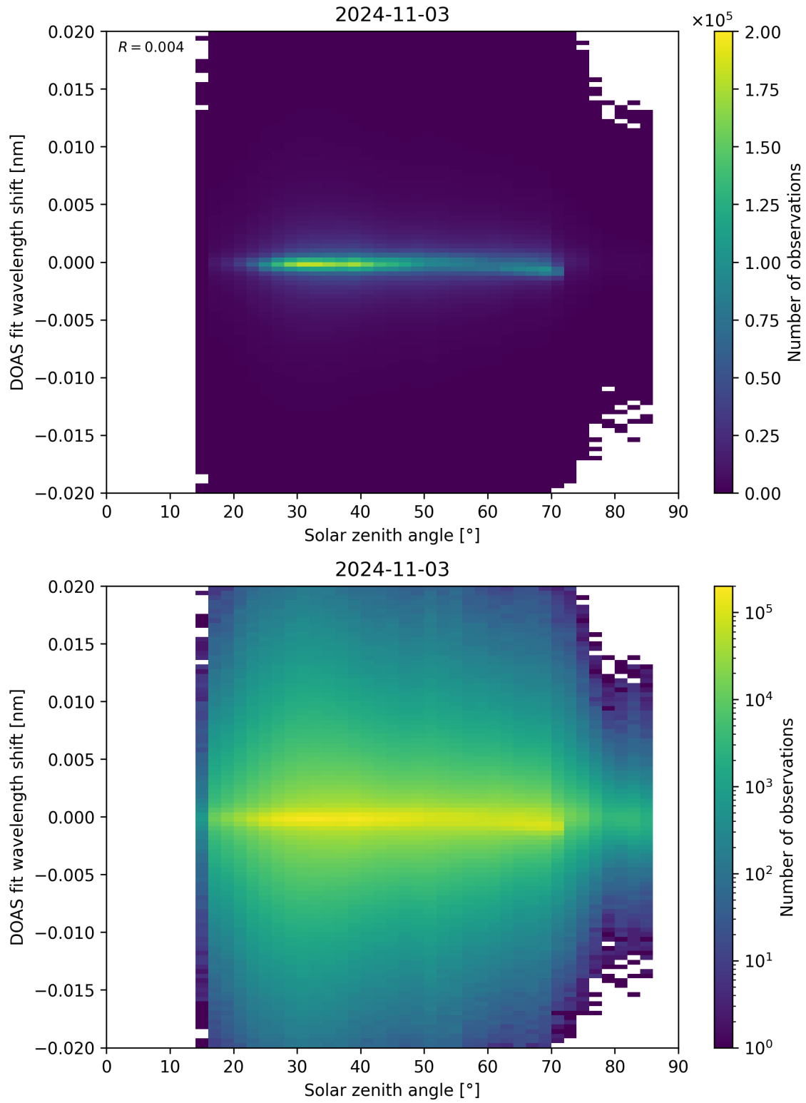
Figure 168: Scatter density plot of “Solar zenith angle” against “DOAS fit wavelength shift” for 2024-11-02 to 2024-11-04.
