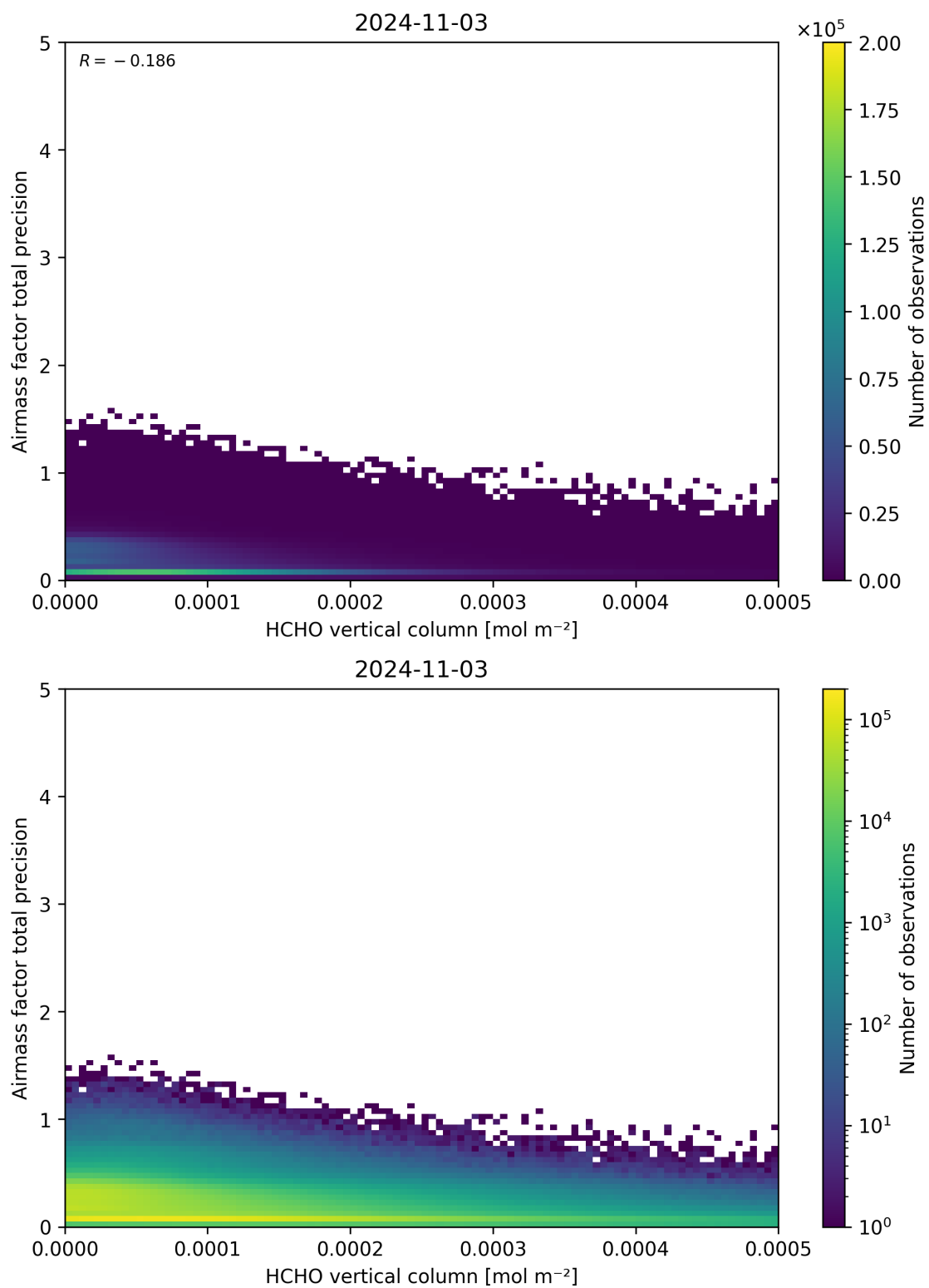
Figure 132: Scatter density plot of “HCHO vertical column” against “Airmass factor total precision” for 2024-11-02 to 2024-11-04.
