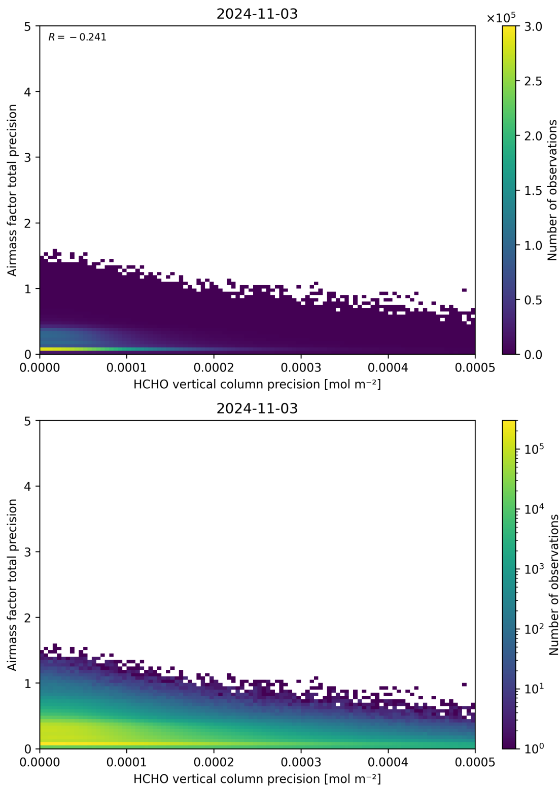
Figure 145: Scatter density plot of “HCHO vertical column precision” against “Airmass factor total precision” for 2024-11-02 to 2024-11-04.
