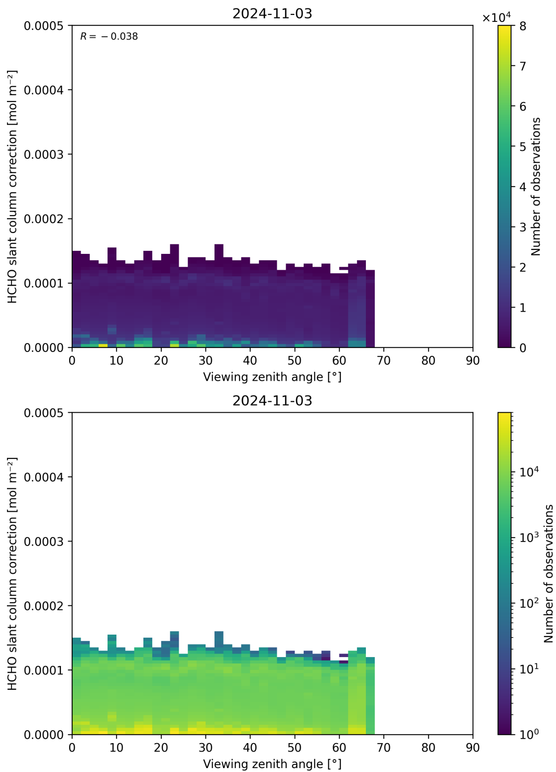
Figure 187: Scatter density plot of “Viewing zenith angle” against “HCHO slant column correction” for 2024-11-02 to 2024-11-04.
