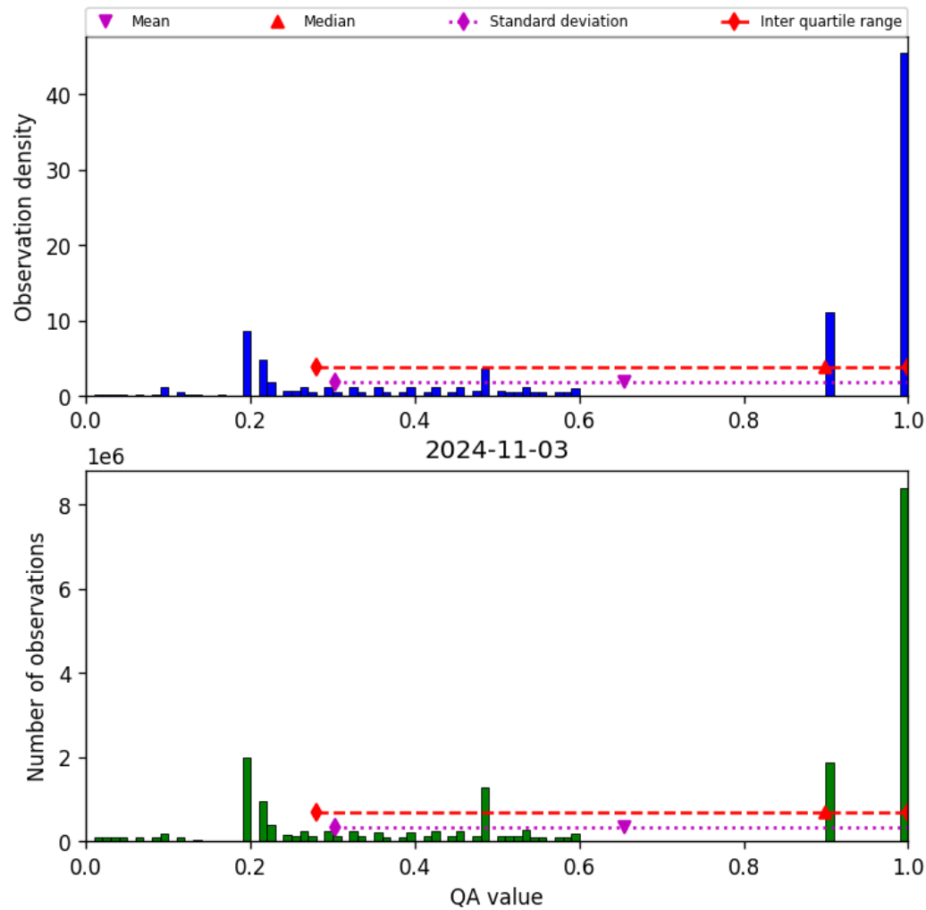
Figure 34: Histogram of “QA value” for 2024-11-02 to 2024-11-04
