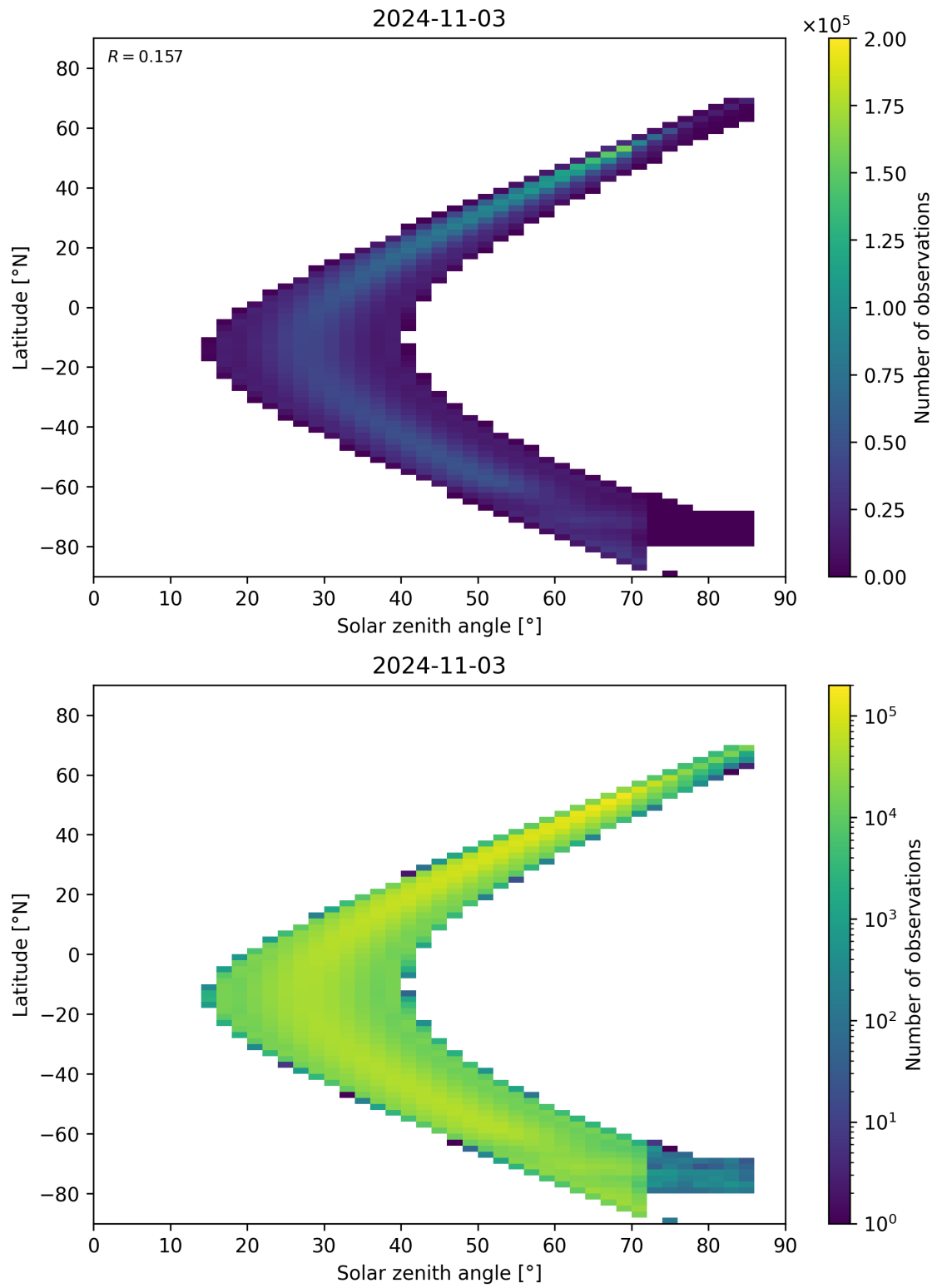
Figure 181: Scatter density plot of “Solar zenith angle” against “Latitude” for 2024-11-02 to 2024-11-04.
