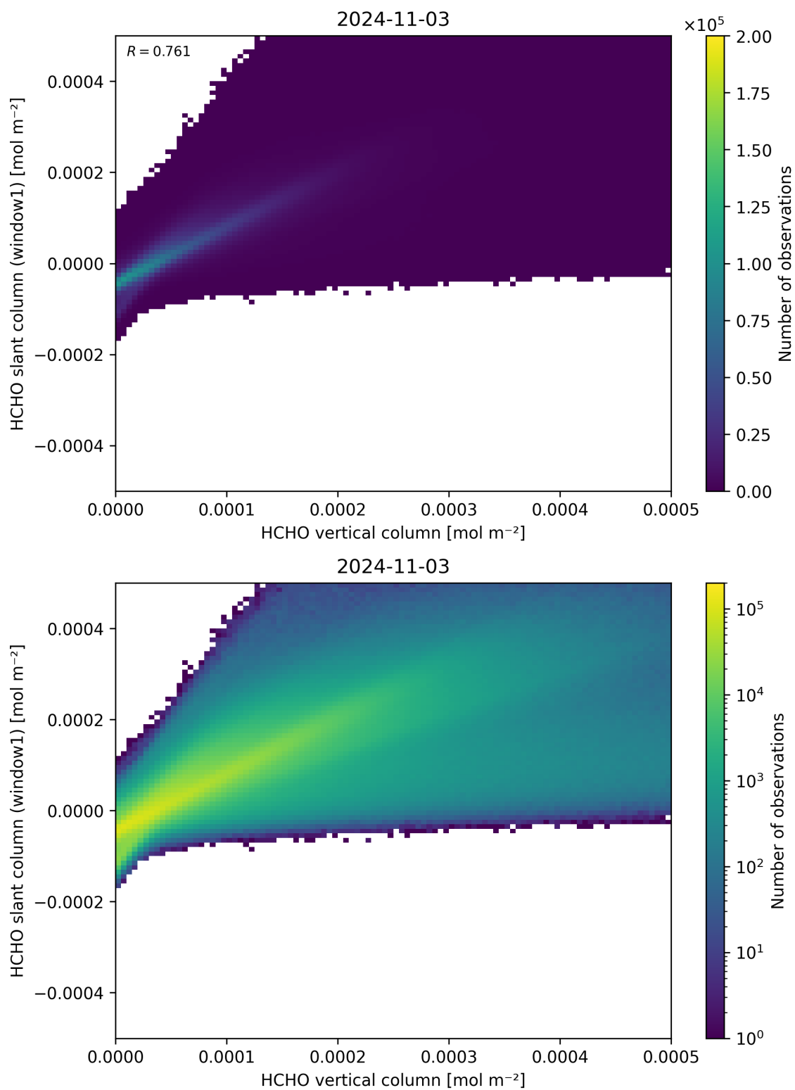
Figure 129: Scatter density plot of “HCHO vertical column” against “HCHO slant column (window1)” for 2024-11-02 to 2024-11-04.
