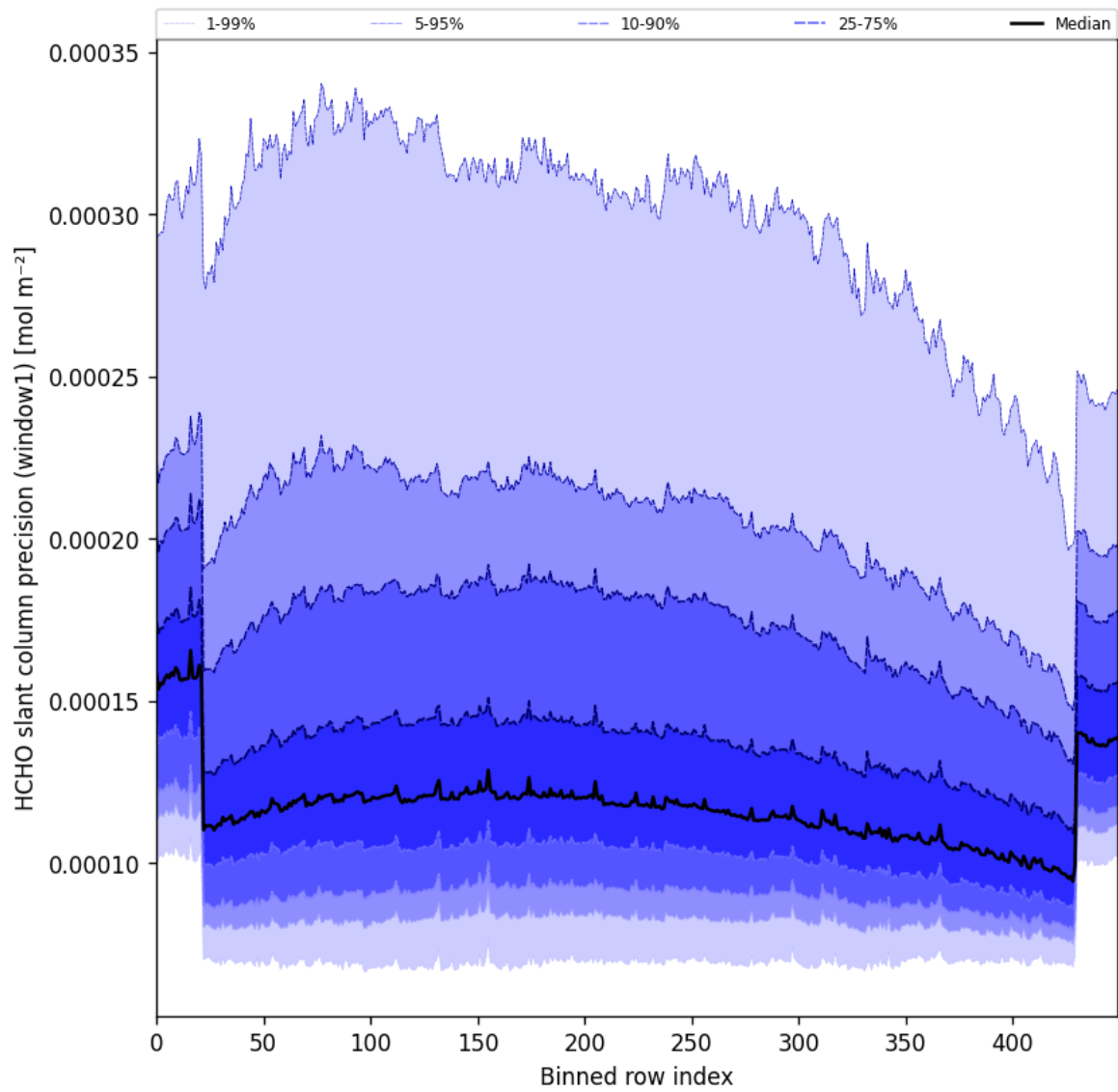
Figure 53: Along track statistics of "HCHO slant column precision (window1)" for 2024-11-02 to 2024-11-04
