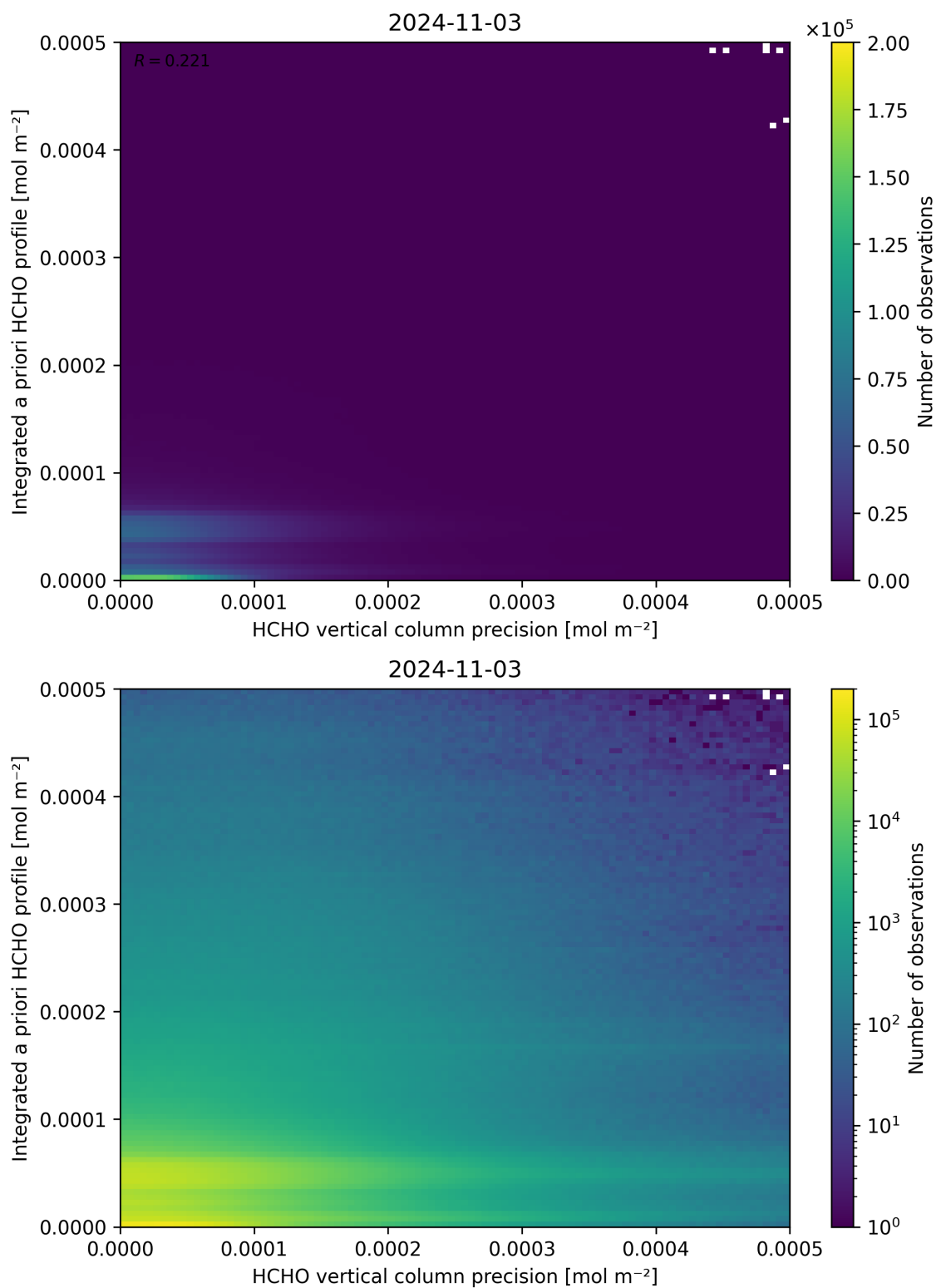
Figure 147: Scatter density plot of “HCHO vertical column precision” against “Integrated a priori HCHO profile” for 2024-11-02 to 2024-11-04.
