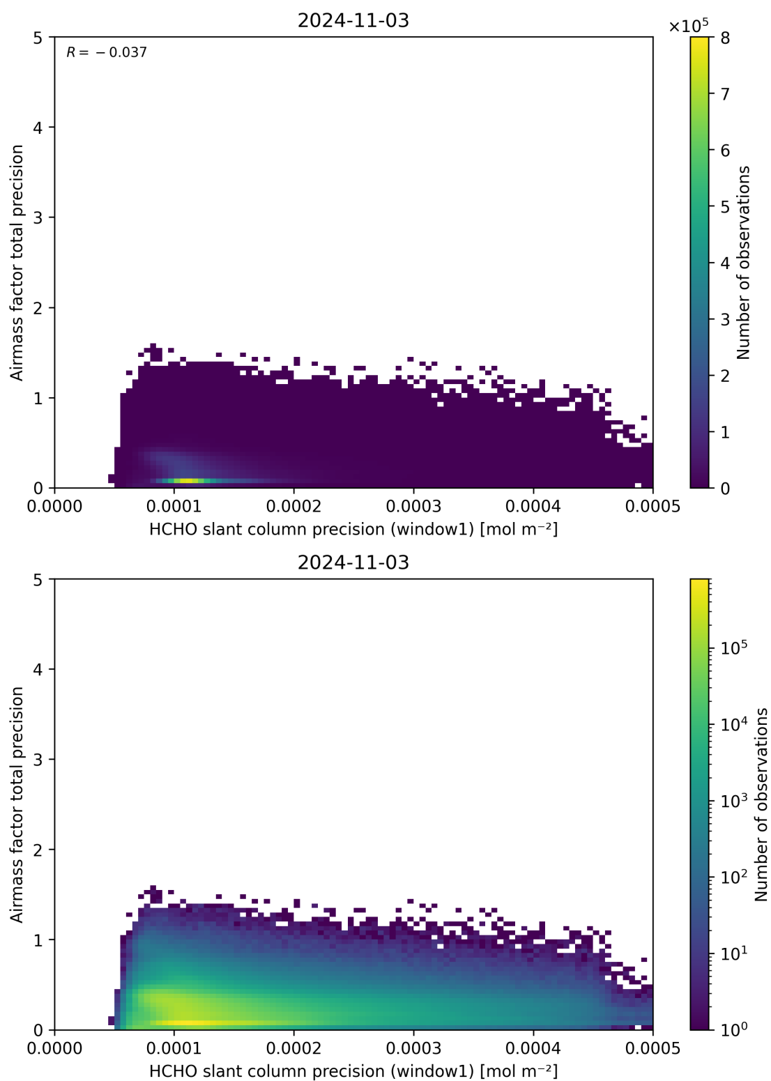
Figure 95: Scatter density plot of “HCHO slant column precision (window1)” against “Airmass factor total precision” for 2024-11-02 to 2024-11-04.
