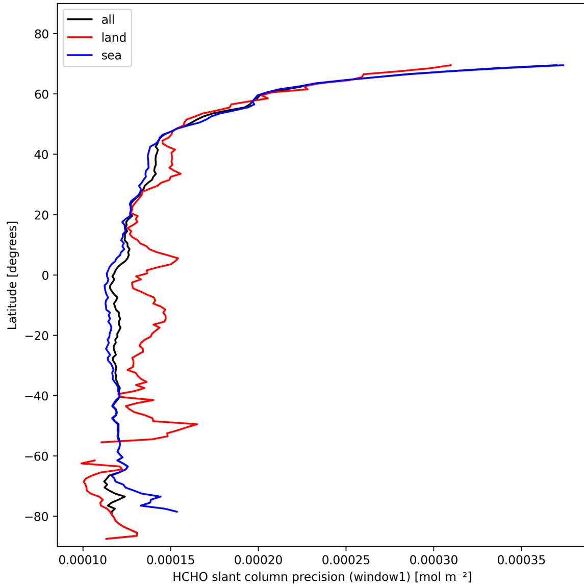
Figure 25: Zonal average of "HCHO slant column precision (window1)" for 2024-11-02 to 2024-11-04.
