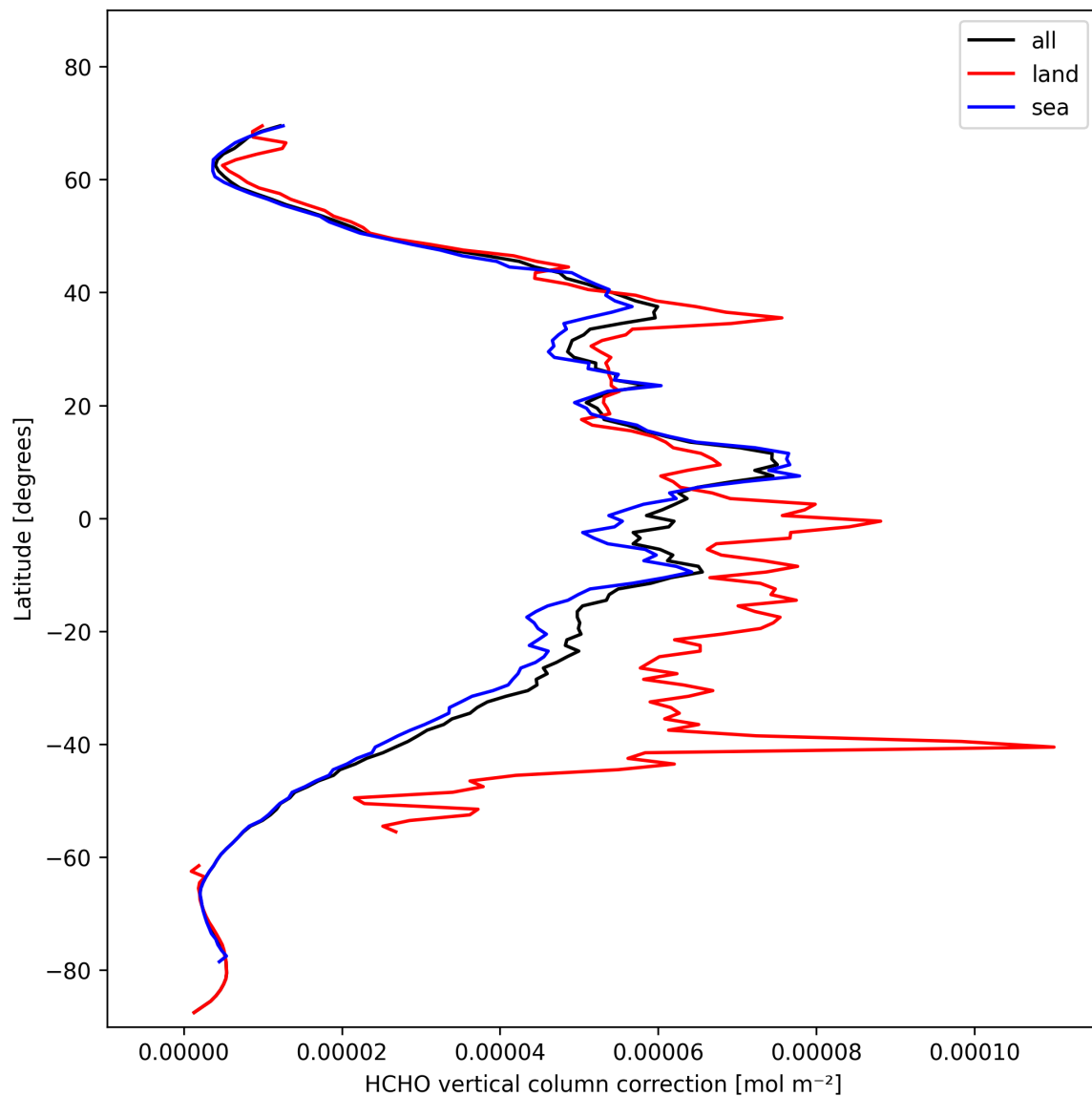
Figure 23: Zonal average of “HCHO vertical column correction” for 2024-11-02 to 2024-11-04.
