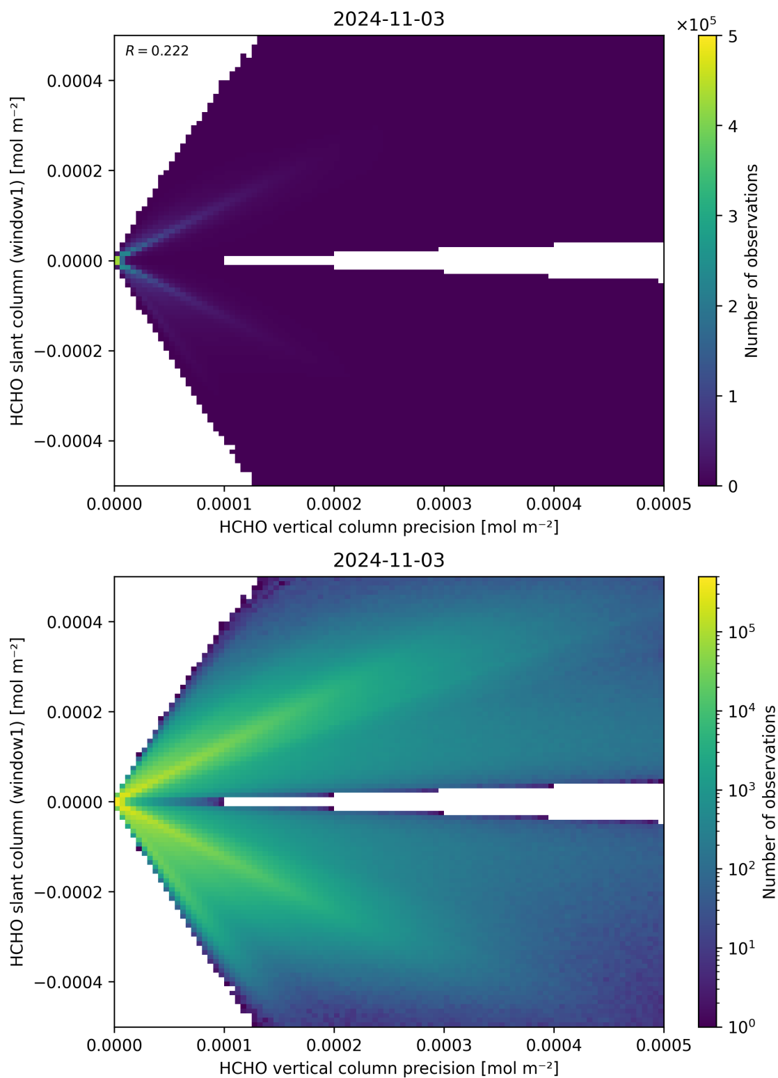
Figure 142: Scatter density plot of “HCHO vertical column precision” against “HCHO slant column (window1)” for 2024-11-02 to 2024-11-04.
