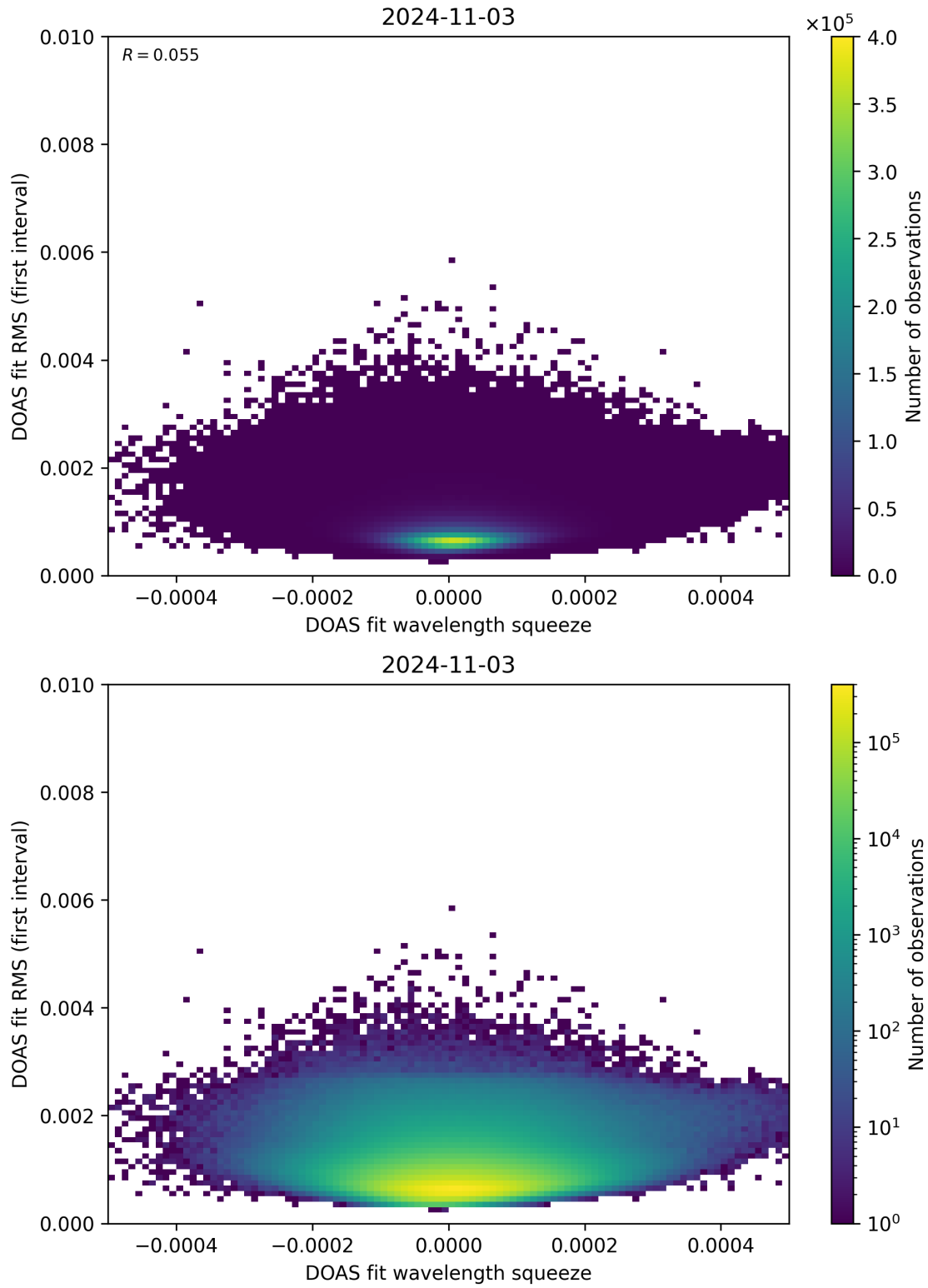
Figure 68: Scatter density plot of “DOAS fit wavelength squeeze” against “DOAS fit RMS (first interval)” for 2024-11-02 to 2024-11-04.
