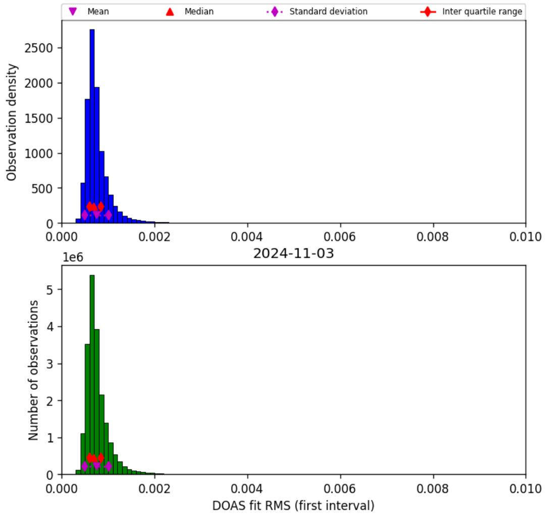
Figure 46: Histogram of “DOAS fit RMS (first interval)” for 2024-11-02 to 2024-11-04
