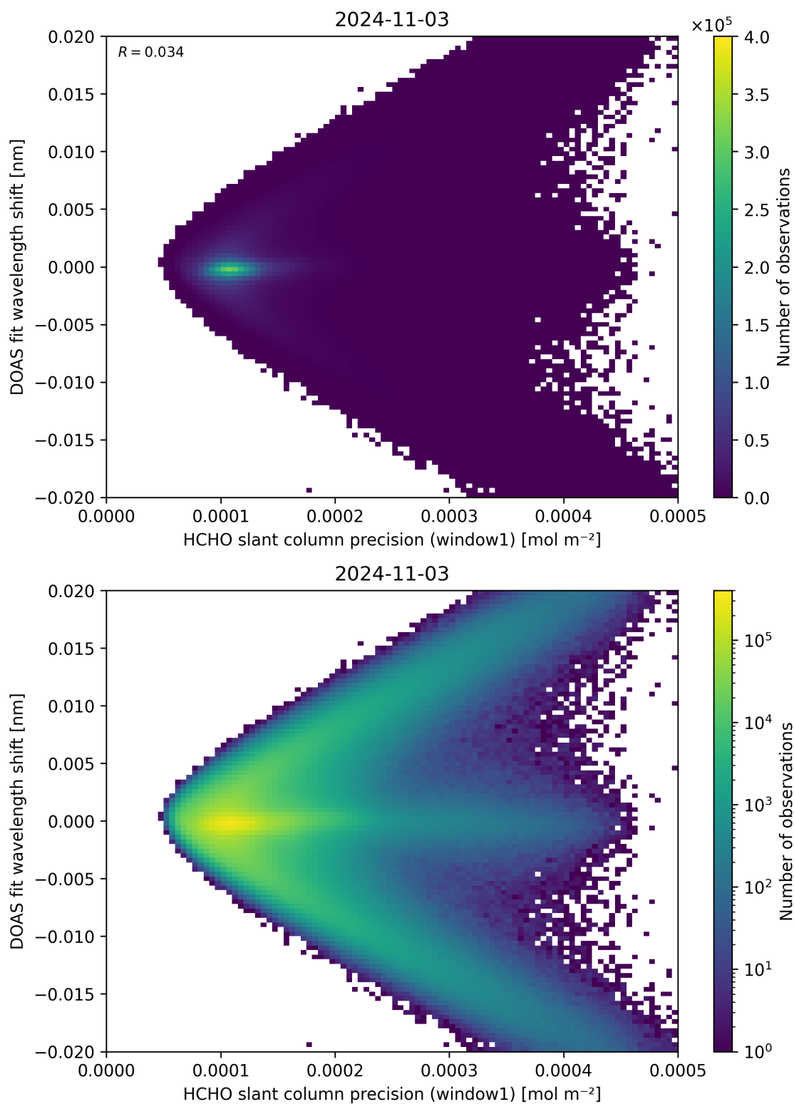
Figure 89: Scatter density plot of “HCHO slant column precision (window1)” against “DOAS fit wavelength shift” for 2024-11-02 to 2024-11-04.
