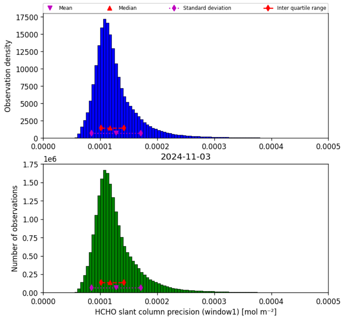
Figure 39: Histogram of “HCHO slant column precision (window1)” for 2024-11-02 to 2024-11-04
