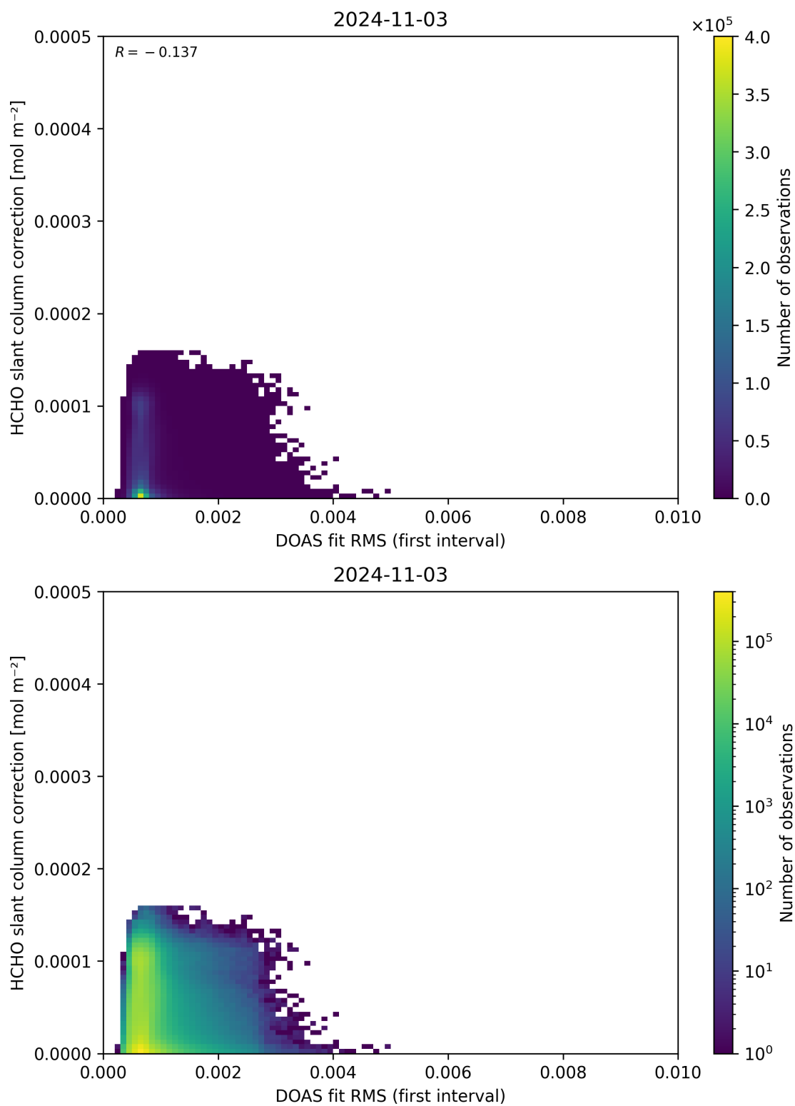
Figure 63: Scatter density plot of “DOAS fit RMS (first interval)” against “HCHO slant column correction” for 2024-11-02 to 2024-11-04.
