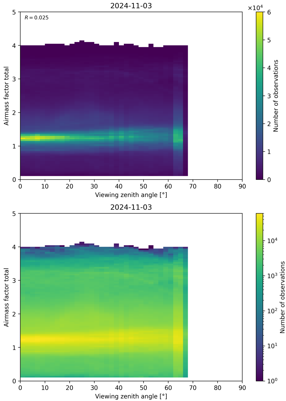
Figure 190: Scatter density plot of “Viewing zenith angle” against “Airmass factor total” for 2024-11-02 to 2024-11-04.
