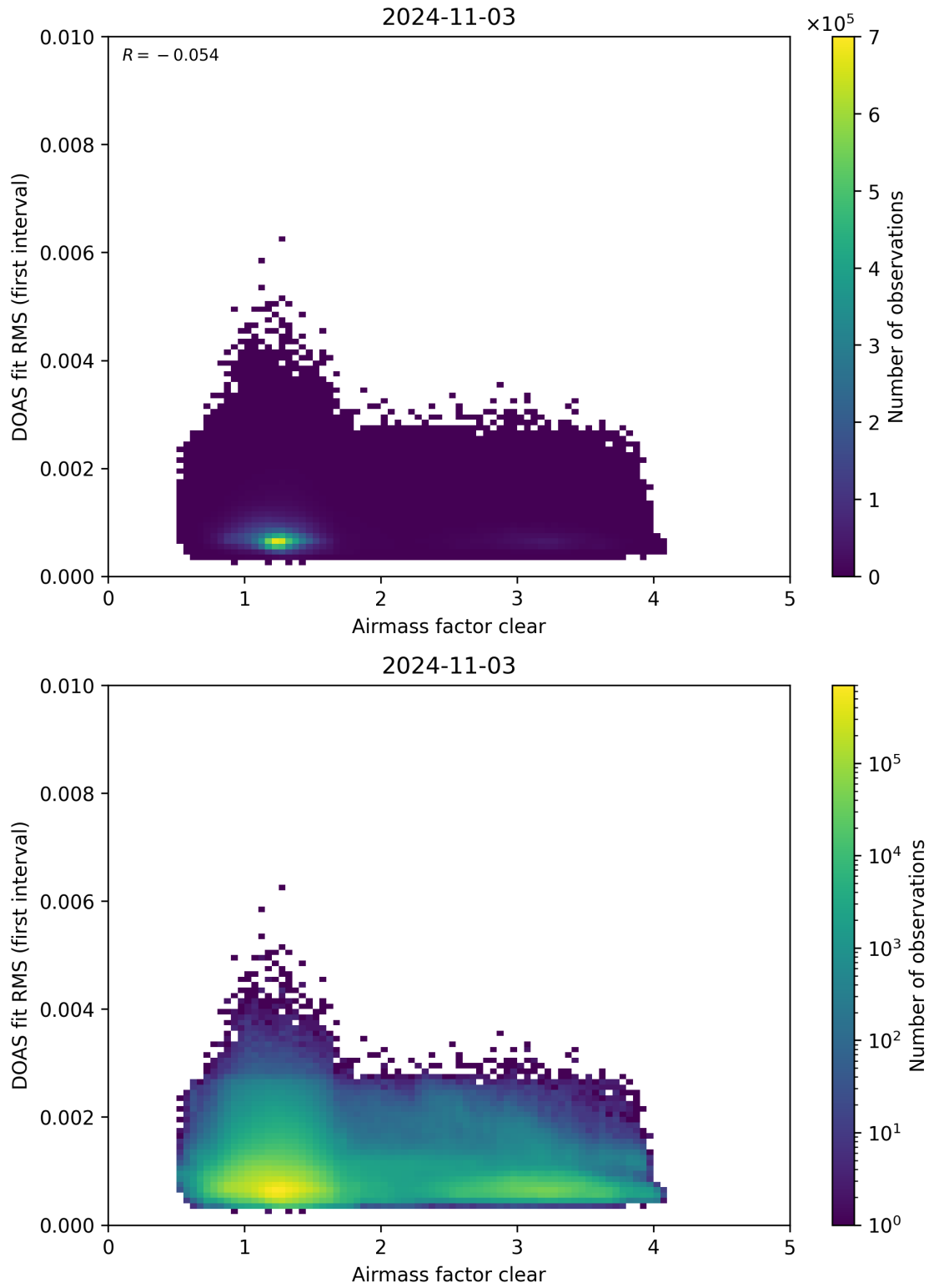
Figure 71: Scatter density plot of “Airmass factor clear” against “DOAS fit RMS (first interval)” for 2024-11-02 to 2024-11-04.
