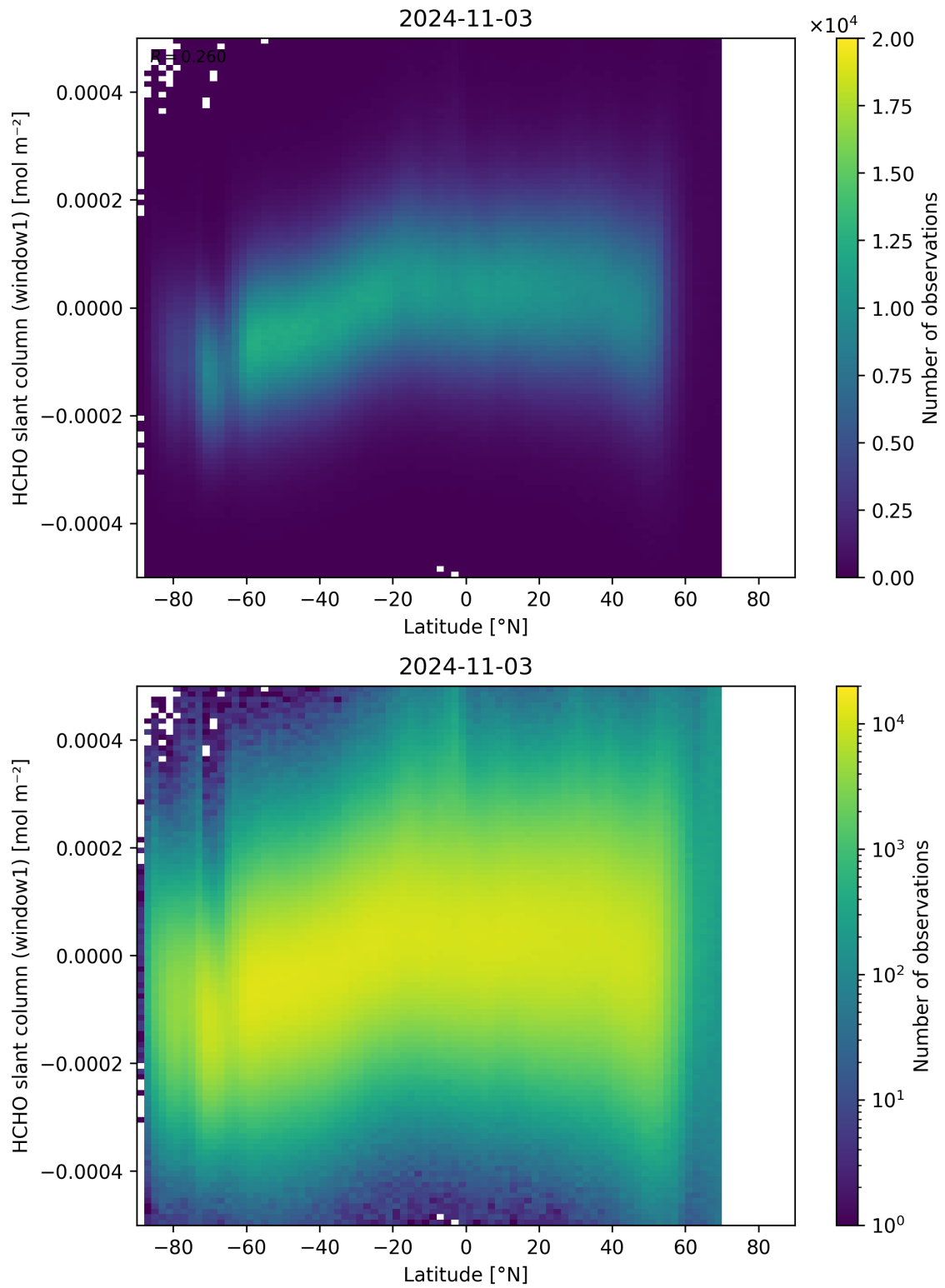
Figure 159: Scatter density plot of “Latitude” against “HCHO slant column (window1)” for 2024-11-02 to 2024-11-04.
