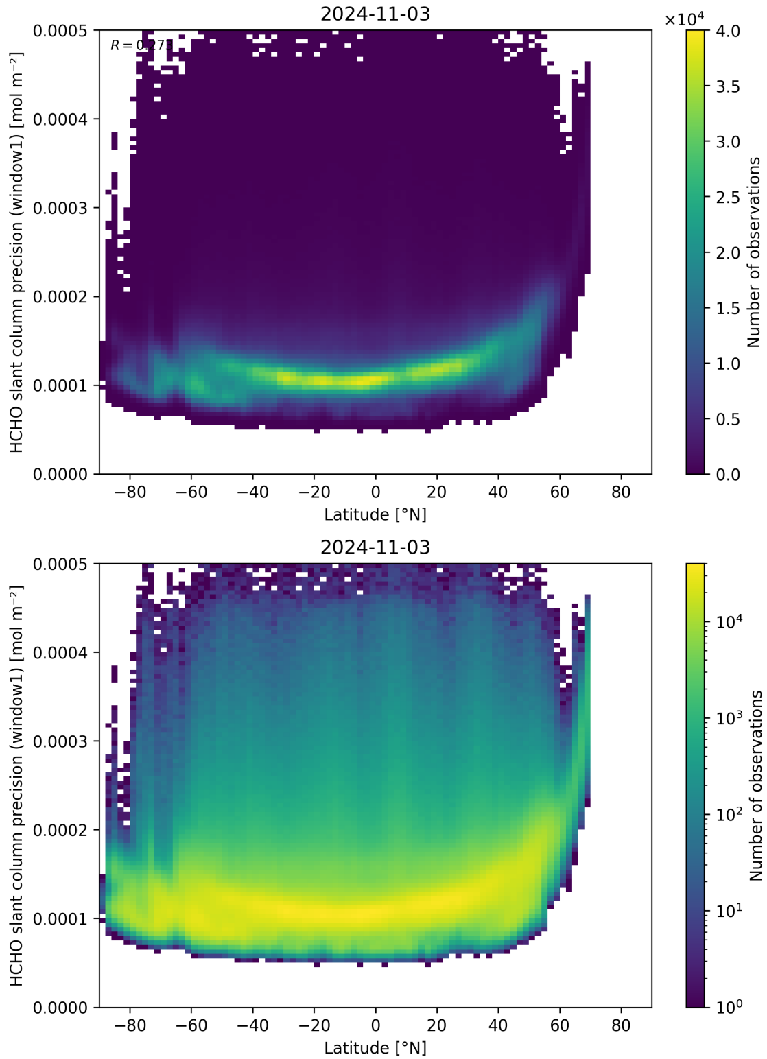
Figure 160: Scatter density plot of “Latitude” against “HCHO slant column precision (window1)” for 2024-11-02 to 2024-11-04.
