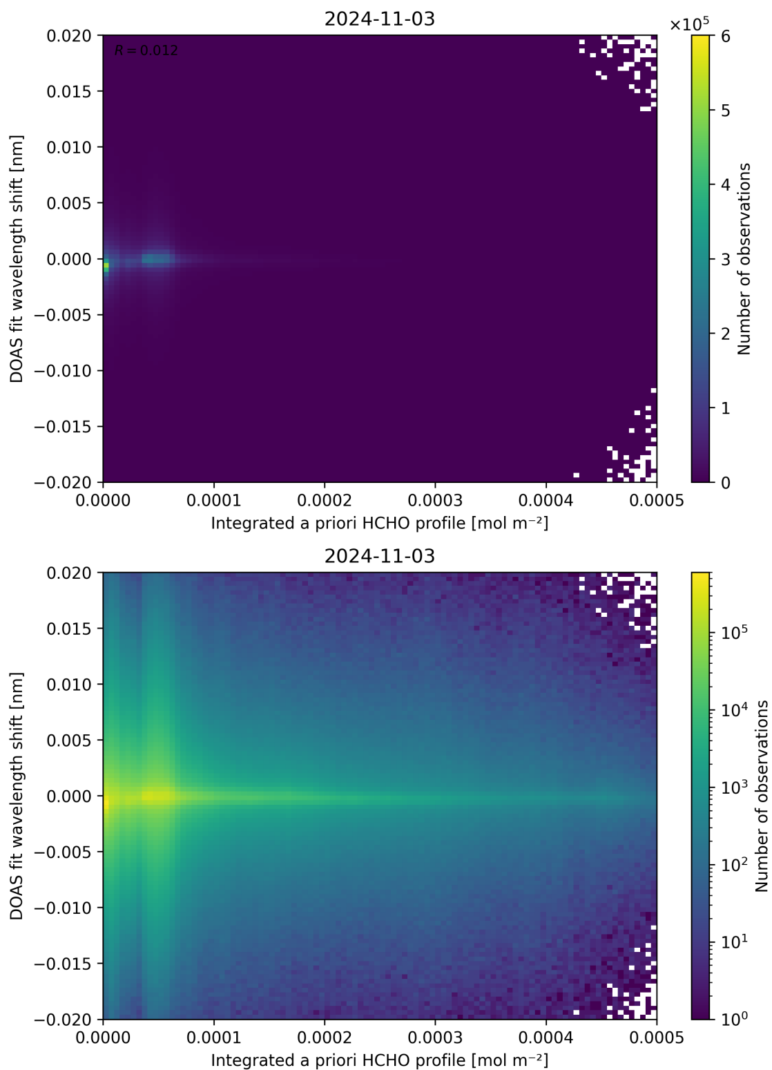
Figure 149: Scatter density plot of “Integrated a priori HCHO profile” against “DOAS fit wavelength shift” for 2024-11-02 to 2024-11-04.
