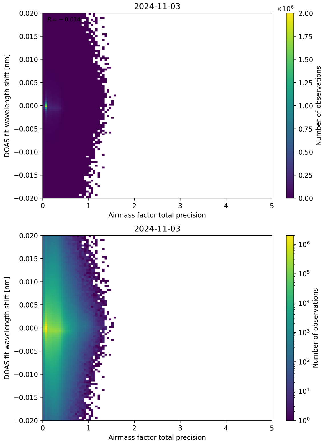
Figure 106: Scatter density plot of “Airmass factor total precision” against “DOAS fit wavelength shift” for 2024-11-02 to 2024-11-04.
