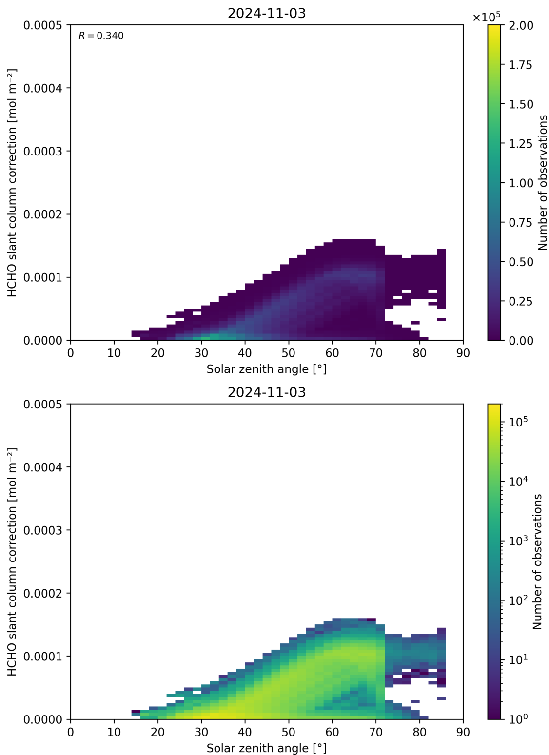
Figure 172: Scatter density plot of “Solar zenith angle” against “HCHO slant column correction” for 2024-11-02 to 2024-11-04.
