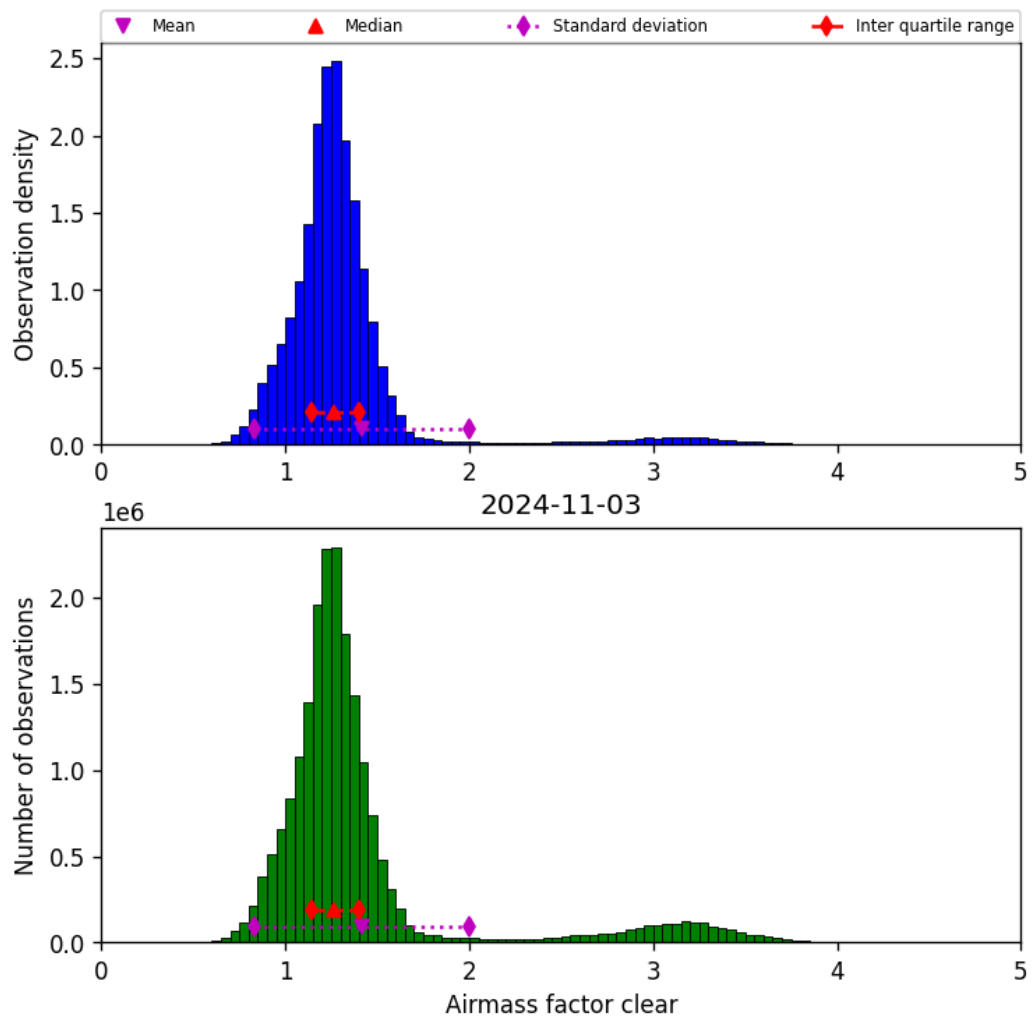
Figure 42: Histogram of “Airmass factor clear” for 2024-11-02 to 2024-11-04
