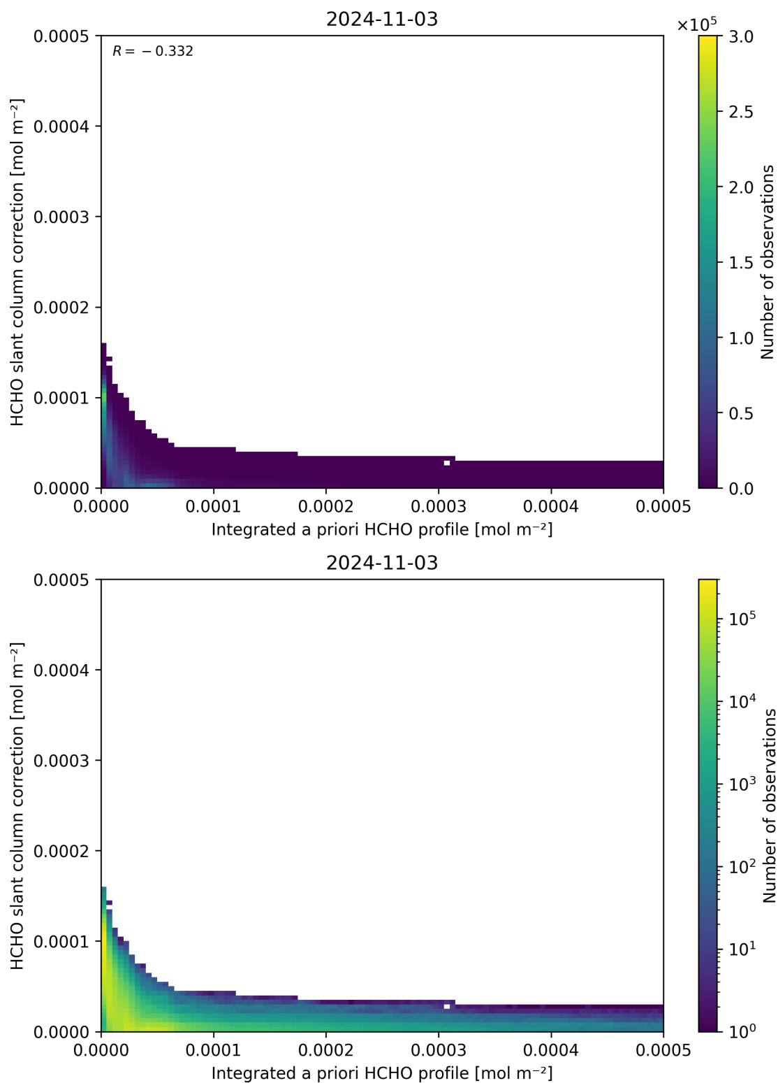
Figure 152: Scatter density plot of “Integrated a priori HCHO profile” against “HCHO slant column correction” for 2024-11-02 to 2024-11-04.
