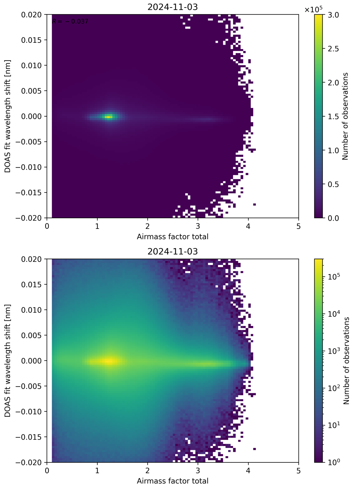
Figure 98: Scatter density plot of “Airmass factor total” against “DOAS fit wavelength shift” for 2024-11-02 to 2024-11-04.
