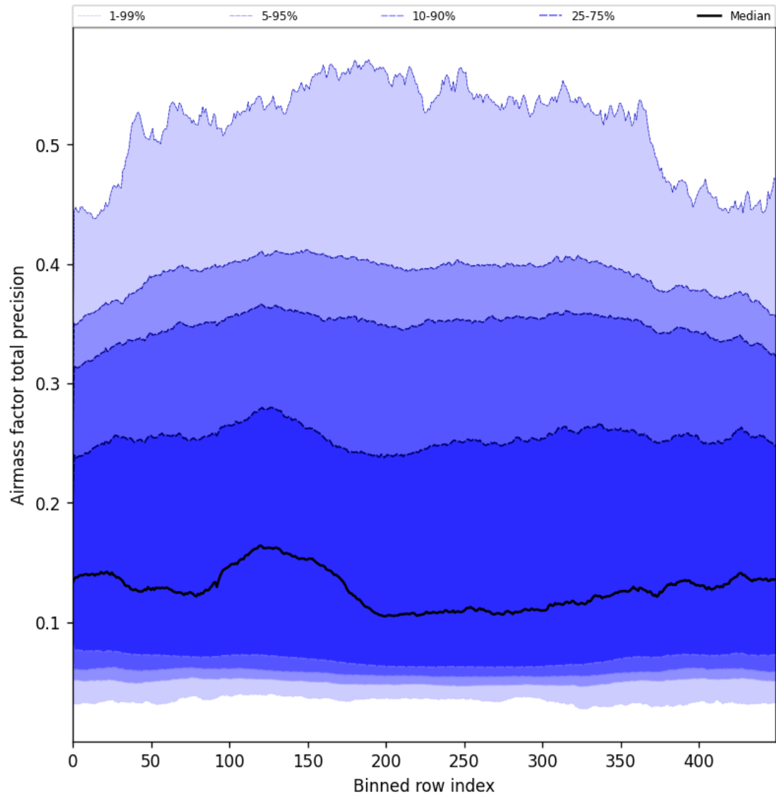
Figure 55: Along track statistics of “Airmass factor total precision” for 2024-11-02 to 2024-11-04
