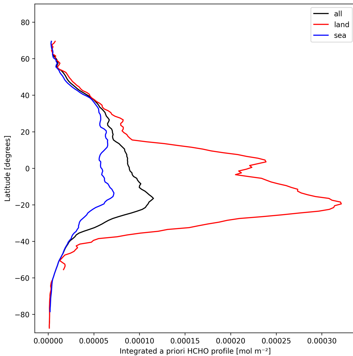
Figure 29: Zonal average of “Integrated a priori HCHO profile” for 2024-11-02 to 2024-11-04.
