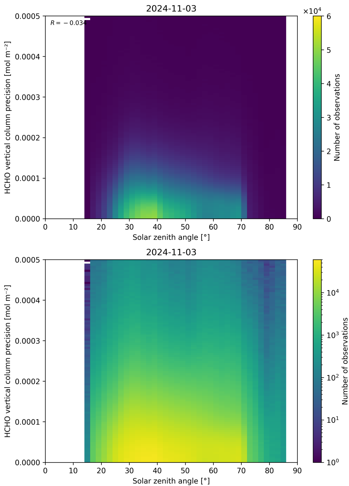
Figure 179: Scatter density plot of “Solar zenith angle” against “HCHO vertical column precision” for 2024-11-02 to 2024-11-04.
