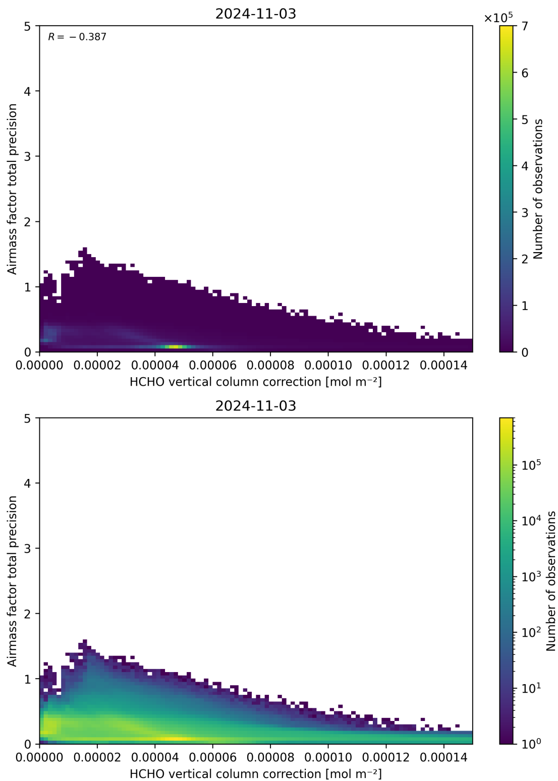
Figure 121: Scatter density plot of “HCHO vertical column correction” against “Airmass factor total precision” for 2024-11-02 to 2024-11-04.
