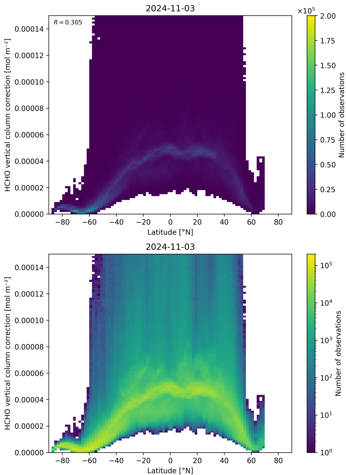
Figure 164: Scatter density plot of “Latitude” against “HCHO vertical column correction” for 2024-11-02 to 2024-11-04.
