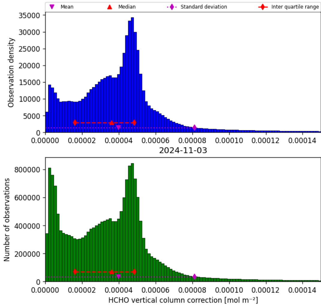
Figure 37: Histogram of “HCHO vertical column correction” for 2024-11-02 to 2024-11-04
