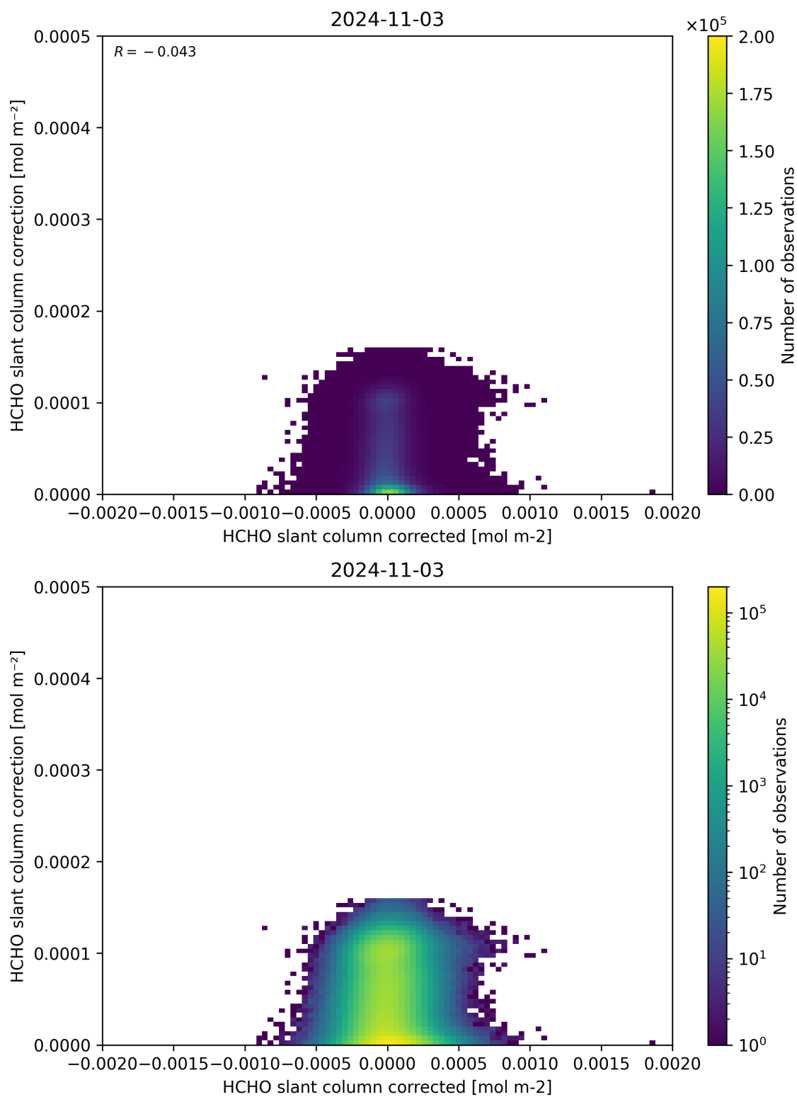
Figure 77: Scatter density plot of “HCHO slant column corrected” against “HCHO slant column correction” for 2024-11-02 to 2024-11-04.
