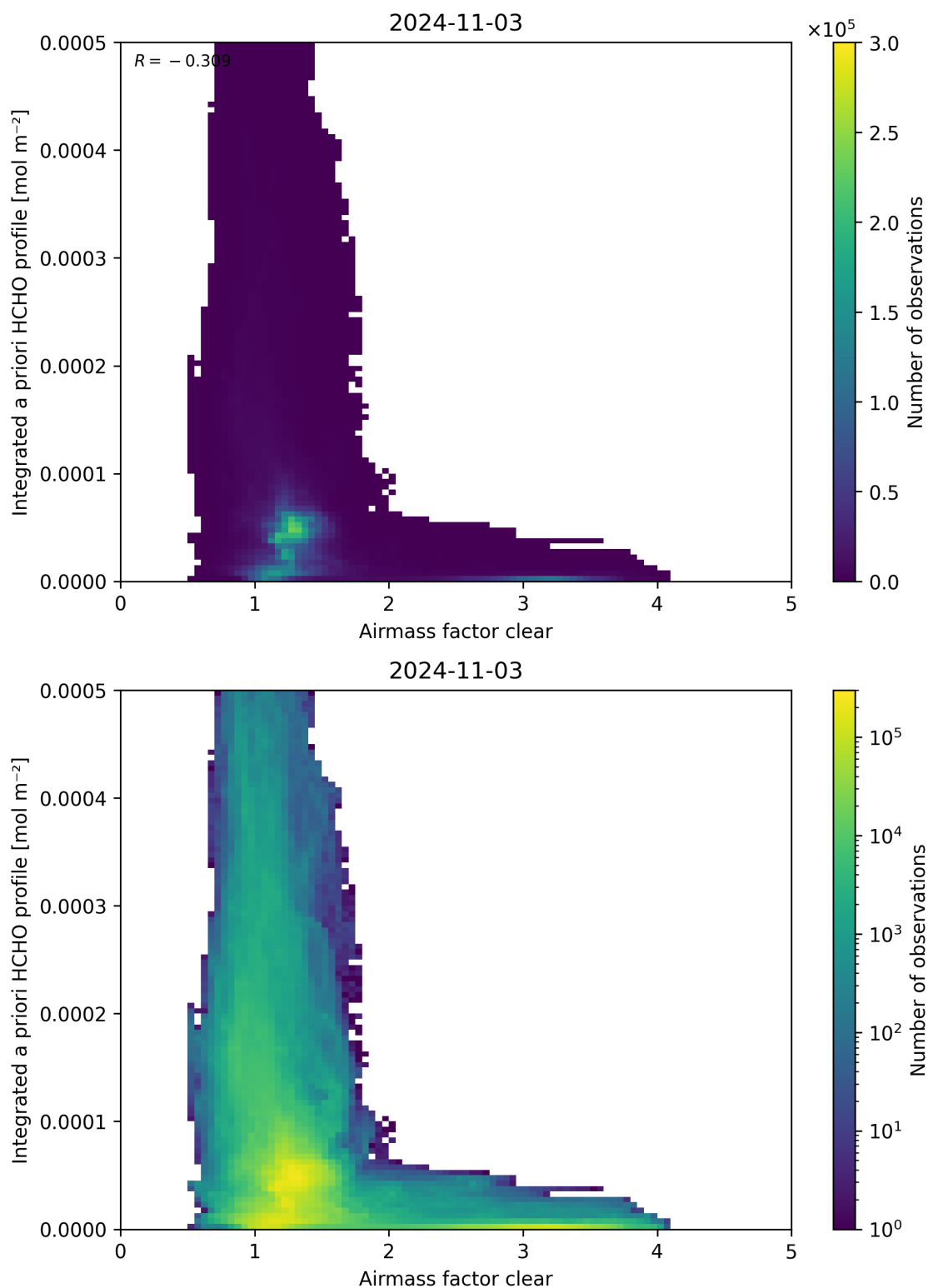
Figure 76: Scatter density plot of “Airmass factor clear” against “Integrated a priori HCHO profile” for 2024-11-02 to 2024-11-04.
