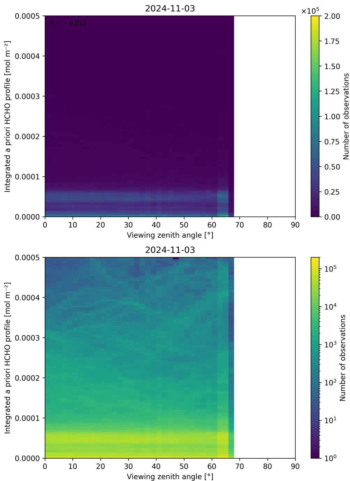
Figure 195: Scatter density plot of “Viewing zenith angle” against “Integrated a priori HCHO profile” for 2024-11-02 to 2024-11-04.
