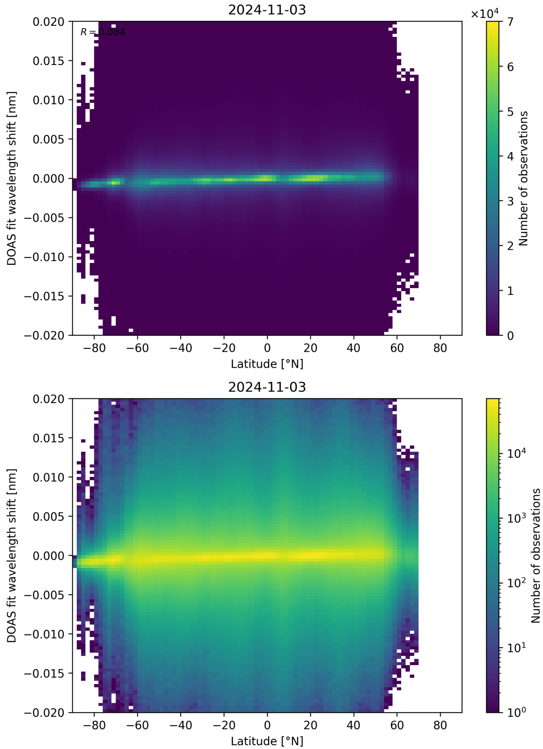
Figure 154: Scatter density plot of “Latitude” against “DOAS fit wavelength shift” for 2024-11-02 to 2024-11-04.
