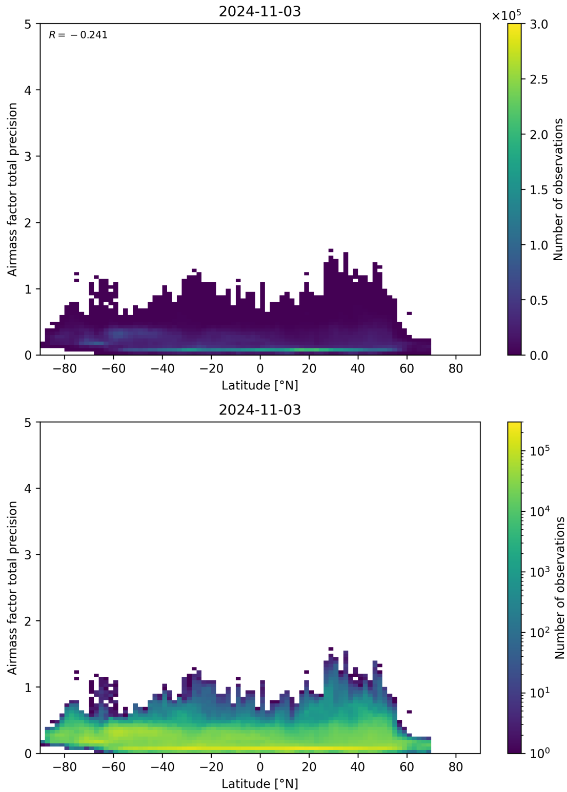
Figure 162: Scatter density plot of “Latitude” against “Airmass factor total precision” for 2024-11-02 to 2024-11-04.
