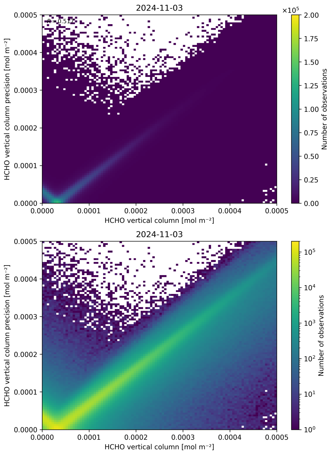
Figure 134: Scatter density plot of “HCHO vertical column” against “HCHO vertical column precision” for 2024-11-02 to 2024-11-04.
