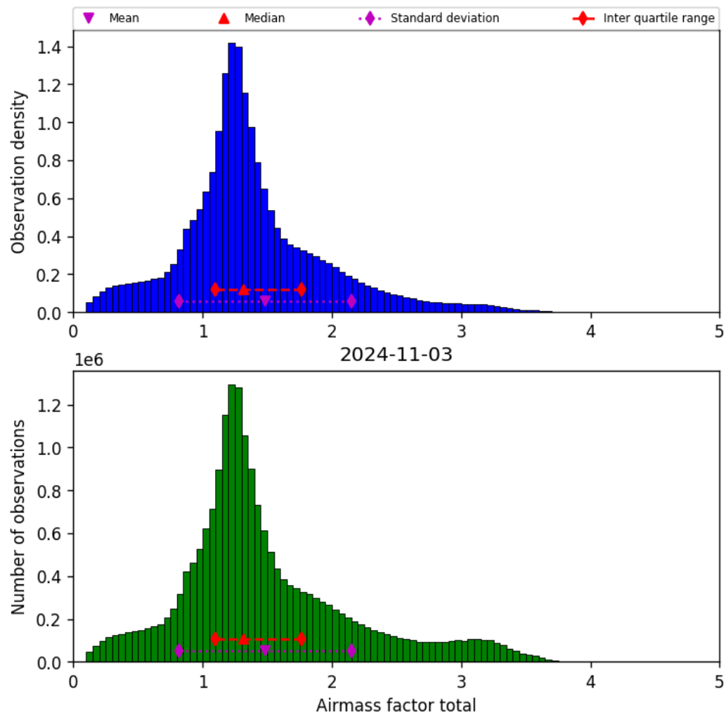
Figure 40: Histogram of “Airmass factor total” for 2024-11-02 to 2024-11-04
