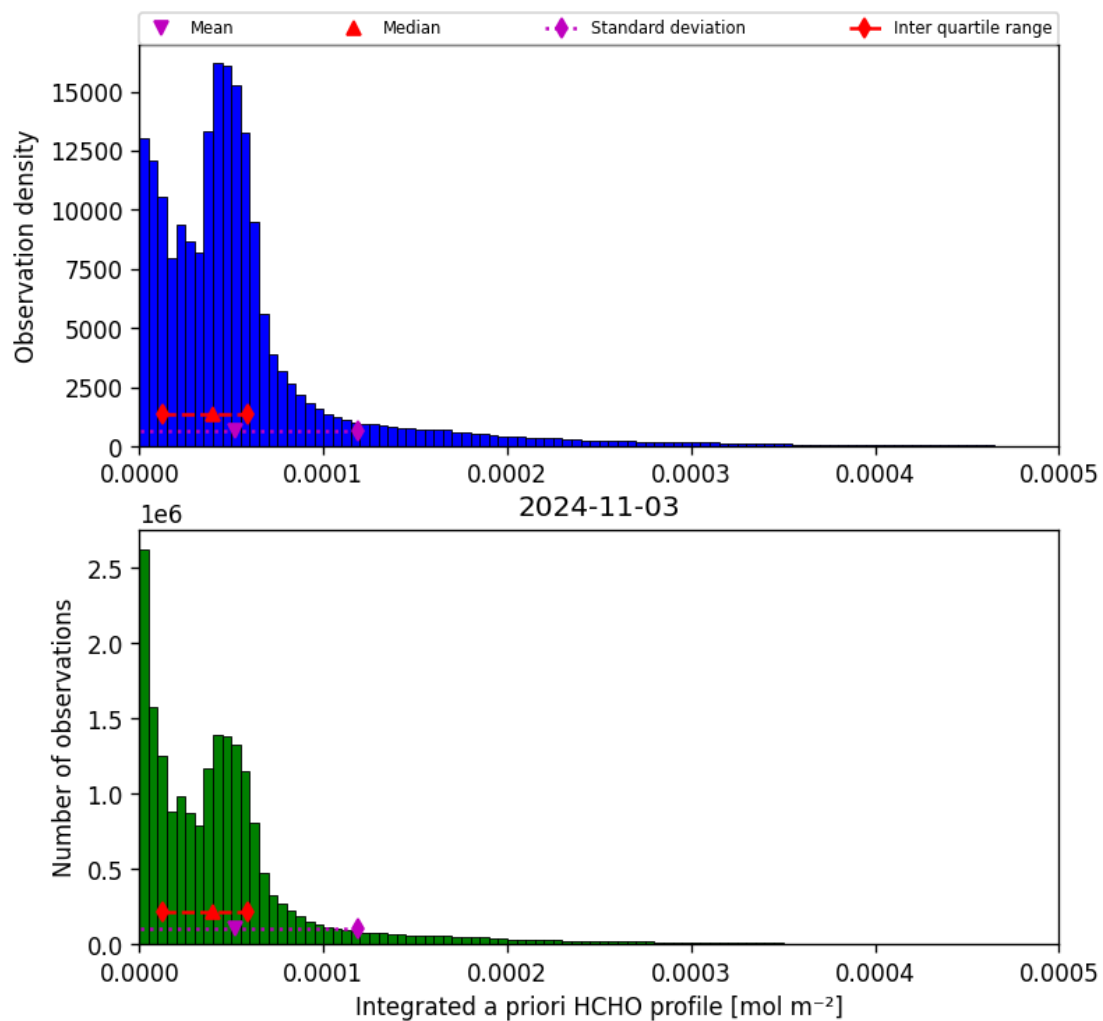
Figure 43: Histogram of “Integrated a priori HCHO profile” for 2024-11-02 to 2024-11-04
