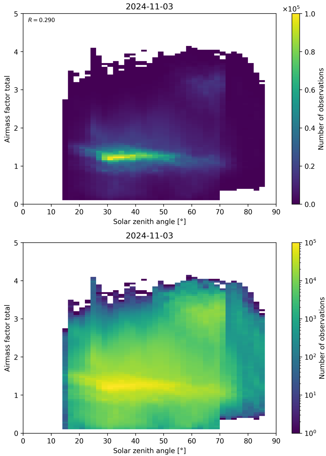
Figure 175: Scatter density plot of “Solar zenith angle” against “Airmass factor total” for 2024-11-02 to 2024-11-04.
