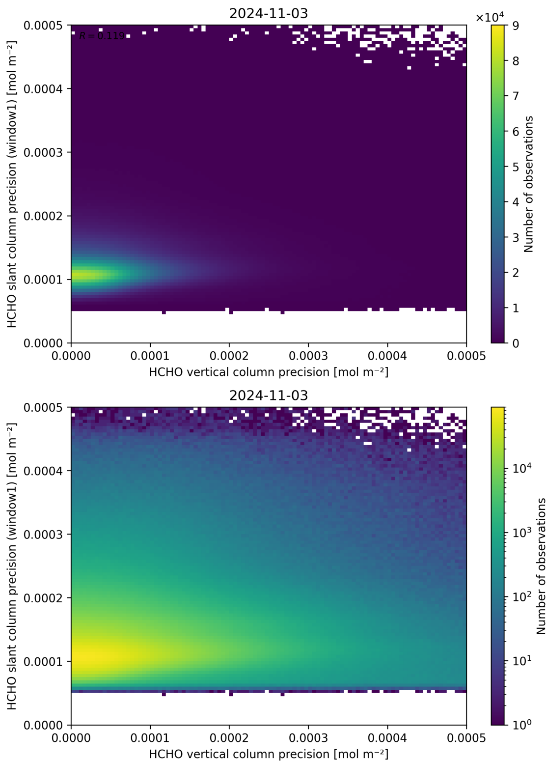
Figure 143: Scatter density plot of “HCHO vertical column precision” against “HCHO slant column precision (window1)” for 2024-11-02 to 2024-11-04.
