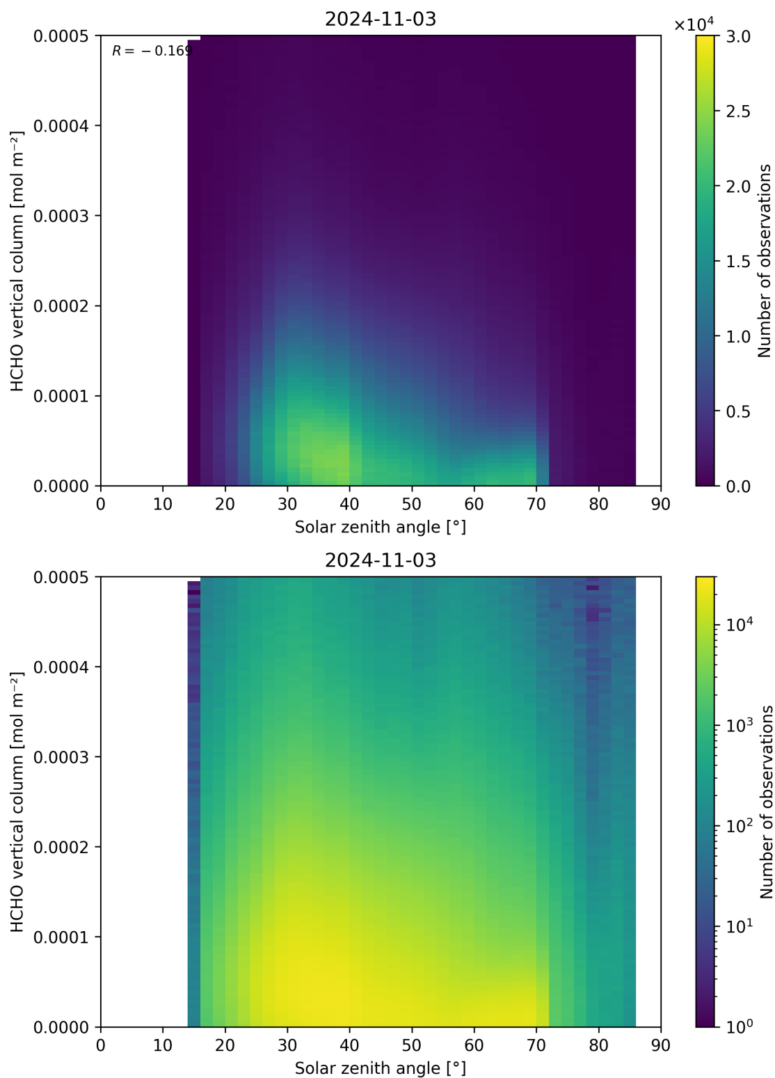
Figure 177: Scatter density plot of “Solar zenith angle” against “HCHO vertical column” for 2024-11-02 to 2024-11-04.
