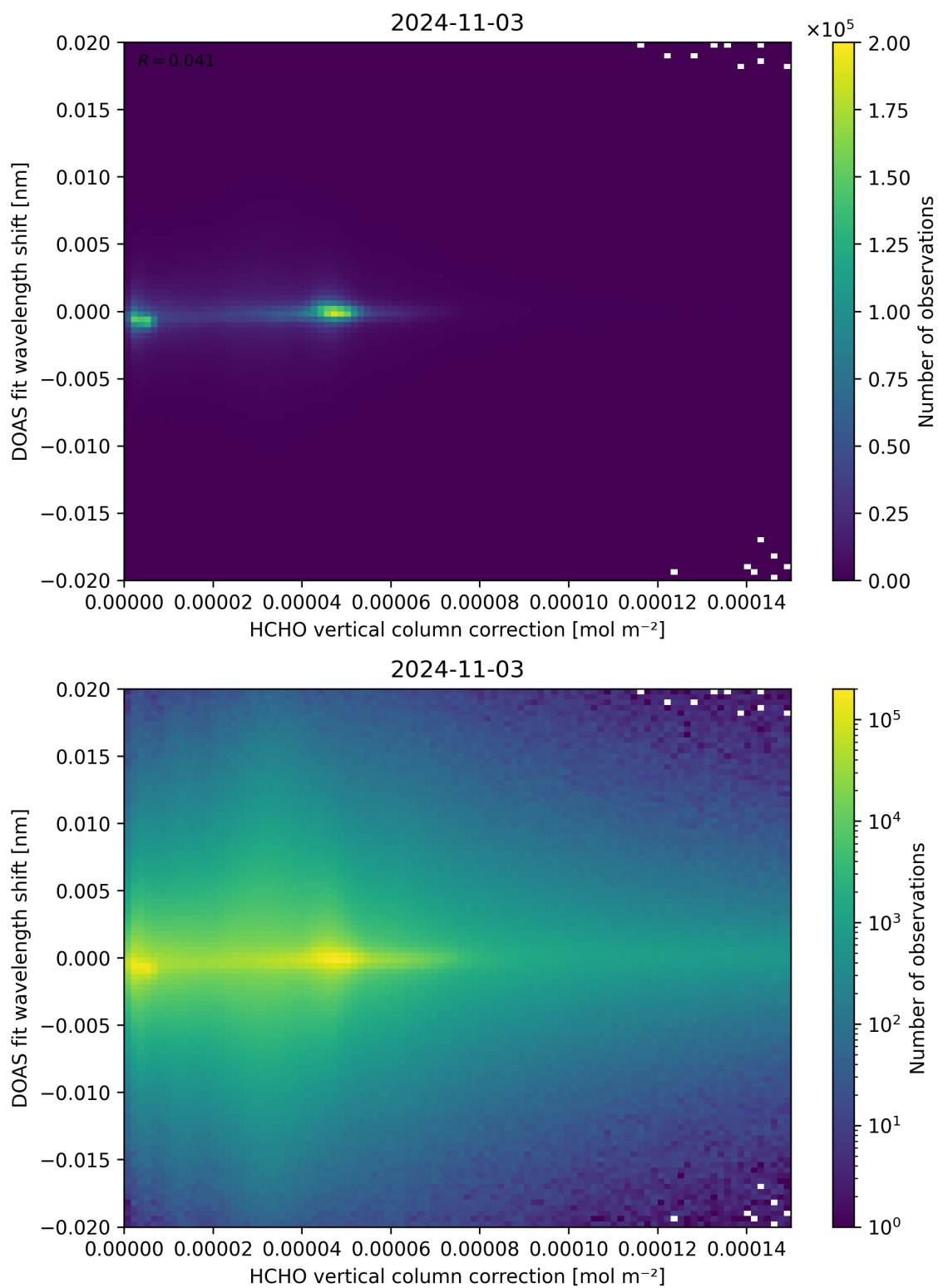
Figure 113: Scatter density plot of “HCHO vertical column correction” against “DOAS fit wavelength shift” for 2024-11-02 to 2024-11-04.
