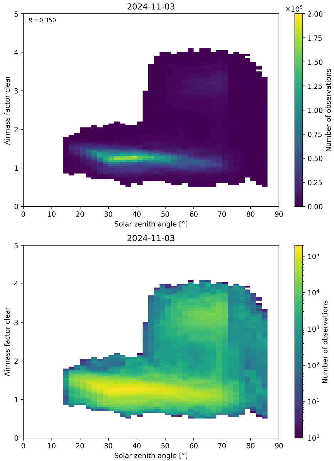
Figure 170: Scatter density plot of “Solar zenith angle” against “Airmass factor clear” for 2024-11-02 to 2024-11-04.
