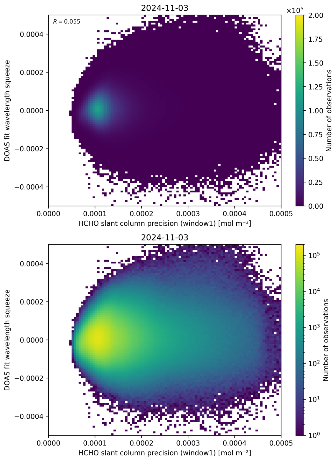
Figure 90: Scatter density plot of “HCHO slant column precision (window1)” against “DOAS fit wavelength squeeze” for 2024-11-02 to 2024-11-04.
