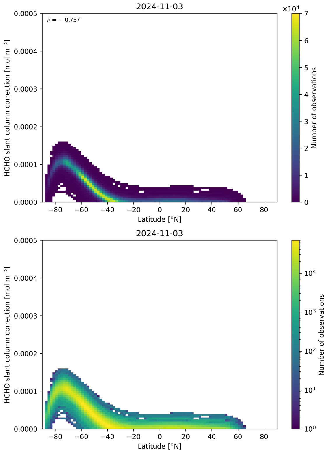
Figure 158: Scatter density plot of “Latitude” against “HCHO slant column correction” for 2024-11-02 to 2024-11-04.
