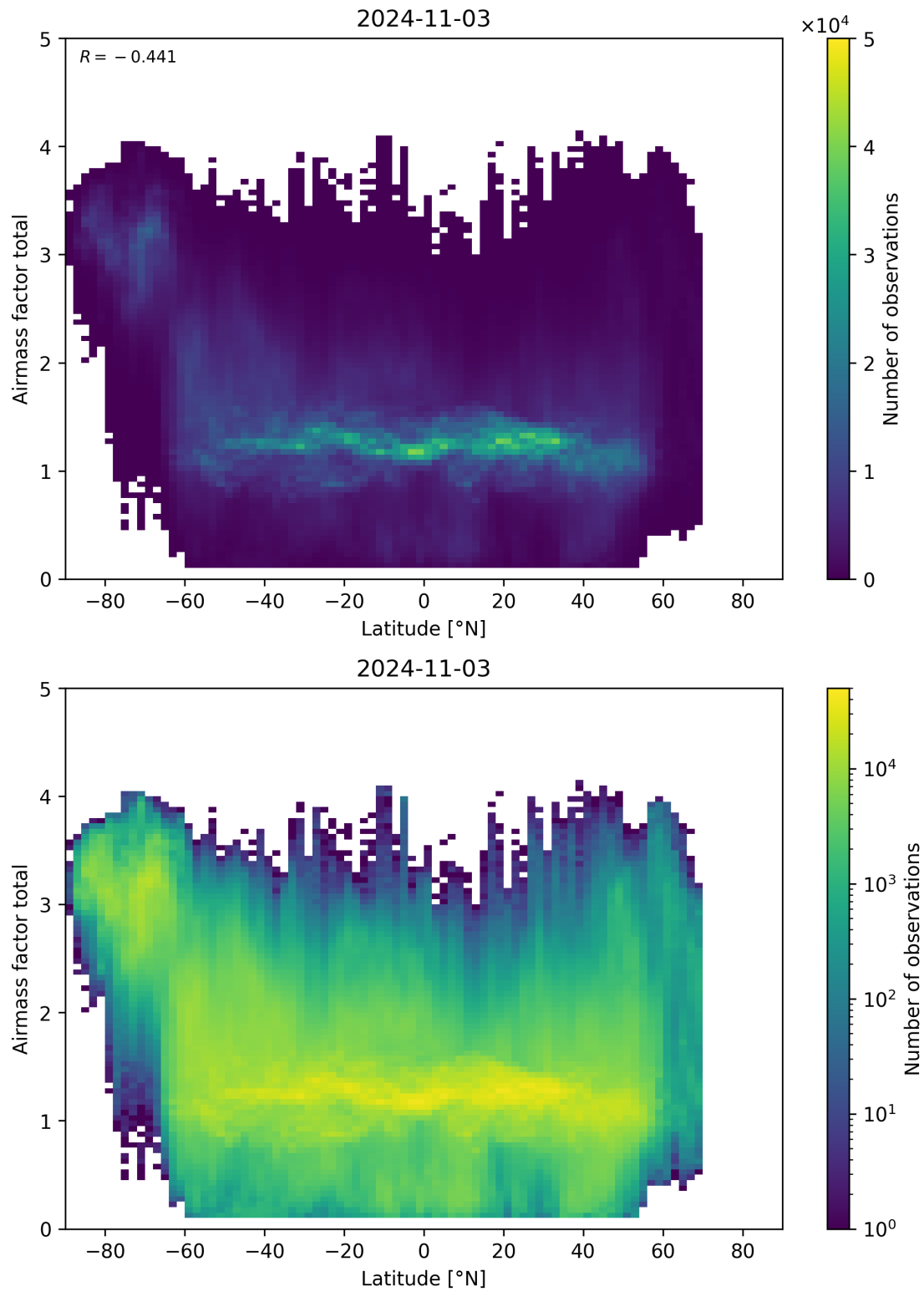
Figure 161: Scatter density plot of “Latitude” against “Airmass factor total” for 2024-11-02 to 2024-11-04.
