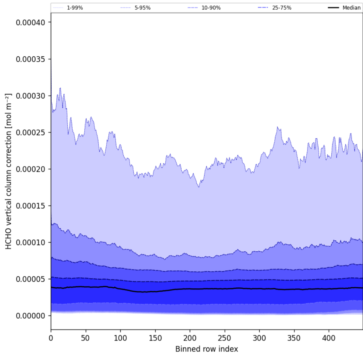
Figure 51: Along track statistics of “HCHO vertical column correction” for 2024-11-02 to 2024-11-04
