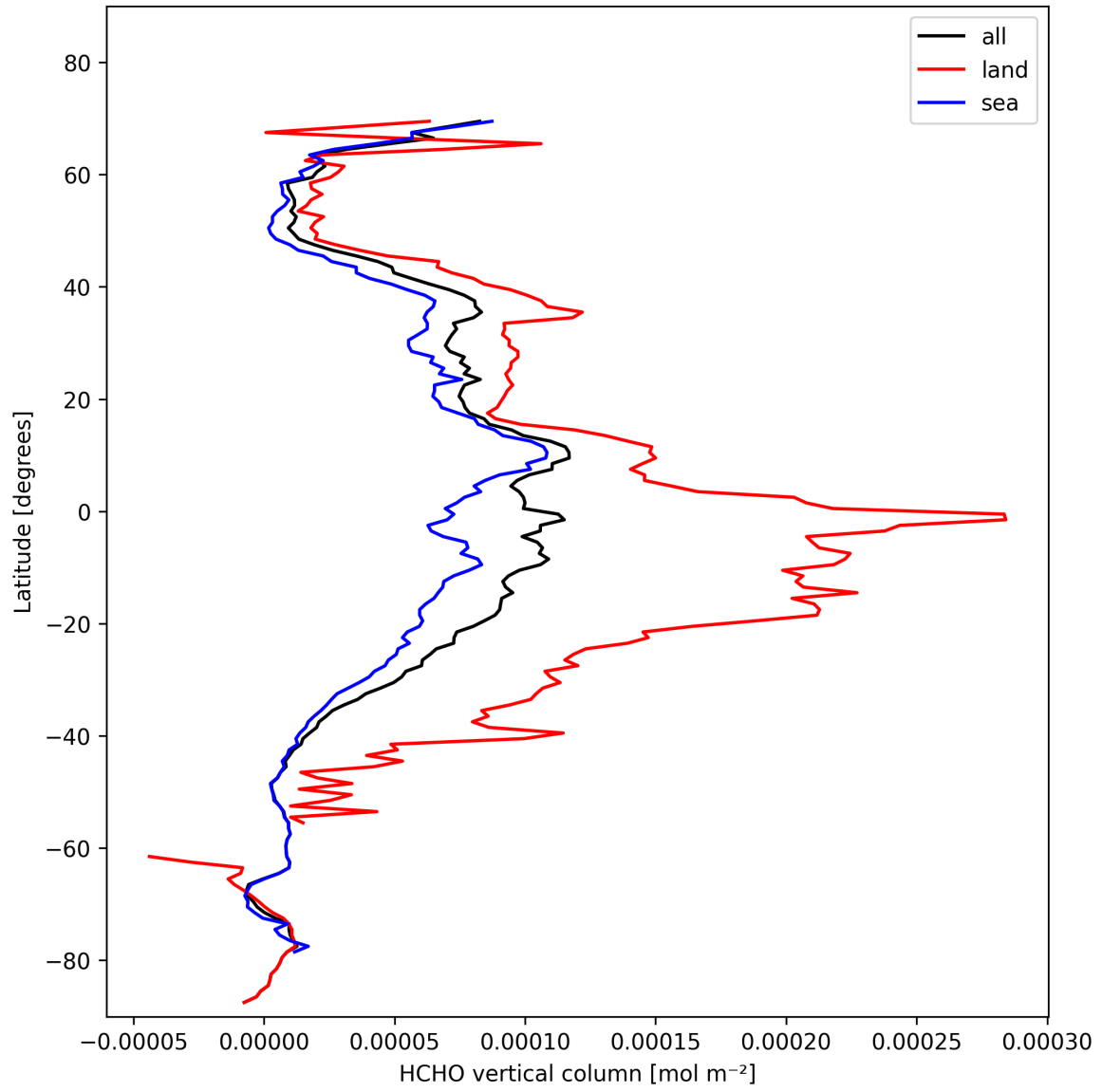
Figure 21: Zonal average of “HCHO vertical column” for 2024-11-02 to 2024-11-04.
