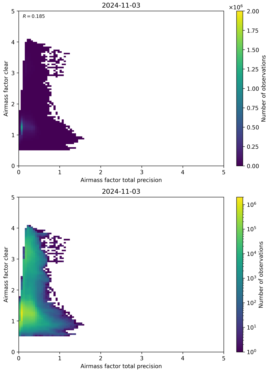
Figure 108: Scatter density plot of “Airmass factor total precision” against “Airmass factor clear” for 2024-11-02 to 2024-11-04.
