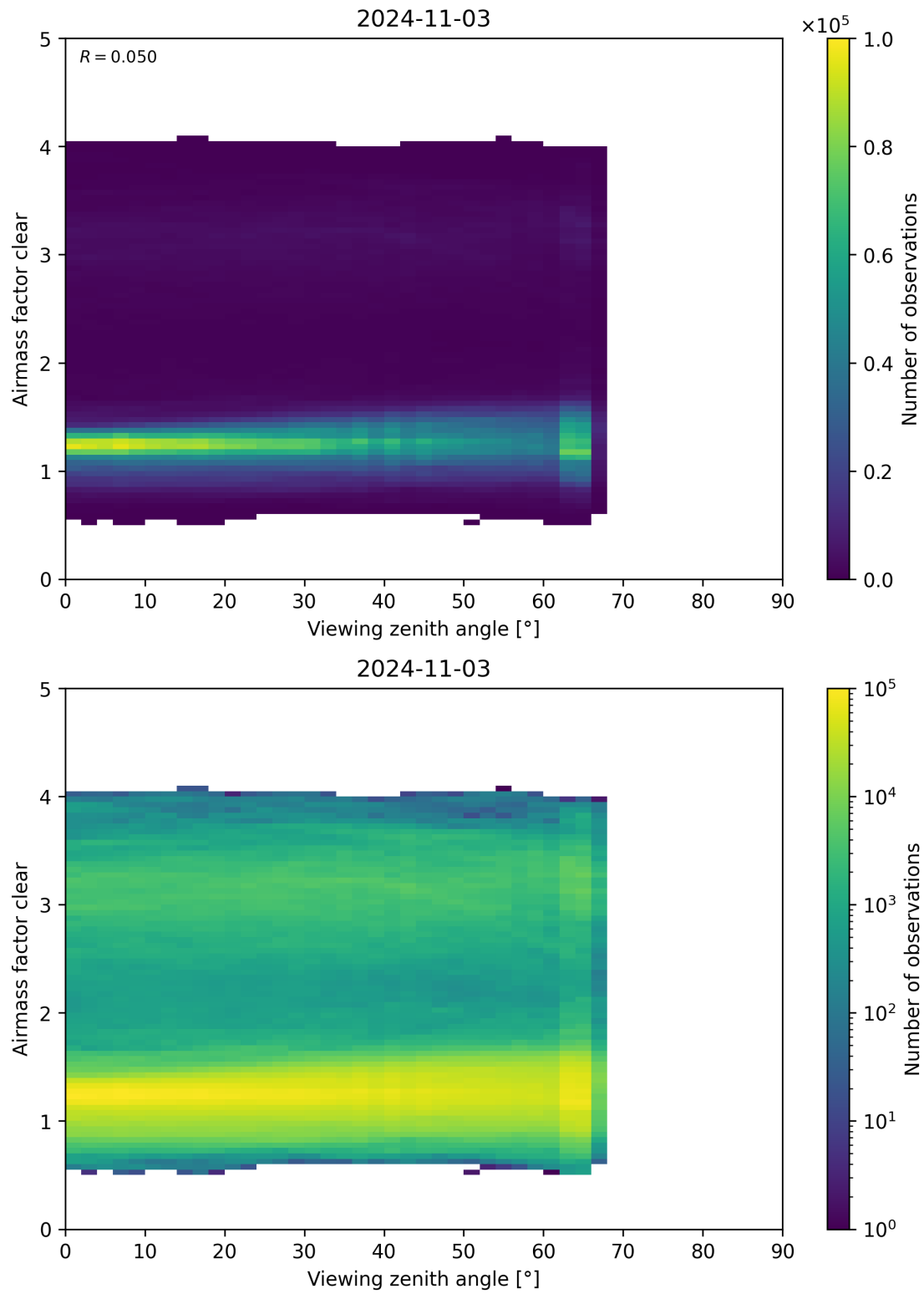
Figure 185: Scatter density plot of “Viewing zenith angle” against “Airmass factor clear” for 2024-11-02 to 2024-11-04.
