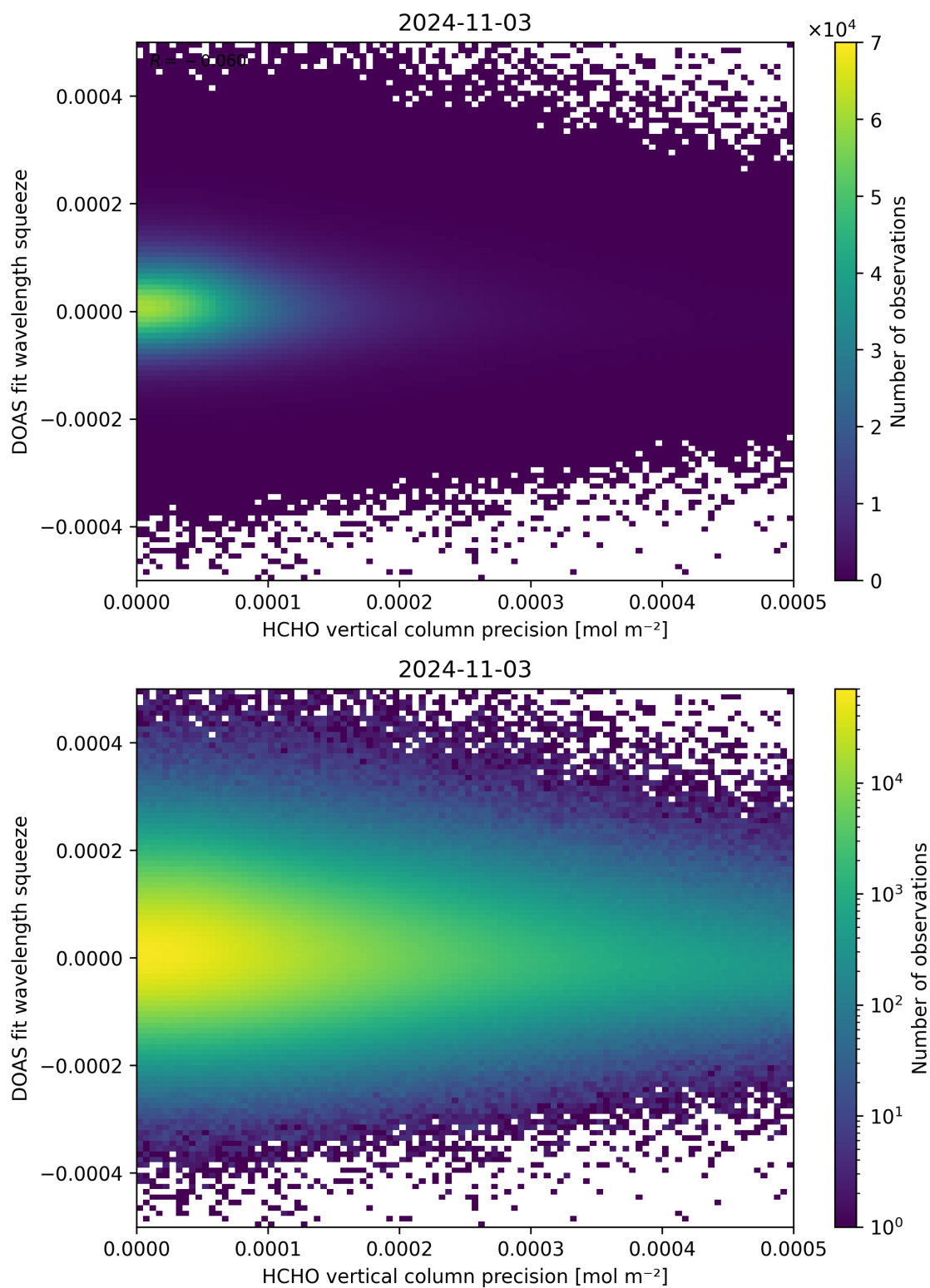
Figure 138: Scatter density plot of “HCHO vertical column precision” against “DOAS fit wavelength squeeze” for 2024-11-02 to 2024-11-04.
