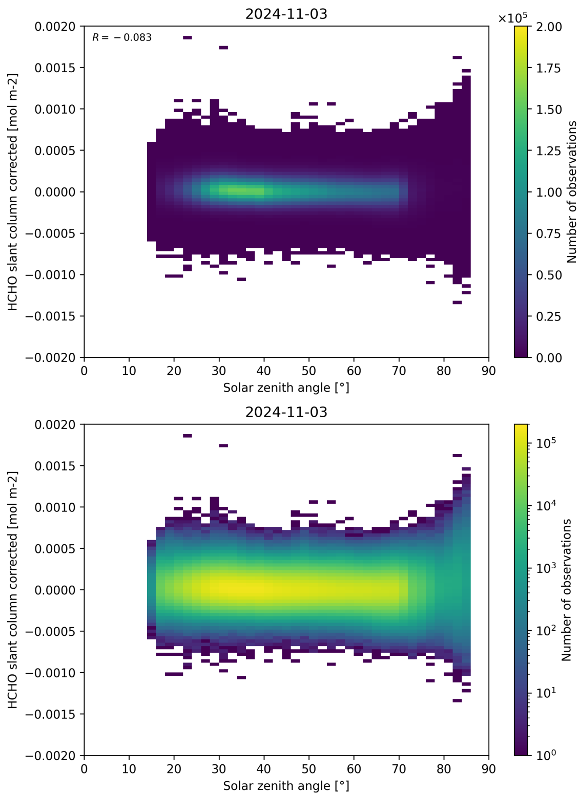
Figure 171: Scatter density plot of “Solar zenith angle” against “HCHO slant column corrected” for 2024-11-02 to 2024-11-04.
