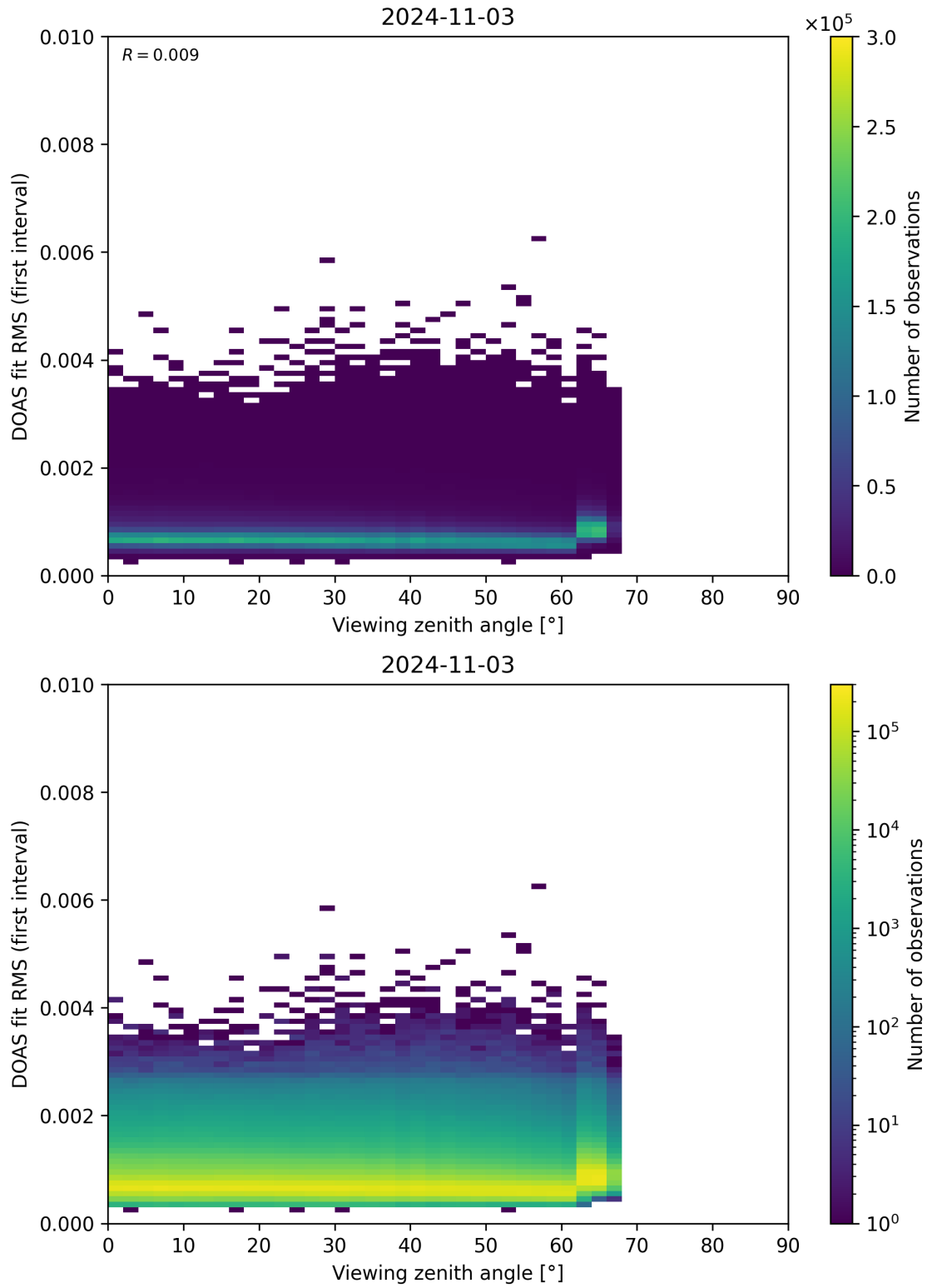
Figure 182: Scatter density plot of “Viewing zenith angle” against “DOAS fit RMS (first interval)” for 2024-11-02 to 2024-11-04.
