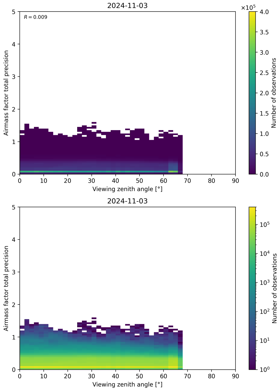
Figure 191: Scatter density plot of “Viewing zenith angle” against “Airmass factor total precision” for 2024-11-02 to 2024-11-04.
