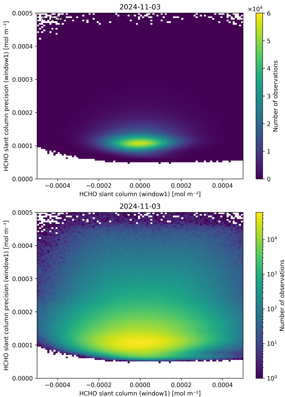
Figure 84: Scatter density plot of “HCHO slant column (window1)” against “HCHO slant column precision (window1)” for 2024-11-02 to 2024-11-04.
