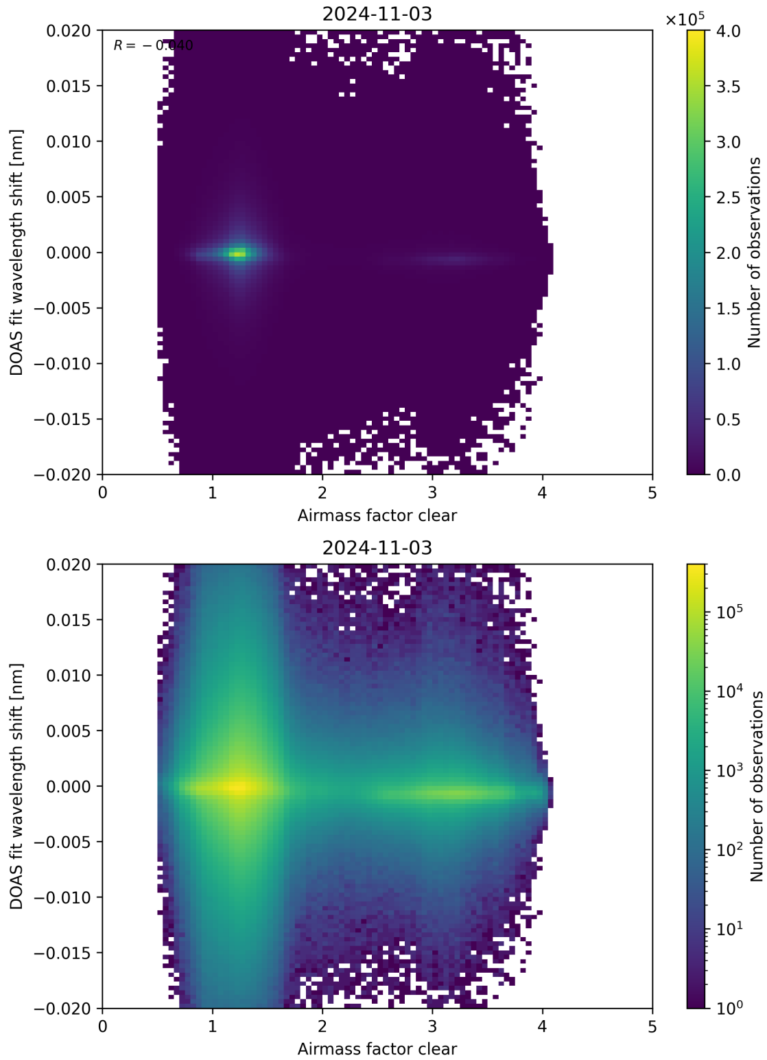
Figure 72: Scatter density plot of “Airmass factor clear” against “DOAS fit wavelength shift” for 2024-11-02 to 2024-11-04.
