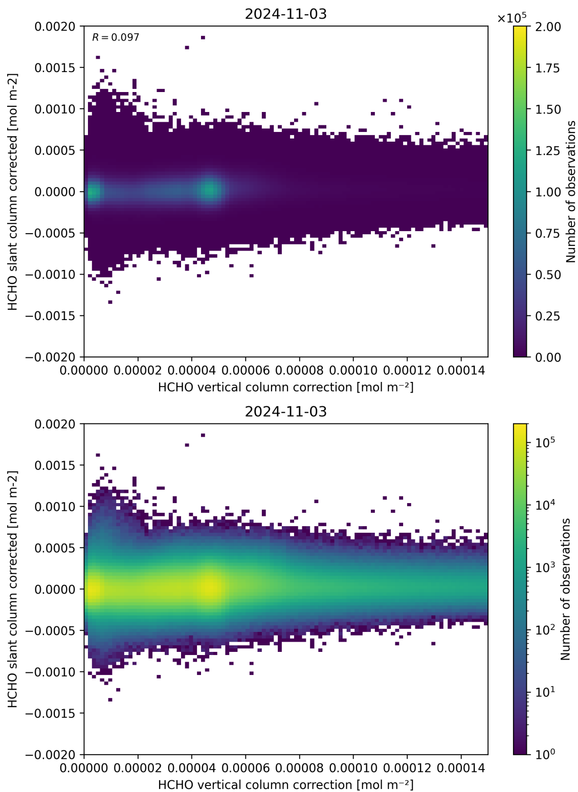
Figure 116: Scatter density plot of “HCHO vertical column correction” against “HCHO slant column corrected” for 2024-11-02 to 2024-11-04.
