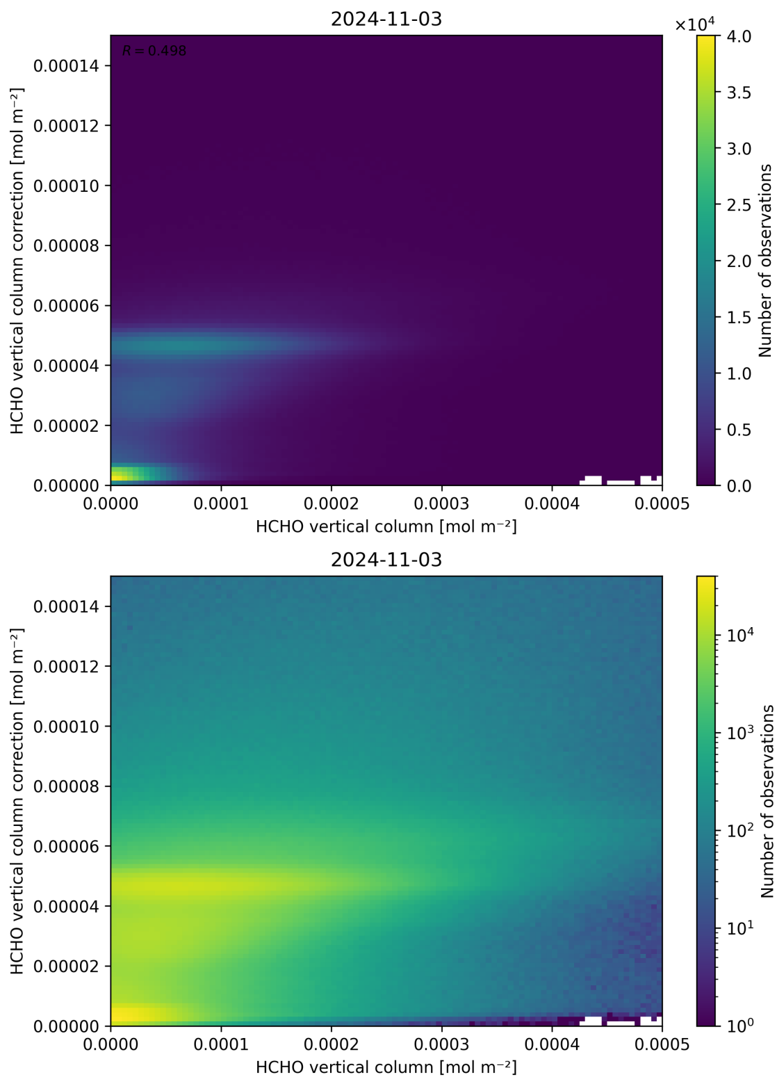
Figure 133: Scatter density plot of “HCHO vertical column” against “HCHO vertical column correction” for 2024-11-02 to 2024-11-04.
