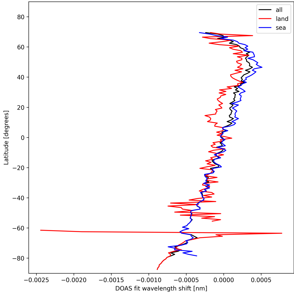
Figure 30: Zonal average of “DOAS fit wavelength shift” for 2024-11-02 to 2024-11-04.
