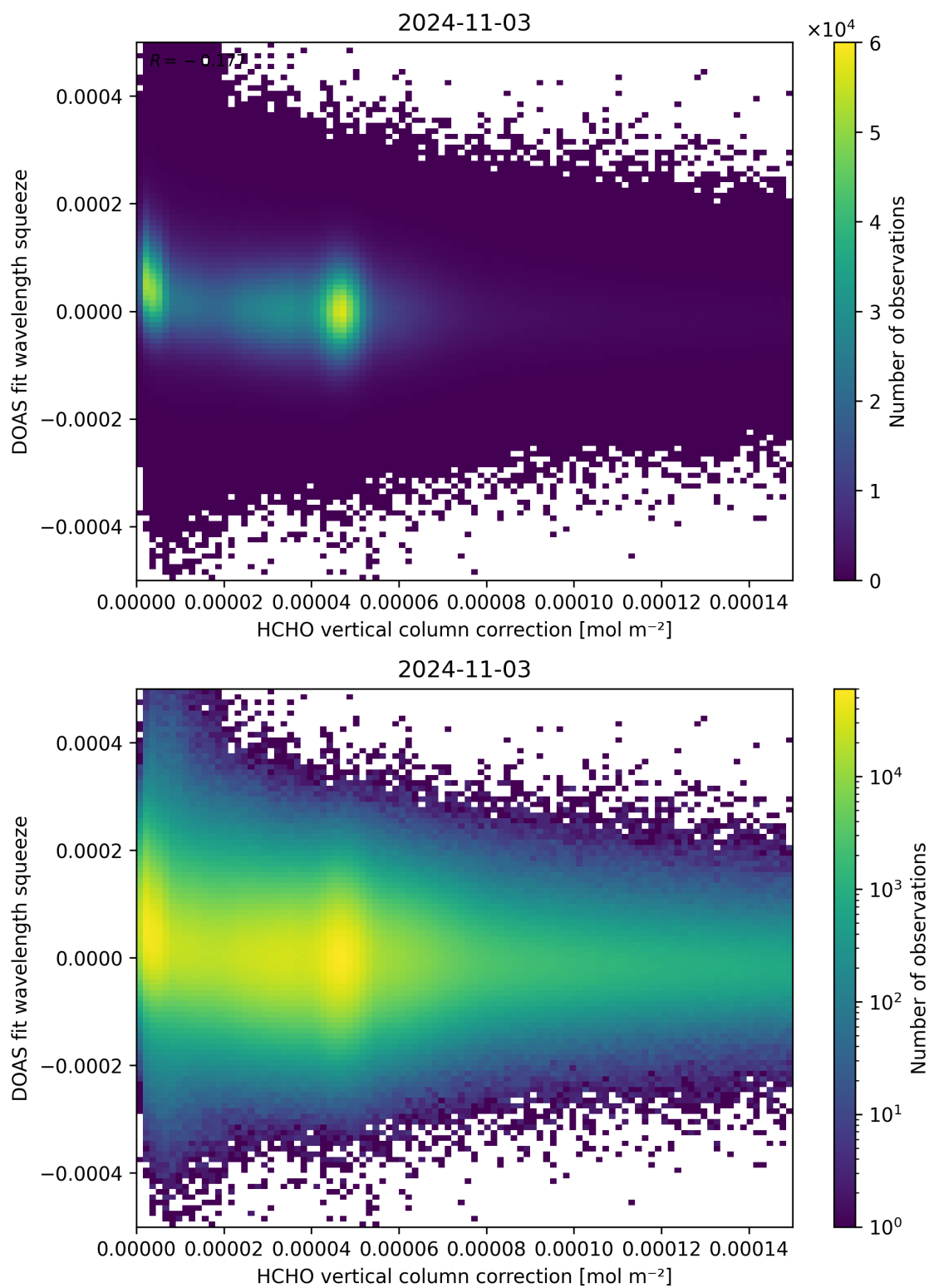
Figure 114: Scatter density plot of “HCHO vertical column correction” against “DOAS fit wavelength squeeze” for 2024-11-02 to 2024-11-04.
