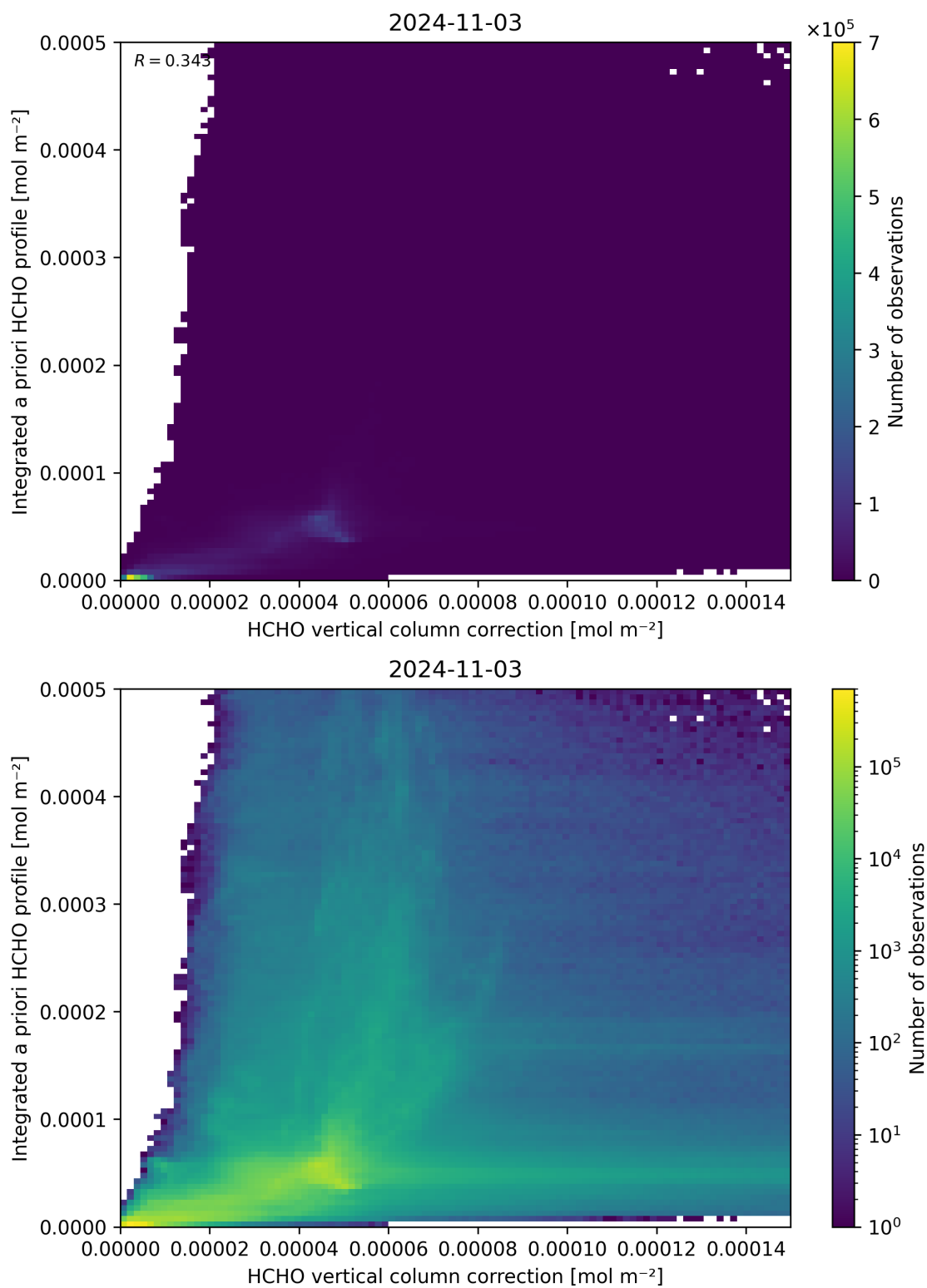
Figure 122: Scatter density plot of “HCHO vertical column correction” against “Integrated a priori HCHO profile” for 2024-11-02 to 2024-11-04.
