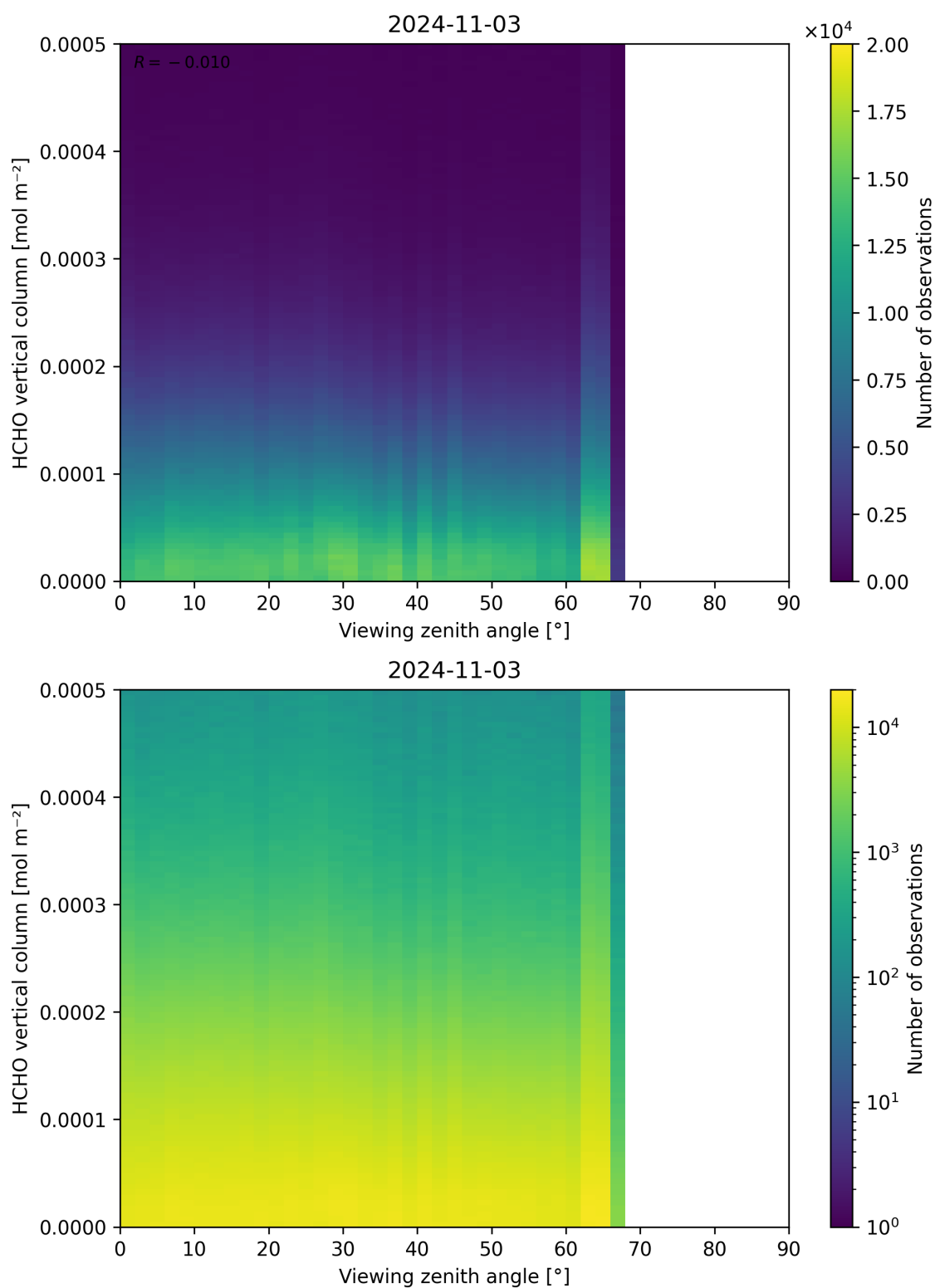
Figure 192: Scatter density plot of “Viewing zenith angle” against “HCHO vertical column” for 2024-11-02 to 2024-11-04.
