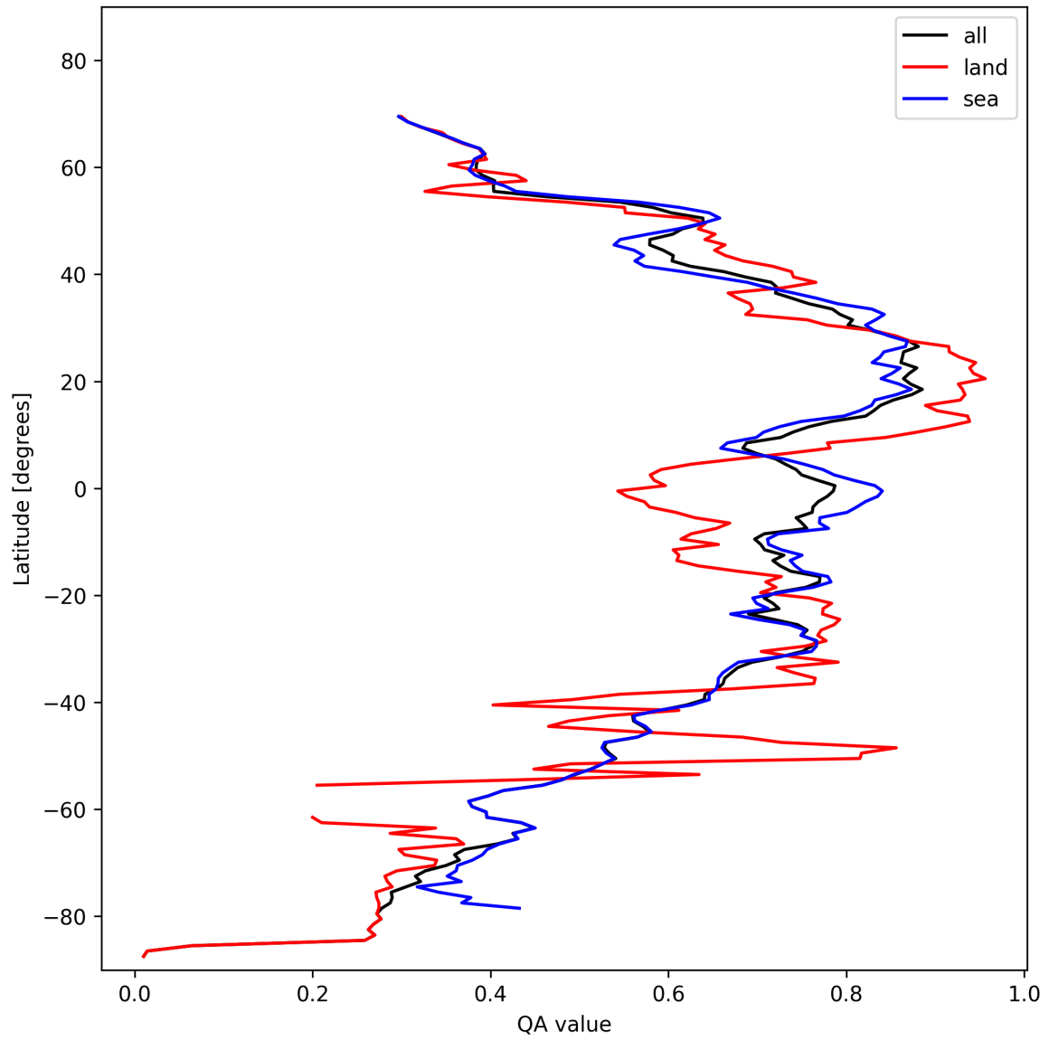
Figure 20: Zonal average of “QA value” for 2024-11-02 to 2024-11-04.
