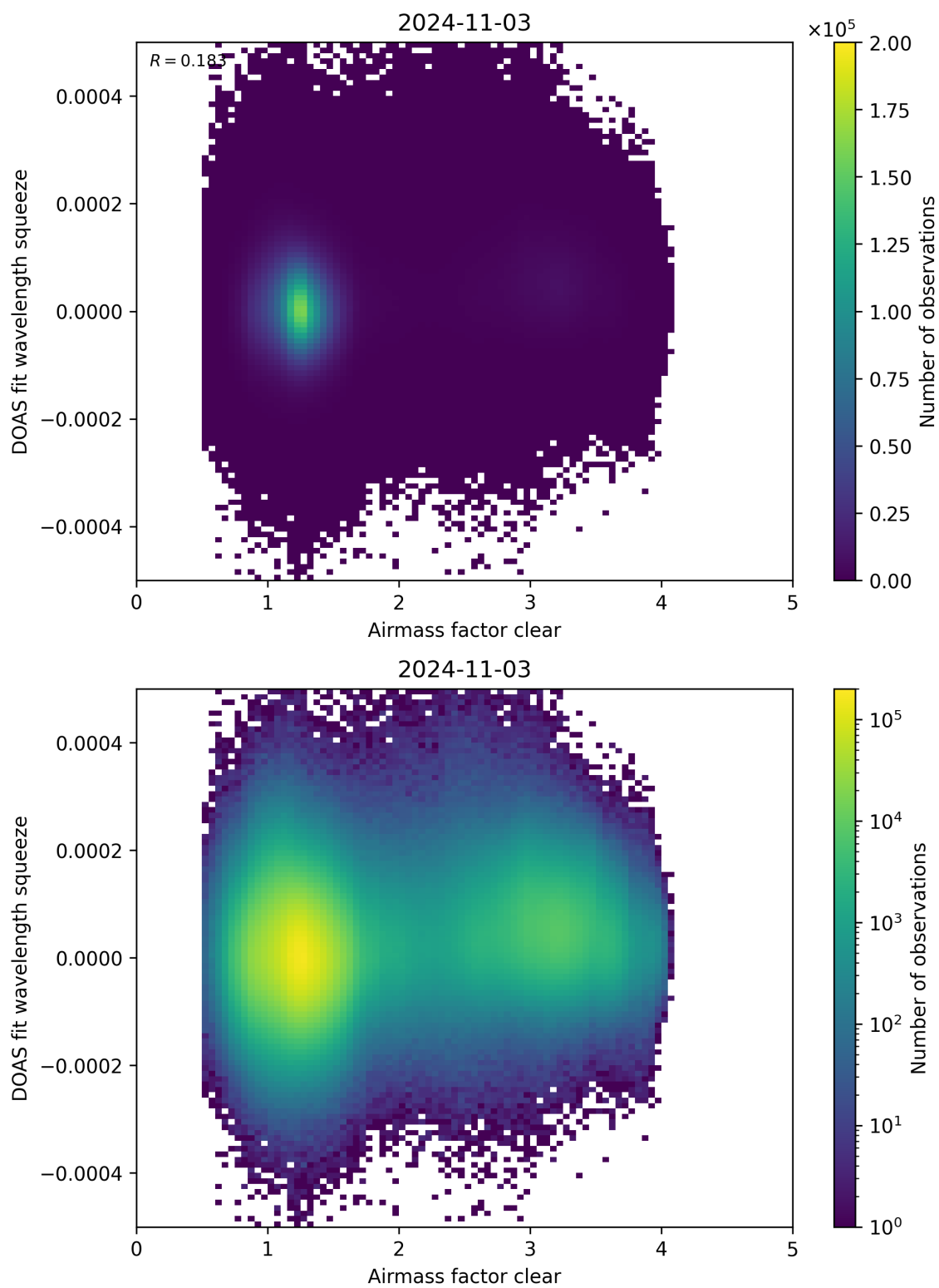
Figure 73: Scatter density plot of “Airmass factor clear” against “DOAS fit wavelength squeeze” for 2024-11-02 to 2024-11-04.
