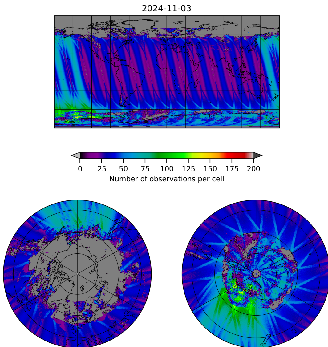
Figure 19: Map of the number of observations for 2024-11-02 to 2024-11-04
