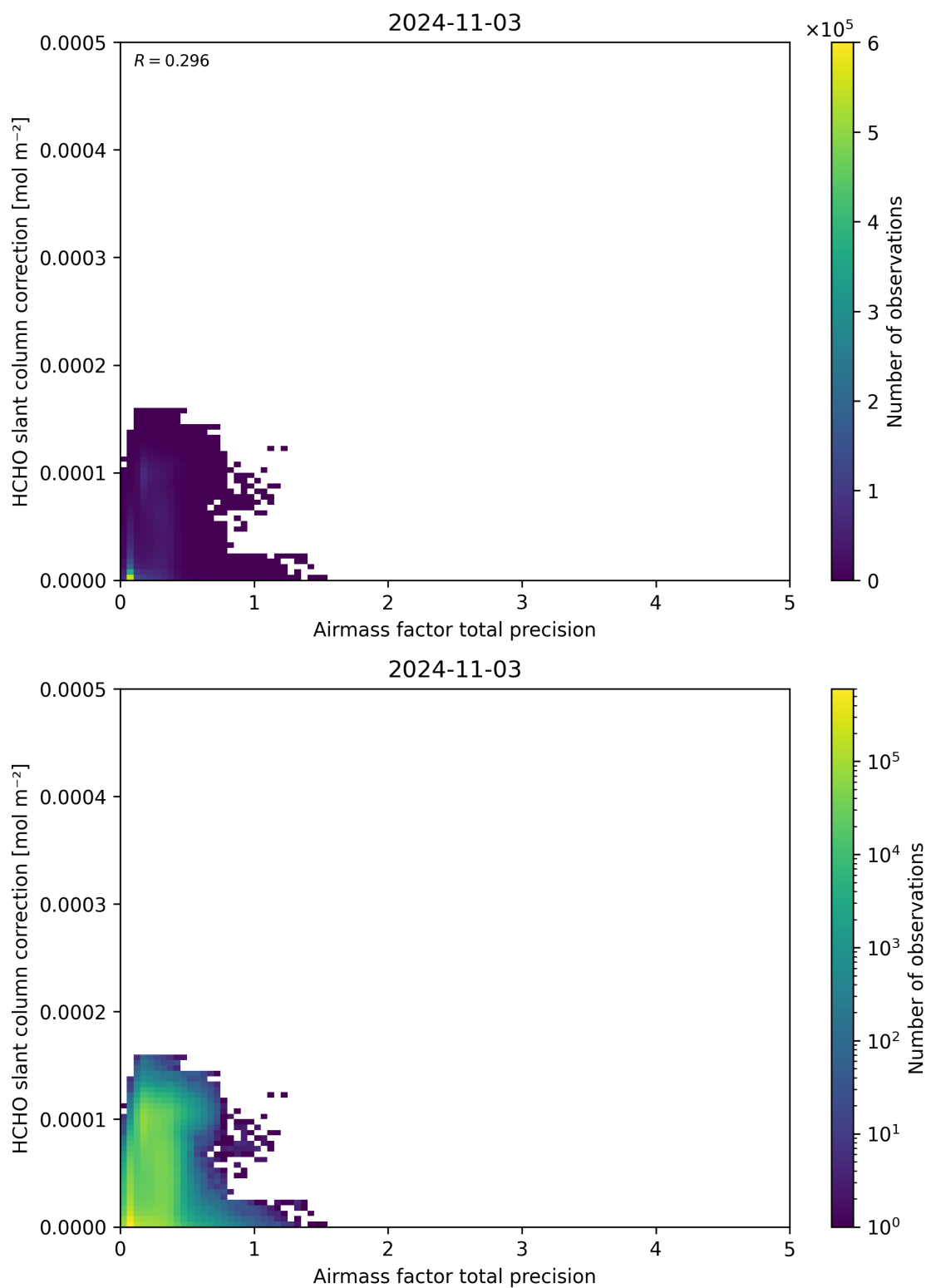
Figure 110: Scatter density plot of “Airmass factor total precision” against “HCHO slant column correction” for 2024-11-02 to 2024-11-04.
