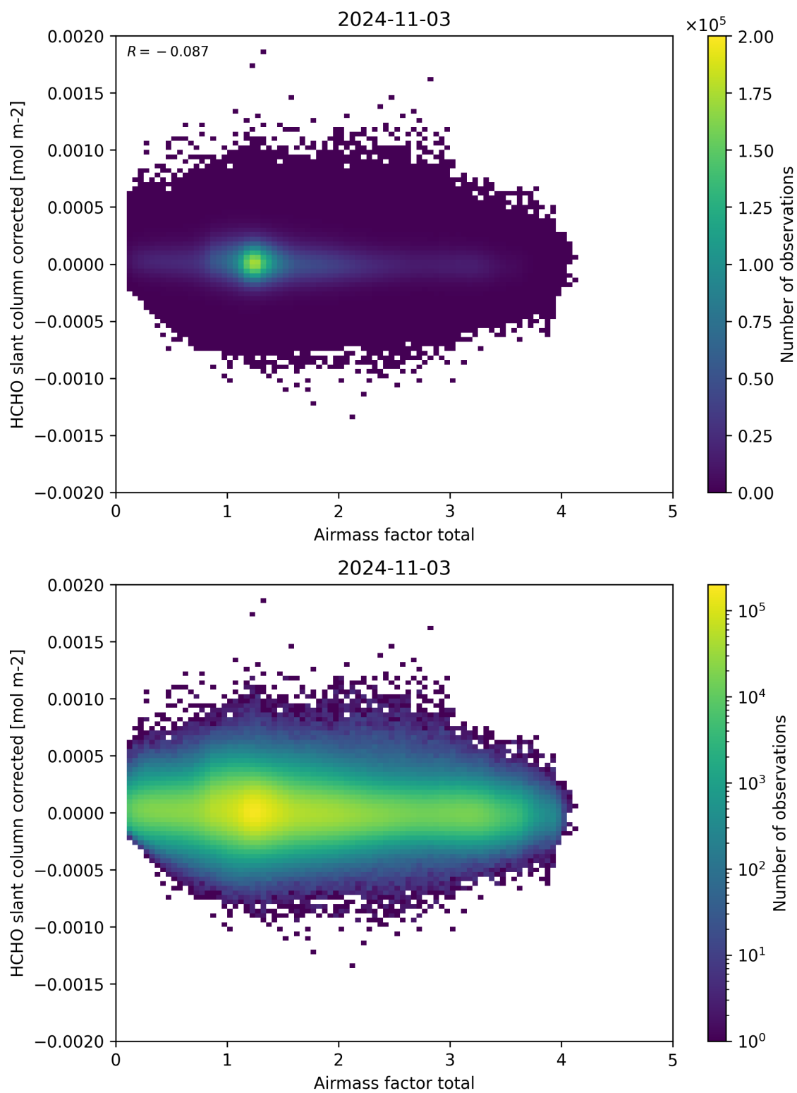
Figure 101: Scatter density plot of “Airmass factor total” against “HCHO slant column corrected” for 2024-11-02 to 2024-11-04.
