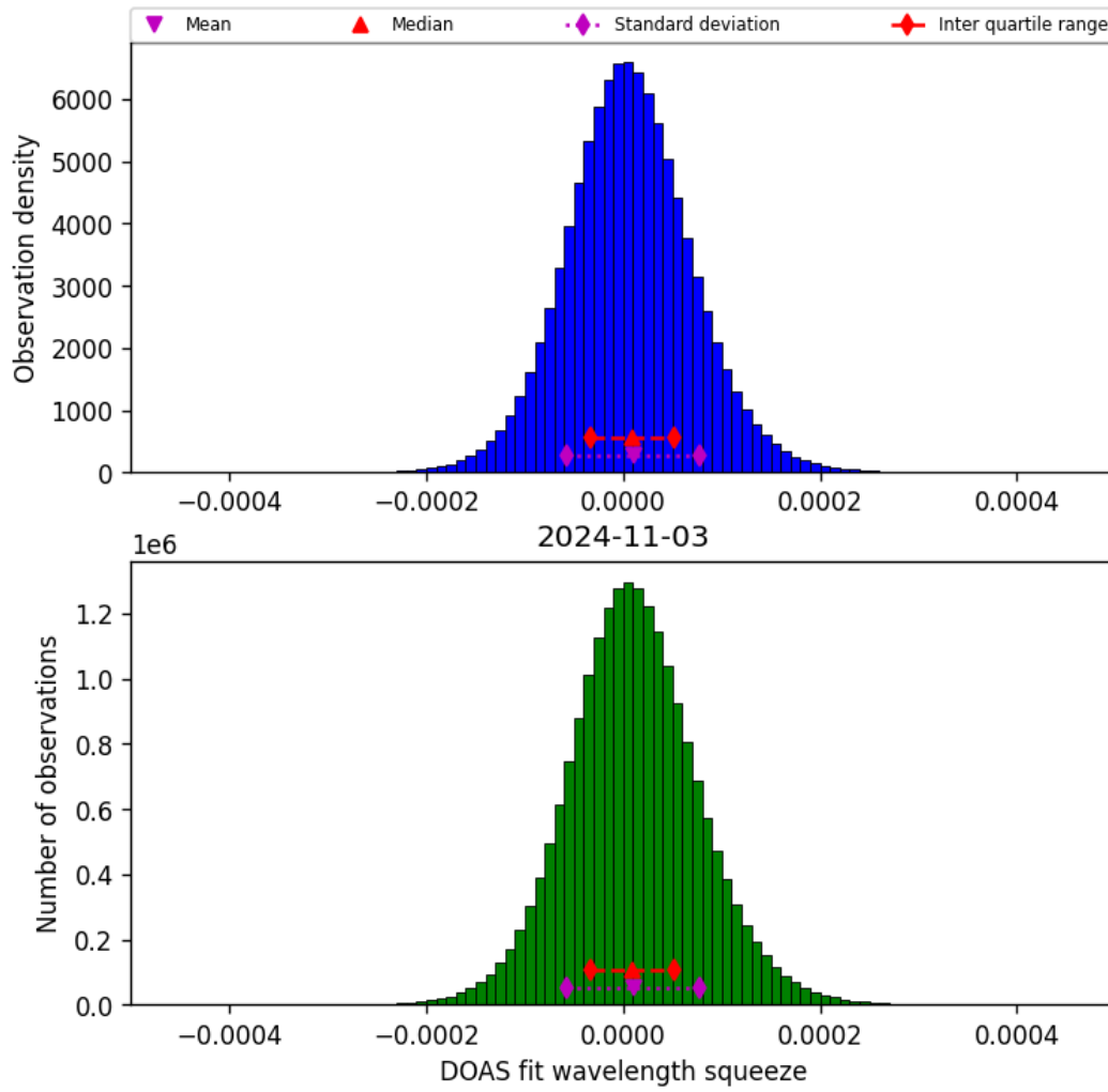
Figure 45: Histogram of “DOAS fit wavelength squeeze” for 2024-11-02 to 2024-11-04
