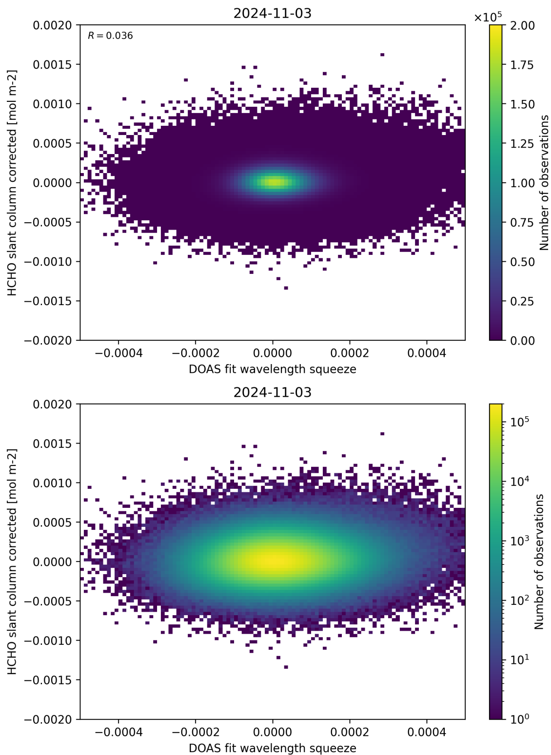
Figure 69: Scatter density plot of “DOAS fit wavelength squeeze” against “HCHO slant column corrected” for 2024-11-02 to 2024-11-04.
