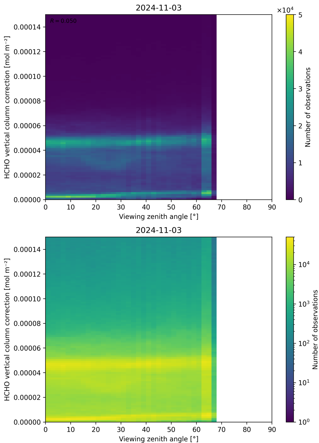
Figure 193: Scatter density plot of “Viewing zenith angle” against “HCHO vertical column correction” for 2024-11-02 to 2024-11-04.
