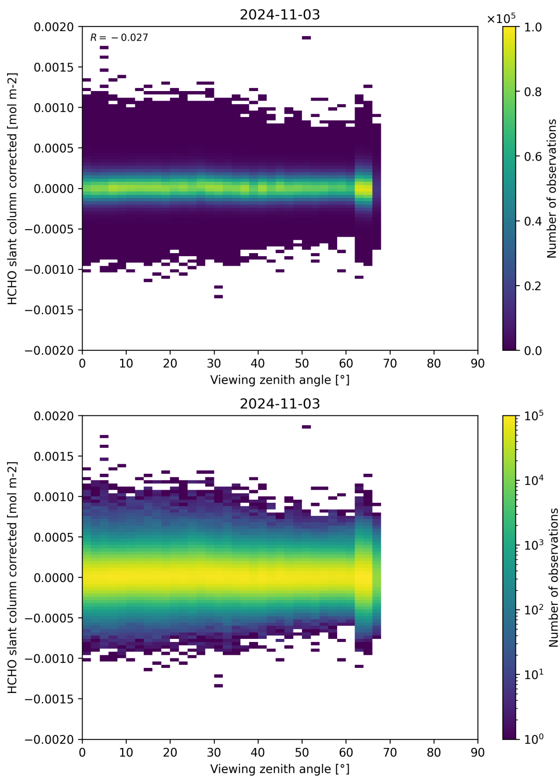
Figure 186: Scatter density plot of “Viewing zenith angle” against “HCHO slant column corrected” for 2024-11-02 to 2024-11-04.
