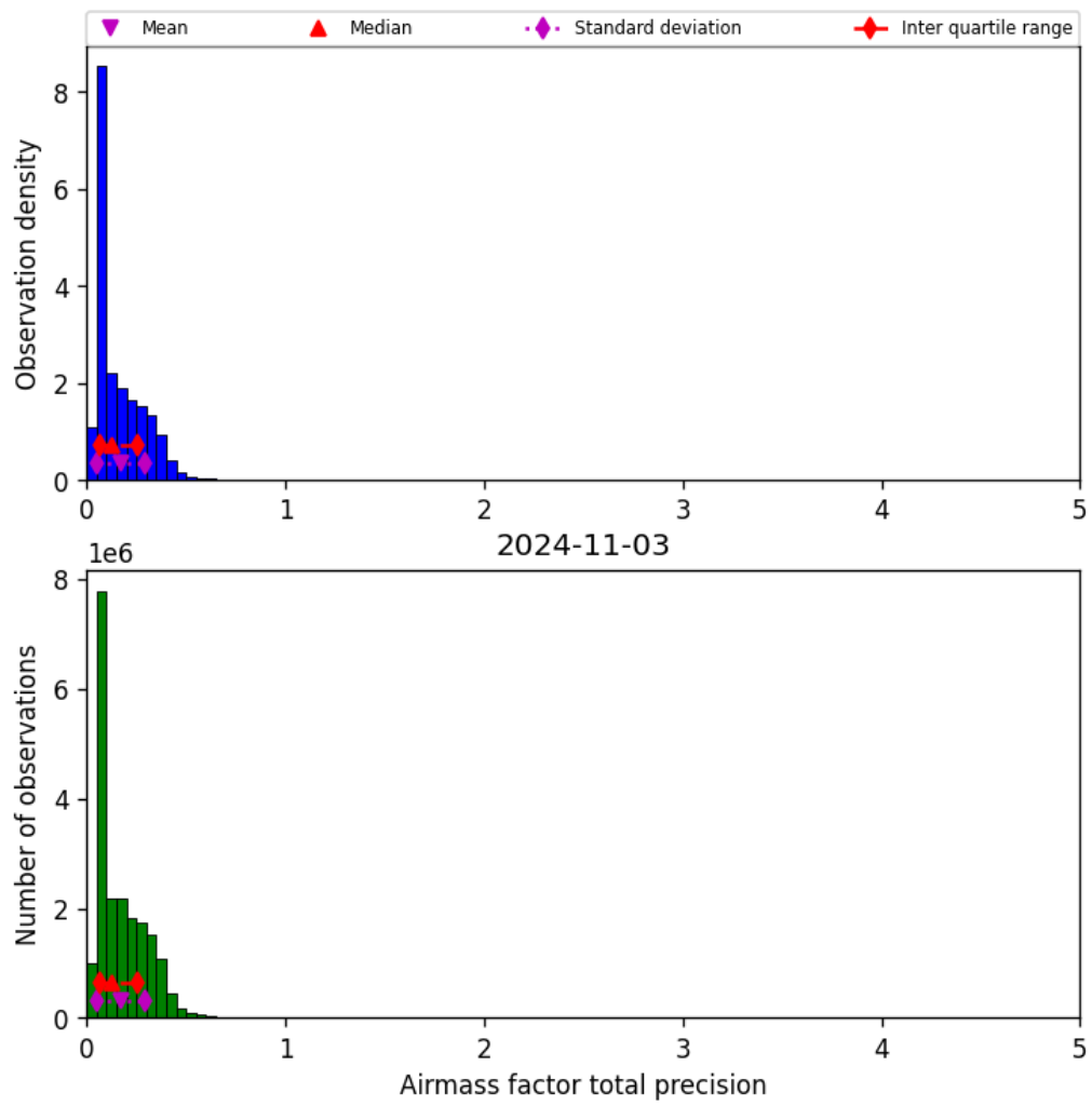
Figure 41: Histogram of “Airmass factor total precision” for 2024-11-02 to 2024-11-04
