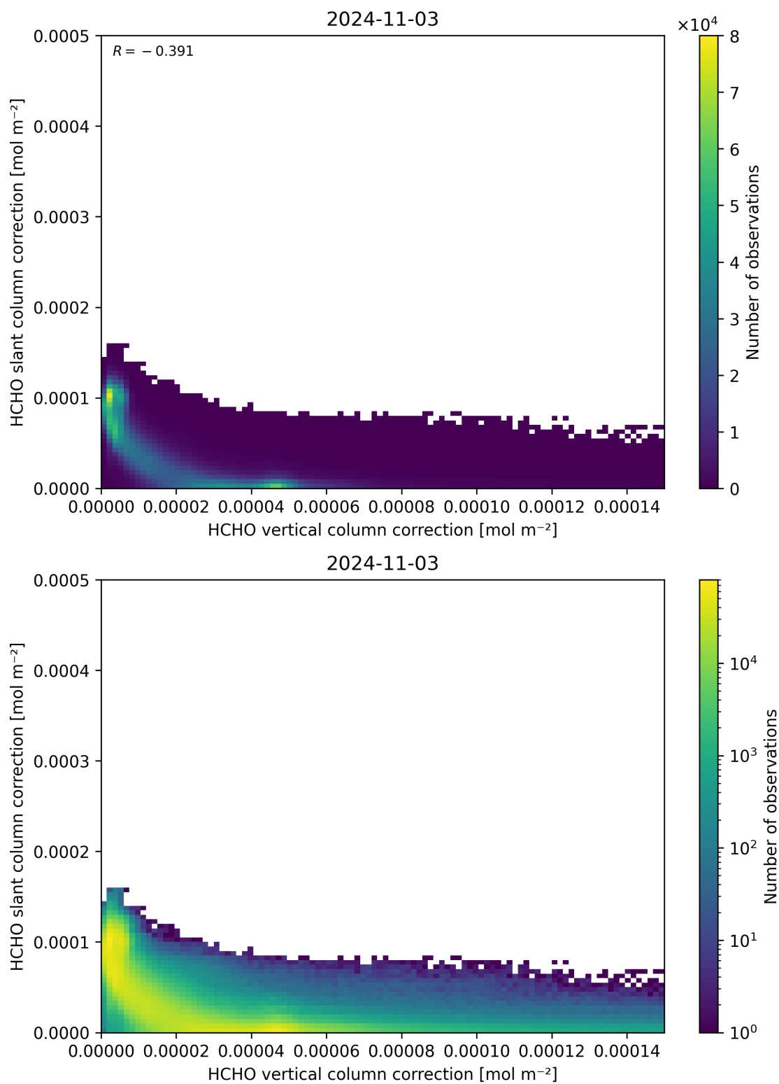
Figure 117: Scatter density plot of “HCHO vertical column correction” against “HCHO slant column correction” for 2024-11-02 to 2024-11-04.
