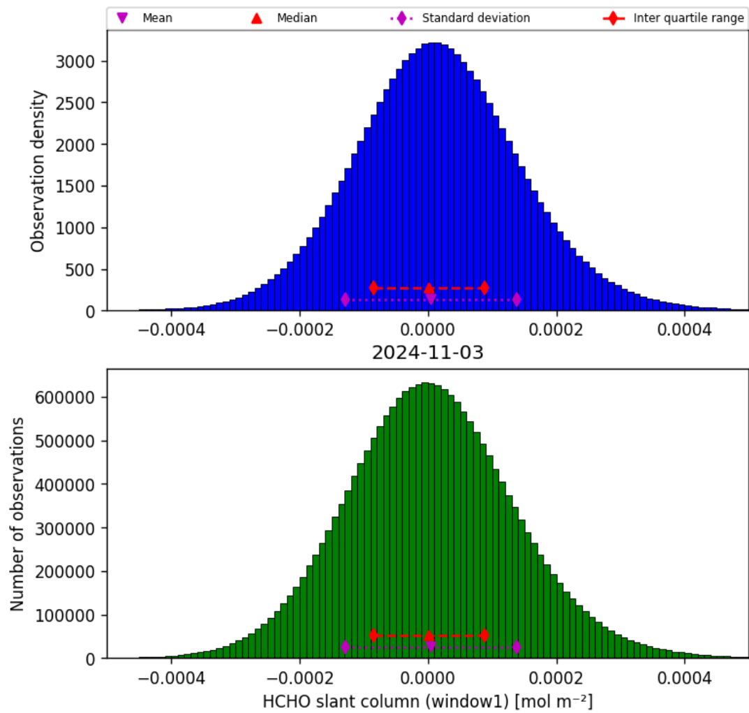
Figure 38: Histogram of “HCHO slant column (window1)” for 2024-11-02 to 2024-11-04
