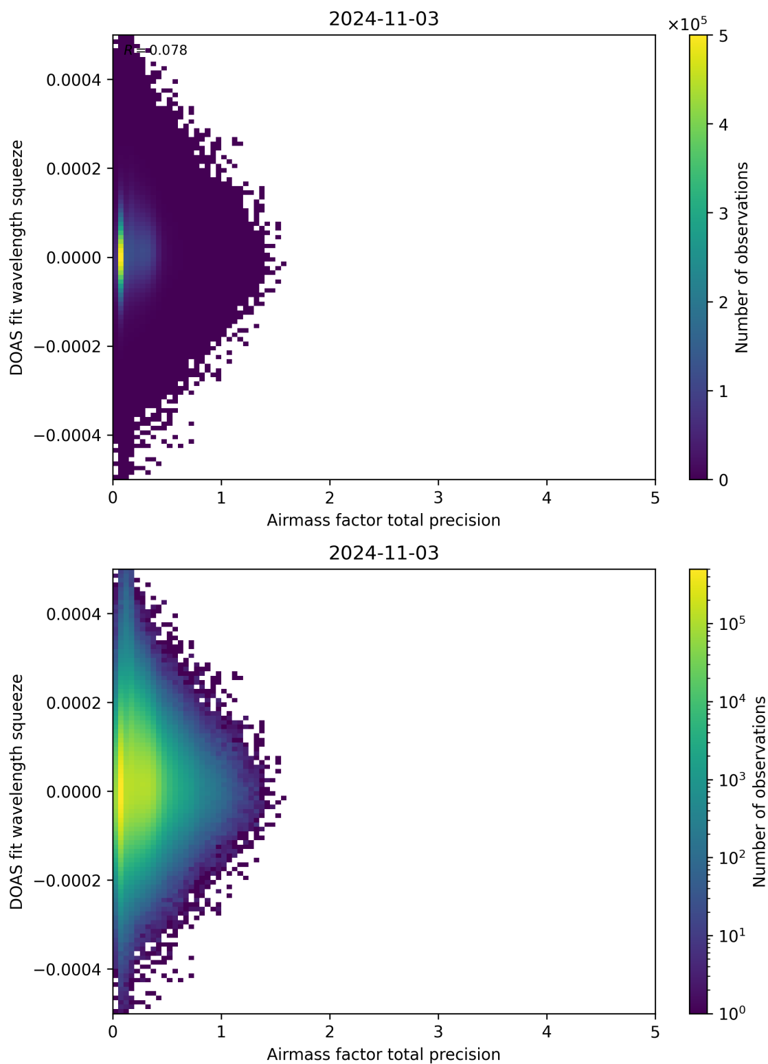
Figure 107: Scatter density plot of “Airmass factor total precision” against “DOAS fit wavelength squeeze” for 2024-11-02 to 2024-11-04.
