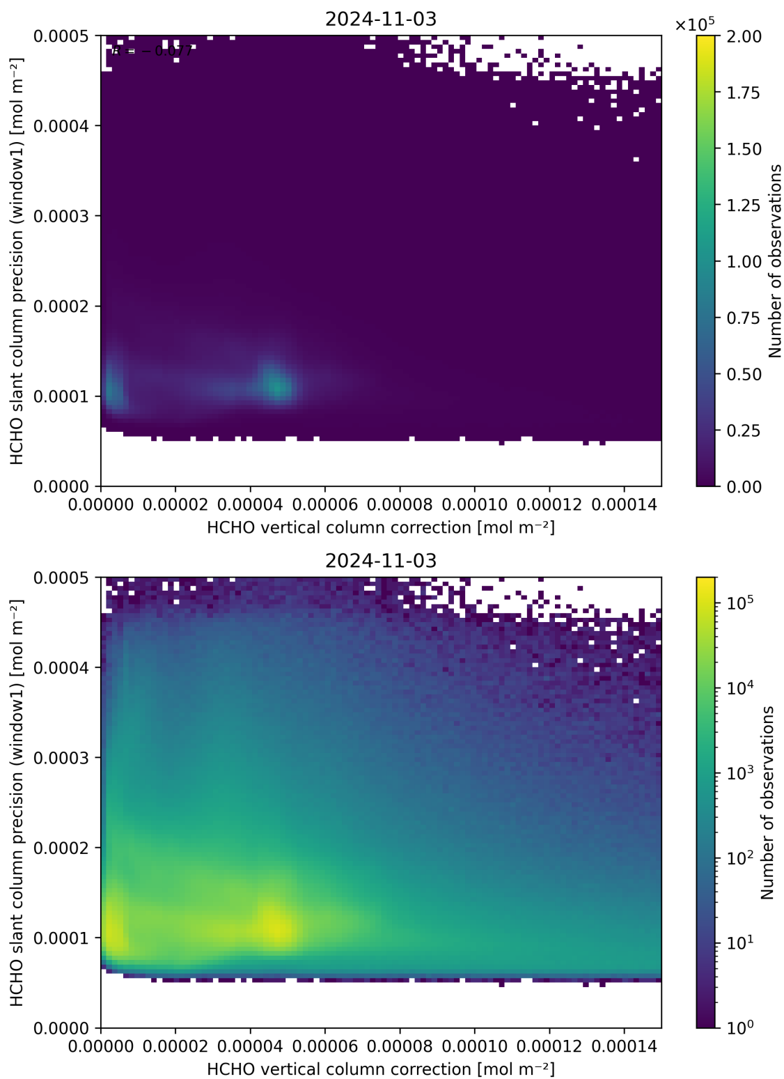
Figure 119: Scatter density plot of “HCHO vertical column correction” against “HCHO slant column precision (window1)” for 2024-11-02 to 2024-11-04.
