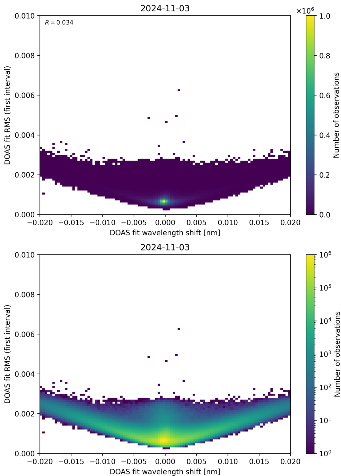
Figure 64: Scatter density plot of “DOAS fit wavelength shift” against “DOAS fit RMS (first interval)” for 2024-11-02 to 2024-11-04.
