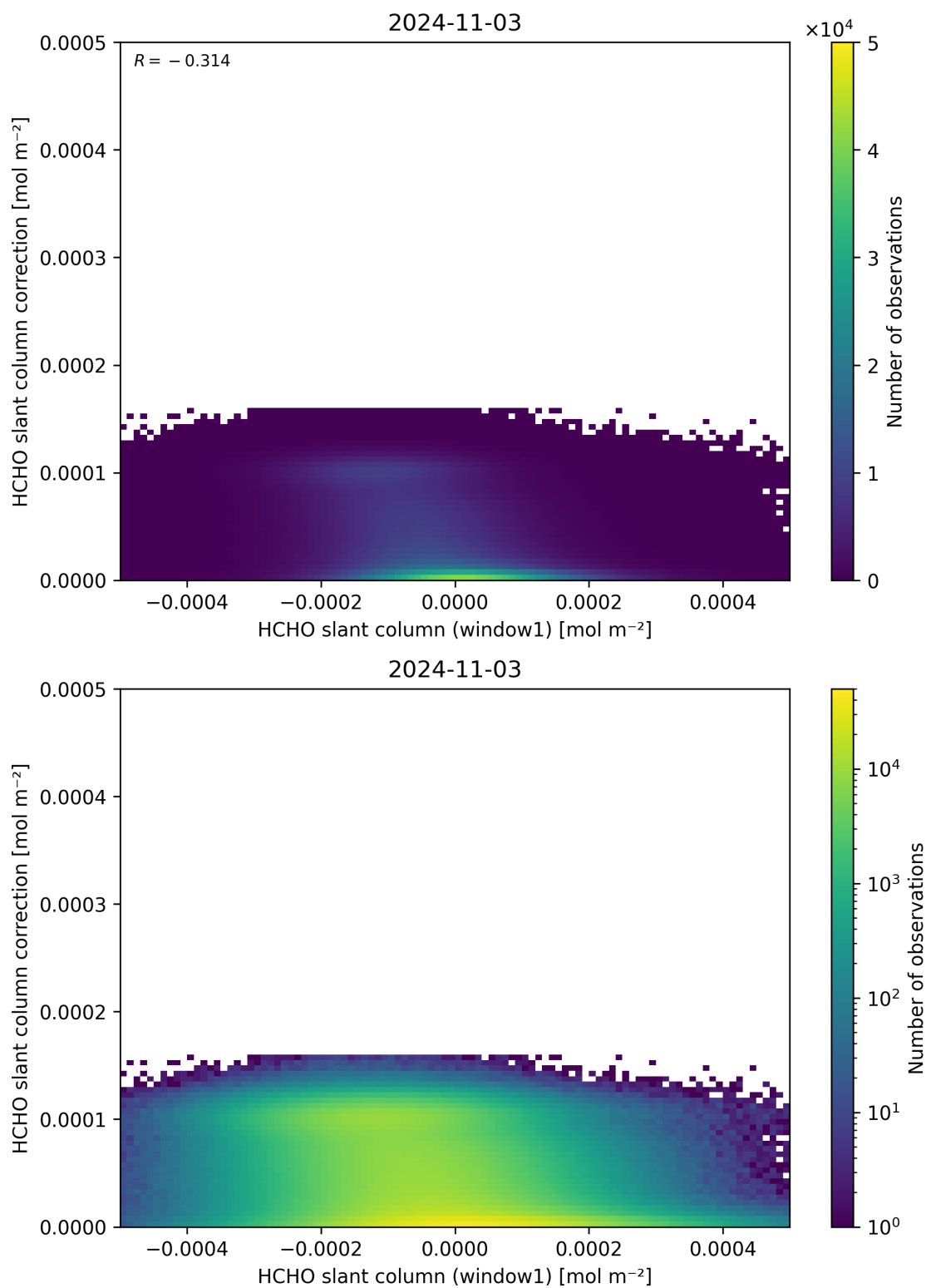
Figure 83: Scatter density plot of “HCHO slant column (window1)” against “HCHO slant column correction” for 2024-11-02 to 2024-11-04.
