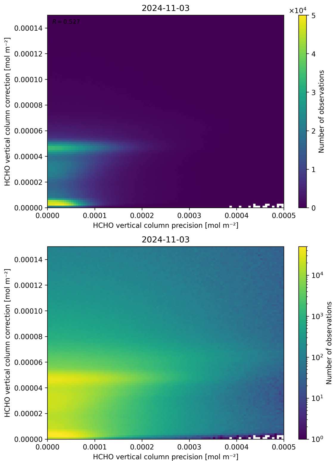
Figure 146: Scatter density plot of “HCHO vertical column precision” against “HCHO vertical column correction” for 2024-11-02 to 2024-11-04.
