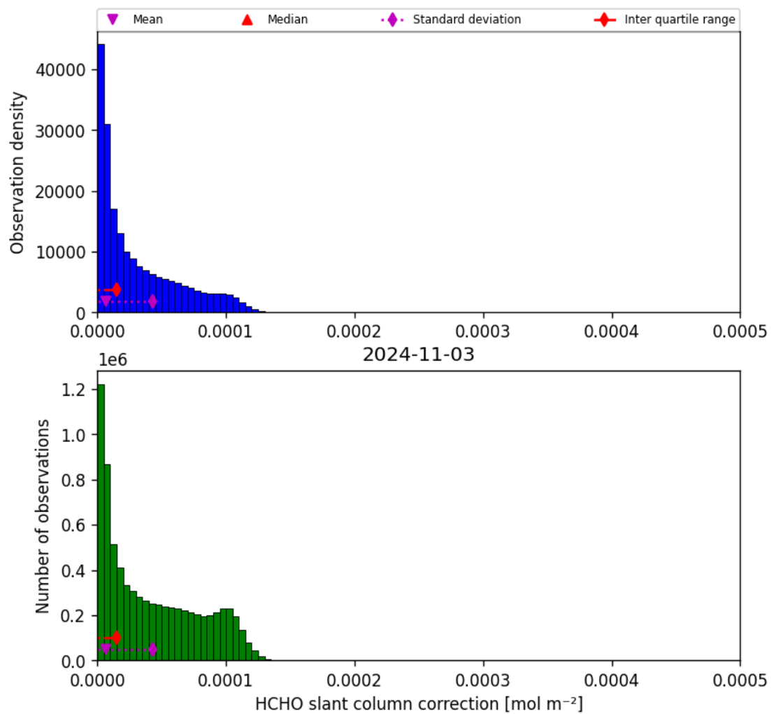
Figure 47: Histogram of “HCHO slant column correction” for 2024-11-02 to 2024-11-04
