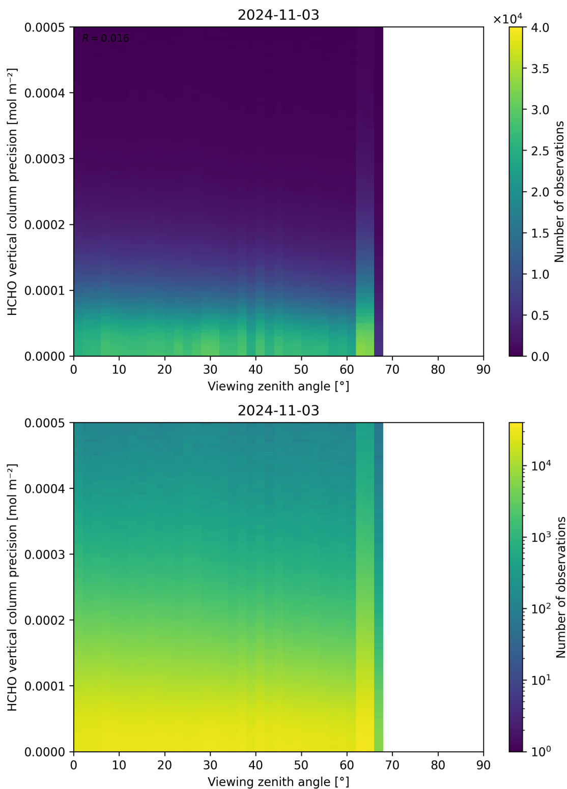
Figure 194: Scatter density plot of “Viewing zenith angle” against “HCHO vertical column precision” for 2024-11-02 to 2024-11-04.
