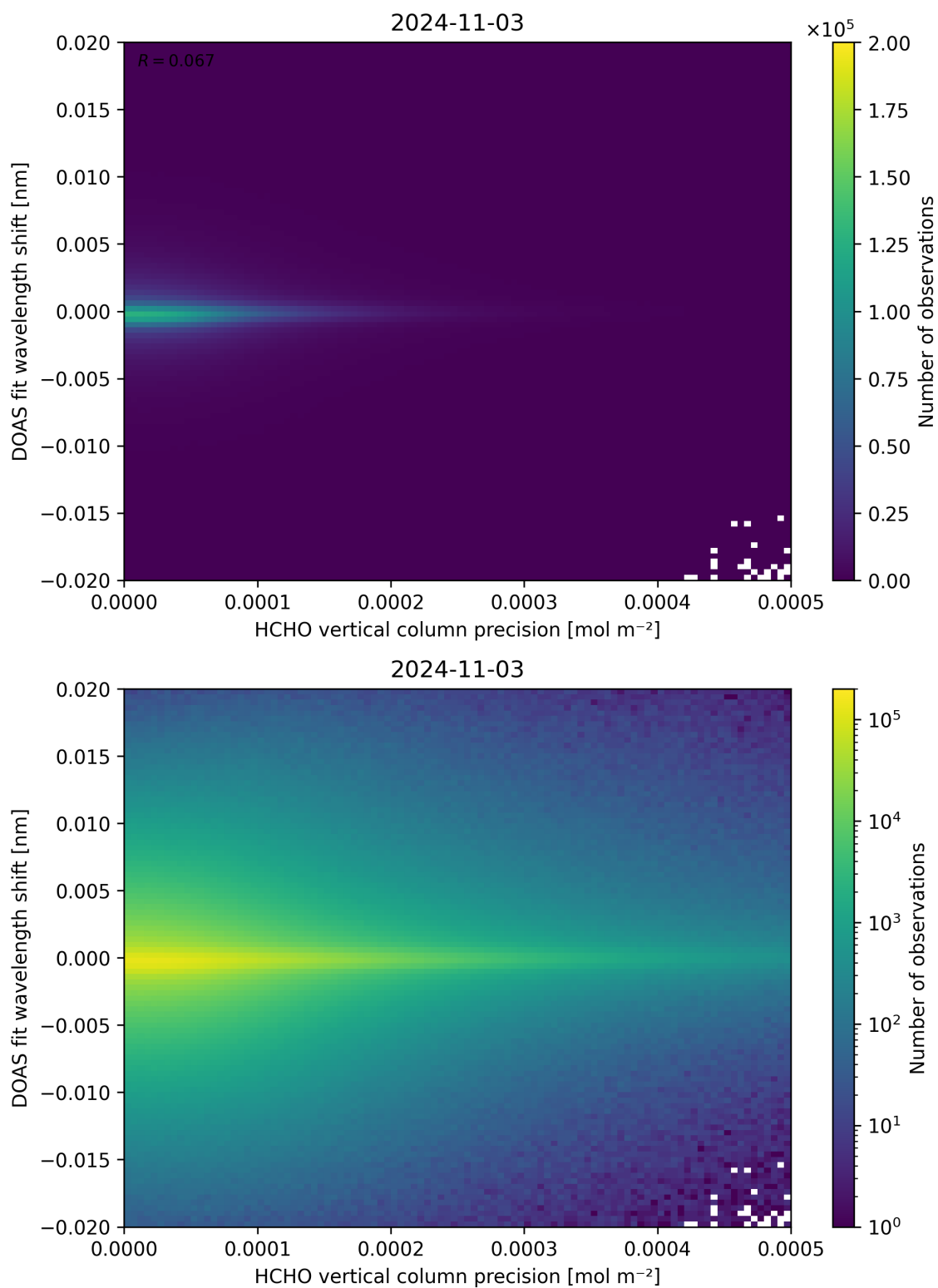
Figure 137: Scatter density plot of “HCHO vertical column precision” against “DOAS fit wavelength shift” for 2024-11-02 to 2024-11-04.
