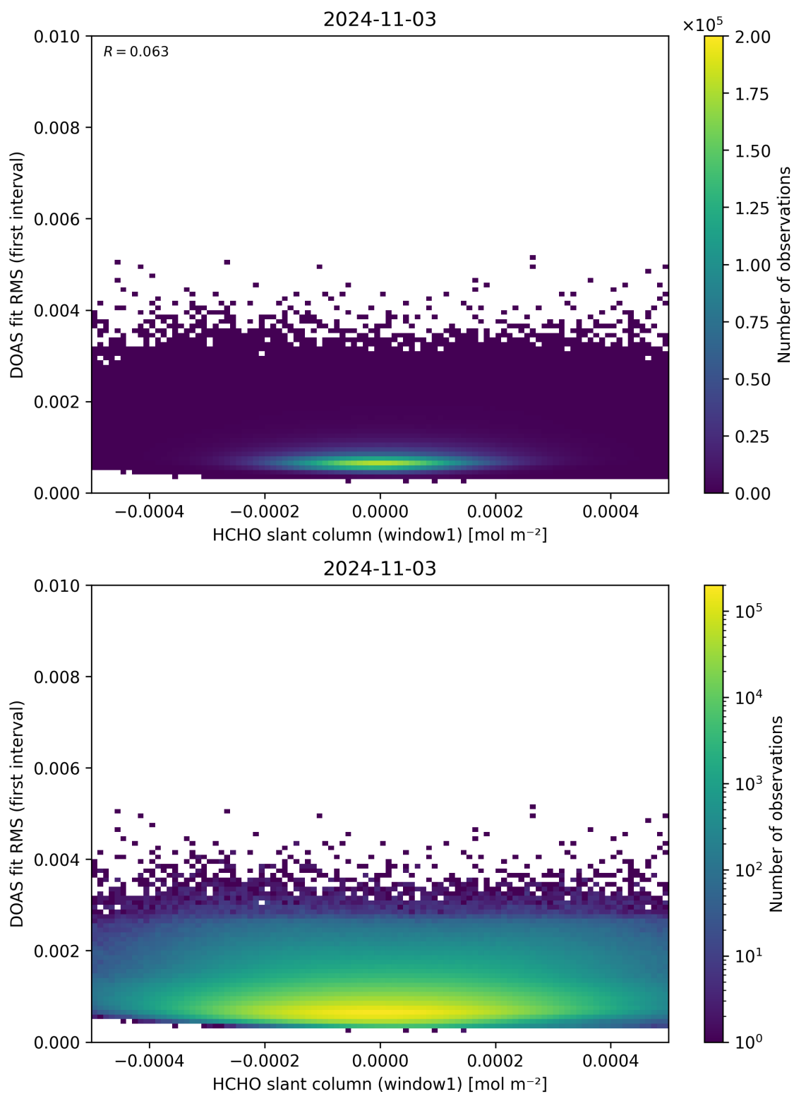
Figure 78: Scatter density plot of “HCHO slant column (window1)” against “DOAS fit RMS (first interval)” for 2024-11-02 to 2024-11-04.
