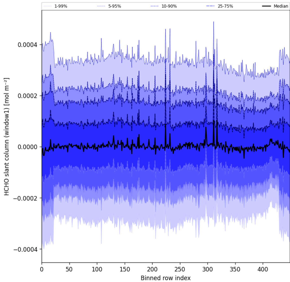
Figure 52: Along track statistics of “HCHO slant column (window1)” for 2024-11-02 to 2024-11-04
