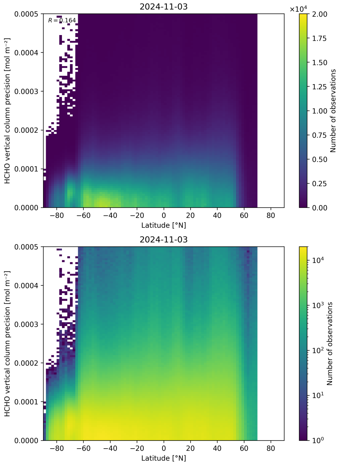
Figure 165: Scatter density plot of “Latitude” against “HCHO vertical column precision” for 2024-11-02 to 2024-11-04.
