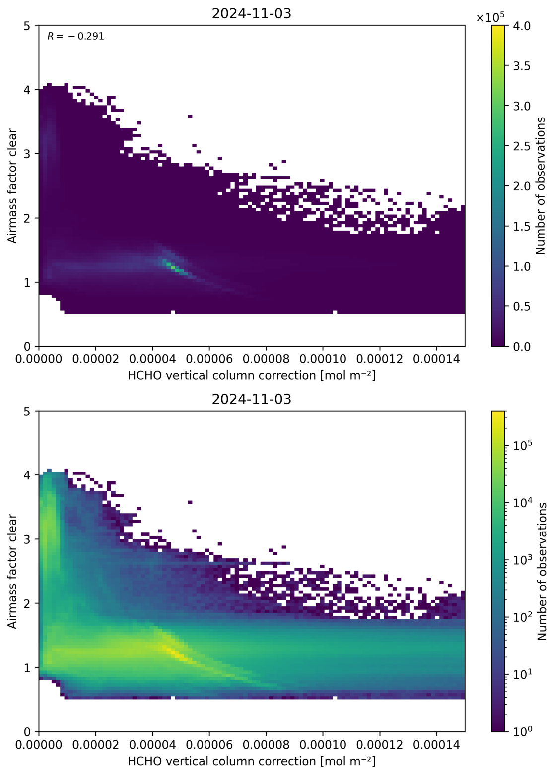
Figure 115: Scatter density plot of “HCHO vertical column correction” against “Airmass factor clear” for 2024-11-02 to 2024-11-04.
