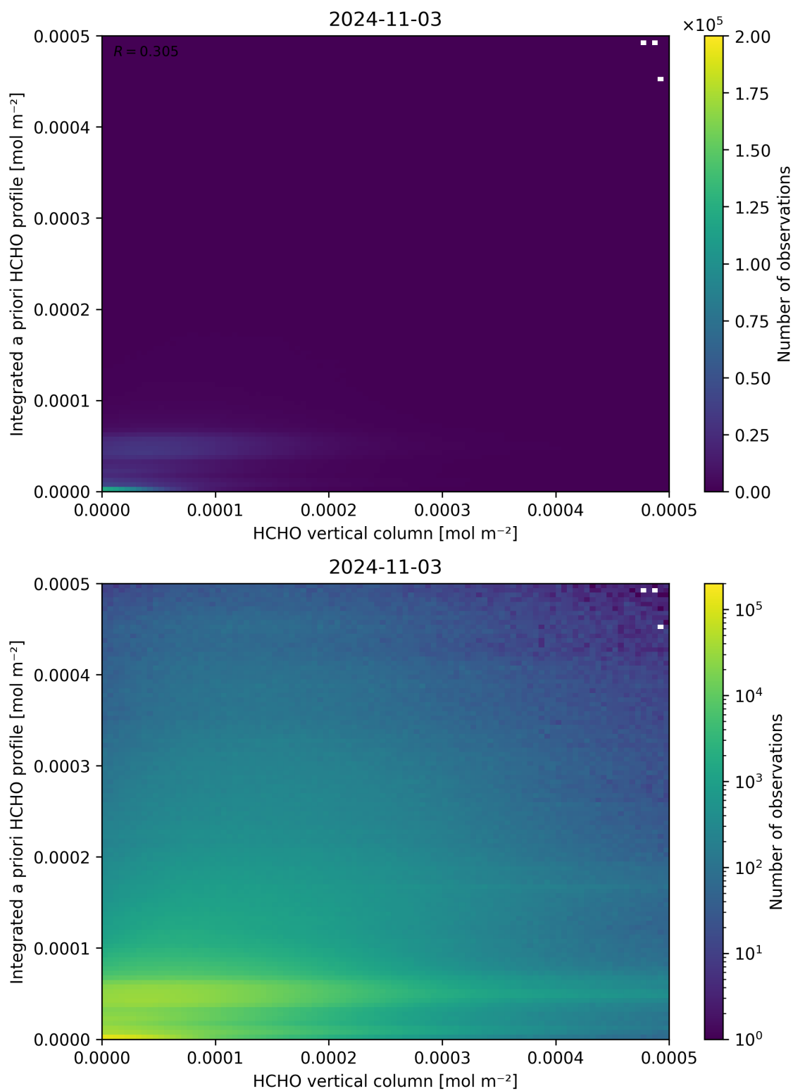
Figure 135: Scatter density plot of “HCHO vertical column” against “Integrated a priori HCHO profile” for 2024-11-02 to 2024-11-04.
