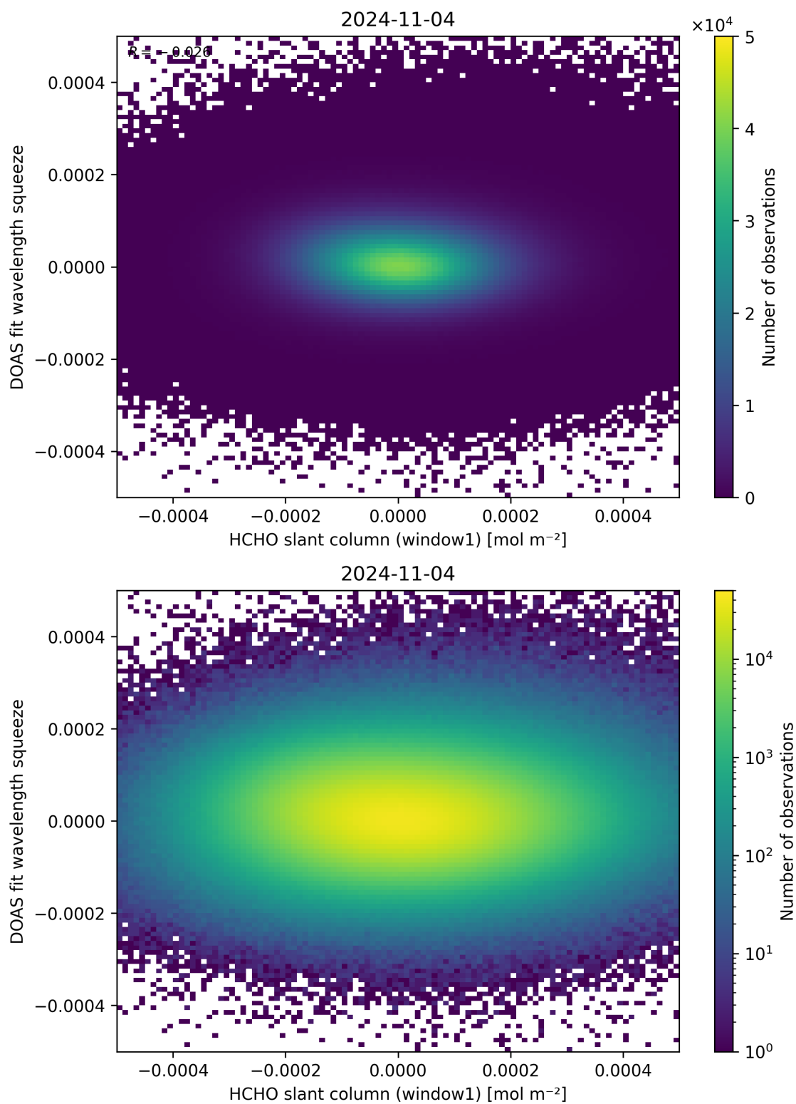
Figure 80: Scatter density plot of “HCHO slant column (window1)” against “DOAS fit wavelength squeeze” for 2024-11-04 to 2024-11-05.
