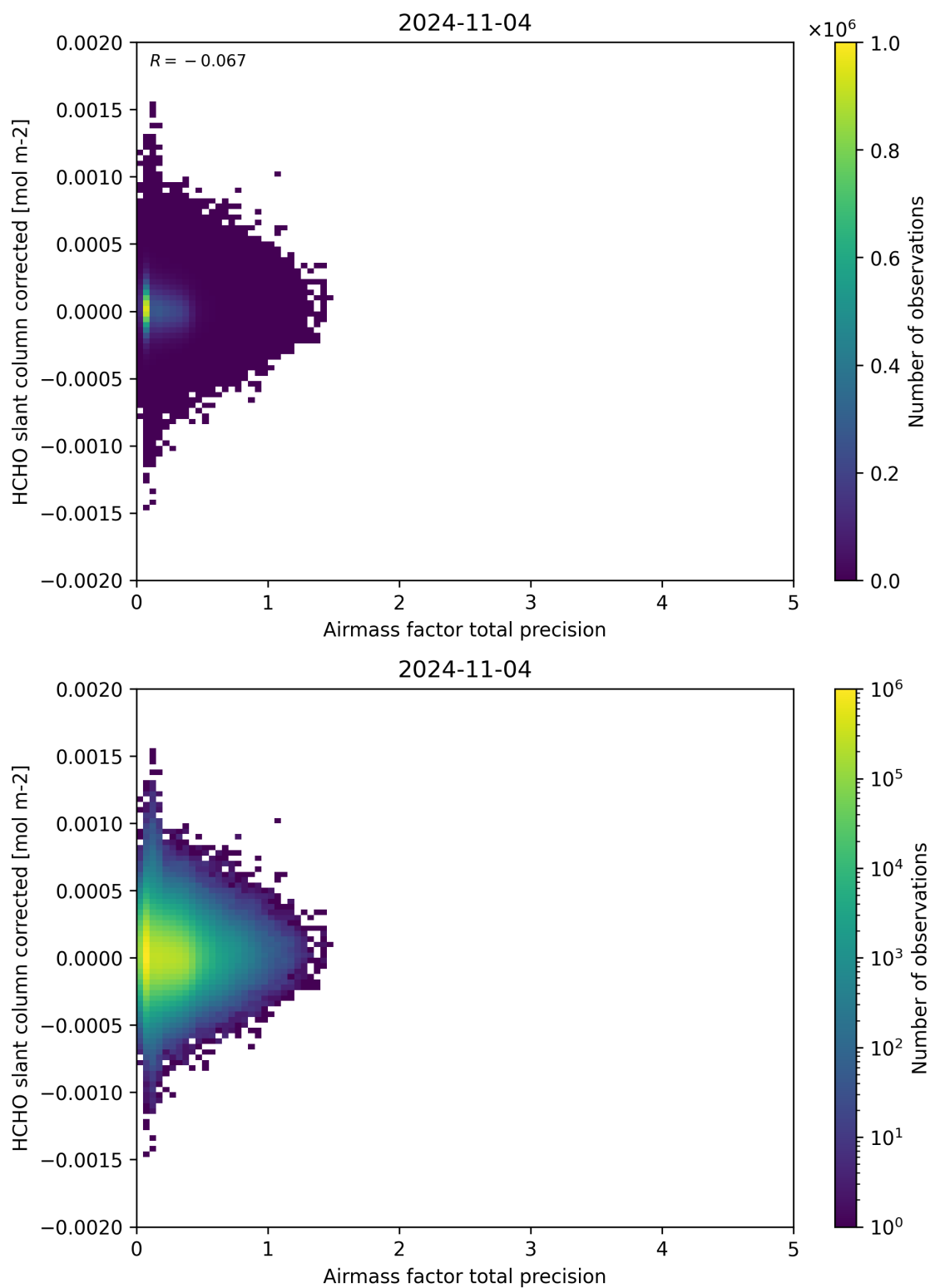
Figure 109: Scatter density plot of “Airmass factor total precision” against “HCHO slant column corrected” for 2024-11-04 to 2024-11-05.
