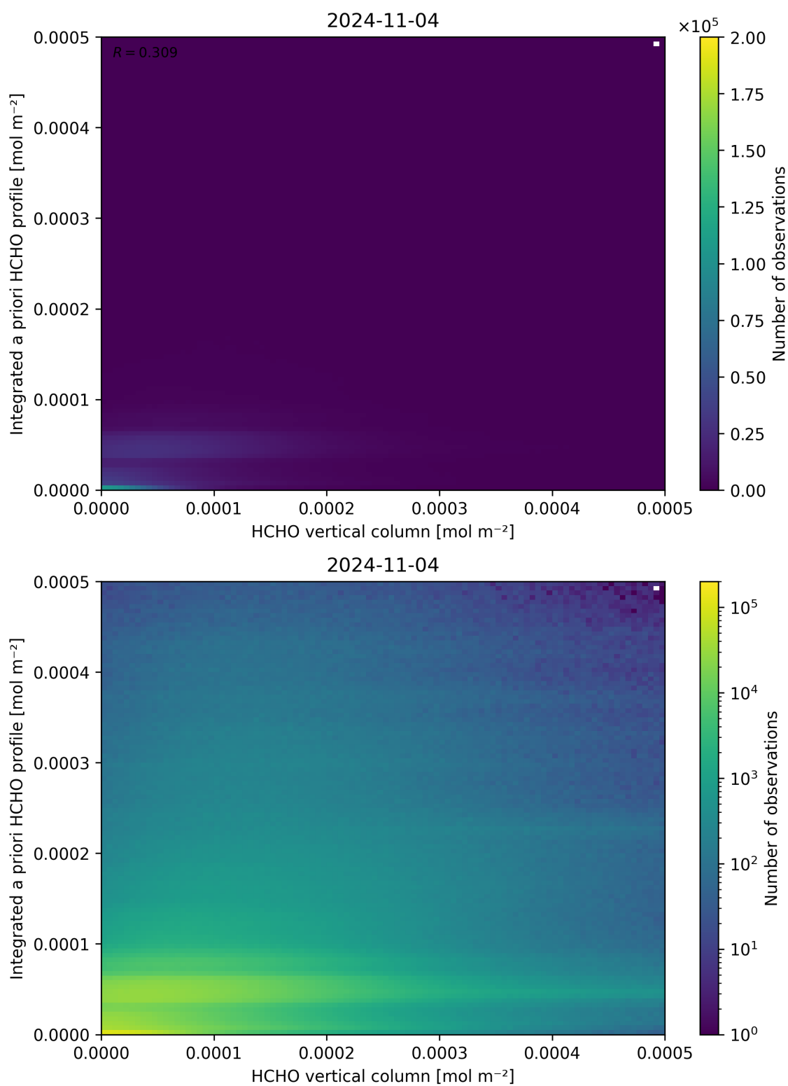
Figure 135: Scatter density plot of “HCHO vertical column” against “Integrated a priori HCHO profile” for 2024-11-04 to 2024-11-05.
