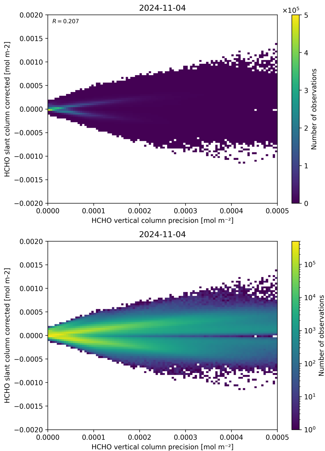
Figure 140: Scatter density plot of “HCHO vertical column precision” against “HCHO slant column corrected” for 2024-11-04 to 2024-11-05.
