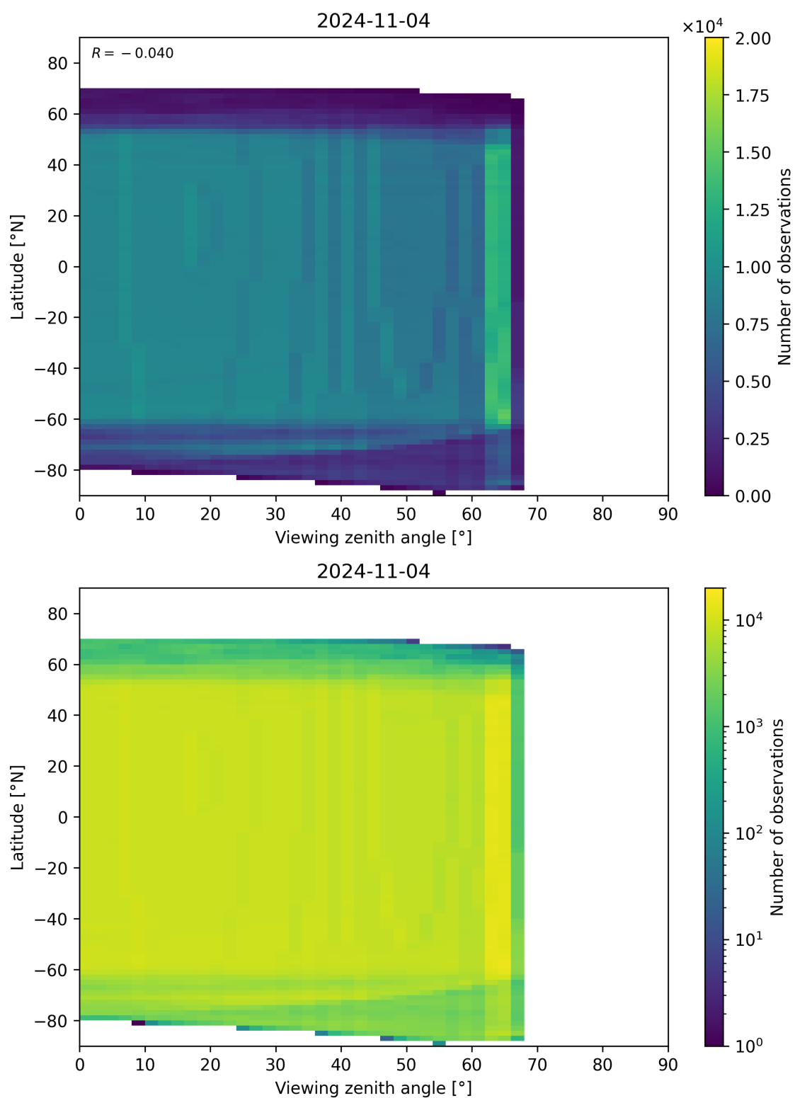
Figure 196: Scatter density plot of “Viewing zenith angle” against “Latitude” for 2024-11-04 to 2024-11-05.
