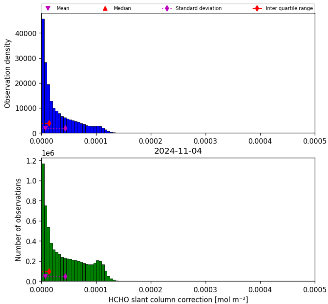
Figure 47: Histogram of “HCHO slant column correction” for 2024-11-04 to 2024-11-05
