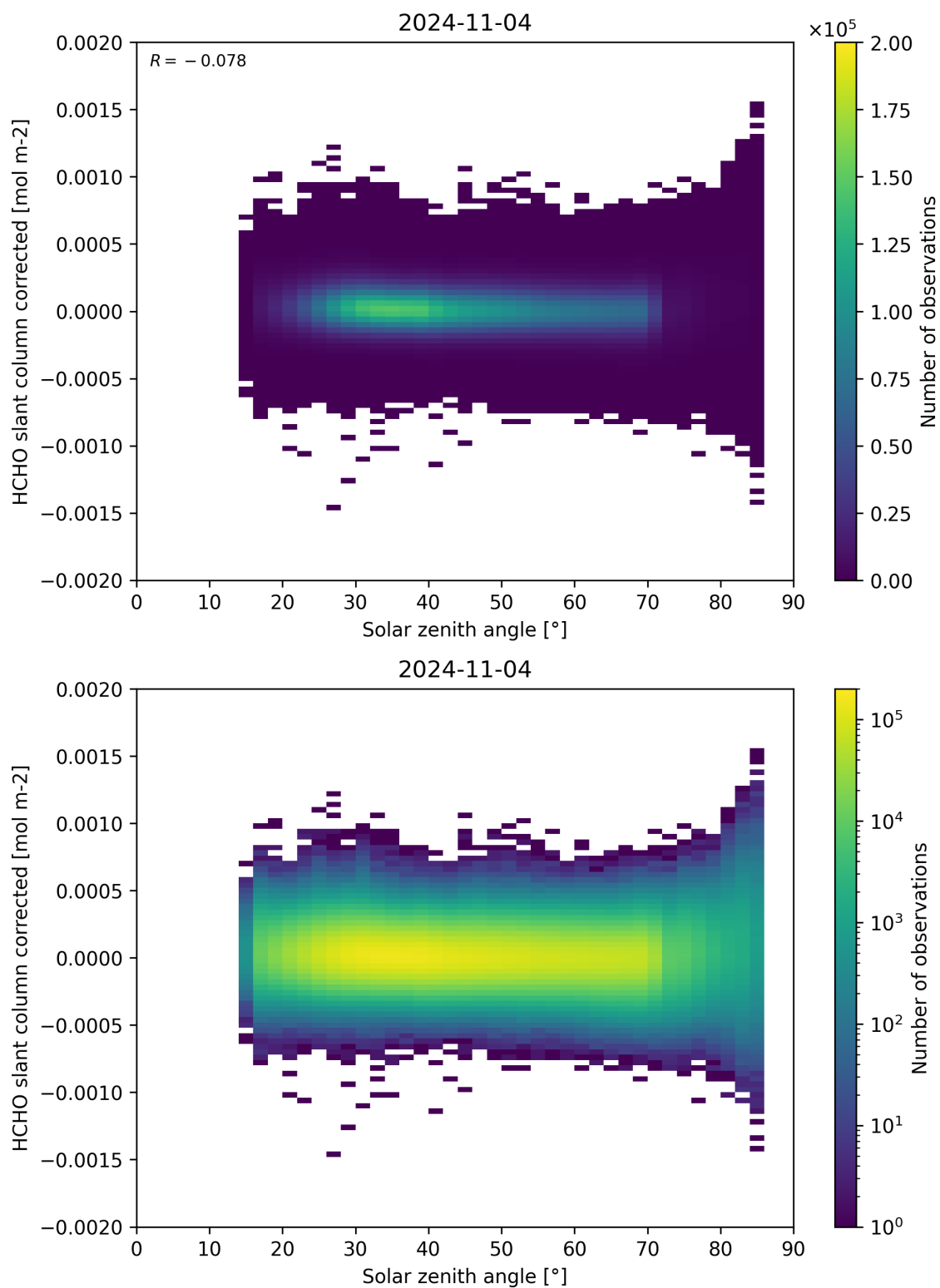
Figure 171: Scatter density plot of “Solar zenith angle” against “HCHO slant column corrected” for 2024-11-04 to 2024-11-05.
