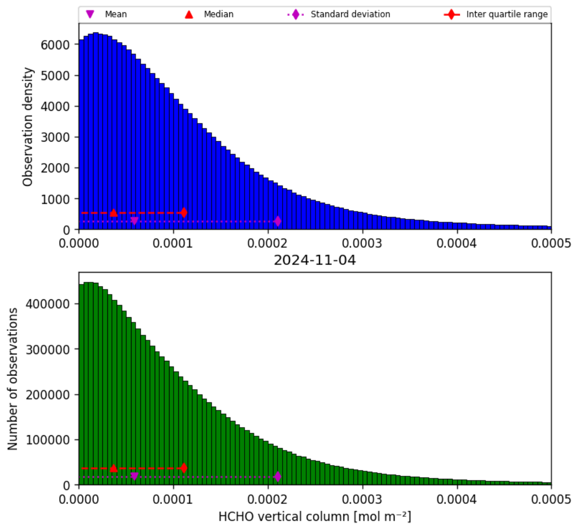
Figure 35: Histogram of “HCHO vertical column” for 2024-11-04 to 2024-11-05
