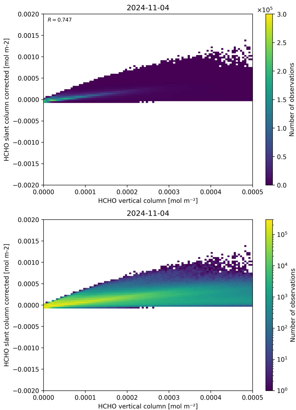
Figure 127: Scatter density plot of “HCHO vertical column” against “HCHO slant column corrected” for 2024-11-04 to 2024-11-05.
