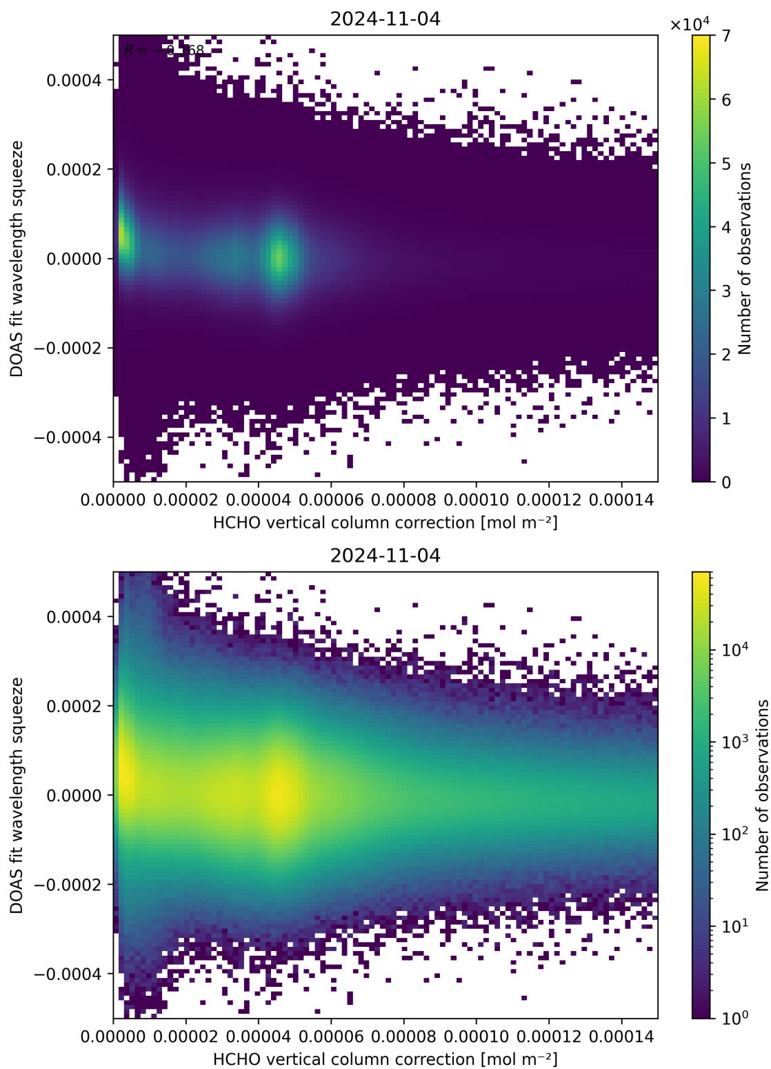
Figure 114: Scatter density plot of “HCHO vertical column correction” against “DOAS fit wavelength squeeze” for 2024-11-04 to 2024-11-05.
