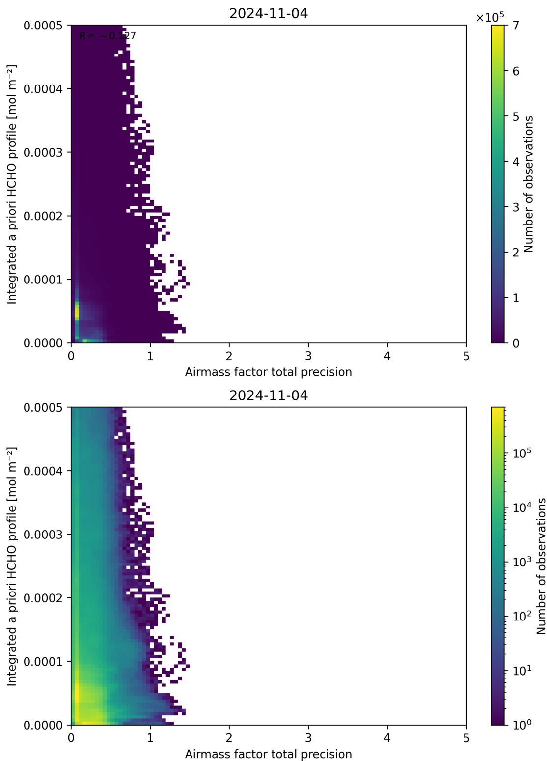
Figure 111: Scatter density plot of “Airmass factor total precision” against “Integrated a priori HCHO profile” for 2024-11-04 to 2024-11-05.
