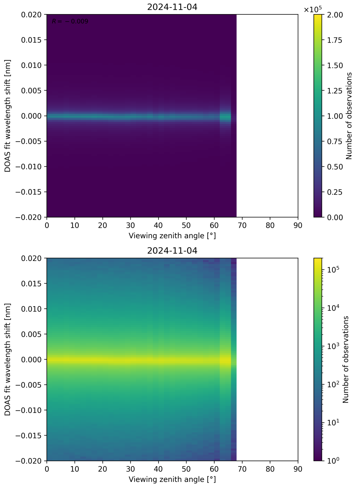
Figure 183: Scatter density plot of “Viewing zenith angle” against “DOAS fit wavelength shift” for 2024-11-04 to 2024-11-05.
