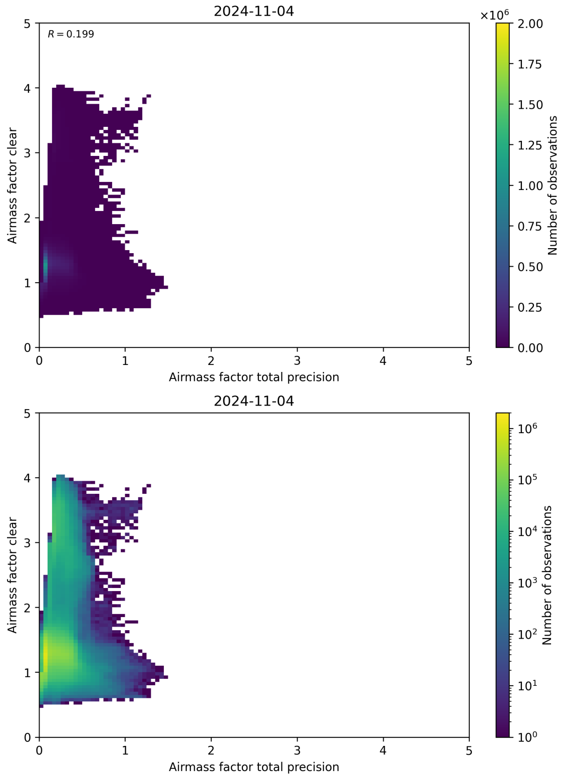
Figure 108: Scatter density plot of “Airmass factor total precision” against “Airmass factor clear” for 2024-11-04 to 2024-11-05.
