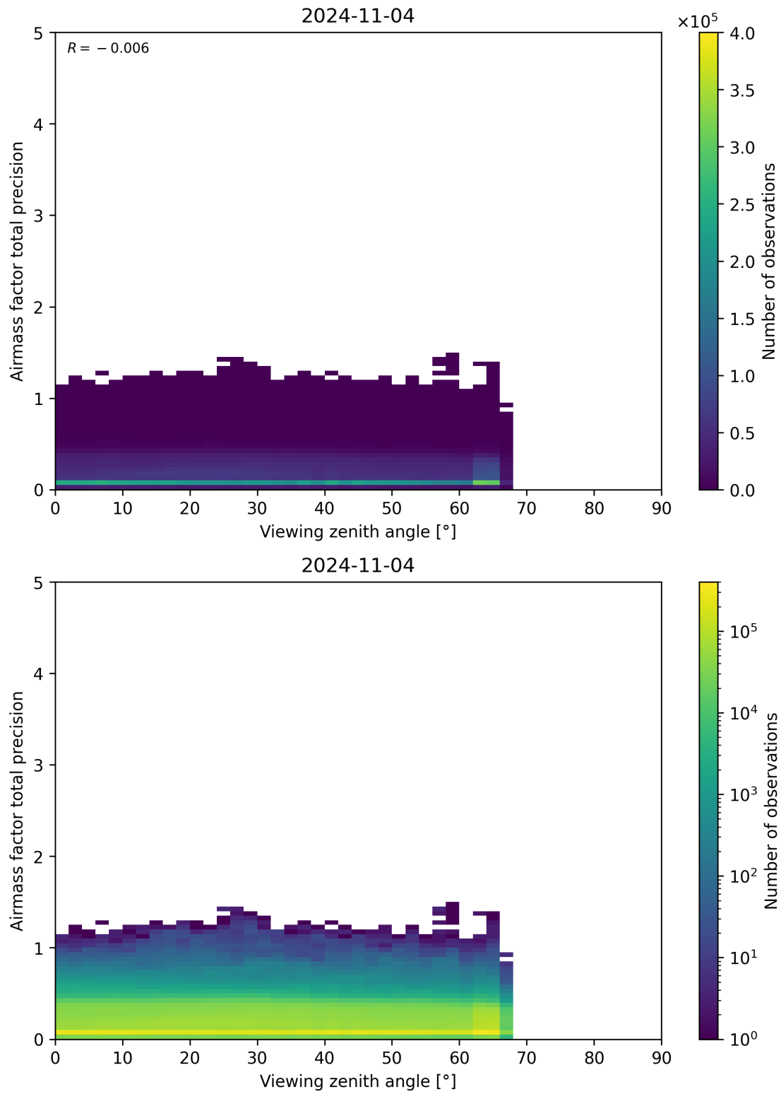
Figure 191: Scatter density plot of “Viewing zenith angle” against “Airmass factor total precision” for 2024-11-04 to 2024-11-05.
