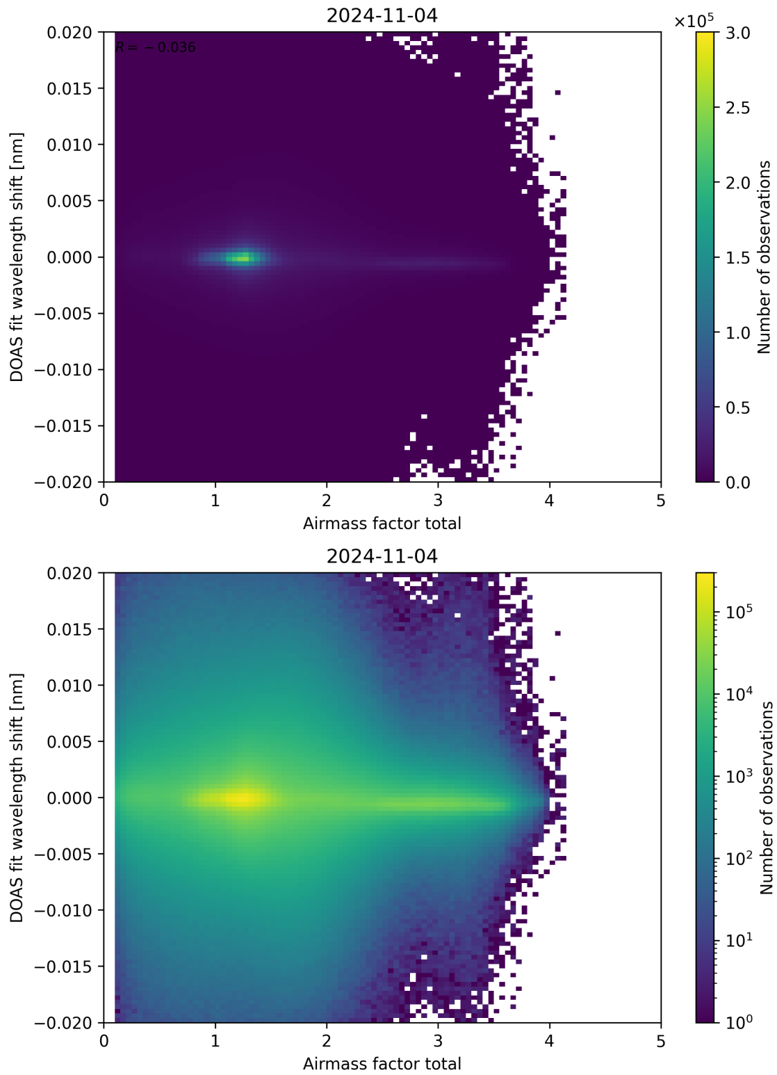
Figure 98: Scatter density plot of “Airmass factor total” against “DOAS fit wavelength shift” for 2024-11-04 to 2024-11-05.
