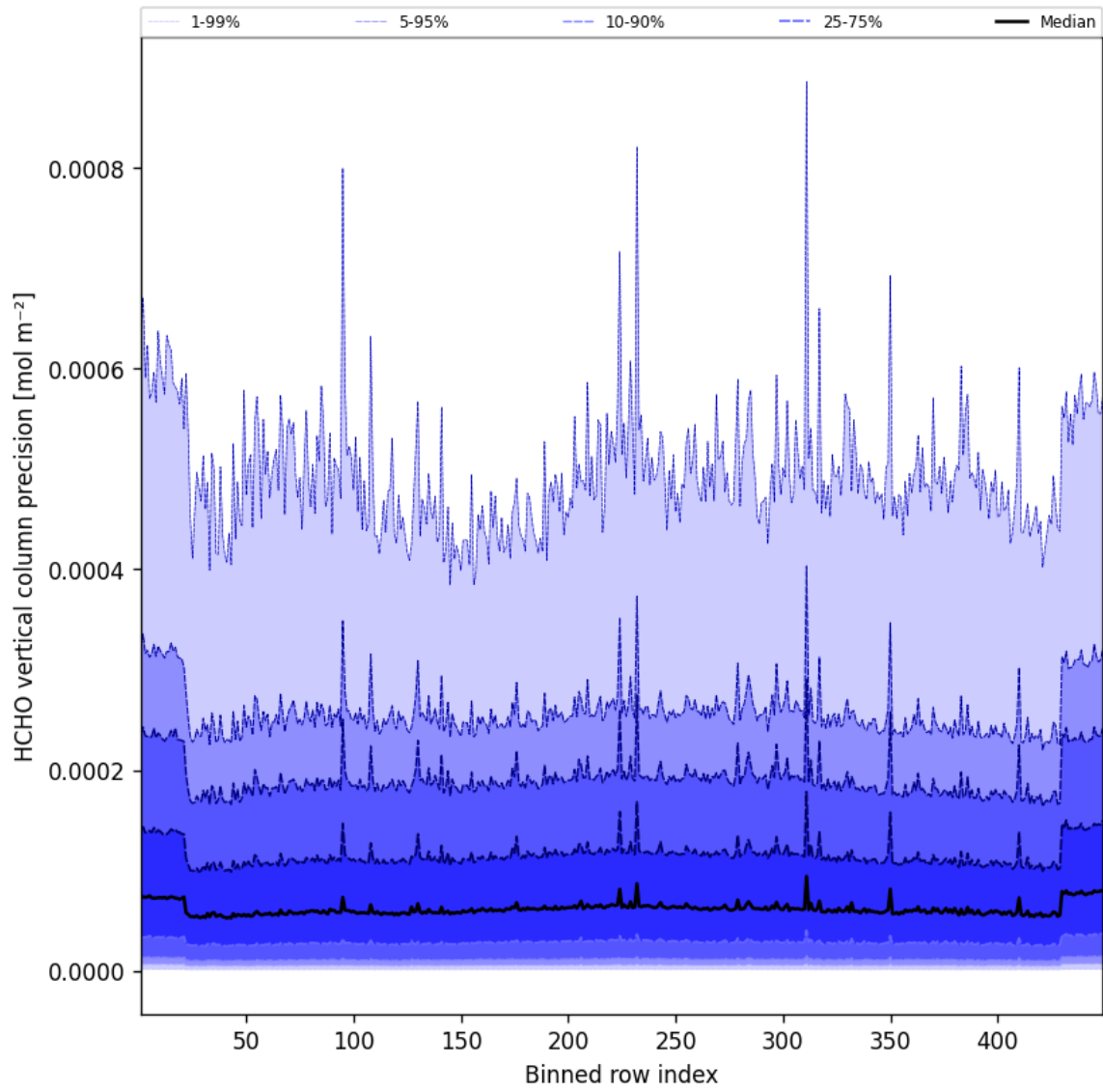
Figure 50: Along track statistics of "HCHO vertical column precision" for 2024-11-04 to 2024-11-05
