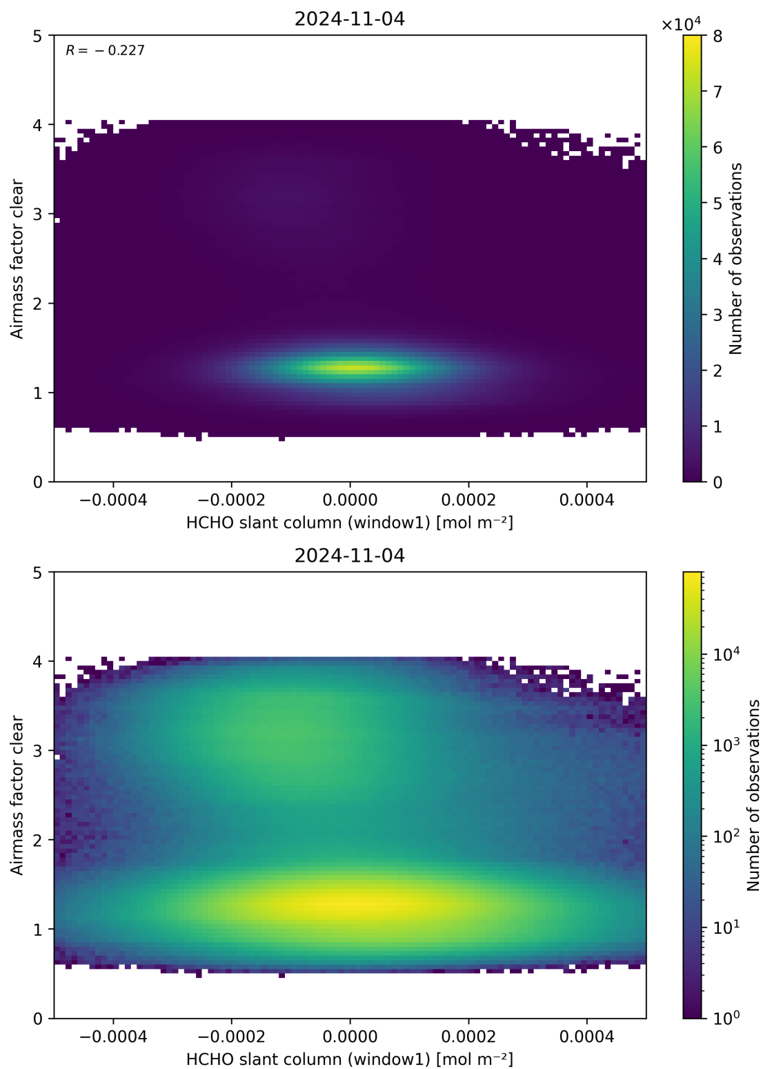
Figure 81: Scatter density plot of “HCHO slant column (window1)” against “Airmass factor clear” for 2024-11-04 to 2024-11-05.
