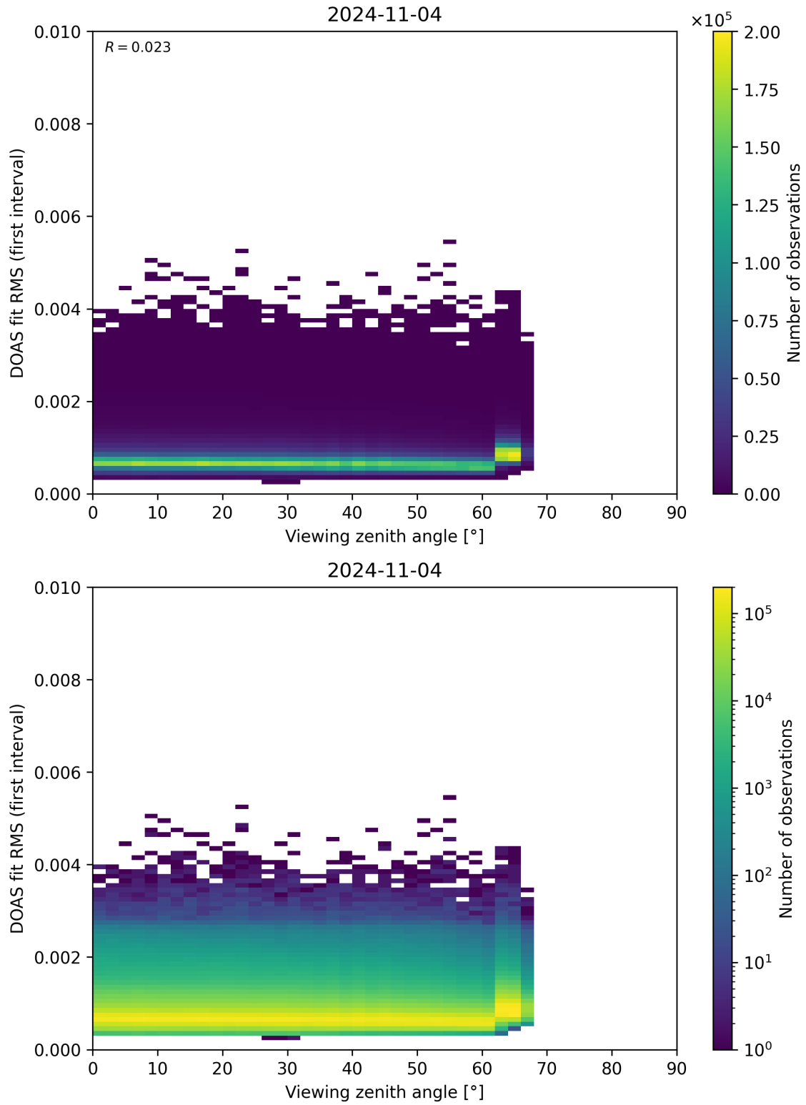
Figure 182: Scatter density plot of “Viewing zenith angle” against “DOAS fit RMS (first interval)” for 2024-11-04 to 2024-11-05.
