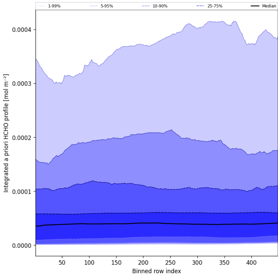
Figure 57: Along track statistics of "Integrated a priori HCHO profile" for 2024-11-04 to 2024-11-05
