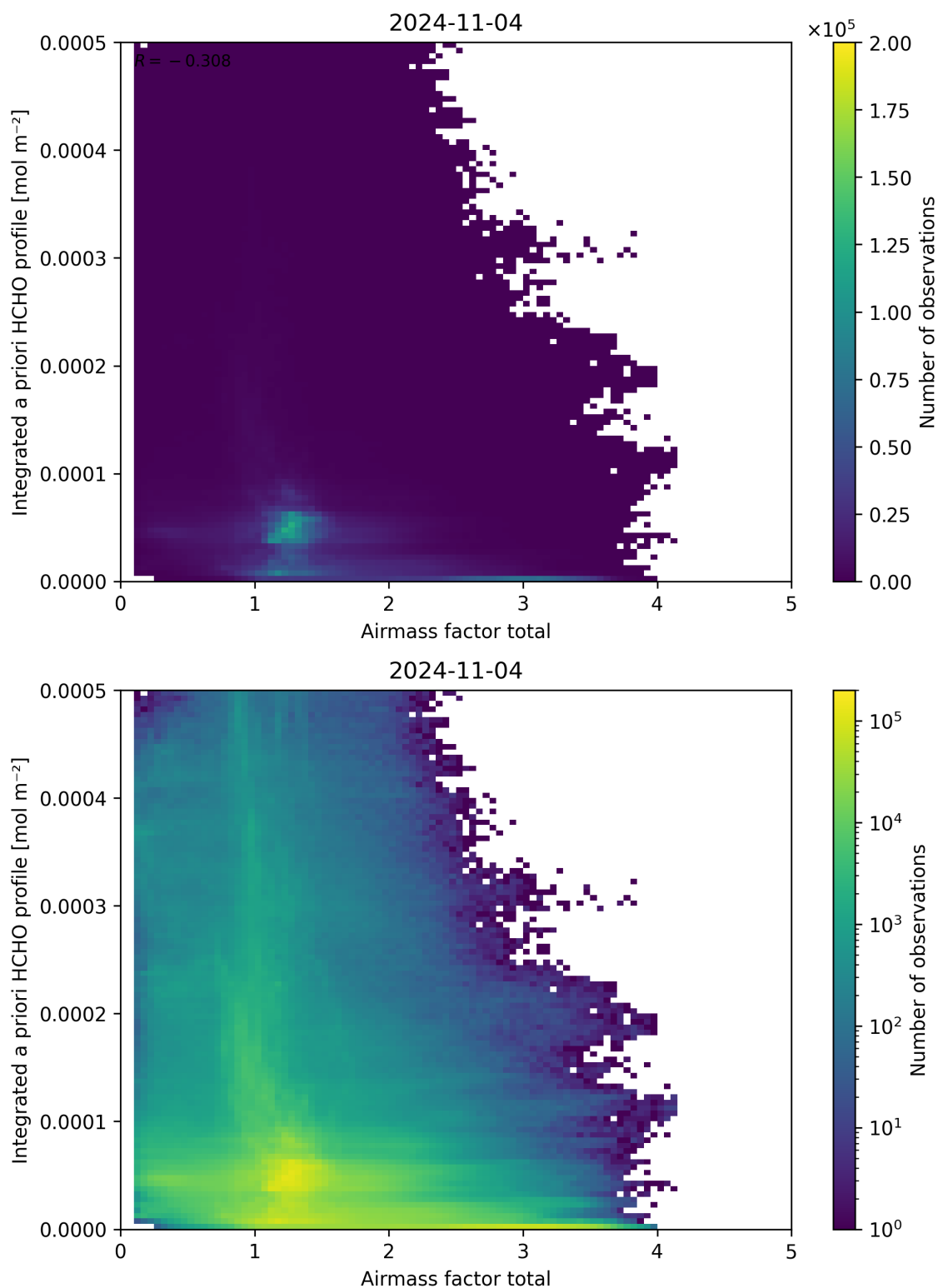
Figure 104: Scatter density plot of “Airmass factor total” against “Integrated a priori HCHO profile” for 2024-11-04 to 2024-11-05.
