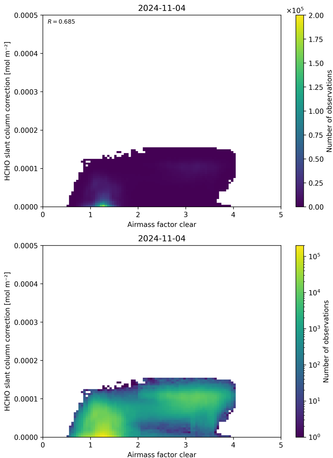
Figure 75: Scatter density plot of “Airmass factor clear” against “HCHO slant column correction” for 2024-11-04 to 2024-11-05.
