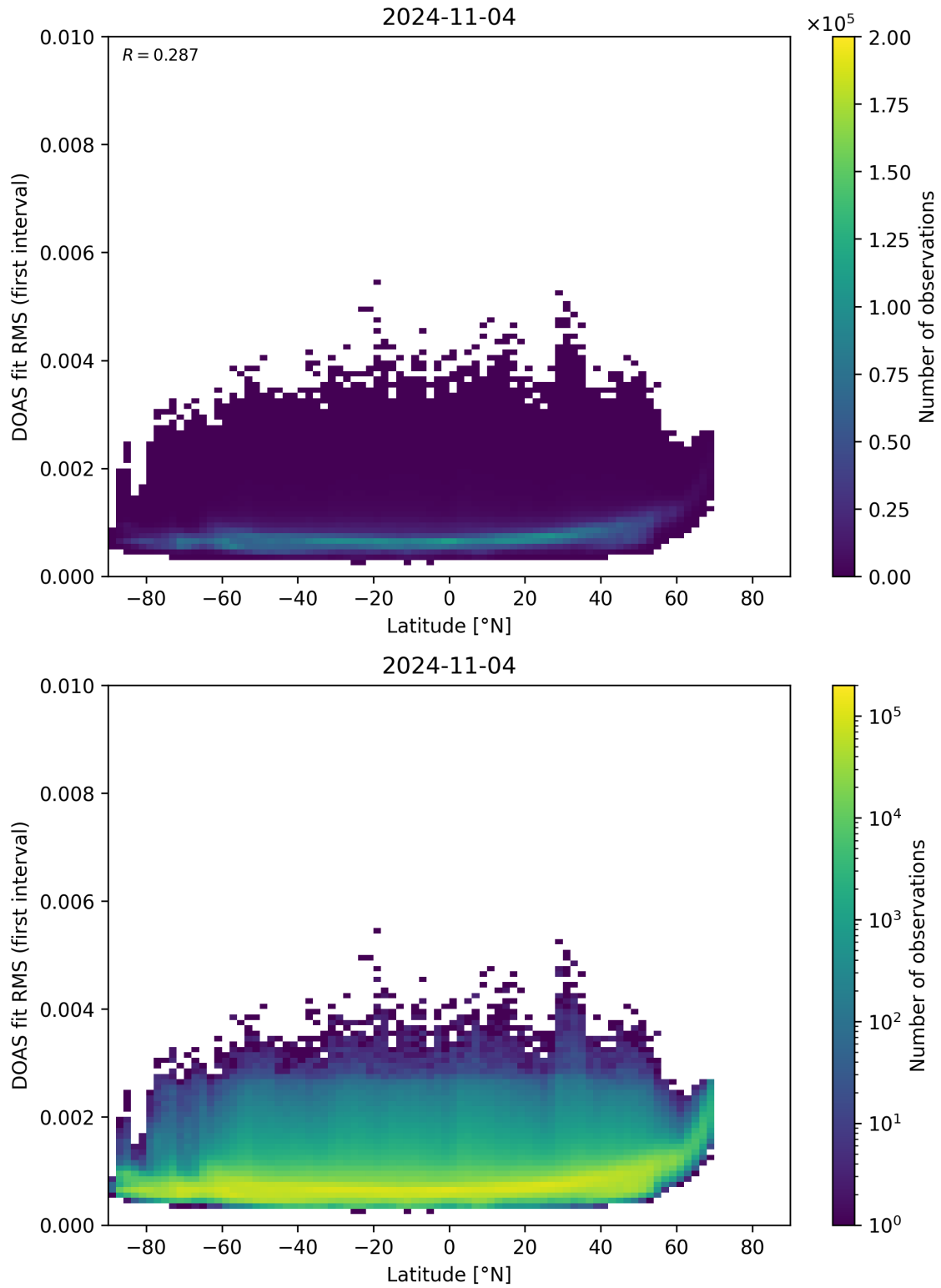
Figure 153: Scatter density plot of “Latitude” against “DOAS fit RMS (first interval)” for 2024-11-04 to 2024-11-05.
