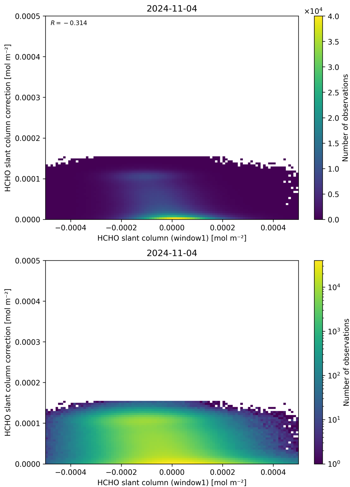
Figure 83: Scatter density plot of “HCHO slant column (window1)” against “HCHO slant column correction” for 2024-11-04 to 2024-11-05.
