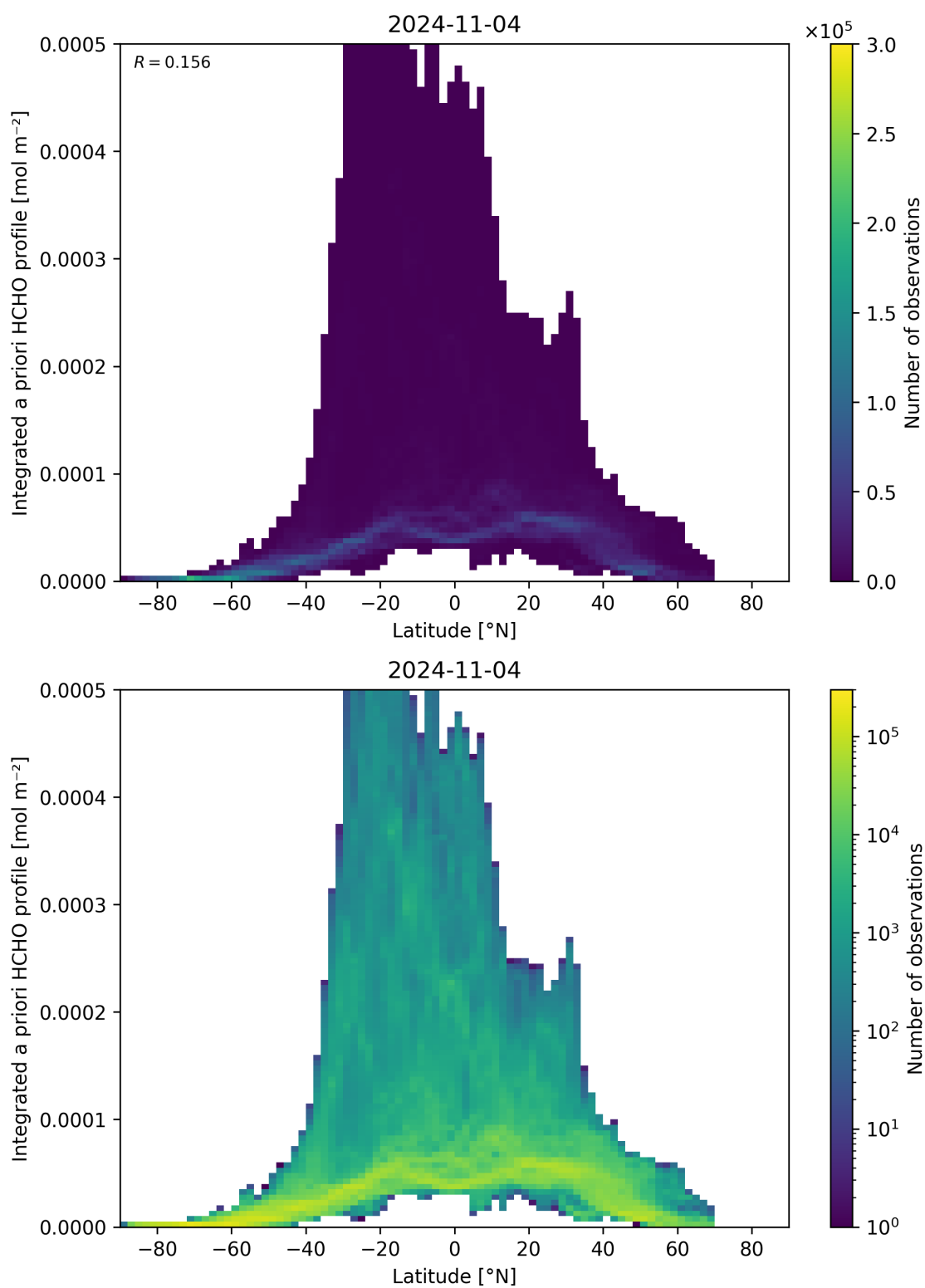
Figure 166: Scatter density plot of “Latitude” against “Integrated a priori HCHO profile” for 2024-11-04 to 2024-11-05.
