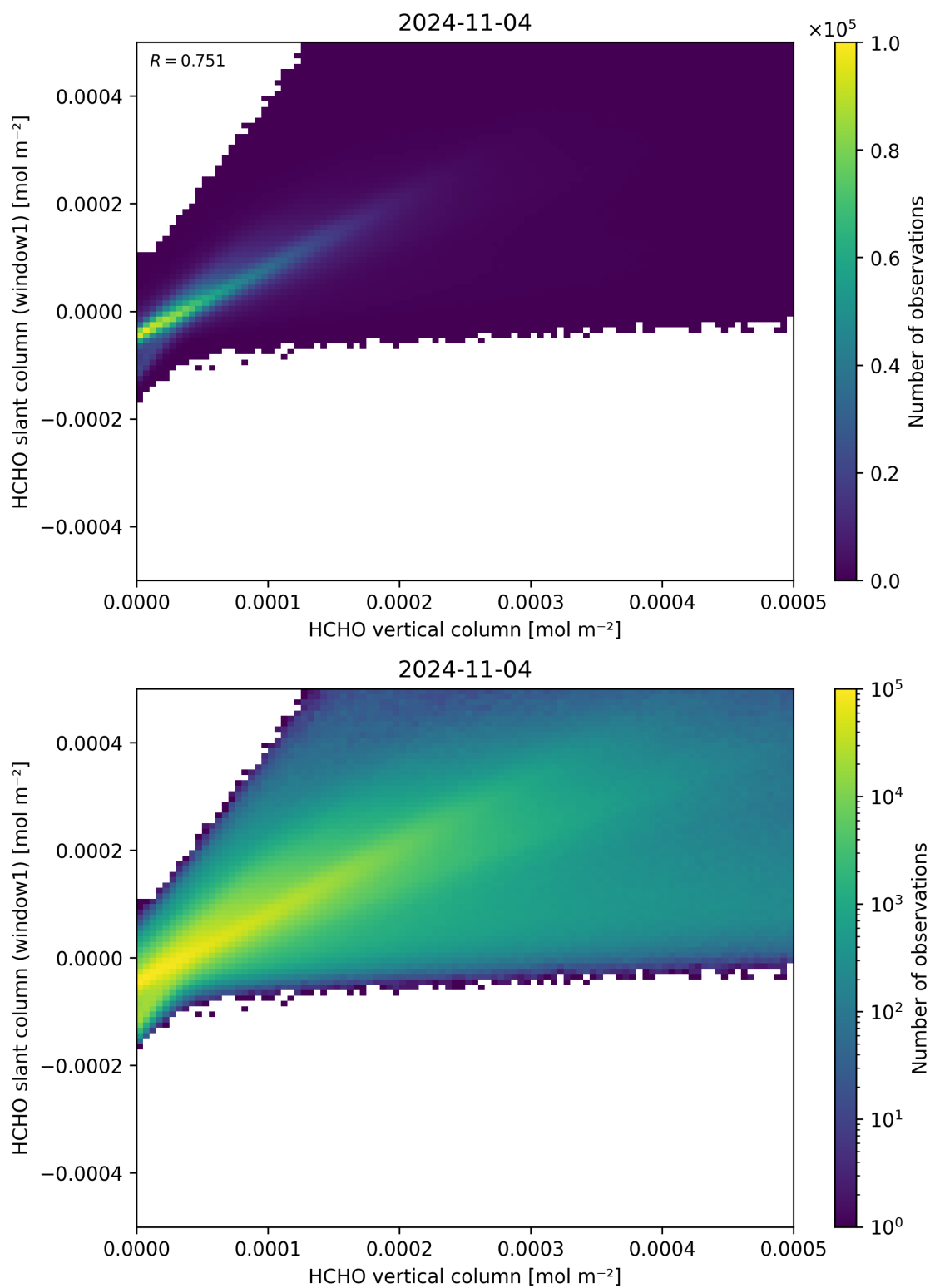
Figure 129: Scatter density plot of “HCHO vertical column” against “HCHO slant column (window1)” for 2024-11-04 to 2024-11-05.
