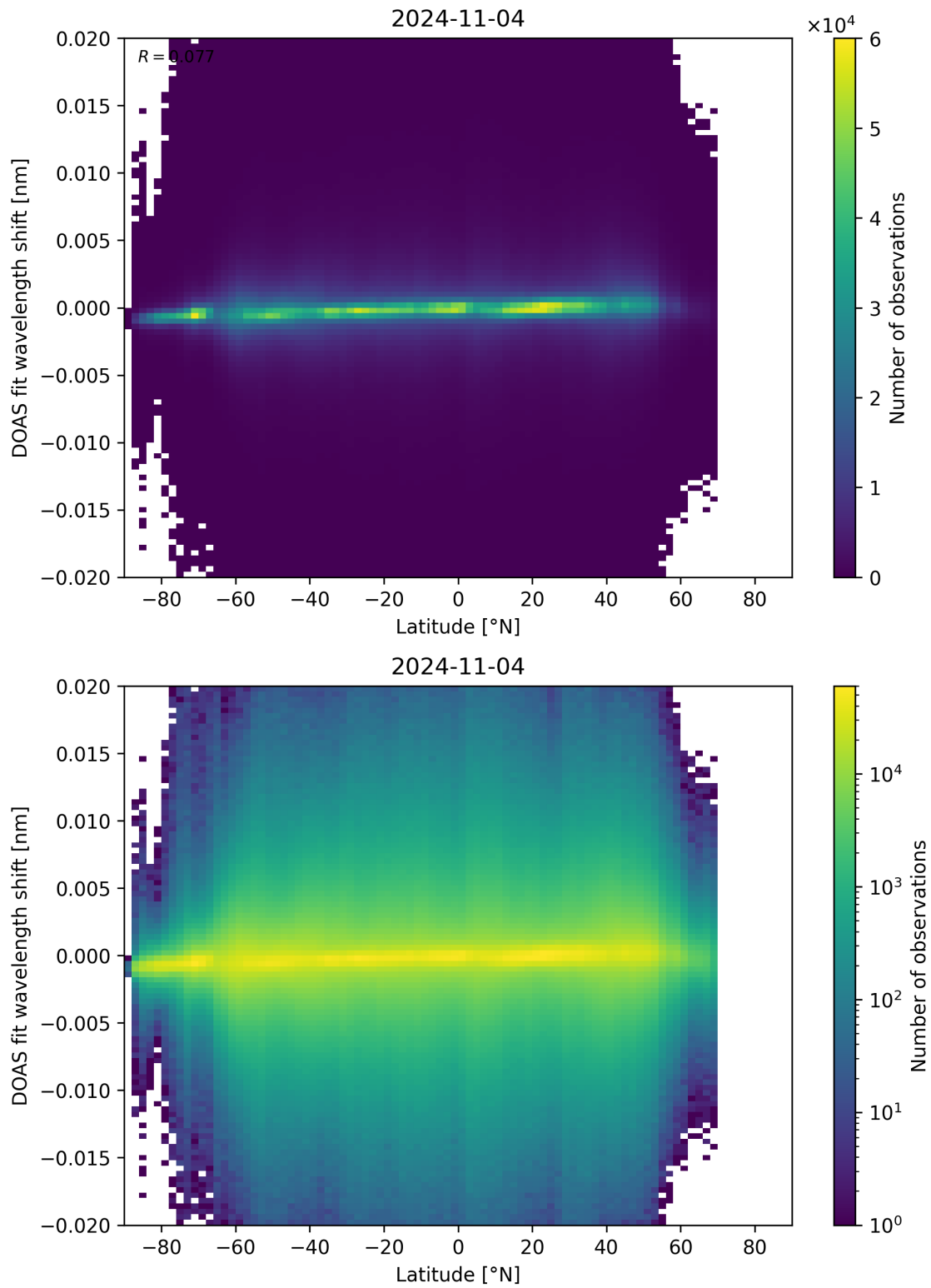
Figure 154: Scatter density plot of “Latitude” against “DOAS fit wavelength shift” for 2024-11-04 to 2024-11-05.
