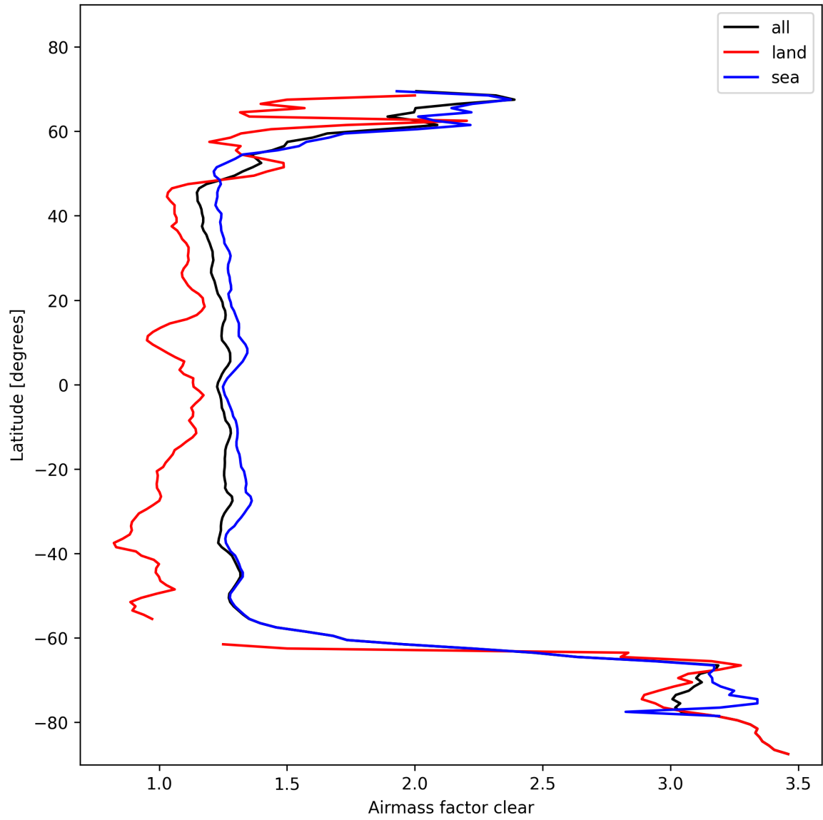
Figure 28: Zonal average of “Airmass factor clear” for 2024-11-04 to 2024-11-05.
