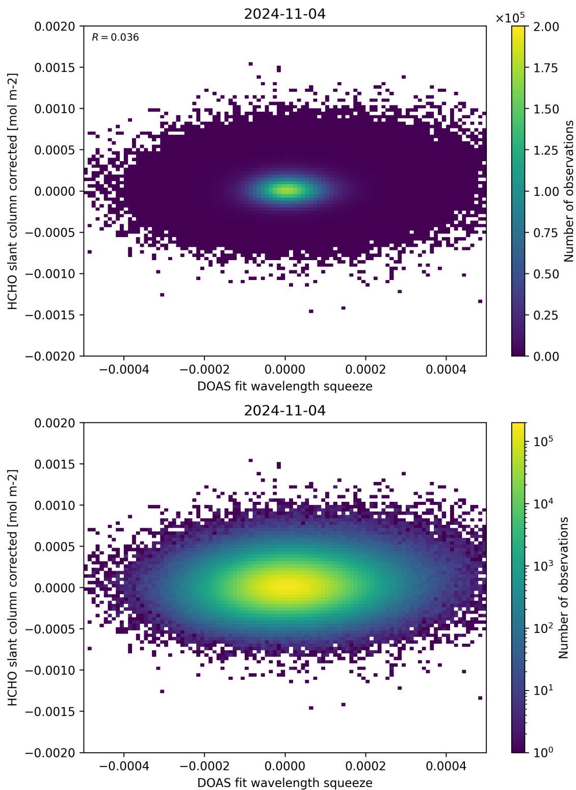
Figure 69: Scatter density plot of “DOAS fit wavelength squeeze” against “HCHO slant column corrected” for 2024-11-04 to 2024-11-05.
