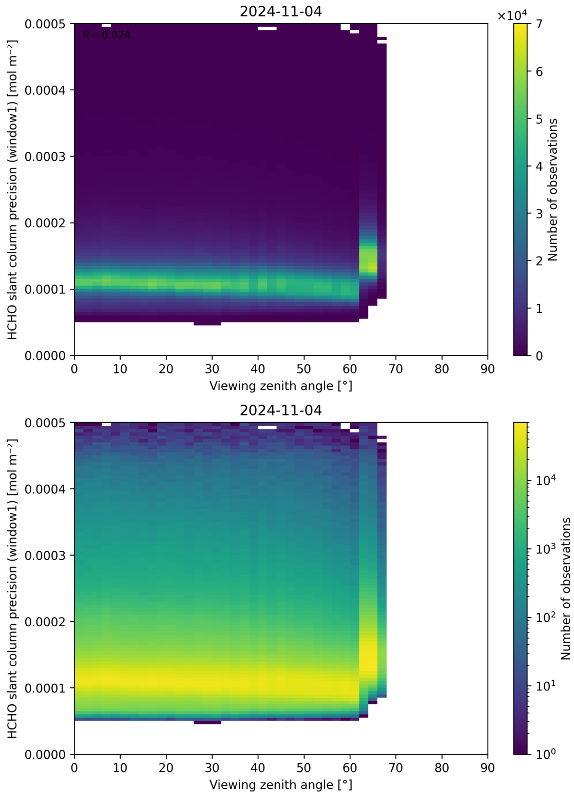
Figure 189: Scatter density plot of “Viewing zenith angle” against “HCHO slant column precision (window1)” for 2024-11-04 to 2024-11-05.
