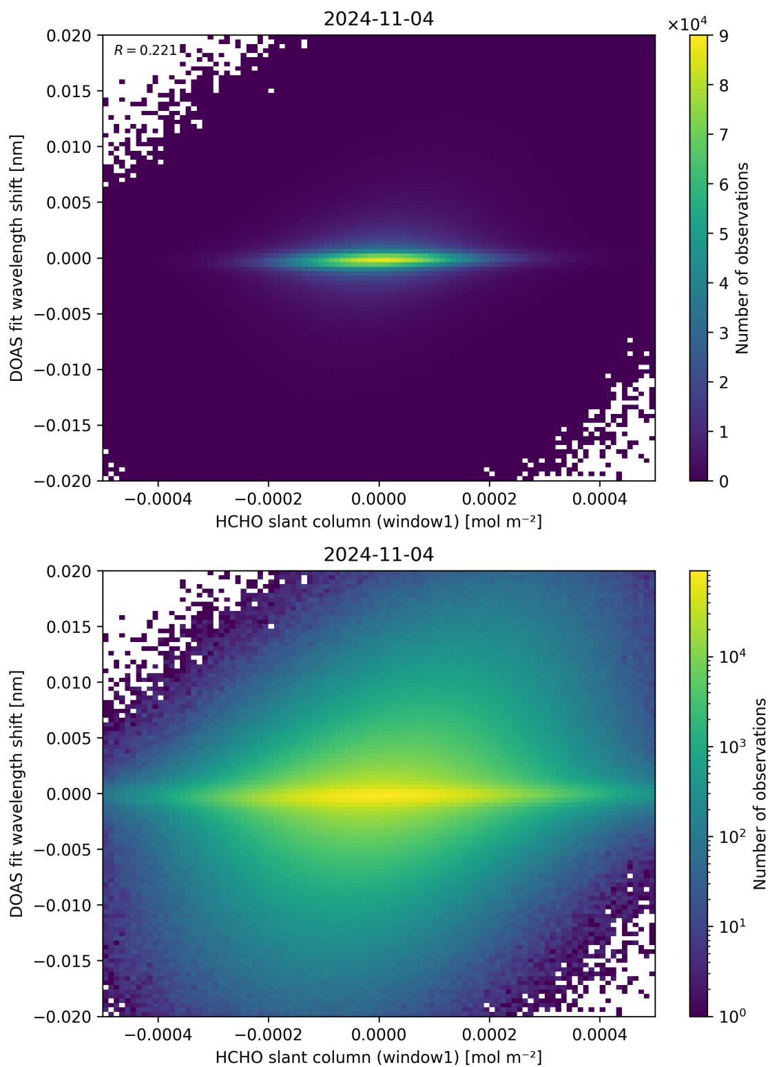
Figure 79: Scatter density plot of “HCHO slant column (window1)” against “DOAS fit wavelength shift” for 2024-11-04 to 2024-11-05.
