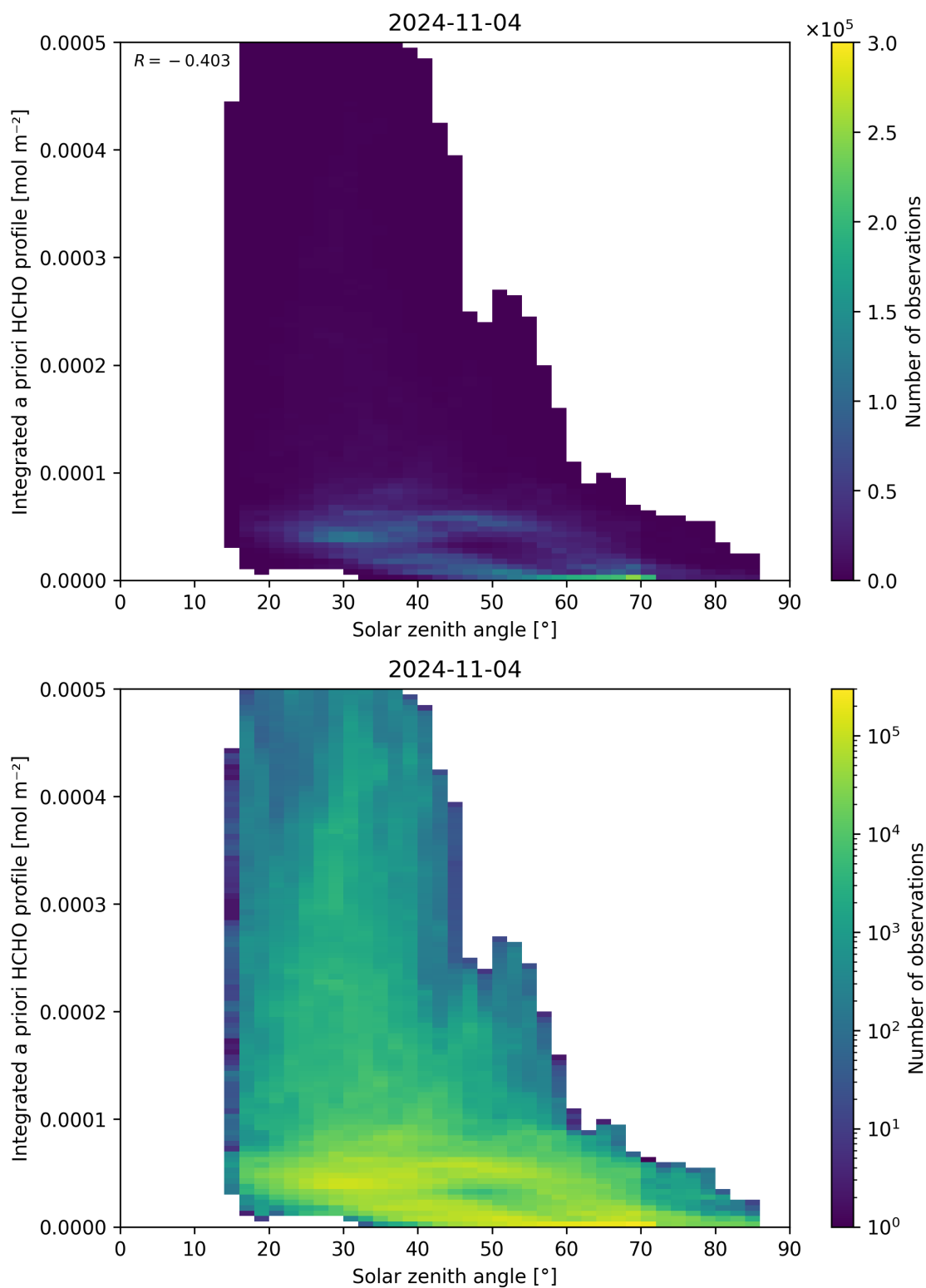
Figure 180: Scatter density plot of “Solar zenith angle” against “Integrated a priori HCHO profile” for 2024-11-04 to 2024-11-05.
