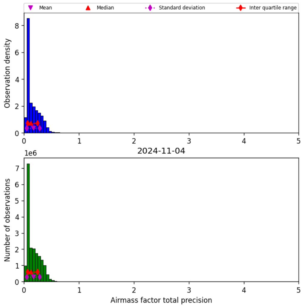
Figure 41: Histogram of “Airmass factor total precision” for 2024-11-04 to 2024-11-05
