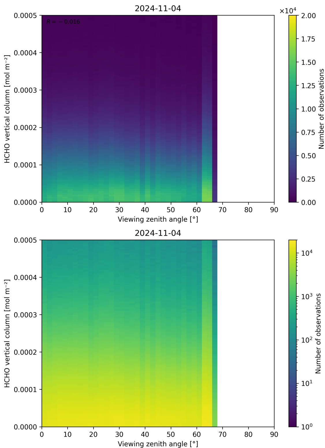
Figure 192: Scatter density plot of “Viewing zenith angle” against “HCHO vertical column” for 2024-11-04 to 2024-11-05.
