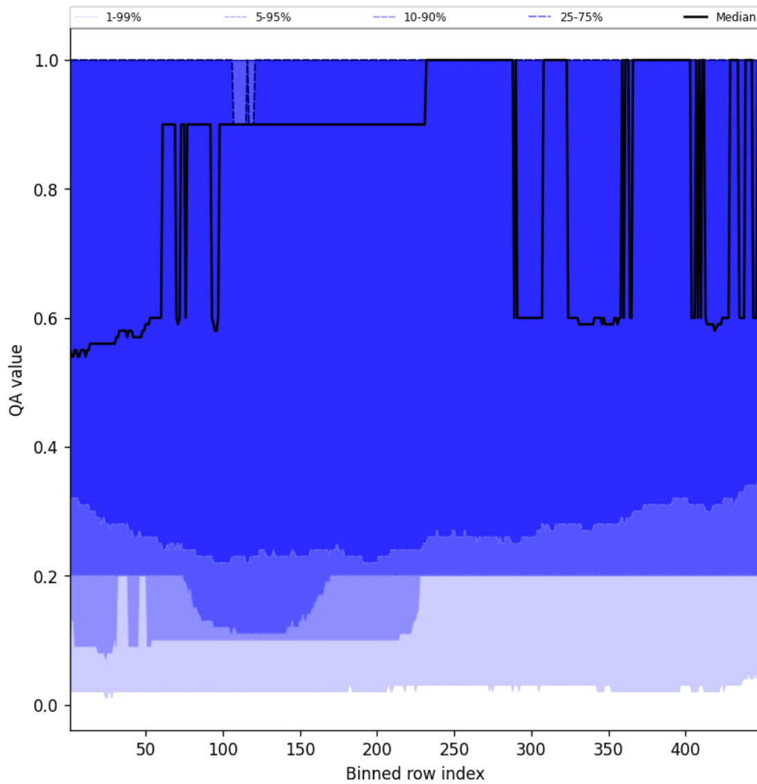
Figure 48: Along track statistics of “QA value” for 2024-11-04 to 2024-11-05
