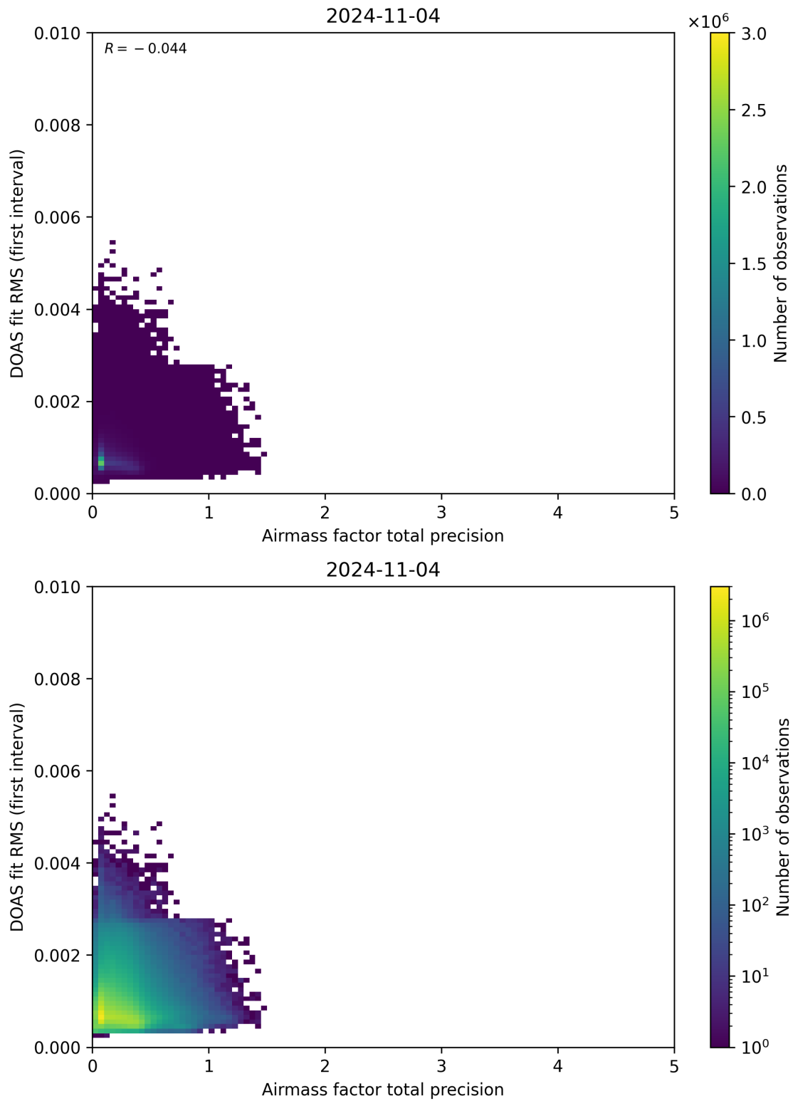
Figure 105: Scatter density plot of “Airmass factor total precision” against “DOAS fit RMS (first interval)” for 2024-11-04 to 2024-11-05.
