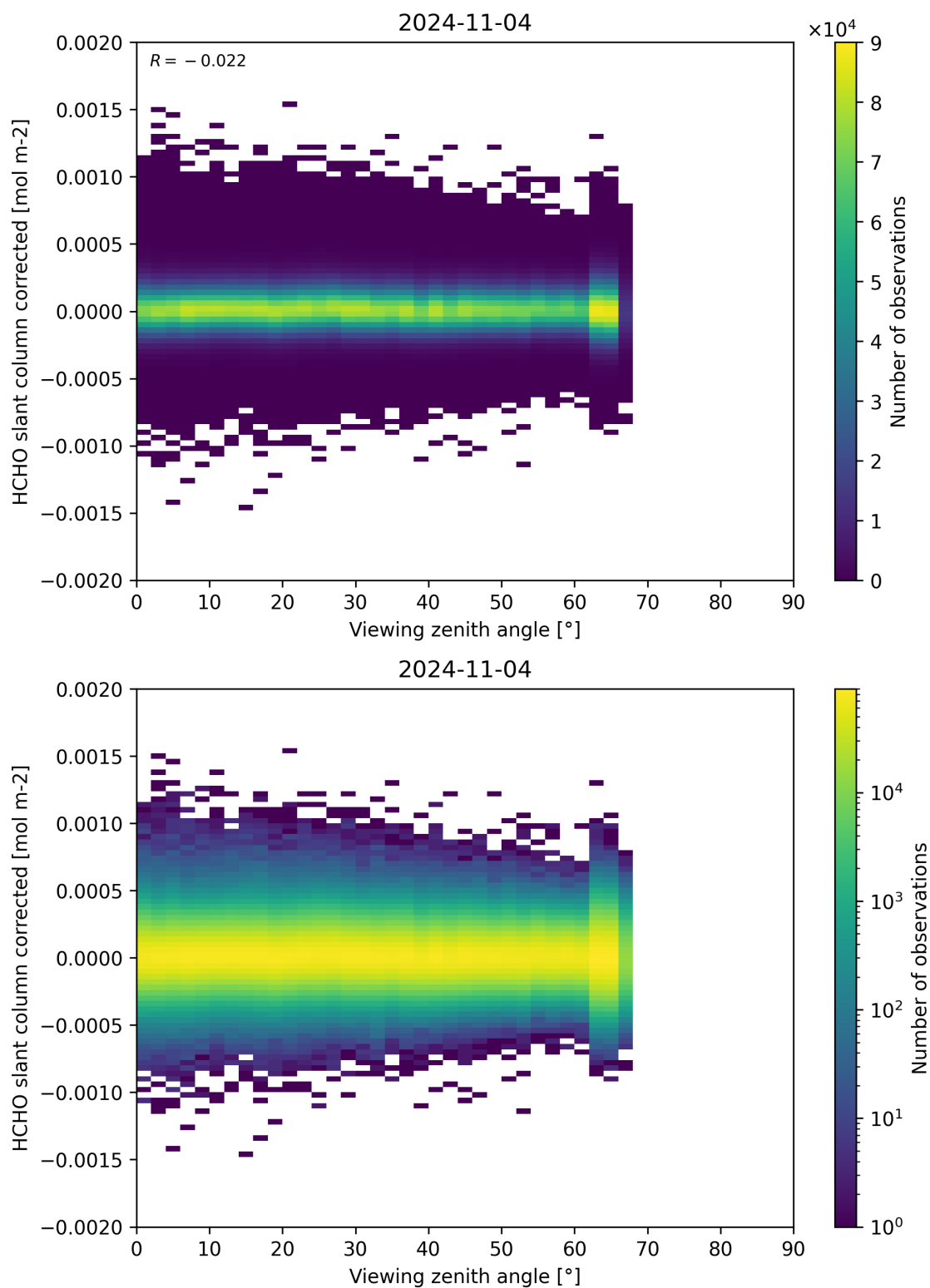
Figure 186: Scatter density plot of “Viewing zenith angle” against “HCHO slant column corrected” for 2024-11-04 to 2024-11-05.
