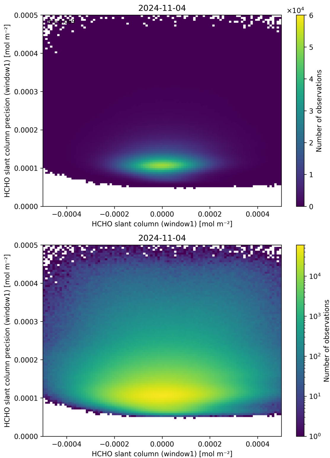
Figure 84: Scatter density plot of “HCHO slant column (window1)” against “HCHO slant column precision (window1)” for 2024-11-04 to 2024-11-05.
