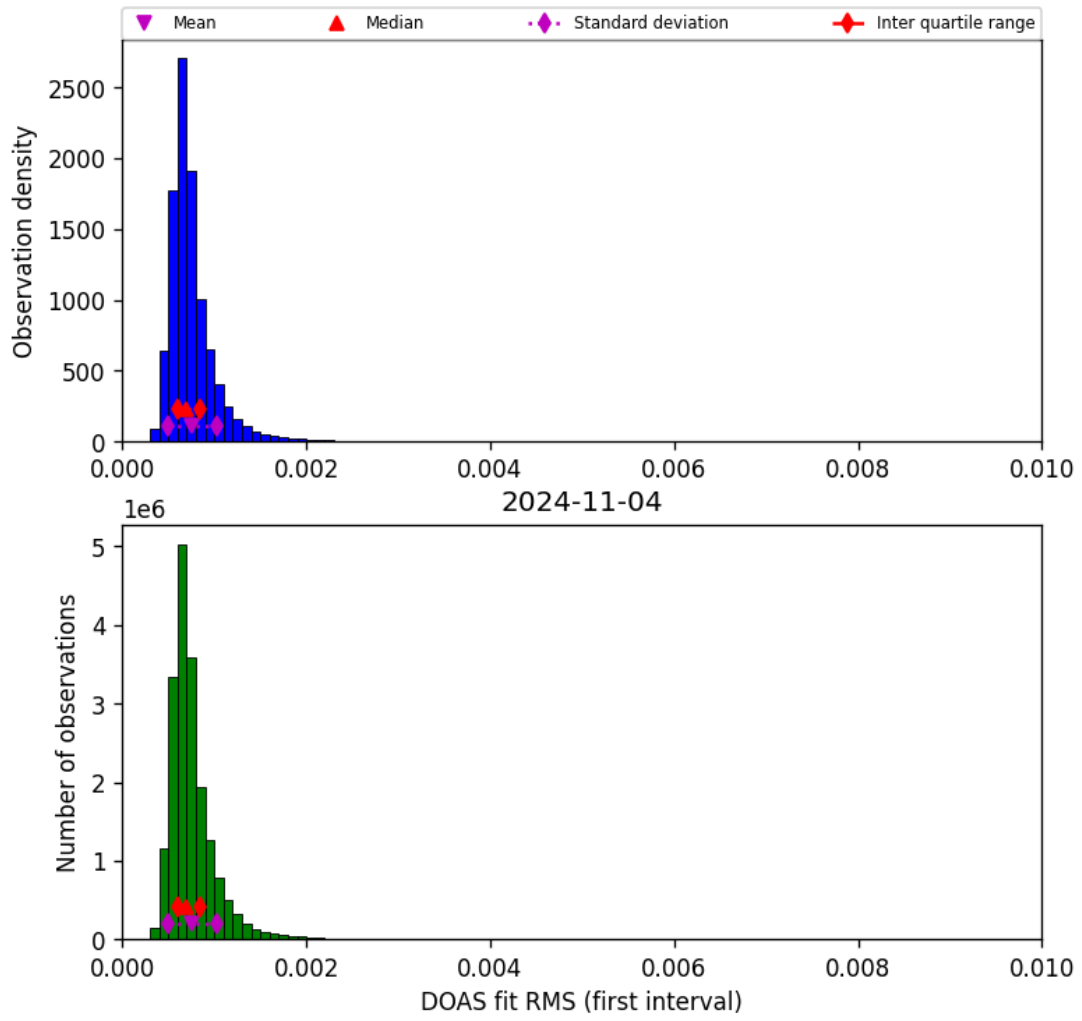
Figure 46: Histogram of “DOAS fit RMS (first interval)” for 2024-11-04 to 2024-11-05
