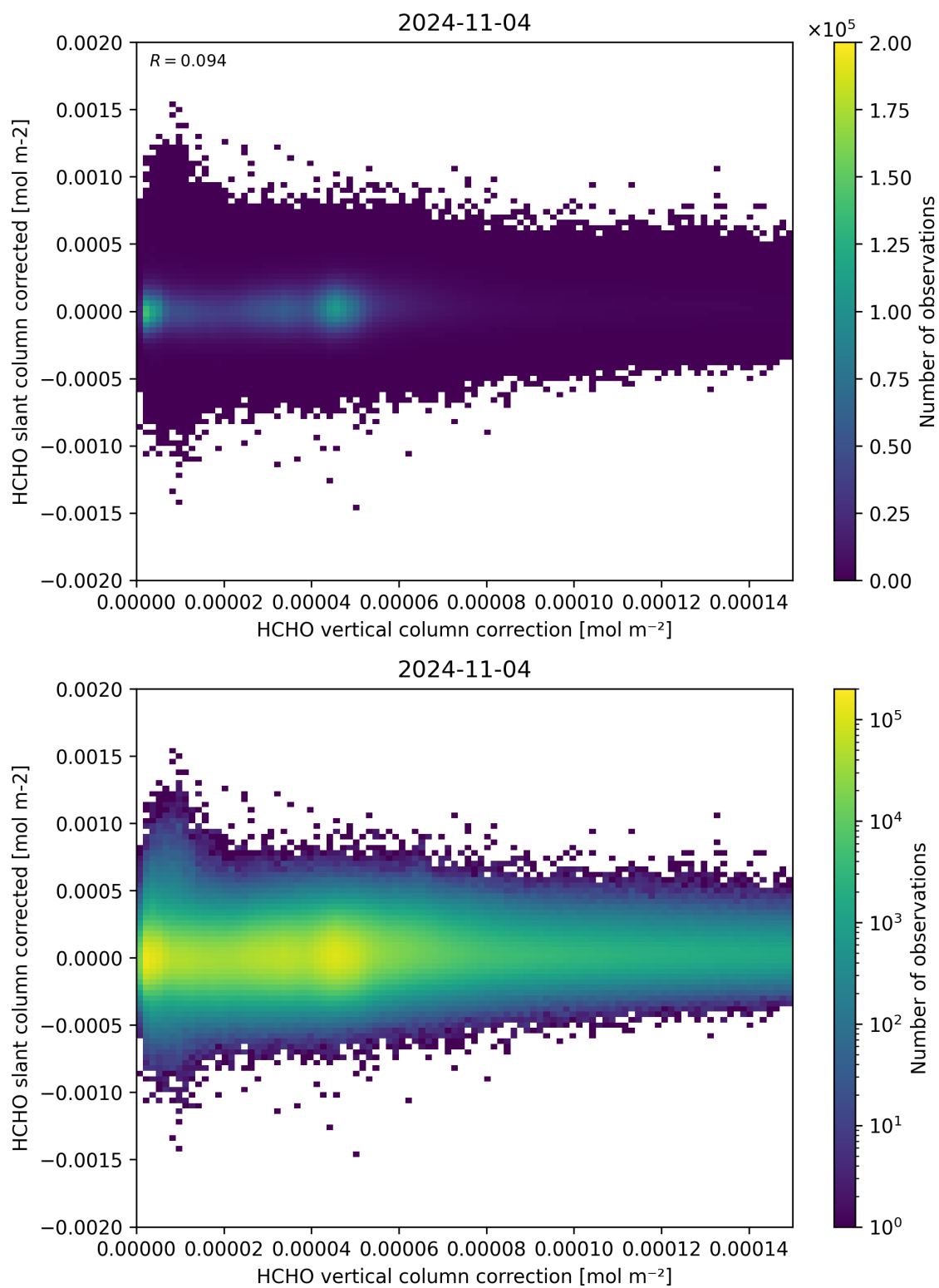
Figure 116: Scatter density plot of “HCHO vertical column correction” against “HCHO slant column corrected” for 2024-11-04 to 2024-11-05.
