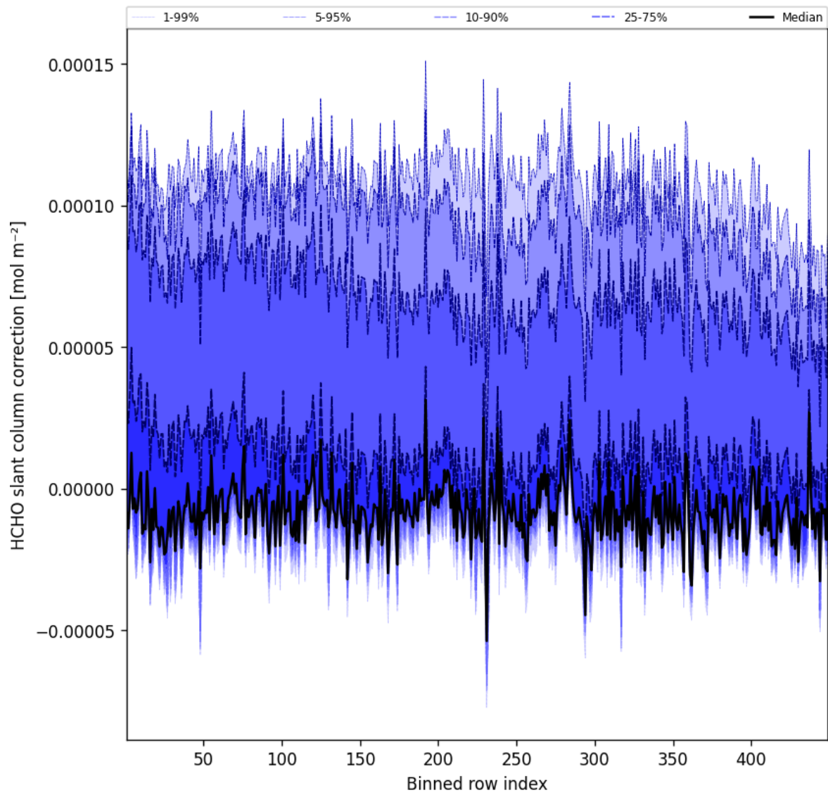
Figure 61: Along track statistics of “HCHO slant column correction” for 2024-11-04 to 2024-11-05
