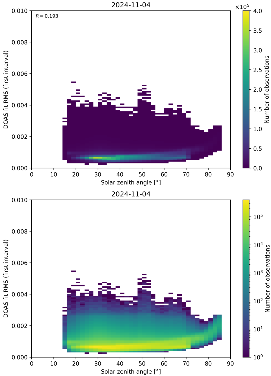
Figure 167: Scatter density plot of “Solar zenith angle” against “DOAS fit RMS (first interval)” for 2024-11-04 to 2024-11-05.
