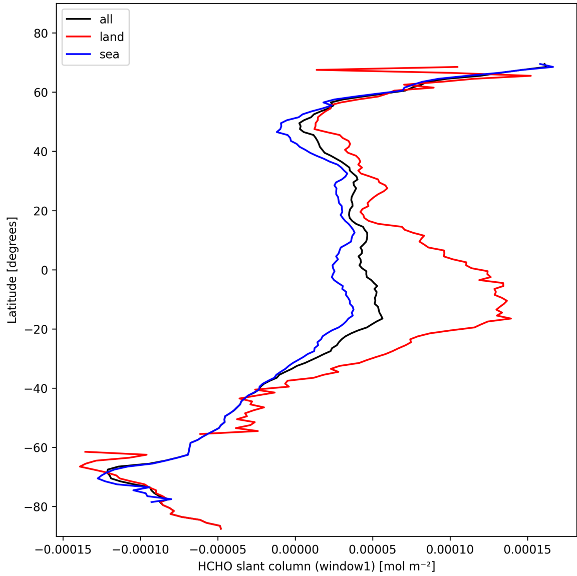
Figure 24: Zonal average of “HCHO slant column (window1)” for 2024-11-04 to 2024-11-05.
