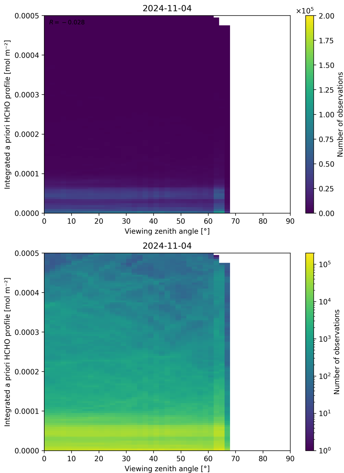
Figure 195: Scatter density plot of “Viewing zenith angle” against “Integrated a priori HCHO profile” for 2024-11-04 to 2024-11-05.
