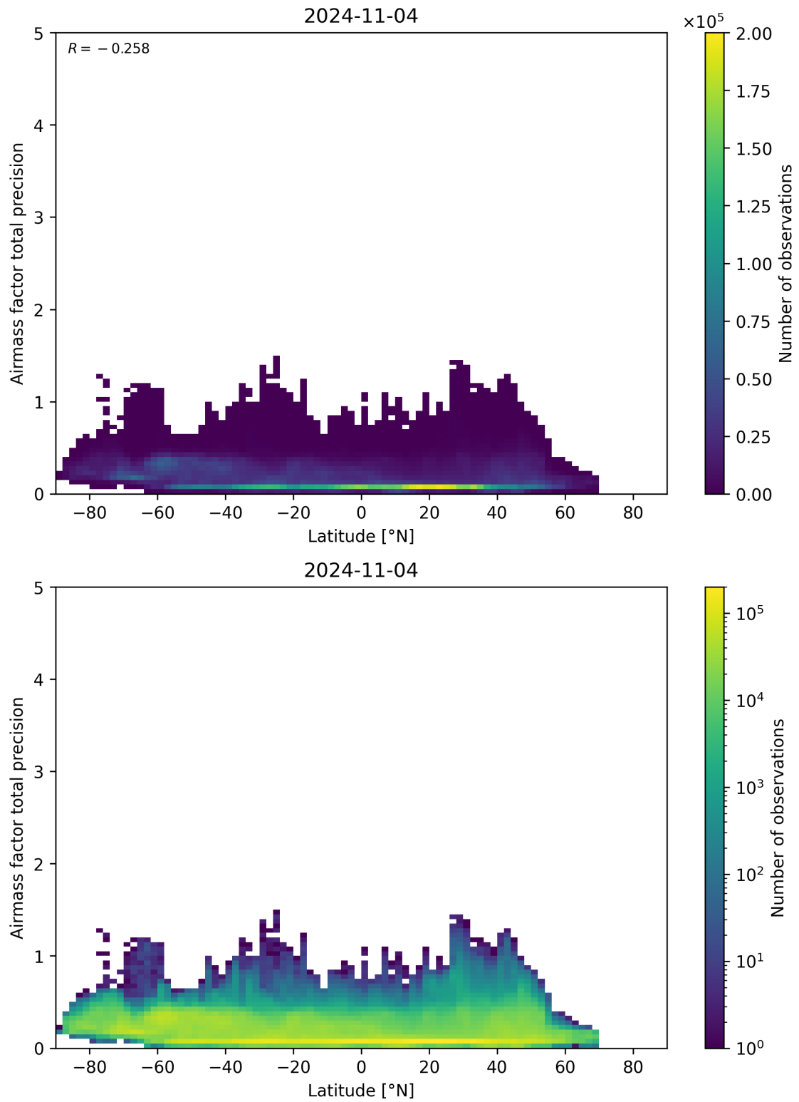
Figure 162: Scatter density plot of “Latitude” against “Airmass factor total precision” for 2024-11-04 to 2024-11-05.
