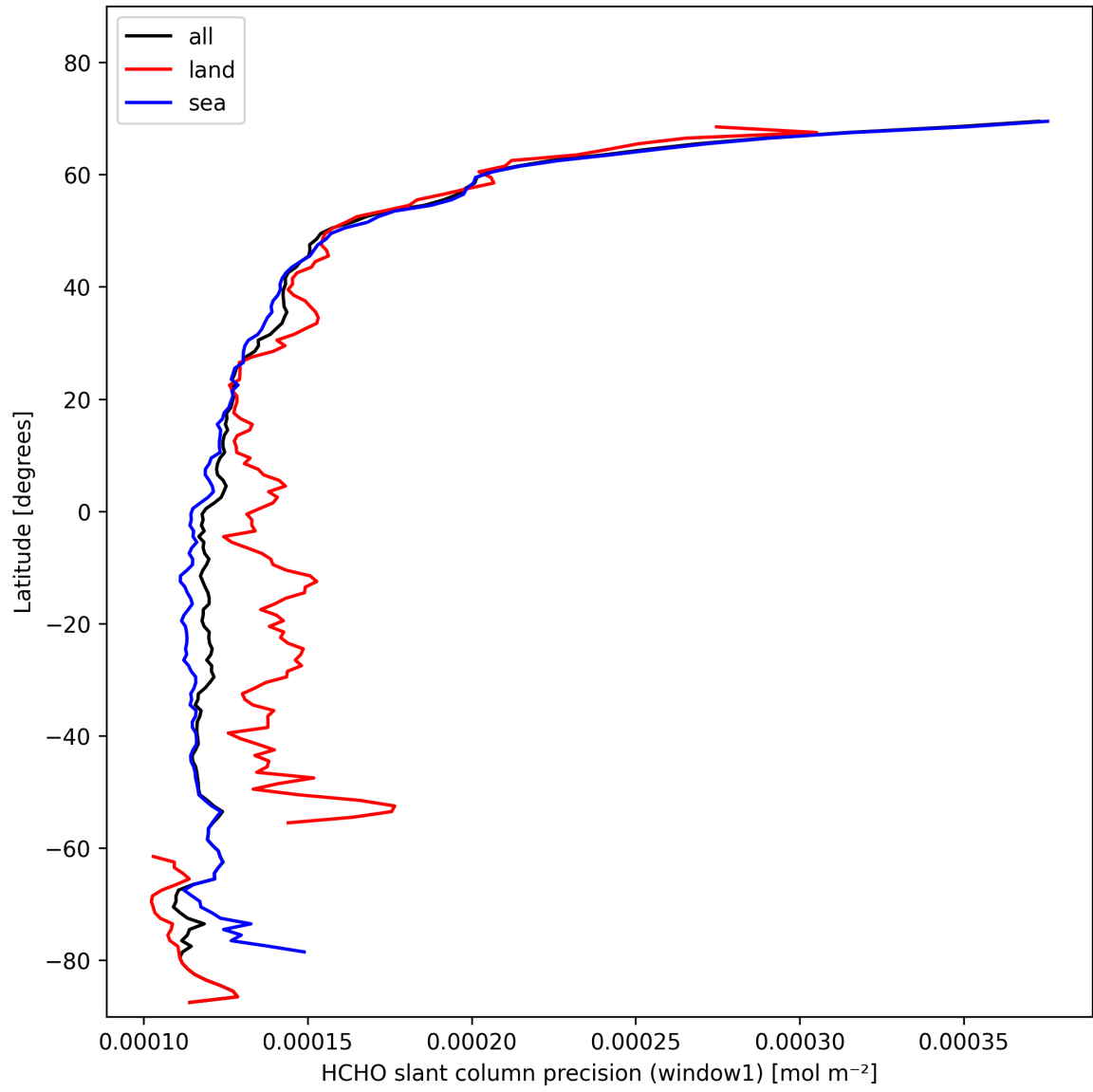
Figure 25: Zonal average of “HCHO slant column precision (window1)” for 2024-11-04 to 2024-11-05.
