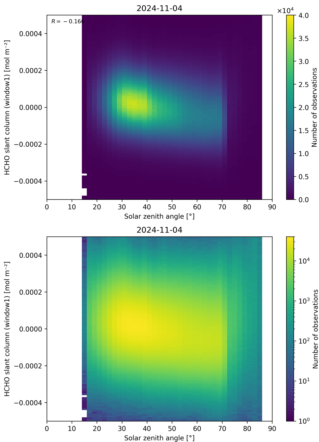
Figure 173: Scatter density plot of “Solar zenith angle” against “HCHO slant column (window1)” for 2024-11-04 to 2024-11-05.
