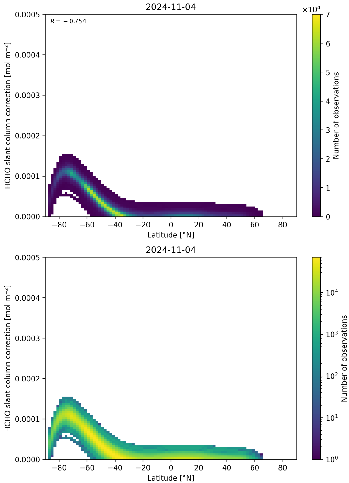
Figure 158: Scatter density plot of “Latitude” against “HCHO slant column correction” for 2024-11-04 to 2024-11-05.
