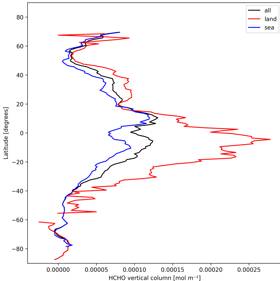
Figure 21: Zonal average of “HCHO vertical column” for 2024-11-04 to 2024-11-05.
