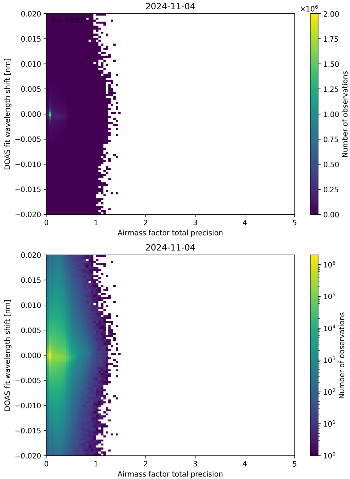
Figure 106: Scatter density plot of “Airmass factor total precision” against “DOAS fit wavelength shift” for 2024-11-04 to 2024-11-05.
