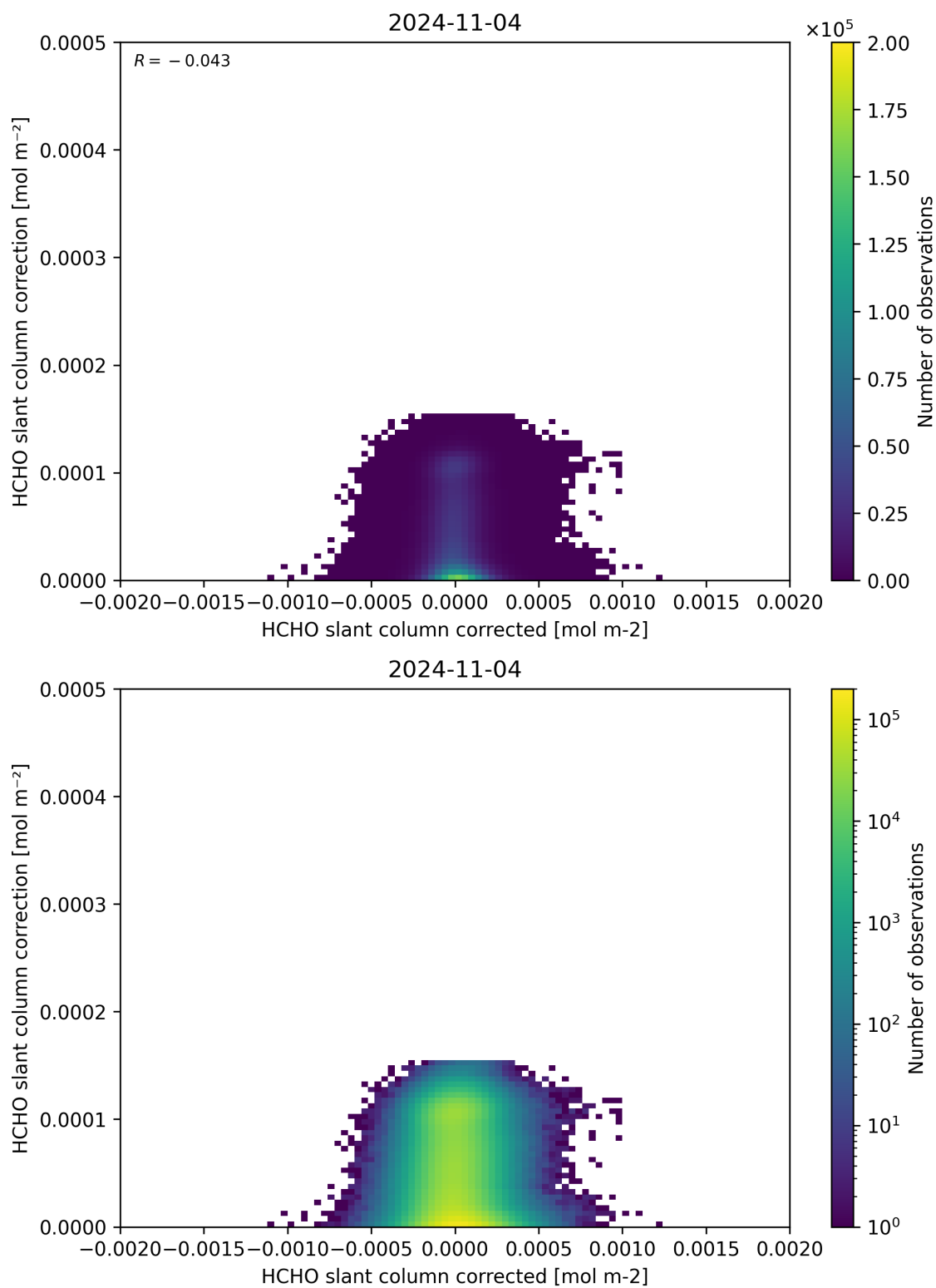
Figure 77: Scatter density plot of “HCHO slant column corrected” against “HCHO slant column correction” for 2024-11-04 to 2024-11-05.
