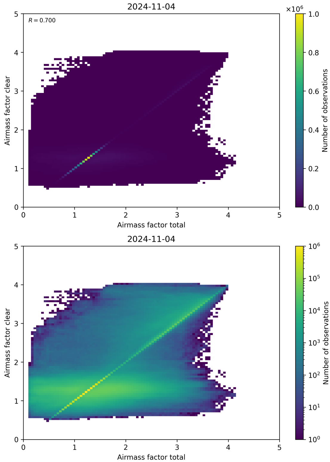
Figure 100: Scatter density plot of “Airmass factor total” against “Airmass factor clear” for 2024-11-04 to 2024-11-05.
