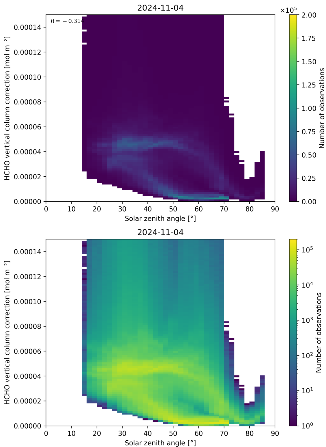
Figure 178: Scatter density plot of “Solar zenith angle” against “HCHO vertical column correction” for 2024-11-04 to 2024-11-05.
