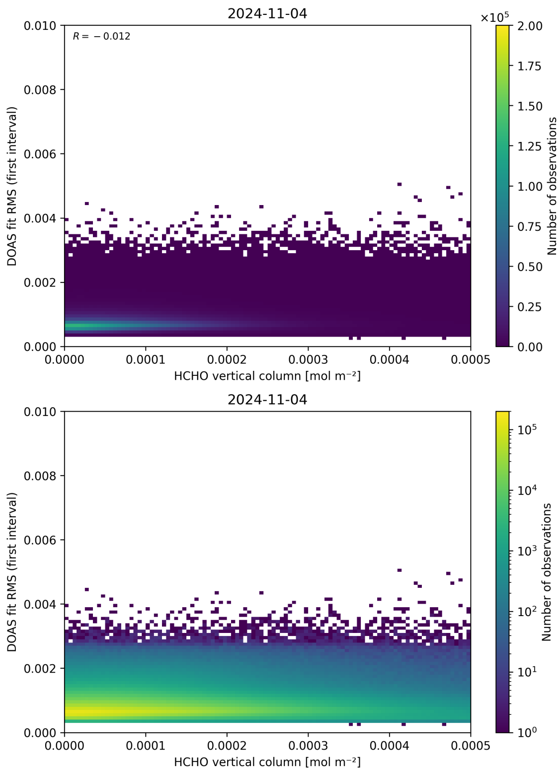
Figure 123: Scatter density plot of “HCHO vertical column” against “DOAS fit RMS (first interval)” for 2024-11-04 to 2024-11-05.
