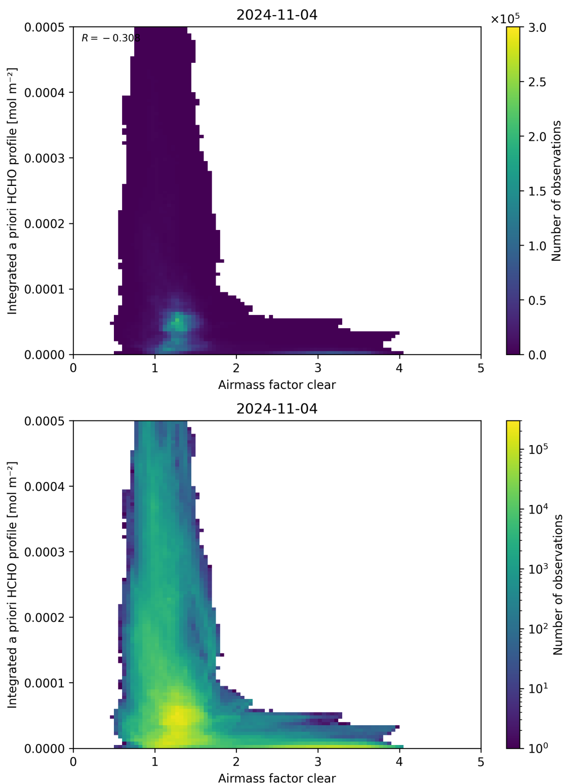
Figure 76: Scatter density plot of “Airmass factor clear” against “Integrated a priori HCHO profile” for 2024-11-04 to 2024-11-05.
