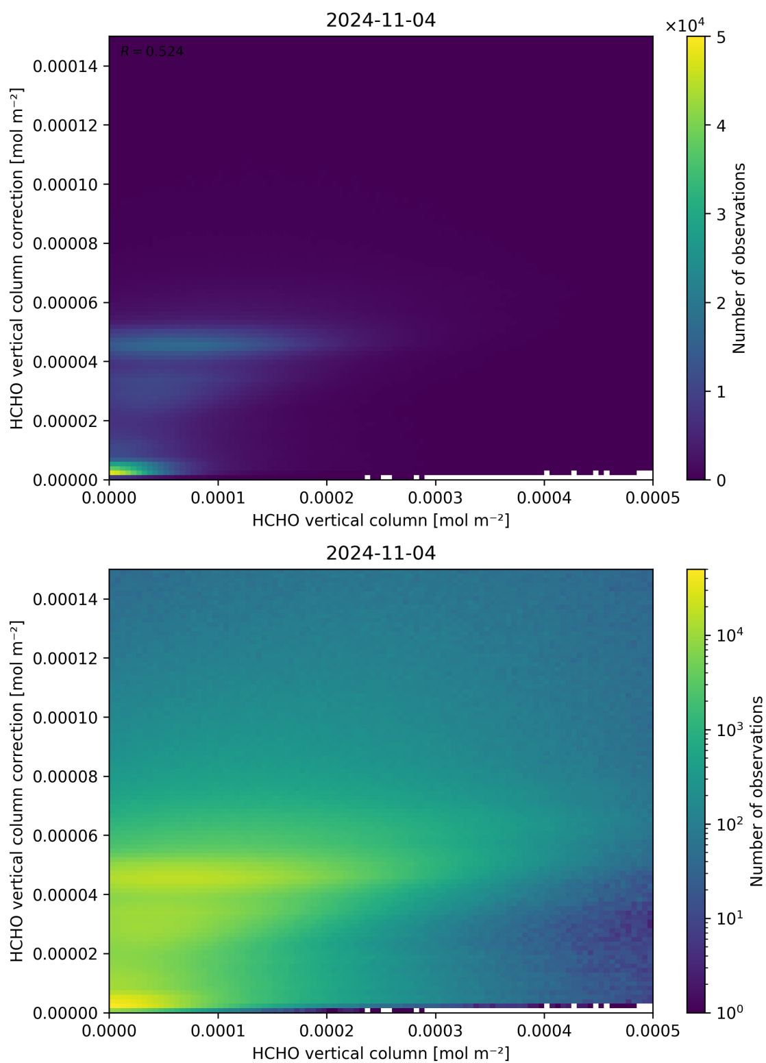
Figure 133: Scatter density plot of “HCHO vertical column” against “HCHO vertical column correction” for 2024-11-04 to 2024-11-05.
