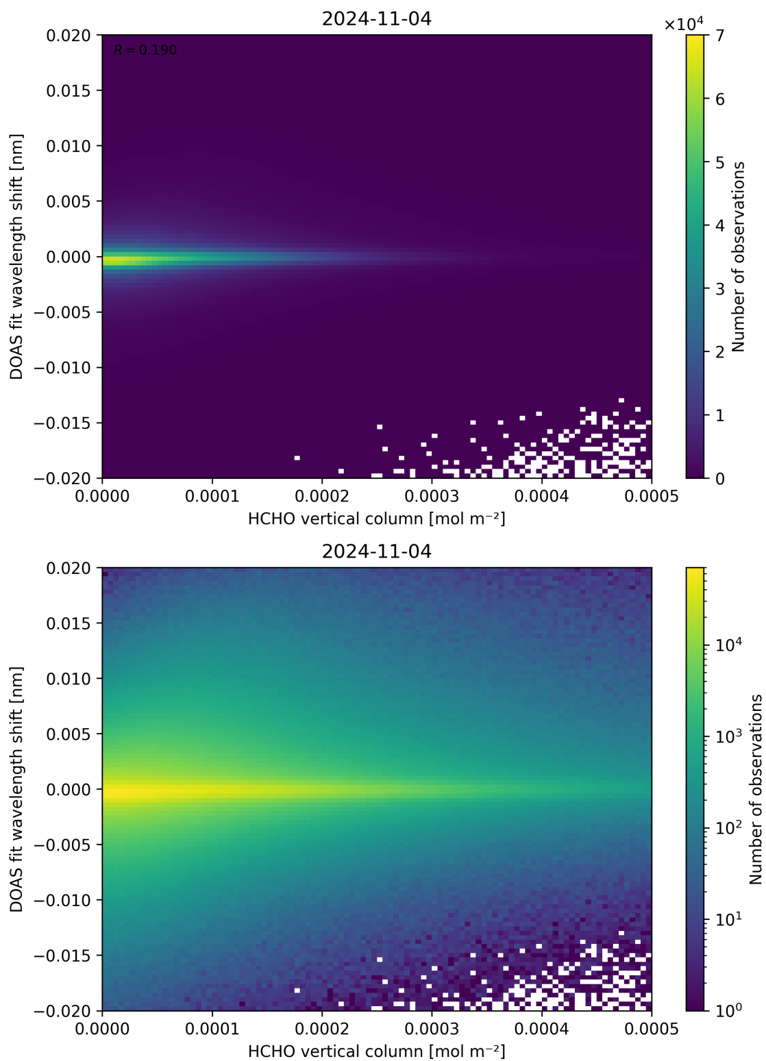
Figure 124: Scatter density plot of “HCHO vertical column” against “DOAS fit wavelength shift” for 2024-11-04 to 2024-11-05.
