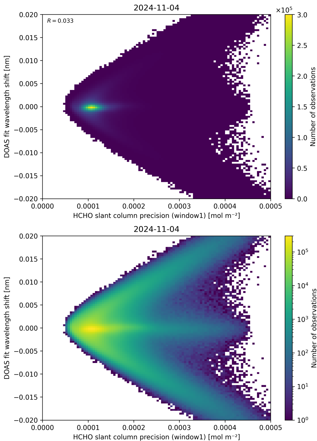
Figure 89: Scatter density plot of “HCHO slant column precision (window1)” against “DOAS fit wavelength shift” for 2024-11-04 to 2024-11-05.
