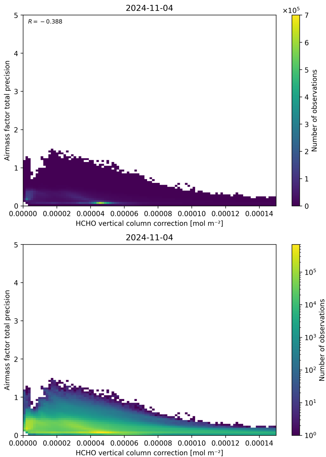
Figure 121: Scatter density plot of “HCHO vertical column correction” against “Airmass factor total precision” for 2024-11-04 to 2024-11-05.
