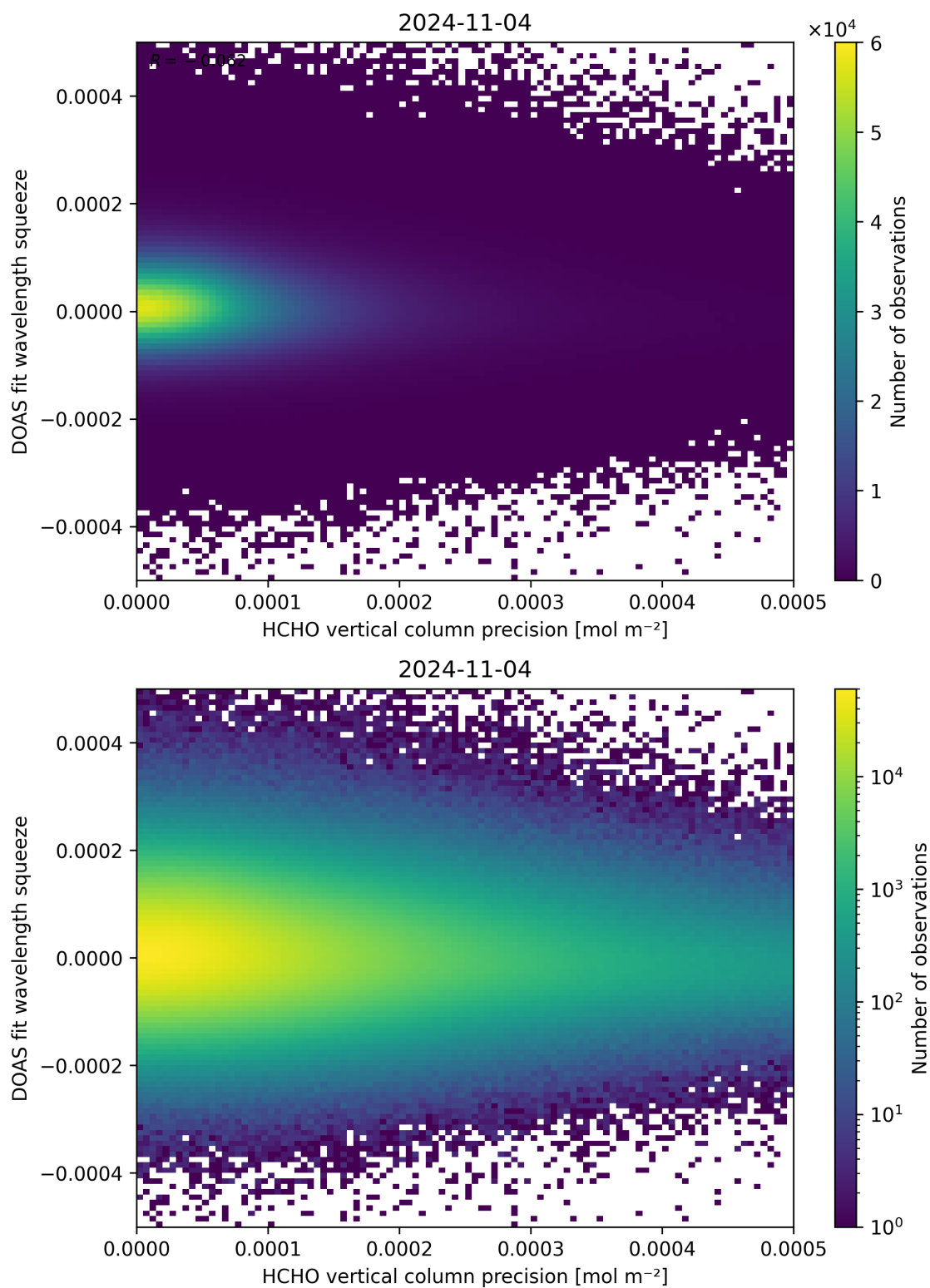
Figure 138: Scatter density plot of “HCHO vertical column precision” against “DOAS fit wavelength squeeze” for 2024-11-04 to 2024-11-05.
