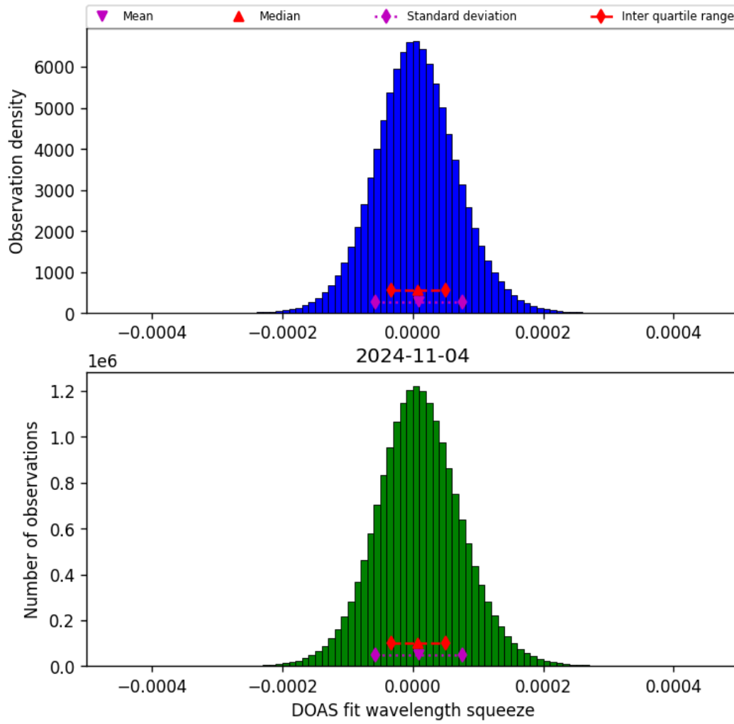
Figure 45: Histogram of “DOAS fit wavelength squeeze” for 2024-11-04 to 2024-11-05
