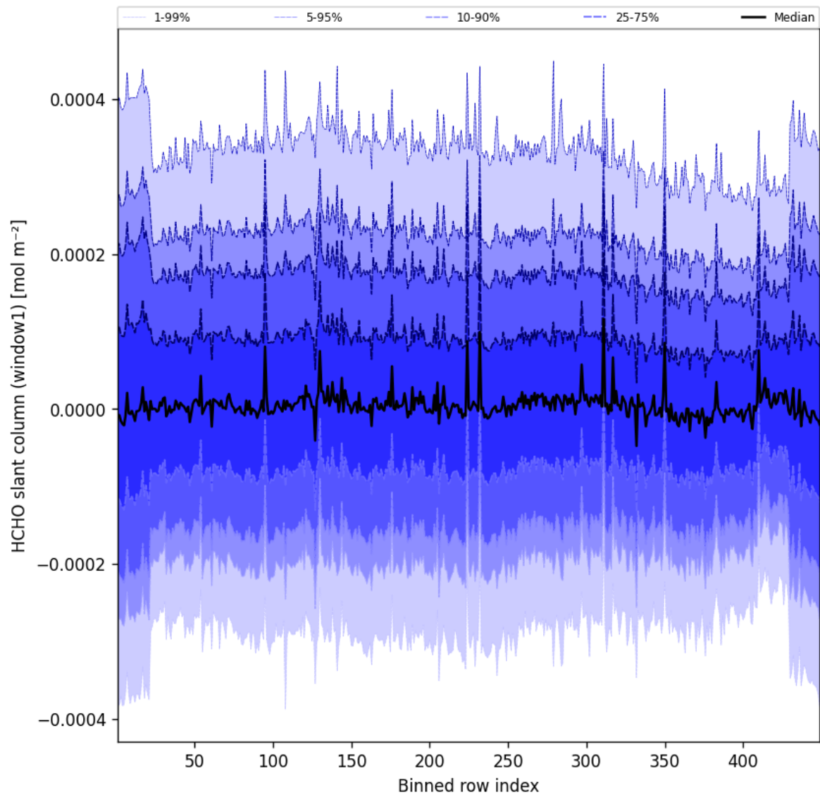
Figure 52: Along track statistics of “HCHO slant column (window1)” for 2024-11-04 to 2024-11-05
