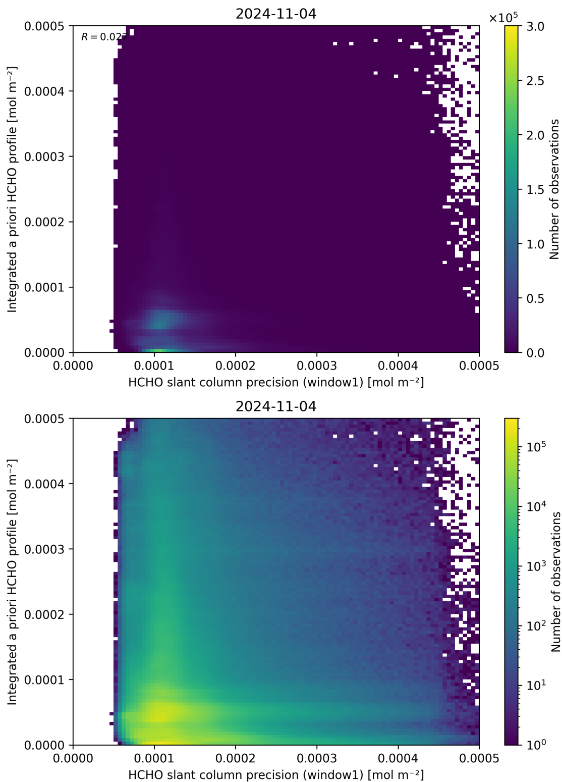
Figure 96: Scatter density plot of “HCHO slant column precision (window1)” against “Integrated a priori HCHO profile” for 2024-11-04 to 2024-11-05.
