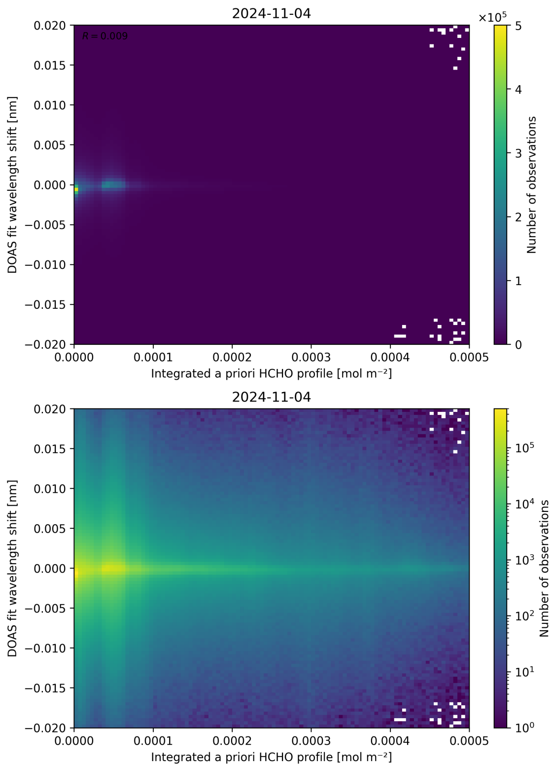
Figure 149: Scatter density plot of “Integrated a priori HCHO profile” against “DOAS fit wavelength shift” for 2024-11-04 to 2024-11-05.
