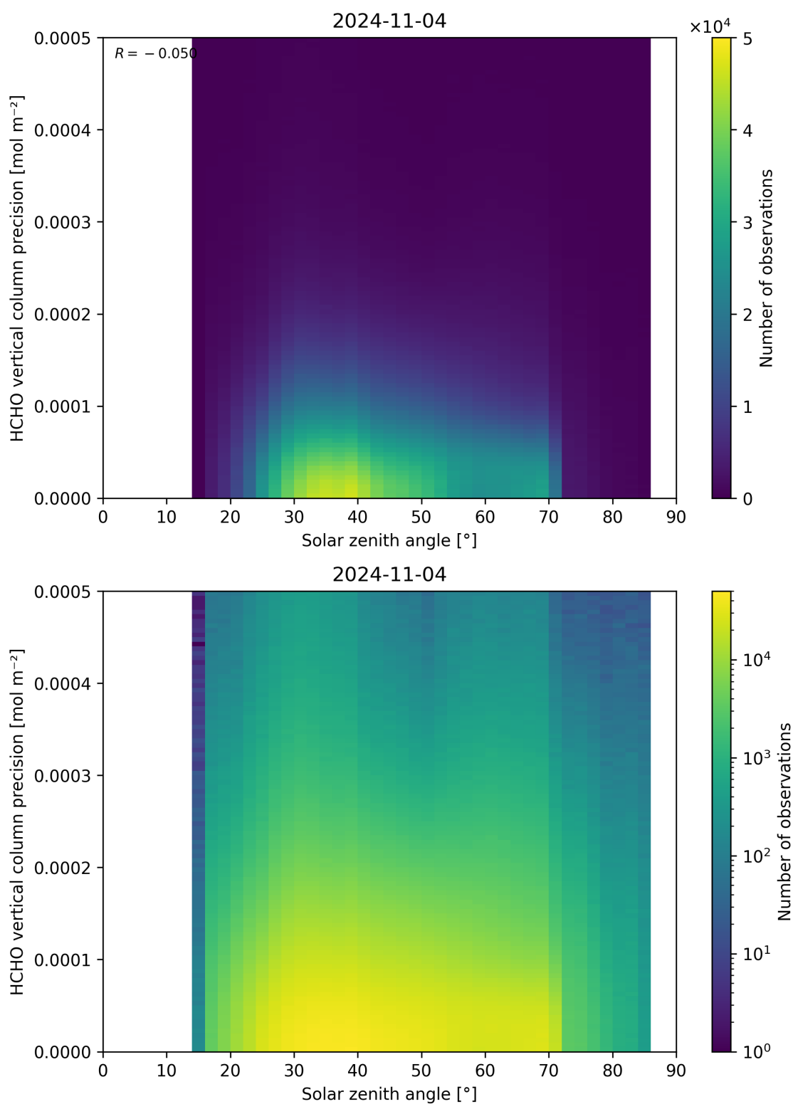
Figure 179: Scatter density plot of “Solar zenith angle” against “HCHO vertical column precision” for 2024-11-04 to 2024-11-05.
