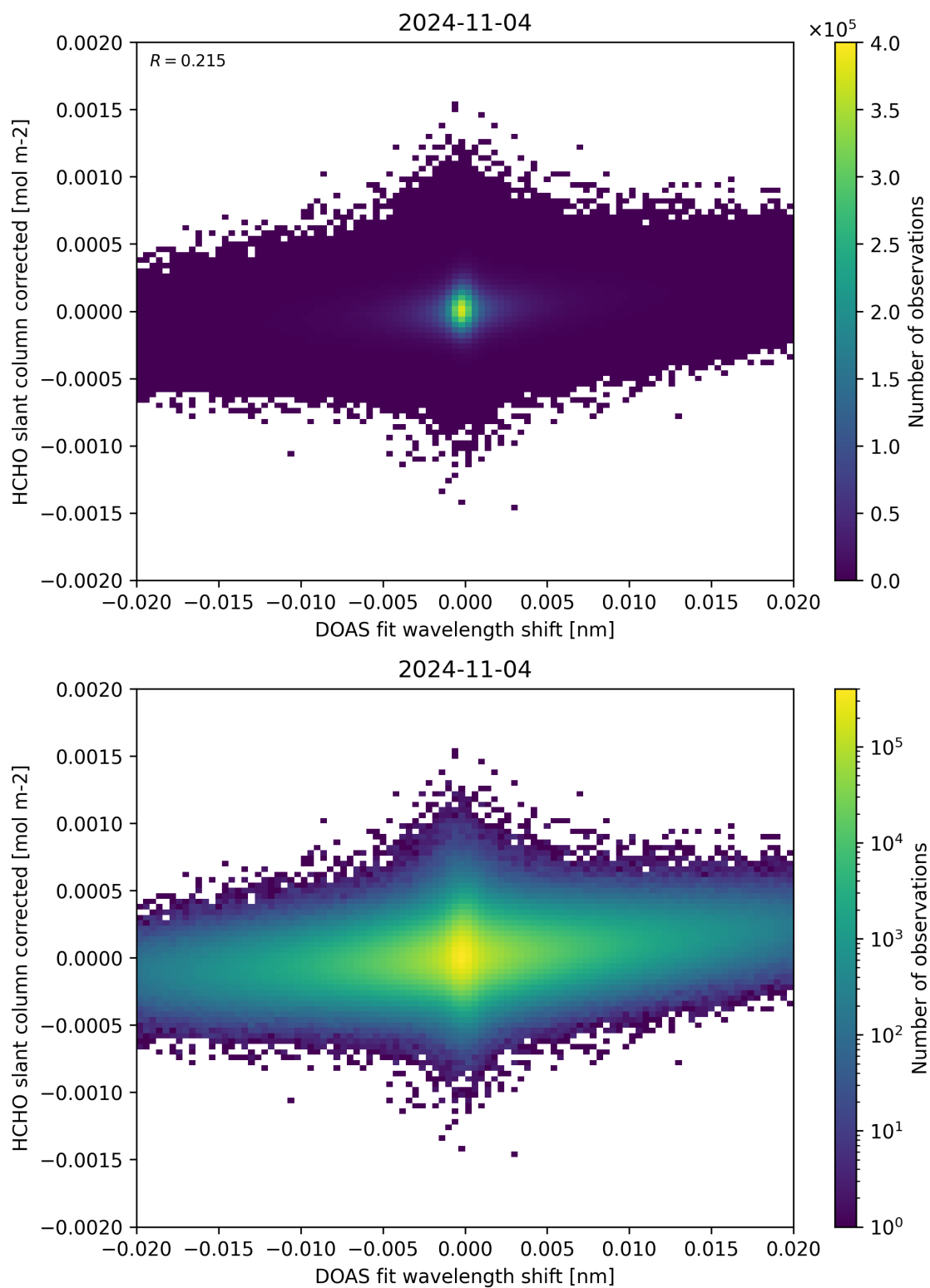
Figure 66: Scatter density plot of “DOAS fit wavelength shift” against “HCHO slant column corrected” for 2024-11-04 to 2024-11-05.
