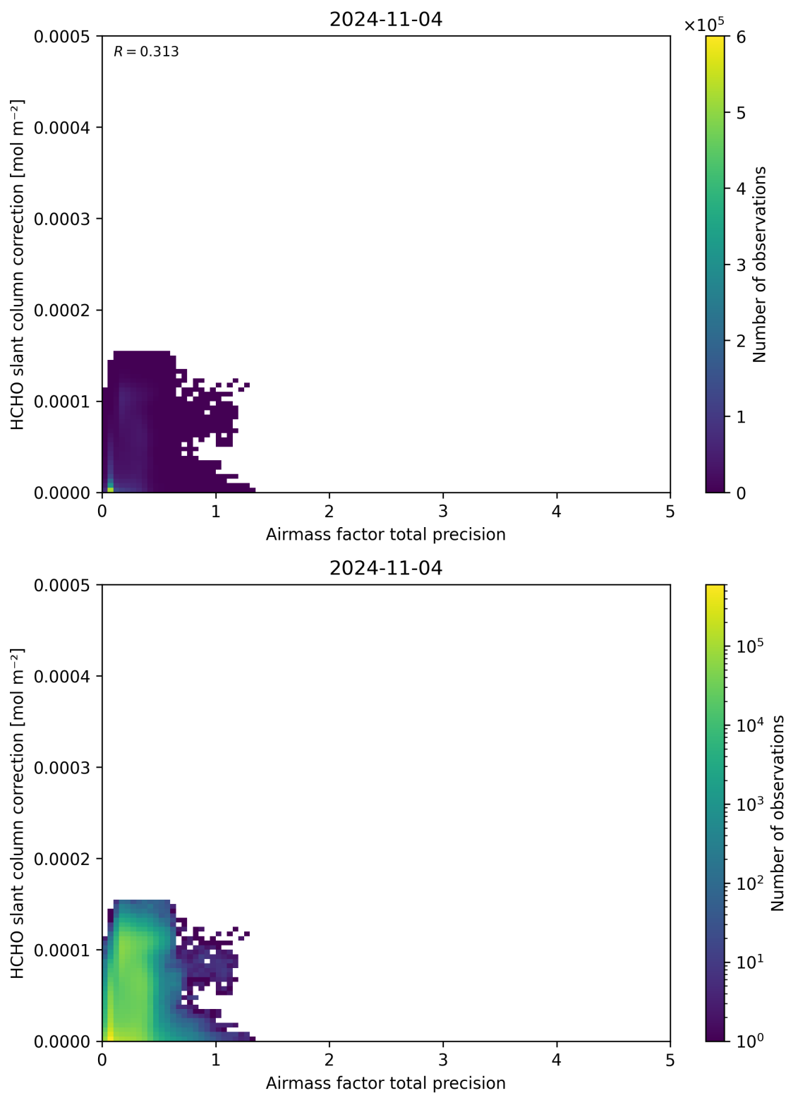
Figure 110: Scatter density plot of “Airmass factor total precision” against “HCHO slant column correction” for 2024-11-04 to 2024-11-05.
