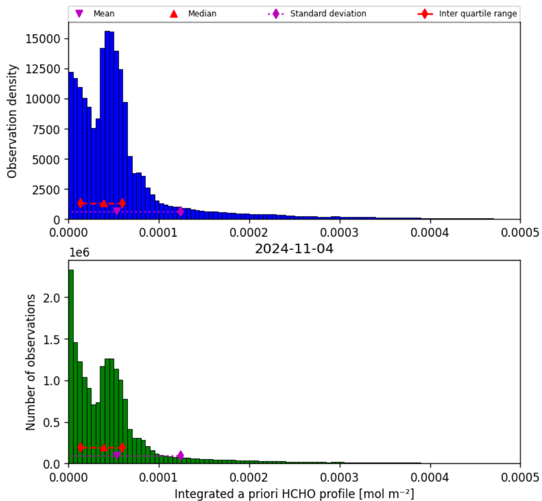
Figure 43: Histogram of “Integrated a priori HCHO profile” for 2024-11-04 to 2024-11-05
