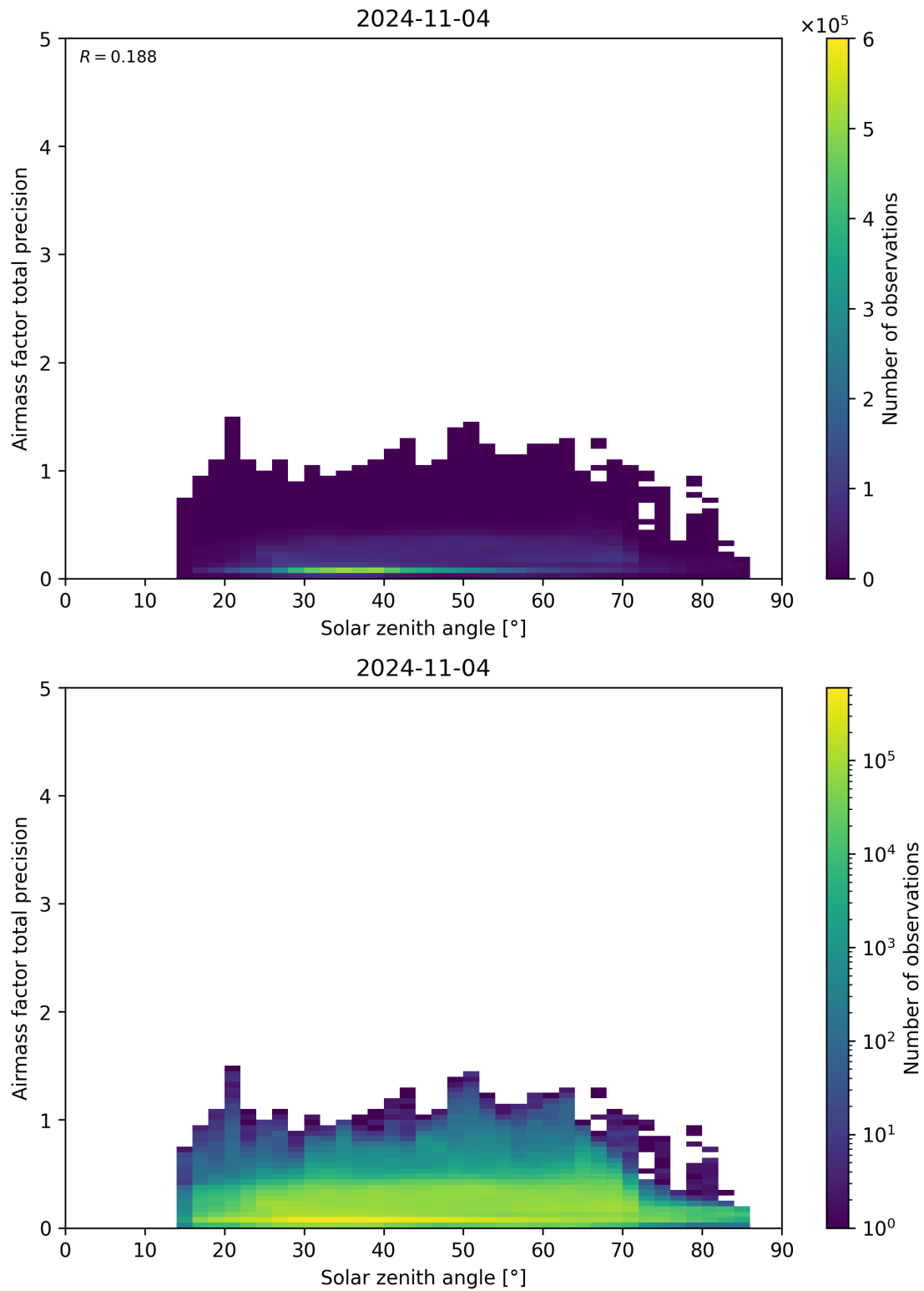
Figure 176: Scatter density plot of “Solar zenith angle” against “Airmass factor total precision” for 2024-11-04 to 2024-11-05.
