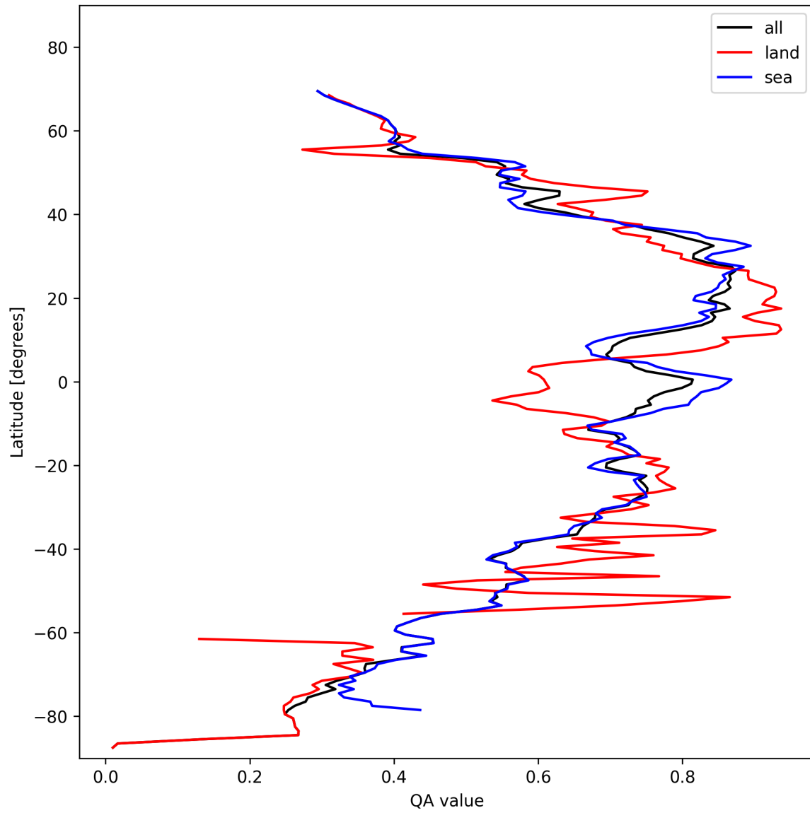
Figure 20: Zonal average of “QA value” for 2024-11-04 to 2024-11-05.
