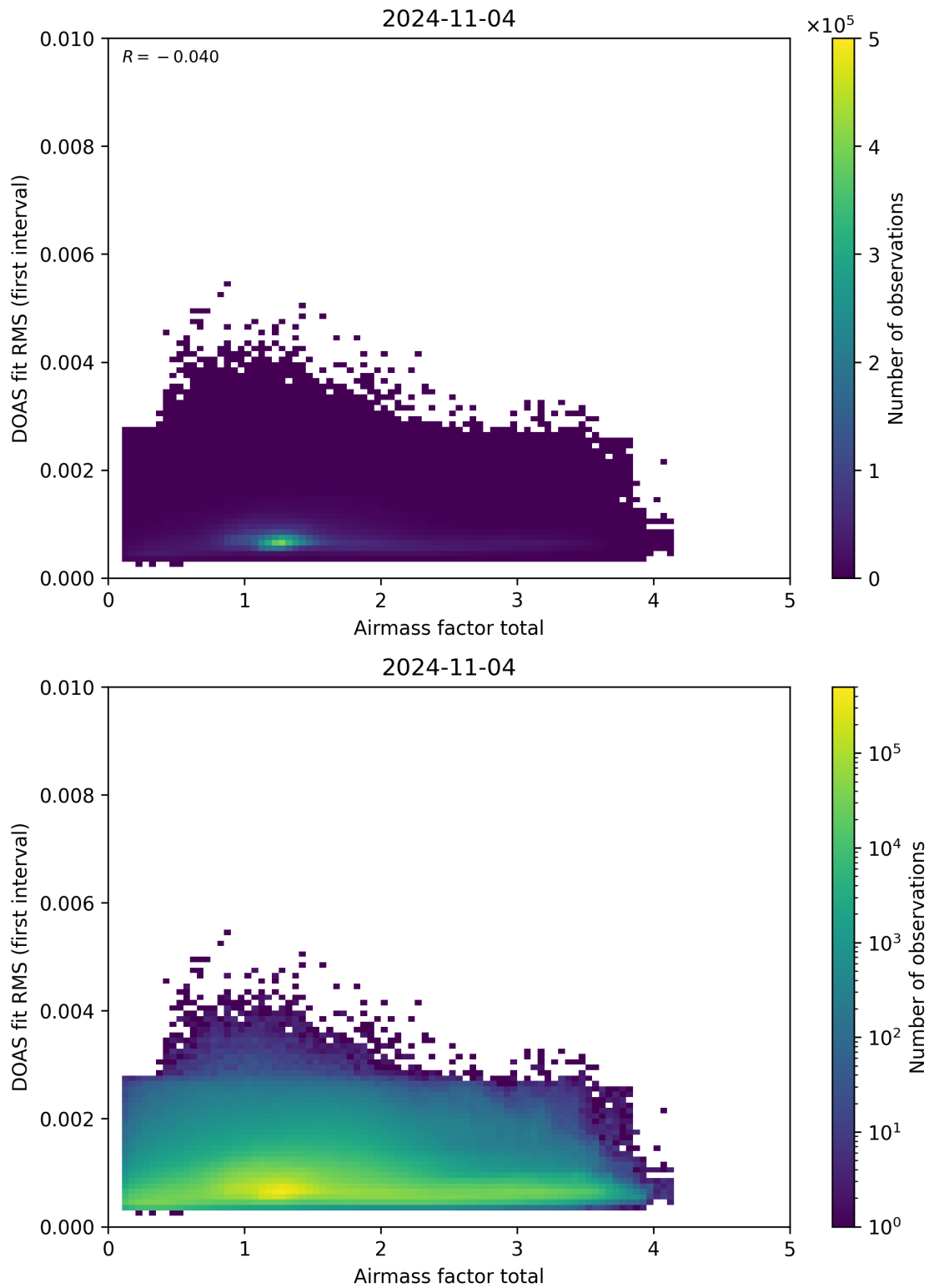
Figure 97: Scatter density plot of “Airmass factor total” against “DOAS fit RMS (first interval)” for 2024-11-04 to 2024-11-05.
