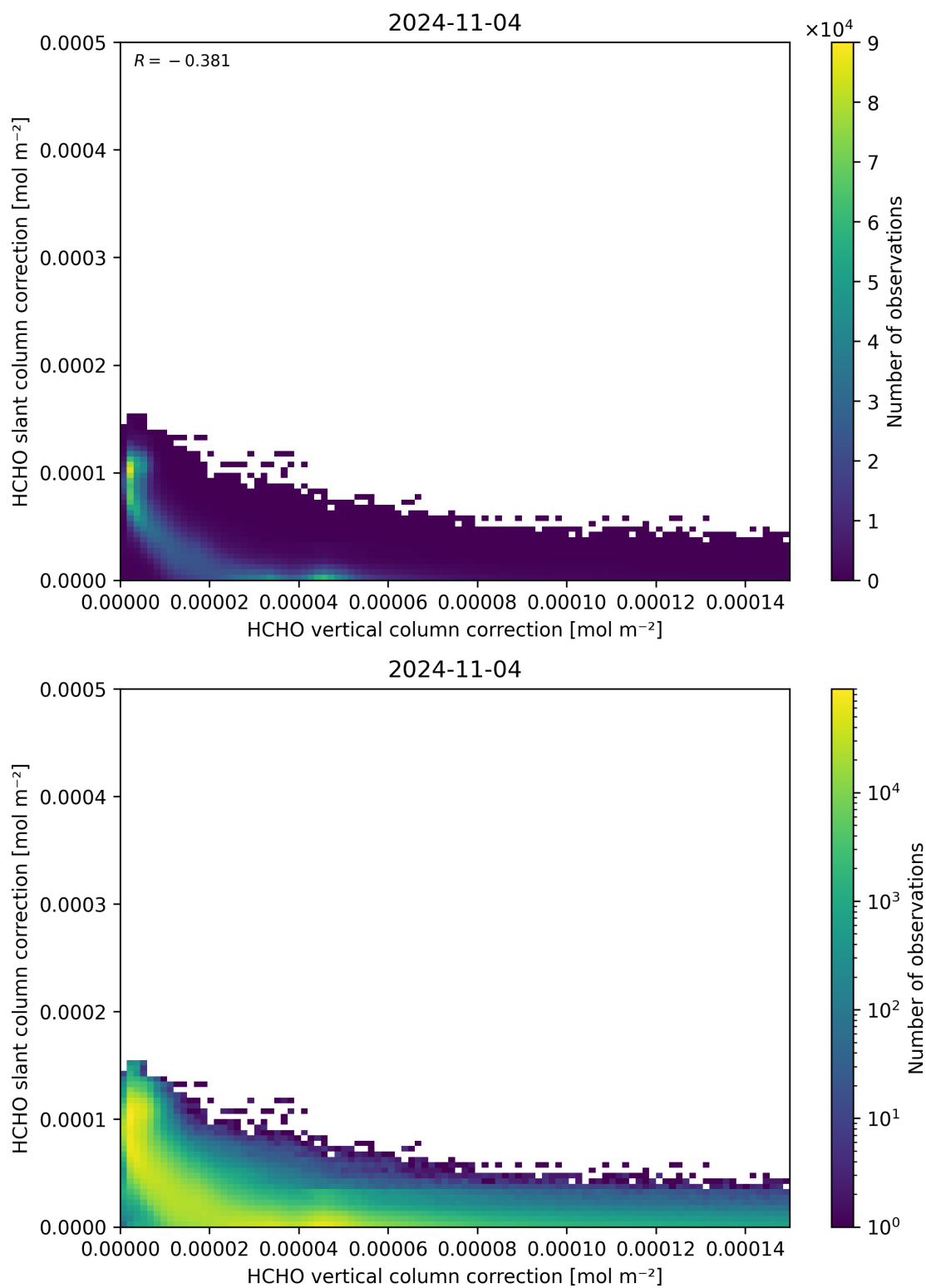
Figure 117: Scatter density plot of “HCHO vertical column correction” against “HCHO slant column correction” for 2024-11-04 to 2024-11-05.
