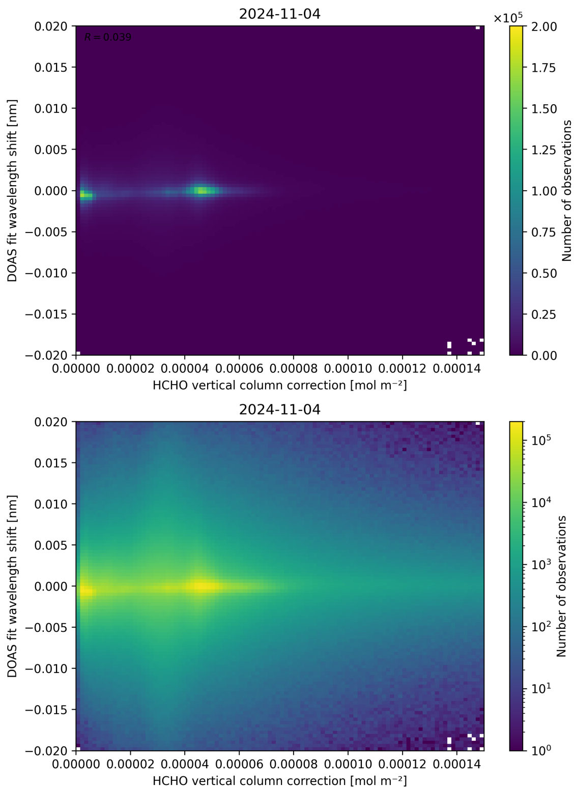
Figure 113: Scatter density plot of “HCHO vertical column correction” against “DOAS fit wavelength shift” for 2024-11-04 to 2024-11-05.
