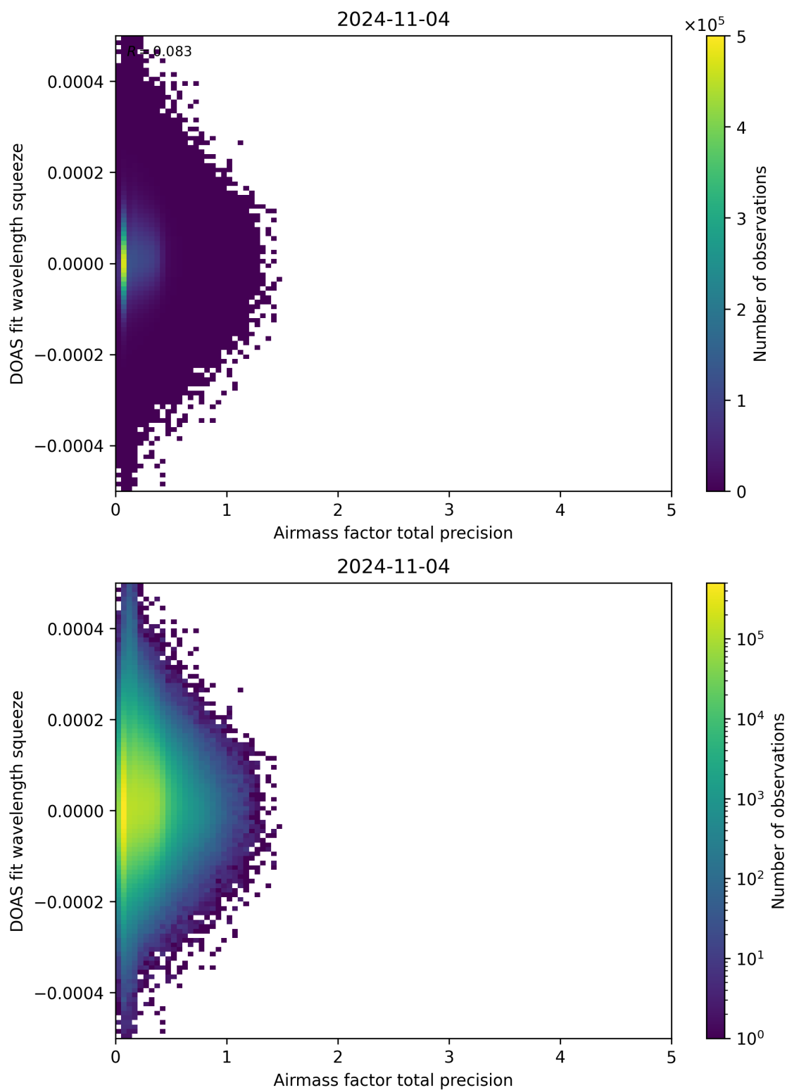
Figure 107: Scatter density plot of “Airmass factor total precision” against “DOAS fit wavelength squeeze” for 2024-11-04 to 2024-11-05.
