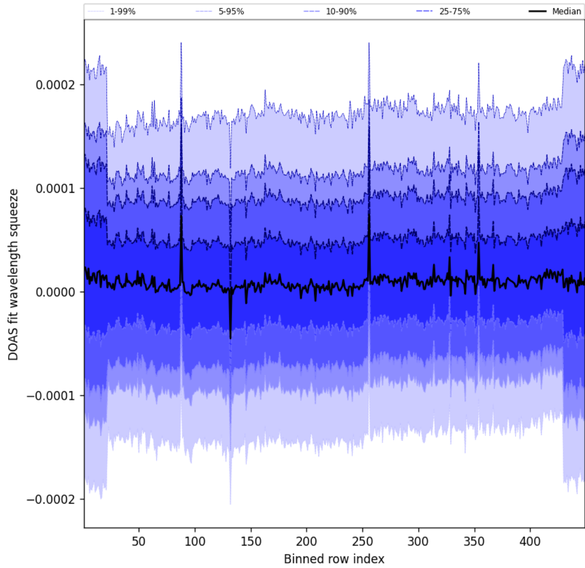
Figure 59: Along track statistics of “DOAS fit wavelength squeeze” for 2024-11-04 to 2024-11-05
