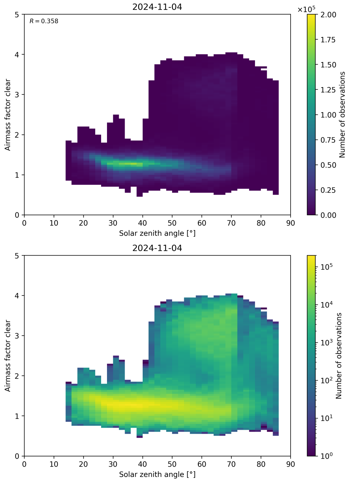
Figure 170: Scatter density plot of “Solar zenith angle” against “Airmass factor clear” for 2024-11-04 to 2024-11-05.
