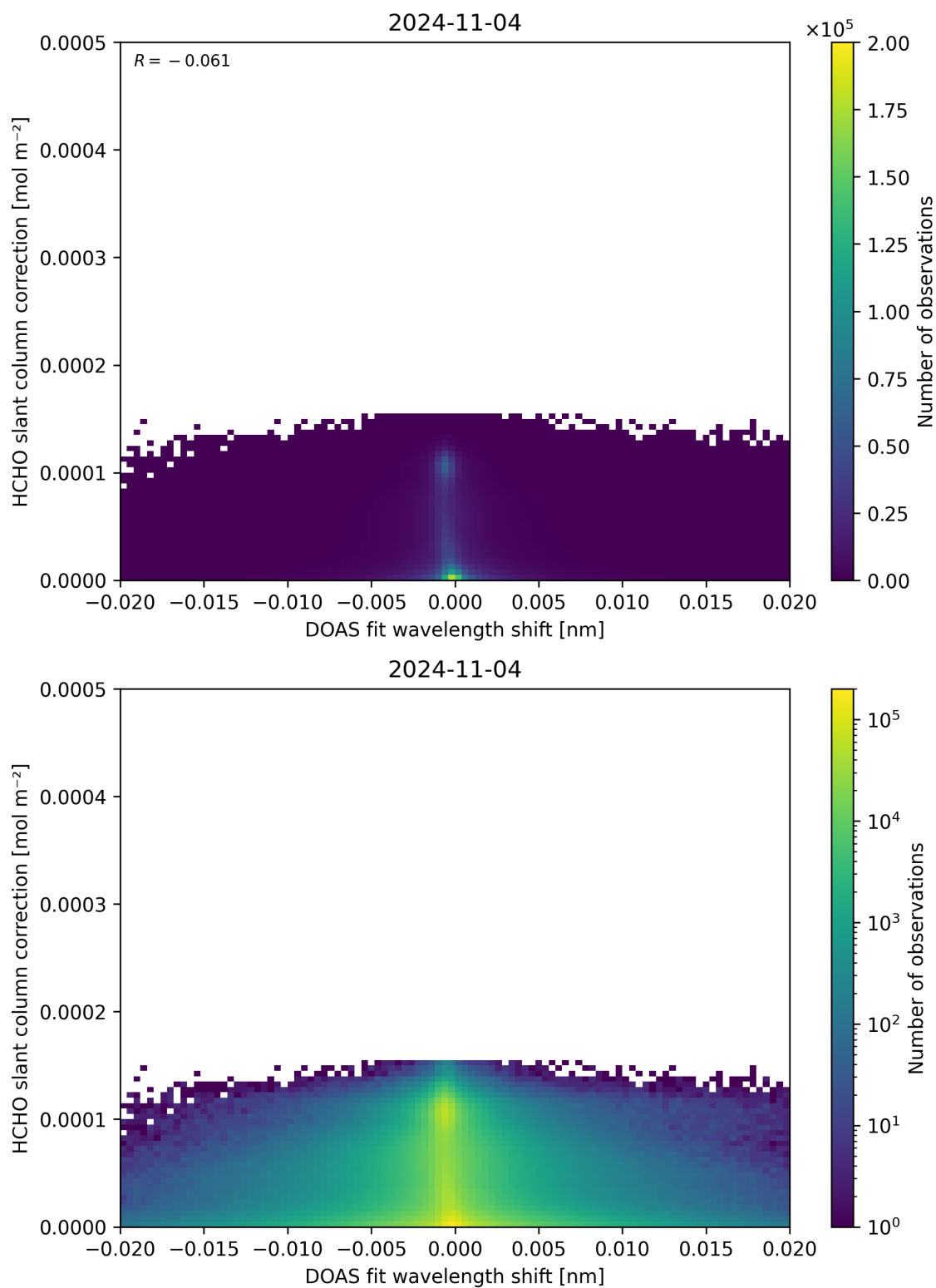
Figure 67: Scatter density plot of “DOAS fit wavelength shift” against “HCHO slant column correction” for 2024-11-04 to 2024-11-05.
