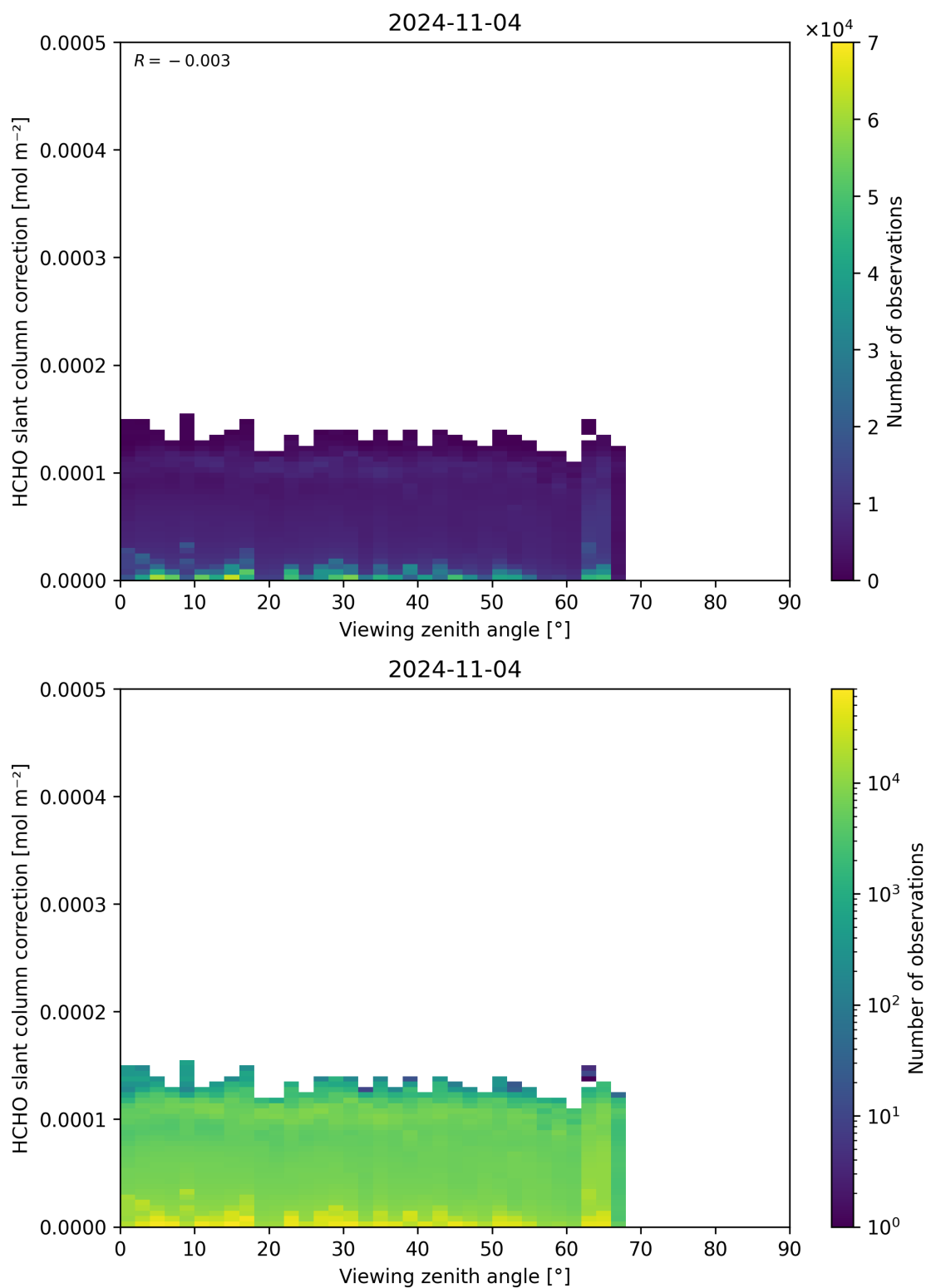
Figure 187: Scatter density plot of “Viewing zenith angle” against “HCHO slant column correction” for 2024-11-04 to 2024-11-05.
