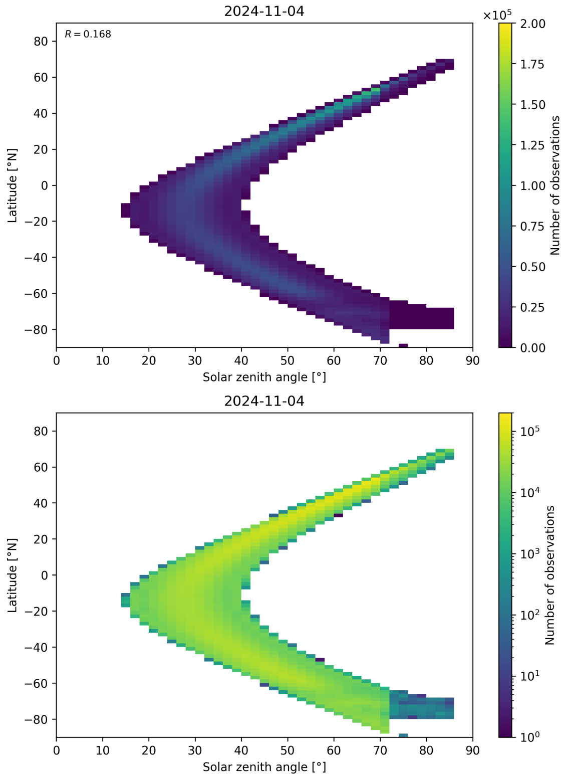
Figure 181: Scatter density plot of “Solar zenith angle” against “Latitude” for 2024-11-04 to 2024-11-05.
