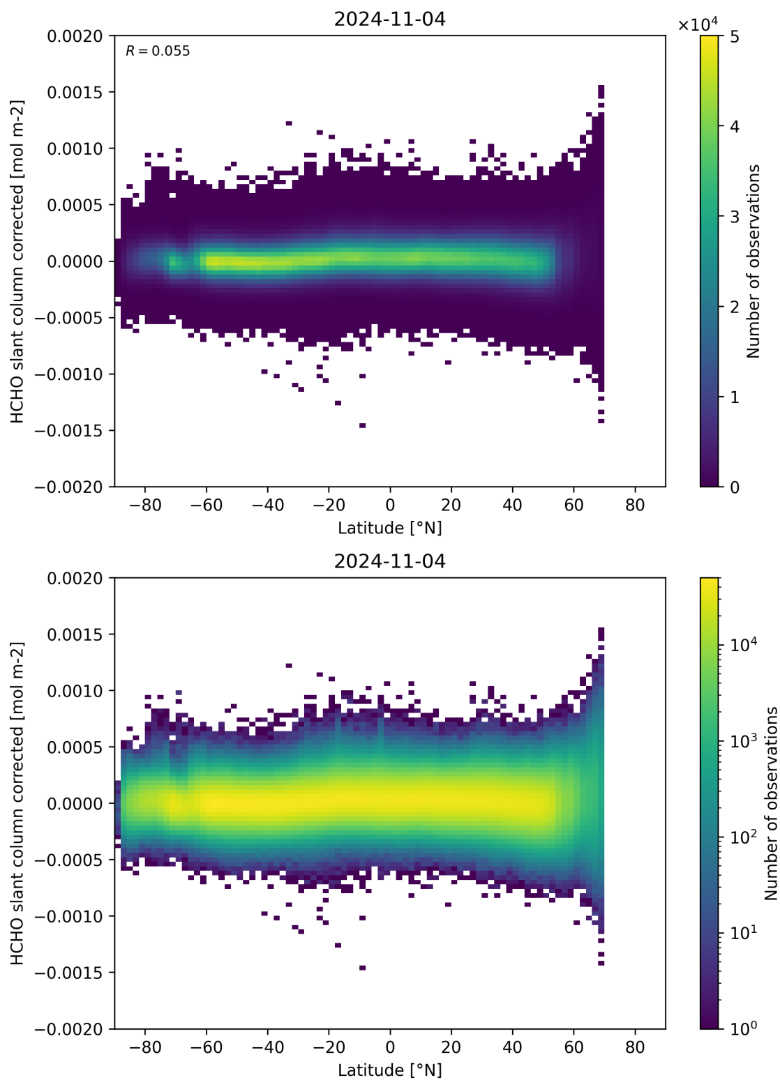
Figure 157: Scatter density plot of “Latitude” against “HCHO slant column corrected” for 2024-11-04 to 2024-11-05.
