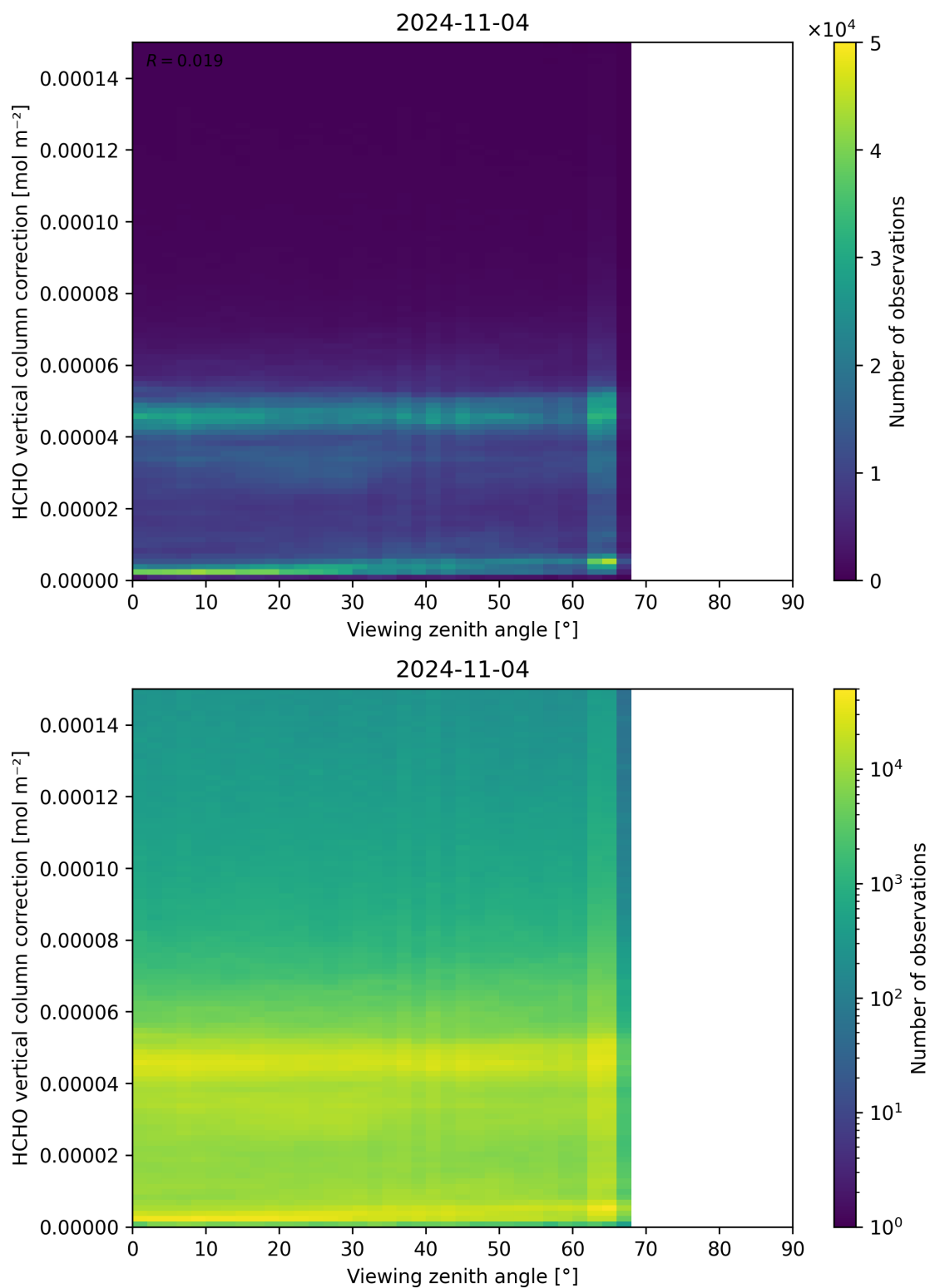
Figure 193: Scatter density plot of “Viewing zenith angle” against “HCHO vertical column correction” for 2024-11-04 to 2024-11-05.
