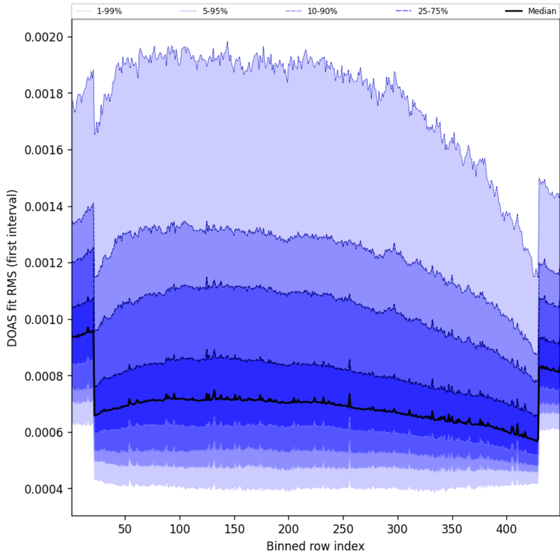
Figure 60: Along track statistics of “DOAS fit RMS (first interval)” for 2024-11-04 to 2024-11-05
