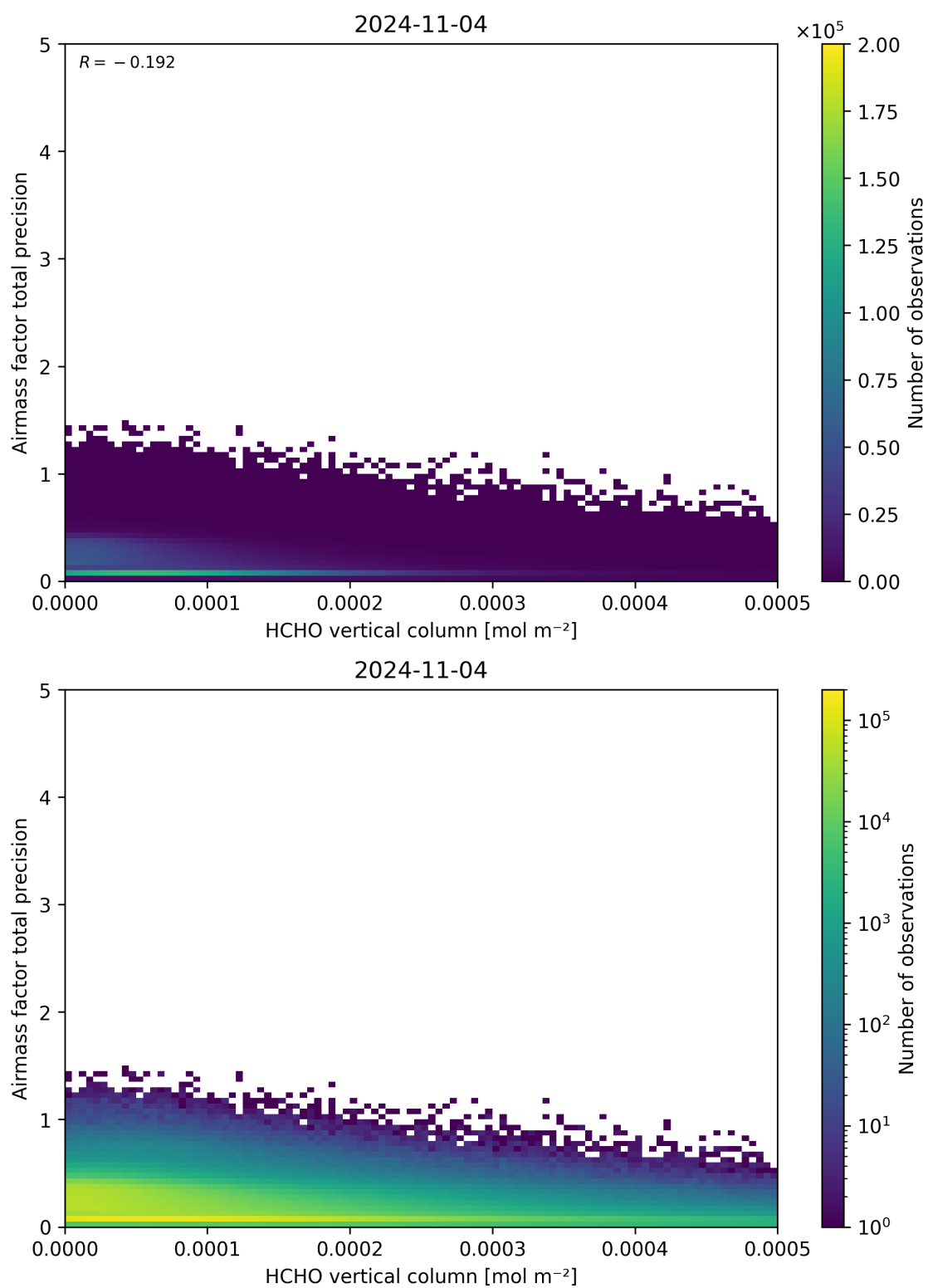
Figure 132: Scatter density plot of “HCHO vertical column” against “Airmass factor total precision” for 2024-11-04 to 2024-11-05.
