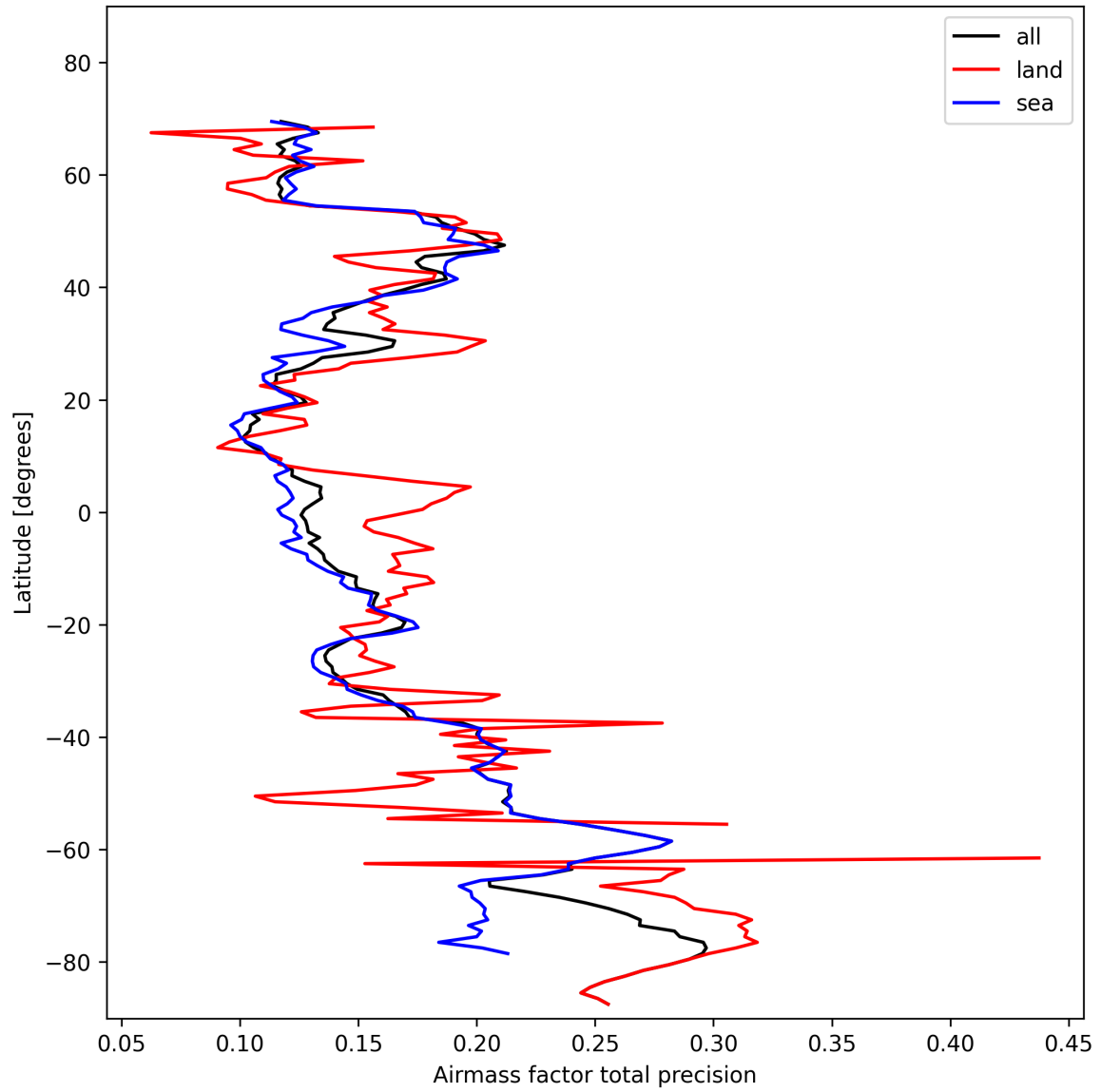
Figure 27: Zonal average of “Airmass factor total precision” for 2024-11-04 to 2024-11-05.
