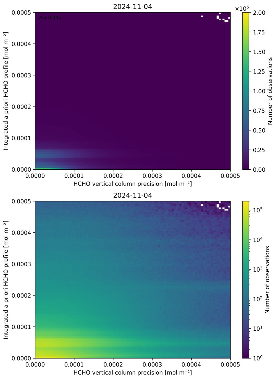
Figure 147: Scatter density plot of “HCHO vertical column precision” against “Integrated a priori HCHO profile” for 2024-11-04 to 2024-11-05.
