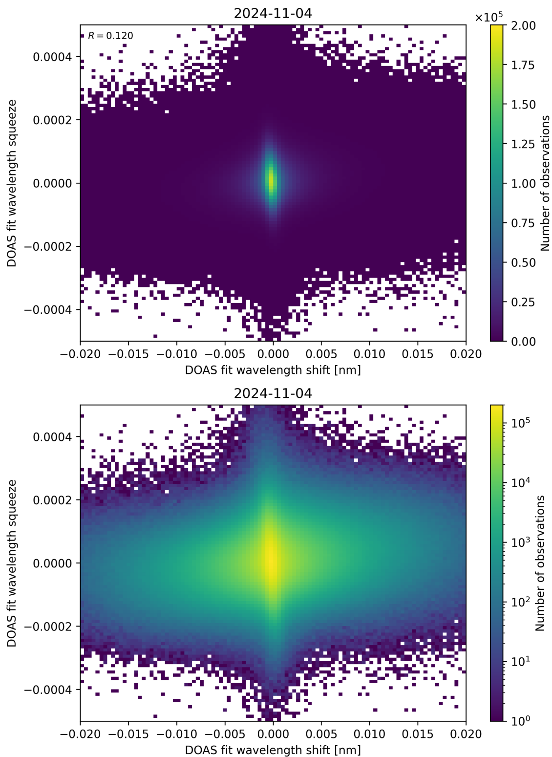
Figure 65: Scatter density plot of “DOAS fit wavelength shift” against “DOAS fit wavelength squeeze” for 2024-11-04 to 2024-11-05.
