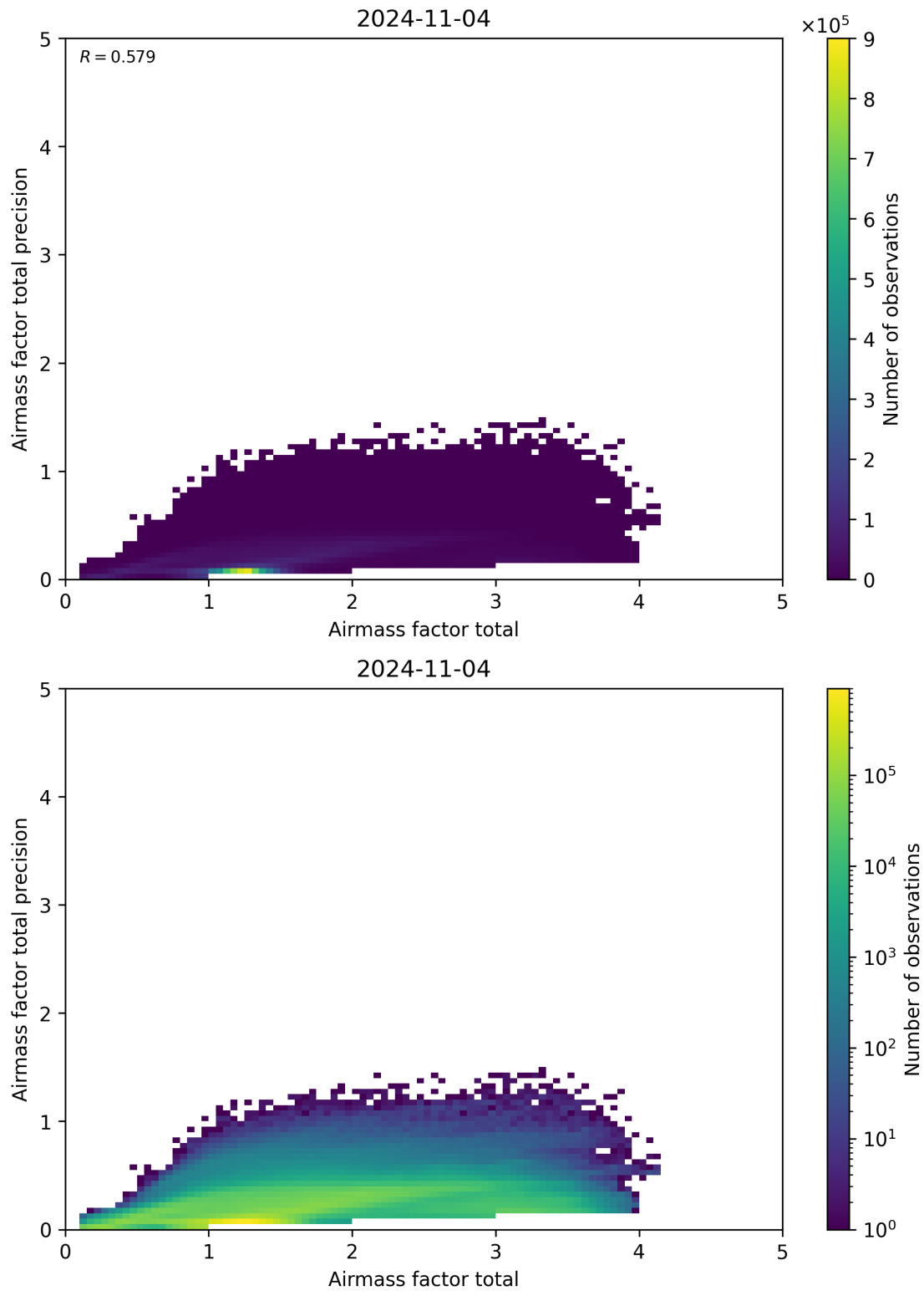
Figure 103: Scatter density plot of “Airmass factor total” against “Airmass factor total precision” for 2024-11-04 to 2024-11-05.
