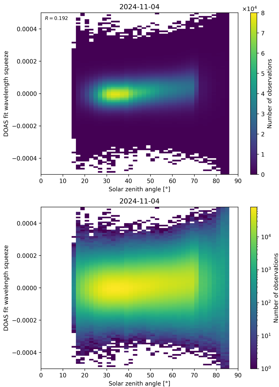
Figure 169: Scatter density plot of “Solar zenith angle” against “DOAS fit wavelength squeeze” for 2024-11-04 to 2024-11-05.
