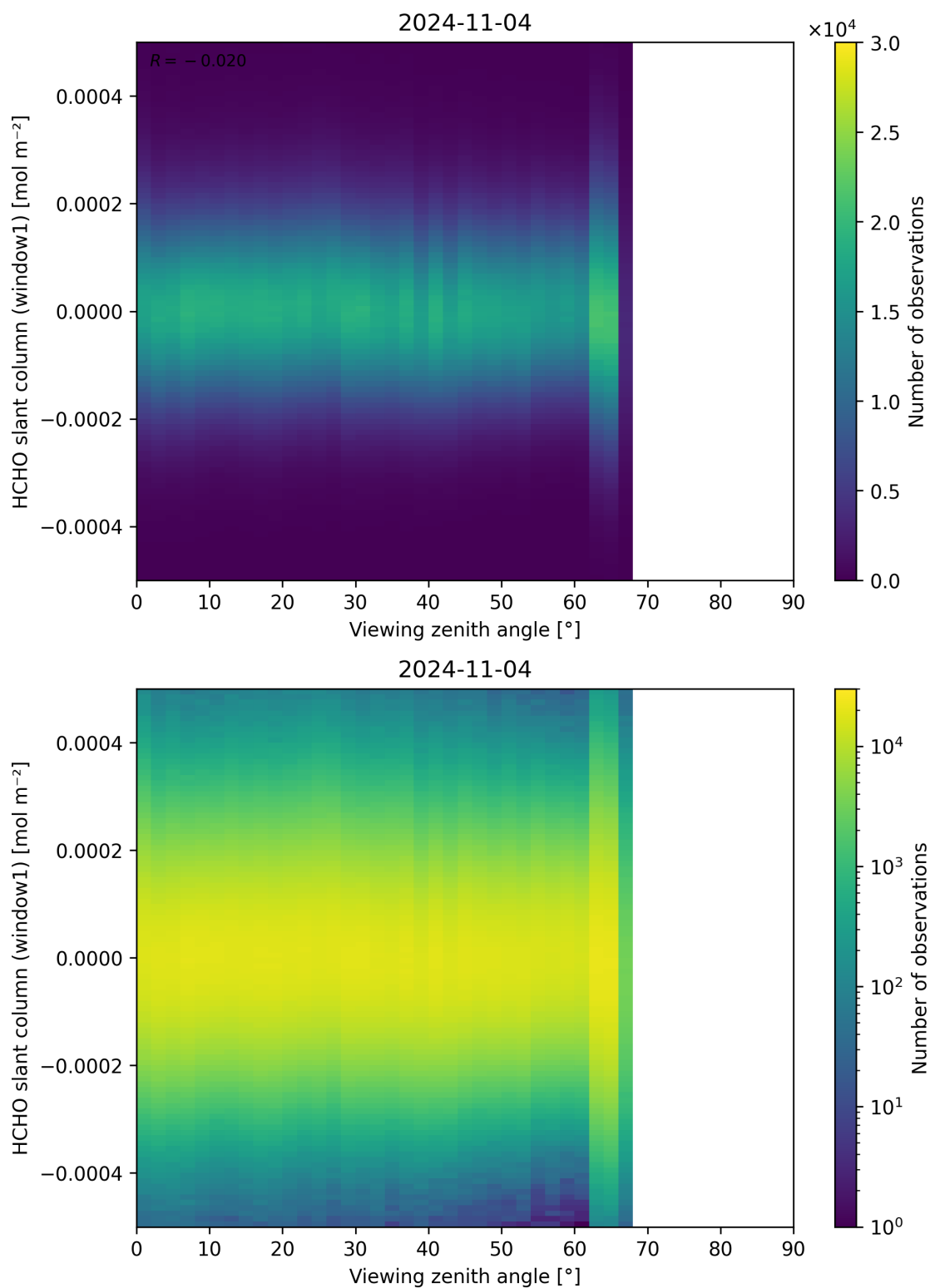
Figure 188: Scatter density plot of “Viewing zenith angle” against “HCHO slant column (window1)” for 2024-11-04 to 2024-11-05.
