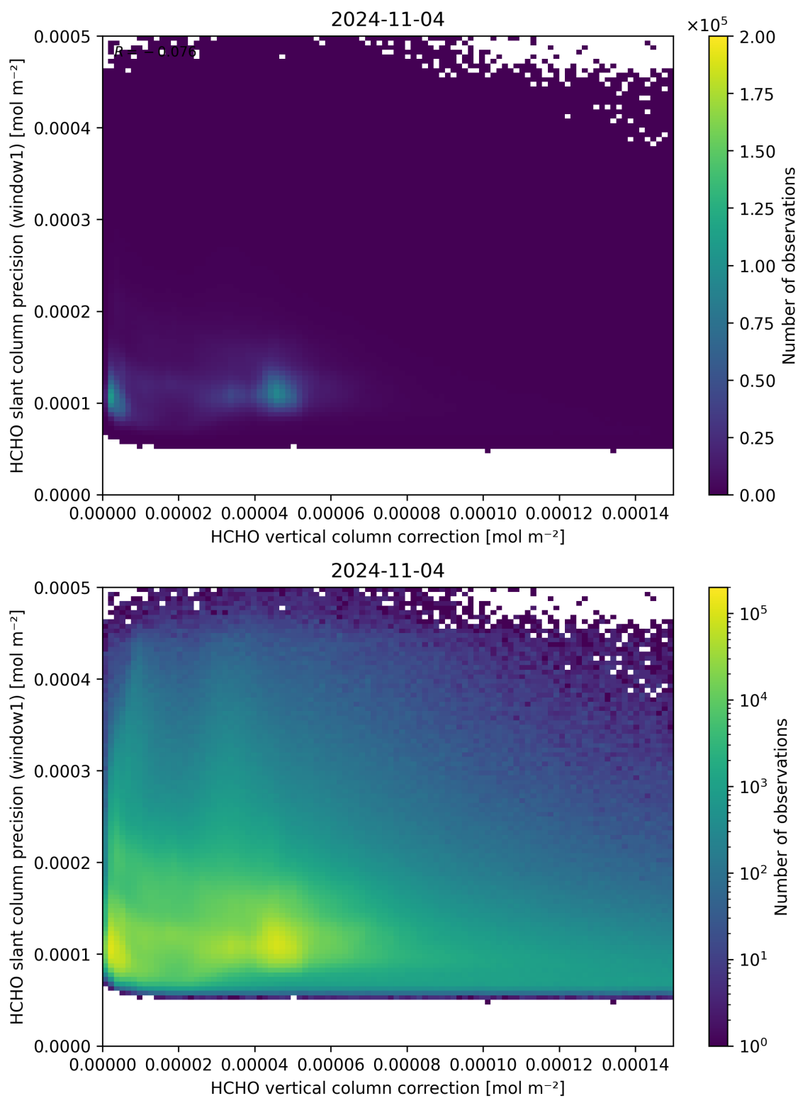
Figure 119: Scatter density plot of “HCHO vertical column correction” against “HCHO slant column precision (window1)” for 2024-11-04 to 2024-11-05.
