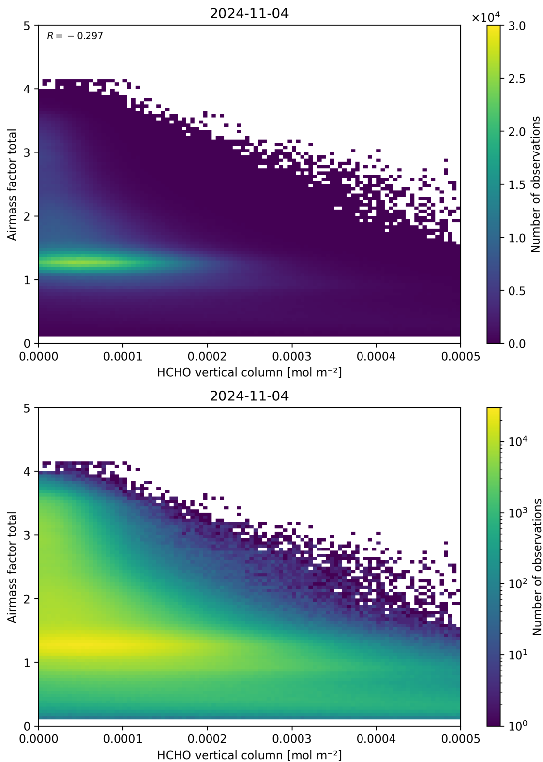
Figure 131: Scatter density plot of “HCHO vertical column” against “Airmass factor total” for 2024-11-04 to 2024-11-05.
