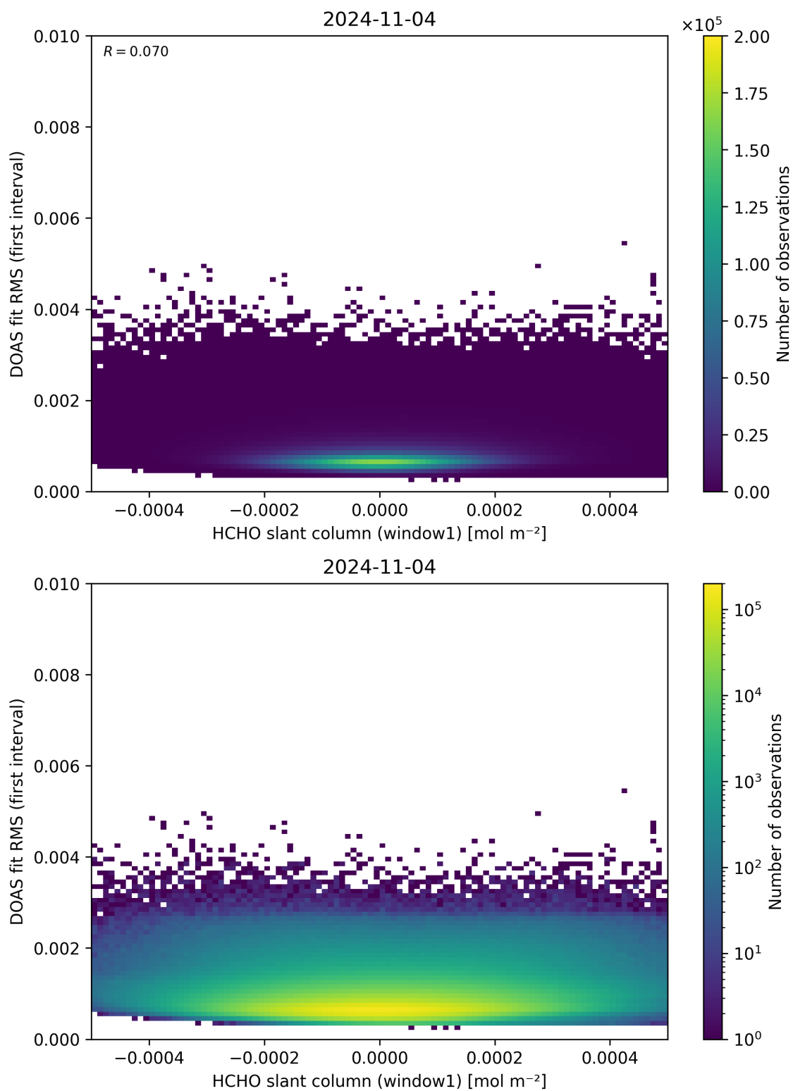
Figure 78: Scatter density plot of “HCHO slant column (window1)” against “DOAS fit RMS (first interval)” for 2024-11-04 to 2024-11-05.
