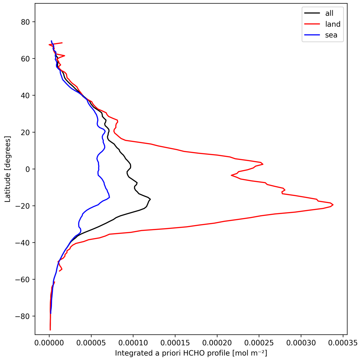
Figure 29: Zonal average of “Integrated a priori HCHO profile” for 2024-11-04 to 2024-11-05.
