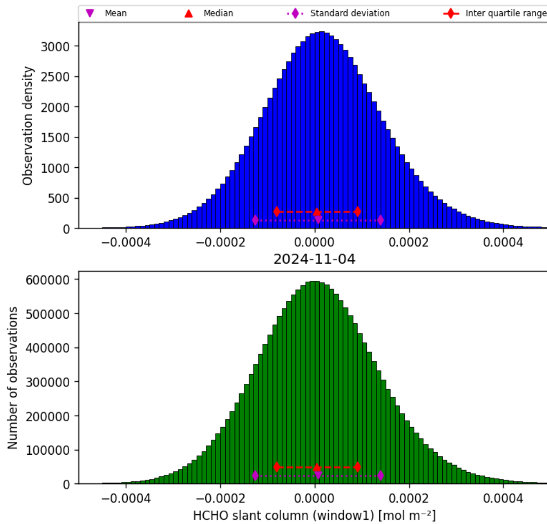
Figure 38: Histogram of “HCHO slant column (window1)” for 2024-11-04 to 2024-11-05
