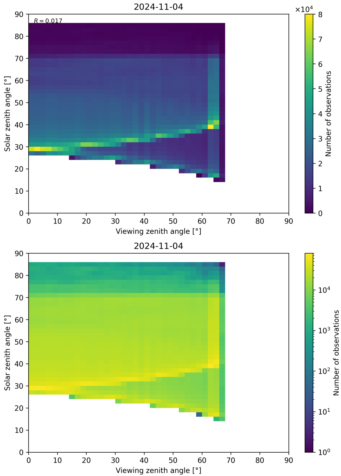
Figure 197: Scatter density plot of “Viewing zenith angle” against “Solar zenith angle” for 2024-11-04 to 2024-11-05.
