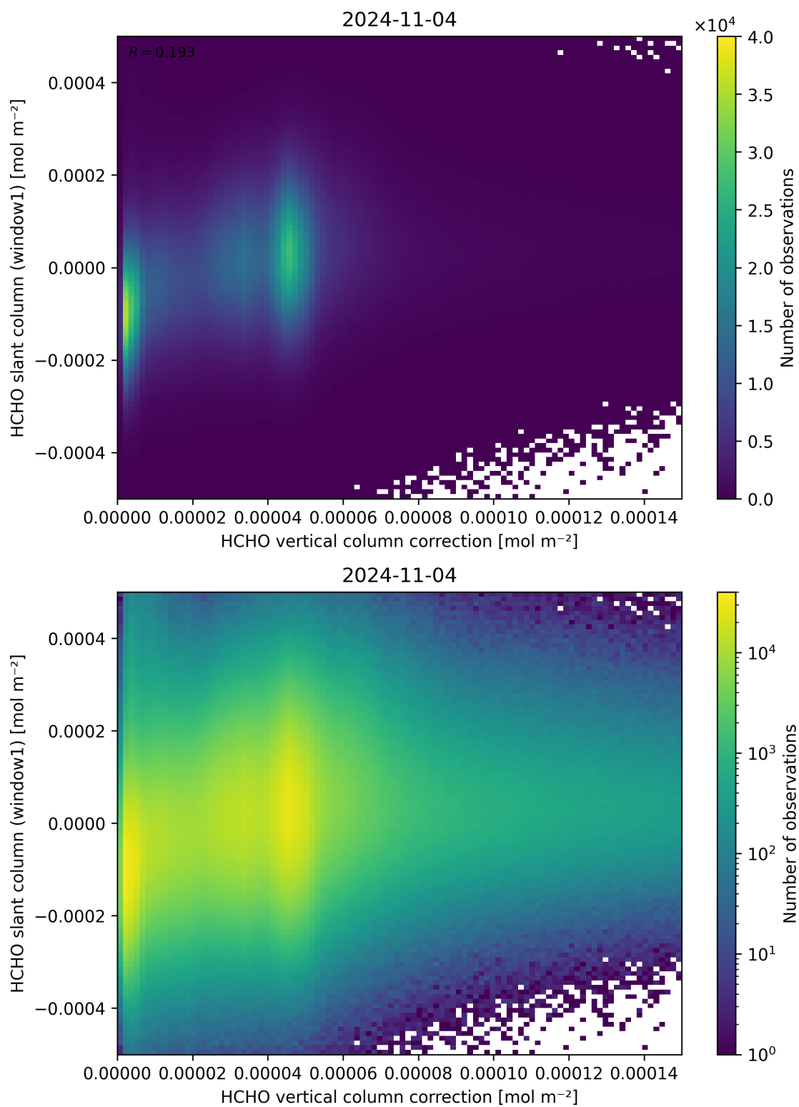
Figure 118: Scatter density plot of “HCHO vertical column correction” against “HCHO slant column (window1)” for 2024-11-04 to 2024-11-05.
