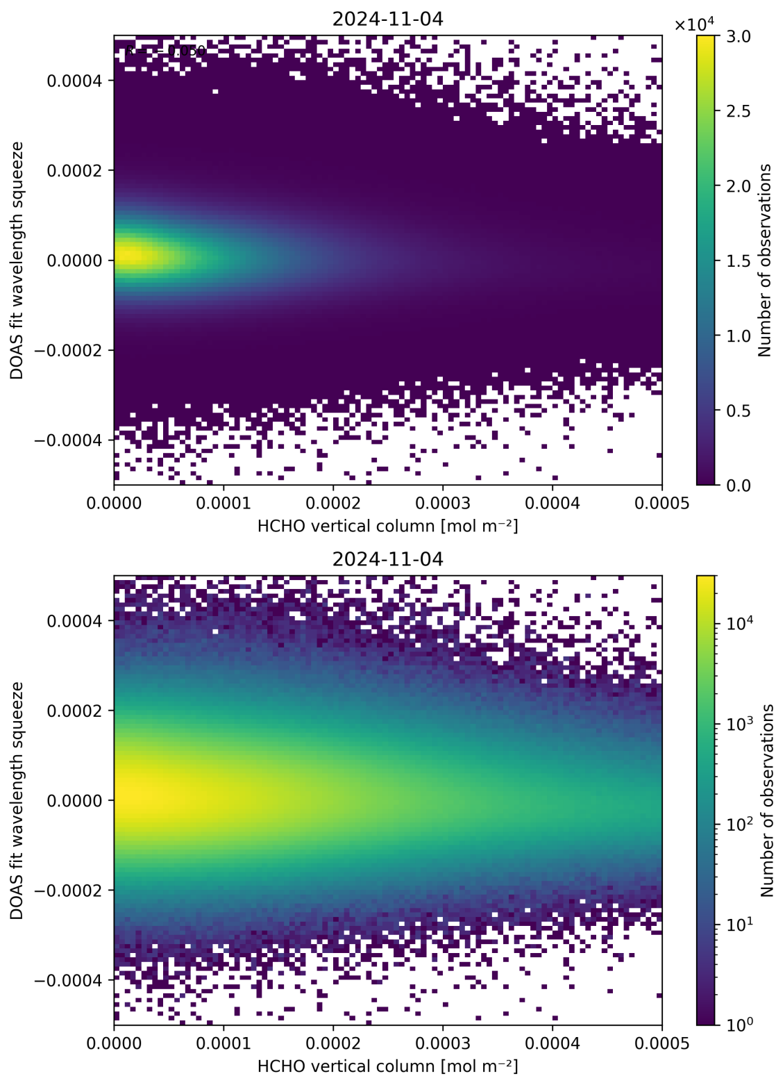
Figure 125: Scatter density plot of “HCHO vertical column” against “DOAS fit wavelength squeeze” for 2024-11-04 to 2024-11-05.
