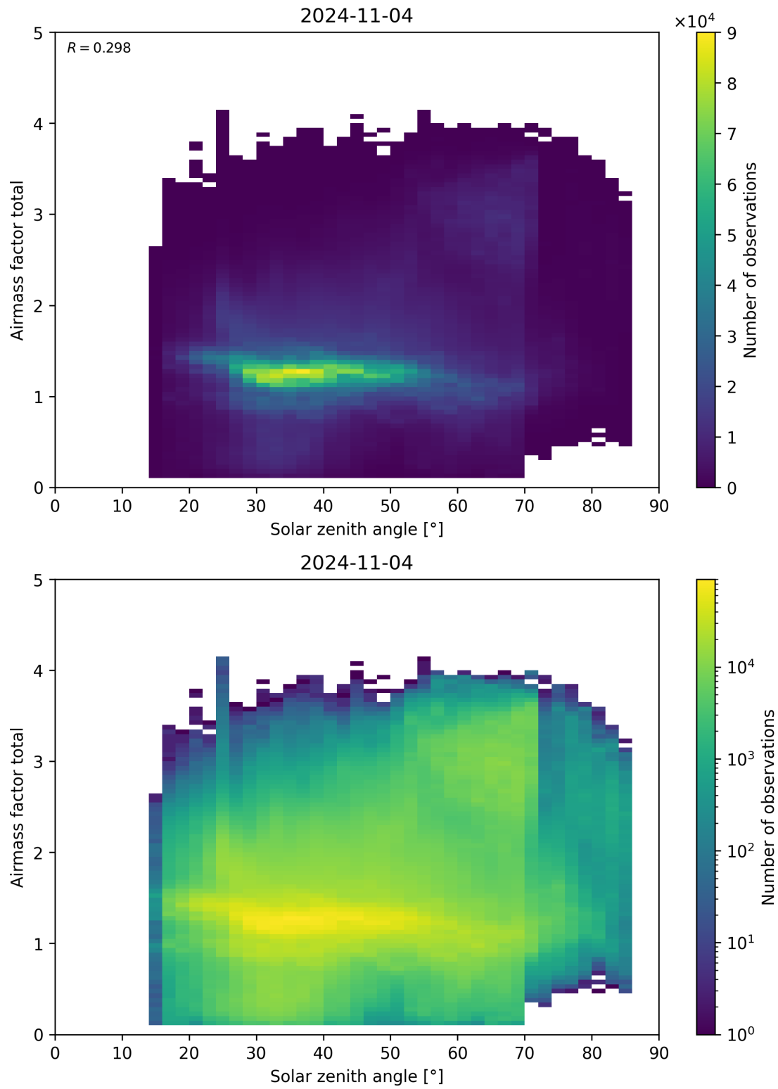
Figure 175: Scatter density plot of “Solar zenith angle” against “Airmass factor total” for 2024-11-04 to 2024-11-05.
