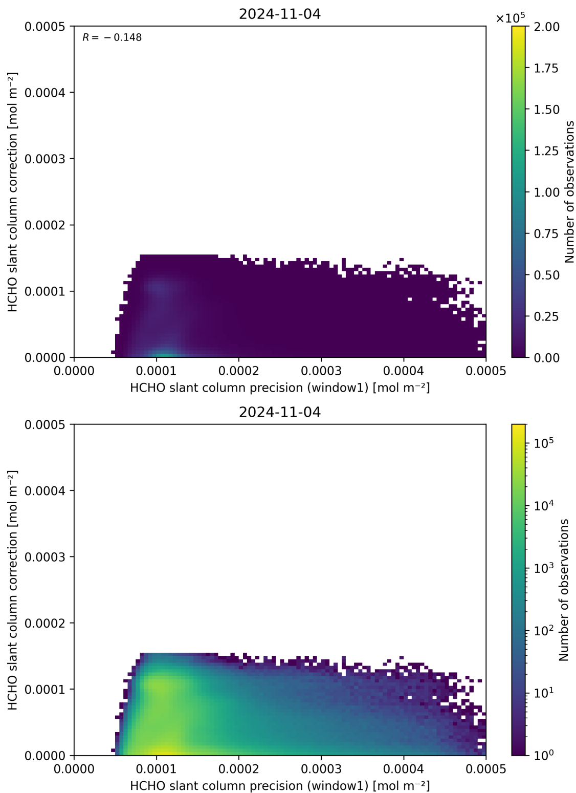
Figure 93: Scatter density plot of “HCHO slant column precision (window1)” against “HCHO slant column correction” for 2024-11-04 to 2024-11-05.
