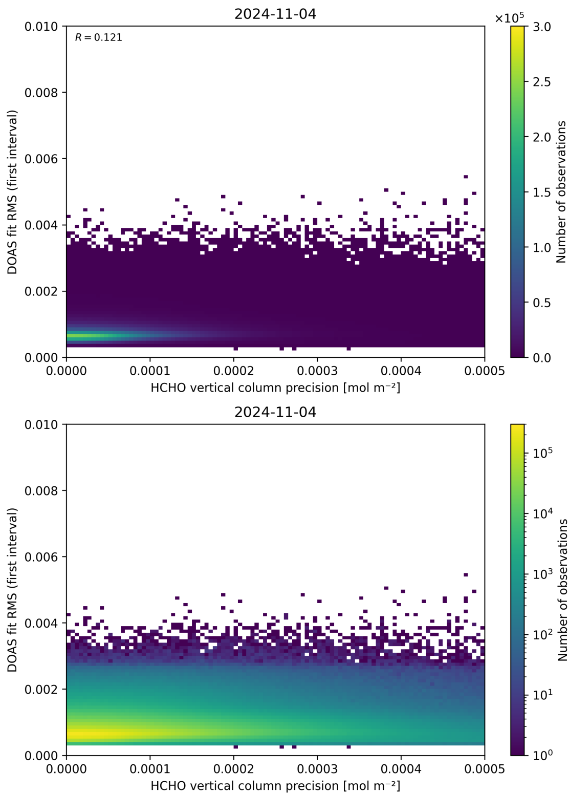
Figure 136: Scatter density plot of “HCHO vertical column precision” against “DOAS fit RMS (first interval)” for 2024-11-04 to 2024-11-05.
