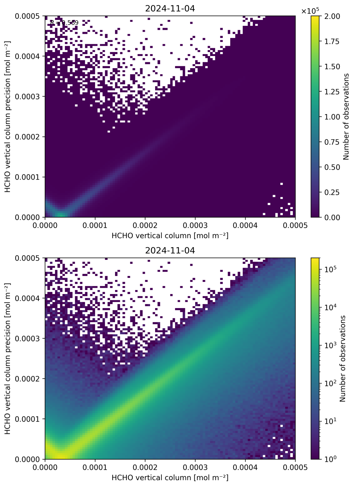
Figure 134: Scatter density plot of “HCHO vertical column” against “HCHO vertical column precision” for 2024-11-04 to 2024-11-05.
