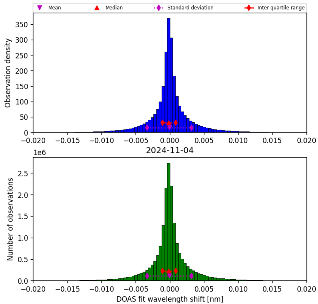
Figure 44: Histogram of “DOAS fit wavelength shift” for 2024-11-04 to 2024-11-05
