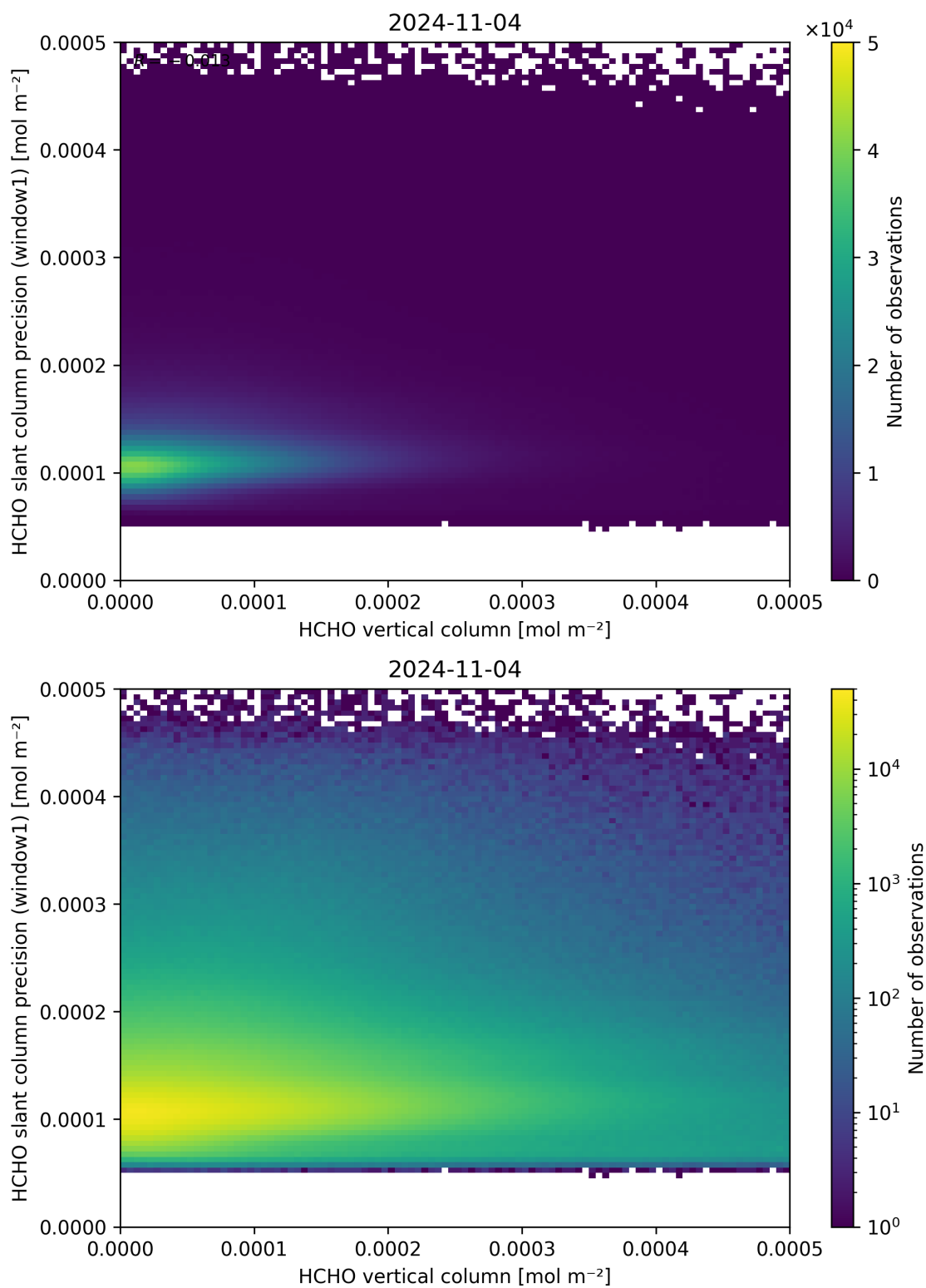
Figure 130: Scatter density plot of “HCHO vertical column” against “HCHO slant column precision (window1)” for 2024-11-04 to 2024-11-05.
