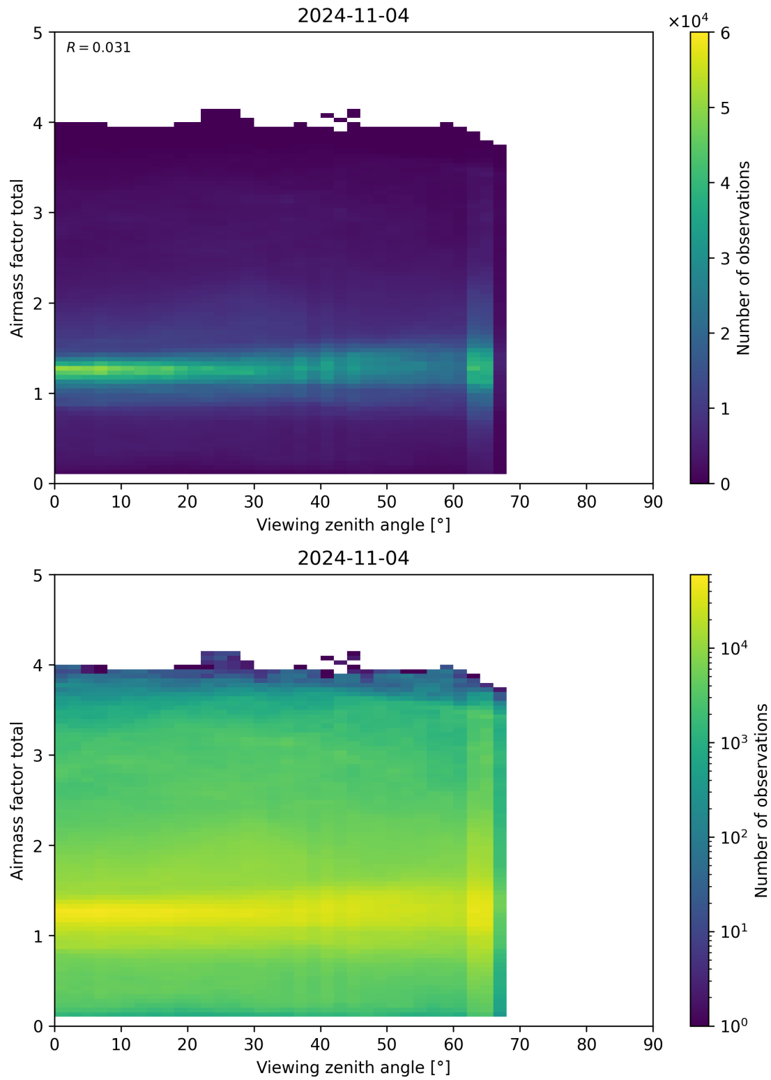
Figure 190: Scatter density plot of “Viewing zenith angle” against “Airmass factor total” for 2024-11-04 to 2024-11-05.
