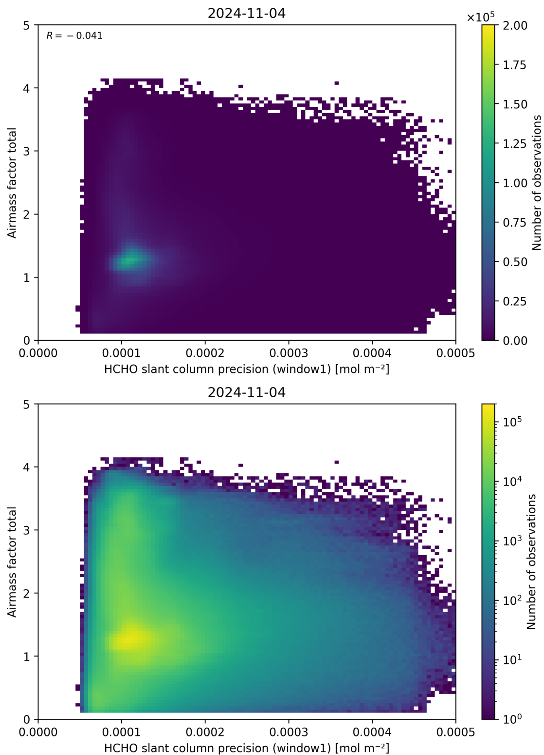
Figure 94: Scatter density plot of “HCHO slant column precision (window1)” against “Airmass factor total” for 2024-11-04 to 2024-11-05.
