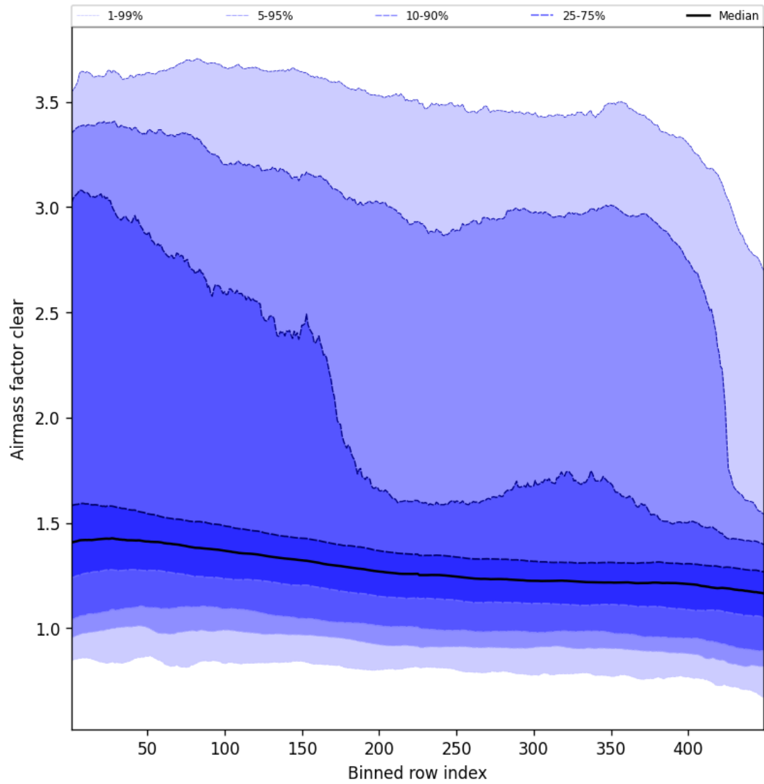
Figure 56: Along track statistics of “Airmass factor clear” for 2024-11-04 to 2024-11-05
