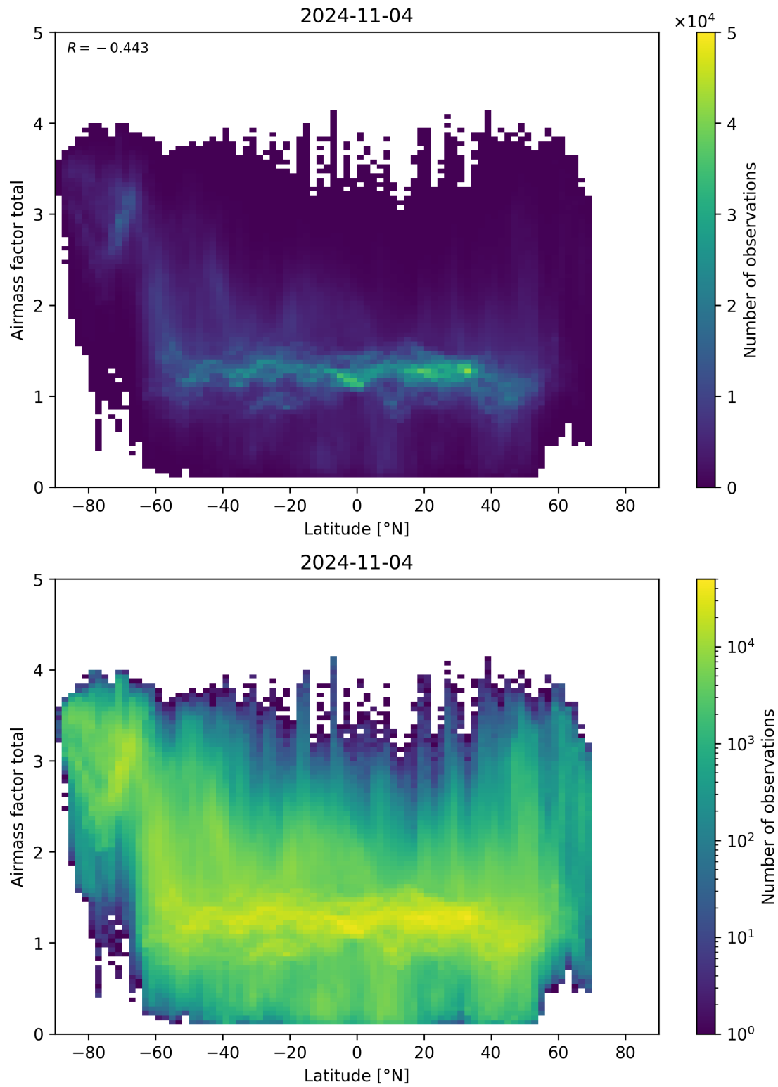
Figure 161: Scatter density plot of “Latitude” against “Airmass factor total” for 2024-11-04 to 2024-11-05.
