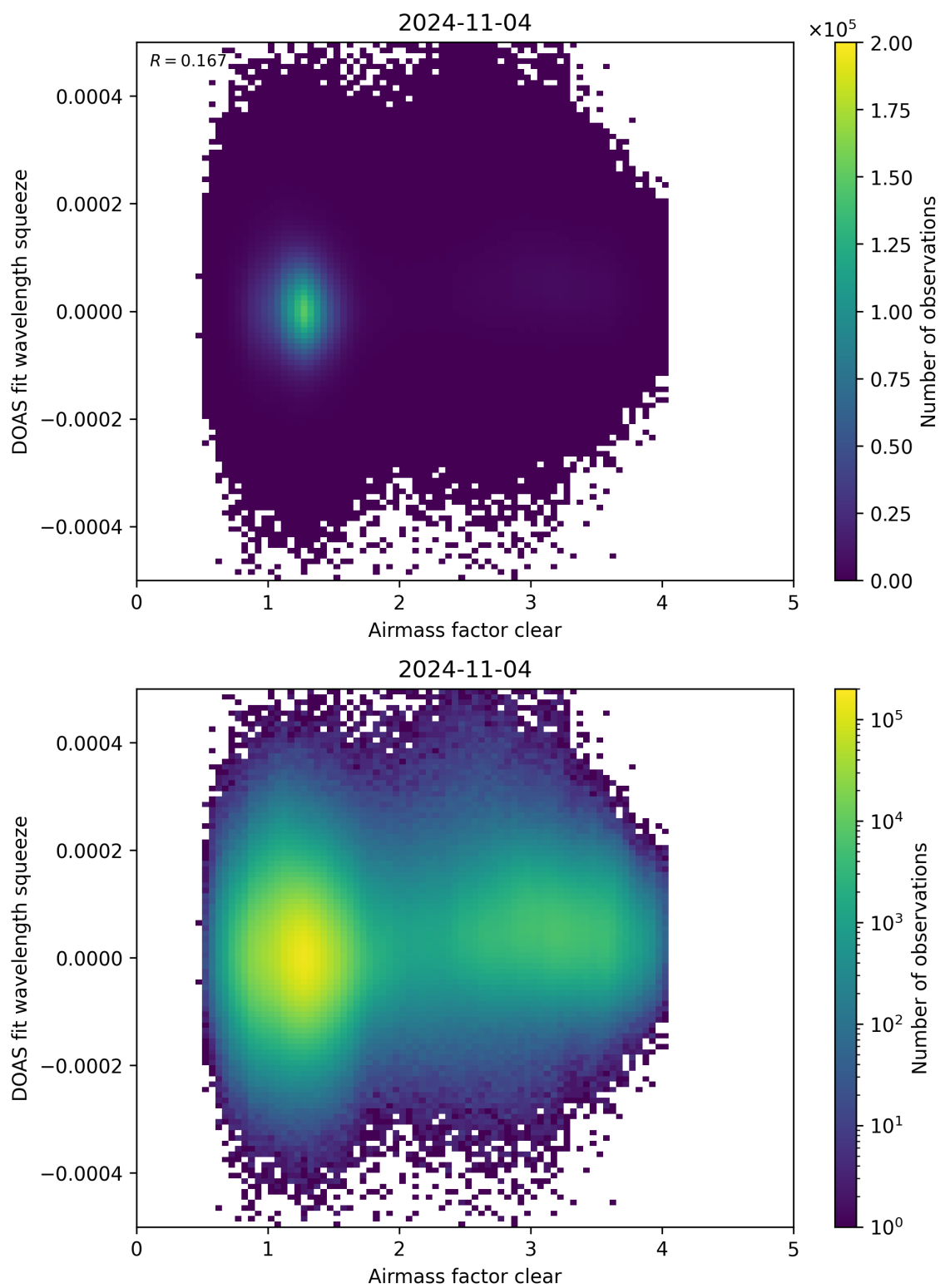
Figure 73: Scatter density plot of “Airmass factor clear” against “DOAS fit wavelength squeeze” for 2024-11-04 to 2024-11-05.
