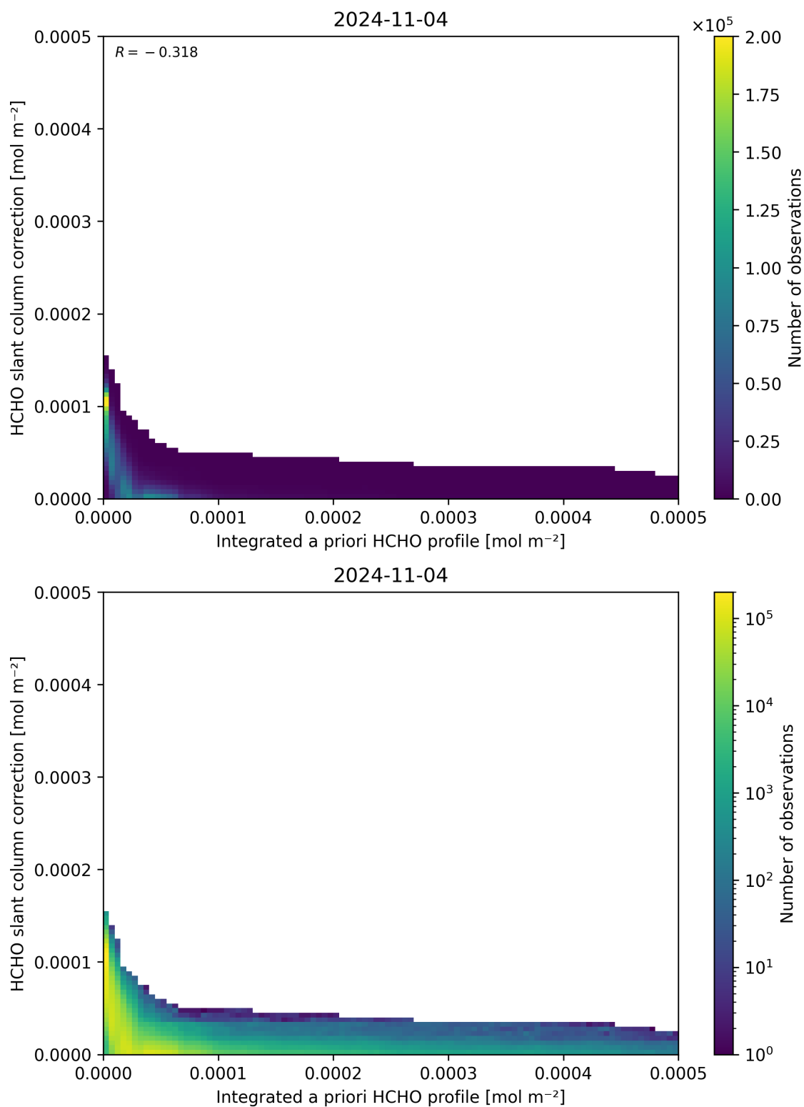
Figure 152: Scatter density plot of “Integrated a priori HCHO profile” against “HCHO slant column correction” for 2024-11-04 to 2024-11-05.
