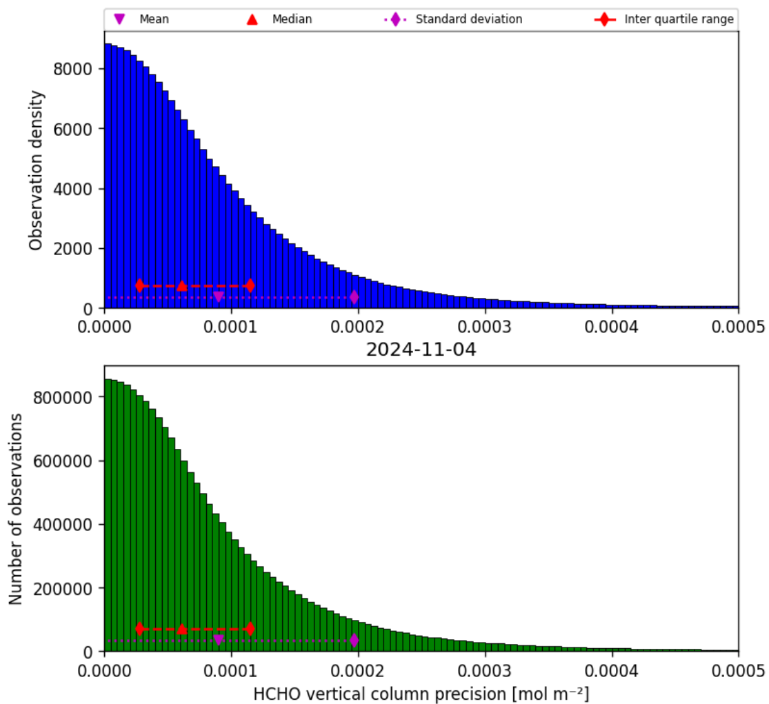
Figure 36: Histogram of “HCHO vertical column precision” for 2024-11-04 to 2024-11-05
