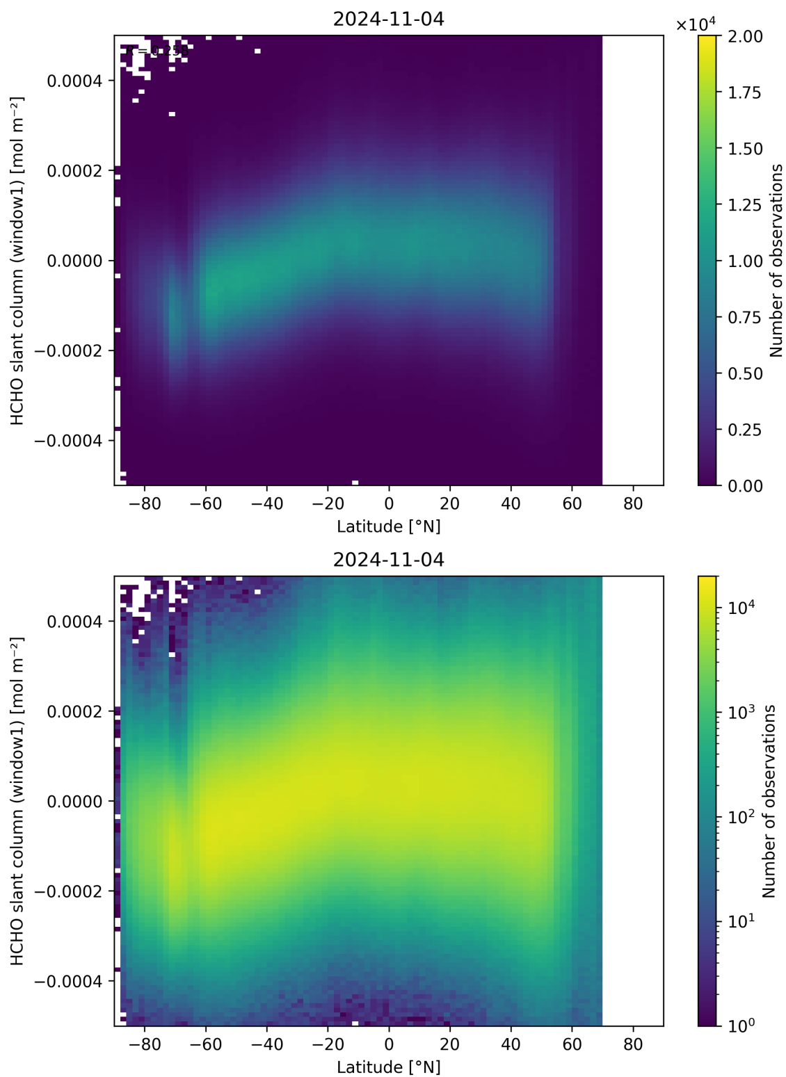
Figure 159: Scatter density plot of “Latitude” against “HCHO slant column (window1)” for 2024-11-04 to 2024-11-05.
