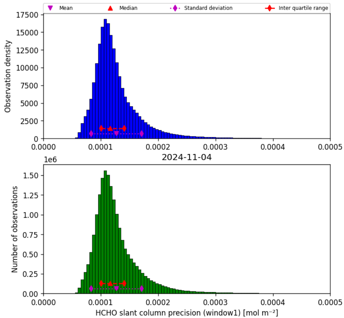
Figure 39: Histogram of “HCHO slant column precision (window1)” for 2024-11-04 to 2024-11-05
