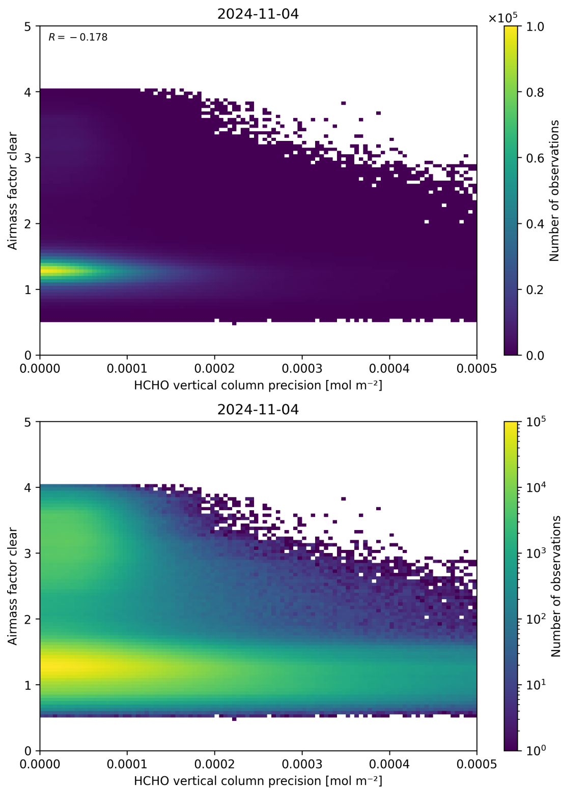
Figure 139: Scatter density plot of “HCHO vertical column precision” against “Airmass factor clear” for 2024-11-04 to 2024-11-05.
