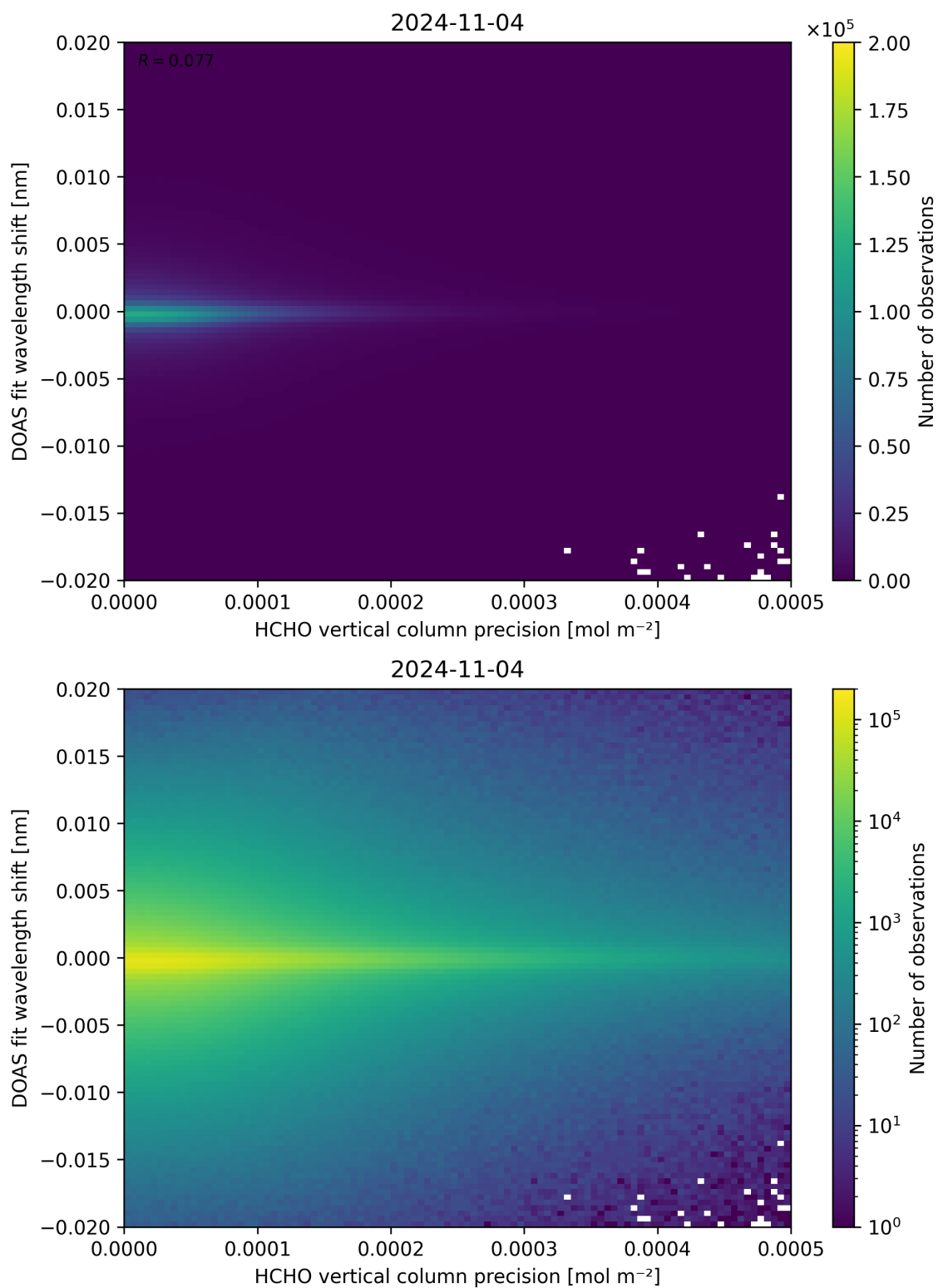
Figure 137: Scatter density plot of “HCHO vertical column precision” against “DOAS fit wavelength shift” for 2024-11-04 to 2024-11-05.
