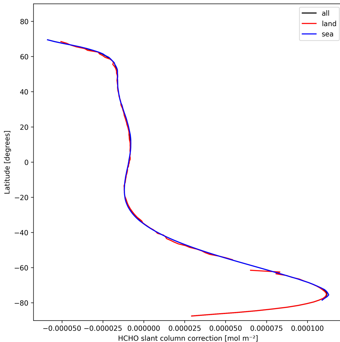
Figure 33: Zonal average of “HCHO slant column correction” for 2024-11-04 to 2024-11-05.
