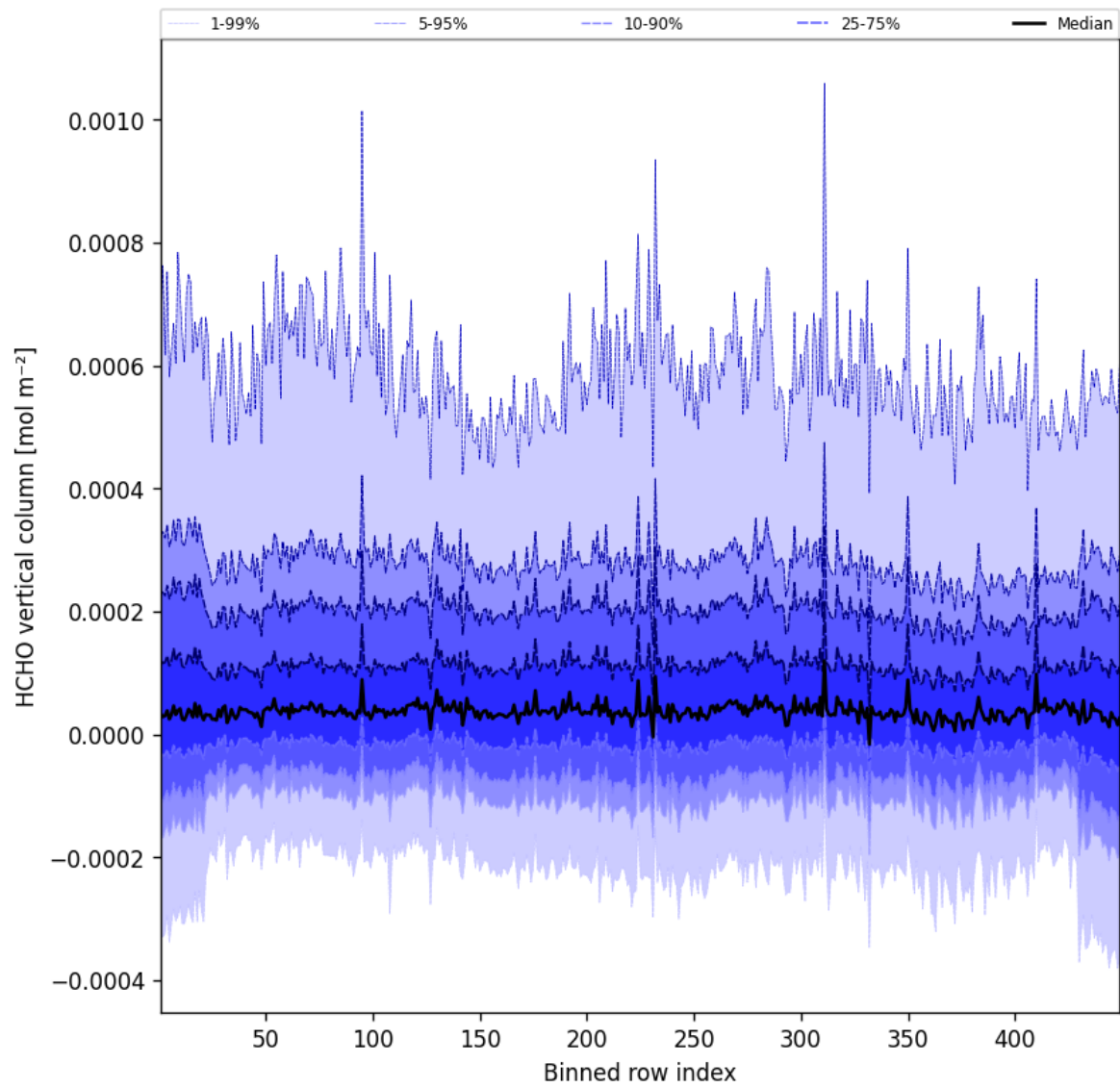
Figure 49: Along track statistics of “HCHO vertical column” for 2024-11-04 to 2024-11-05
