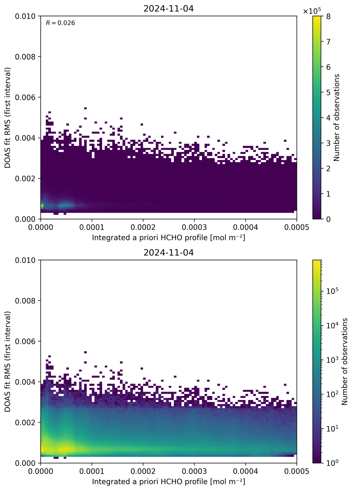
Figure 148: Scatter density plot of “Integrated a priori HCHO profile” against “DOAS fit RMS (first interval)” for 2024-11-04 to 2024-11-05.
