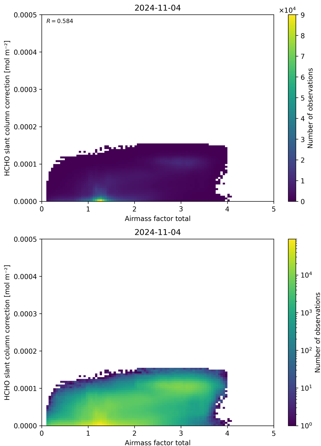
Figure 102: Scatter density plot of “Airmass factor total” against “HCHO slant column correction” for 2024-11-04 to 2024-11-05.
