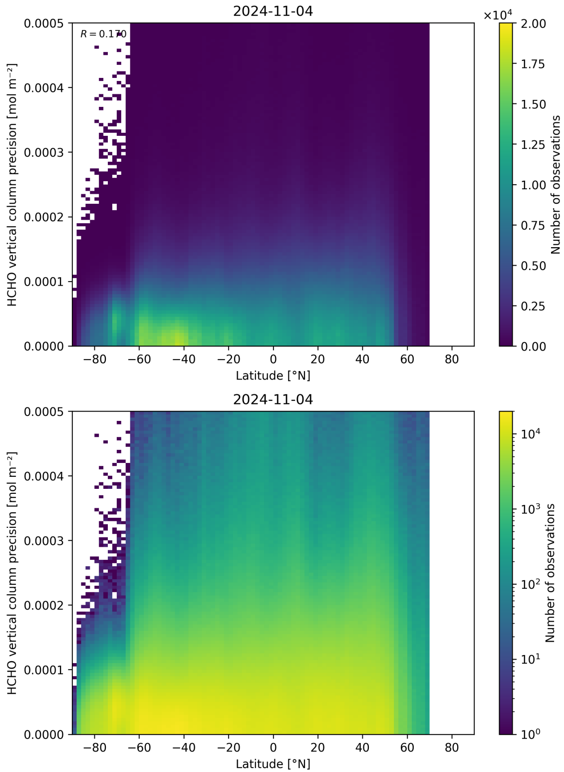
Figure 165: Scatter density plot of “Latitude” against “HCHO vertical column precision” for 2024-11-04 to 2024-11-05.
