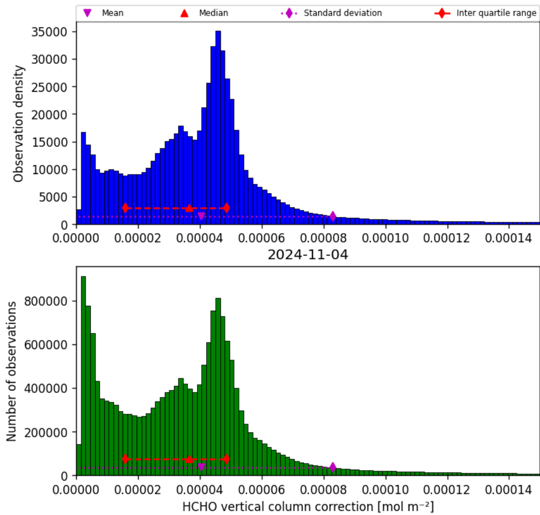
Figure 37: Histogram of “HCHO vertical column correction” for 2024-11-04 to 2024-11-05
