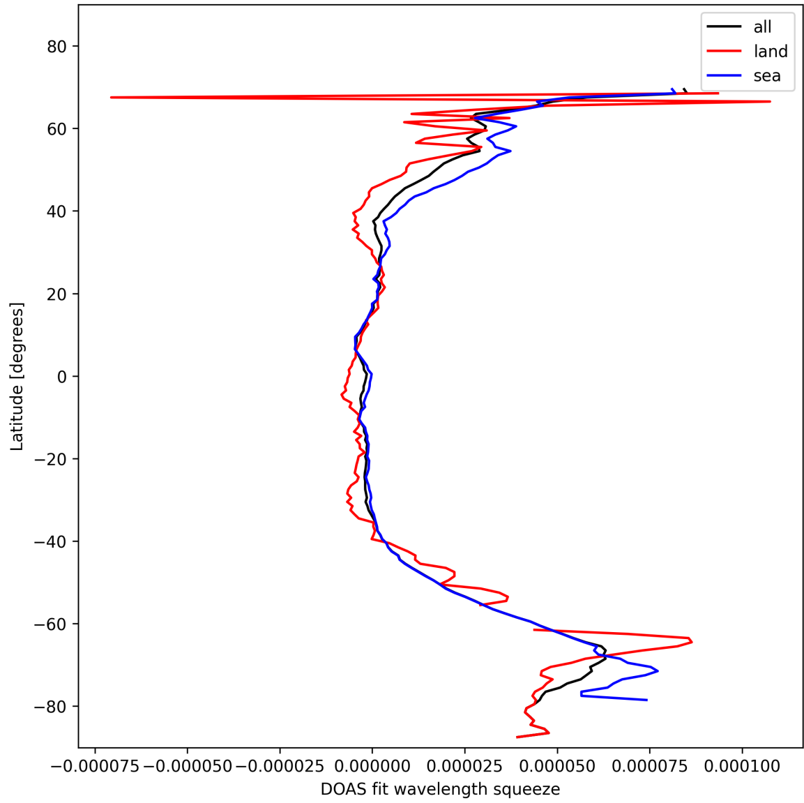
Figure 31: Zonal average of “DOAS fit wavelength squeeze” for 2024-11-04 to 2024-11-05.
