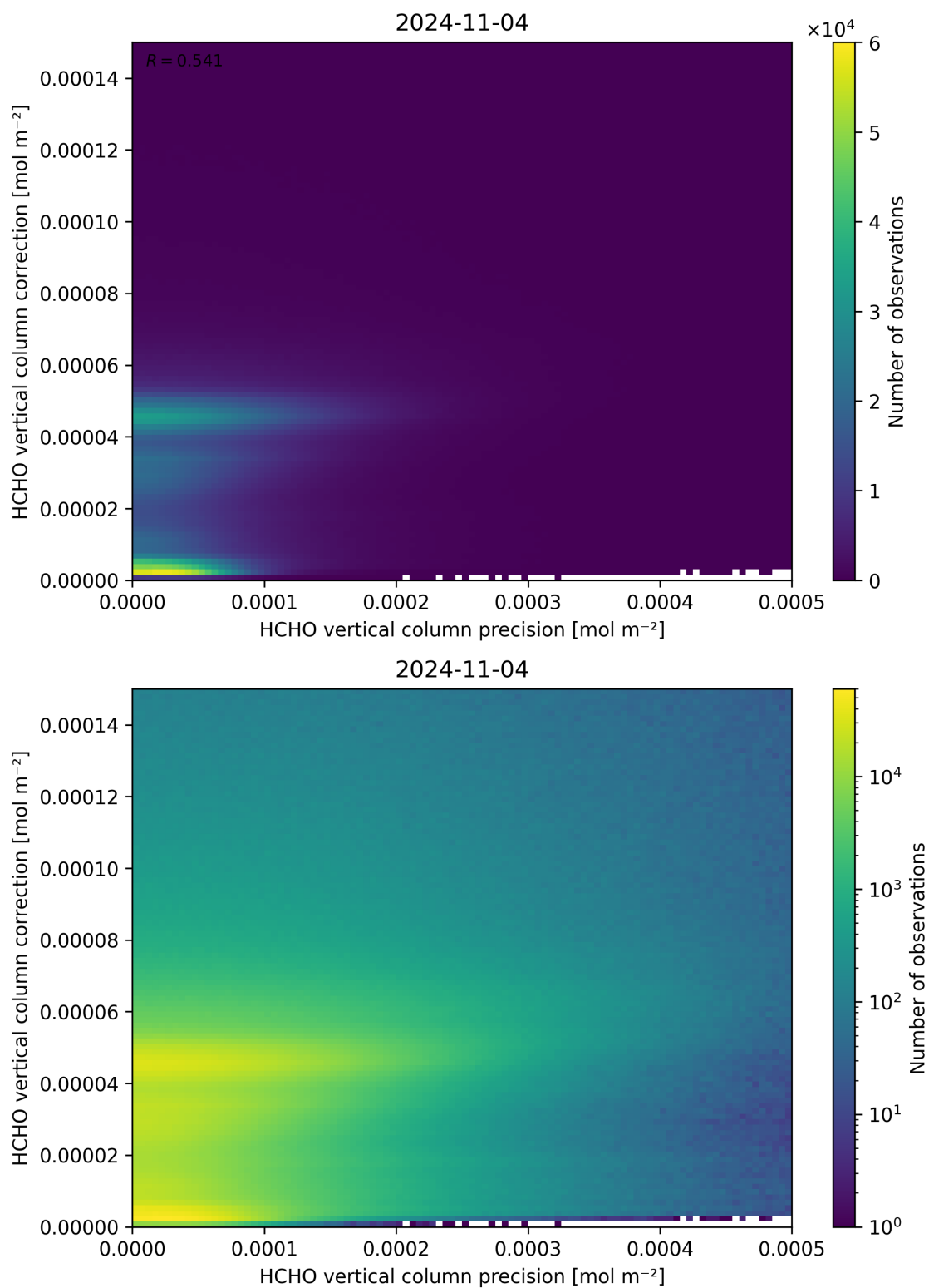
Figure 146: Scatter density plot of “HCHO vertical column precision” against “HCHO vertical column correction” for 2024-11-04 to 2024-11-05.
