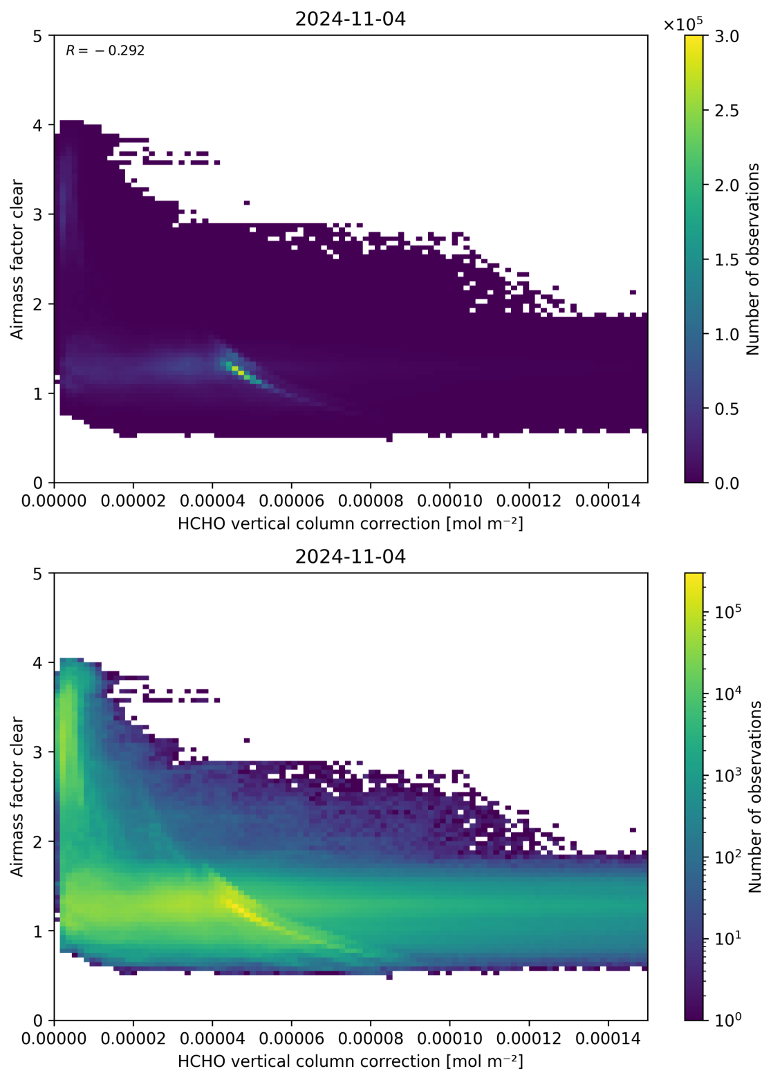
Figure 115: Scatter density plot of “HCHO vertical column correction” against “Airmass factor clear” for 2024-11-04 to 2024-11-05.
