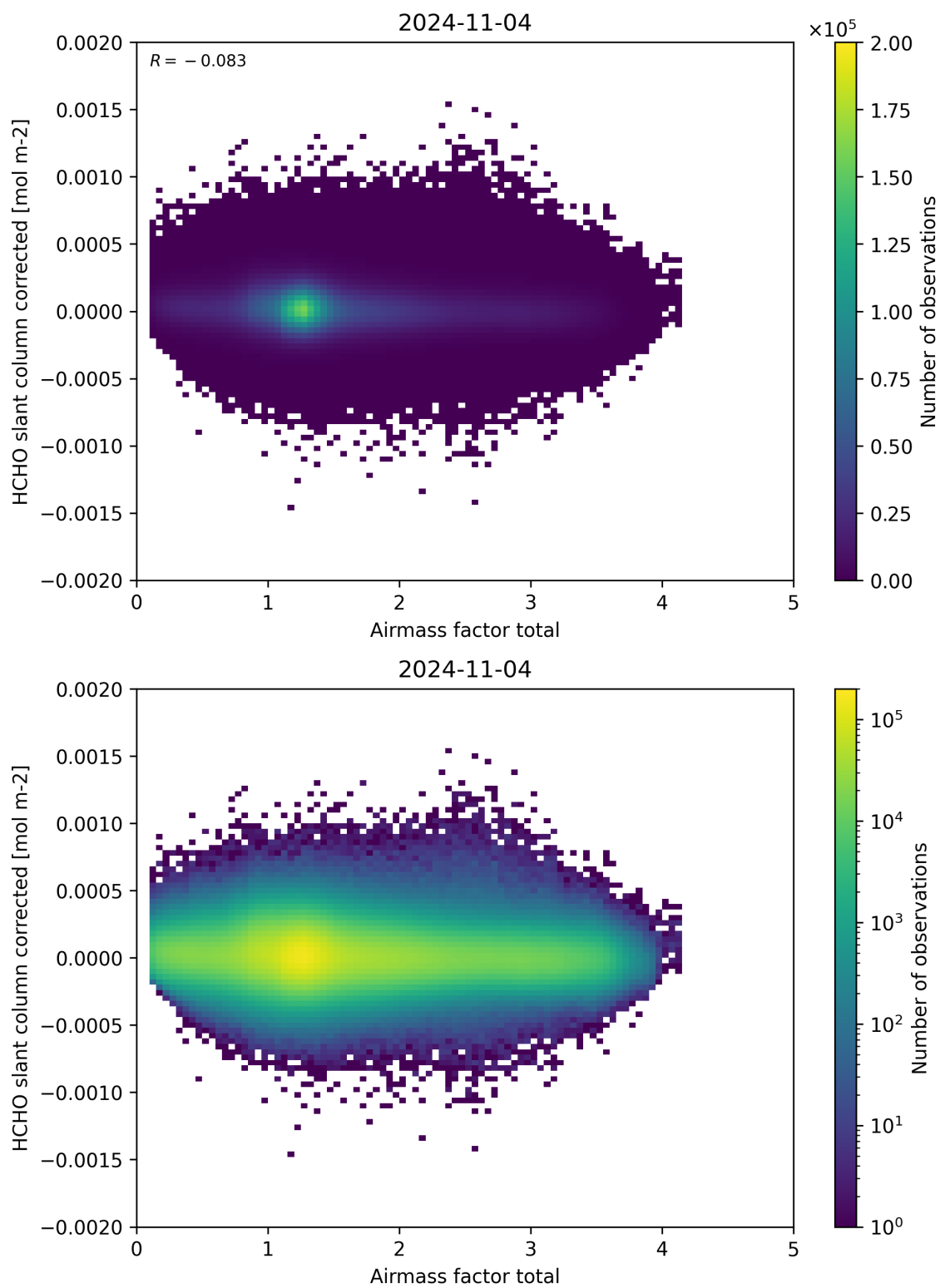
Figure 101: Scatter density plot of “Airmass factor total” against “HCHO slant column corrected” for 2024-11-04 to 2024-11-05.
