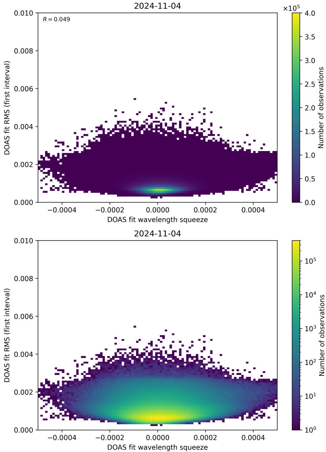
Figure 68: Scatter density plot of “DOAS fit wavelength squeeze” against “DOAS fit RMS (first interval)” for 2024-11-04 to 2024-11-05.
