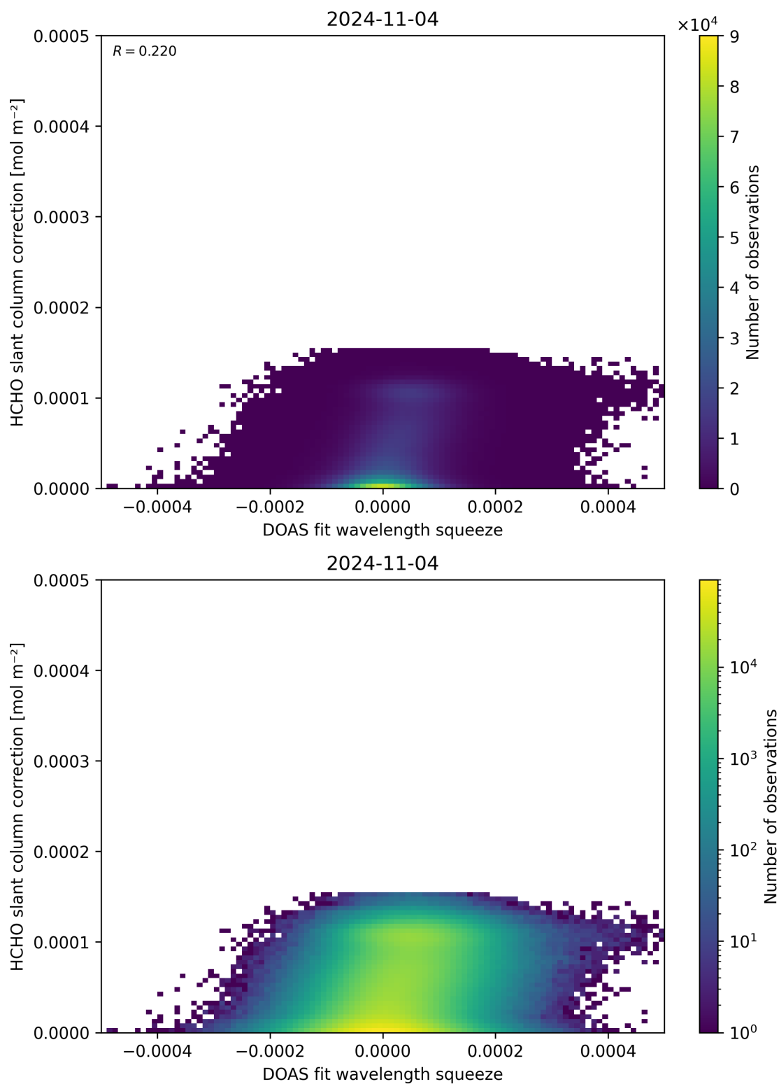
Figure 70: Scatter density plot of “DOAS fit wavelength squeeze” against “HCHO slant column correction” for 2024-11-04 to 2024-11-05.
