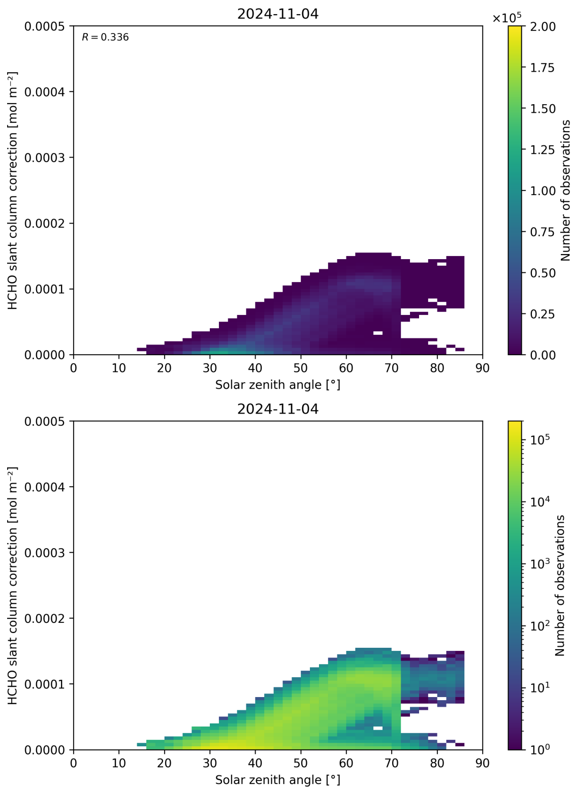
Figure 172: Scatter density plot of “Solar zenith angle” against “HCHO slant column correction” for 2024-11-04 to 2024-11-05.
