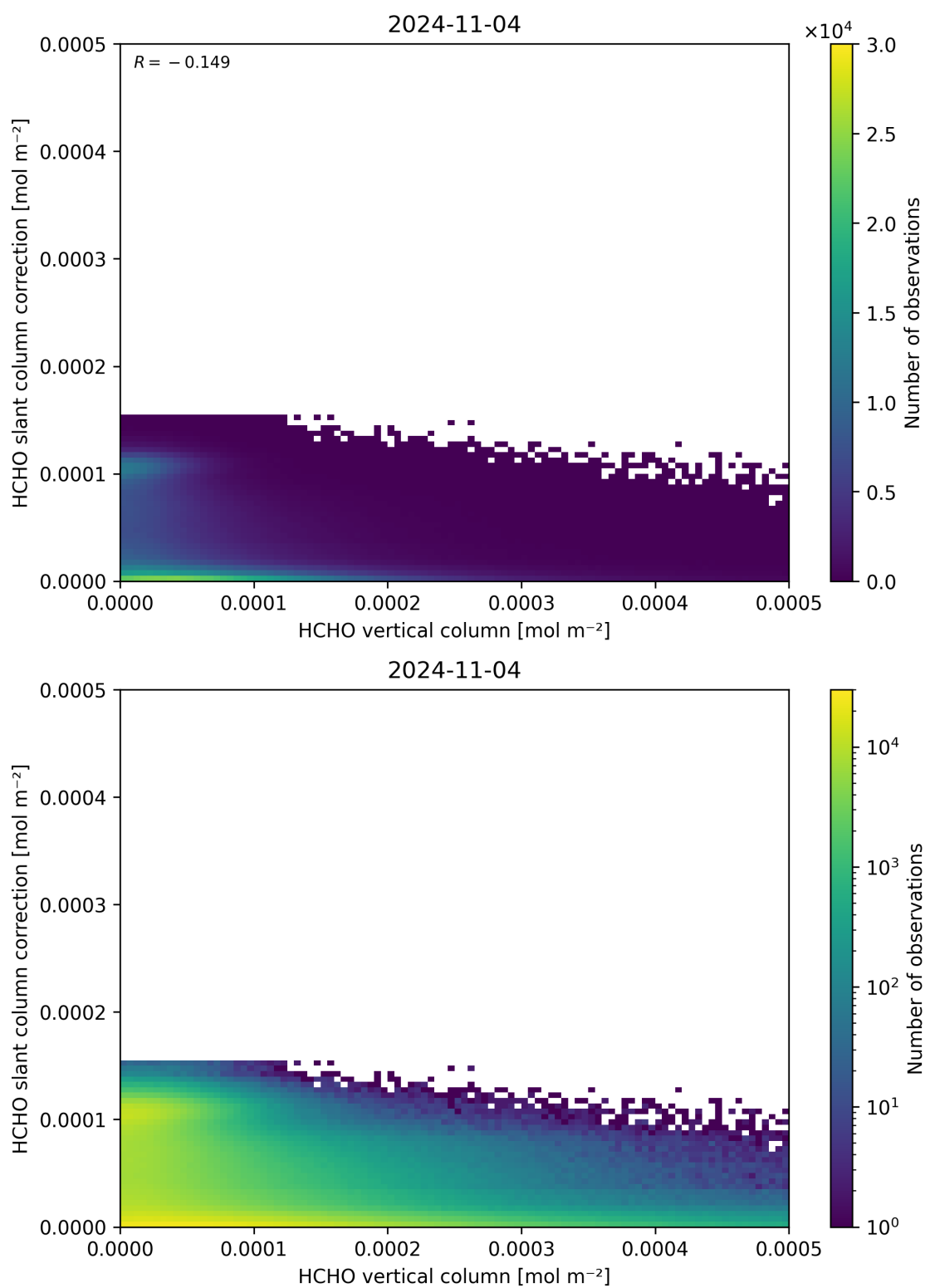
Figure 128: Scatter density plot of “HCHO vertical column” against “HCHO slant column correction” for 2024-11-04 to 2024-11-05.
