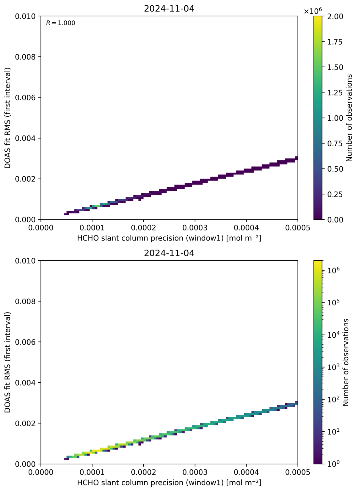
Figure 88: Scatter density plot of “HCHO slant column precision (window1)” against “DOAS fit RMS (first interval)” for 2024-11-04 to 2024-11-05.
