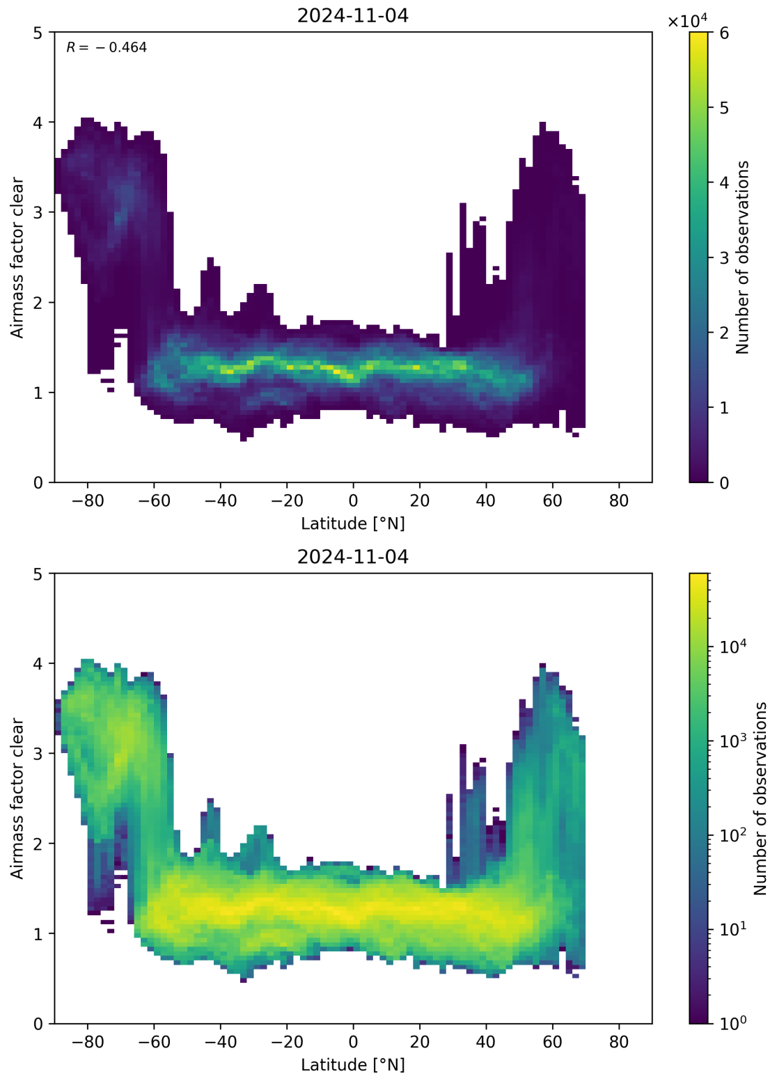
Figure 156: Scatter density plot of “Latitude” against “Airmass factor clear” for 2024-11-04 to 2024-11-05.
