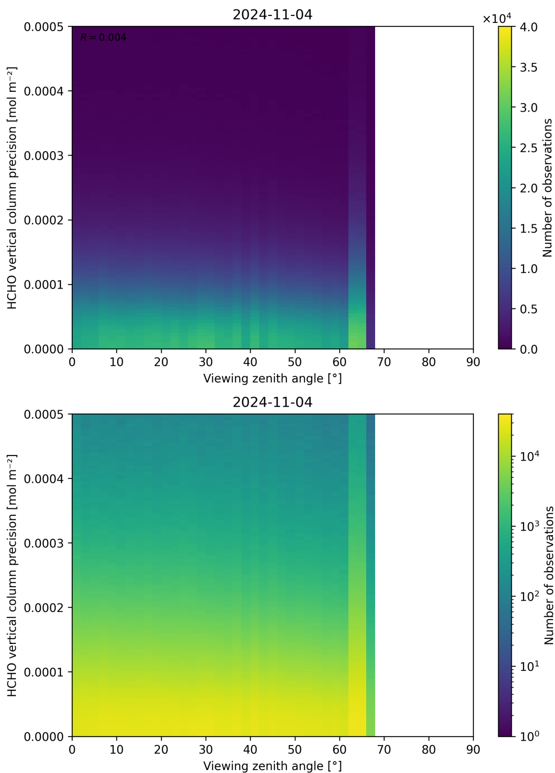
Figure 194: Scatter density plot of “Viewing zenith angle” against “HCHO vertical column precision” for 2024-11-04 to 2024-11-05.
