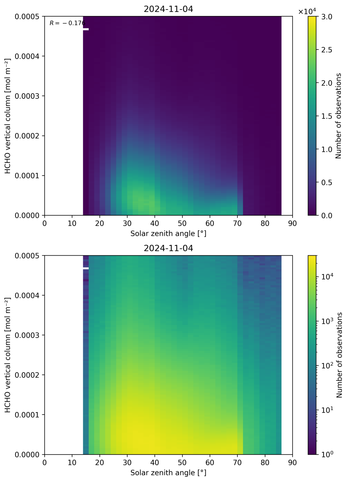
Figure 177: Scatter density plot of “Solar zenith angle” against “HCHO vertical column” for 2024-11-04 to 2024-11-05.
