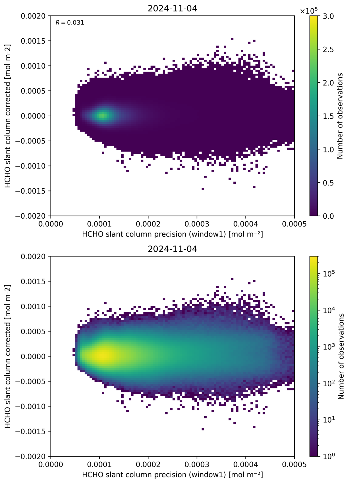
Figure 92: Scatter density plot of “HCHO slant column precision (window1)” against “HCHO slant column corrected” for 2024-11-04 to 2024-11-05.
