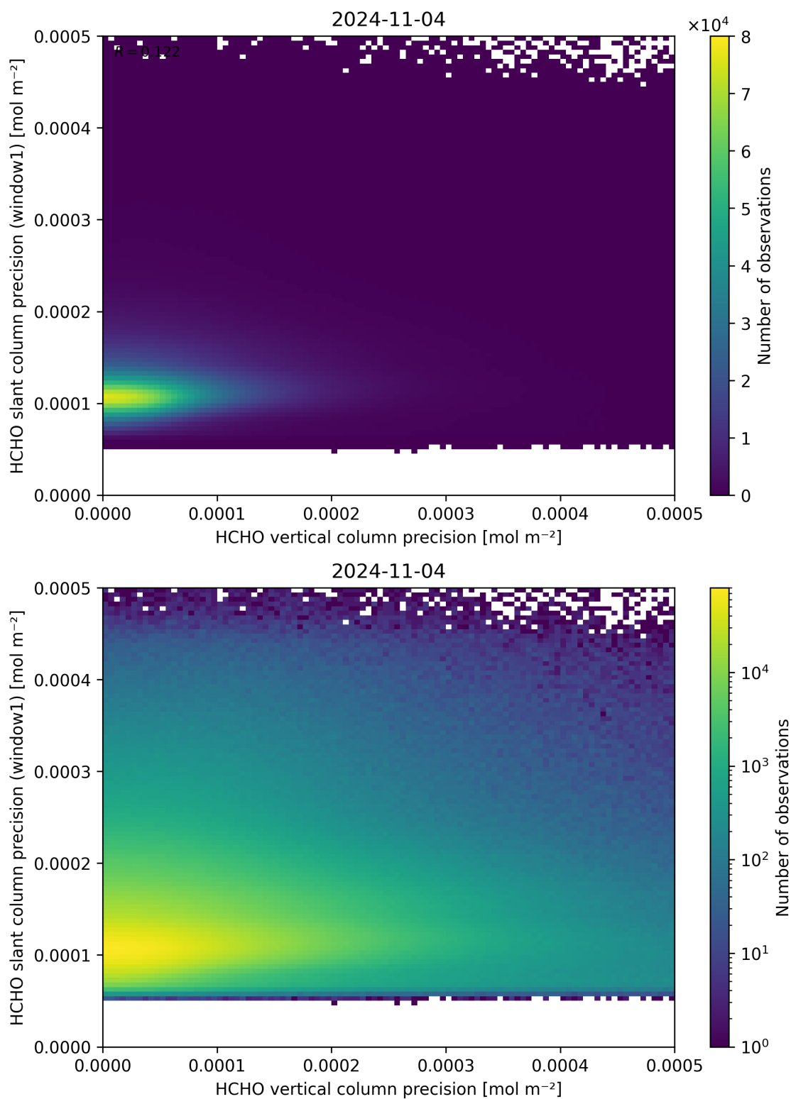
Figure 143: Scatter density plot of “HCHO vertical column precision” against “HCHO slant column precision (window1)” for 2024-11-04 to 2024-11-05.
