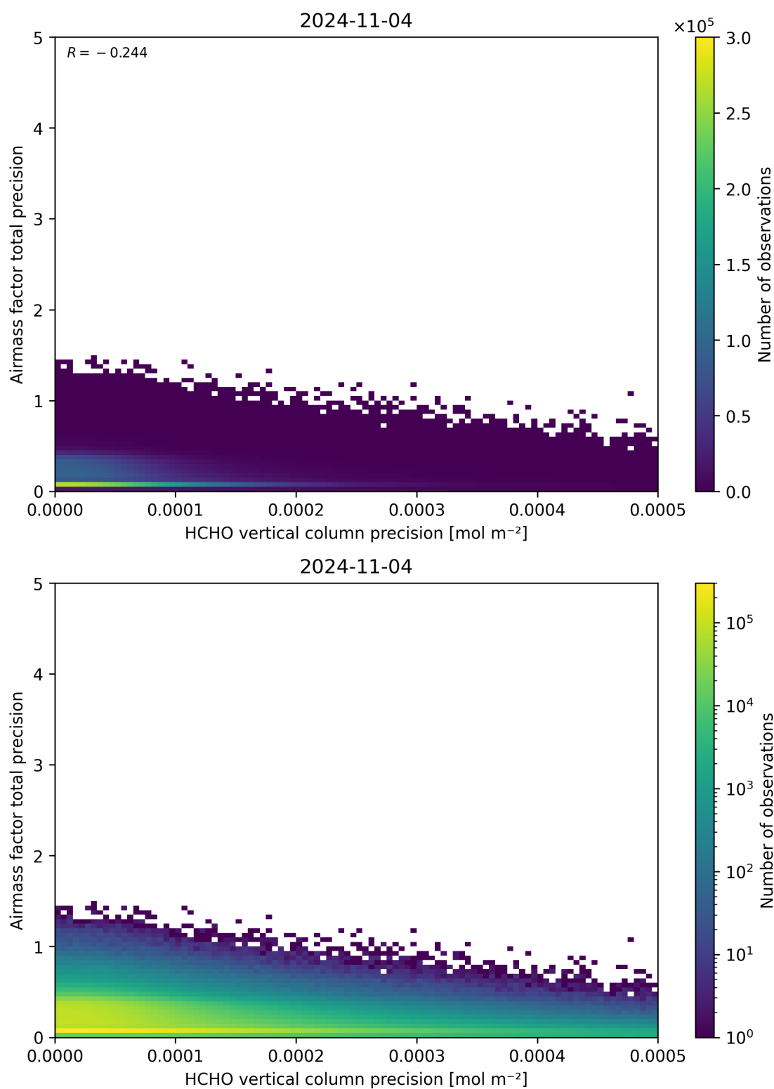
Figure 145: Scatter density plot of “HCHO vertical column precision” against “Airmass factor total precision” for 2024-11-04 to 2024-11-05.
