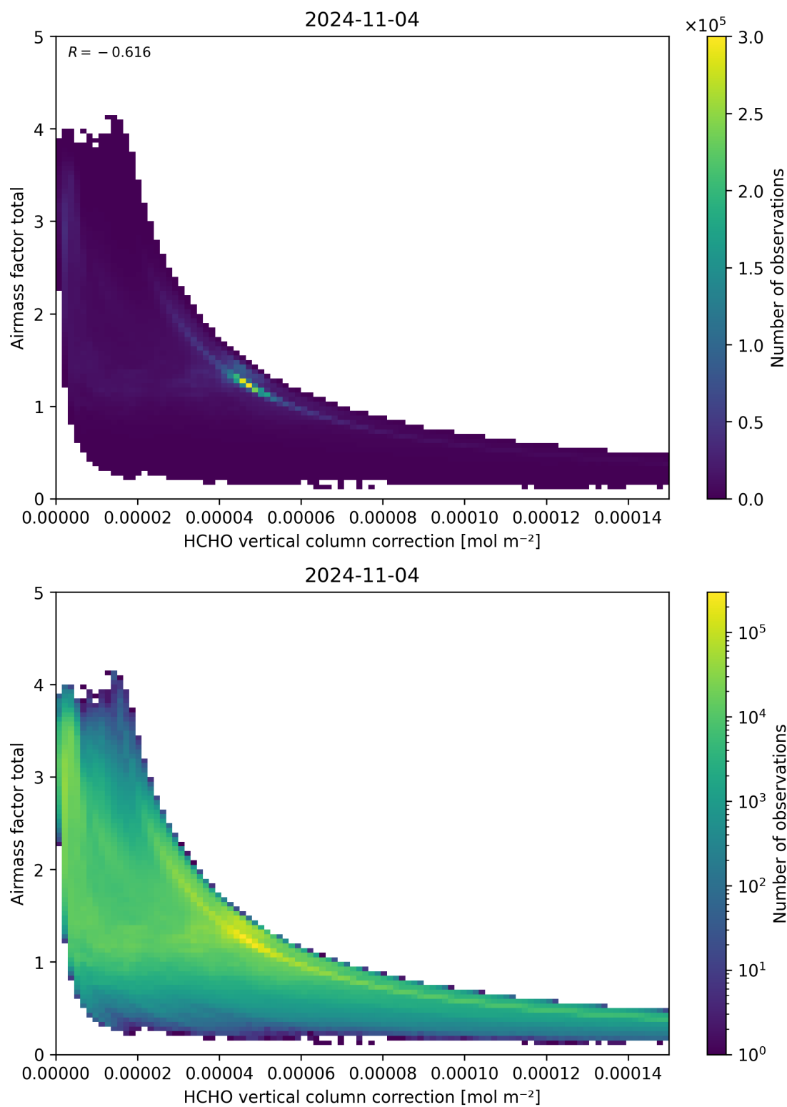
Figure 120: Scatter density plot of “HCHO vertical column correction” against “Airmass factor total” for 2024-11-04 to 2024-11-05.
