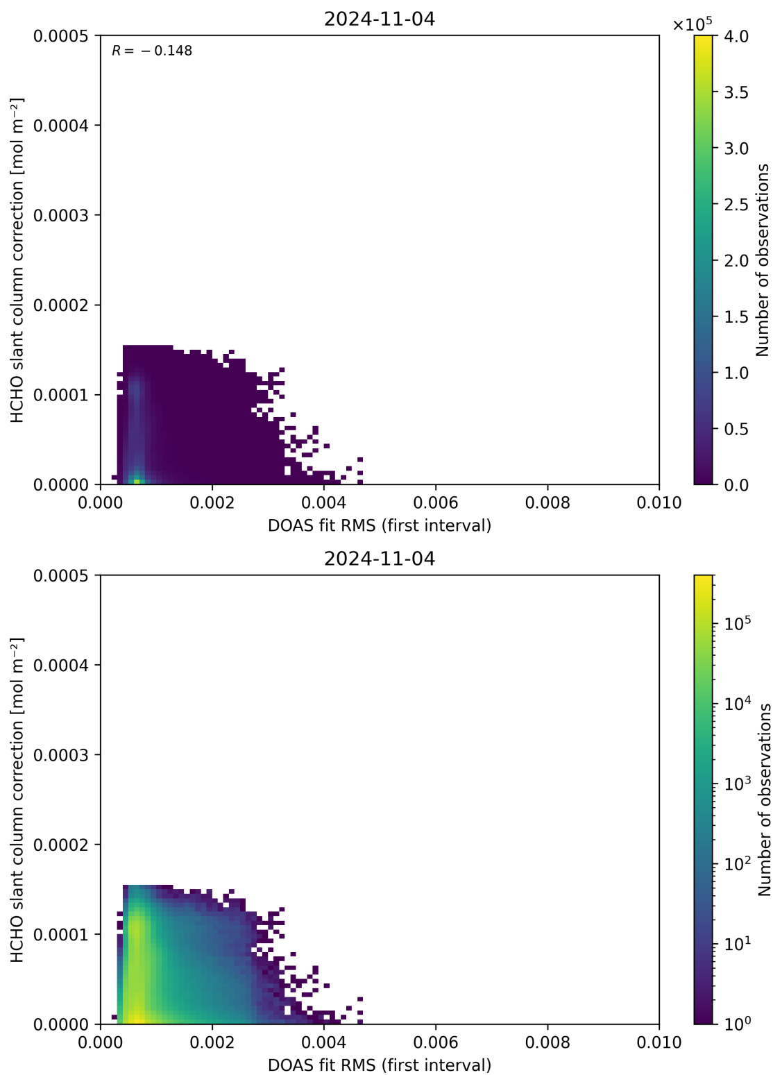
Figure 63: Scatter density plot of “DOAS fit RMS (first interval)” against “HCHO slant column correction” for 2024-11-04 to 2024-11-05.
