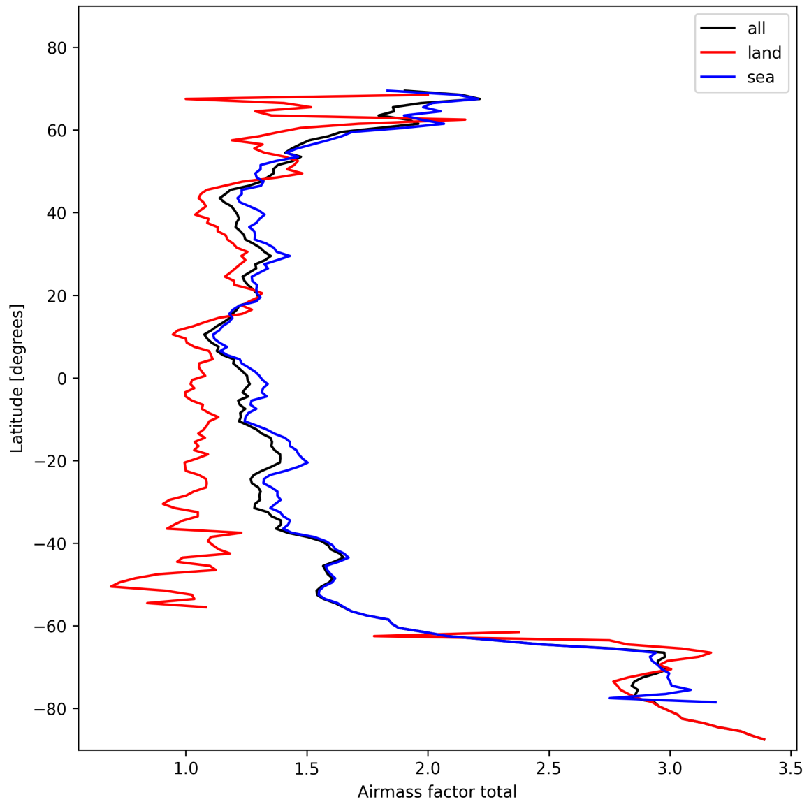
Figure 26: Zonal average of “Airmass factor total” for 2024-11-04 to 2024-11-05.
