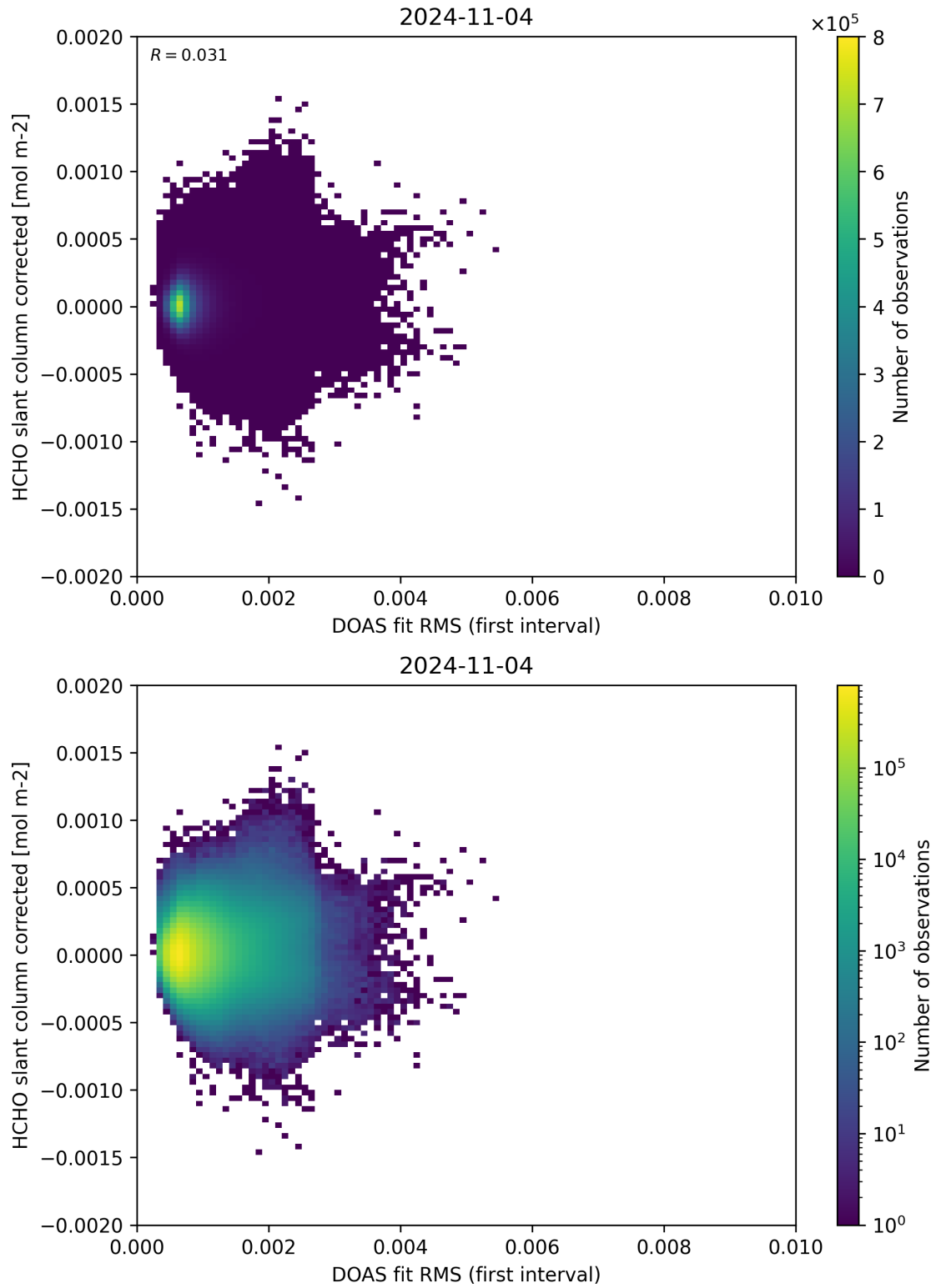
Figure 62: Scatter density plot of “DOAS fit RMS (first interval)” against “HCHO slant column corrected” for 2024-11-04 to 2024-11-05.
