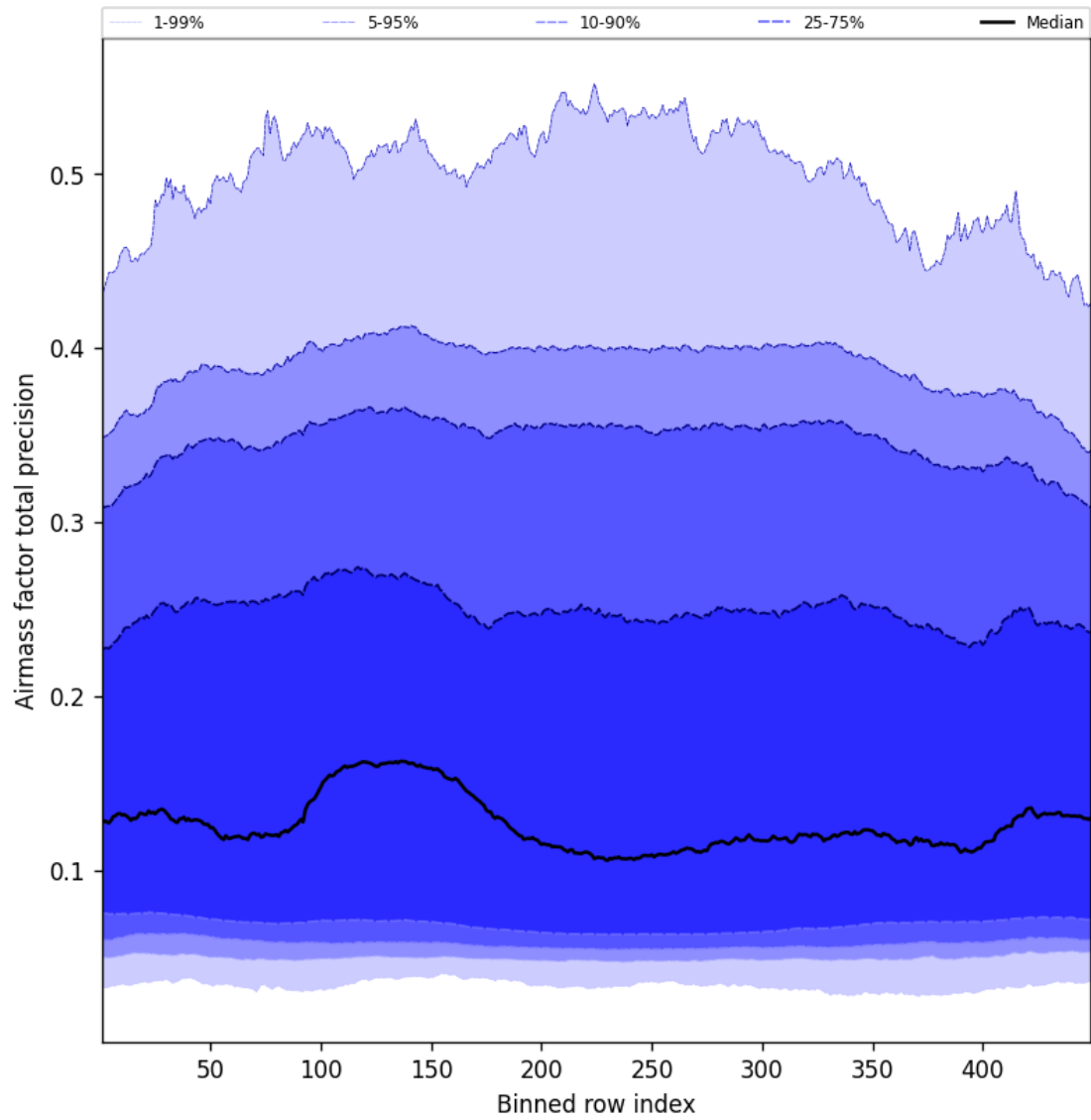
Figure 55: Along track statistics of “Airmass factor total precision” for 2024-11-04 to 2024-11-05
