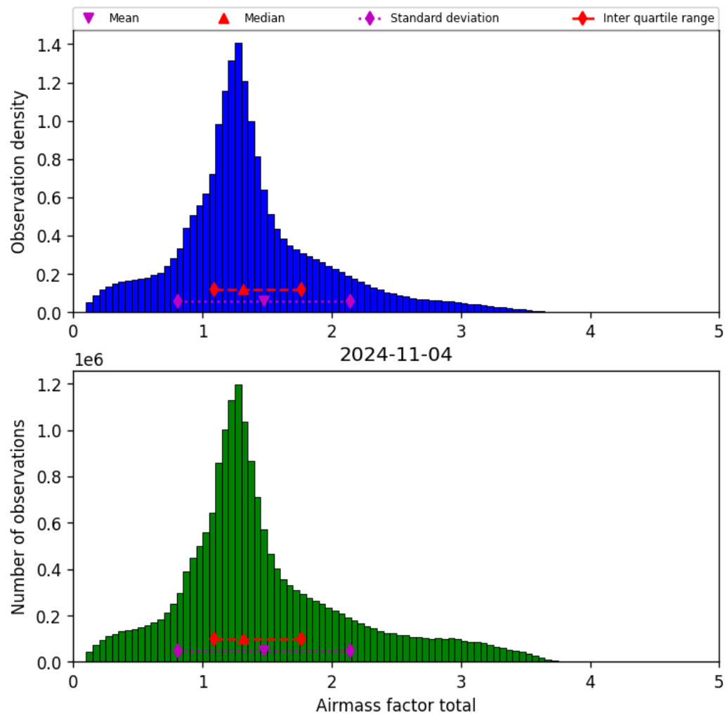
Figure 40: Histogram of “Airmass factor total” for 2024-11-04 to 2024-11-05
