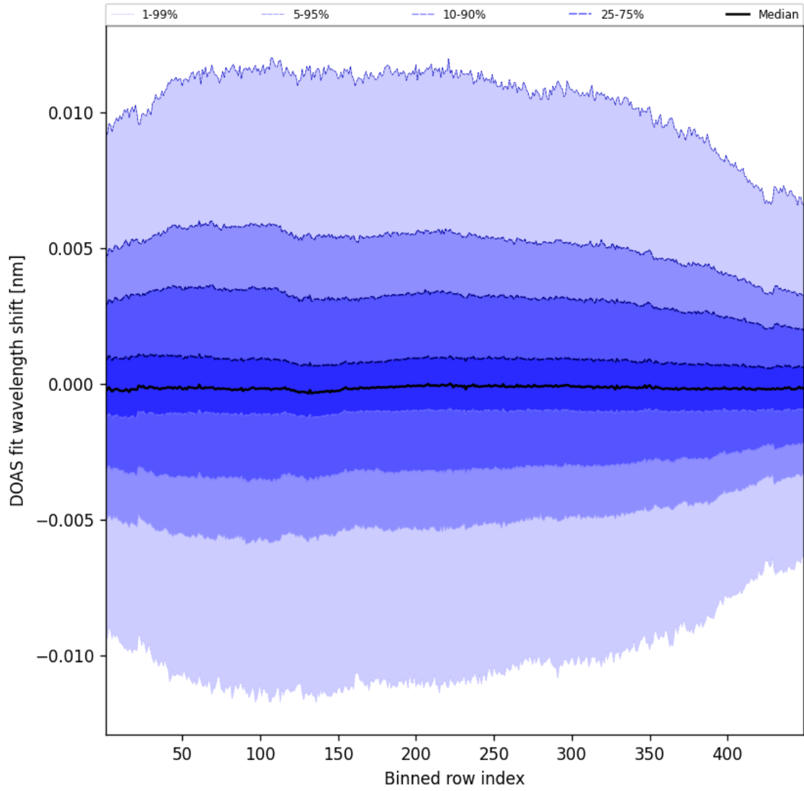
Figure 58: Along track statistics of “DOAS fit wavelength shift” for 2024-11-04 to 2024-11-05
