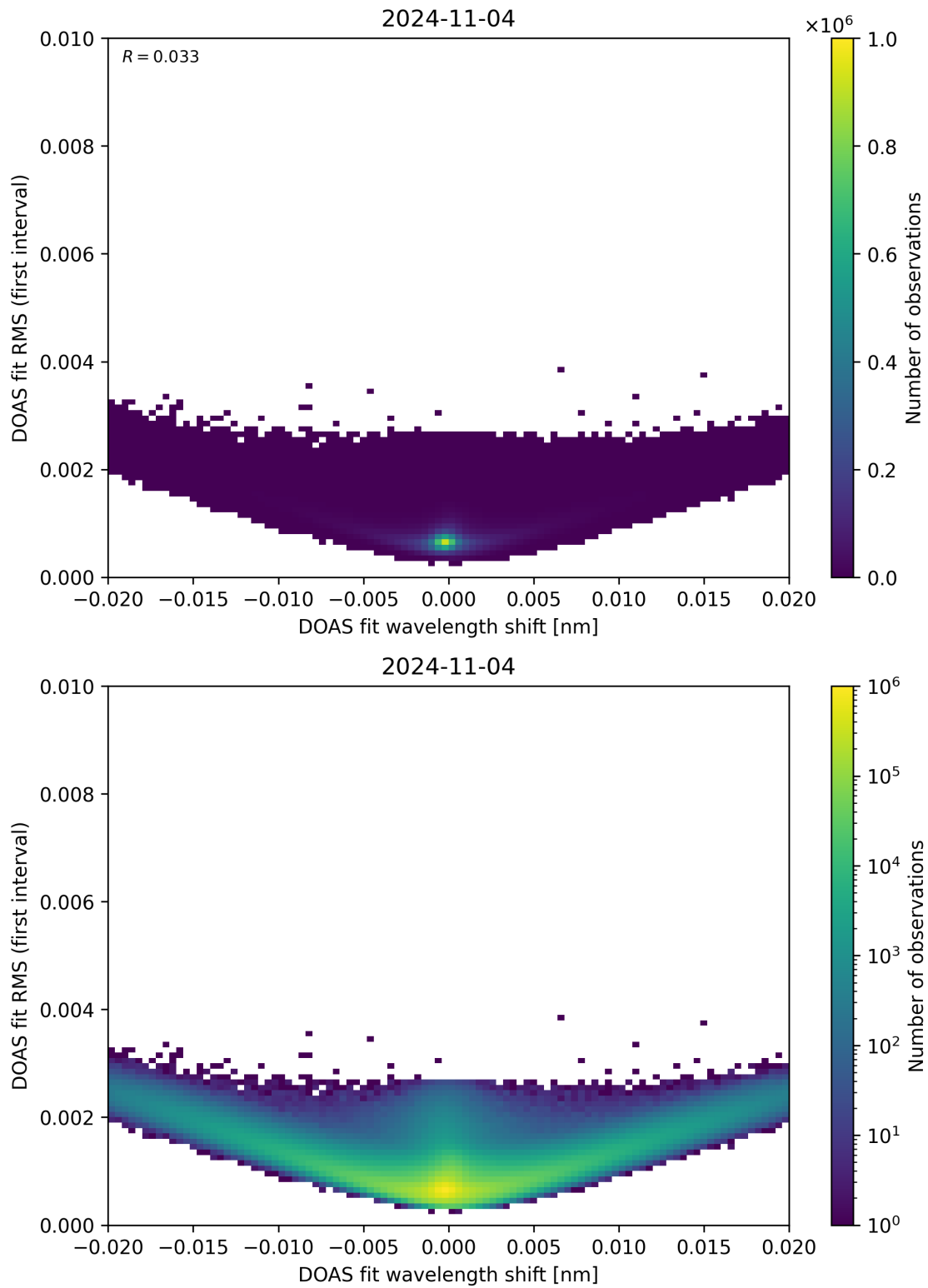
Figure 64: Scatter density plot of “DOAS fit wavelength shift” against “DOAS fit RMS (first interval)” for 2024-11-04 to 2024-11-05.
