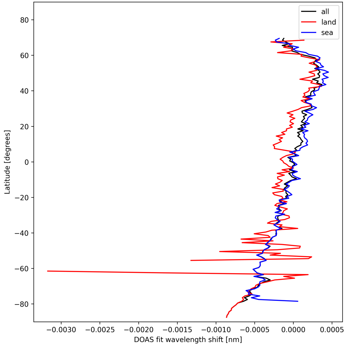
Figure 30: Zonal average of “DOAS fit wavelength shift” for 2024-11-04 to 2024-11-05.
