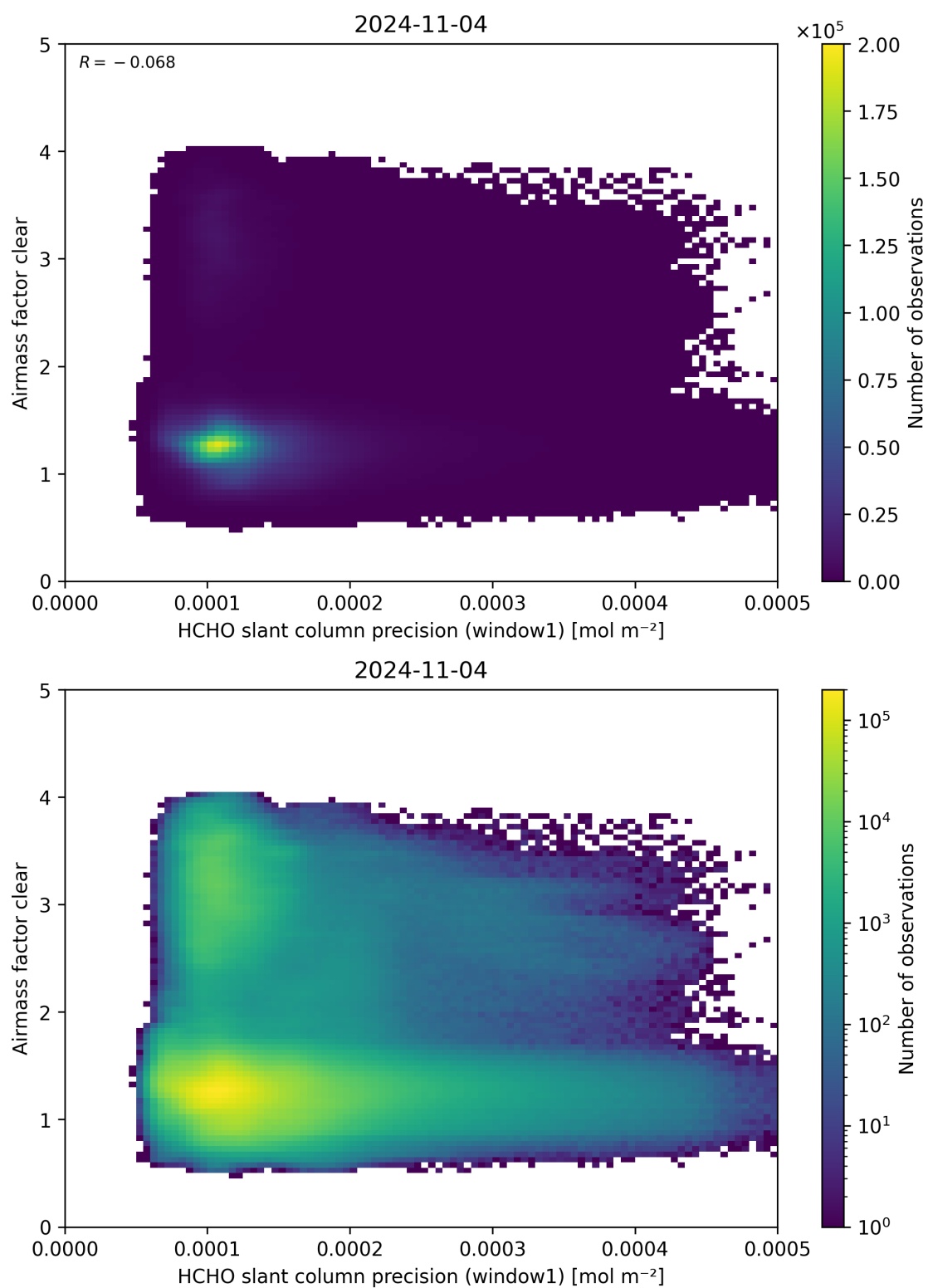
Figure 91: Scatter density plot of “HCHO slant column precision (window1)” against “Airmass factor clear” for 2024-11-04 to 2024-11-05.
