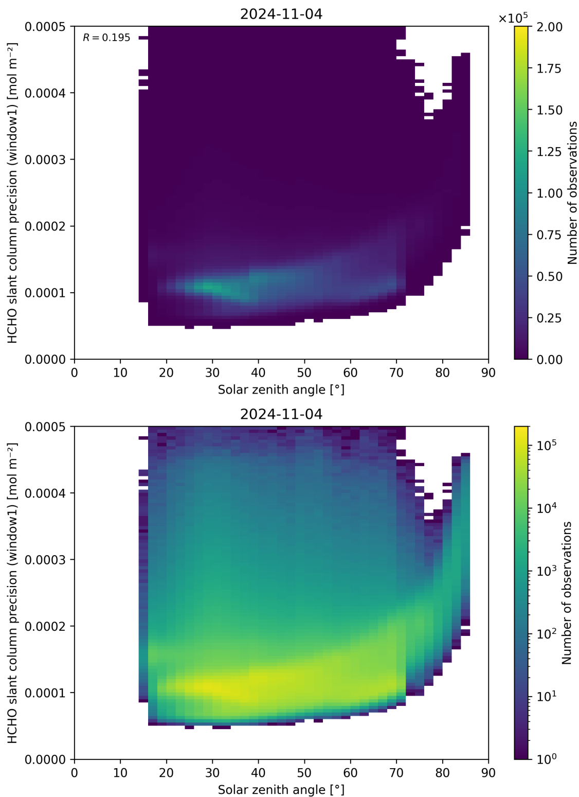
Figure 174: Scatter density plot of “Solar zenith angle” against “HCHO slant column precision (window1)” for 2024-11-04 to 2024-11-05.
