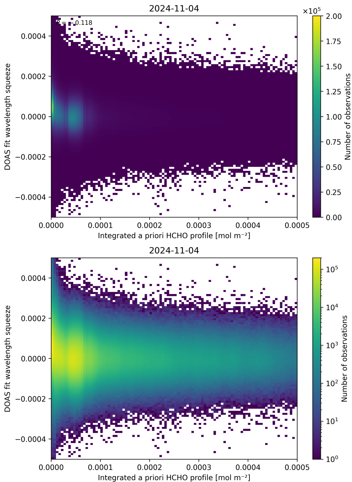
Figure 150: Scatter density plot of “Integrated a priori HCHO profile” against “DOAS fit wavelength squeeze” for 2024-11-04 to 2024-11-05.
