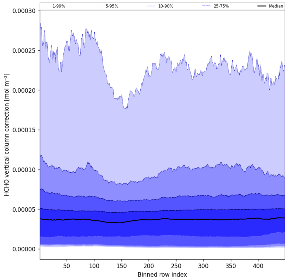
Figure 51: Along track statistics of “HCHO vertical column correction” for 2024-11-04 to 2024-11-05
