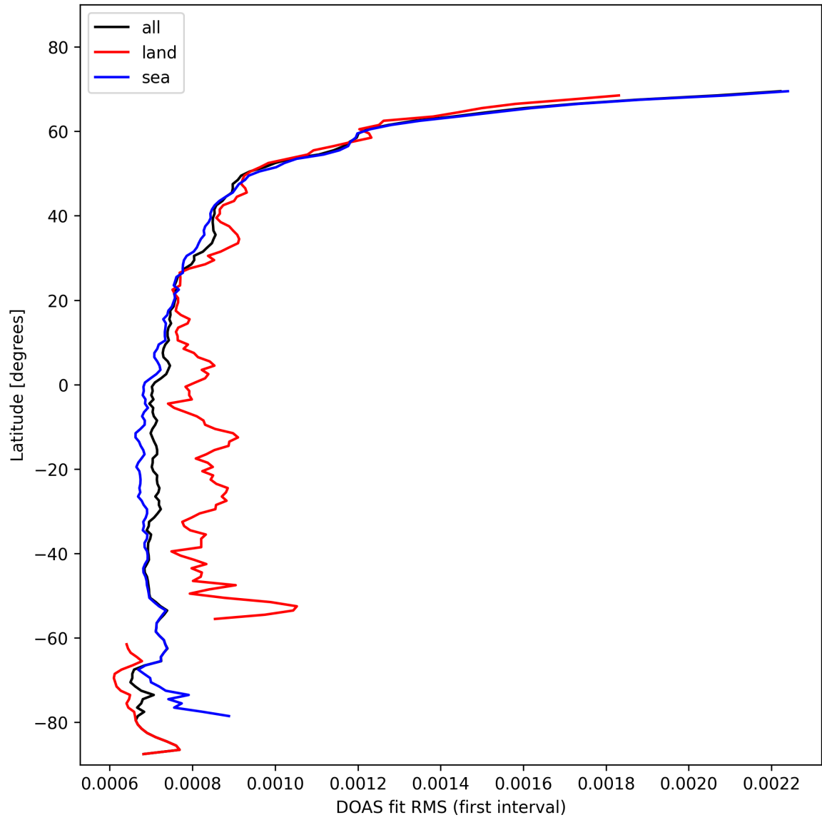
Figure 32: Zonal average of “DOAS fit RMS (first interval)” for 2024-11-04 to 2024-11-05.
