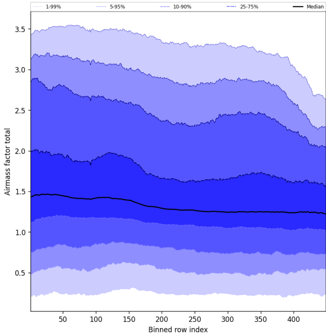
Figure 54: Along track statistics of “Airmass factor total” for 2024-11-04 to 2024-11-05
