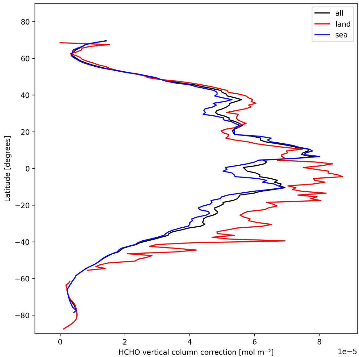
Figure 23: Zonal average of "HCHO vertical column correction" for 2024-11-04 to 2024-11-05.
