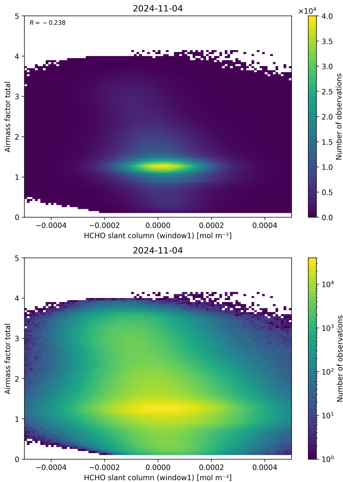
Figure 85: Scatter density plot of “HCHO slant column (window1)” against “Airmass factor total” for 2024-11-04 to 2024-11-05.
