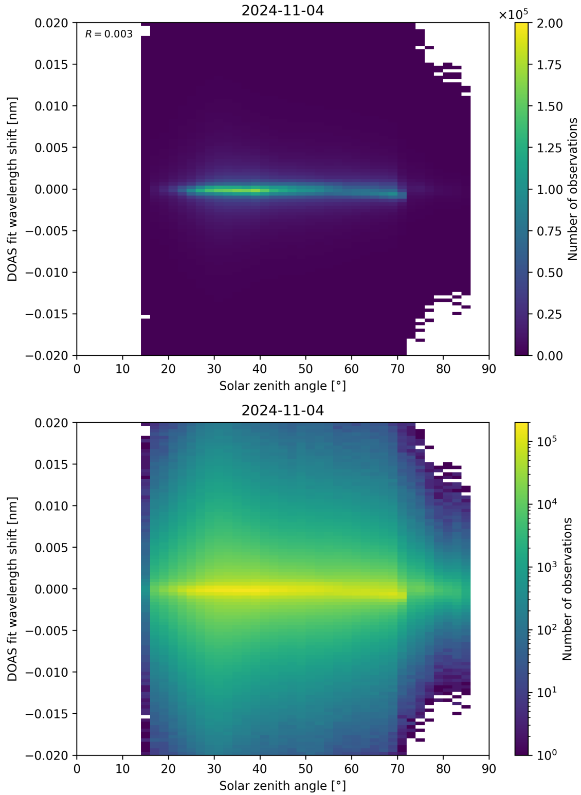
Figure 168: Scatter density plot of “Solar zenith angle” against “DOAS fit wavelength shift” for 2024-11-04 to 2024-11-05.
