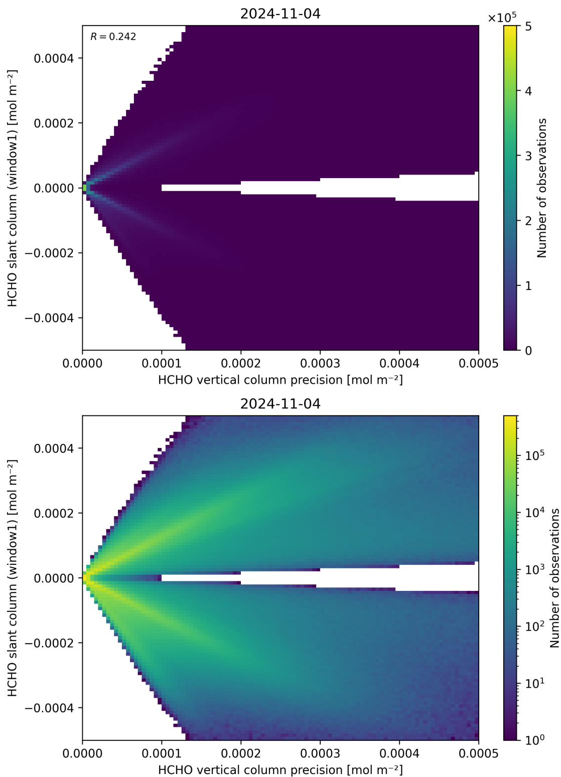
Figure 142: Scatter density plot of “HCHO vertical column precision” against “HCHO slant column (window1)” for 2024-11-04 to 2024-11-05.
