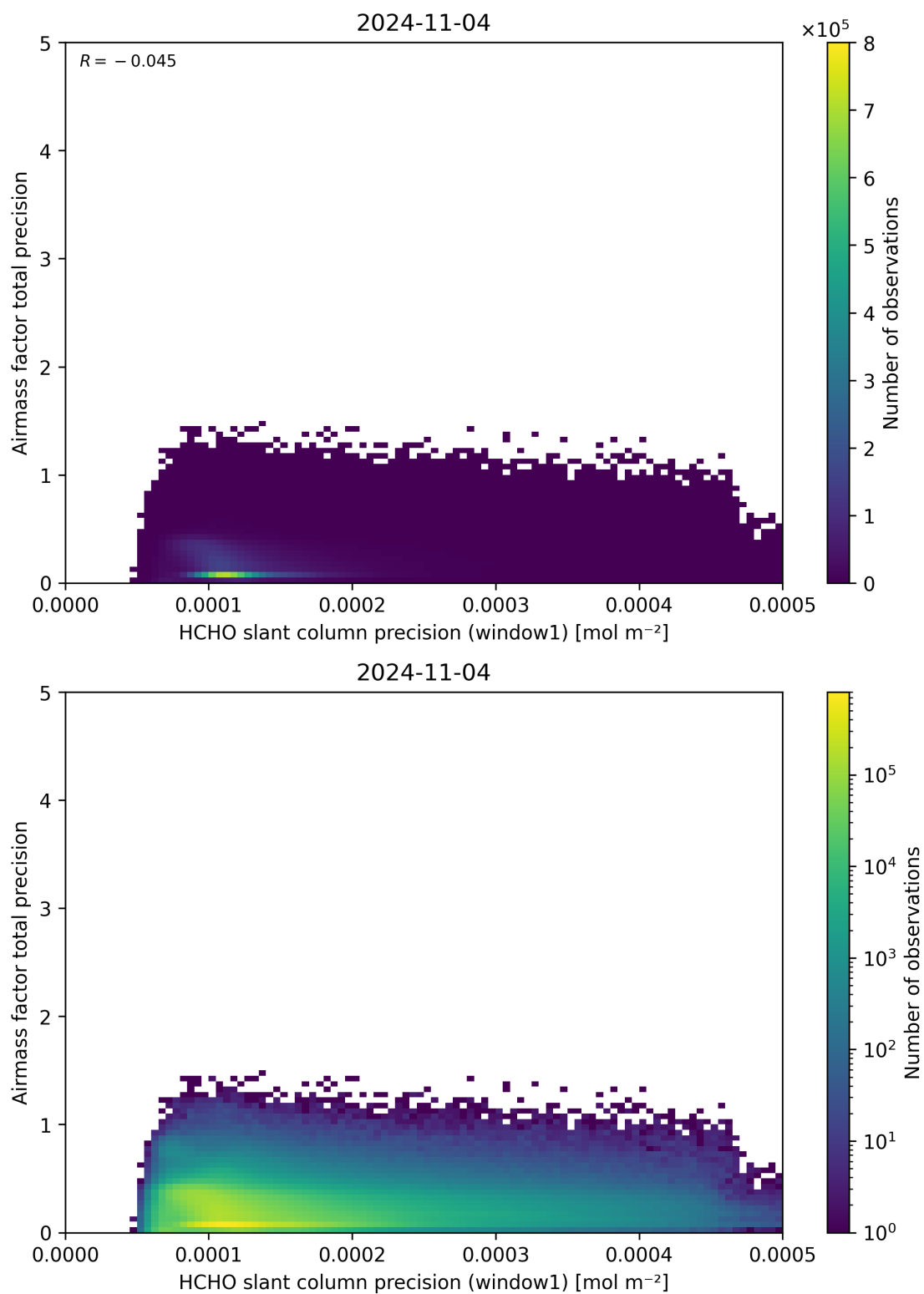
Figure 95: Scatter density plot of “HCHO slant column precision (window1)” against “Airmass factor total precision” for 2024-11-04 to 2024-11-05.
