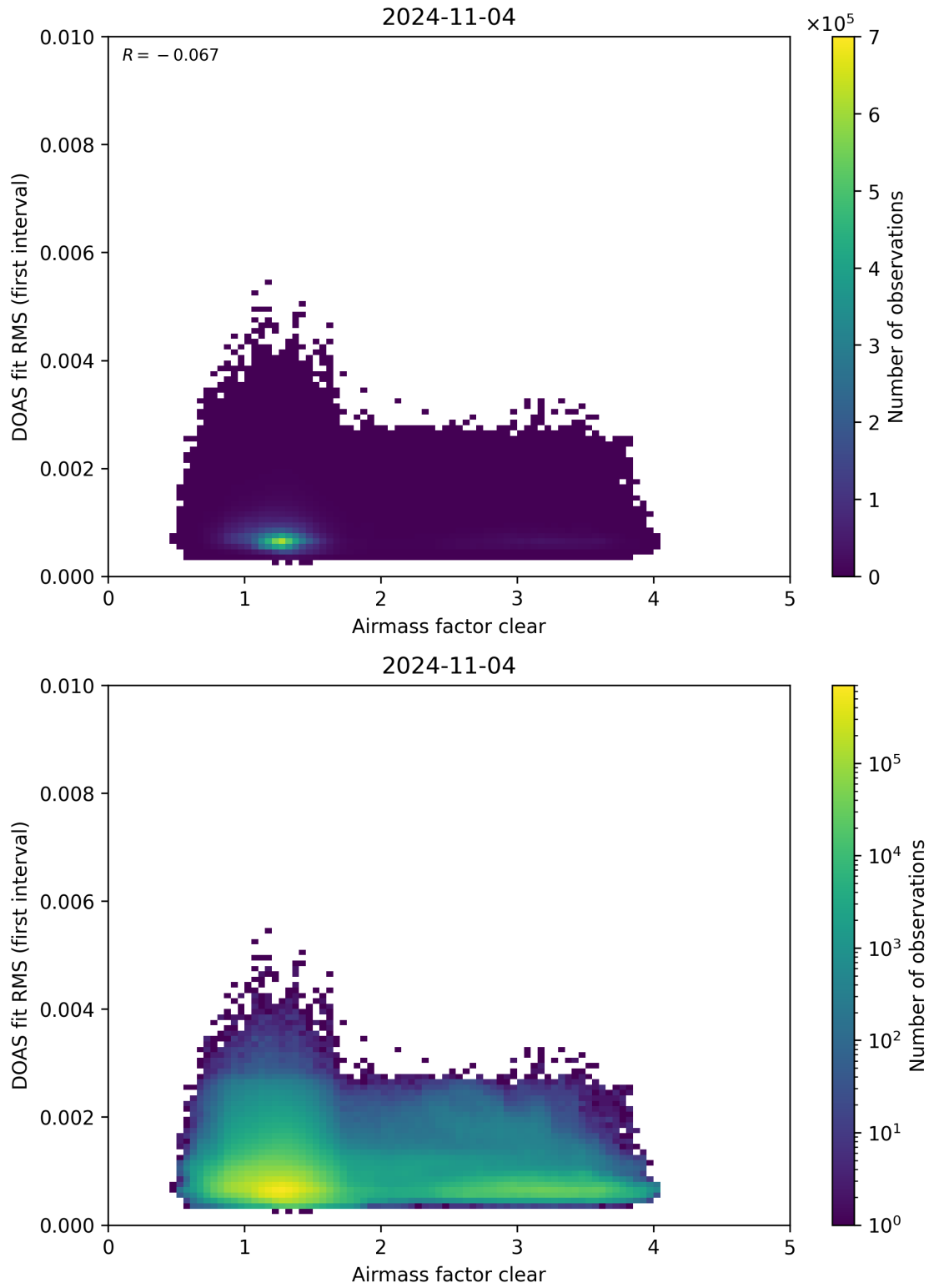
Figure 71: Scatter density plot of “Airmass factor clear” against “DOAS fit RMS (first interval)” for 2024-11-04 to 2024-11-05.
