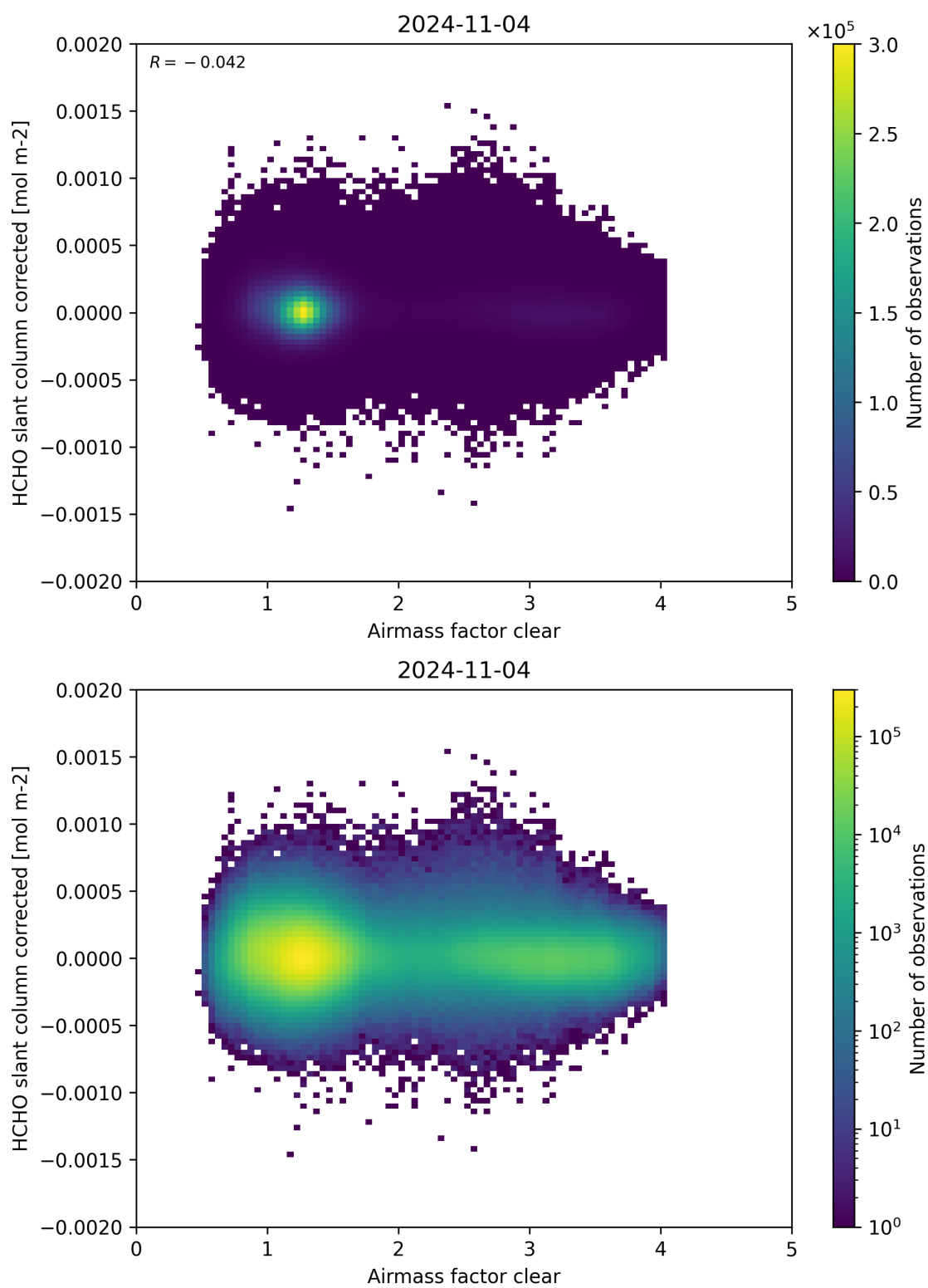
Figure 74: Scatter density plot of “Airmass factor clear” against “HCHO slant column corrected” for 2024-11-04 to 2024-11-05.
