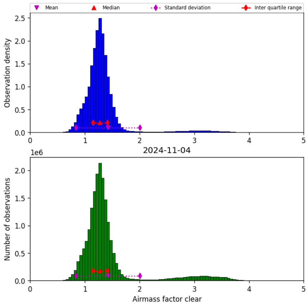
Figure 42: Histogram of “Airmass factor clear” for 2024-11-04 to 2024-11-05
