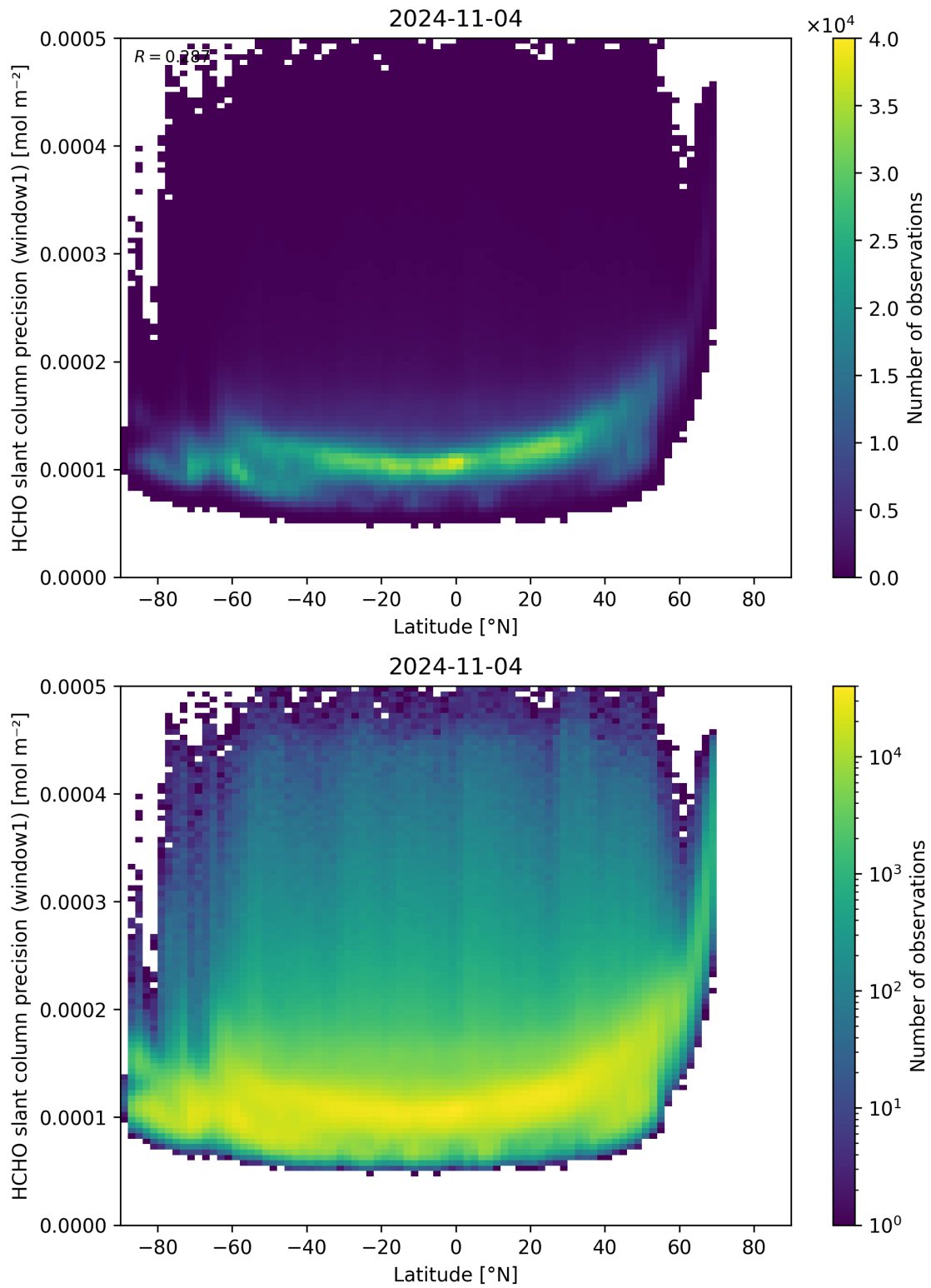
Figure 160: Scatter density plot of “Latitude” against “HCHO slant column precision (window1)” for 2024-11-04 to 2024-11-05.
