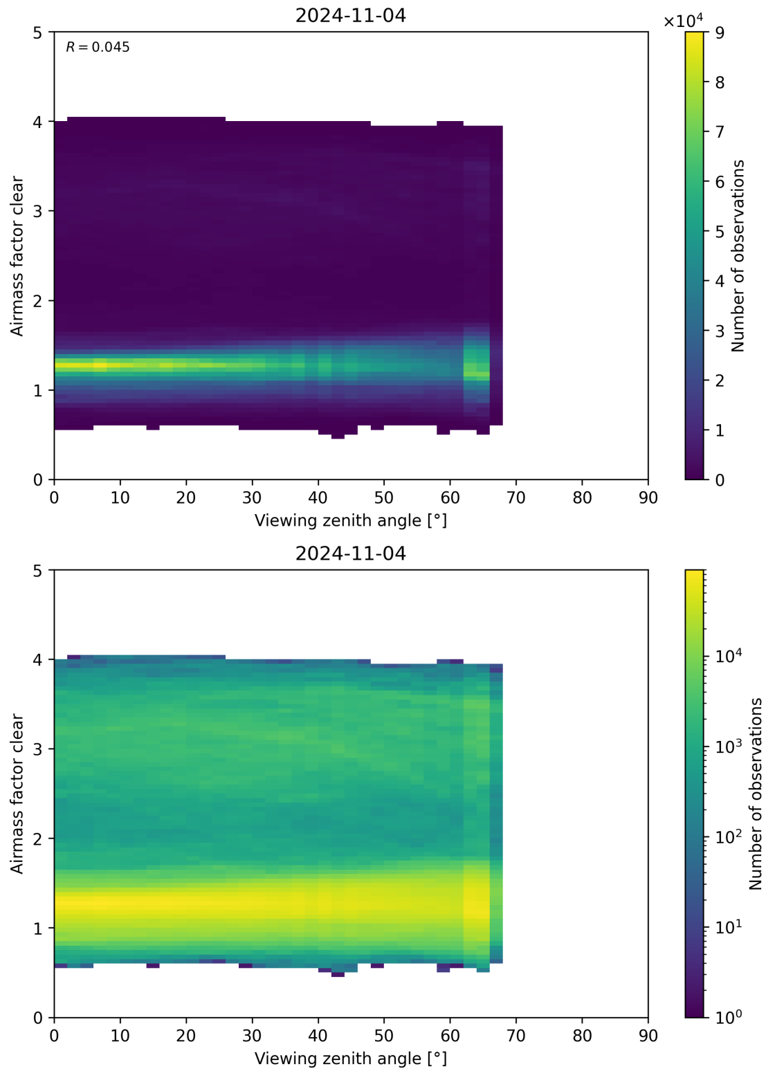
Figure 185: Scatter density plot of “Viewing zenith angle” against “Airmass factor clear” for 2024-11-04 to 2024-11-05.
