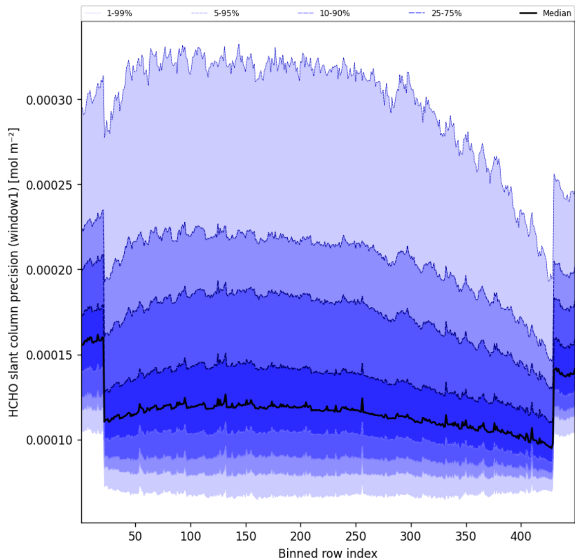
Figure 53: Along track statistics of “HCHO slant column precision (window1)” for 2024-11-04 to 2024-11-05
