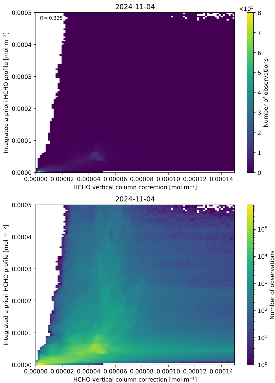
Figure 122: Scatter density plot of “HCHO vertical column correction” against “Integrated a priori HCHO profile” for 2024-11-04 to 2024-11-05.
