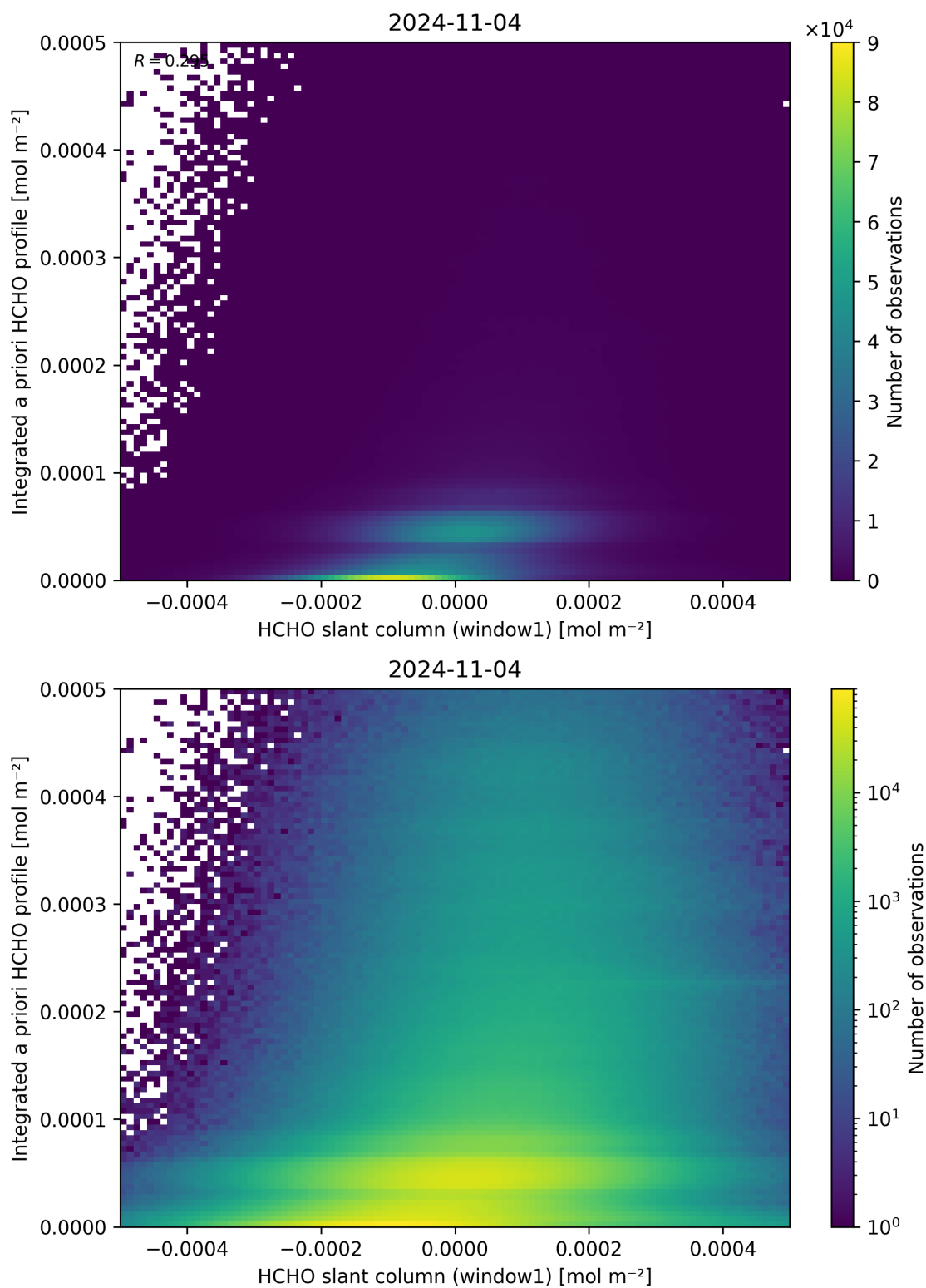
Figure 87: Scatter density plot of “HCHO slant column (window1)” against “Integrated a priori HCHO profile” for 2024-11-04 to 2024-11-05.
