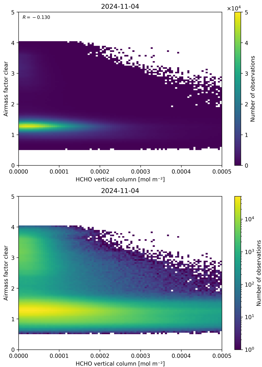
Figure 126: Scatter density plot of “HCHO vertical column” against “Airmass factor clear” for 2024-11-04 to 2024-11-05.
