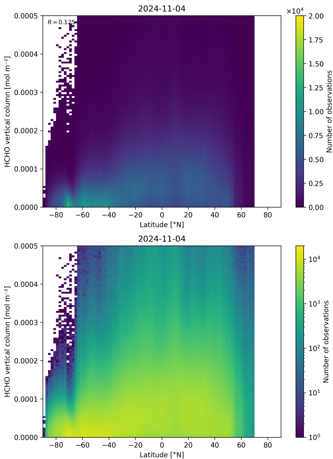
Figure 163: Scatter density plot of “Latitude” against “HCHO vertical column” for 2024-11-04 to 2024-11-05.
