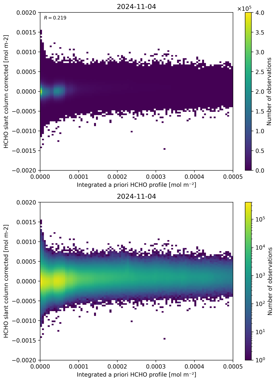
Figure 151: Scatter density plot of “Integrated a priori HCHO profile” against “HCHO slant column corrected” for 2024-11-04 to 2024-11-05.
