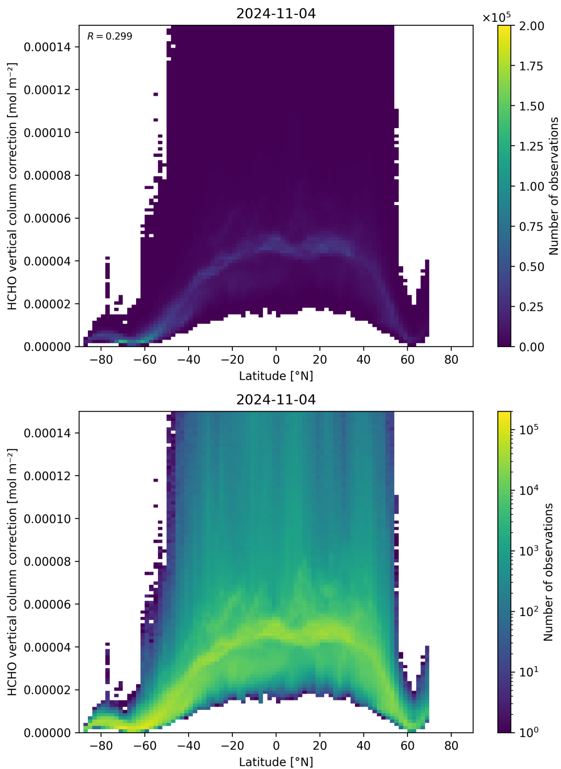
Figure 164: Scatter density plot of “Latitude” against “HCHO vertical column correction” for 2024-11-04 to 2024-11-05.
