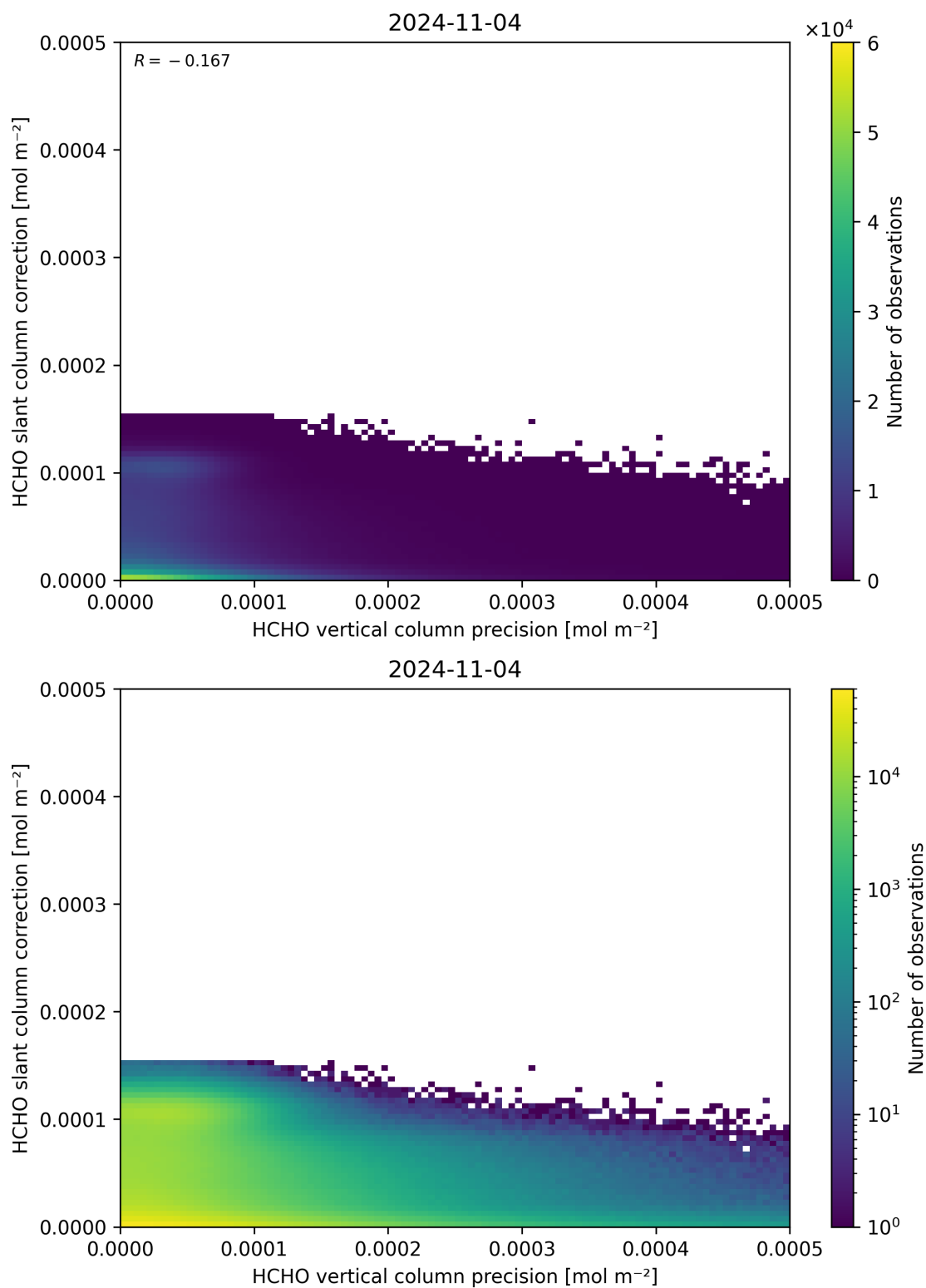
Figure 141: Scatter density plot of “HCHO vertical column precision” against “HCHO slant column correction” for 2024-11-04 to 2024-11-05.
