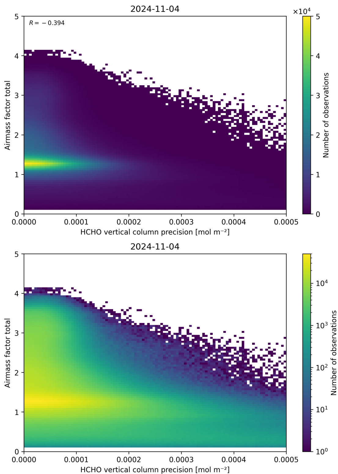
Figure 144: Scatter density plot of “HCHO vertical column precision” against “Airmass factor total” for 2024-11-04 to 2024-11-05.
