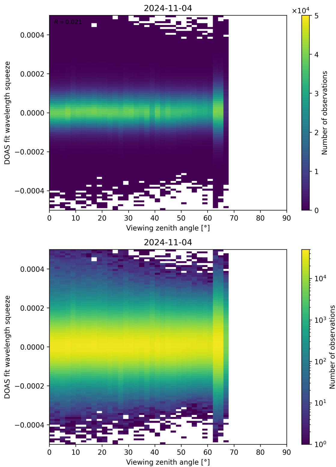
Figure 184: Scatter density plot of “Viewing zenith angle” against “DOAS fit wavelength squeeze” for 2024-11-04 to 2024-11-05.
