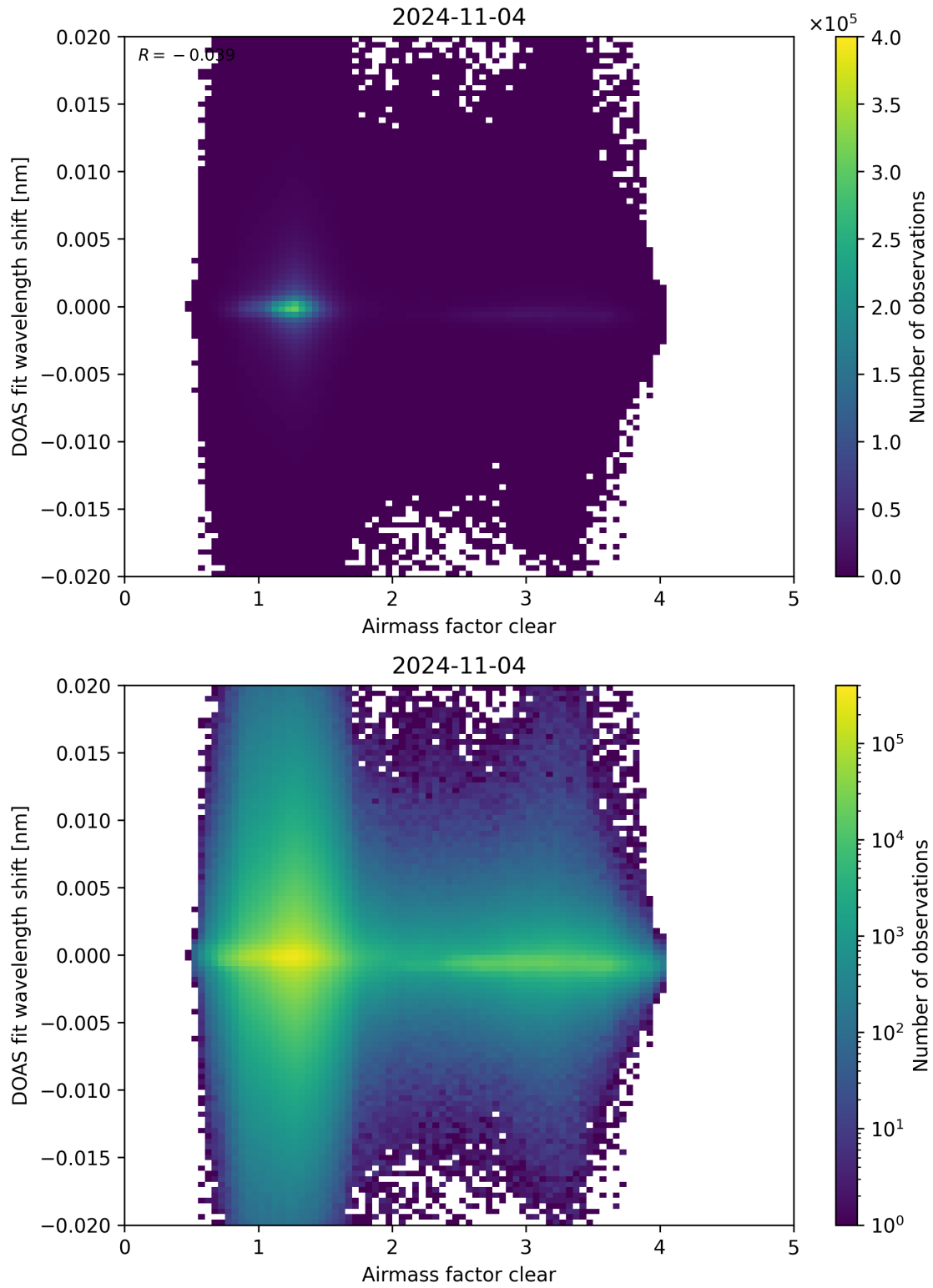
Figure 72: Scatter density plot of “Airmass factor clear” against “DOAS fit wavelength shift” for 2024-11-04 to 2024-11-05.
