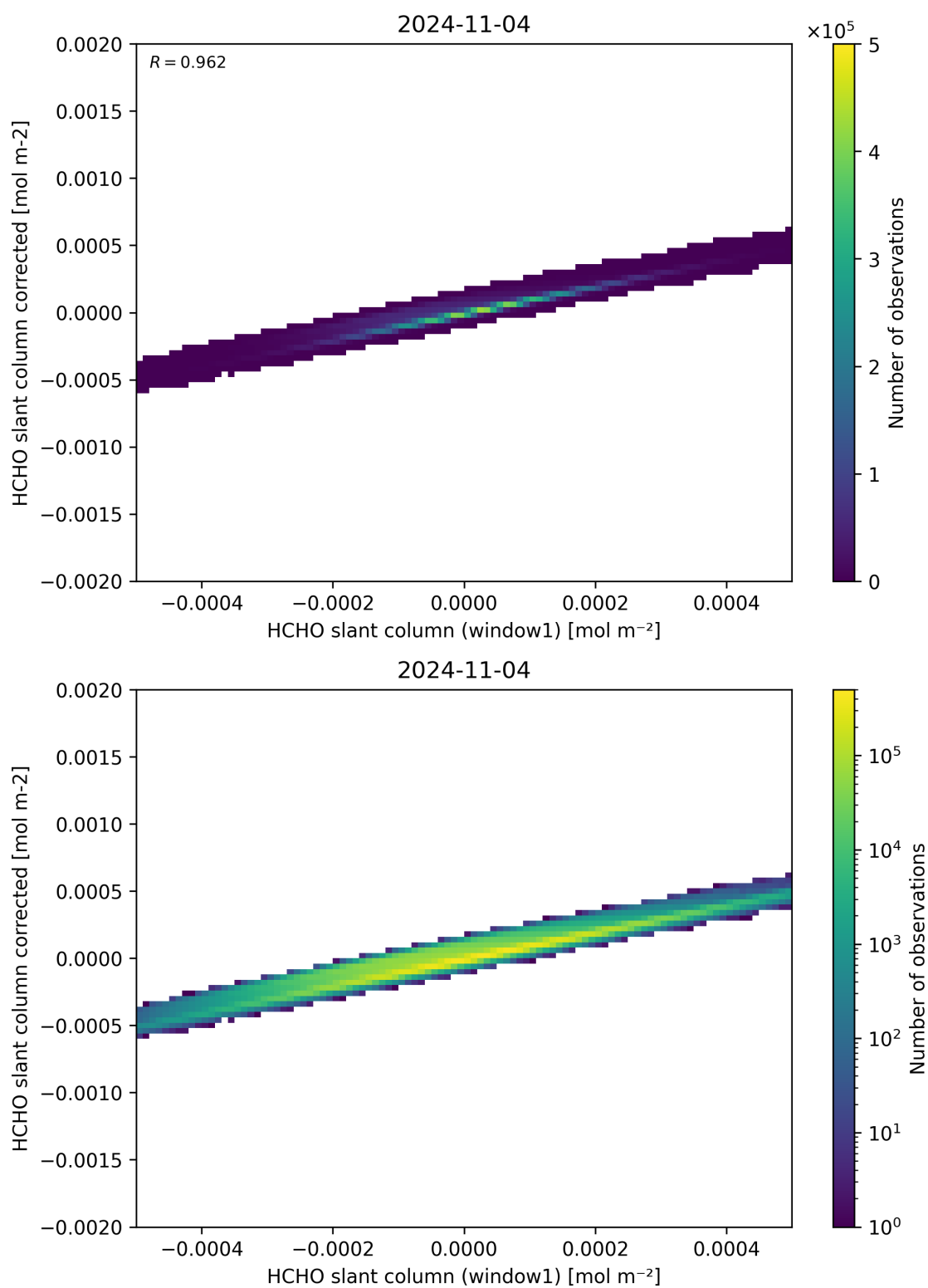
Figure 82: Scatter density plot of “HCHO slant column (window1)” against “HCHO slant column corrected” for 2024-11-04 to 2024-11-05.
