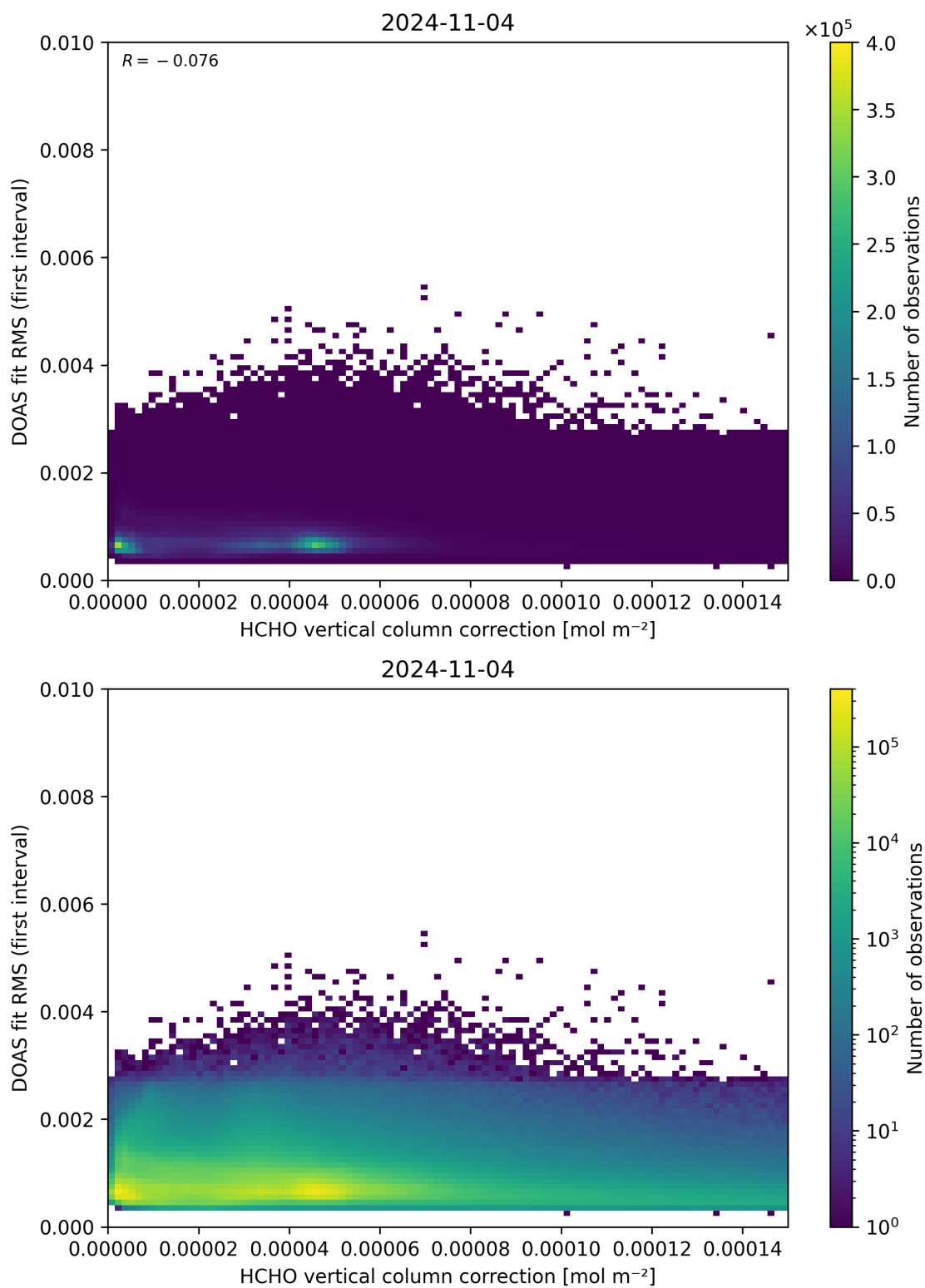
Figure 112: Scatter density plot of “HCHO vertical column correction” against “DOAS fit RMS (first interval)” for 2024-11-04 to 2024-11-05.
