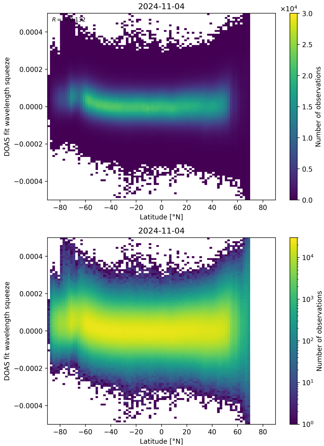
Figure 155: Scatter density plot of “Latitude” against “DOAS fit wavelength squeeze” for 2024-11-04 to 2024-11-05.
