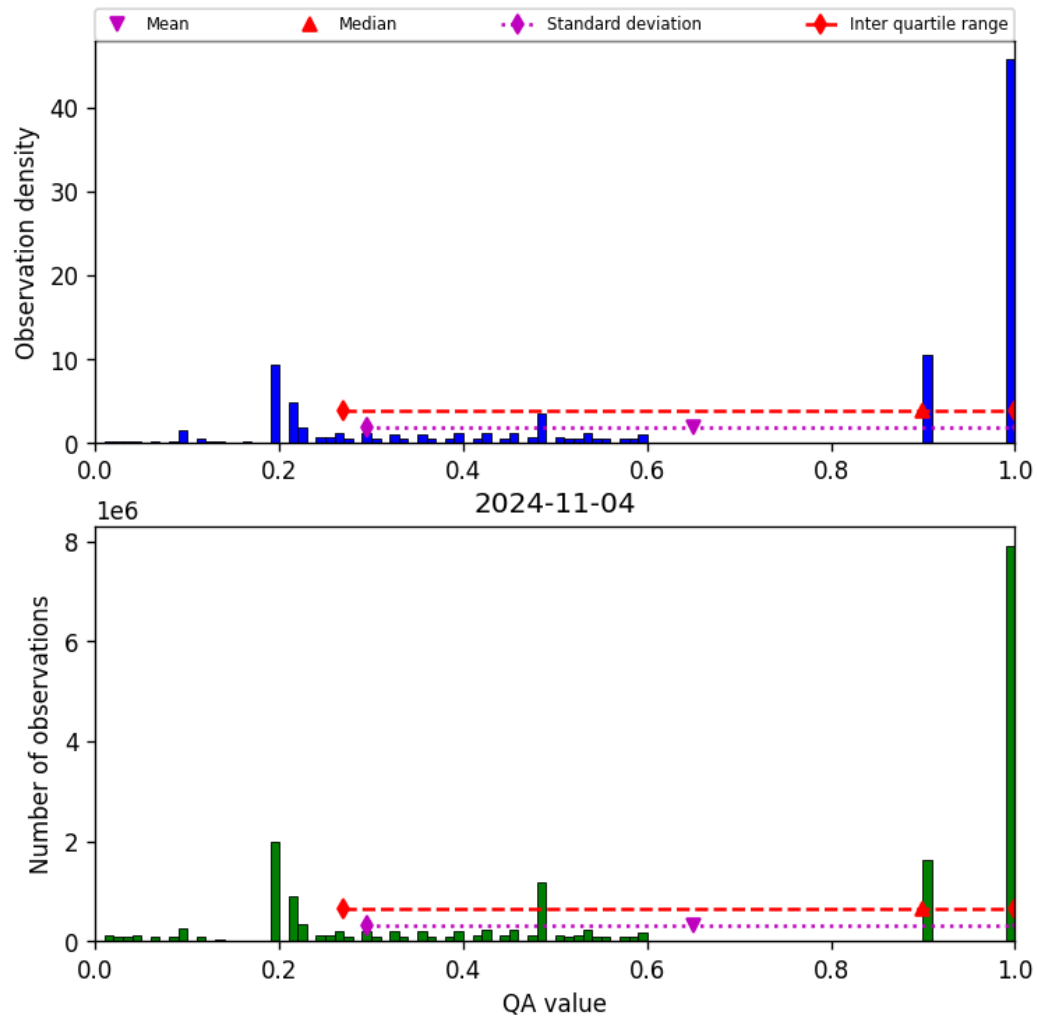
Figure 34: Histogram of “QA value” for 2024-11-04 to 2024-11-05
