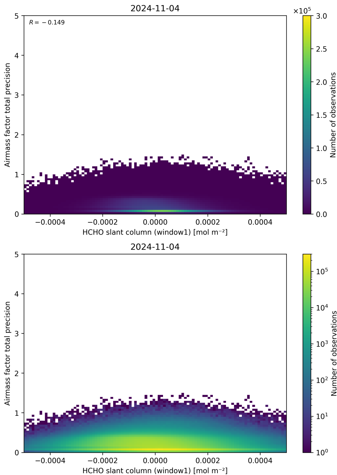
Figure 86: Scatter density plot of “HCHO slant column (window1)” against “Airmass factor total precision” for 2024-11-04 to 2024-11-05.
