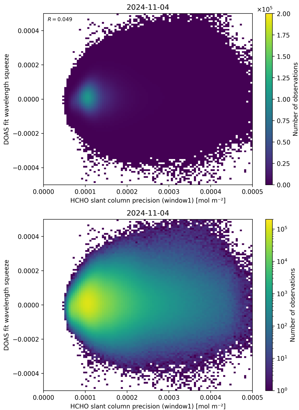
Figure 90: Scatter density plot of “HCHO slant column precision (window1)” against “DOAS fit wavelength squeeze” for 2024-11-04 to 2024-11-05.
