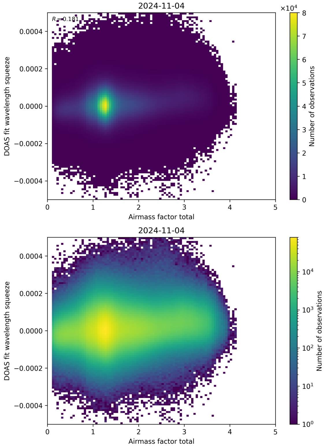
Figure 99: Scatter density plot of “Airmass factor total” against “DOAS fit wavelength squeeze” for 2024-11-04 to 2024-11-05.
