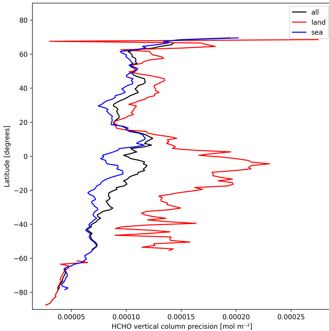
Figure 22: Zonal average of “HCHO vertical column precision” for 2024-11-04 to 2024-11-05.
