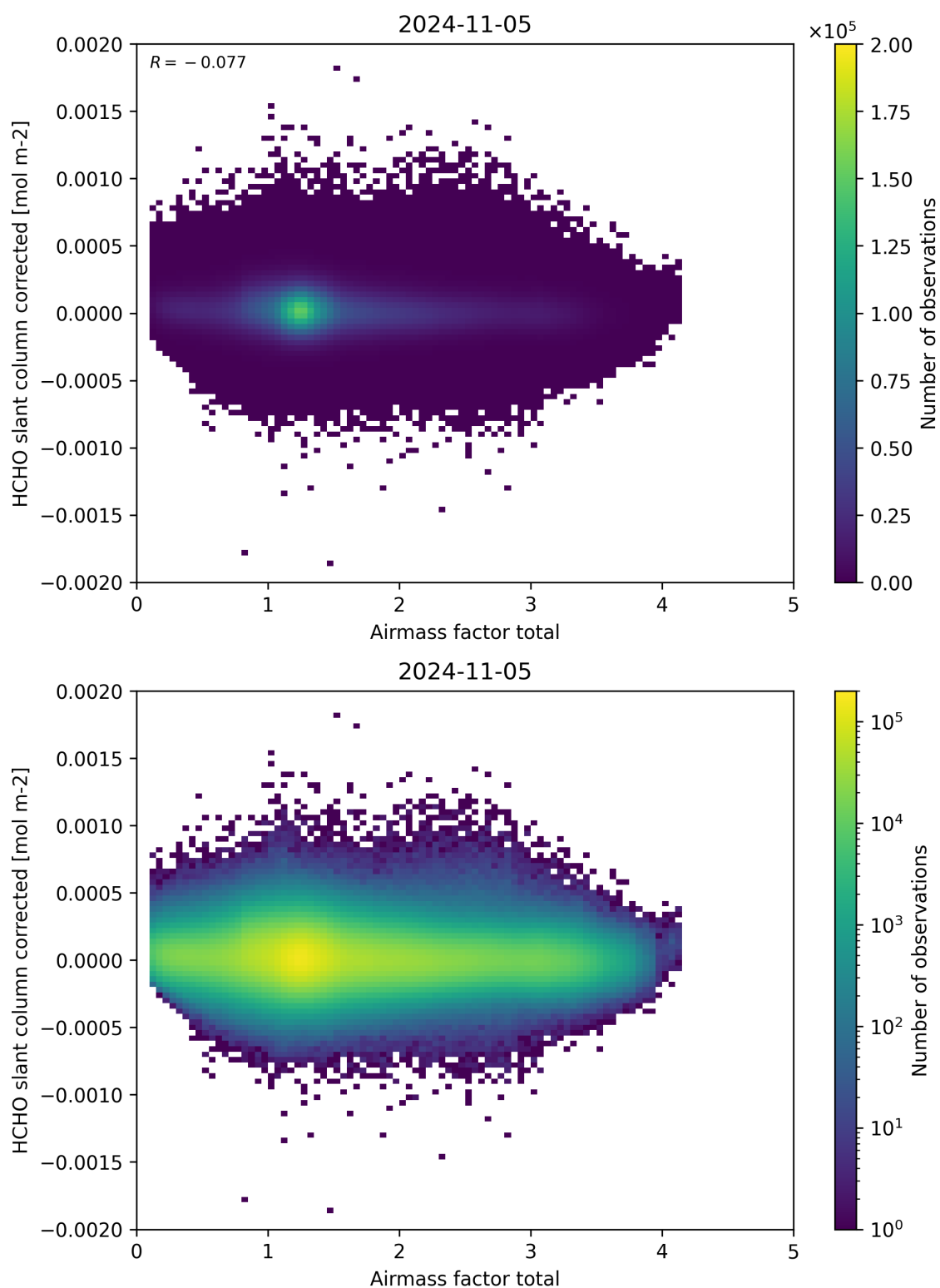
Figure 101: Scatter density plot of “Airmass factor total” against “HCHO slant column corrected” for 2024-11-04 to 2024-11-06.
