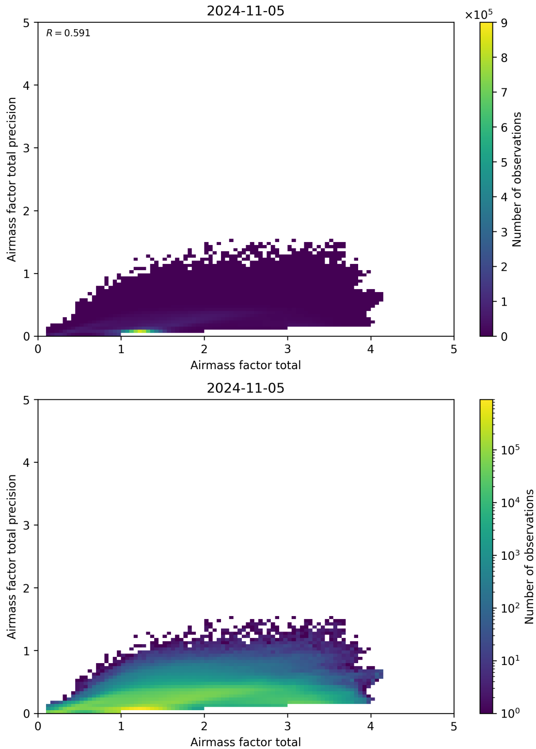
Figure 103: Scatter density plot of “Airmass factor total” against “Airmass factor total precision” for 2024-11-04 to 2024-11-06.
