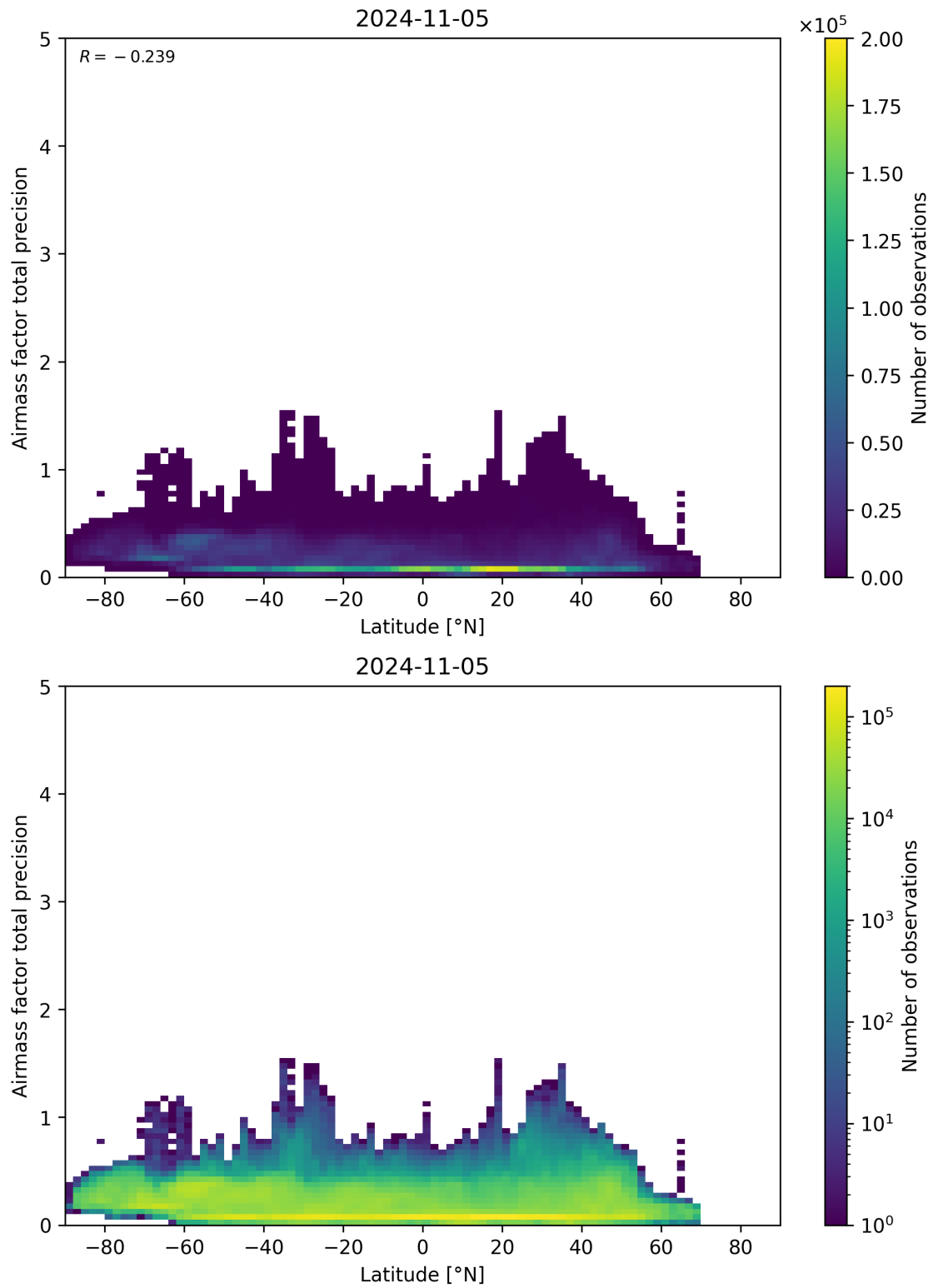
Figure 162: Scatter density plot of “Latitude” against “Airmass factor total precision” for 2024-11-04 to 2024-11-06.
