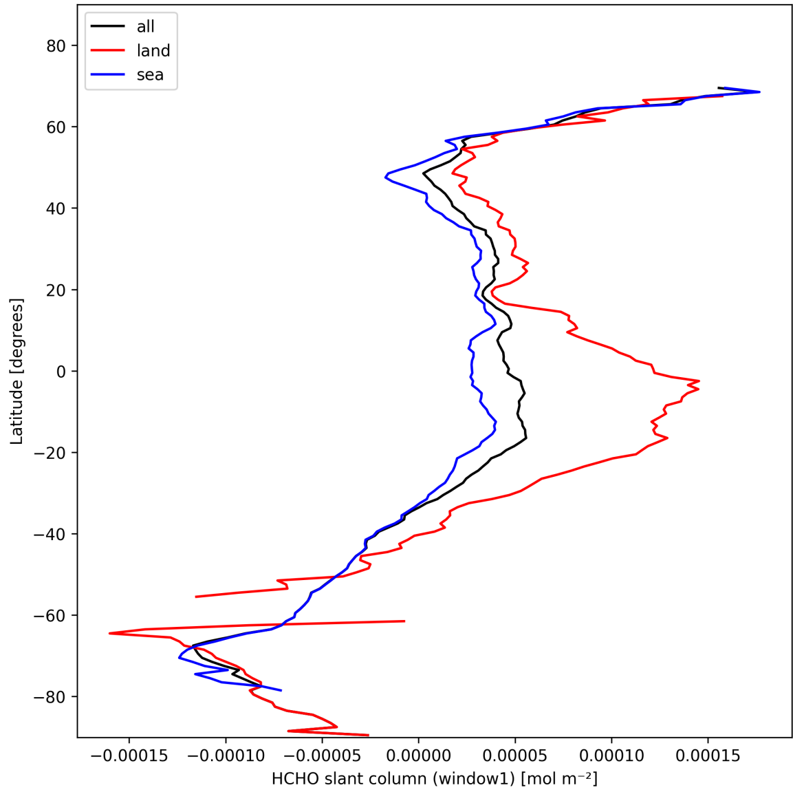
Figure 24: Zonal average of “HCHO slant column (window1)” for 2024-11-04 to 2024-11-06.
