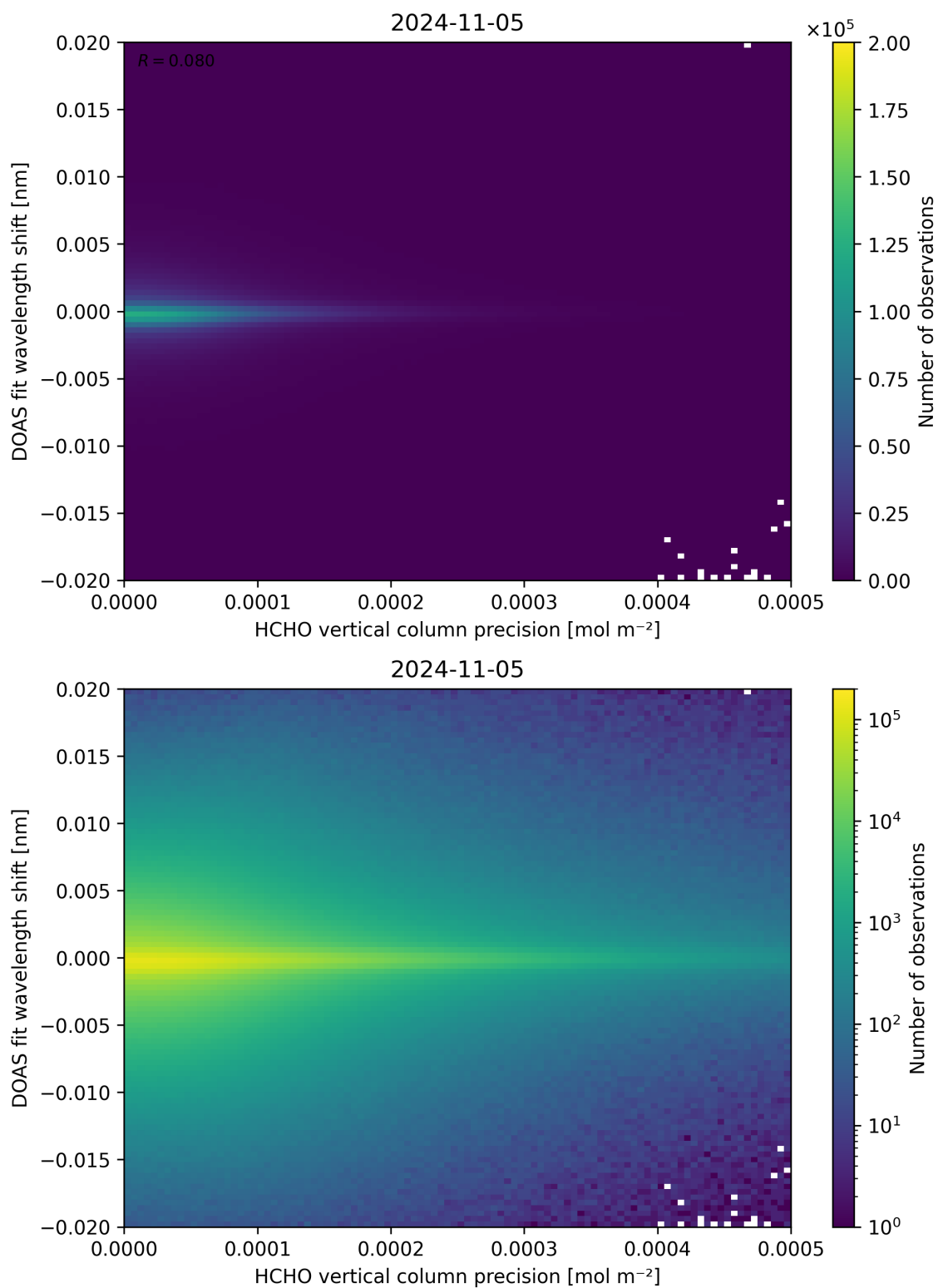
Figure 137: Scatter density plot of “HCHO vertical column precision” against “DOAS fit wavelength shift” for 2024-11-04 to 2024-11-06.
