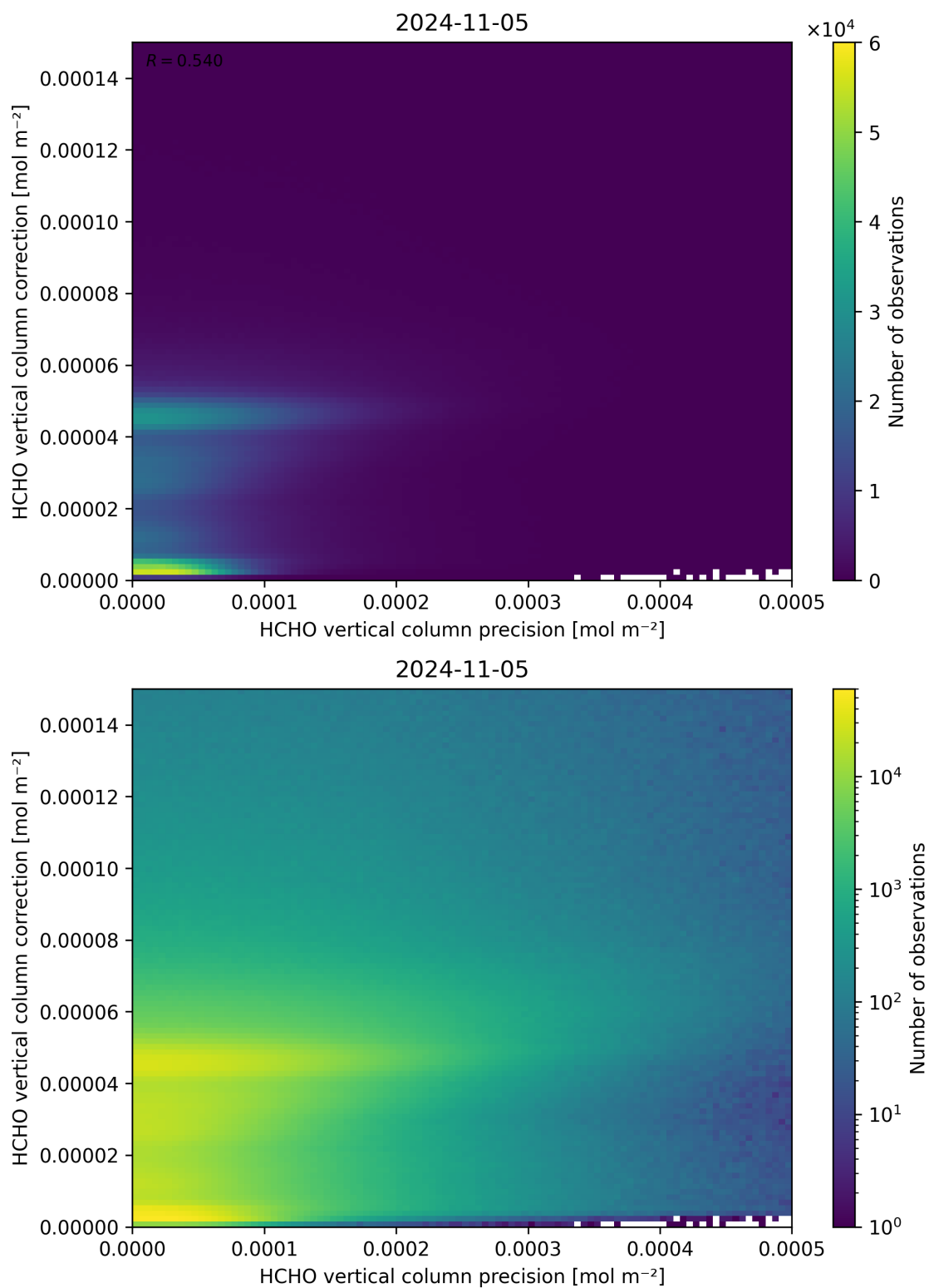
Figure 146: Scatter density plot of “HCHO vertical column precision” against “HCHO vertical column correction” for 2024-11-04 to 2024-11-06.
