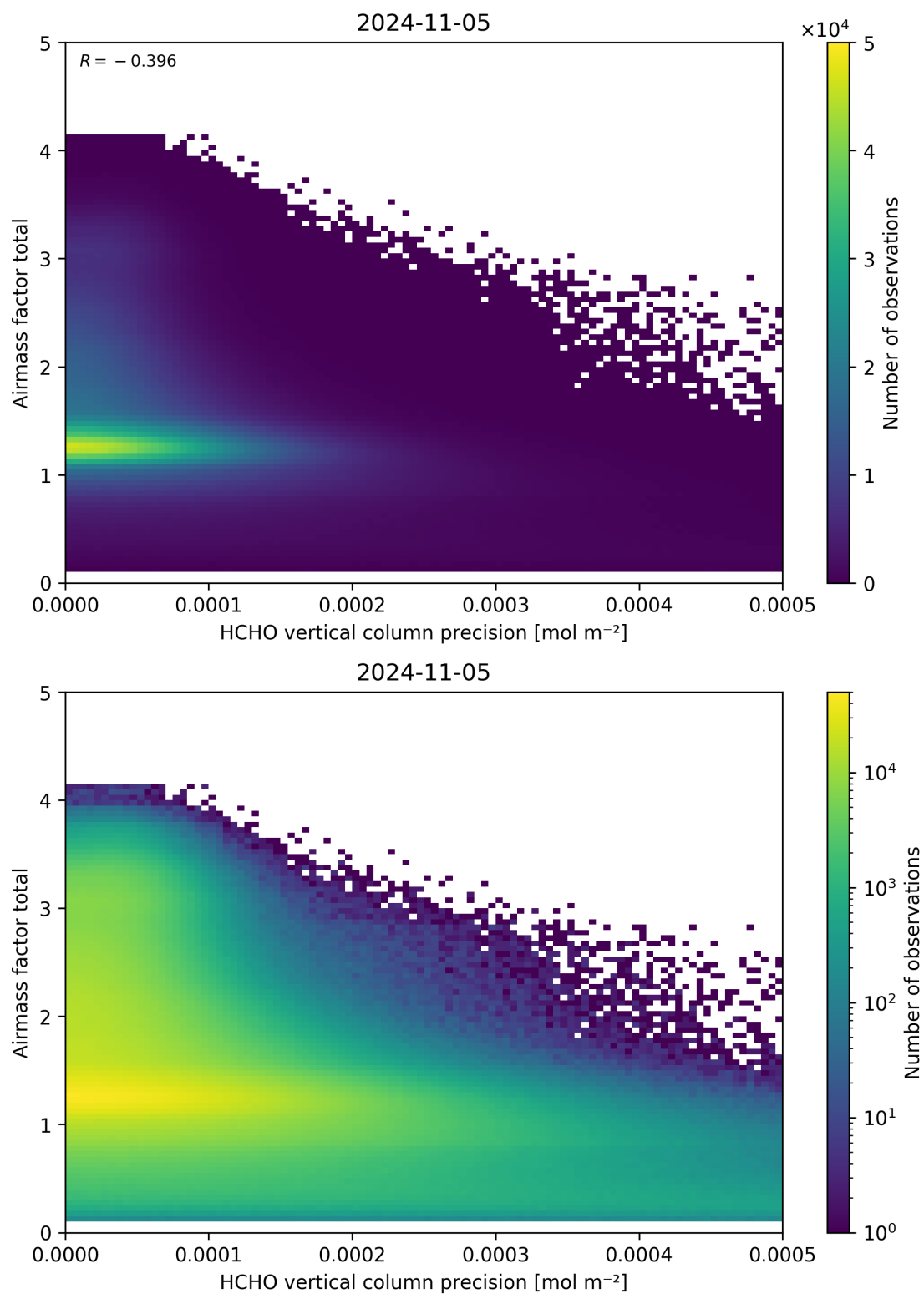
Figure 144: Scatter density plot of “HCHO vertical column precision” against “Airmass factor total” for 2024-11-04 to 2024-11-06.
