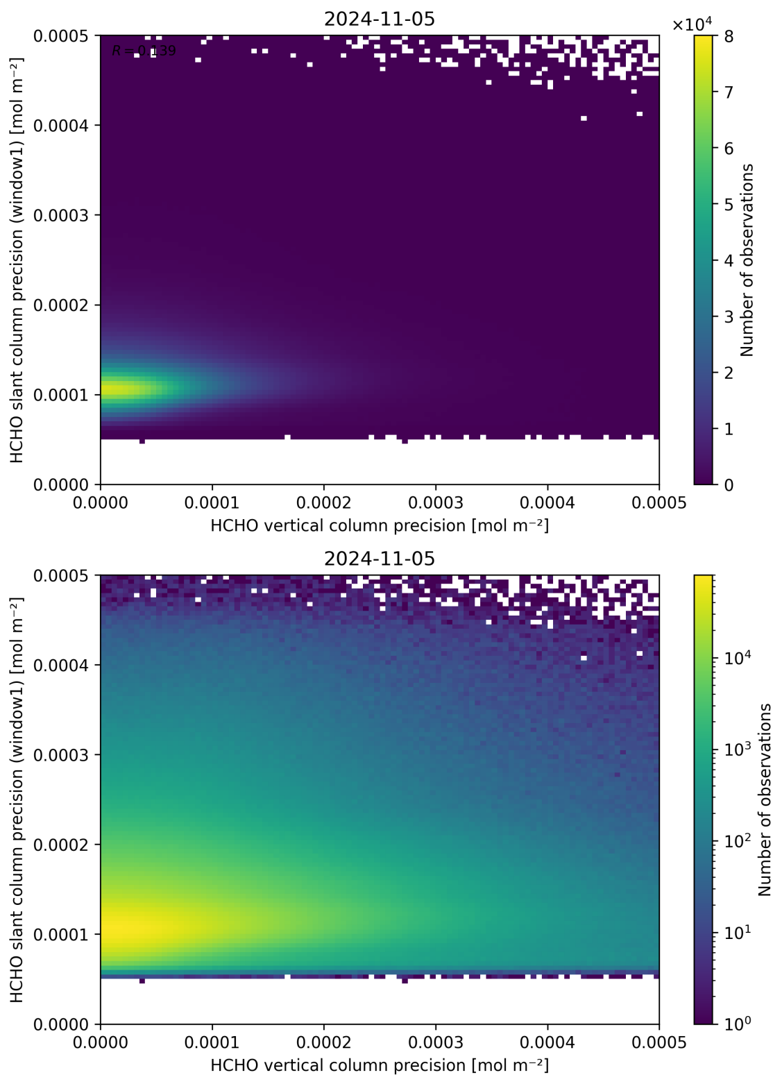
Figure 143: Scatter density plot of “HCHO vertical column precision” against “HCHO slant column precision (window1)” for 2024-11-04 to 2024-11-06.
