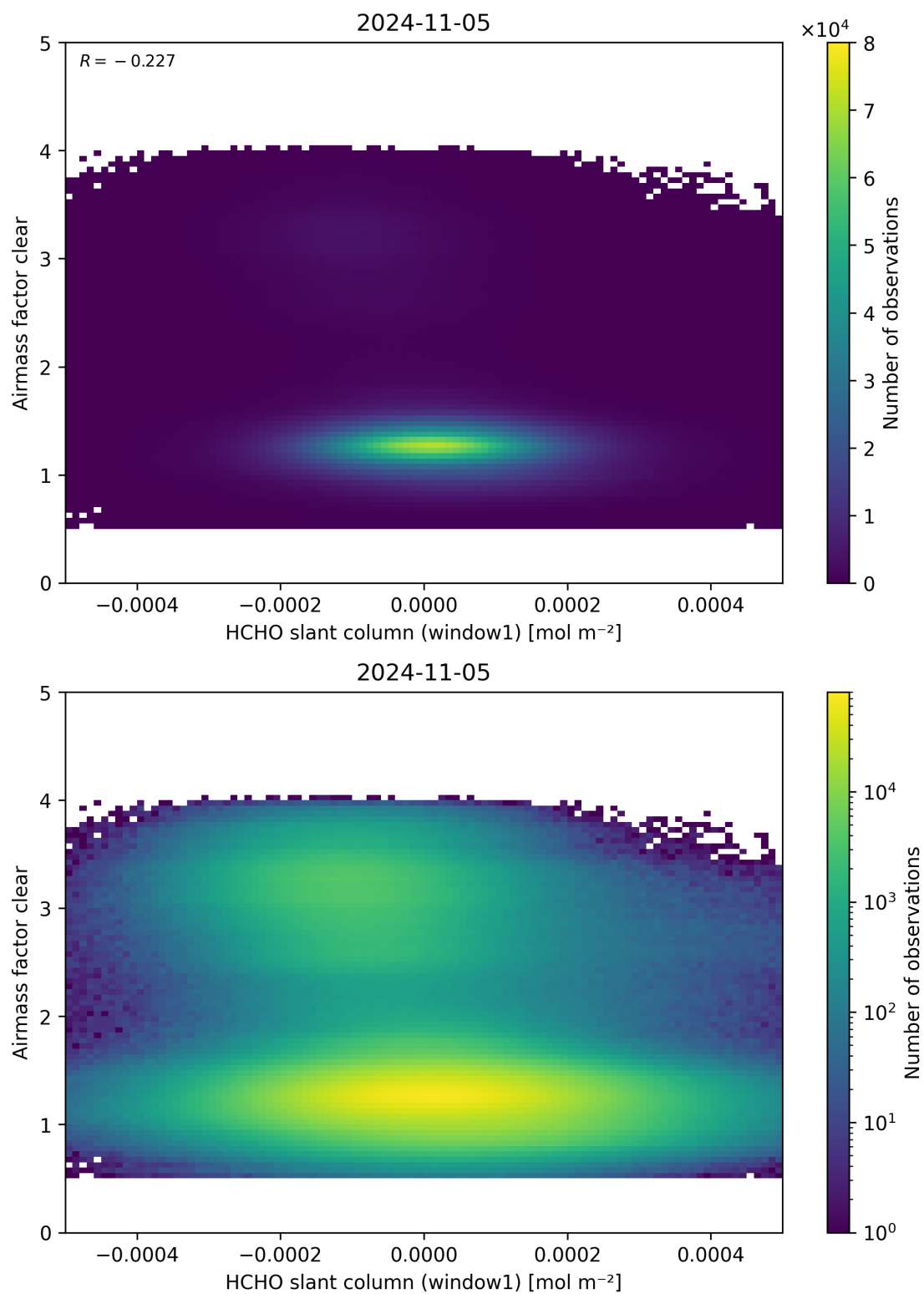
Figure 81: Scatter density plot of “HCHO slant column (window1)” against “Airmass factor clear” for 2024-11-04 to 2024-11-06.
