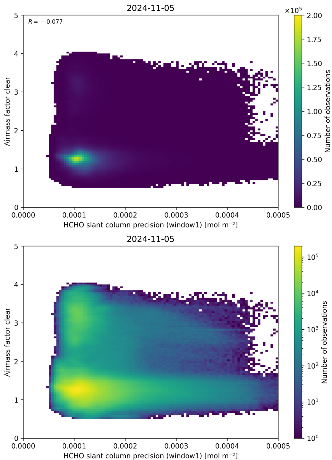
Figure 91: Scatter density plot of “HCHO slant column precision (window1)” against “Airmass factor clear” for 2024-11-04 to 2024-11-06.
