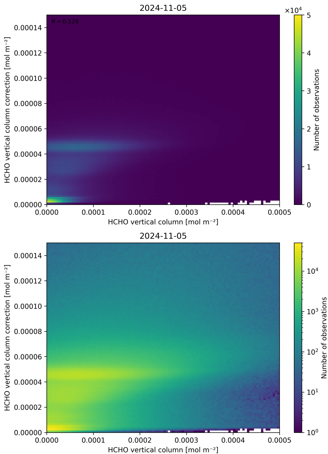
Figure 133: Scatter density plot of “HCHO vertical column” against “HCHO vertical column correction” for 2024-11-04 to 2024-11-06.
