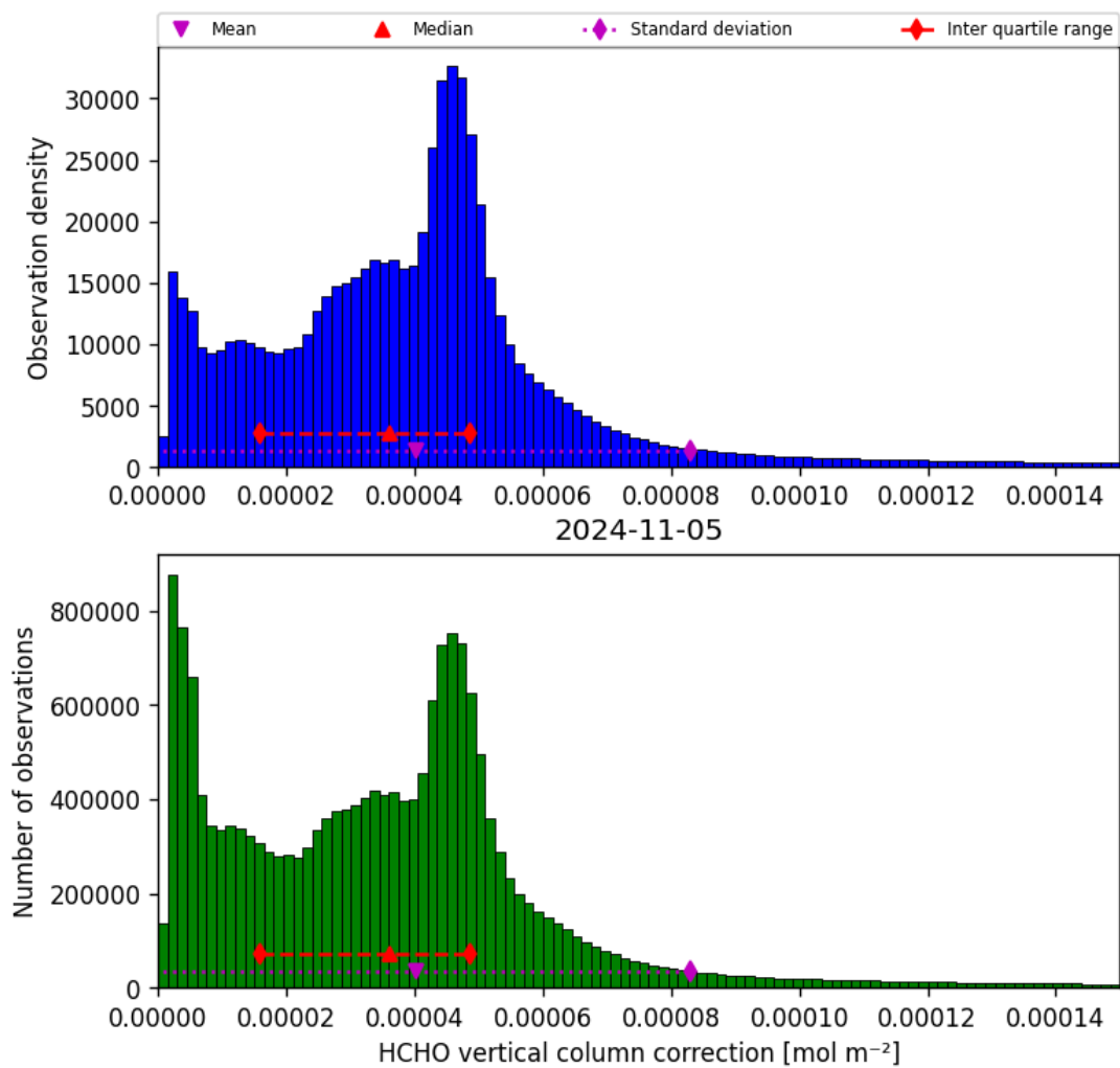
Figure 37: Histogram of “HCHO vertical column correction” for 2024-11-04 to 2024-11-06
