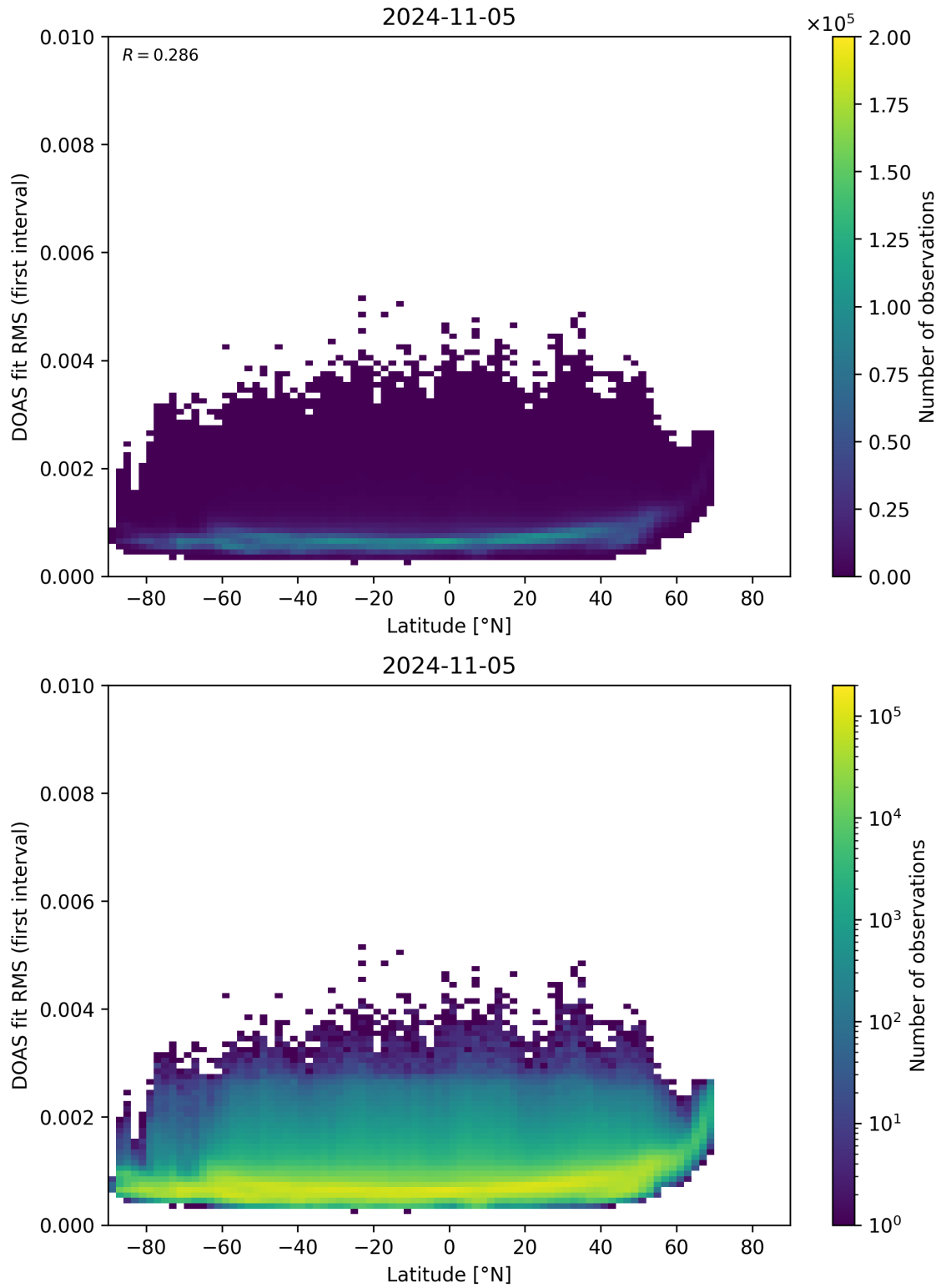
Figure 153: Scatter density plot of “Latitude” against “DOAS fit RMS (first interval)” for 2024-11-04 to 2024-11-06.
