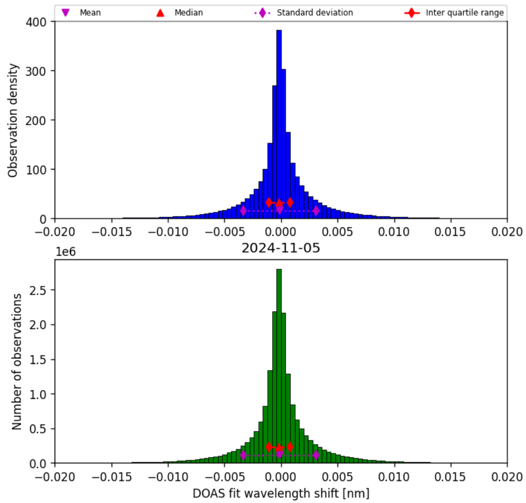
Figure 44: Histogram of “DOAS fit wavelength shift” for 2024-11-04 to 2024-11-06
