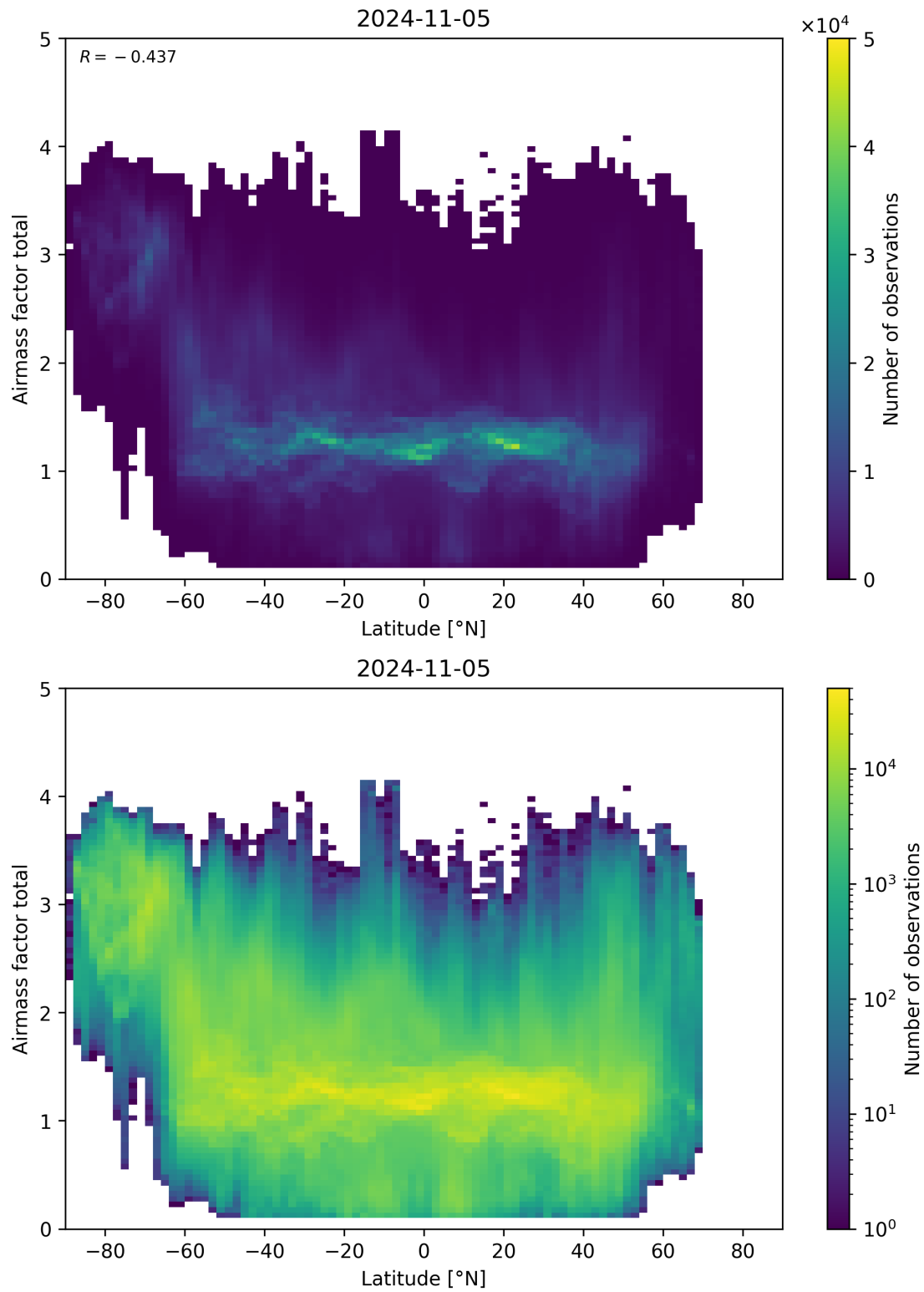
Figure 161: Scatter density plot of “Latitude” against “Airmass factor total” for 2024-11-04 to 2024-11-06.
