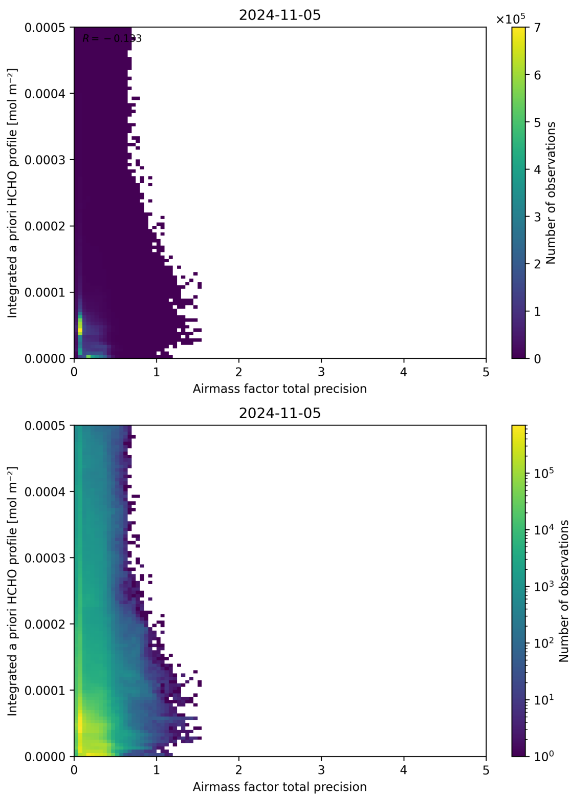
Figure 111: Scatter density plot of “Airmass factor total precision” against “Integrated a priori HCHO profile” for 2024-11-04 to 2024-11-06.
