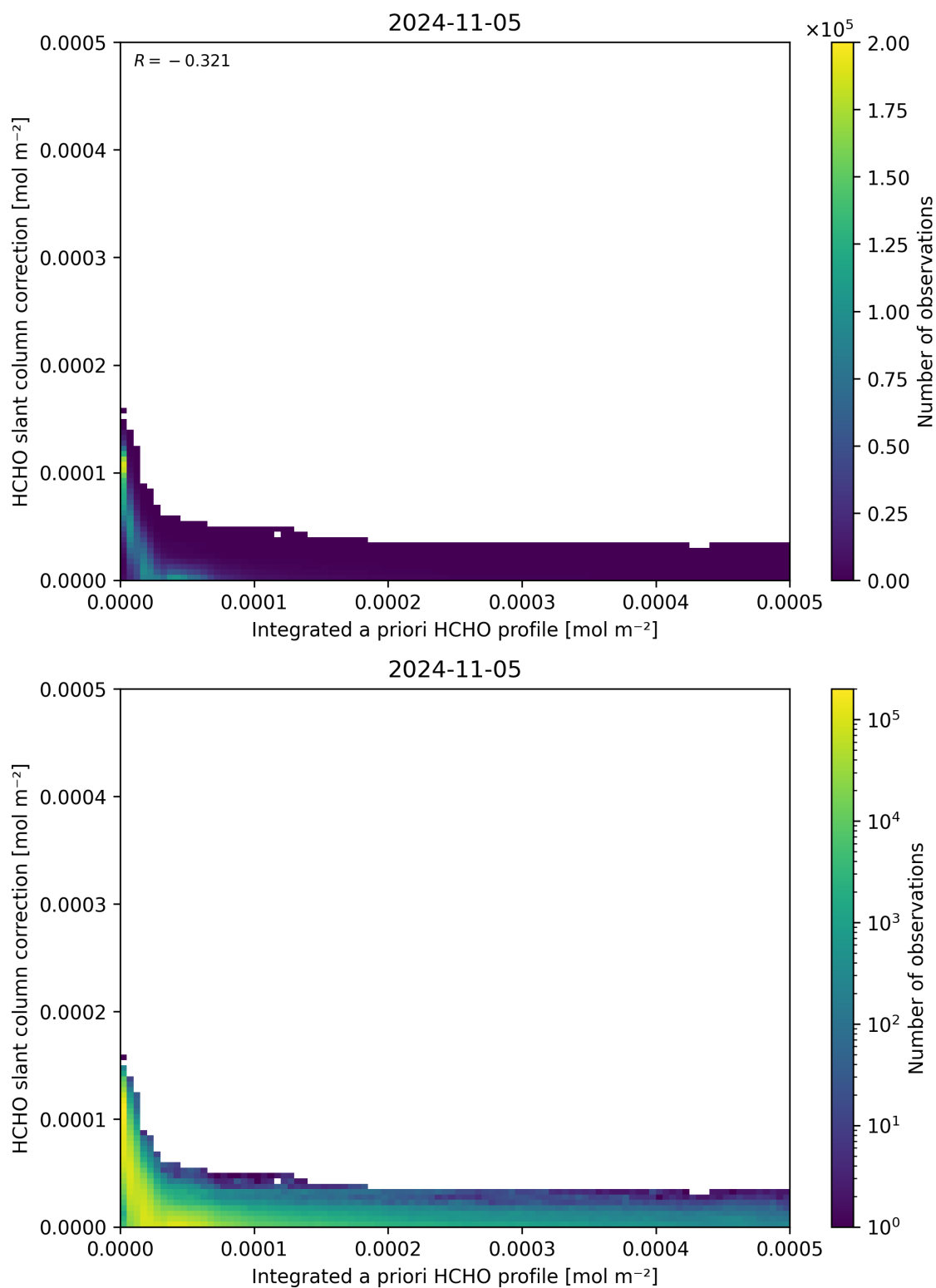
Figure 152: Scatter density plot of “Integrated a priori HCHO profile” against “HCHO slant column correction” for 2024-11-04 to 2024-11-06.
