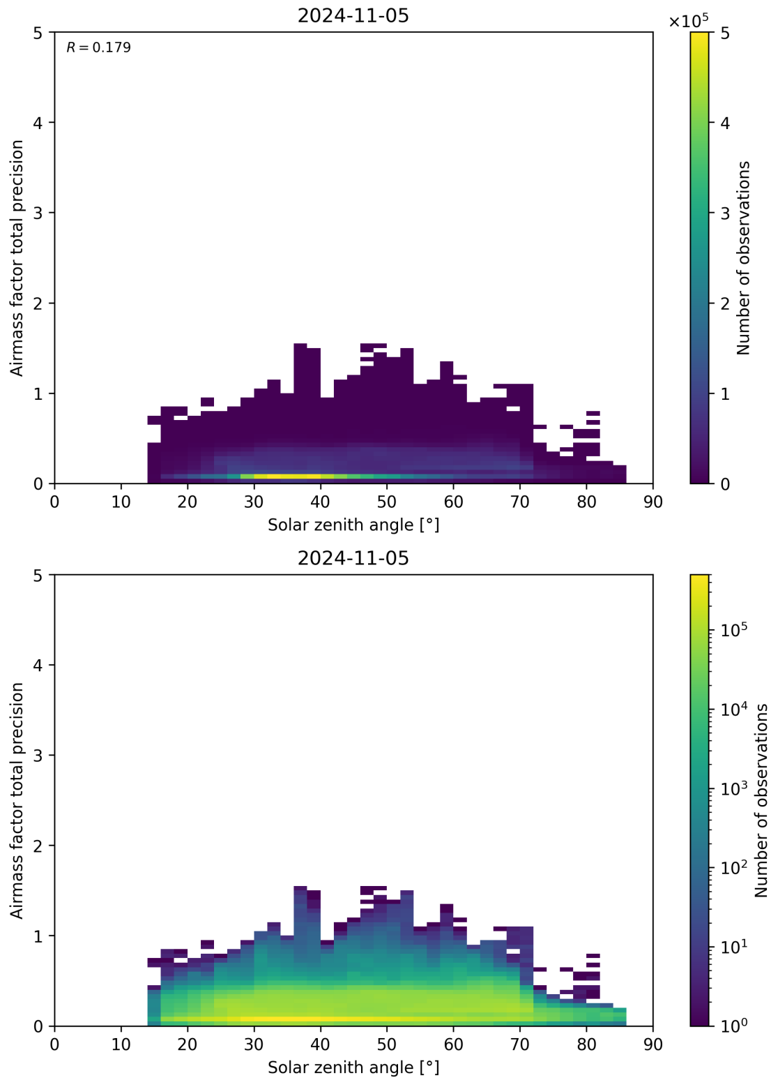
Figure 176: Scatter density plot of “Solar zenith angle” against “Airmass factor total precision” for 2024-11-04 to 2024-11-06.
