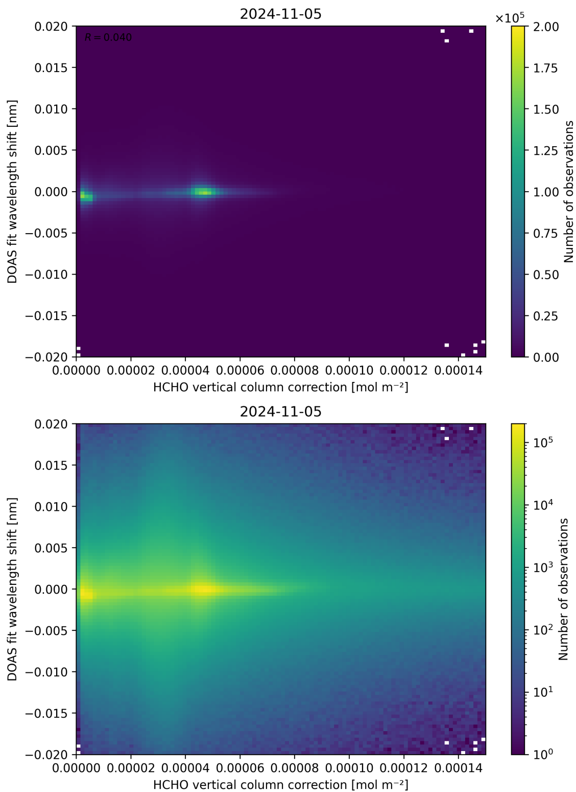
Figure 113: Scatter density plot of “HCHO vertical column correction” against “DOAS fit wavelength shift” for 2024-11-04 to 2024-11-06.
