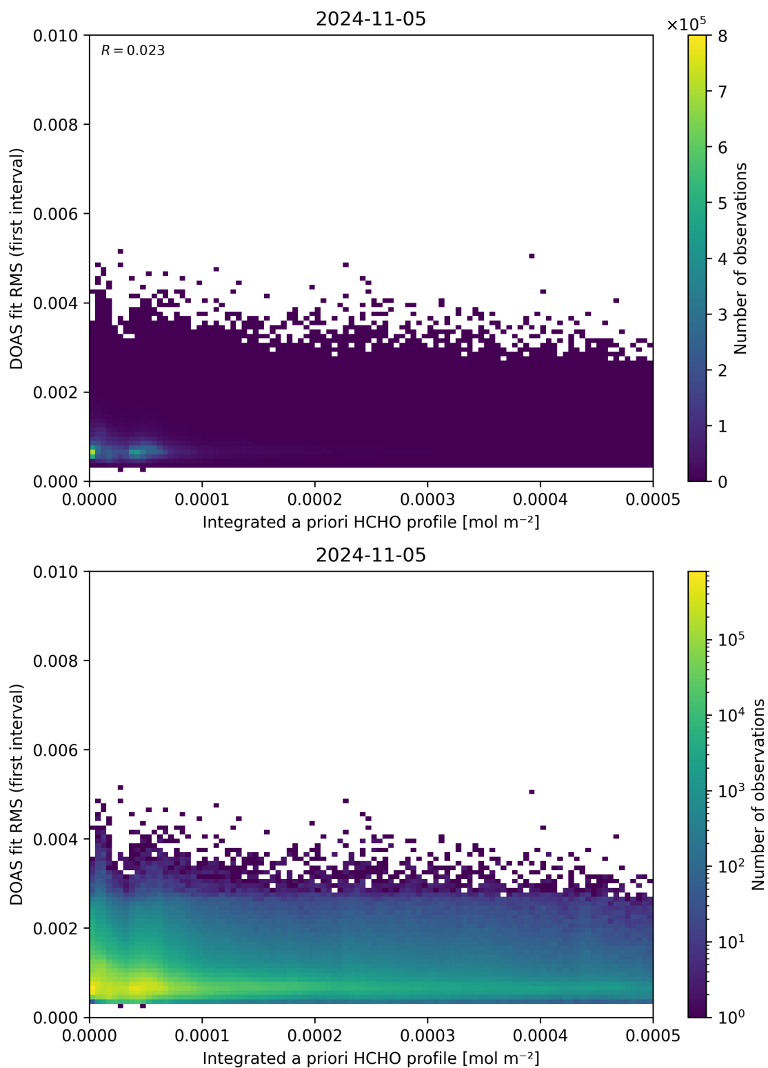
Figure 148: Scatter density plot of “Integrated a priori HCHO profile” against “DOAS fit RMS (first interval)” for 2024-11-04 to 2024-11-06.
