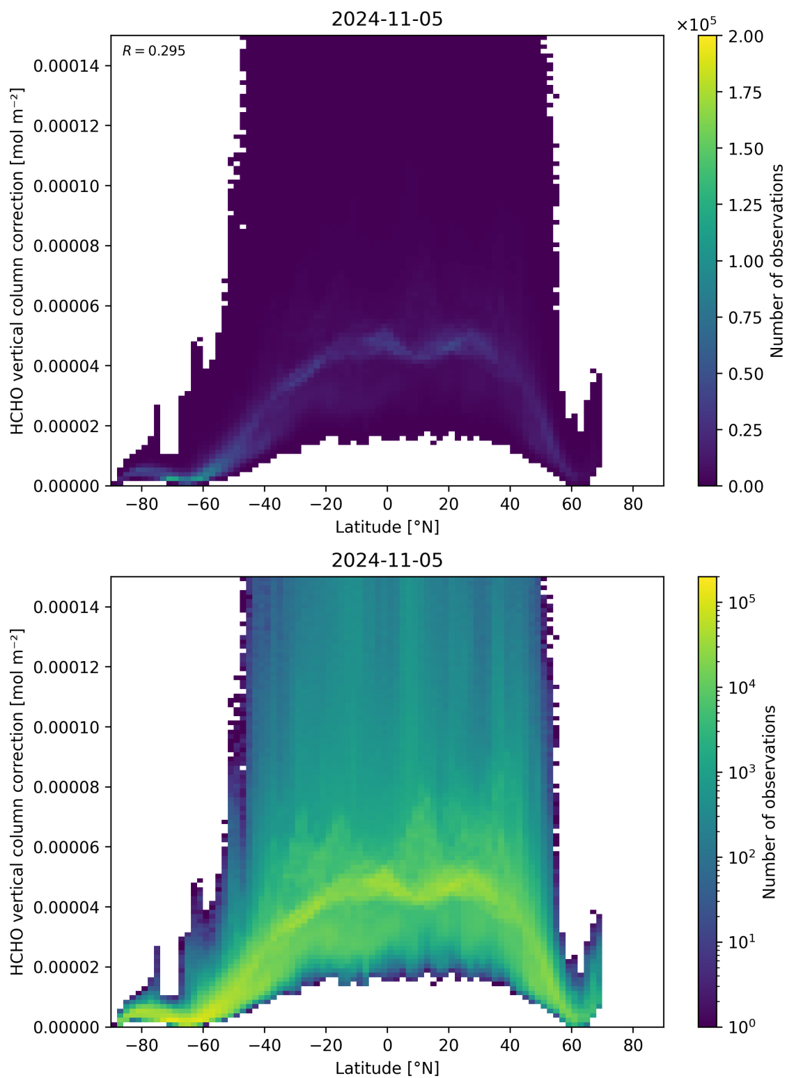
Figure 164: Scatter density plot of “Latitude” against “HCHO vertical column correction” for 2024-11-04 to 2024-11-06.
