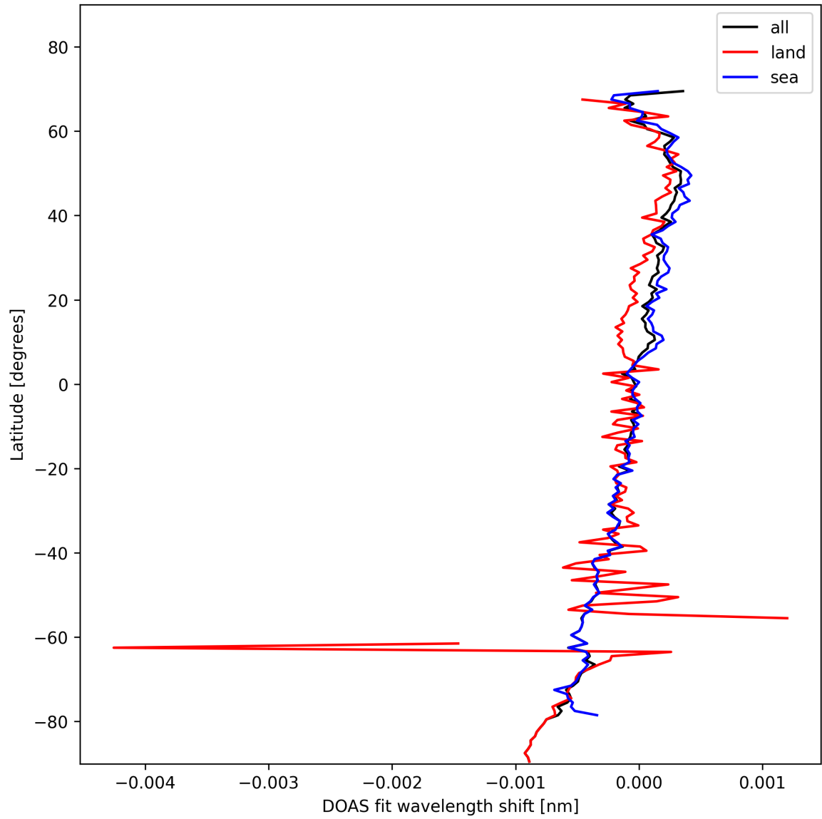
Figure 30: Zonal average of “DOAS fit wavelength shift” for 2024-11-04 to 2024-11-06.
