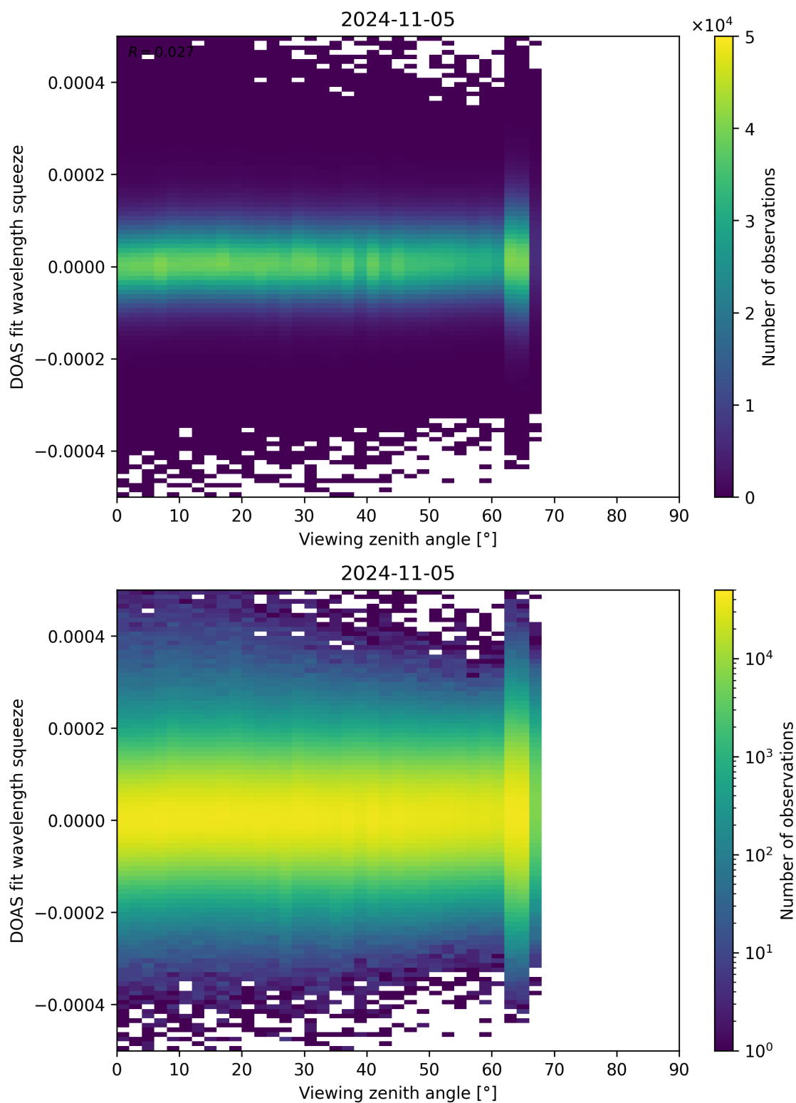
Figure 184: Scatter density plot of “Viewing zenith angle” against “DOAS fit wavelength squeeze” for 2024-11-04 to 2024-11-06.
