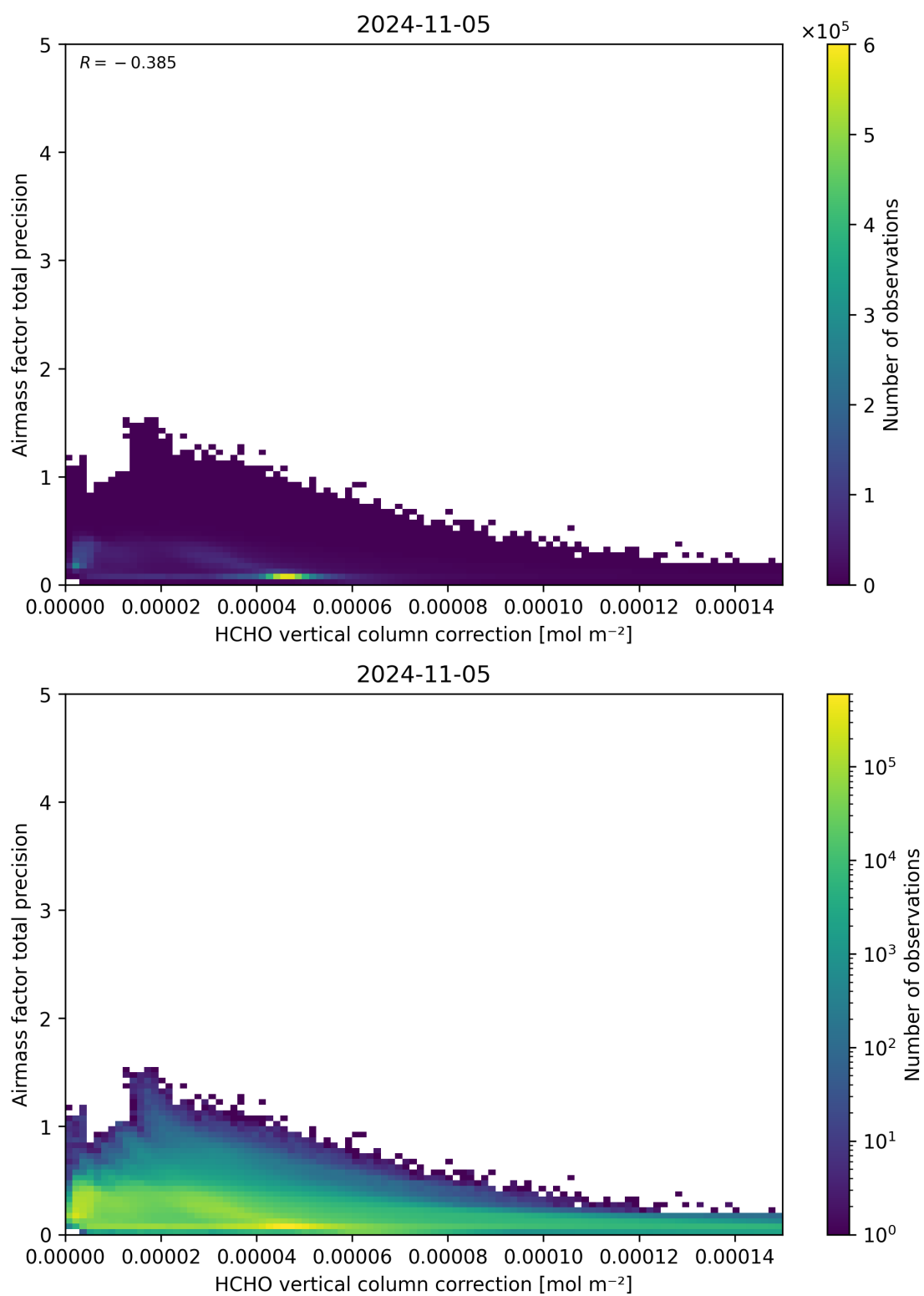
Figure 121: Scatter density plot of “HCHO vertical column correction” against “Airmass factor total precision” for 2024-11-04 to 2024-11-06.
