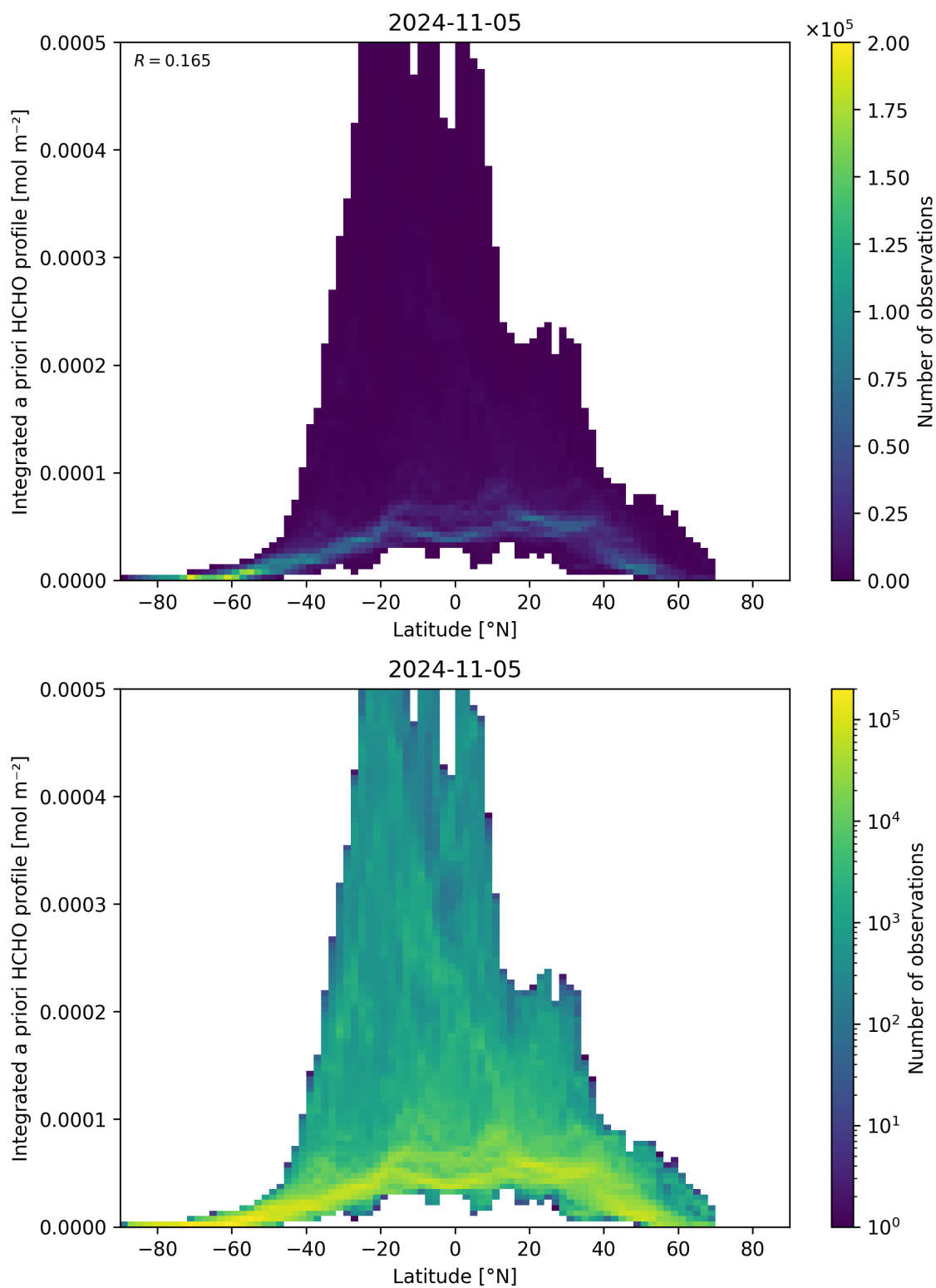
Figure 166: Scatter density plot of “Latitude” against “Integrated a priori HCHO profile” for 2024-11-04 to 2024-11-06.
