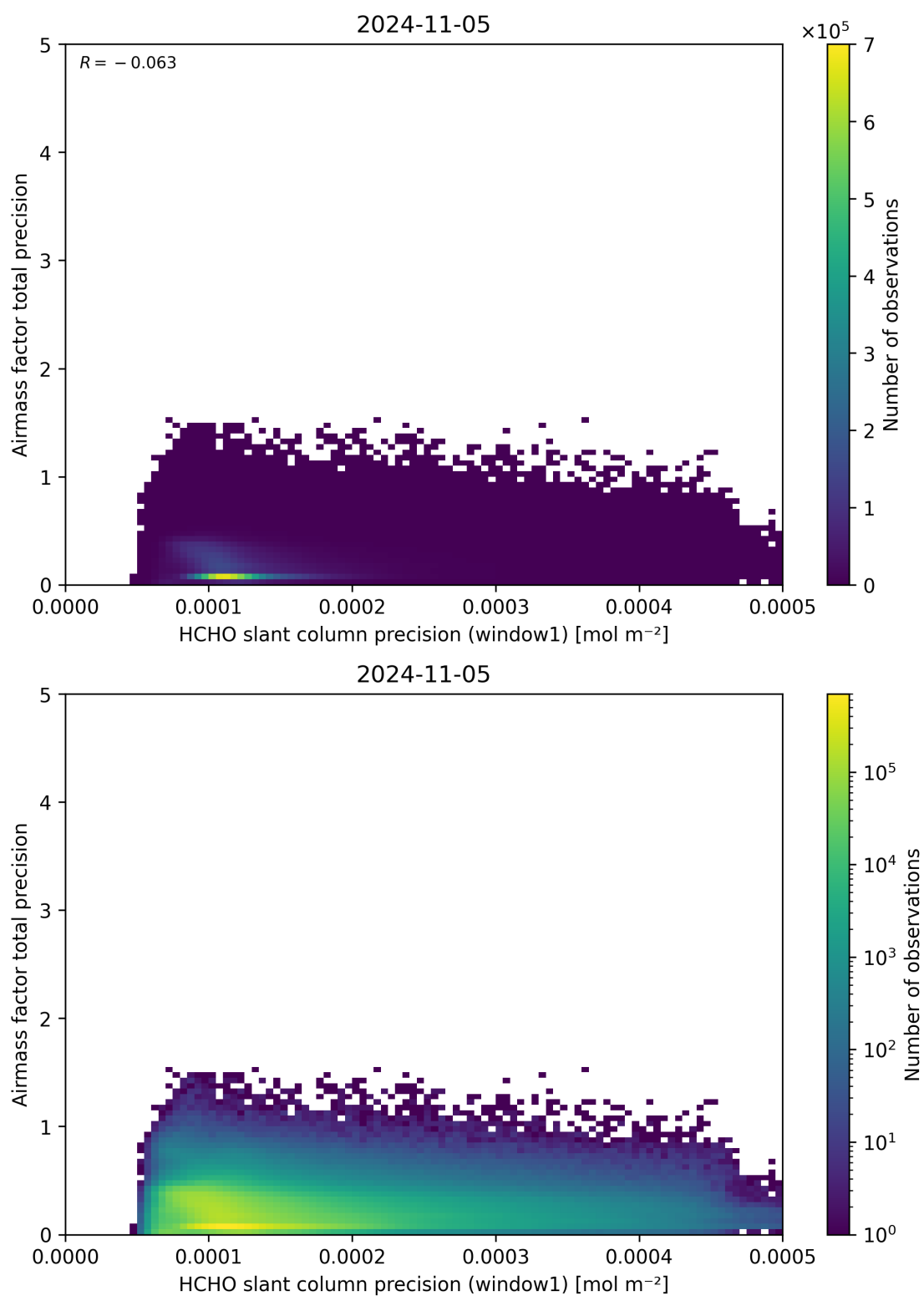
Figure 95: Scatter density plot of “HCHO slant column precision (window1)” against “Airmass factor total precision” for 2024-11-04 to 2024-11-06.
