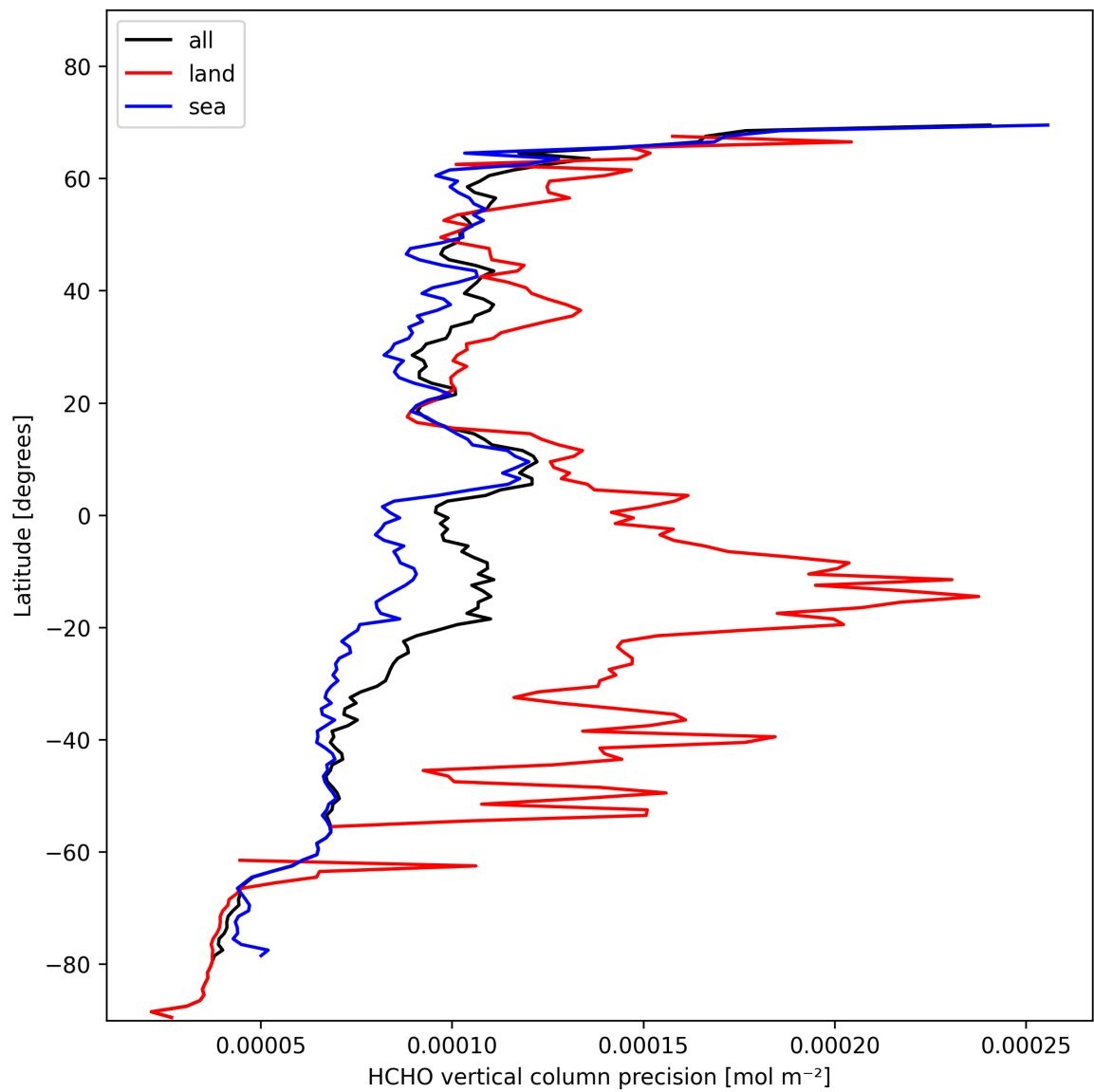
Figure 22: Zonal average of “HCHO vertical column precision” for 2024-11-04 to 2024-11-06.
