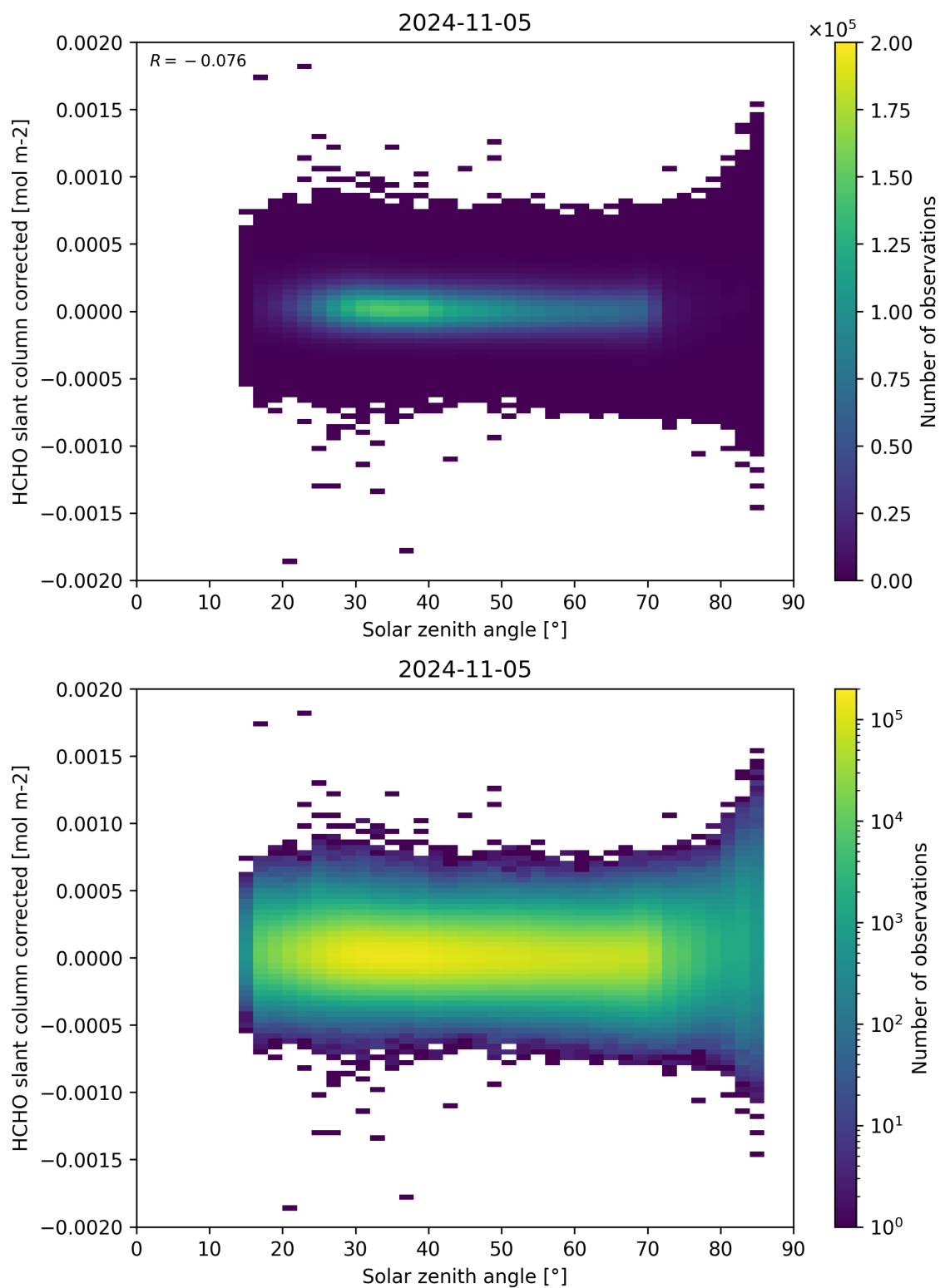
Figure 171: Scatter density plot of “Solar zenith angle” against “HCHO slant column corrected” for 2024-11-04 to 2024-11-06.
