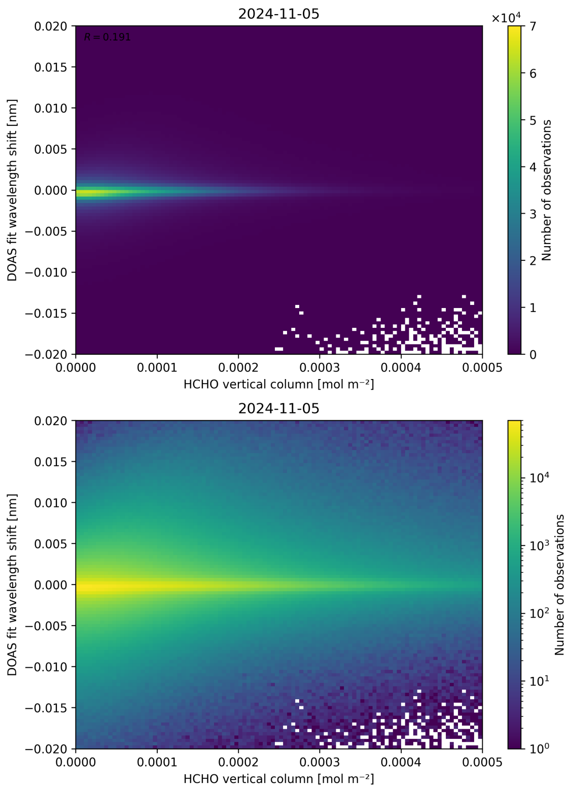
Figure 124: Scatter density plot of “HCHO vertical column” against “DOAS fit wavelength shift” for 2024-11-04 to 2024-11-06.
