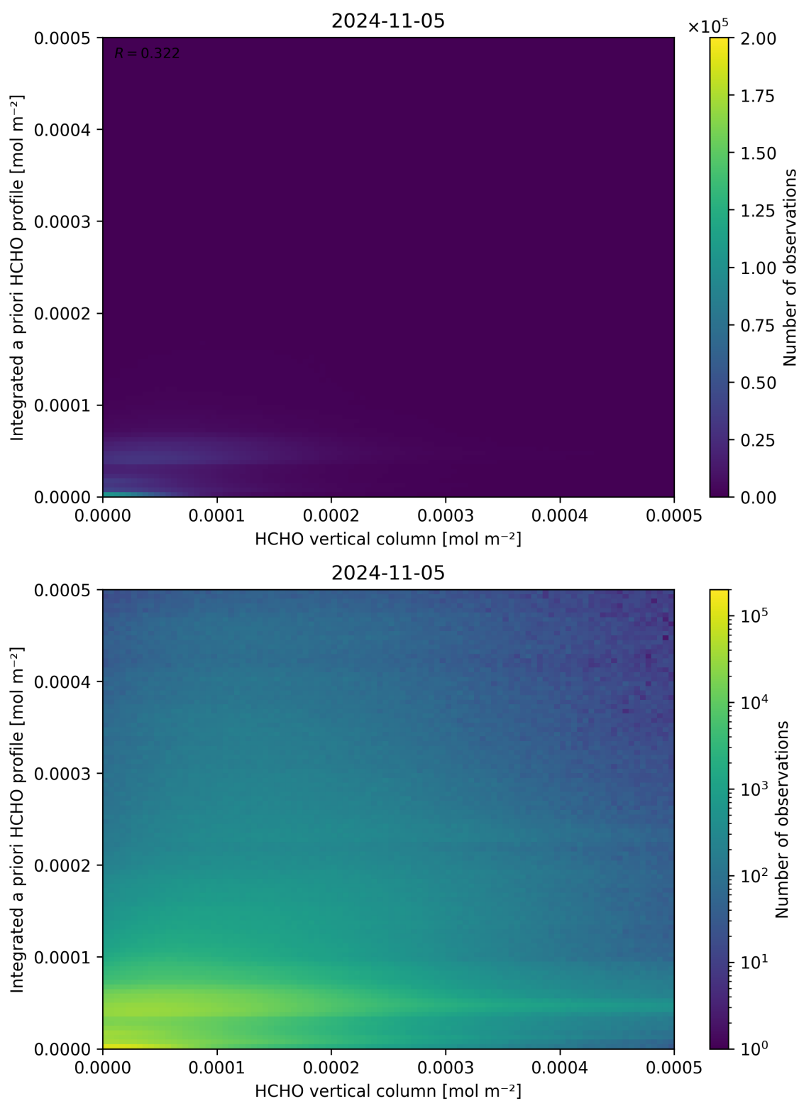
Figure 135: Scatter density plot of “HCHO vertical column” against “Integrated a priori HCHO profile” for 2024-11-04 to 2024-11-06.
