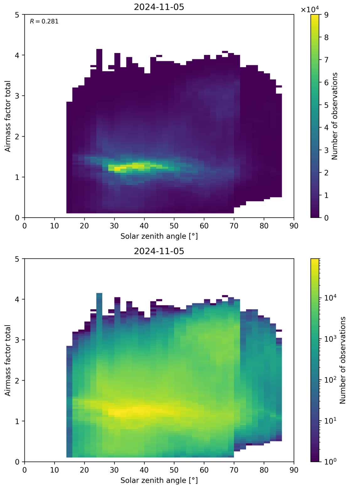
Figure 175: Scatter density plot of “Solar zenith angle” against “Airmass factor total” for 2024-11-04 to 2024-11-06.
