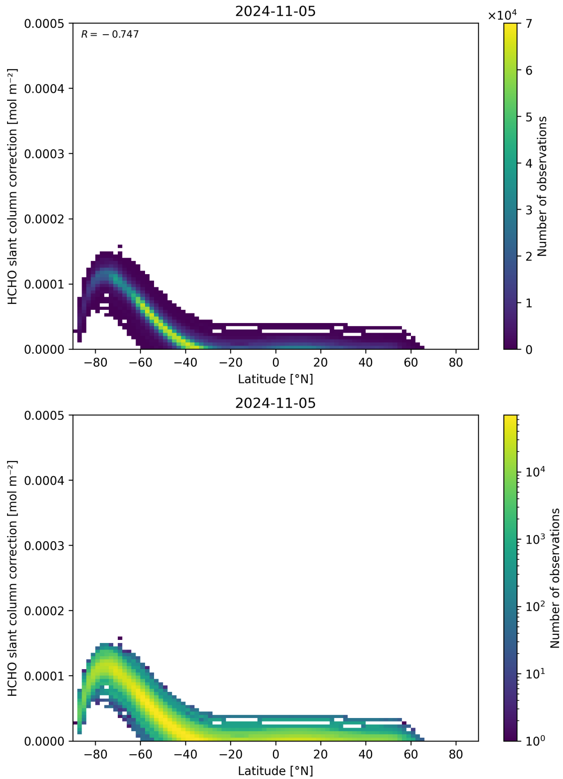
Figure 158: Scatter density plot of “Latitude” against “HCHO slant column correction” for 2024-11-04 to 2024-11-06.
