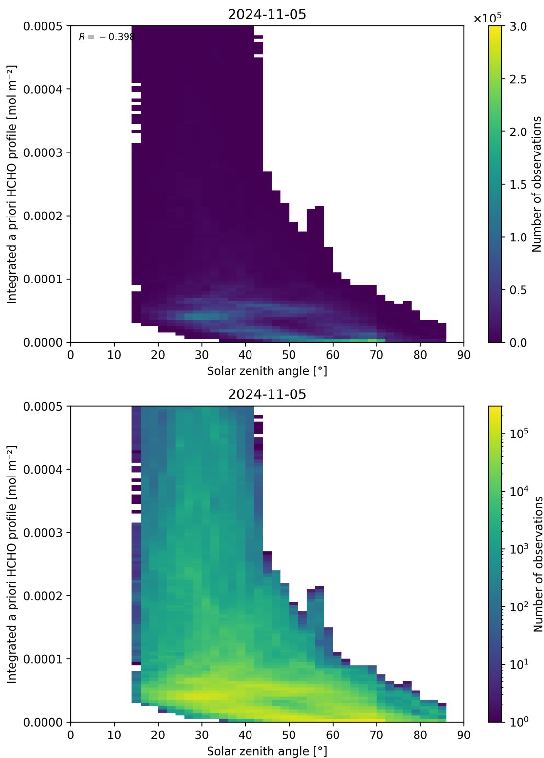
Figure 180: Scatter density plot of “Solar zenith angle” against “Integrated a priori HCHO profile” for 2024-11-04 to 2024-11-06.
