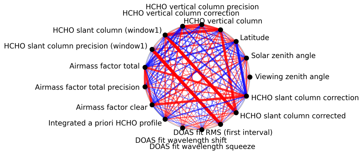
Figure 1: Map of correlation graph for 2024-11-04 to 2024-11-06.
