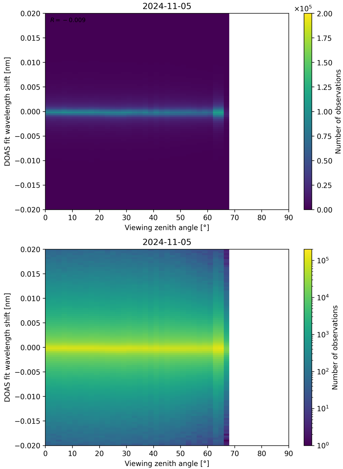
Figure 183: Scatter density plot of “Viewing zenith angle” against “DOAS fit wavelength shift” for 2024-11-04 to 2024-11-06.
