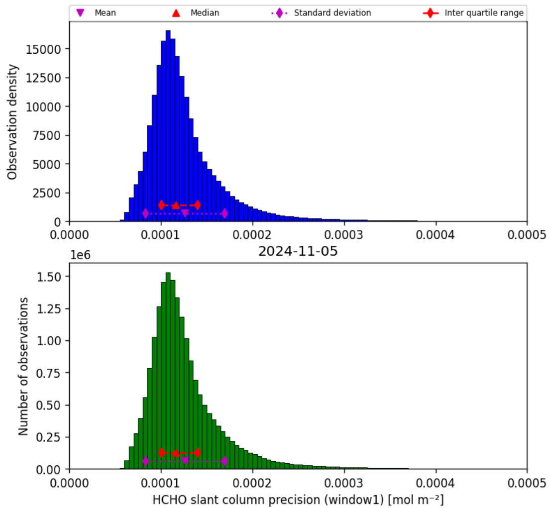
Figure 39: Histogram of “HCHO slant column precision (window1)” for 2024-11-04 to 2024-11-06
