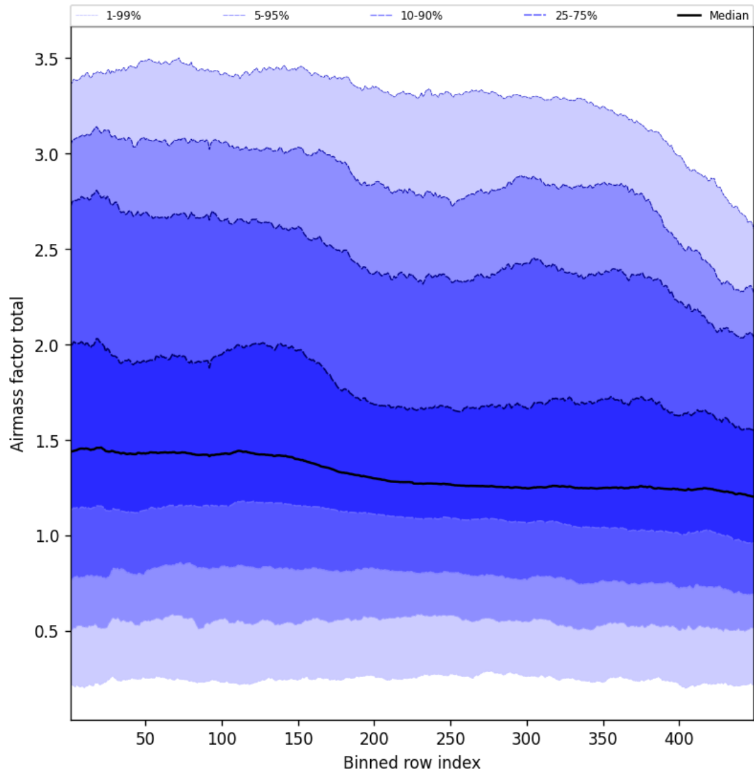
Figure 54: Along track statistics of “Airmass factor total” for 2024-11-04 to 2024-11-06
