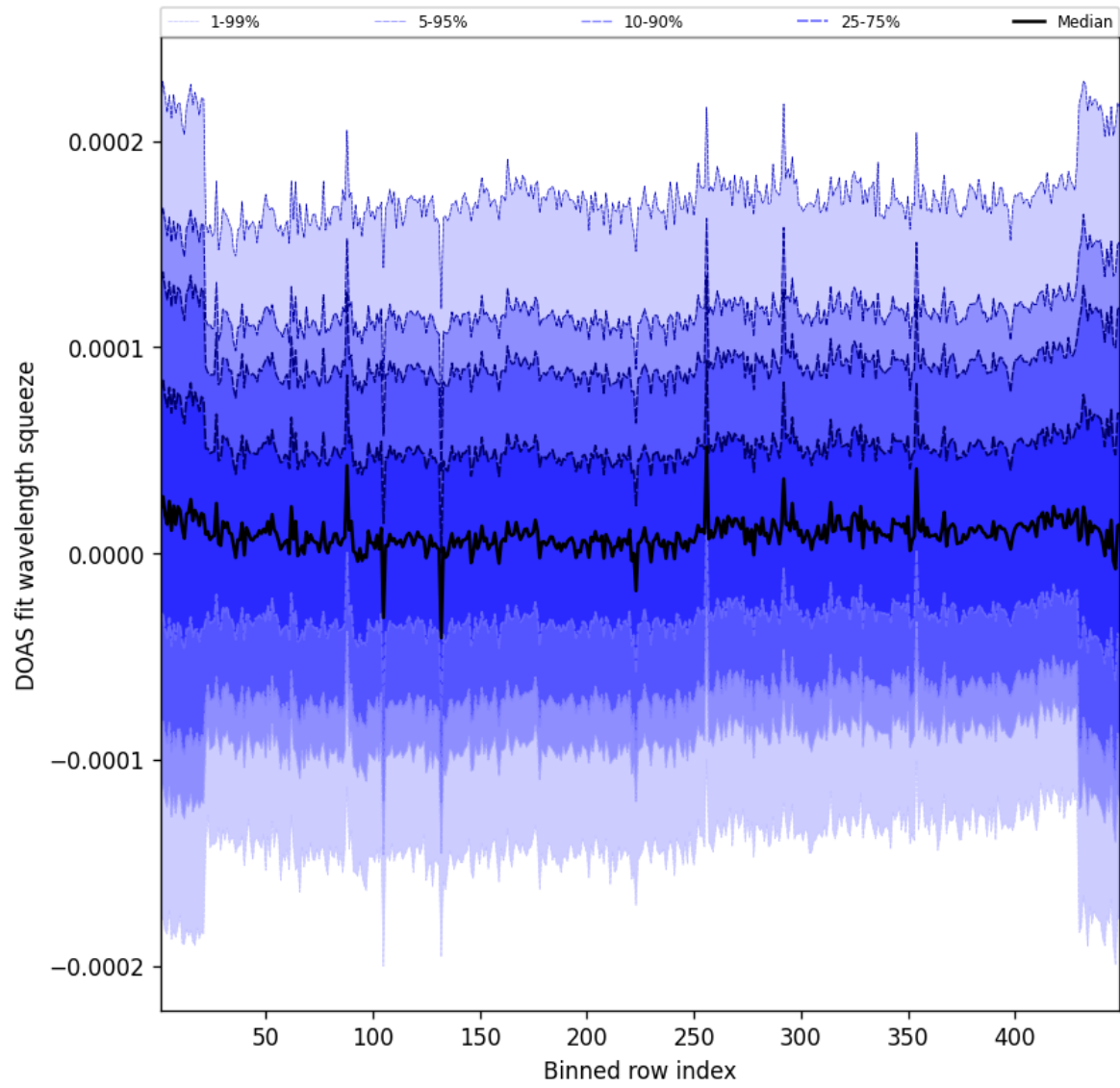
Figure 59: Along track statistics of “DOAS fit wavelength squeeze” for 2024-11-04 to 2024-11-06
