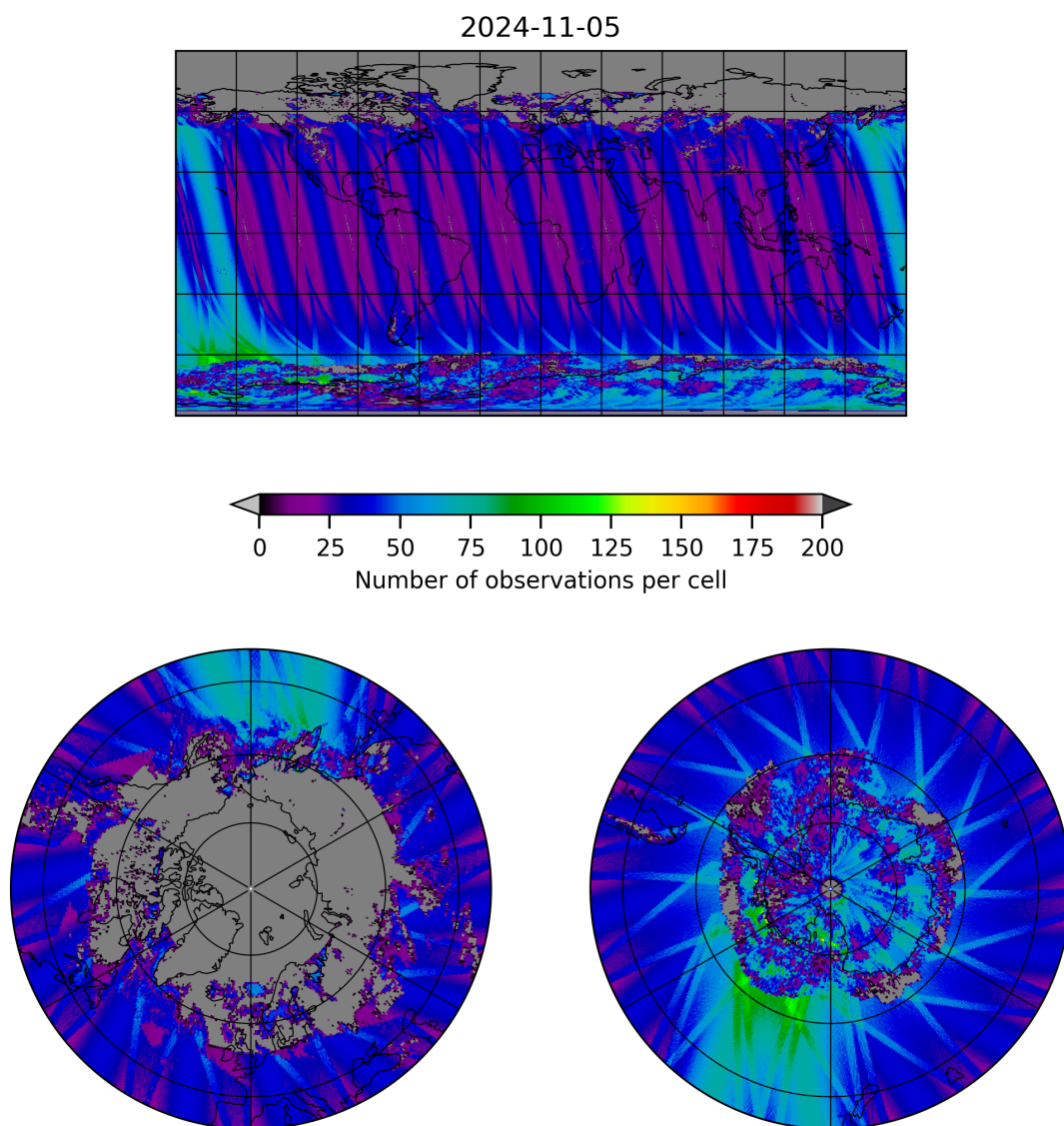
Figure 19: Map of the number of observations for 2024-11-04 to 2024-11-06
