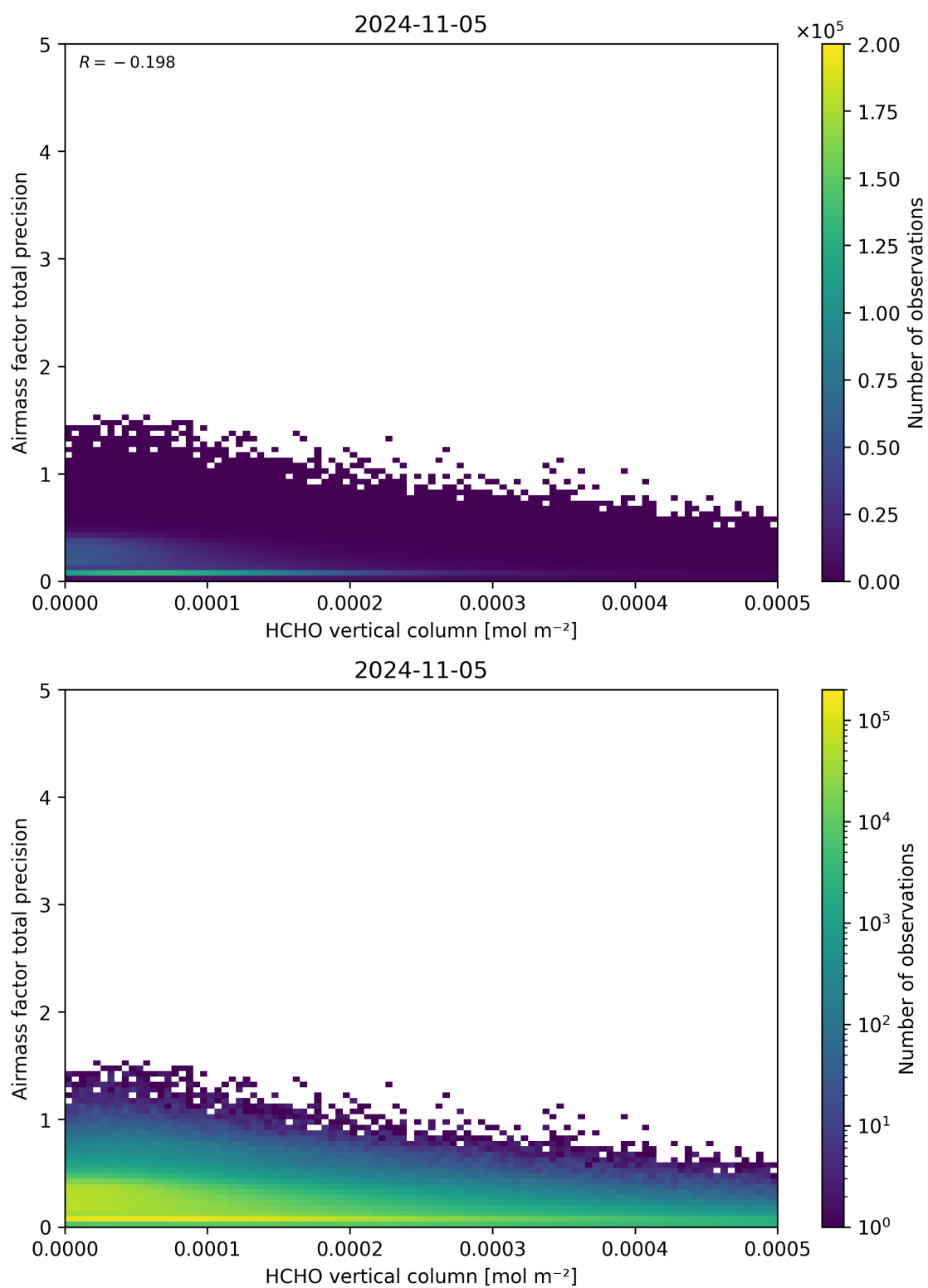
Figure 132: Scatter density plot of “HCHO vertical column” against “Airmass factor total precision” for 2024-11-04 to 2024-11-06.
