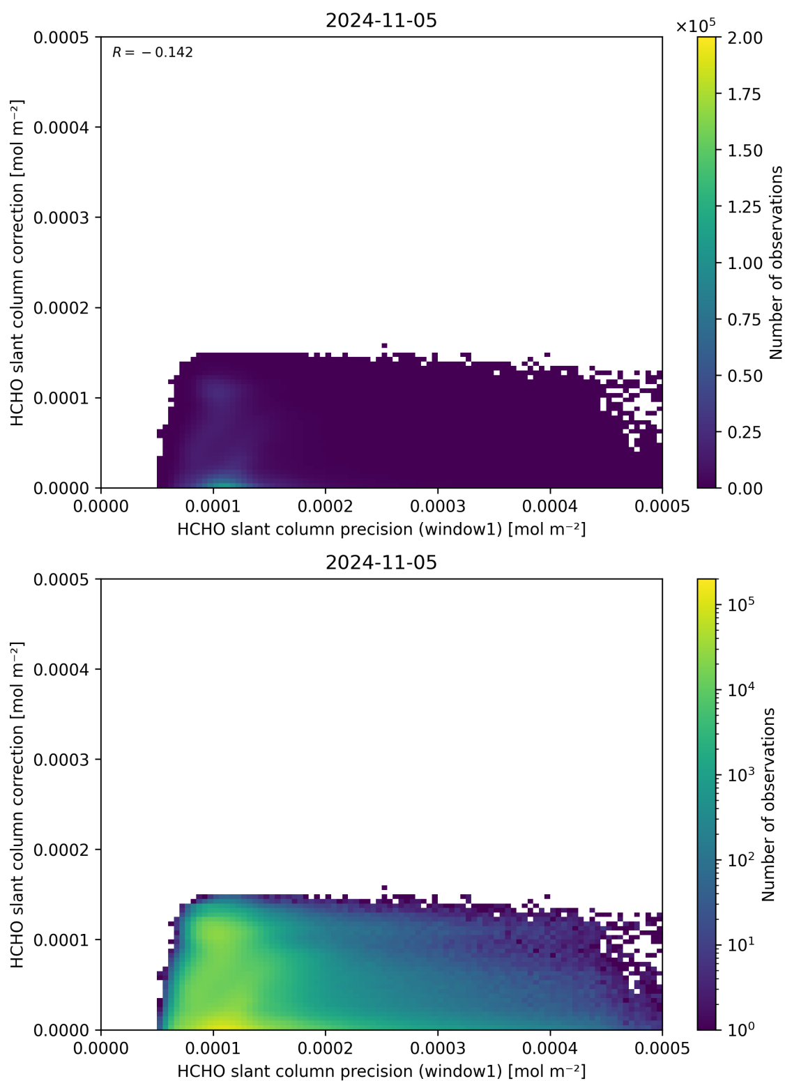
Figure 93: Scatter density plot of “HCHO slant column precision (window1)” against “HCHO slant column correction” for 2024-11-04 to 2024-11-06.
