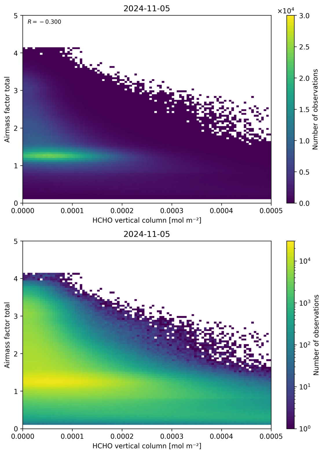
Figure 131: Scatter density plot of “HCHO vertical column” against “Airmass factor total” for 2024-11-04 to 2024-11-06.
