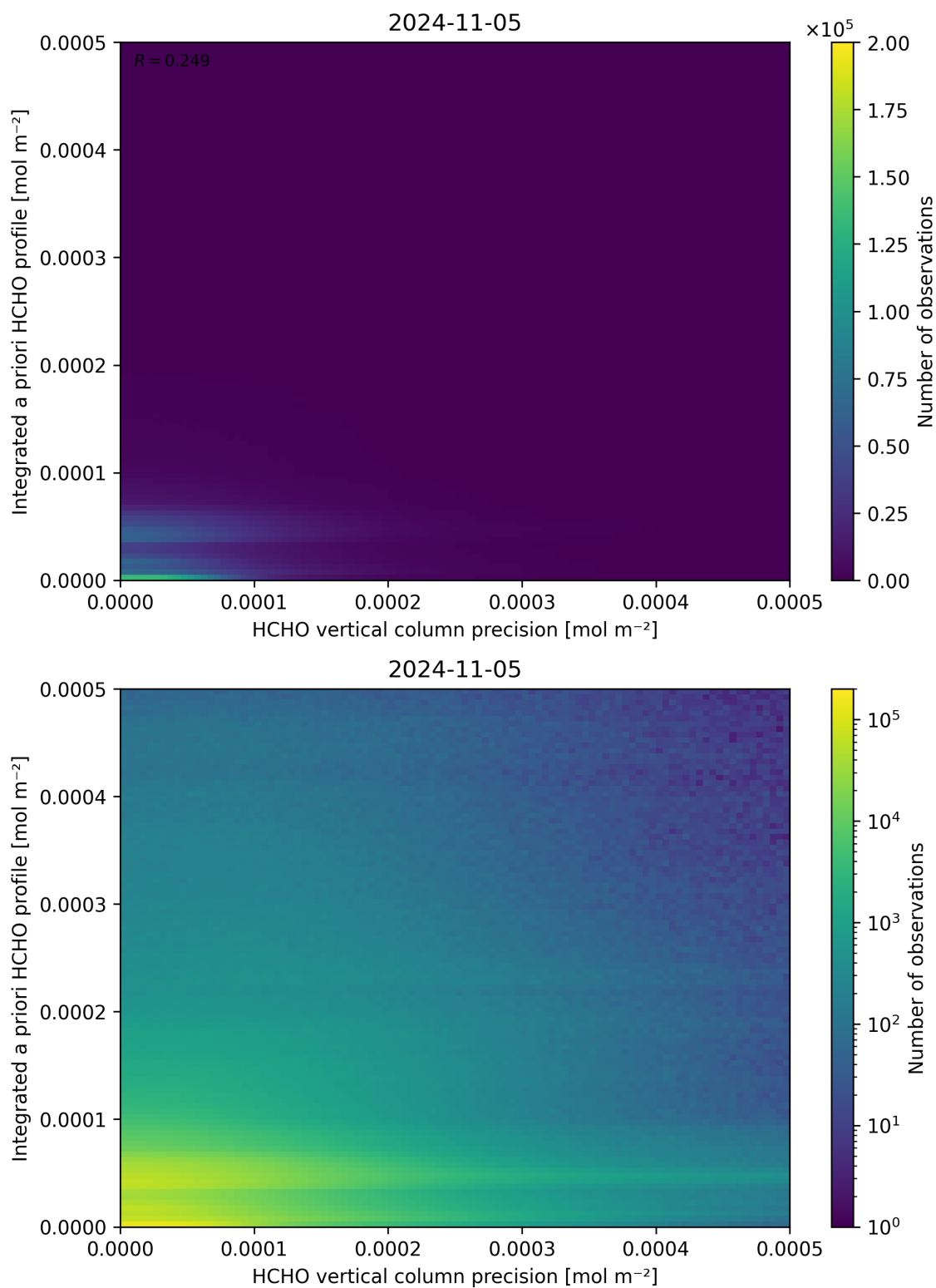
Figure 147: Scatter density plot of “HCHO vertical column precision” against “Integrated a priori HCHO profile” for 2024-11-04 to 2024-11-06.
