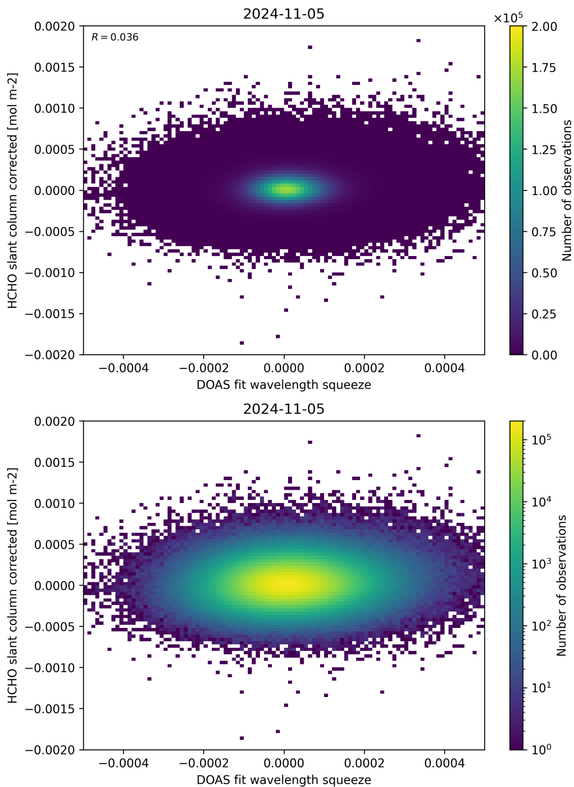
Figure 69: Scatter density plot of “DOAS fit wavelength squeeze” against “HCHO slant column corrected” for 2024-11-04 to 2024-11-06.
