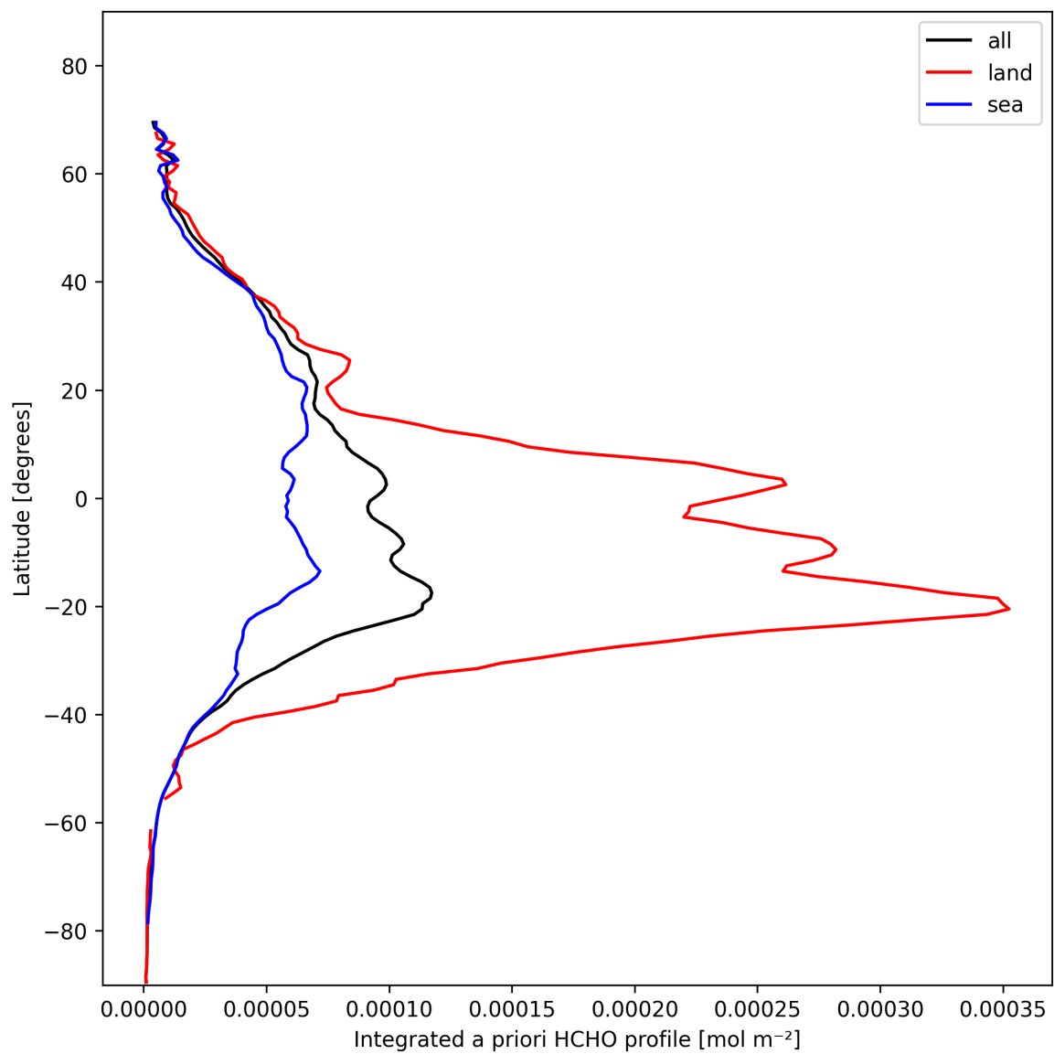
Figure 29: Zonal average of “Integrated a priori HCHO profile” for 2024-11-04 to 2024-11-06.
