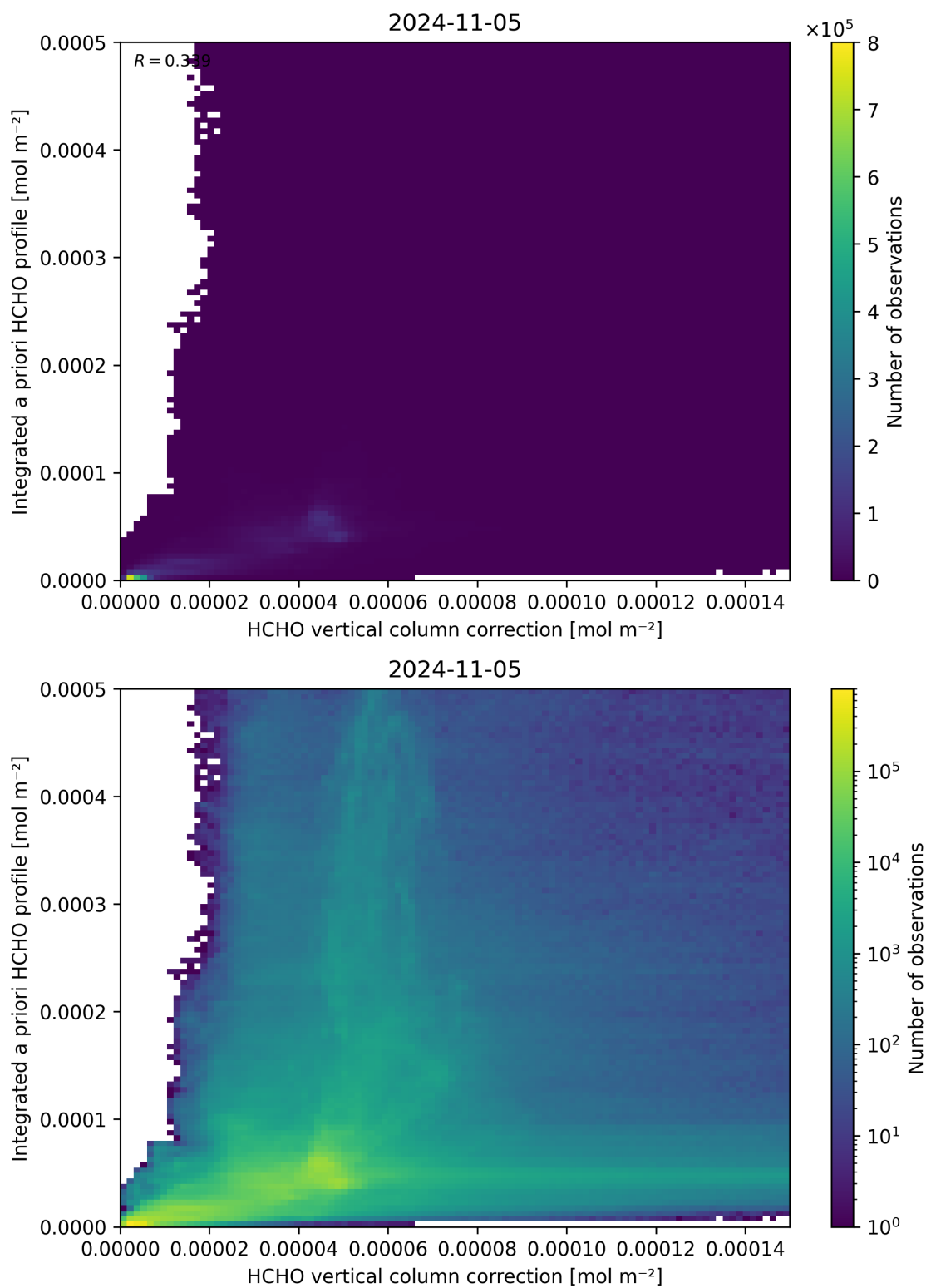
Figure 122: Scatter density plot of “HCHO vertical column correction” against “Integrated a priori HCHO profile” for 2024-11-04 to 2024-11-06.
