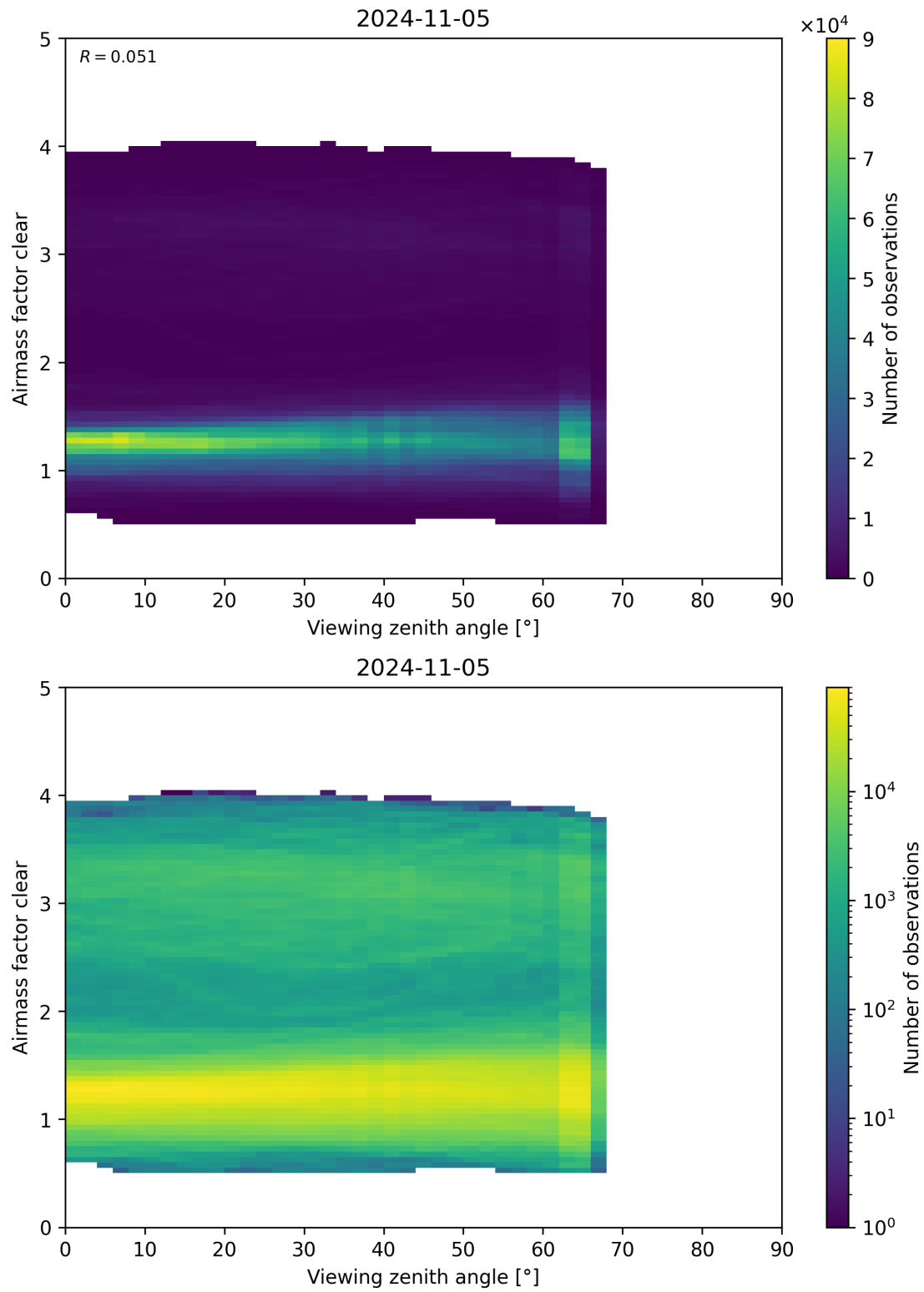
Figure 185: Scatter density plot of “Viewing zenith angle” against “Airmass factor clear” for 2024-11-04 to 2024-11-06.
