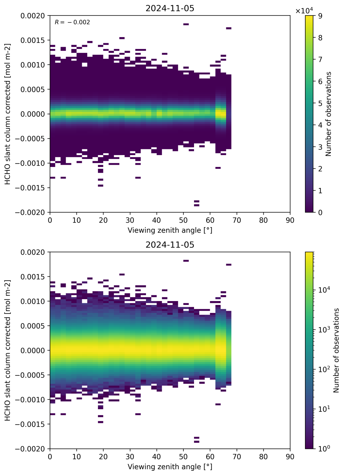
Figure 186: Scatter density plot of “Viewing zenith angle” against “HCHO slant column corrected” for 2024-11-04 to 2024-11-06.
