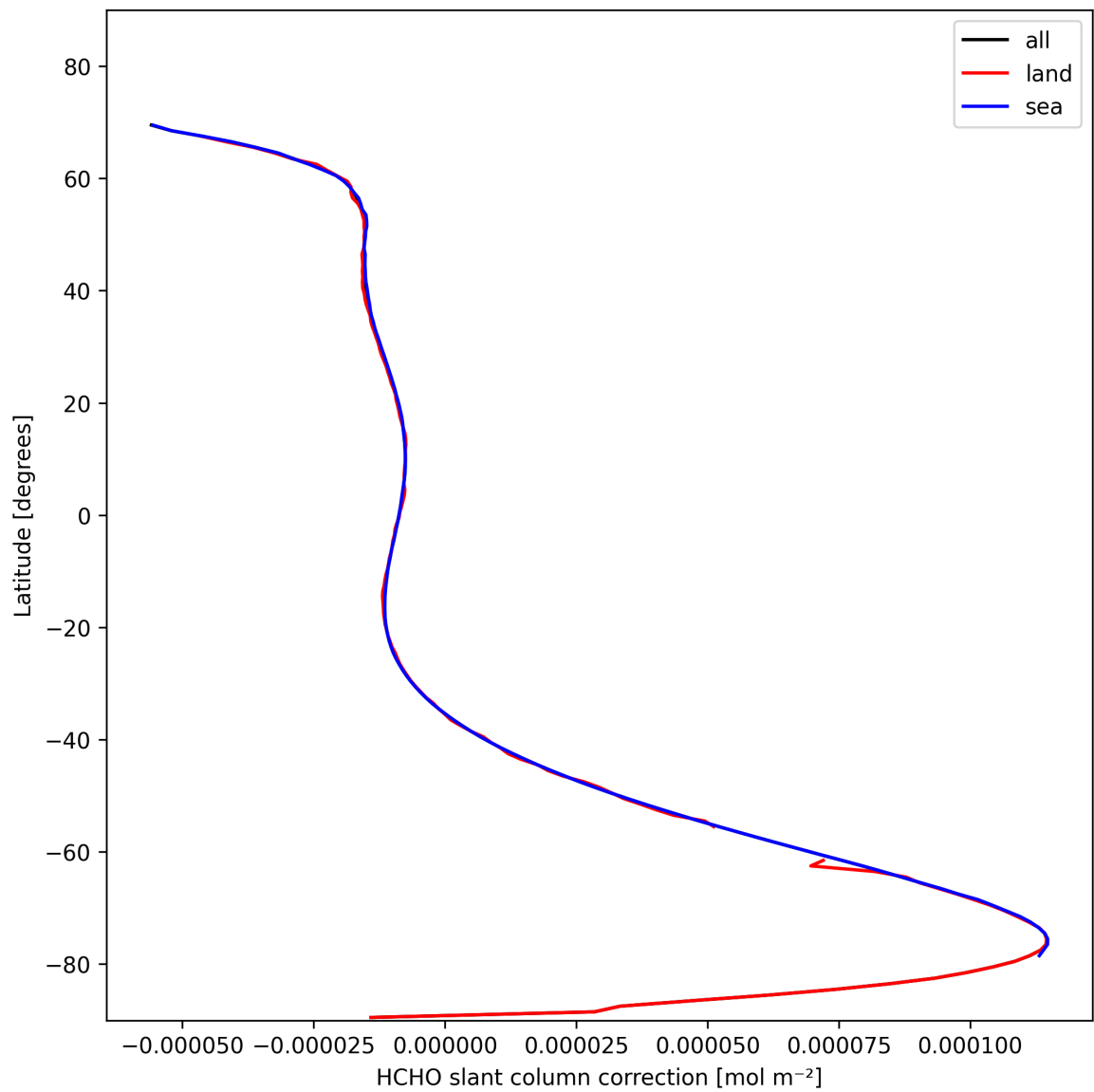
Figure 33: Zonal average of “HCHO slant column correction” for 2024-11-04 to 2024-11-06.
