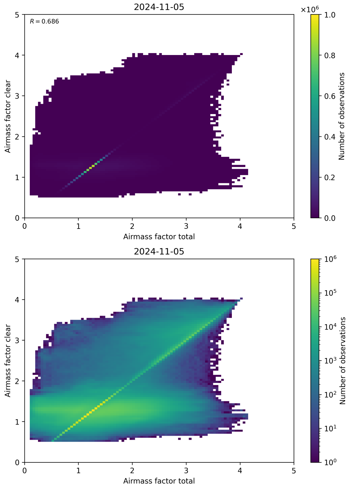
Figure 100: Scatter density plot of “Airmass factor total” against “Airmass factor clear” for 2024-11-04 to 2024-11-06.
