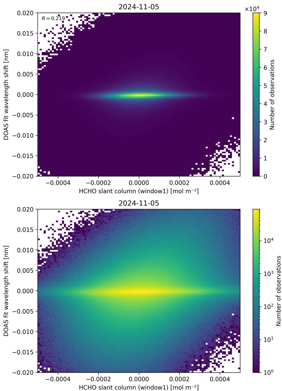
Figure 79: Scatter density plot of “HCHO slant column (window1)” against “DOAS fit wavelength shift” for 2024-11-04 to 2024-11-06.
