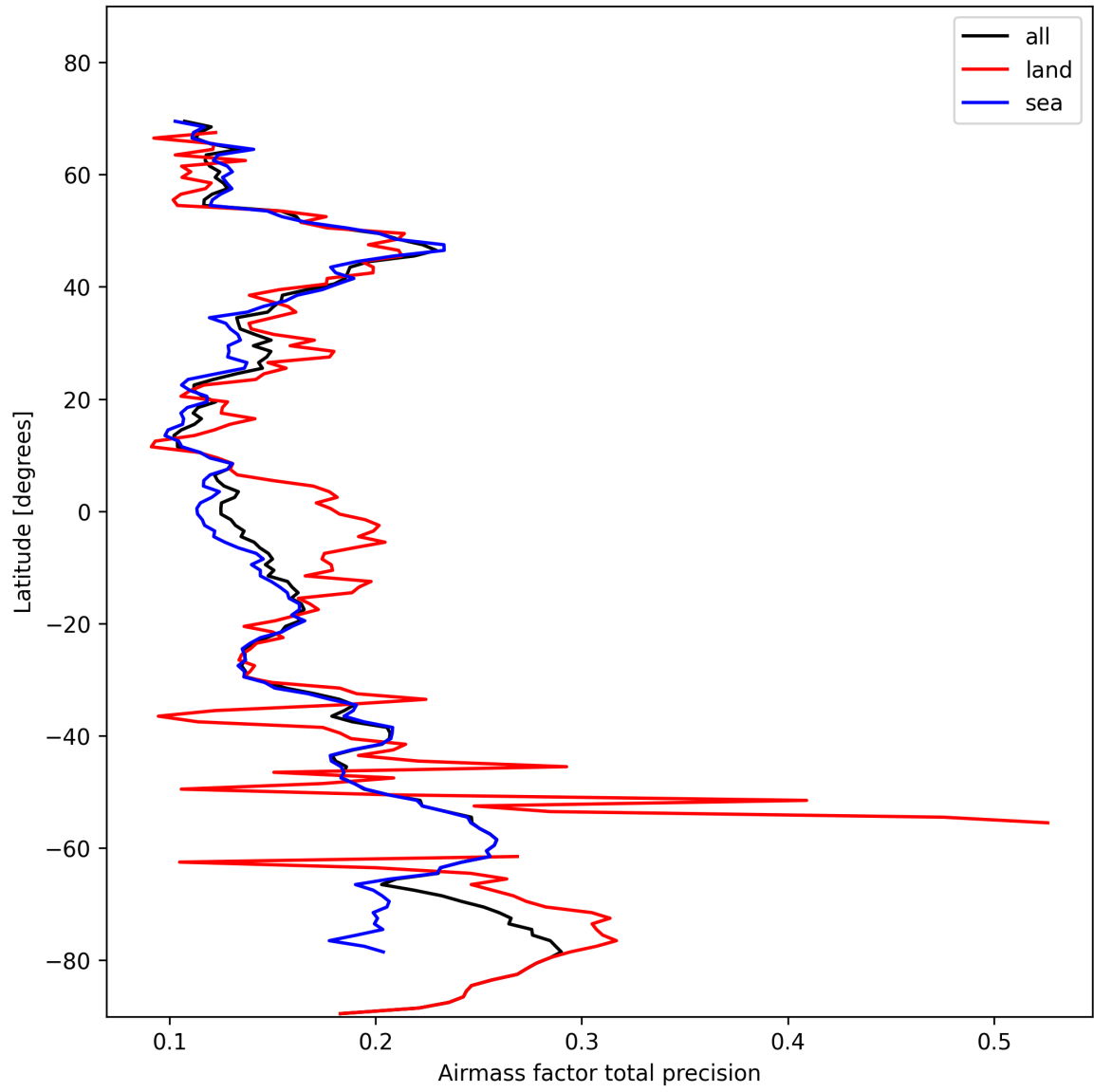
Figure 27: Zonal average of “Airmass factor total precision” for 2024-11-04 to 2024-11-06.
