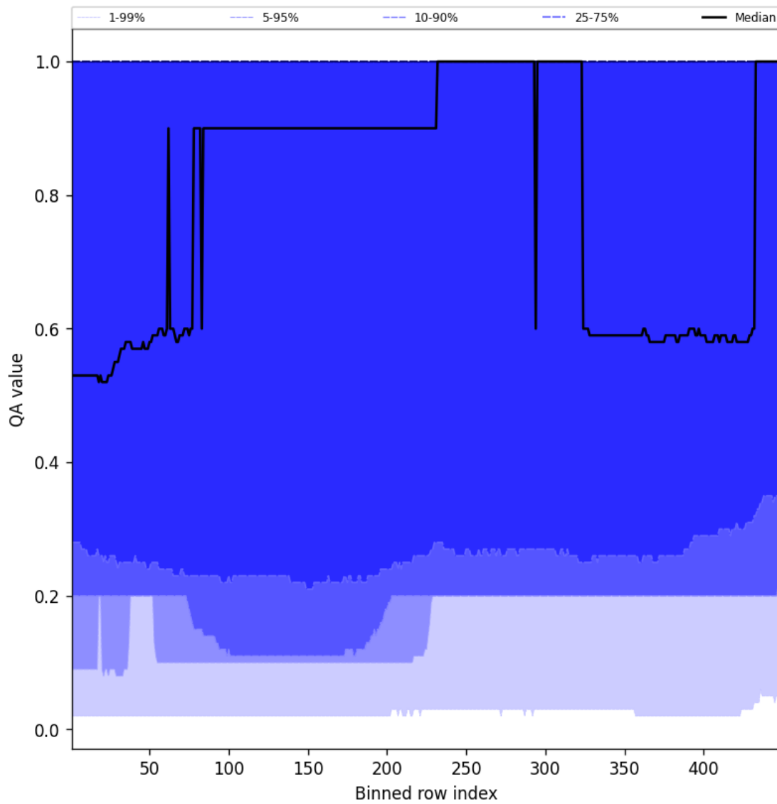
Figure 48: Along track statistics of “QA value” for 2024-11-04 to 2024-11-06
