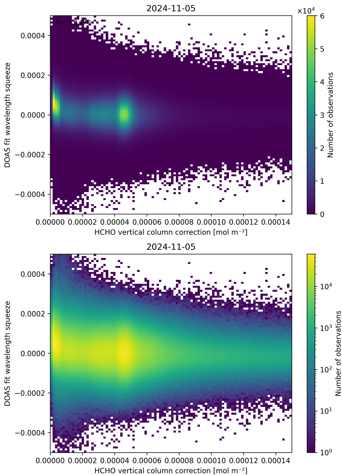
Figure 114: Scatter density plot of “HCHO vertical column correction” against “DOAS fit wavelength squeeze” for 2024-11-04 to 2024-11-06.
