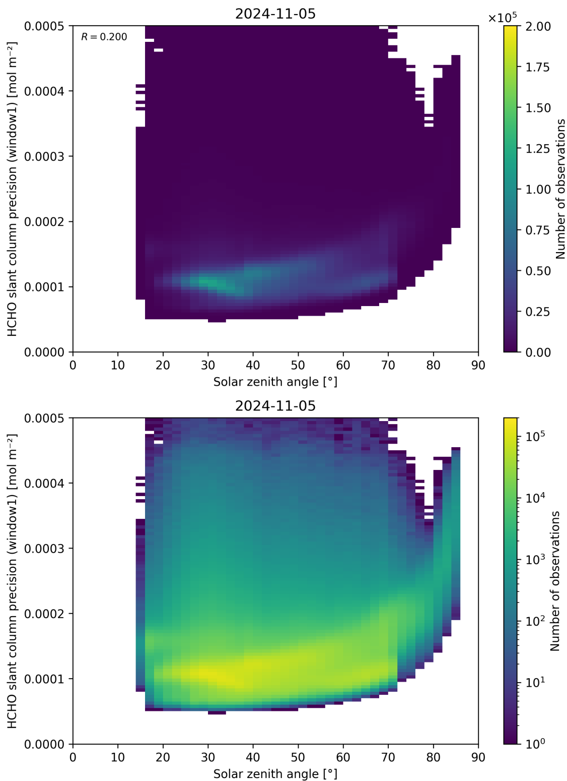
Figure 174: Scatter density plot of “Solar zenith angle” against “HCHO slant column precision (window1)” for 2024-11-04 to 2024-11-06.
