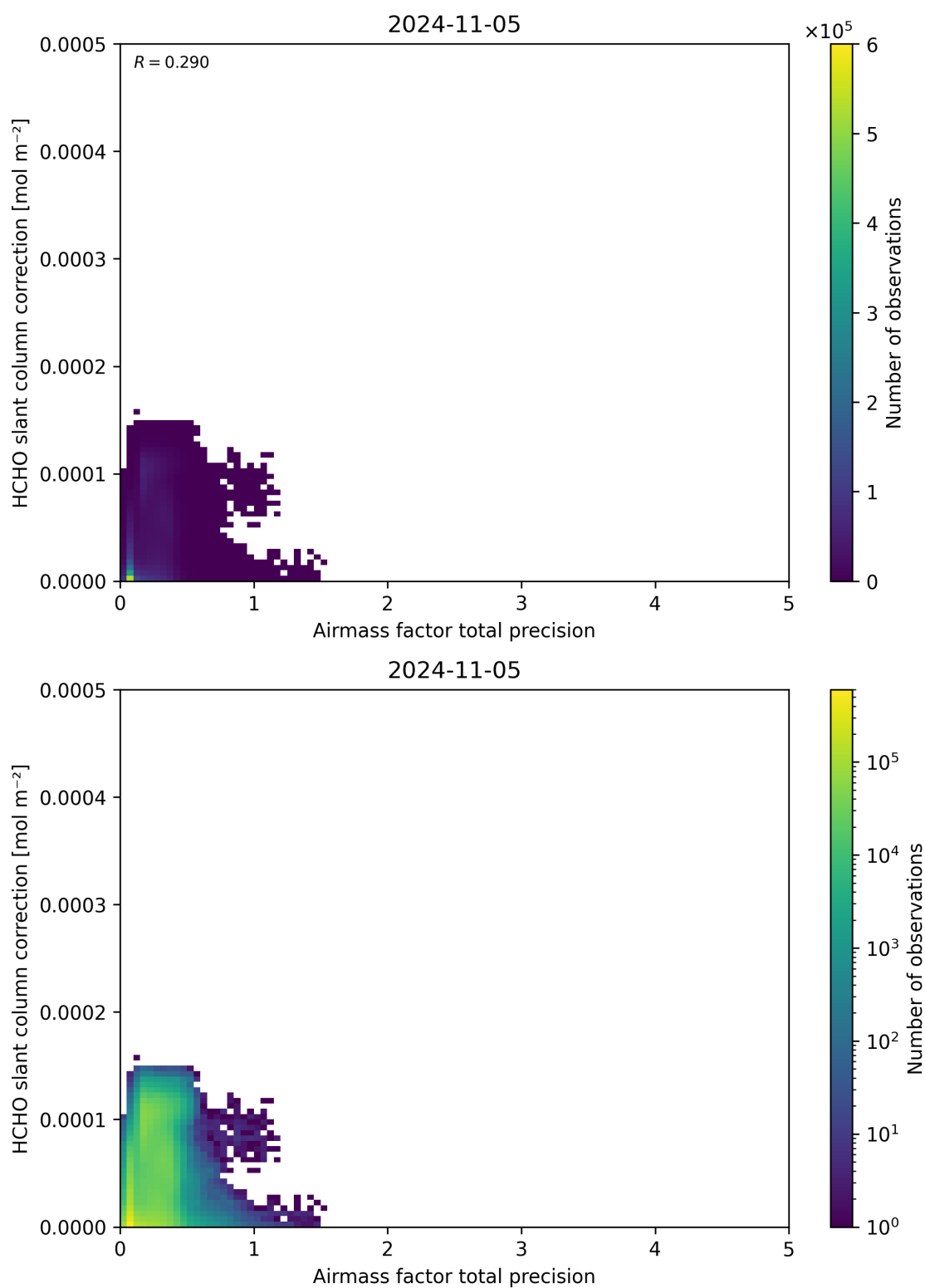
Figure 110: Scatter density plot of “Airmass factor total precision” against “HCHO slant column correction” for 2024-11-04 to 2024-11-06.
