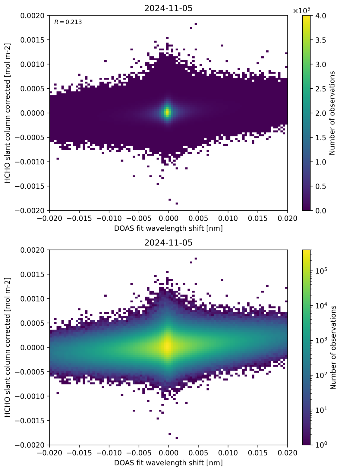
Figure 66: Scatter density plot of “DOAS fit wavelength shift” against “HCHO slant column corrected” for 2024-11-04 to 2024-11-06.
