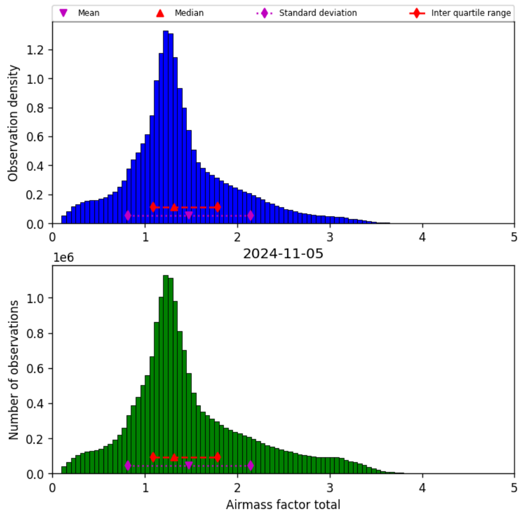
Figure 40: Histogram of “Airmass factor total” for 2024-11-04 to 2024-11-06
