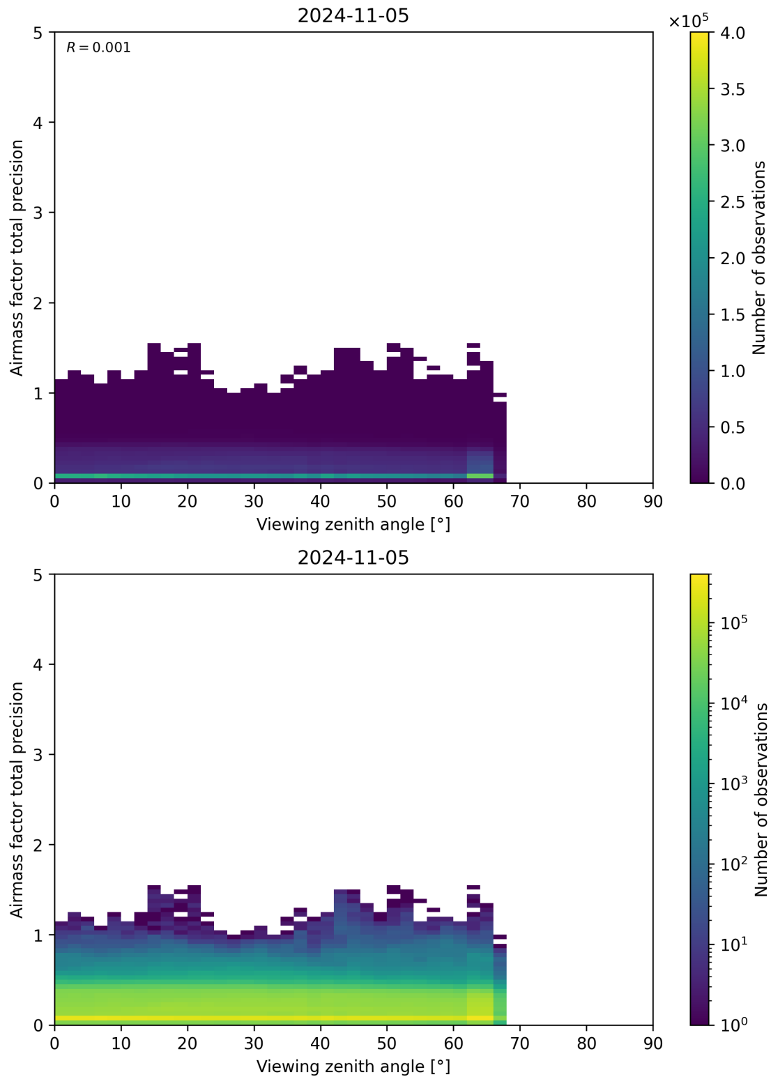
Figure 191: Scatter density plot of “Viewing zenith angle” against “Airmass factor total precision” for 2024-11-04 to 2024-11-06.
