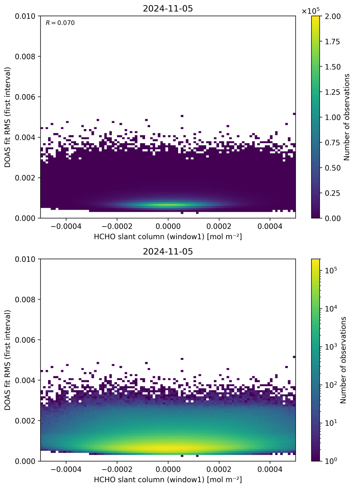
Figure 78: Scatter density plot of “HCHO slant column (window1)” against “DOAS fit RMS (first interval)” for 2024-11-04 to 2024-11-06.
