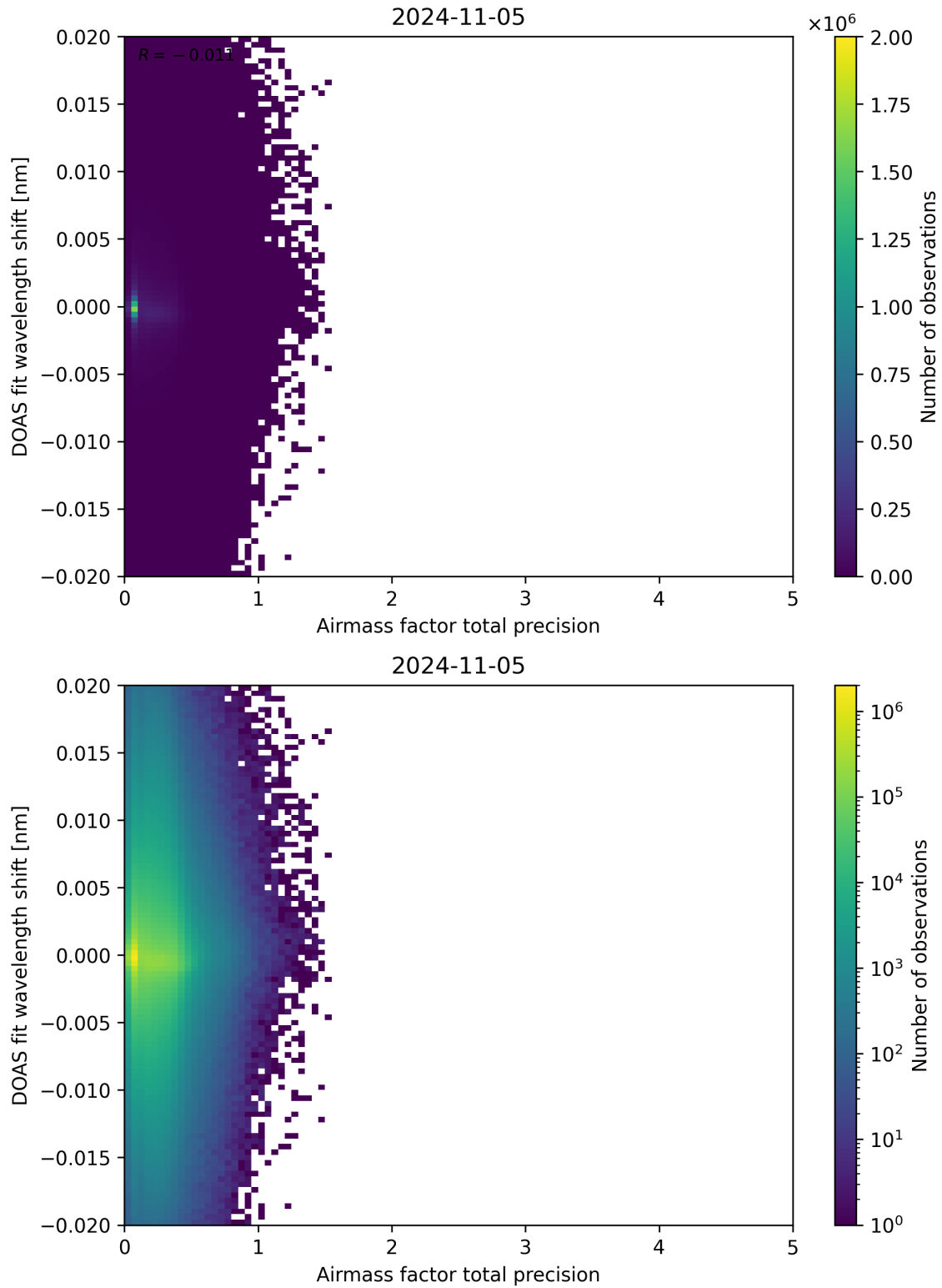
Figure 106: Scatter density plot of “Airmass factor total precision” against “DOAS fit wavelength shift” for 2024-11-04 to 2024-11-06.
