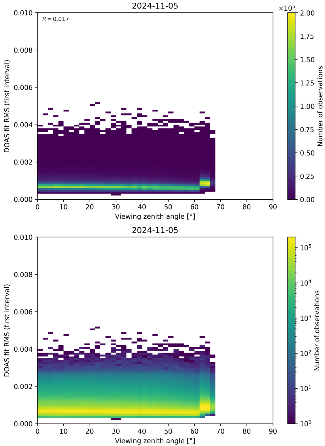
Figure 182: Scatter density plot of “Viewing zenith angle” against “DOAS fit RMS (first interval)” for 2024-11-04 to 2024-11-06.
