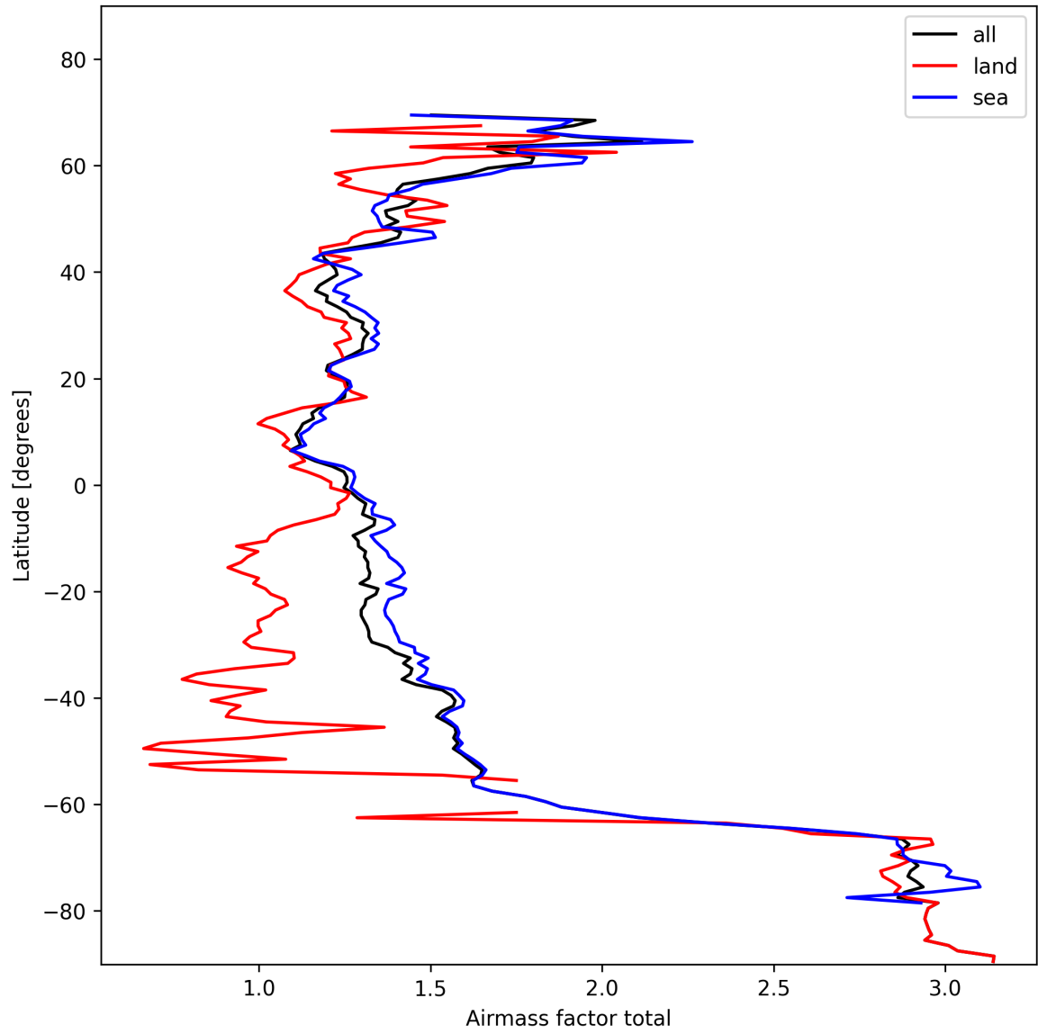
Figure 26: Zonal average of “Airmass factor total” for 2024-11-04 to 2024-11-06.
