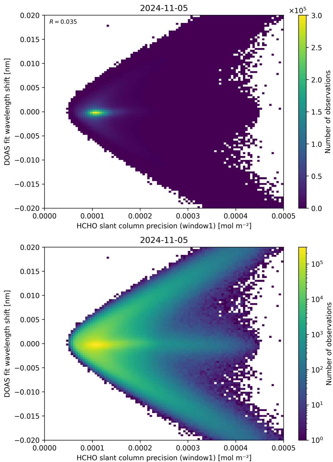
Figure 89: Scatter density plot of “HCHO slant column precision (window1)” against “DOAS fit wavelength shift” for 2024-11-04 to 2024-11-06.
