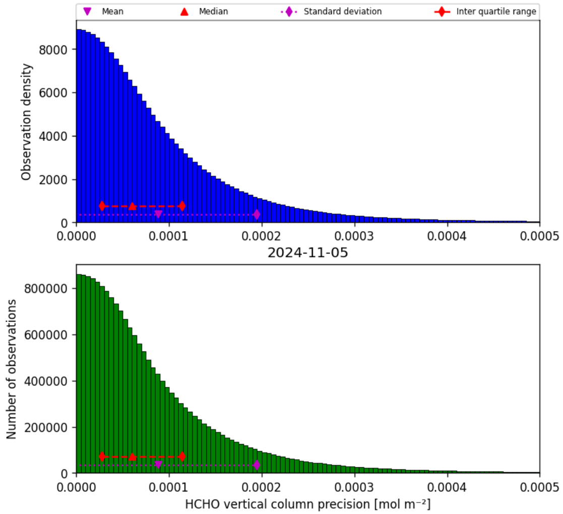
Figure 36: Histogram of “HCHO vertical column precision” for 2024-11-04 to 2024-11-06
