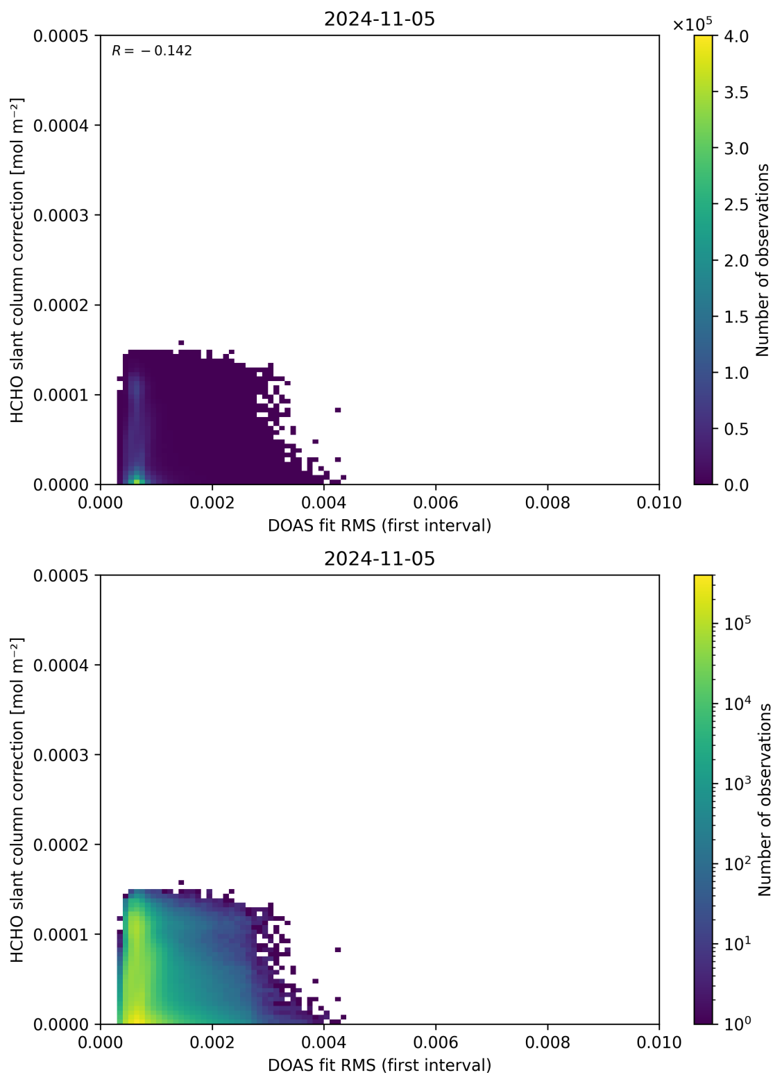
Figure 63: Scatter density plot of “DOAS fit RMS (first interval)” against “HCHO slant column correction” for 2024-11-04 to 2024-11-06.
