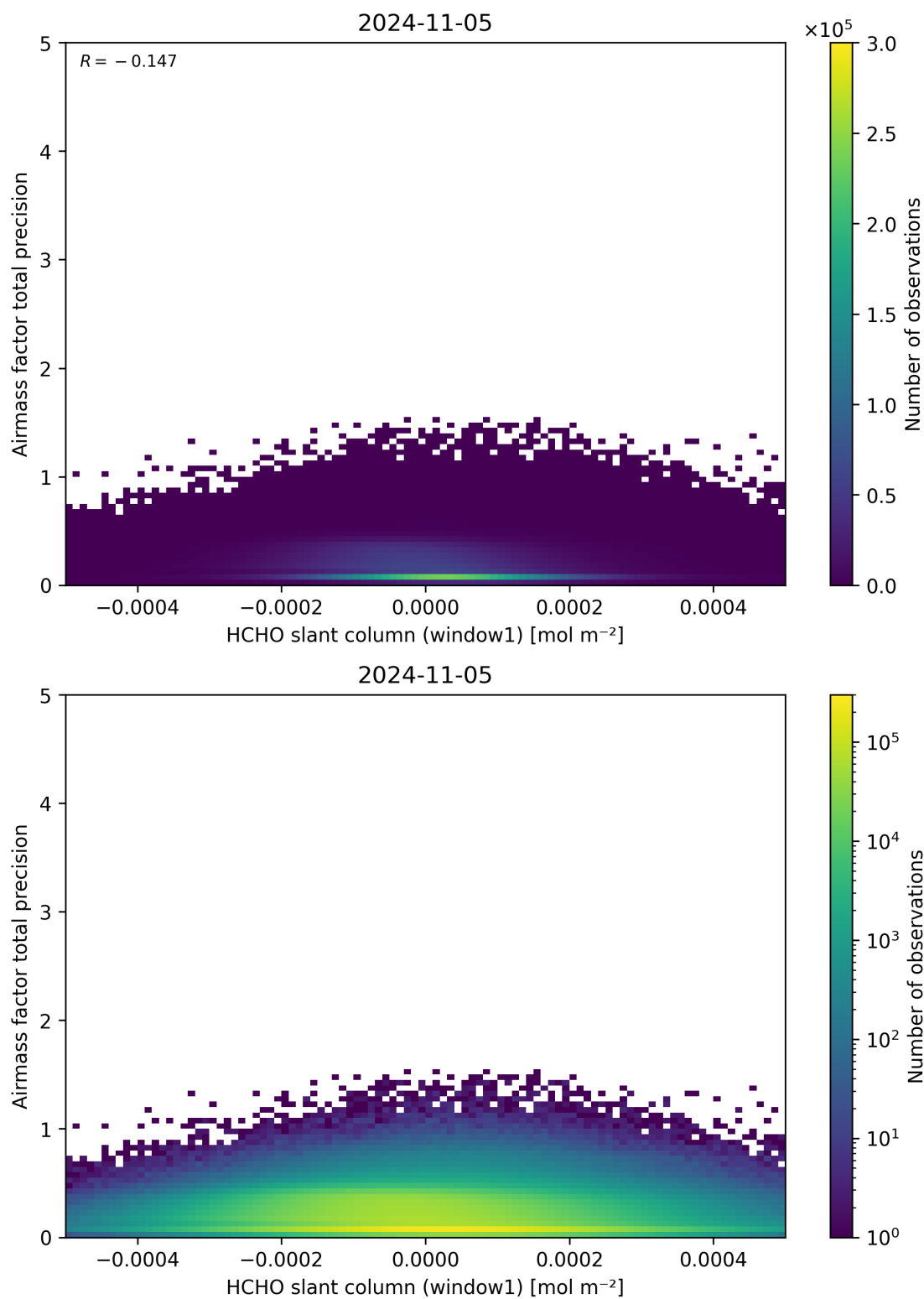
Figure 86: Scatter density plot of “HCHO slant column (window1)” against “Airmass factor total precision” for 2024-11-04 to 2024-11-06.
