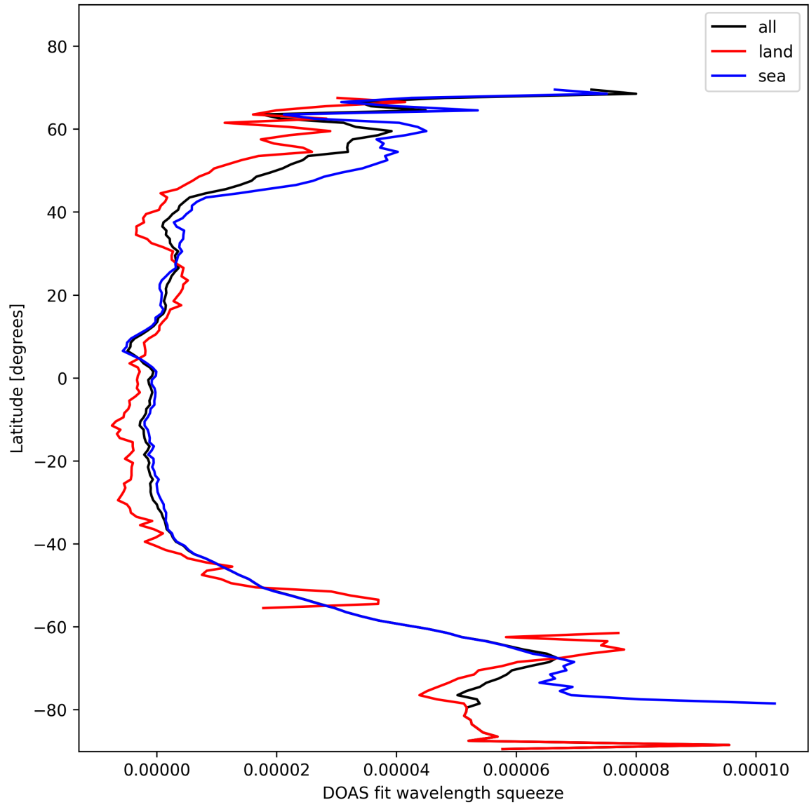
Figure 31: Zonal average of “DOAS fit wavelength squeeze” for 2024-11-04 to 2024-11-06.
