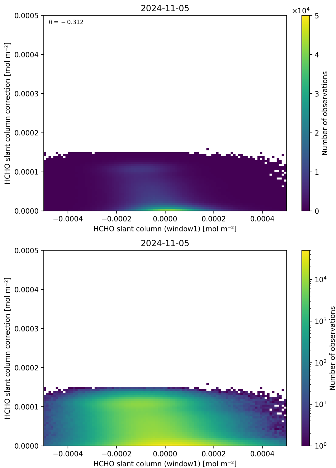
Figure 83: Scatter density plot of “HCHO slant column (window1)” against “HCHO slant column correction” for 2024-11-04 to 2024-11-06.
