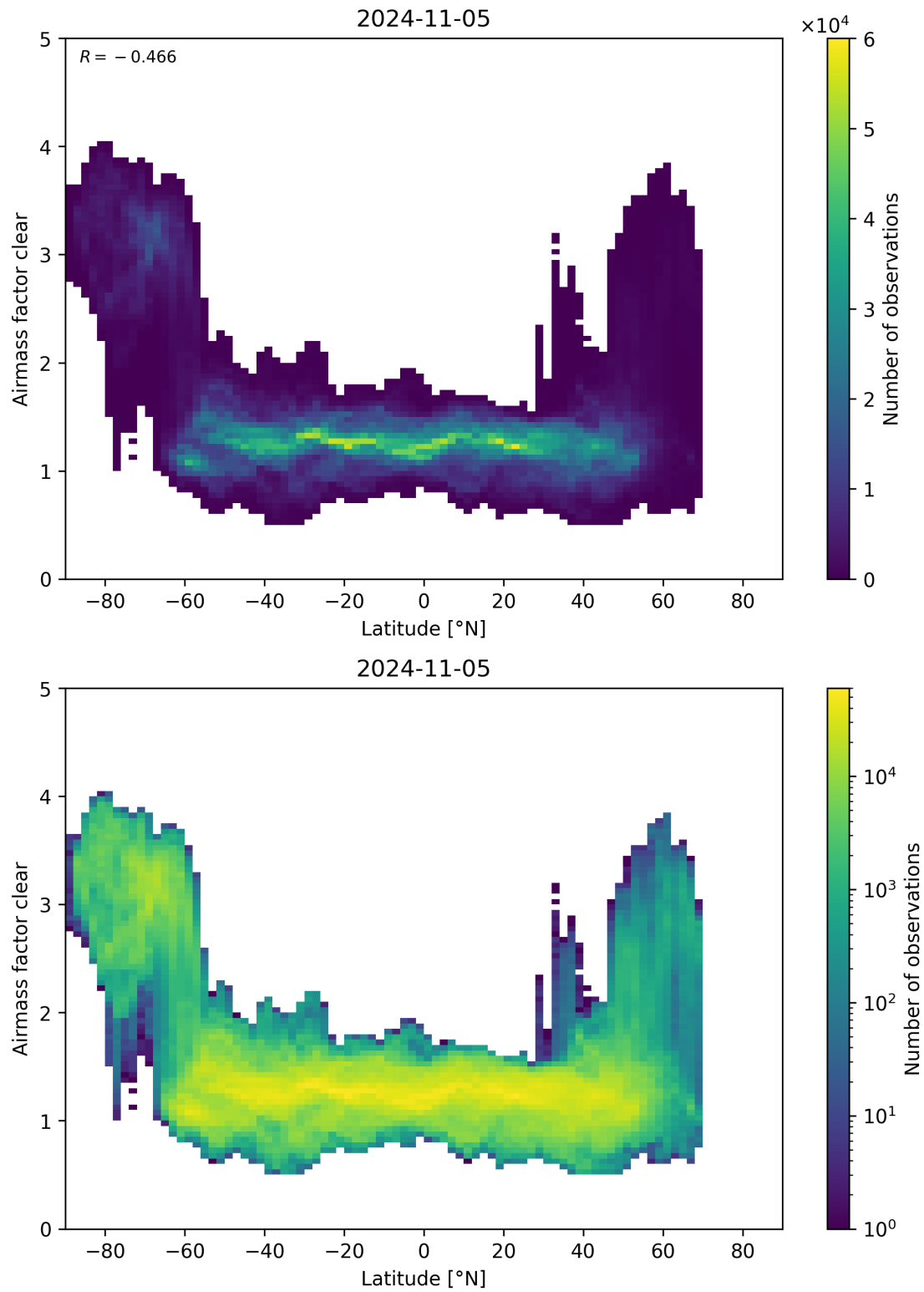
Figure 156: Scatter density plot of “Latitude” against “Airmass factor clear” for 2024-11-04 to 2024-11-06.
