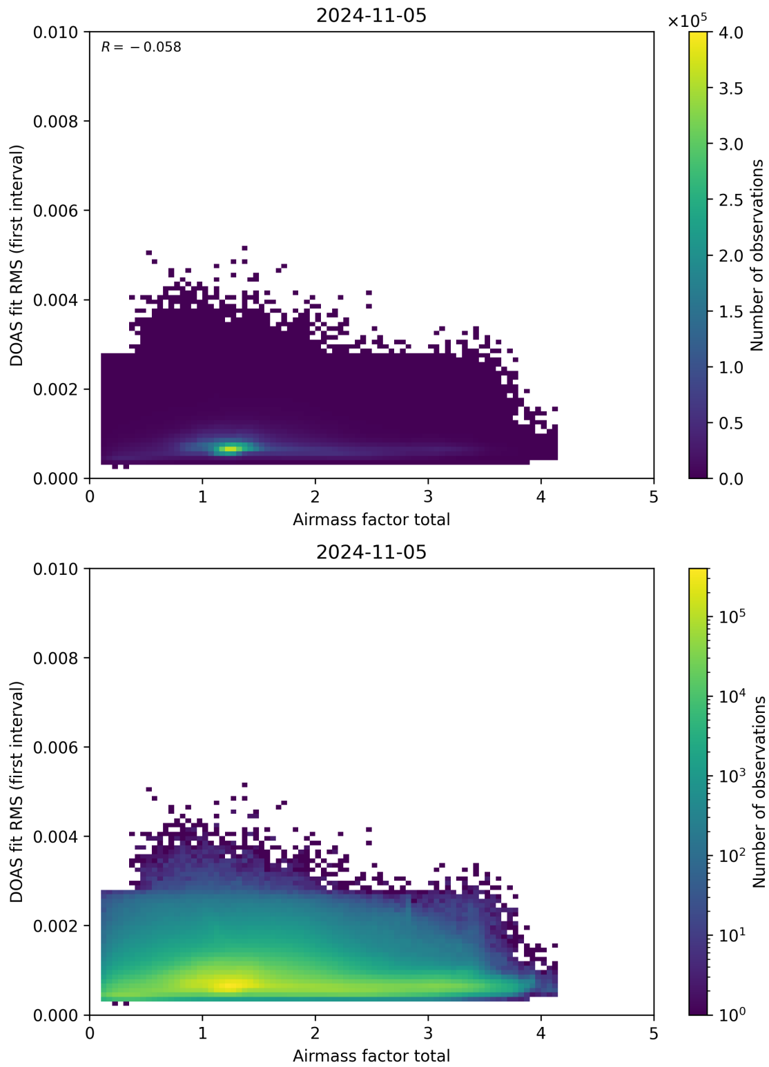
Figure 97: Scatter density plot of “Airmass factor total” against “DOAS fit RMS (first interval)” for 2024-11-04 to 2024-11-06.
