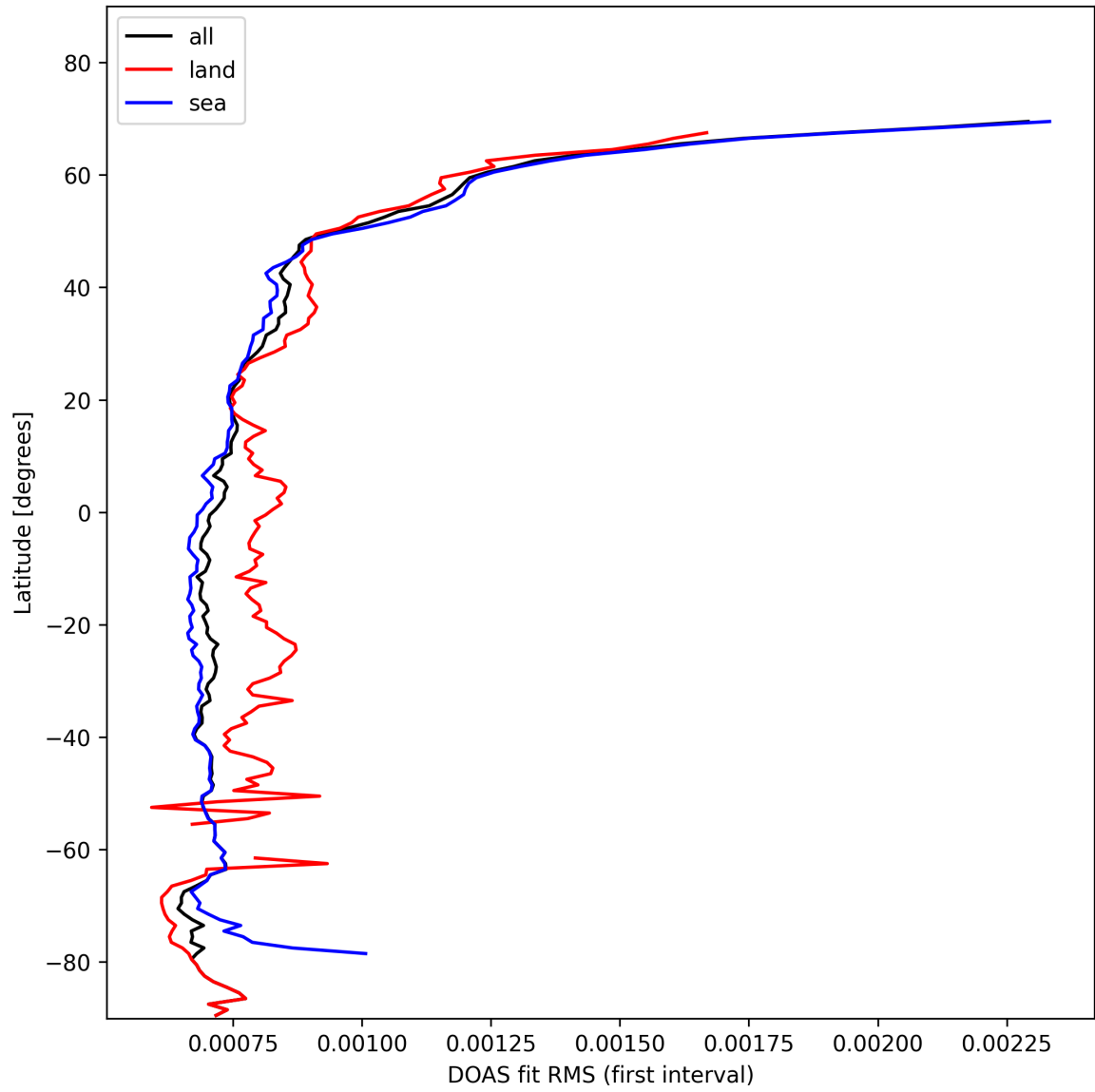
Figure 32: Zonal average of “DOAS fit RMS (first interval)” for 2024-11-04 to 2024-11-06.
