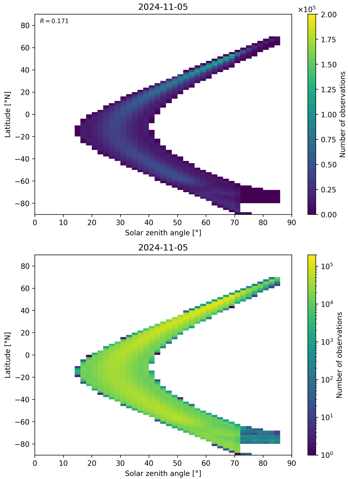
Figure 181: Scatter density plot of “Solar zenith angle” against “Latitude” for 2024-11-04 to 2024-11-06.
