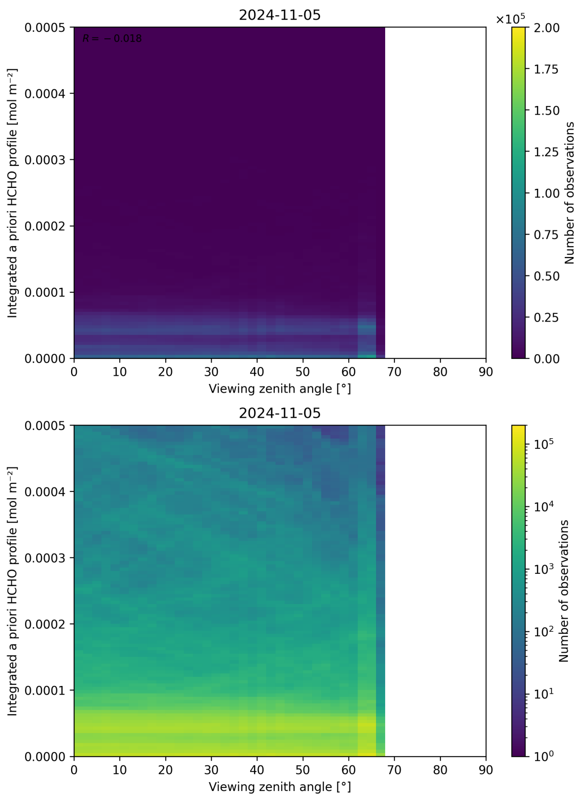
Figure 195: Scatter density plot of “Viewing zenith angle” against “Integrated a priori HCHO profile” for 2024-11-04 to 2024-11-06.
