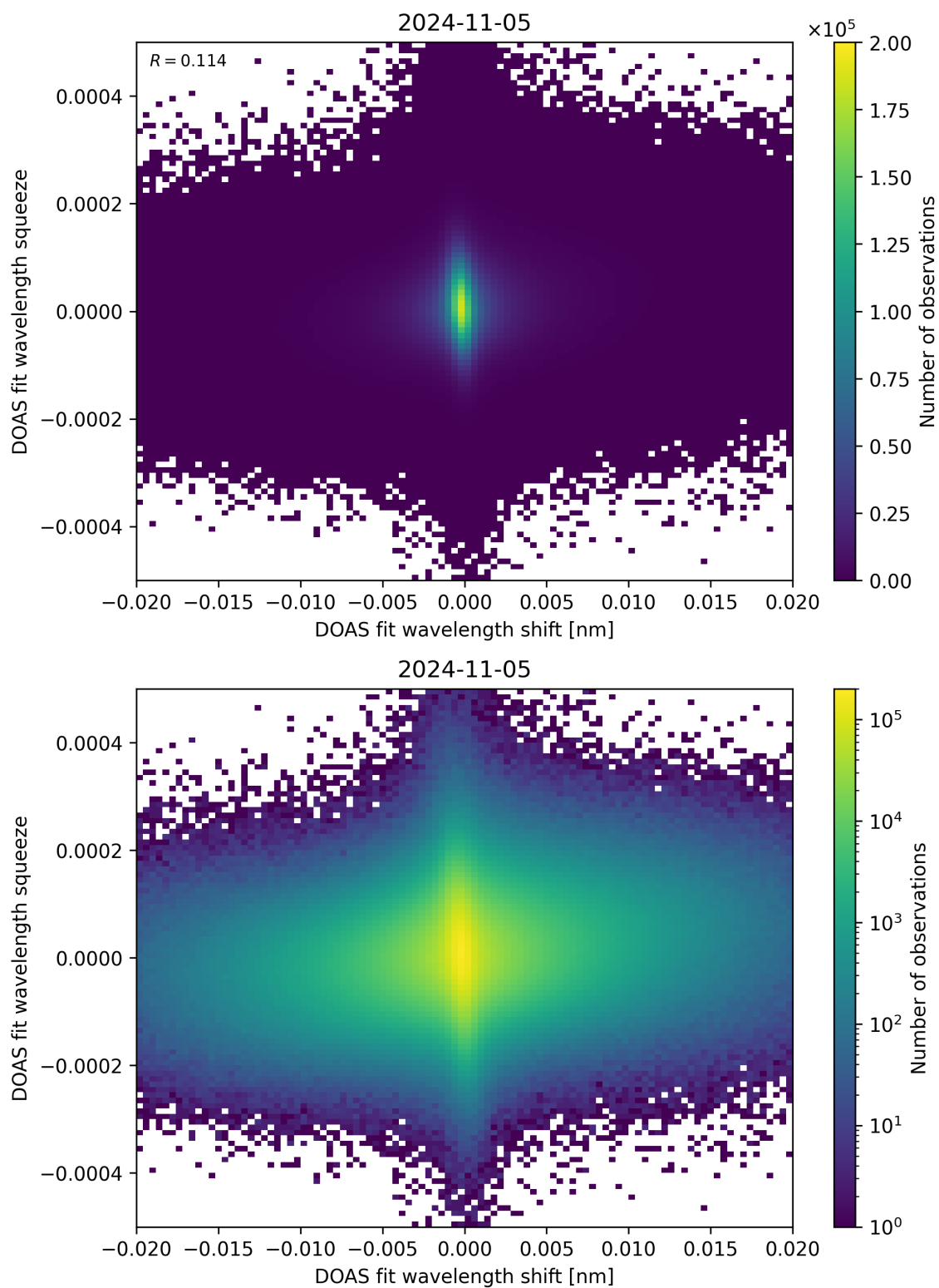
Figure 65: Scatter density plot of “DOAS fit wavelength shift” against “DOAS fit wavelength squeeze” for 2024-11-04 to 2024-11-06.
