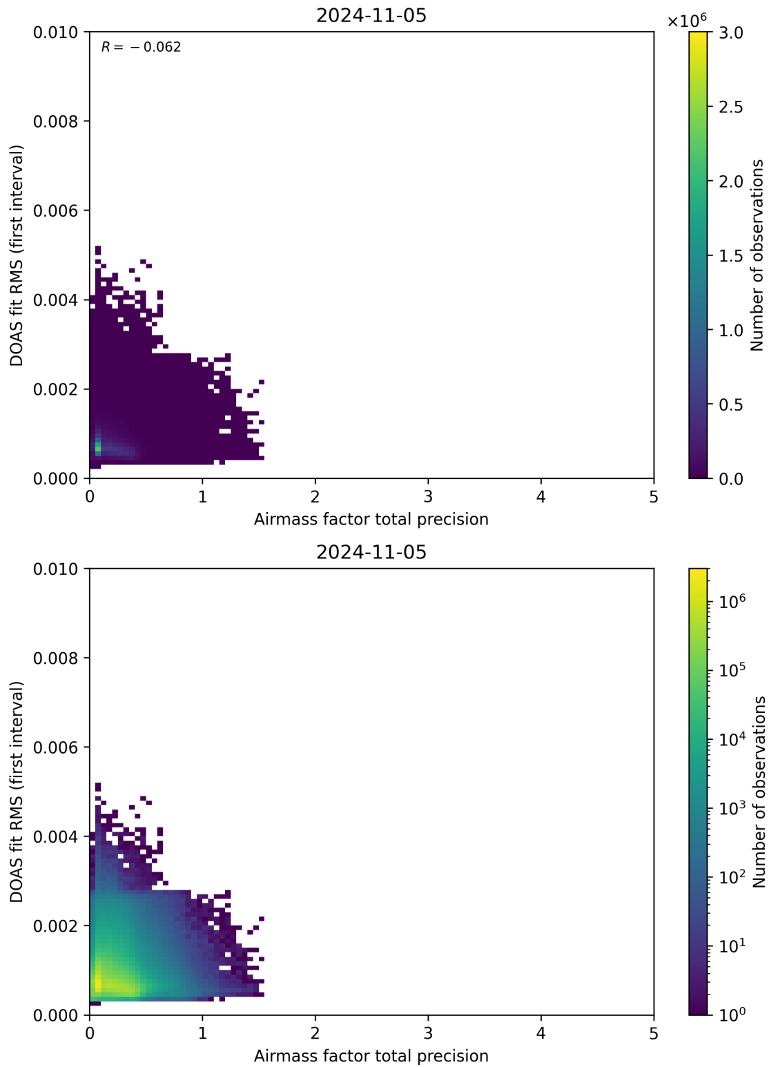
Figure 105: Scatter density plot of “Airmass factor total precision” against “DOAS fit RMS (first interval)” for 2024-11-04 to 2024-11-06.
