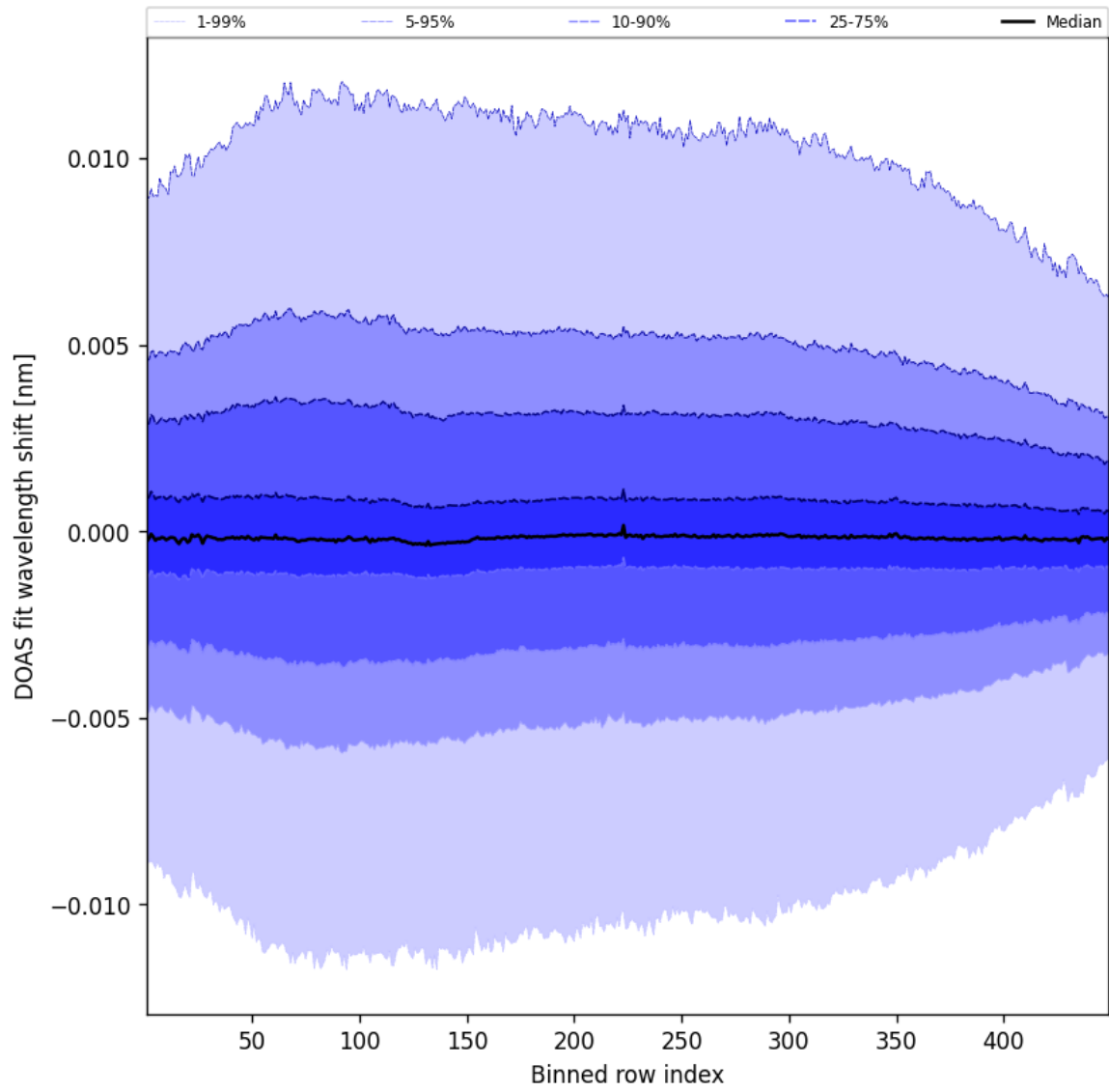
Figure 58: Along track statistics of “DOAS fit wavelength shift” for 2024-11-04 to 2024-11-06
