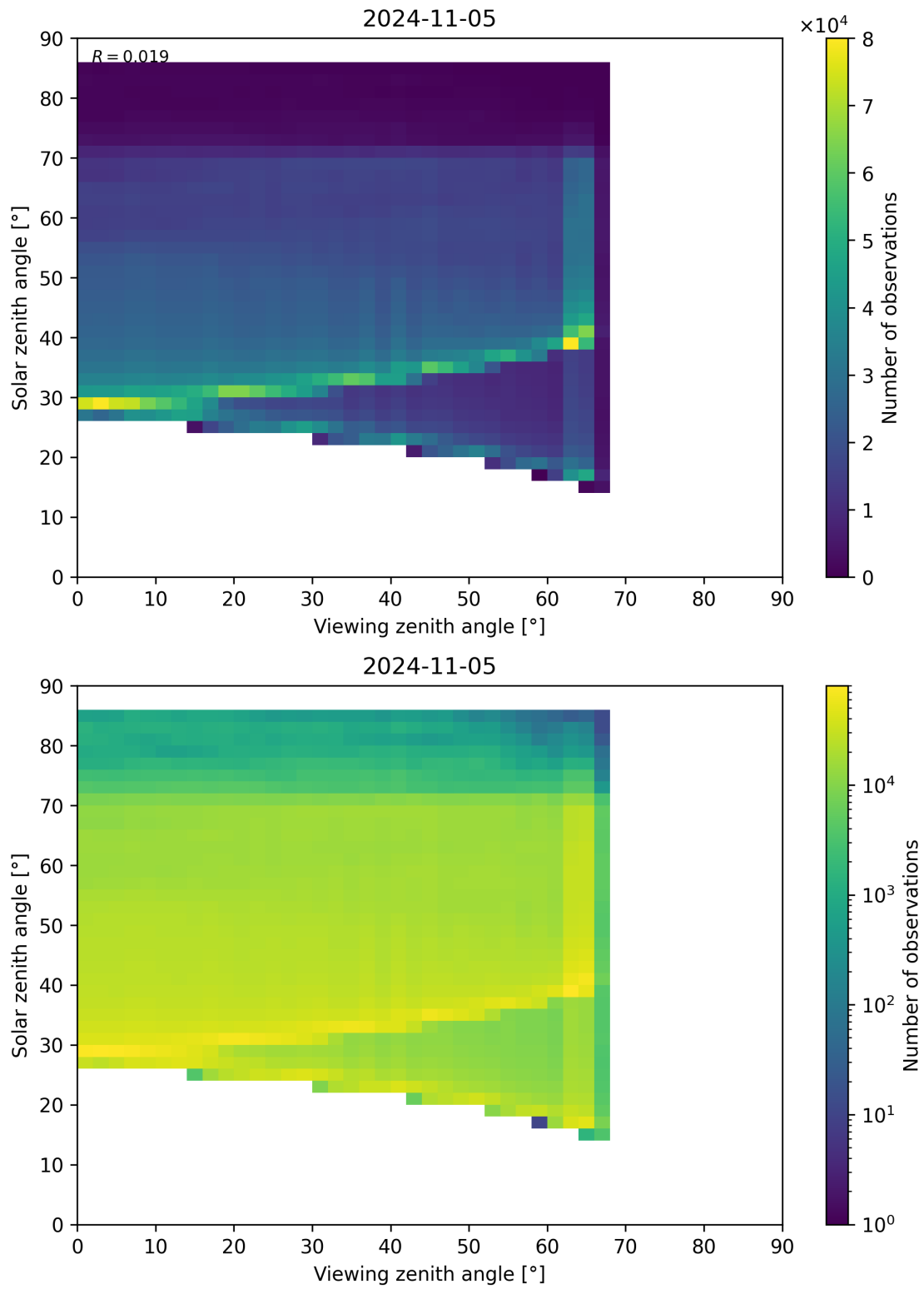
Figure 197: Scatter density plot of “Viewing zenith angle” against “Solar zenith angle” for 2024-11-04 to 2024-11-06.
