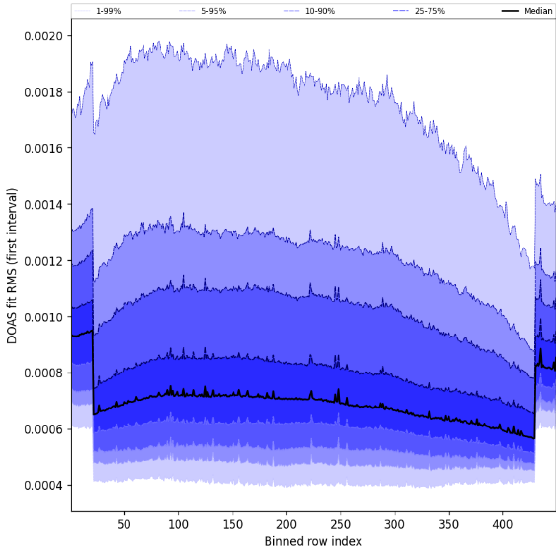
Figure 60: Along track statistics of “DOAS fit RMS (first interval)” for 2024-11-04 to 2024-11-06
