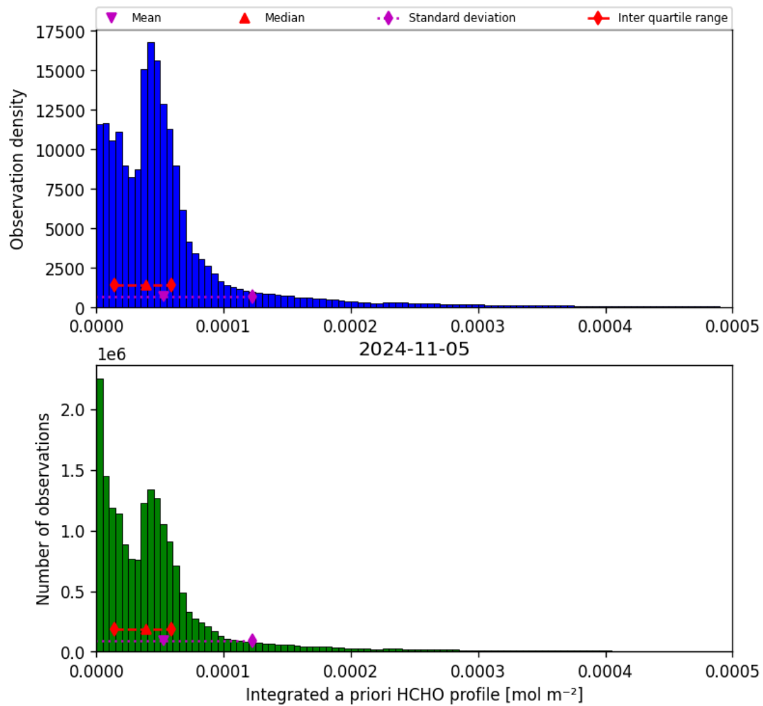
Figure 43: Histogram of “Integrated a priori HCHO profile” for 2024-11-04 to 2024-11-06
