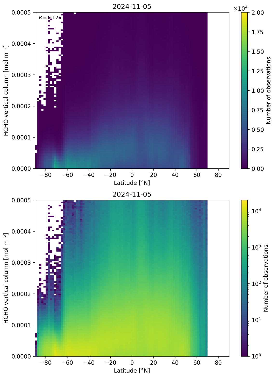
Figure 163: Scatter density plot of “Latitude” against “HCHO vertical column” for 2024-11-04 to 2024-11-06.
