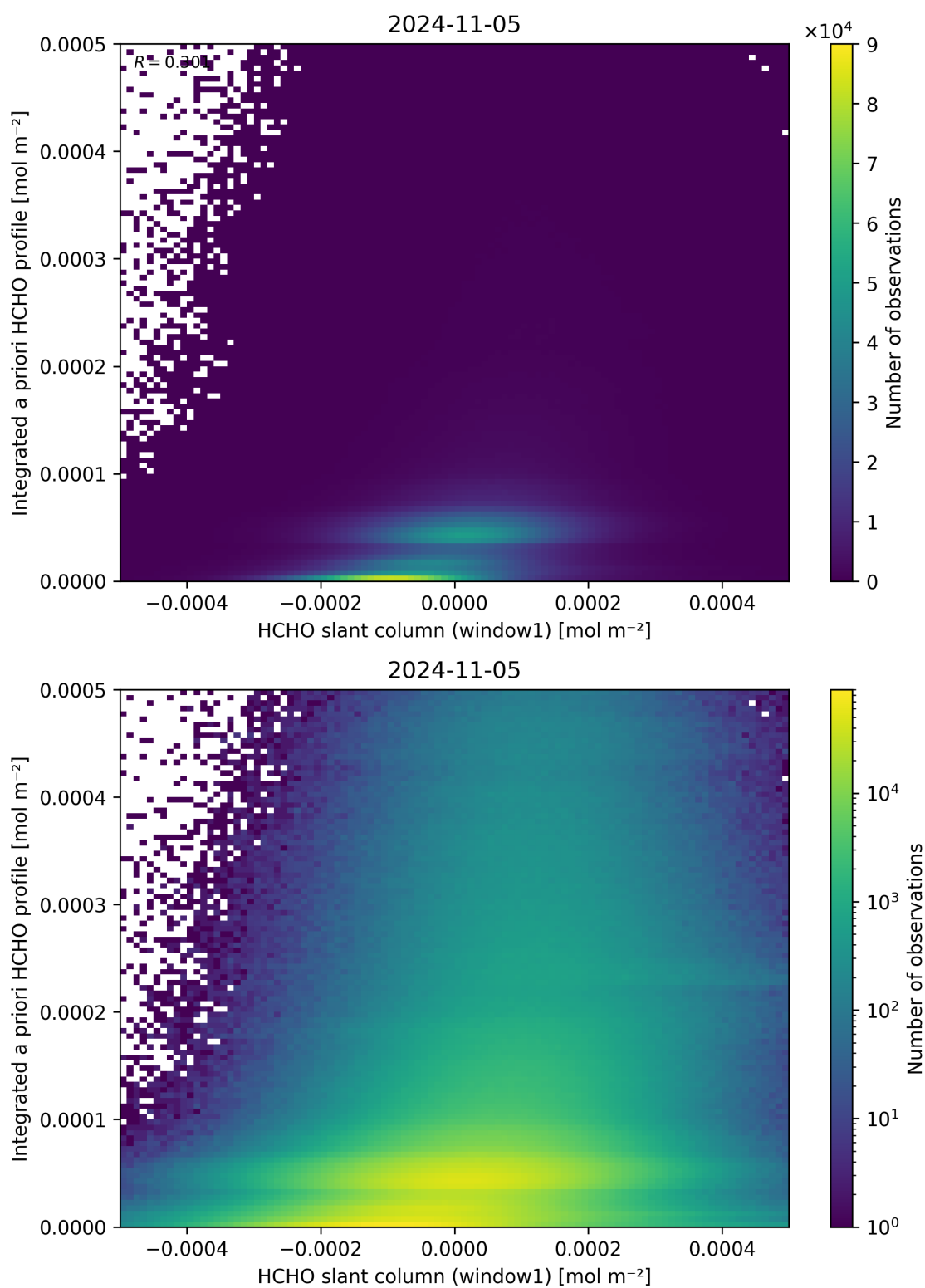
Figure 87: Scatter density plot of “HCHO slant column (window1)” against “Integrated a priori HCHO profile” for 2024-11-04 to 2024-11-06.
