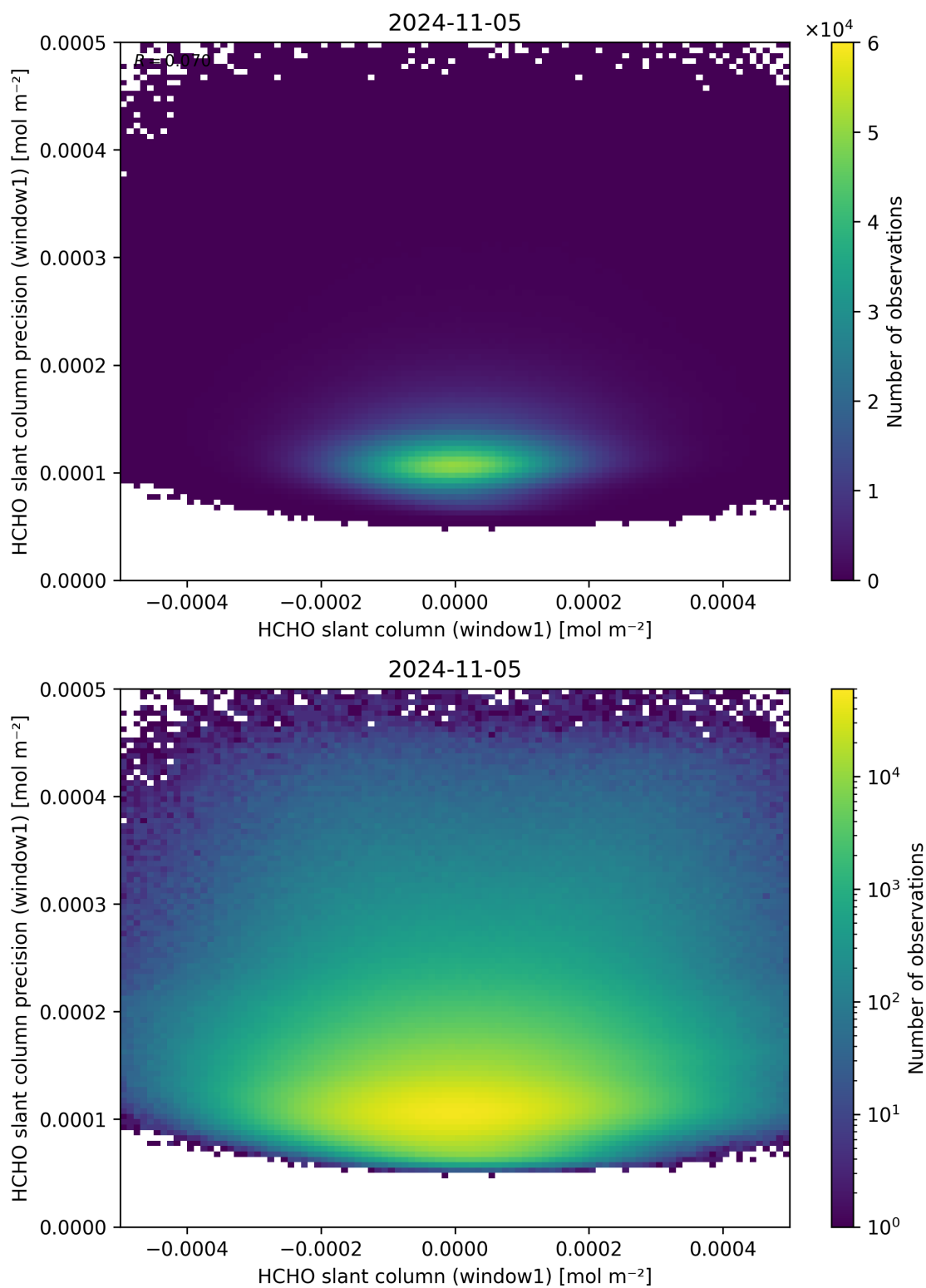
Figure 84: Scatter density plot of “HCHO slant column (window1)” against “HCHO slant column precision (window1)” for 2024-11-04 to 2024-11-06.
