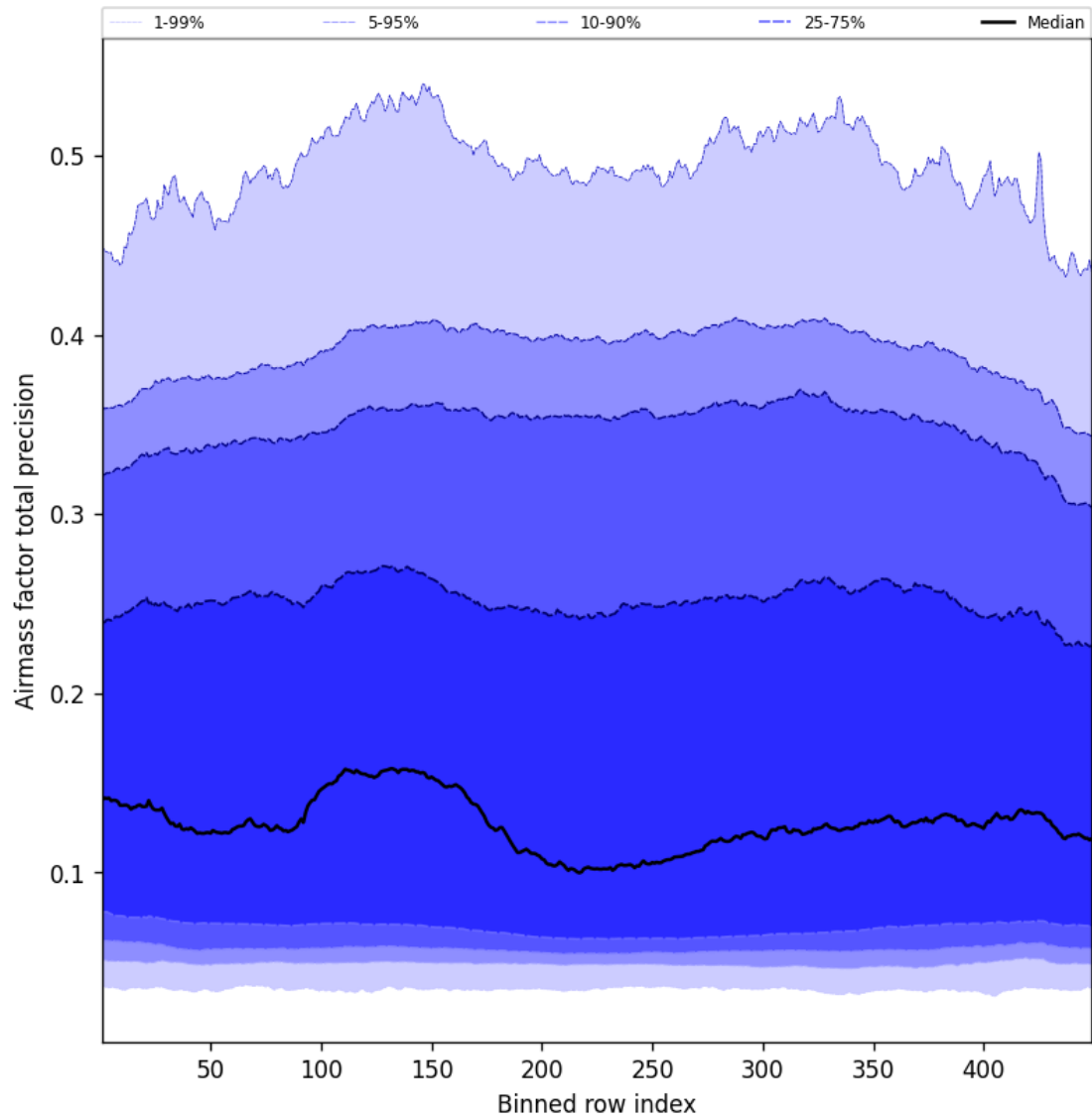
Figure 55: Along track statistics of “Airmass factor total precision” for 2024-11-04 to 2024-11-06
