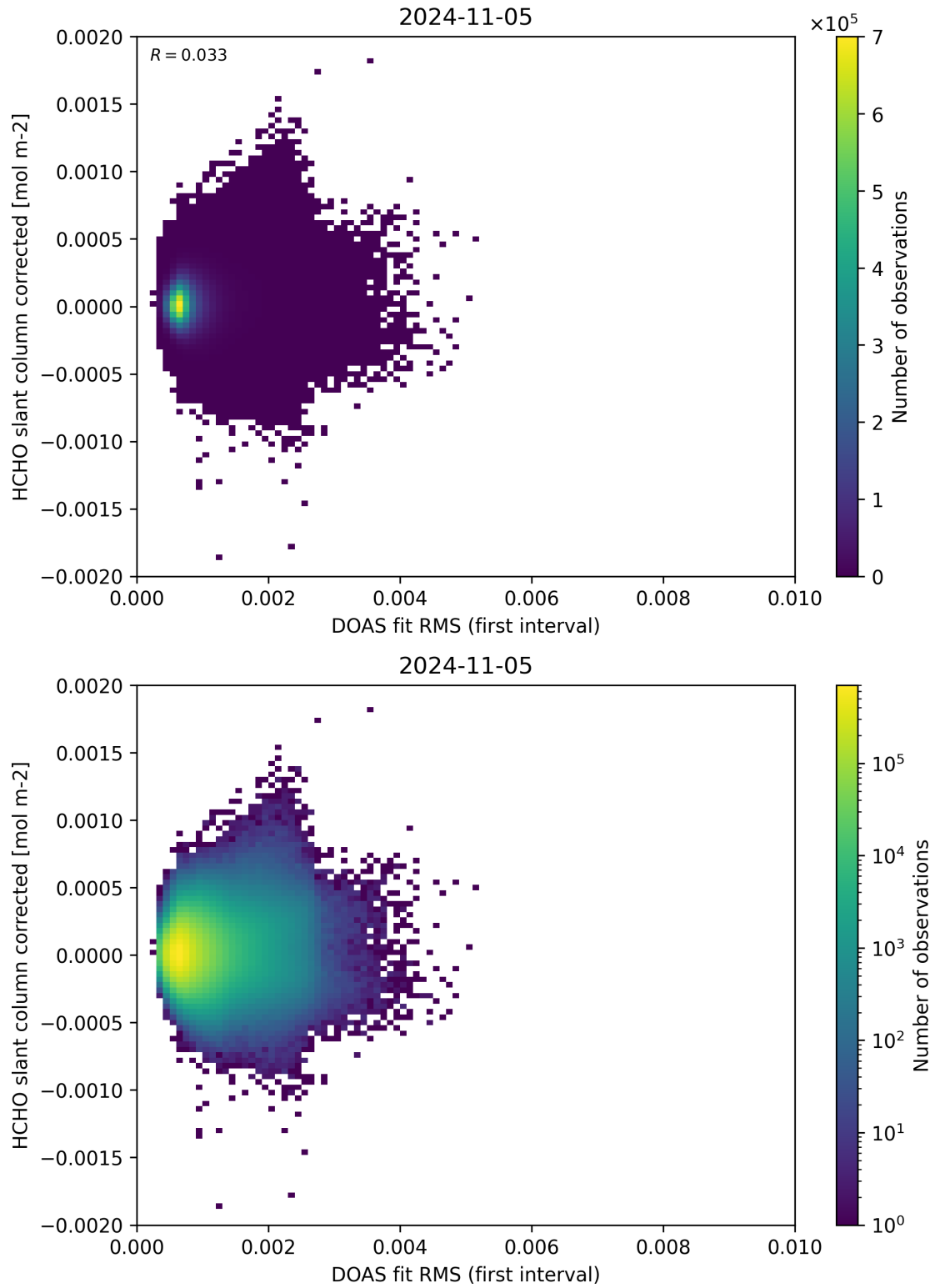
Figure 62: Scatter density plot of “DOAS fit RMS (first interval)” against “HCHO slant column corrected” for 2024-11-04 to 2024-11-06.
