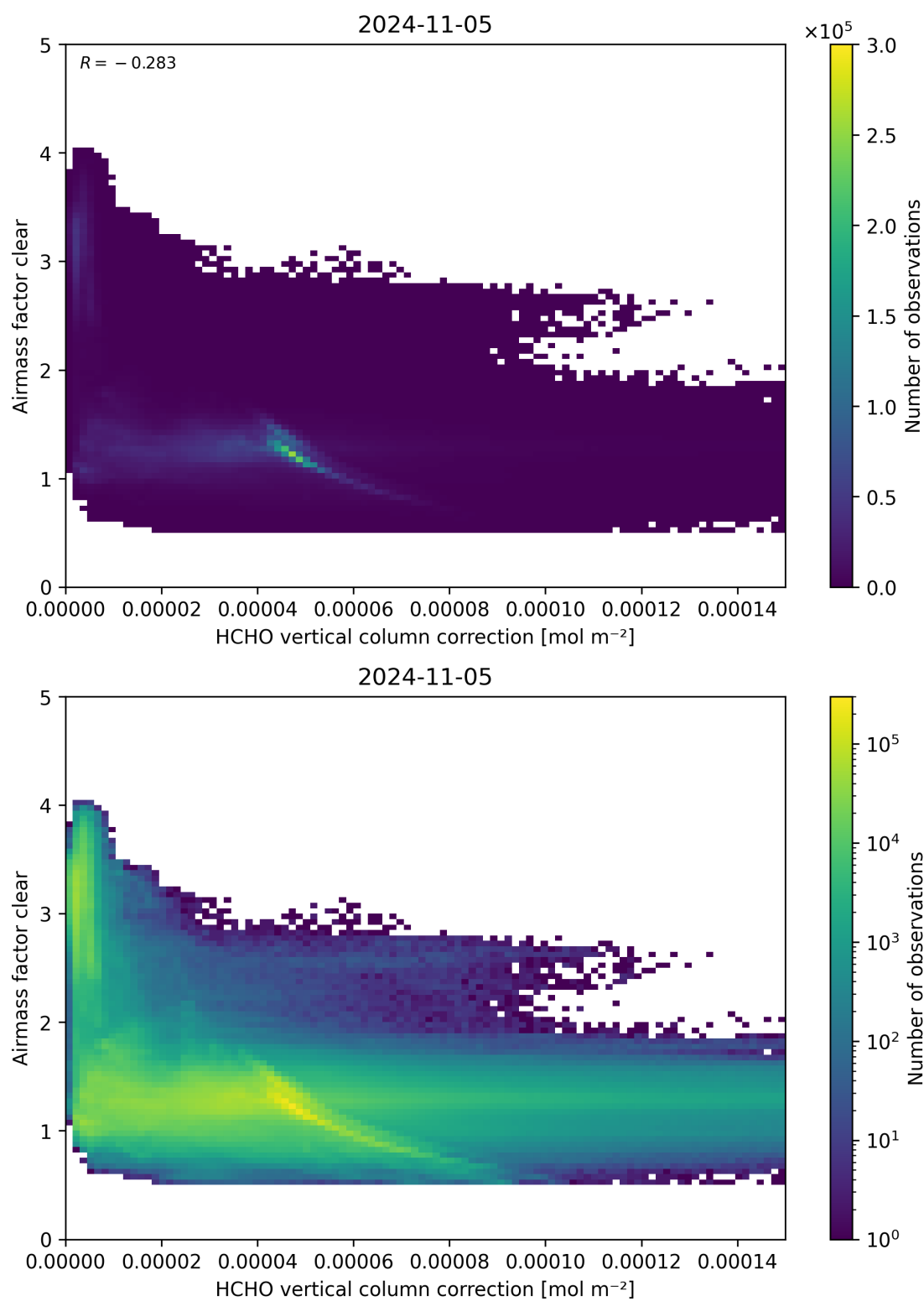
Figure 115: Scatter density plot of “HCHO vertical column correction” against “Airmass factor clear” for 2024-11-04 to 2024-11-06.
