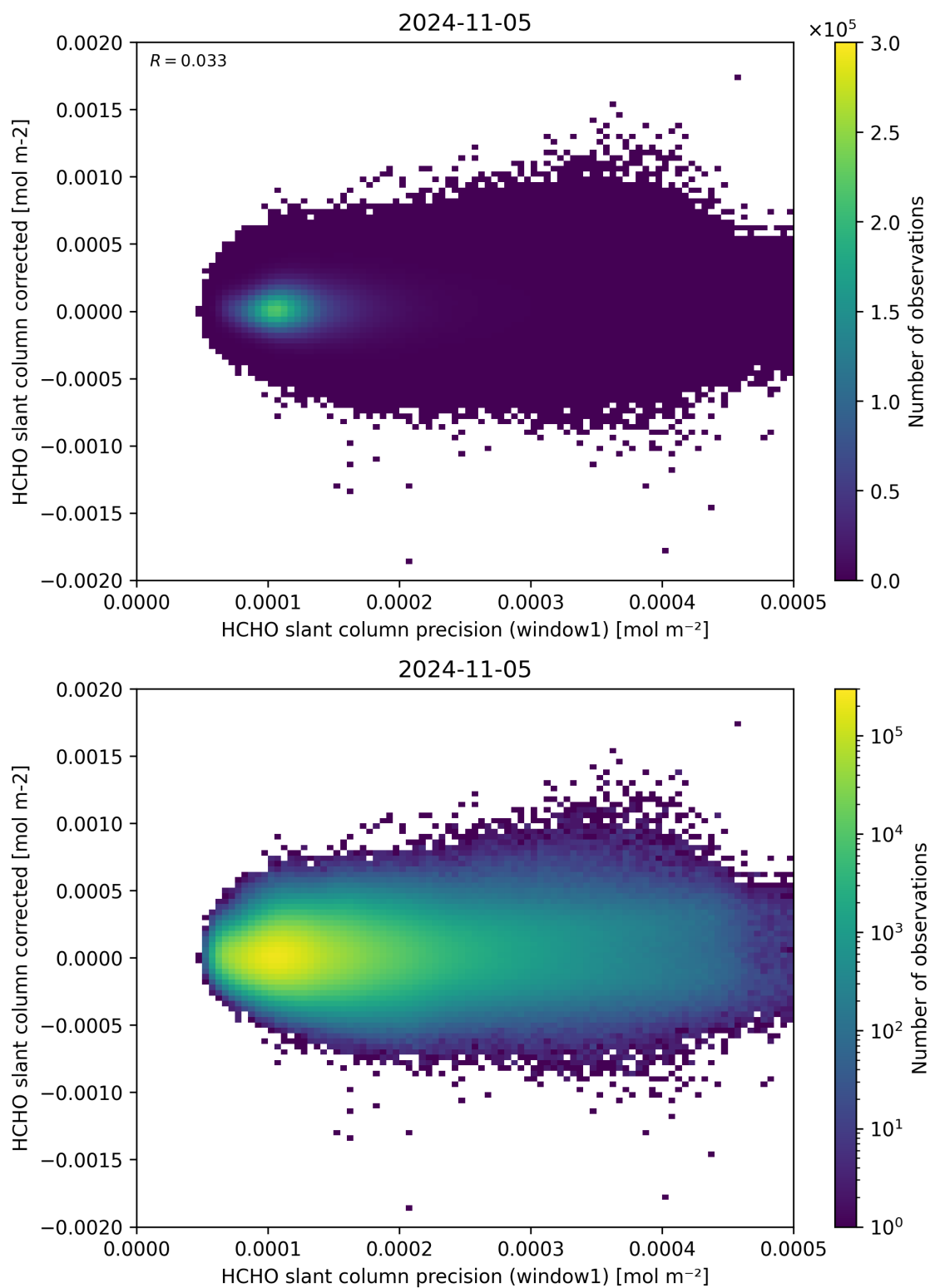
Figure 92: Scatter density plot of “HCHO slant column precision (window1)” against “HCHO slant column corrected” for 2024-11-04 to 2024-11-06.
