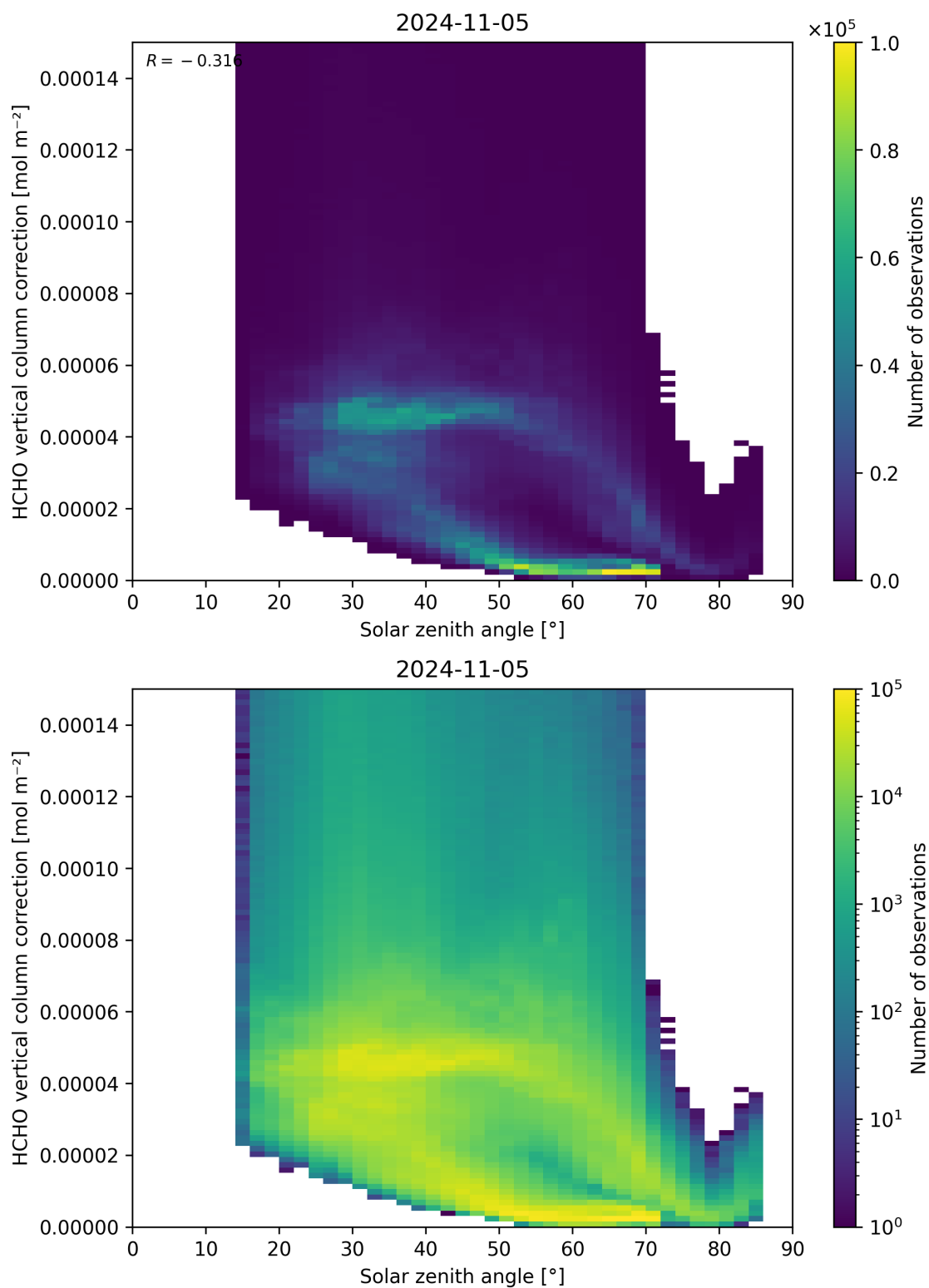
Figure 178: Scatter density plot of “Solar zenith angle” against “HCHO vertical column correction” for 2024-11-04 to 2024-11-06.
