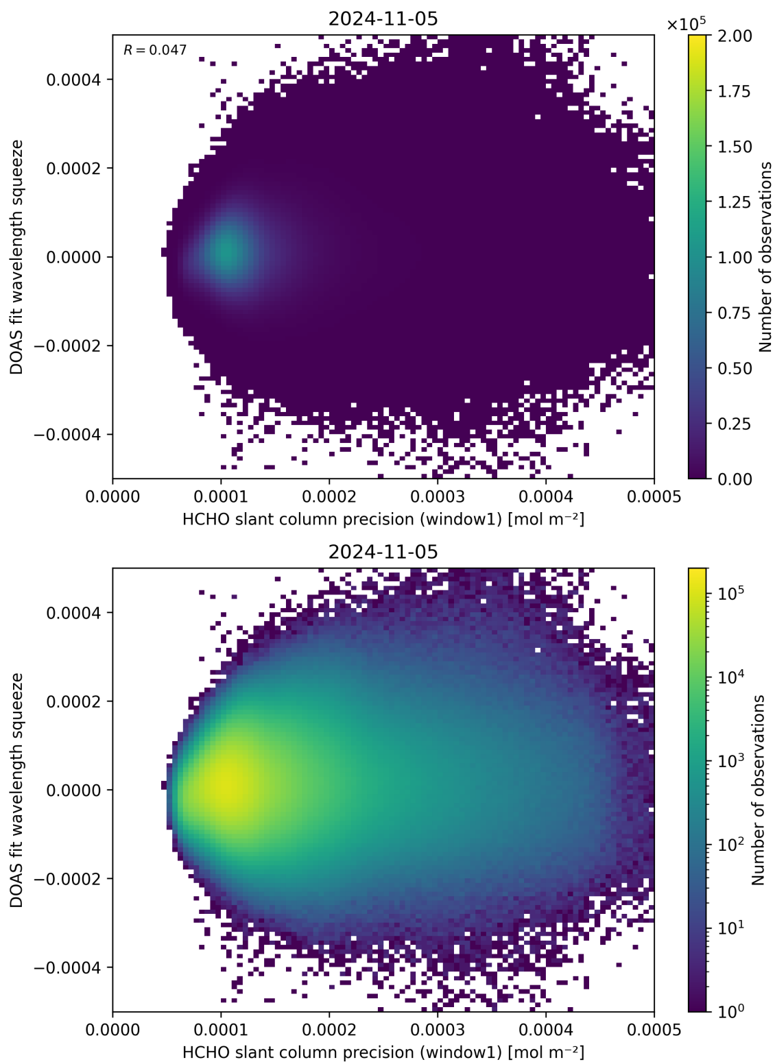
Figure 90: Scatter density plot of “HCHO slant column precision (window1)” against “DOAS fit wavelength squeeze” for 2024-11-04 to 2024-11-06.
