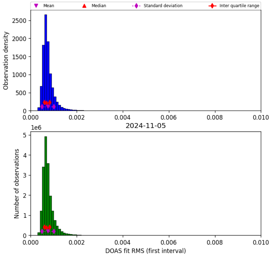
Figure 46: Histogram of “DOAS fit RMS (first interval)” for 2024-11-04 to 2024-11-06
