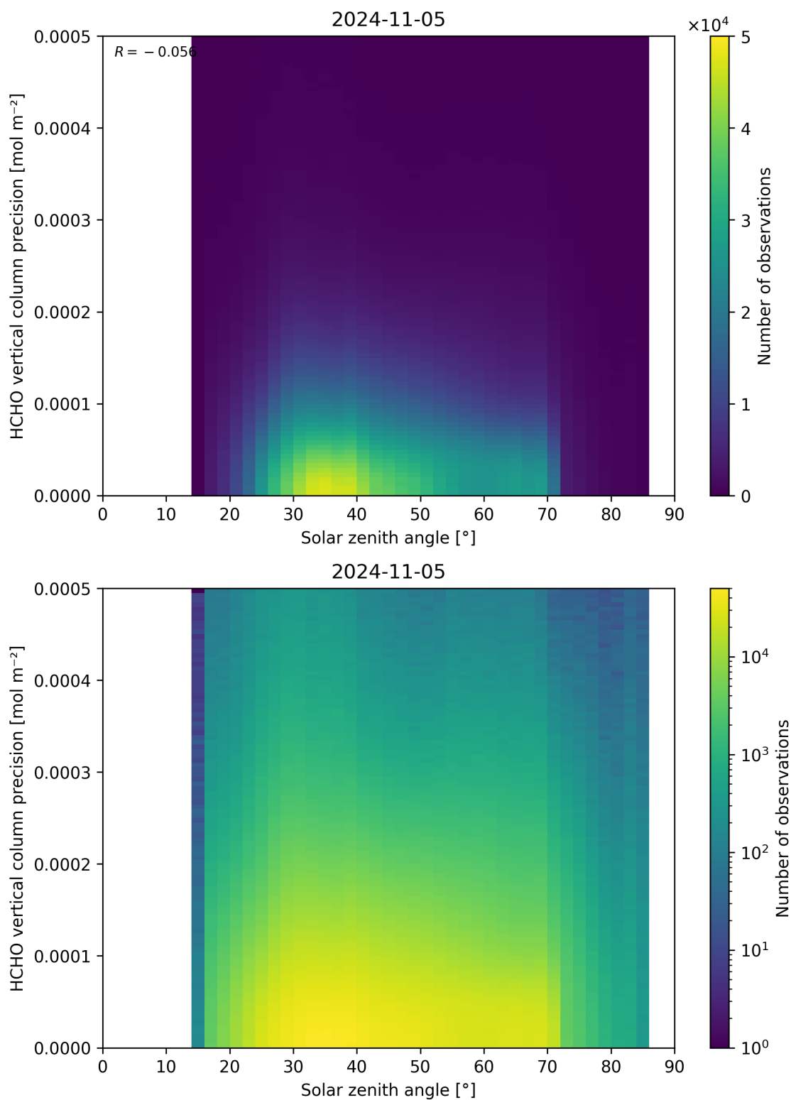
Figure 179: Scatter density plot of “Solar zenith angle” against “HCHO vertical column precision” for 2024-11-04 to 2024-11-06.
