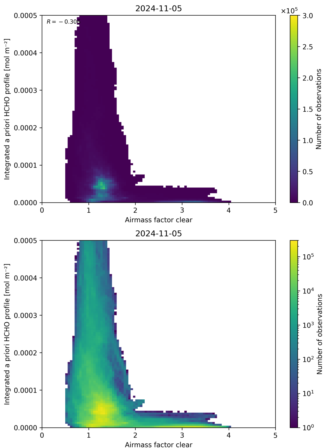
Figure 76: Scatter density plot of “Airmass factor clear” against “Integrated a priori HCHO profile” for 2024-11-04 to 2024-11-06.
