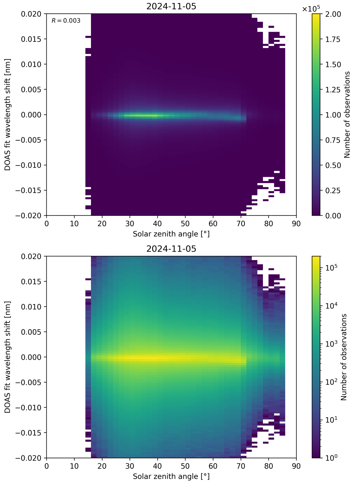
Figure 168: Scatter density plot of “Solar zenith angle” against “DOAS fit wavelength shift” for 2024-11-04 to 2024-11-06.
