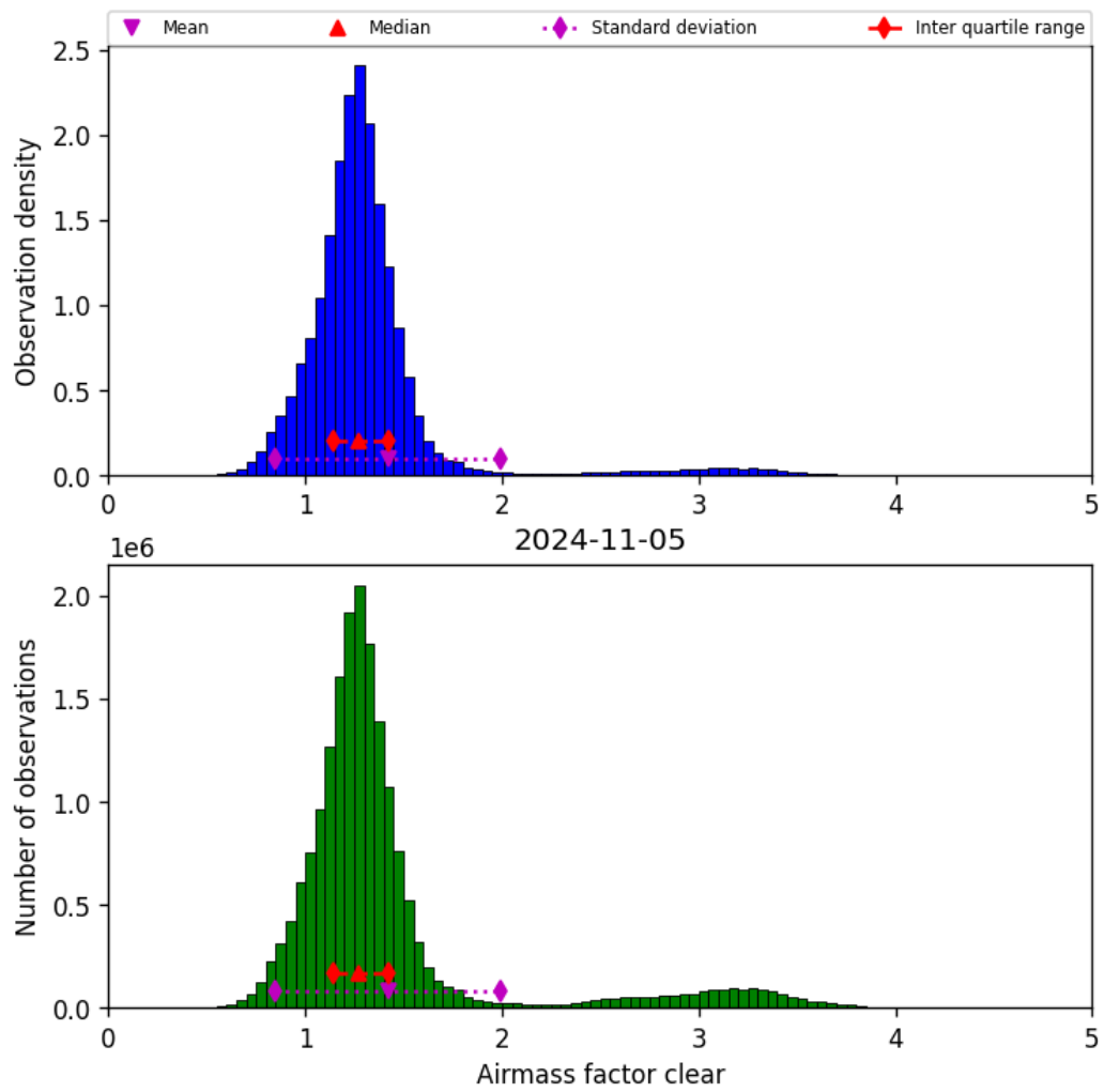
Figure 42: Histogram of “Airmass factor clear” for 2024-11-04 to 2024-11-06
