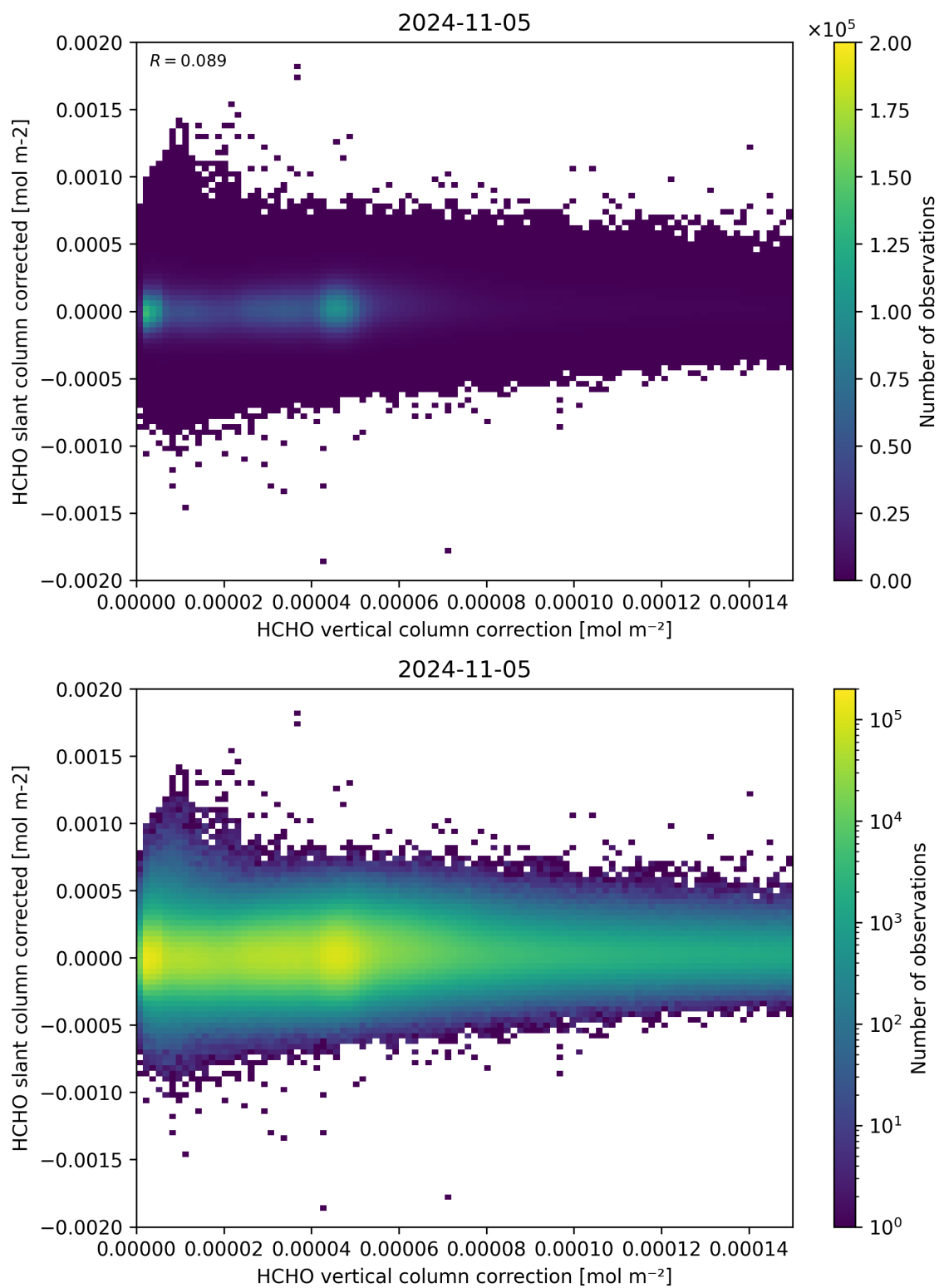
Figure 116: Scatter density plot of “HCHO vertical column correction” against “HCHO slant column corrected” for 2024-11-04 to 2024-11-06.
