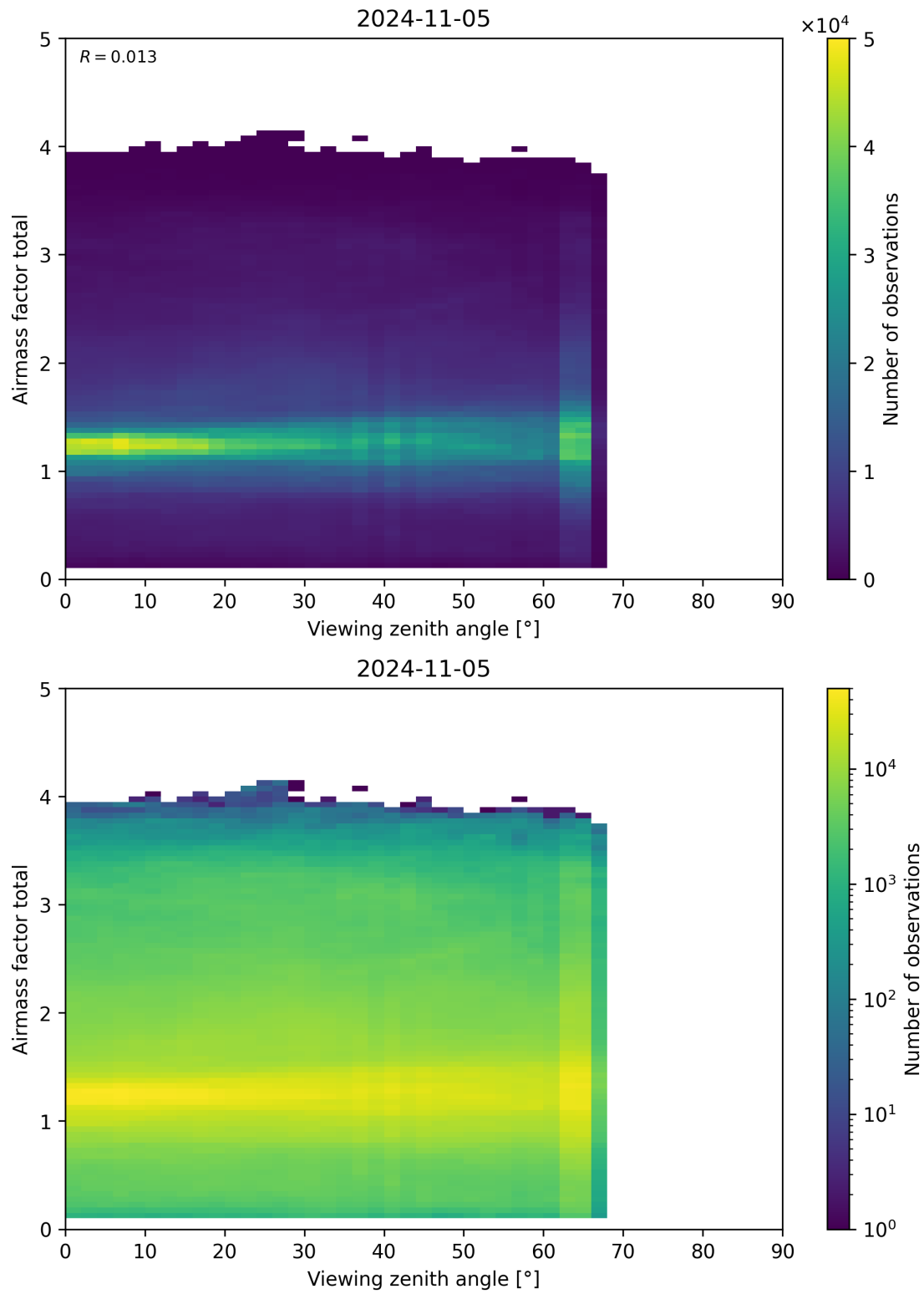
Figure 190: Scatter density plot of “Viewing zenith angle” against “Airmass factor total” for 2024-11-04 to 2024-11-06.
