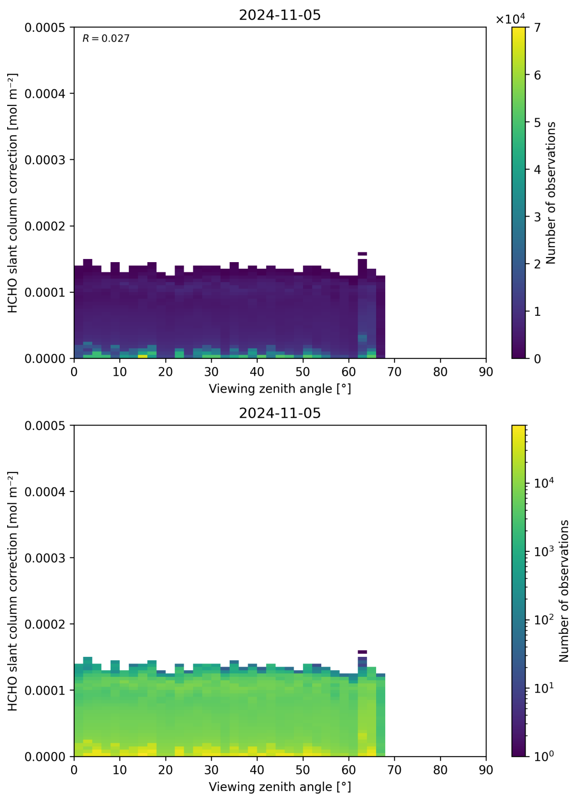
Figure 187: Scatter density plot of “Viewing zenith angle” against “HCHO slant column correction” for 2024-11-04 to 2024-11-06.
