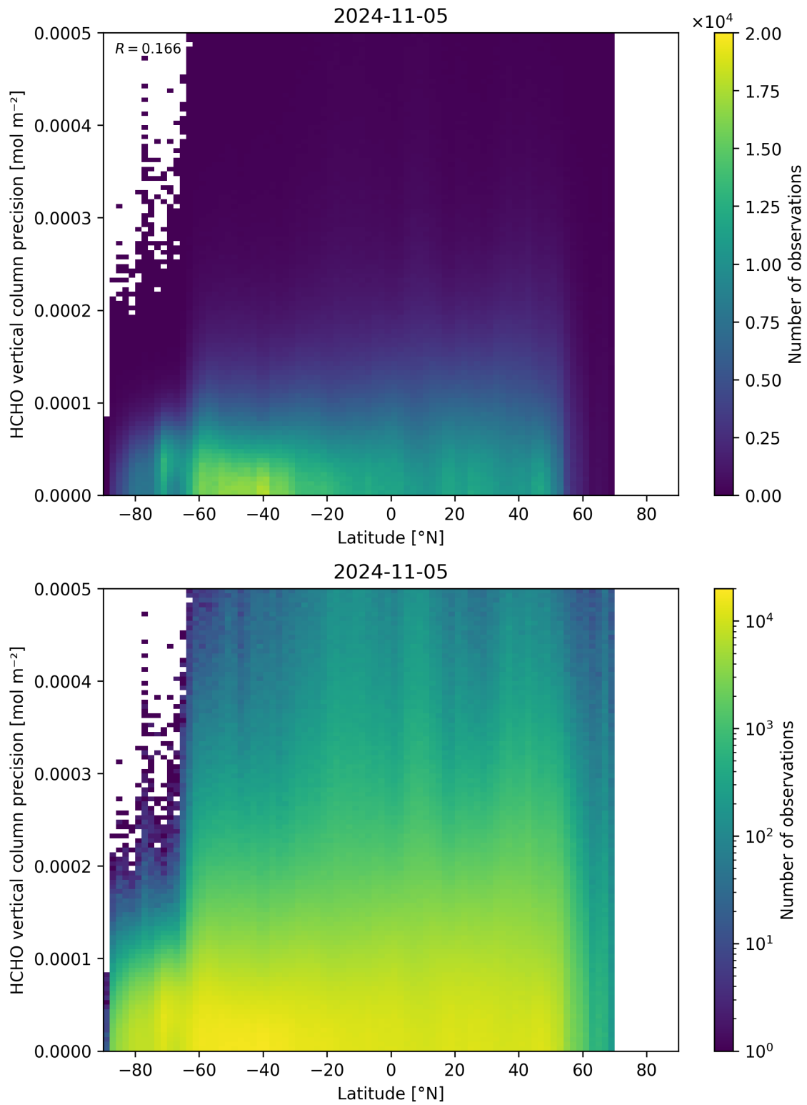
Figure 165: Scatter density plot of “Latitude” against “HCHO vertical column precision” for 2024-11-04 to 2024-11-06.
