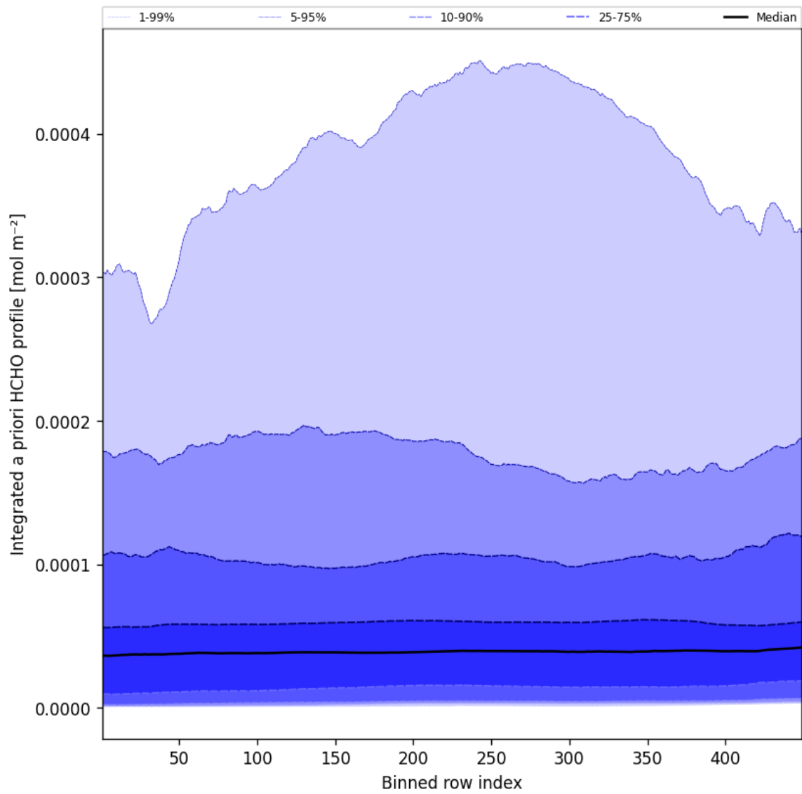
Figure 57: Along track statistics of "Integrated a priori HCHO profile" for 2024-11-04 to 2024-11-06
