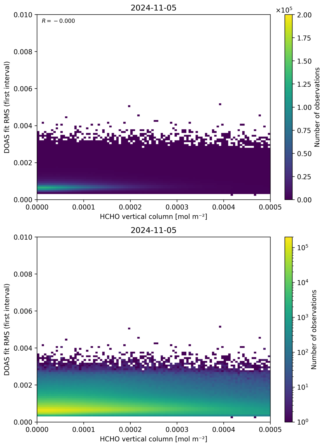
Figure 123: Scatter density plot of “HCHO vertical column” against “DOAS fit RMS (first interval)” for 2024-11-04 to 2024-11-06.
