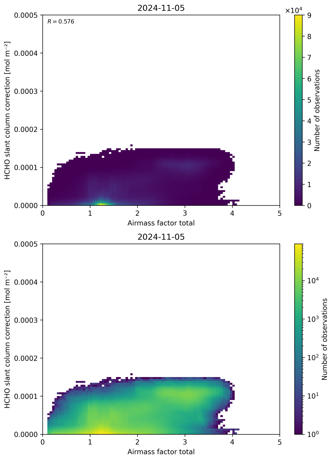
Figure 102: Scatter density plot of “Airmass factor total” against “HCHO slant column correction” for 2024-11-04 to 2024-11-06.
