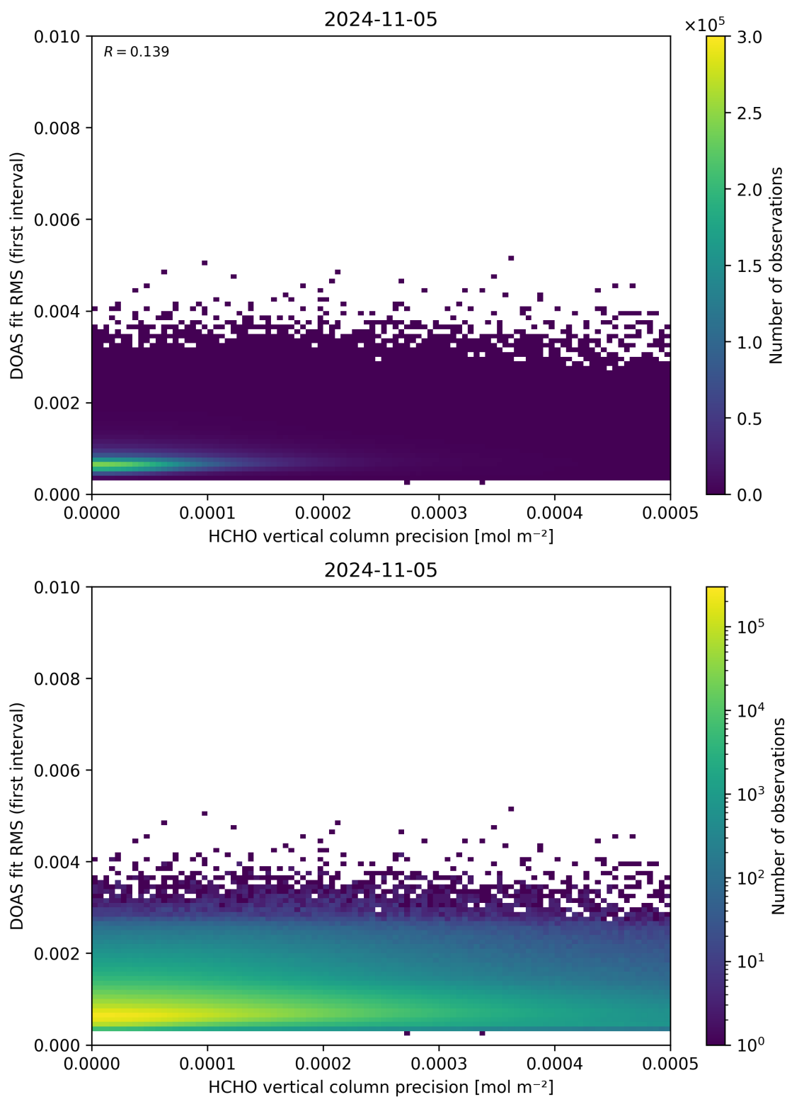
Figure 136: Scatter density plot of “HCHO vertical column precision” against “DOAS fit RMS (first interval)” for 2024-11-04 to 2024-11-06.
