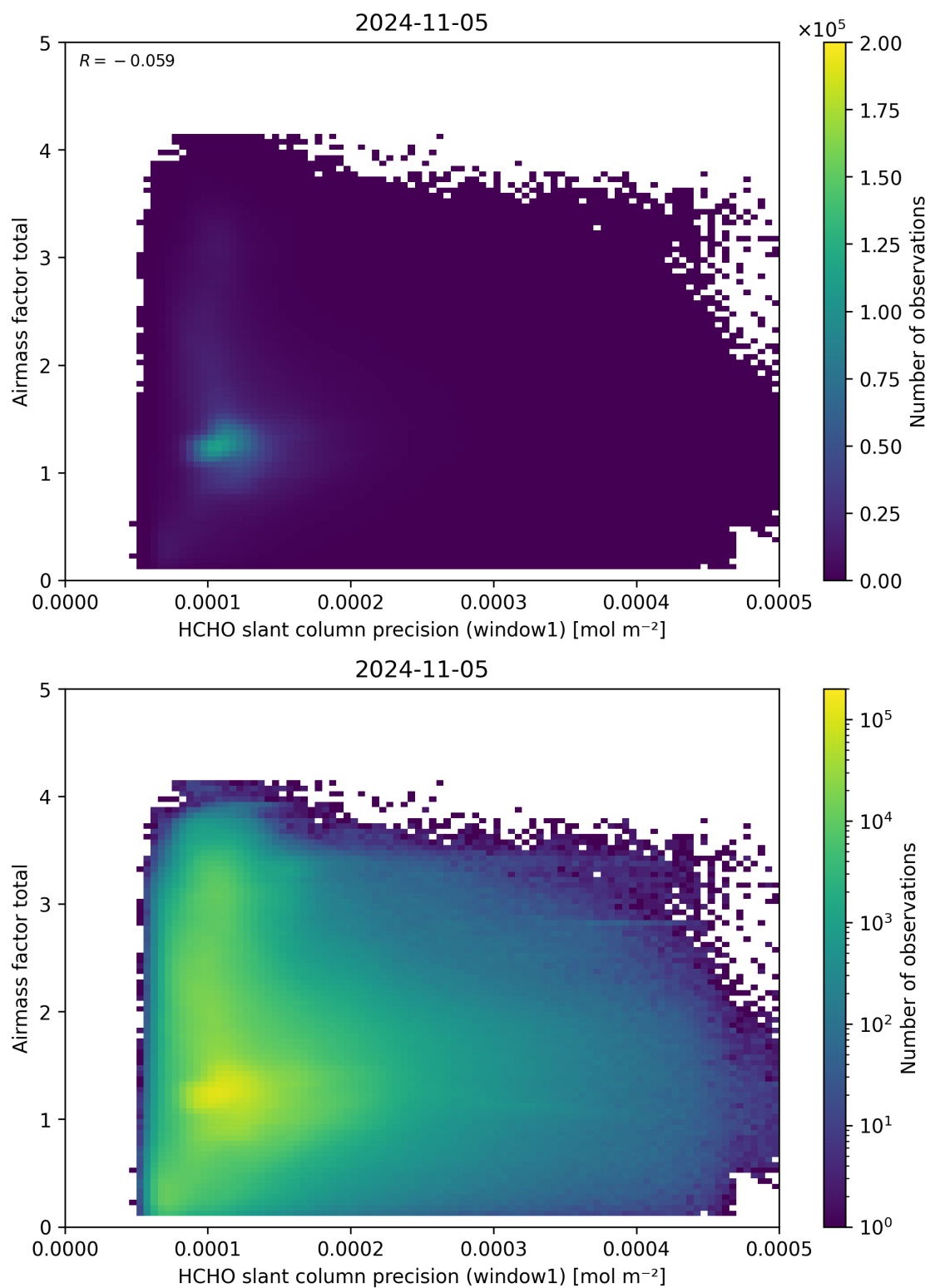
Figure 94: Scatter density plot of “HCHO slant column precision (window1)” against “Airmass factor total” for 2024-11-04 to 2024-11-06.
