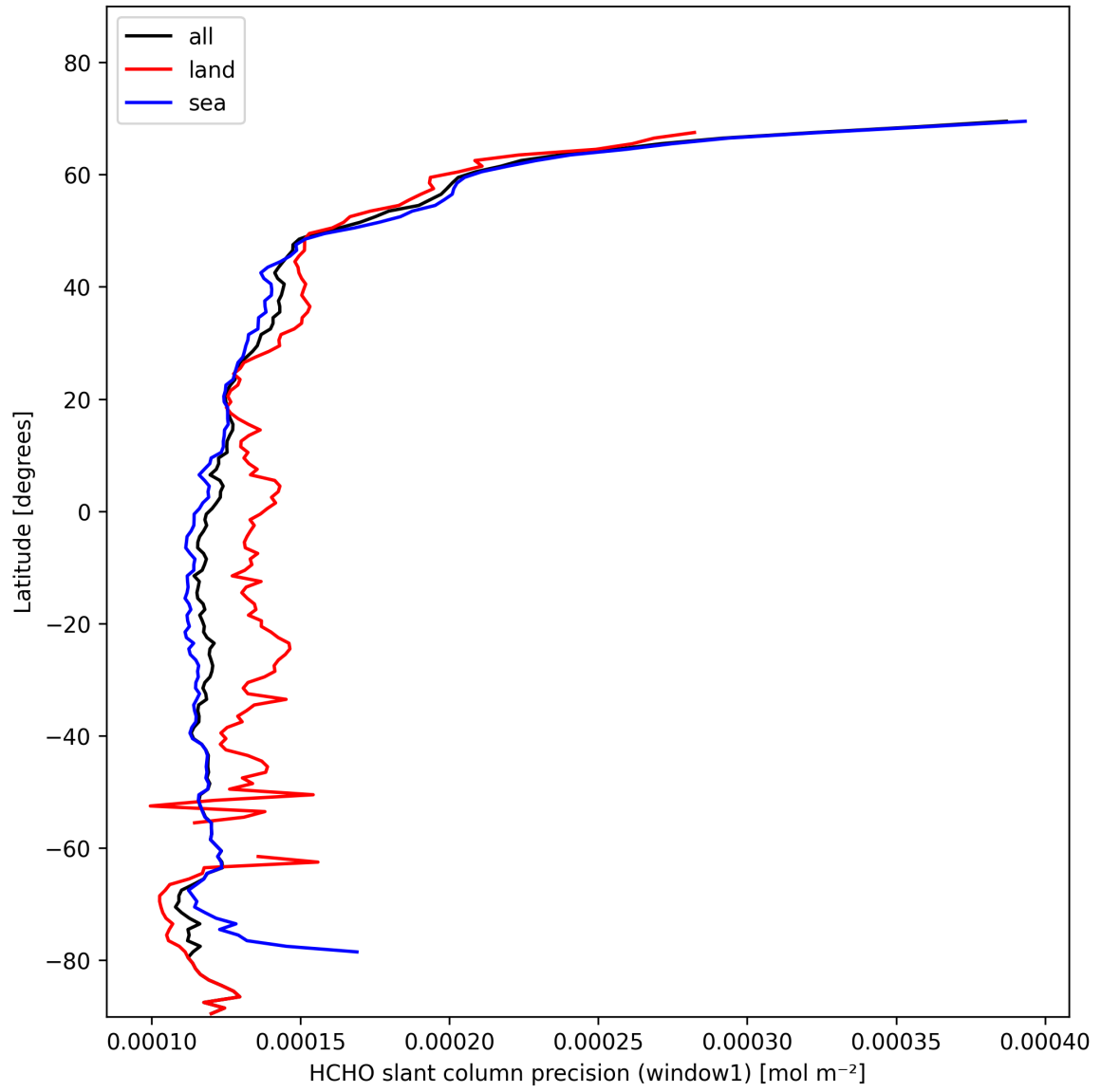
Figure 25: Zonal average of "HCHO slant column precision (window1)" for 2024-11-04 to 2024-11-06.
