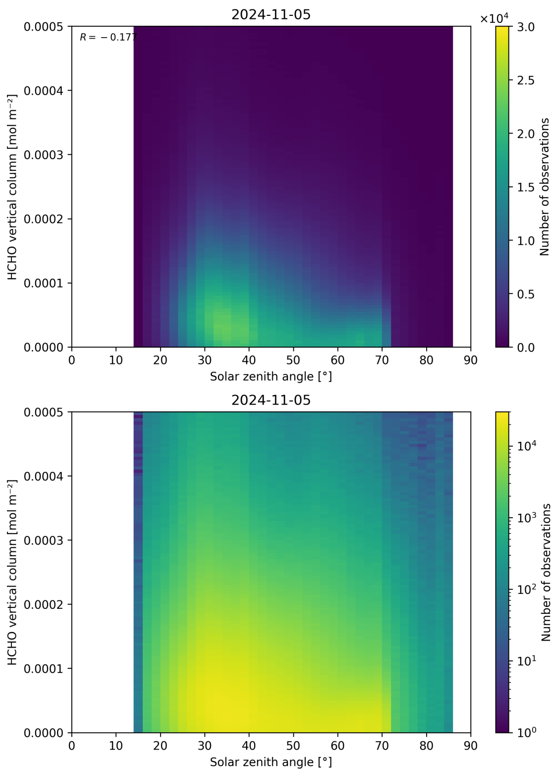
Figure 177: Scatter density plot of “Solar zenith angle” against “HCHO vertical column” for 2024-11-04 to 2024-11-06.
