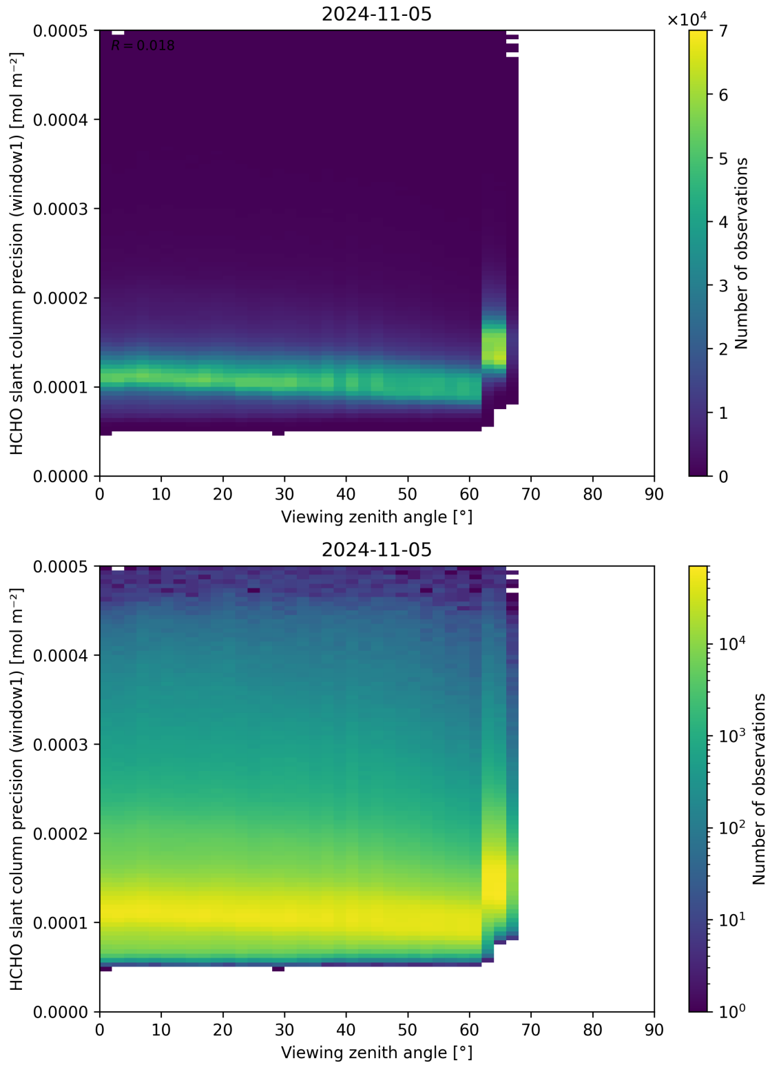
Figure 189: Scatter density plot of “Viewing zenith angle” against “HCHO slant column precision (window1)” for 2024-11-04 to 2024-11-06.
