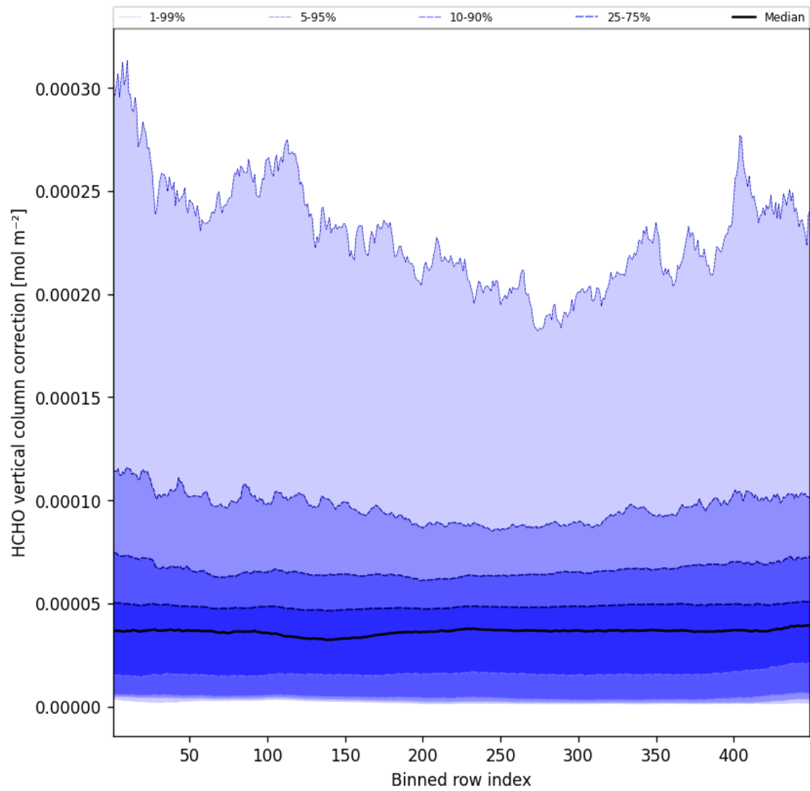
Figure 51: Along track statistics of “HCHO vertical column correction” for 2024-11-04 to 2024-11-06
