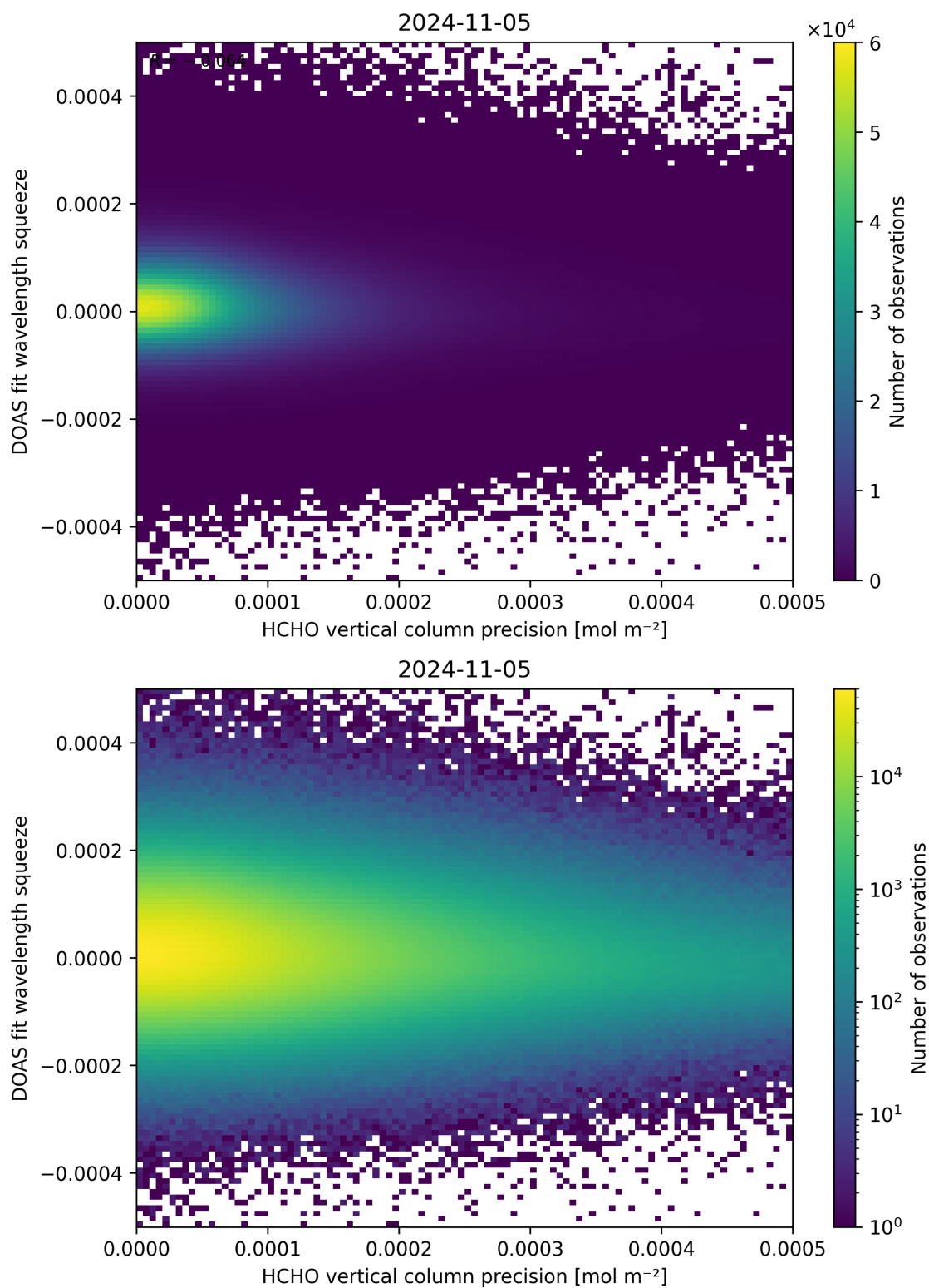
Figure 138: Scatter density plot of “HCHO vertical column precision” against “DOAS fit wavelength squeeze” for 2024-11-04 to 2024-11-06.
