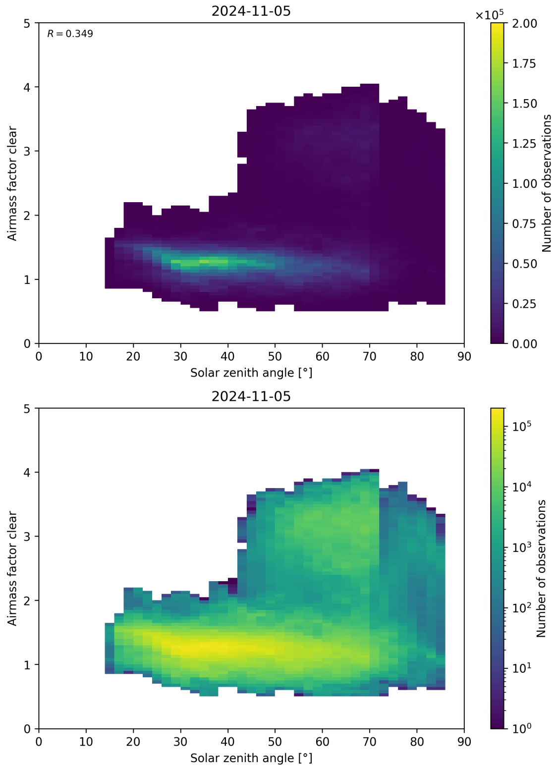
Figure 170: Scatter density plot of “Solar zenith angle” against “Airmass factor clear” for 2024-11-04 to 2024-11-06.
