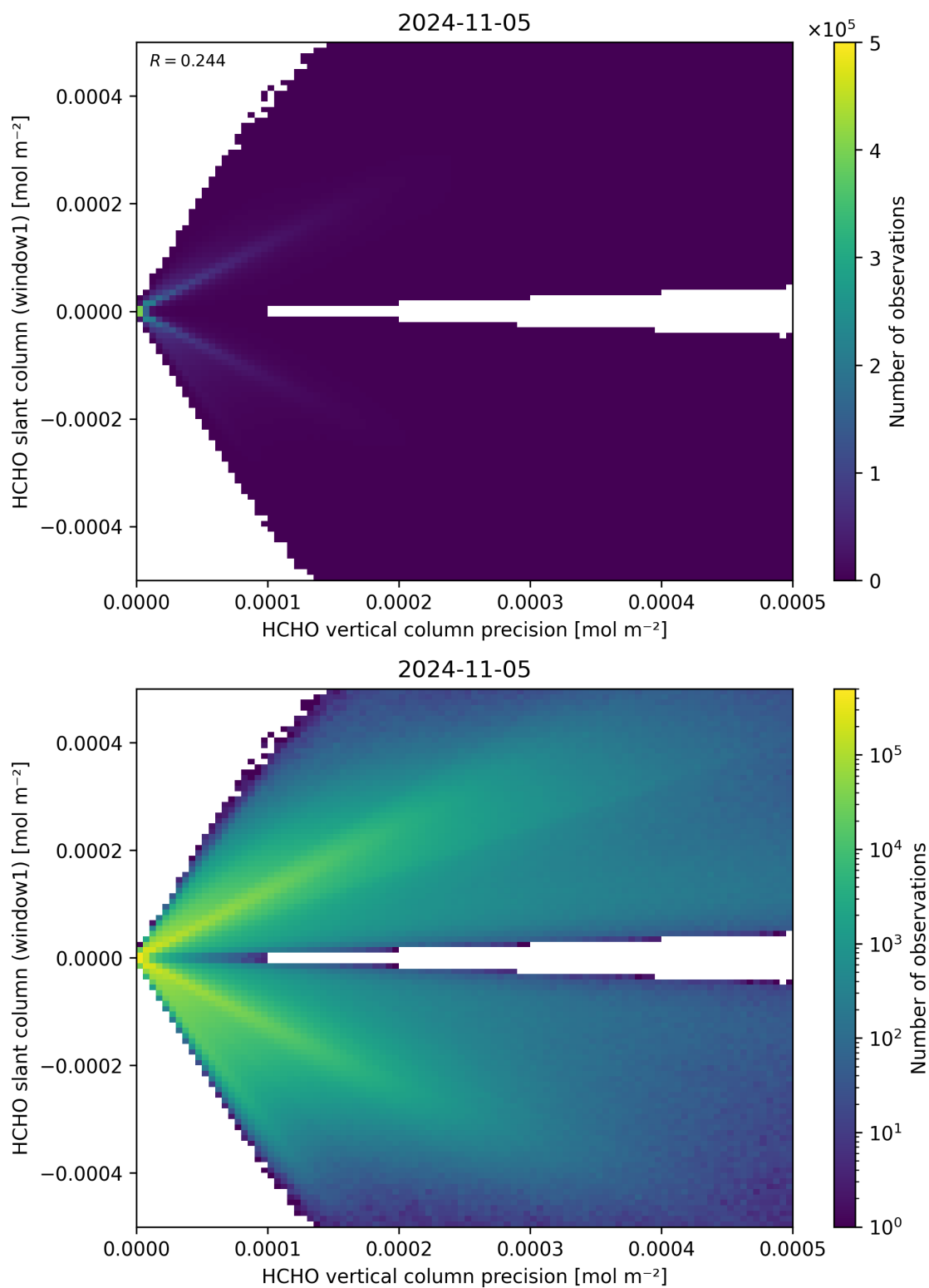
Figure 142: Scatter density plot of “HCHO vertical column precision” against “HCHO slant column (window1)” for 2024-11-04 to 2024-11-06.
