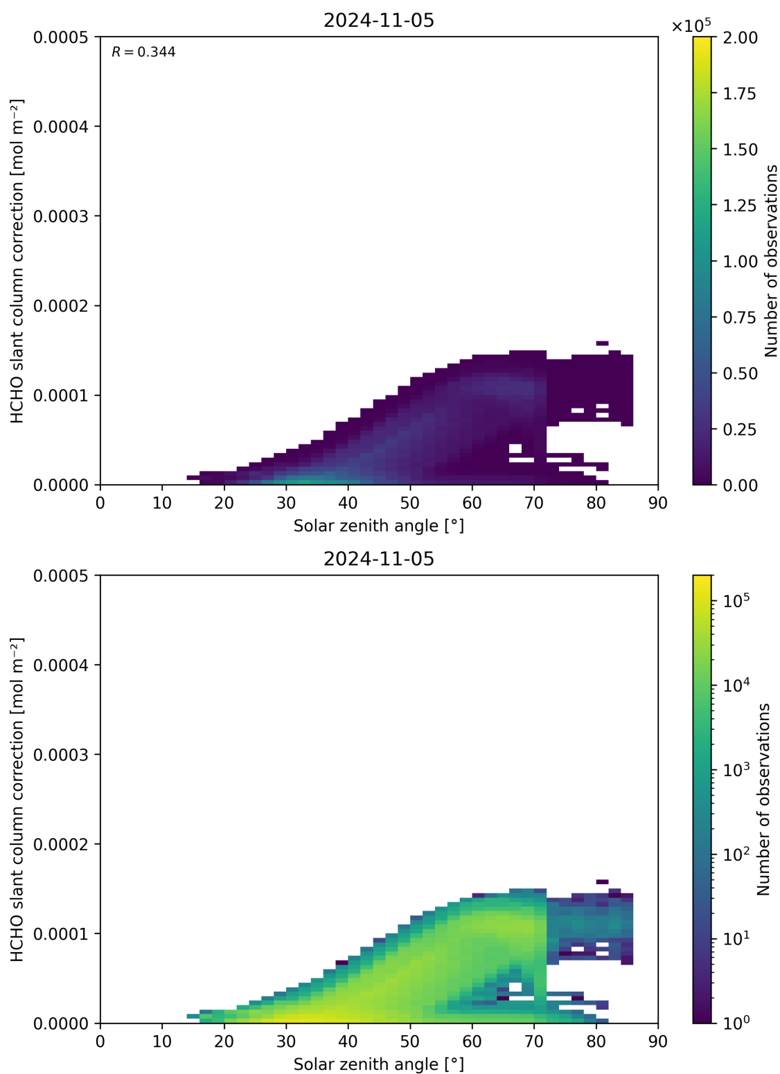
Figure 172: Scatter density plot of “Solar zenith angle” against “HCHO slant column correction” for 2024-11-04 to 2024-11-06.
