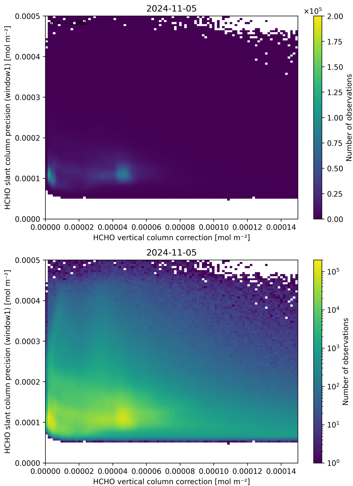
Figure 119: Scatter density plot of “HCHO vertical column correction” against “HCHO slant column precision (window1)” for 2024-11-04 to 2024-11-06.
