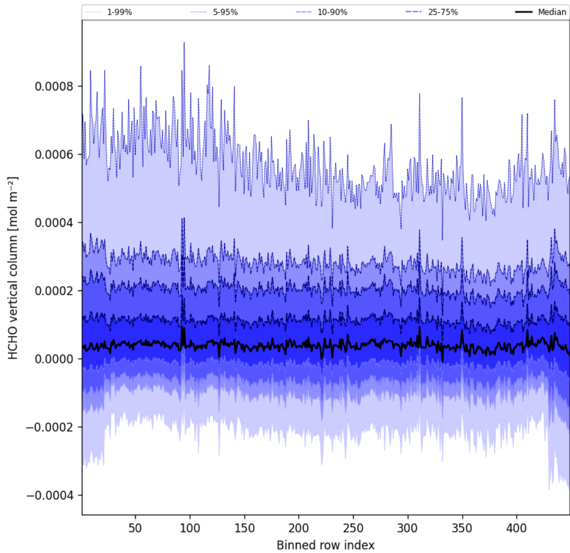
Figure 49: Along track statistics of “HCHO vertical column” for 2024-11-04 to 2024-11-06
