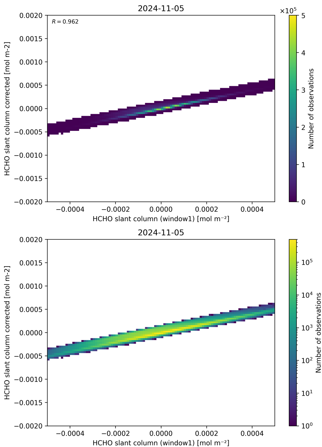
Figure 82: Scatter density plot of “HCHO slant column (window1)” against “HCHO slant column corrected” for 2024-11-04 to 2024-11-06.
